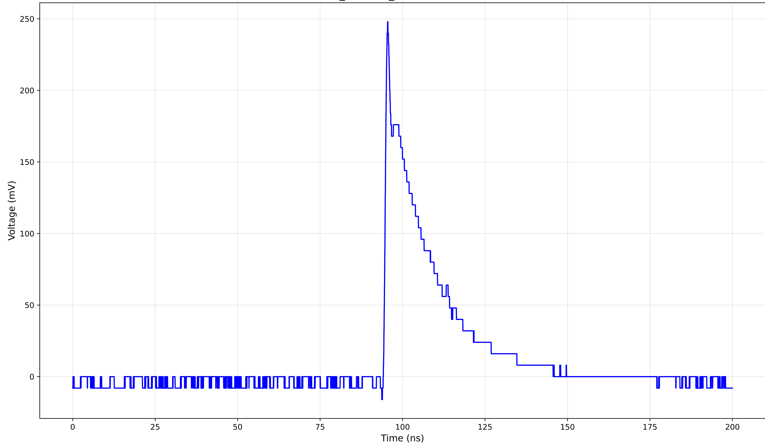
TCT Pulse Waveform - Run 3_80: 1cm_42-Position3 (80.0 V) - Rise Time: 0.87 ns
