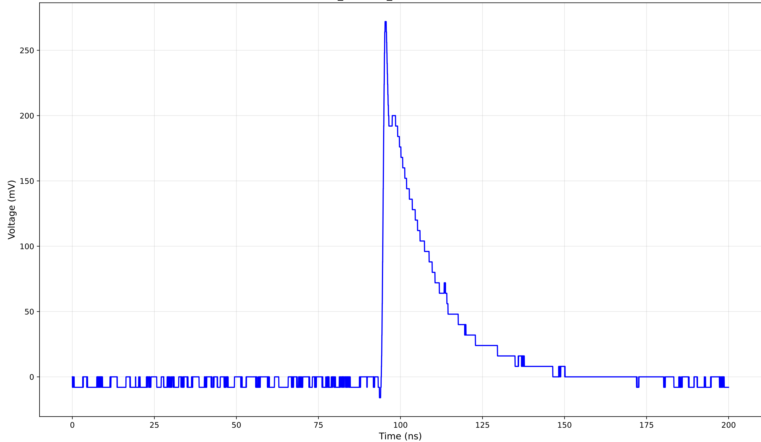
TCT Pulse Waveform - Run 3_90: 1cm_42-Position3 (90.0 V) - Rise Time: 0.82 ns
