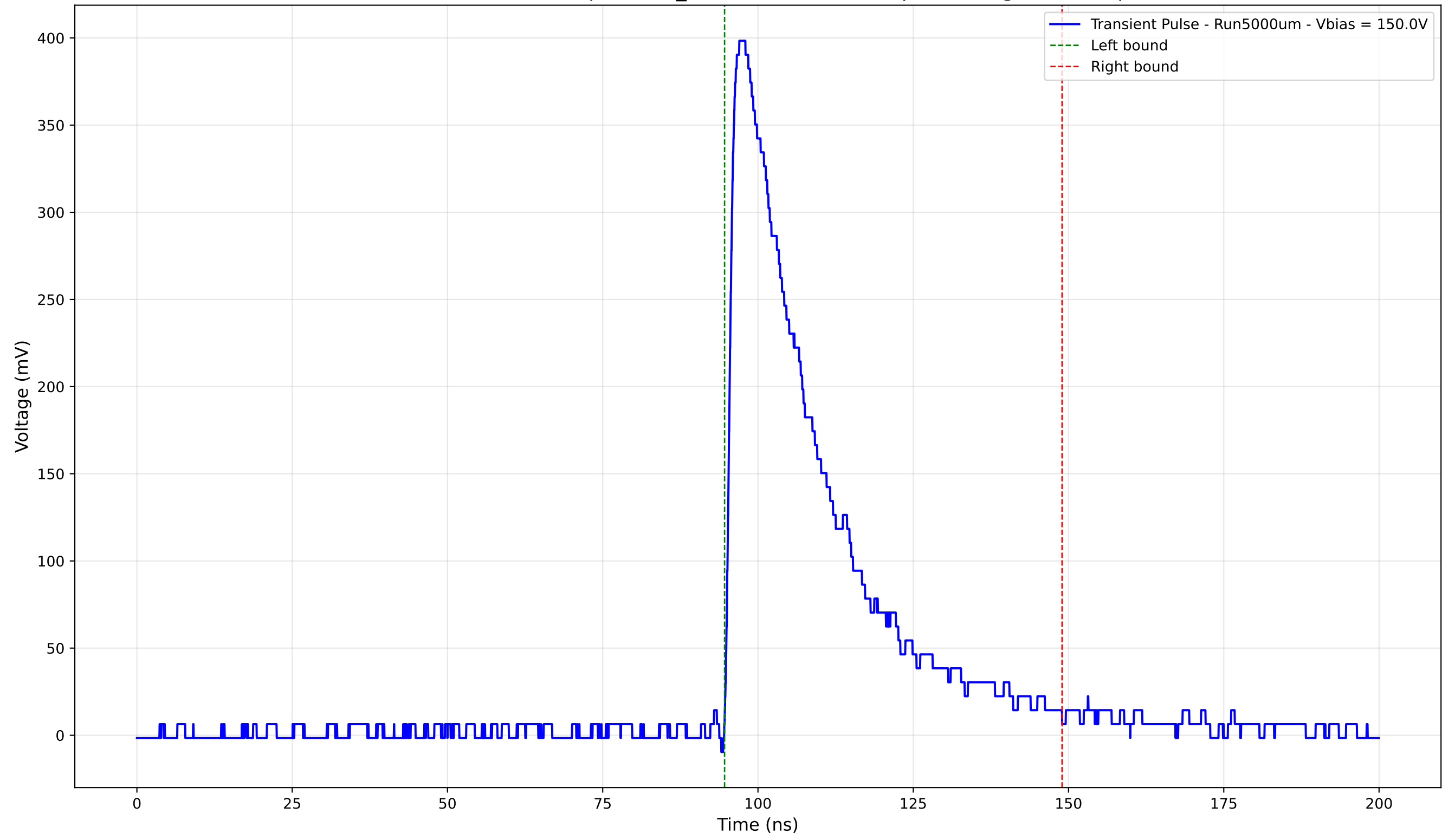
Transient Pulse - Sample: 1cm_42 - Position: 1075.0 \mu\text{m} - Charge: 124.59 pC
