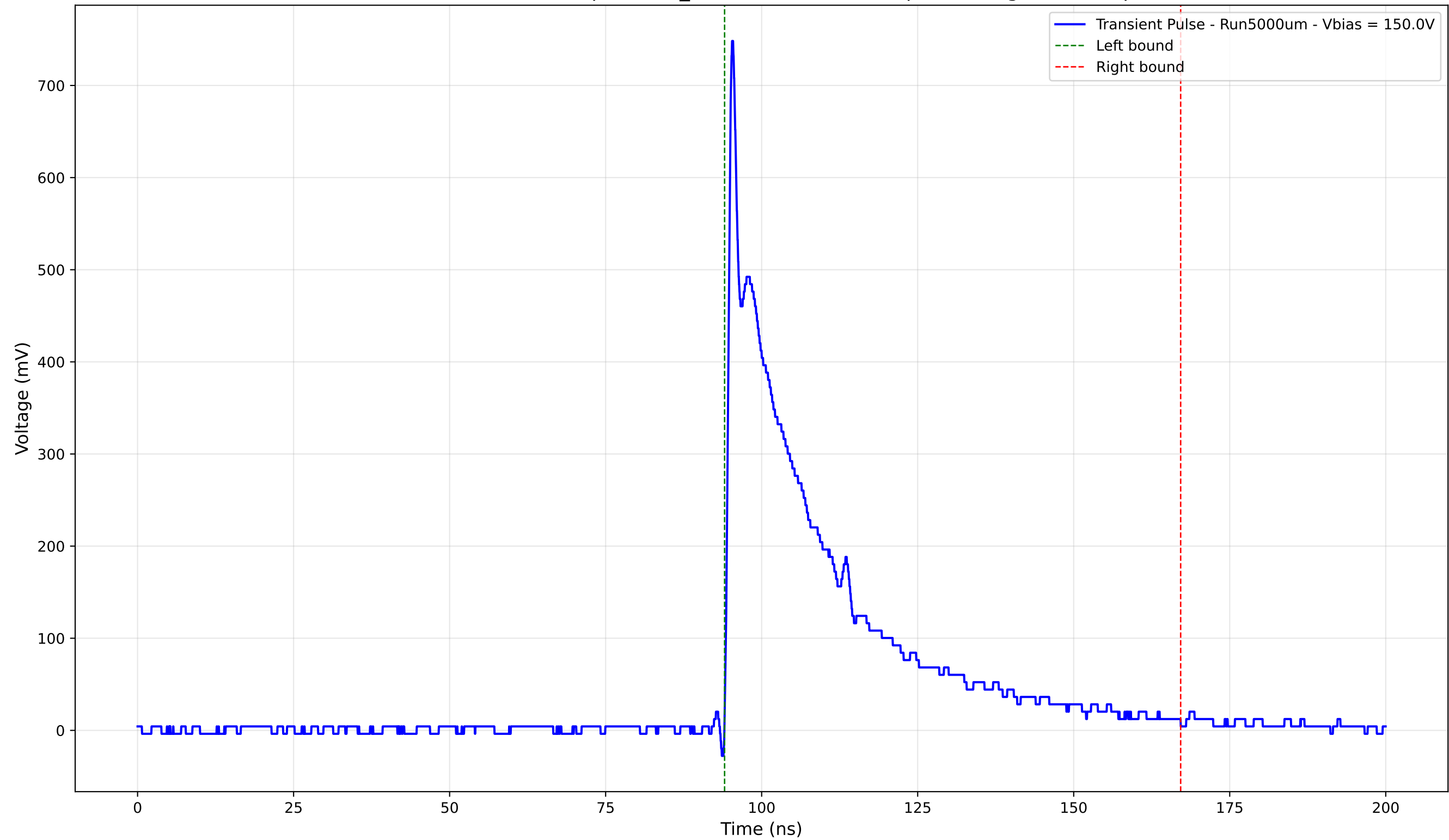
Transient Pulse - Sample: 1cm_42 - Position: 2730.0 \mu\text{m} - Charge: 181.82 pC
