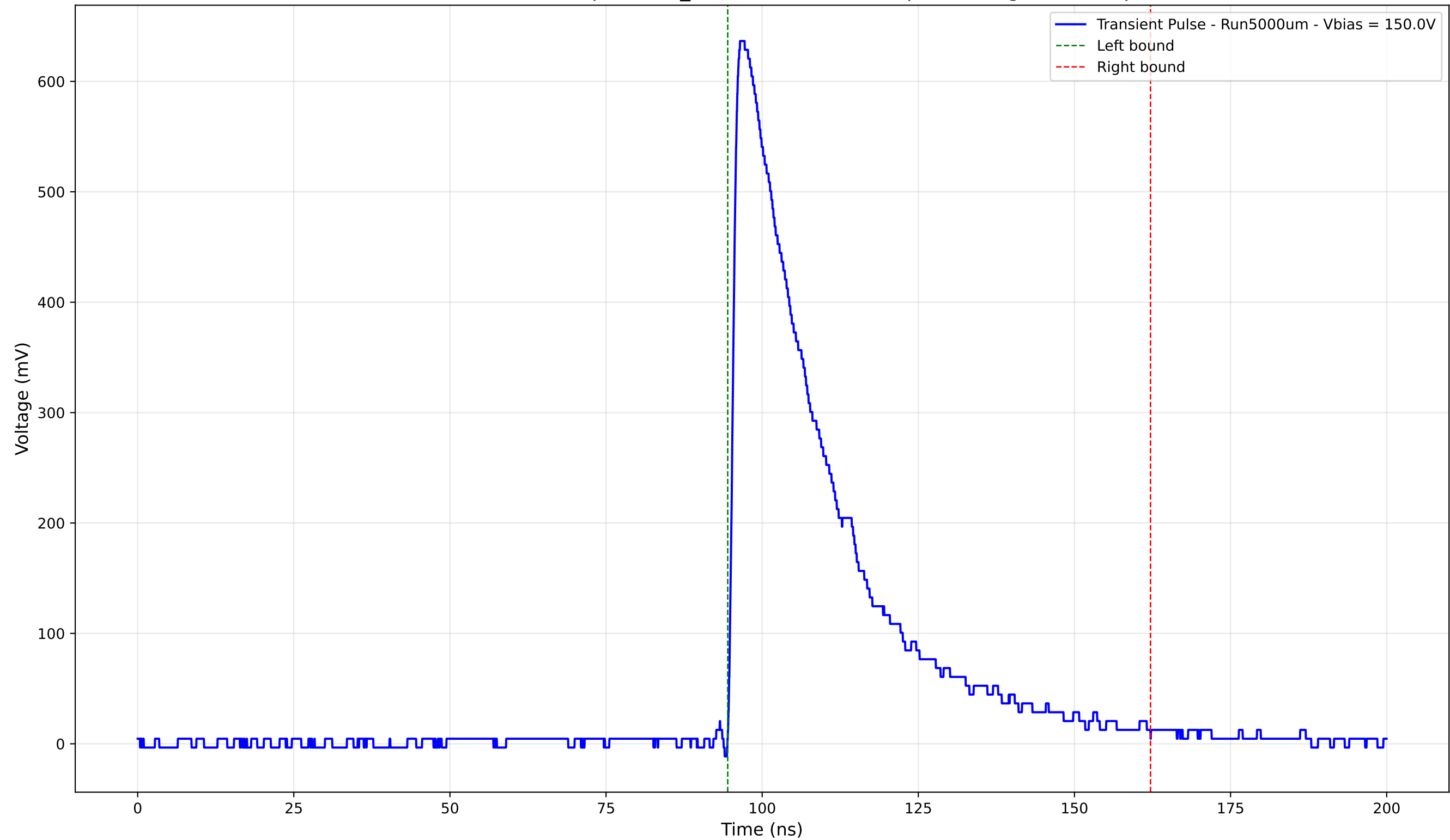
Transient Pulse - Sample: 1cm_42 - Position: 3785.0 \mu\text{m} - Charge: 207.79 pC
