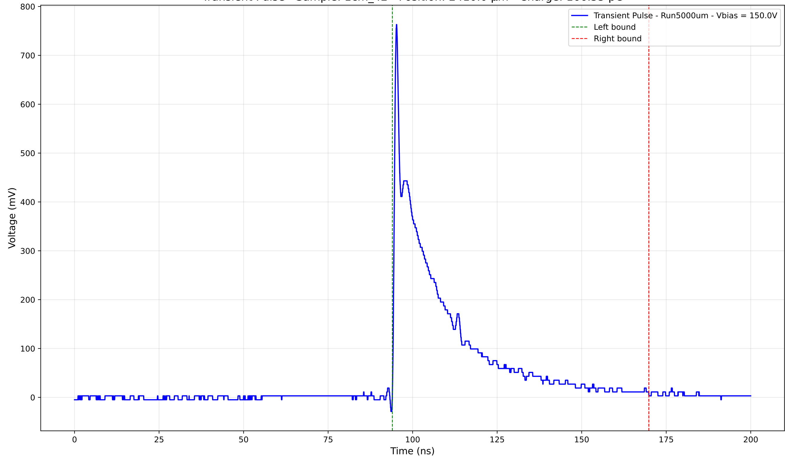
Transient Pulse - Sample: 1cm_42 - Position: 2410.0 \mu\text{m} - Charge: 166.55 pC
