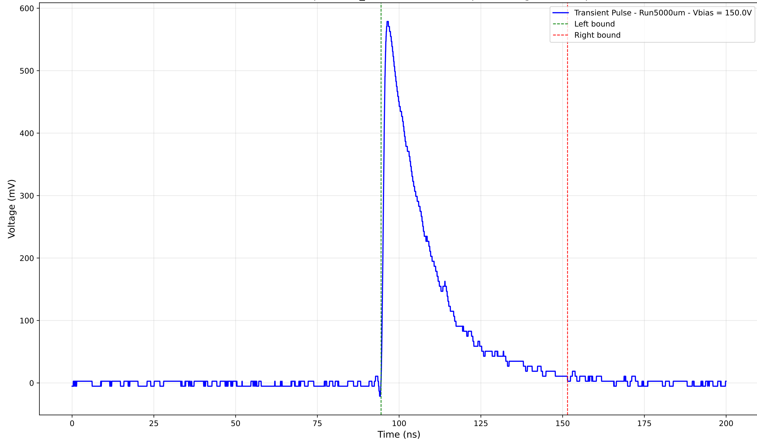
Transient Pulse - Sample: 1cm_42 - Position: 610.0 \mu\text{m} - Charge: 163.13 pC
