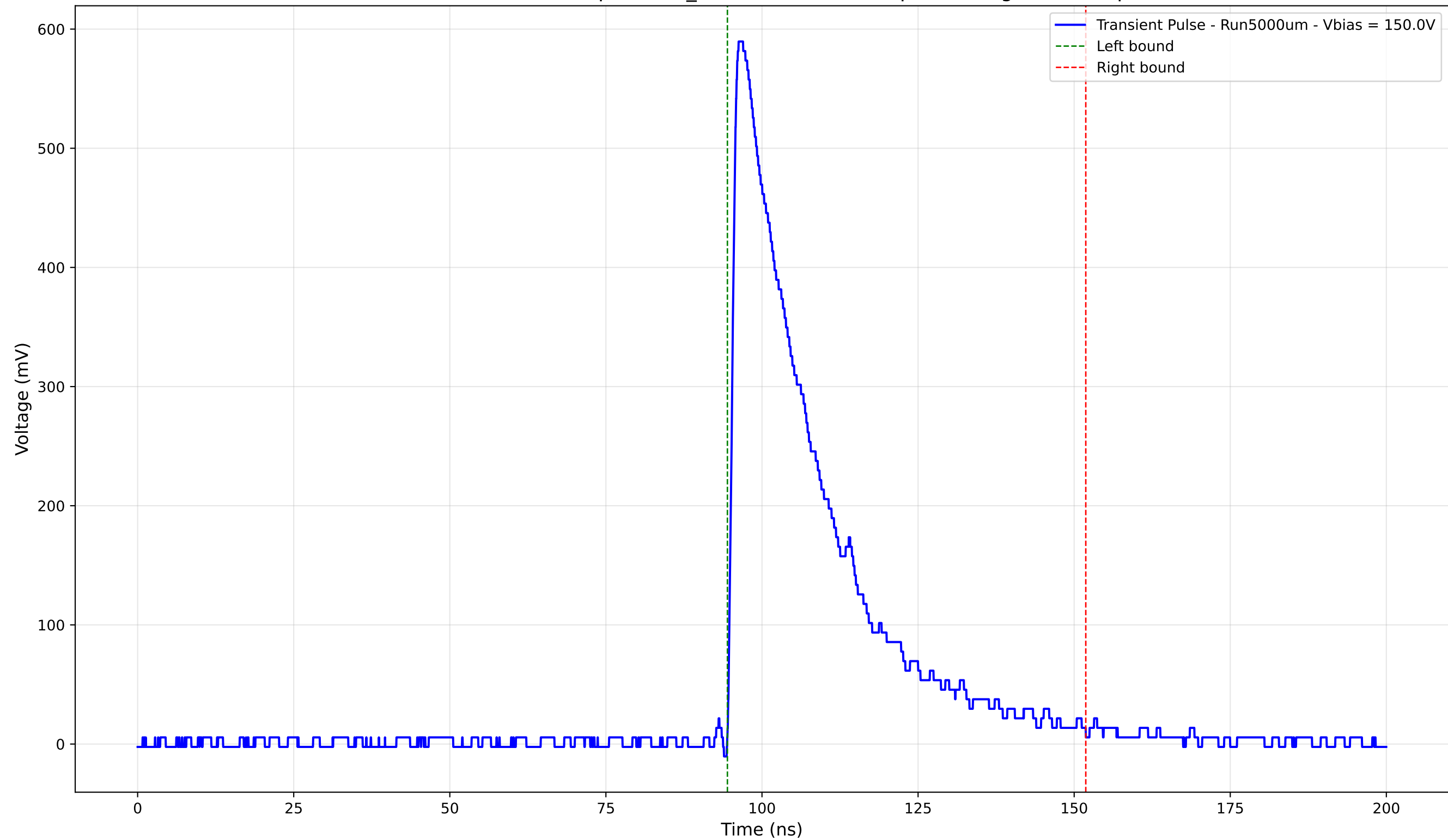
Transient Pulse - Sample: 1cm_42 - Position: 635.0 \mu\text{m} - Charge: 171.45 pC
