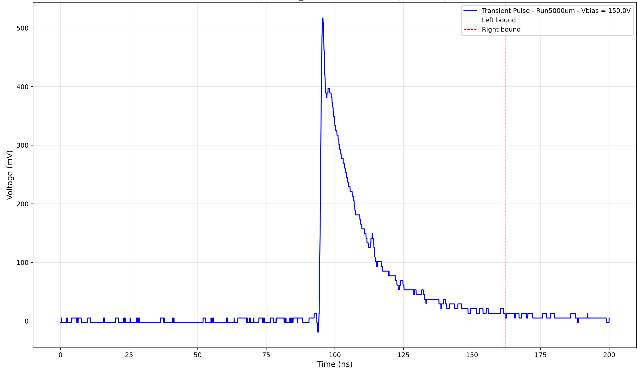
Transient Pulse - Sample: 1cm_42 - Position: 2965.0 \mu\text{m} - Charge: 142.05 pC
