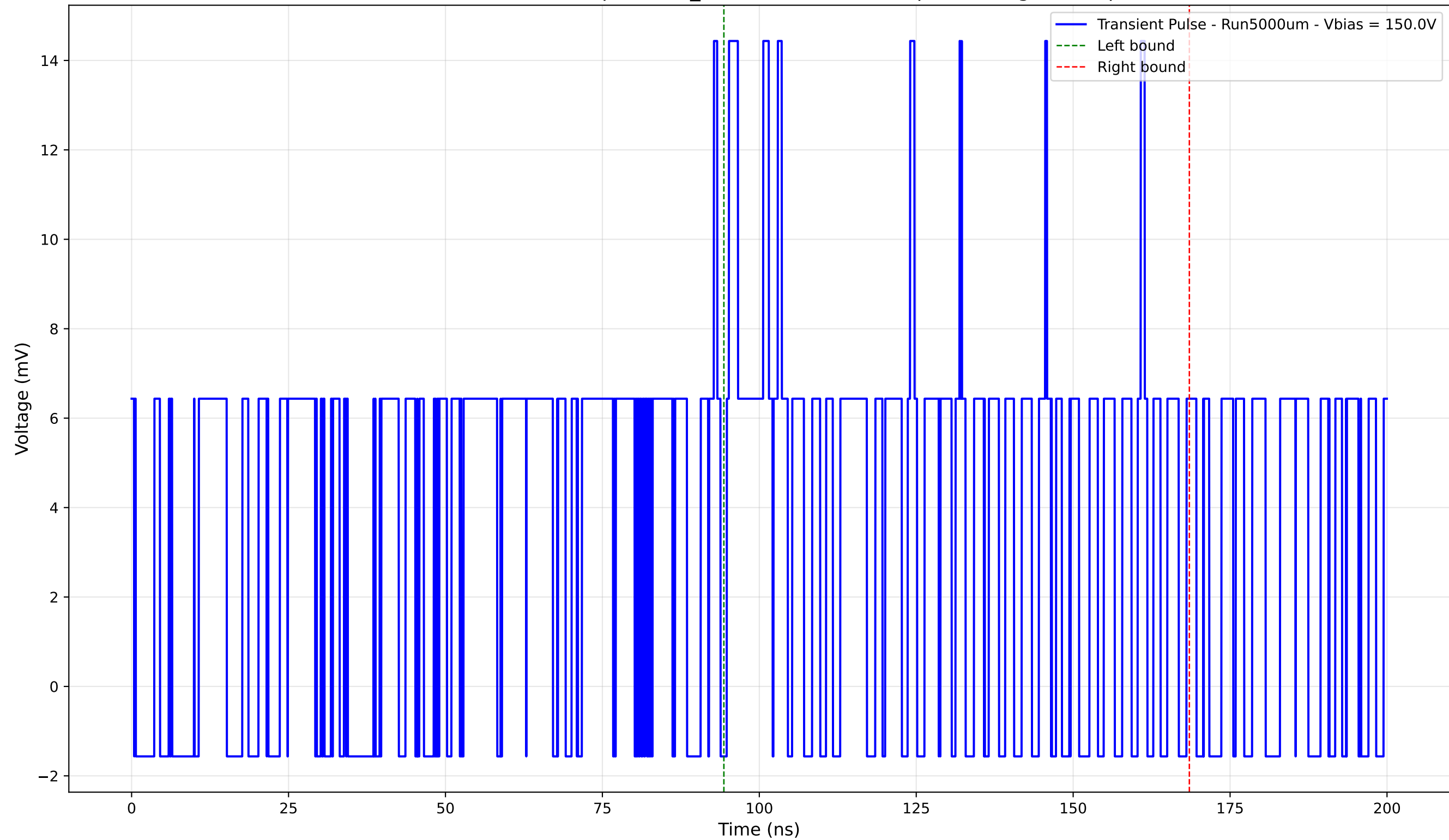
Transient Pulse - Sample: 1cm_42 - Position: 4970.0 \mu\text{m} - Charge: 6.35 pC
