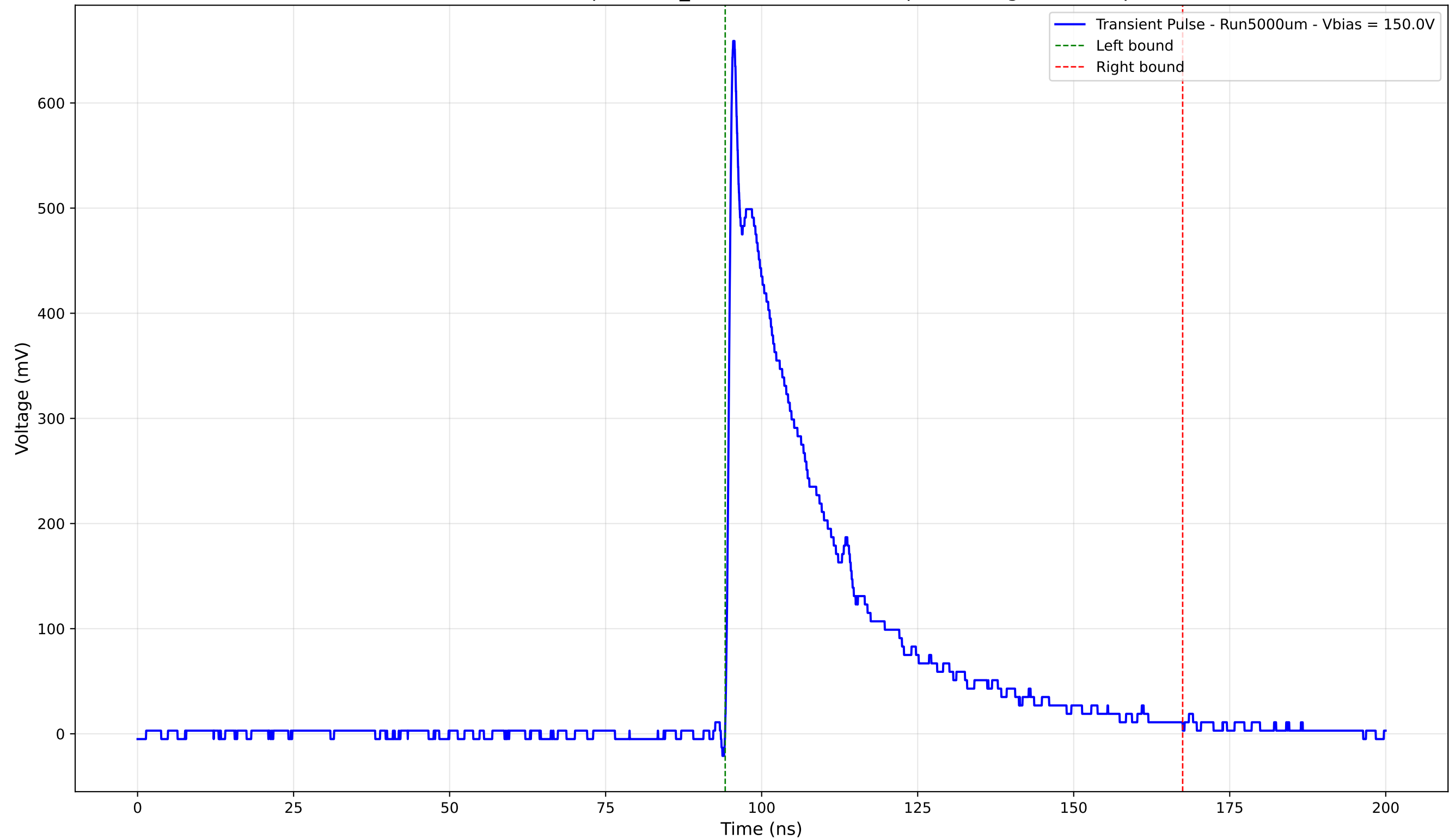
Transient Pulse - Sample: 1cm_42 - Position: 2145.0 \mu\text{m} - Charge: 182.87 pC
