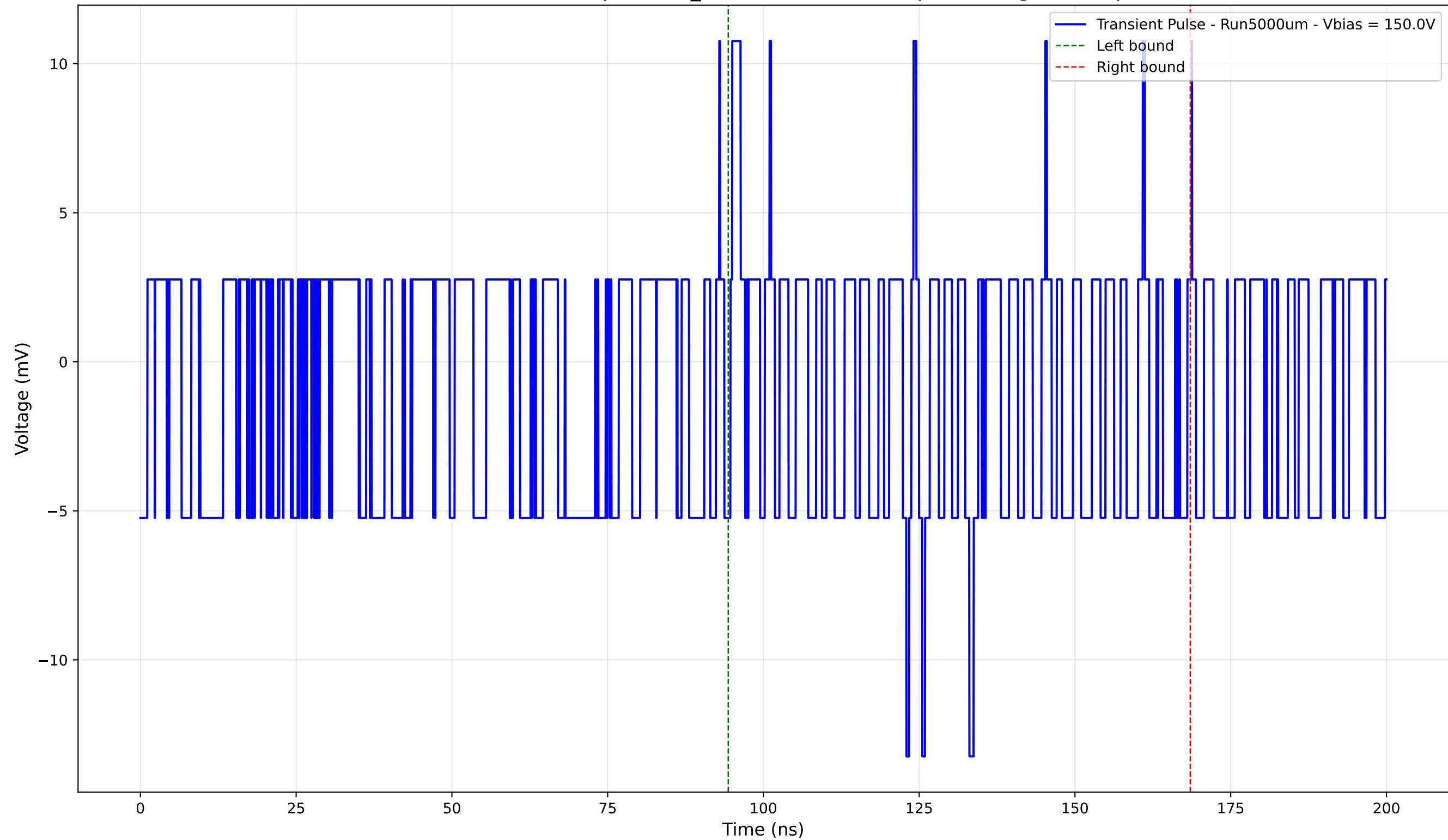
Transient Pulse - Sample: 1cm_42 - Position: 5005.0 \mu\text{m} - Charge: -1.22 pC
