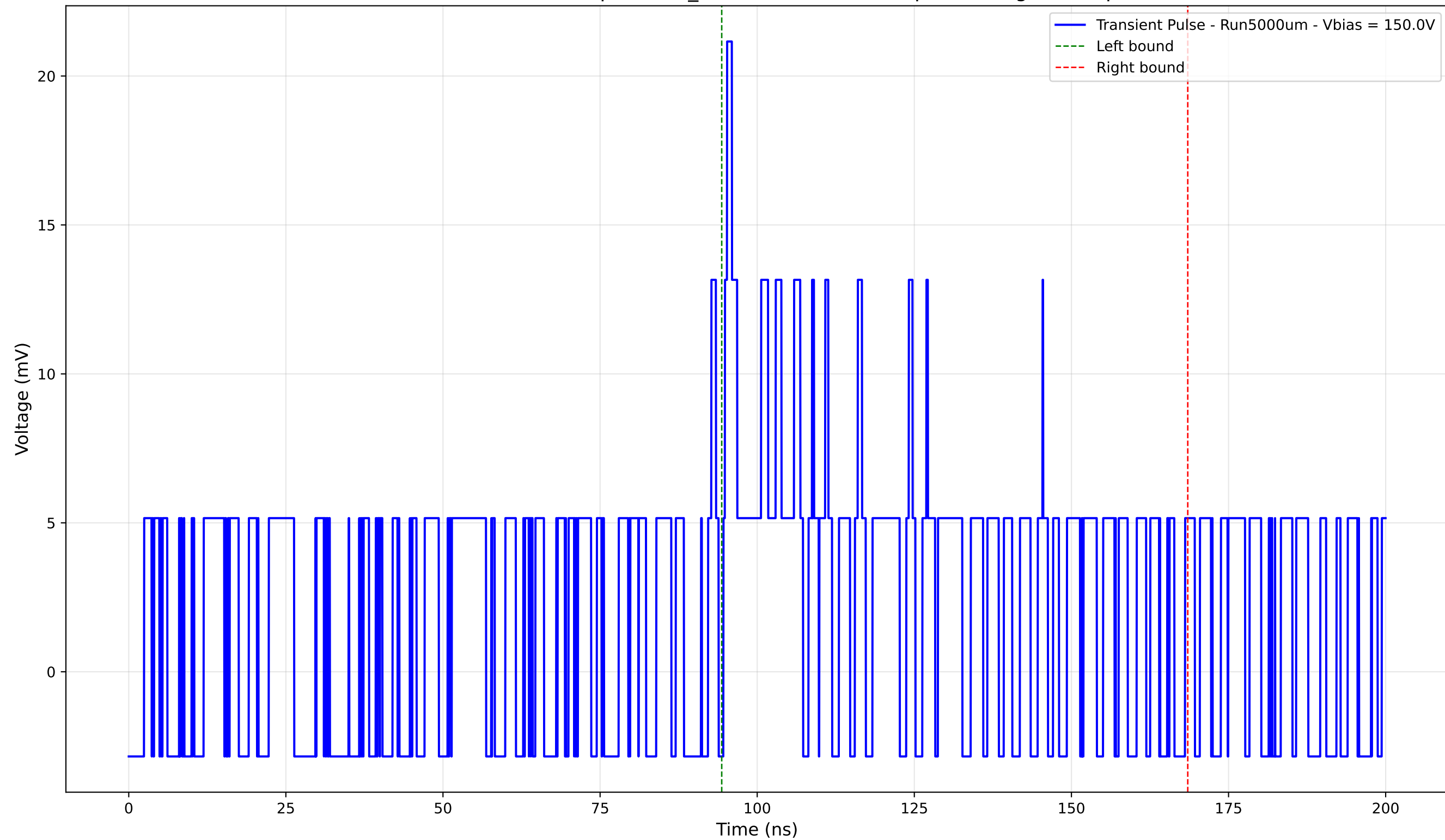
Transient Pulse - Sample: 1cm_42 - Position: 5065.0 \mu\text{m} - Charge: 5.57 pC
