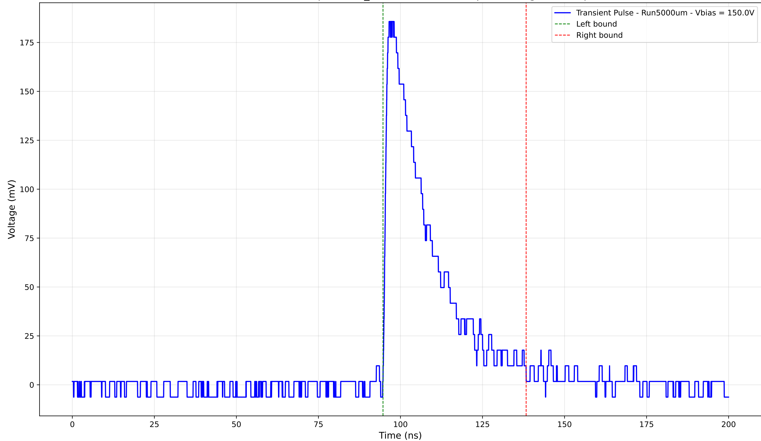
Transient Pulse - Sample: 1cm_42 -Position: 975.0 \mu\text{m} - Charge: 54.09 pC
