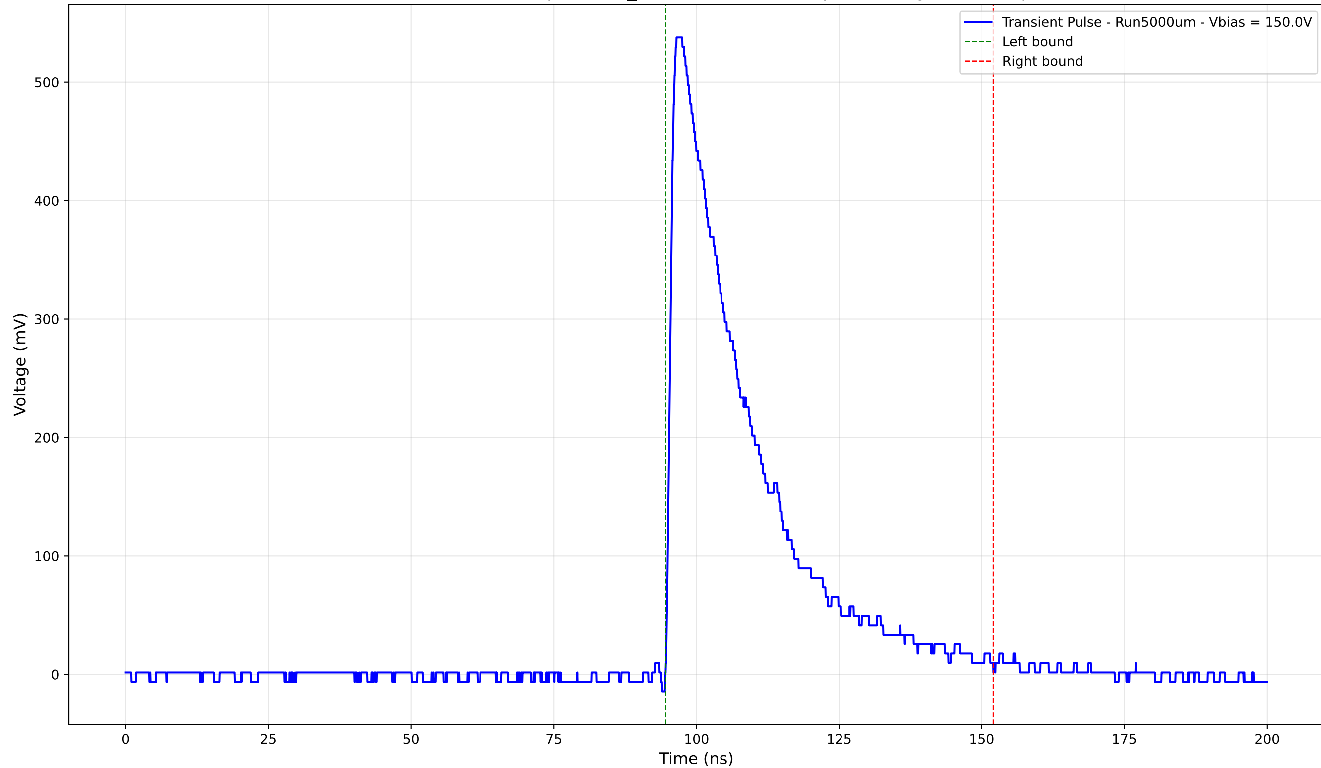
Transient Pulse - Sample: 1cm_42 - Position: 815.0 \mu\text{m} - Charge: 160.16 pC
