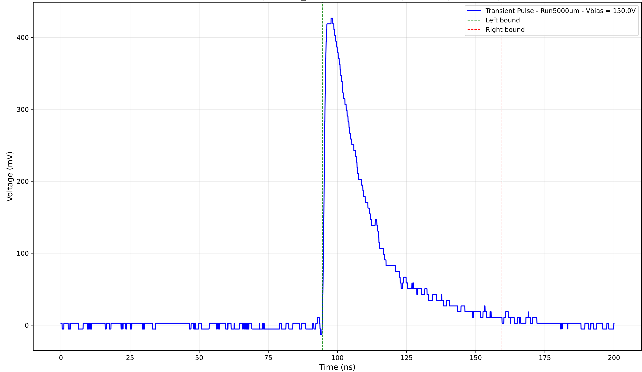
Transient Pulse - Sample: 1cm_42 - Position: 1590.0 \mu\text{m} - Charge: 143.86 pC
