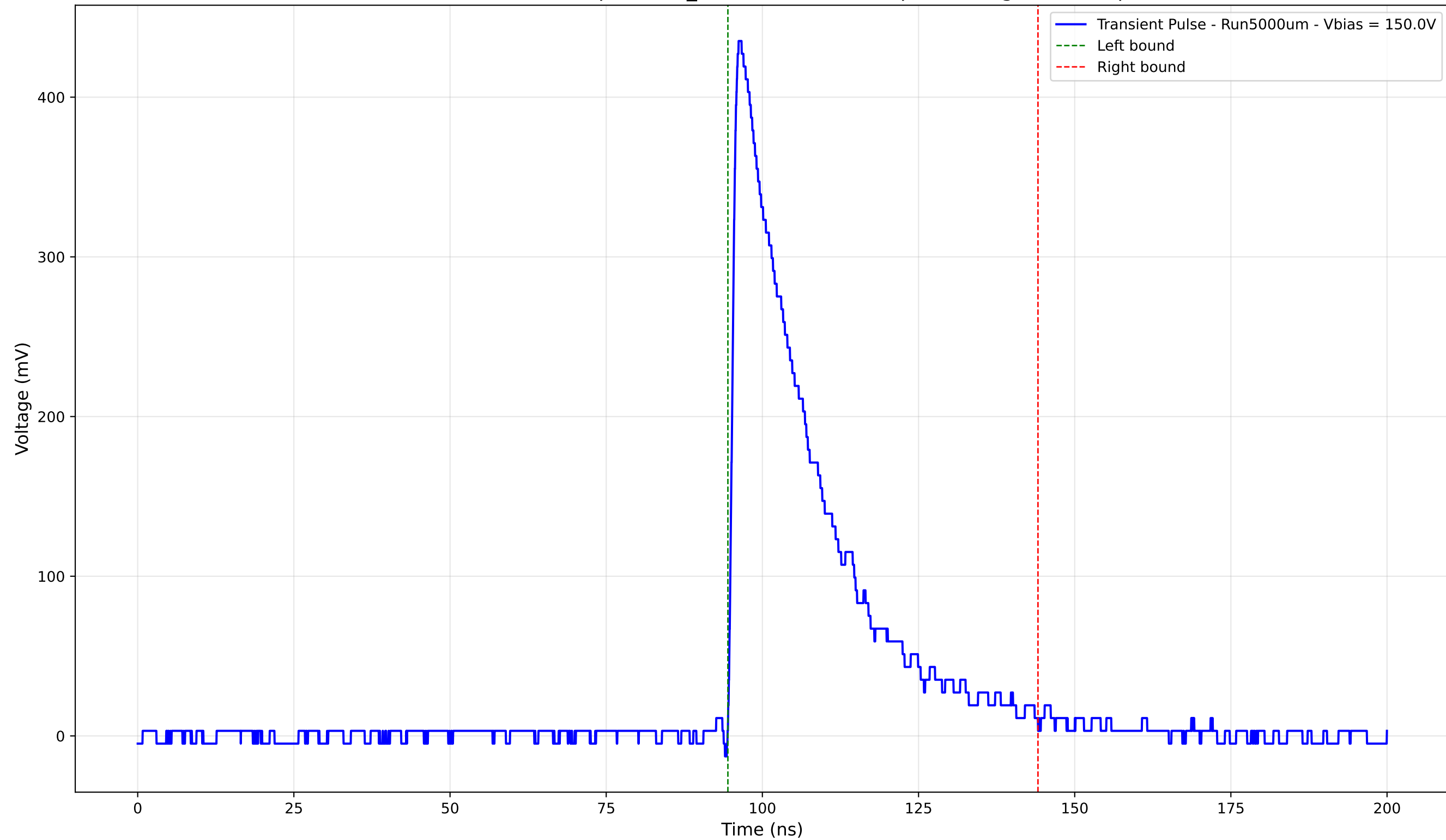
Transient Pulse - Sample: 1cm_42 - Position: 570.0 \mu\text{m} - Charge: 119.26 pC
