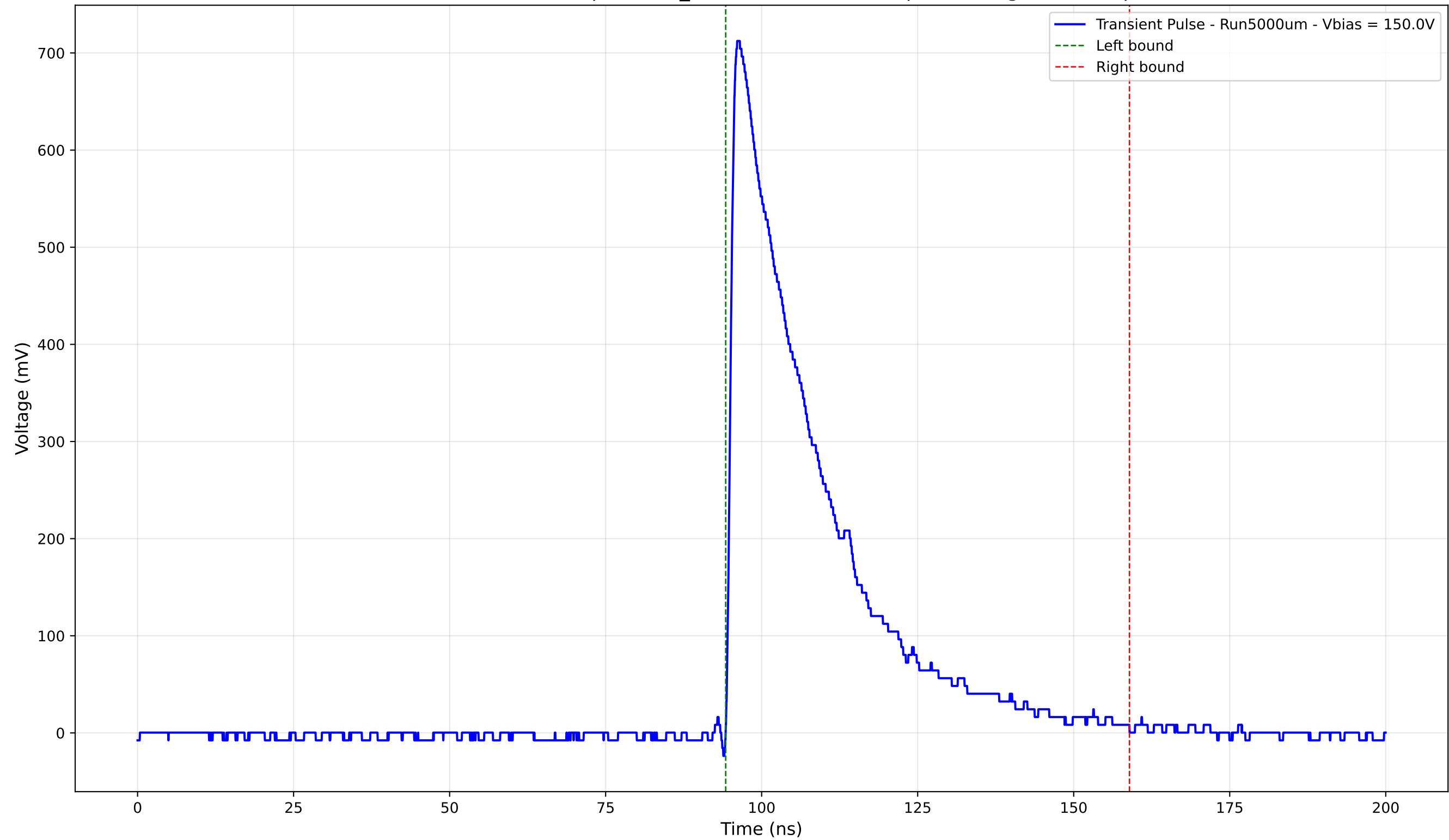
Transient Pulse - Sample: 1cm_42 - Position: 4360.0 \mu\text{m} - Charge: 209.12 pC
