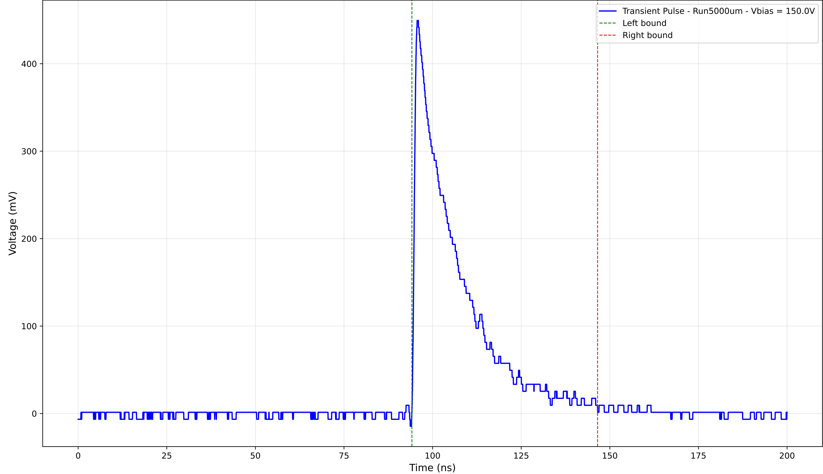
Transient Pulse - Sample: 1cm_42 - Position: 4600.0 \mu\text{m} - Charge: 113.30 pC
