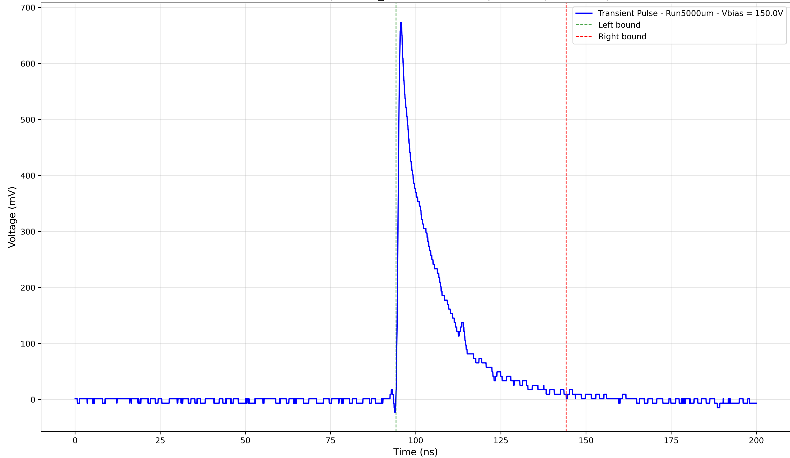
Transient Pulse - Sample: 1cm_42 - Position: 95.0 \mu\text{m} - Charge: 139.25 pC
