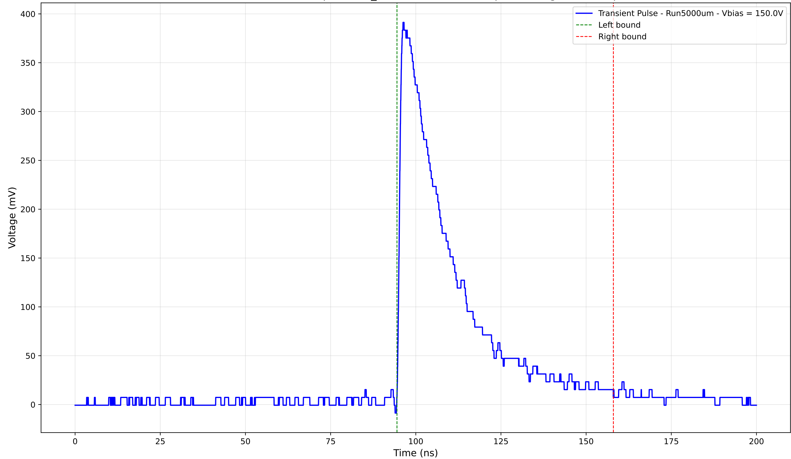
Transient Pulse - Sample: 1cm_42 - Position: 3475.0 \mu\text{m} - Charge: 128.79 pC
