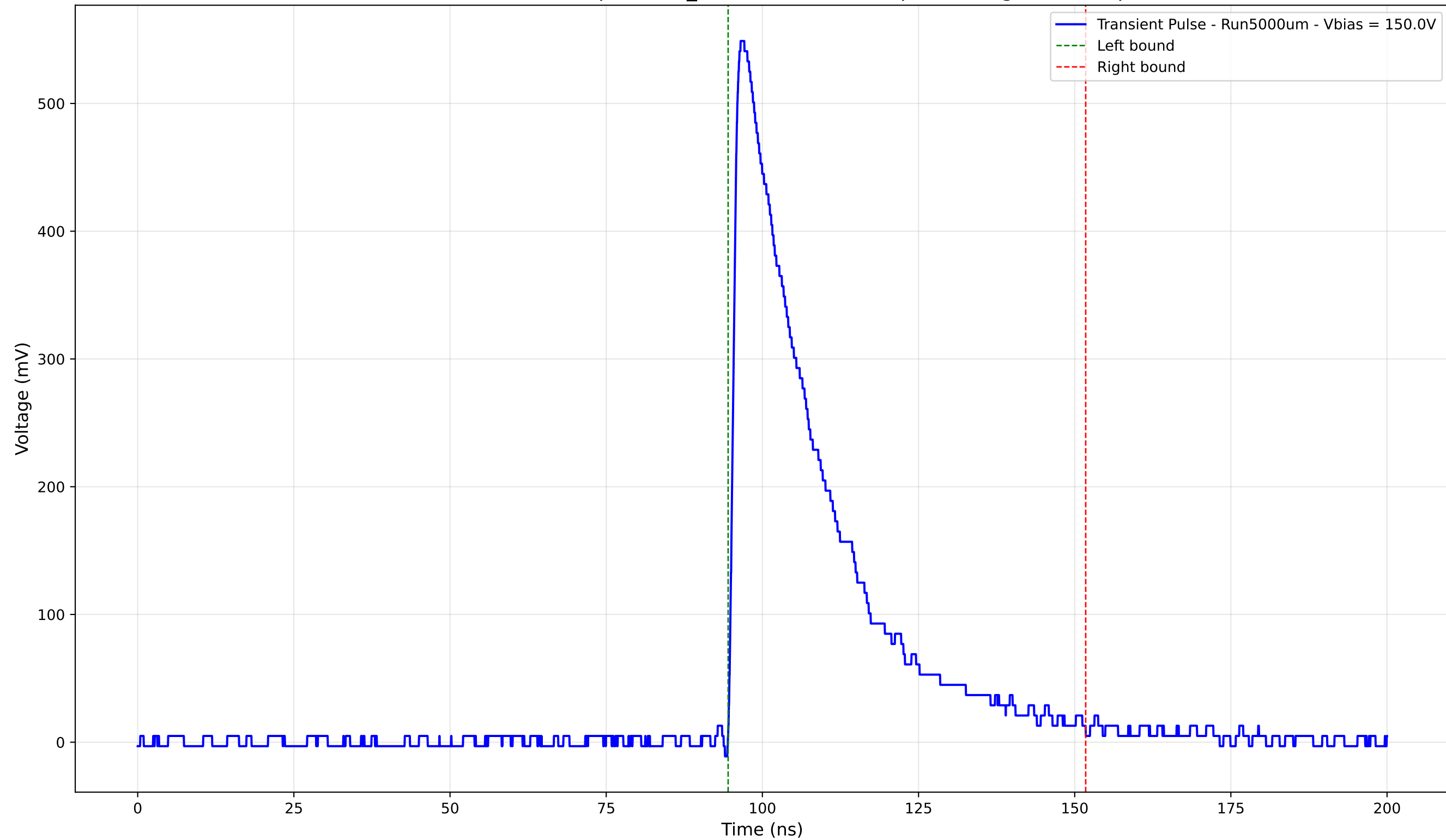
Transient Pulse - Sample: 1cm_42 - Position: 765.0 \mu\text{m} - Charge: 162.82 pC
