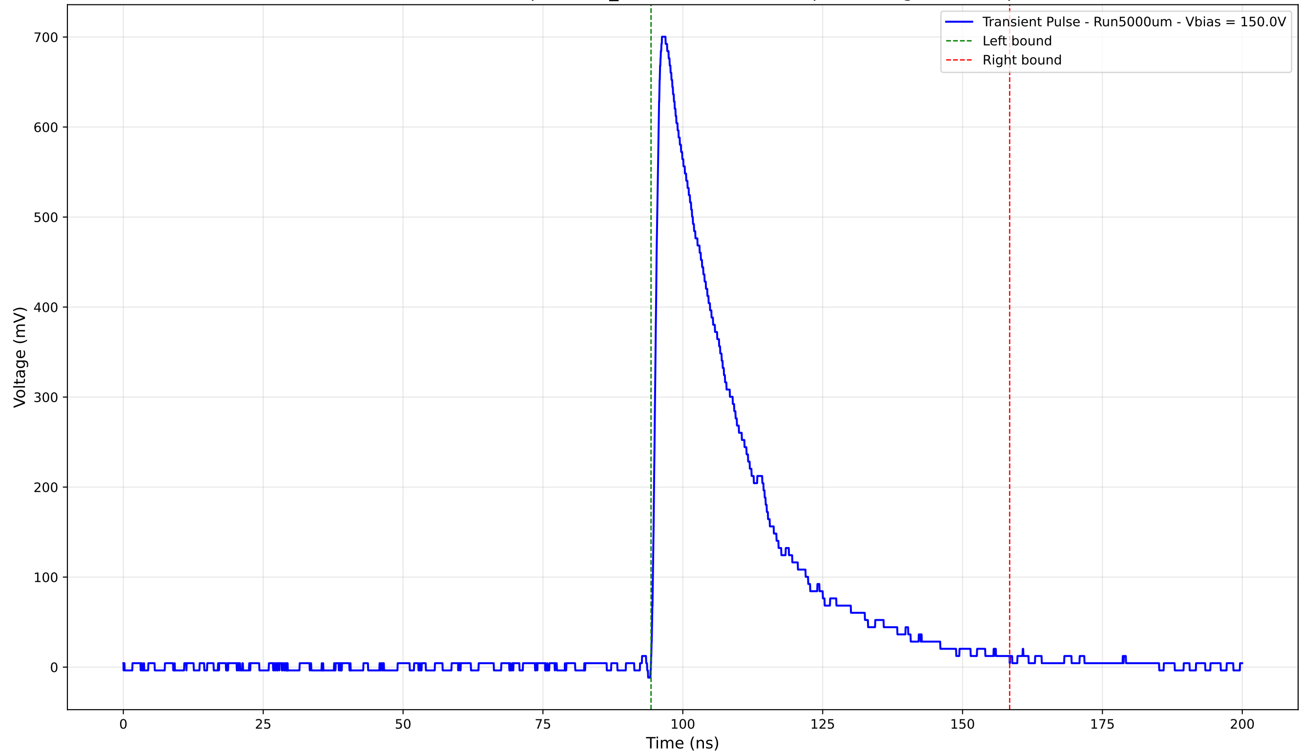
Transient Pulse - Sample: 1cm_42 - Position: 4225.0 \mu\text{m} - Charge: 214.58 pC
