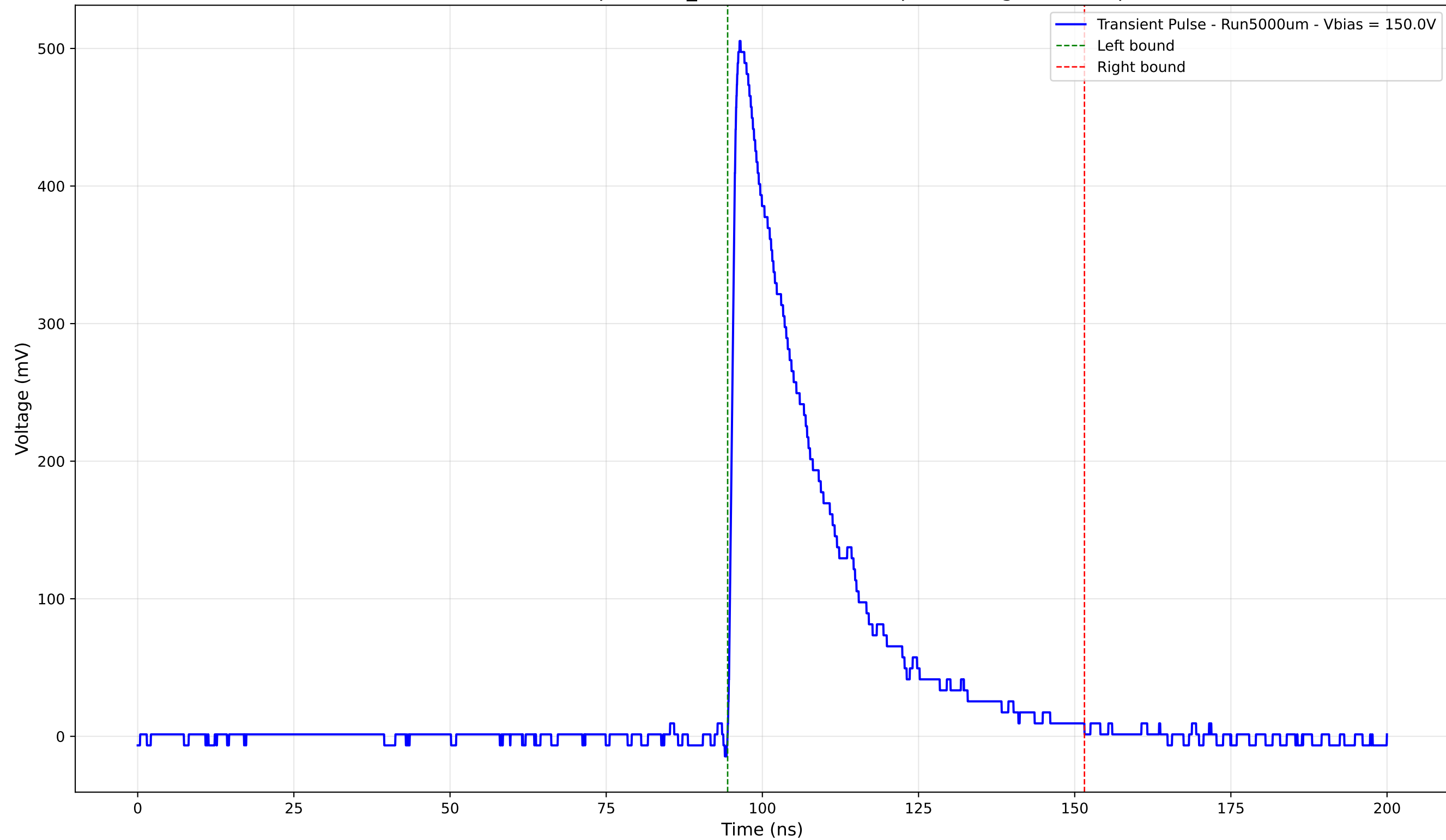
Transient Pulse - Sample: 1cm_42 - Position: 585.0 \mu\text{m} - Charge: 139.59 pC
