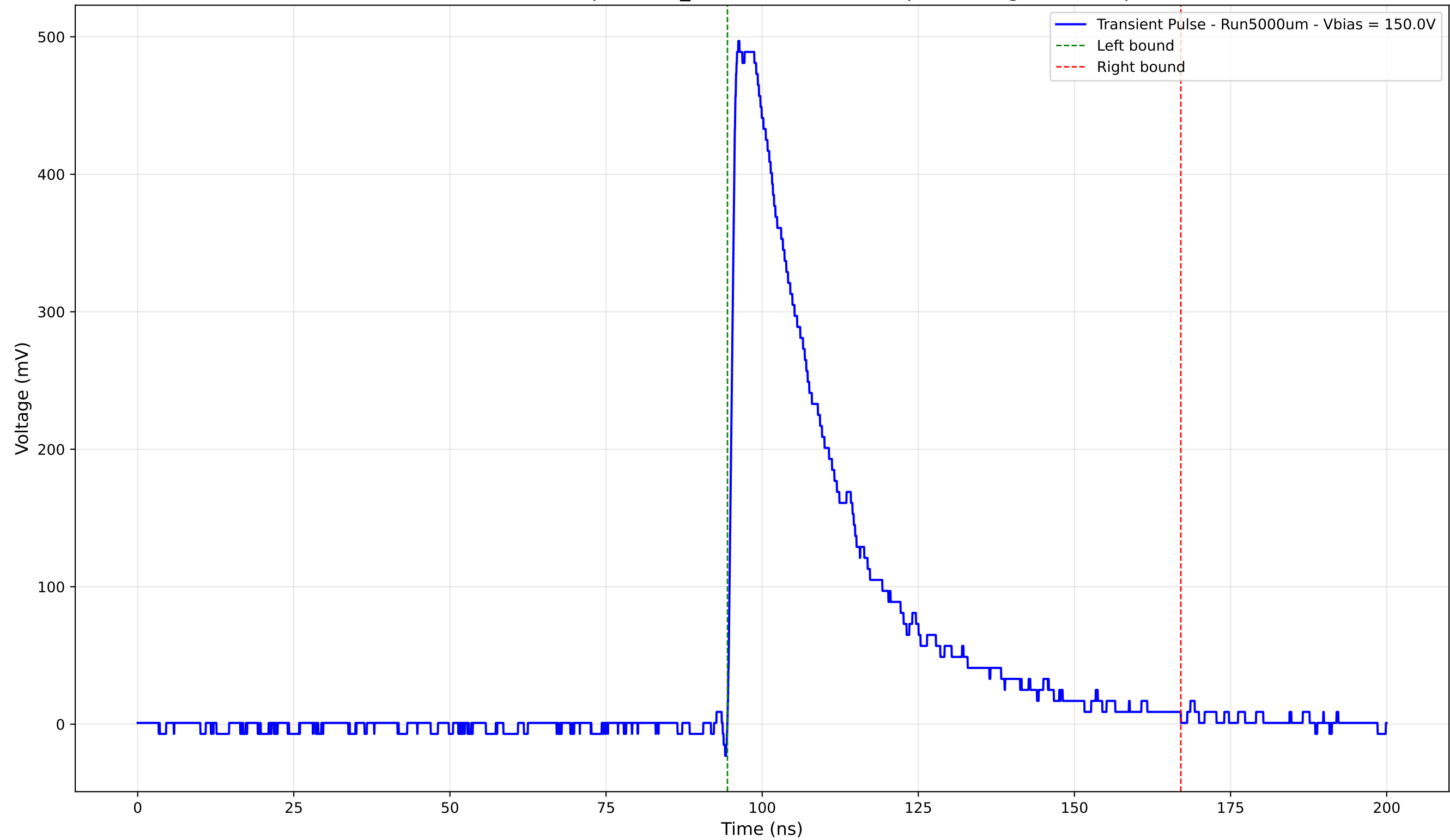
Transient Pulse - Sample: 1cm_42 - Position: 1695.0 \mu\text{m} - Charge: 169.15 pC
