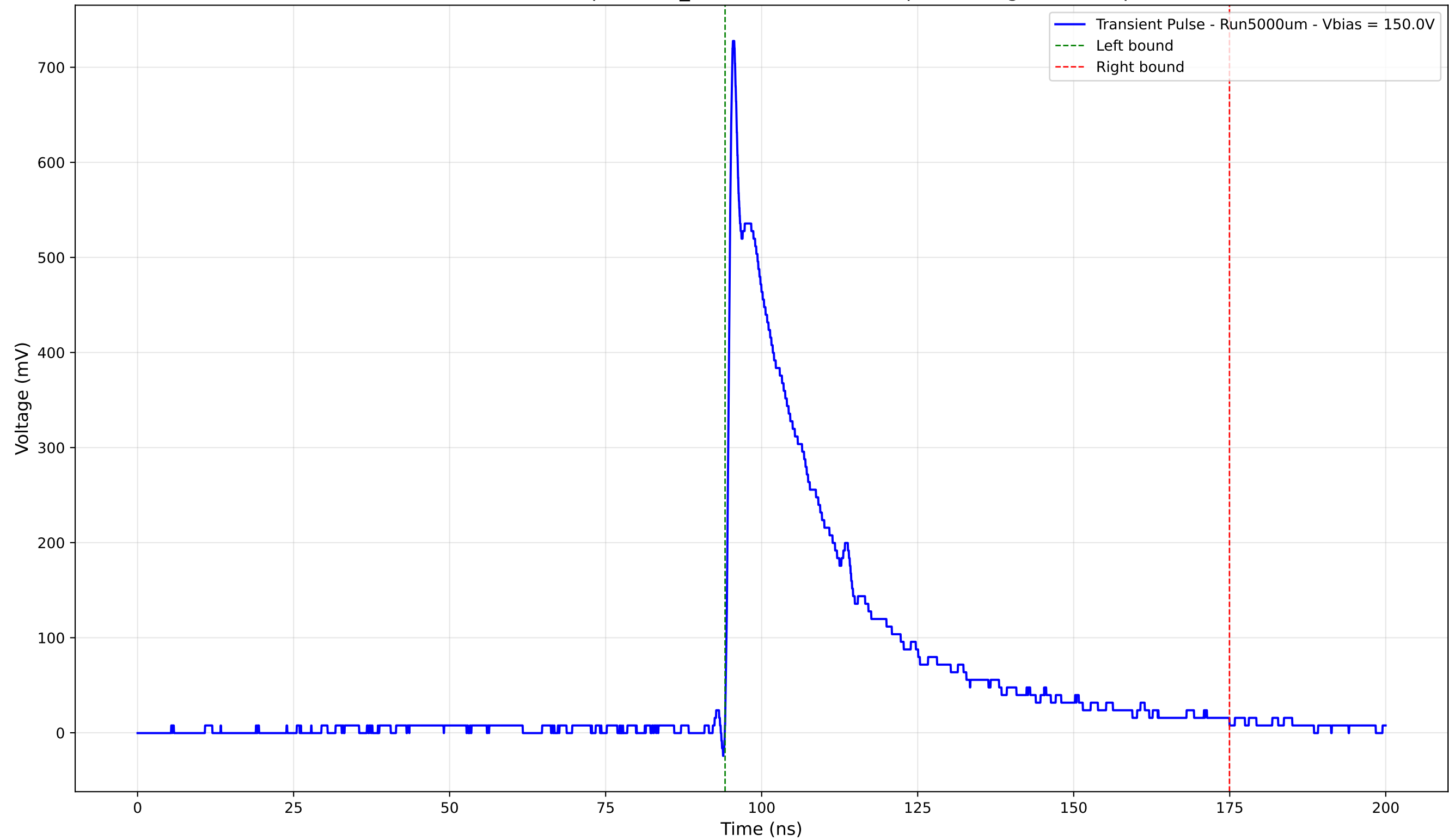
Transient Pulse - Sample: 1cm_42 - Position: 2865.0 \mu\text{m} - Charge: 205.21 pC
