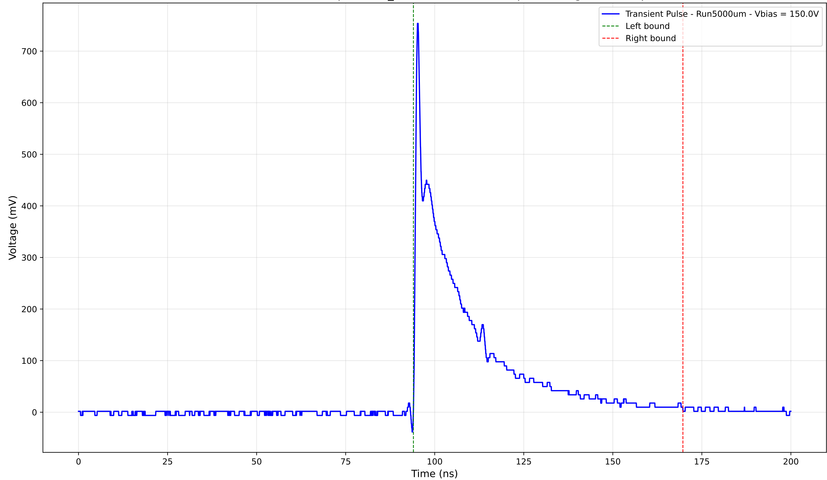
Transient Pulse - Sample: 1cm_42 - Position: 2405.0 \mu\text{m} - Charge: 164.27 pC
