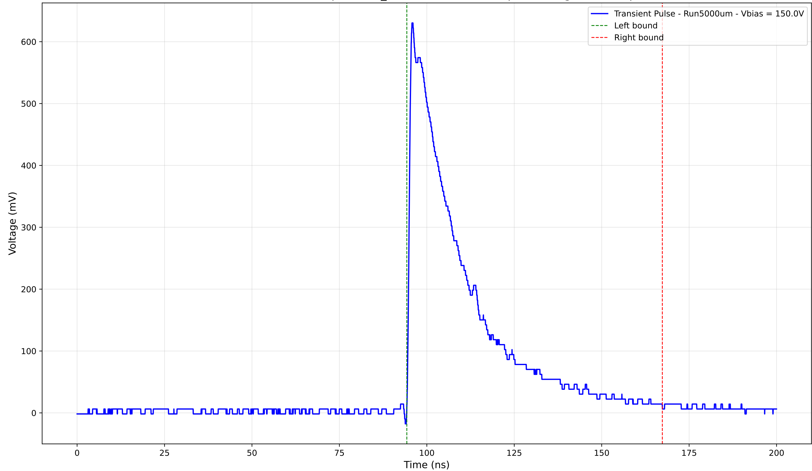
Transient Pulse - Sample: 1cm_42 - Position: 3155.0 \mu\text{m} - Charge: 206.55 pC
