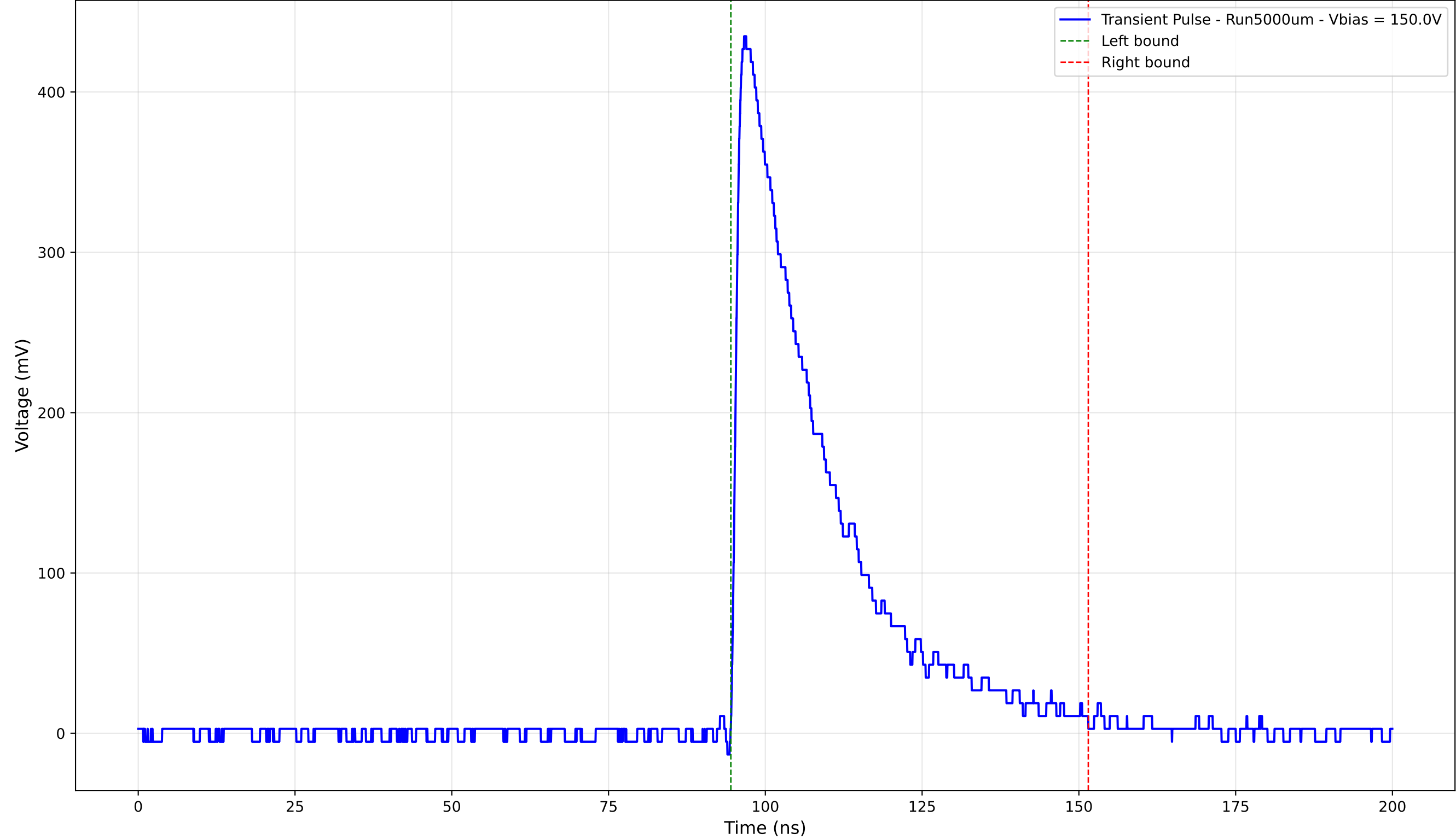
Transient Pulse - Sample: 1cm_42 - Position: 3980.0 \mu\text{m} - Charge: 130.49 pC
