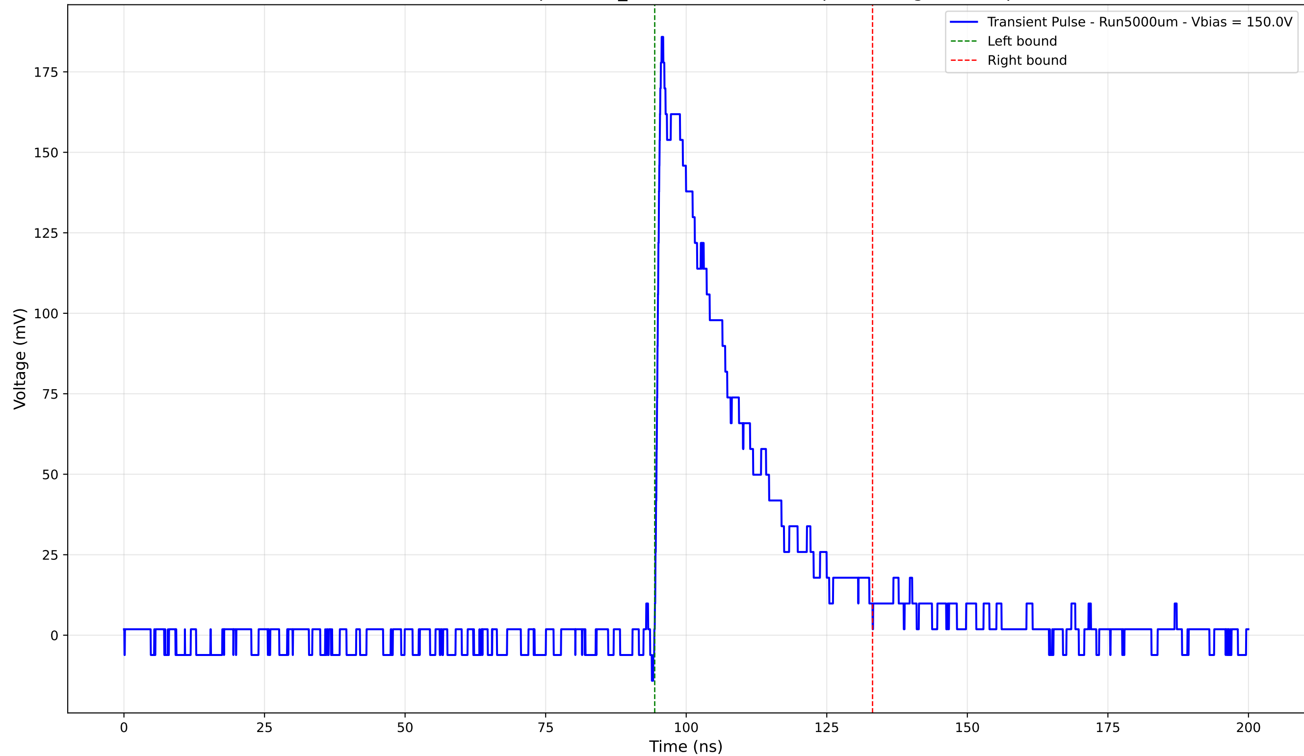
Transient Pulse - Sample: 1cm_42 - Position: 3060.0 \mu\text{m} - Charge: 50.82 pC
