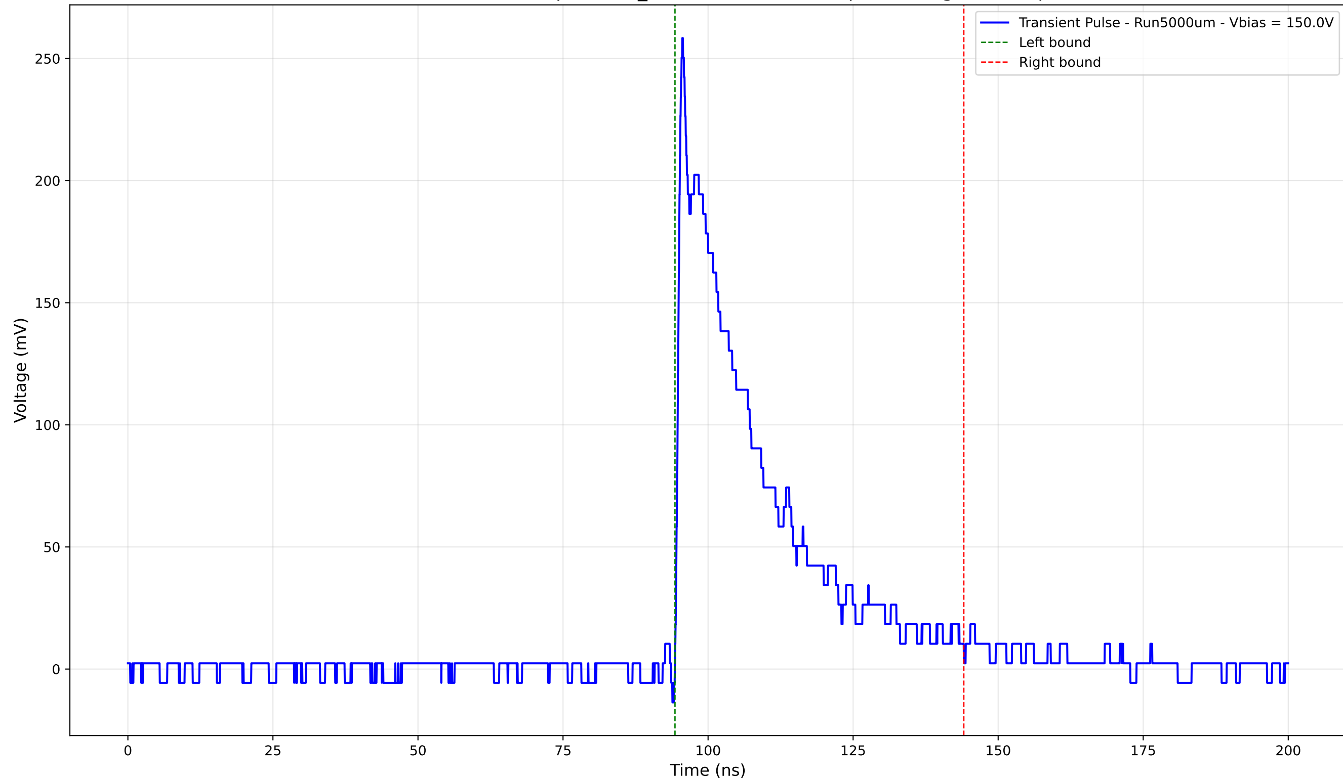
Transient Pulse - Sample: 1cm_42 - Position: 2055.0 \mu\text{m} - Charge: 67.33 pC
