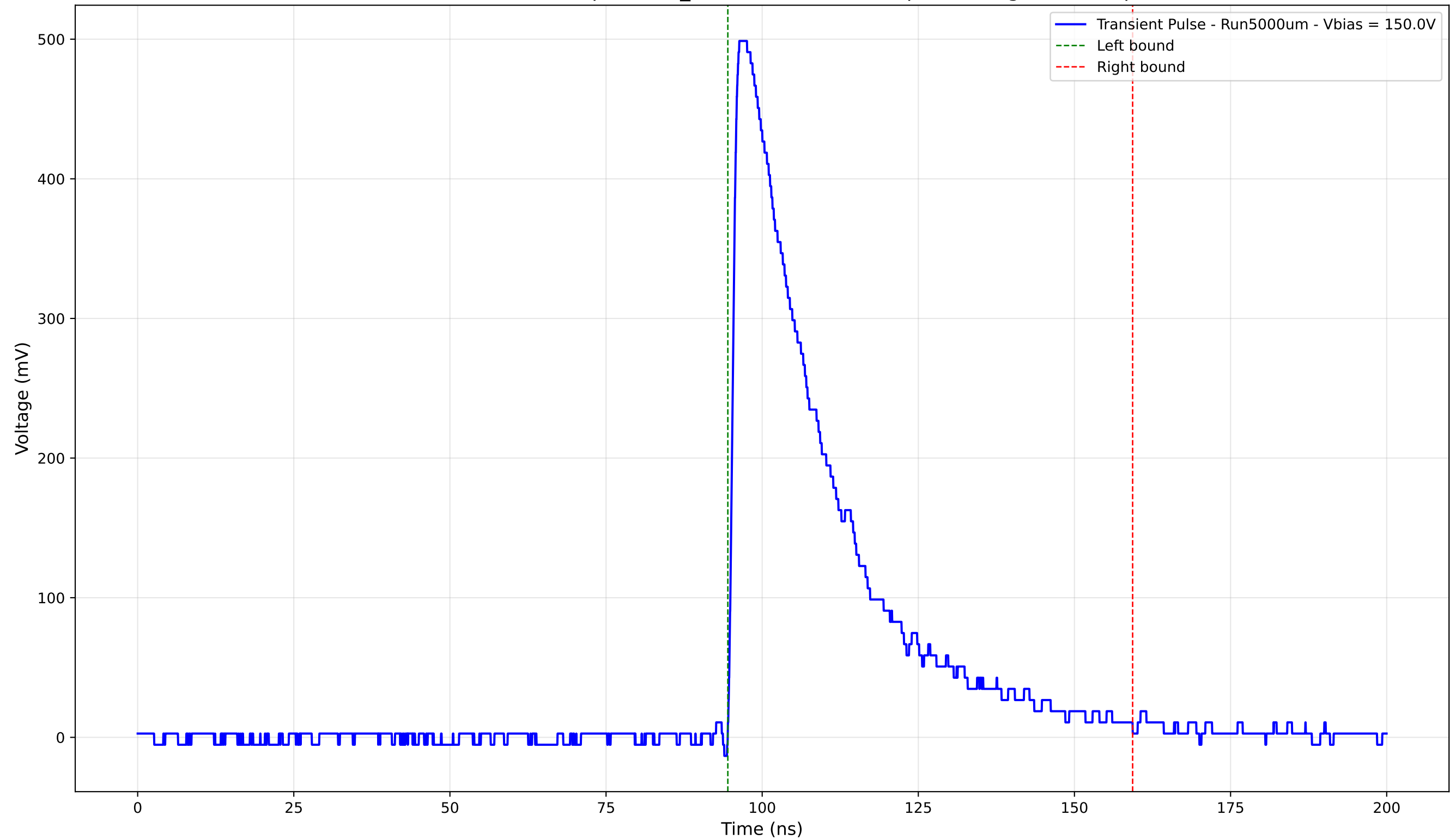
Transient Pulse - Sample: 1cm_42 - Position: 3610.0 \mu\text{m} - Charge: 162.40 pC
