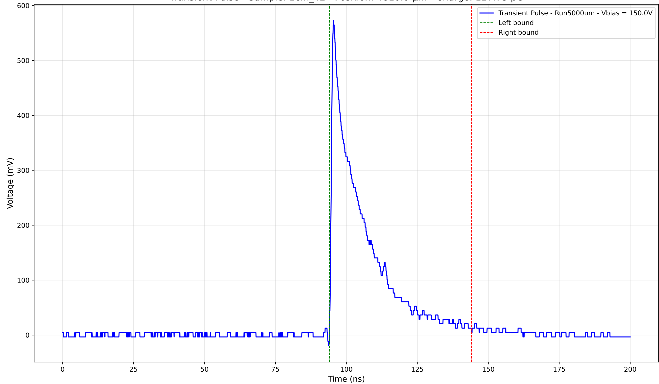
Transient Pulse - Sample: 1cm_42 - Position: 4810.0 \mu\text{m} - Charge: 127.75 pC
