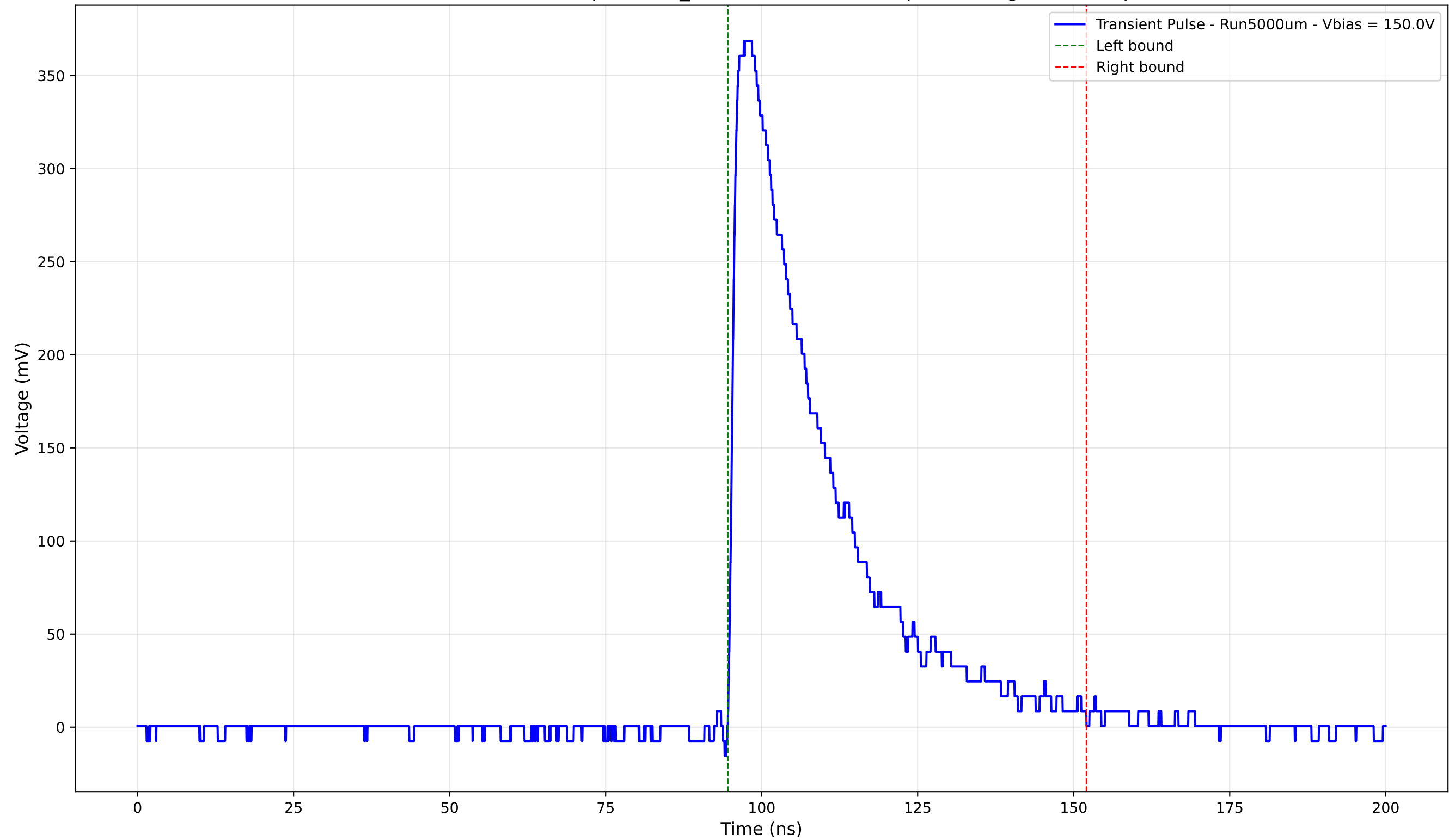
Transient Pulse - Sample: 1cm_42 - Position: 1445.0 \mu\text{m} - Charge: 117.28 pC
