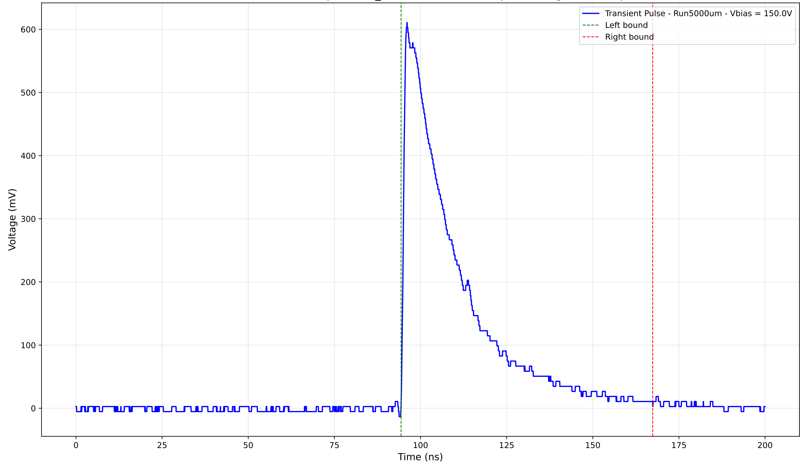
Transient Pulse - Sample: 1cm_42 - Position: 3265.0 \mu\text{m} - Charge: 199.72 pC
