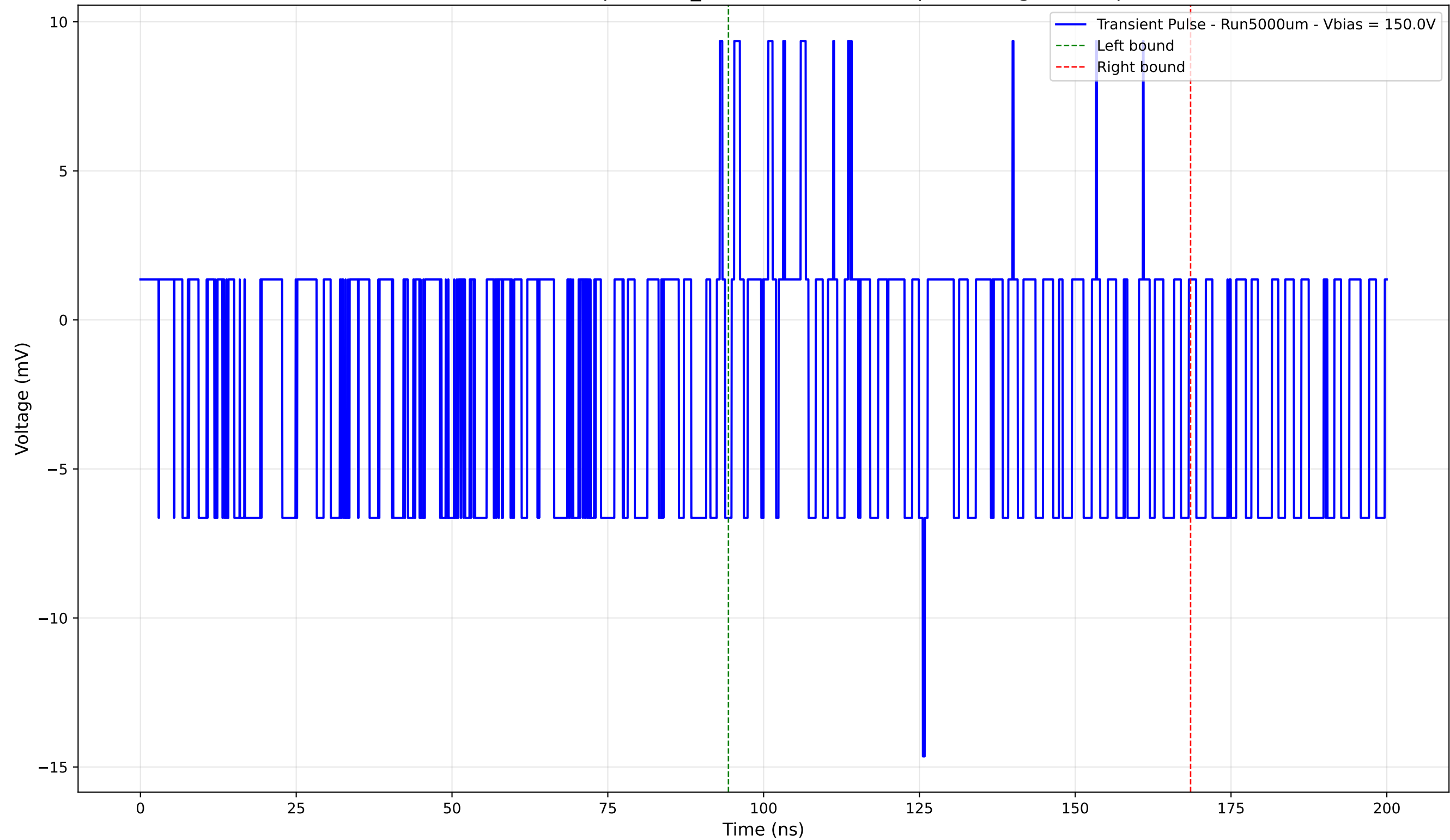
Transient Pulse - Sample: 1cm_42 - Position: 4985.0 \mu\text{m} - Charge: -1.71 pC
