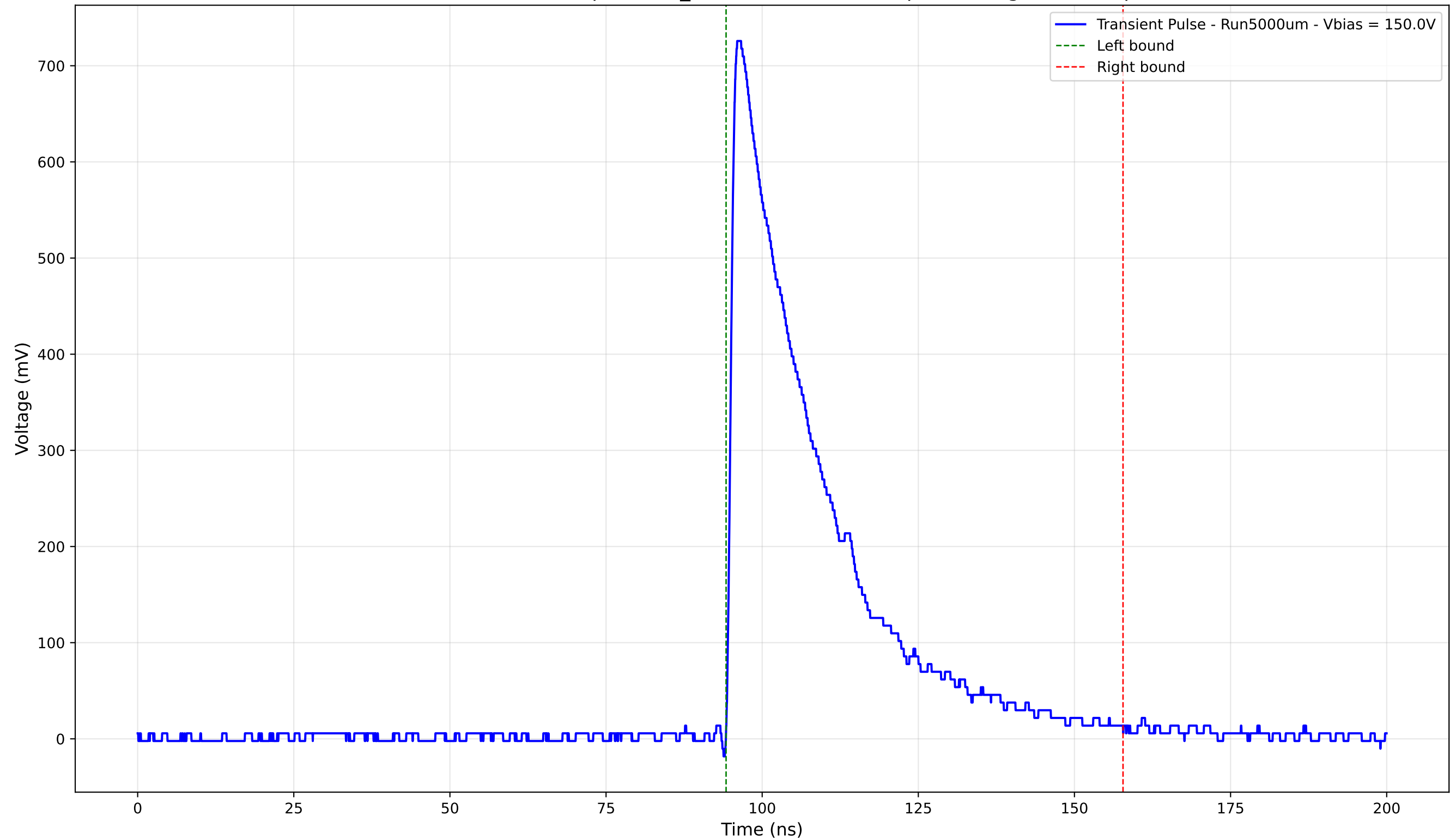
Transient Pulse - Sample: 1cm_42 - Position: 4385.0 \mu\text{m} - Charge: 217.16 pC
