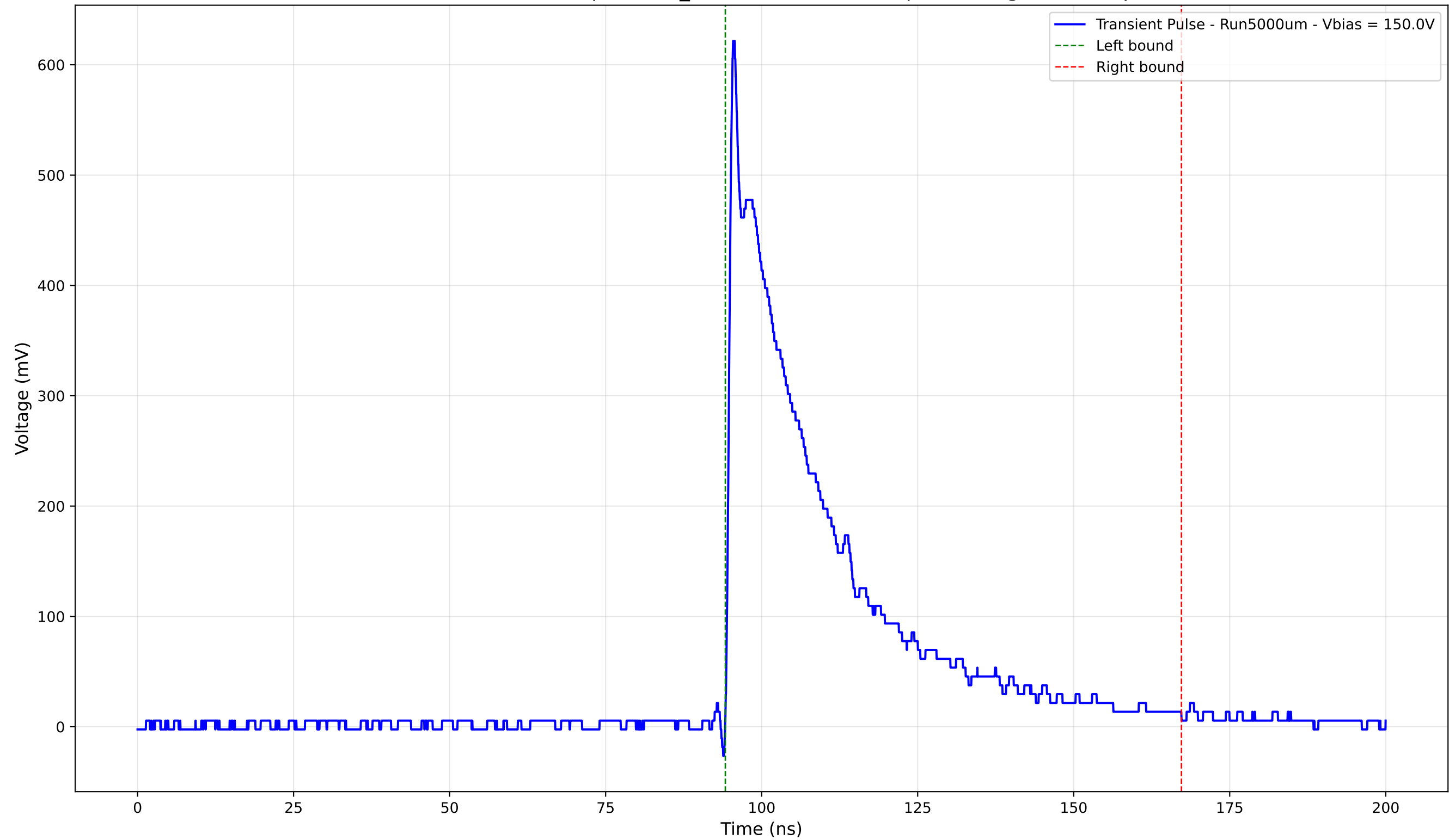
Transient Pulse - Sample: 1cm_42 - Position: 2125.0 \mu\text{m} - Charge: 176.02 pC
