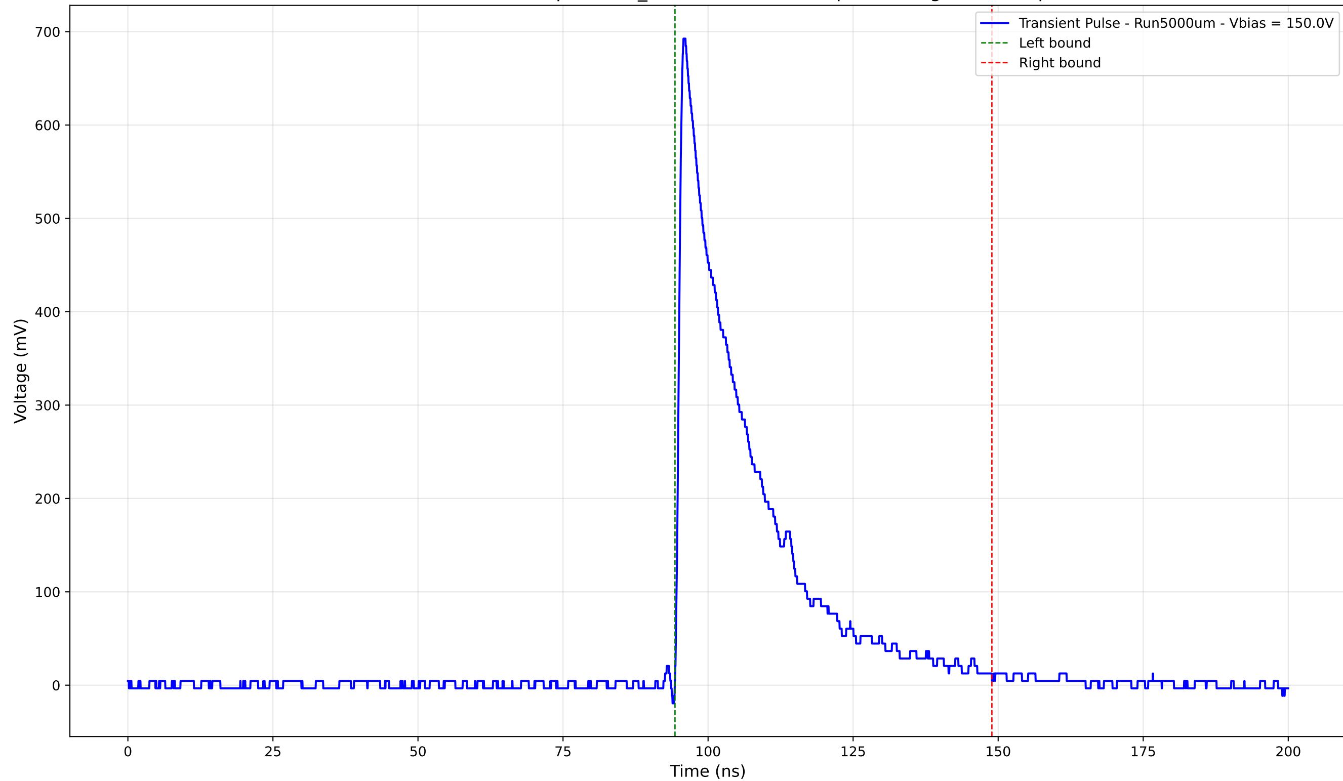
Transient Pulse - Sample: 1cm_42 - Position: 285.0 \mu\text{m} - Charge: 170.36 pC
