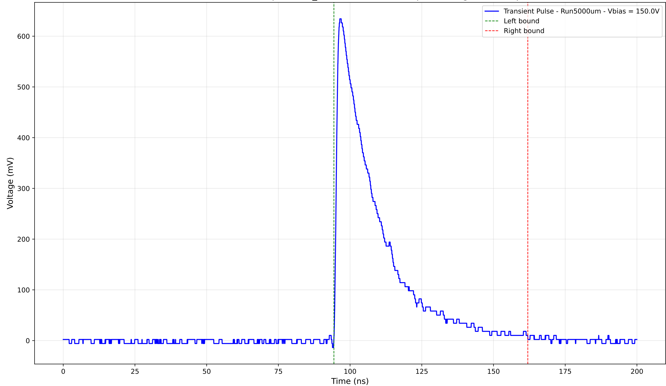
Transient Pulse - Sample: 1cm_42 - Position: 4130.0 \mu\text{m} - Charge: 193.73 pC
