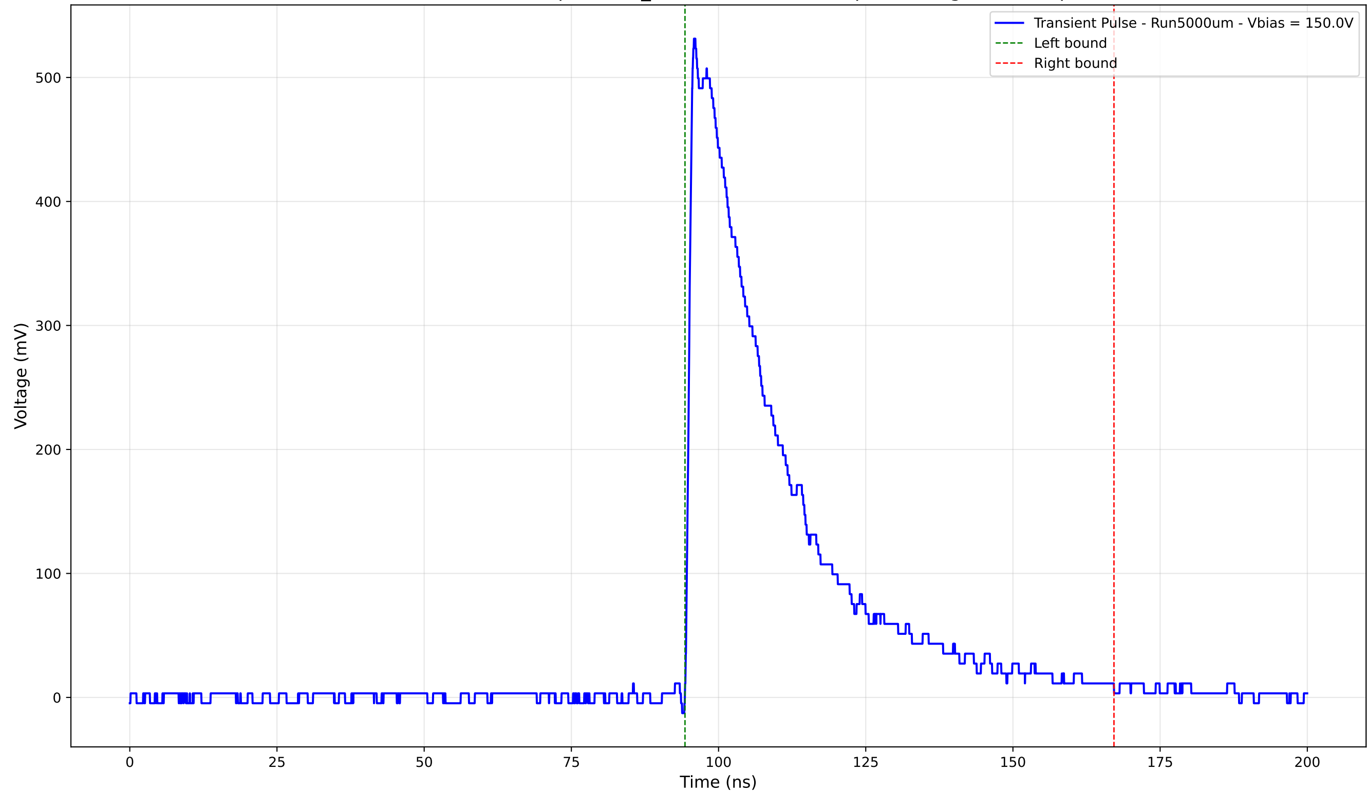
Transient Pulse - Sample: 1cm_42 - Position: 1840.0 \mu\text{m} - Charge: 176.85 pC
