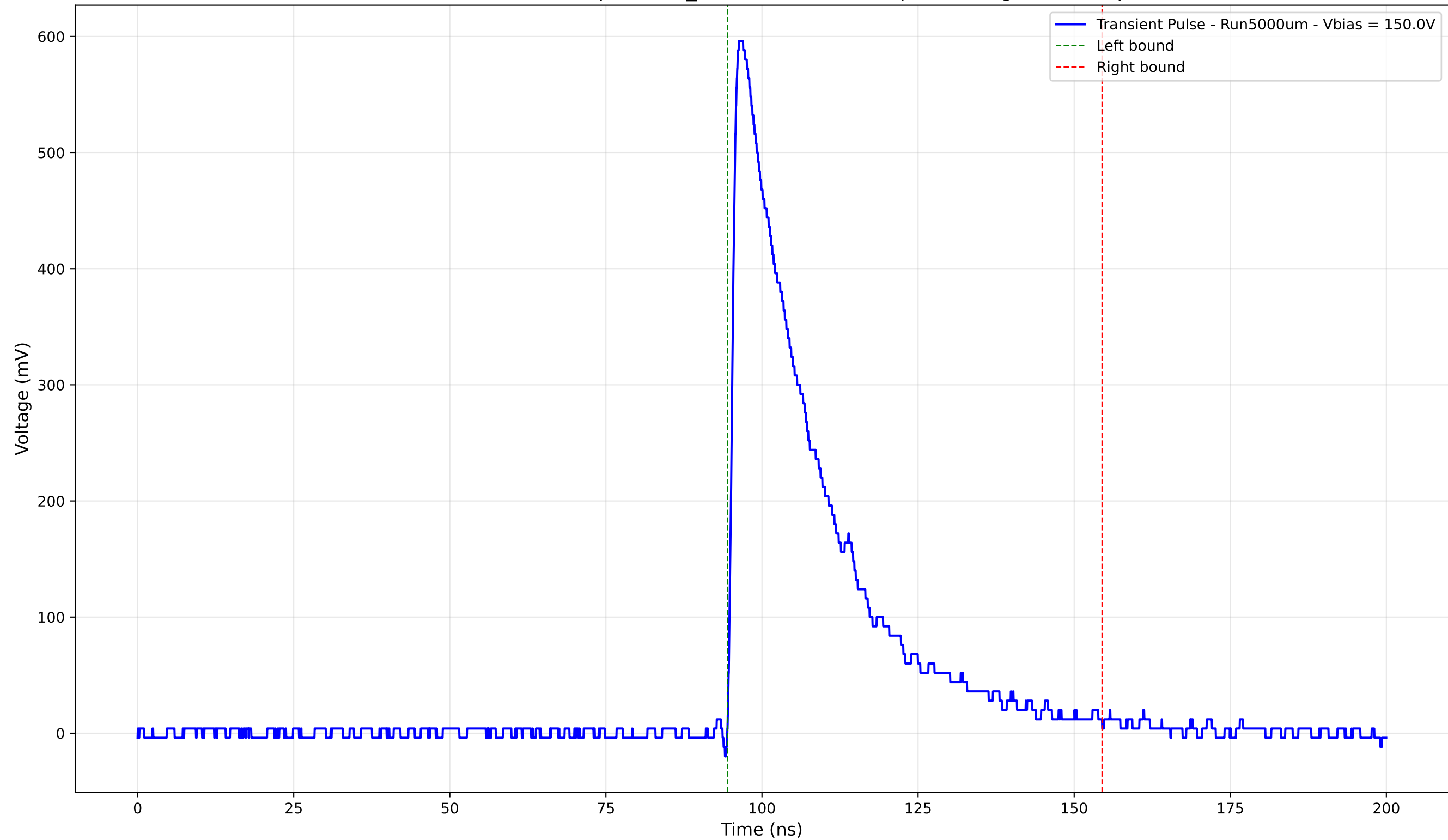
Transient Pulse - Sample: 1cm_42 - Position: 640.0 \mu\text{m} - Charge: 171.62 pC
