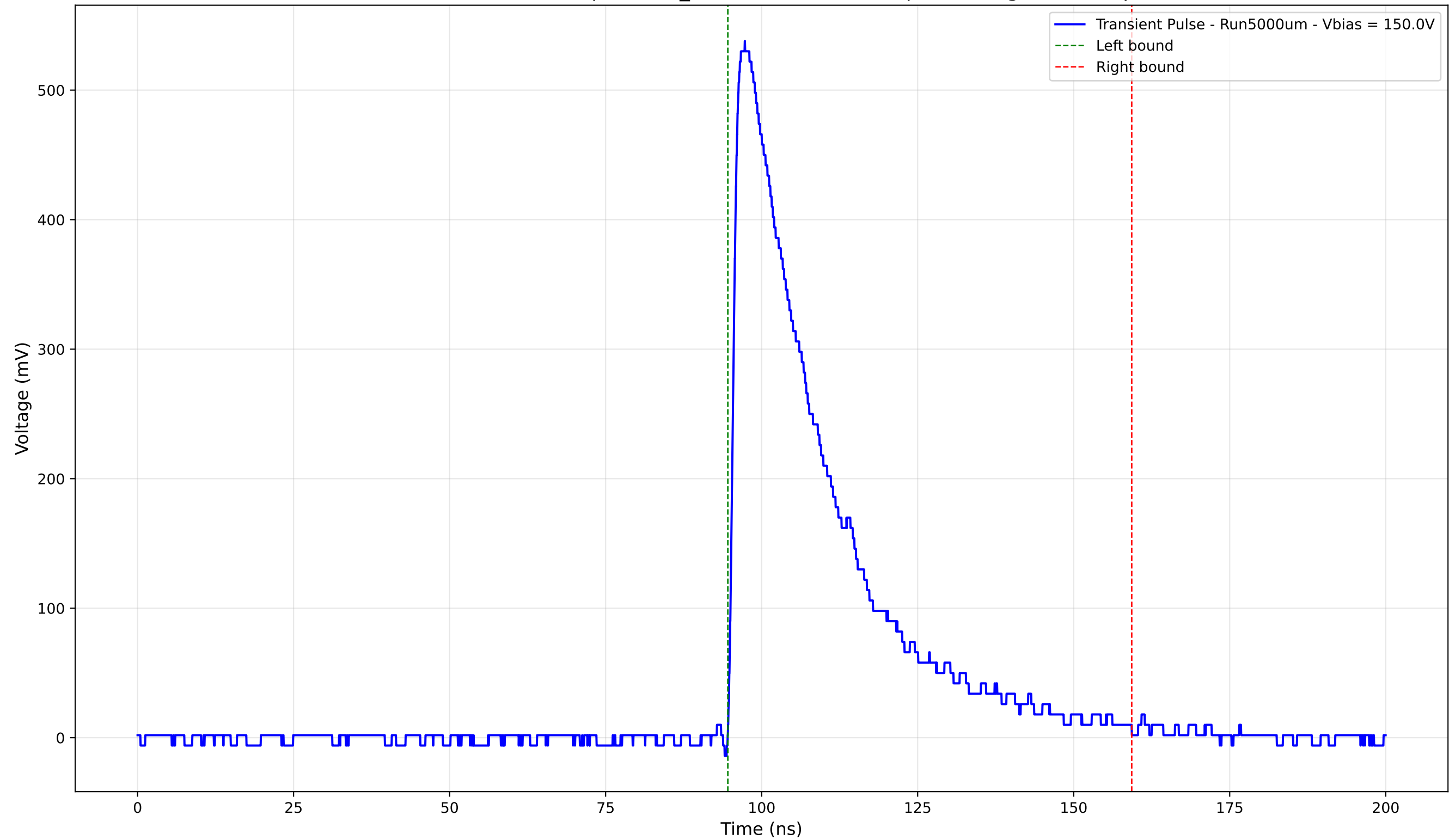
Transient Pulse - Sample: 1cm_42 - Position: 1125.0 \mu\text{m} - Charge: 169.04 pC
