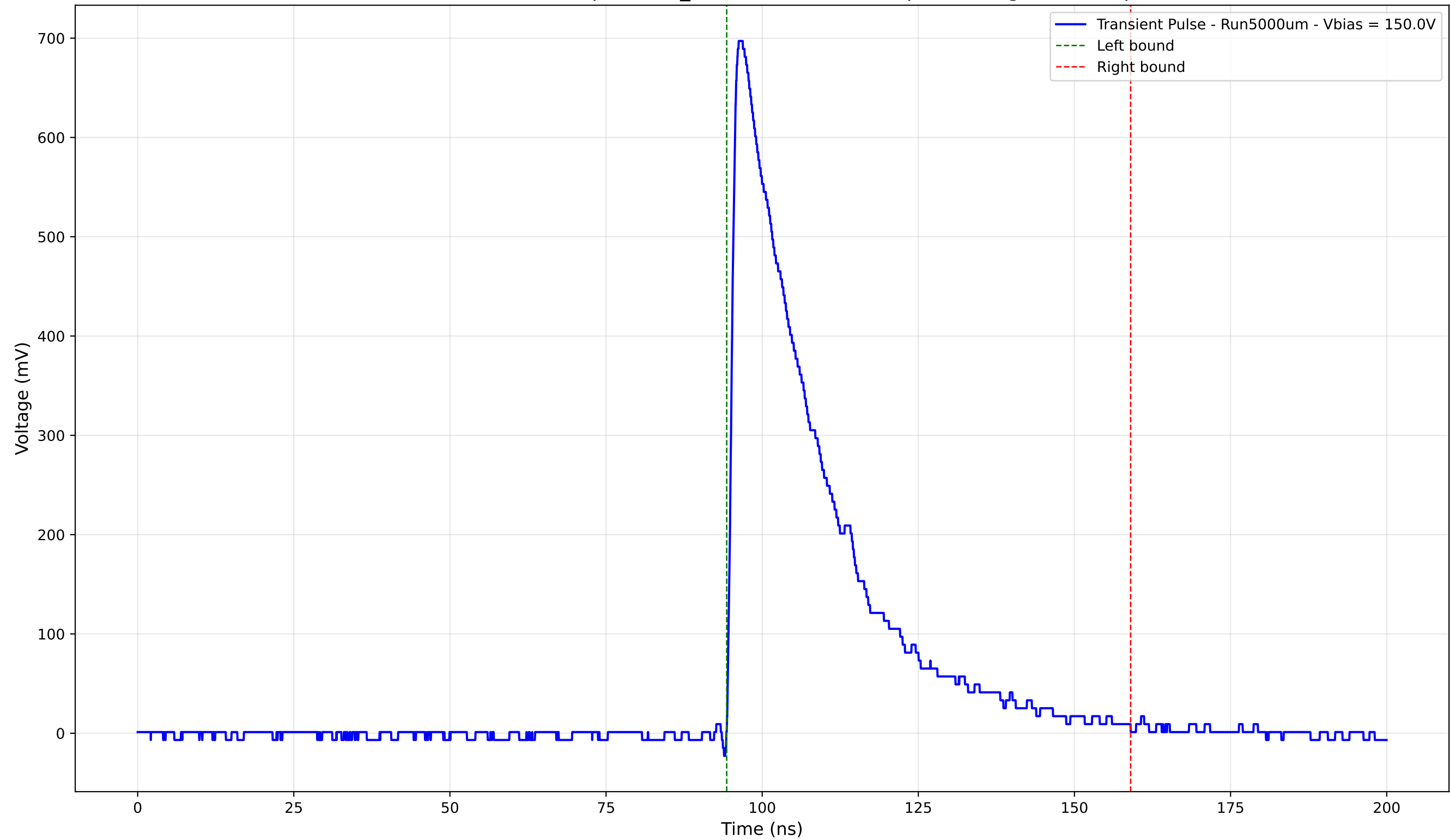
Transient Pulse - Sample: 1cm_42 - Position: 4260.0 \mu\text{m} - Charge: 209.47 pC
