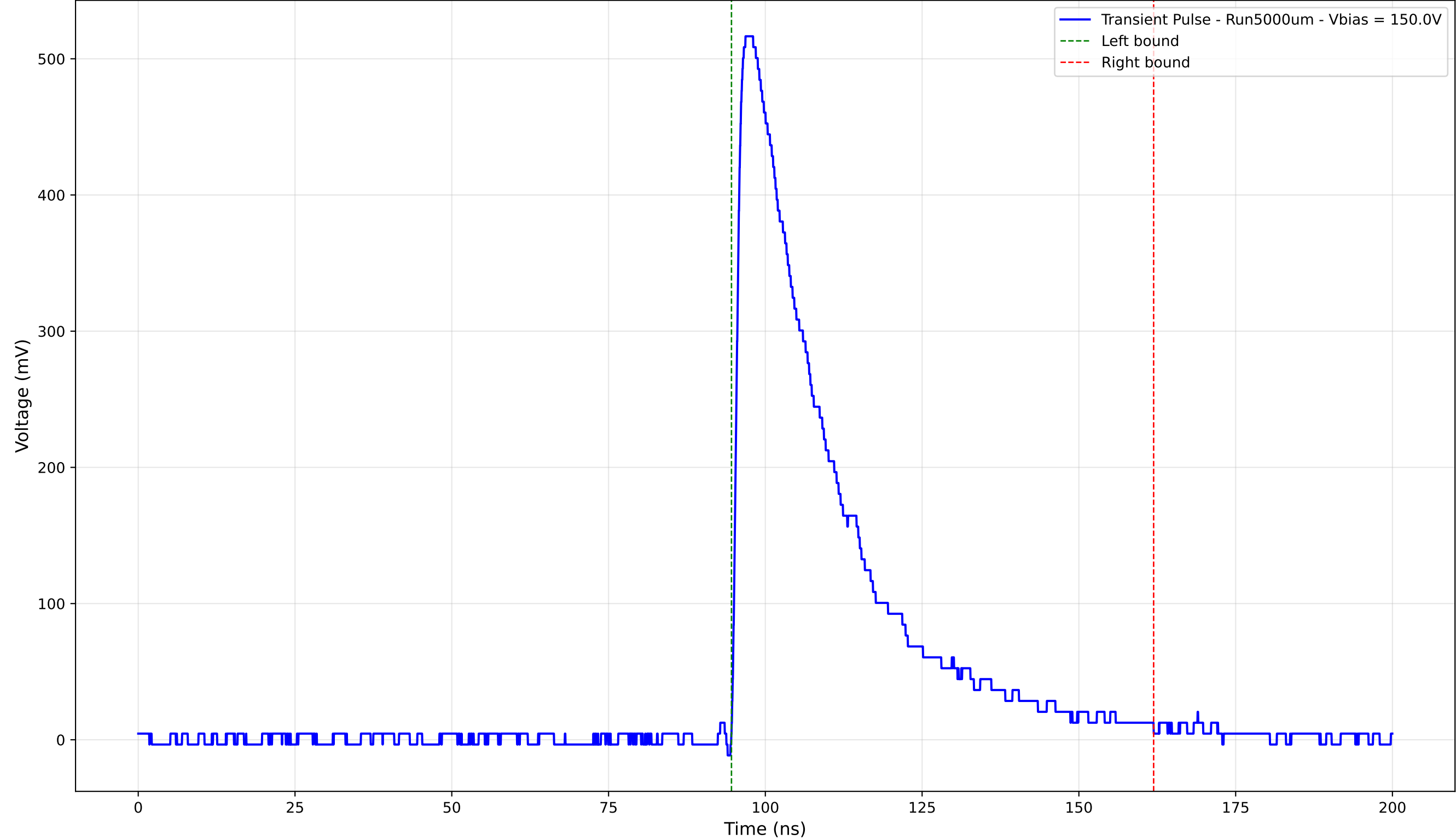
Transient Pulse - Sample: 1cm_42 - Position: 1235.0 \mu\text{m} - Charge: 169.53 pC
