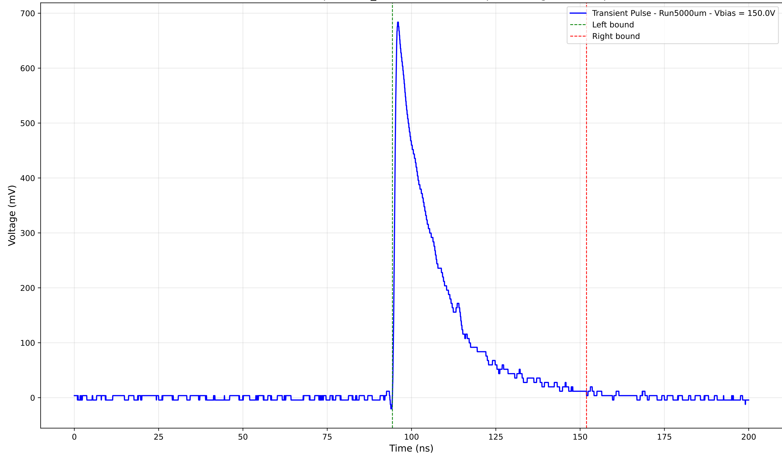
Transient Pulse - Sample: 1cm_42 - Position: 335.0 \mu\text{m} - Charge: 173.20 pC
