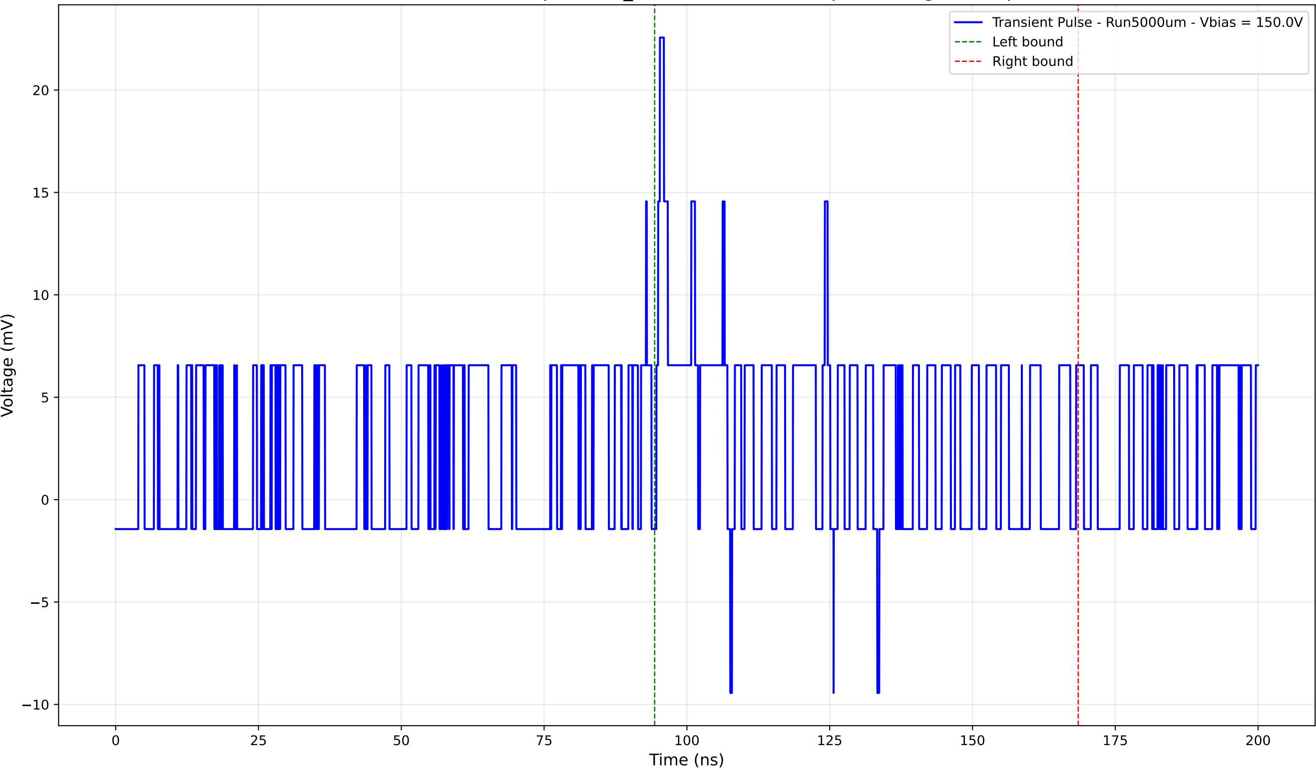
Transient Pulse - Sample: 1cm_42 - Position: 5045.0 \mu\text{m} - Charge: 5.37 pC
