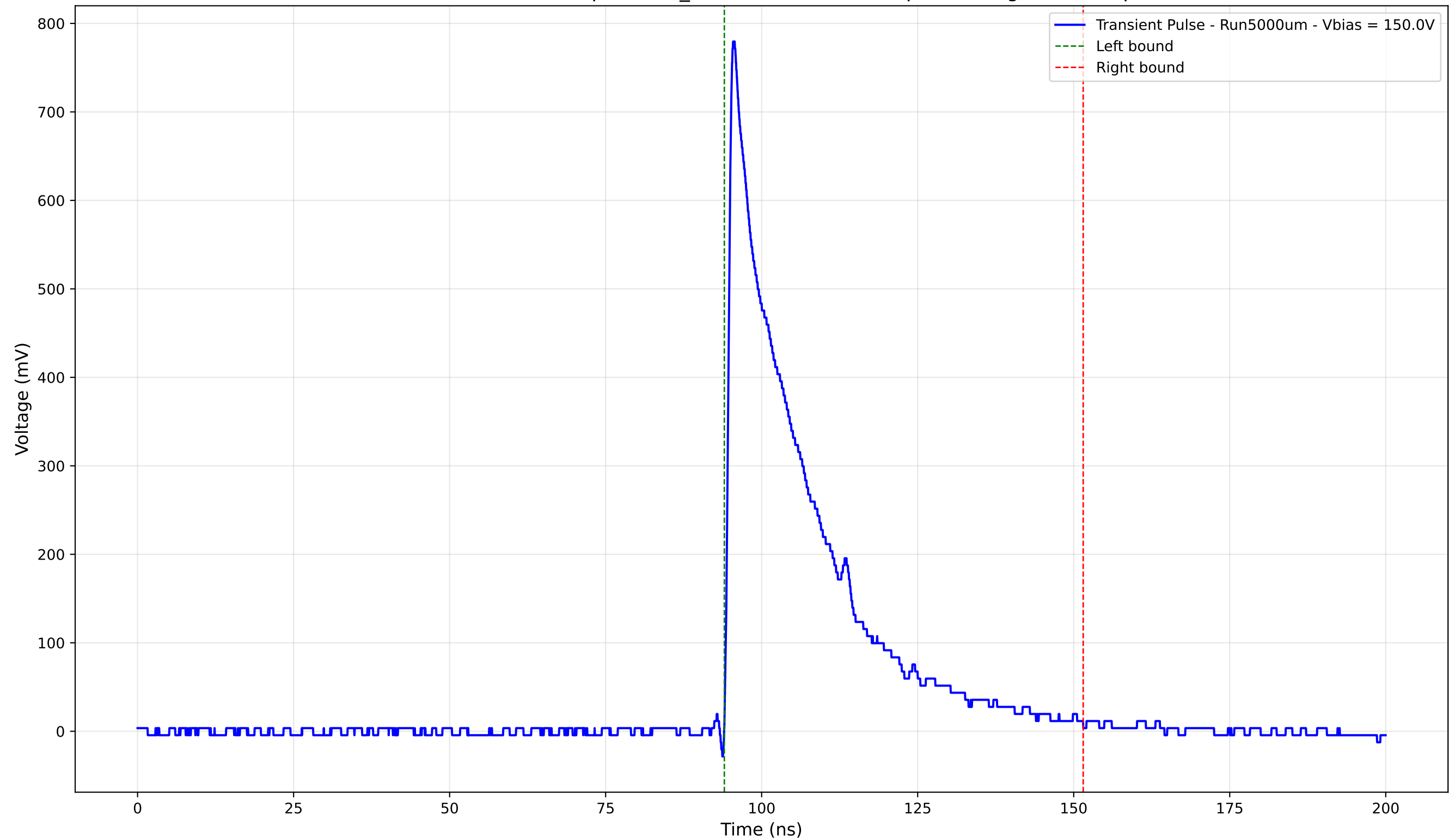
Transient Pulse - Sample: 1cm_42 - Position: 4765.0 \mu\text{m} - Charge: 189.57 pC
