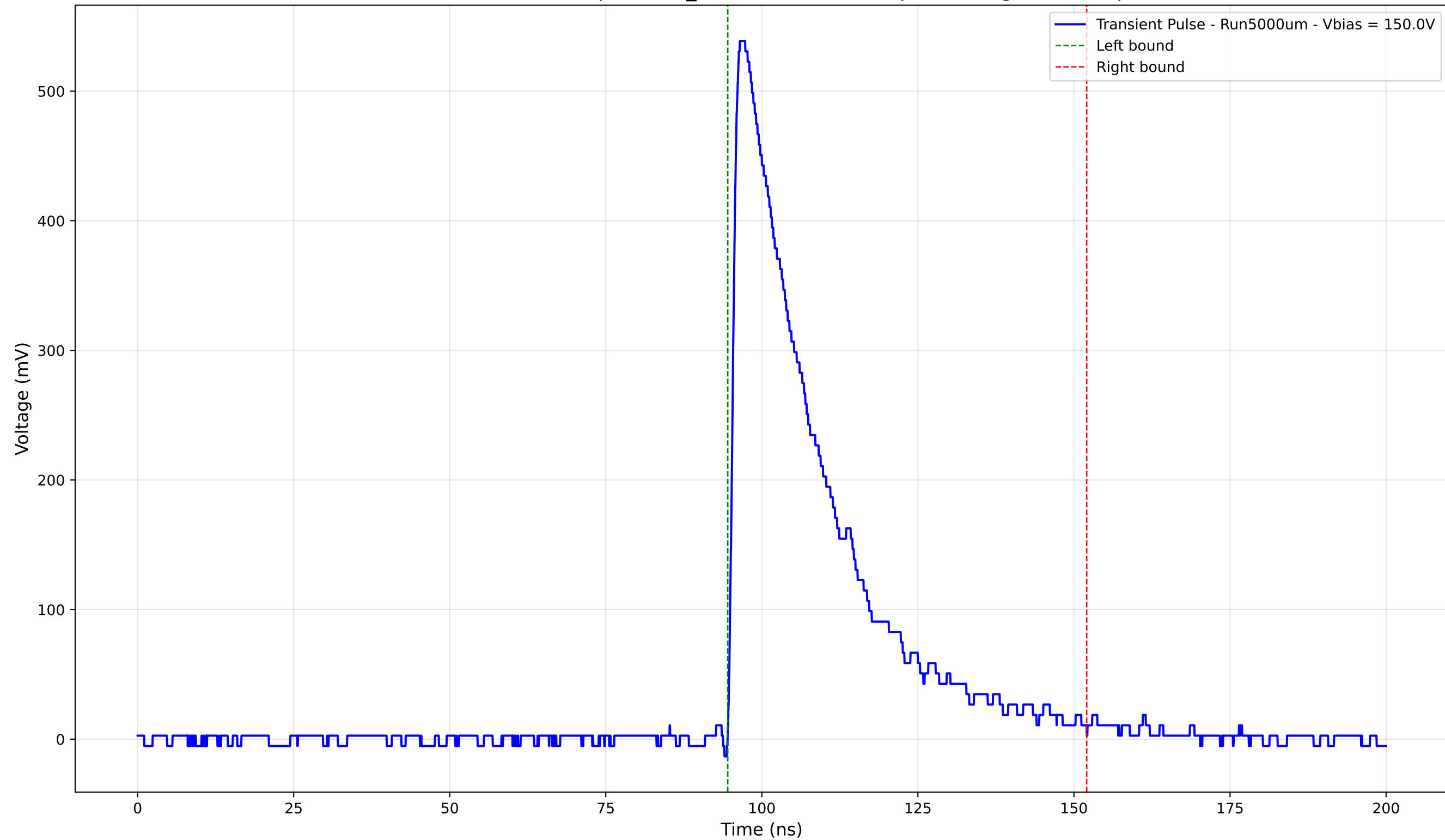
Transient Pulse - Sample: 1cm_42 - Position: 805.0 \mu\text{m} - Charge: 161.16 pC
