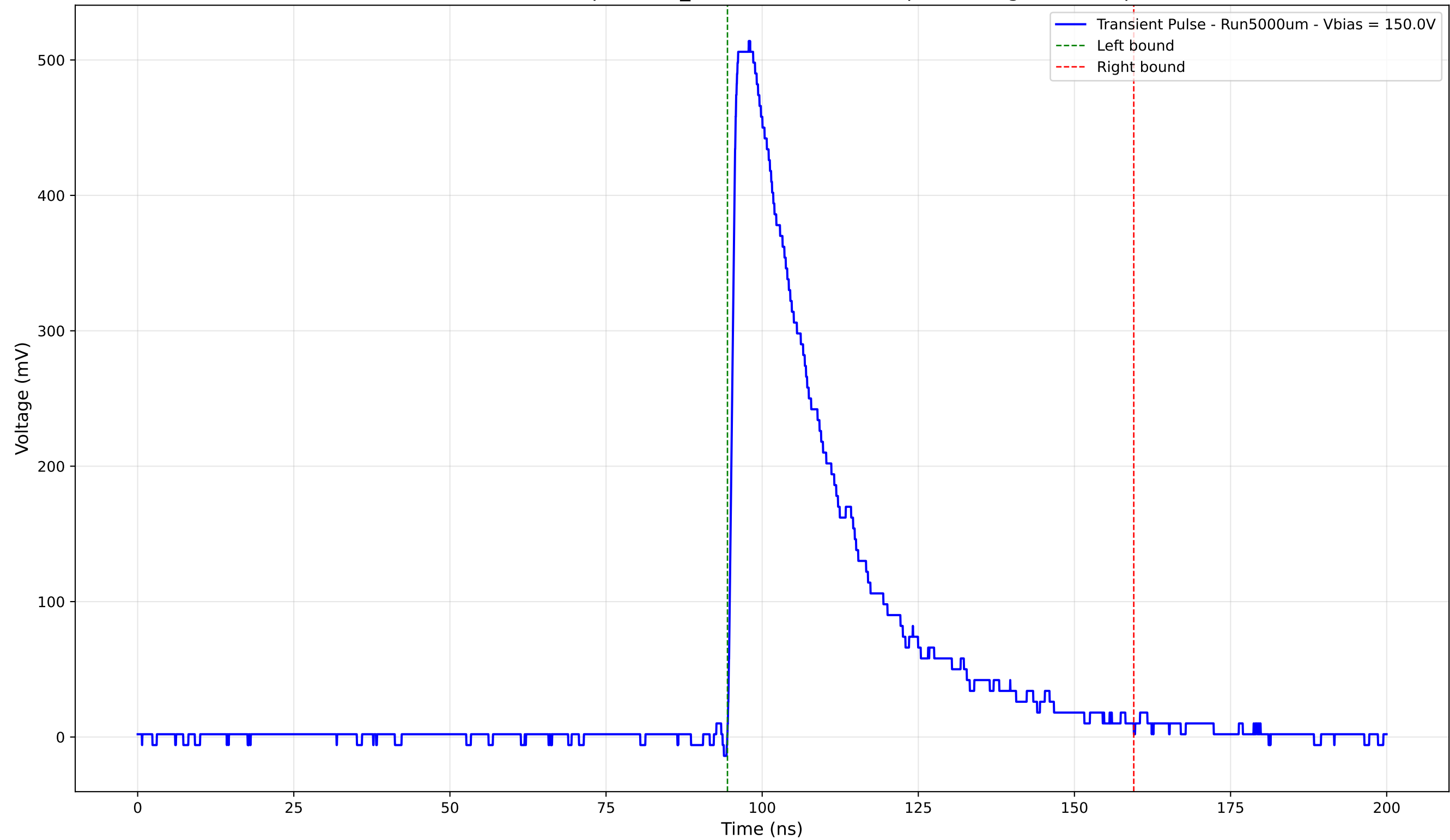
Transient Pulse - Sample: 1cm_42 - Position: 1635.0 \mu\text{m} - Charge: 171.69 pC
