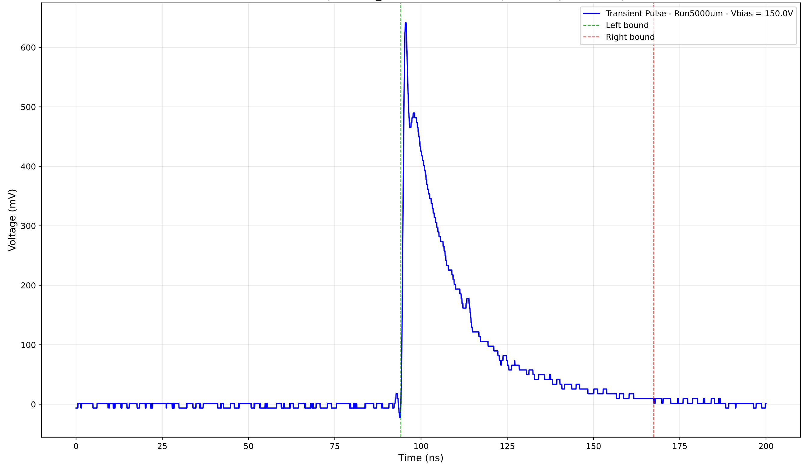
Transient Pulse - Sample: 1cm_42 - Position: 2135.0 \mu\text{m} - Charge: 175.98 pC
