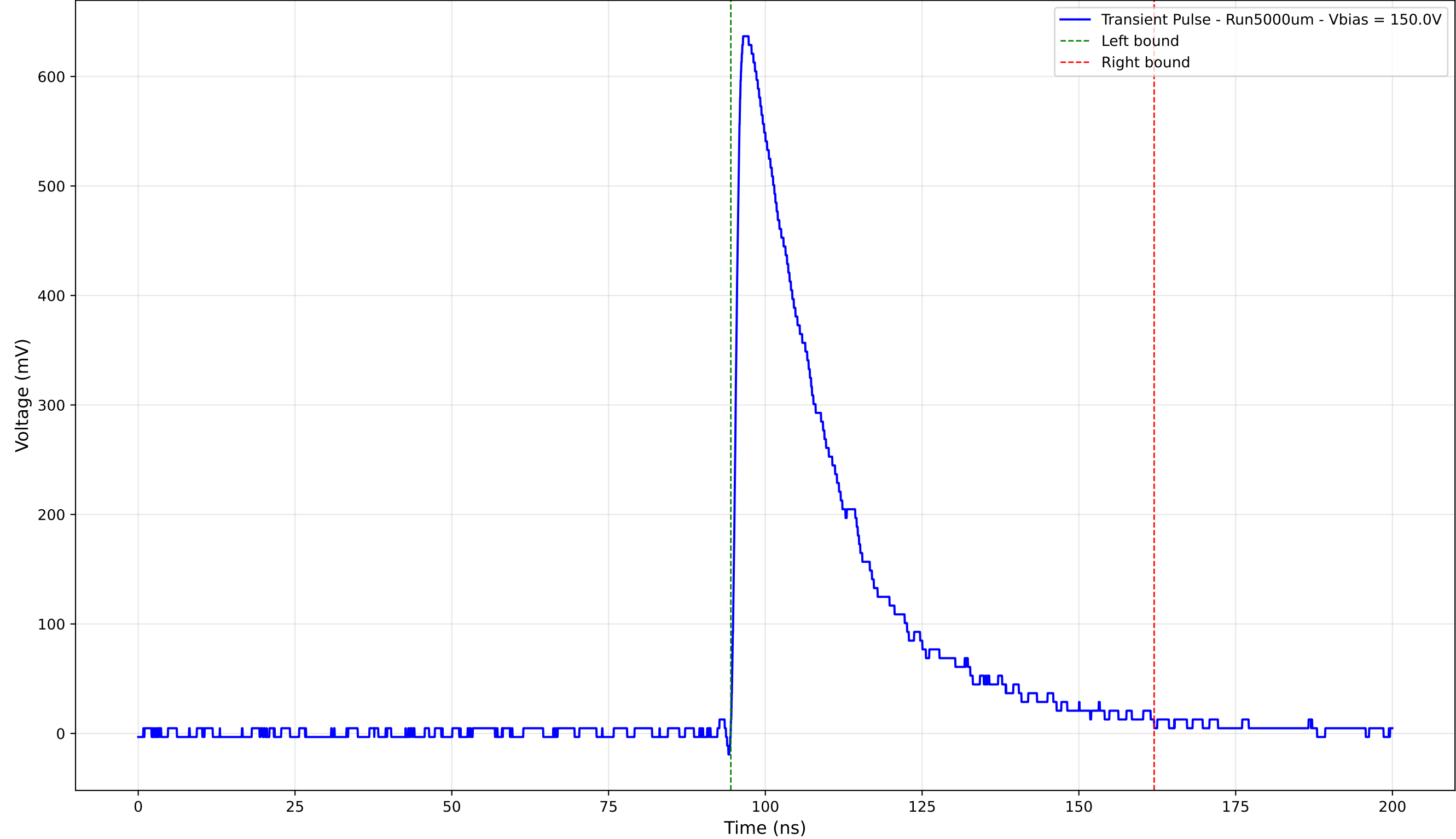
Transient Pulse - Sample: 1cm_42 - Position: 3755.0 \mu\text{m} - Charge: 208.17 pC
