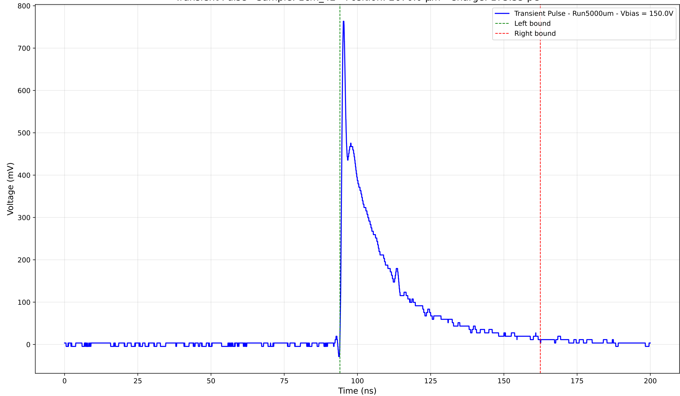
Transient Pulse - Sample: 1cm_42 - Position: 2670.0 \mu\text{m} - Charge: 173.35 pC
