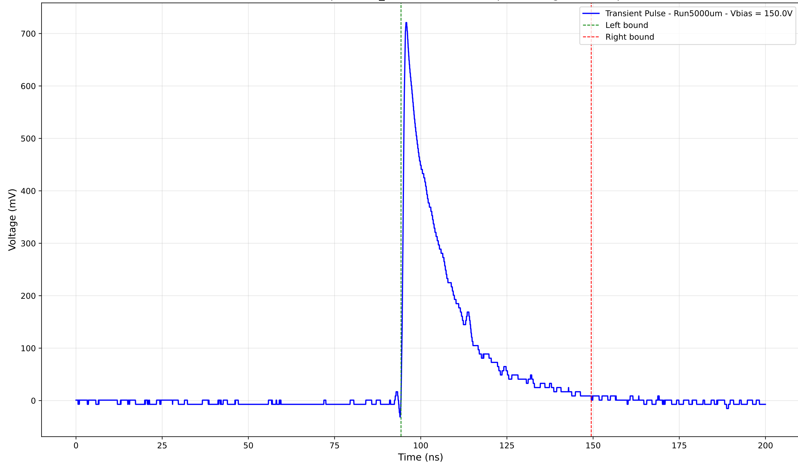
Transient Pulse - Sample: 1cm_42 - Position: 220.0 \mu\text{m} - Charge: 167.65 pC
