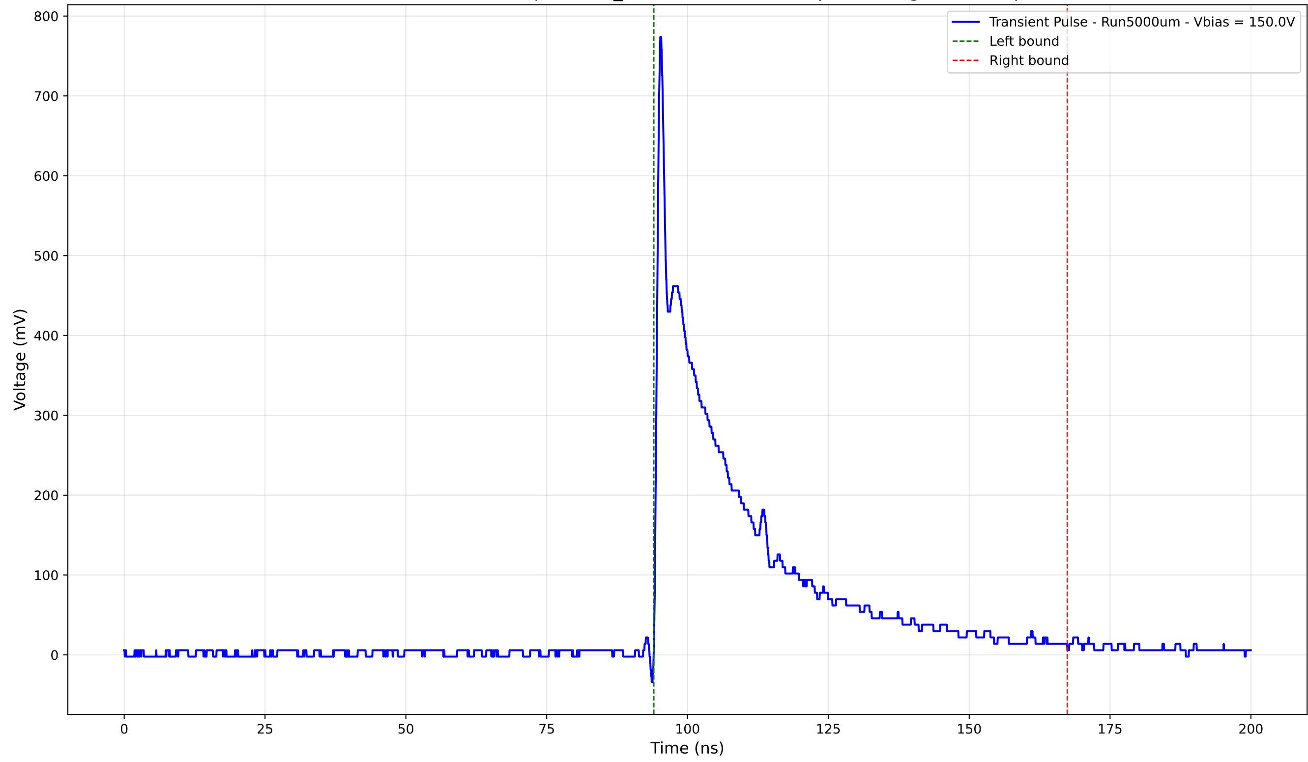
Transient Pulse - Sample: 1cm_42 - Position: 2635.0 \mu\text{m} - Charge: 174.76 pC
