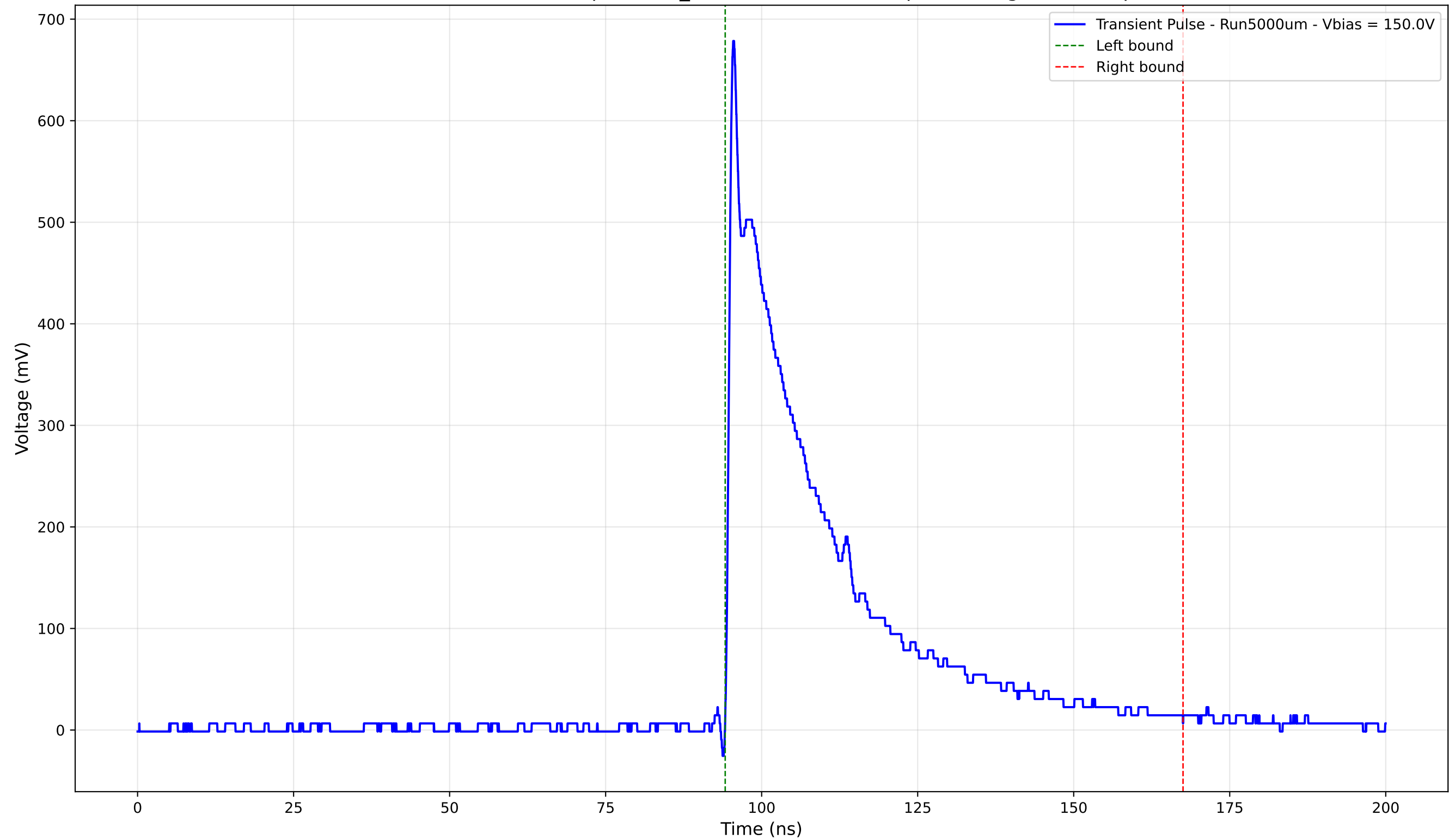
Transient Pulse - Sample: 1cm_42 - Position: 2165.0 \mu\text{m} - Charge: 187.94 pC
