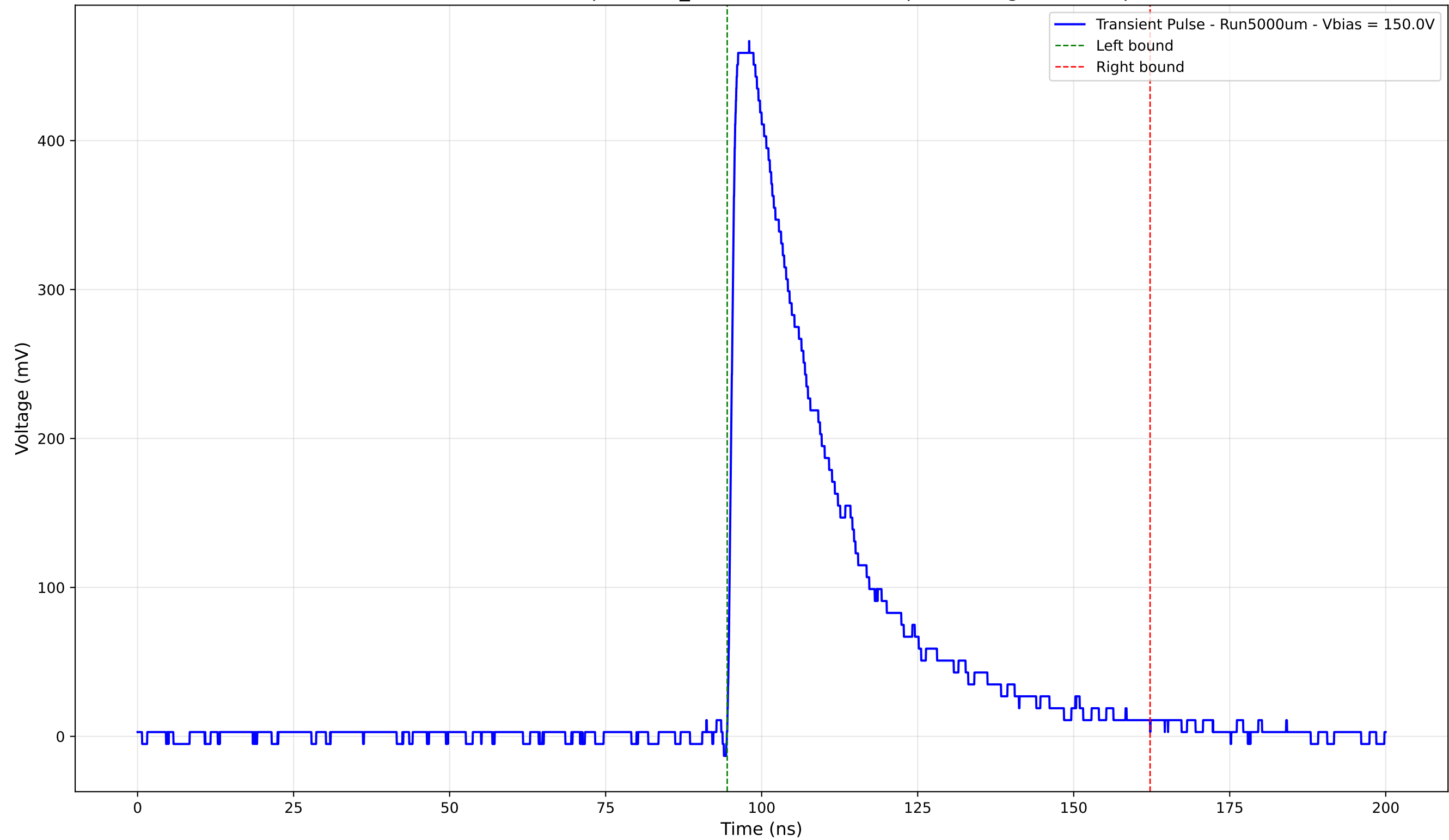
Transient Pulse - Sample: 1cm_42 - Position: 1600.0 \mu\text{m} - Charge: 157.38 pC
