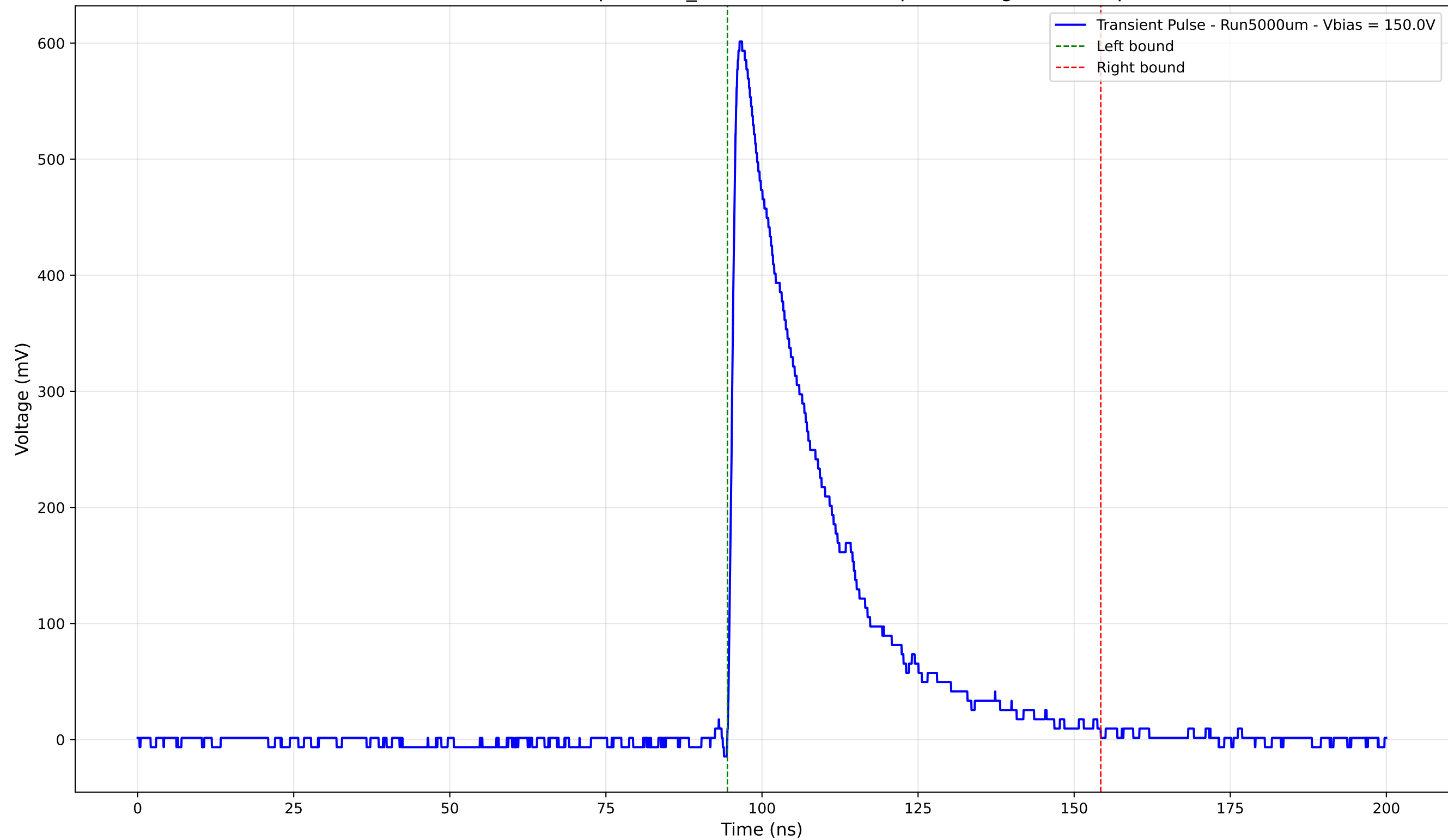
Transient Pulse - Sample: 1cm_42 - Position: 650.0 \mu\text{m} - Charge: 171.85 pC
