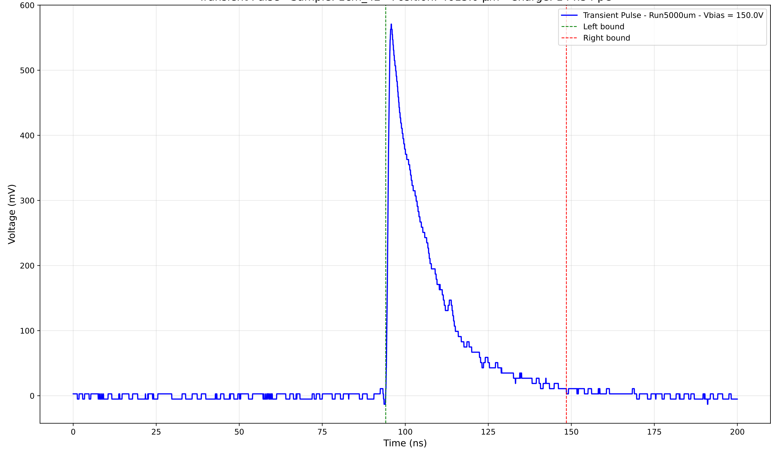
Transient Pulse - Sample: 1cm_42 - Position: 4615.0 \mu\text{m} - Charge: 144.54 pC
