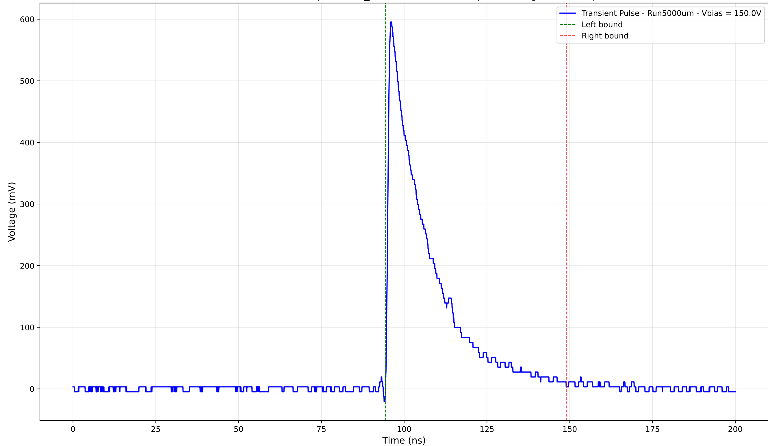
Transient Pulse - Sample: 1cm_42 - Position: 410.0 \mu\text{m} - Charge: 152.72 pC
