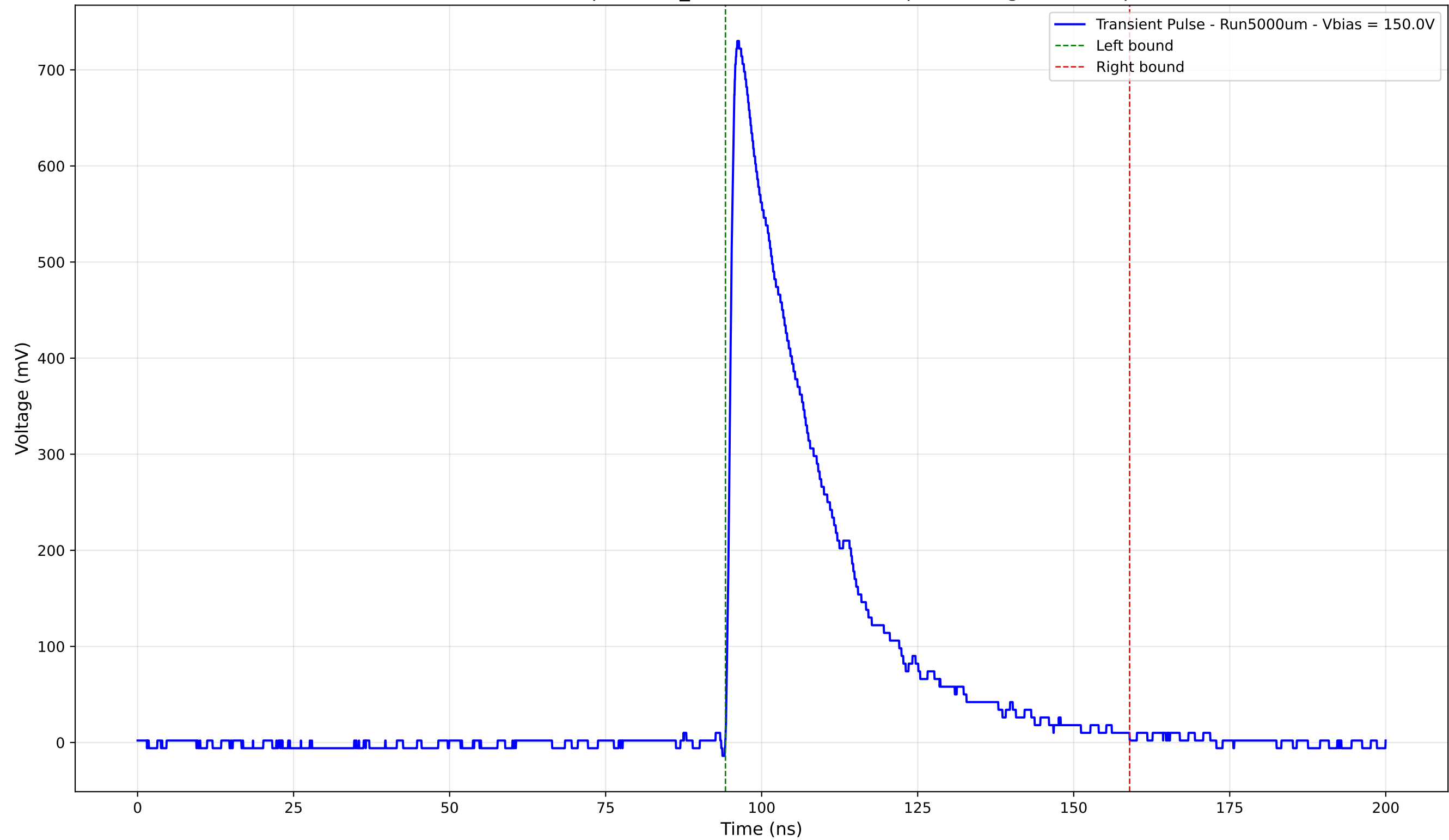
Transient Pulse - Sample: 1cm_42 - Position: 4390.0 \mu\text{m} - Charge: 214.50 pC
