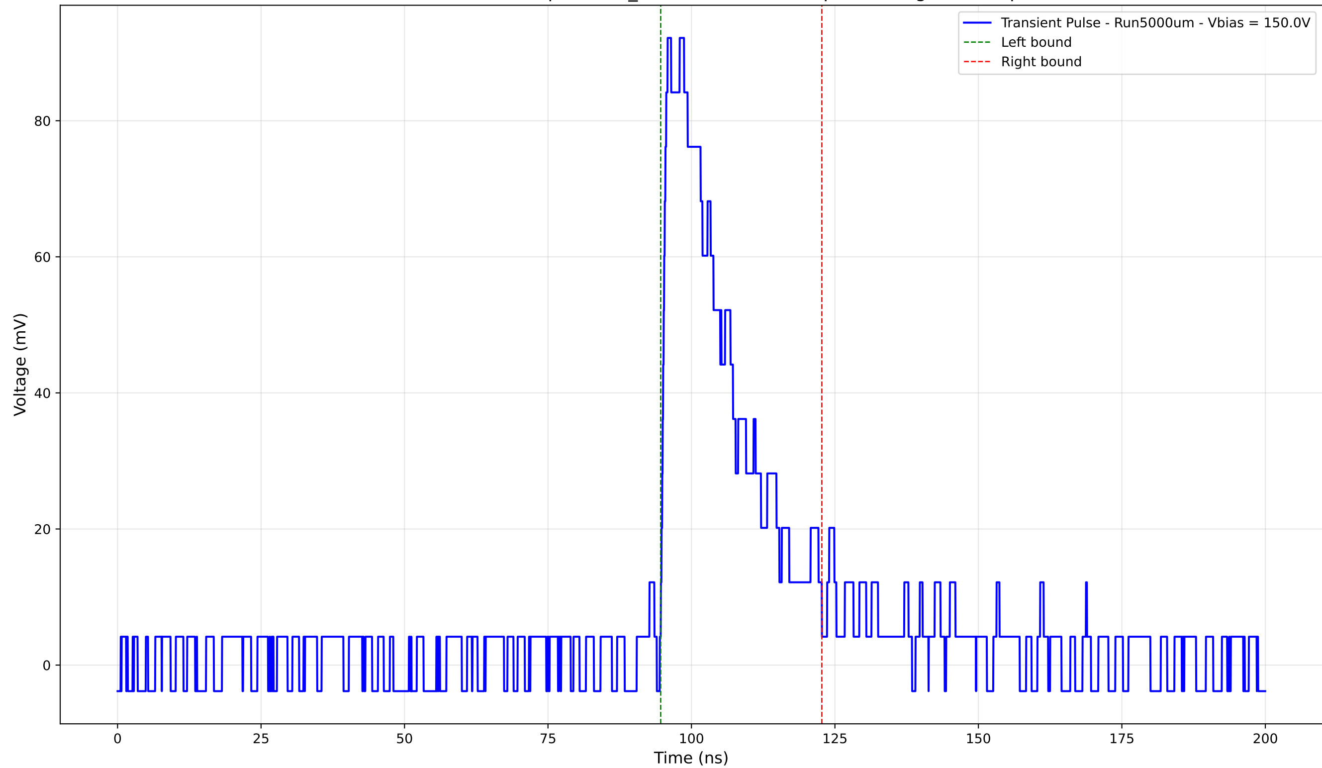
Transient Pulse - Sample: 1cm_42 - Position: 505.0 \mu\text{m} - Charge: 23.88 pC
