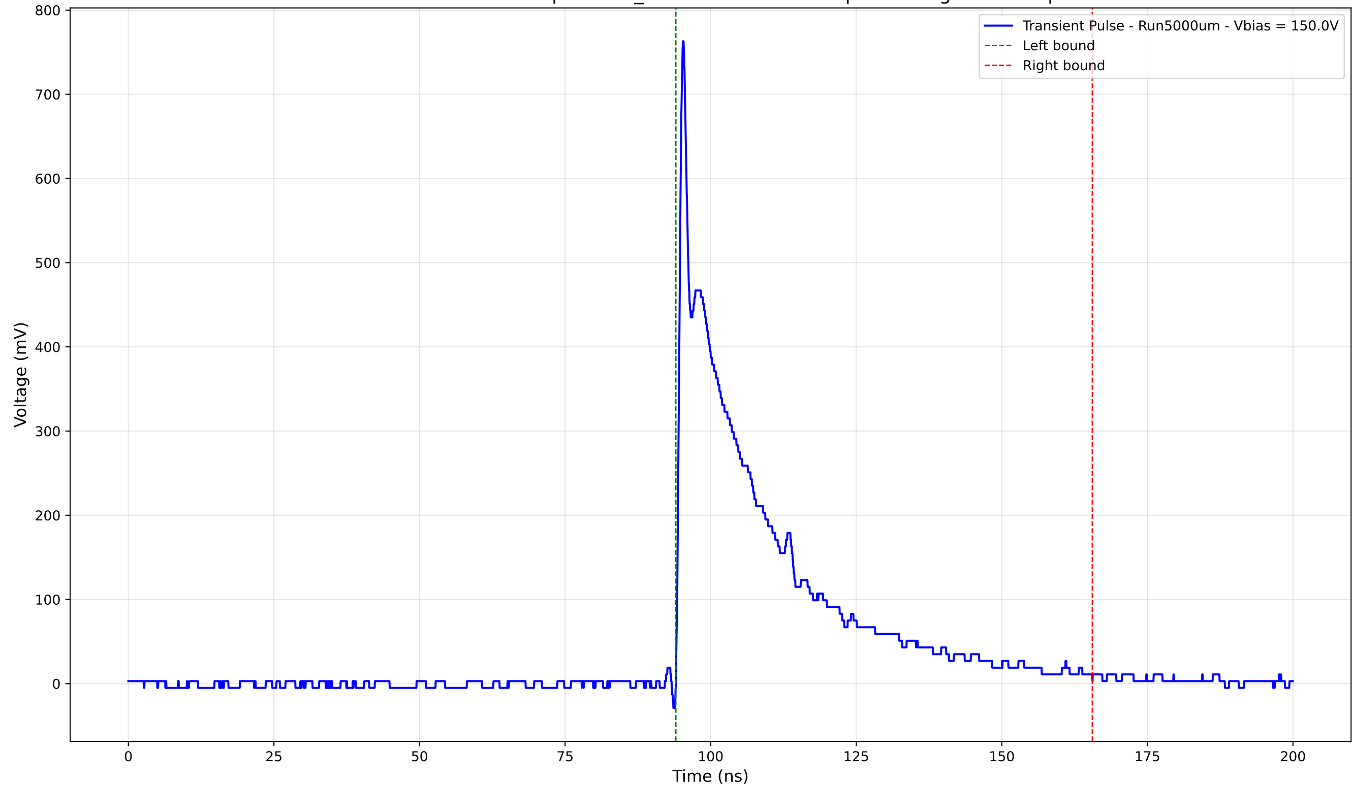
Transient Pulse - Sample: 1cm_42 - Position: 2365.0 \mu\text{m} - Charge: 174.05 pC
