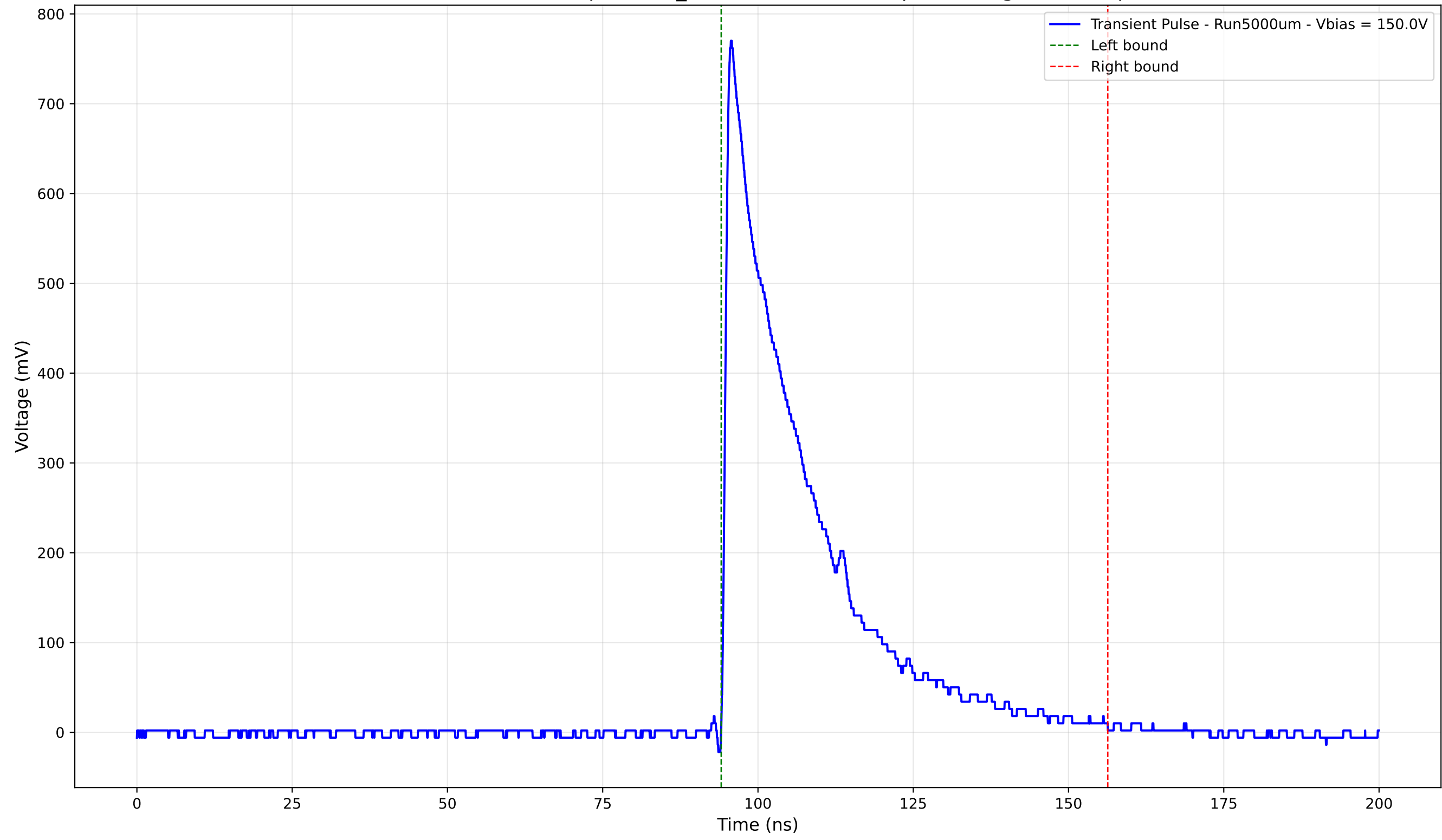
Transient Pulse - Sample: 1cm_42 - Position: 4670.0 \mu\text{m} - Charge: 200.33 pC
