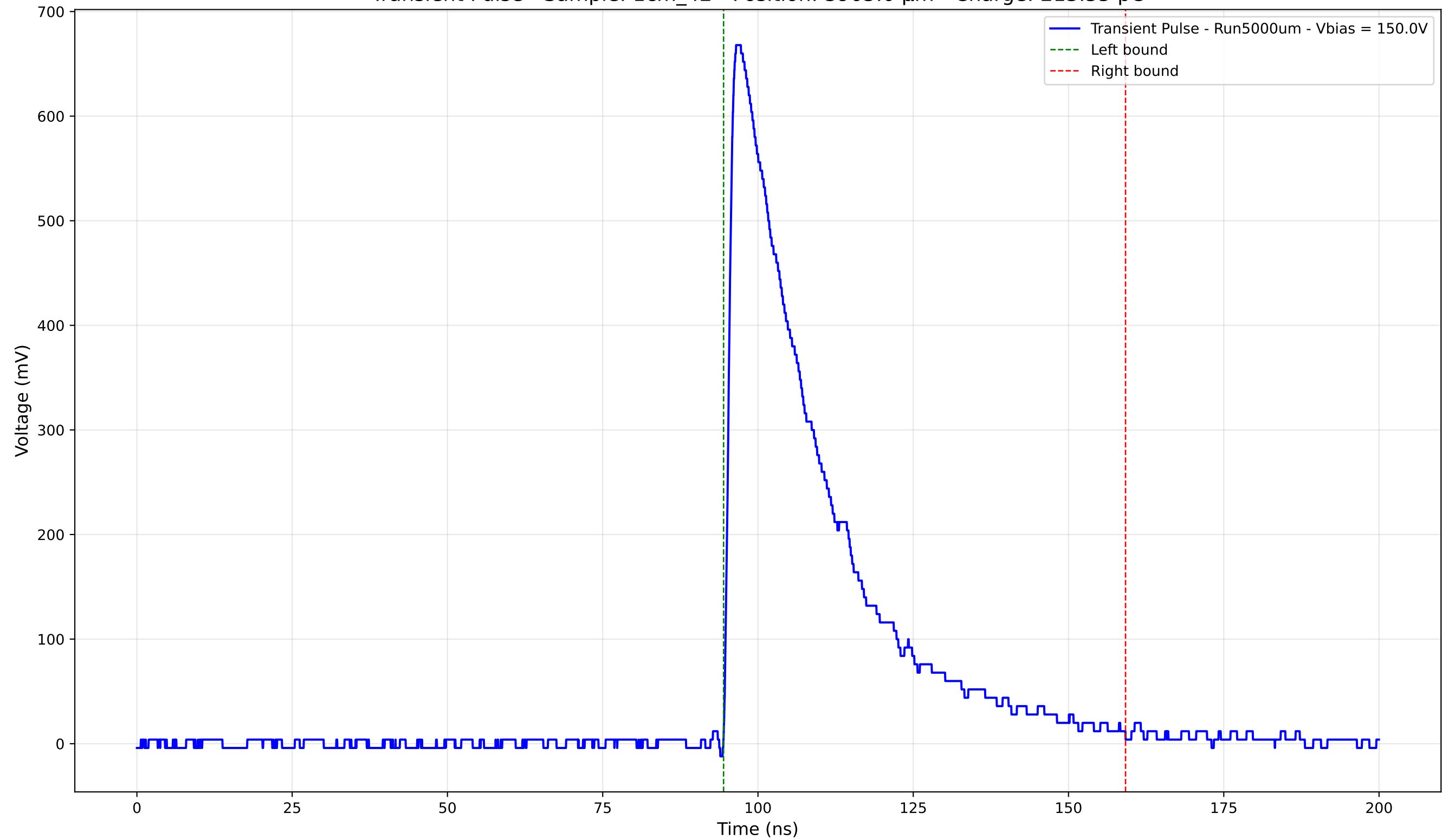
Transient Pulse - Sample: 1cm_42 - Position: 3905.0 \mu\text{m} - Charge: 213.55 pC
