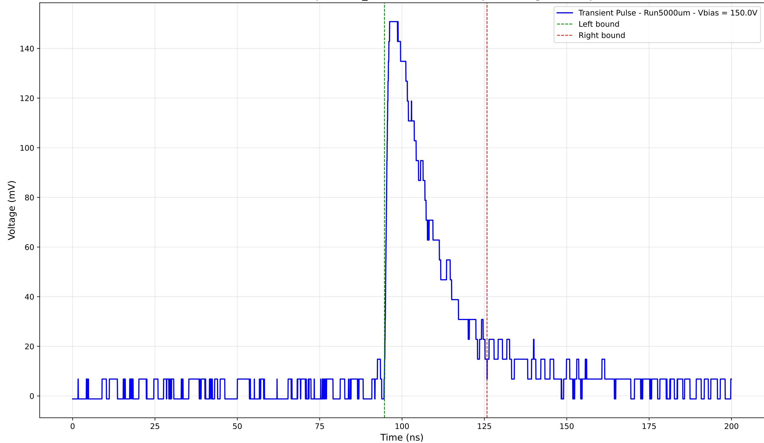
Transient Pulse - Sample: 1cm_42 - Position: 4020.0 \mu\text{m} - Charge: 44.78 pC
