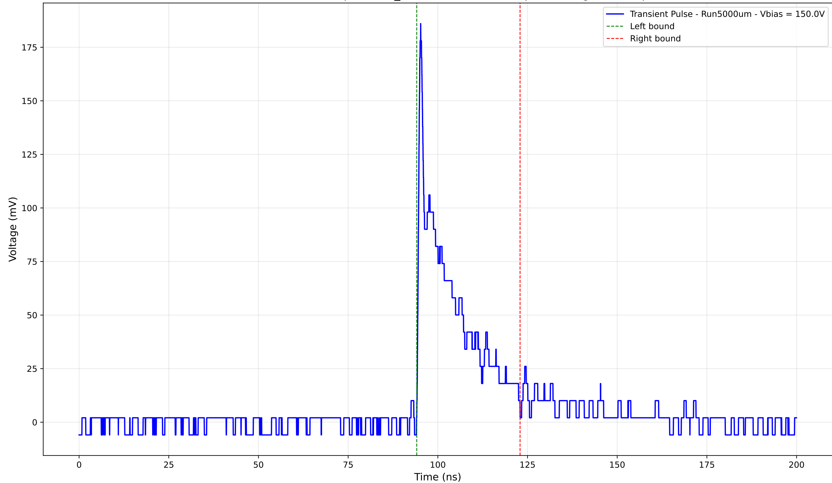
Transient Pulse - Sample: 1cm_42 - Position: 2510.0 \mu\text{m} - Charge: 29.91 pC
