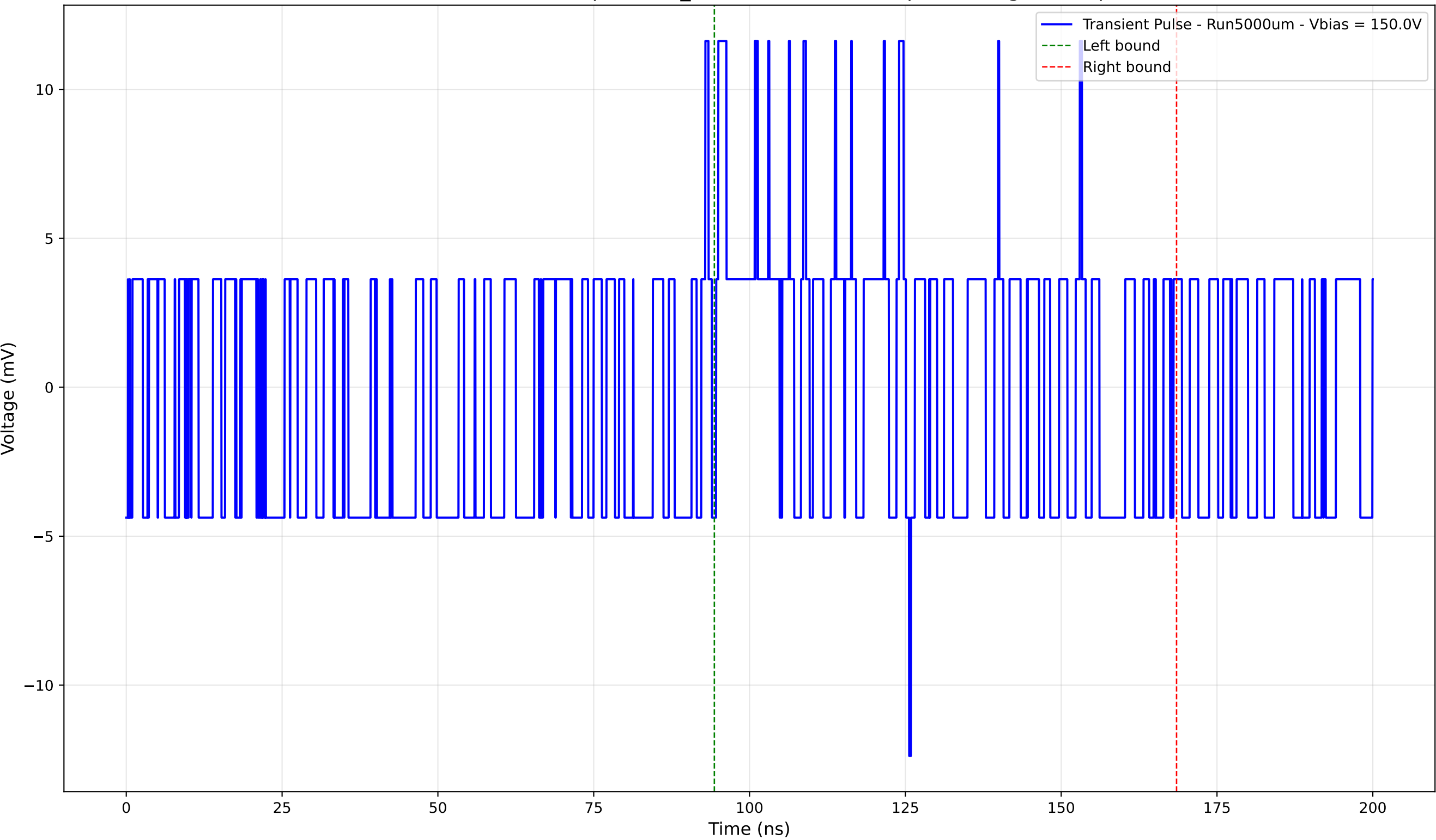
Transient Pulse - Sample: 1cm_42 - Position: 5020.0 \mu\text{m} - Charge: 1.66 pC
