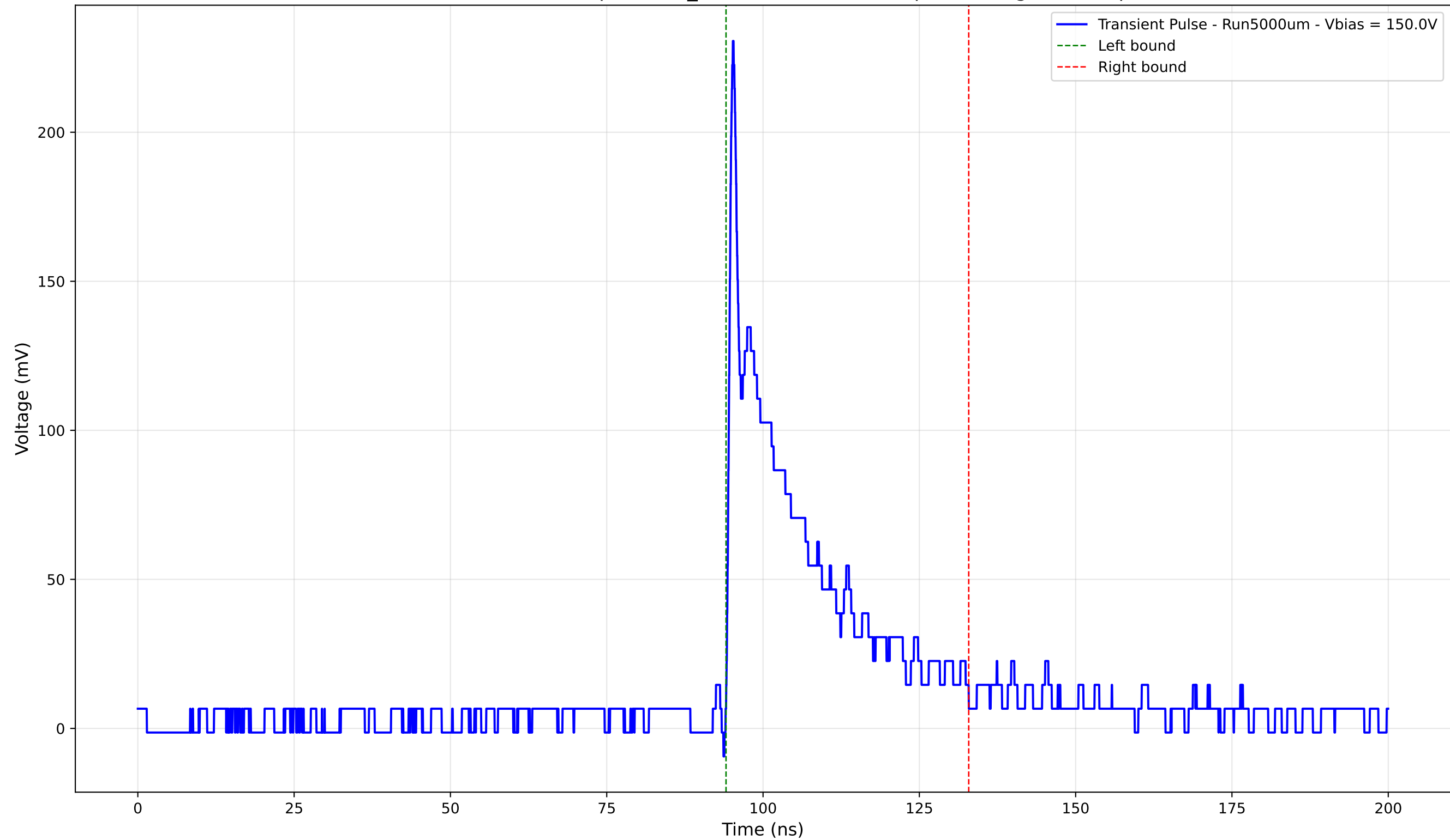
Transient Pulse - Sample: 1cm_42 - Position: 2545.0 \mu\text{m} - Charge: 43.47 pC
