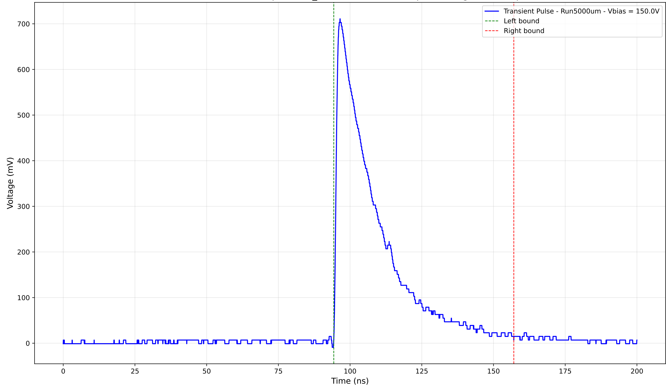
Transient Pulse - Sample: 1cm_42 - Position: 4250.0 \mu\text{m} - Charge: 217.69 pC
