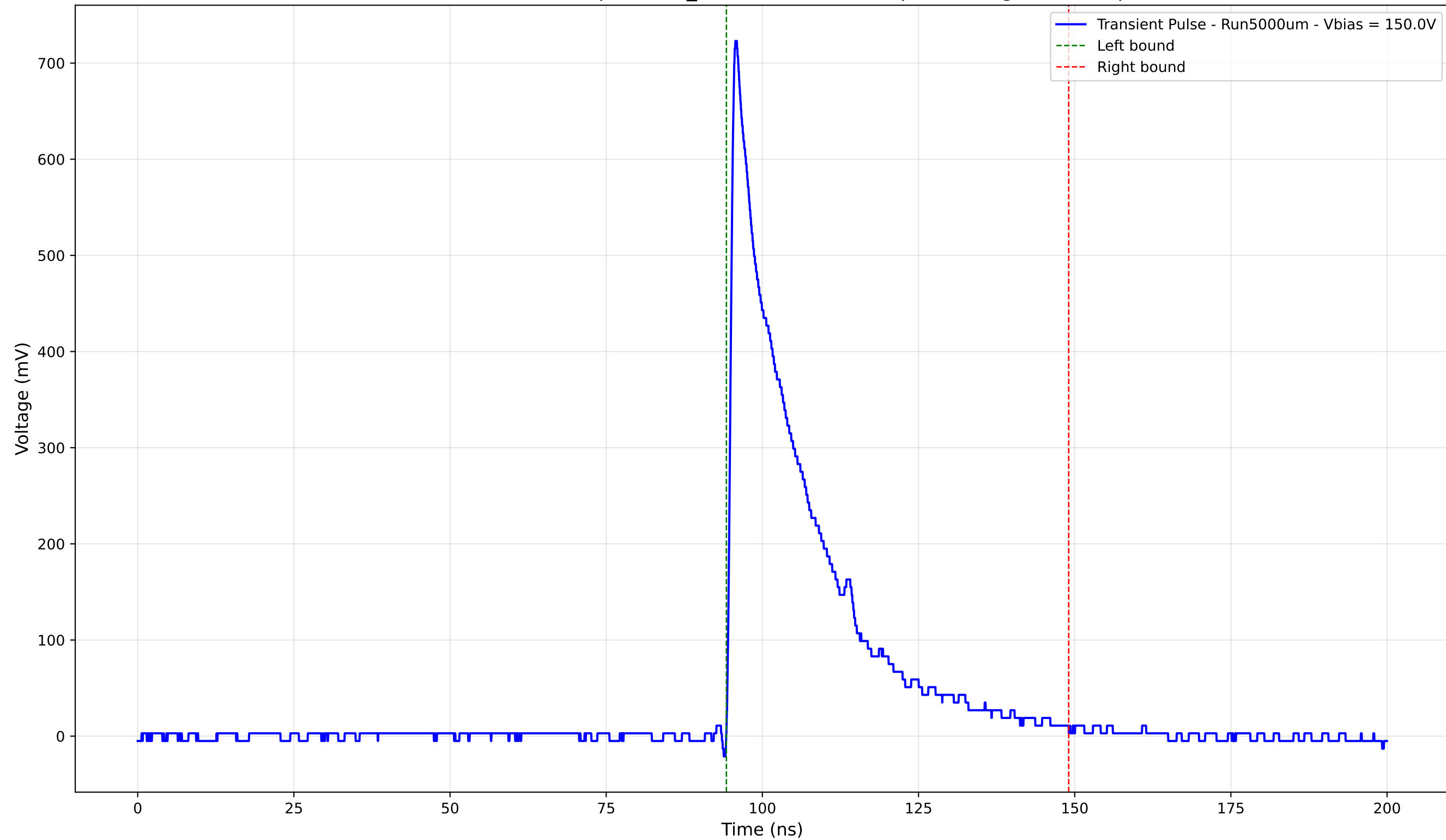
Transient Pulse - Sample: 1cm_42 - Position: 205.0 \mu\text{m} - Charge: 167.09 pC
