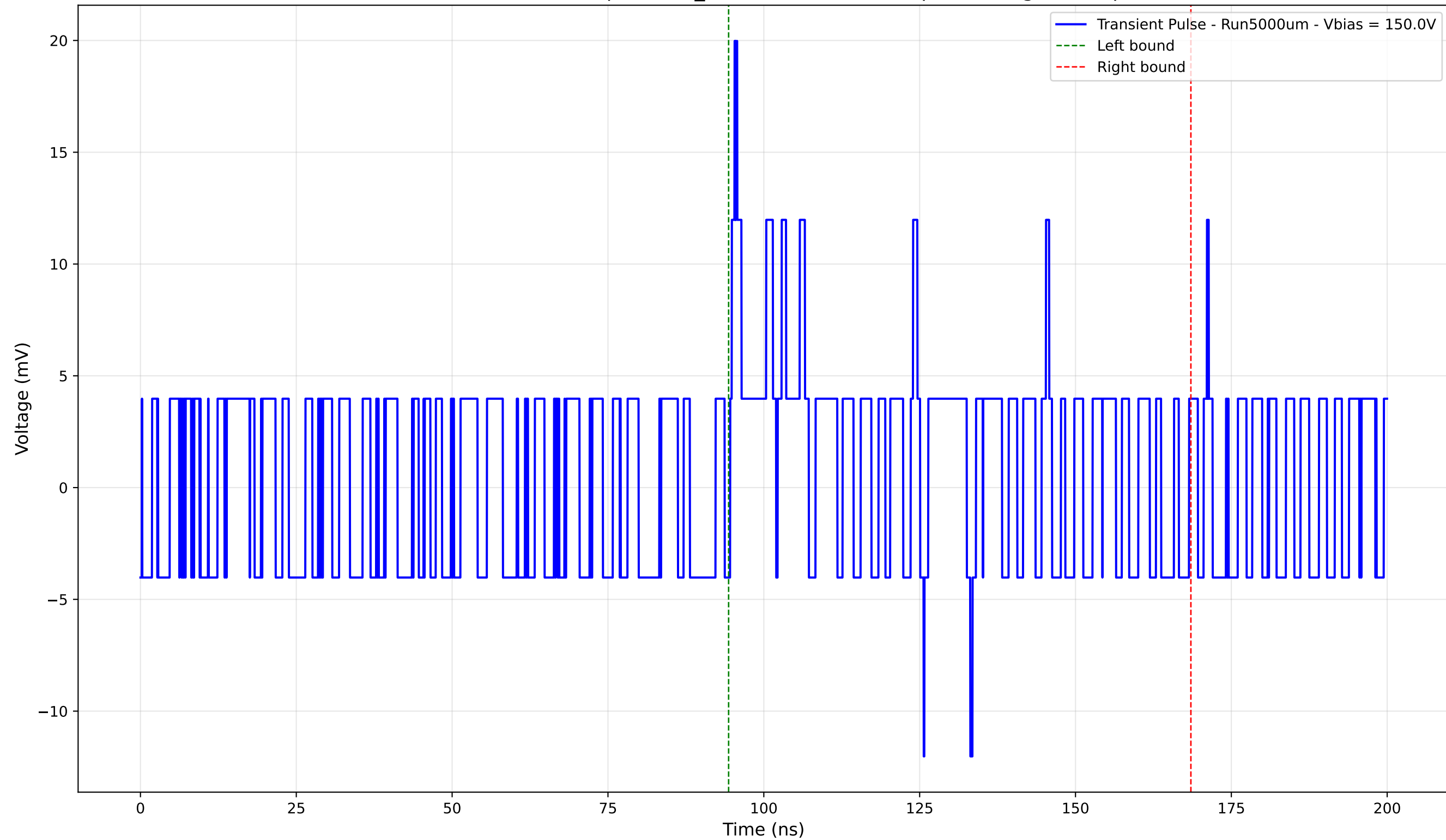
Transient Pulse - Sample: 1cm_42 - Position: 5030.0 \mu\text{m} - Charge: 2.89 pC
