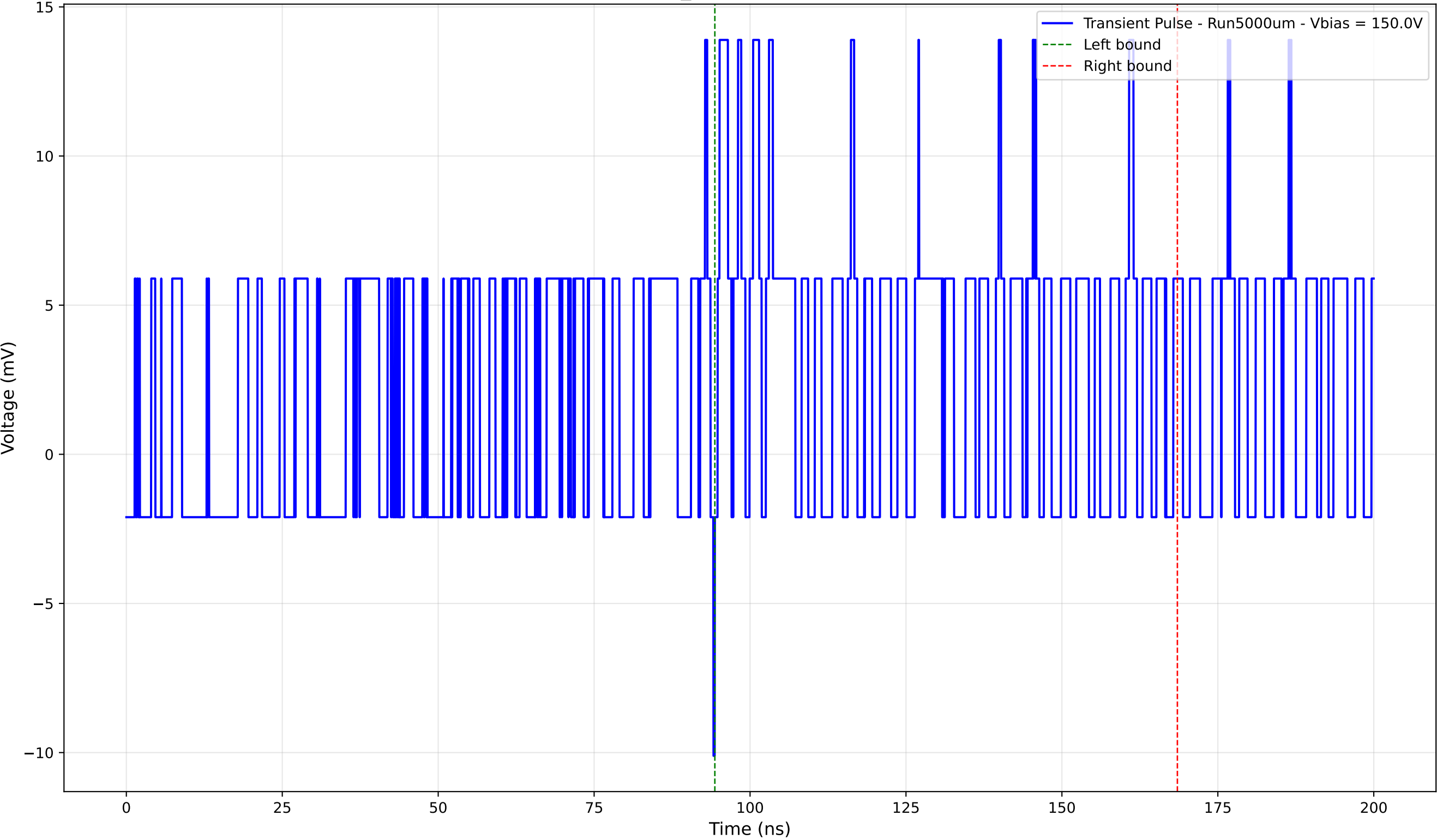
Transient Pulse - Sample: 1cm_42 - Position: 5000.0 \mu\text{m} - Charge: 5.36 pC
