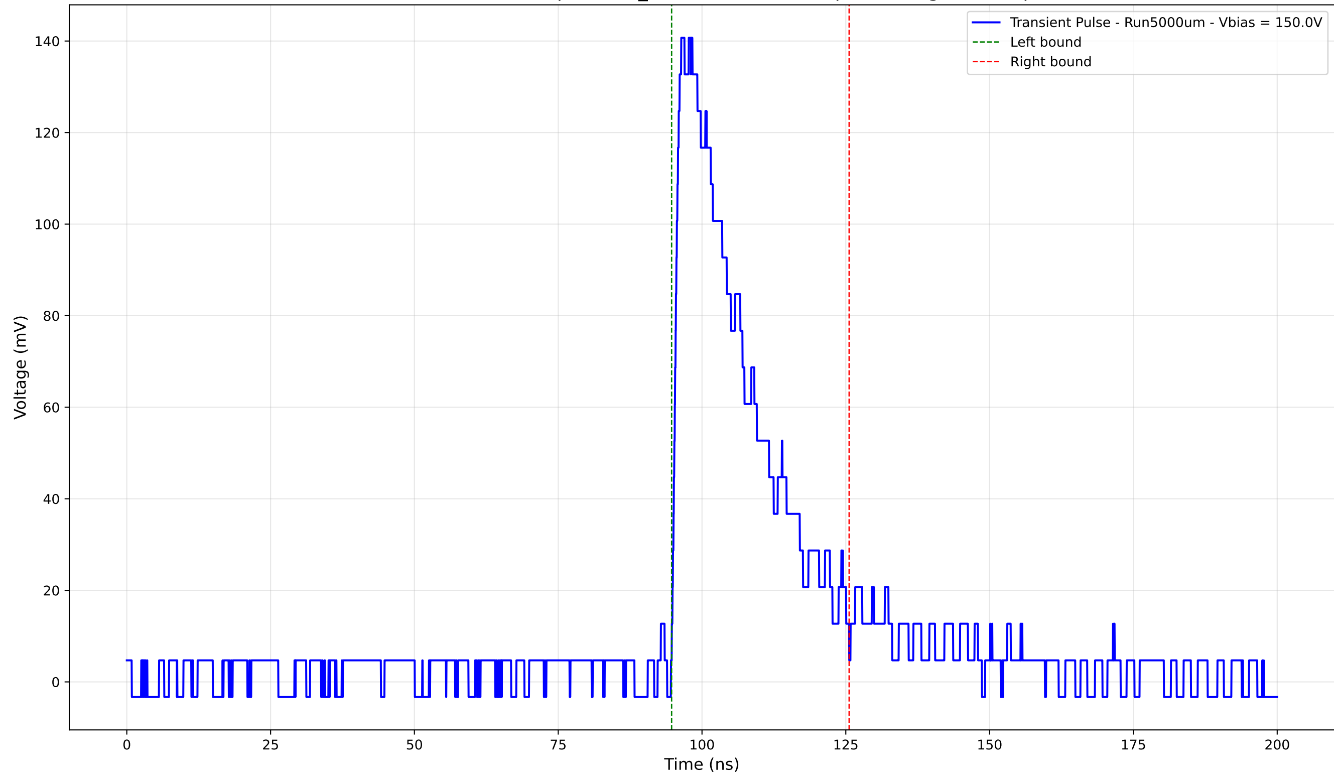
Transient Pulse - Sample: 1cm_42 -Position: 985.0 \mu\text{m} - Charge: 39.51 pC
