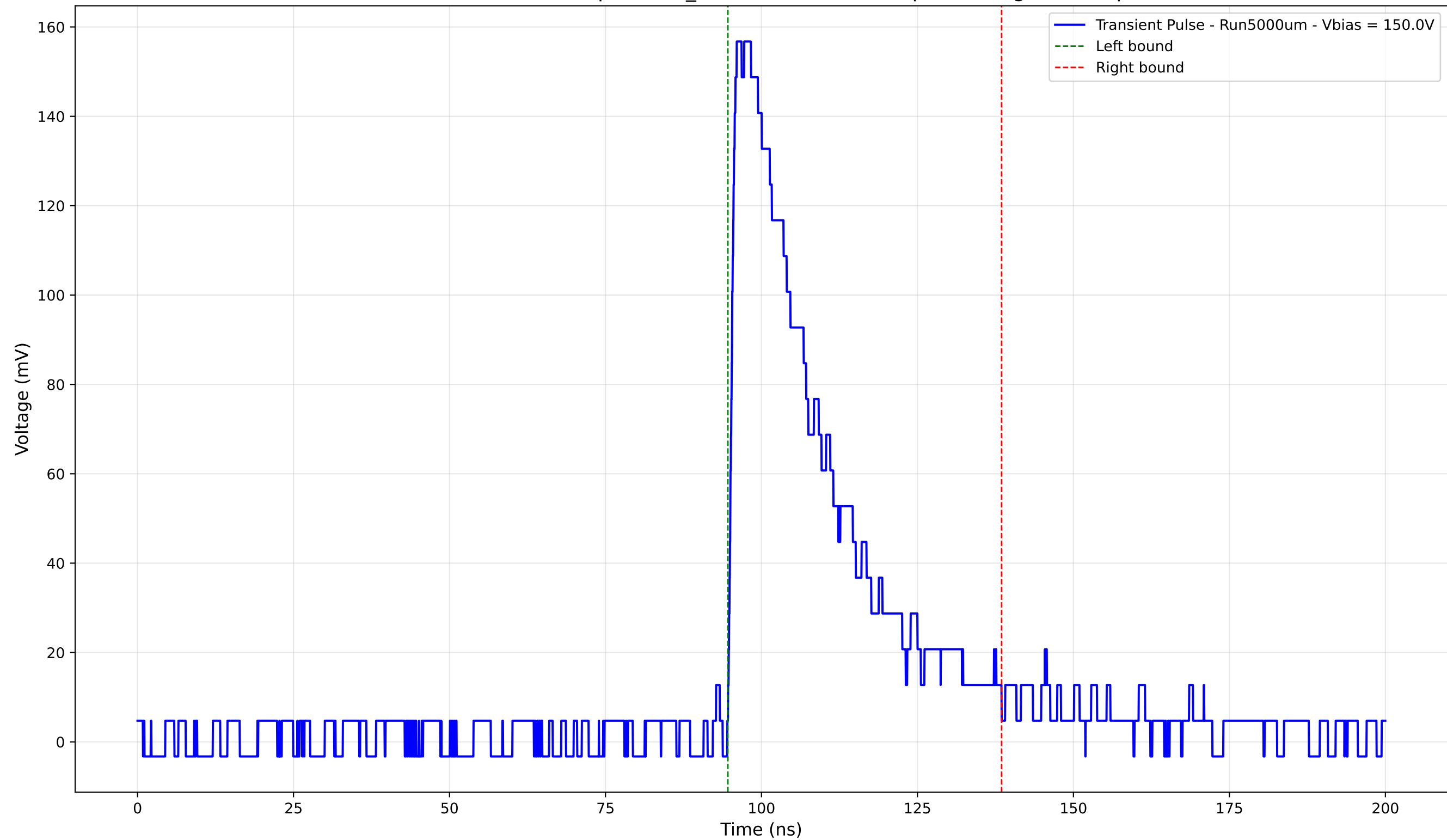
Transient Pulse - Sample: 1cm_42 - Position: 3510.0 \mu\text{m} - Charge: 50.44 pC
