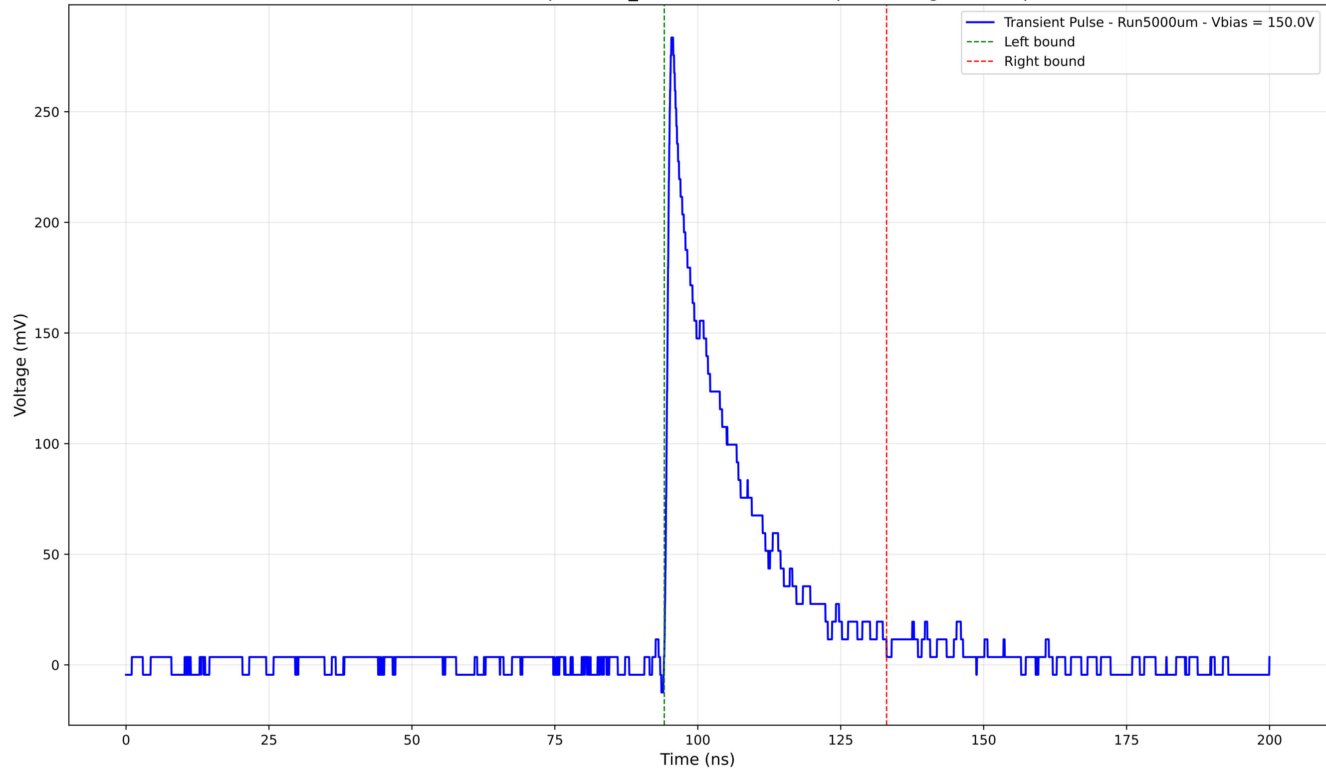
Transient Pulse - Sample: 1cm_42 - Position: 4840.0 \mu\text{m} - Charge: 58.15 pC
