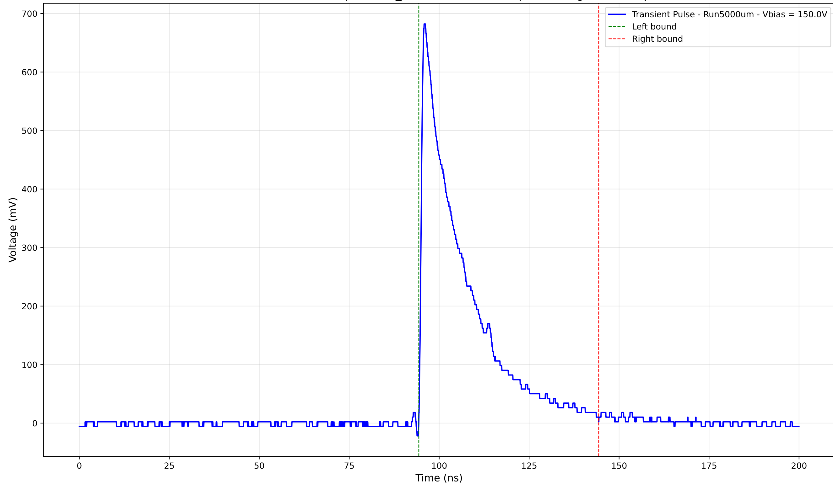
Transient Pulse - Sample: 1cm_42 - Position: 315.0 \mu\text{m} - Charge: 167.75 pC
