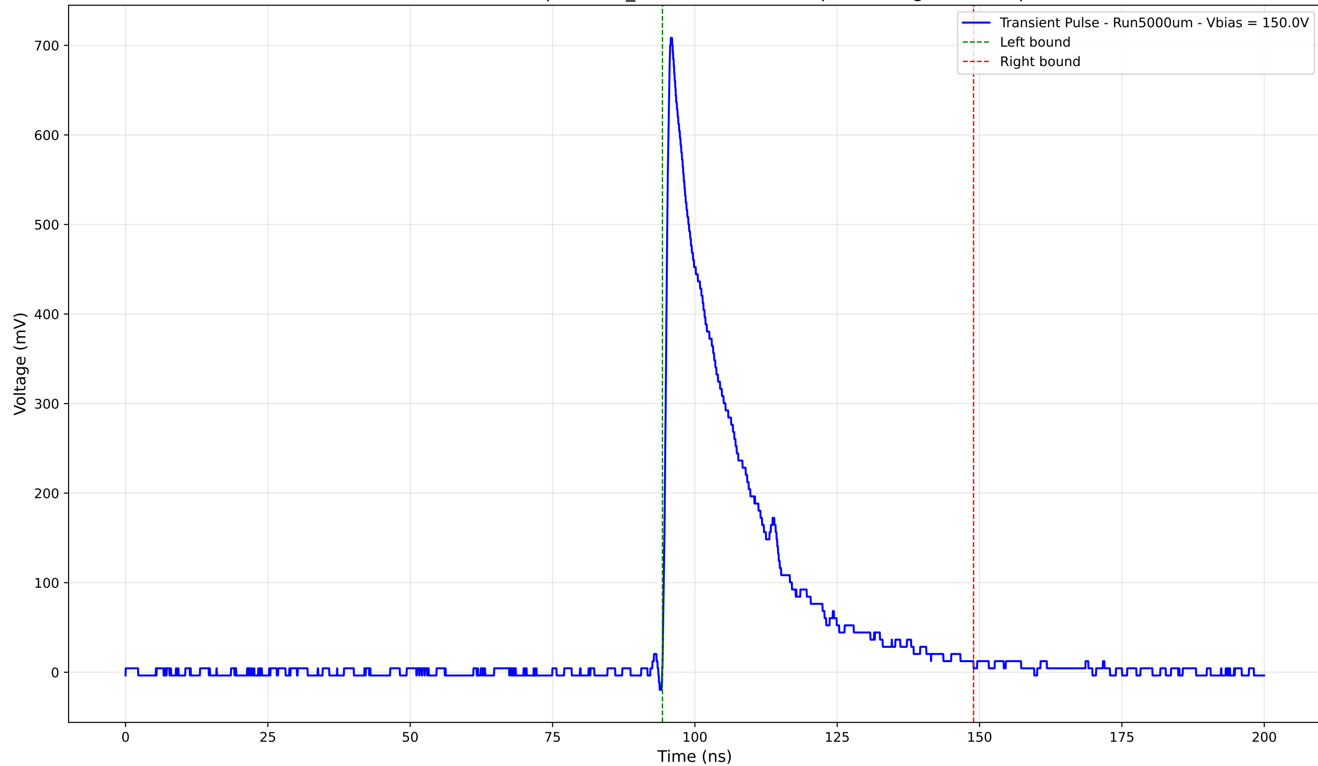
Transient Pulse - Sample: 1cm_42 - Position: 255.0 \mu\text{m} - Charge: 170.06 pC
