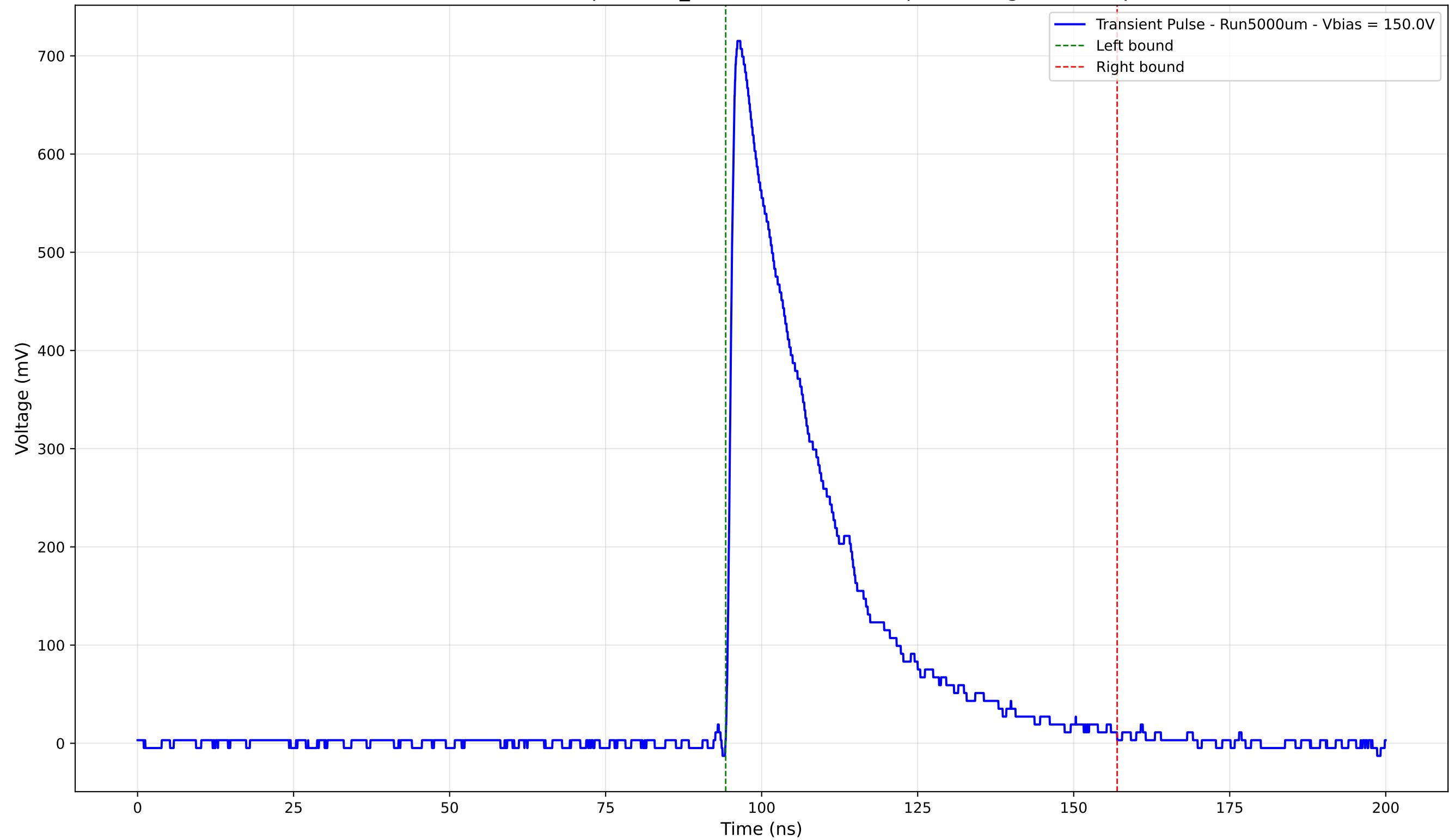
Transient Pulse - Sample: 1cm_42 - Position: 4345.0 \mu\text{m} - Charge: 213.34 pC
