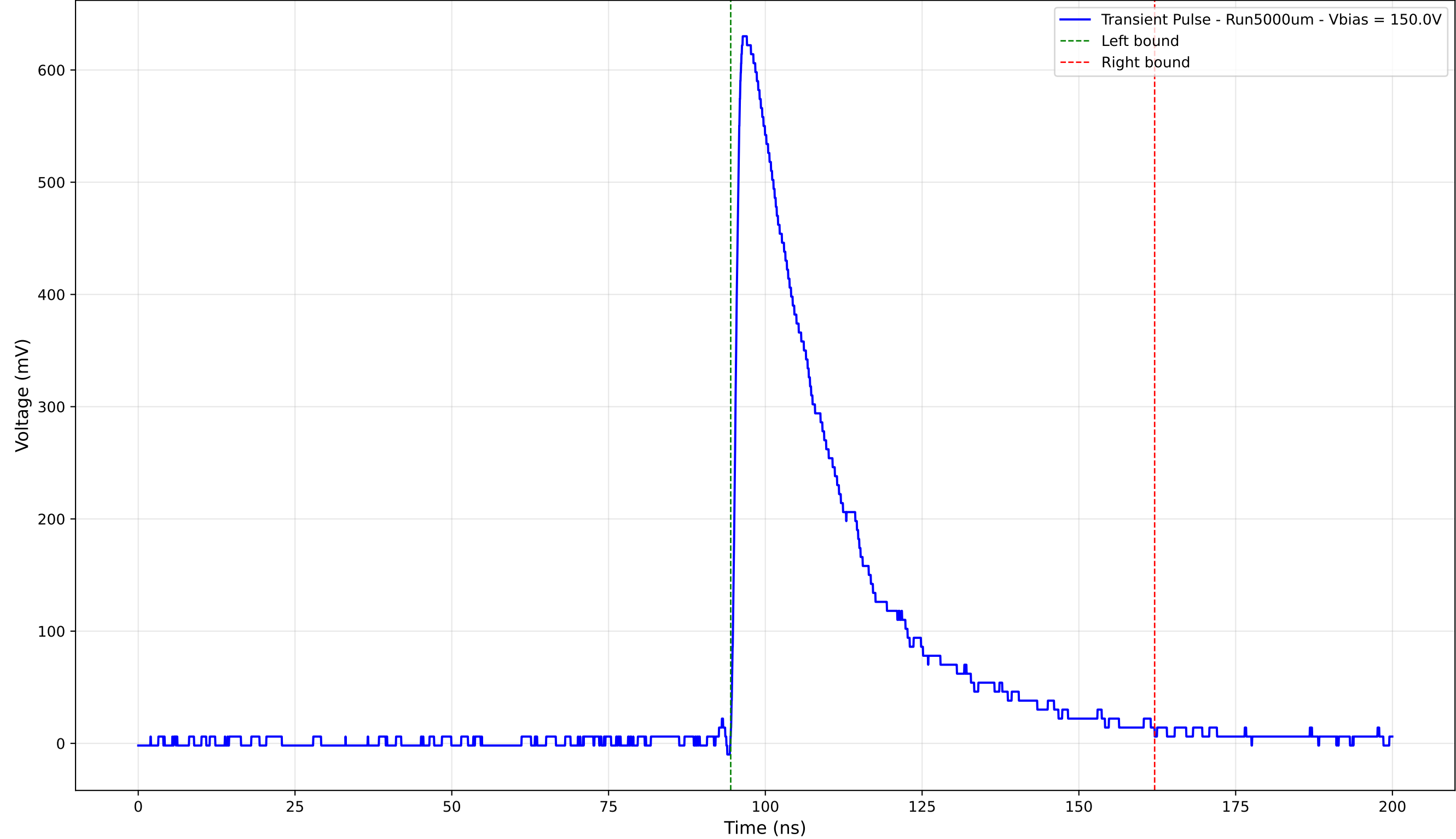
Transient Pulse - Sample: 1cm_42 - Position: 3650.0 \mu\text{m} - Charge: 209.55 pC
