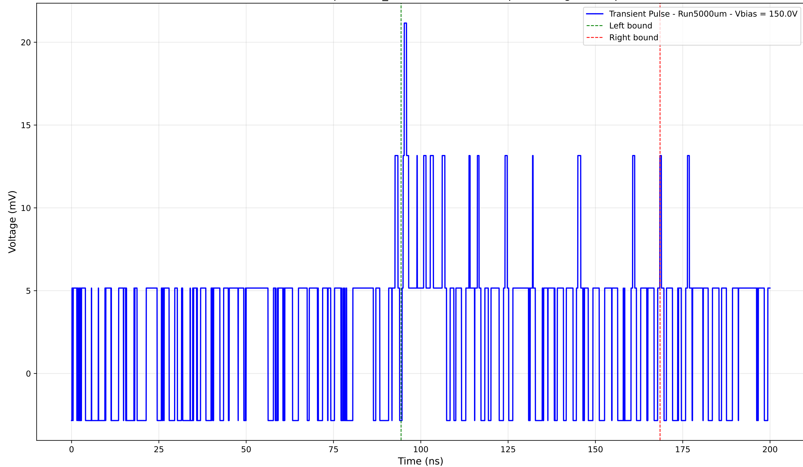
Transient Pulse - Sample: 1cm_42 - Position: 5035.0 \mu\text{m} - Charge: 5.34 pC
