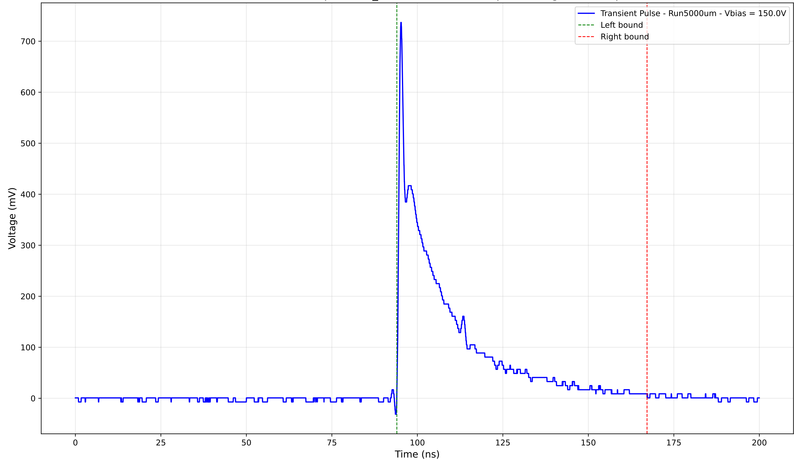
Transient Pulse - Sample: 1cm_42 - Position: 2430.0 \mu\text{m} - Charge: 153.56 pC
