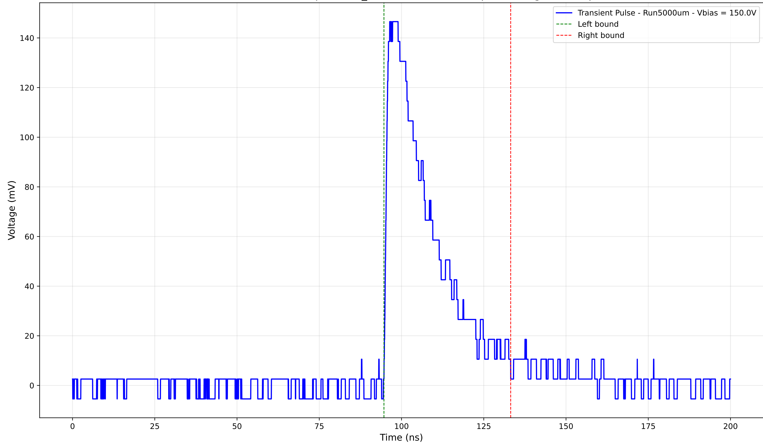
Transient Pulse - Sample: 1cm_42 - Position: 1485.0 \mu\text{m} - Charge: 44.82 pC
