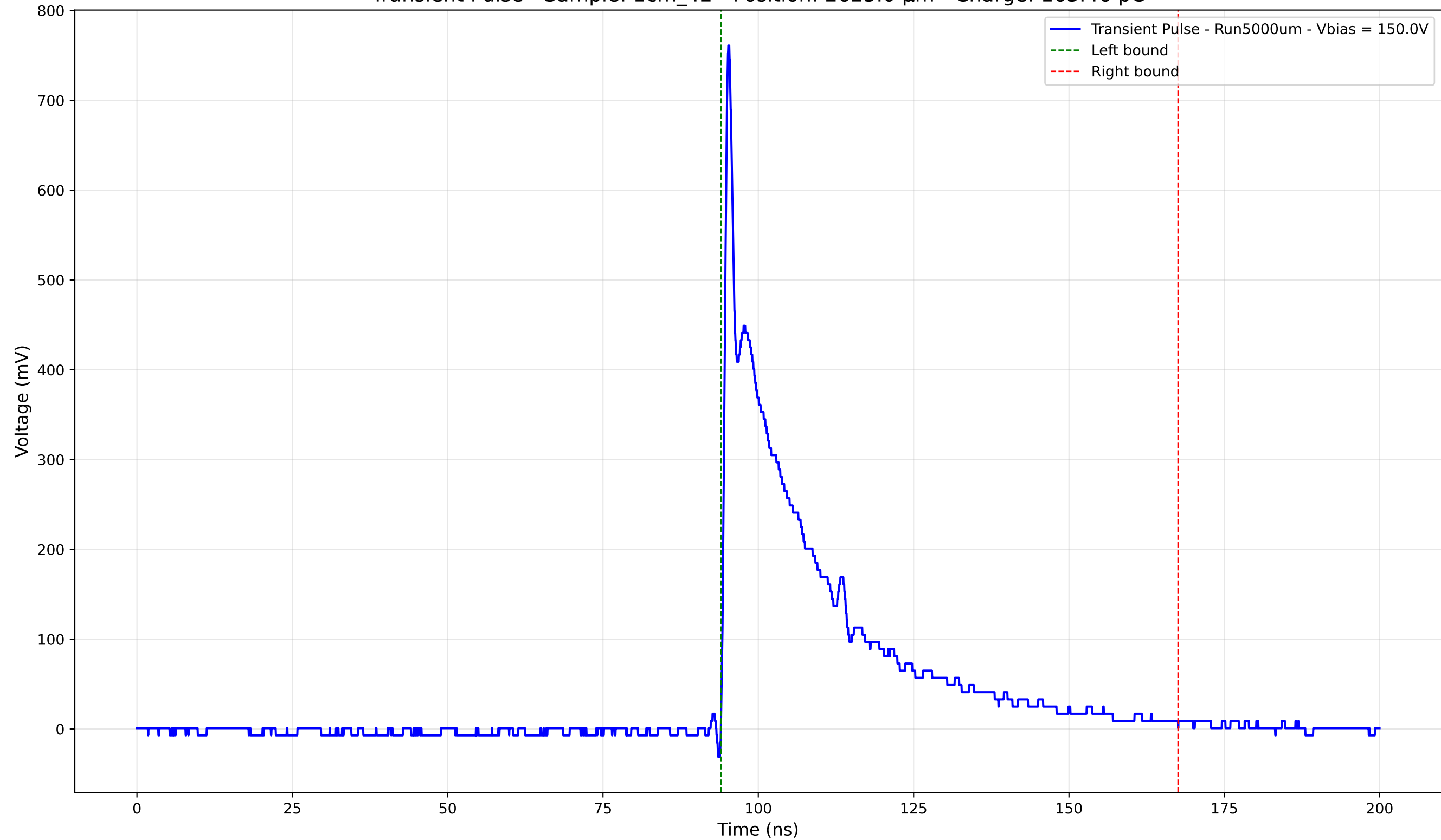
Transient Pulse - Sample: 1cm_42 - Position: 2625.0 \mu\text{m} - Charge: 163.46 pC
