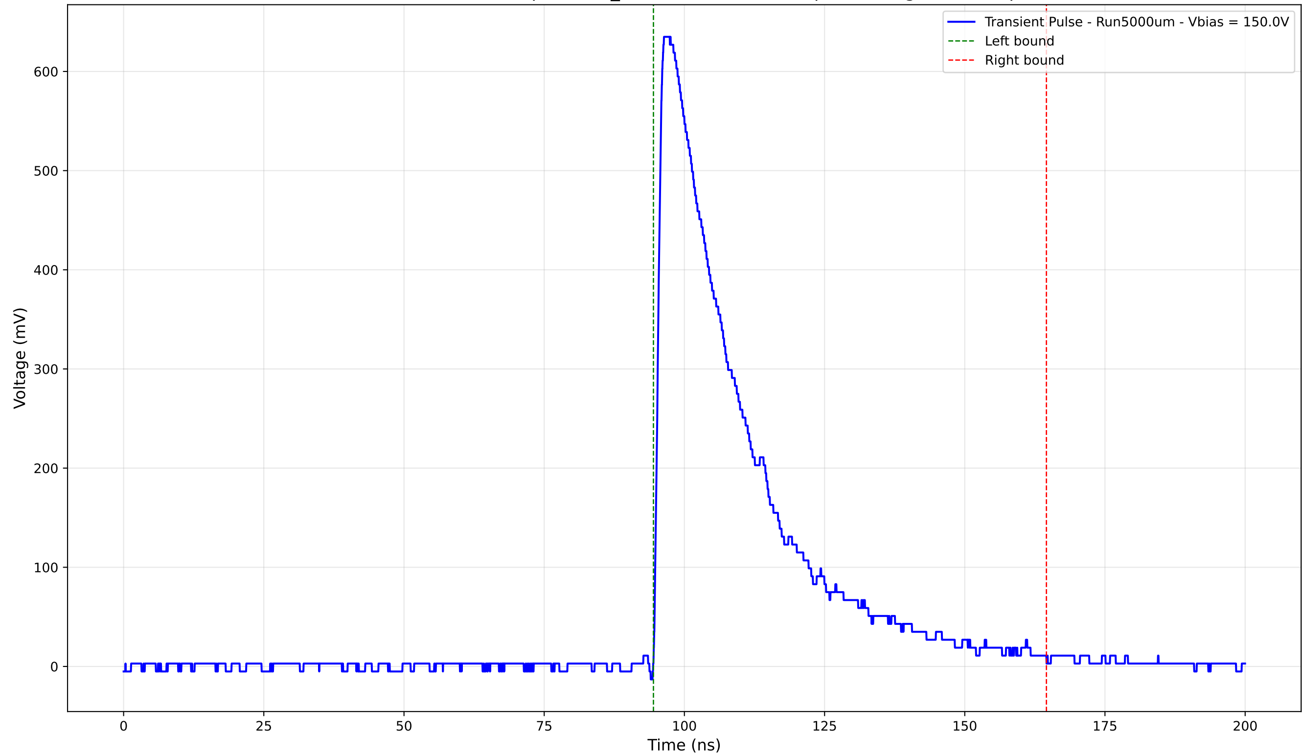
Transient Pulse - Sample: 1cm_42 - Position: 3665.0 \mu\text{m} - Charge: 210.12 pC
