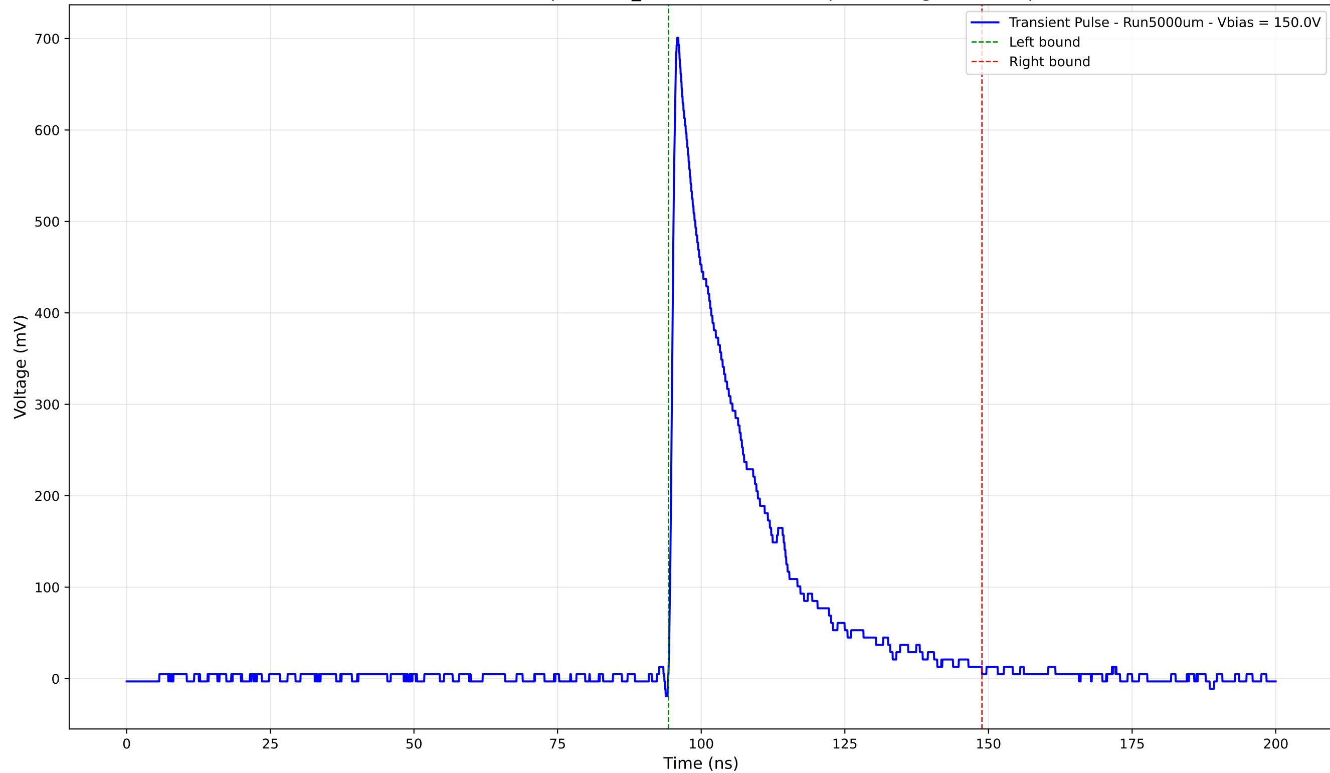
Transient Pulse - Sample: 1cm_42 - Position: 275.0 \mu\text{m} - Charge: 169.96 pC
