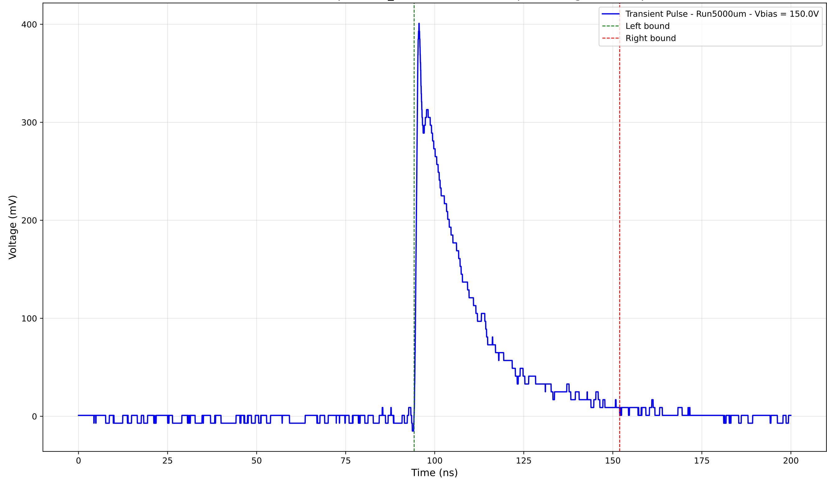
Transient Pulse - Sample: 1cm_42 - Position: 2075.0 \mu\text{m} - Charge: 104.98 pC
