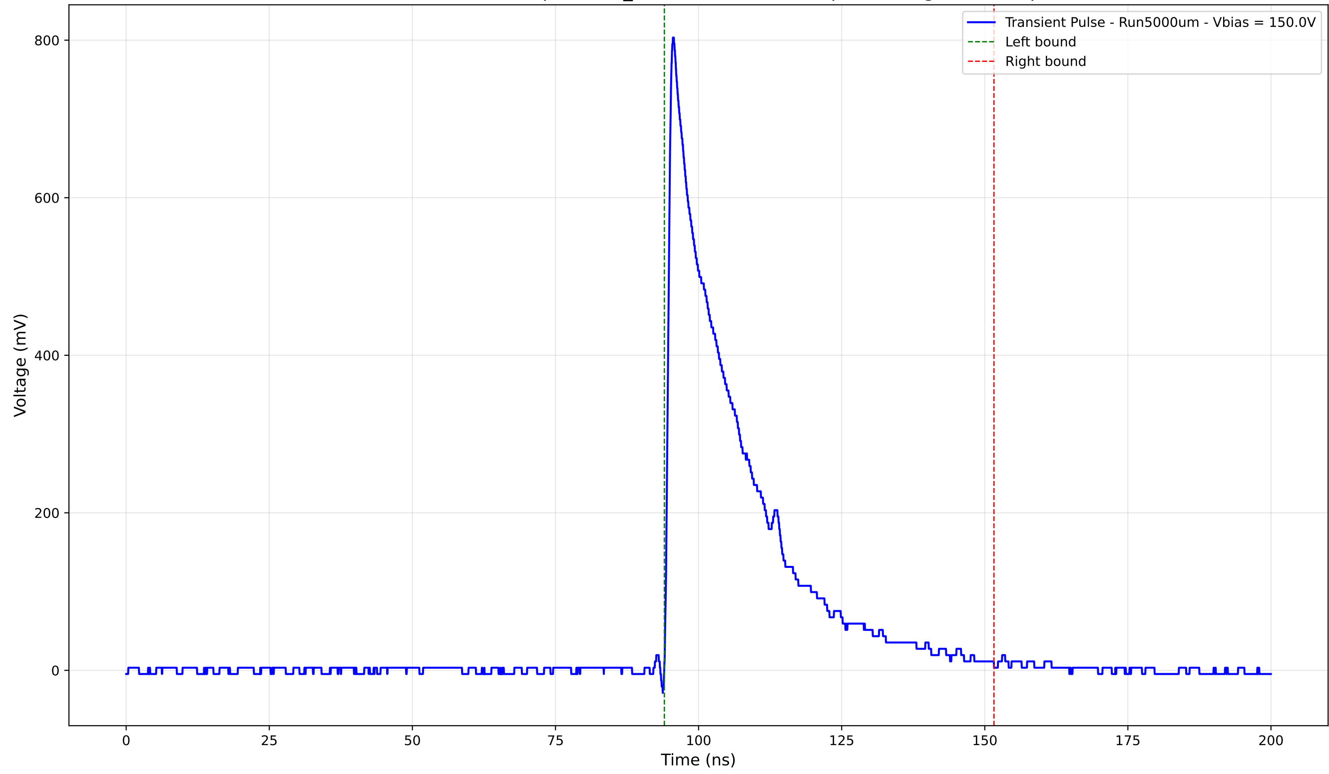
Transient Pulse - Sample: 1cm_42 - Position: 4740.0 \mu\text{m} - Charge: 199.73 pC
