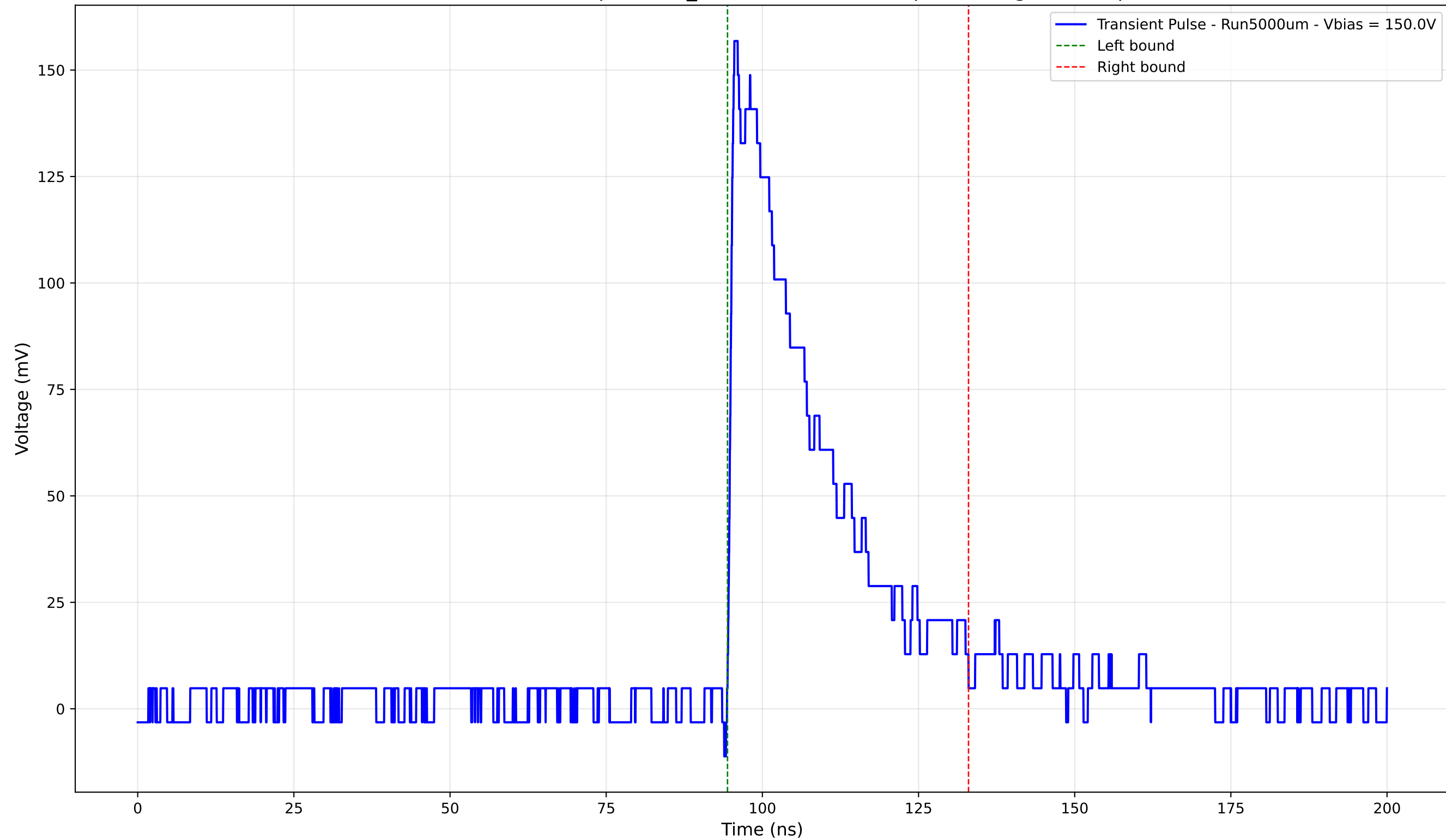
Transient Pulse - Sample: 1cm_42 - Position: 3055.0 \mu\text{m} - Charge: 45.91 pC
