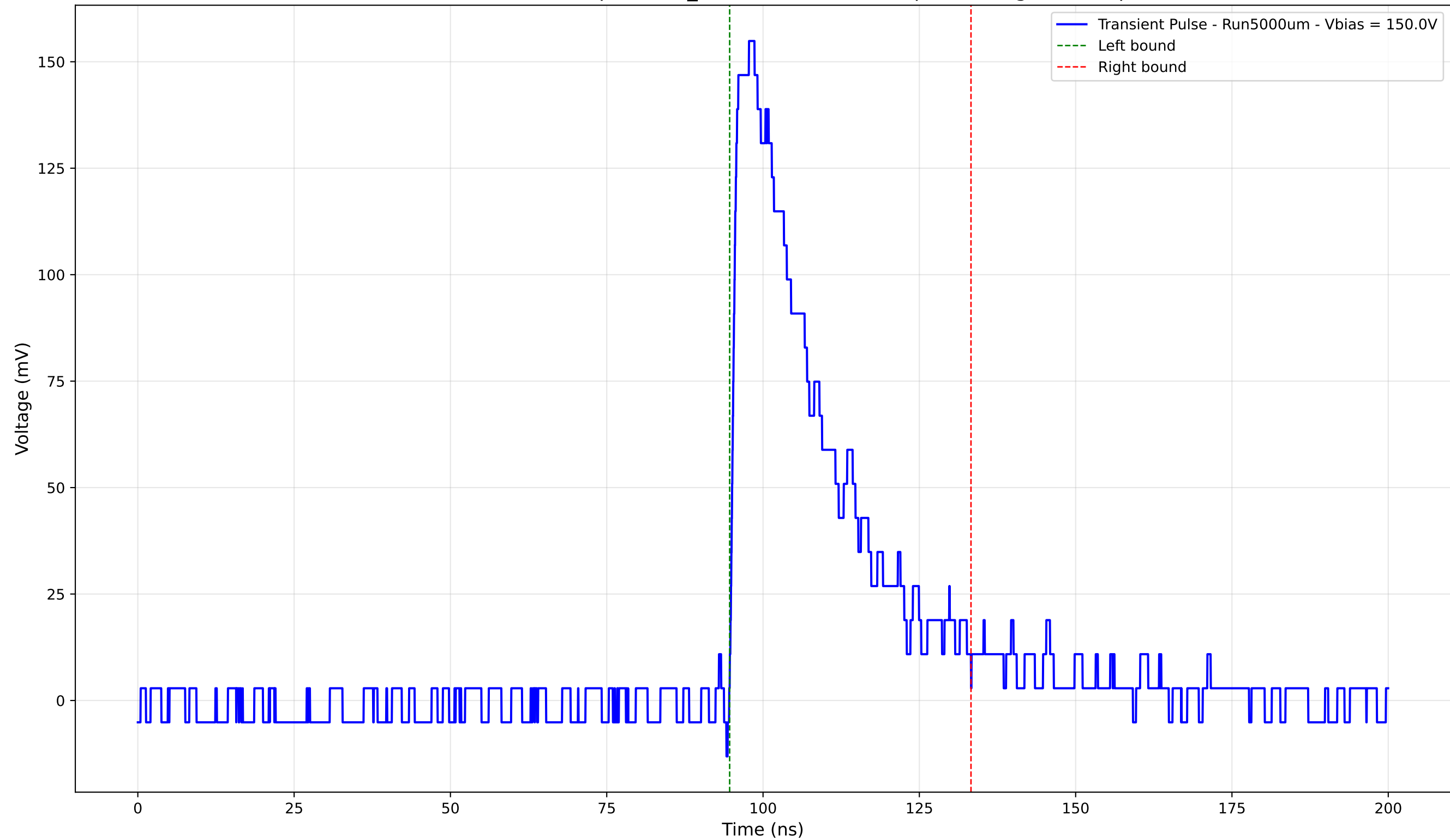
Transient Pulse - Sample: 1cm_42 - Position: 3555.0 \mu\text{m} - Charge: 46.93 pC
