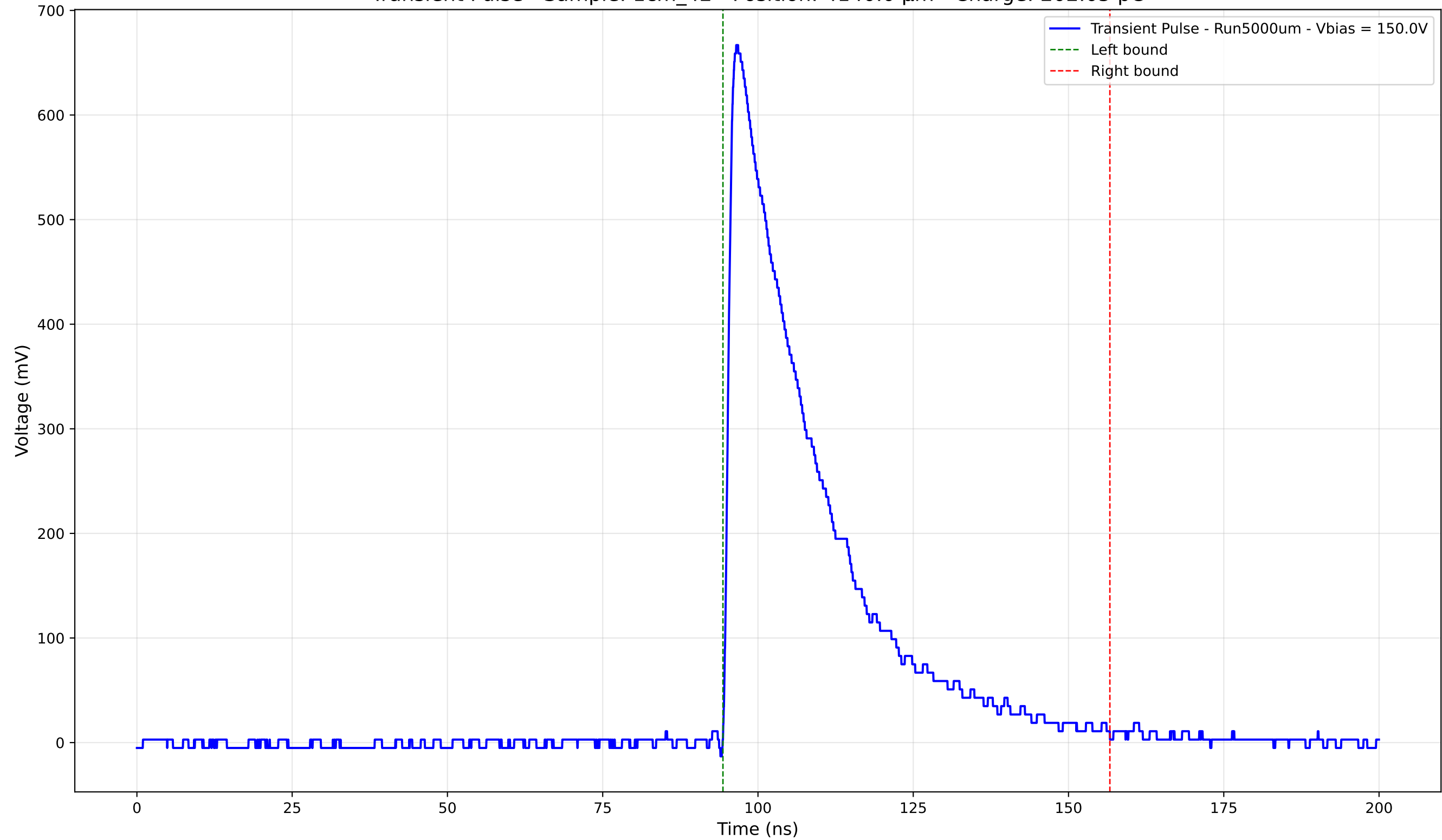
Transient Pulse - Sample: 1cm_42 - Position: 4140.0 \mu\text{m} - Charge: 202.05 pC
