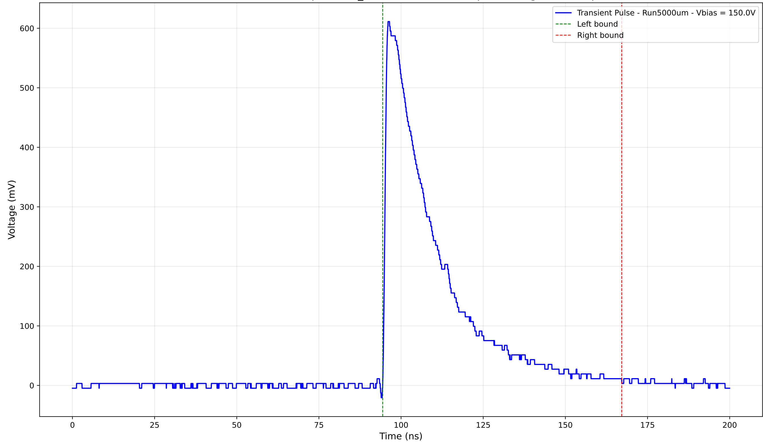
Transient Pulse - Sample: 1cm_42 - Position: 3350.0 \mu\text{m} - Charge: 203.90 pC
