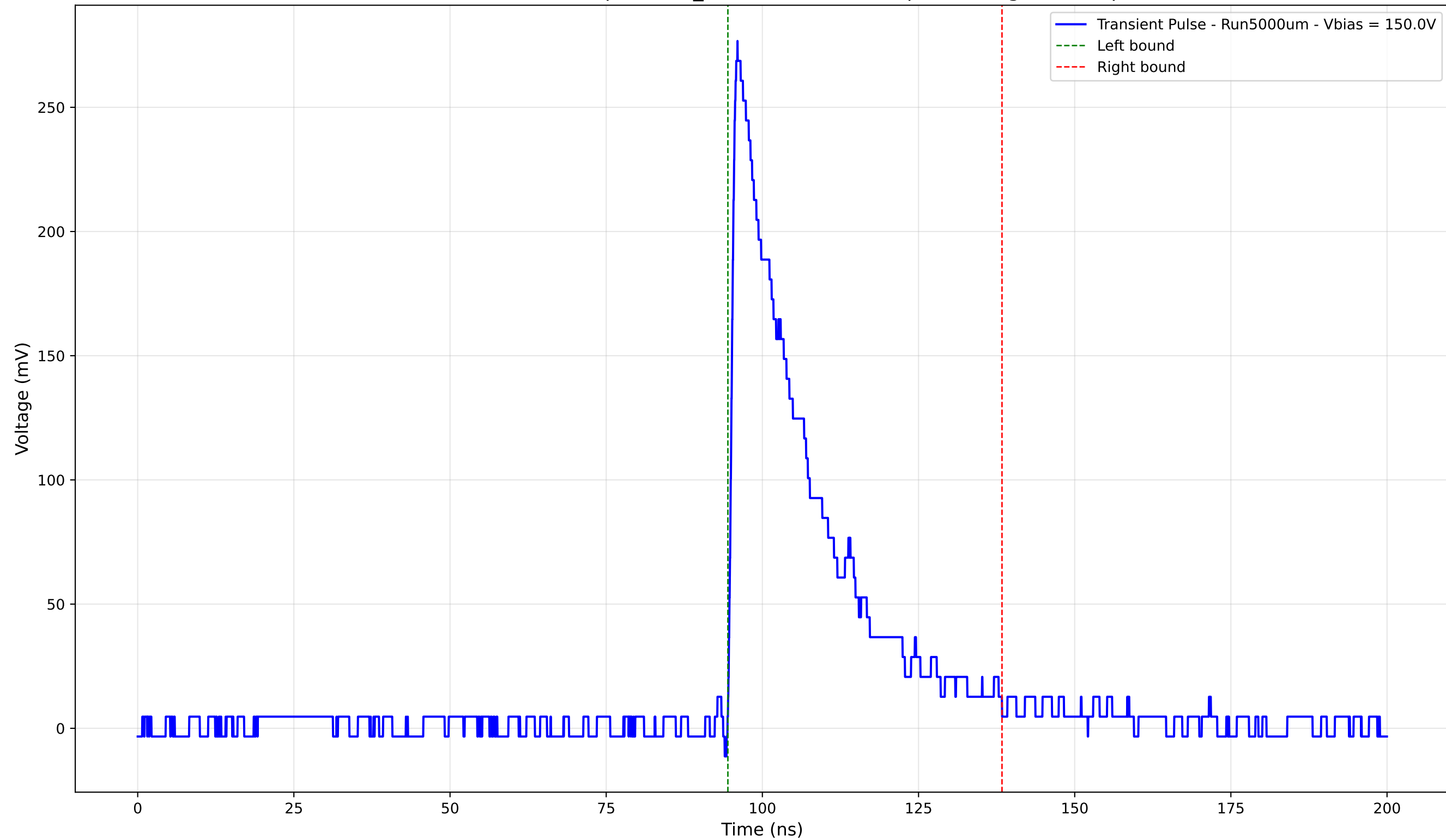
Transient Pulse - Sample: 1cm_42 -Position: 460.0 \mu\text{m} - Charge: 69.43 pC
