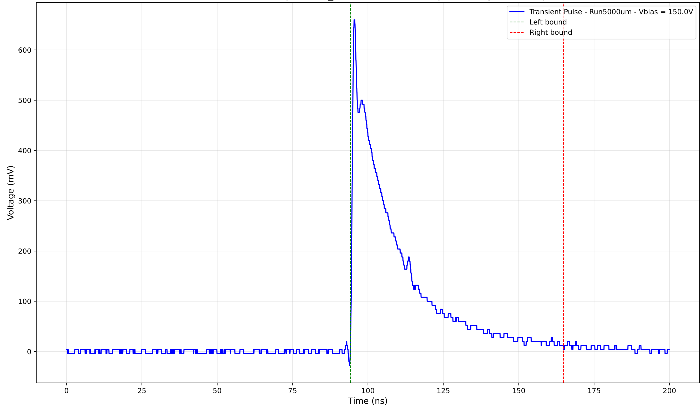
Transient Pulse - Sample: 1cm_42 - Position: 2150.0 \mu\text{m} - Charge: 182.72 pC
