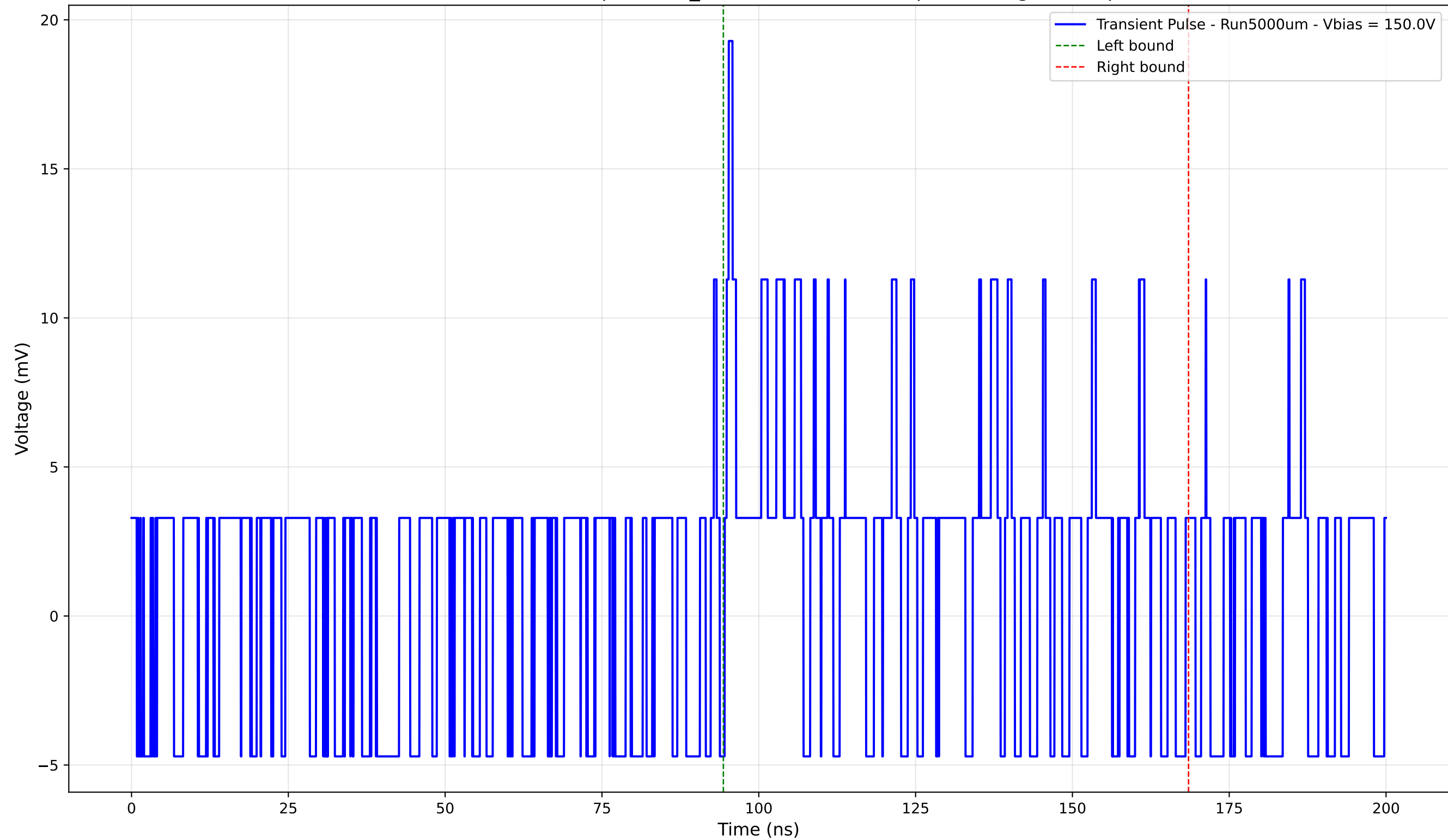
Transient Pulse - Sample: 1cm_42 - Position: 4935.0 \mu\text{m} - Charge: 3.82 pC
