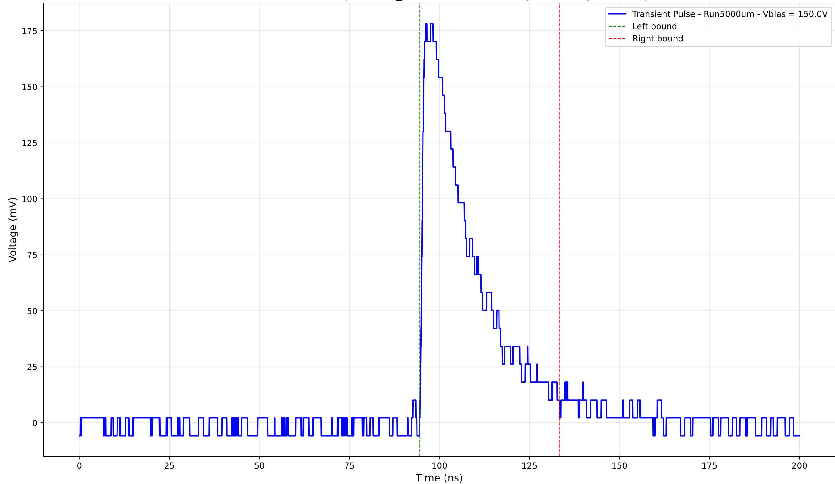
Transient Pulse - Sample: 1cm_42 - Position: 3505.0 \mu\text{m} - Charge: 53.20 pC
