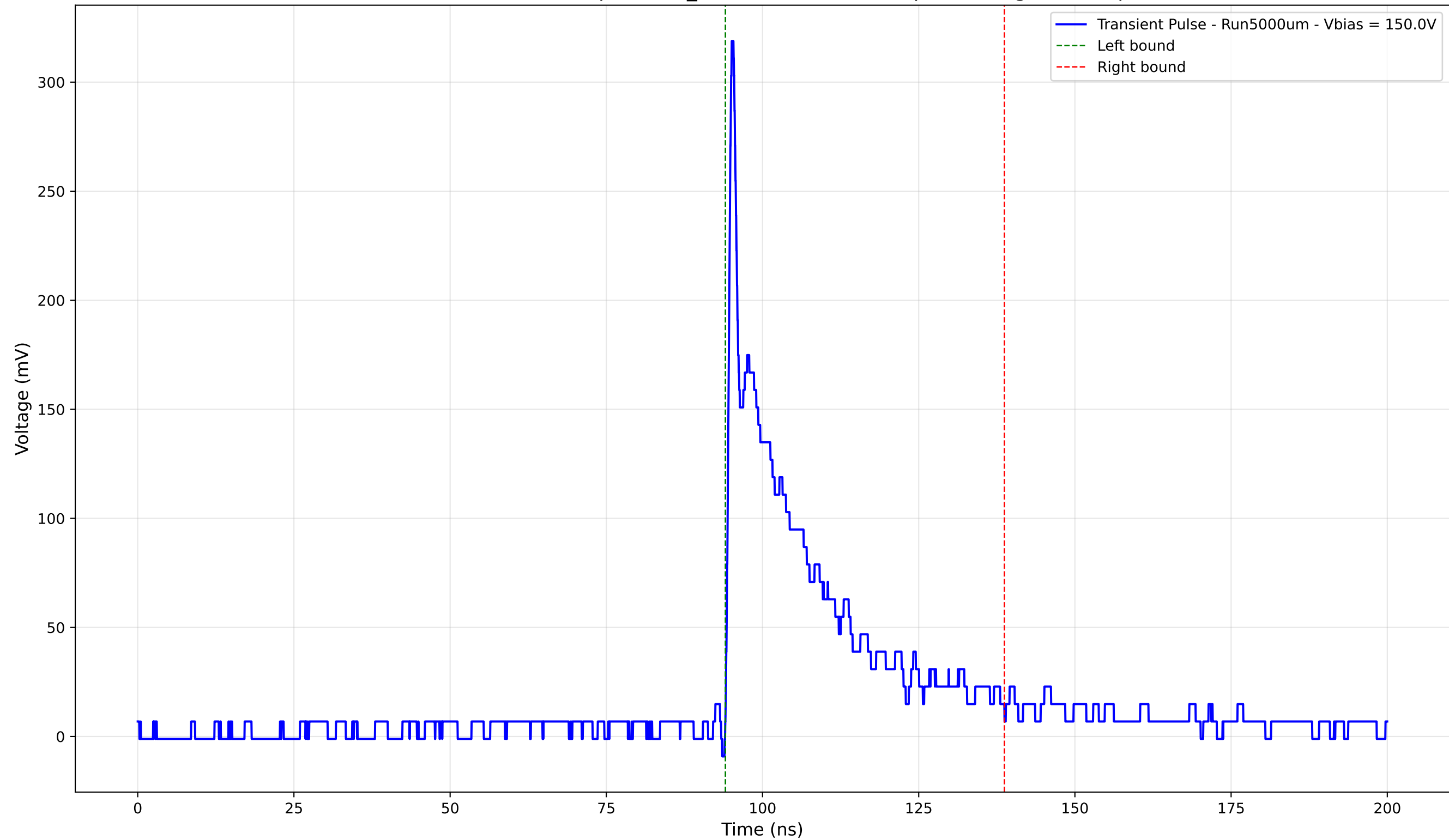
Transient Pulse - Sample: 1cm_42 - Position: 2490.0 \mu\text{m} - Charge: 59.52 pC
