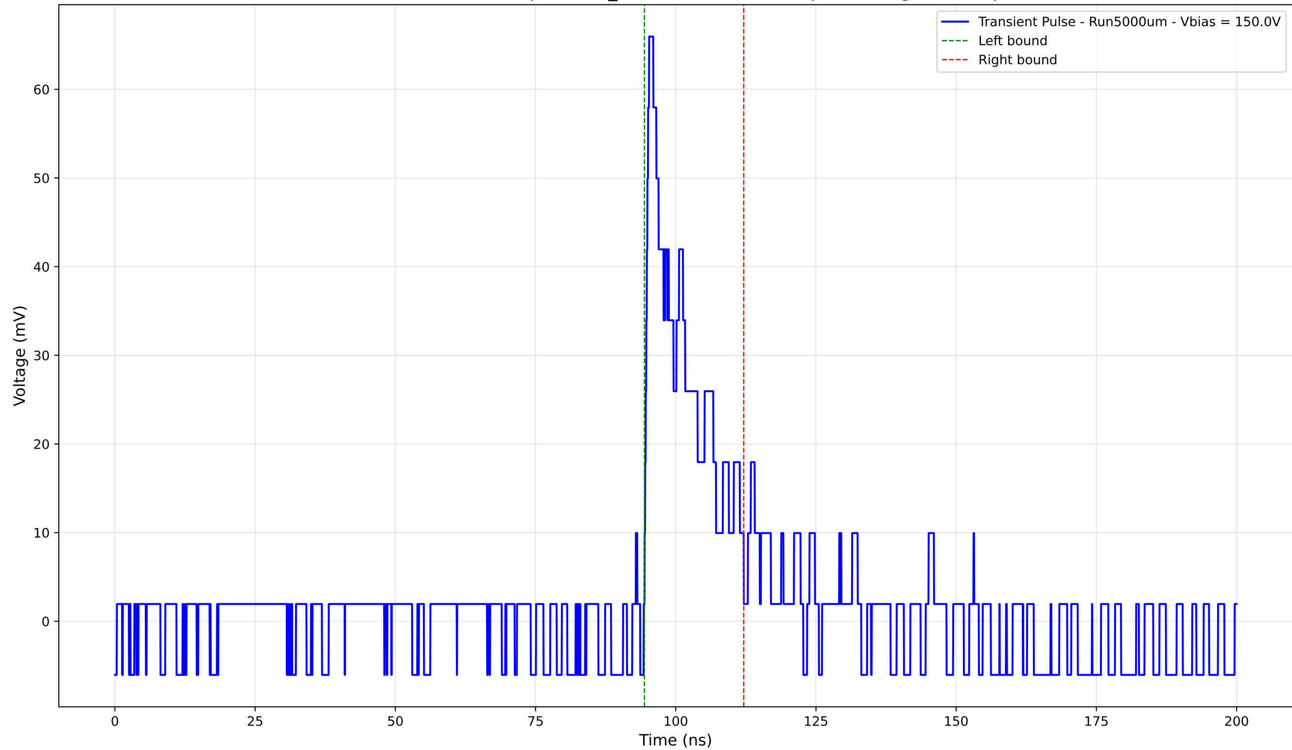
Transient Pulse - Sample: 1cm_42 - Position: 4875.0 \mu\text{m} - Charge: 10.01 pC
