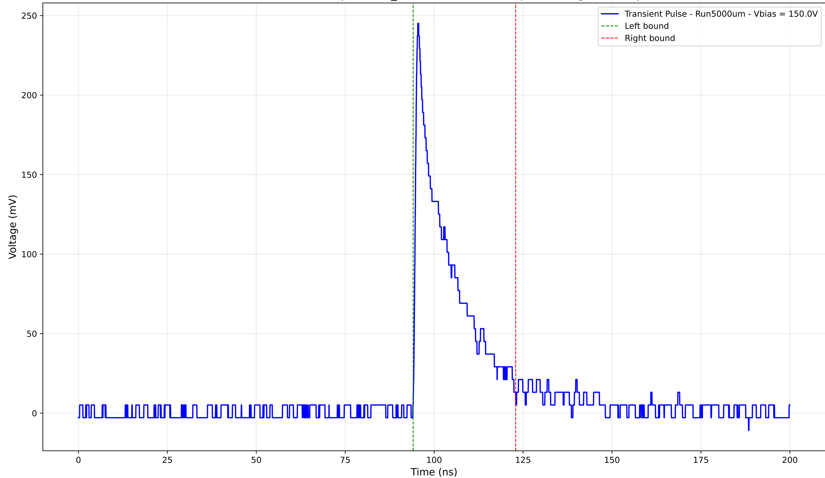
Transient Pulse - Sample: 1cm_42 - Position: 4845.0 \mu\text{m} - Charge: 48.02 pC
