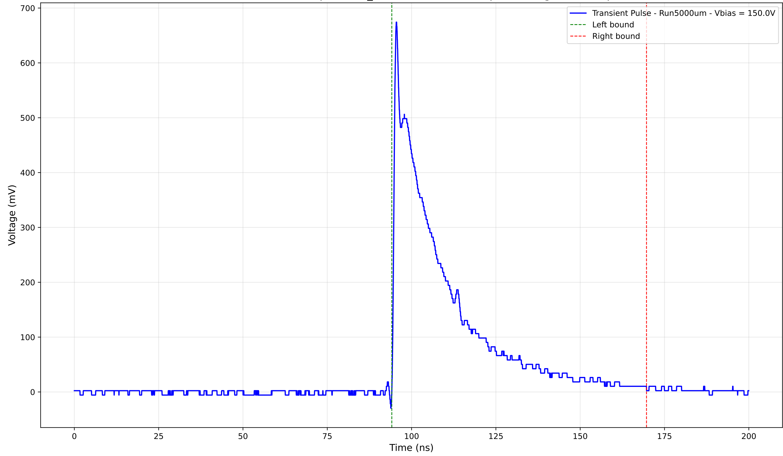
Transient Pulse - Sample: 1cm_42 - Position: 2155.0 \mu\text{m} - Charge: 183.41 pC
