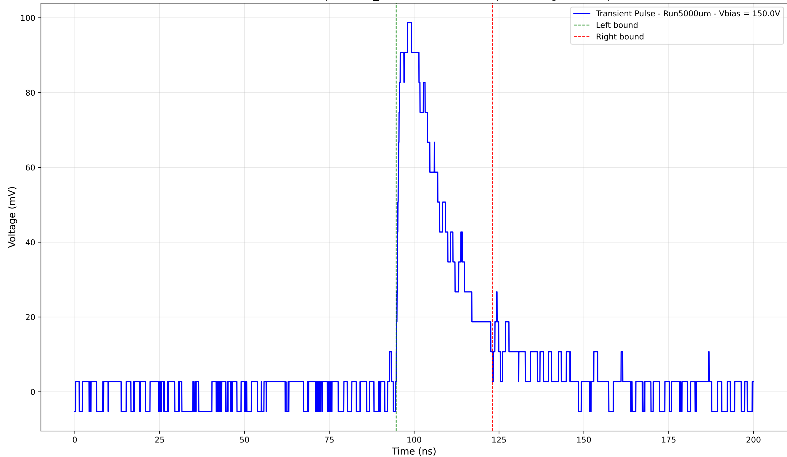
Transient Pulse - Sample: 1cm_42 - Position: 1525.0 \mu\text{m} - Charge: 28.48 pC
