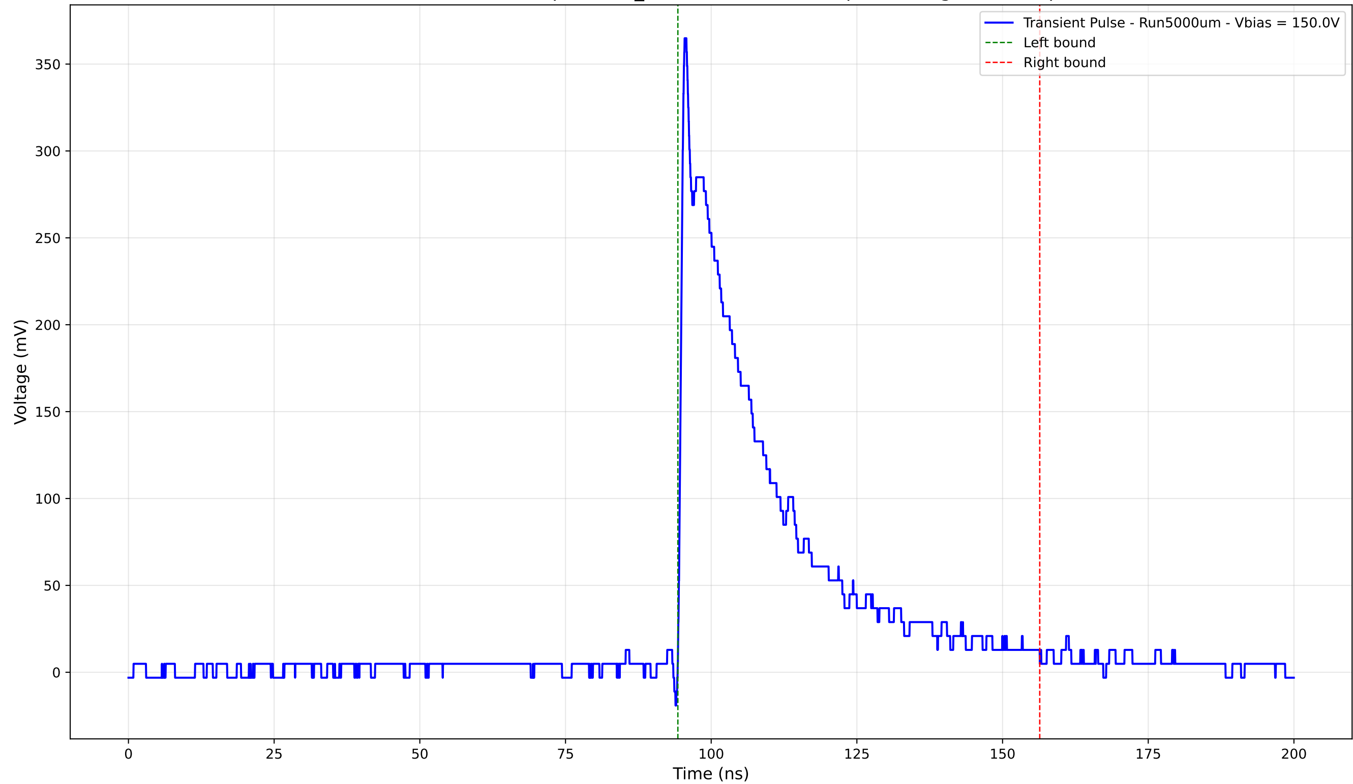
Transient Pulse - Sample: 1cm_42 - Position: 2070.0 \mu\text{m} - Charge: 101.81 pC
