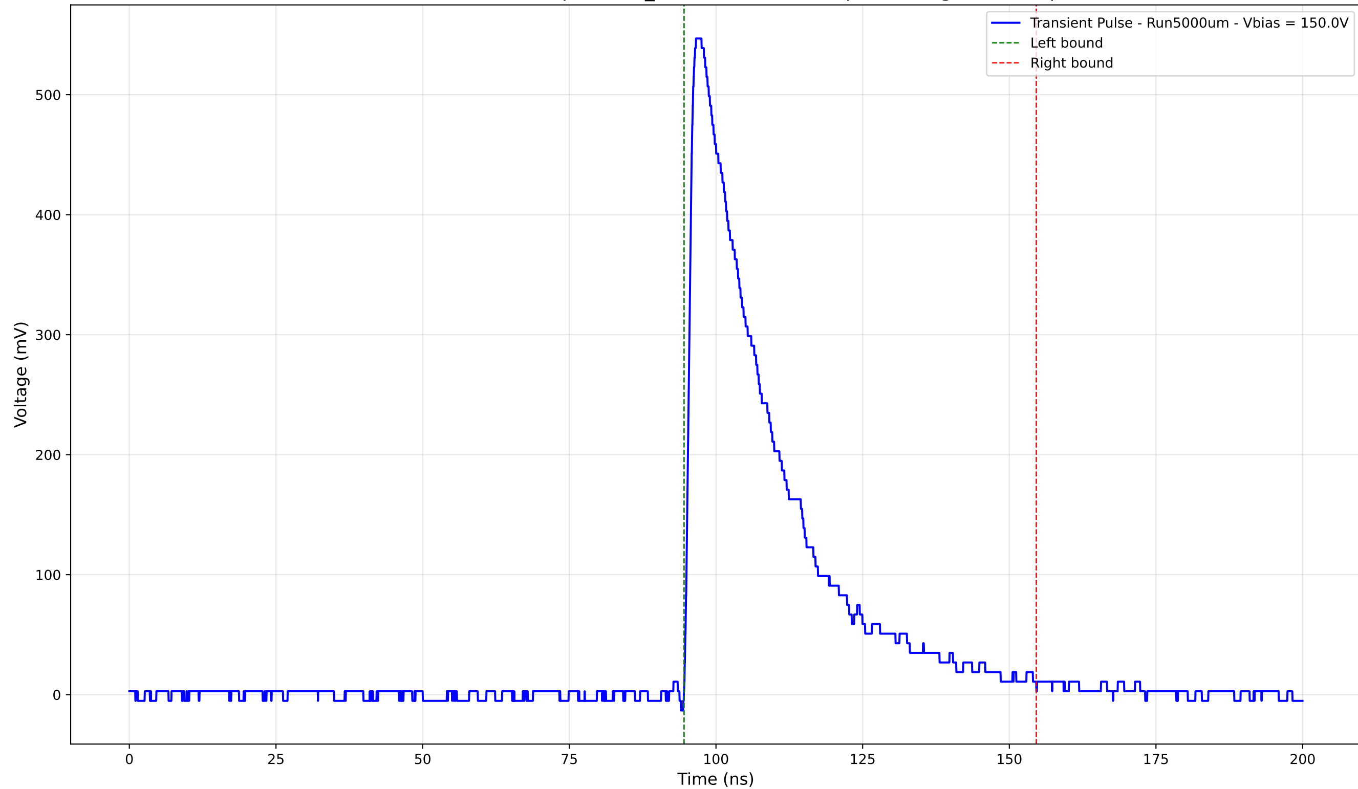
Transient Pulse - Sample: 1cm_42 - Position: 895.0 \mu\text{m} - Charge: 166.64 pC
