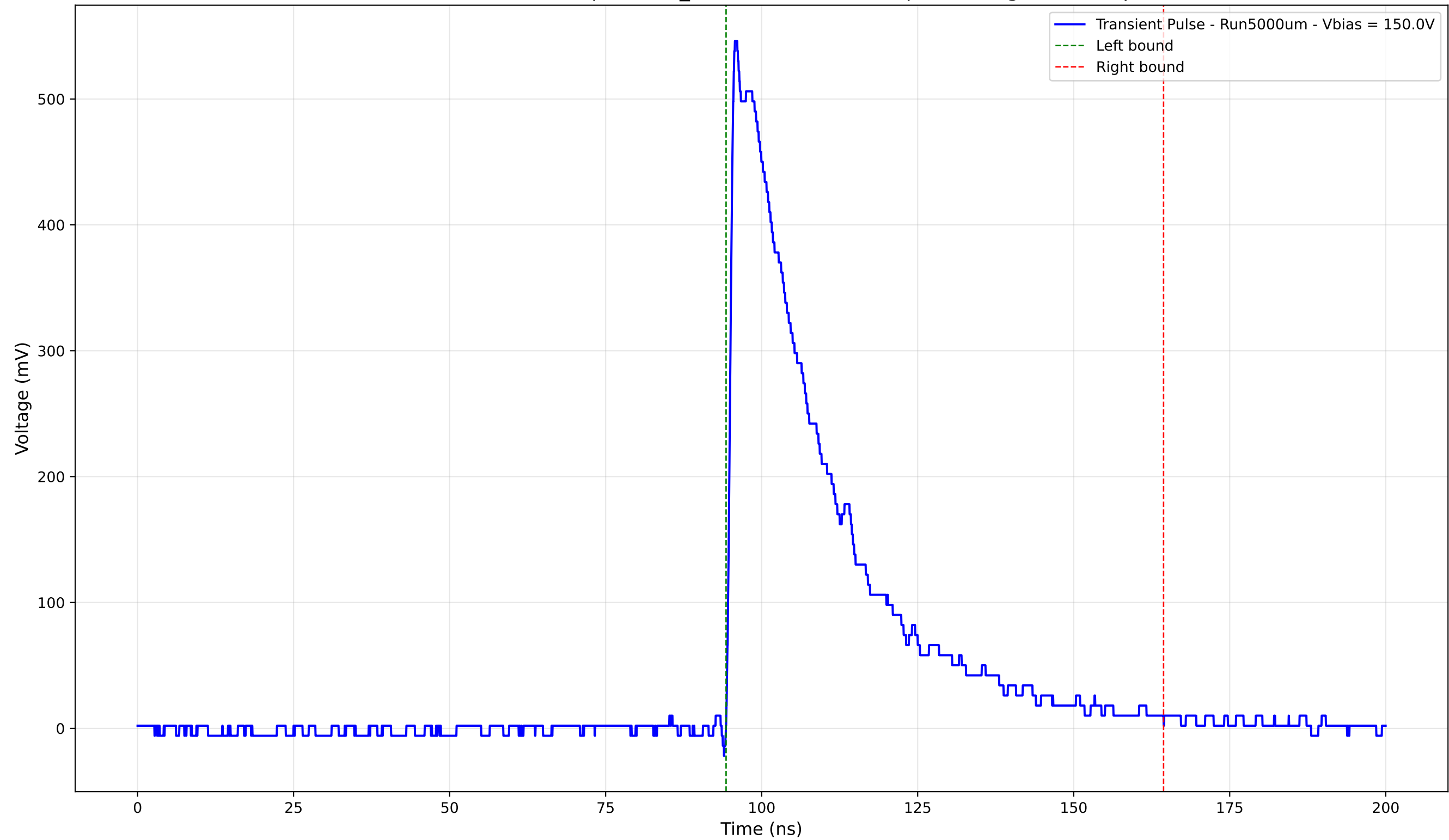
Transient Pulse - Sample: 1cm_42 - Position: 1875.0 \mu\text{m} - Charge: 176.38 pC
