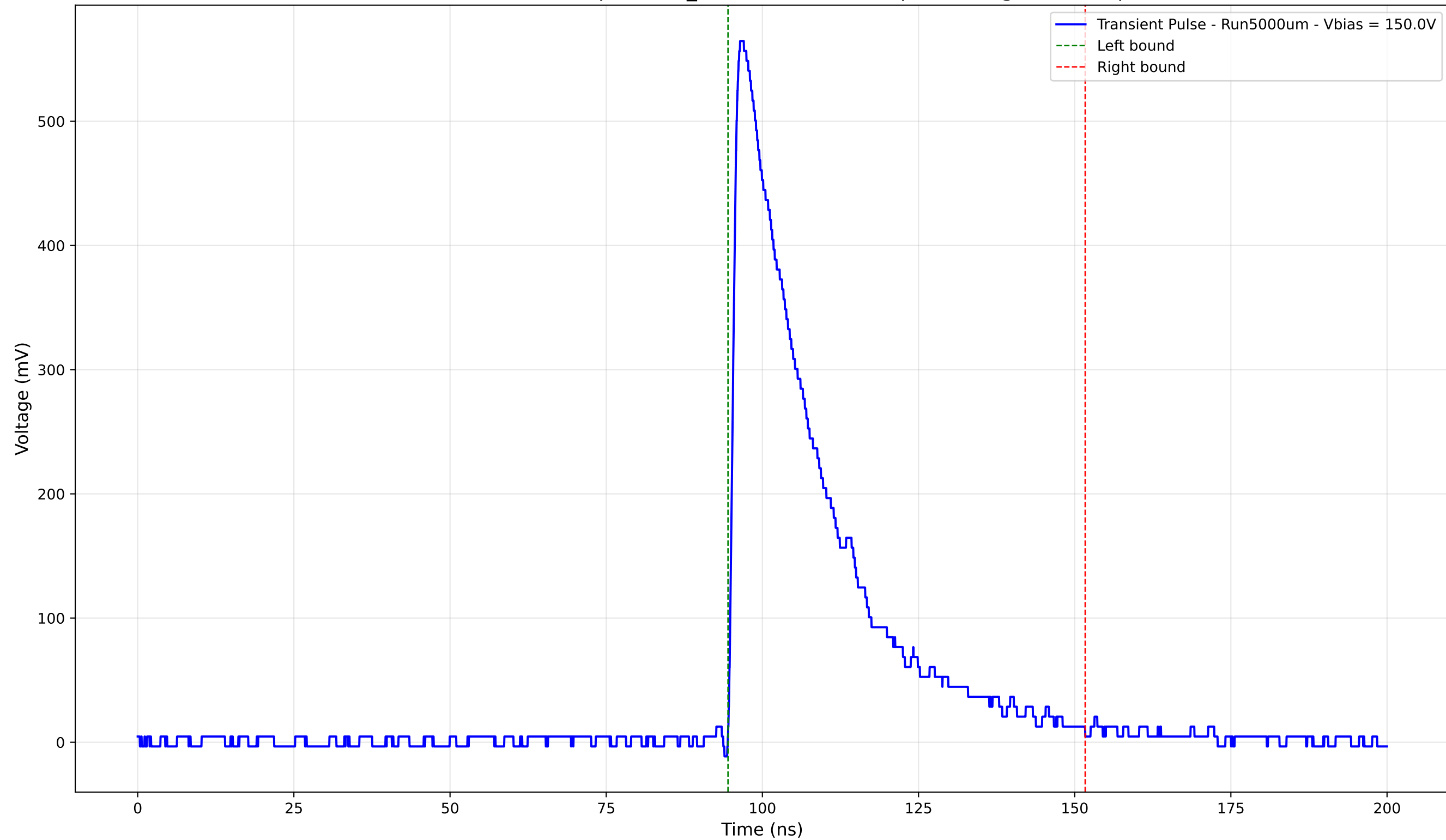
Transient Pulse - Sample: 1cm_42 - Position: 715.0 \mu\text{m} - Charge: 165.74 pC
