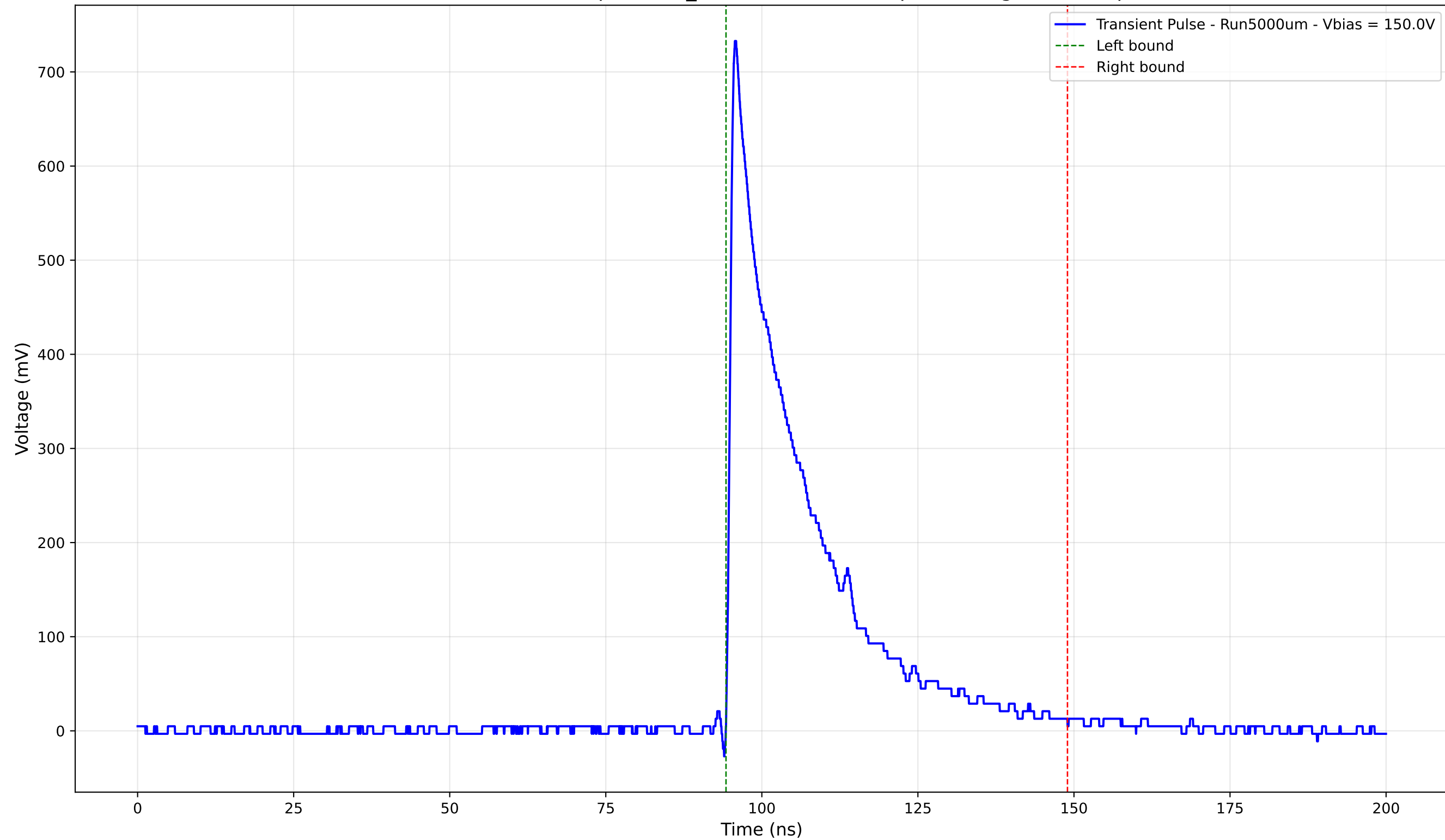
Transient Pulse - Sample: 1cm_42 - Position: 195.0 \mu\text{m} - Charge: 170.73 pC
