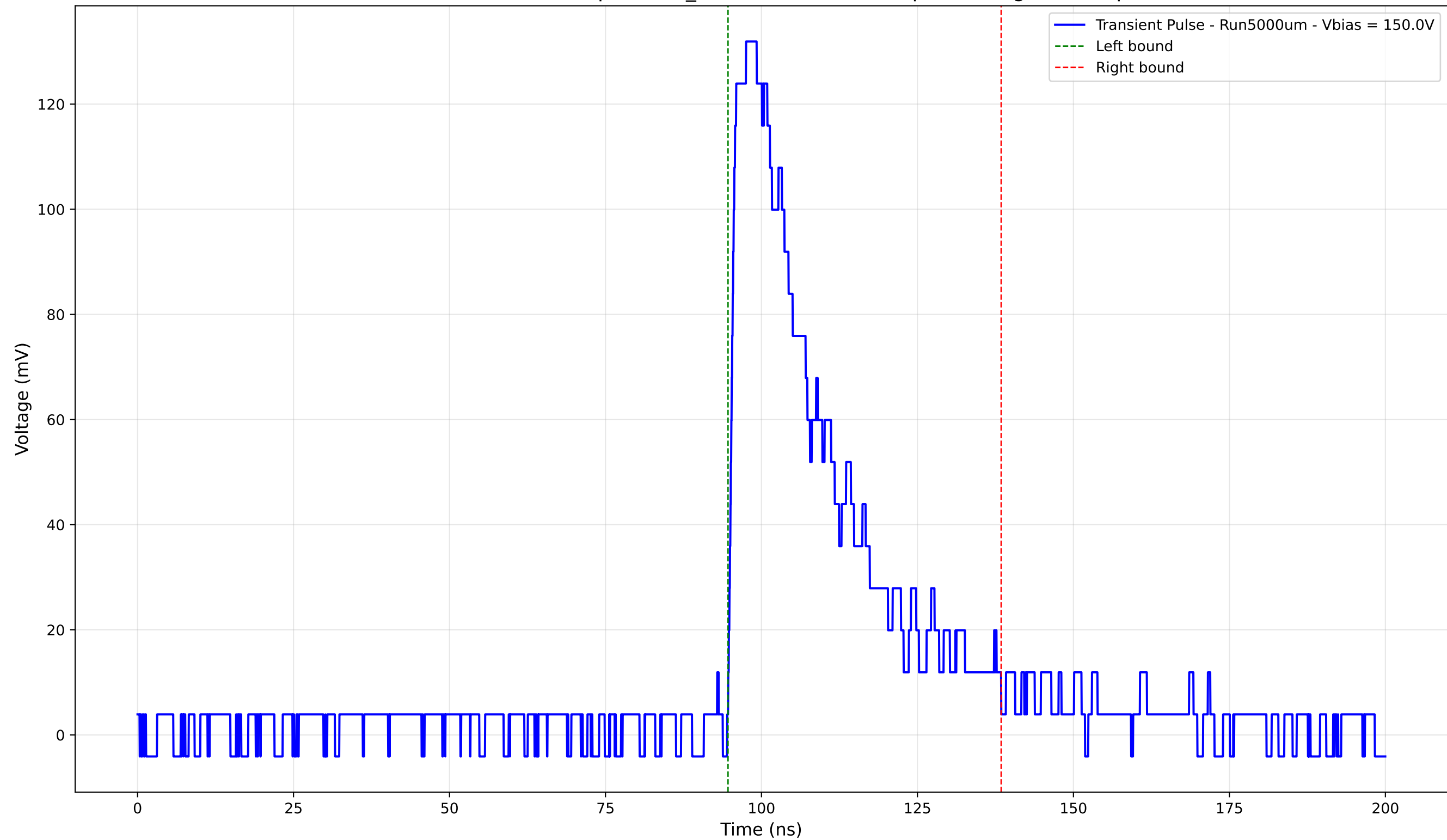
Transient Pulse - Sample: 1cm_42 - Position: 1535.0 \mu\text{m} - Charge: 43.58 pC
