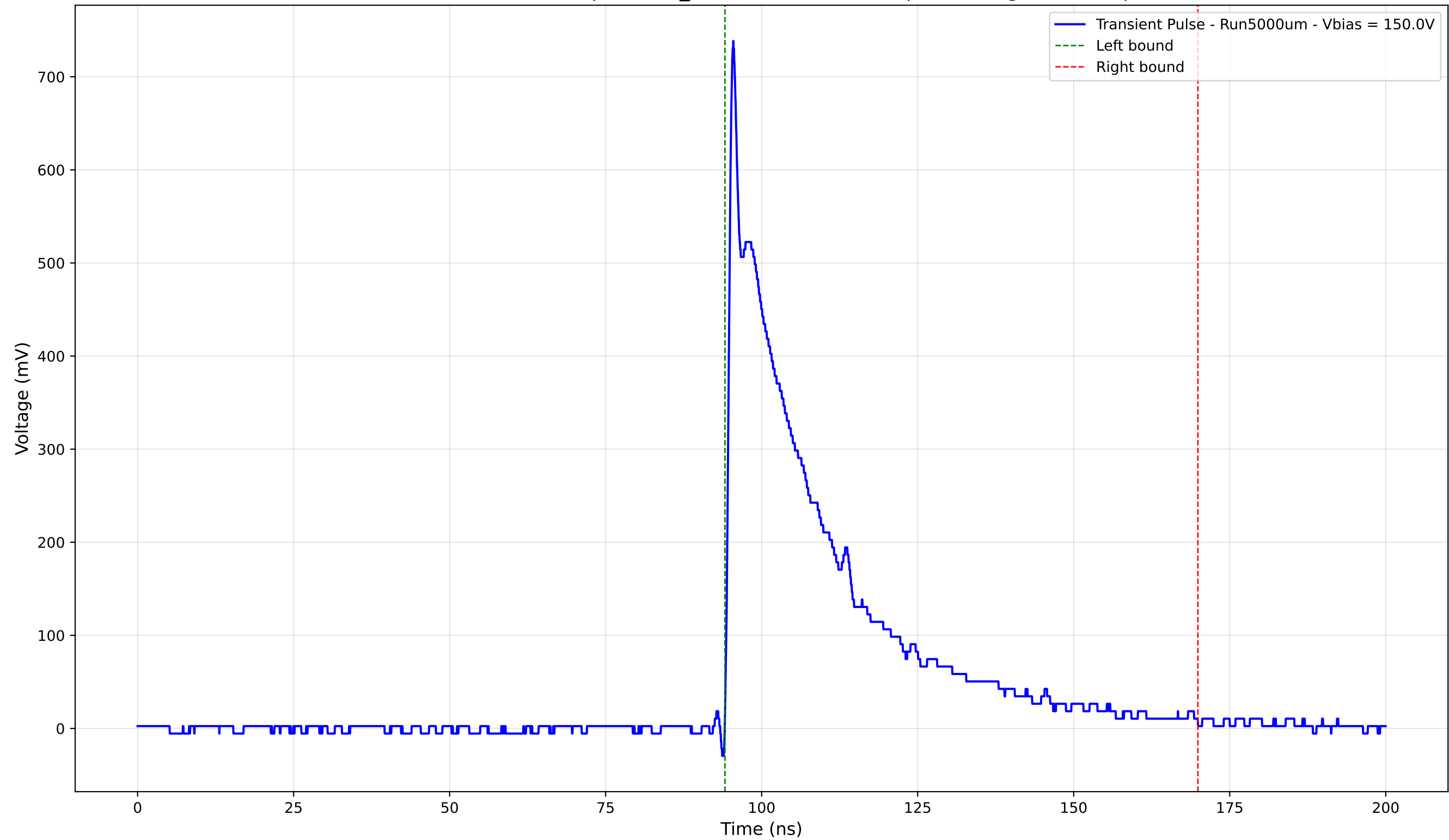
Transient Pulse - Sample: 1cm_42 - Position: 2830.0 \mu\text{m} - Charge: 192.23 pC
