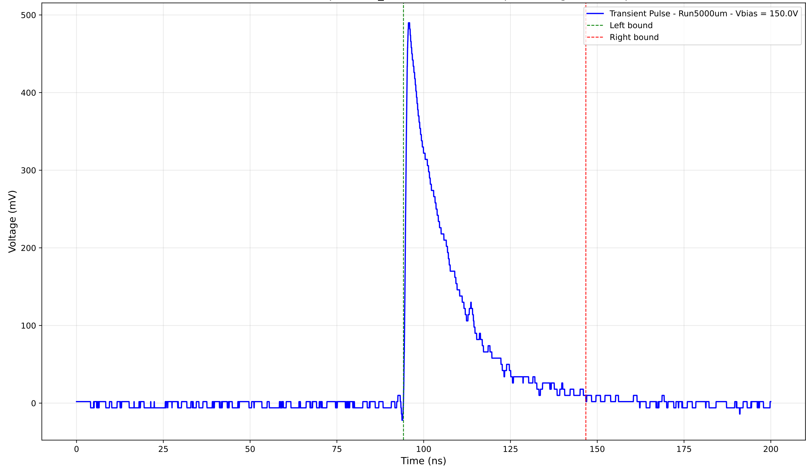
Transient Pulse - Sample: 1cm_42 - Position: 4605.0 \mu\text{m} - Charge: 123.28 pC
