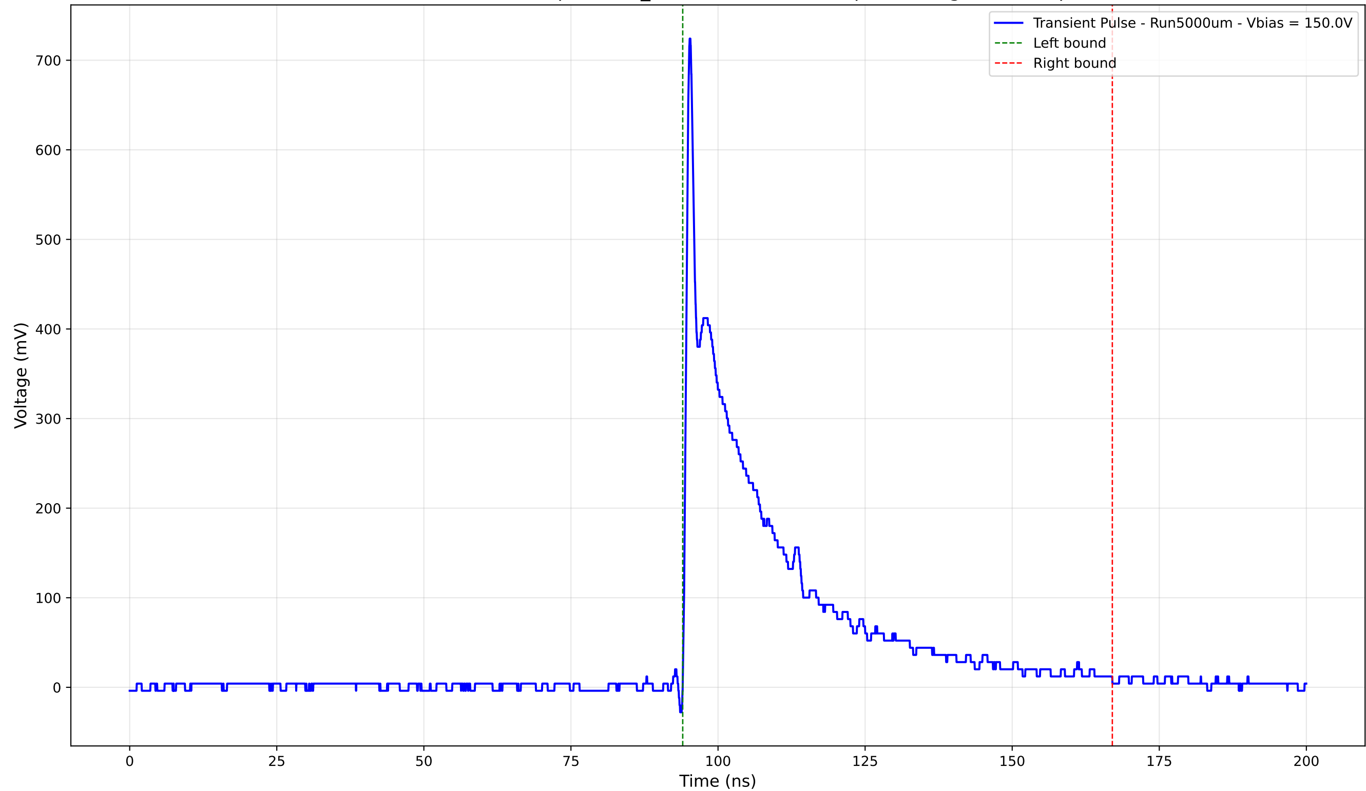
Transient Pulse - Sample: 1cm_42 - Position: 2435.0 \mu\text{m} - Charge: 155.07 pC
