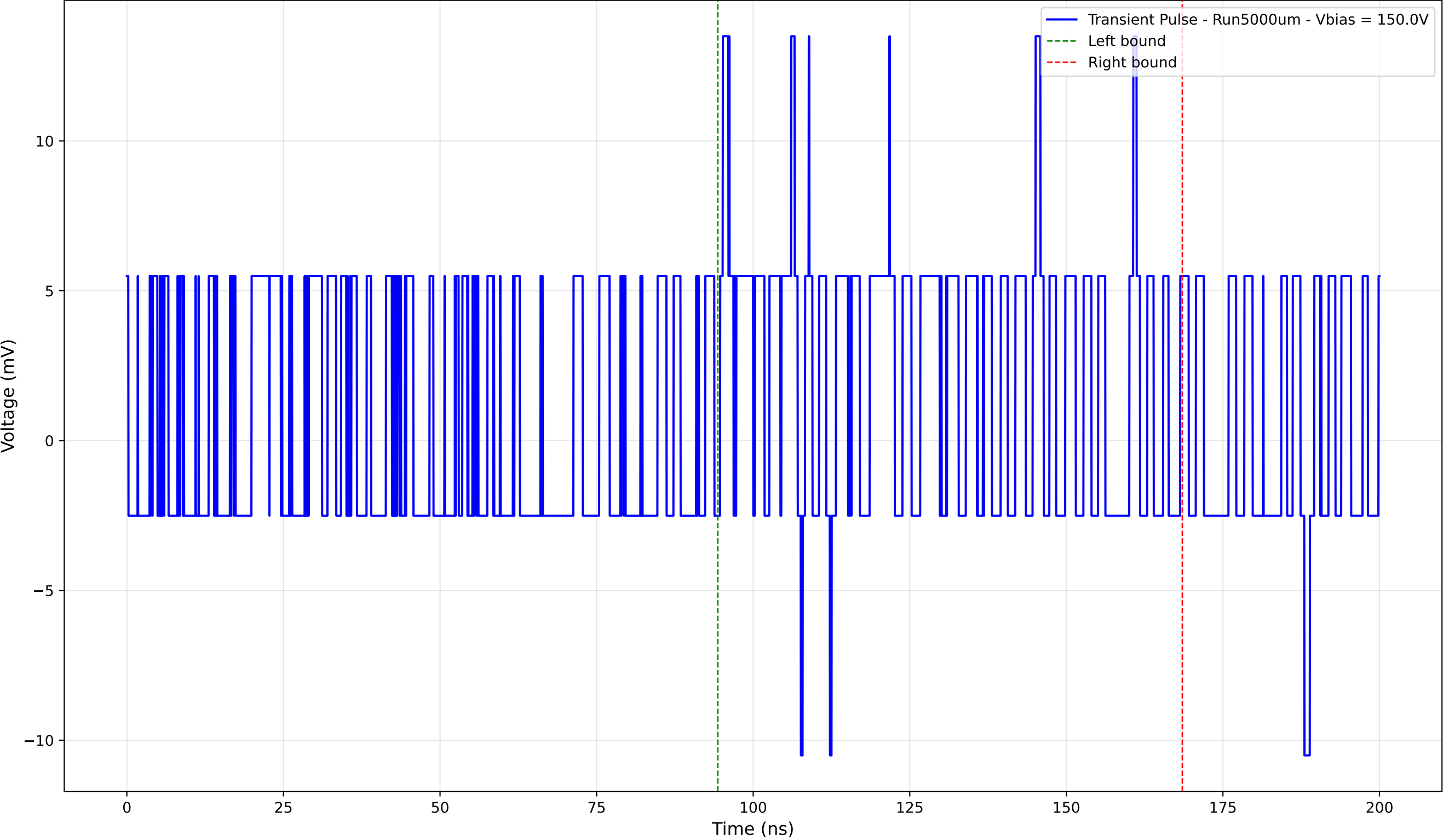
Transient Pulse - Sample: 1cm_42 - Position: 4975.0 \mu\text{m} - Charge: 3.71 pC
