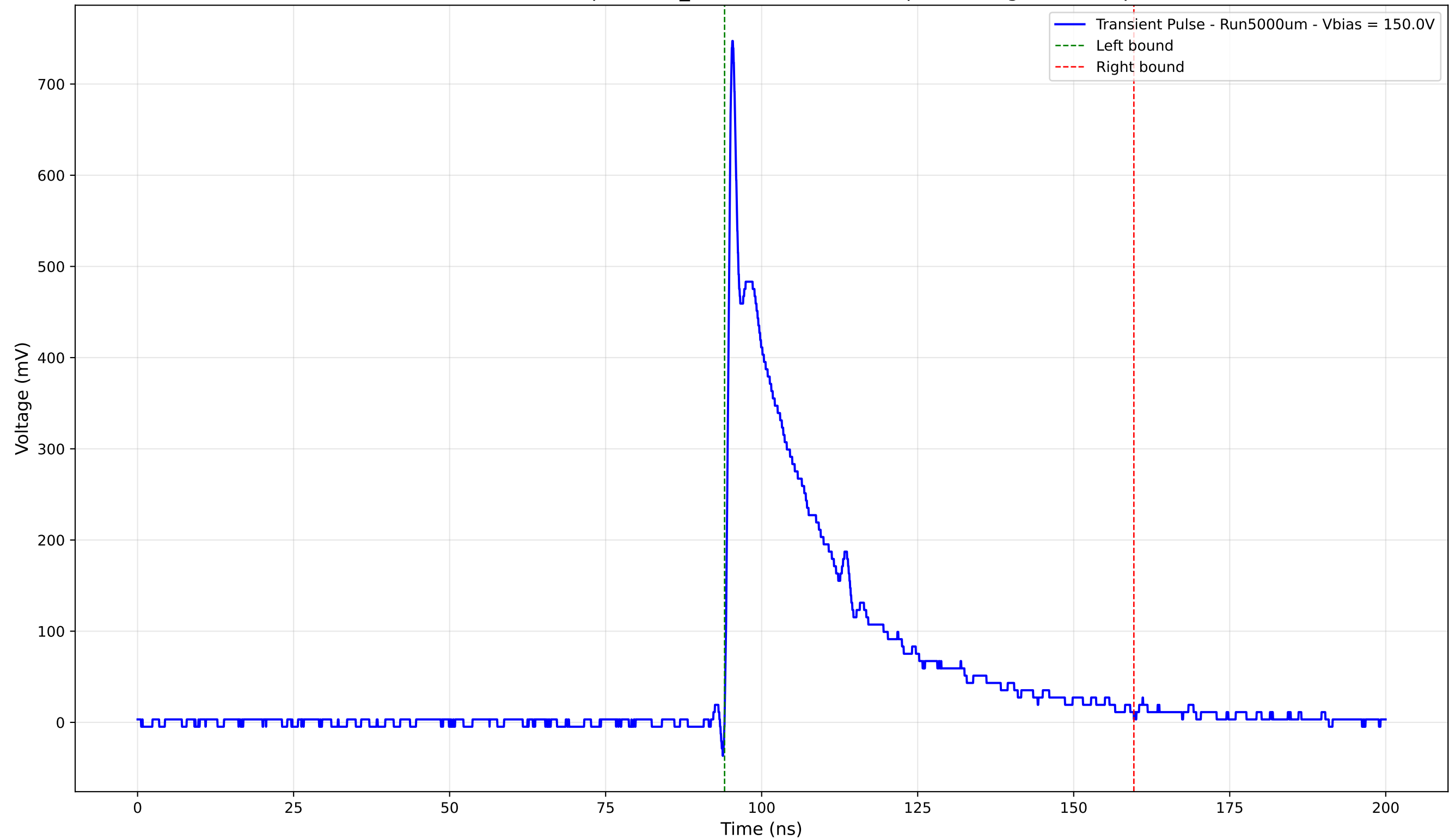
Transient Pulse - Sample: 1cm_42 - Position: 2305.0 \mu\text{m} - Charge: 178.06 pC
