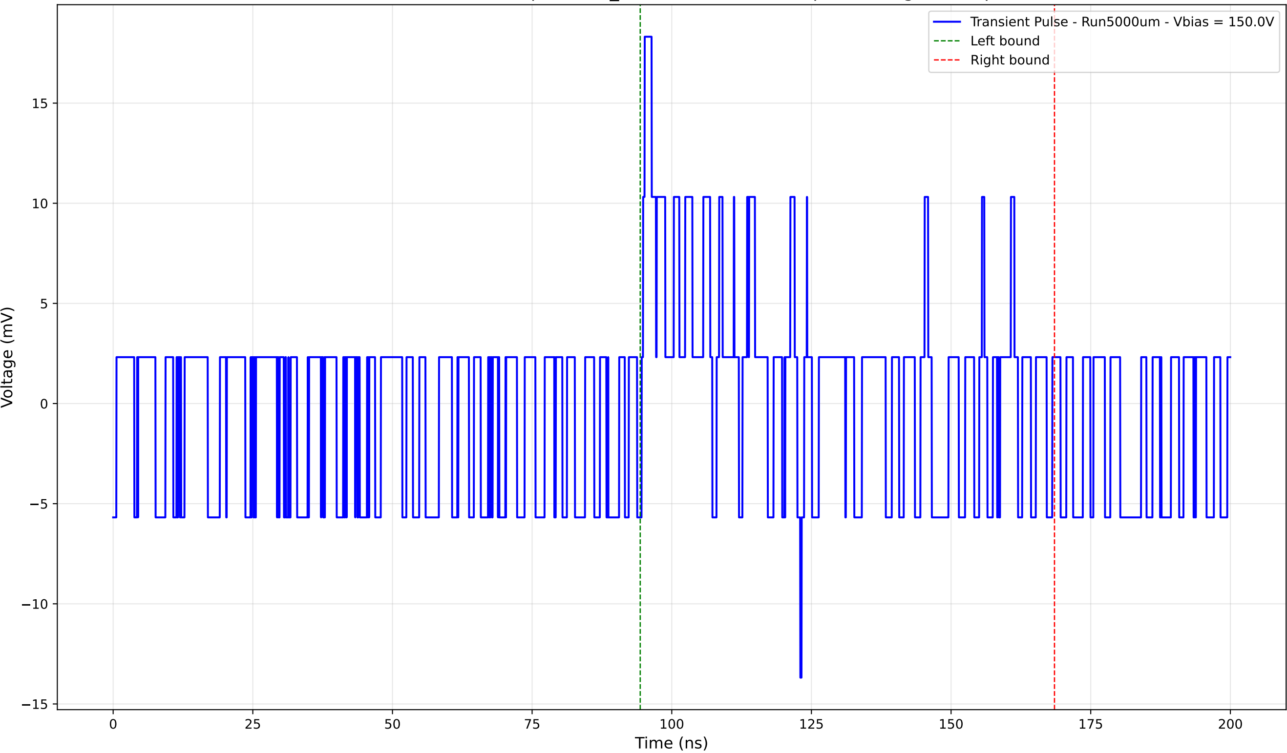
Transient Pulse - Sample: 1cm_42 - Position: 4910.0 \mu\text{m} - Charge: 2.47 pC
