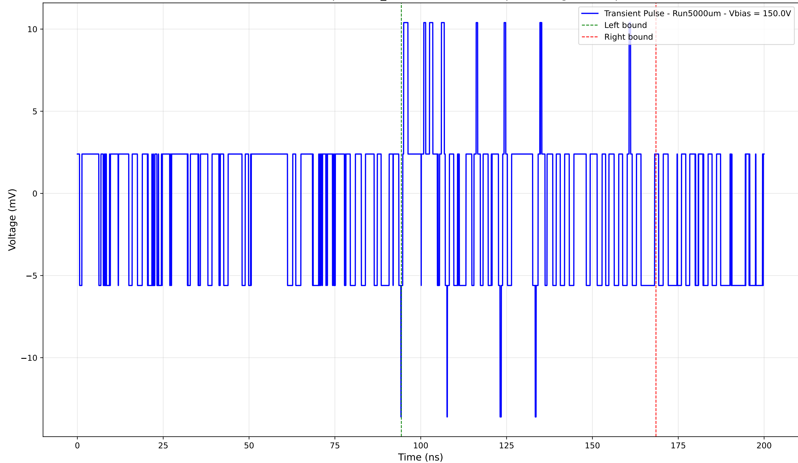
Transient Pulse - Sample: 1cm_42 - Position: 4945.0 \mu\text{m} - Charge: -0.03 pC
