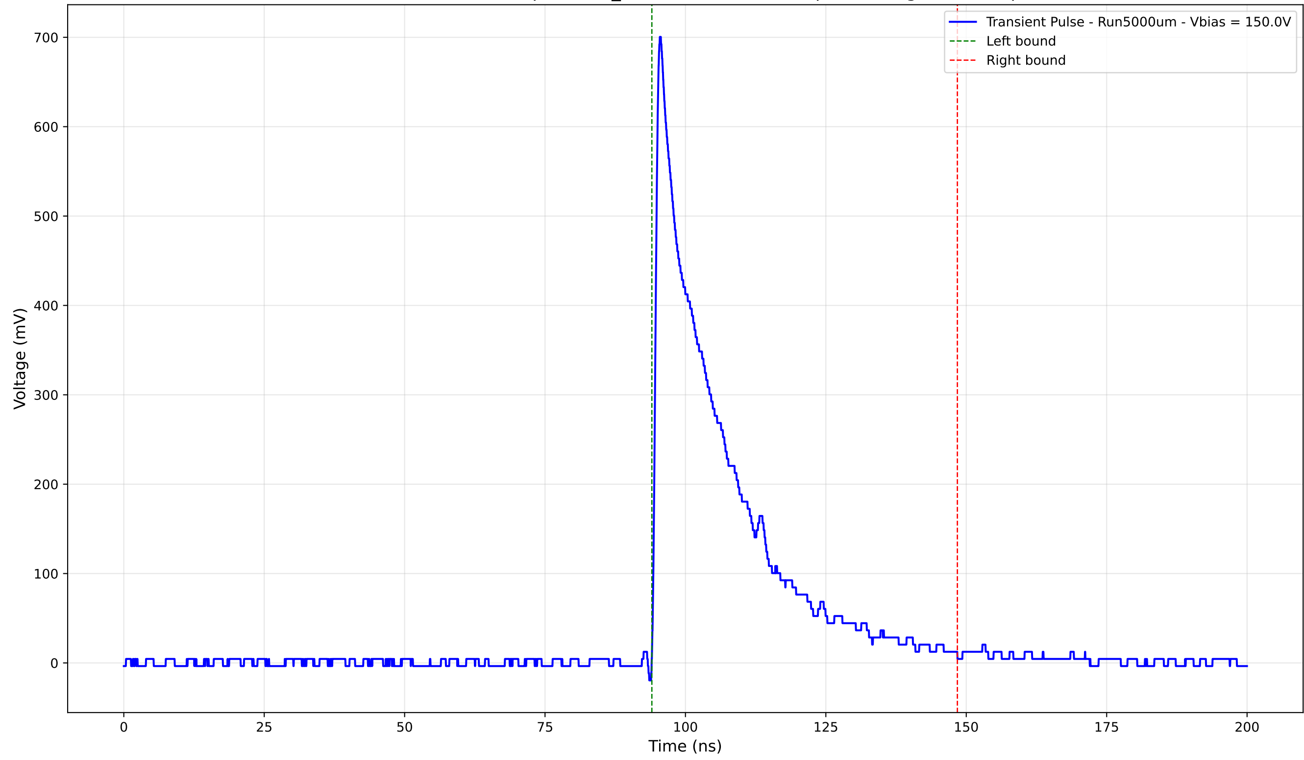
Transient Pulse - Sample: 1cm_42 - Position: 4790.0 \mu\text{m} - Charge: 163.50 pC
