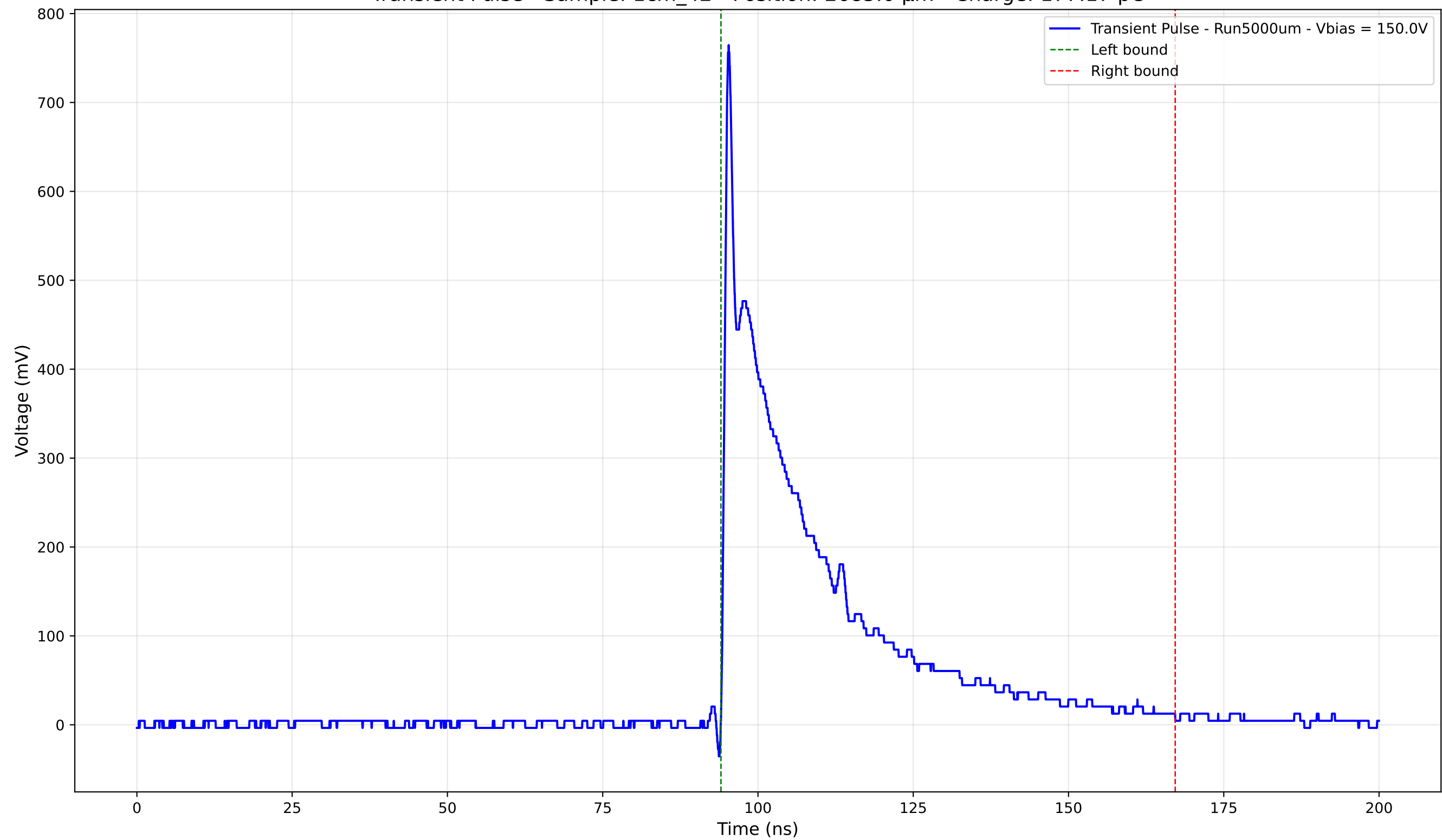
Transient Pulse - Sample: 1cm_42 - Position: 2685.0 \mu\text{m} - Charge: 177.17 pC
