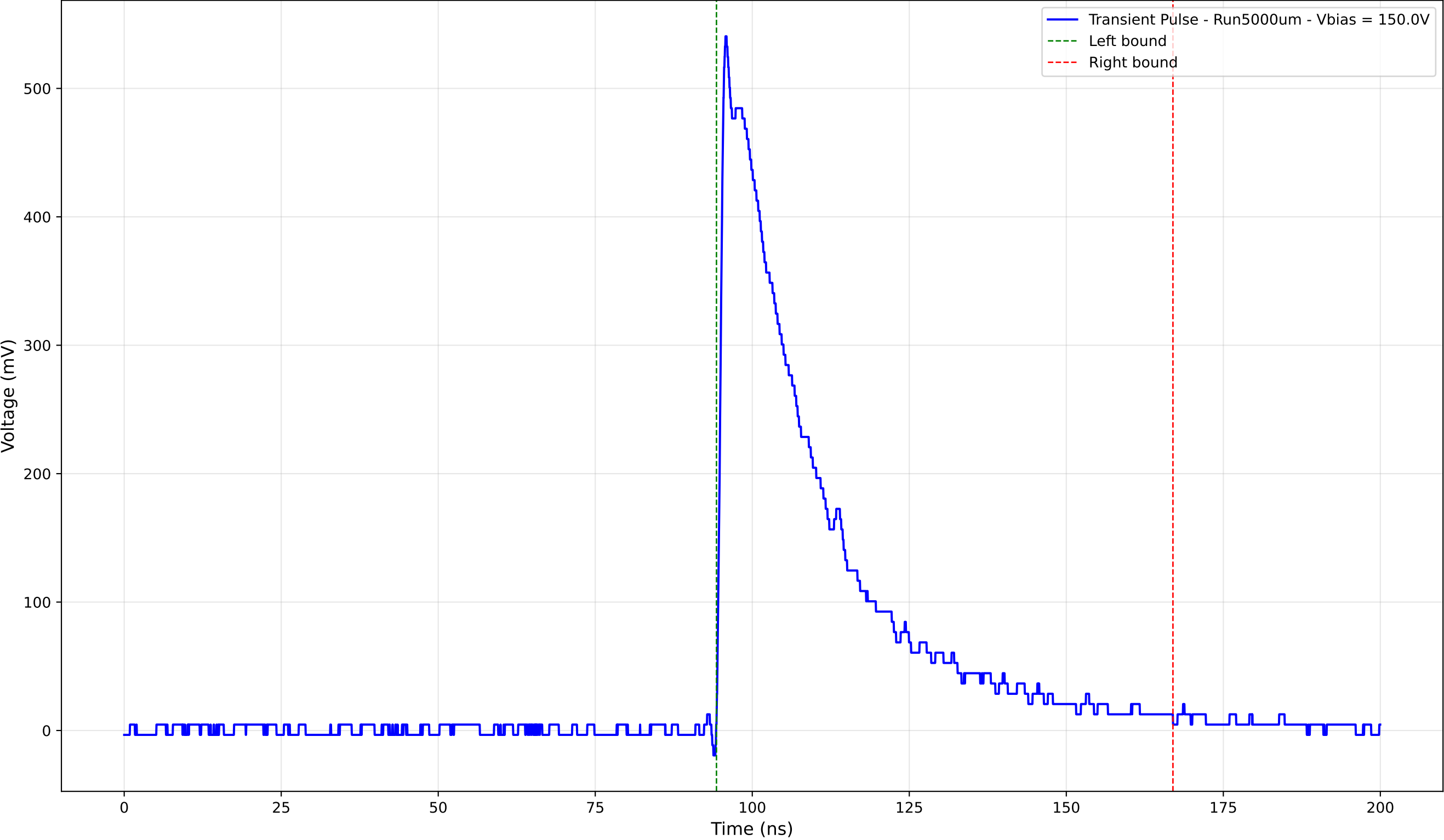
Transient Pulse - Sample: 1cm_42 - Position: 1905.0 \mu\text{m} - Charge: 173.11 pC
