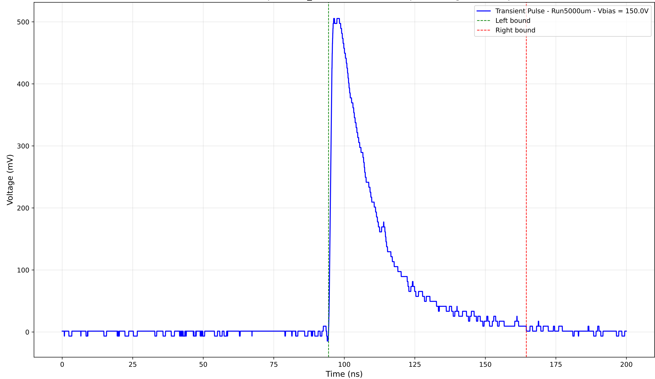
Transient Pulse - Sample: 1cm_42 - Position: 1650.0 \mu\text{m} - Charge: 171.80 pC
