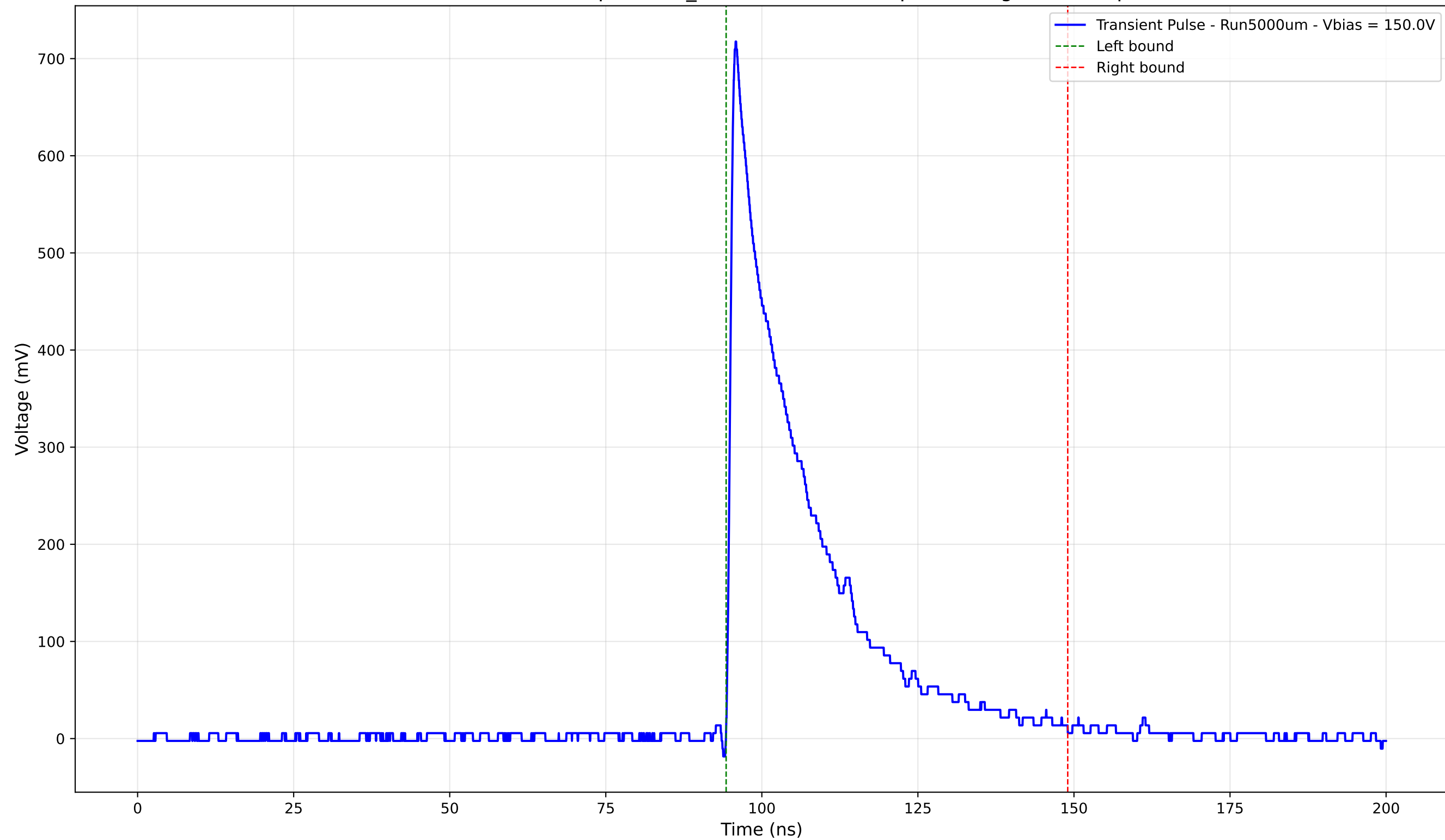
Transient Pulse - Sample: 1cm_42 - Position: 235.0 \mu\text{m} - Charge: 170.93 pC
