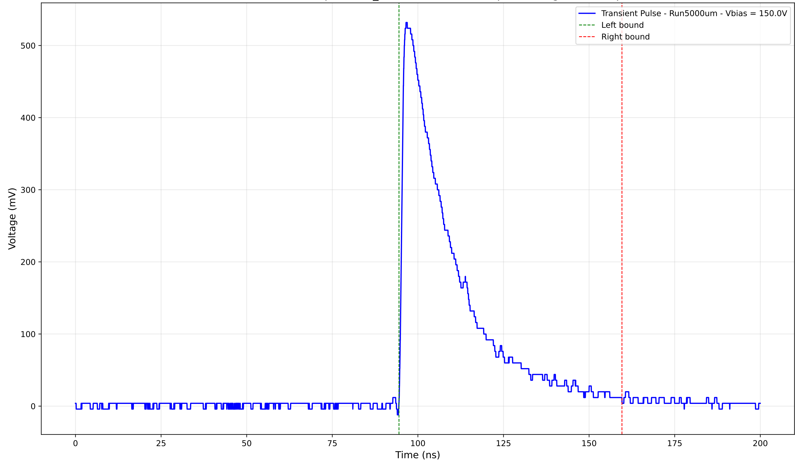
Transient Pulse - Sample: 1cm_42 - Position: 3615.0 \mu\text{m} - Charge: 173.30 pC
