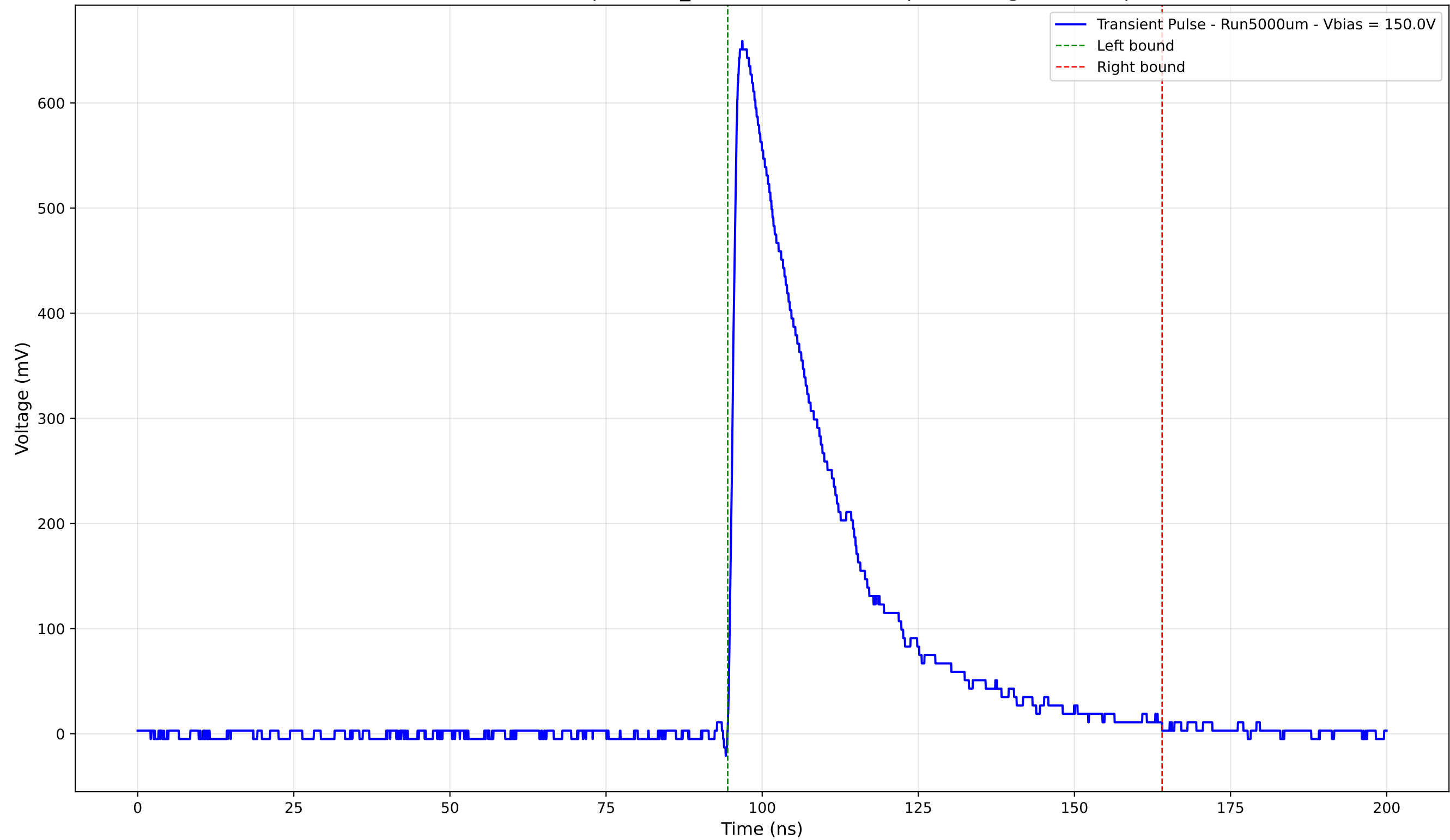
Transient Pulse - Sample: 1cm_42 - Position: 3865.0 \mu\text{m} - Charge: 210.56 pC
