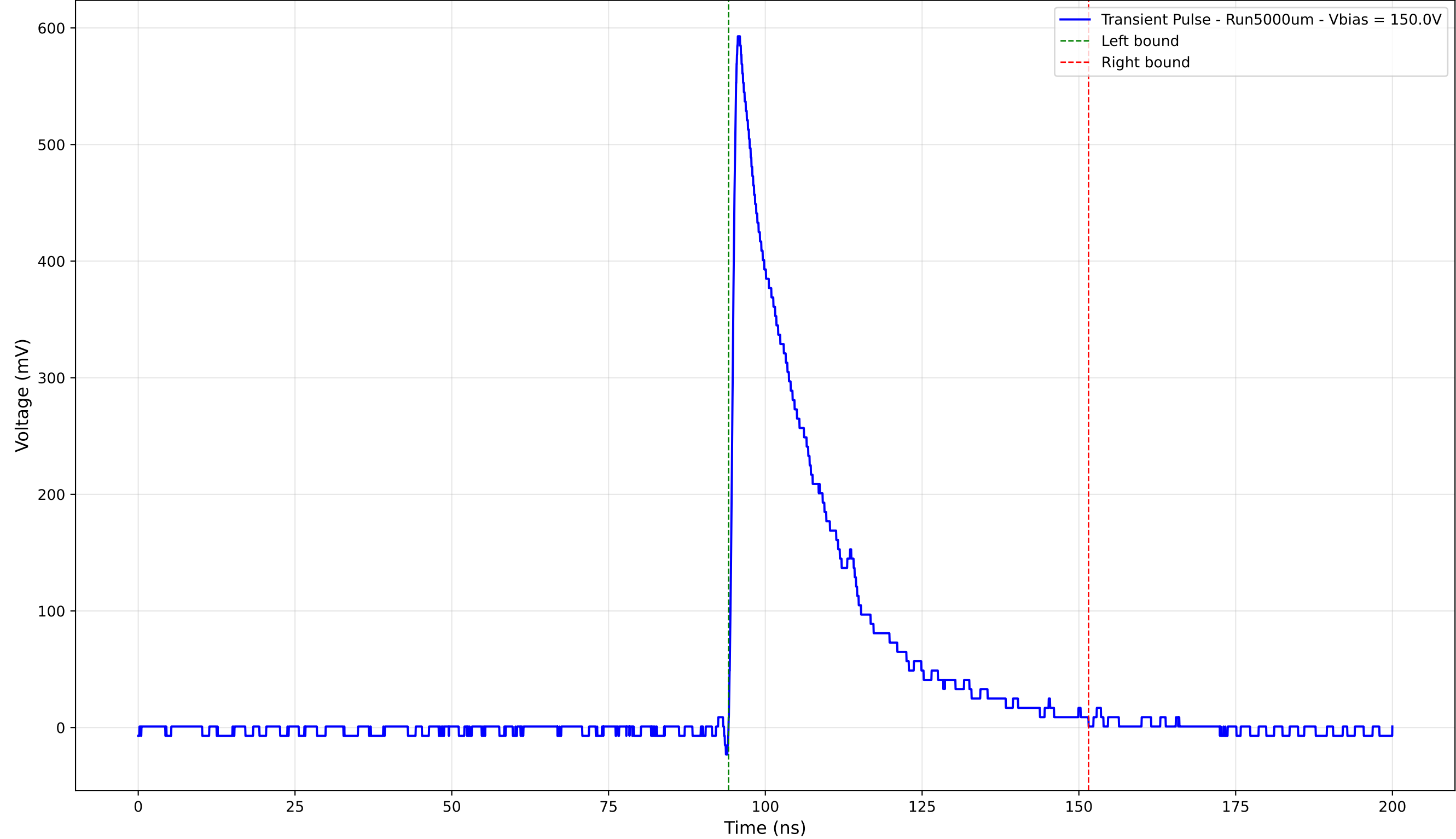
Transient Pulse - Sample: 1cm_42 - Position: 4620.0 \mu\text{m} - Charge: 150.37 pC
