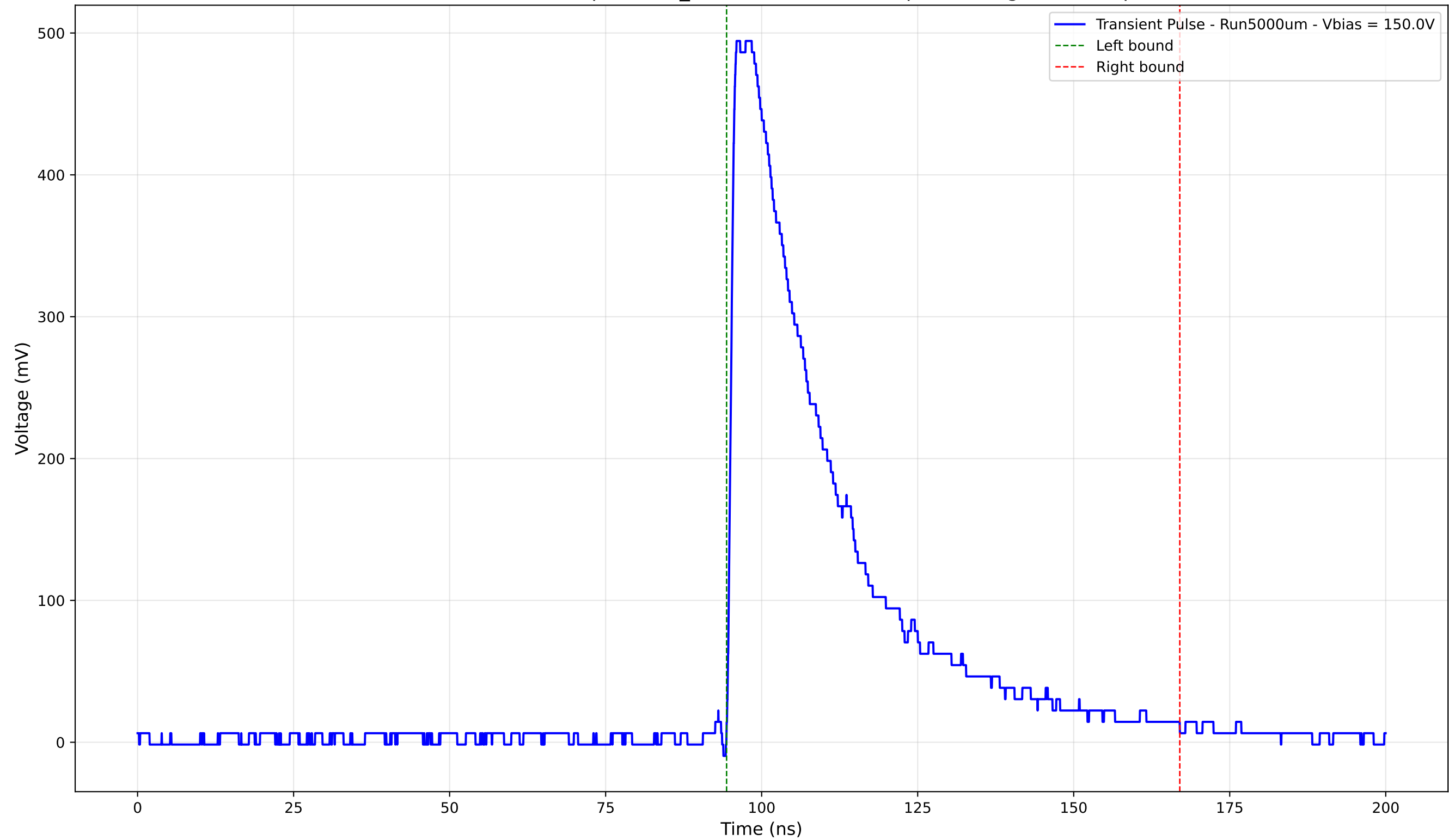
Transient Pulse - Sample: 1cm_42 - Position: 1730.0 \mu\text{m} - Charge: 175.47 pC
