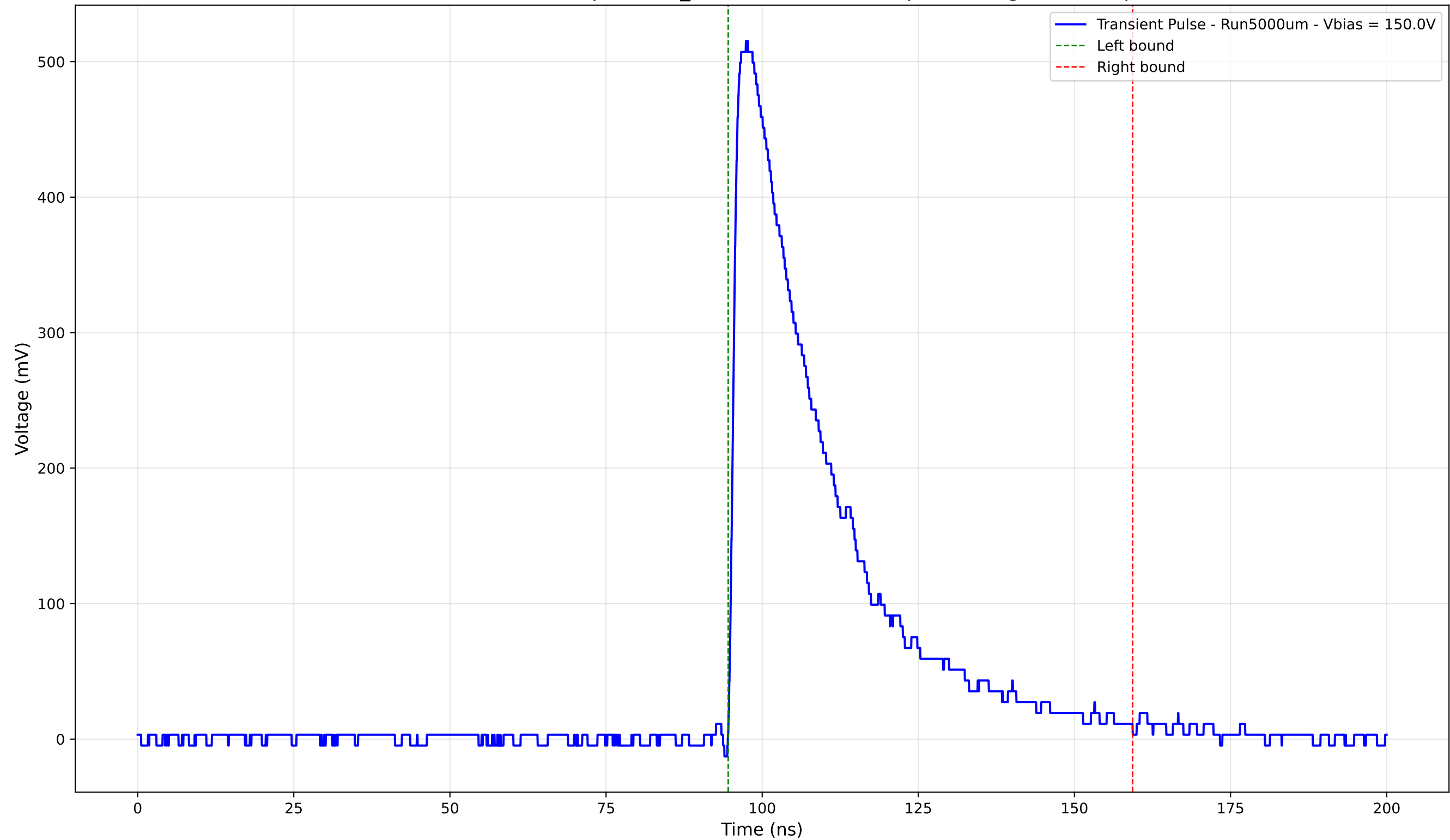
Transient Pulse - Sample: 1cm_42 - Position: 1355.0 \mu\text{m} - Charge: 168.66 pC
