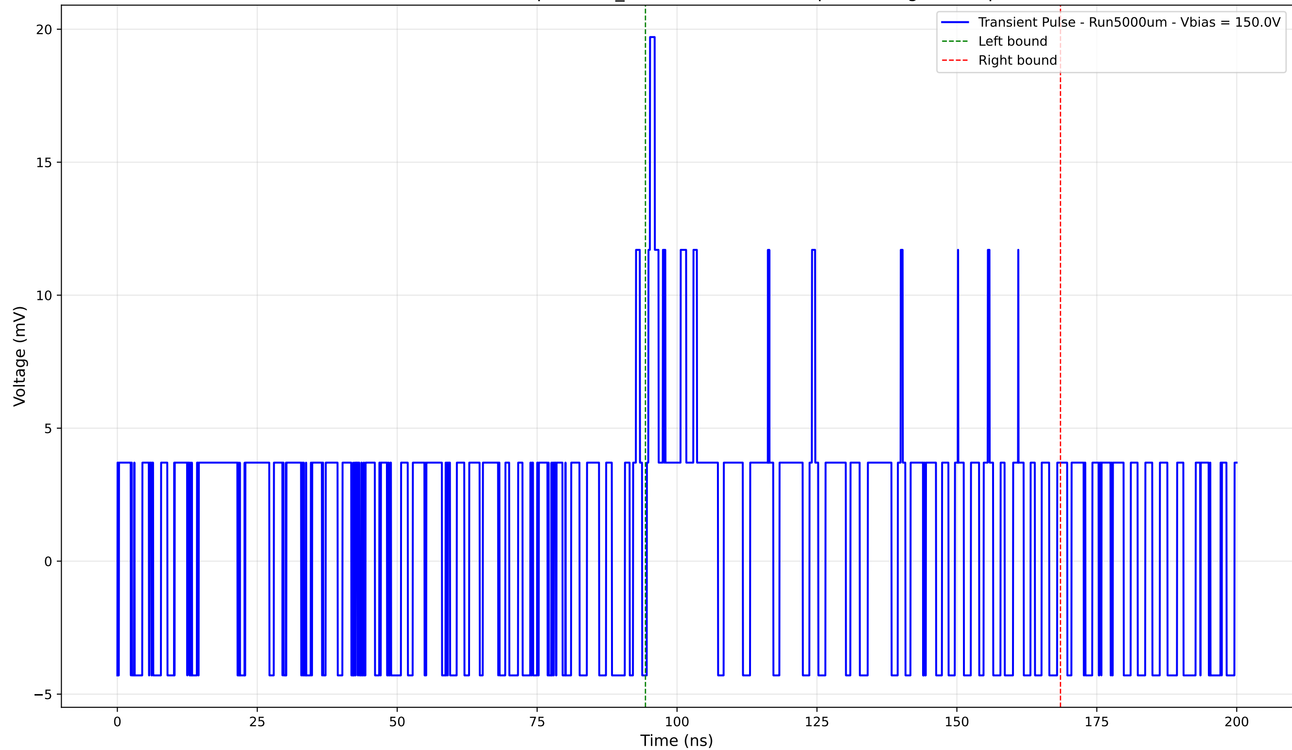
Transient Pulse - Sample: 1cm_42 - Position: 5060.0 \mu\text{m} - Charge: 3.01 pC
