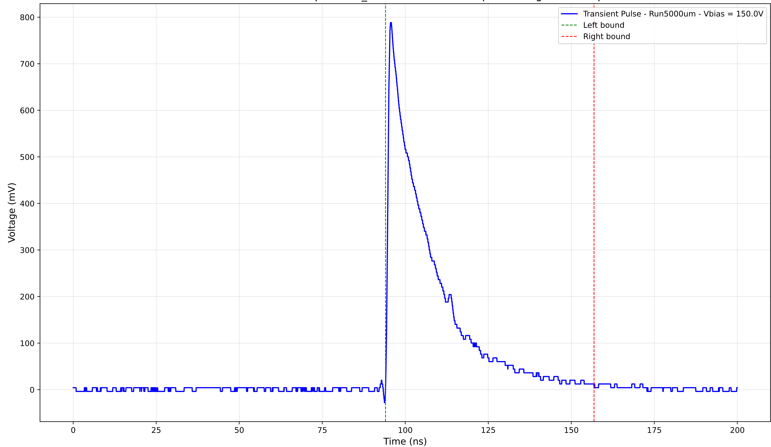
Transient Pulse - Sample: 1cm_42 - Position: 4690.0 \mu\text{m} - Charge: 205.64 pC
