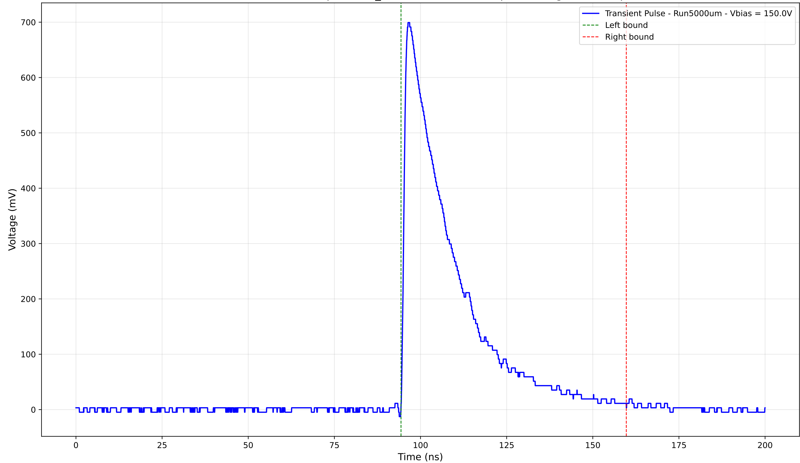
Transient Pulse - Sample: 1cm_42 - Position: 4175.0 \mu\text{m} - Charge: 214.10 pC
