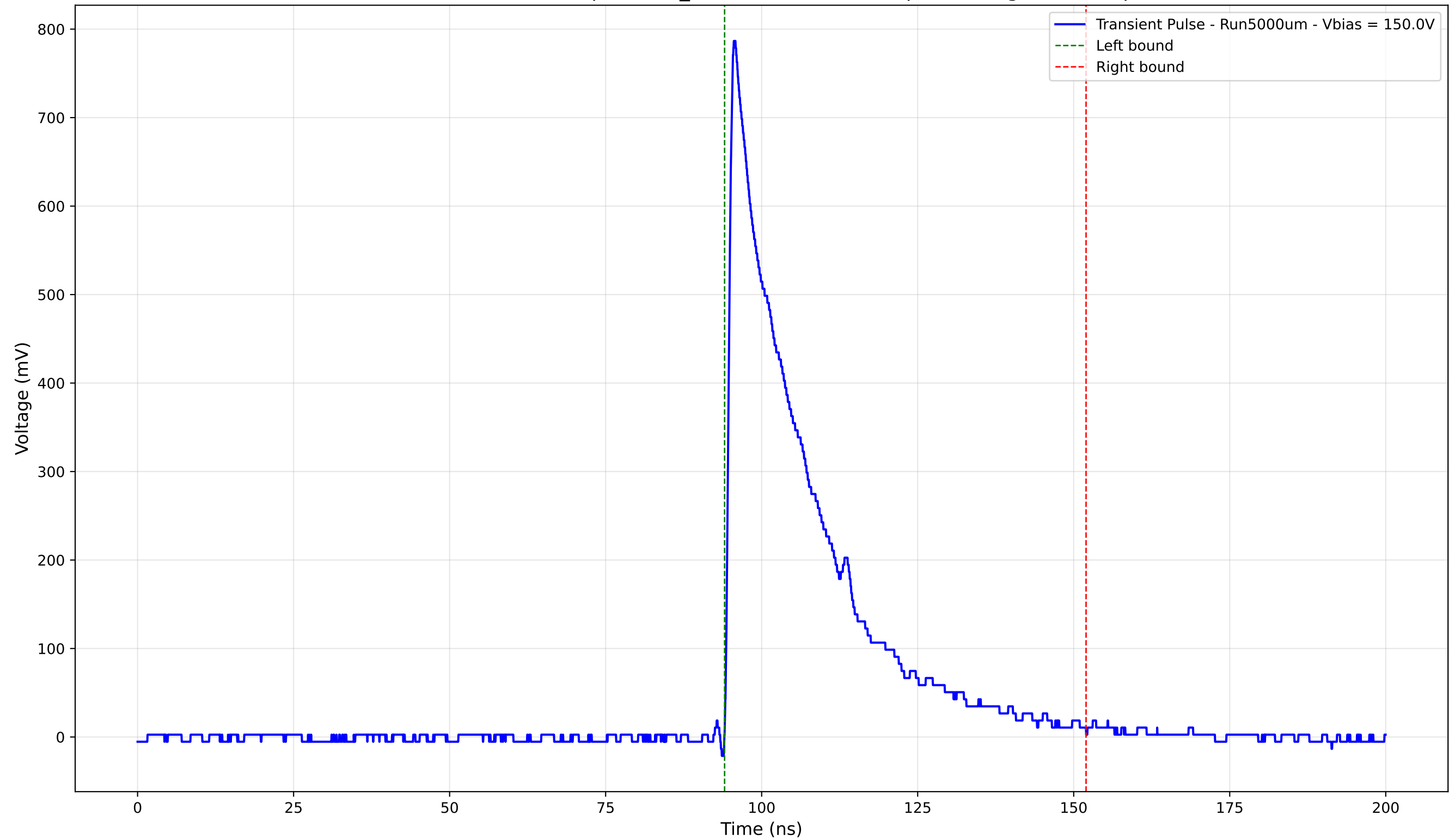
Transient Pulse - Sample: 1cm_42 - Position: 4695.0 \mu\text{m} - Charge: 200.44 pC
