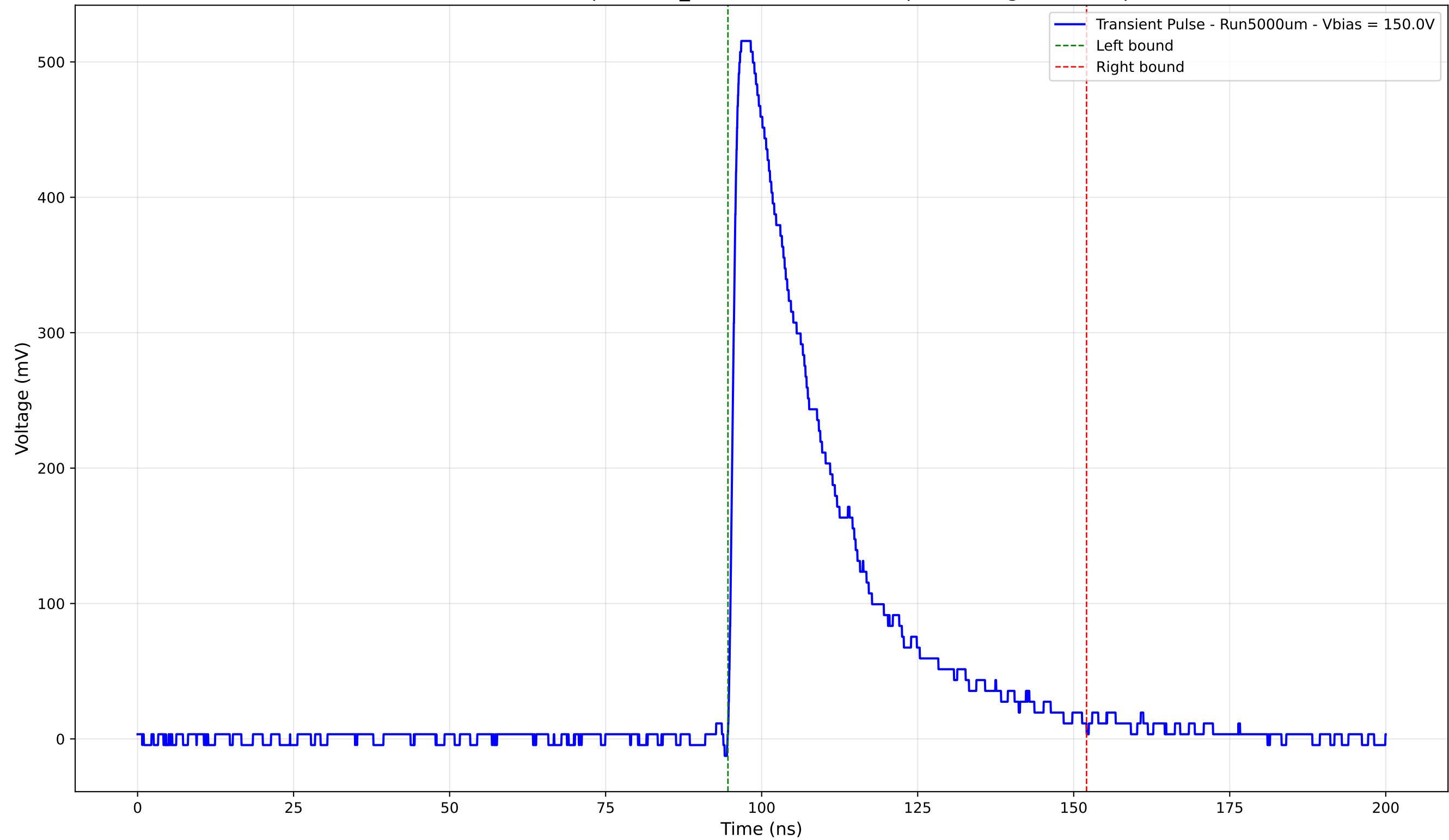
Transient Pulse - Sample: 1cm_42 - Position: 1240.0 \mu\text{m} - Charge: 166.07 pC
