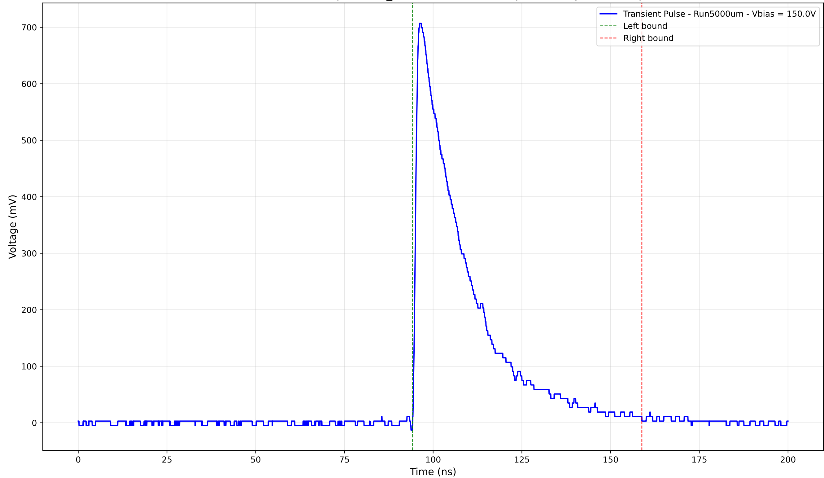
Transient Pulse - Sample: 1cm_42 - Position: 4325.0 \mu\text{m} - Charge: 212.81 pC
