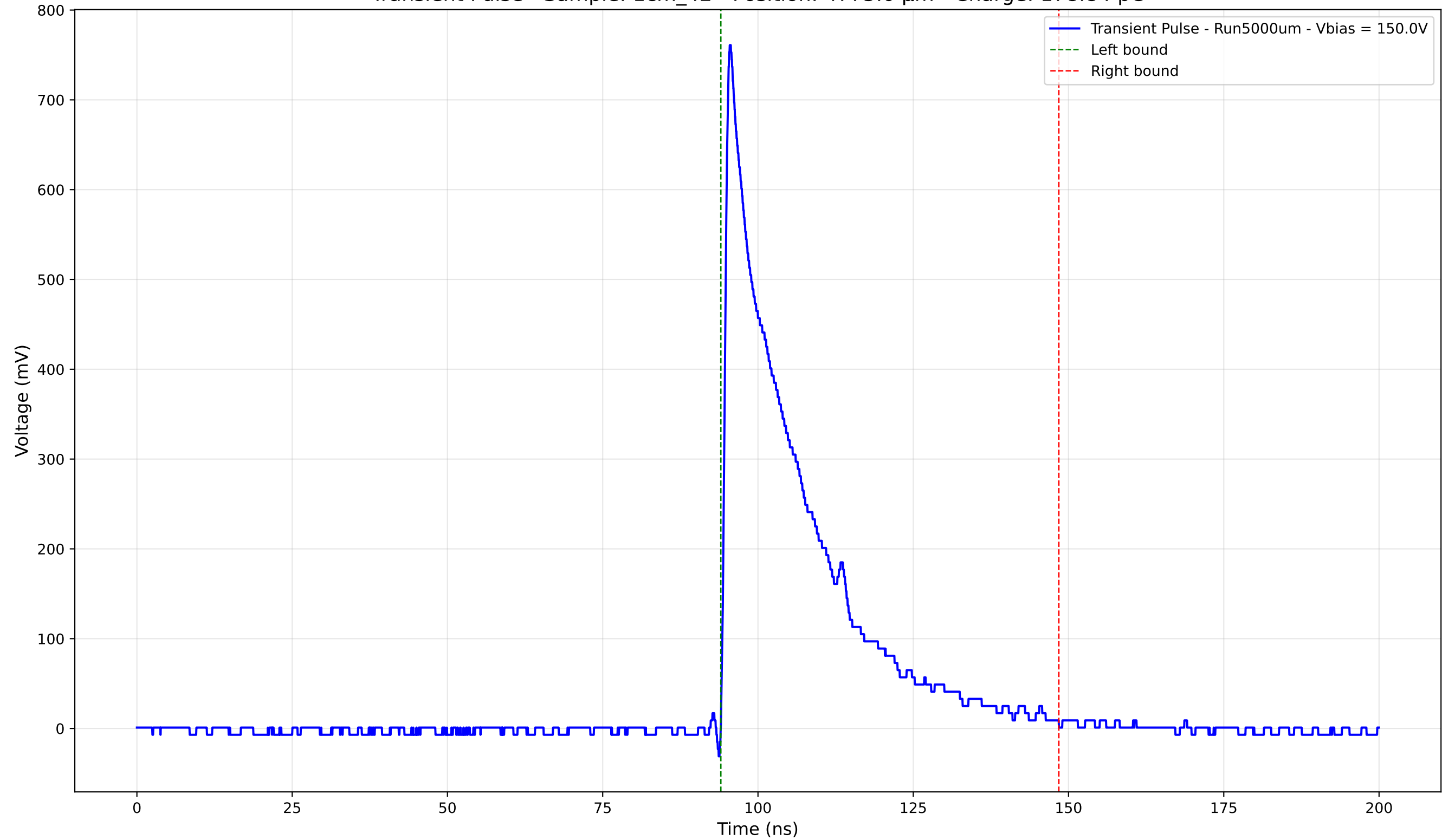
Transient Pulse - Sample: 1cm_42 - Position: 4775.0 \mu\text{m} - Charge: 178.84 pC
