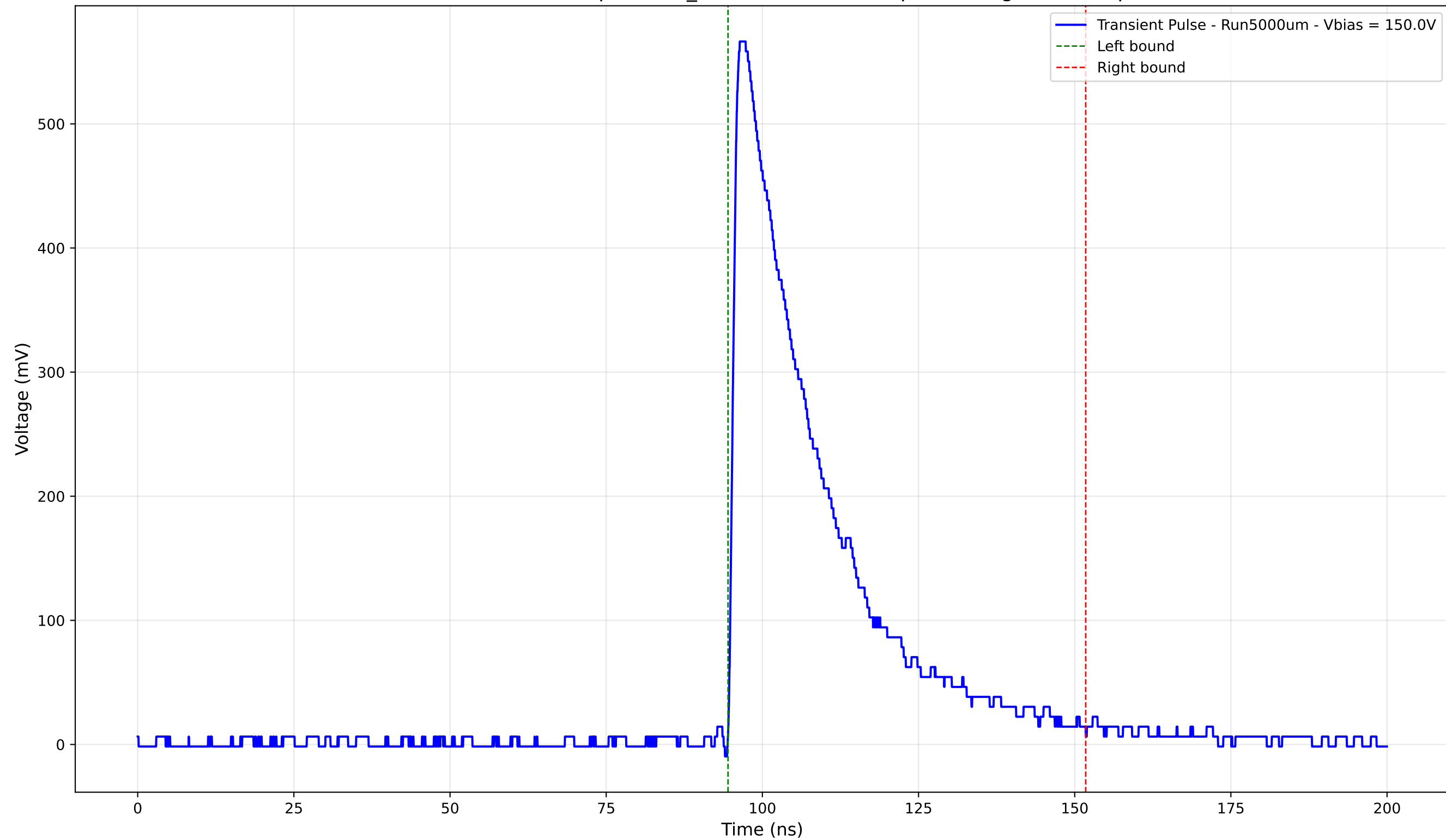
Transient Pulse - Sample: 1cm_42 - Position: 710.0 \mu\text{m} - Charge: 169.30 pC
