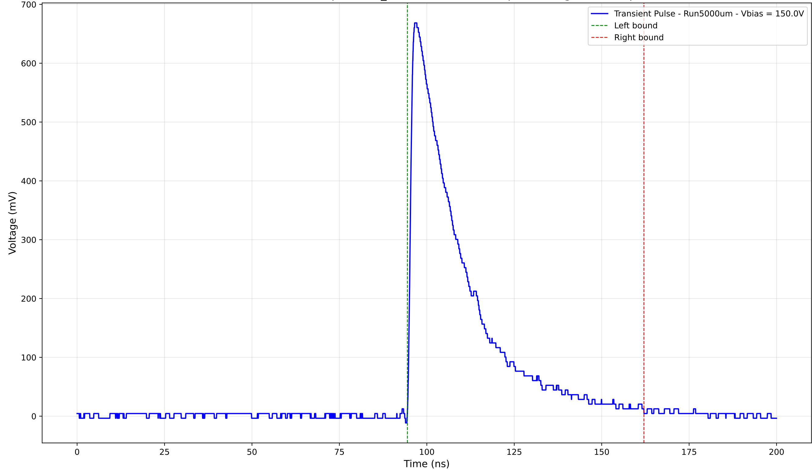
Transient Pulse - Sample: 1cm_42 - Position: 3895.0 \mu\text{m} - Charge: 214.25 pC
