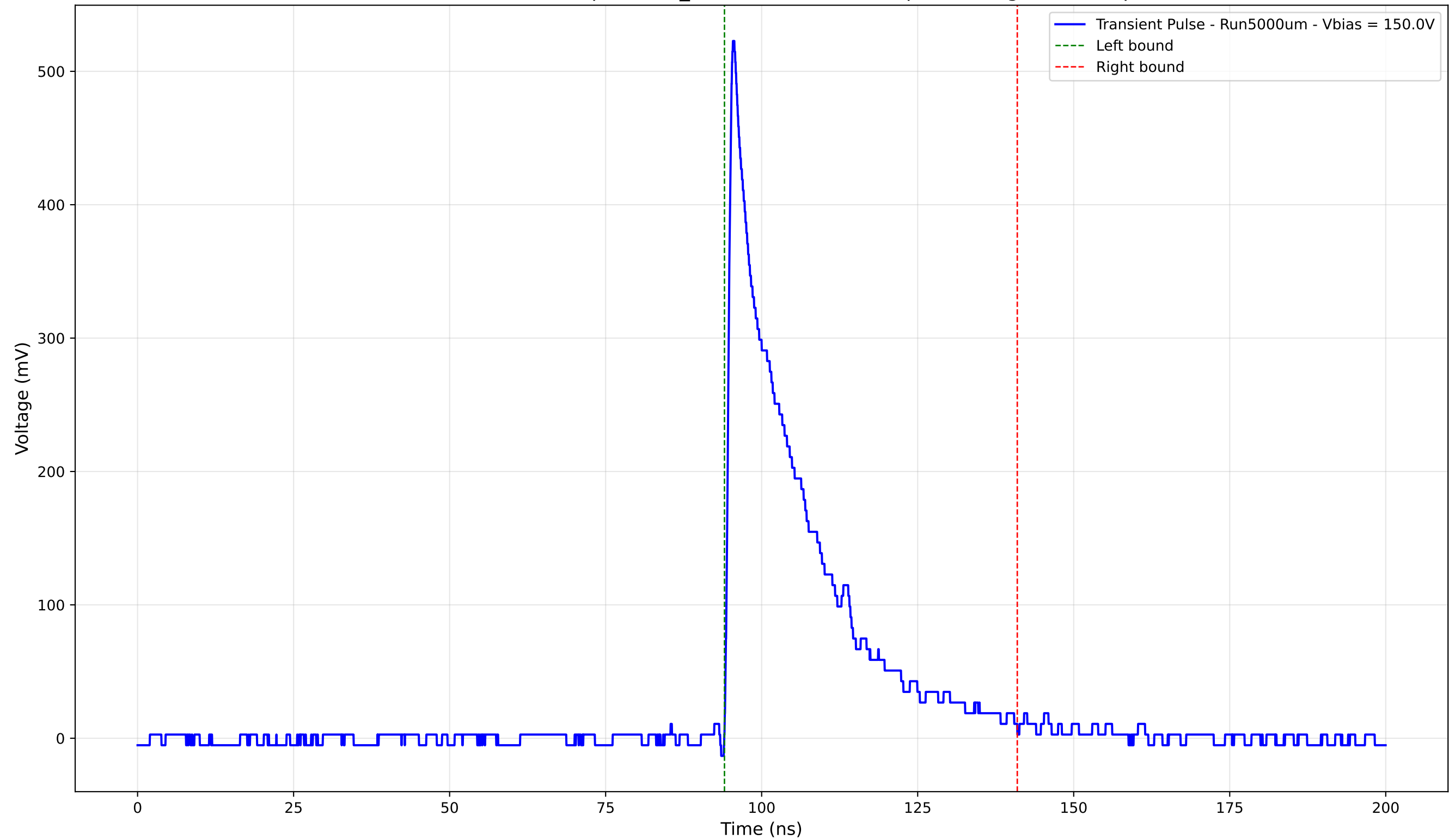
Transient Pulse - Sample: 1cm_42 - Position: 4815.0 \mu\text{m} - Charge: 114.43 pC
