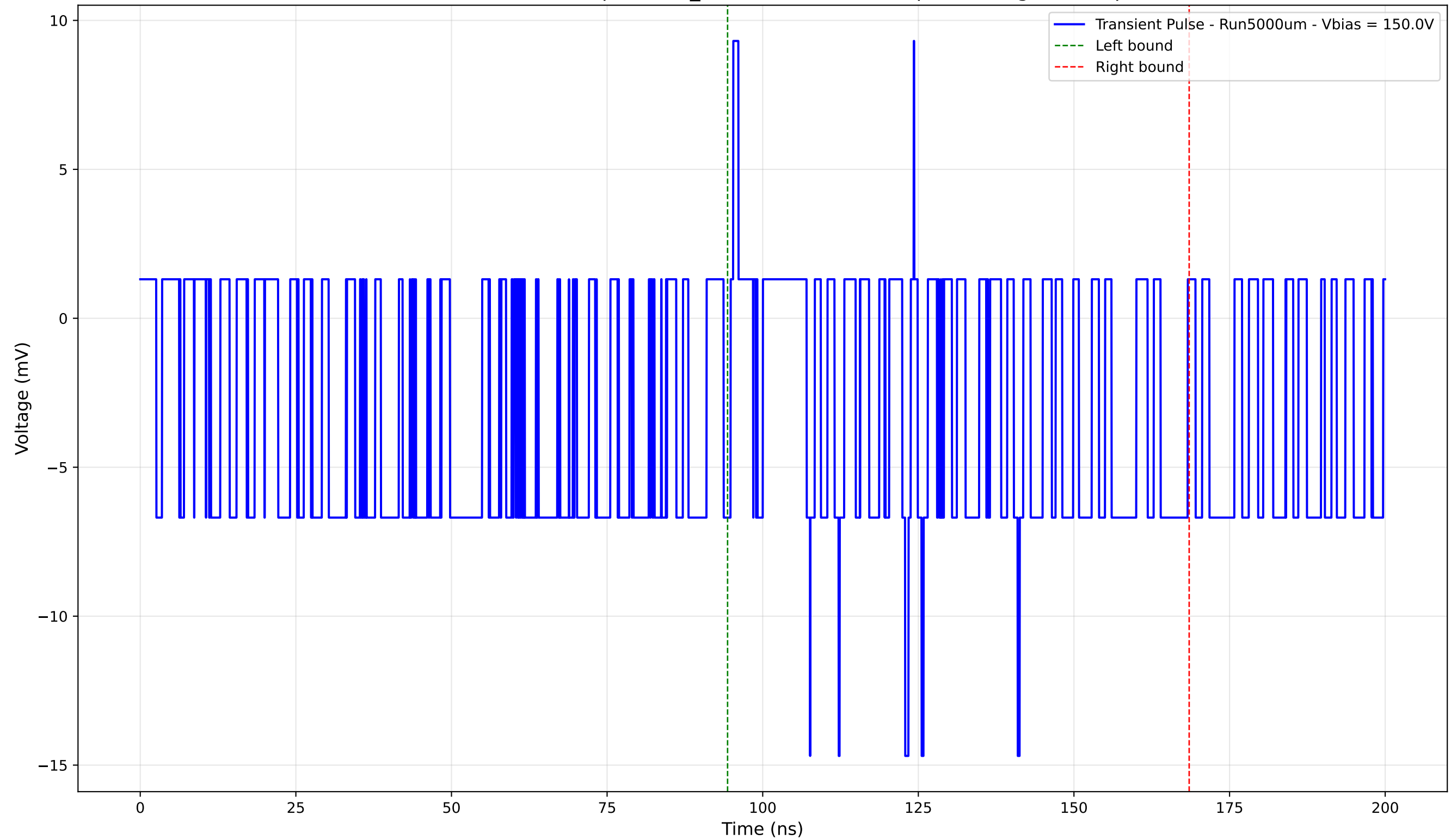
Transient Pulse - Sample: 1cm_42 - Position: 4990.0 \mu\text{m} - Charge: -3.69 pC
