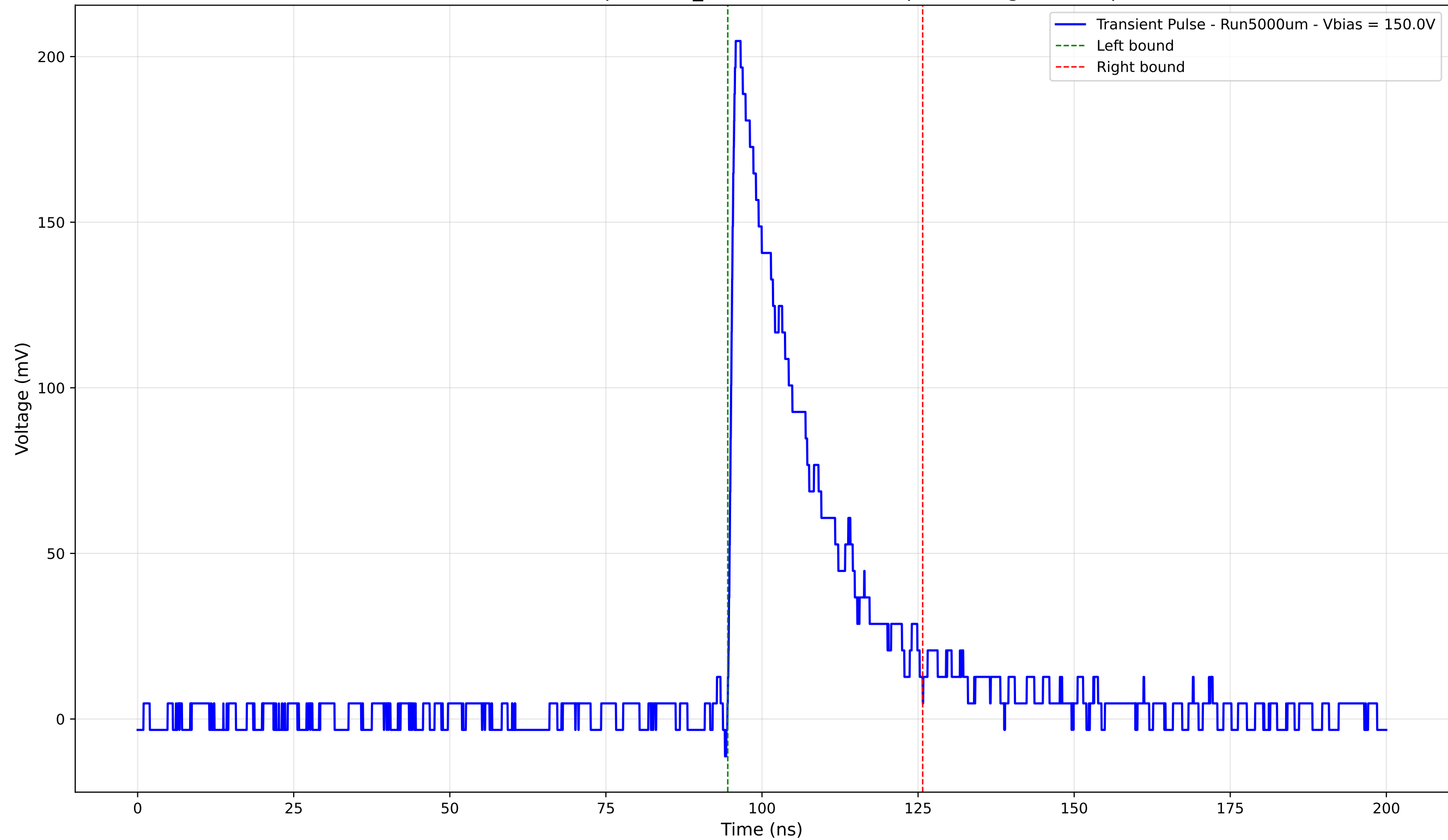
Transient Pulse - Sample: 1cm_42 - Position: 470.0 \mu\text{m} - Charge: 49.21 pC
