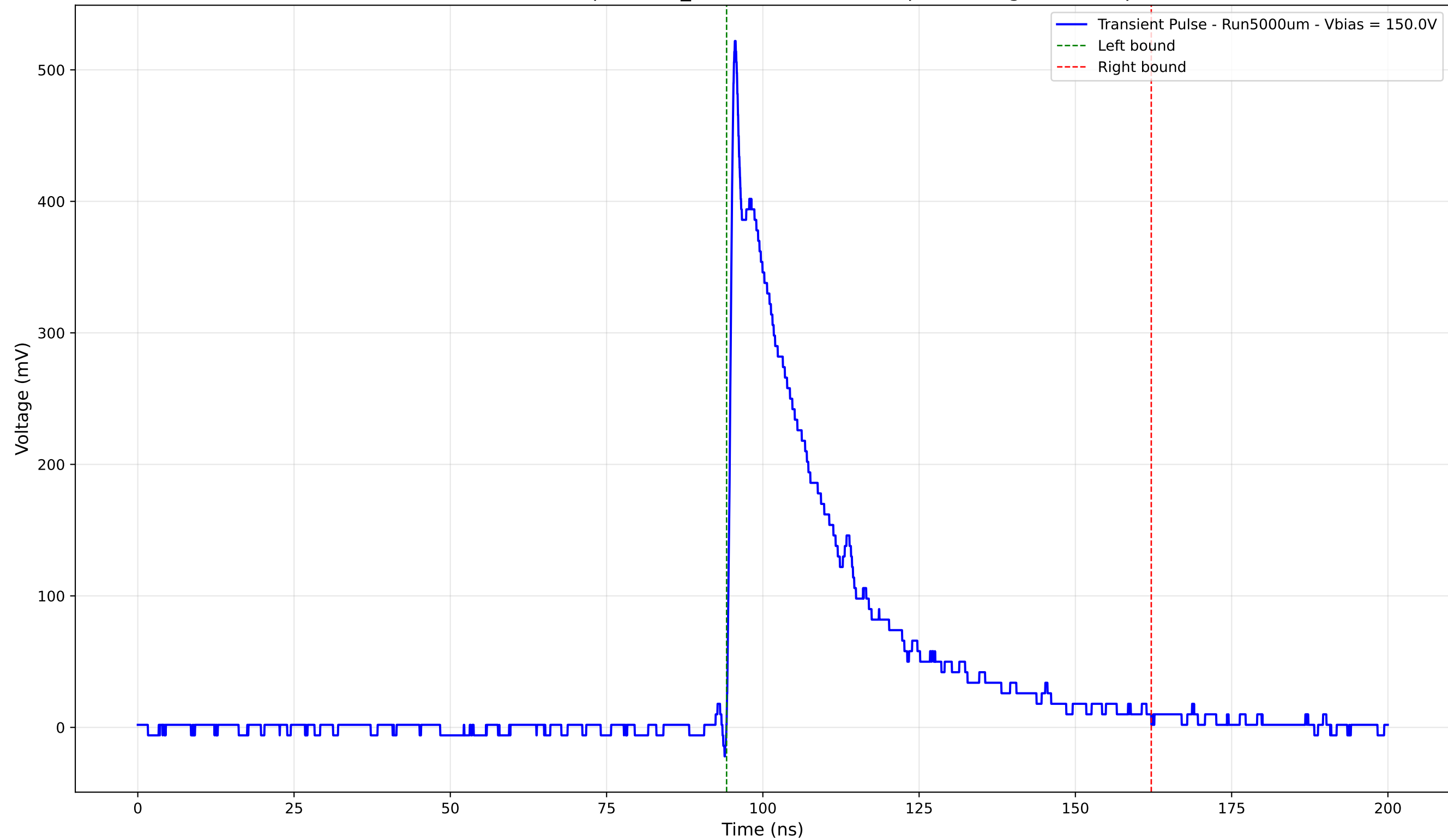
Transient Pulse - Sample: 1cm_42 - Position: 2095.0 \mu\text{m} - Charge: 142.02 pC
