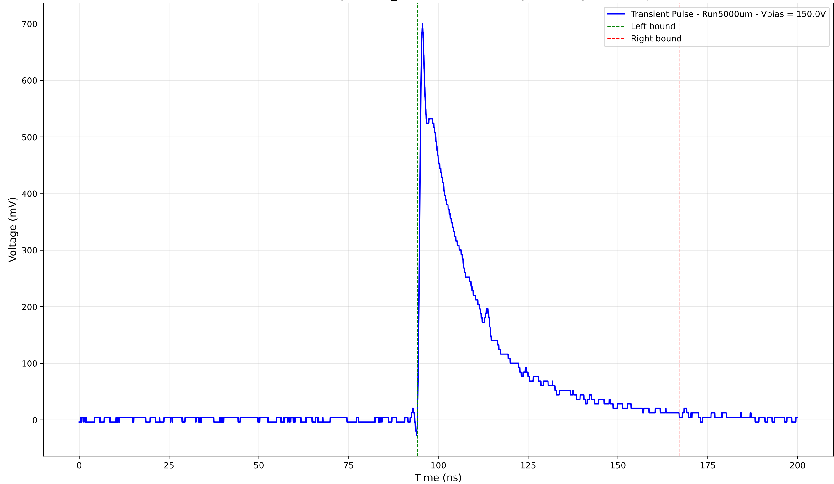
Transient Pulse - Sample: 1cm_42 - Position: 2920.0 \mu\text{m} - Charge: 193.96 pC
