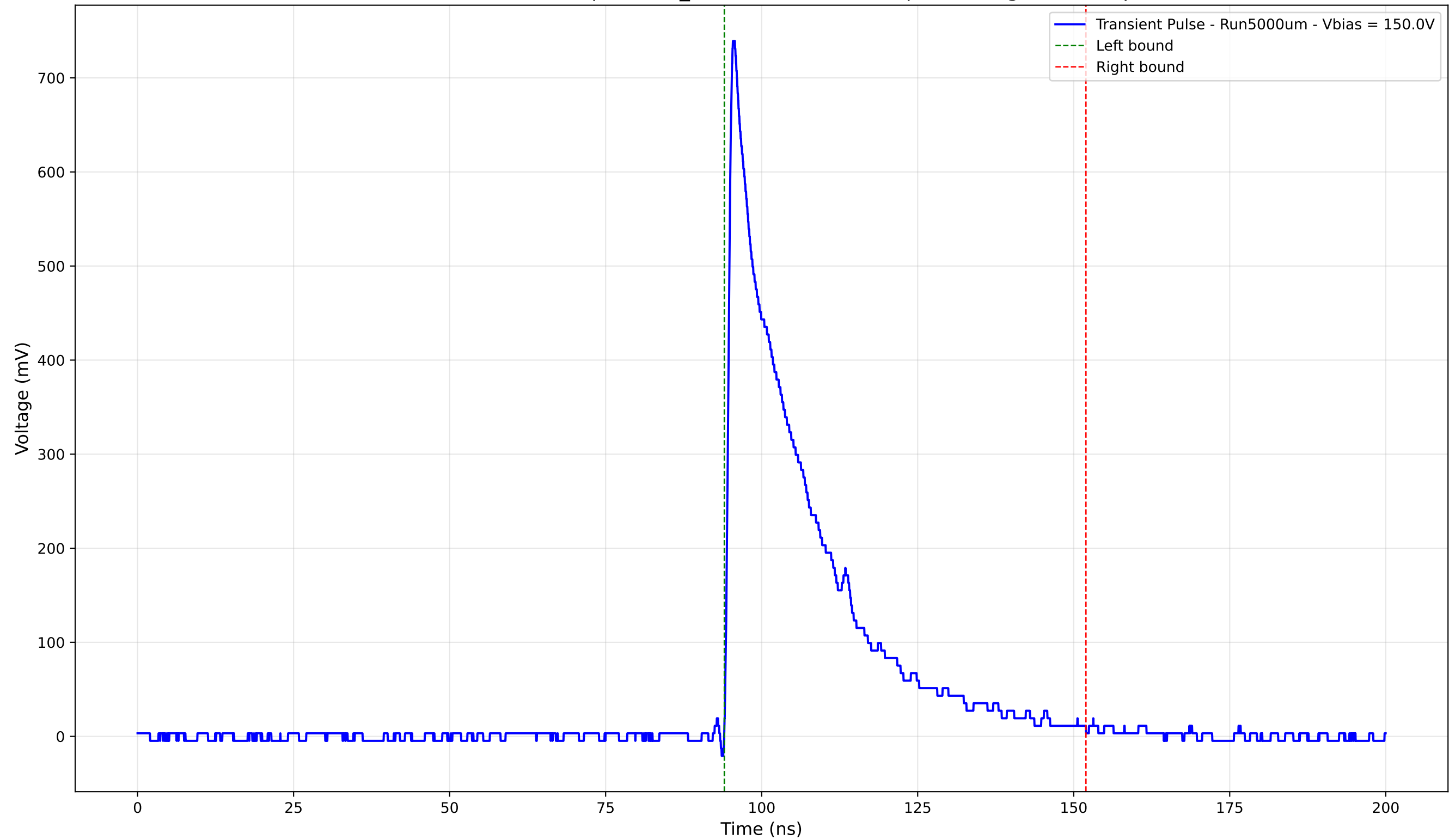
Transient Pulse - Sample: 1cm_42 - Position: 4780.0 \mu\text{m} - Charge: 176.78 pC
