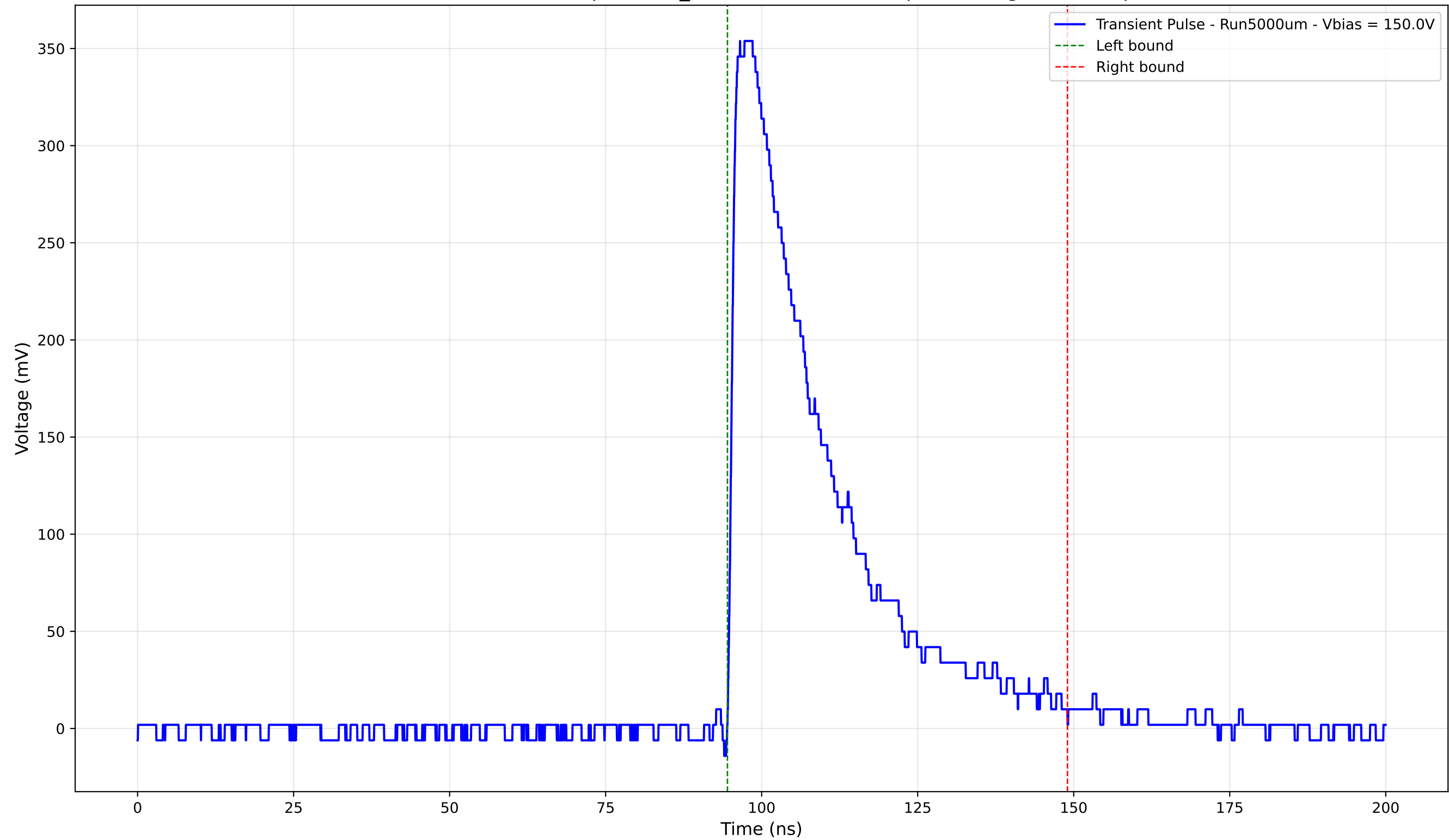
Transient Pulse - Sample: 1cm_42 - Position: 1575.0 \mu\text{m} - Charge: 115.39 pC
