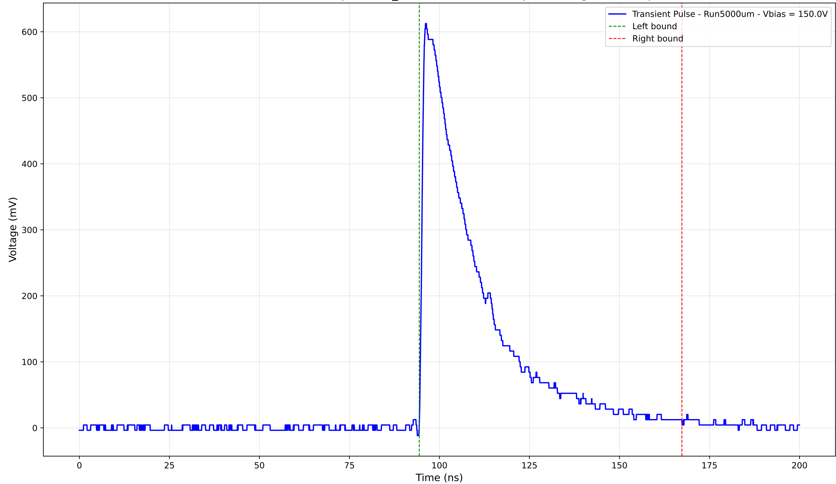
Transient Pulse - Sample: 1cm_42 - Position: 3355.0 \mu\text{m} - Charge: 204.95 pC
