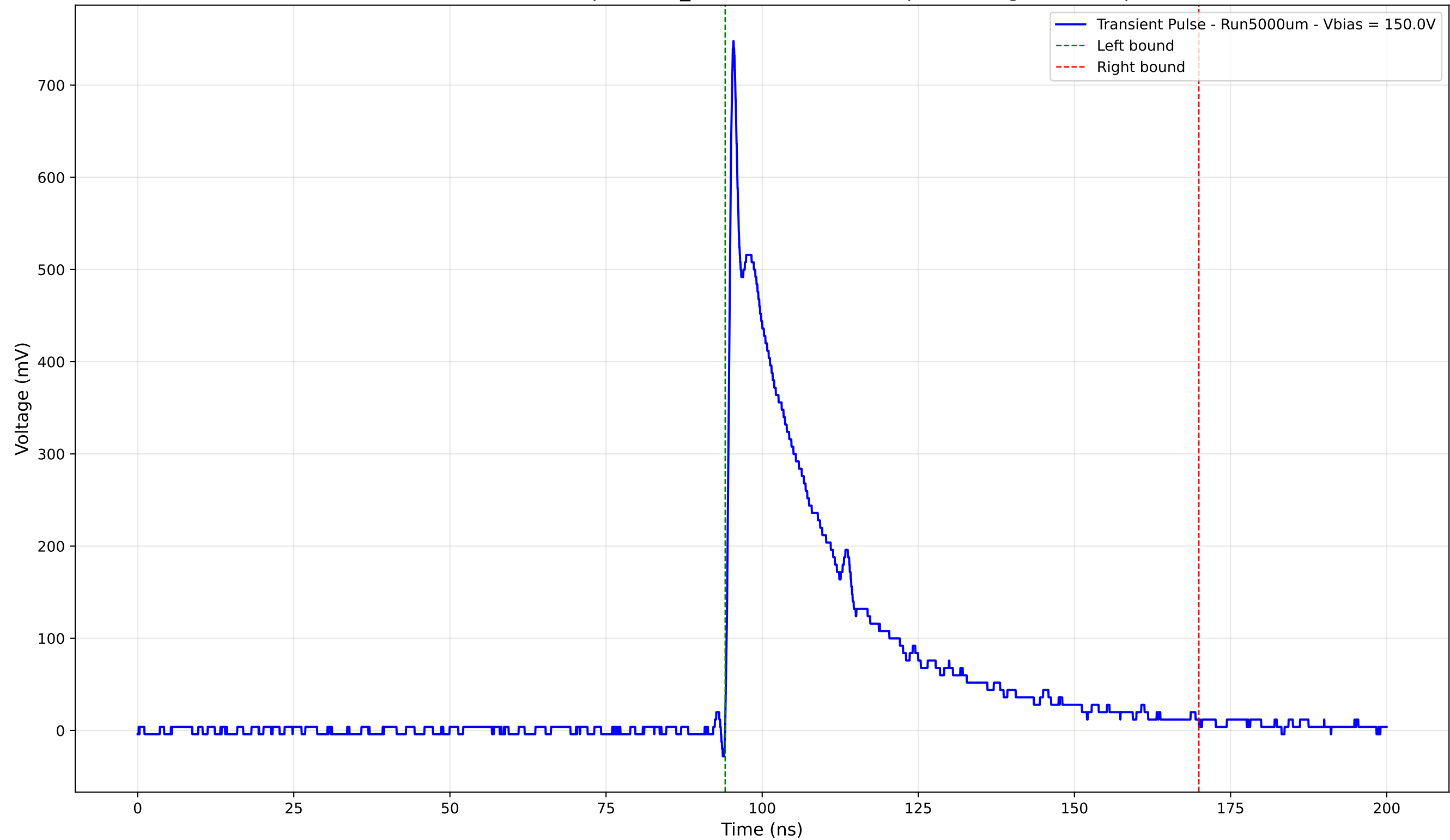
Transient Pulse - Sample: 1cm_42 - Position: 2795.0 \mu\text{m} - Charge: 191.79 pC
