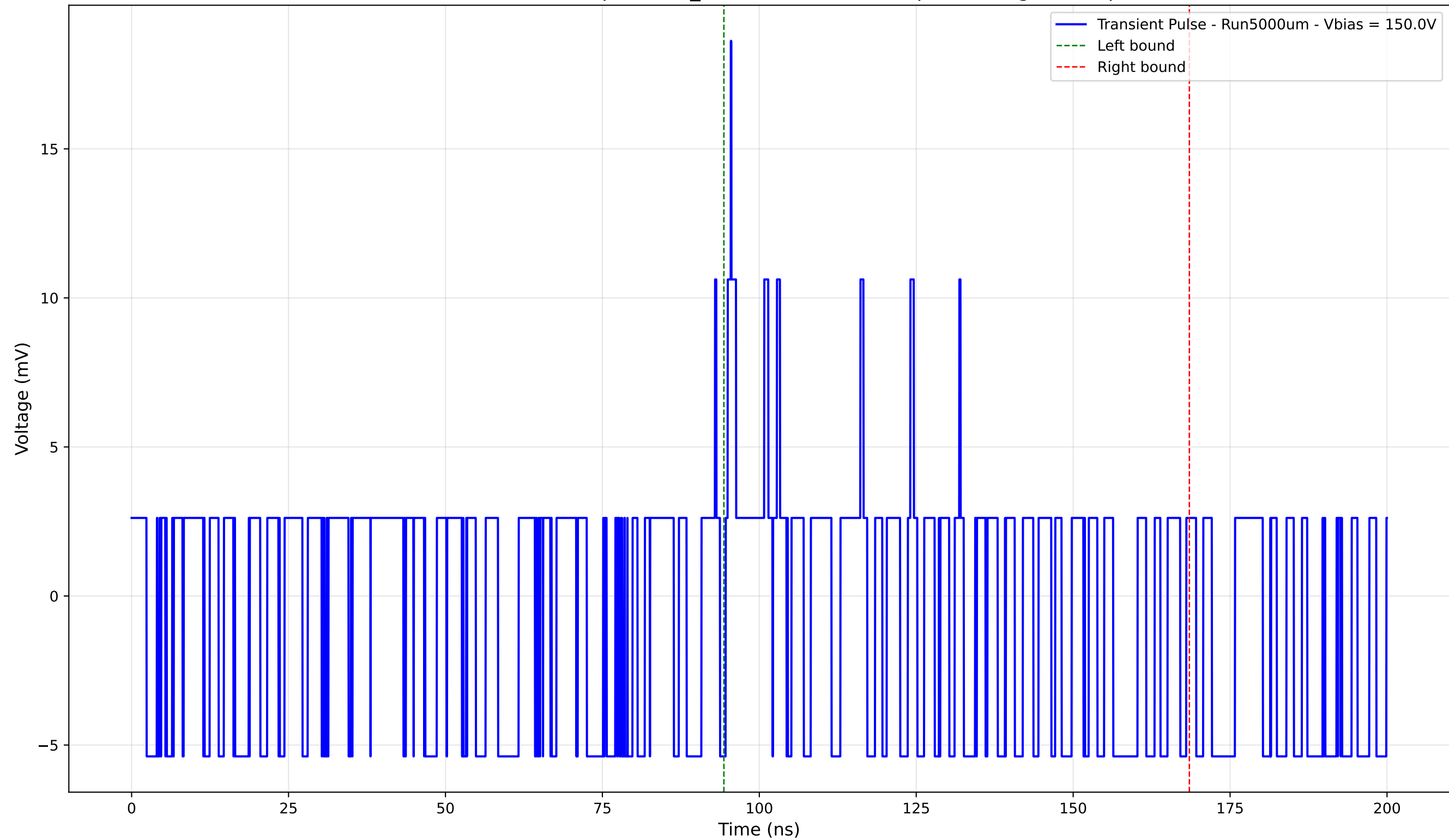
Transient Pulse - Sample: 1cm_42 - Position: 5015.0 \mu\text{m} - Charge: 0.27 pC
