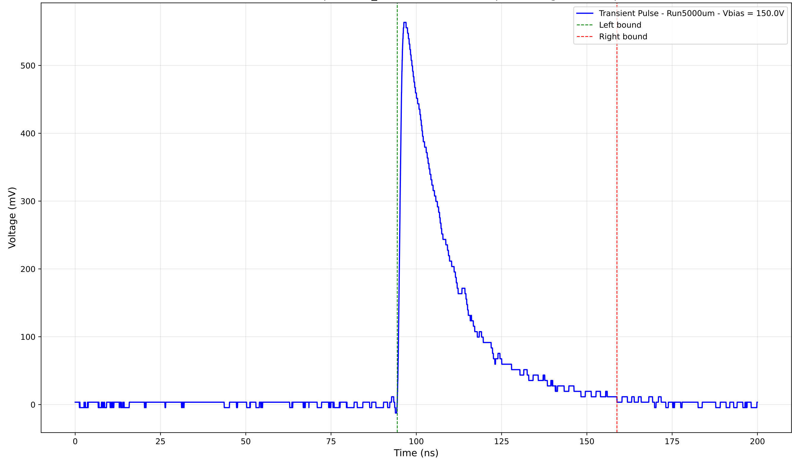
Transient Pulse - Sample: 1cm_42 - Position: 4115.0 \mu\text{m} - Charge: 172.65 pC
