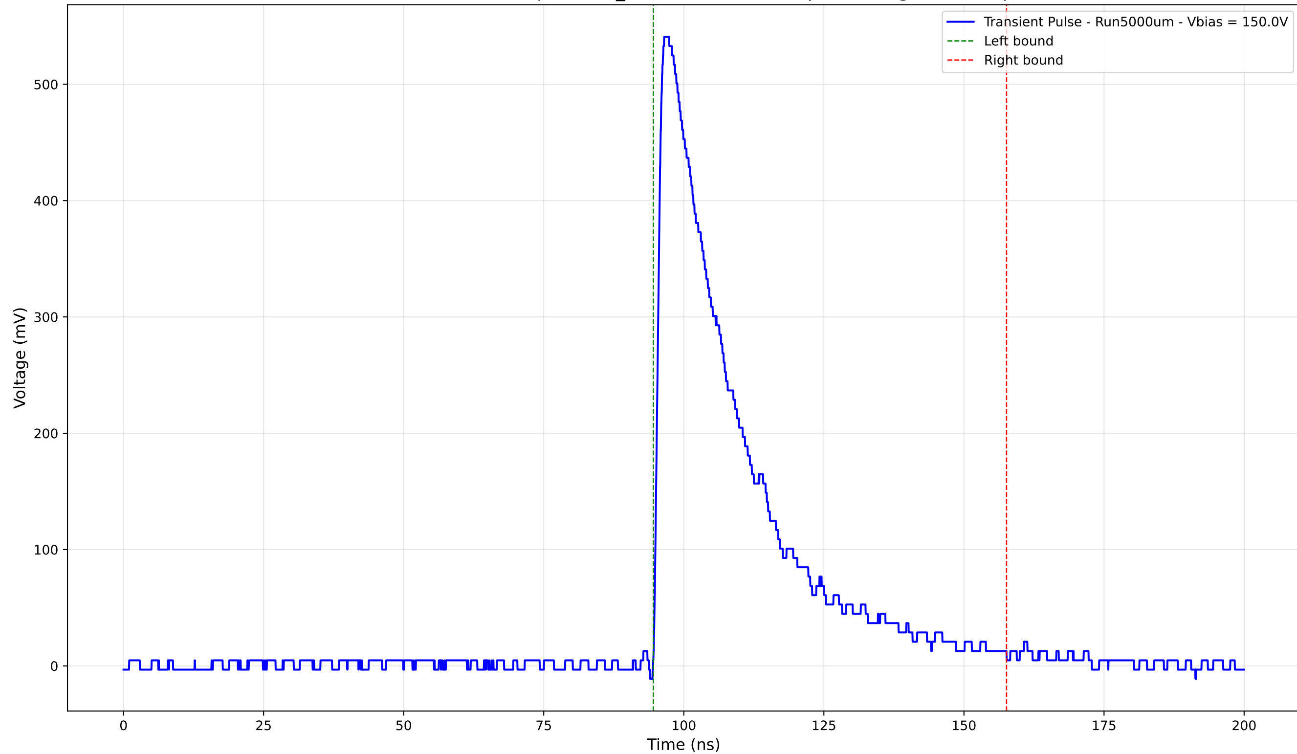
Transient Pulse - Sample: 1cm_42 - Position: 835.0 \mu\text{m} - Charge: 167.38 pC
