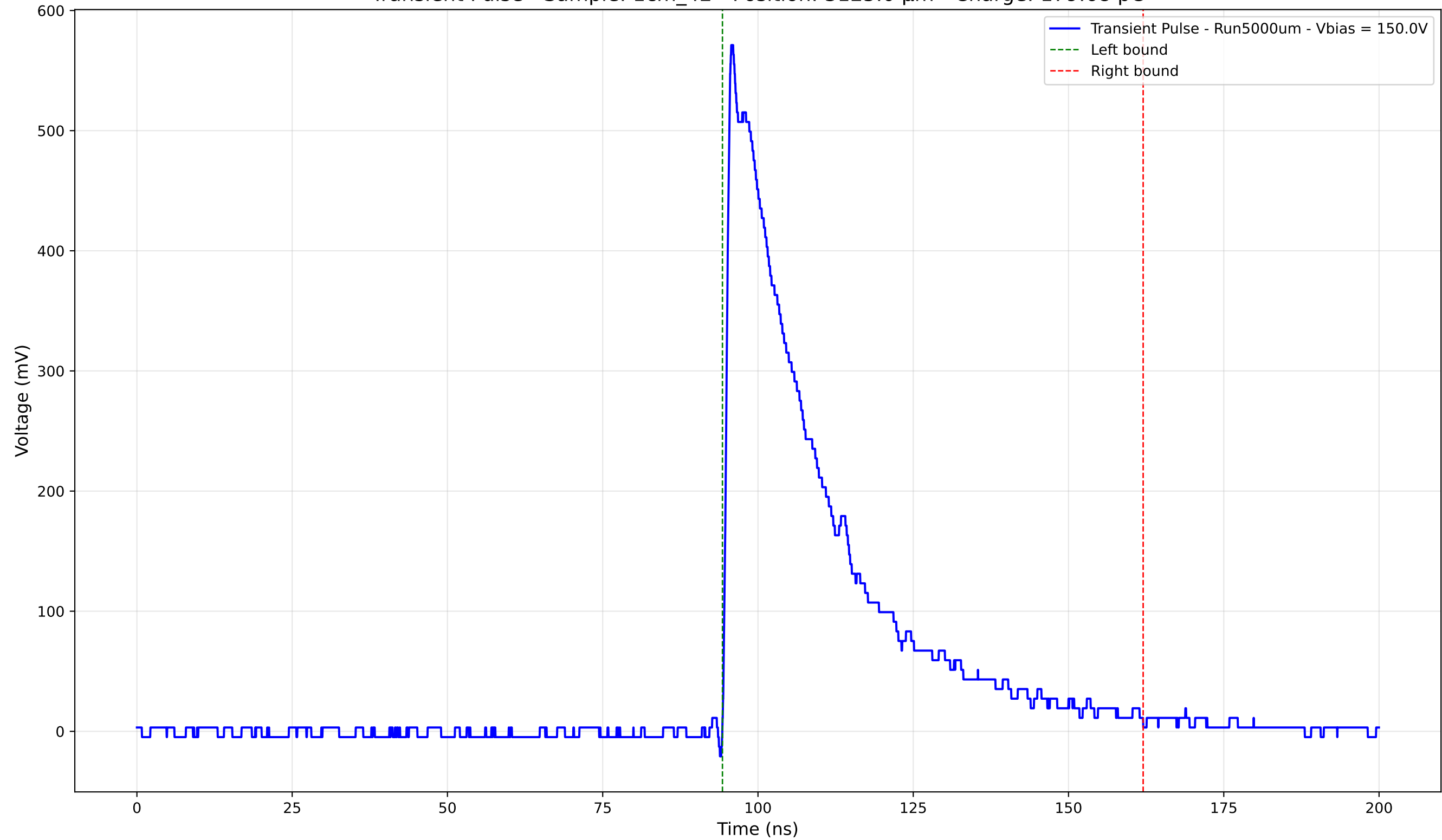
Transient Pulse - Sample: 1cm_42 - Position: 3125.0 \mu\text{m} - Charge: 179.68 pC
