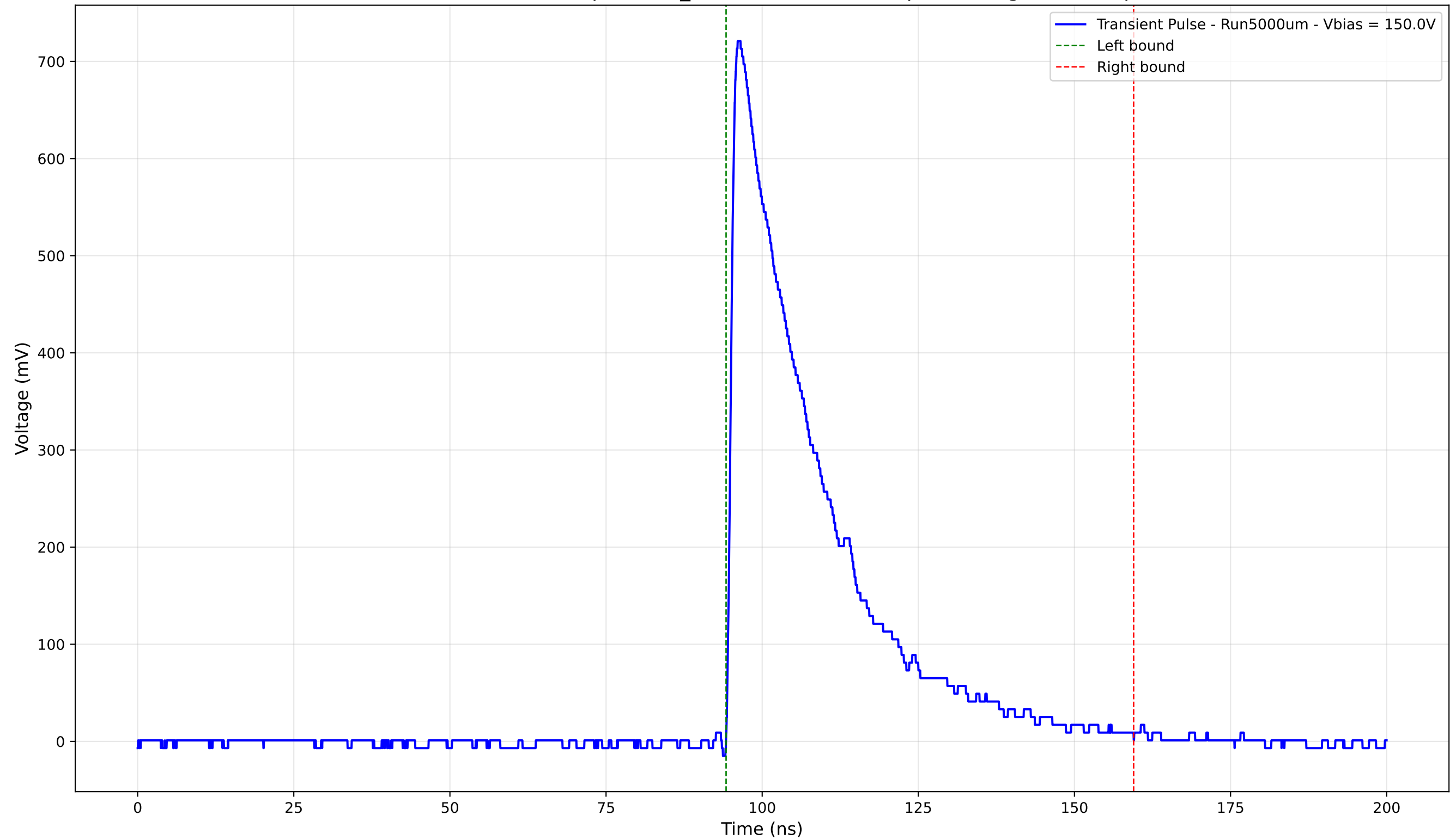
Transient Pulse - Sample: 1cm_42 - Position: 4375.0 \mu\text{m} - Charge: 211.68 pC
