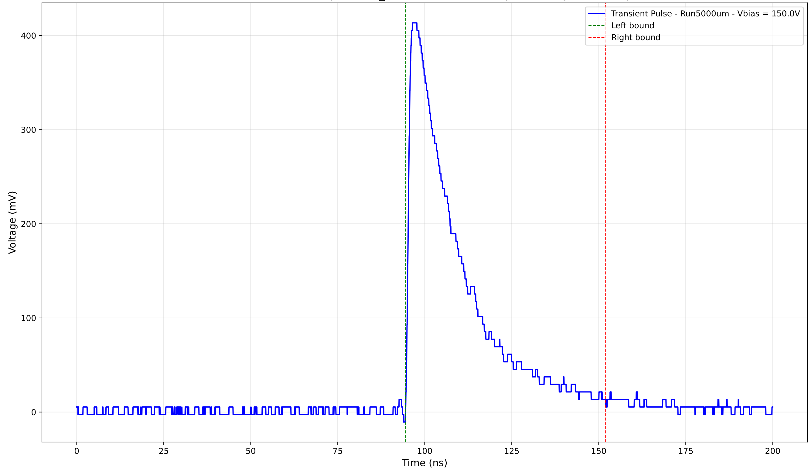
Transient Pulse - Sample: 1cm_42 - Position: 3595.0 \mu\text{m} - Charge: 133.38 pC
