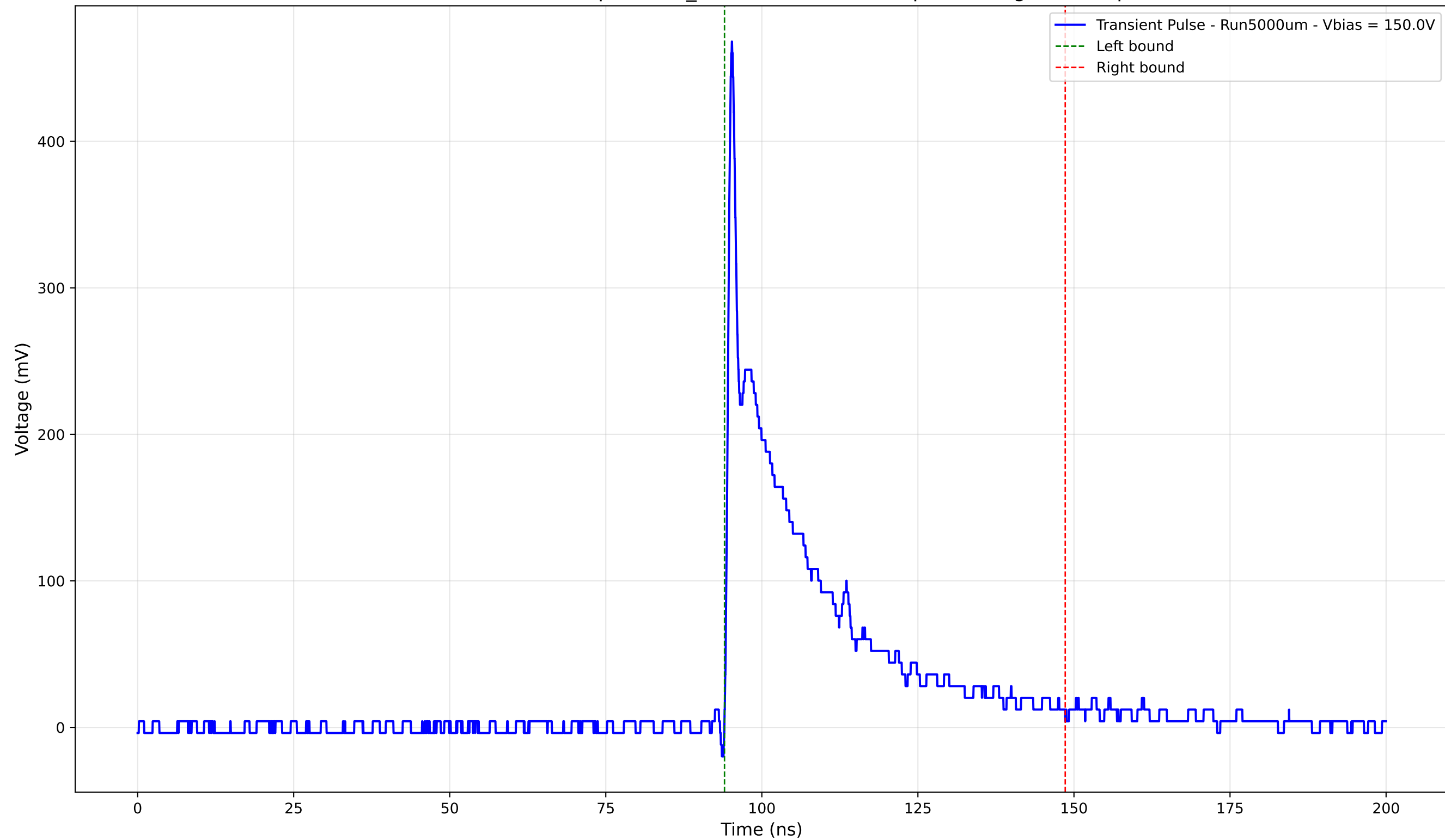
Transient Pulse - Sample: 1cm_42 - Position: 2475.0 \mu\text{m} - Charge: 87.80 pC
