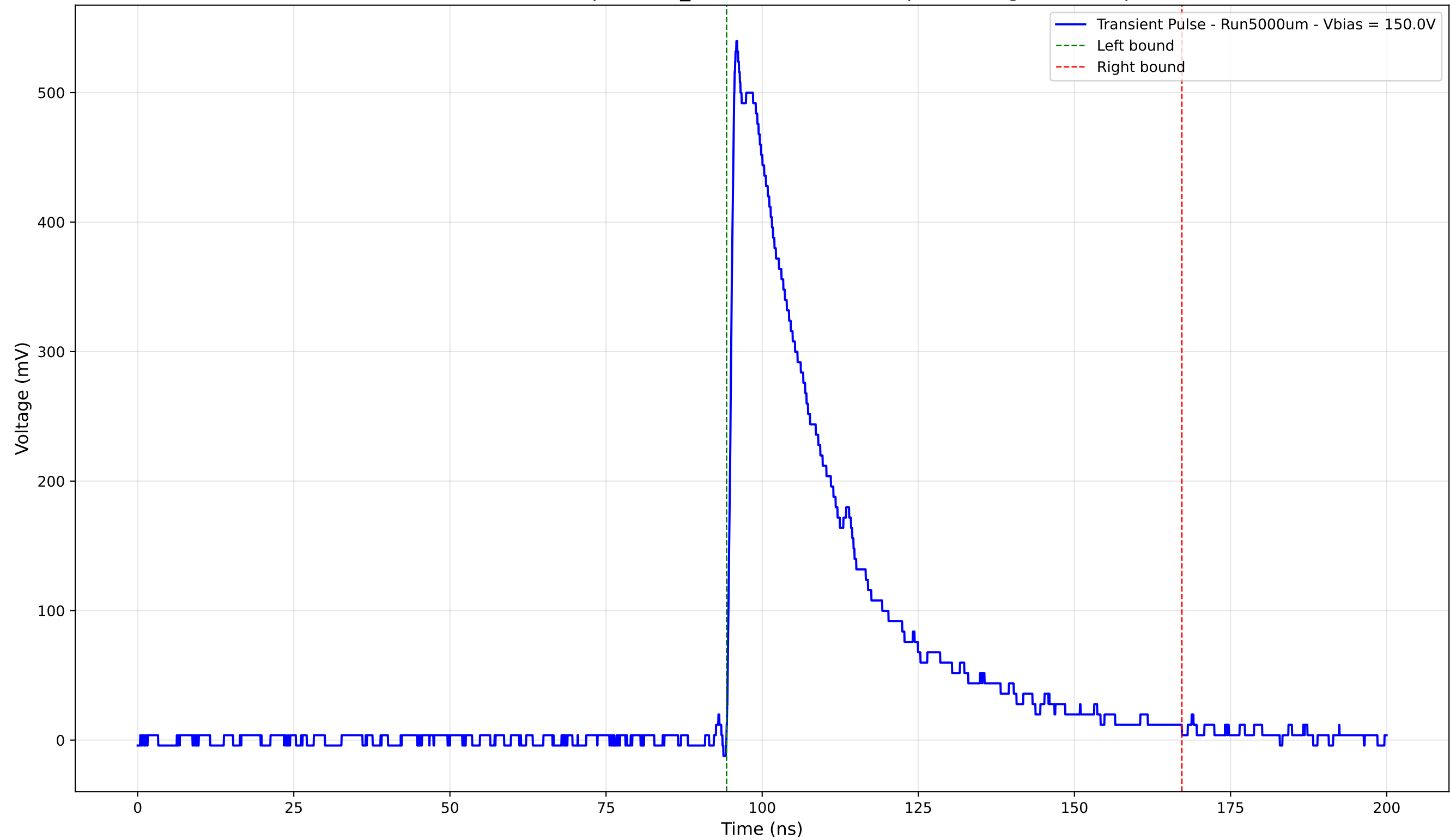
Transient Pulse - Sample: 1cm_42 - Position: 1855.0 \mu\text{m} - Charge: 178.35 pC
