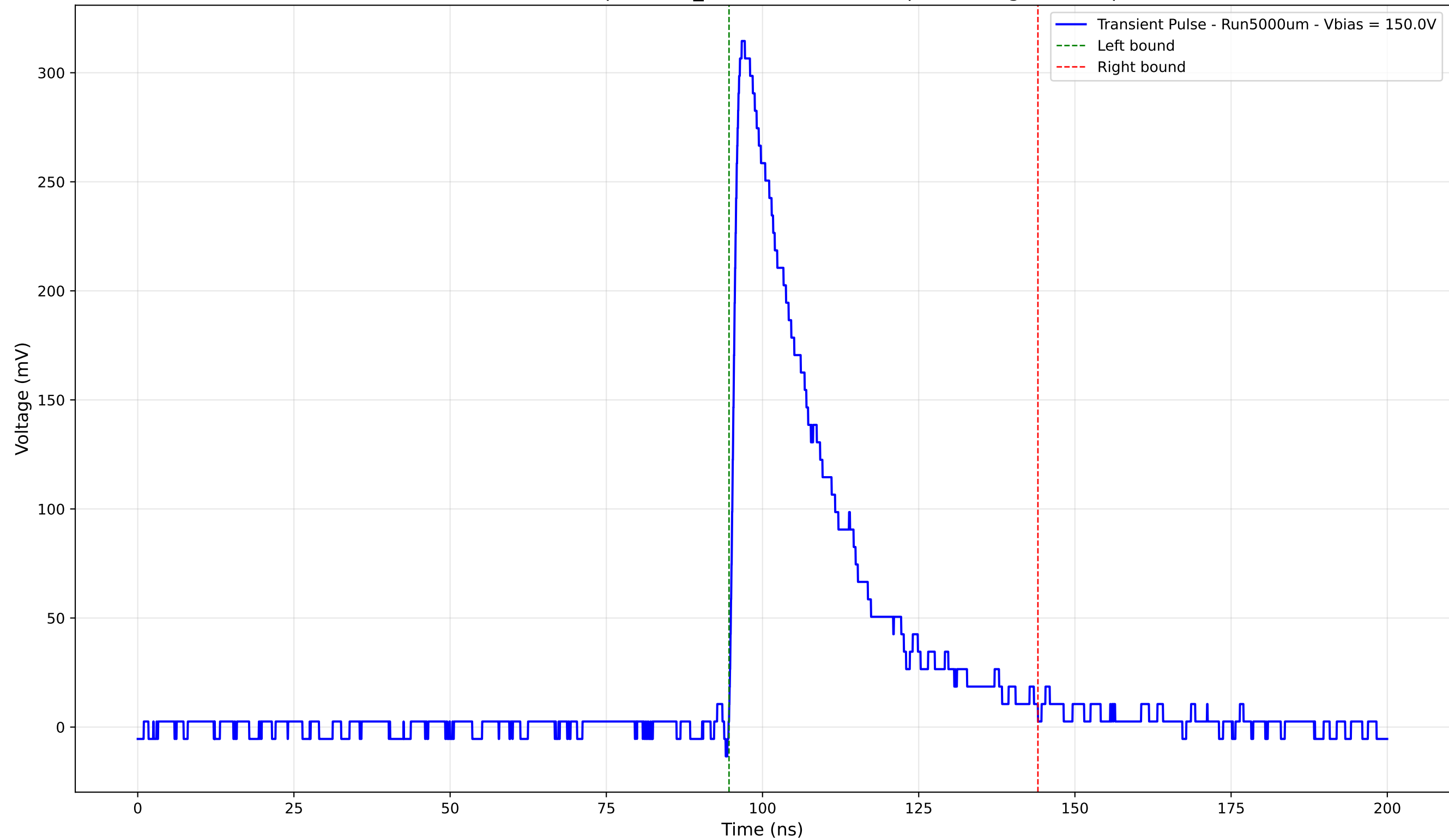
Transient Pulse - Sample: 1cm_42 -Position: 955.0 \mu\text{m} - Charge: 91.37 pC
