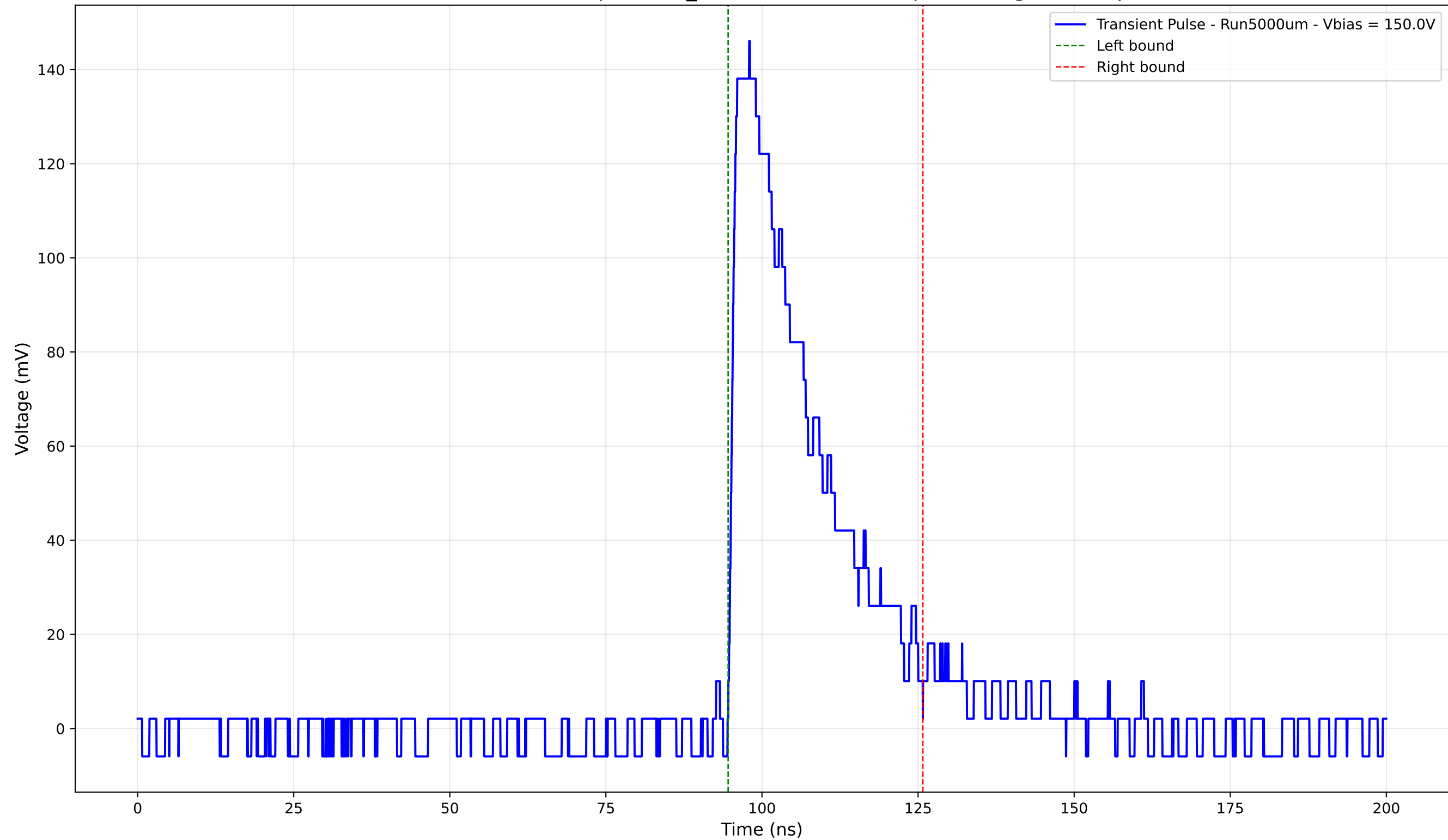
Transient Pulse - Sample: 1cm_42 - Position: 4055.0 \mu\text{m} - Charge: 40.00 pC
