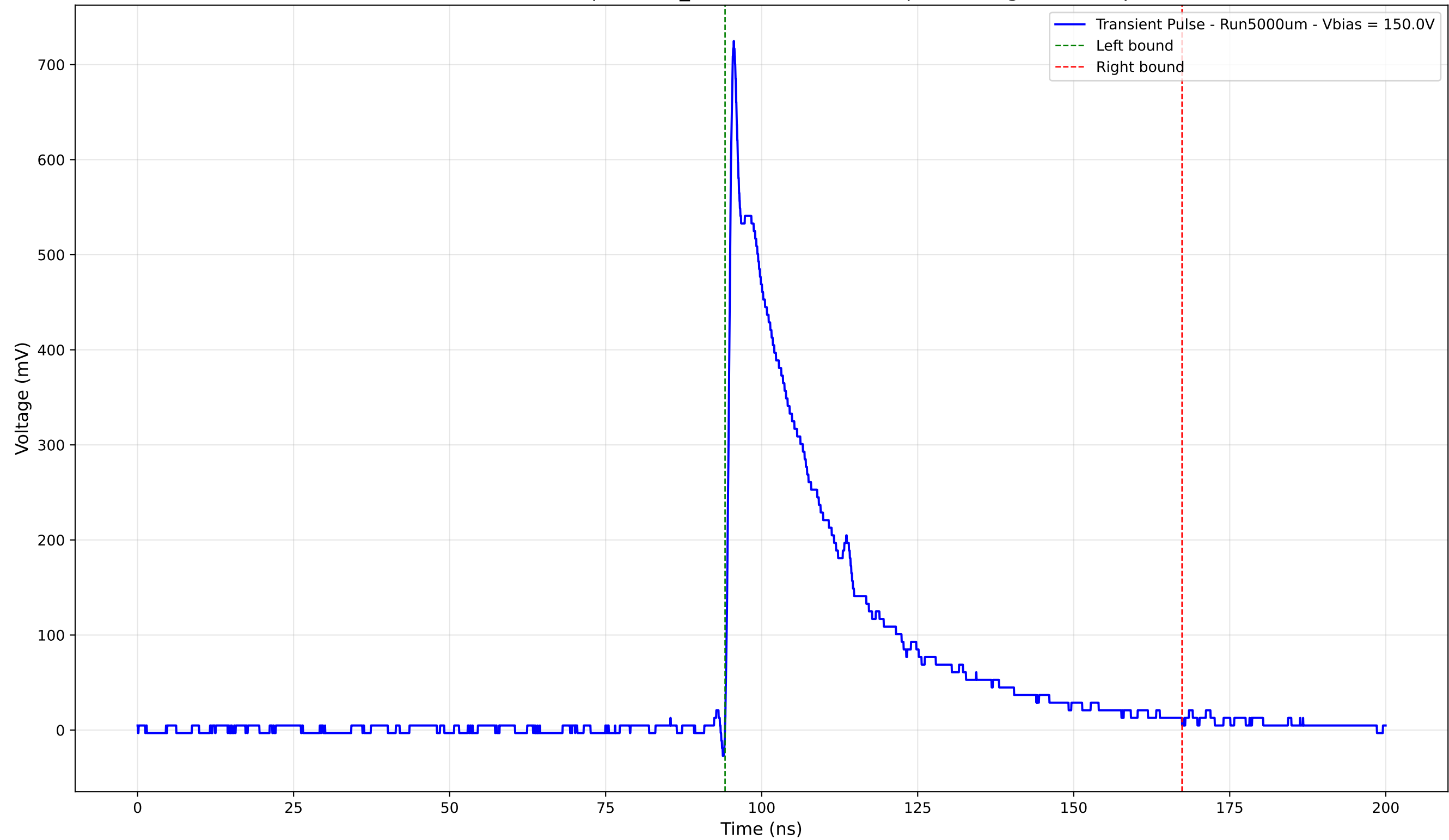
Transient Pulse - Sample: 1cm_42 - Position: 2895.0 \mu\text{m} - Charge: 199.77 pC
