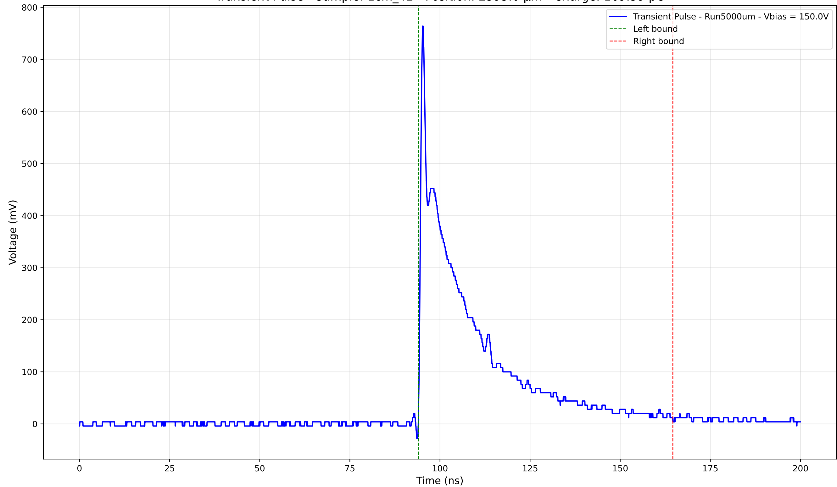
Transient Pulse - Sample: 1cm_42 - Position: 2395.0 \mu\text{m} - Charge: 169.59 pC
