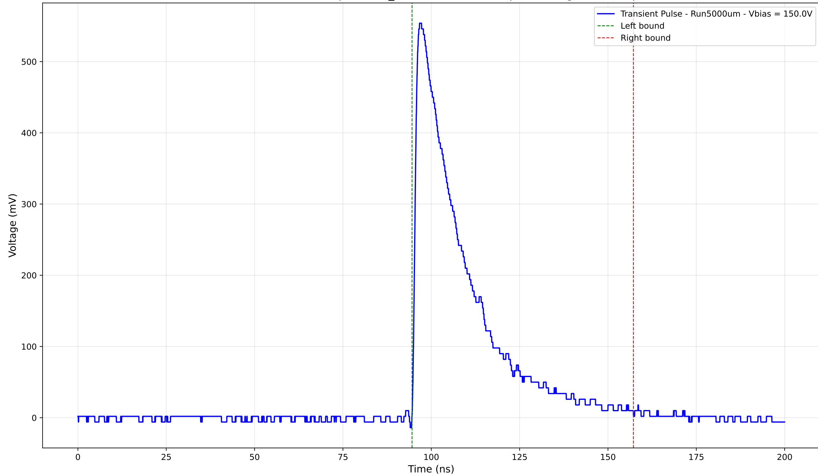
Transient Pulse - Sample: 1cm_42 - Position: 885.0 \mu\text{m} - Charge: 167.62 pC
