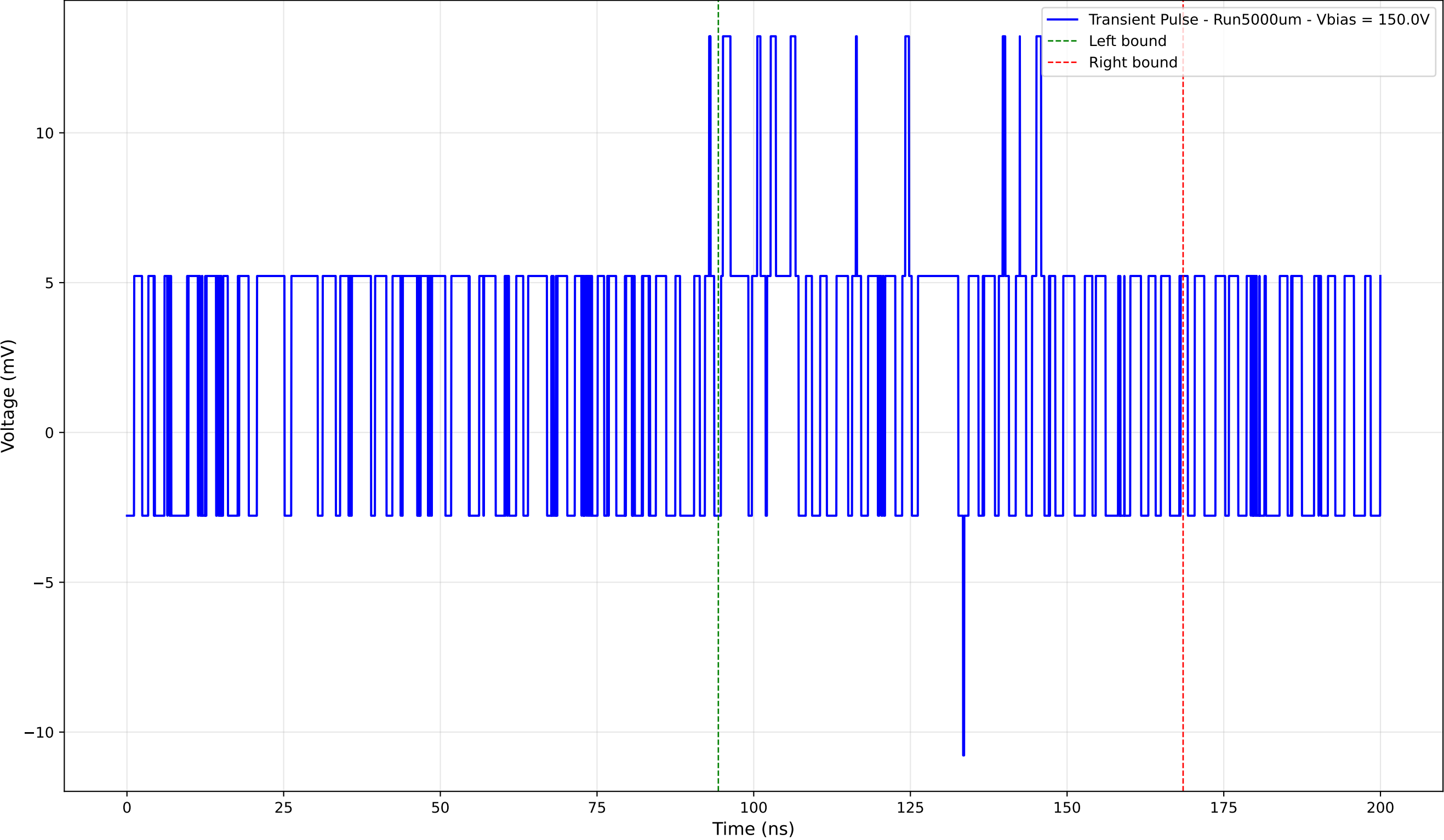
Transient Pulse - Sample: 1cm_42 - Position: 4960.0 \mu\text{m} - Charge: 4.36 pC
