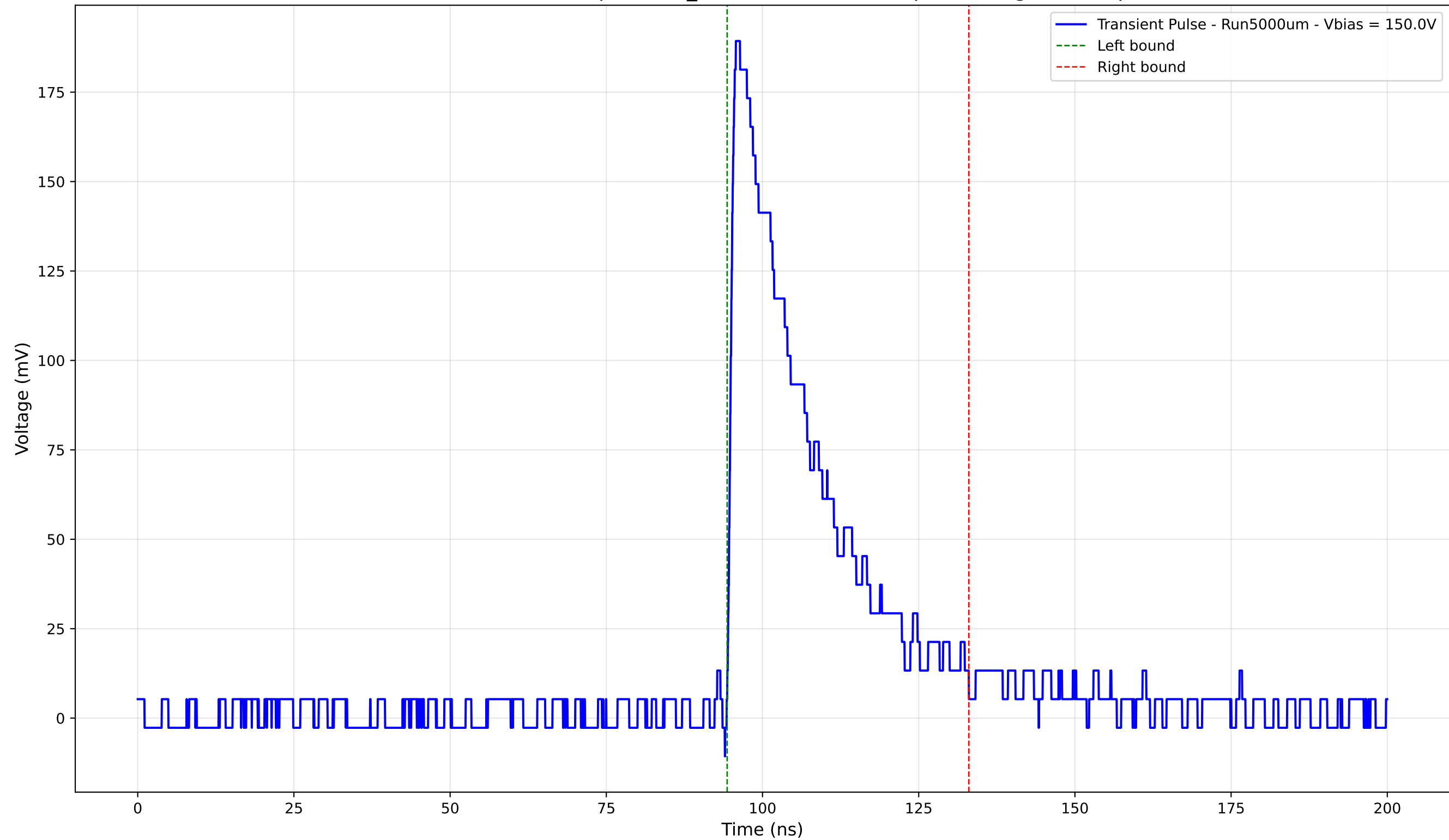
Transient Pulse - Sample: 1cm_42 - Position: 4520.0 \mu\text{m} - Charge: 51.33 pC
