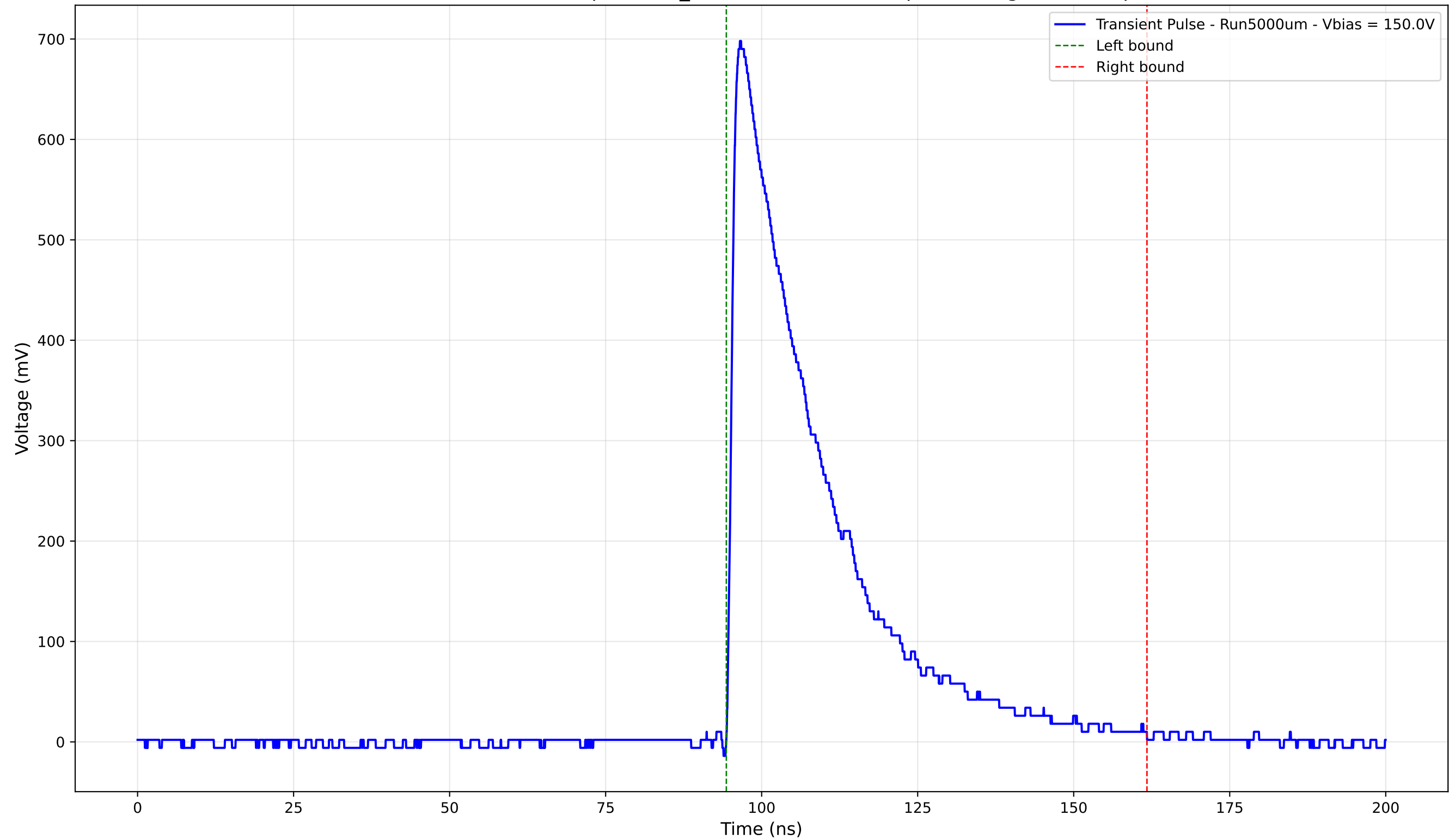
Transient Pulse - Sample: 1cm_42 - Position: 4165.0 \mu\text{m} - Charge: 213.06 pC
