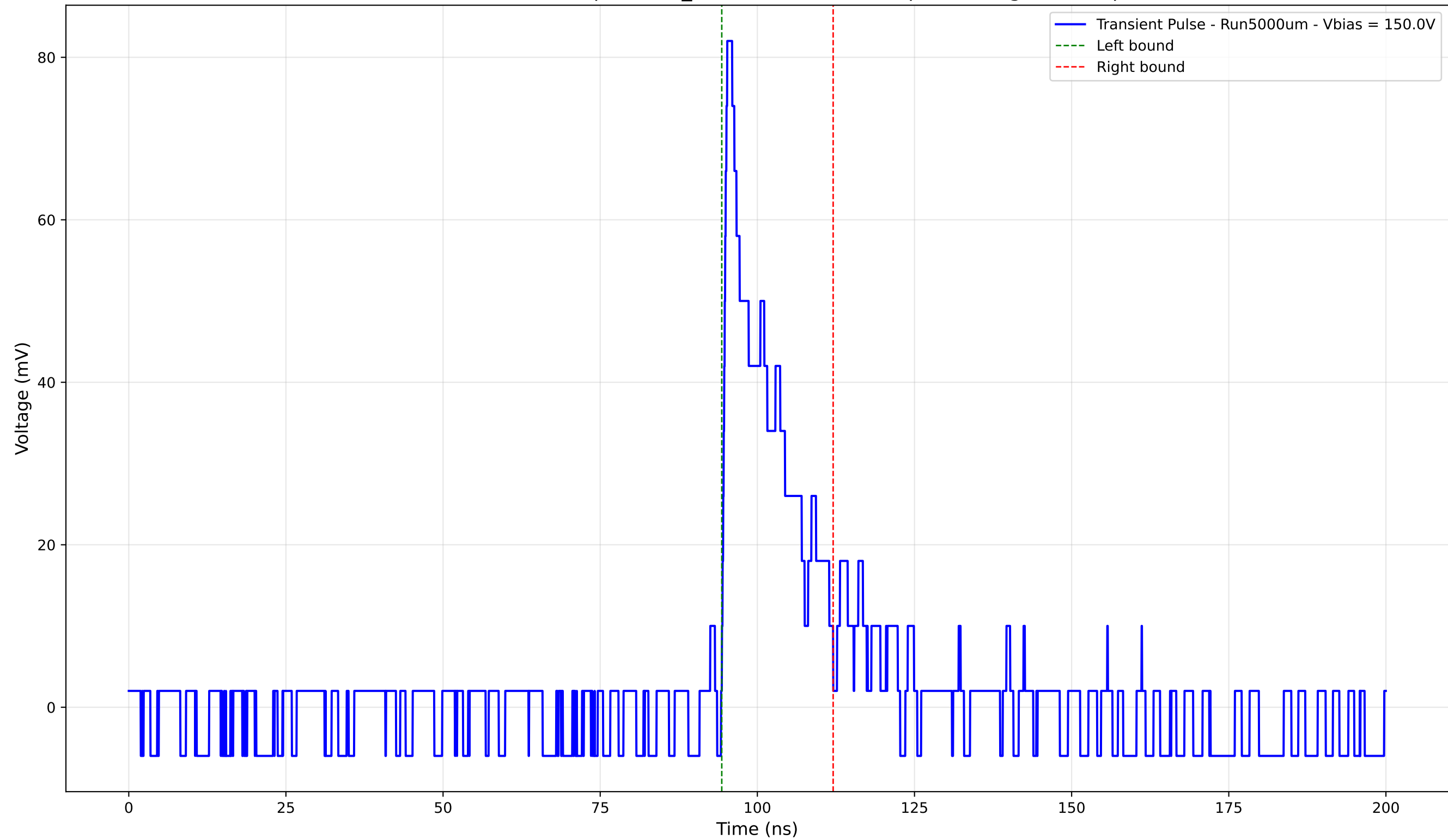
Transient Pulse - Sample: 1cm_42 - Position: 4870.0 \mu\text{m} - Charge: 12.75 pC
