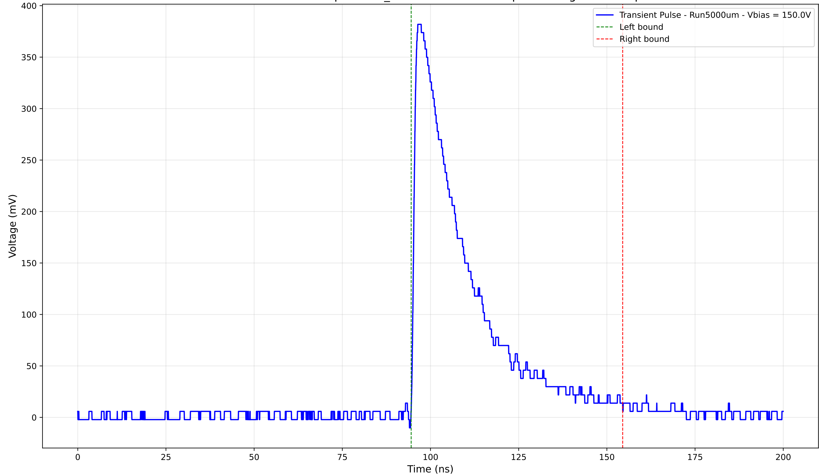
Transient Pulse - Sample: 1cm_42 - Position: 3590.0 \mu\text{m} - Charge: 123.74 pC
