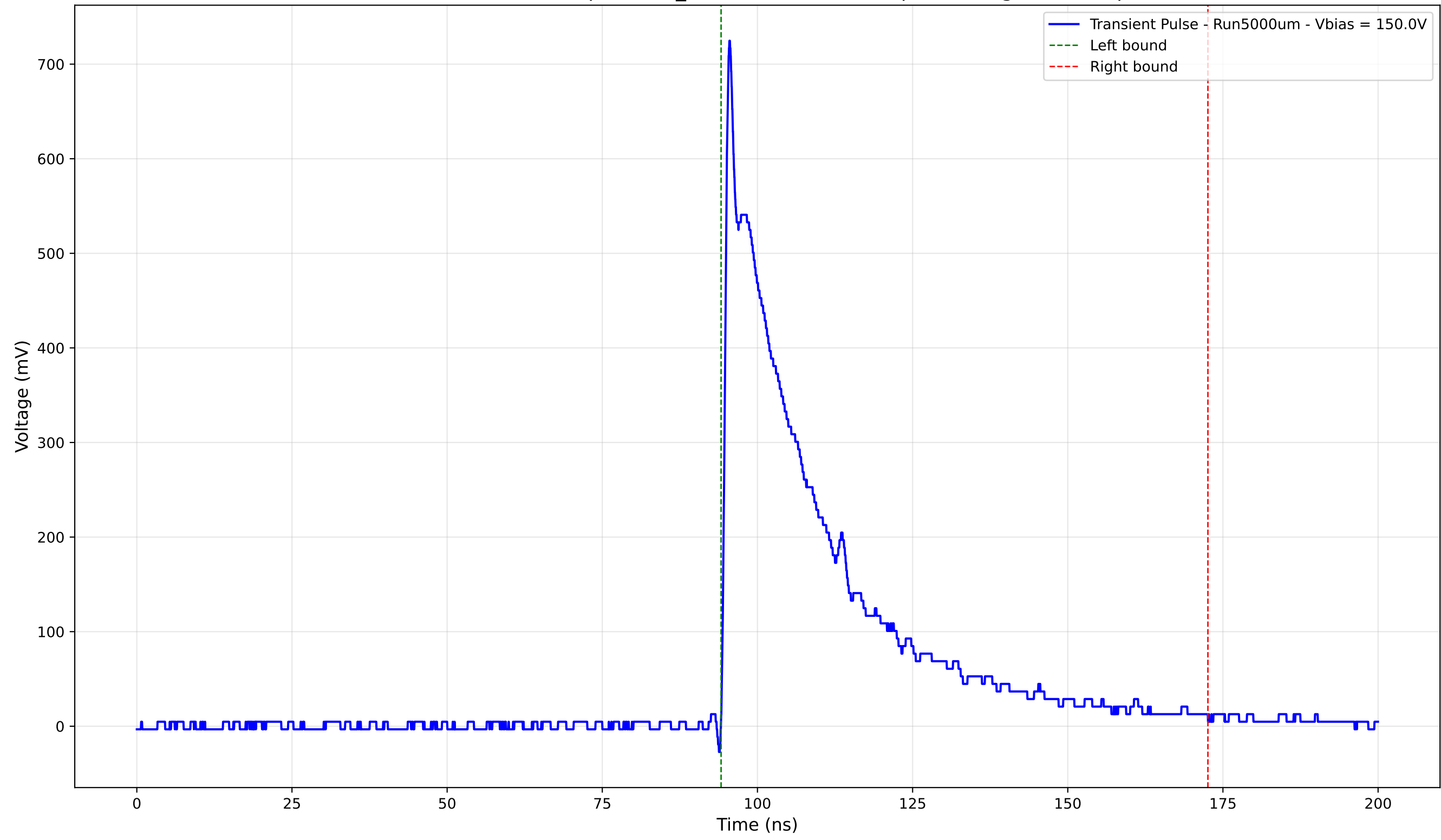
Transient Pulse - Sample: 1cm_42 - Position: 2885.0 \mu\text{m} - Charge: 200.21 pC
