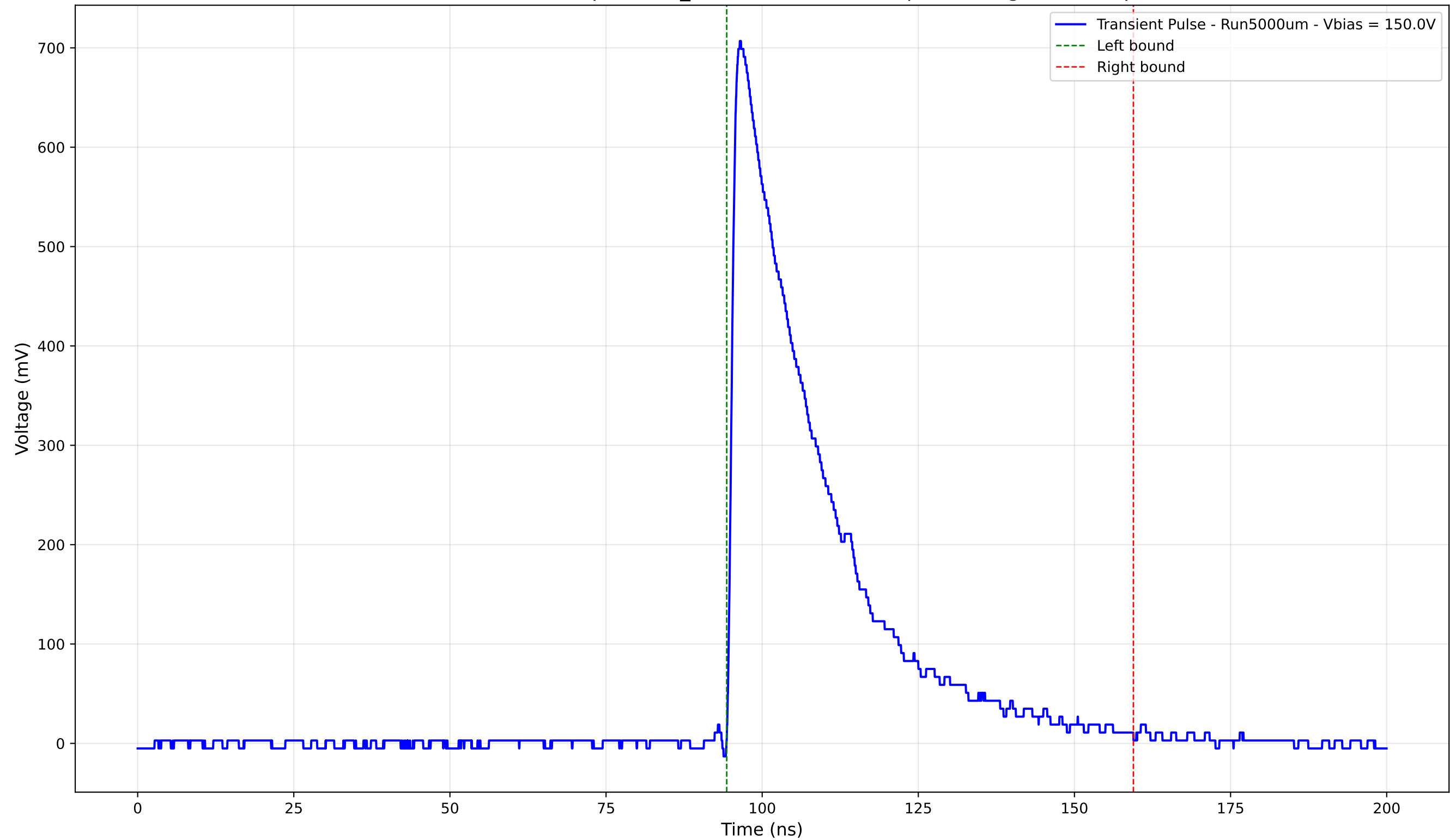
Transient Pulse - Sample: 1cm_42 - Position: 4235.0 \mu\text{m} - Charge: 214.29 pC
