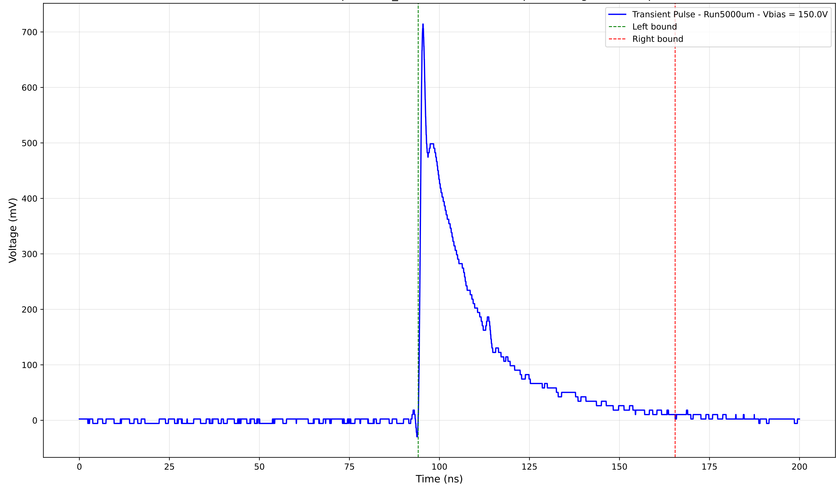
Transient Pulse - Sample: 1cm_42 - Position: 2220.0 \mu\text{m} - Charge: 182.71 pC
