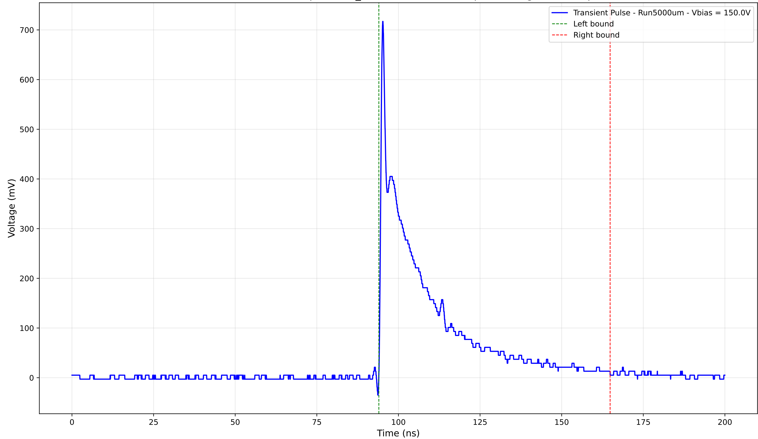
Transient Pulse - Sample: 1cm_42 - Position: 2605.0 \mu\text{m} - Charge: 151.41 pC
