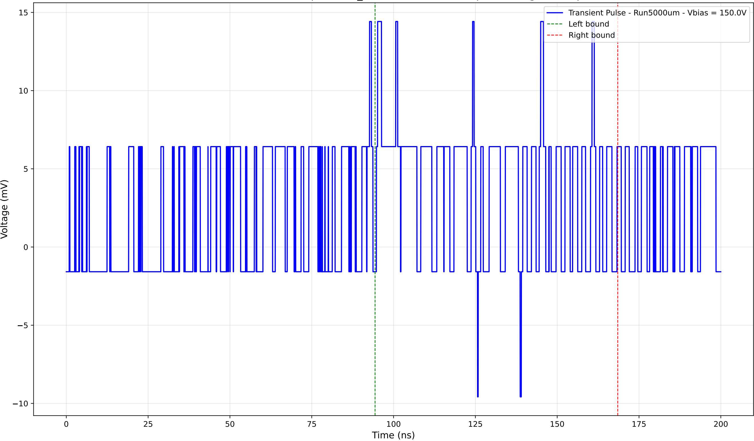
Transient Pulse - Sample: 1cm_42 - Position: 4955.0 \mu\text{m} - Charge: 6.00 pC
