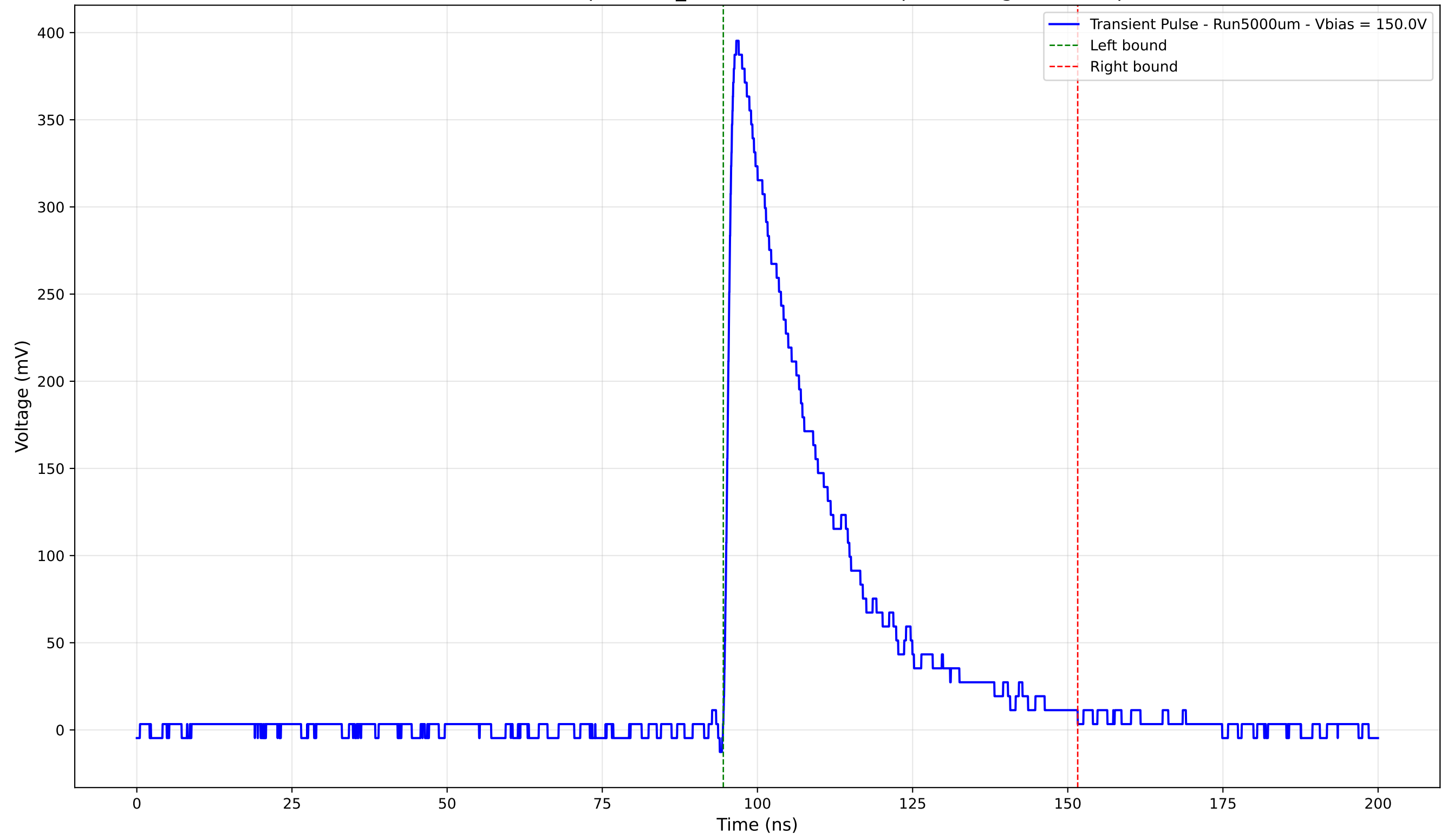
Transient Pulse - Sample: 1cm_42 - Position: 3985.0 \mu\text{m} - Charge: 119.39 pC
