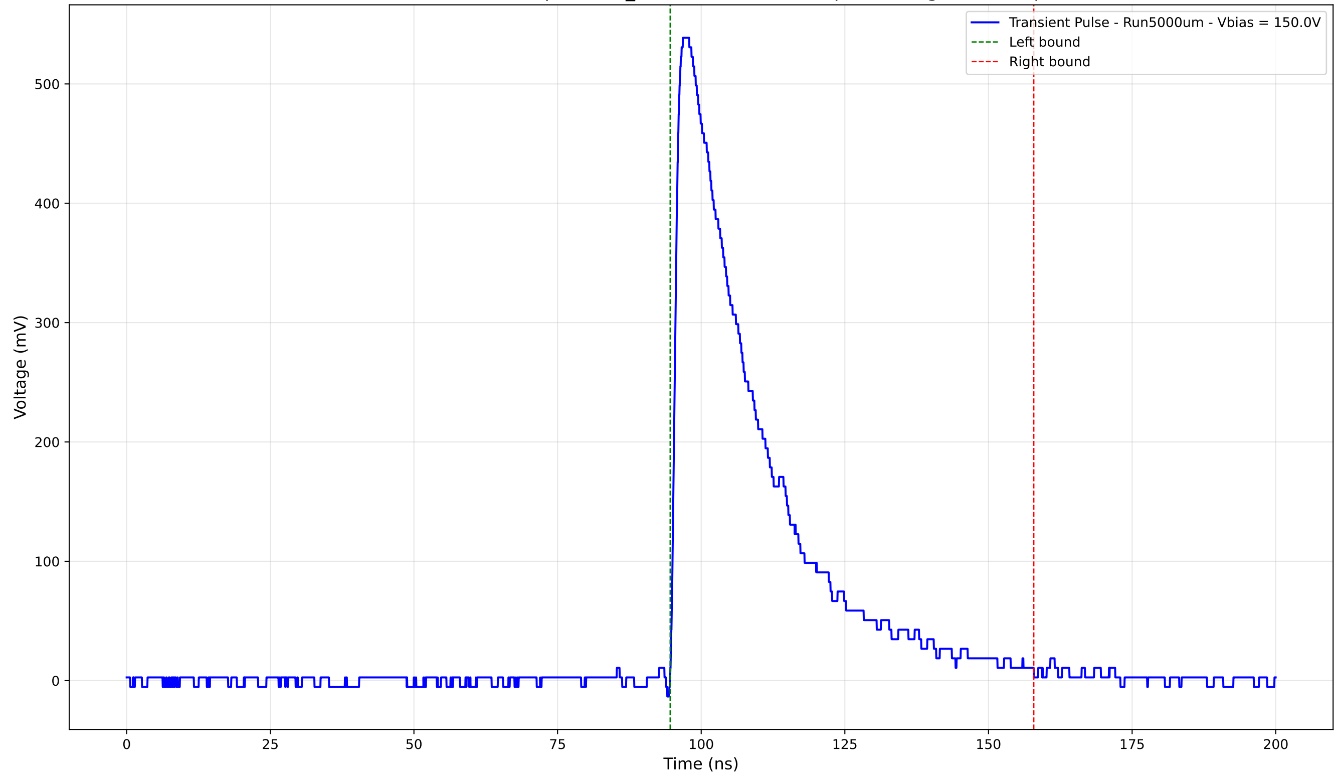
Transient Pulse - Sample: 1cm_42 - Position: 1160.0 \mu\text{m} - Charge: 170.98 pC
