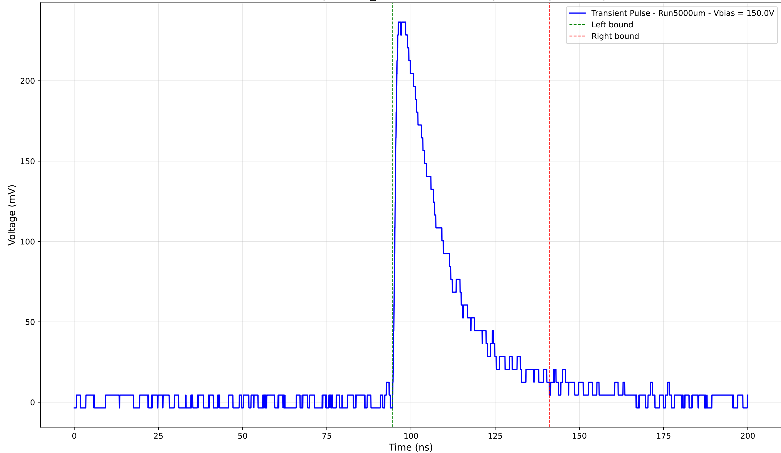
Transient Pulse - Sample: 1cm_42 - Position: 3570.0 \mu\text{m} - Charge: 74.46 pC
