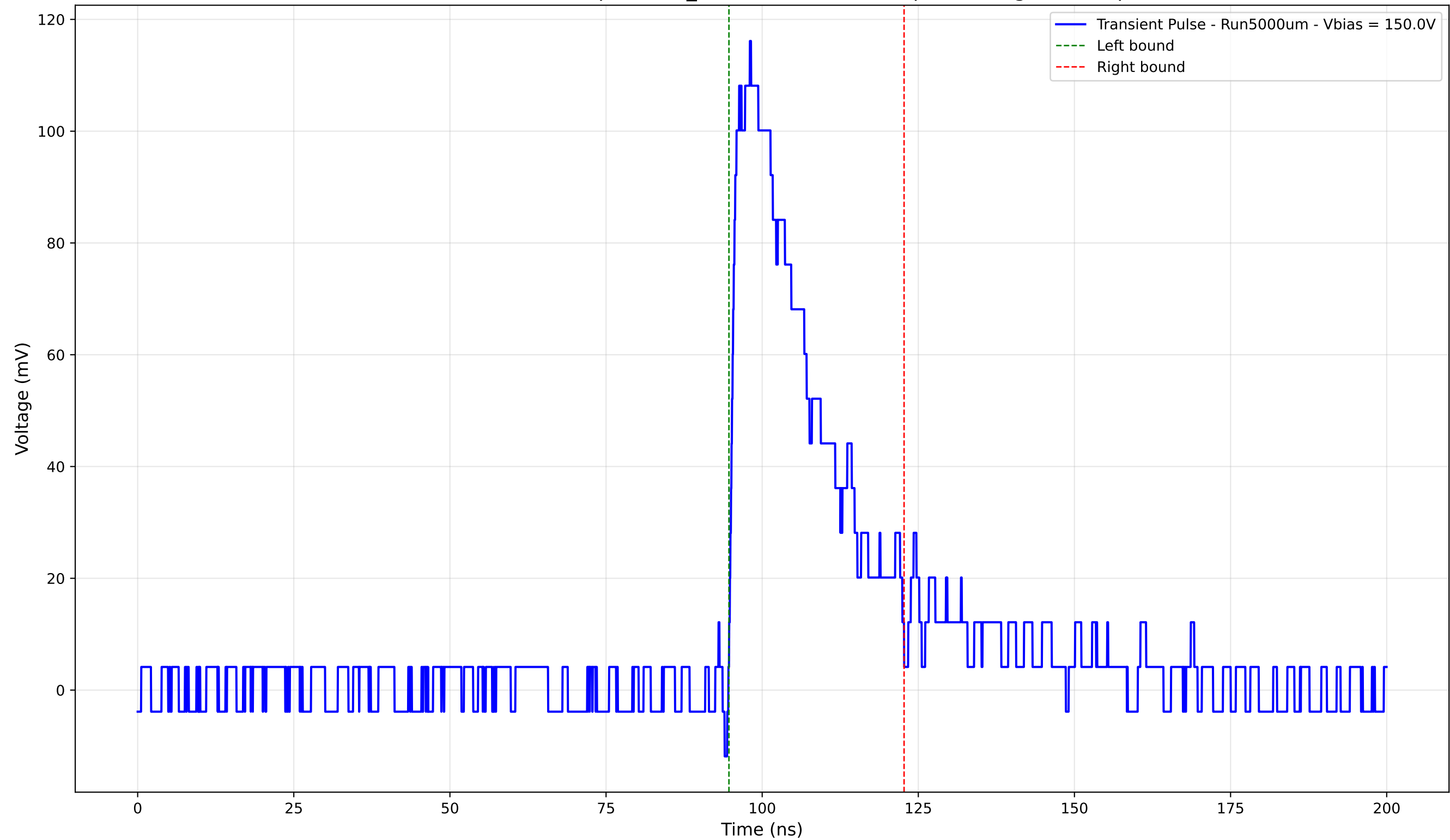
Transient Pulse - Sample: 1cm_42 - Position: 4045.0 \mu\text{m} - Charge: 31.66 pC
