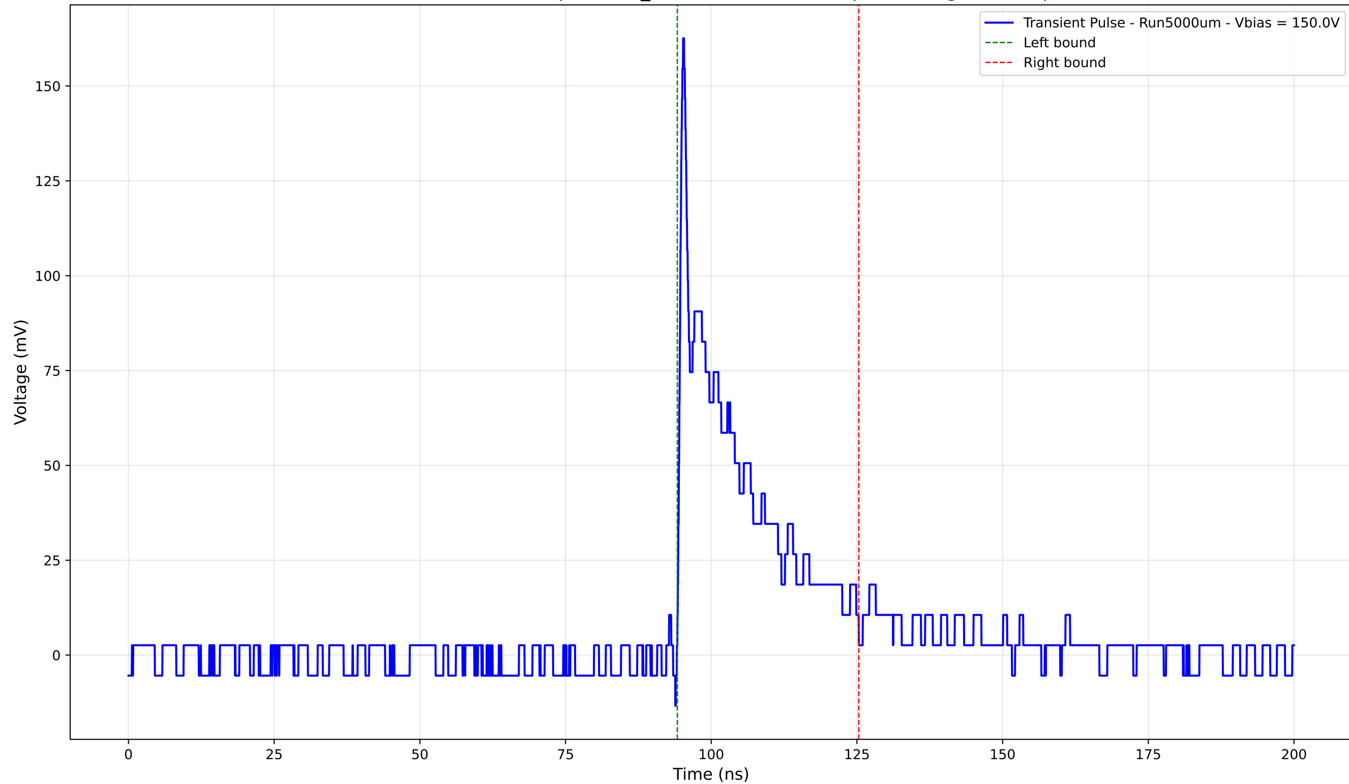
Transient Pulse - Sample: 1cm_42 - Position: 2535.0 \mu\text{m} - Charge: 27.42 pC
