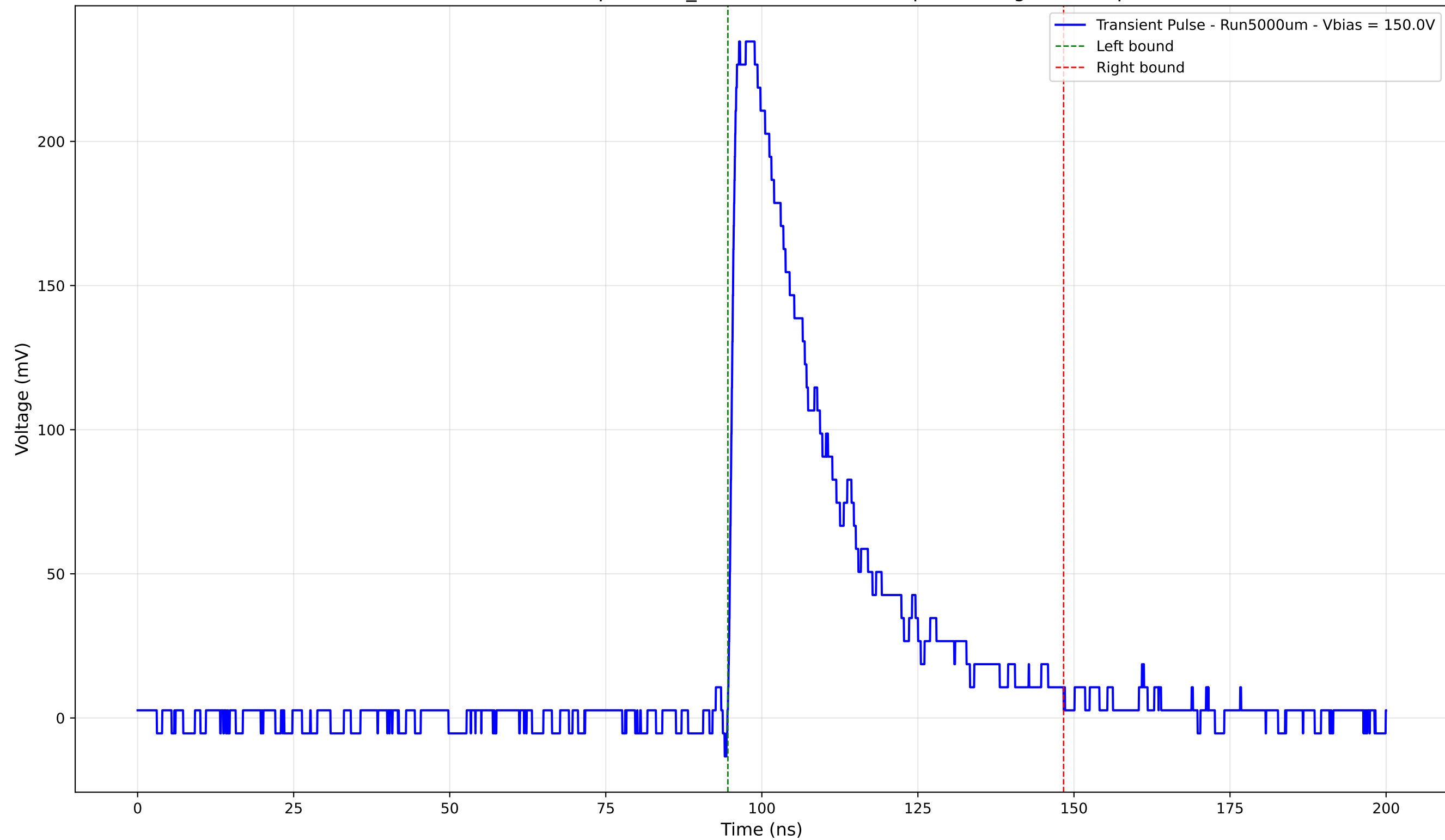
Transient Pulse - Sample: 1cm_42 - Position: 1555.0 \mu\text{m} - Charge: 77.00 pC
