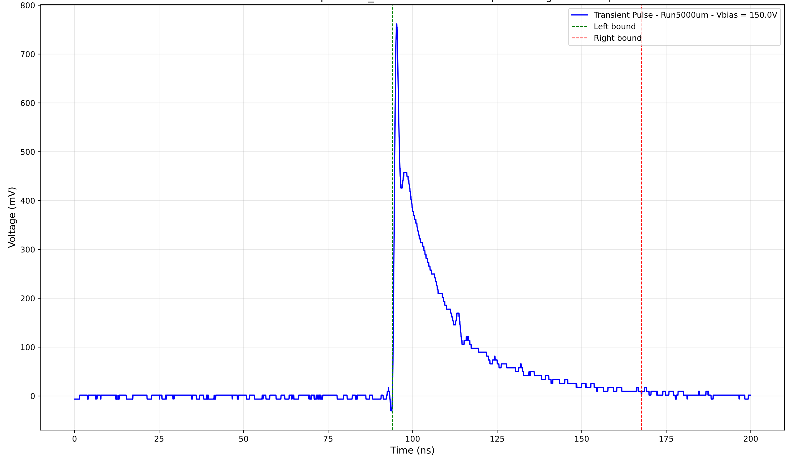
Transient Pulse - Sample: 1cm_42 - Position: 2385.0 \mu\text{m} - Charge: 169.44 pC
