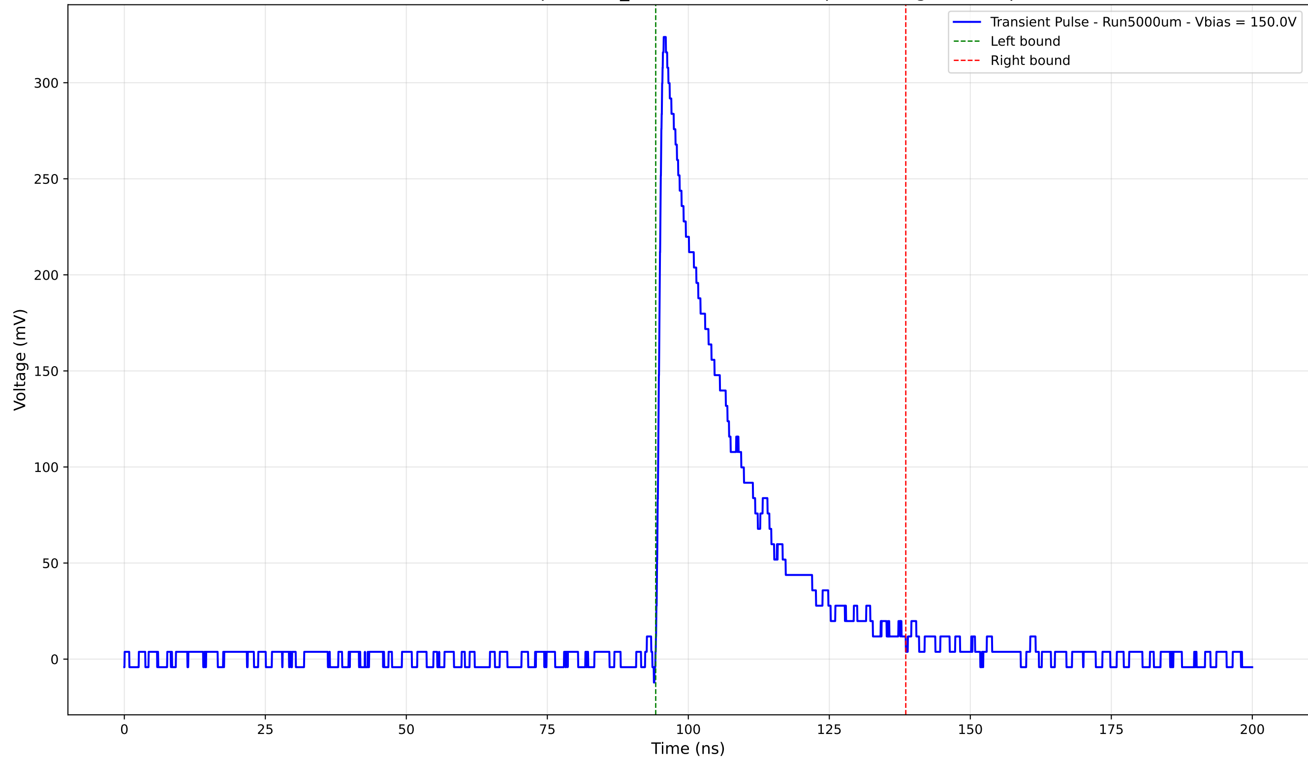
Transient Pulse - Sample: 1cm_42 - Position: 4585.0 \mu\text{m} - Charge: 80.77 pC
