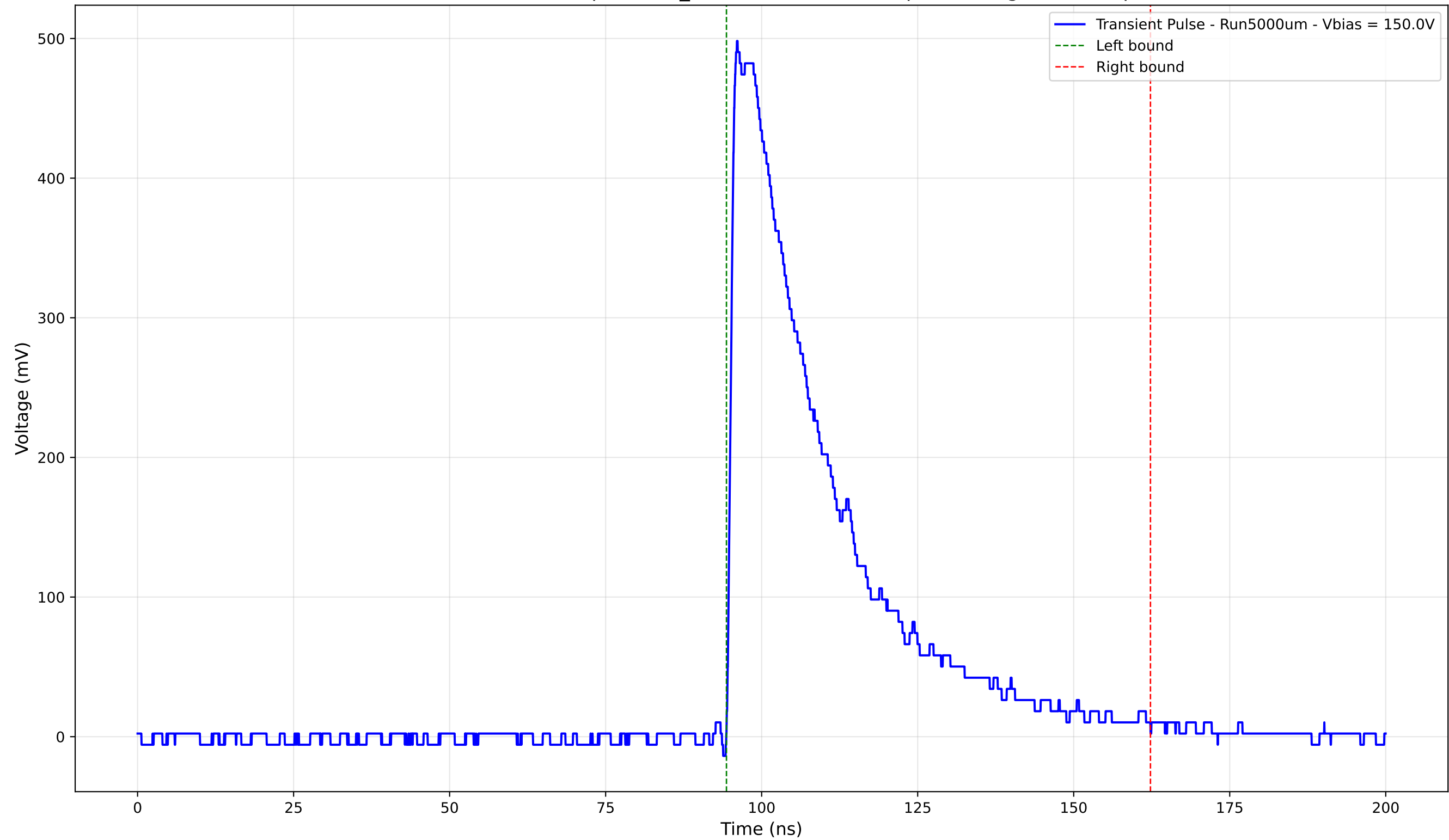
Transient Pulse - Sample: 1cm_42 - Position: 1760.0 \mu\text{m} - Charge: 166.62 pC
