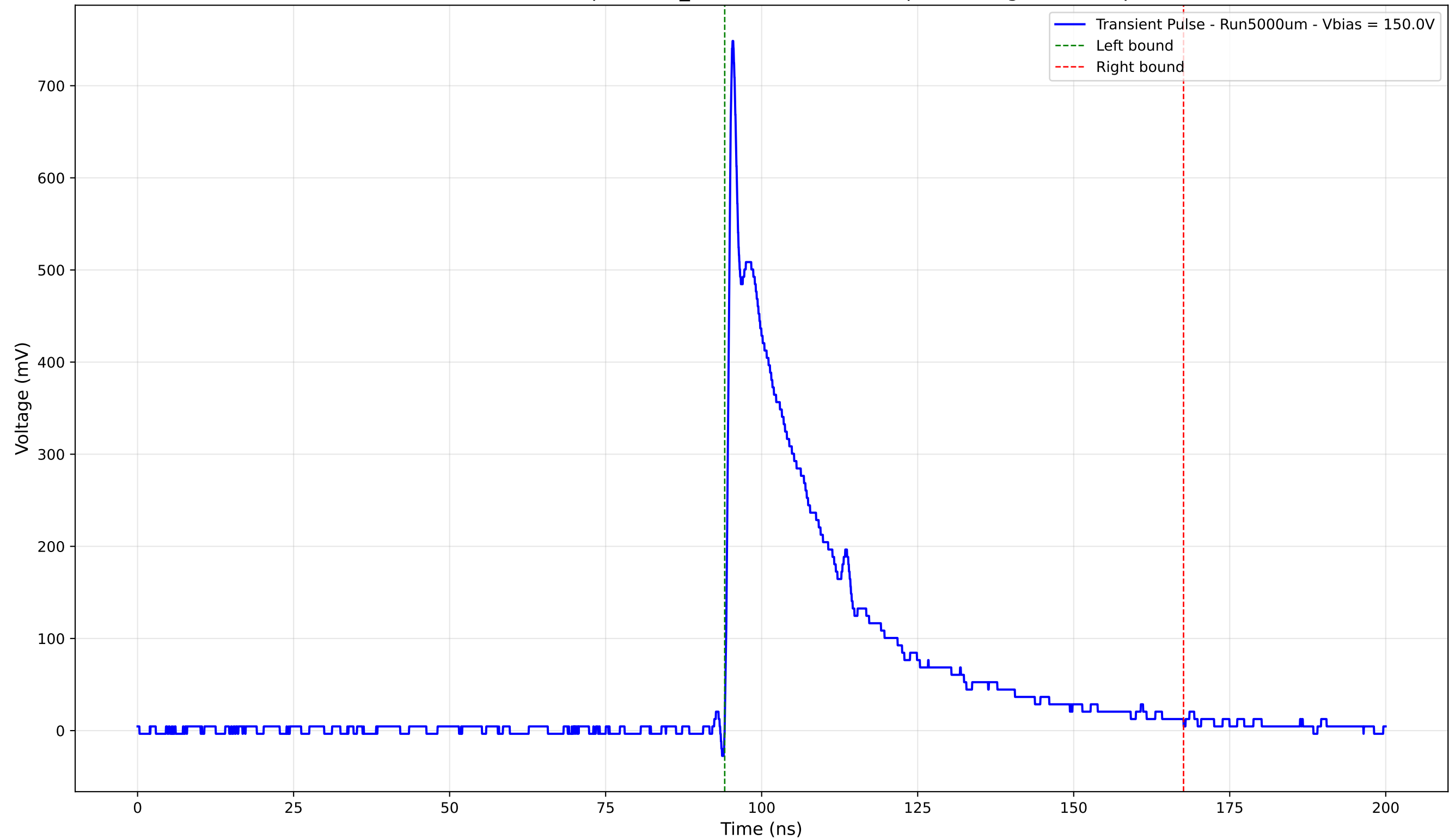
Transient Pulse - Sample: 1cm_42 - Position: 2775.0 \mu\text{m} - Charge: 189.69 pC
