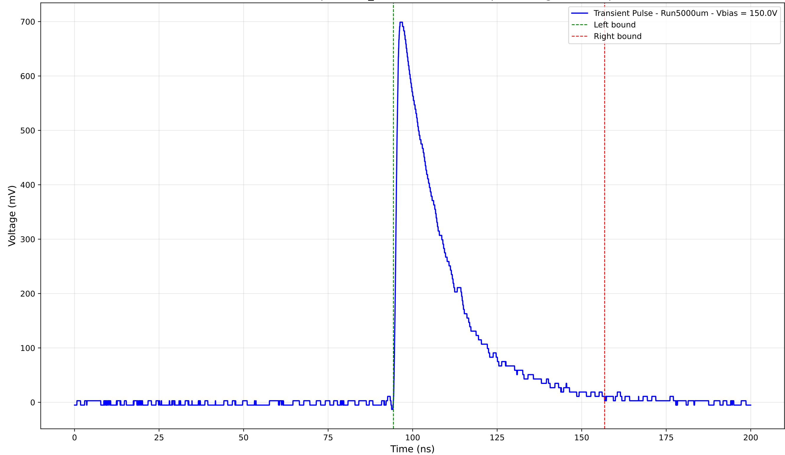
Transient Pulse - Sample: 1cm_42 - Position: 4205.0 \mu\text{m} - Charge: 213.83 pC
