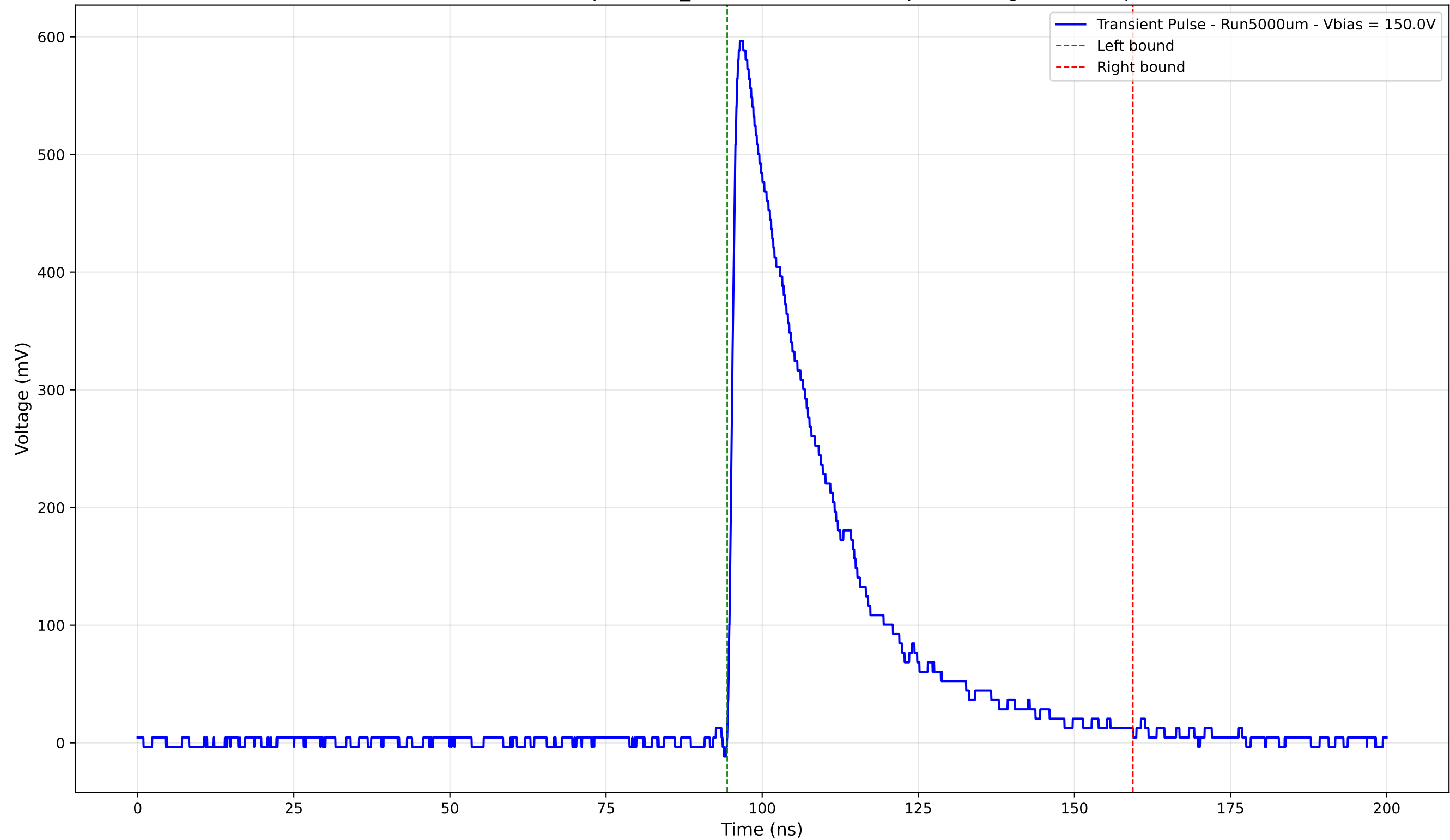
Transient Pulse - Sample: 1cm_42 - Position: 4120.0 \mu\text{m} - Charge: 183.57 pC
