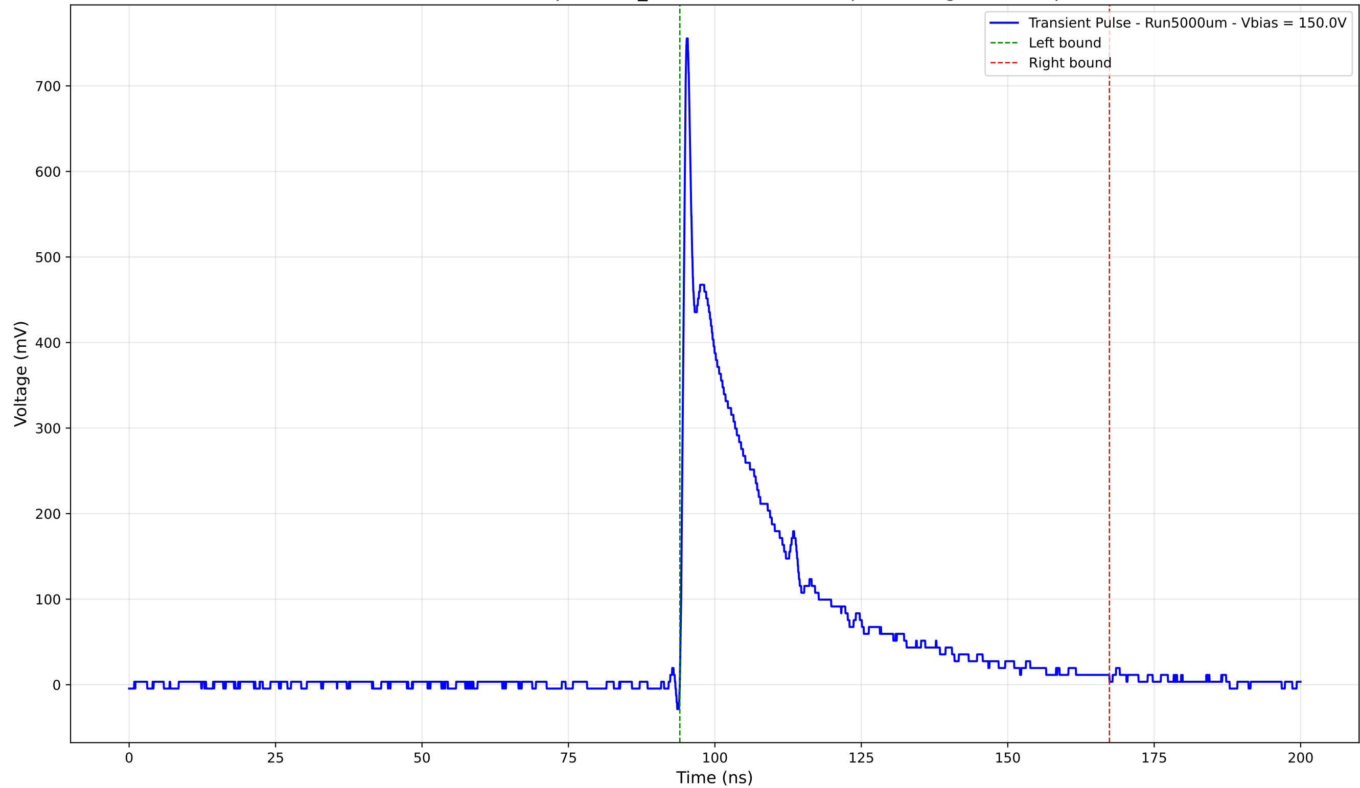
Transient Pulse - Sample: 1cm_42 - Position: 2370.0 \mu\text{m} - Charge: 173.29 pC
