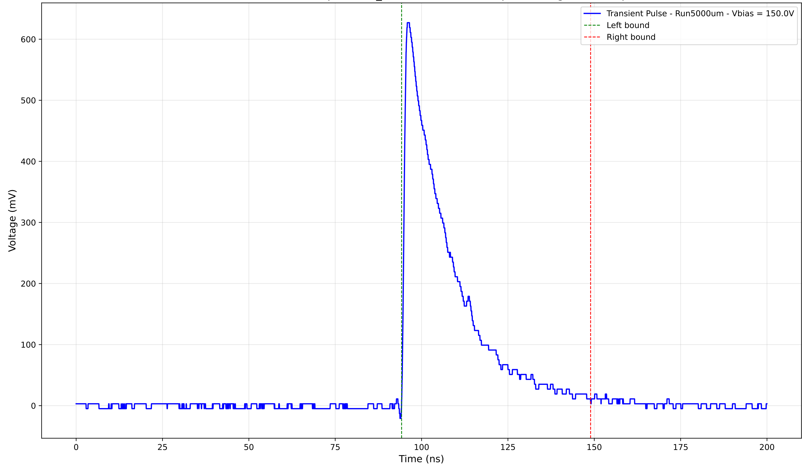
Transient Pulse - Sample: 1cm_42 - Position: 4460.0 \mu\text{m} - Charge: 175.09 pC
