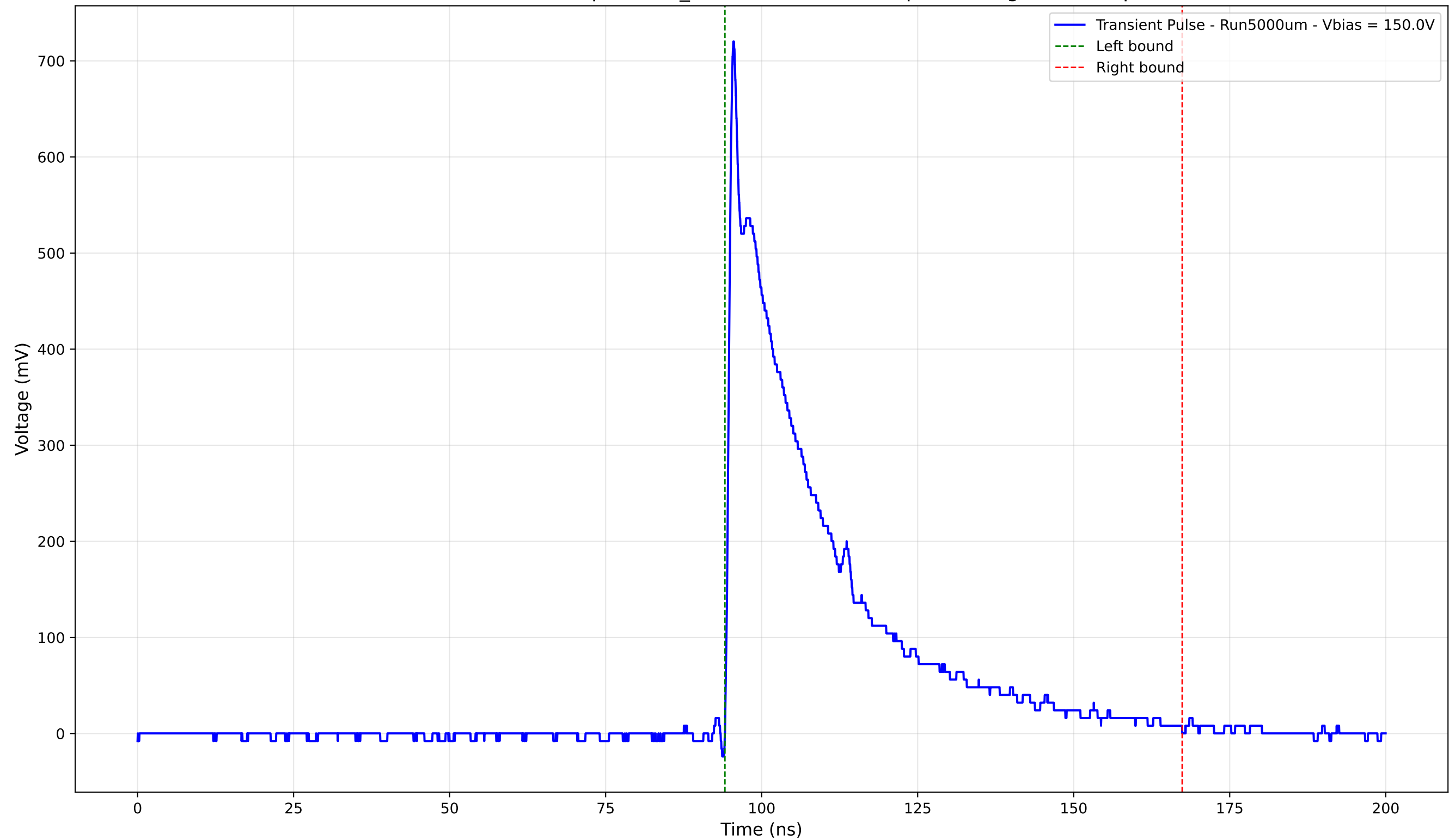
Transient Pulse - Sample: 1cm_42 - Position: 2875.0 \mu\text{m} - Charge: 193.10 pC
