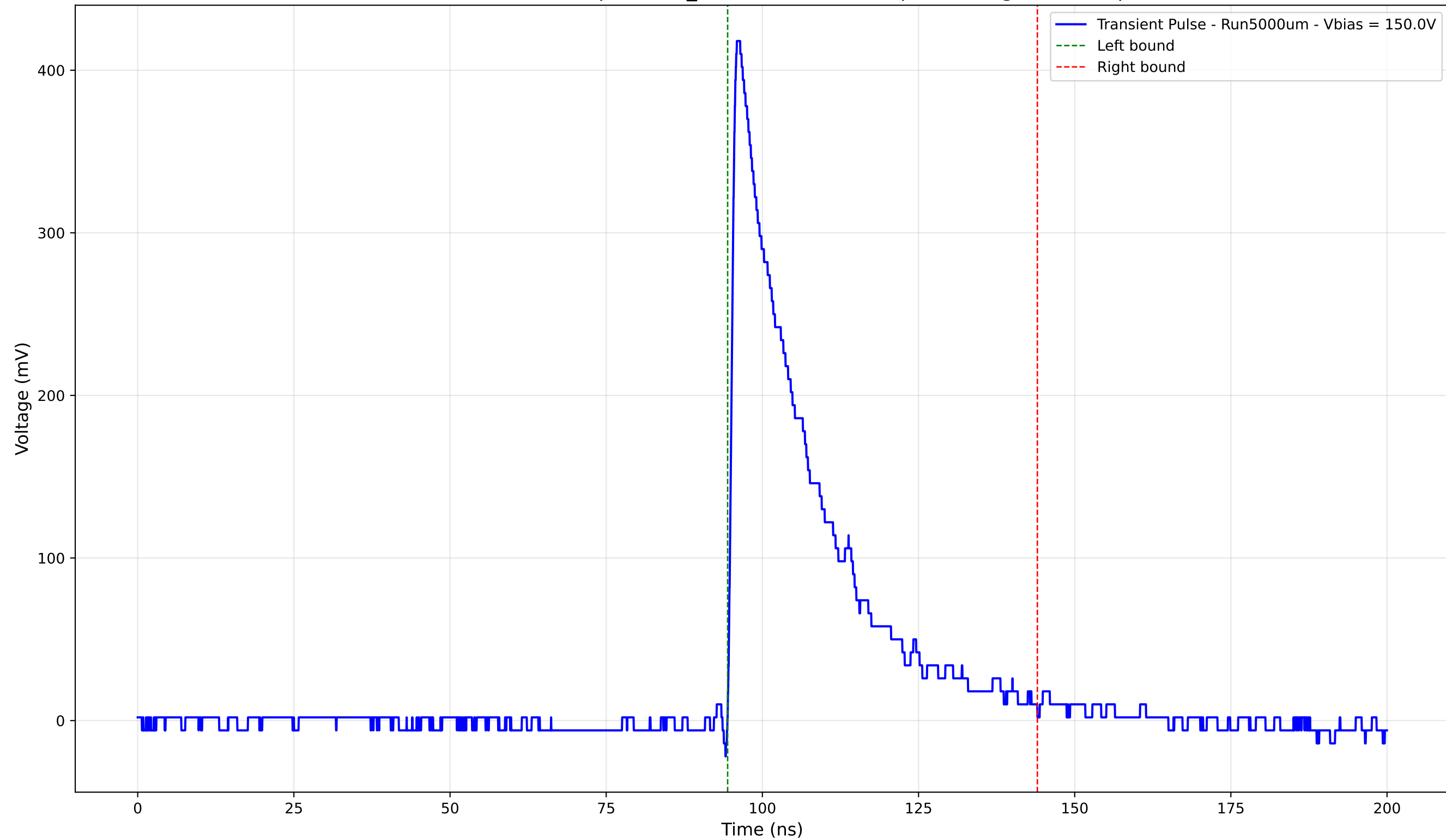
Transient Pulse - Sample: 1cm_42 - Position: 440.0 \mu\text{m} - Charge: 106.64 pC
