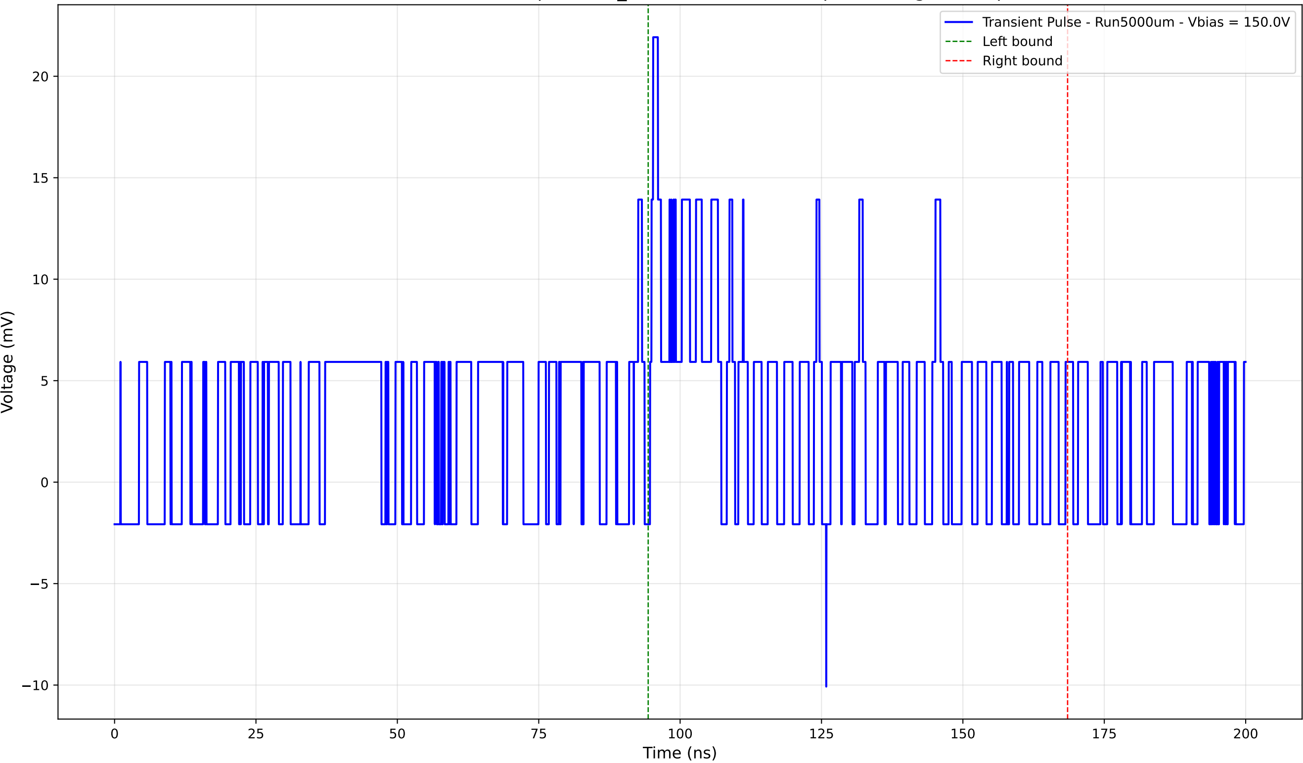
Transient Pulse - Sample: 1cm_42 - Position: 4920.0 \mu\text{m} - Charge: 6.08 pC
