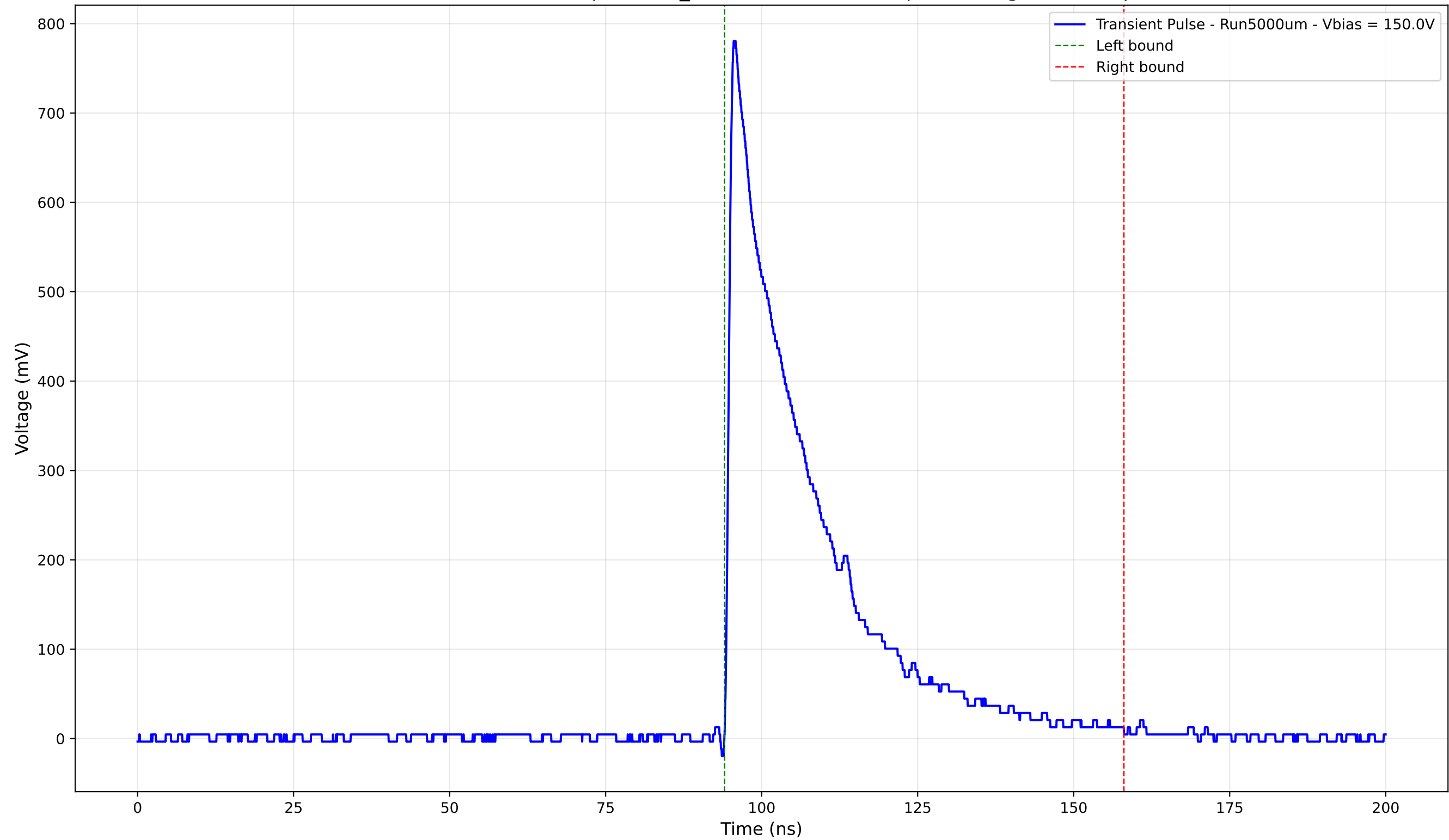
Transient Pulse - Sample: 1cm_42 - Position: 4685.0 \mu\text{m} - Charge: 205.73 pC
