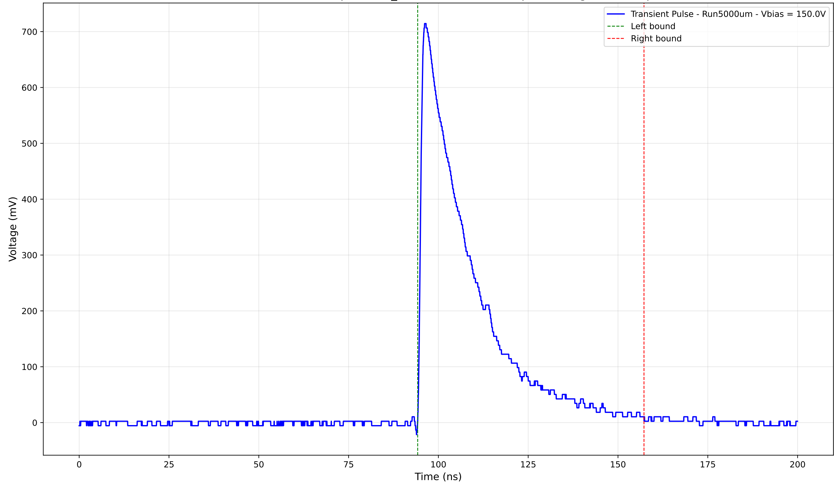
Transient Pulse - Sample: 1cm_42 - Position: 4340.0 \mu\text{m} - Charge: 212.70 pC
