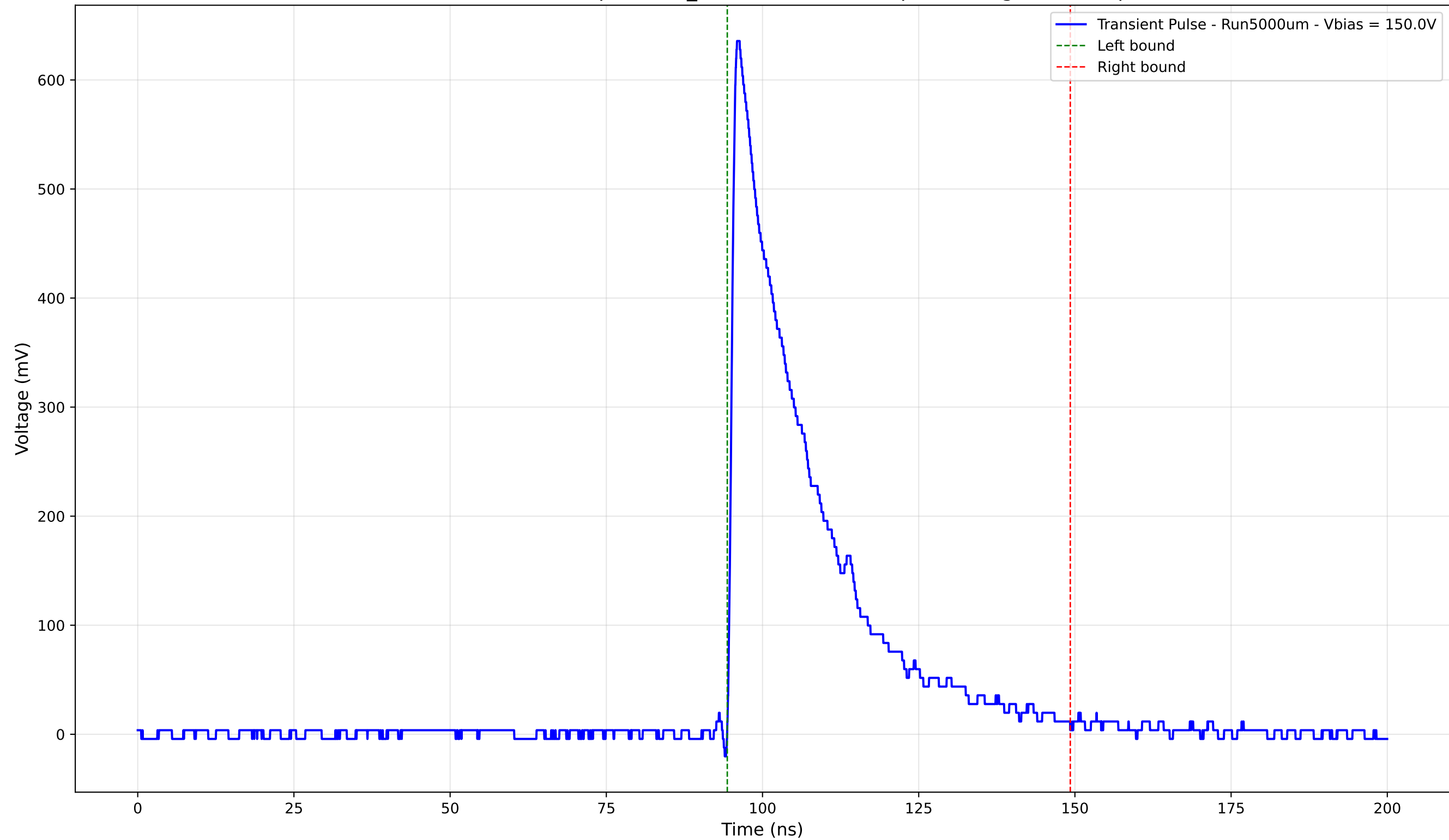
Transient Pulse - Sample: 1cm_42 - Position: 395.0 \mu\text{m} - Charge: 165.29 pC
