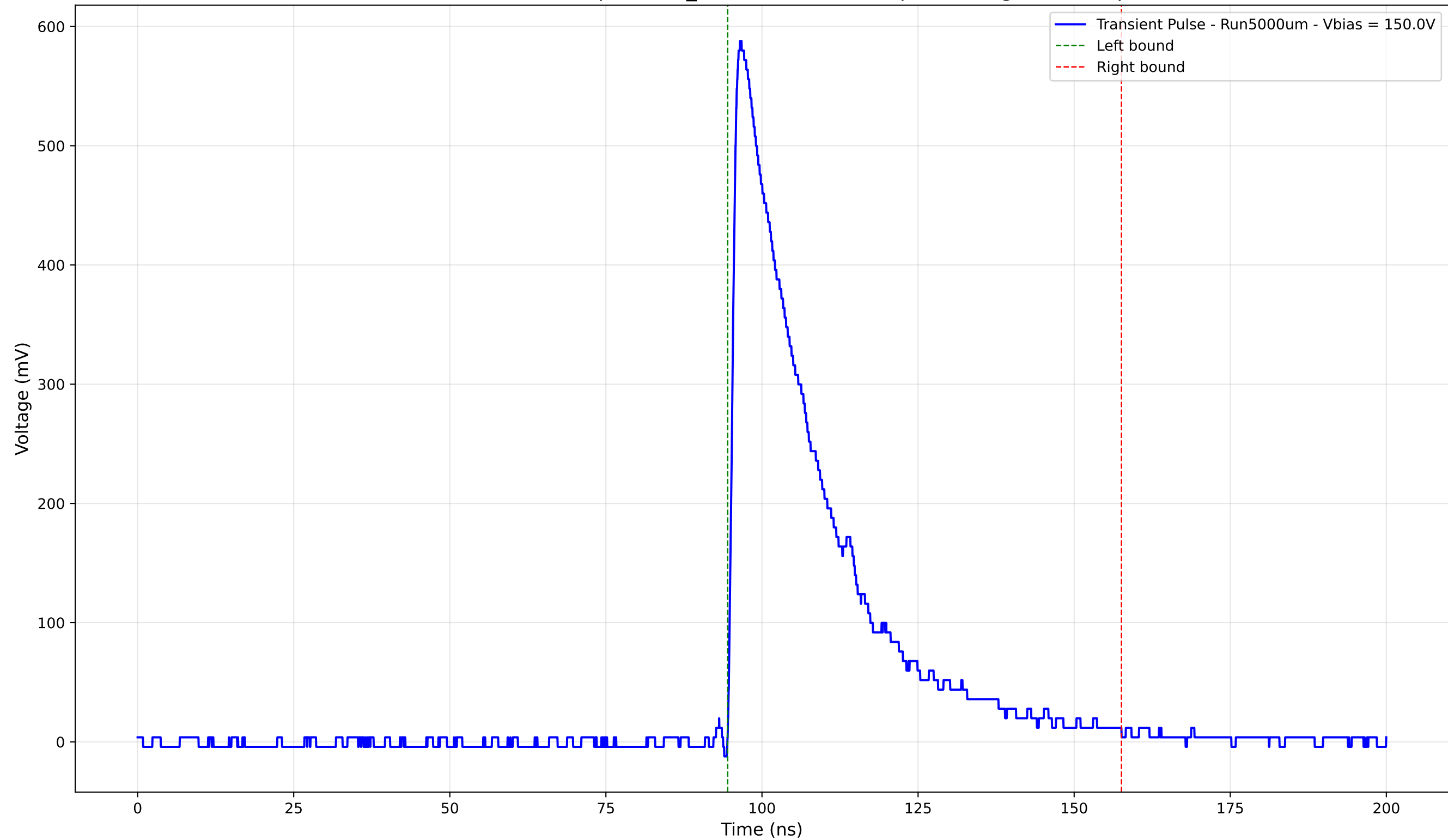
Transient Pulse - Sample: 1cm_42 - Position: 675.0 \mu\text{m} - Charge: 171.17 pC
