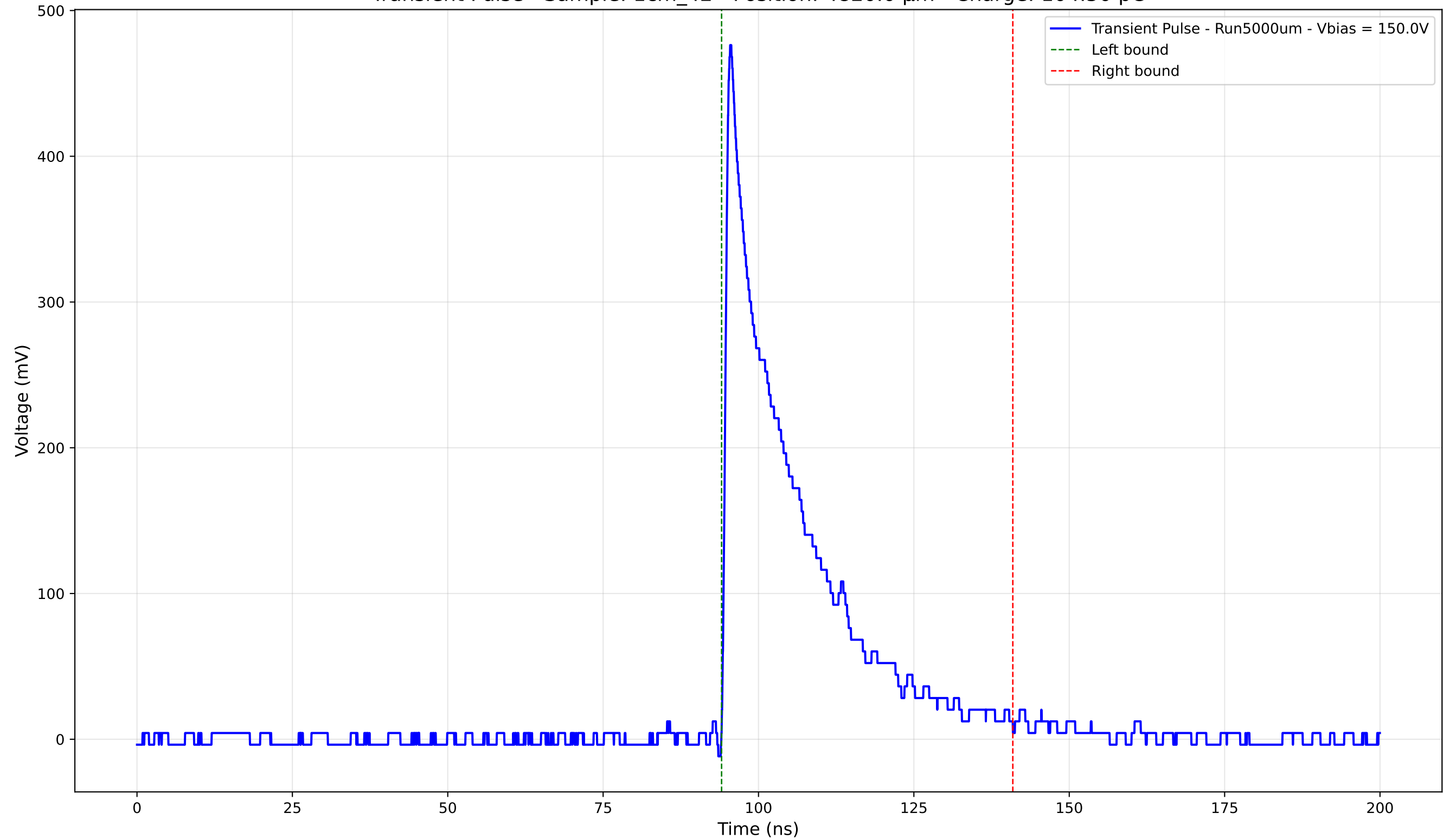
Transient Pulse - Sample: 1cm_42 - Position: 4820.0 \mu\text{m} - Charge: 104.50 pC
