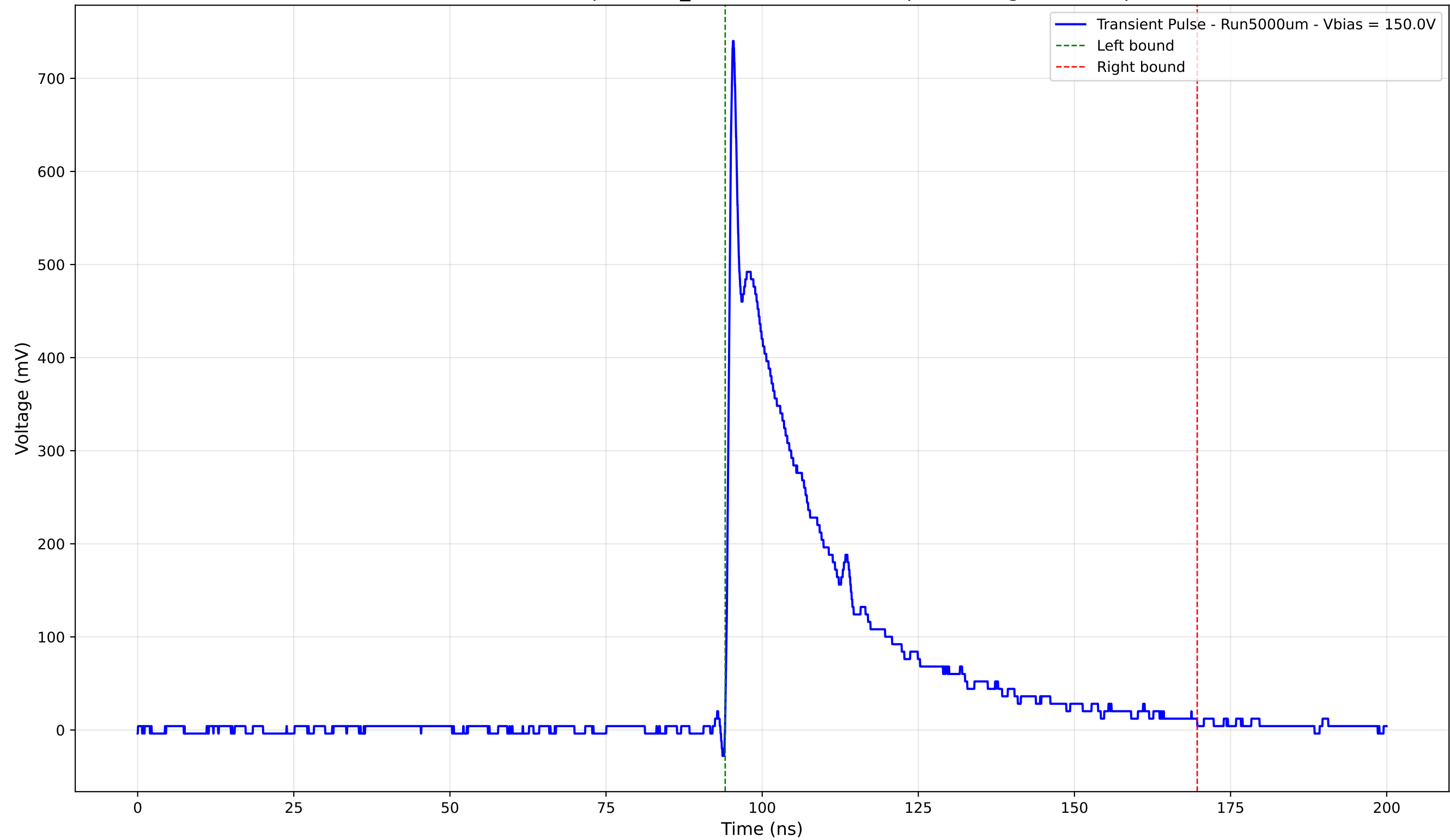
Transient Pulse - Sample: 1cm_42 - Position: 2280.0 \mu\text{m} - Charge: 184.34 pC
