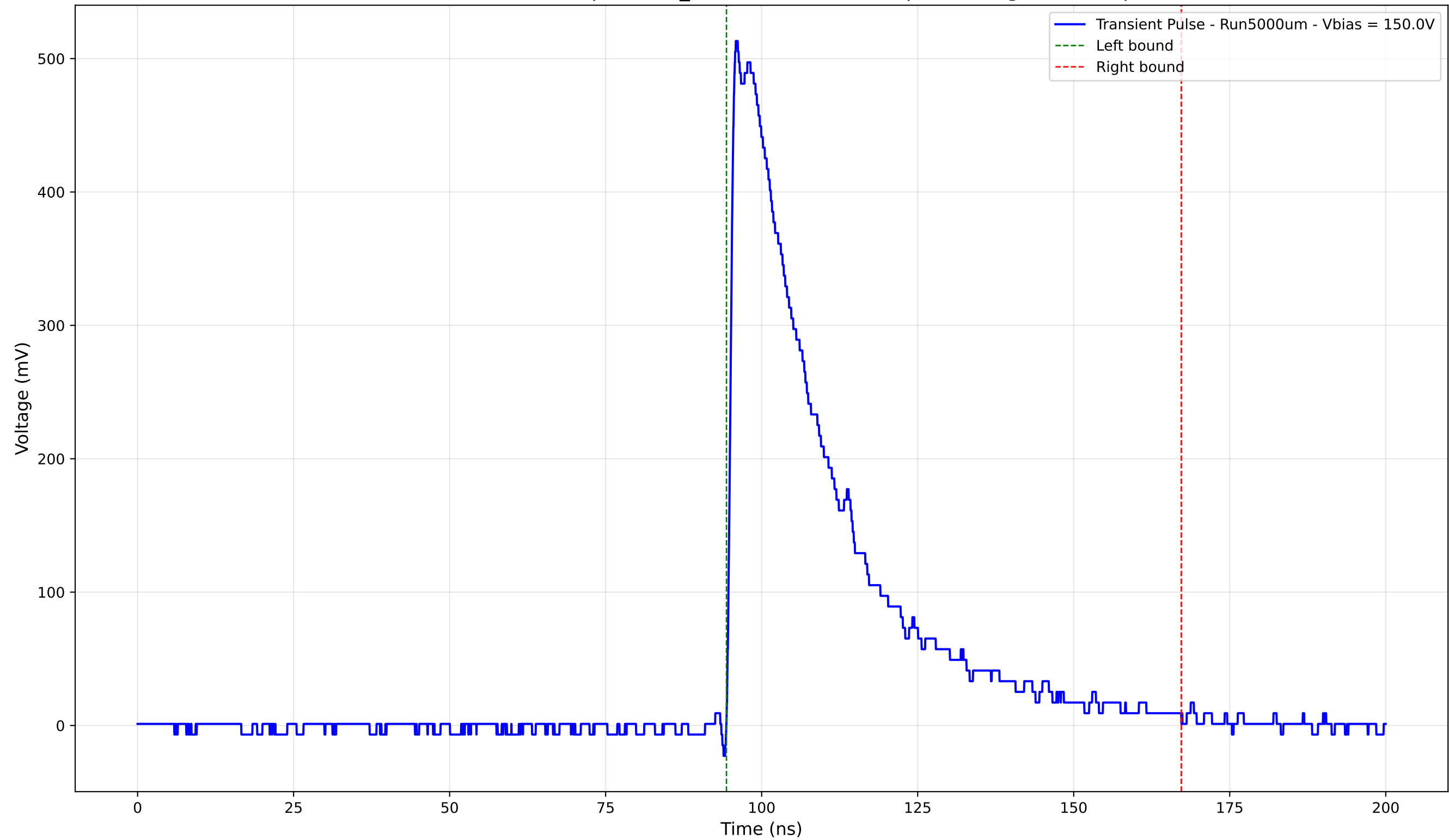
Transient Pulse - Sample: 1cm_42 - Position: 1810.0 \mu\text{m} - Charge: 171.59 pC
