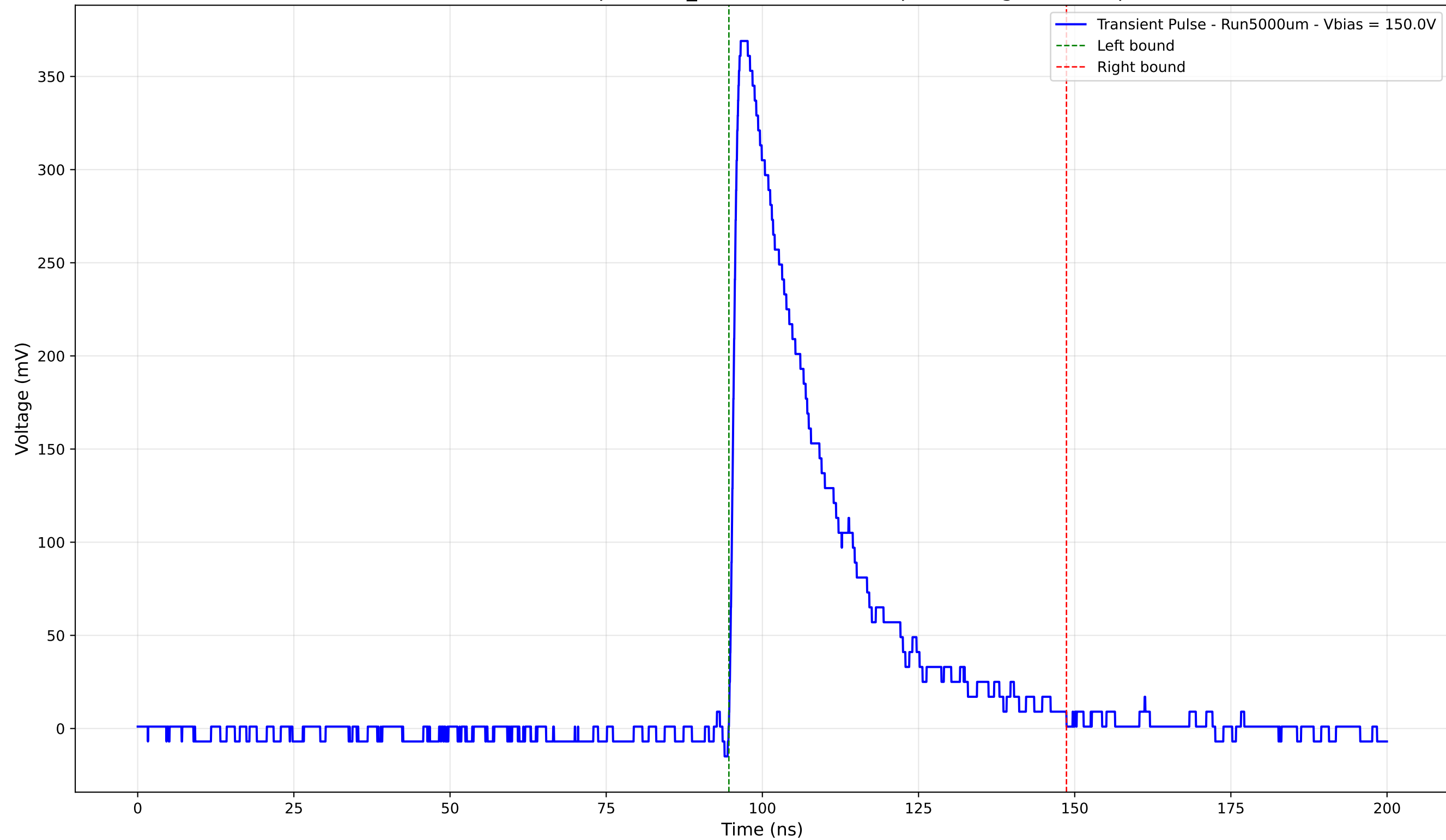
Transient Pulse - Sample: 1cm_42 - Position: 945.0 \mu\text{m} - Charge: 107.73 pC
