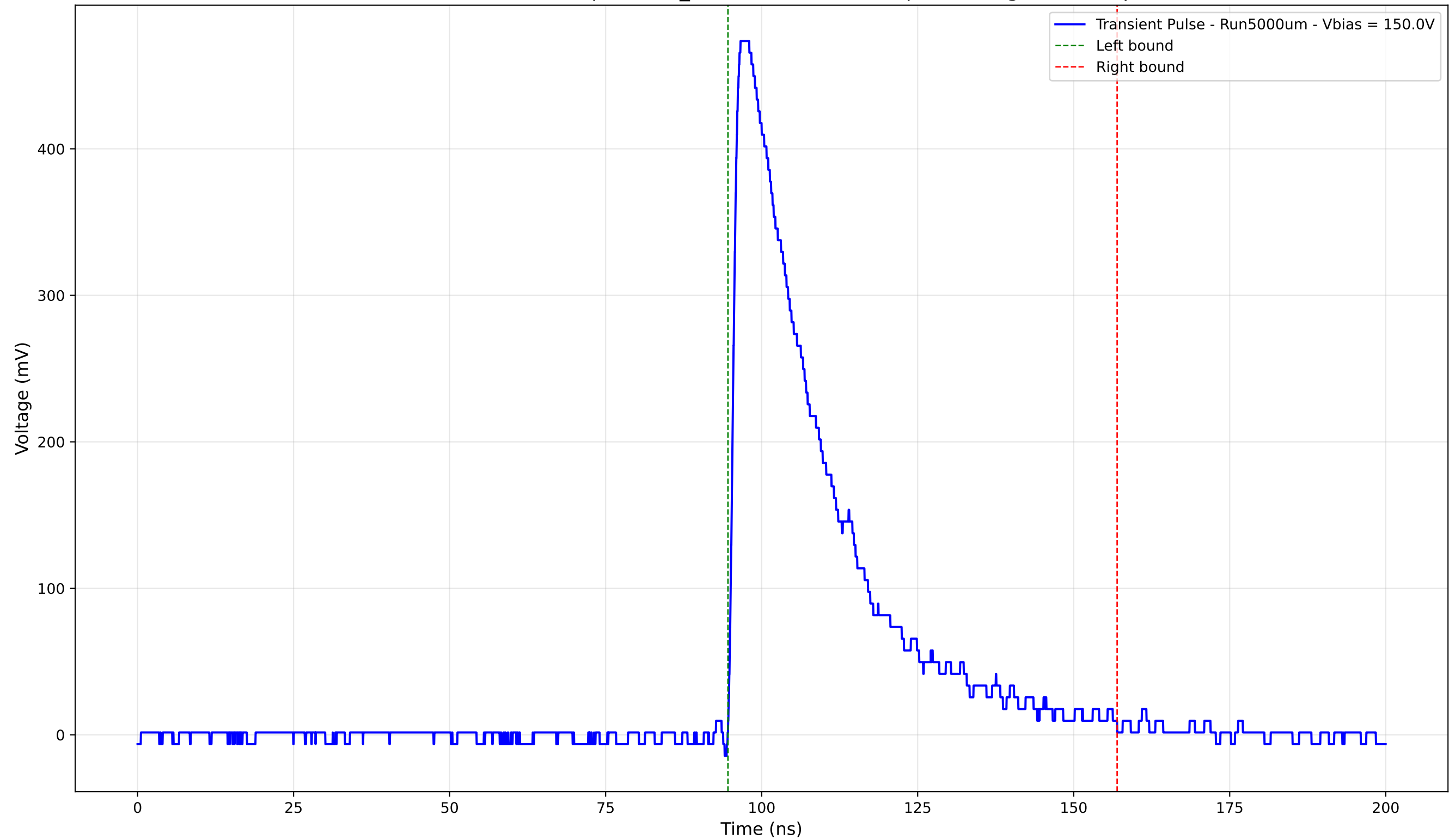
Transient Pulse - Sample: 1cm_42 - Position: 1095.0 \mu\text{m} - Charge: 149.01 pC
