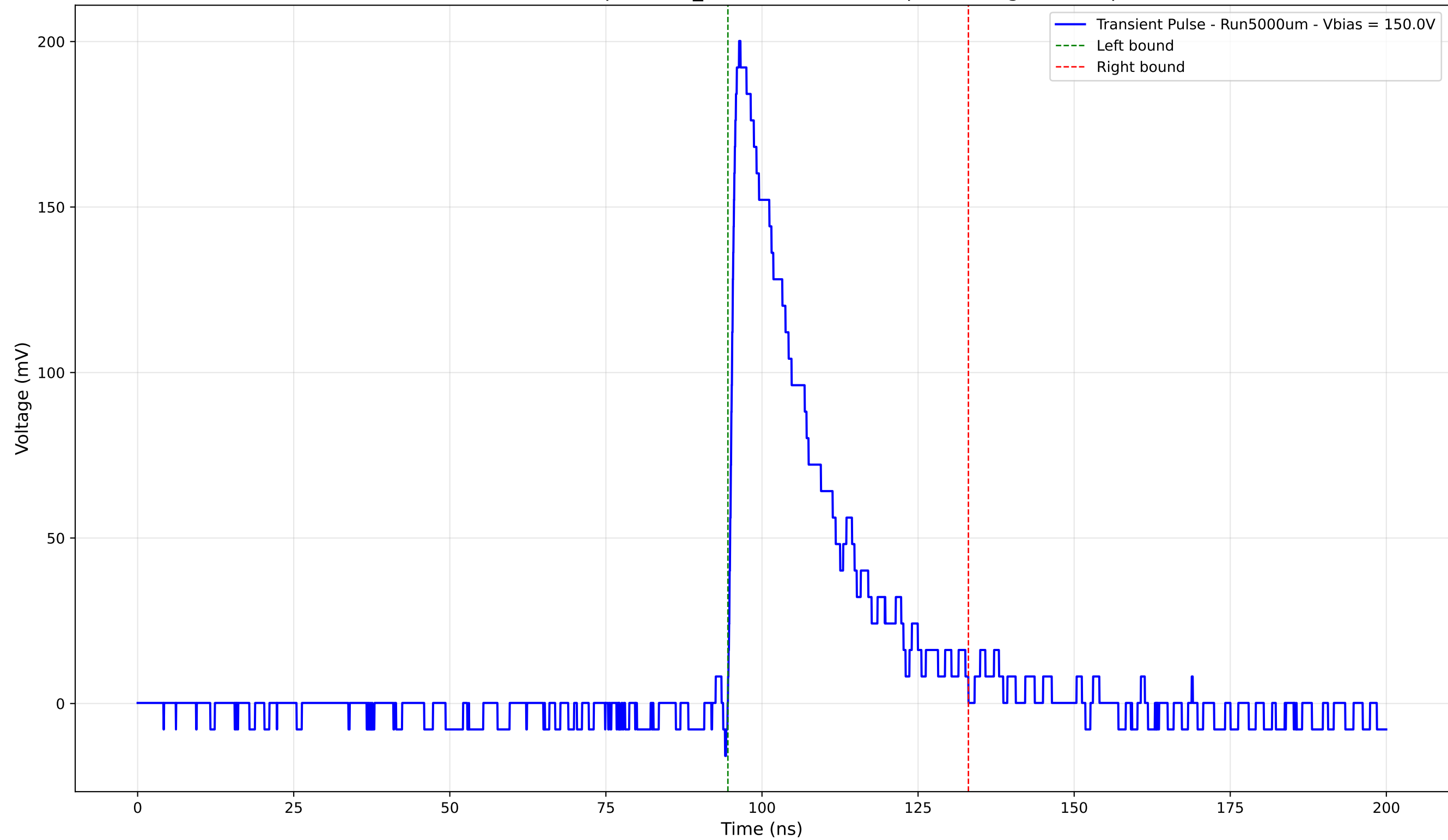
Transient Pulse - Sample: 1cm_42 -Position: 535.0 \mu\text{m} - Charge: 51.35 pC
