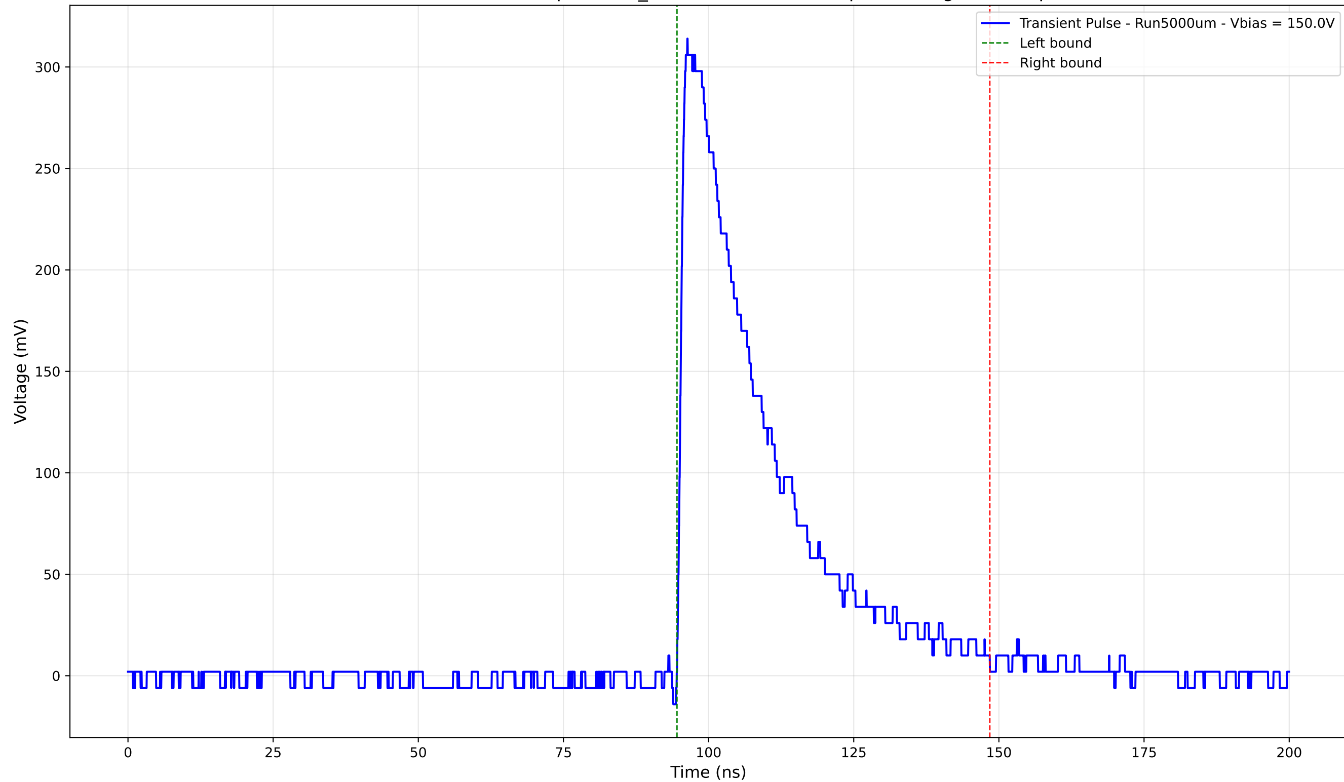
Transient Pulse - Sample: 1cm_42 - Position: 3485.0 \mu\text{m} - Charge: 97.51 pC
