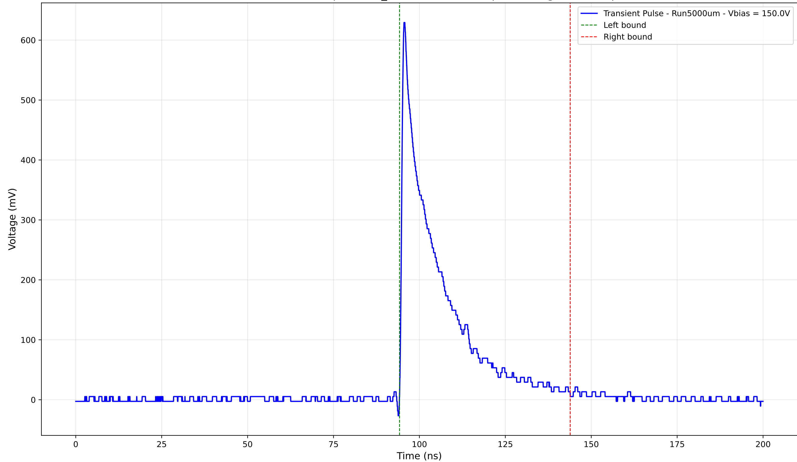
Transient Pulse - Sample: 1cm_42 - Position: 85.0 \mu\text{m} - Charge: 132.35 pC
