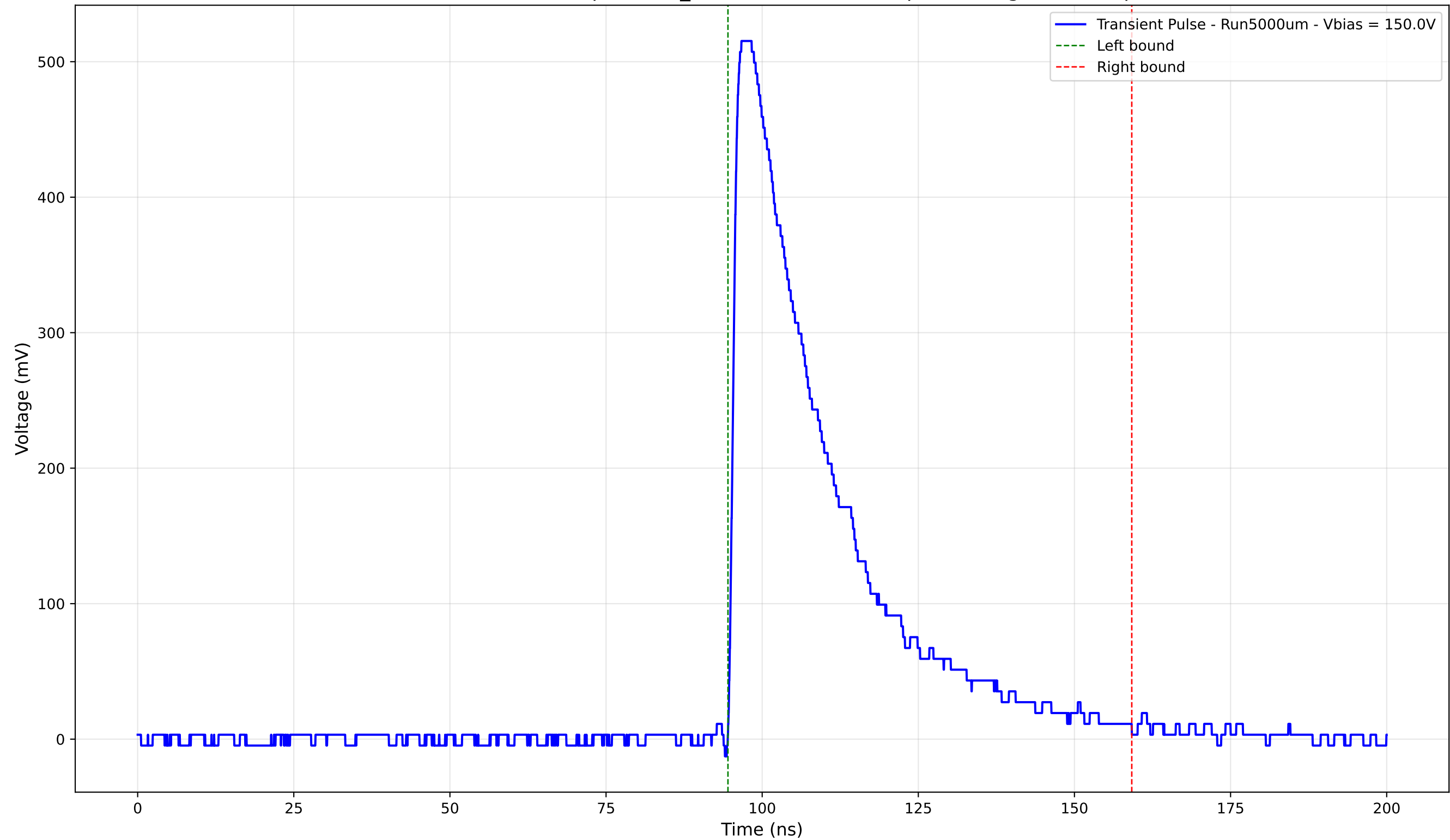
Transient Pulse - Sample: 1cm_42 - Position: 1390.0 \mu\text{m} - Charge: 171.22 pC
