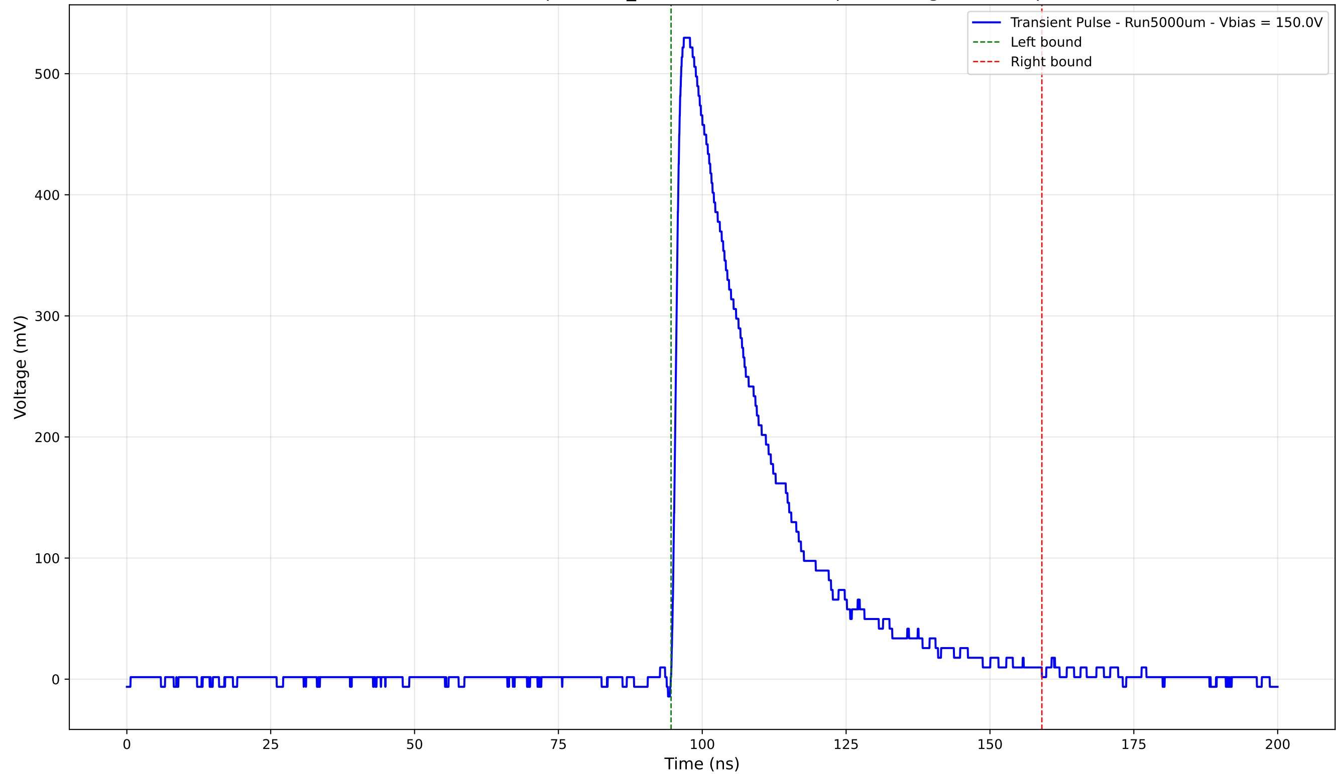
Transient Pulse - Sample: 1cm_42 - Position: 1190.0 \mu\text{m} - Charge: 167.56 pC
