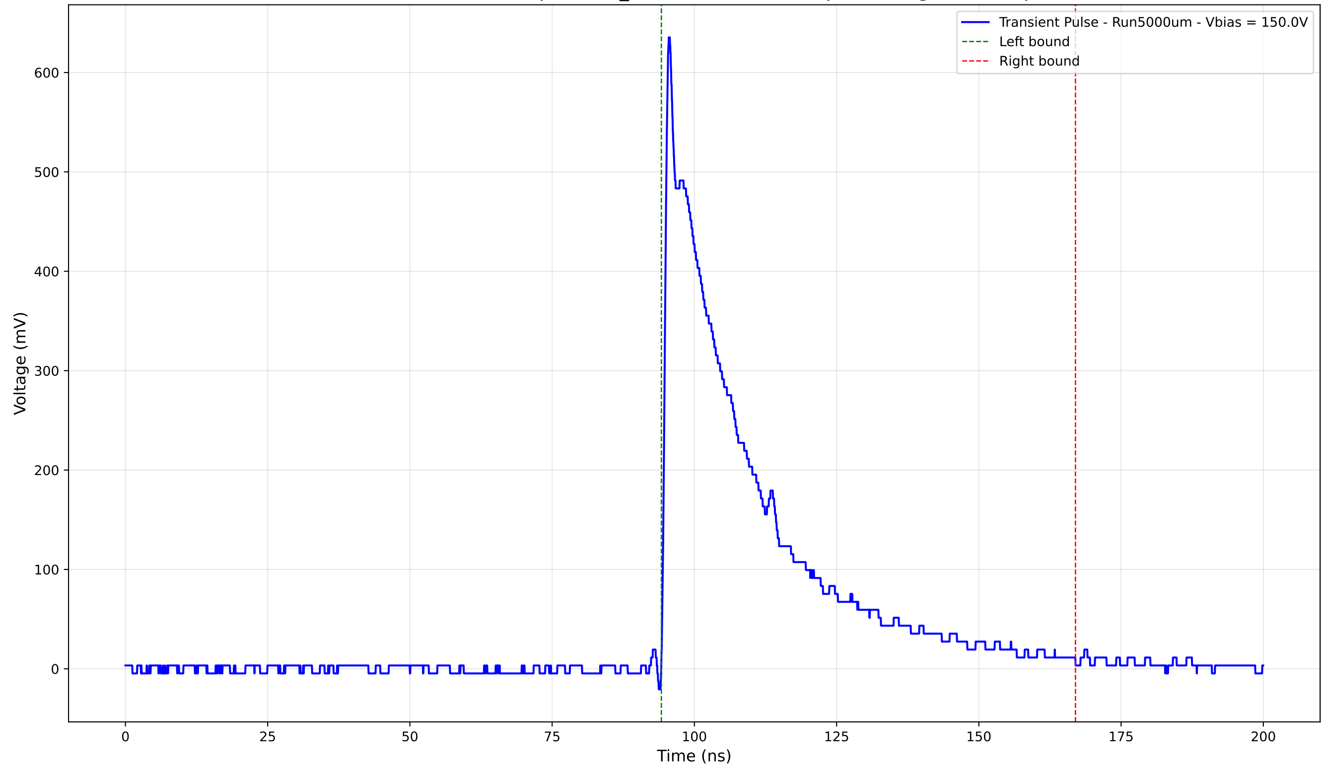
Transient Pulse - Sample: 1cm_42 - Position: 2945.0 \mu\text{m} - Charge: 178.08 pC
