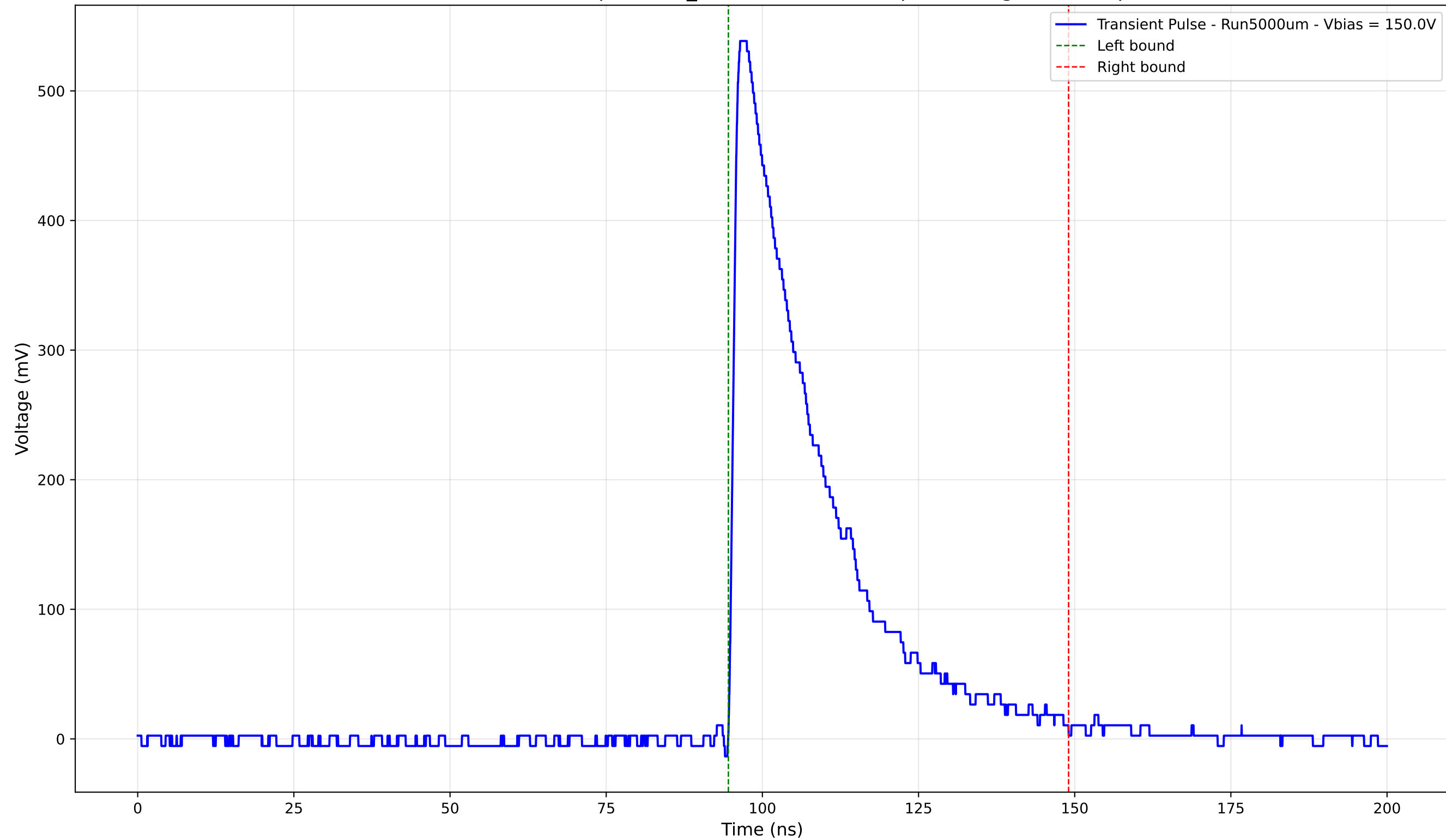
Transient Pulse - Sample: 1cm_42 - Position: 785.0 \mu\text{m} - Charge: 159.21 pC
