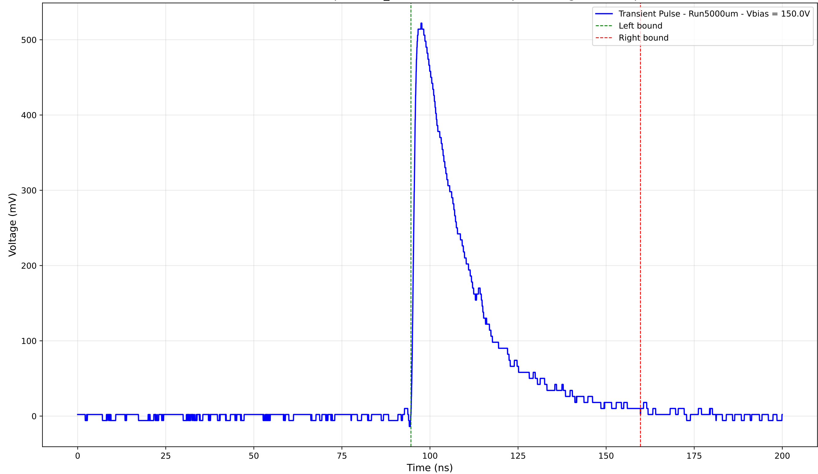
Transient Pulse - Sample: 1cm_42 - Position: 1220.0 \mu\text{m} - Charge: 166.65 pC
