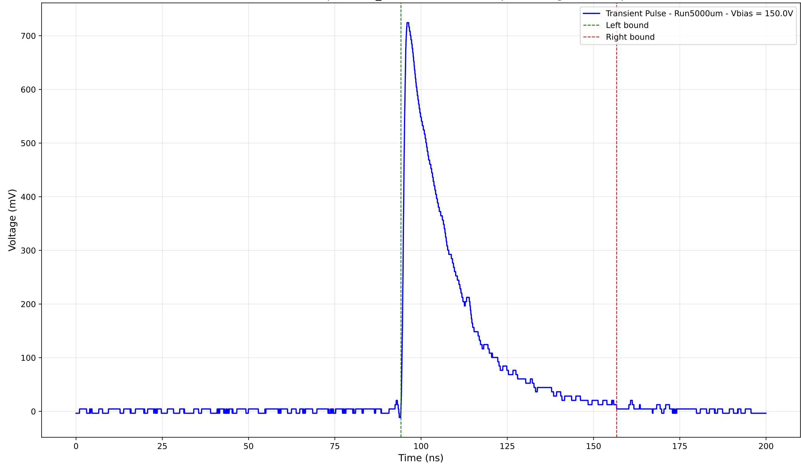
Transient Pulse - Sample: 1cm_42 - Position: 4430.0 \mu\text{m} - Charge: 211.49 pC
