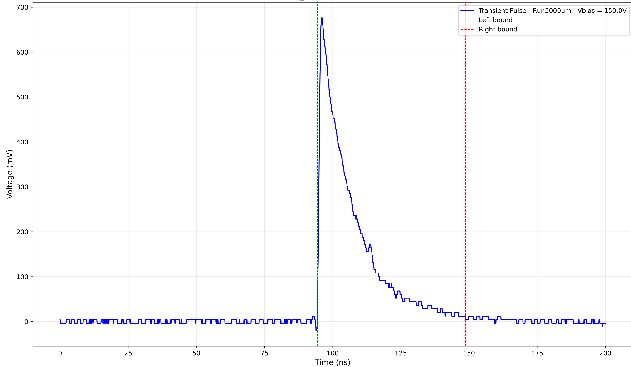
Transient Pulse - Sample: 1cm_42 - Position: 340.0 \mu\text{m} - Charge: 170.44 pC
