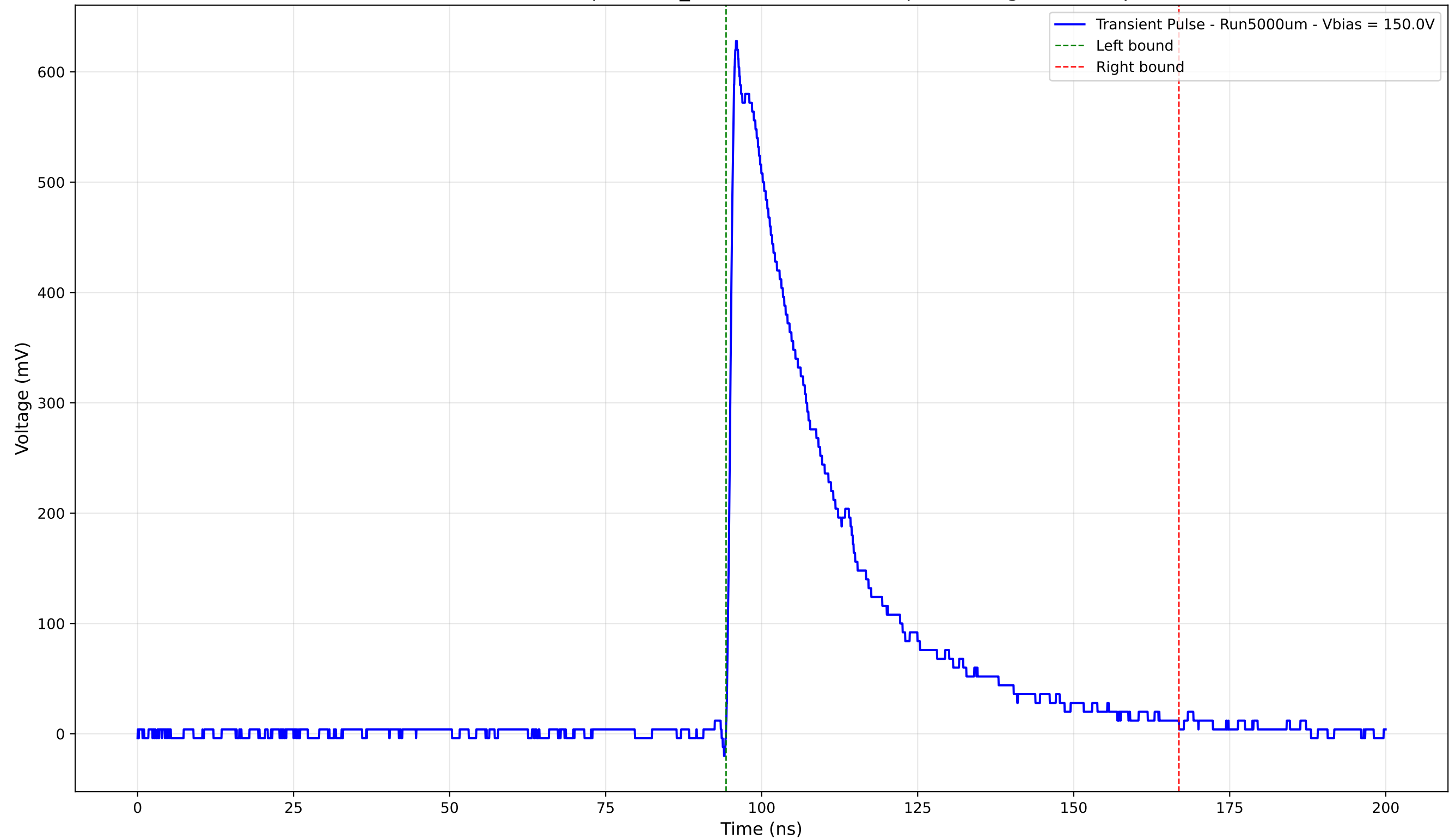
Transient Pulse - Sample: 1cm_42 - Position: 3205.0 \mu\text{m} - Charge: 204.80 pC
