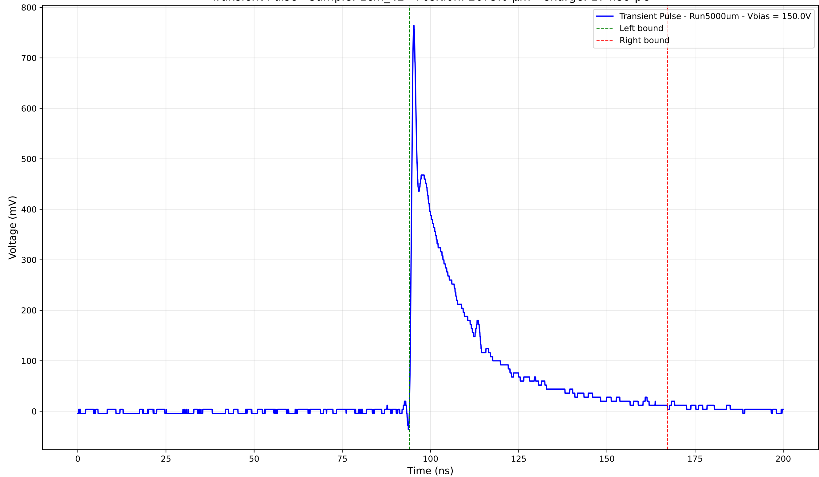
Transient Pulse - Sample: 1cm_42 - Position: 2675.0 \mu\text{m} - Charge: 174.39 pC
