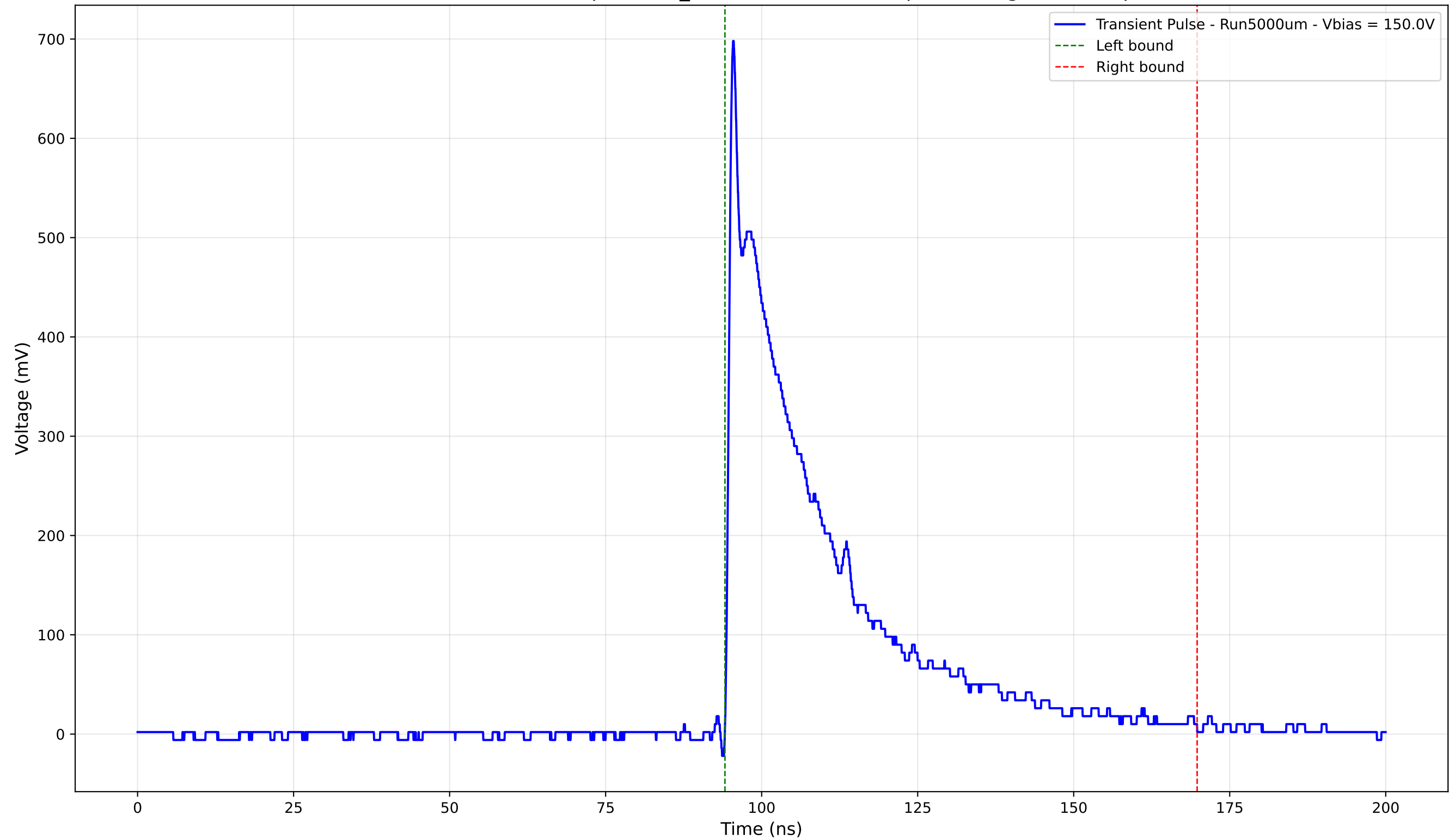
Transient Pulse - Sample: 1cm_42 - Position: 2195.0 \mu\text{m} - Charge: 185.82 pC
