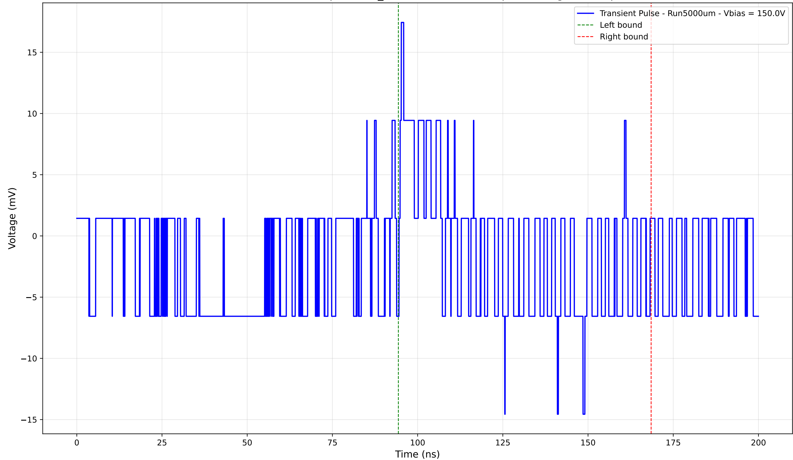
Transient Pulse - Sample: 1cm_42 - Position: 4915.0 \mu\text{m} - Charge: -1.46 pC
