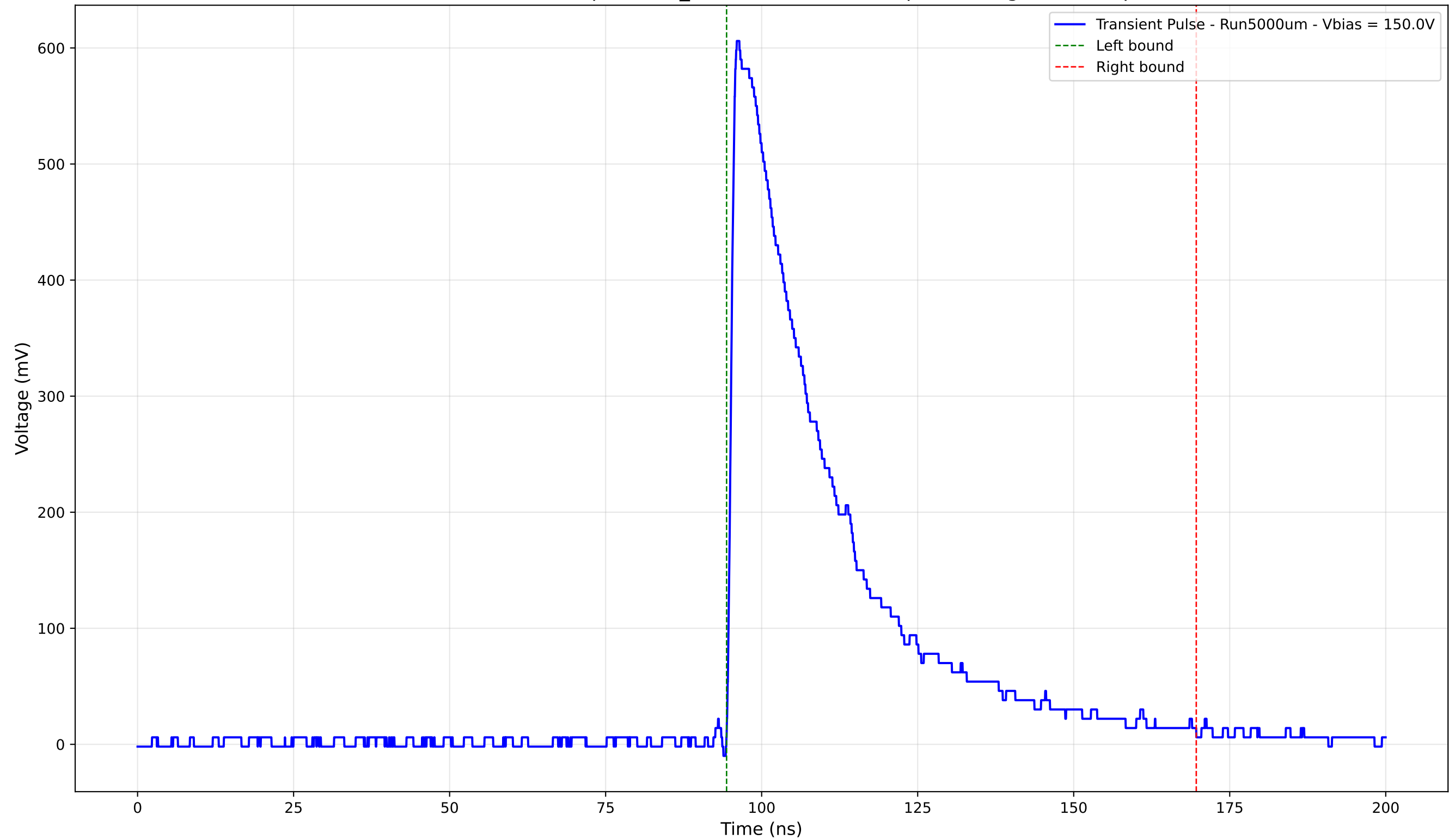
Transient Pulse - Sample: 1cm_42 - Position: 3325.0 \mu\text{m} - Charge: 206.72 pC
