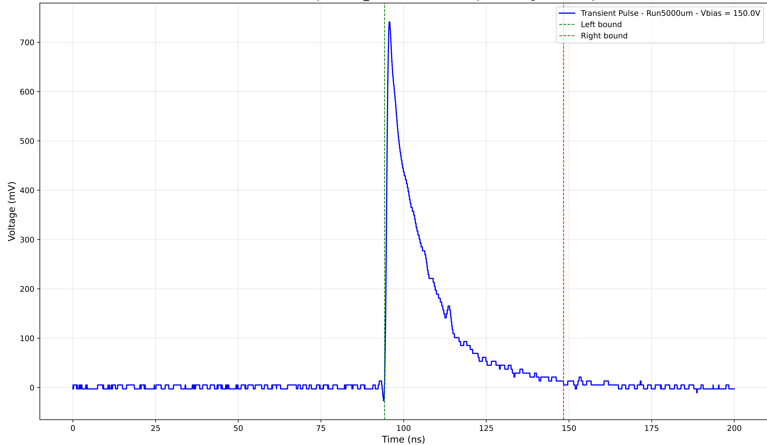
Transient Pulse - Sample: 1cm_42 - Position: 155.0 \mu\text{m} - Charge: 167.30 pC
