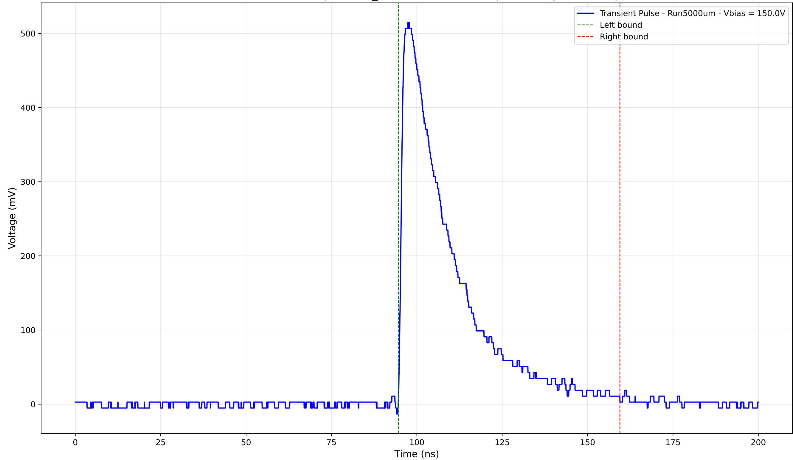
Transient Pulse - Sample: 1cm_42 - Position: 1260.0 \mu\text{m} - Charge: 166.23 pC
