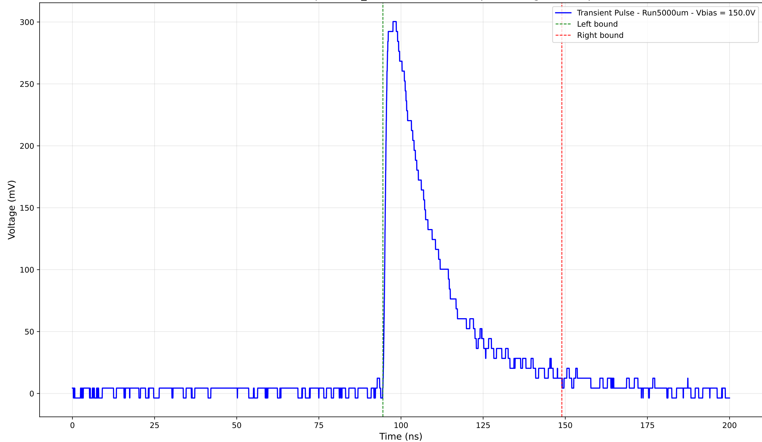
Transient Pulse - Sample: 1cm_42 - Position: 1565.0 \mu\text{m} - Charge: 99.23 pC
