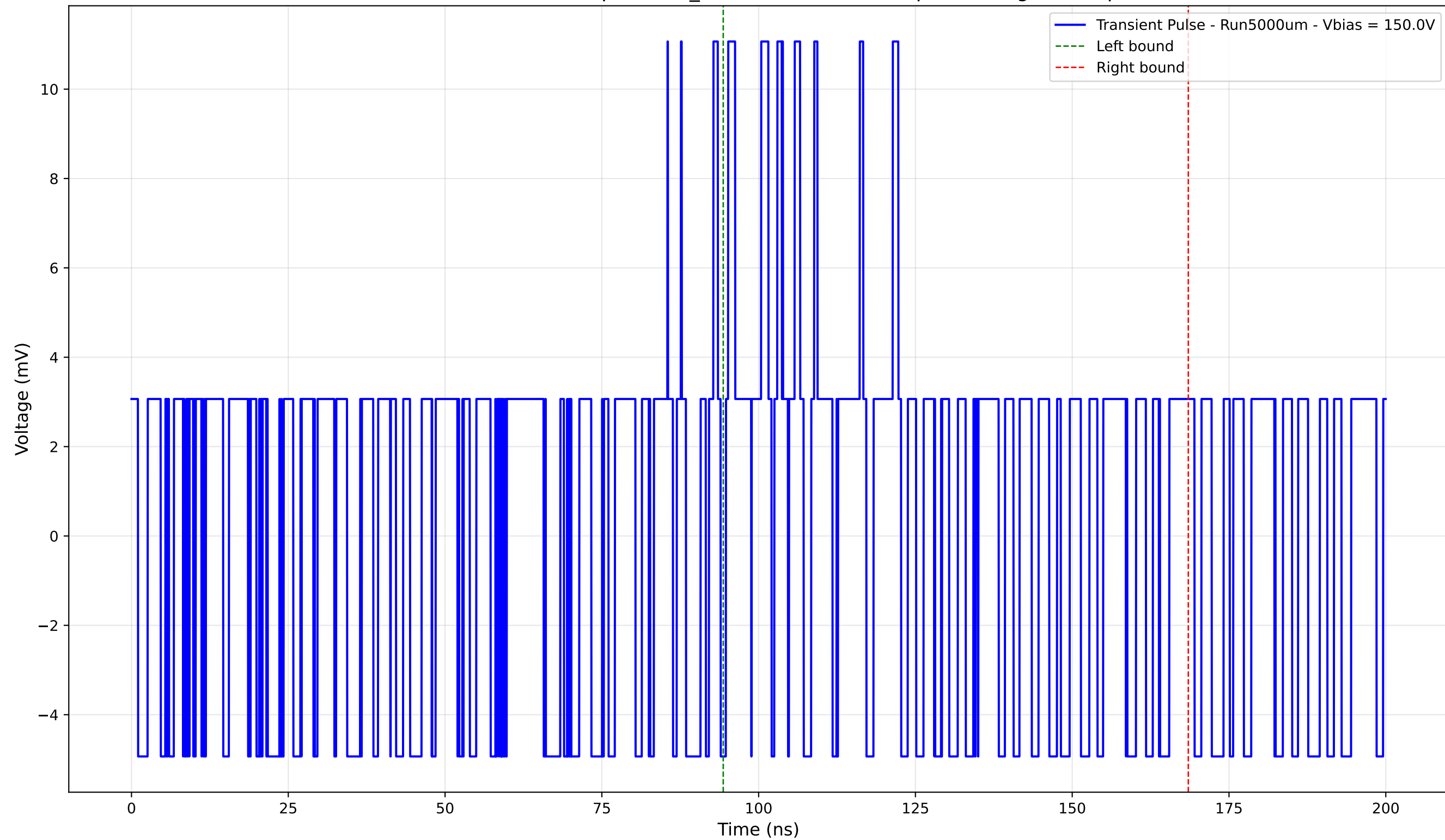
Transient Pulse - Sample: 1cm_42 - Position: 4995.0 \mu\text{m} - Charge: 1.89 pC
