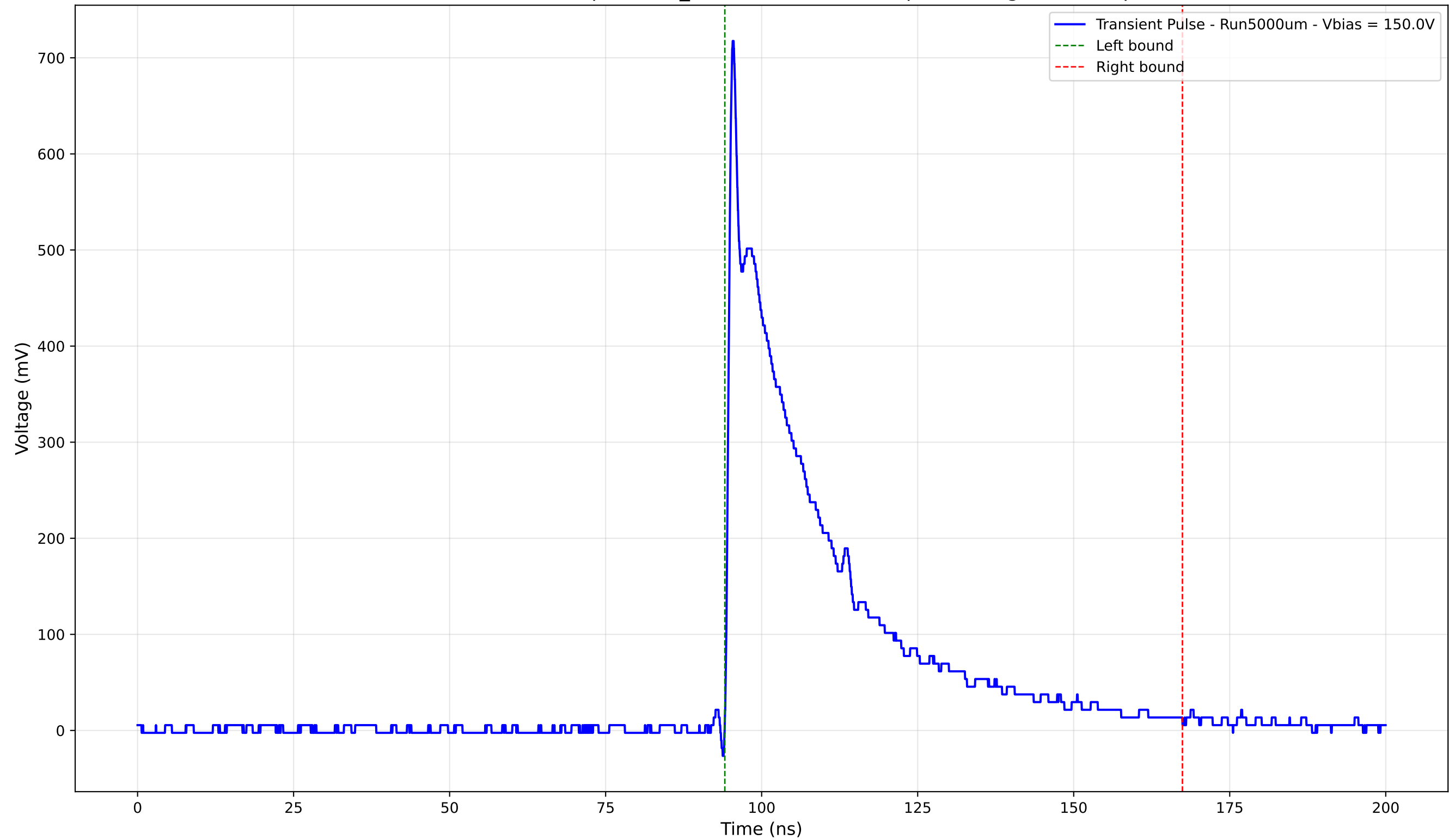
Transient Pulse - Sample: 1cm_42 - Position: 2230.0 \mu\text{m} - Charge: 188.07 pC
