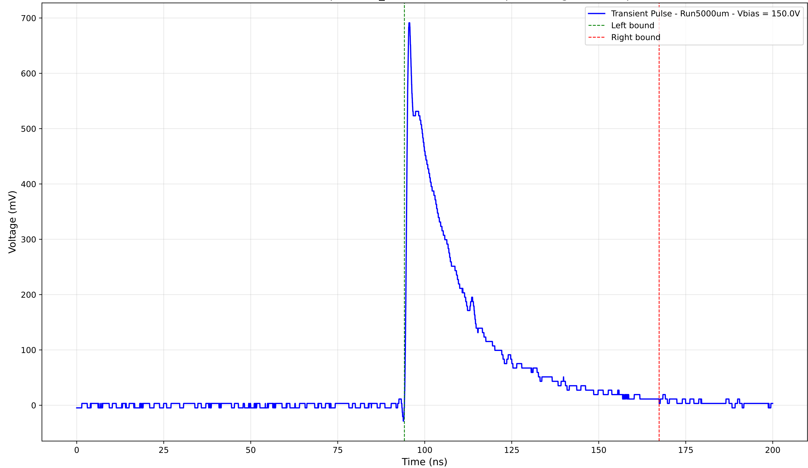
Transient Pulse - Sample: 1cm_42 - Position: 2925.0 \mu\text{m} - Charge: 192.67 pC
