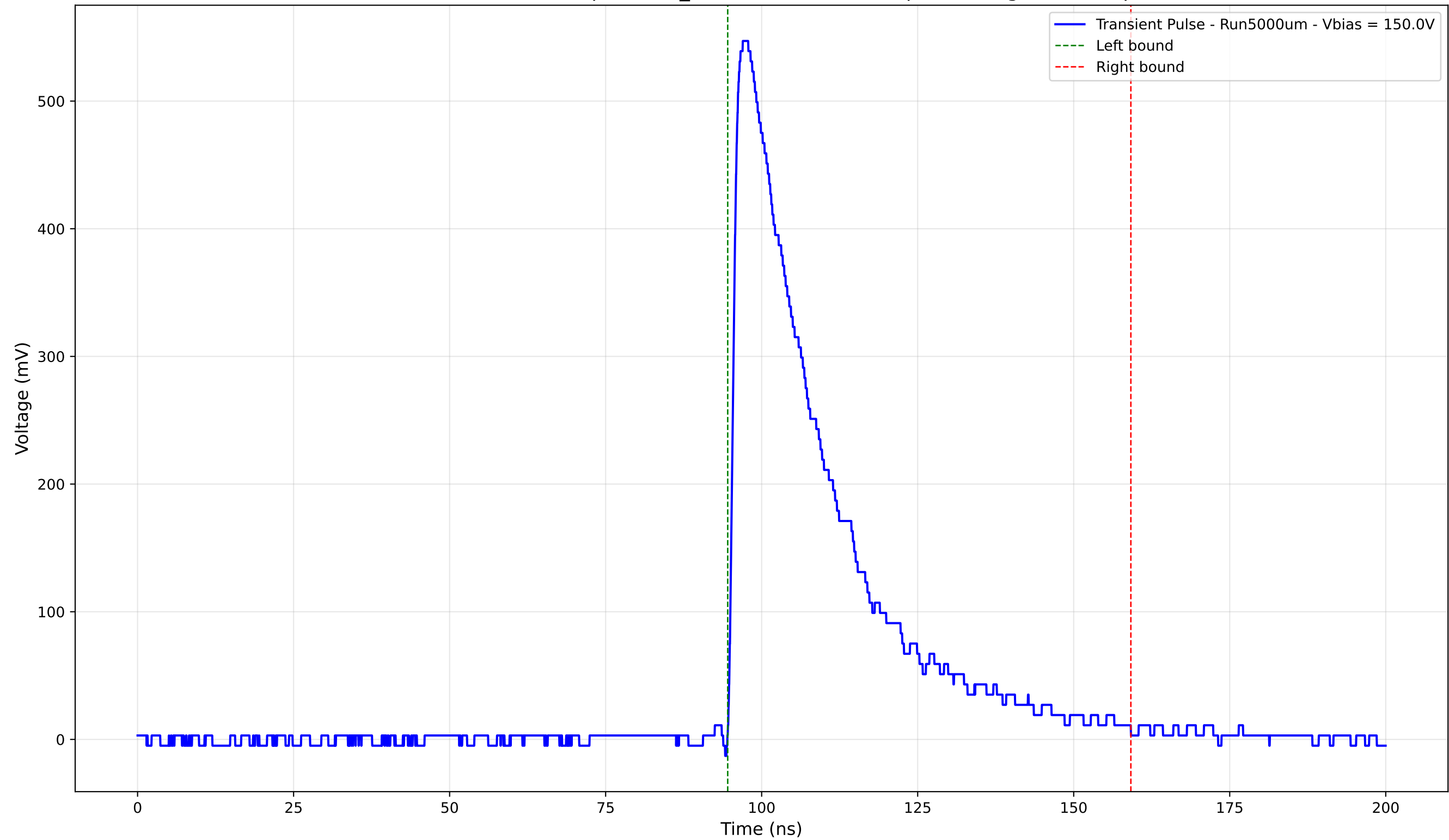
Transient Pulse - Sample: 1cm_42 - Position: 1140.0 \mu\text{m} - Charge: 174.00 pC
