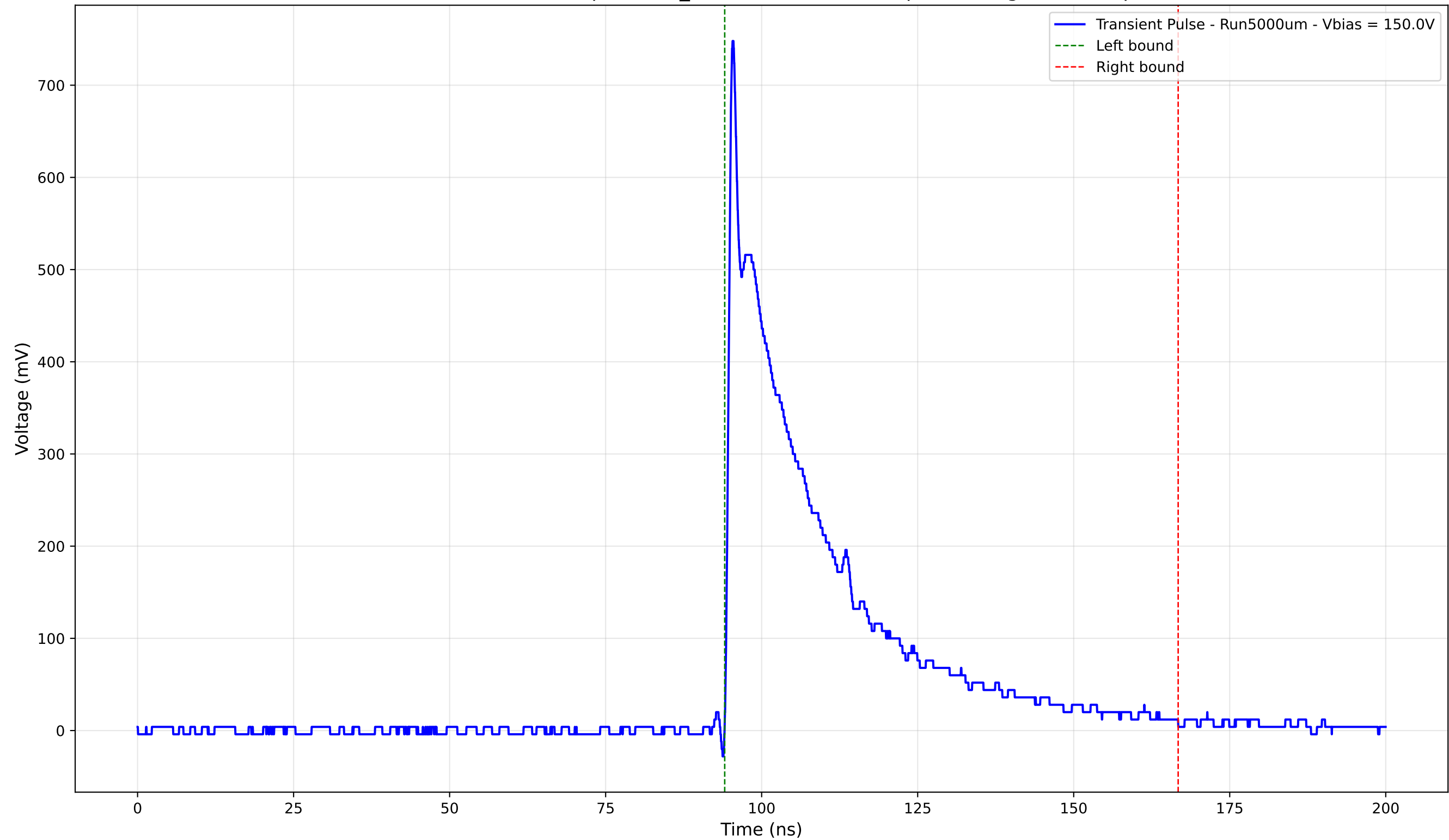
Transient Pulse - Sample: 1cm_42 - Position: 2790.0 \mu\text{m} - Charge: 190.69 pC
