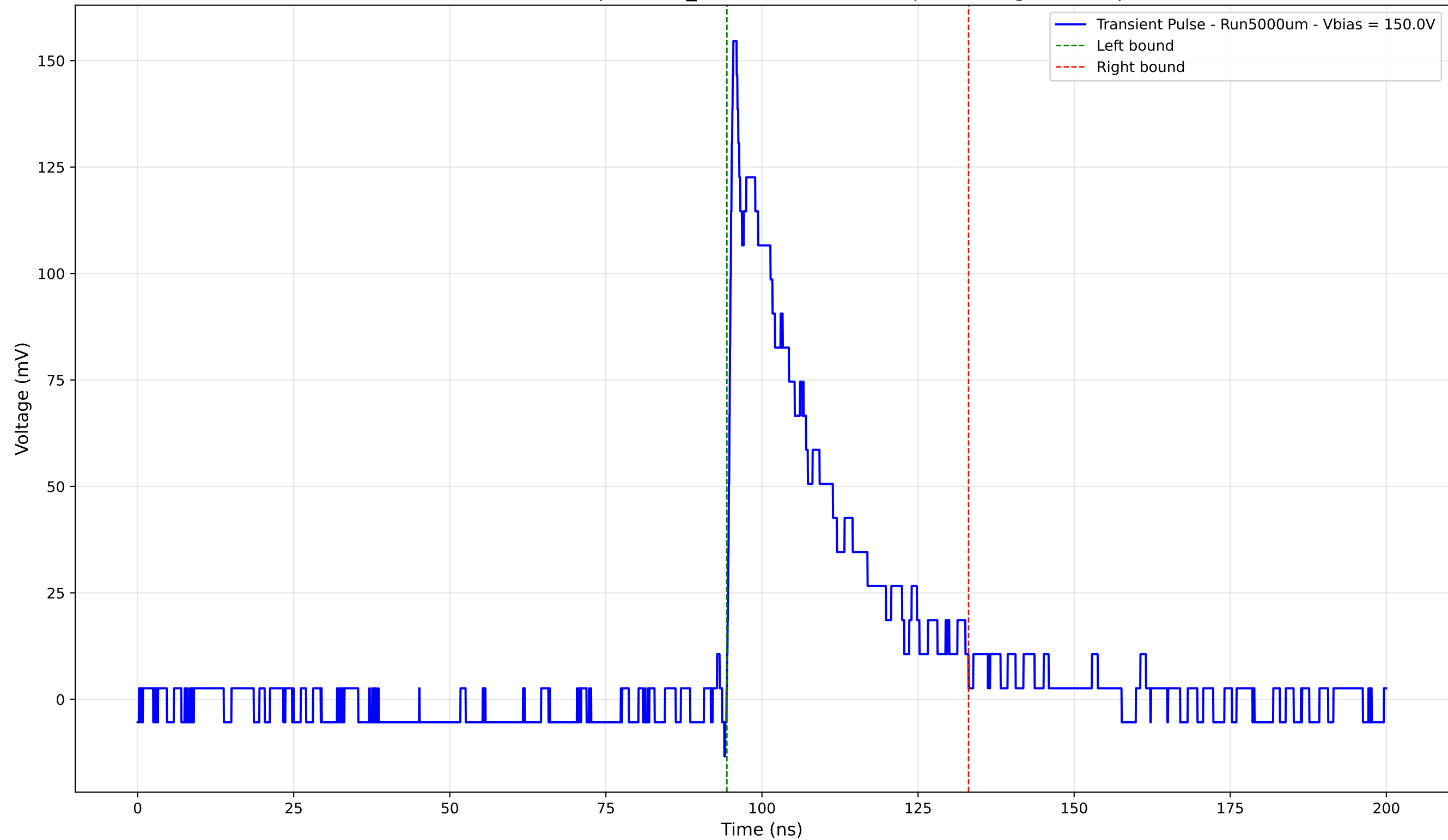
Transient Pulse - Sample: 1cm_42 - Position: 3015.0 \mu\text{m} - Charge: 39.53 pC
