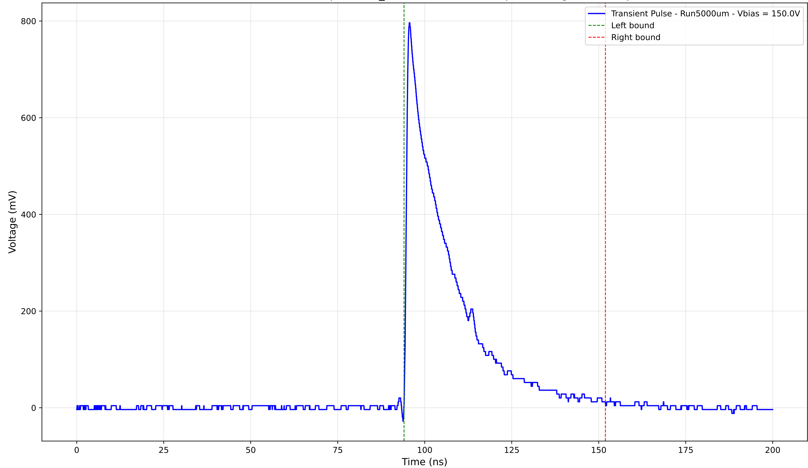
Transient Pulse - Sample: 1cm_42 - Position: 4705.0 \mu\text{m} - Charge: 202.79 pC
