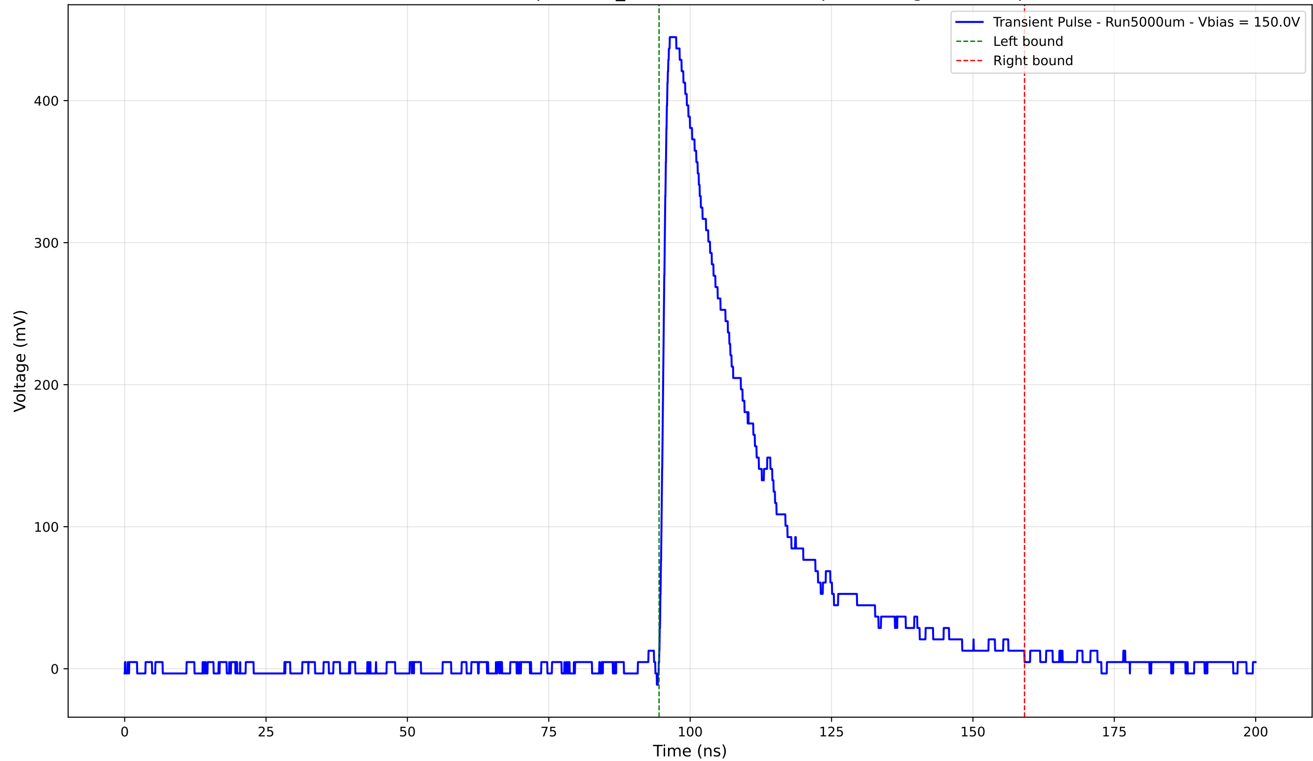
Transient Pulse - Sample: 1cm_42 - Position: 3600.0 \mu\text{m} - Charge: 145.51 pC
