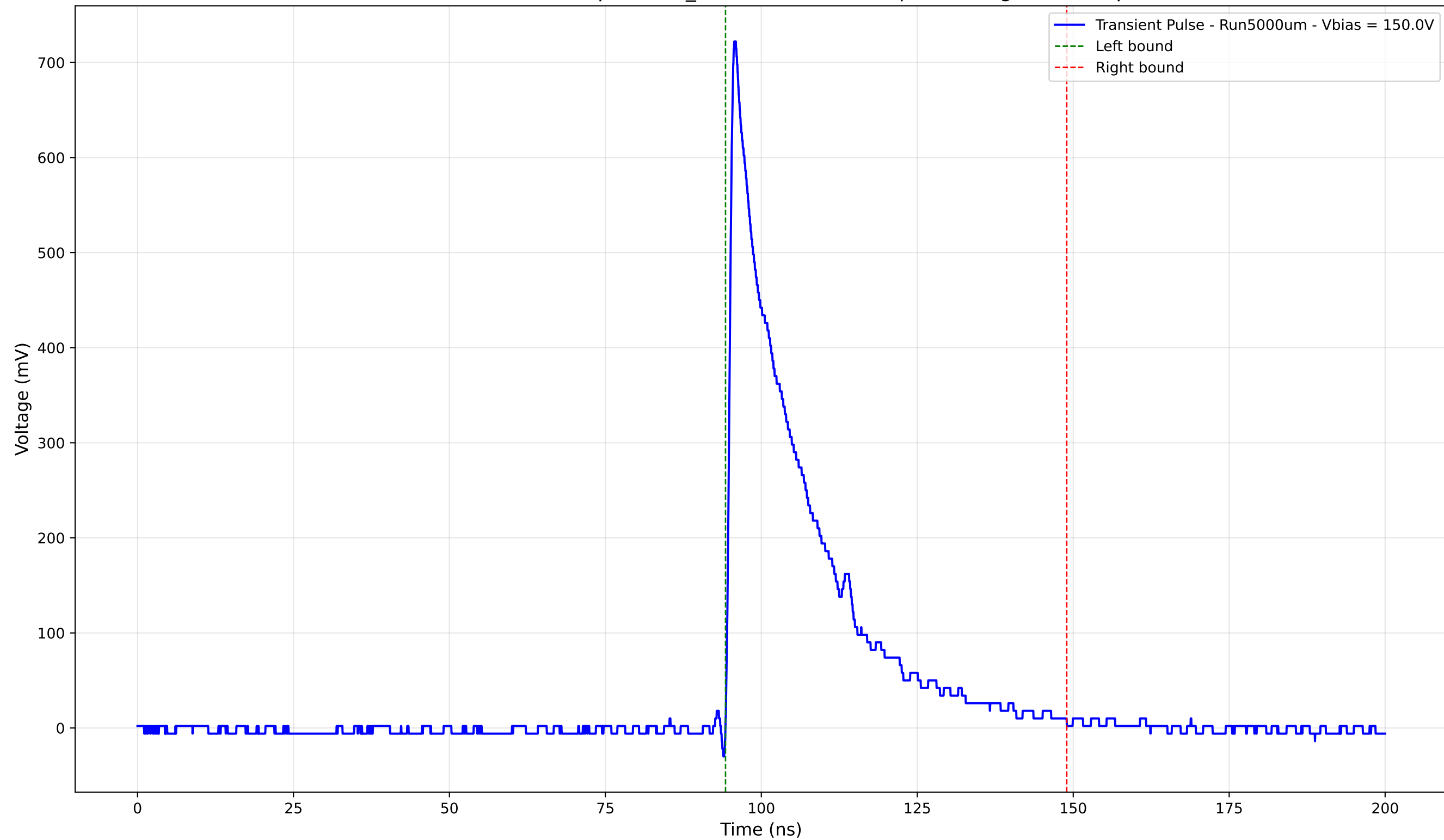
Transient Pulse - Sample: 1cm_42 - Position: 200.0 \mu\text{m} - Charge: 165.28 pC
