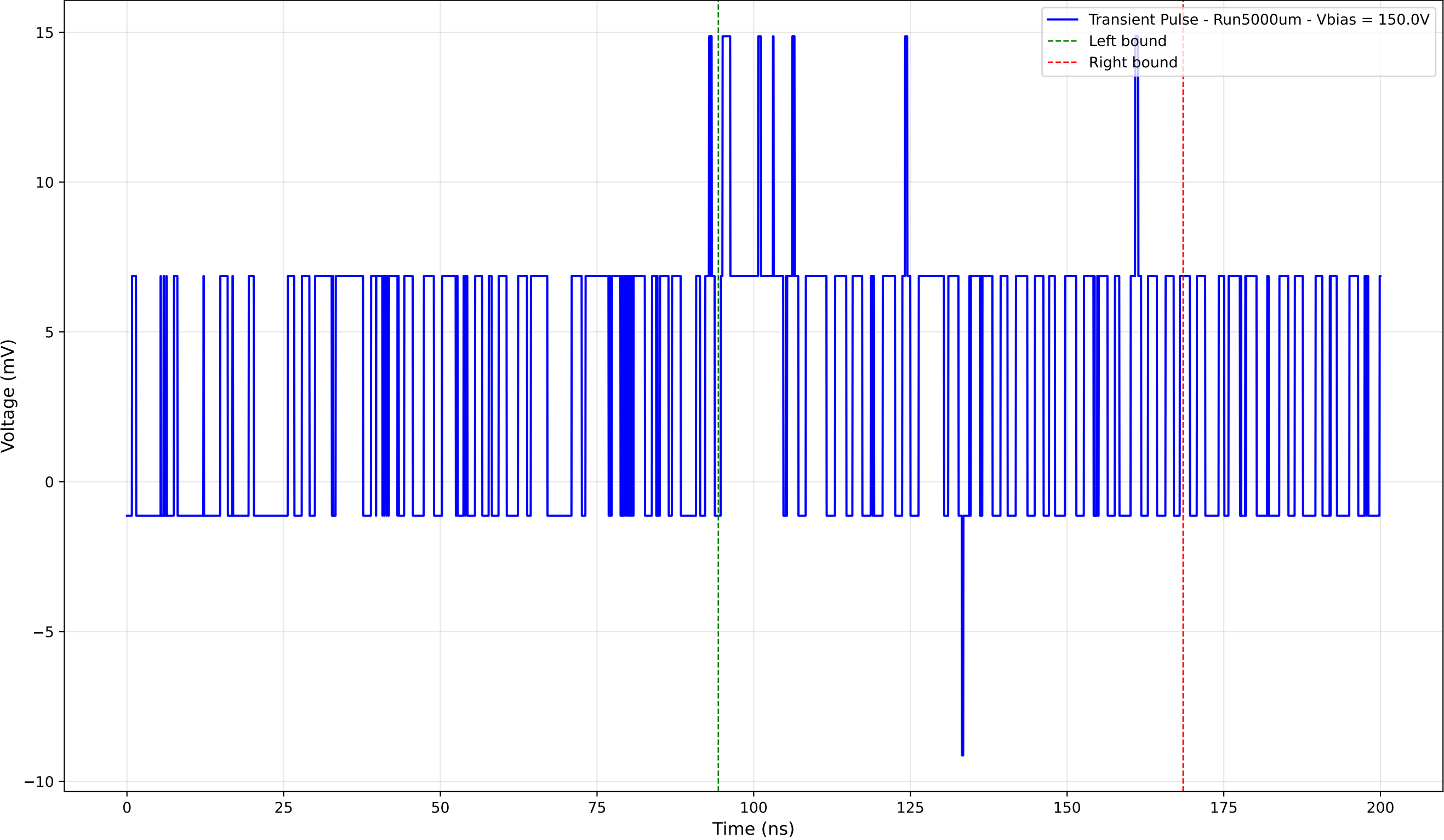
Transient Pulse - Sample: 1cm_42 - Position: 5040.0 \mu\text{m} - Charge: 6.30 pC
