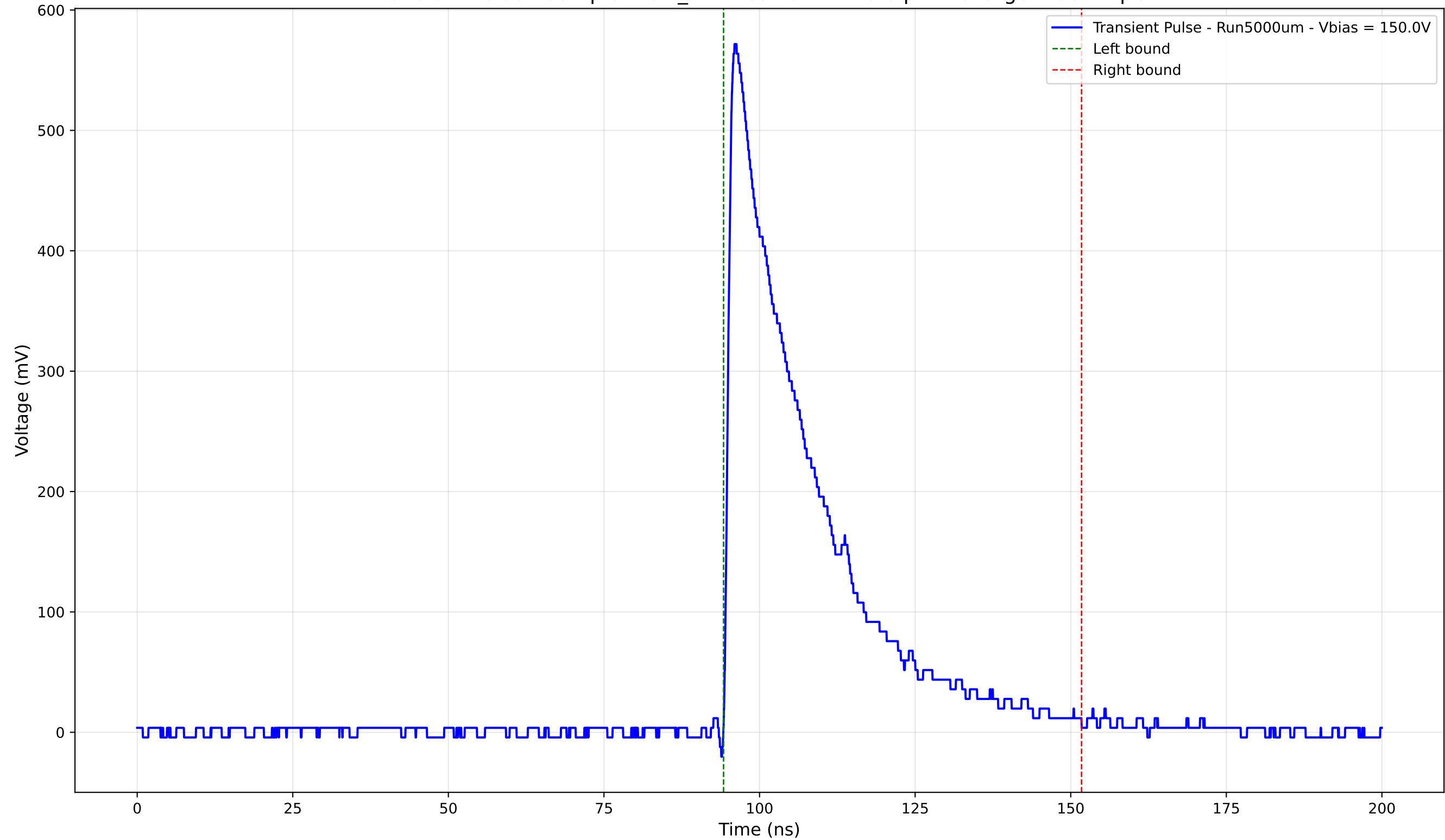
Transient Pulse - Sample: 1cm_42 - Position: 4470.0 \mu\text{m} - Charge: 158.71 pC
