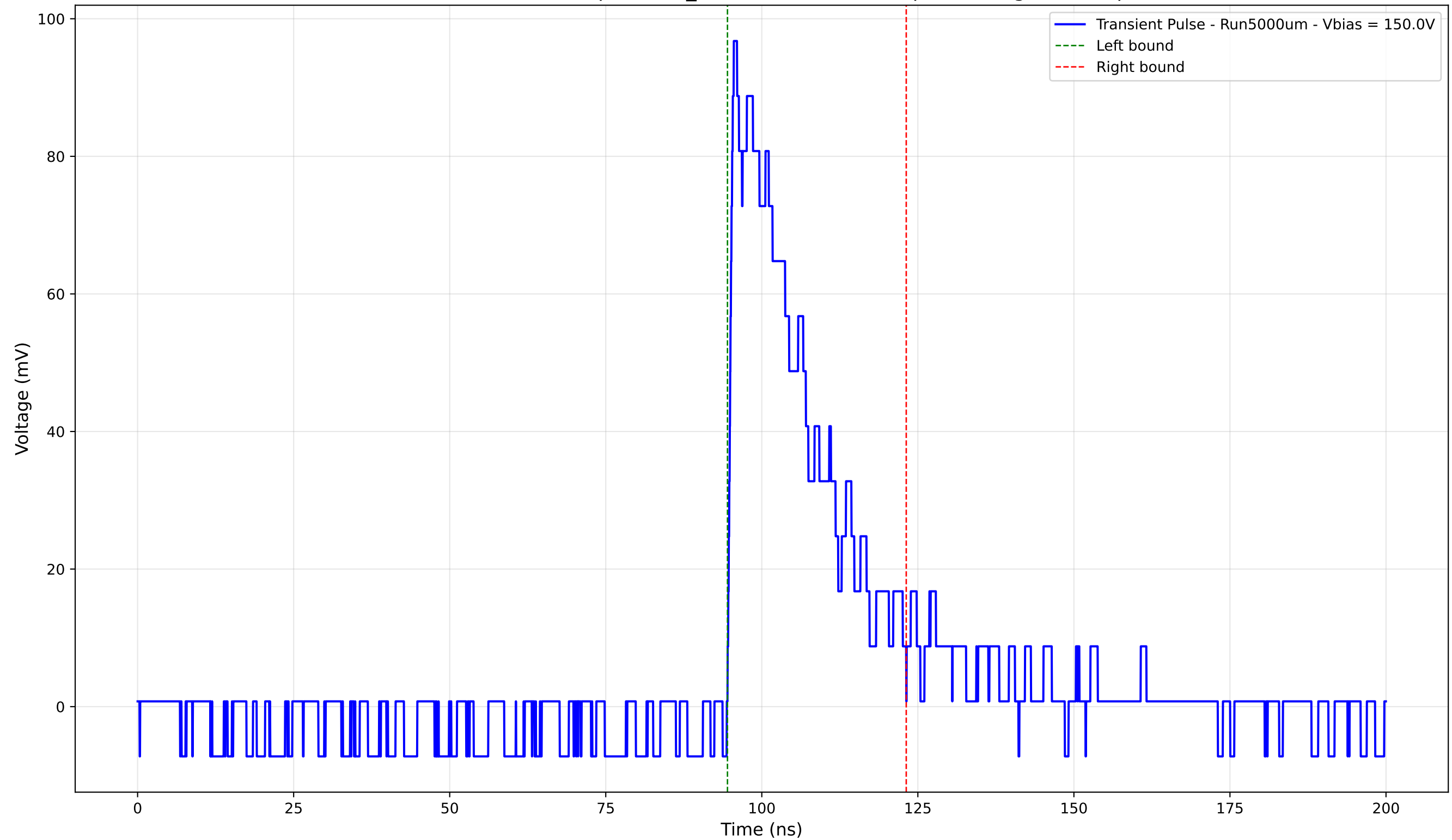
Transient Pulse - Sample: 1cm_42 - Position: 2005.0 \mu\text{m} - Charge: 24.74 pC
