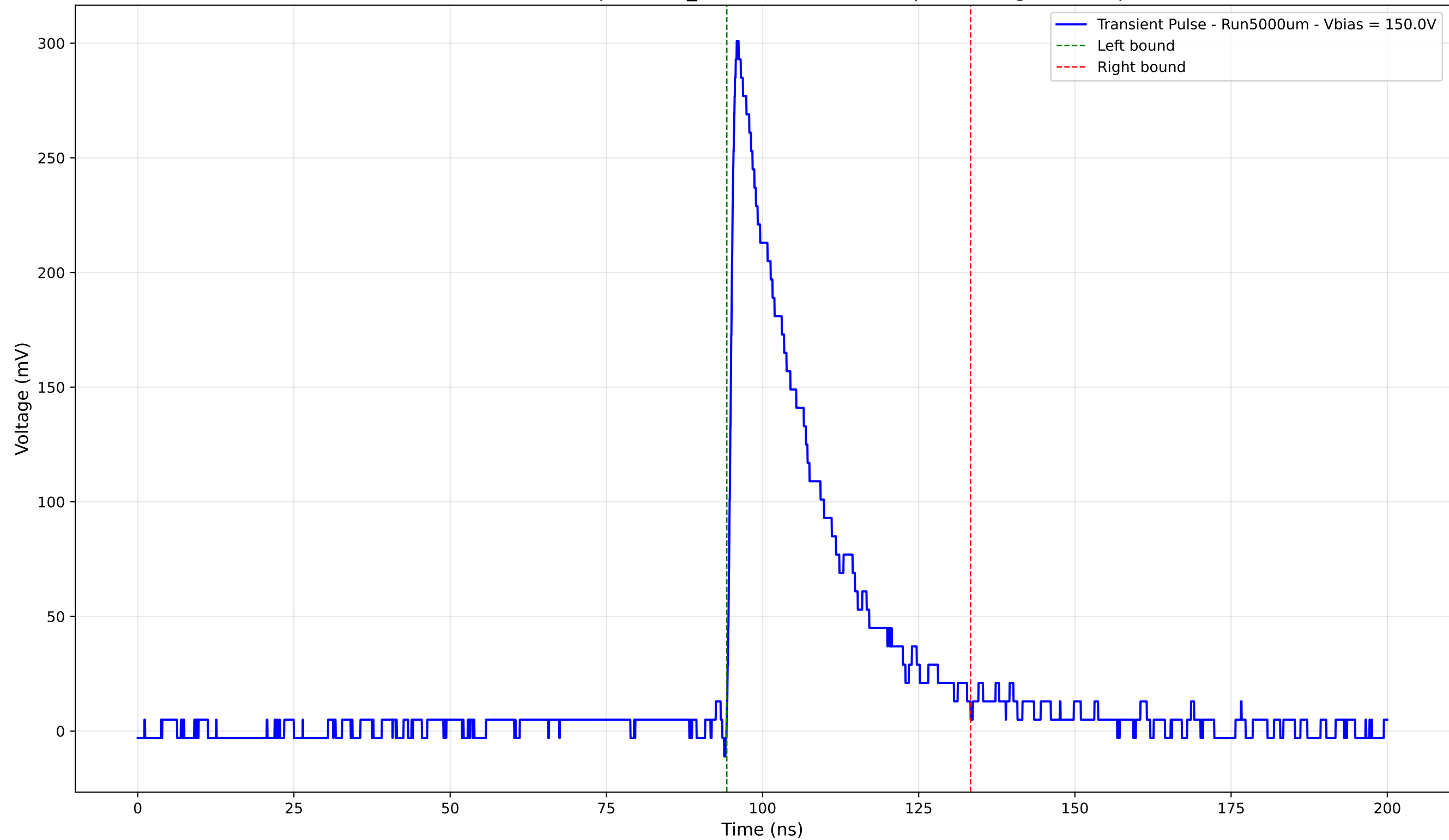
Transient Pulse - Sample: 1cm_42 - Position: 4505.0 \mu\text{m} - Charge: 76.94 pC
