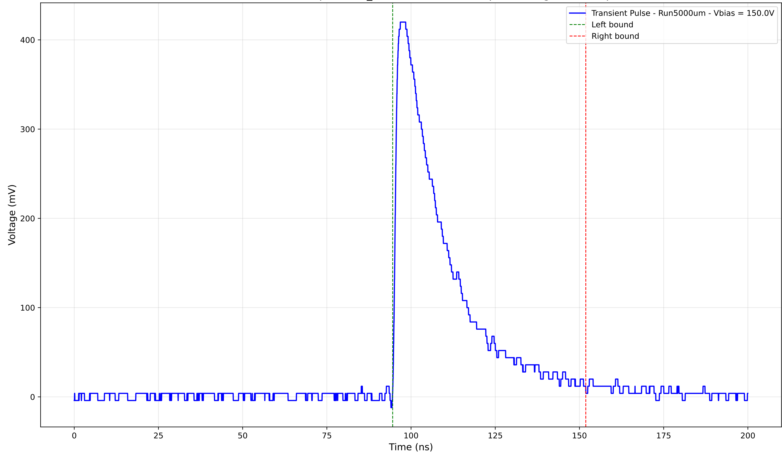
Transient Pulse - Sample: 1cm_42 - Position: 1435.0 \mu\text{m} - Charge: 137.67 pC
