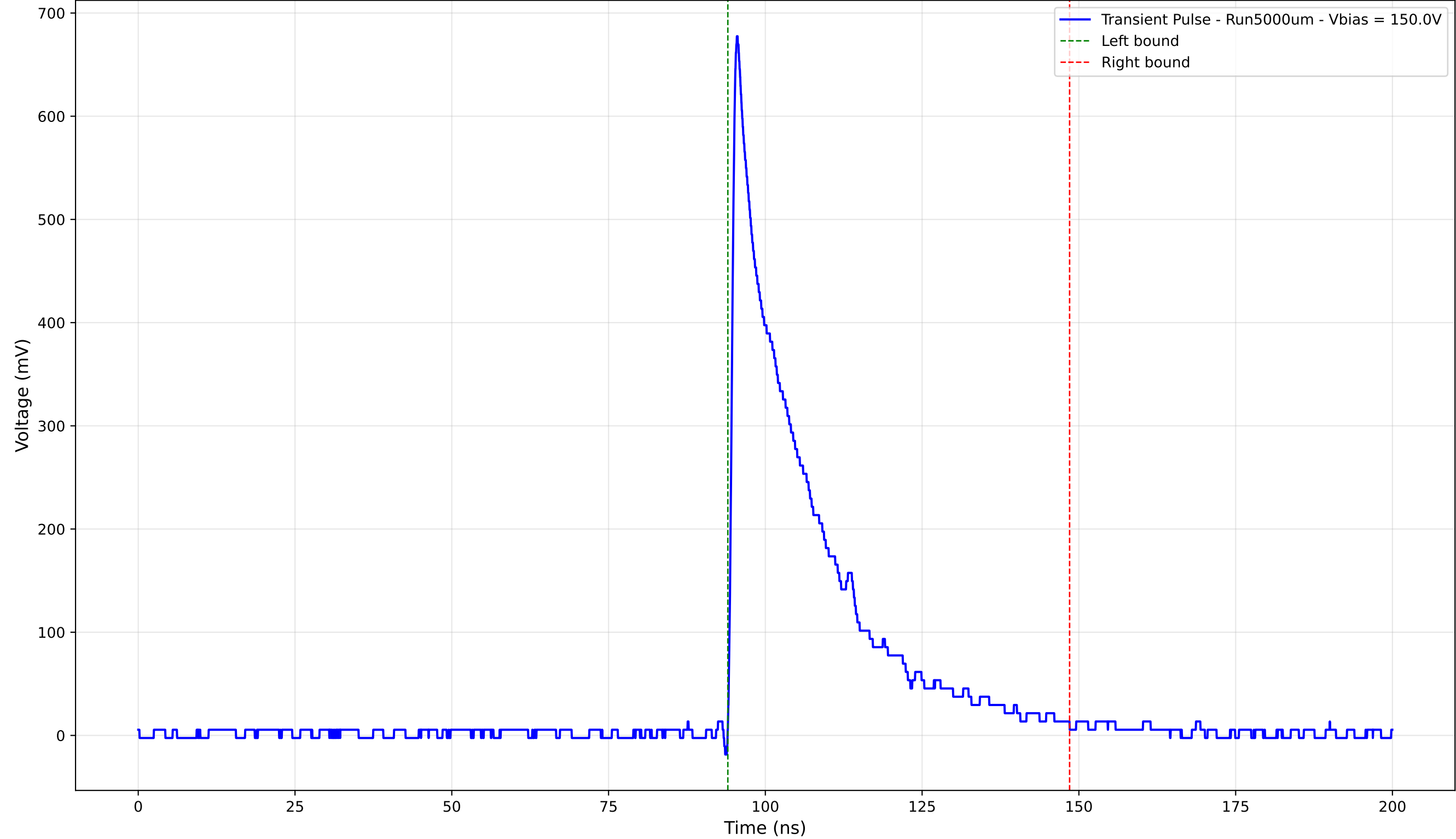
Transient Pulse - Sample: 1cm_42 - Position: 4795.0 \mu\text{m} - Charge: 158.62 pC
