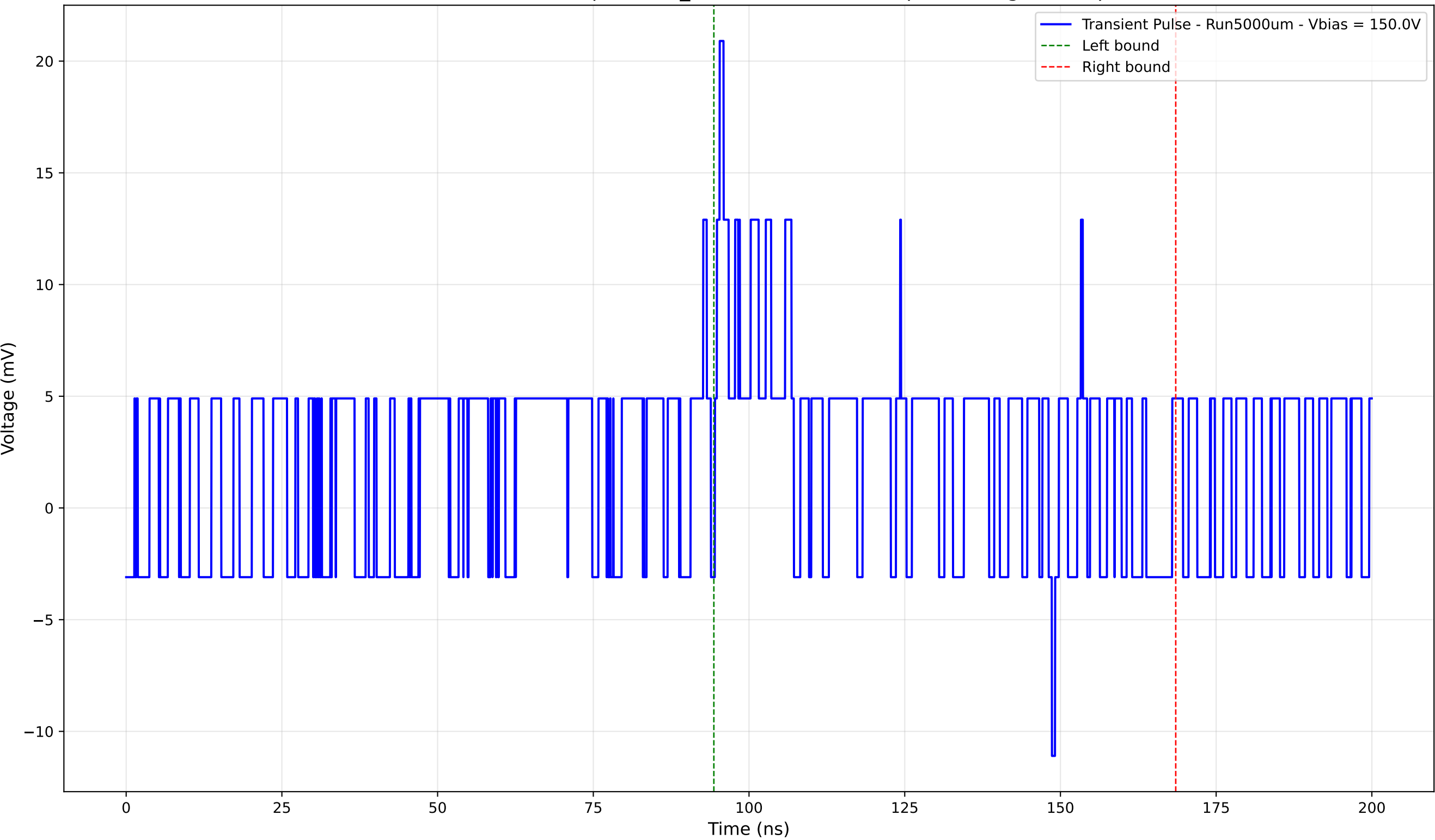
Transient Pulse - Sample: 1cm_42 - Position: 4925.0 \mu\text{m} - Charge: 4.62 pC
