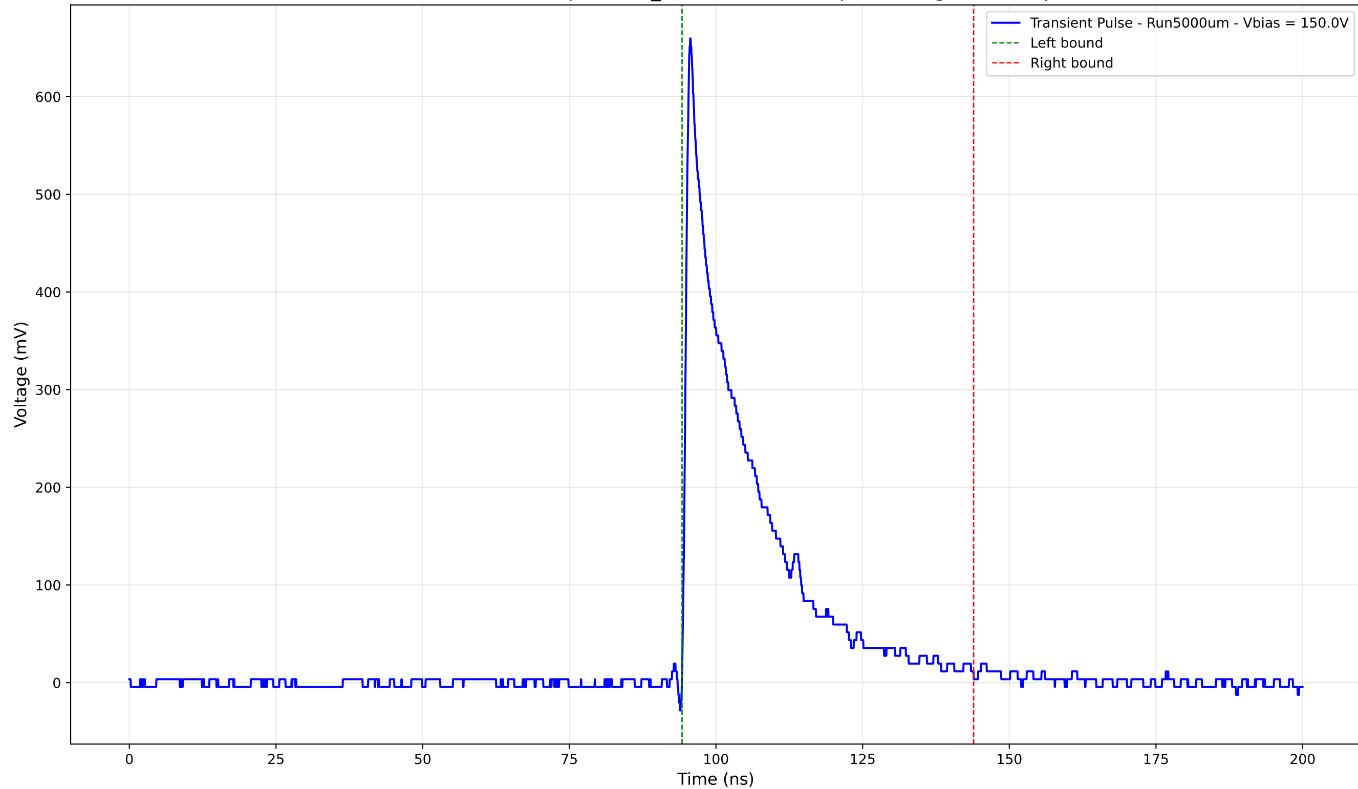
Transient Pulse - Sample: 1cm_42 - Position: 90.0 \mu\text{m} - Charge: 136.35 pC
