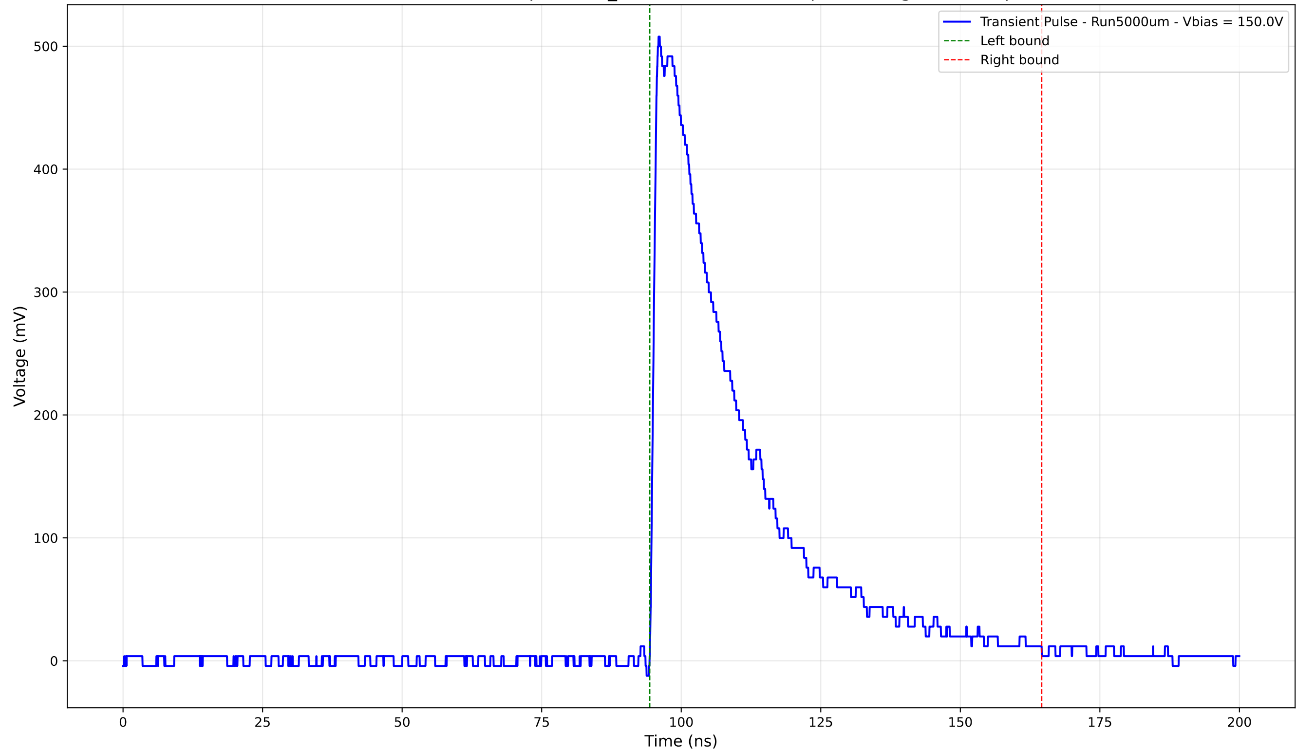
Transient Pulse - Sample: 1cm_42 - Position: 1795.0 \mu\text{m} - Charge: 172.06 pC
