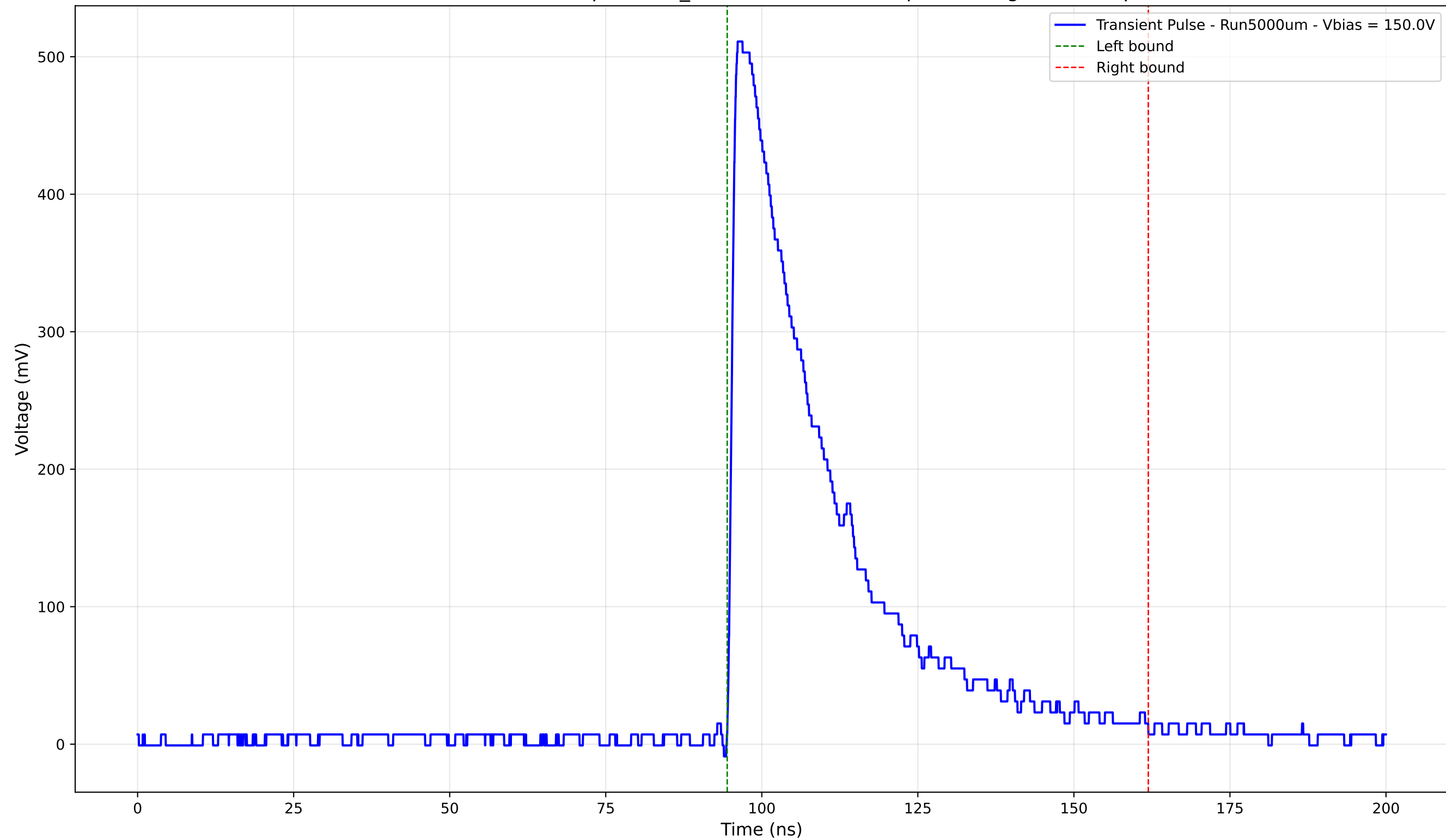
Transient Pulse - Sample: 1cm_42 - Position: 3455.0 \mu\text{m} - Charge: 171.98 pC
