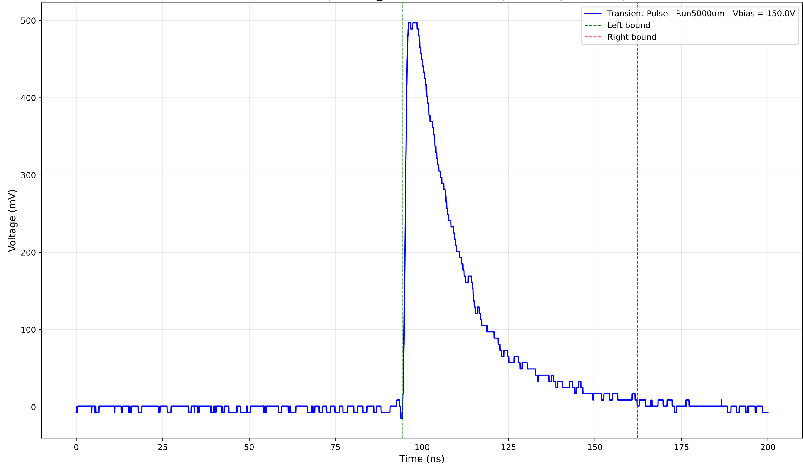
Transient Pulse - Sample: 1cm_42 - Position: 1670.0 \mu\text{m} - Charge: 168.76 pC
