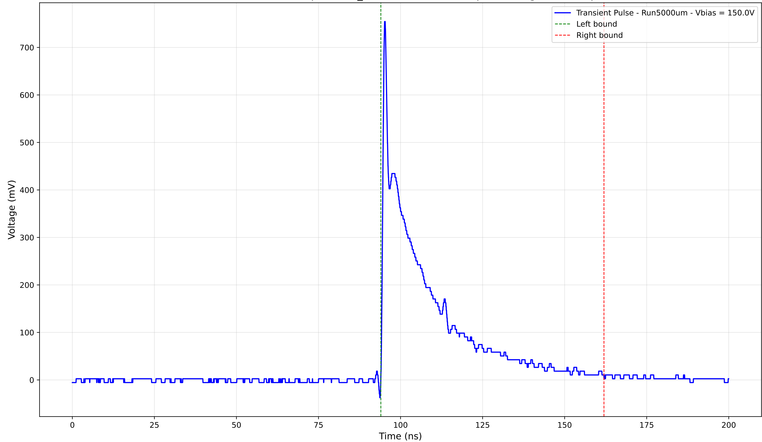
Transient Pulse - Sample: 1cm_42 - Position: 2420.0 \mu\text{m} - Charge: 160.61 pC
