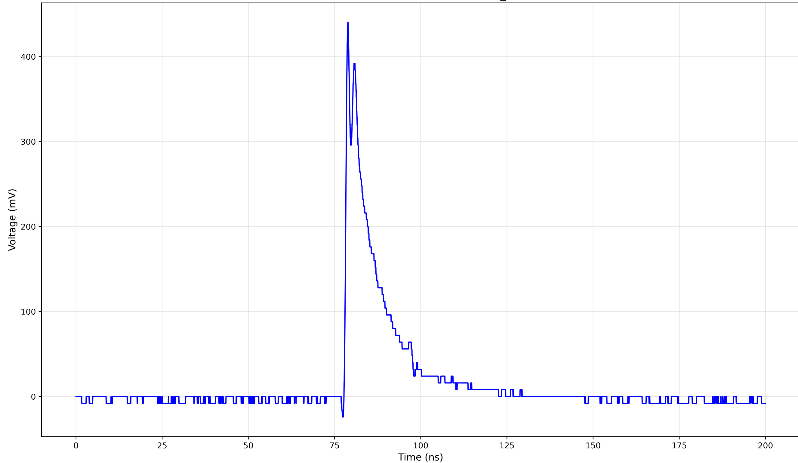
TCT Pulse Waveform - Run 5mm)old: 5mm_old (100.0 V)
