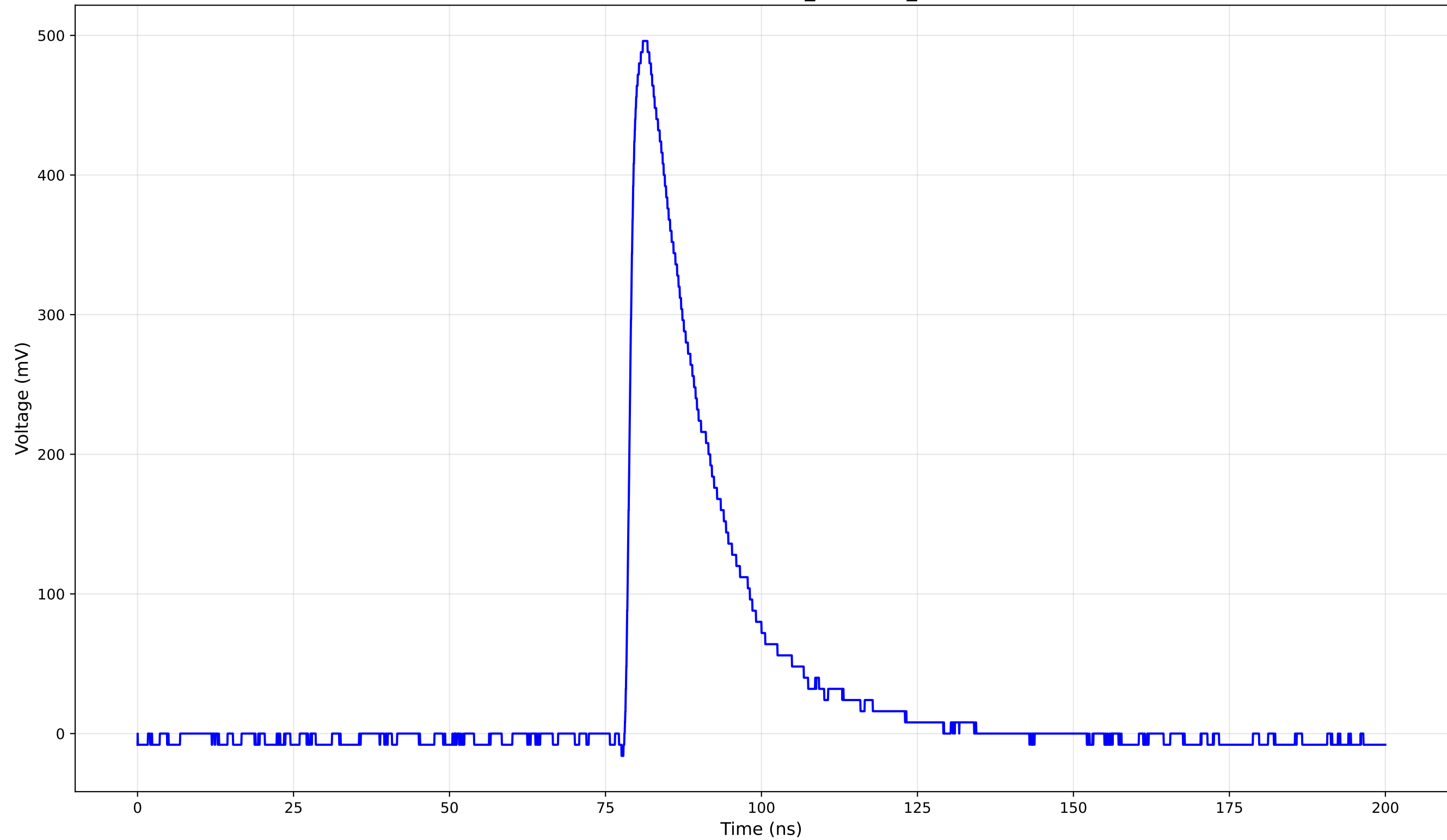
TCT Pulse Waveform - Run 5mm_23: 5mm_23 (150.0 V)
