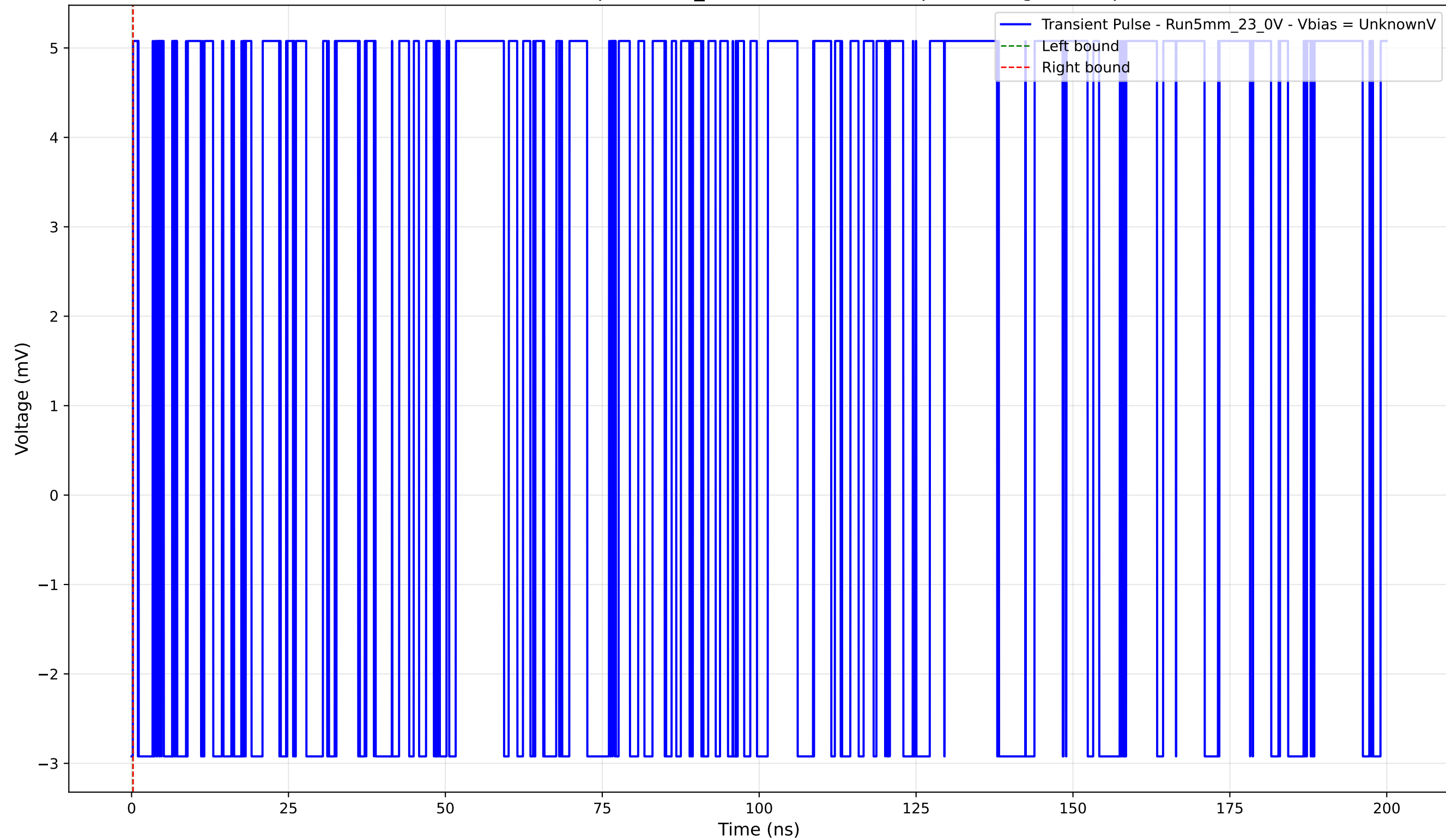
Transient Pulse - Sample: 5mm_23 - Position: 2665.0 \mu\text{m} - Charge: 0.00 pC
