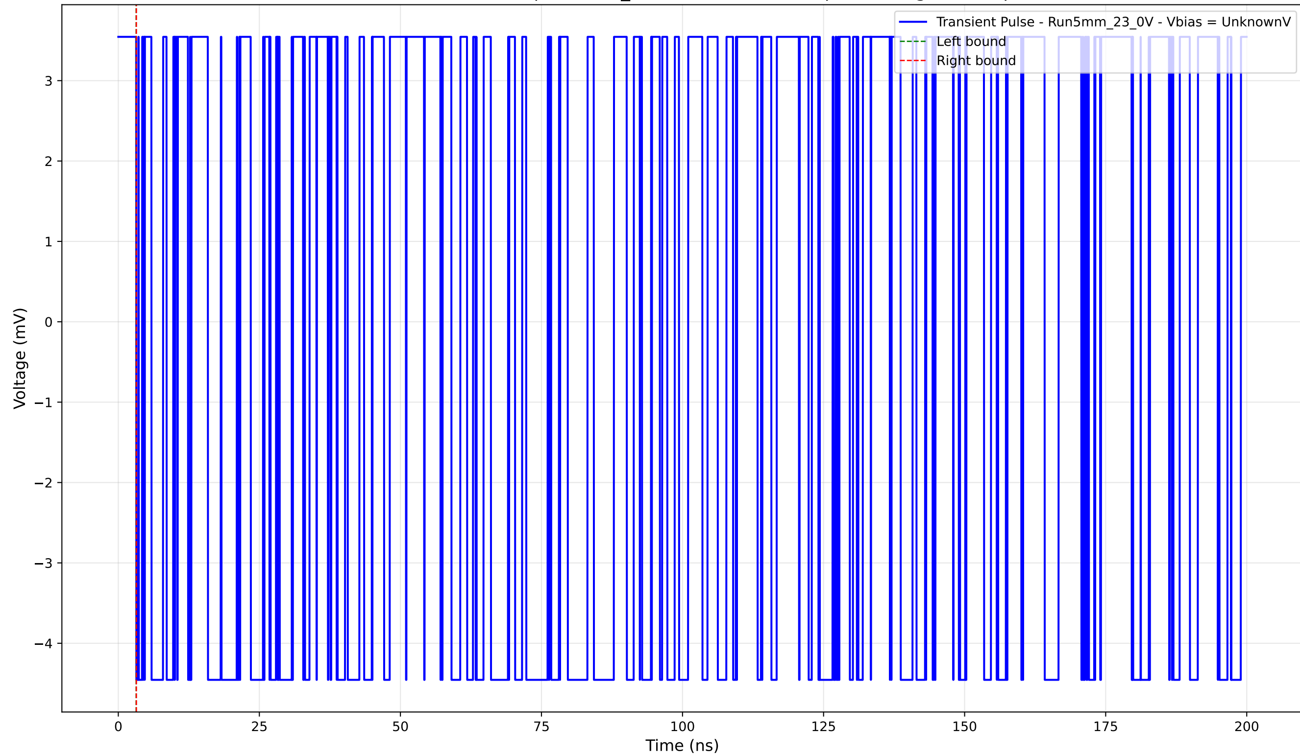
Transient Pulse - Sample: 5mm_23 - Position: 2910.0 \mu\text{m} - Charge: -0.00 pC
