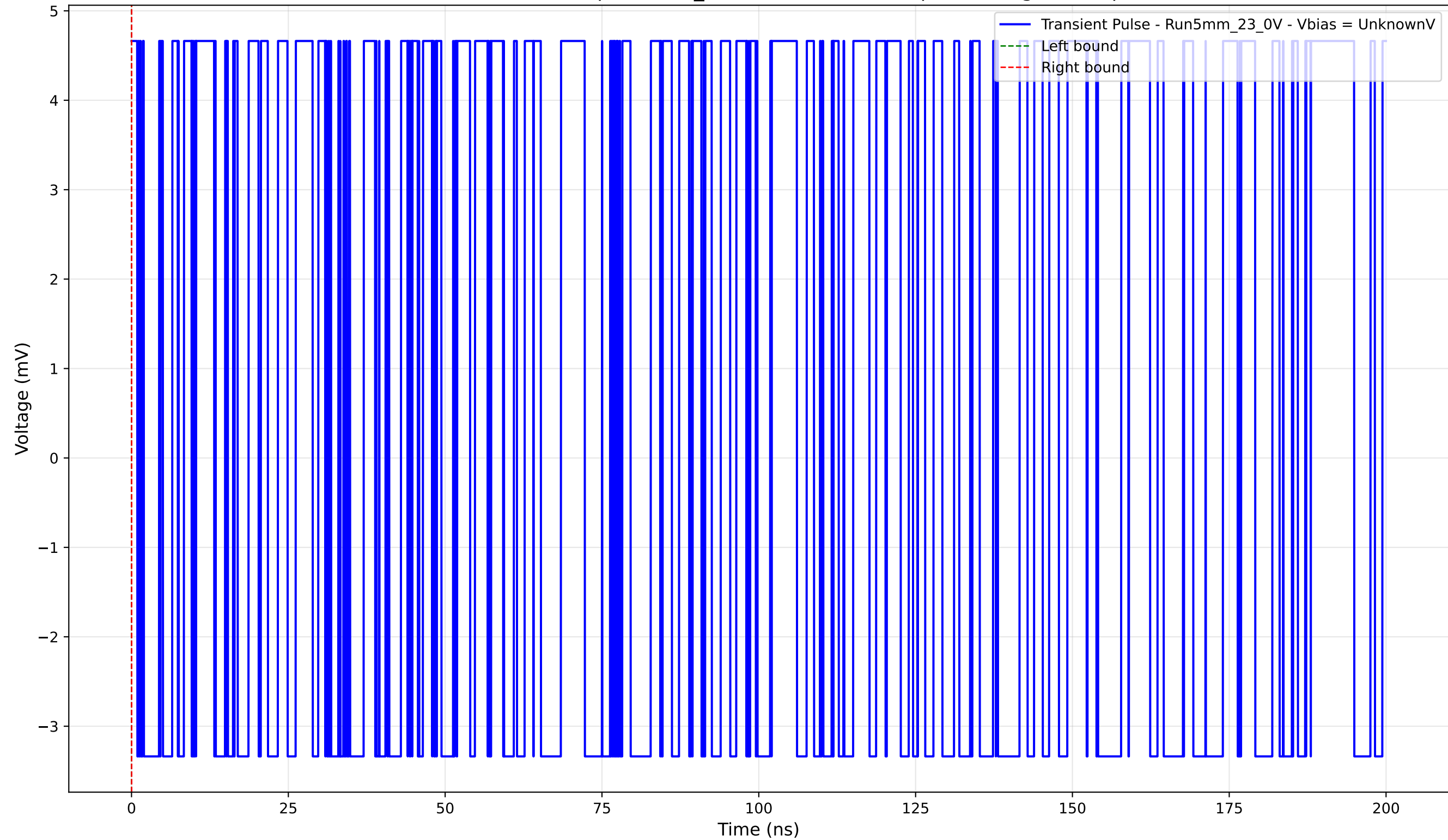
Transient Pulse - Sample: 5mm_23 - Position: 4770.0 \mu\text{m} - Charge: 0.00 pC
