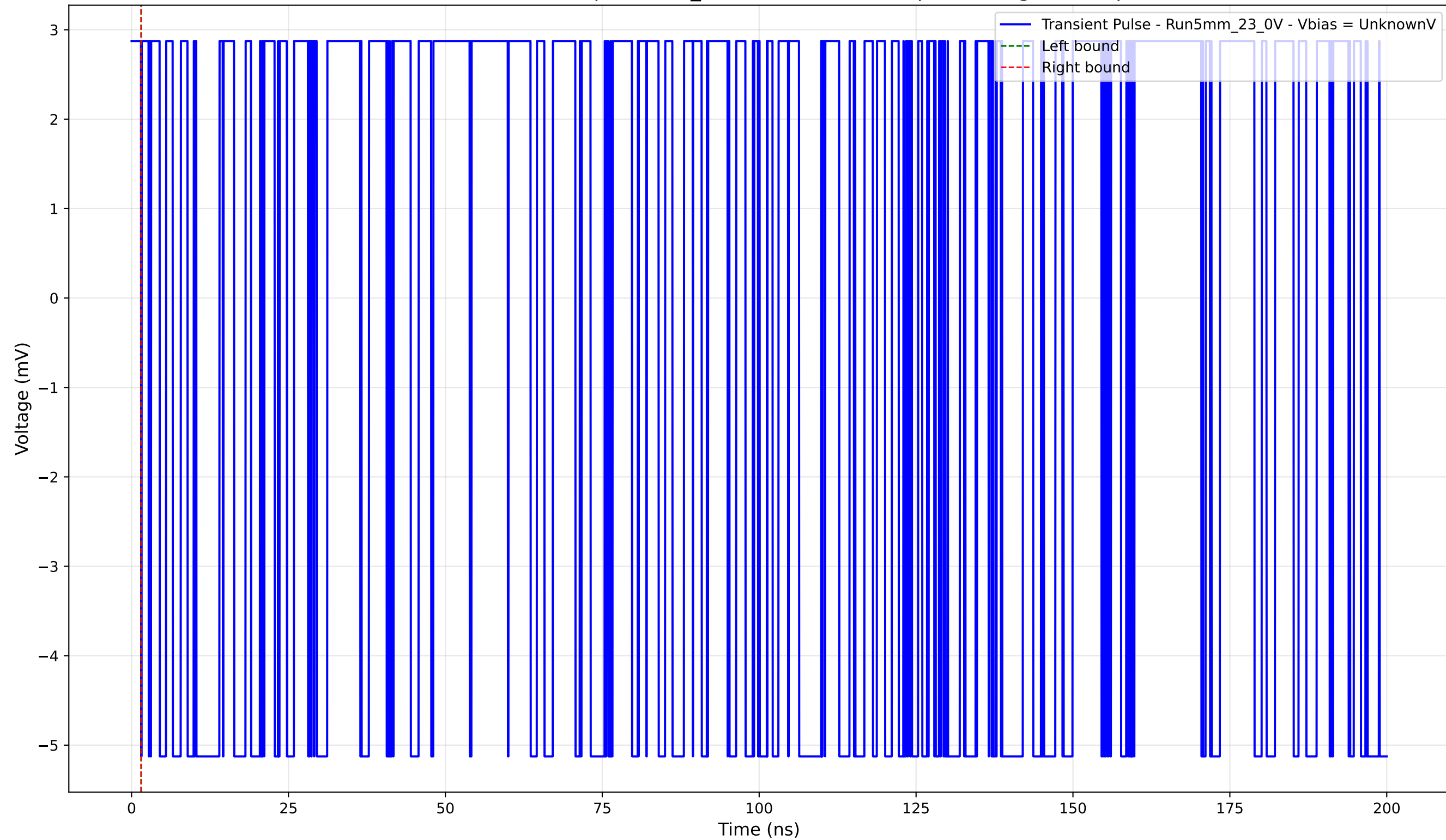
Transient Pulse - Sample: 5mm_23 - Position: 3640.0 \mu\text{m} - Charge: -0.00 pC
