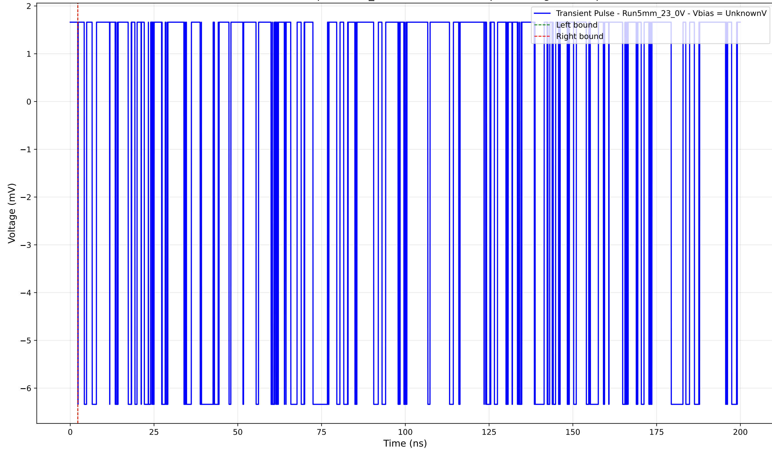
Transient Pulse - Sample: 5mm_23 - Position: 3410.0 \mu\text{m} - Charge: -0.00 pC
