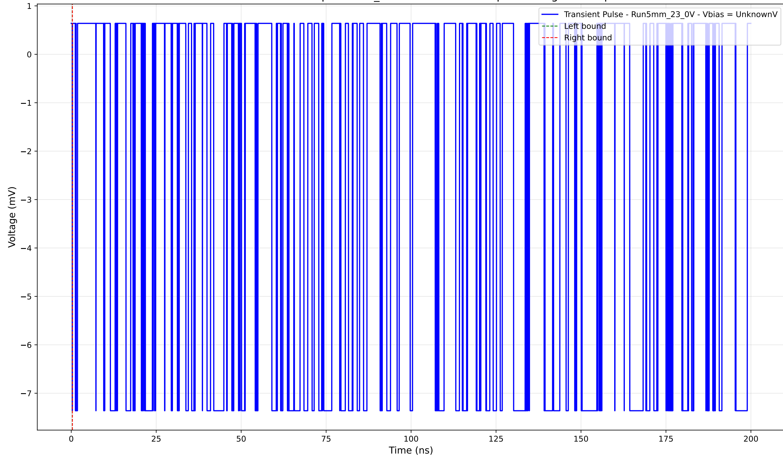
Transient Pulse - Sample: 5mm_23 - Position: 5030.0 \mu\text{m} - Charge: -0.00 pC
