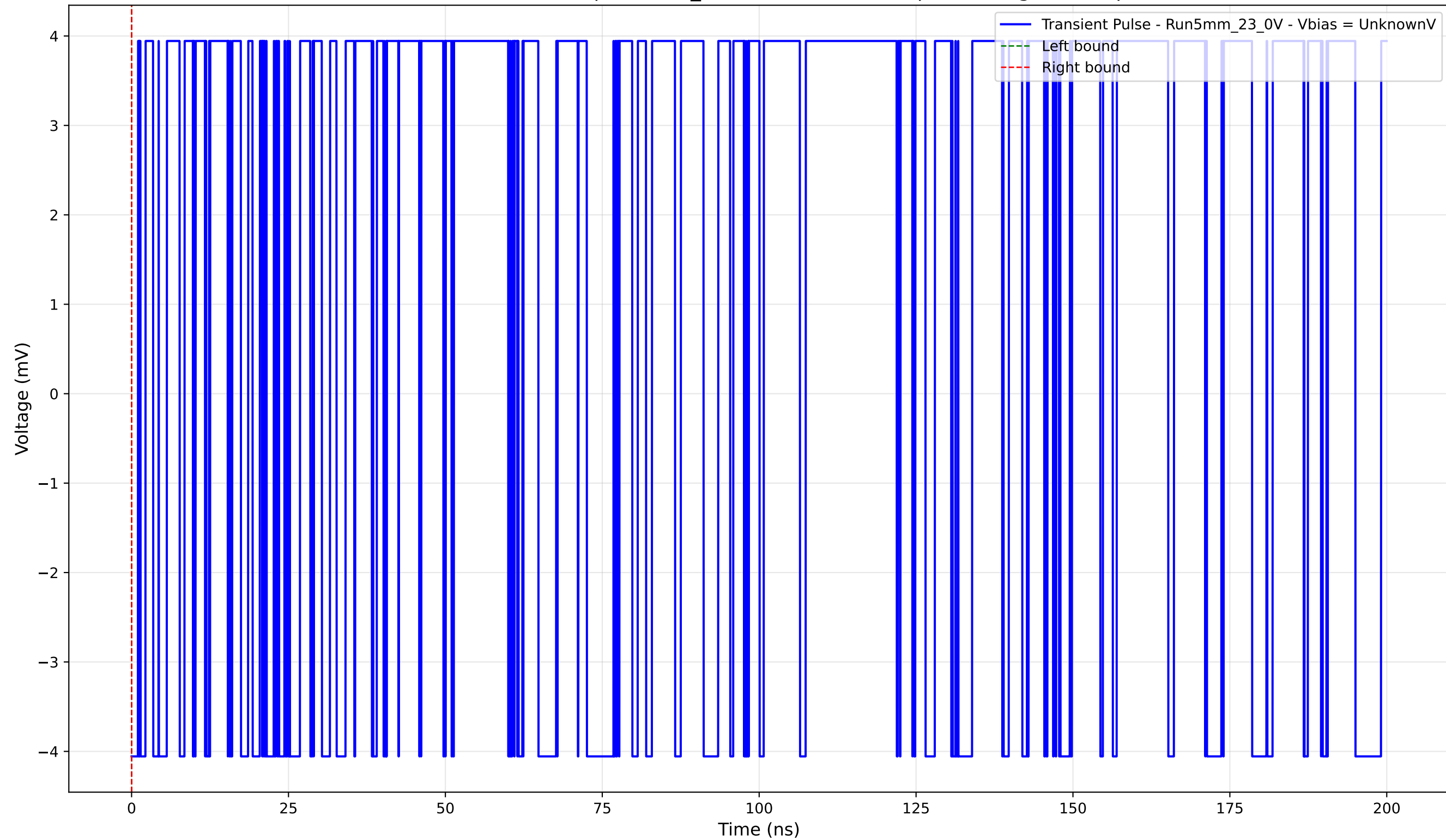
Transient Pulse - Sample: 5mm_23 - Position: 2880.0 \mu\text{m} - Charge: -0.00 pC
