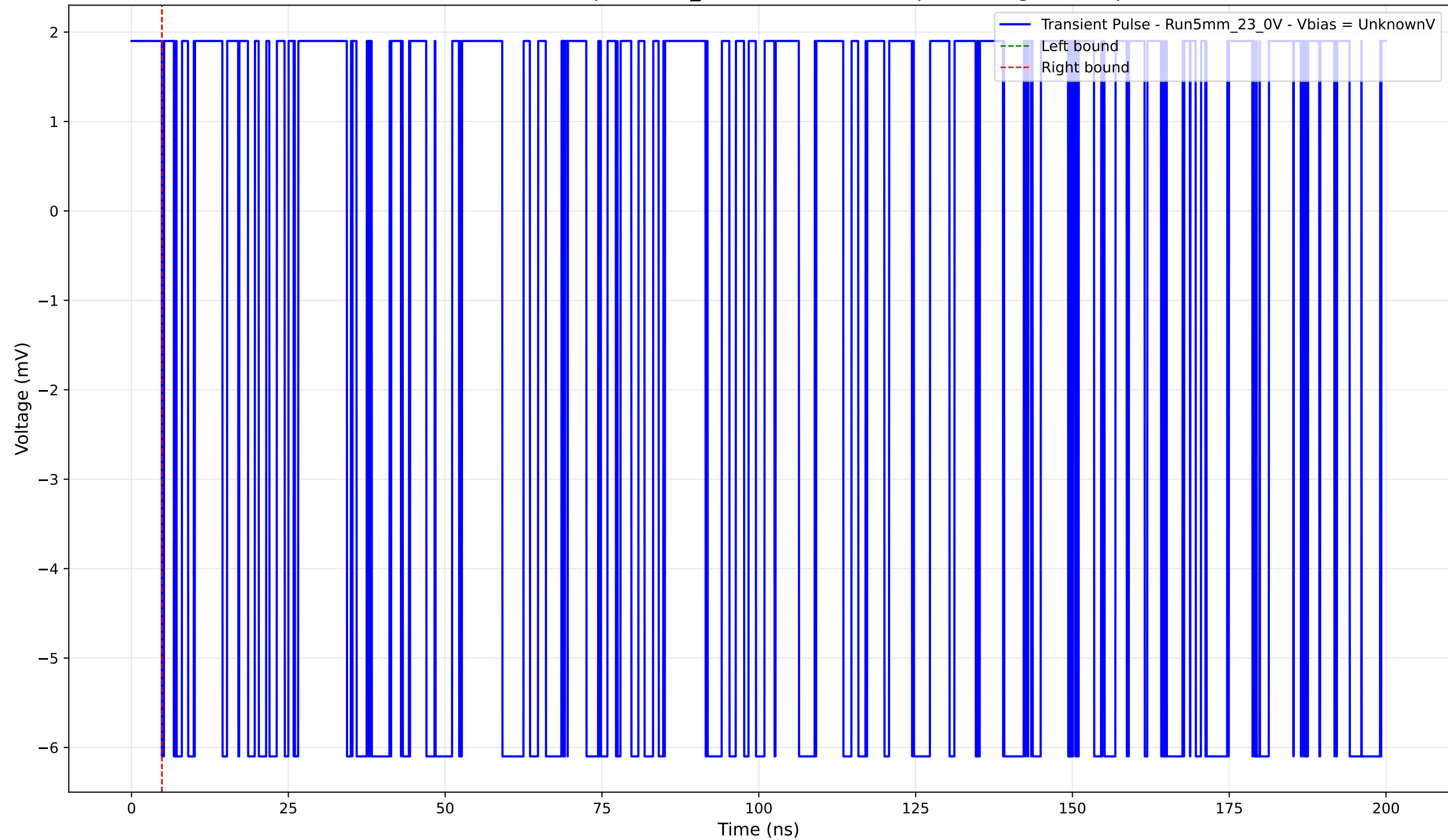
Transient Pulse - Sample: 5mm_23 - Position: 2540.0 \mu\text{m} - Charge: -0.00 pC
