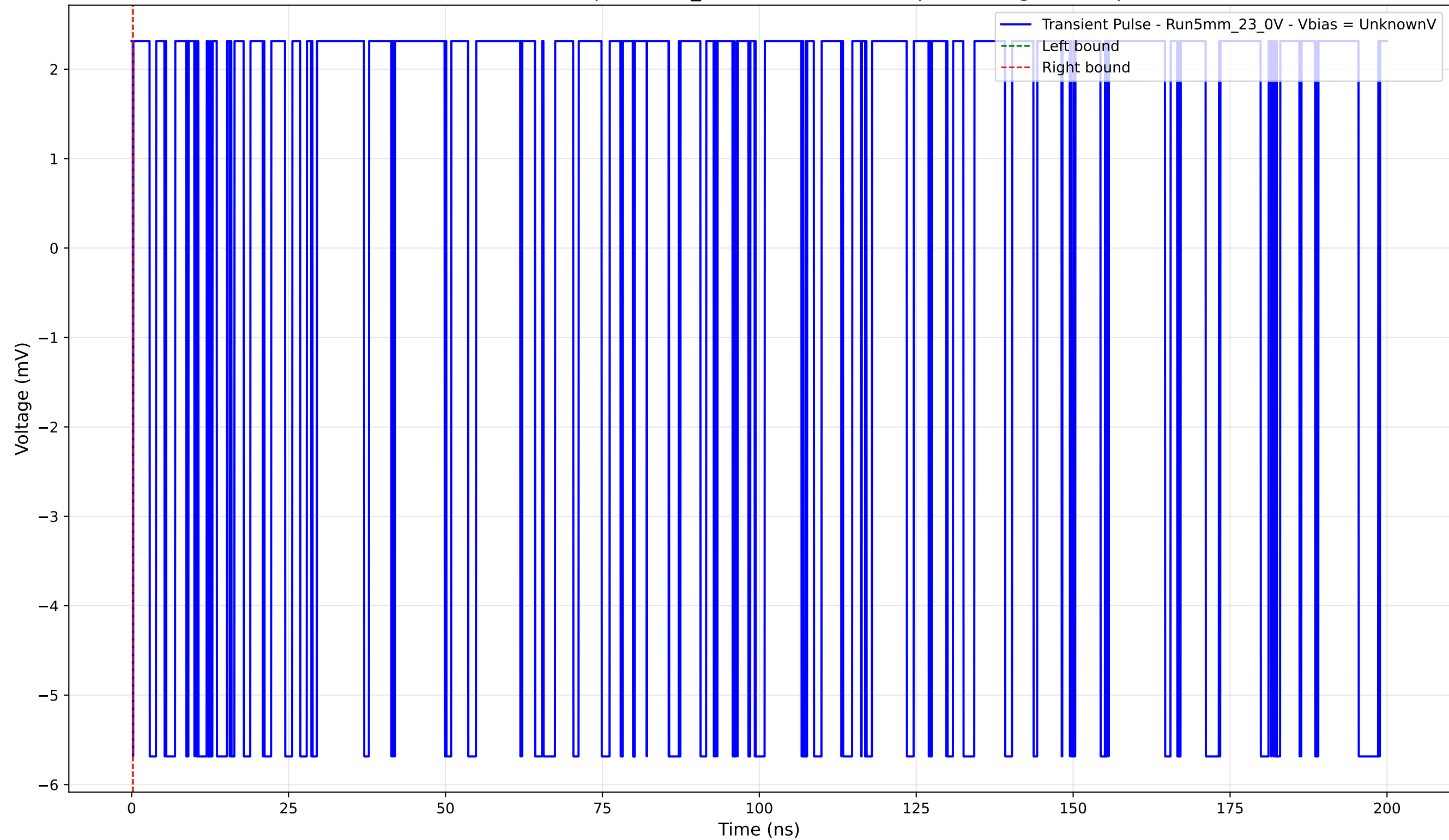
Transient Pulse - Sample: 5mm_23 - Position: 1195.0 \mu\text{m} - Charge: -0.00 pC
