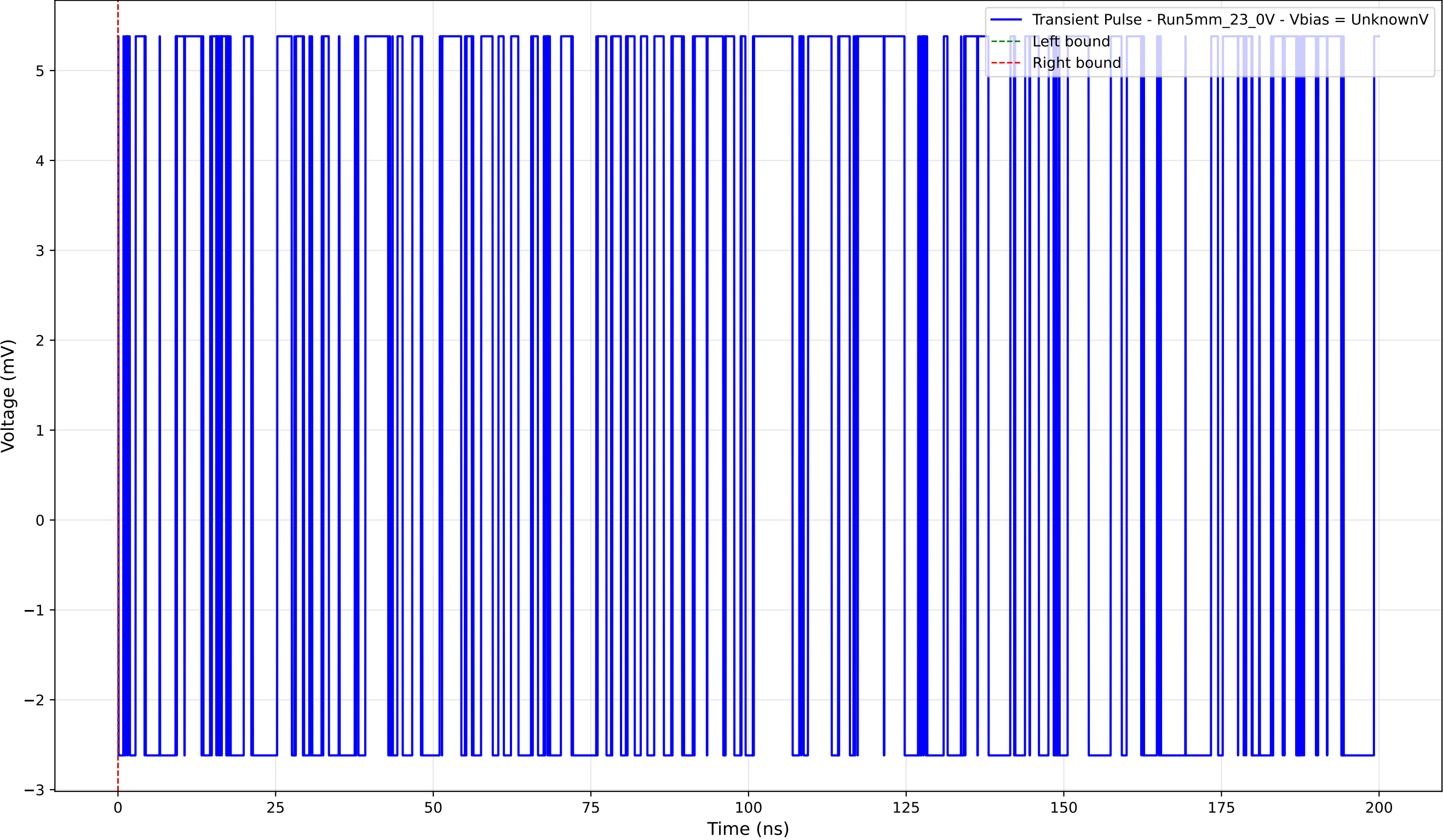
Transient Pulse - Sample: 5mm_23 - Position: 110.0 \mu\text{m} - Charge: 0.00 pC
