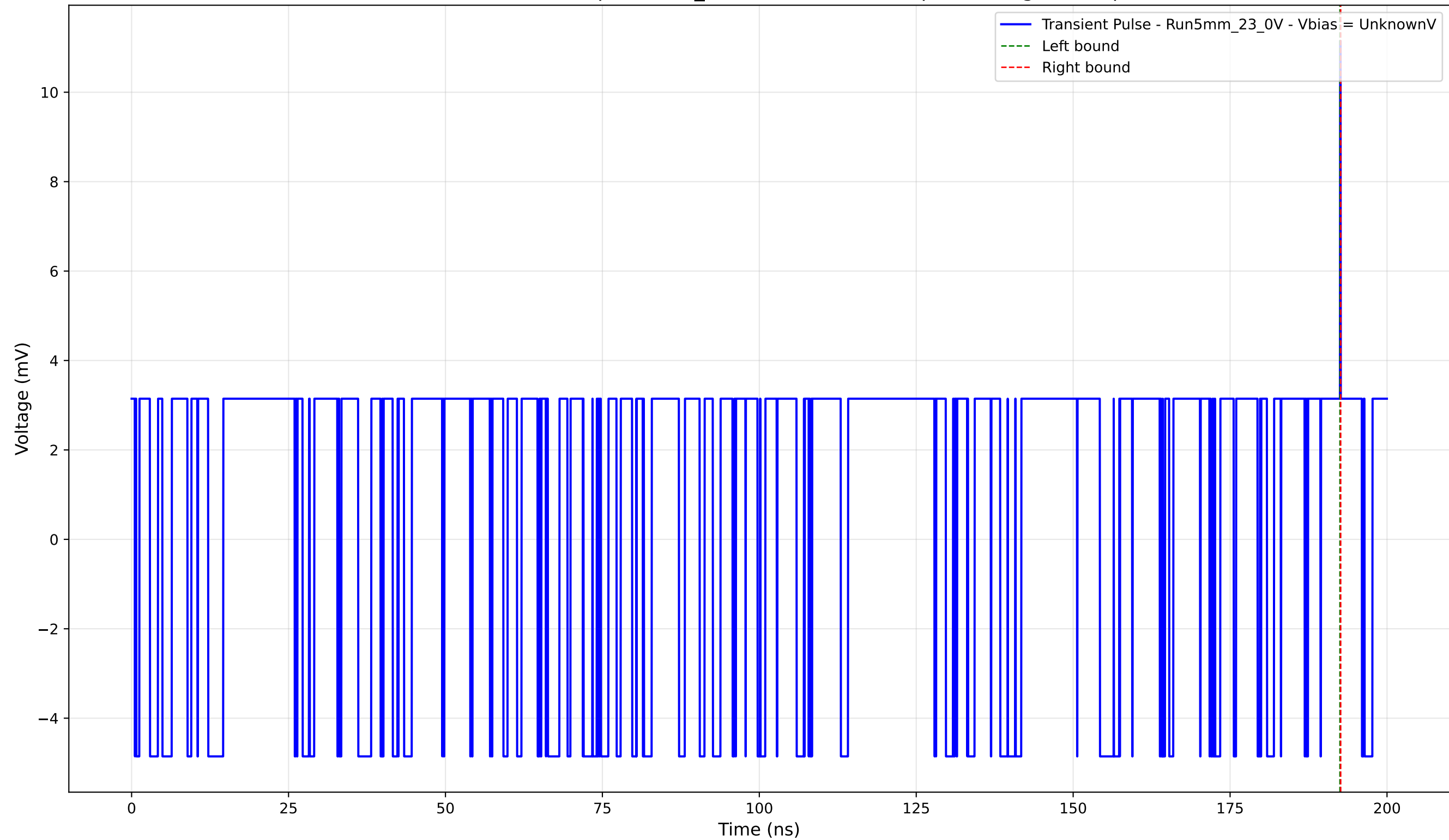
Transient Pulse - Sample: 5mm_23 - Position: 2845.0 \mu\text{m} - Charge: 0.02 pC
