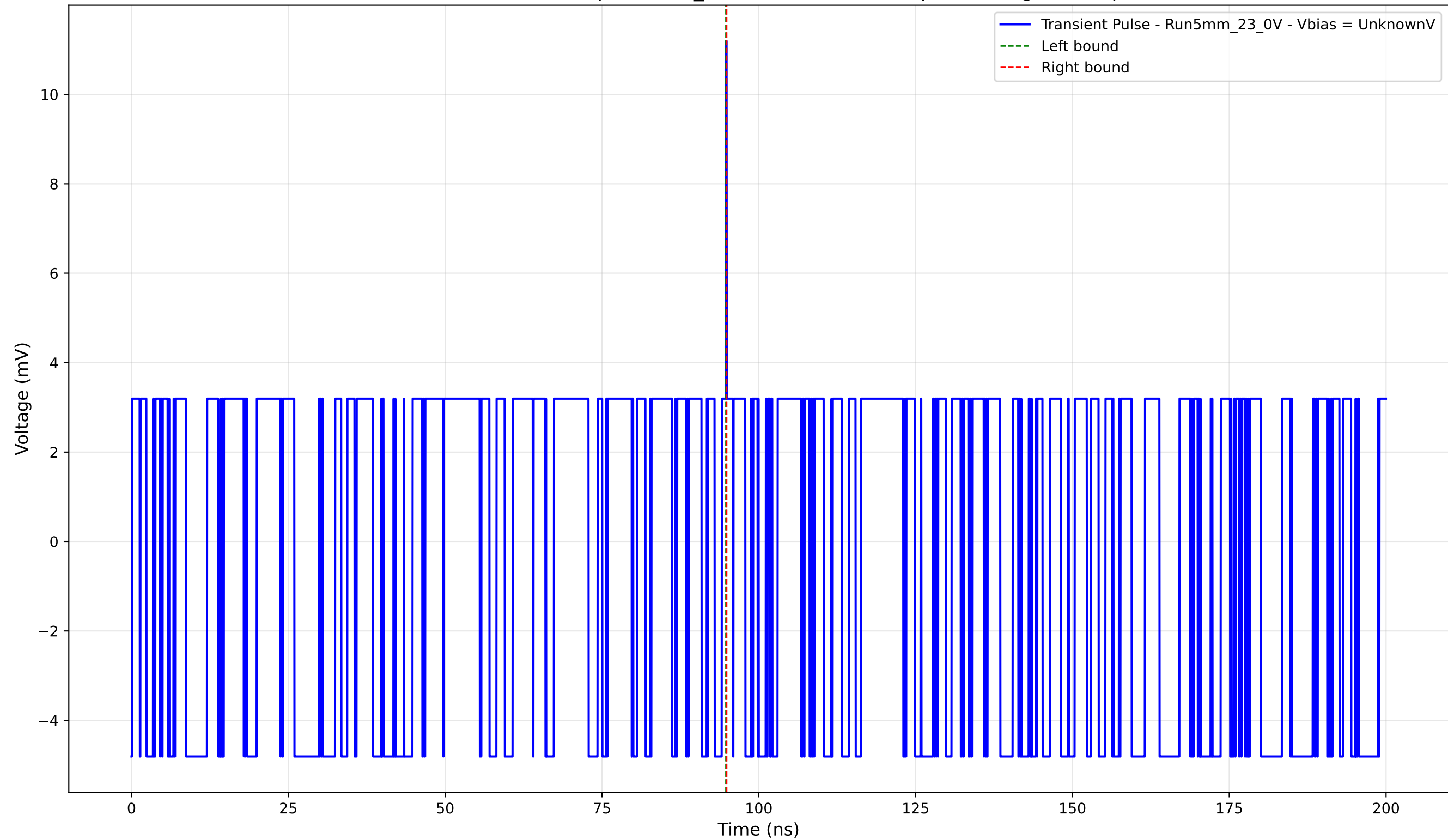
Transient Pulse - Sample: 5mm_23 - Position: 4930.0 \mu\text{m} - Charge: 0.02 pC
