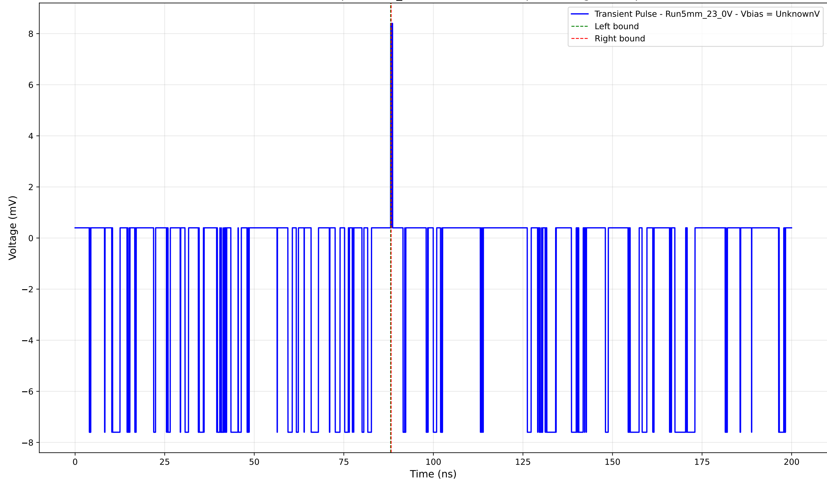
Transient Pulse - Sample: 5mm_23 - Position: 2925.0 \mu\text{m} - Charge: 0.02 pC
