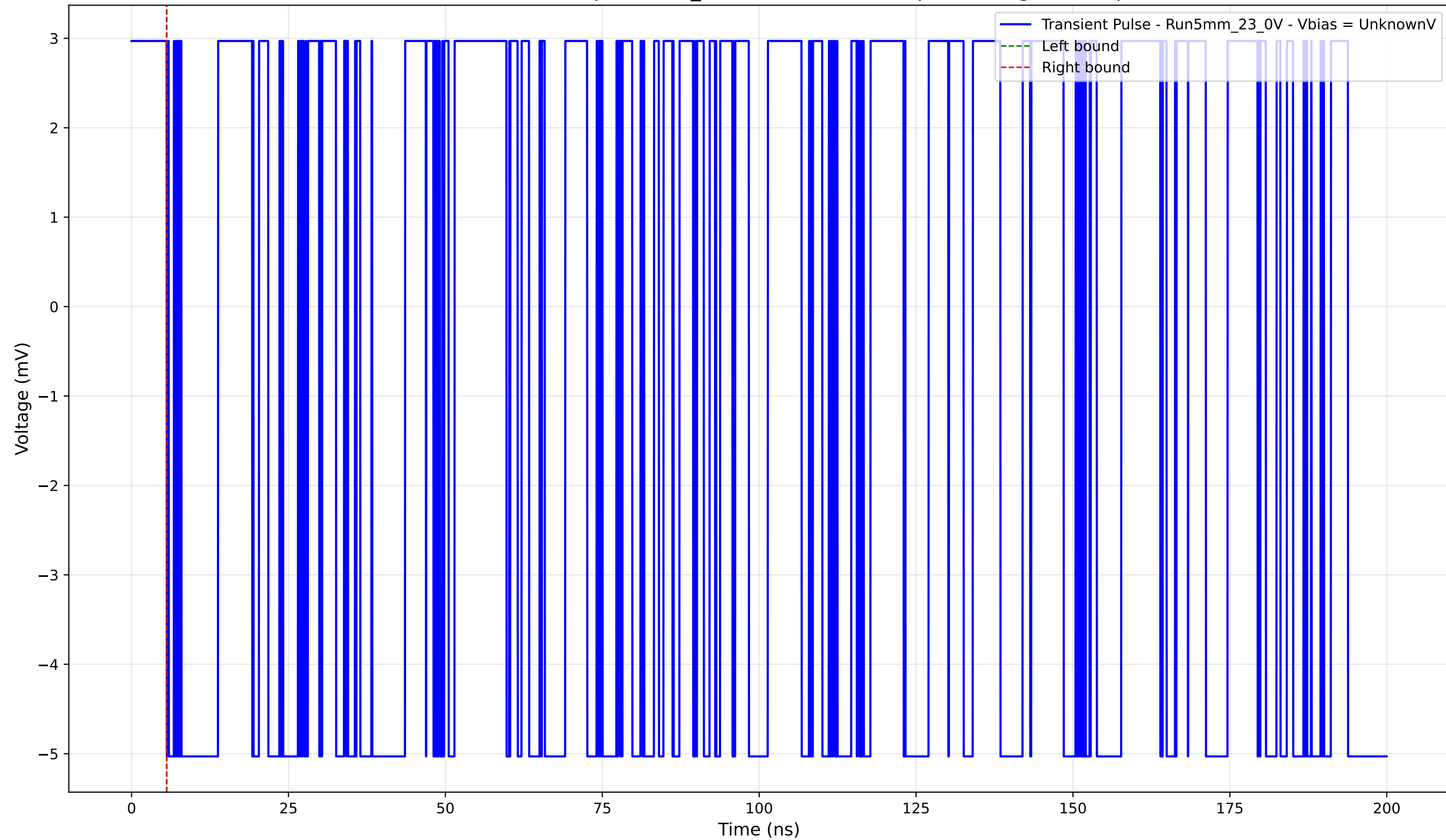
Transient Pulse - Sample: 5mm_23 - Position: 1460.0 \mu\text{m} - Charge: -0.00 pC
