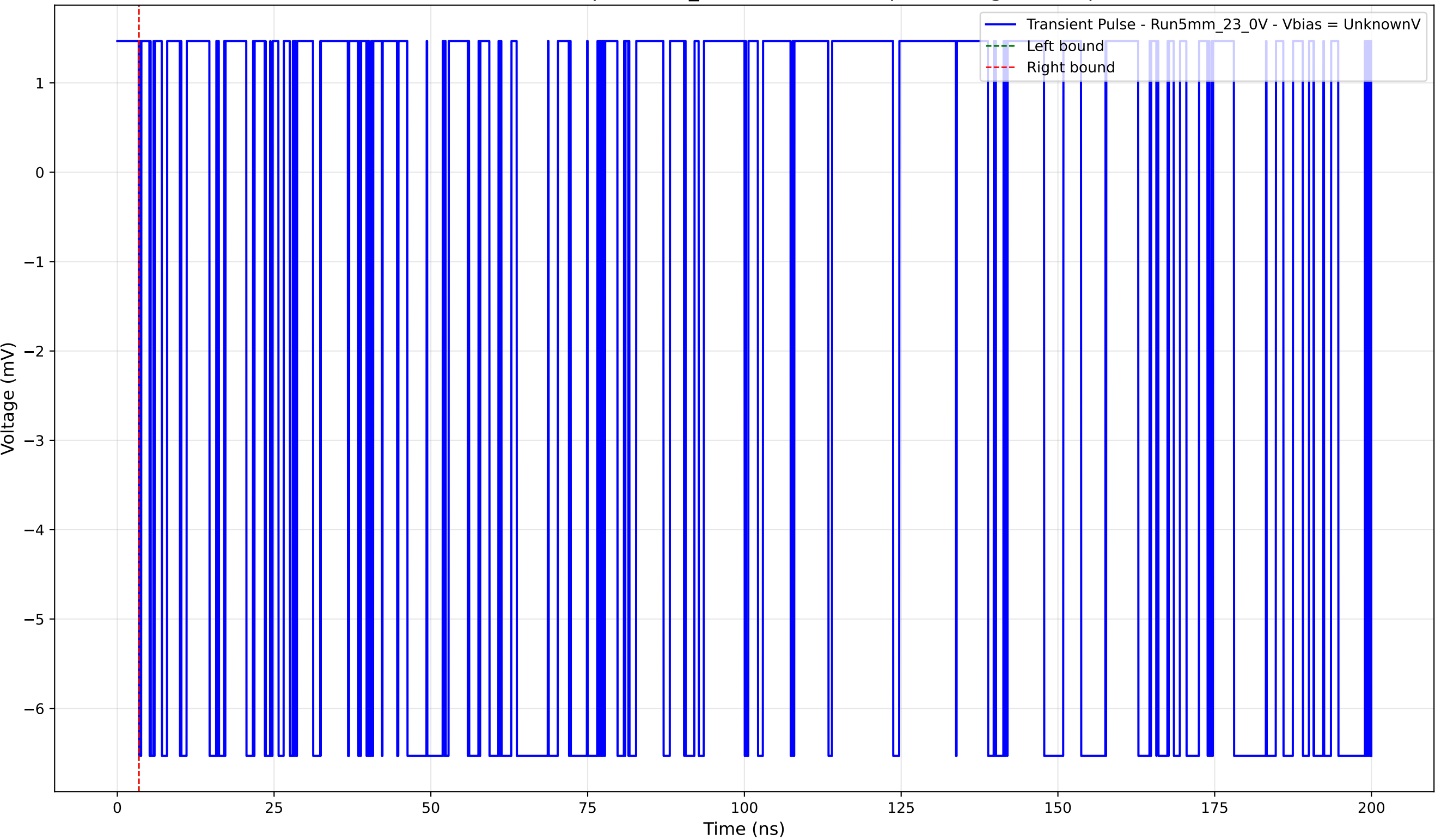
Transient Pulse - Sample: 5mm_23 - Position: 20.0 \mu\text{m} - Charge: -0.00 pC
