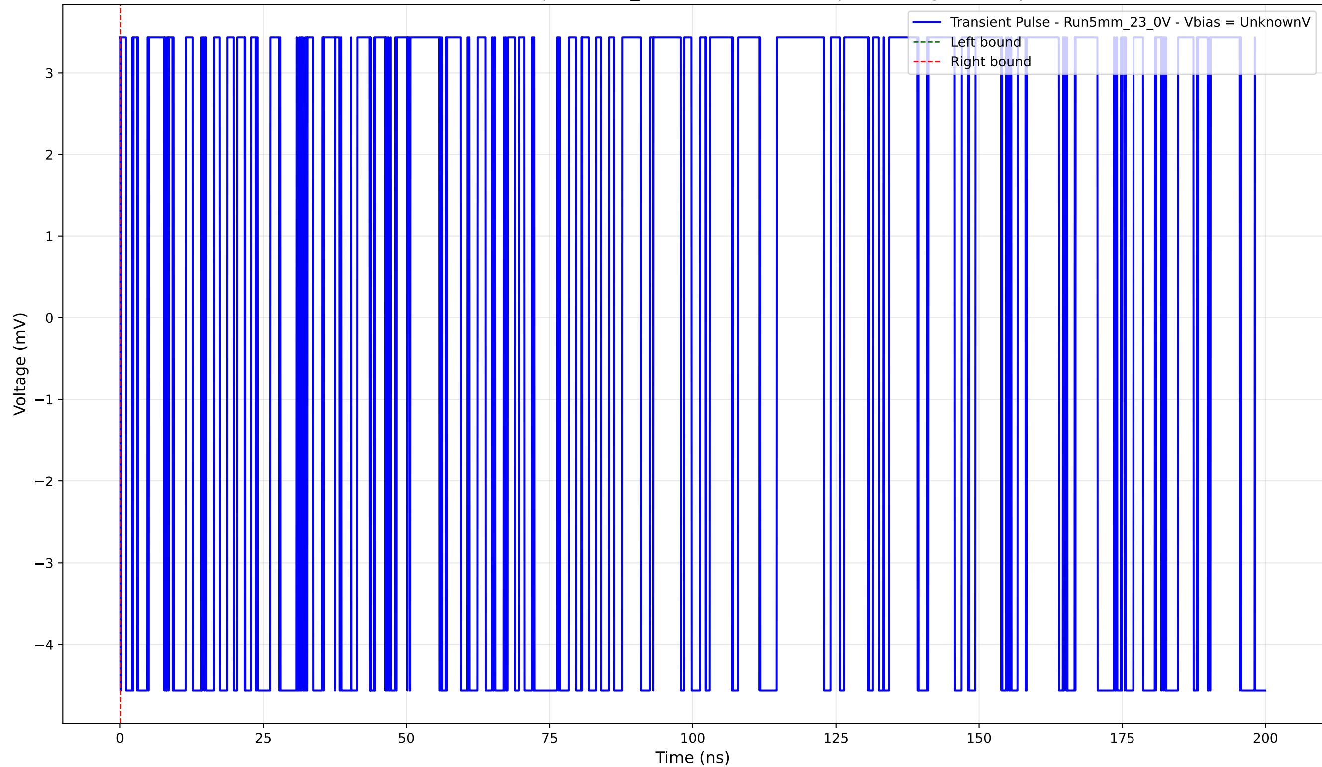
Transient Pulse - Sample: 5mm_23 - Position: 4100.0 \mu\text{m} - Charge: -0.00 pC
