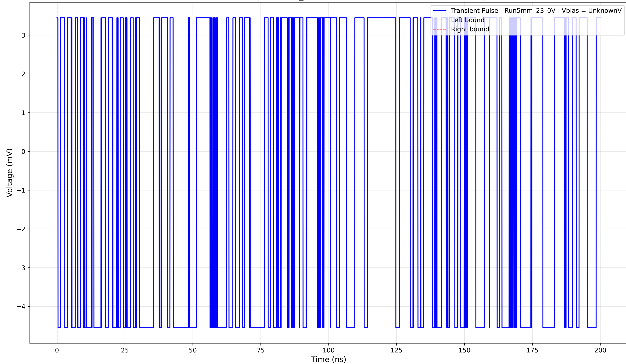
Transient Pulse - Sample: 5mm_23 - Position: 3415.0 \mu\text{m} - Charge: -0.00 pC
