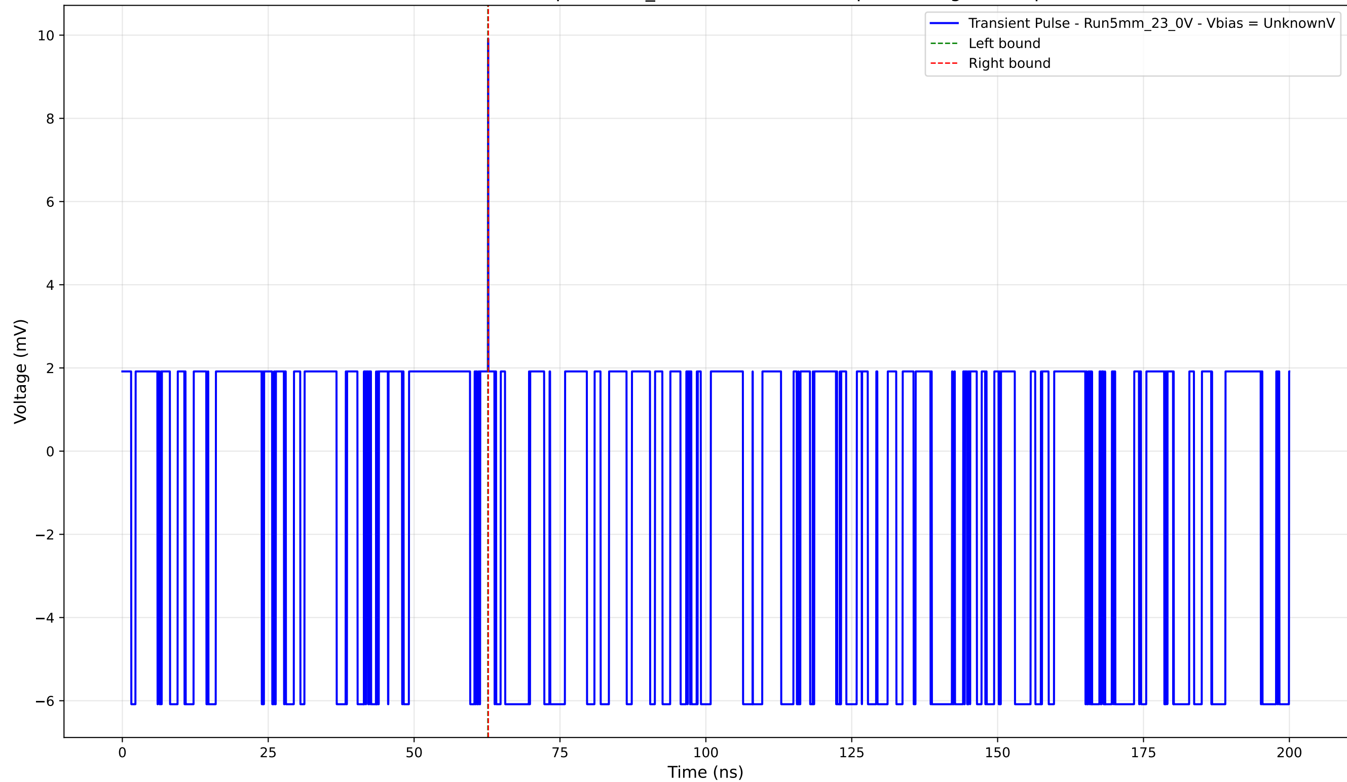
Transient Pulse - Sample: 5mm_23 - Position: 2950.0 \mu\text{m} - Charge: 0.01 pC
