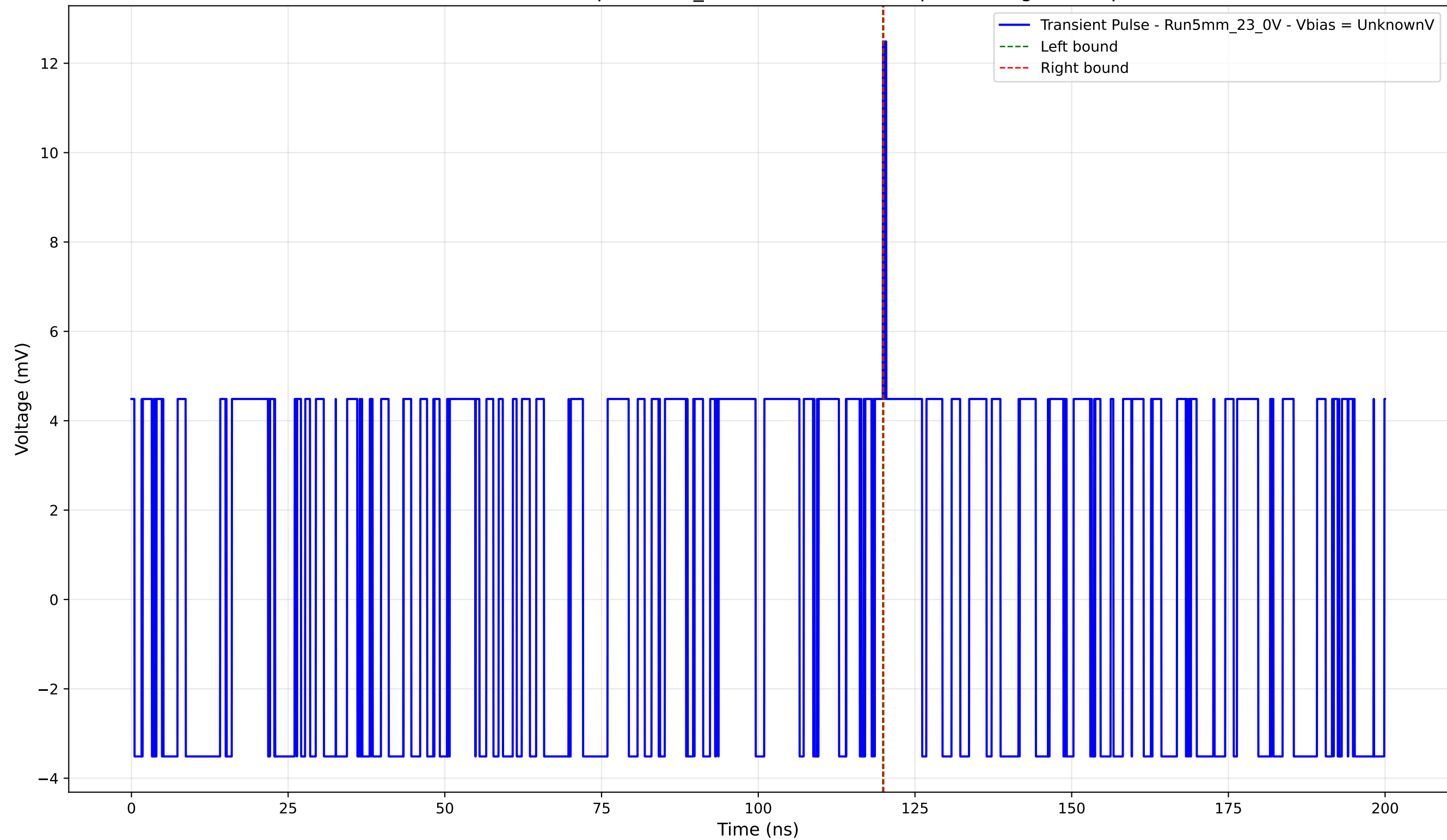
Transient Pulse - Sample: 5mm_23 - Position: 4165.0 \mu\text{m} - Charge: 0.03 pC
