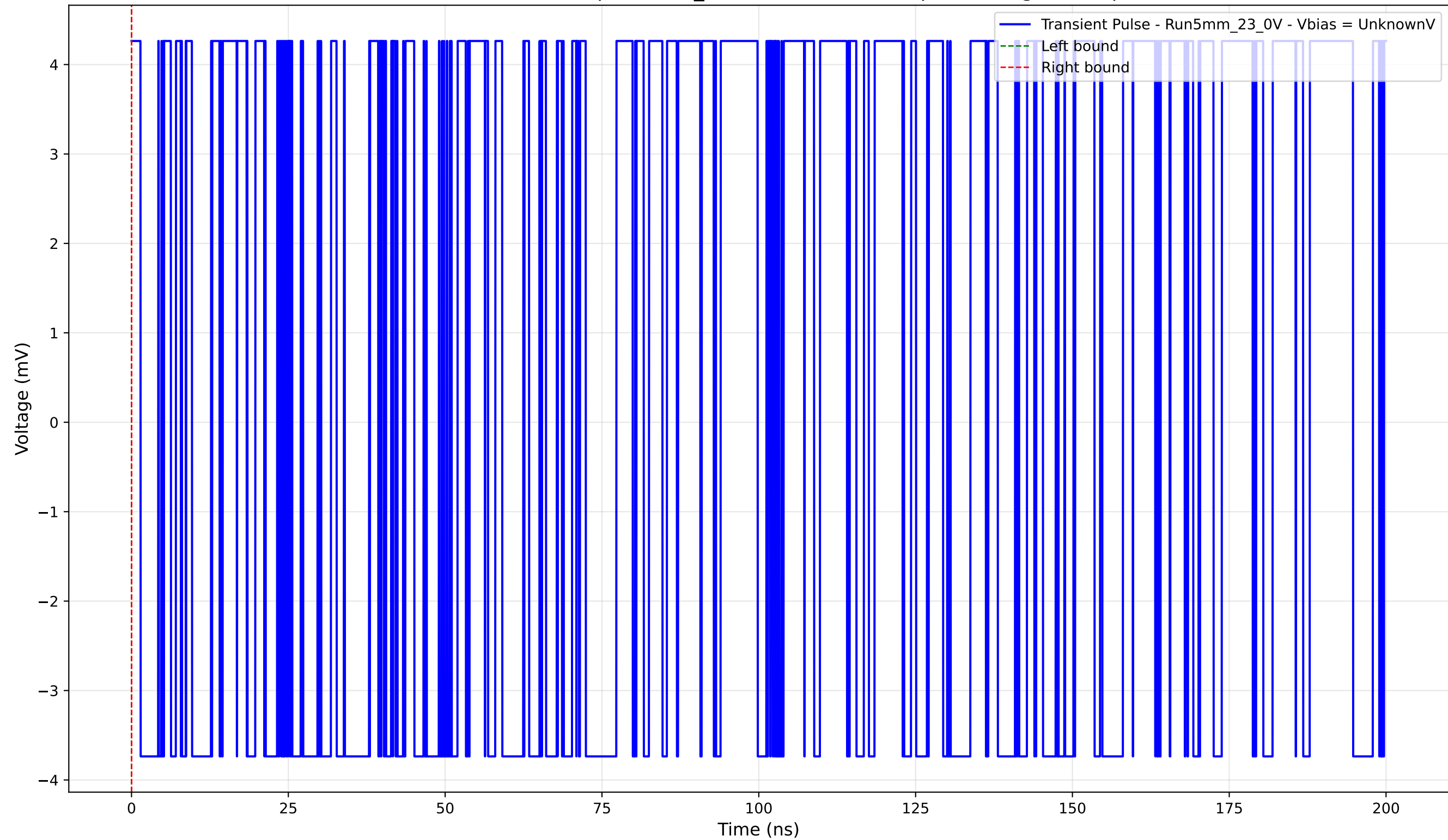
Transient Pulse - Sample: 5mm_23 - Position: 1285.0 \mu\text{m} - Charge: 0.00 pC
