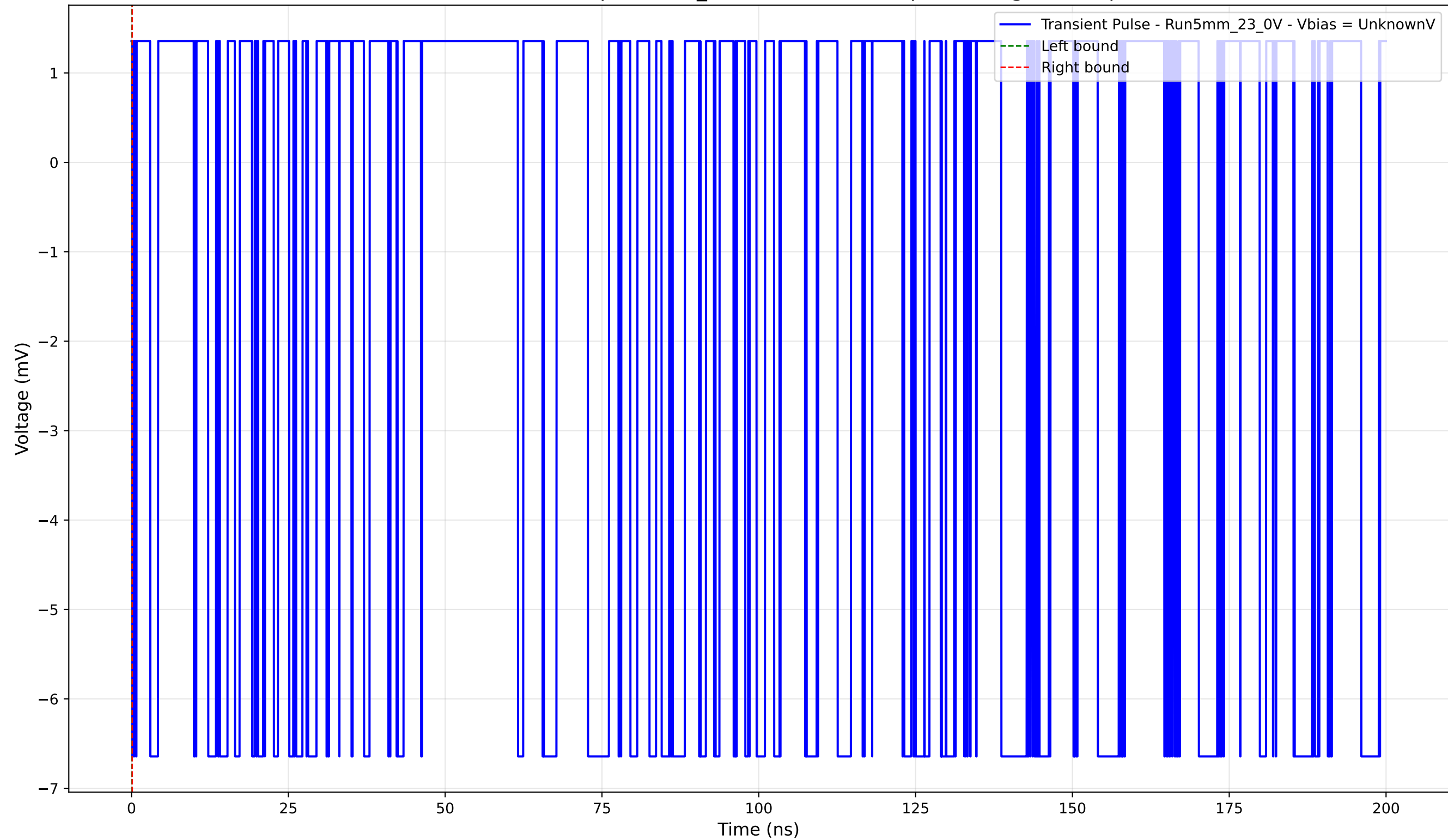
Transient Pulse - Sample: 5mm_23 - Position: 130.0 \mu\text{m} - Charge: -0.00 pC
