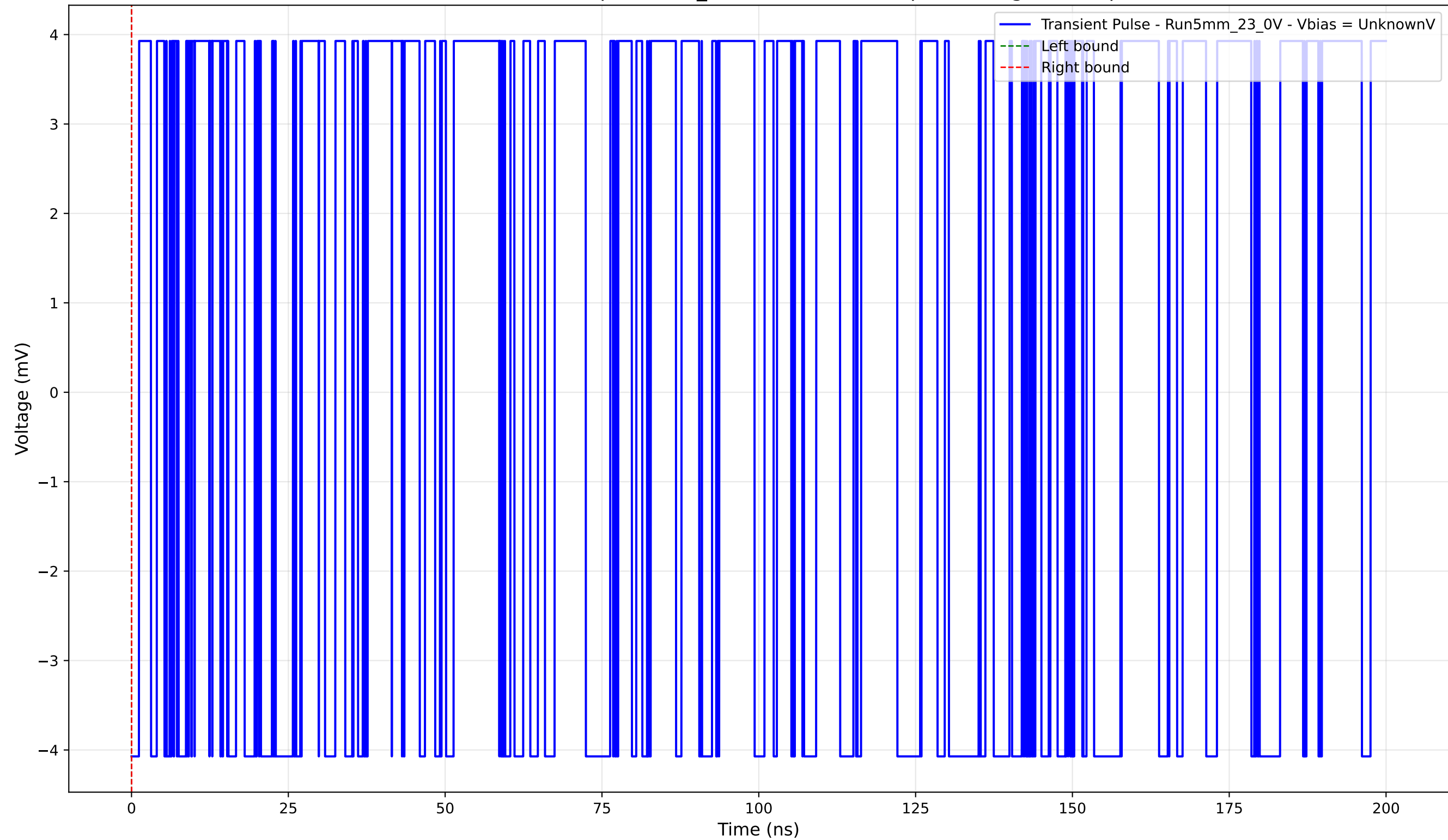
Transient Pulse - Sample: 5mm_23 - Position: 845.0 \mu\text{m} - Charge: -0.00 pC
