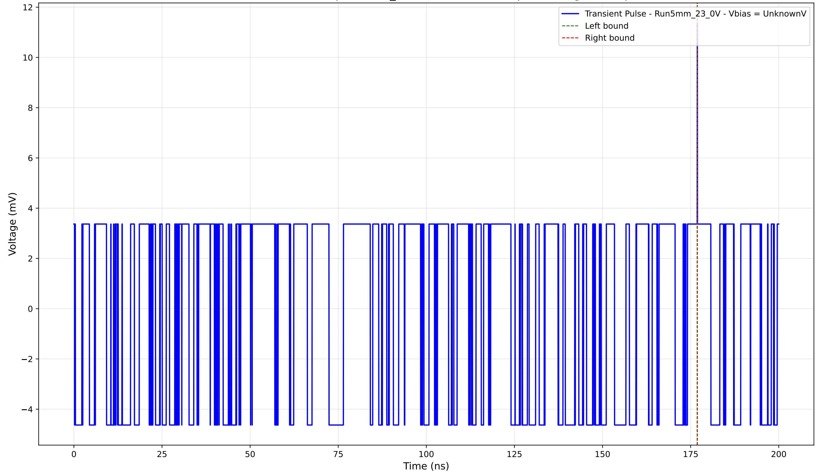
Transient Pulse - Sample: 5mm_23 - Position: 3730.0 \mu\text{m} - Charge: 0.01 pC
