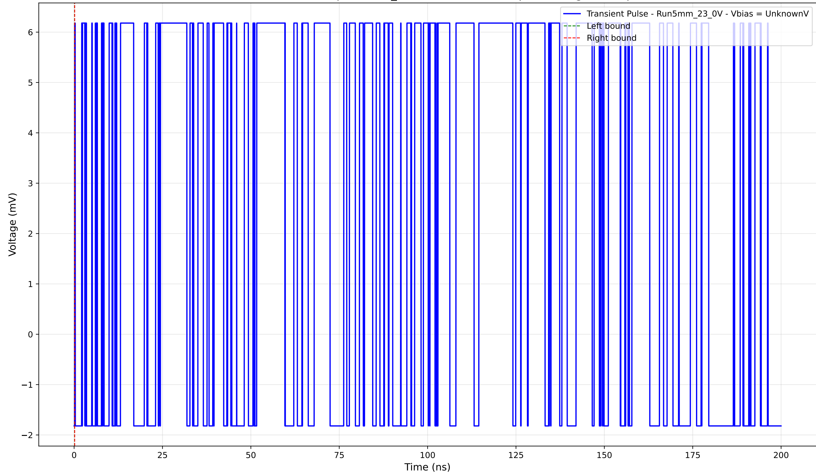
Transient Pulse - Sample: 5mm_23 - Position: 4725.0 \mu\text{m} - Charge: 0.00 pC
