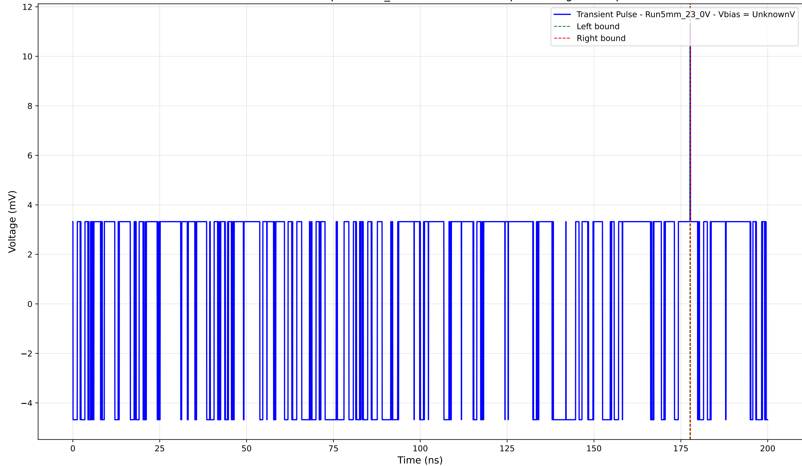
Transient Pulse - Sample: 5mm_23 - Position: 3515.0 \mu\text{m} - Charge: 0.03 pC
