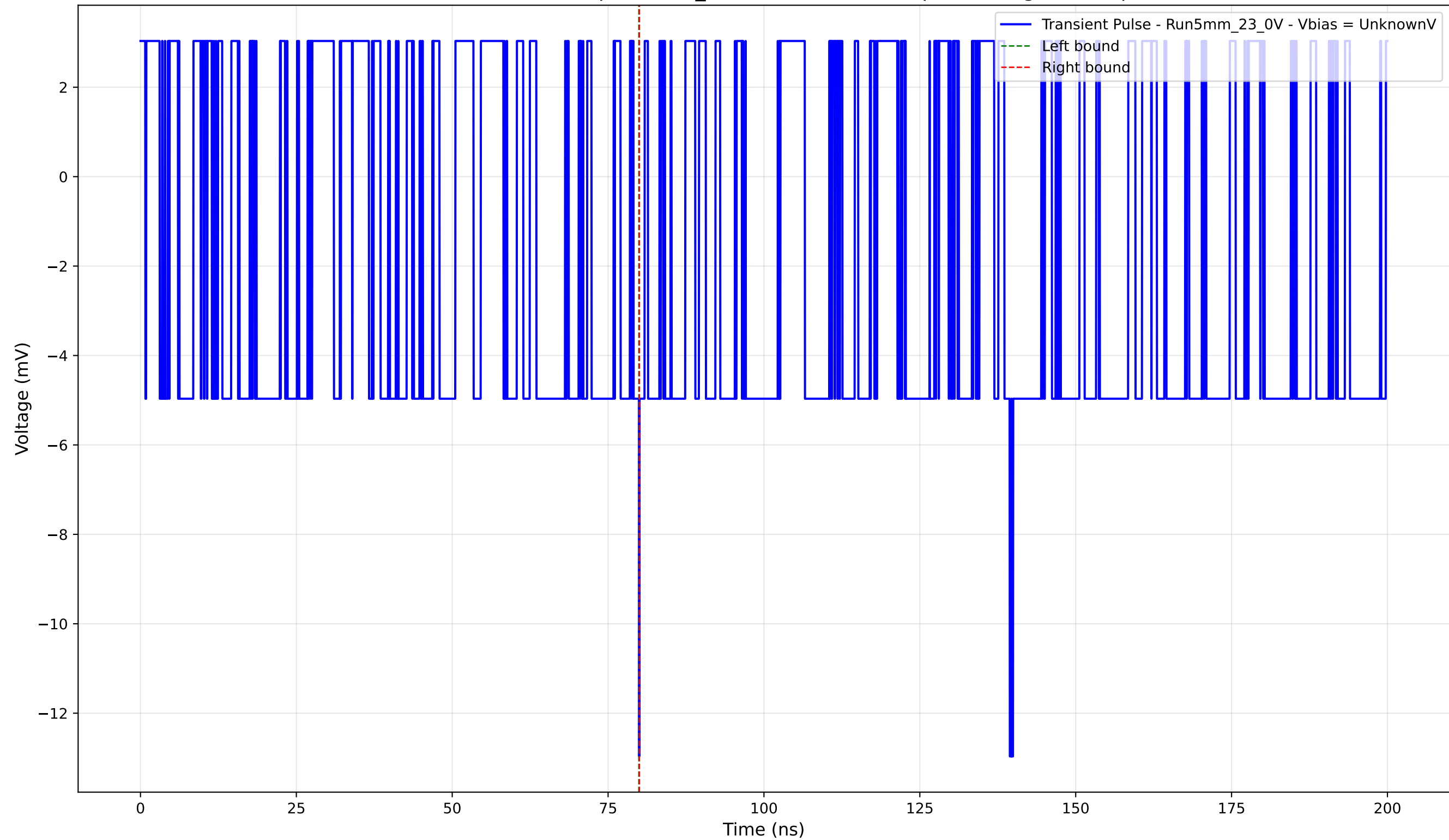
Transient Pulse - Sample: 5mm_23 - Position: 1725.0 \mu\text{m} - Charge: -0.02 pC
