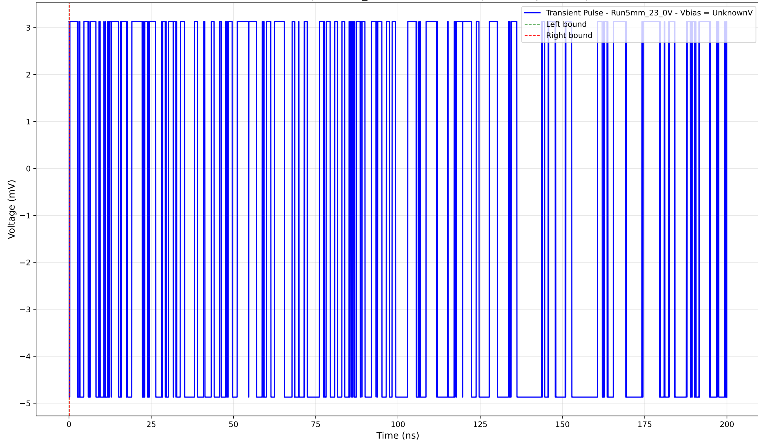
Transient Pulse - Sample: 5mm_23 - Position: 4395.0 \mu\text{m} - Charge: -0.00 pC
