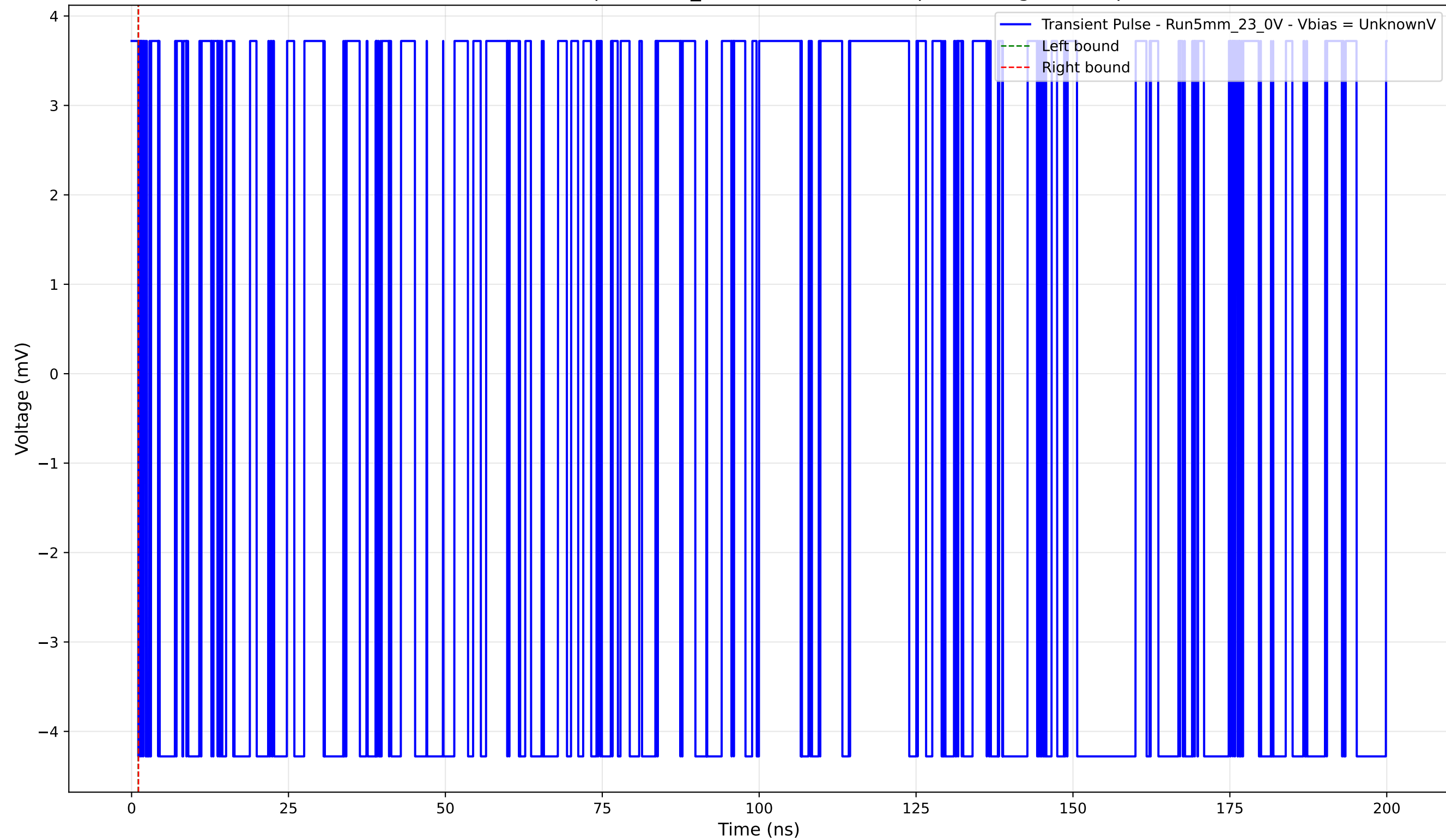
Transient Pulse - Sample: 5mm_23 - Position: 1325.0 \mu\text{m} - Charge: -0.00 pC
