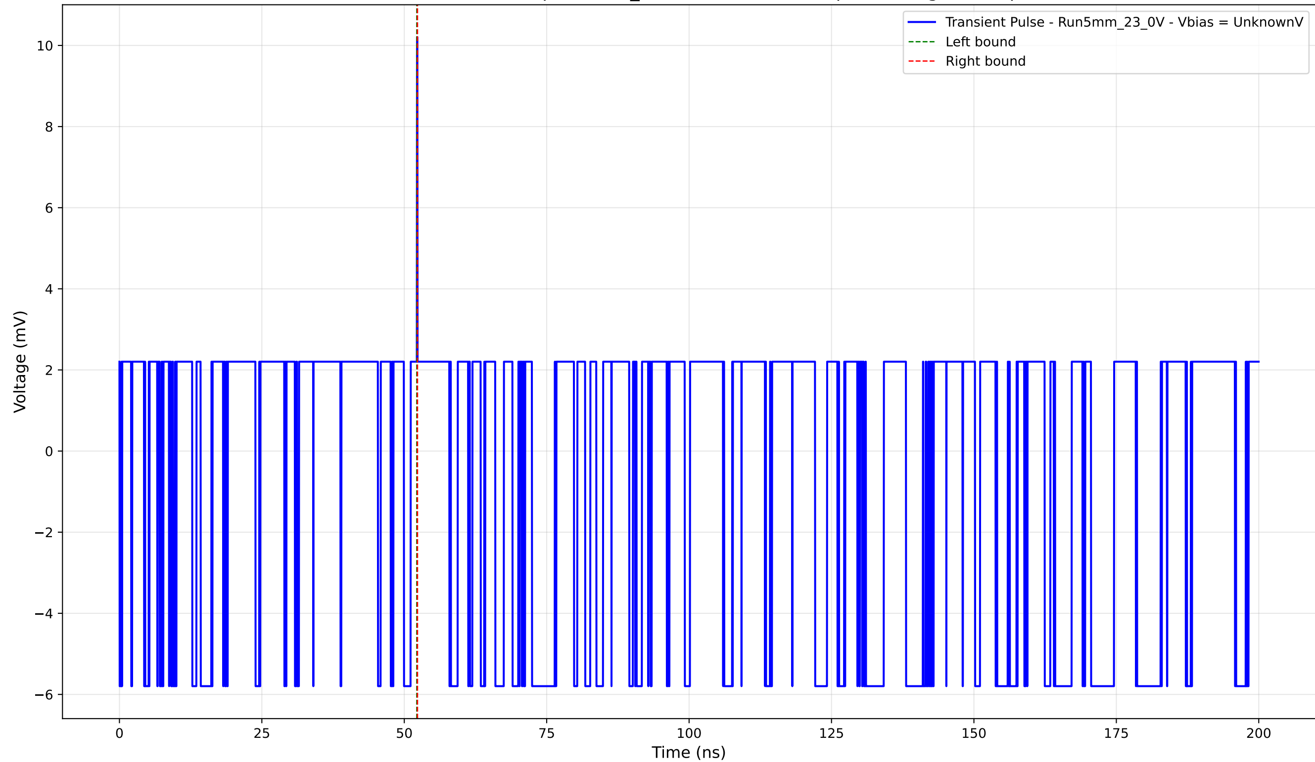
Transient Pulse - Sample: 5mm_23 - Position: 3815.0 \mu\text{m} - Charge: 0.02 pC
