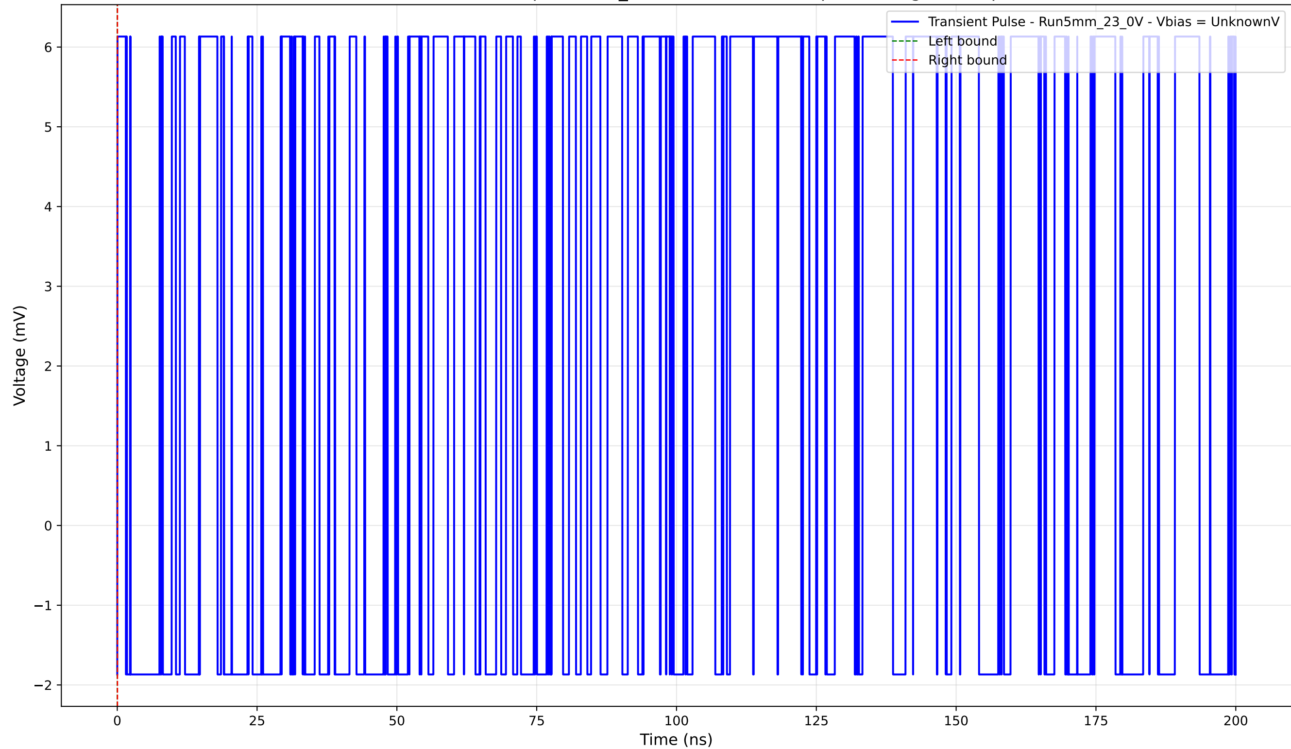
Transient Pulse - Sample: 5mm_23 - Position: 2080.0 \mu\text{m} - Charge: 0.00 pC
