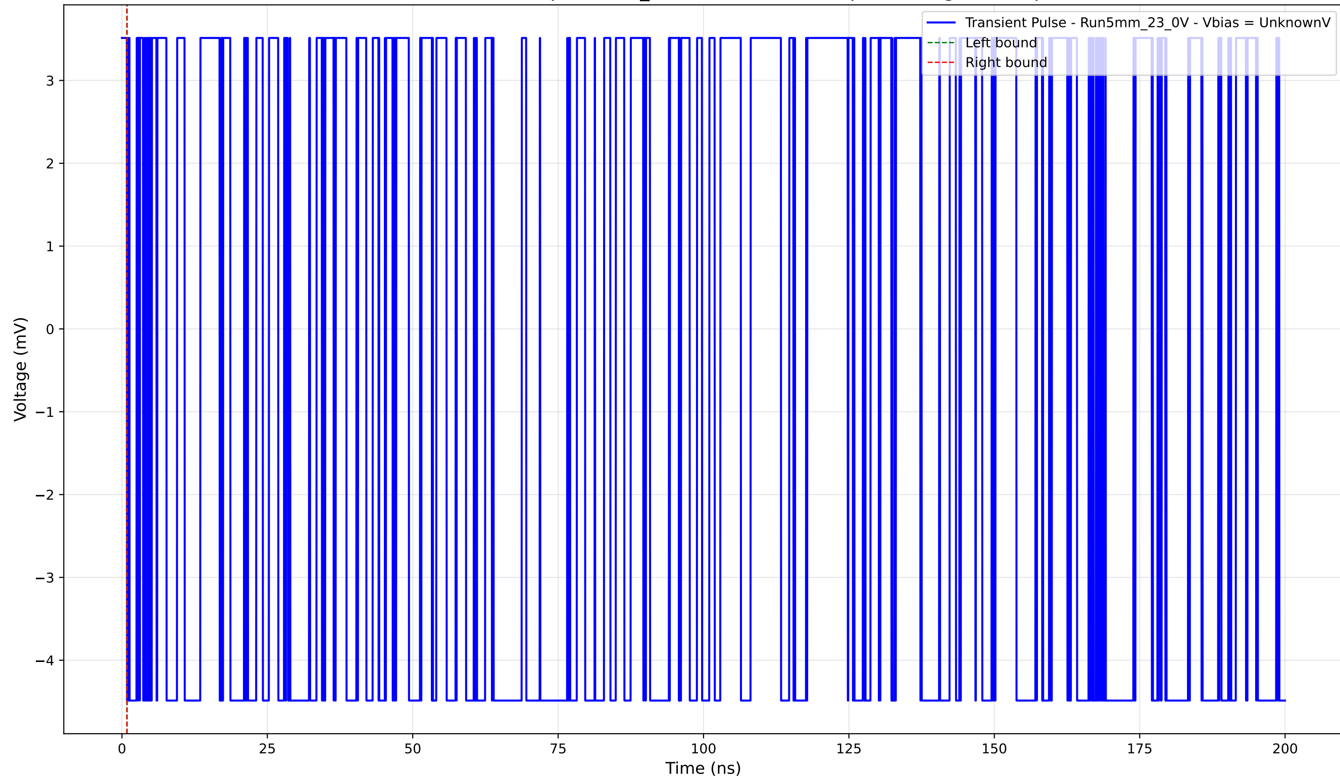
Transient Pulse - Sample: 5mm_23 - Position: 4050.0 \mu\text{m} - Charge: -0.00 pC
