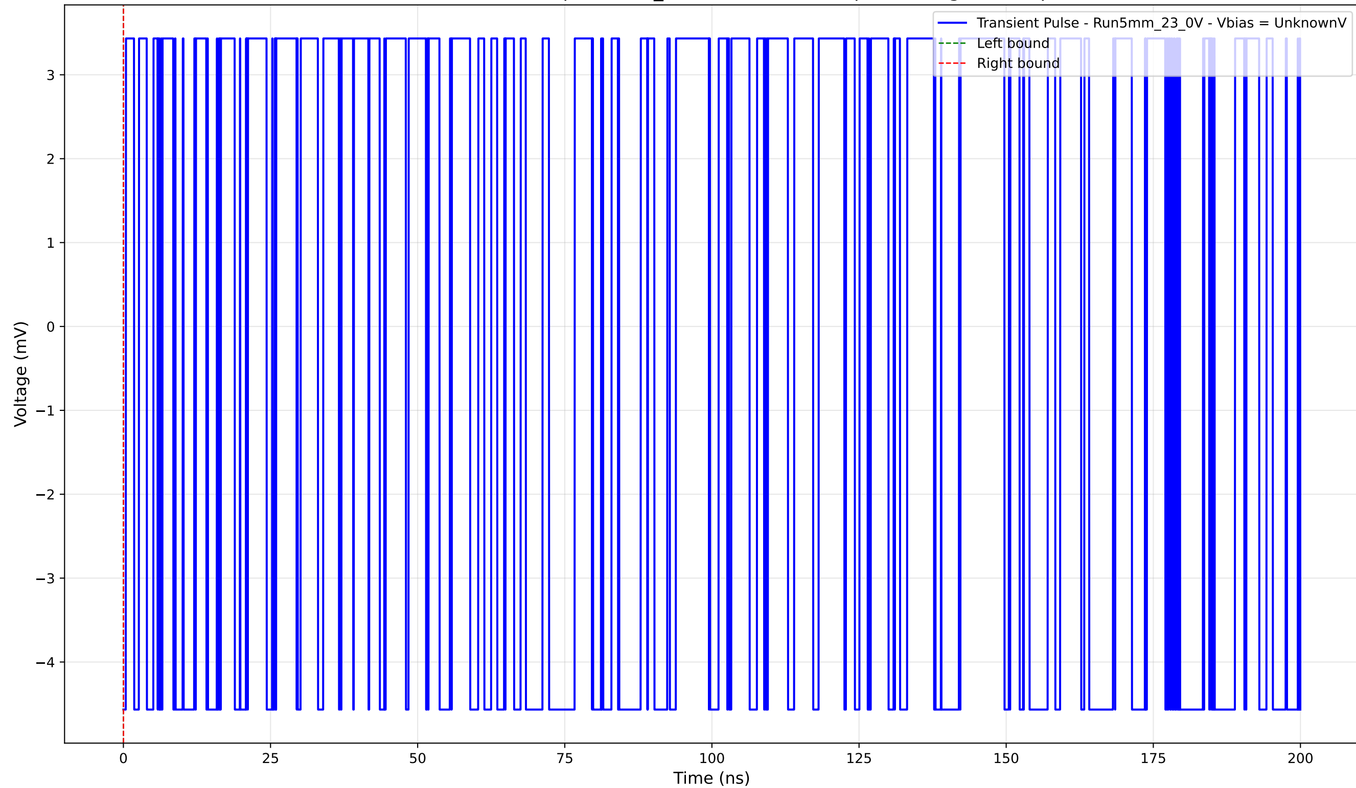
Transient Pulse - Sample: 5mm_23 - Position: 735.0 \mu\text{m} - Charge: -0.00 pC
