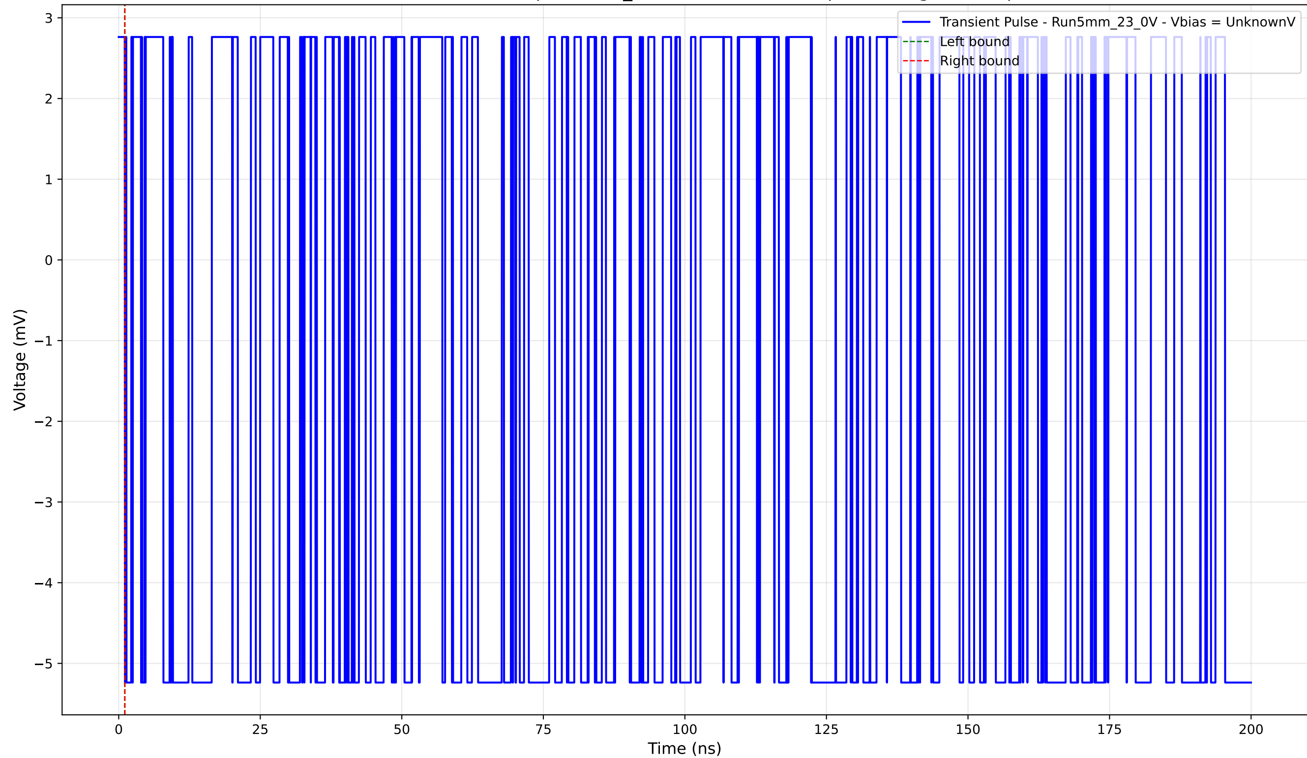
Transient Pulse - Sample: 5mm_23 - Position: 1680.0 \mu\text{m} - Charge: -0.00 pC
