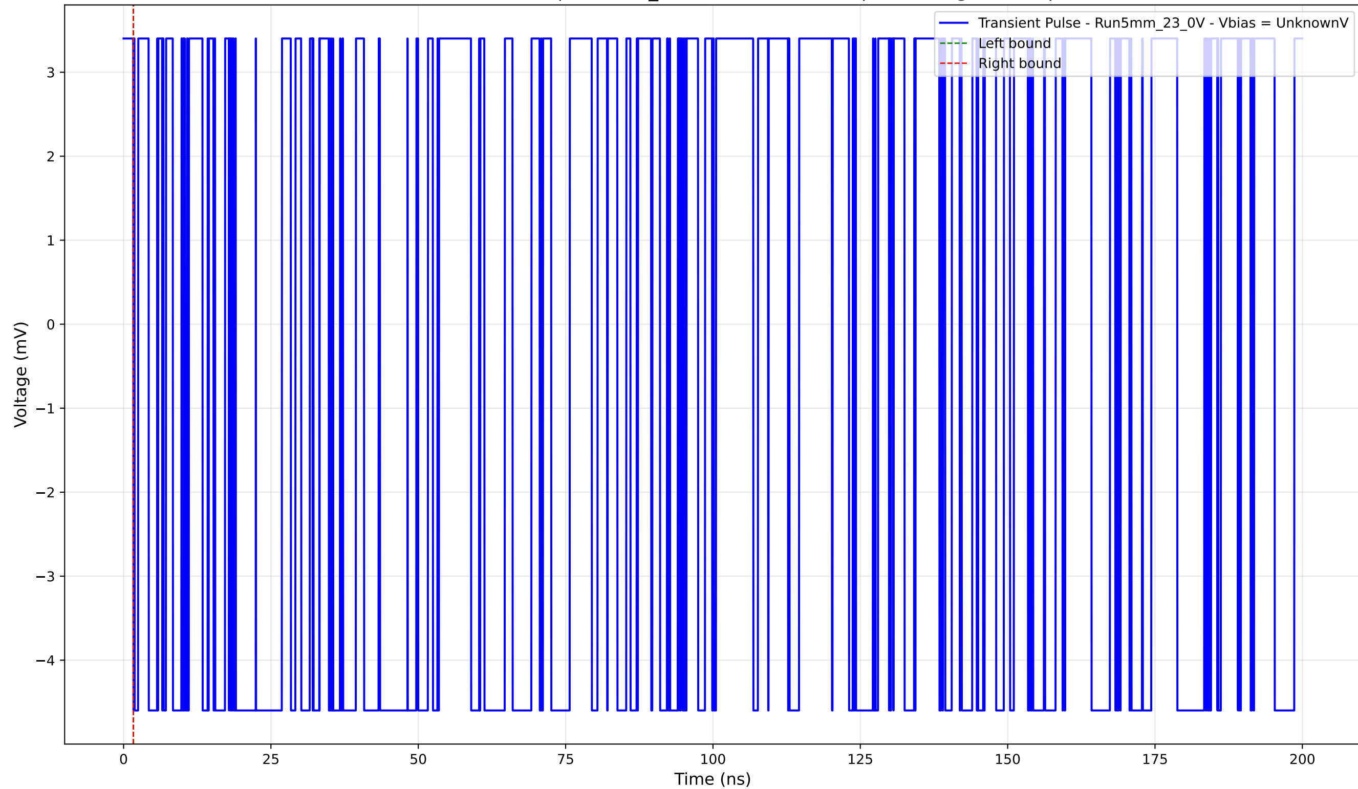
Transient Pulse - Sample: 5mm_23 - Position: 2915.0 \mu\text{m} - Charge: -0.00 pC
