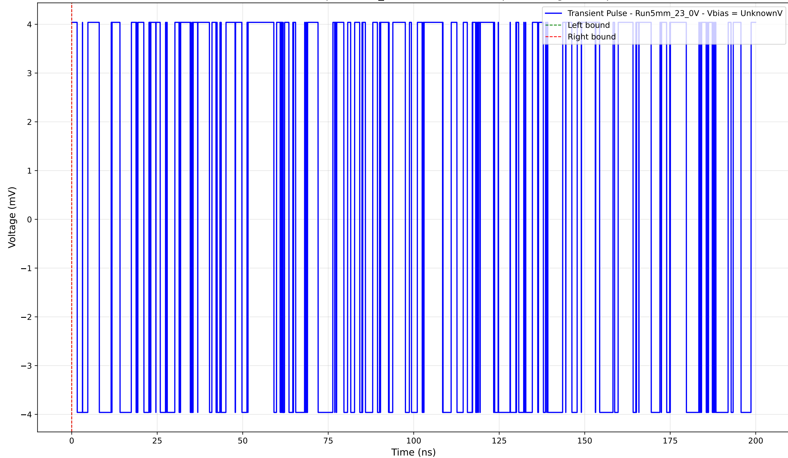
Transient Pulse - Sample: 5mm_23 - Position: 5010.0 \mu\text{m} - Charge: 0.00 pC
