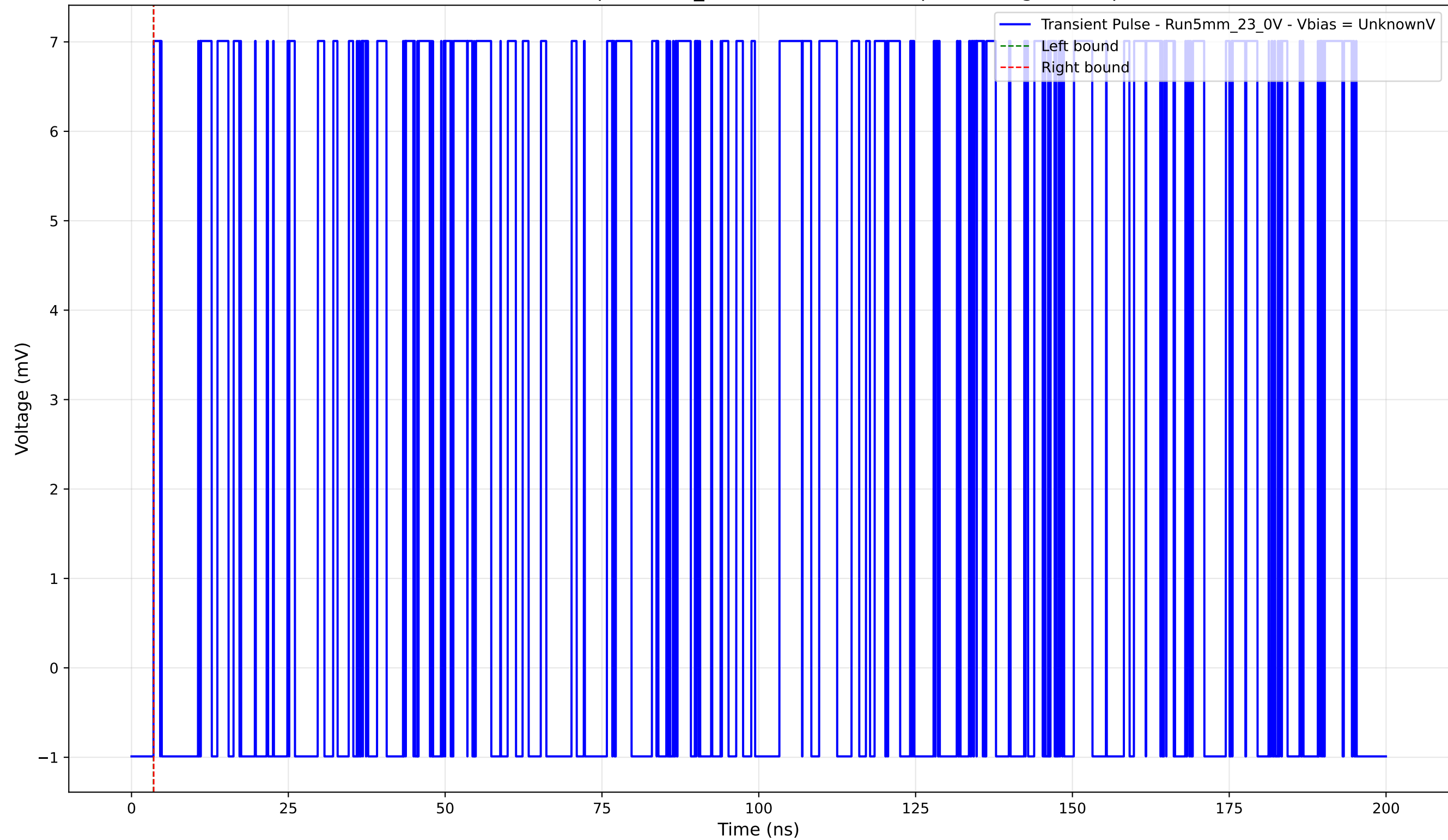
Transient Pulse - Sample: 5mm_23 - Position: 1390.0 \mu\text{m} - Charge: 0.00 pC
