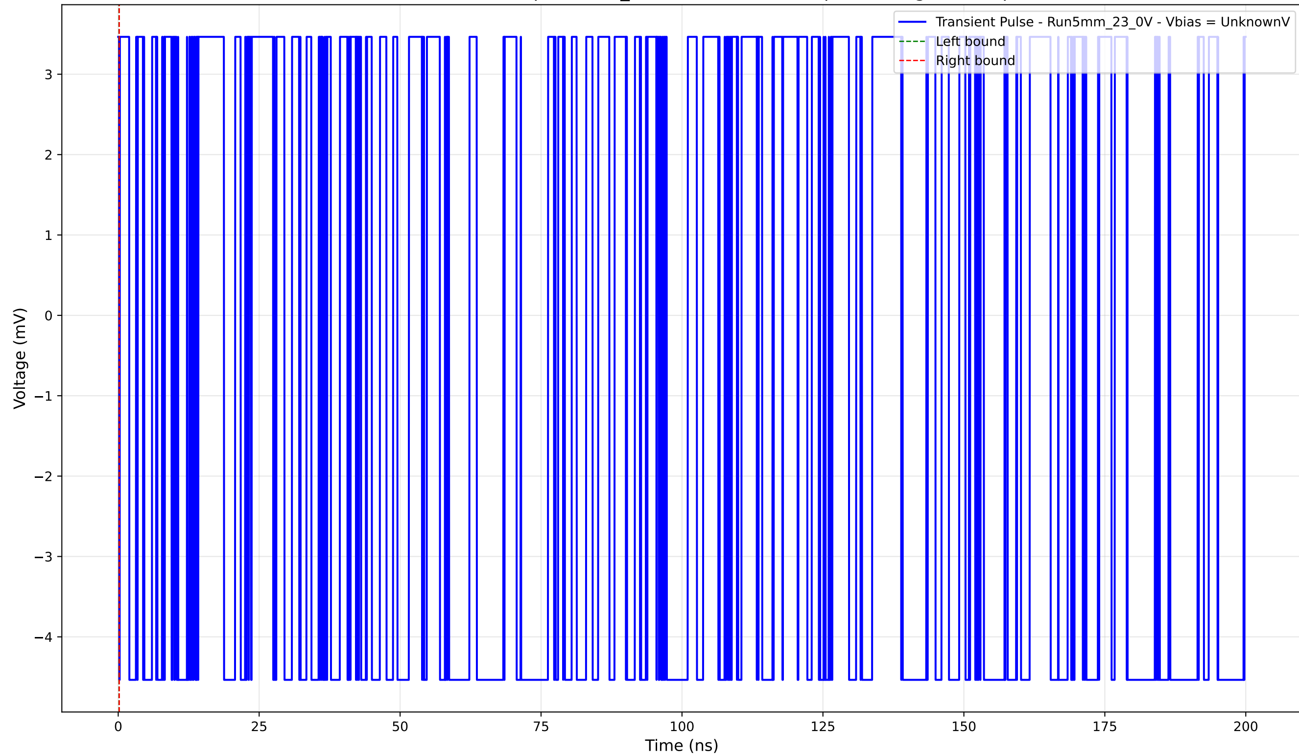
Transient Pulse - Sample: 5mm_23 - Position: 1600.0 \mu\text{m} - Charge: -0.00 pC
