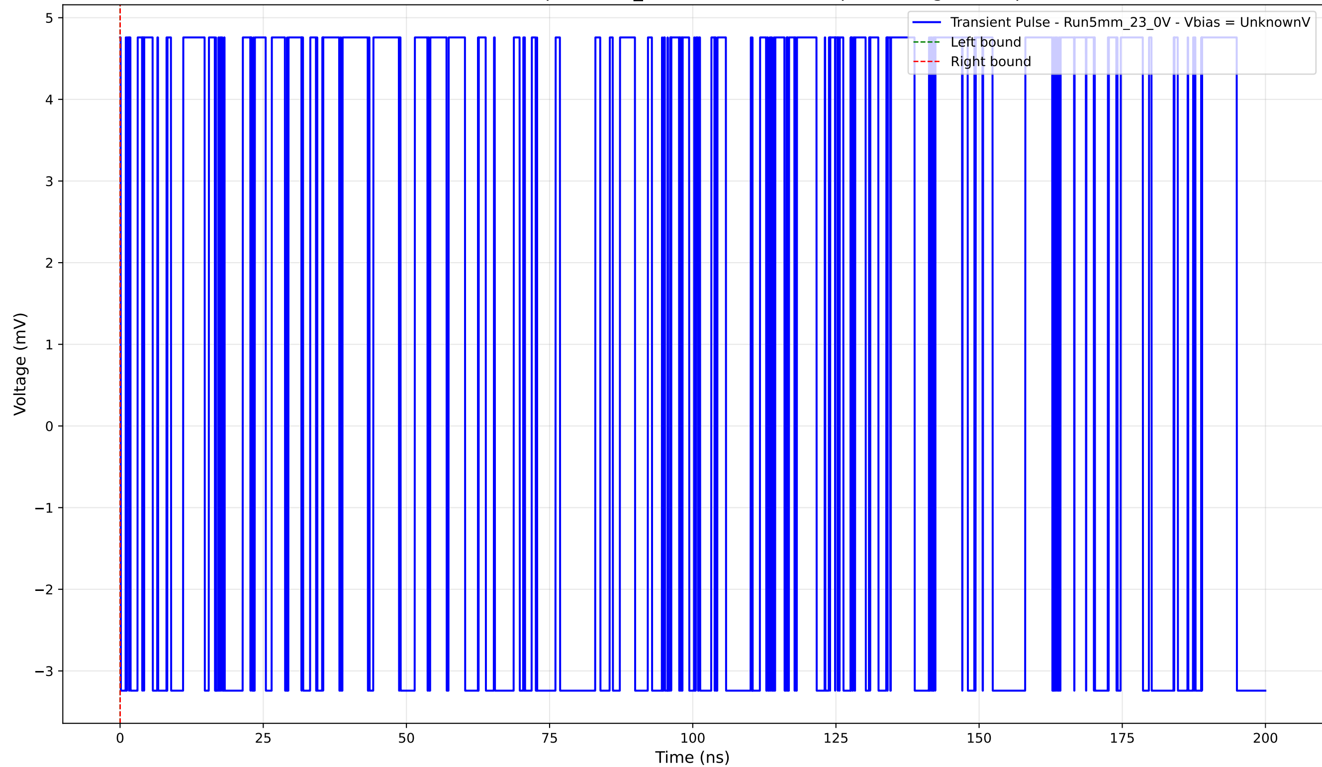
Transient Pulse - Sample: 5mm_23 - Position: 4995.0 \mu\text{m} - Charge: 0.00 pC
