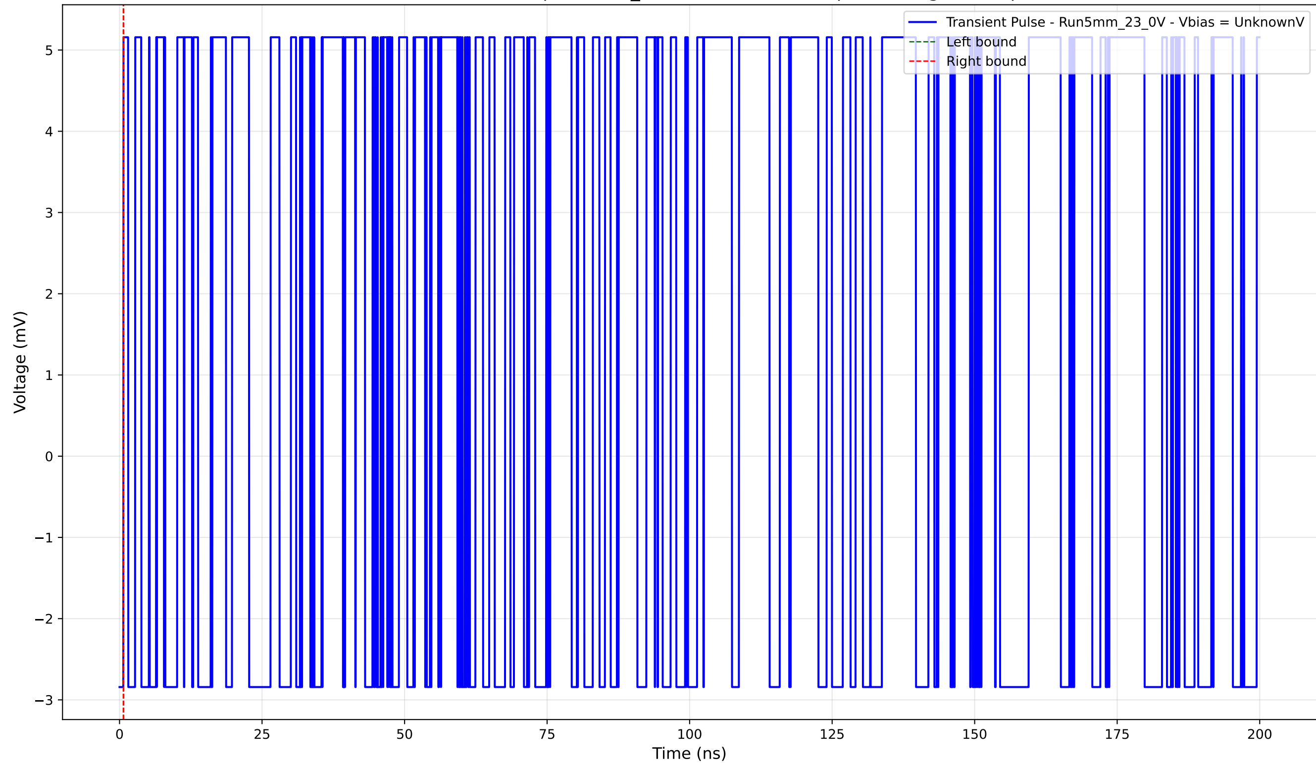
Transient Pulse - Sample: 5mm_23 - Position: 3155.0 \mu\text{m} - Charge: 0.00 pC
