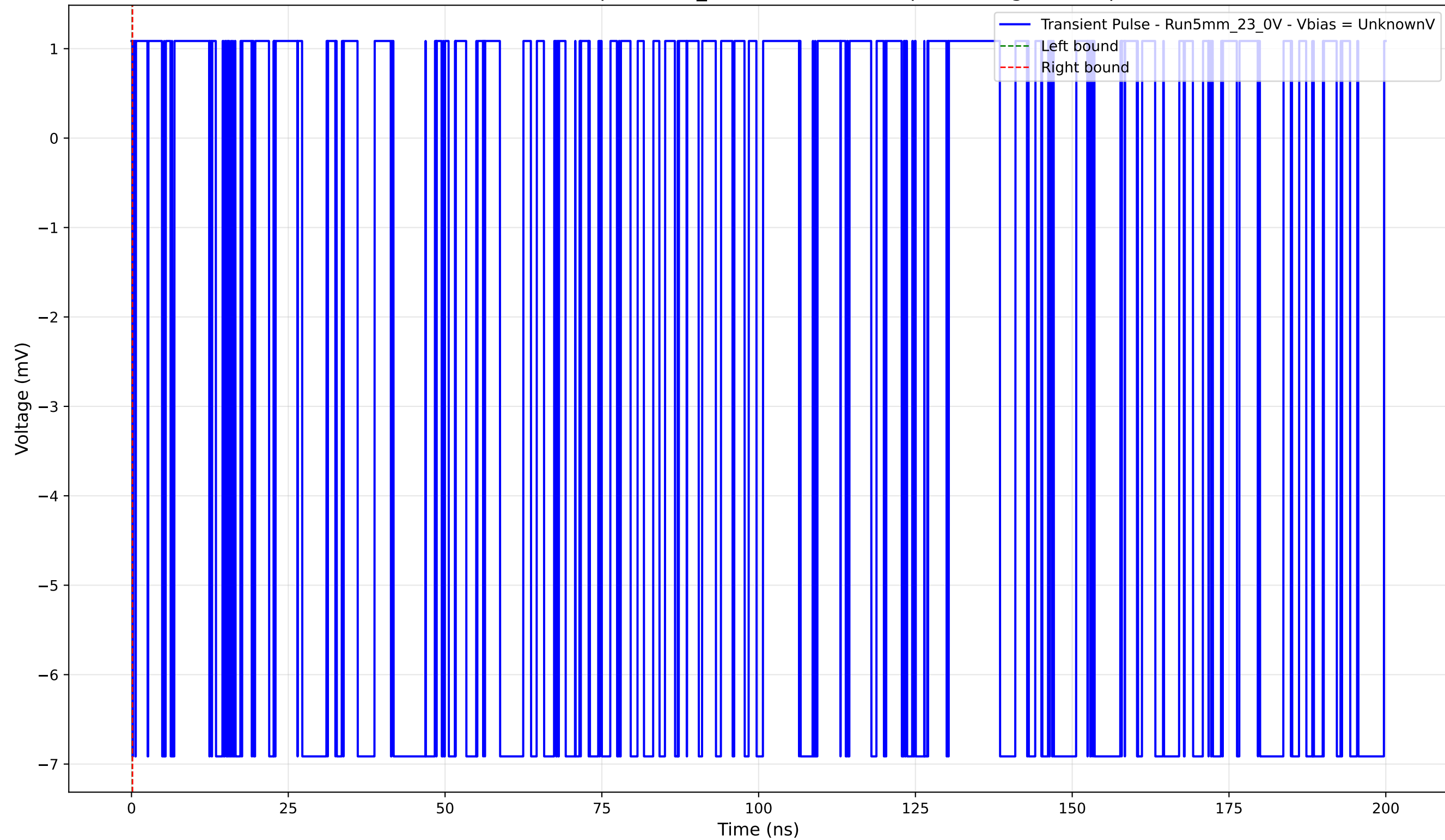
Transient Pulse - Sample: 5mm_23 - Position: 215.0 \mu\text{m} - Charge: -0.00 pC
