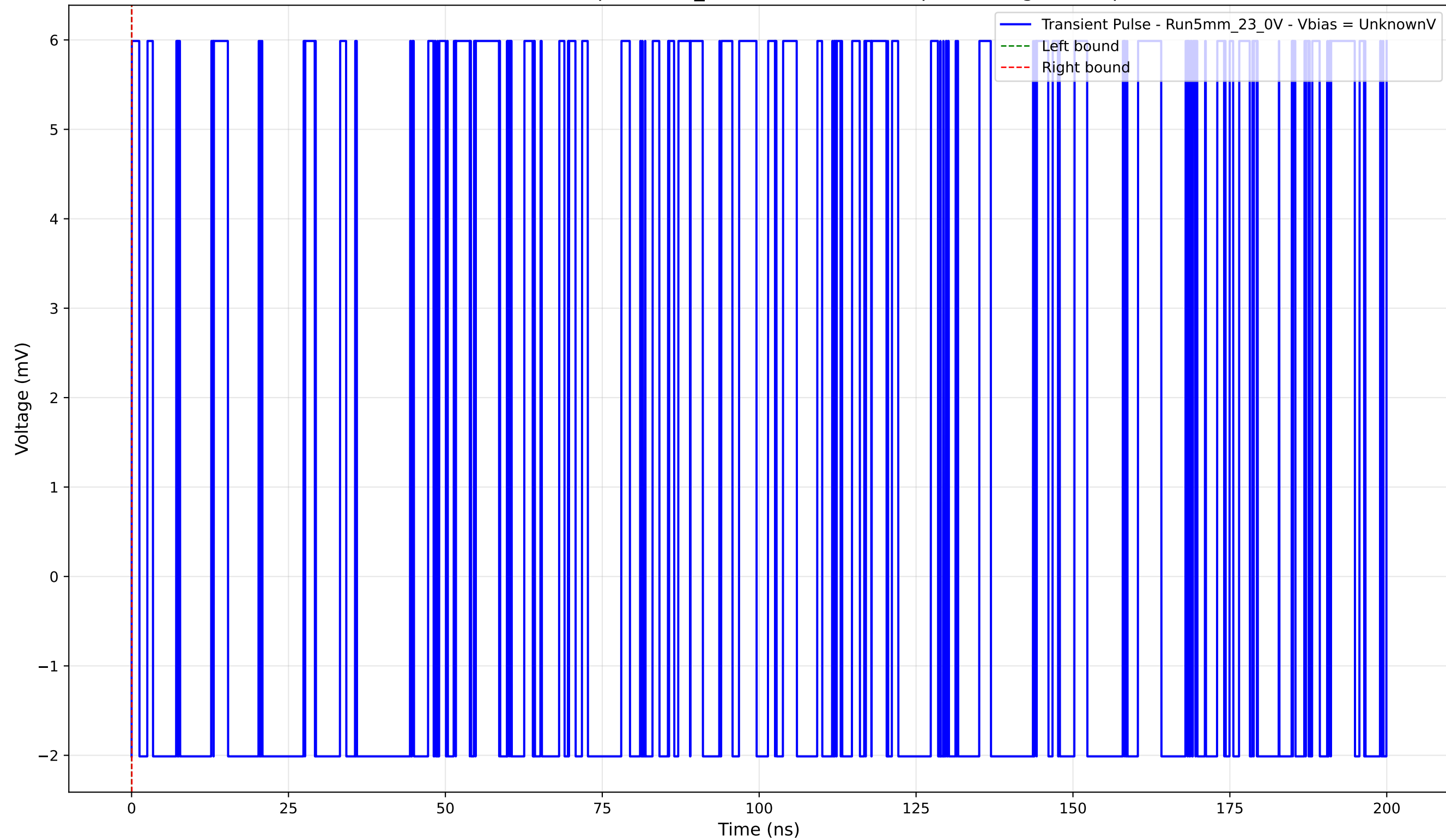
Transient Pulse - Sample: 5mm_23 - Position: 2705.0 \mu\text{m} - Charge: 0.00 pC
