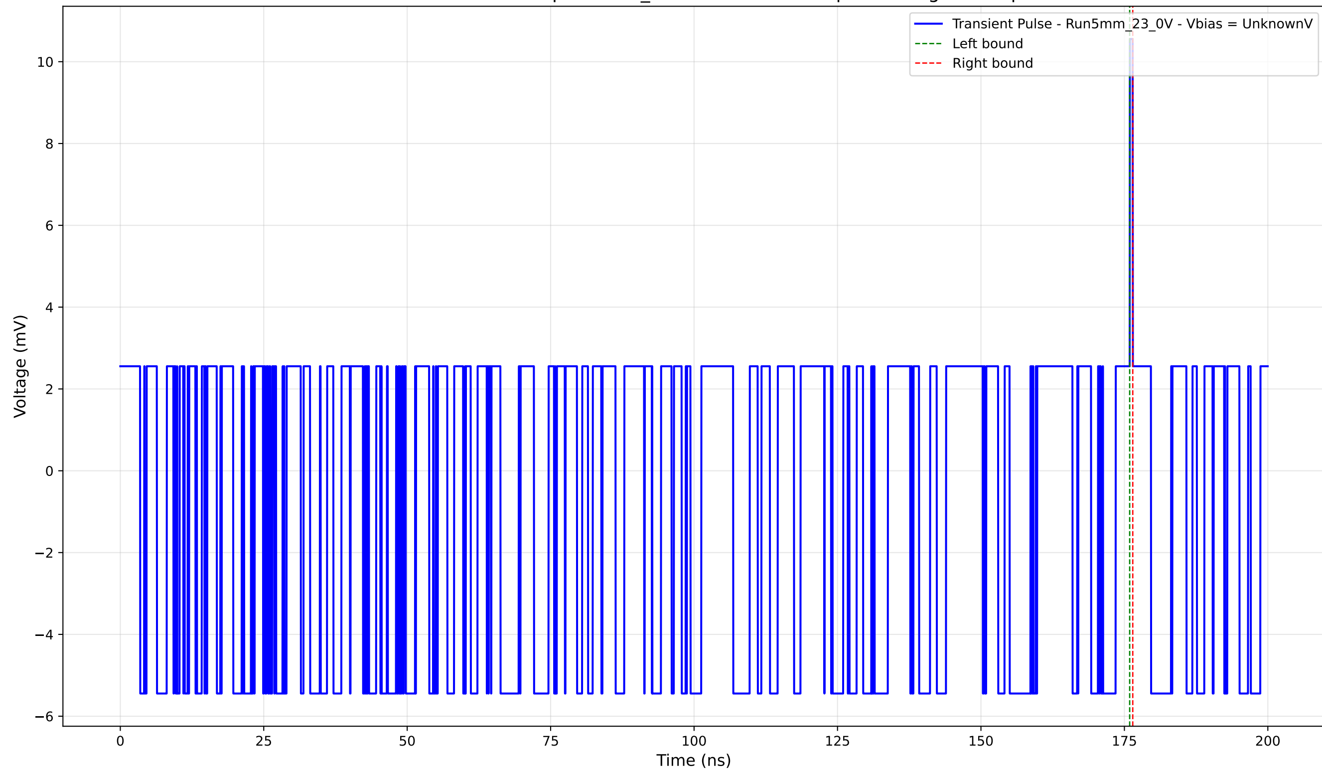
Transient Pulse - Sample: 5mm_23 - Position: 185.0 \mu\text{m} - Charge: 0.11 pC
