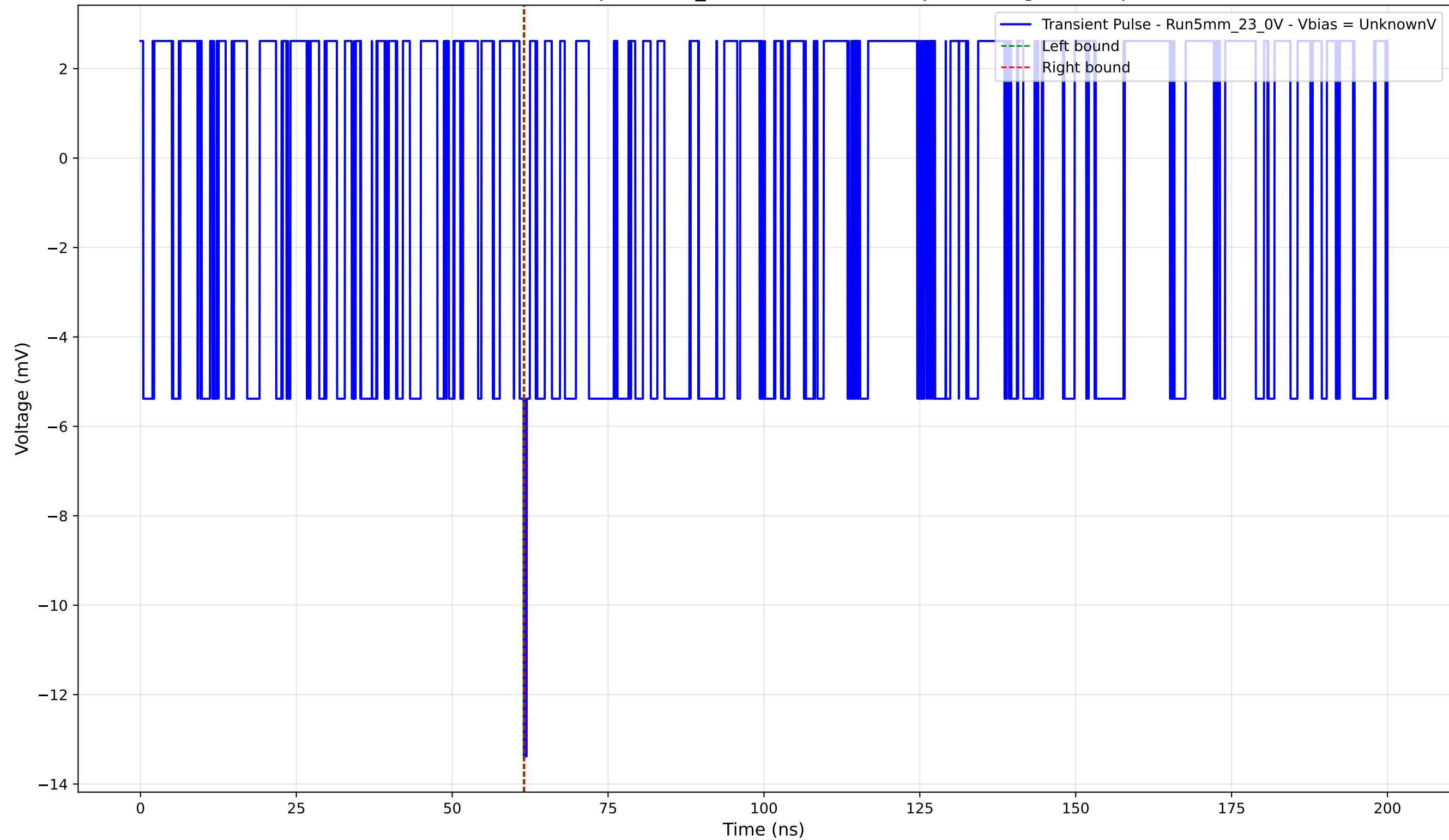
Transient Pulse - Sample: 5mm_23 - Position: 4690.0 \mu\text{m} - Charge: -0.04 pC
