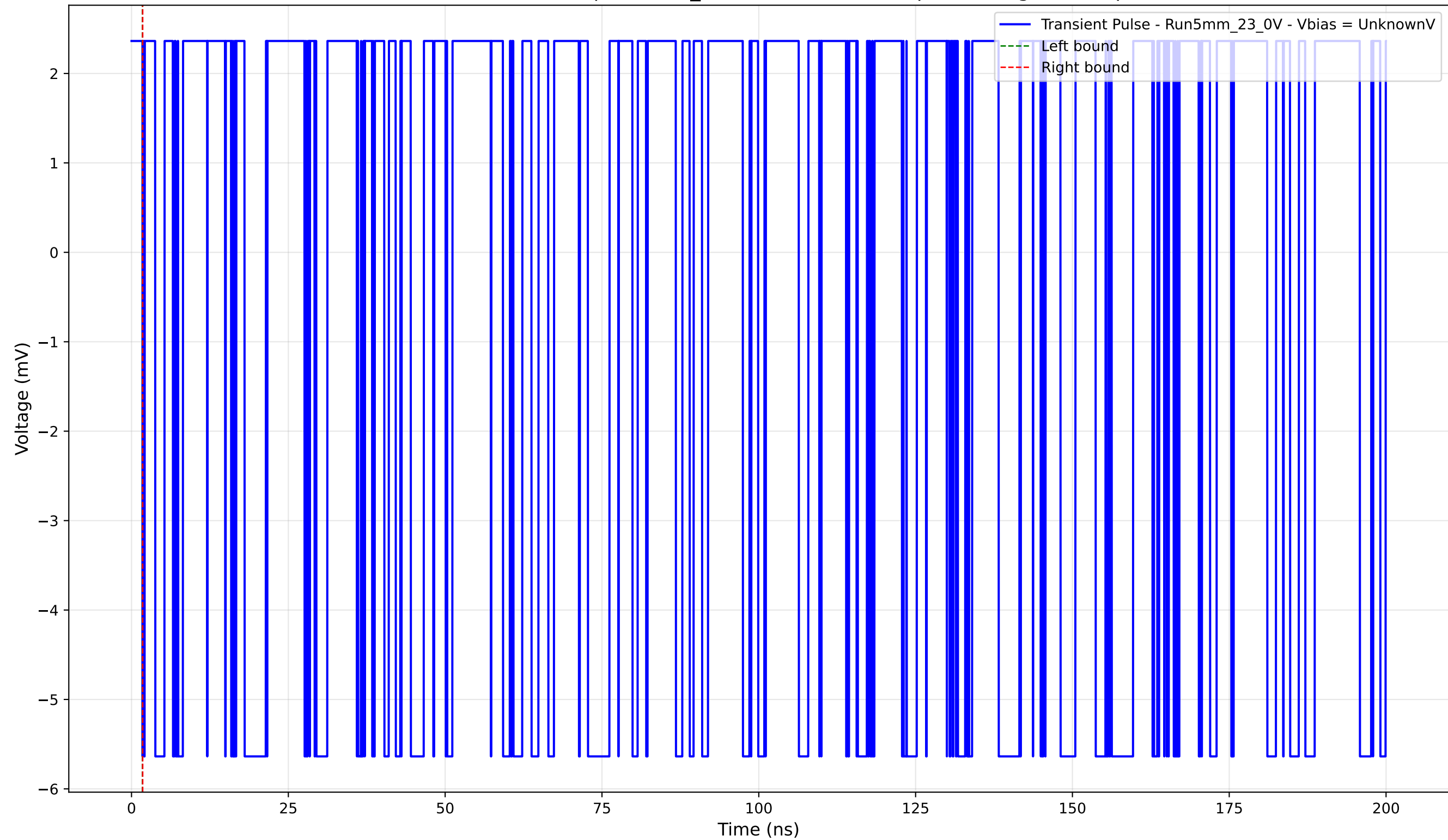
Transient Pulse - Sample: 5mm_23 - Position: 1070.0 \mu\text{m} - Charge: -0.00 pC
