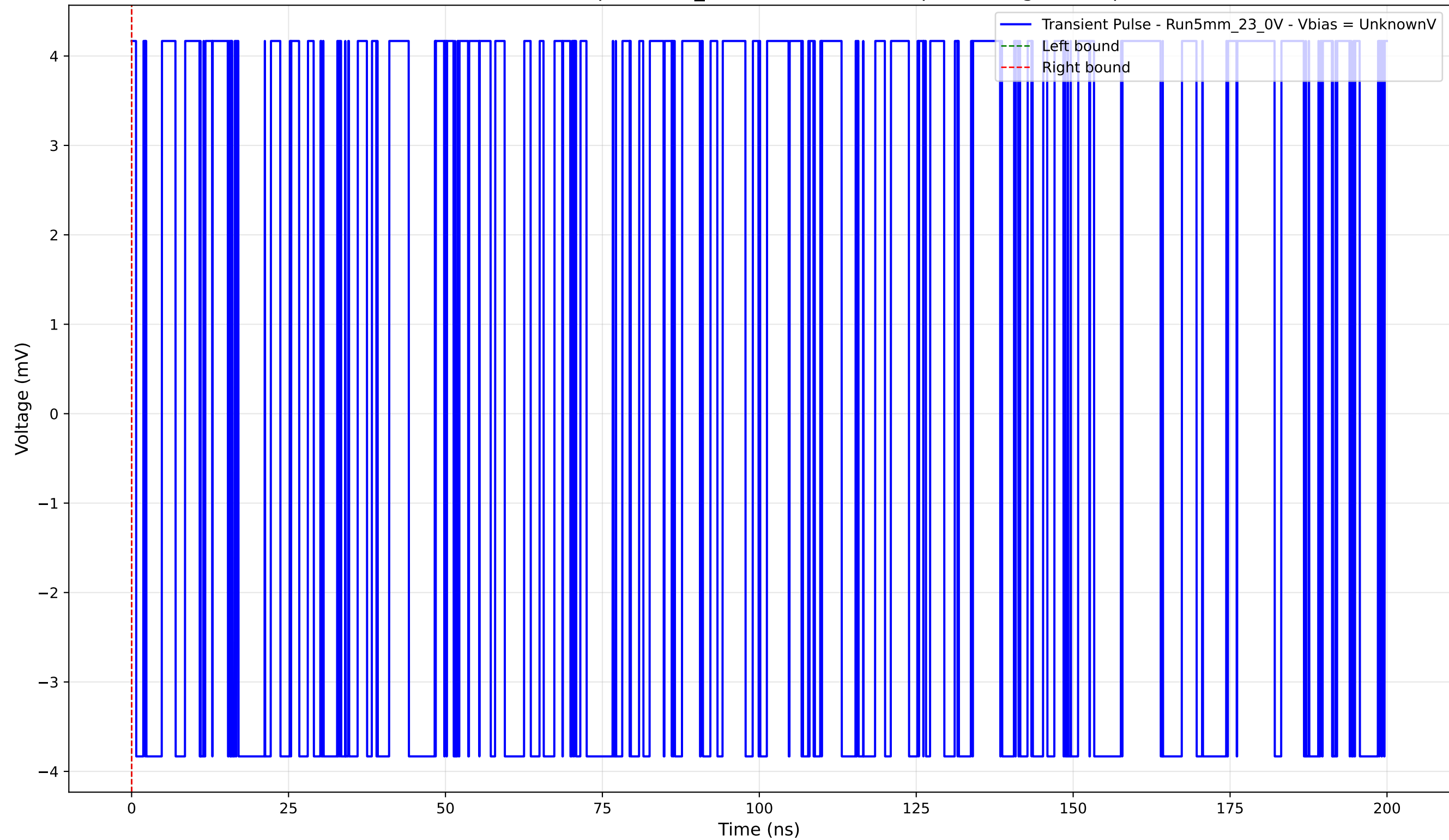
Transient Pulse - Sample: 5mm_23 - Position: 1445.0 \mu\text{m} - Charge: 0.00 pC
