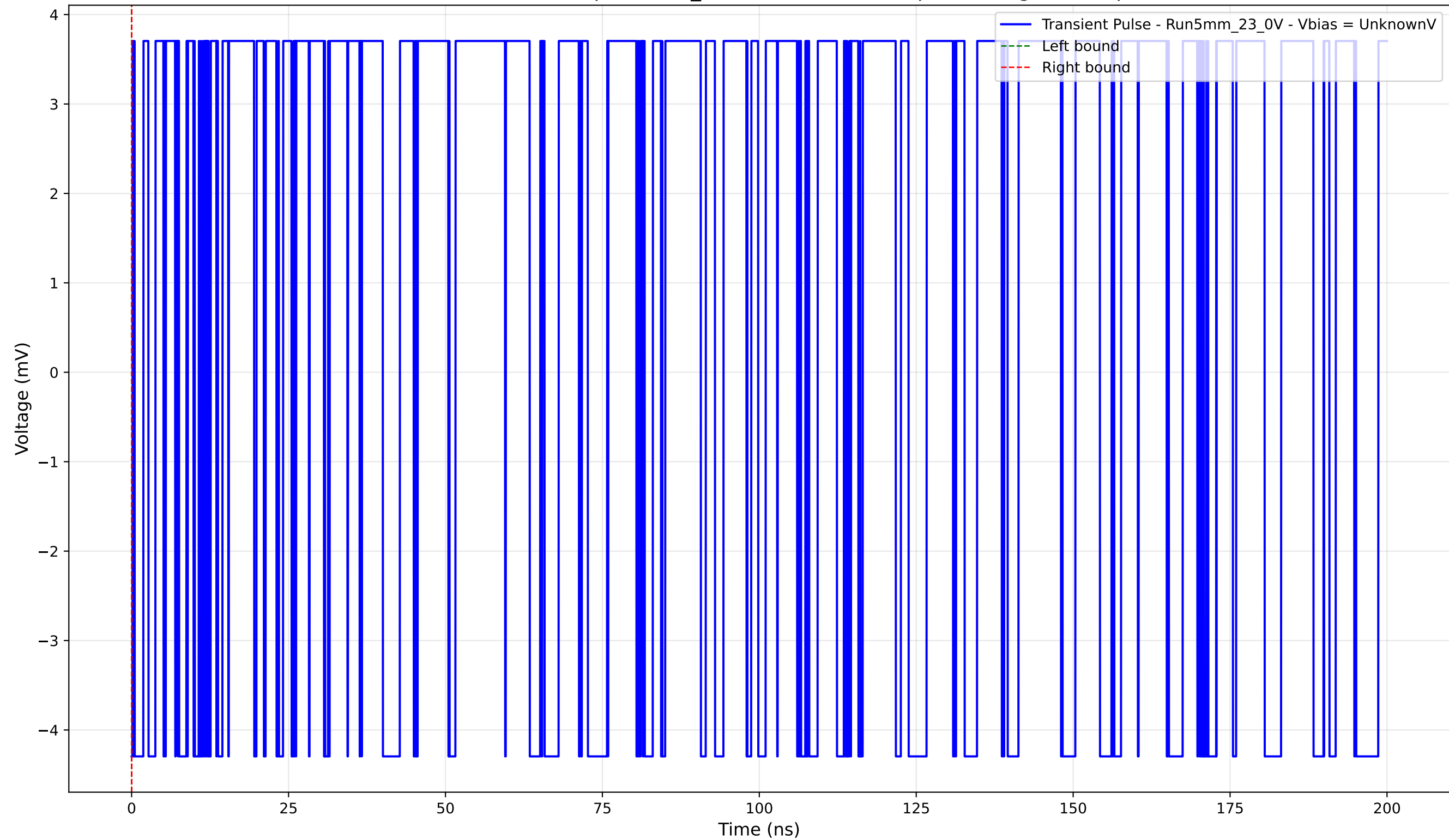
Transient Pulse - Sample: 5mm_23 - Position: 2945.0 \mu\text{m} - Charge: -0.00 pC
