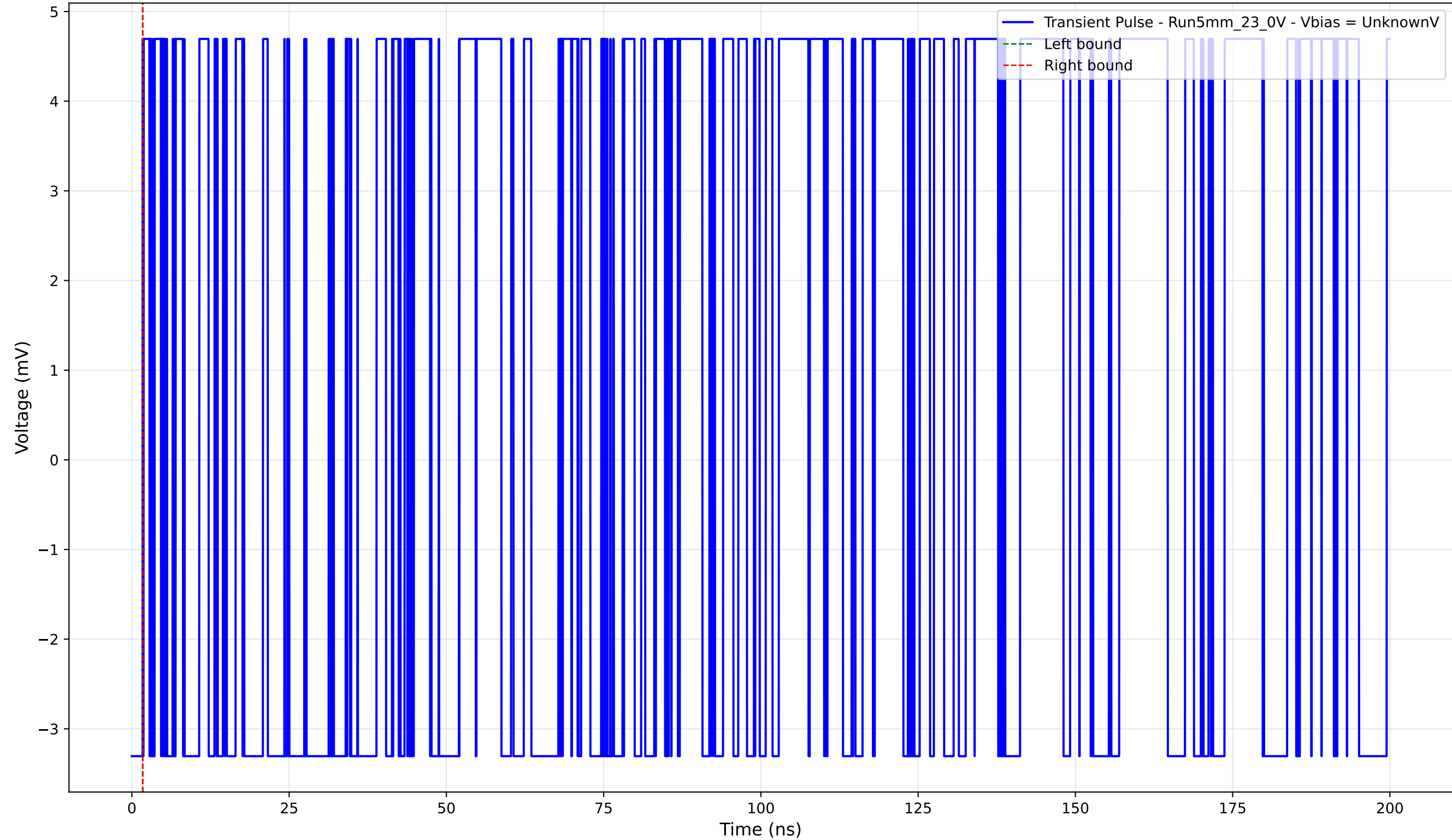
Transient Pulse - Sample: 5mm_23 - Position: 2350.0 \mu\text{m} - Charge: 0.00 pC
