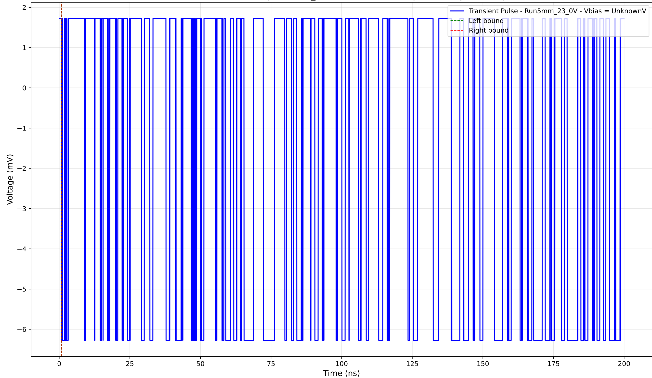
Transient Pulse - Sample: 5mm_23 - Position: 2645.0 \mu\text{m} - Charge: -0.00 pC
