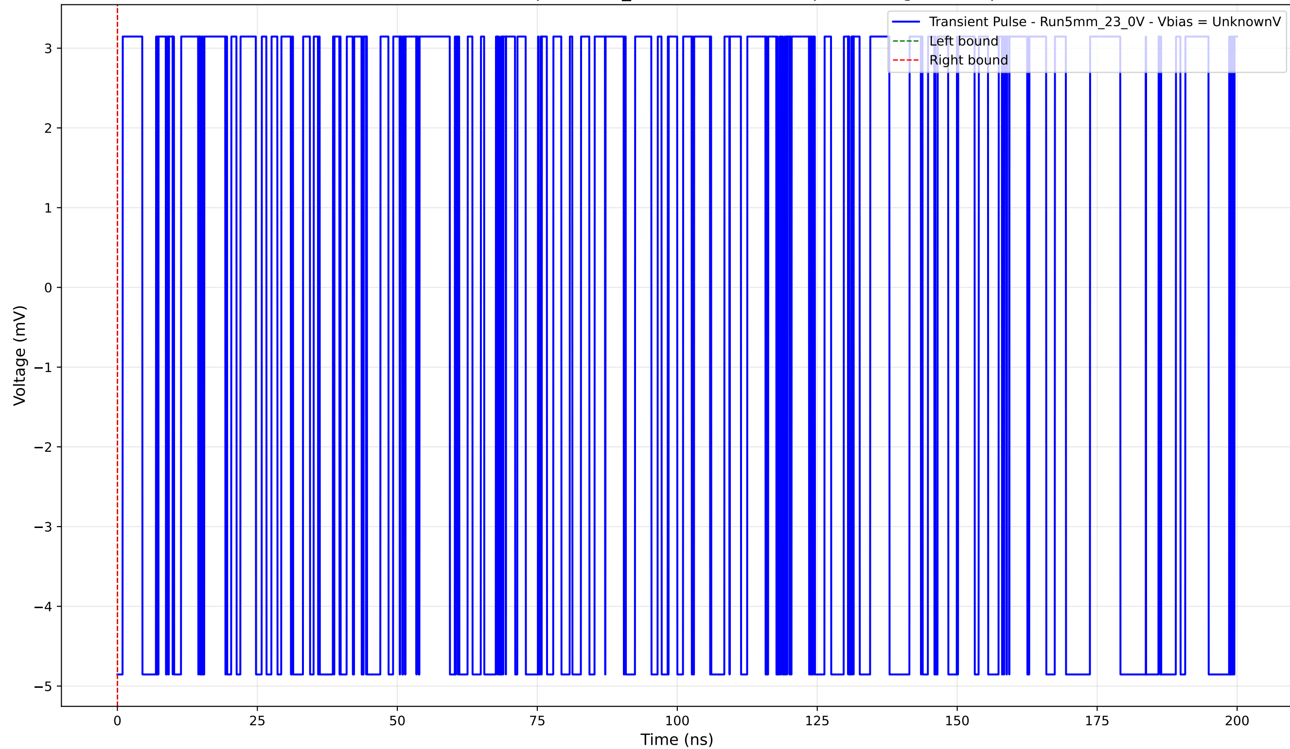
Transient Pulse - Sample: 5mm_23 - Position: 390.0 \mu\text{m} - Charge: -0.00 pC
