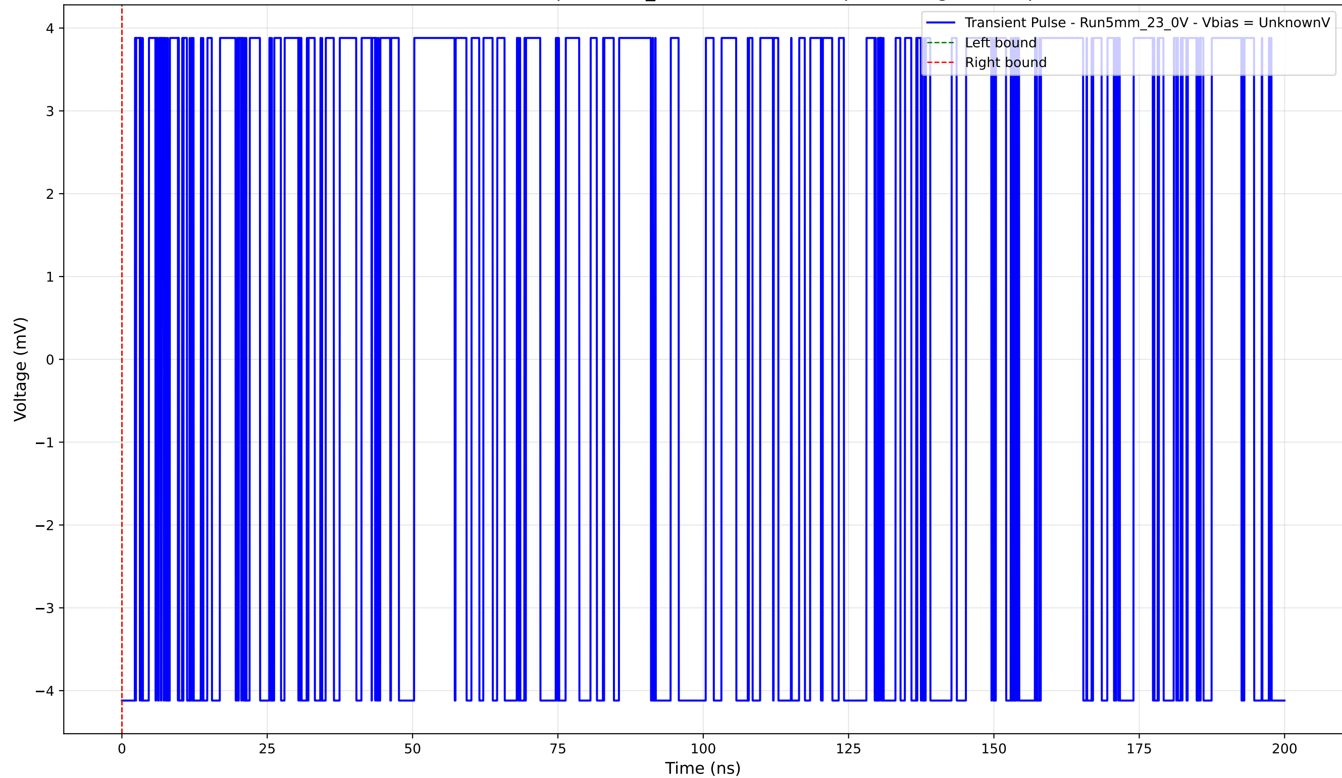
Transient Pulse - Sample: 5mm_23 - Position: 950.0 \mu\text{m} - Charge: -0.00 pC
