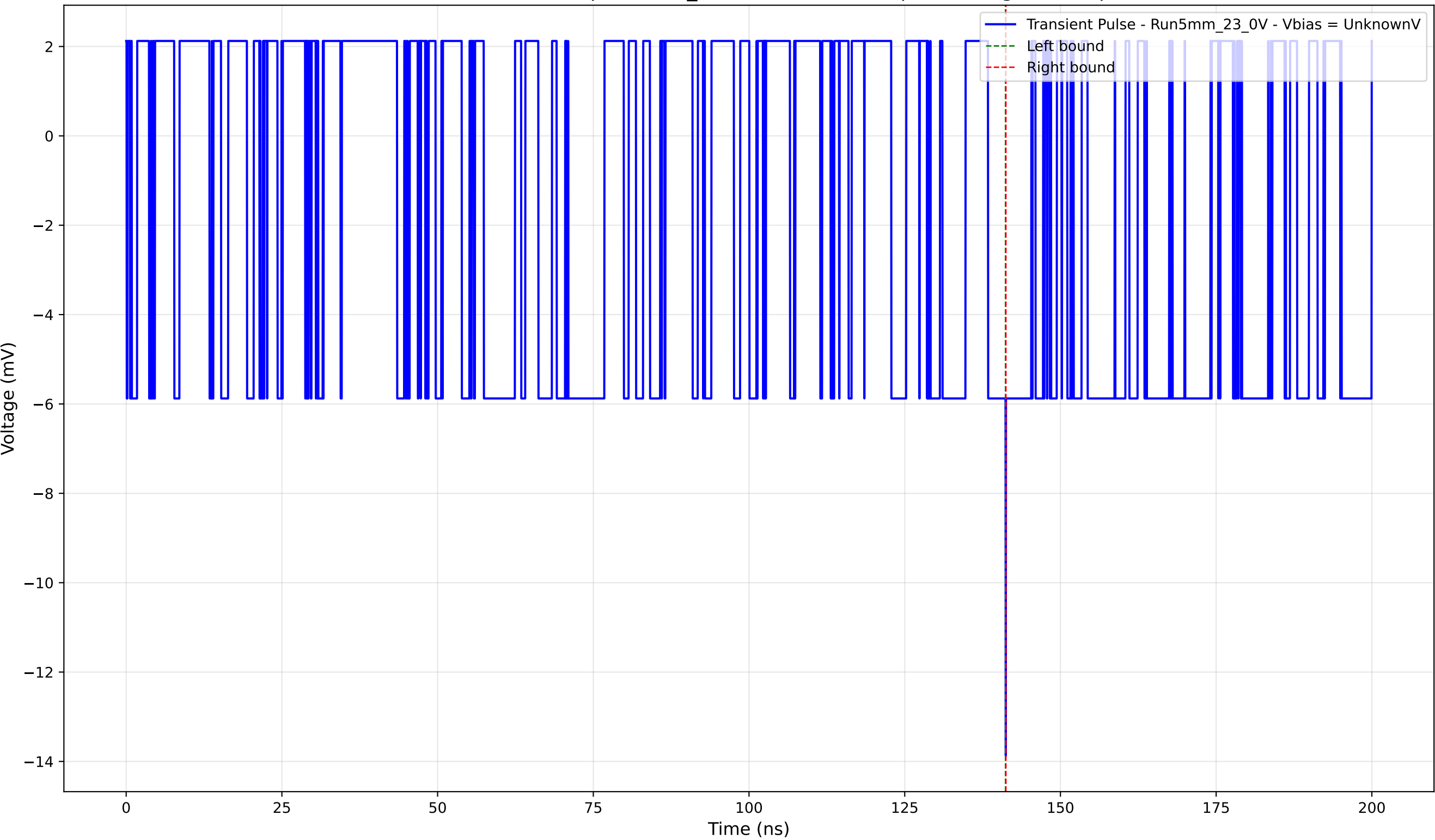
Transient Pulse - Sample: 5mm_23 - Position: 415.0 \mu\text{m} - Charge: -0.01 pC
