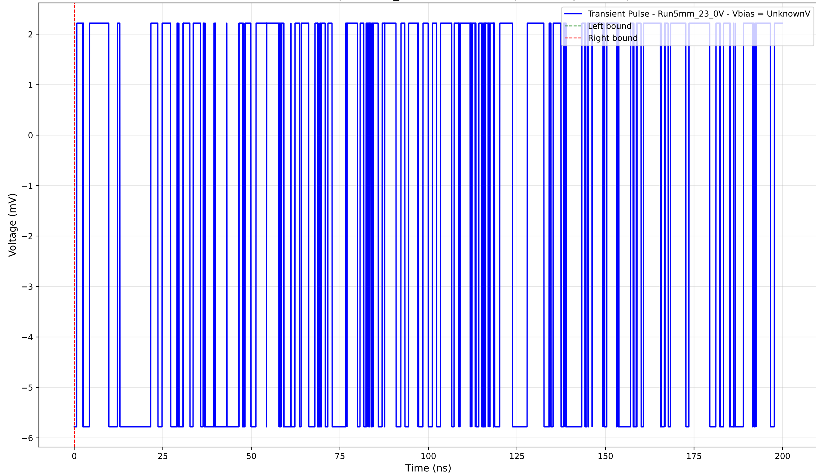
Transient Pulse - Sample: 5mm_23 - Position: 870.0 \mu\text{m} - Charge: -0.00 pC
