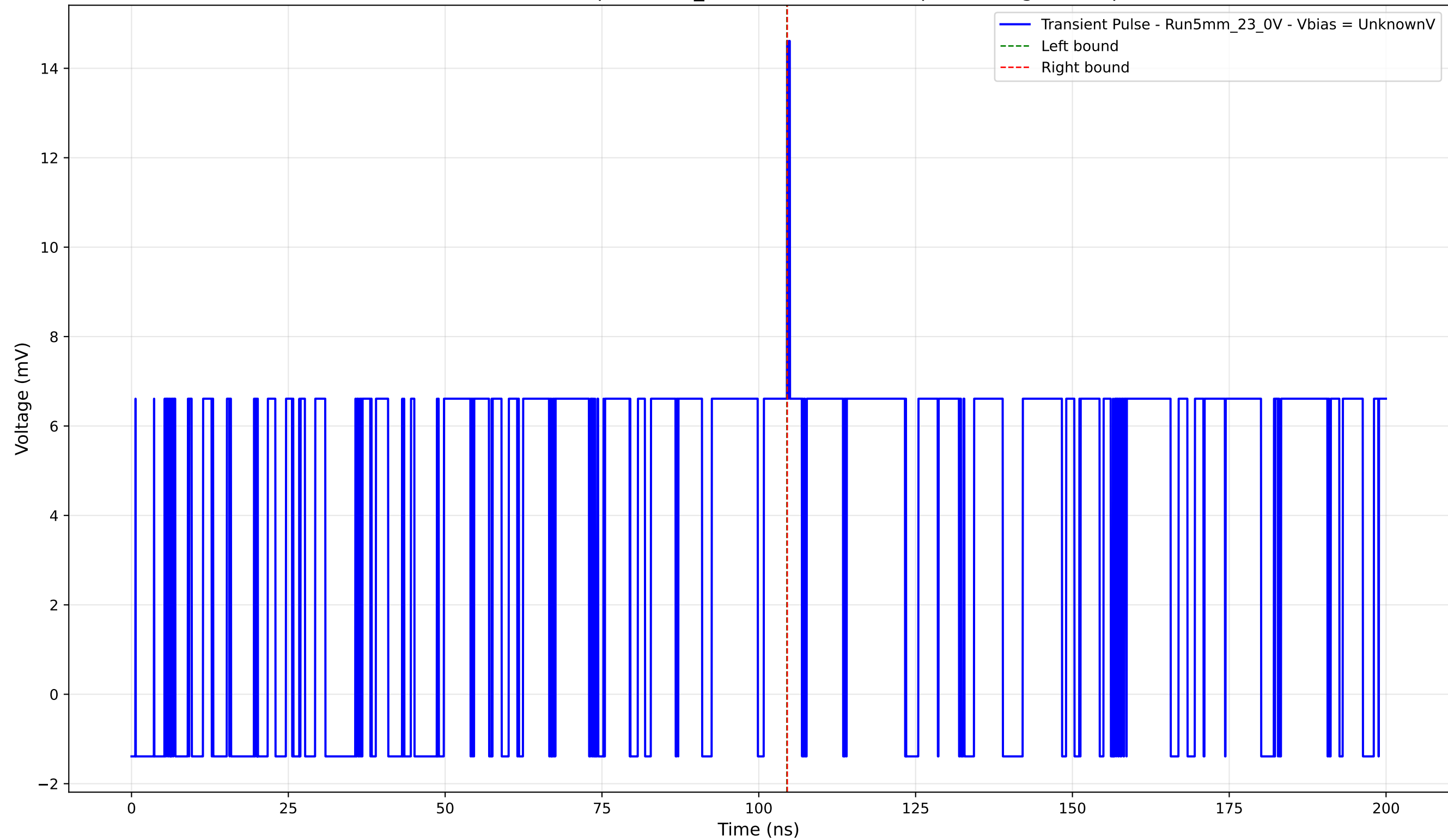
Transient Pulse - Sample: 5mm_23 - Position: 3090.0 \mu\text{m} - Charge: 0.01 pC
