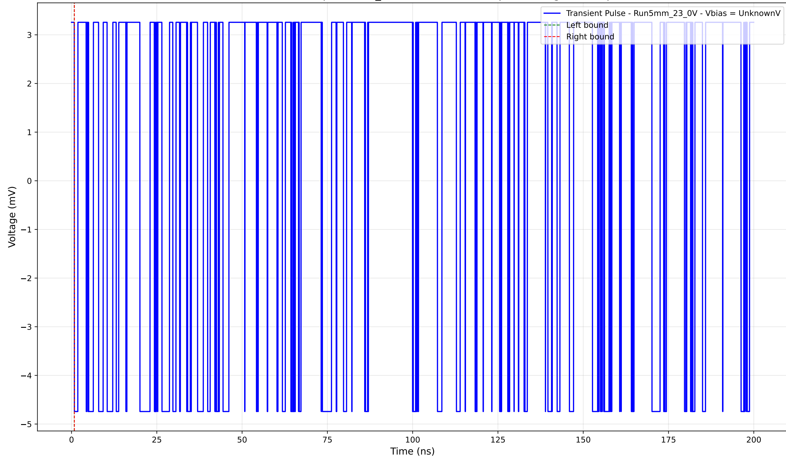
Transient Pulse - Sample: 5mm_23 - Position: 3935.0 \mu\text{m} - Charge: -0.00 pC
