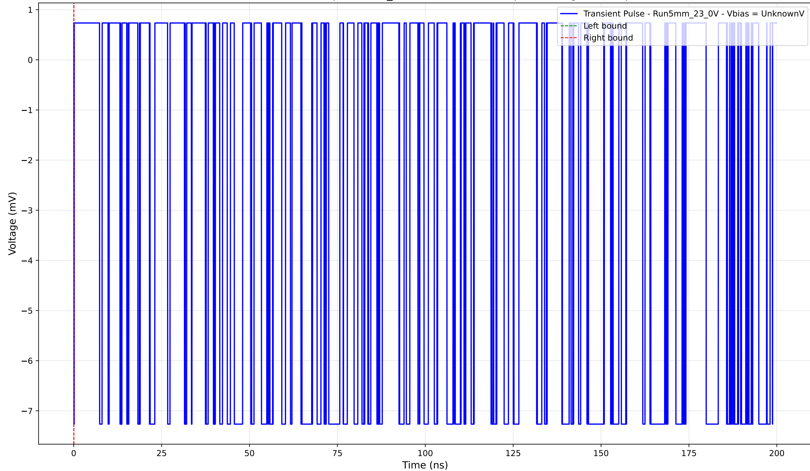
Transient Pulse - Sample: 5mm_23 - Position: 3740.0 \mu\text{m} - Charge: -0.00 pC
