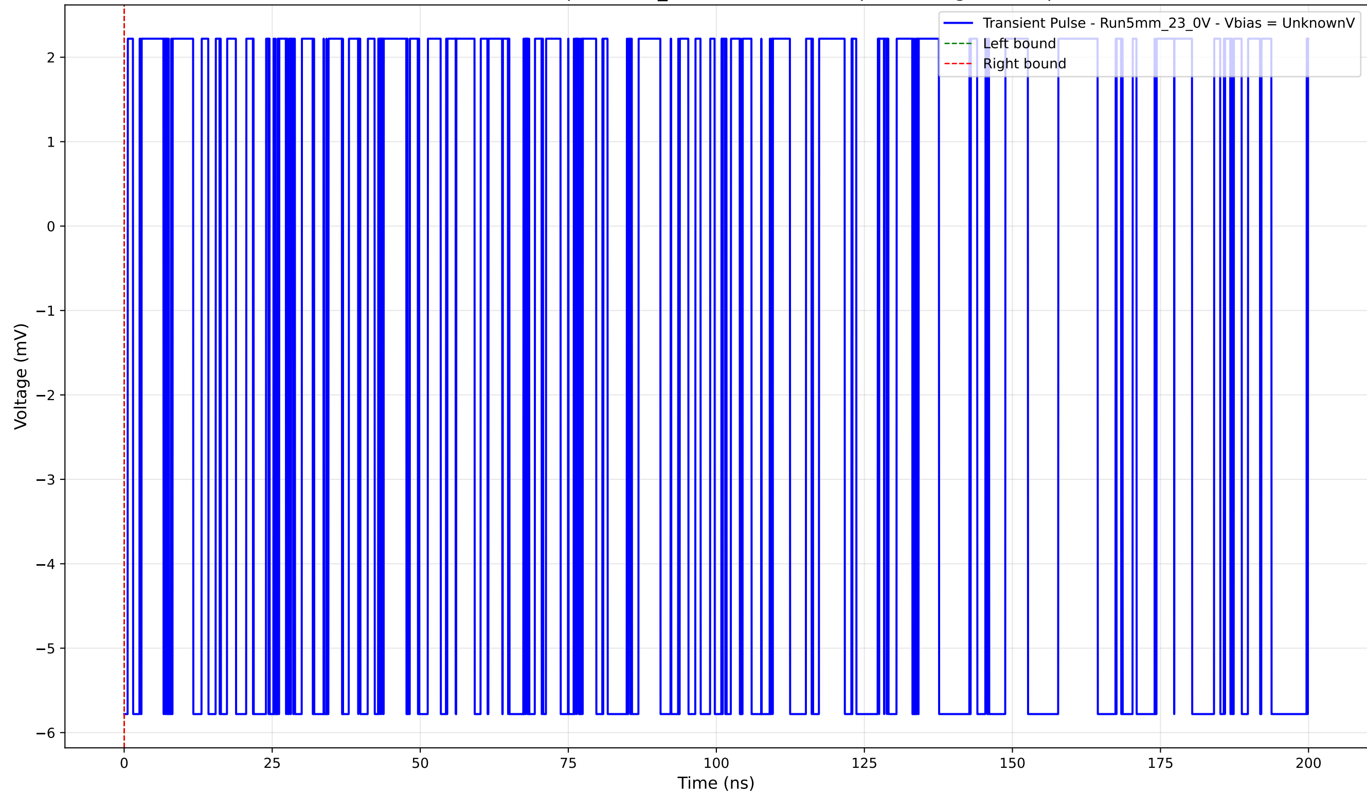
Transient Pulse - Sample: 5mm_23 - Position: 445.0 \mu\text{m} - Charge: -0.00 pC
