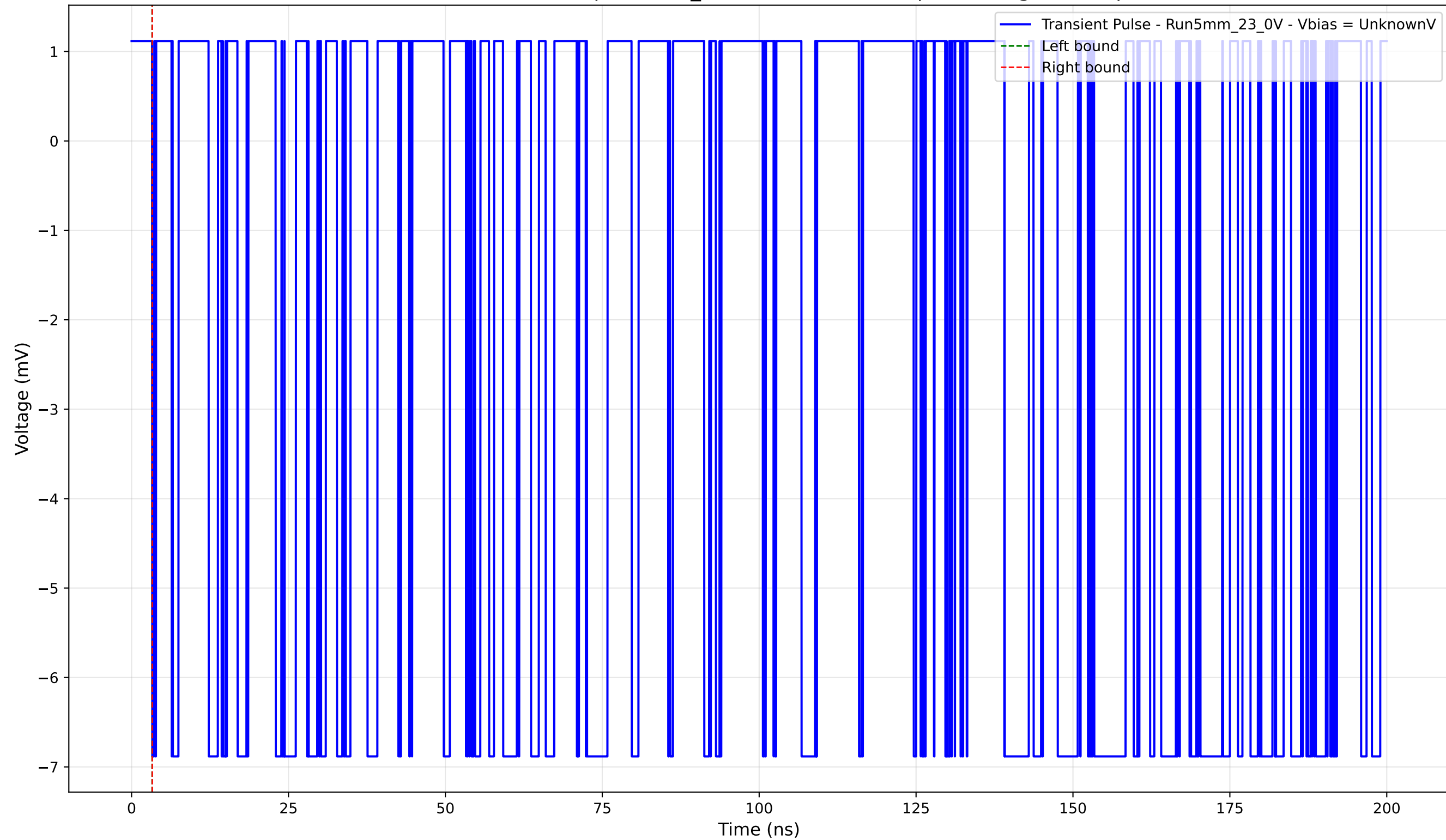
Transient Pulse - Sample: 5mm_23 - Position: 3960.0 \mu\text{m} - Charge: -0.00 pC
