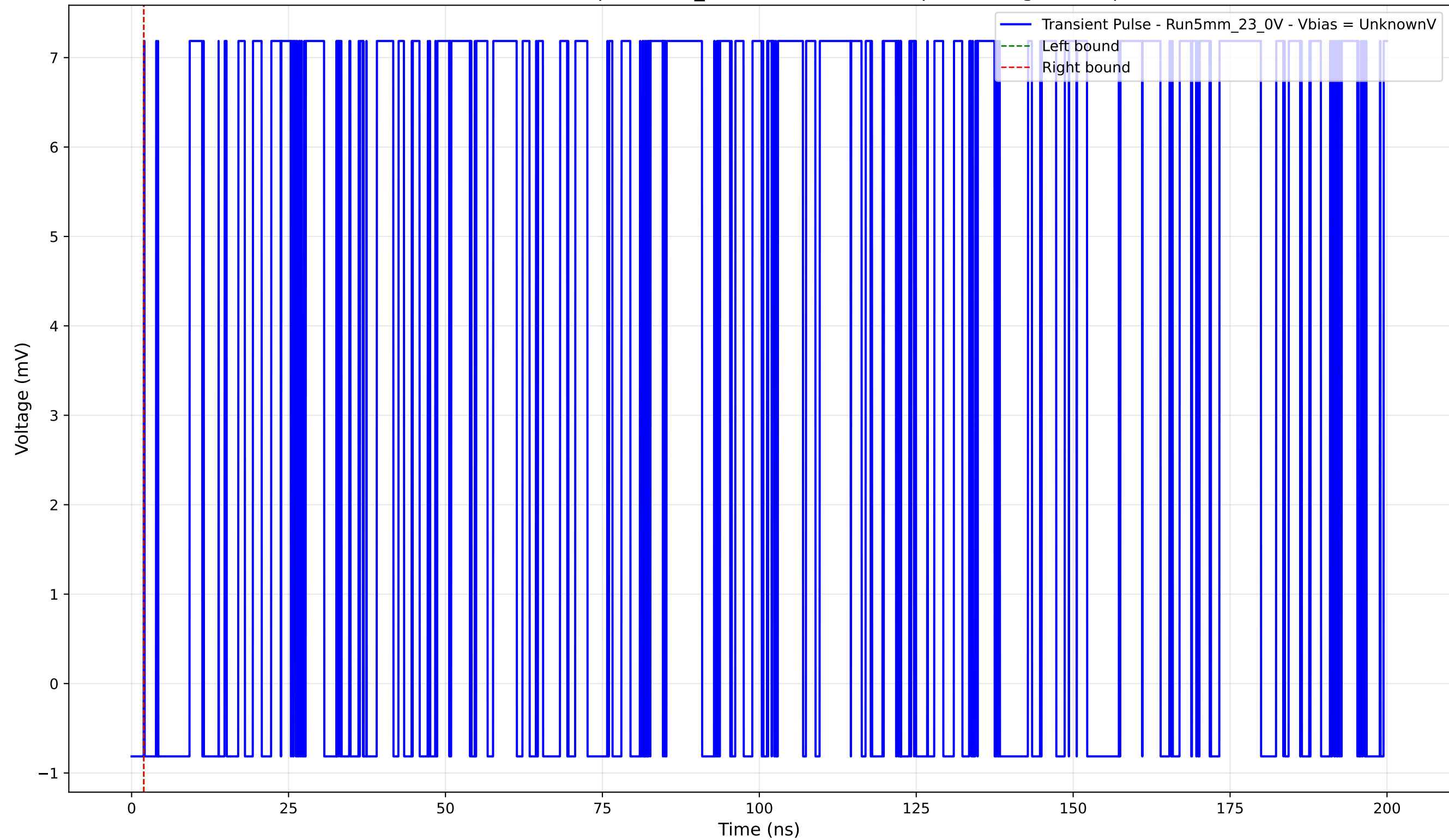
Transient Pulse - Sample: 5mm_23 - Position: 1805.0 \mu\text{m} - Charge: 0.00 pC
