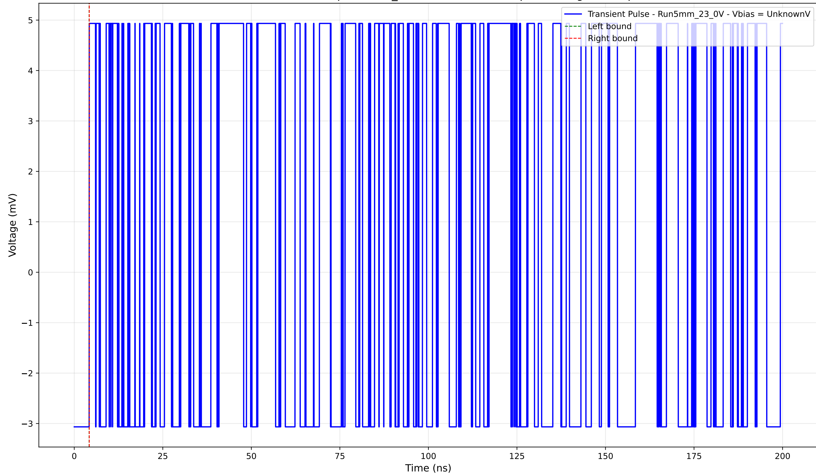
Transient Pulse - Sample: 5mm_23 - Position: 3655.0 \mu\text{m} - Charge: 0.00 pC
