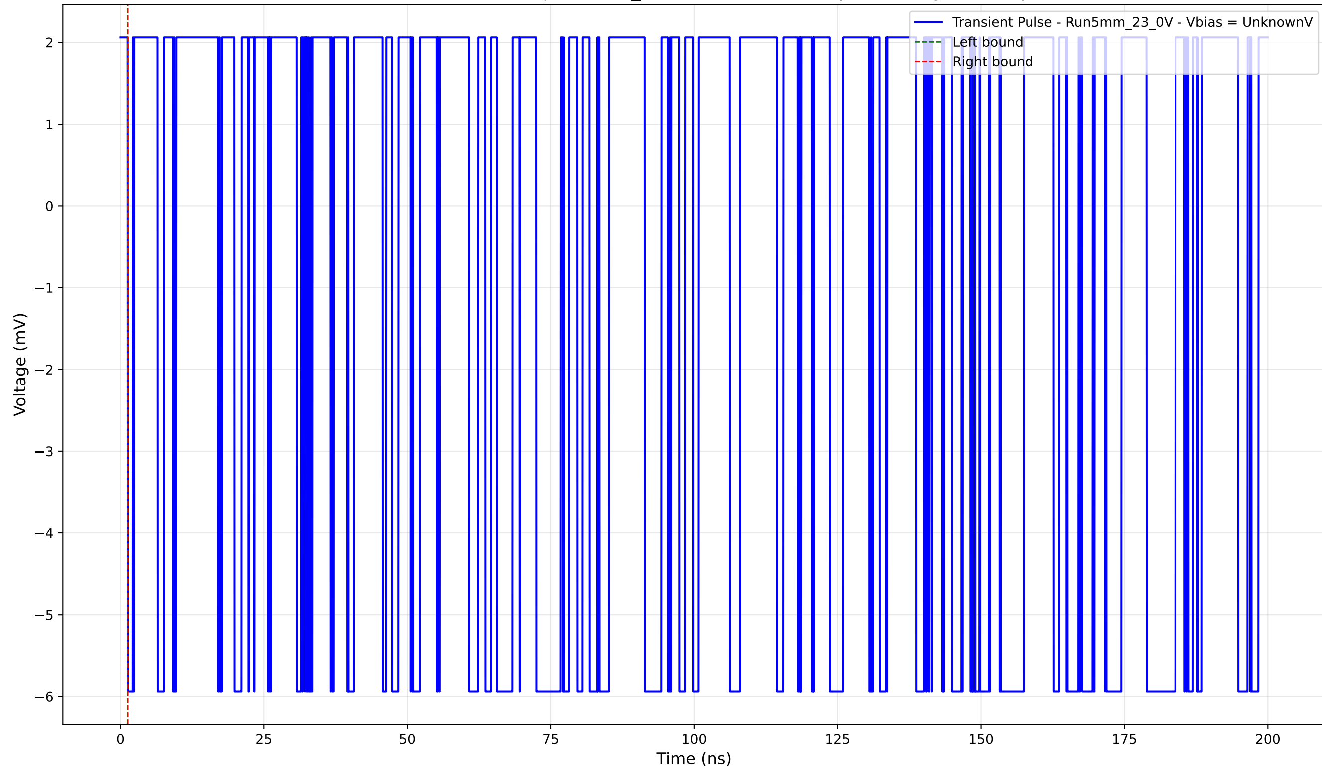
Transient Pulse - Sample: 5mm_23 - Position: 2265.0 \mu\text{m} - Charge: -0.00 pC
