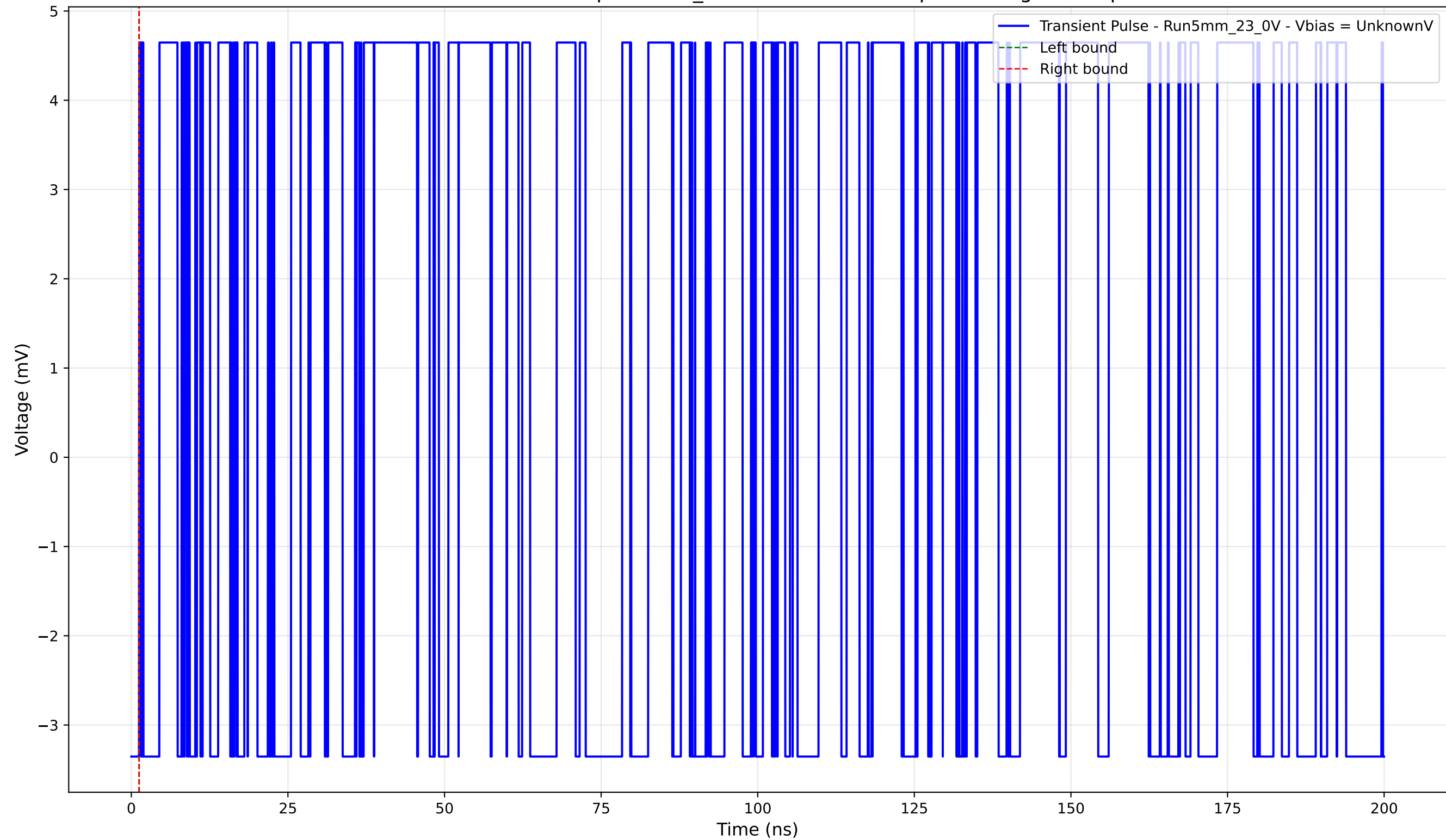
Transient Pulse - Sample: 5mm_23 - Position: 4105.0 \mu\text{m} - Charge: 0.00 pC
