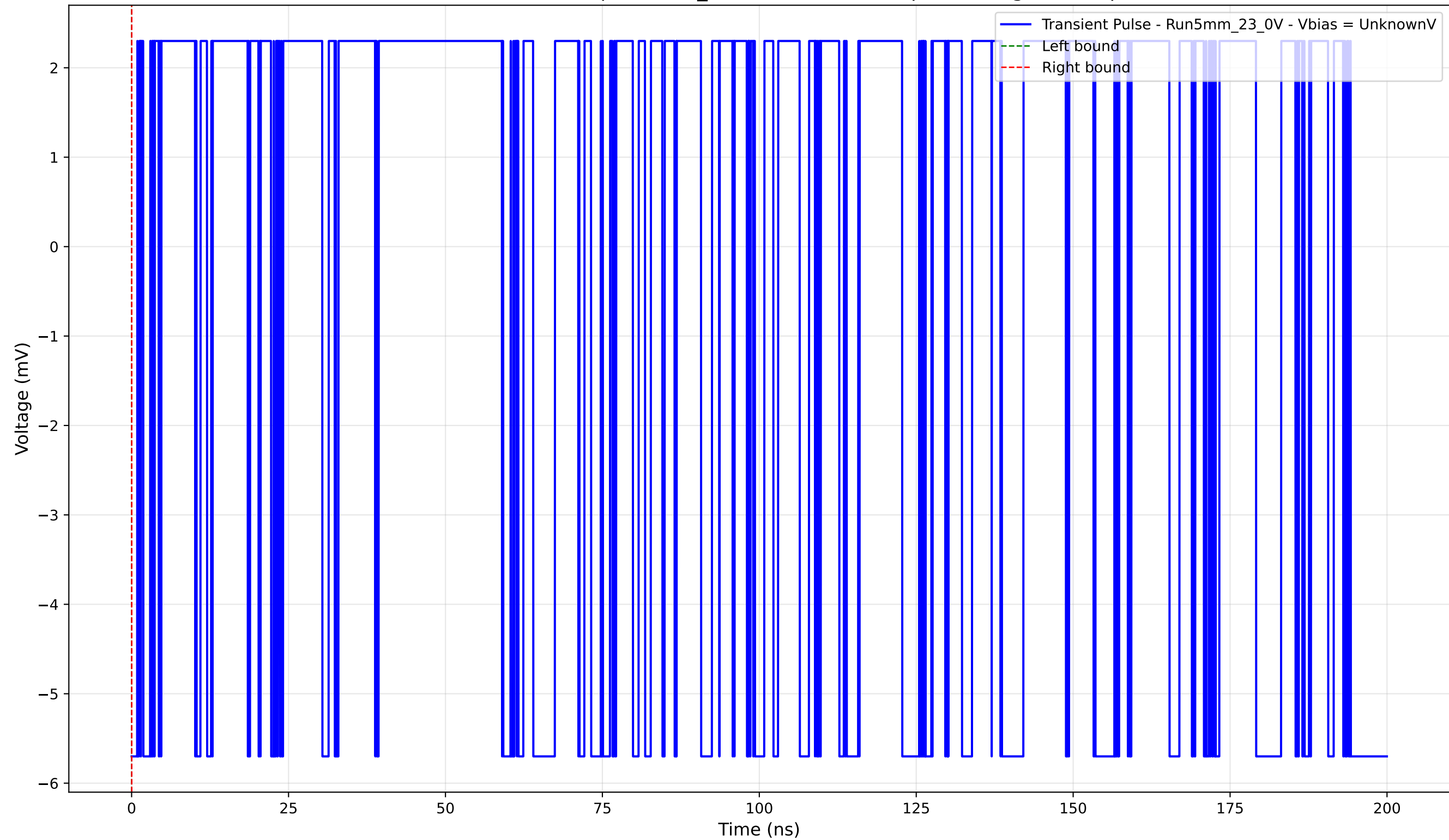
Transient Pulse - Sample: 5mm_23 - Position: 255.0 \mu\text{m} - Charge: -0.00 pC
