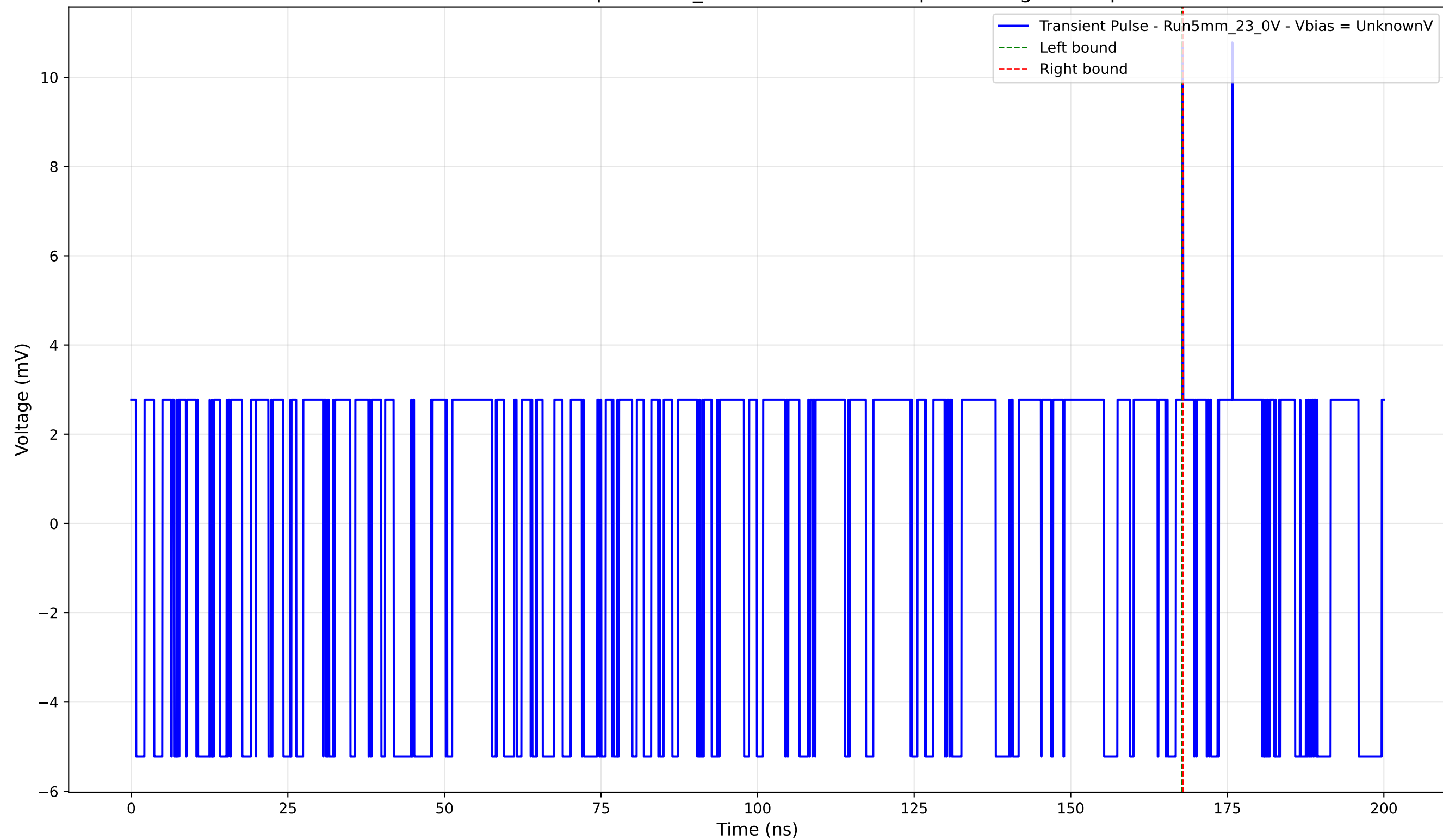
Transient Pulse - Sample: 5mm_23 - Position: 1435.0 \mu\text{m} - Charge: 0.03 pC
