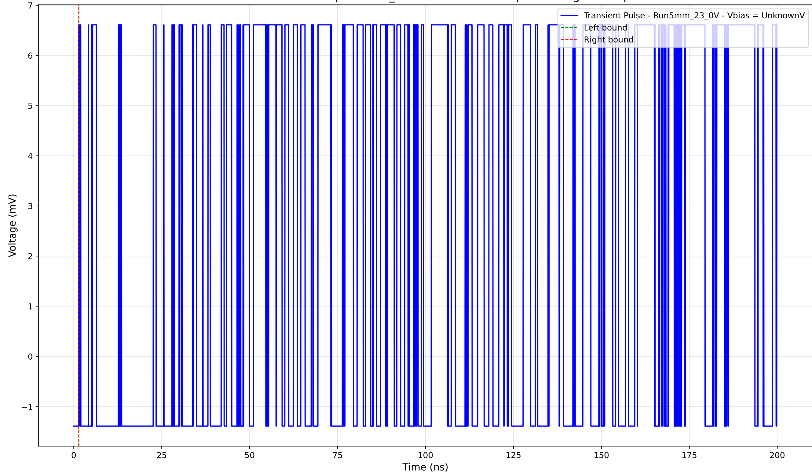
Transient Pulse - Sample: 5mm_23 - Position: 4705.0 \mu\text{m} - Charge: 0.00 pC
