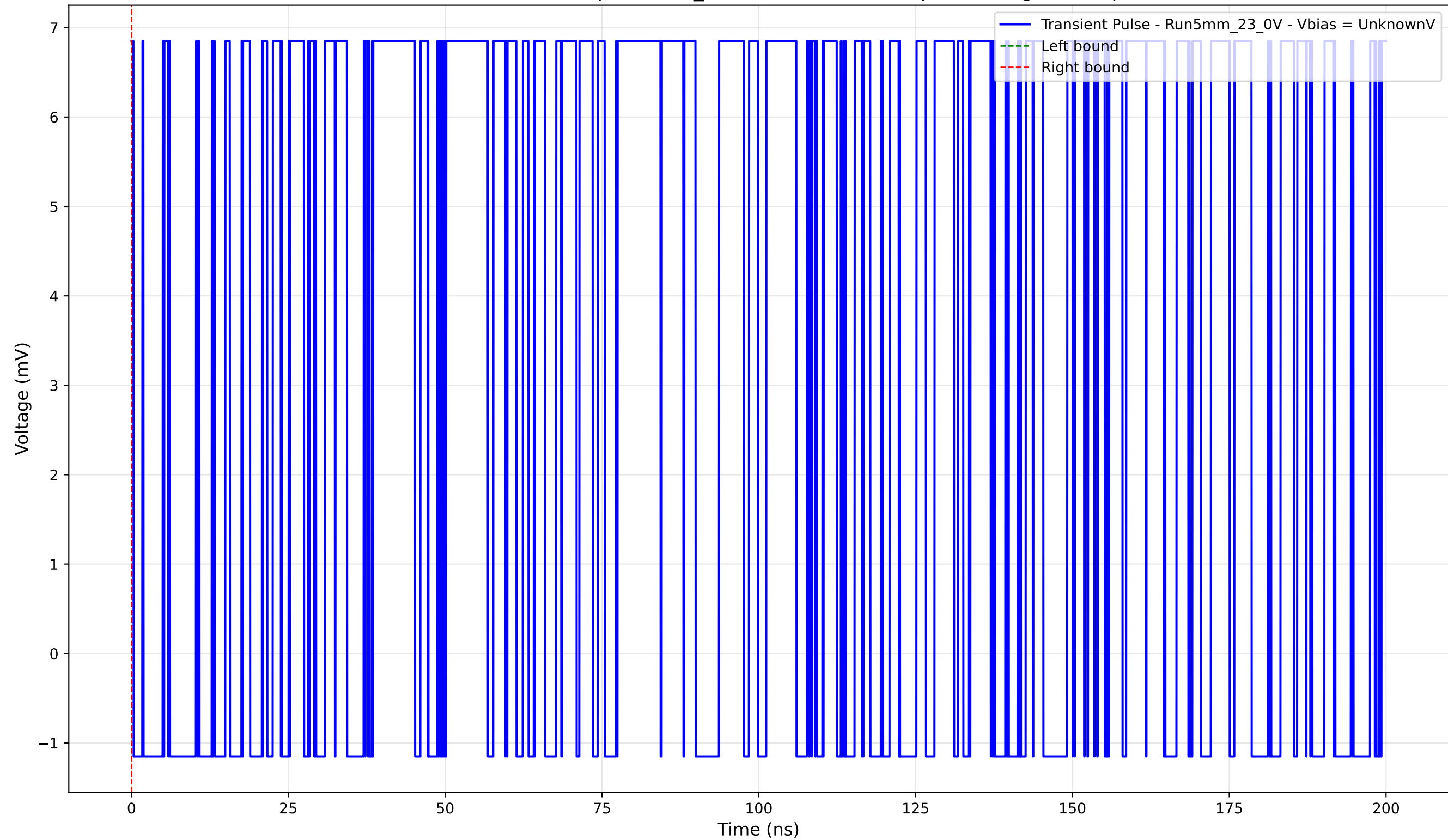
Transient Pulse - Sample: 5mm_23 - Position: 4985.0 \mu\text{m} - Charge: 0.00 pC
