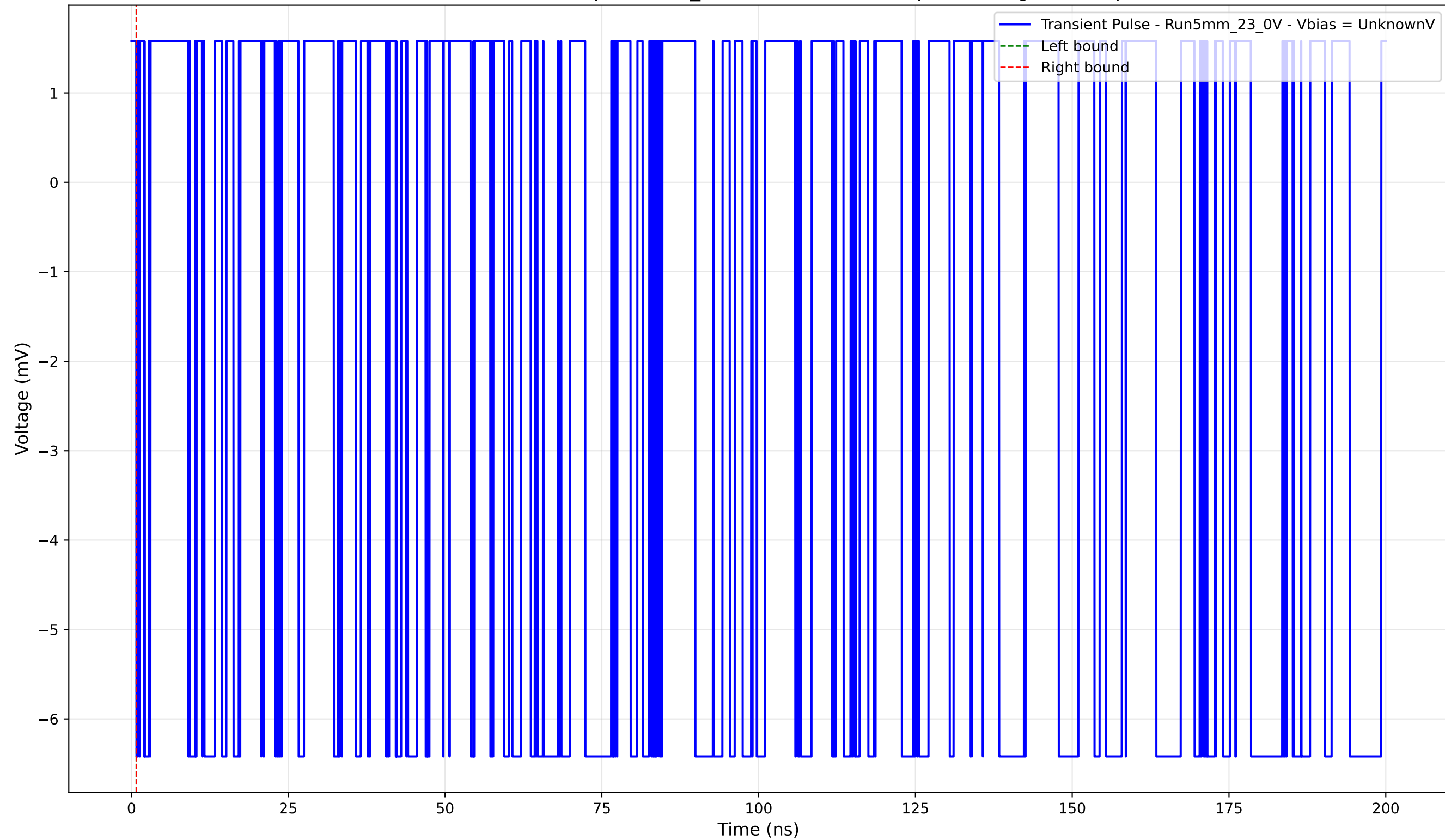
Transient Pulse - Sample: 5mm_23 - Position: 1040.0 \mu\text{m} - Charge: -0.00 pC
