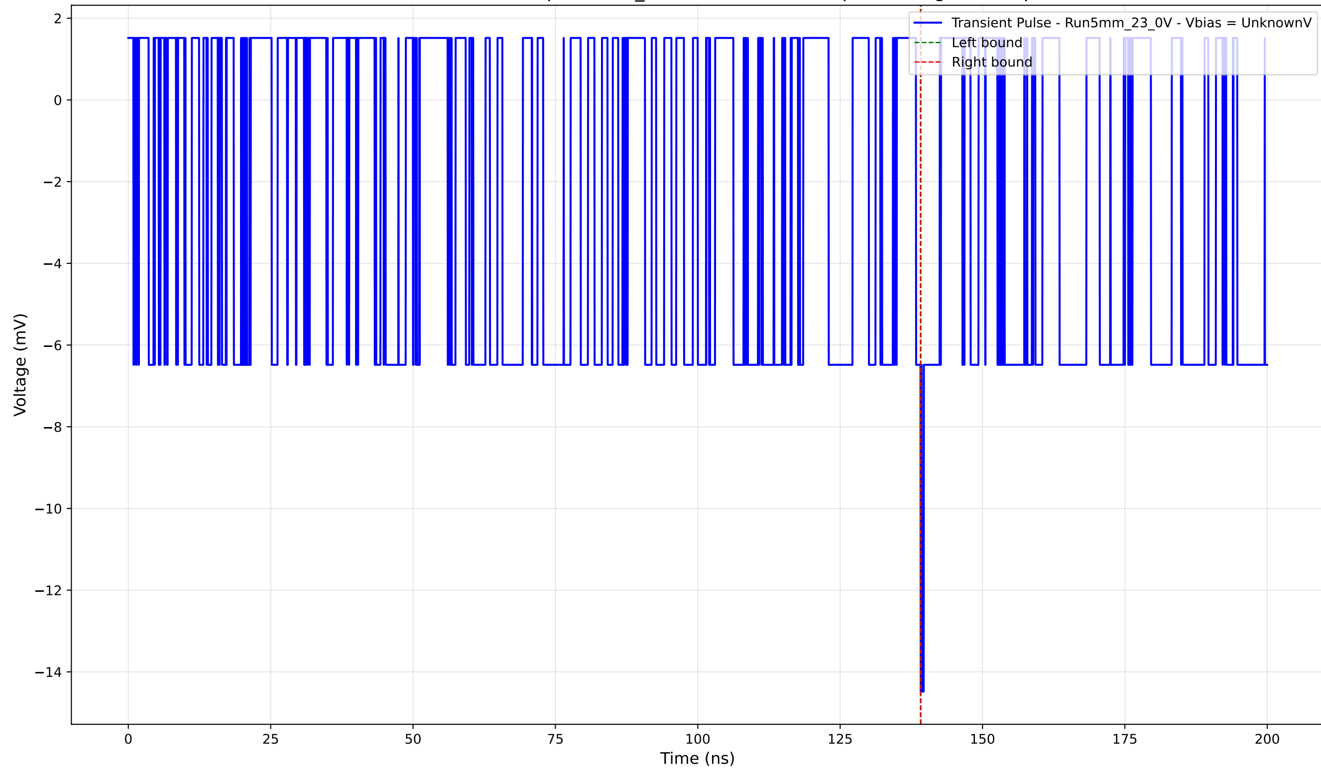
Transient Pulse - Sample: 5mm_23 - Position: 1575.0 \mu\text{m} - Charge: -0.02 pC
