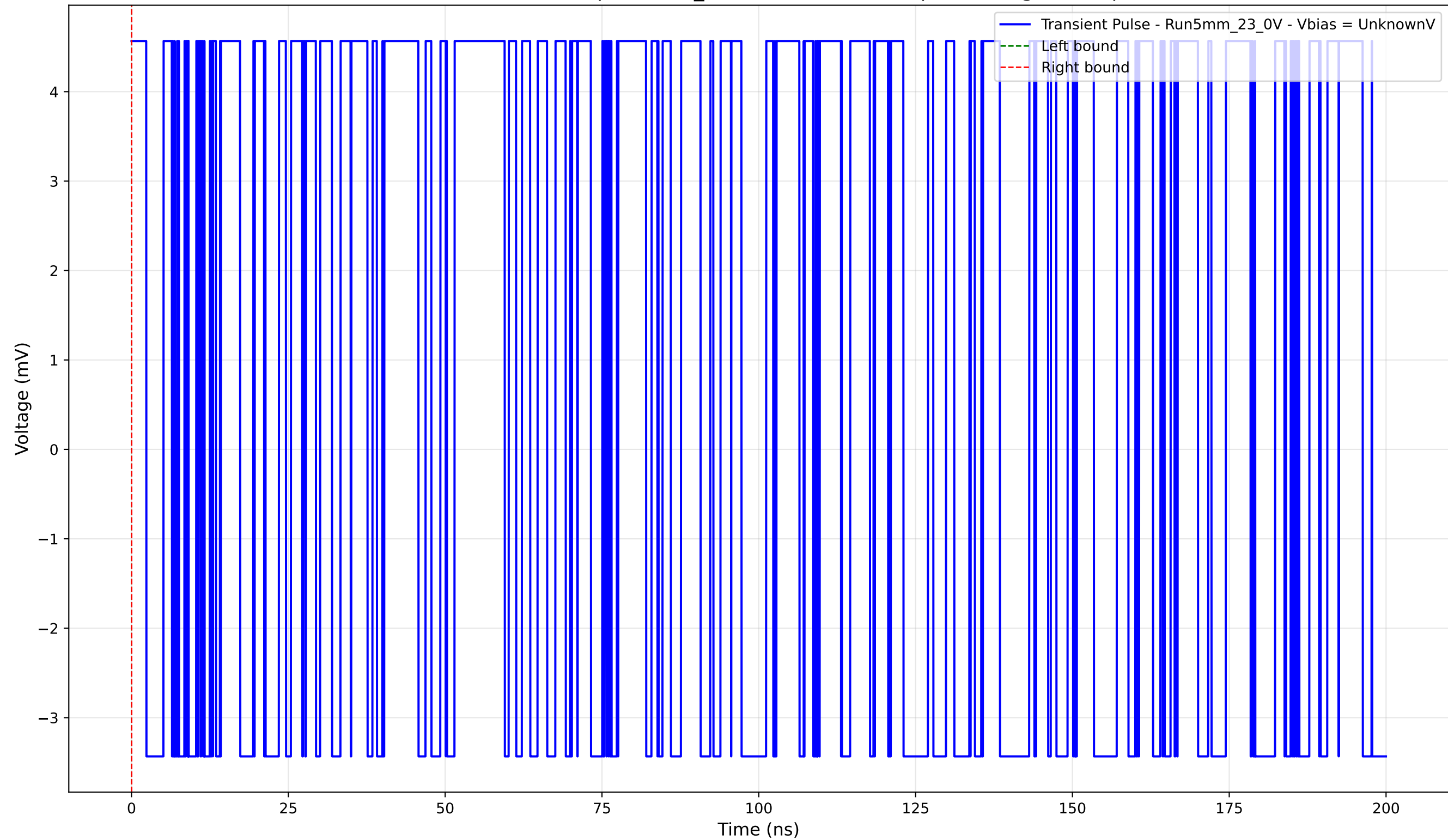
Transient Pulse - Sample: 5mm_23 - Position: 2500.0 \mu\text{m} - Charge: 0.00 pC
