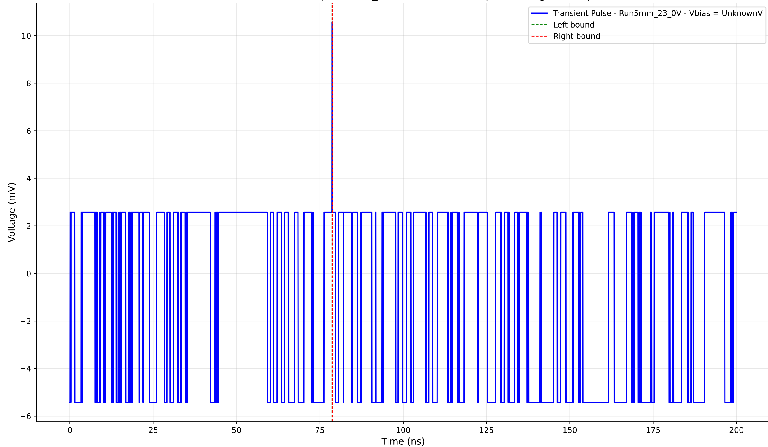
Transient Pulse - Sample: 5mm_23 - Position: 410.0 \mu\text{m} - Charge: 0.01 pC
