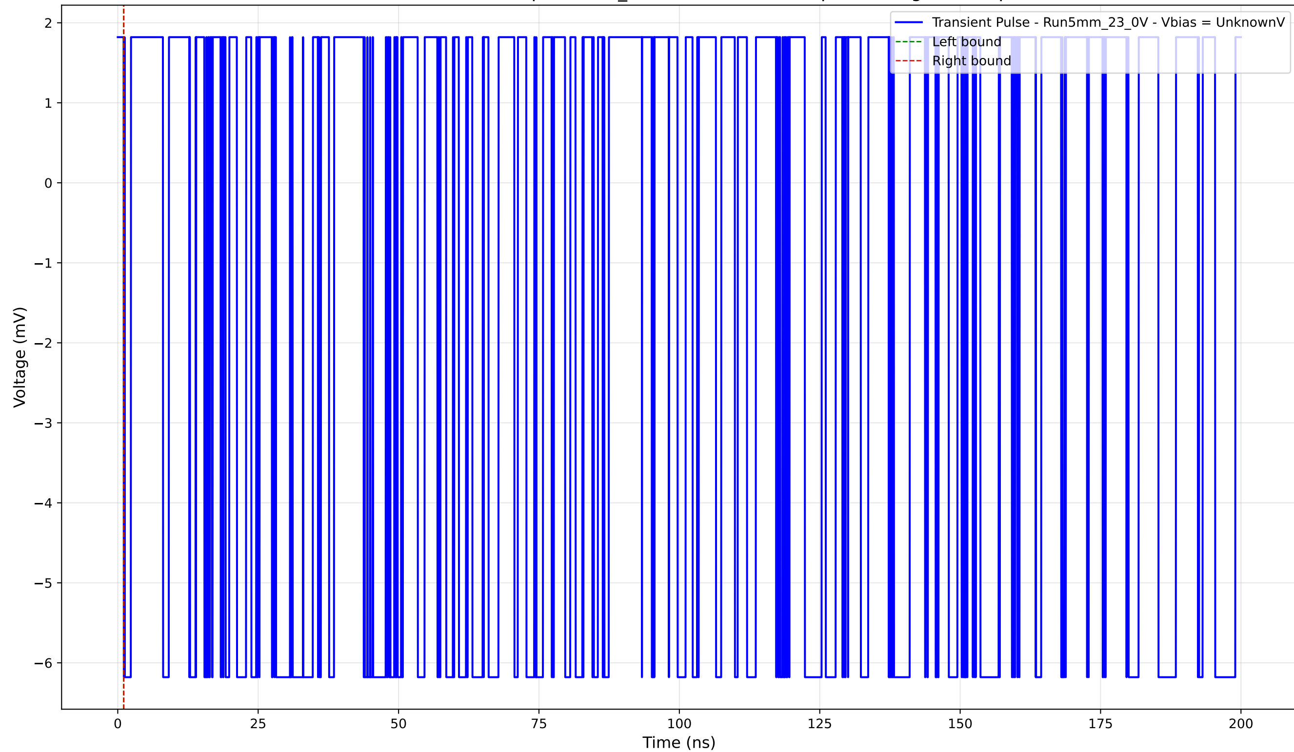
Transient Pulse - Sample: 5mm_23 - Position: 3775.0 \mu\text{m} - Charge: -0.00 pC
