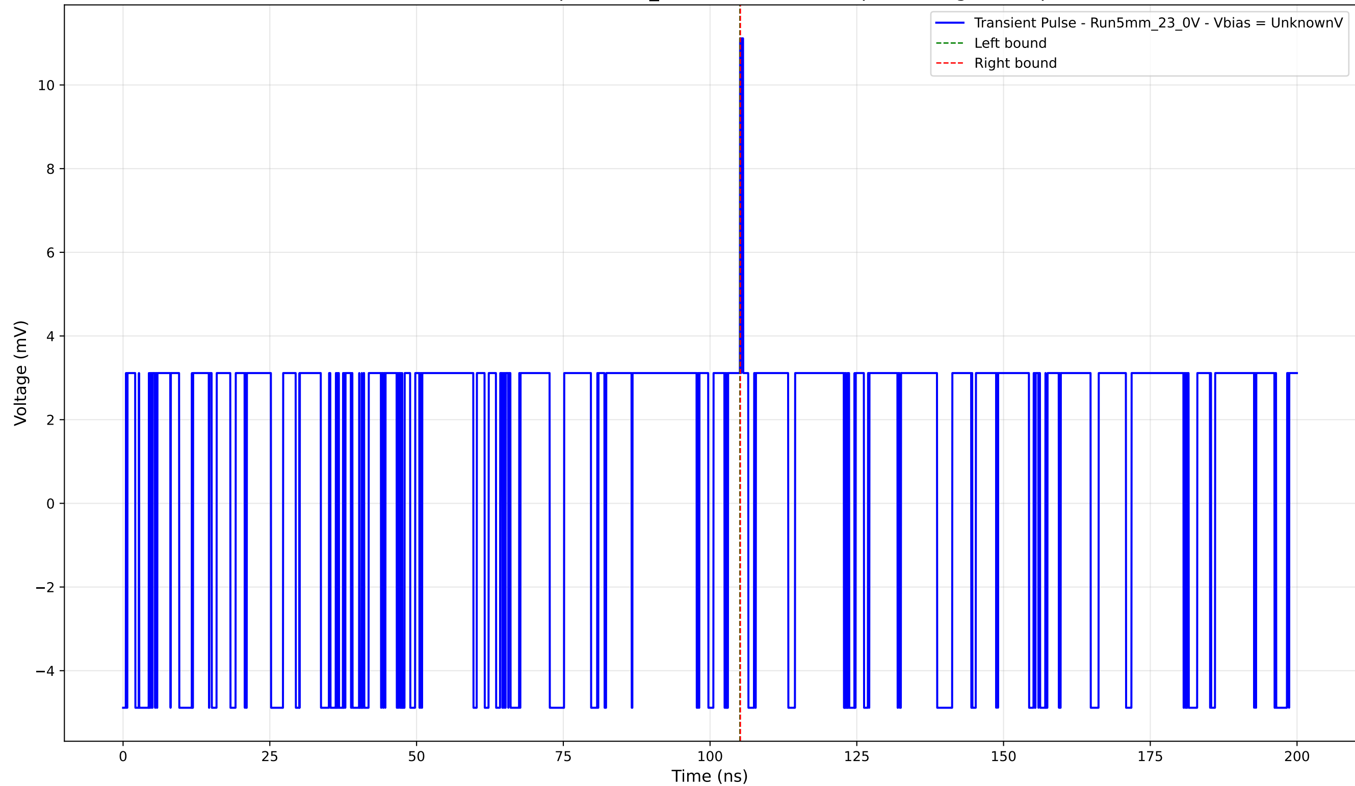
Transient Pulse - Sample: 5mm_23 - Position: 2600.0 \mu\text{m} - Charge: 0.01 pC
