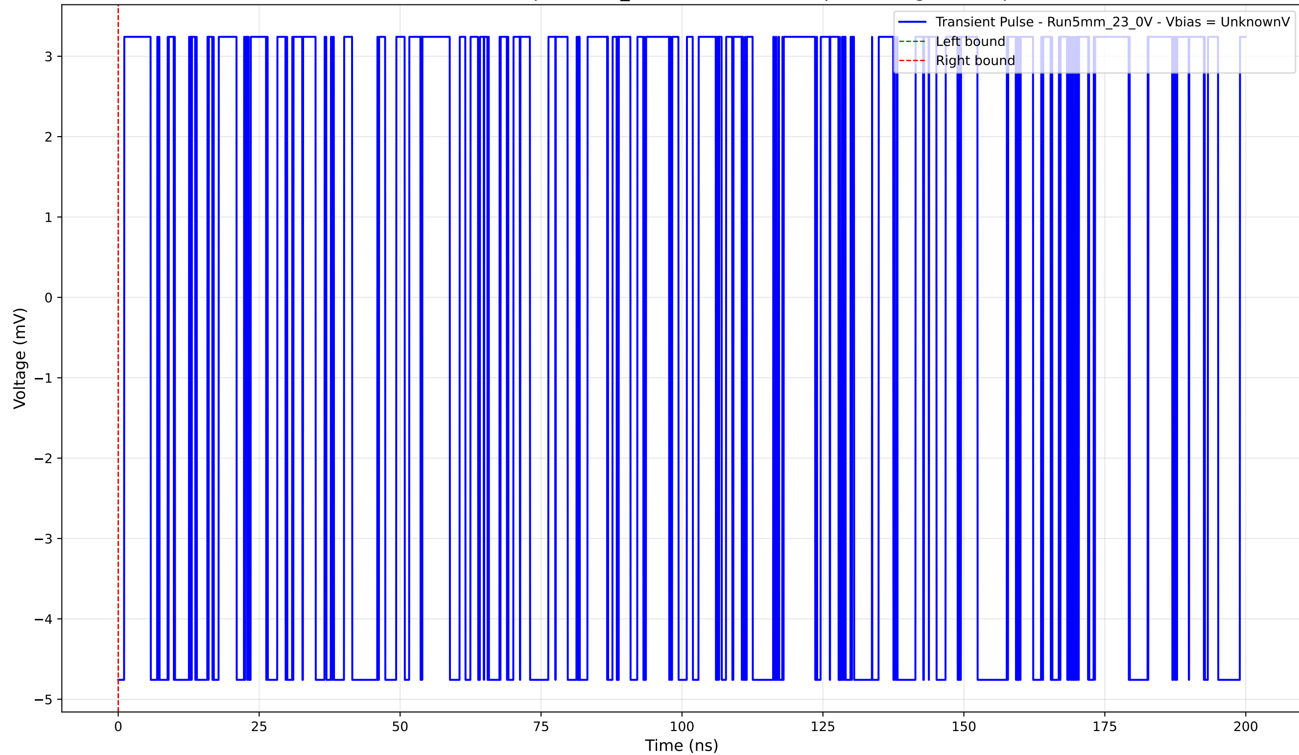
Transient Pulse - Sample: 5mm_23 - Position: 3300.0 \mu\text{m} - Charge: -0.00 pC
