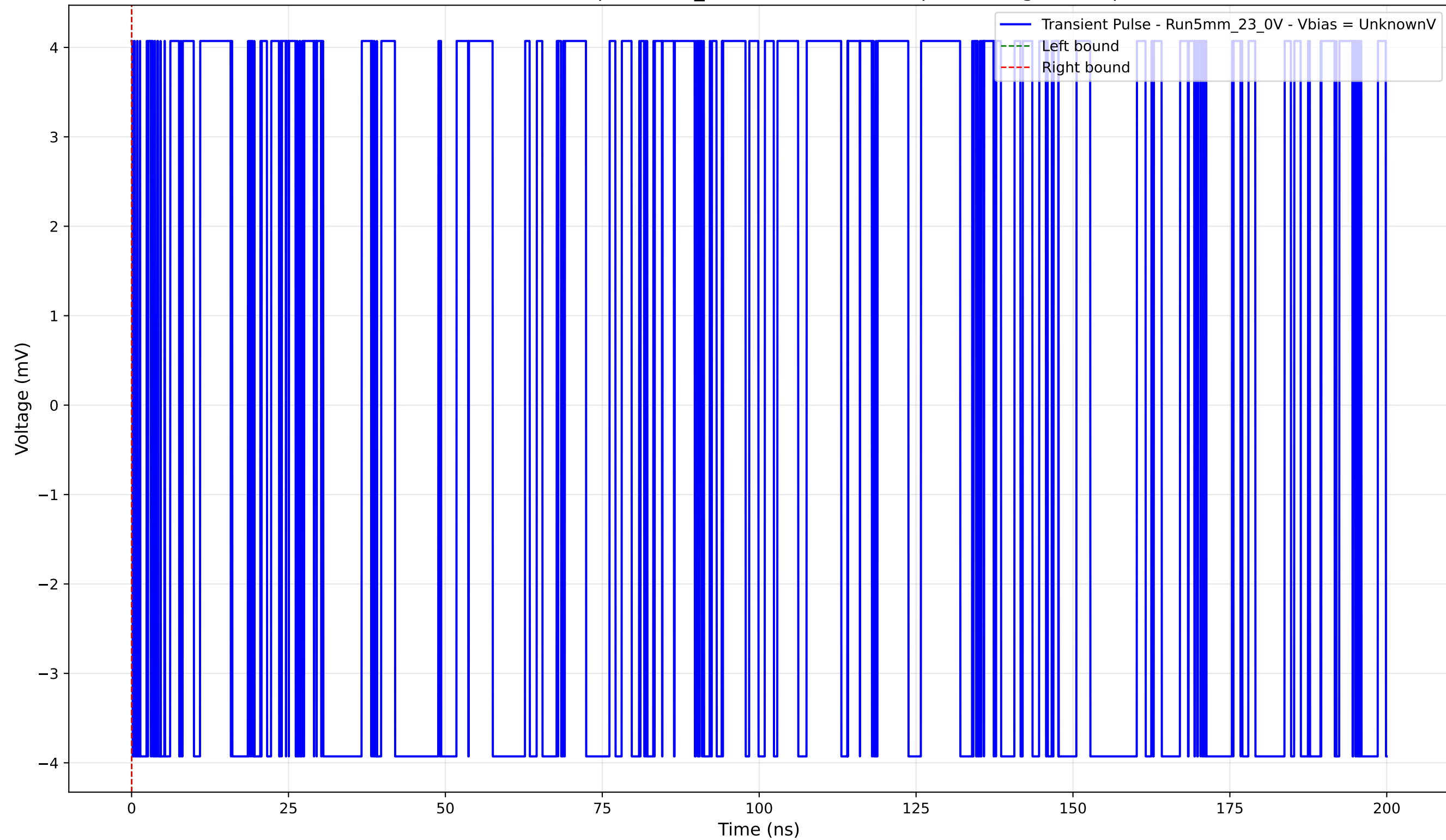
Transient Pulse - Sample: 5mm_23 - Position: 1620.0 \mu\text{m} - Charge: 0.00 pC
