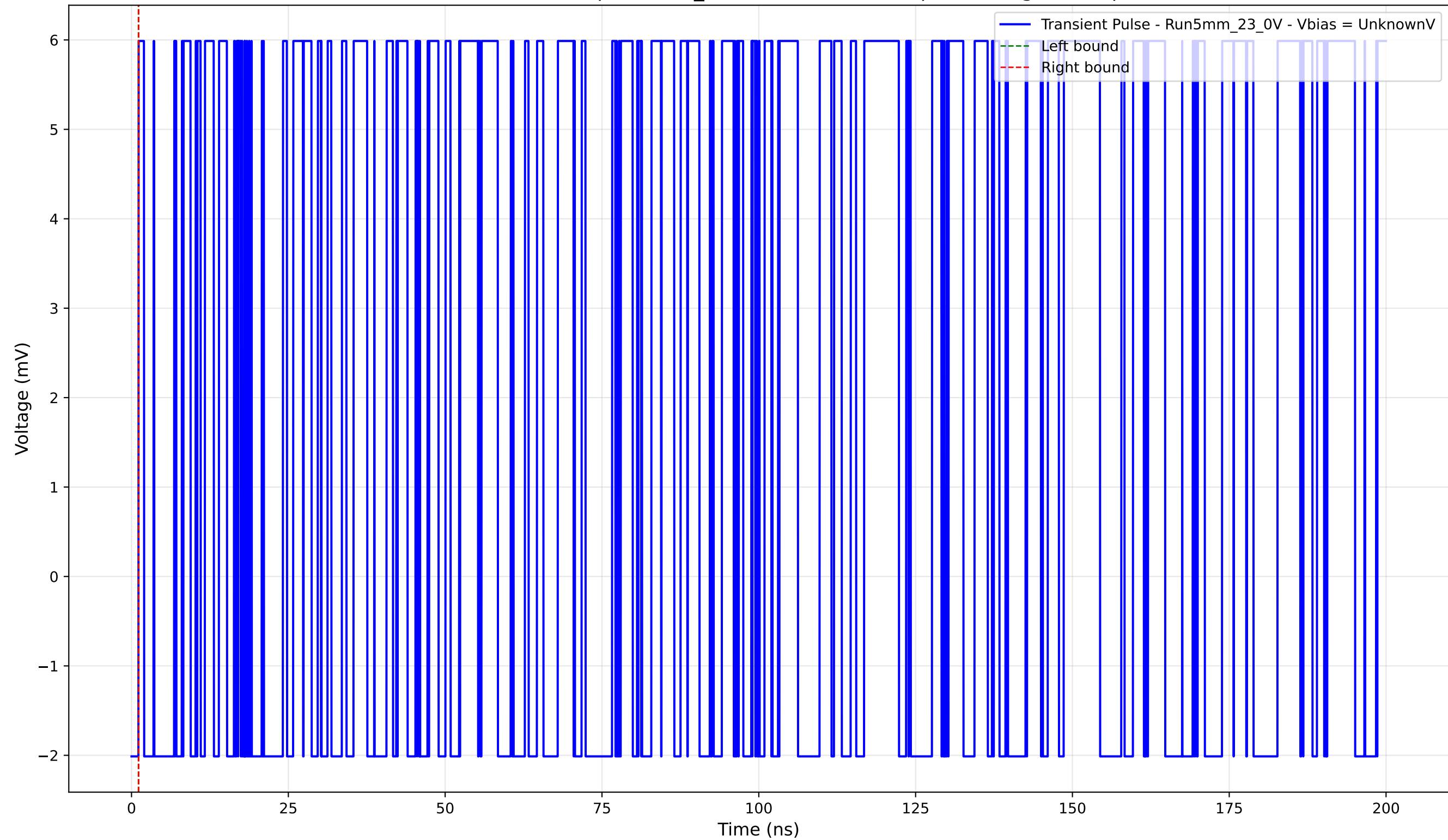
Transient Pulse - Sample: 5mm_23 - Position: 2185.0 \mu\text{m} - Charge: 0.00 pC
