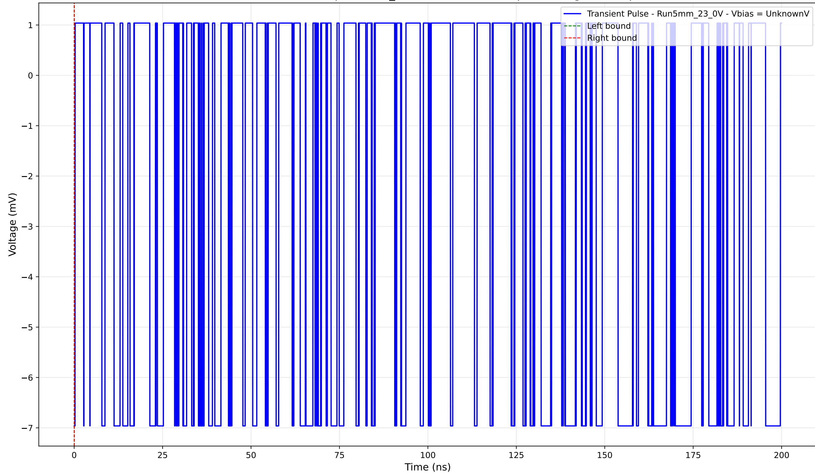
Transient Pulse - Sample: 5mm_23 - Position: 1800.0 \mu\text{m} - Charge: -0.00 pC
