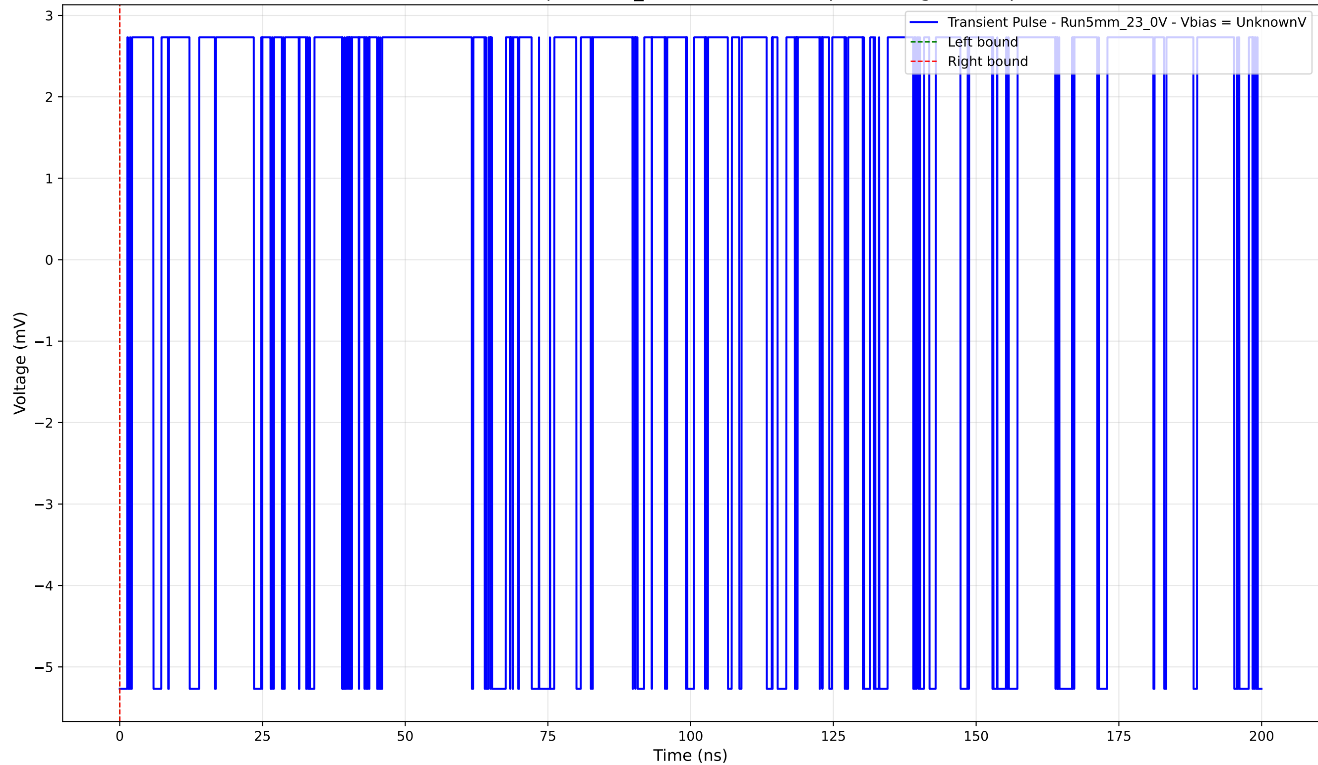
Transient Pulse - Sample: 5mm_23 - Position: 920.0 \mu\text{m} - Charge: -0.00 pC
