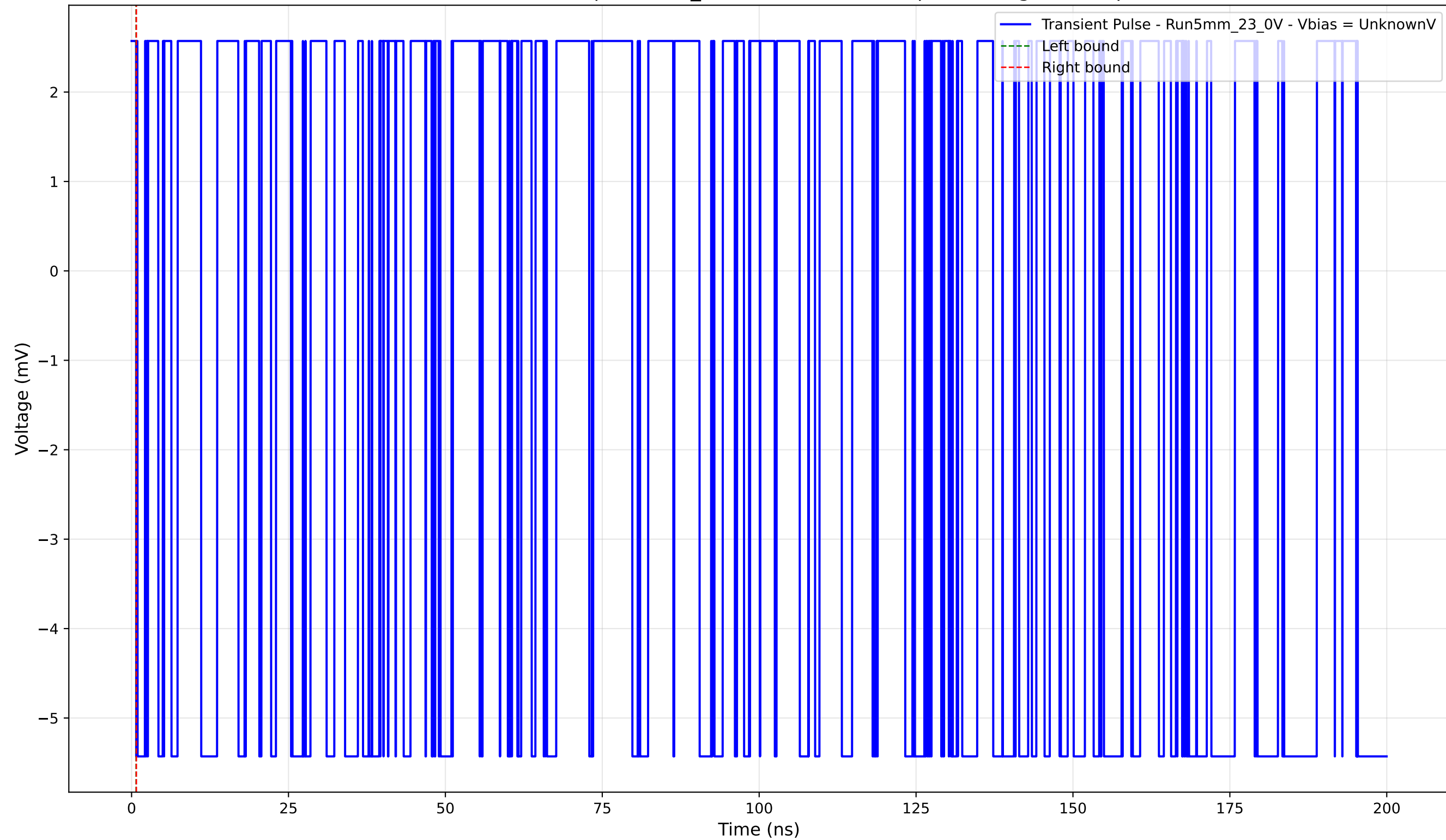
Transient Pulse - Sample: 5mm_23 - Position: 2685.0 \mu\text{m} - Charge: -0.00 pC
