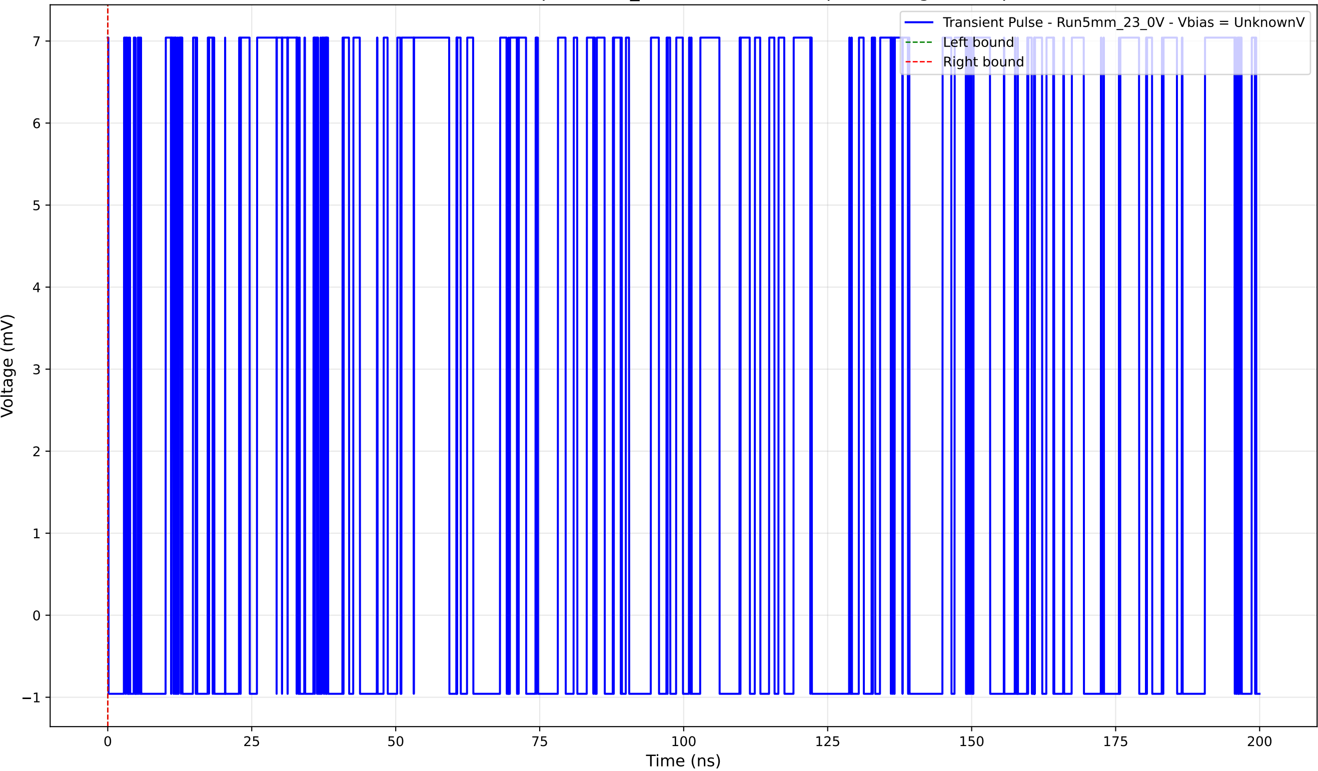
Transient Pulse - Sample: 5mm_23 - Position: 970.0 \mu\text{m} - Charge: 0.00 pC
