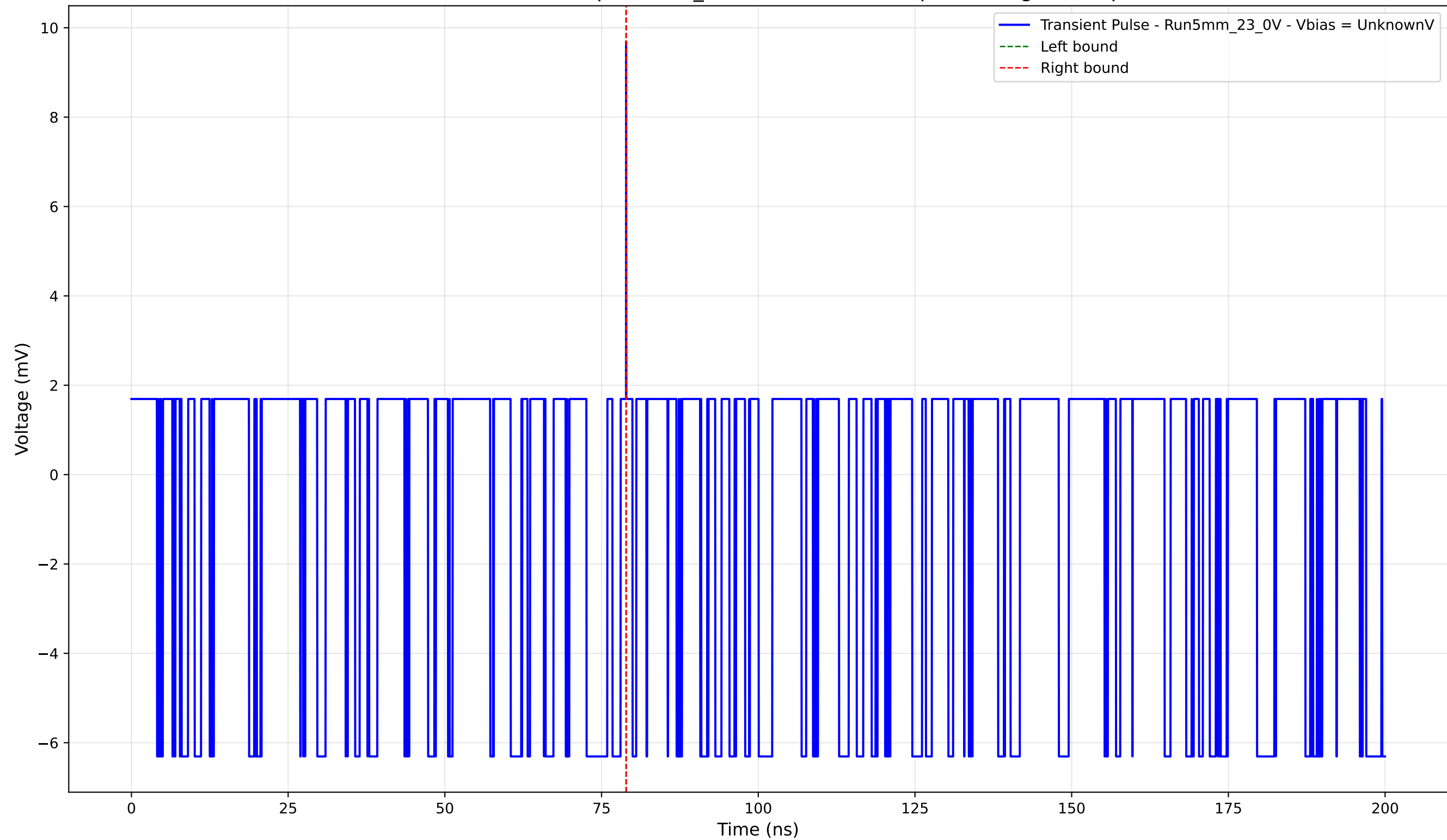
Transient Pulse - Sample: 5mm_23 - Position: 3550.0 \mu\text{m} - Charge: 0.00 pC
