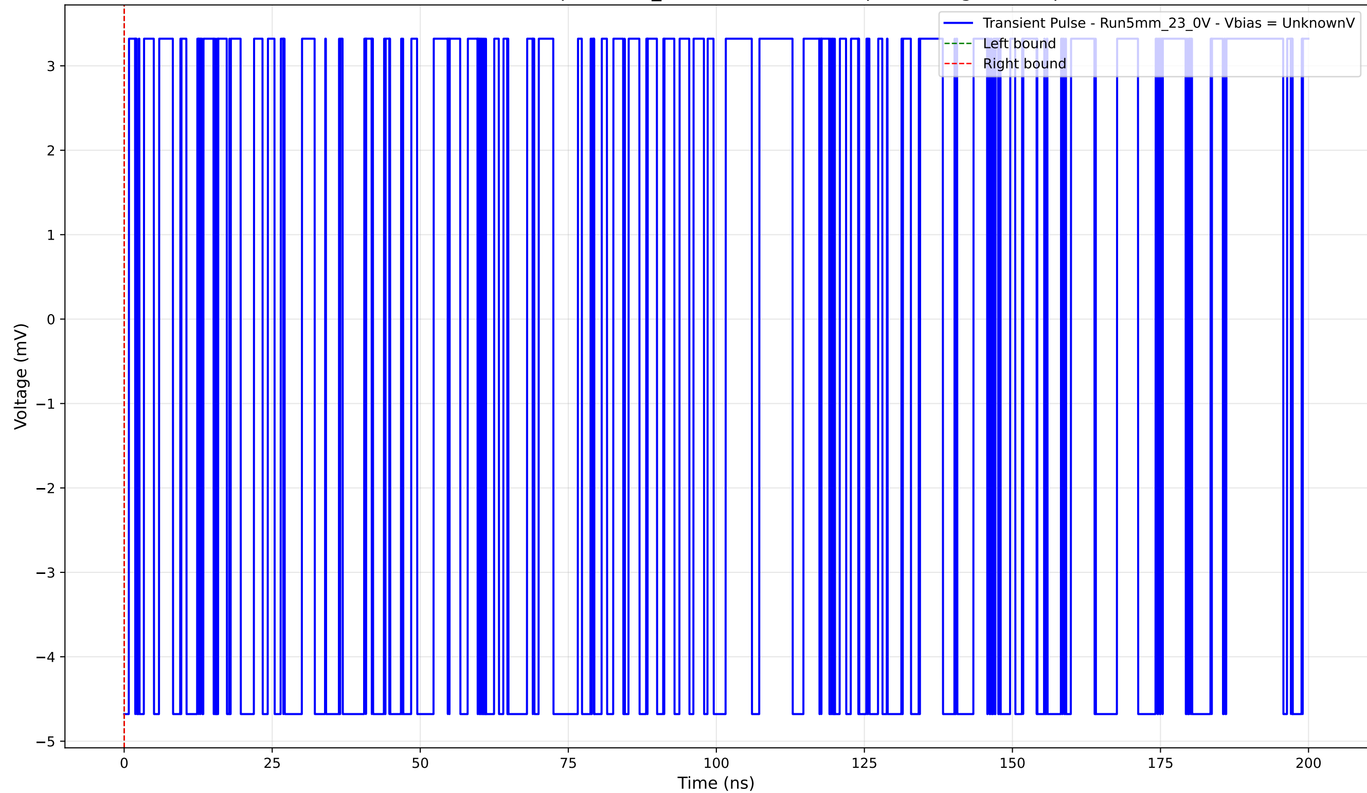
Transient Pulse - Sample: 5mm_23 - Position: 4015.0 \mu\text{m} - Charge: -0.00 pC
