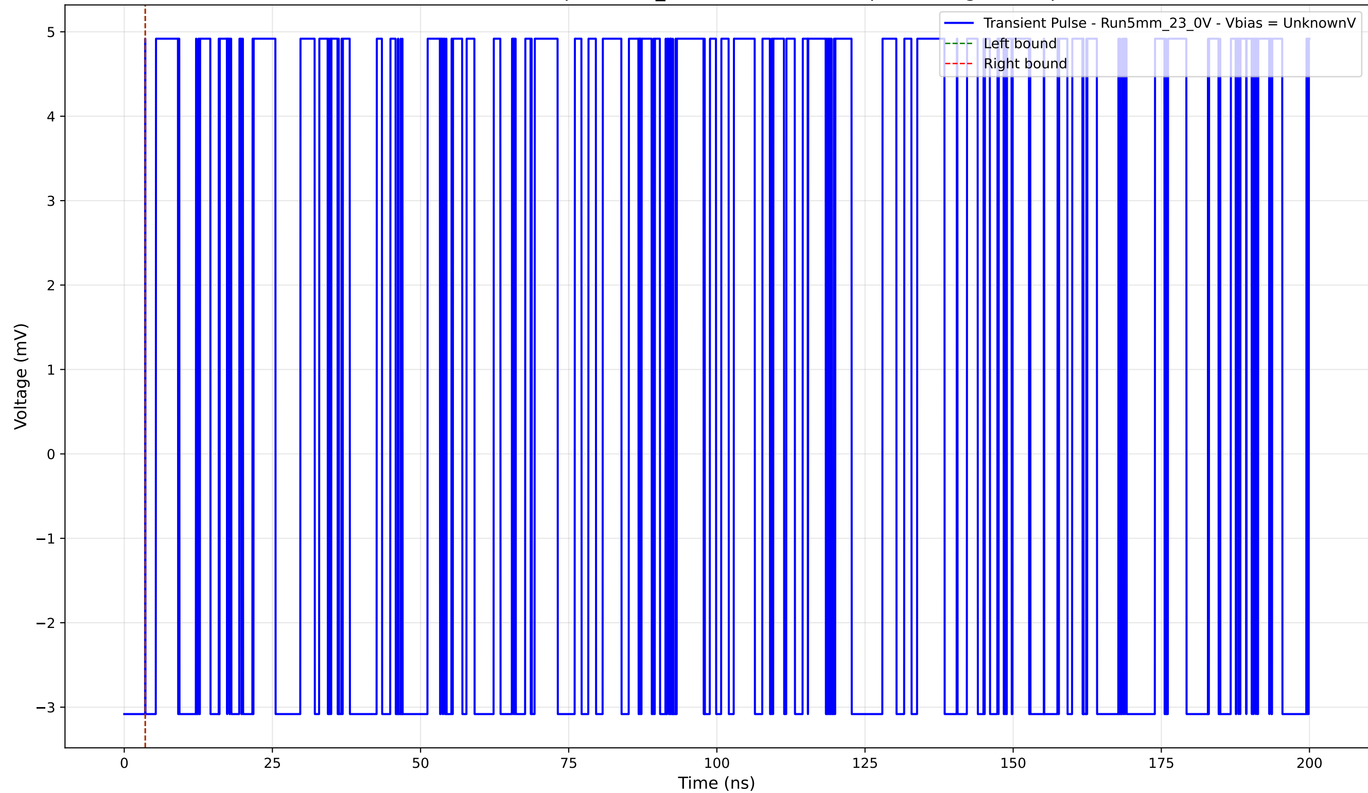
Transient Pulse - Sample: 5mm_23 - Position: 4905.0 \mu\text{m} - Charge: 0.00 pC
