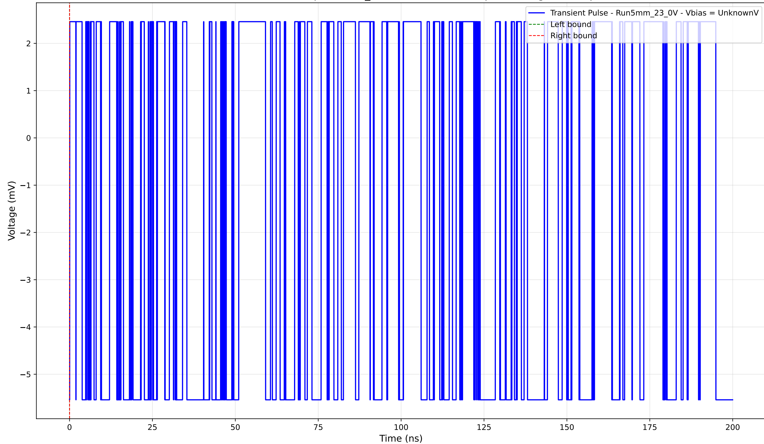
Transient Pulse - Sample: 5mm_23 - Position: 4740.0 \mu\text{m} - Charge: -0.00 pC
