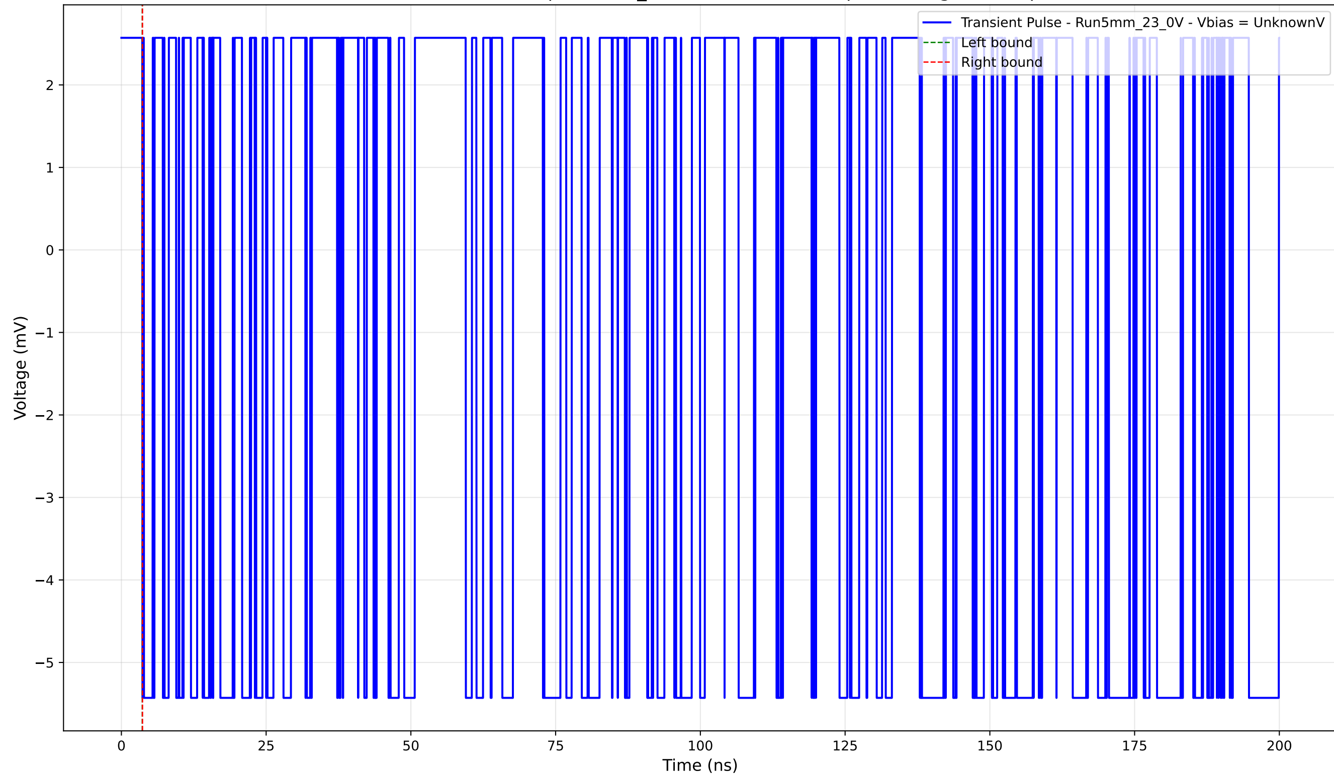
Transient Pulse - Sample: 5mm_23 - Position: 2430.0 \mu\text{m} - Charge: -0.00 pC
