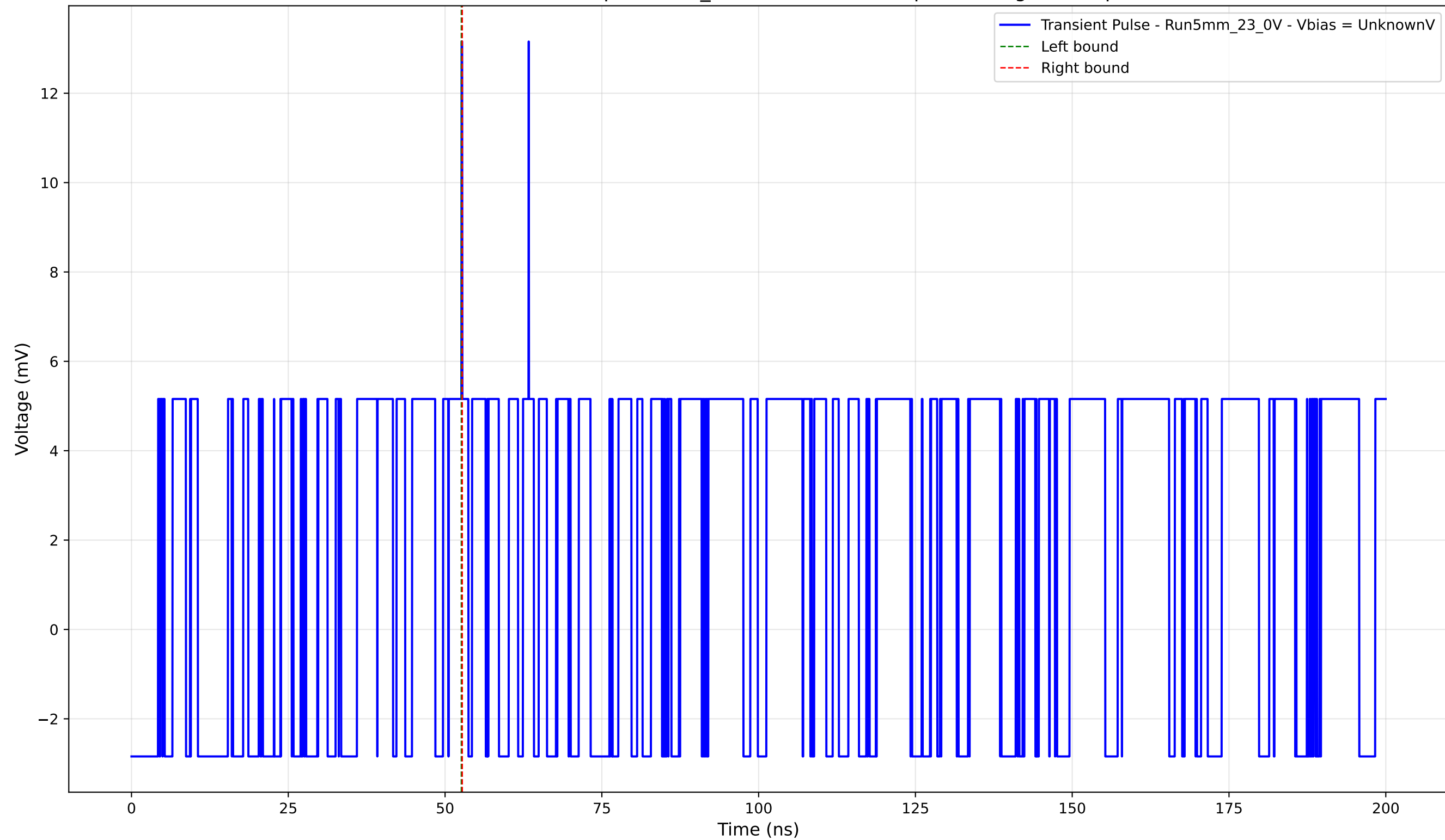
Transient Pulse - Sample: 5mm_23 - Position: 195.0 \mu\text{m} - Charge: 0.03 pC
