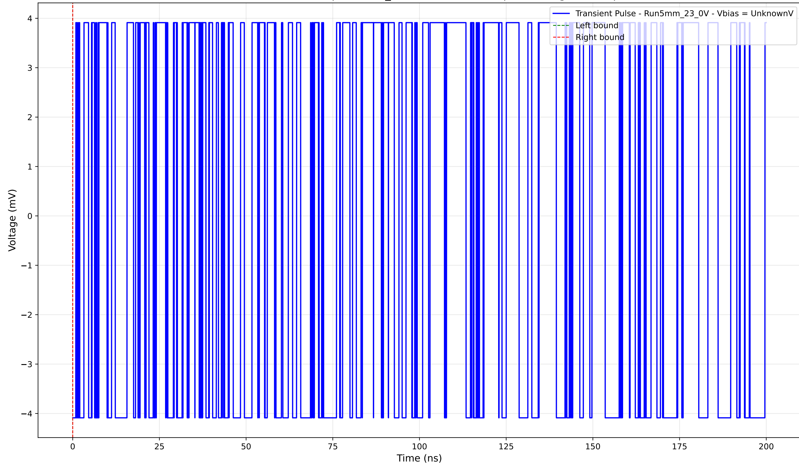
Transient Pulse - Sample: 5mm_23 - Position: 530.0 \mu\text{m} - Charge: -0.00 pC
