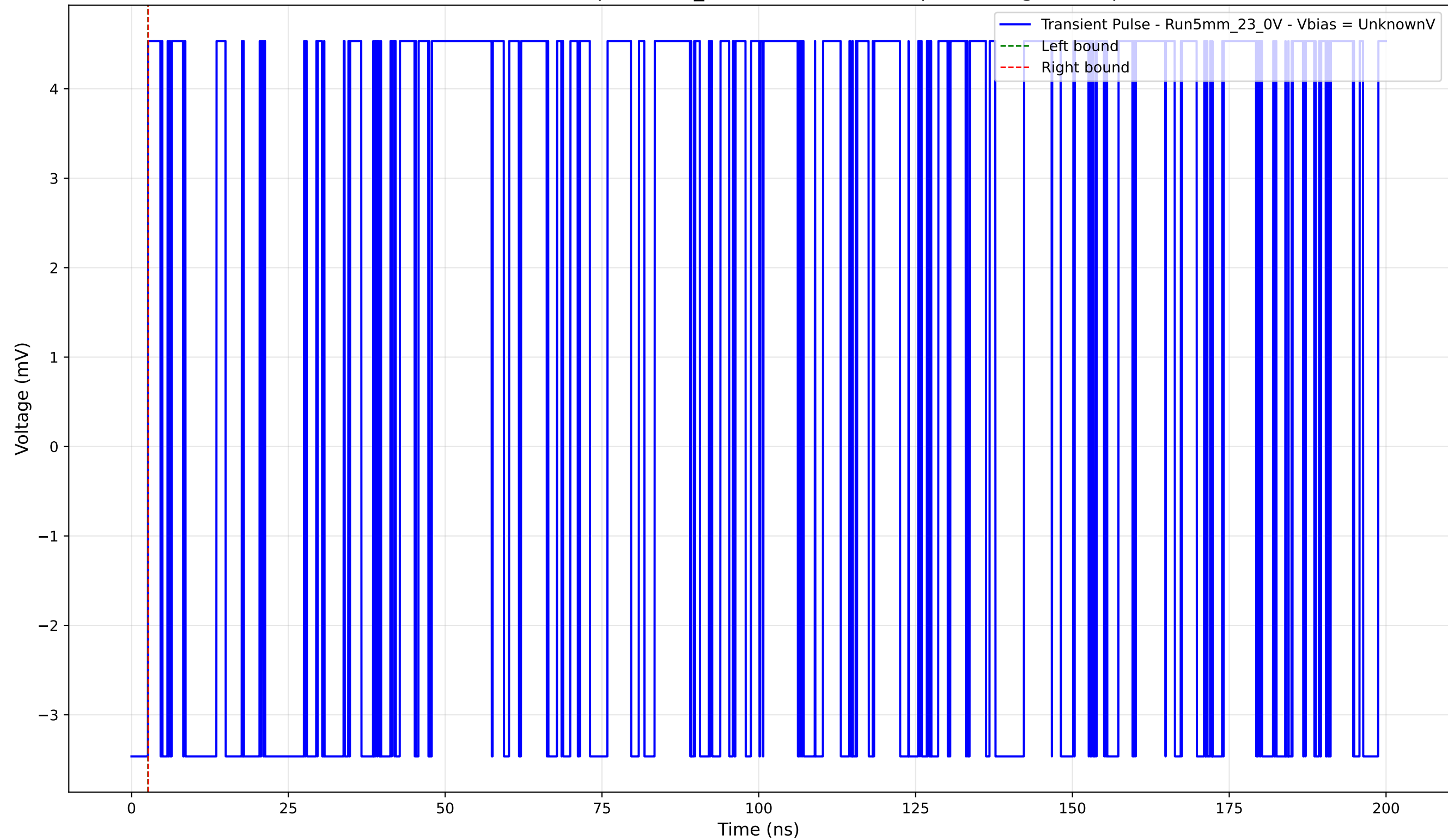
Transient Pulse - Sample: 5mm_23 - Position: 1750.0 \mu\text{m} - Charge: 0.00 pC
