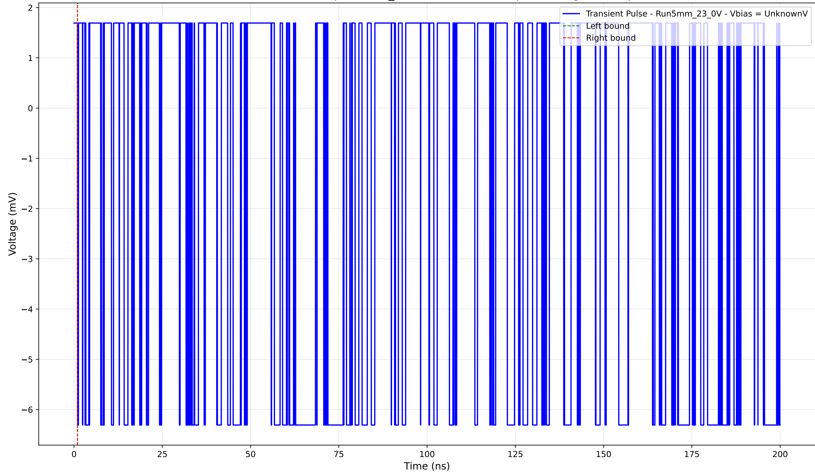
Transient Pulse - Sample: 5mm_23 - Position: 4480.0 \mu\text{m} - Charge: -0.00 pC
