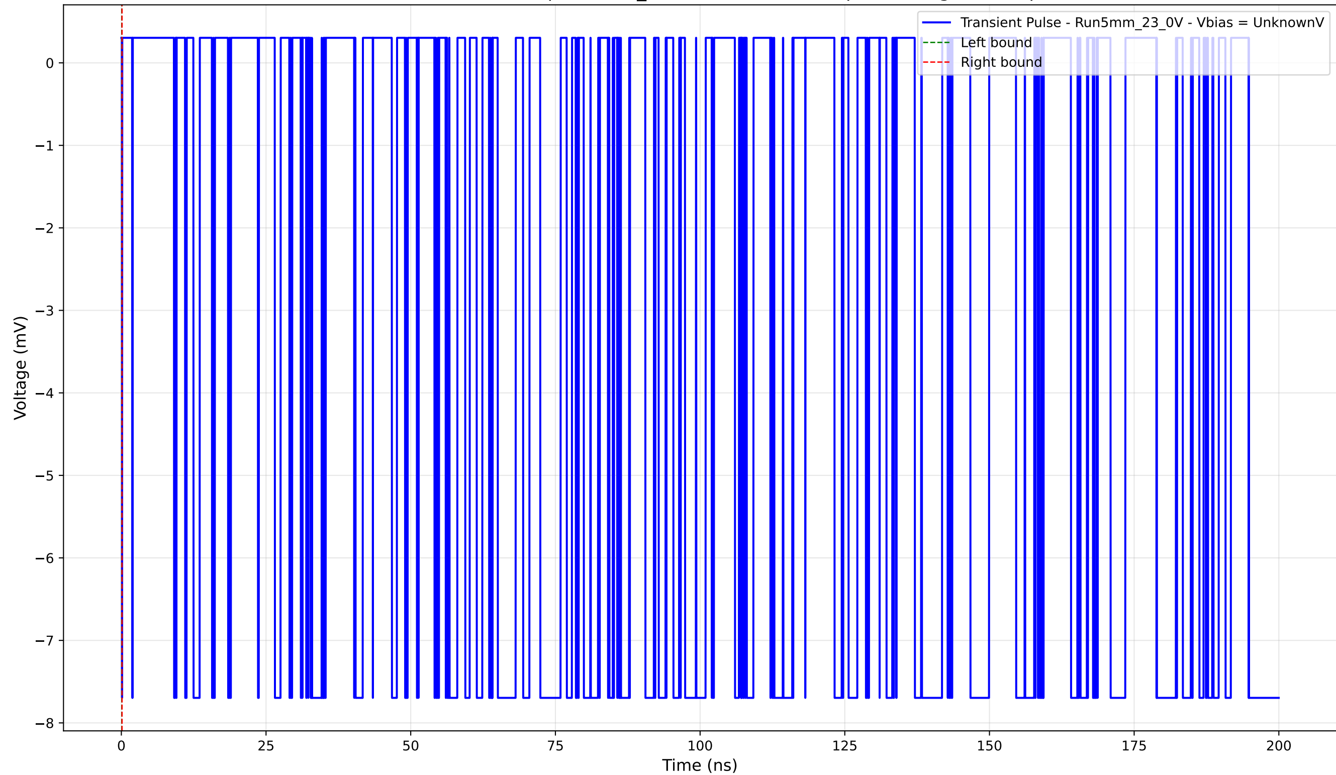
Transient Pulse - Sample: 5mm_23 - Position: 3745.0 \mu\text{m} - Charge: -0.00 pC
