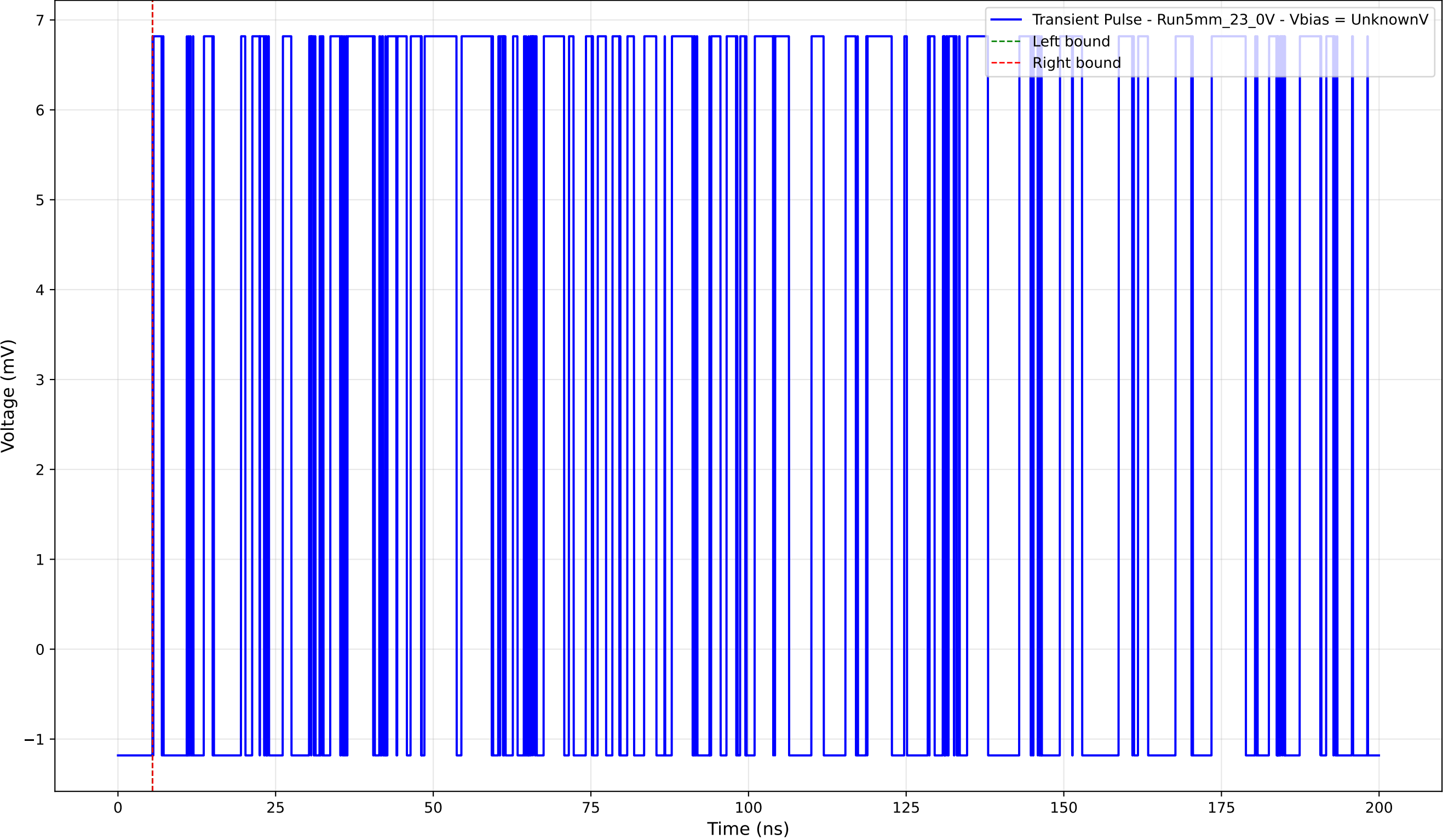
Transient Pulse - Sample: 5mm_23 - Position: 790.0 \mu\text{m} - Charge: 0.00 pC
