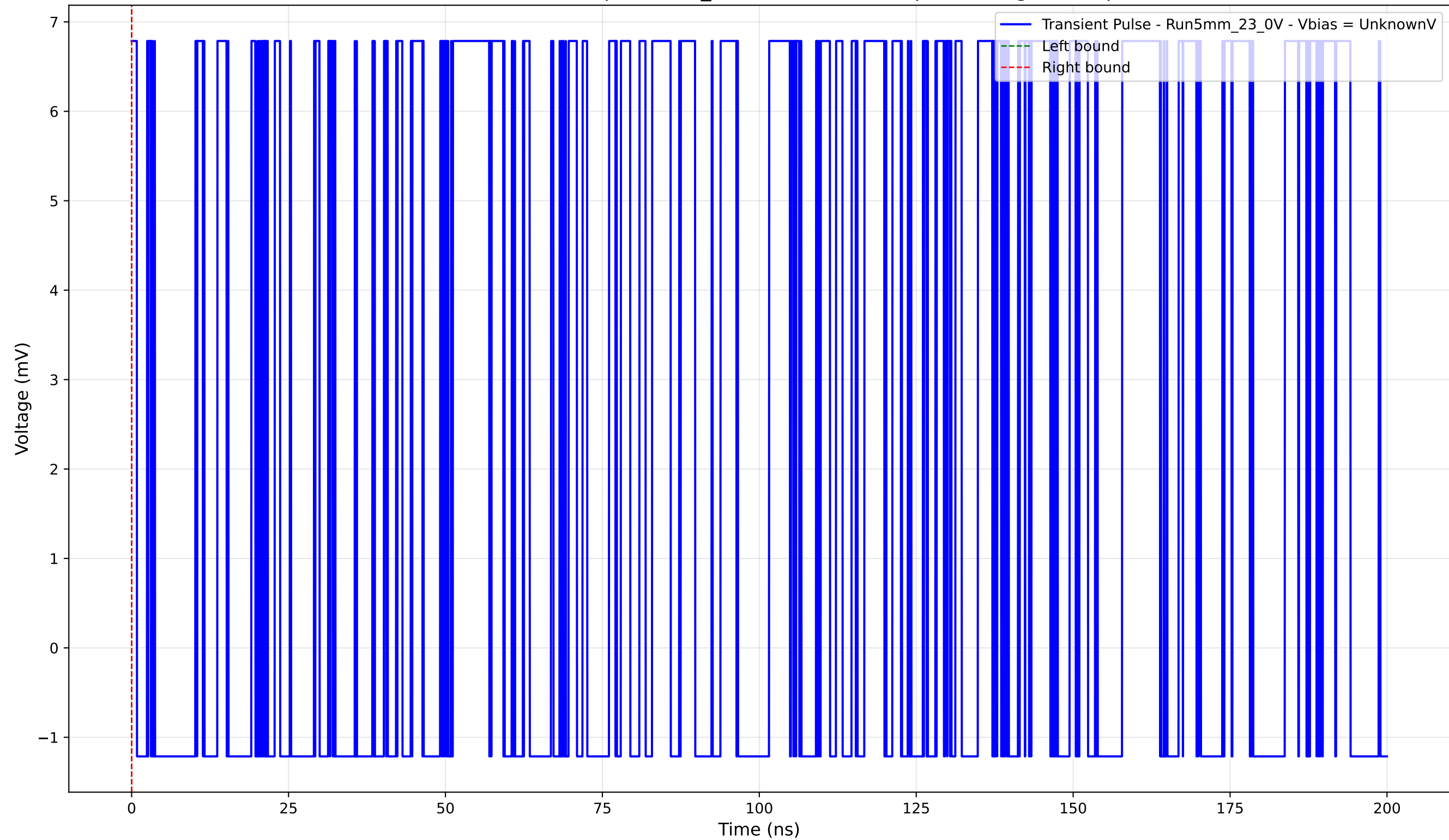
Transient Pulse - Sample: 5mm_23 - Position: 915.0 \mu\text{m} - Charge: 0.00 pC
