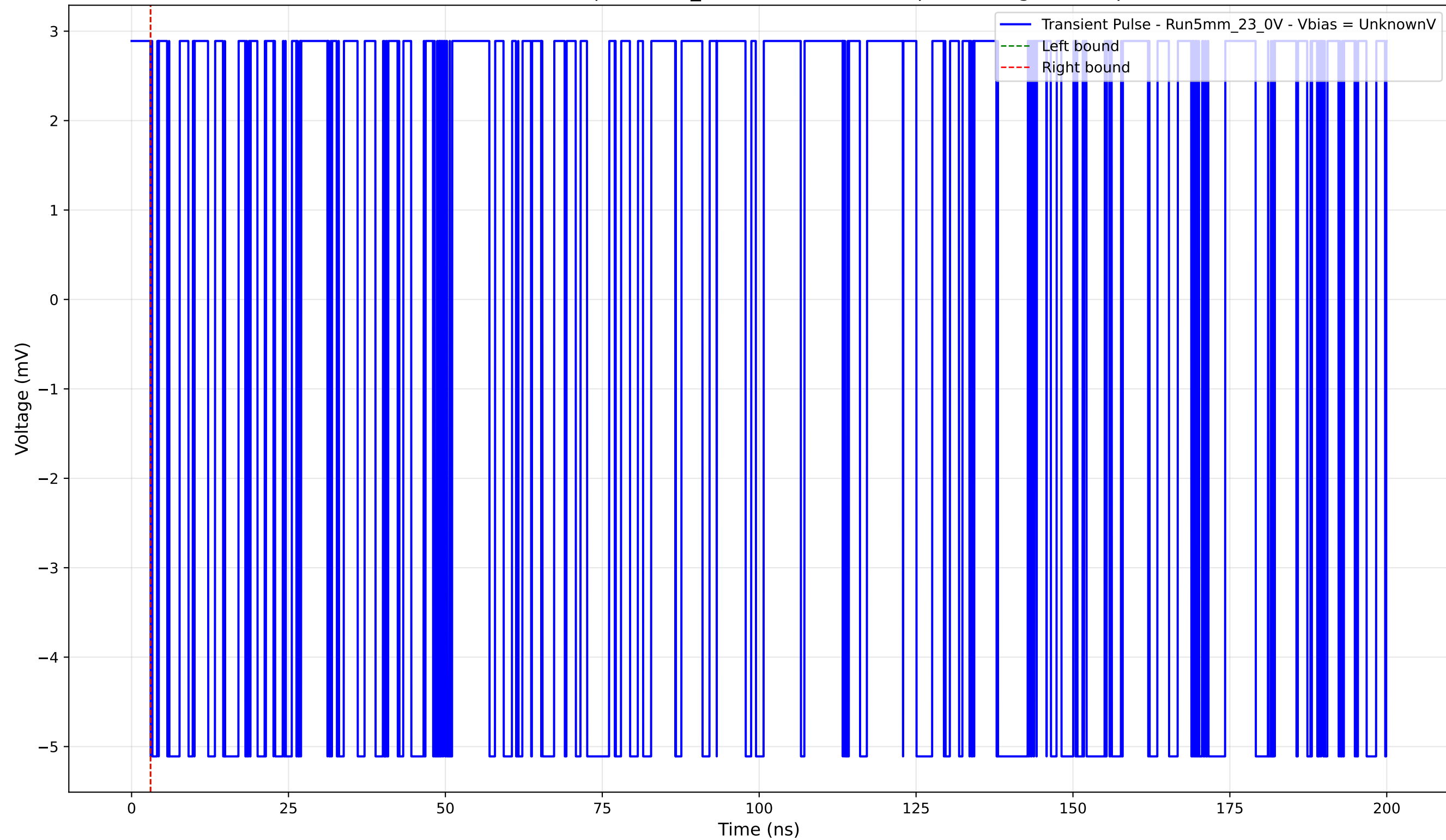
Transient Pulse - Sample: 5mm_23 - Position: 4365.0 \mu\text{m} - Charge: -0.00 pC
