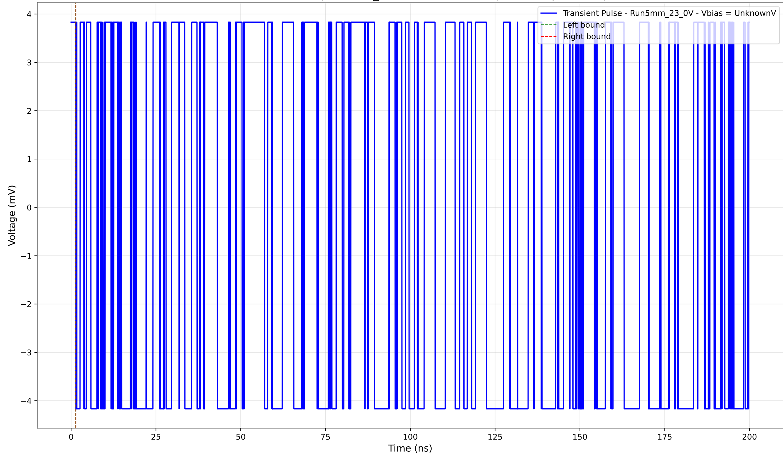
Transient Pulse - Sample: 5mm_23 - Position: 1335.0 \mu\text{m} - Charge: -0.00 pC
