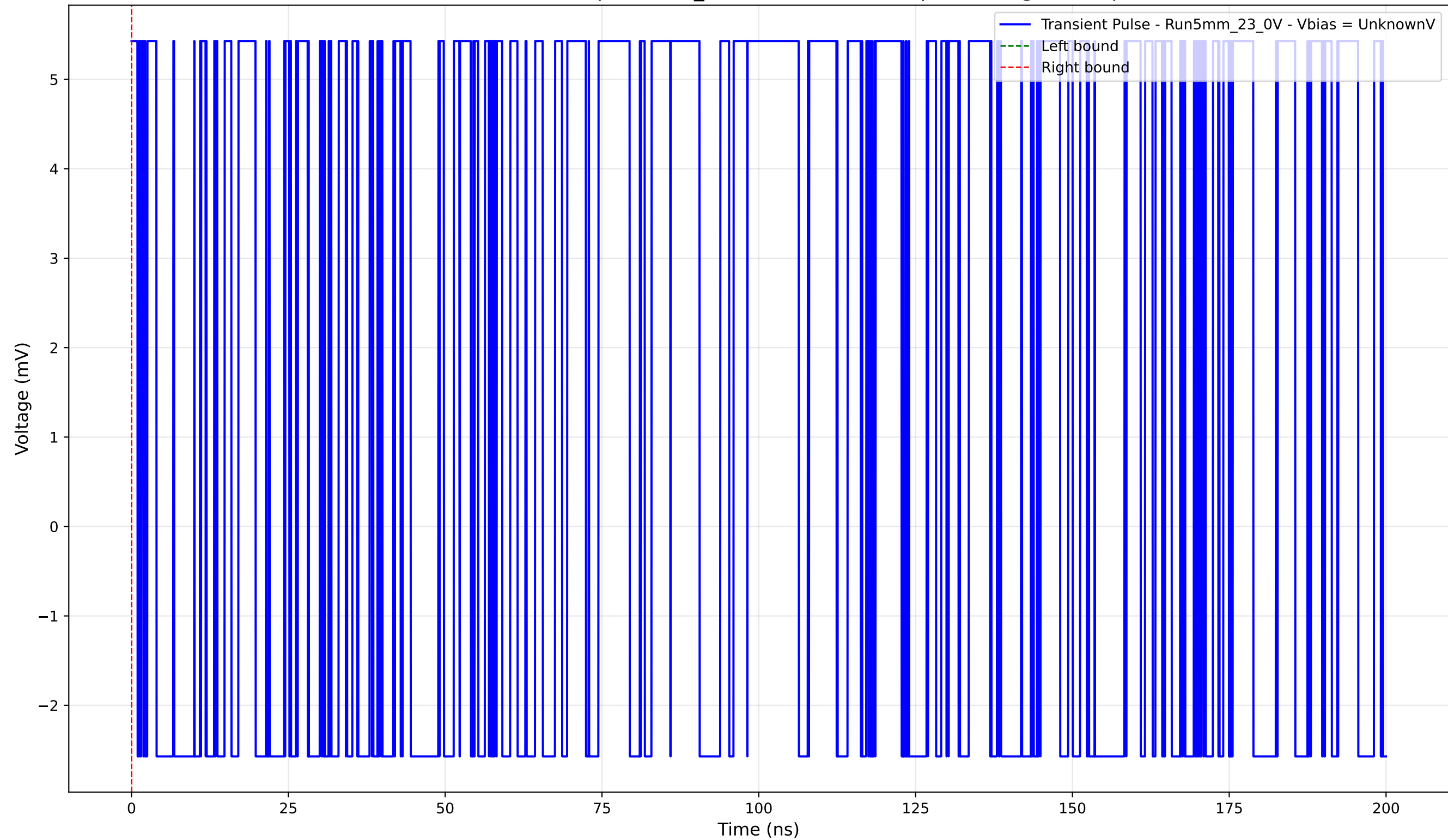
Transient Pulse - Sample: 5mm_23 - Position: 4325.0 \mu\text{m} - Charge: 0.00 pC
