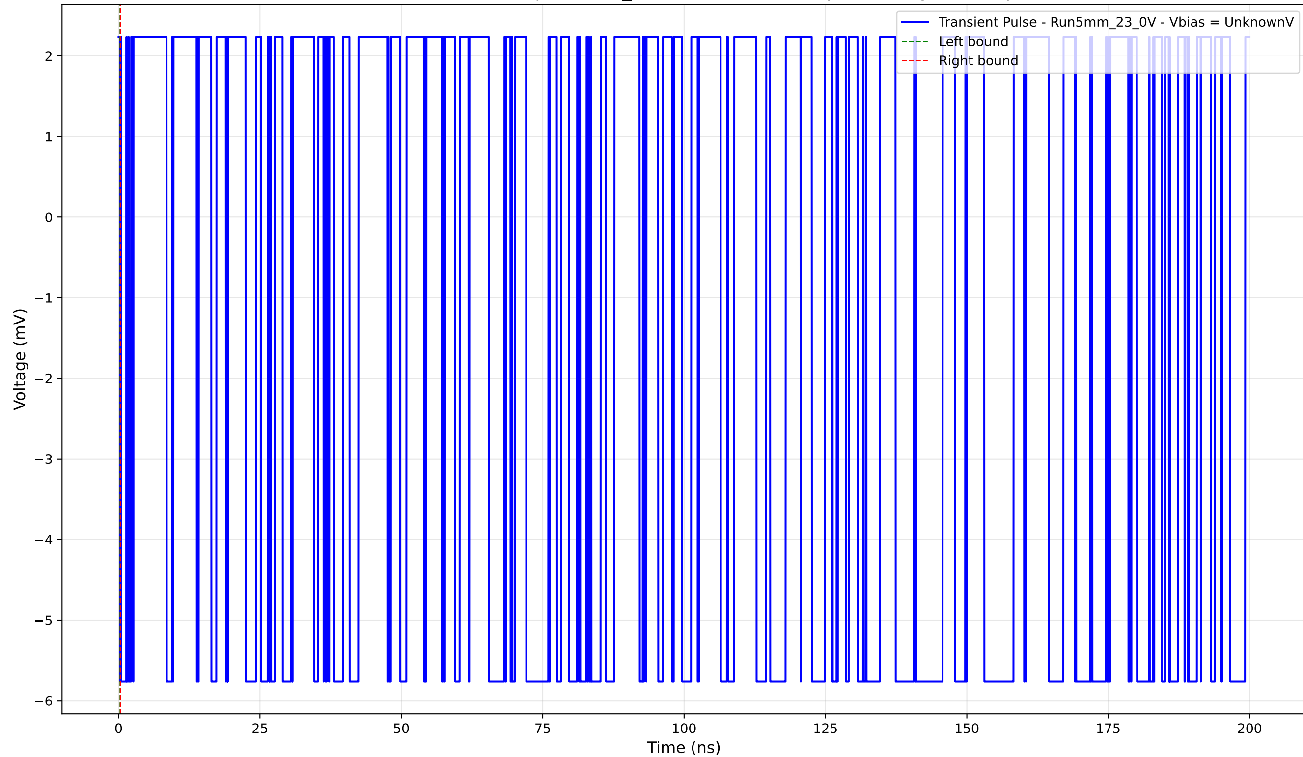
Transient Pulse - Sample: 5mm_23 - Position: 2860.0 \mu\text{m} - Charge: -0.00 pC
