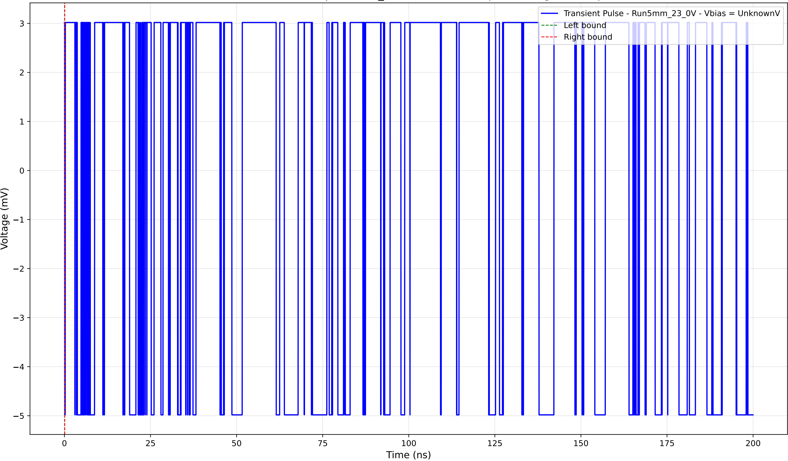
Transient Pulse - Sample: 5mm_23 - Position: 50.0 \mu\text{m} - Charge: -0.00 pC
