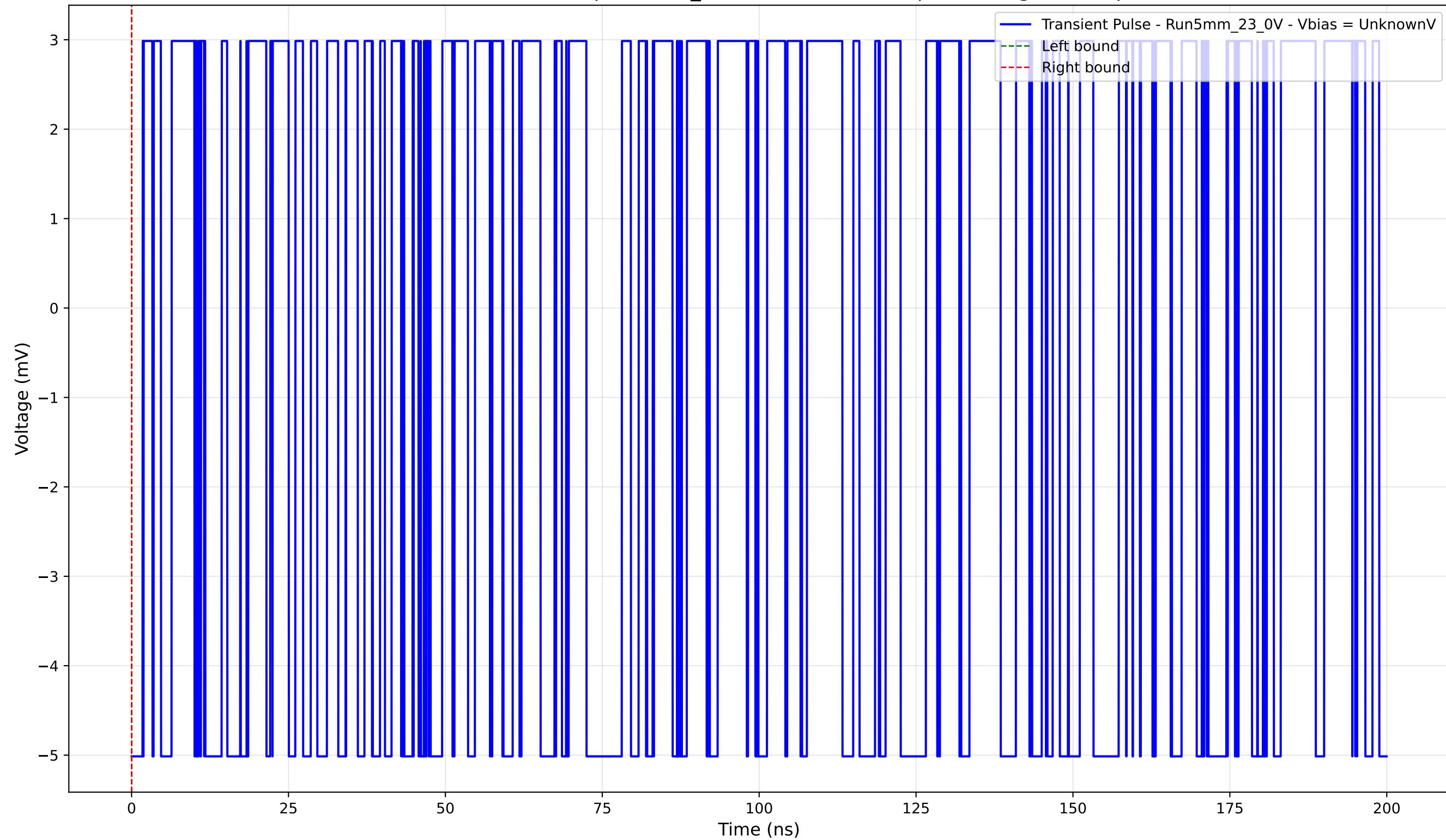
Transient Pulse - Sample: 5mm_23 - Position: 3140.0 \mu\text{m} - Charge: -0.00 pC
