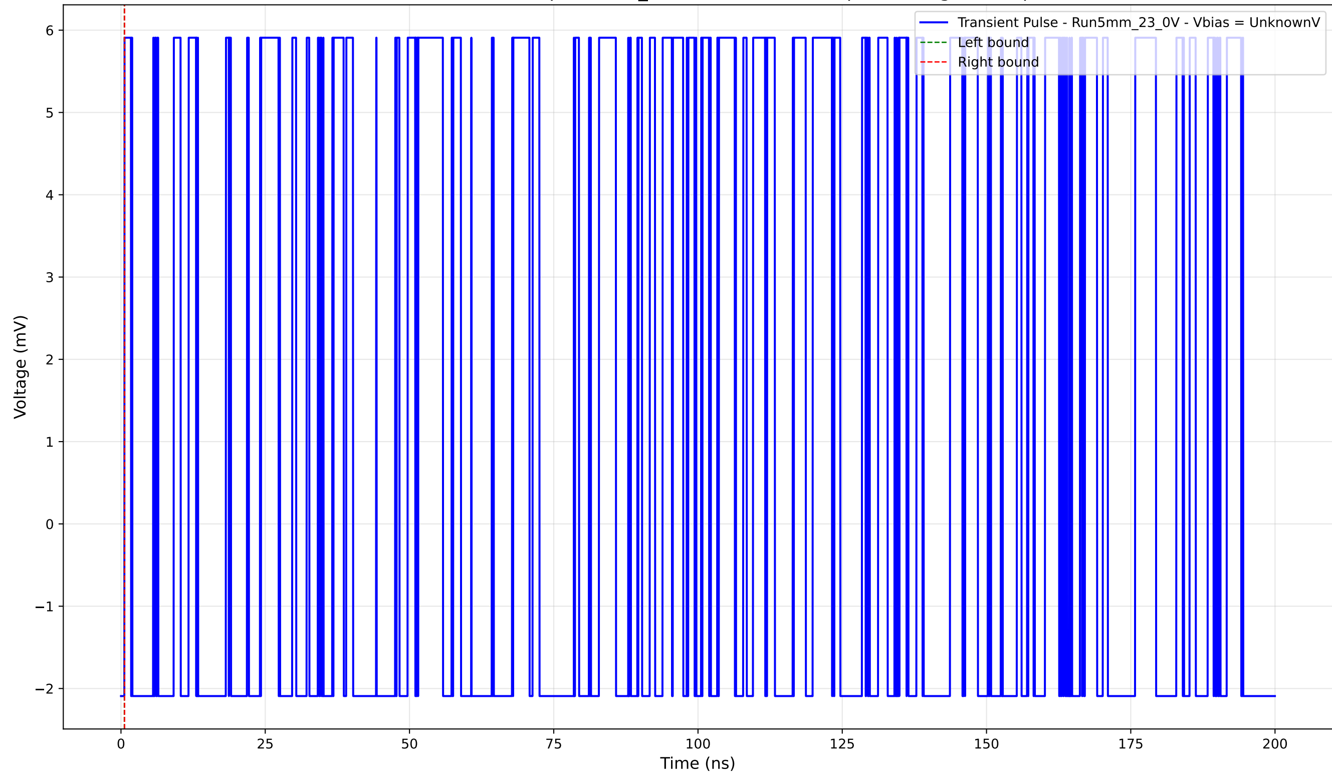
Transient Pulse - Sample: 5mm_23 - Position: 5075.0 \mu\text{m} - Charge: 0.00 pC
