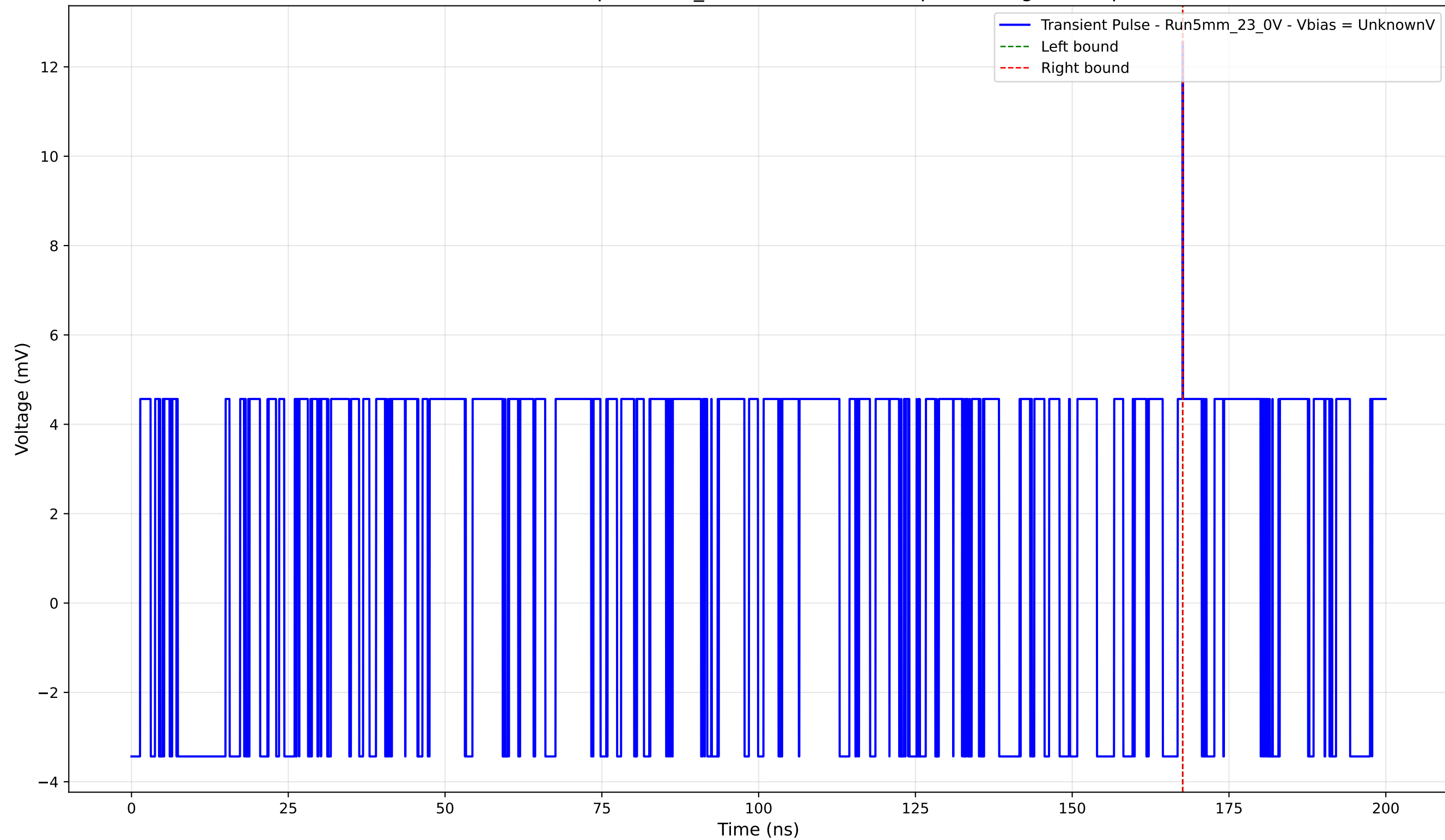
Transient Pulse - Sample: 5mm_23 - Position: 2390.0 \mu\text{m} - Charge: 0.01 pC
