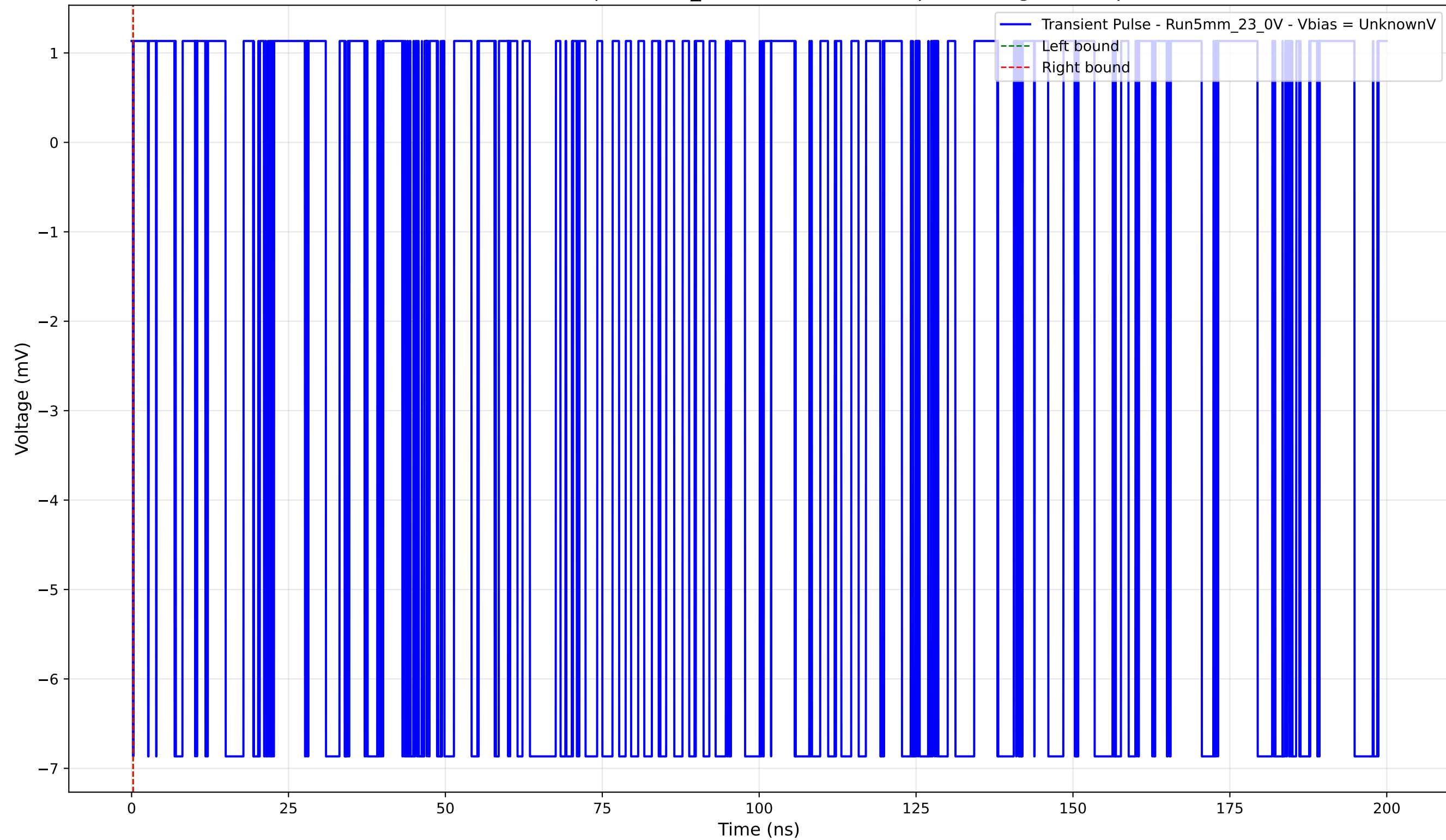
Transient Pulse - Sample: 5mm_23 - Position: 1085.0 \mu\text{m} - Charge: -0.00 pC
