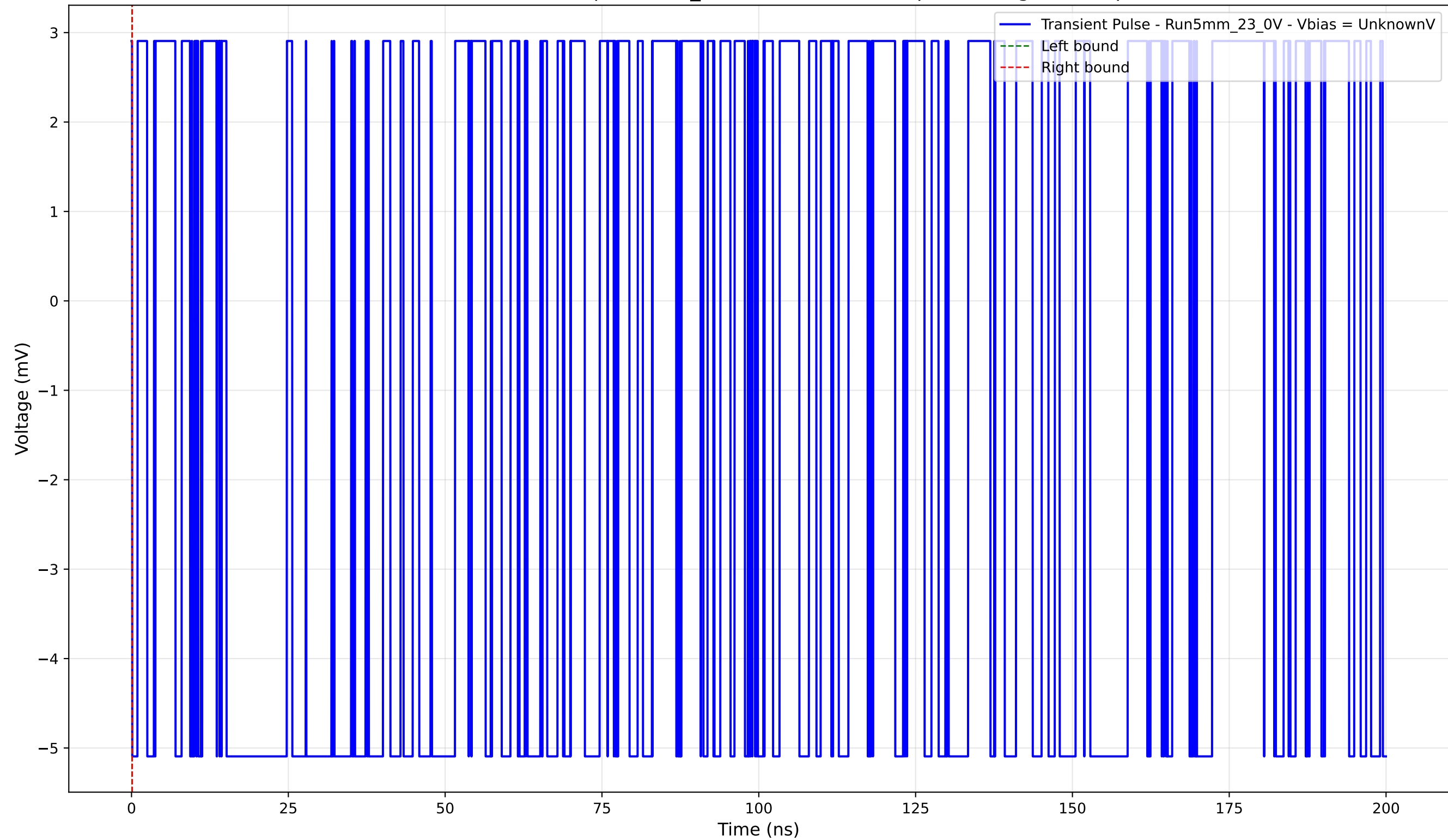
Transient Pulse - Sample: 5mm_23 - Position: 4855.0 \mu\text{m} - Charge: -0.00 pC
