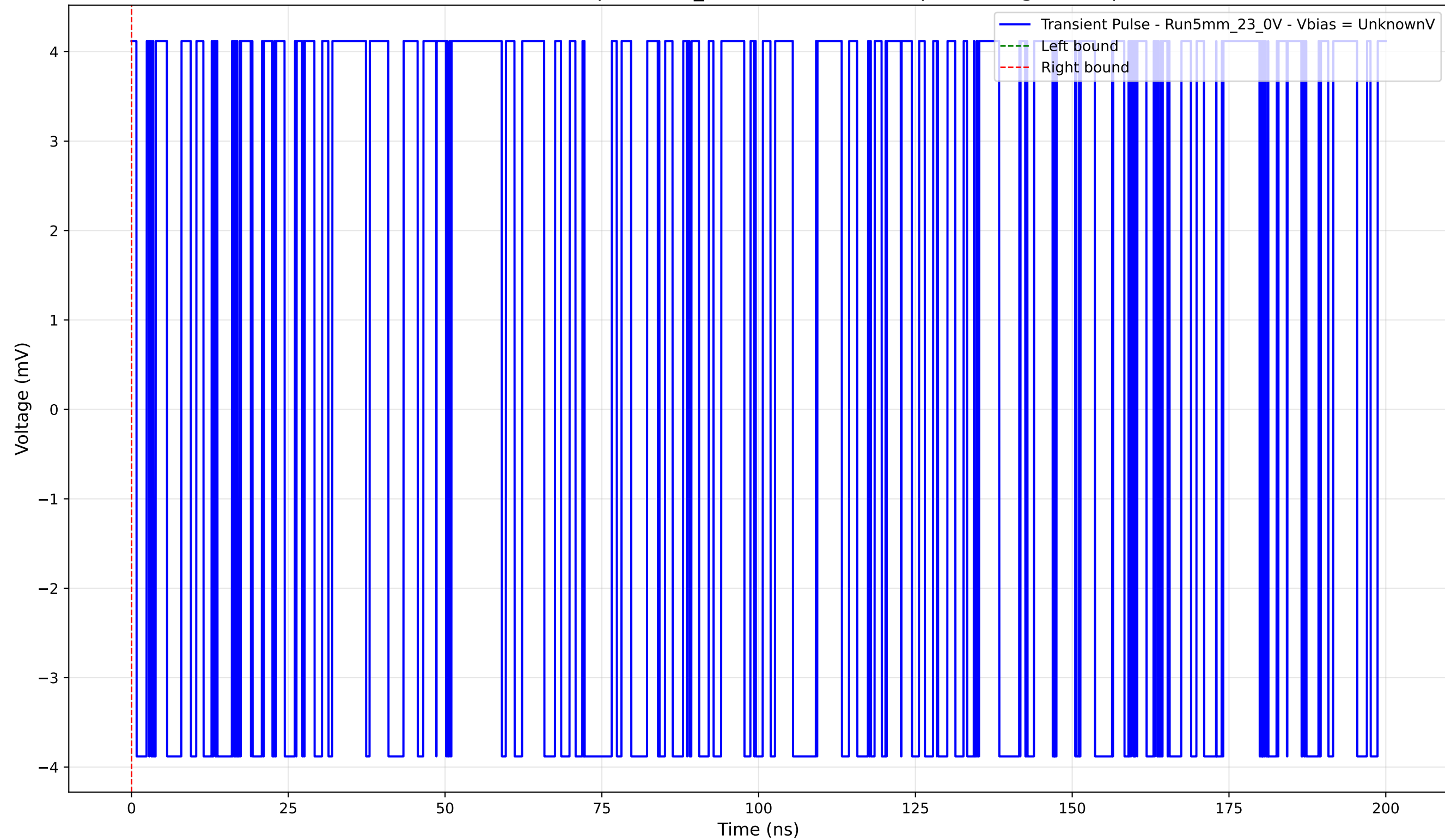
Transient Pulse - Sample: 5mm_23 - Position: 2555.0 \mu\text{m} - Charge: 0.00 pC
