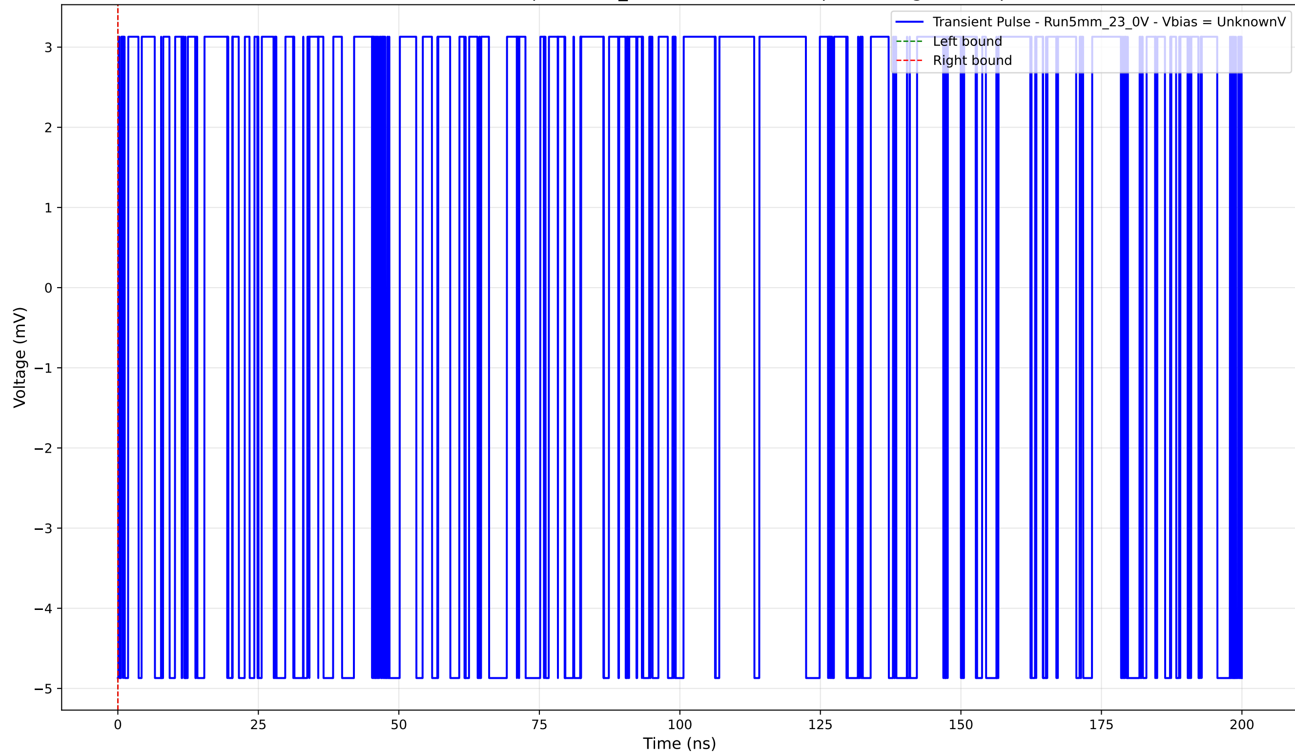
Transient Pulse - Sample: 5mm_23 - Position: 4605.0 \mu\text{m} - Charge: -0.00 pC
