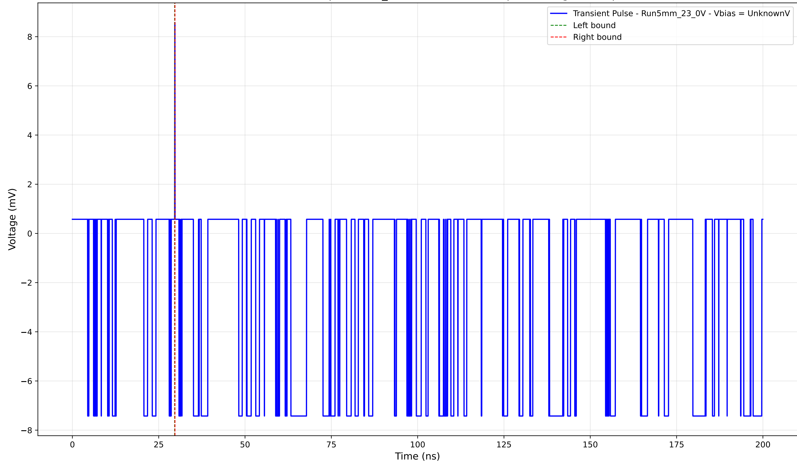
Transient Pulse - Sample: 5mm_23 - Position: 2960.0 \mu\text{m} - Charge: 0.01 pC
