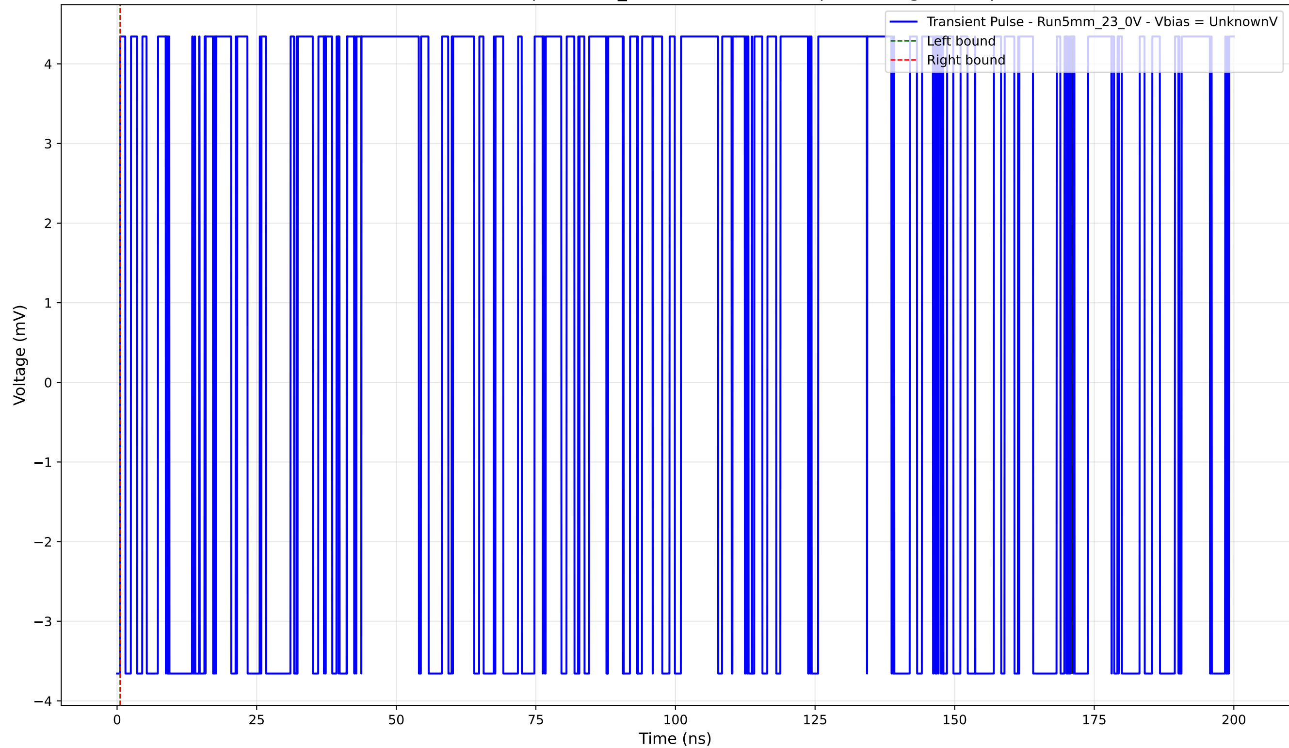
Transient Pulse - Sample: 5mm_23 - Position: 3360.0 \mu\text{m} - Charge: 0.00 pC
