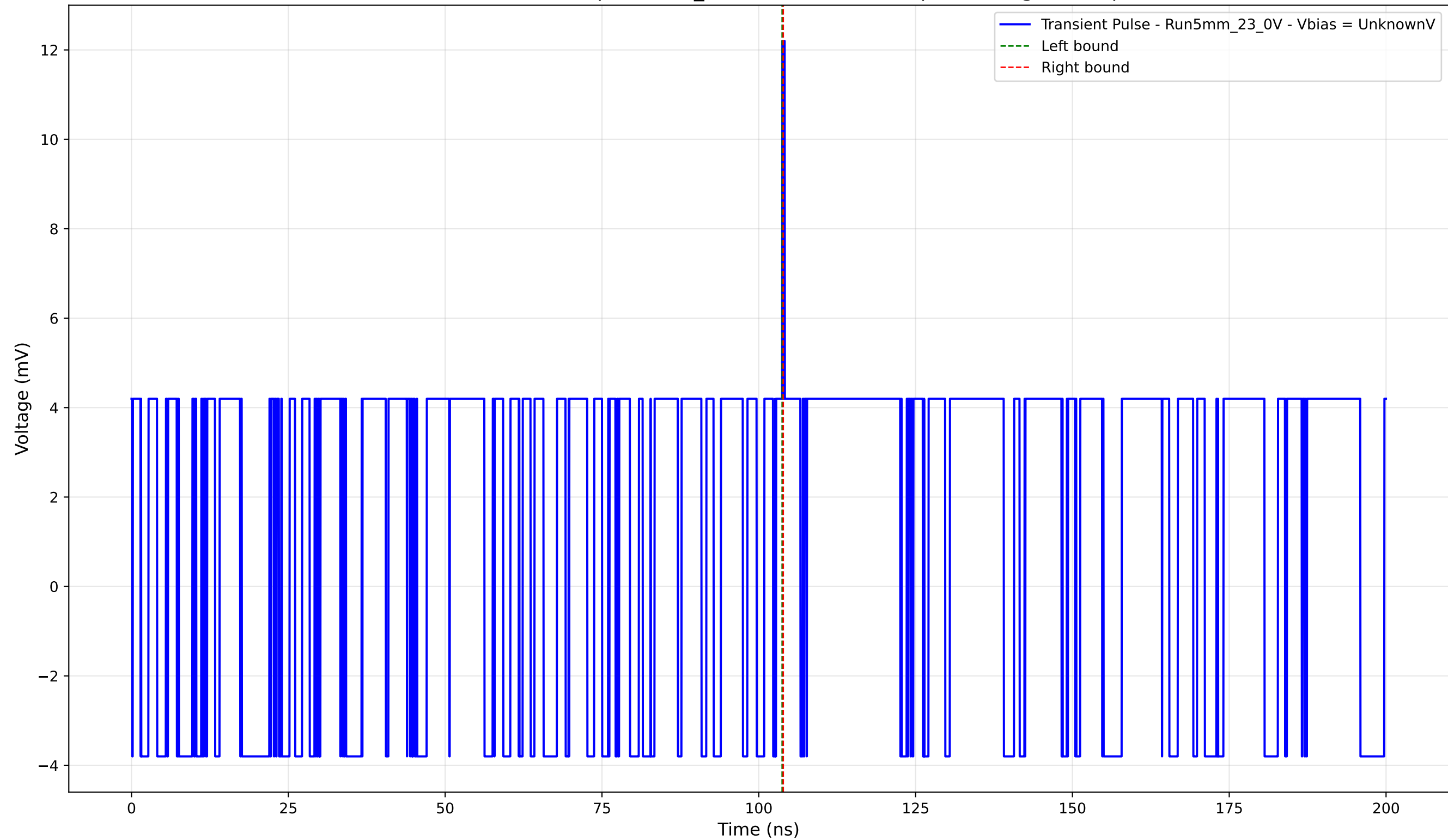
Transient Pulse - Sample: 5mm_23 - Position: 2585.0 \mu\text{m} - Charge: 0.04 pC
