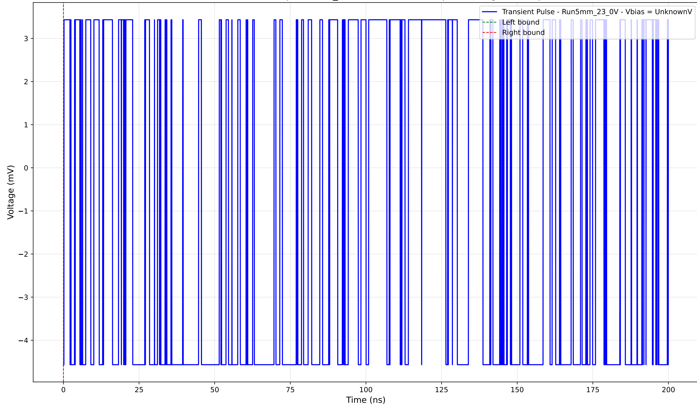
Transient Pulse - Sample: 5mm_23 - Position: 3955.0 \mu\text{m} - Charge: -0.00 pC
