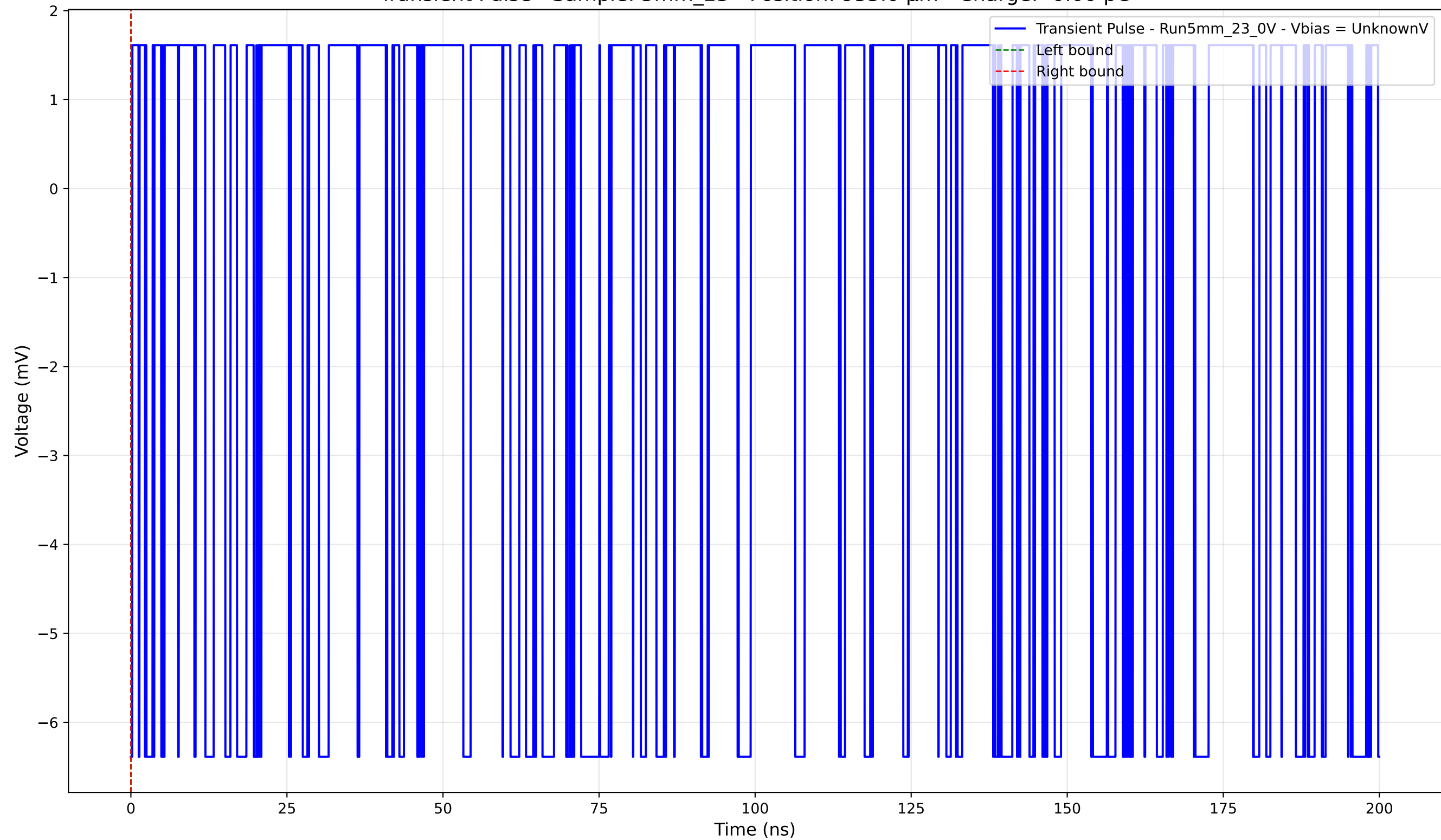
Transient Pulse - Sample: 5mm_23 - Position: 955.0 \mu\text{m} - Charge: -0.00 pC
