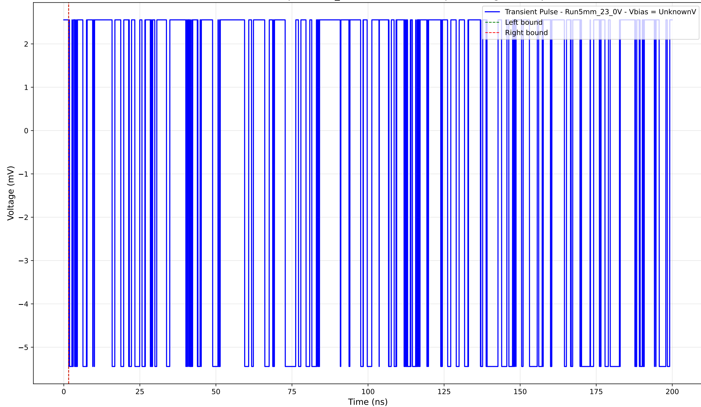
Transient Pulse - Sample: 5mm_23 - Position: 2810.0 \mu\text{m} - Charge: -0.00 pC
