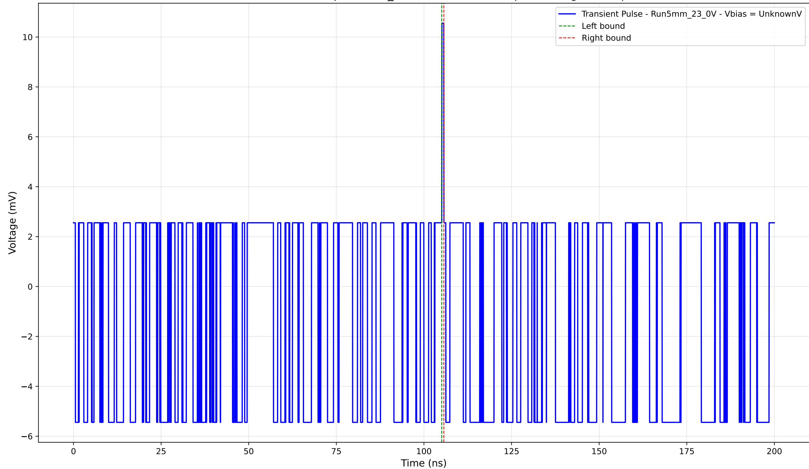
Transient Pulse - Sample: 5mm_23 - Position: 4285.0 \mu\text{m} - Charge: 0.12 pC
