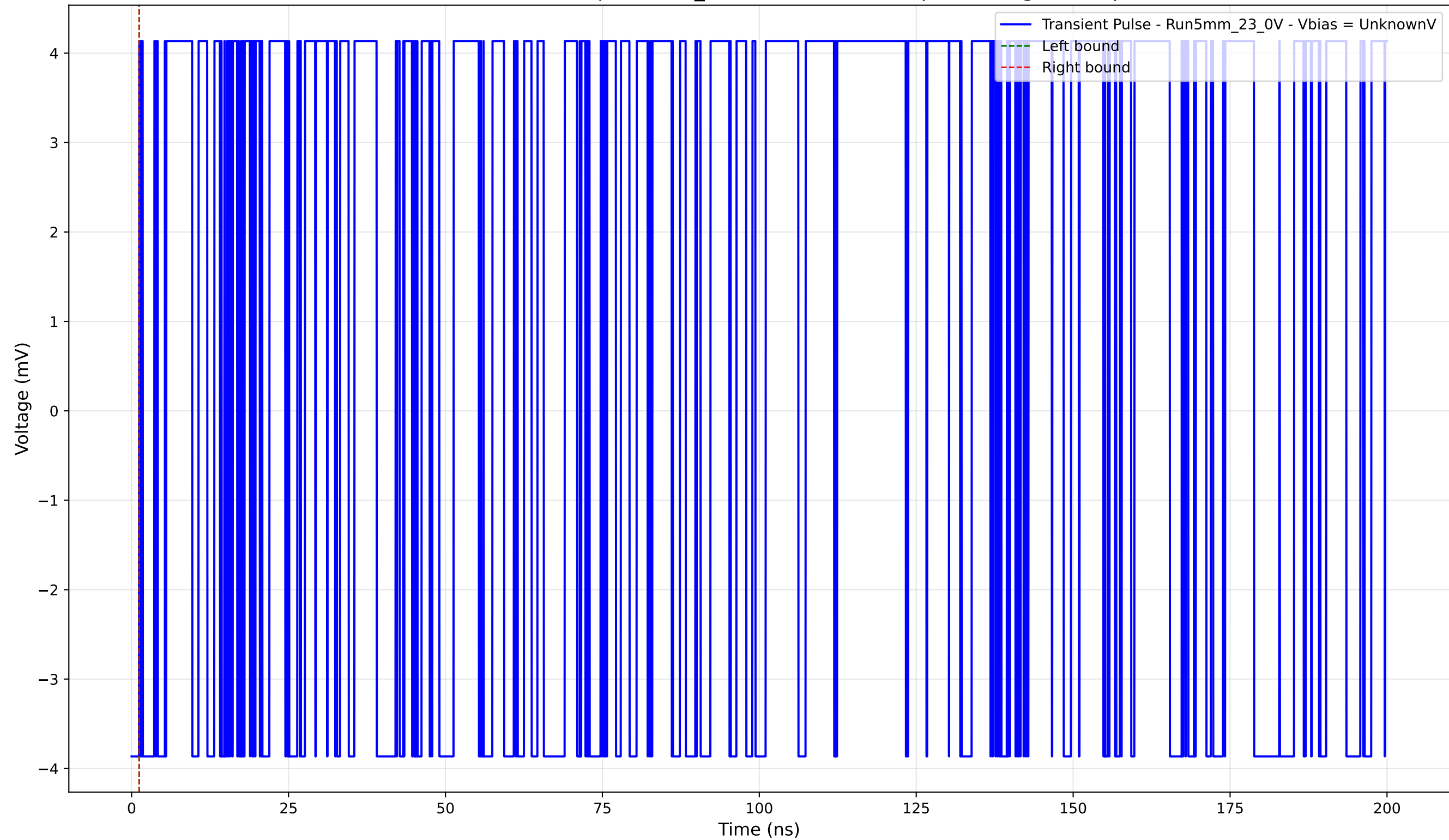
Transient Pulse - Sample: 5mm_23 - Position: 4645.0 \mu\text{m} - Charge: 0.00 pC
