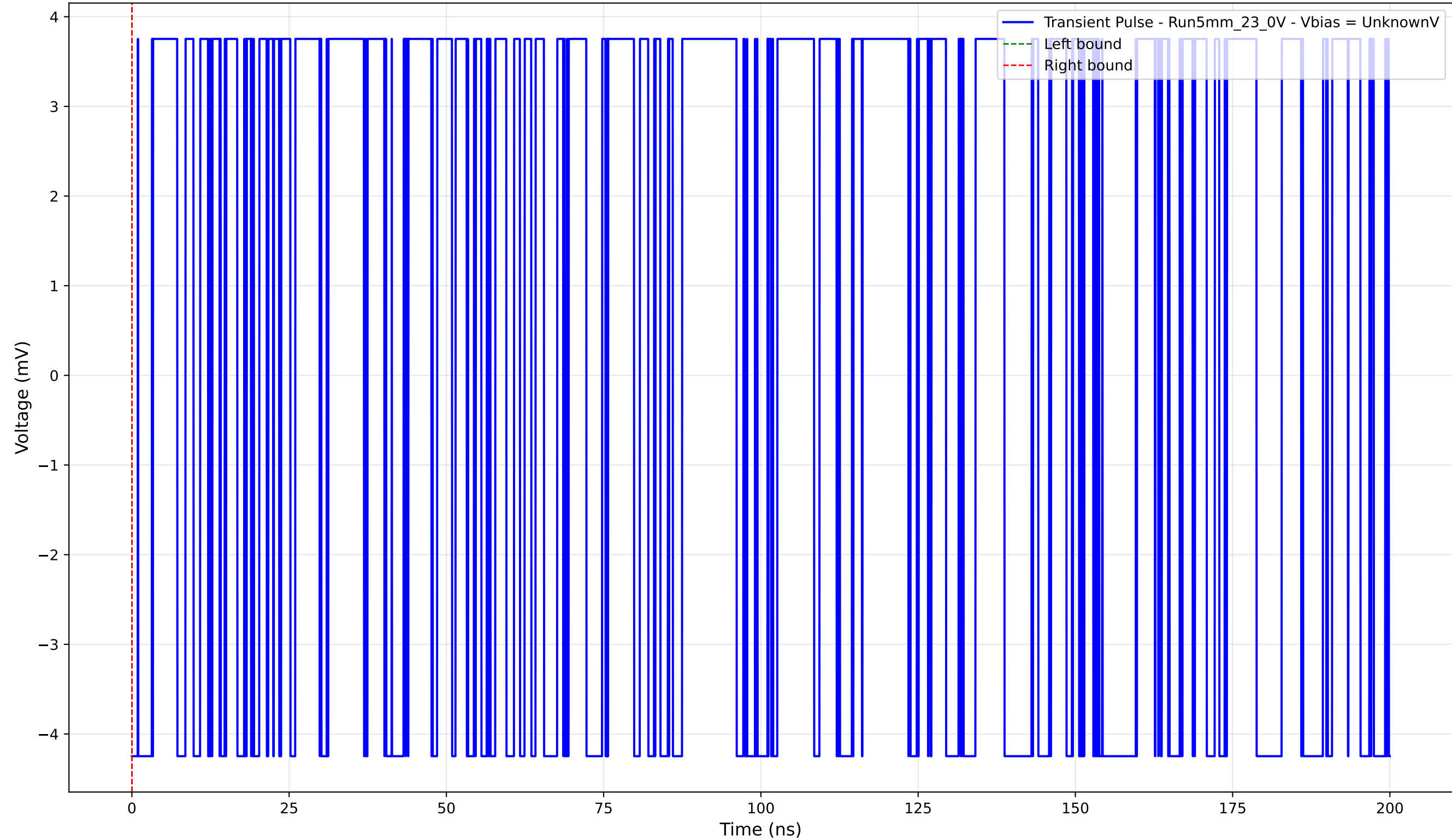
Transient Pulse - Sample: 5mm_23 - Position: 1900.0 \mu\text{m} - Charge: -0.00 pC
