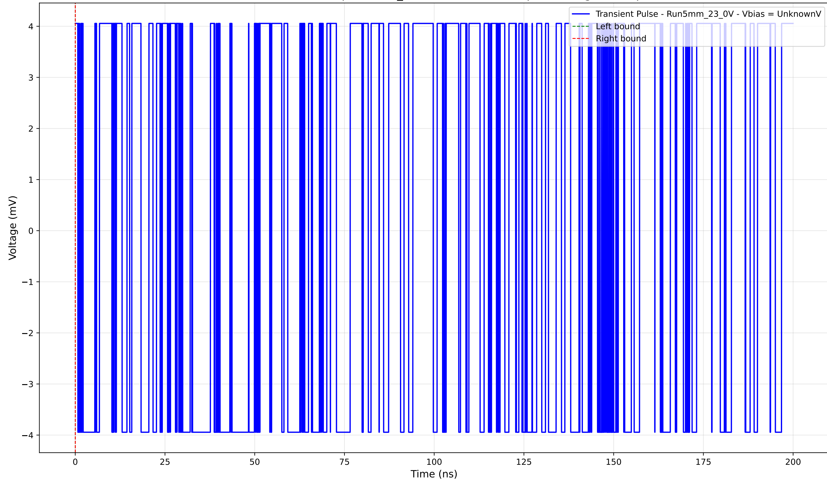
Transient Pulse - Sample: 5mm_23 - Position: 4385.0 \mu\text{m} - Charge: 0.00 pC
