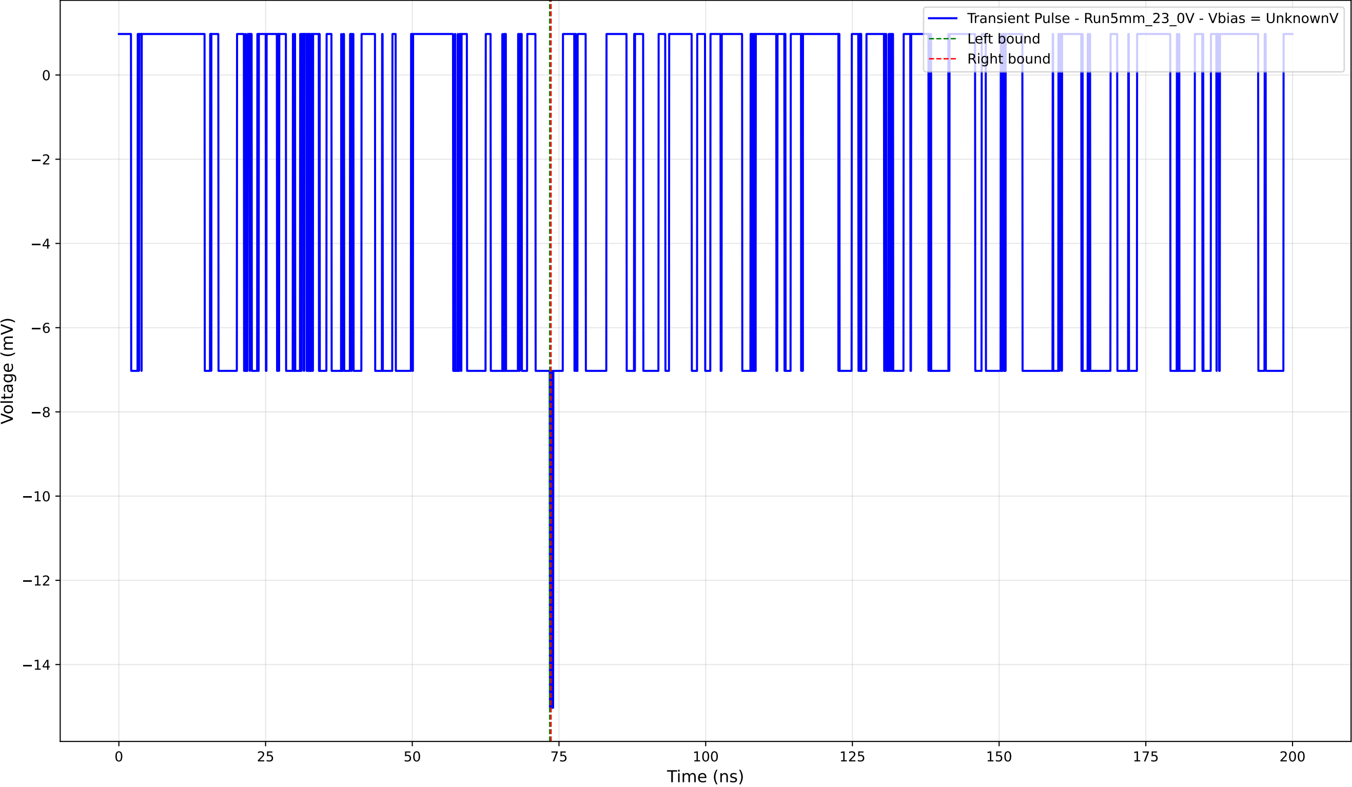
Transient Pulse - Sample: 5mm_23 - Position: 555.0 \mu\text{m} - Charge: -0.06 pC
