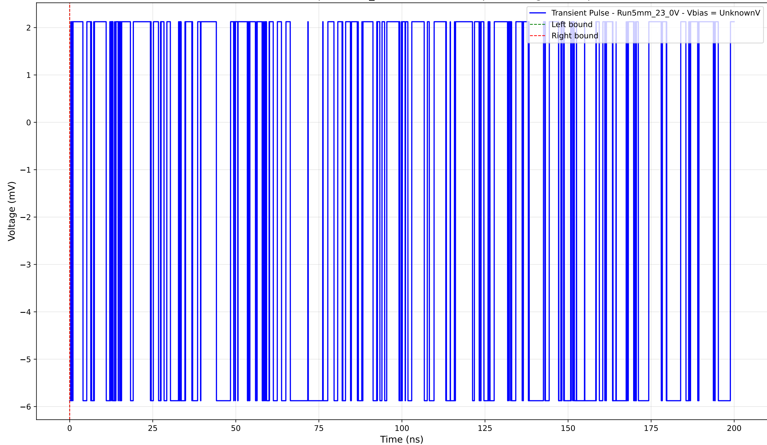
Transient Pulse - Sample: 5mm_23 - Position: 995.0 \mu\text{m} - Charge: -0.00 pC
