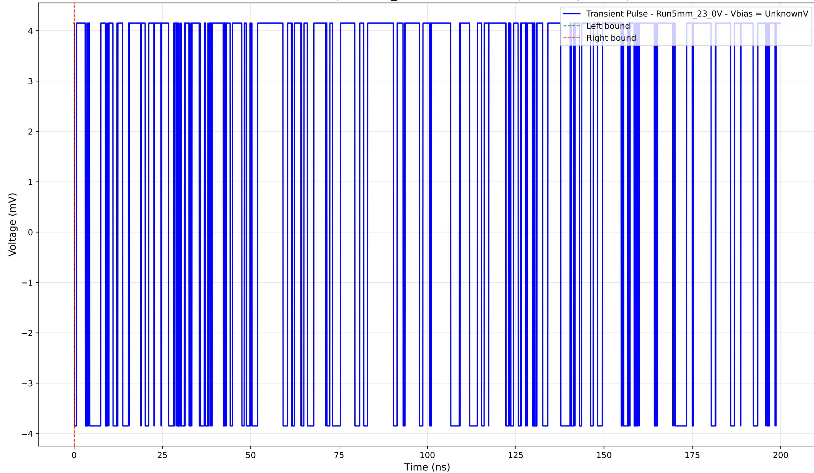
Transient Pulse - Sample: 5mm_23 - Position: 2970.0 \mu\text{m} - Charge: 0.00 pC
