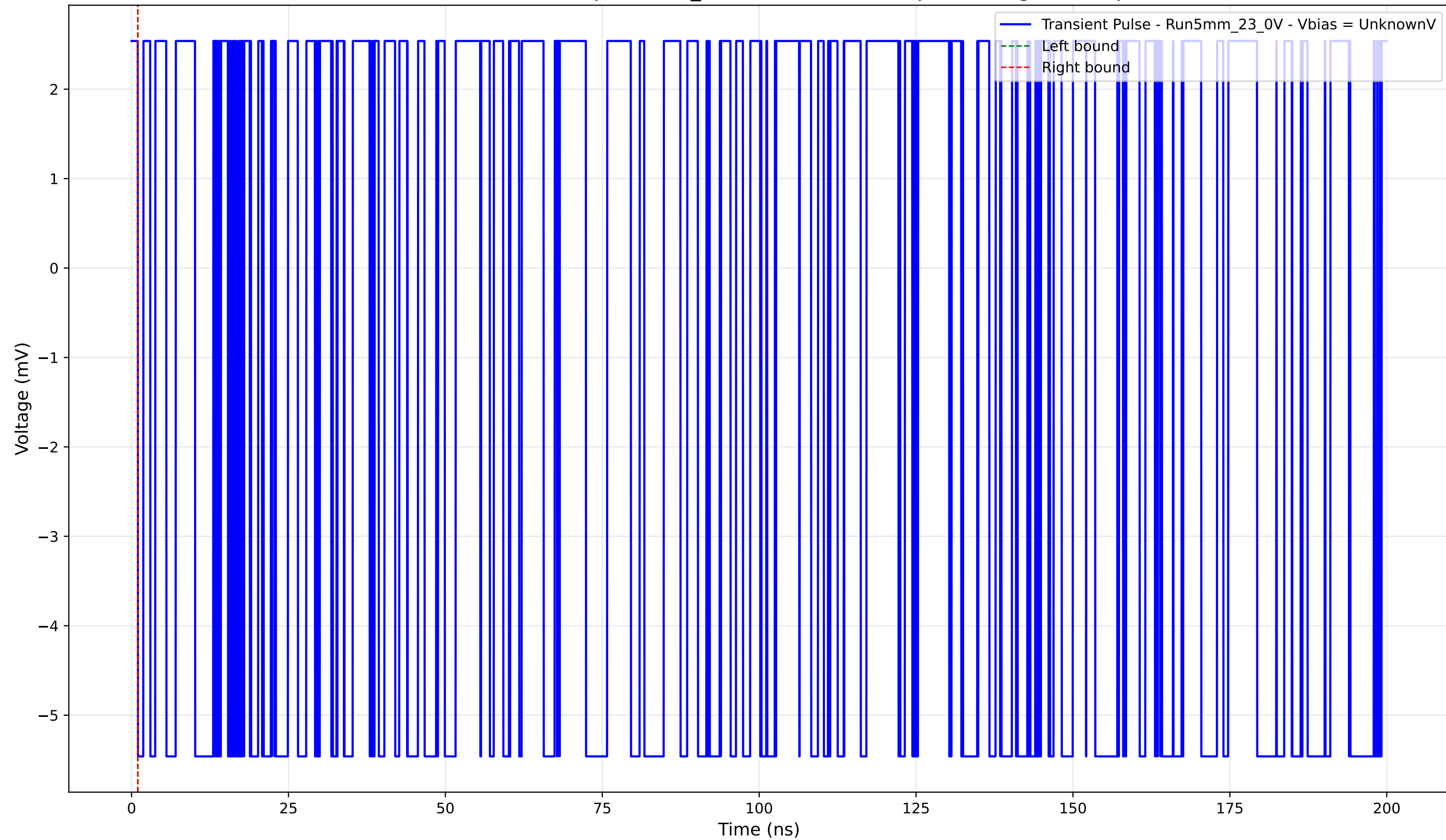
Transient Pulse - Sample: 5mm_23 - Position: 4970.0 \mu\text{m} - Charge: -0.00 pC
