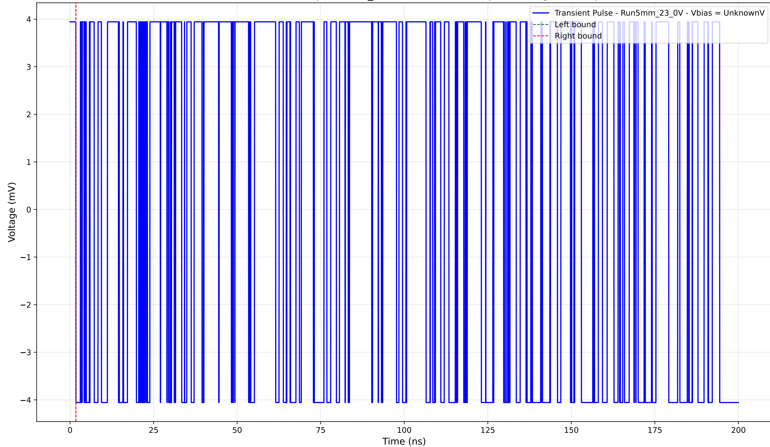
Transient Pulse - Sample: 5mm_23 - Position: 3480.0 \mu\text{m} - Charge: -0.00 pC
