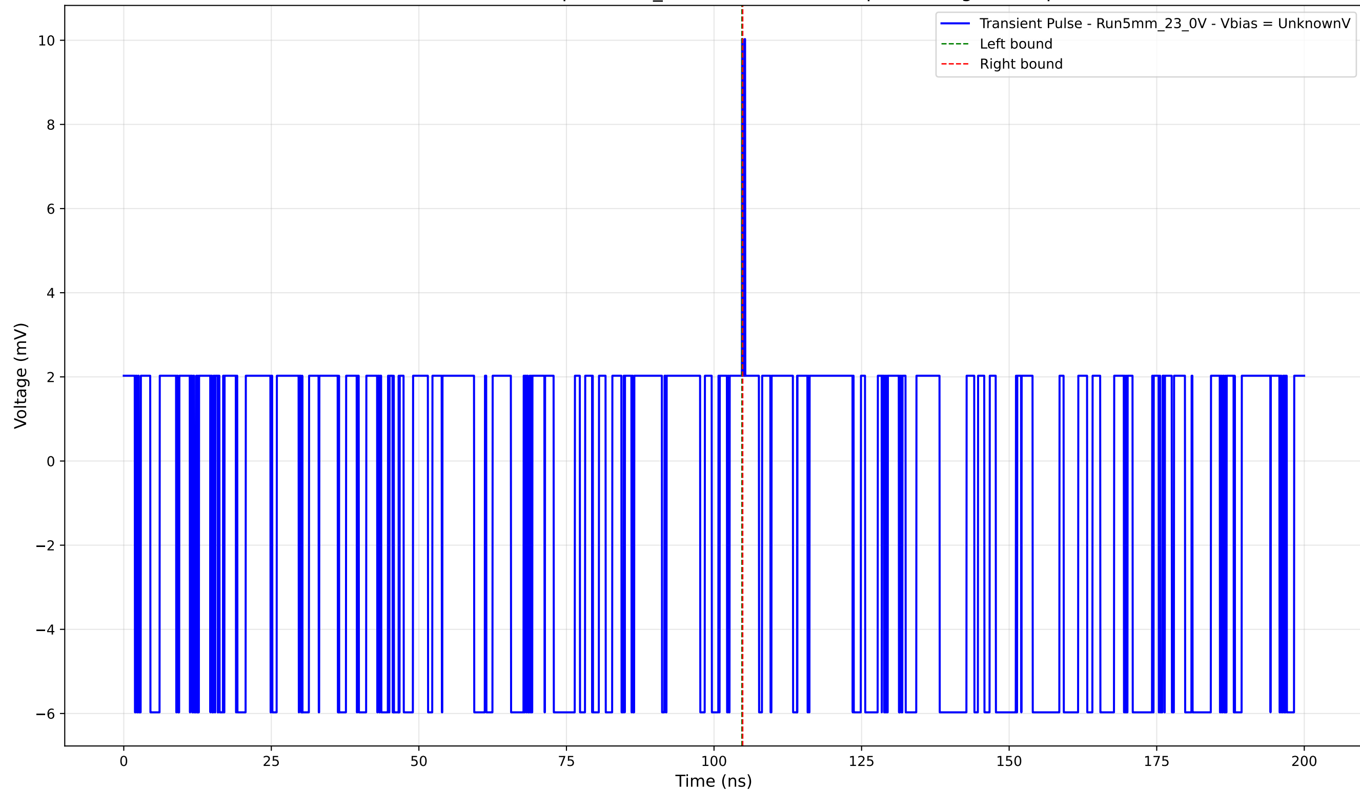
Transient Pulse - Sample: 5mm_23 - Position: 1585.0 \mu\text{m} - Charge: 0.02 pC
