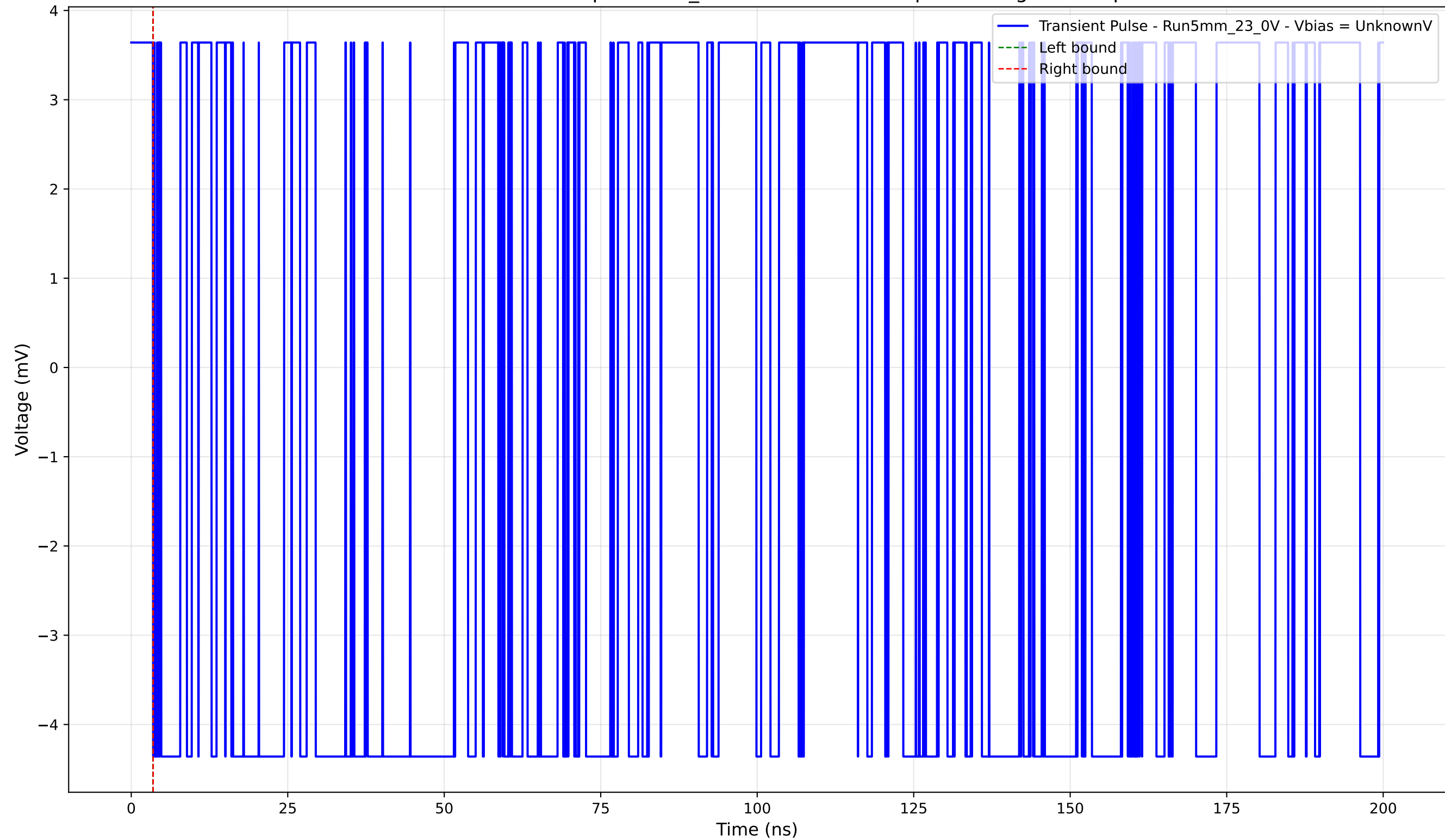
Transient Pulse - Sample: 5mm_23 - Position: 1915.0 \mu\text{m} - Charge: -0.00 pC
