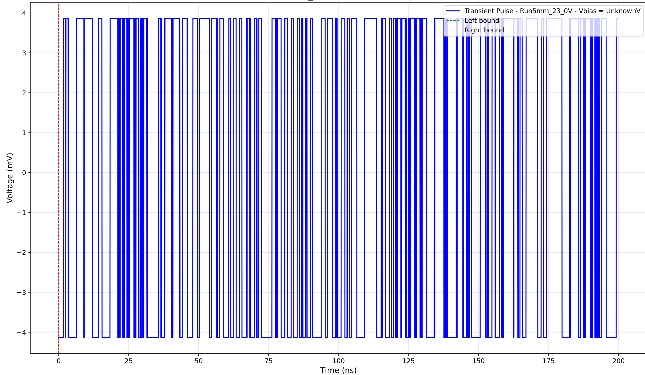
Transient Pulse - Sample: 5mm_23 - Position: 1570.0 \mu\text{m} - Charge: -0.00 pC
