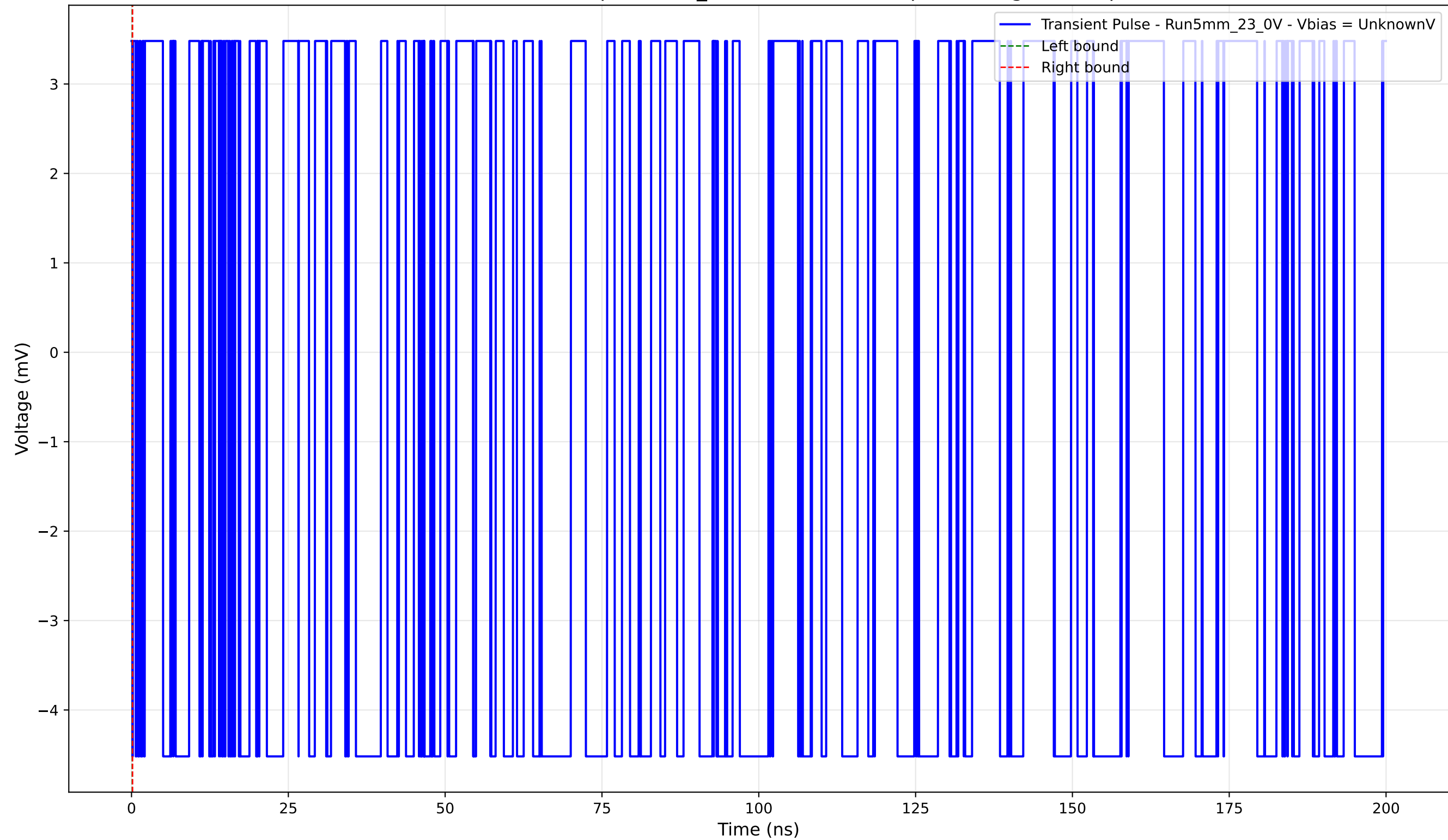
Transient Pulse - Sample: 5mm_23 - Position: 465.0 \mu\text{m} - Charge: -0.00 pC
