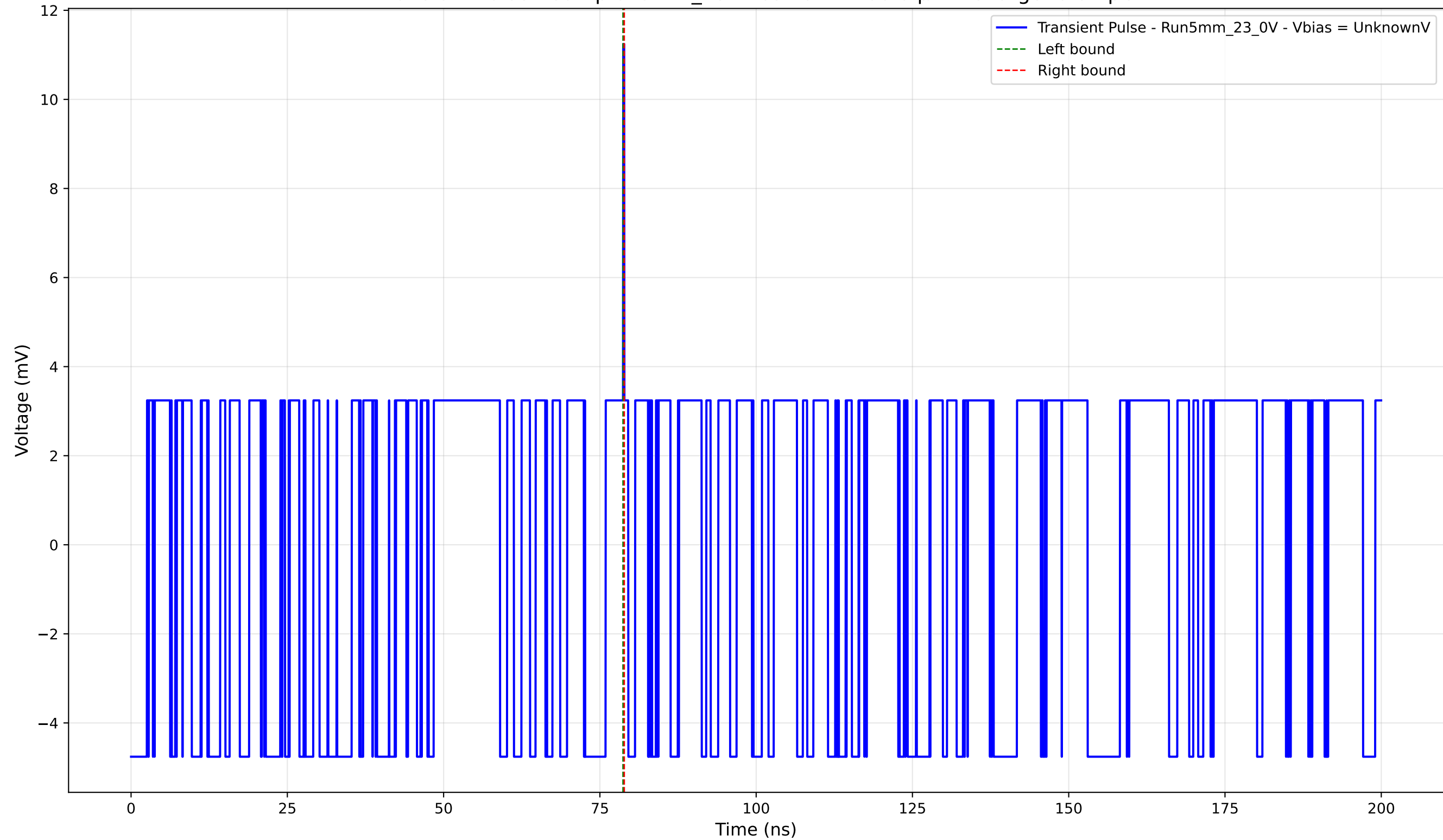
Transient Pulse - Sample: 5mm_23 - Position: 1200.0 \mu\text{m} - Charge: 0.04 pC
