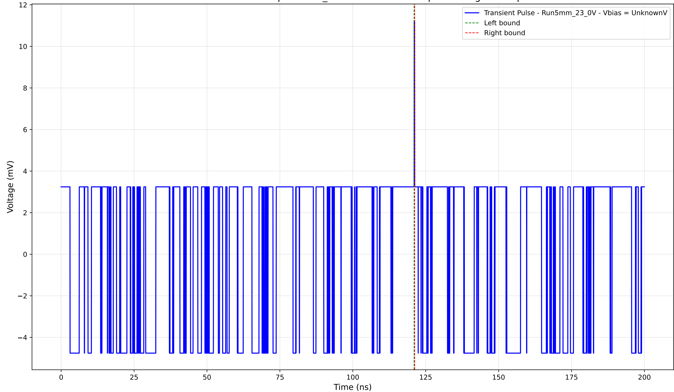
Transient Pulse - Sample: 5mm_23 - Position: 3430.0 \mu\text{m} - Charge: 0.04 pC
