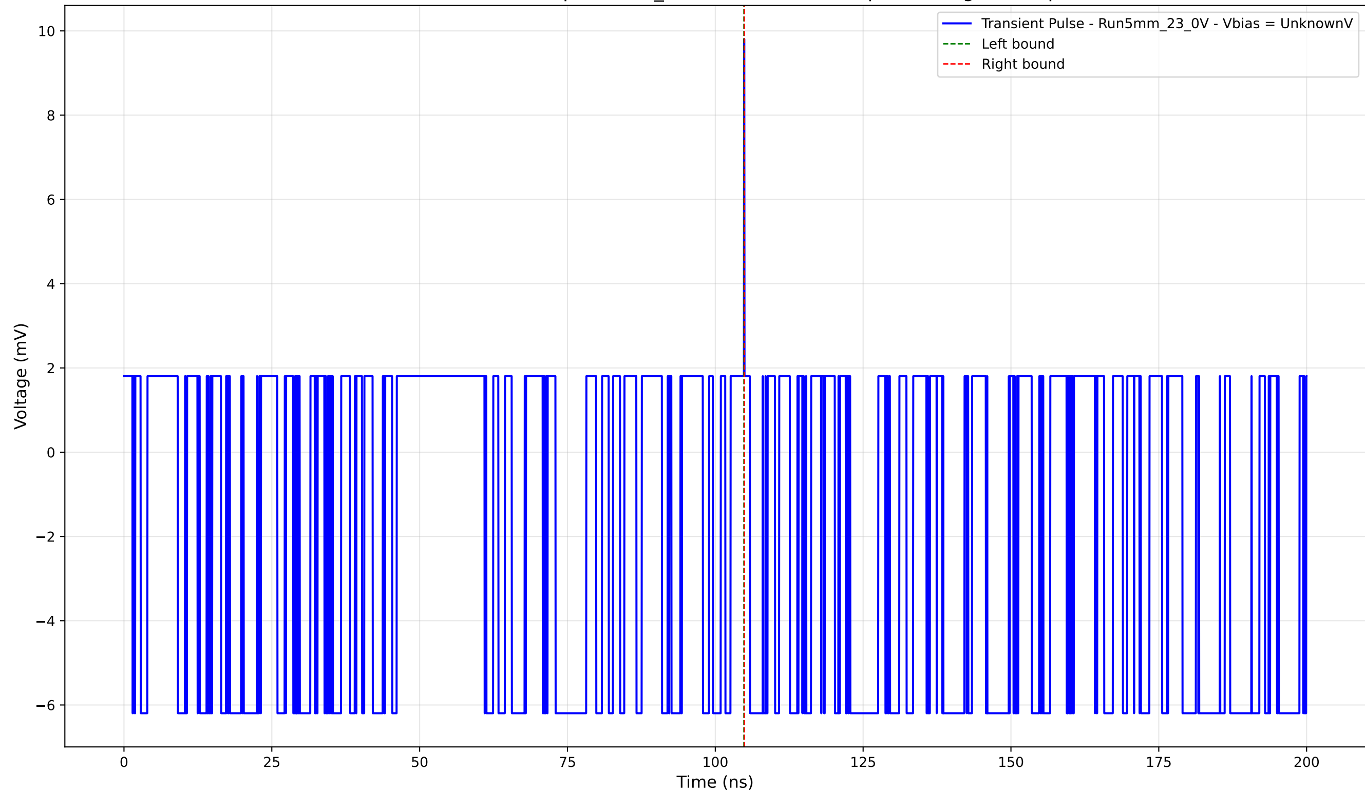
Transient Pulse - Sample: 5mm_23 - Position: 2275.0 \mu\text{m} - Charge: 0.01 pC
