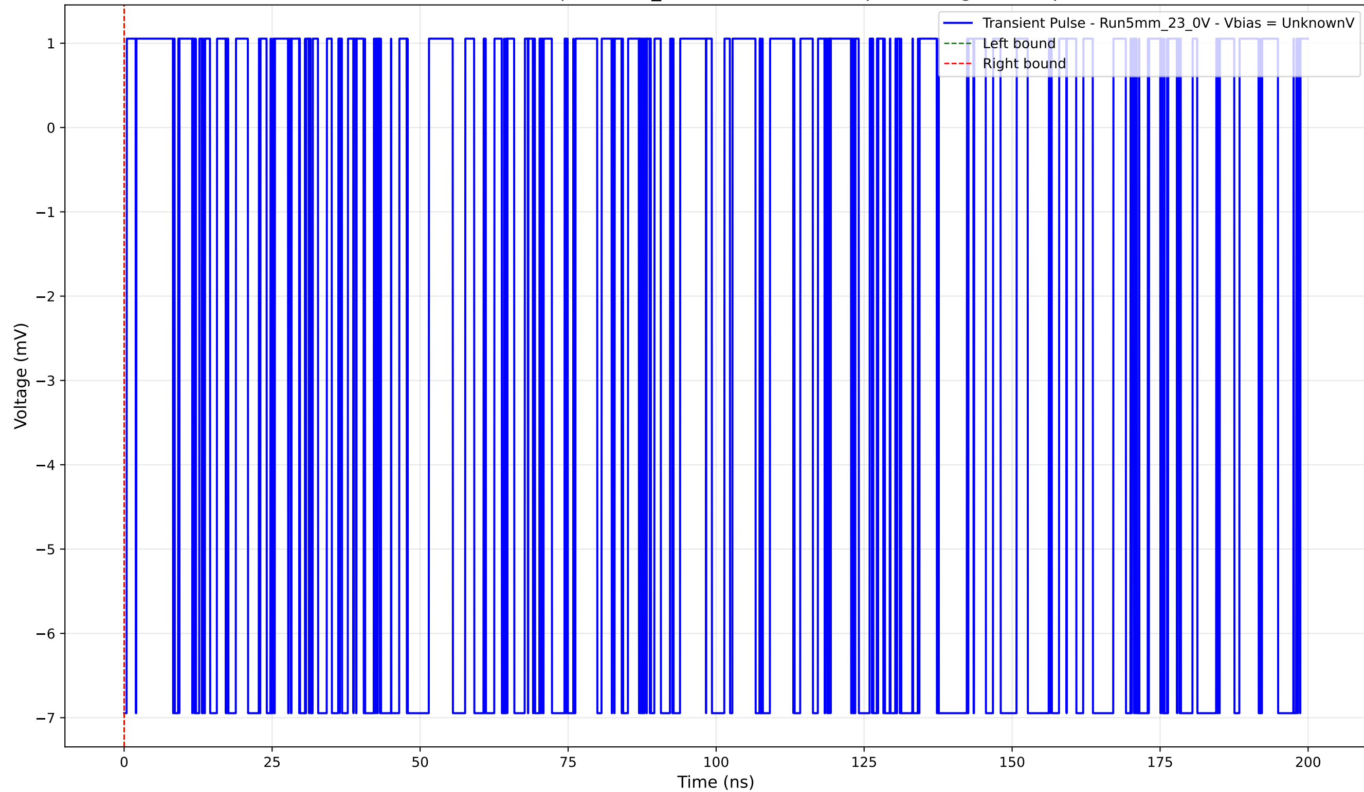
Transient Pulse - Sample: 5mm_23 - Position: 1730.0 \mu\text{m} - Charge: -0.00 pC
