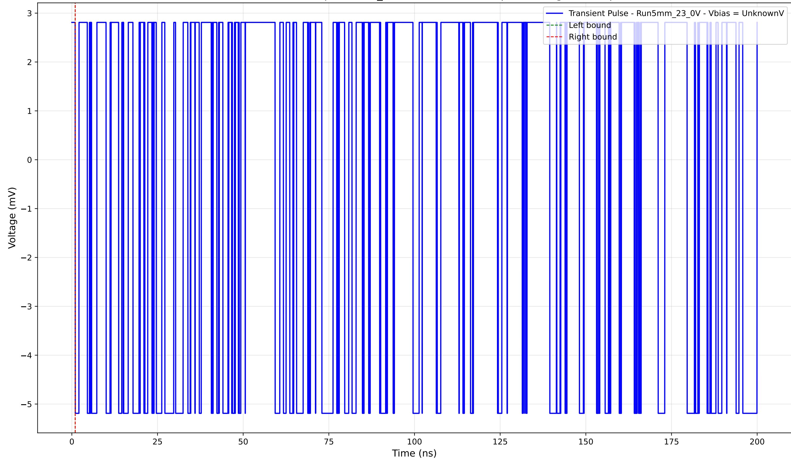
Transient Pulse - Sample: 5mm_23 - Position: 1135.0 \mu\text{m} - Charge: -0.00 pC
