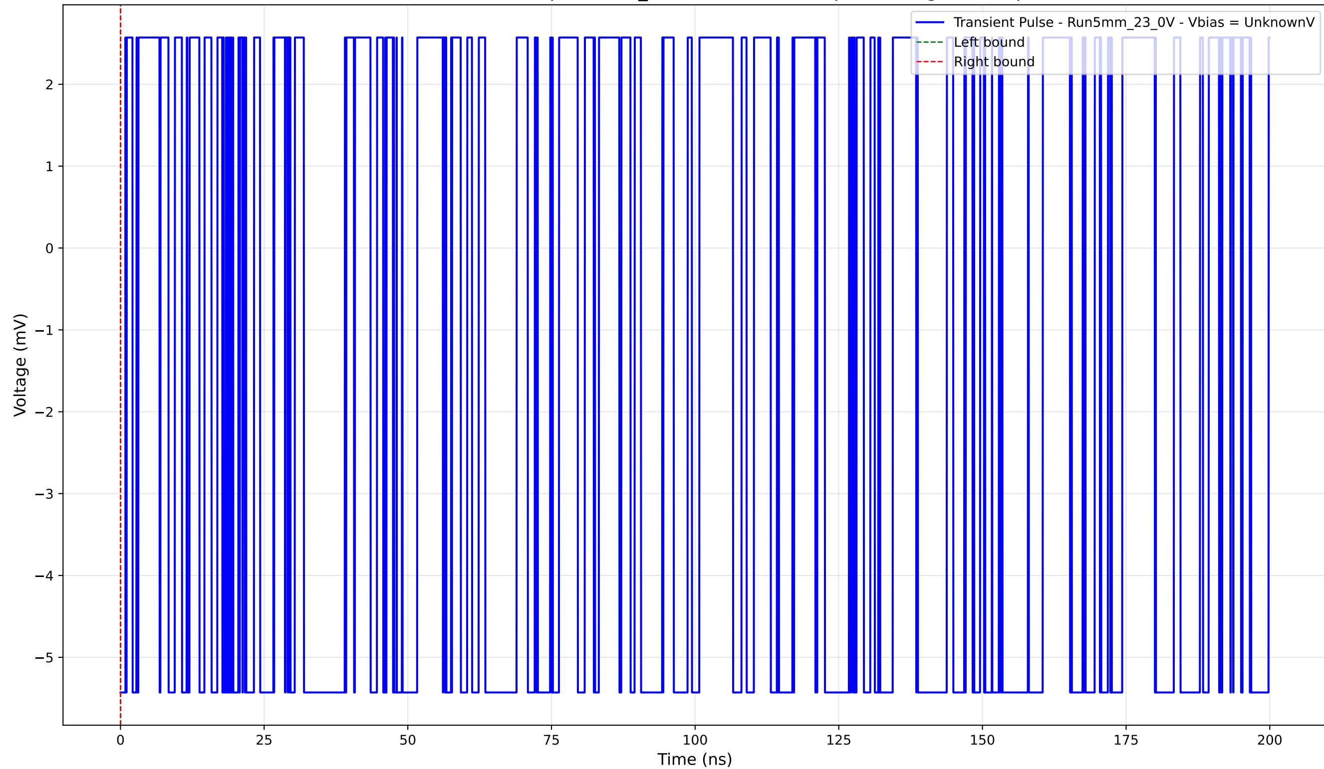
Transient Pulse - Sample: 5mm_23 - Position: 900.0 \mu\text{m} - Charge: -0.00 pC
