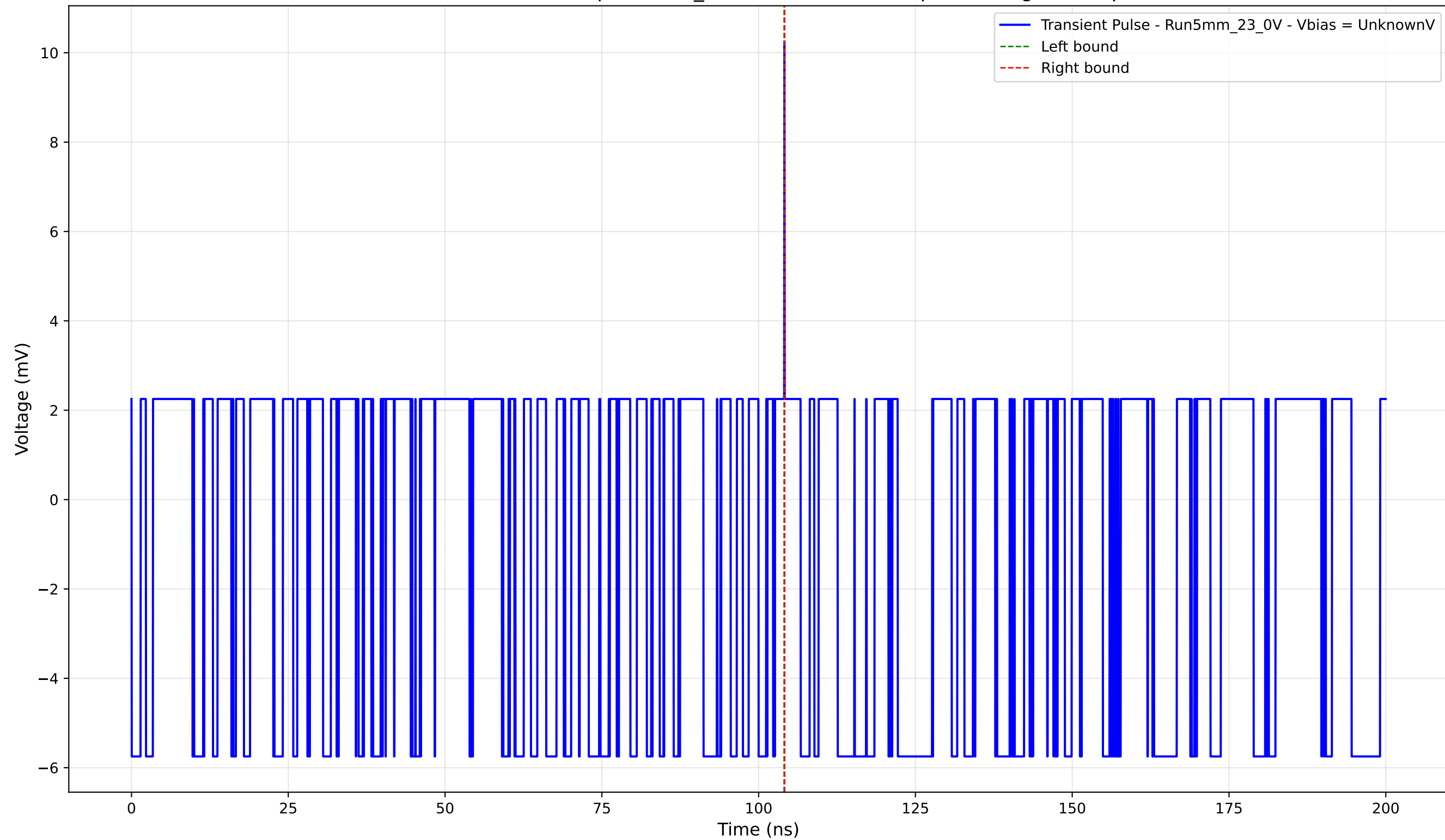
Transient Pulse - Sample: 5mm_23 - Position: 1885.0 \mu\text{m} - Charge: 0.01 pC
