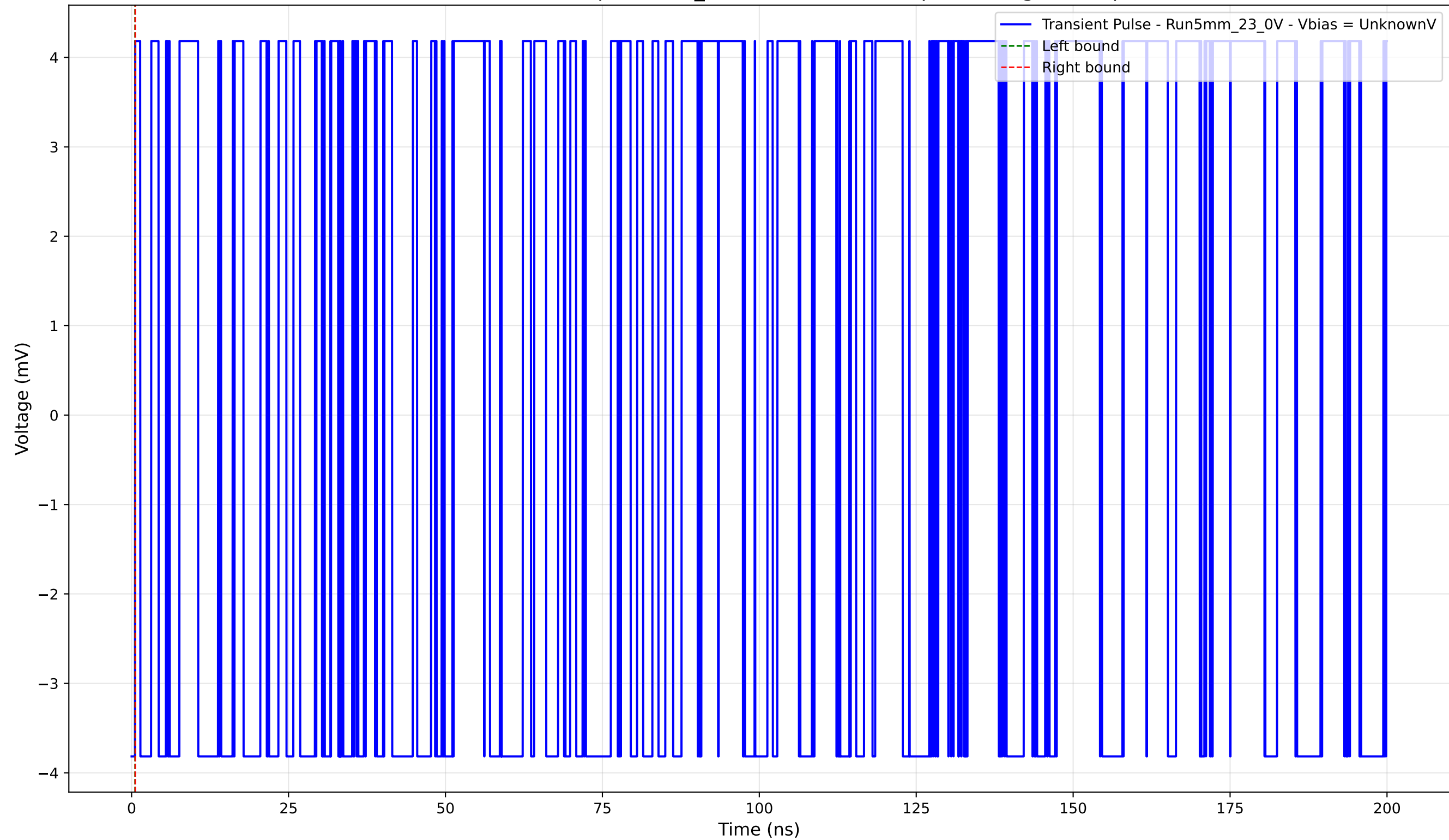
Transient Pulse - Sample: 5mm_23 - Position: 1170.0 \mu\text{m} - Charge: 0.00 pC
