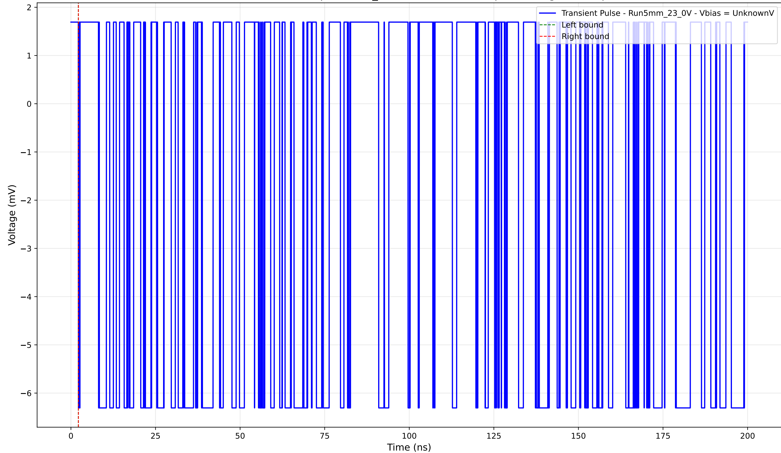
Transient Pulse - Sample: 5mm_23 - Position: 3120.0 \mu\text{m} - Charge: -0.00 pC
