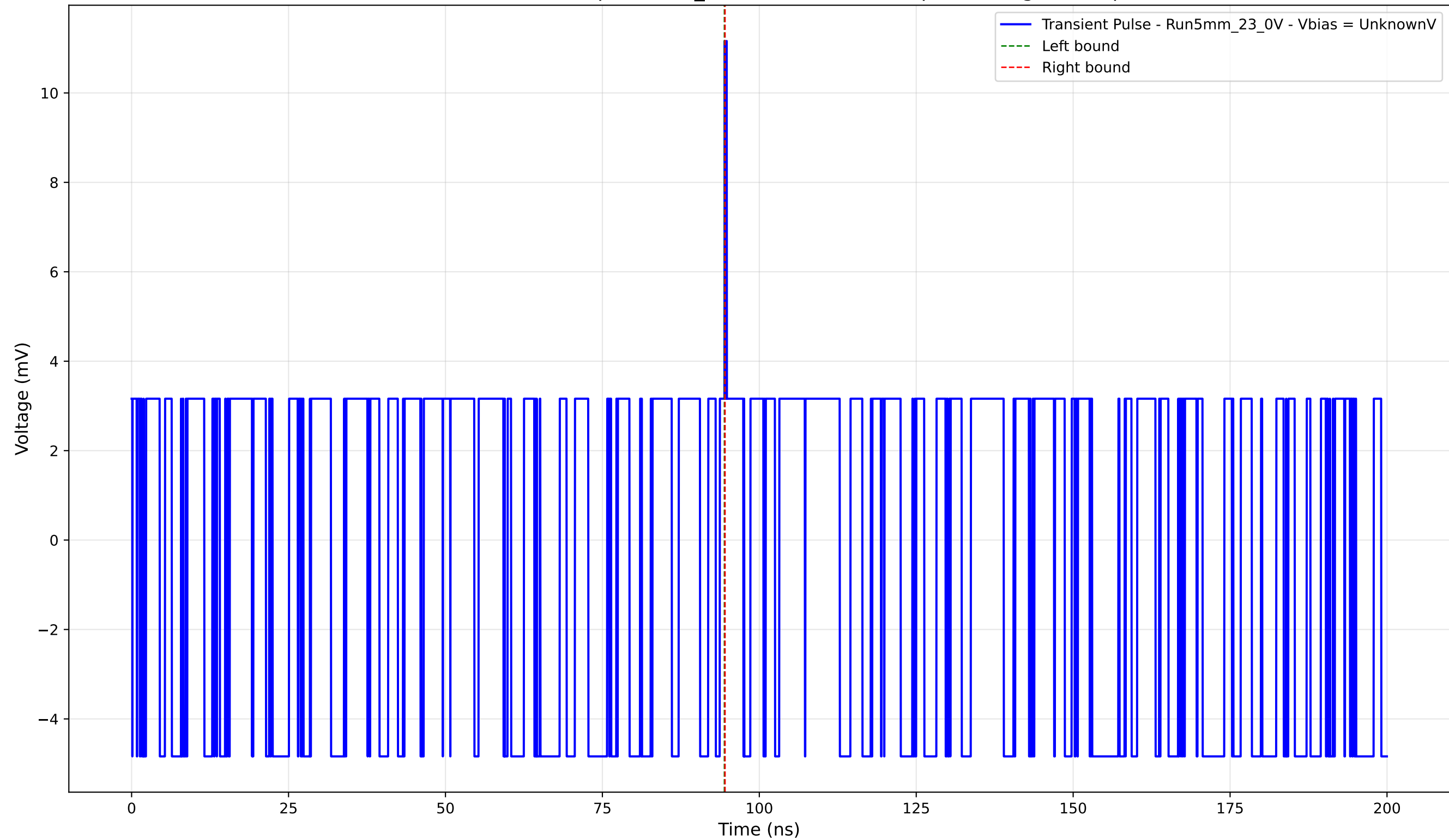
Transient Pulse - Sample: 5mm_23 - Position: 4720.0 \mu\text{m} - Charge: 0.02 pC
