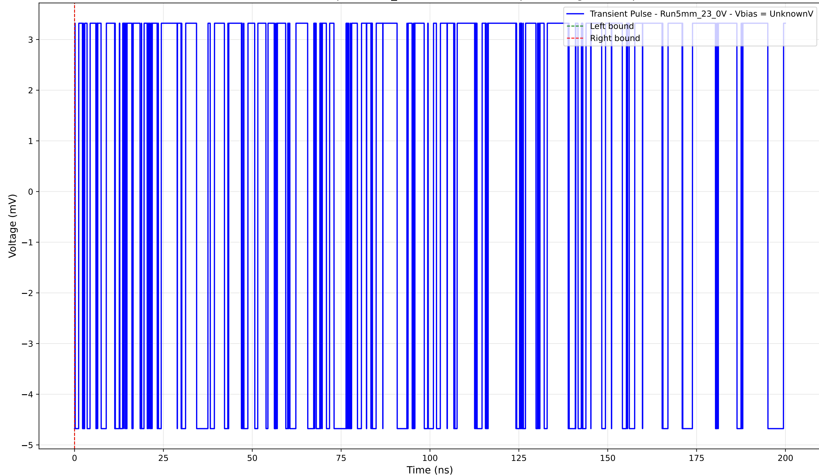
Transient Pulse - Sample: 5mm_23 - Position: 2630.0 \mu\text{m} - Charge: -0.00 pC
