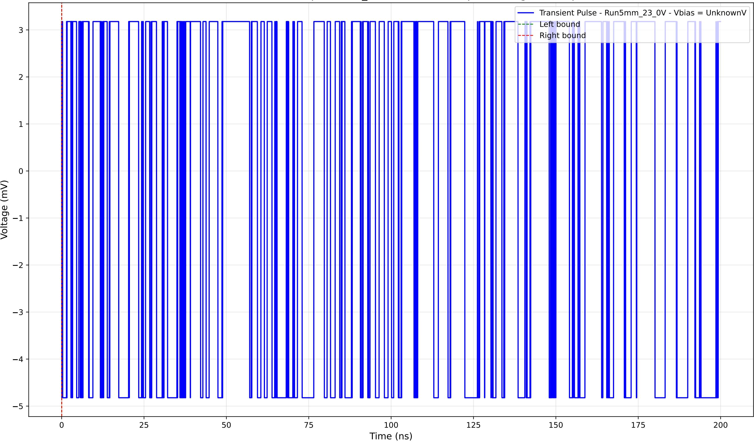
Transient Pulse - Sample: 5mm_23 - Position: 30.0 \mu\text{m} - Charge: -0.00 pC
