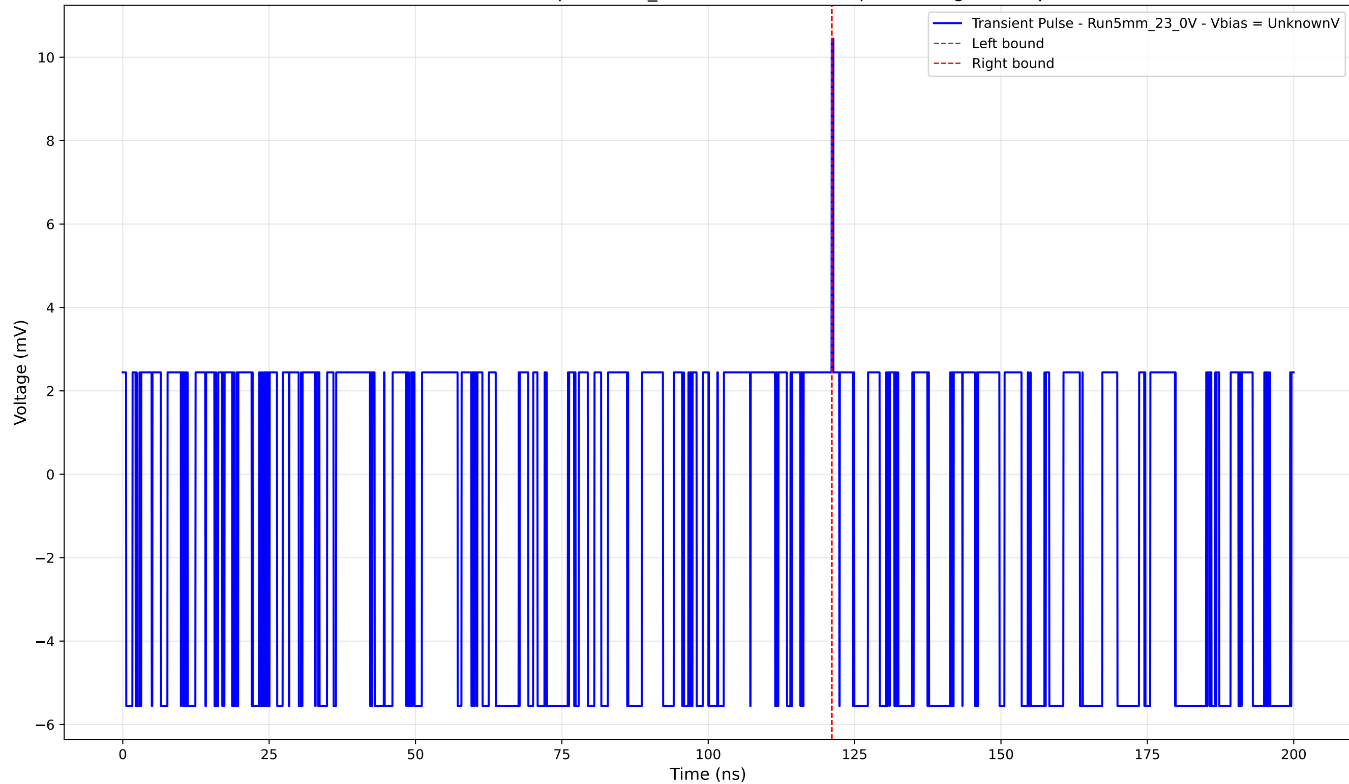
Transient Pulse - Sample: 5mm_23 - Position: 3285.0 \mu\text{m} - Charge: 0.01 pC
