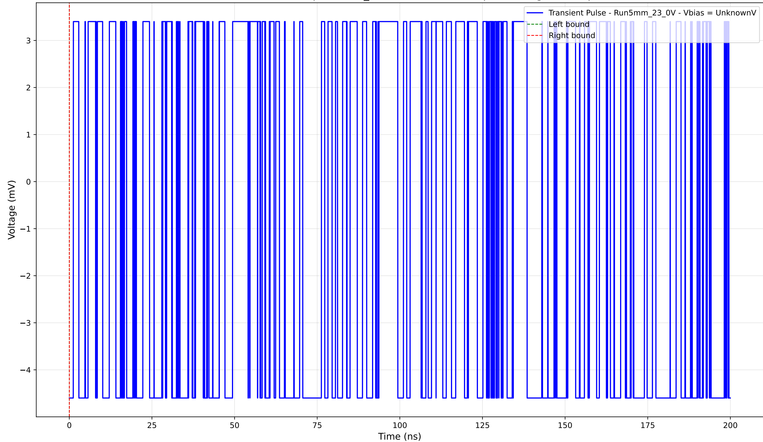
Transient Pulse - Sample: 5mm_23 - Position: 4545.0 \mu\text{m} - Charge: -0.00 pC
