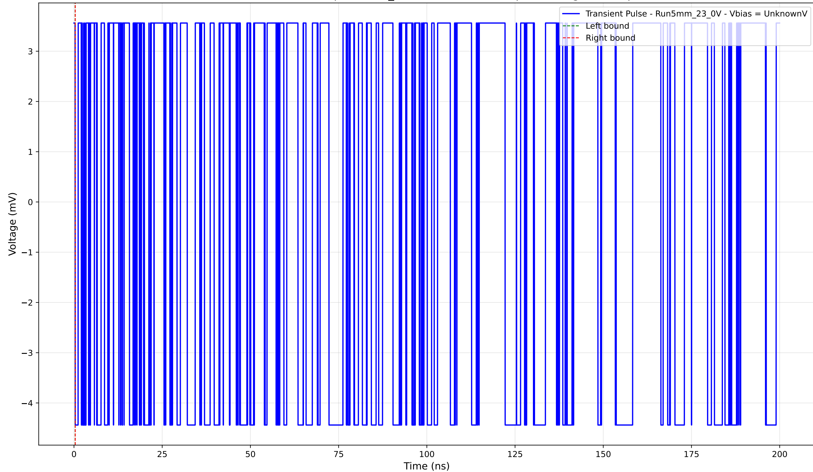
Transient Pulse - Sample: 5mm_23 - Position: 1985.0 \mu\text{m} - Charge: -0.00 pC
