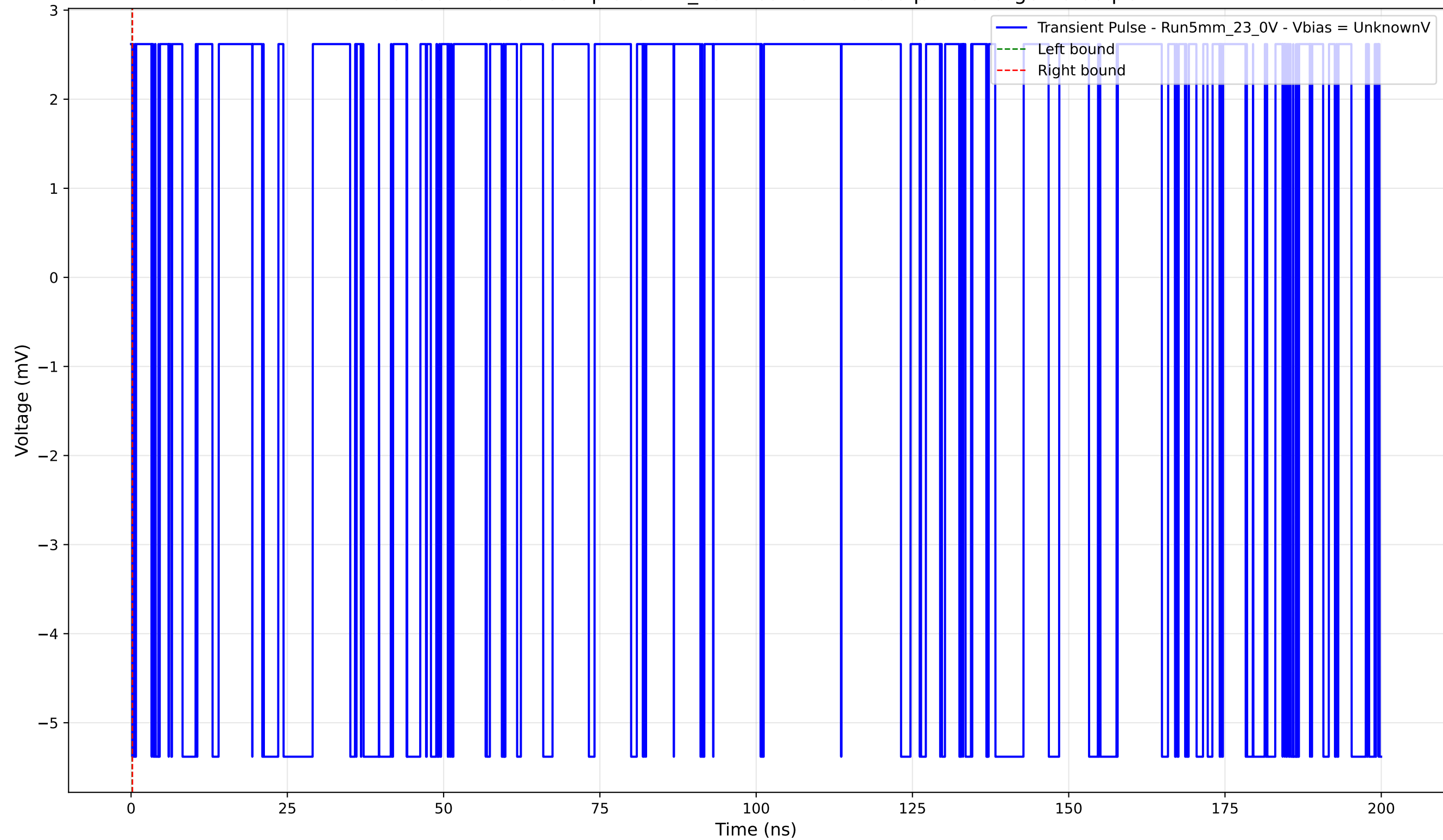
Transient Pulse - Sample: 5mm_23 - Position: 4900.0 \mu\text{m} - Charge: -0.00 pC
