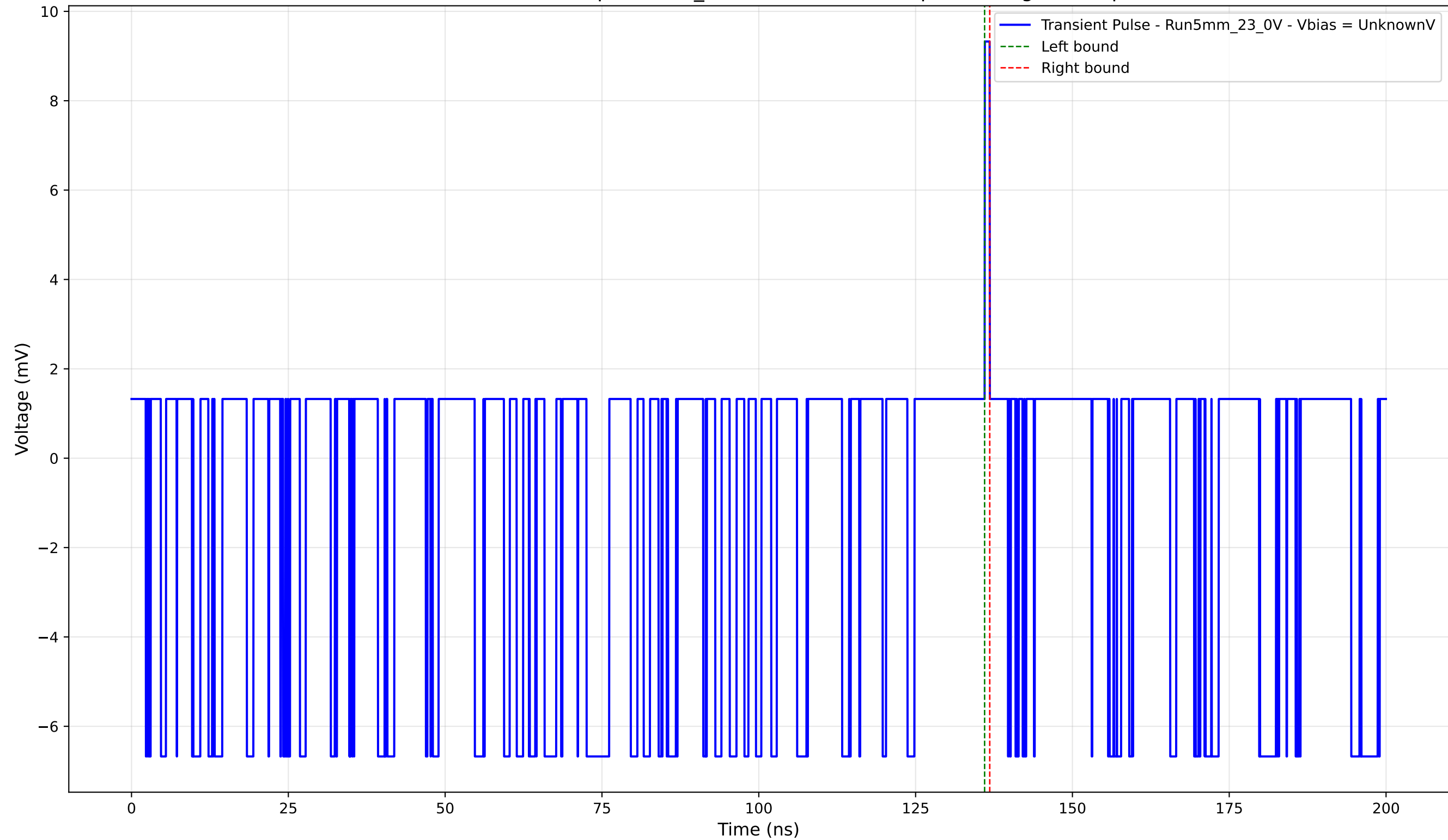
Transient Pulse - Sample: 5mm_23 - Position: 3280.0 \mu\text{m} - Charge: 0.15 pC
