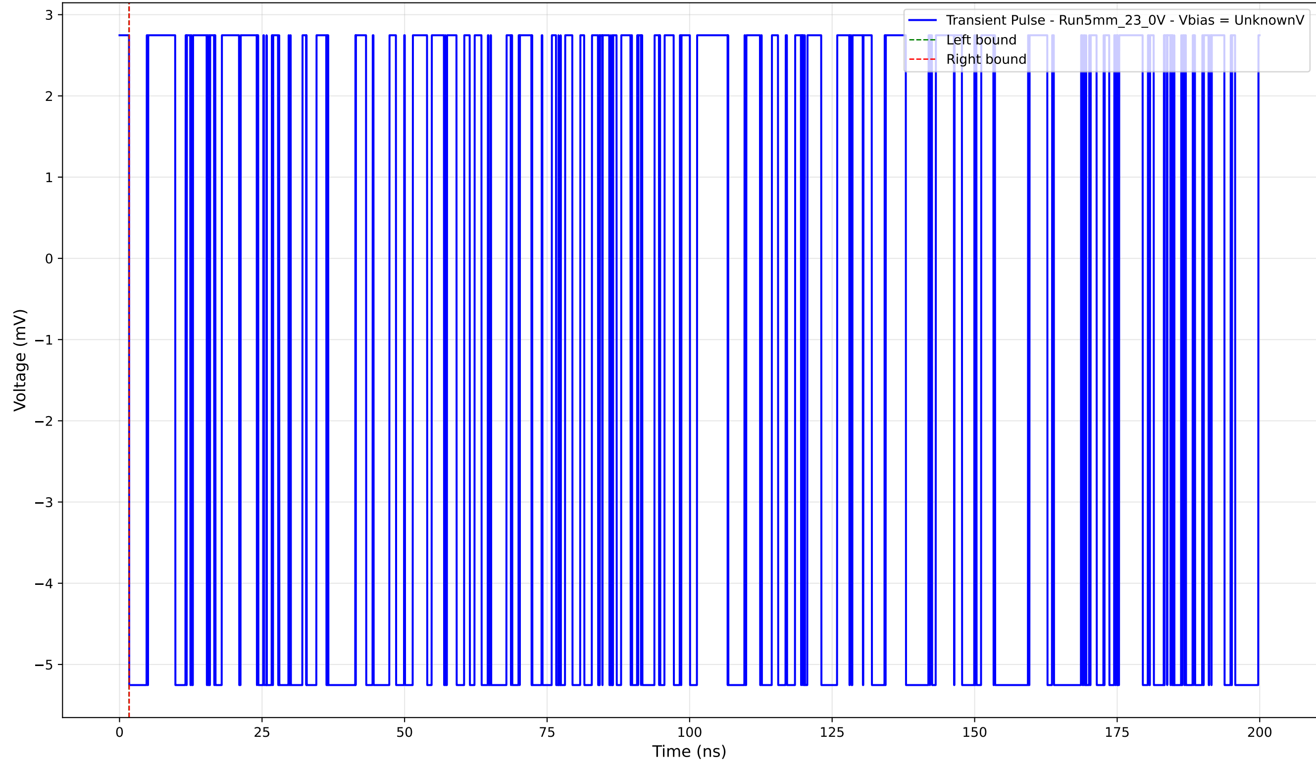
Transient Pulse - Sample: 5mm_23 - Position: 3265.0 \mu\text{m} - Charge: -0.00 pC
