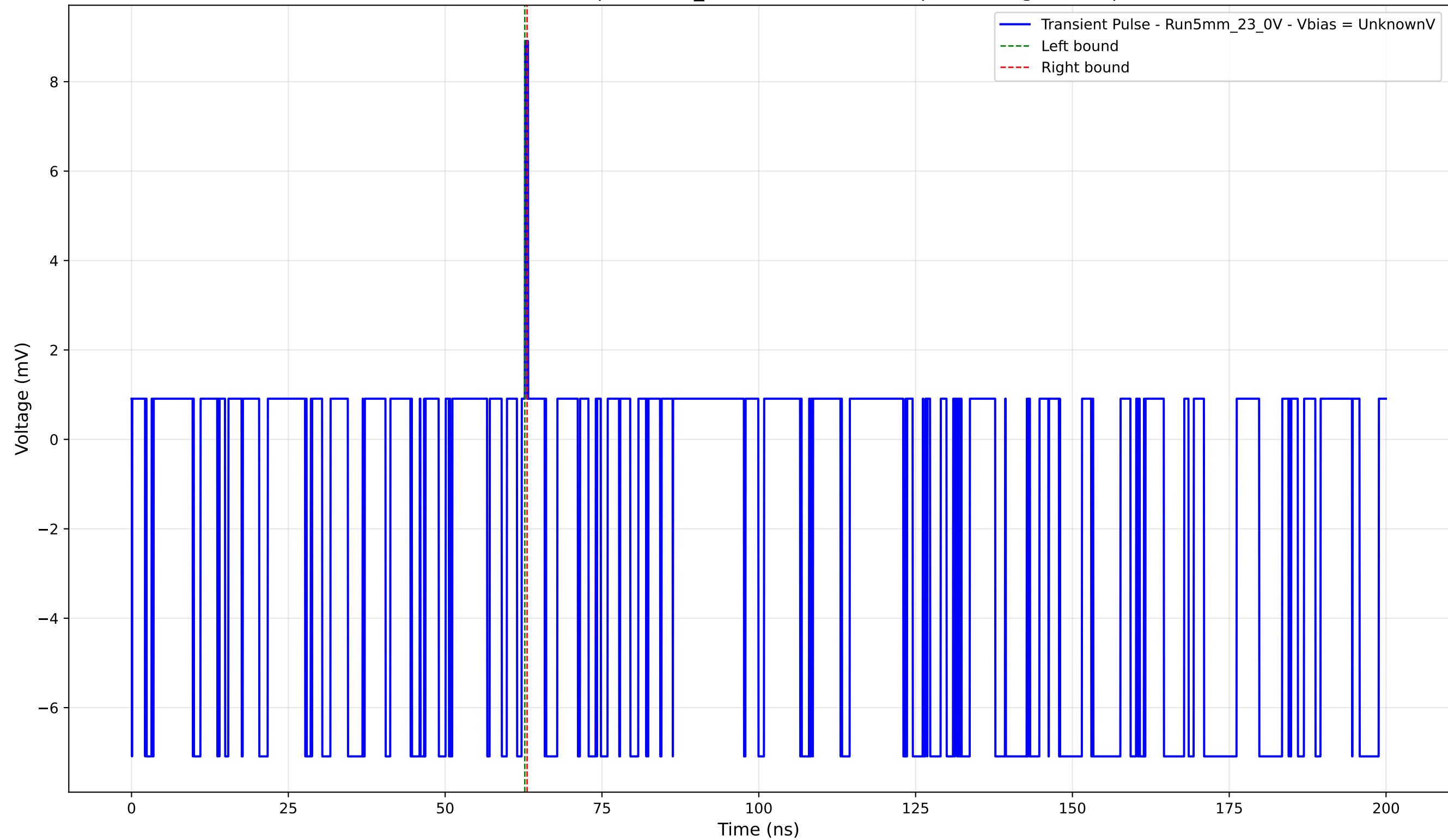
Transient Pulse - Sample: 5mm_23 - Position: 3125.0 \mu\text{m} - Charge: 0.06 pC
