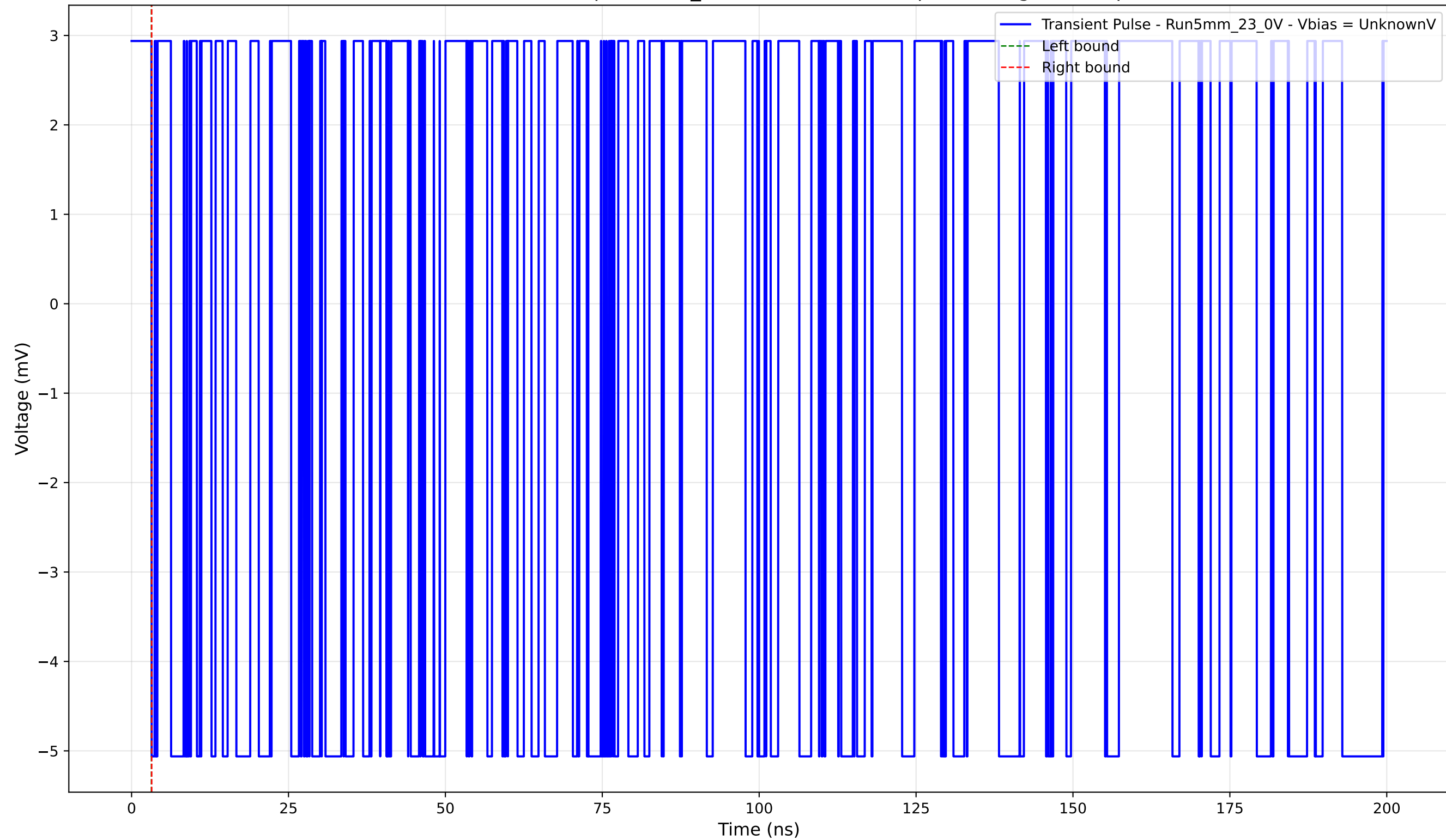
Transient Pulse - Sample: 5mm_23 - Position: 2190.0 \mu\text{m} - Charge: -0.00 pC
