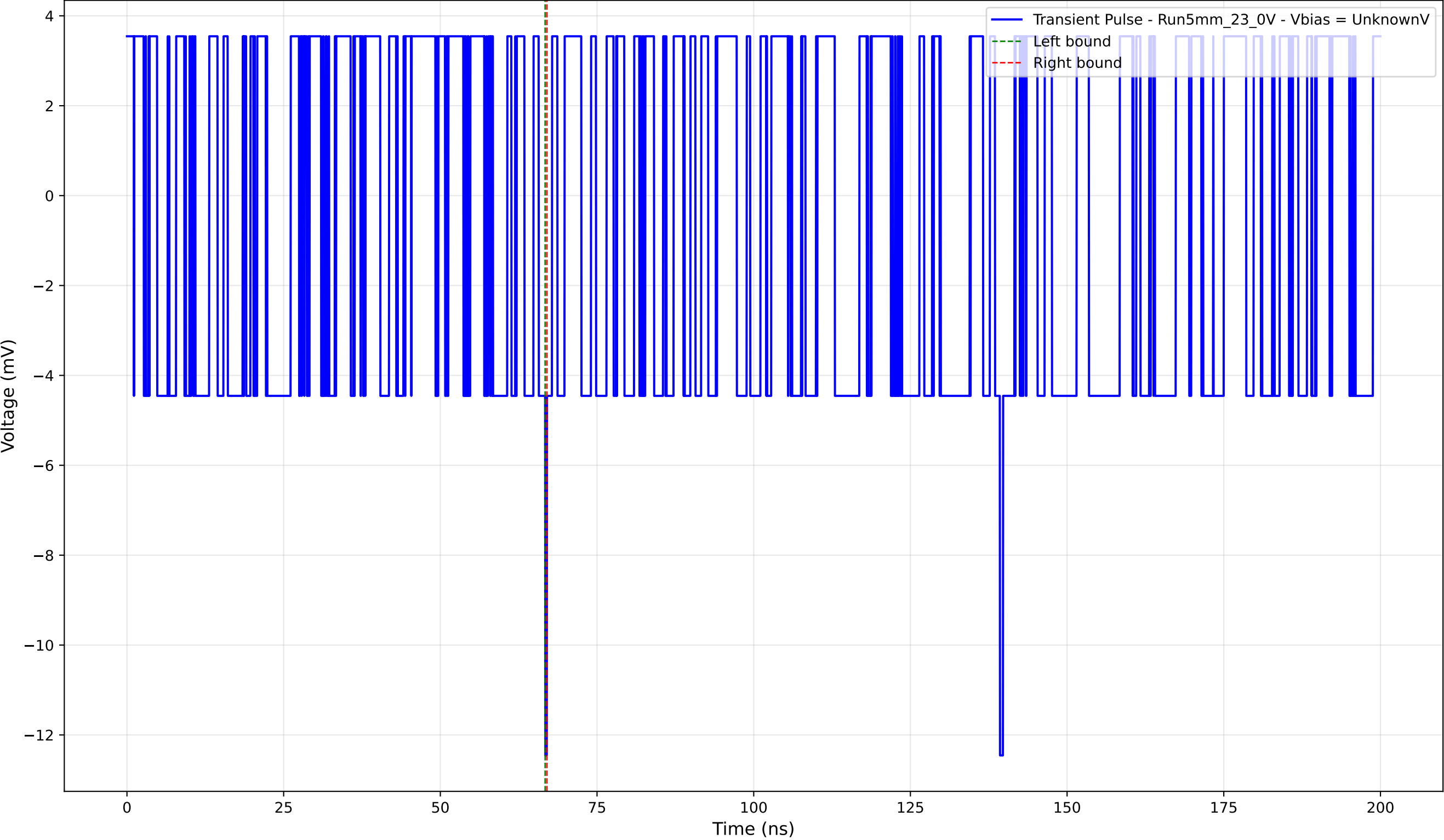
Transient Pulse - Sample: 5mm_23 - Position: 840.0 \mu\text{m} - Charge: -0.07 pC
