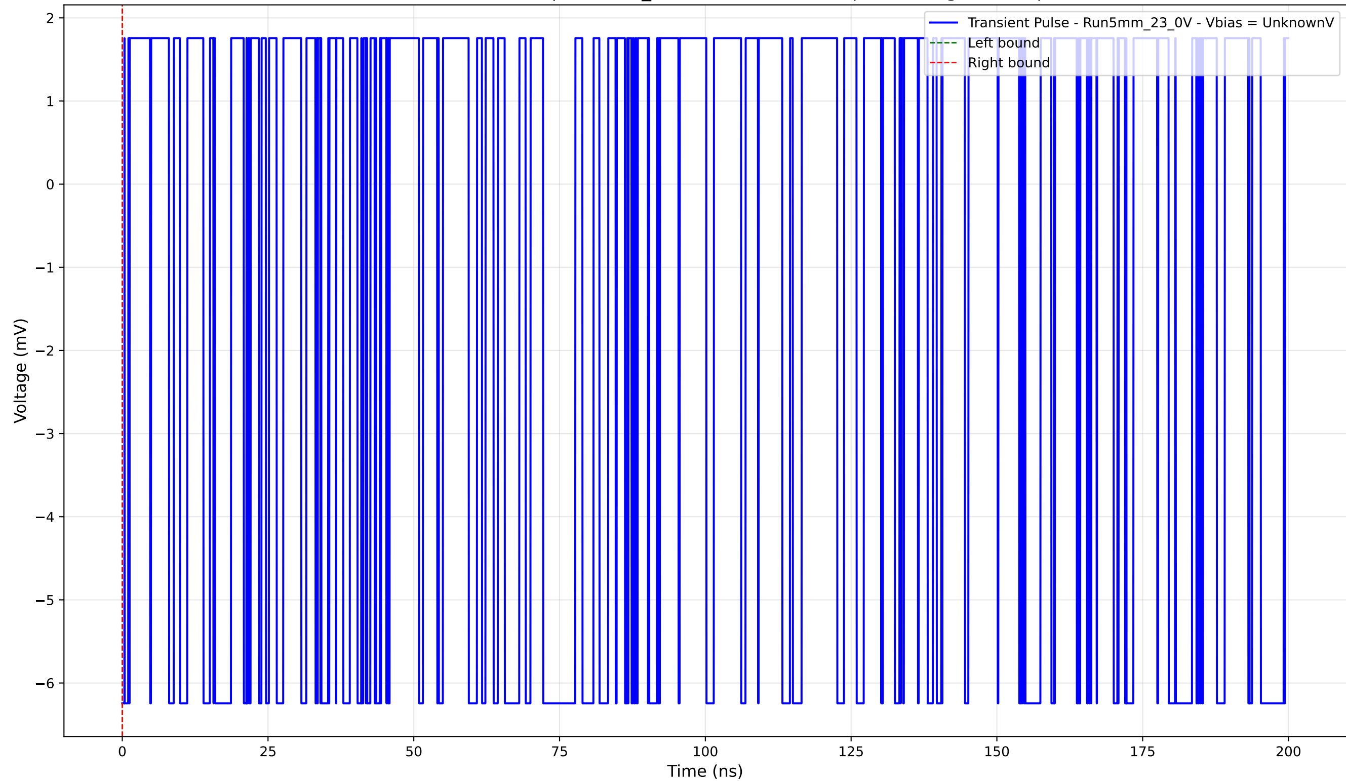
Transient Pulse - Sample: 5mm_23 - Position: 3015.0 \mu\text{m} - Charge: -0.00 pC
