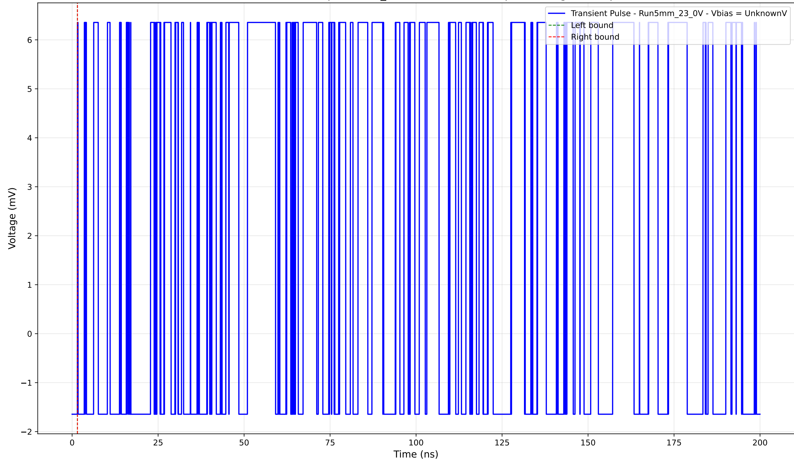
Transient Pulse - Sample: 5mm_23 - Position: 4760.0 \mu\text{m} - Charge: 0.00 pC
