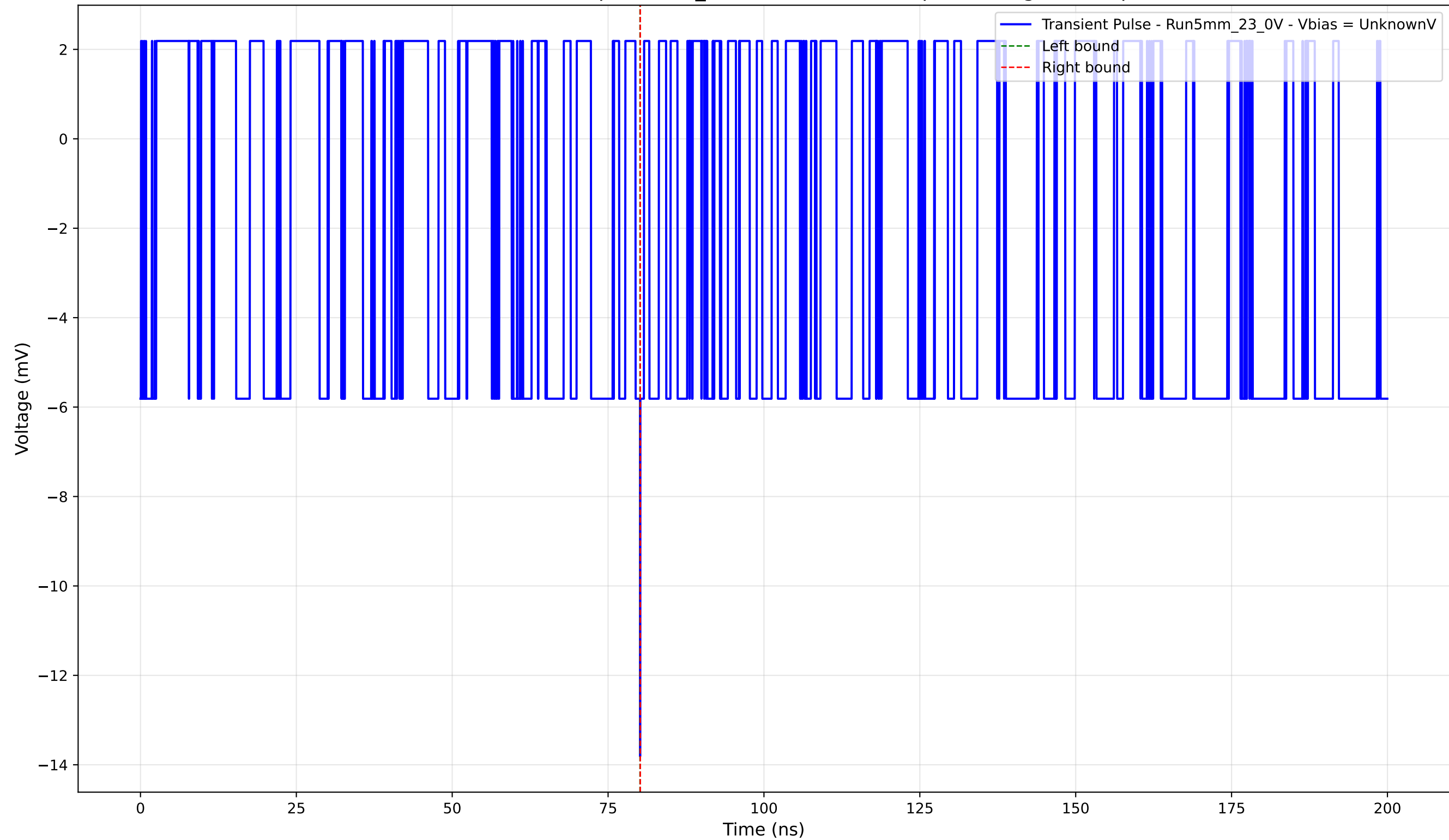
Transient Pulse - Sample: 5mm_23 - Position: 3335.0 \mu\text{m} - Charge: -0.01 pC
