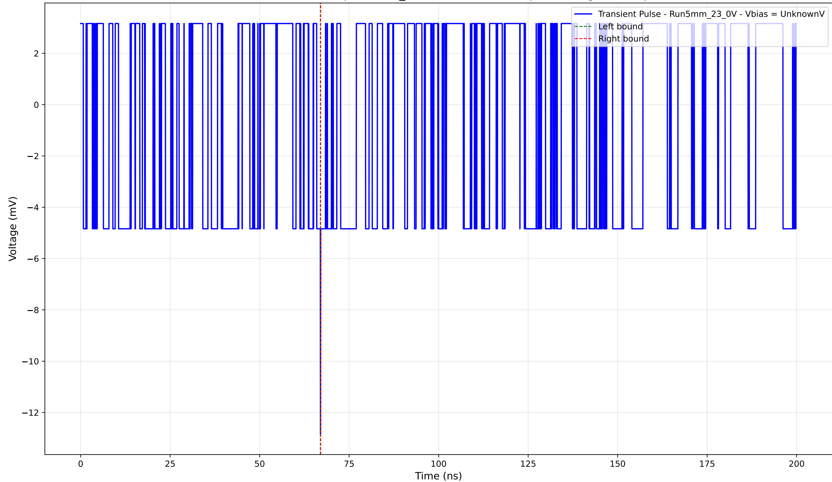
Transient Pulse - Sample: 5mm_23 - Position: 1485.0 \mu\text{m} - Charge: -0.02 pC
