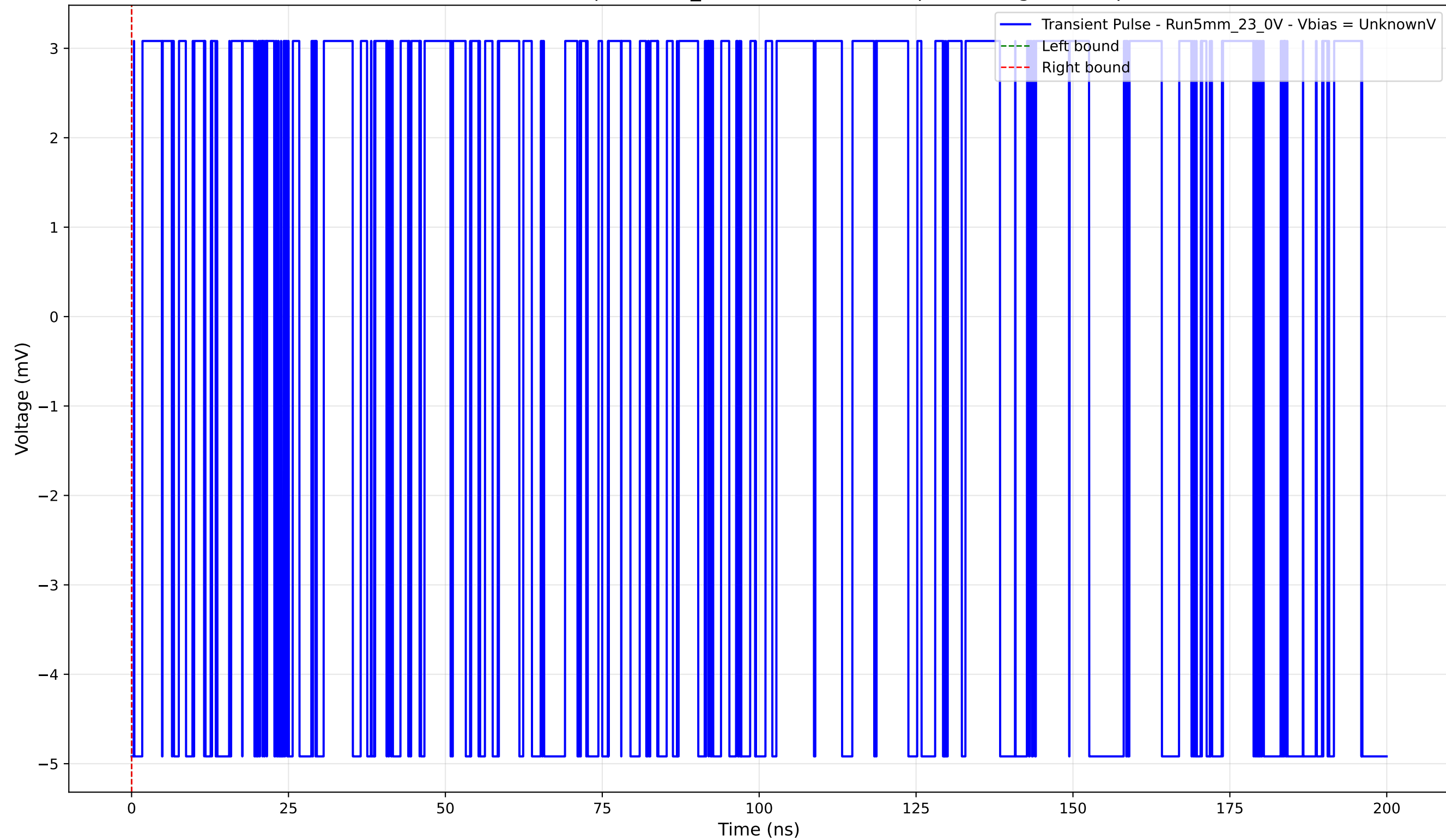
Transient Pulse - Sample: 5mm_23 - Position: 1395.0 \mu\text{m} - Charge: -0.00 pC
