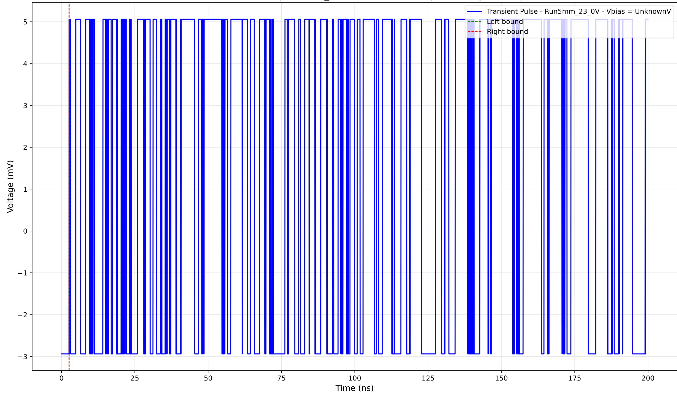
Transient Pulse - Sample: 5mm_23 - Position: 1625.0 \mu\text{m} - Charge: 0.00 pC
