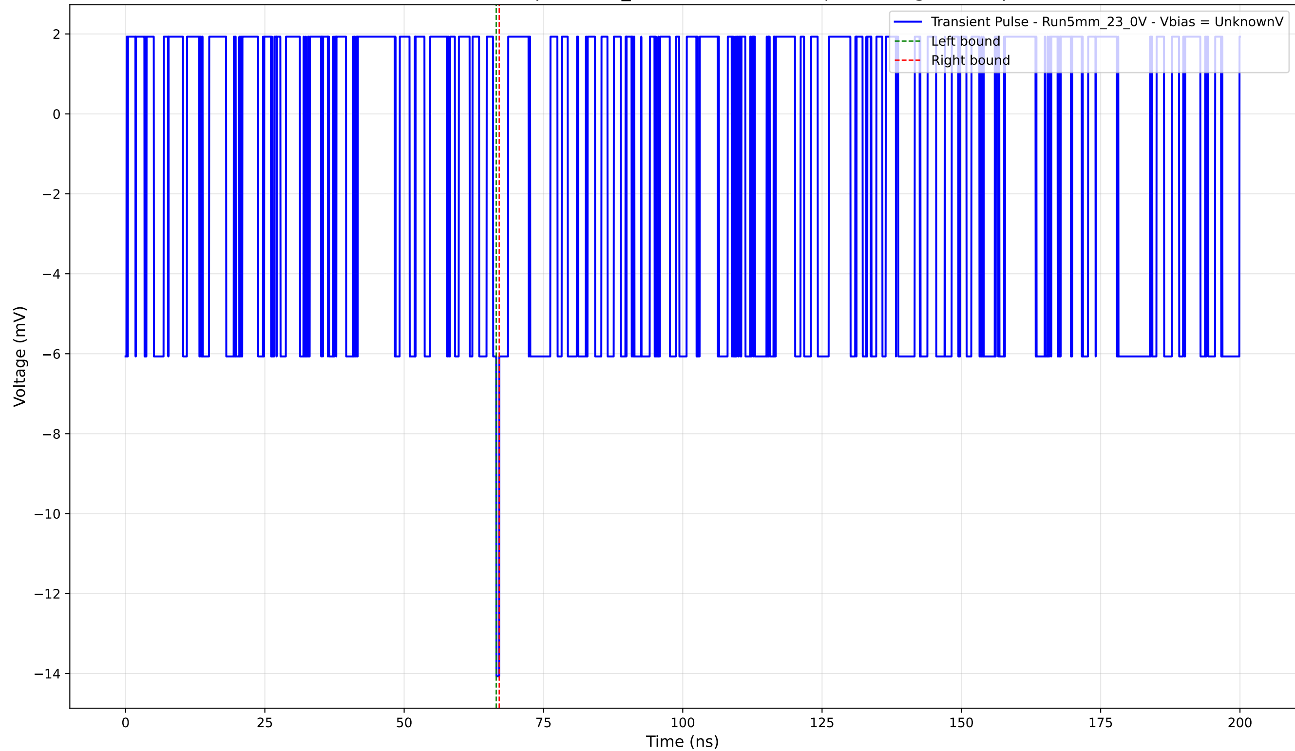
Transient Pulse - Sample: 5mm_23 - Position: 1720.0 \mu\text{m} - Charge: -0.15 pC
