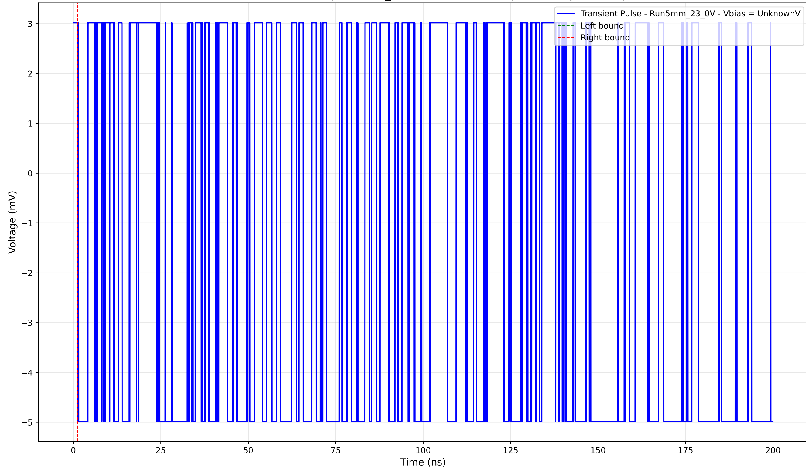
Transient Pulse - Sample: 5mm_23 - Position: 1150.0 \mu\text{m} - Charge: -0.00 pC
