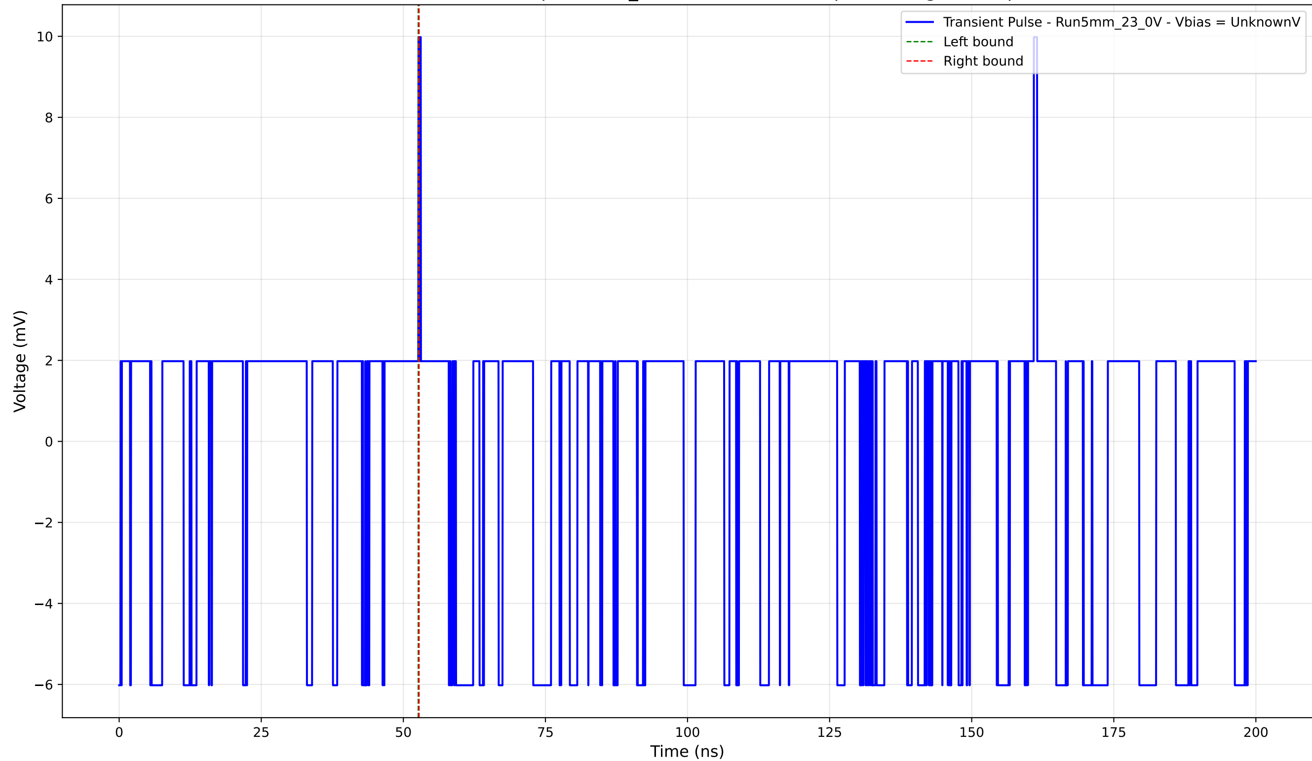
Transient Pulse - Sample: 5mm_23 - Position: 2720.0 \mu\text{m} - Charge: 0.02 pC
