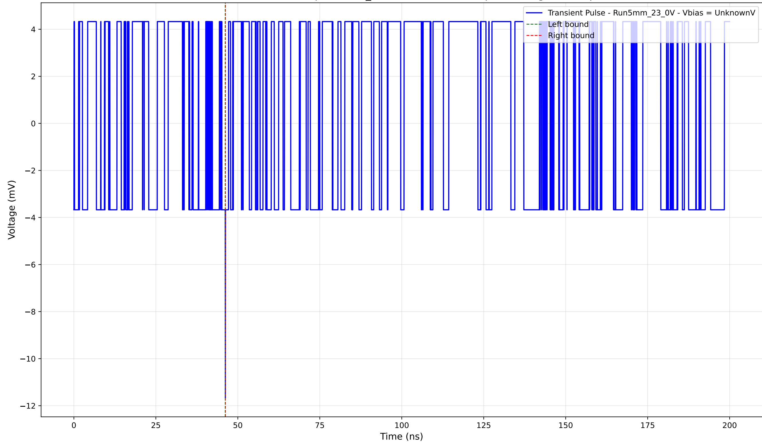
Transient Pulse - Sample: 5mm_23 - Position: 3890.0 \mu\text{m} - Charge: -0.01 pC
