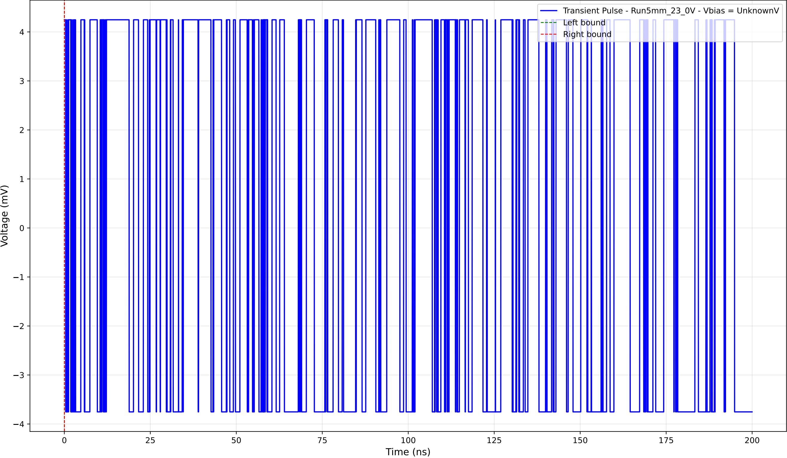
Transient Pulse - Sample: 5mm_23 - Position: 730.0 \mu\text{m} - Charge: 0.00 pC
