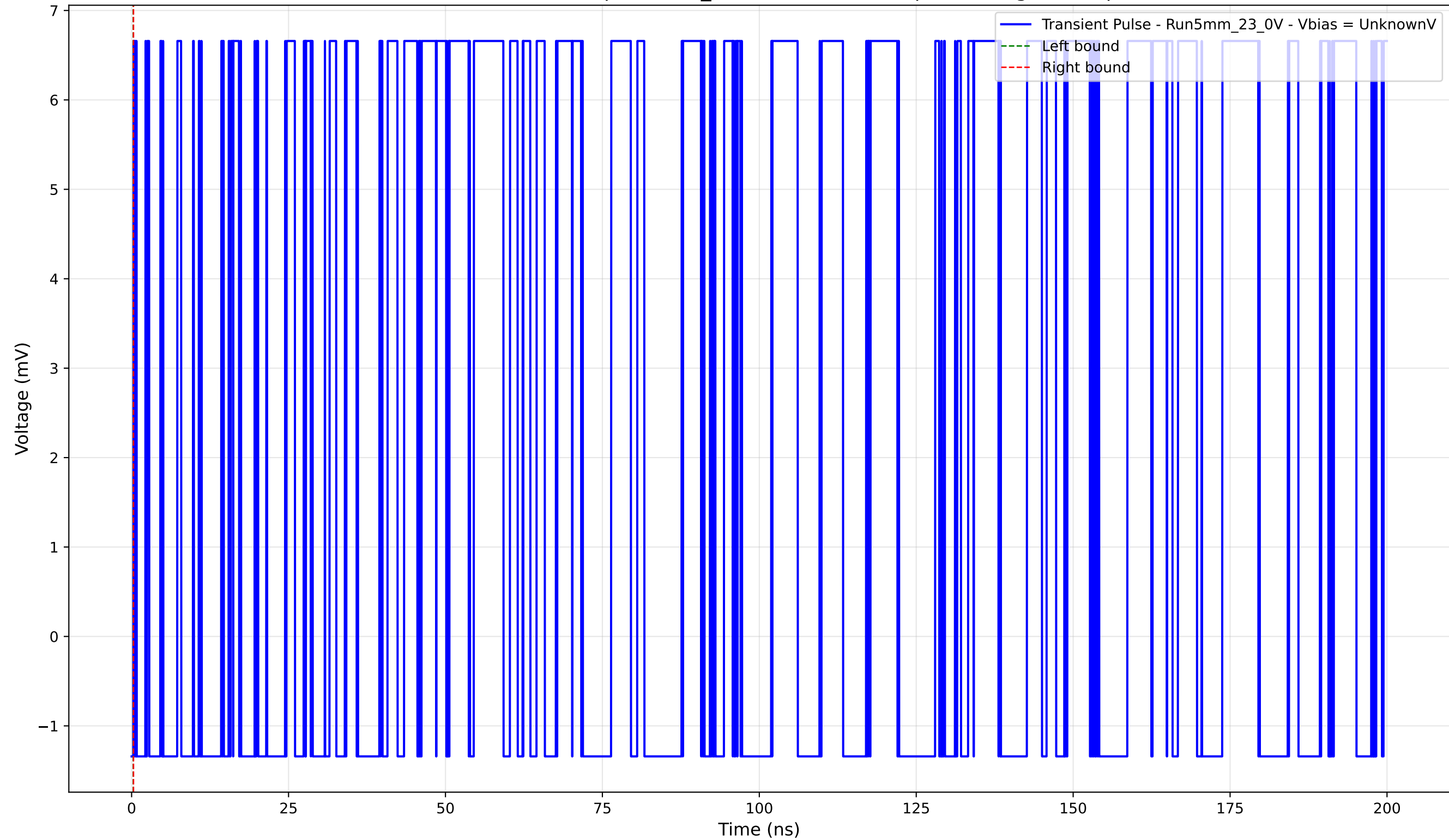
Transient Pulse - Sample: 5mm_23 - Position: 320.0 \mu\text{m} - Charge: 0.00 pC
