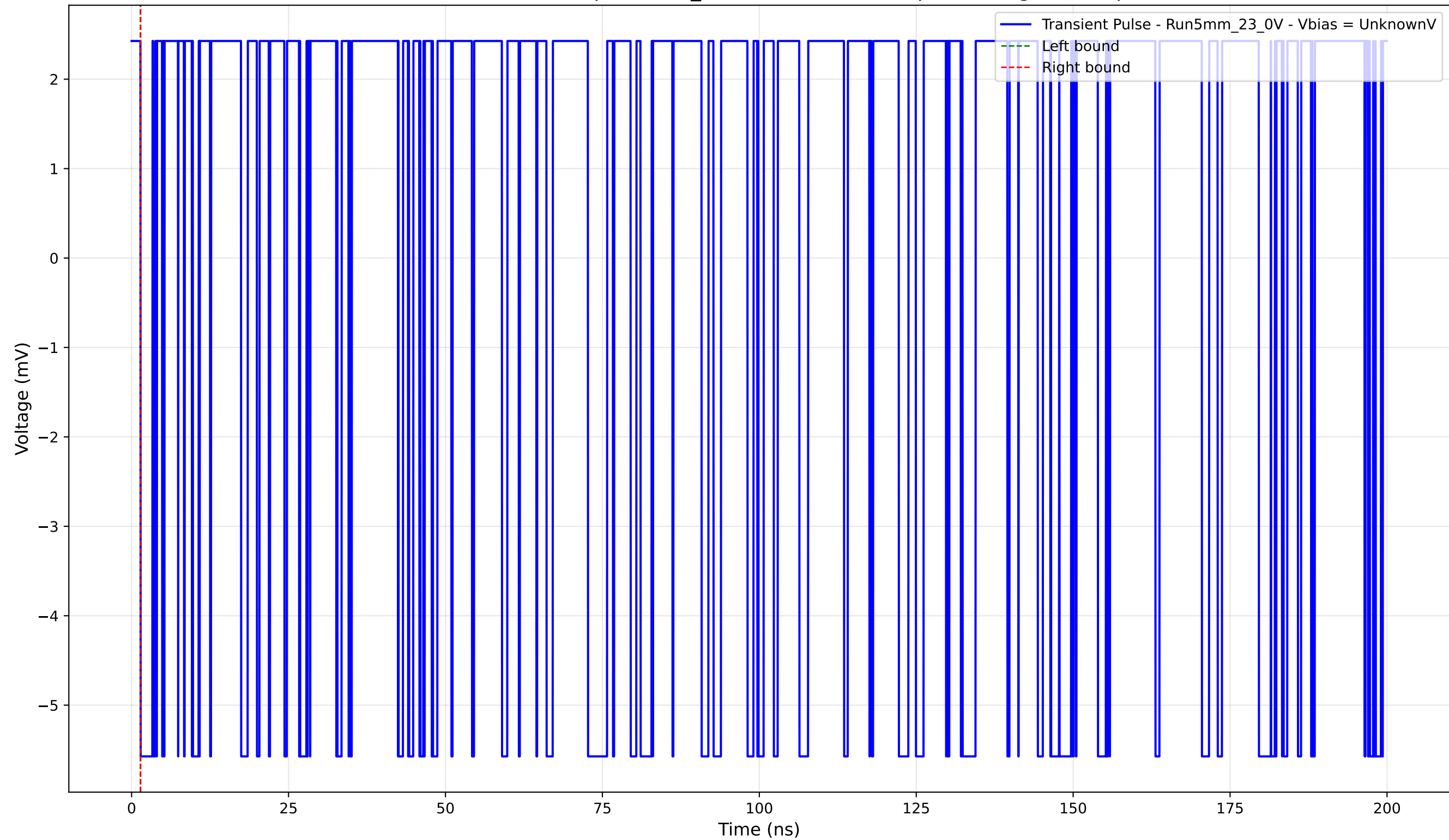
Transient Pulse - Sample: 5mm_23 - Position: 3485.0 \mu\text{m} - Charge: -0.00 pC
