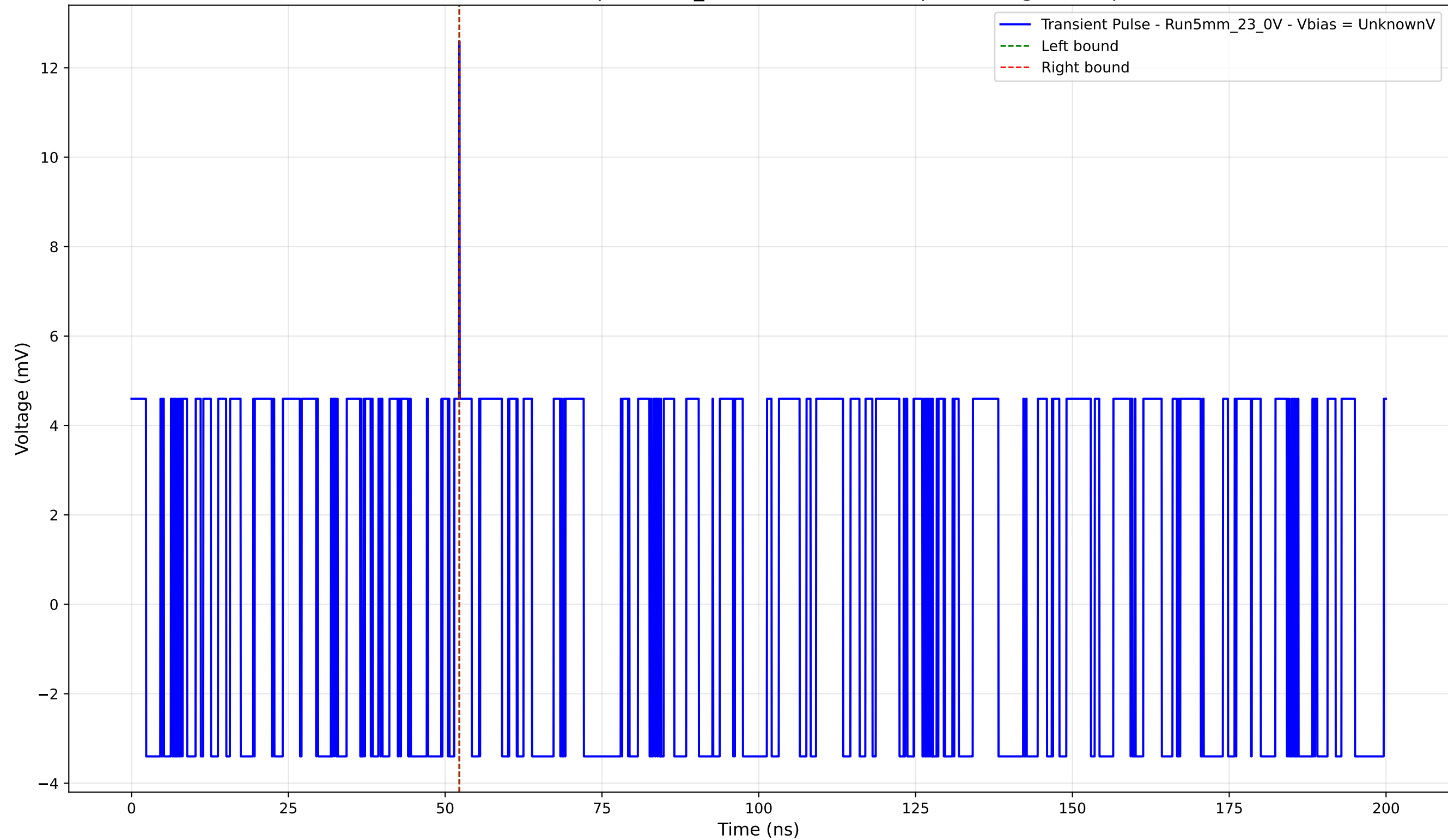
Transient Pulse - Sample: 5mm_23 - Position: 1760.0 \mu\text{m} - Charge: 0.02 pC
