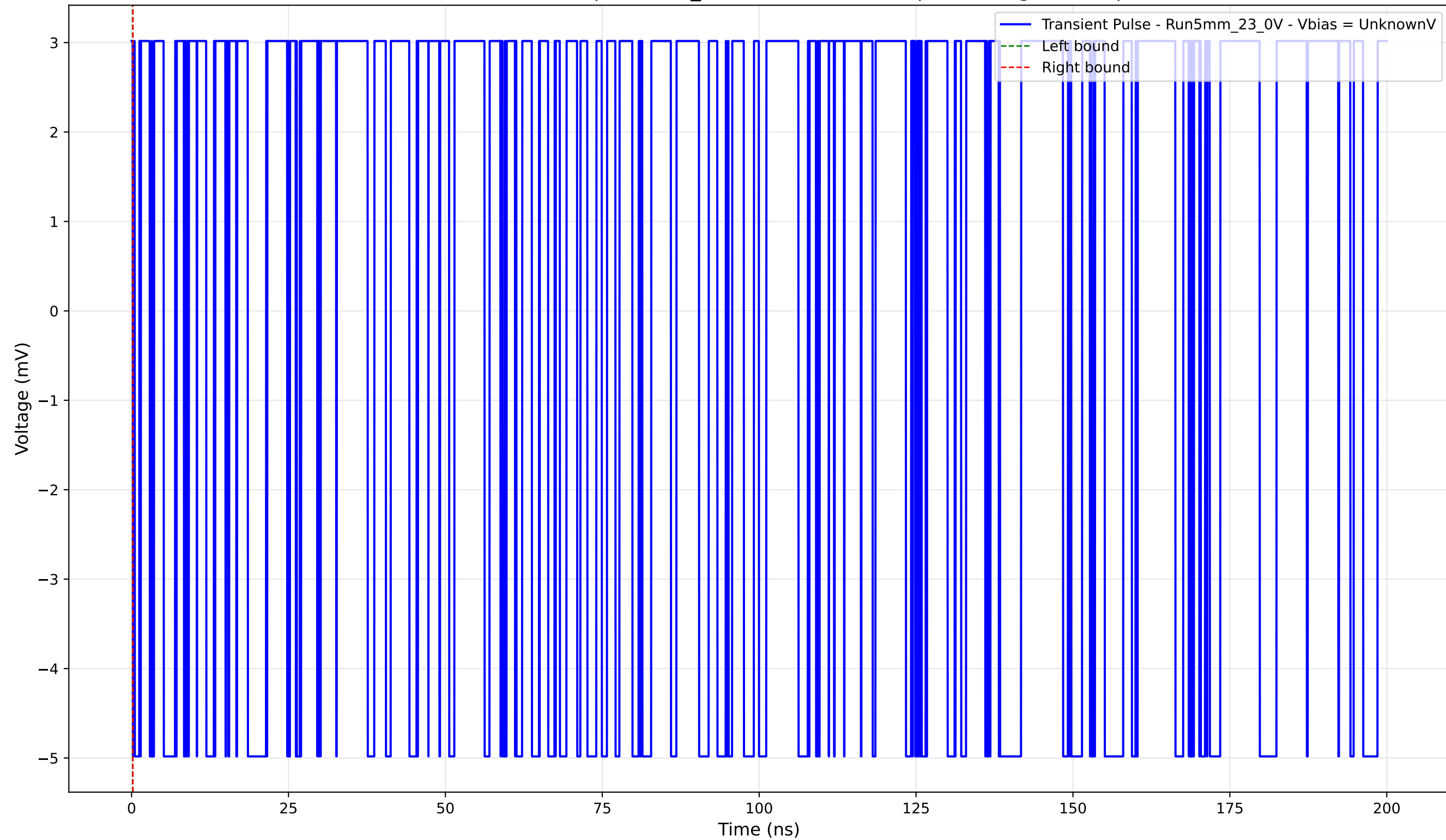
Transient Pulse - Sample: 5mm_23 - Position: 3690.0 \mu\text{m} - Charge: -0.00 pC
