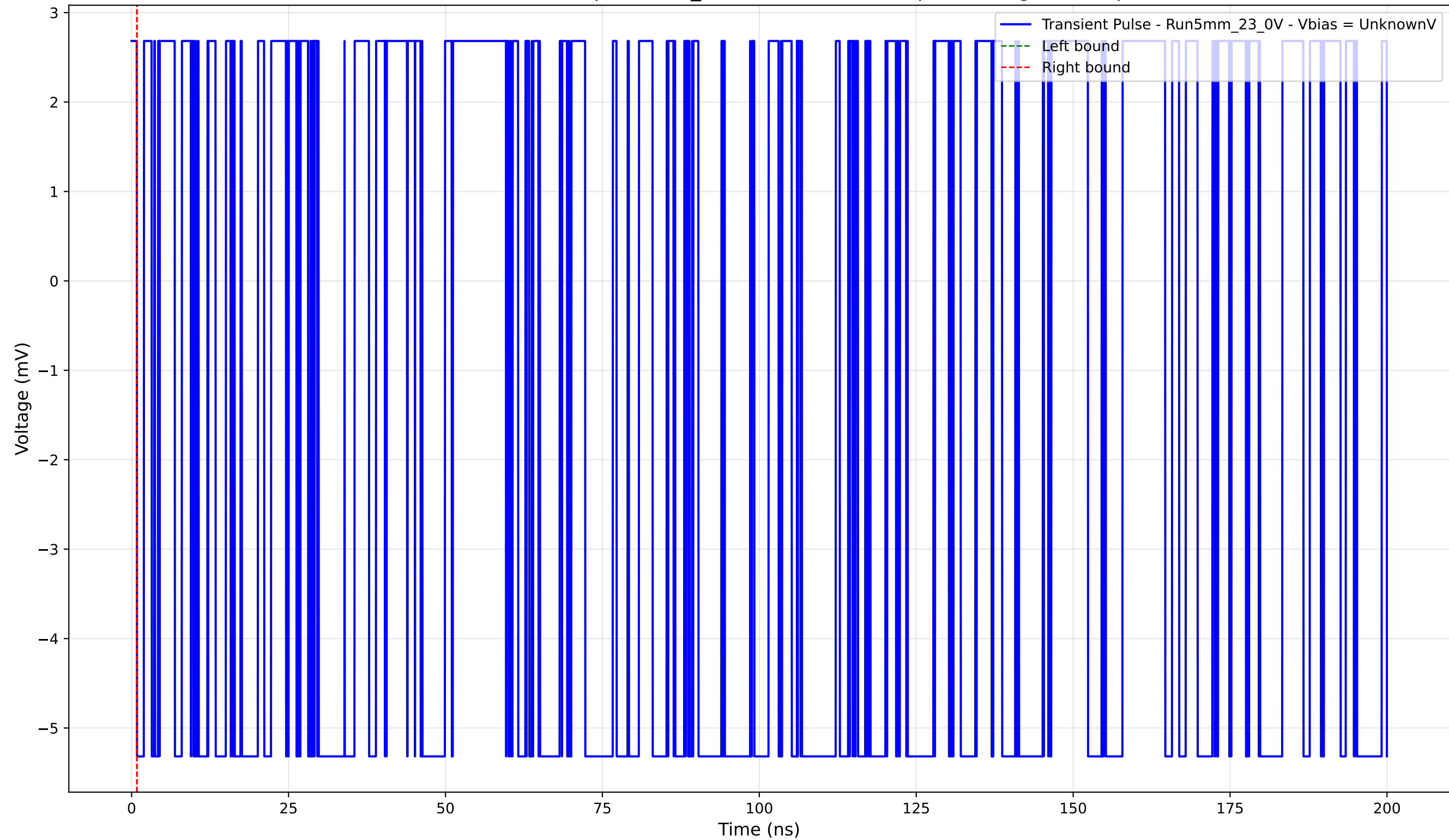
Transient Pulse - Sample: 5mm_23 - Position: 4450.0 \mu\text{m} - Charge: -0.00 pC
