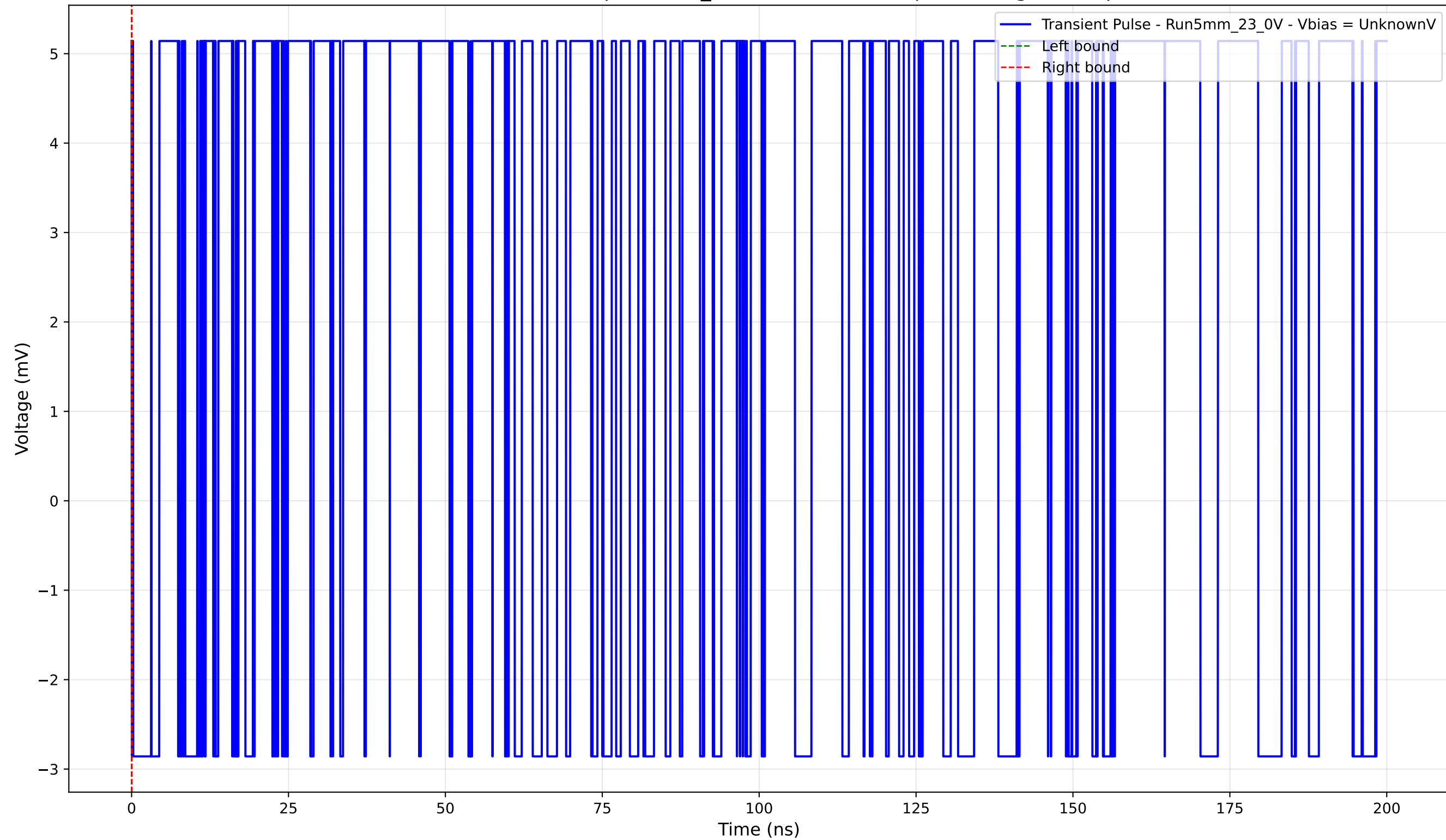
Transient Pulse - Sample: 5mm_23 - Position: 490.0 \mu\text{m} - Charge: 0.00 pC
