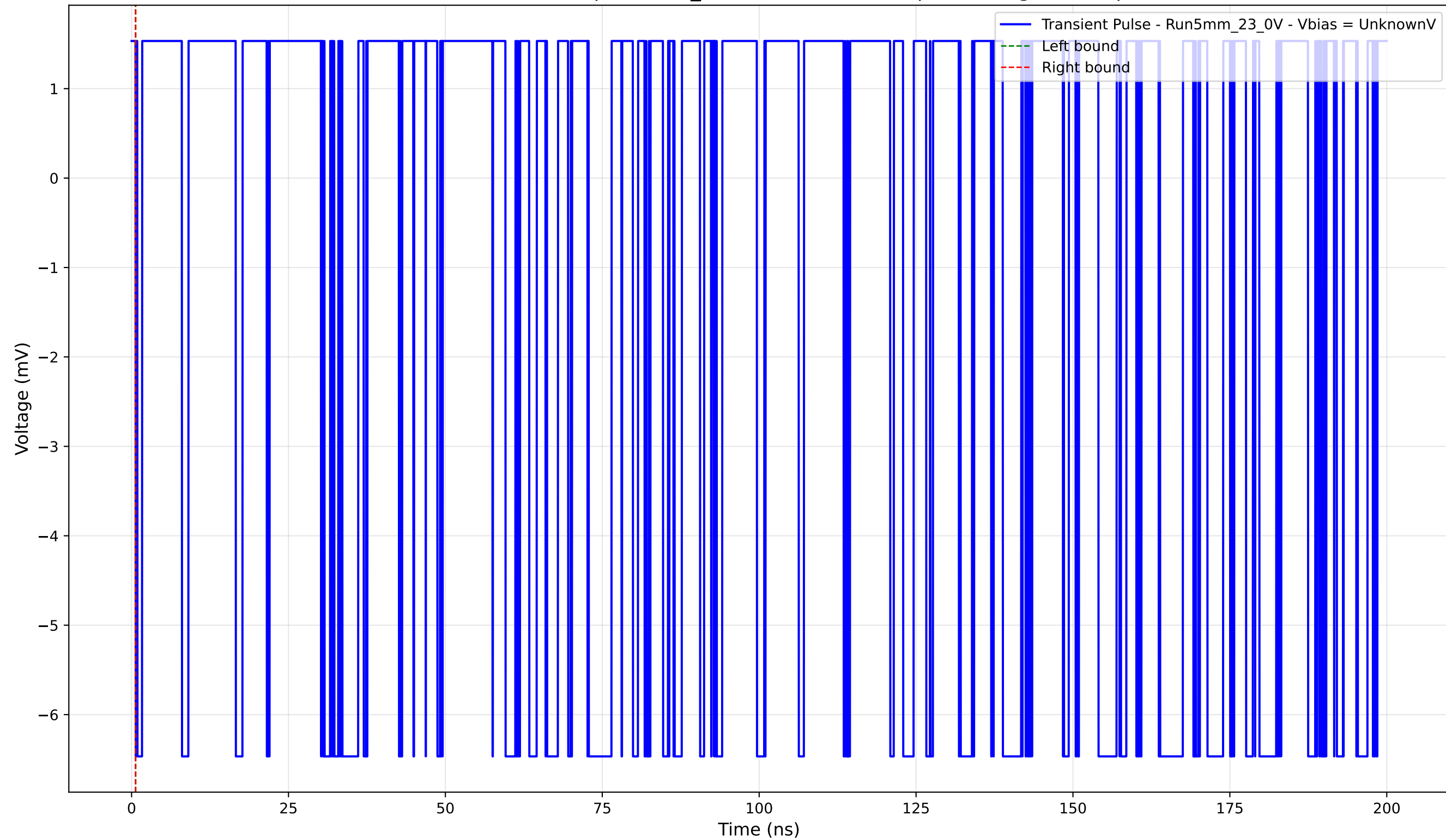
Transient Pulse - Sample: 5mm_23 - Position: 3255.0 \mu\text{m} - Charge: -0.00 pC
