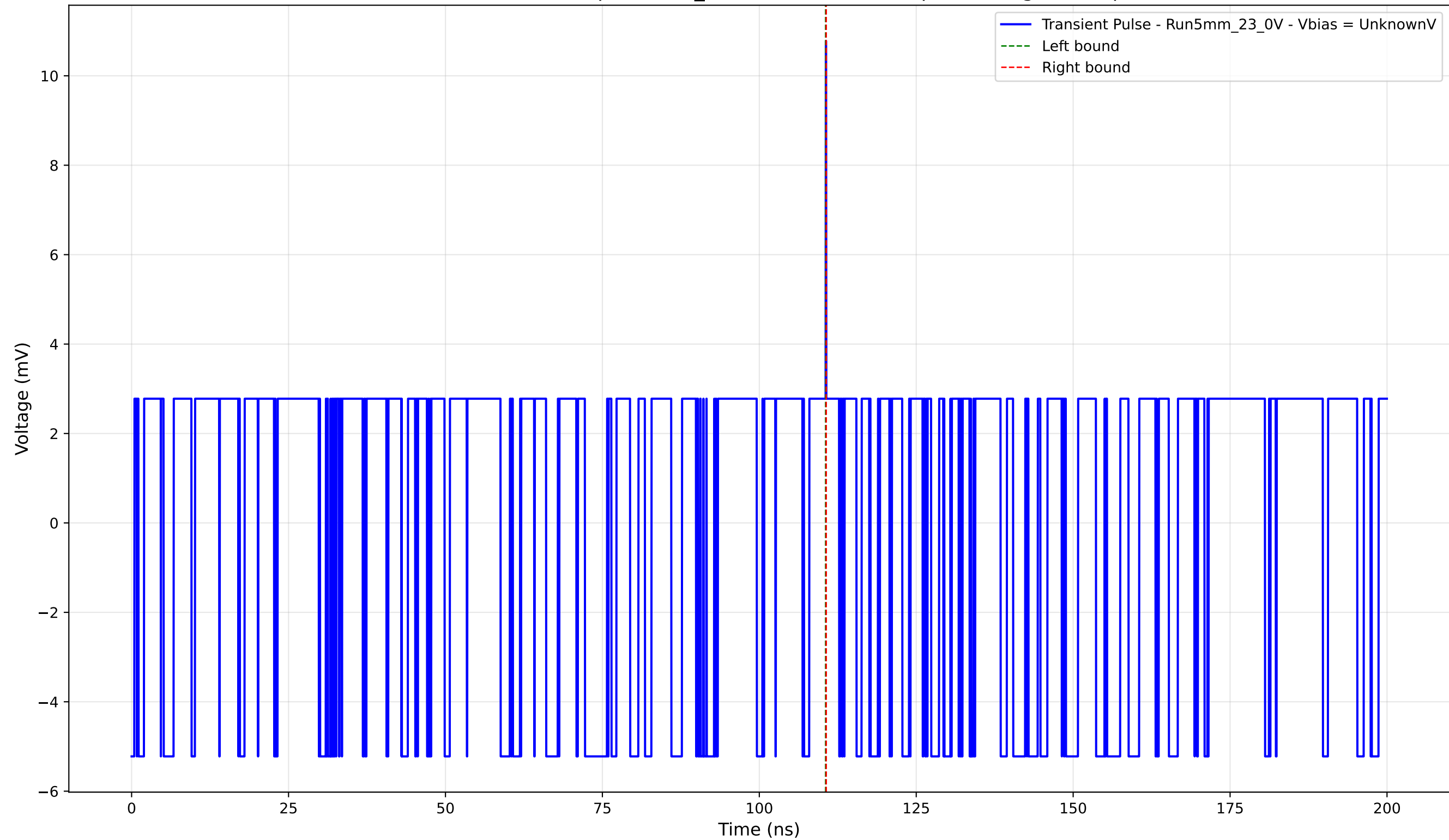
Transient Pulse - Sample: 5mm_23 - Position: 3350.0 \mu\text{m} - Charge: 0.02 pC
