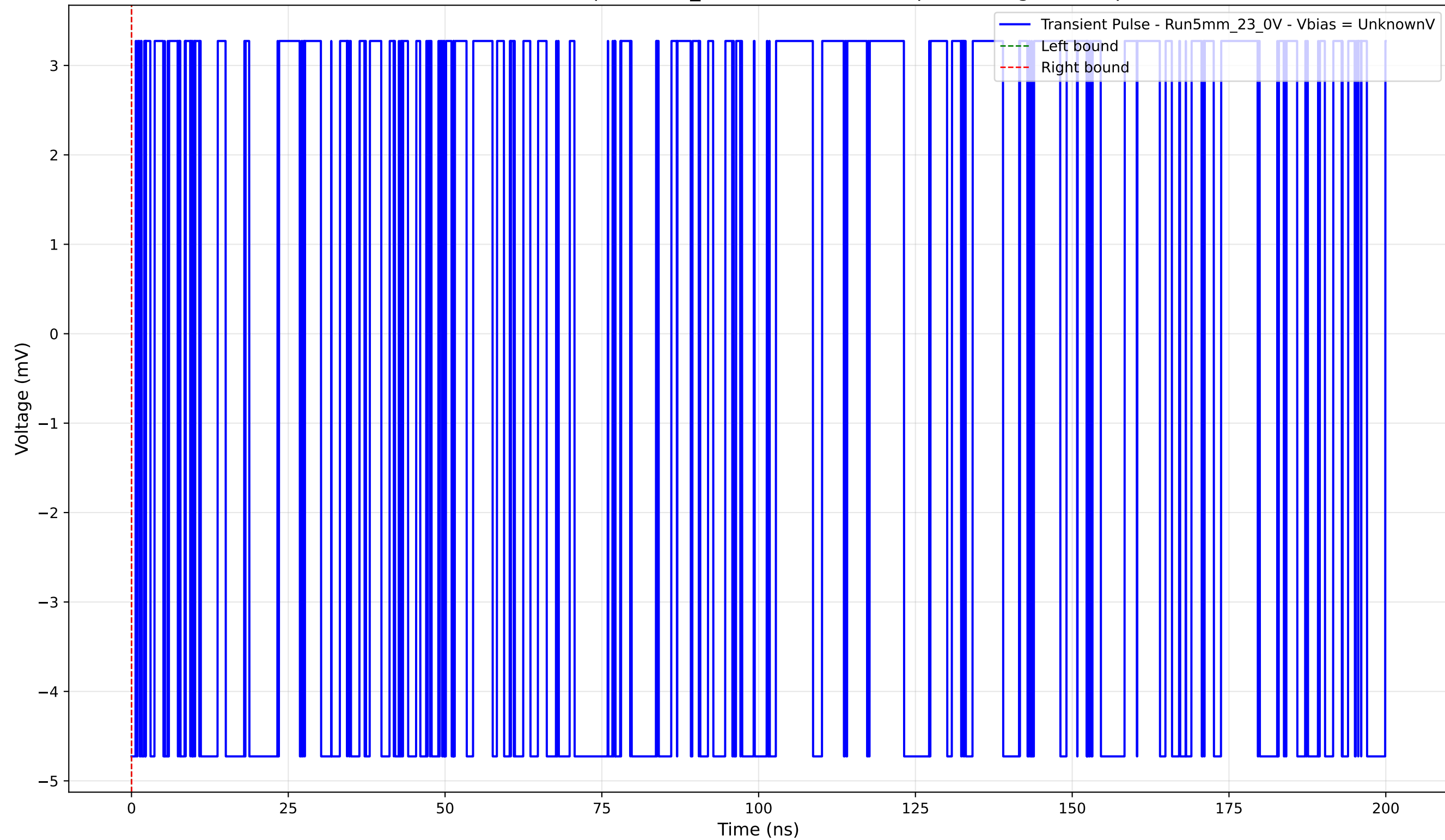
Transient Pulse - Sample: 5mm_23 - Position: 1045.0 \mu\text{m} - Charge: -0.00 pC
