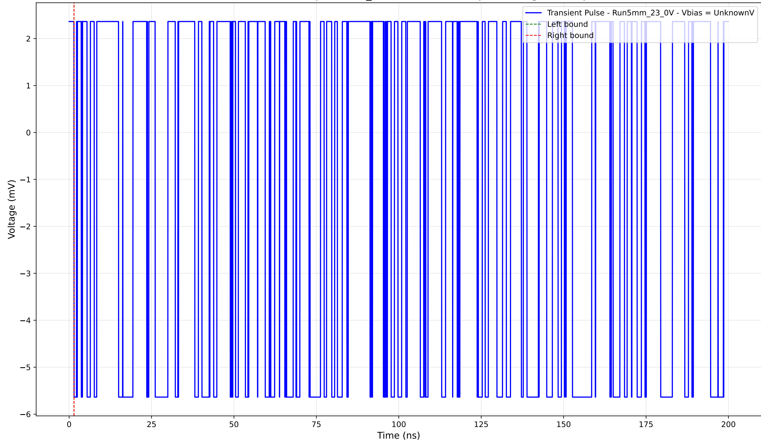
Transient Pulse - Sample: 5mm_23 - Position: 680.0 \mu\text{m} - Charge: -0.00 pC
