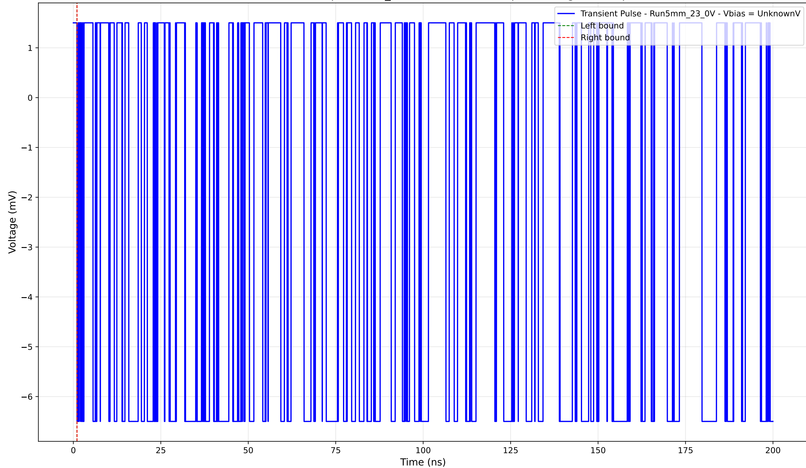
Transient Pulse - Sample: 5mm_23 - Position: 3725.0 \mu\text{m} - Charge: -0.00 pC
