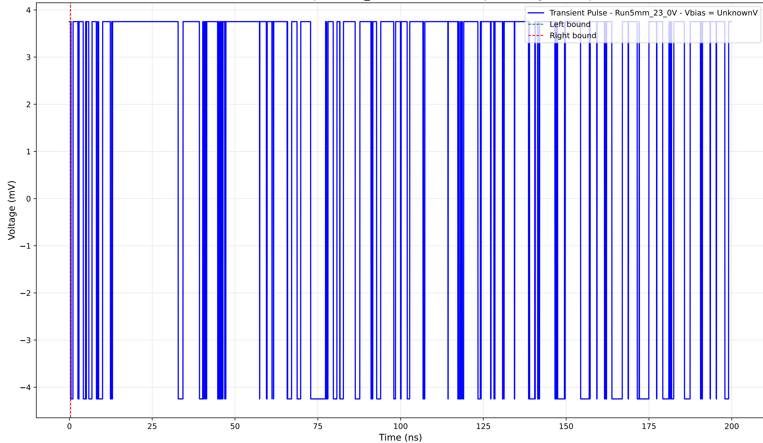
Transient Pulse - Sample: 5mm_23 - Position: 2655.0 \mu\text{m} - Charge: -0.00 pC
