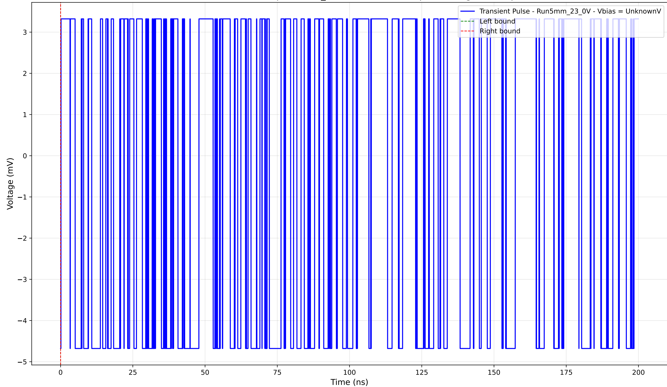
Transient Pulse - Sample: 5mm_23 - Position: 780.0 \mu\text{m} - Charge: -0.00 pC
