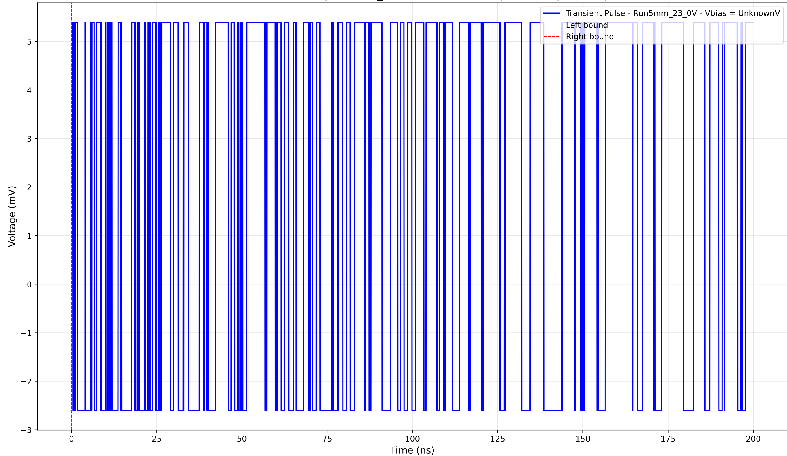
Transient Pulse - Sample: 5mm_23 - Position: 3465.0 \mu\text{m} - Charge: 0.00 pC
