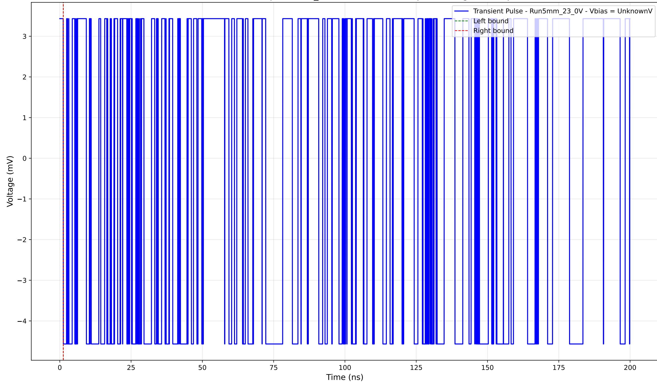
Transient Pulse - Sample: 5mm_23 - Position: 1060.0 \mu\text{m} - Charge: -0.00 pC
