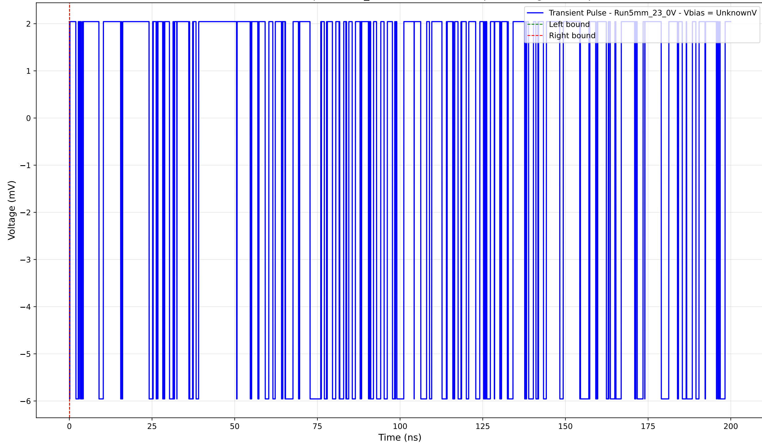
Transient Pulse - Sample: 5mm_23 - Position: 2805.0 \mu\text{m} - Charge: -0.00 pC
