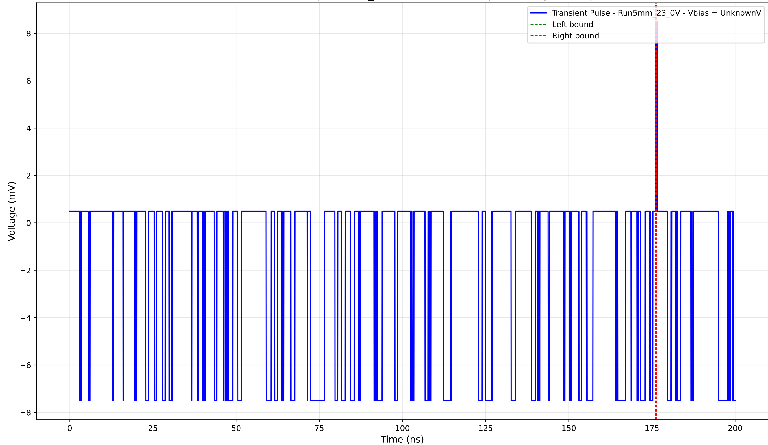
Transient Pulse - Sample: 5mm_23 - Position: 2680.0 \mu\text{m} - Charge: 0.07 pC
