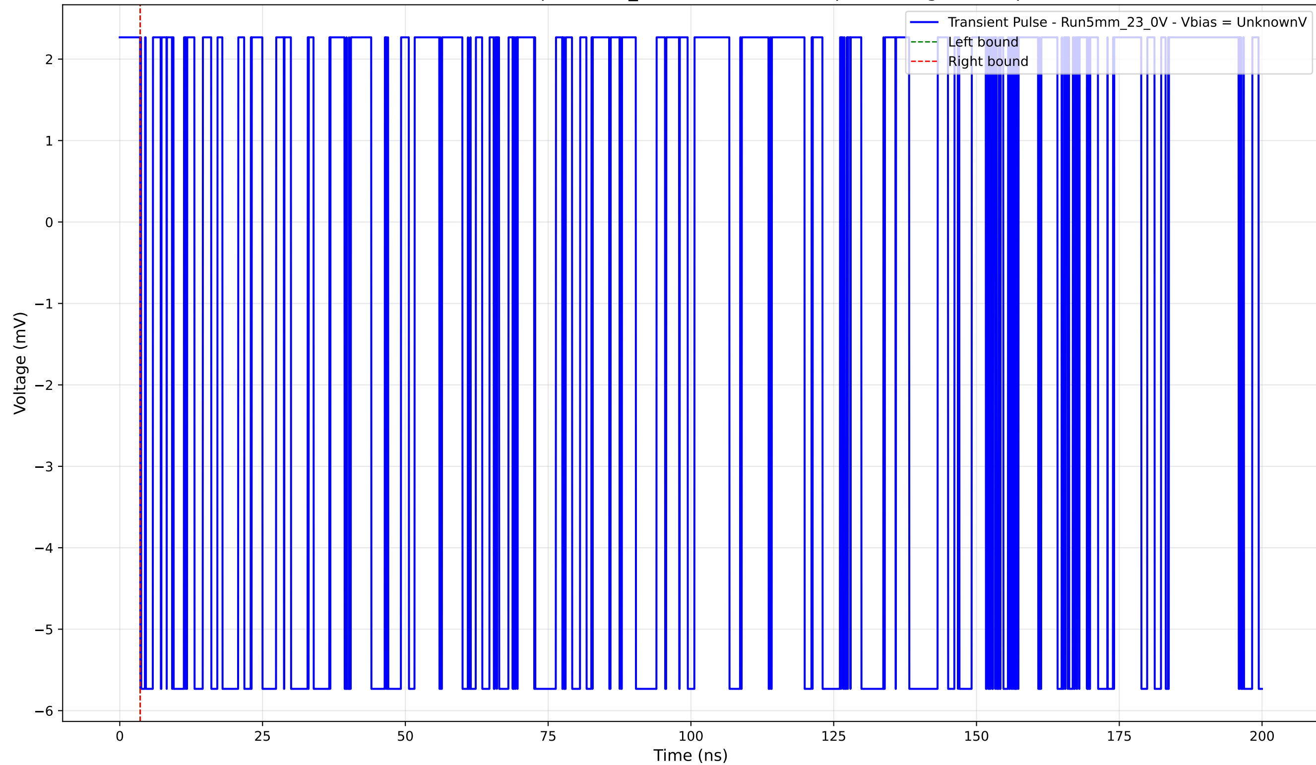
Transient Pulse - Sample: 5mm_23 - Position: 3555.0 \mu\text{m} - Charge: -0.00 pC
