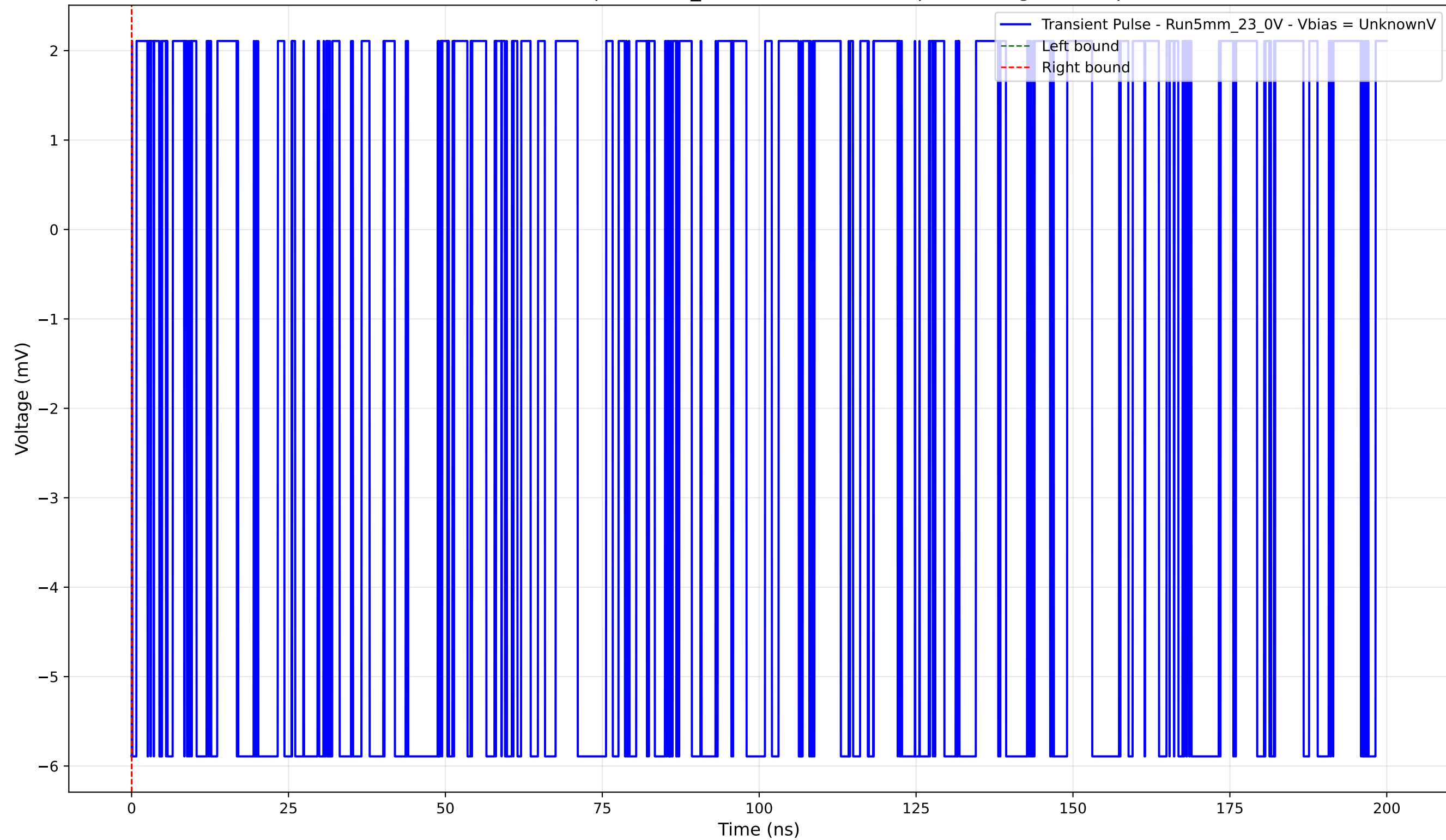
Transient Pulse - Sample: 5mm_23 - Position: 4350.0 \mu\text{m} - Charge: -0.00 pC
