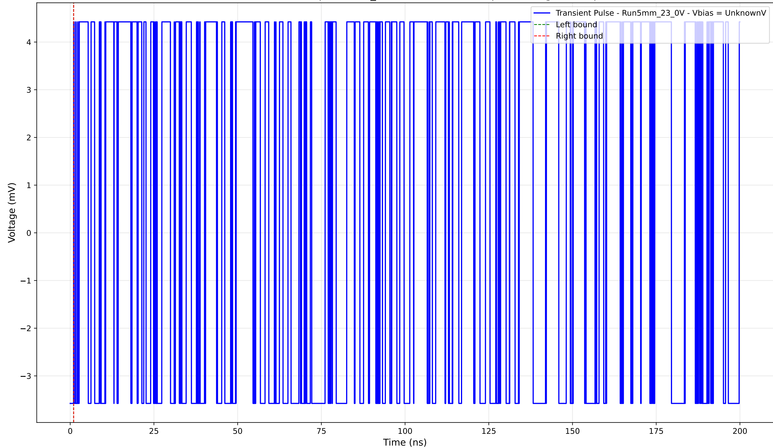
Transient Pulse - Sample: 5mm_23 - Position: 3520.0 \mu\text{m} - Charge: 0.00 pC
