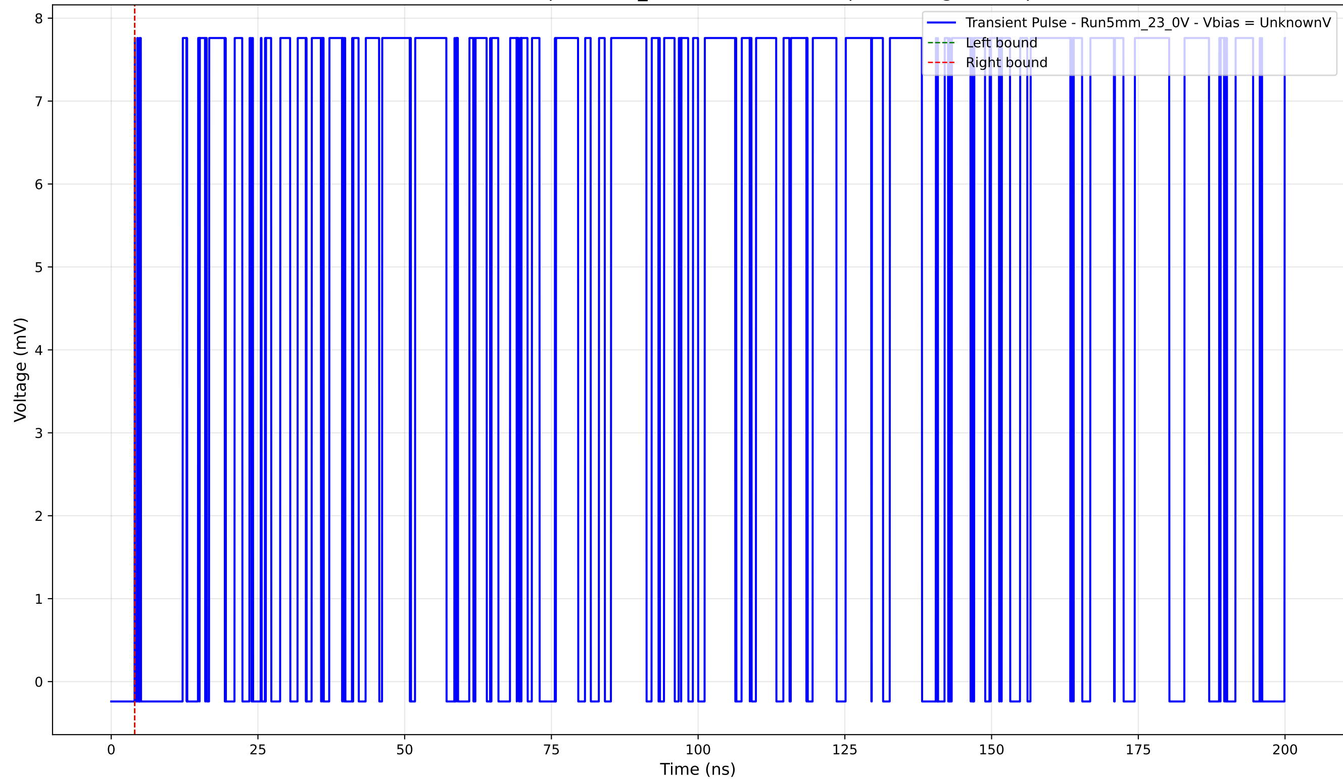
Transient Pulse - Sample: 5mm_23 - Position: 2325.0 \mu\text{m} - Charge: 0.00 pC
