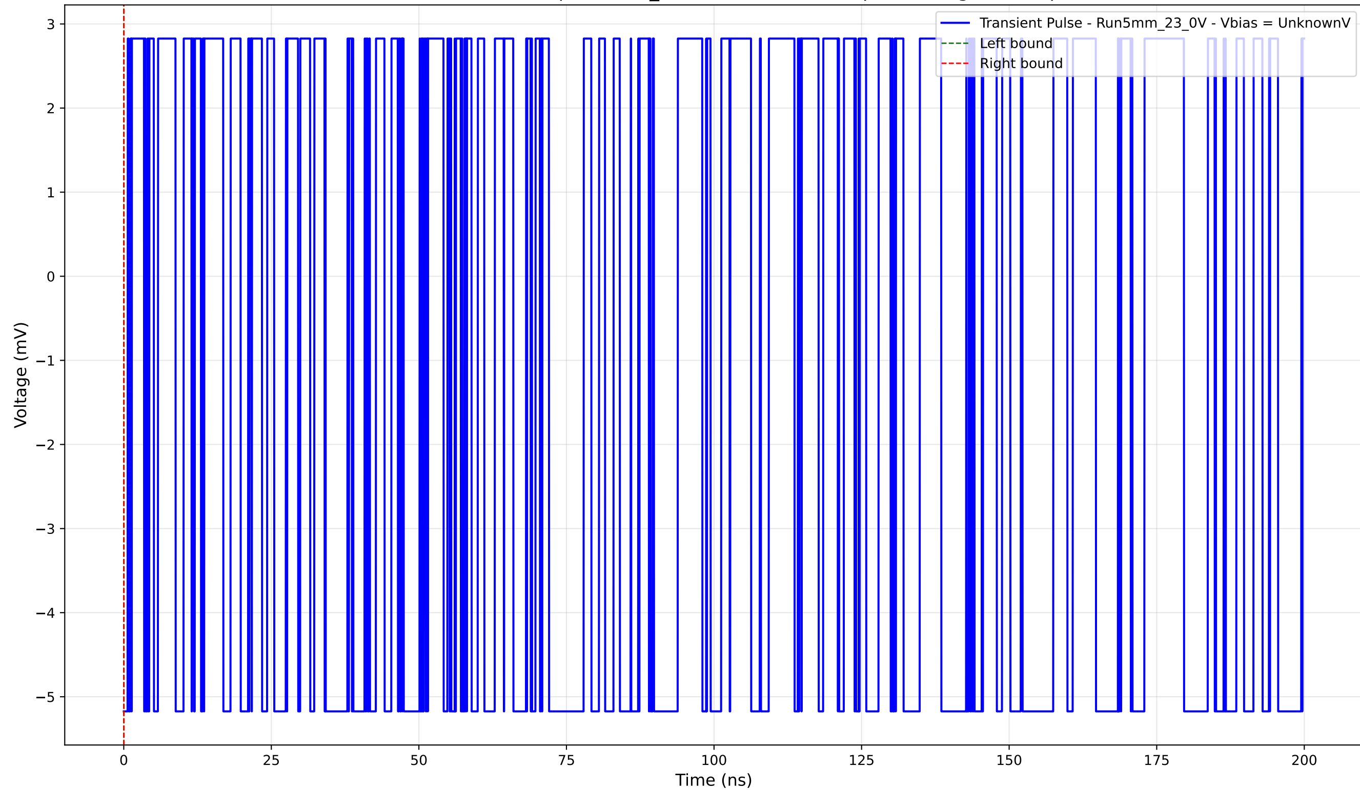
Transient Pulse - Sample: 5mm_23 - Position: 4405.0 \mu\text{m} - Charge: -0.00 pC
