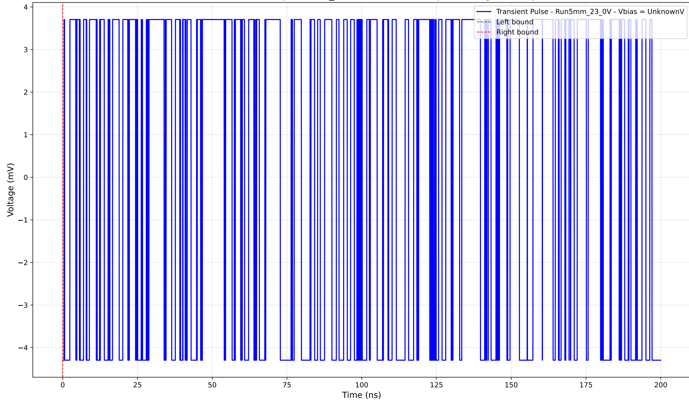
Transient Pulse - Sample: 5mm_23 - Position: 4630.0 \mu\text{m} - Charge: -0.00 pC
