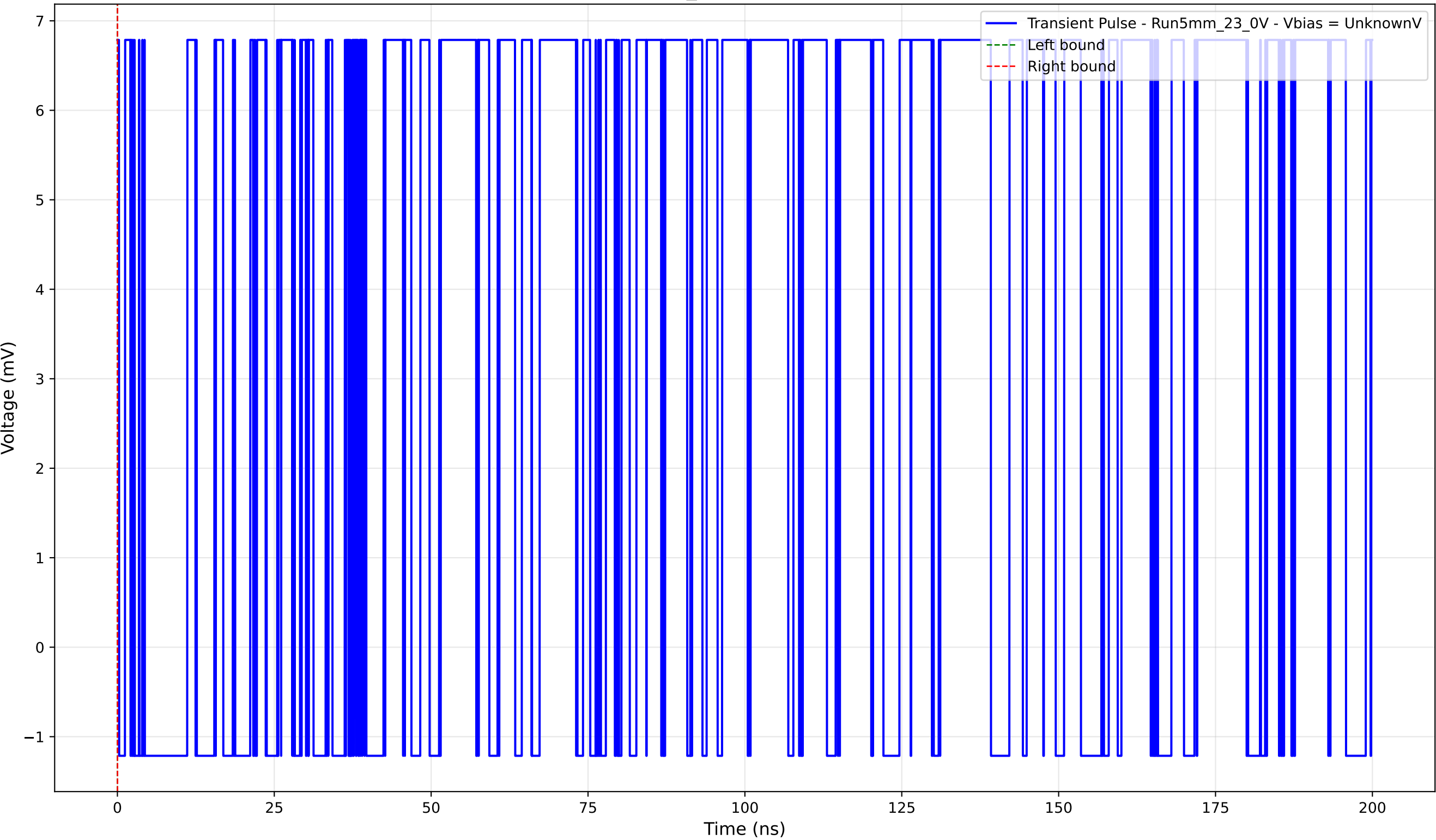
Transient Pulse - Sample: 5mm_23 - Position: 745.0 \mu\text{m} - Charge: 0.00 pC
