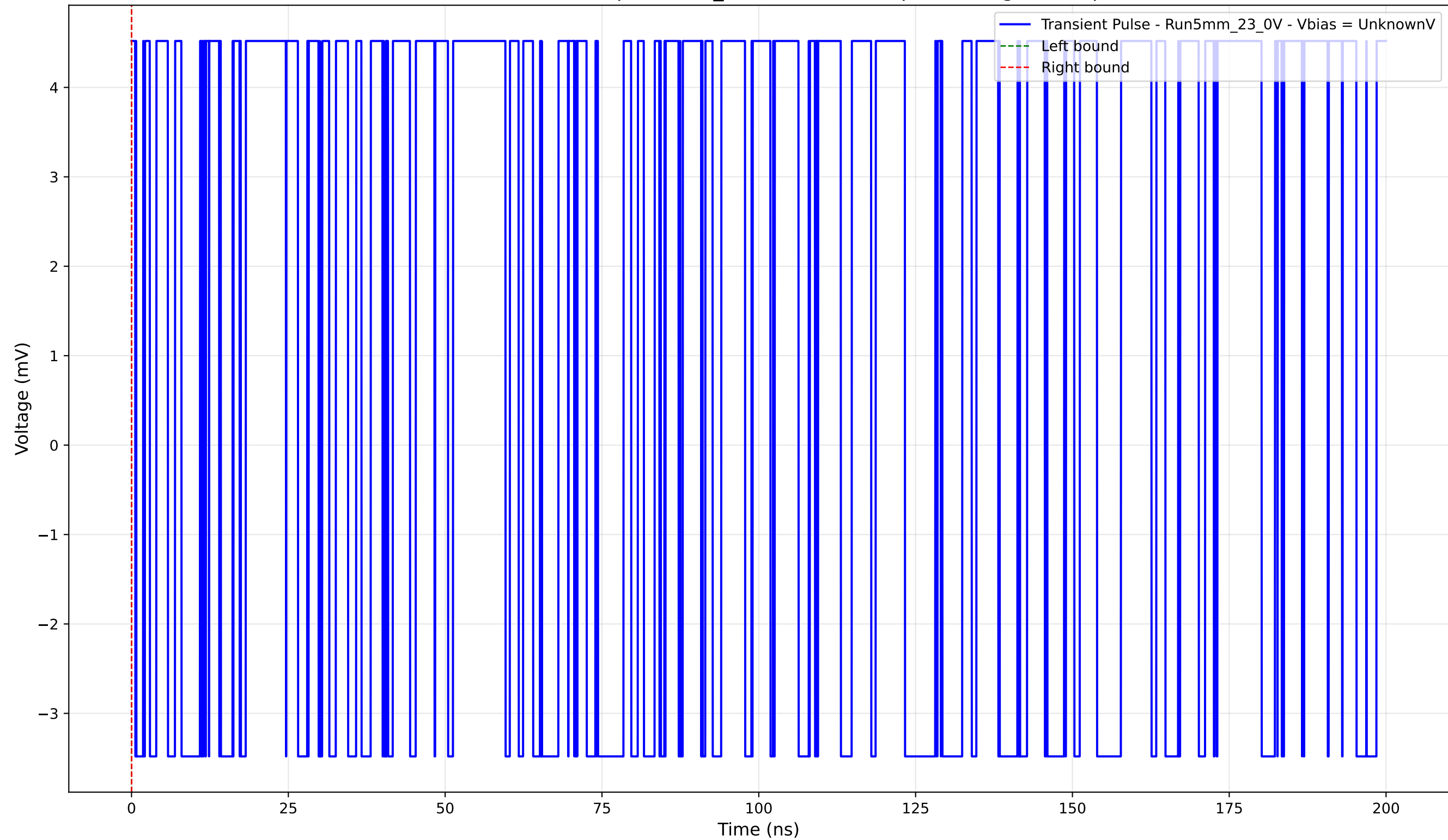
Transient Pulse - Sample: 5mm_23 - Position: 5.0 \mu\text{m} - Charge: 0.00 pC
