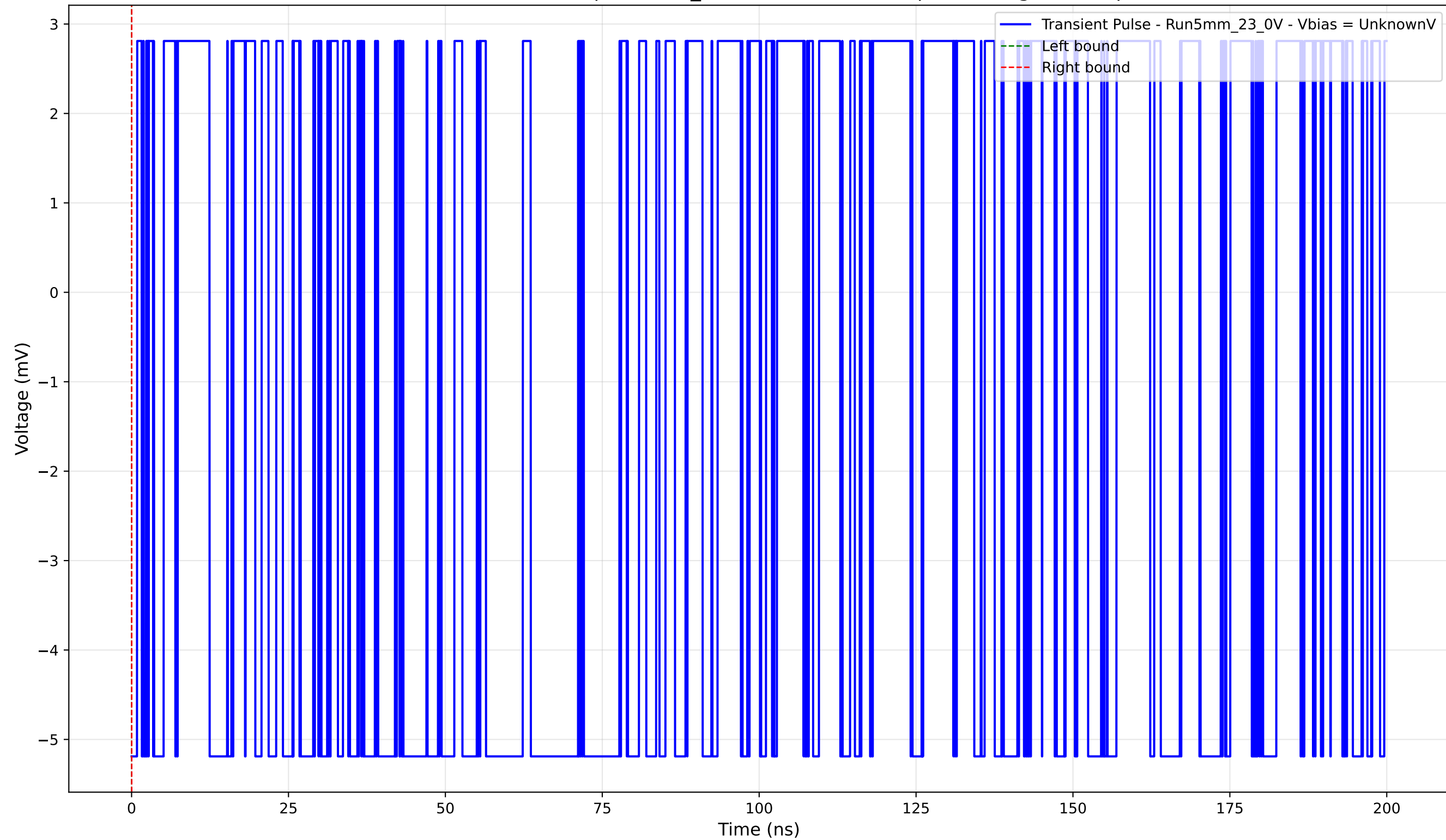
Transient Pulse - Sample: 5mm_23 - Position: 4600.0 \mu\text{m} - Charge: -0.00 pC
