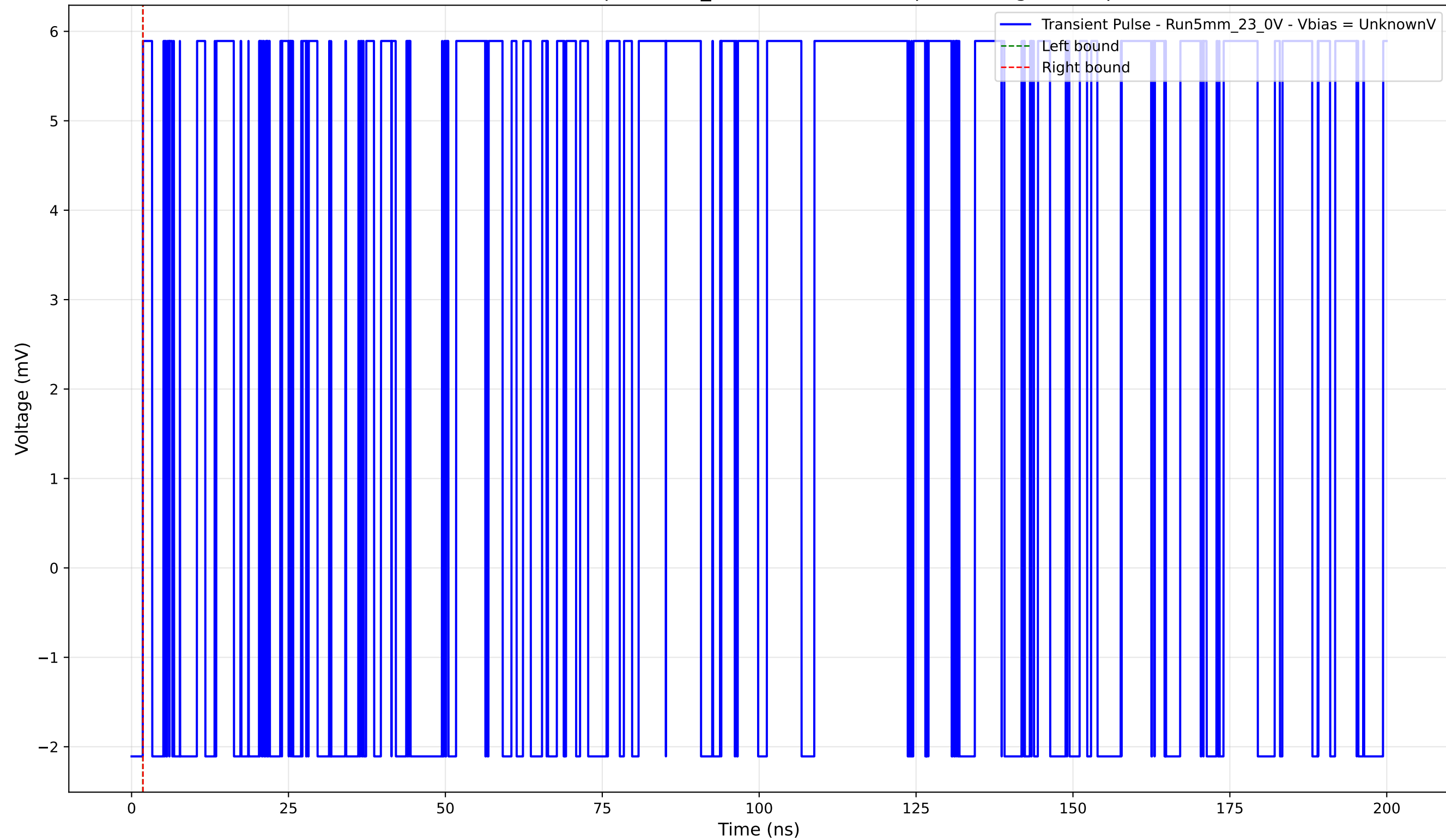
Transient Pulse - Sample: 5mm_23 - Position: 455.0 \mu\text{m} - Charge: 0.00 pC
