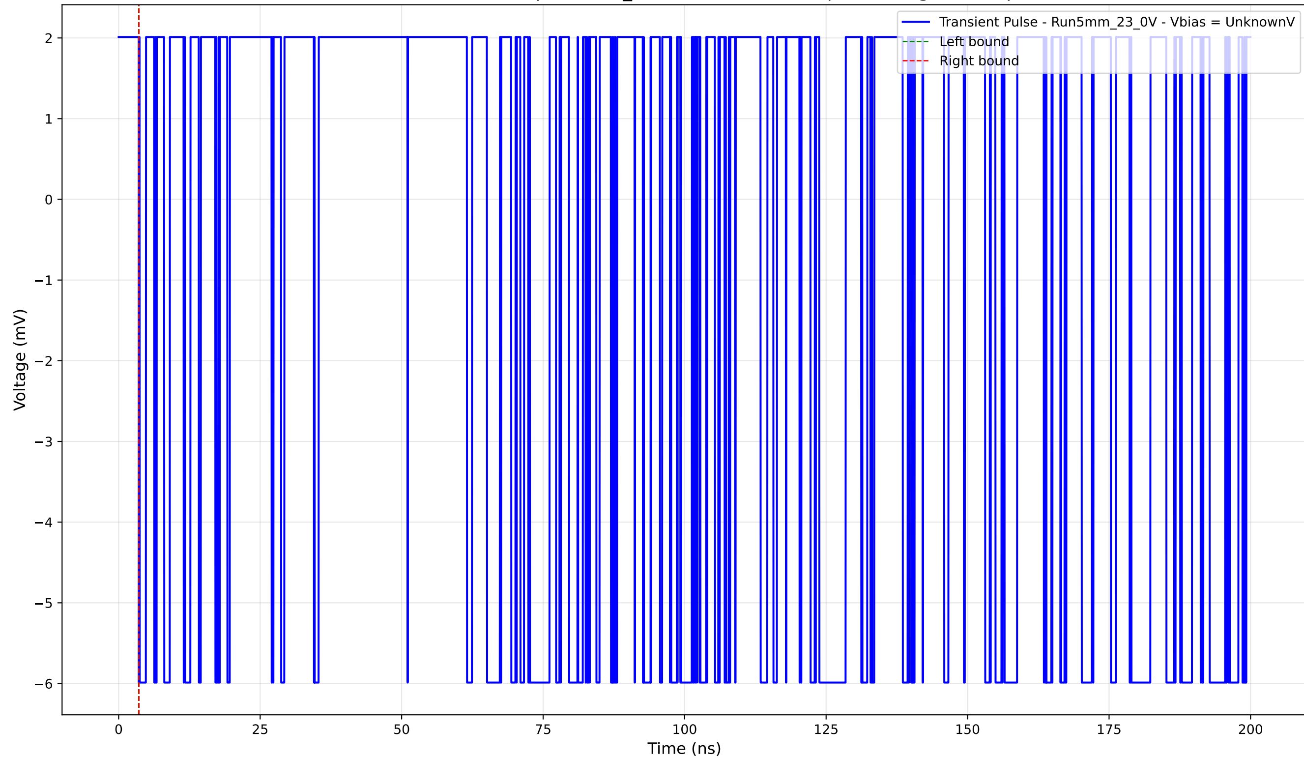
Transient Pulse - Sample: 5mm_23 - Position: 3940.0 \mu\text{m} - Charge: -0.00 pC
