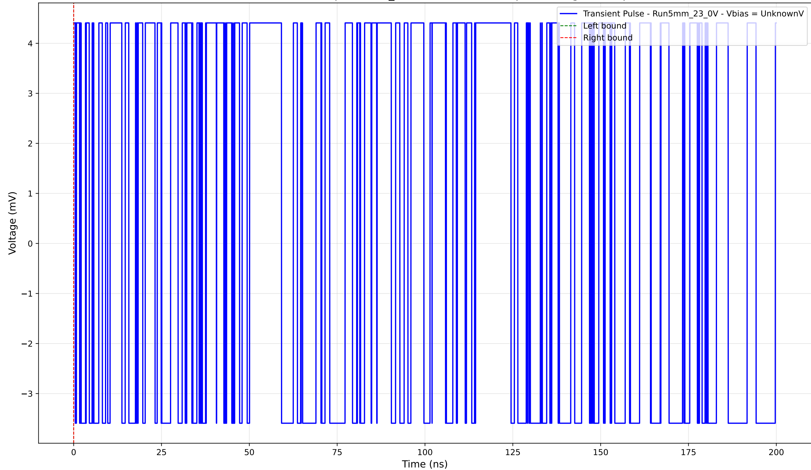
Transient Pulse - Sample: 5mm_23 - Position: 3030.0 \mu\text{m} - Charge: 0.00 pC
