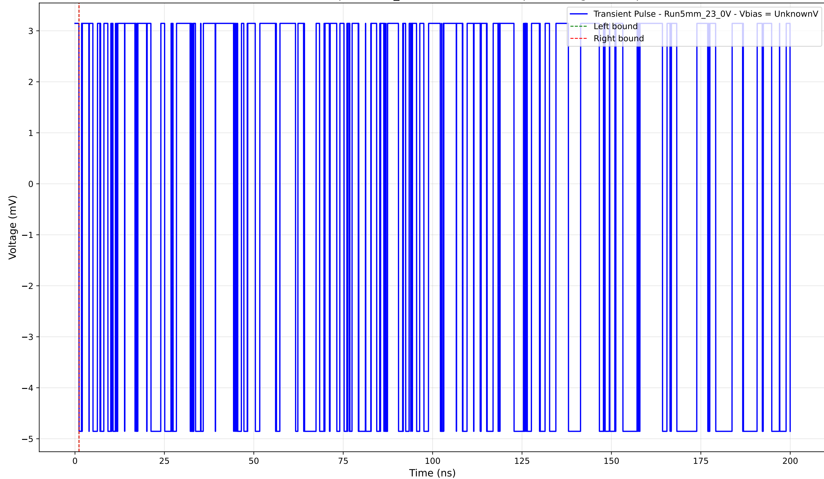
Transient Pulse - Sample: 5mm_23 - Position: 5045.0 \mu\text{m} - Charge: -0.00 pC
