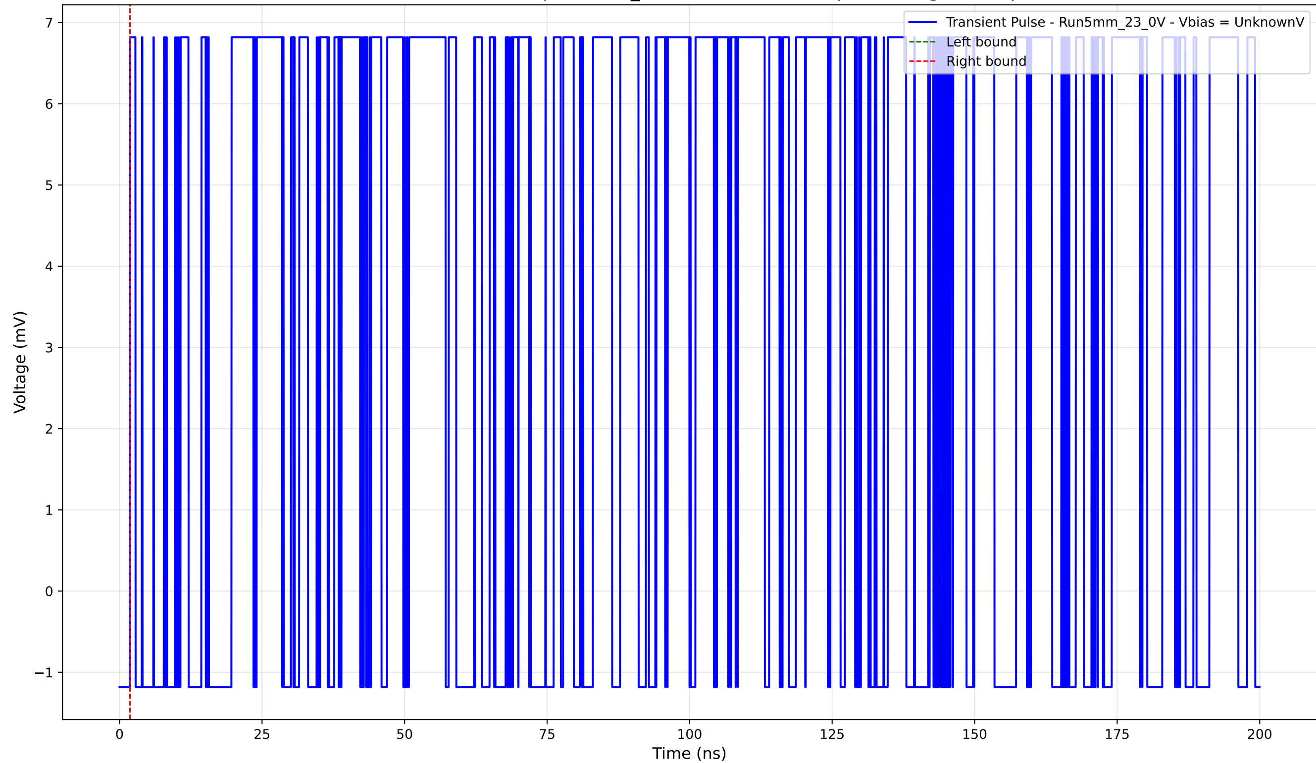
Transient Pulse - Sample: 5mm_23 - Position: 1665.0 \mu\text{m} - Charge: 0.00 pC
