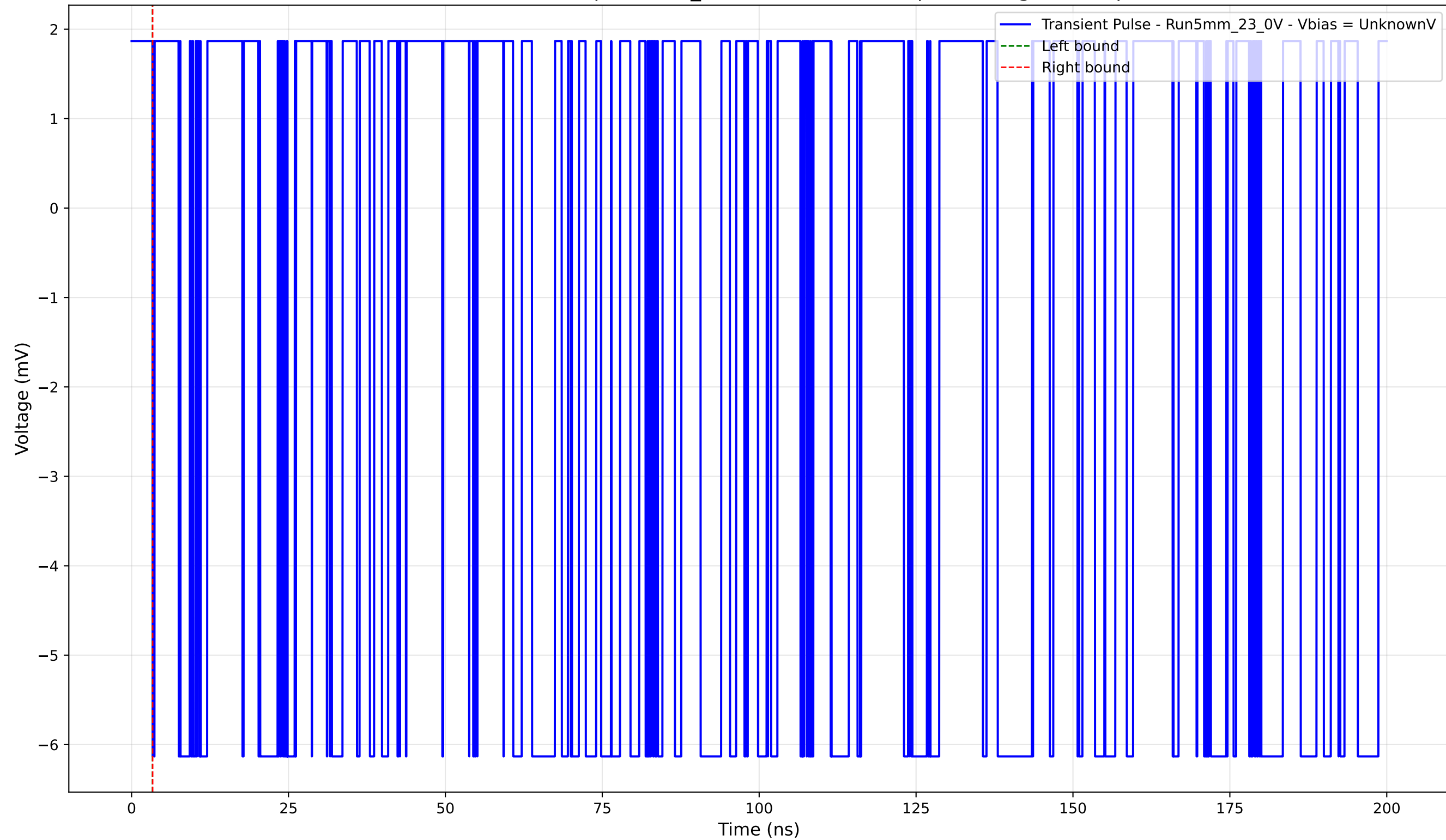
Transient Pulse - Sample: 5mm_23 - Position: 2490.0 \mu\text{m} - Charge: -0.00 pC
