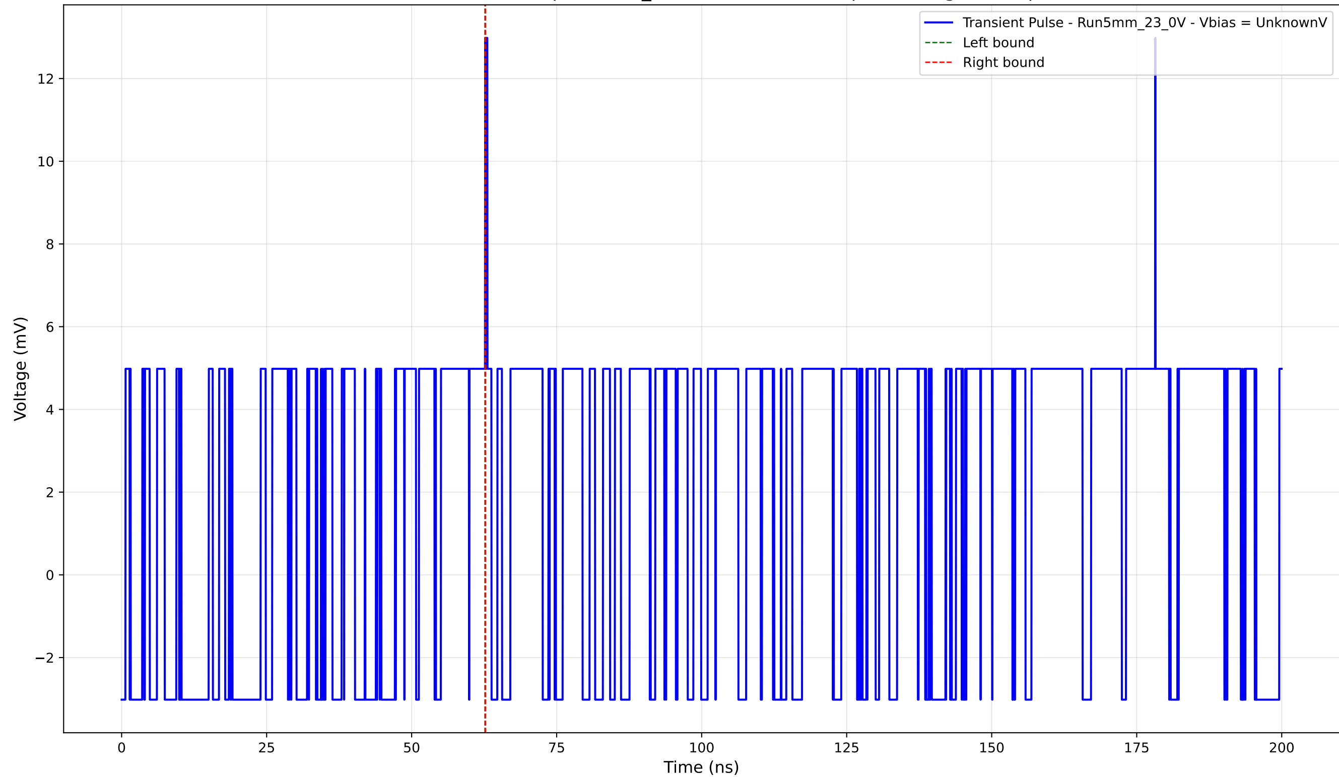
Transient Pulse - Sample: 5mm_23 - Position: 1015.0 \mu\text{m} - Charge: 0.02 pC
