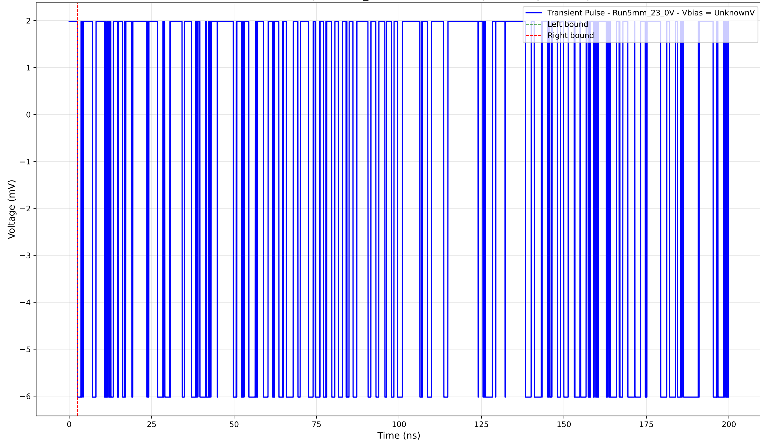
Transient Pulse - Sample: 5mm_23 - Position: 3810.0 \mu\text{m} - Charge: -0.00 pC
