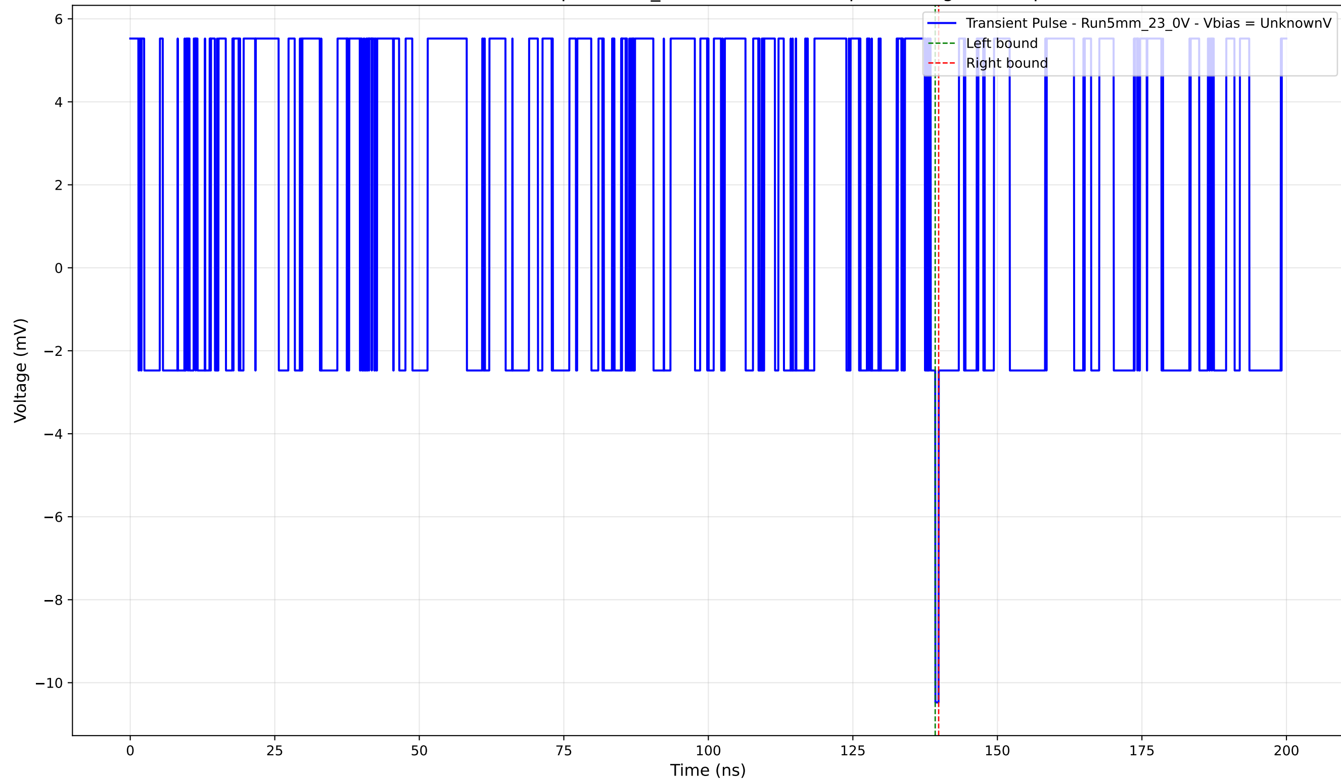
Transient Pulse - Sample: 5mm_23 - Position: 150.0 \mu\text{m} - Charge: -0.12 pC
