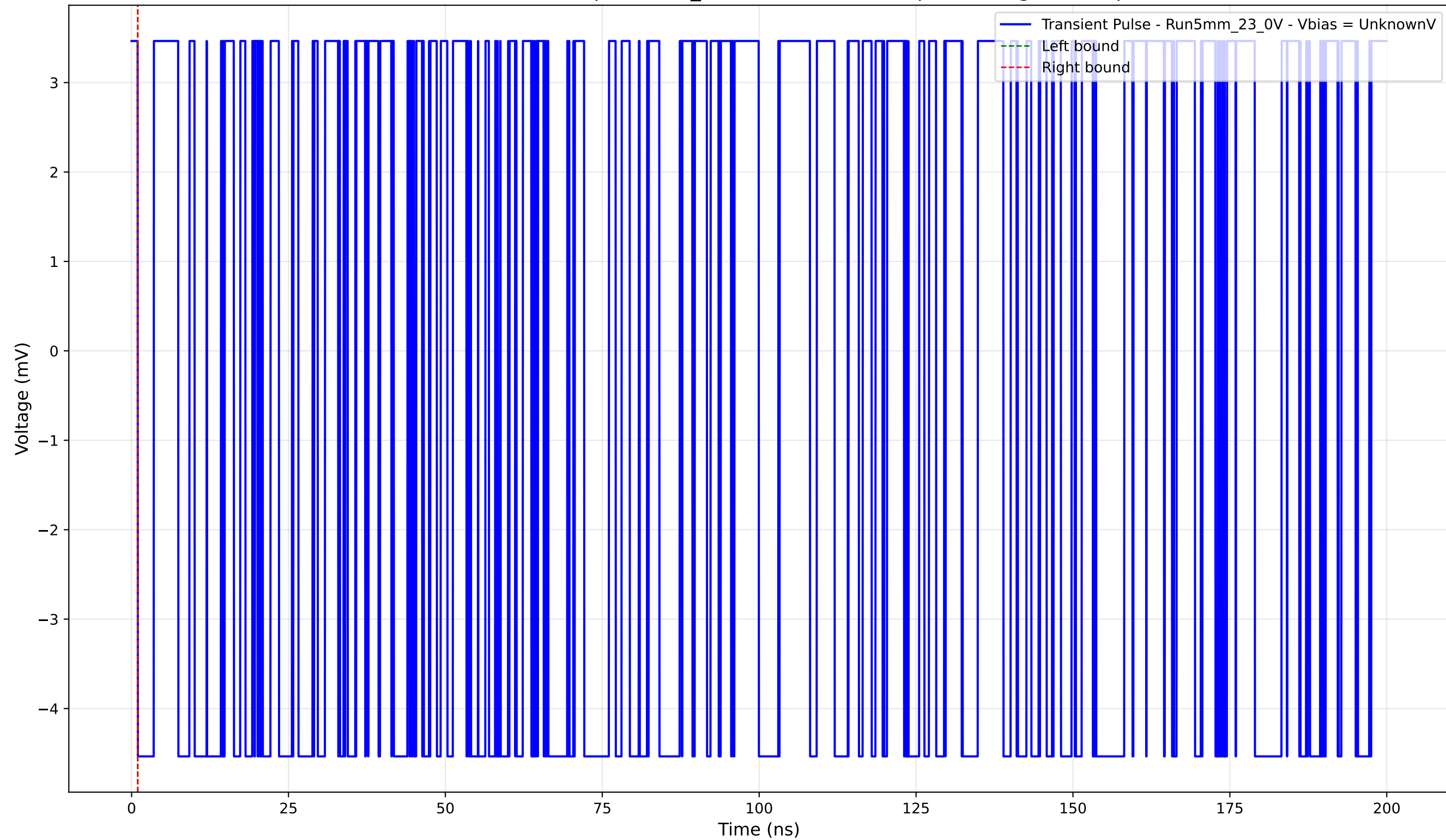
Transient Pulse - Sample: 5mm_23 - Position: 2465.0 \mu\text{m} - Charge: -0.00 pC
