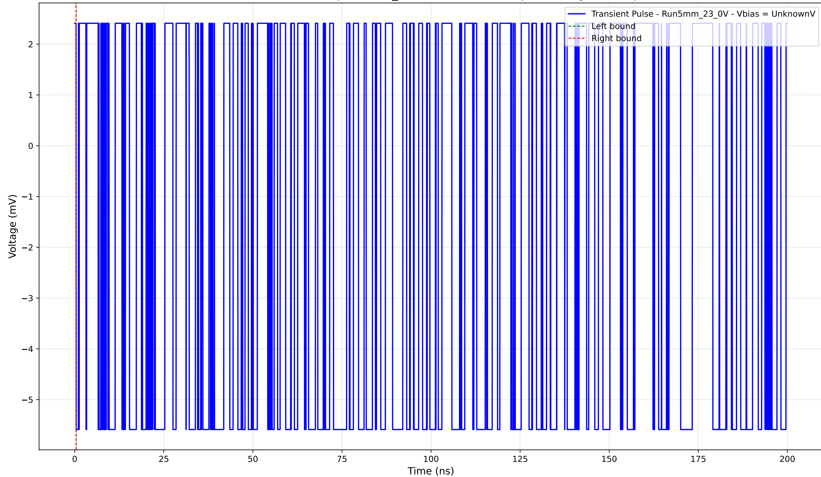
Transient Pulse - Sample: 5mm_23 - Position: 3425.0 \mu\text{m} - Charge: -0.00 pC
