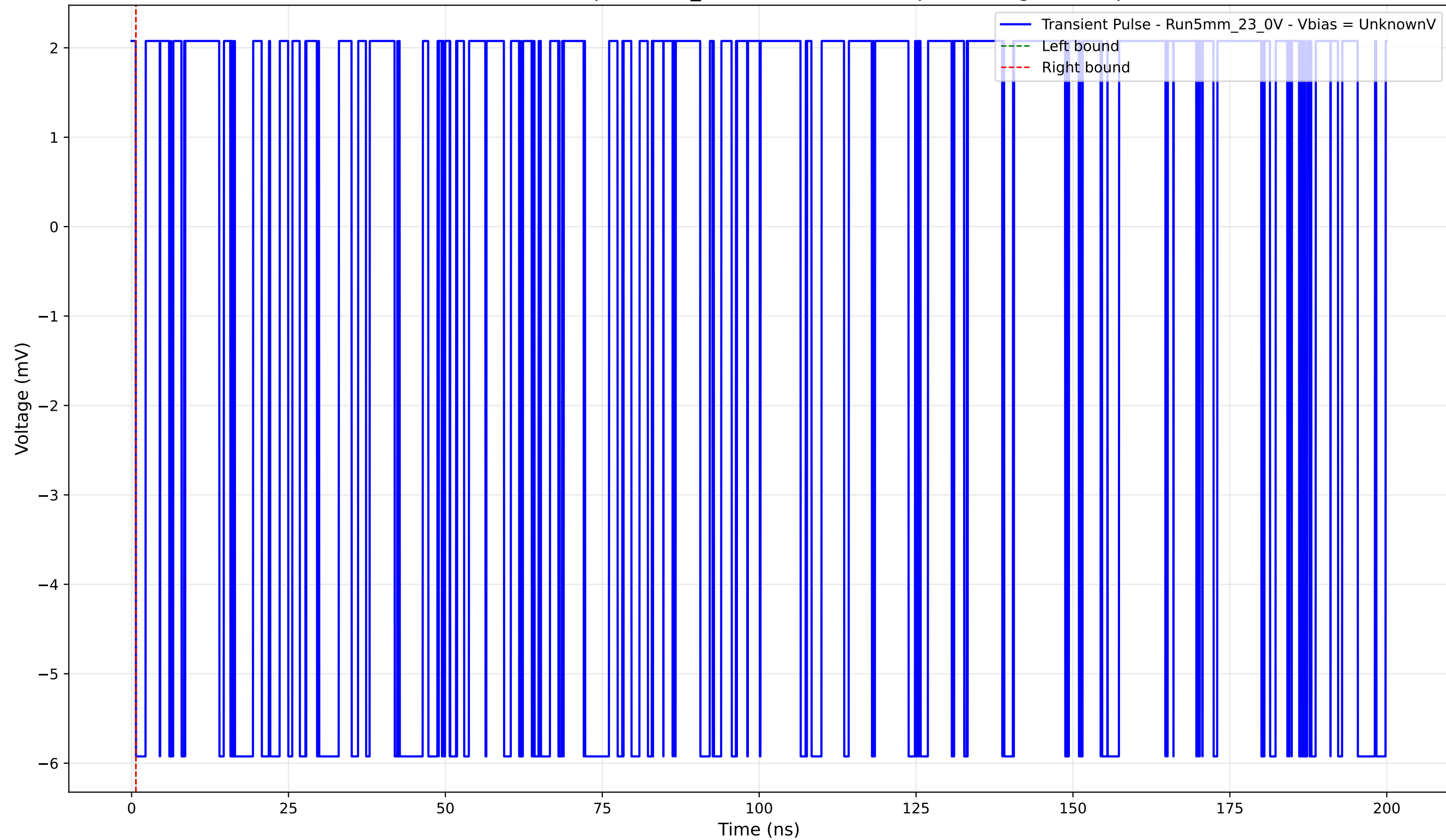
Transient Pulse - Sample: 5mm_23 - Position: 2590.0 \mu\text{m} - Charge: -0.00 pC
