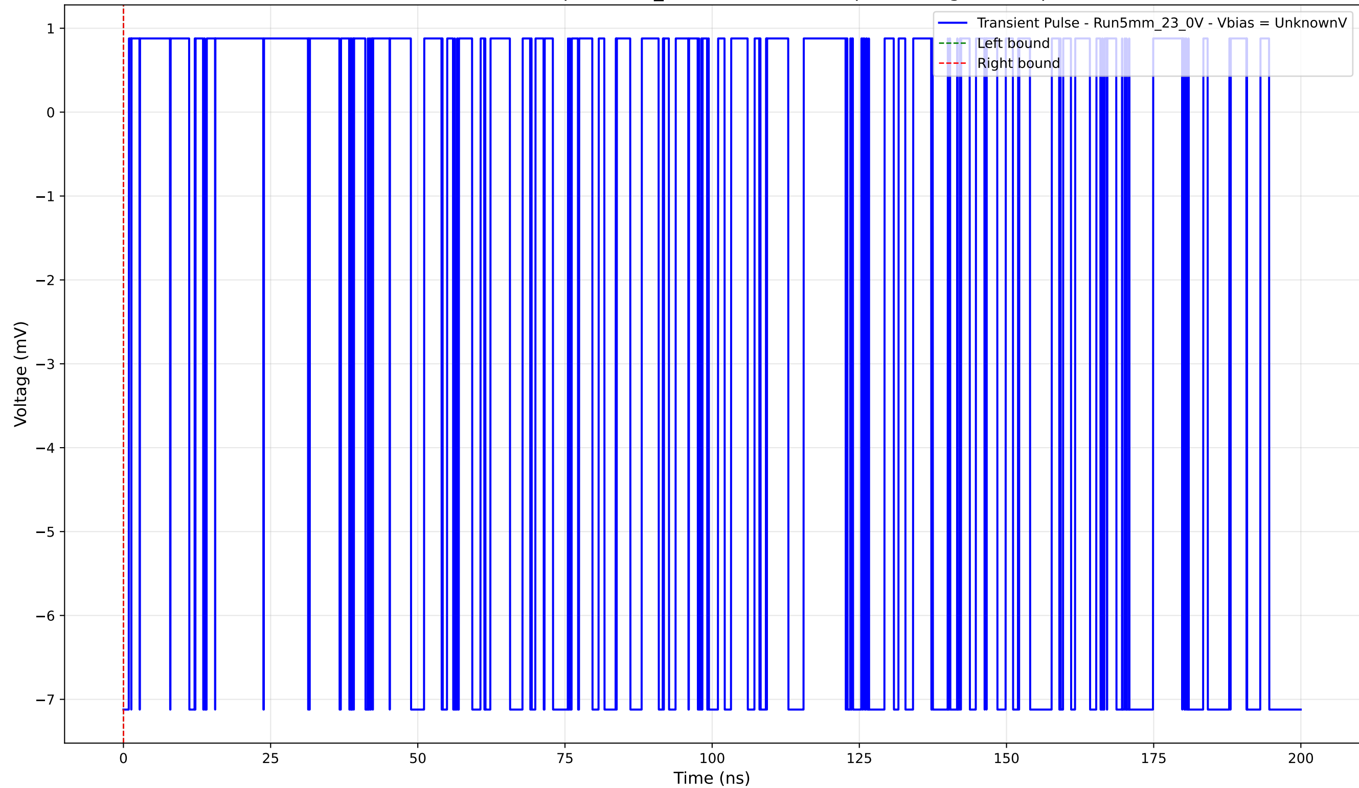
Transient Pulse - Sample: 5mm_23 - Position: 830.0 \mu\text{m} - Charge: -0.00 pC
