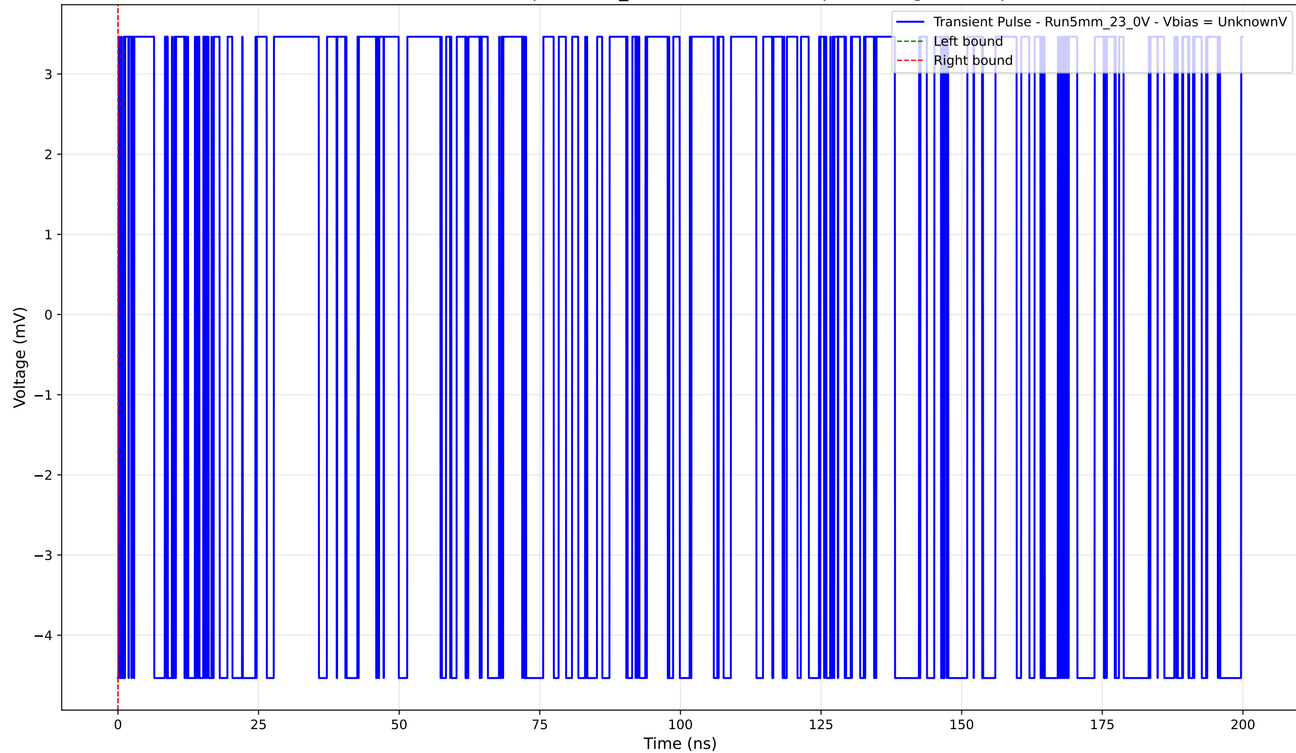
Transient Pulse - Sample: 5mm_23 - Position: 1630.0 \mu\text{m} - Charge: -0.00 pC
