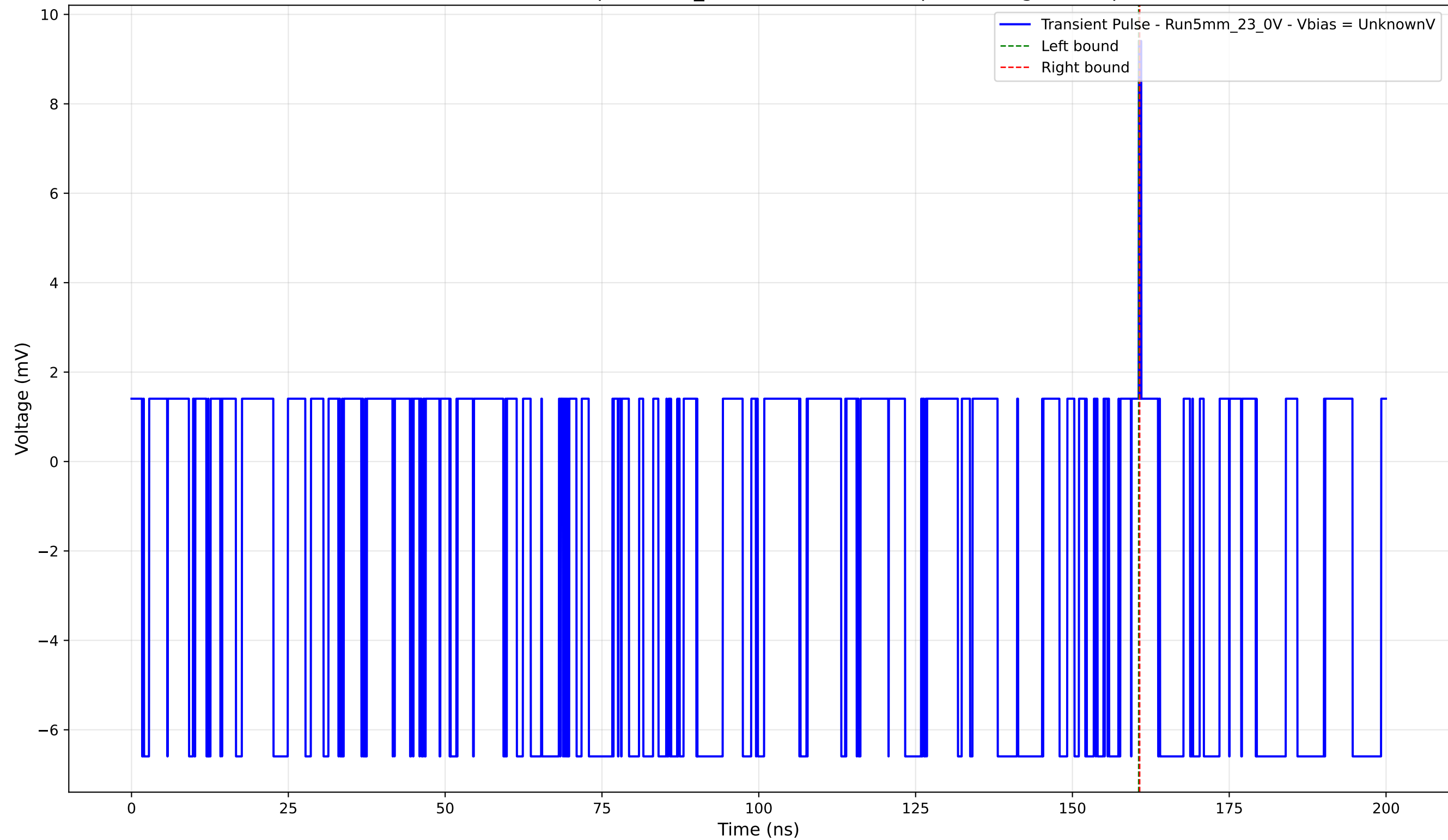
Transient Pulse - Sample: 5mm_23 - Position: 1555.0 \mu\text{m} - Charge: 0.03 pC
