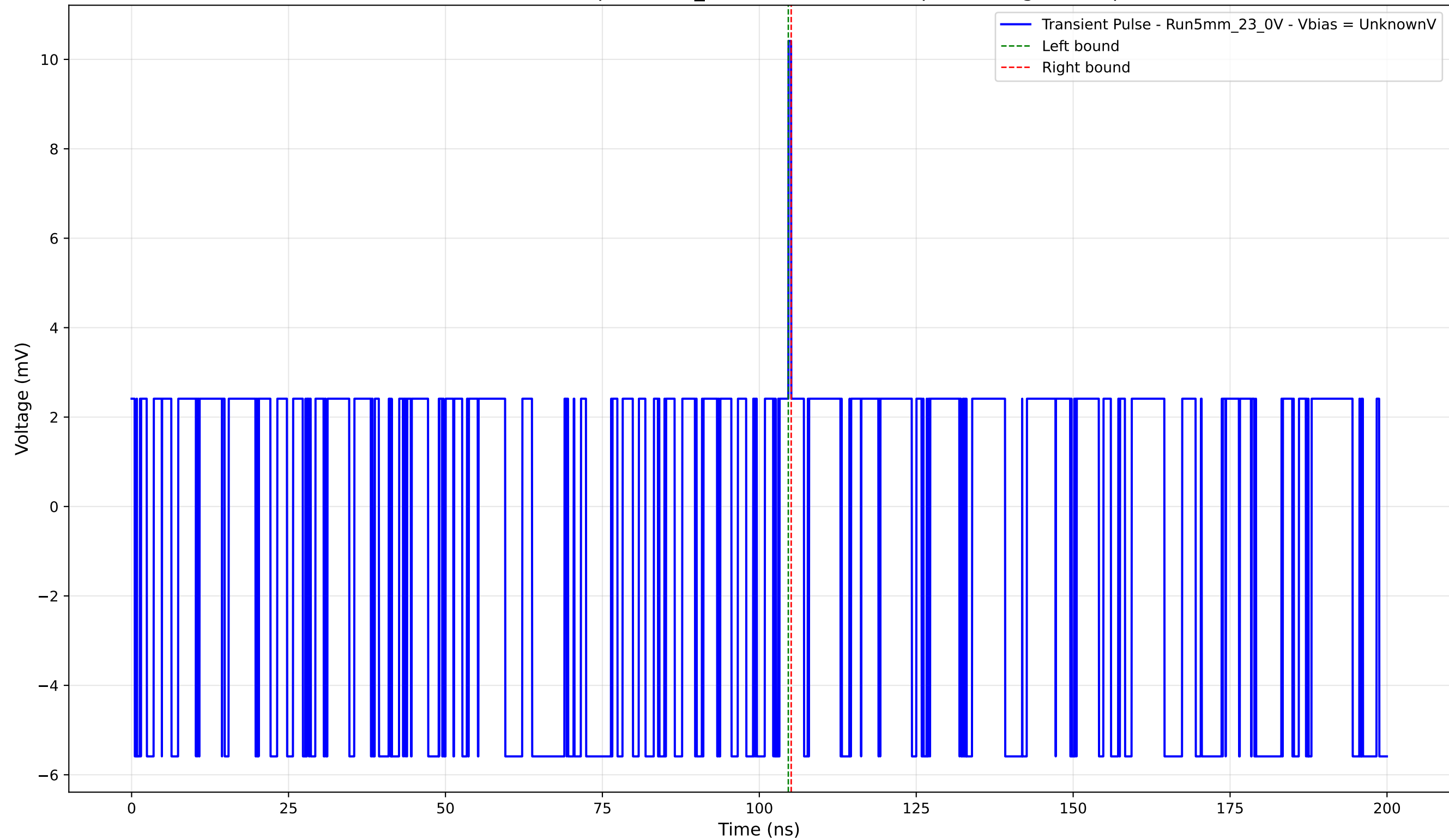
Transient Pulse - Sample: 5mm_23 - Position: 4160.0 \mu\text{m} - Charge: 0.09 pC
