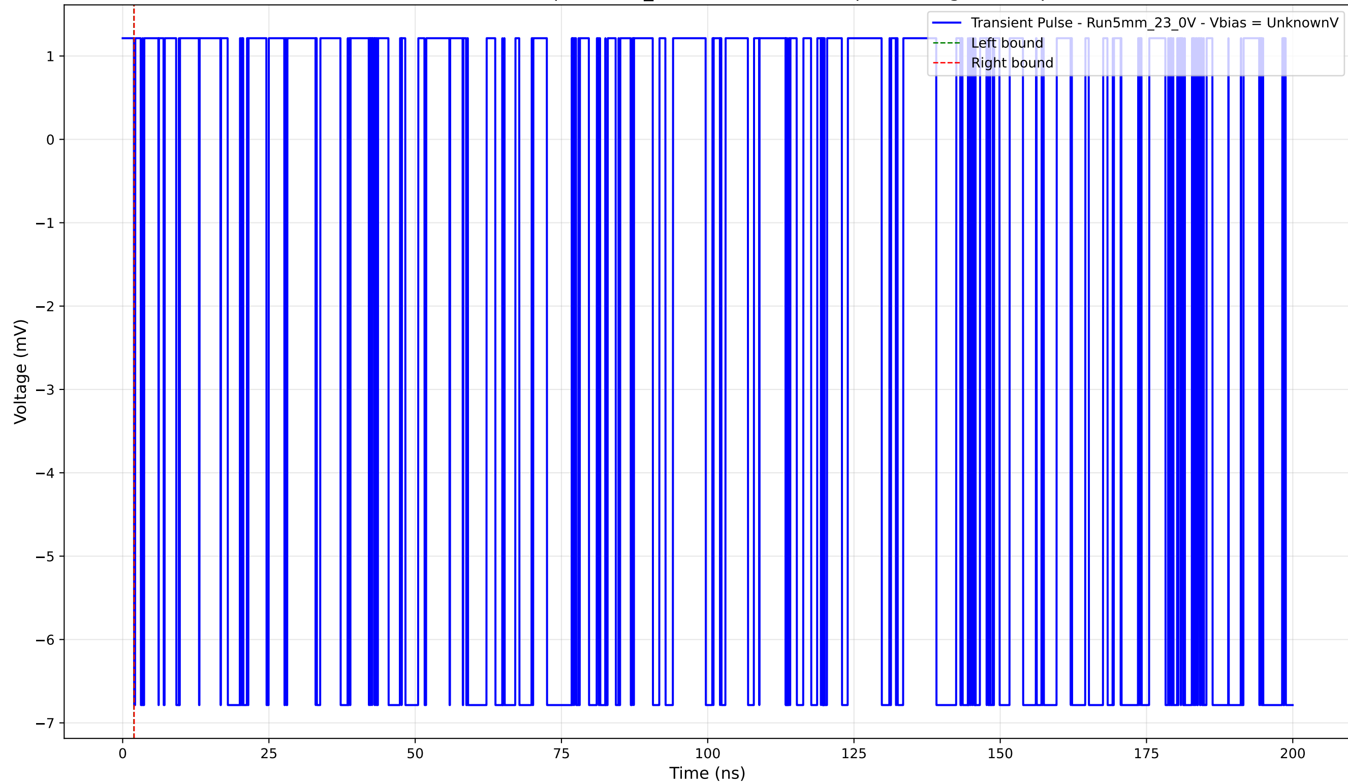
Transient Pulse - Sample: 5mm_23 - Position: 4145.0 \mu\text{m} - Charge: -0.00 pC
