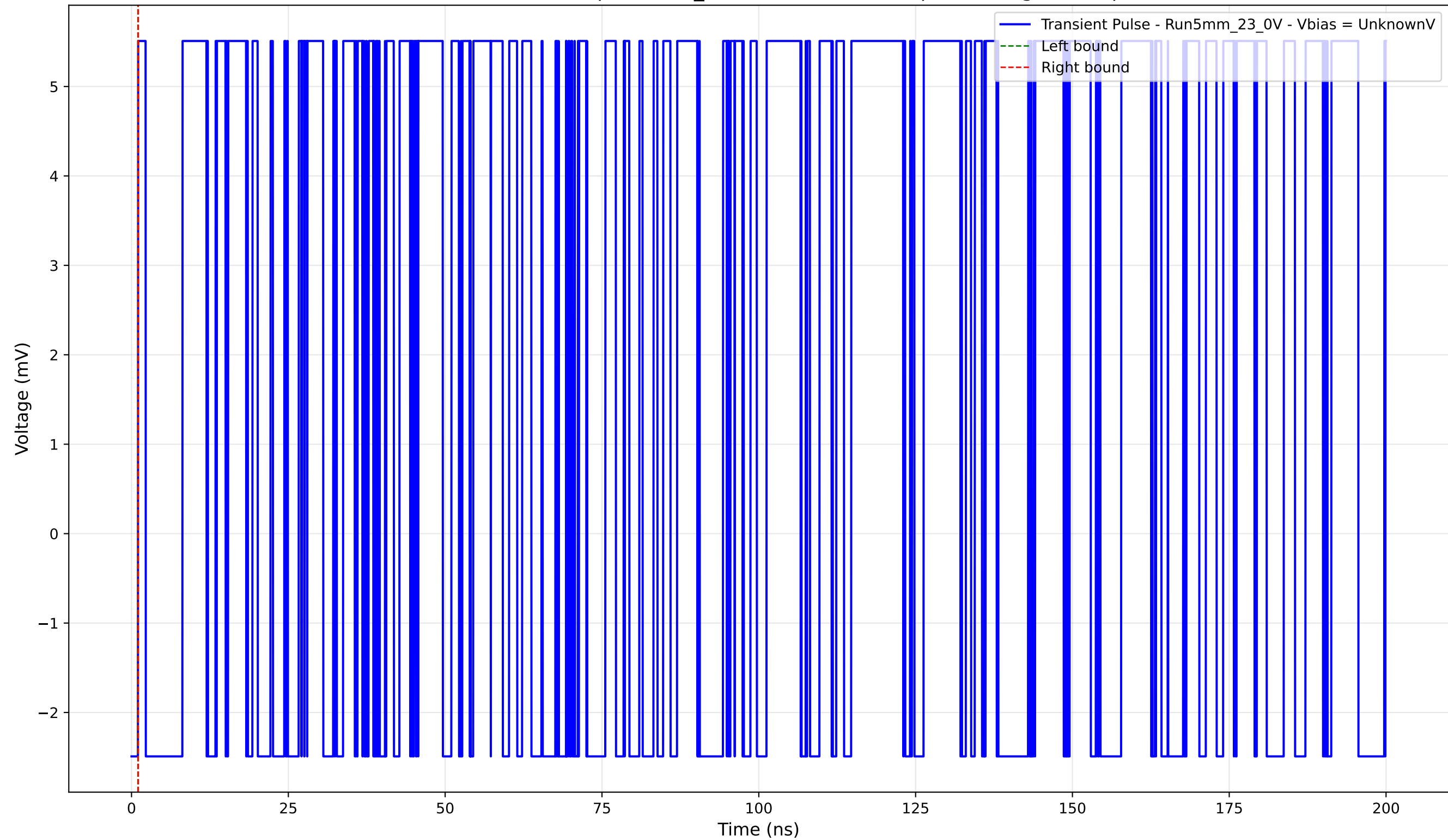
Transient Pulse - Sample: 5mm_23 - Position: 2875.0 \mu\text{m} - Charge: 0.00 pC
