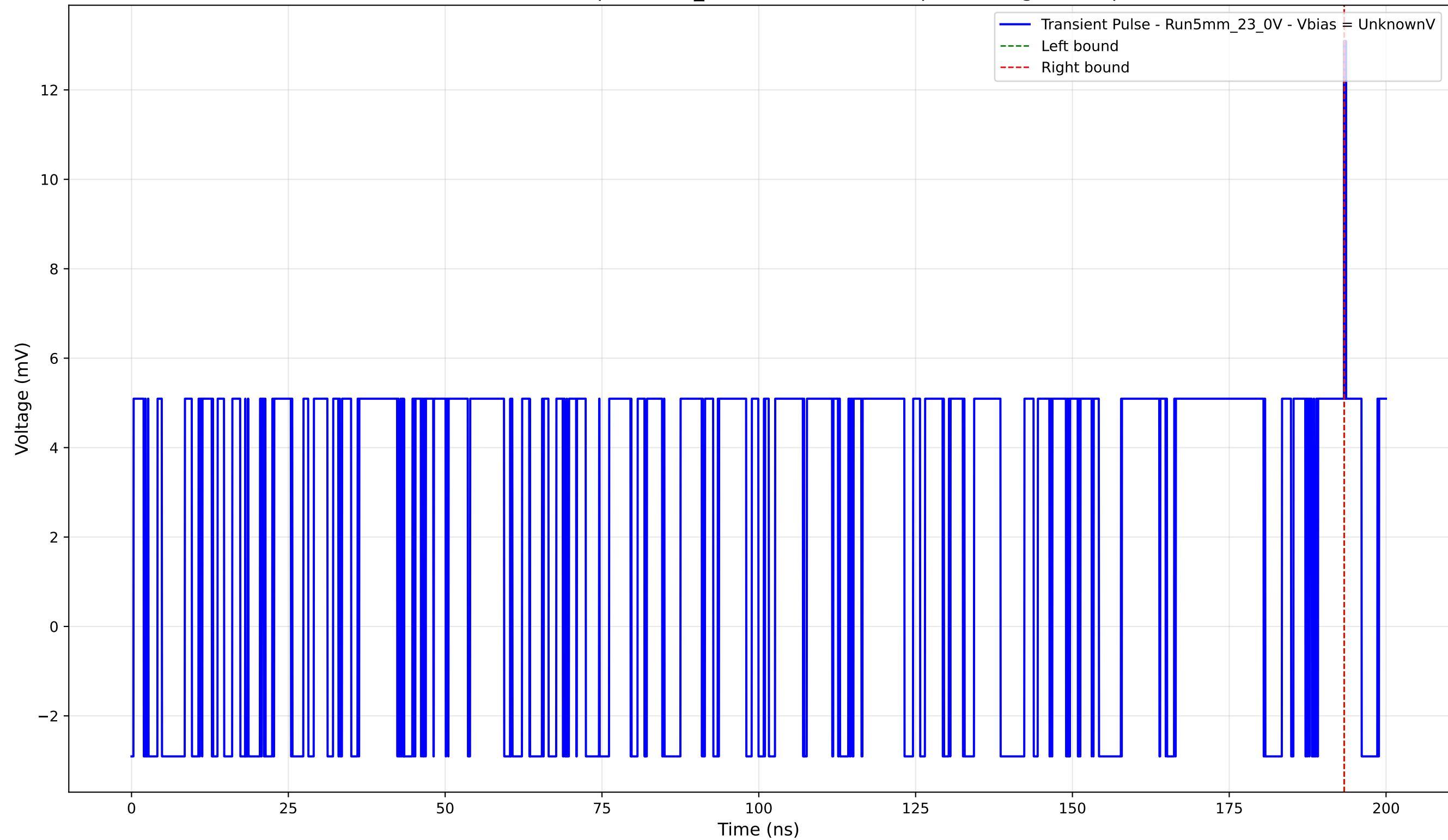
Transient Pulse - Sample: 5mm_23 - Position: 4550.0 \mu\text{m} - Charge: 0.01 pC
