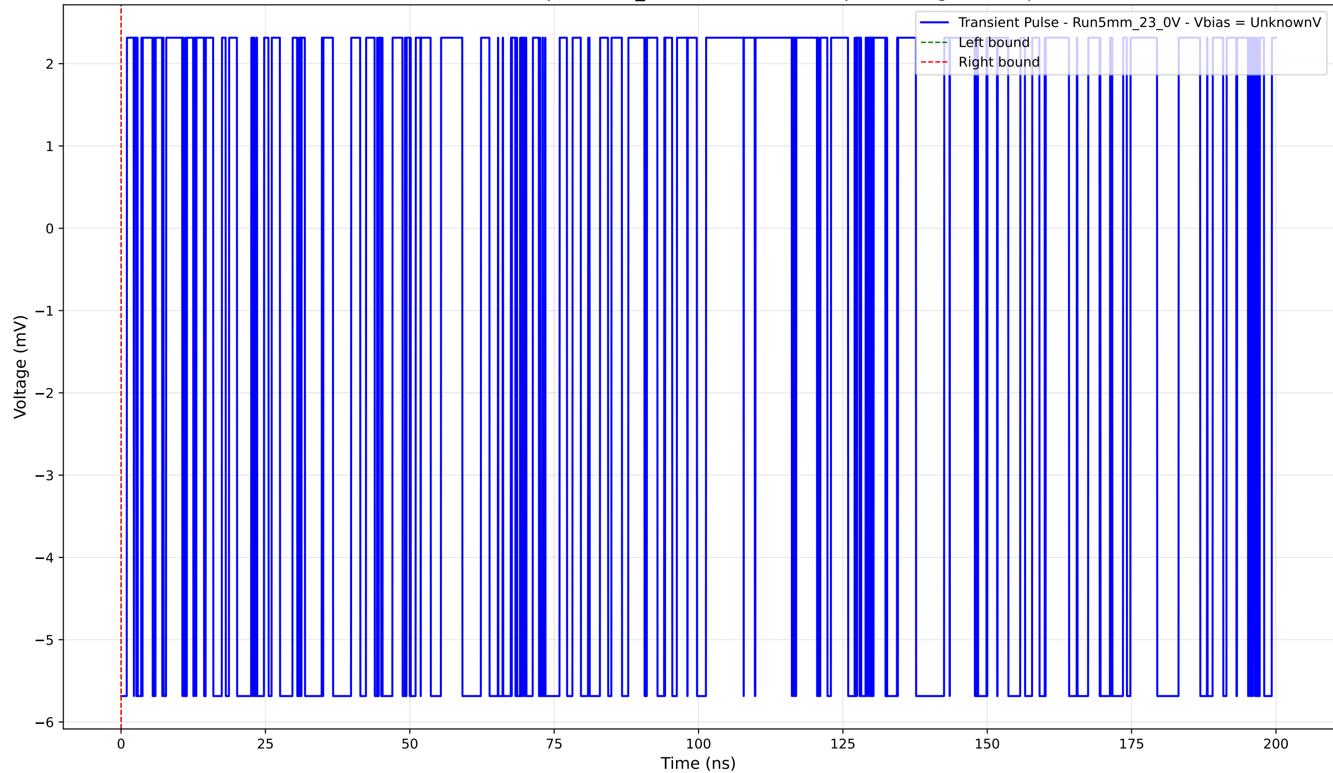
Transient Pulse - Sample: 5mm_23 - Position: 3370.0 \mu\text{m} - Charge: -0.00 pC
