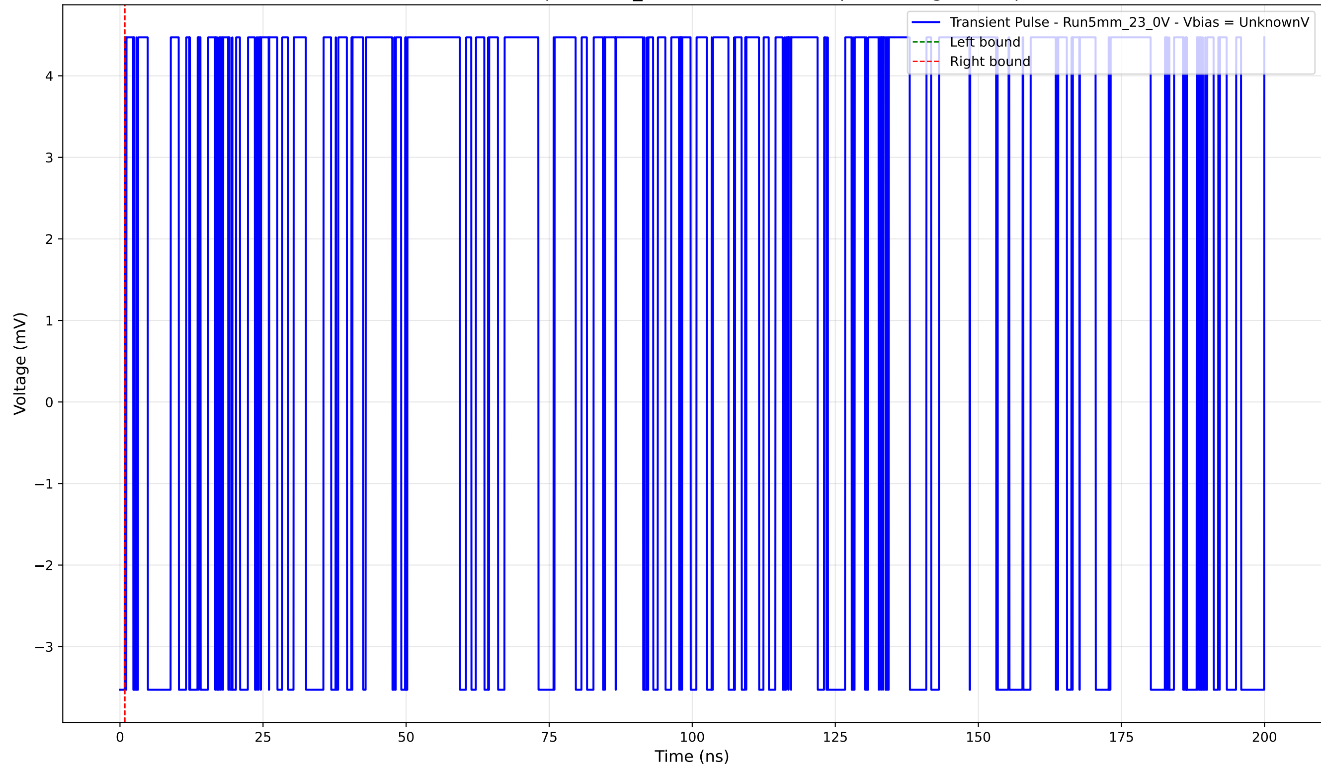
Transient Pulse - Sample: 5mm_23 - Position: 1815.0 \mu\text{m} - Charge: 0.00 pC
