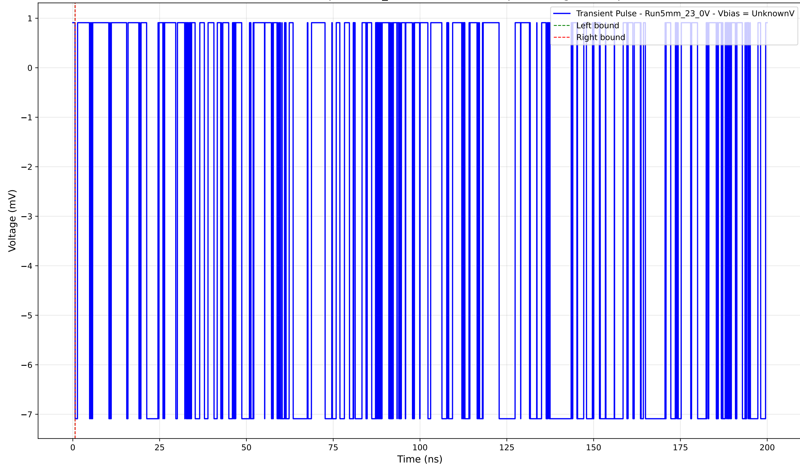
Transient Pulse - Sample: 5mm_23 - Position: 4655.0 \mu\text{m} - Charge: -0.00 pC
