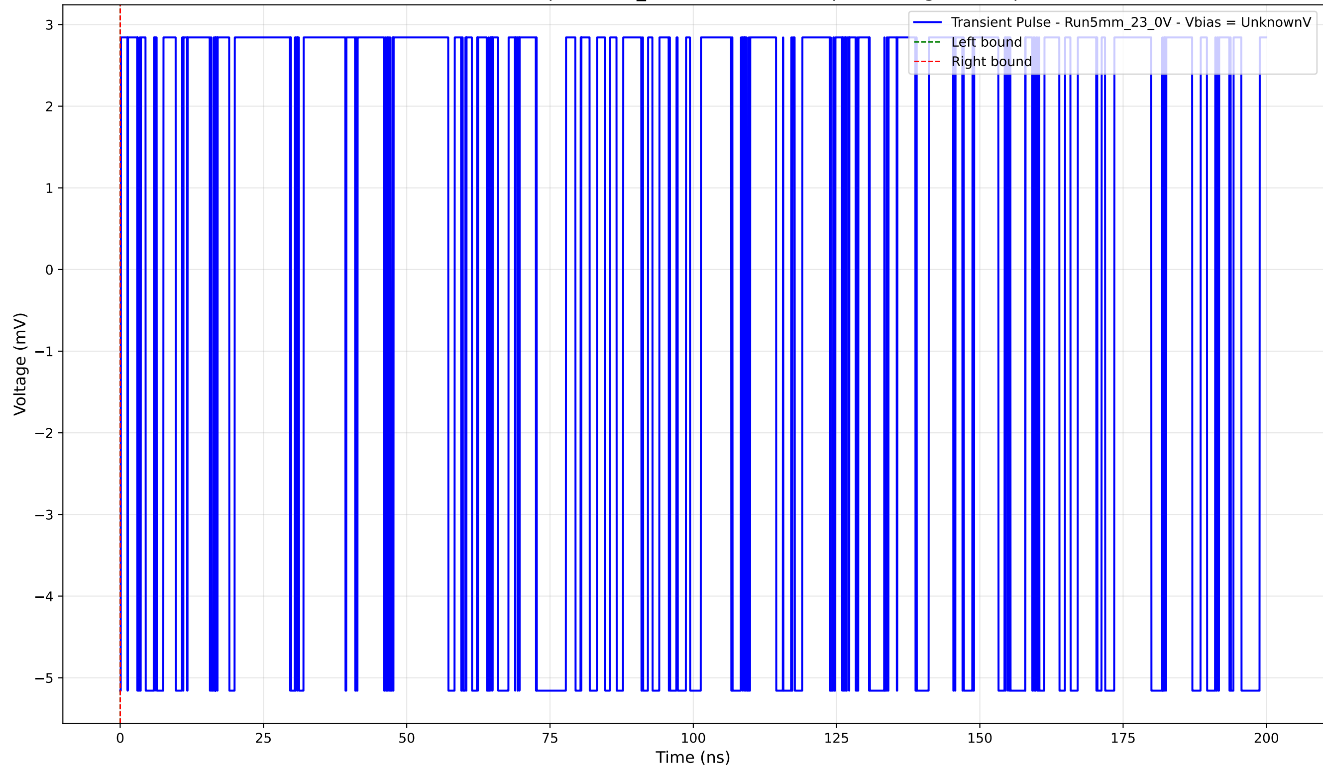
Transient Pulse - Sample: 5mm_23 - Position: 715.0 \mu\text{m} - Charge: -0.00 pC
