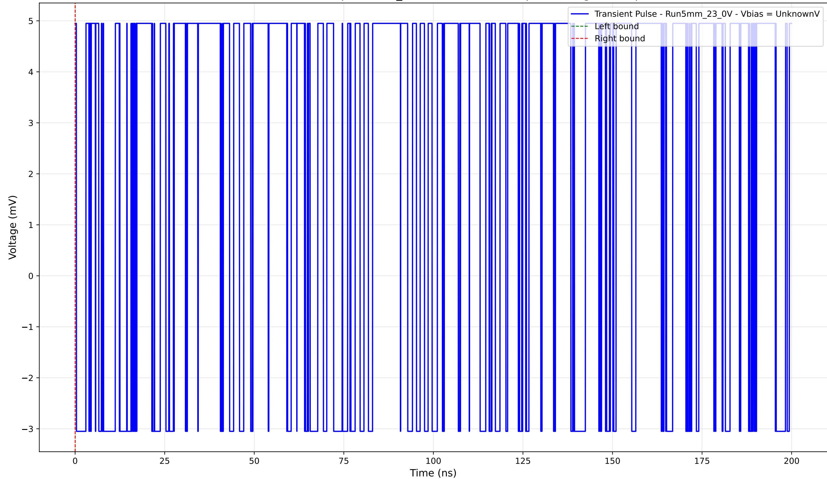
Transient Pulse - Sample: 5mm_23 - Position: 2105.0 \mu\text{m} - Charge: 0.00 pC
