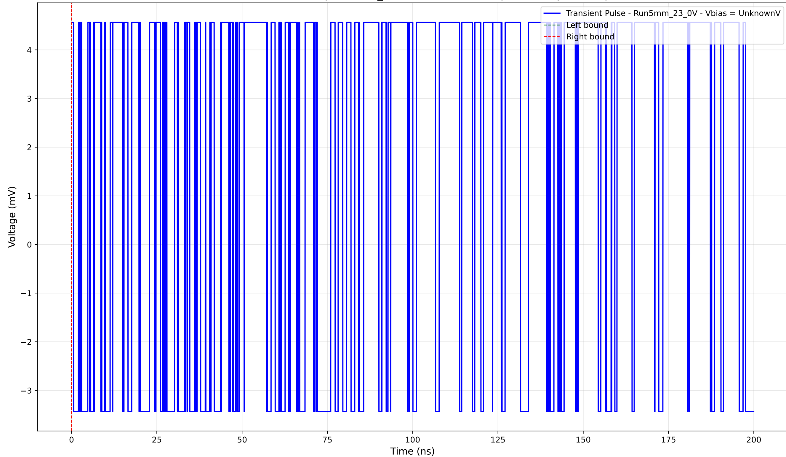
Transient Pulse - Sample: 5mm_23 - Position: 2395.0 \mu\text{m} - Charge: 0.00 pC
