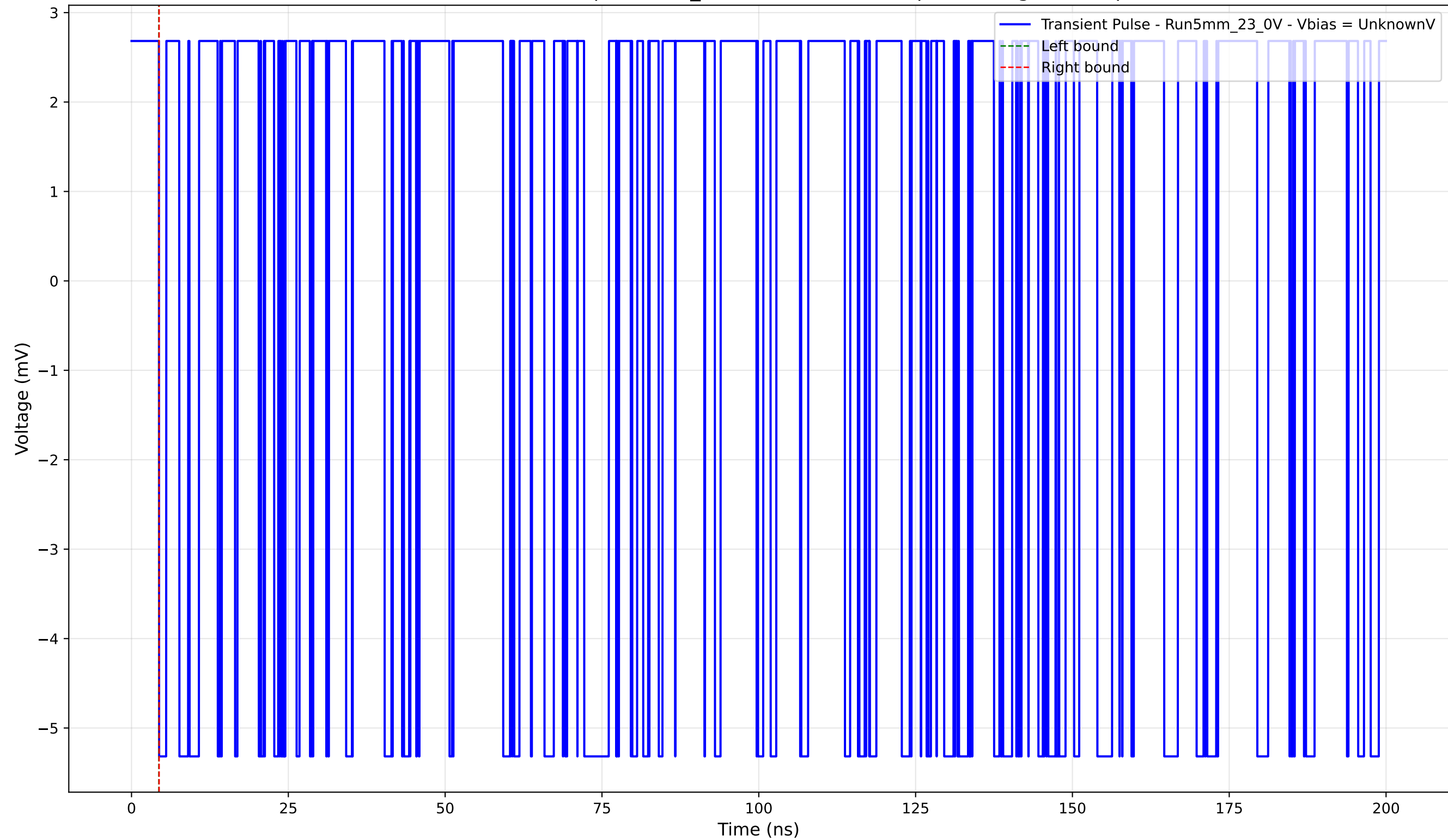
Transient Pulse - Sample: 5mm_23 - Position: 2765.0 \mu\text{m} - Charge: -0.00 pC
