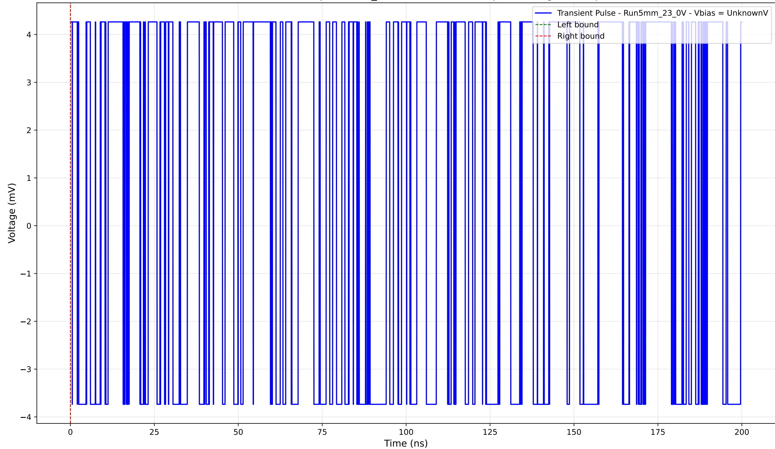
Transient Pulse - Sample: 5mm_23 - Position: 1225.0 \mu\text{m} - Charge: 0.00 pC
