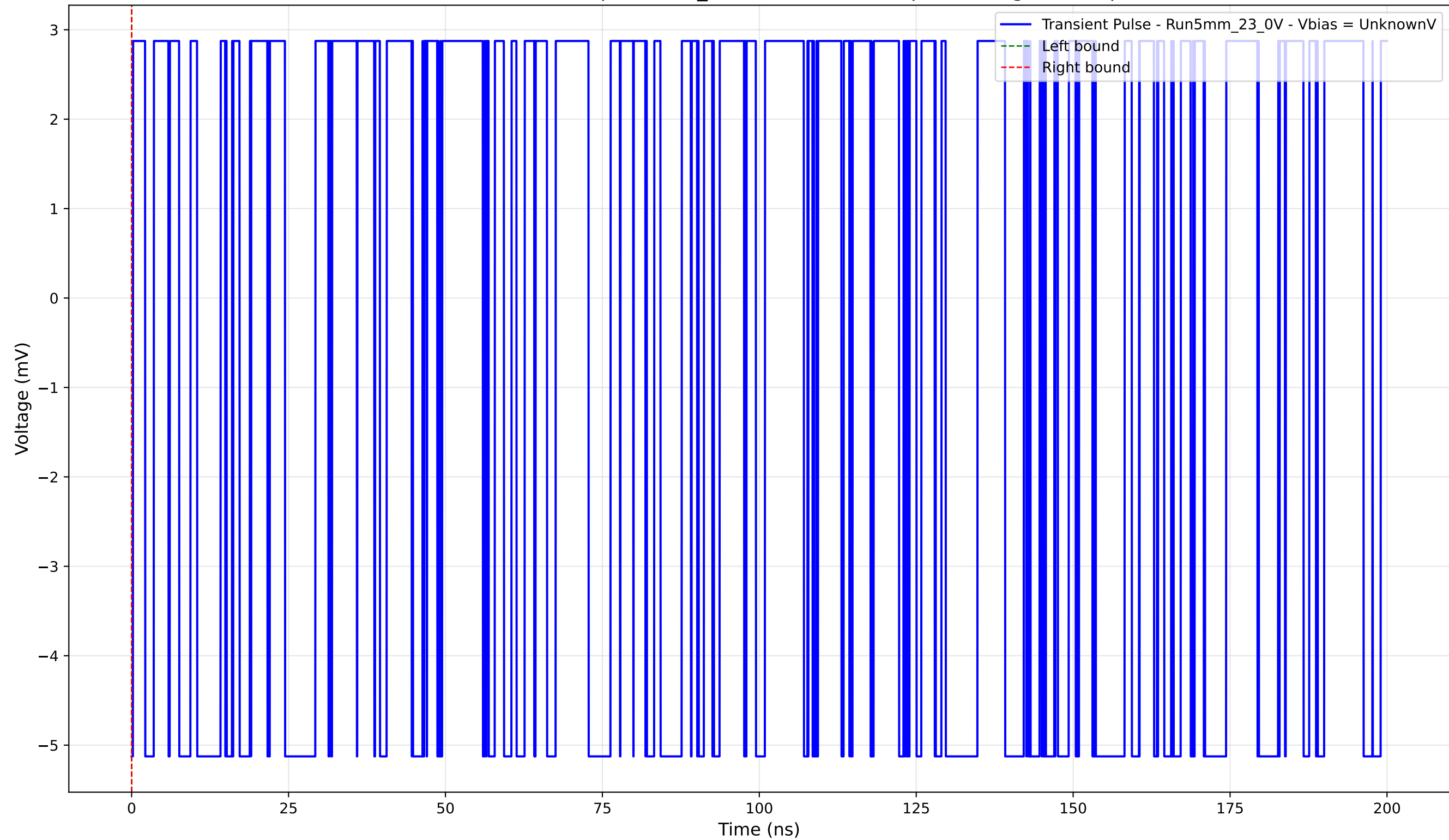
Transient Pulse - Sample: 5mm_23 - Position: 305.0 \mu\text{m} - Charge: -0.00 pC
