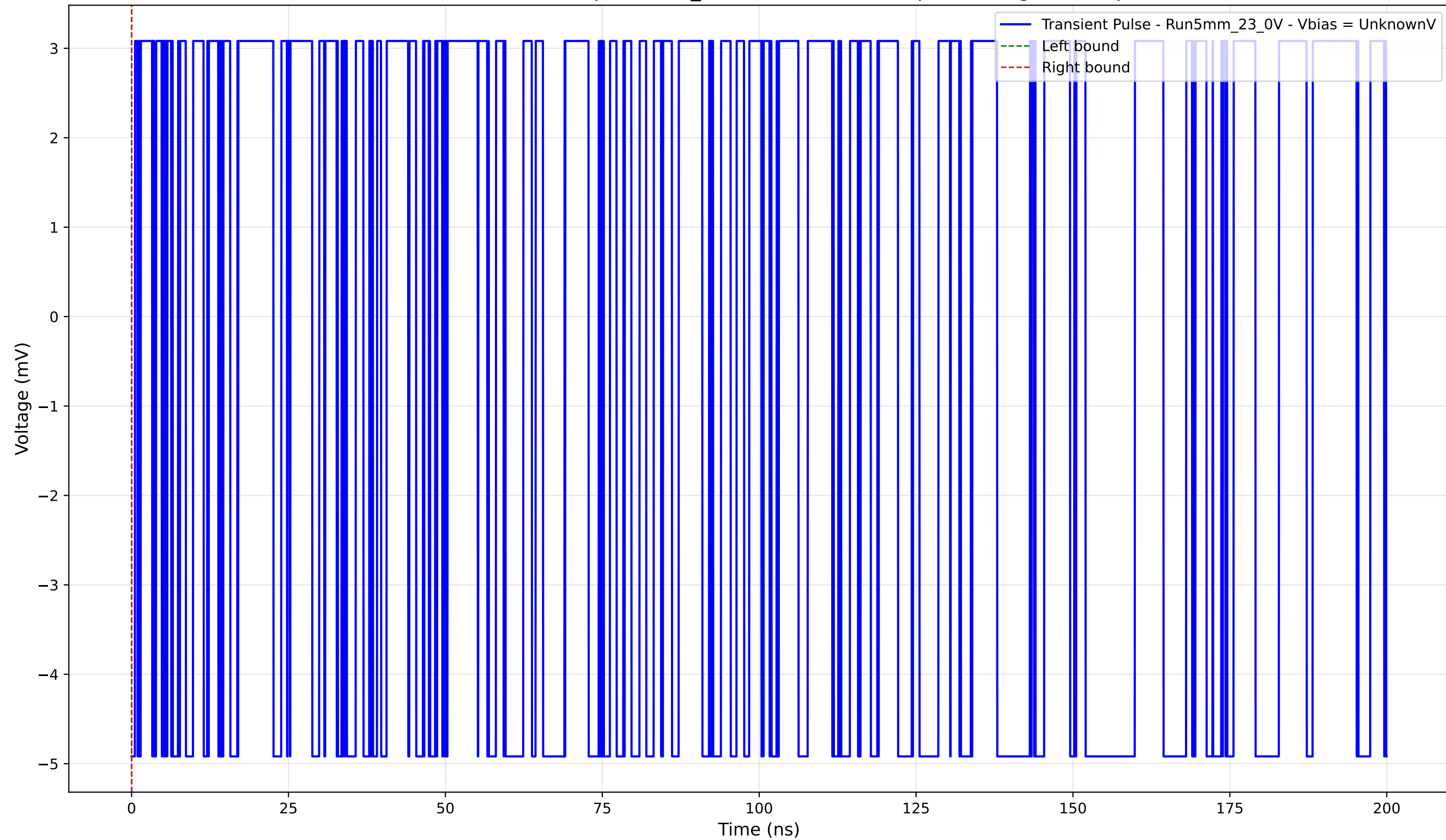
Transient Pulse - Sample: 5mm_23 - Position: 1165.0 \mu\text{m} - Charge: -0.00 pC
