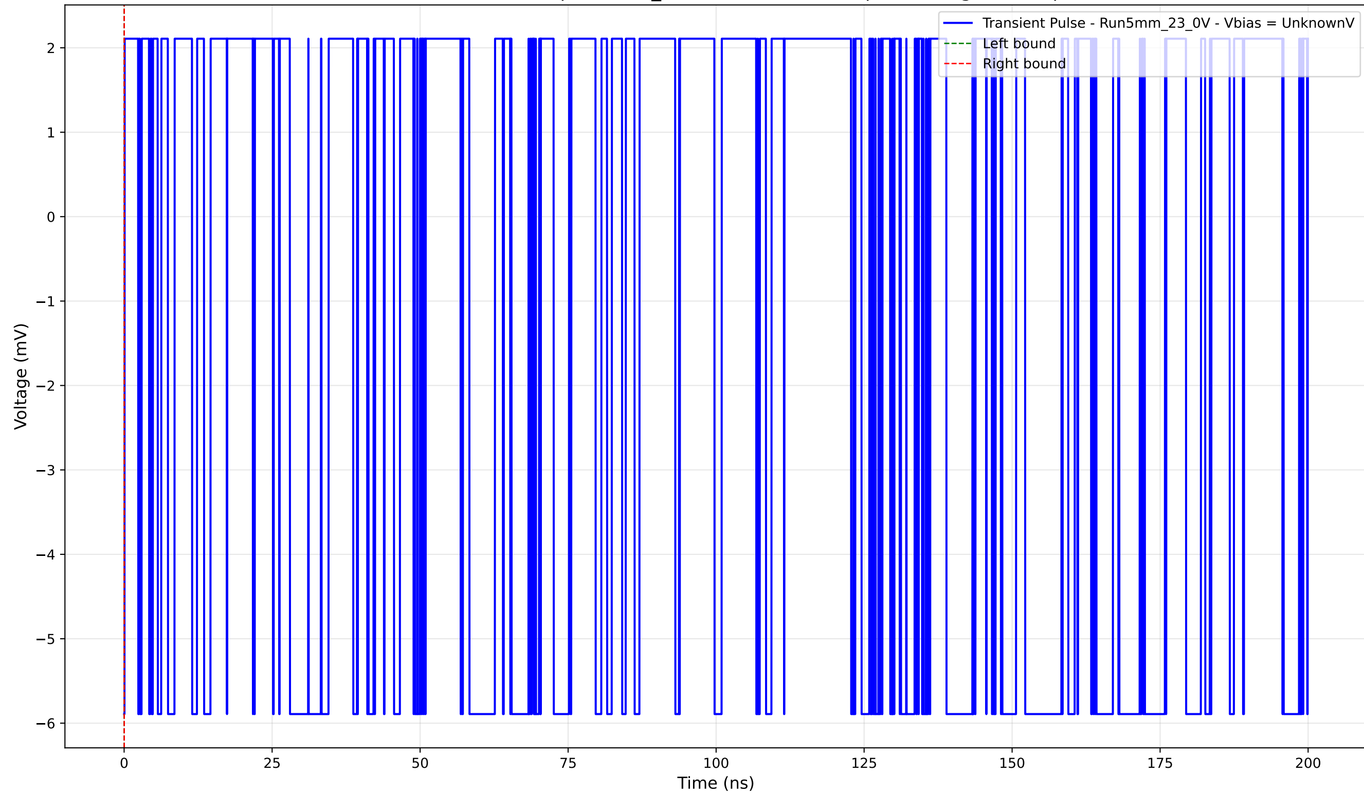
Transient Pulse - Sample: 5mm_23 - Position: 4775.0 \mu\text{m} - Charge: -0.00 pC
