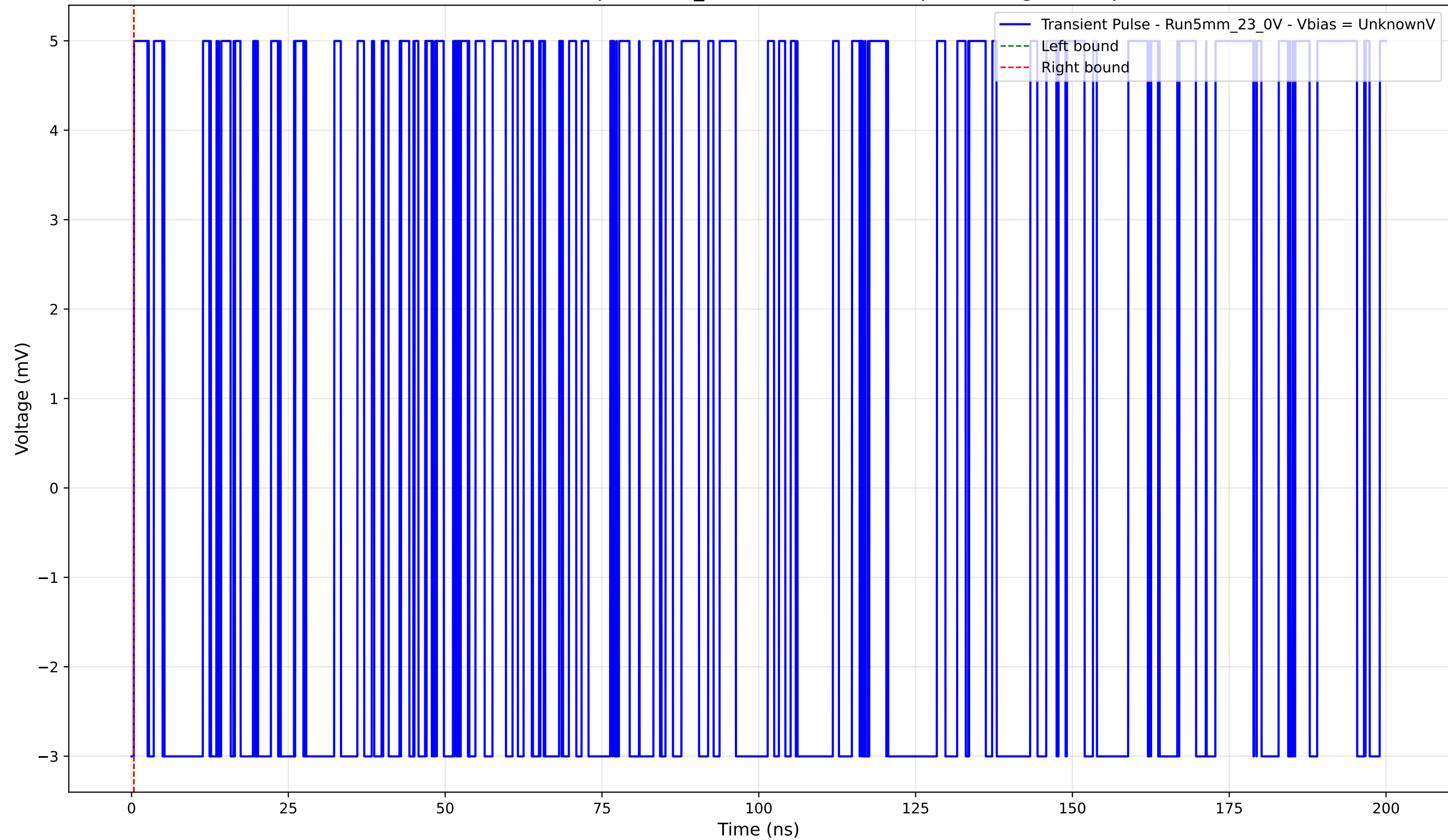
Transient Pulse - Sample: 5mm_23 - Position: 5085.0 \mu\text{m} - Charge: 0.00 pC
