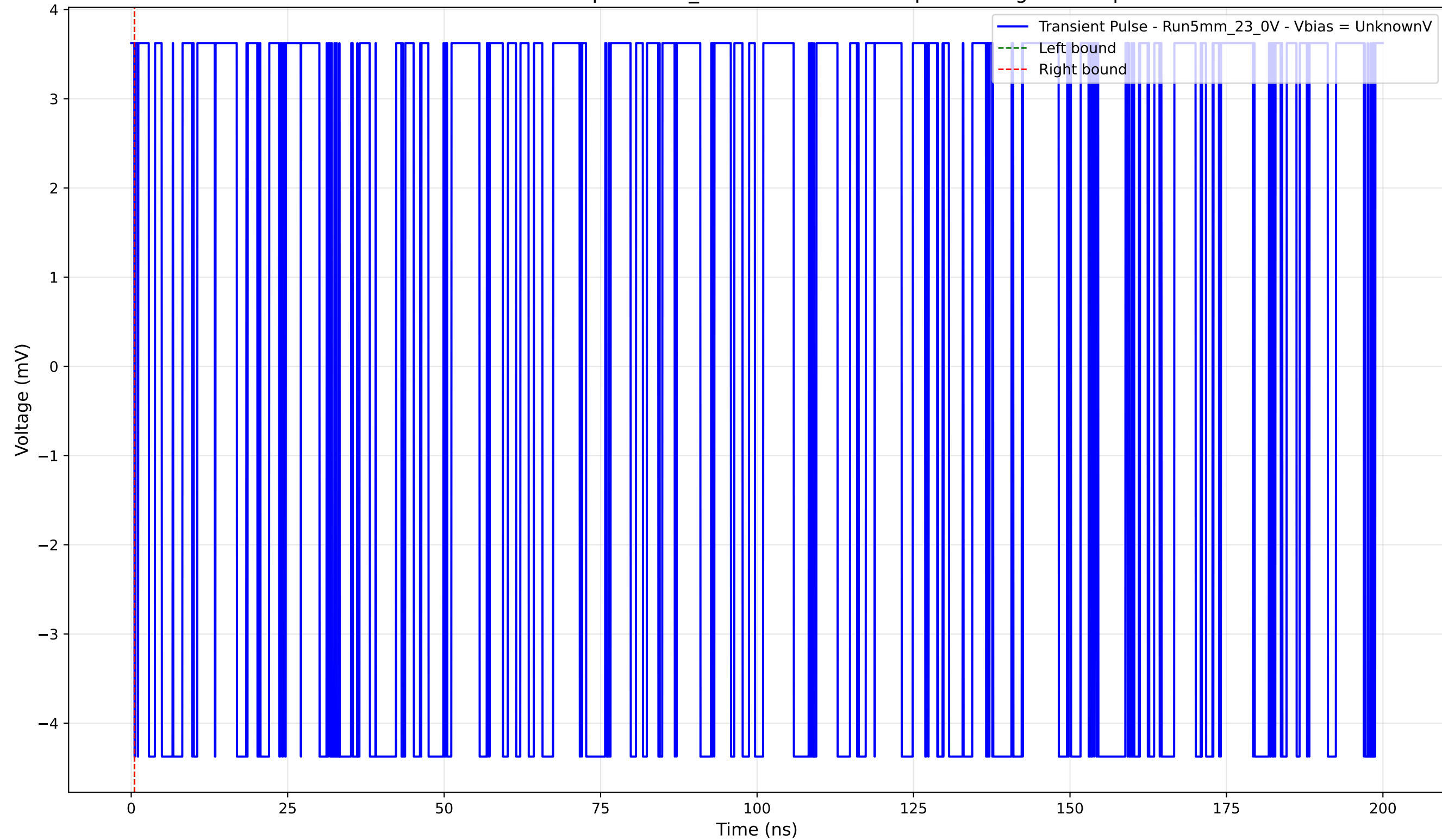
Transient Pulse - Sample: 5mm_23 - Position: 3925.0 \mu\text{m} - Charge: -0.00 pC
