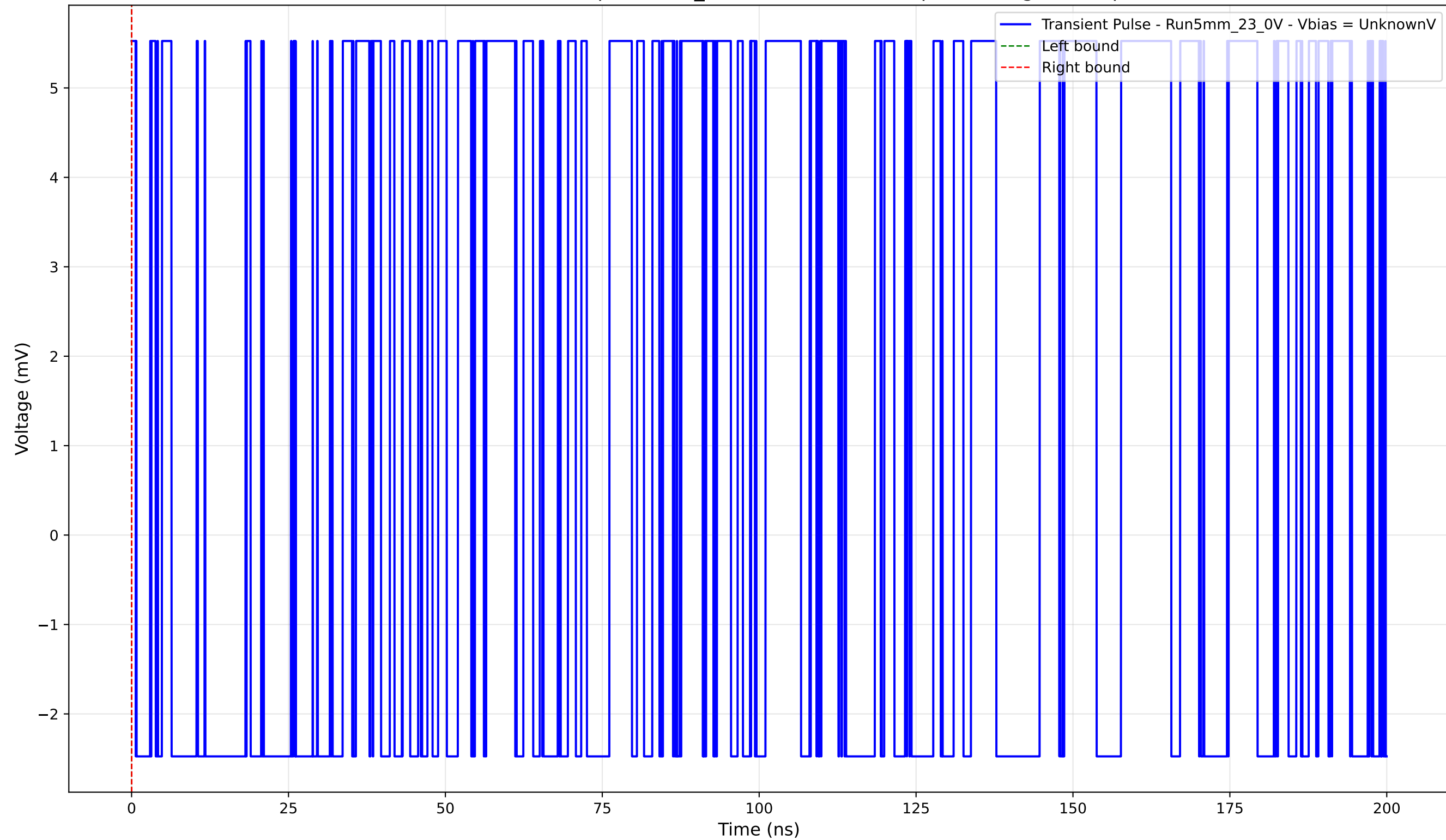
Transient Pulse - Sample: 5mm_23 - Position: 1525.0 \mu\text{m} - Charge: 0.00 pC
