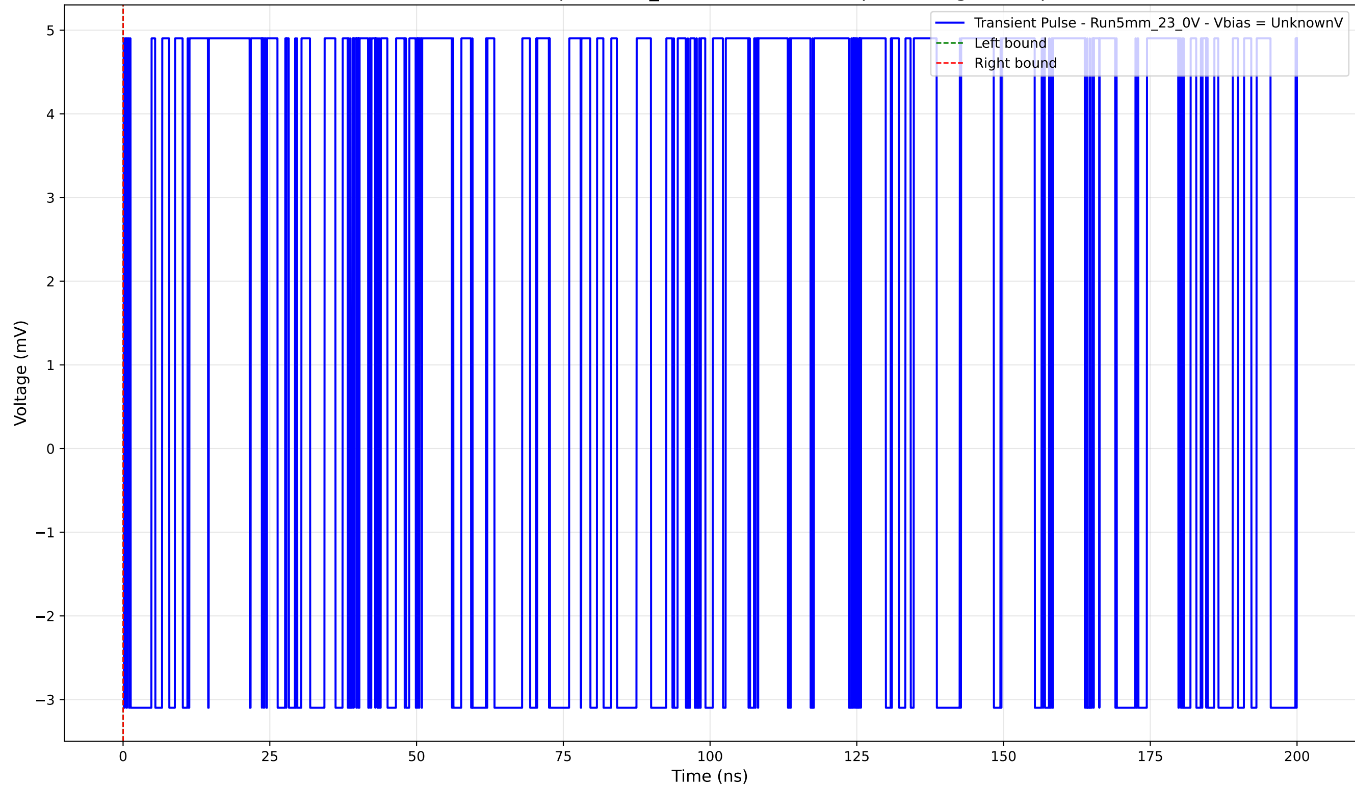
Transient Pulse - Sample: 5mm_23 - Position: 1075.0 \mu\text{m} - Charge: 0.00 pC
