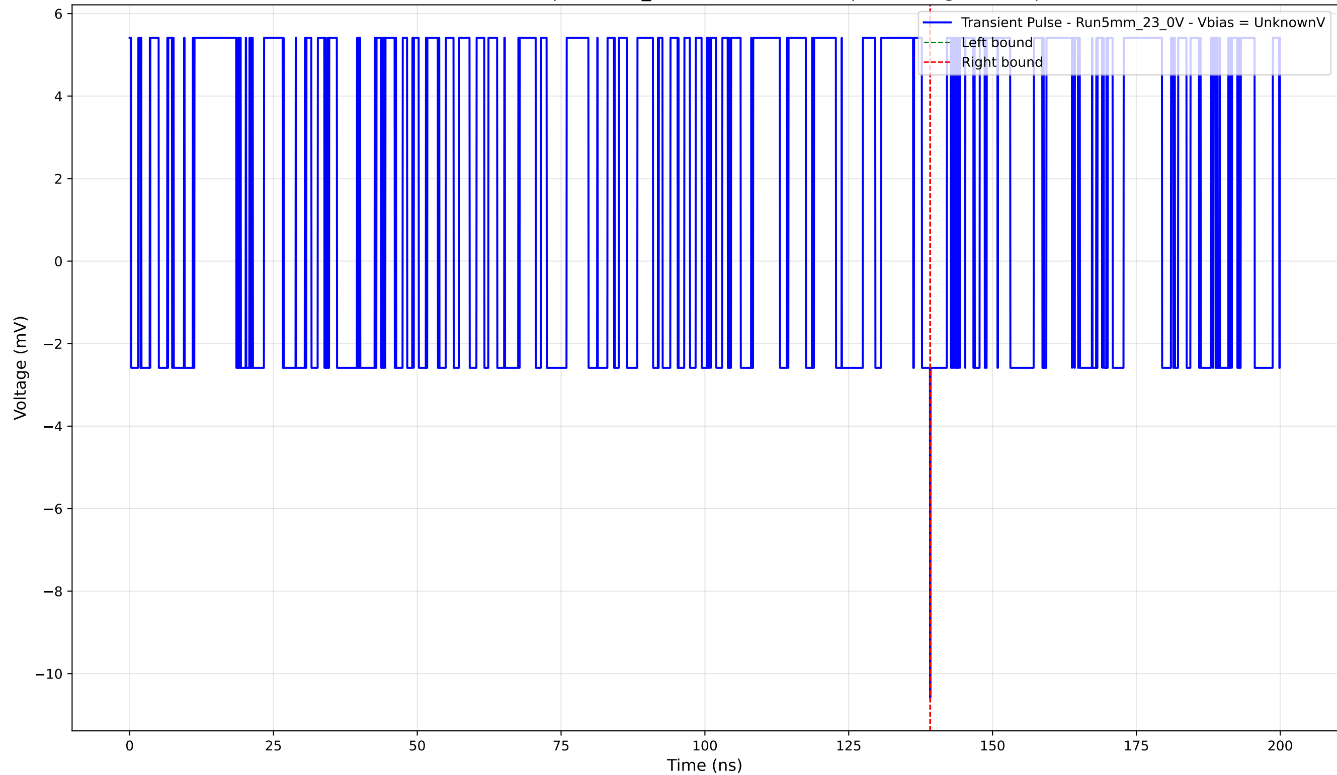
Transient Pulse - Sample: 5mm_23 - Position: 3895.0 \mu\text{m} - Charge: -0.01 pC
