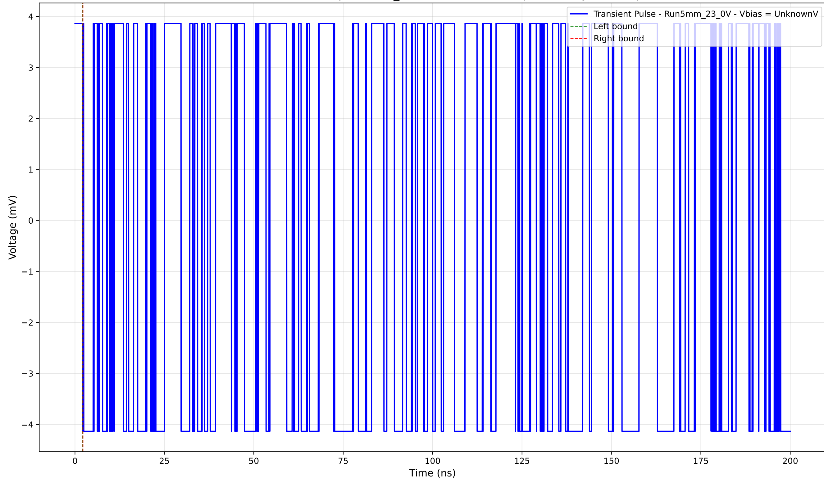
Transient Pulse - Sample: 5mm_23 - Position: 1080.0 \mu\text{m} - Charge: -0.00 pC
