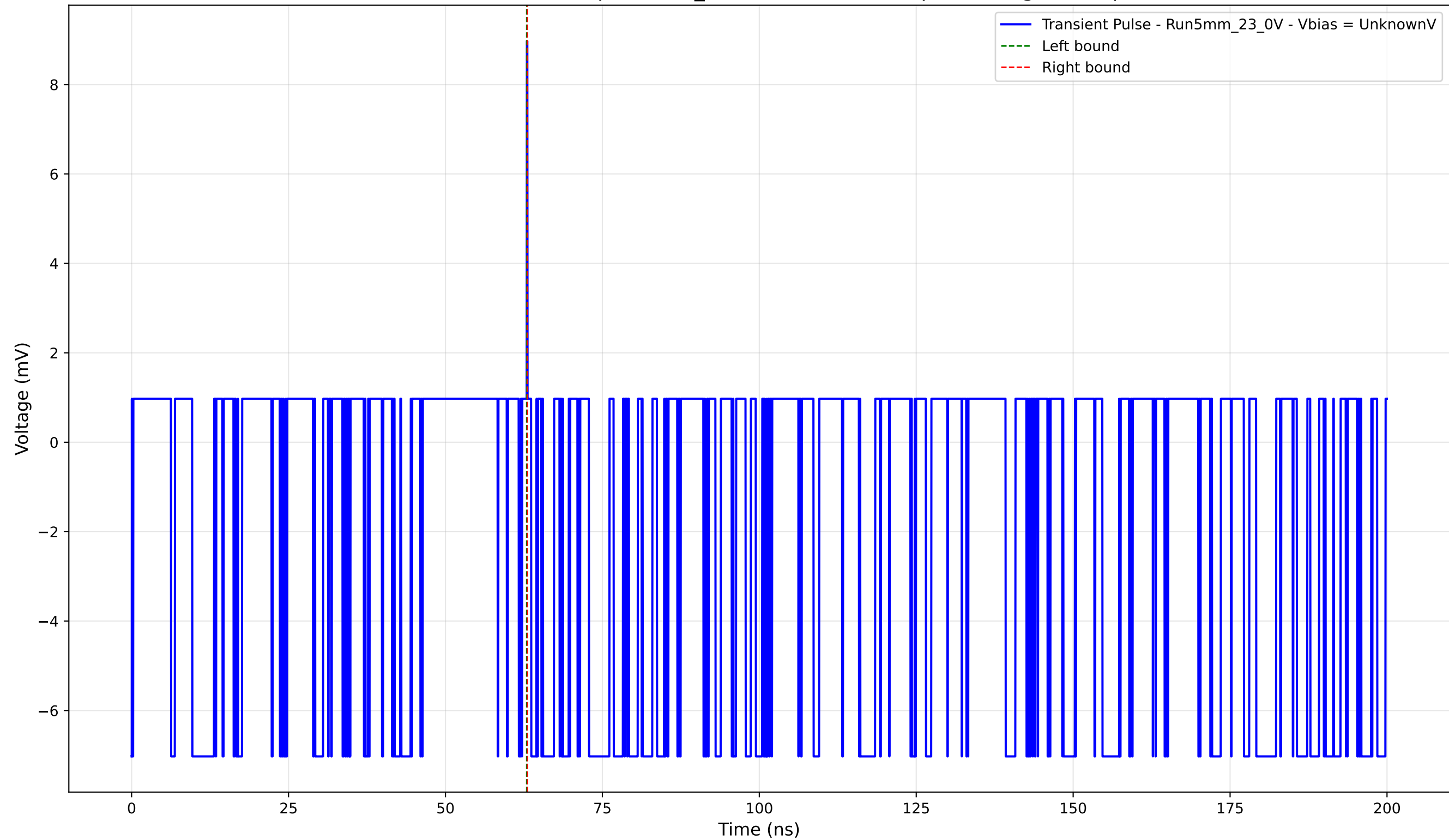
Transient Pulse - Sample: 5mm_23 - Position: 3160.0 \mu\text{m} - Charge: 0.02 pC
