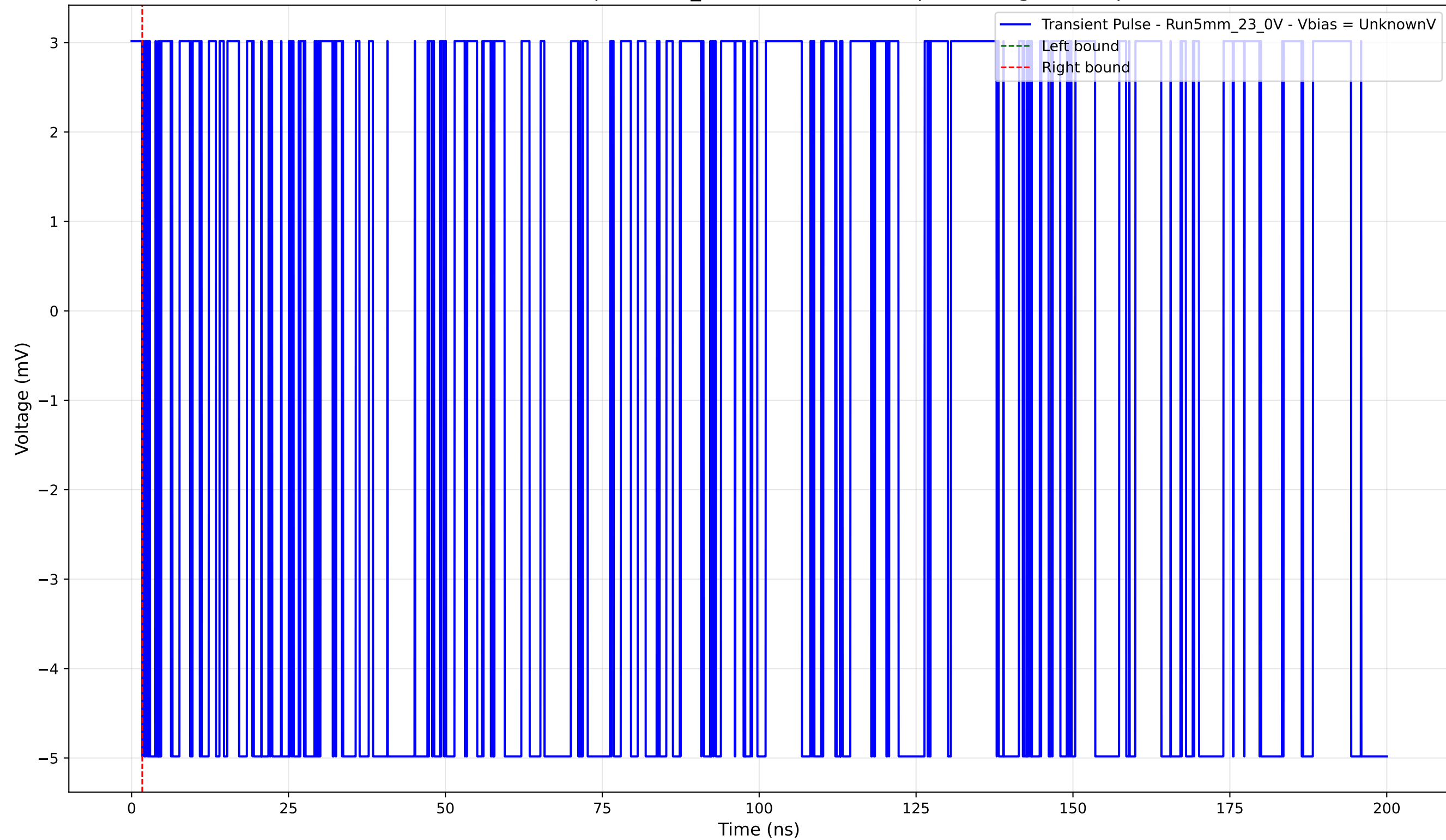
Transient Pulse - Sample: 5mm_23 - Position: 1370.0 \mu\text{m} - Charge: -0.00 pC
