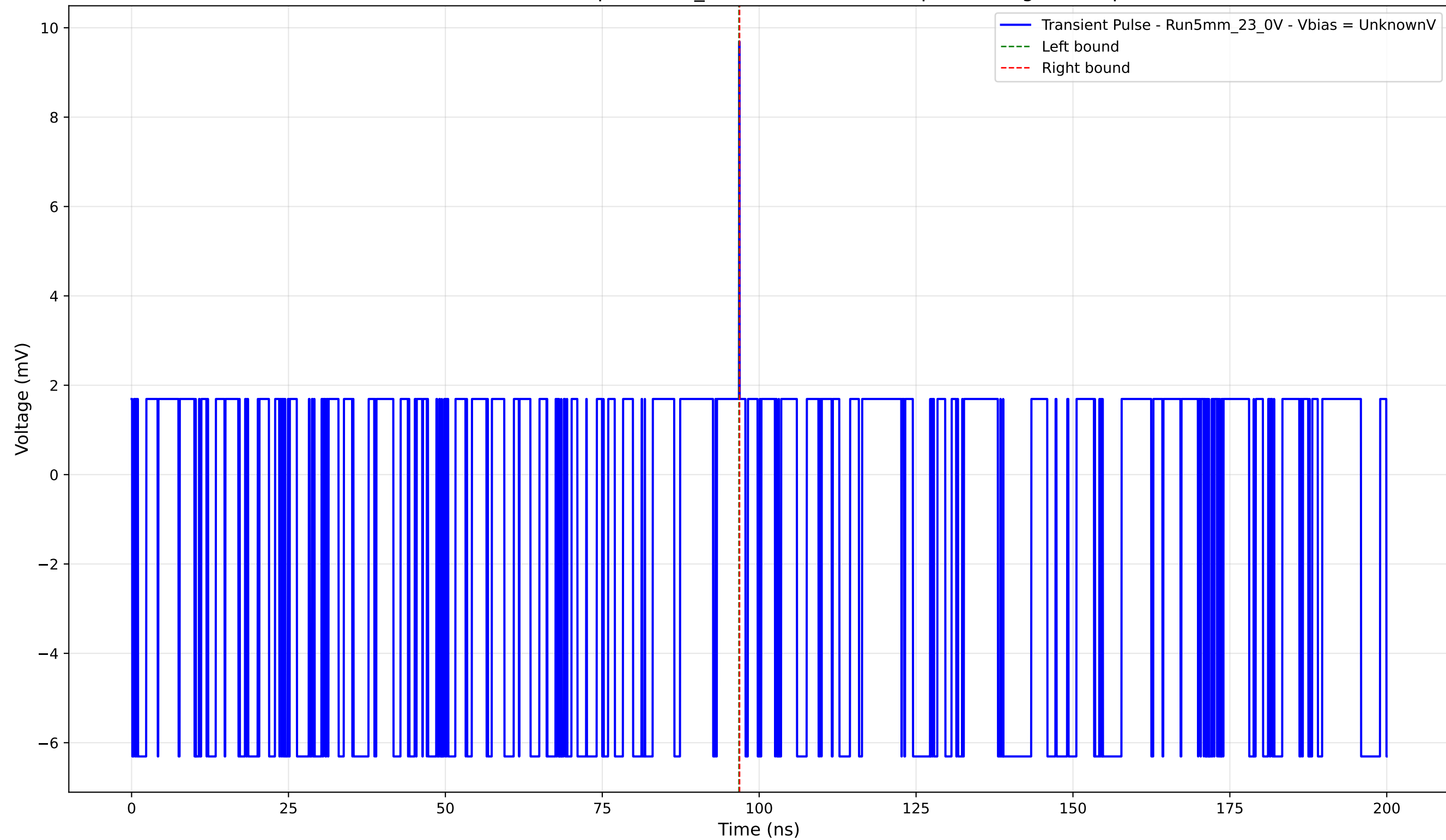
Transient Pulse - Sample: 5mm_23 - Position: 3970.0 \mu\text{m} - Charge: 0.02 pC
