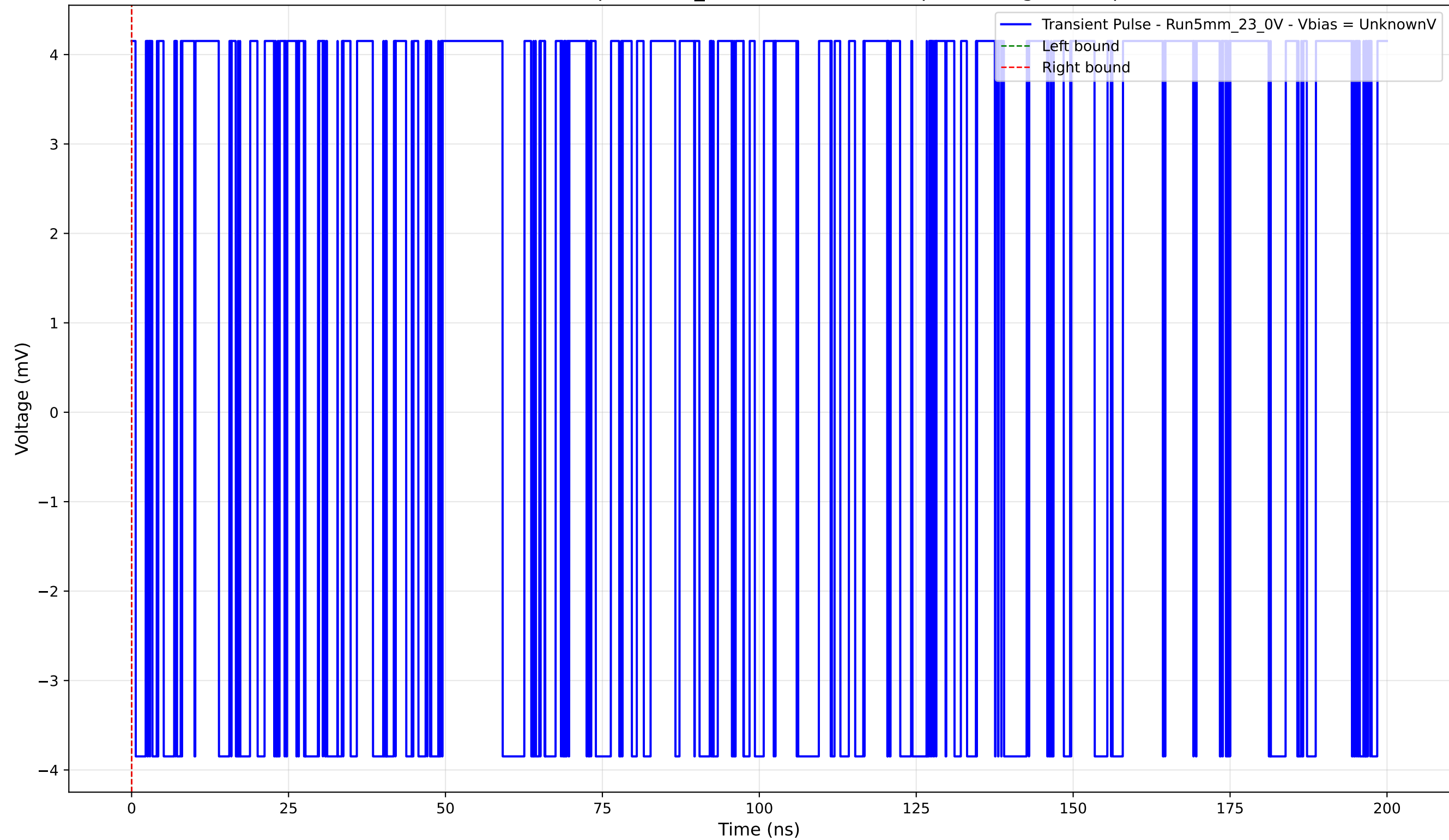
Transient Pulse - Sample: 5mm_23 - Position: 3615.0 \mu\text{m} - Charge: 0.00 pC
