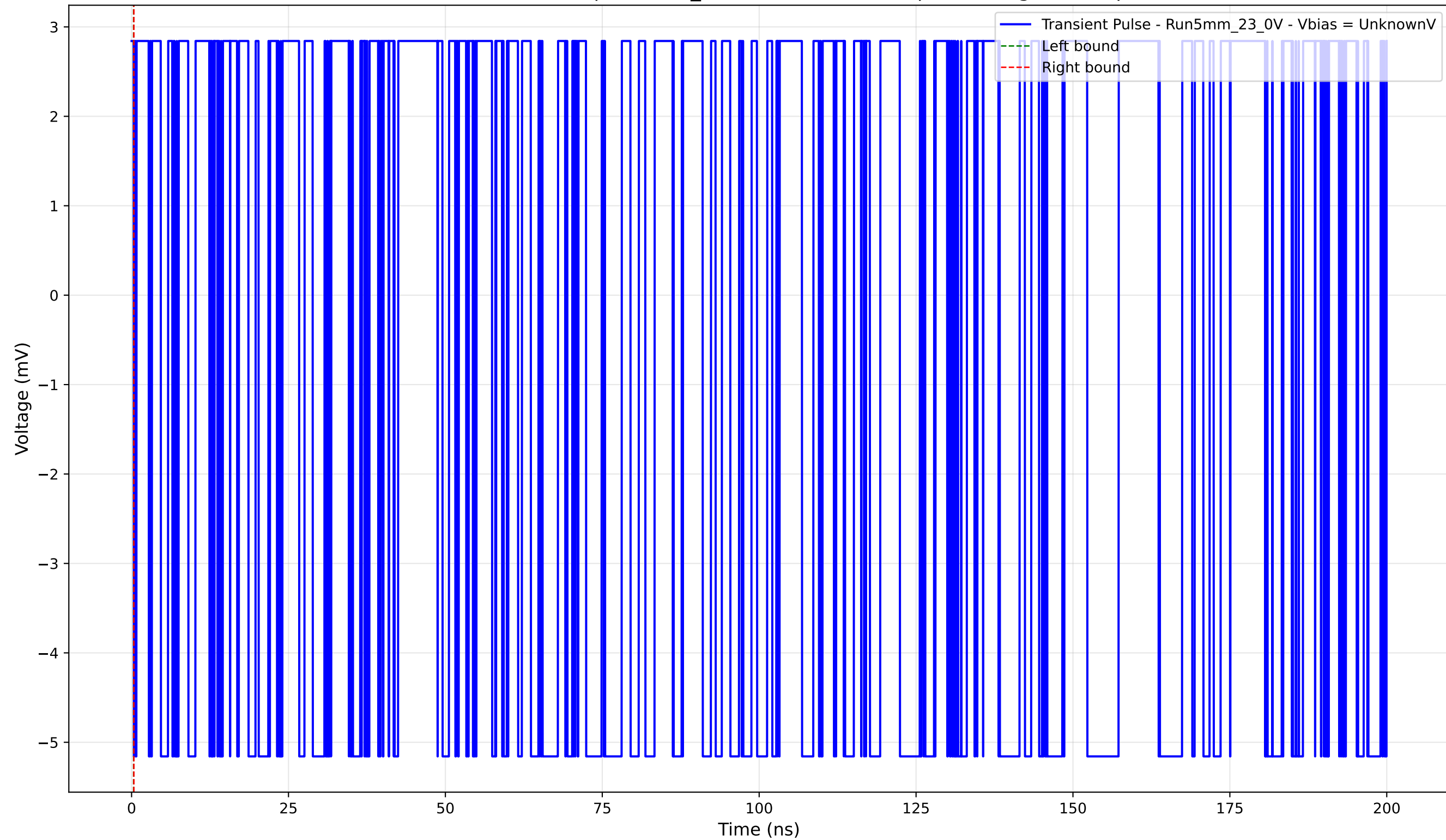
Transient Pulse - Sample: 5mm_23 - Position: 1530.0 \mu\text{m} - Charge: -0.00 pC
