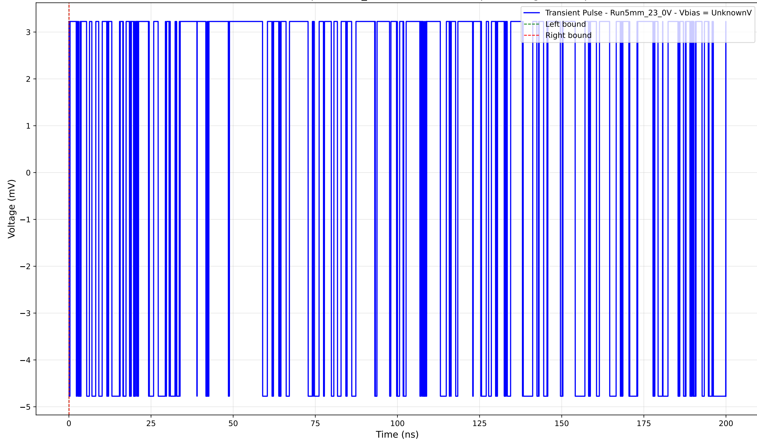
Transient Pulse - Sample: 5mm_23 - Position: 4475.0 \mu\text{m} - Charge: -0.00 pC
