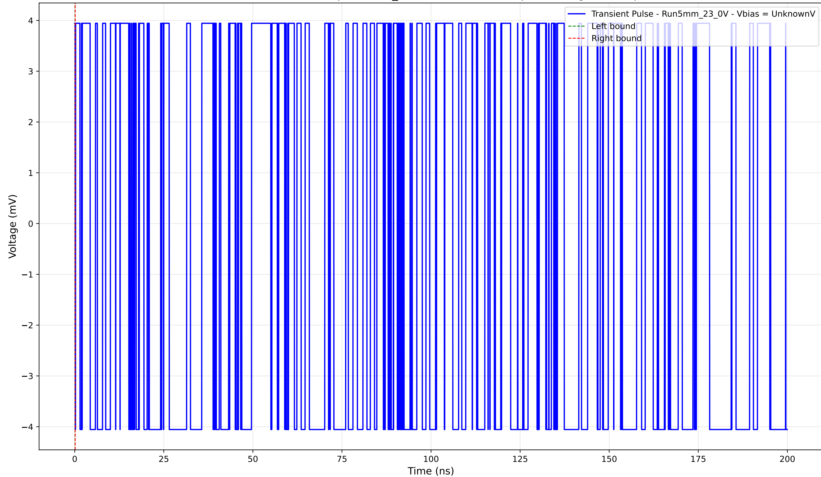
Transient Pulse - Sample: 5mm_23 - Position: 2085.0 \mu\text{m} - Charge: -0.00 pC
