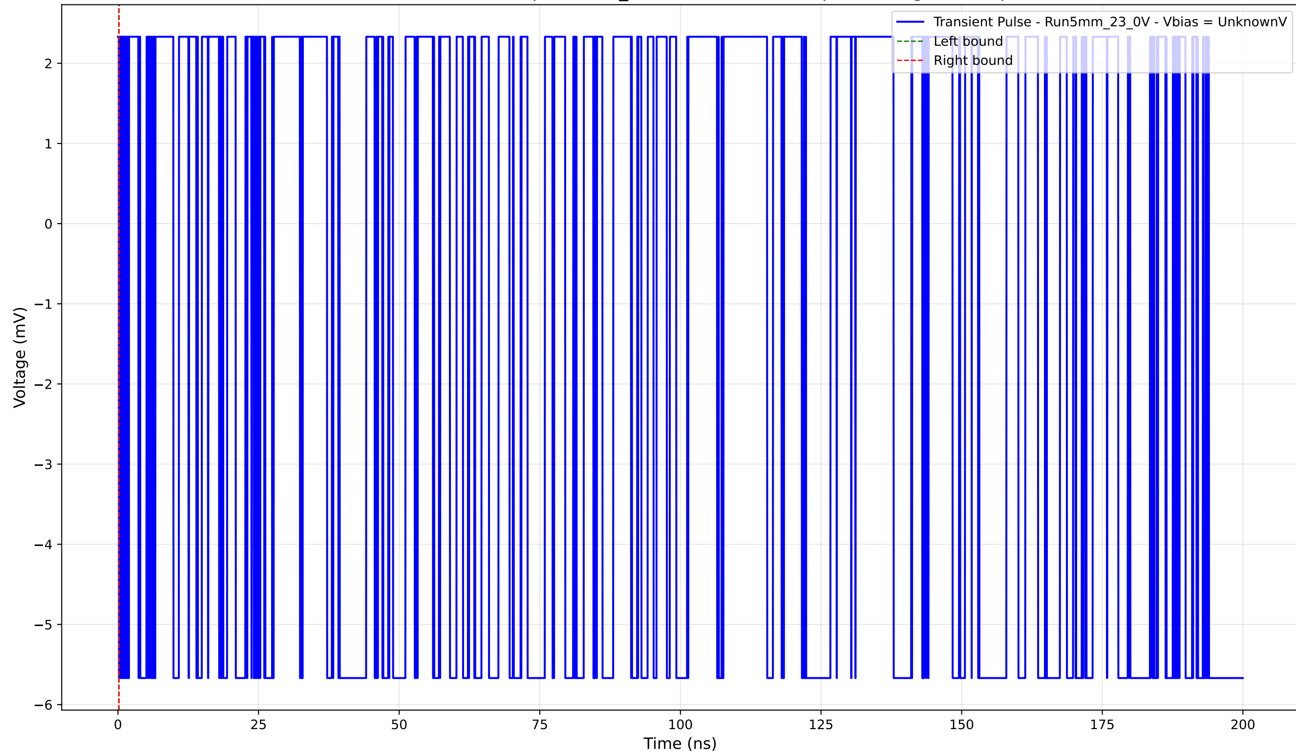
Transient Pulse - Sample: 5mm_23 - Position: 4795.0 \mu\text{m} - Charge: -0.00 pC
