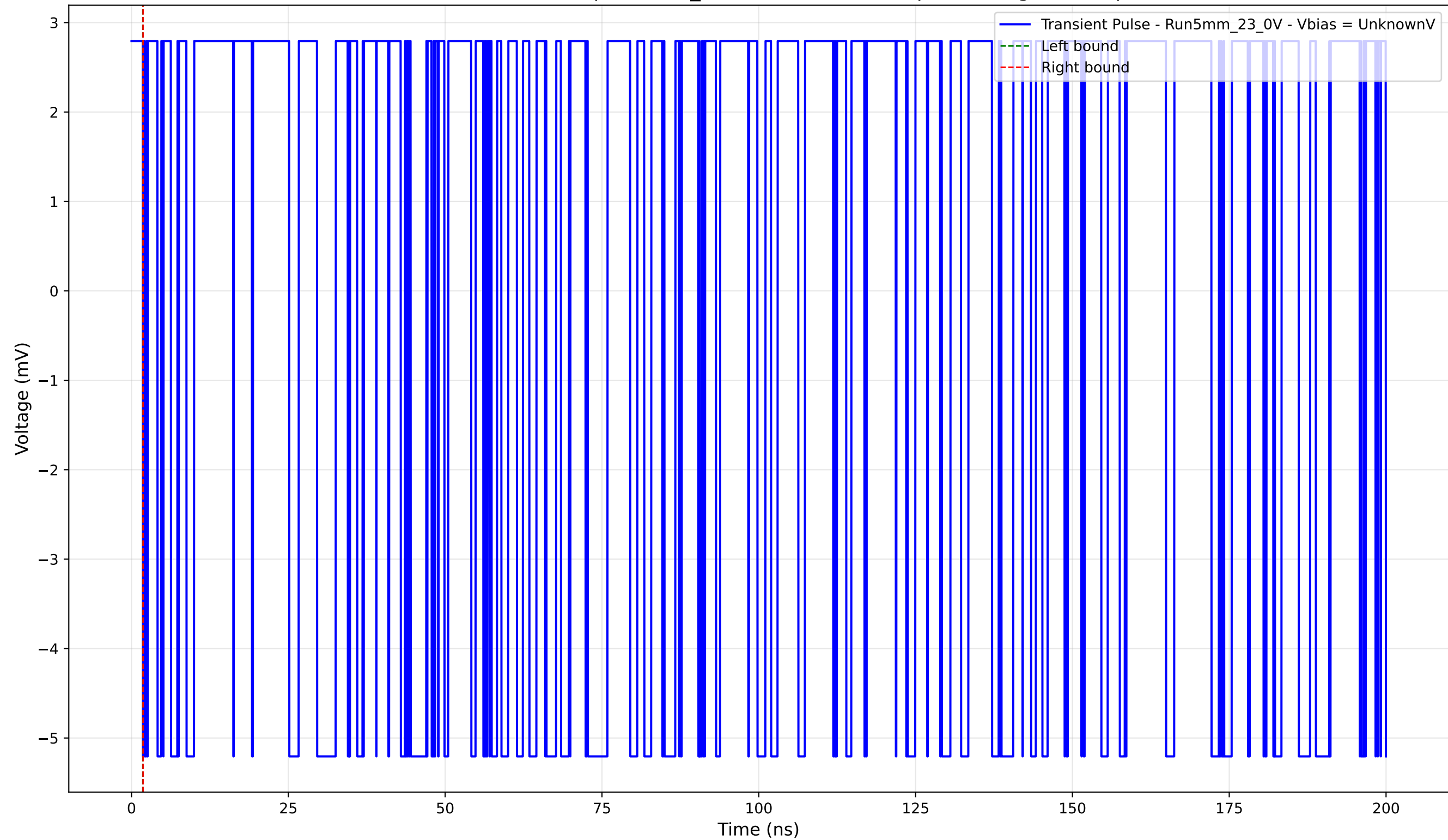
Transient Pulse - Sample: 5mm_23 - Position: 2375.0 \mu\text{m} - Charge: -0.00 pC
