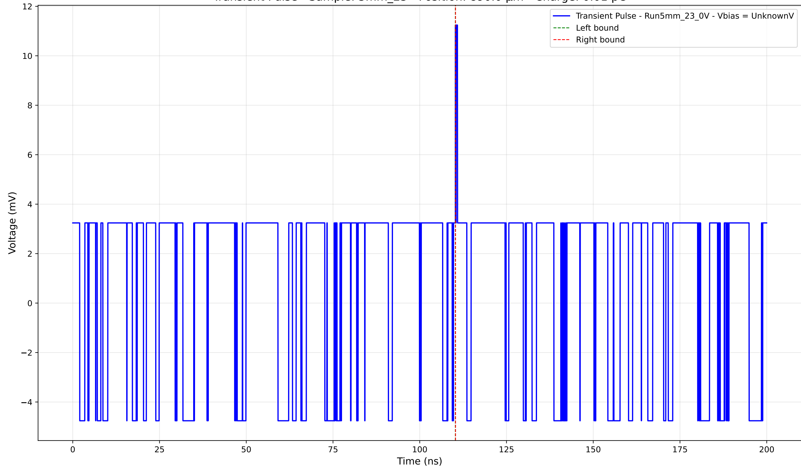
Transient Pulse - Sample: 5mm_23 - Position: 890.0 \mu\text{m} - Charge: 0.01 pC
