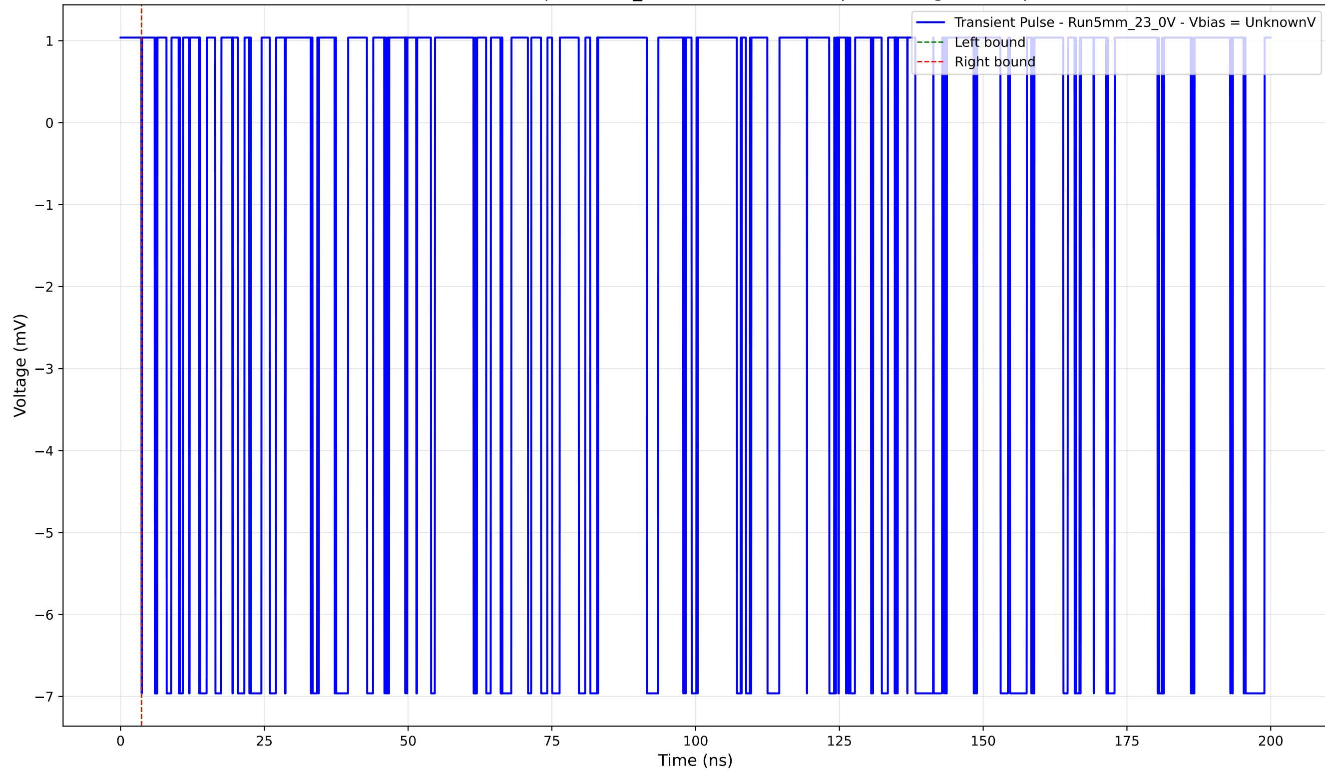
Transient Pulse - Sample: 5mm_23 - Position: 2710.0 \mu\text{m} - Charge: -0.00 pC
