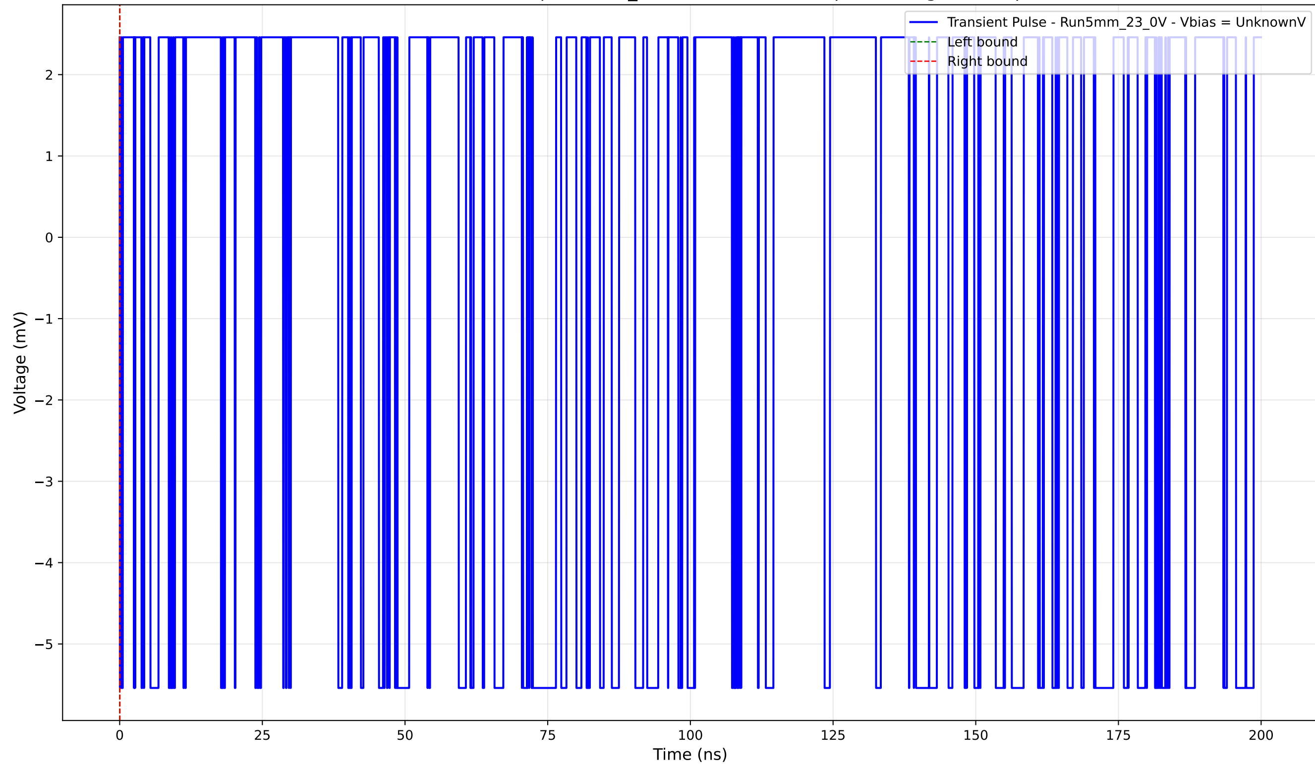
Transient Pulse - Sample: 5mm_23 - Position: 2830.0 \mu\text{m} - Charge: -0.00 pC
