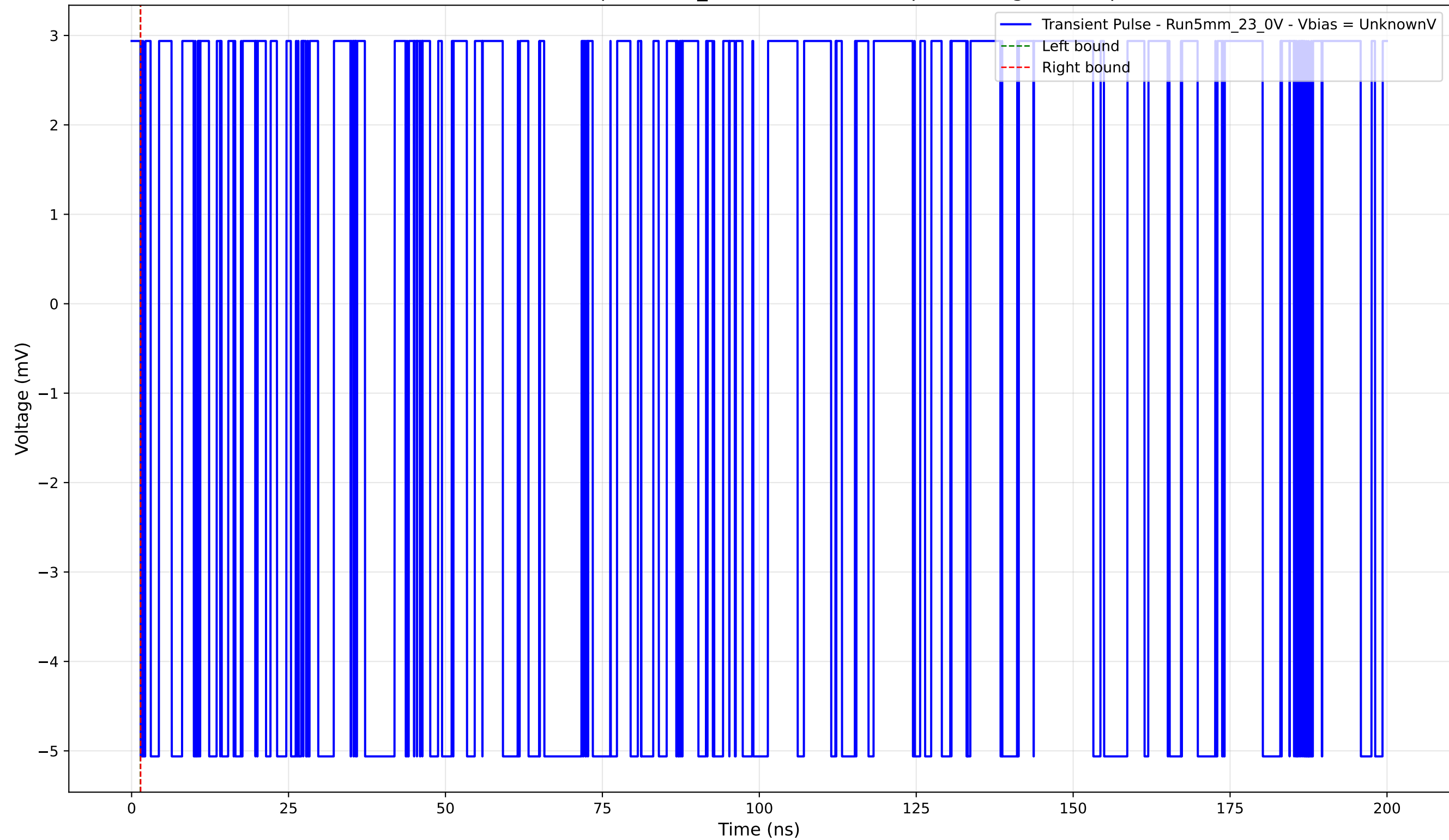
Transient Pulse - Sample: 5mm_23 - Position: 525.0 \mu\text{m} - Charge: -0.00 pC
