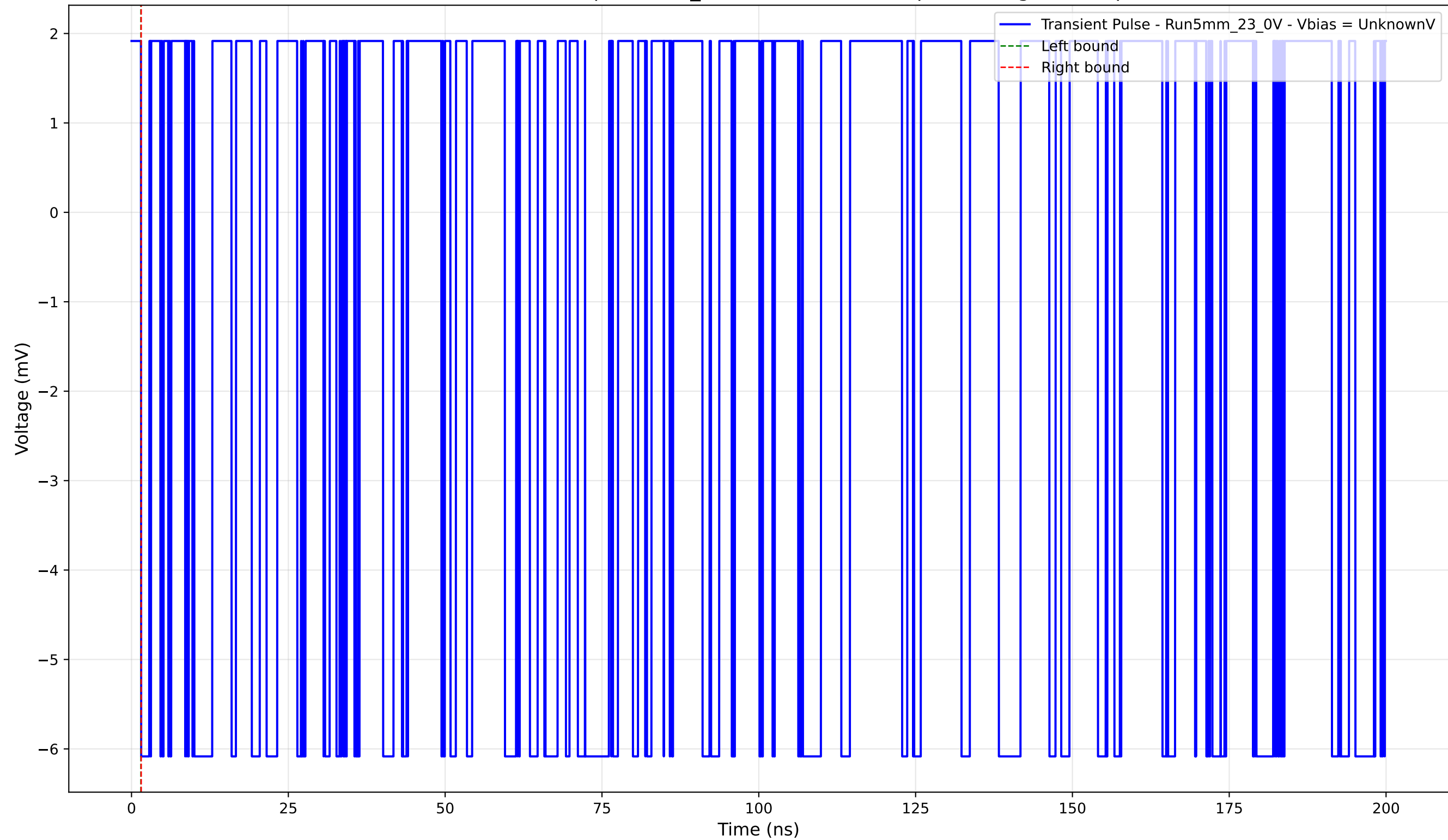
Transient Pulse - Sample: 5mm_23 - Position: 2625.0 \mu\text{m} - Charge: -0.00 pC
