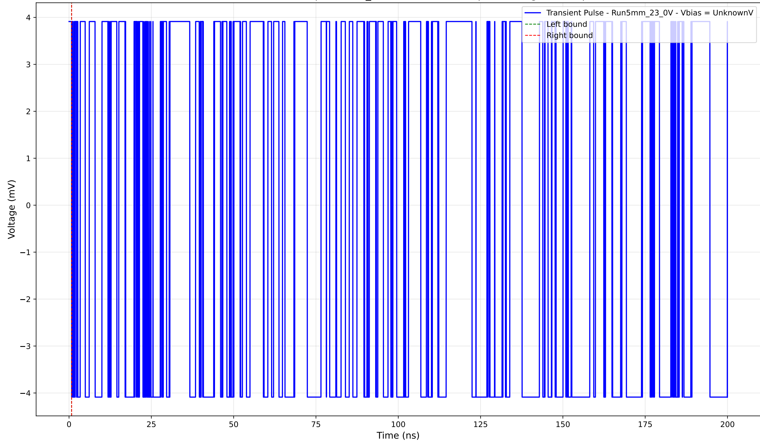
Transient Pulse - Sample: 5mm_23 - Position: 440.0 \mu\text{m} - Charge: -0.00 pC
