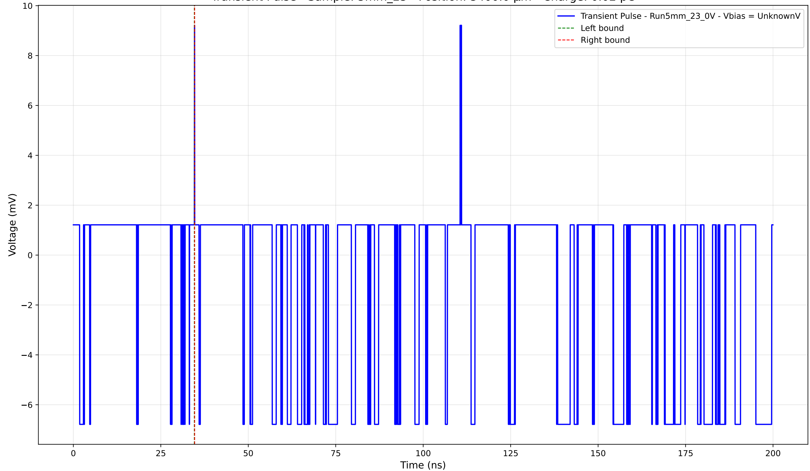
Transient Pulse - Sample: 5mm_23 - Position: 3400.0 \mu\text{m} - Charge: 0.02 pC
