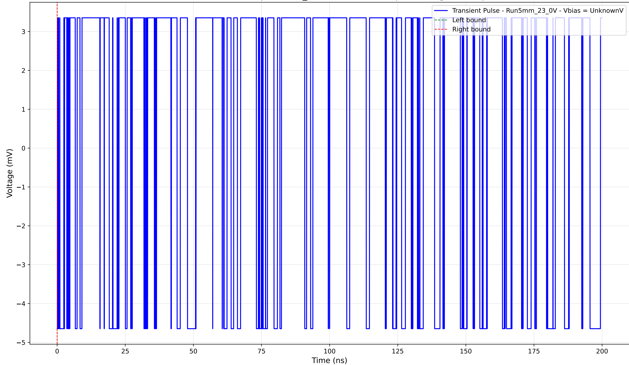
Transient Pulse - Sample: 5mm_23 - Position: 285.0 \mu\text{m} - Charge: -0.00 pC
