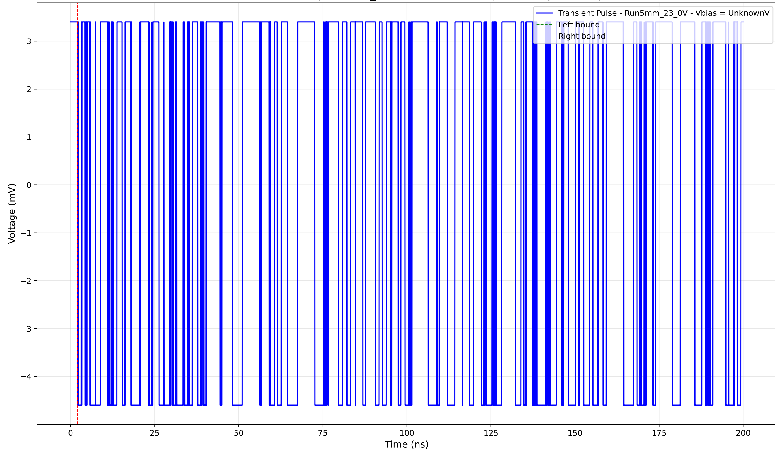
Transient Pulse - Sample: 5mm_23 - Position: 2380.0 \mu\text{m} - Charge: -0.00 pC
