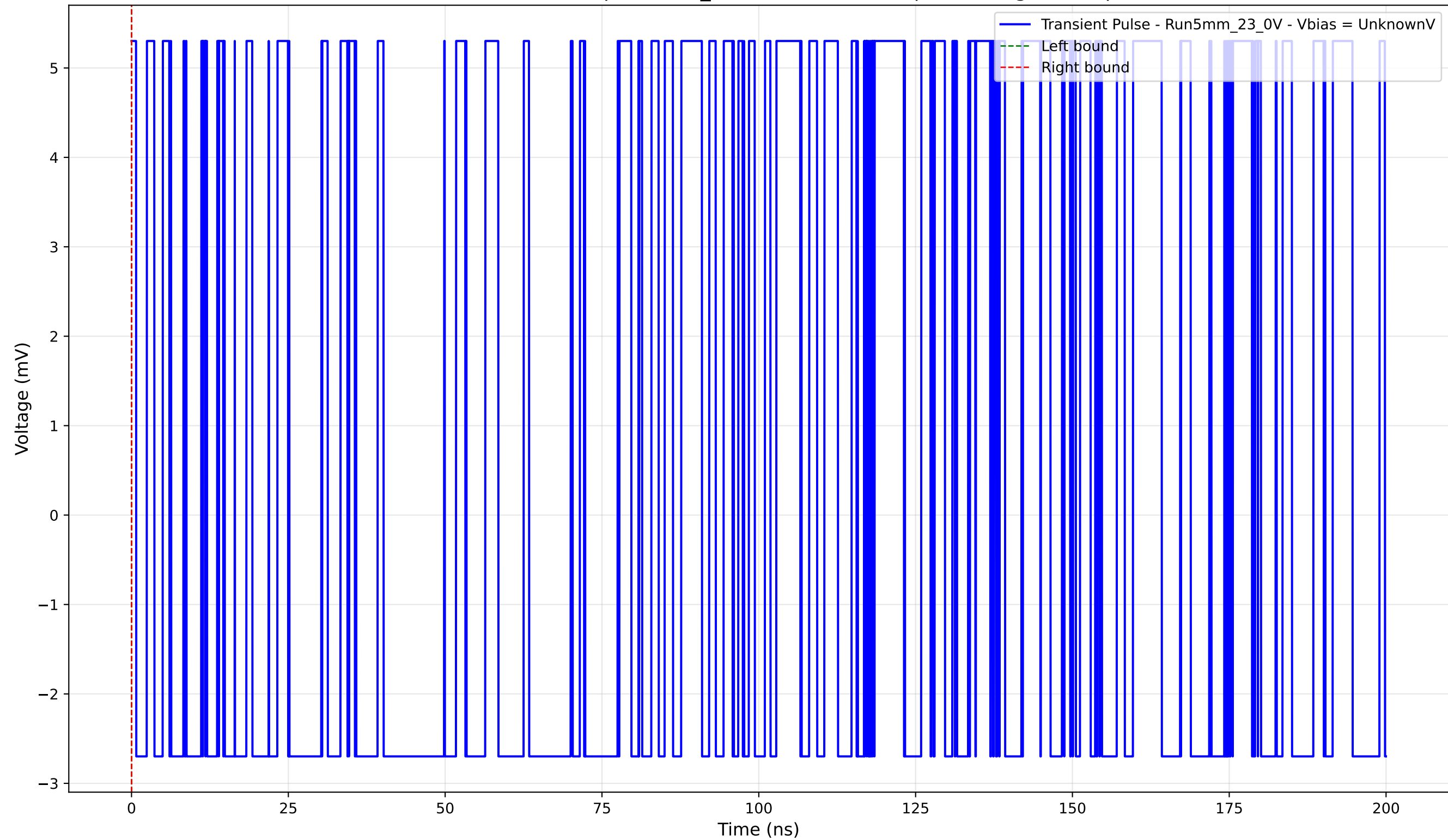
Transient Pulse - Sample: 5mm_23 - Position: 170.0 \mu\text{m} - Charge: 0.00 pC
