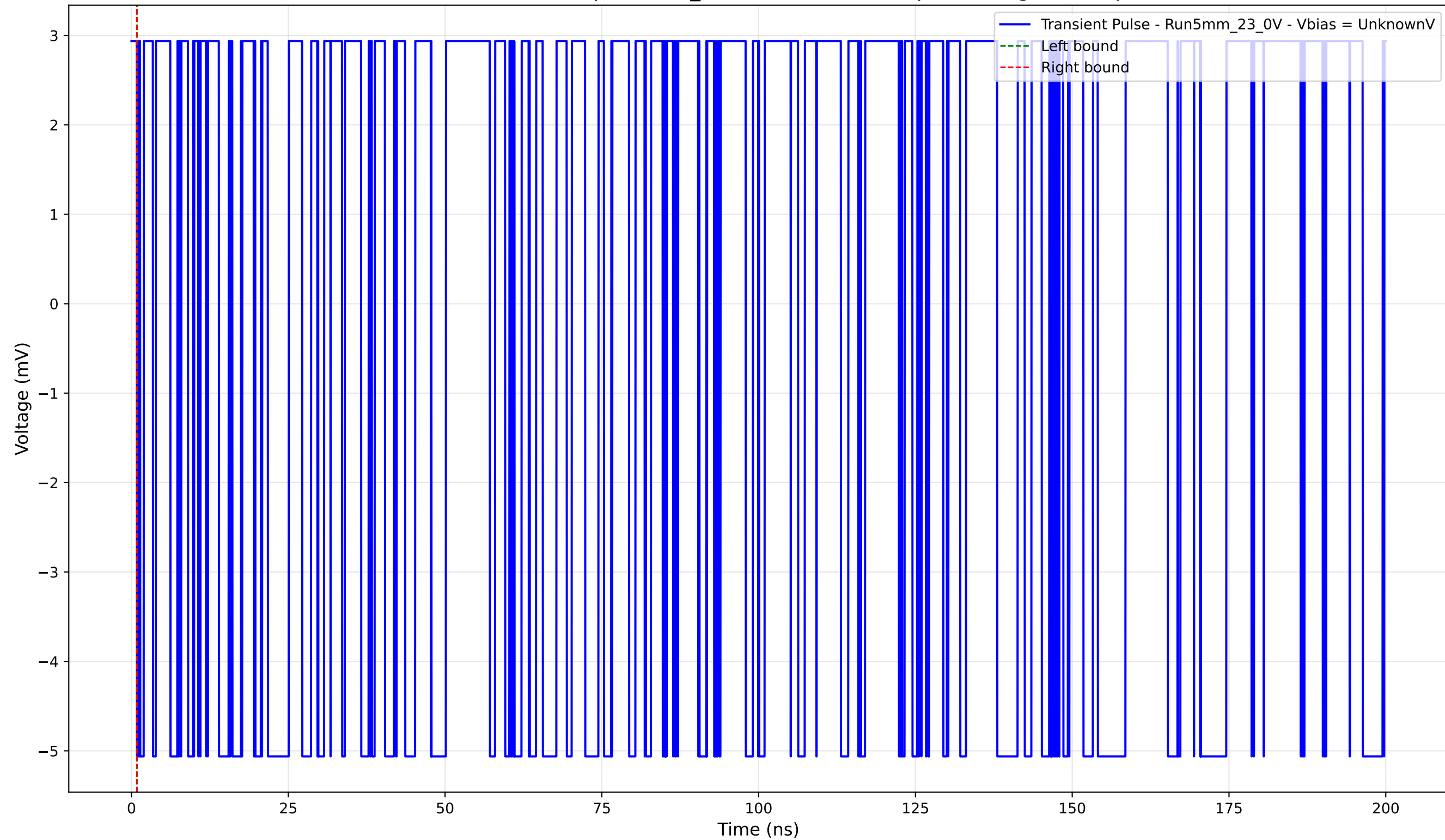
Transient Pulse - Sample: 5mm_23 - Position: 2930.0 \mu\text{m} - Charge: -0.00 pC
