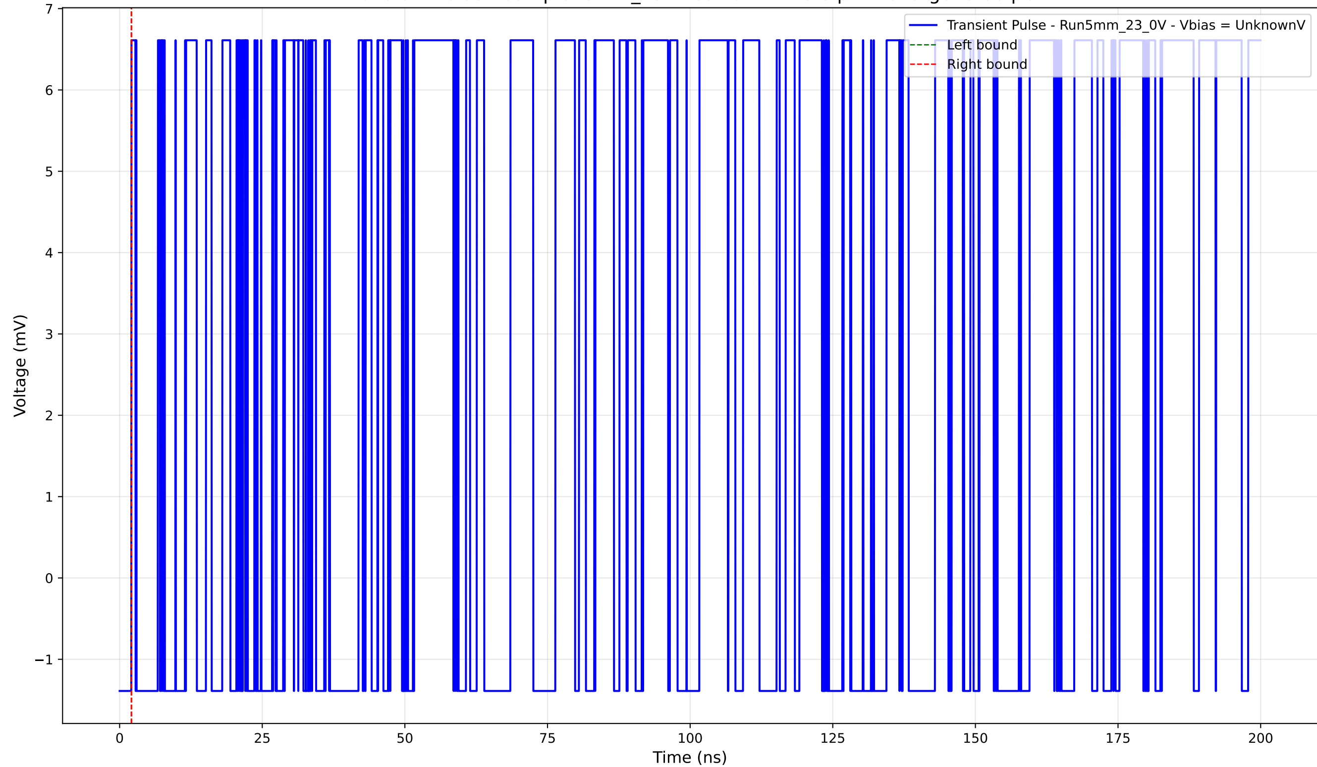
Transient Pulse - Sample: 5mm_23 - Position: 1740.0 \mu\text{m} - Charge: 0.00 pC
