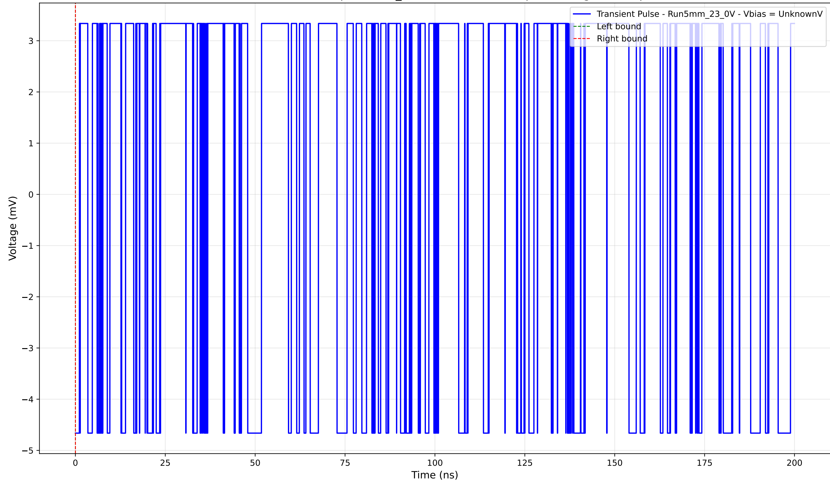
Transient Pulse - Sample: 5mm_23 - Position: 4815.0 \mu\text{m} - Charge: -0.00 pC
