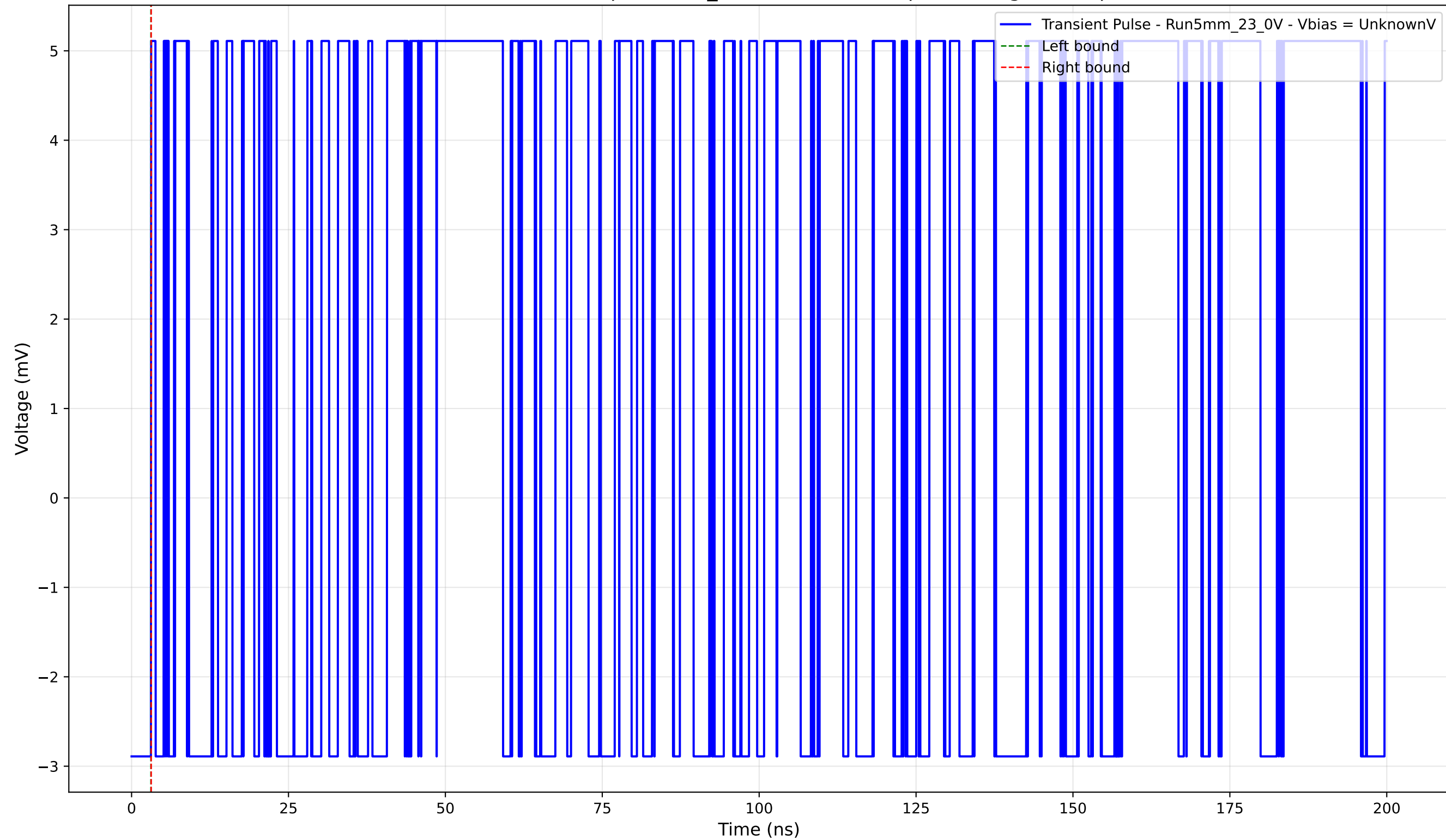
Transient Pulse - Sample: 5mm_23 - Position: 75.0 \mu\text{m} - Charge: 0.00 pC
