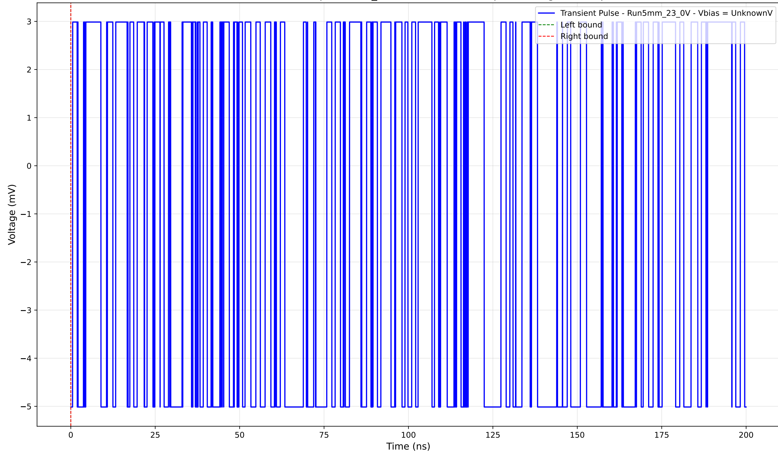
Transient Pulse - Sample: 5mm_23 - Position: 3525.0 \mu\text{m} - Charge: -0.00 pC
