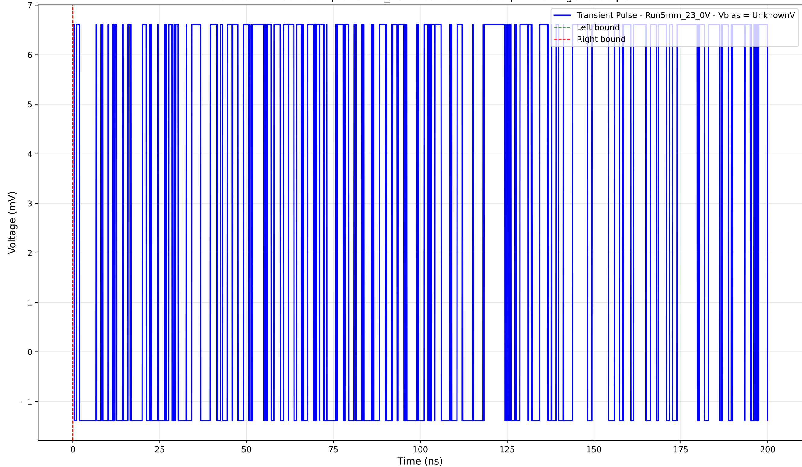
Transient Pulse - Sample: 5mm_23 - Position: 4840.0 \mu\text{m} - Charge: 0.00 pC
