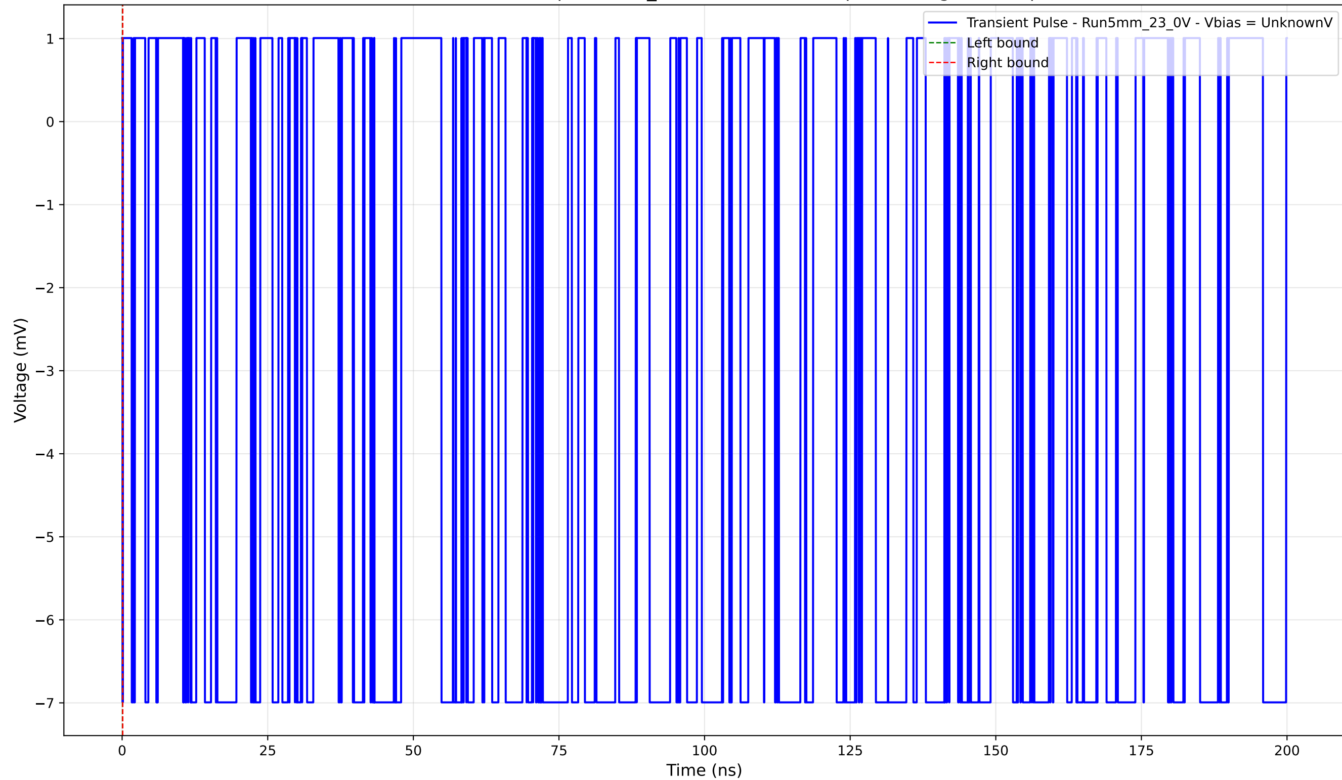
Transient Pulse - Sample: 5mm_23 - Position: 535.0 \mu\text{m} - Charge: -0.00 pC
