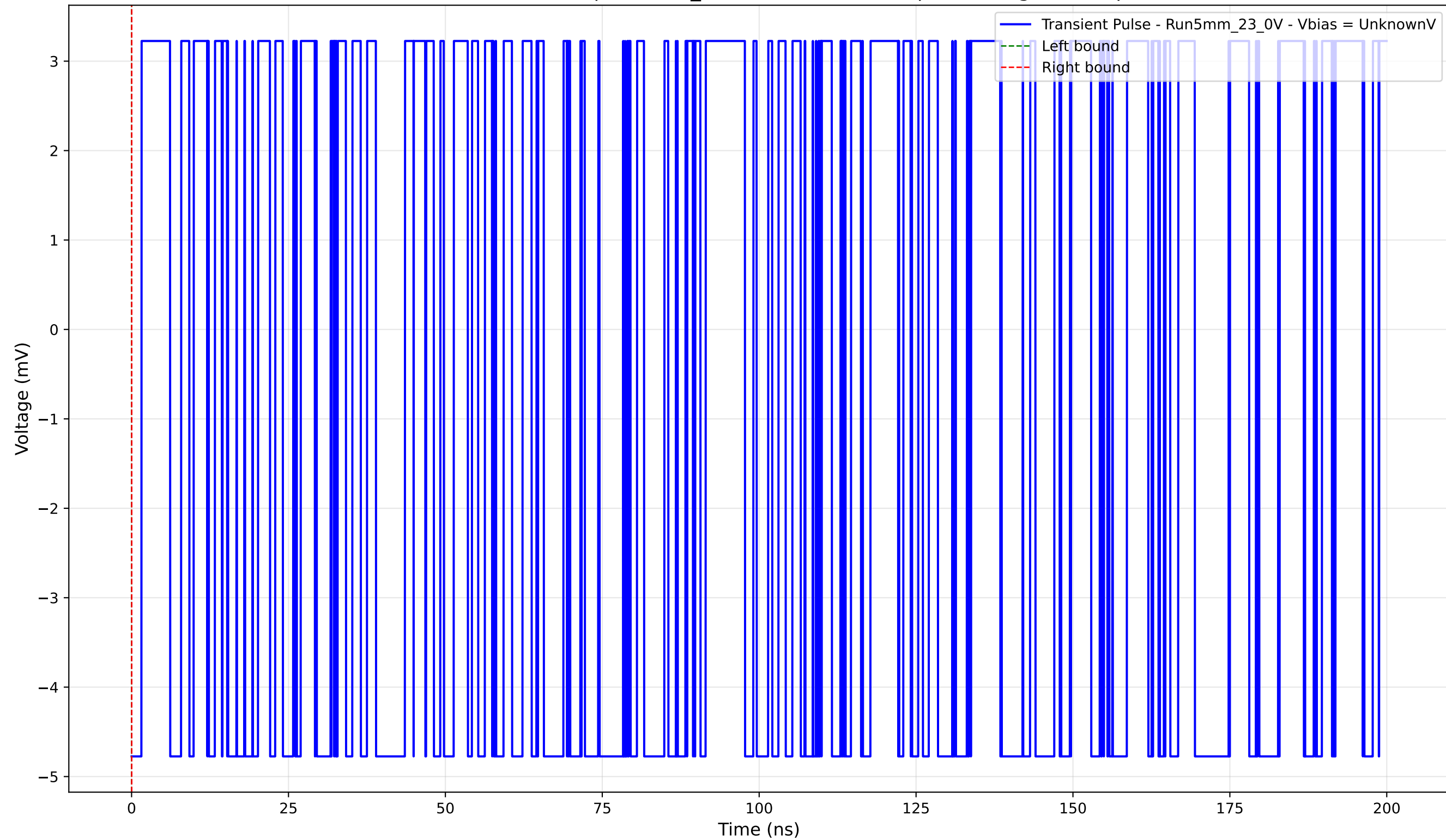
Transient Pulse - Sample: 5mm_23 - Position: 3585.0 \mu\text{m} - Charge: -0.00 pC
