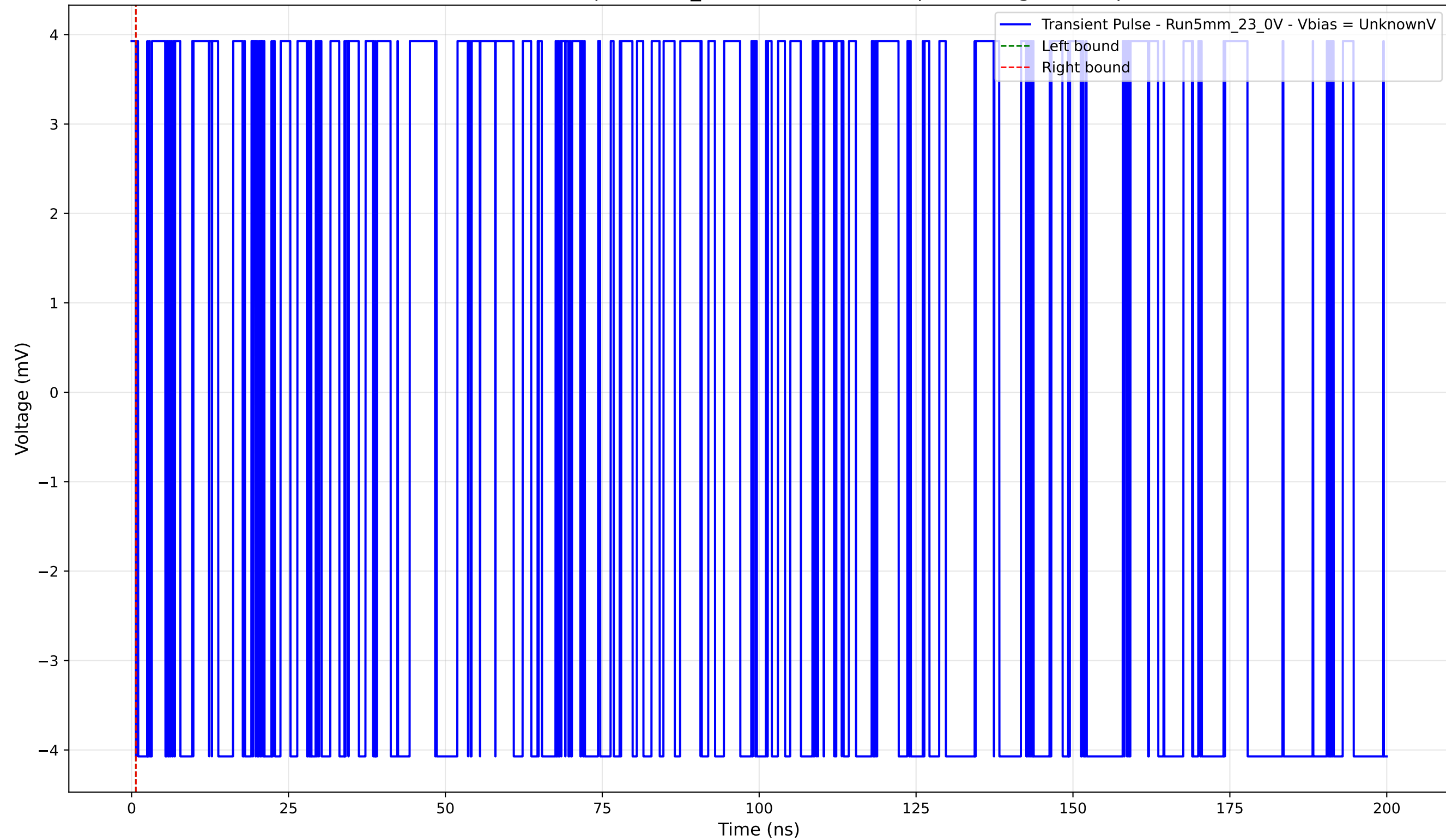
Transient Pulse - Sample: 5mm_23 - Position: 2015.0 \mu\text{m} - Charge: -0.00 pC
