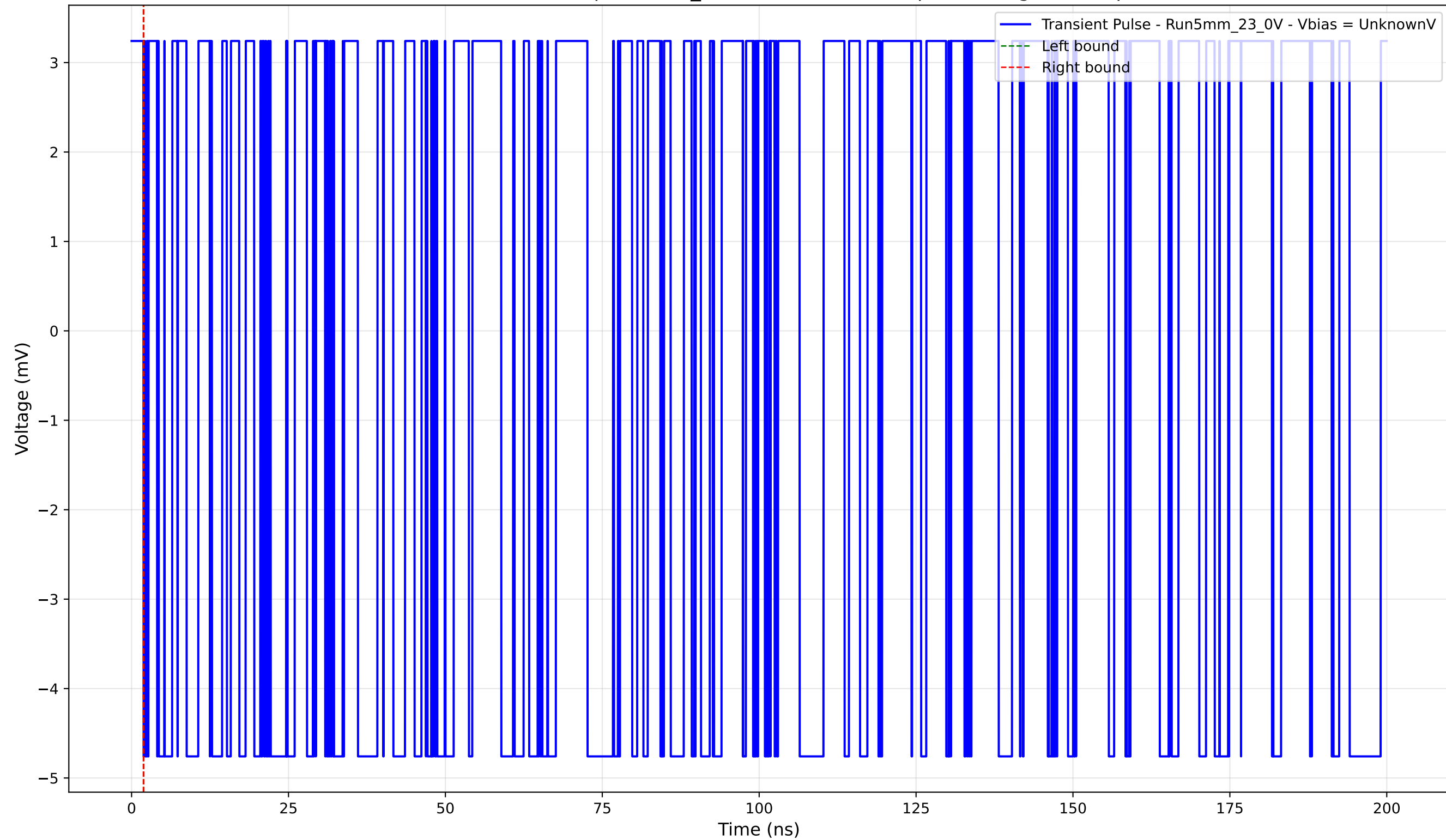
Transient Pulse - Sample: 5mm_23 - Position: 3450.0 \mu\text{m} - Charge: -0.00 pC
