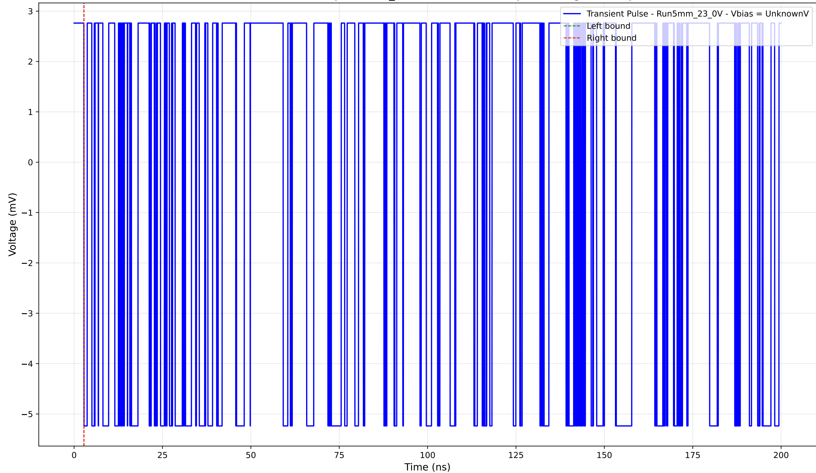
Transient Pulse - Sample: 5mm_23 - Position: 3965.0 \mu\text{m} - Charge: -0.00 pC
