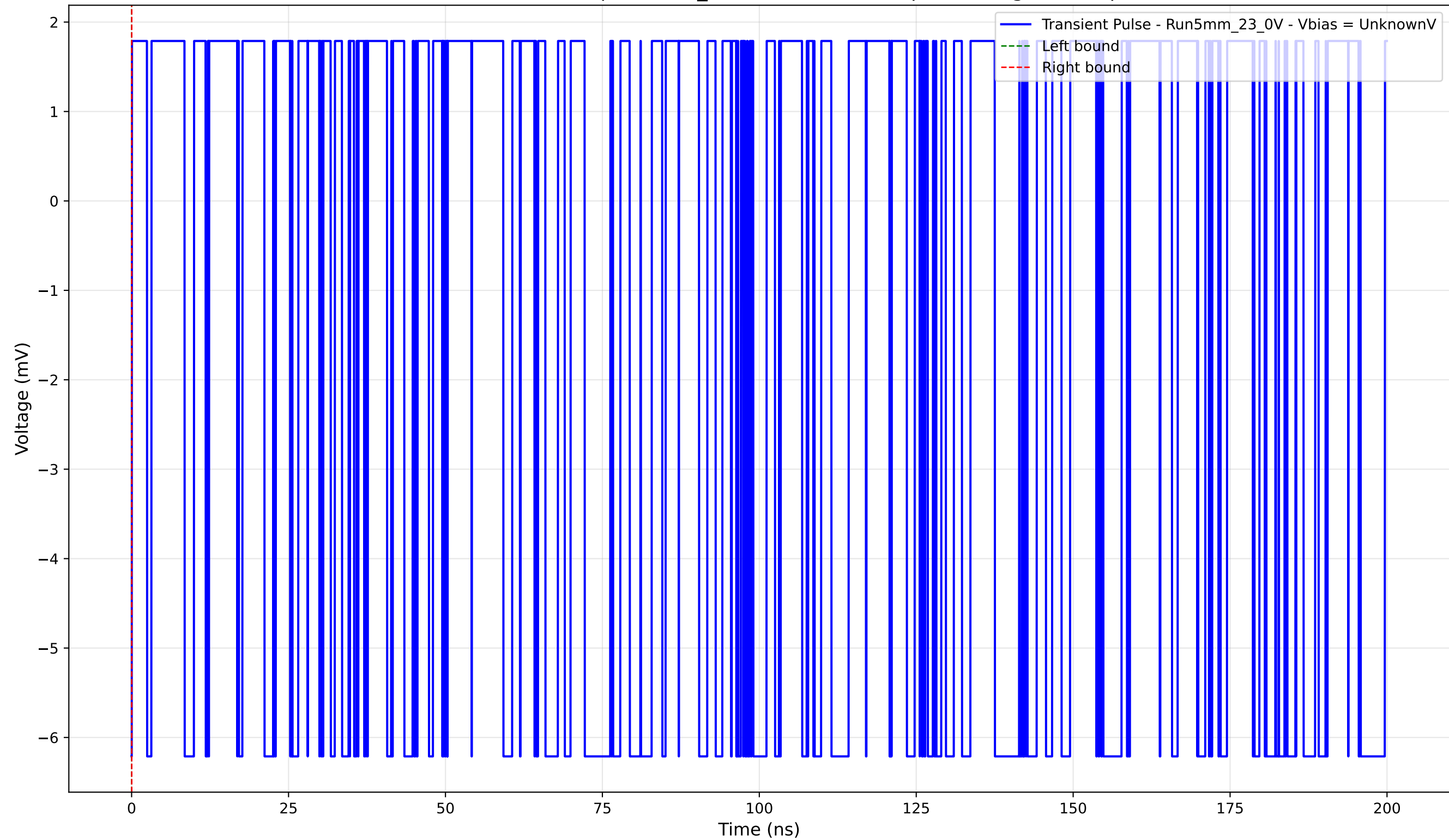
Transient Pulse - Sample: 5mm_23 - Position: 980.0 \mu\text{m} - Charge: -0.00 pC
