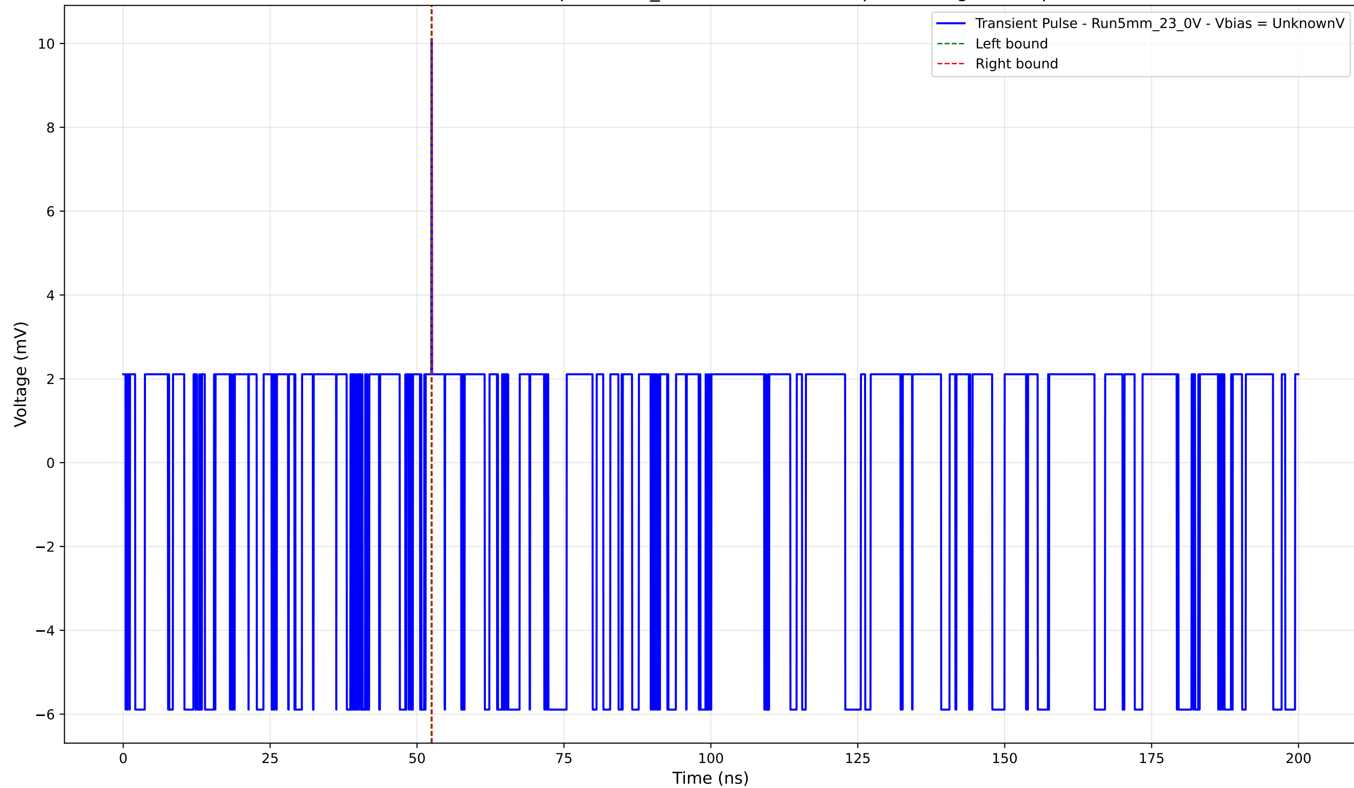
Transient Pulse - Sample: 5mm_23 - Position: 1245.0 \mu\text{m} - Charge: 0.02 pC
