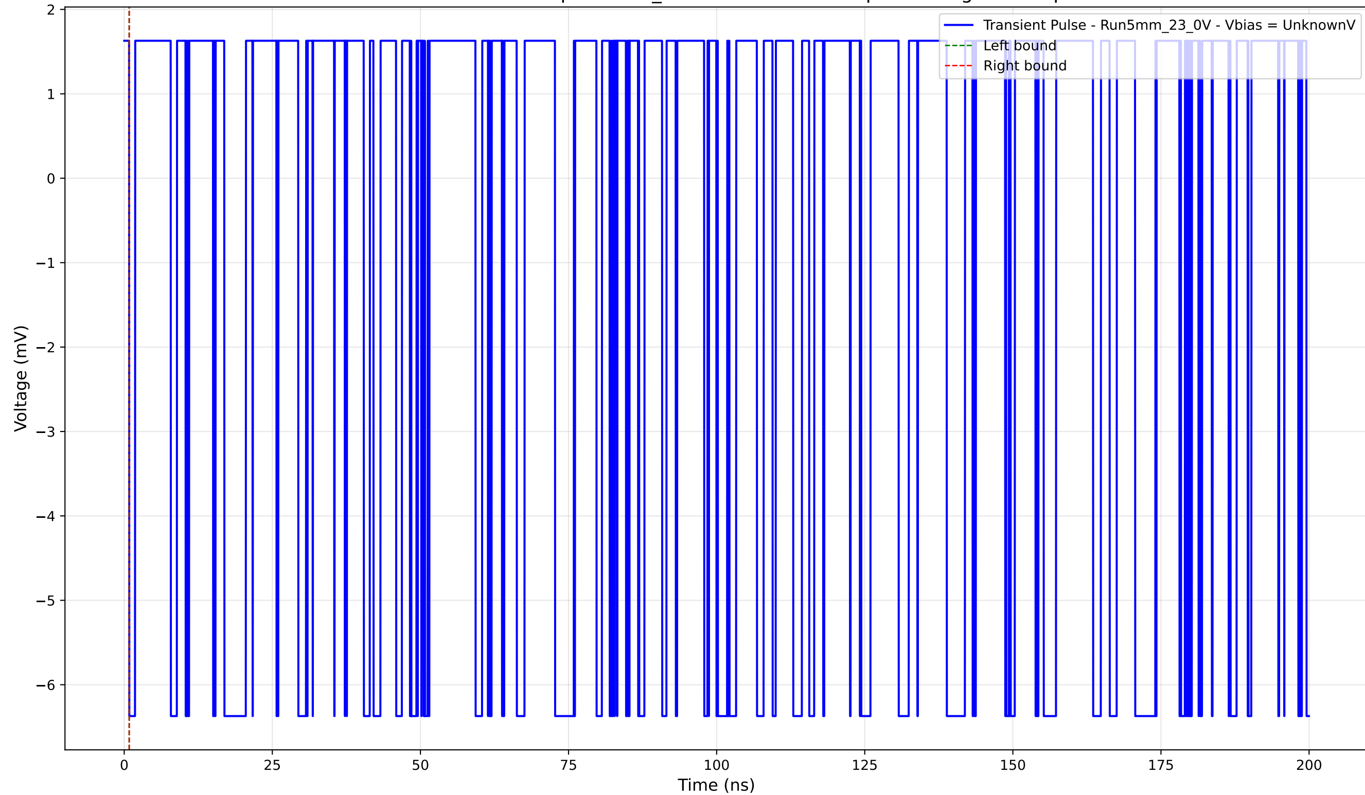
Transient Pulse - Sample: 5mm_23 - Position: 3215.0 \mu\text{m} - Charge: -0.00 pC
