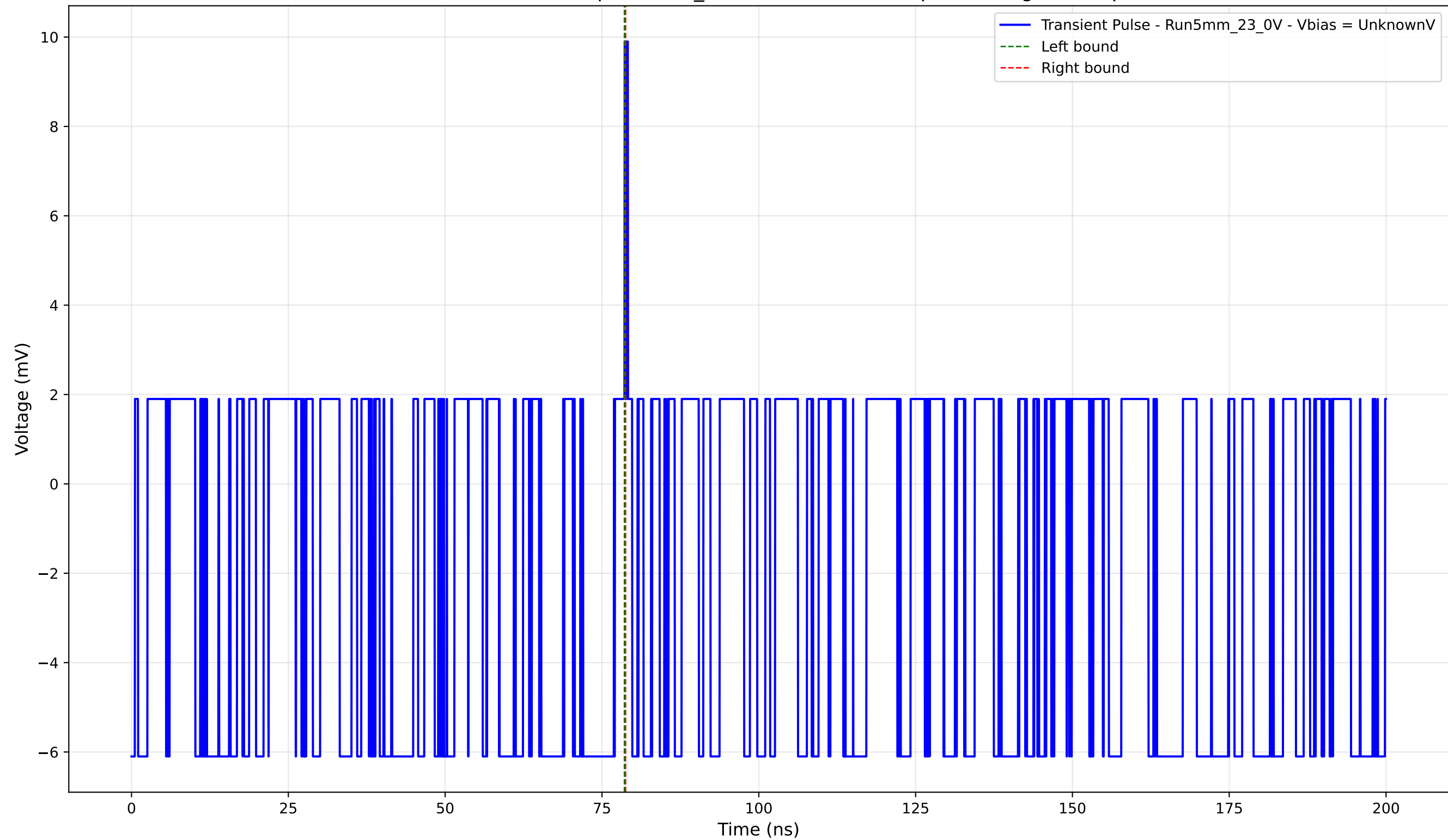
Transient Pulse - Sample: 5mm_23 - Position: 2415.0 \mu\text{m} - Charge: 0.03 pC
