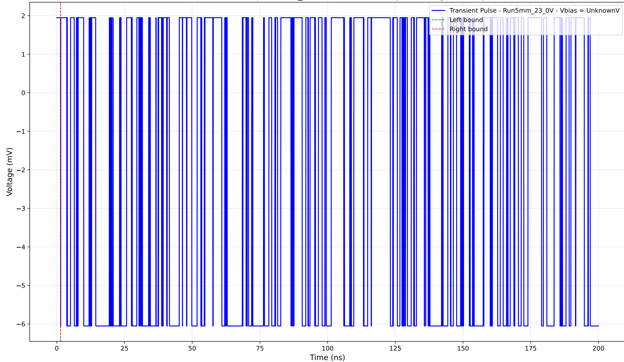
Transient Pulse - Sample: 5mm_23 - Position: 1500.0 \mu\text{m} - Charge: -0.00 pC
