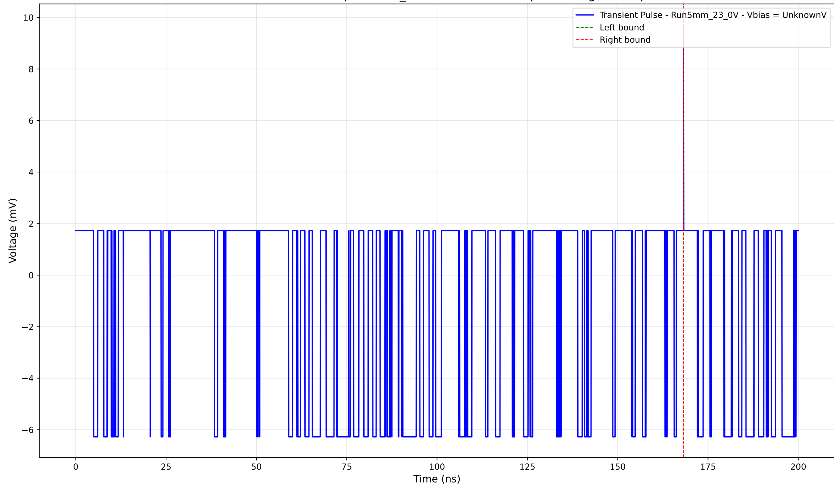
Transient Pulse - Sample: 5mm_23 - Position: 2310.0 \mu\text{m} - Charge: 0.00 pC
