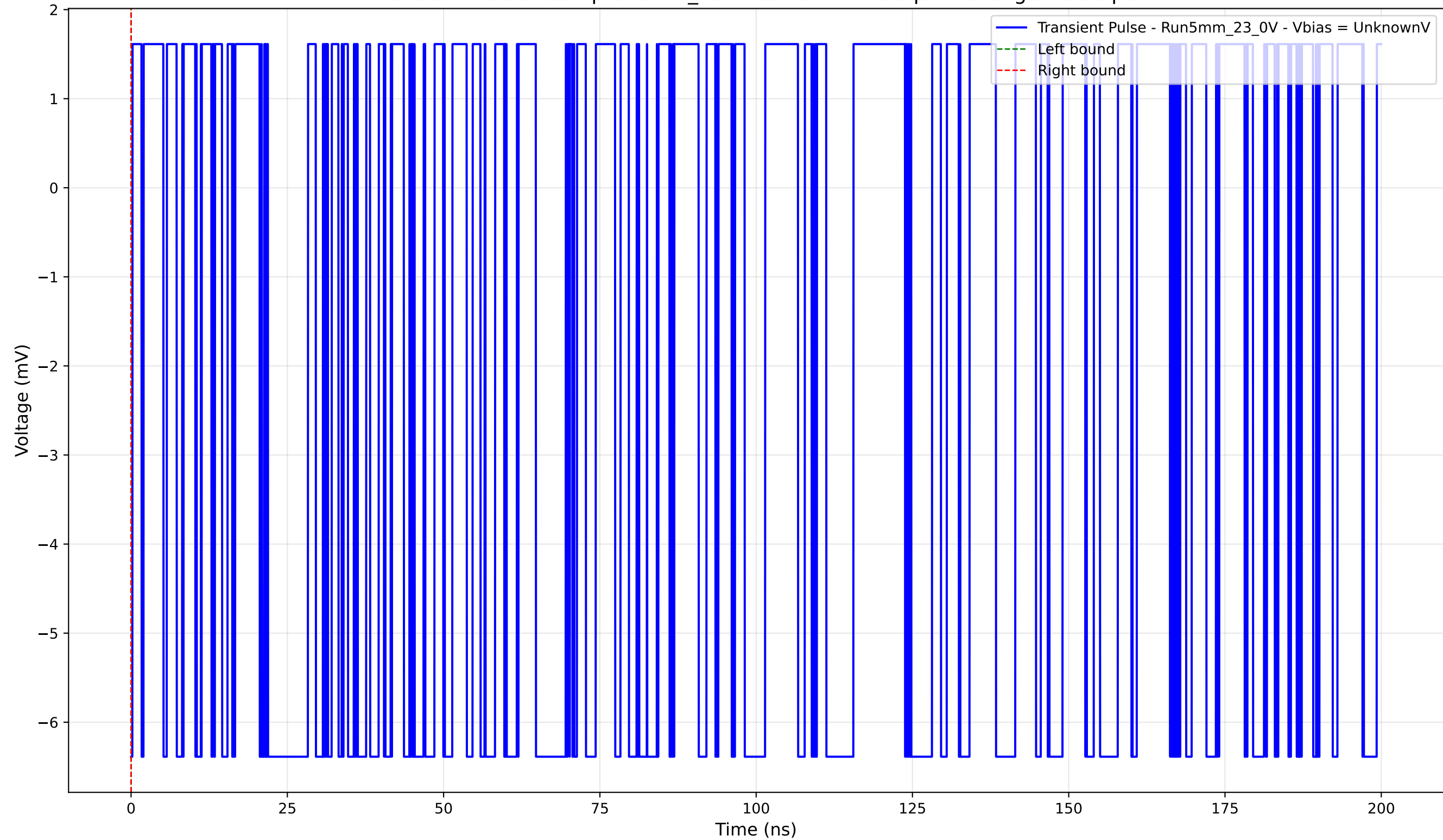
Transient Pulse - Sample: 5mm_23 - Position: 2240.0 \mu\text{m} - Charge: -0.00 pC
