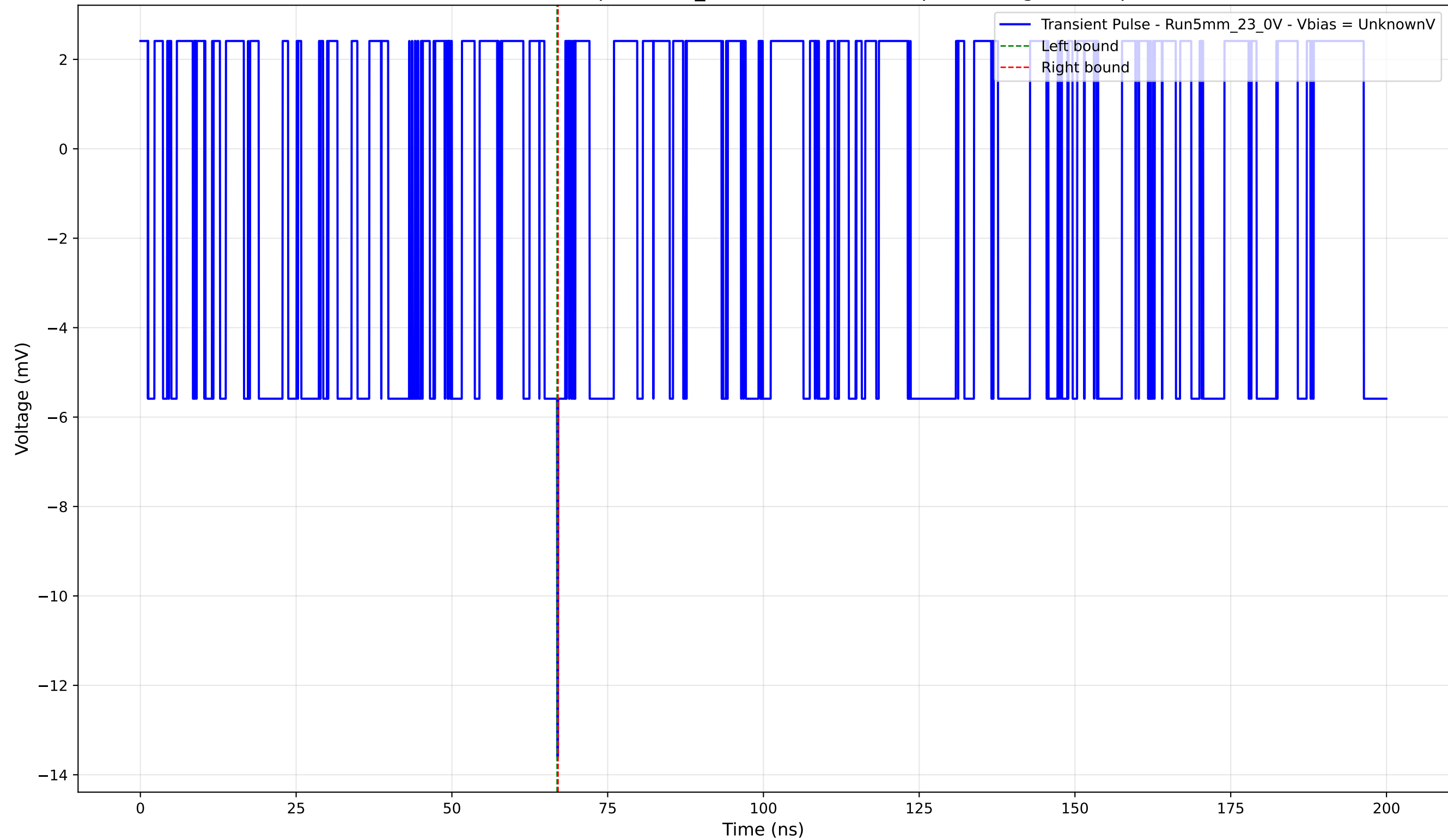
Transient Pulse - Sample: 5mm_23 - Position: 2370.0 \mu\text{m} - Charge: -0.04 pC
