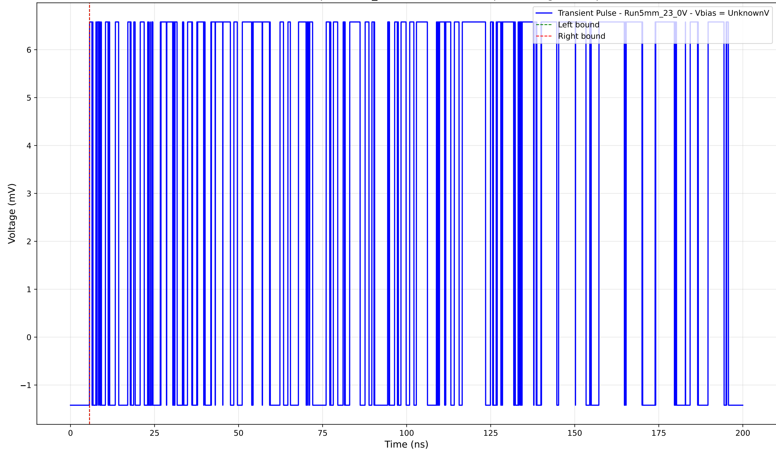
Transient Pulse - Sample: 5mm_23 - Position: 2195.0 \mu\text{m} - Charge: 0.00 pC
