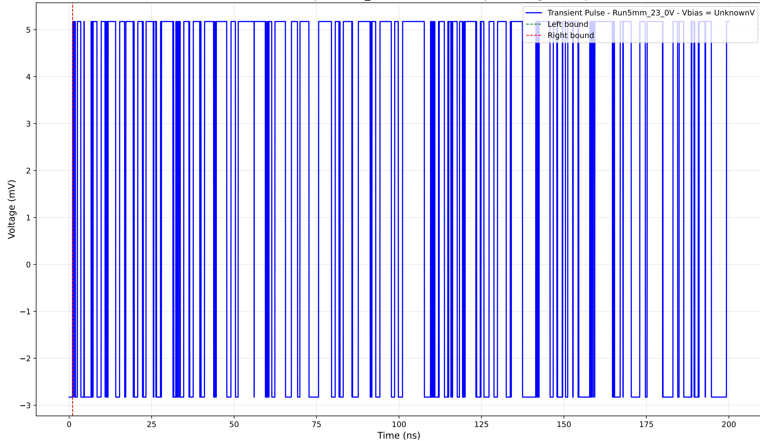
Transient Pulse - Sample: 5mm_23 - Position: 1320.0 \mu\text{m} - Charge: 0.00 pC
