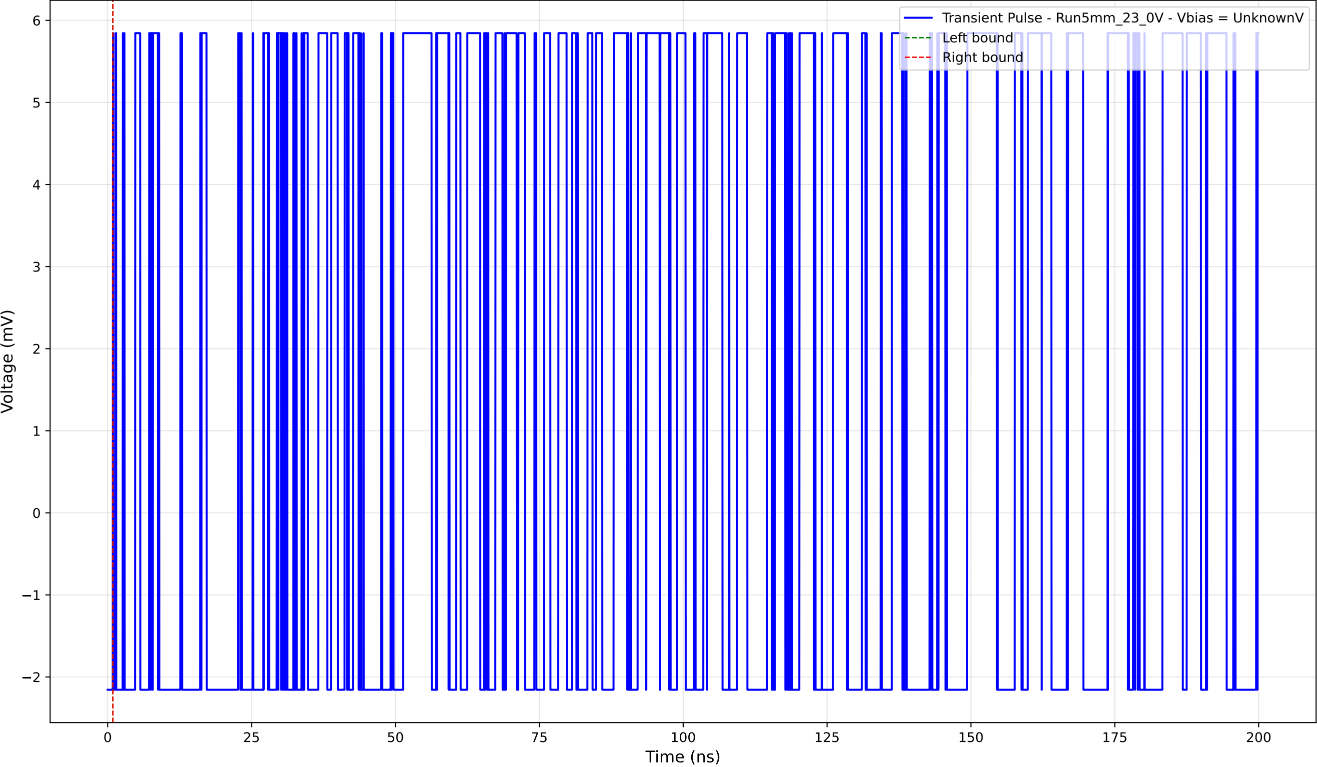
Transient Pulse - Sample: 5mm_23 -Position: 795.0 \mu\text{m} - Charge: 0.00 pC
