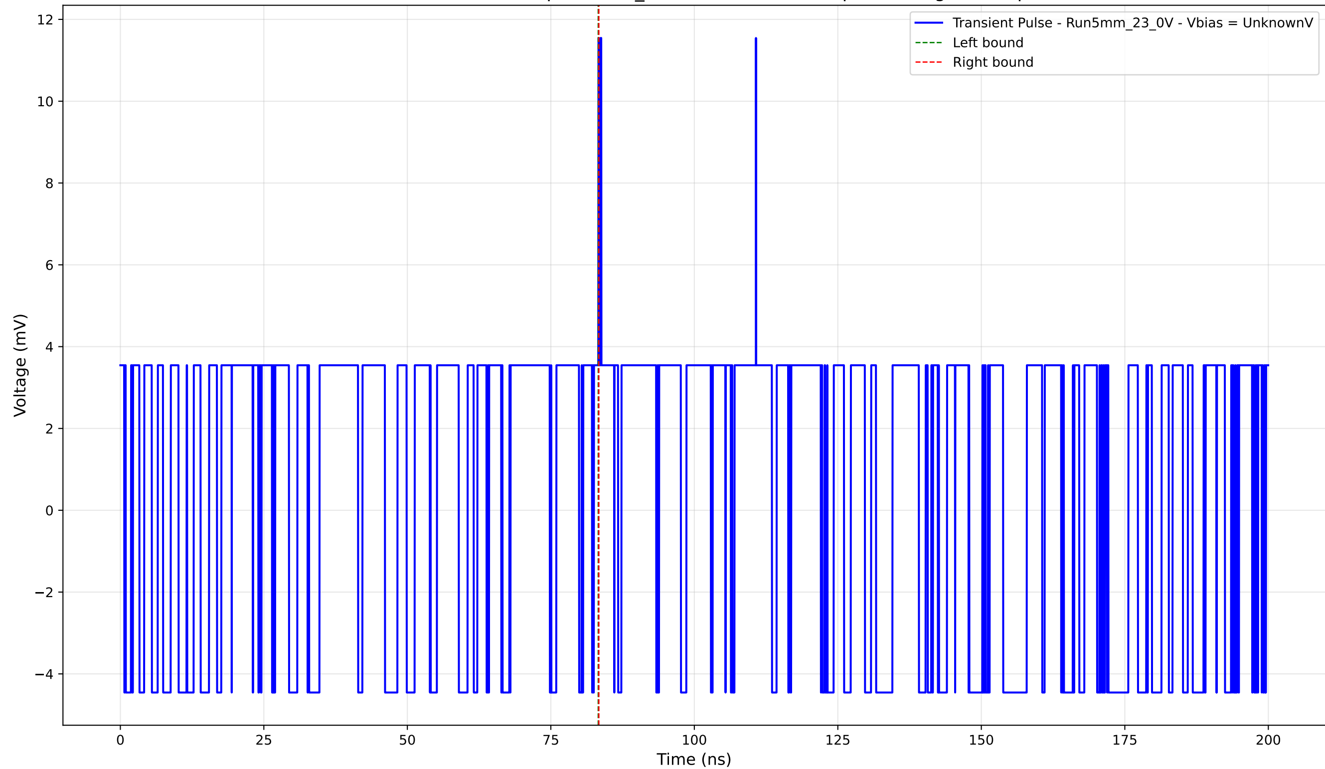
Transient Pulse - Sample: 5mm_23 - Position: 4920.0 \mu\text{m} - Charge: 0.02 pC
