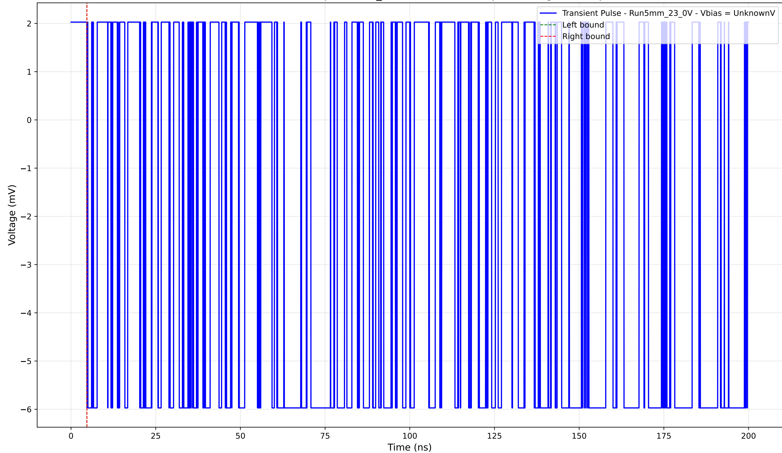
Transient Pulse - Sample: 5mm_23 - Position: 515.0 \mu\text{m} - Charge: -0.00 pC
