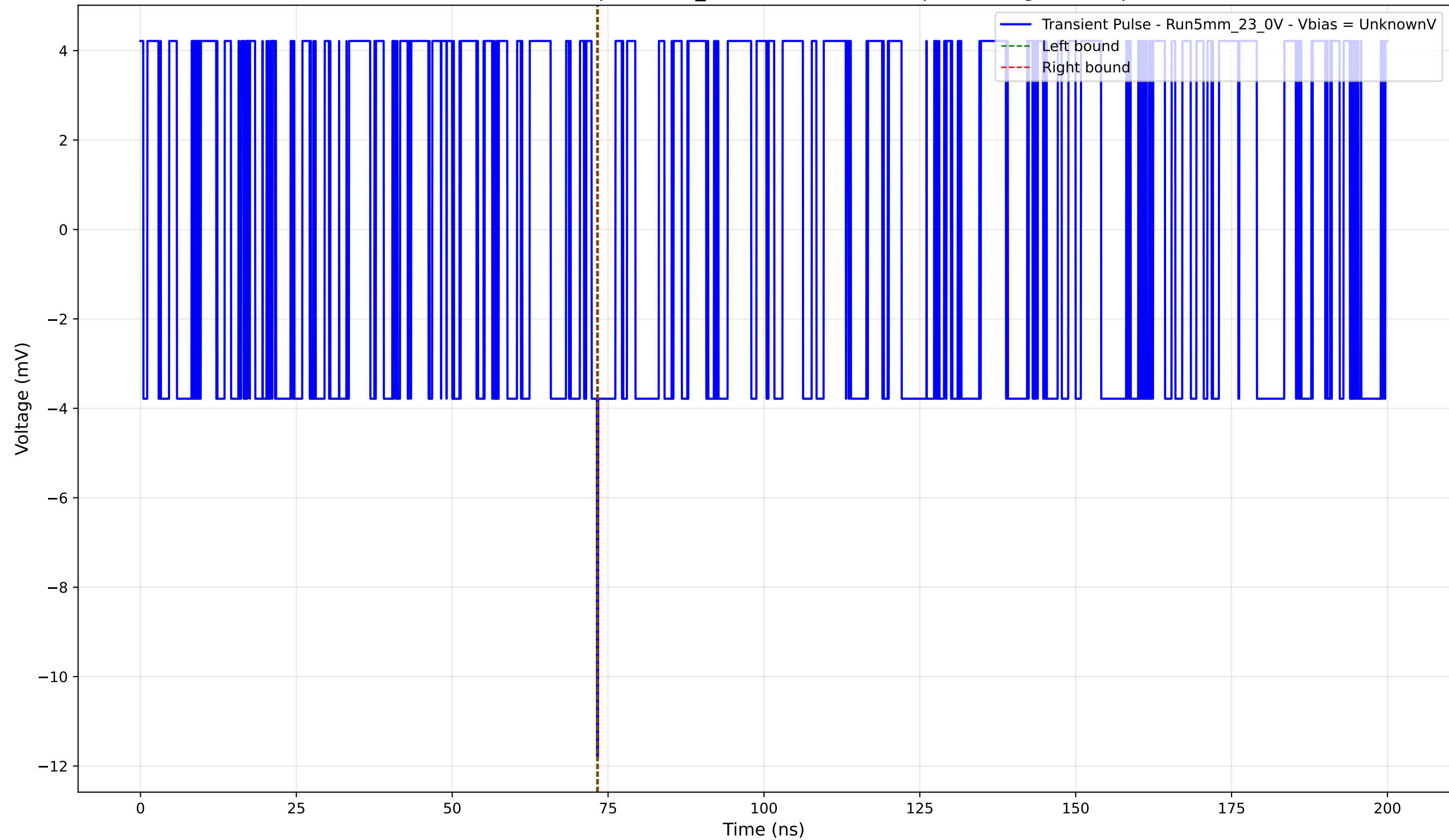
Transient Pulse - Sample: 5mm_23 - Position: 1850.0 \mu\text{m} - Charge: -0.04 pC
