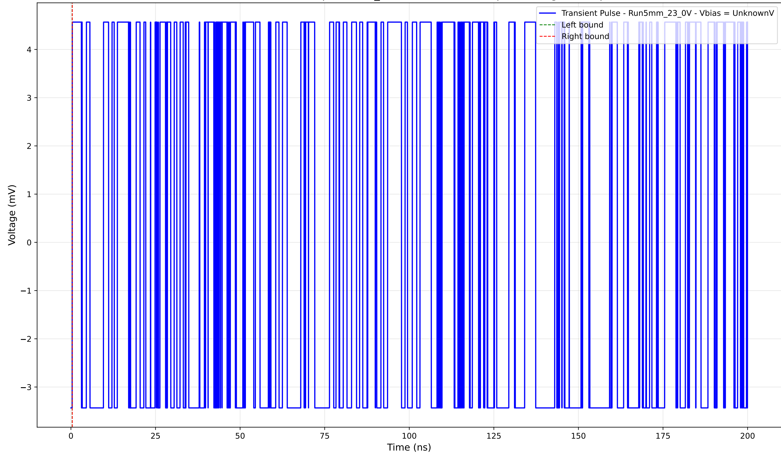
Transient Pulse - Sample: 5mm_23 - Position: 2210.0 \mu\text{m} - Charge: 0.00 pC
