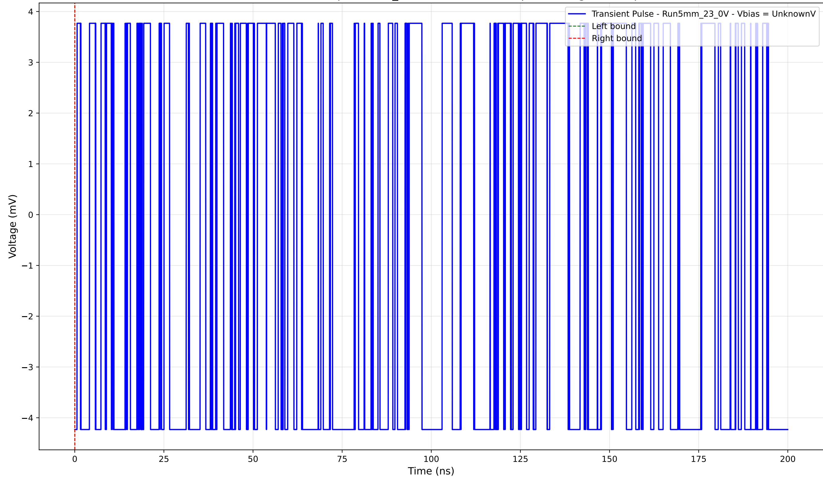
Transient Pulse - Sample: 5mm_23 - Position: 4060.0 \mu\text{m} - Charge: -0.00 pC
