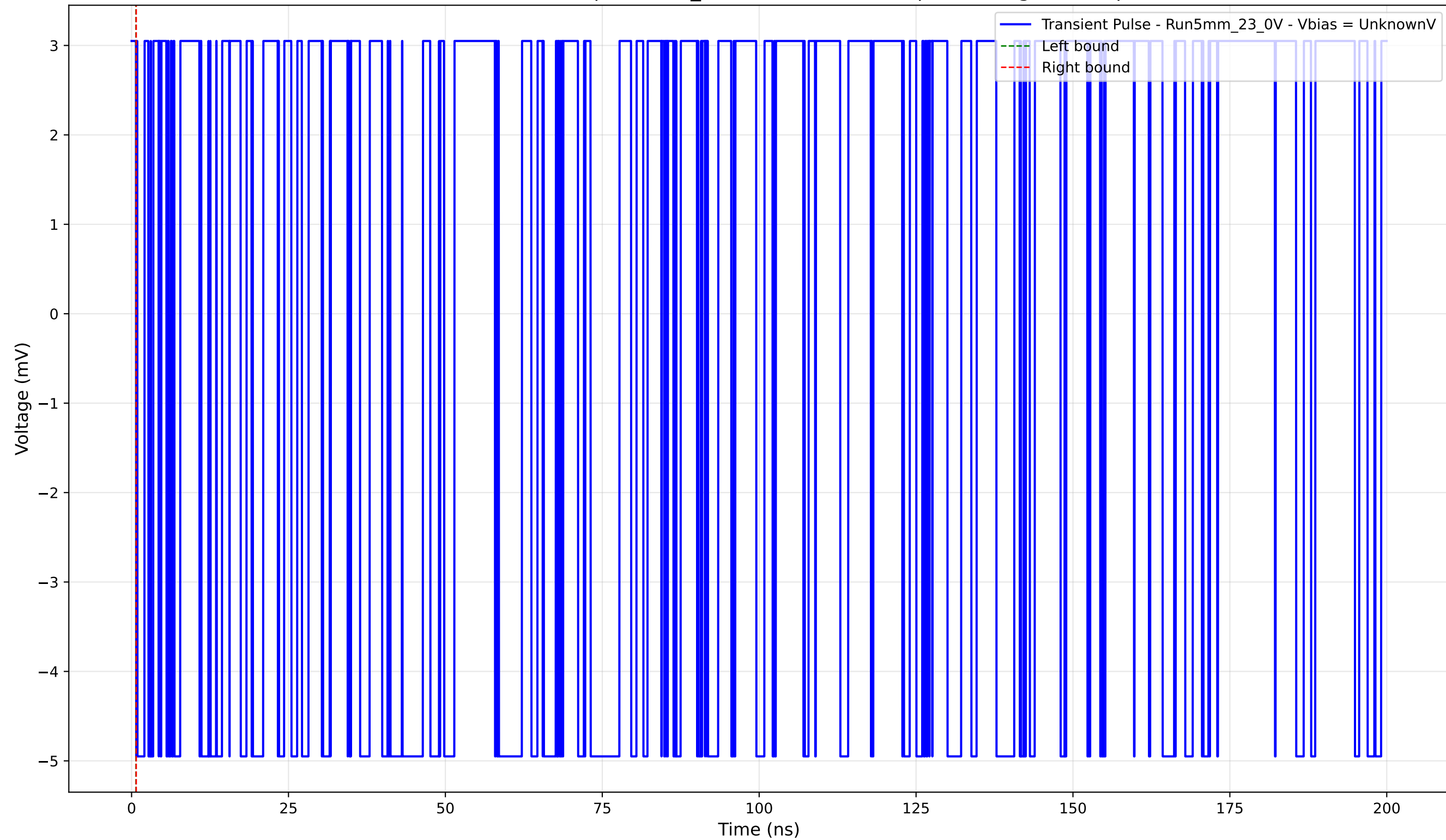
Transient Pulse - Sample: 5mm_23 - Position: 3570.0 \mu\text{m} - Charge: -0.00 pC
