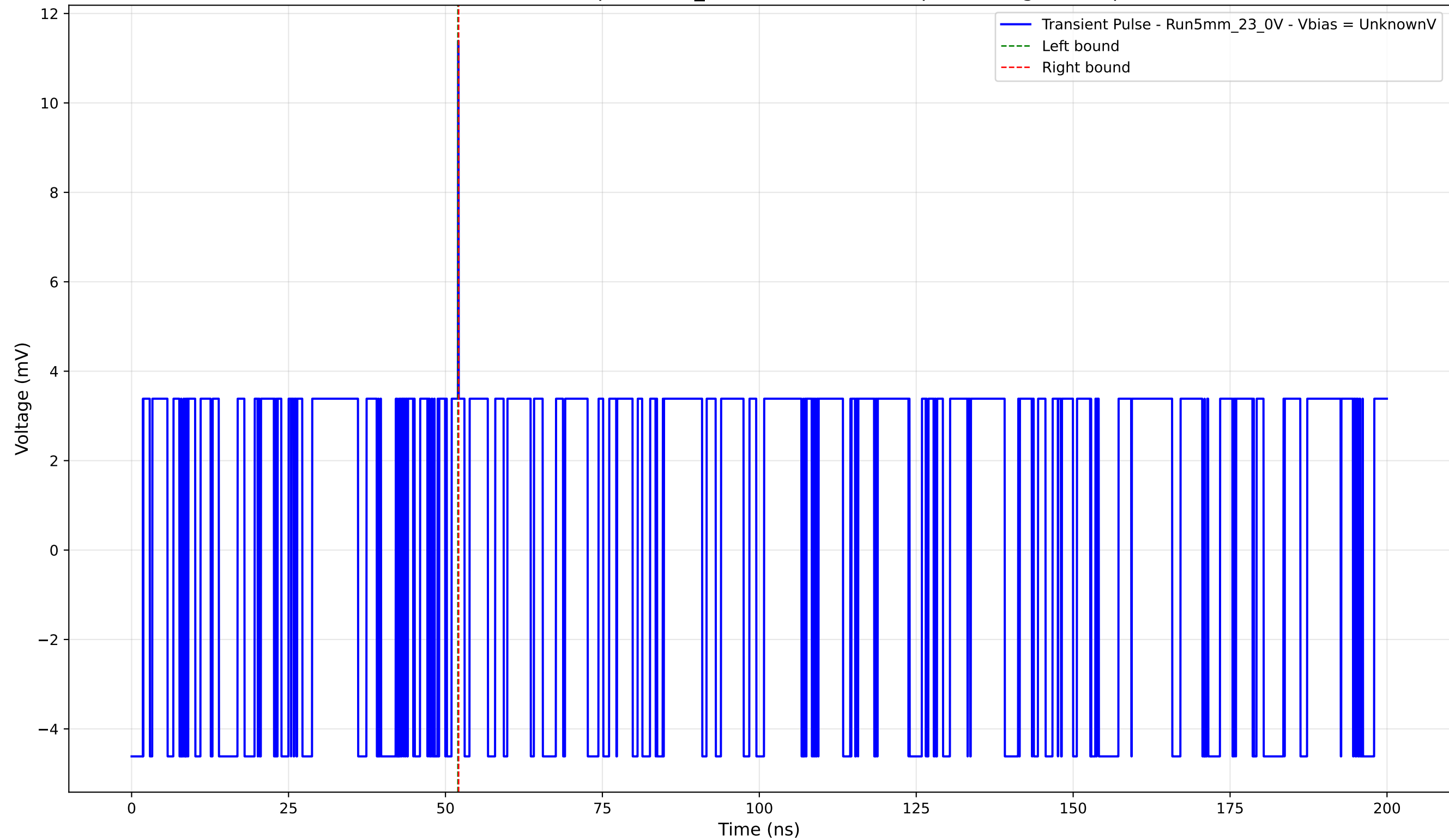
Transient Pulse - Sample: 5mm_23 - Position: 2920.0 \mu\text{m} - Charge: 0.02 pC
