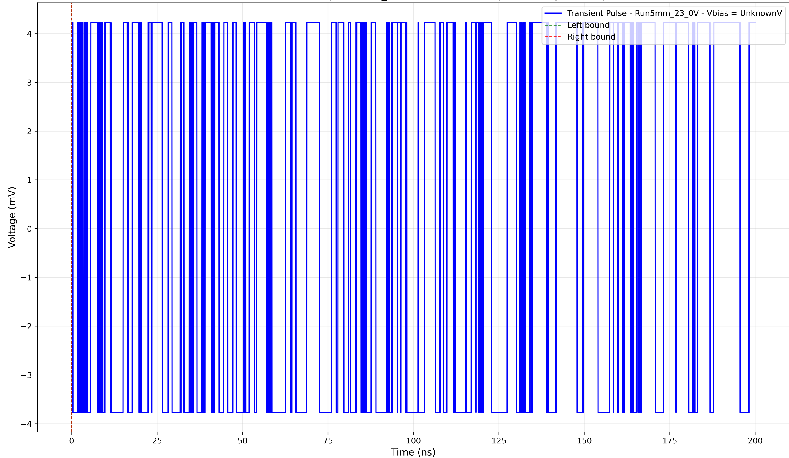
Transient Pulse - Sample: 5mm_23 - Position: 835.0 \mu\text{m} - Charge: 0.00 pC
