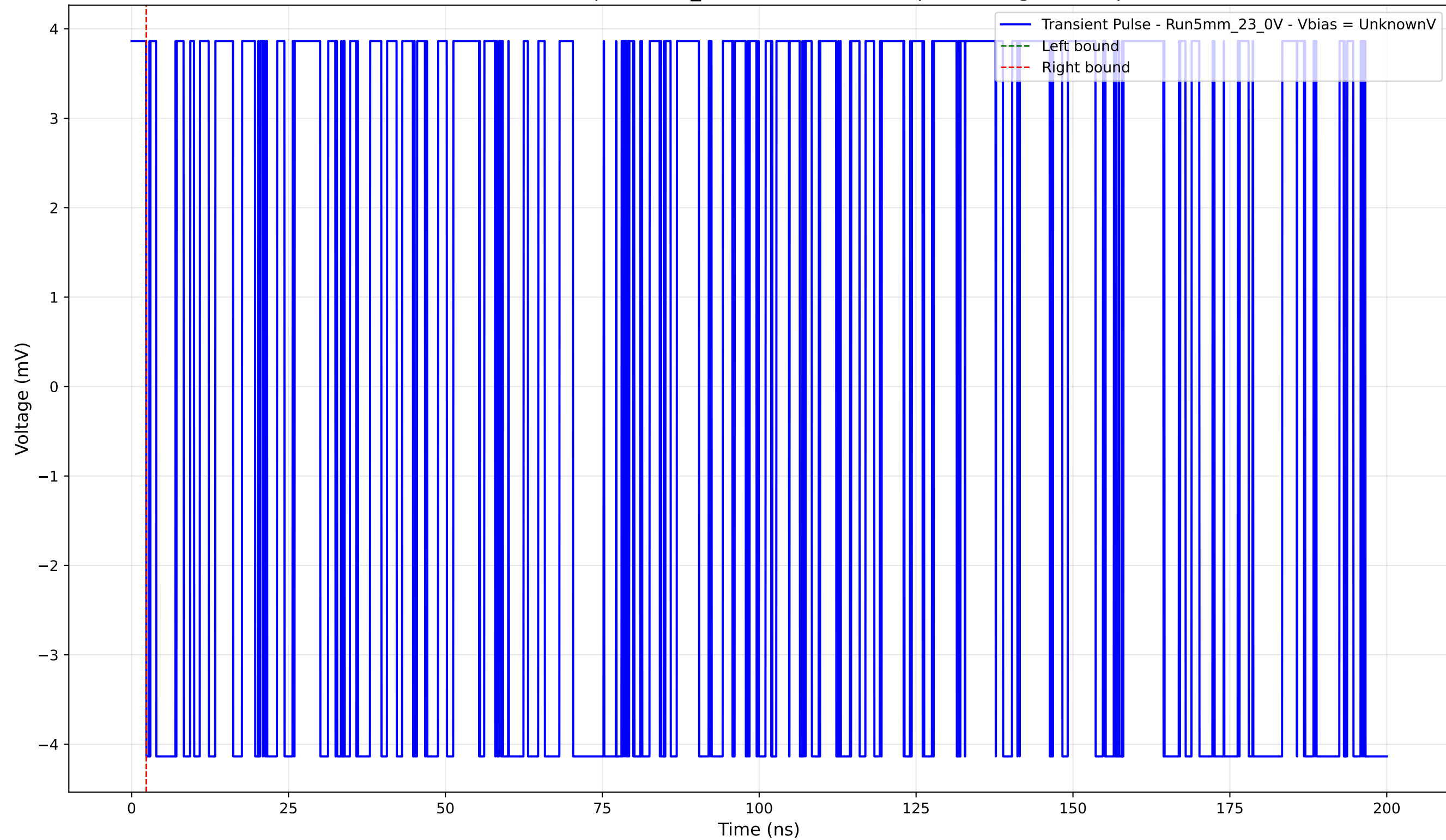
Transient Pulse - Sample: 5mm_23 - Position: 4410.0 \mu\text{m} - Charge: -0.00 pC
