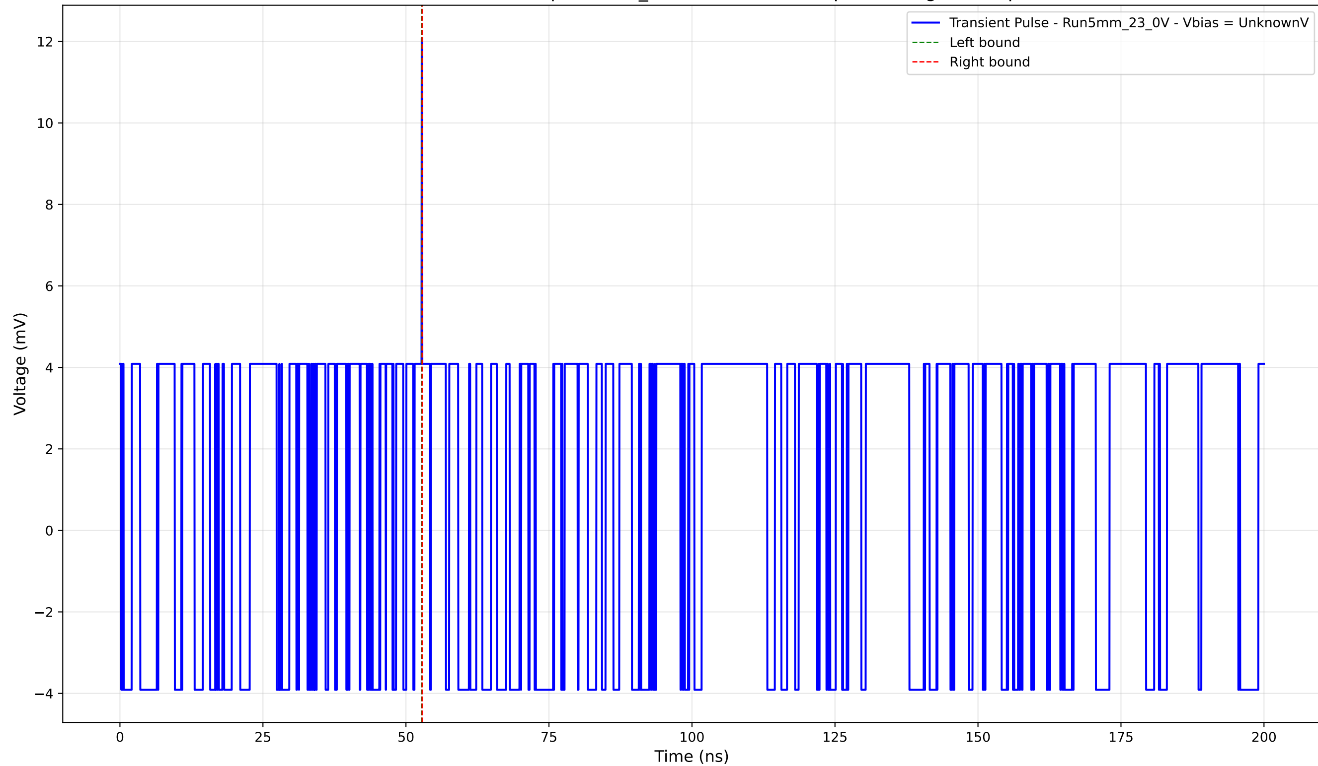
Transient Pulse - Sample: 5mm_23 - Position: 985.0 \mu\text{m} - Charge: 0.03 pC
