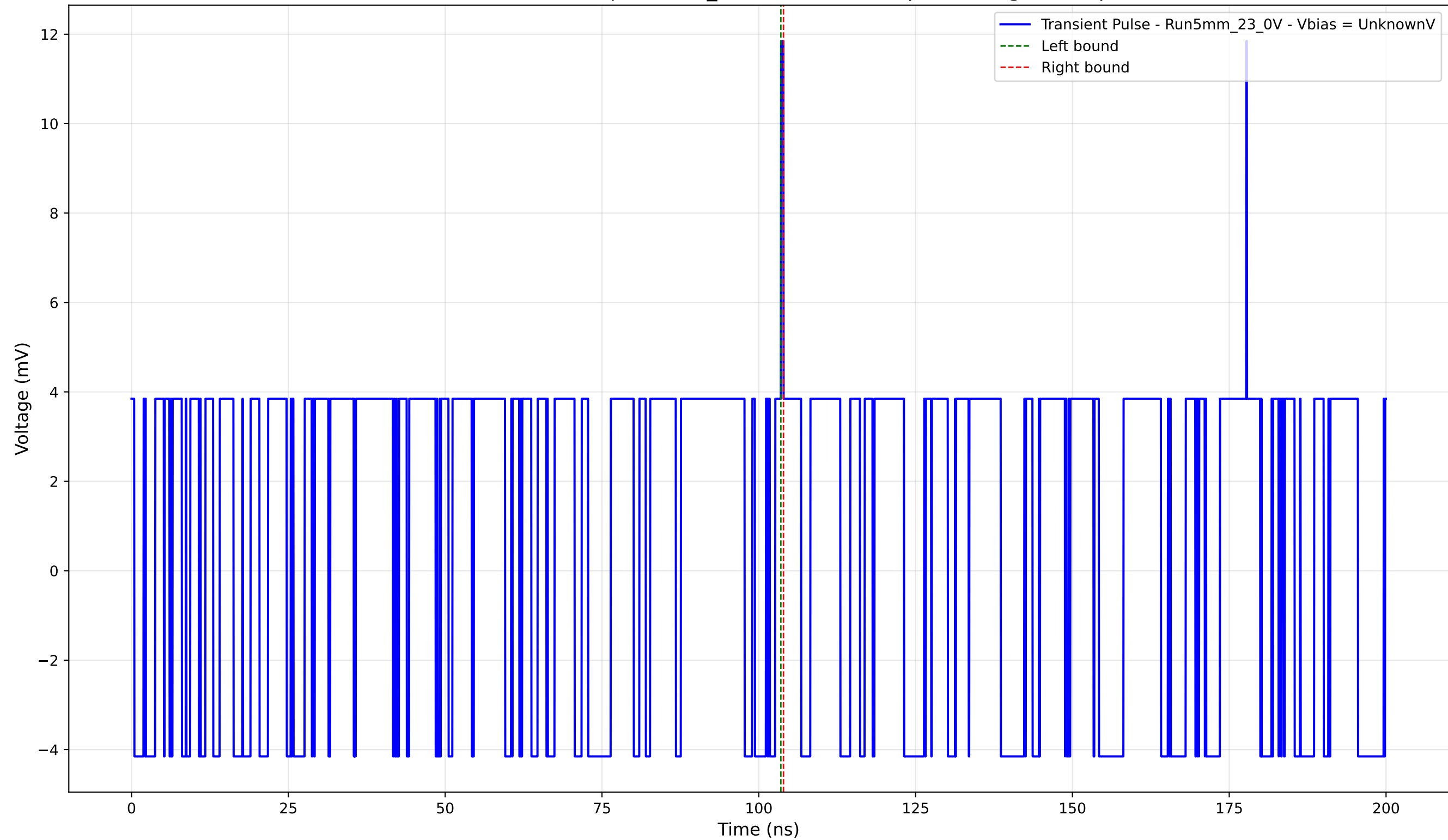
Transient Pulse - Sample: 5mm_23 - Position: 15.0 \mu\text{m} - Charge: 0.10 pC
