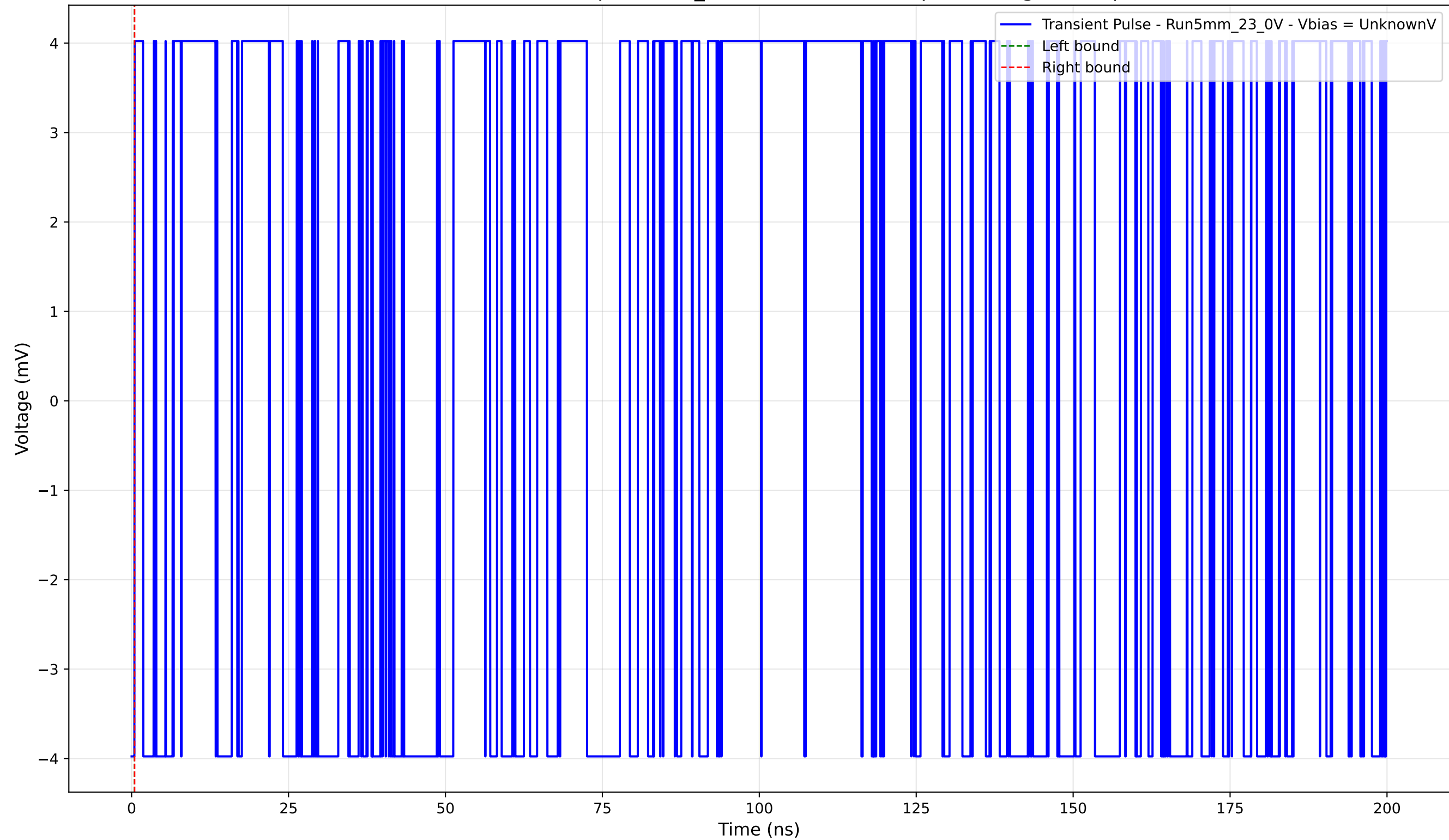
Transient Pulse - Sample: 5mm_23 - Position: 2475.0 \mu\text{m} - Charge: 0.00 pC
