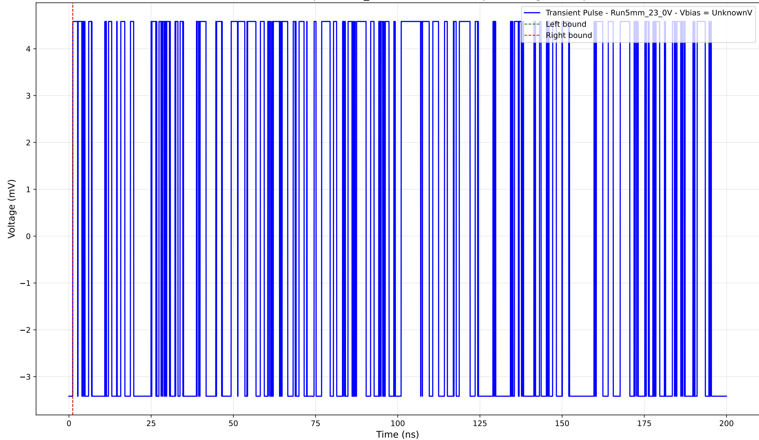
Transient Pulse - Sample: 5mm_23 - Position: 4830.0 \mu\text{m} - Charge: 0.00 pC
