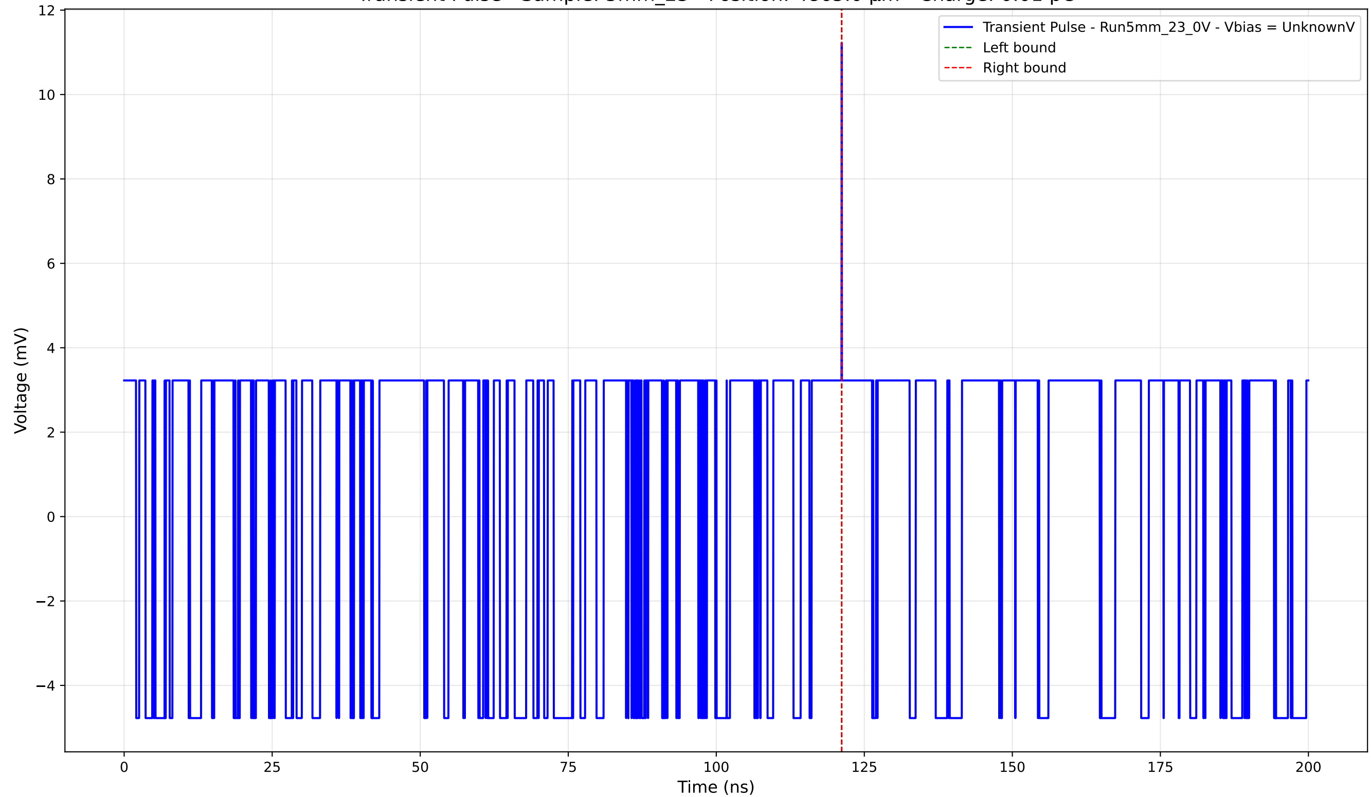
Transient Pulse - Sample: 5mm_23 - Position: 4865.0 \mu\text{m} - Charge: 0.01 pC
