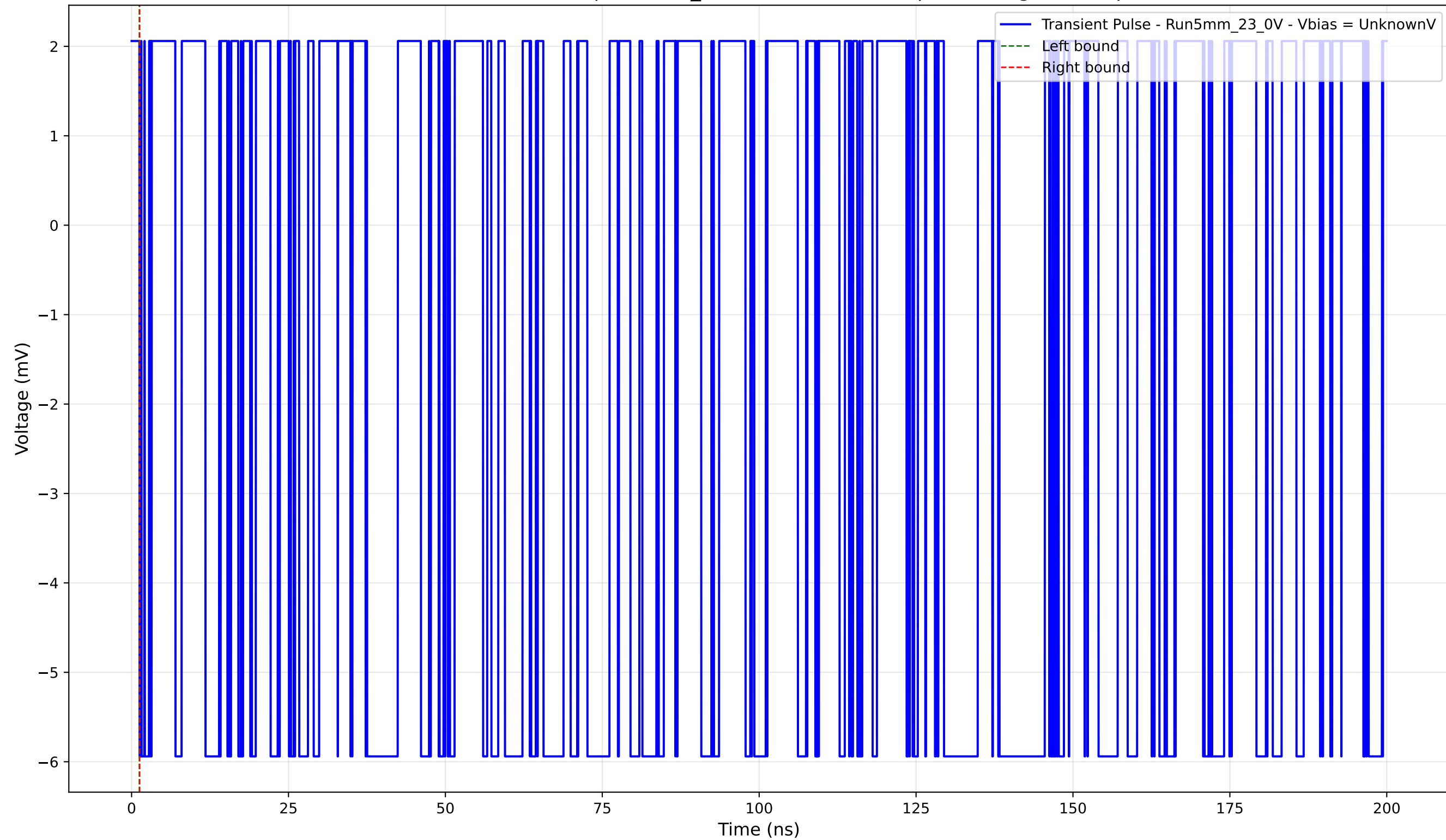
Transient Pulse - Sample: 5mm_23 - Position: 3055.0 \mu\text{m} - Charge: -0.00 pC
