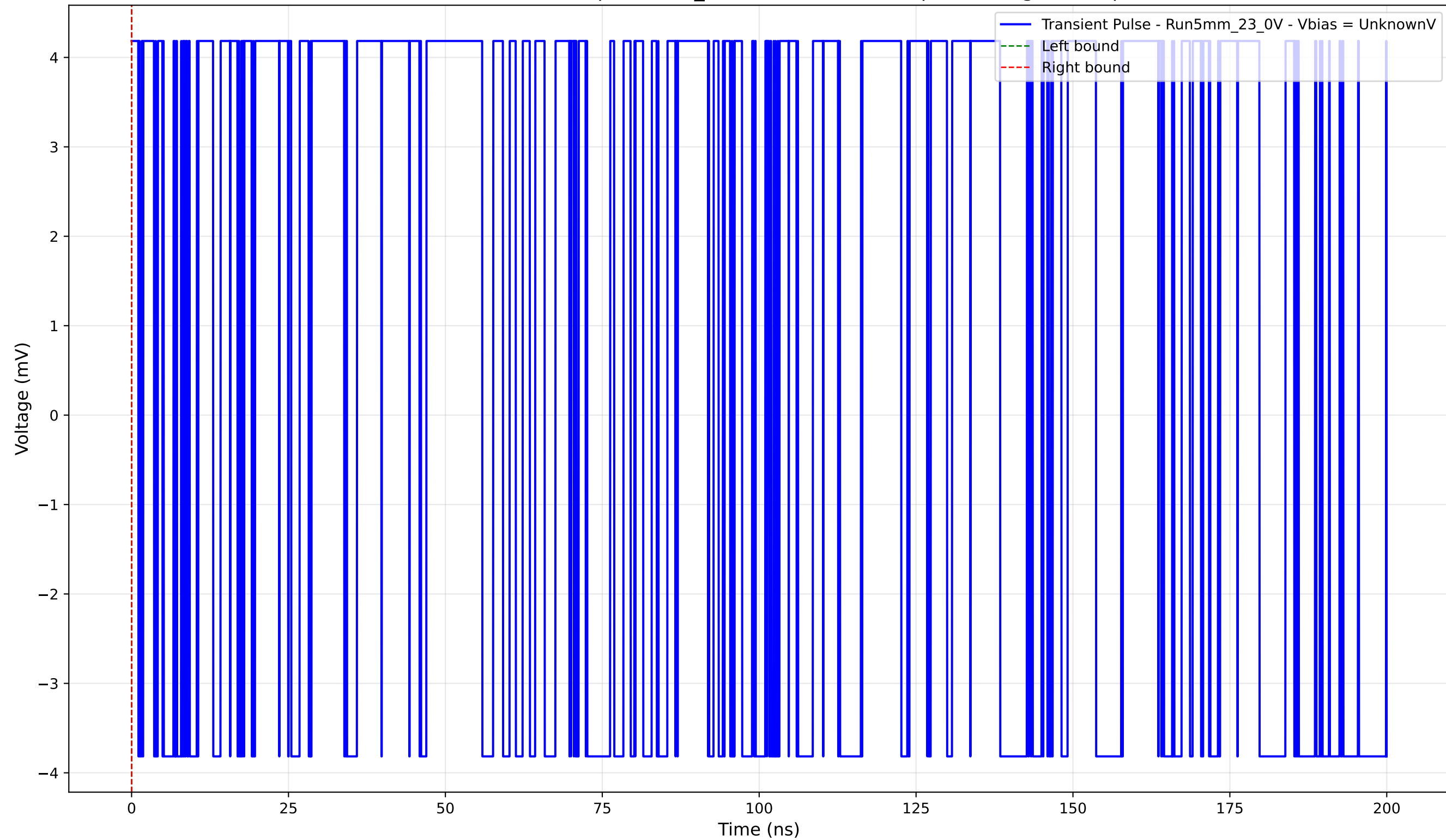
Transient Pulse - Sample: 5mm_23 - Position: 1590.0 \mu\text{m} - Charge: 0.00 pC
