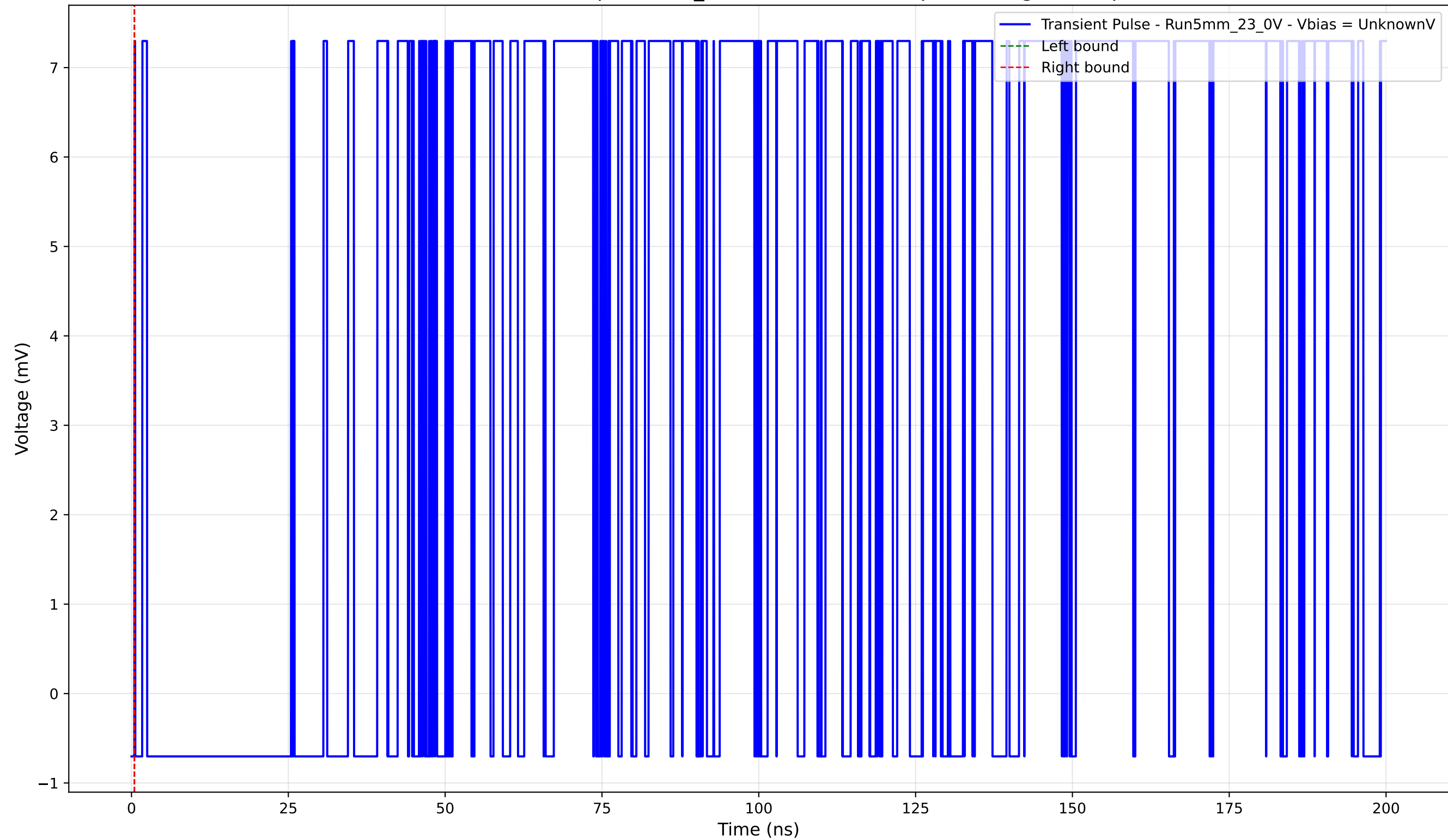
Transient Pulse - Sample: 5mm_23 - Position: 3595.0 \mu\text{m} - Charge: 0.00 pC
