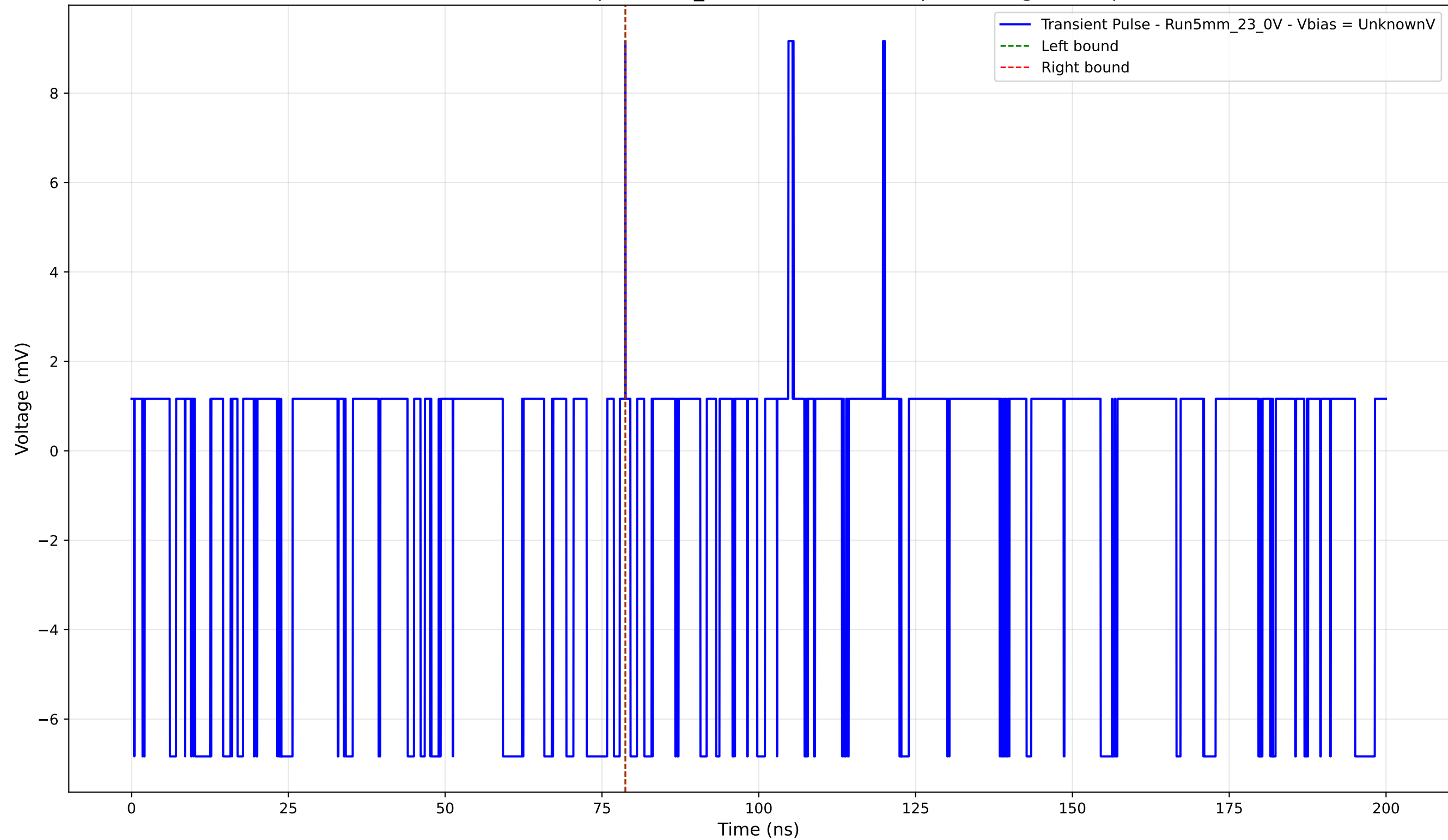
Transient Pulse - Sample: 5mm_23 - Position: 2595.0 \mu\text{m} - Charge: 0.01 pC
