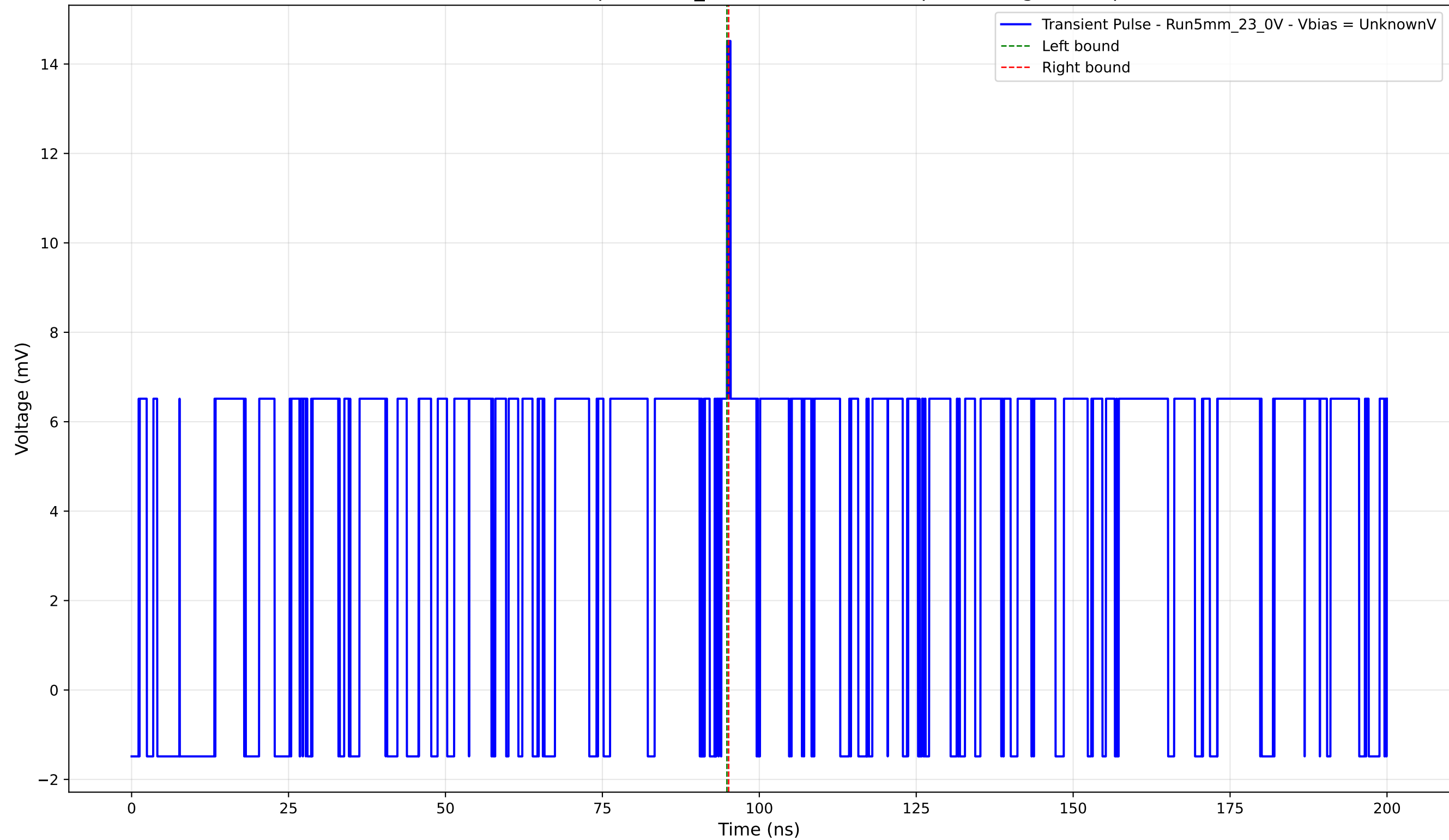
Transient Pulse - Sample: 5mm_23 - Position: 4260.0 \mu\text{m} - Charge: 0.08 pC
