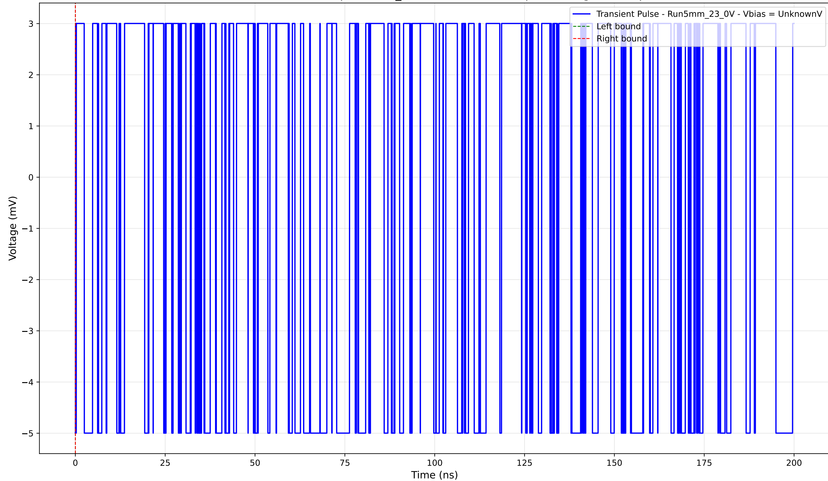
Transient Pulse - Sample: 5mm_23 - Position: 4355.0 \mu\text{m} - Charge: -0.00 pC
