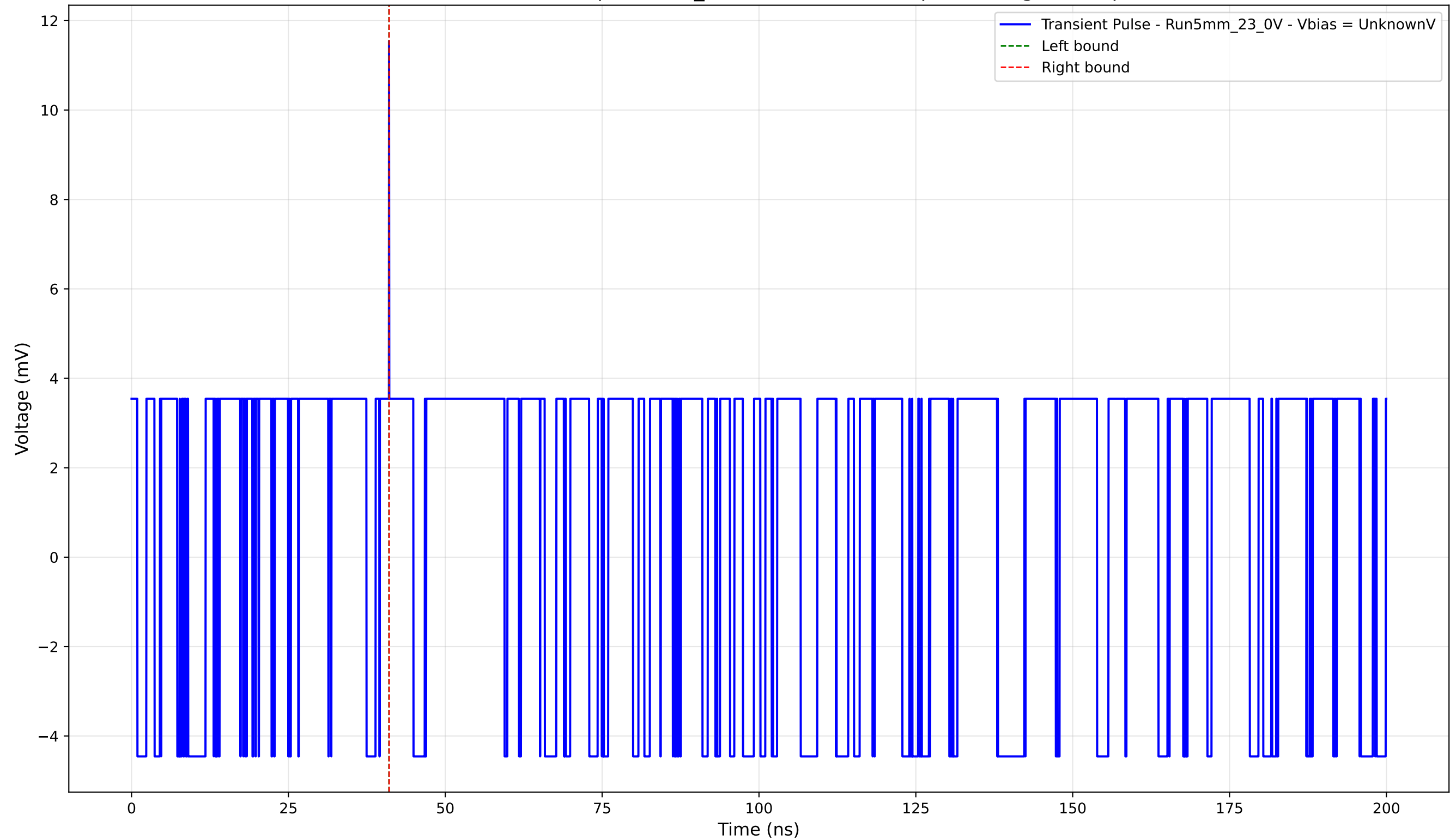
Transient Pulse - Sample: 5mm_23 - Position: 3700.0 \mu\text{m} - Charge: 0.01 pC
