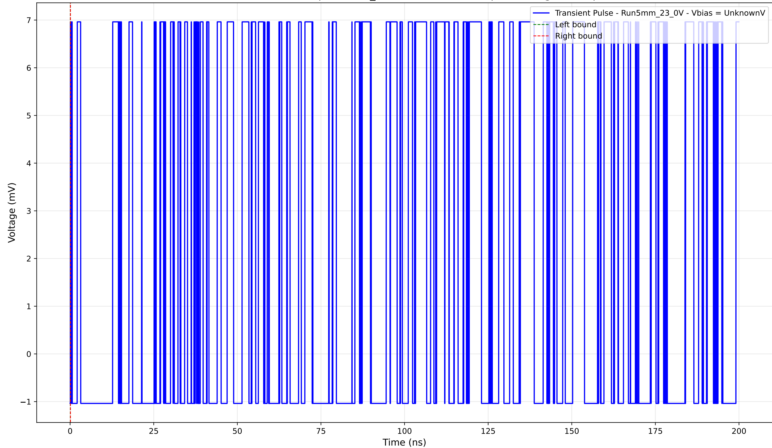
Transient Pulse - Sample: 5mm_23 - Position: 1855.0 \mu\text{m} - Charge: 0.00 pC
