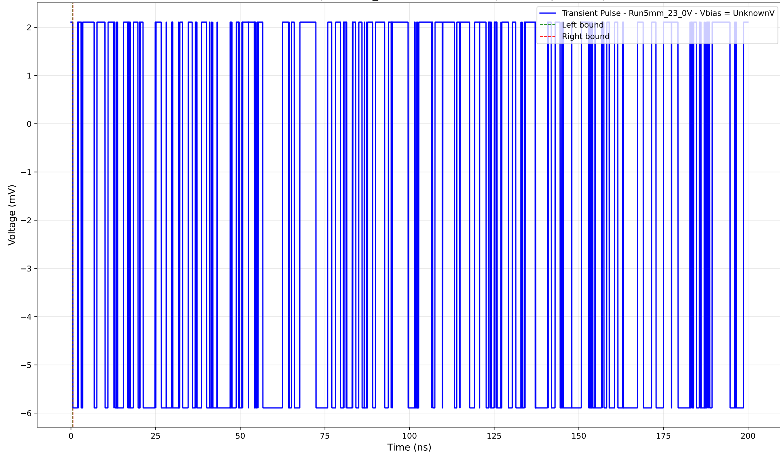
Transient Pulse - Sample: 5mm_23 - Position: 4695.0 \mu\text{m} - Charge: -0.00 pC
