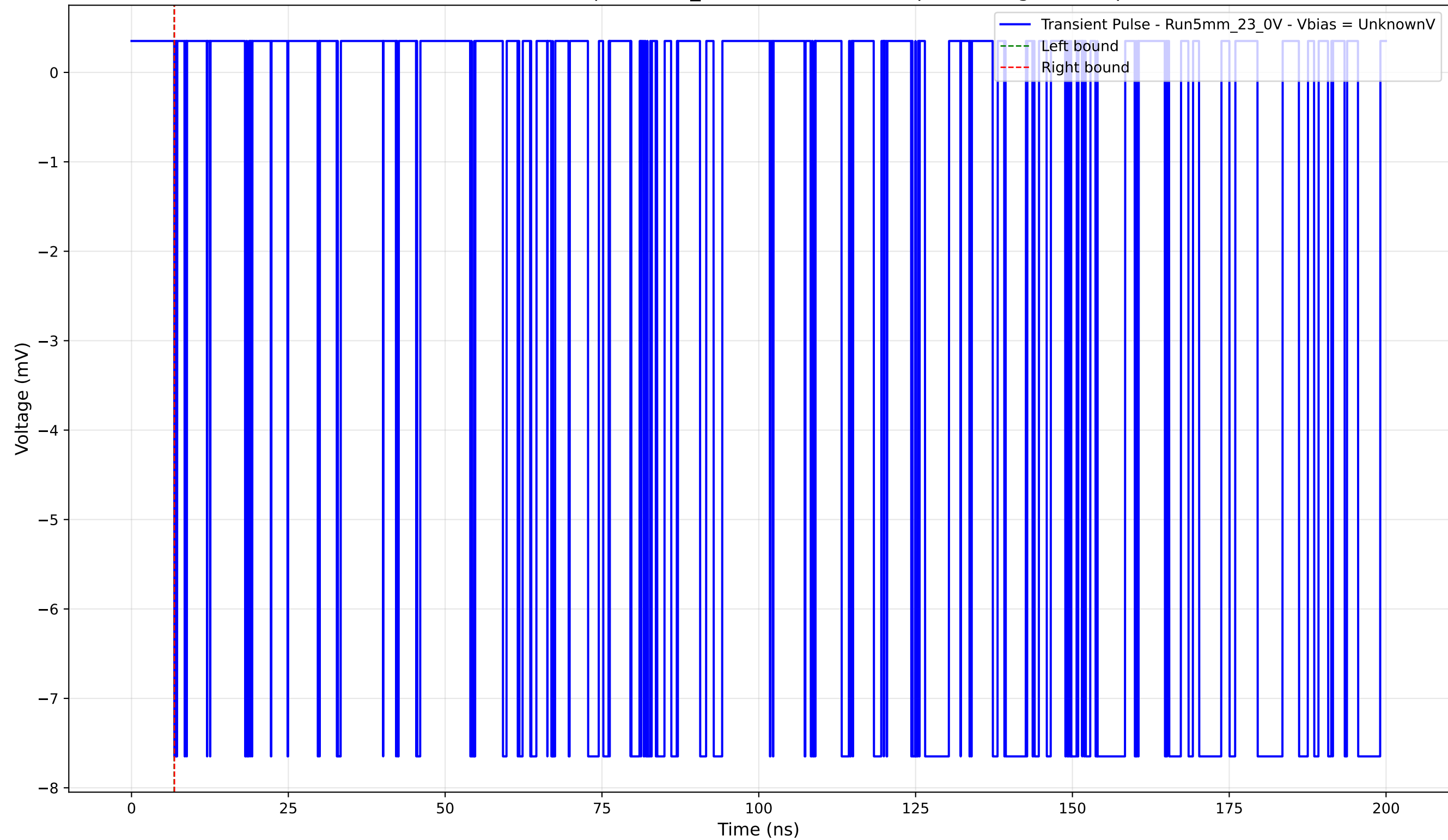
Transient Pulse - Sample: 5mm_23 - Position: 3170.0 \mu\text{m} - Charge: -0.00 pC
