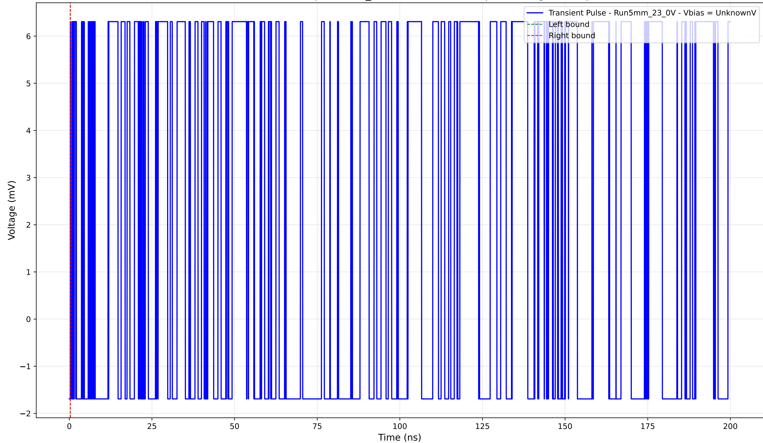
Transient Pulse - Sample: 5mm_23 - Position: 1005.0 \mu\text{m} - Charge: 0.00 pC
