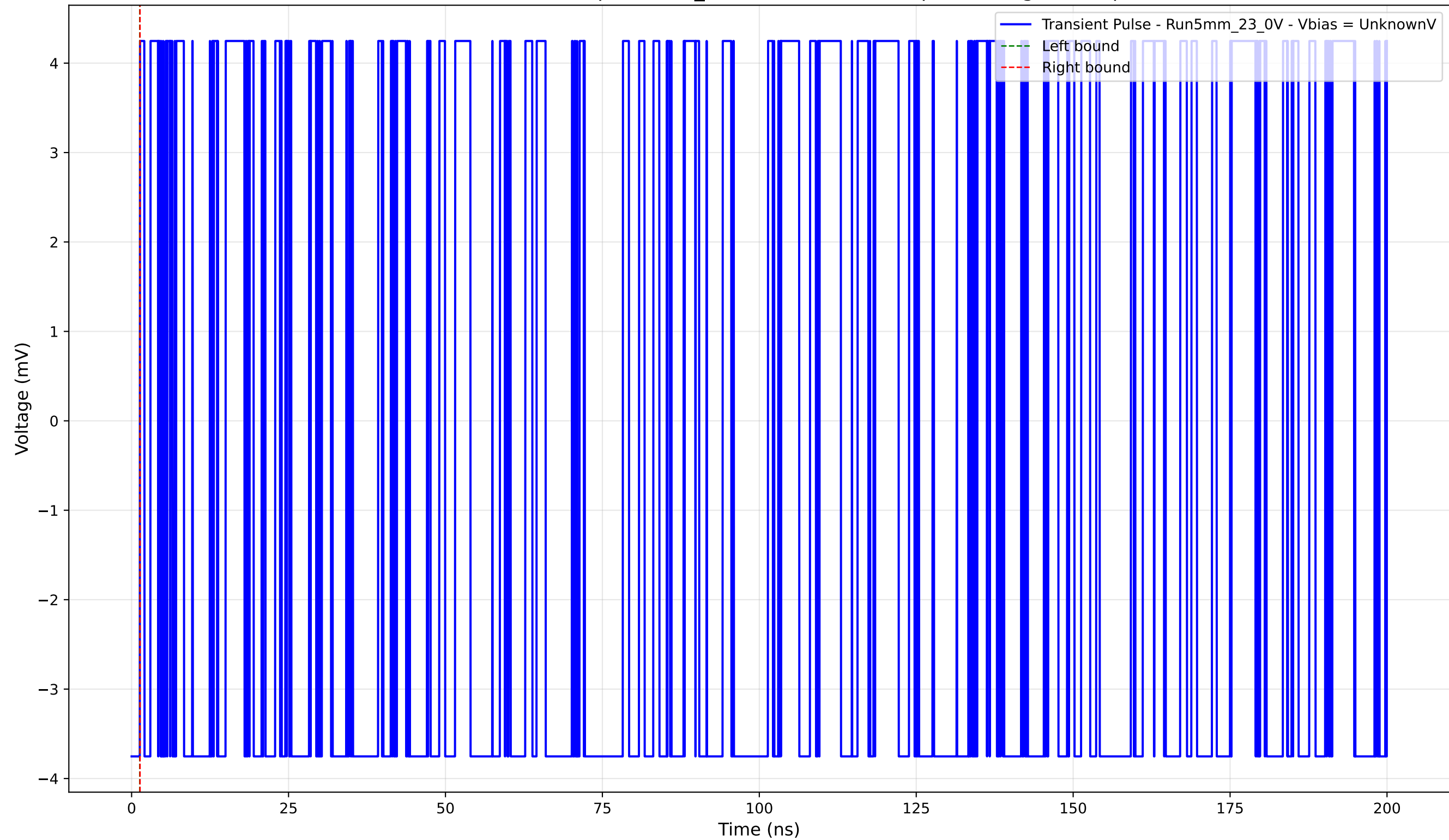
Transient Pulse - Sample: 5mm_23 - Position: 1470.0 \mu\text{m} - Charge: 0.00 pC
