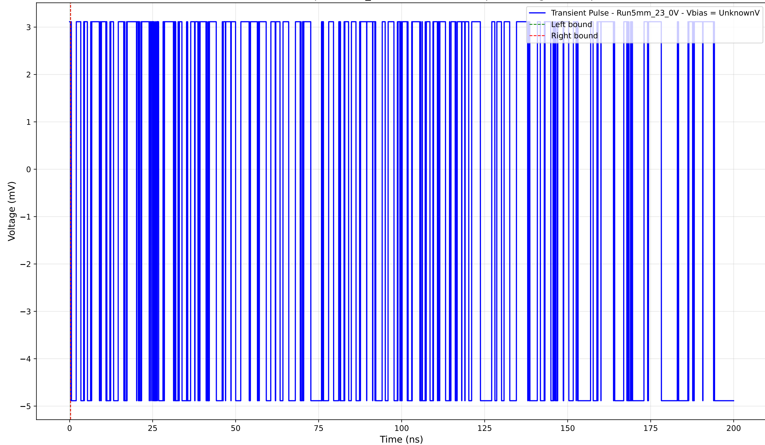
Transient Pulse - Sample: 5mm_23 - Position: 4230.0 \mu\text{m} - Charge: -0.00 pC
