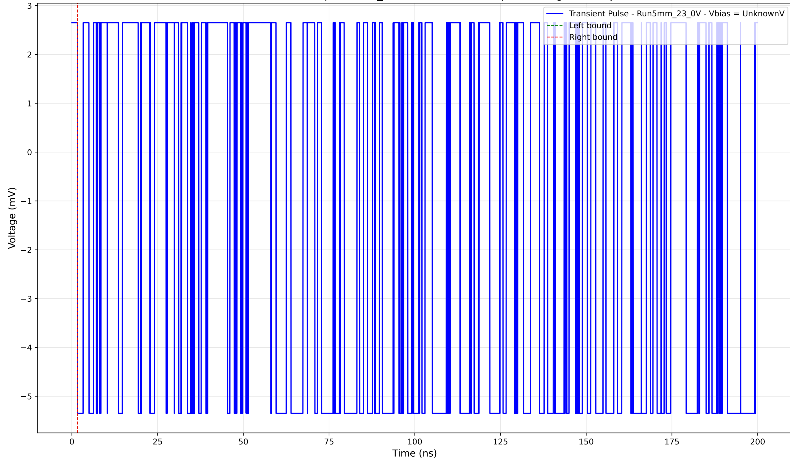
Transient Pulse - Sample: 5mm_23 - Position: 1770.0 \mu\text{m} - Charge: -0.00 pC
