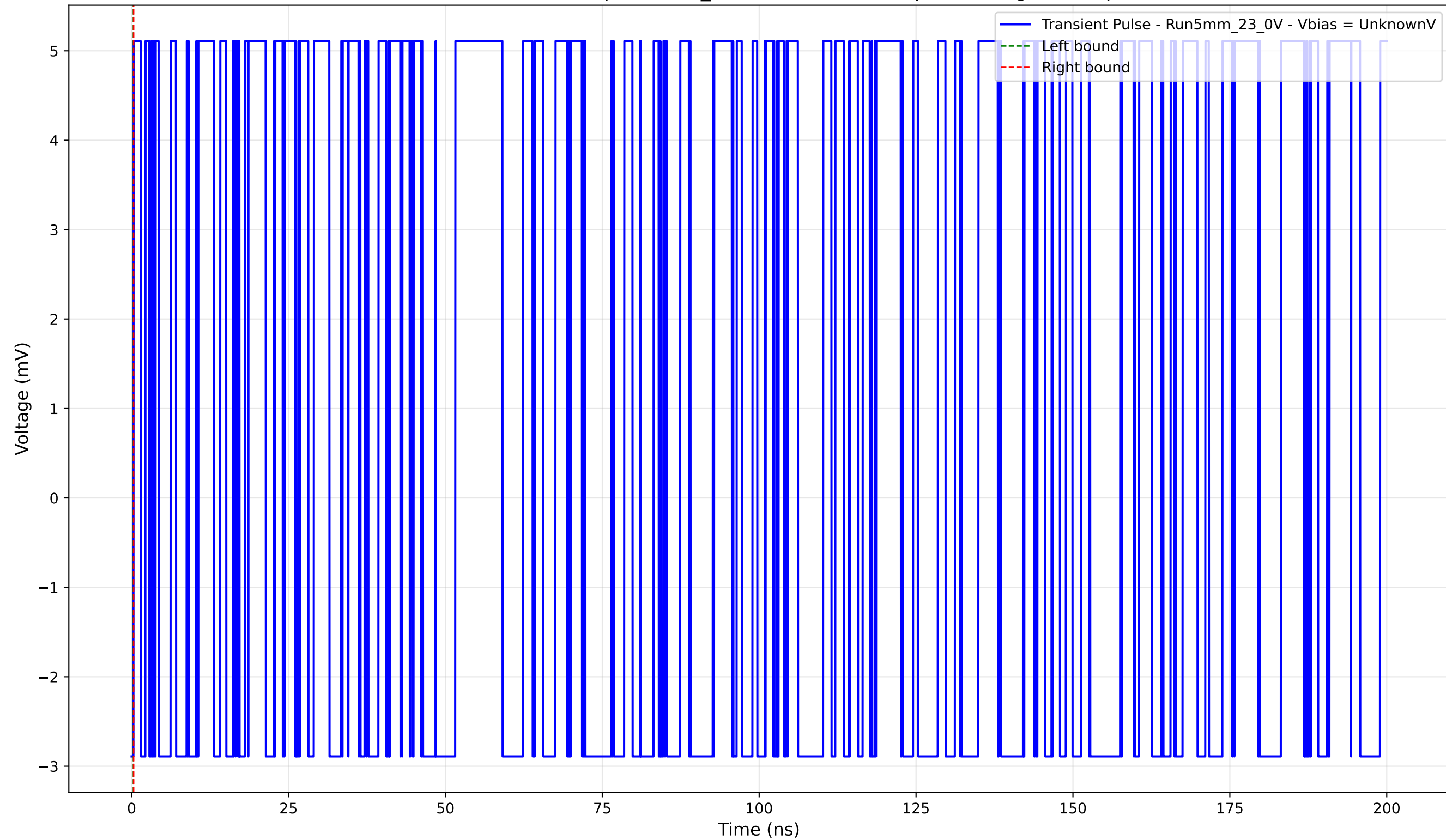
Transient Pulse - Sample: 5mm_23 - Position: 115.0 \mu\text{m} - Charge: 0.00 pC
