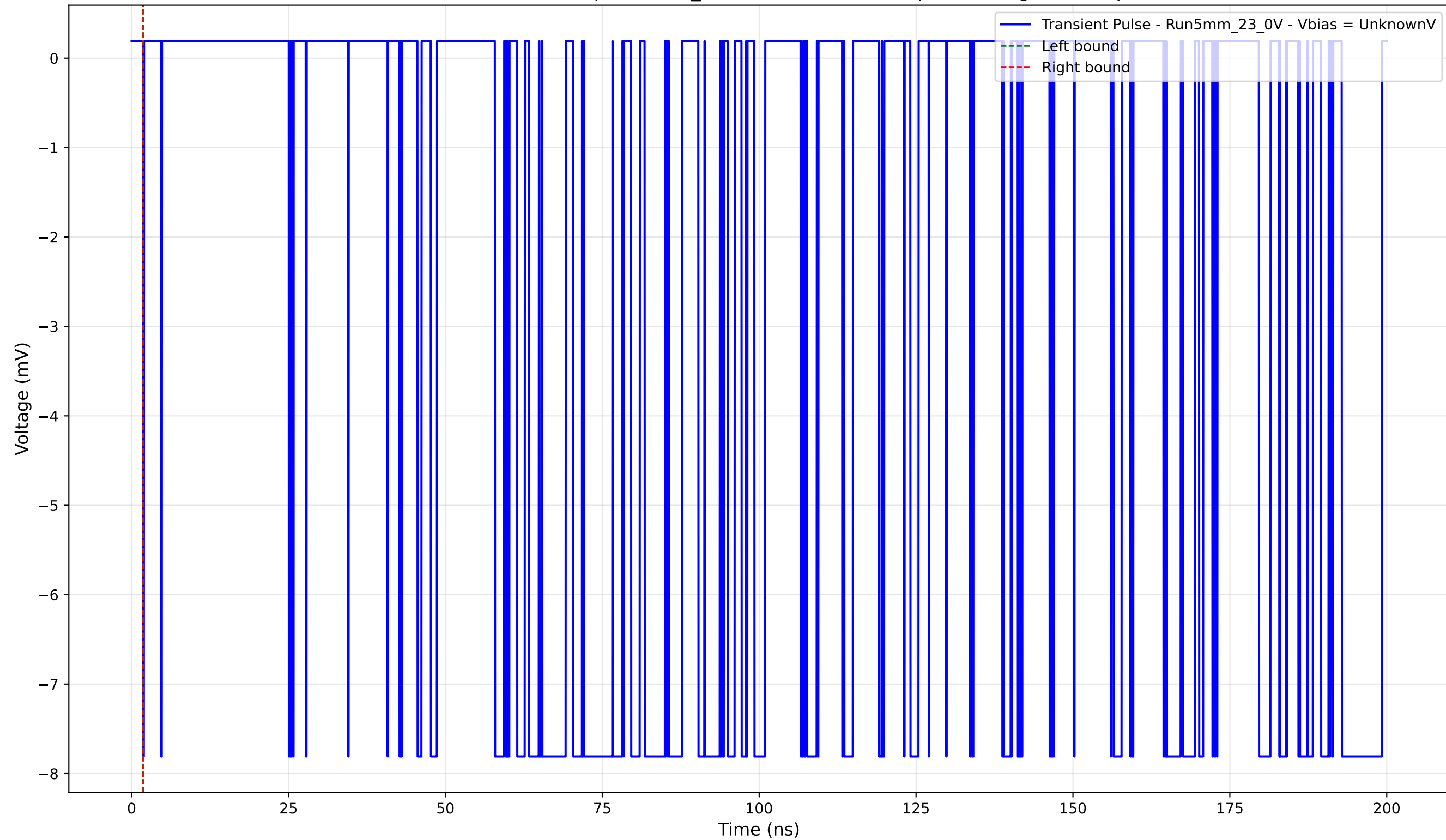
Transient Pulse - Sample: 5mm_23 - Position: 3475.0 \mu\text{m} - Charge: -0.00 pC
