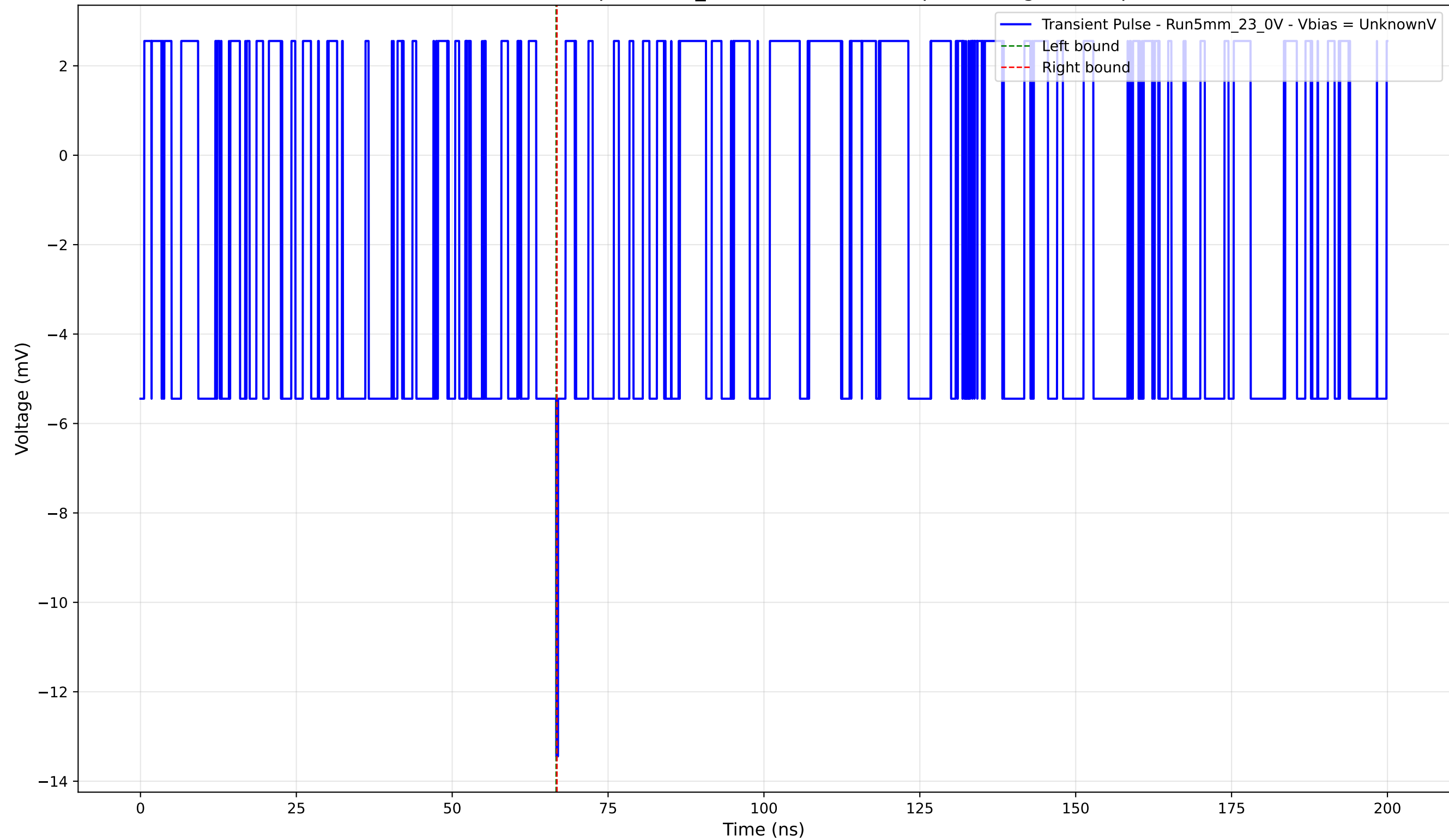
Transient Pulse - Sample: 5mm_23 - Position: 4620.0 \mu\text{m} - Charge: -0.03 pC
