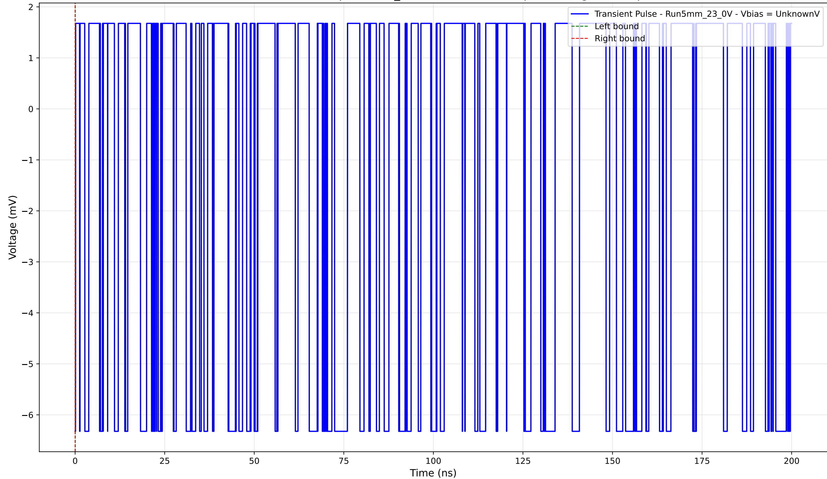
Transient Pulse - Sample: 5mm_23 - Position: 2280.0 \mu\text{m} - Charge: -0.00 pC
