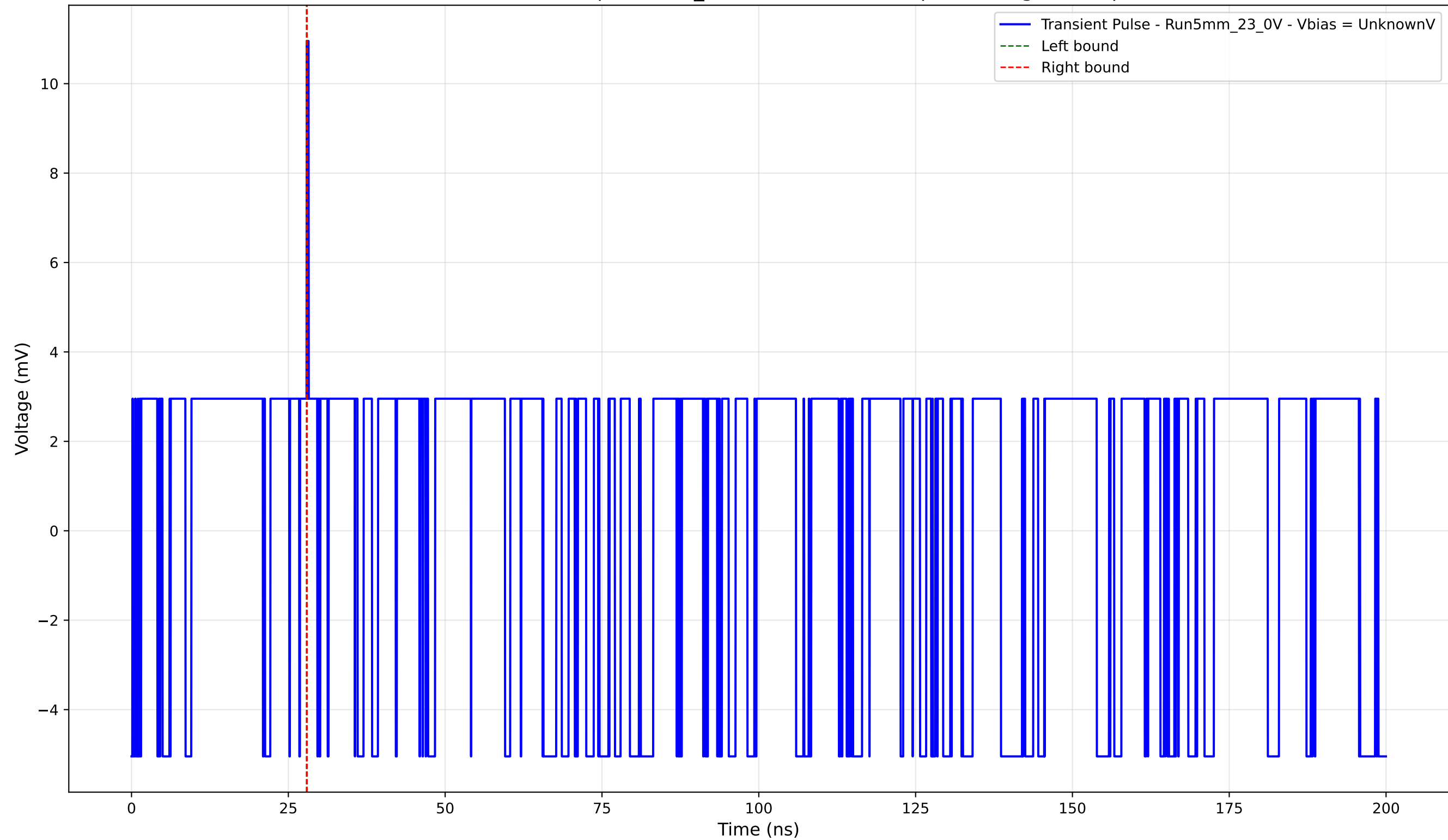
Transient Pulse - Sample: 5mm_23 - Position: 2255.0 \mu\text{m} - Charge: 0.01 pC
