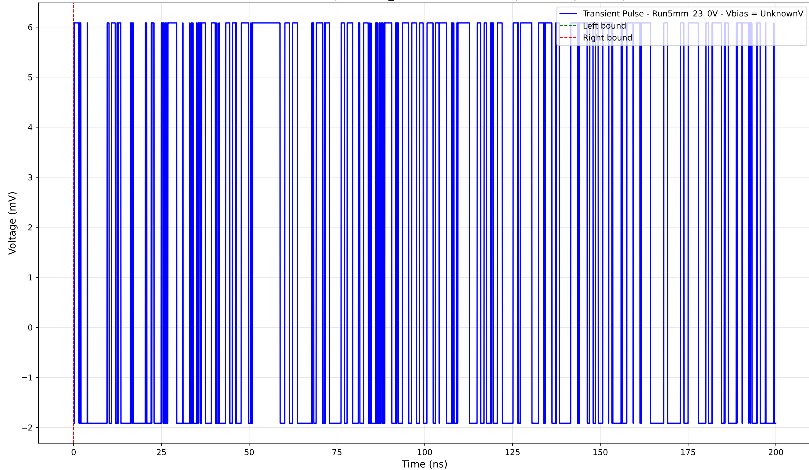
Transient Pulse - Sample: 5mm_23 - Position: 1265.0 \mu\text{m} - Charge: 0.00 pC
