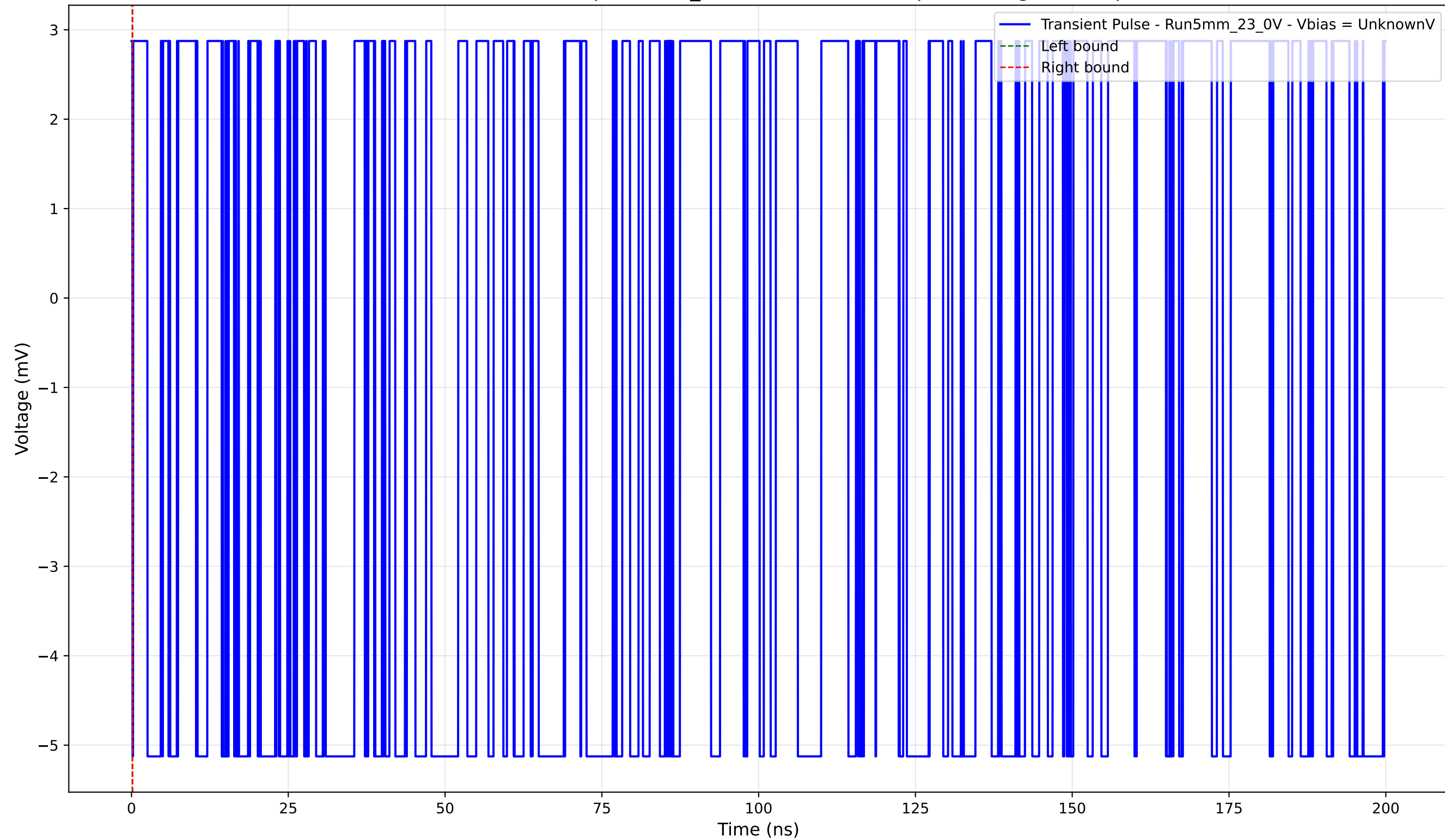
Transient Pulse - Sample: 5mm_23 - Position: 2955.0 \mu\text{m} - Charge: -0.00 pC
