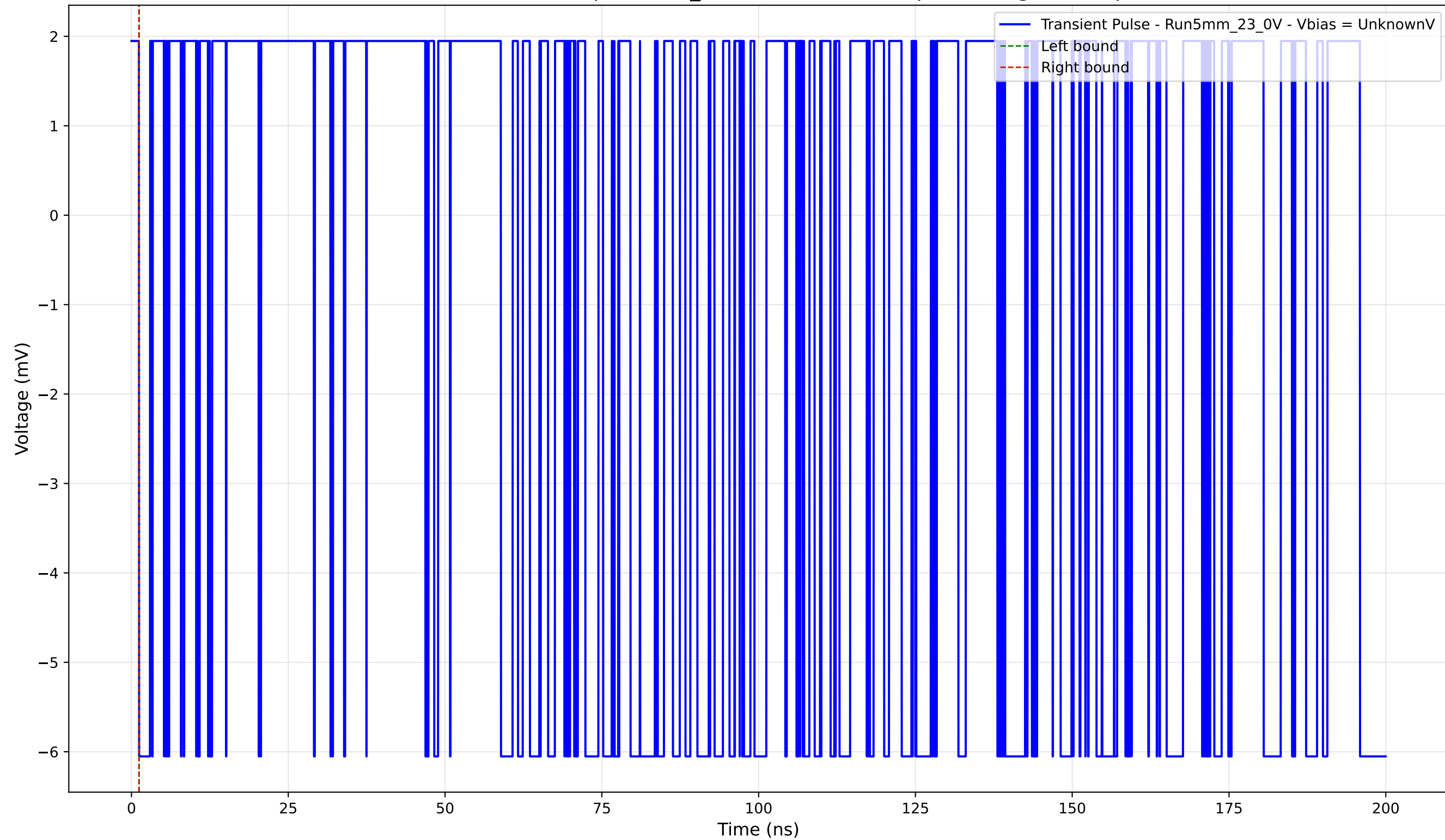
Transient Pulse - Sample: 5mm_23 - Position: 3545.0 \mu\text{m} - Charge: -0.00 pC
