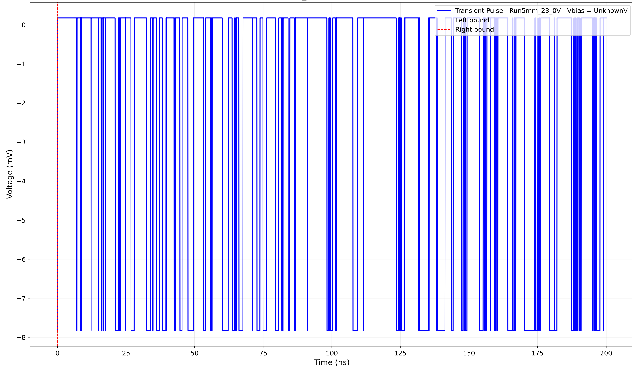
Transient Pulse - Sample: 5mm_23 - Position: 2735.0 \mu\text{m} - Charge: -0.00 pC
