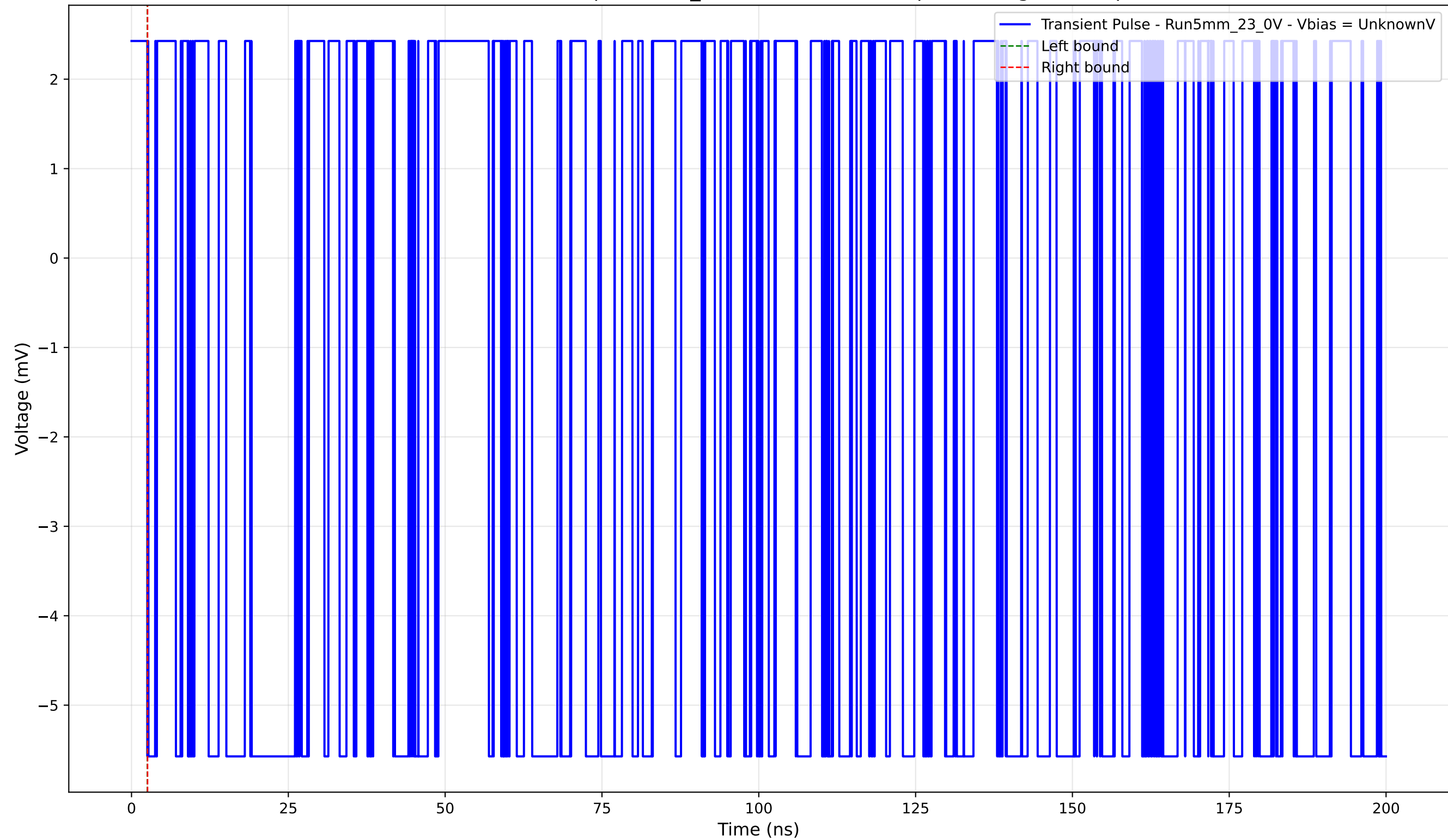
Transient Pulse - Sample: 5mm_23 - Position: 4035.0 \mu\text{m} - Charge: -0.00 pC
