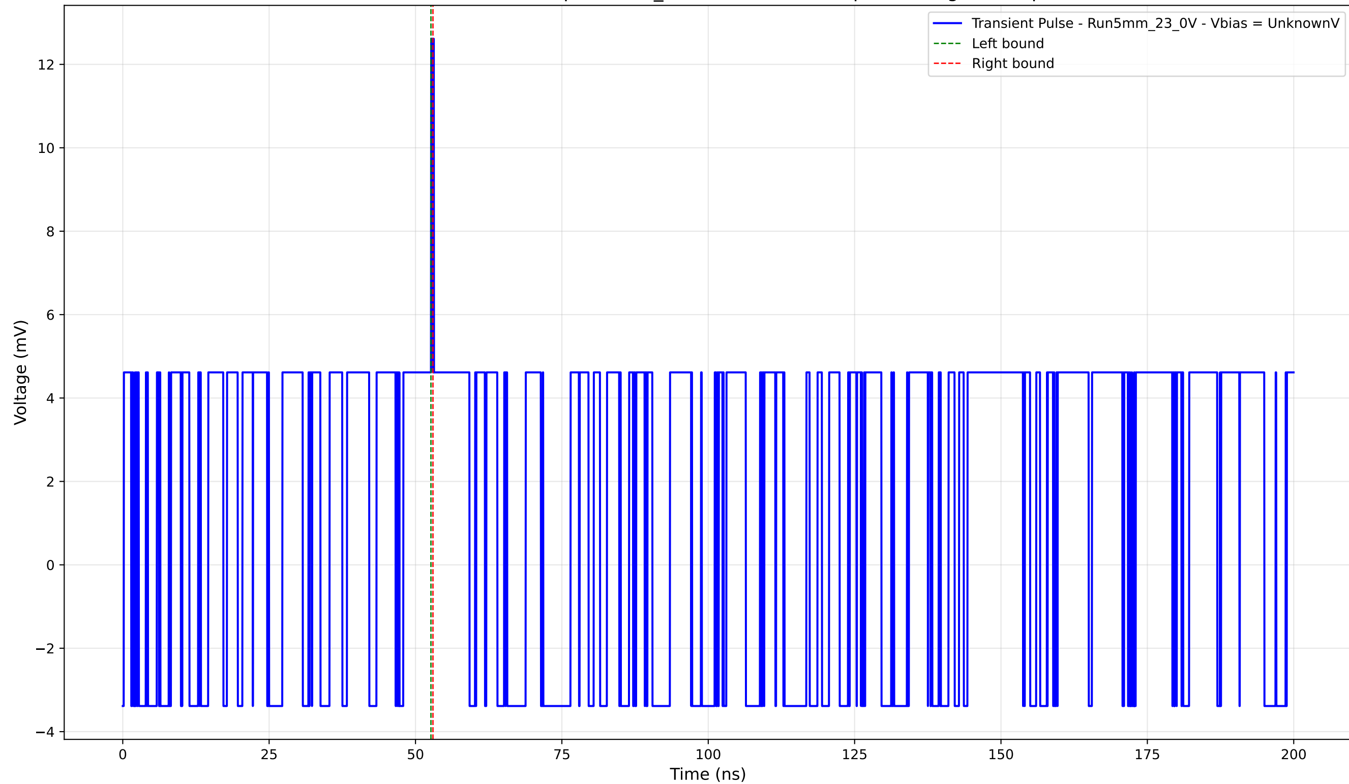
Transient Pulse - Sample: 5mm_23 - Position: 710.0 \mu\text{m} - Charge: 0.08 pC
