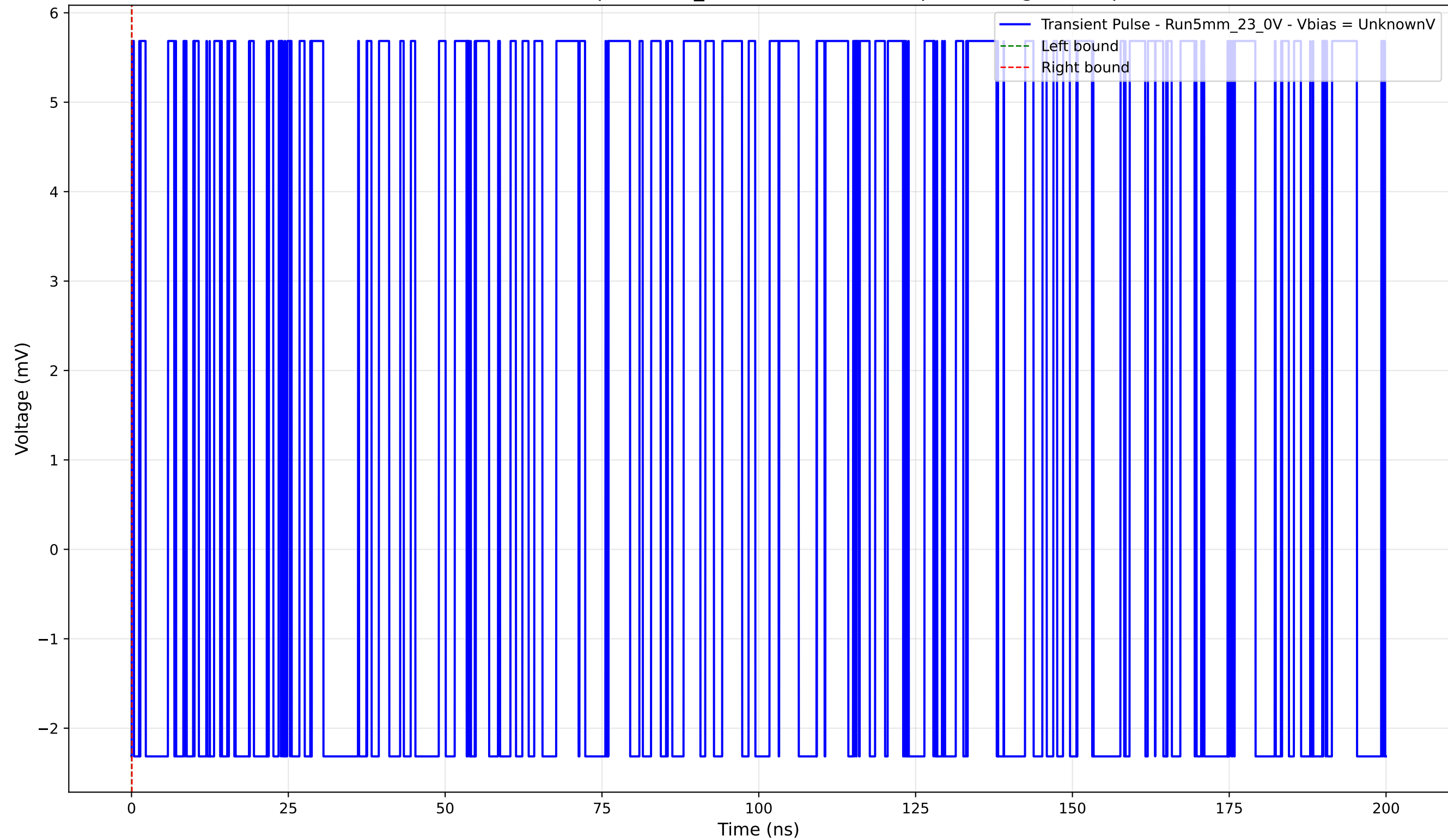
Transient Pulse - Sample: 5mm_23 - Position: 1140.0 \mu\text{m} - Charge: 0.00 pC
