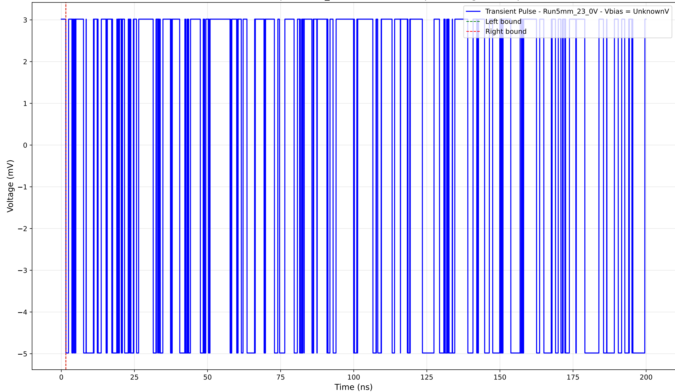
Transient Pulse - Sample: 5mm_23 - Position: 635.0 \mu\text{m} - Charge: -0.00 pC
