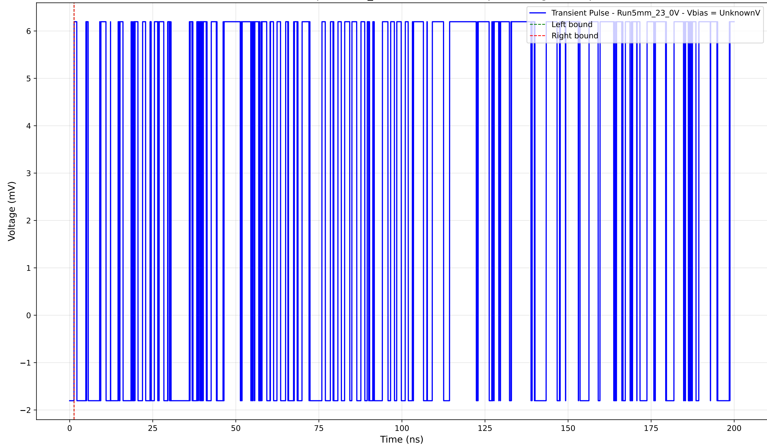
Transient Pulse - Sample: 5mm_23 - Position: 4390.0 \mu\text{m} - Charge: 0.00 pC
