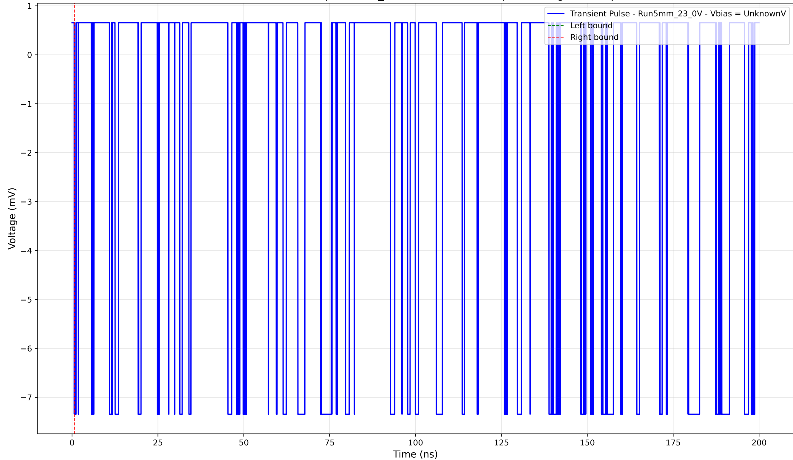
Transient Pulse - Sample: 5mm_23 - Position: 3560.0 \mu\text{m} - Charge: -0.00 pC
