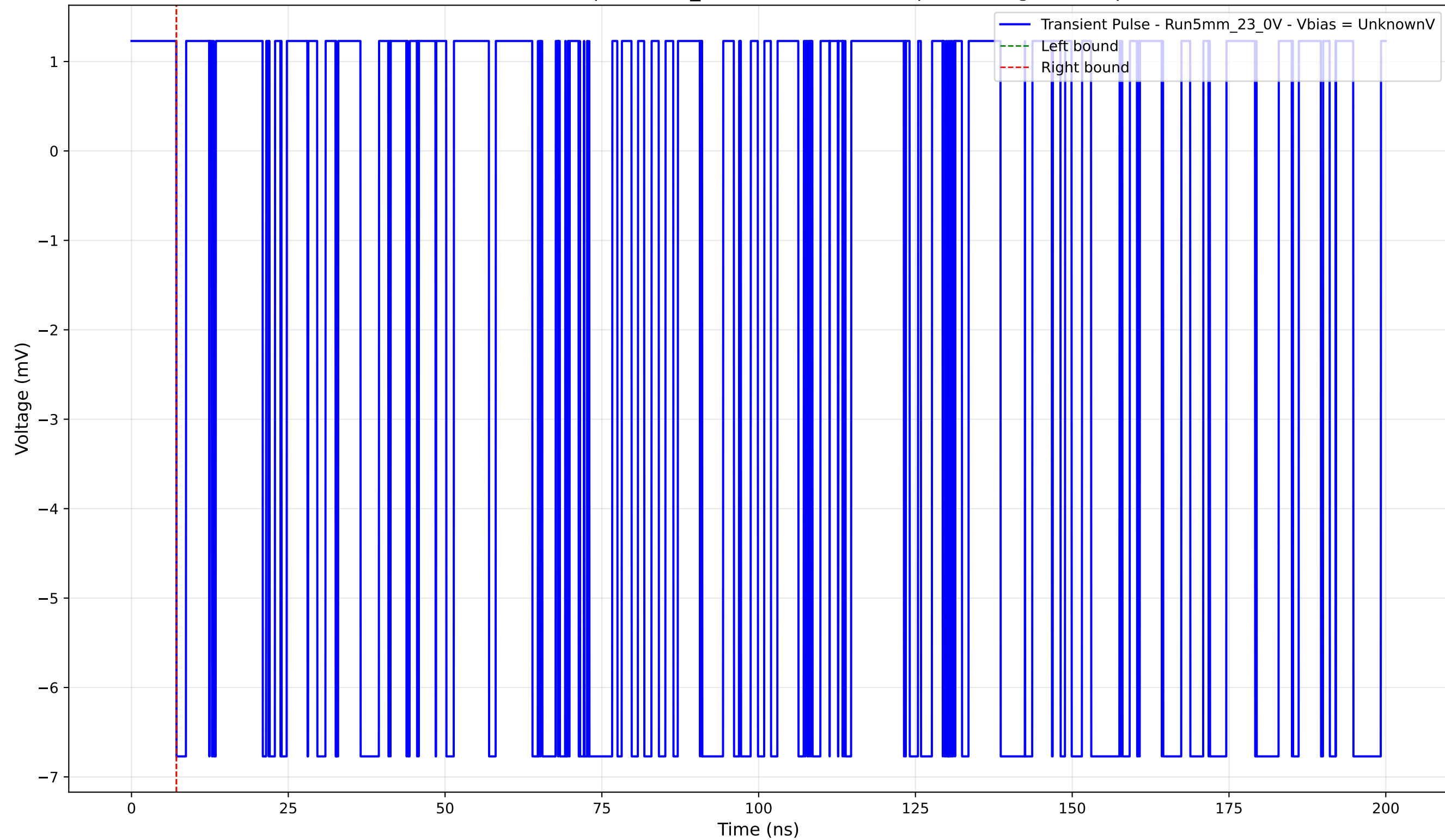
Transient Pulse - Sample: 5mm_23 - Position: 2800.0 \mu\text{m} - Charge: -0.00 pC
