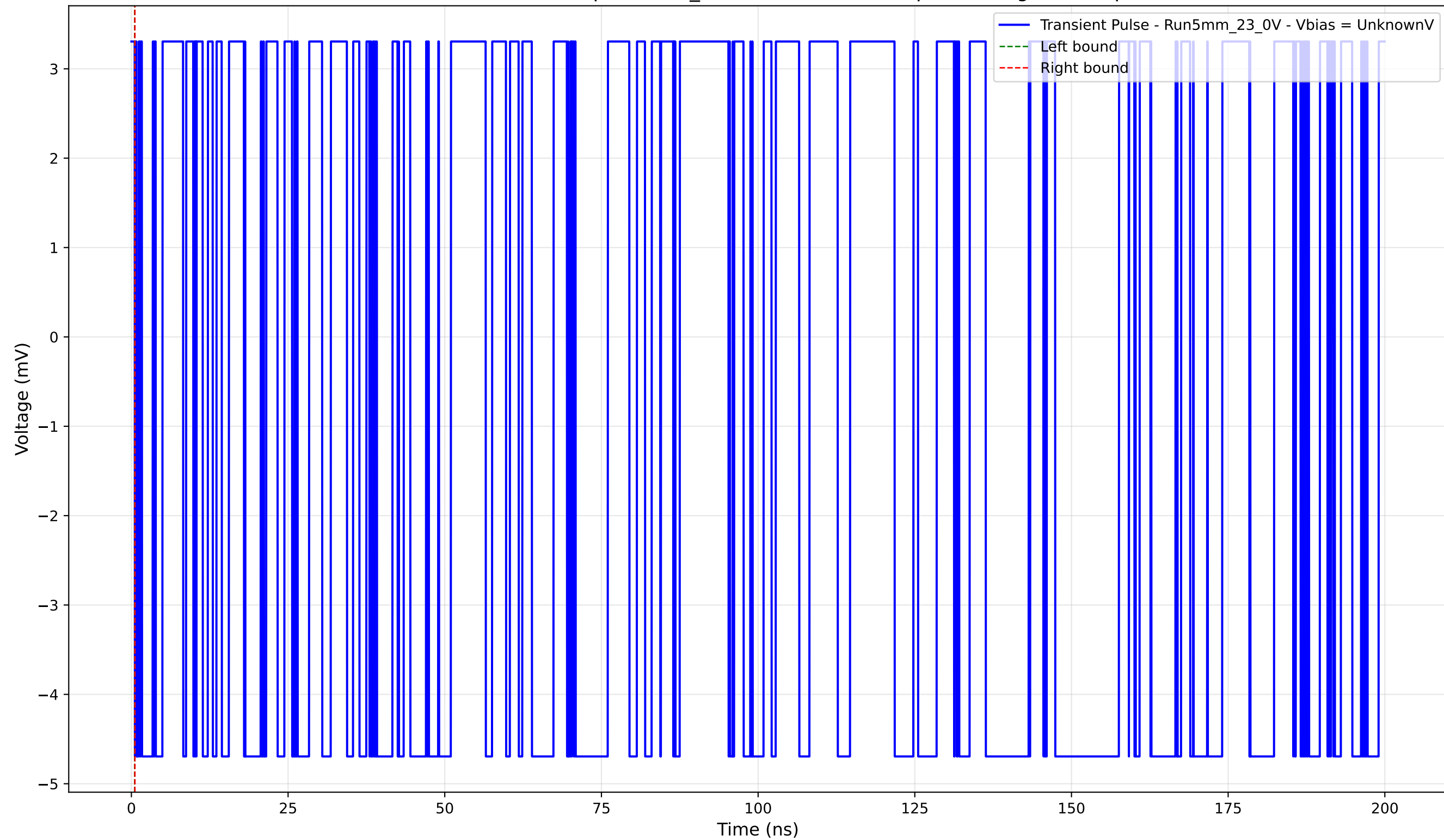
Transient Pulse - Sample: 5mm_23 - Position: 5040.0 \mu\text{m} - Charge: -0.00 pC
