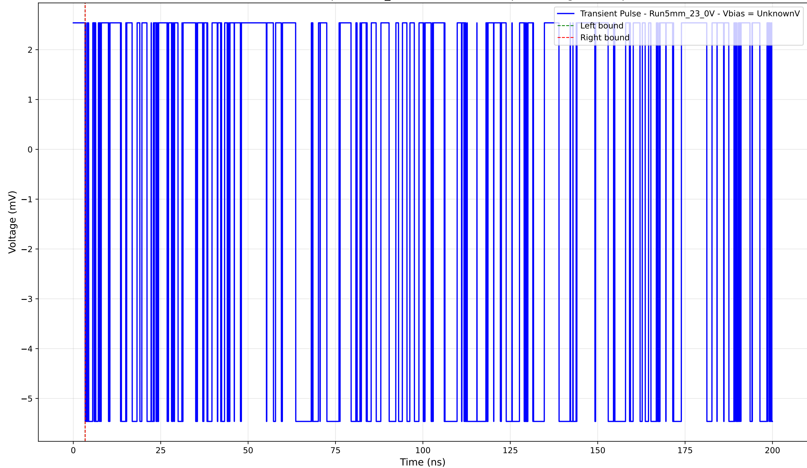
Transient Pulse - Sample: 5mm_23 - Position: 2000.0 \mu\text{m} - Charge: -0.00 pC
