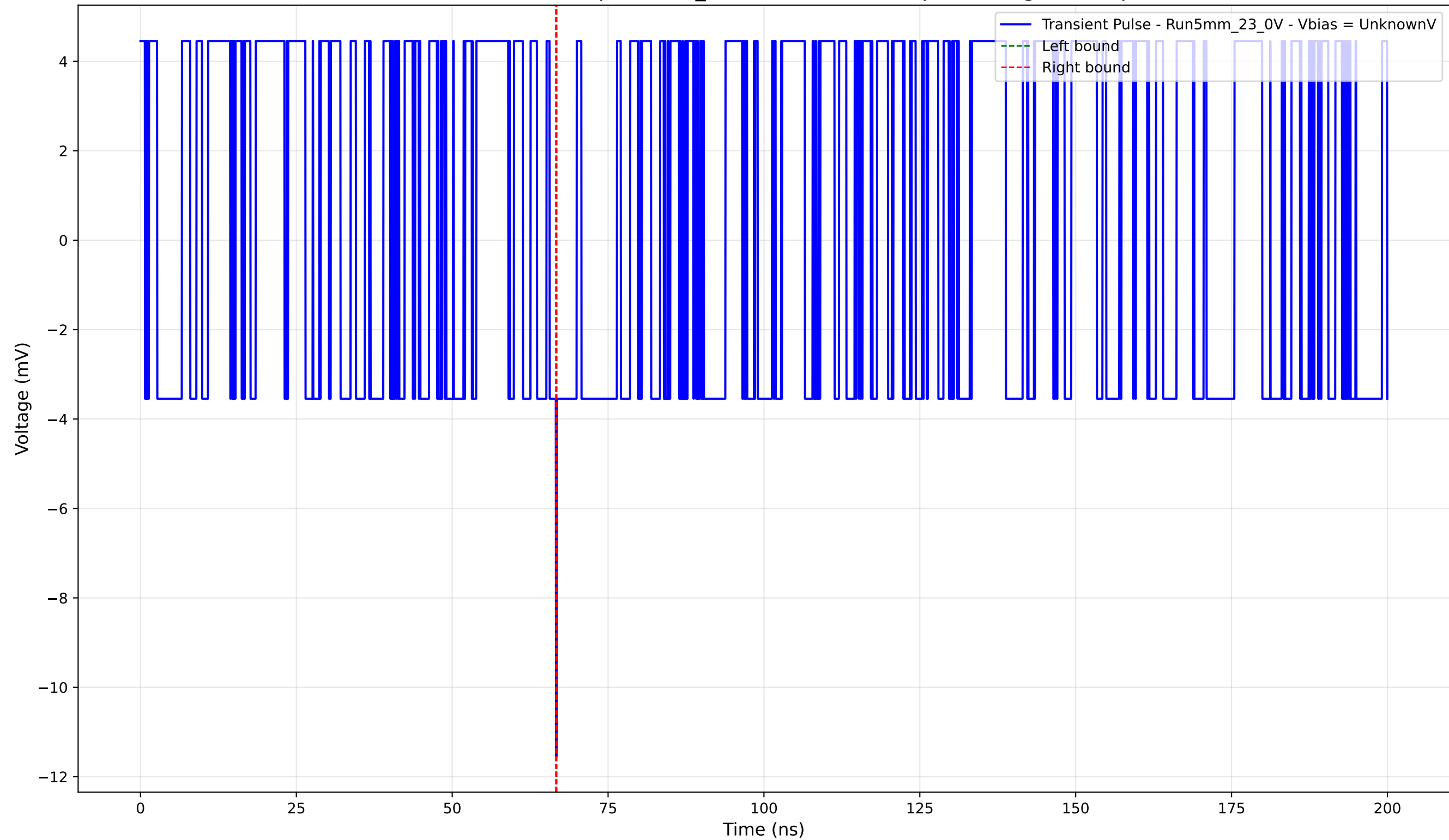
Transient Pulse - Sample: 5mm_23 - Position: 4560.0 \mu\text{m} - Charge: -0.03 pC
