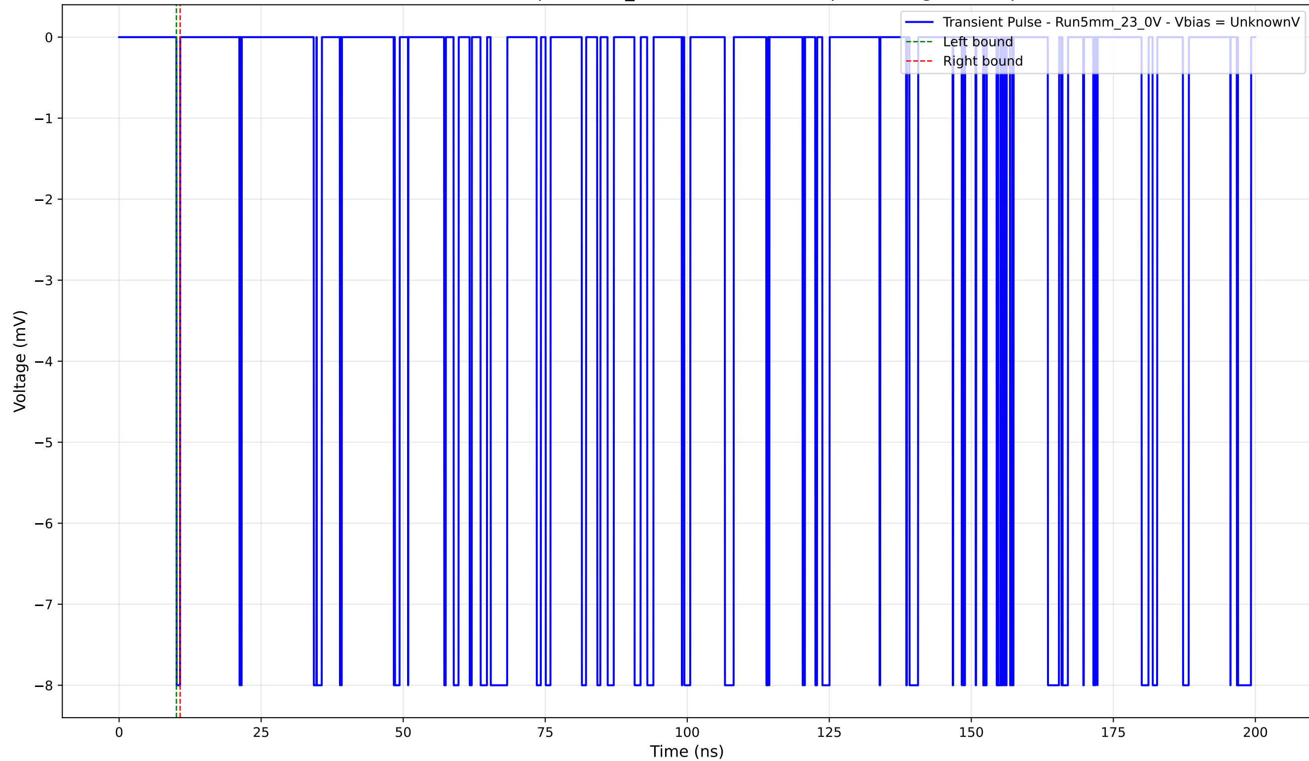
Transient Pulse - Sample: 5mm_23 - Position: 2260.0 \mu\text{m} - Charge: -0.10 pC
