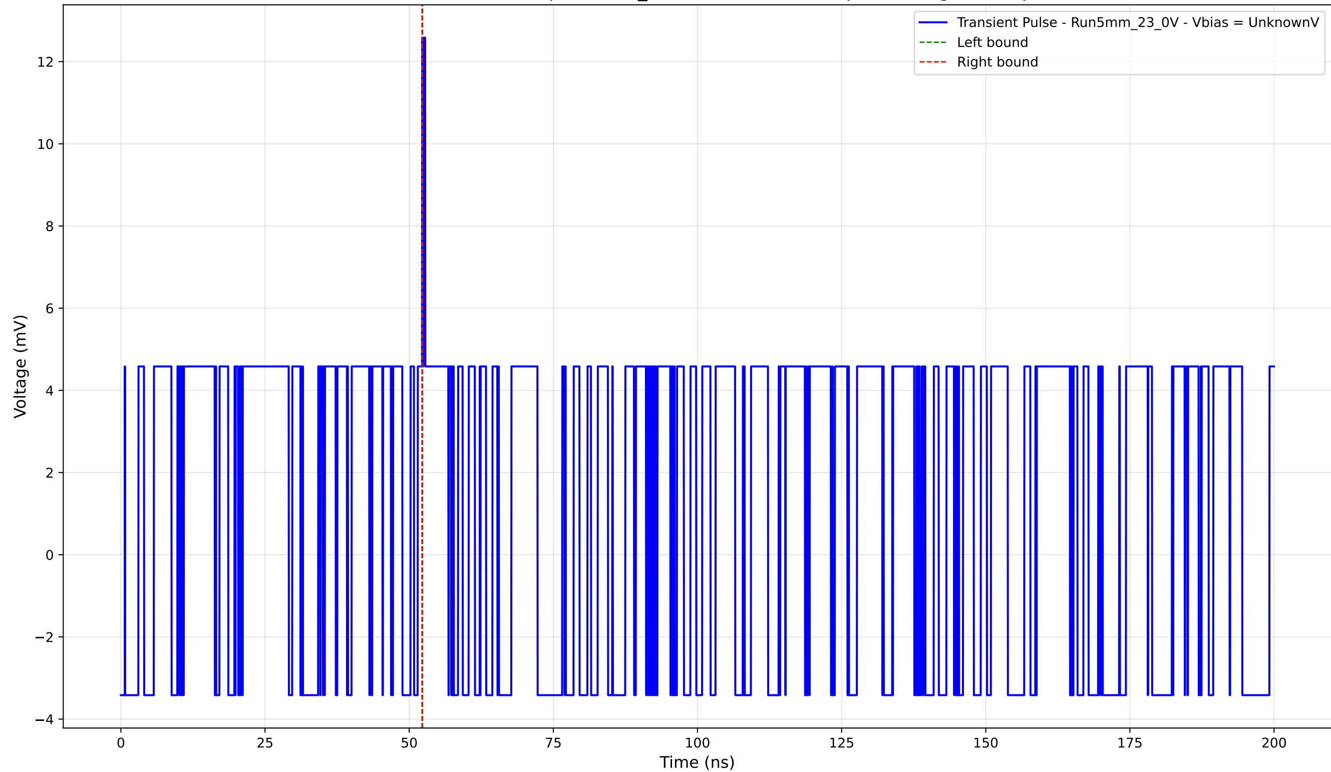
Transient Pulse - Sample: 5mm_23 - Position: 2230.0 \mu\text{m} - Charge: 0.02 pC
