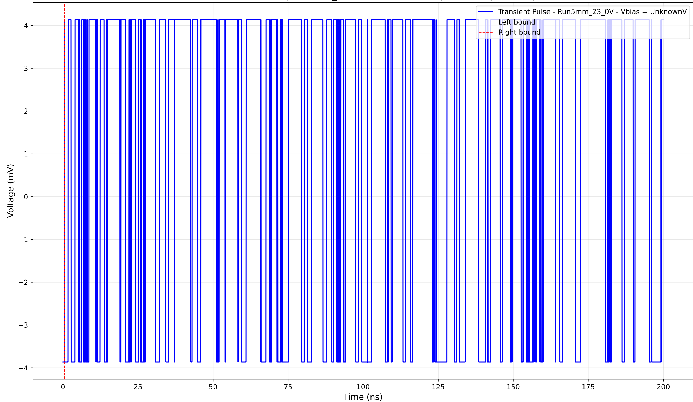
Transient Pulse - Sample: 5mm_23 - Position: 3220.0 \mu\text{m} - Charge: 0.00 pC
