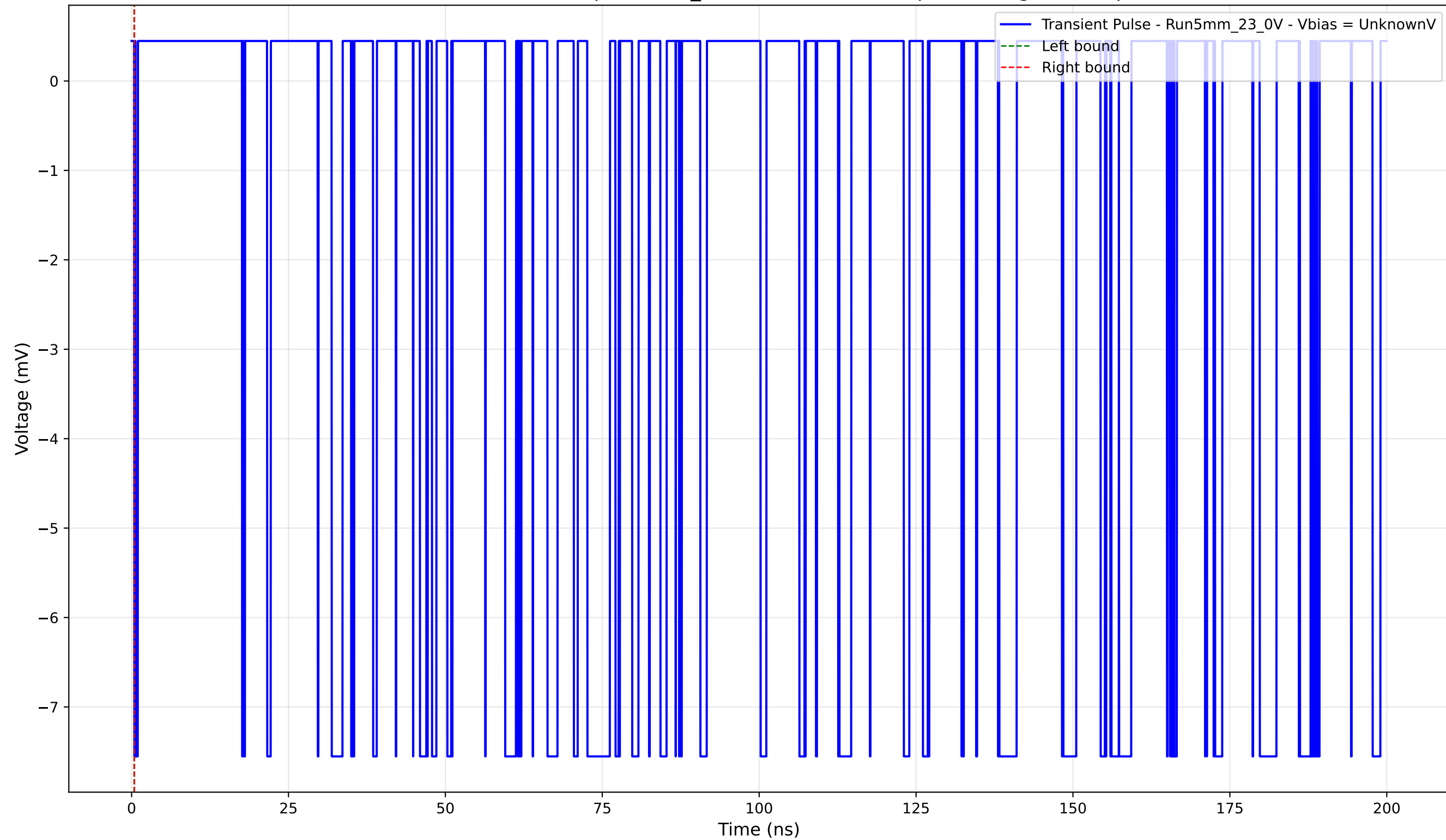
Transient Pulse - Sample: 5mm_23 - Position: 2785.0 \mu\text{m} - Charge: -0.00 pC
