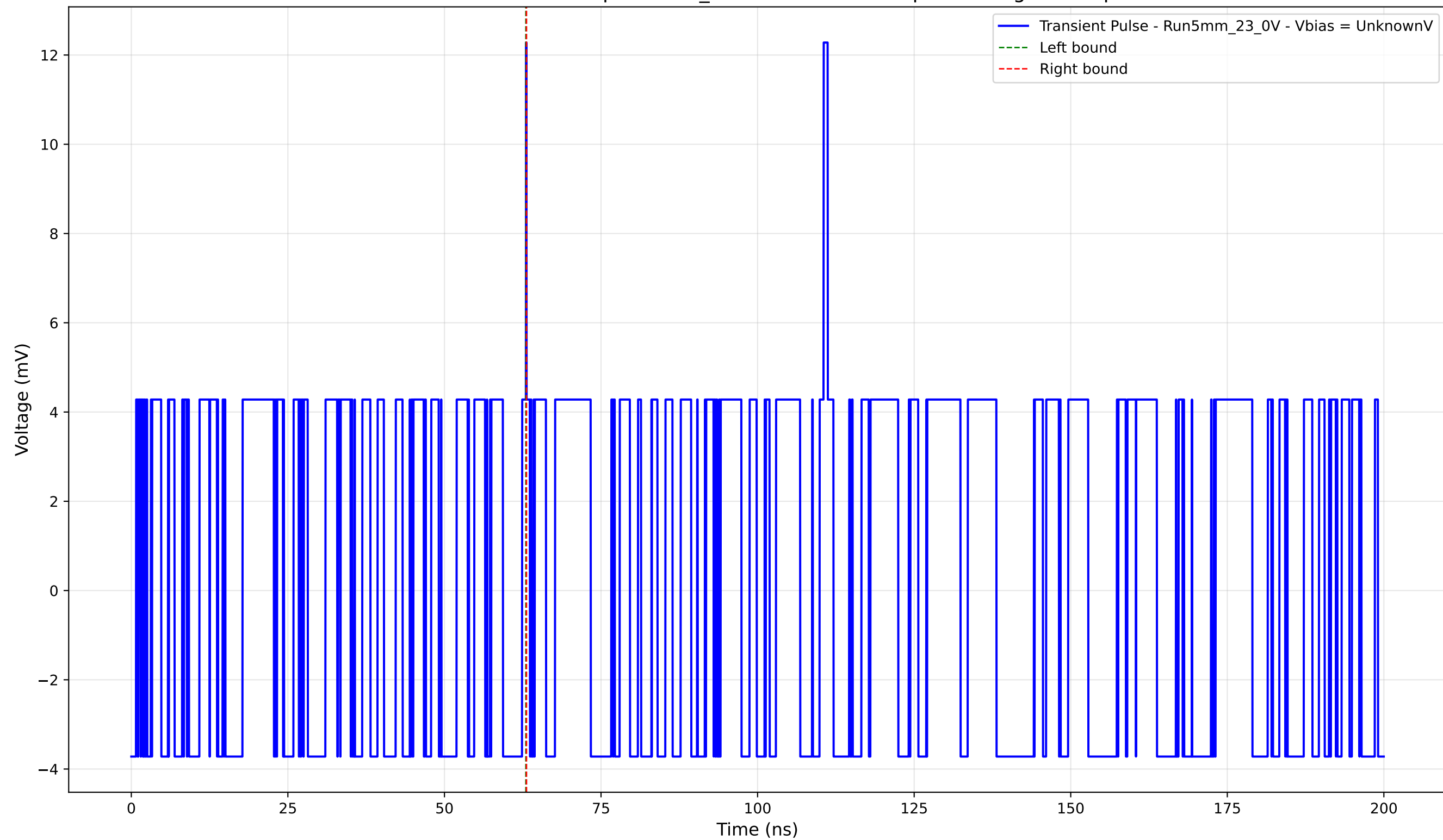
Transient Pulse - Sample: 5mm_23 - Position: 175.0 \mu\text{m} - Charge: 0.02 pC
