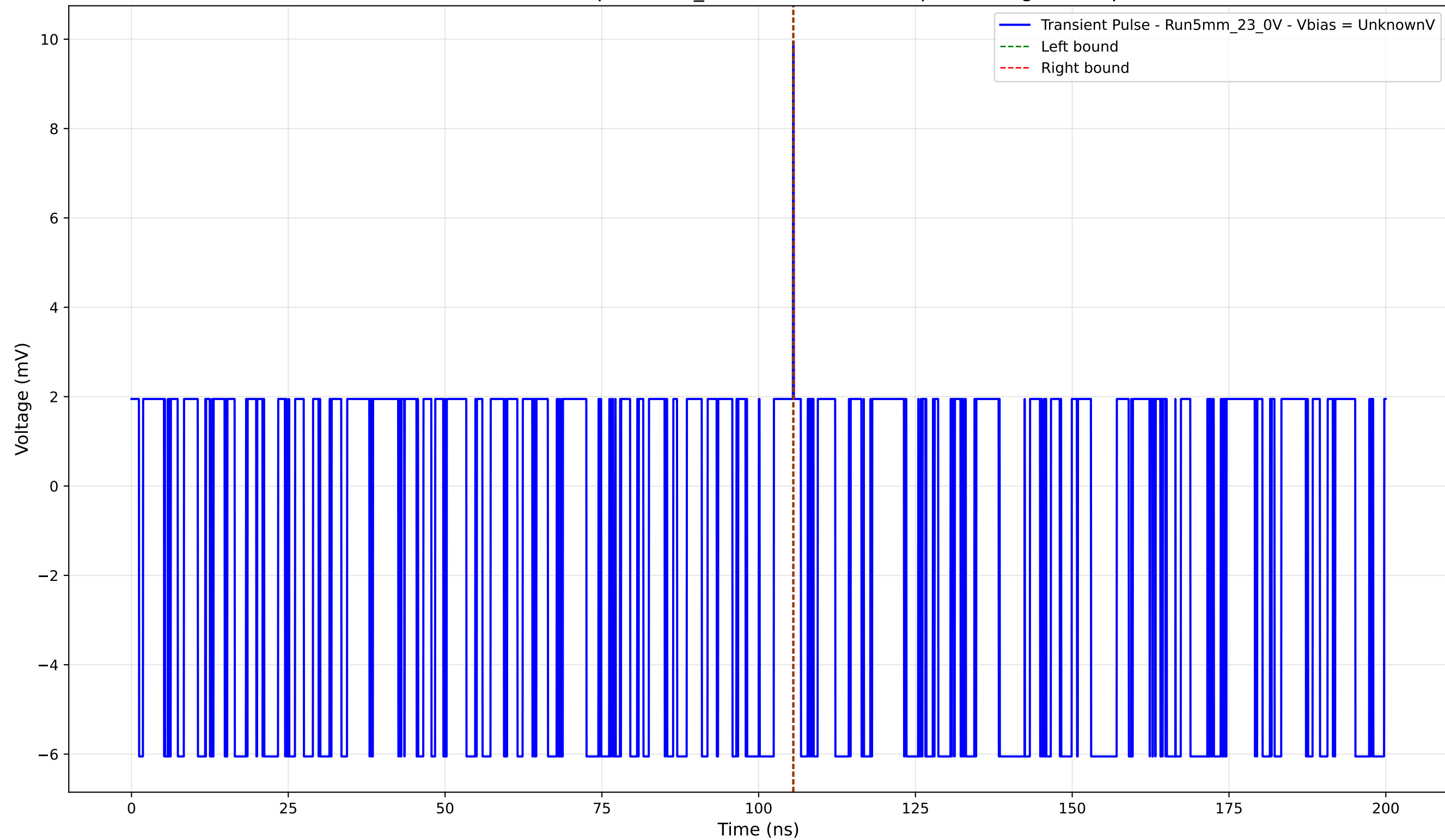
Transient Pulse - Sample: 5mm_23 - Position: 2160.0 \mu\text{m} - Charge: 0.02 pC
