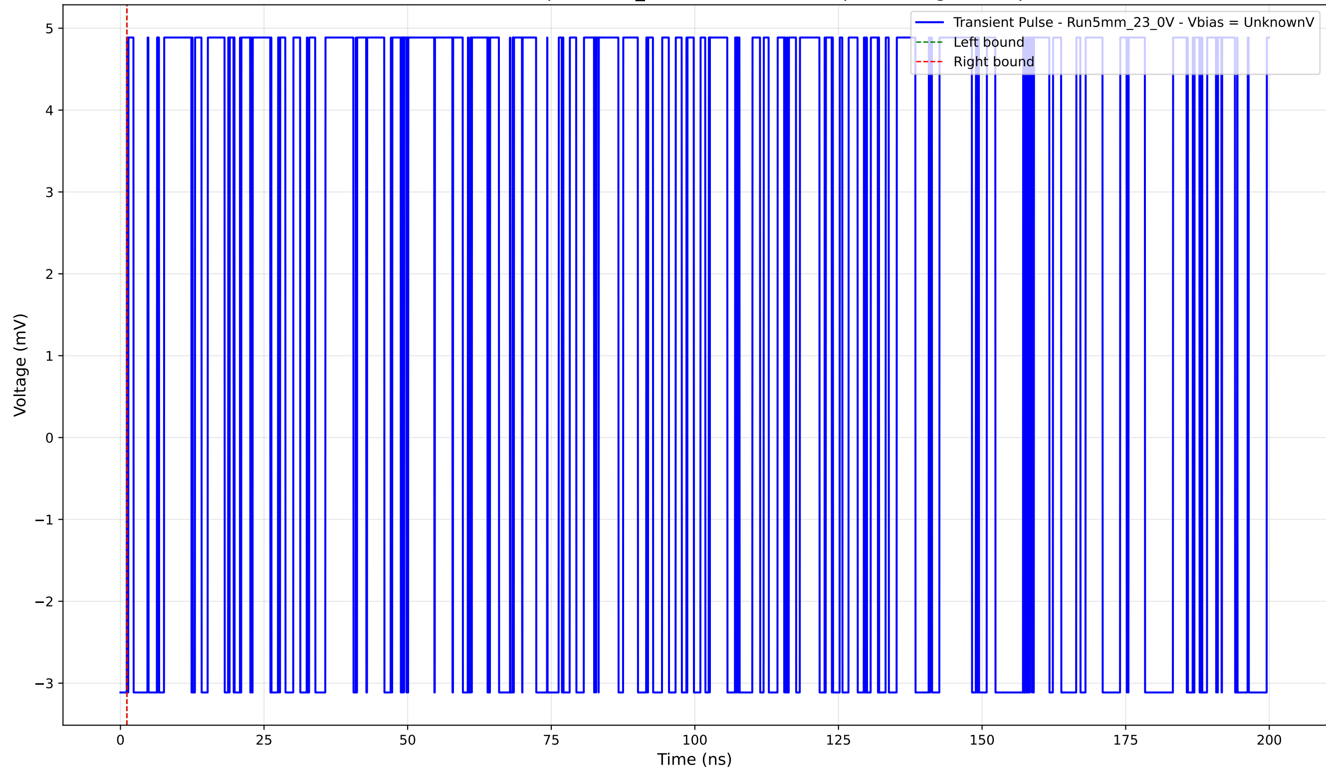
Transient Pulse - Sample: 5mm_23 - Position: 4640.0 \mu\text{m} - Charge: 0.00 pC
