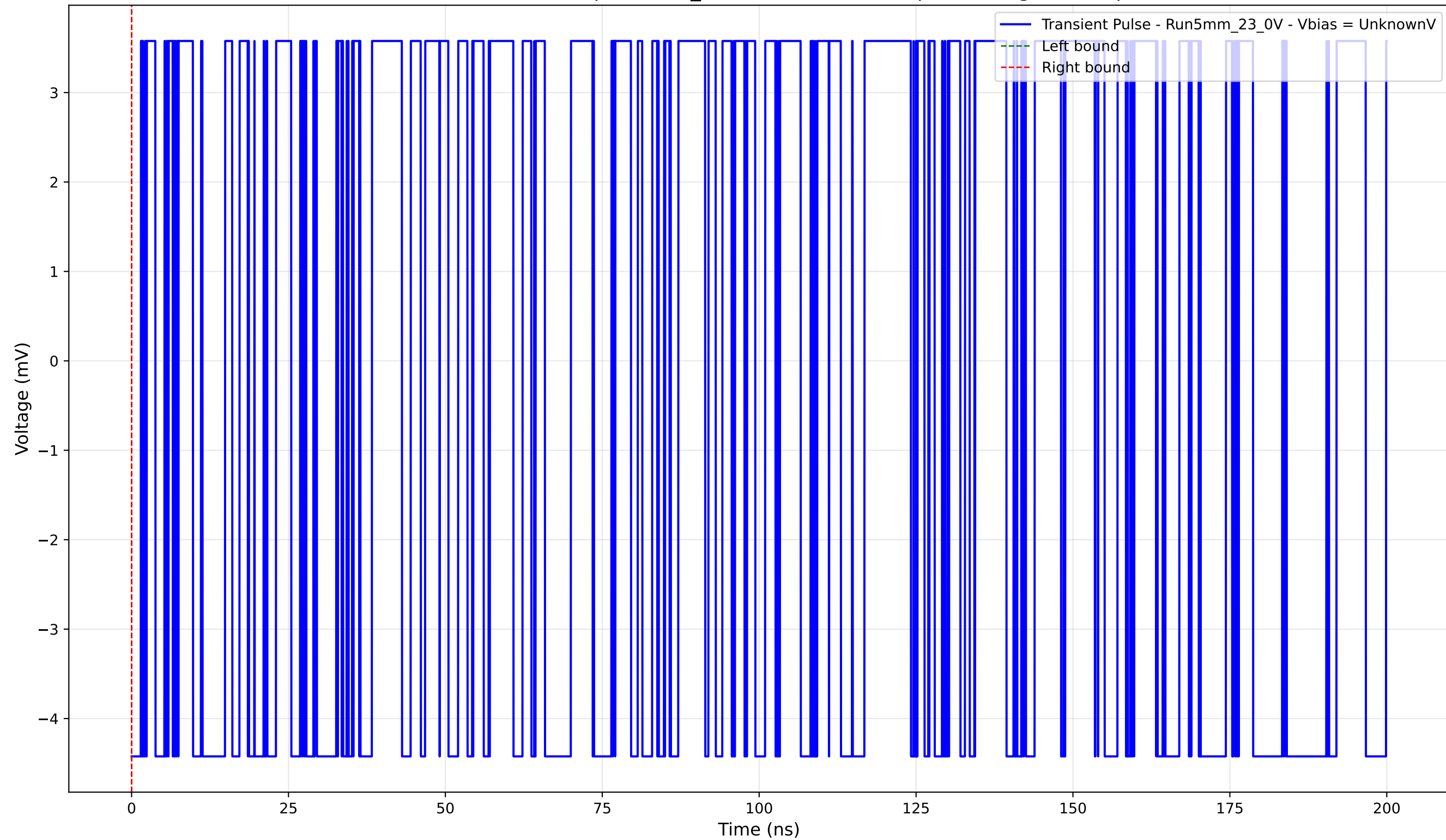
Transient Pulse - Sample: 5mm_23 - Position: 5055.0 \mu\text{m} - Charge: -0.00 pC
