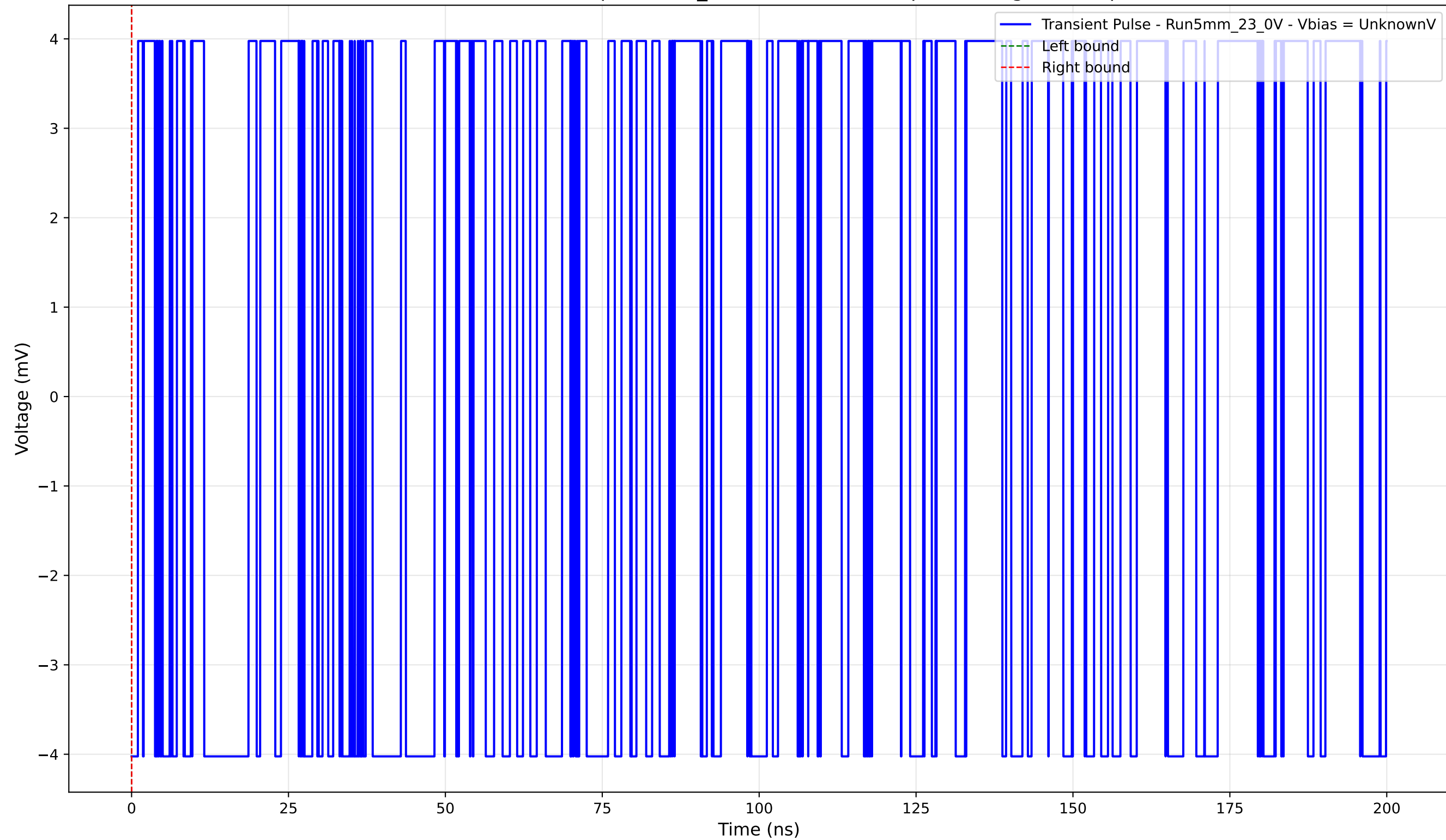
Transient Pulse - Sample: 5mm_23 - Position: 765.0 \mu\text{m} - Charge: -0.00 pC
