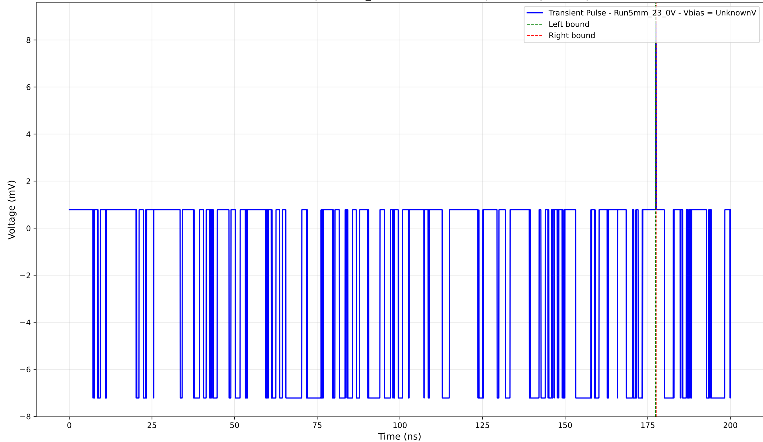
Transient Pulse - Sample: 5mm_23 - Position: 2700.0 \mu\text{m} - Charge: 0.02 pC
