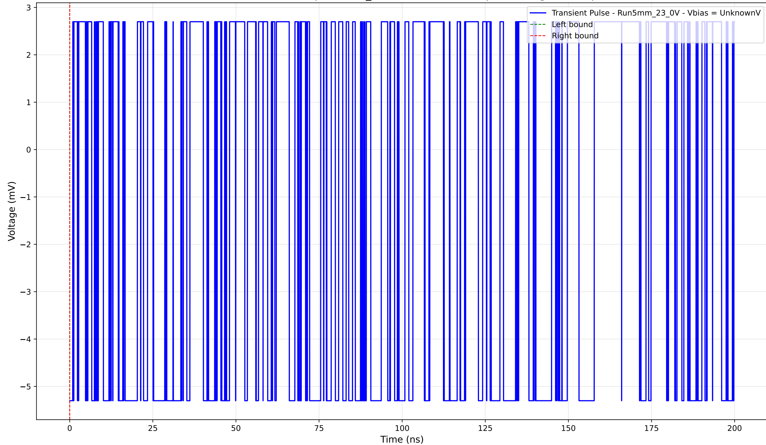
Transient Pulse - Sample: 5mm_23 - Position: 3000.0 \mu\text{m} - Charge: -0.00 pC
