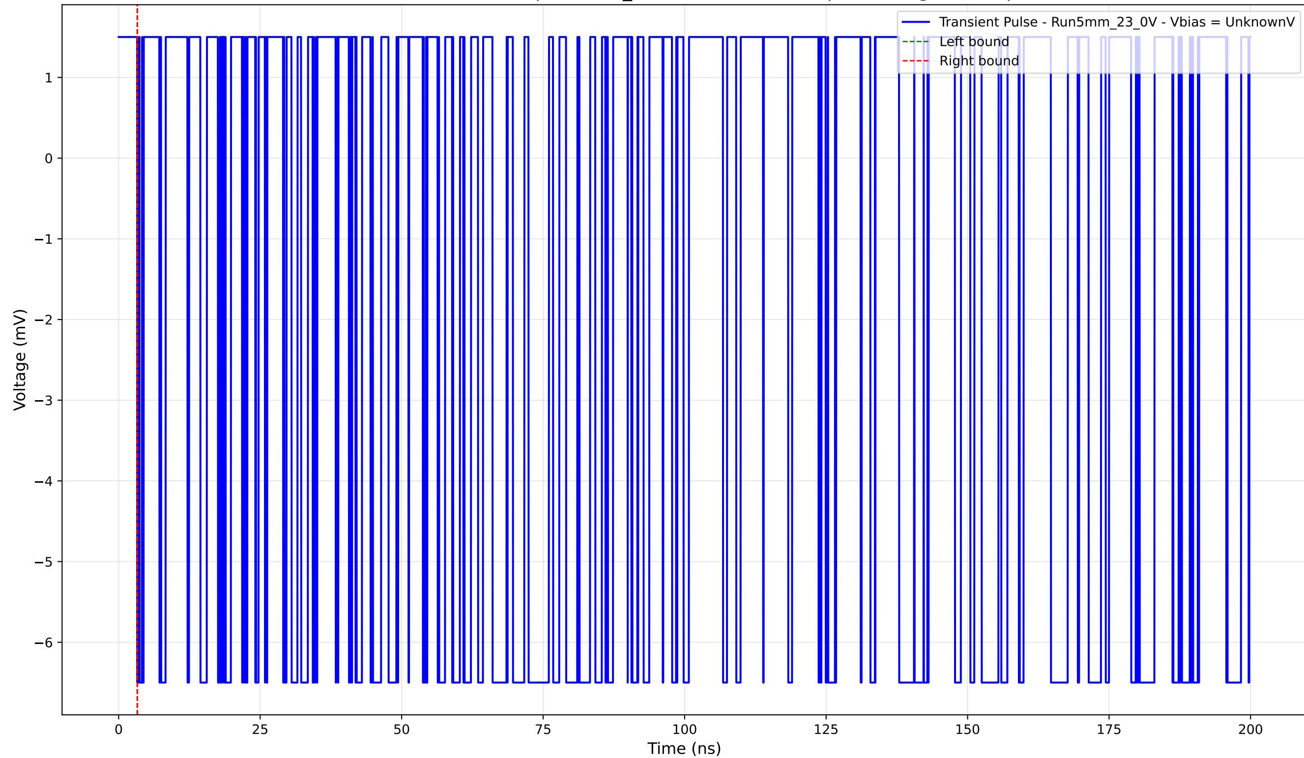
Transient Pulse - Sample: 5mm_23 - Position: 3805.0 \mu\text{m} - Charge: -0.00 pC
