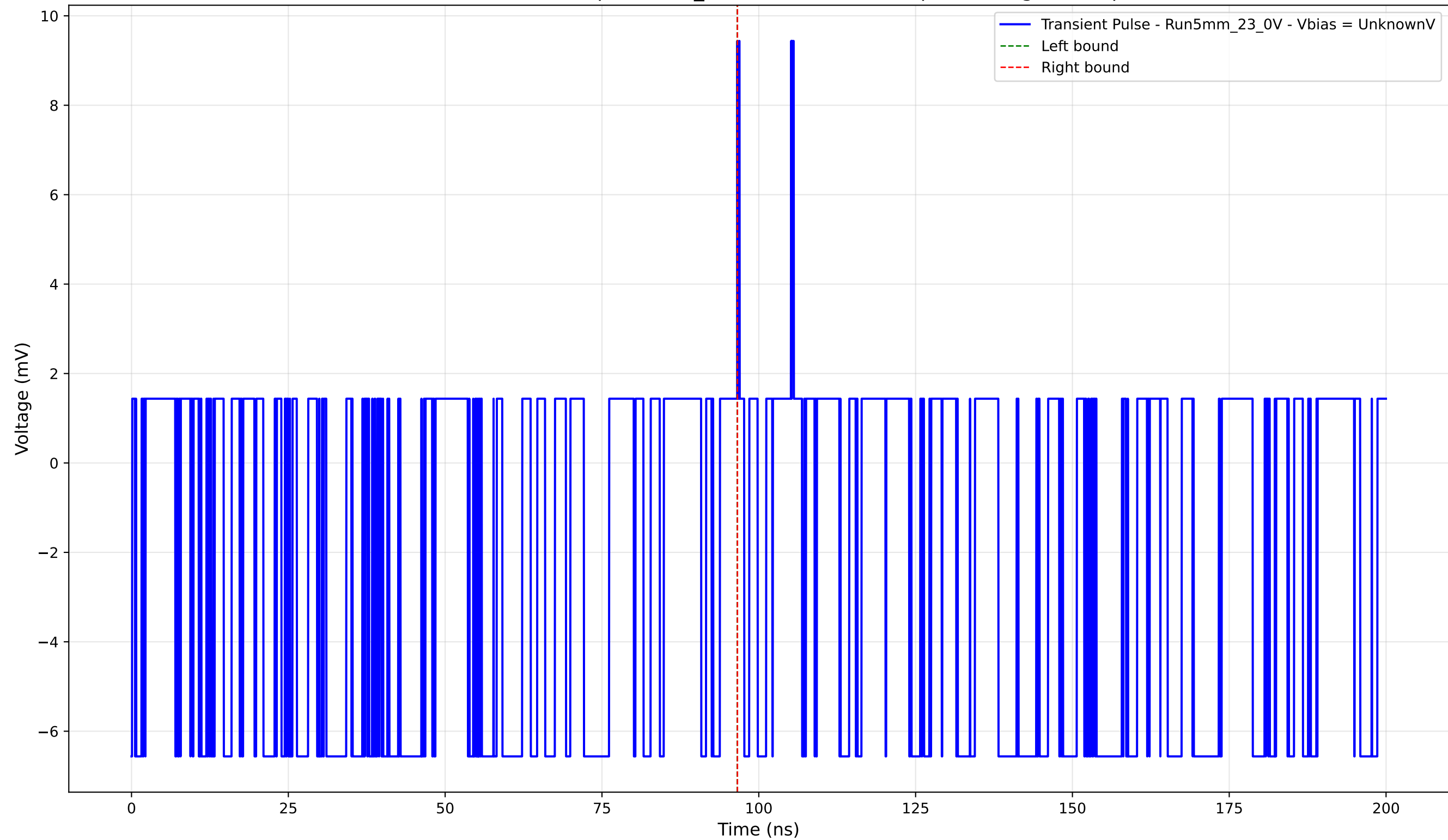
Transient Pulse - Sample: 5mm_23 - Position: 2165.0 \mu\text{m} - Charge: 0.00 pC
