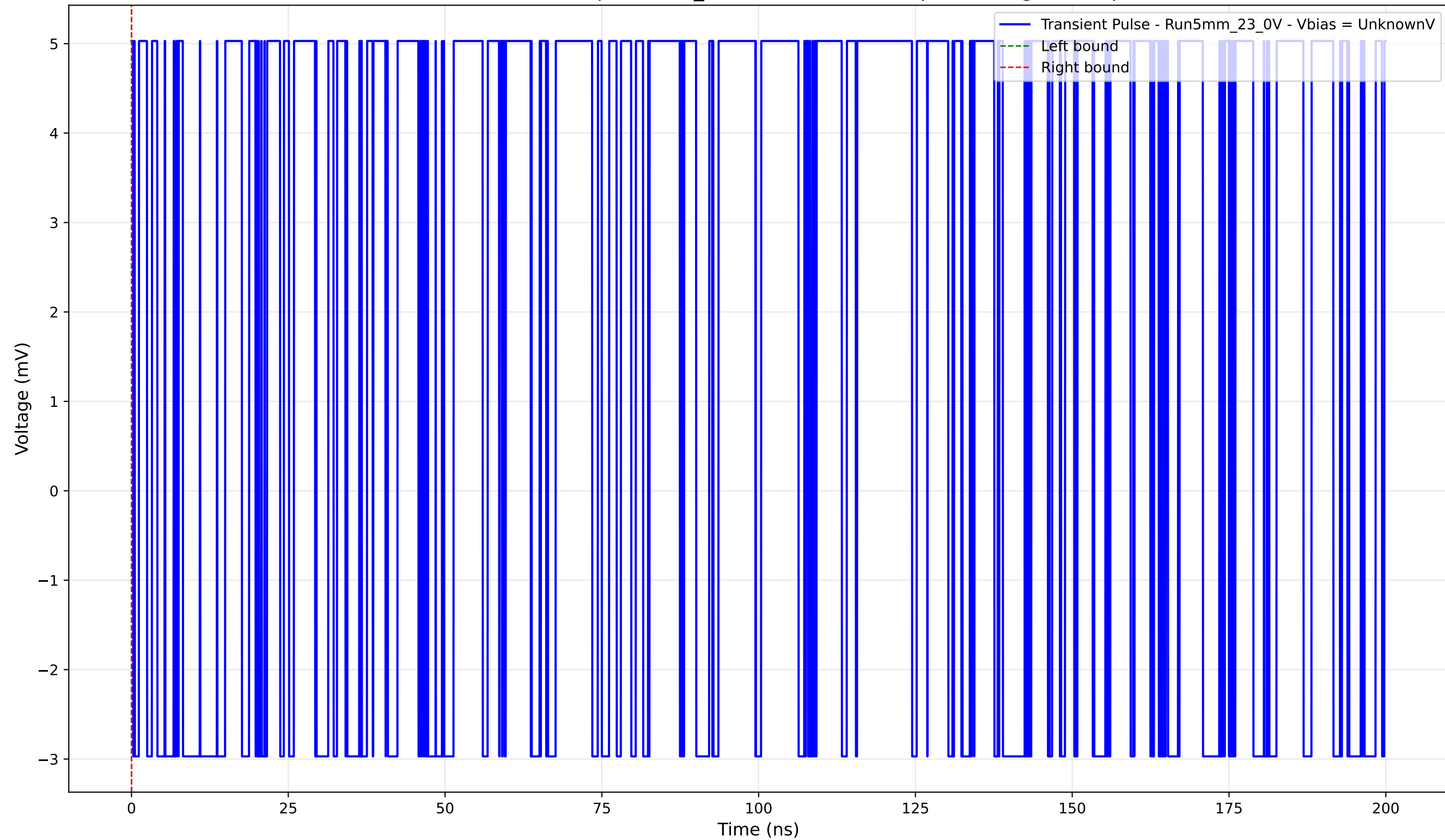
Transient Pulse - Sample: 5mm_23 - Position: 4950.0 \mu\text{m} - Charge: 0.00 pC
