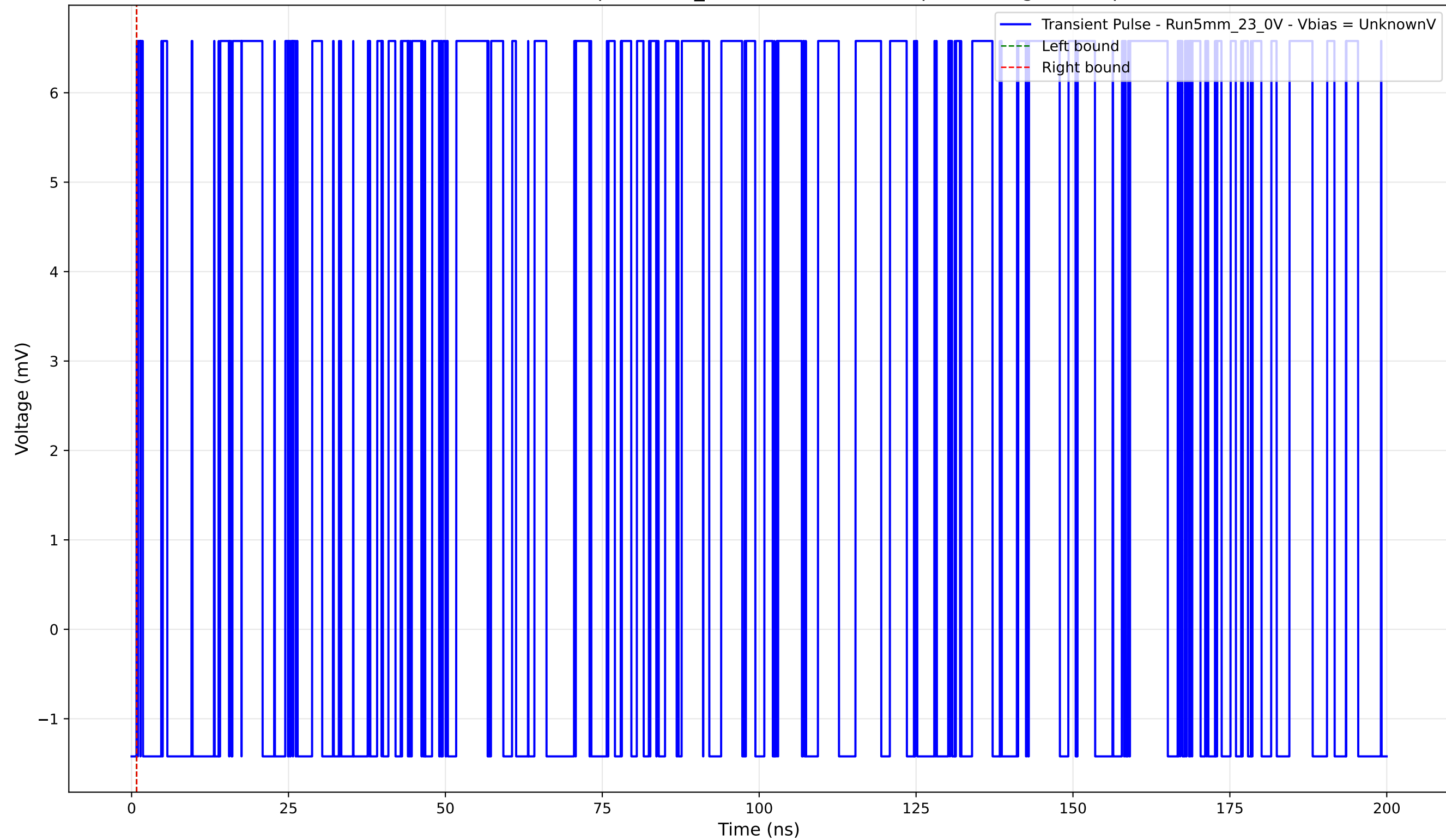
Transient Pulse - Sample: 5mm_23 - Position: 2245.0 \mu\text{m} - Charge: 0.00 pC
