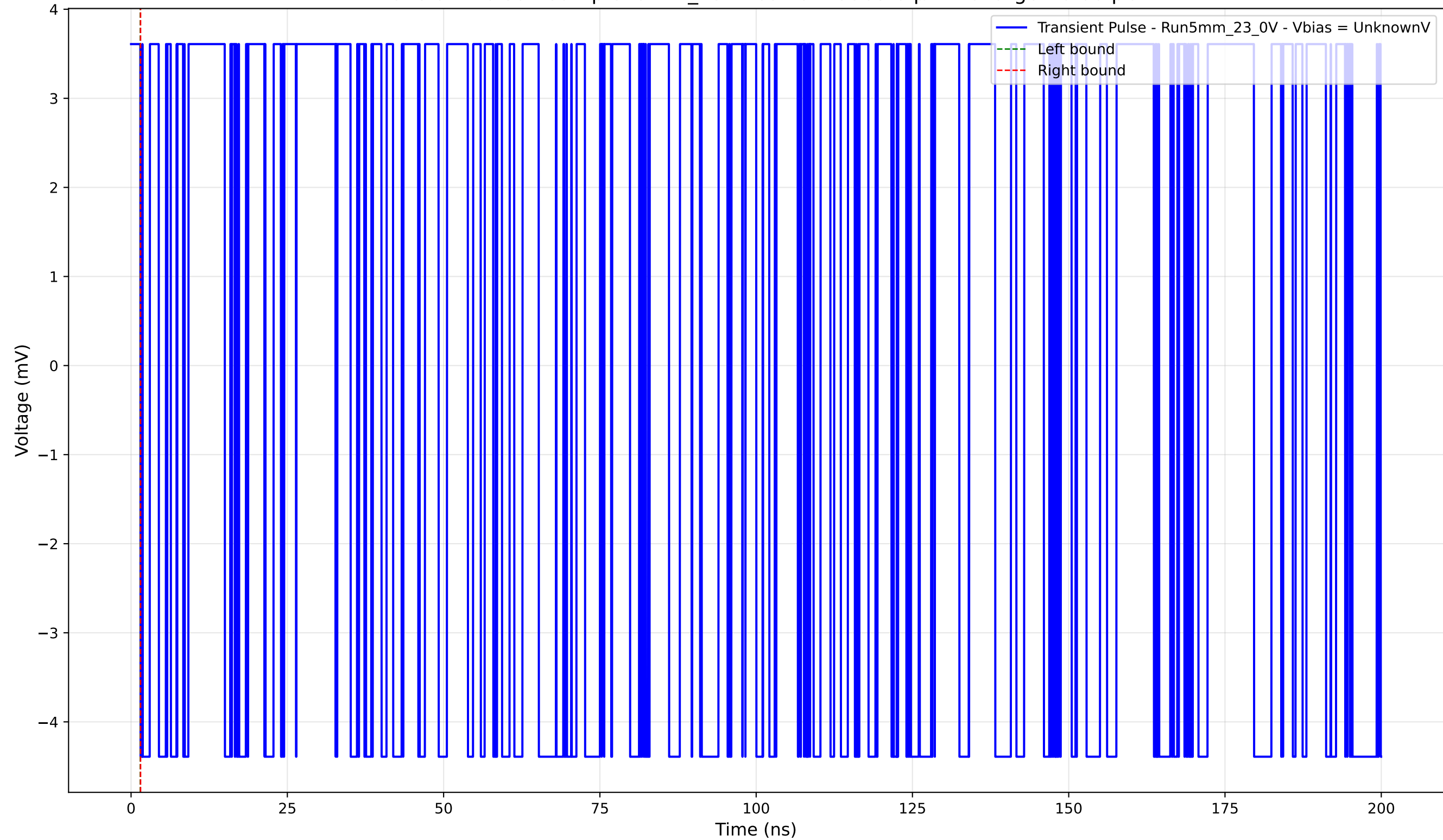
Transient Pulse - Sample: 5mm_23 - Position: 3565.0 \mu\text{m} - Charge: -0.00 pC
