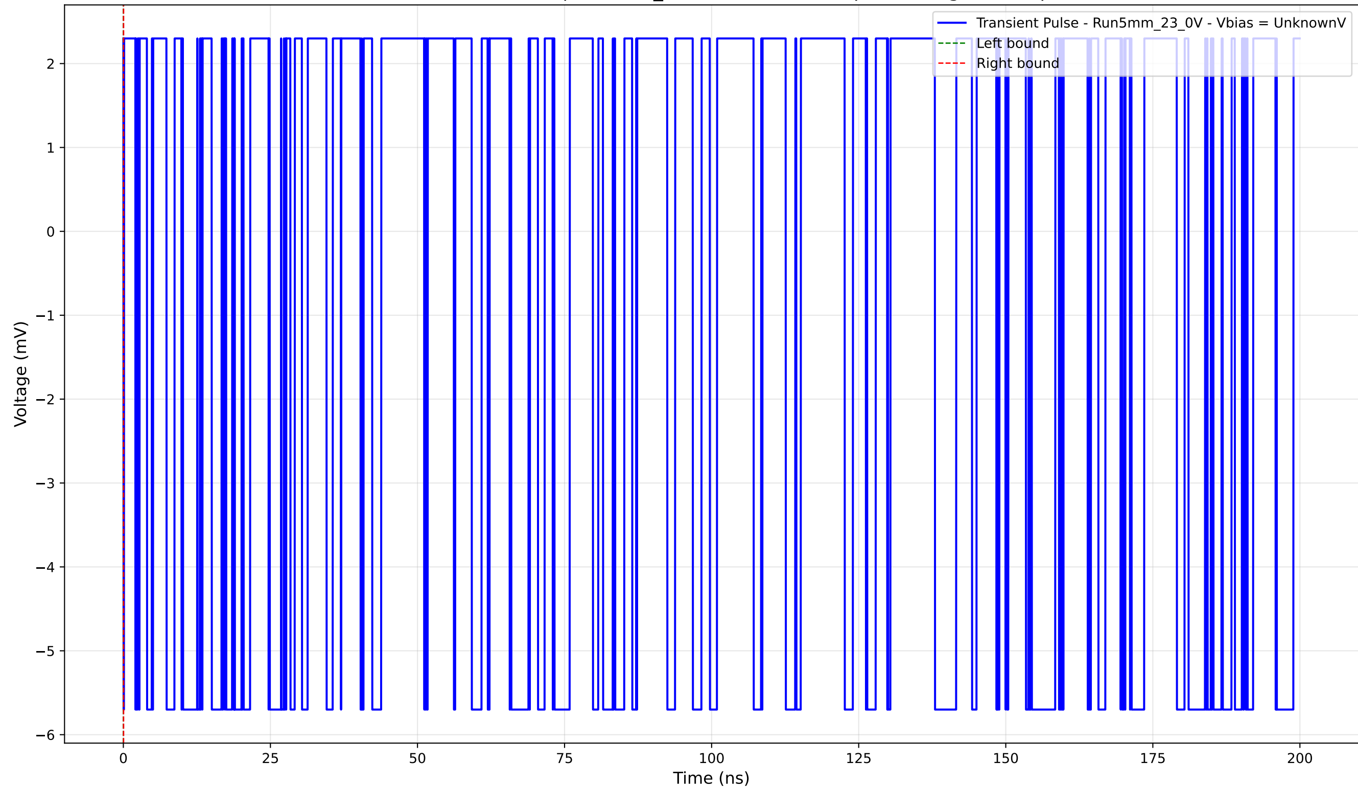
Transient Pulse - Sample: 5mm_23 - Position: 300.0 \mu\text{m} - Charge: -0.00 pC
