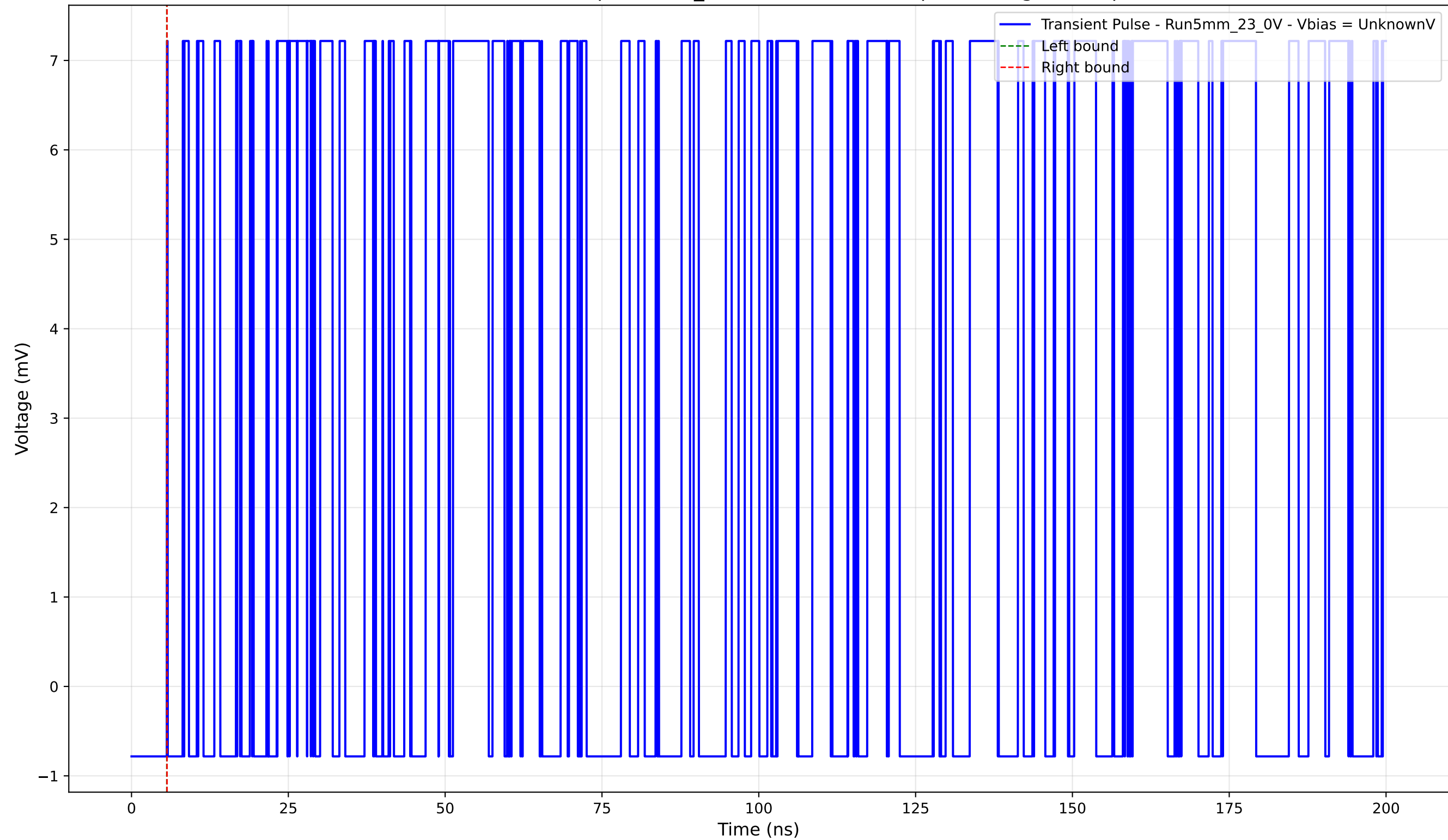
Transient Pulse - Sample: 5mm_23 - Position: 2440.0 \mu\text{m} - Charge: 0.00 pC
