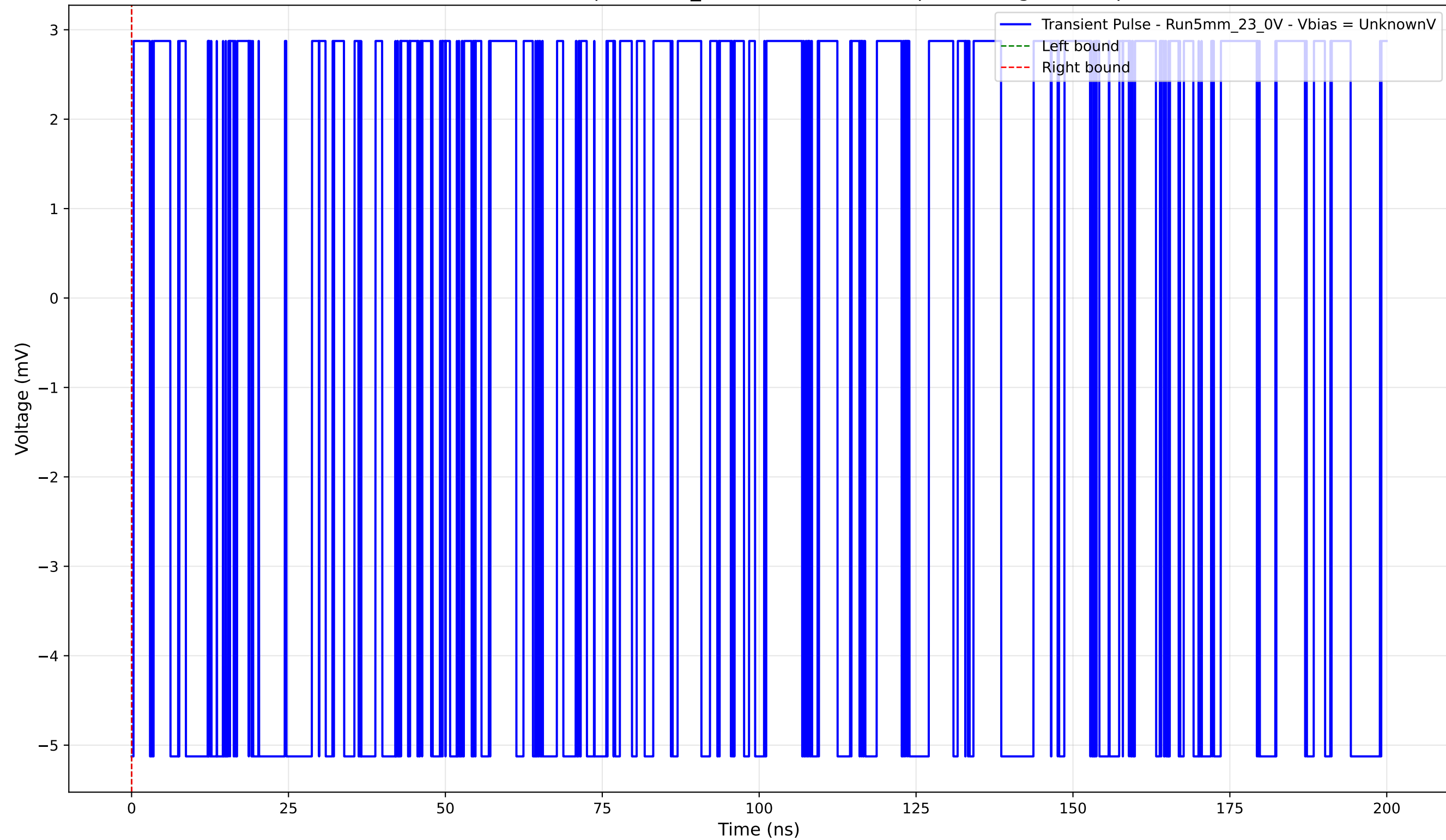
Transient Pulse - Sample: 5mm_23 - Position: 1820.0 \mu\text{m} - Charge: -0.00 pC
