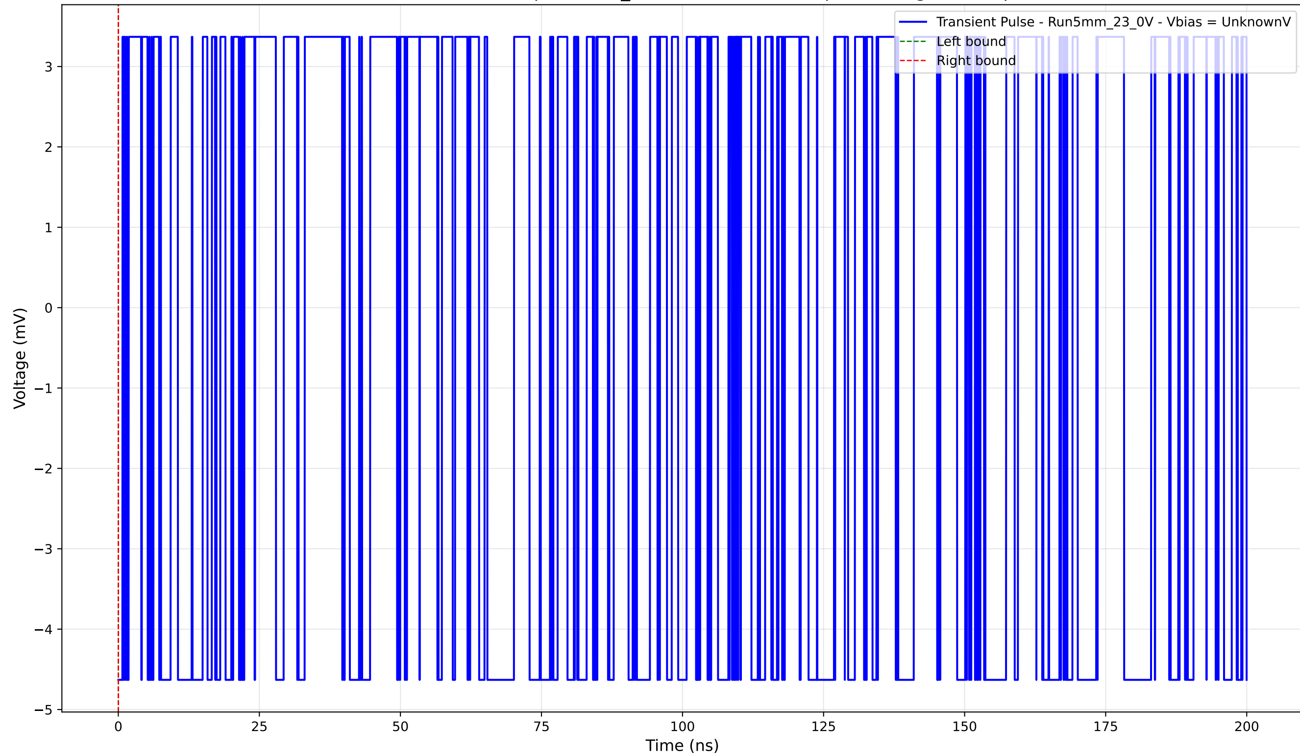
Transient Pulse - Sample: 5mm_23 - Position: 4185.0 \mu\text{m} - Charge: -0.00 pC
