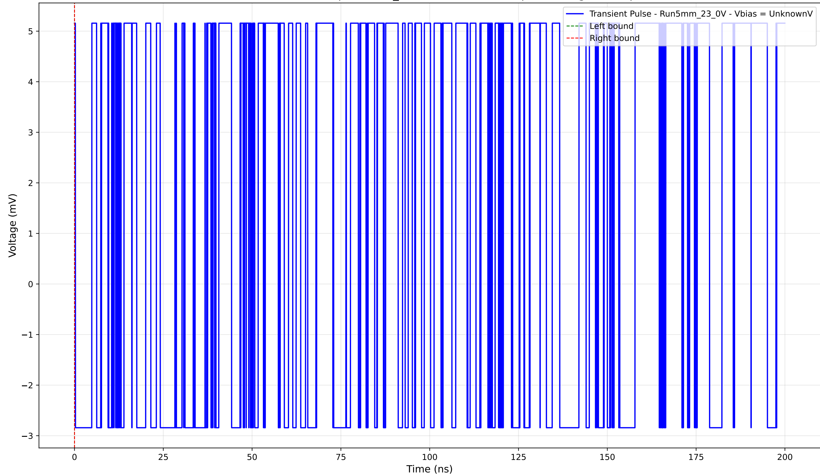
Transient Pulse - Sample: 5mm_23 - Position: 3830.0 \mu\text{m} - Charge: 0.00 pC
