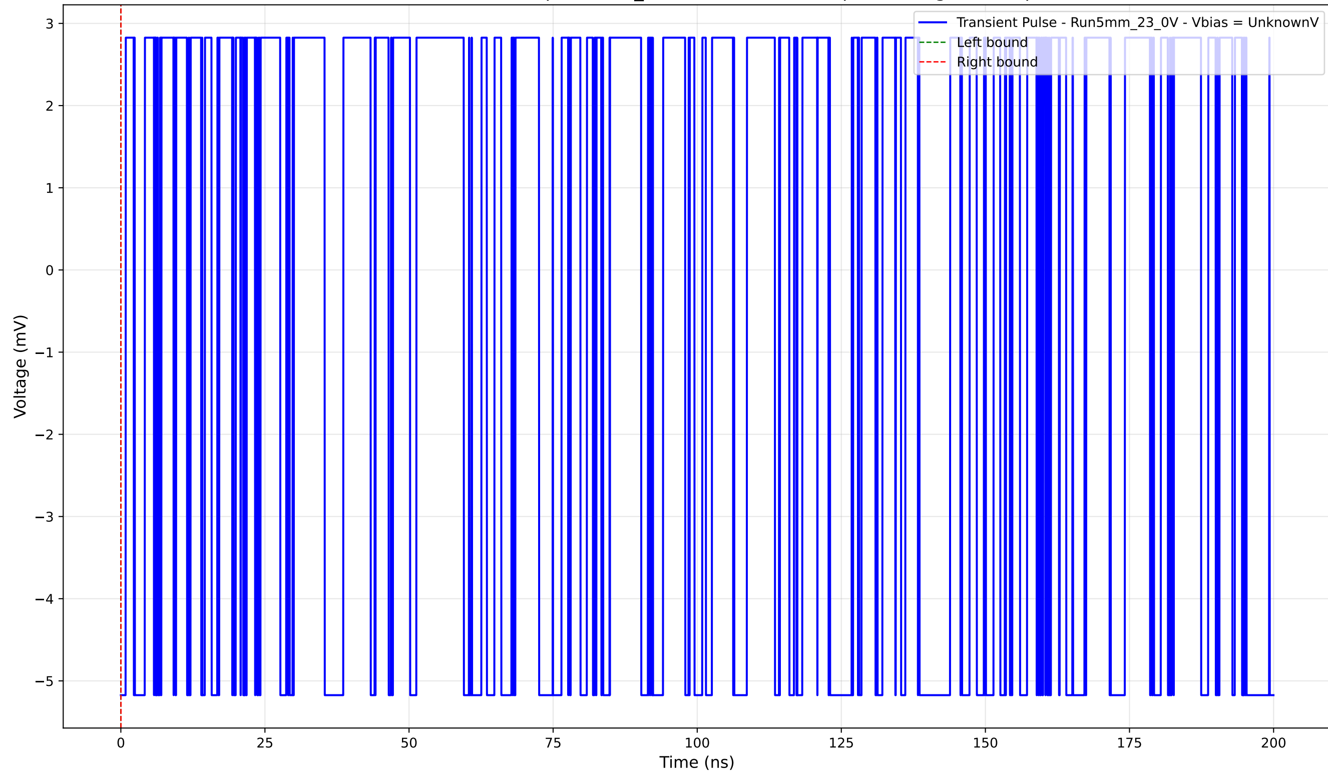
Transient Pulse - Sample: 5mm_23 - Position: 1115.0 \mu\text{m} - Charge: -0.00 pC
