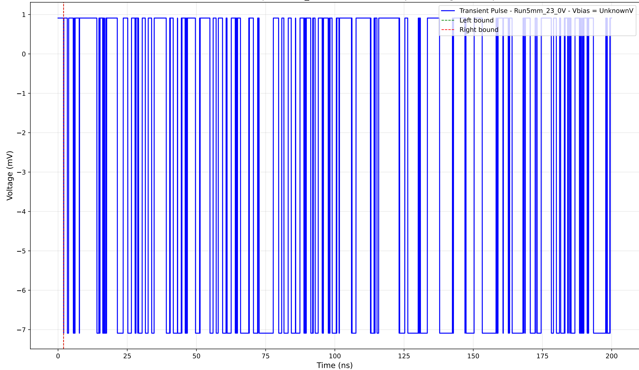
Transient Pulse - Sample: 5mm_23 - Position: 2285.0 \mu\text{m} - Charge: -0.00 pC
