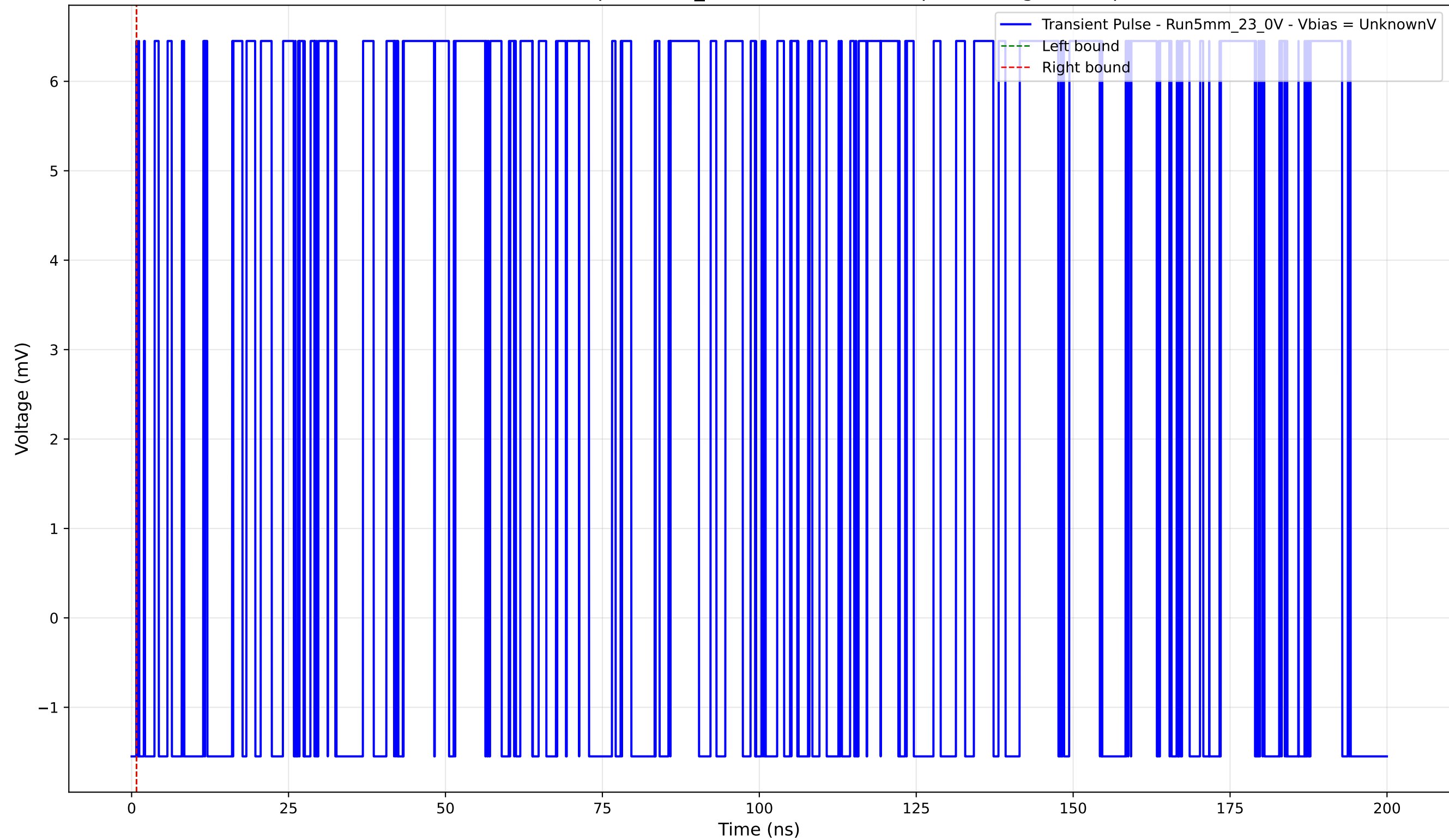
Transient Pulse - Sample: 5mm_23 - Position: 2070.0 \mu\text{m} - Charge: 0.00 pC
