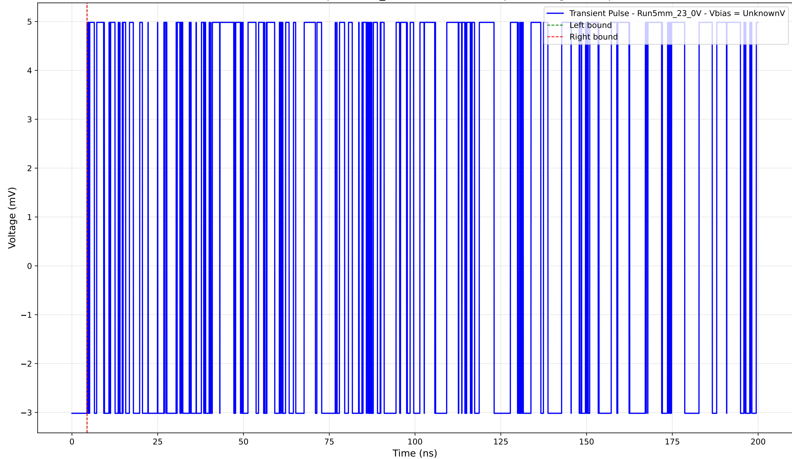
Transient Pulse - Sample: 5mm_23 - Position: 1365.0 \mu\text{m} - Charge: 0.00 pC
