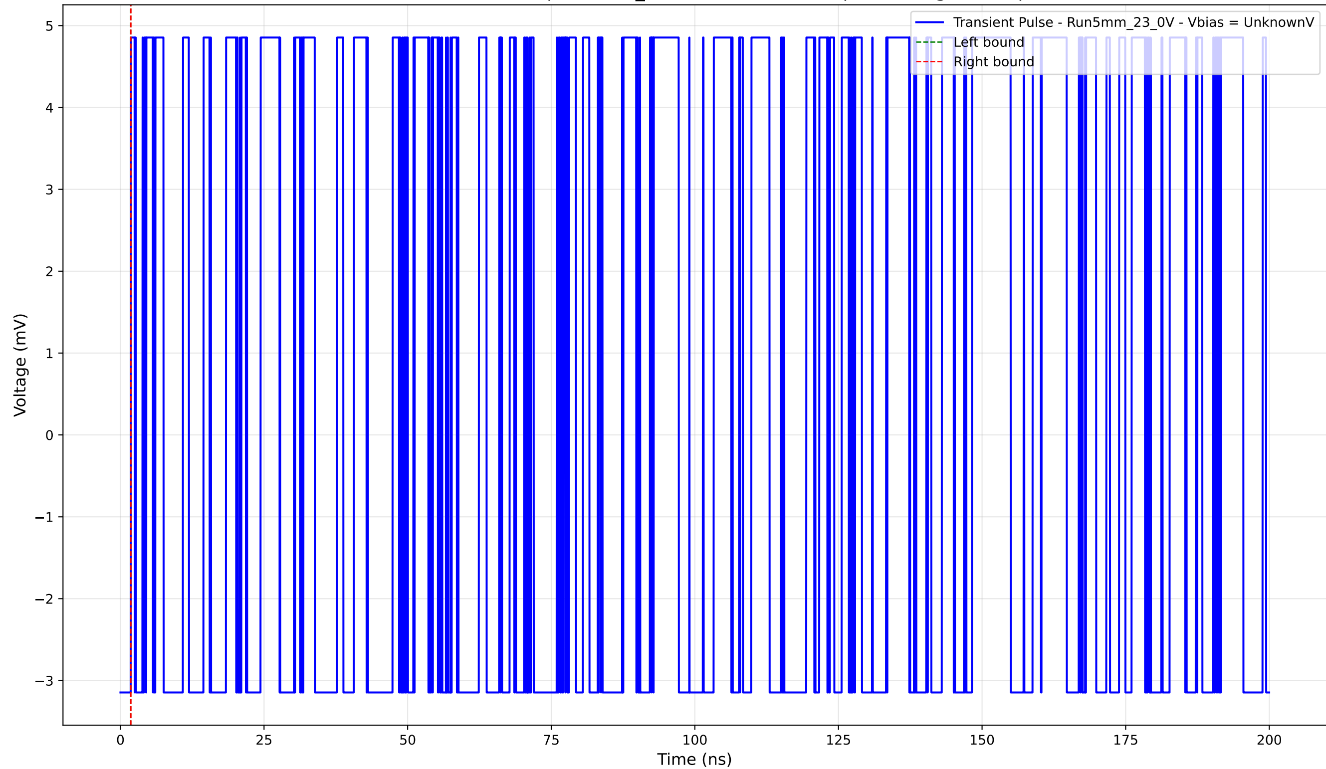
Transient Pulse - Sample: 5mm_23 - Position: 4665.0 \mu\text{m} - Charge: 0.00 pC
