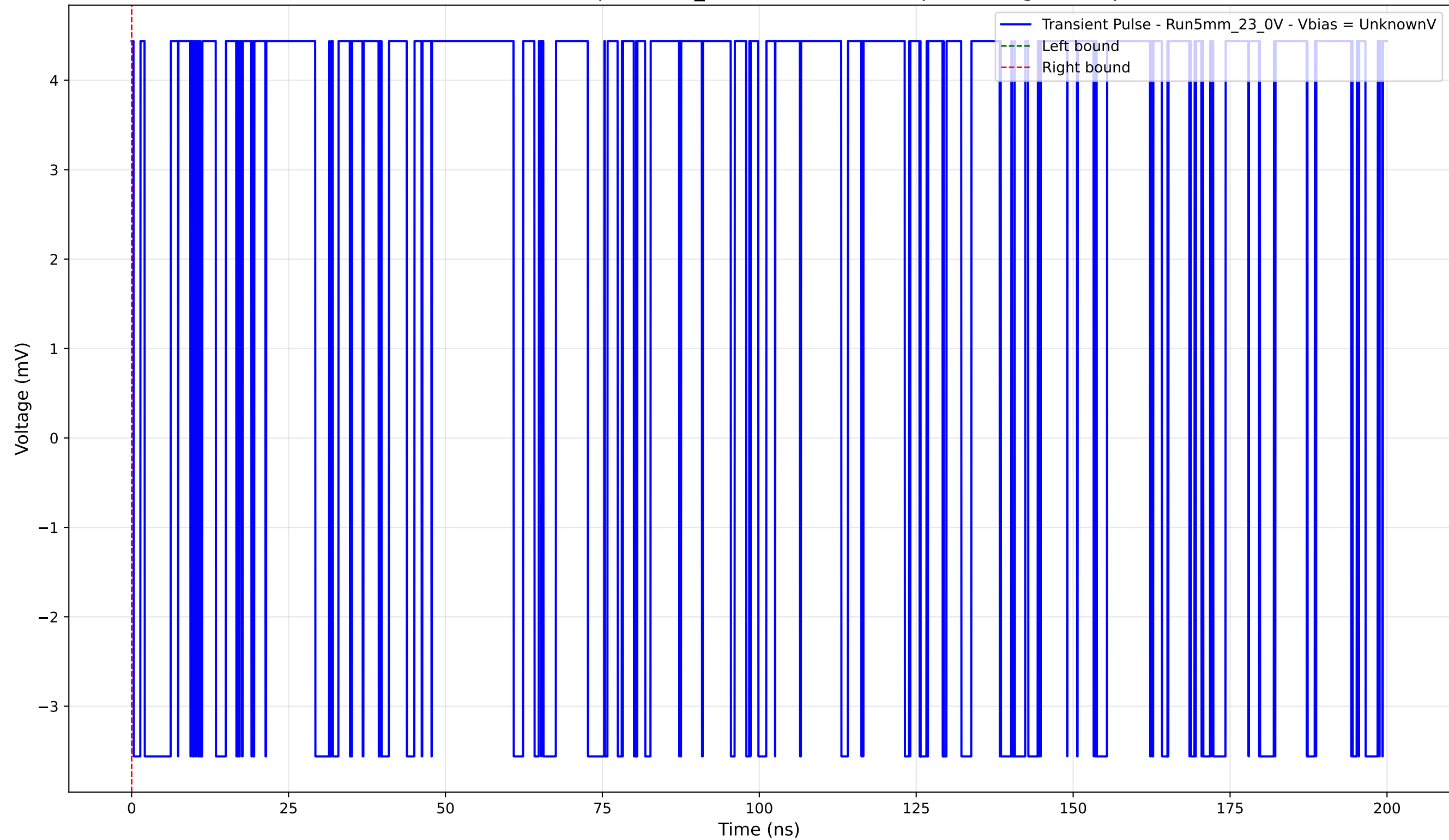
Transient Pulse - Sample: 5mm_23 - Position: 3075.0 \mu\text{m} - Charge: 0.00 pC
