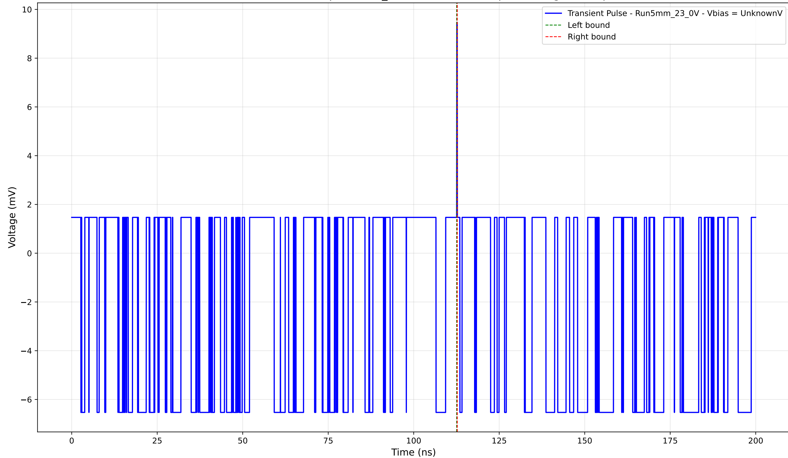
Transient Pulse - Sample: 5mm_23 - Position: 425.0 \mu\text{m} - Charge: 0.03 pC
