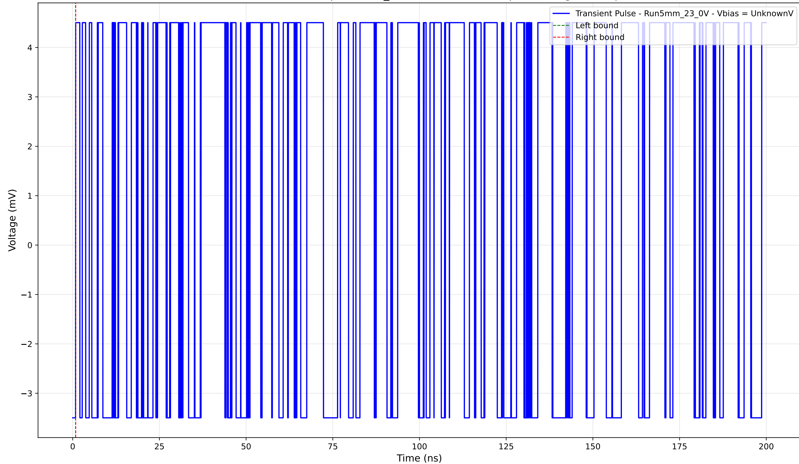
Transient Pulse - Sample: 5mm_23 - Position: 3240.0 \mu\text{m} - Charge: 0.00 pC
