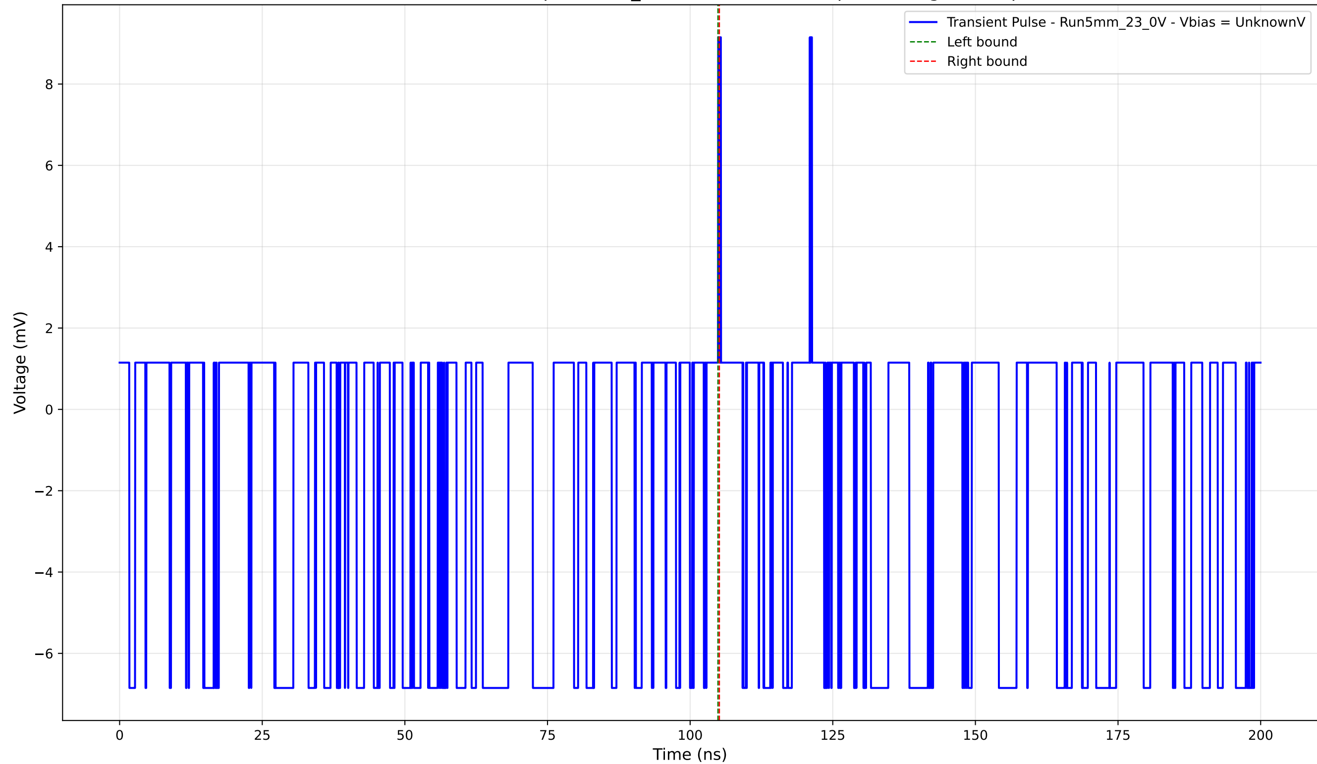
Transient Pulse - Sample: 5mm_23 - Position: 2580.0 \mu\text{m} - Charge: 0.04 pC
