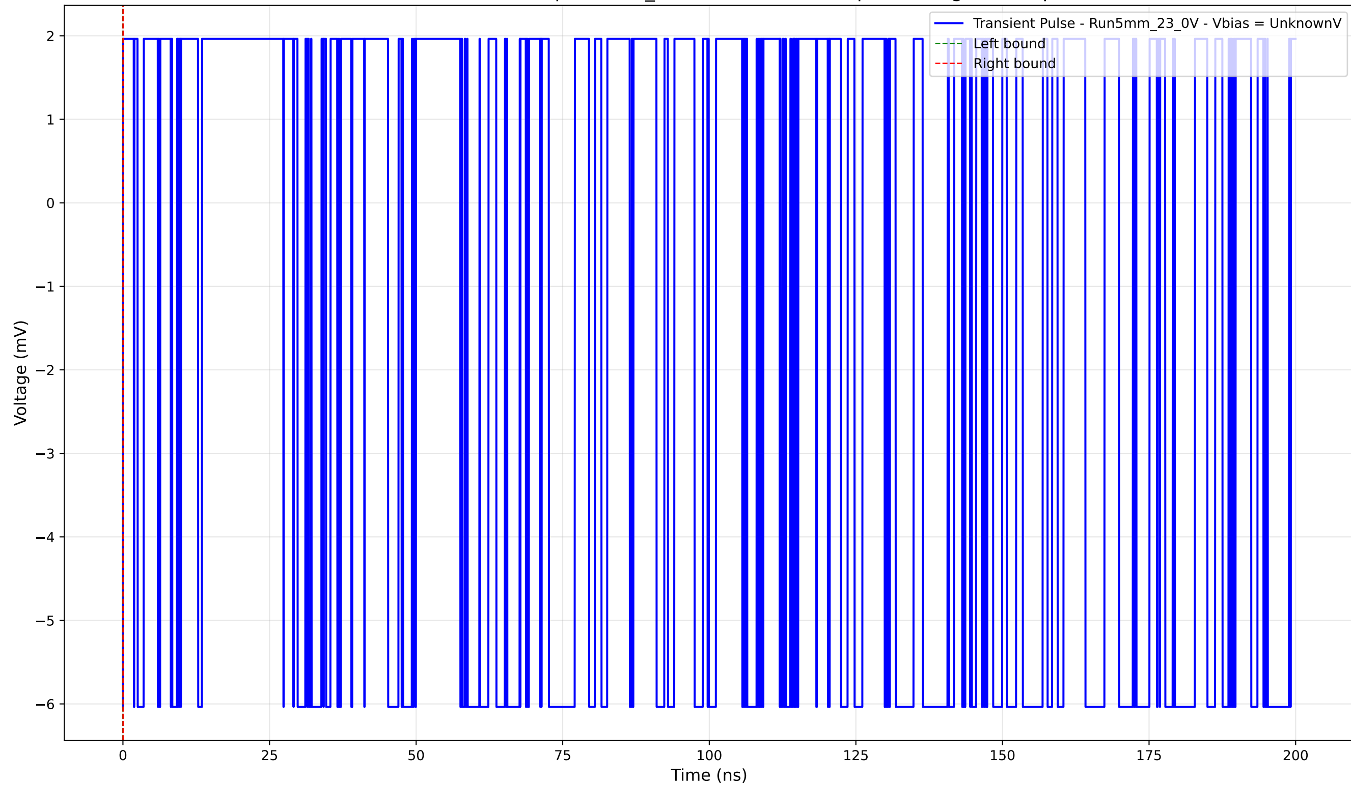
Transient Pulse - Sample: 5mm_23 - Position: 2055.0 \mu\text{m} - Charge: -0.00 pC
