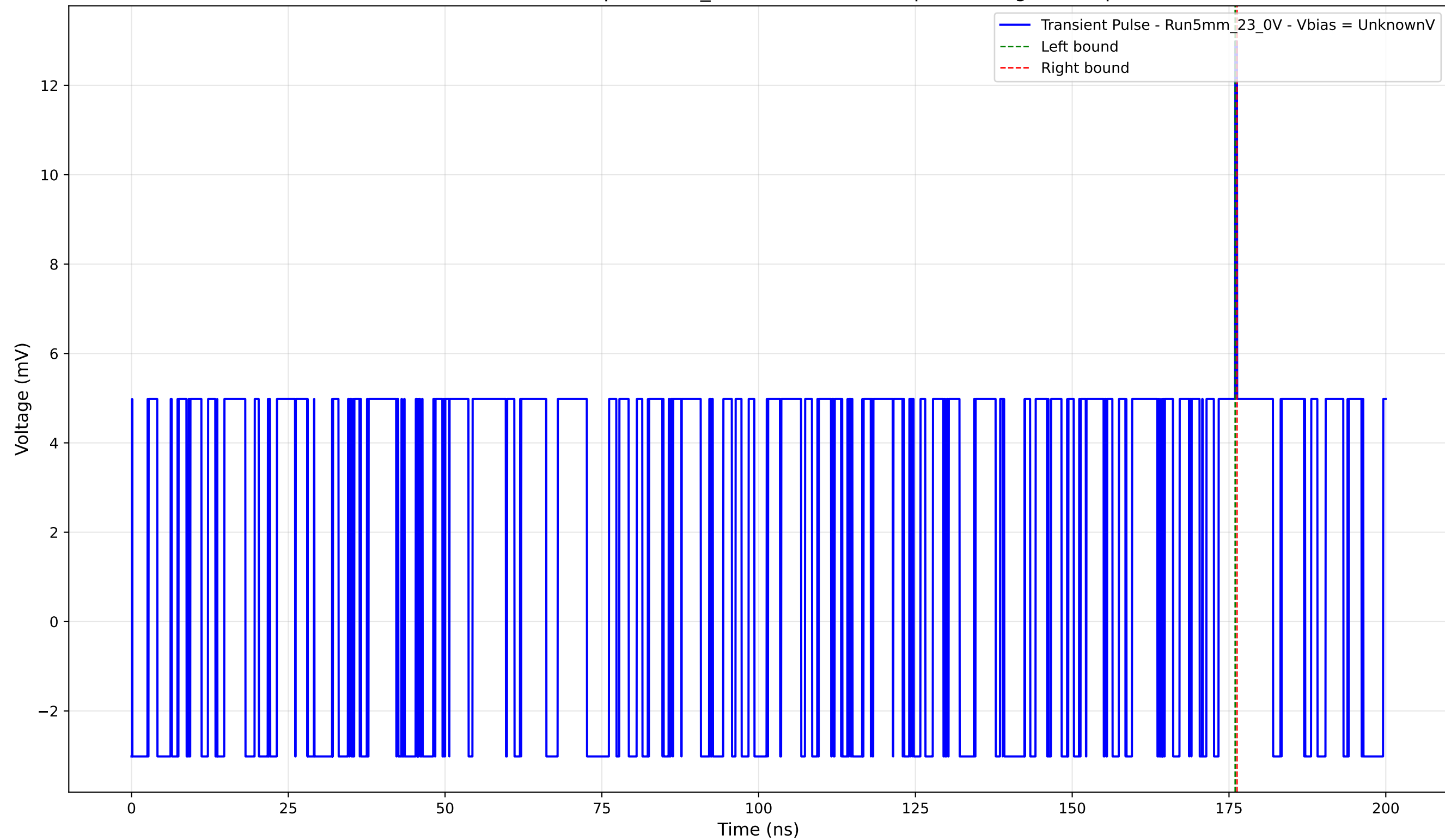
Transient Pulse - Sample: 5mm_23 - Position: 940.0 \mu\text{m} - Charge: 0.07 pC
