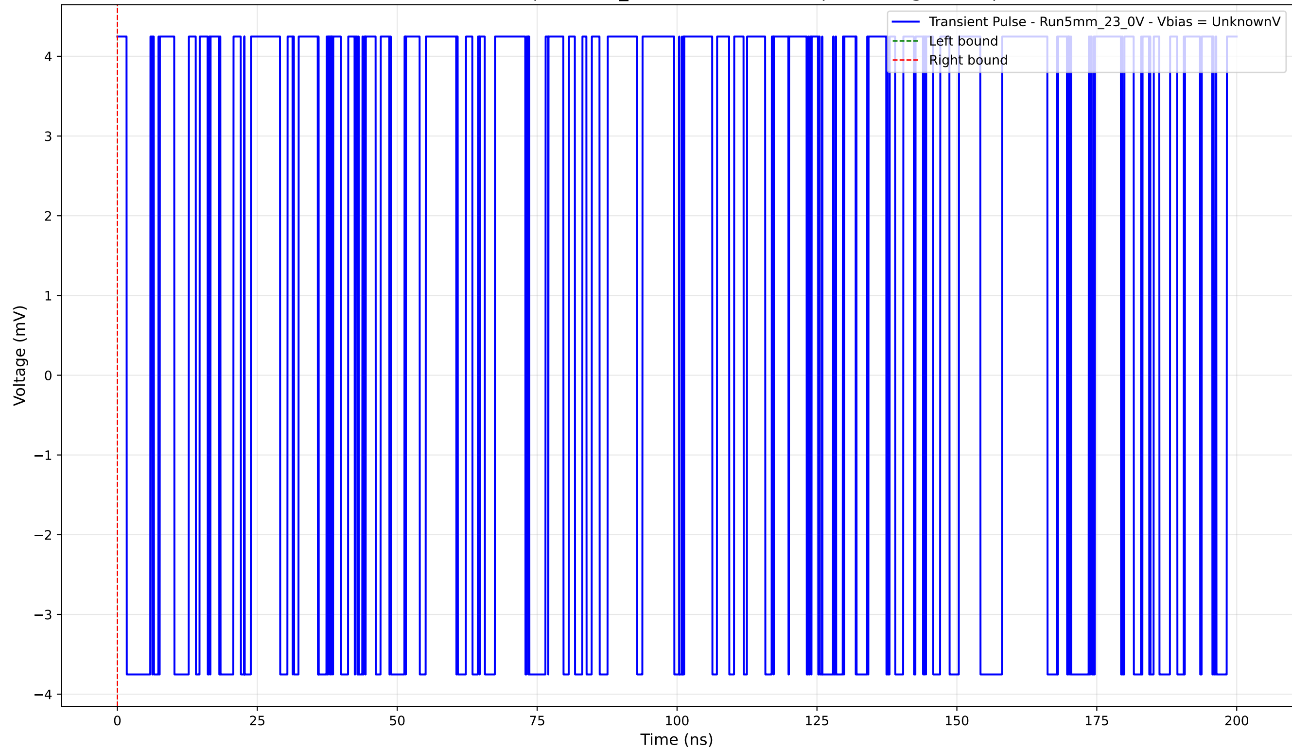
Transient Pulse - Sample: 5mm_23 - Position: 3845.0 \mu\text{m} - Charge: 0.00 pC
