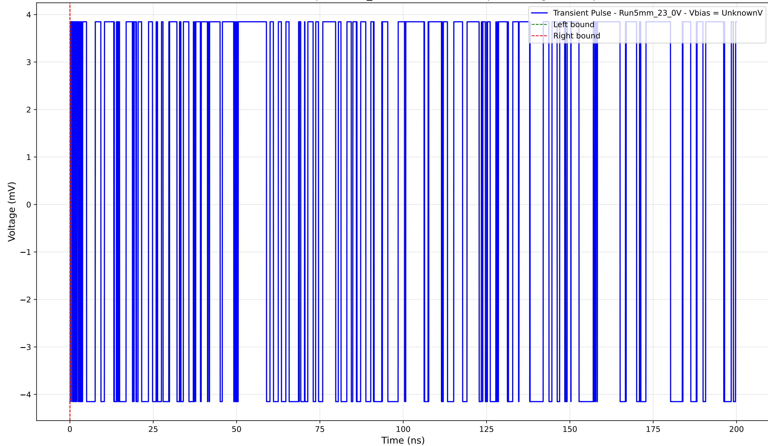
Transient Pulse - Sample: 5mm_23 - Position: 1890.0 \mu\text{m} - Charge: -0.00 pC
