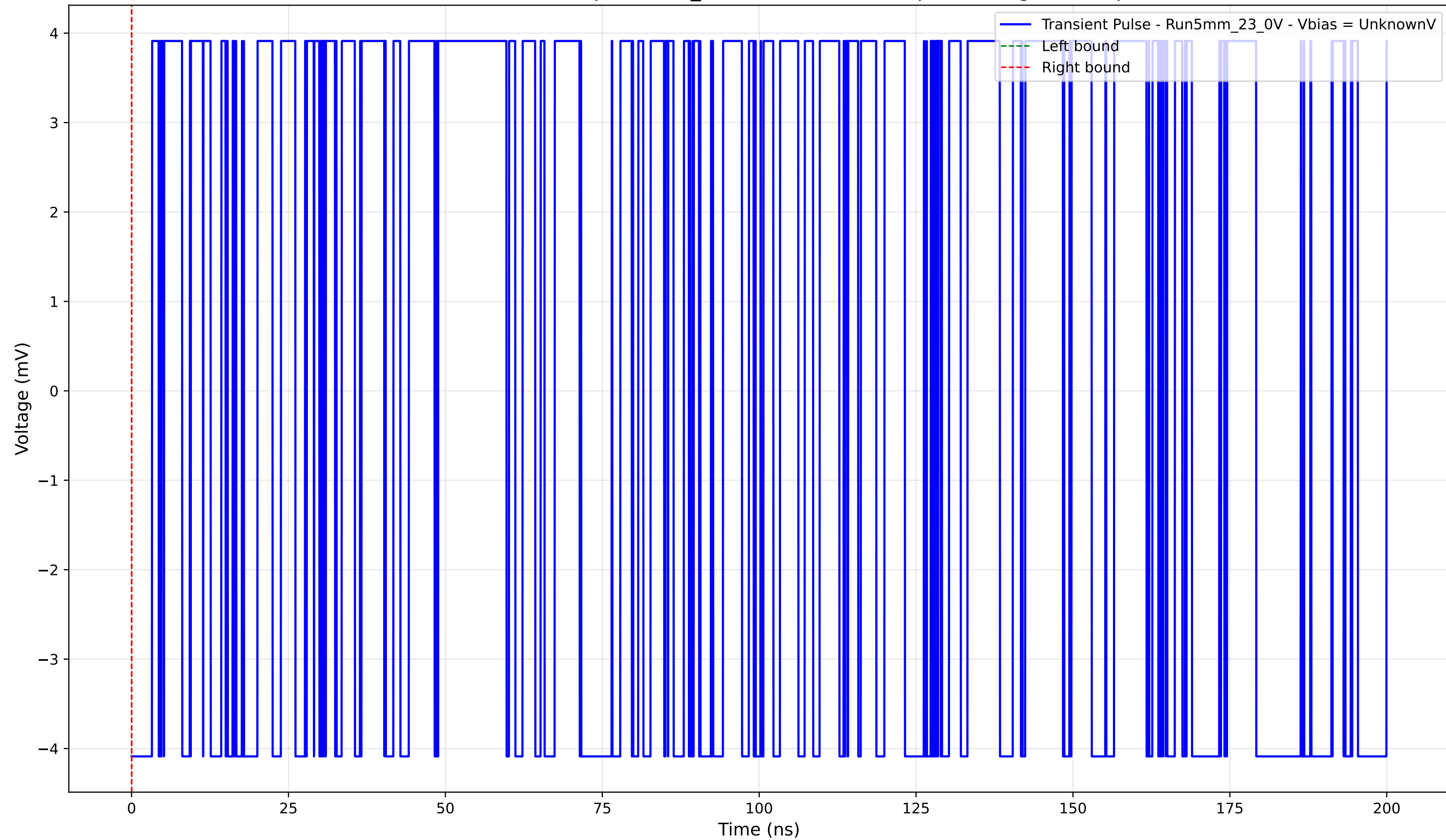
Transient Pulse - Sample: 5mm_23 - Position: 4510.0 \mu\text{m} - Charge: -0.00 pC
