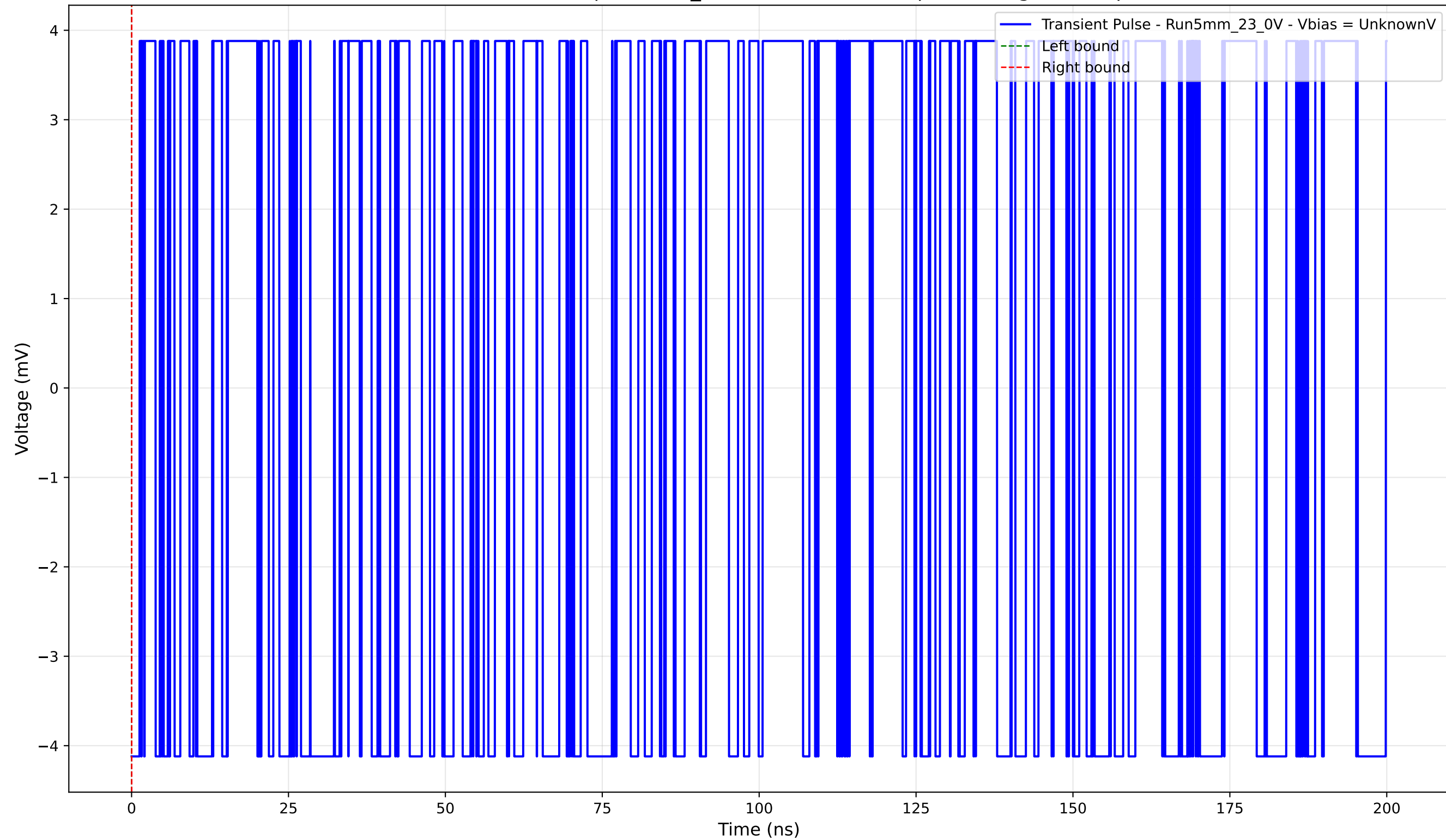
Transient Pulse - Sample: 5mm_23 - Position: 4595.0 \mu\text{m} - Charge: -0.00 pC
