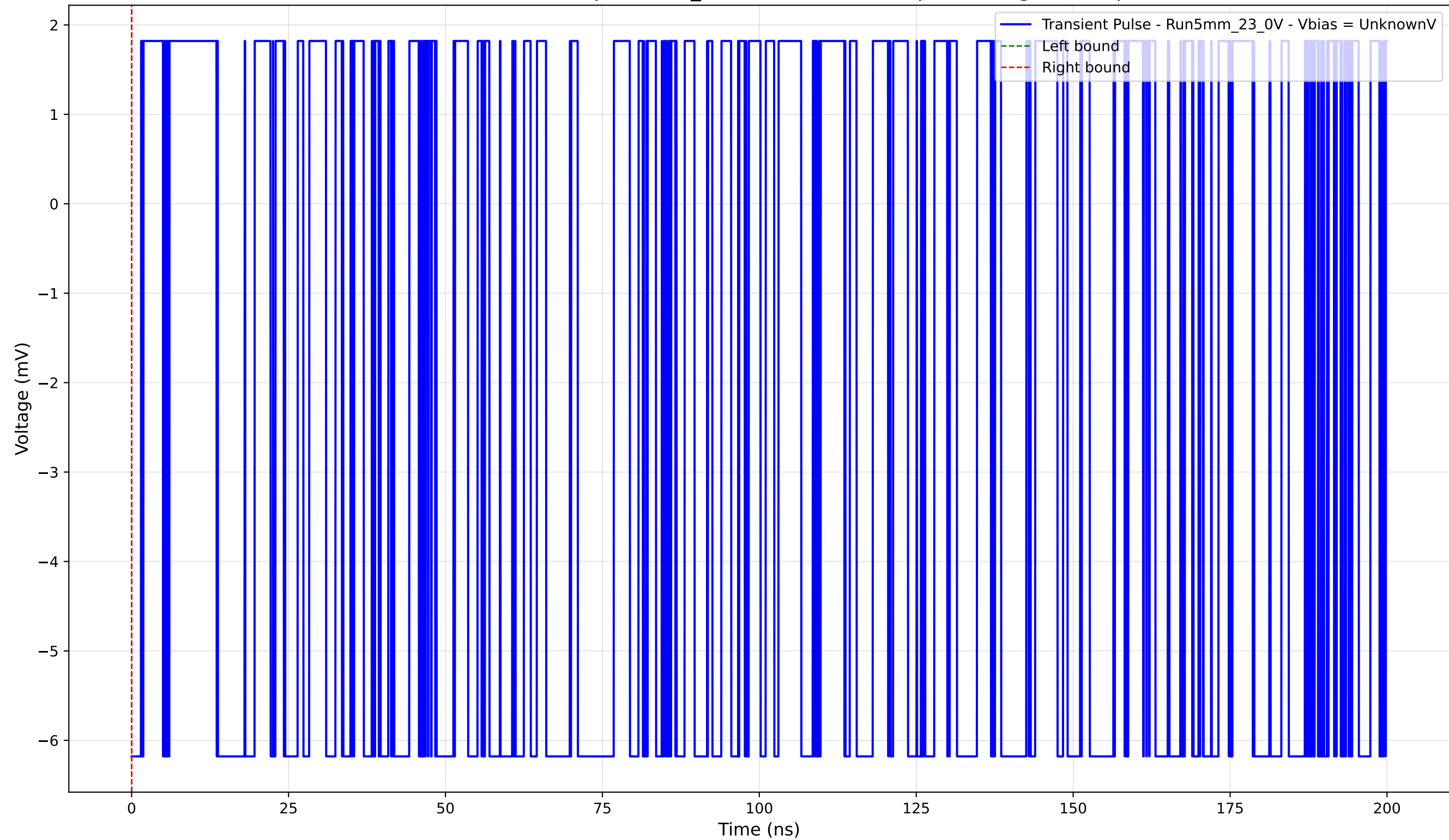
Transient Pulse - Sample: 5mm_23 - Position: 1685.0 \mu\text{m} - Charge: -0.00 pC
