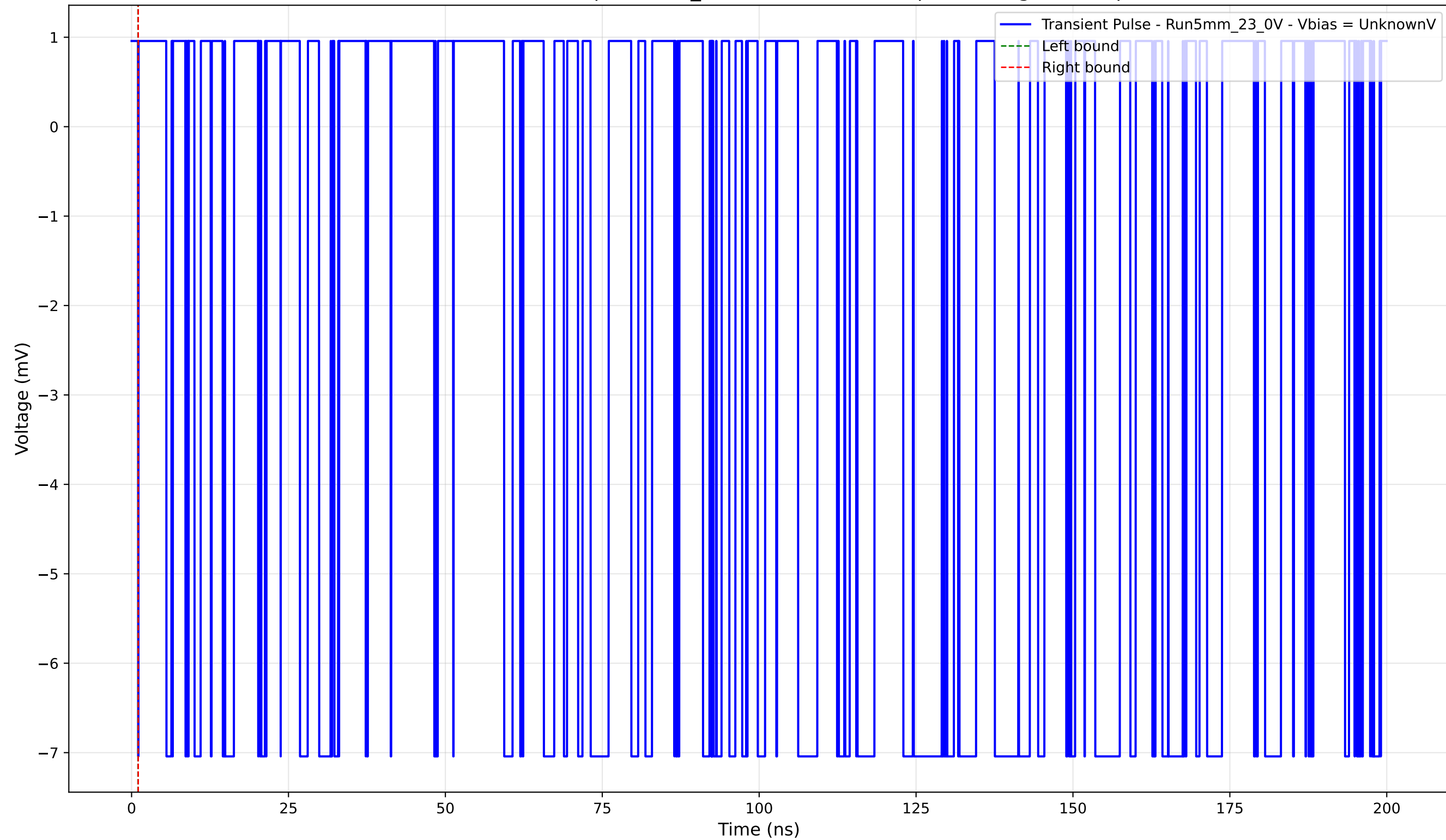
Transient Pulse - Sample: 5mm_23 - Position: 3820.0 \mu\text{m} - Charge: -0.00 pC
