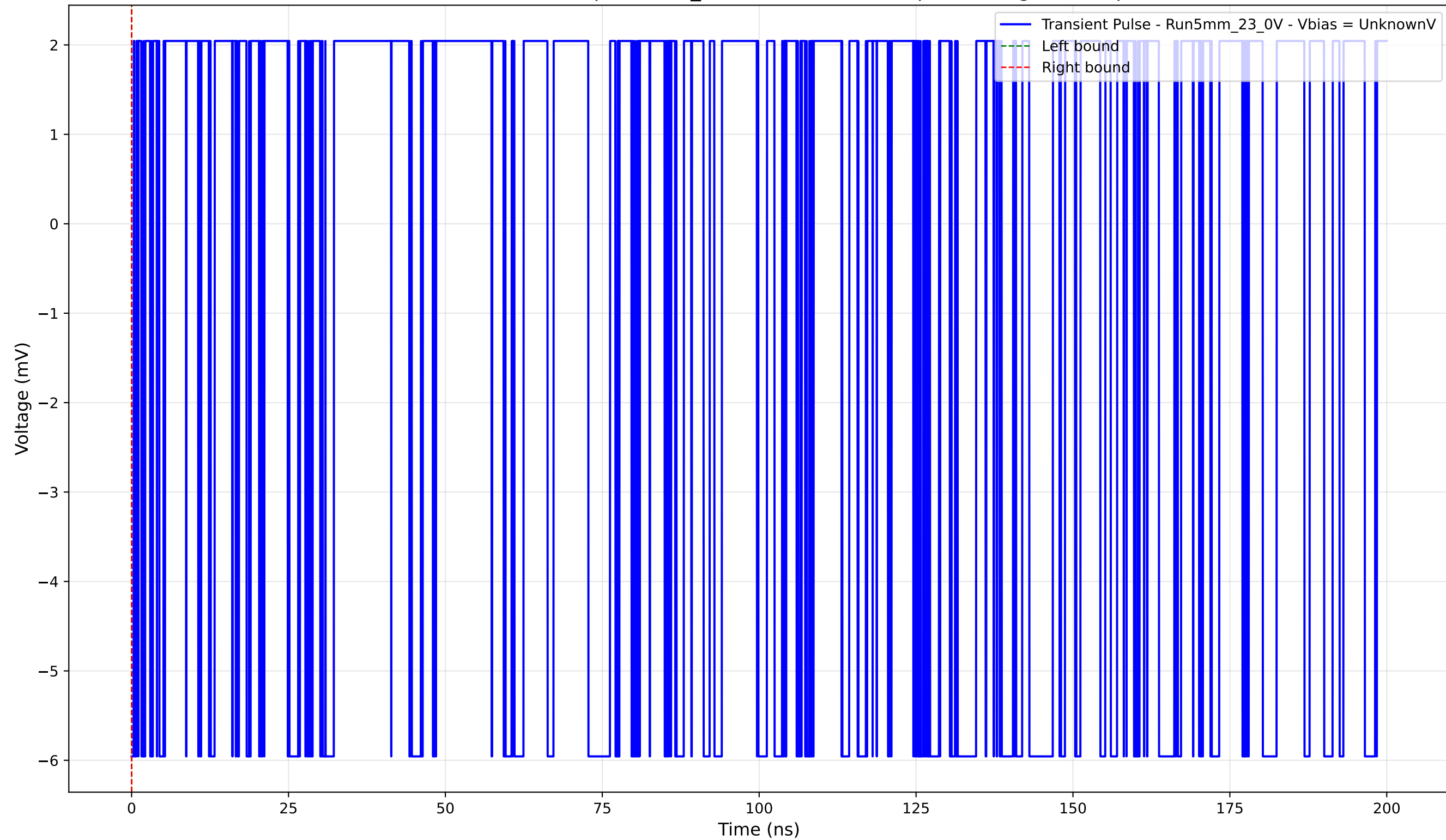
Transient Pulse - Sample: 5mm_23 - Position: 4210.0 \mu\text{m} - Charge: -0.00 pC
