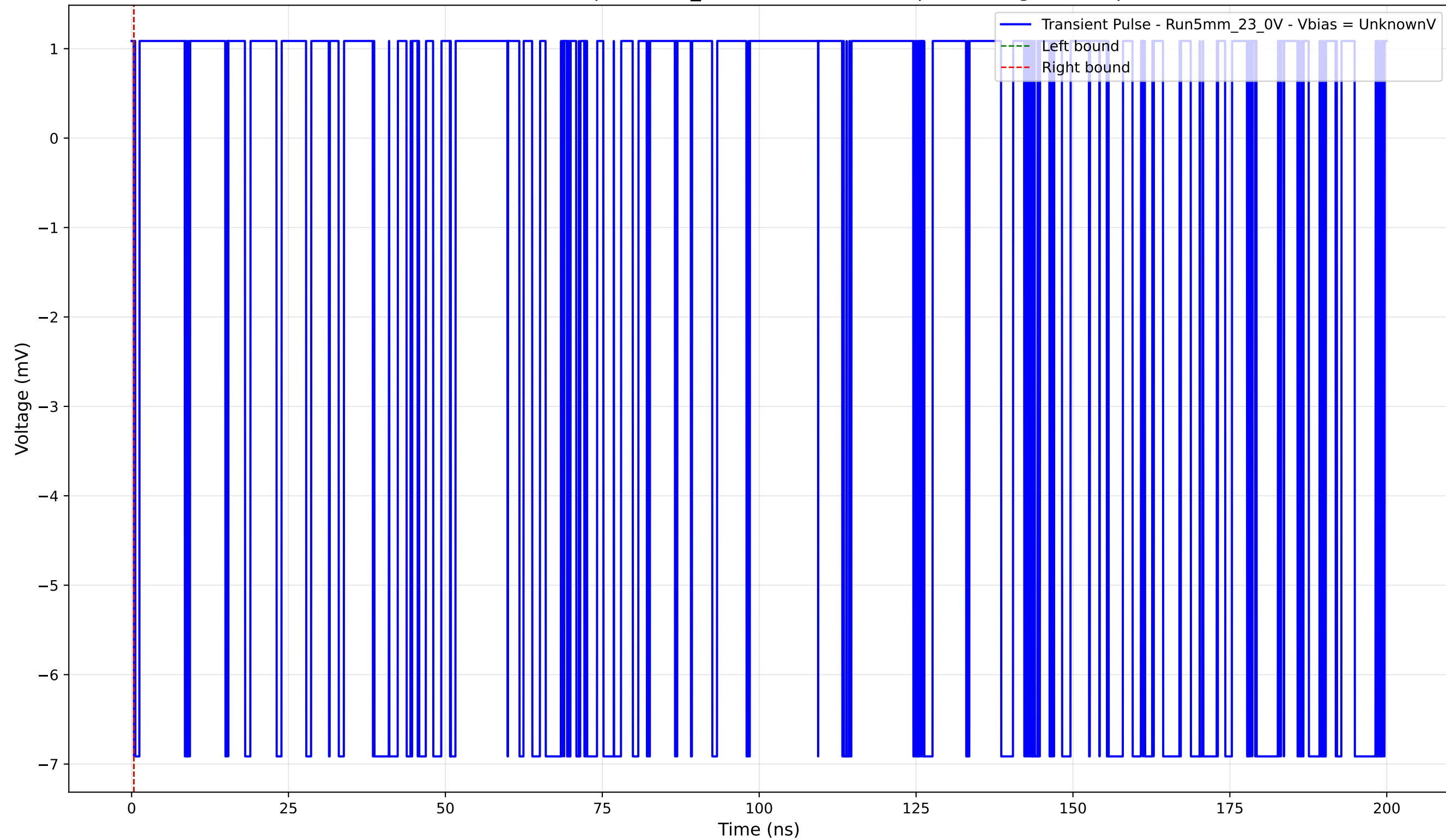
Transient Pulse - Sample: 5mm_23 - Position: 3795.0 \mu\text{m} - Charge: -0.00 pC
