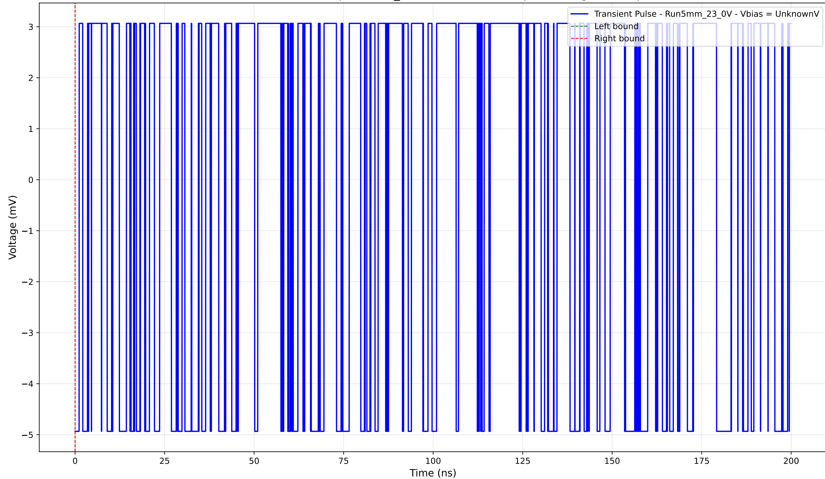
Transient Pulse - Sample: 5mm_23 - Position: 1950.0 \mu\text{m} - Charge: -0.00 pC
