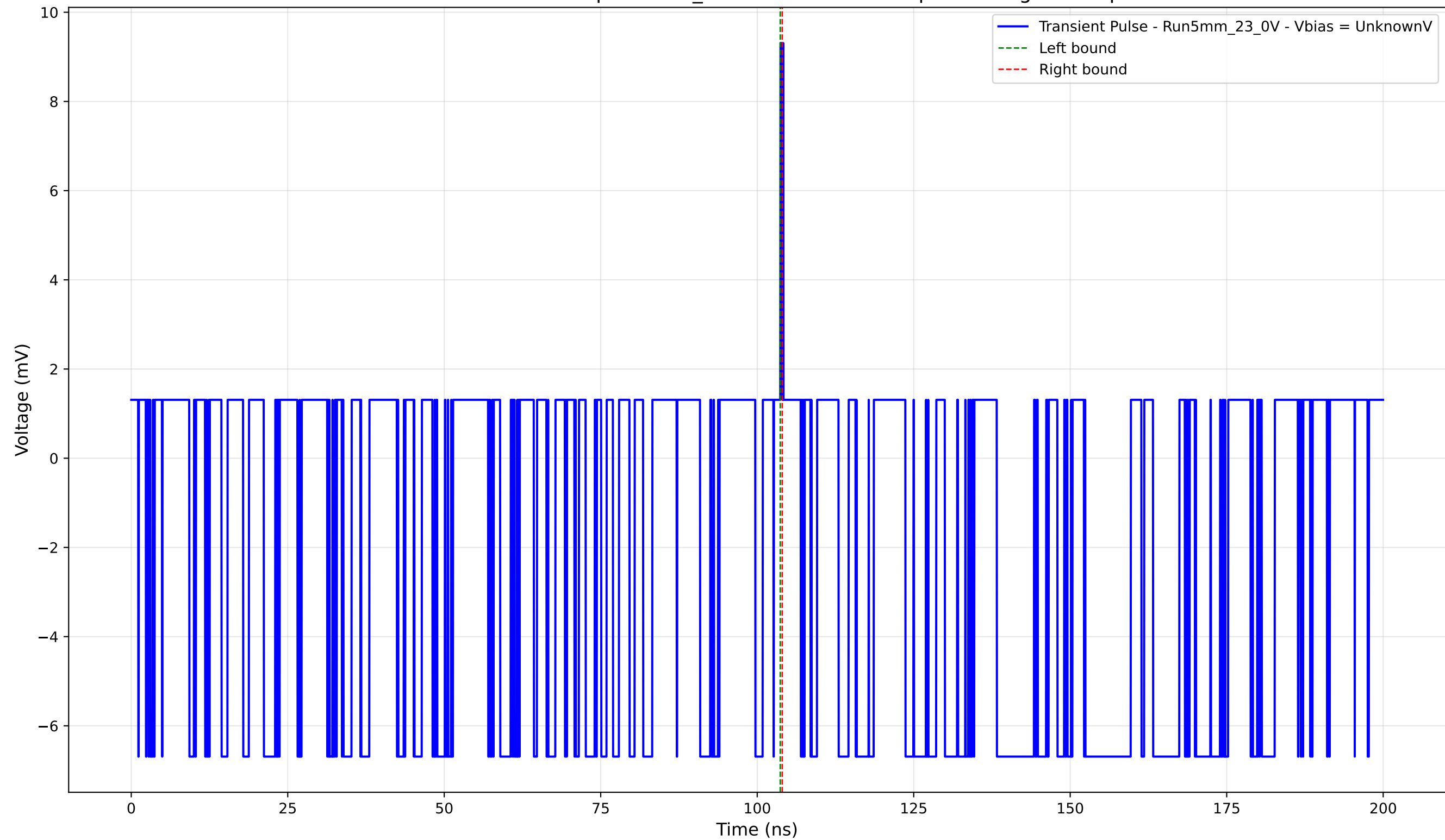
Transient Pulse - Sample: 5mm_23 - Position: 1300.0 \mu\text{m} - Charge: 0.06 pC
