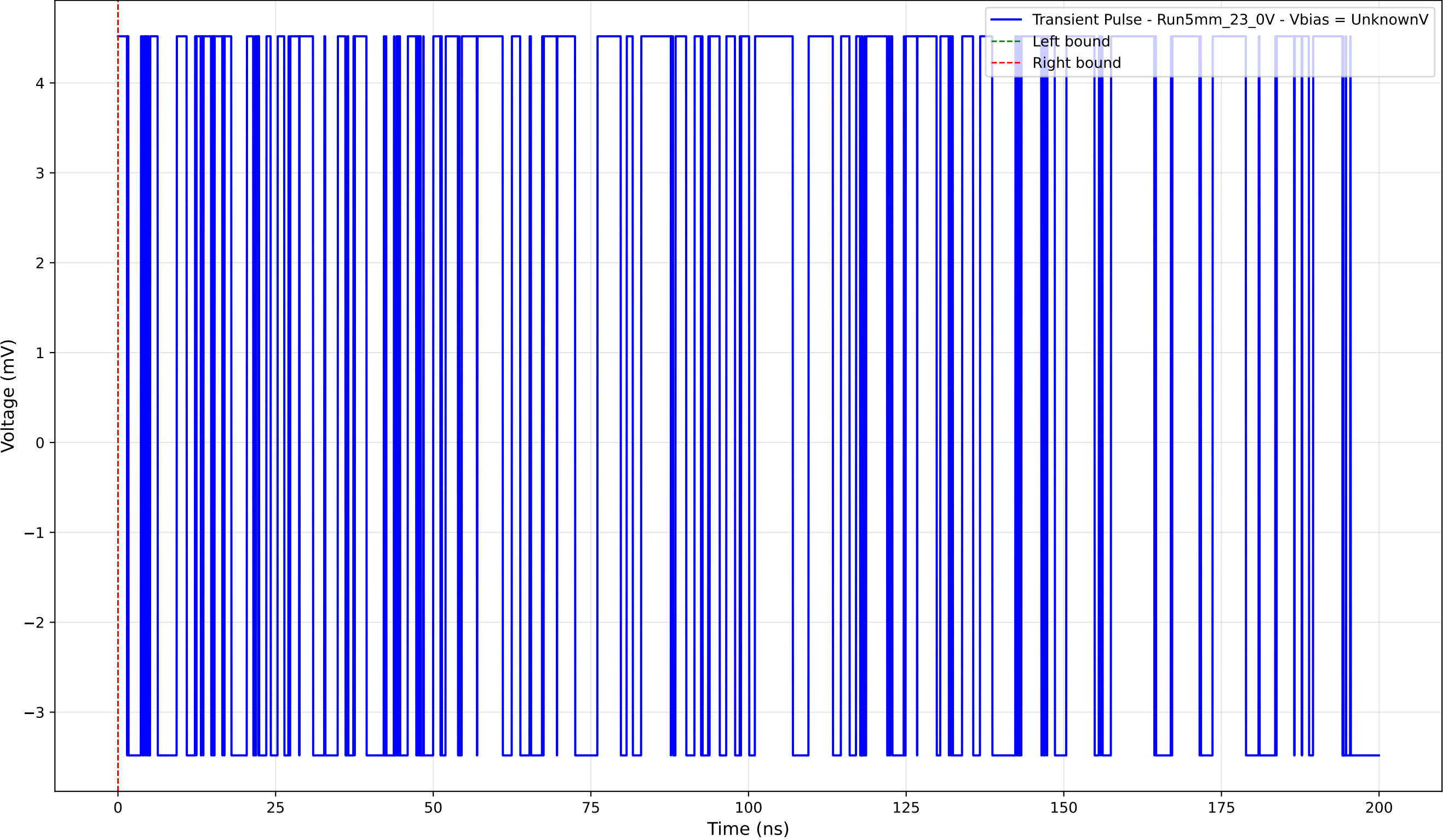
Transient Pulse - Sample: 5mm_23 - Position: 660.0 \mu\text{m} - Charge: 0.00 pC
