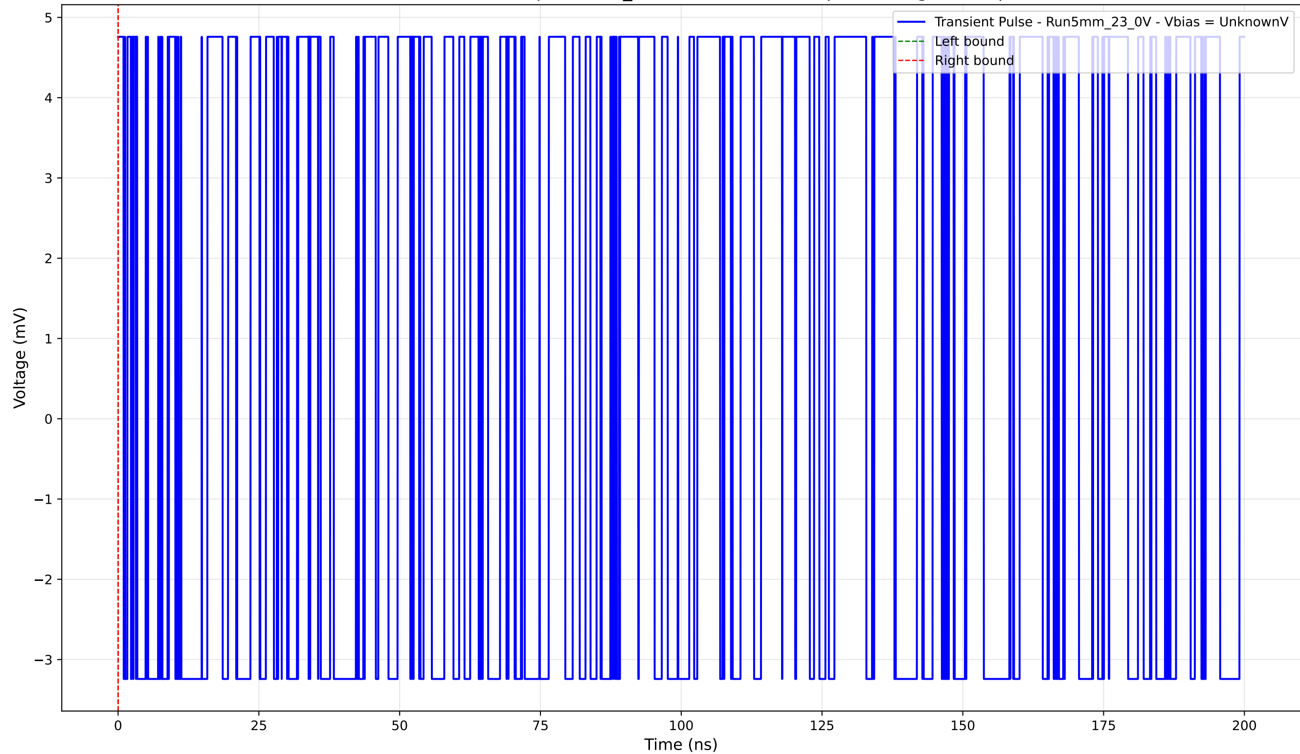
Transient Pulse - Sample: 5mm_23 - Position: 4445.0 \mu\text{m} - Charge: 0.00 pC
