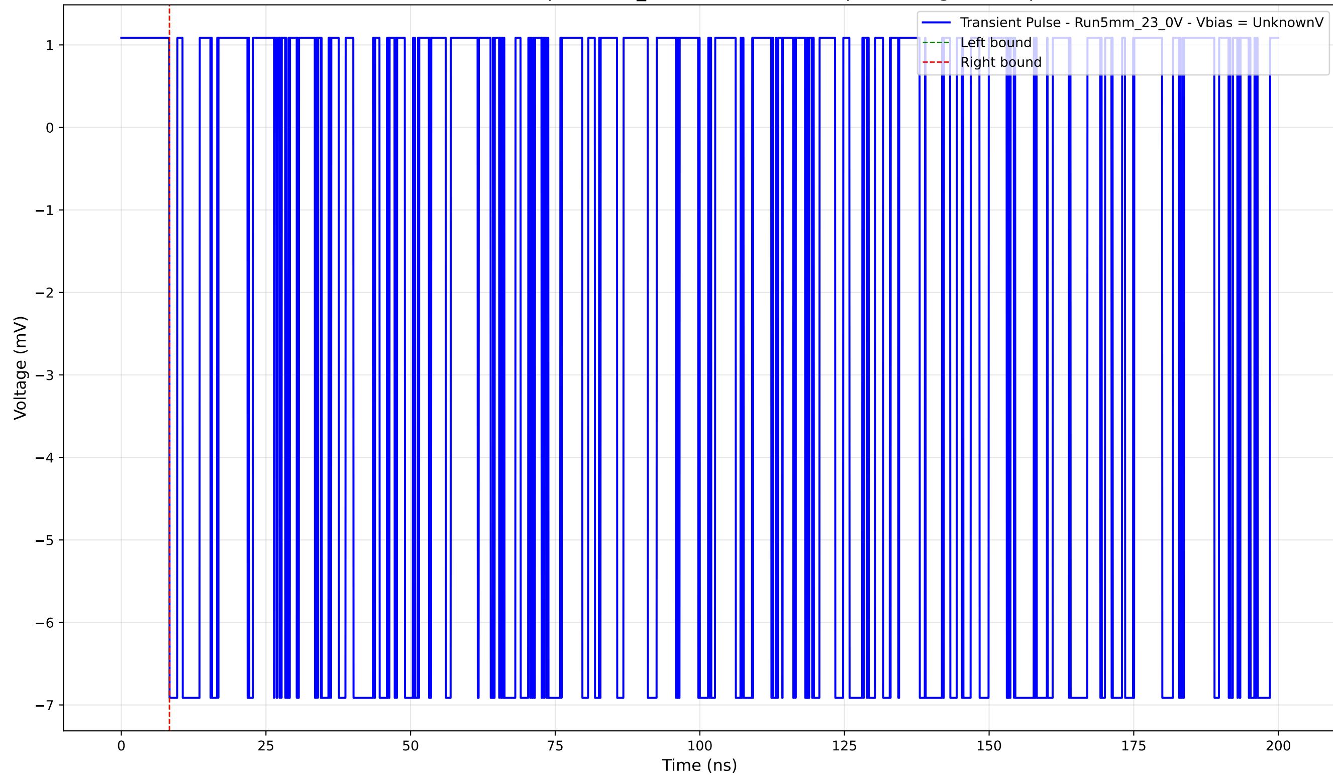
Transient Pulse - Sample: 5mm_23 - Position: 3785.0 \mu\text{m} - Charge: -0.00 pC
