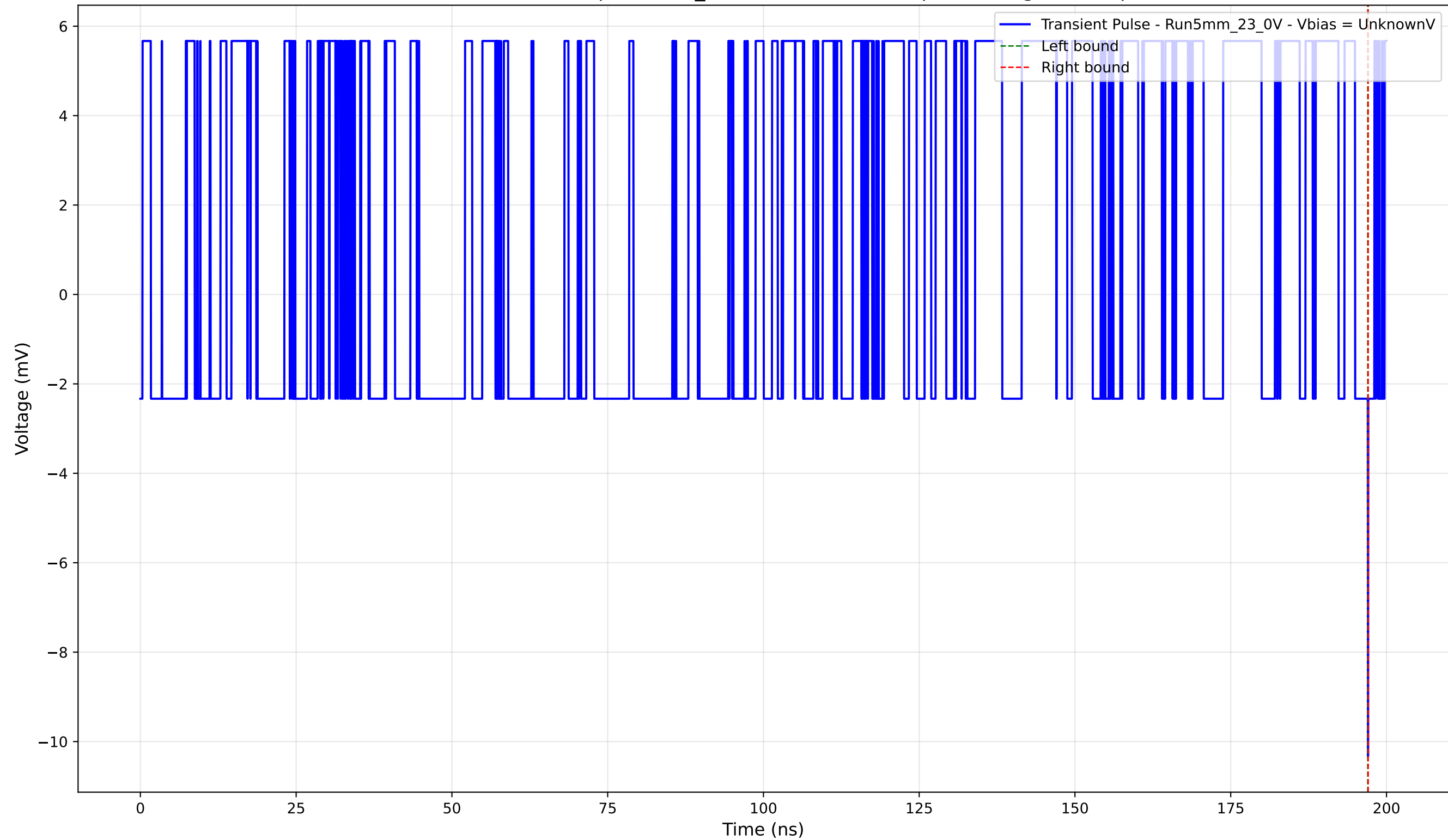
Transient Pulse - Sample: 5mm_23 - Position: 1450.0 \mu\text{m} - Charge: -0.01 pC
