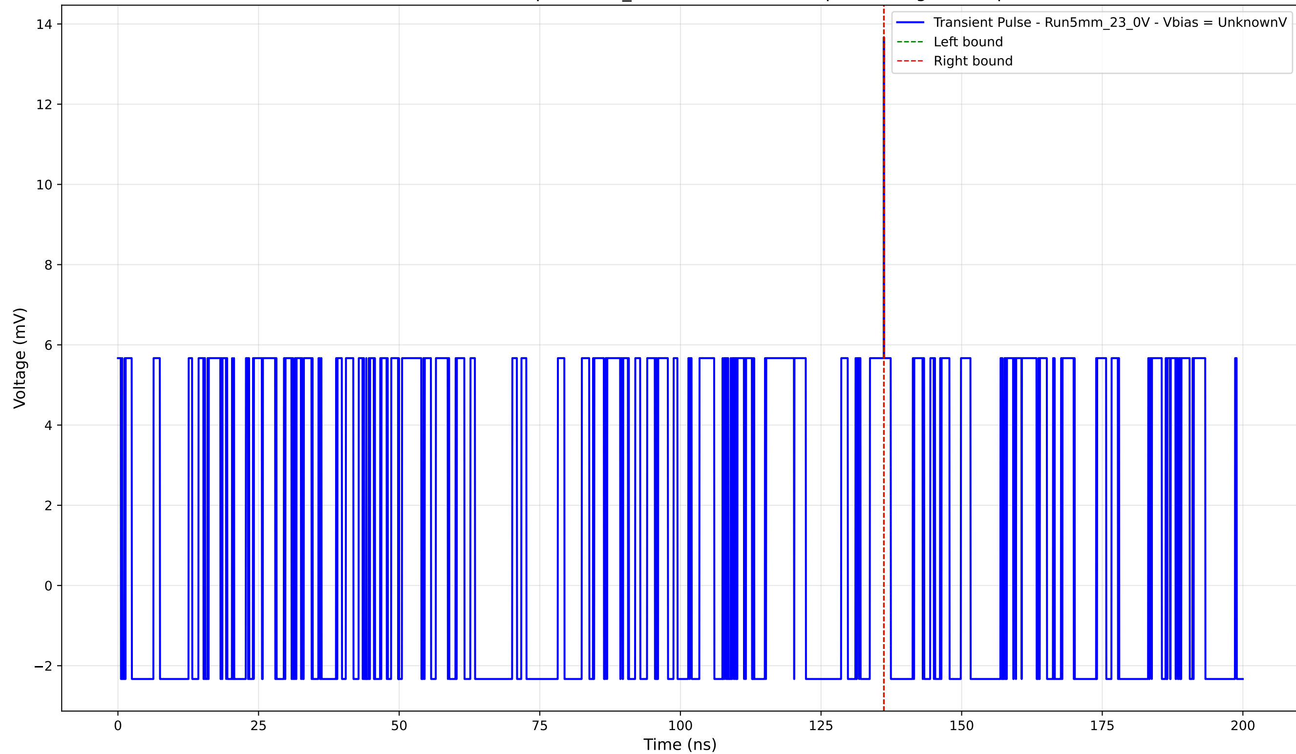
Transient Pulse - Sample: 5mm_23 - Position: 2040.0 \mu\text{m} - Charge: 0.01 pC
