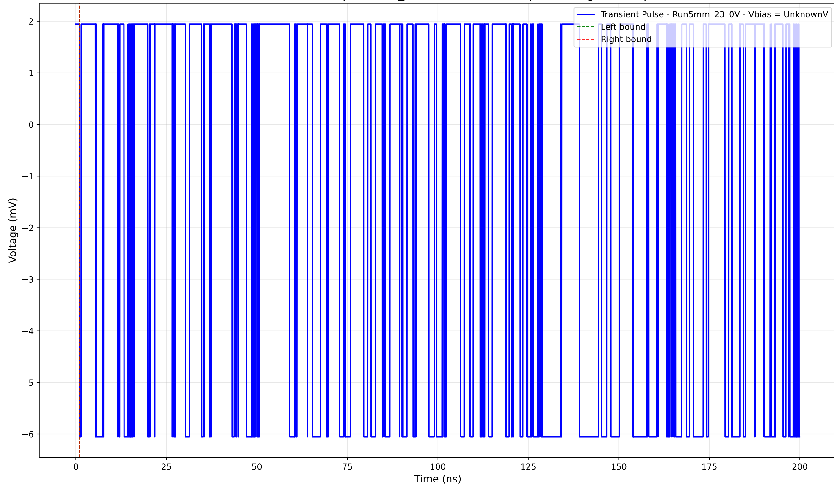
Transient Pulse - Sample: 5mm_23 - Position: 2690.0 \mu\text{m} - Charge: -0.00 pC
