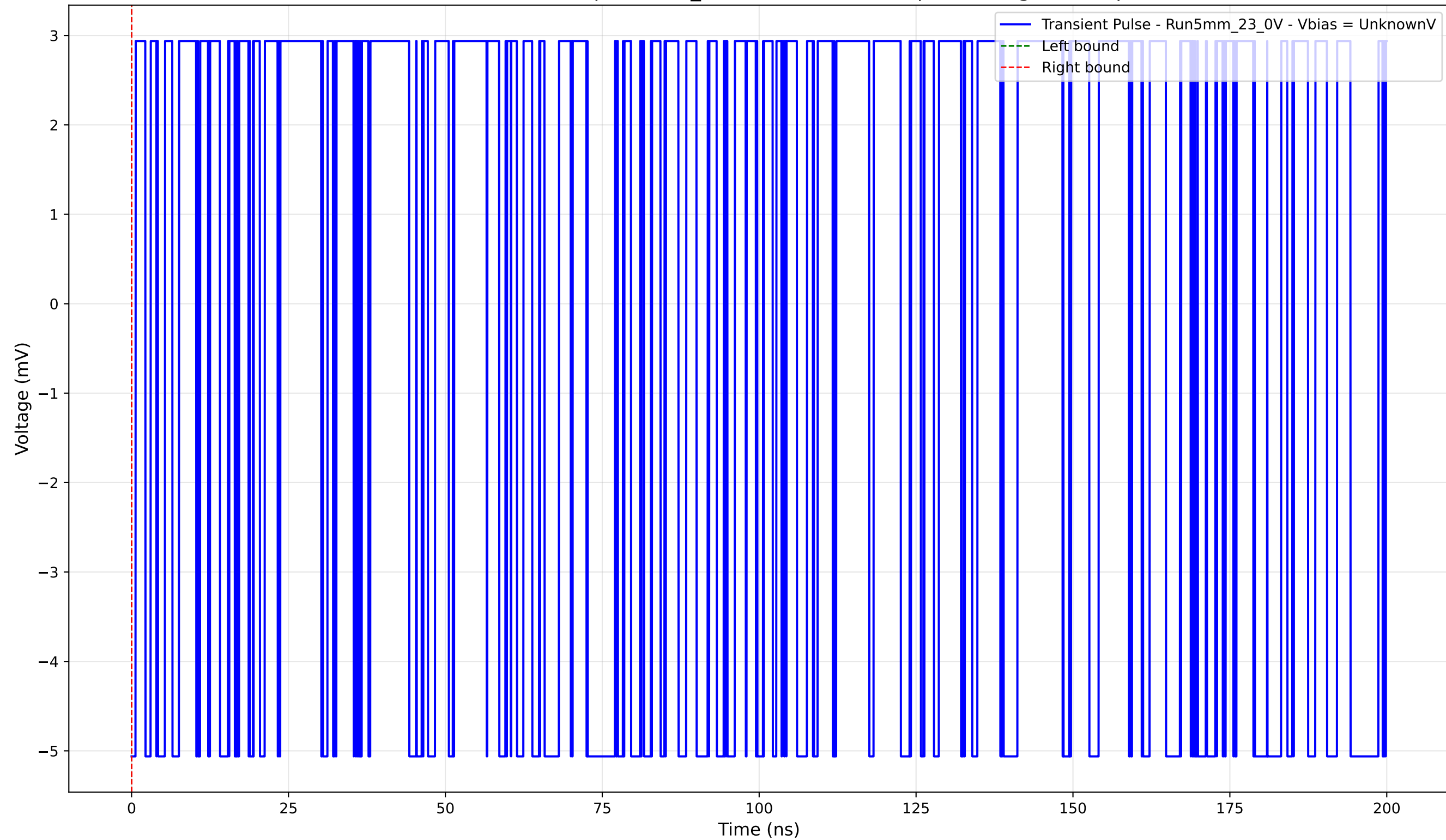
Transient Pulse - Sample: 5mm_23 - Position: 2640.0 \mu\text{m} - Charge: -0.00 pC
