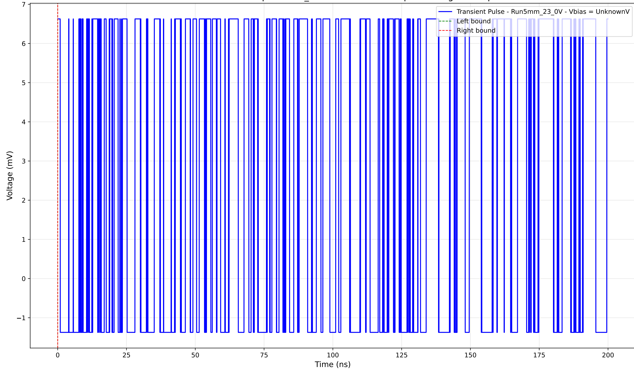
Transient Pulse - Sample: 5mm_23 - Position: 1780.0 \mu\text{m} - Charge: 0.00 pC
