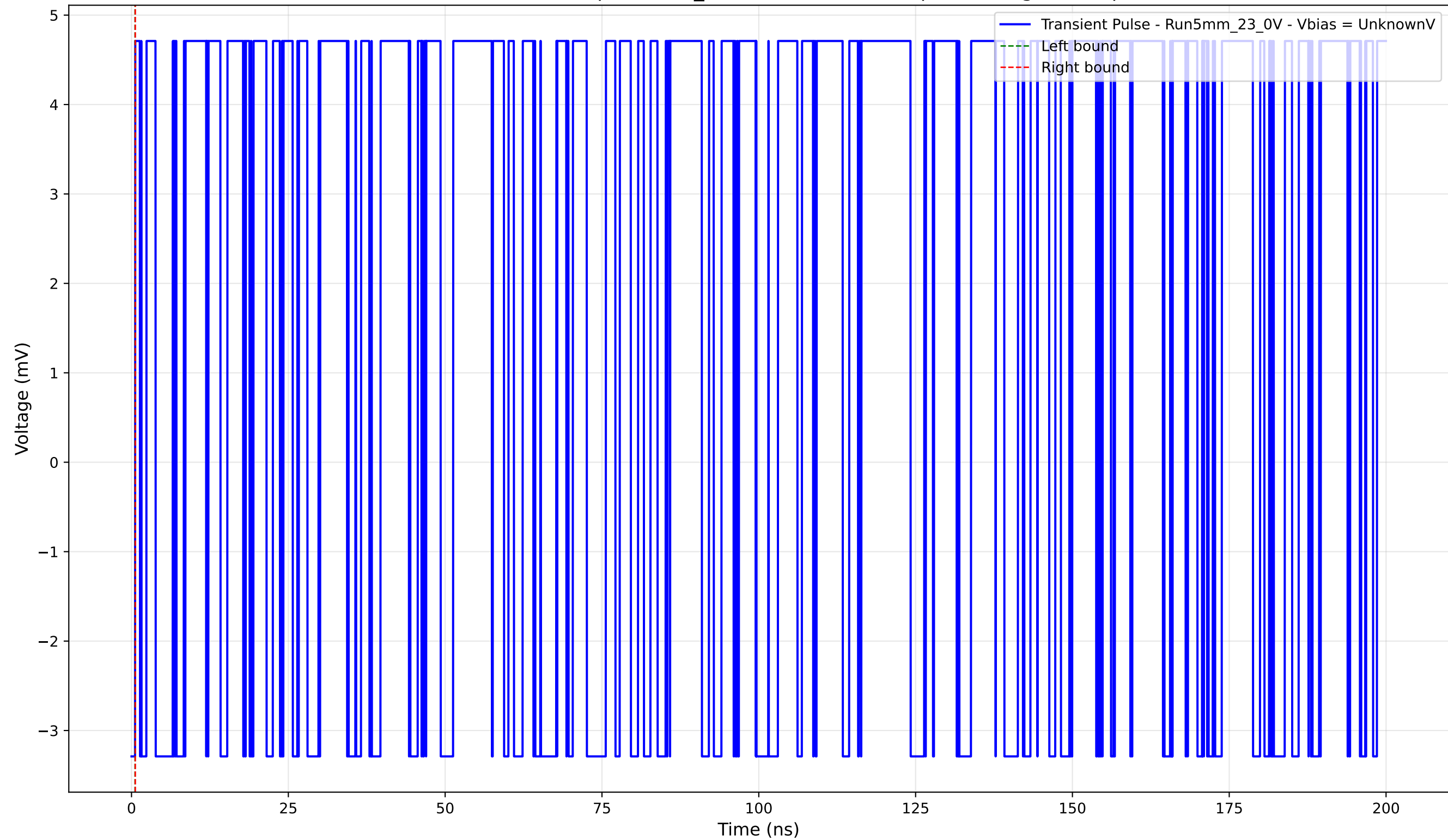
Transient Pulse - Sample: 5mm_23 - Position: 2770.0 \mu\text{m} - Charge: 0.00 pC
