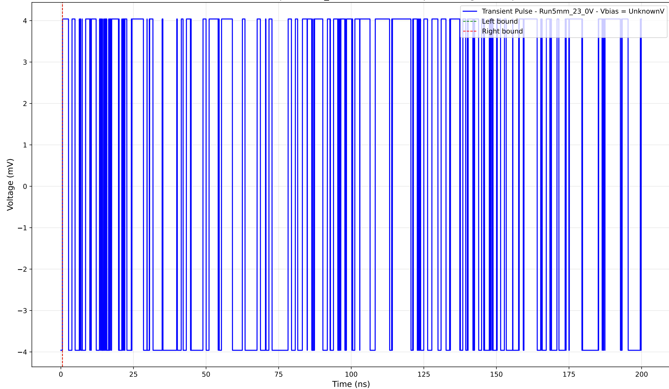
Transient Pulse - Sample: 5mm_23 - Position: 550.0 \mu\text{m} - Charge: 0.00 pC
