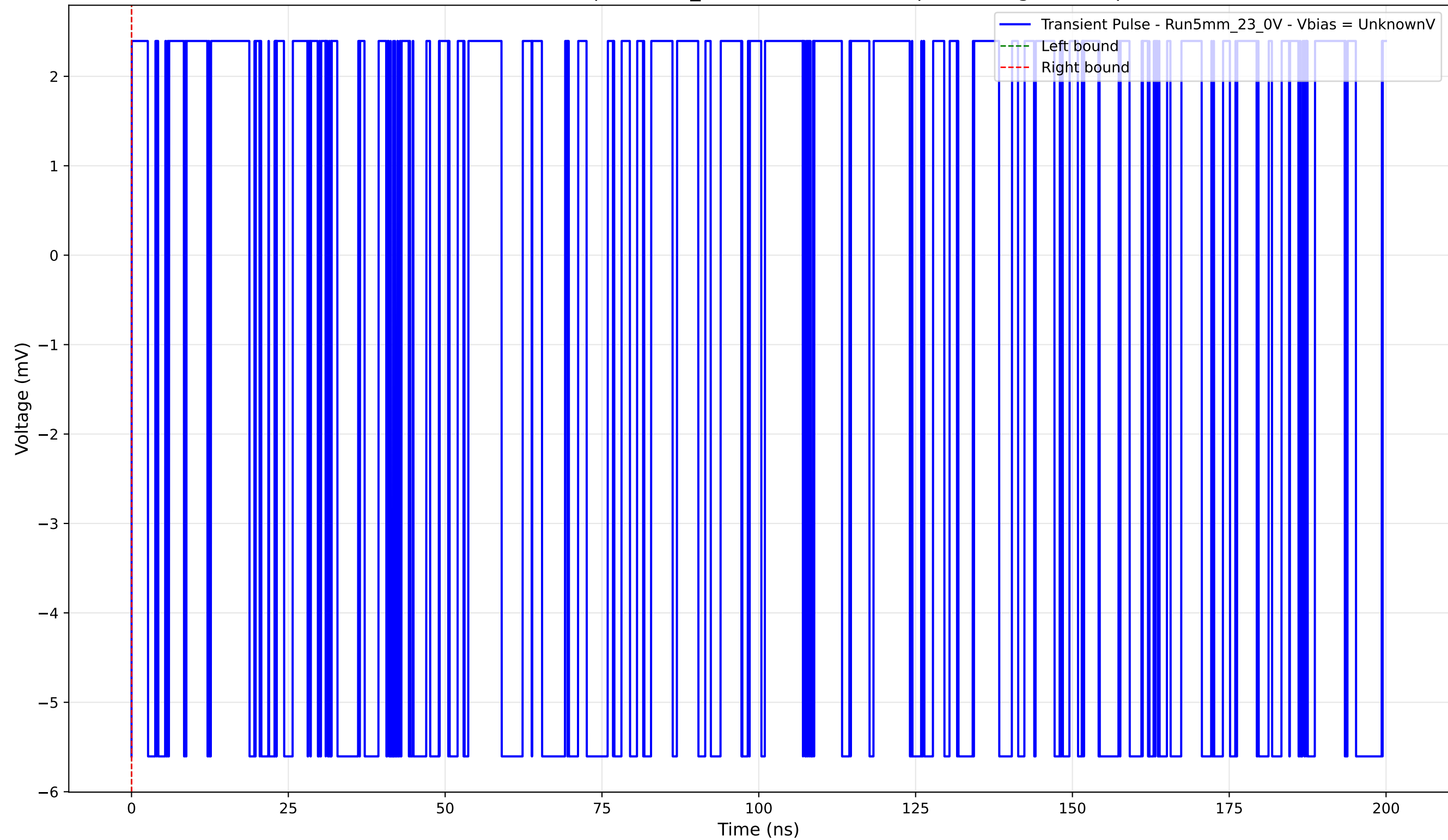
Transient Pulse - Sample: 5mm_23 - Position: 2855.0 \mu\text{m} - Charge: -0.00 pC
