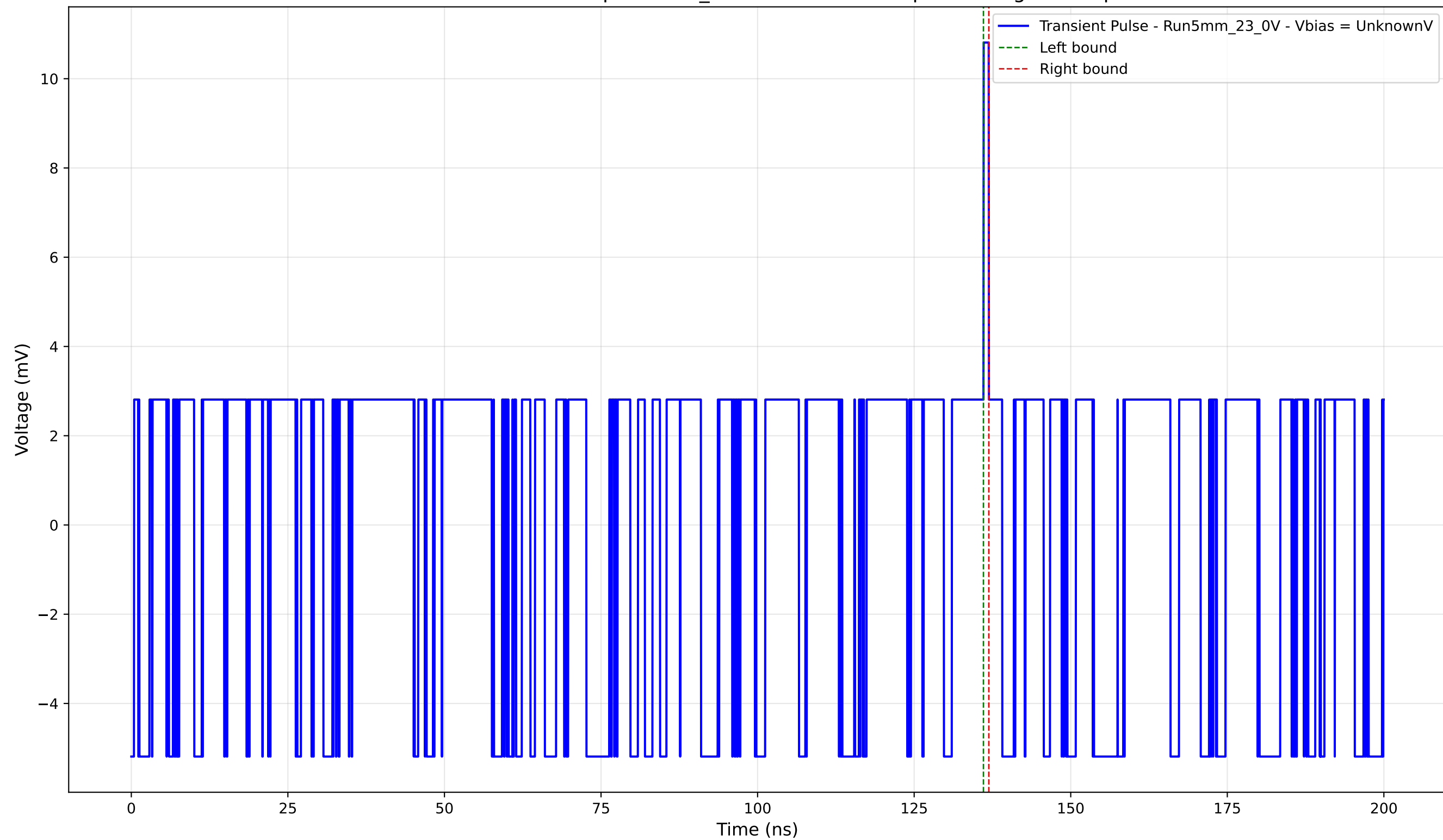
Transient Pulse - Sample: 5mm_23 - Position: 360.0 \mu\text{m} - Charge: 0.18 pC
