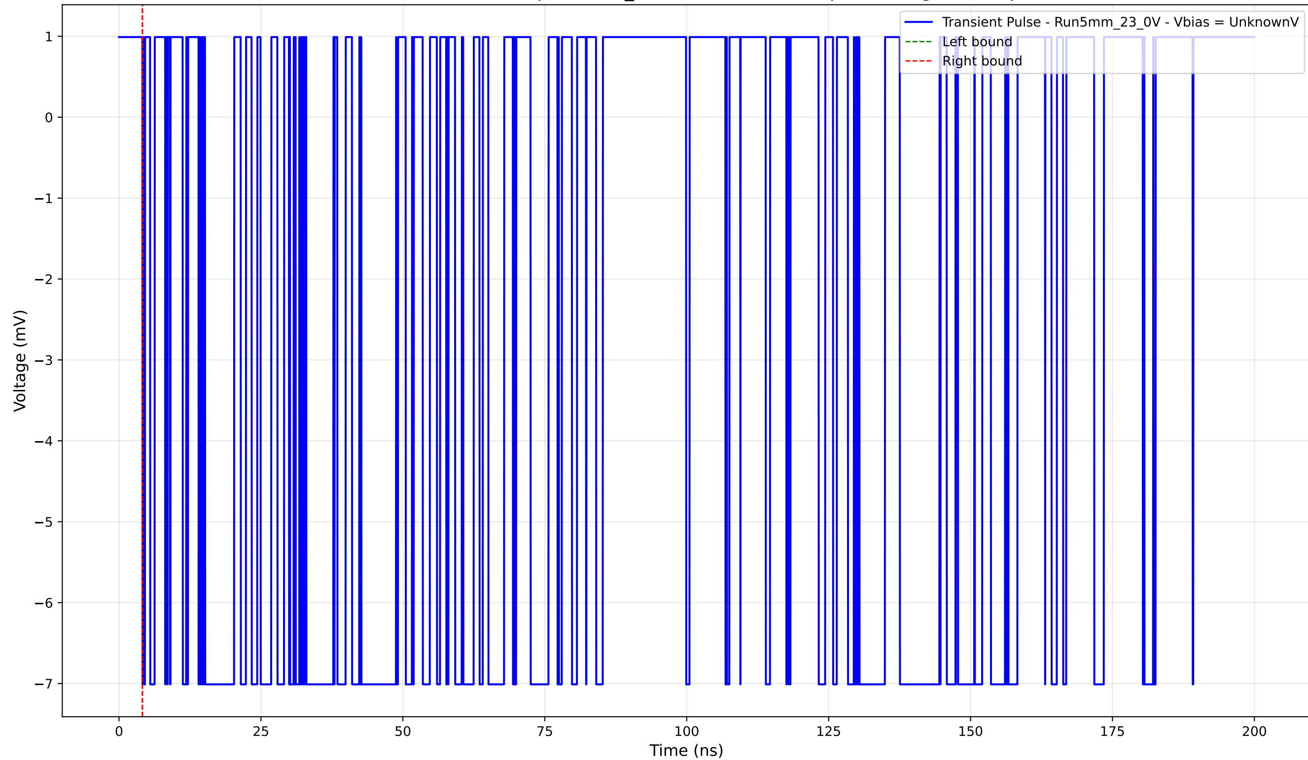
Transient Pulse - Sample: 5mm_23 - Position: 1275.0 \mu\text{m} - Charge: -0.00 pC
