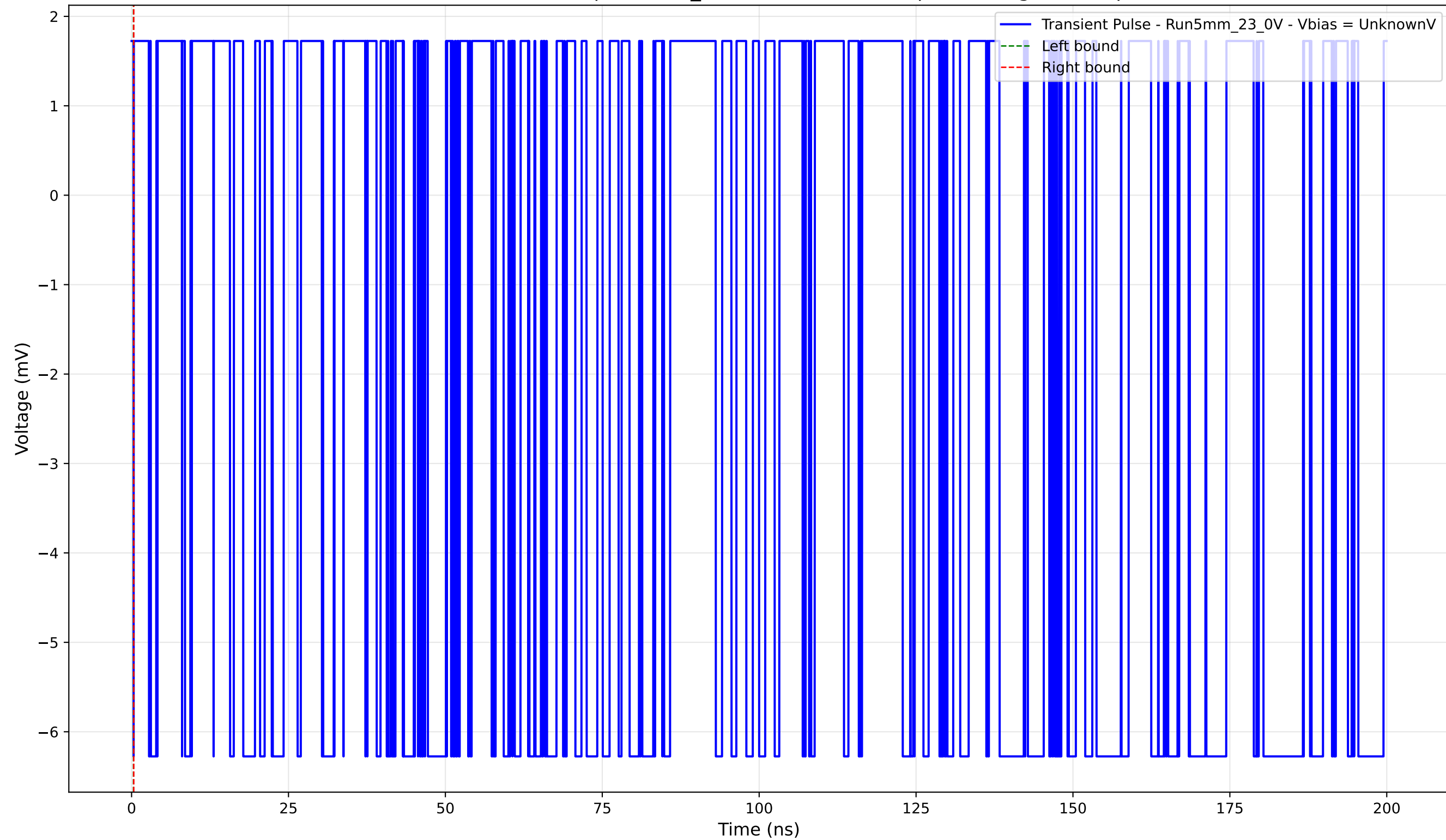
Transient Pulse - Sample: 5mm_23 - Position: 5005.0 \mu\text{m} - Charge: -0.00 pC
