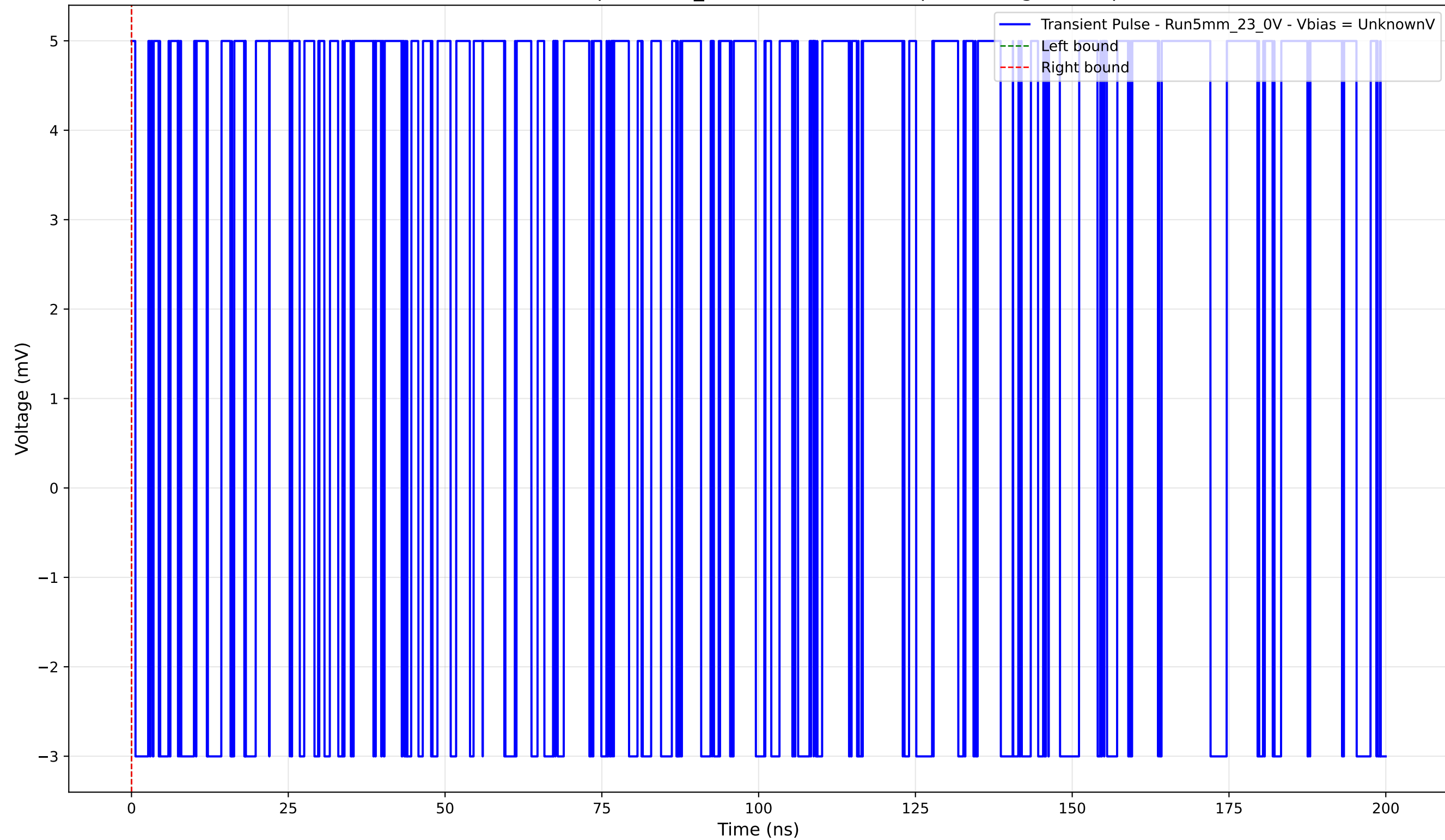
Transient Pulse - Sample: 5mm_23 - Position: 4125.0 \mu\text{m} - Charge: 0.00 pC
