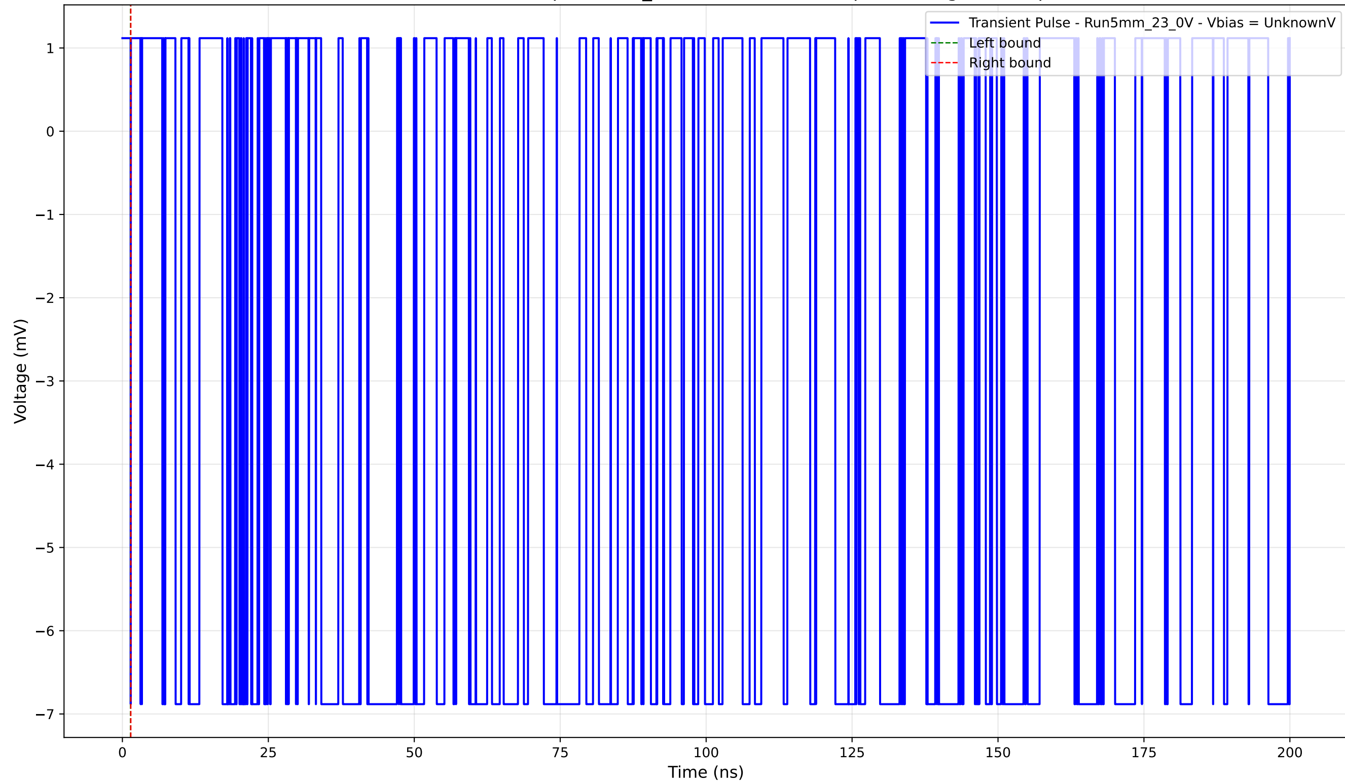
Transient Pulse - Sample: 5mm_23 - Position: 2315.0 \mu\text{m} - Charge: -0.00 pC
