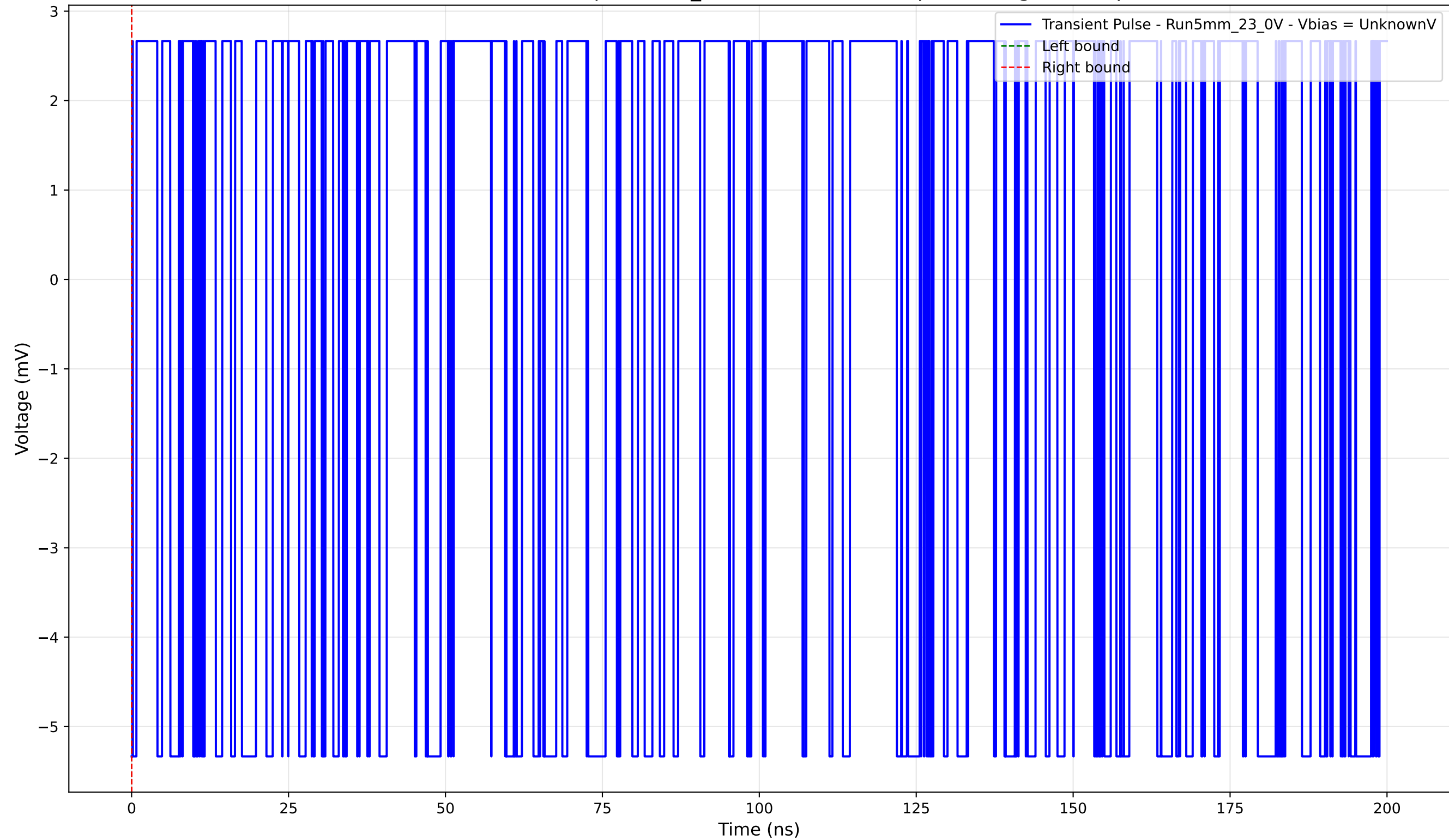
Transient Pulse - Sample: 5mm_23 - Position: 3470.0 \mu\text{m} - Charge: -0.00 pC
