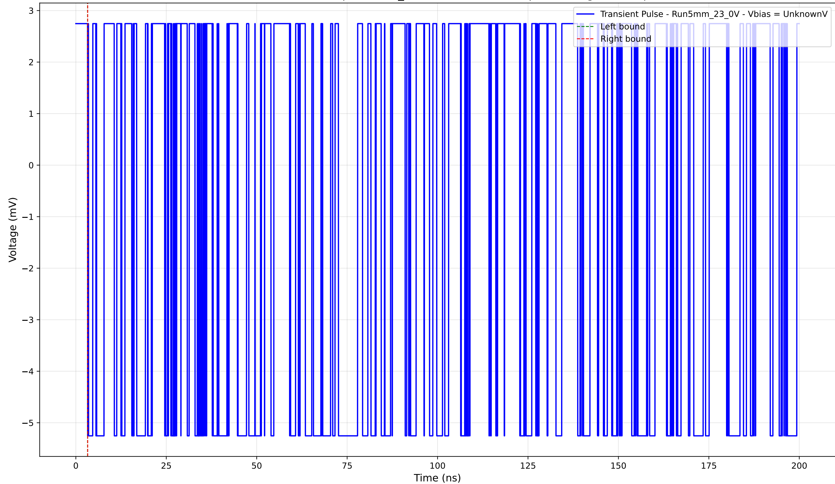
Transient Pulse - Sample: 5mm_23 - Position: 1380.0 \mu\text{m} - Charge: -0.00 pC
