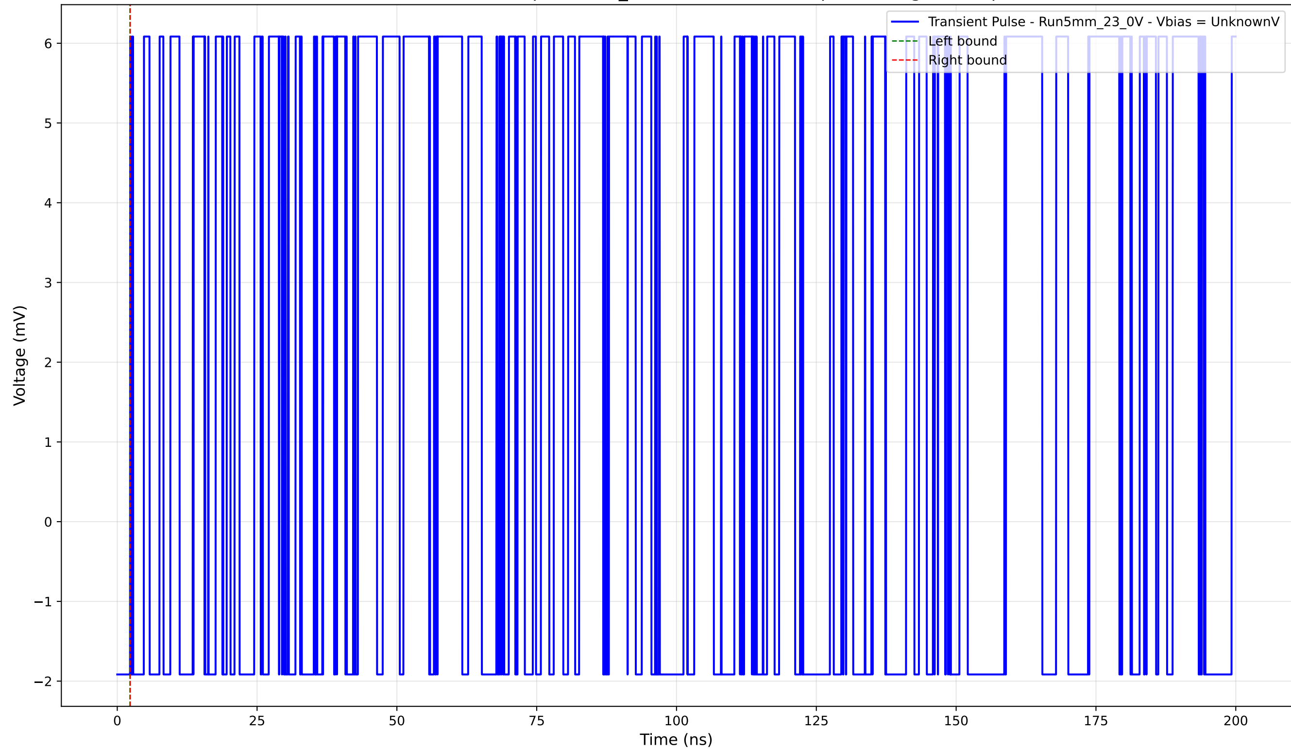
Transient Pulse - Sample: 5mm_23 - Position: 2120.0 \mu\text{m} - Charge: 0.00 pC
