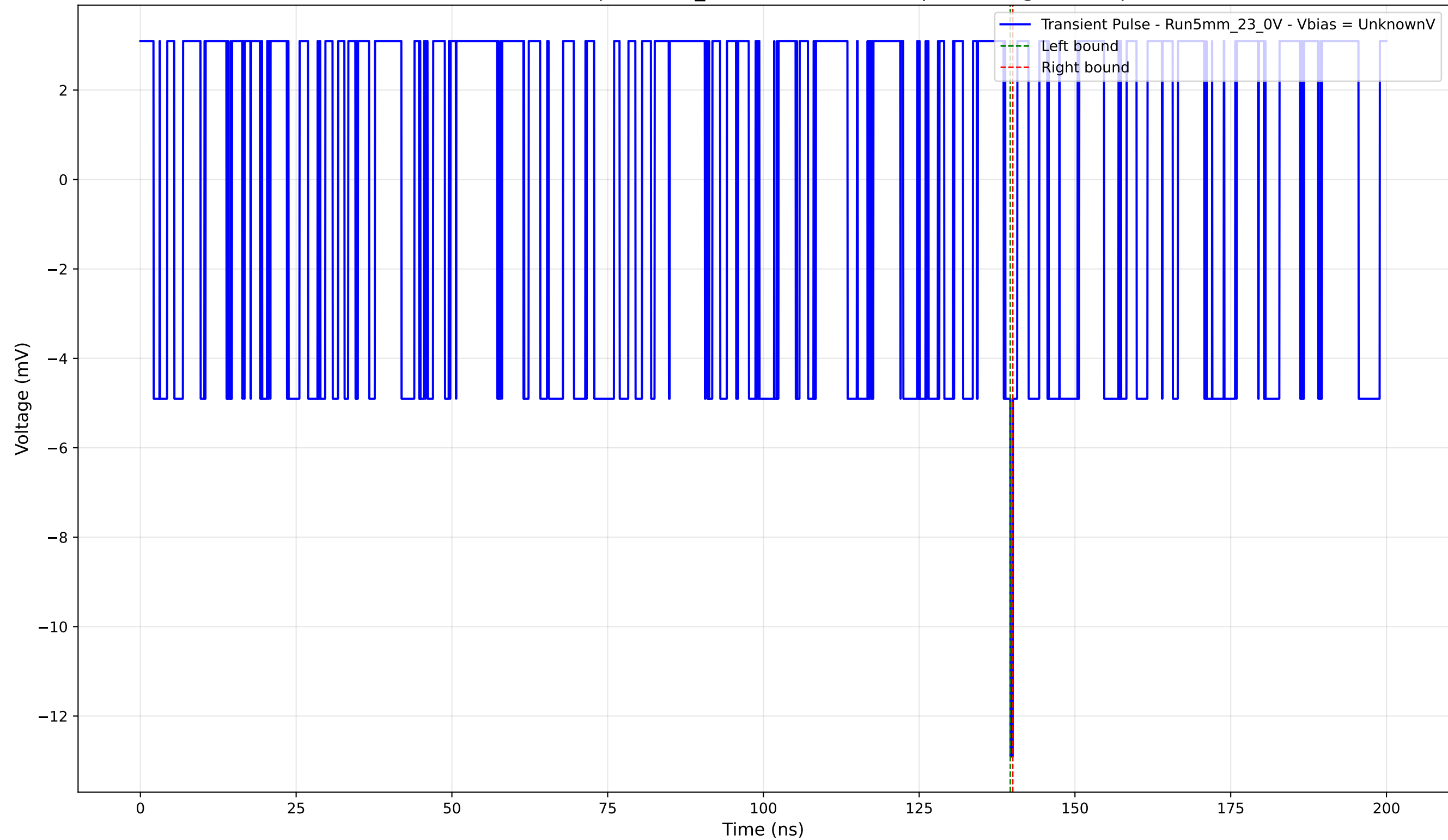
Transient Pulse - Sample: 5mm_23 - Position: 2410.0 \mu\text{m} - Charge: -0.10 pC
