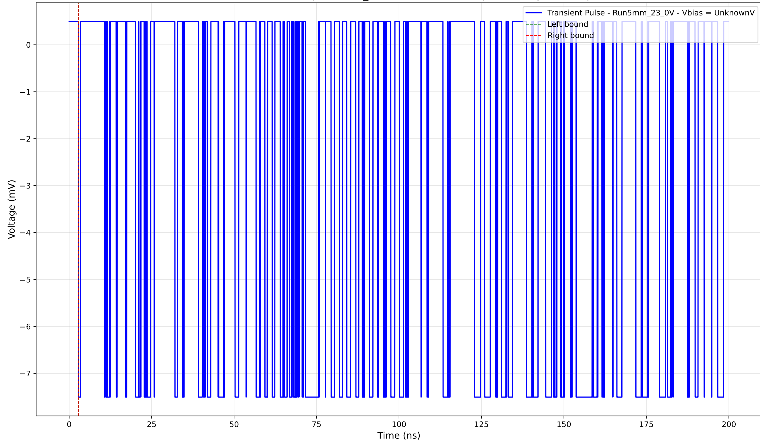
Transient Pulse - Sample: 5mm_23 - Position: 4715.0 \mu\text{m} - Charge: -0.00 pC
