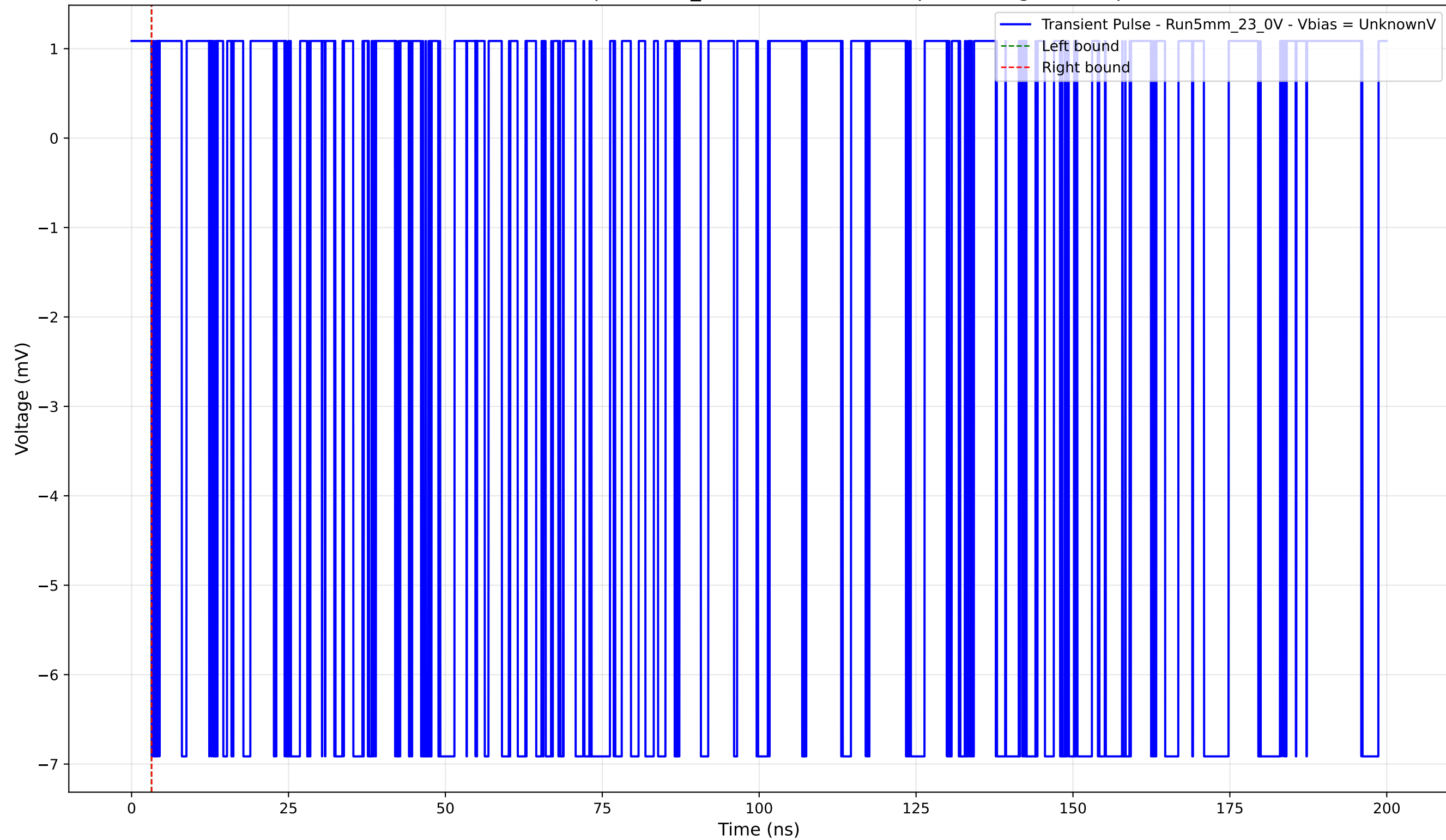
Transient Pulse - Sample: 5mm_23 - Position: 1695.0 \mu\text{m} - Charge: -0.00 pC
