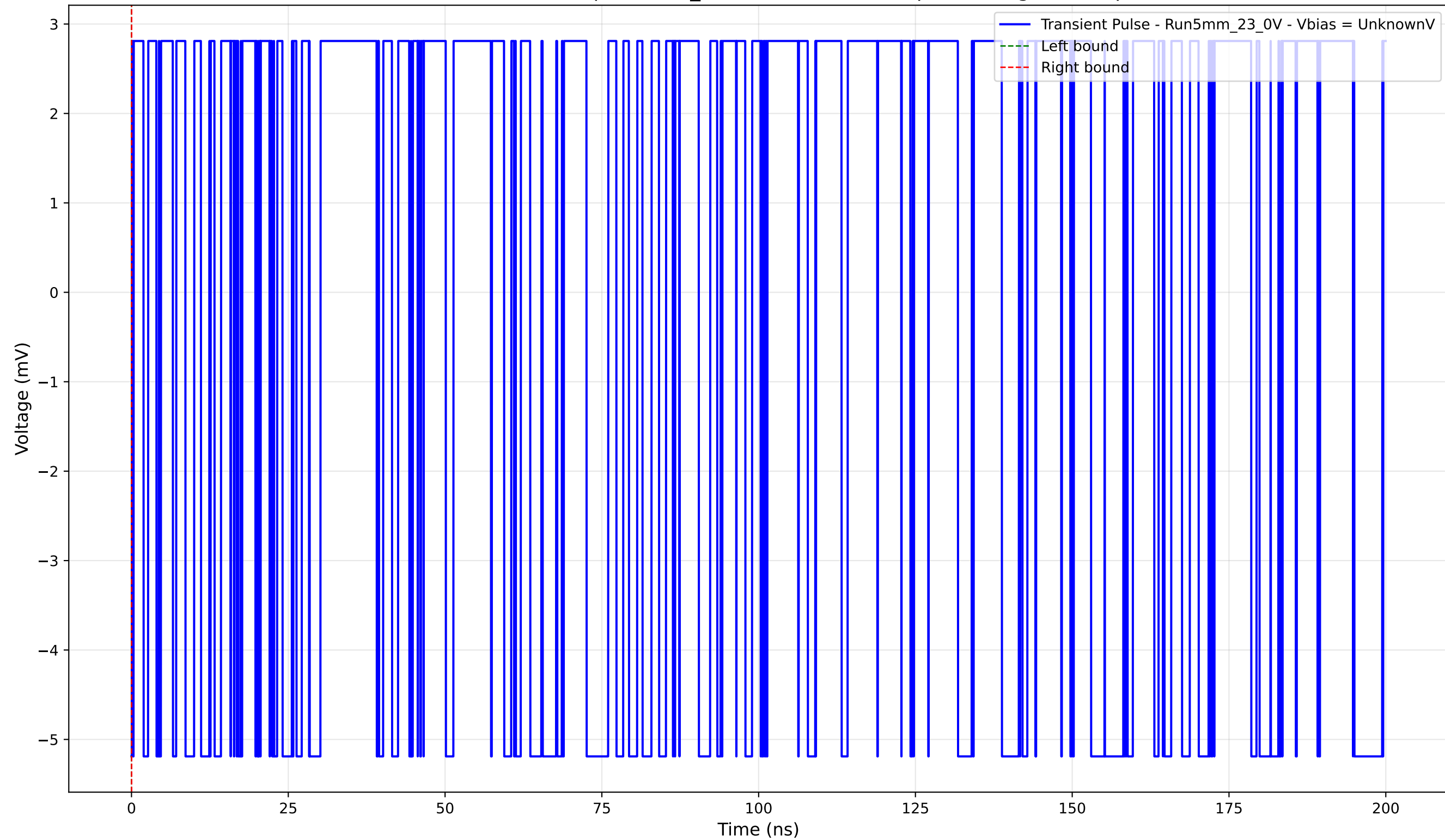
Transient Pulse - Sample: 5mm_23 - Position: 4345.0 \mu\text{m} - Charge: -0.00 pC
