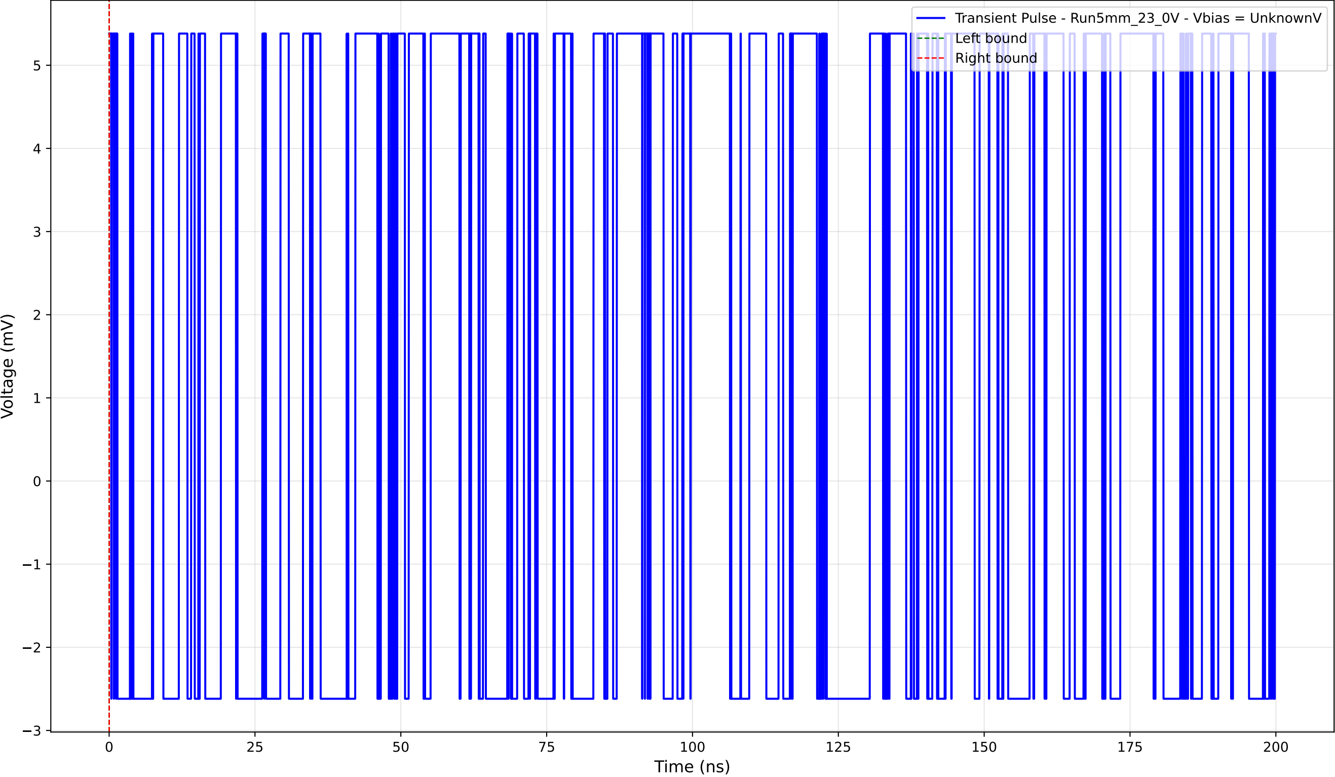
Transient Pulse - Sample: 5mm_23 - Position: 975.0 \mu\text{m} - Charge: 0.00 pC
