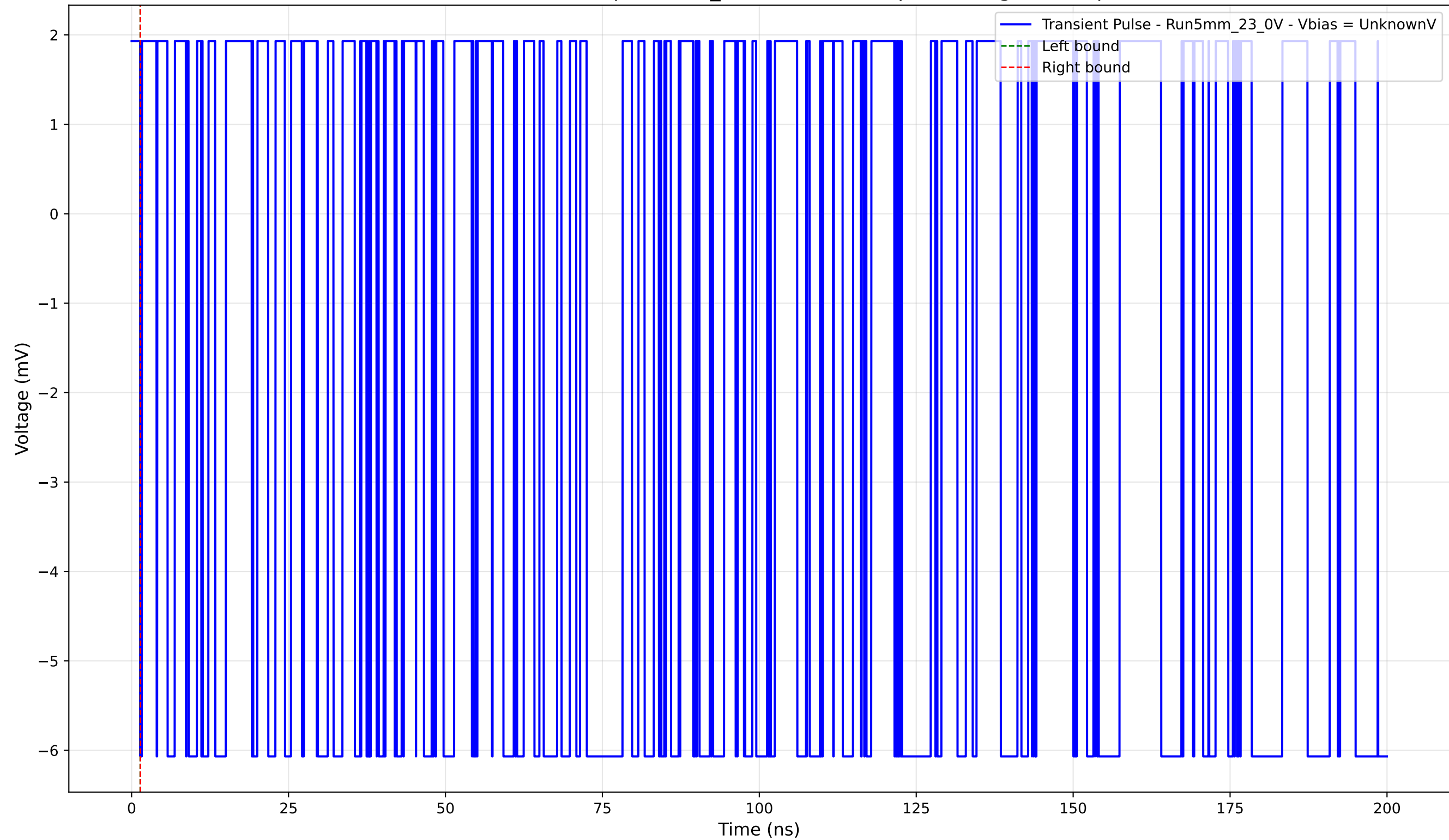
Transient Pulse - Sample: 5mm_23 - Position: 0.0 \mu\text{m} - Charge: -0.00 pC
