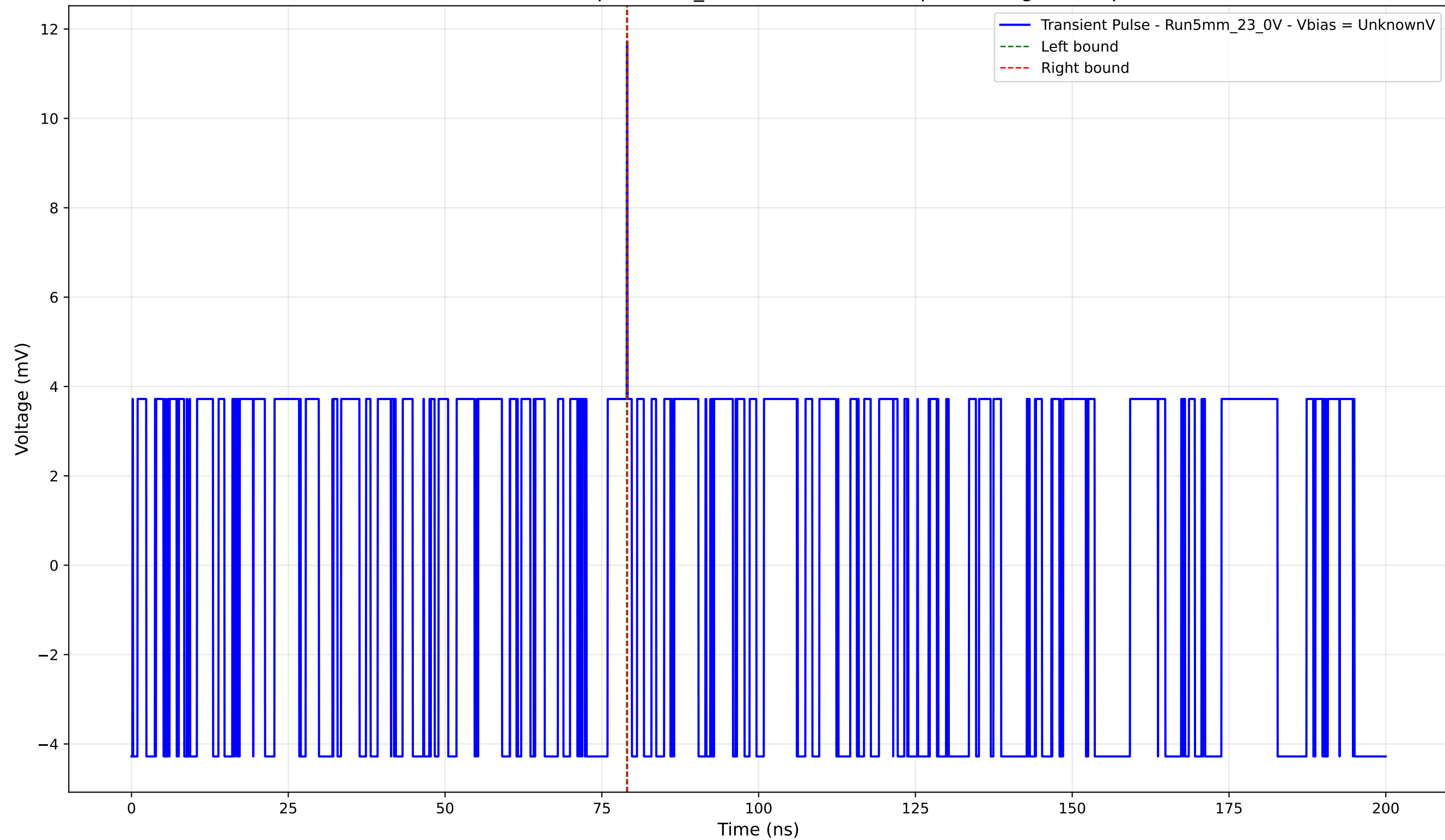
Transient Pulse - Sample: 5mm_23 - Position: 2570.0 \mu\text{m} - Charge: 0.02 pC
