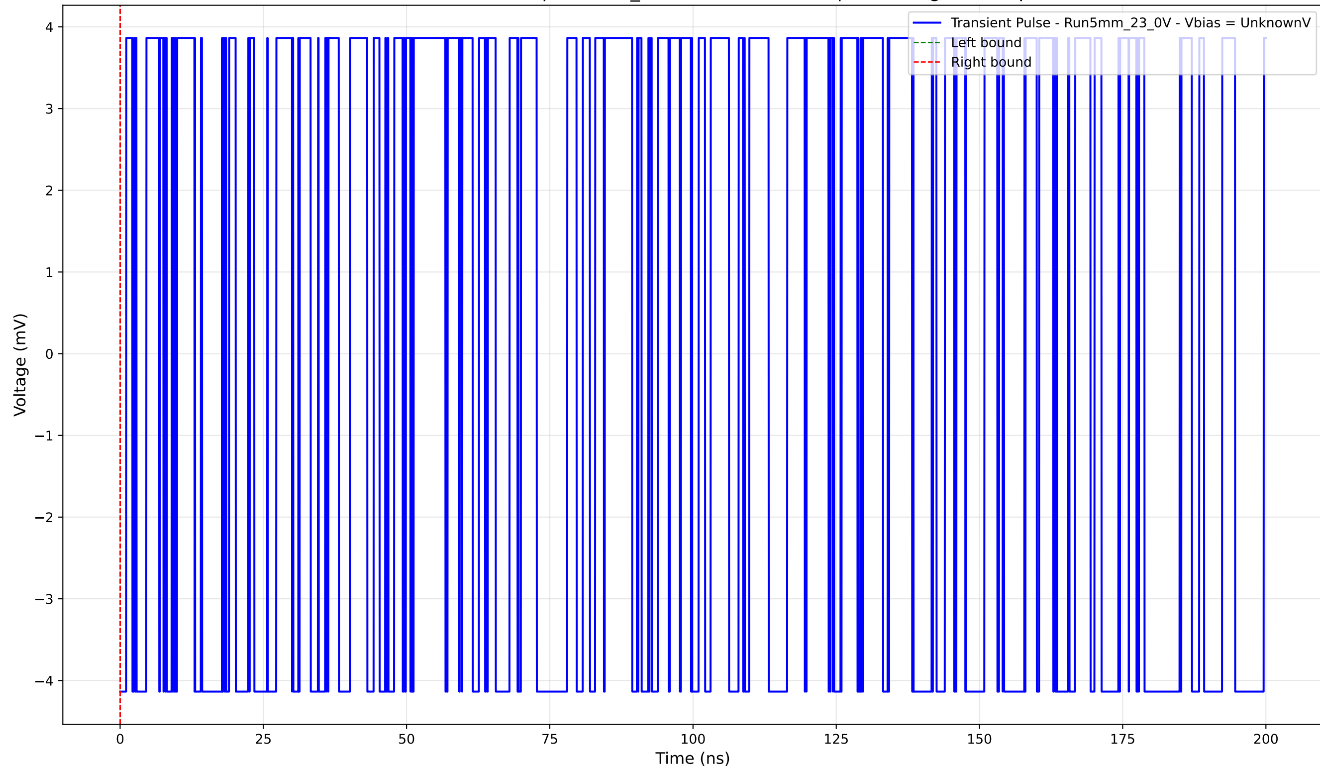
Transient Pulse - Sample: 5mm_23 - Position: 2940.0 \mu\text{m} - Charge: -0.00 pC
