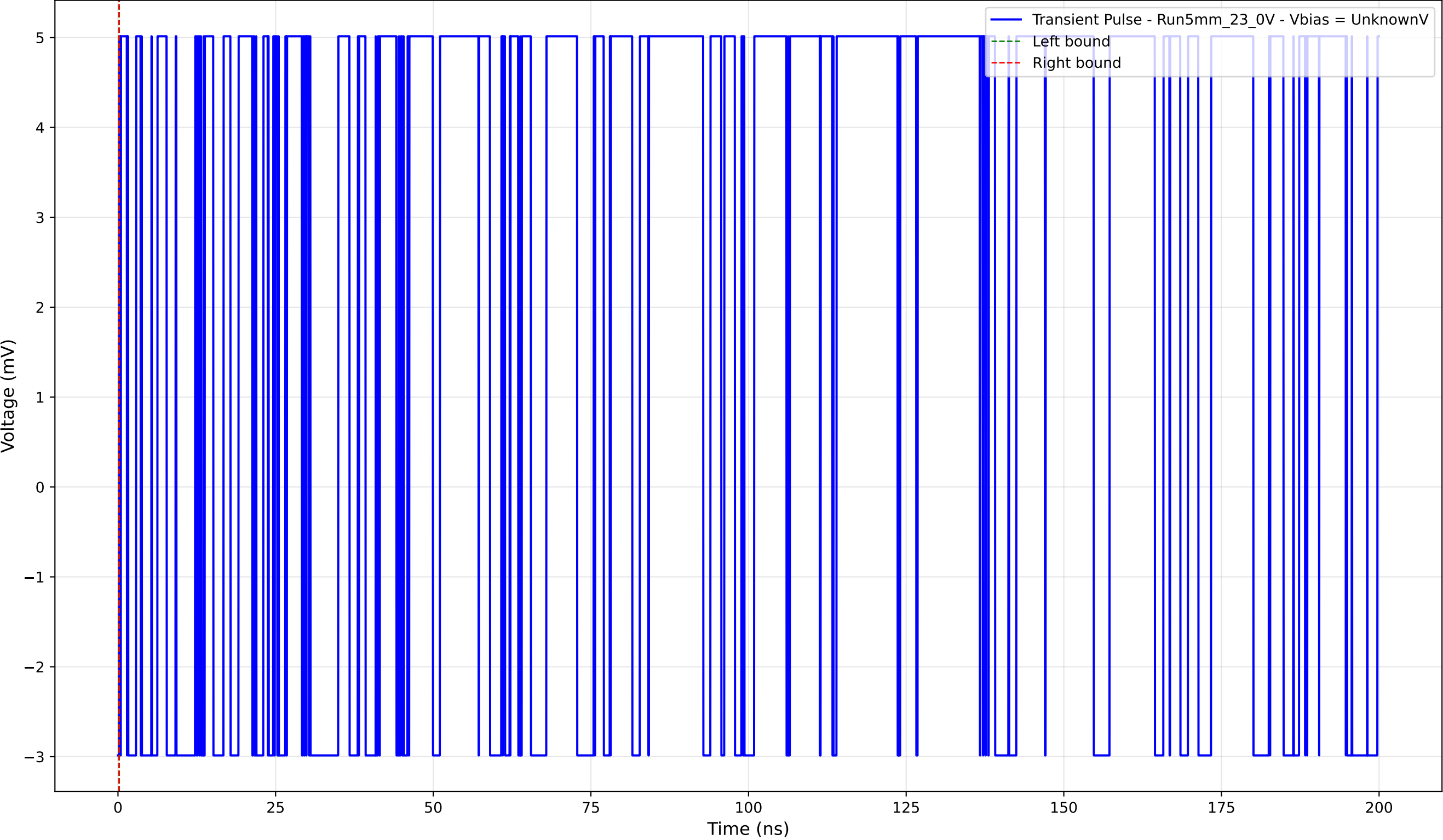
Transient Pulse - Sample: 5mm_23 - Position: 700.0 \mu\text{m} - Charge: 0.00 pC
