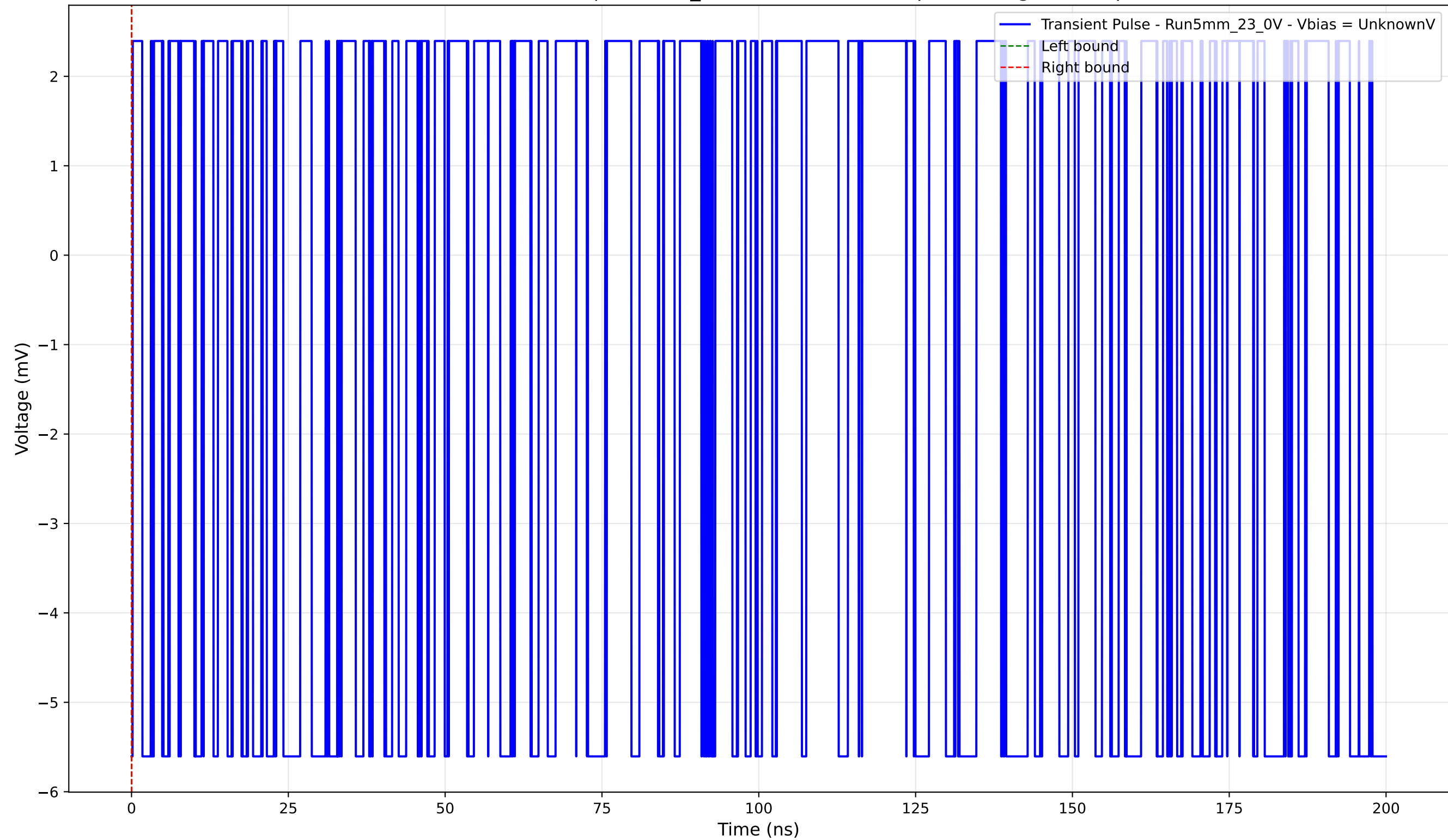
Transient Pulse - Sample: 5mm_23 - Position: 4895.0 \mu\text{m} - Charge: -0.00 pC
