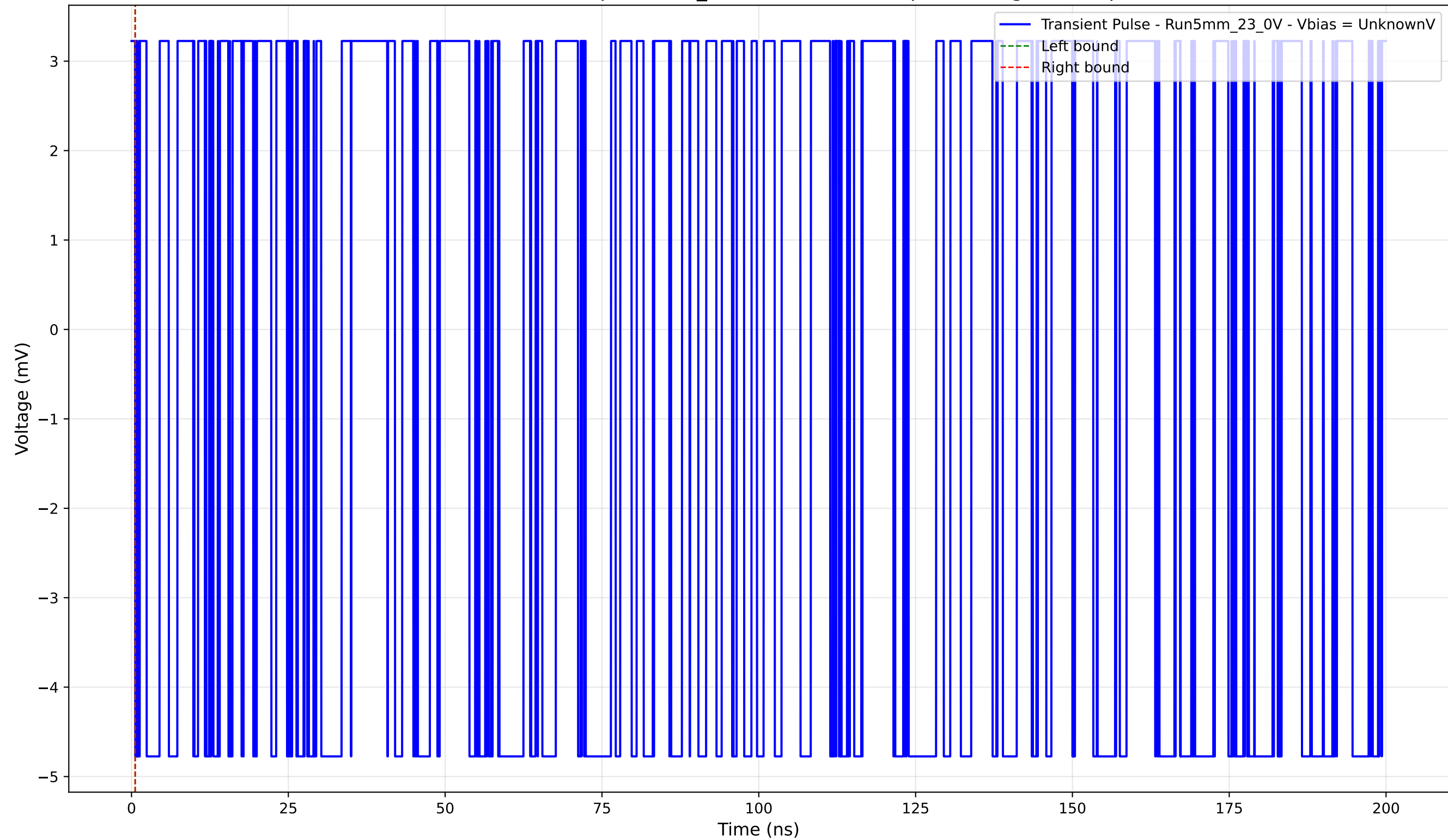
Transient Pulse - Sample: 5mm_23 - Position: 585.0 \mu\text{m} - Charge: -0.00 pC
