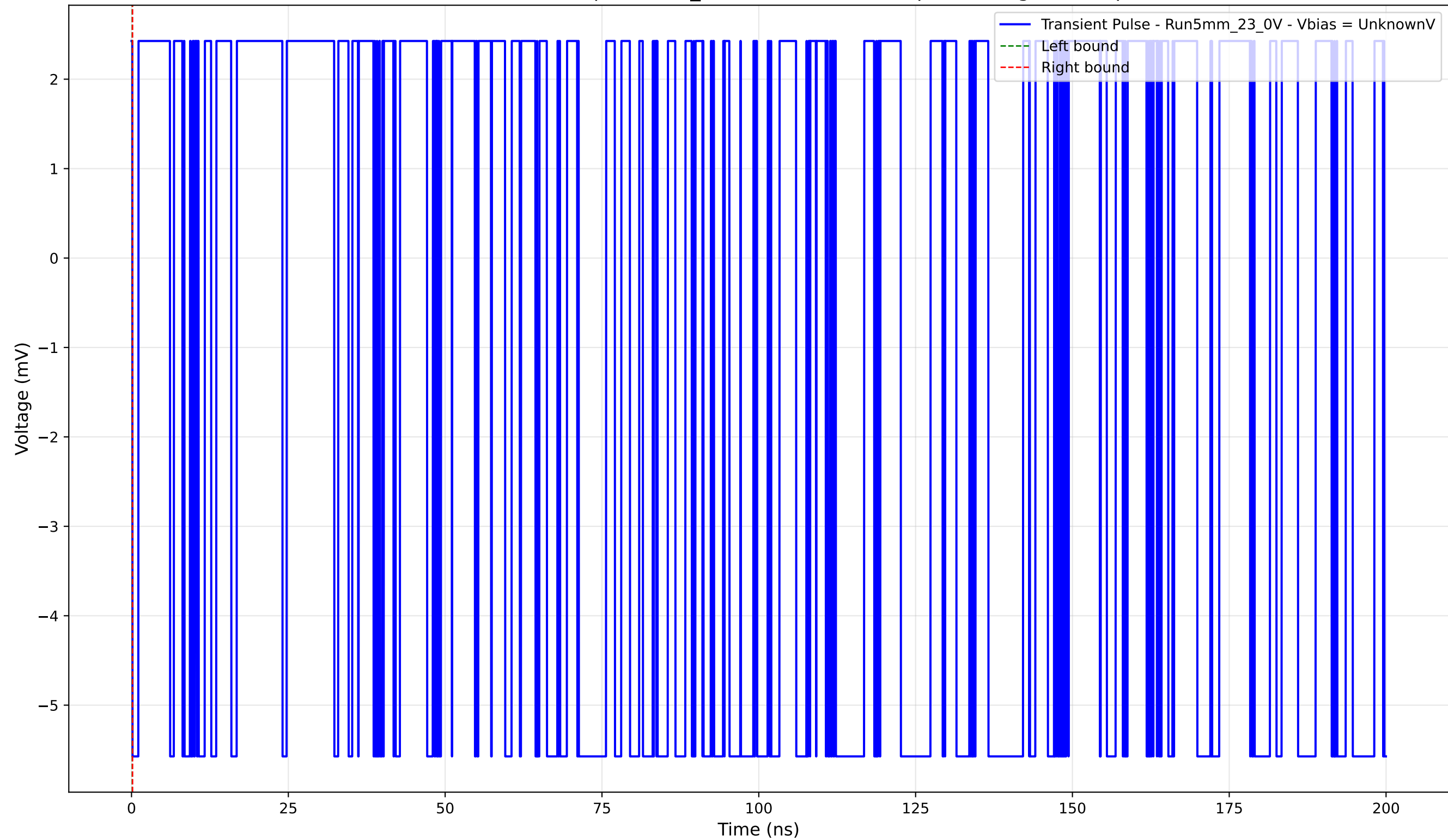
Transient Pulse - Sample: 5mm_23 - Position: 1505.0 \mu\text{m} - Charge: -0.00 pC
