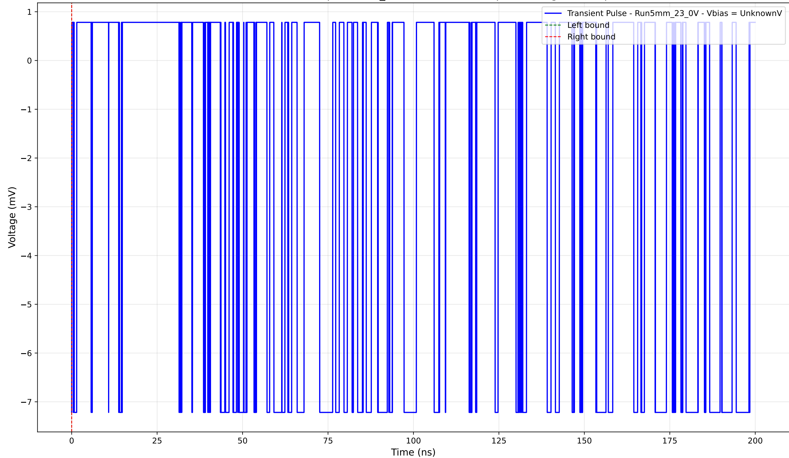
Transient Pulse - Sample: 5mm_23 - Position: 805.0 \mu\text{m} - Charge: -0.00 pC
