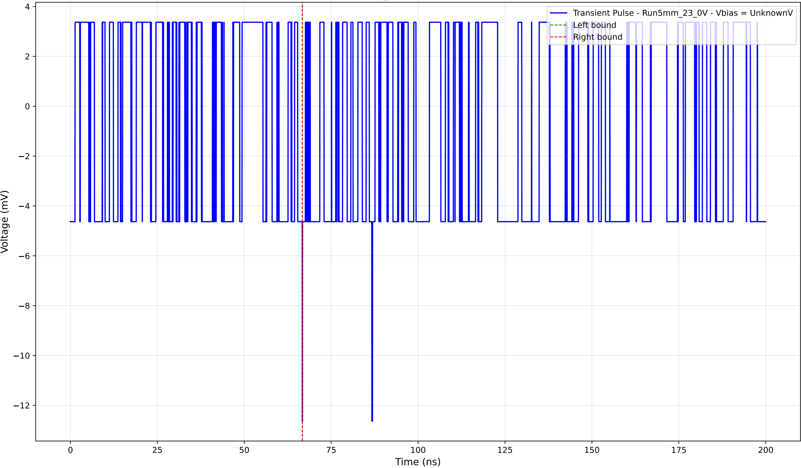
Transient Pulse - Sample: 5mm_23 - Position: 720.0 \mu\text{m} - Charge: -0.02 pC
