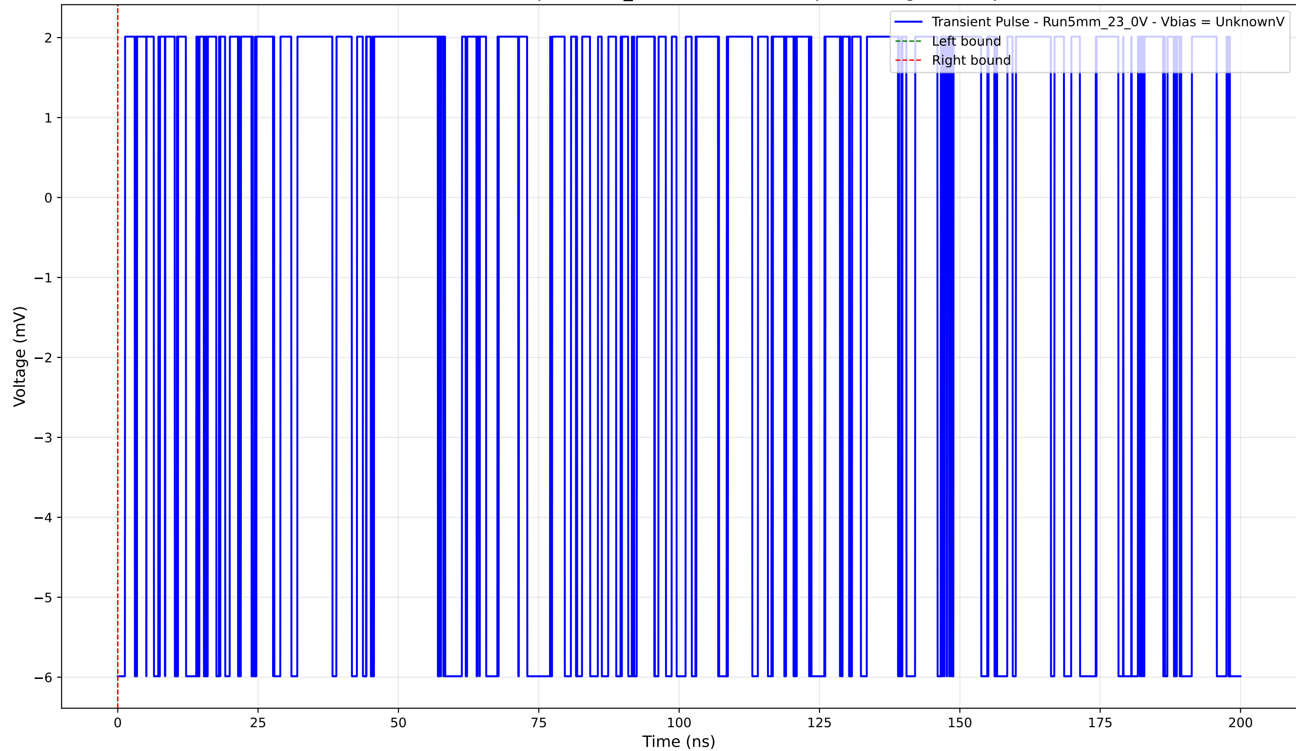
Transient Pulse - Sample: 5mm_23 - Position: 145.0 \mu\text{m} - Charge: -0.00 pC
