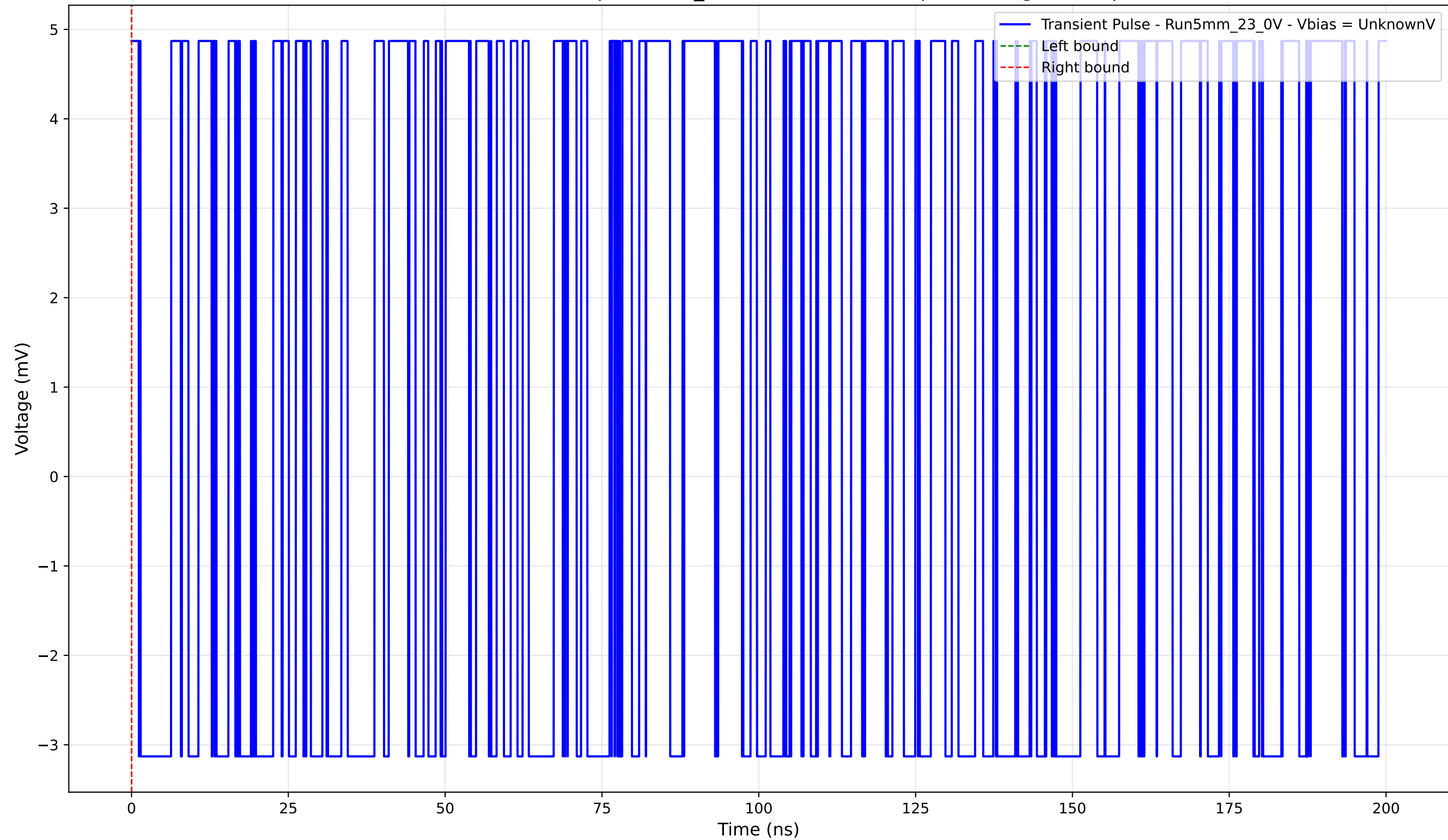
Transient Pulse - Sample: 5mm_23 - Position: 2835.0 \mu\text{m} - Charge: 0.00 pC
