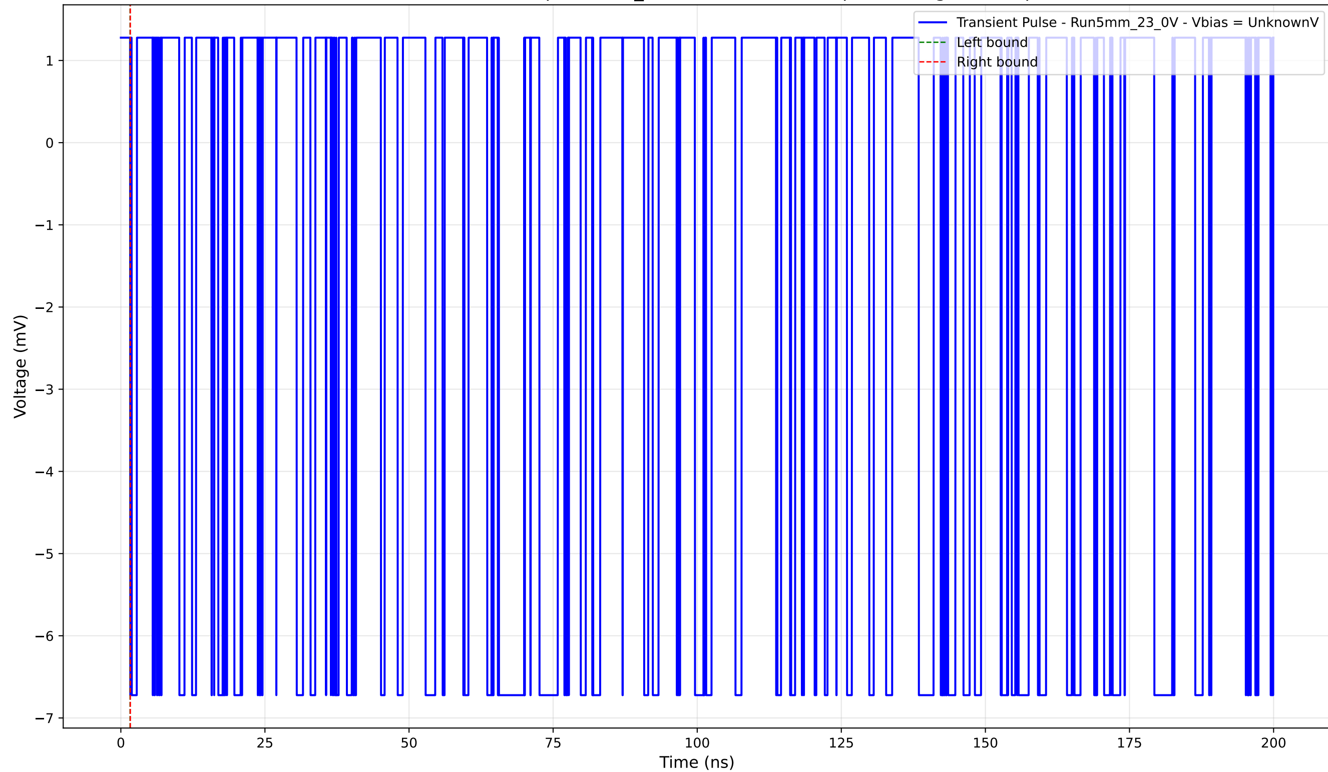
Transient Pulse - Sample: 5mm_23 - Position: 2750.0 \mu\text{m} - Charge: -0.00 pC
