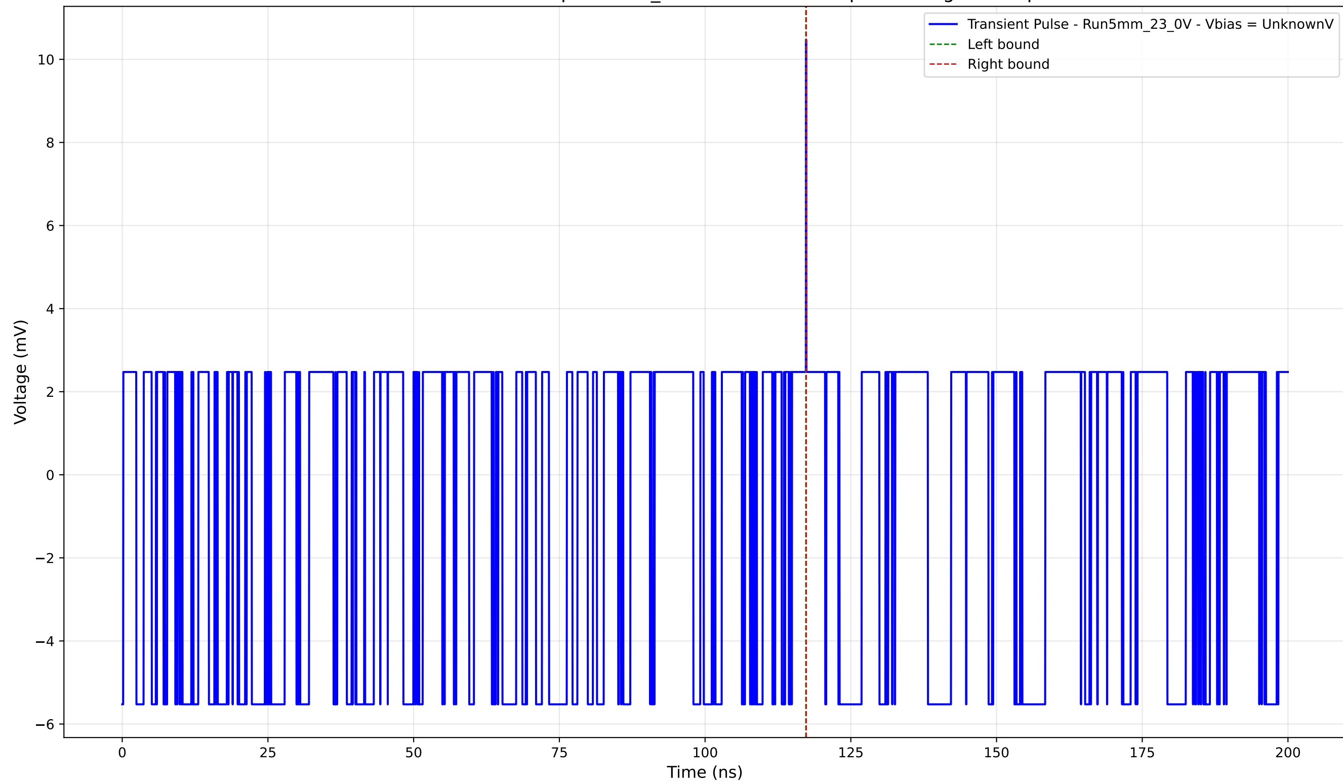
Transient Pulse - Sample: 5mm_23 - Position: 630.0 \mu\text{m} - Charge: 0.01 pC
