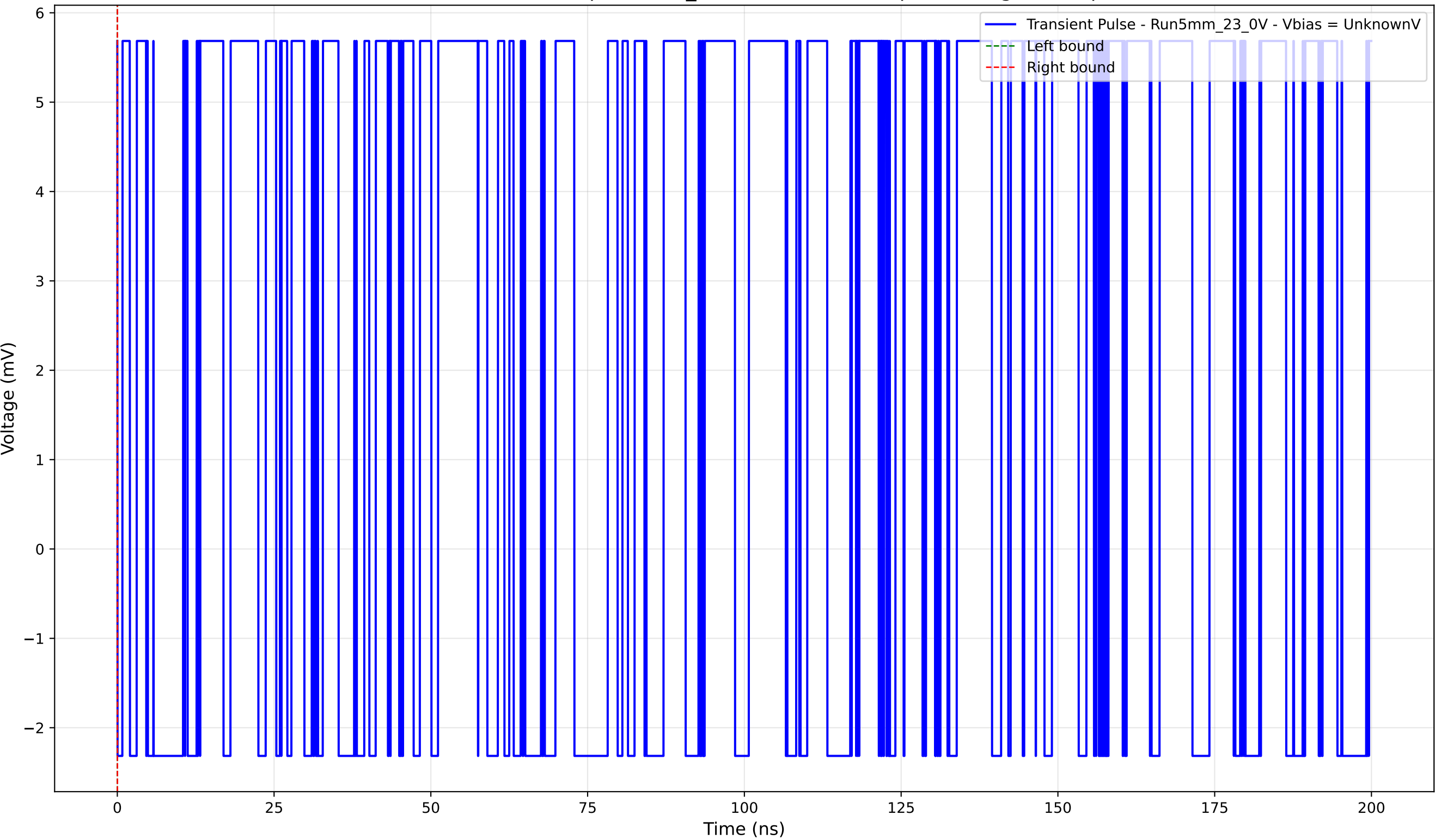
Transient Pulse - Sample: 5mm_23 - Position: 405.0 \mu\text{m} - Charge: 0.00 pC
