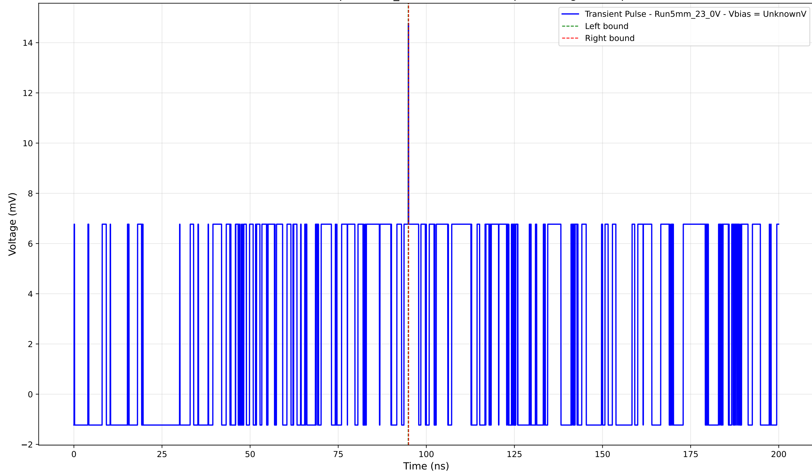
Transient Pulse - Sample: 5mm_23 - Position: 570.0 \mu\text{m} - Charge: 0.03 pC
