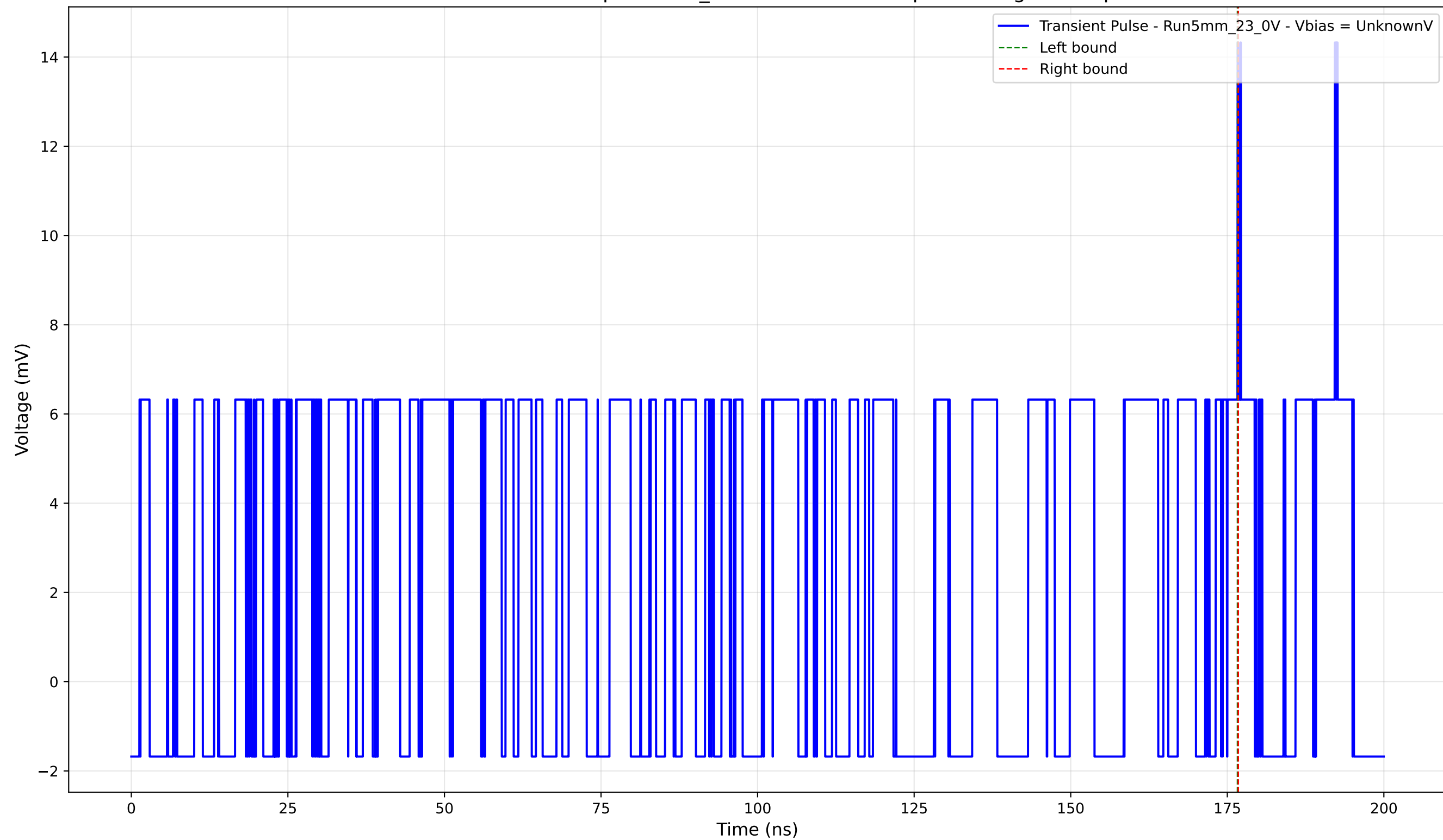
Transient Pulse - Sample: 5mm_23 - Position: 190.0 \mu\text{m} - Charge: 0.04 pC
