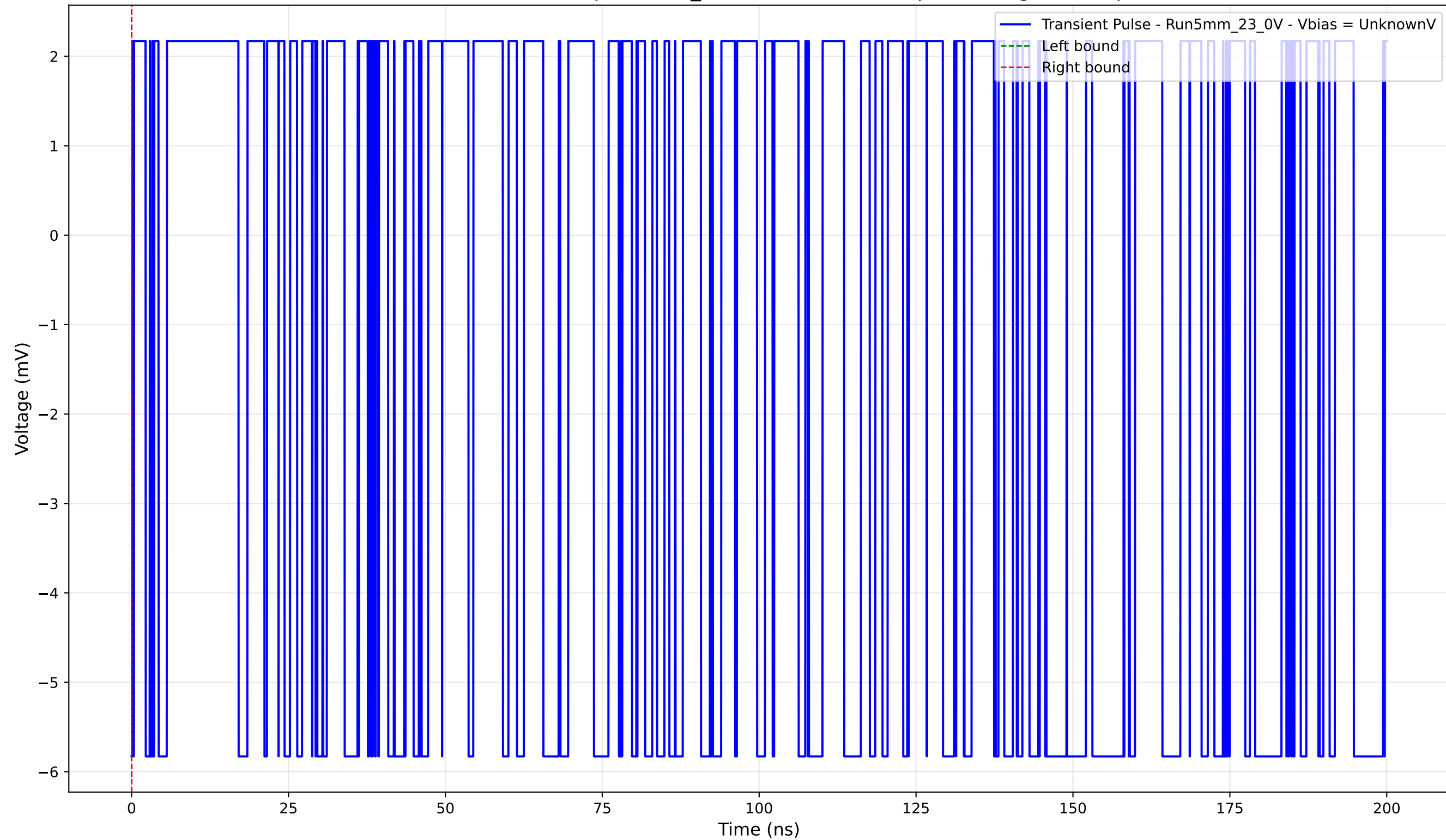
Transient Pulse - Sample: 5mm_23 - Position: 3145.0 \mu\text{m} - Charge: -0.00 pC
