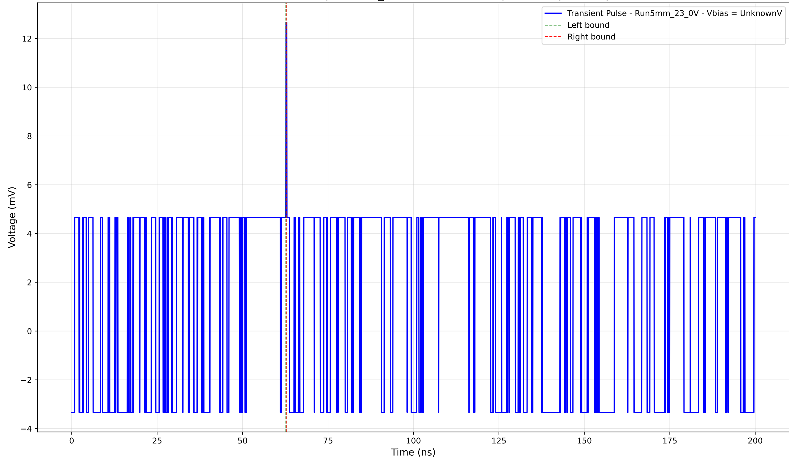
Transient Pulse - Sample: 5mm_23 - Position: 2470.0 \mu\text{m} - Charge: 0.07 pC
