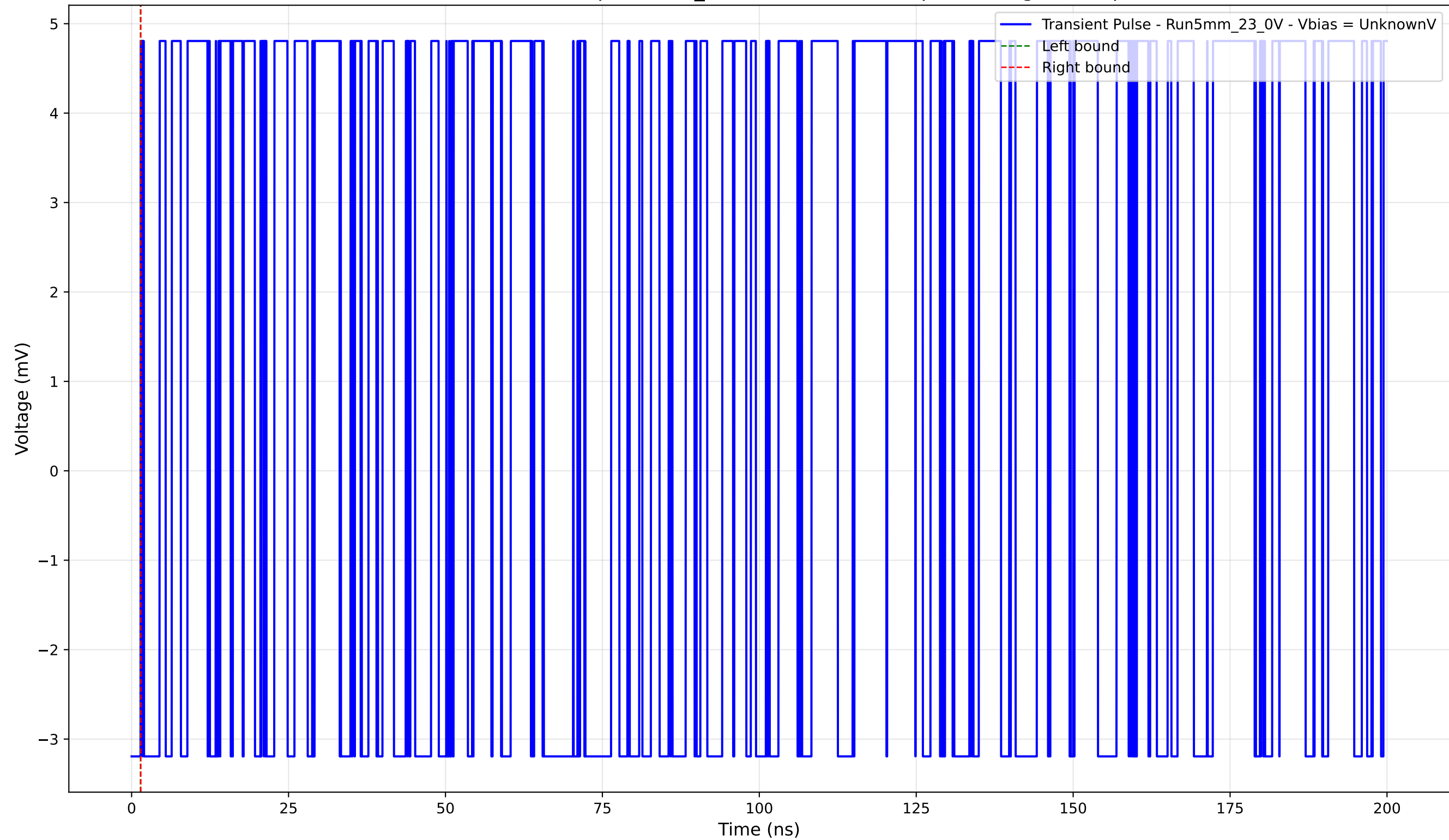
Transient Pulse - Sample: 5mm_23 - Position: 3445.0 \mu\text{m} - Charge: 0.00 pC
