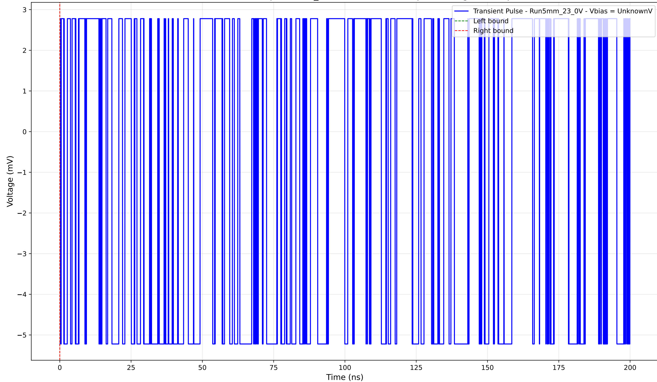
Transient Pulse - Sample: 5mm_23 - Position: 1615.0 \mu\text{m} - Charge: -0.00 pC
