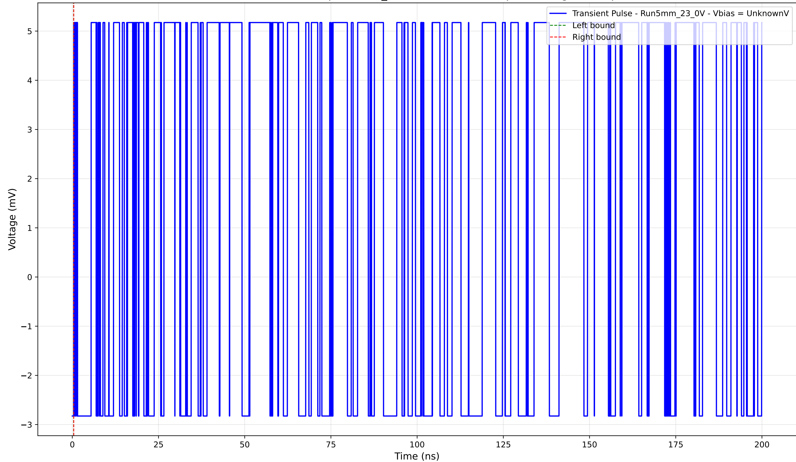
Transient Pulse - Sample: 5mm_23 - Position: 2510.0 \mu\text{m} - Charge: 0.00 pC
