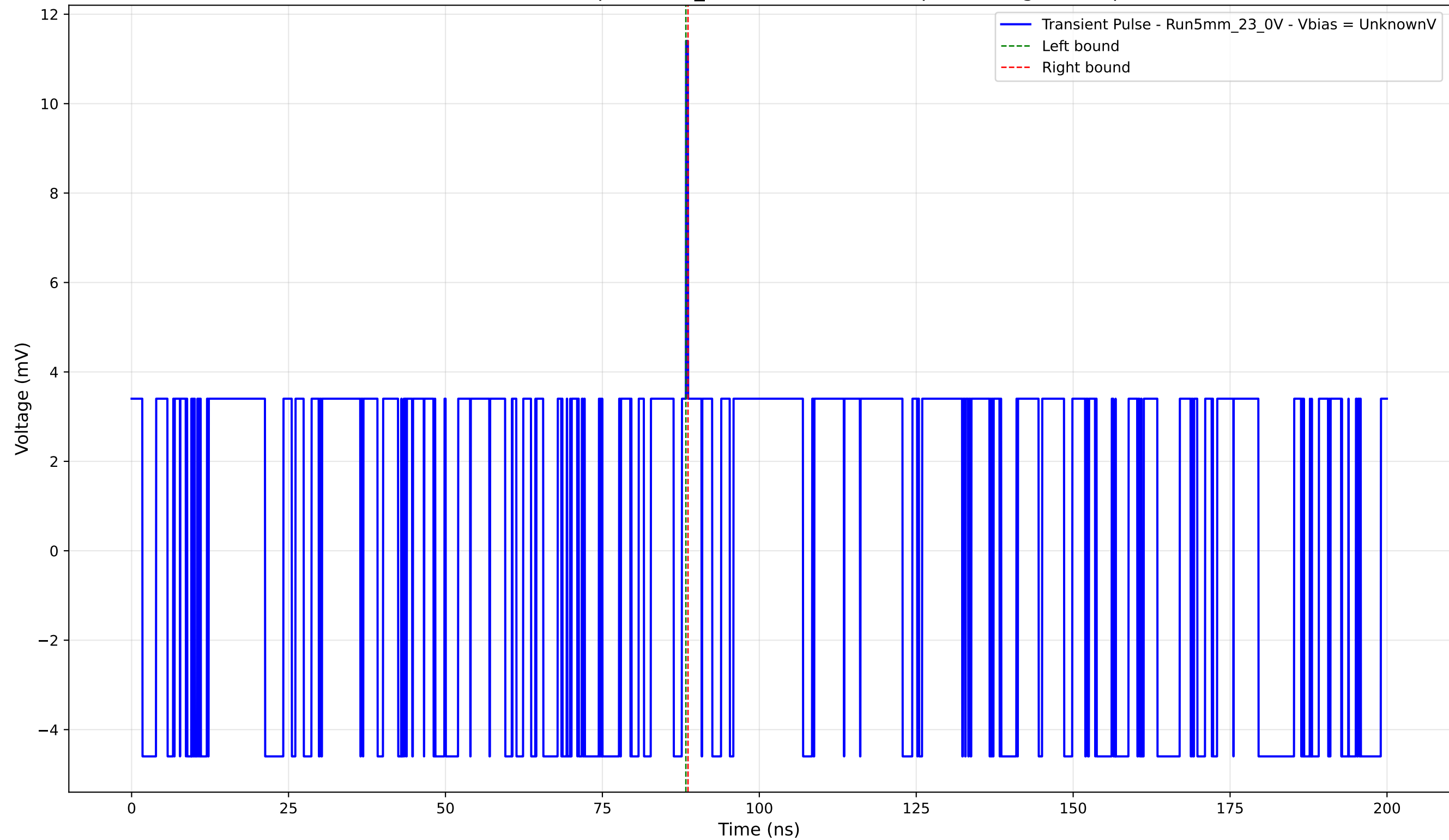
Transient Pulse - Sample: 5mm_23 - Position: 4175.0 \mu\text{m} - Charge: 0.07 pC
