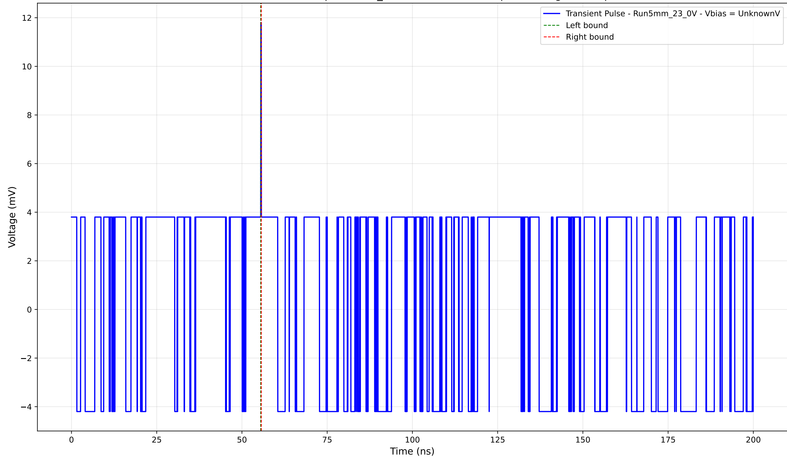
Transient Pulse - Sample: 5mm_23 - Position: 1945.0 \mu\text{m} - Charge: 0.04 pC
