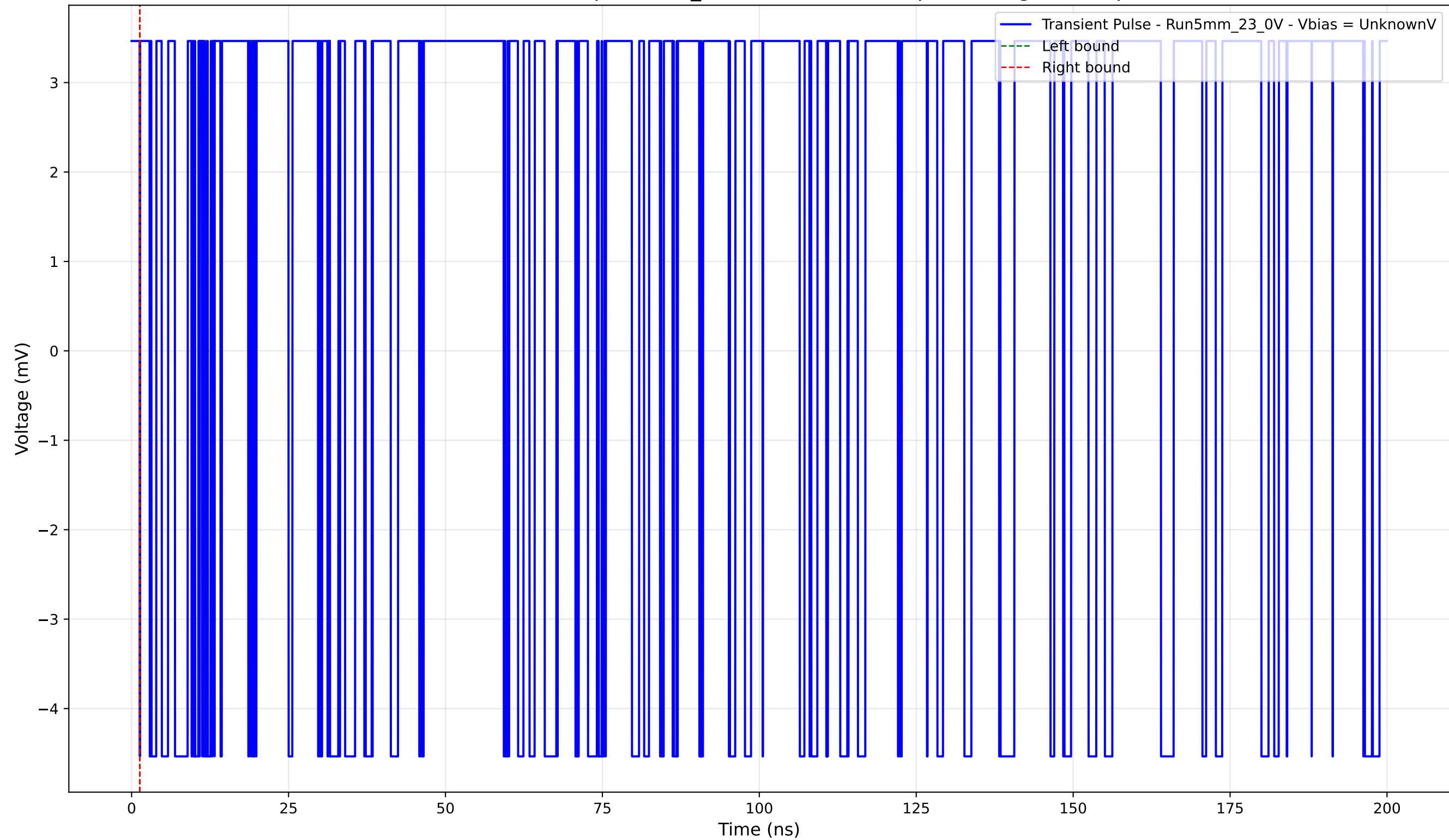
Transient Pulse - Sample: 5mm_23 - Position: 2670.0 \mu\text{m} - Charge: -0.00 pC
