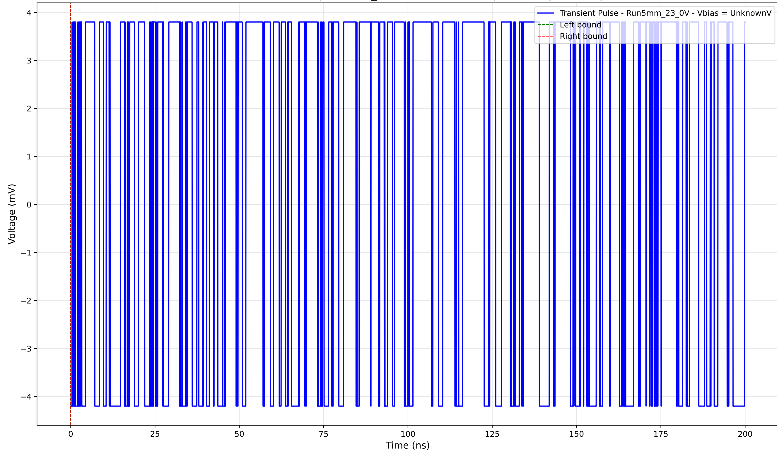
Transient Pulse - Sample: 5mm_23 - Position: 4860.0 \mu\text{m} - Charge: -0.00 pC
