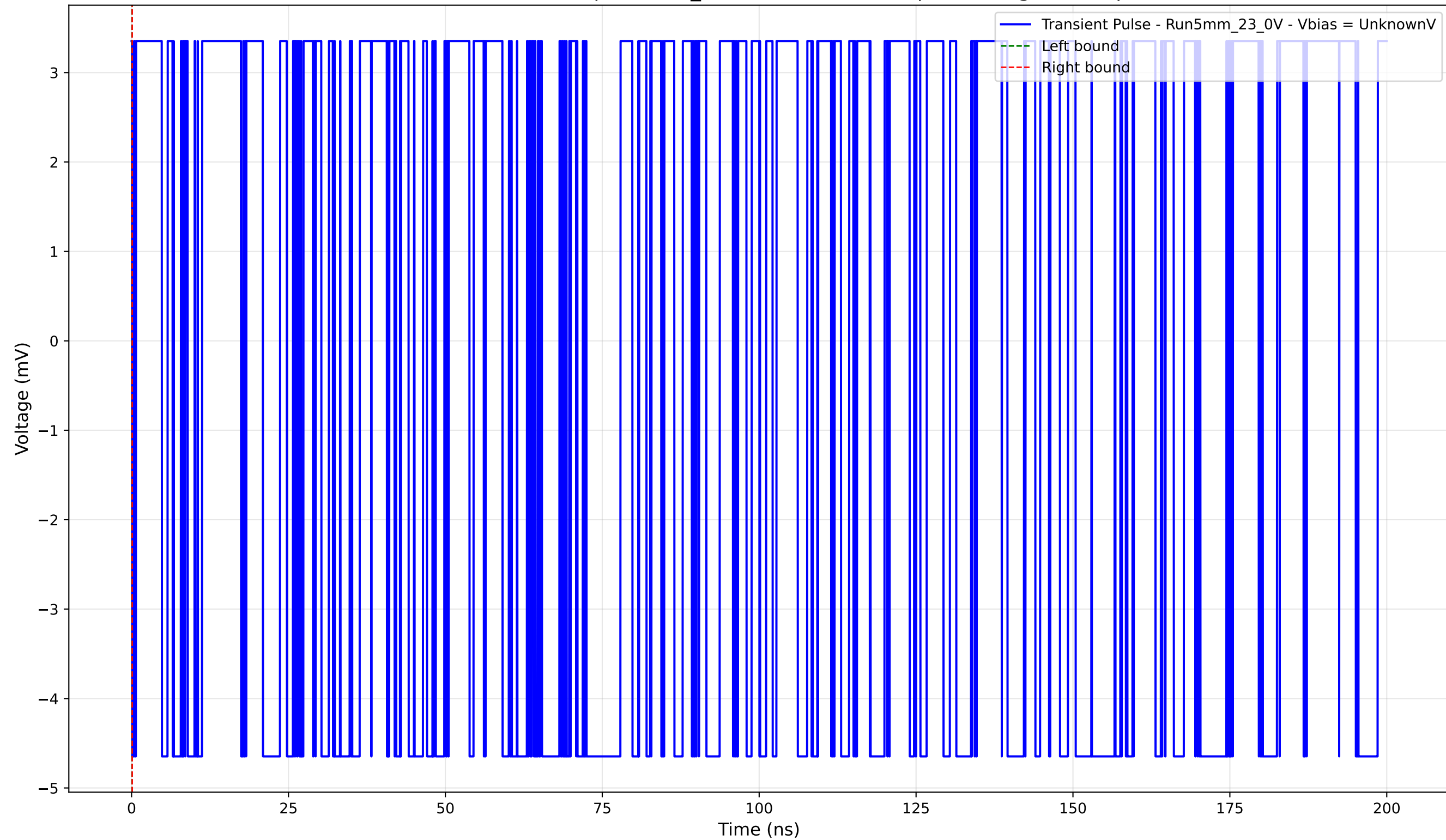
Transient Pulse - Sample: 5mm_23 - Position: 3605.0 \mu\text{m} - Charge: -0.00 pC
