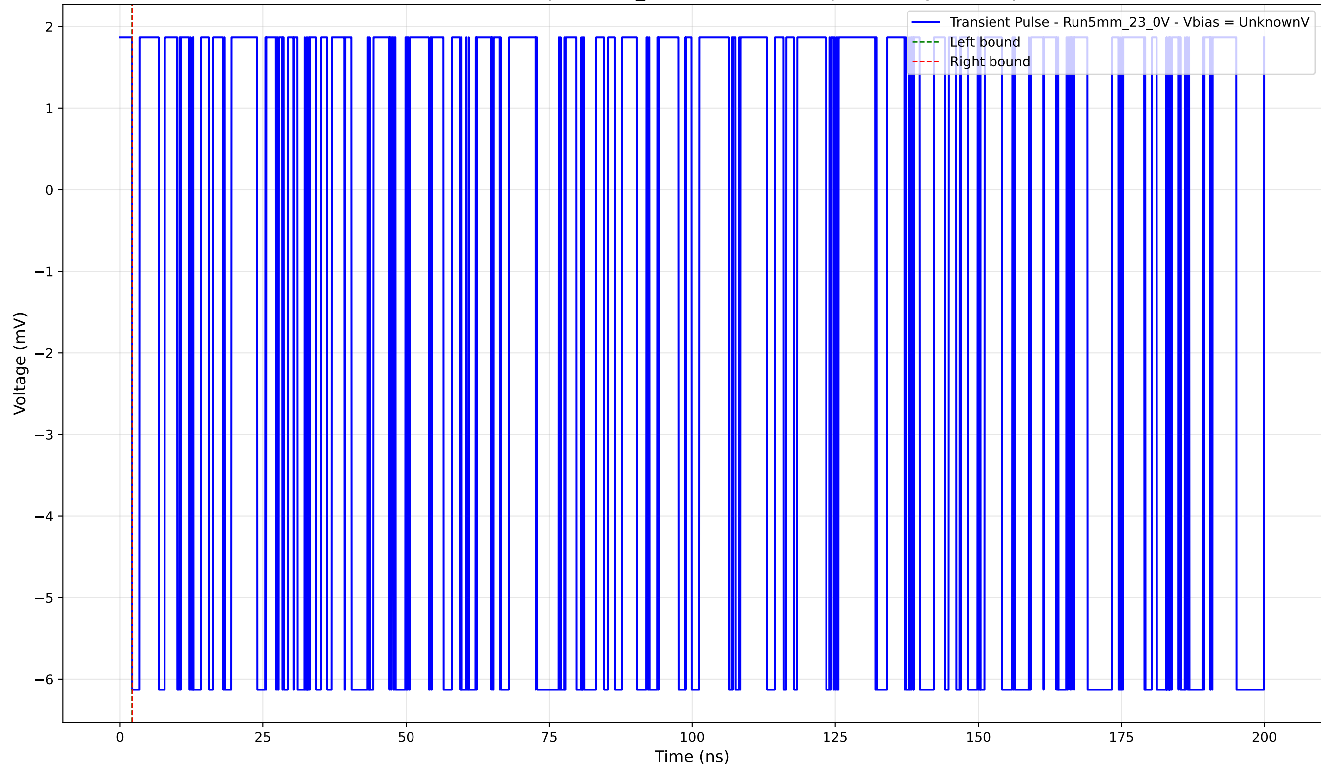
Transient Pulse - Sample: 5mm_23 - Position: 280.0 \mu\text{m} - Charge: -0.00 pC
