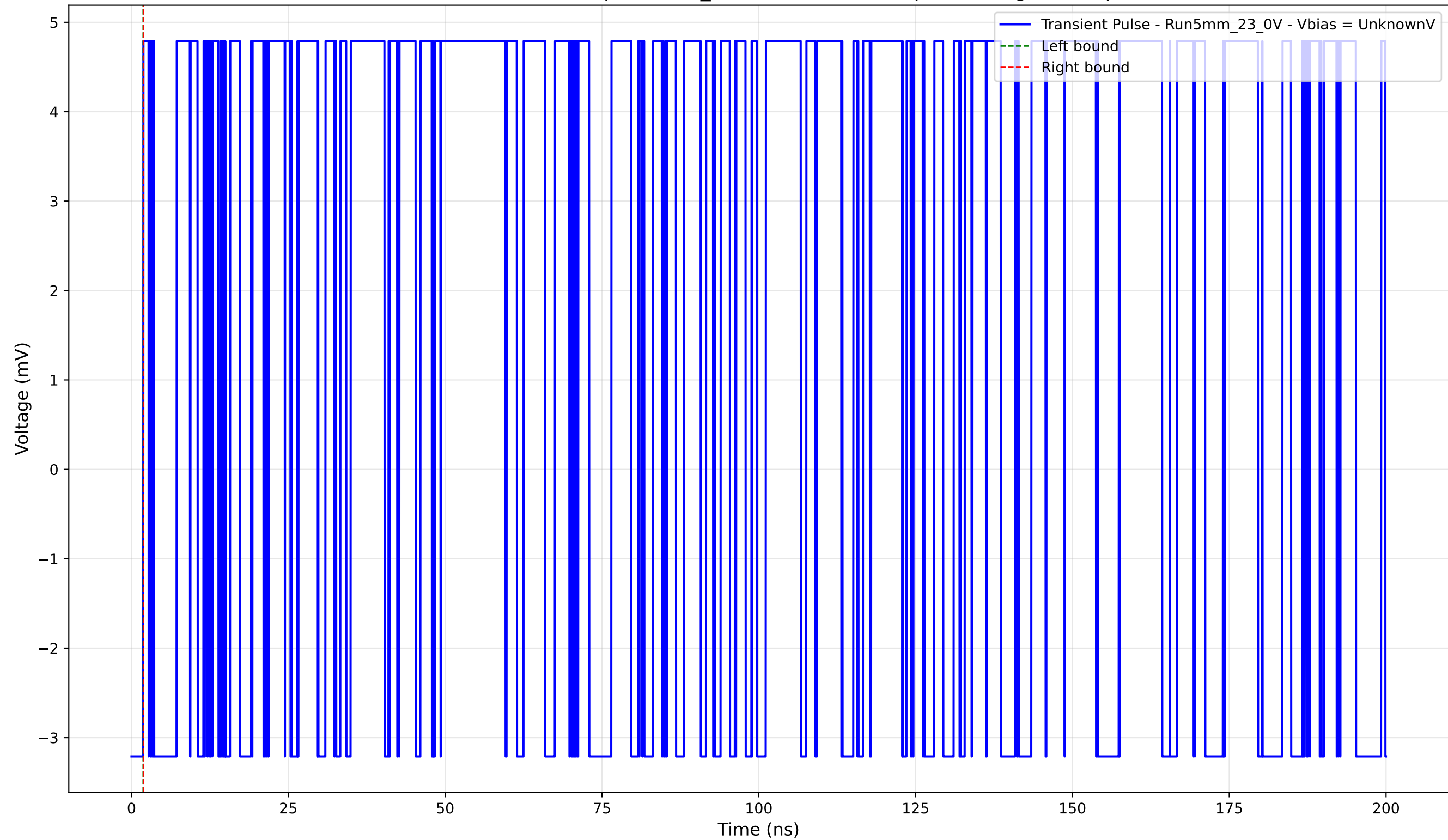
Transient Pulse - Sample: 5mm_23 - Position: 670.0 \mu\text{m} - Charge: 0.00 pC
