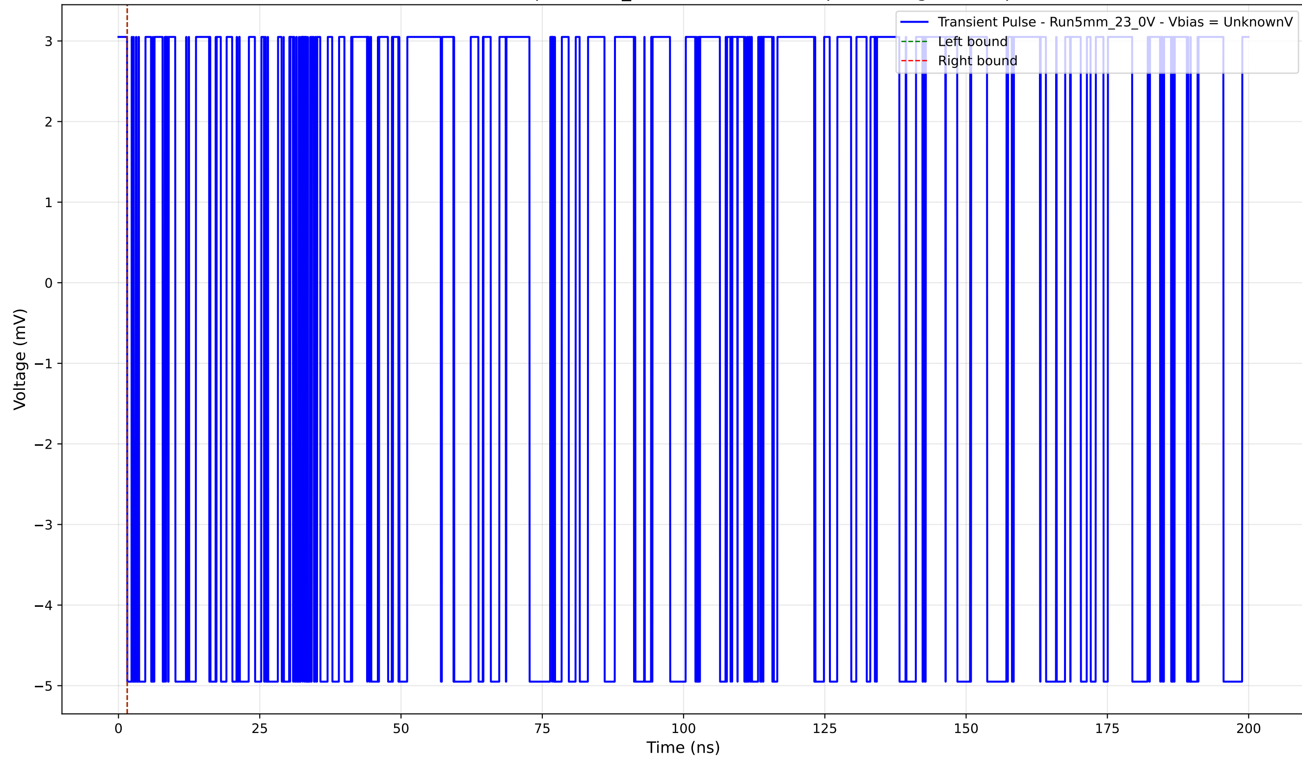
Transient Pulse - Sample: 5mm_23 - Position: 4825.0 \mu\text{m} - Charge: -0.00 pC
