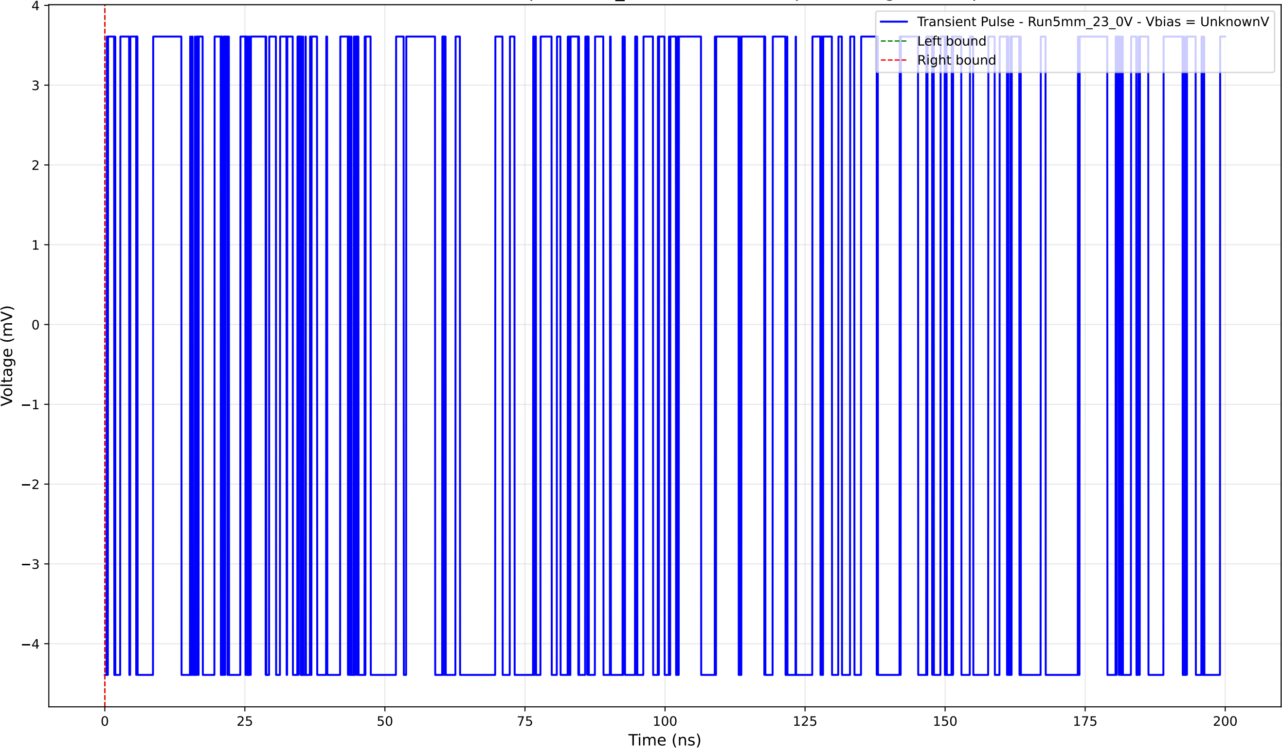
Transient Pulse - Sample: 5mm_23 - Position: 95.0 \mu\text{m} - Charge: -0.00 pC
