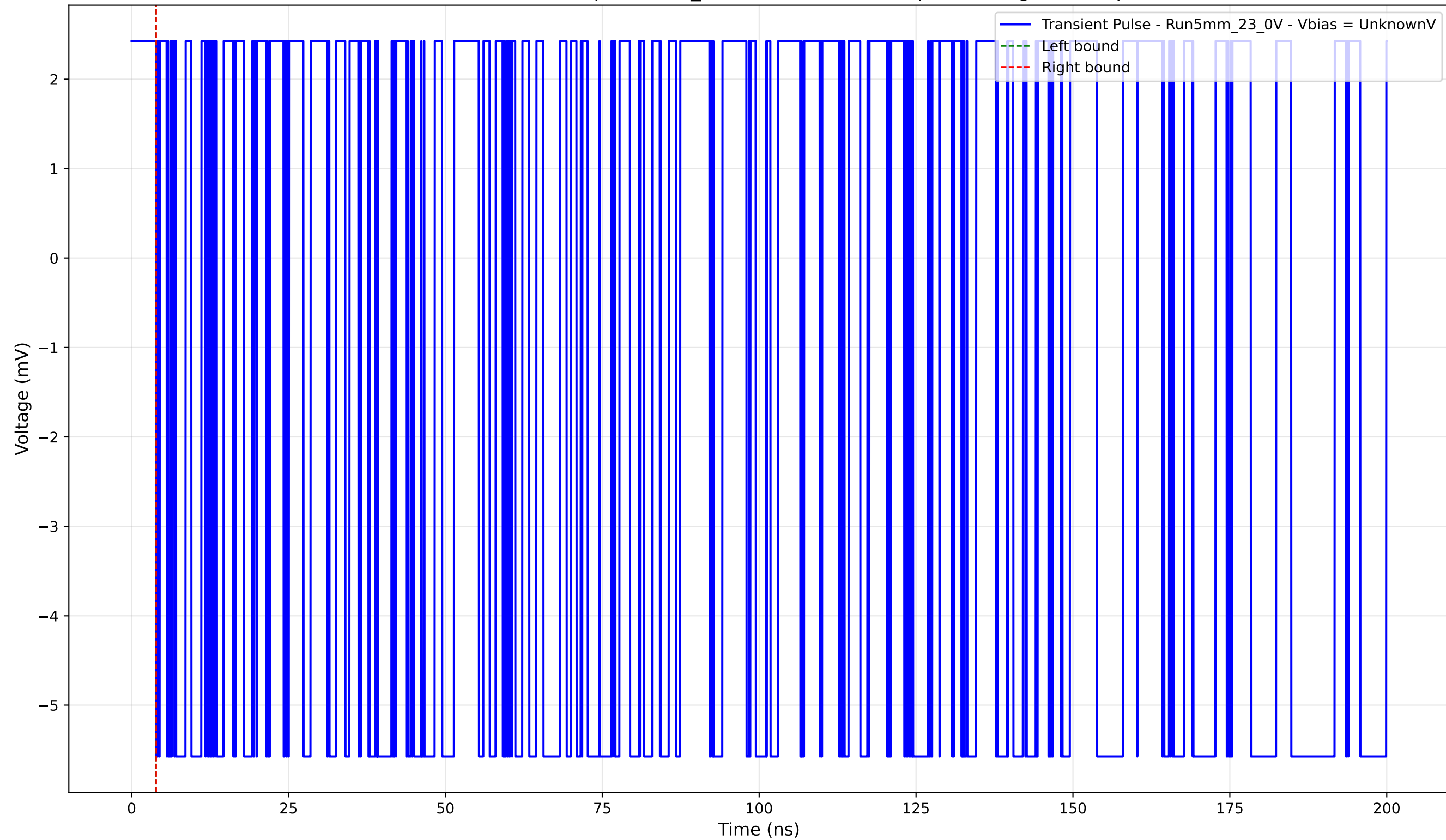
Transient Pulse - Sample: 5mm_23 - Position: 3765.0 \mu\text{m} - Charge: -0.00 pC
