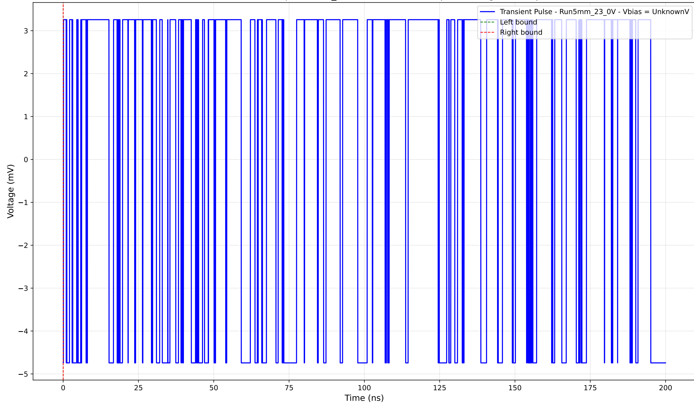
Transient Pulse - Sample: 5mm_23 - Position: 1190.0 \mu\text{m} - Charge: -0.00 pC
