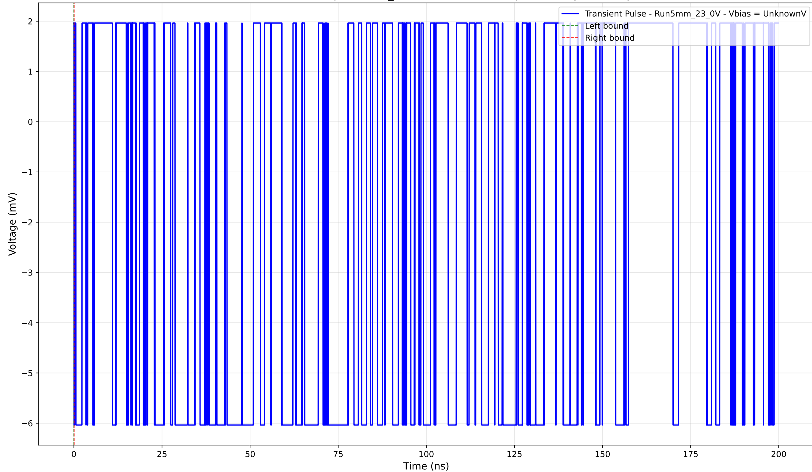
Transient Pulse - Sample: 5mm_23 - Position: 3510.0 \mu\text{m} - Charge: -0.00 pC
