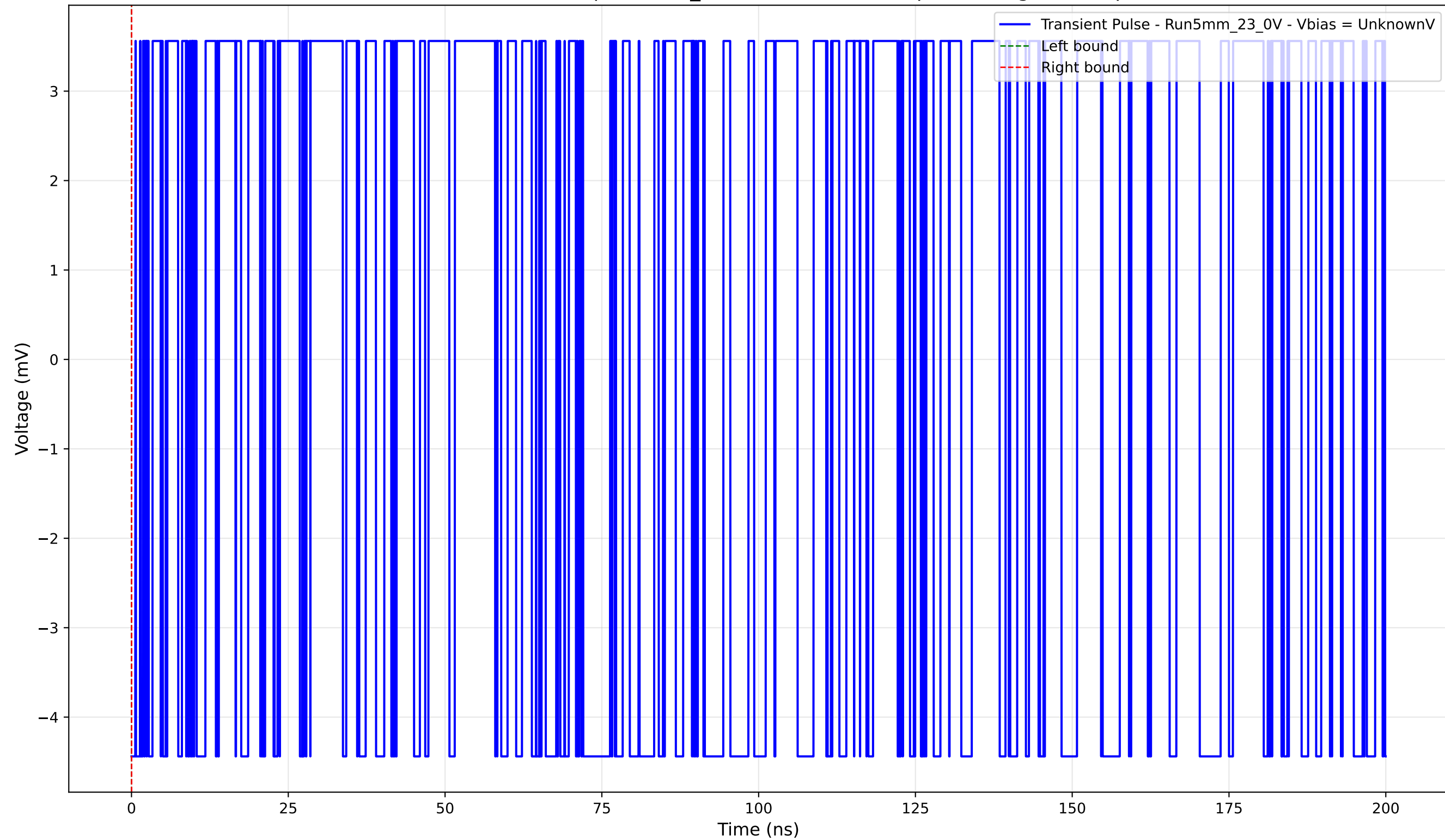
Transient Pulse - Sample: 5mm_23 - Position: 2340.0 \mu\text{m} - Charge: -0.00 pC
