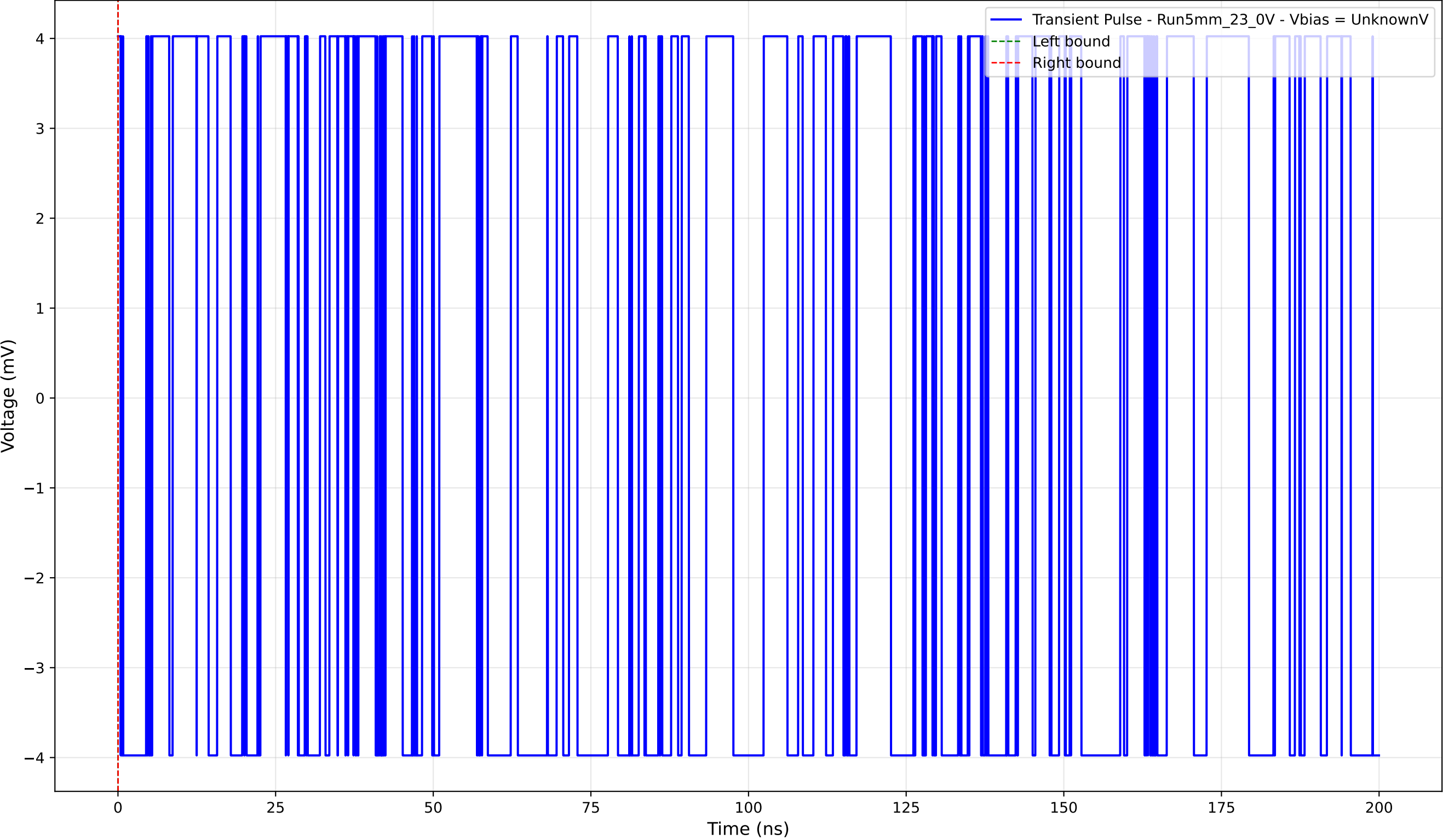
Transient Pulse - Sample: 5mm_23 - Position: 460.0 \mu\text{m} - Charge: 0.00 pC
