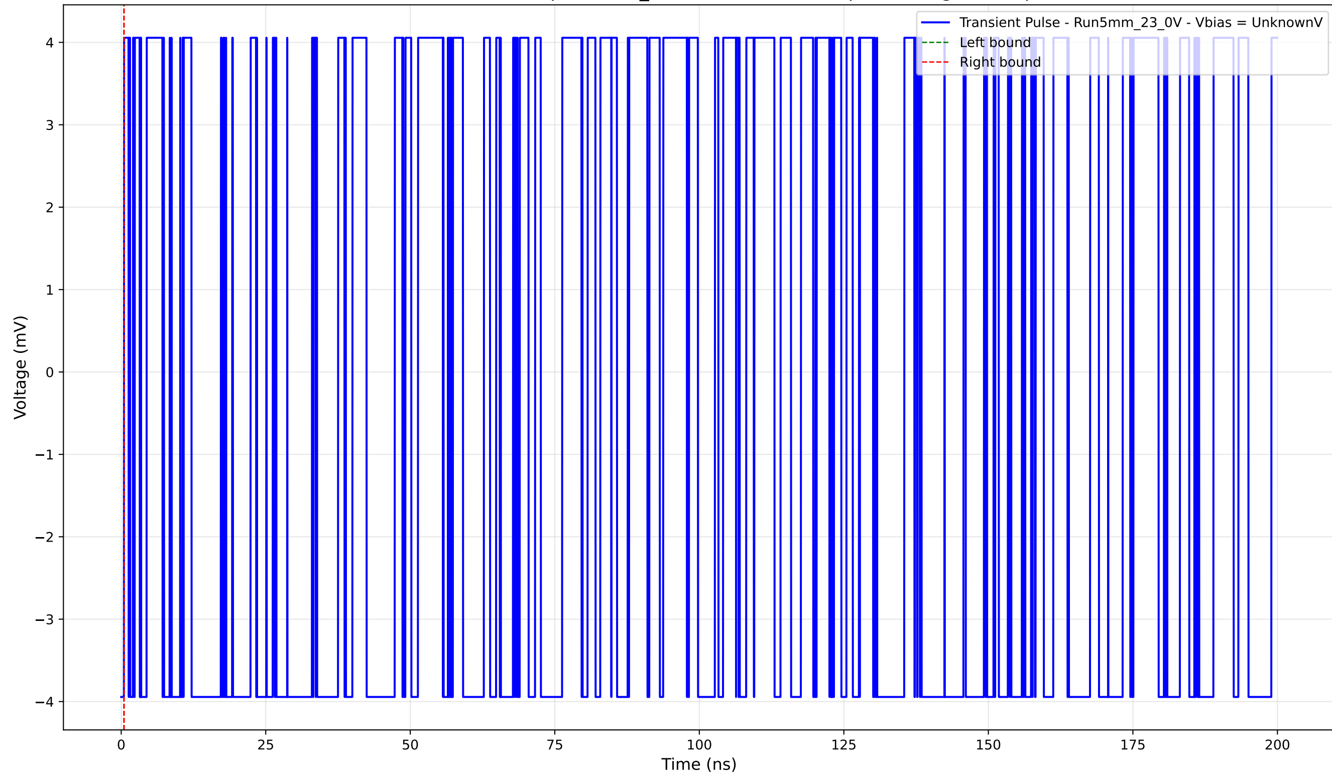
Transient Pulse - Sample: 5mm_23 - Position: 2745.0 \mu\text{m} - Charge: 0.00 pC
