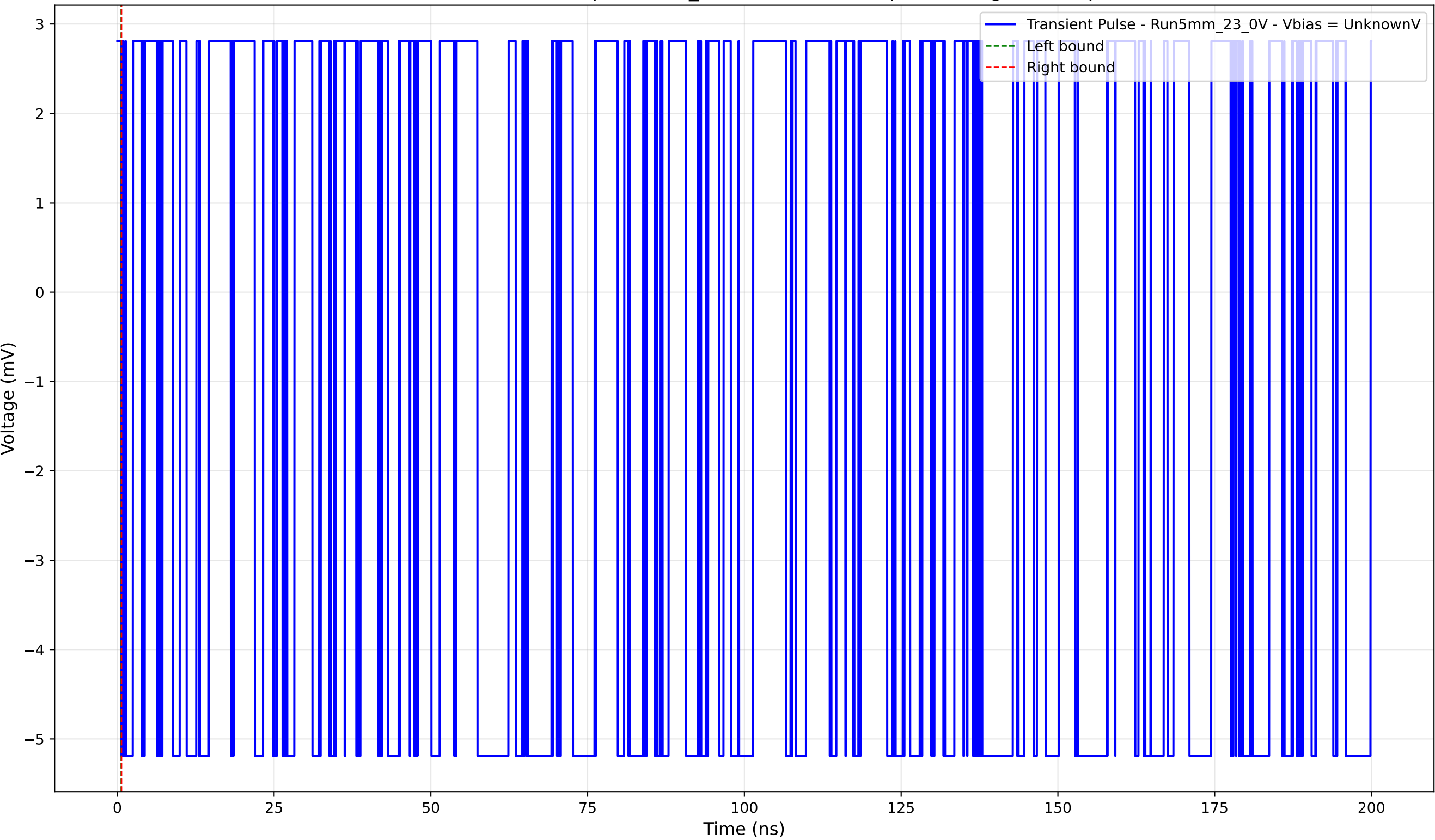
Transient Pulse - Sample: 5mm_23 - Position: 65.0 \mu\text{m} - Charge: -0.00 pC
