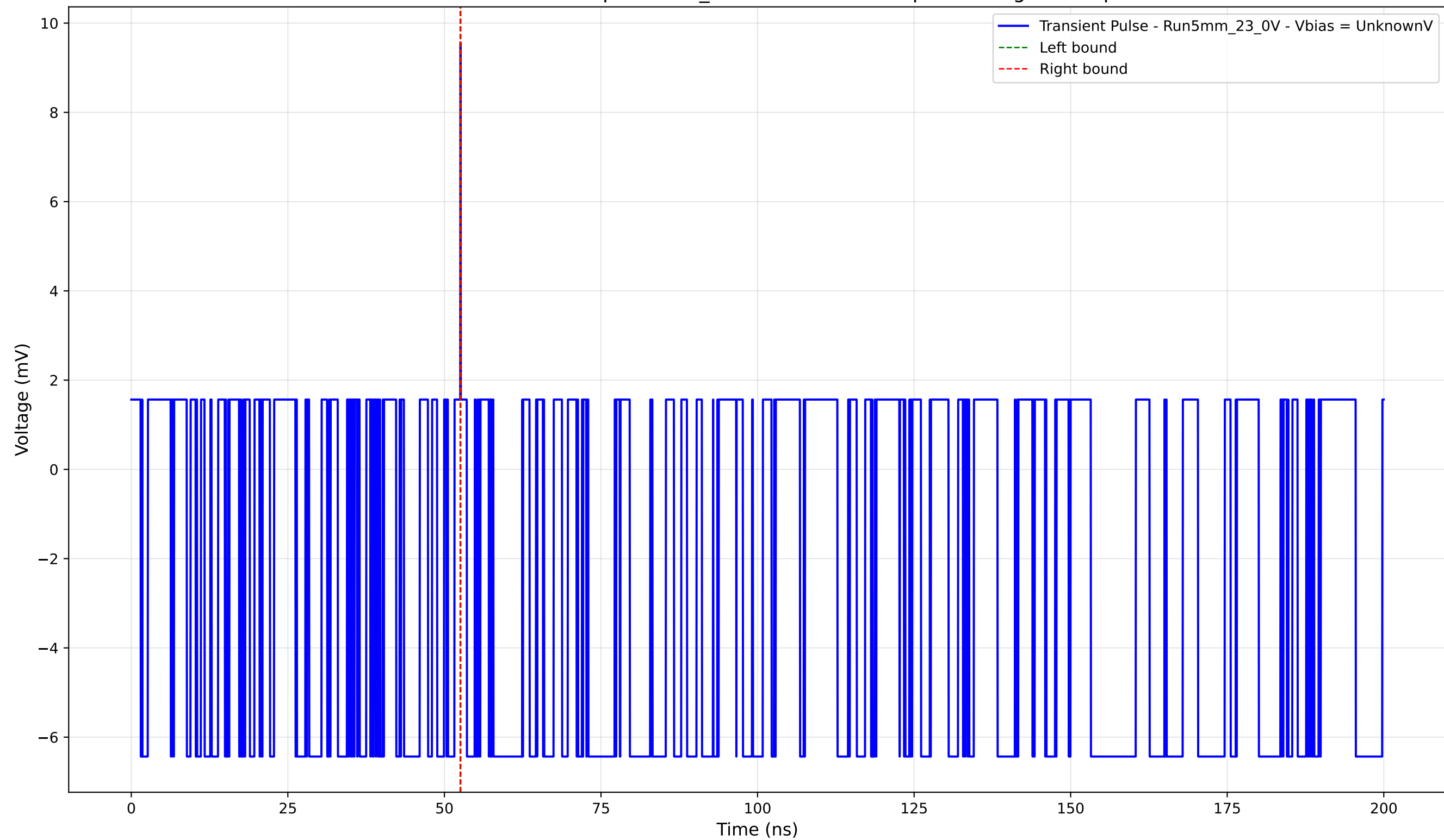
Transient Pulse - Sample: 5mm_23 - Position: 385.0 \mu\text{m} - Charge: 0.01 pC
