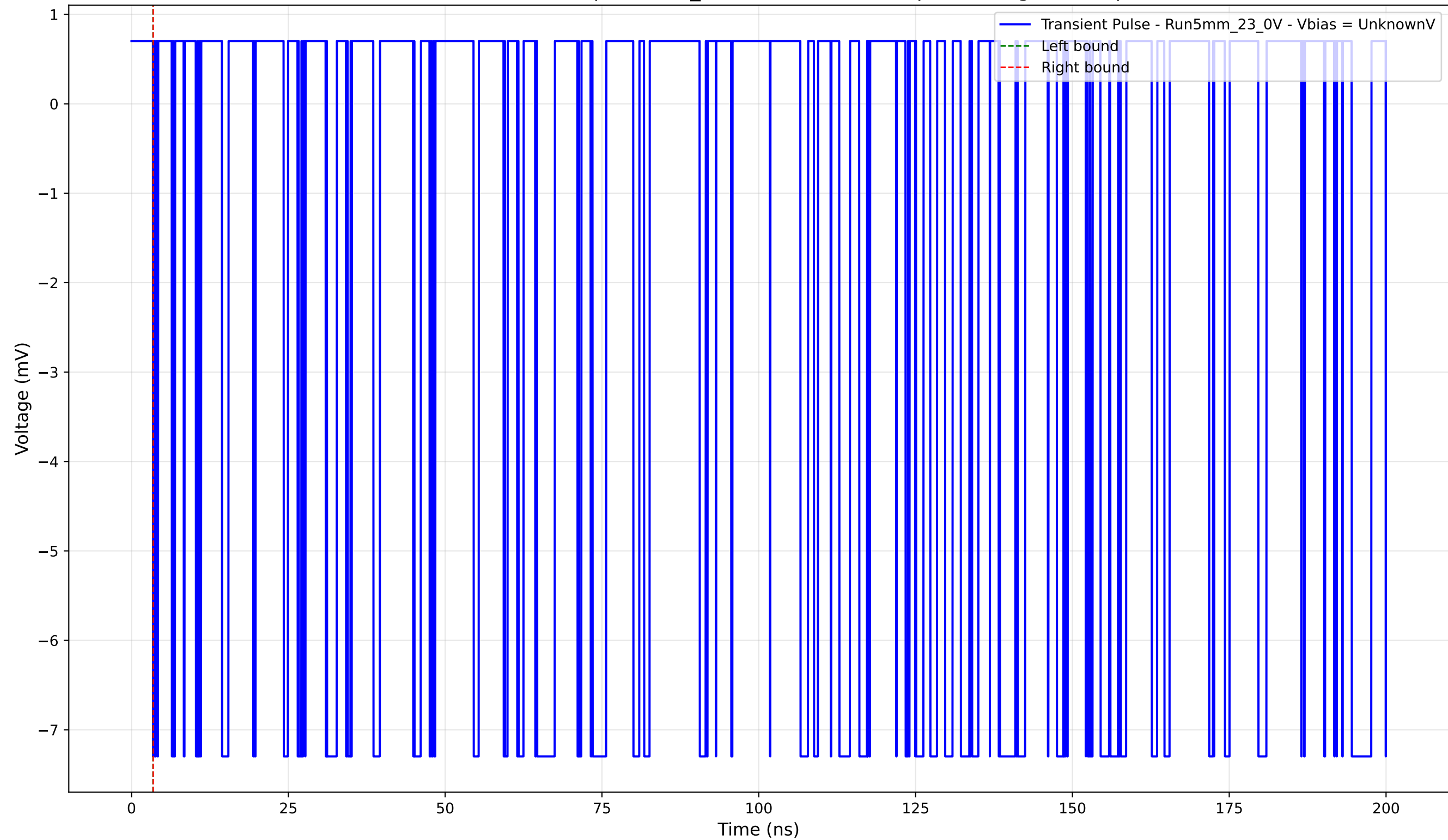
Transient Pulse - Sample: 5mm_23 - Position: 3340.0 \mu\text{m} - Charge: -0.00 pC
