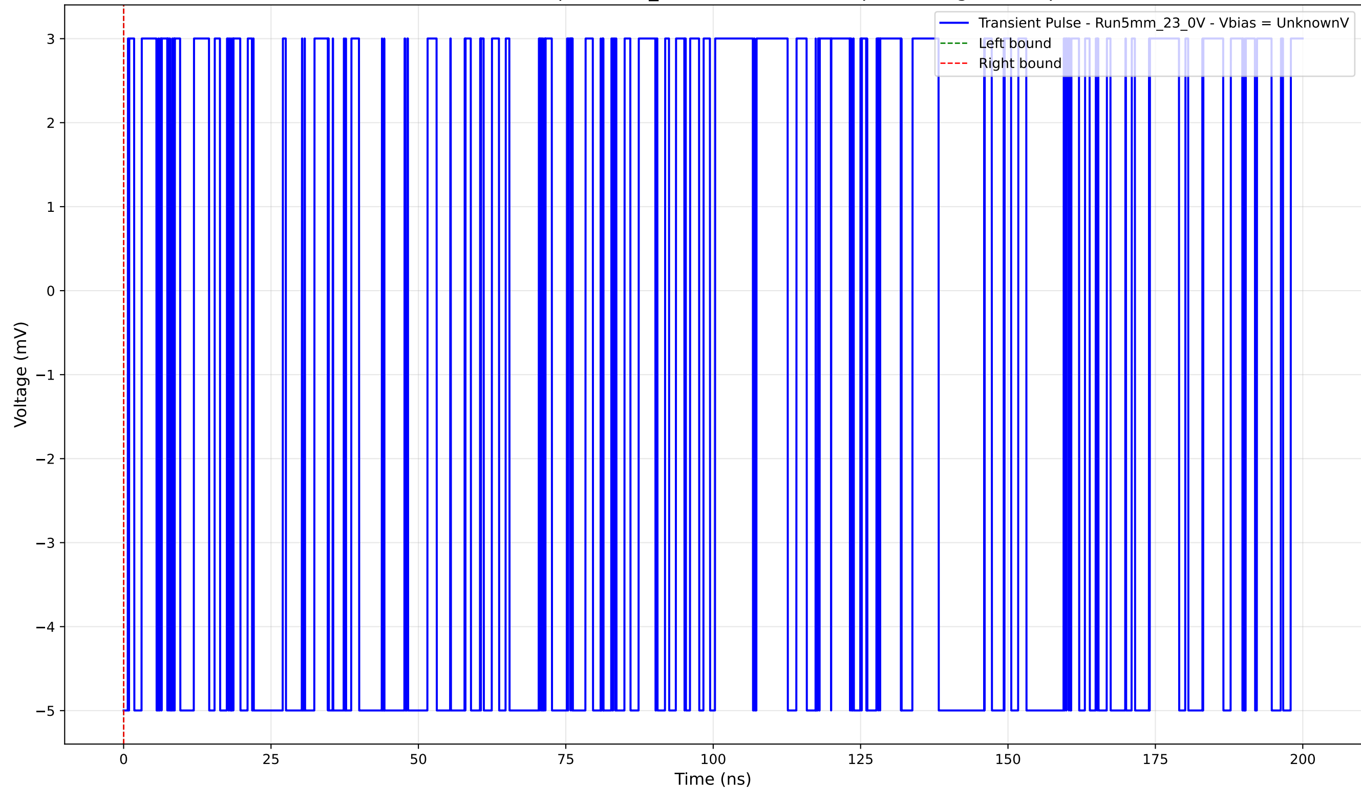
Transient Pulse - Sample: 5mm_23 - Position: 4990.0 \mu\text{m} - Charge: -0.00 pC
