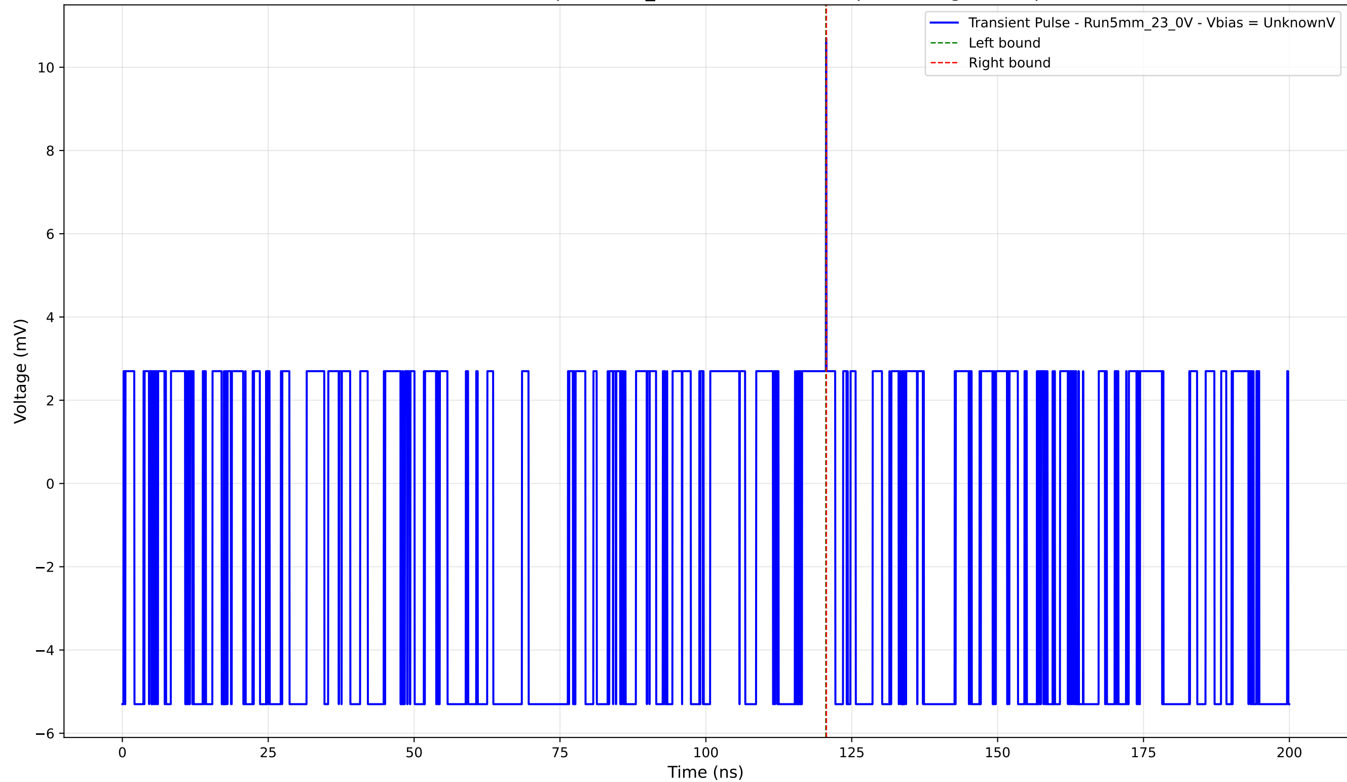
Transient Pulse - Sample: 5mm_23 - Position: 4685.0 \mu\text{m} - Charge: 0.02 pC
