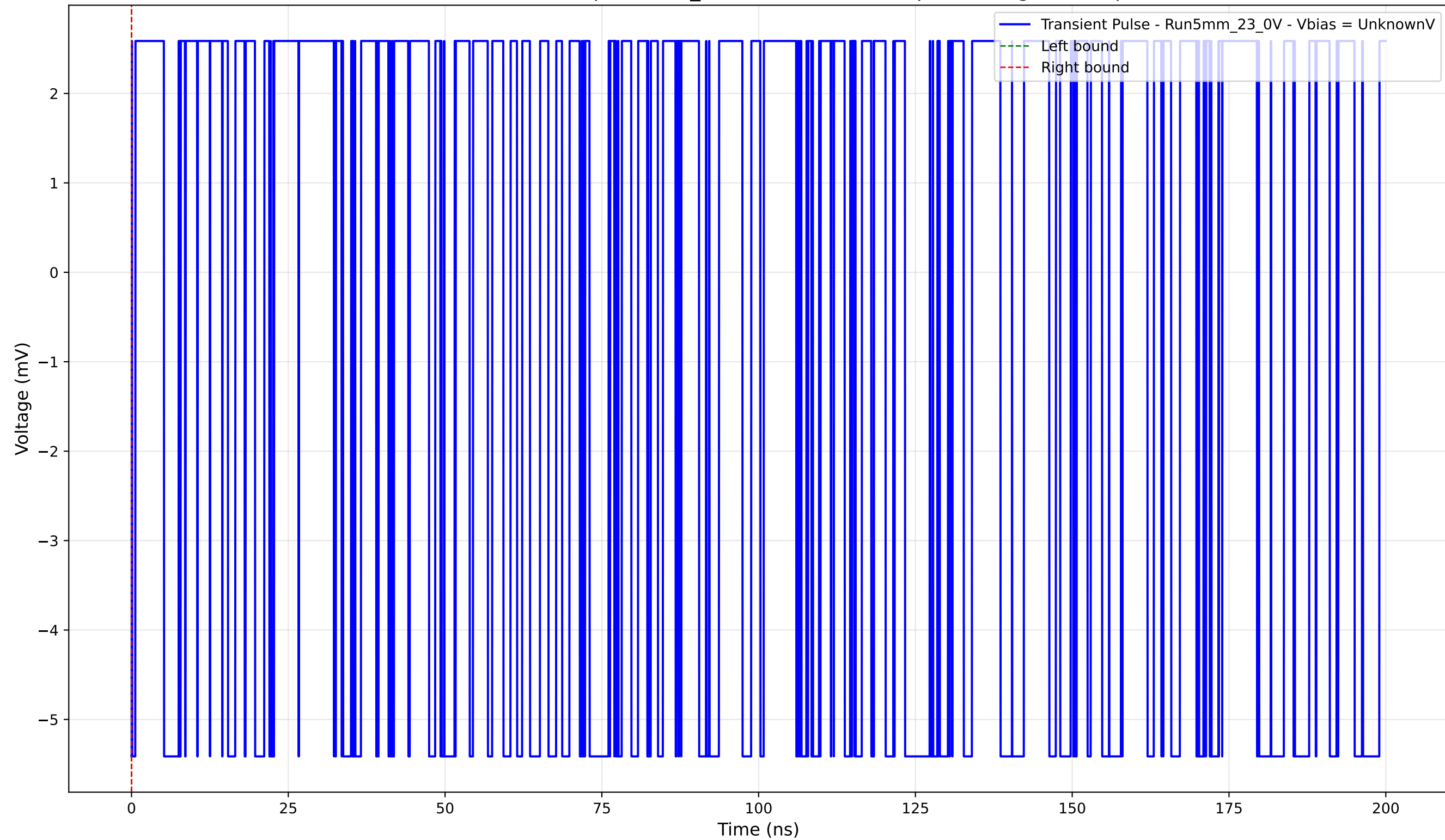
Transient Pulse - Sample: 5mm_23 - Position: 1735.0 \mu\text{m} - Charge: -0.00 pC
