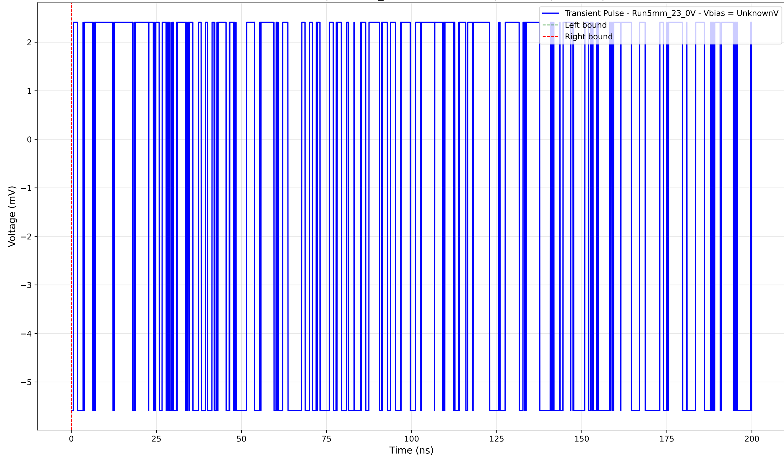
Transient Pulse - Sample: 5mm_23 - Position: 125.0 \mu\text{m} - Charge: -0.00 pC
