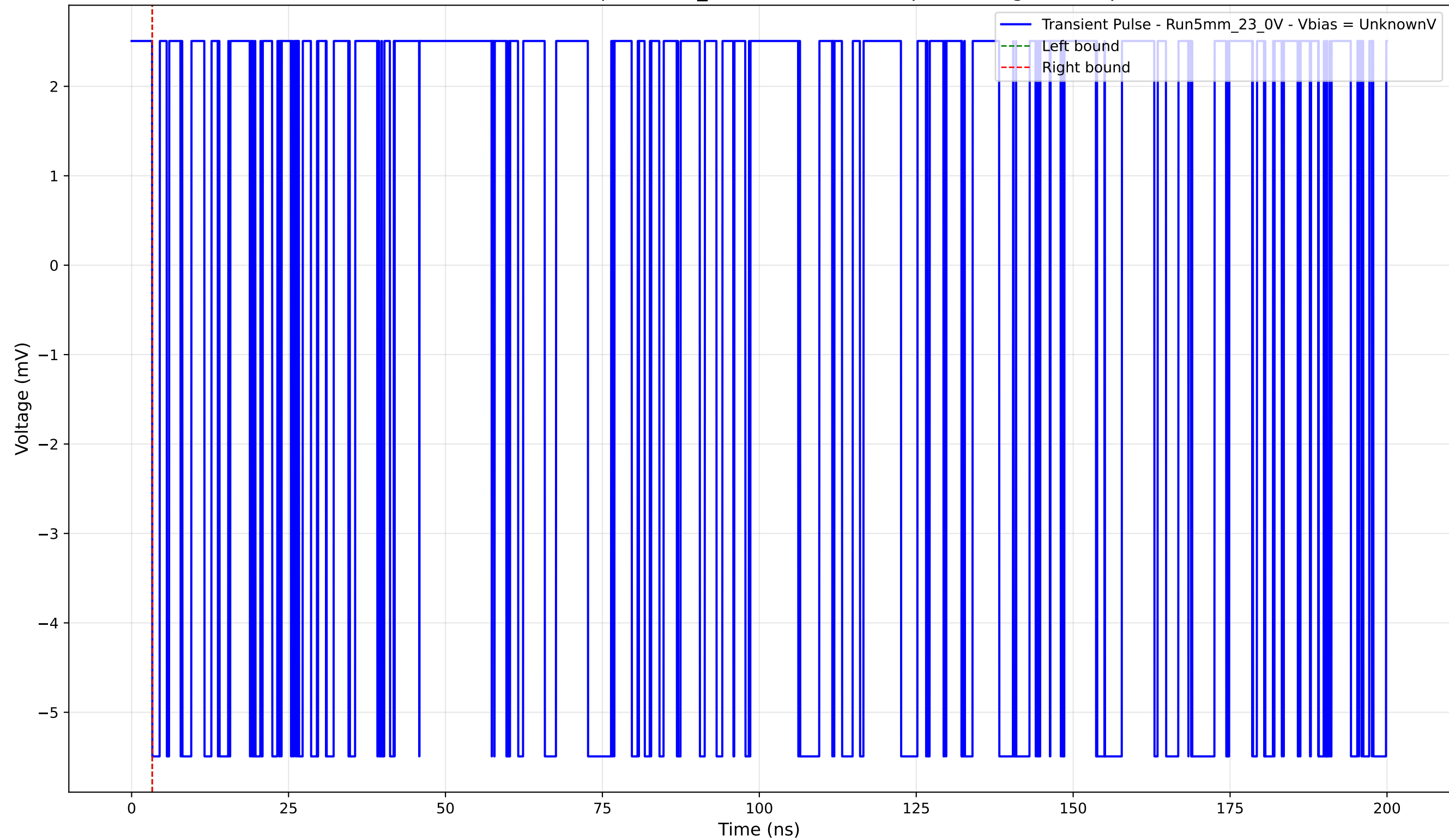
Transient Pulse - Sample: 5mm_23 - Position: 240.0 \mu\text{m} - Charge: -0.00 pC
