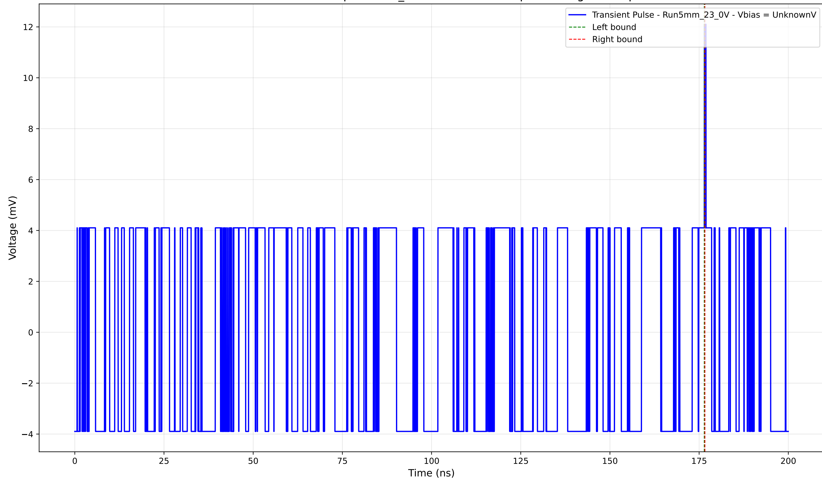
Transient Pulse - Sample: 5mm_23 - Position: 590.0 \mu\text{m} - Charge: 0.04 pC
