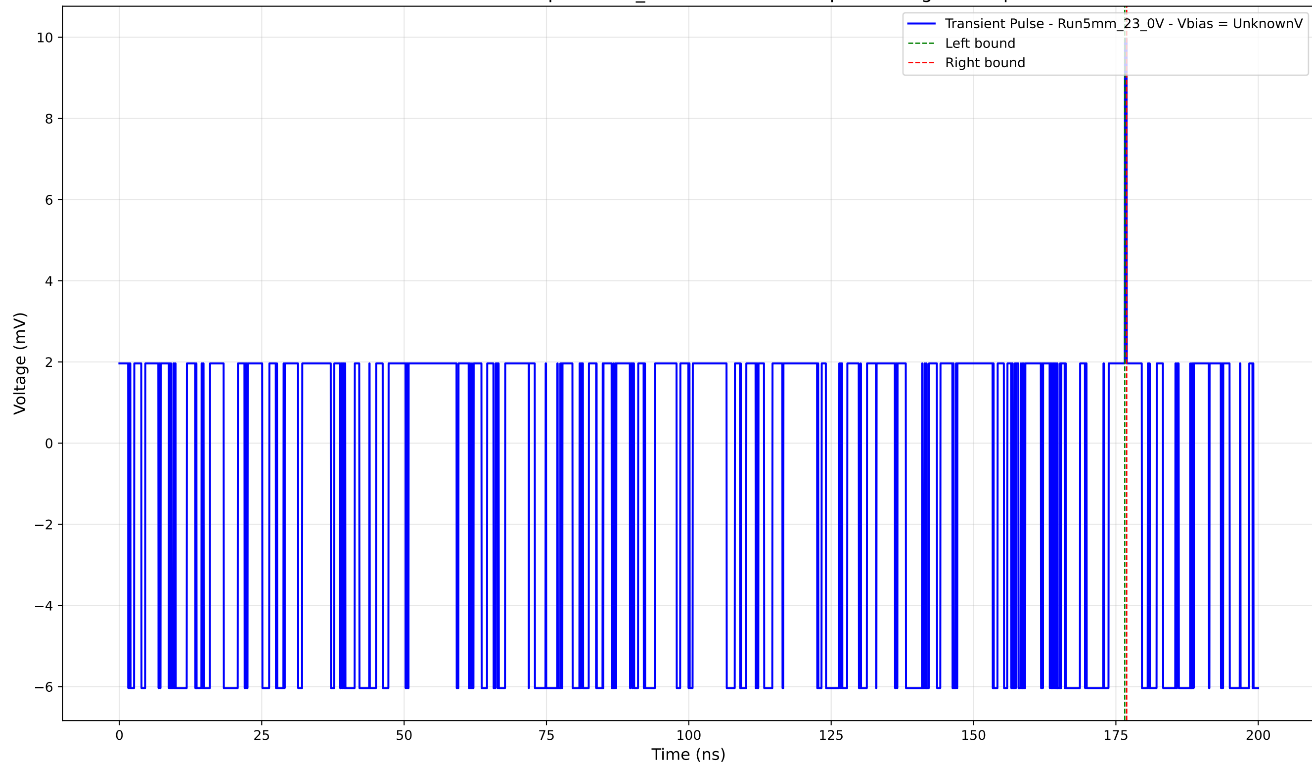
Transient Pulse - Sample: 5mm_23 - Position: 105.0 \mu\text{m} - Charge: 0.06 pC
