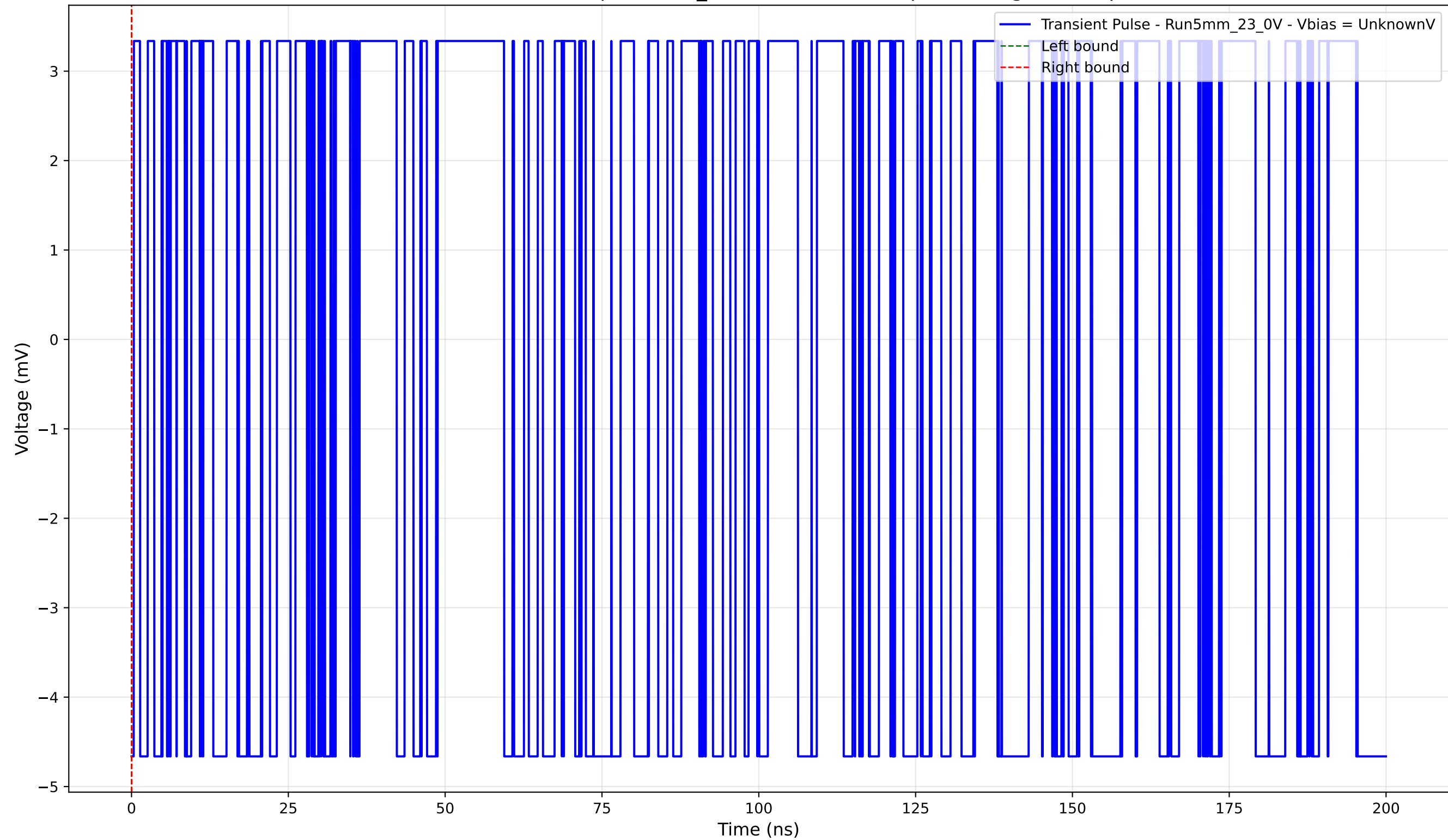
Transient Pulse - Sample: 5mm_23 - Position: 420.0 \mu\text{m} - Charge: -0.00 pC
