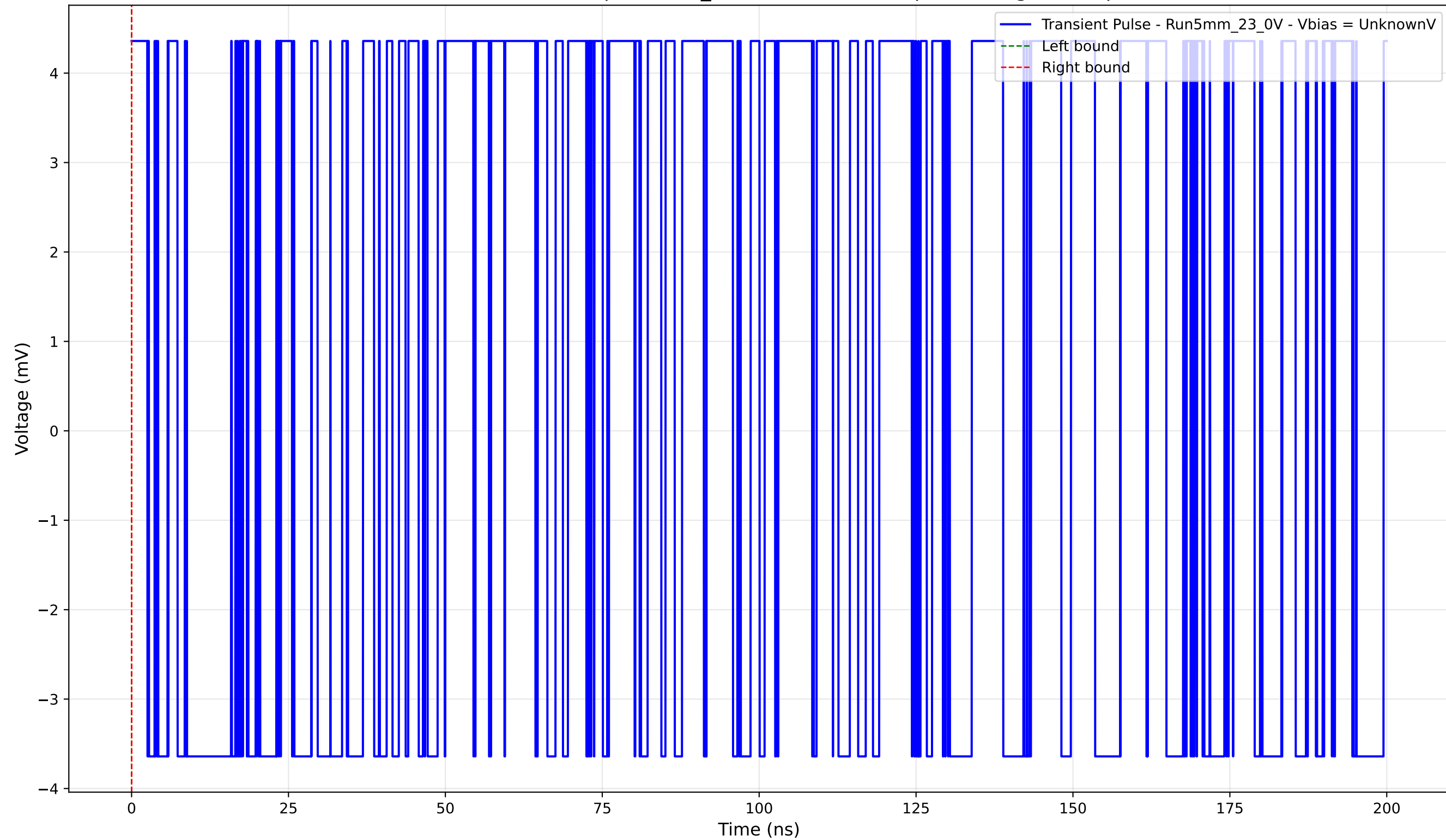
Transient Pulse - Sample: 5mm_23 - Position: 645.0 \mu\text{m} - Charge: 0.00 pC
