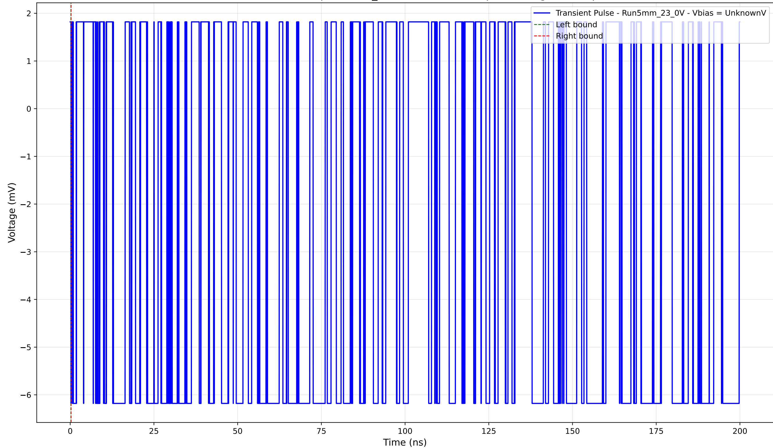
Transient Pulse - Sample: 5mm_23 - Position: 500.0 \mu\text{m} - Charge: -0.00 pC
