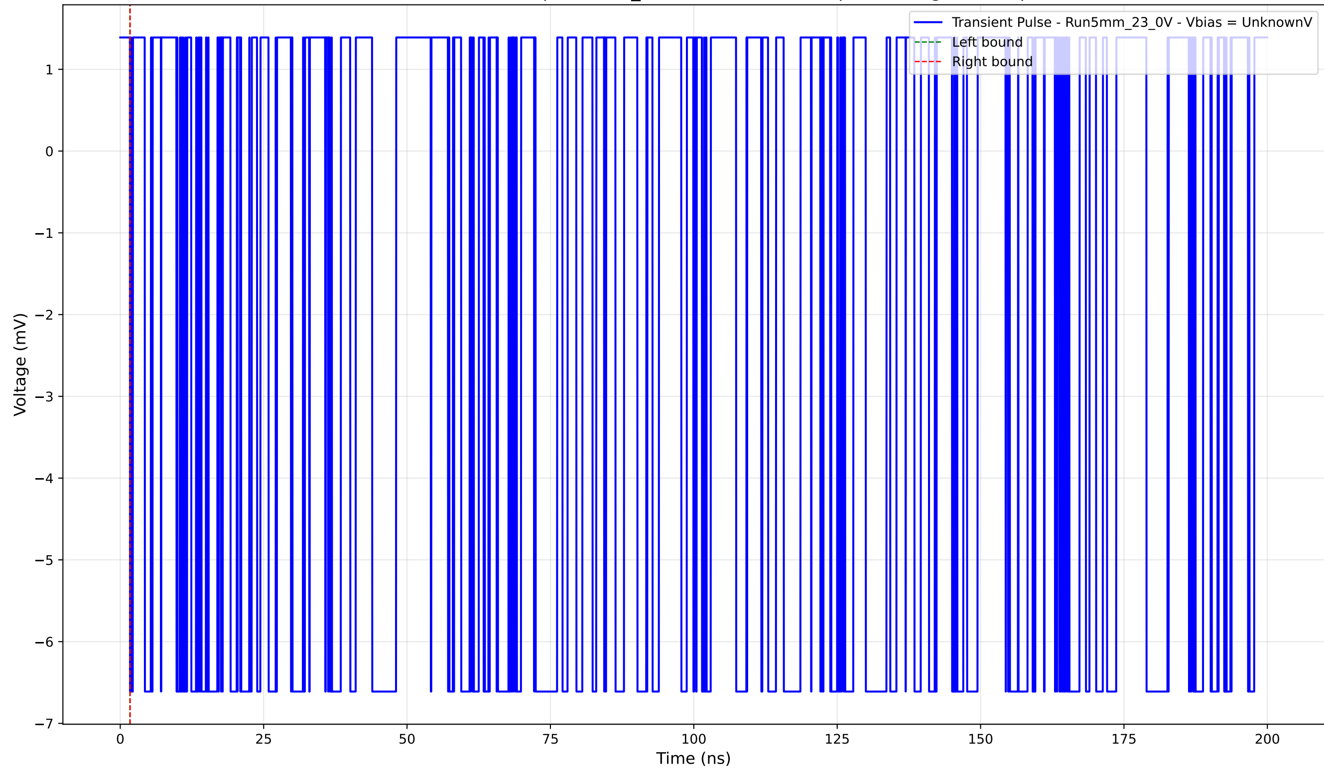
Transient Pulse - Sample: 5mm_23 - Position: 1710.0 \mu\text{m} - Charge: -0.00 pC
