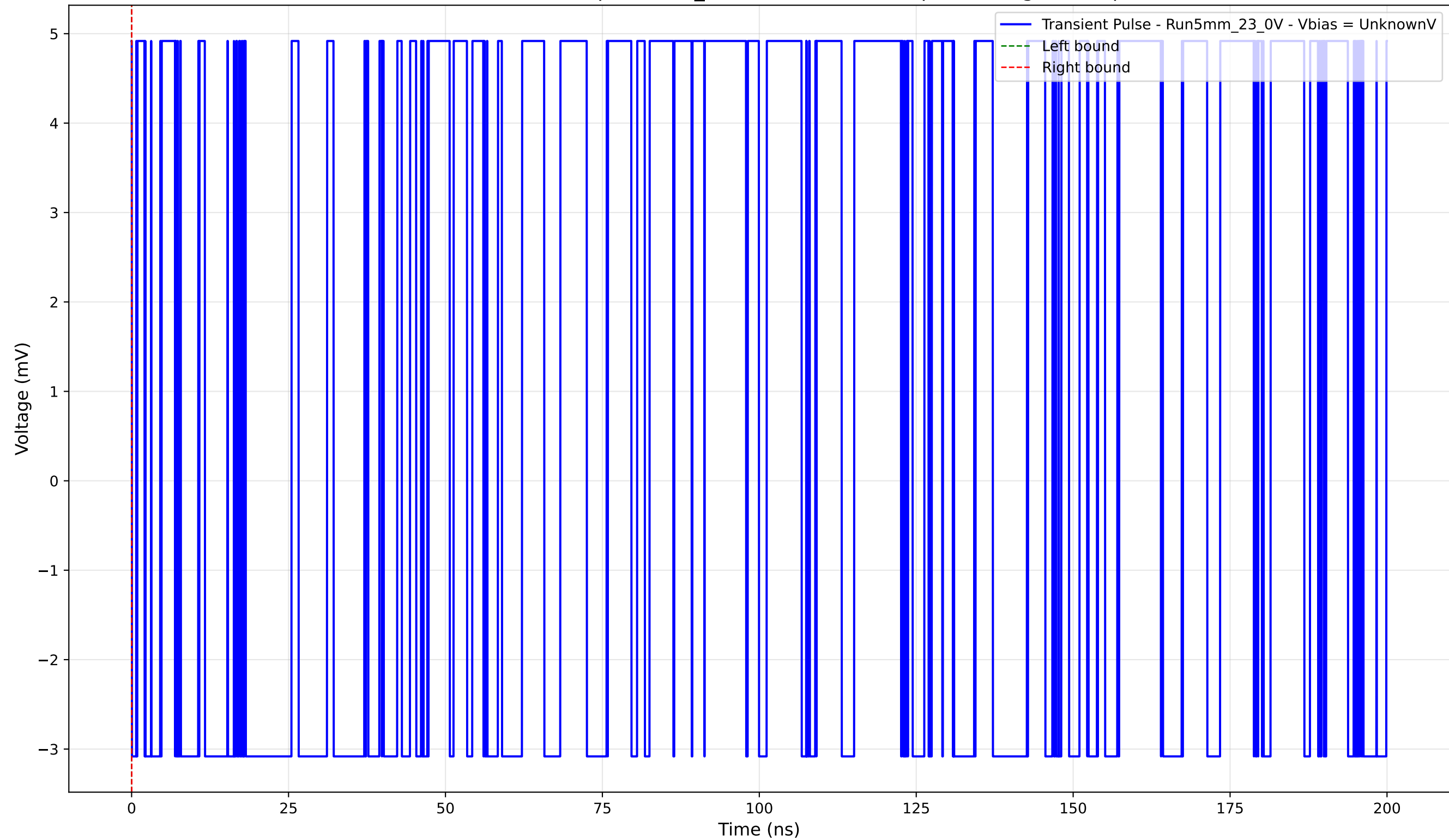
Transient Pulse - Sample: 5mm_23 - Position: 3040.0 \mu\text{m} - Charge: 0.00 pC
