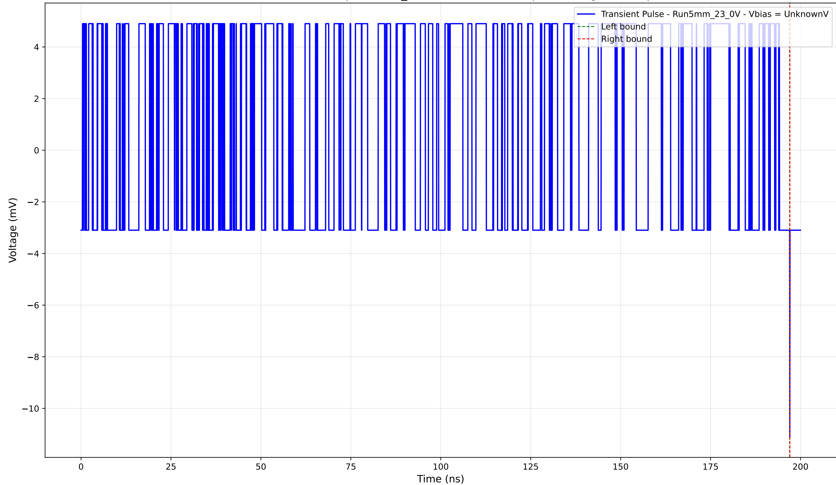
Transient Pulse - Sample: 5mm_23 - Position: 1290.0 \mu\text{m} - Charge: -0.01 pC
