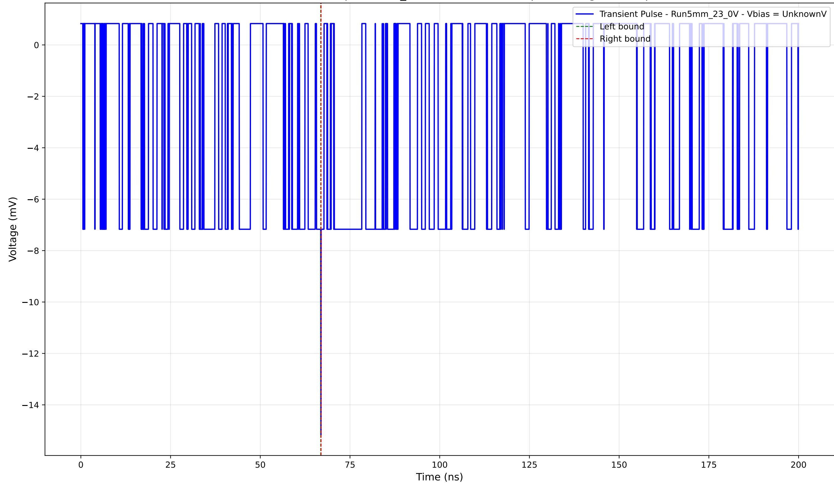
Transient Pulse - Sample: 5mm_23 - Position: 2795.0 \mu\text{m} - Charge: -0.03 pC
