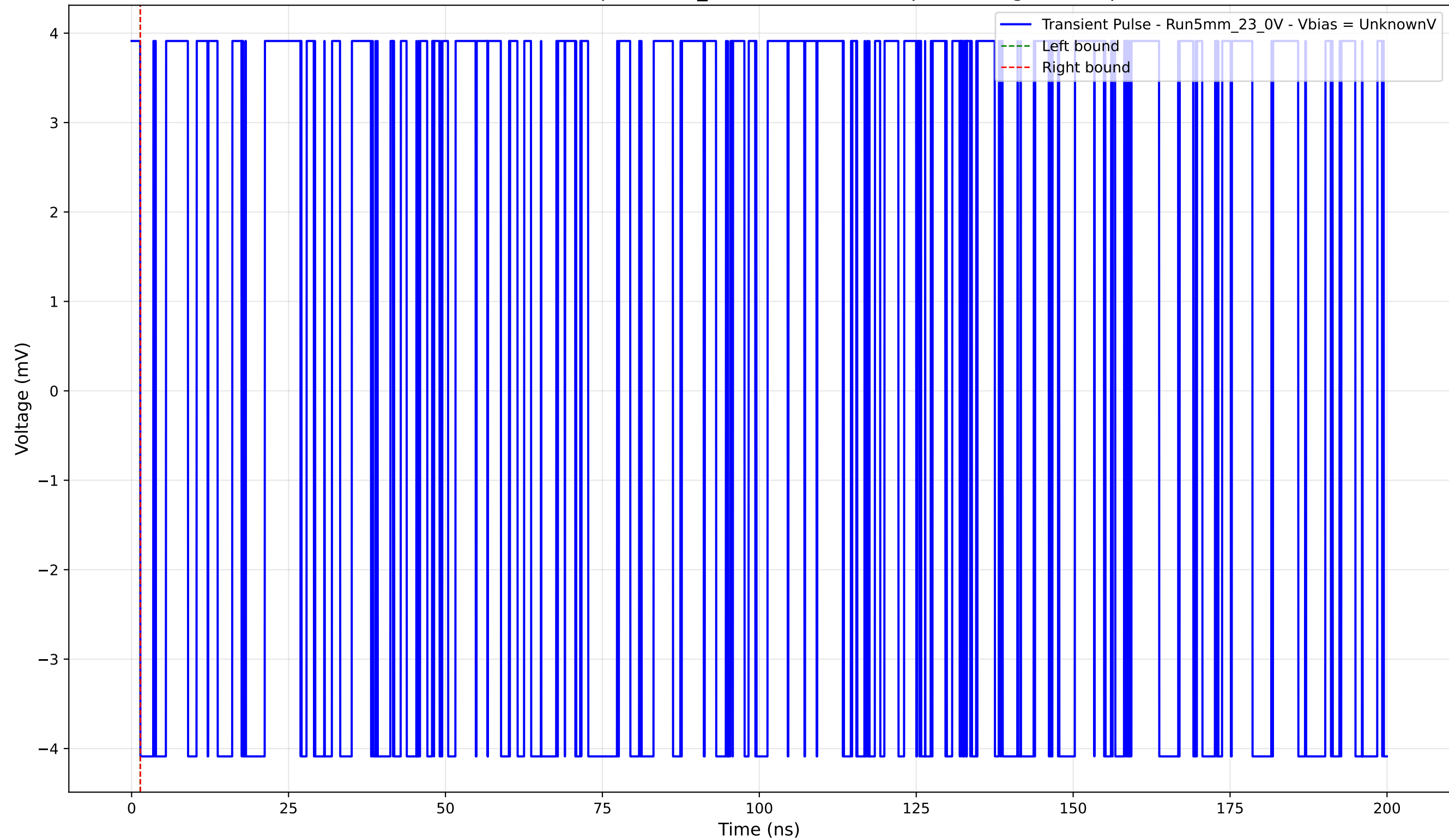
Transient Pulse - Sample: 5mm_23 - Position: 470.0 \mu\text{m} - Charge: -0.00 pC
