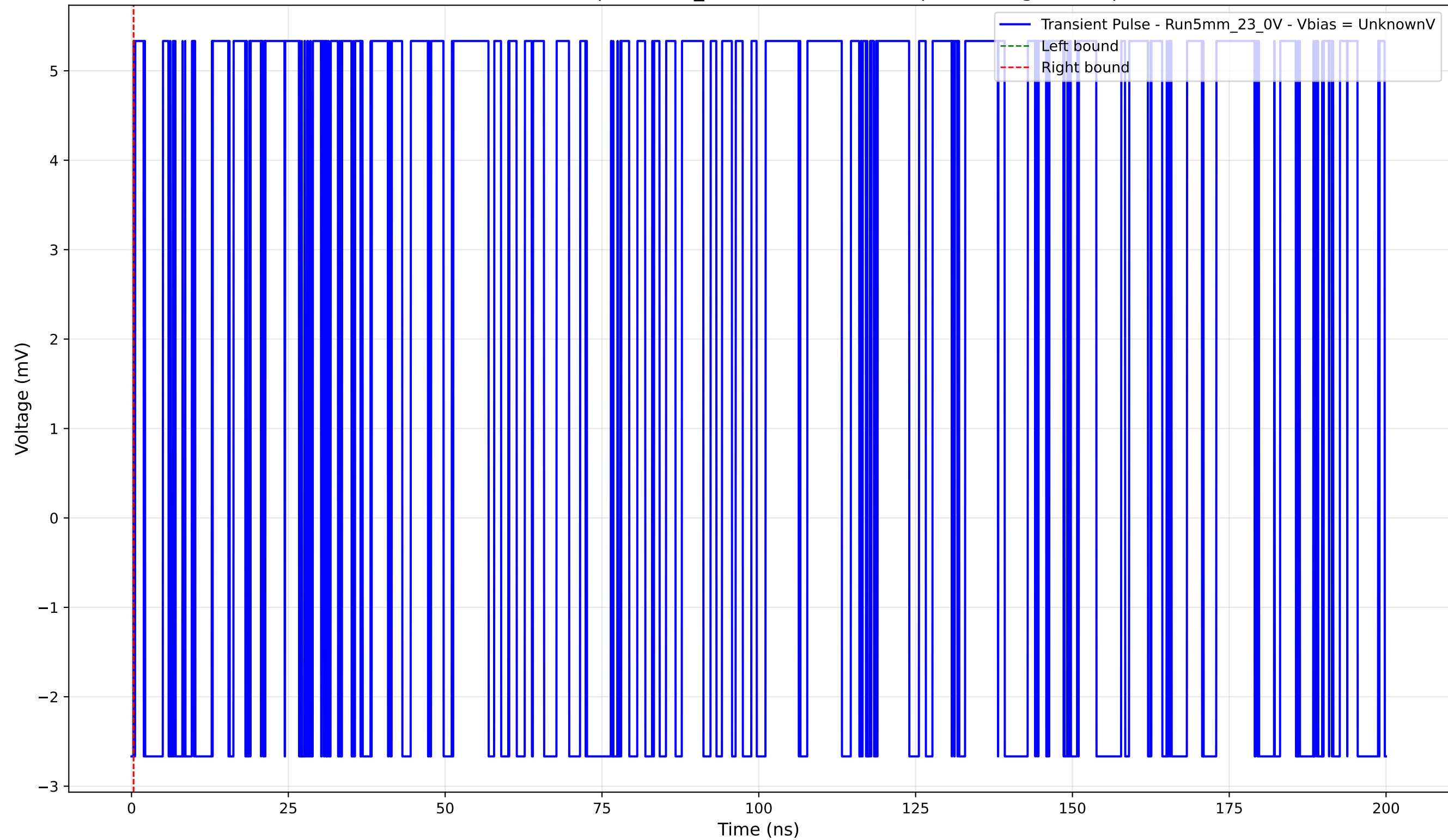
Transient Pulse - Sample: 5mm_23 - Position: 4980.0 \mu\text{m} - Charge: 0.00 pC
