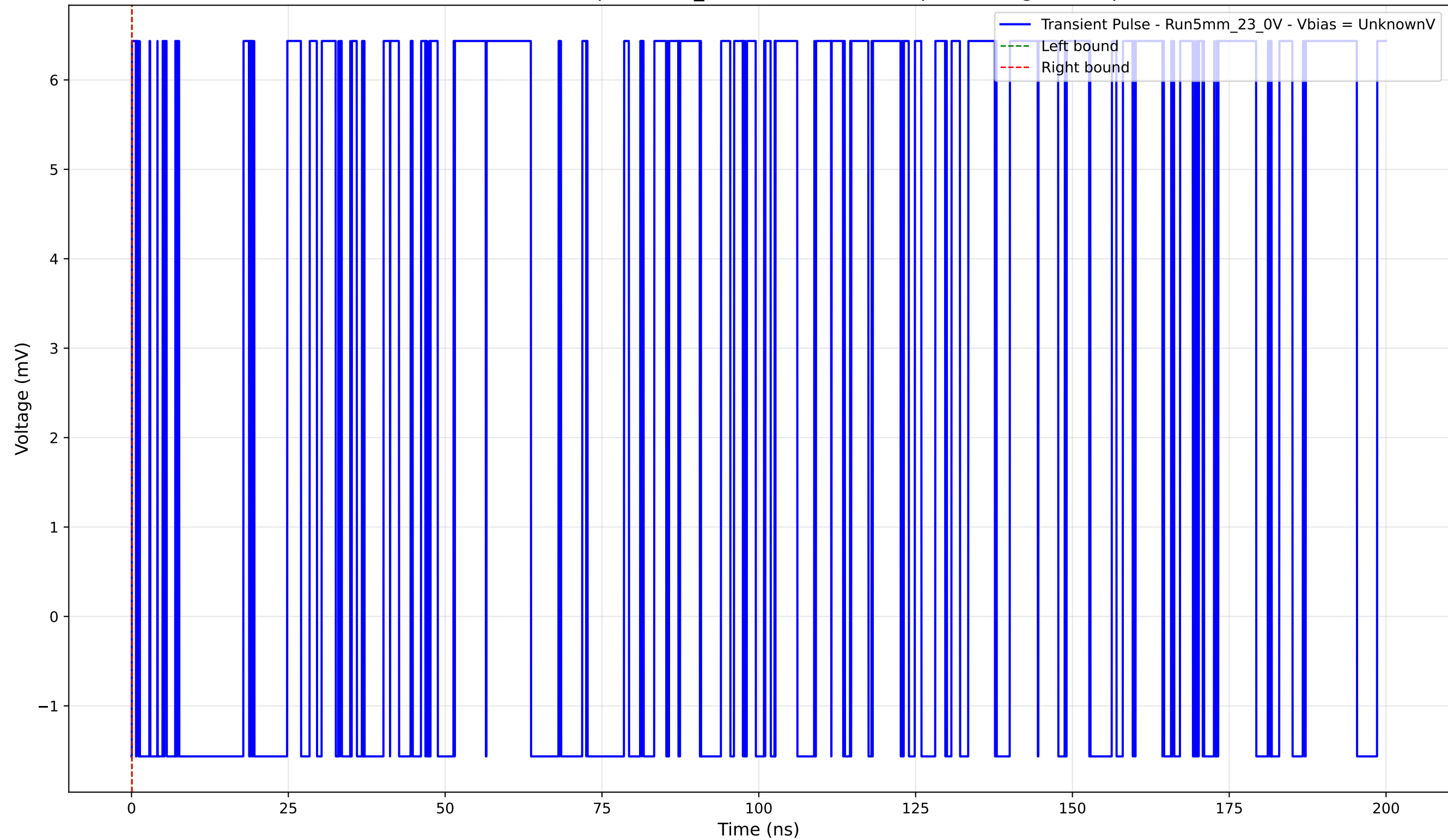
Transient Pulse - Sample: 5mm_23 - Position: 4030.0 \mu\text{m} - Charge: 0.00 pC
