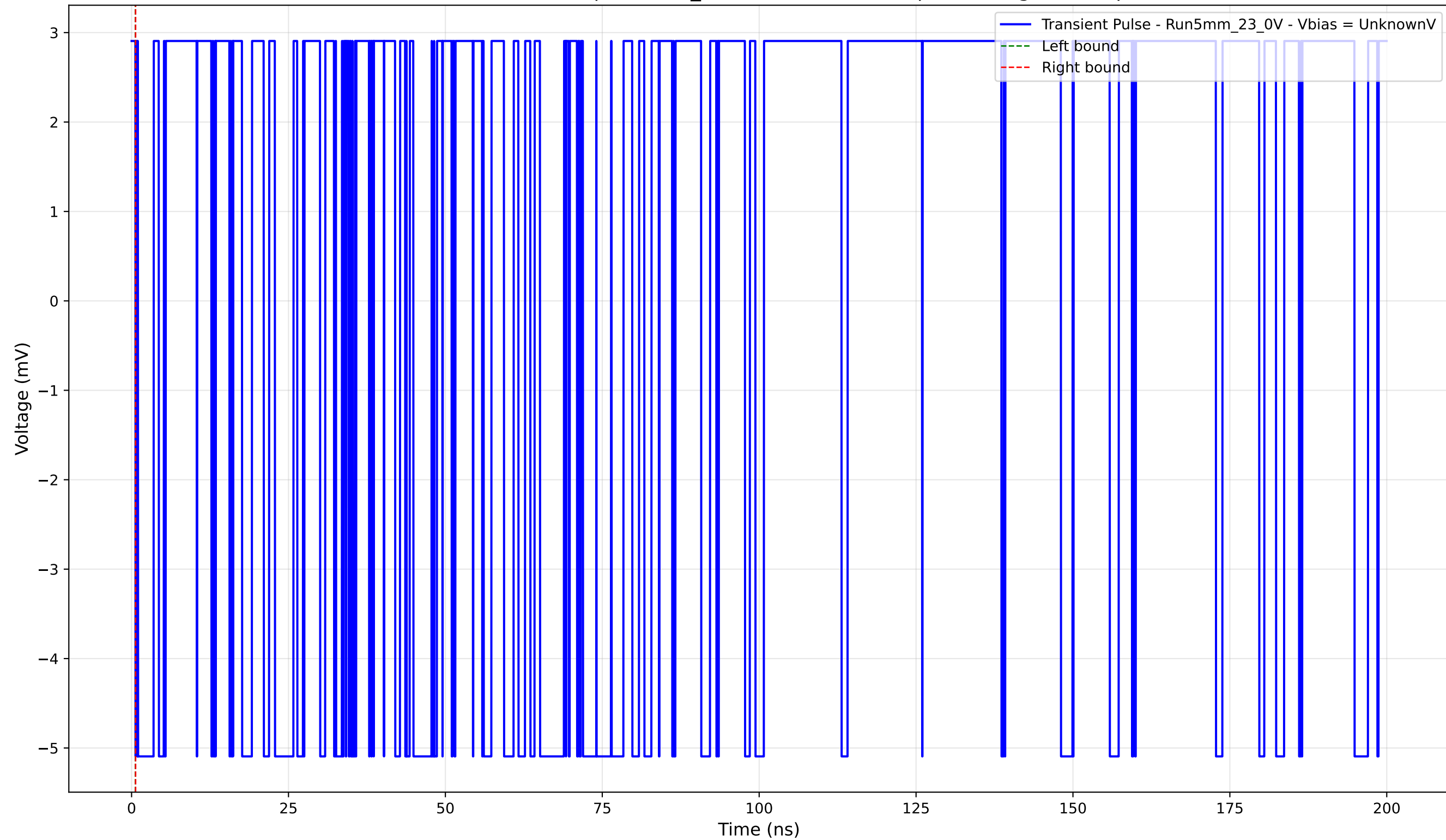
Transient Pulse - Sample: 5mm_23 - Position: 2820.0 \mu\text{m} - Charge: -0.00 pC
