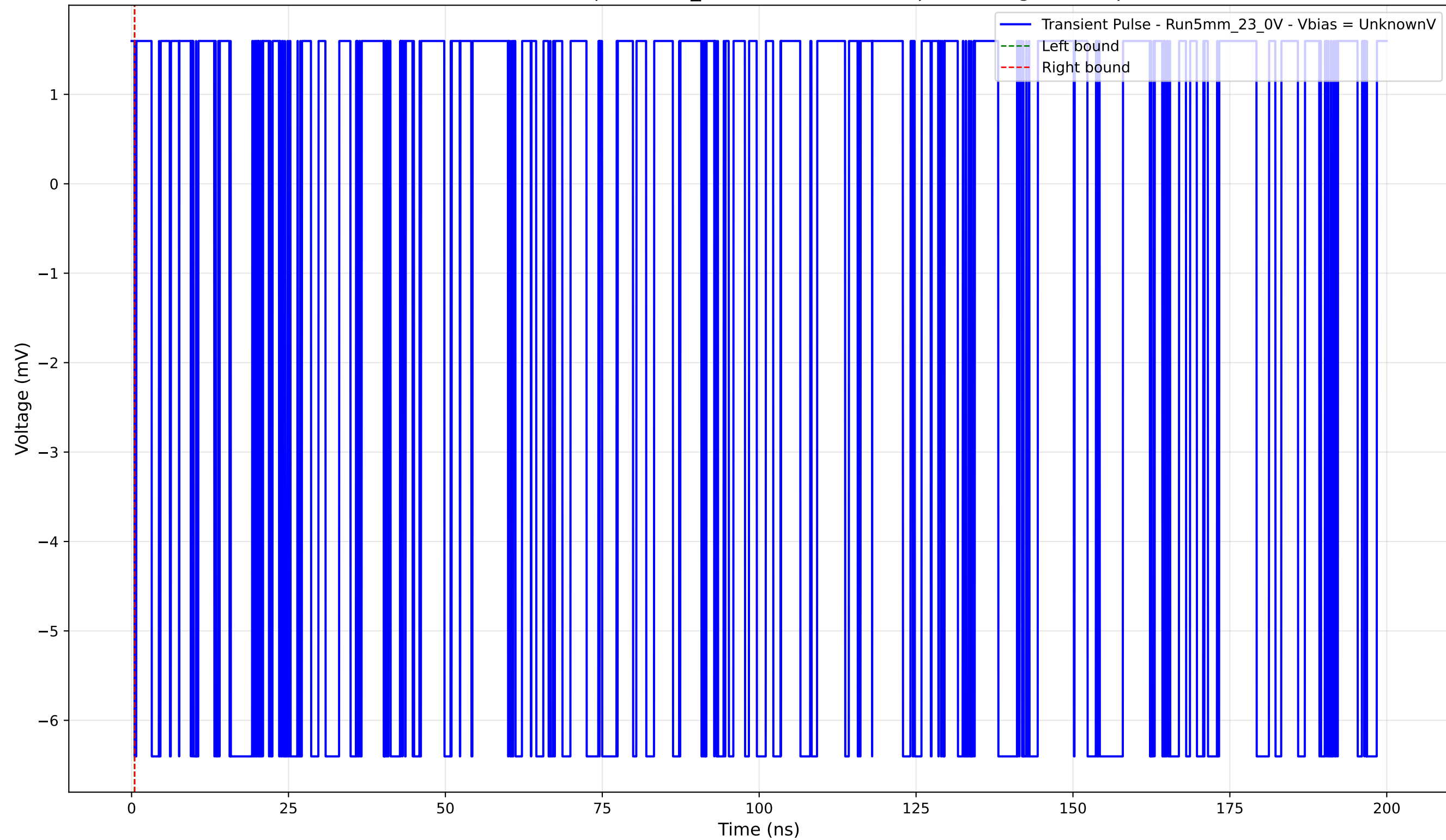
Transient Pulse - Sample: 5mm_23 - Position: 4275.0 \mu\text{m} - Charge: -0.00 pC
