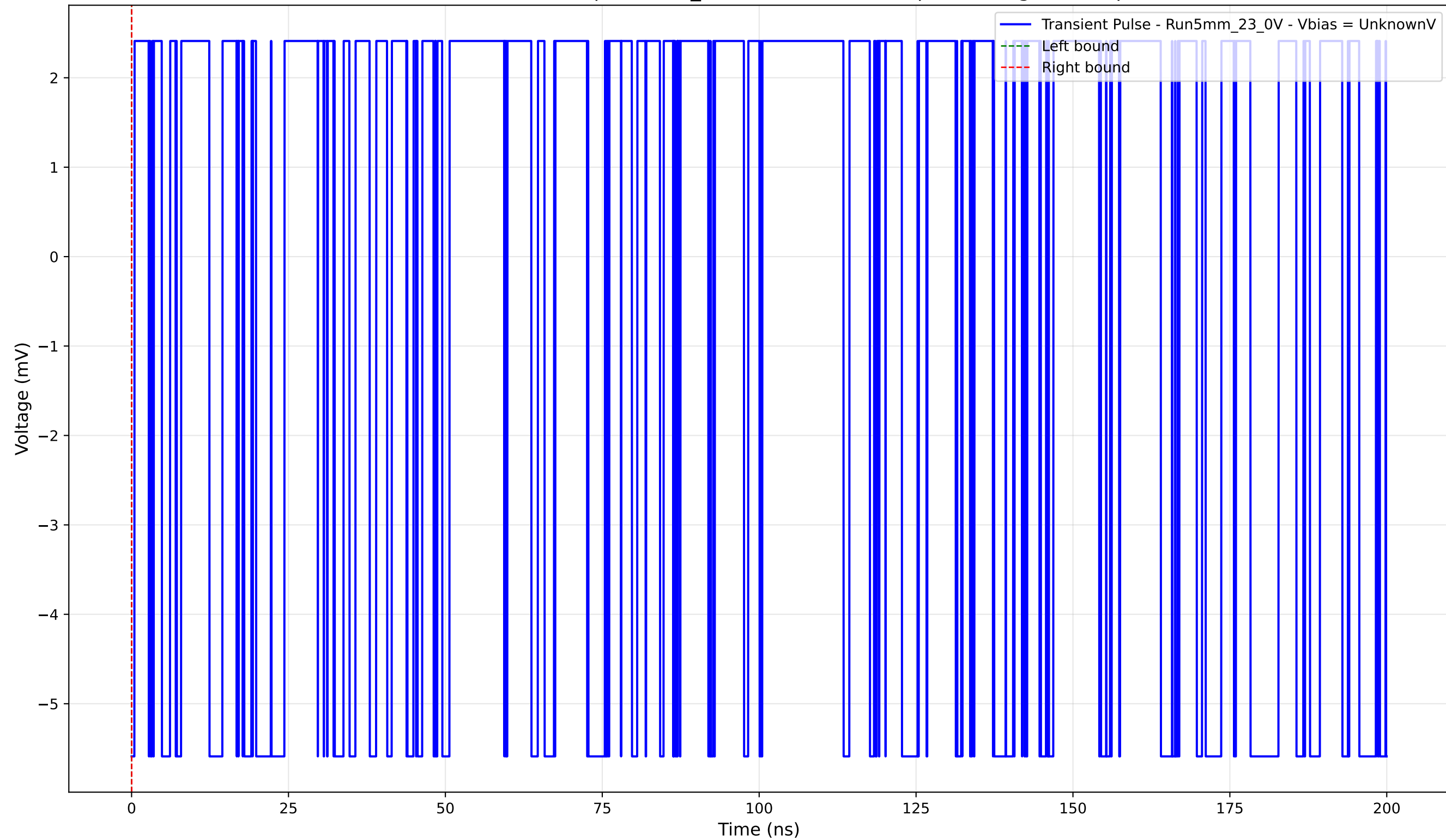
Transient Pulse - Sample: 5mm_23 - Position: 3135.0 \mu\text{m} - Charge: -0.00 pC
