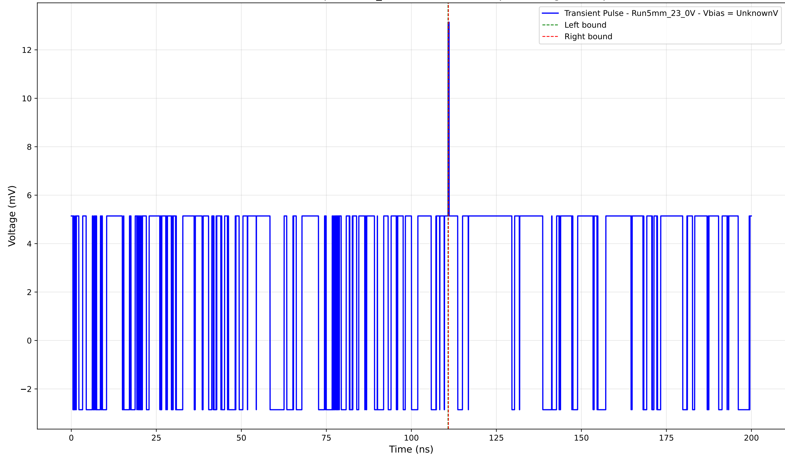
Transient Pulse - Sample: 5mm_23 - Position: 3930.0 \mu\text{m} - Charge: 0.03 pC
