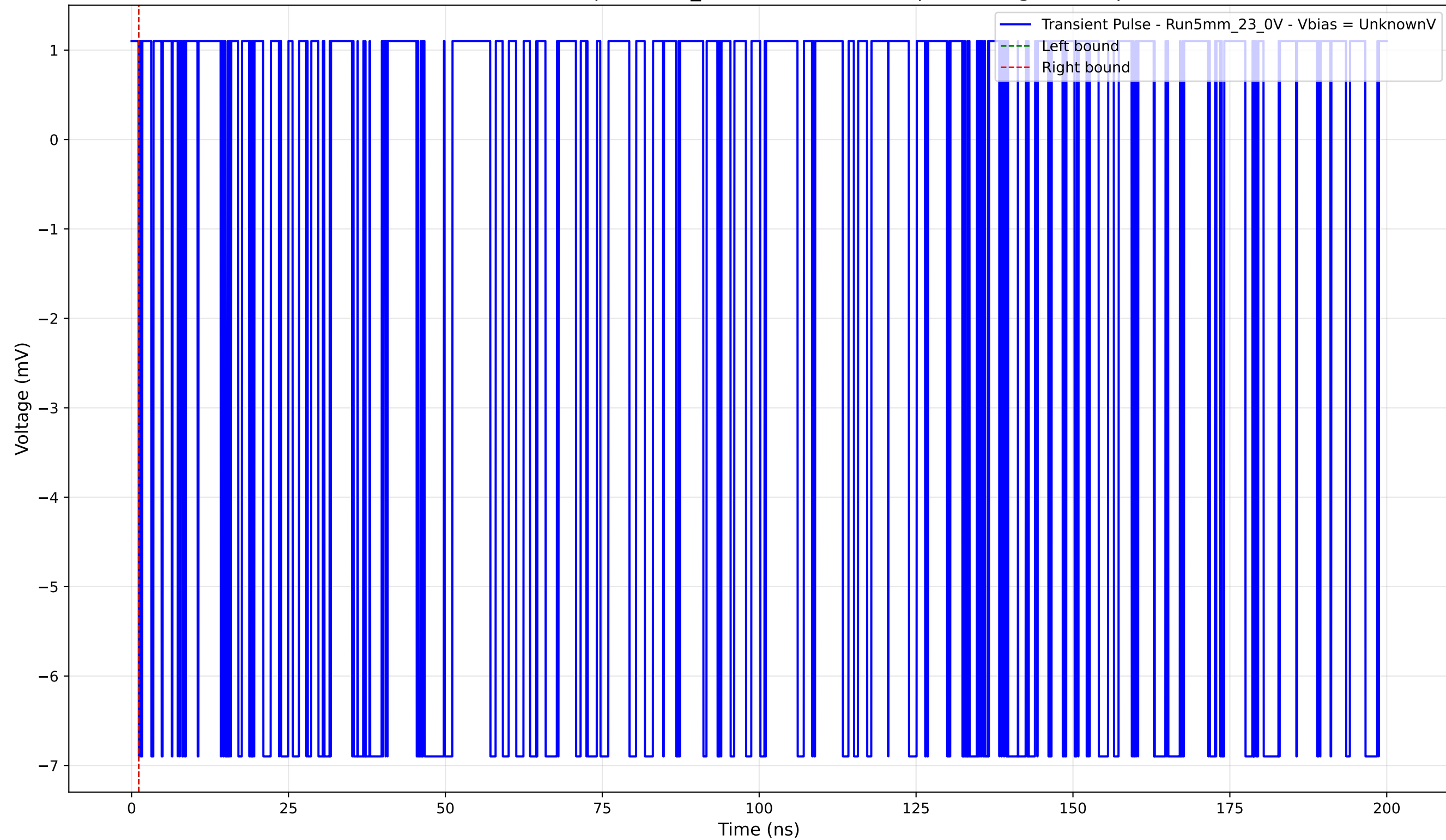
Transient Pulse - Sample: 5mm_23 - Position: 2900.0 \mu\text{m} - Charge: -0.00 pC
