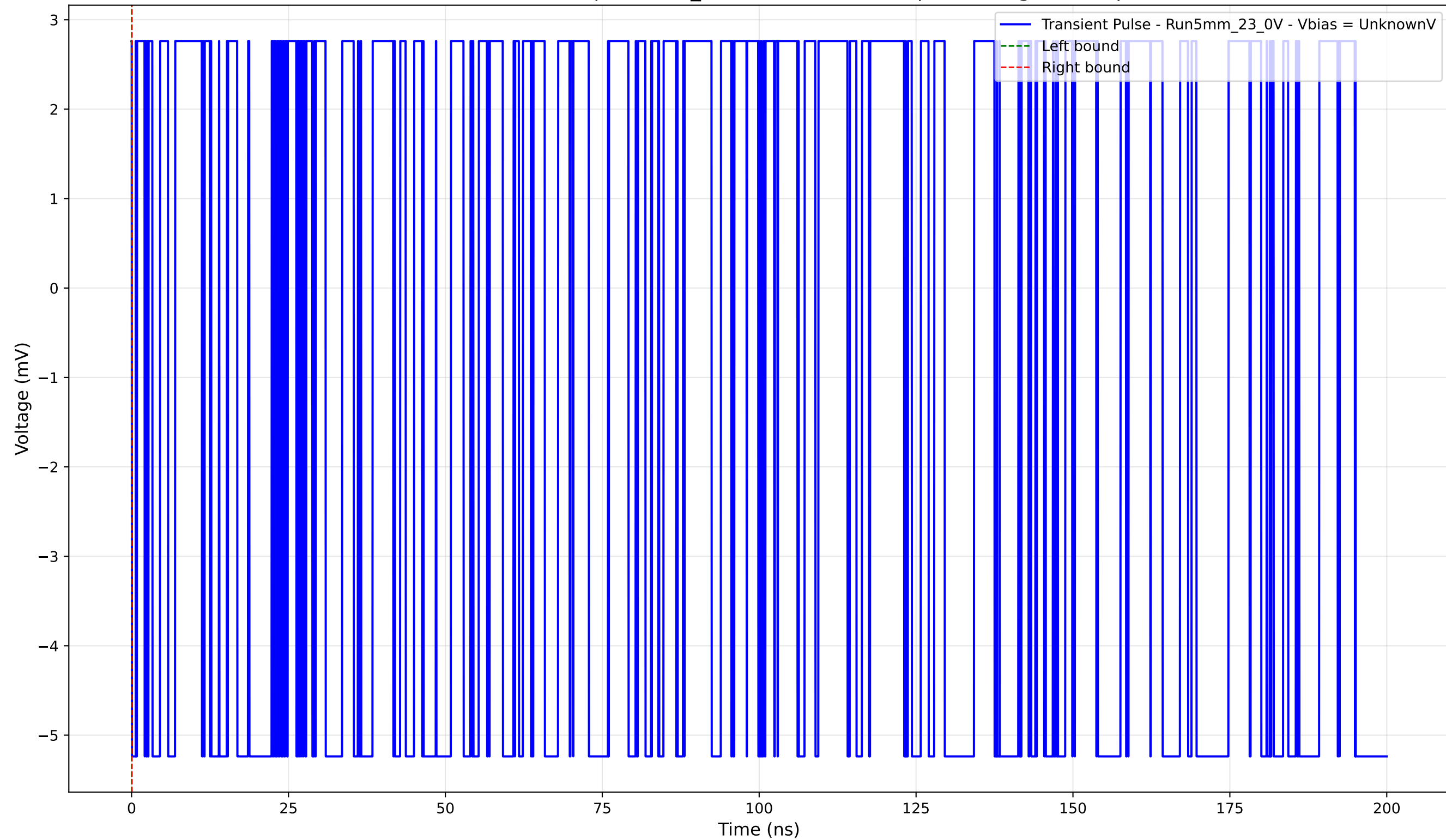
Transient Pulse - Sample: 5mm_23 - Position: 4845.0 \mu\text{m} - Charge: -0.00 pC
