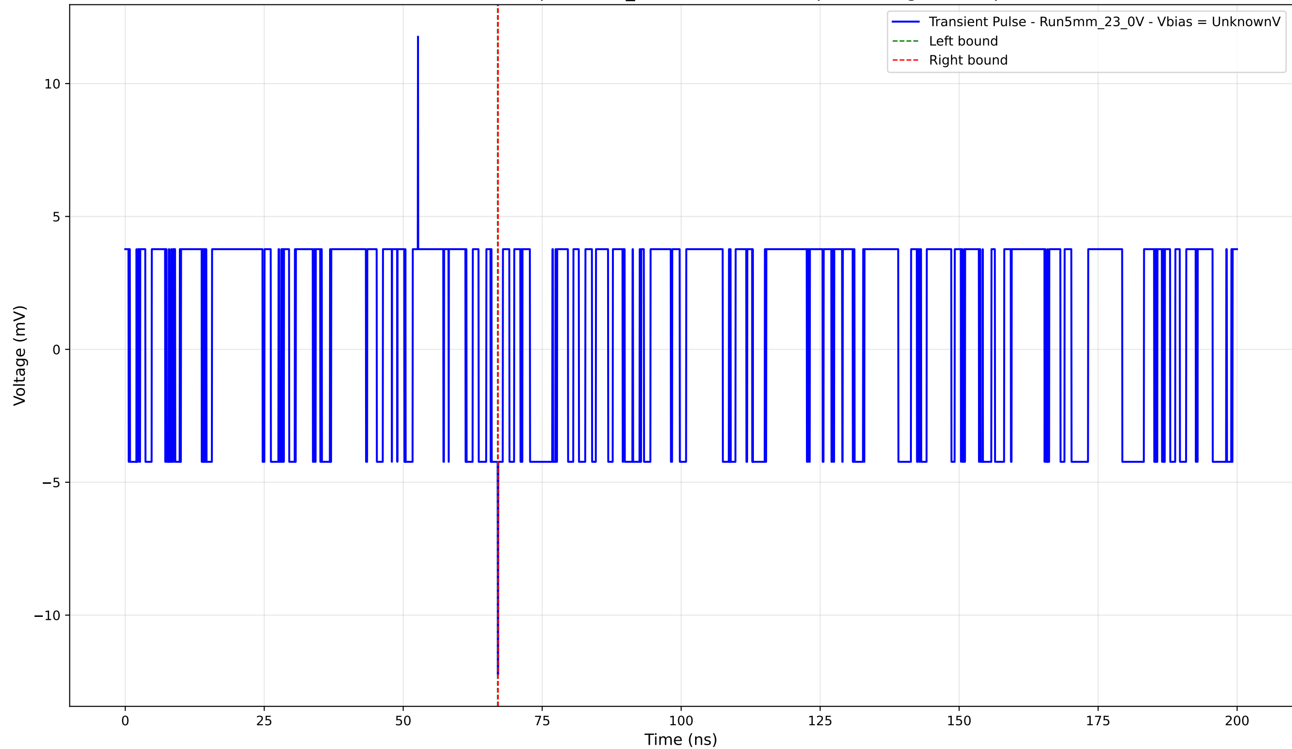
Transient Pulse - Sample: 5mm_23 - Position: 705.0 \mu\text{m} - Charge: -0.02 pC
