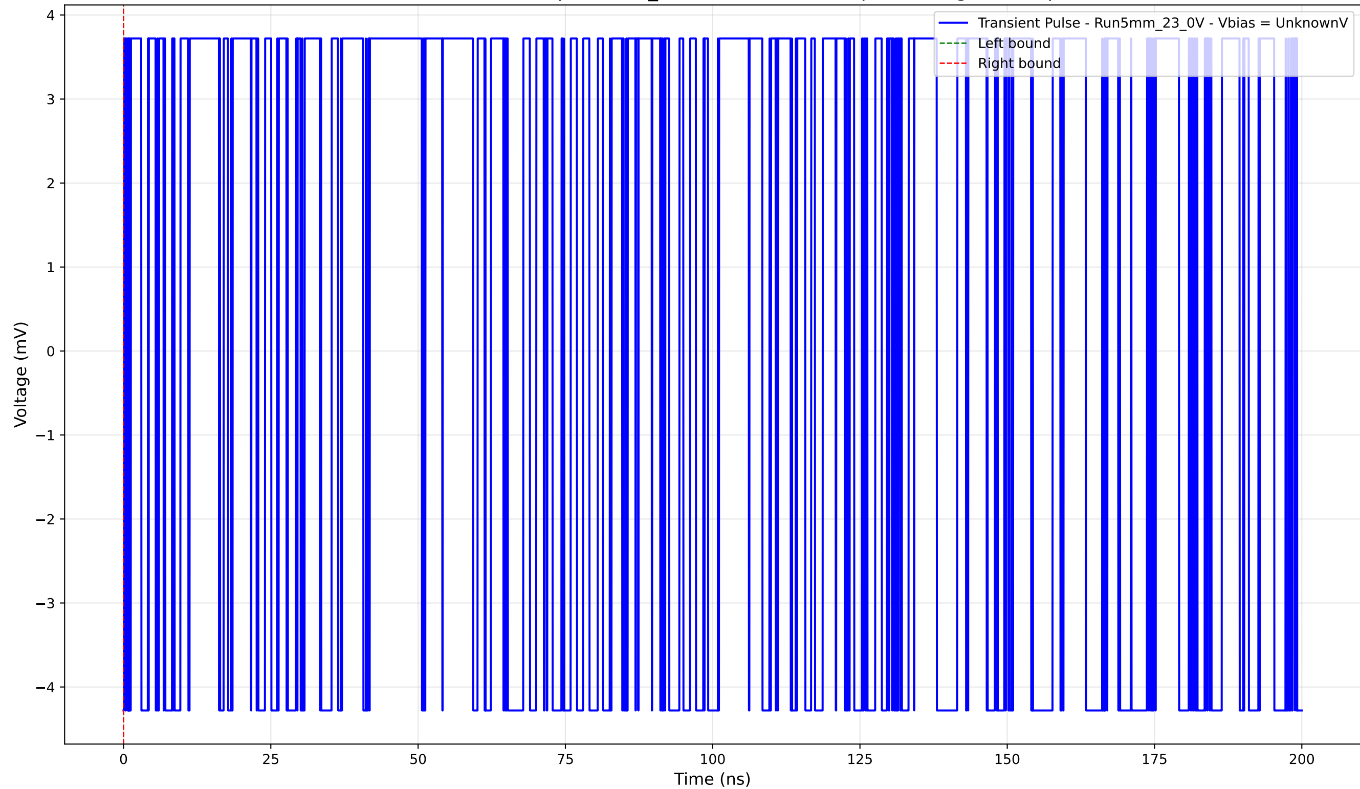
Transient Pulse - Sample: 5mm_23 - Position: 5090.0 \mu\text{m} - Charge: -0.00 pC
