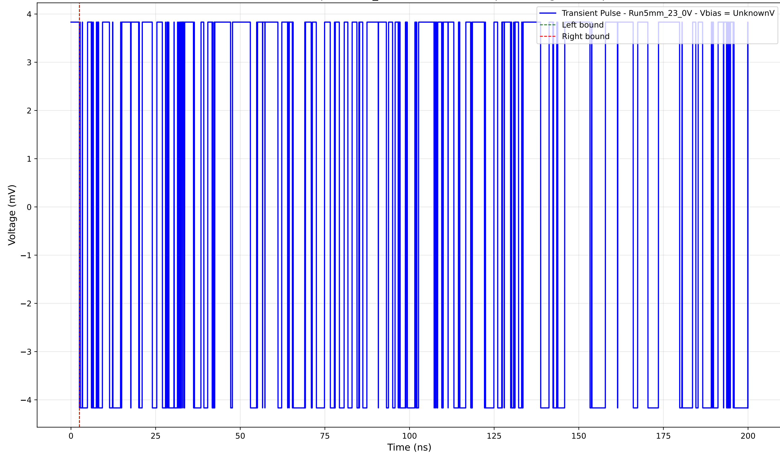
Transient Pulse - Sample: 5mm_23 - Position: 2660.0 \mu\text{m} - Charge: -0.00 pC
