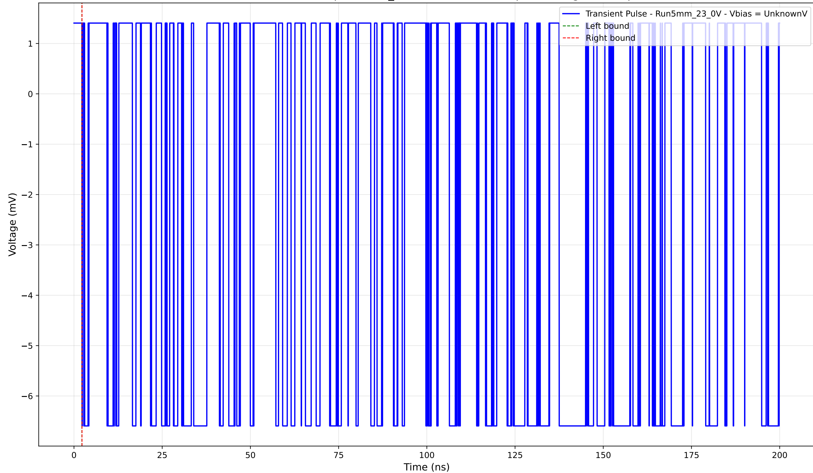
Transient Pulse - Sample: 5mm_23 - Position: 3210.0 \mu\text{m} - Charge: -0.00 pC
