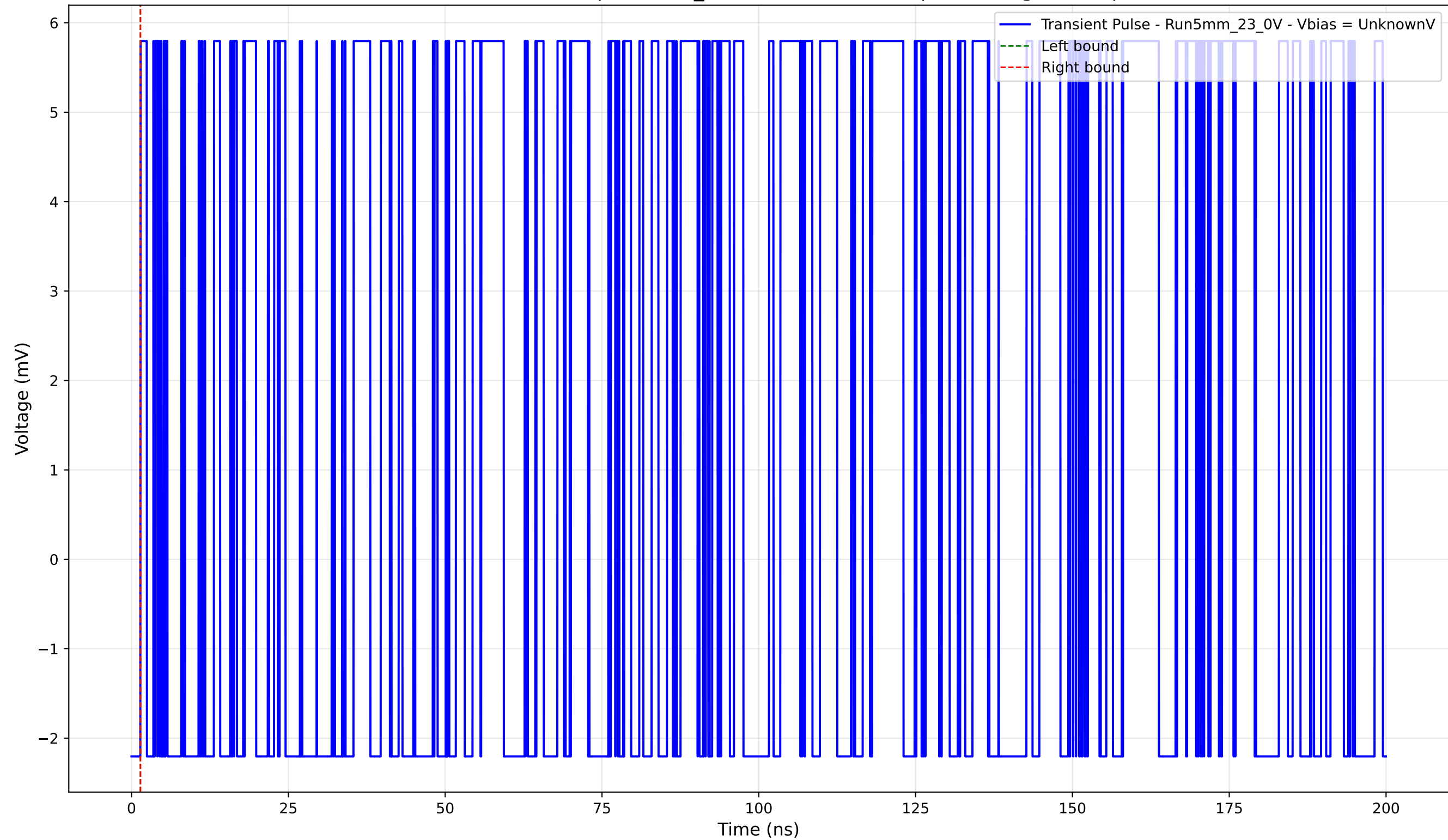
Transient Pulse - Sample: 5mm_23 - Position: 4135.0 \mu\text{m} - Charge: 0.00 pC
