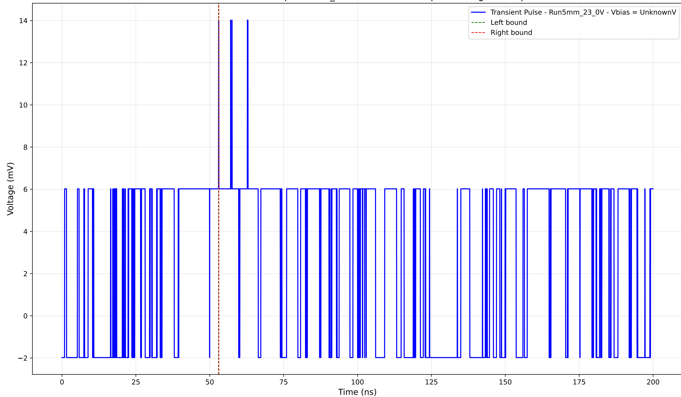
Transient Pulse - Sample: 5mm_23 - Position: 725.0 \mu\text{m} - Charge: 0.03 pC
