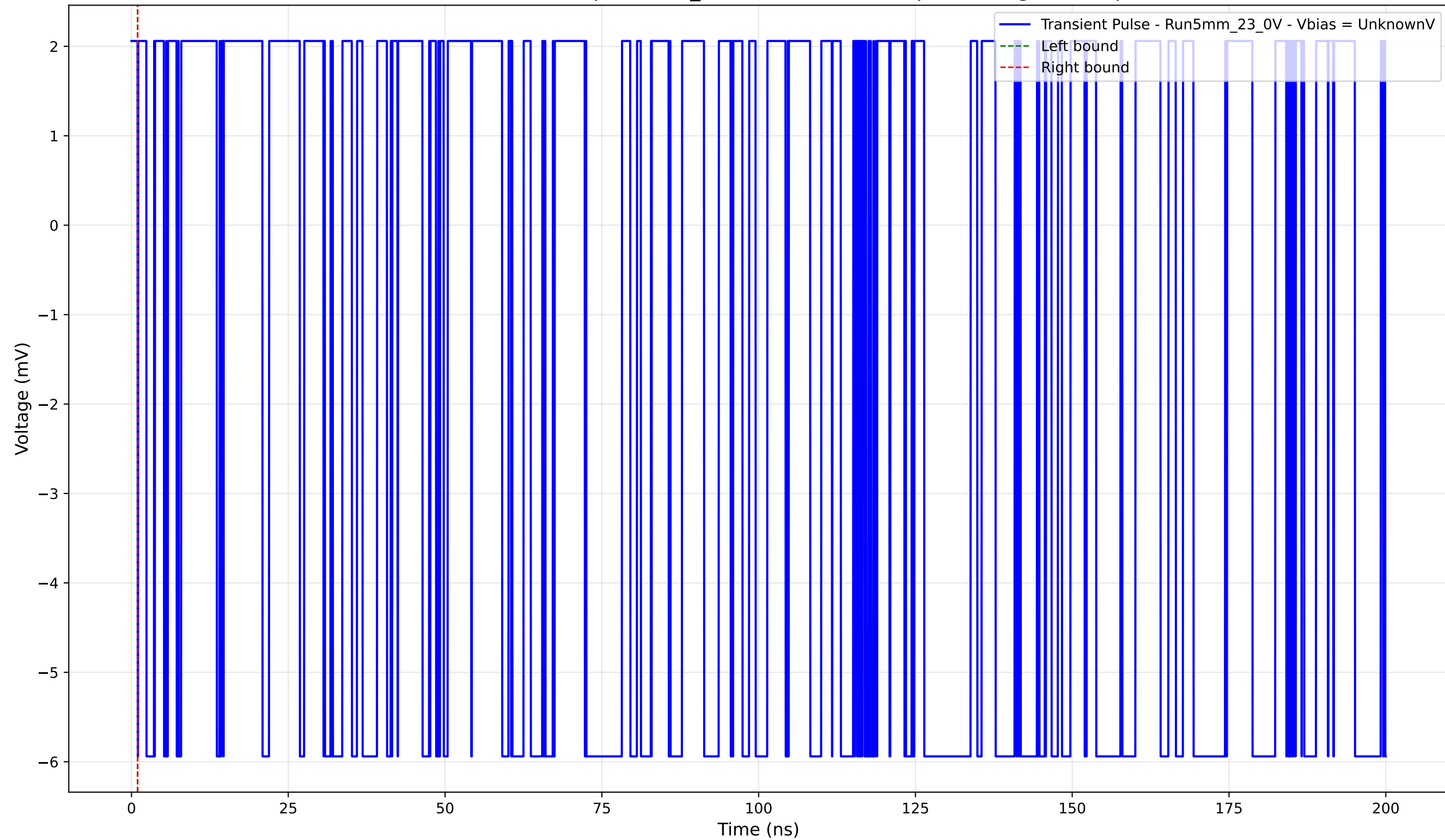
Transient Pulse - Sample: 5mm_23 - Position: 2295.0 \mu\text{m} - Charge: -0.00 pC
