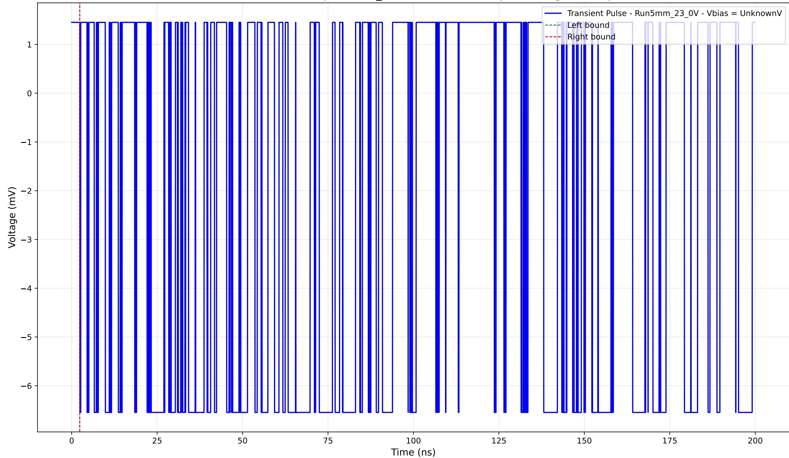
Transient Pulse - Sample: 5mm_23 - Position: 1905.0 \mu\text{m} - Charge: -0.00 pC
