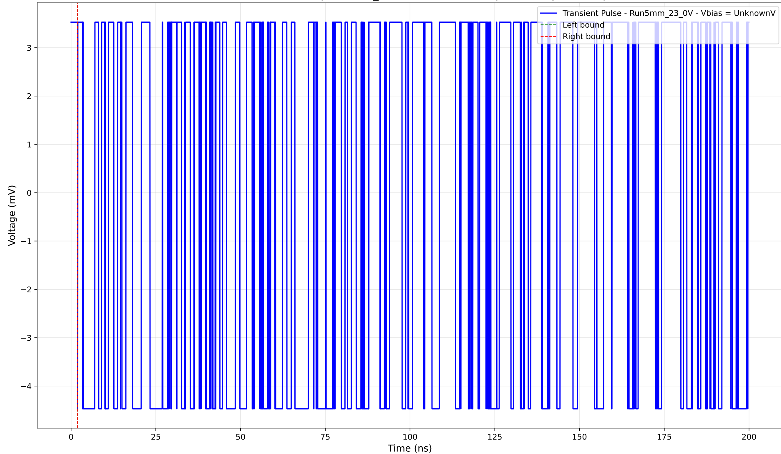
Transient Pulse - Sample: 5mm_23 - Position: 1410.0 \mu\text{m} - Charge: -0.00 pC
