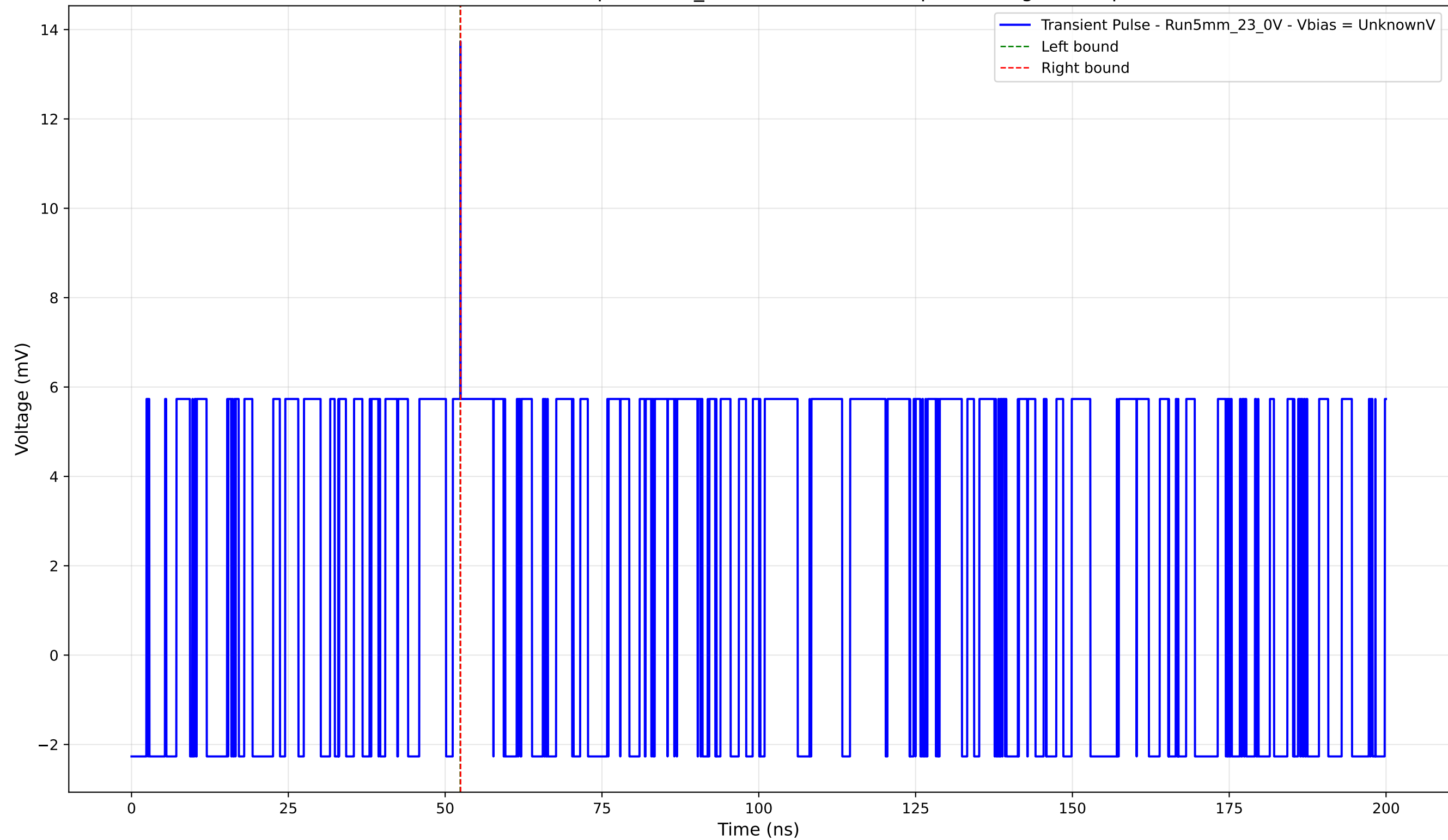
Transient Pulse - Sample: 5mm_23 - Position: 4190.0 \mu\text{m} - Charge: 0.01 pC
