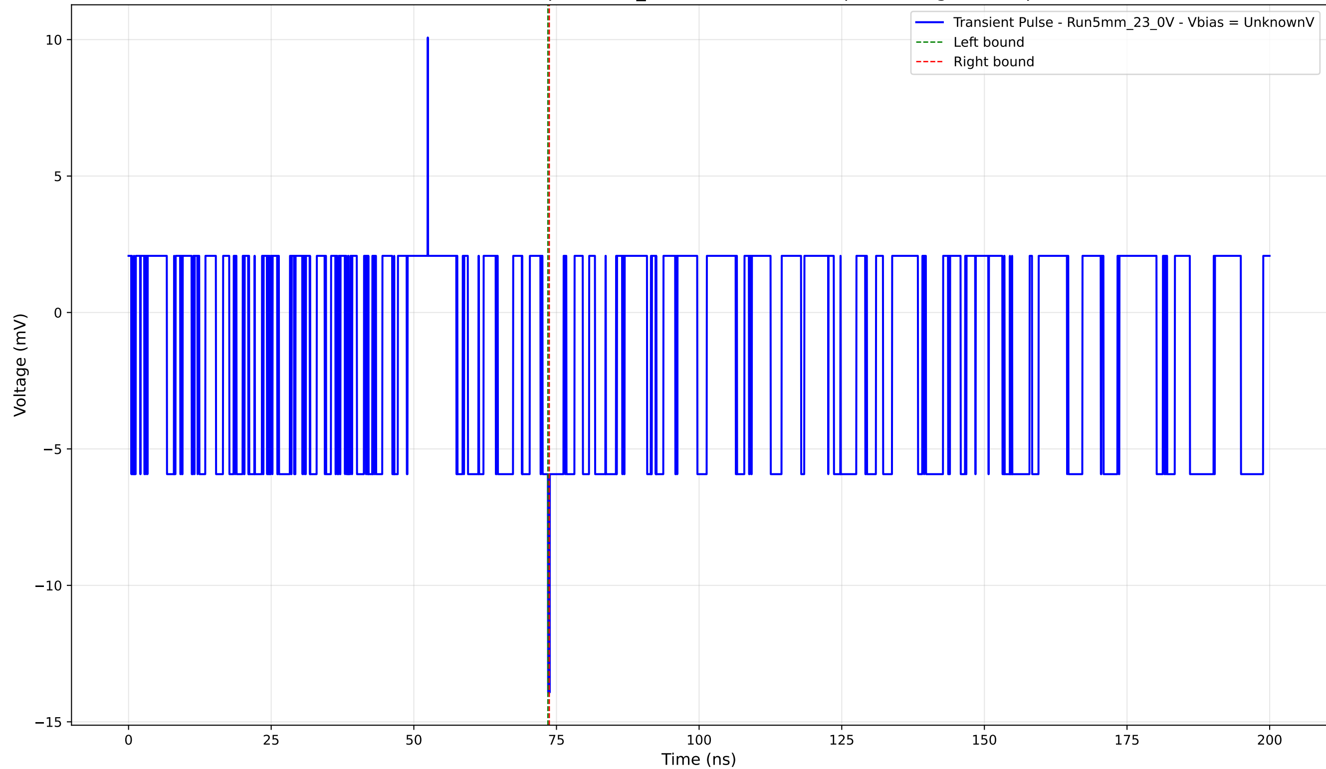
Transient Pulse - Sample: 5mm_23 - Position: 2460.0 \mu\text{m} - Charge: -0.06 pC
