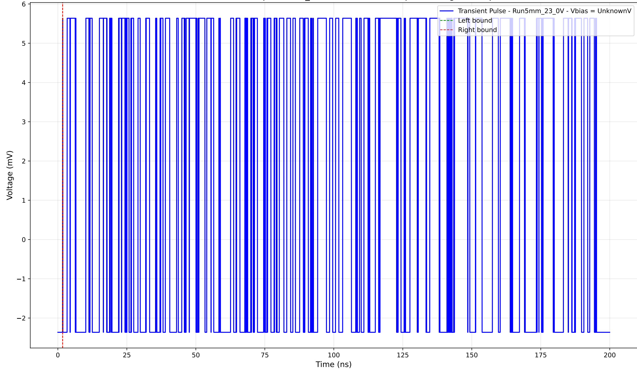
Transient Pulse - Sample: 5mm_23 - Position: 3405.0 \mu\text{m} - Charge: 0.00 pC
