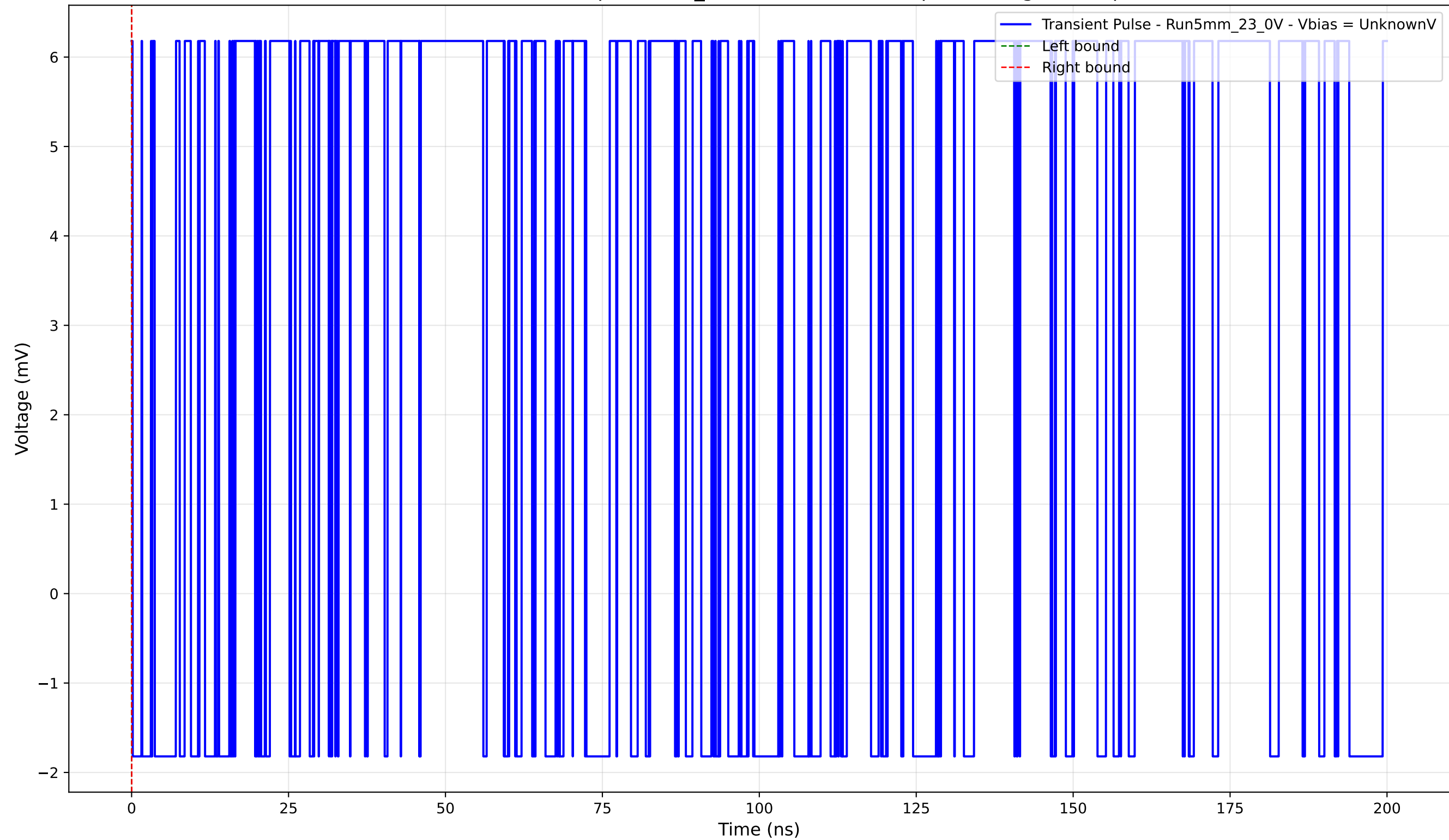
Transient Pulse - Sample: 5mm_23 - Position: 1910.0 \mu\text{m} - Charge: 0.00 pC
