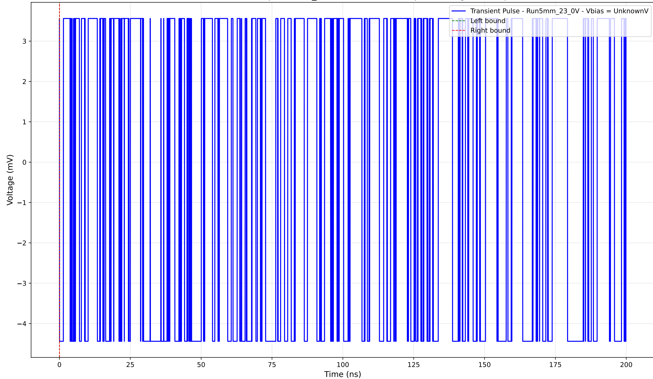
Transient Pulse - Sample: 5mm_23 - Position: 1420.0 \mu\text{m} - Charge: -0.00 pC
