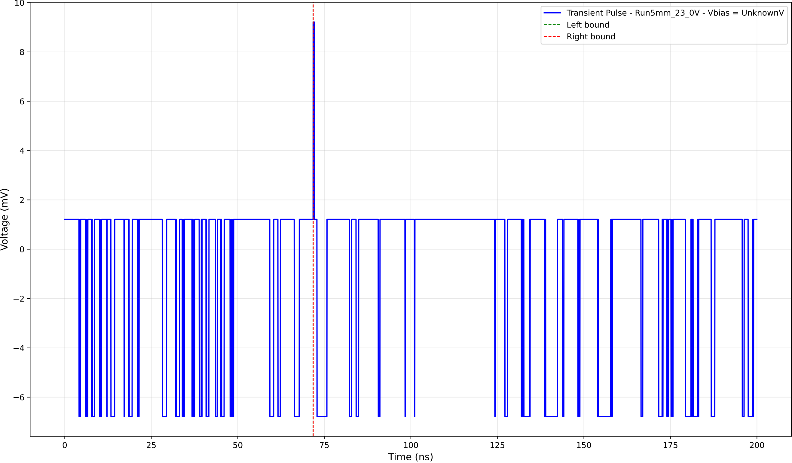
Transient Pulse - Sample: 5mm_23 - Position: 200.0 \mu\text{m} - Charge: 0.00 pC
