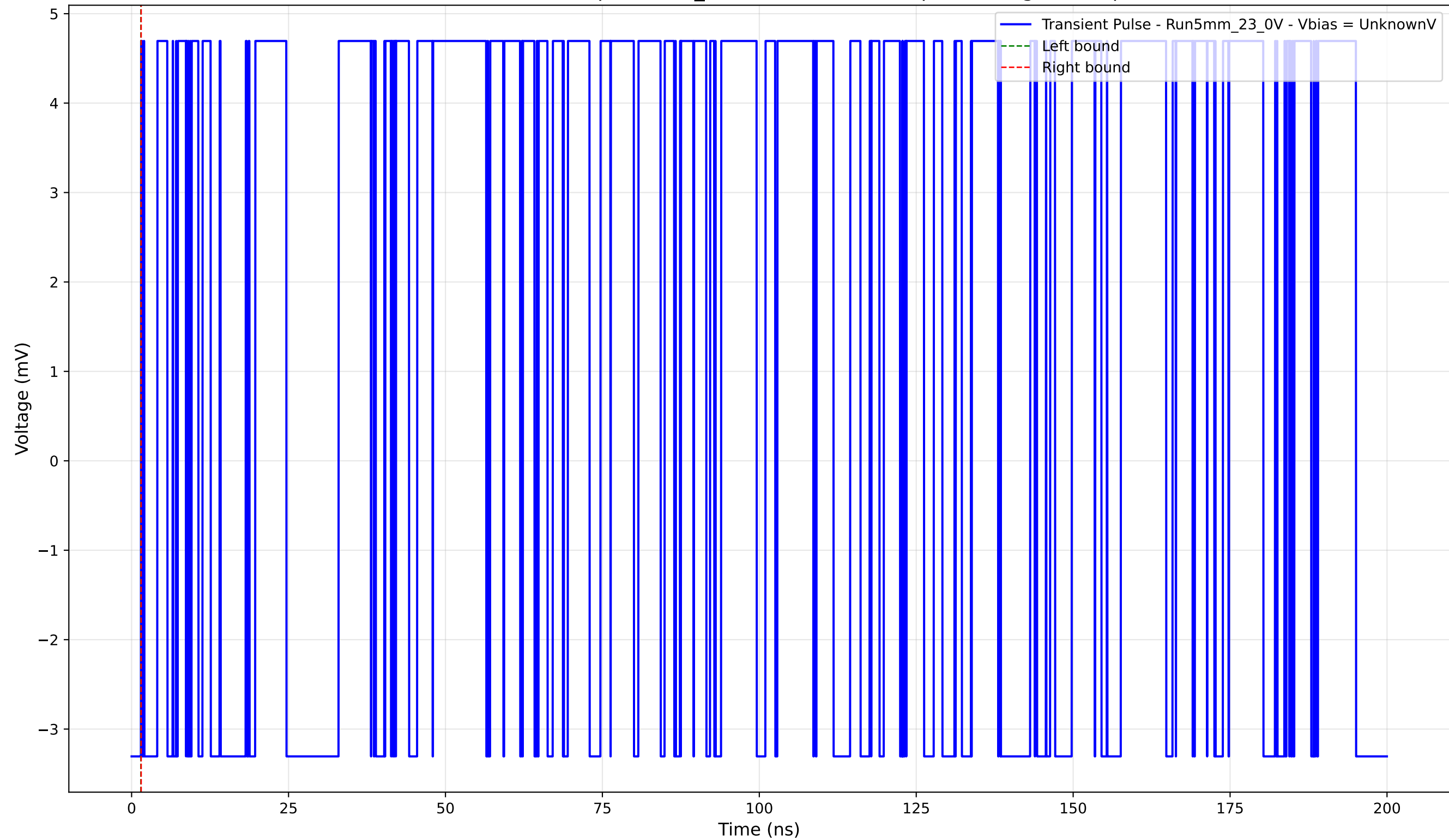
Transient Pulse - Sample: 5mm_23 - Position: 4420.0 \mu\text{m} - Charge: 0.00 pC
