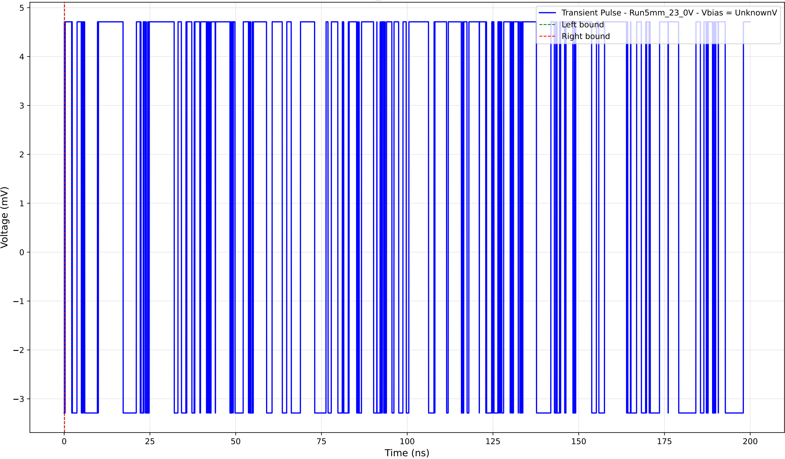
Transient Pulse - Sample: 5mm_23 - Position: 910.0 \mu\text{m} - Charge: 0.00 pC
