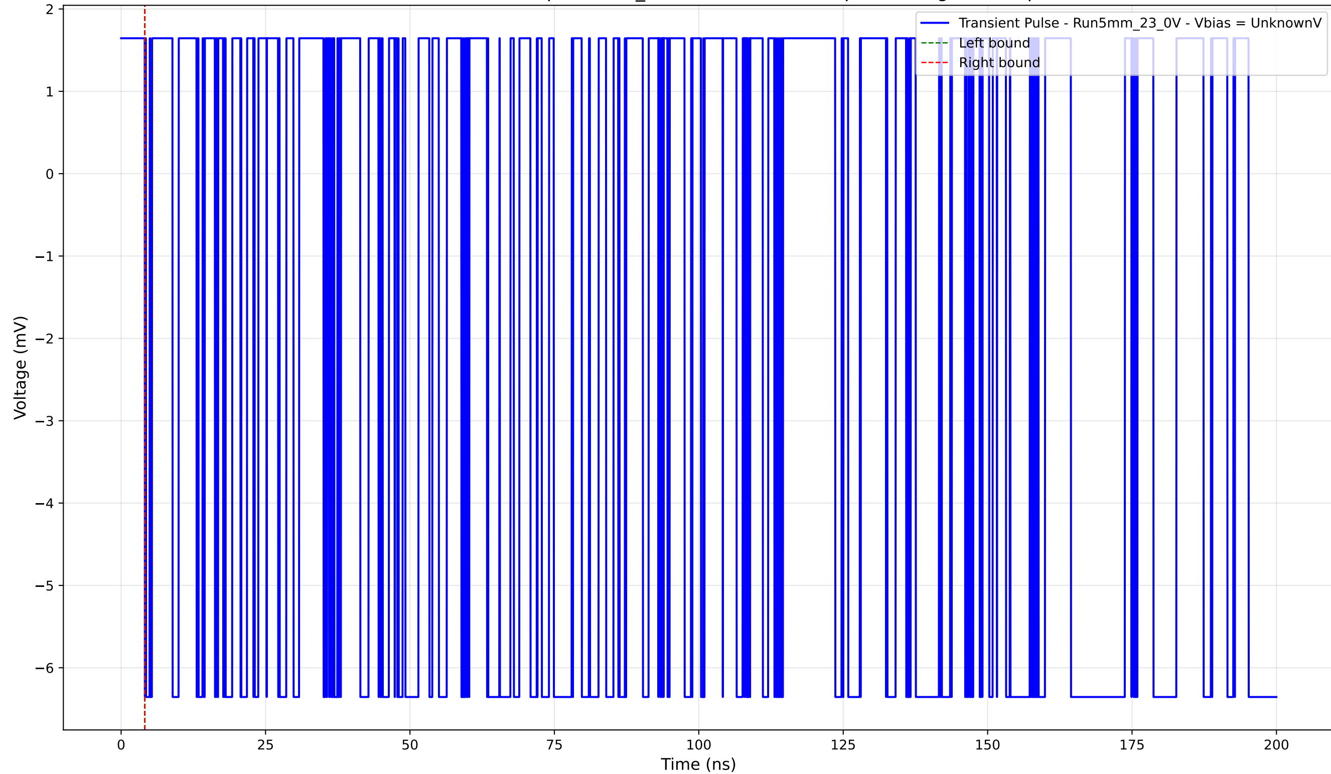
Transient Pulse - Sample: 5mm_23 - Position: 2730.0 \mu\text{m} - Charge: -0.00 pC
