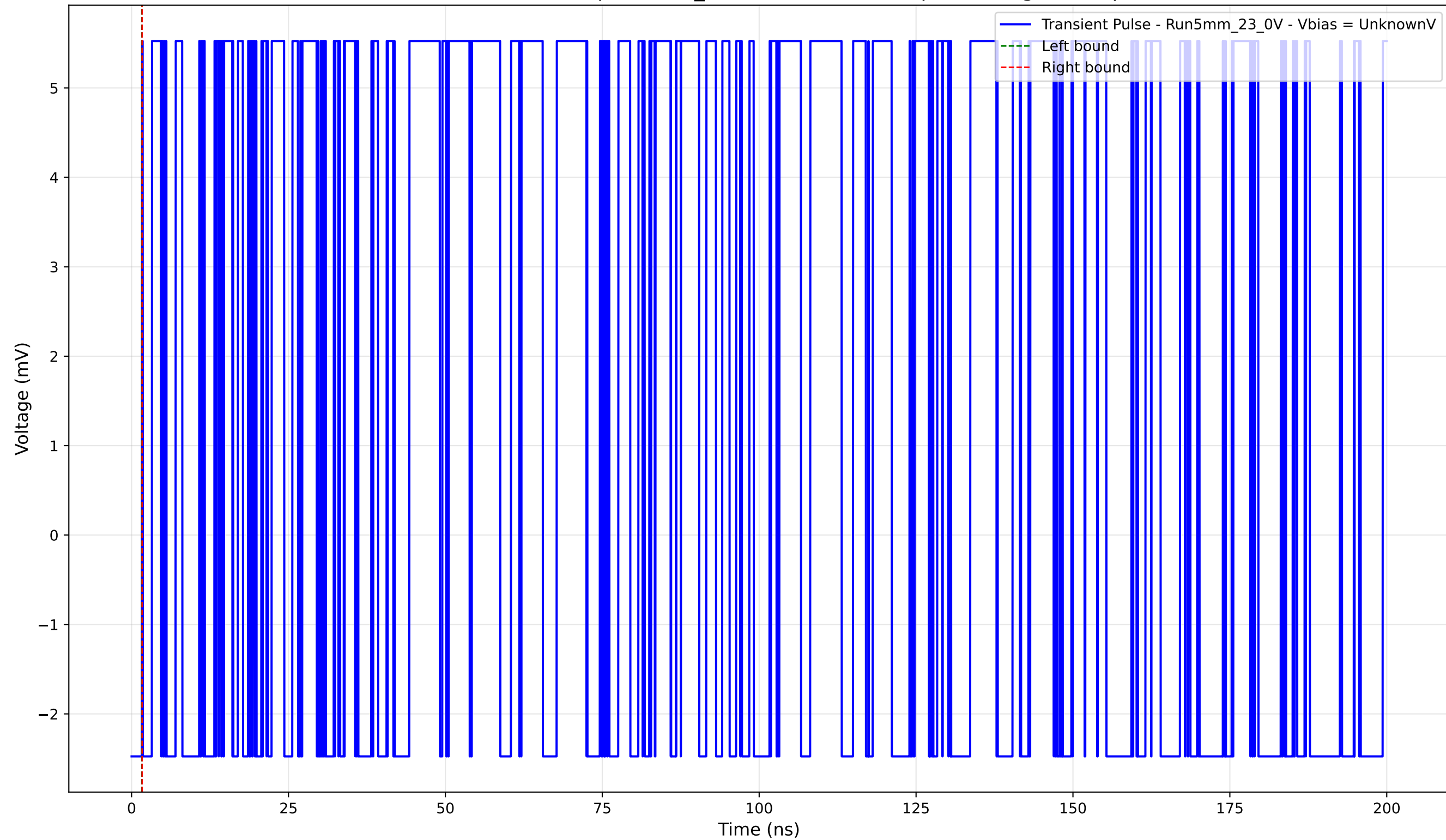
Transient Pulse - Sample: 5mm_23 - Position: 3600.0 \mu\text{m} - Charge: 0.00 pC
