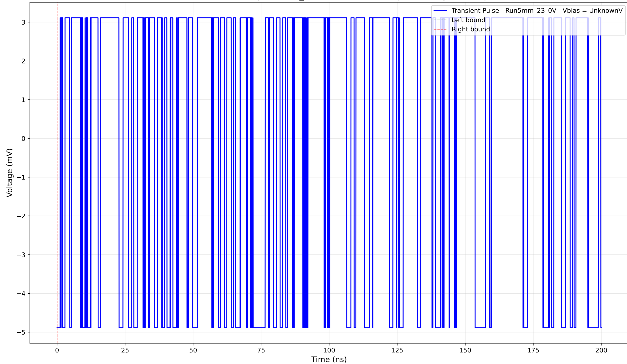
Transient Pulse - Sample: 5mm_23 - Position: 2650.0 \mu\text{m} - Charge: -0.00 pC
