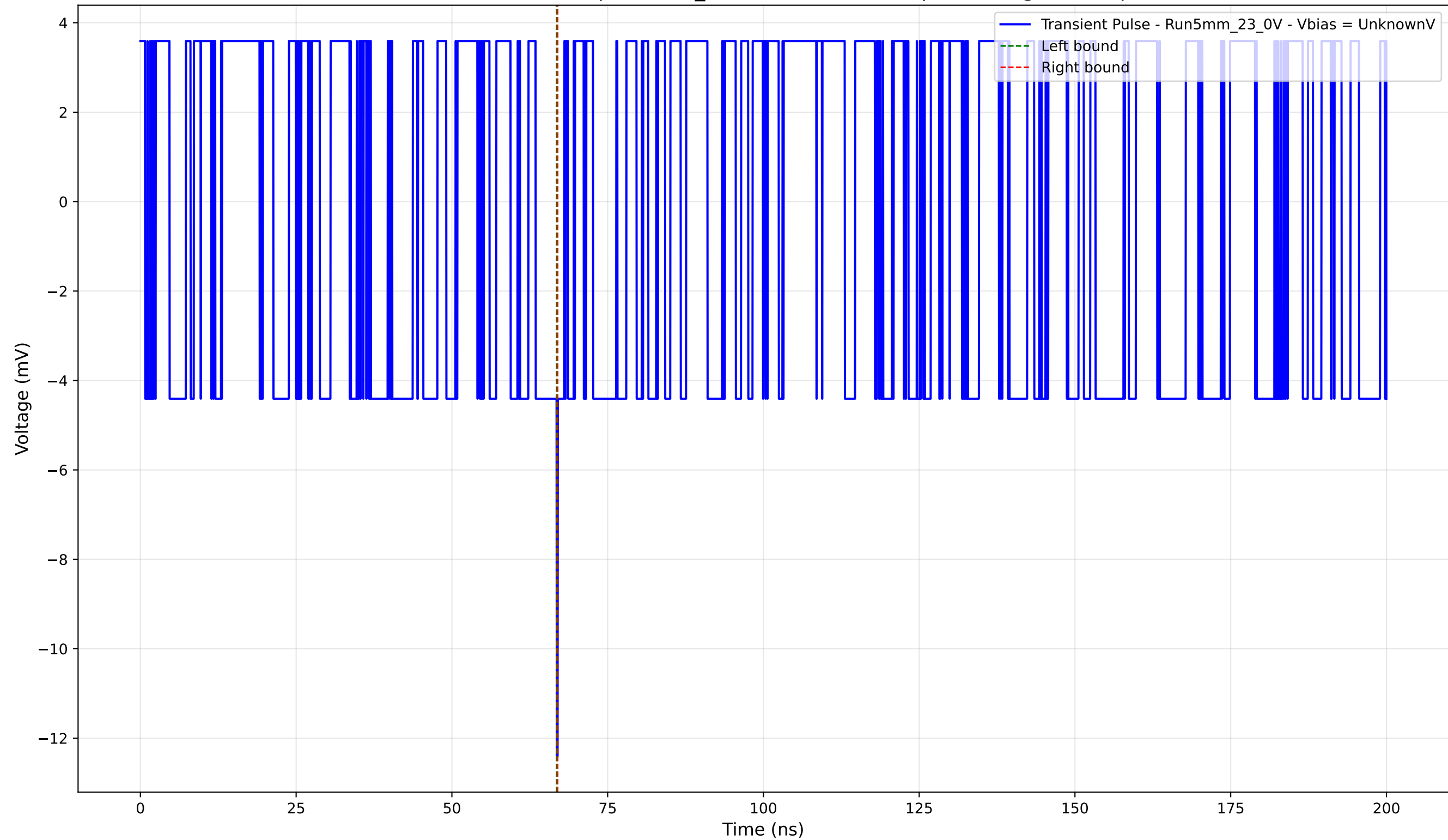
Transient Pulse - Sample: 5mm_23 - Position: 4615.0 \mu\text{m} - Charge: -0.04 pC
