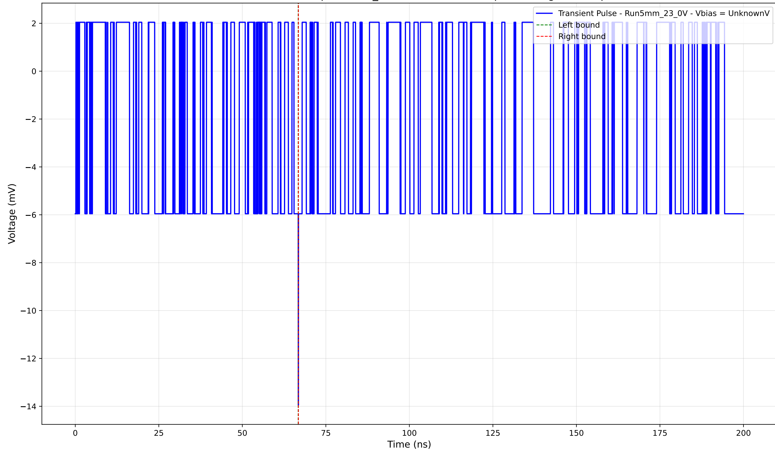
Transient Pulse - Sample: 5mm_23 - Position: 1700.0 \mu\text{m} - Charge: -0.02 pC
