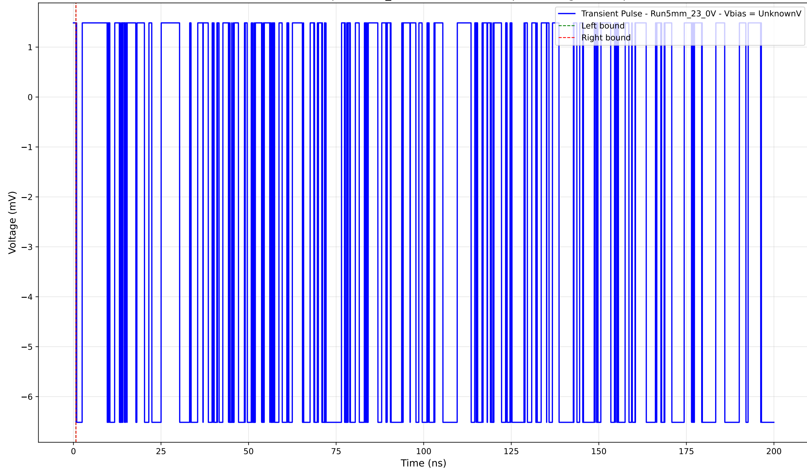
Transient Pulse - Sample: 5mm_23 - Position: 1350.0 \mu\text{m} - Charge: -0.00 pC
