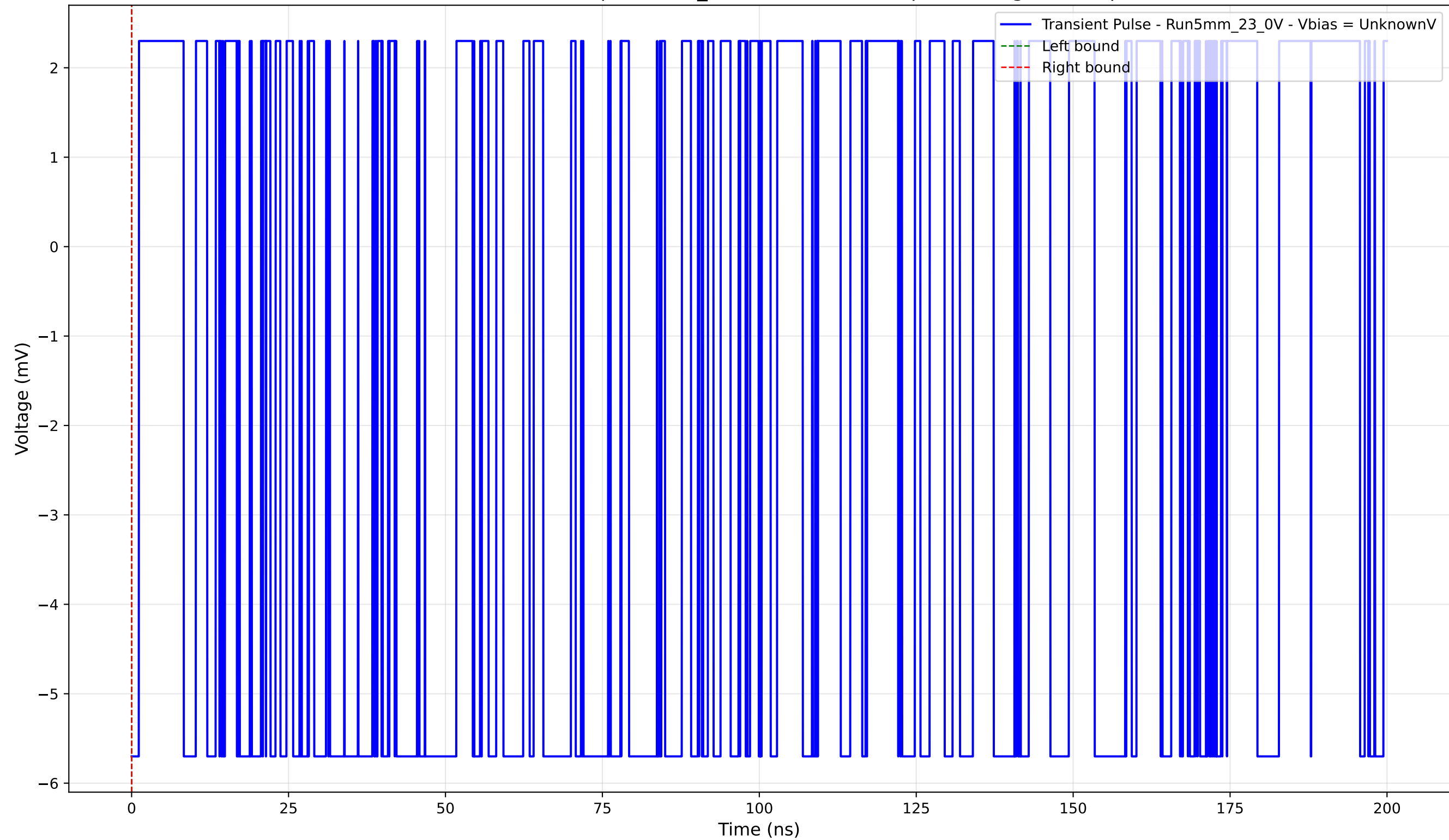
Transient Pulse - Sample: 5mm_23 - Position: 230.0 \mu\text{m} - Charge: -0.00 pC
