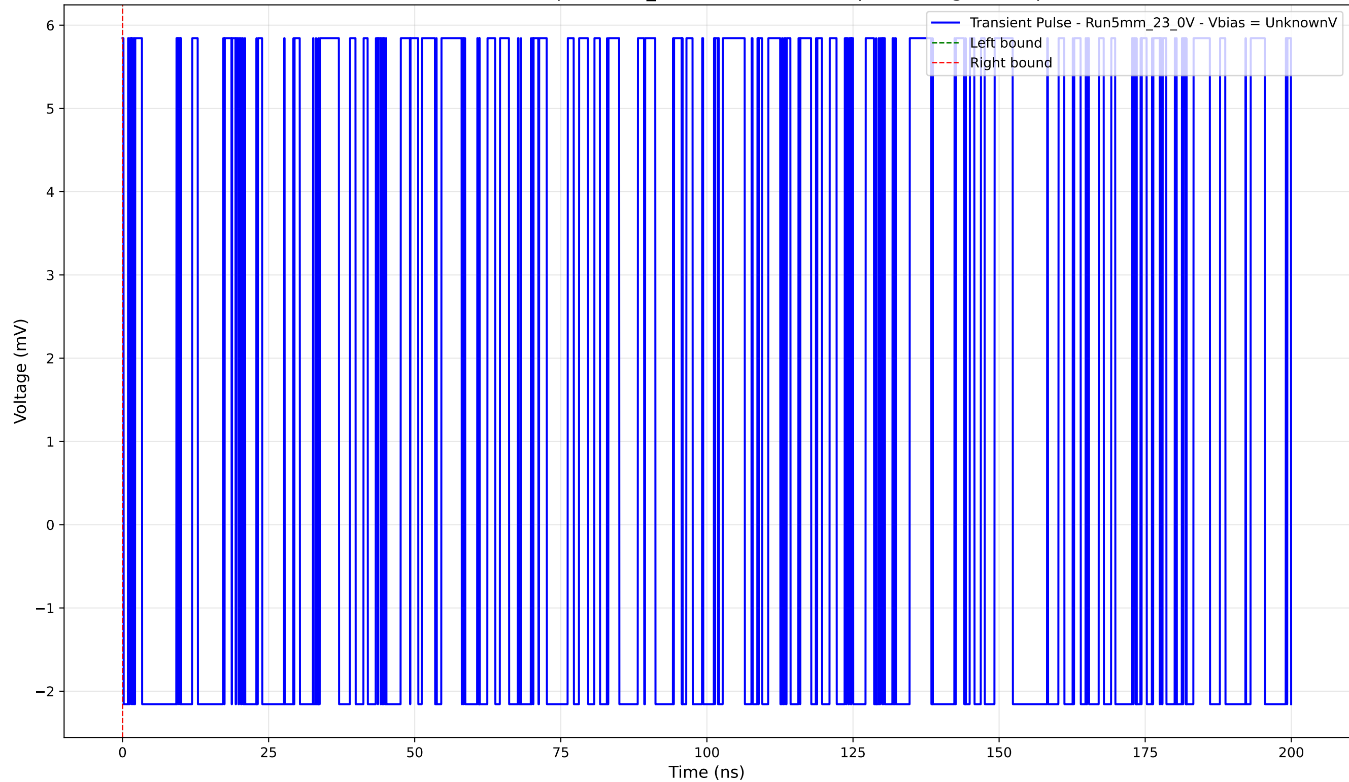
Transient Pulse - Sample: 5mm_23 - Position: 1215.0 \mu\text{m} - Charge: 0.00 pC
