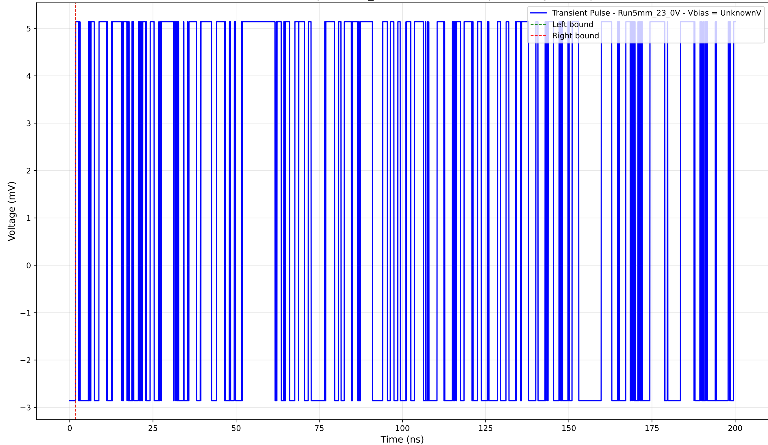
Transient Pulse - Sample: 5mm_23 - Position: 1775.0 \mu\text{m} - Charge: 0.00 pC
