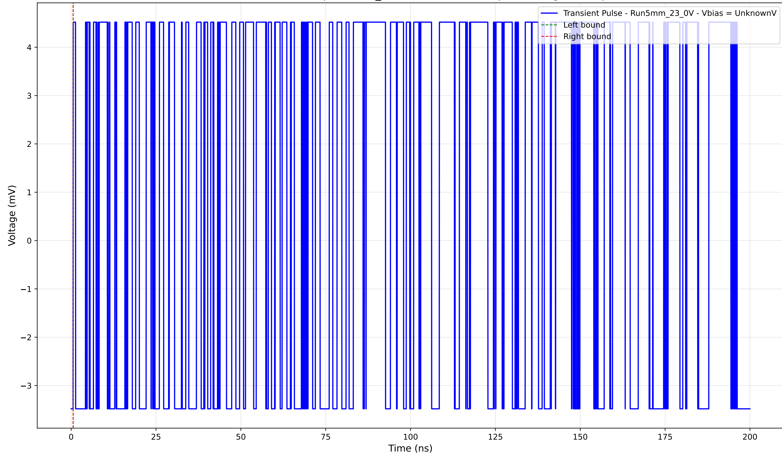
Transient Pulse - Sample: 5mm_23 - Position: 2610.0 \mu\text{m} - Charge: 0.00 pC
