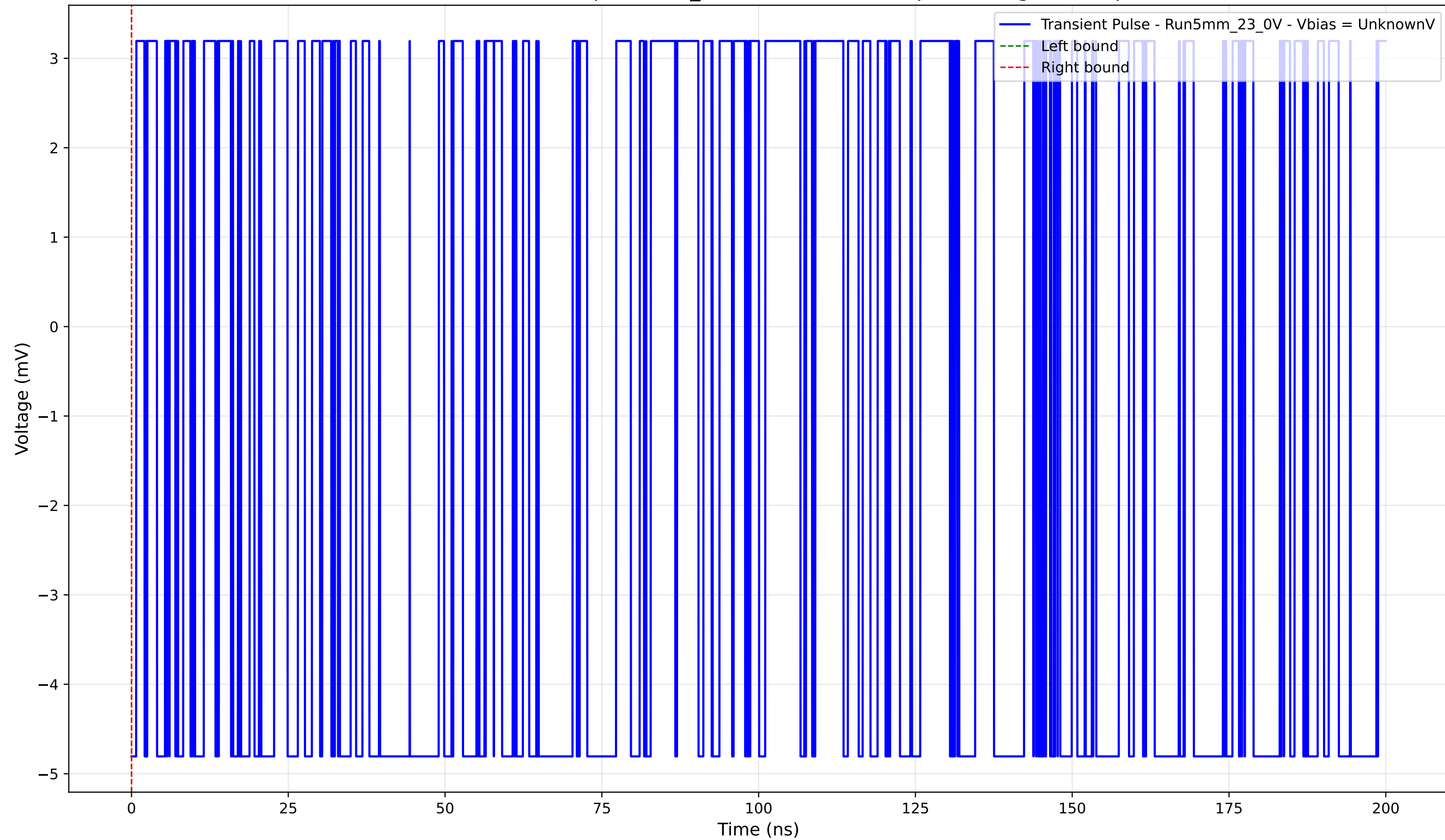
Transient Pulse - Sample: 5mm_23 - Position: 1260.0 \mu\text{m} - Charge: -0.00 pC
