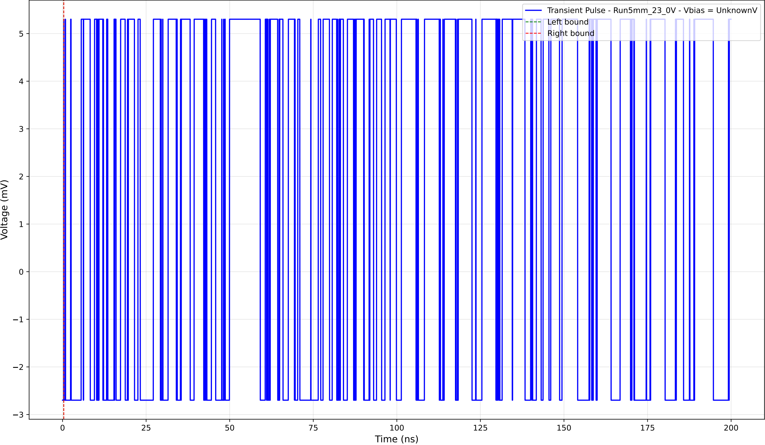
Transient Pulse - Sample: 5mm_23 - Position: 155.0 \mu\text{m} - Charge: 0.00 pC
