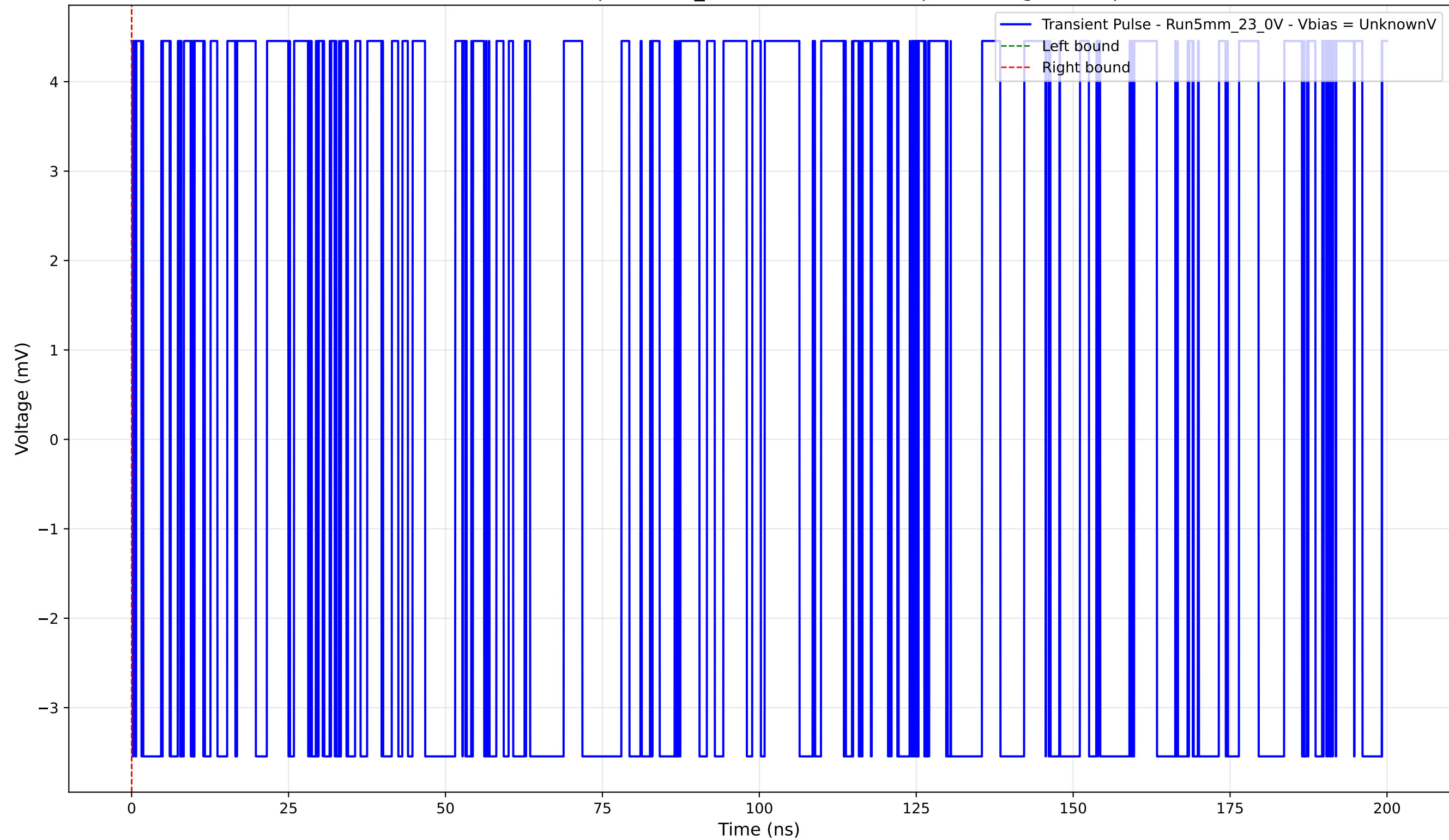
Transient Pulse - Sample: 5mm_23 - Position: 1560.0 \mu\text{m} - Charge: 0.00 pC
