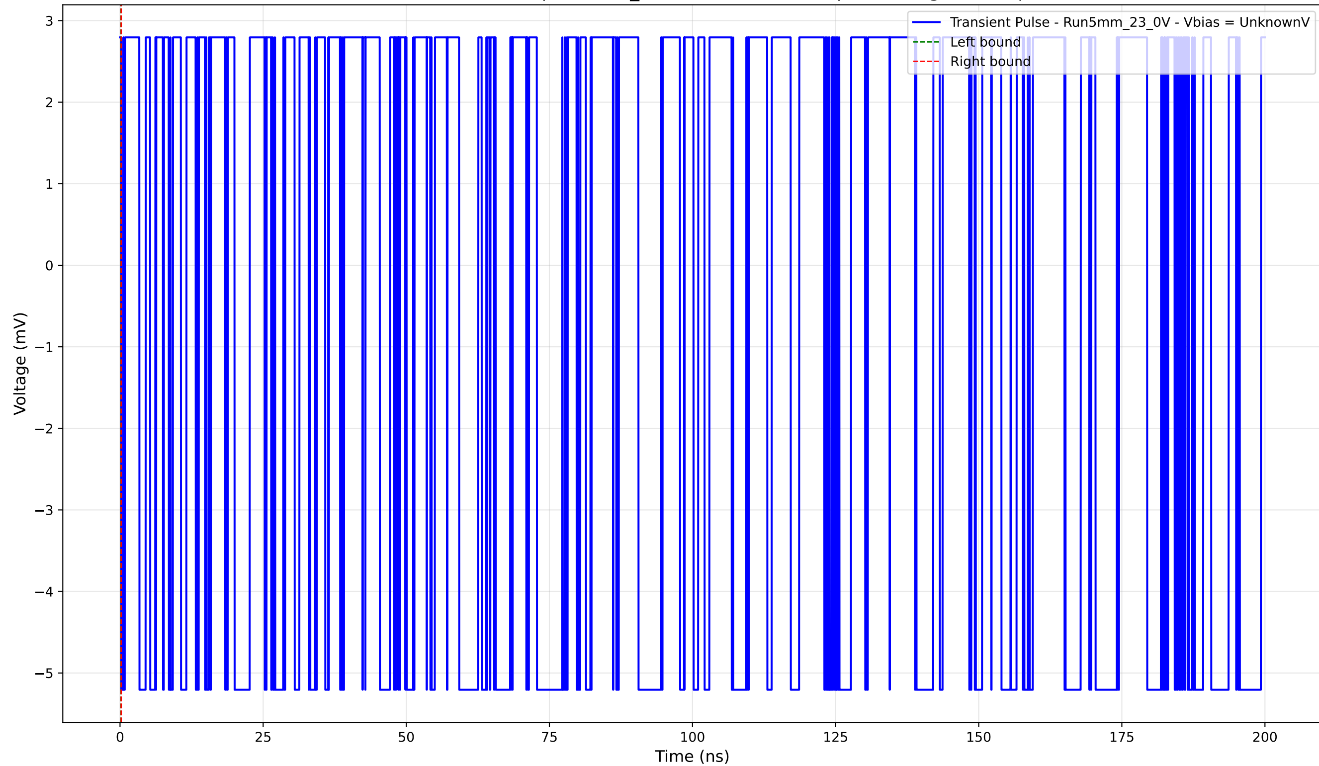
Transient Pulse - Sample: 5mm_23 - Position: 2130.0 \mu\text{m} - Charge: -0.00 pC
