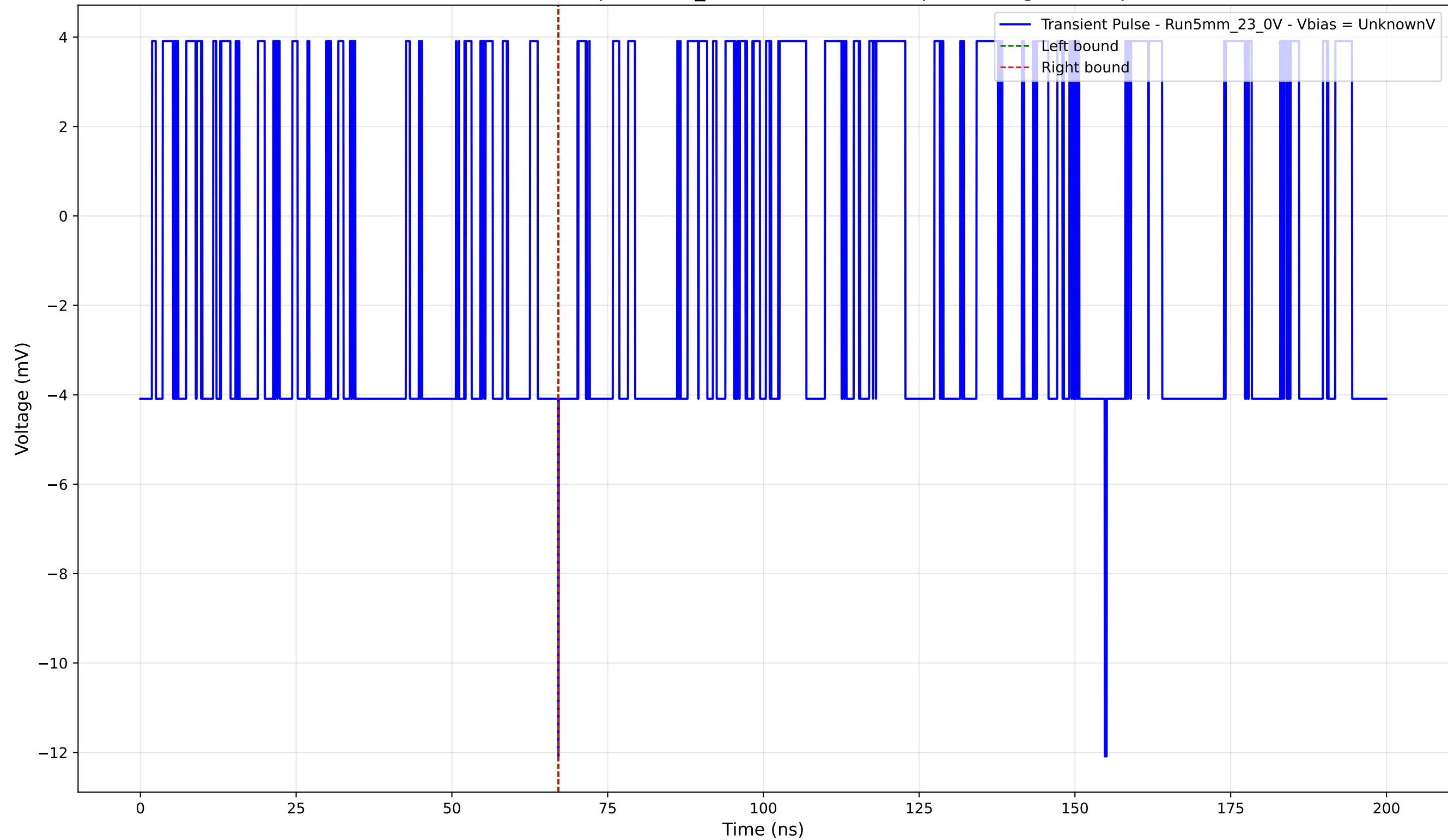
Transient Pulse - Sample: 5mm_23 - Position: 1495.0 \mu\text{m} - Charge: -0.03 pC
