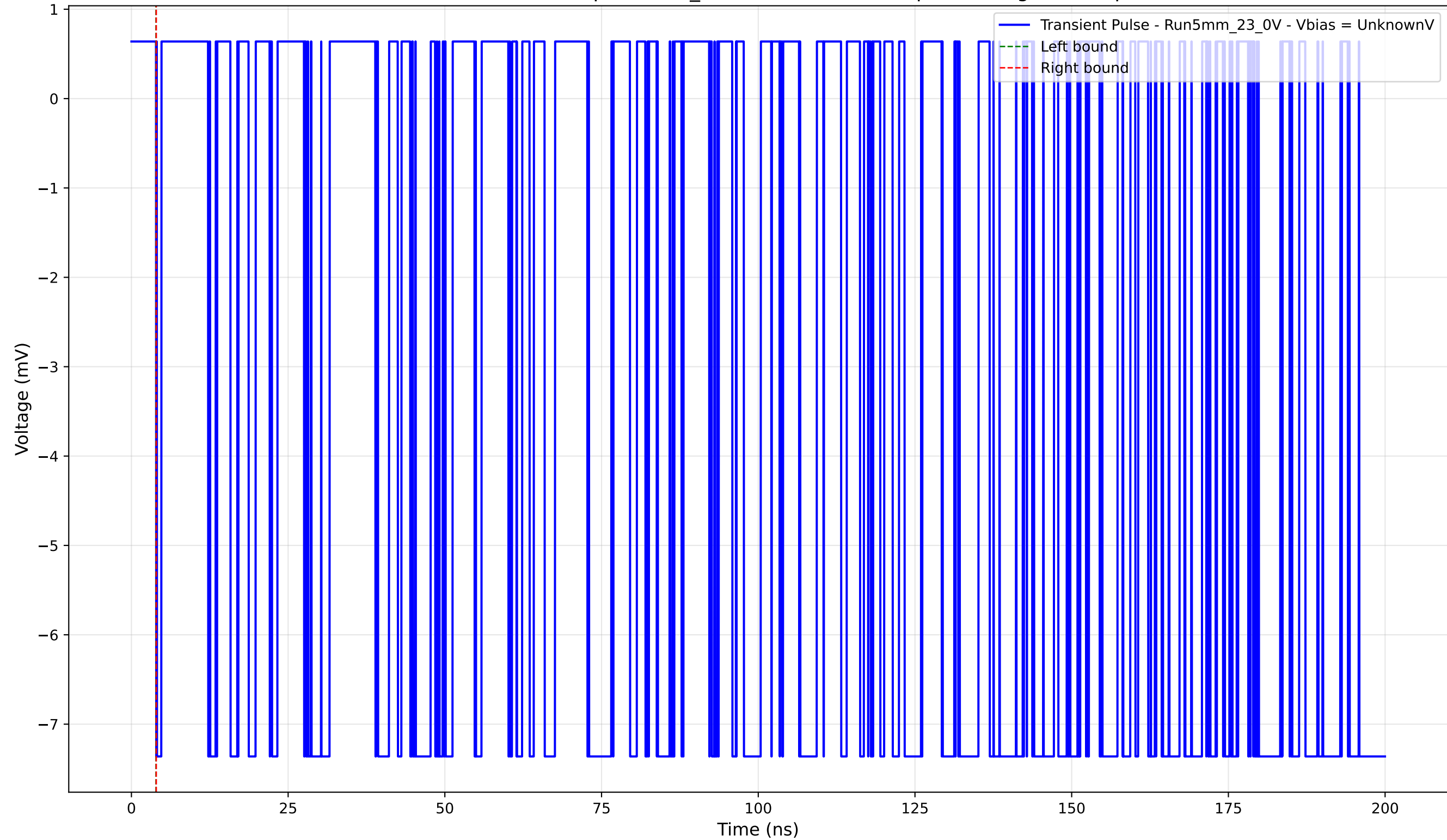
Transient Pulse - Sample: 5mm_23 - Position: 4960.0 \mu\text{m} - Charge: -0.00 pC
