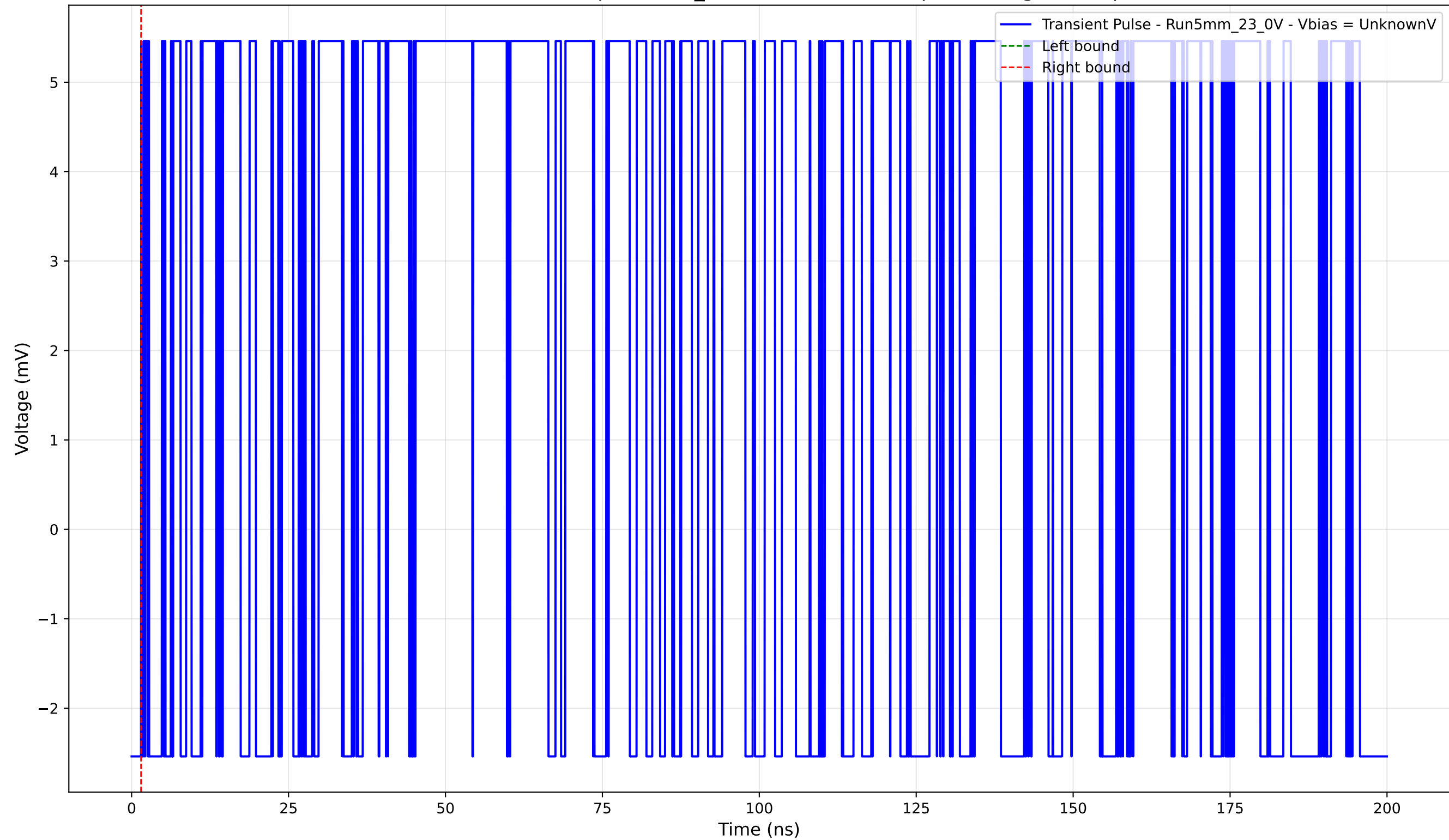
Transient Pulse - Sample: 5mm_23 - Position: 3230.0 \mu\text{m} - Charge: 0.00 pC
