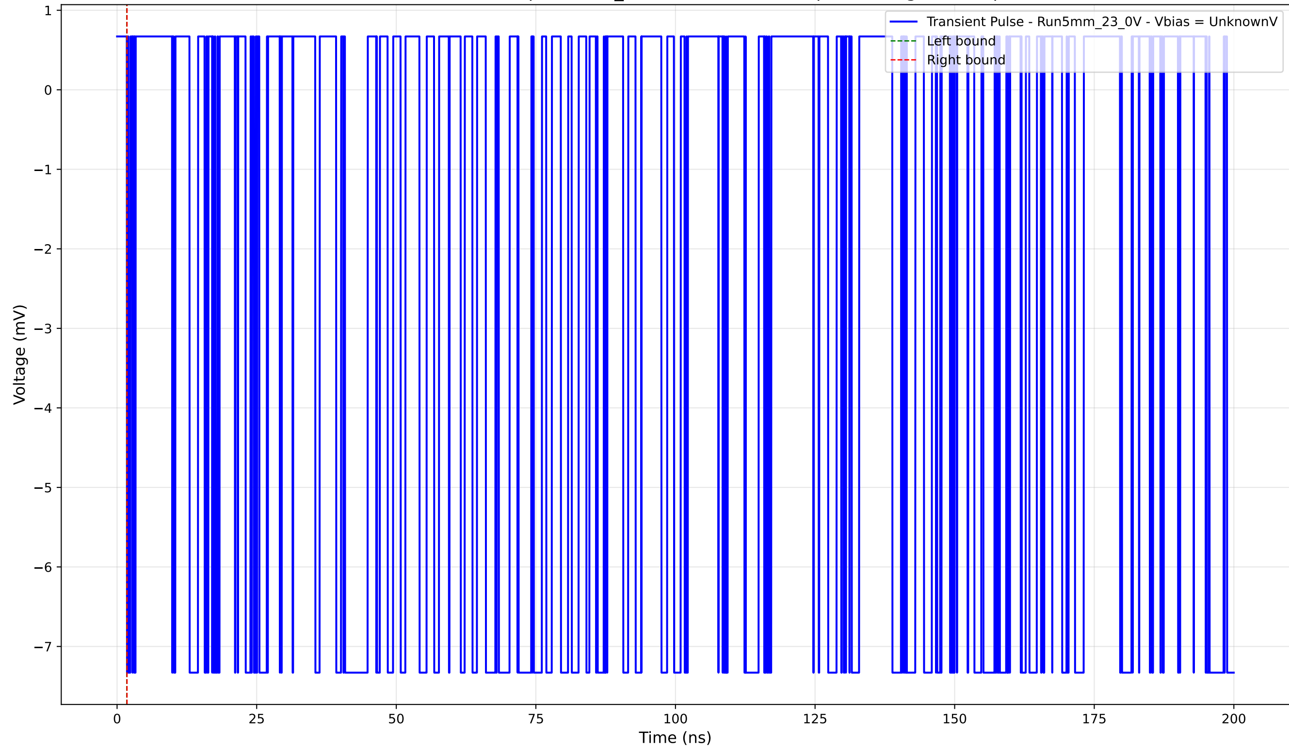
Transient Pulse - Sample: 5mm_23 - Position: 2530.0 \mu\text{m} - Charge: -0.00 pC
