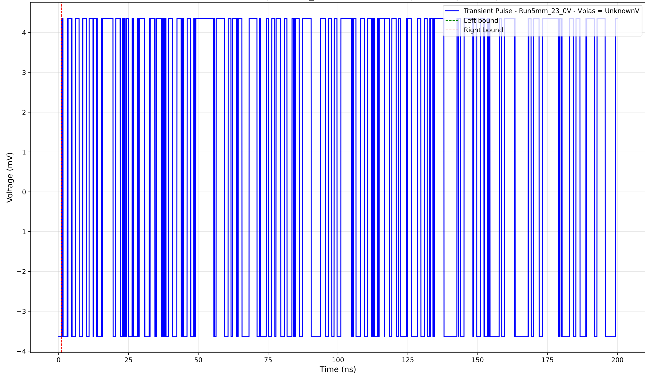
Transient Pulse - Sample: 5mm_23 - Position: 3580.0 \mu\text{m} - Charge: 0.00 pC
