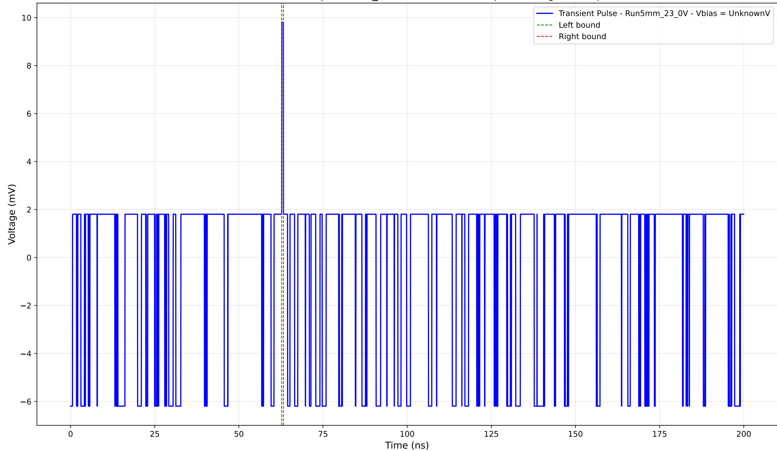
Transient Pulse - Sample: 5mm_23 - Position: 3325.0 \mu\text{m} - Charge: 0.10 pC
