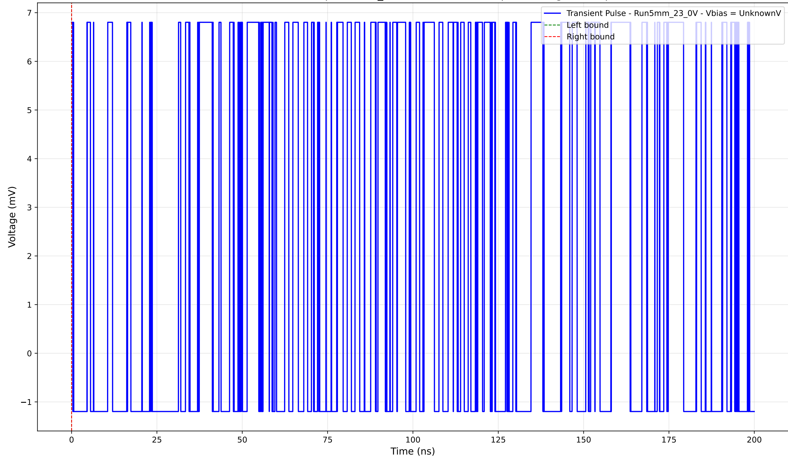
Transient Pulse - Sample: 5mm_23 - Position: 1840.0 \mu\text{m} - Charge: 0.00 pC
