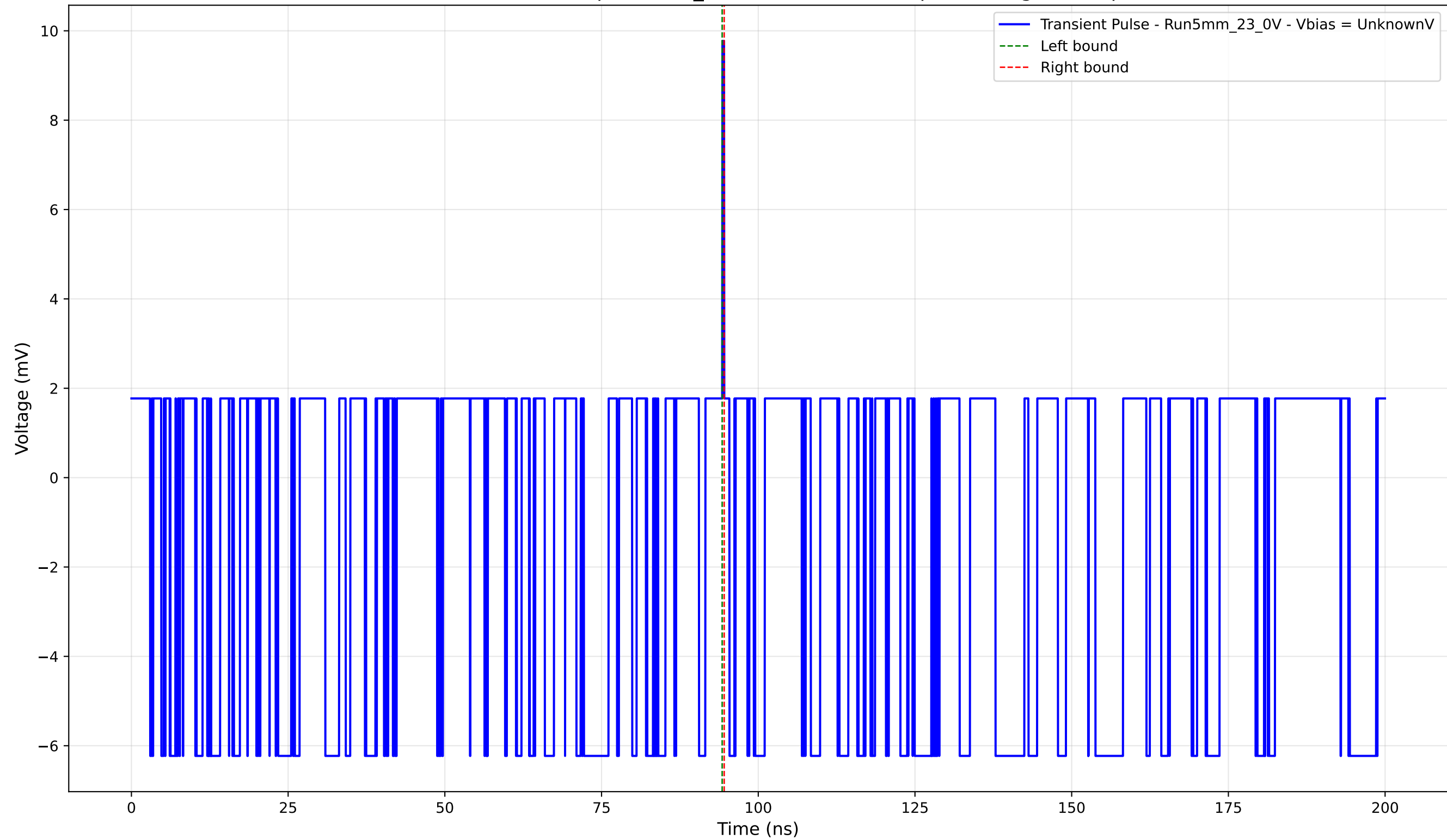
Transient Pulse - Sample: 5mm_23 - Position: 1880.0 \mu\text{m} - Charge: 0.06 pC
