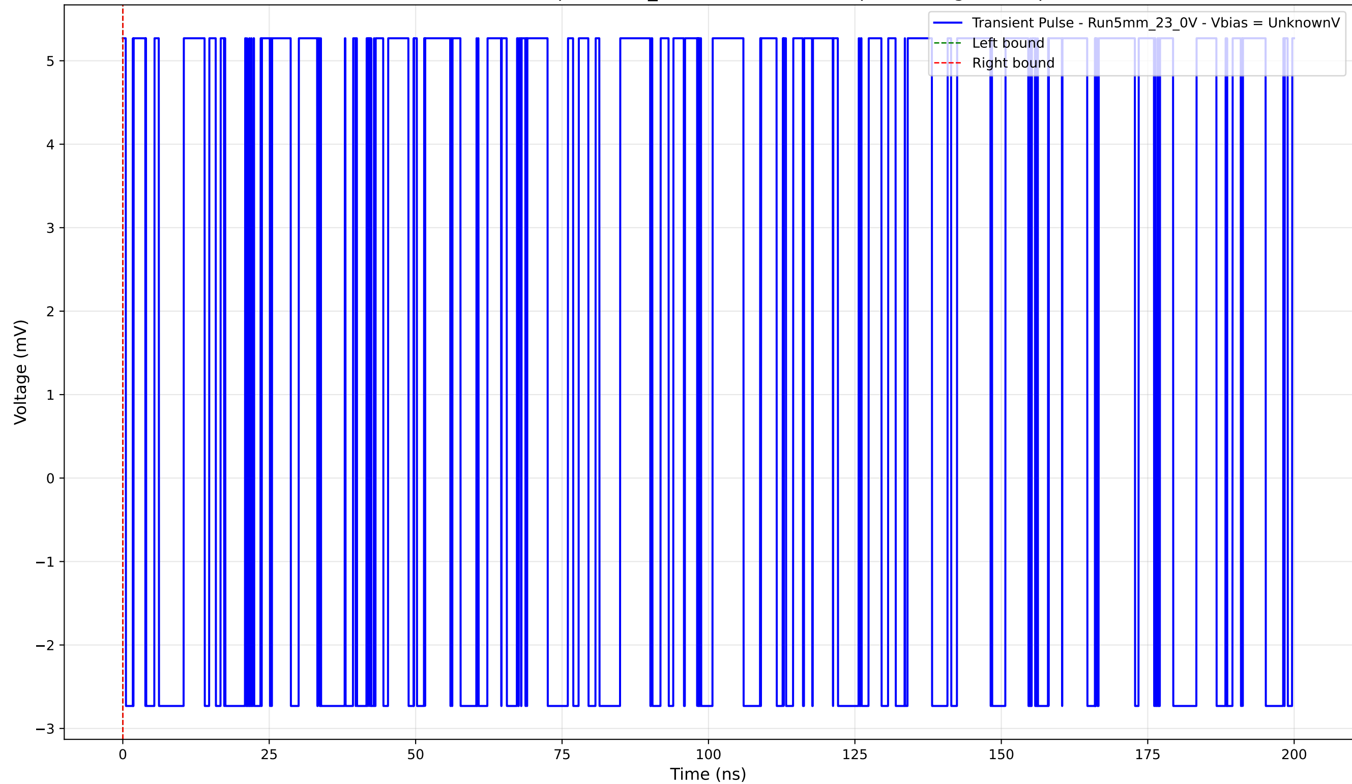
Transient Pulse - Sample: 5mm_23 - Position: 2335.0 \mu\text{m} - Charge: 0.00 pC
