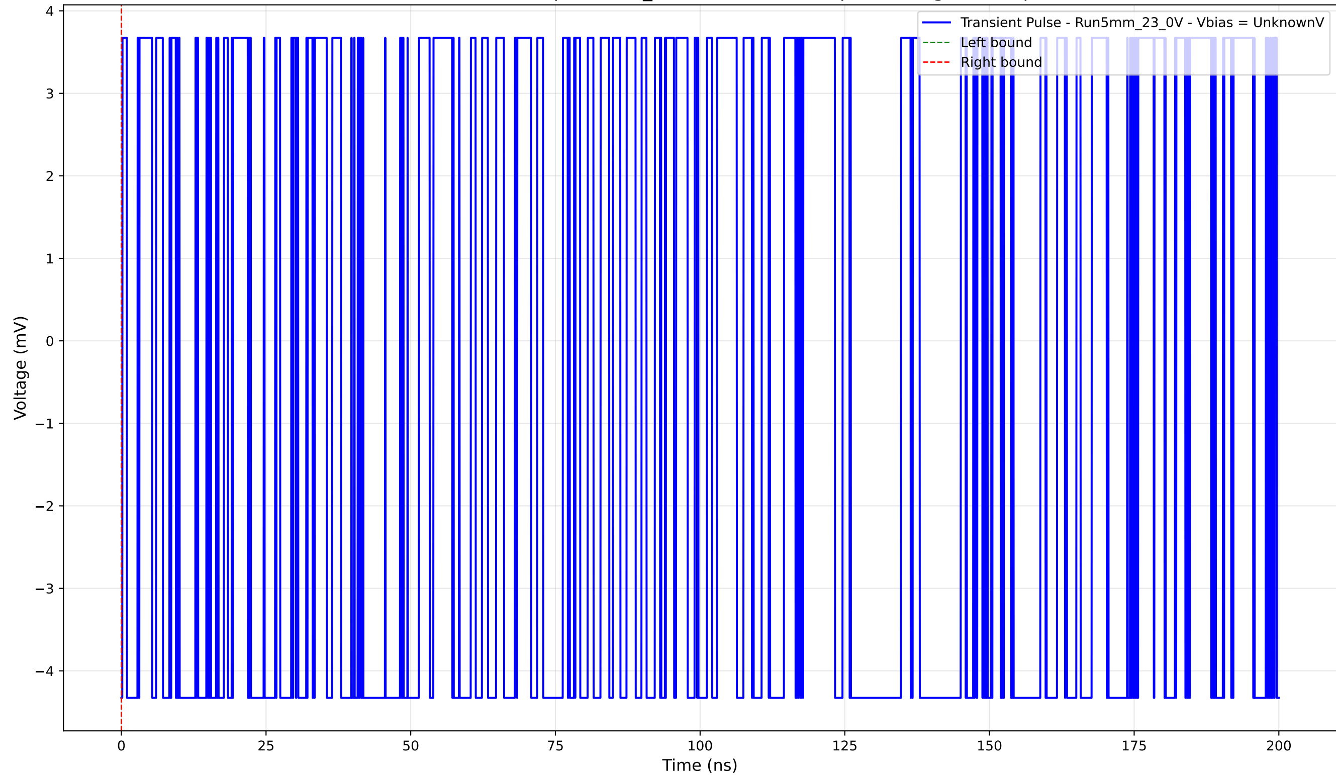
Transient Pulse - Sample: 5mm_23 - Position: 450.0 \mu\text{m} - Charge: -0.00 pC
