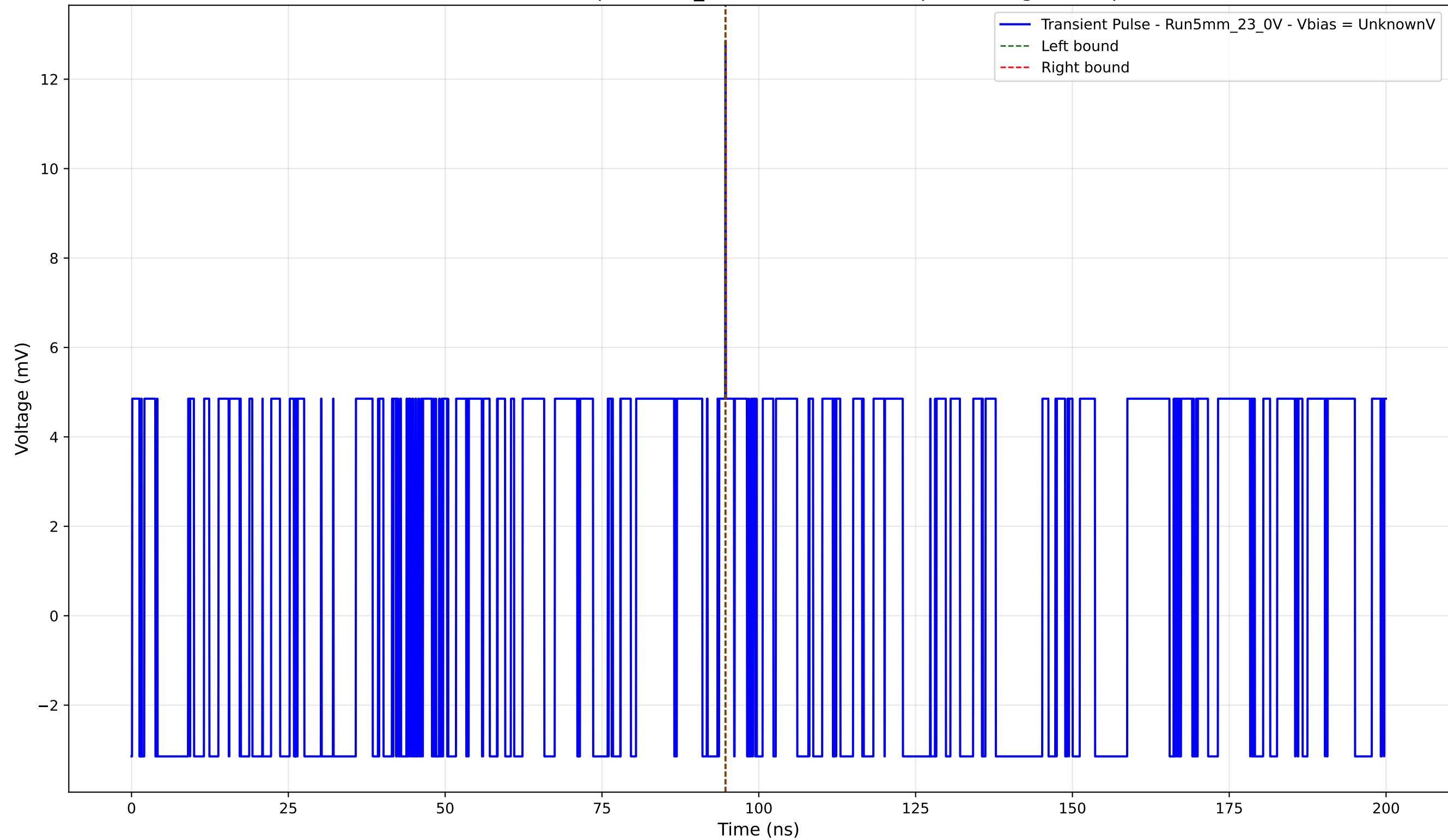
Transient Pulse - Sample: 5mm_23 - Position: 2905.0 \mu\text{m} - Charge: 0.02 pC
