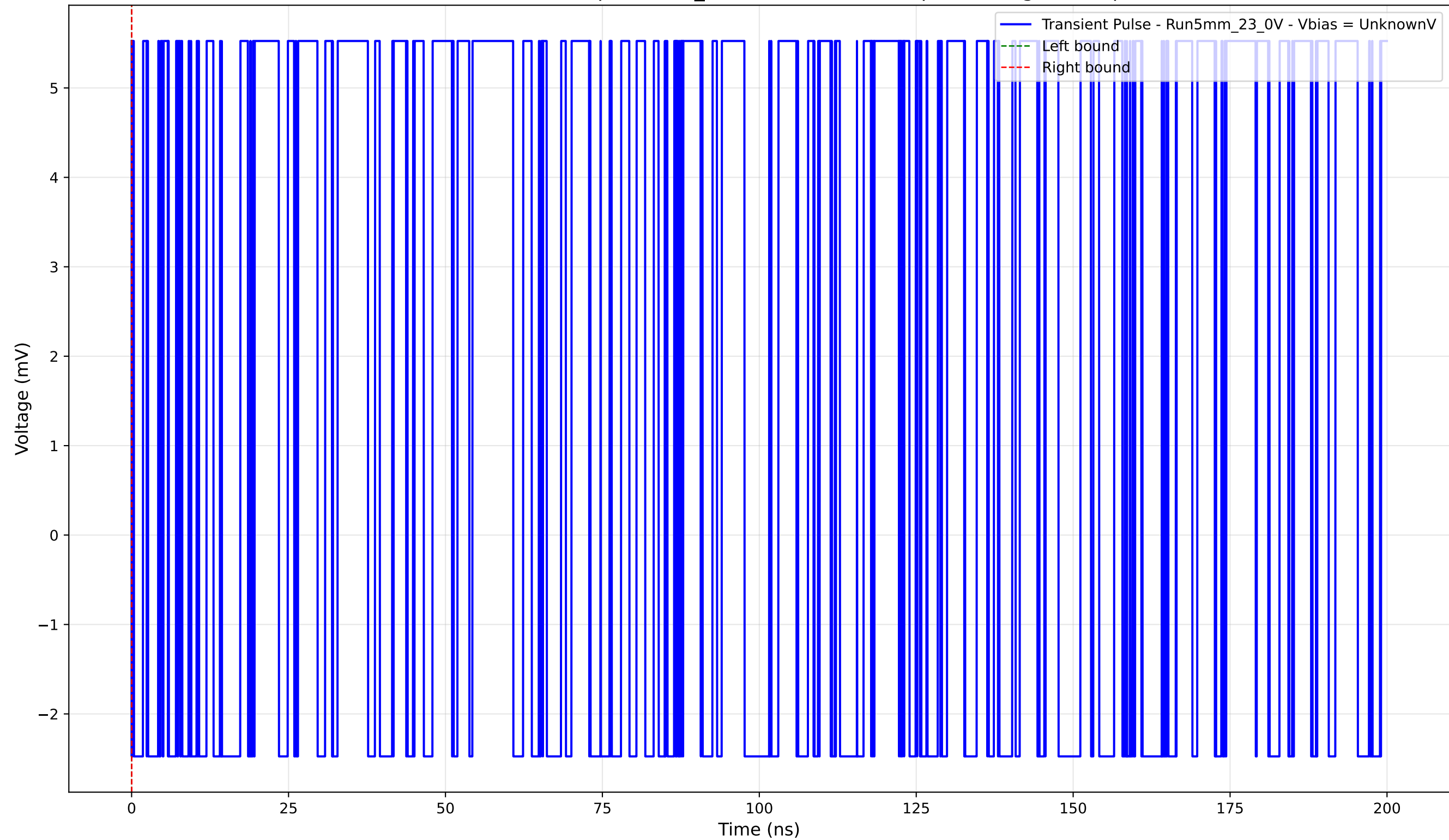
Transient Pulse - Sample: 5mm_23 - Position: 4120.0 \mu\text{m} - Charge: 0.00 pC
