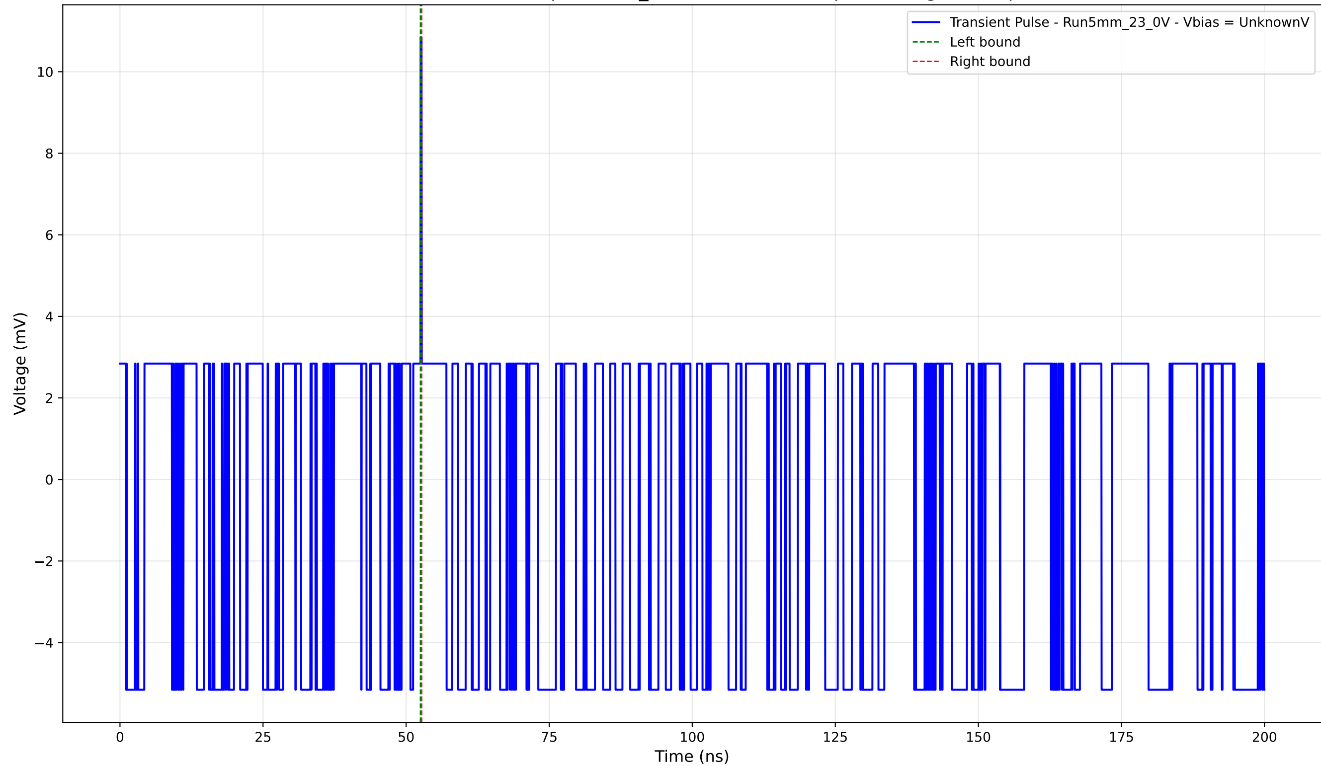
Transient Pulse - Sample: 5mm_23 - Position: 315.0 \mu\text{m} - Charge: 0.04 pC
