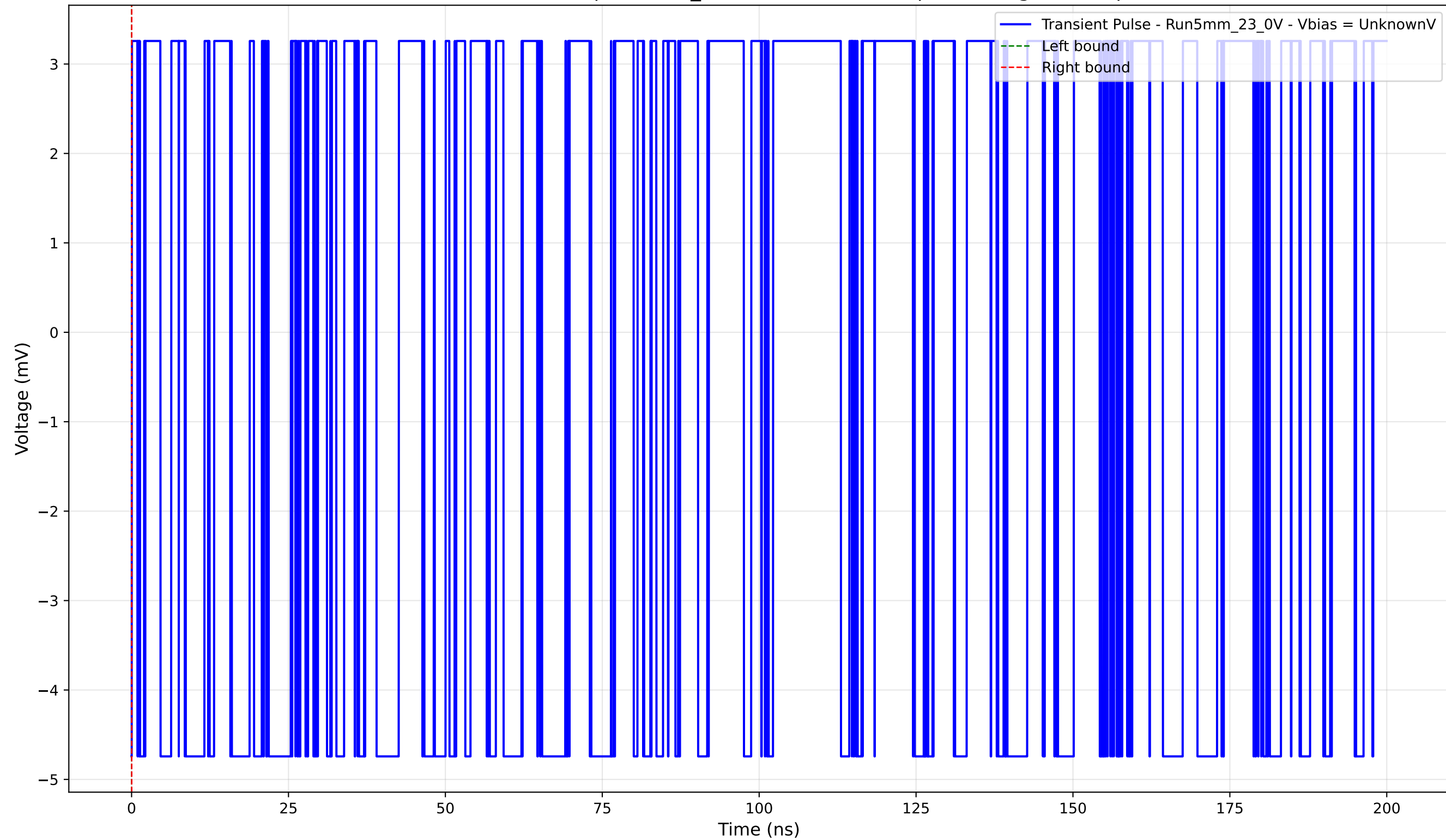
Transient Pulse - Sample: 5mm_23 - Position: 4790.0 \mu\text{m} - Charge: -0.00 pC
