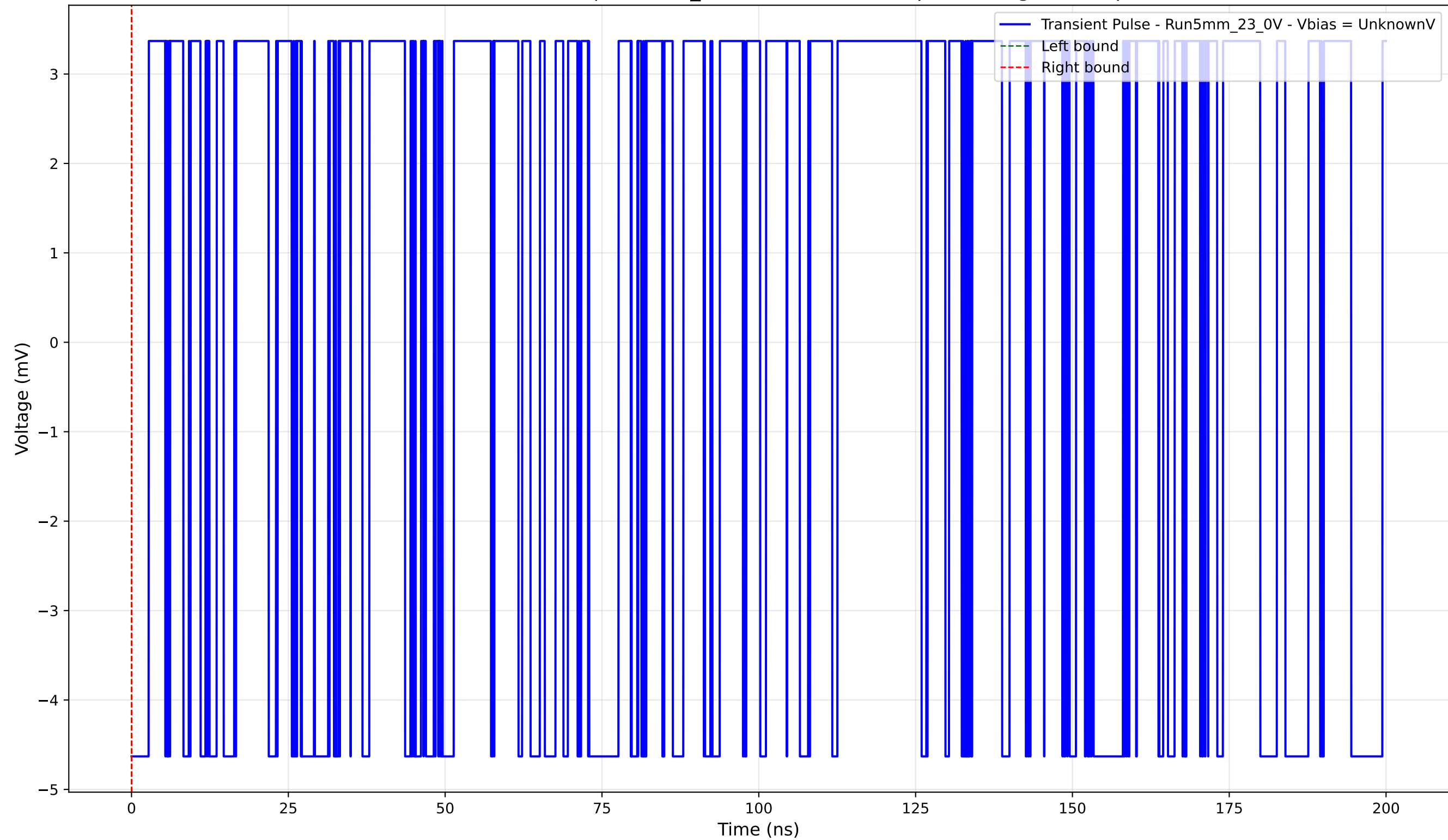
Transient Pulse - Sample: 5mm_23 - Position: 3750.0 \mu\text{m} - Charge: -0.00 pC
