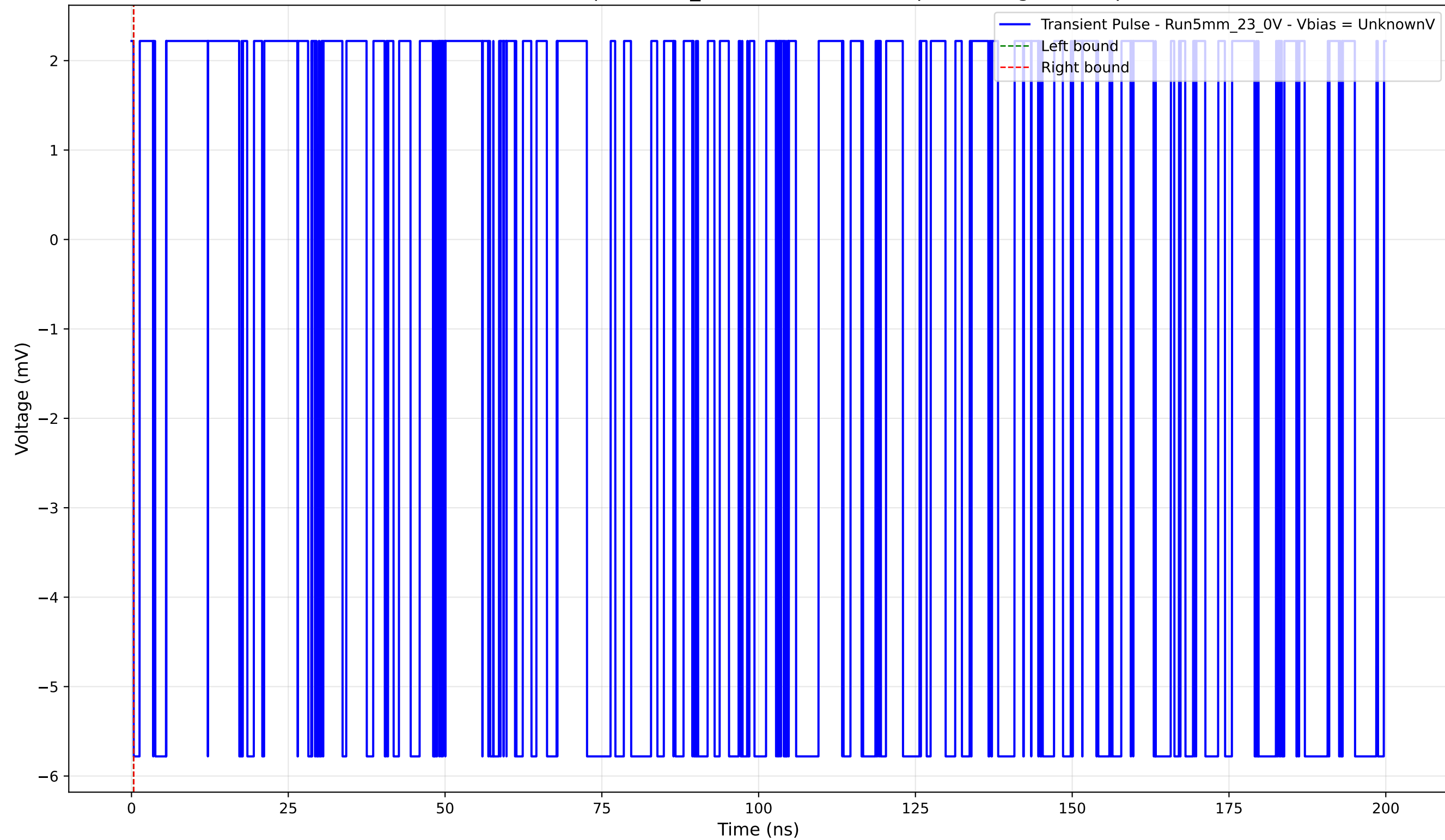
Transient Pulse - Sample: 5mm_23 - Position: 3715.0 \mu\text{m} - Charge: -0.00 pC
