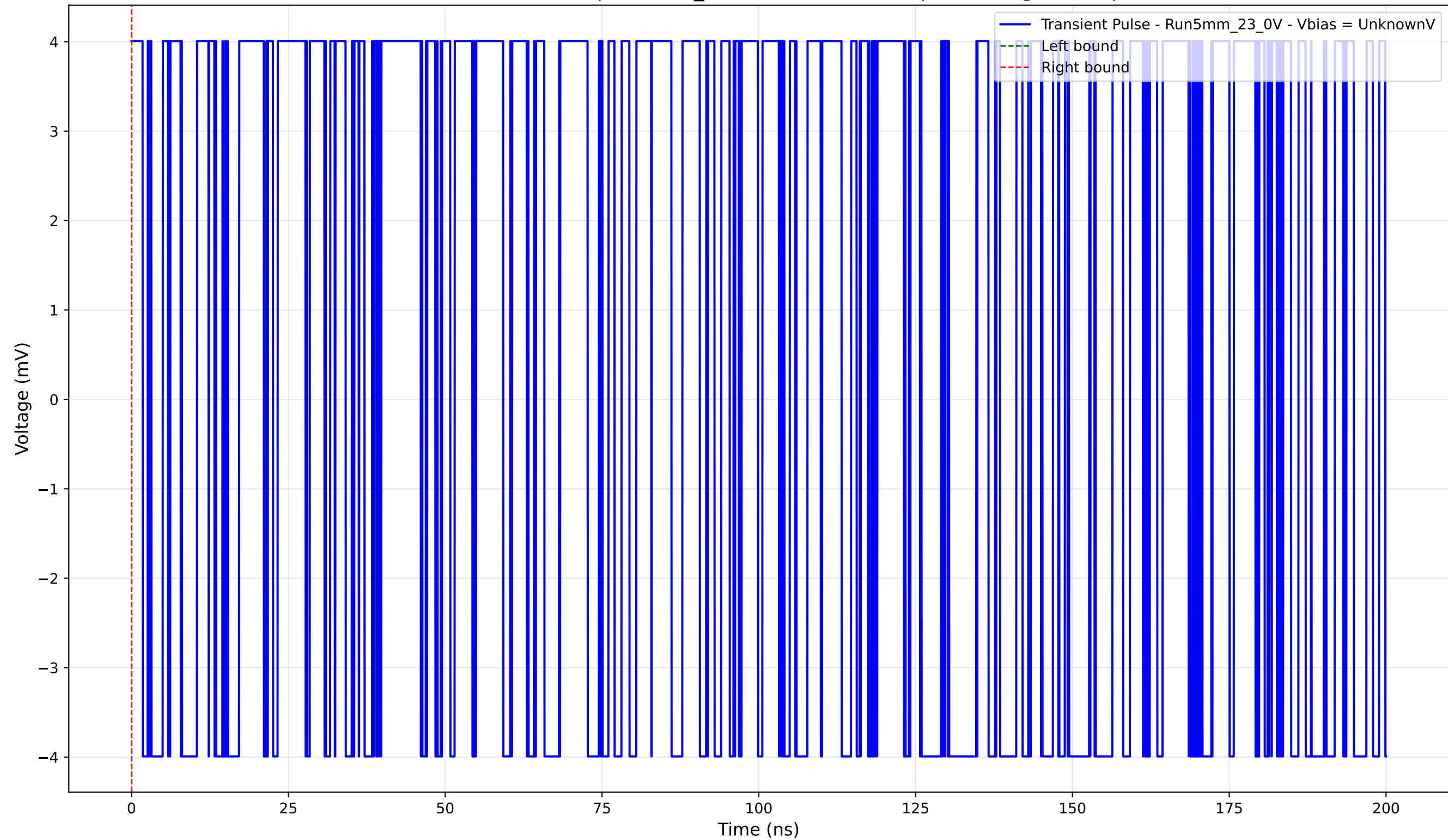
Transient Pulse - Sample: 5mm_23 - Position: 4250.0 \mu\text{m} - Charge: 0.00 pC
