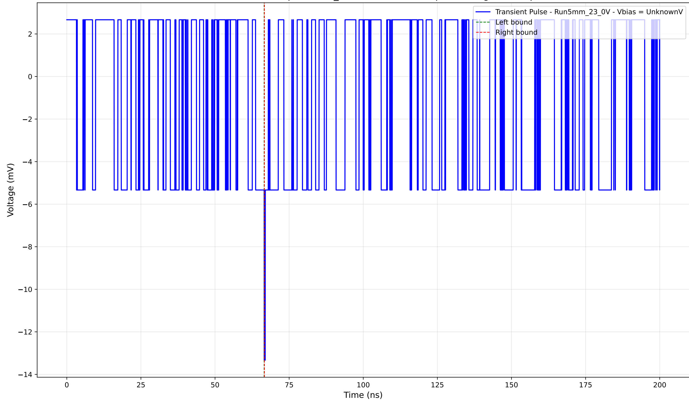
Transient Pulse - Sample: 5mm_23 - Position: 895.0 \mu\text{m} - Charge: -0.02 pC
