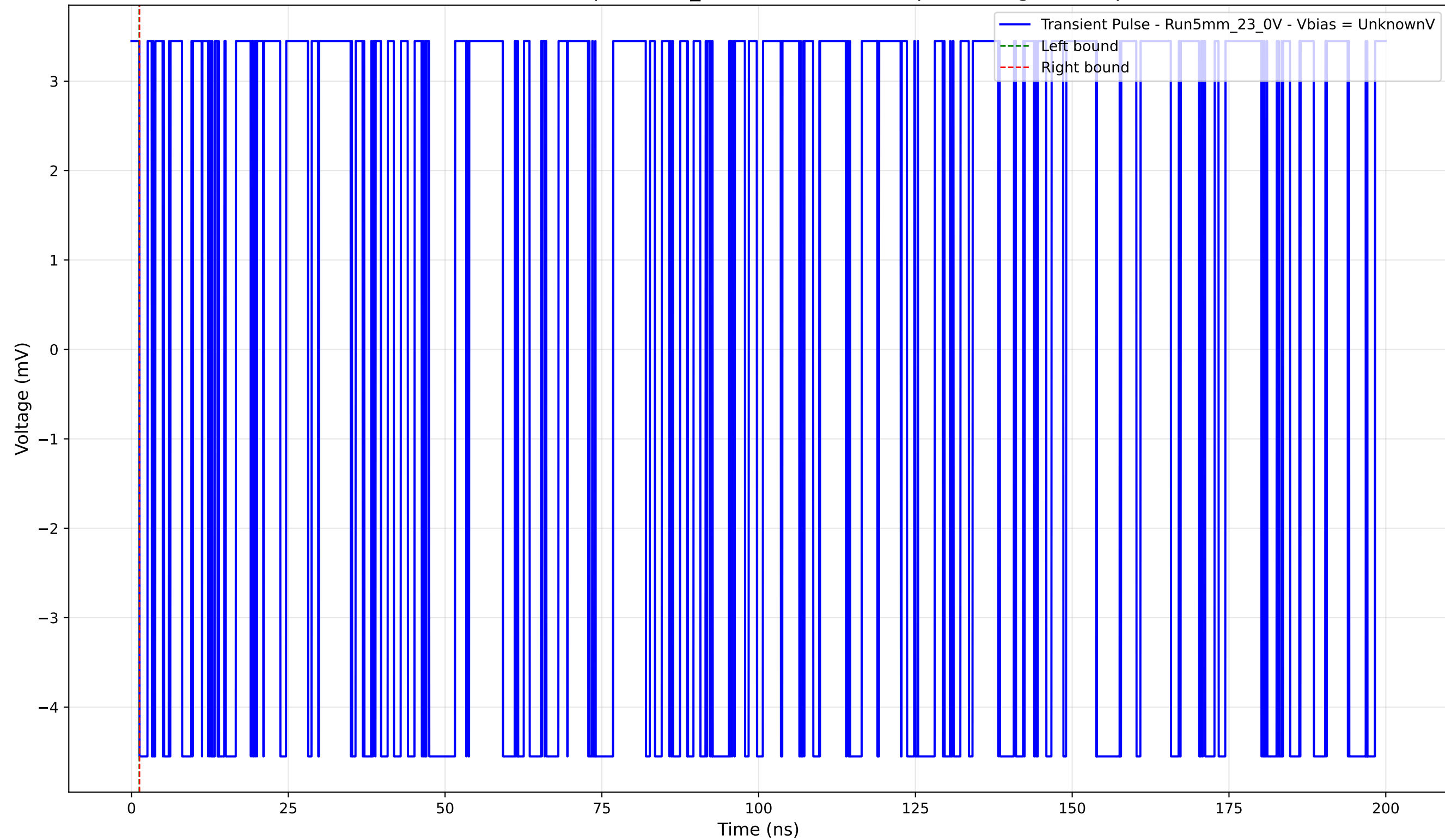
Transient Pulse - Sample: 5mm_23 - Position: 4150.0 \mu\text{m} - Charge: -0.00 pC
