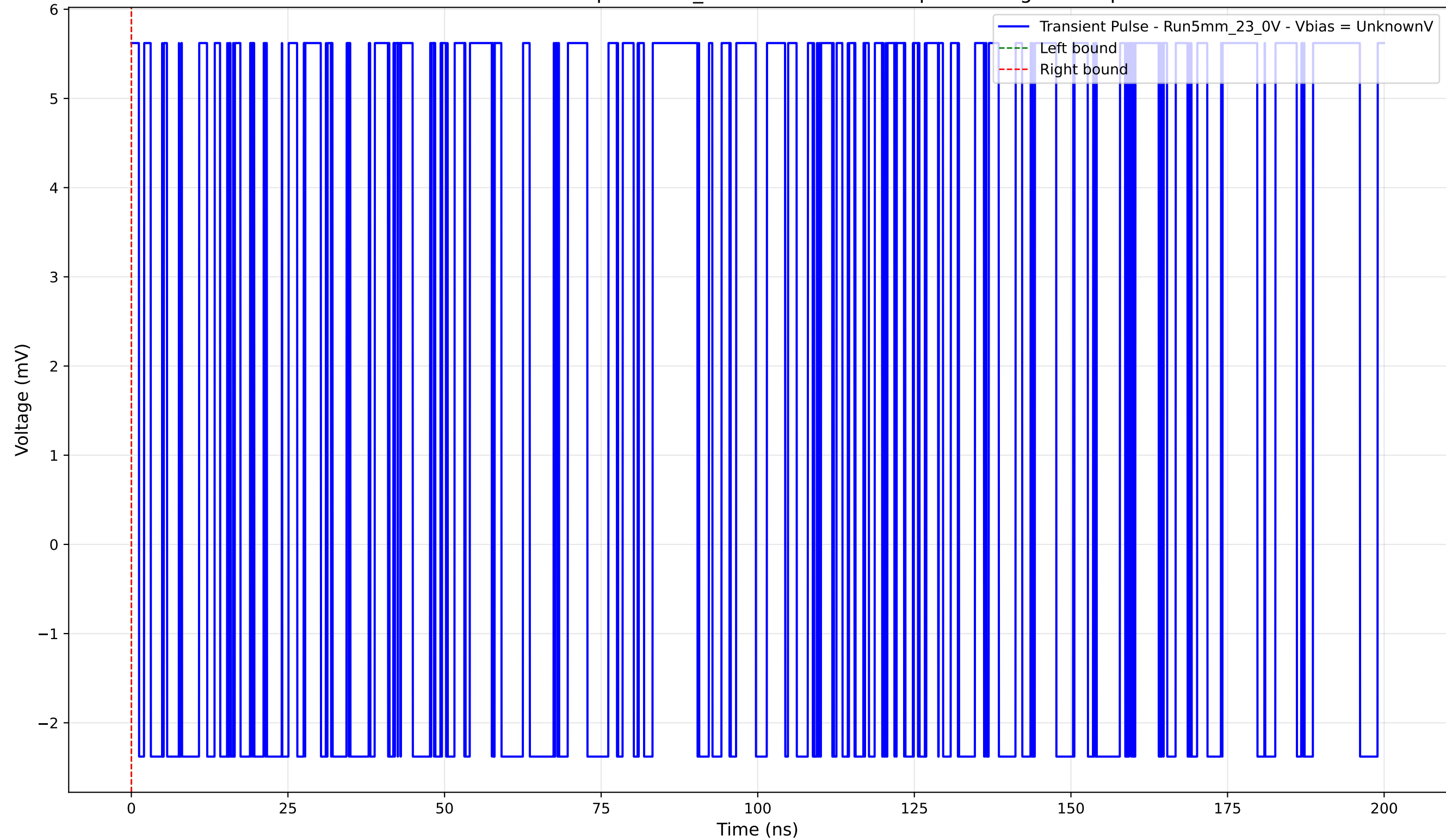
Transient Pulse - Sample: 5mm_23 - Position: 1935.0 \mu\text{m} - Charge: 0.00 pC
