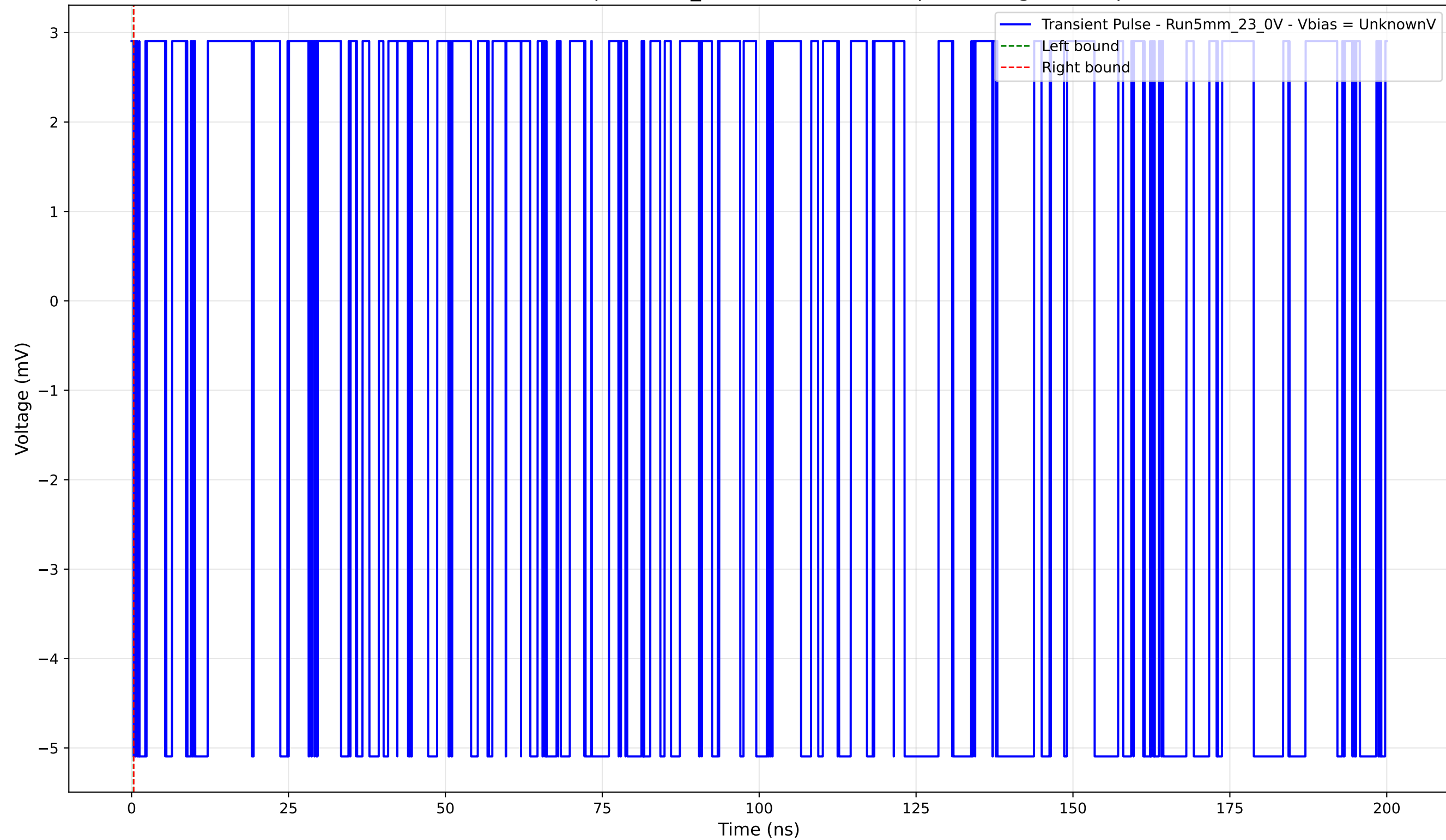
Transient Pulse - Sample: 5mm_23 - Position: 5000.0 \mu\text{m} - Charge: -0.00 pC
