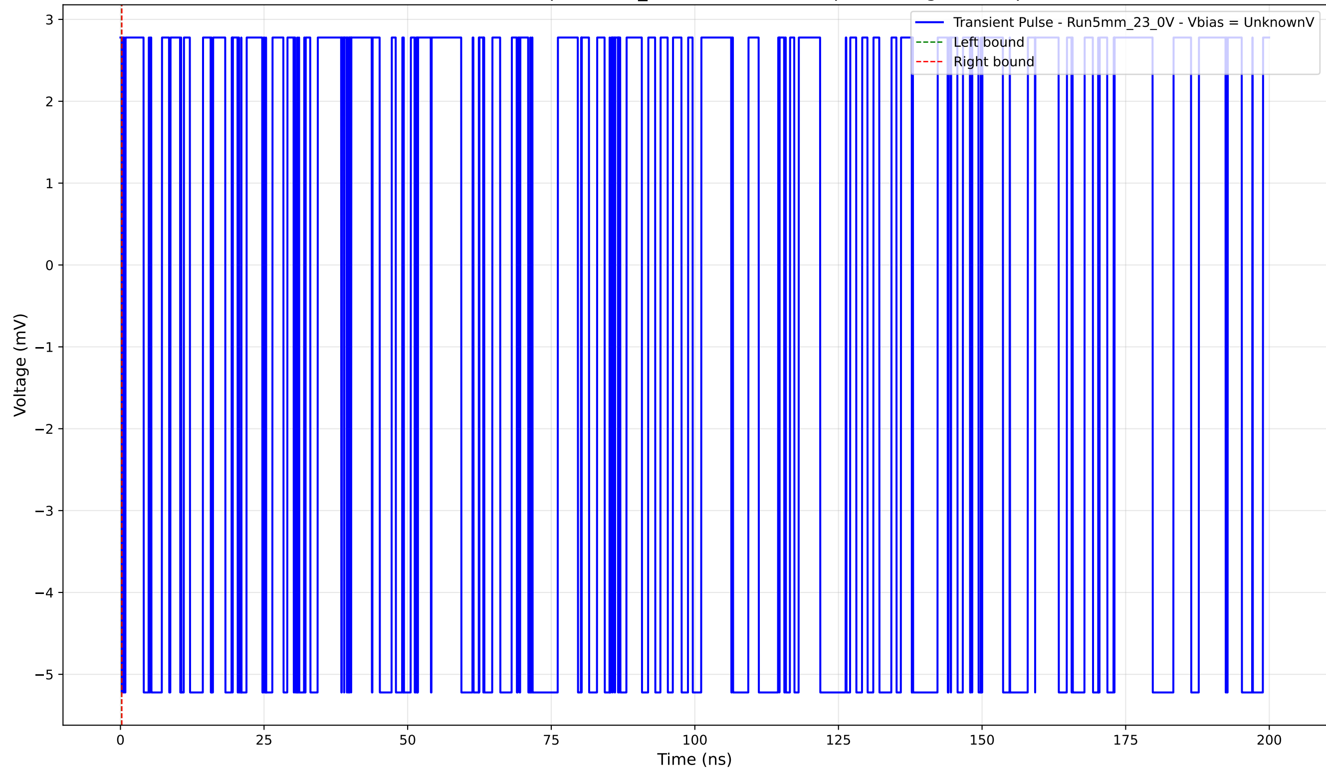
Transient Pulse - Sample: 5mm_23 - Position: 760.0 \mu\text{m} - Charge: -0.00 pC
