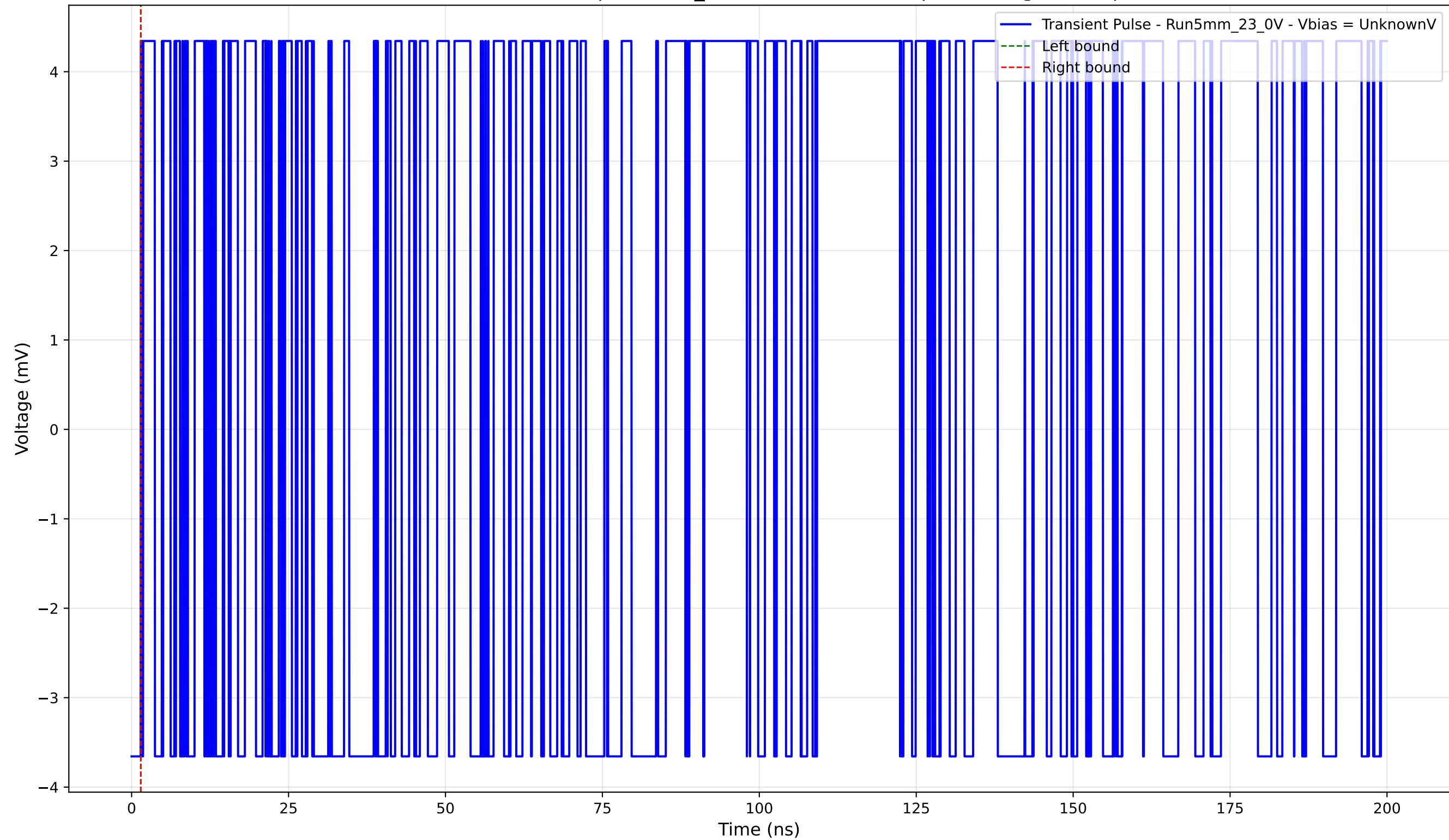
Transient Pulse - Sample: 5mm_23 - Position: 4115.0 \mu\text{m} - Charge: 0.00 pC
