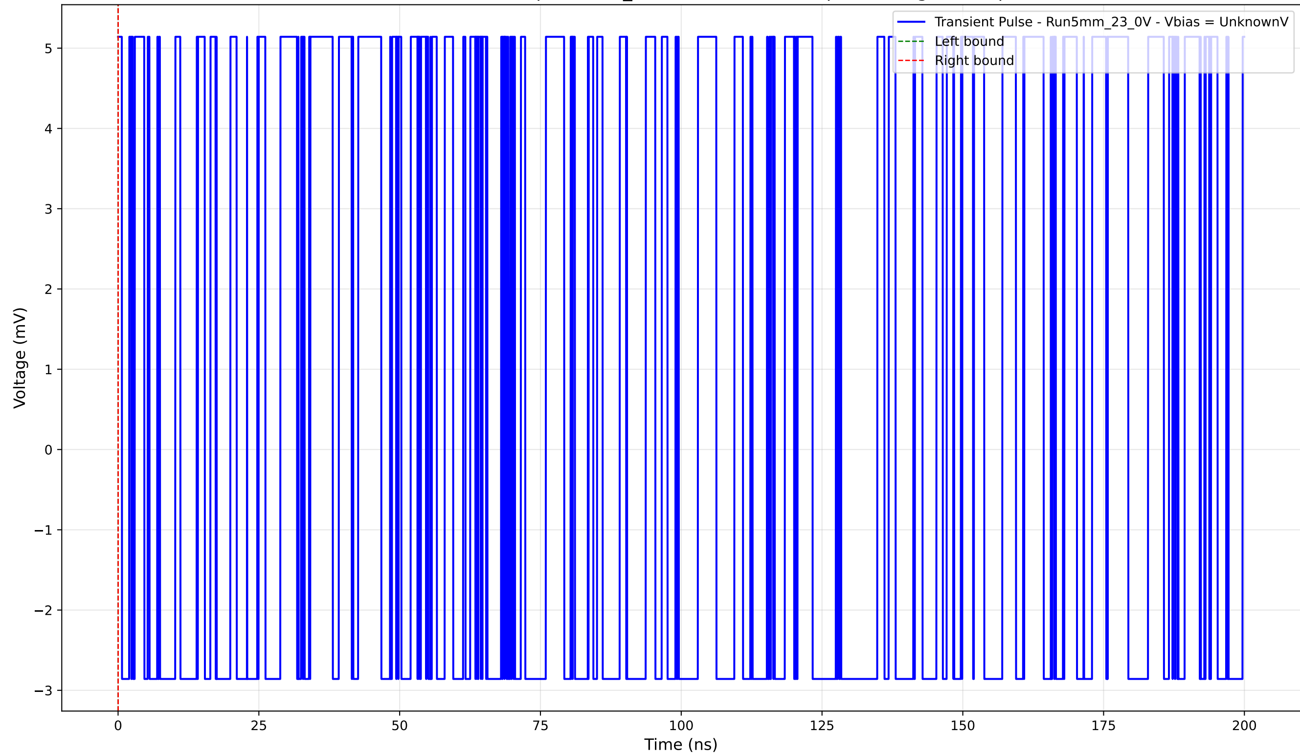
Transient Pulse - Sample: 5mm_23 - Position: 4755.0 \mu\text{m} - Charge: 0.00 pC
