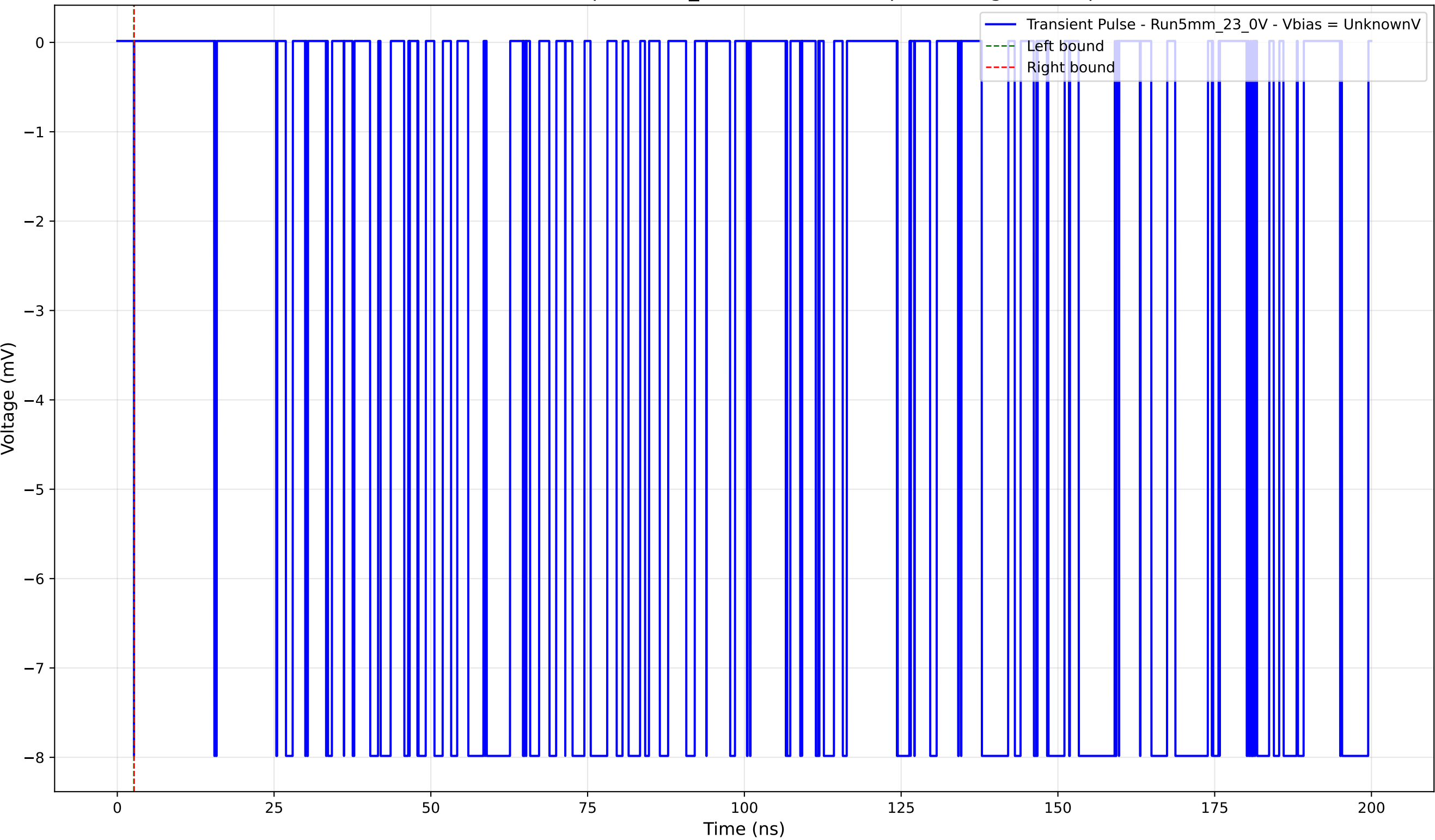
Transient Pulse - Sample: 5mm_23 - Position: 90.0 \mu\text{m} - Charge: -0.00 pC
