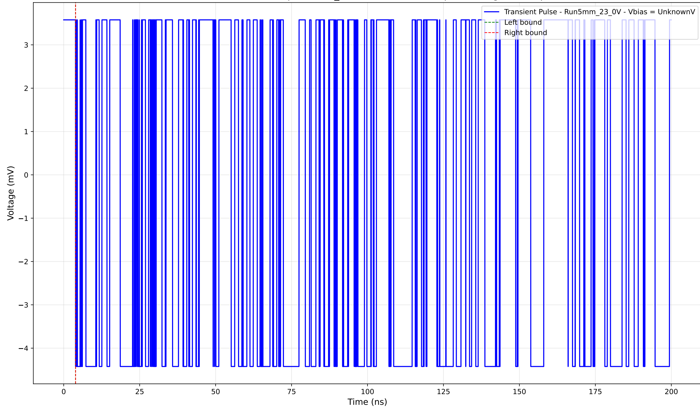
Transient Pulse - Sample: 5mm_23 - Position: 2010.0 \mu\text{m} - Charge: -0.00 pC
