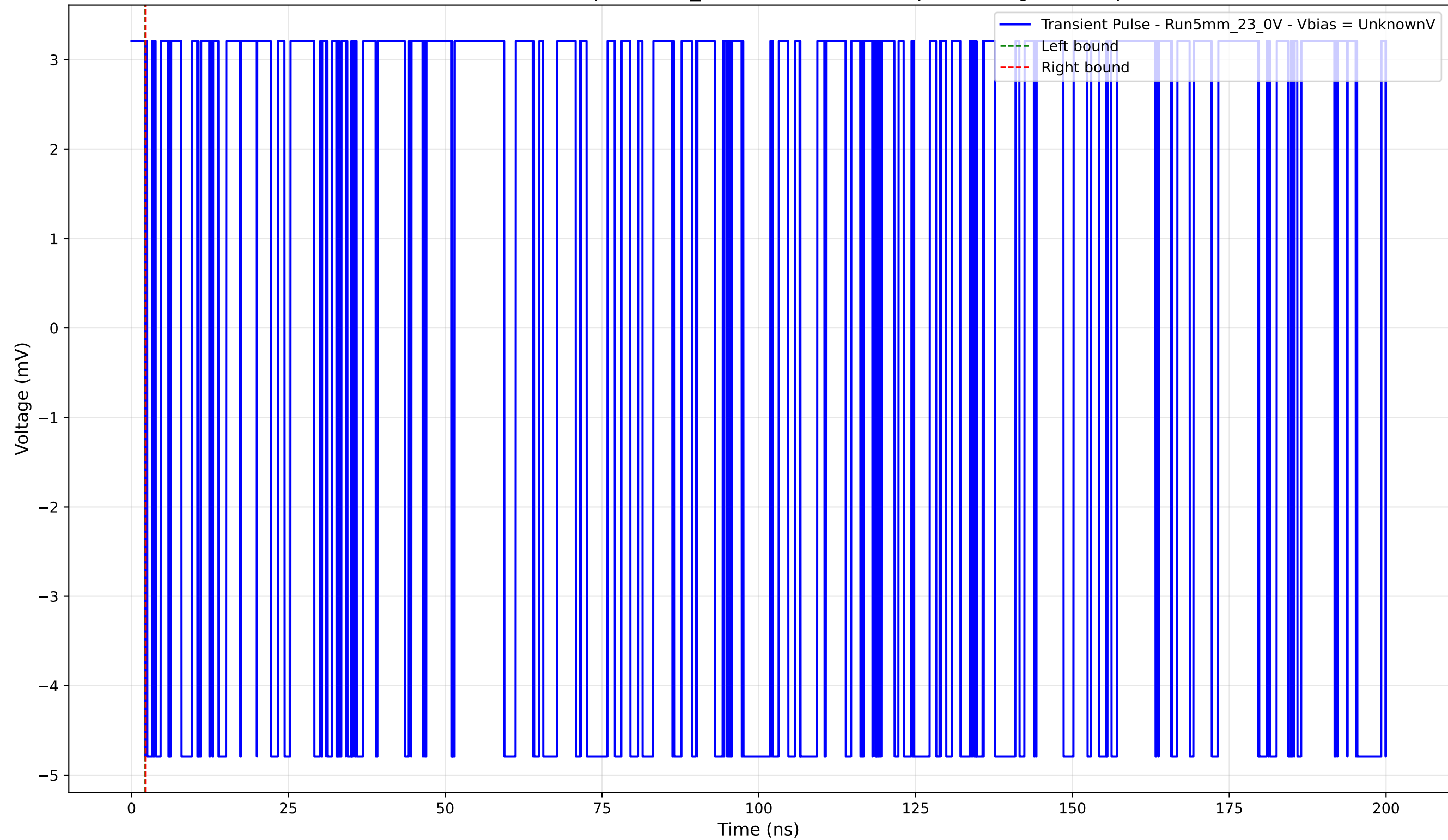
Transient Pulse - Sample: 5mm_23 - Position: 3020.0 \mu\text{m} - Charge: -0.00 pC
