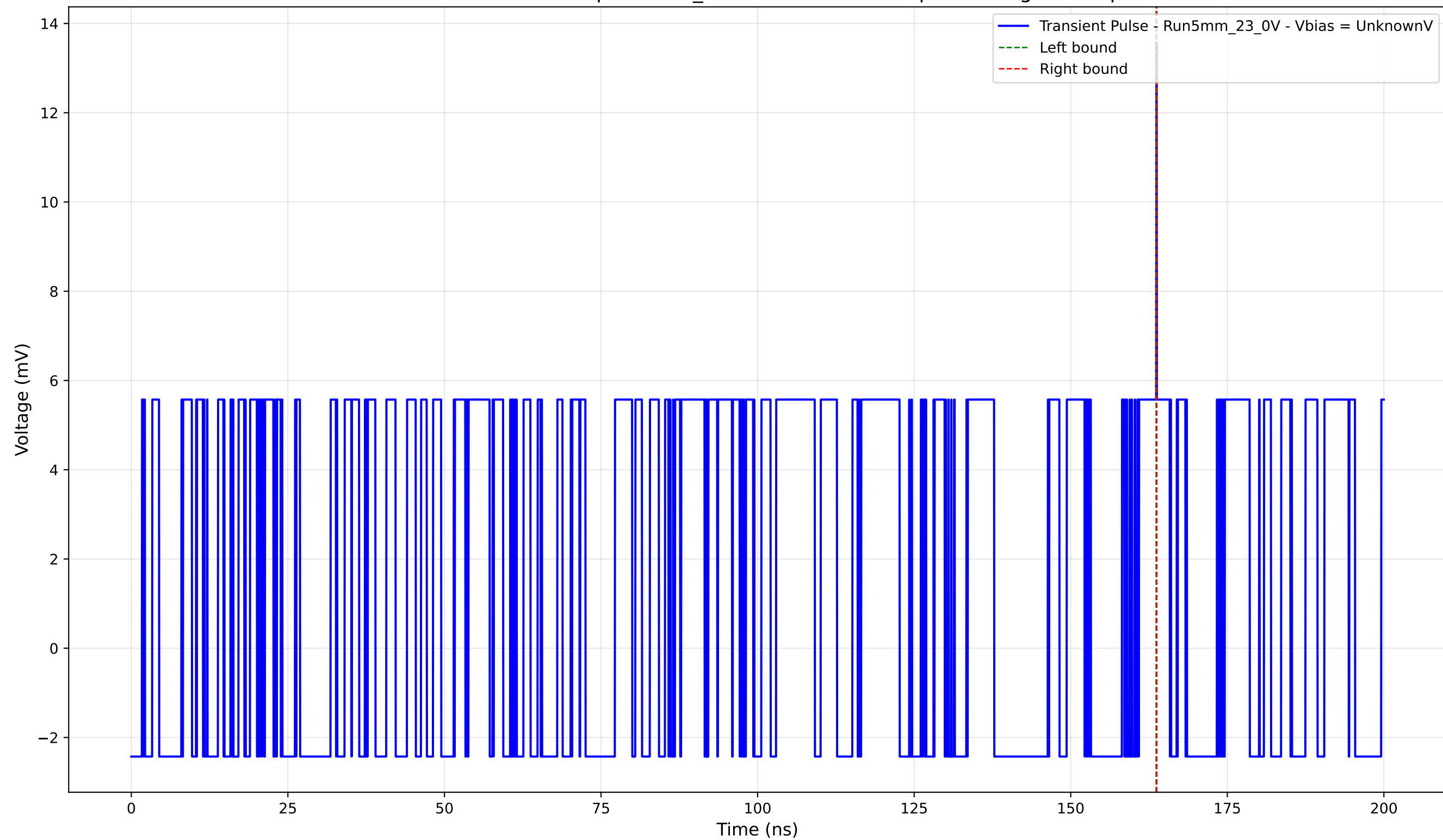
Transient Pulse - Sample: 5mm_23 - Position: 1330.0 \mu\text{m} - Charge: 0.02 pC
