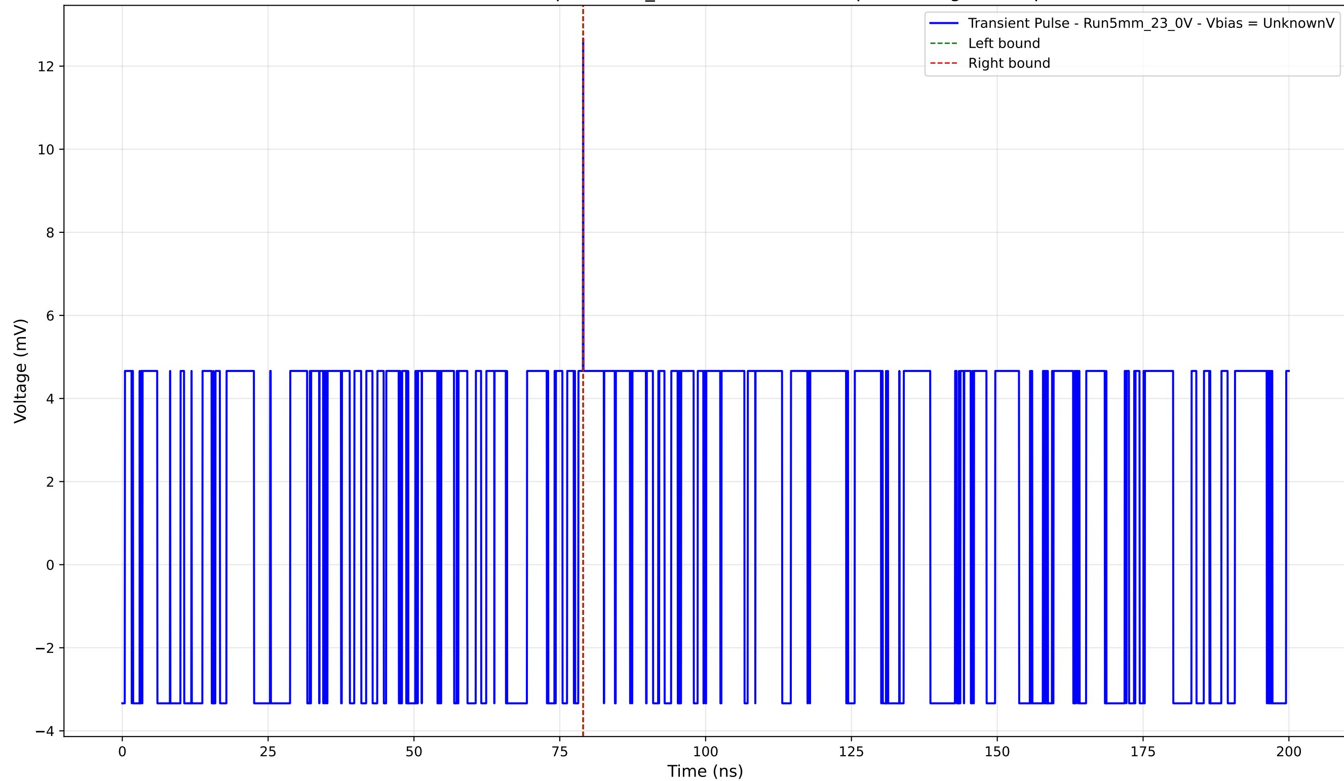
Transient Pulse - Sample: 5mm_23 - Position: 4785.0 \mu\text{m} - Charge: 0.02 pC
