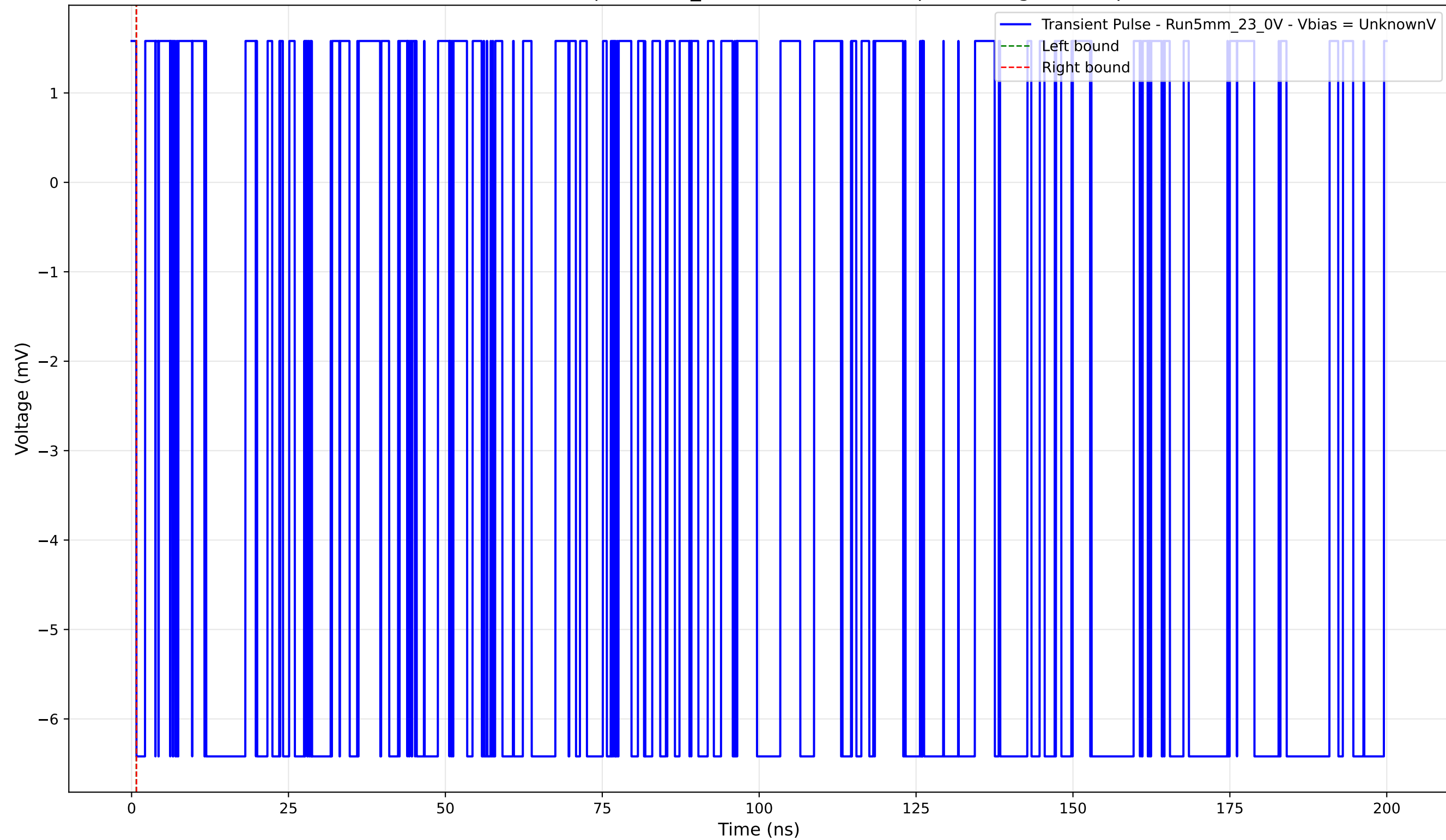
Transient Pulse - Sample: 5mm_23 - Position: 1745.0 \mu\text{m} - Charge: -0.00 pC
