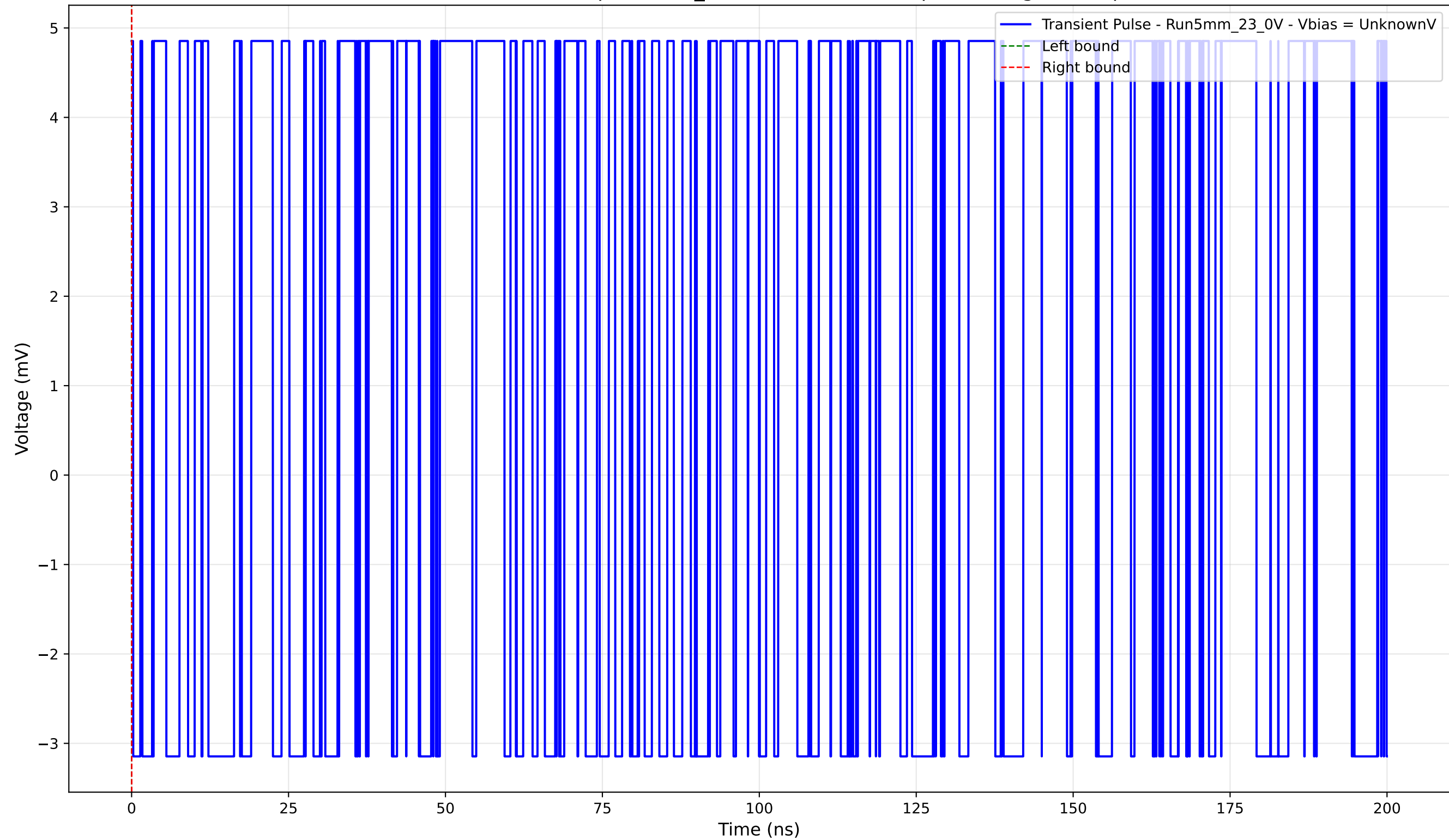
Transient Pulse - Sample: 5mm_23 - Position: 2400.0 \mu\text{m} - Charge: 0.00 pC
