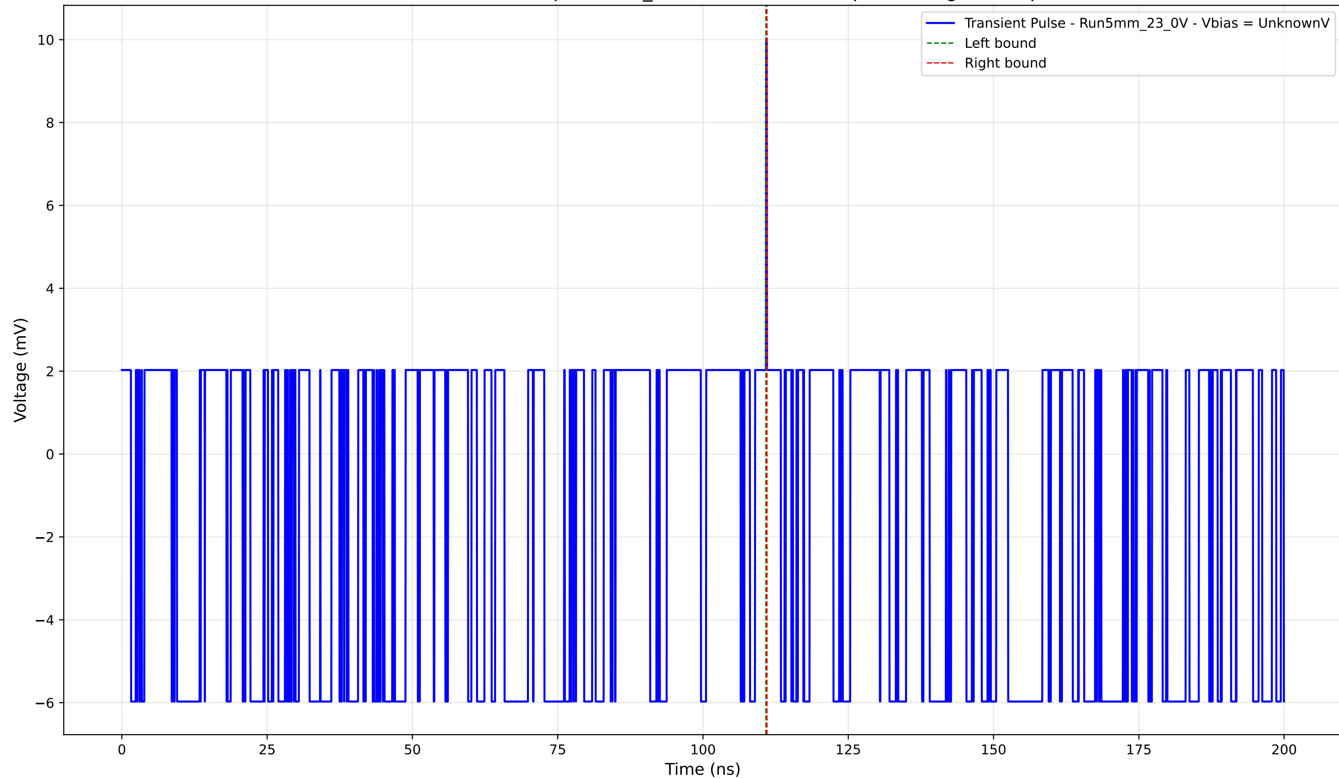
Transient Pulse - Sample: 5mm_23 - Position: 3540.0 \mu\text{m} - Charge: 0.03 pC
