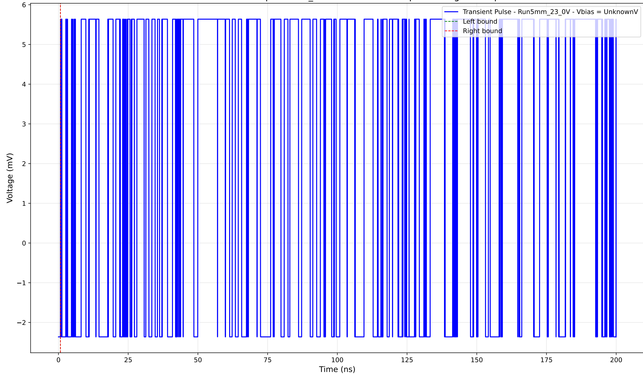
Transient Pulse - Sample: 5mm_23 - Position: 4610.0 \mu\text{m} - Charge: 0.00 pC
