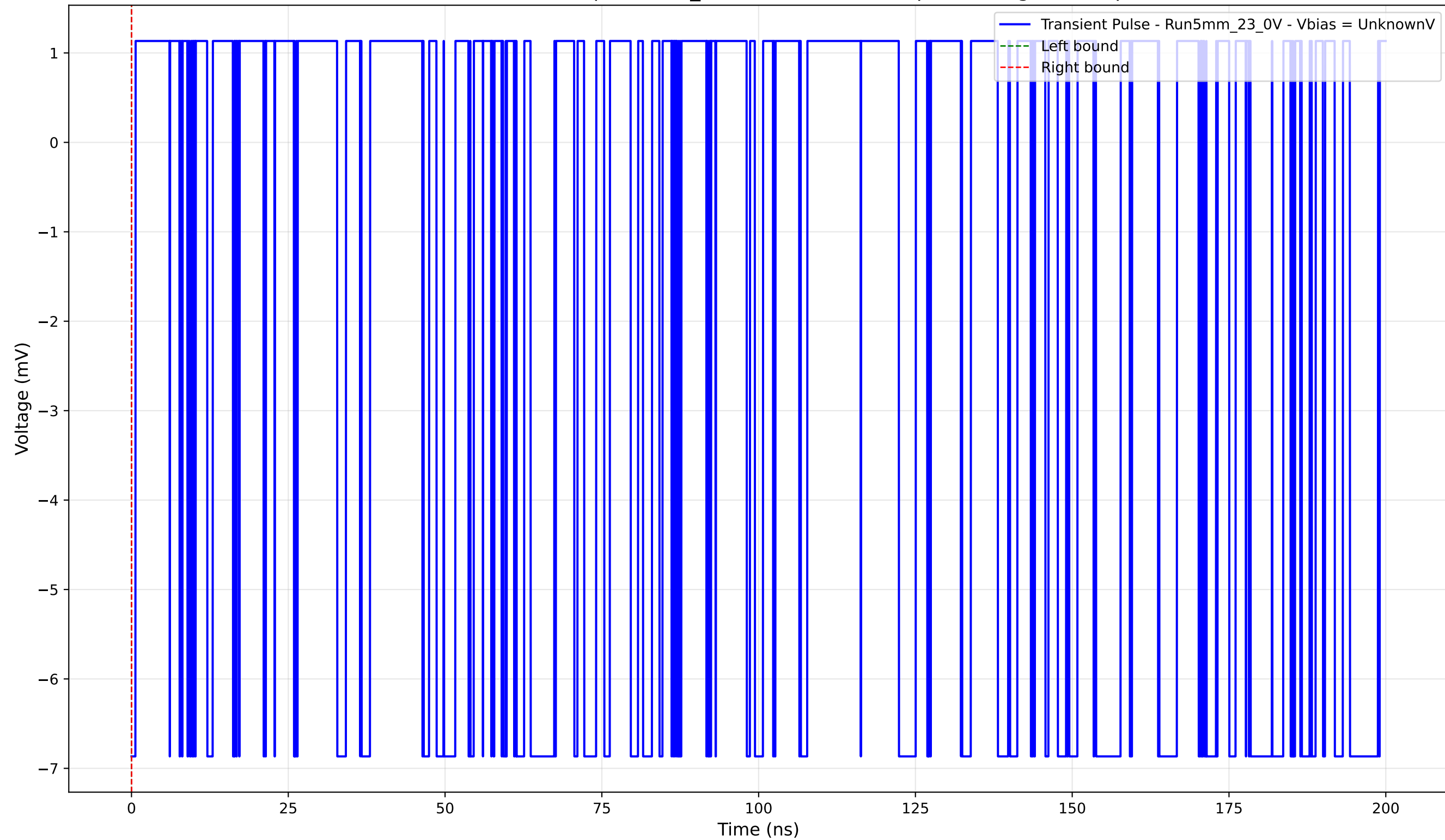
Transient Pulse - Sample: 5mm_23 - Position: 2575.0 \mu\text{m} - Charge: -0.00 pC
