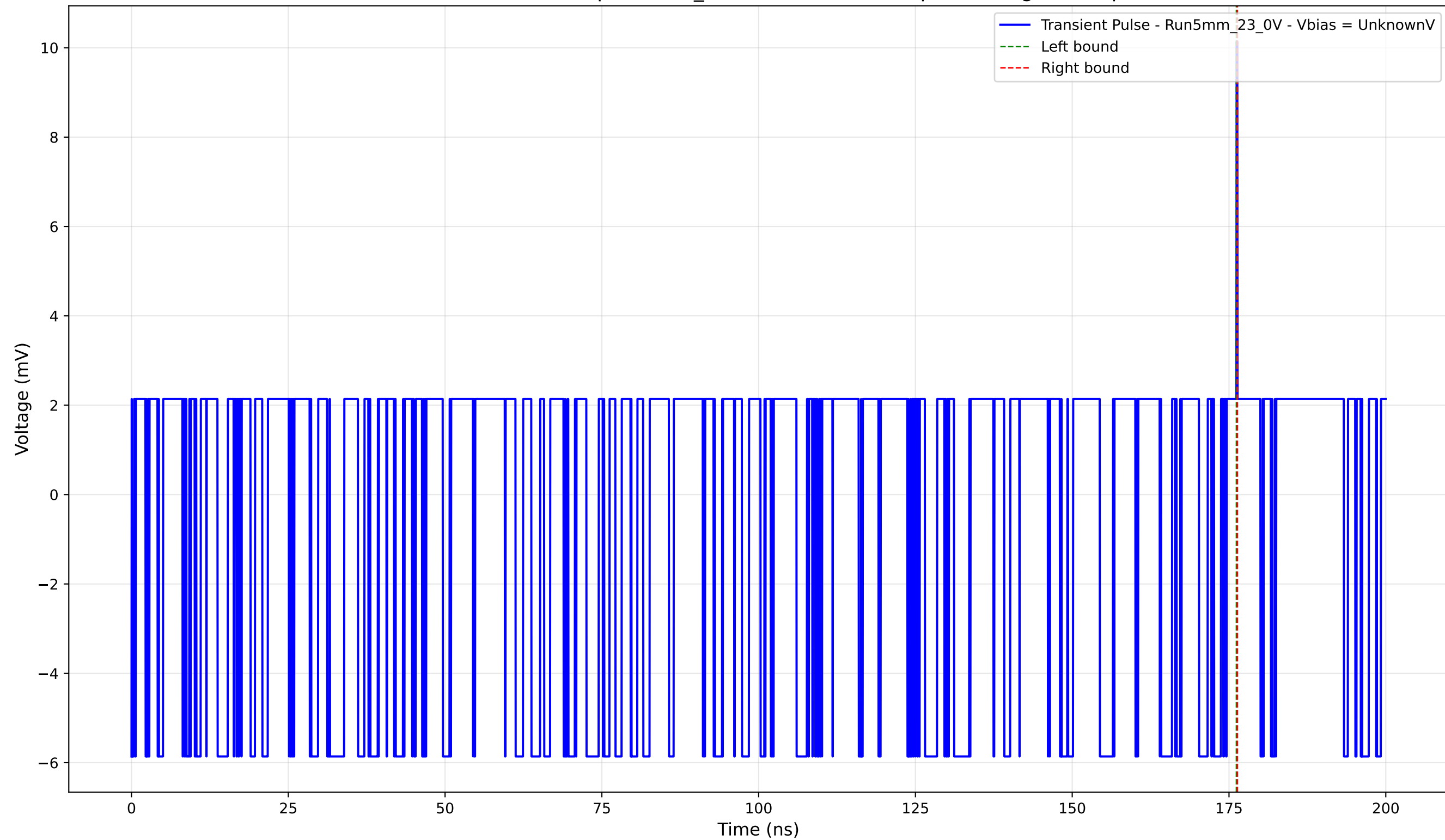
Transient Pulse - Sample: 5mm_23 - Position: 4270.0 \mu\text{m} - Charge: 0.03 pC
