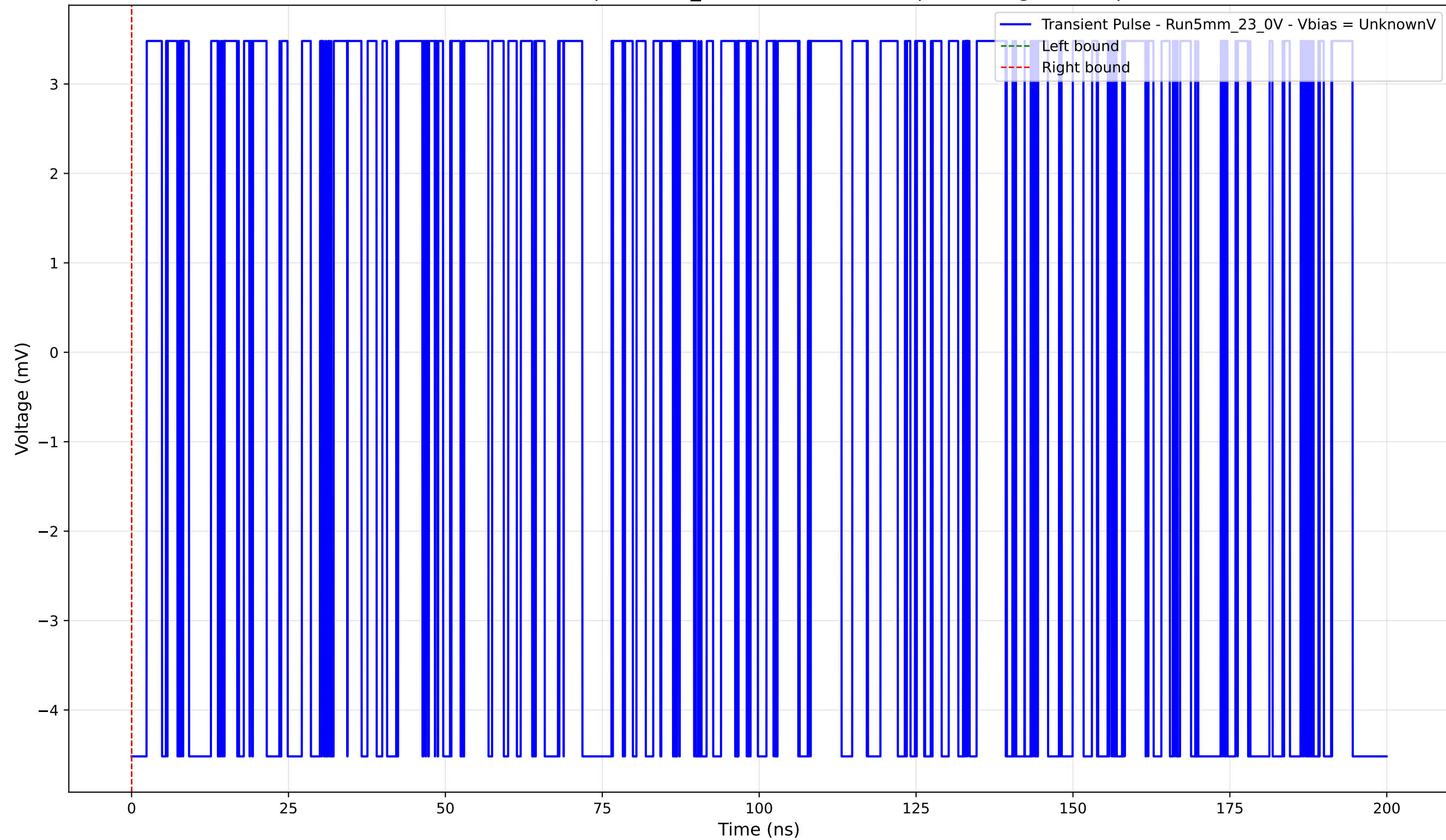
Transient Pulse - Sample: 5mm_23 - Position: 3505.0 \mu\text{m} - Charge: -0.00 pC
