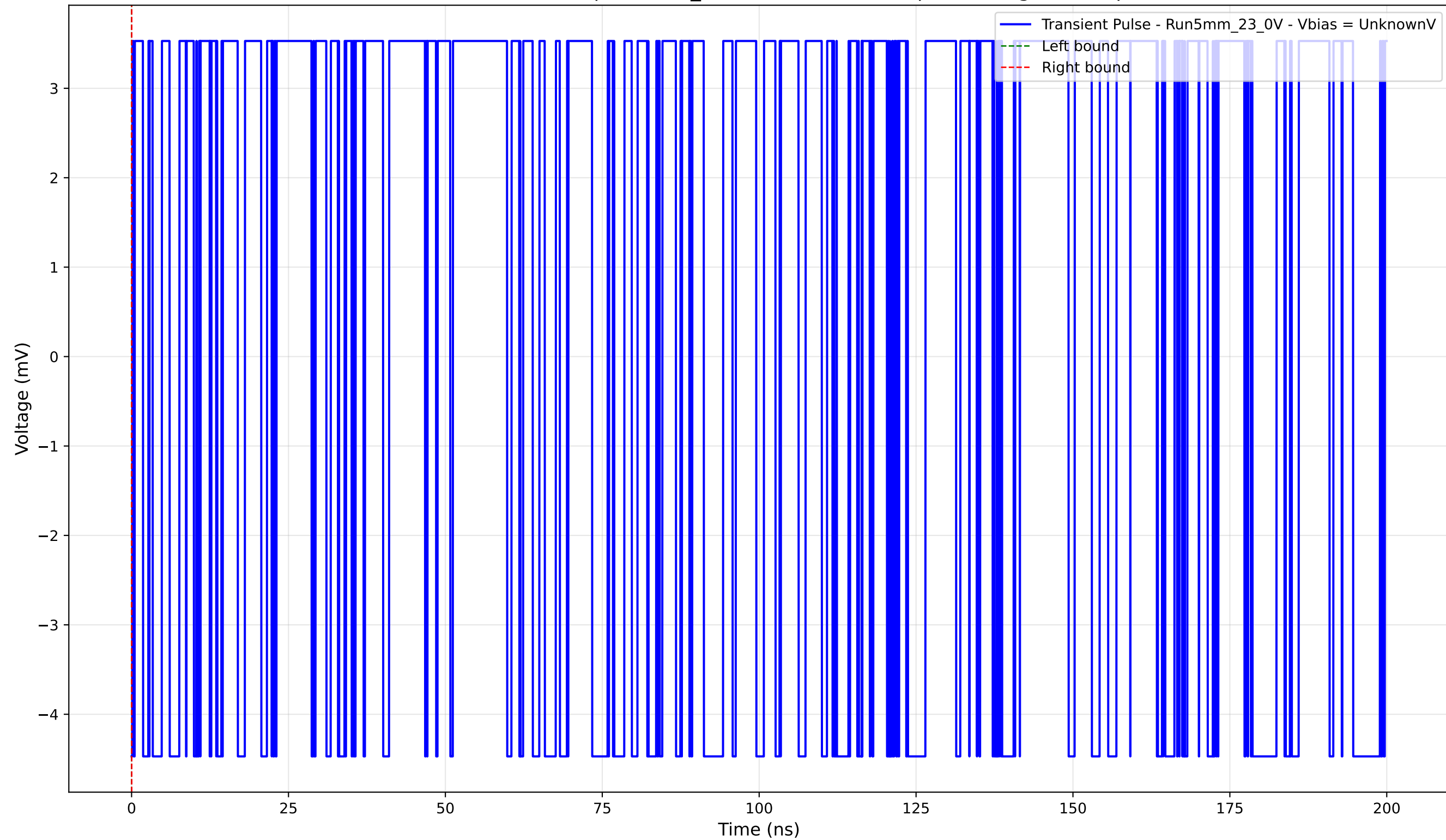
Transient Pulse - Sample: 5mm_23 - Position: 2225.0 \mu\text{m} - Charge: -0.00 pC
