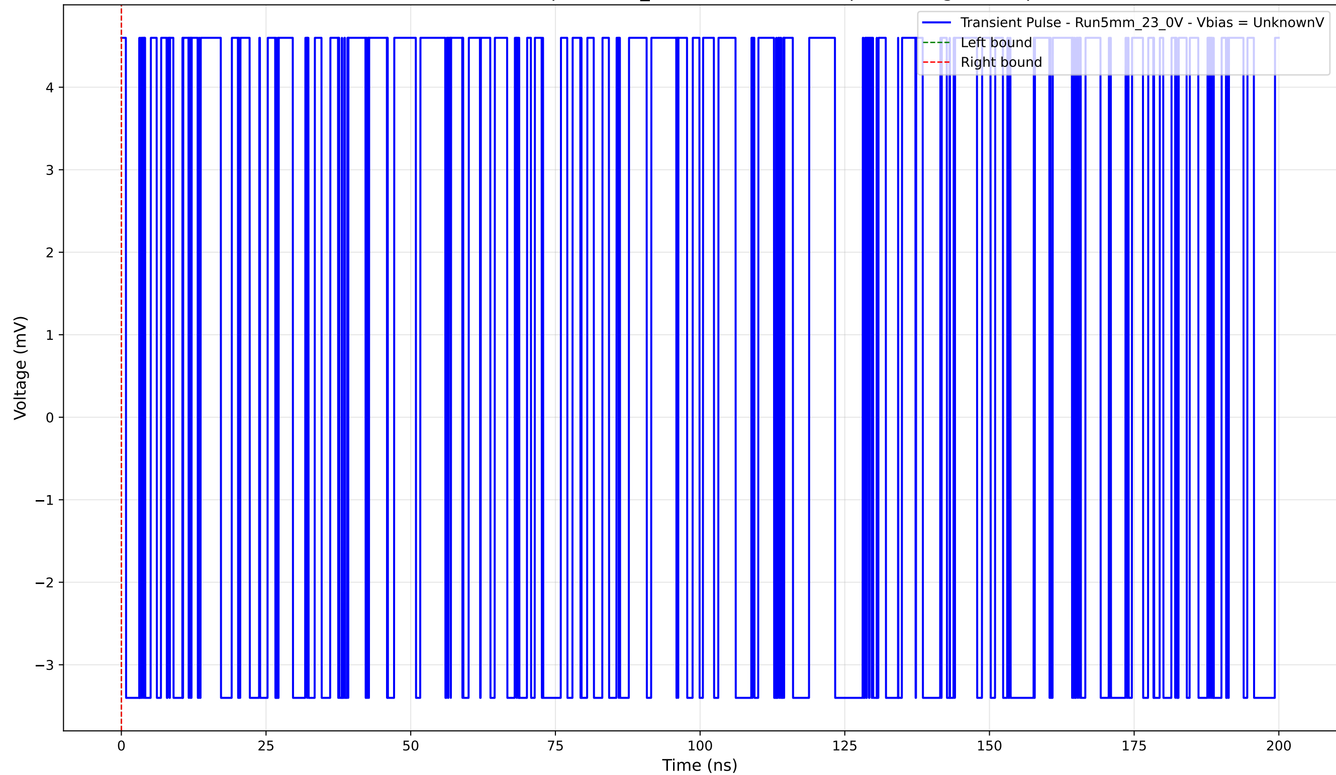
Transient Pulse - Sample: 5mm_23 - Position: 2405.0 \mu\text{m} - Charge: 0.00 pC
