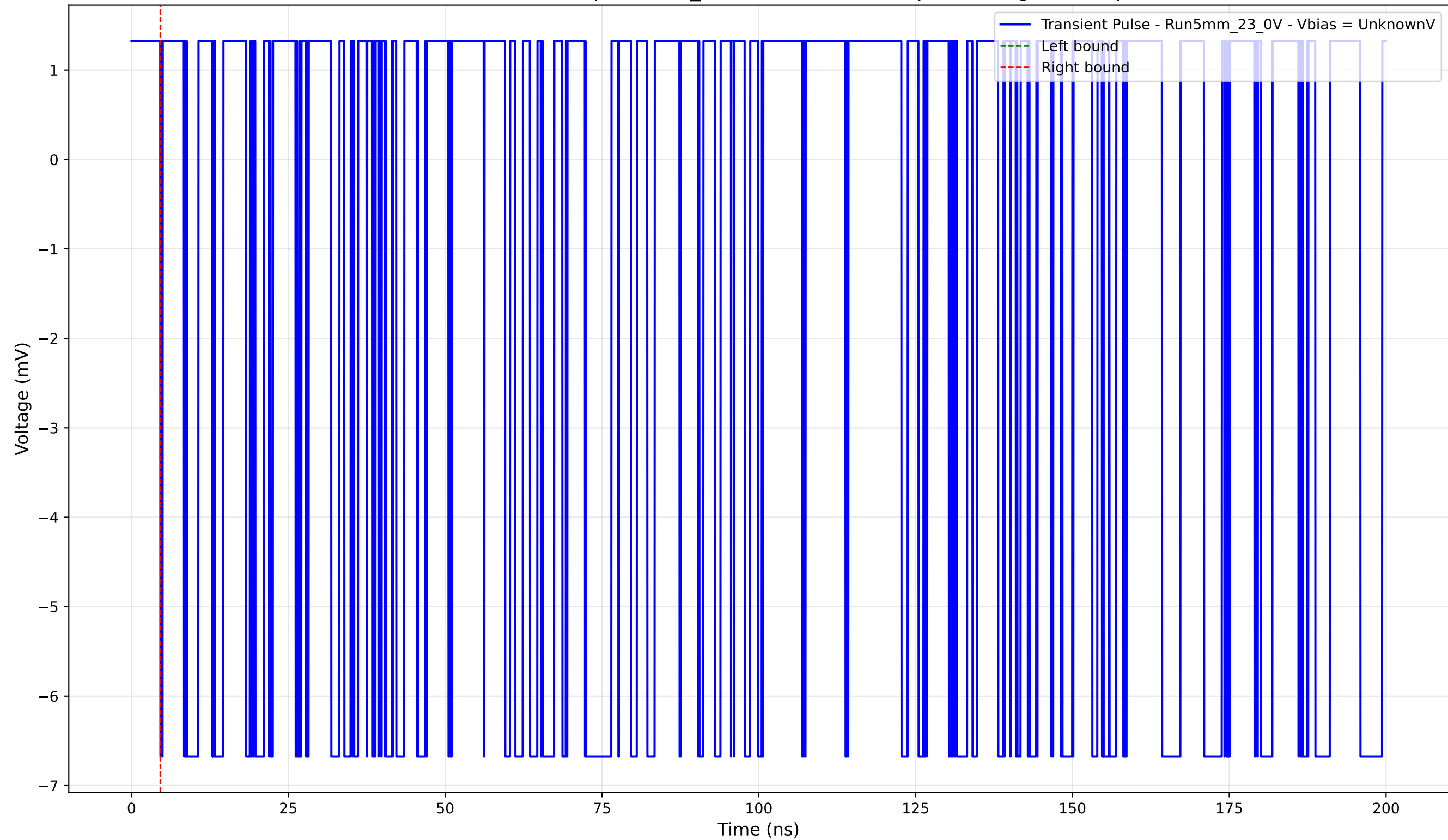
Transient Pulse - Sample: 5mm_23 - Position: 3205.0 \mu\text{m} - Charge: -0.00 pC
