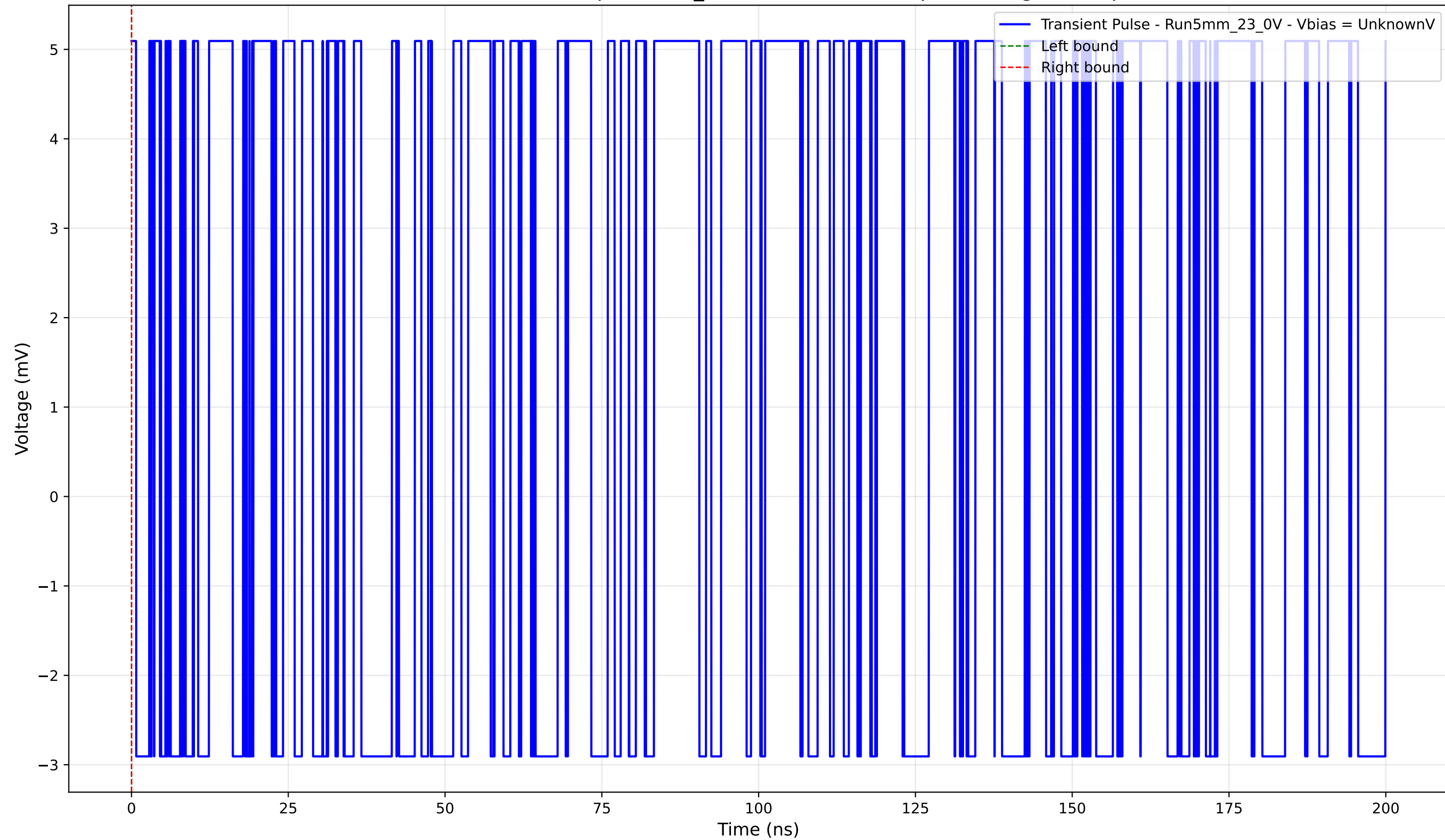
Transient Pulse - Sample: 5mm_23 - Position: 2075.0 \mu\text{m} - Charge: 0.00 pC
