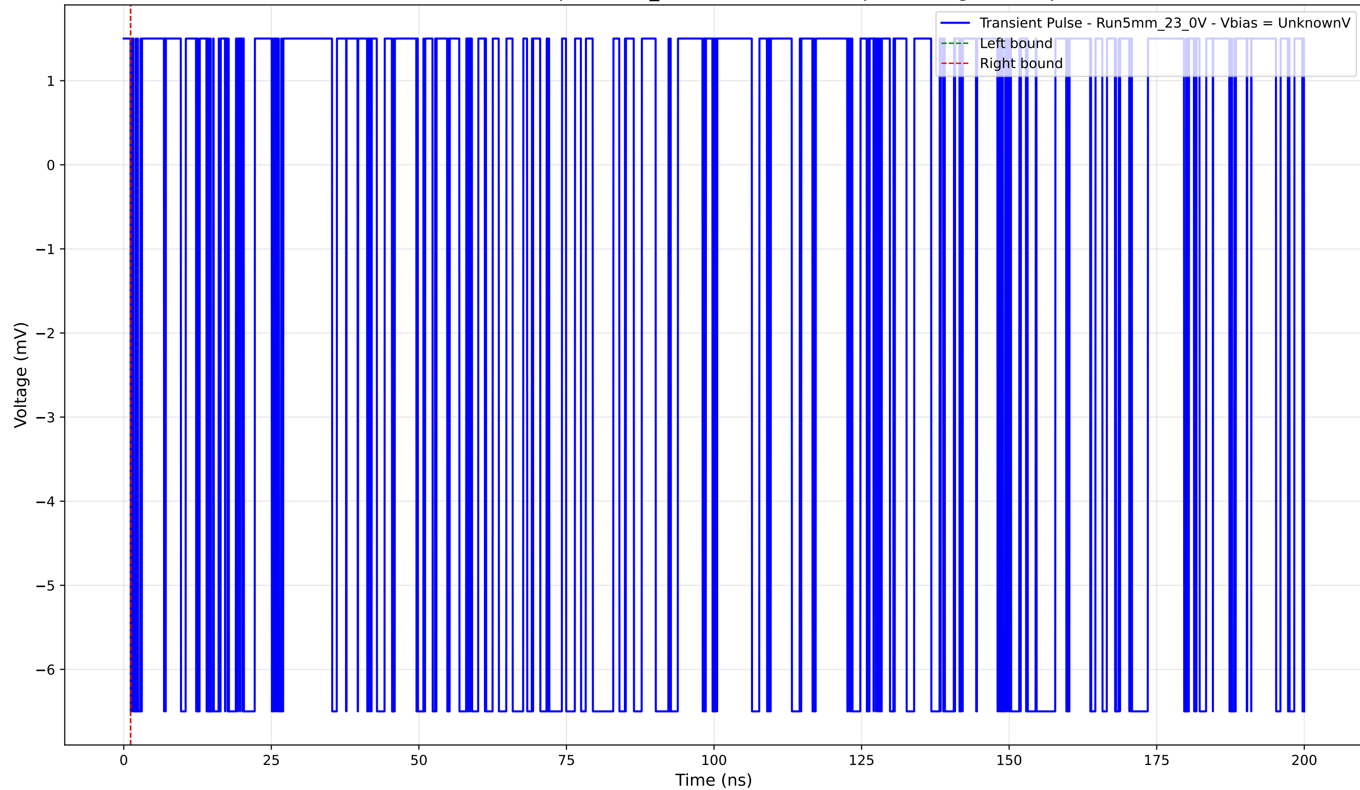
Transient Pulse - Sample: 5mm_23 - Position: 3085.0 \mu\text{m} - Charge: -0.00 pC
