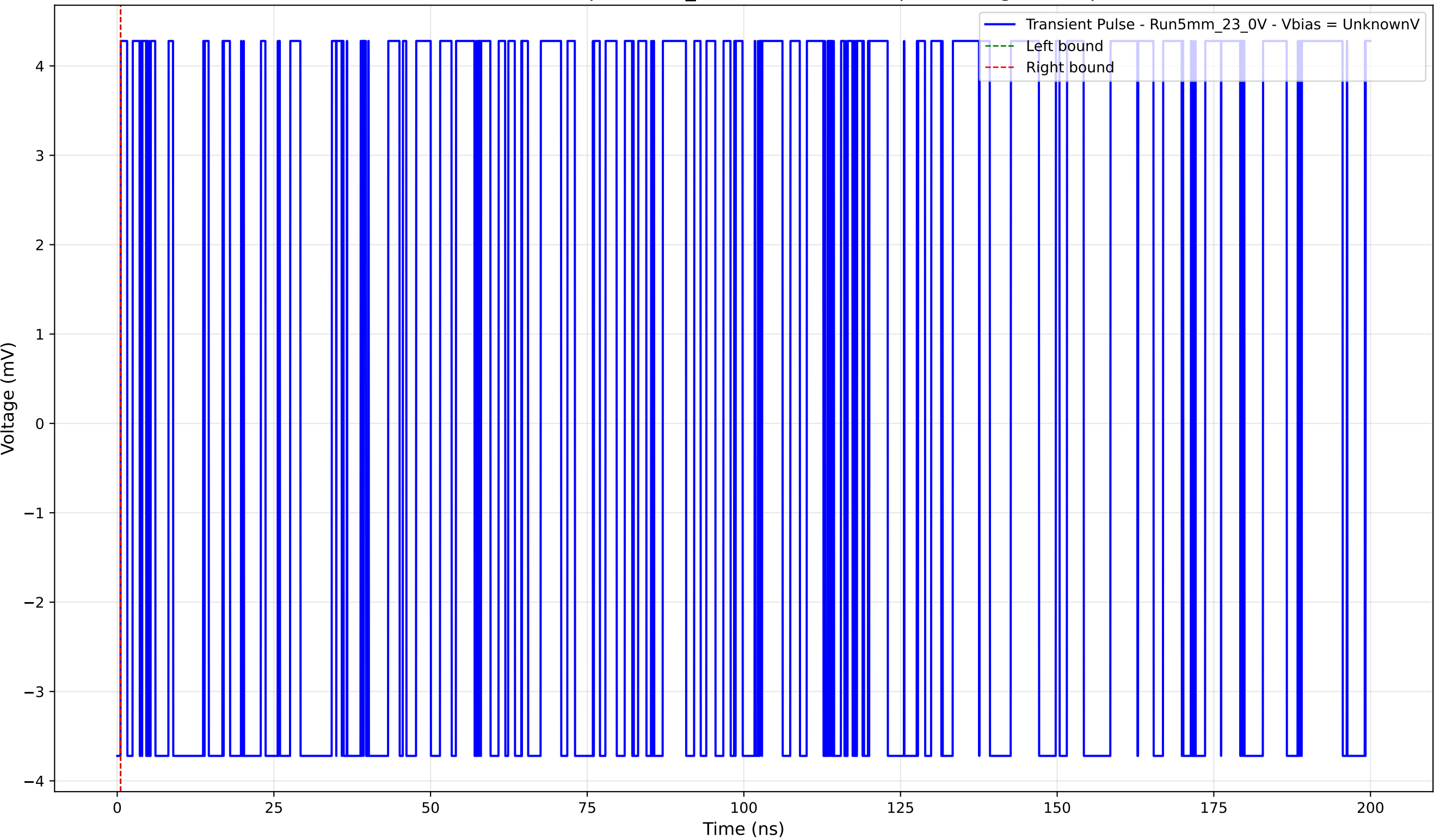
Transient Pulse - Sample: 5mm_23 - Position: 990.0 \mu\text{m} - Charge: 0.00 pC
