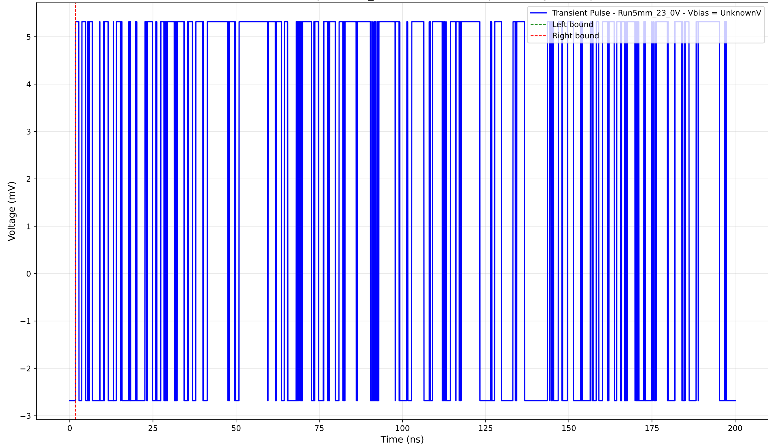
Transient Pulse - Sample: 5mm_23 - Position: 1510.0 \mu\text{m} - Charge: 0.00 pC
