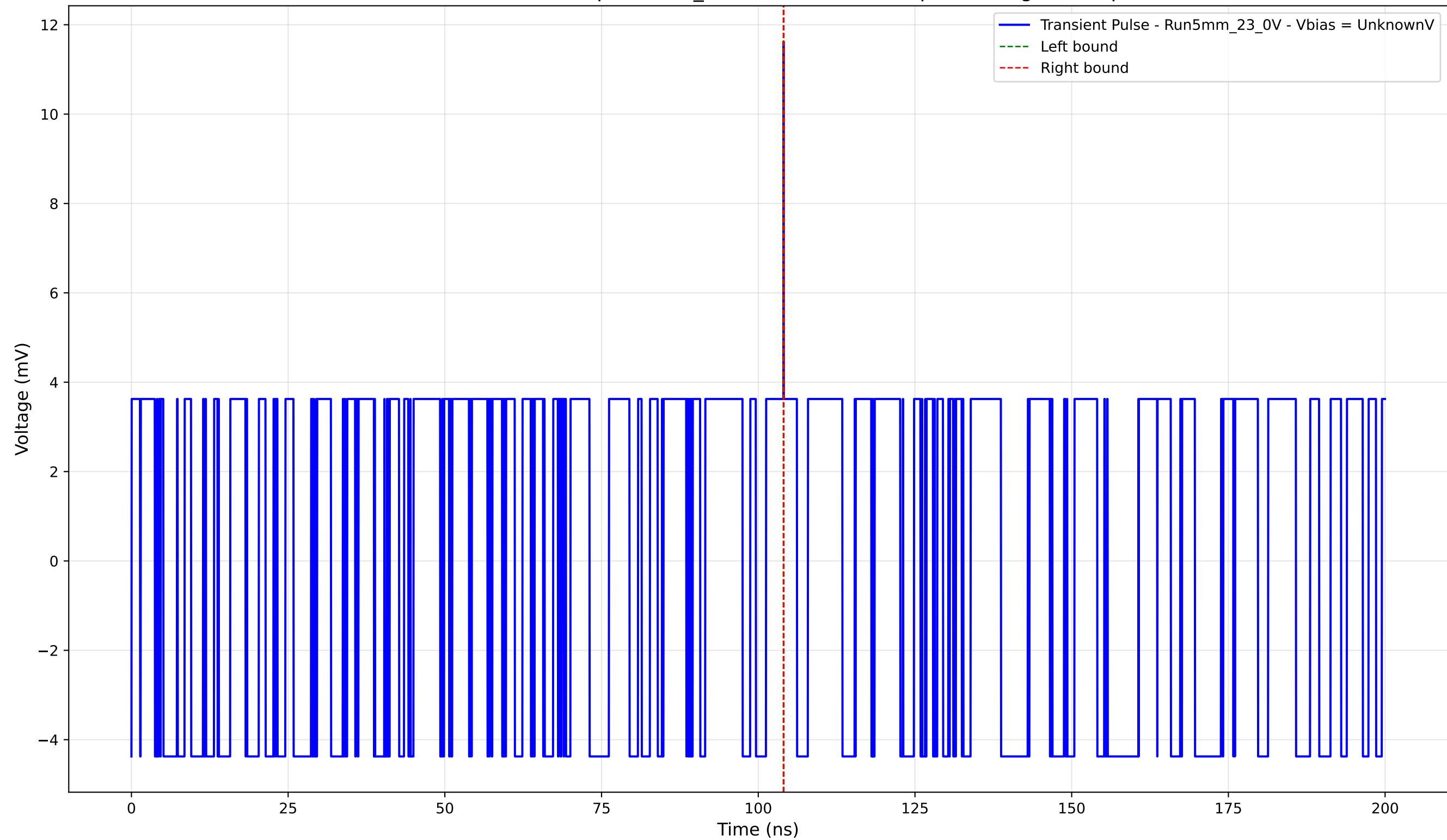
Transient Pulse - Sample: 5mm_23 - Position: 2760.0 \mu\text{m} - Charge: 0.01 pC
