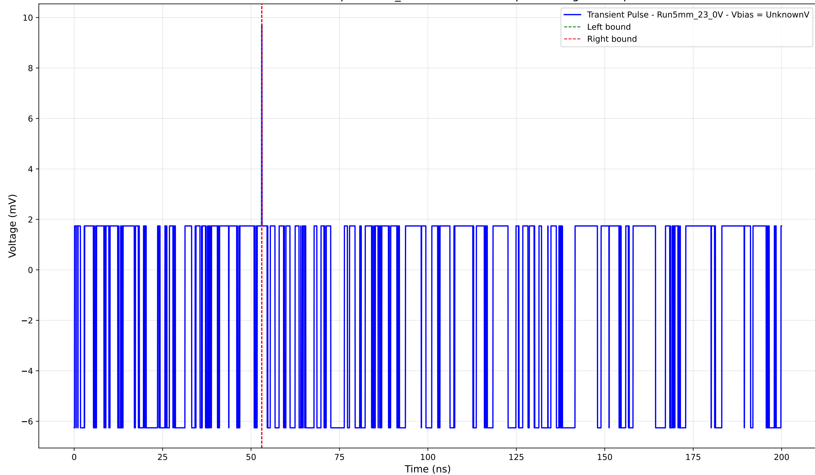
Transient Pulse - Sample: 5mm_23 - Position: 350.0 \mu\text{m} - Charge: 0.02 pC
