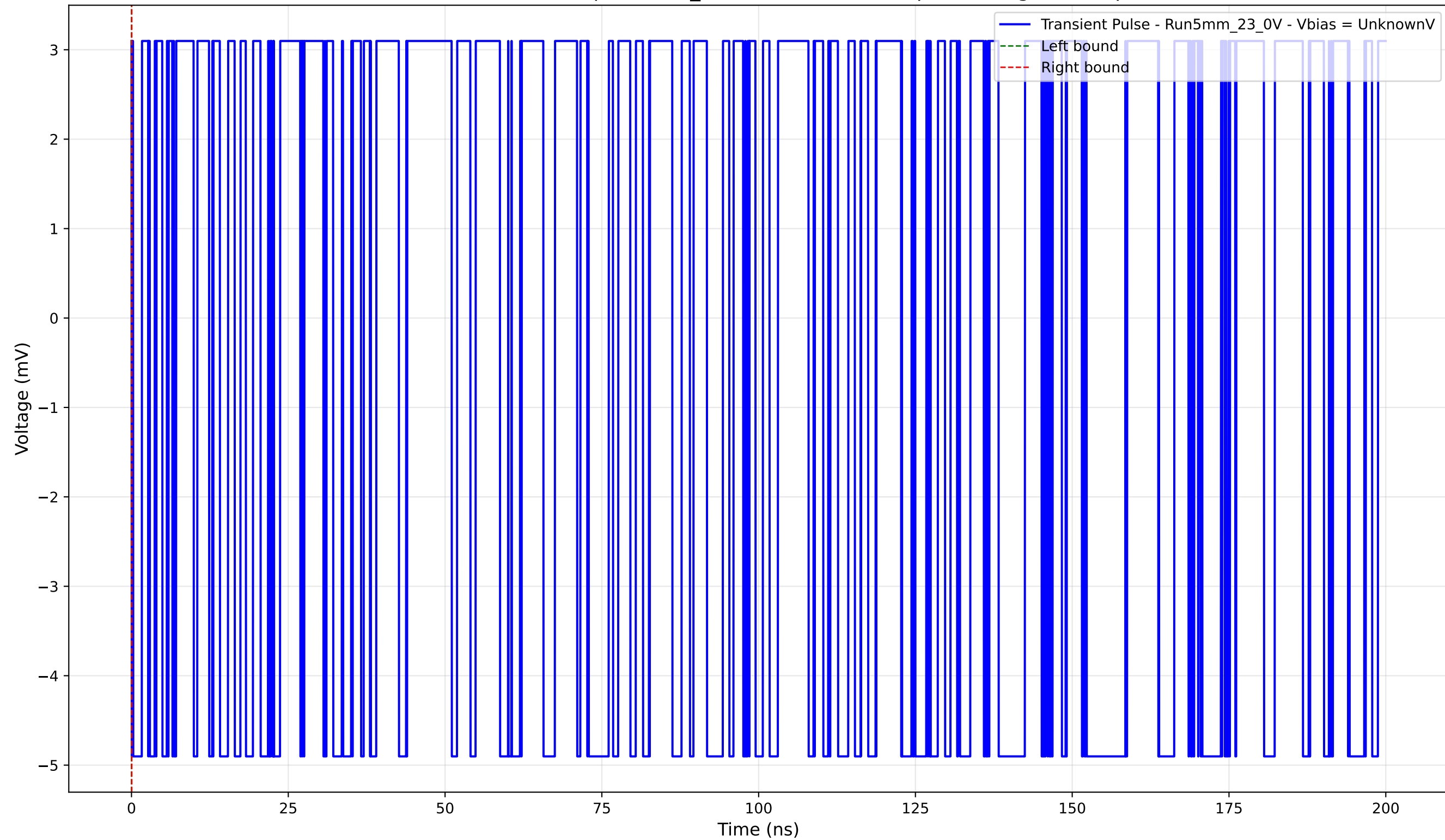
Transient Pulse - Sample: 5mm_23 - Position: 4590.0 \mu\text{m} - Charge: -0.00 pC
