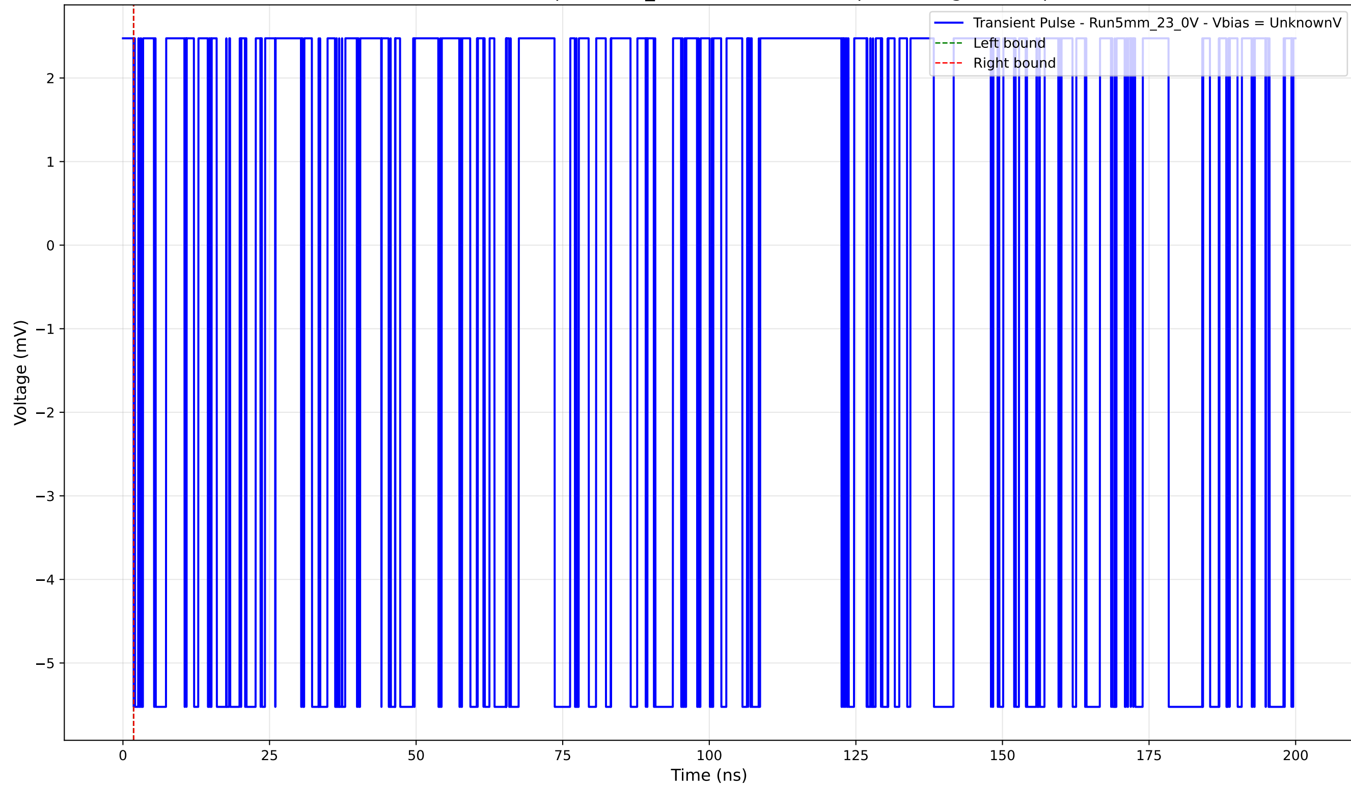
Transient Pulse - Sample: 5mm_23 - Position: 1145.0 \mu\text{m} - Charge: -0.00 pC
