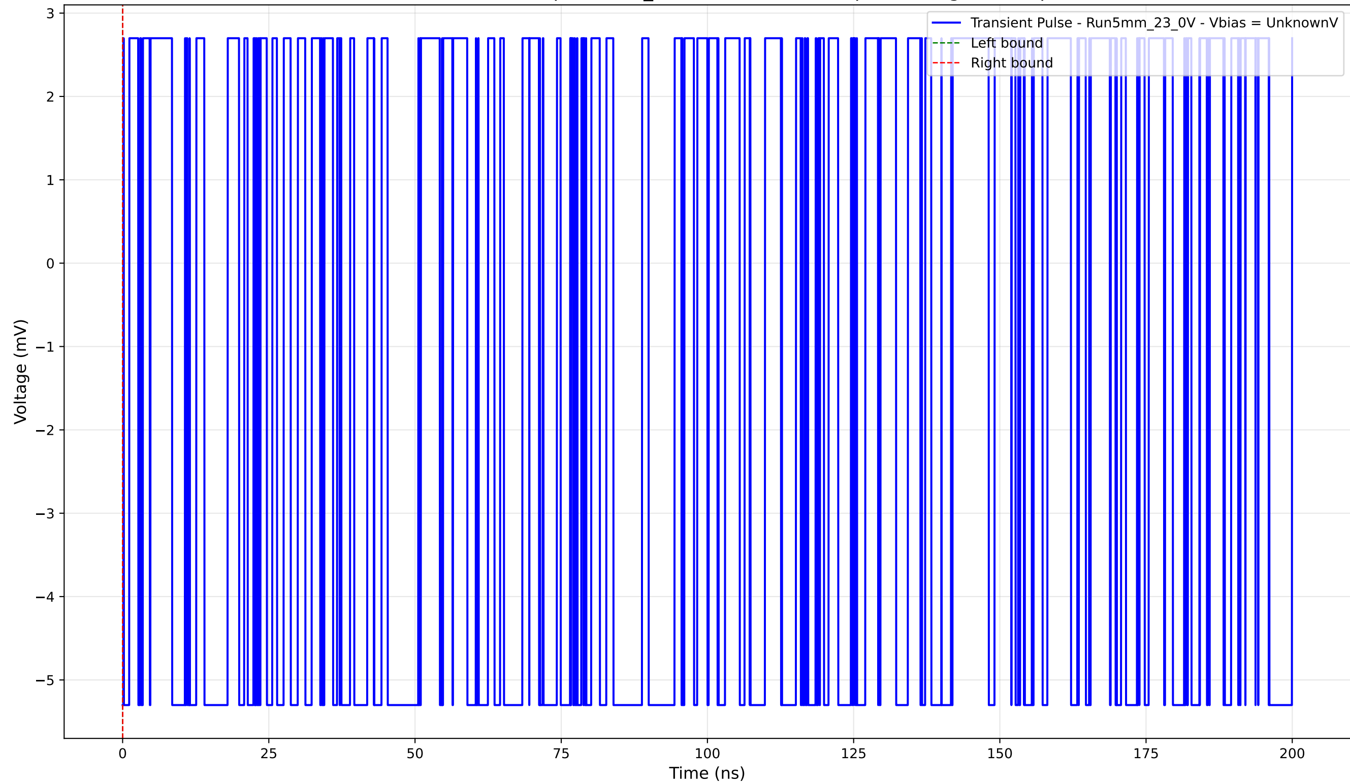
Transient Pulse - Sample: 5mm_23 - Position: 4850.0 \mu\text{m} - Charge: -0.00 pC
