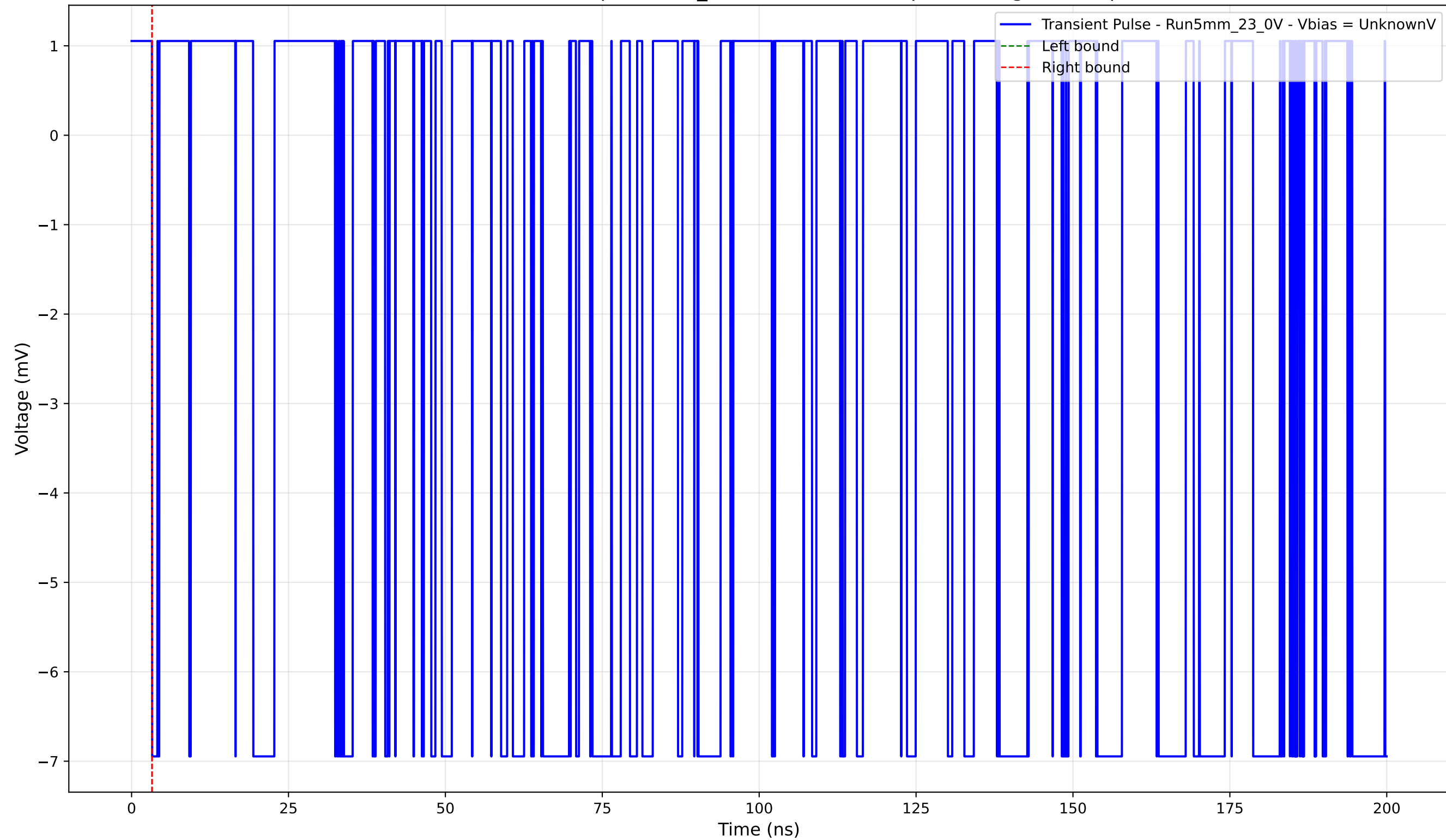
Transient Pulse - Sample: 5mm_23 - Position: 615.0 \mu\text{m} - Charge: -0.00 pC
