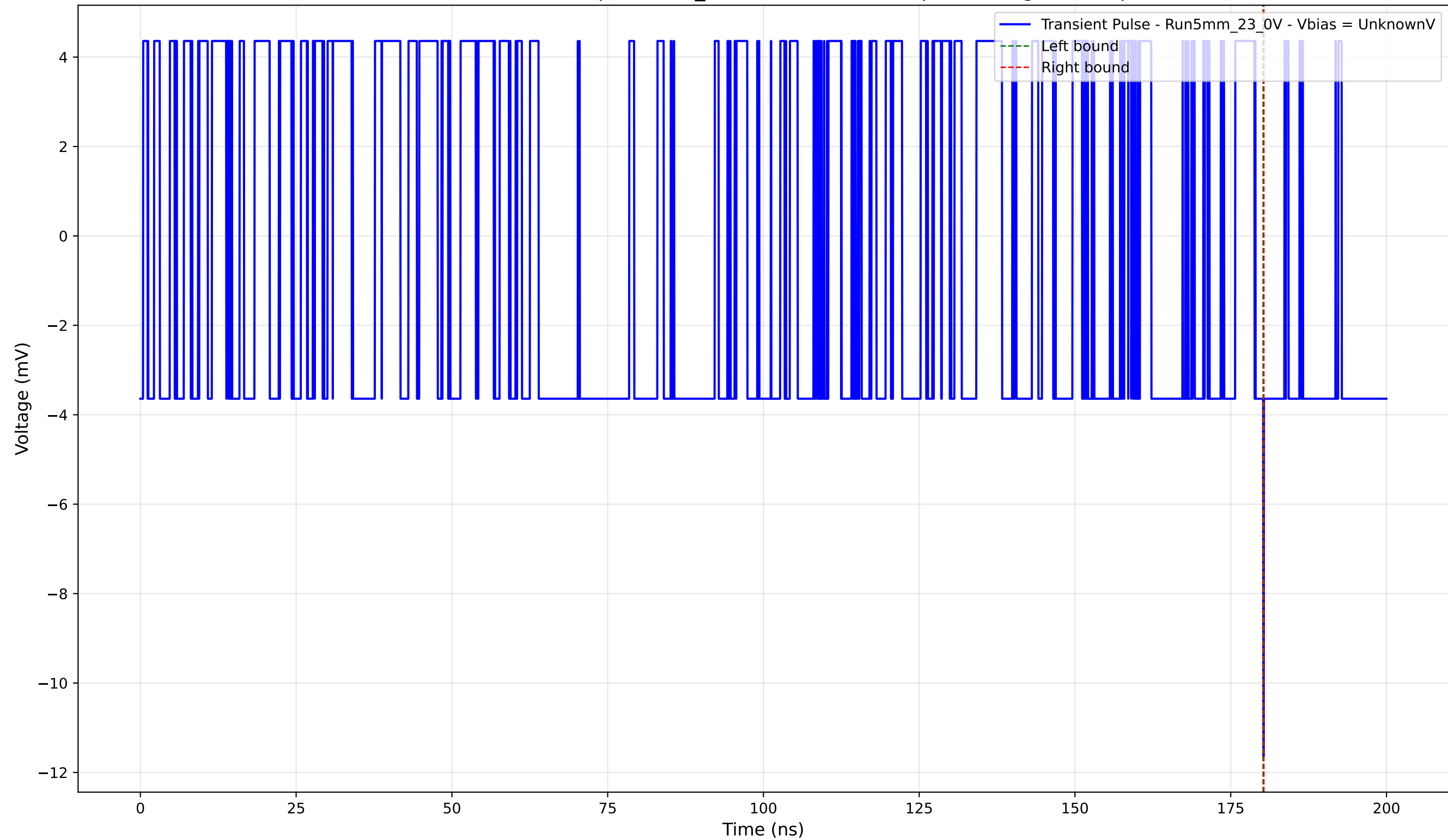
Transient Pulse - Sample: 5mm_23 - Position: 3345.0 \mu\text{m} - Charge: -0.02 pC
