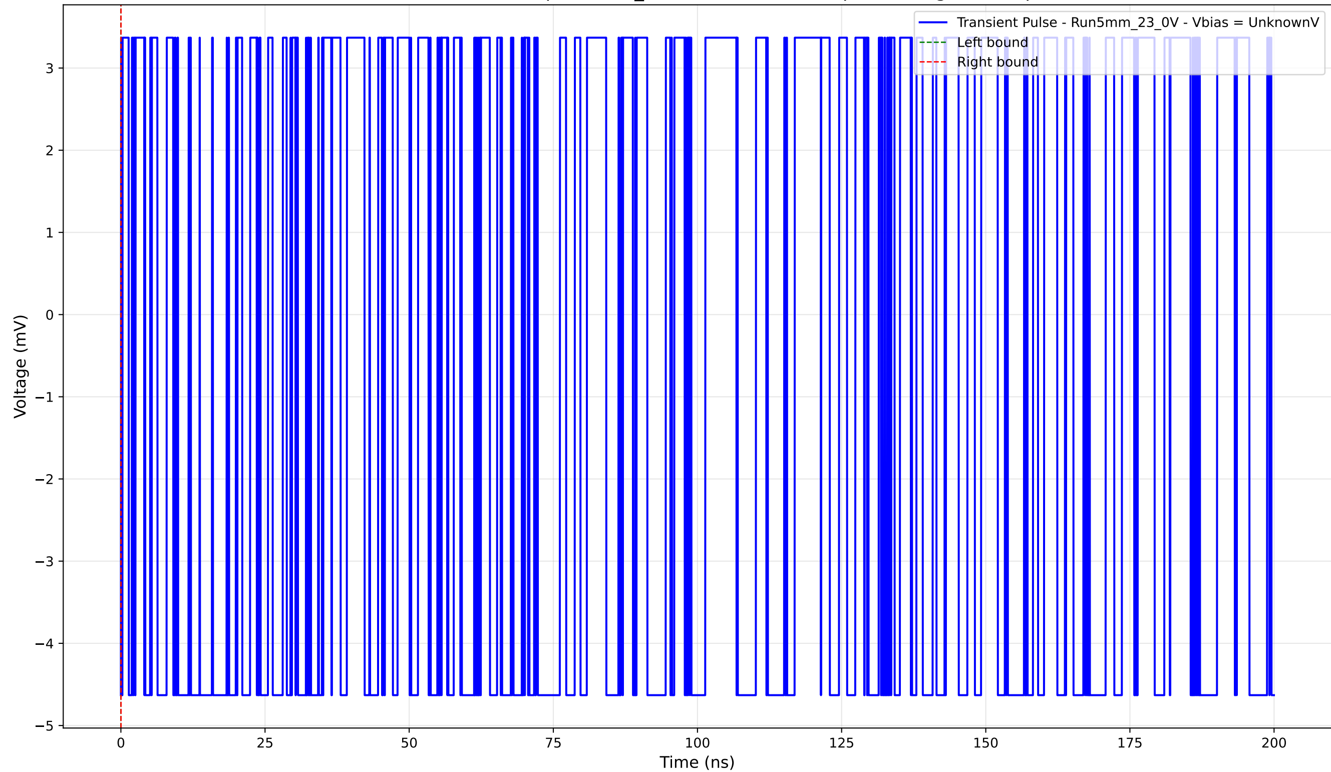
Transient Pulse - Sample: 5mm_23 - Position: 2485.0 \mu\text{m} - Charge: -0.00 pC
