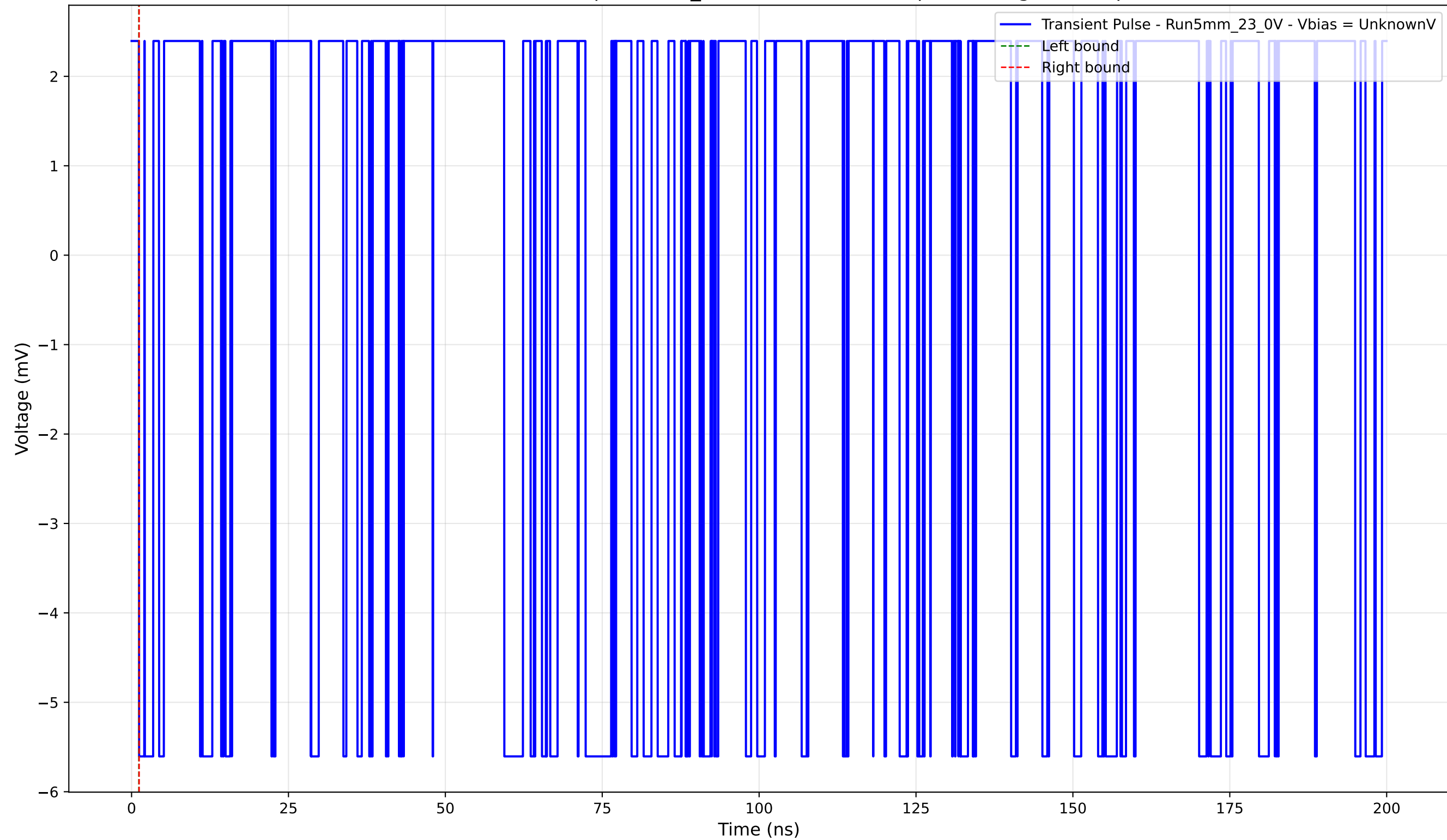
Transient Pulse - Sample: 5mm_23 - Position: 2890.0 \mu\text{m} - Charge: -0.00 pC
