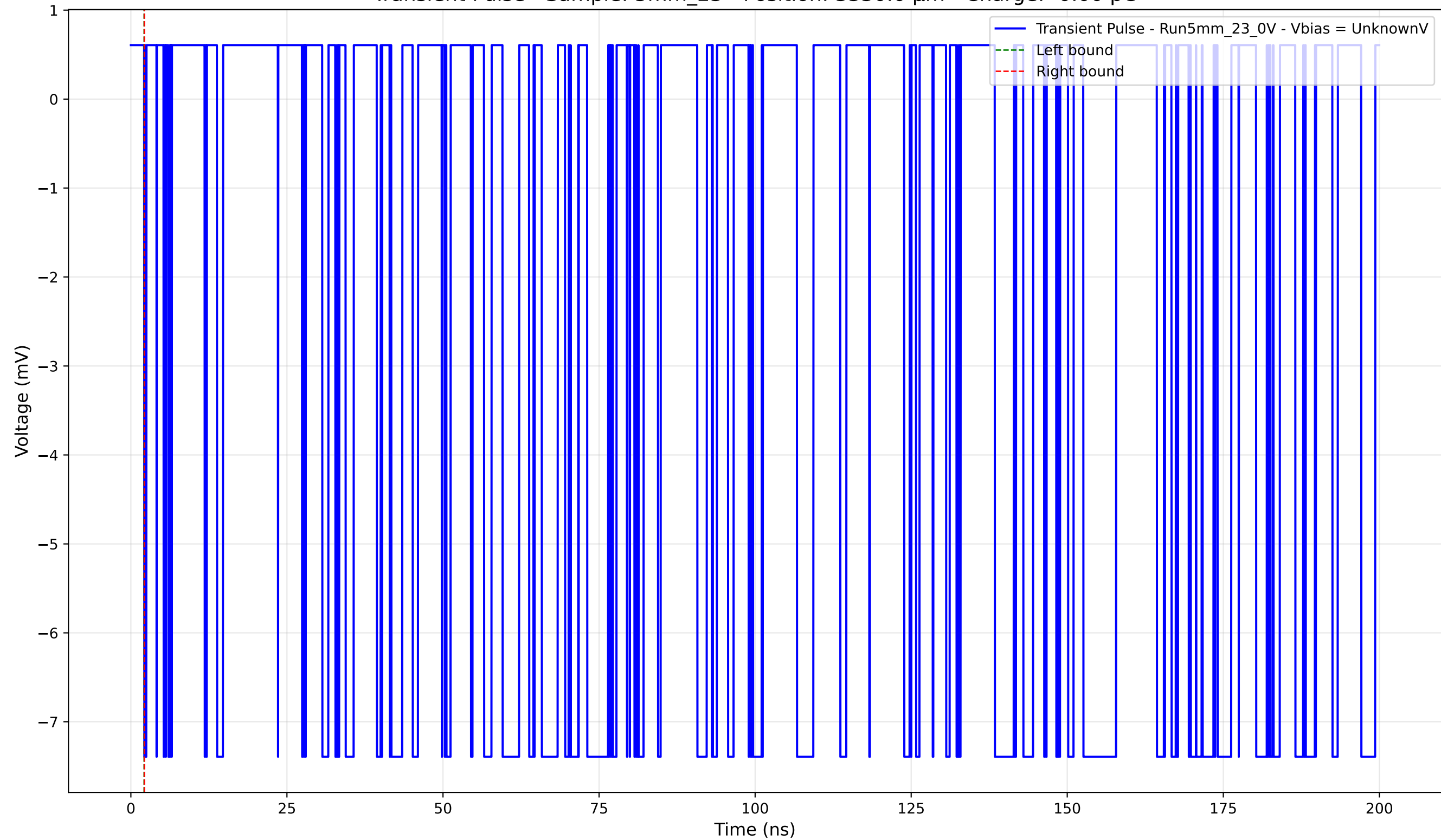
Transient Pulse - Sample: 5mm_23 - Position: 3330.0 \mu\text{m} - Charge: -0.00 pC
