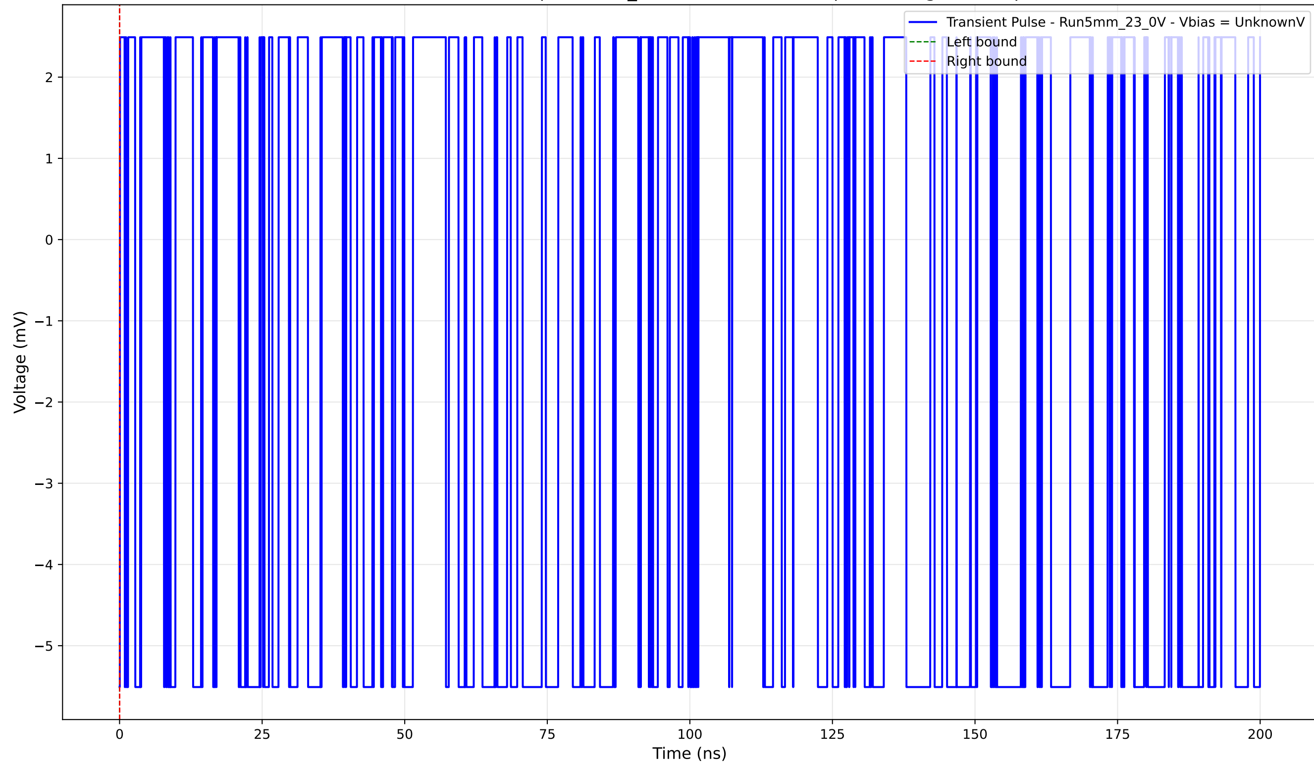
Transient Pulse - Sample: 5mm_23 - Position: 1425.0 \mu\text{m} - Charge: -0.00 pC
