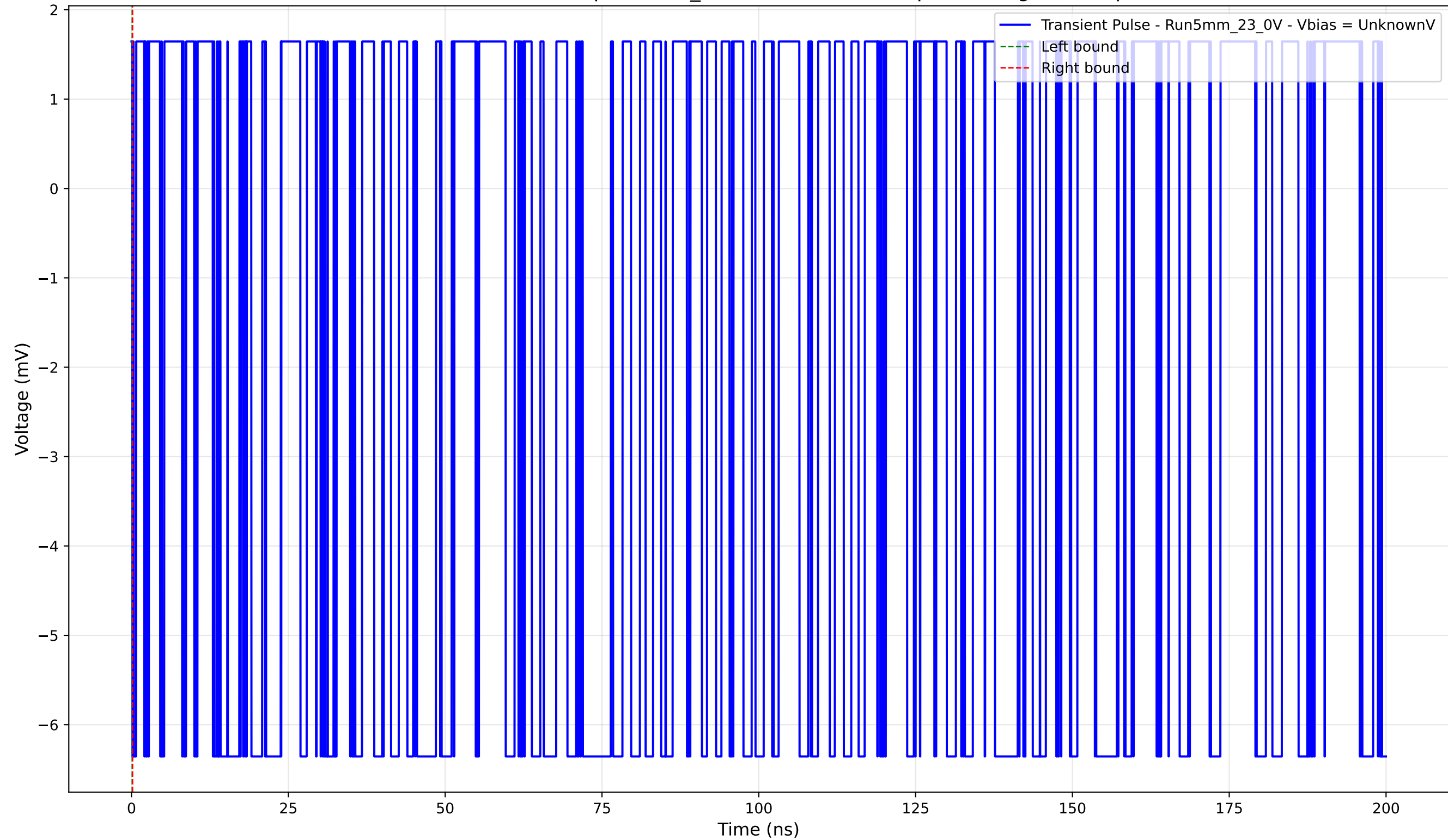
Transient Pulse - Sample: 5mm_23 - Position: 1055.0 \mu\text{m} - Charge: -0.00 pC
