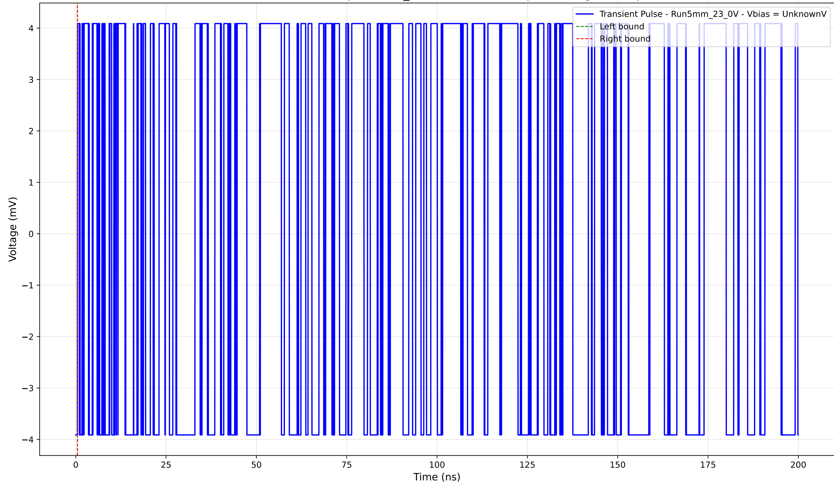
Transient Pulse - Sample: 5mm_23 -Position: 370.0 \mu\text{m} - Charge: 0.00 pC
