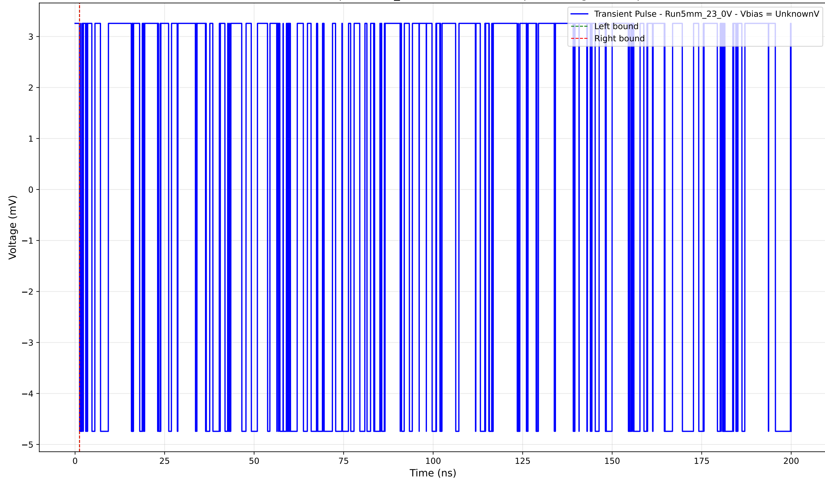
Transient Pulse - Sample: 5mm_23 - Position: 2615.0 \mu\text{m} - Charge: -0.00 pC
