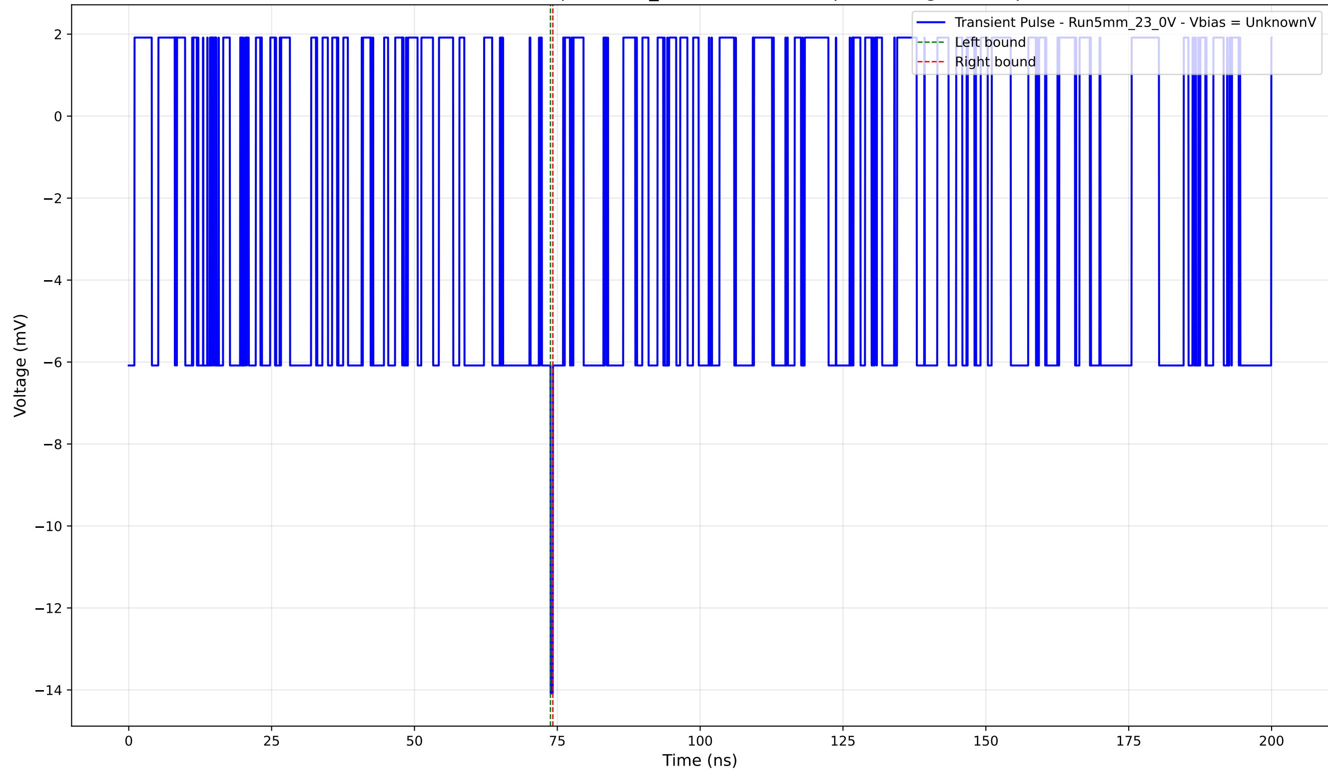
Transient Pulse - Sample: 5mm_23 - Position: 80.0 \mu\text{m} - Charge: -0.12 pC
