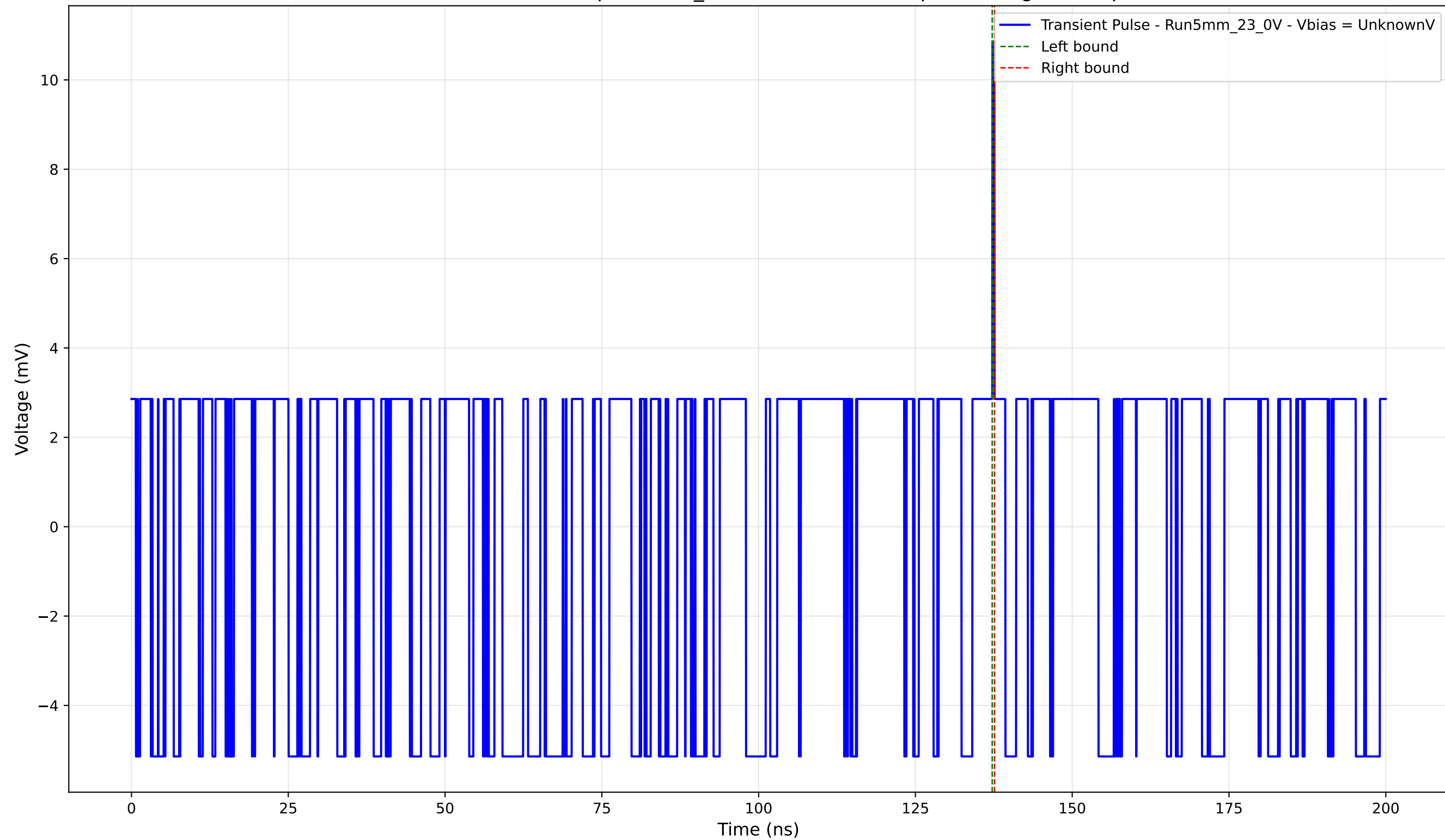
Transient Pulse - Sample: 5mm_23 - Position: 1415.0 \mu\text{m} - Charge: 0.07 pC
