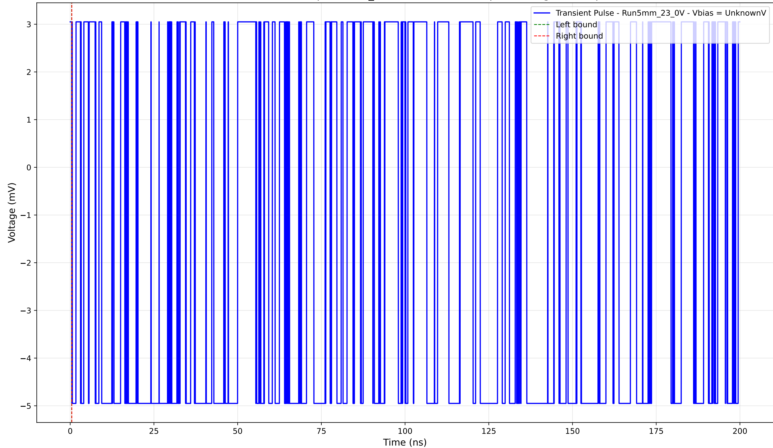
Transient Pulse - Sample: 5mm_23 - Position: 4370.0 \mu\text{m} - Charge: -0.00 pC
