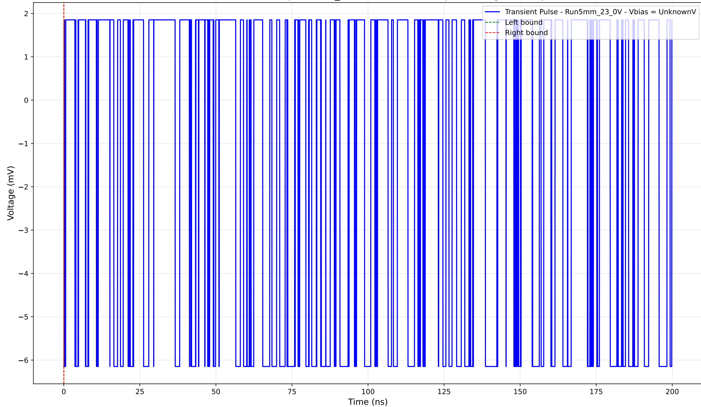
Transient Pulse - Sample: 5mm_23 - Position: 3105.0 \mu\text{m} - Charge: -0.00 pC
