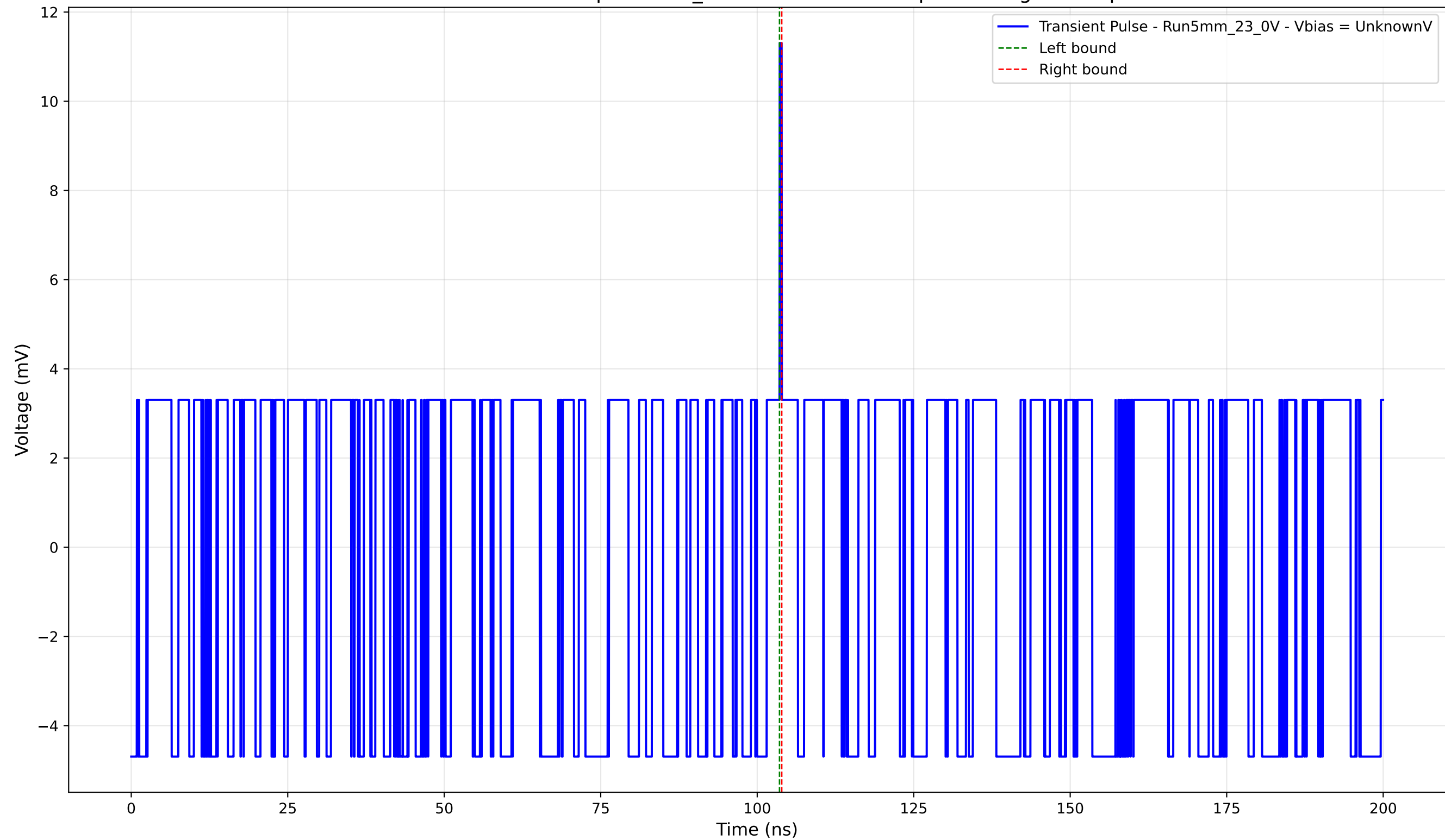
Transient Pulse - Sample: 5mm_23 - Position: 2520.0 \mu\text{m} - Charge: 0.08 pC
