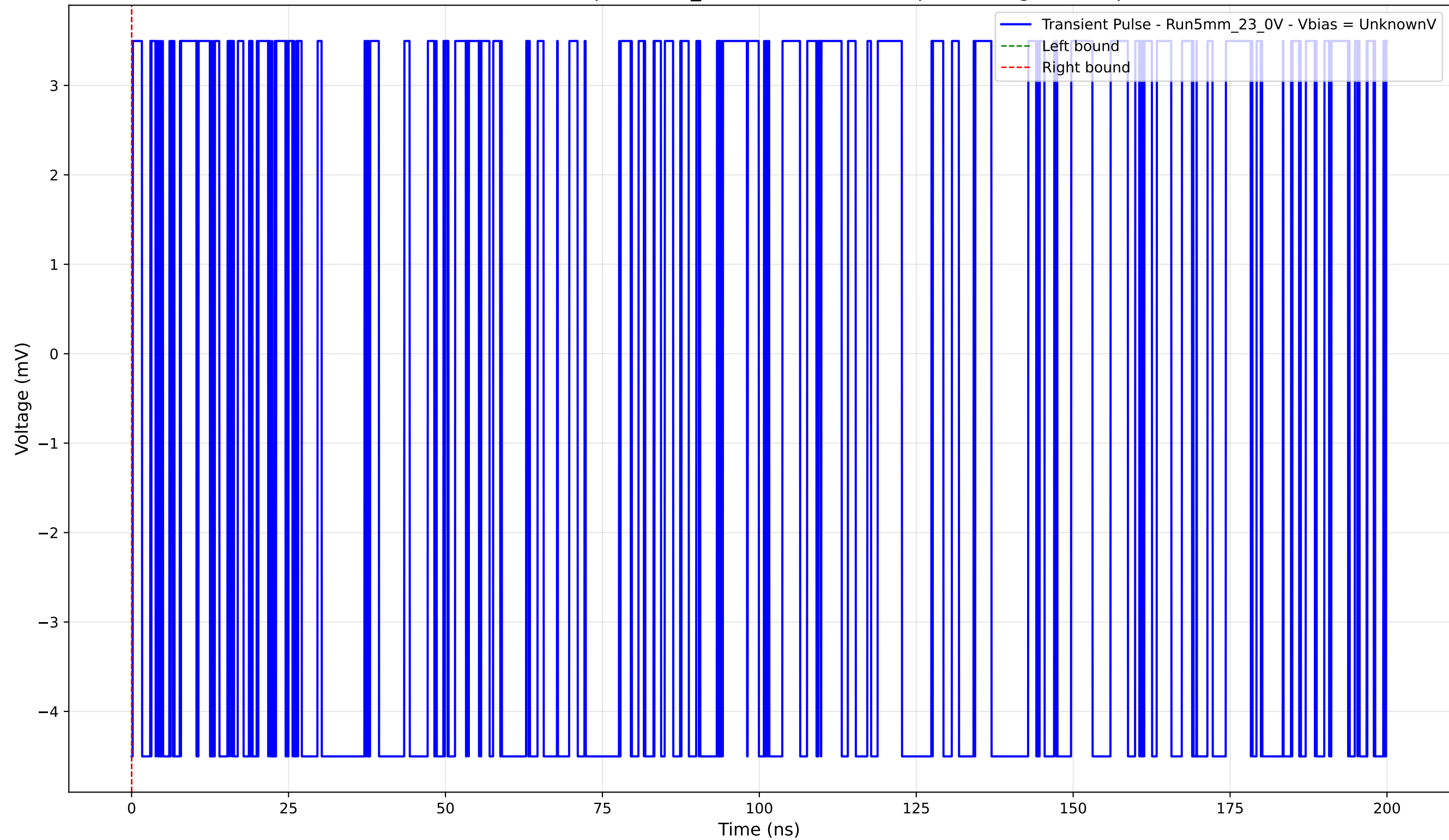
Transient Pulse - Sample: 5mm_23 - Position: 4290.0 \mu\text{m} - Charge: -0.00 pC
