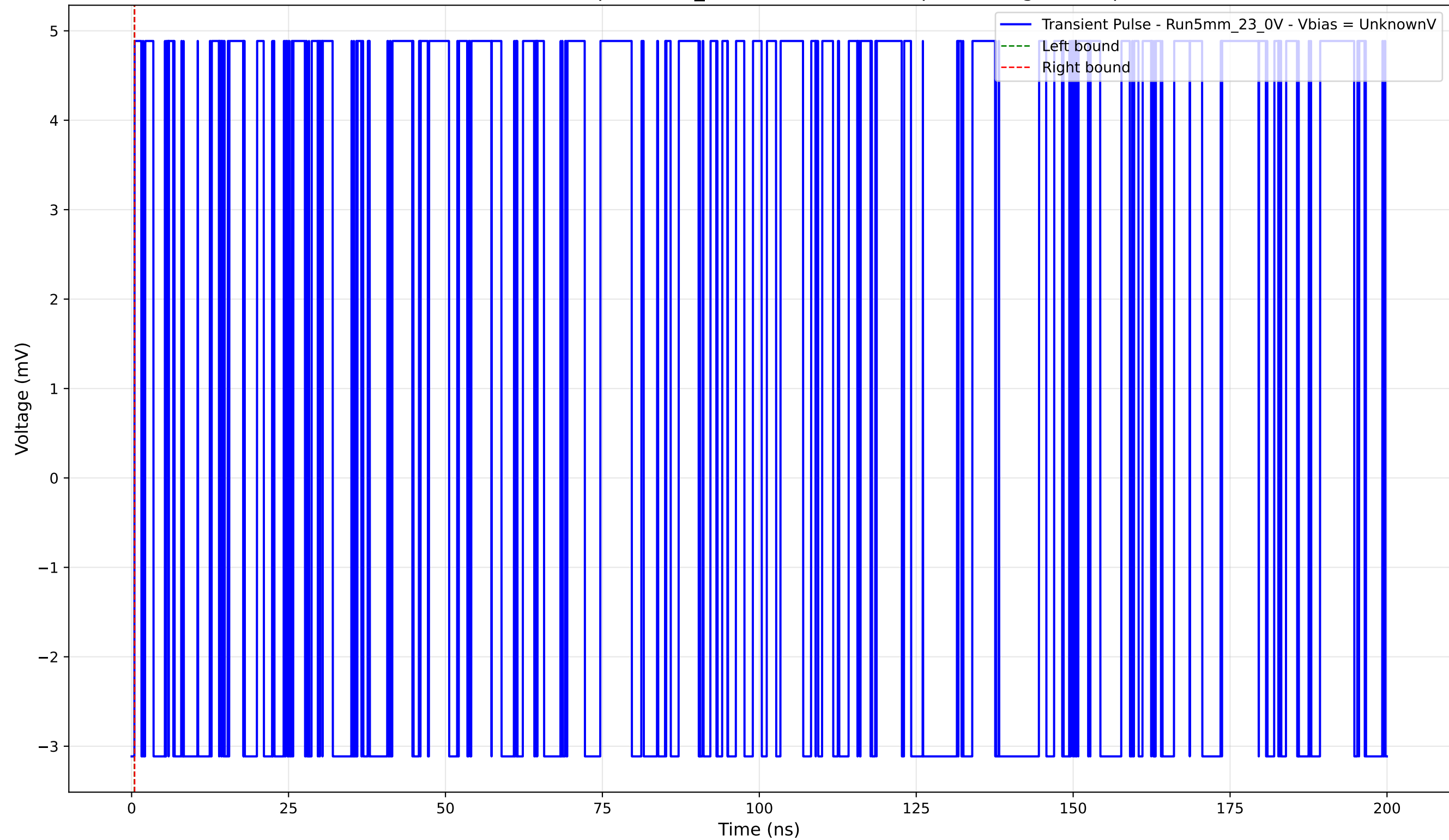
Transient Pulse - Sample: 5mm_23 - Position: 1610.0 \mu\text{m} - Charge: 0.00 pC
