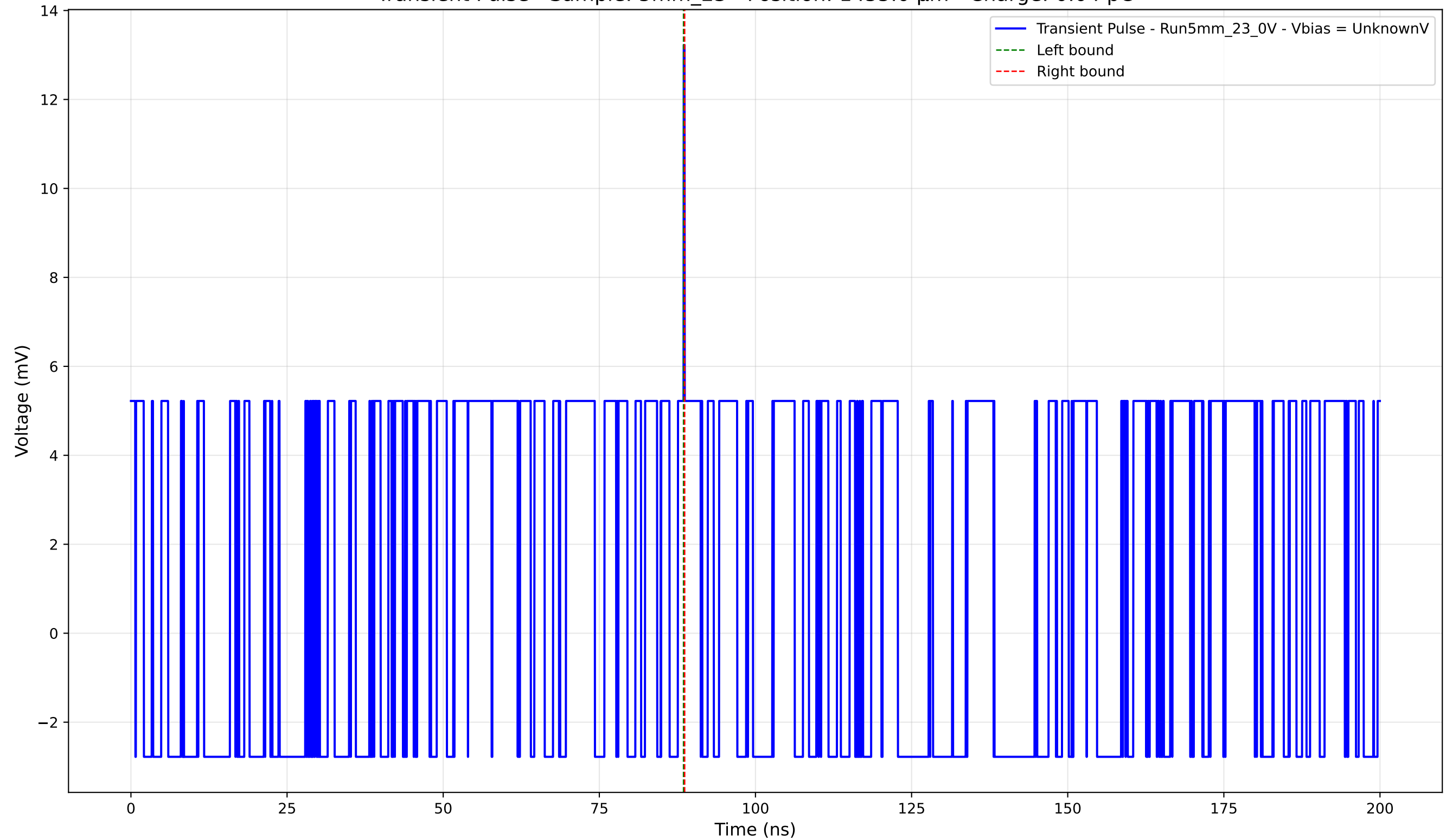
Transient Pulse - Sample: 5mm_23 - Position: 1455.0 \mu\text{m} - Charge: 0.04 pC
