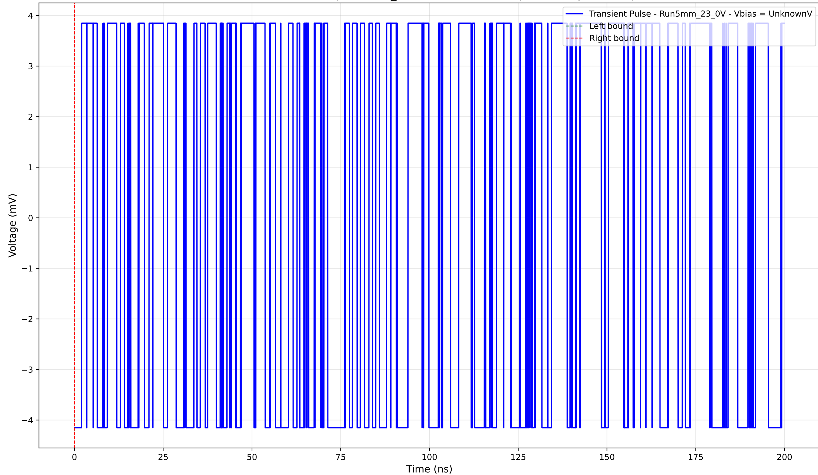
Transient Pulse - Sample: 5mm_23 - Position: 2060.0 \mu\text{m} - Charge: -0.00 pC
