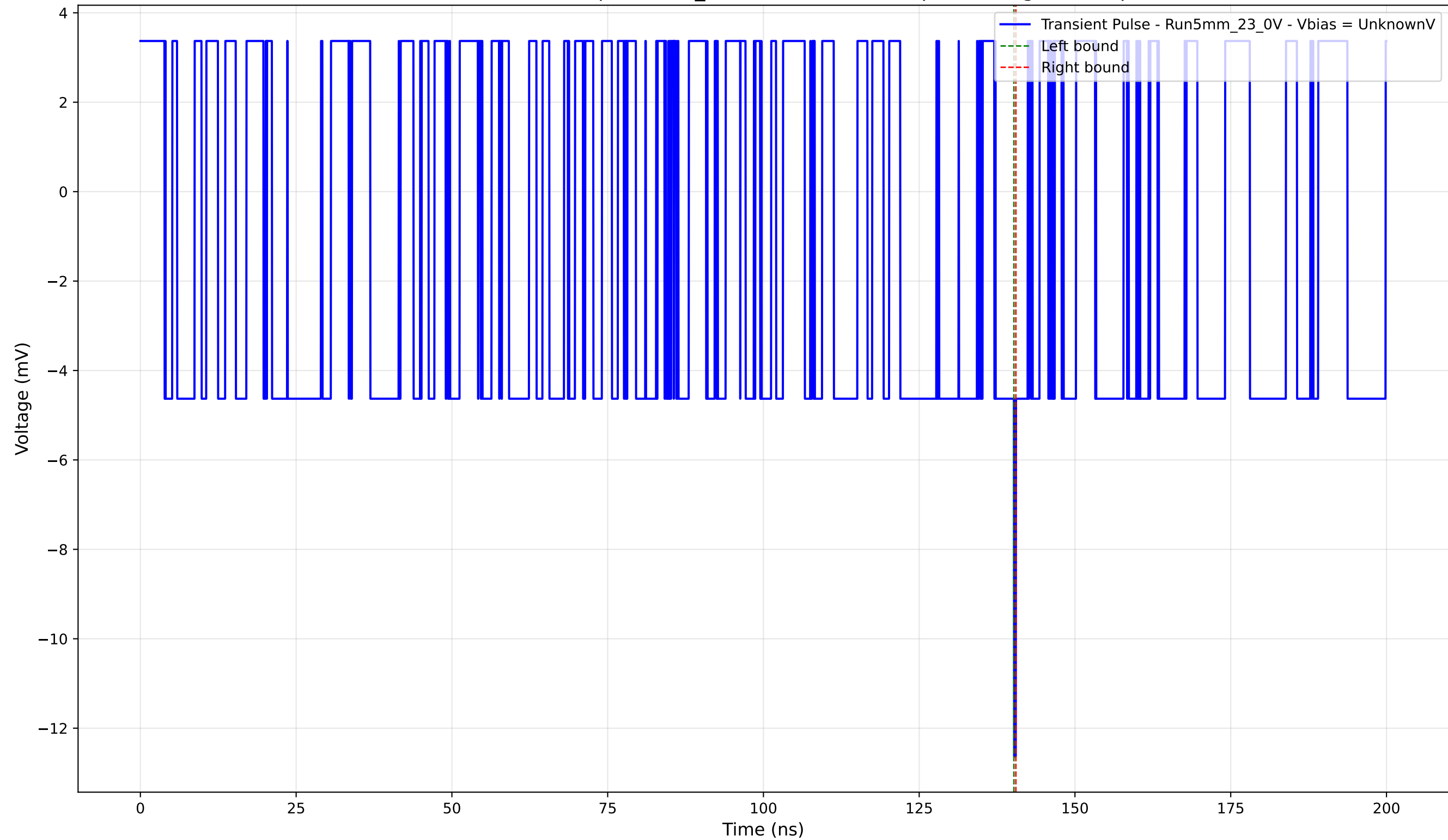
Transient Pulse - Sample: 5mm_23 - Position: 1715.0 \mu\text{m} - Charge: -0.08 pC
