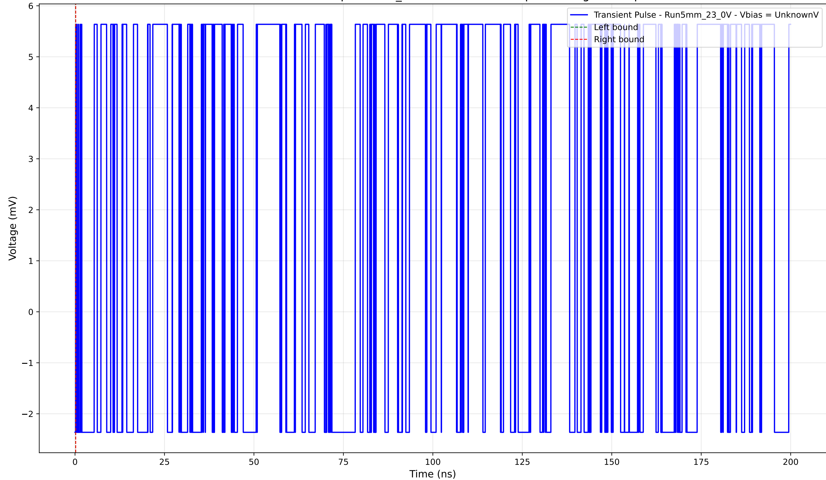
Transient Pulse - Sample: 5mm_23 - Position: 4300.0 \mu\text{m} - Charge: 0.00 pC
