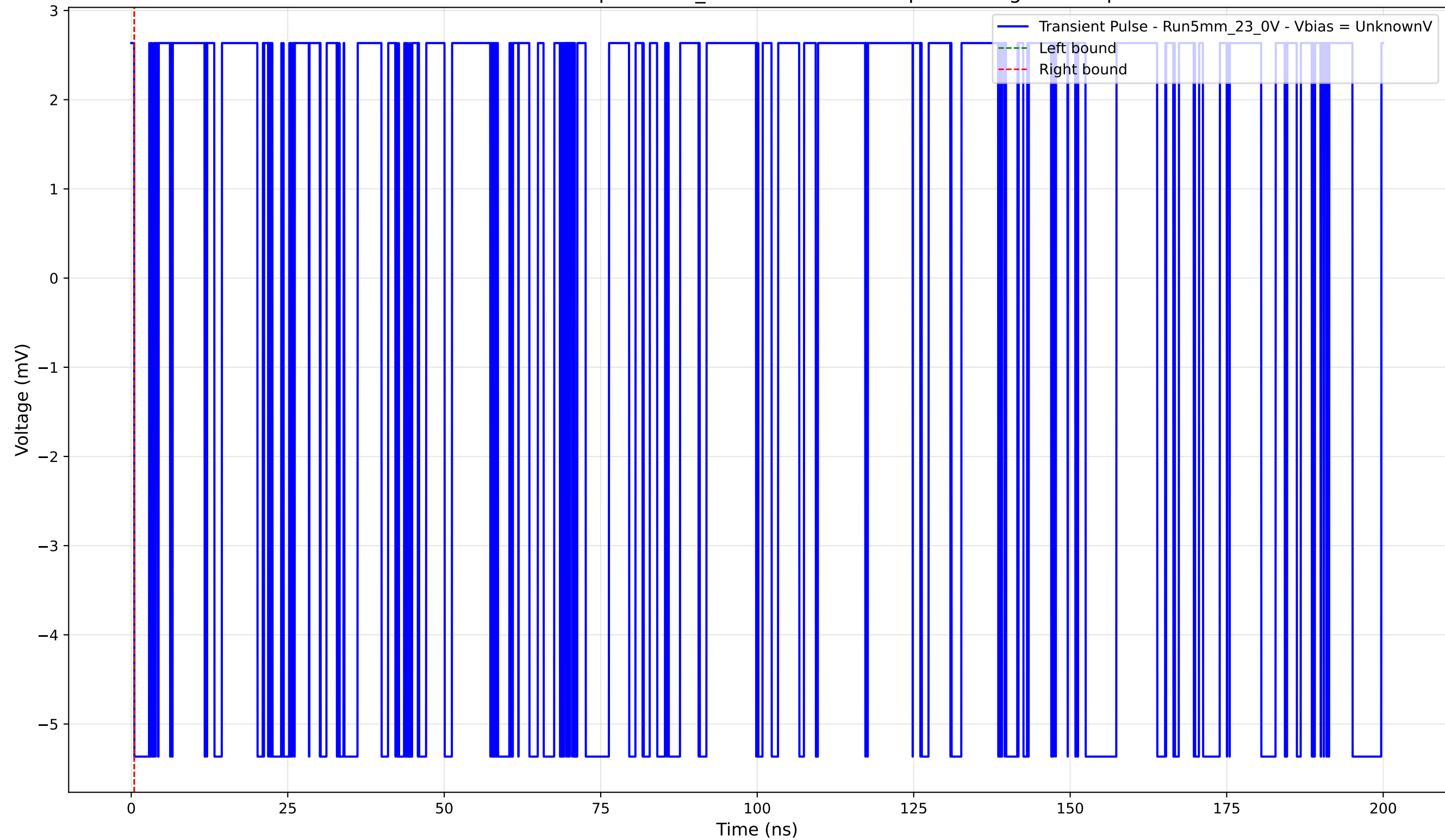
Transient Pulse - Sample: 5mm_23 - Position: 750.0 \mu\text{m} - Charge: -0.00 pC
