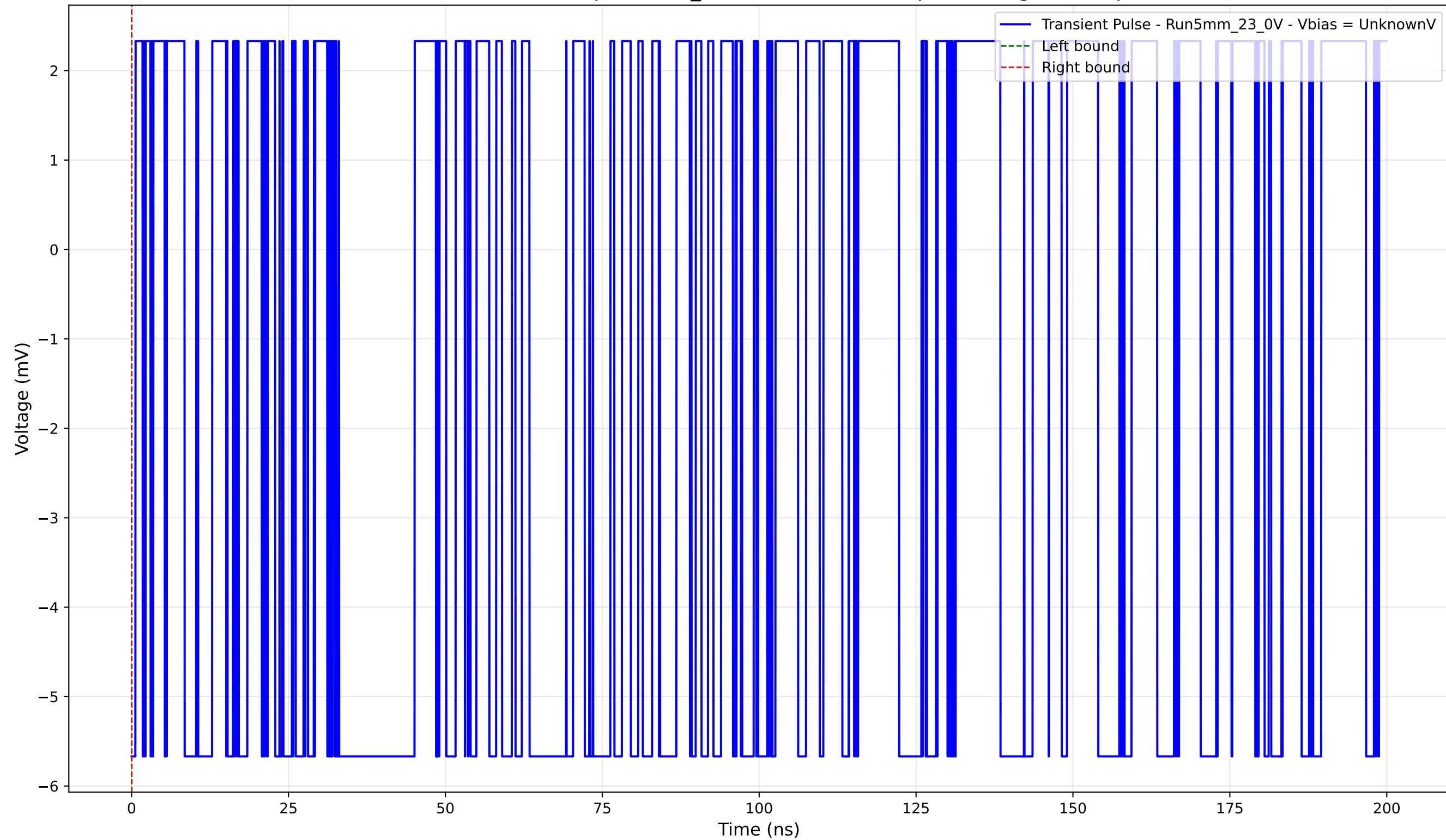
Transient Pulse - Sample: 5mm_23 - Position: 2425.0 \mu\text{m} - Charge: -0.00 pC
