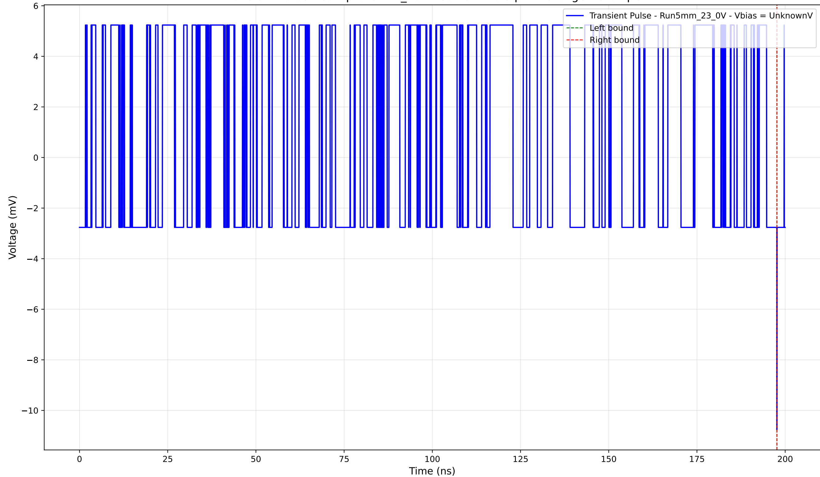
Transient Pulse - Sample: 5mm_23 - Position: 40.0 \mu\text{m} - Charge: -0.01 pC
