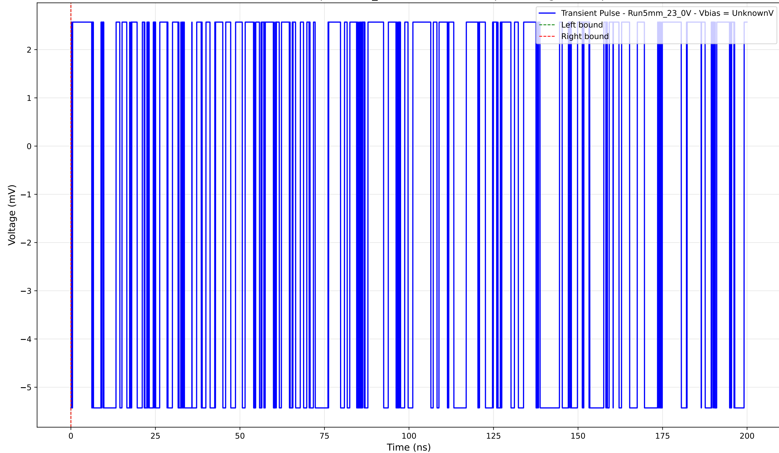
Transient Pulse - Sample: 5mm_23 - Position: 3270.0 \mu\text{m} - Charge: -0.00 pC
