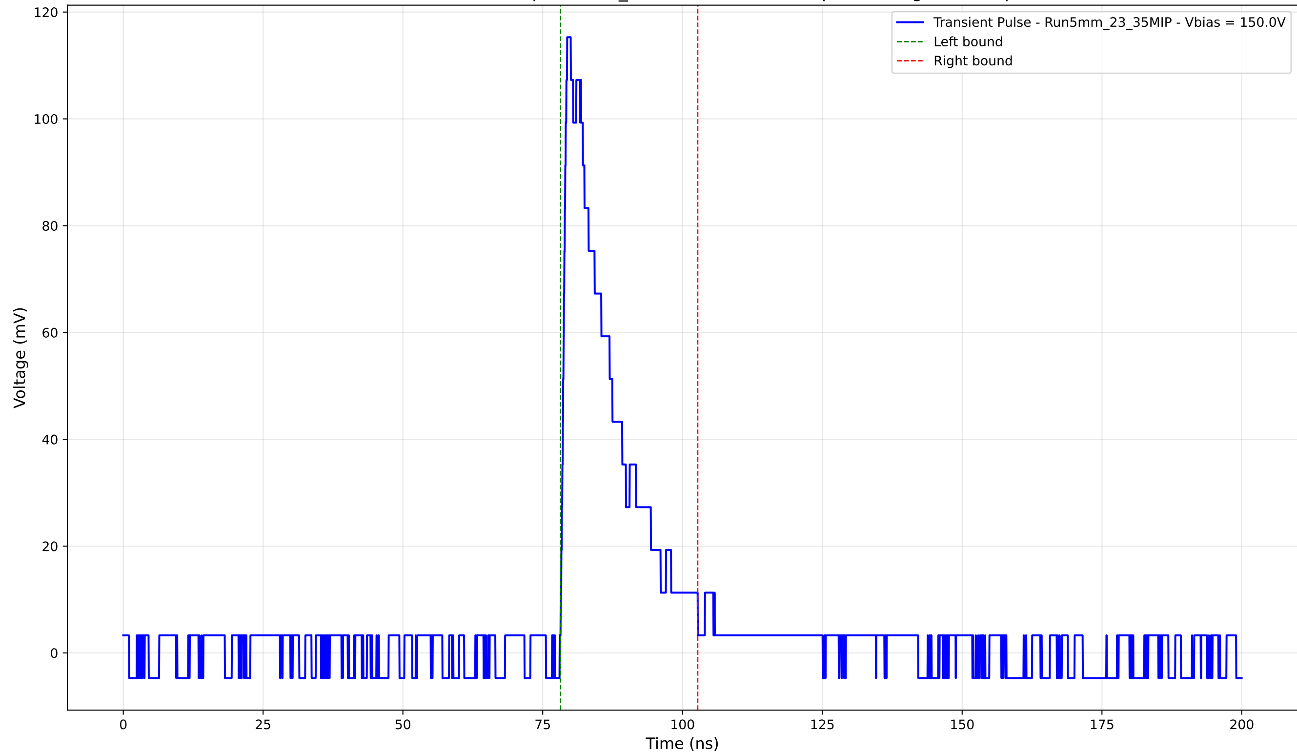
Transient Pulse - Sample: 5mm_23 - Position: 4170.0 \mu\text{m} - Charge: 21.61 pC
