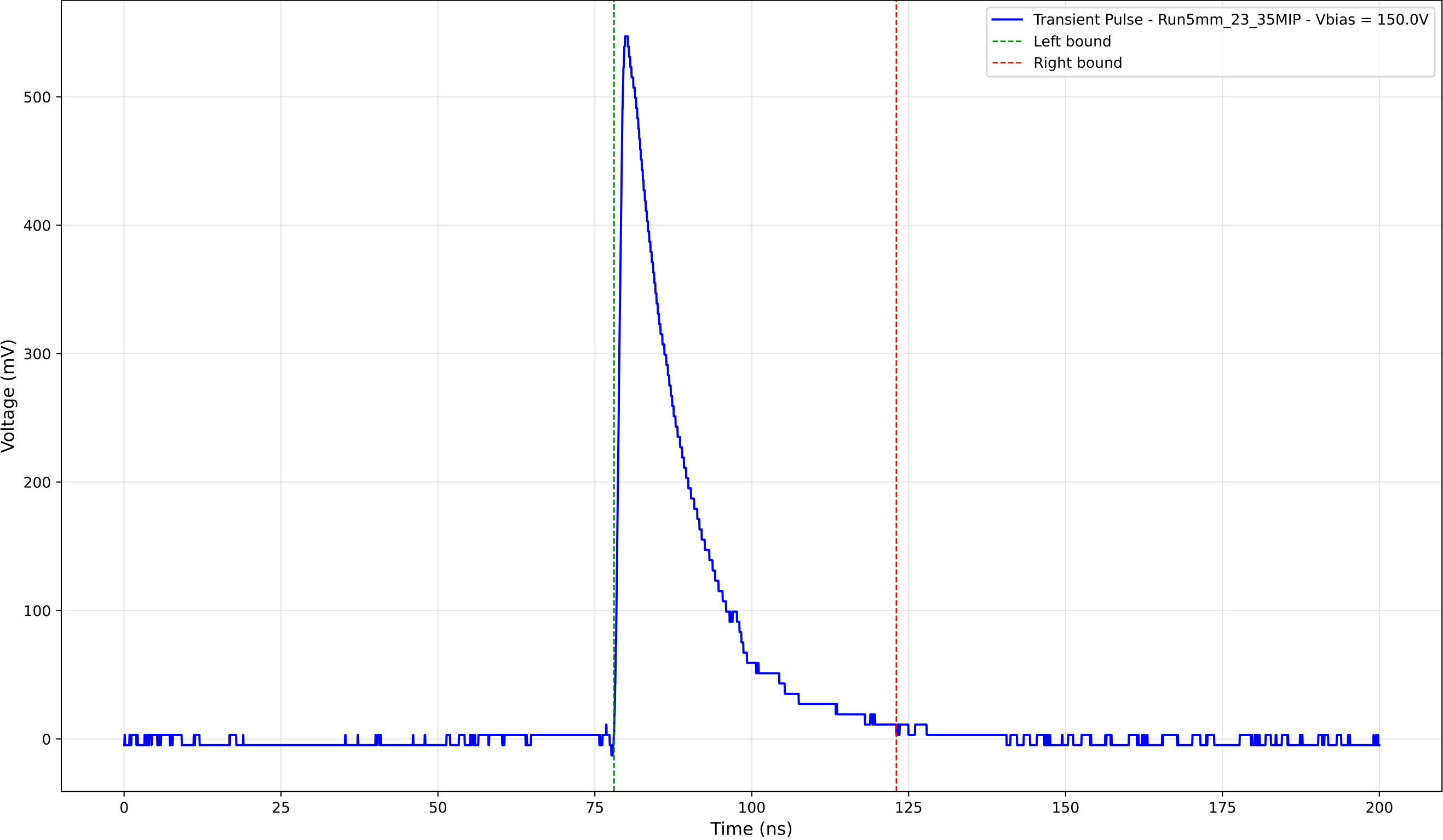
Transient Pulse - Sample: 5mm_23 - Position: 3870.0 \mu\text{m} - Charge: 120.63 pC
