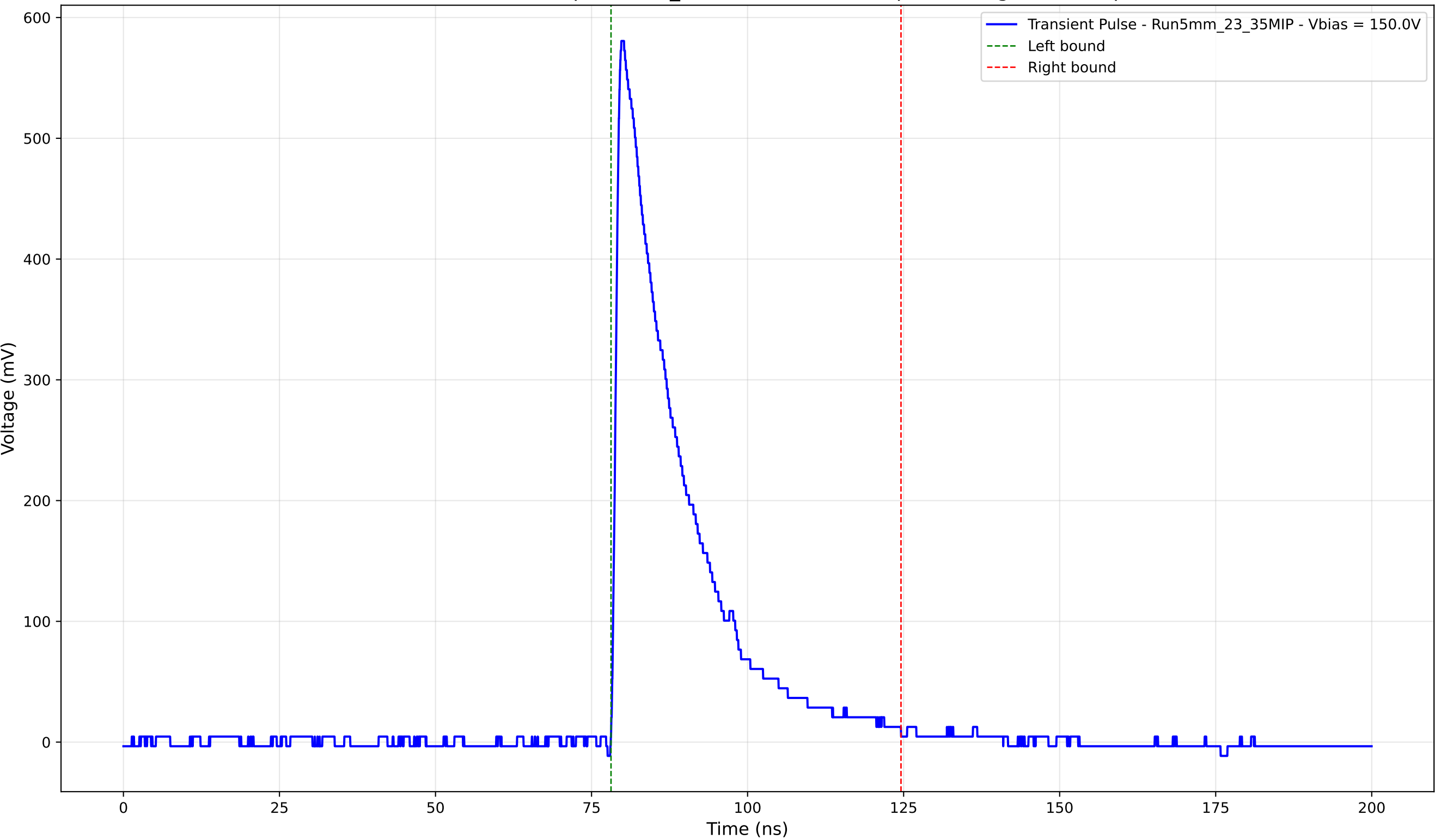
Transient Pulse - Sample: 5mm_23 - Position: 1345.0 \mu\text{m} - Charge: 130.58 pC
