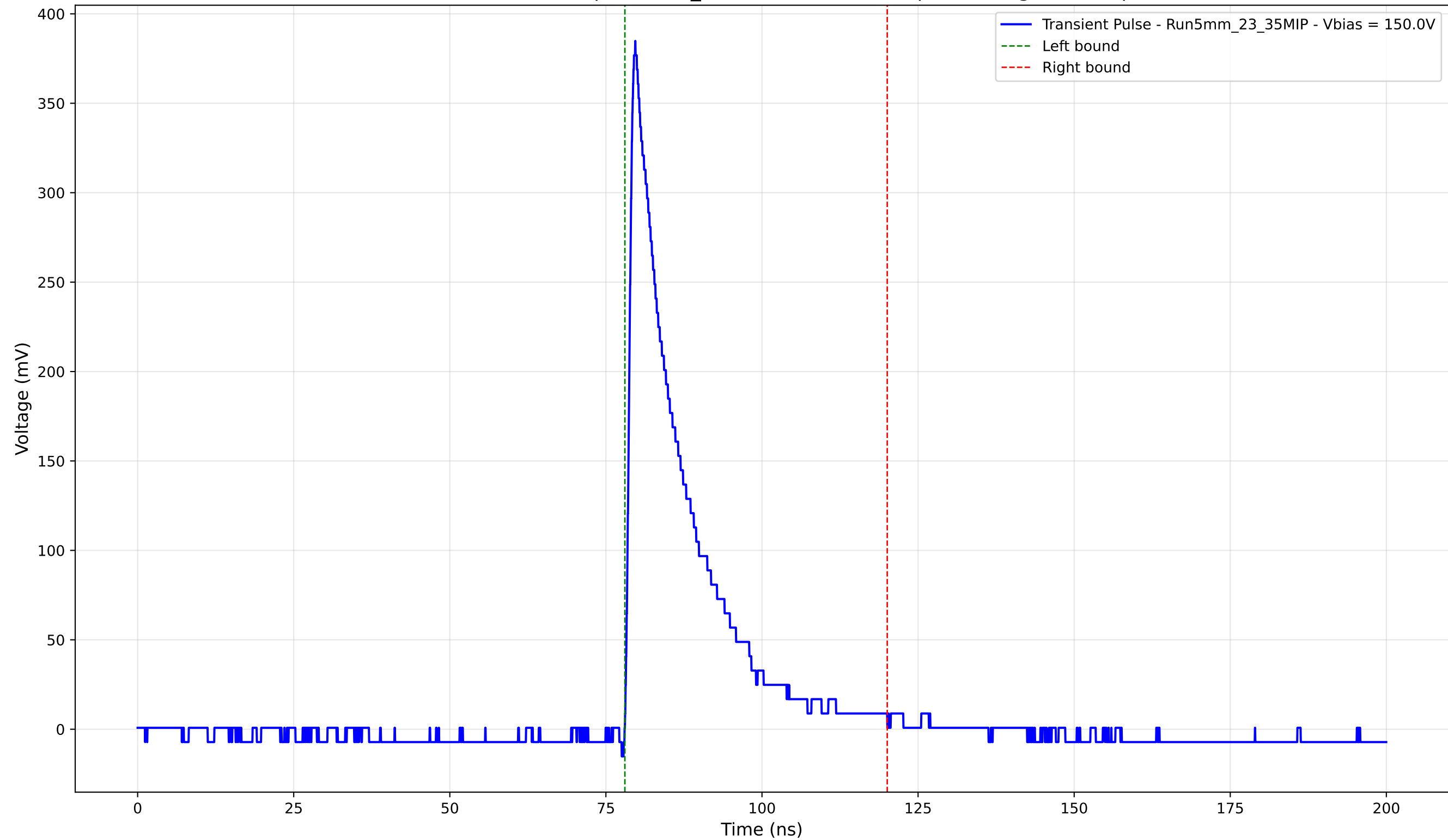
Transient Pulse - Sample: 5mm_23 - Position: 4215.0 \mu\text{m} - Charge: 68.59 pC
