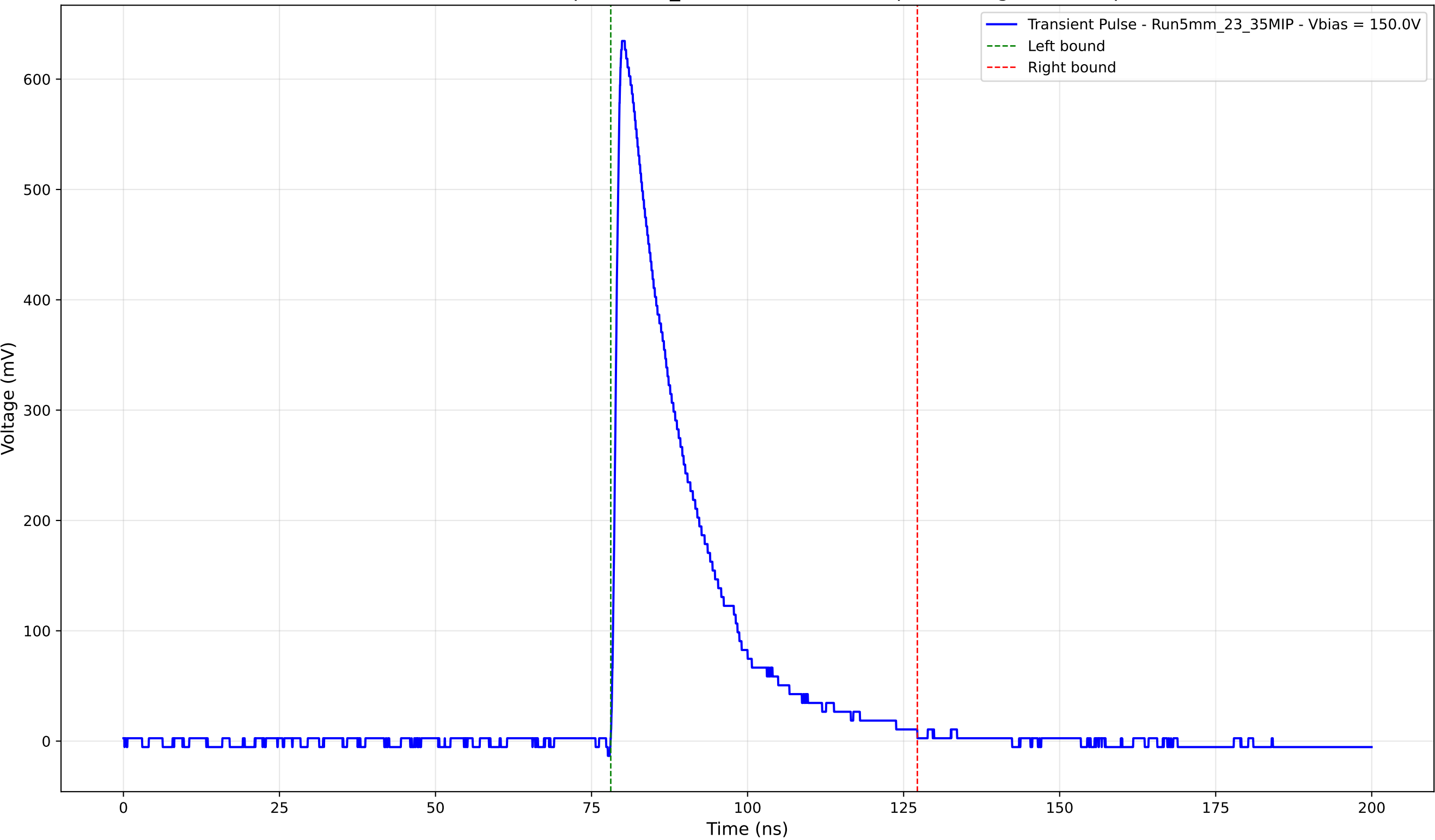
Transient Pulse - Sample: 5mm_23 - Position: 1465.0 \mu\text{m} - Charge: 149.31 pC
