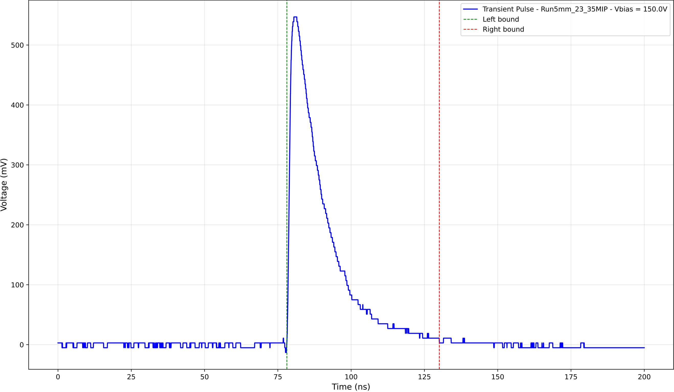
Transient Pulse - Sample: 5mm_23 - Position: 1990.0 \mu\text{m} - Charge: 144.93 pC
