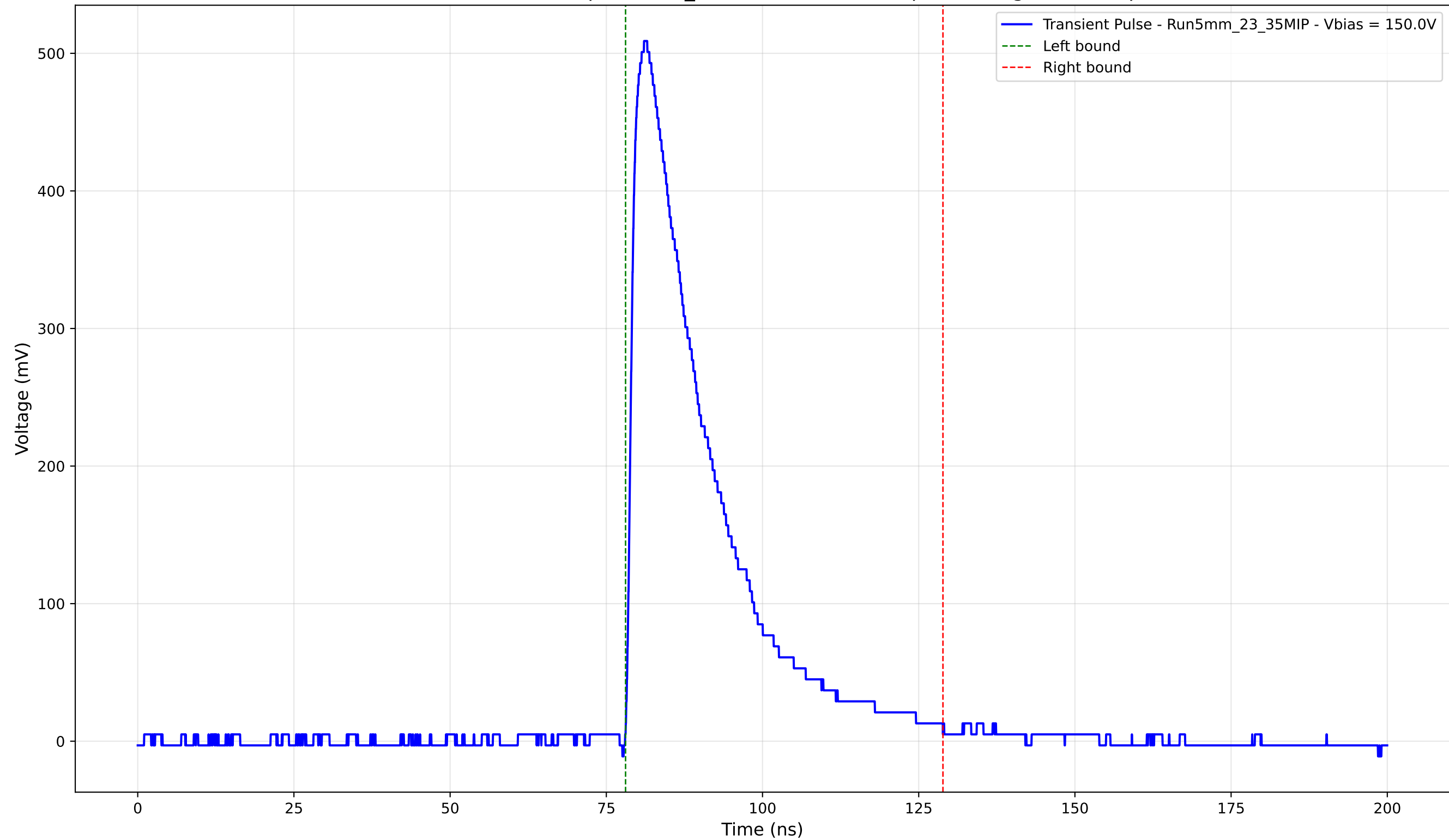
Transient Pulse - Sample: 5mm_23 - Position: 2475.0 \mu\text{m} - Charge: 138.97 pC
