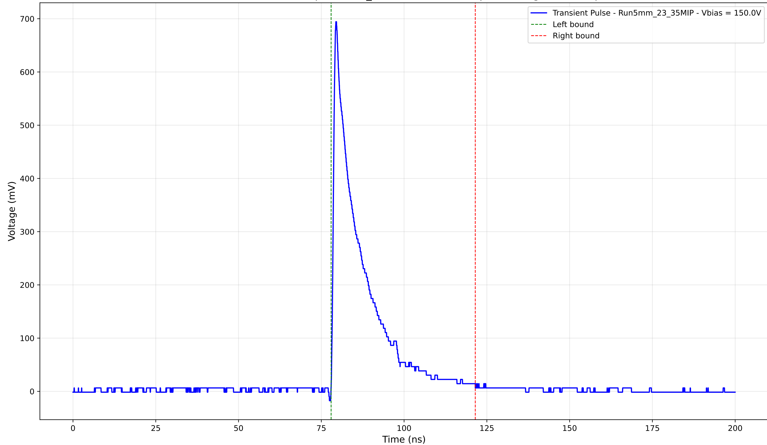
Transient Pulse - Sample: 5mm_23 - Position: 790.0 \mu\text{m} - Charge: 121.65 pC
