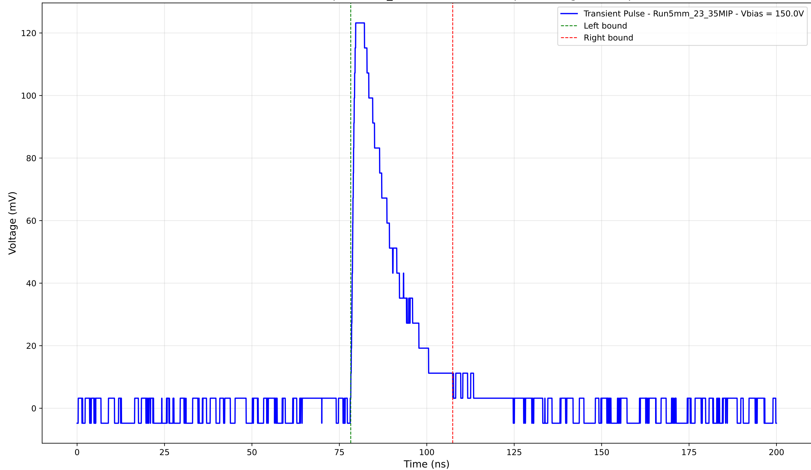
Transient Pulse - Sample: 5mm_23 - Position: 3635.0 \mu\text{m} - Charge: 29.11 pC
