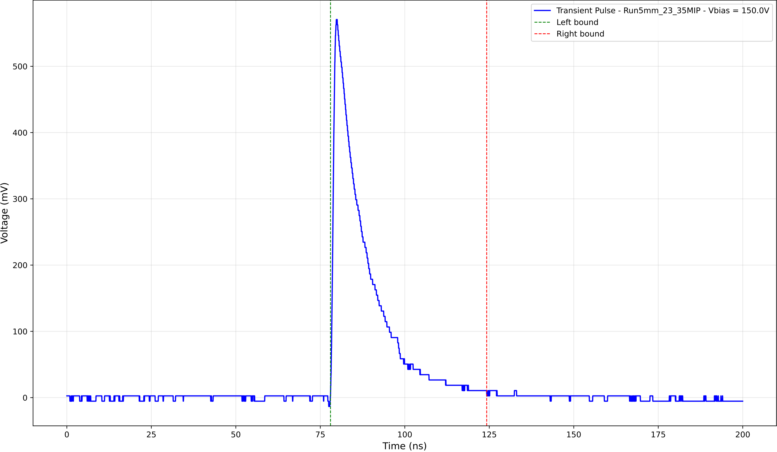
Transient Pulse - Sample: 5mm_23 - Position: 4030.0 \mu\text{m} - Charge: 117.01 pC
