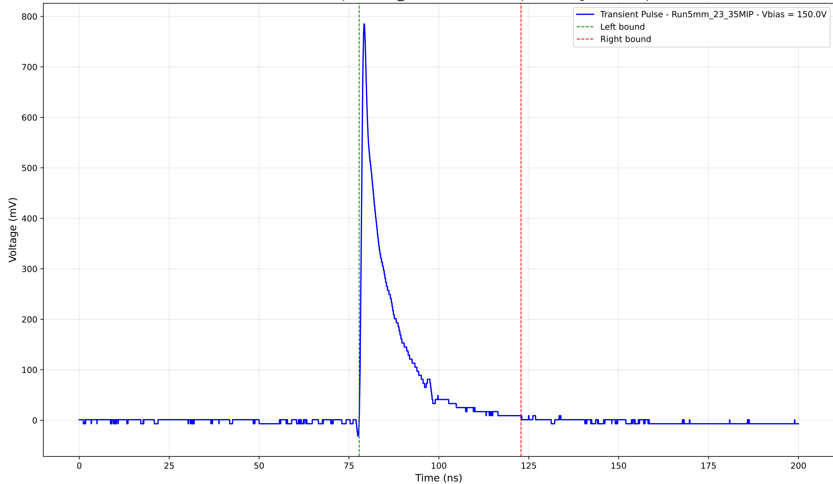
Transient Pulse - Sample: 5mm_23 - Position: 510.0 \mu\text{m} - Charge: 113.19 pC
