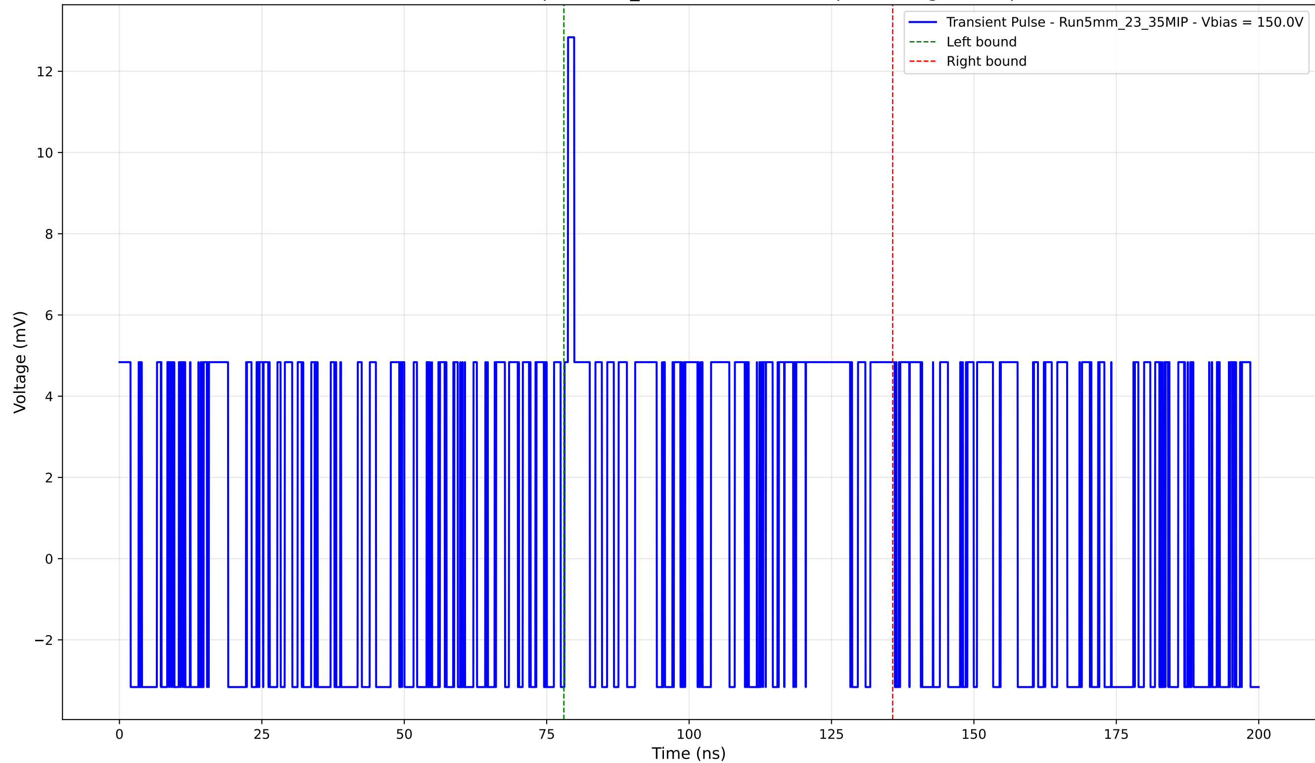
Transient Pulse - Sample: 5mm_23 - Position: 5205.0 \mu\text{m} - Charge: 3.20 pC
