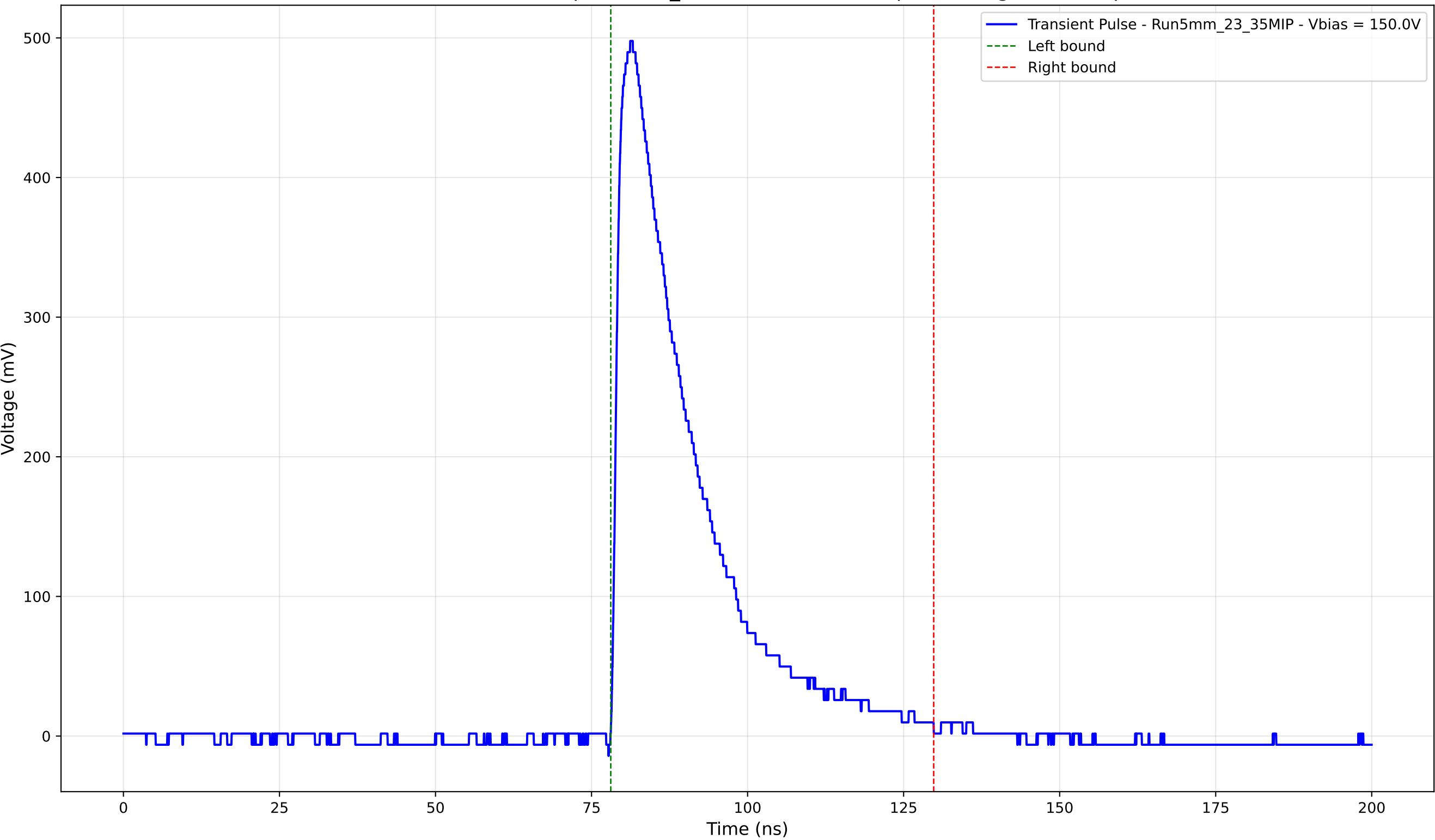
Transient Pulse - Sample: 5mm_23 - Position: 2895.0 \mu\text{m} - Charge: 134.18 pC
