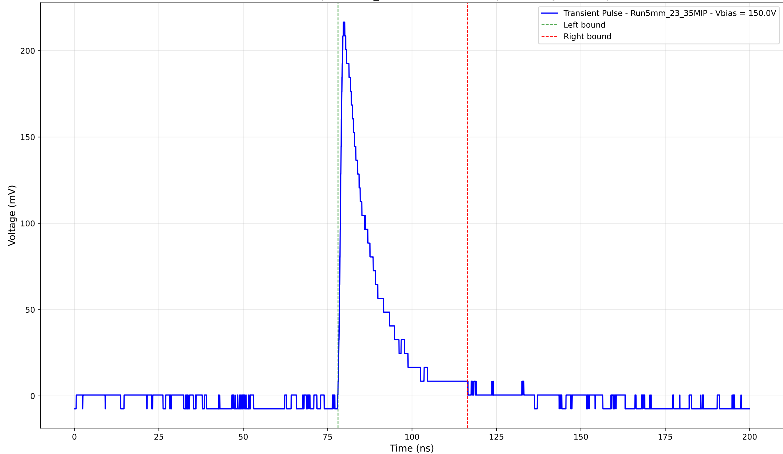
Transient Pulse - Sample: 5mm_23 - Position: 4125.0 \mu\text{m} - Charge: 40.60 pC
