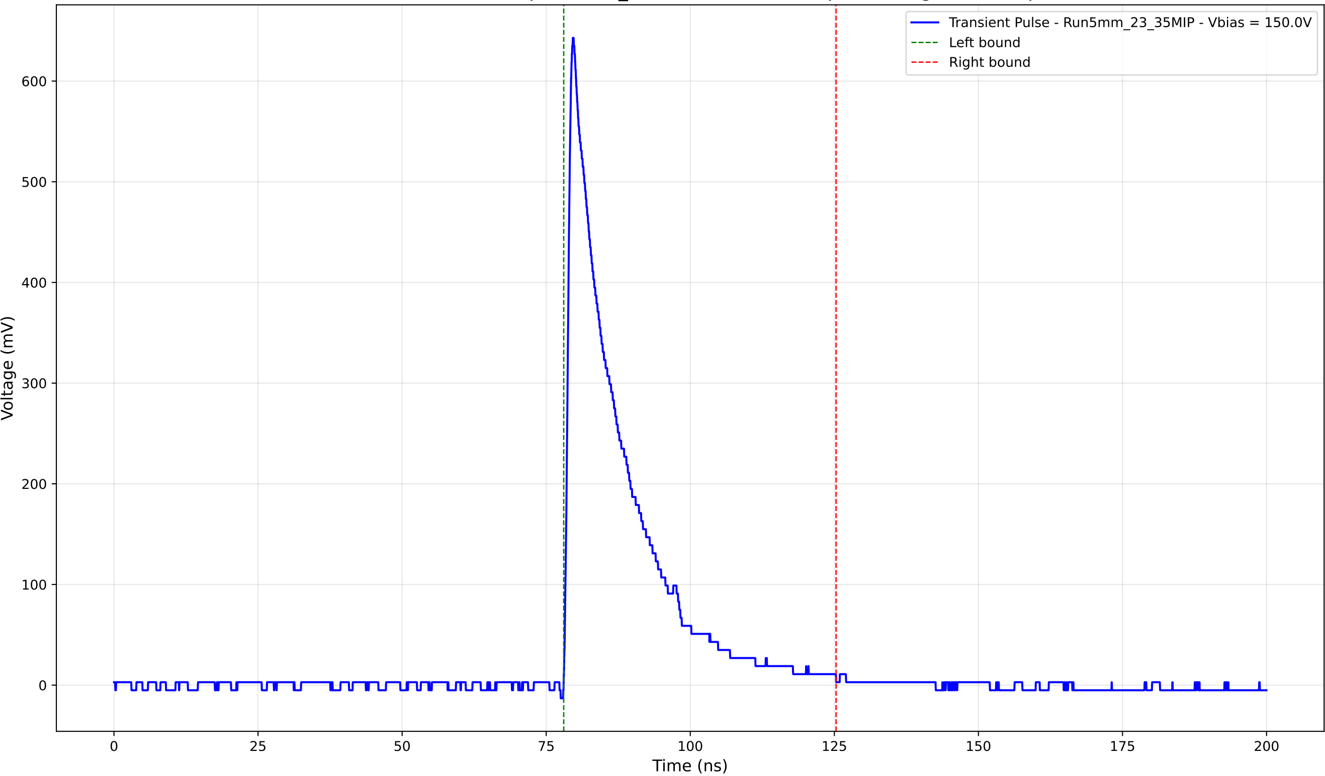
Transient Pulse - Sample: 5mm_23 - Position: 1005.0 \mu\text{m} - Charge: 123.00 pC
