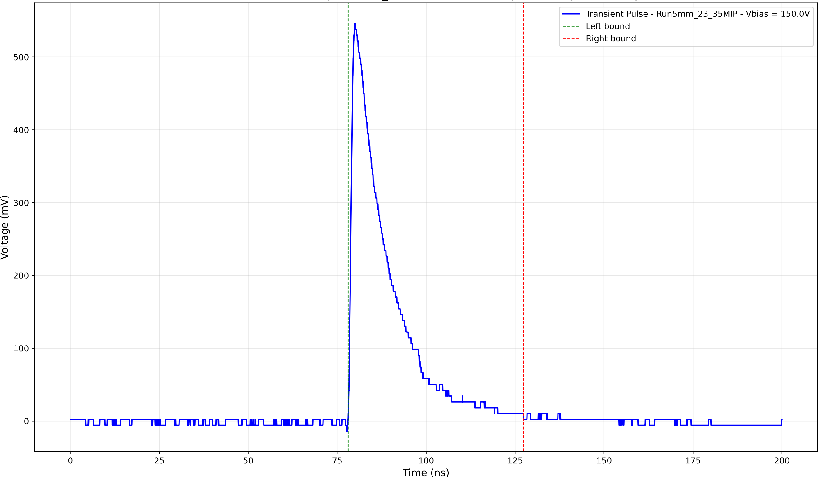
Transient Pulse - Sample: 5mm_23 - Position: 3820.0 \mu\text{m} - Charge: 121.56 pC
