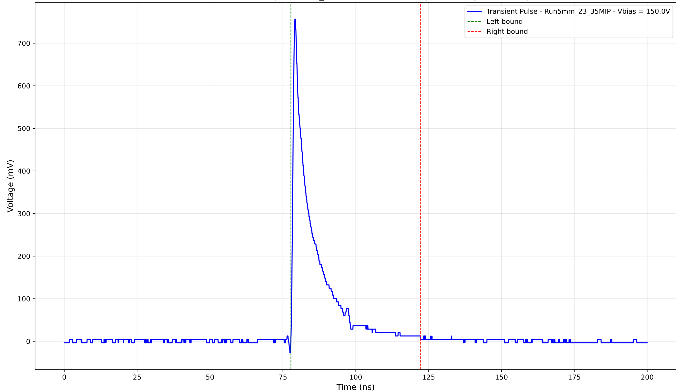
Transient Pulse - Sample: 5mm_23 - Position: 4755.0 \mu\text{m} - Charge: 107.31 pC
