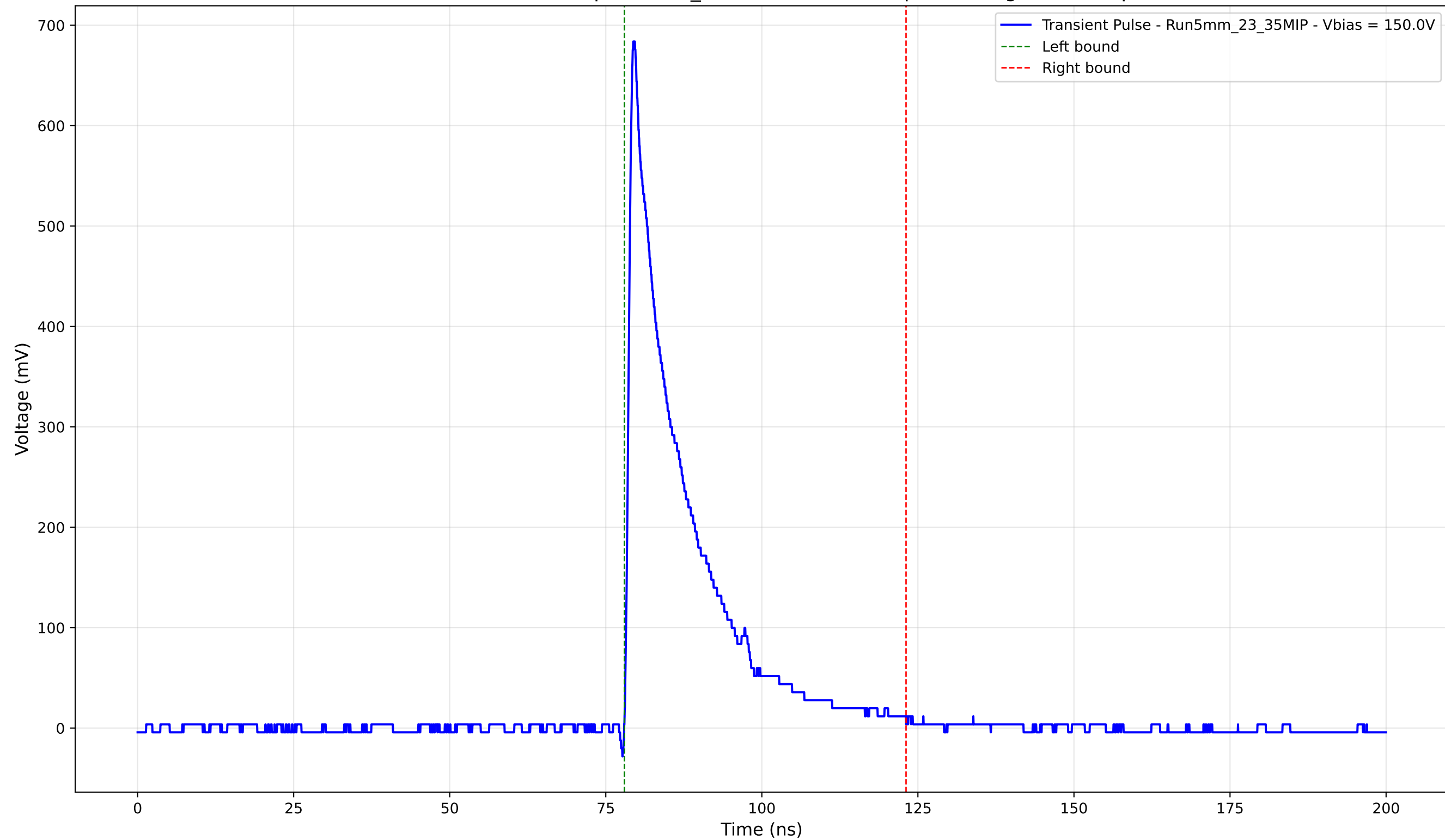
Transient Pulse - Sample: 5mm_23 - Position: 820.0 \mu\text{m} - Charge: 122.26 pC
