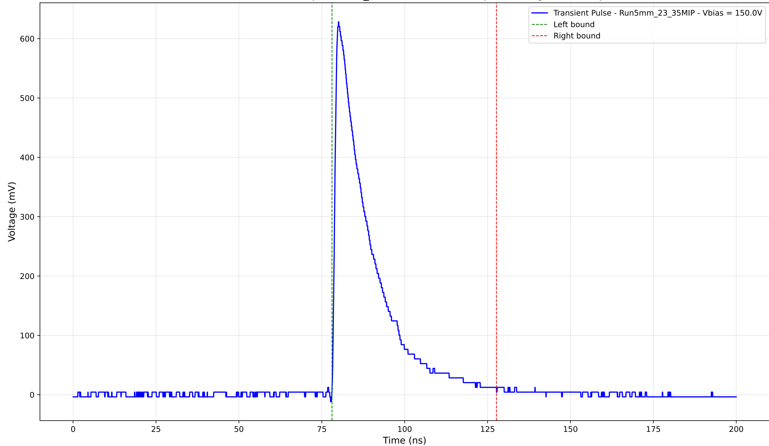
Transient Pulse - Sample: 5mm_23 - Position: 1480.0 \mu\text{m} - Charge: 148.20 pC
