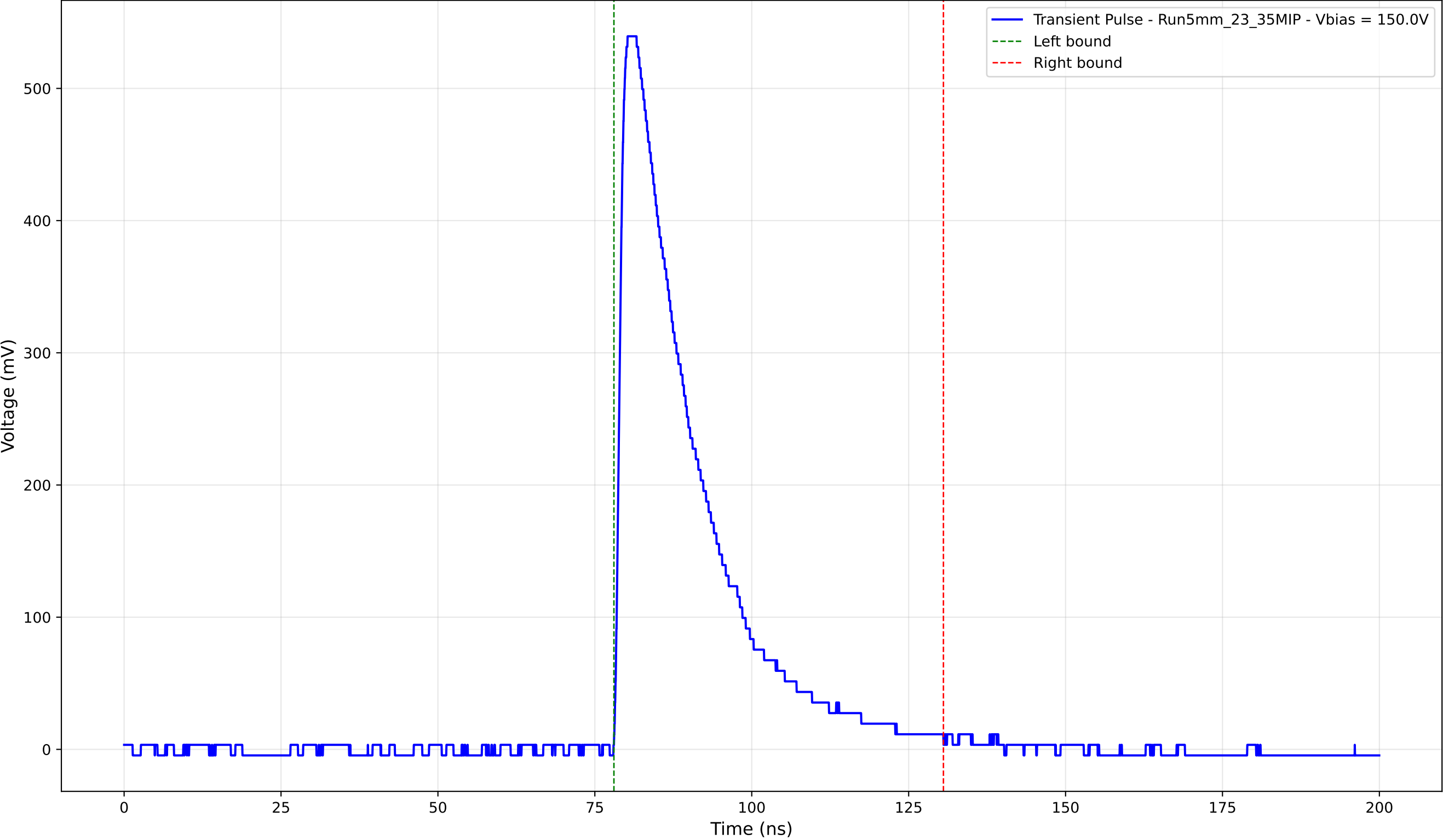
Transient Pulse - Sample: 5mm_23 - Position: 2025.0 \mu\text{m} - Charge: 143.99 pC
