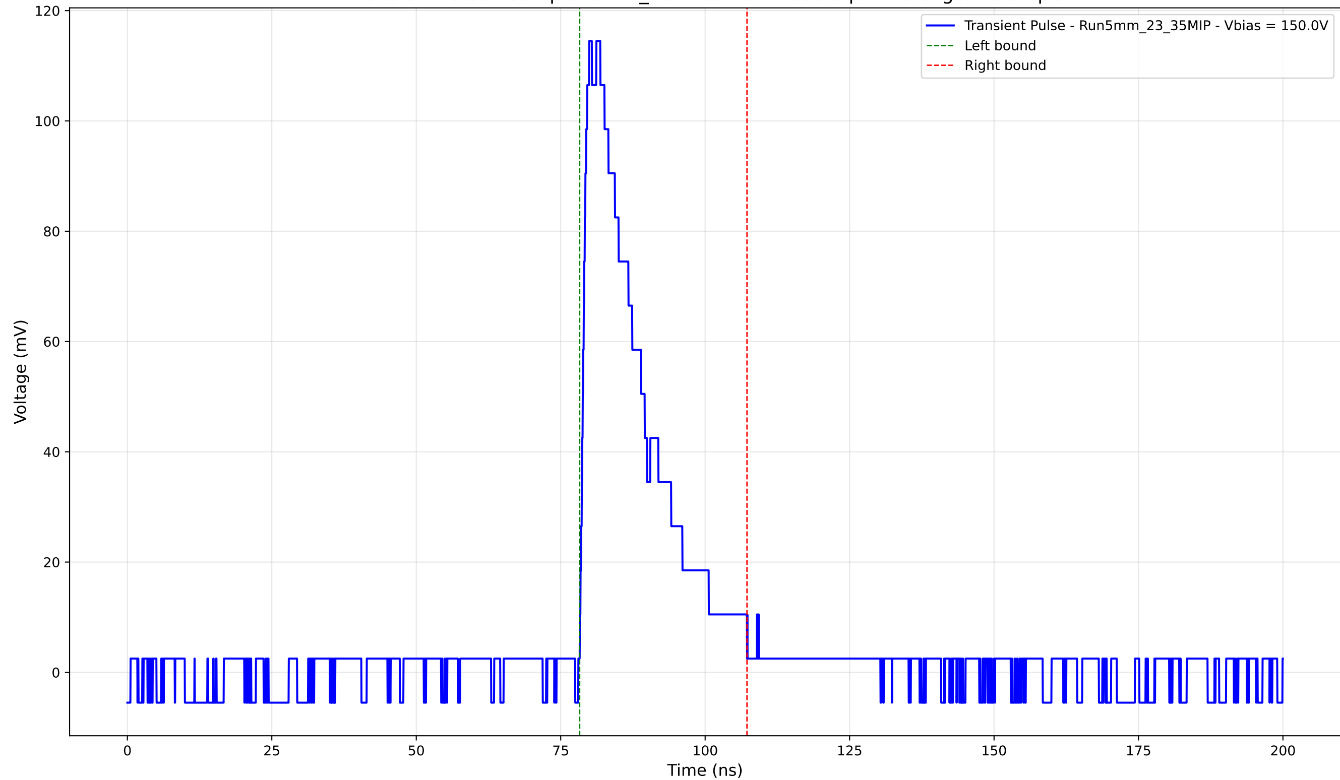
Transient Pulse - Sample: 5mm_23 - Position: 1605.0 \mu\text{m} - Charge: 25.87 pC
