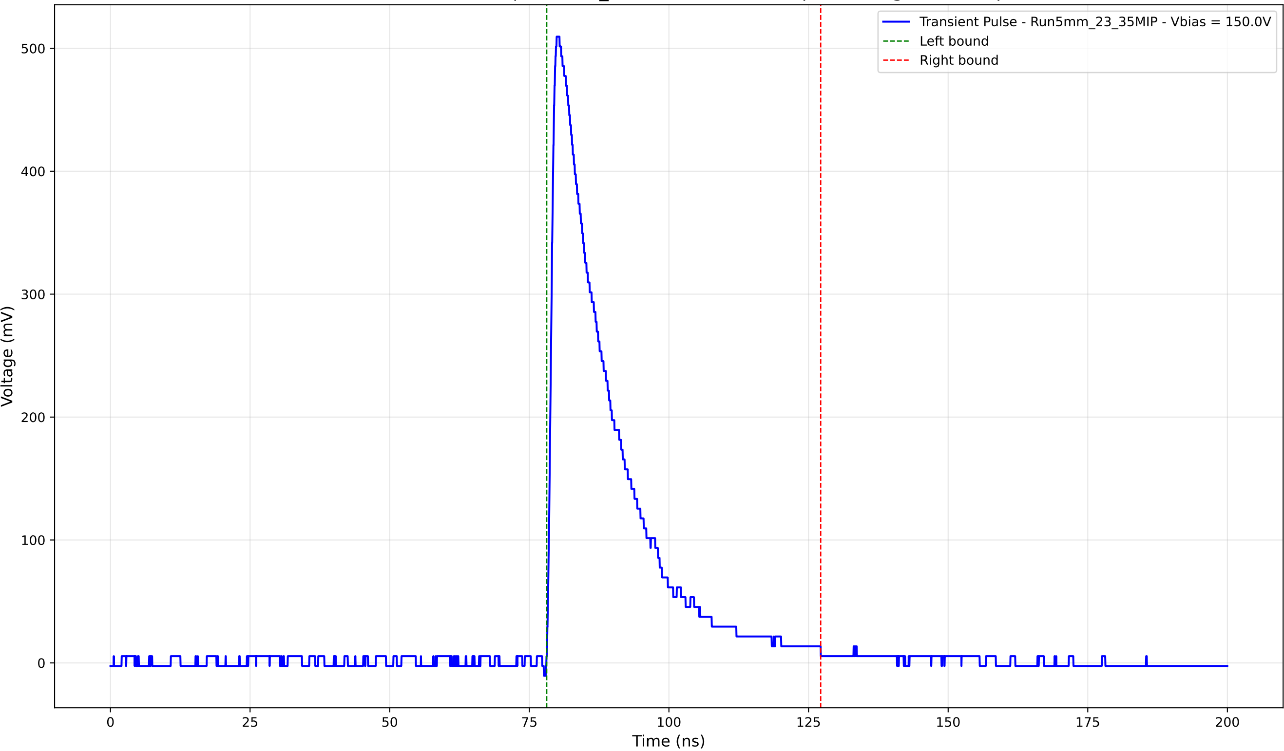
Transient Pulse - Sample: 5mm_23 - Position: 1540.0 \mu\text{m} - Charge: 120.58 pC
