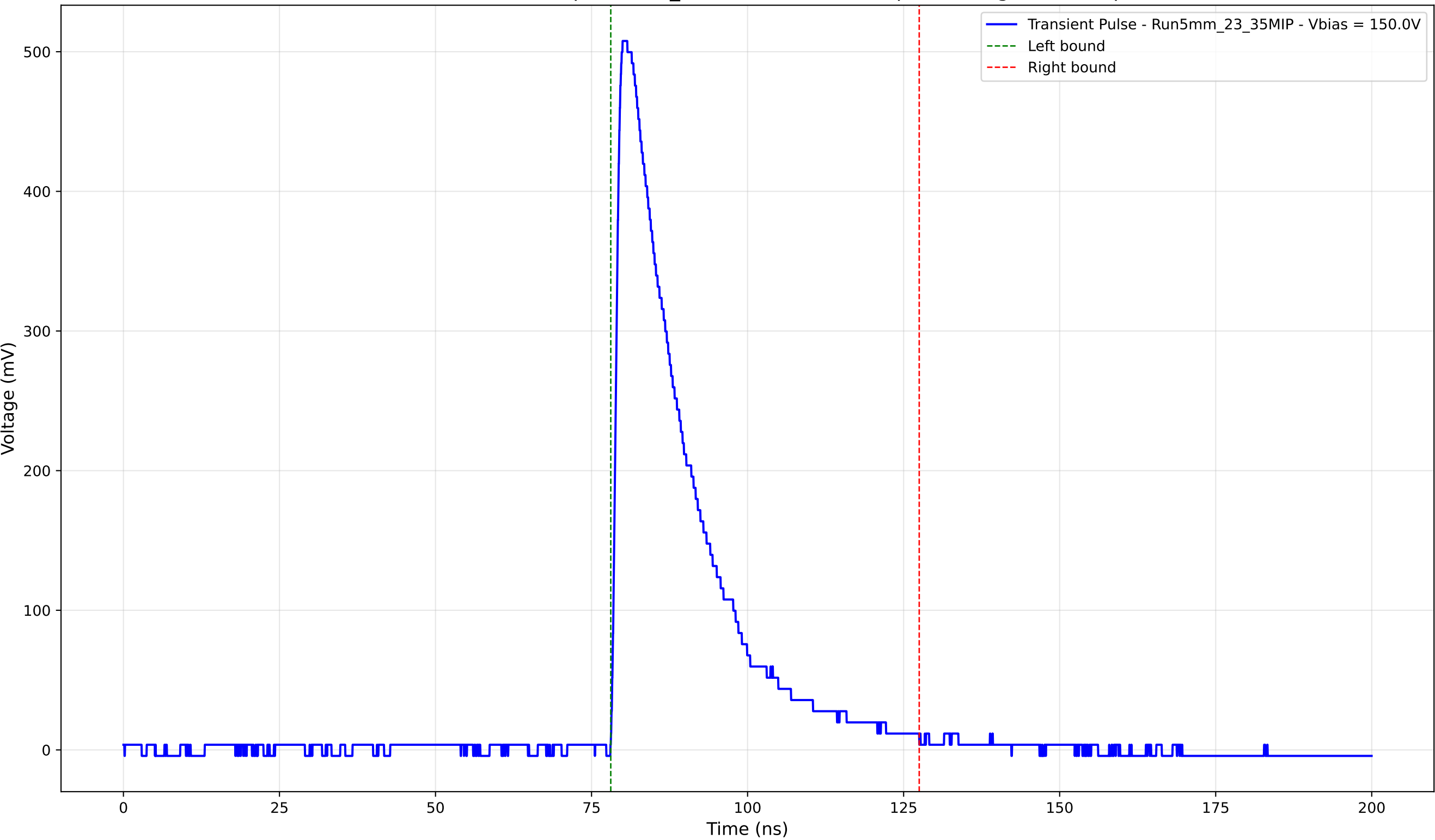
Transient Pulse - Sample: 5mm_23 - Position: 1725.0 \mu\text{m} - Charge: 127.43 pC
