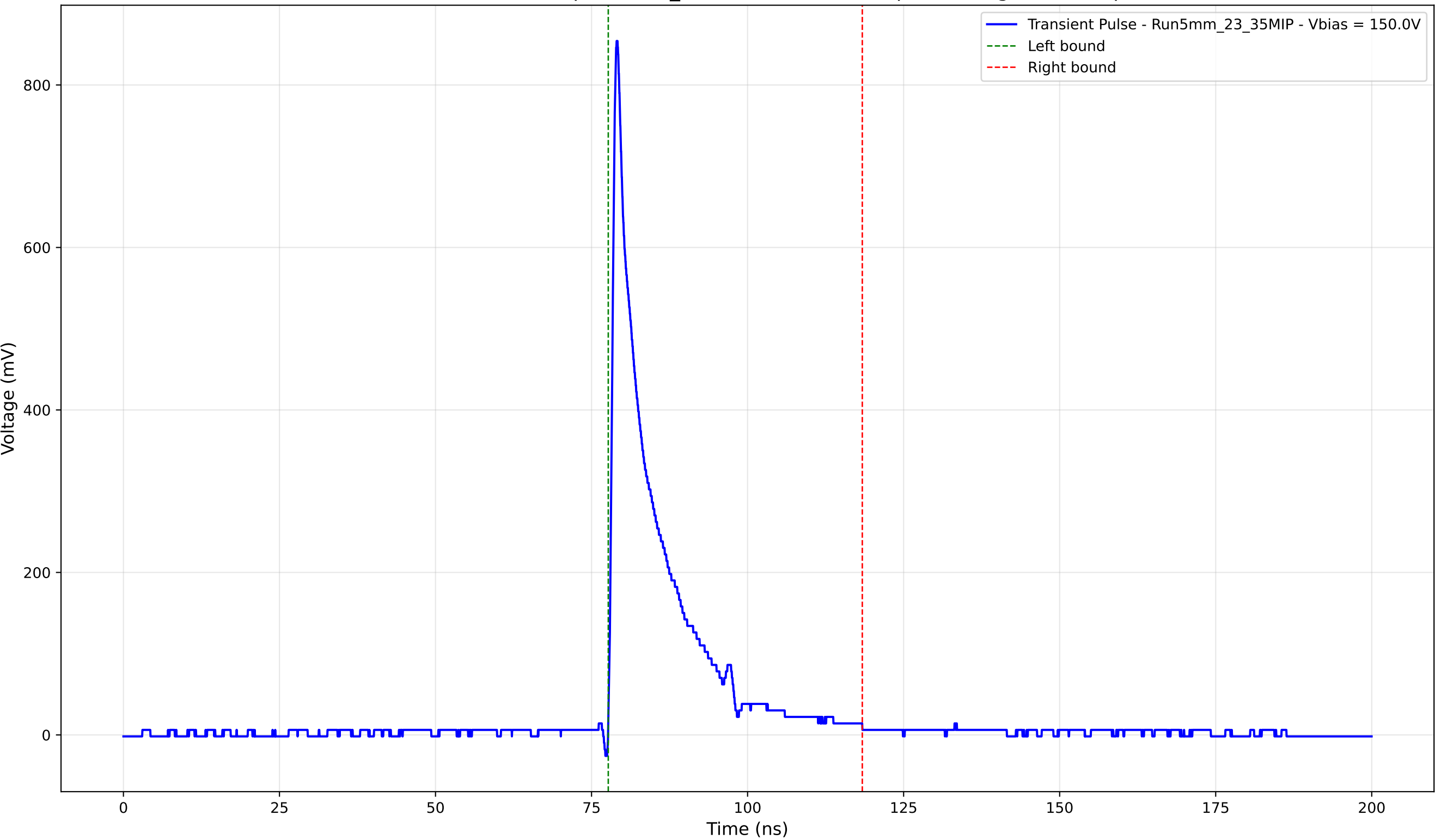
Transient Pulse - Sample: 5mm_23 - Position: 4880.0 \mu\text{m} - Charge: 115.56 pC
