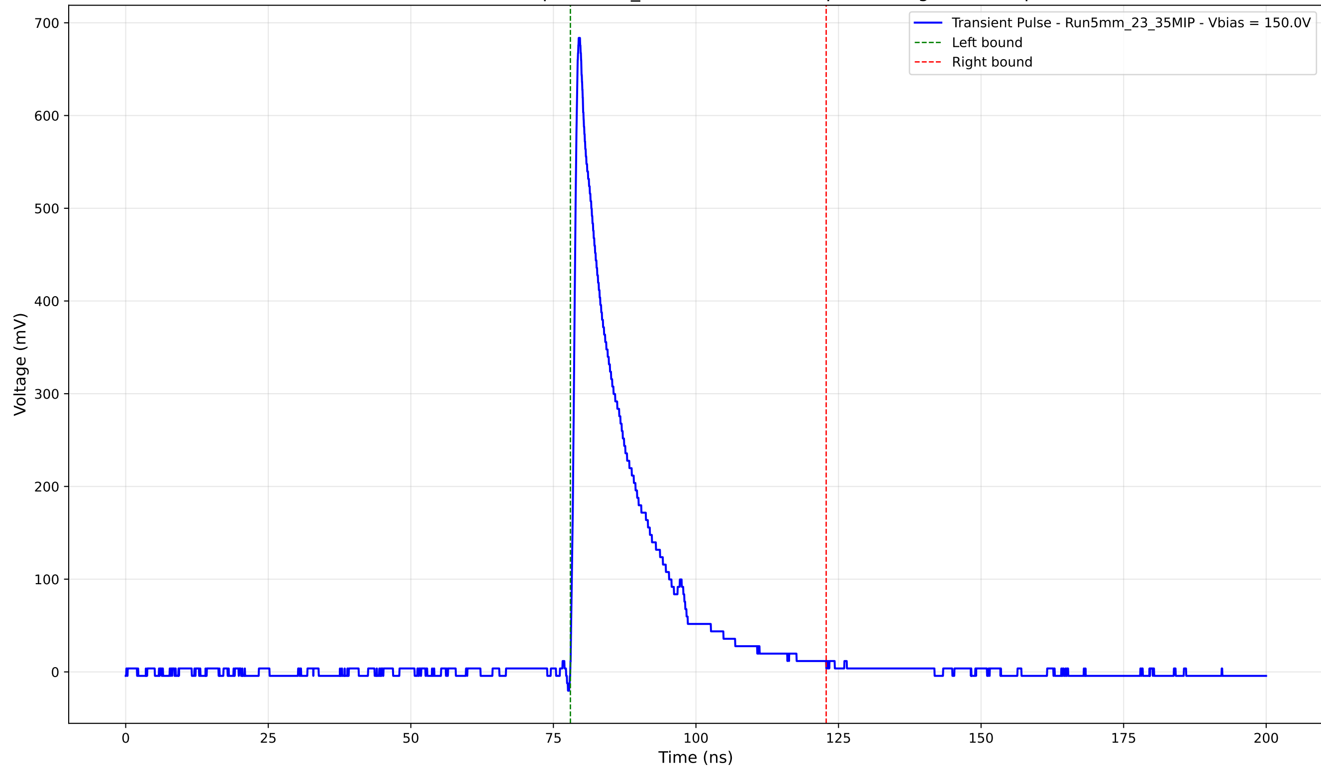
Transient Pulse - Sample: 5mm_23 - Position: 845.0 \mu\text{m} - Charge: 122.80 pC
