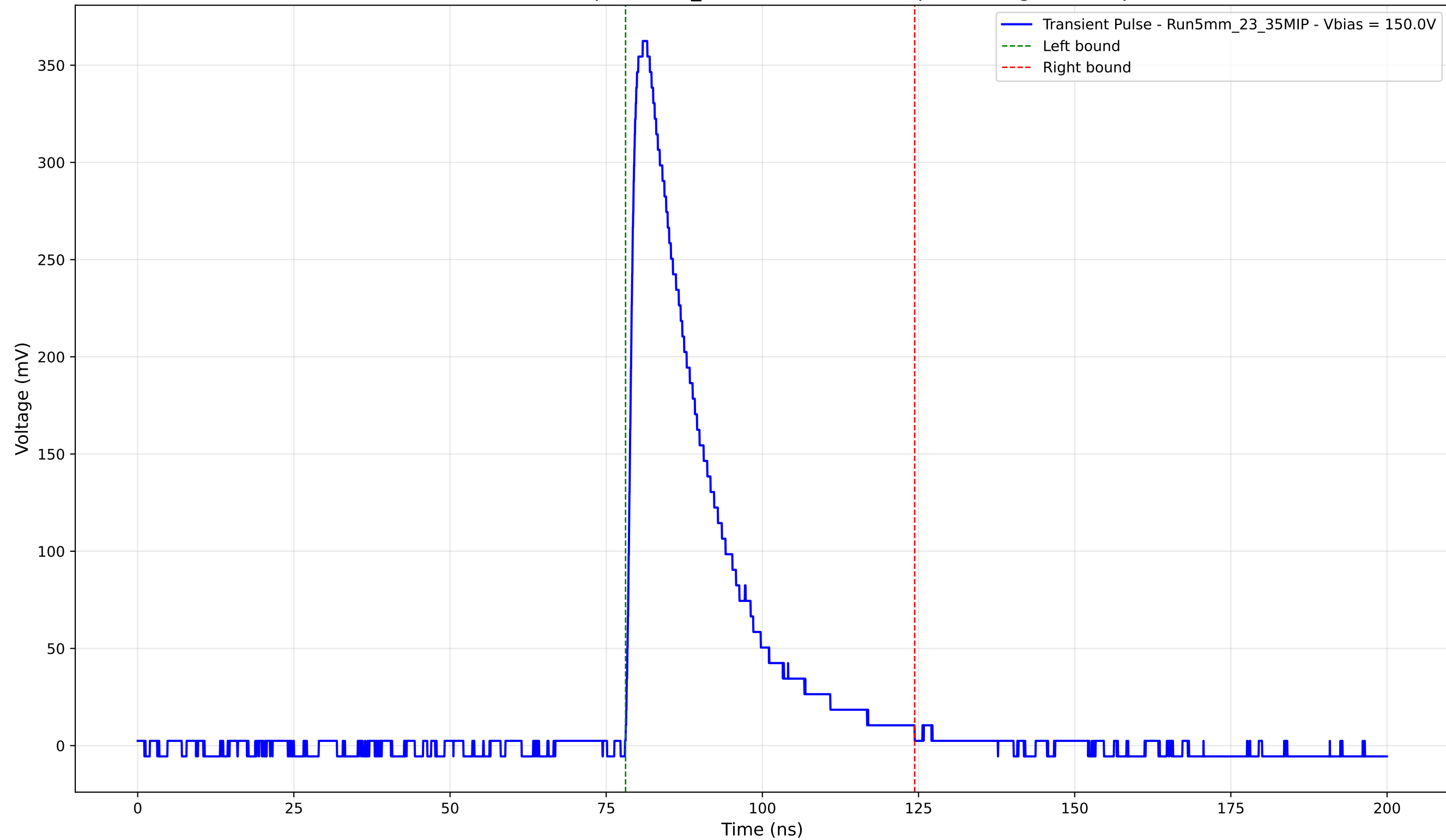
Transient Pulse - Sample: 5mm_23 - Position: 3205.0 \mu\text{m} - Charge: 92.09 pC
