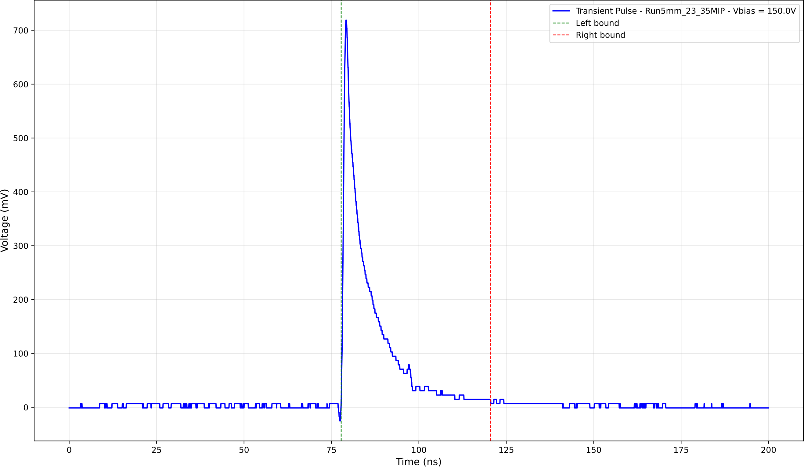
Transient Pulse - Sample: 5mm_23 - Position: 4745.0 \mu\text{m} - Charge: 101.08 pC
