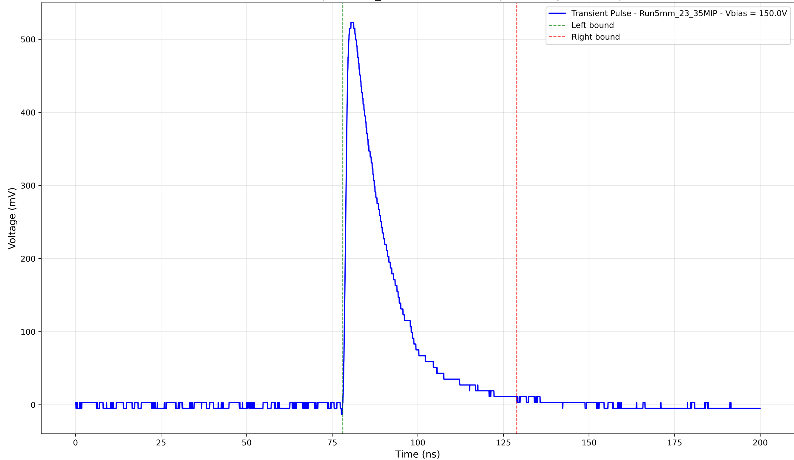
Transient Pulse - Sample: 5mm_23 - Position: 1840.0 \mu\text{m} - Charge: 134.17 pC
