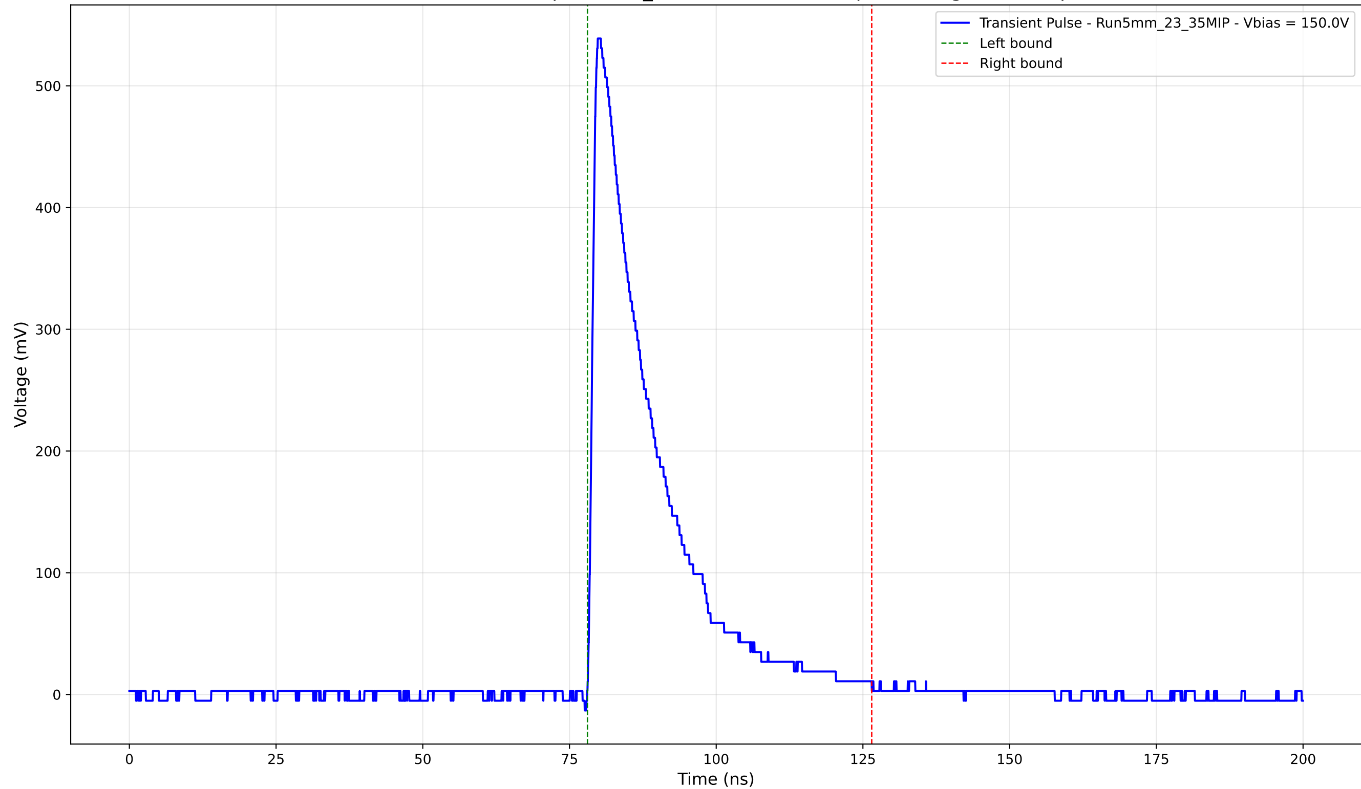
Transient Pulse - Sample: 5mm_23 - Position: 3815.0 \mu\text{m} - Charge: 122.09 pC
