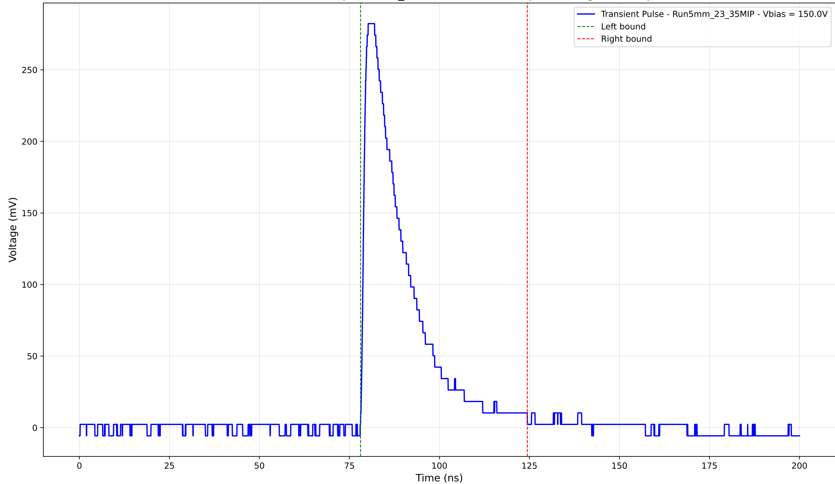
Transient Pulse - Sample: 5mm_23 - Position: 2090.0 \mu\text{m} - Charge: 72.25 pC
