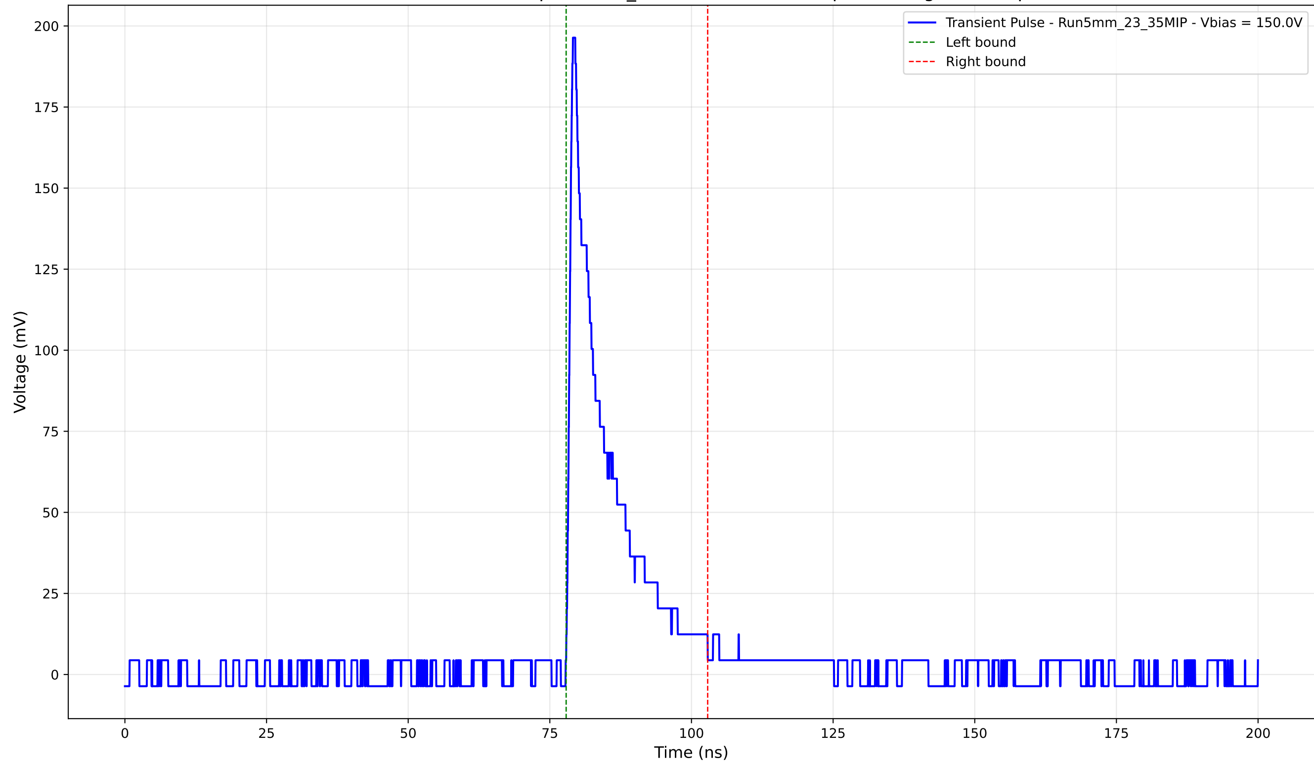
Transient Pulse - Sample: 5mm_23 - Position: 4685.0 \mu\text{m} - Charge: 26.88 pC
