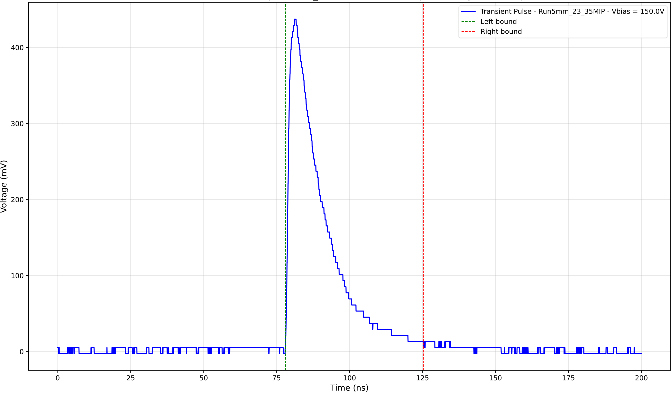
Transient Pulse - Sample: 5mm_23 - Position: 2725.0 \mu\text{m} - Charge: 117.25 pC
