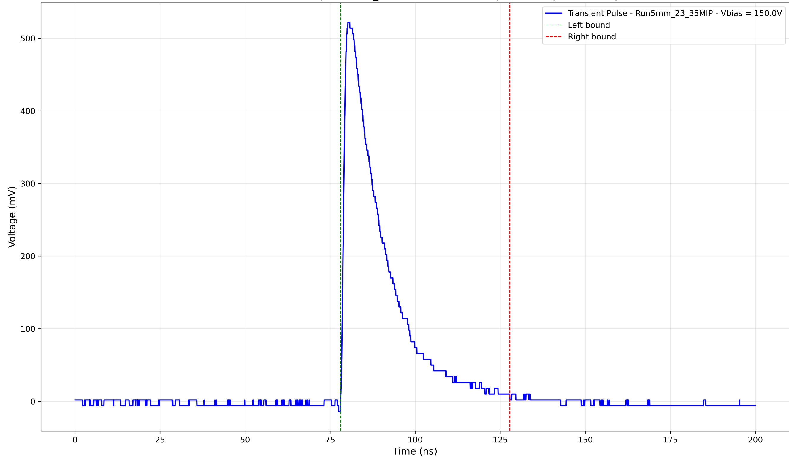
Transient Pulse - Sample: 5mm_23 - Position: 1830.0 \mu\text{m} - Charge: 133.53 pC
