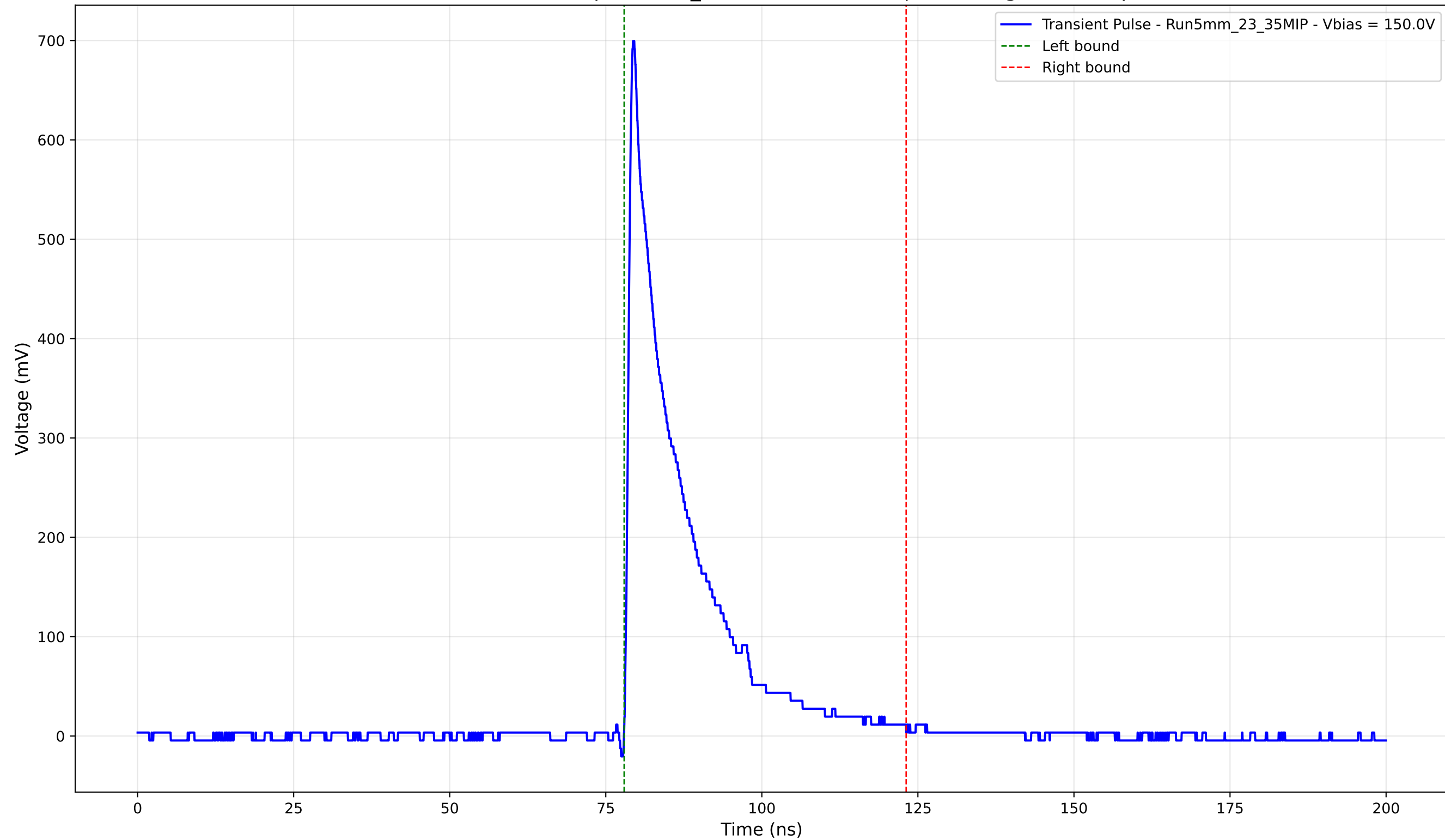
Transient Pulse - Sample: 5mm_23 - Position: 760.0 \mu\text{m} - Charge: 120.15 pC
