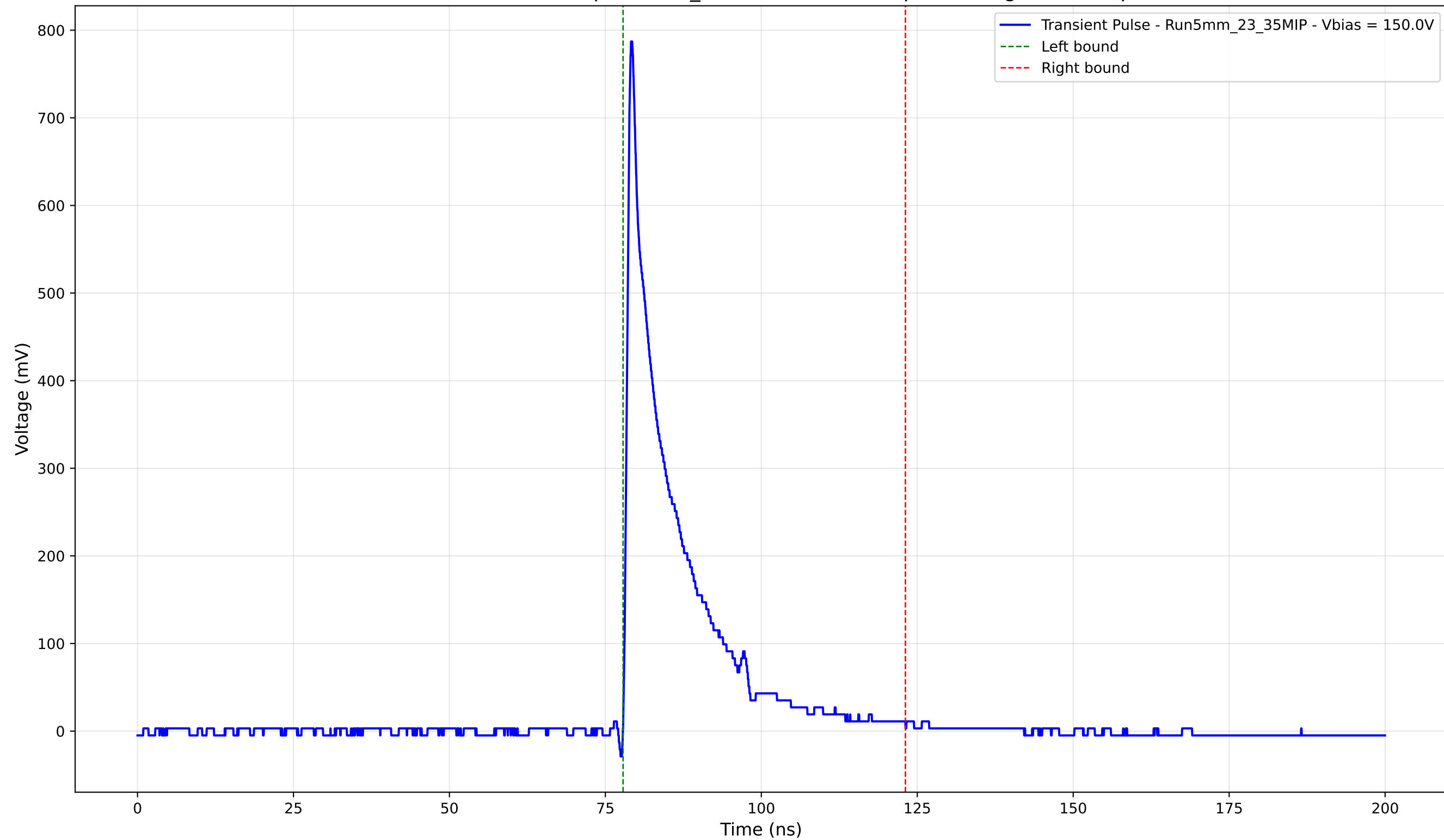
Transient Pulse - Sample: 5mm_23 - Position: 495.0 \mu\text{m} - Charge: 114.81 pC
