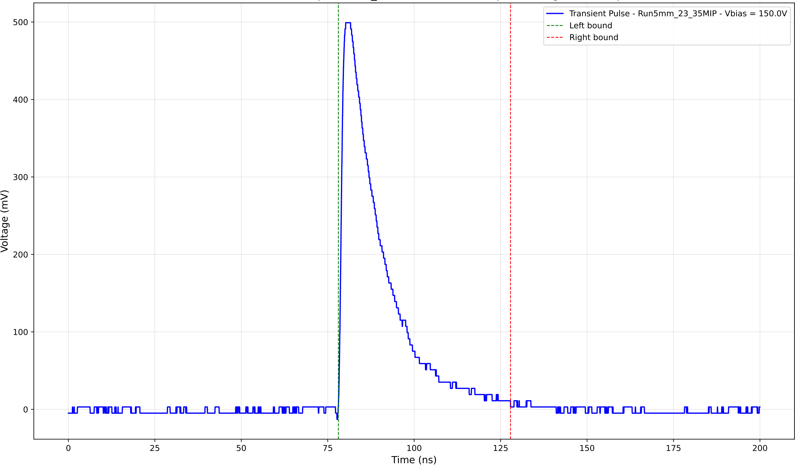
Transient Pulse - Sample: 5mm_23 - Position: 3355.0 \mu\text{m} - Charge: 129.85 pC
