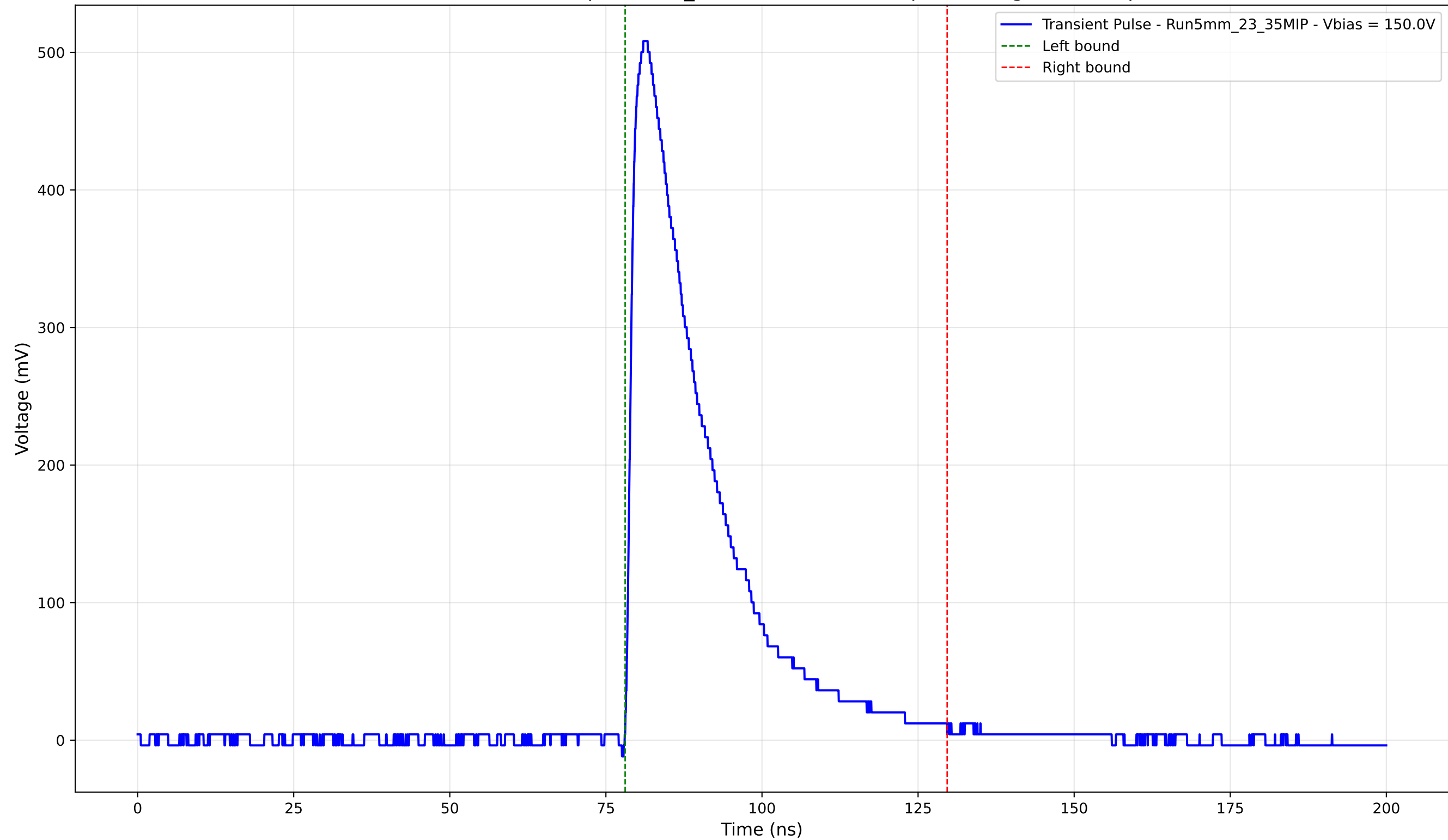
Transient Pulse - Sample: 5mm_23 - Position: 2490.0 \mu\text{m} - Charge: 138.16 pC
