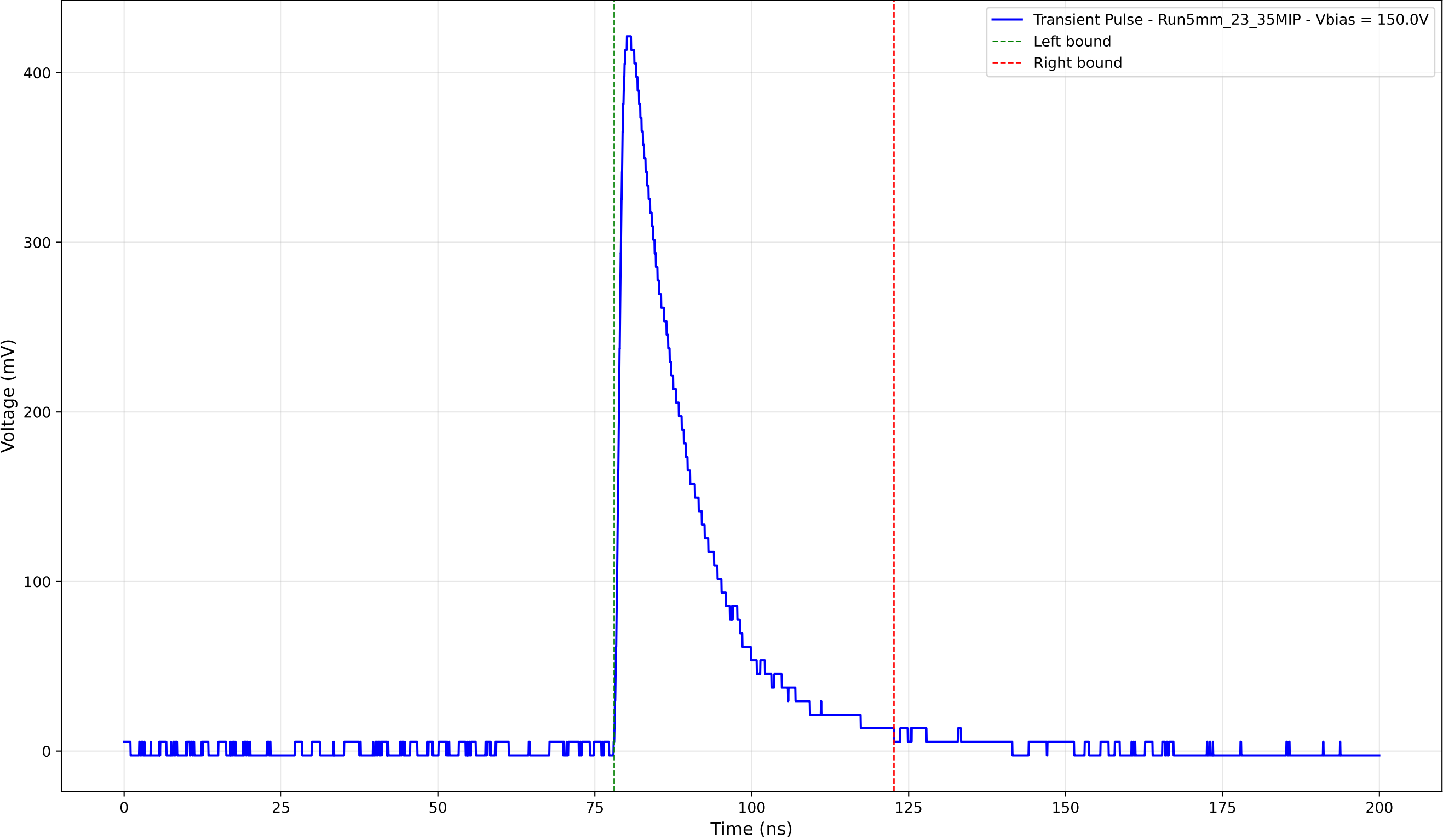
Transient Pulse - Sample: 5mm_23 - Position: 3585.0 \mu\text{m} - Charge: 101.03 pC
