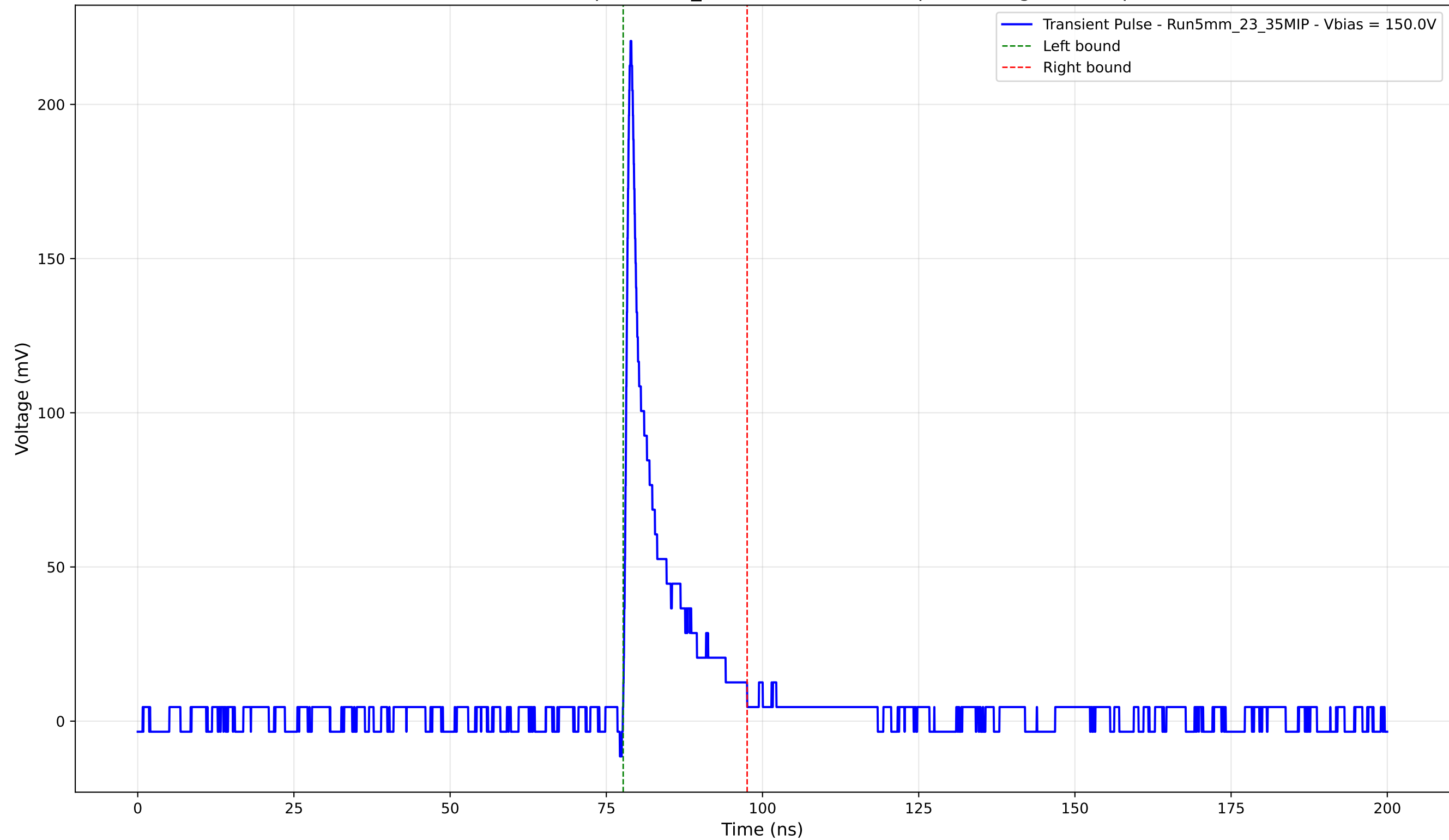
Transient Pulse - Sample: 5mm_23 - Position: 5090.0 \mu\text{m} - Charge: 20.33 pC
