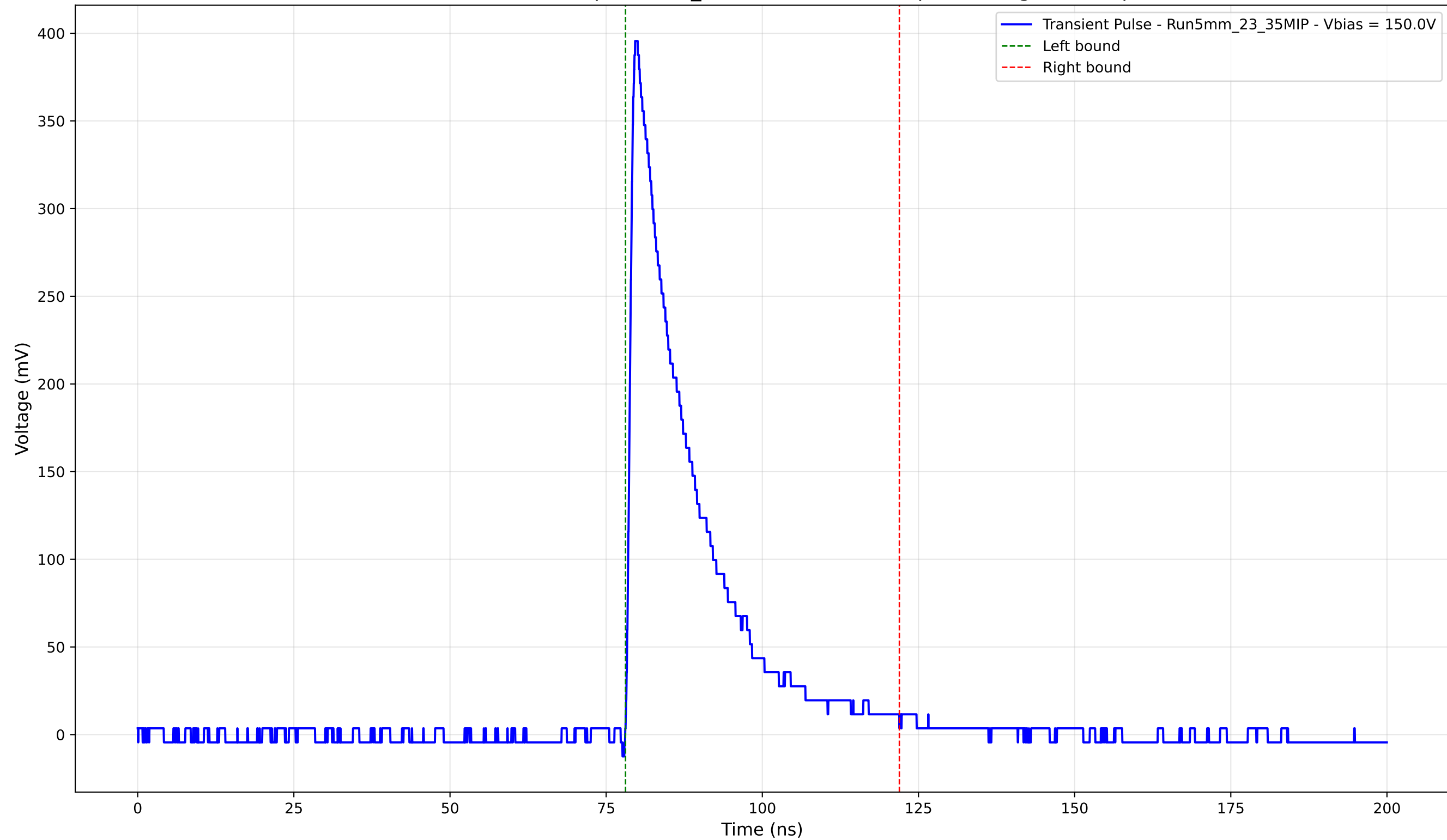
Transient Pulse - Sample: 5mm_23 - Position: 1180.0 \mu\text{m} - Charge: 82.24 pC
