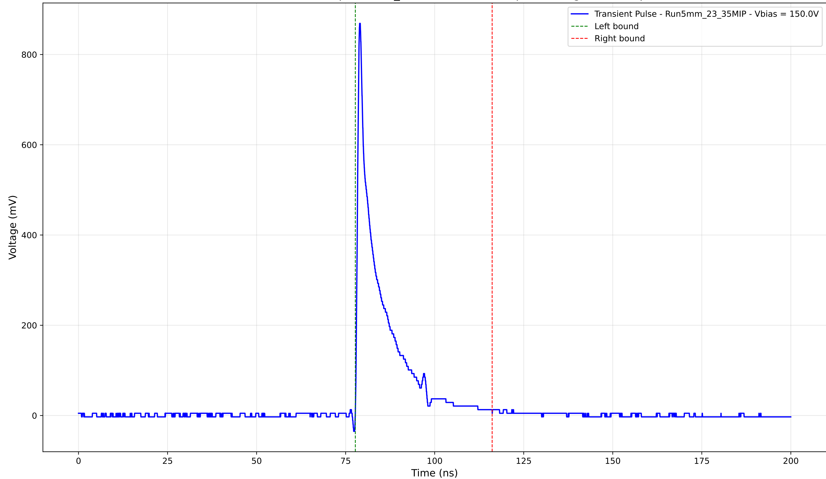
Transient Pulse - Sample: 5mm_23 - Position: 265.0 \mu\text{m} - Charge: 109.68 pC
