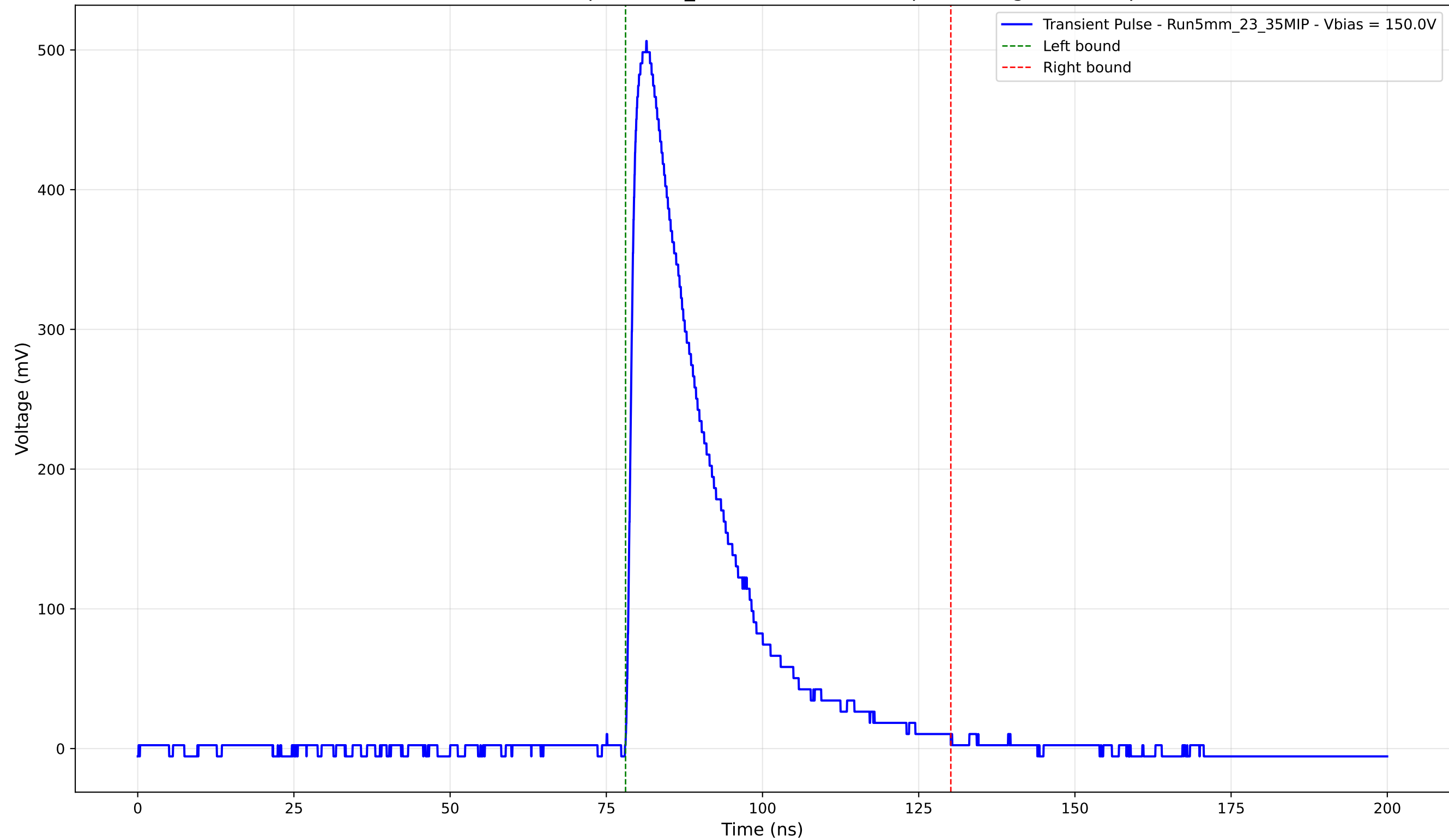
Transient Pulse - Sample: 5mm_23 - Position: 2410.0 \mu\text{m} - Charge: 135.77 pC
