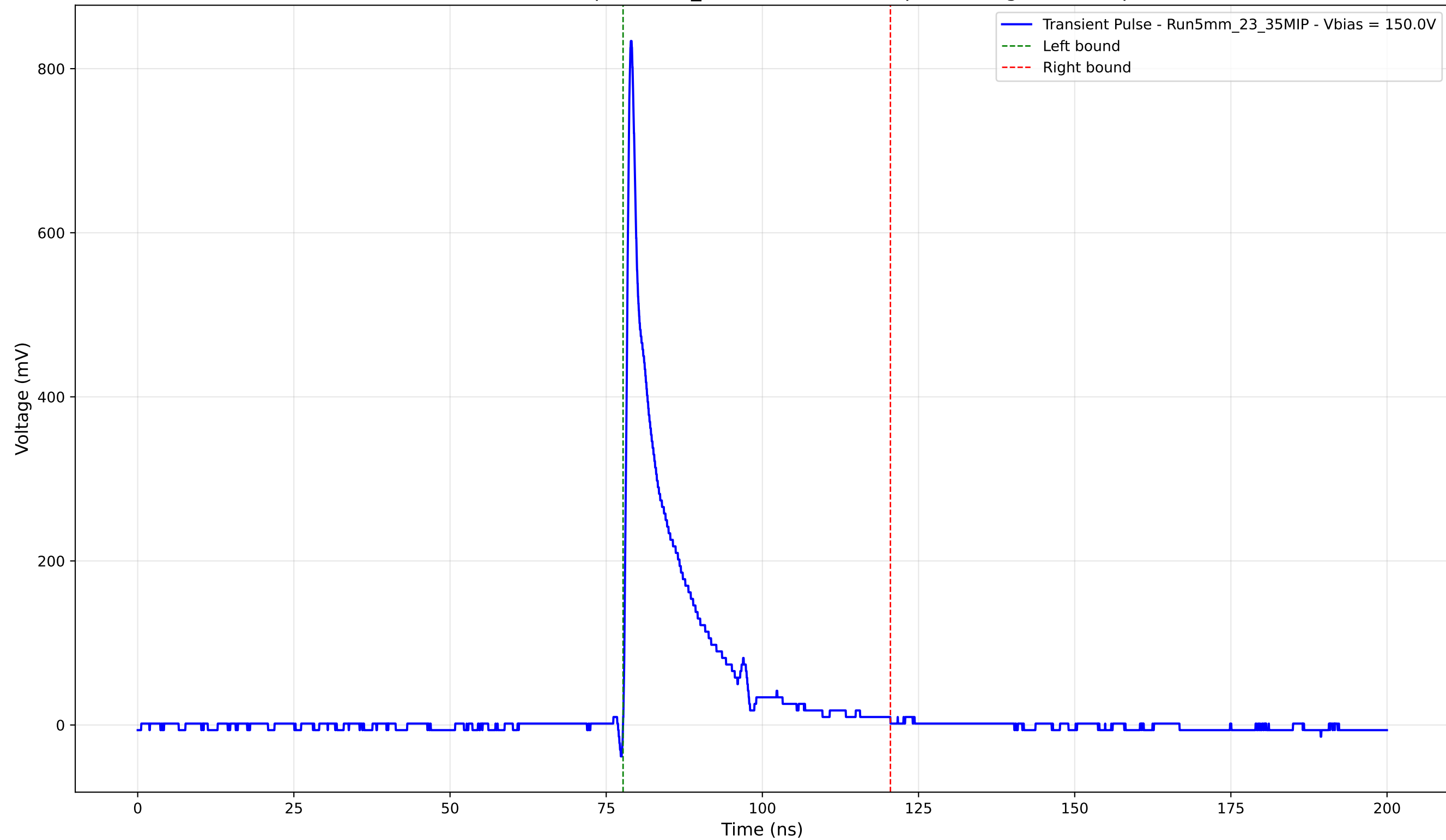
Transient Pulse - Sample: 5mm_23 - Position: 250.0 \mu\text{m} - Charge: 101.25 pC
