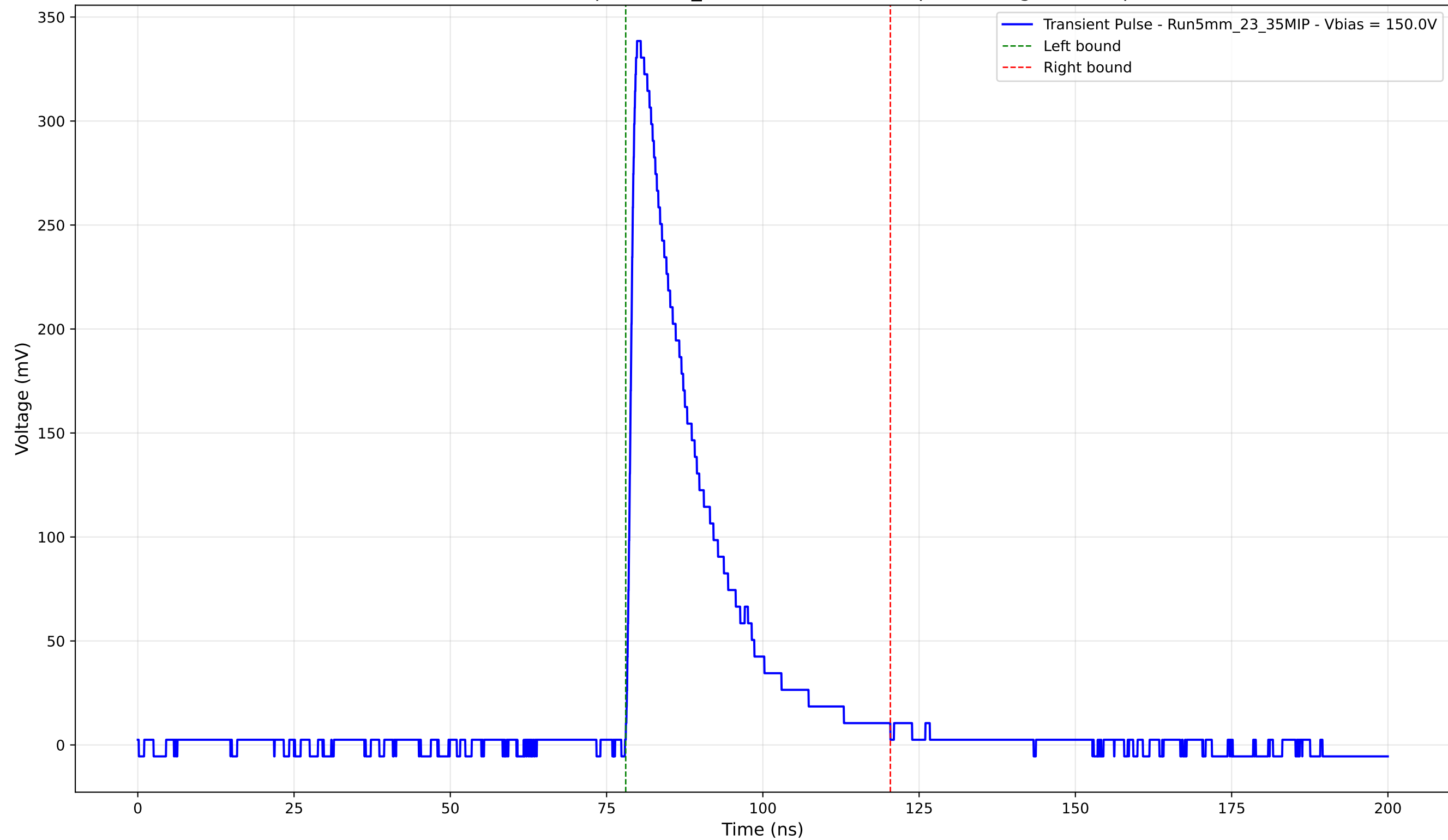
Transient Pulse - Sample: 5mm_23 - Position: 3705.0 \mu\text{m} - Charge: 76.84 pC
