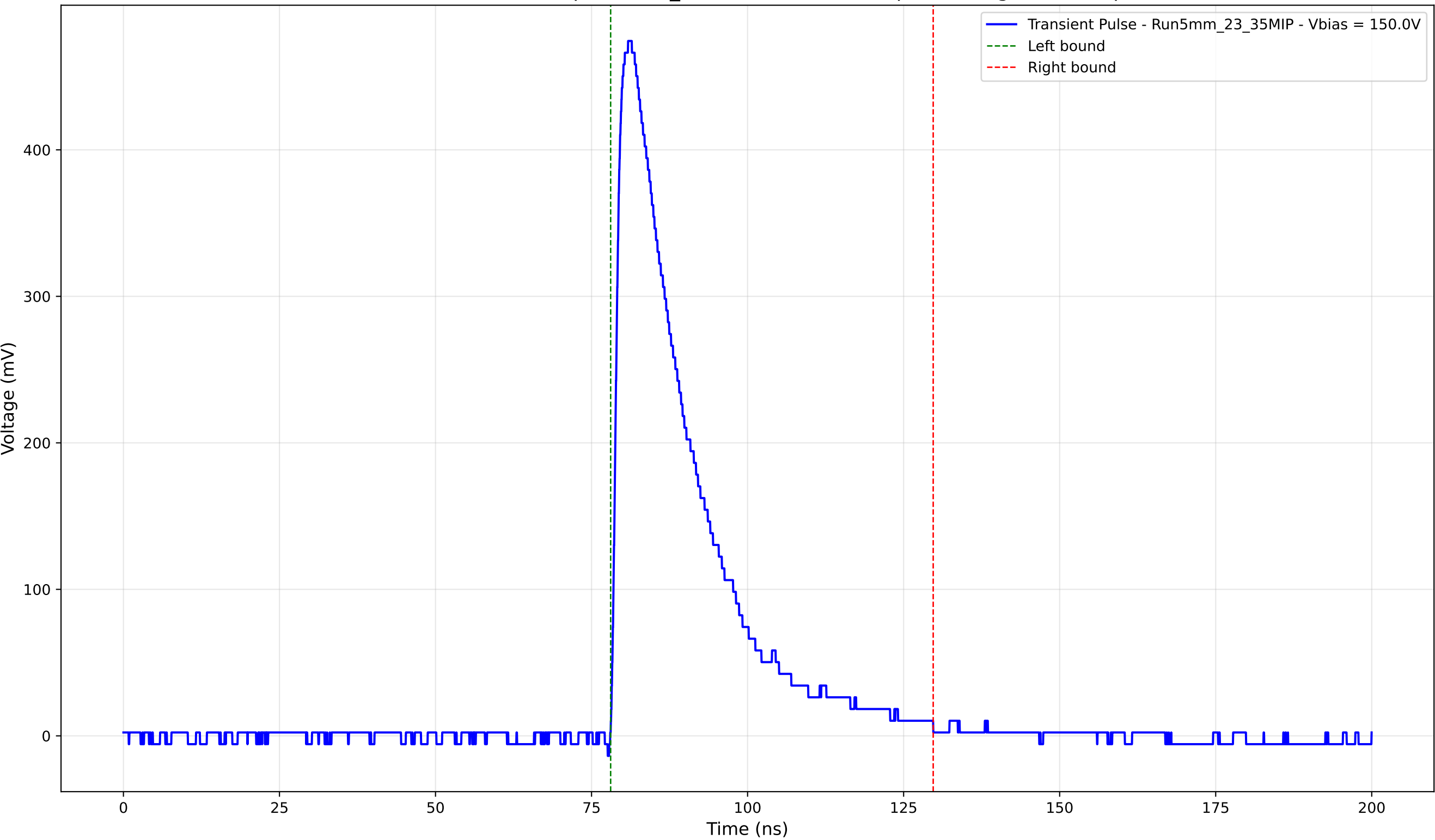
Transient Pulse - Sample: 5mm_23 - Position: 3060.0 \mu\text{m} - Charge: 124.52 pC
