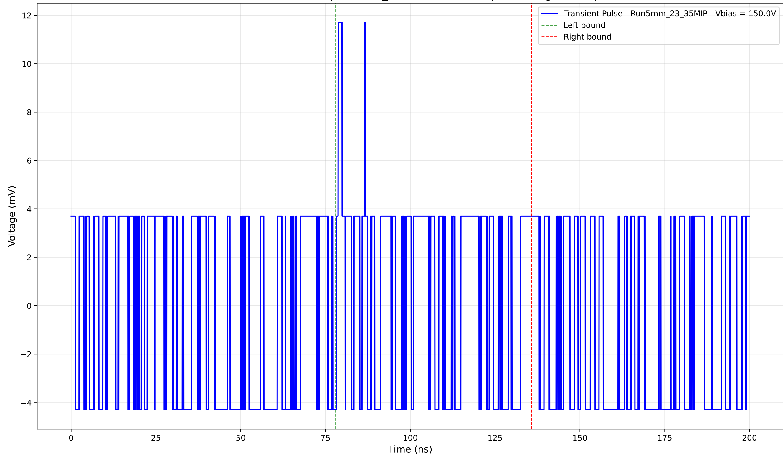
Transient Pulse - Sample: 5mm_23 - Position: 85.0 \mu\text{m} - Charge: 1.16 pC
