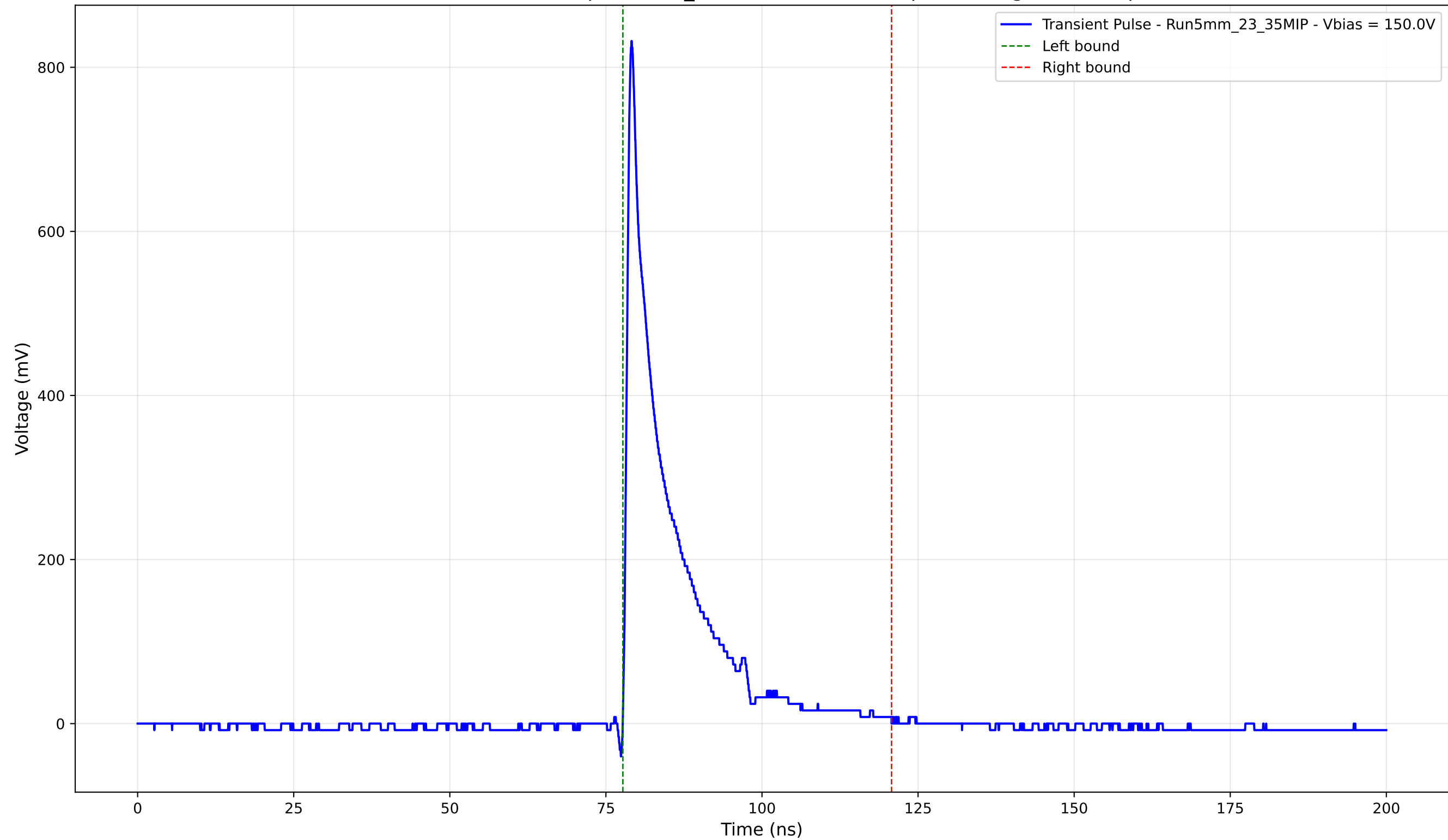
Transient Pulse - Sample: 5mm_23 - Position: 4840.0 \mu\text{m} - Charge: 111.57 pC
