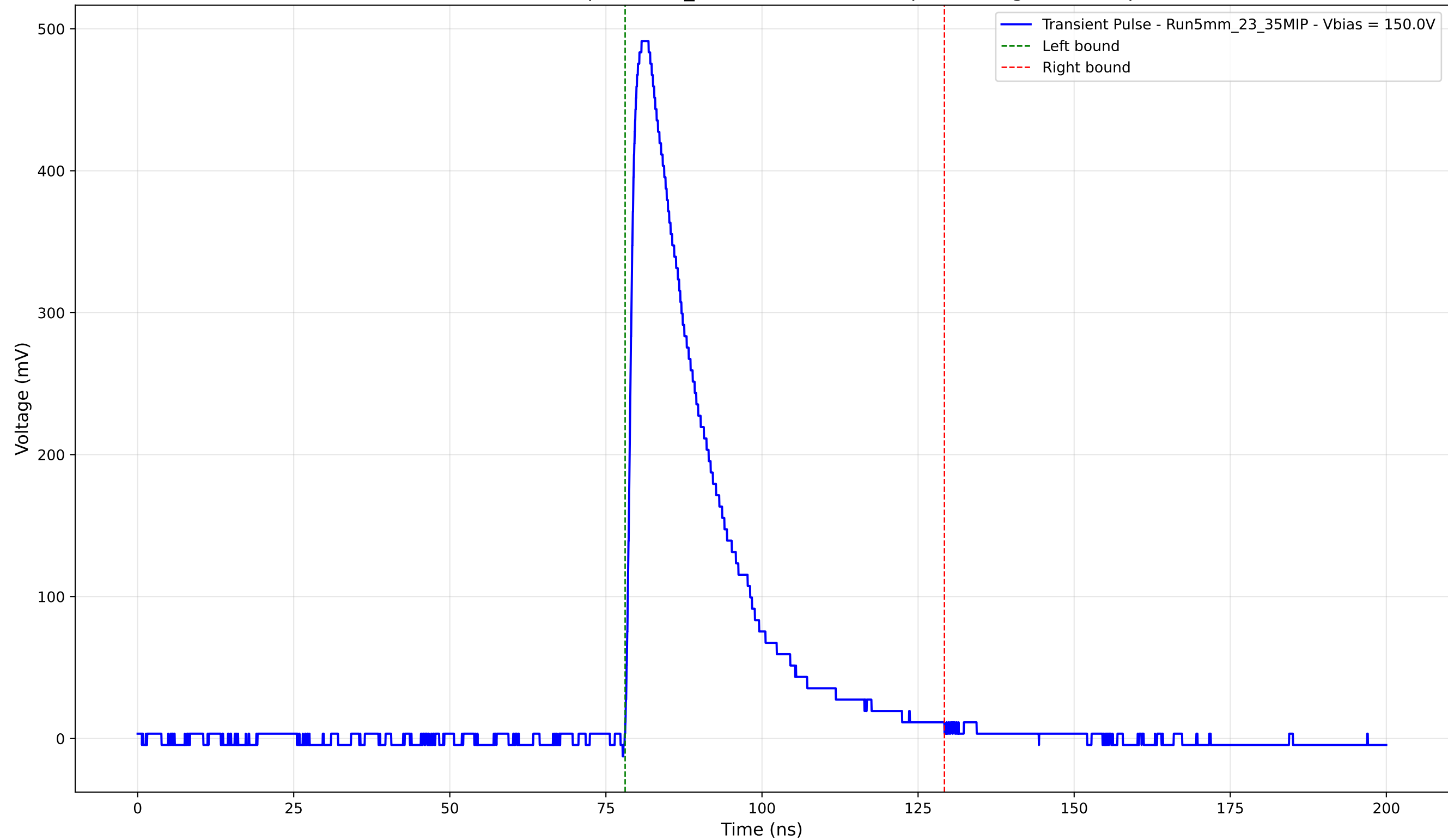
Transient Pulse - Sample: 5mm_23 - Position: 3020.0 \mu\text{m} - Charge: 131.52 pC
