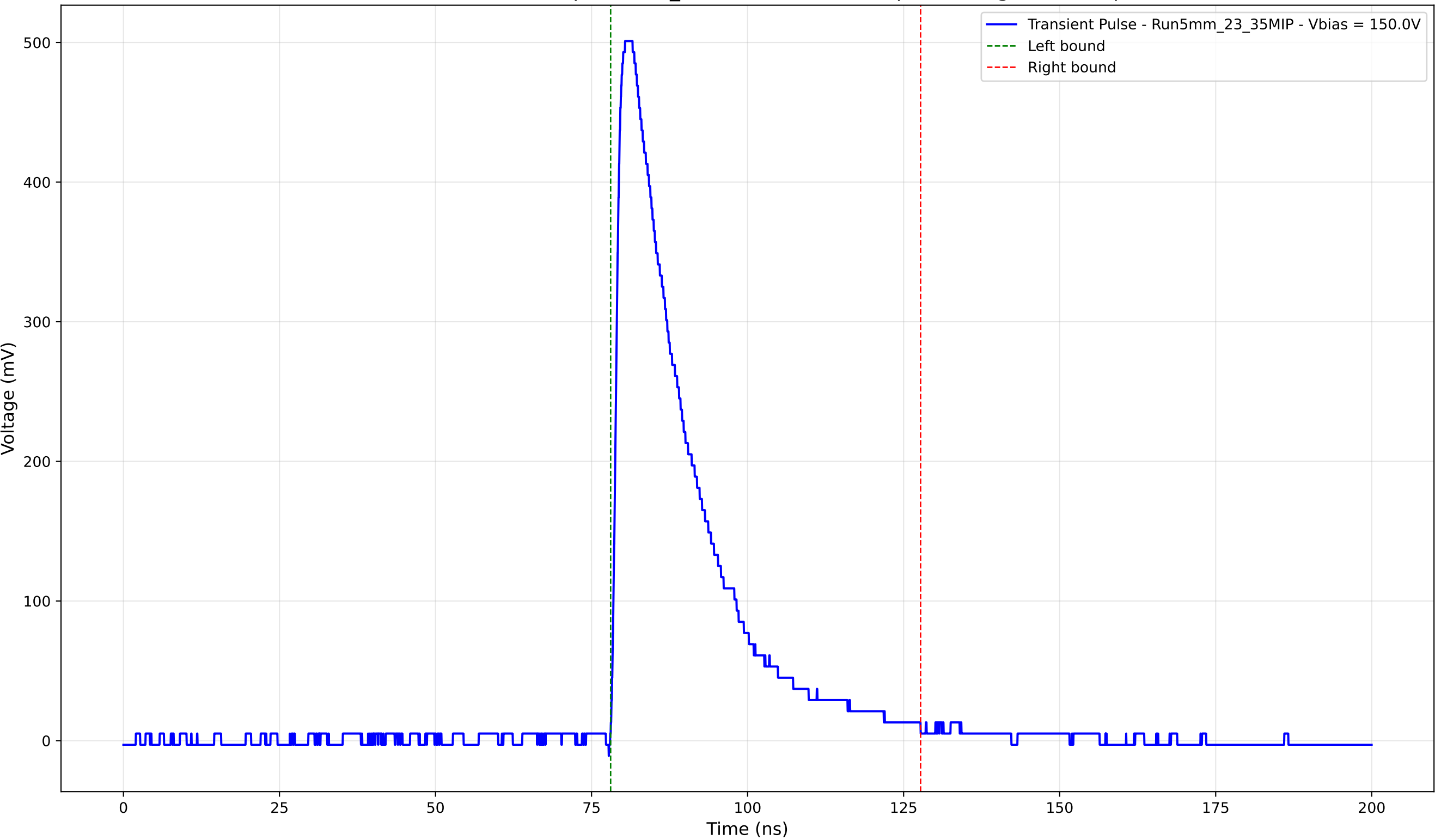
Transient Pulse - Sample: 5mm_23 - Position: 3340.0 \mu\text{m} - Charge: 130.05 pC
