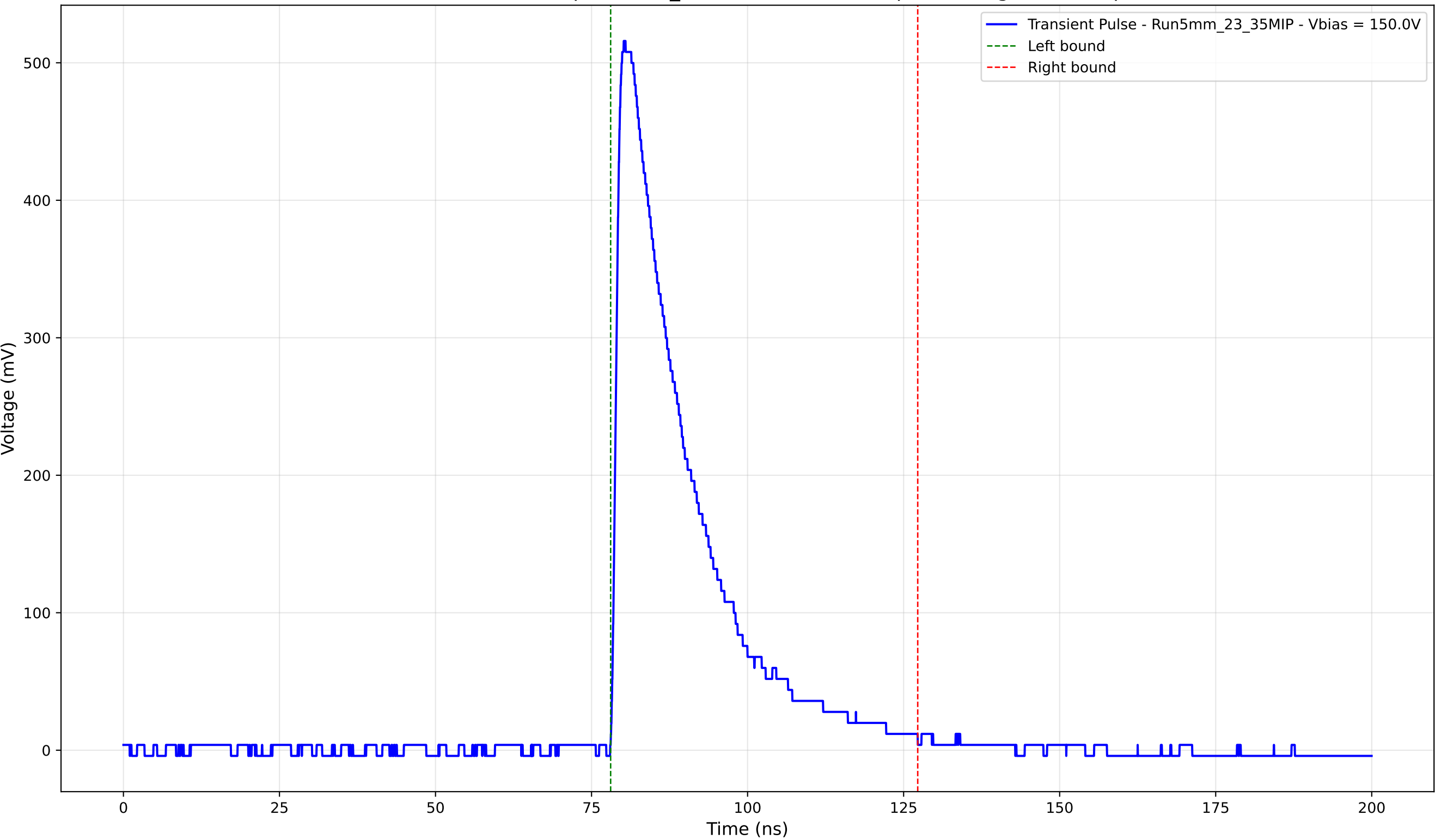
Transient Pulse - Sample: 5mm_23 - Position: 1730.0 \mu\text{m} - Charge: 130.10 pC
