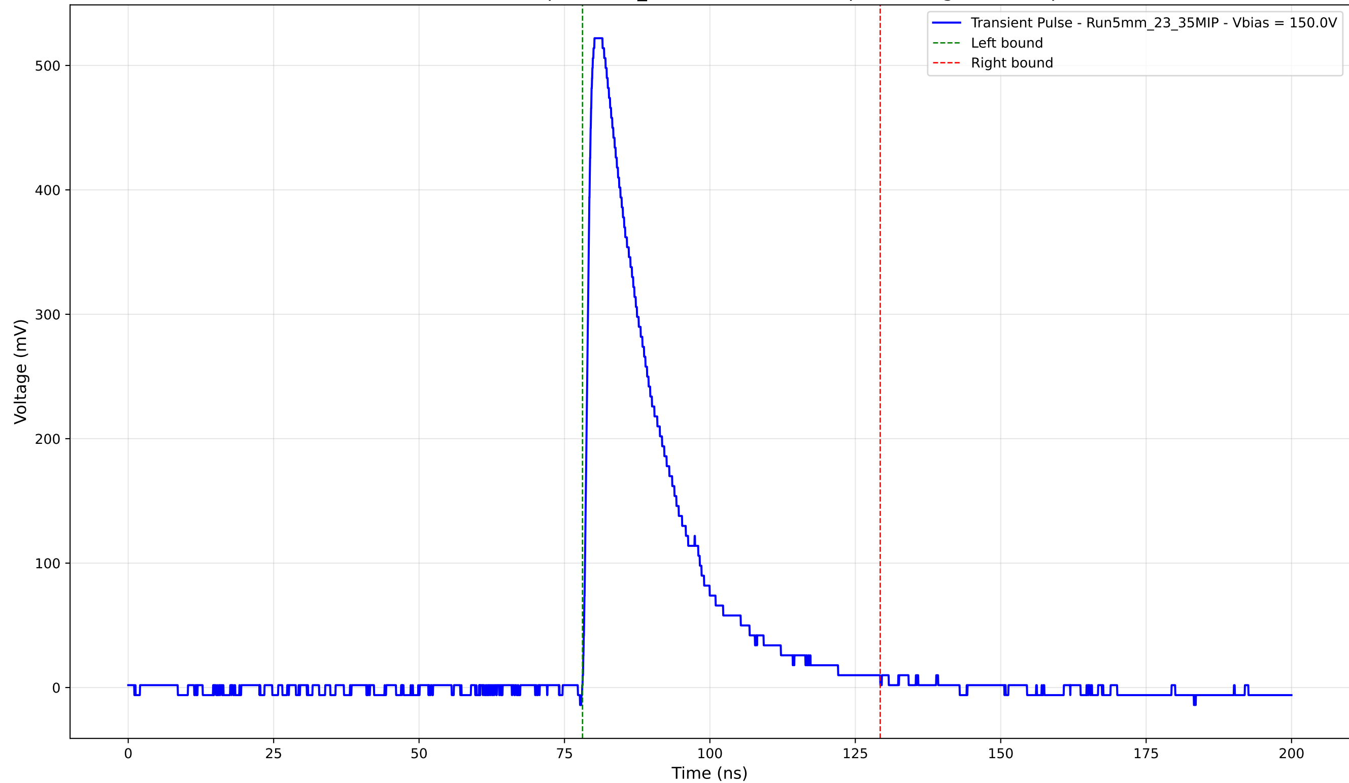
Transient Pulse - Sample: 5mm_23 - Position: 1890.0 \mu\text{m} - Charge: 135.54 pC
