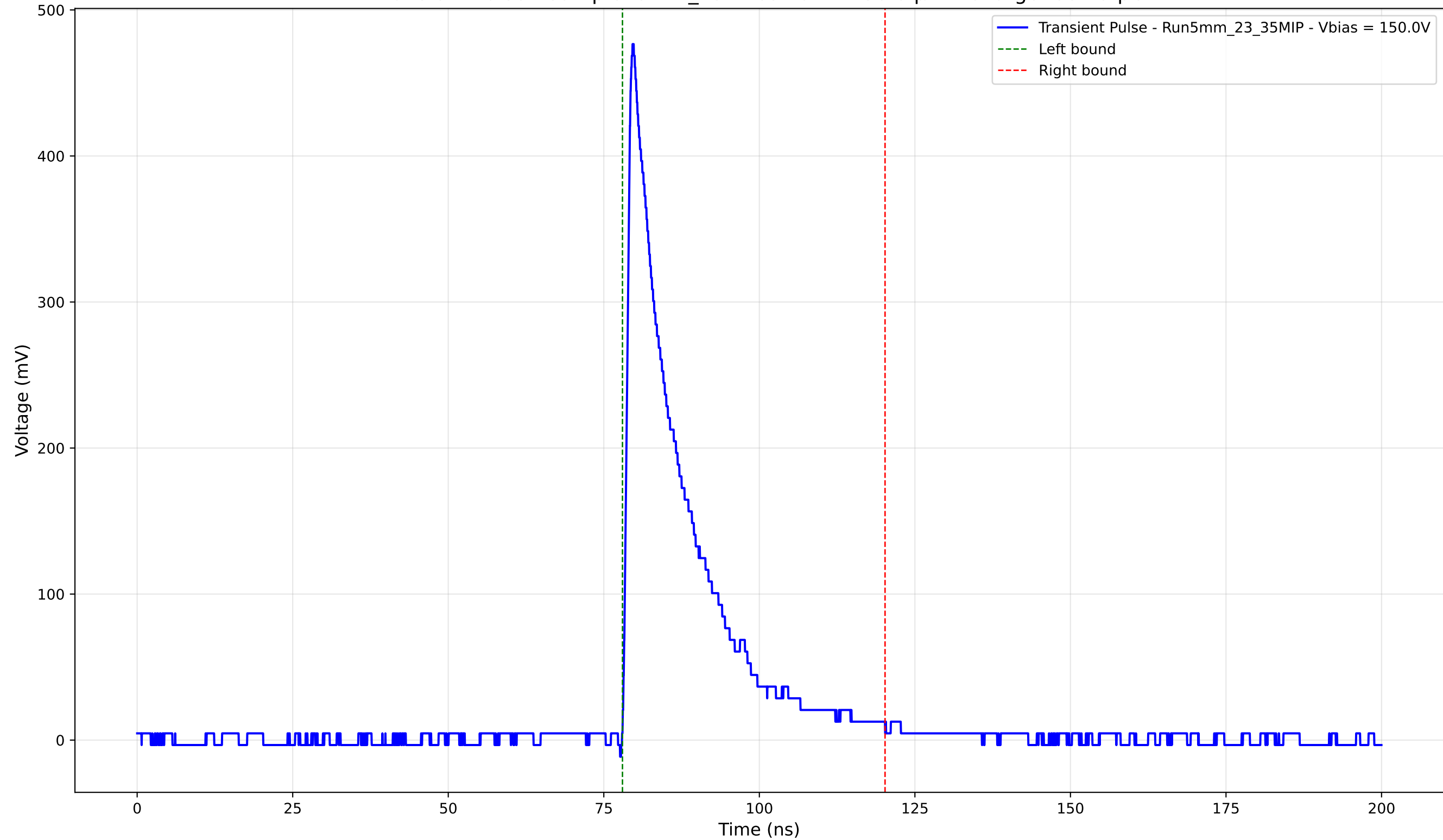
Transient Pulse - Sample: 5mm_23 - Position: 4230.0 \mu\text{m} - Charge: 88.79 pC
