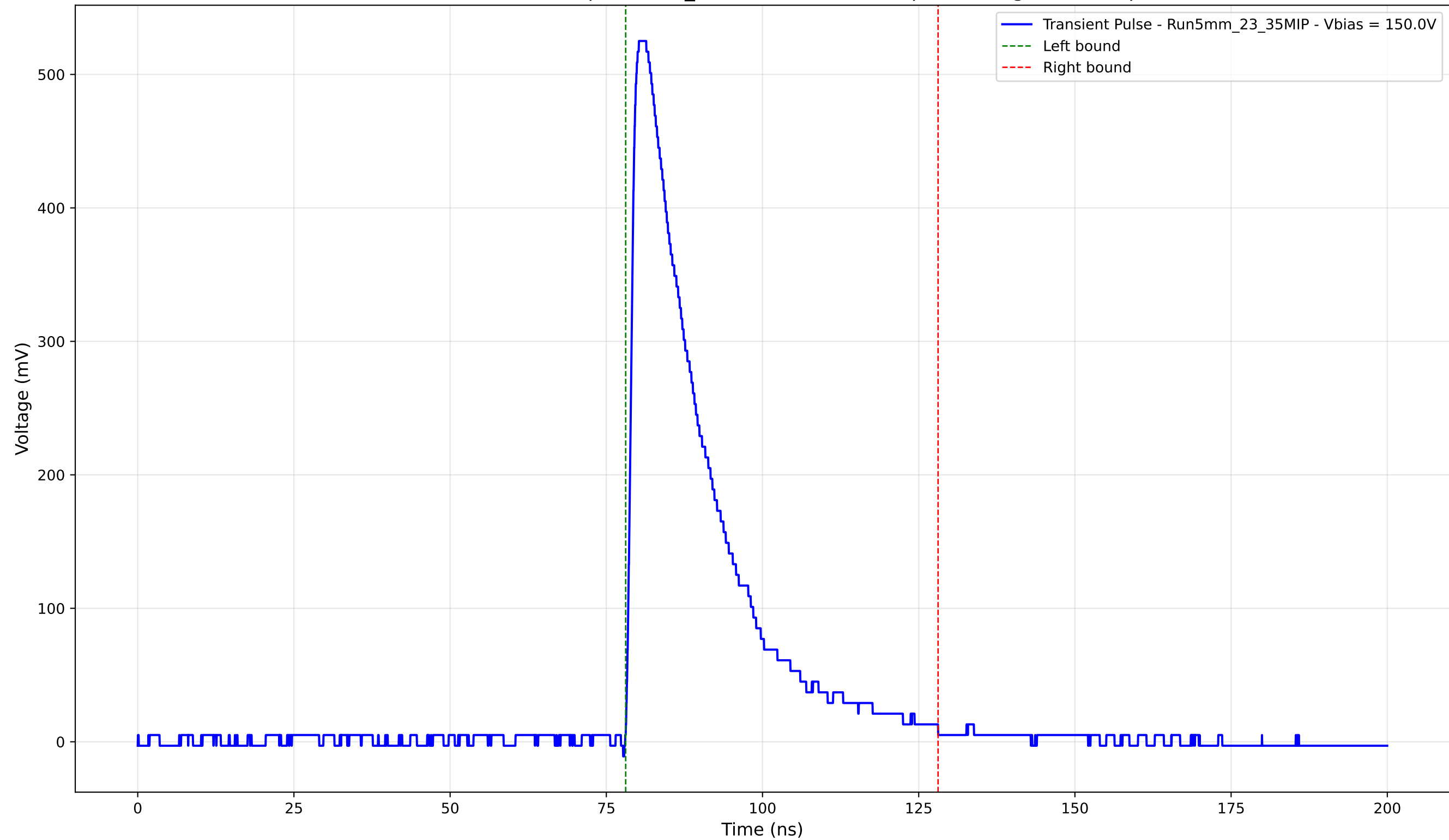
Transient Pulse - Sample: 5mm_23 - Position: 1850.0 \mu\text{m} - Charge: 137.16 pC
