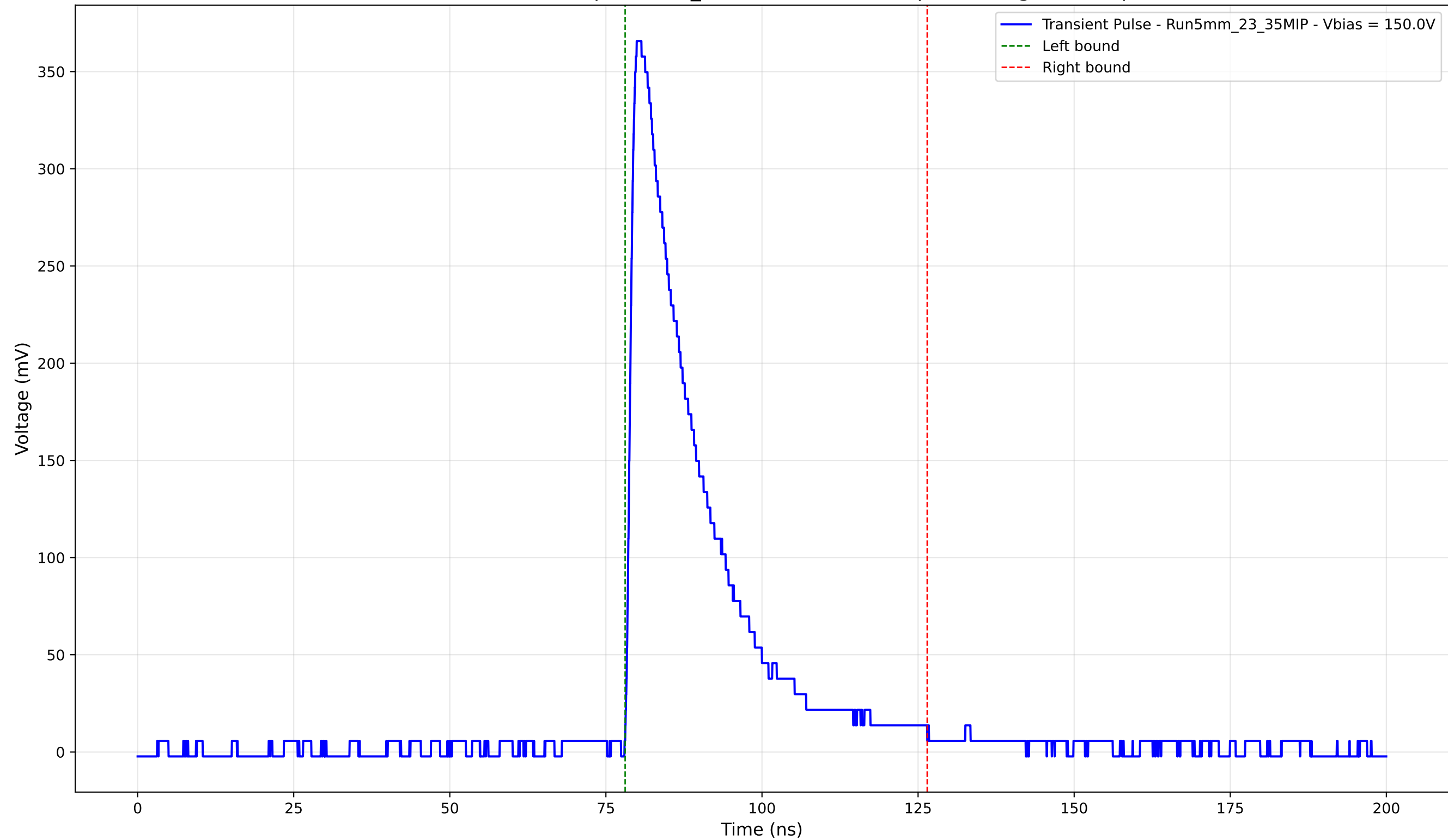
Transient Pulse - Sample: 5mm_23 - Position: 3595.0 \mu\text{m} - Charge: 89.24 pC
