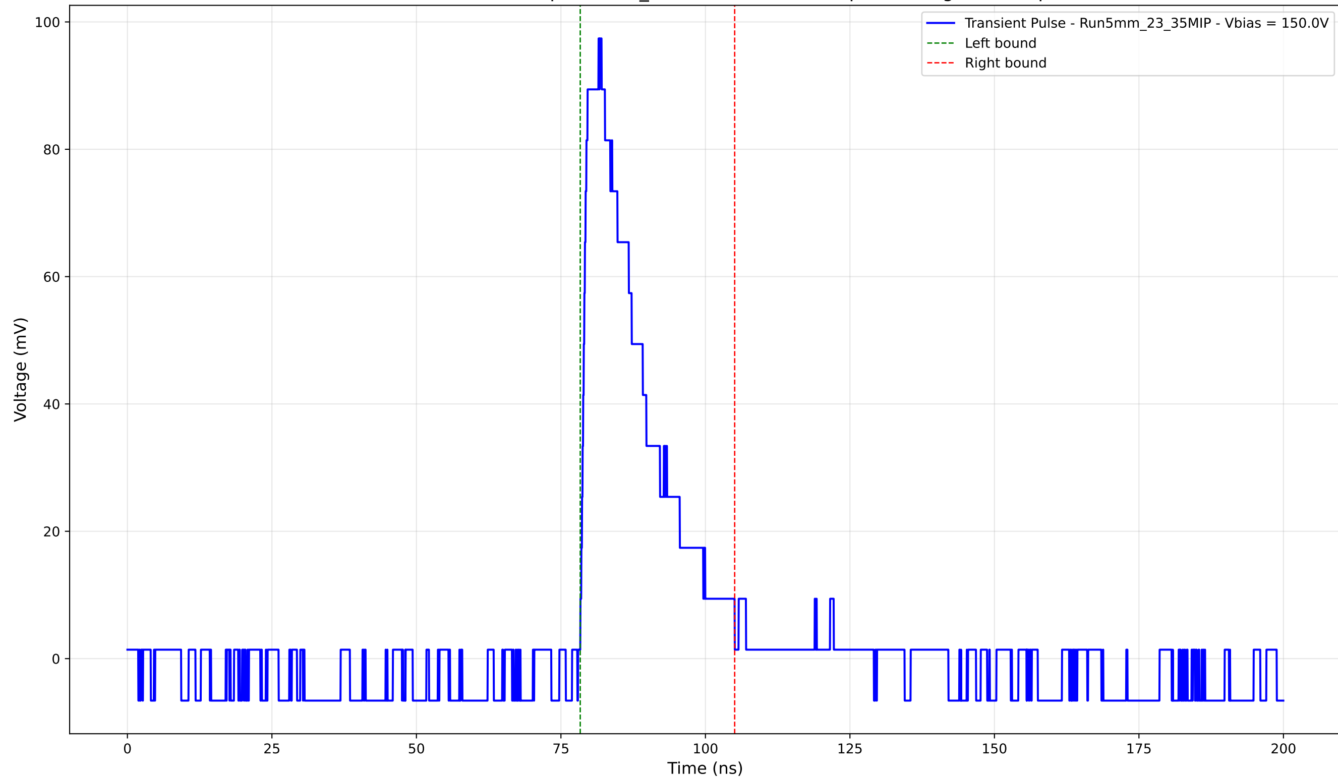
Transient Pulse - Sample: 5mm_23 - Position: 1610.0 \mu\text{m} - Charge: 21.36 pC
