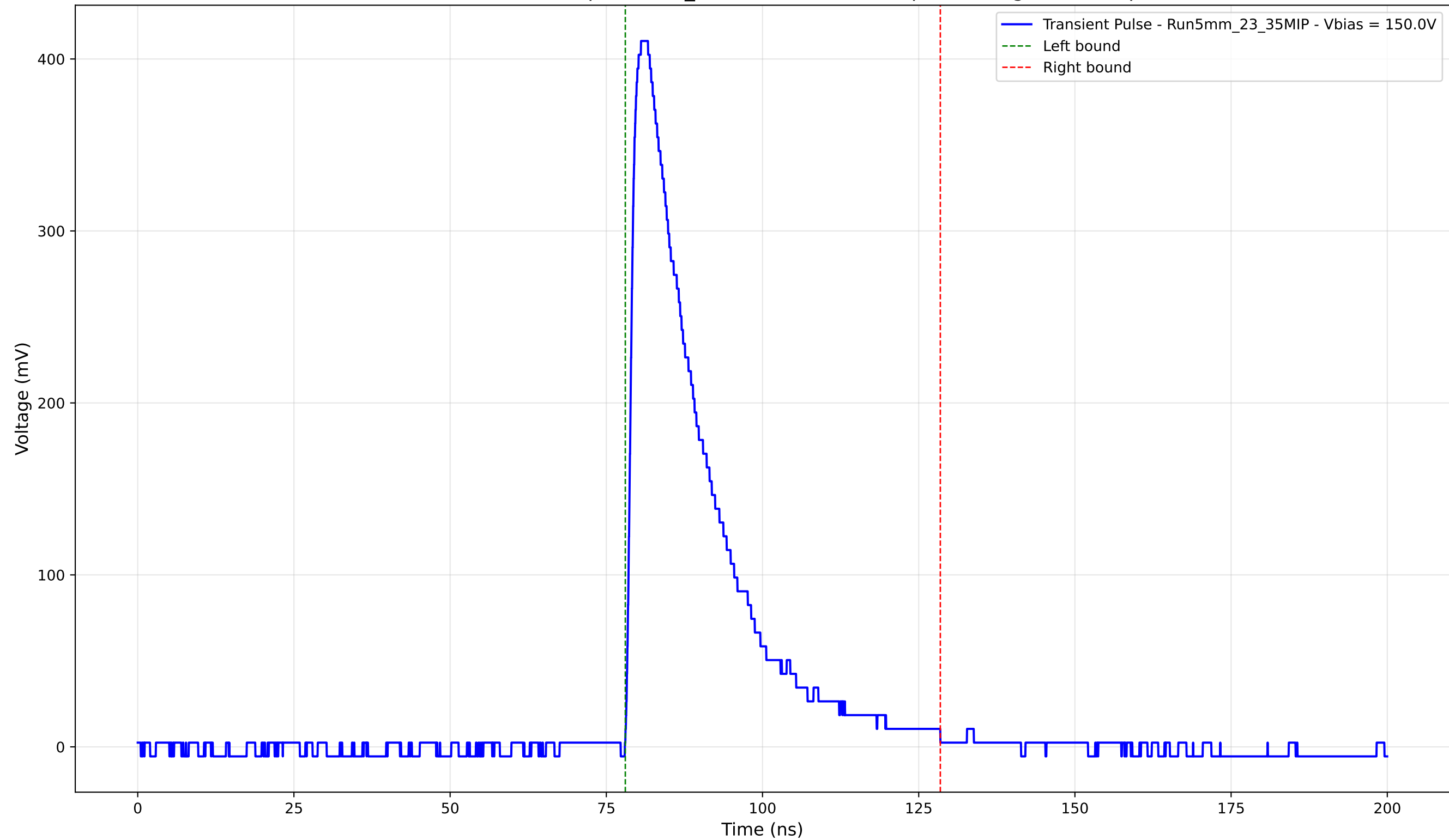
Transient Pulse - Sample: 5mm_23 - Position: 3215.0 \mu\text{m} - Charge: 106.11 pC
