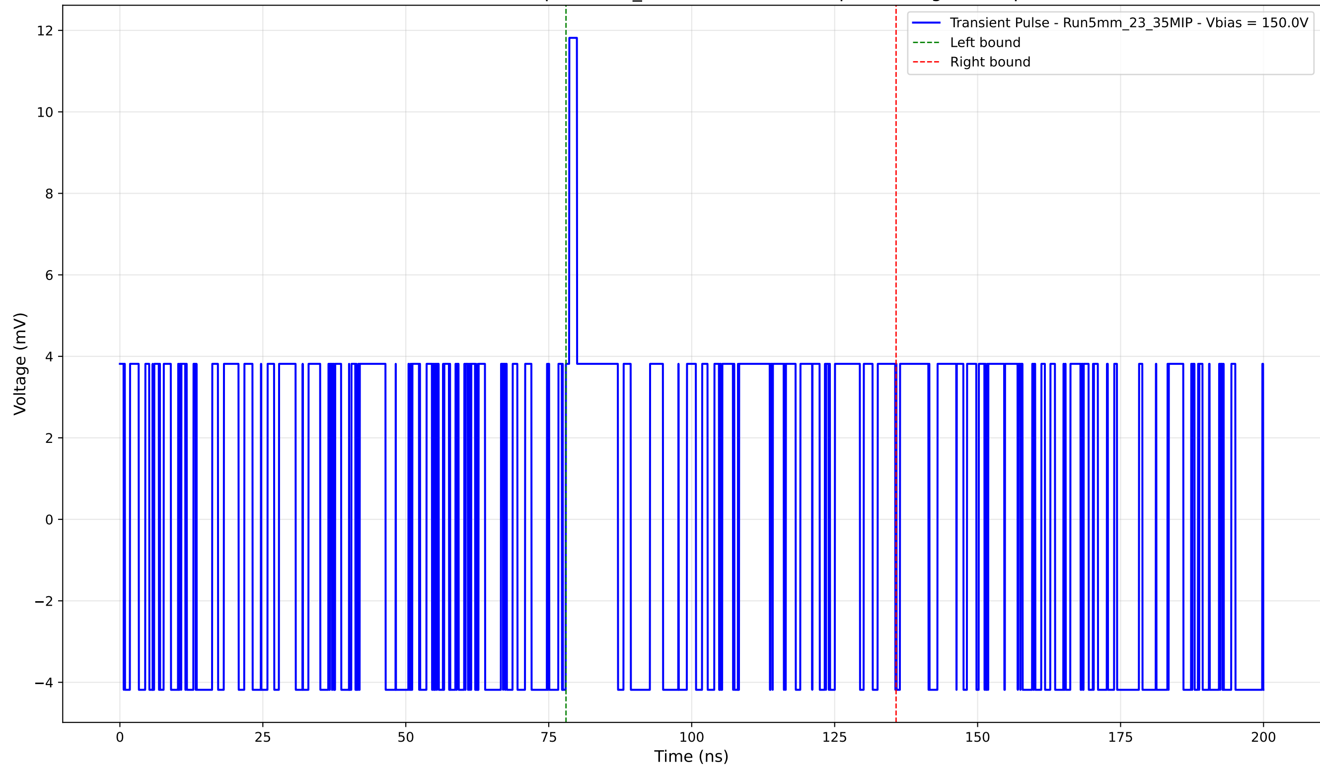
Transient Pulse - Sample: 5mm_23 - Position: 5190.0 \mu\text{m} - Charge: 1.94 pC
