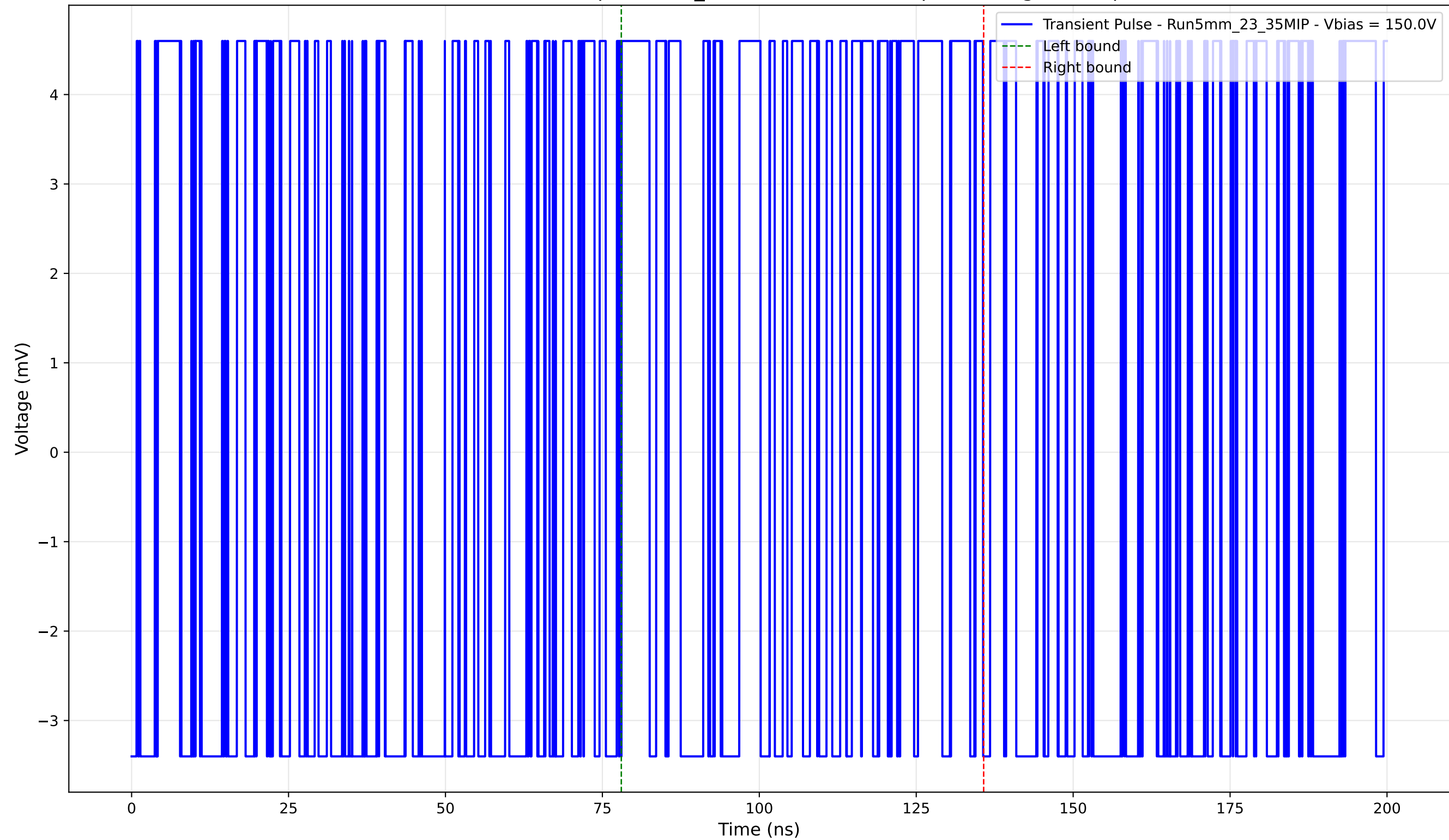
Transient Pulse - Sample: 5mm_23 - Position: 5270.0 \mu\text{m} - Charge: 1.84 pC
