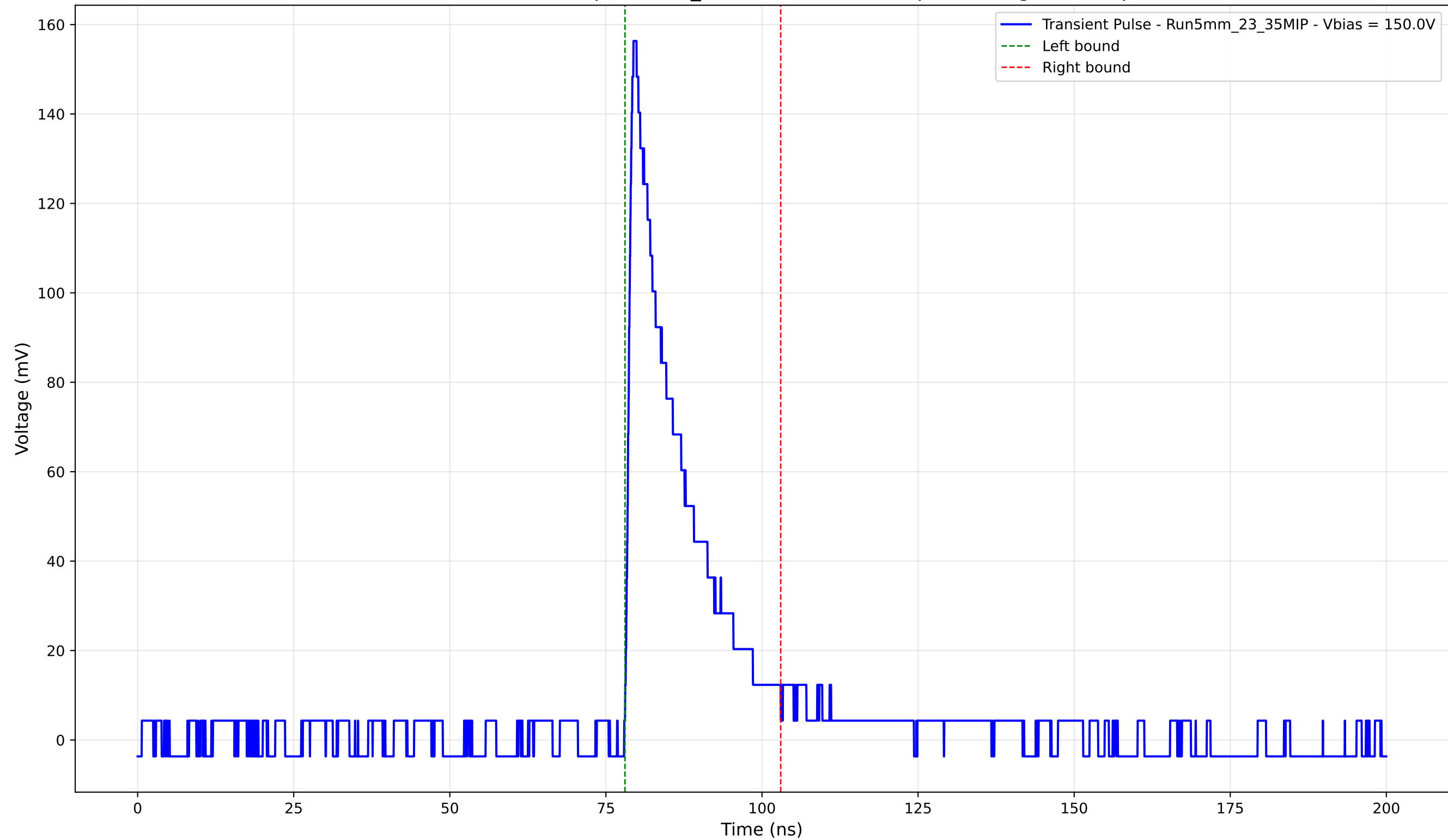
Transient Pulse - Sample: 5mm_23 - Position: 4490.0 \mu\text{m} - Charge: 26.89 pC
