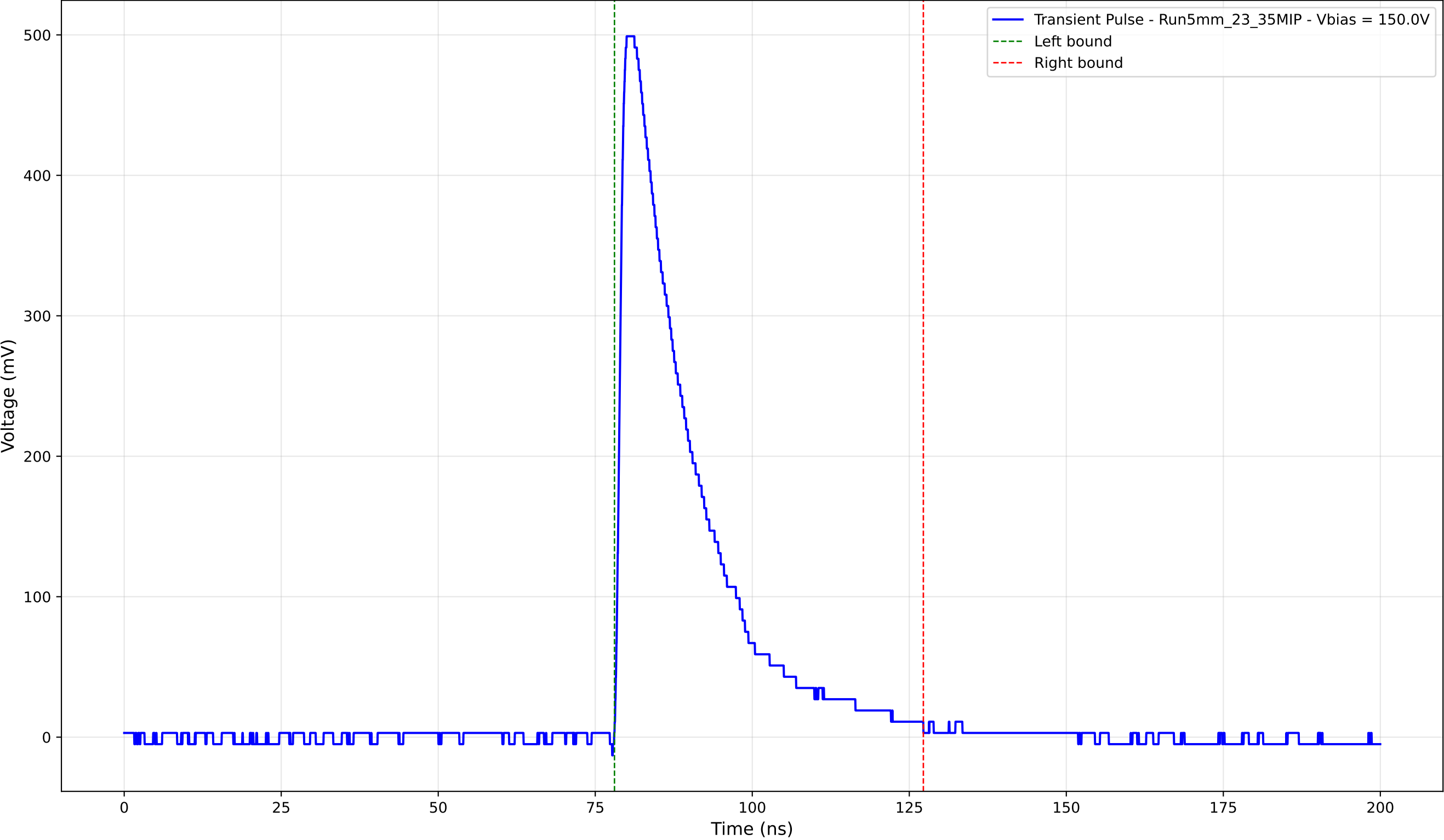
Transient Pulse - Sample: 5mm_23 - Position: 3505.0 \mu\text{m} - Charge: 125.42 pC
