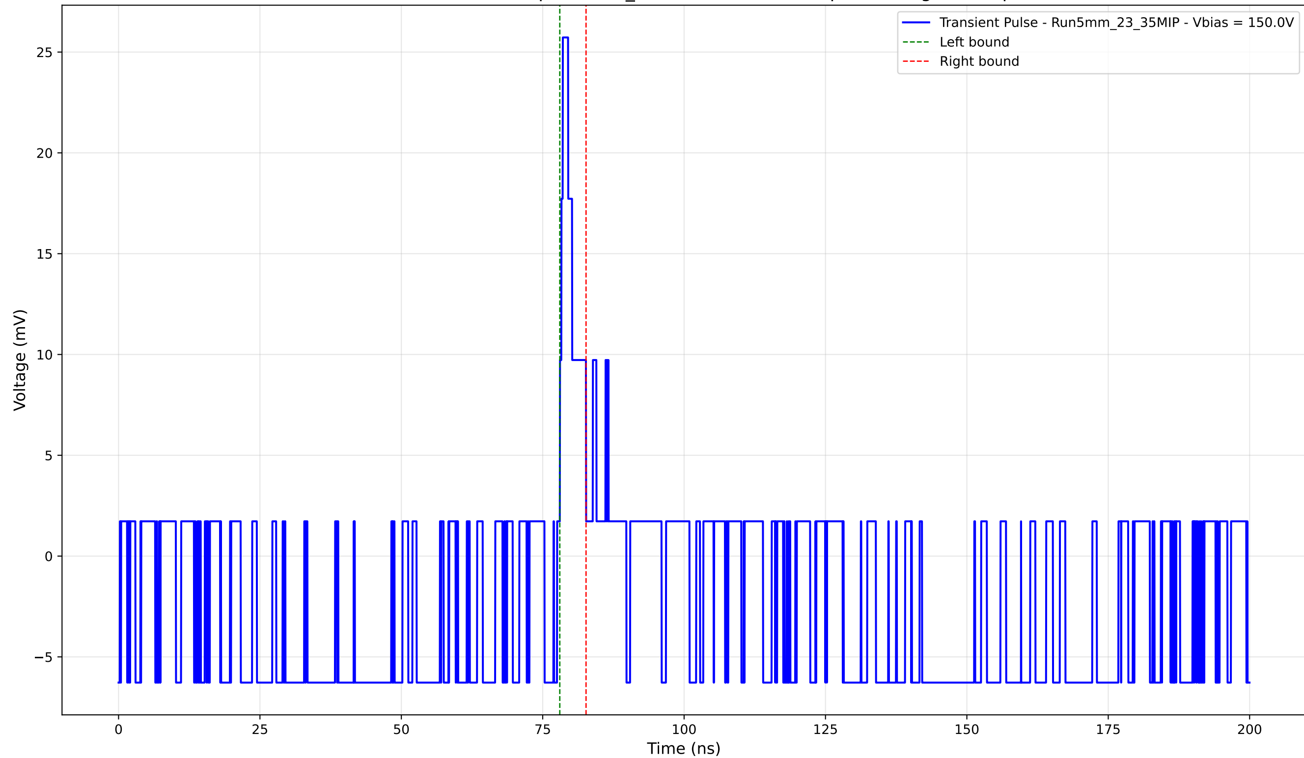
Transient Pulse - Sample: 5mm_23 - Position: 5160.0 \mu\text{m} - Charge: 1.36 pC
