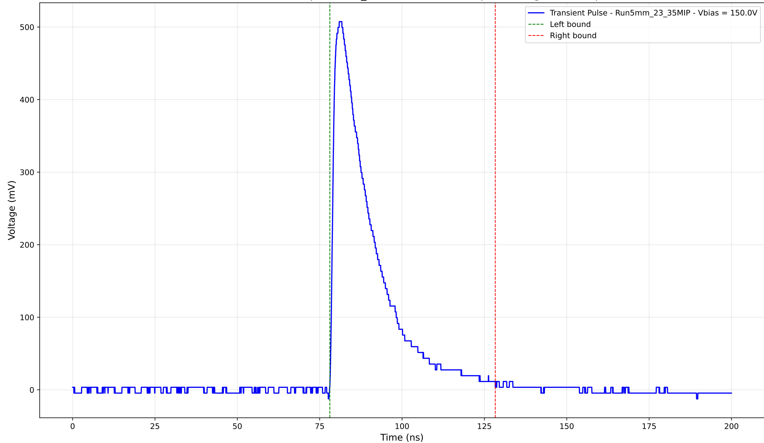
Transient Pulse - Sample: 5mm_23 - Position: 2305.0 \mu\text{m} - Charge: 136.17 pC
