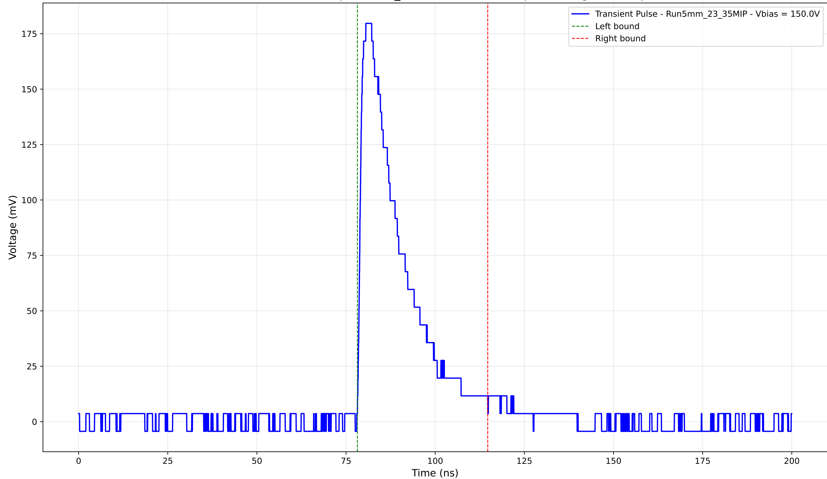
Transient Pulse - Sample: 5mm_23 - Position: 3175.0 \mu\text{m} - Charge: 46.09 pC
