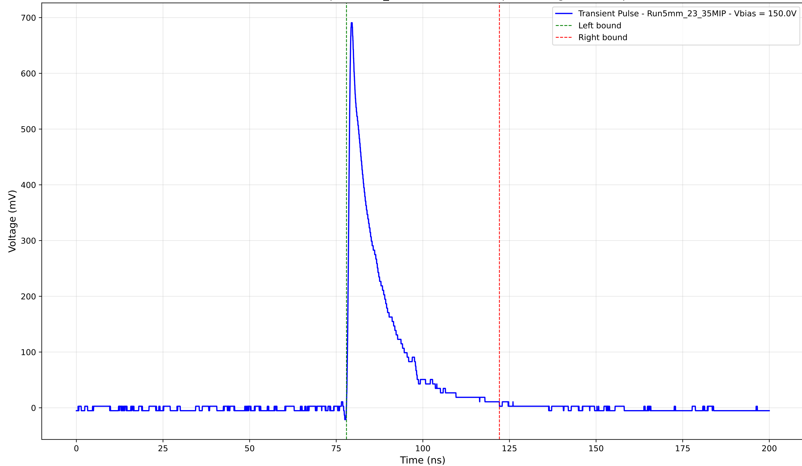
Transient Pulse - Sample: 5mm_23 - Position: 765.0 \mu\text{m} - Charge: 117.86 pC
