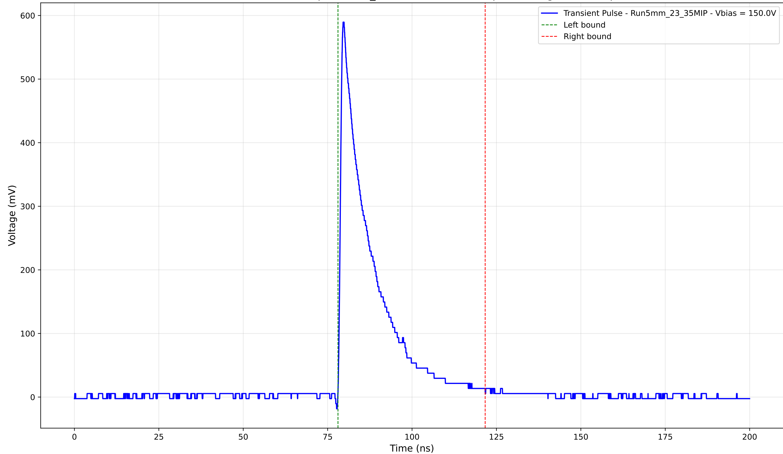
Transient Pulse - Sample: 5mm_23 - Position: 1040.0 \mu\text{m} - Charge: 114.43 pC
