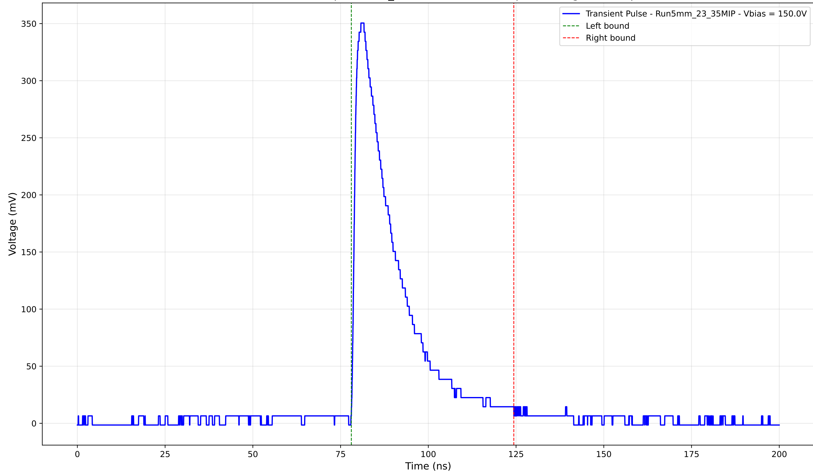
Transient Pulse - Sample: 5mm_23 - Position: 3090.0 \mu\text{m} - Charge: 92.24 pC
