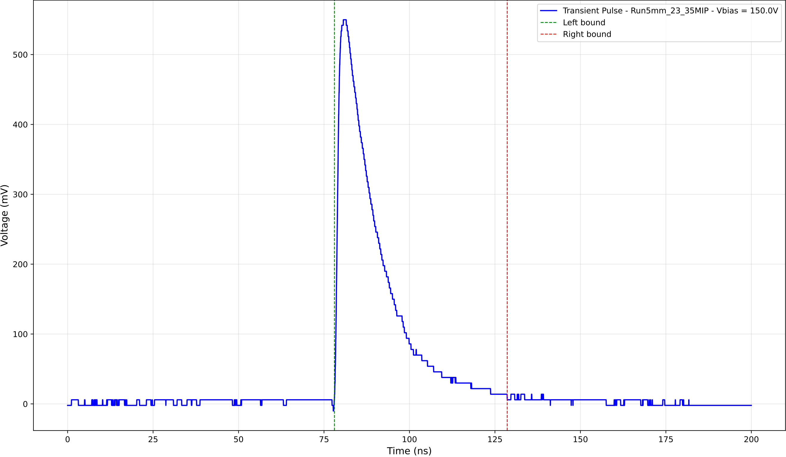
Transient Pulse - Sample: 5mm_23 - Position: 2020.0 \mu\text{m} - Charge: 147.36 pC
