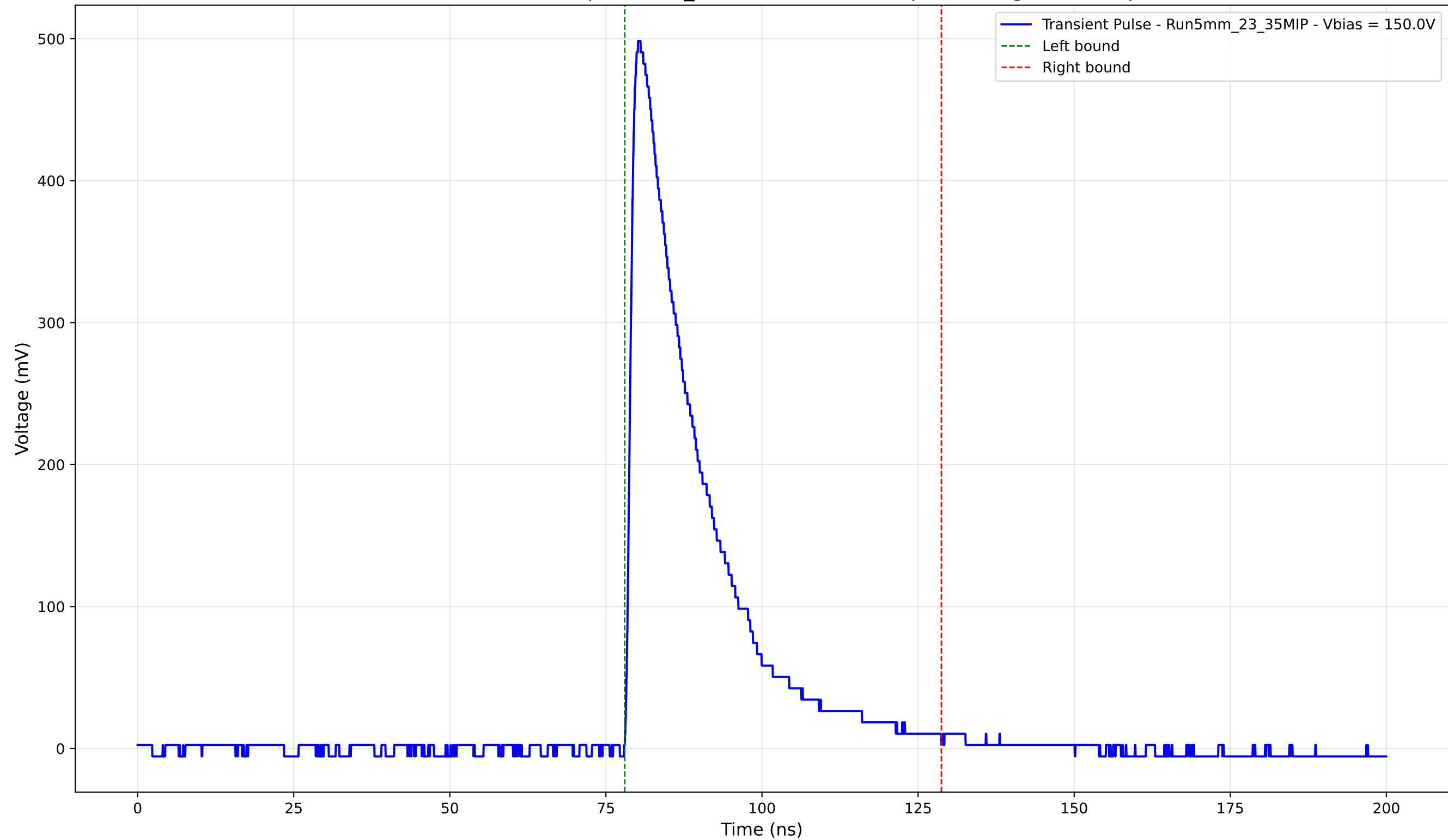
Transient Pulse - Sample: 5mm_23 - Position: 3560.0 \mu\text{m} - Charge: 120.75 pC
