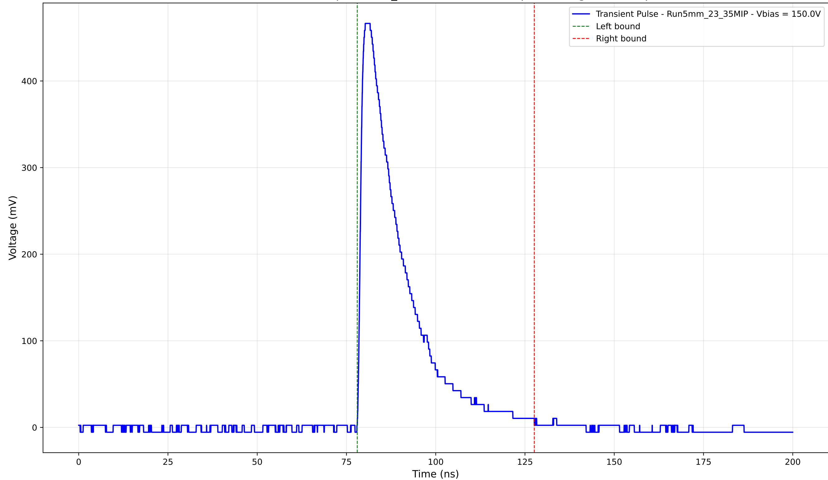
Transient Pulse - Sample: 5mm_23 - Position: 3235.0 \mu\text{m} - Charge: 121.16 pC
