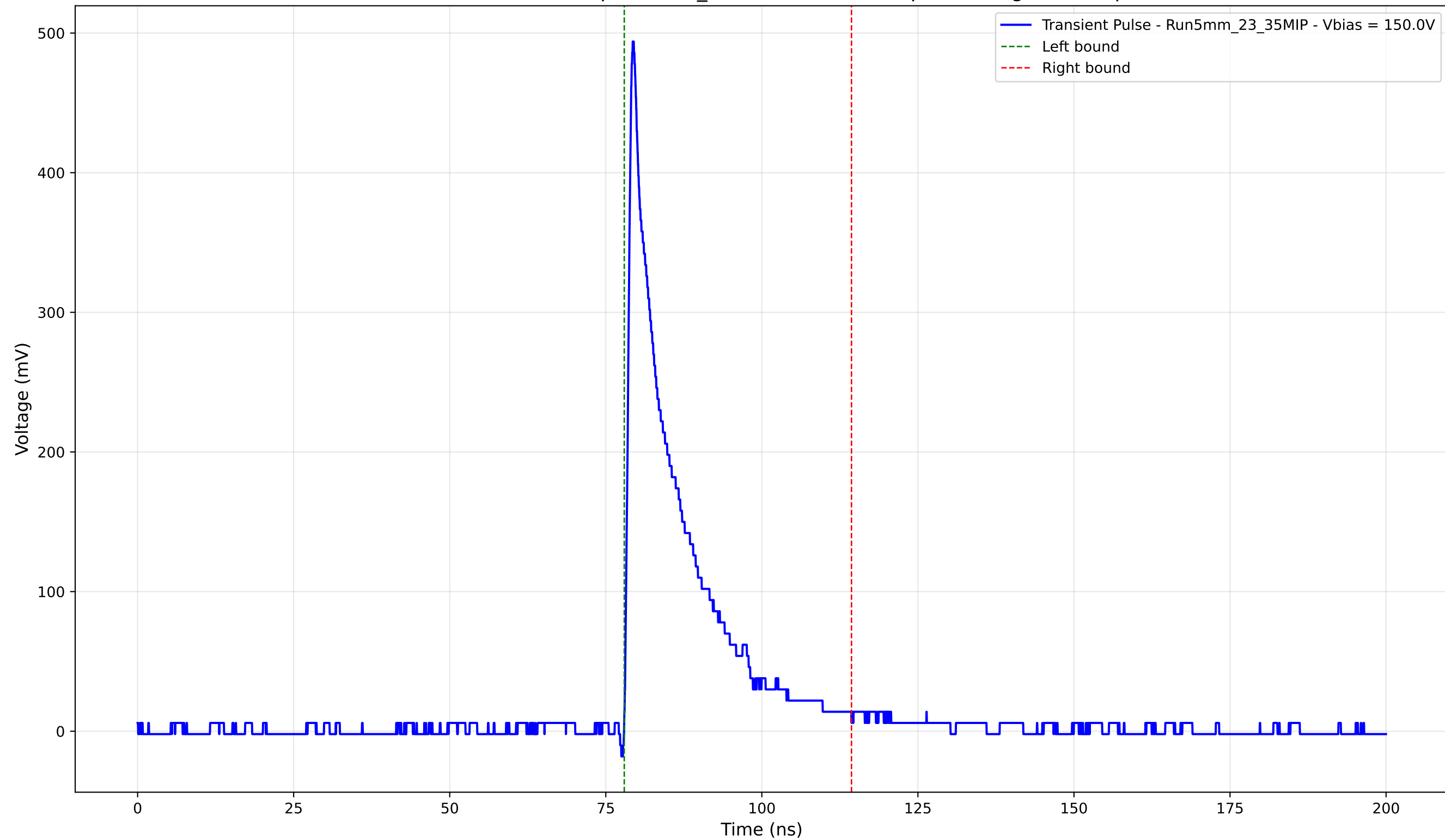
Transient Pulse - Sample: 5mm_23 - Position: 675.0 \mu\text{m} - Charge: 77.60 pC
