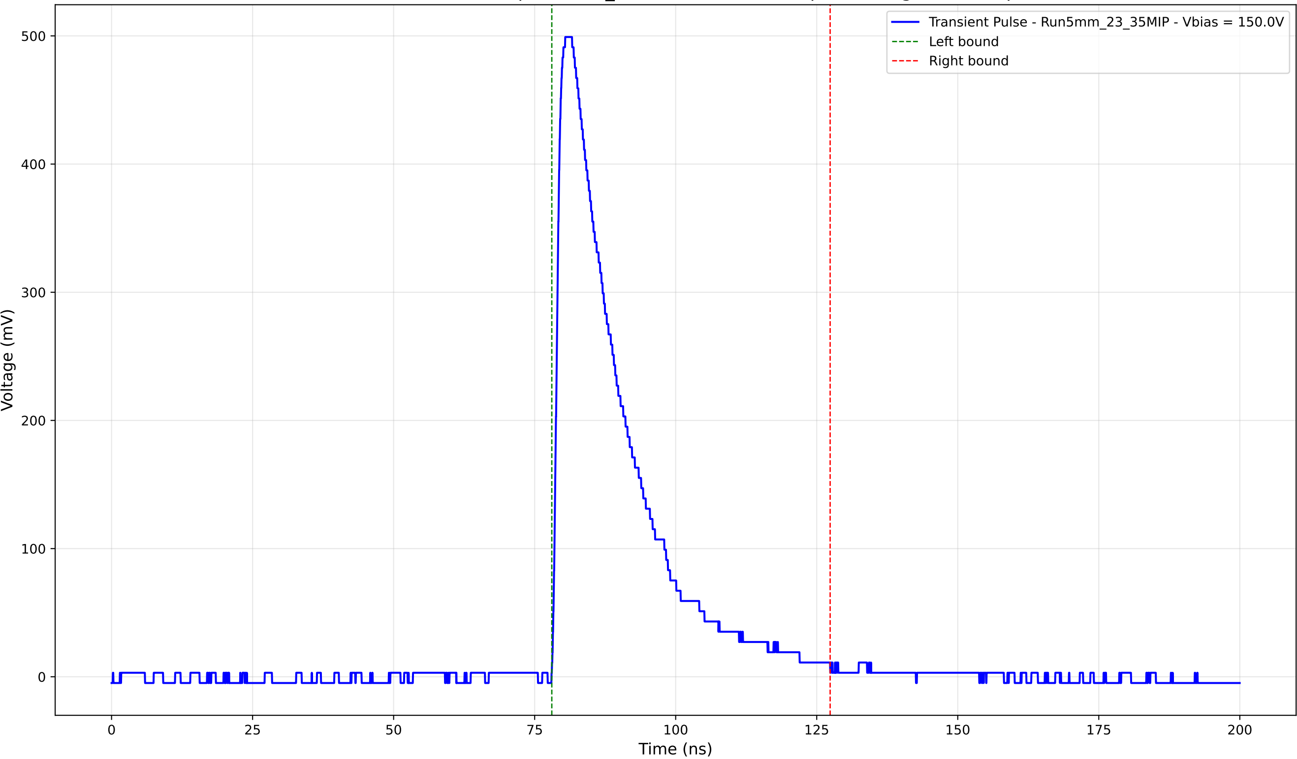
Transient Pulse - Sample: 5mm_23 - Position: 3310.0 \mu\text{m} - Charge: 129.39 pC
