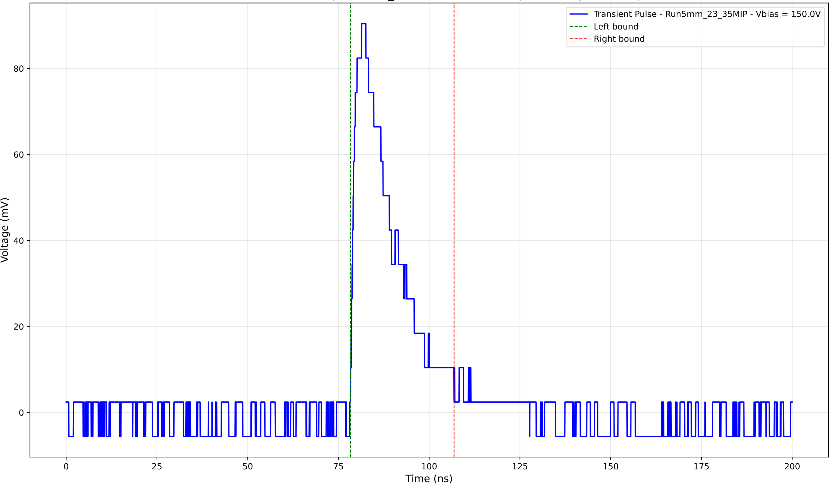
Transient Pulse - Sample: 5mm_23 - Position: 3140.0 \mu\text{m} - Charge: 21.79 pC
