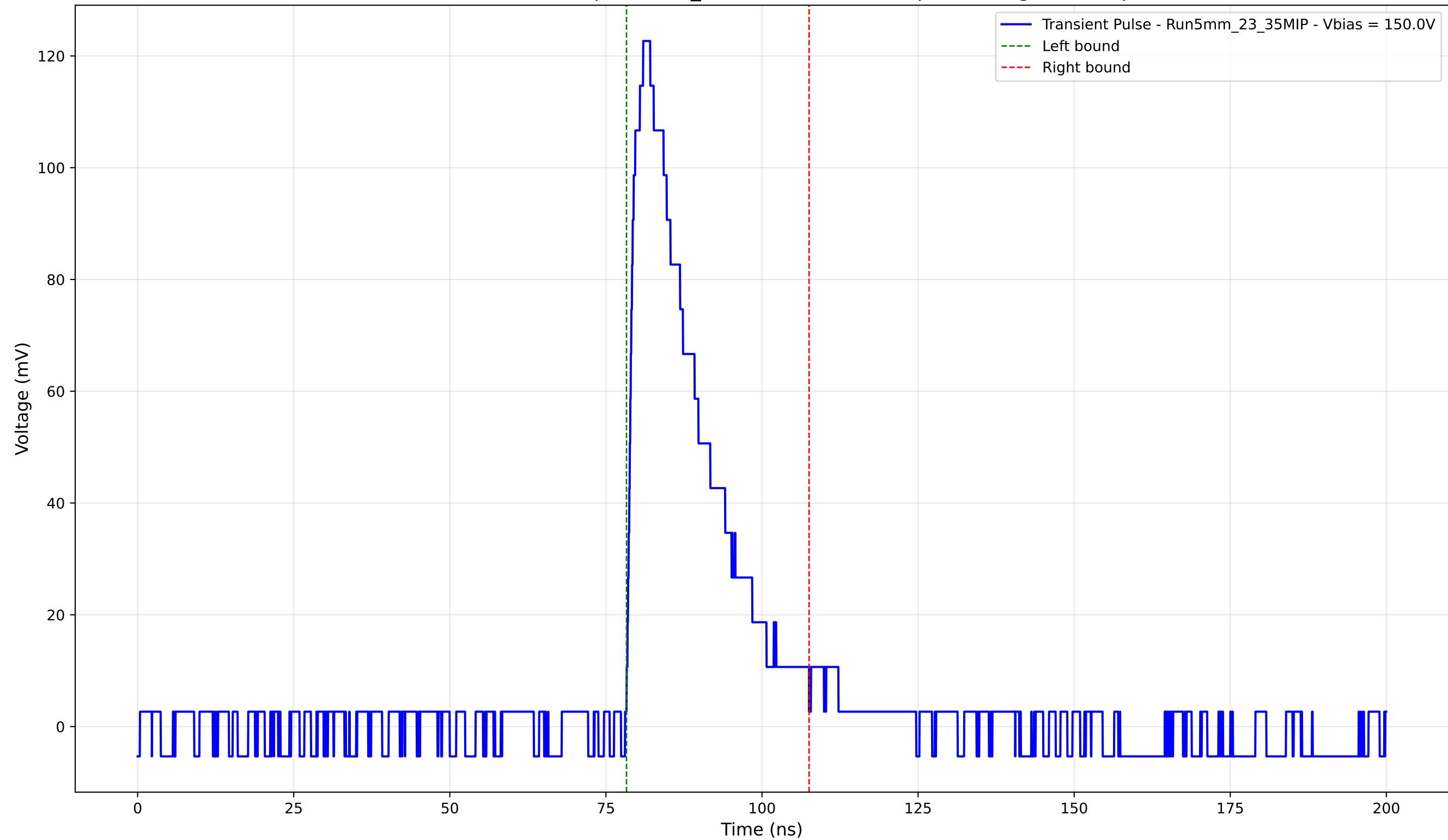
Transient Pulse - Sample: 5mm_23 - Position: 2120.0 \mu\text{m} - Charge: 29.24 pC
