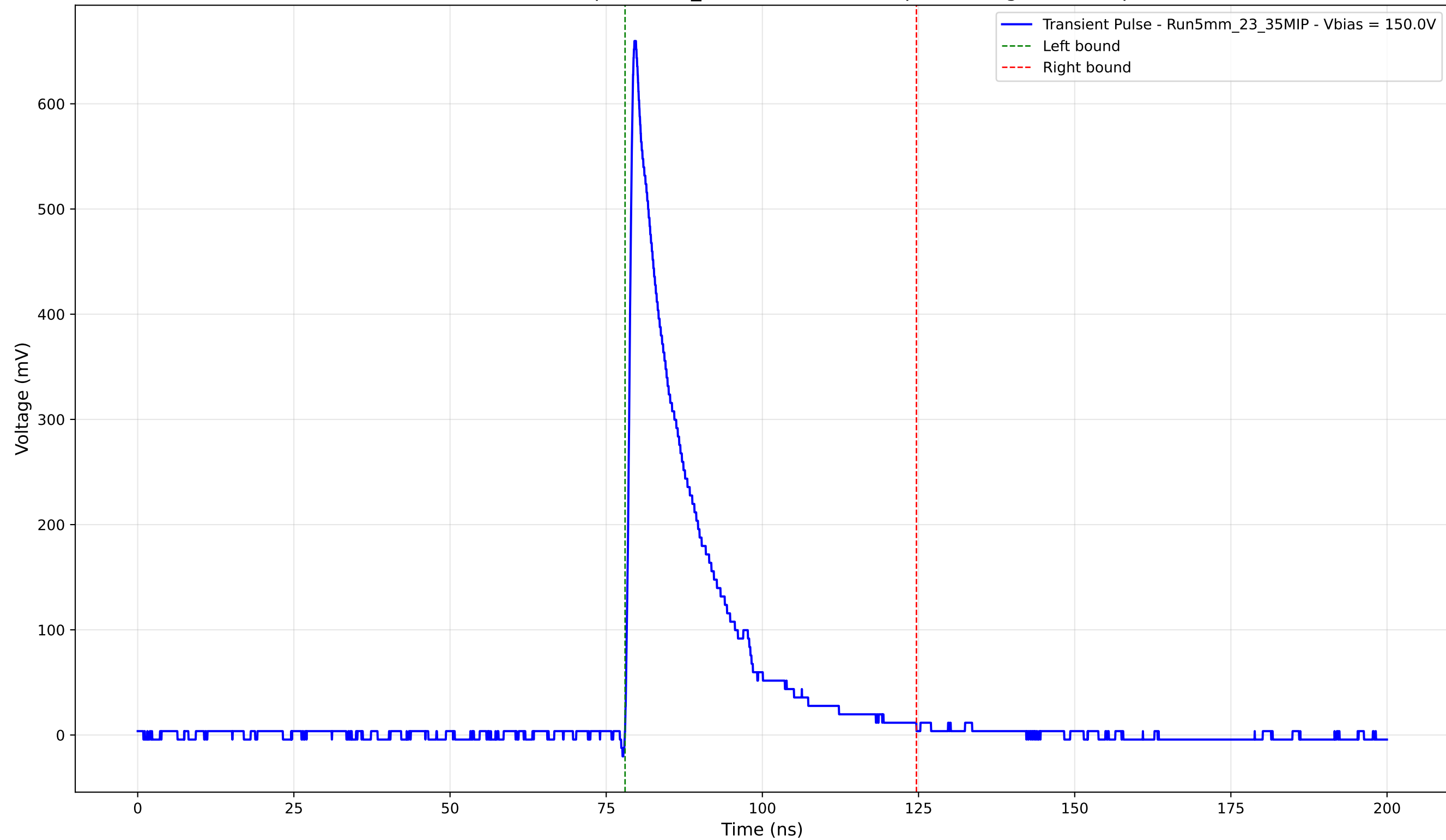
Transient Pulse - Sample: 5mm_23 - Position: 940.0 \mu\text{m} - Charge: 124.92 pC
