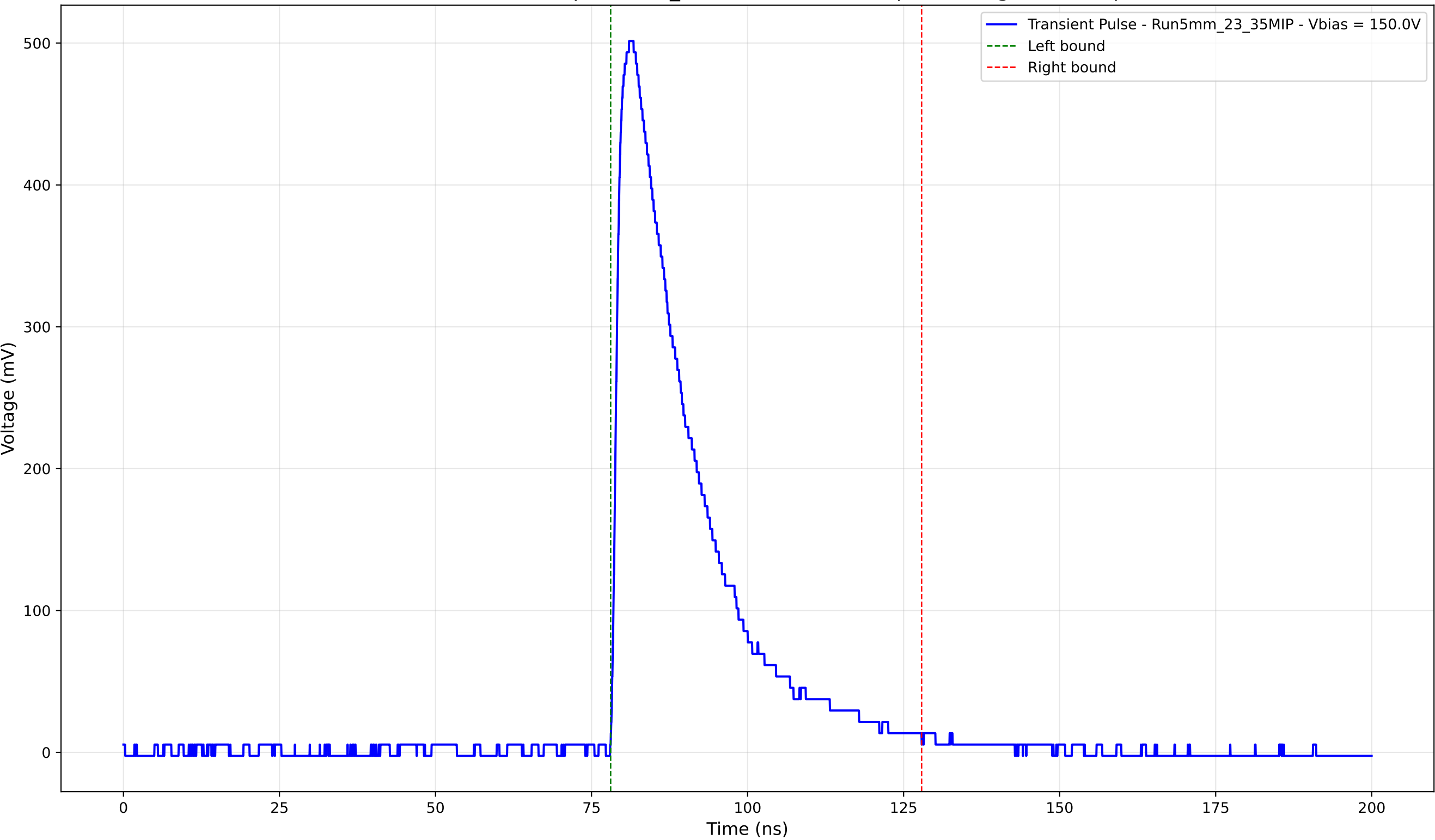
Transient Pulse - Sample: 5mm_23 - Position: 2805.0 \mu\text{m} - Charge: 136.70 pC
