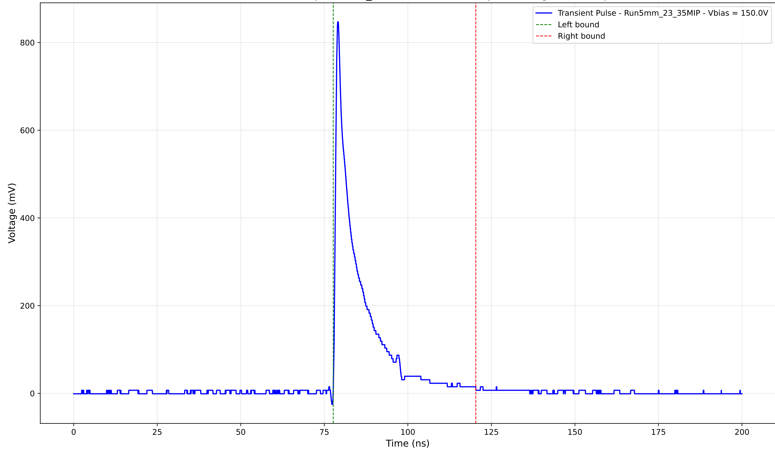
Transient Pulse - Sample: 5mm_23 - Position: 4870.0 \mu\text{m} - Charge: 117.07 pC
