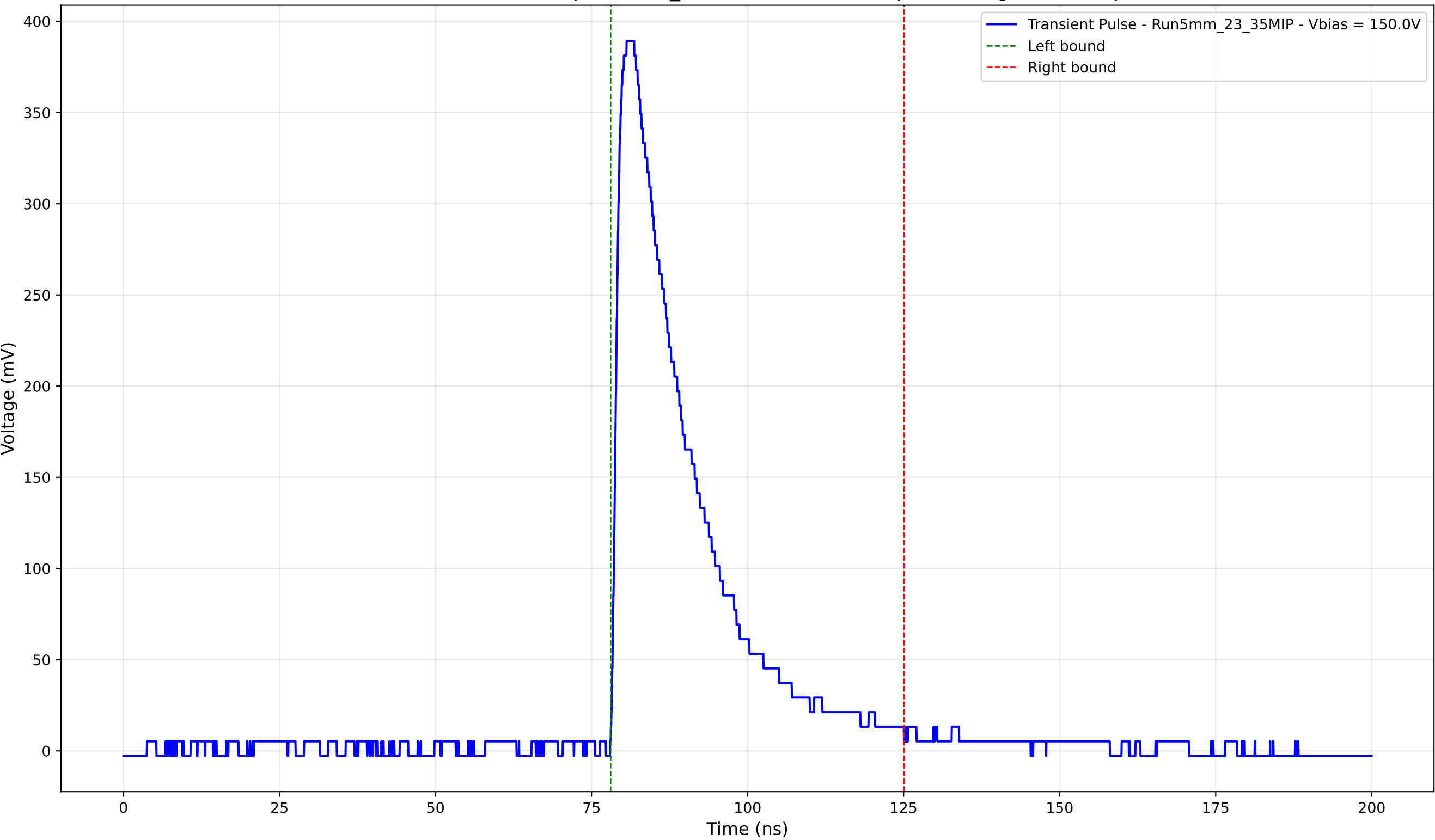
Transient Pulse - Sample: 5mm_23 - Position: 3210.0 \mu\text{m} - Charge: 101.86 pC
