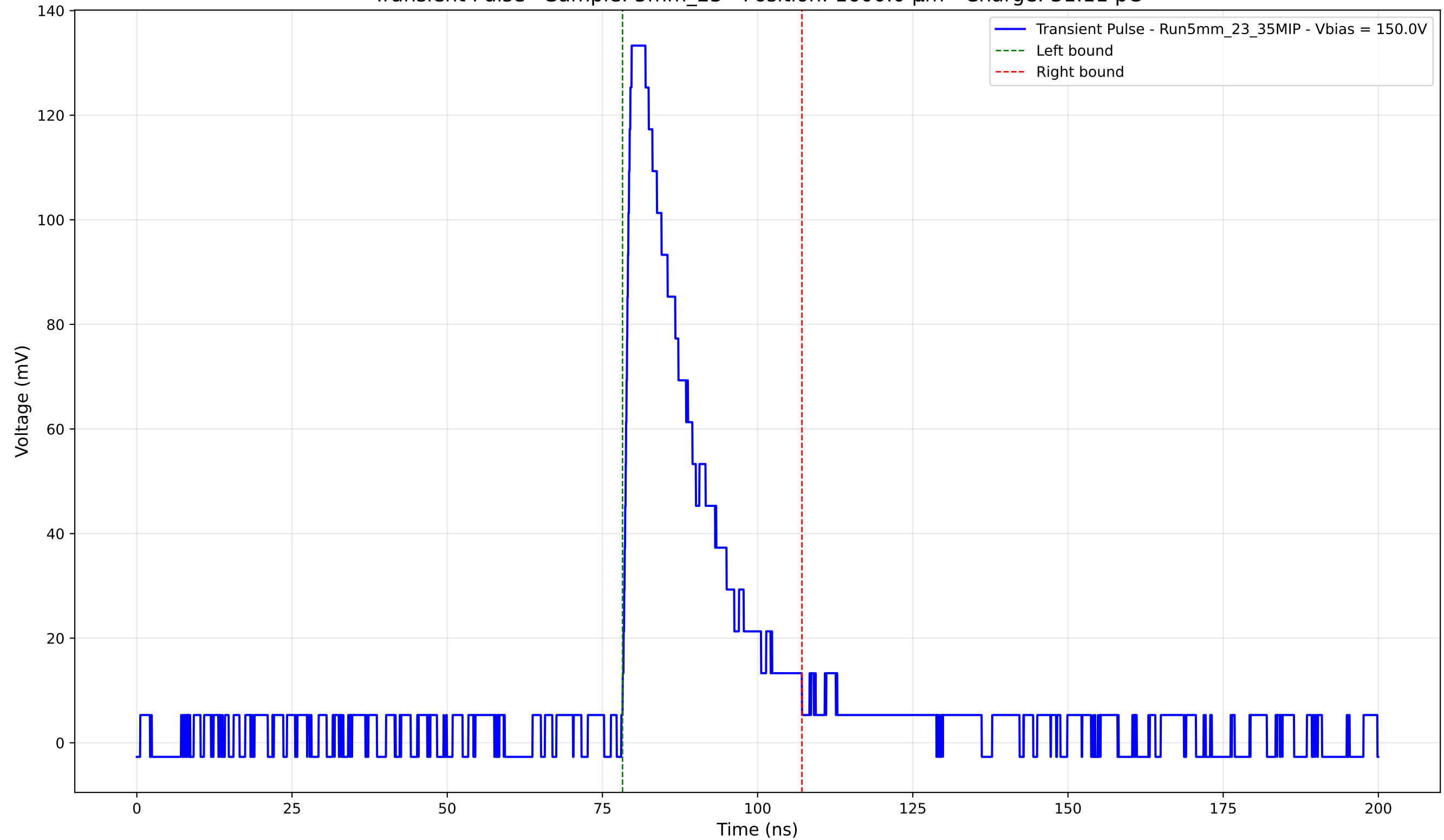
Transient Pulse - Sample: 5mm_23 - Position: 1600.0 \mu\text{m} - Charge: 31.11 pC
