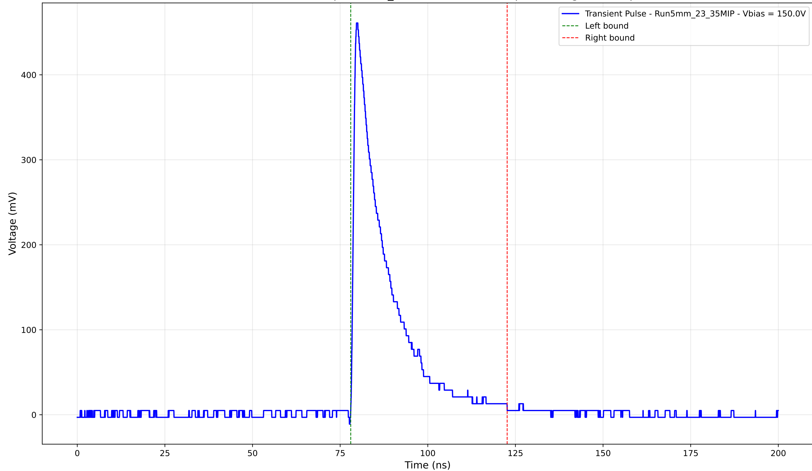
Transient Pulse - Sample: 5mm_23 - Position: 4090.0 \mu\text{m} - Charge: 92.99 pC
