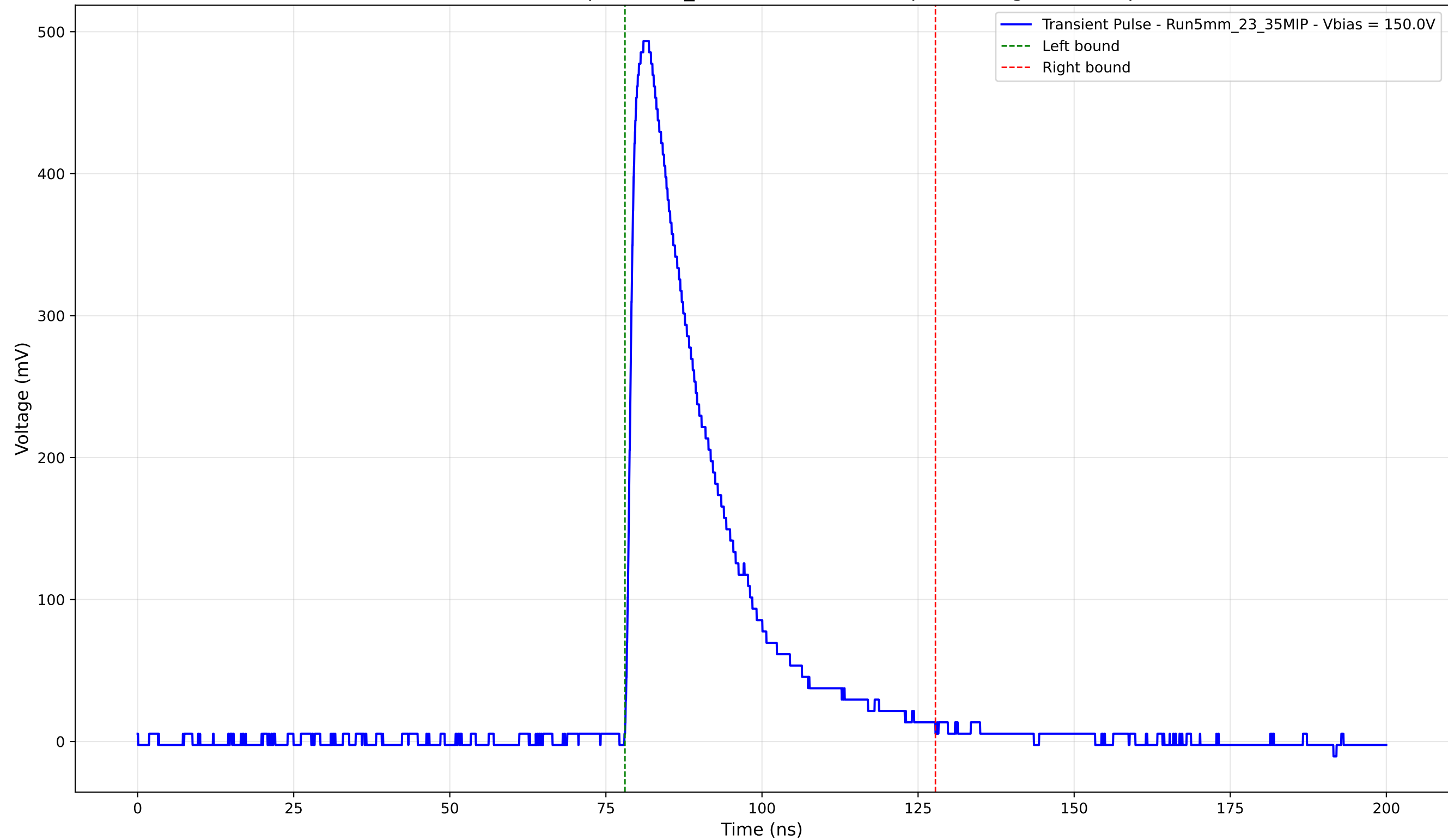
Transient Pulse - Sample: 5mm_23 - Position: 2765.0 \mu\text{m} - Charge: 135.44 pC
