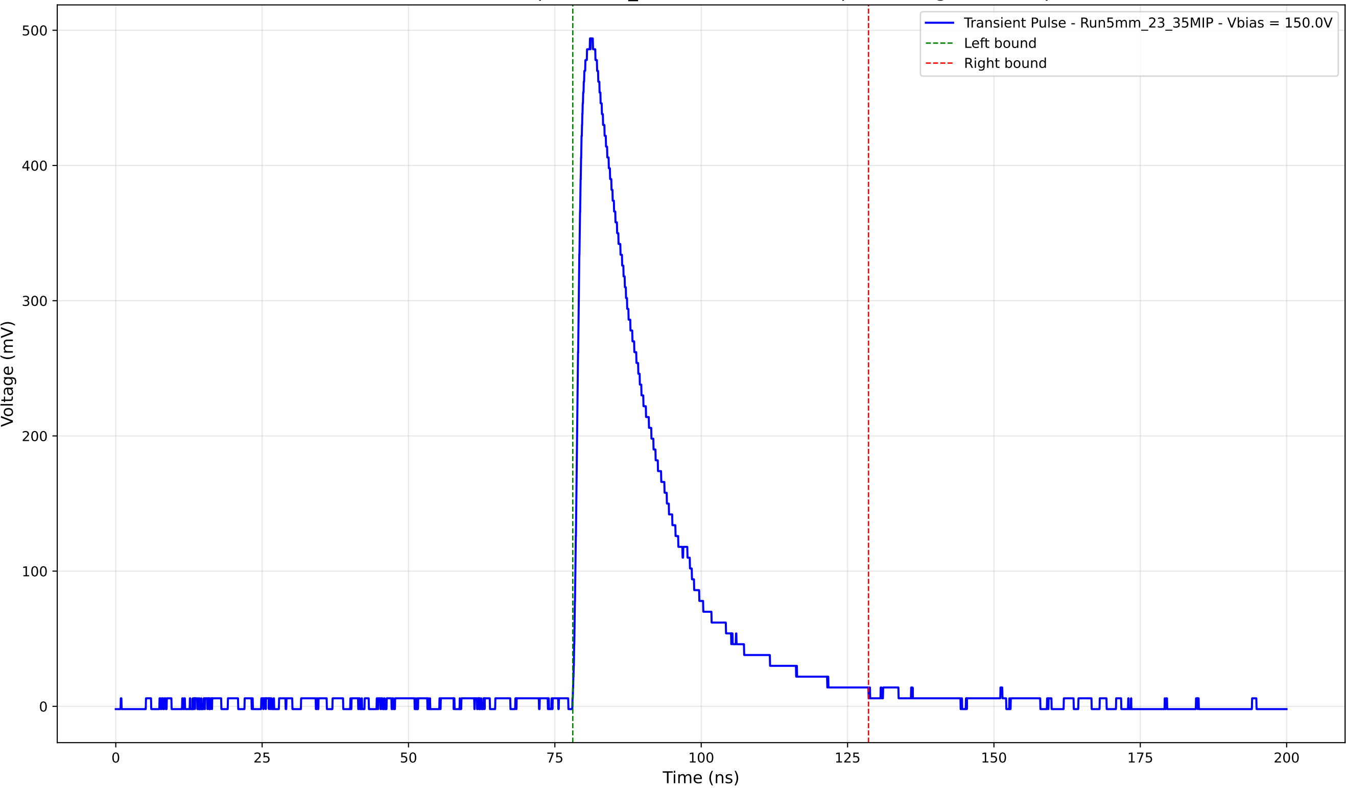
Transient Pulse - Sample: 5mm_23 - Position: 2235.0 \mu\text{m} - Charge: 132.83 pC
