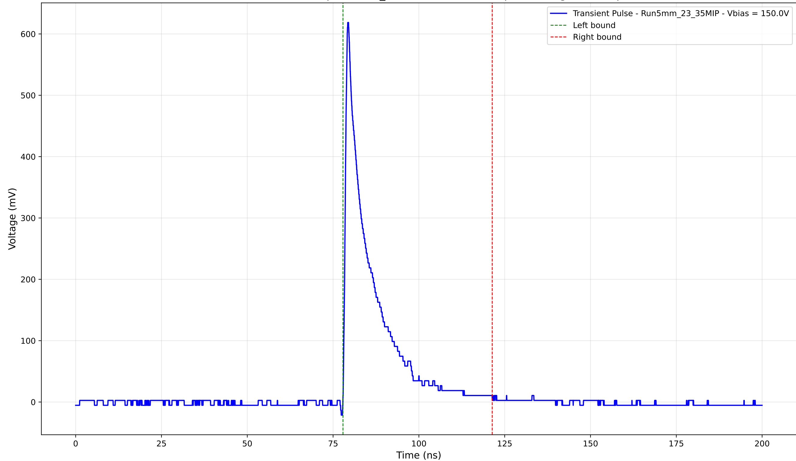
Transient Pulse - Sample: 5mm_23 - Position: 4590.0 \mu\text{m} - Charge: 94.67 pC
