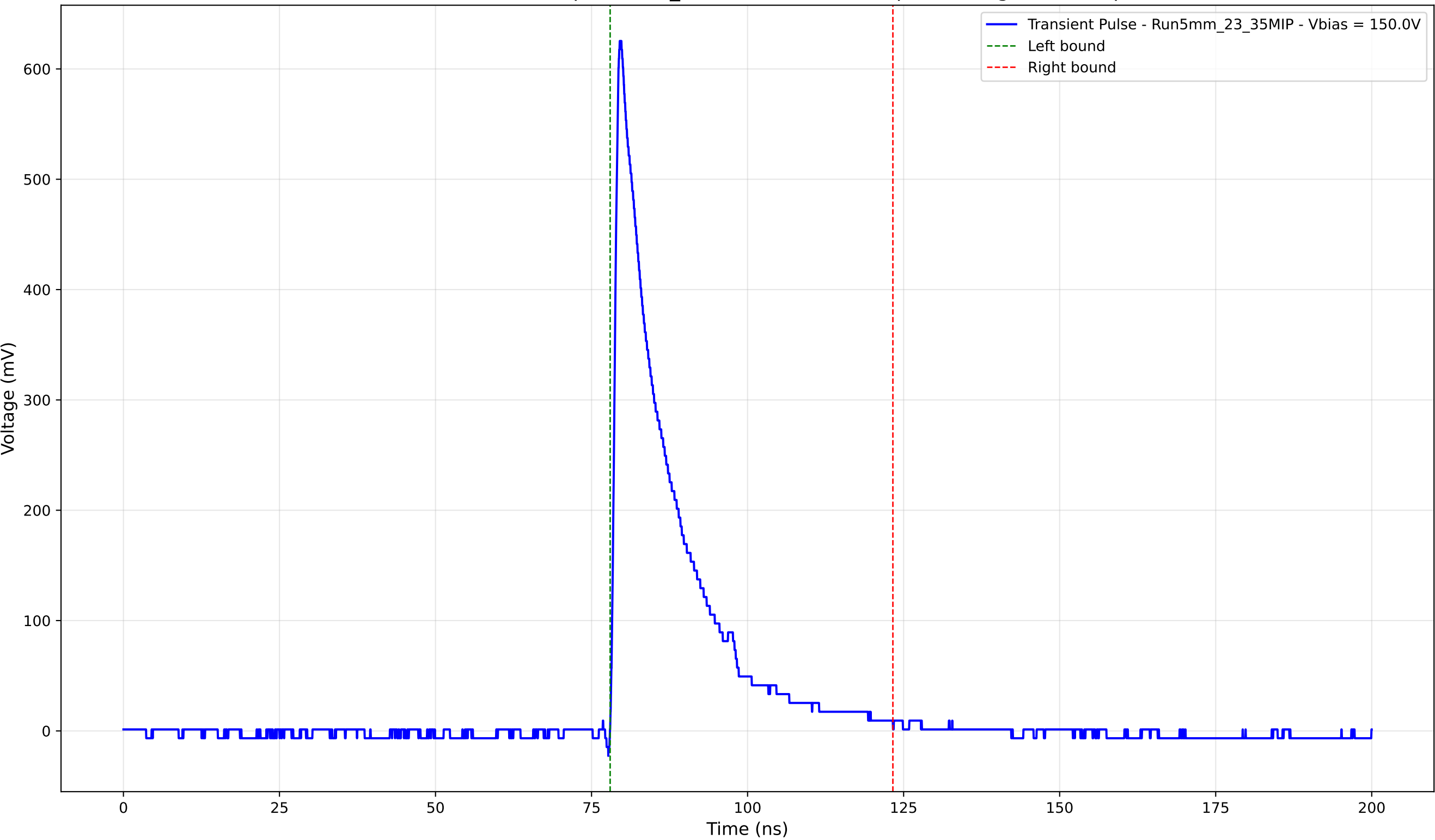
Transient Pulse - Sample: 5mm_23 - Position: 4300.0 \mu\text{m} - Charge: 114.73 pC
