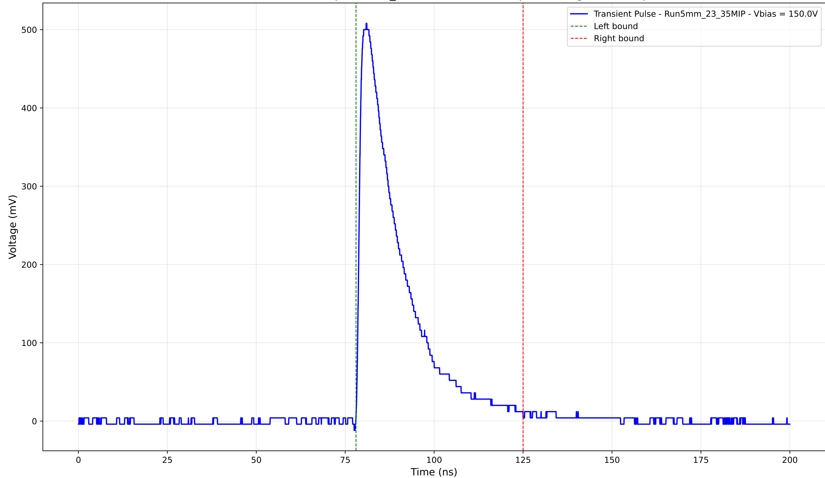
Transient Pulse - Sample: 5mm_23 - Position: 3270.0 \mu\text{m} - Charge: 130.71 pC
