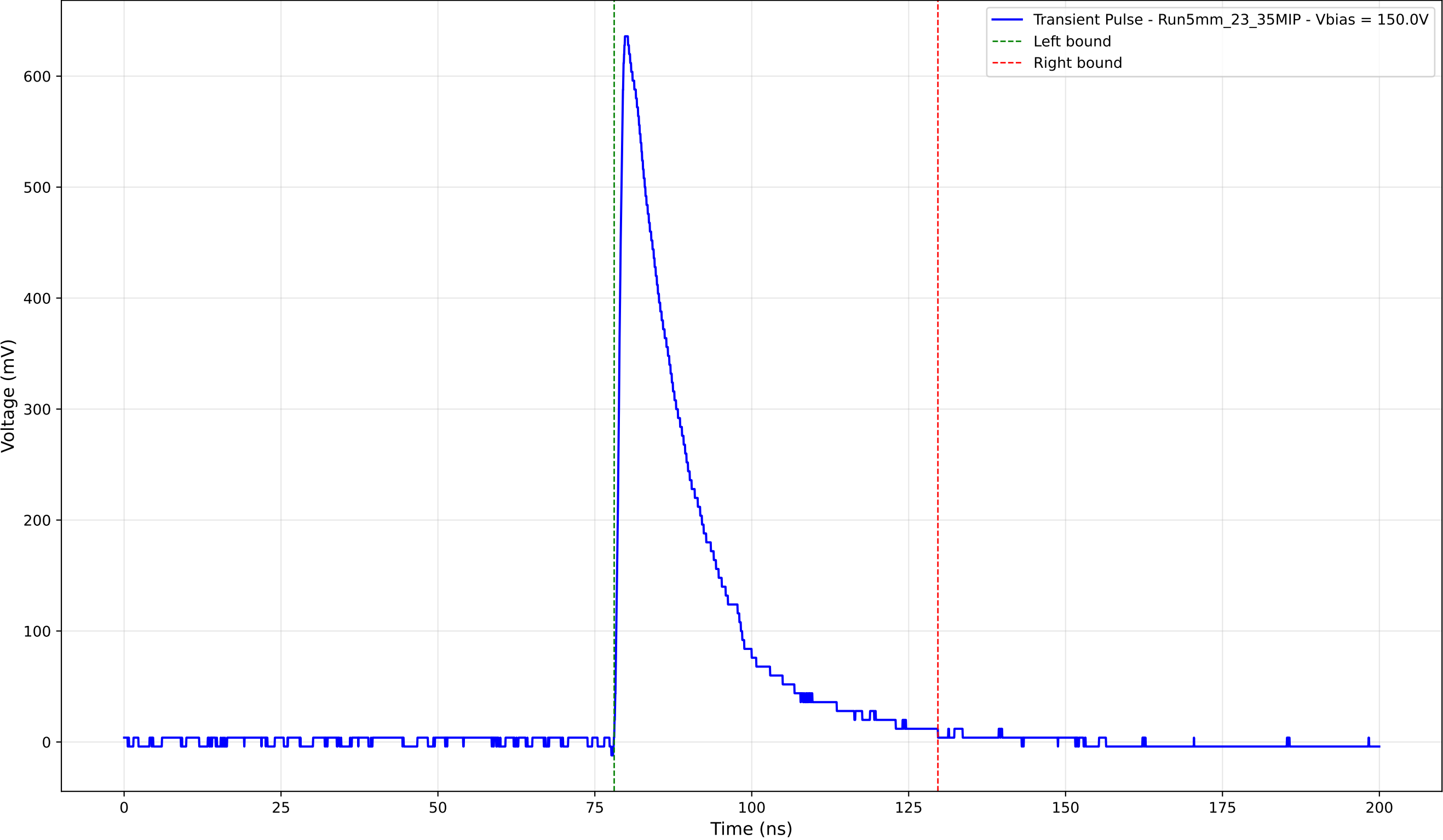
Transient Pulse - Sample: 5mm_23 - Position: 1415.0 \mu\text{m} - Charge: 149.74 pC
