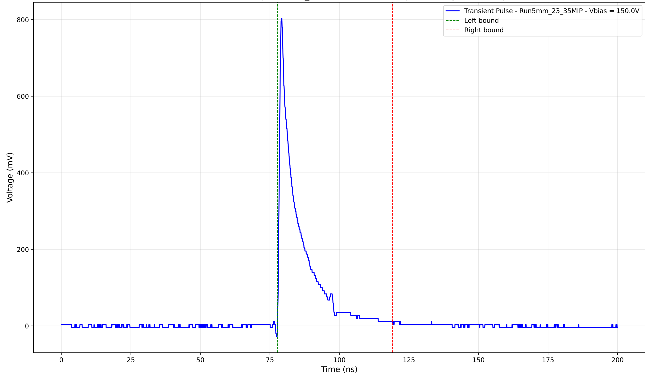
Transient Pulse - Sample: 5mm_23 - Position: 4790.0 \mu\text{m} - Charge: 112.44 pC
