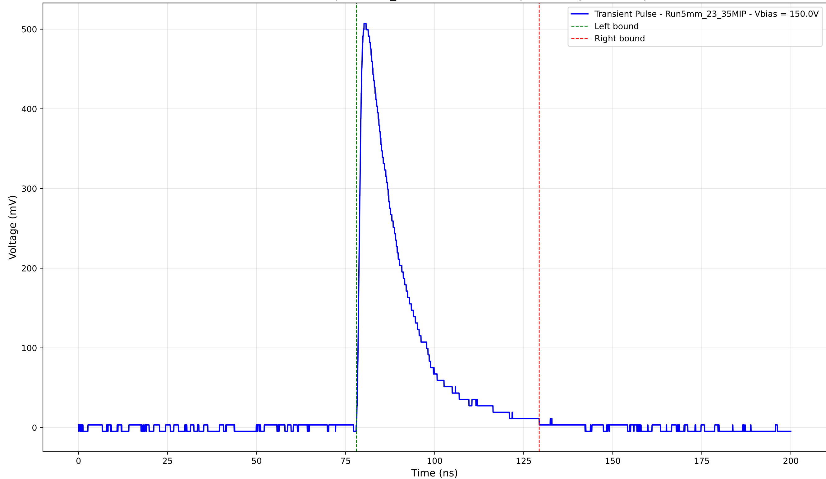
Transient Pulse - Sample: 5mm_23 - Position: 3495.0 \mu\text{m} - Charge: 127.18 pC
