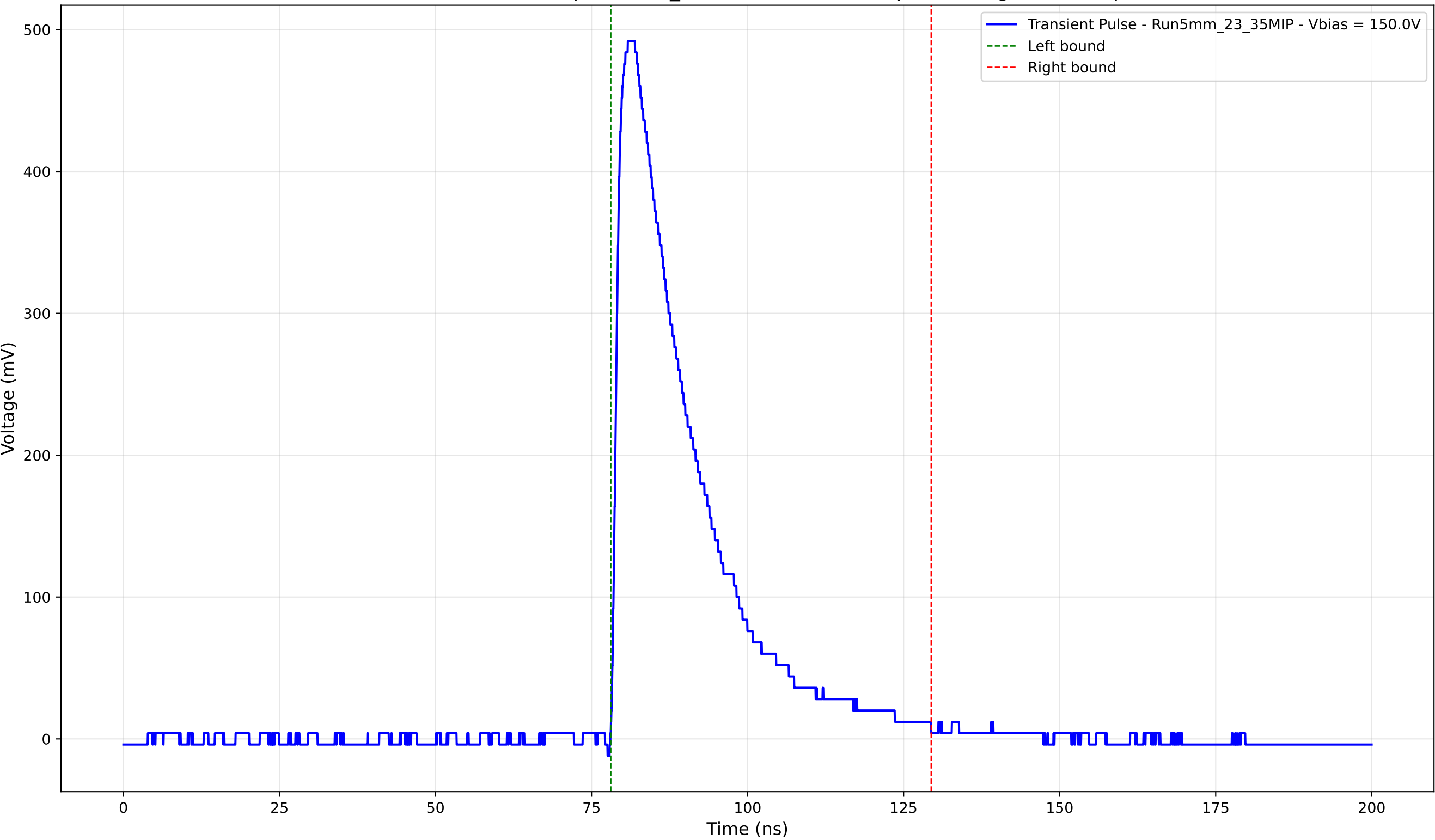
Transient Pulse - Sample: 5mm_23 - Position: 2810.0 \mu\text{m} - Charge: 134.03 pC
