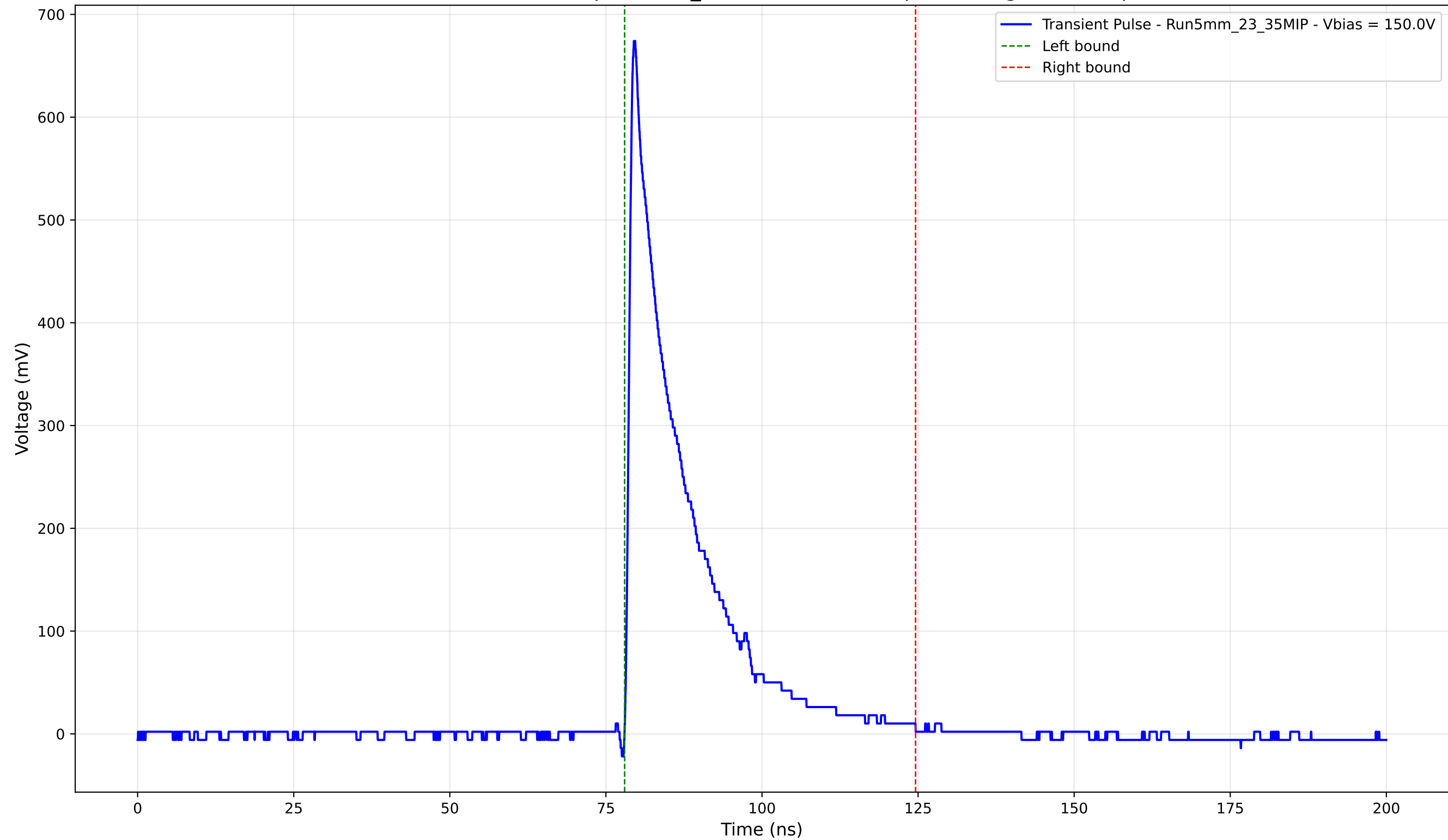
Transient Pulse - Sample: 5mm_23 - Position: 880.0 \mu\text{m} - Charge: 122.54 pC
