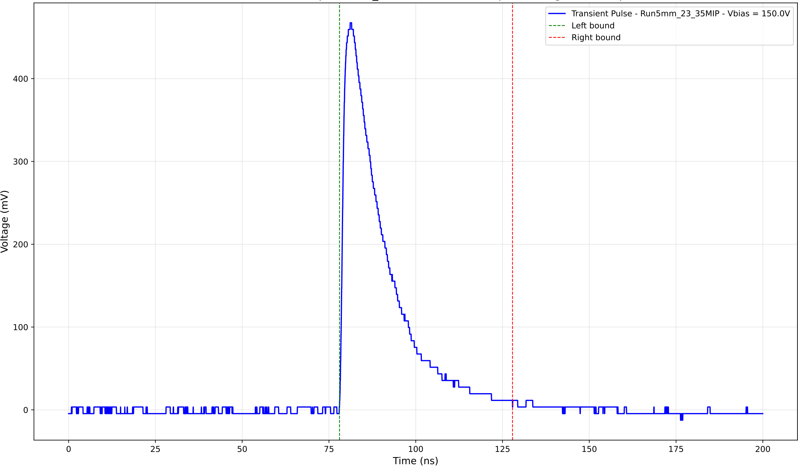
Transient Pulse - Sample: 5mm_23 - Position: 2560.0 \mu\text{m} - Charge: 125.75 pC
