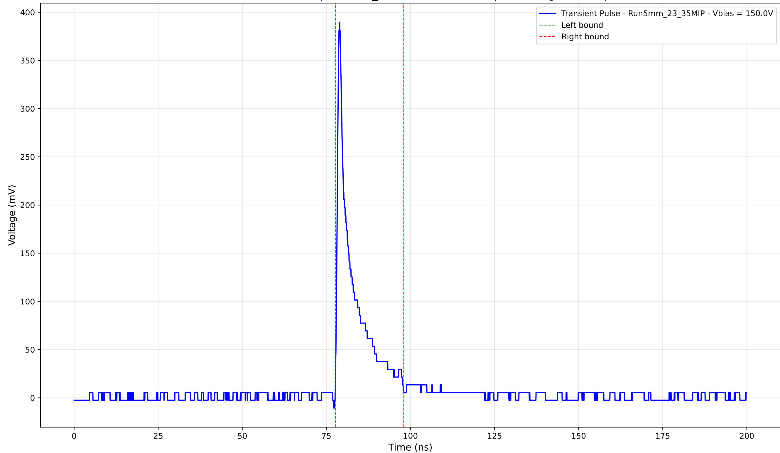
Transient Pulse - Sample: 5mm_23 - Position: 5075.0 \mu\text{m} - Charge: 36.99 pC
