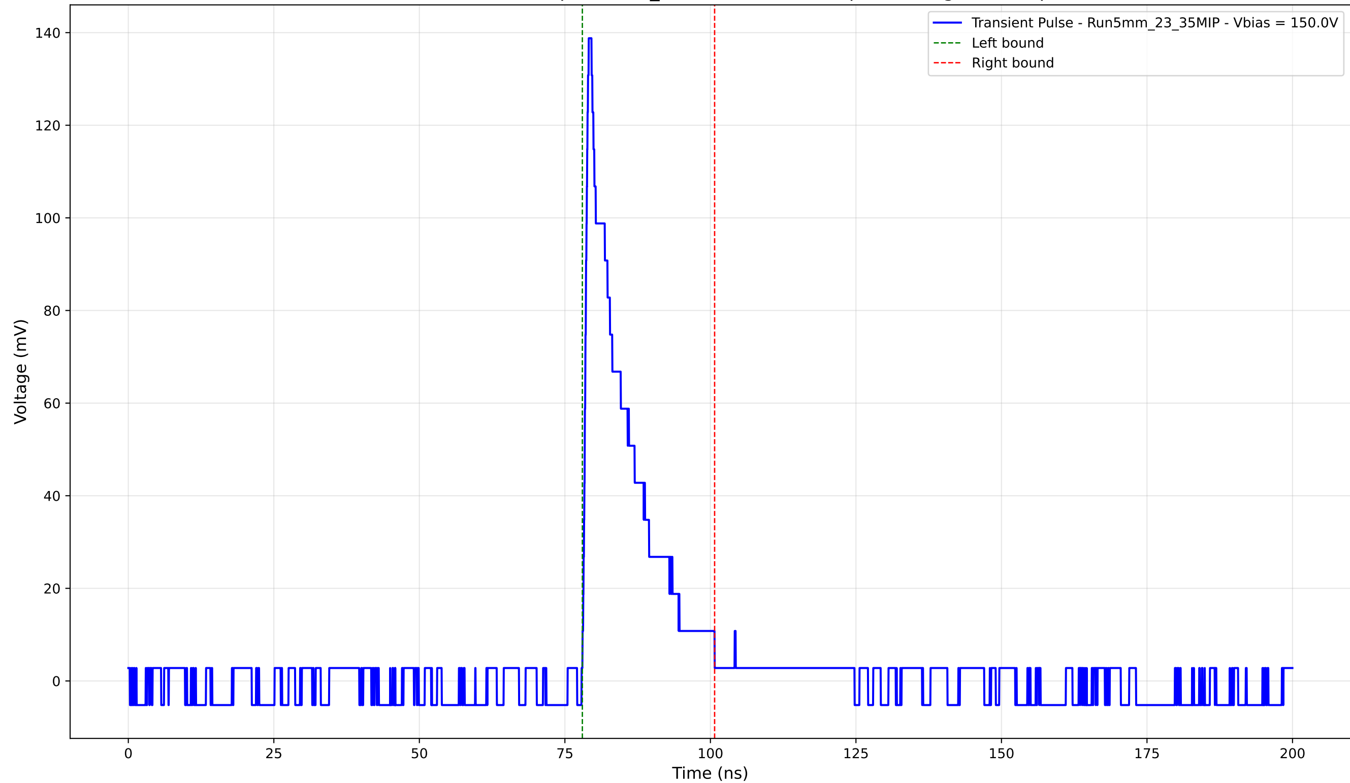
Transient Pulse - Sample: 5mm_23 - Position: 610.0 \mu\text{m} - Charge: 20.26 pC
