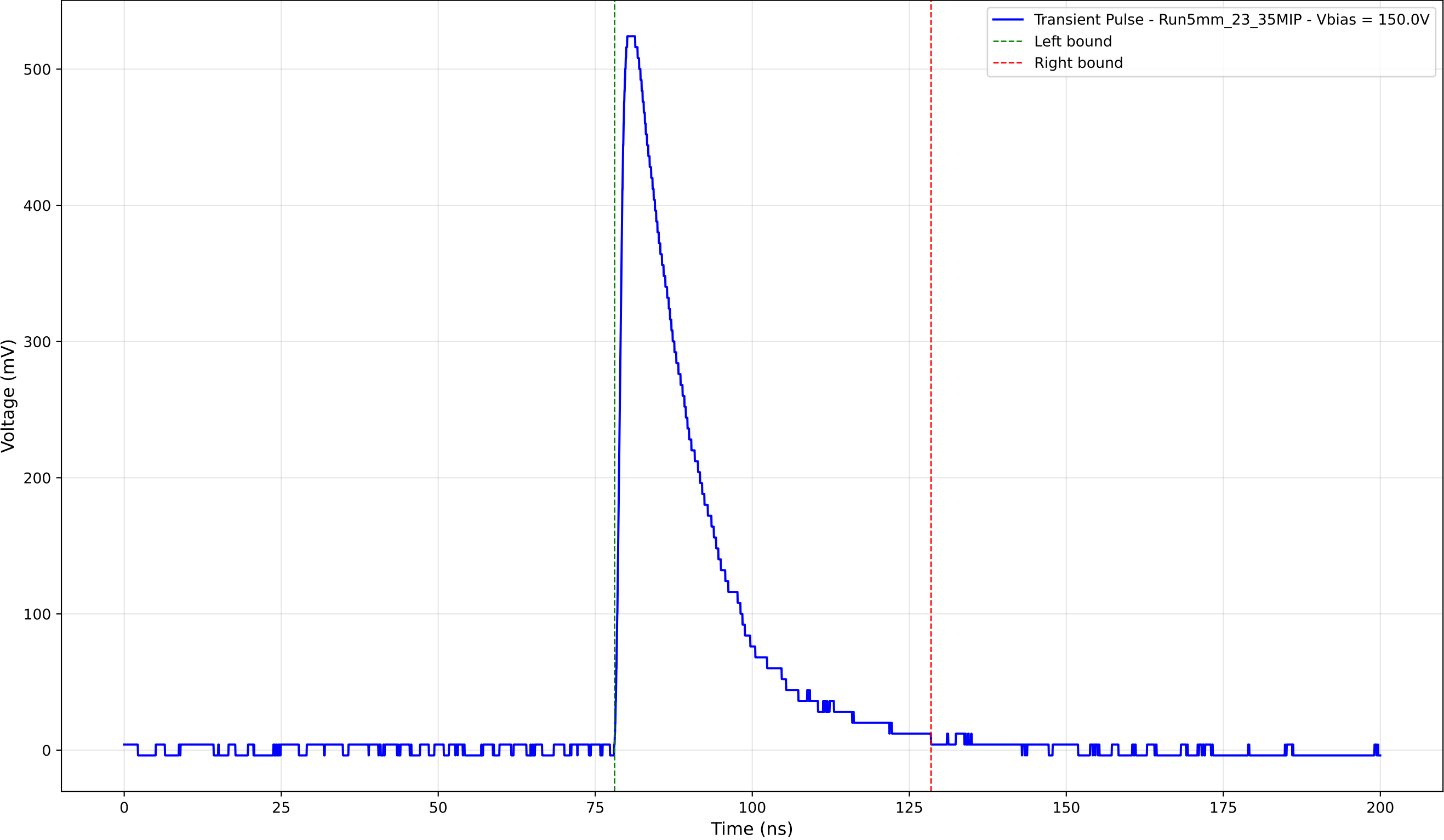
Transient Pulse - Sample: 5mm_23 - Position: 1825.0 \mu\text{m} - Charge: 135.84 pC
