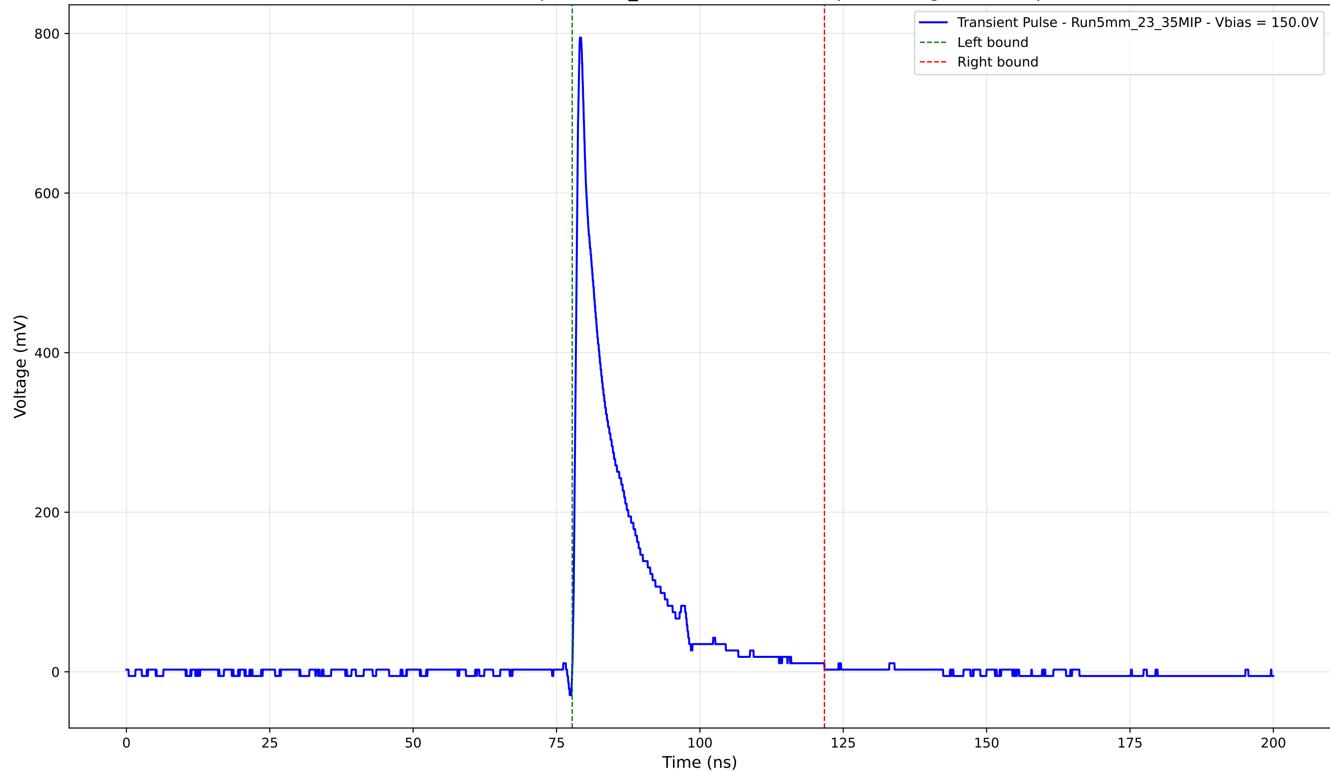
Transient Pulse - Sample: 5mm_23 - Position: 4780.0 \mu\text{m} - Charge: 112.34 pC
