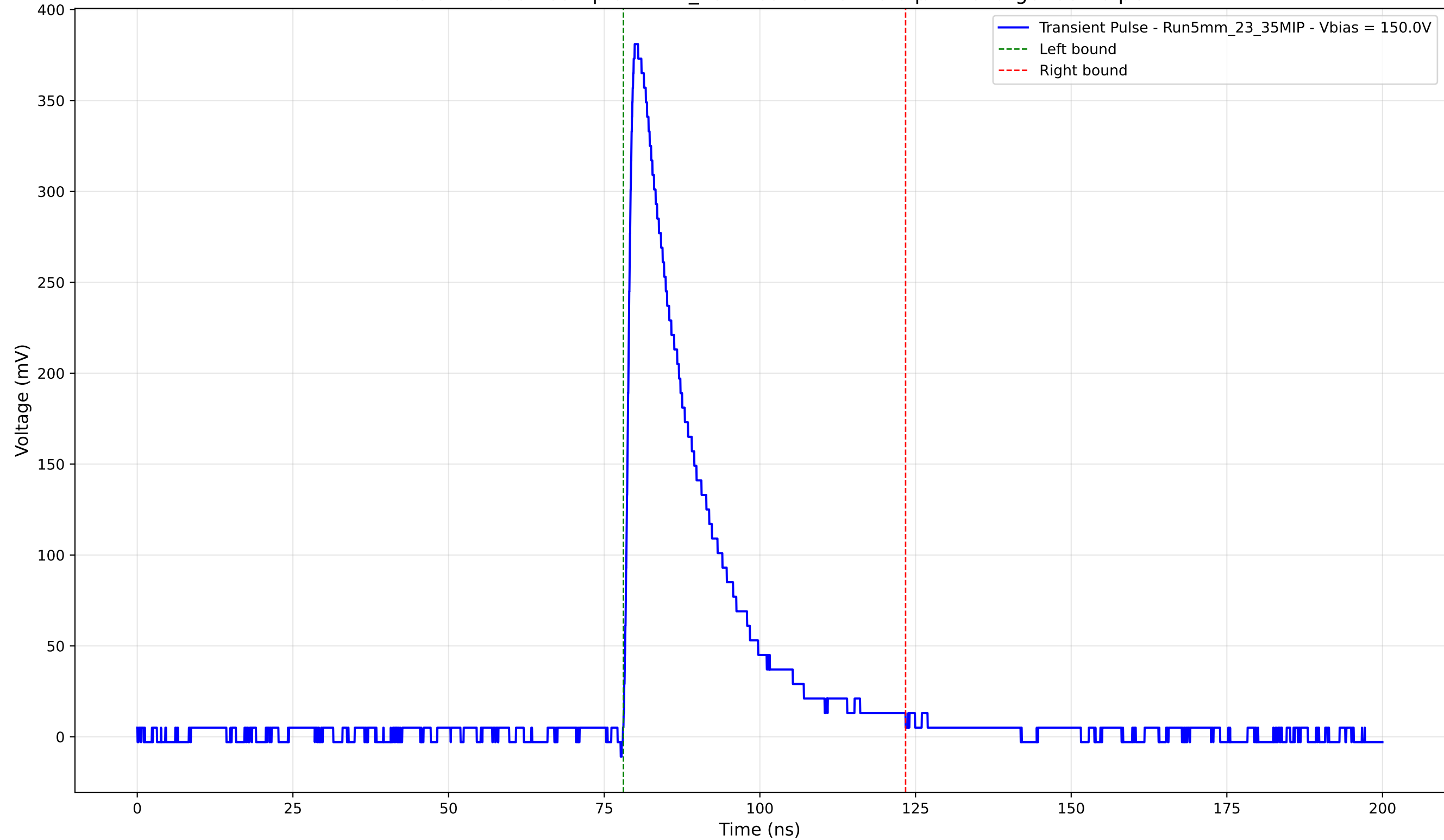
Transient Pulse - Sample: 5mm_23 - Position: 3710.0 \mu\text{m} - Charge: 88.26 pC
