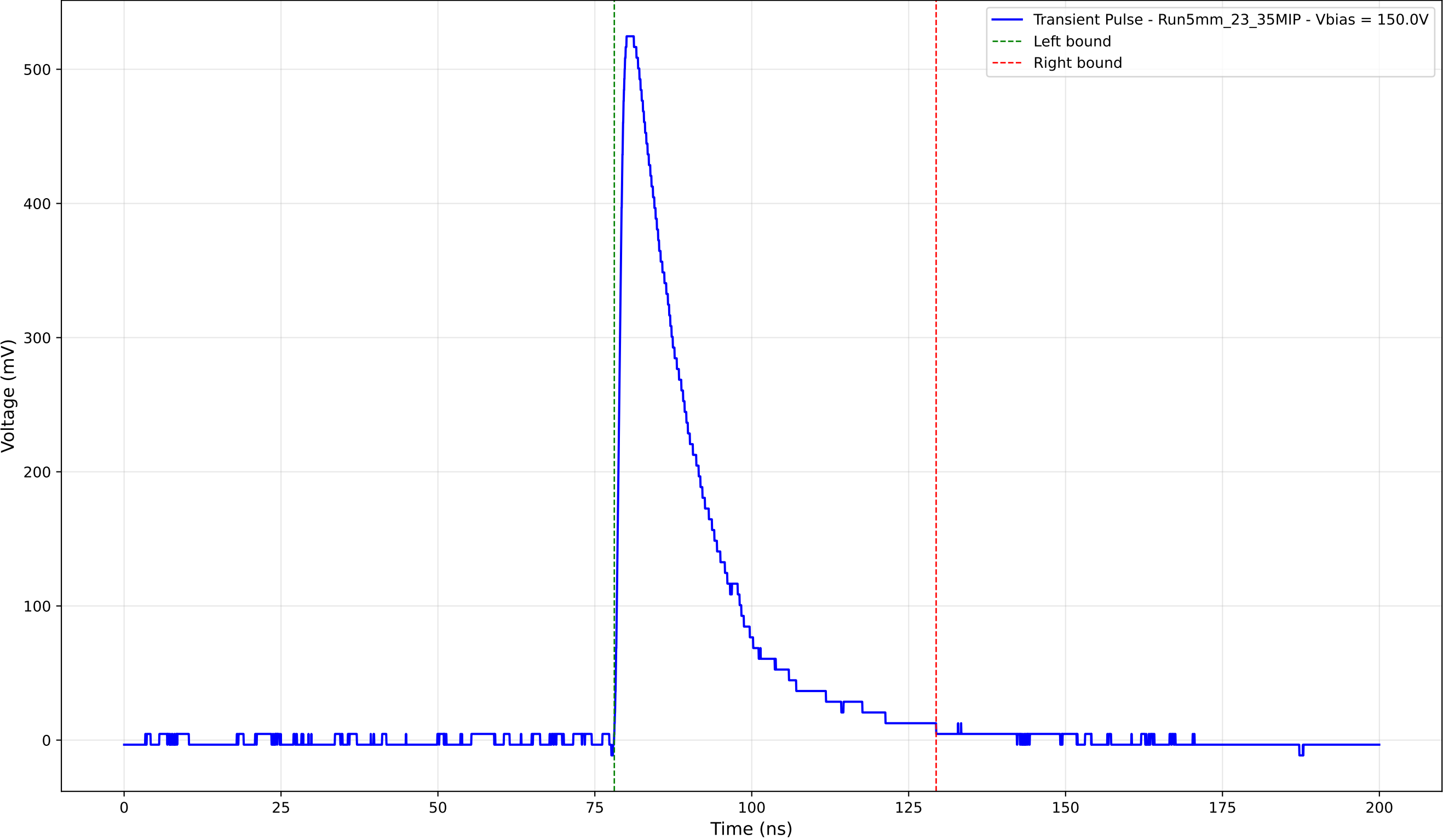
Transient Pulse - Sample: 5mm_23 - Position: 1785.0 \mu\text{m} - Charge: 135.30 pC
