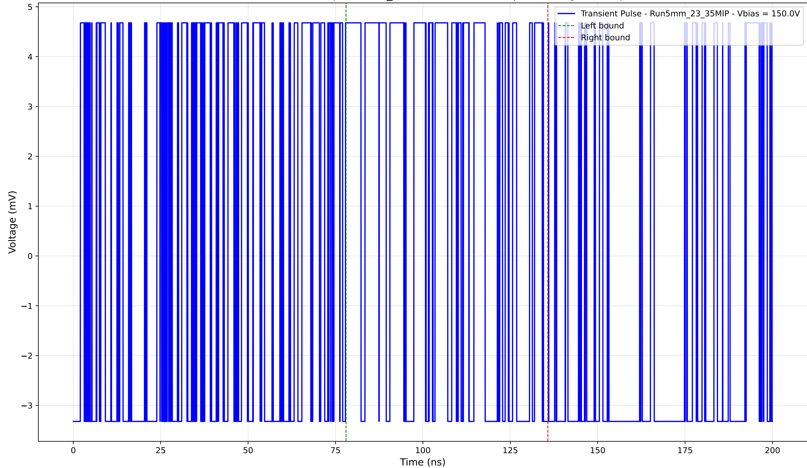
Transient Pulse - Sample: 5mm_23 - Position: 5255.0 \mu\text{m} - Charge: 1.92 pC
