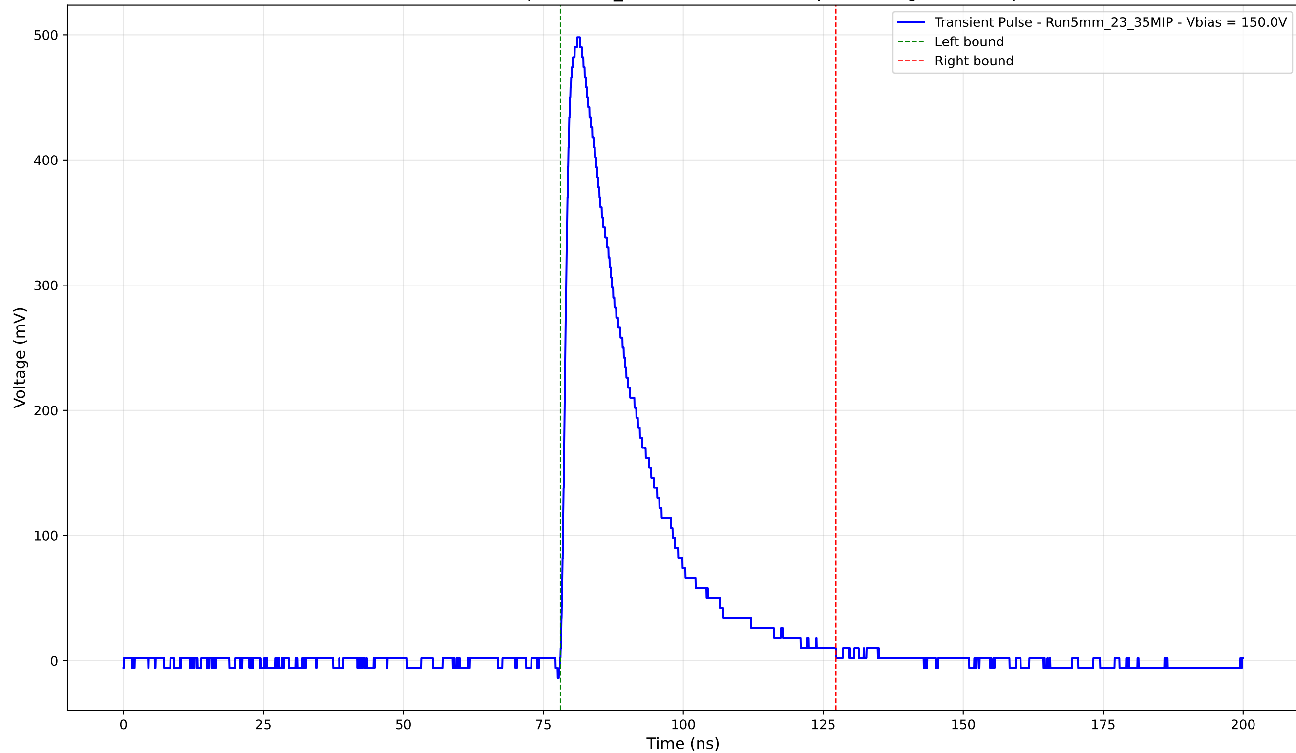
Transient Pulse - Sample: 5mm_23 - Position: 3010.0 \mu\text{m} - Charge: 130.61 pC
