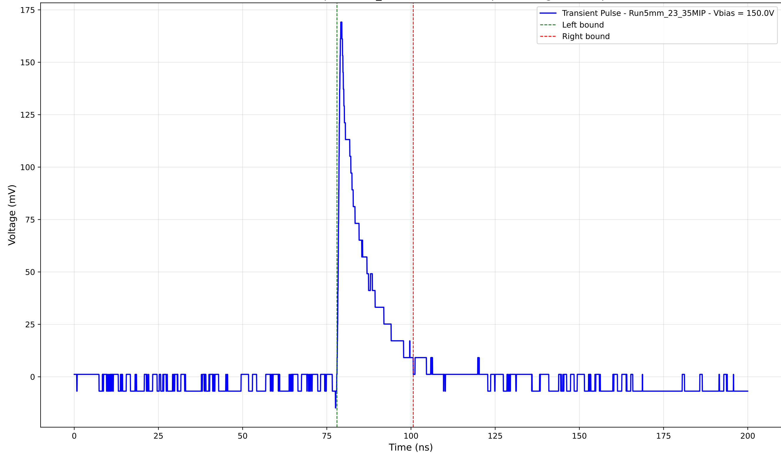
Transient Pulse - Sample: 5mm_23 - Position: 605.0 \mu\text{m} - Charge: 23.12 pC
