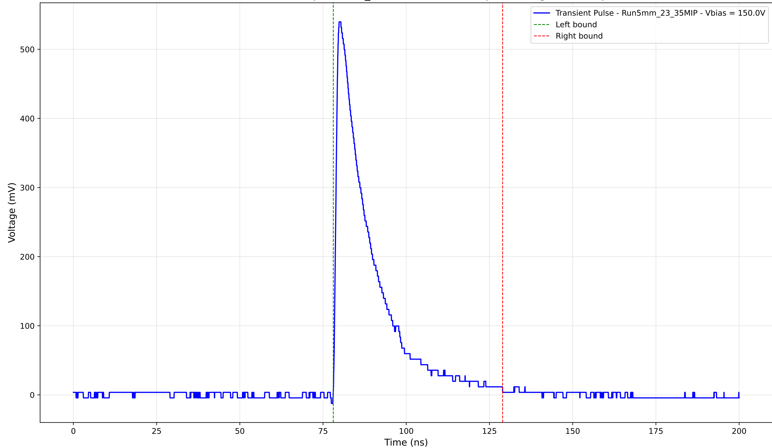
Transient Pulse - Sample: 5mm_23 - Position: 3830.0 \mu\text{m} - Charge: 123.87 pC
