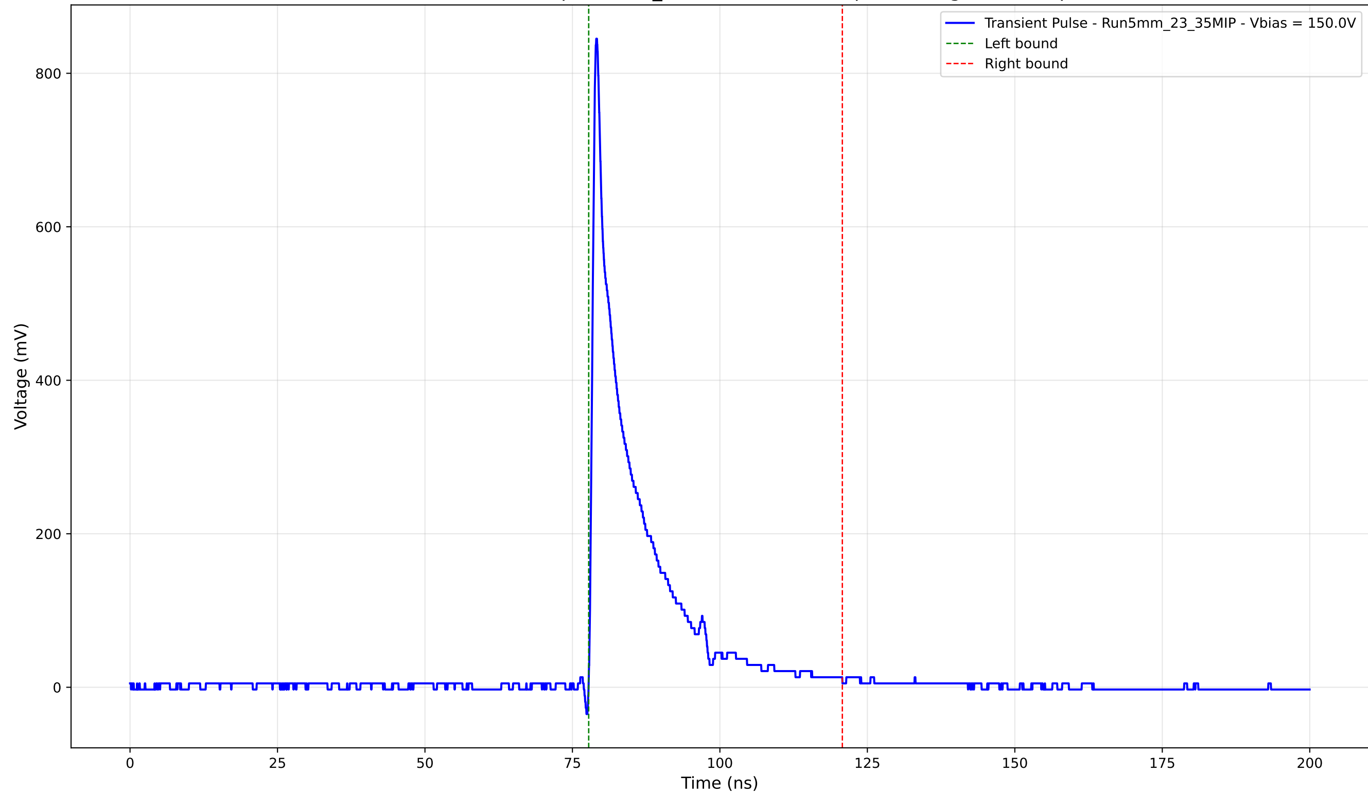
Transient Pulse - Sample: 5mm_23 - Position: 365.0 \mu\text{m} - Charge: 115.78 pC
