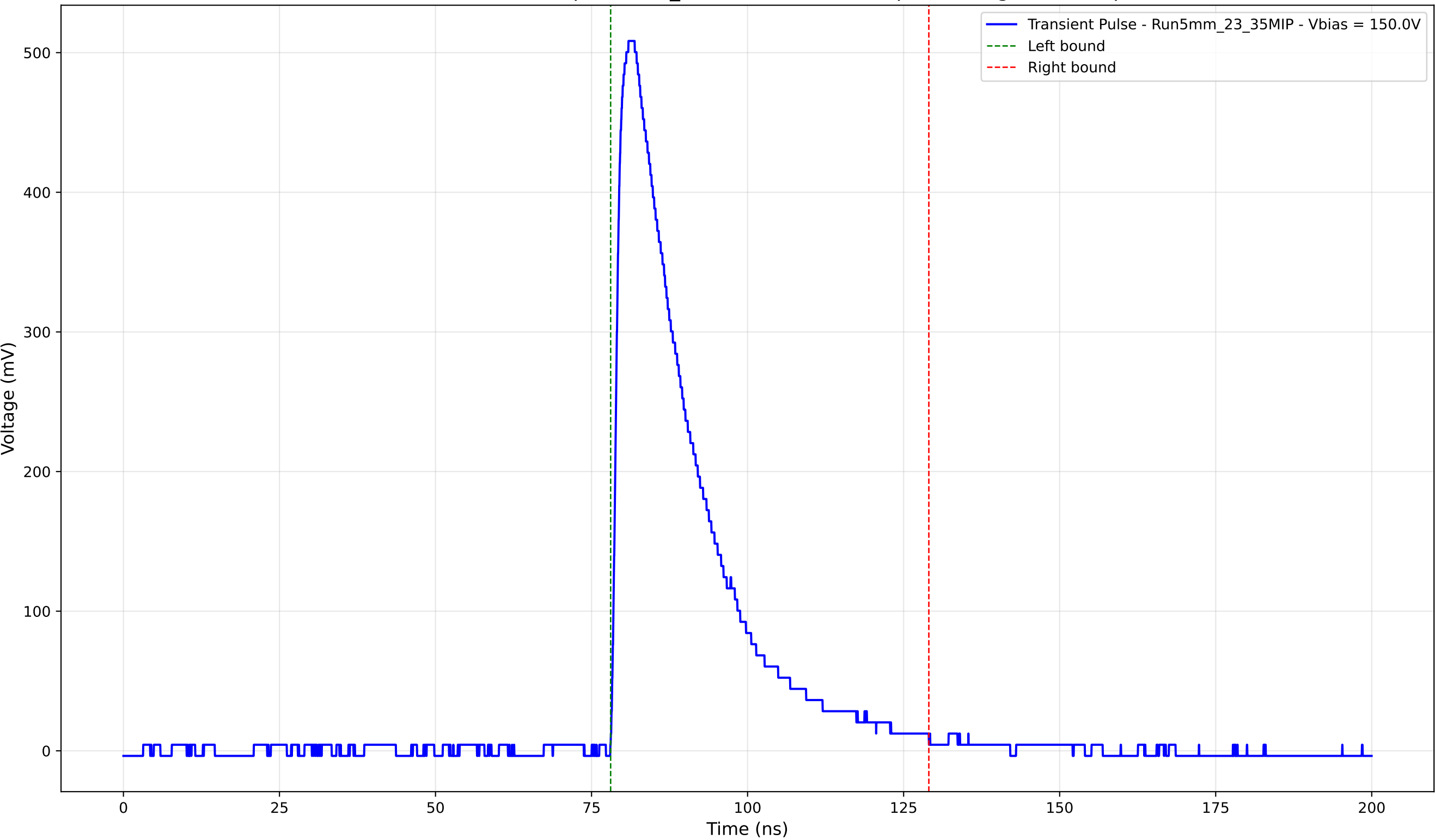
Transient Pulse - Sample: 5mm_23 - Position: 2485.0 \mu\text{m} - Charge: 139.06 pC
