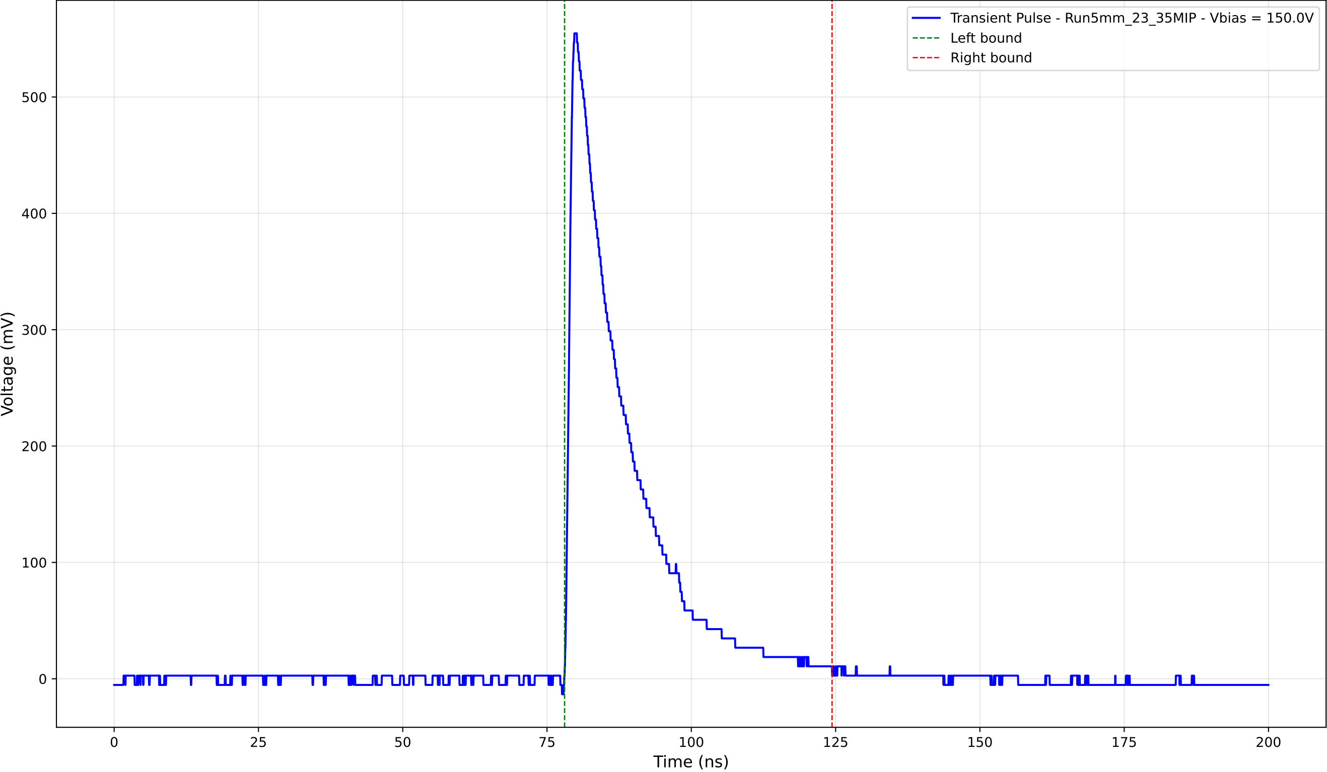
Transient Pulse - Sample: 5mm_23 - Position: 3965.0 \mu\text{m} - Charge: 118.13 pC
