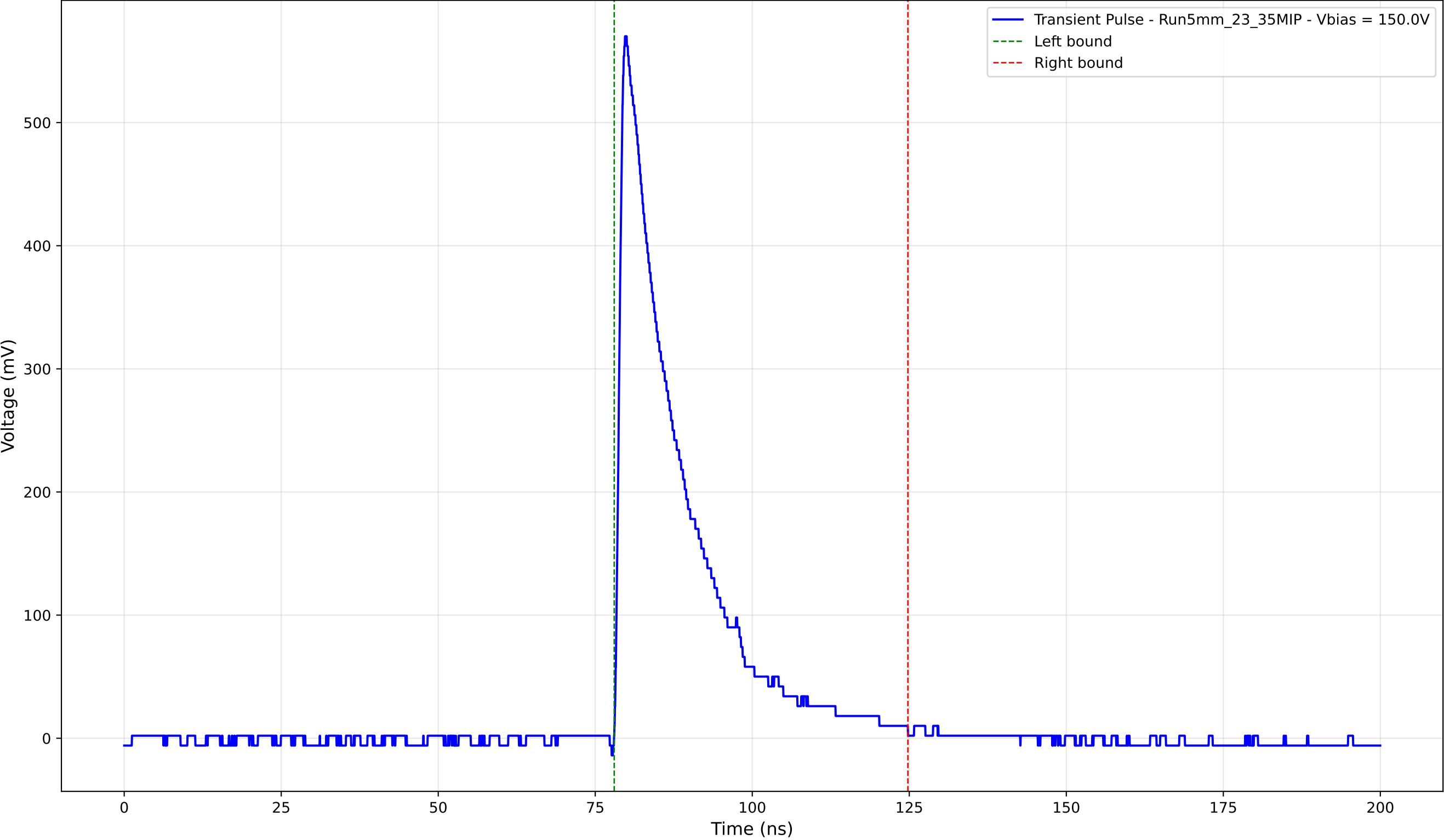
Transient Pulse - Sample: 5mm_23 - Position: 4015.0 \mu\text{m} - Charge: 119.14 pC
