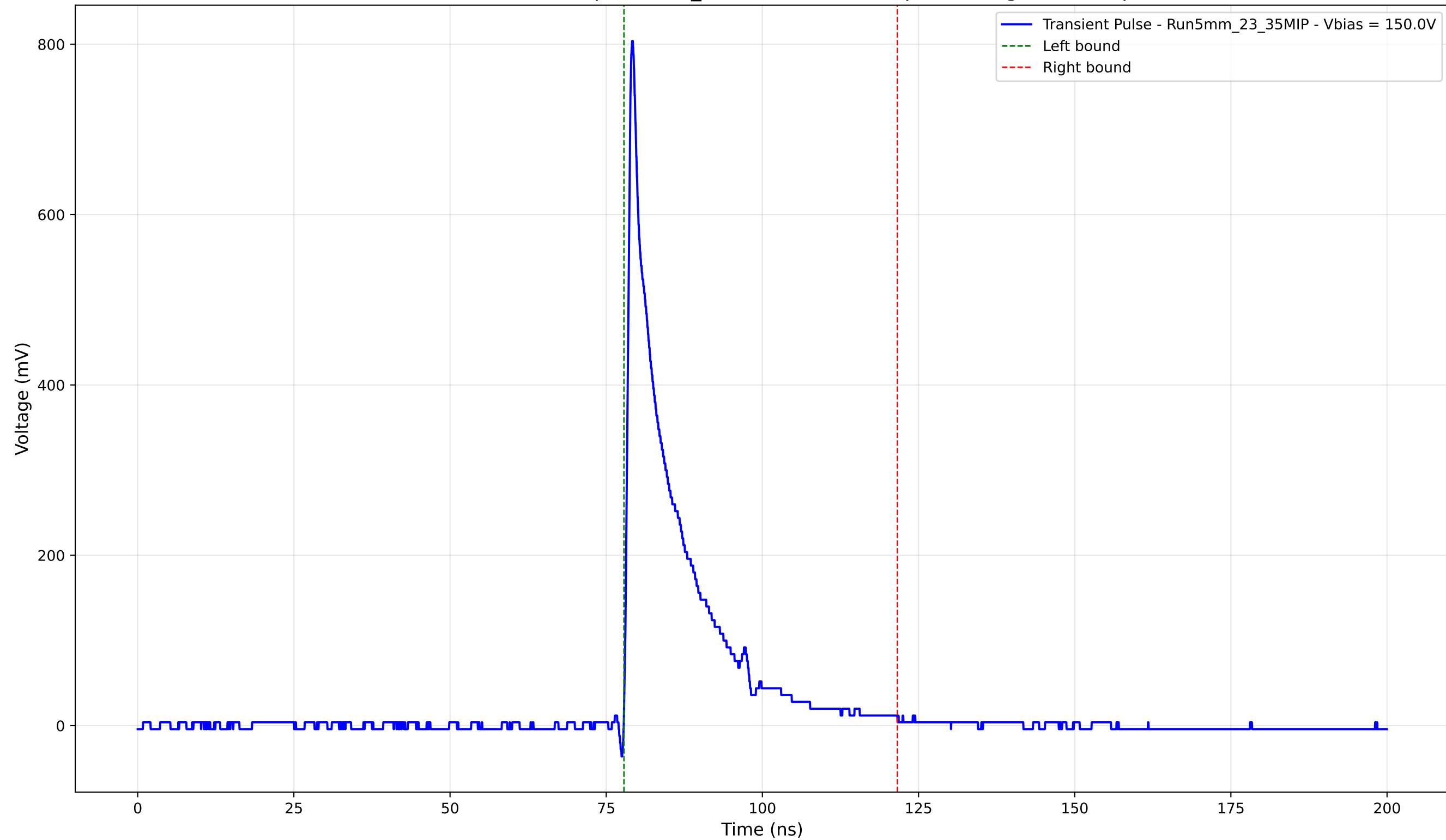
Transient Pulse - Sample: 5mm_23 - Position: 465.0 \mu\text{m} - Charge: 115.52 pC
