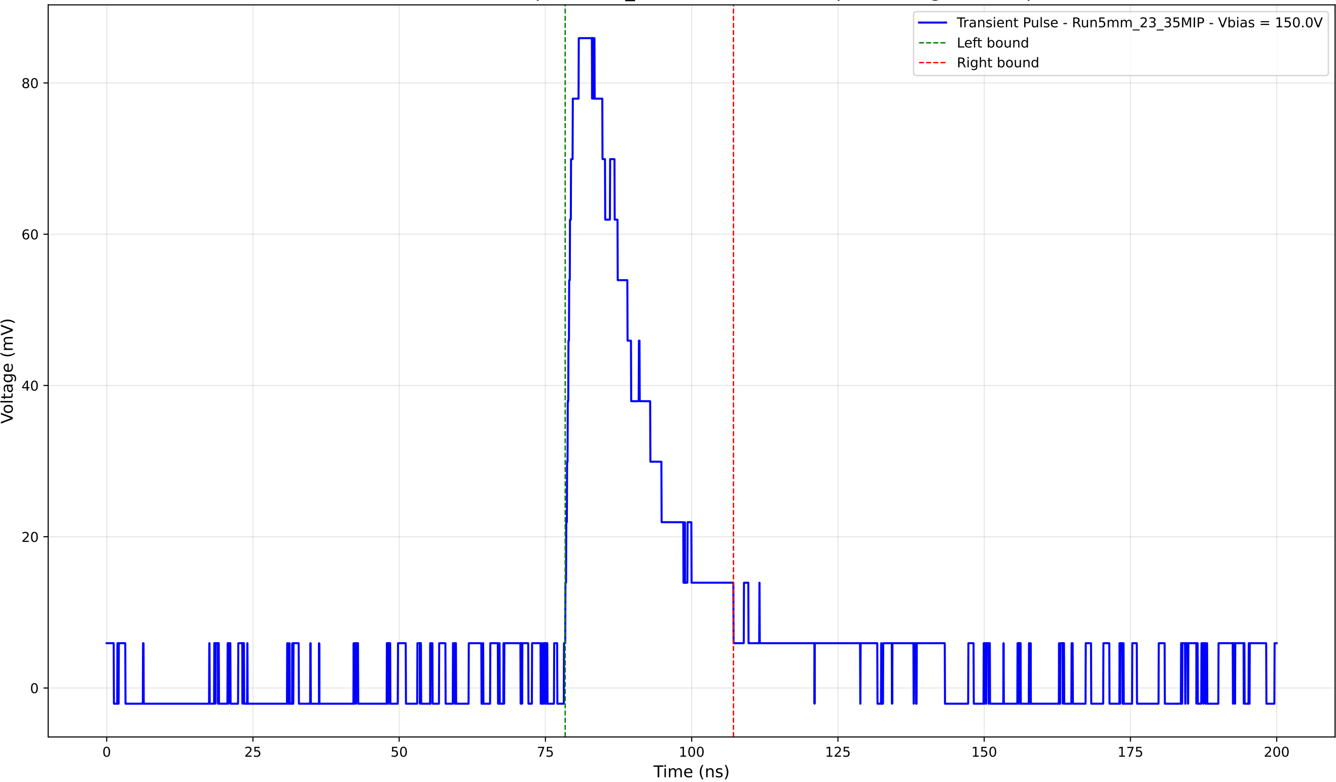
Transient Pulse - Sample: 5mm_23 - Position: 2135.0 \mu\text{m} - Charge: 23.09 pC
