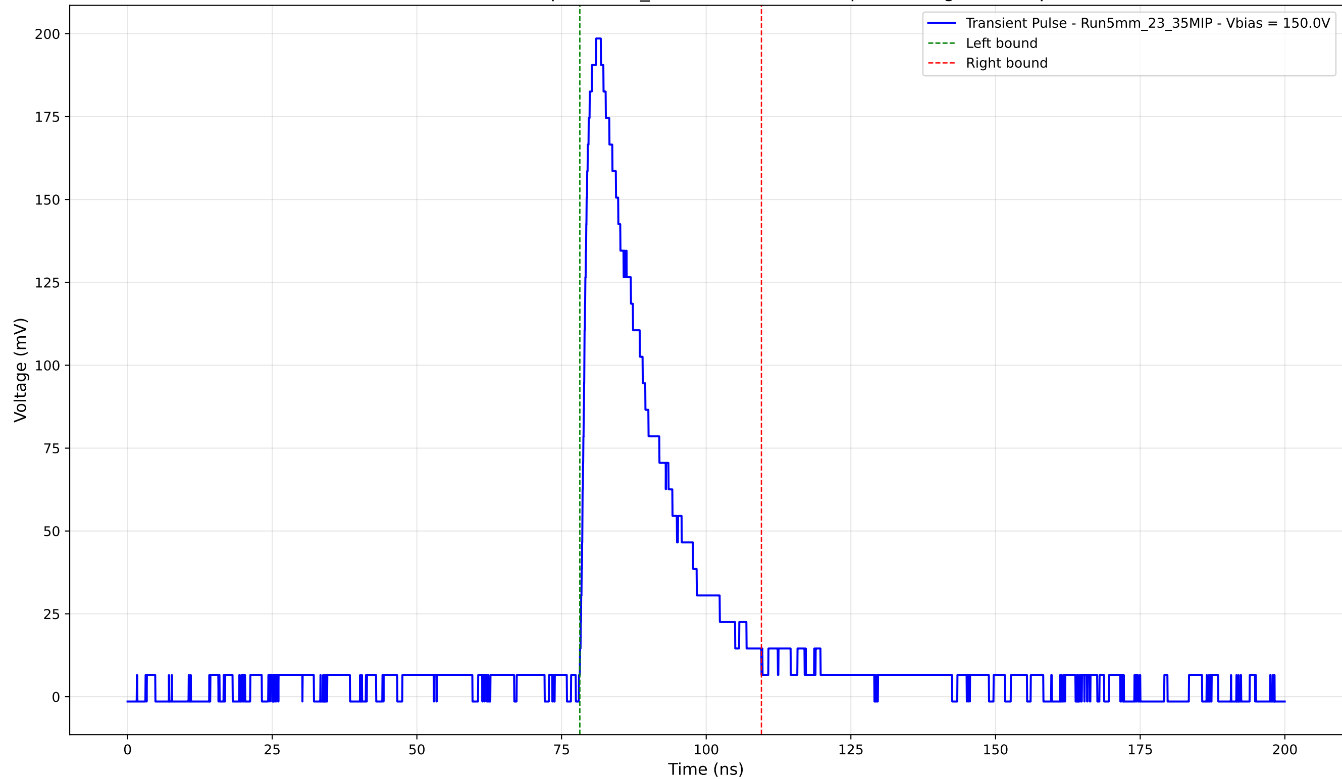
Transient Pulse - Sample: 5mm_23 - Position: 2105.0 \mu\text{m} - Charge: 48.42 pC
