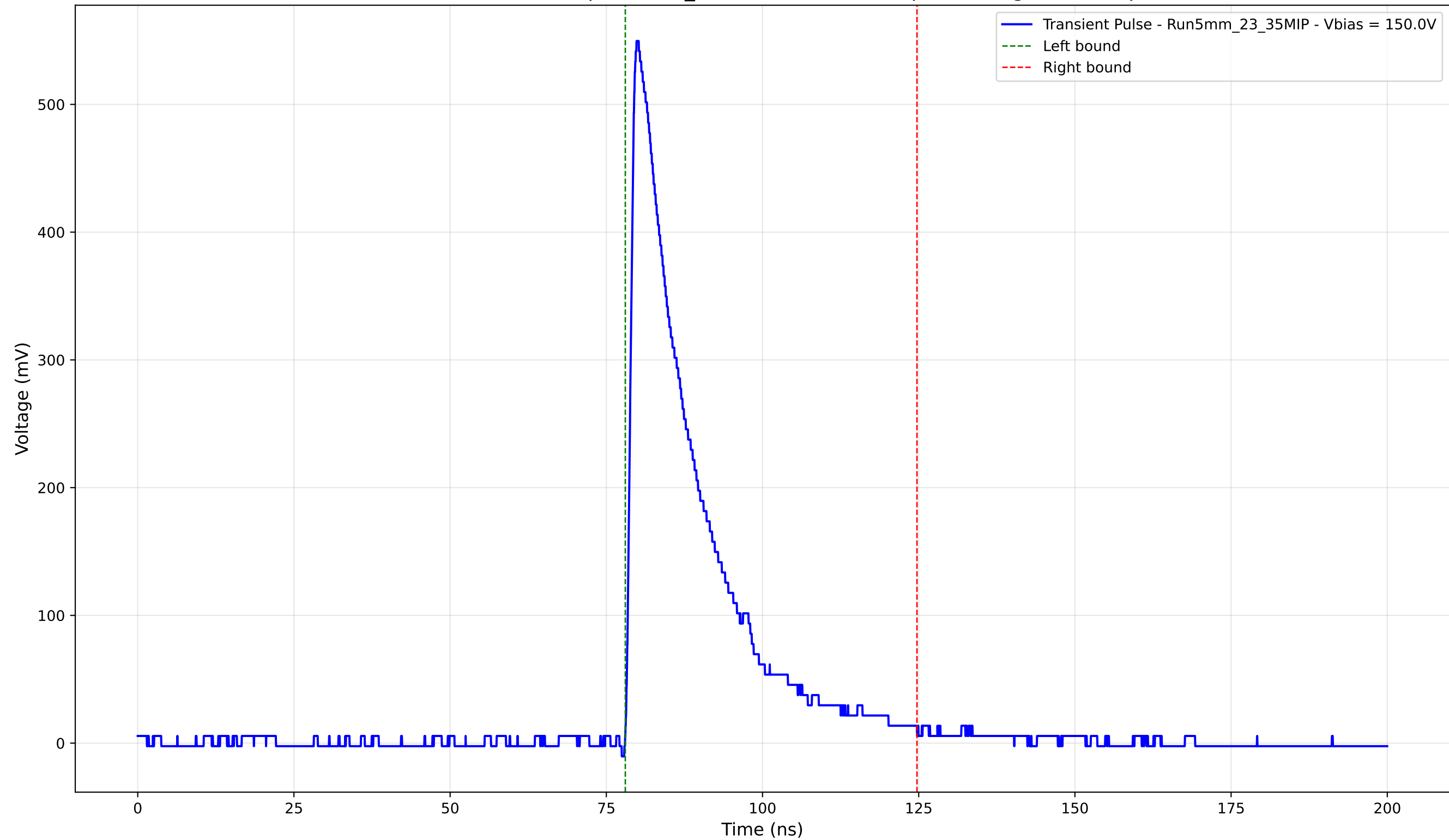
Transient Pulse - Sample: 5mm_23 - Position: 3895.0 \mu\text{m} - Charge: 122.79 pC
