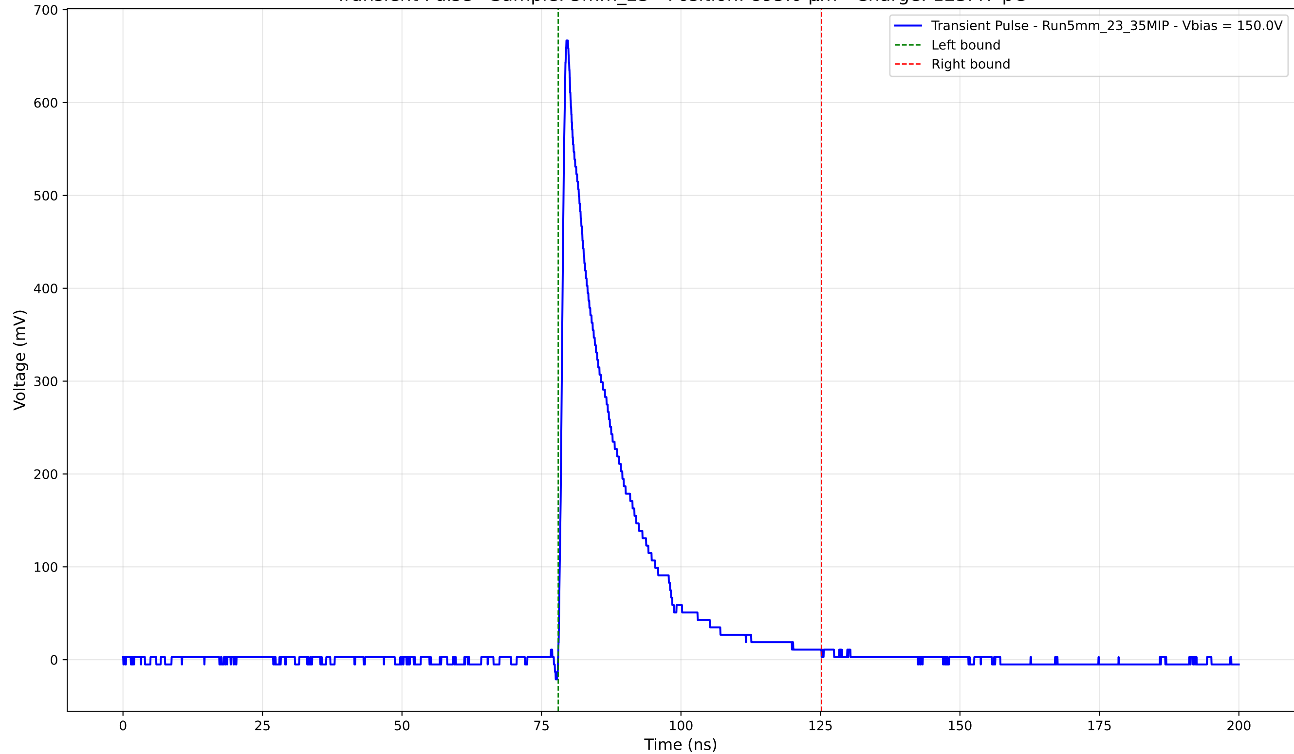
Transient Pulse - Sample: 5mm_23 - Position: 895.0 \mu\text{m} - Charge: 123.47 pC
