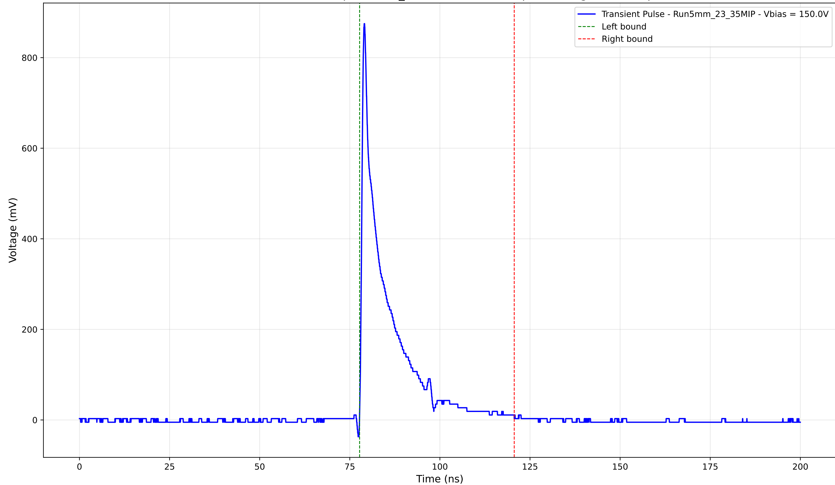
Transient Pulse - Sample: 5mm_23 - Position: 305.0 \mu\text{m} - Charge: 115.64 pC
