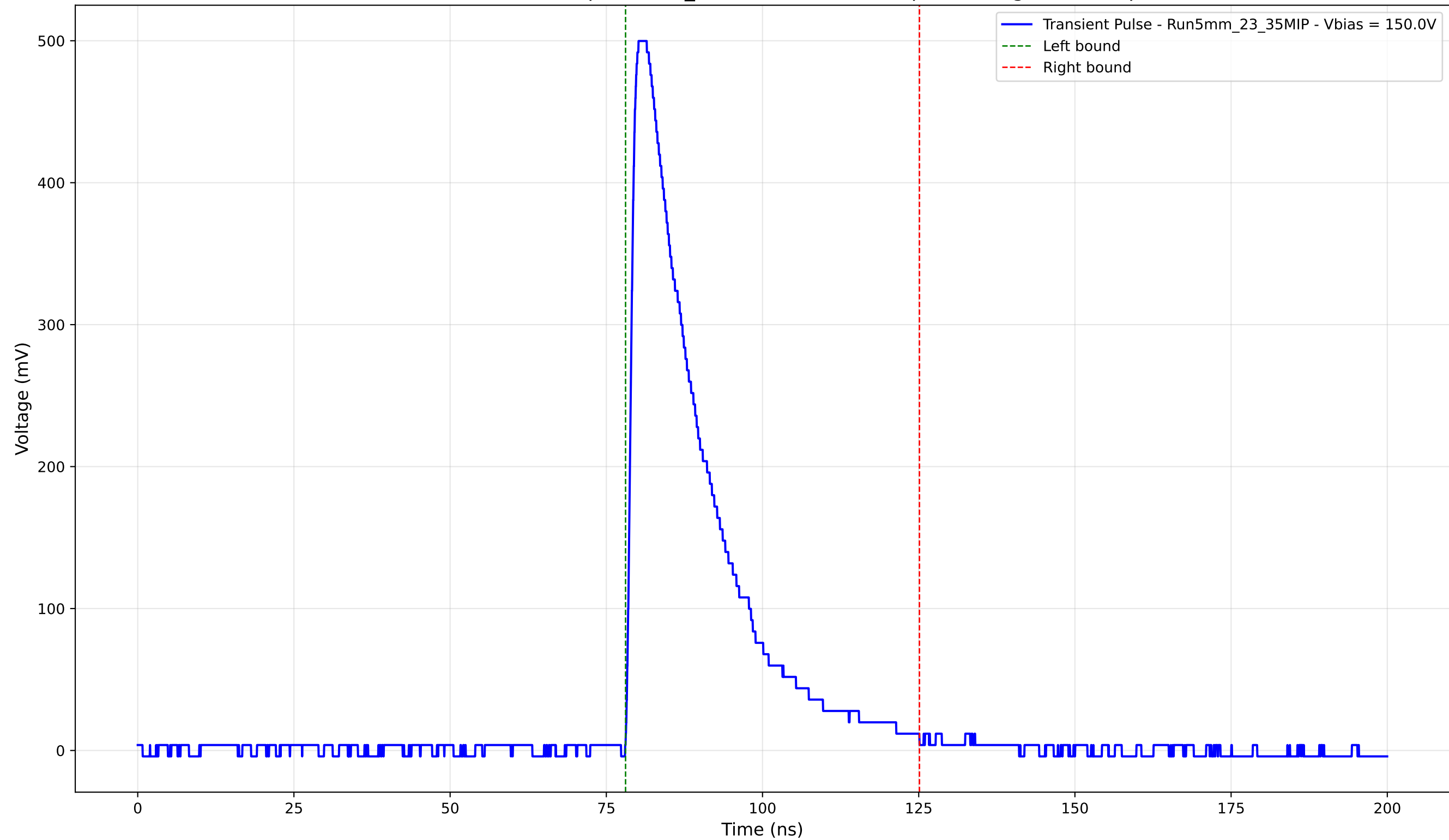
Transient Pulse - Sample: 5mm_23 - Position: 3390.0 \mu\text{m} - Charge: 127.67 pC
