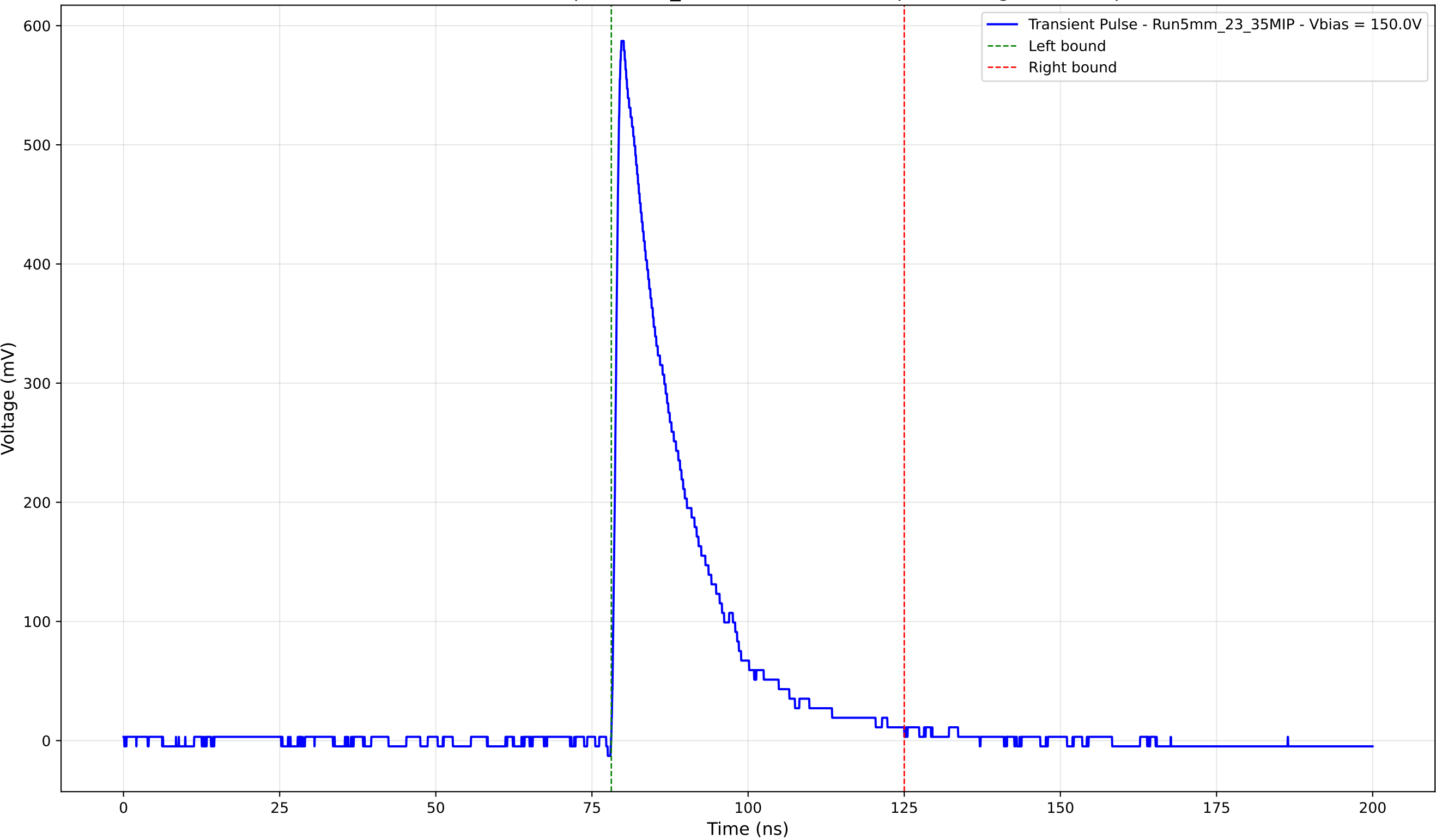
Transient Pulse - Sample: 5mm_23 - Position: 1270.0 \mu\text{m} - Charge: 127.73 pC
