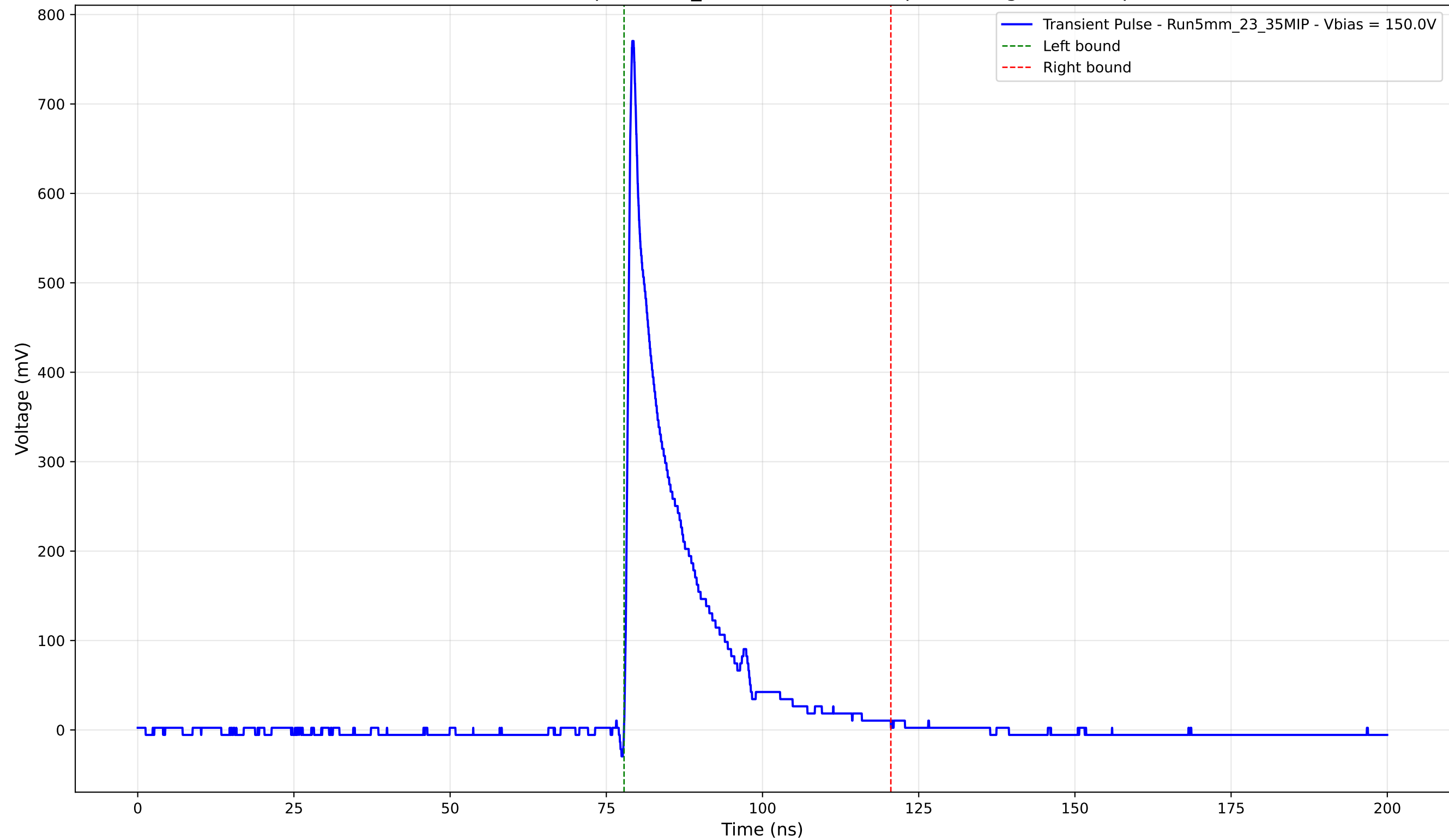
Transient Pulse - Sample: 5mm_23 - Position: 520.0 \mu\text{m} - Charge: 112.55 pC
