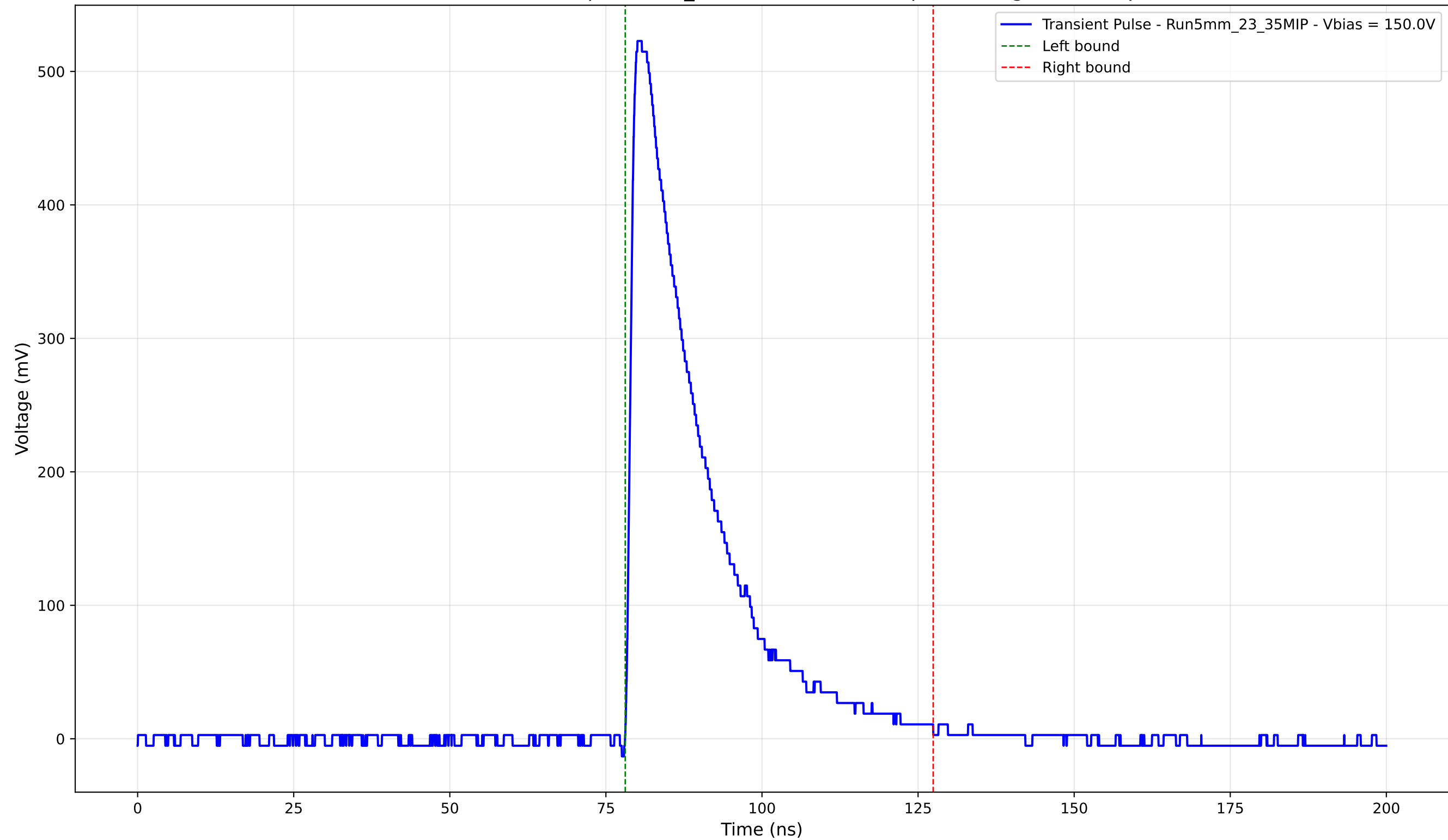
Transient Pulse - Sample: 5mm_23 - Position: 1750.0 \mu\text{m} - Charge: 132.39 pC
