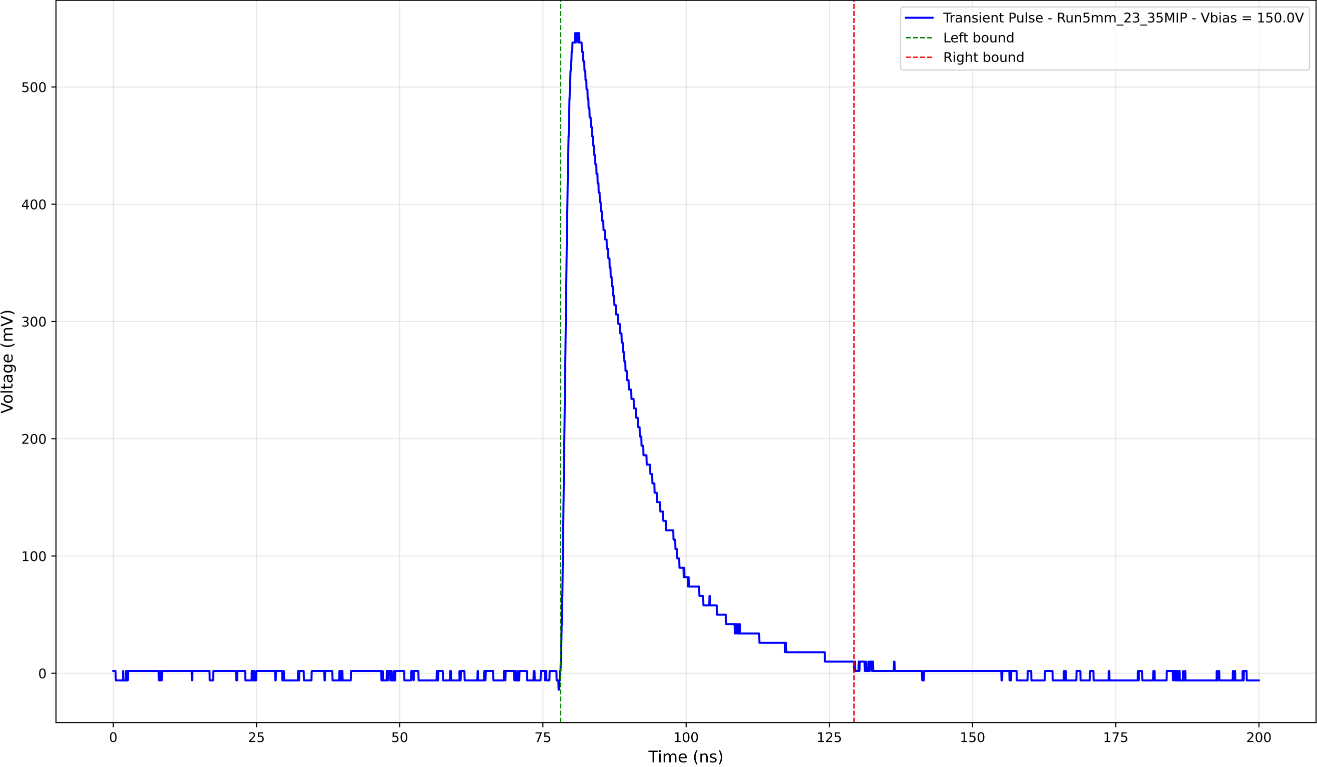
Transient Pulse - Sample: 5mm_23 - Position: 1980.0 \mu\text{m} - Charge: 142.65 pC
