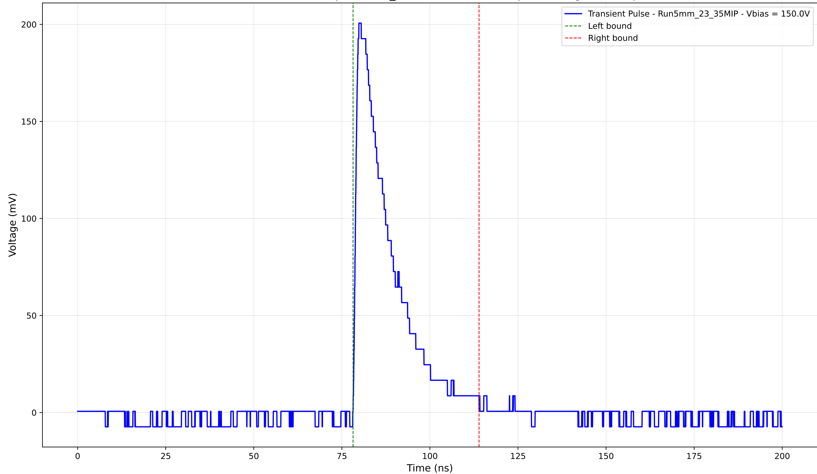
Transient Pulse - Sample: 5mm_23 - Position: 3685.0 \mu\text{m} - Charge: 43.84 pC
