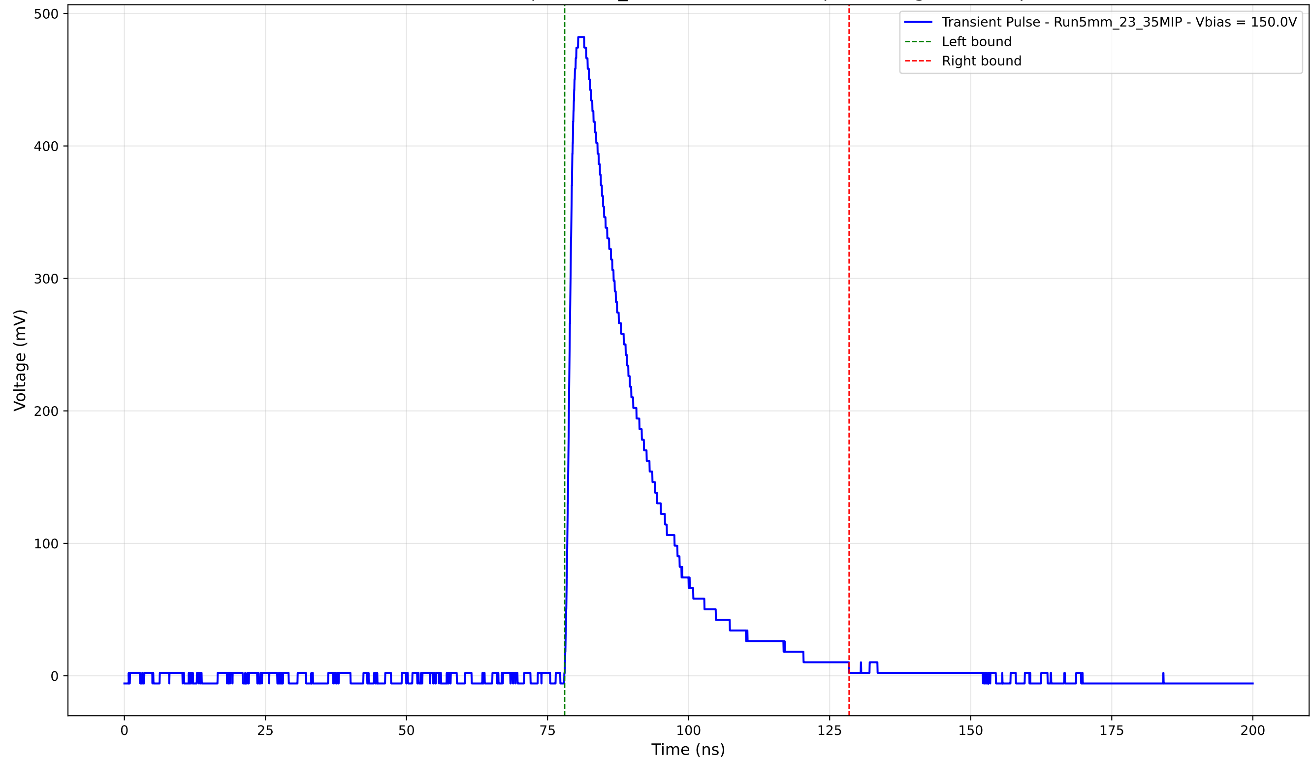
Transient Pulse - Sample: 5mm_23 - Position: 3240.0 \mu\text{m} - Charge: 124.34 pC
