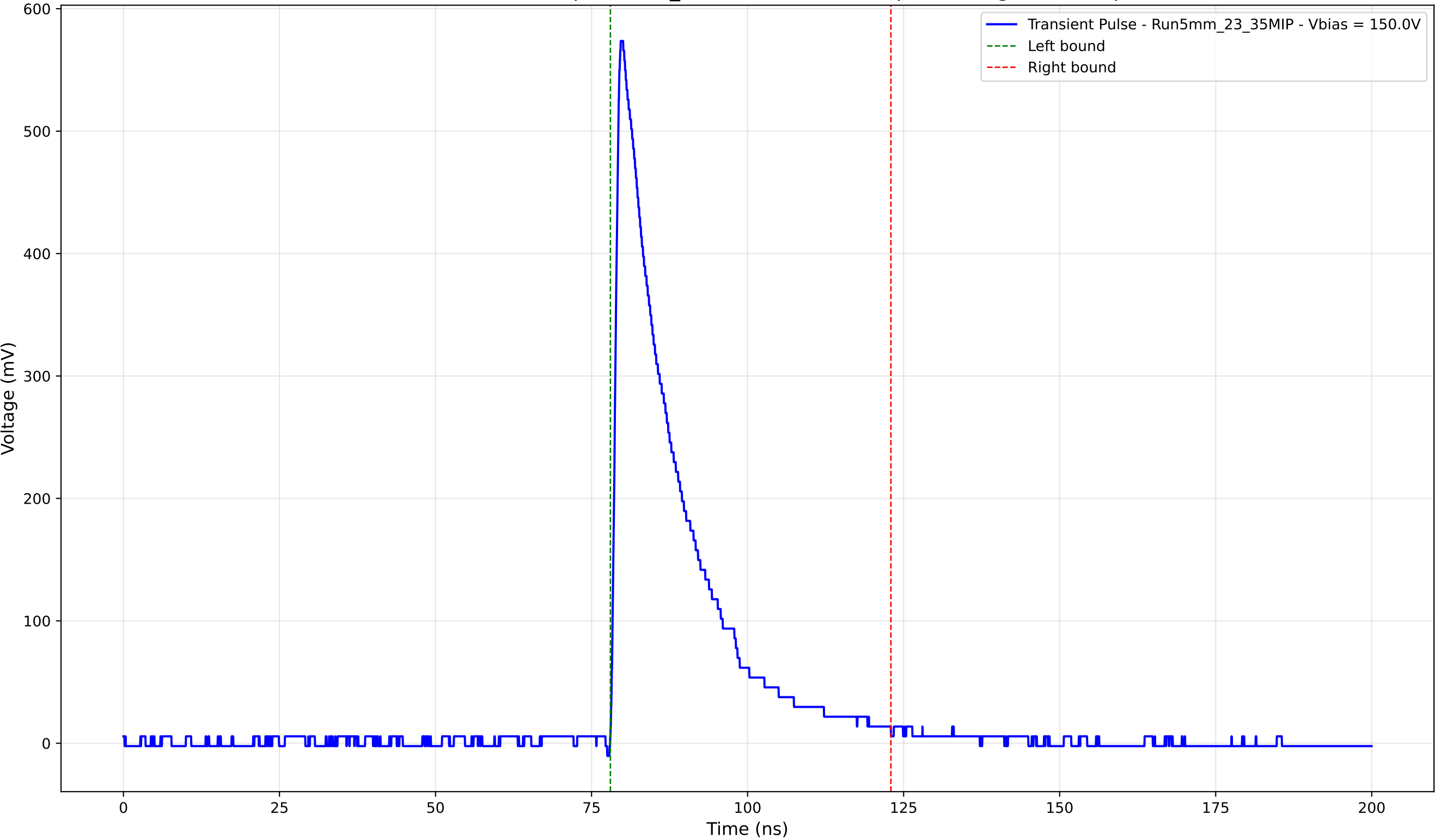
Transient Pulse - Sample: 5mm_23 - Position: 4025.0 \mu\text{m} - Charge: 120.97 pC
