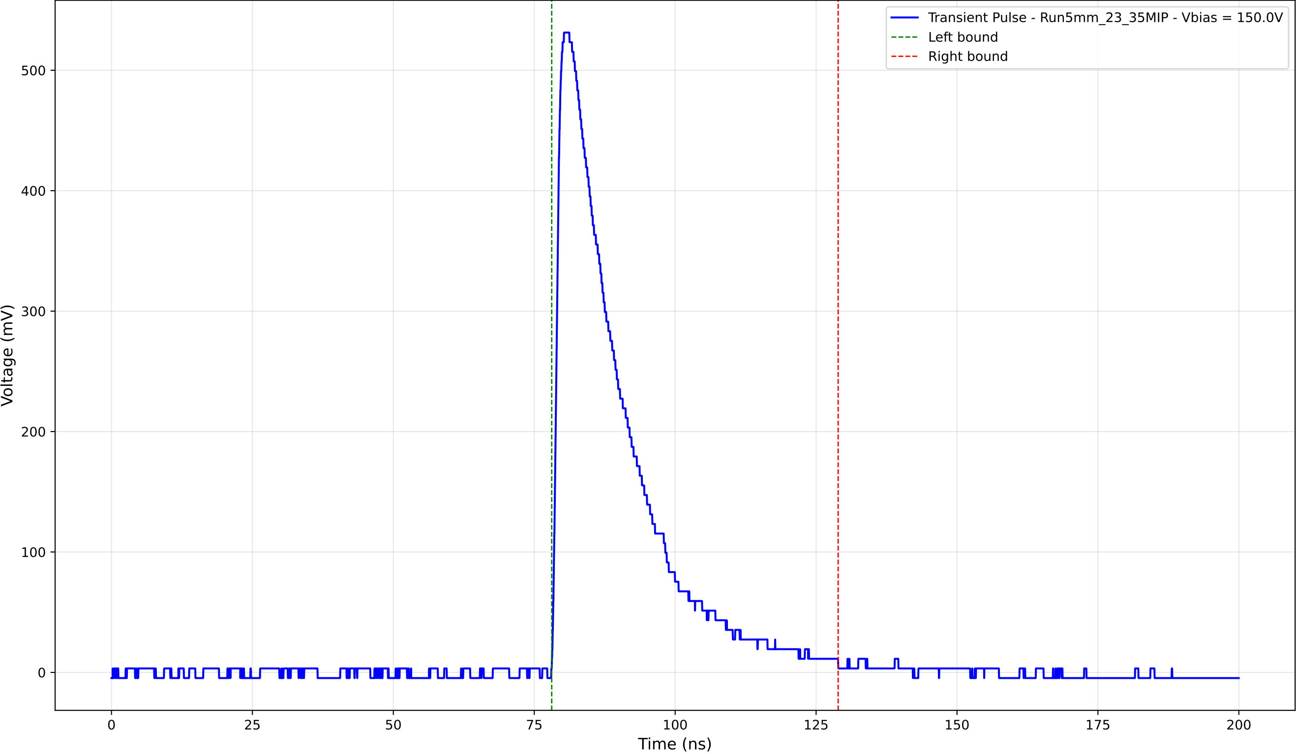
Transient Pulse - Sample: 5mm_23 - Position: 1910.0 \mu\text{m} - Charge: 138.13 pC
