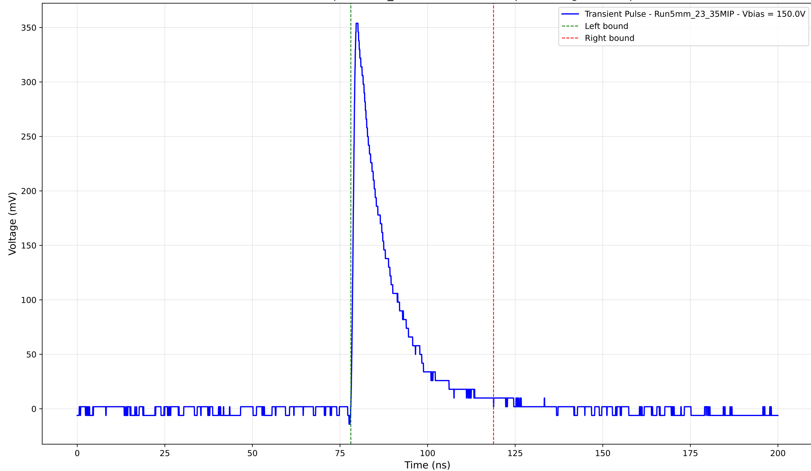
Transient Pulse - Sample: 5mm_23 - Position: 1175.0 \mu\text{m} - Charge: 71.87 pC
