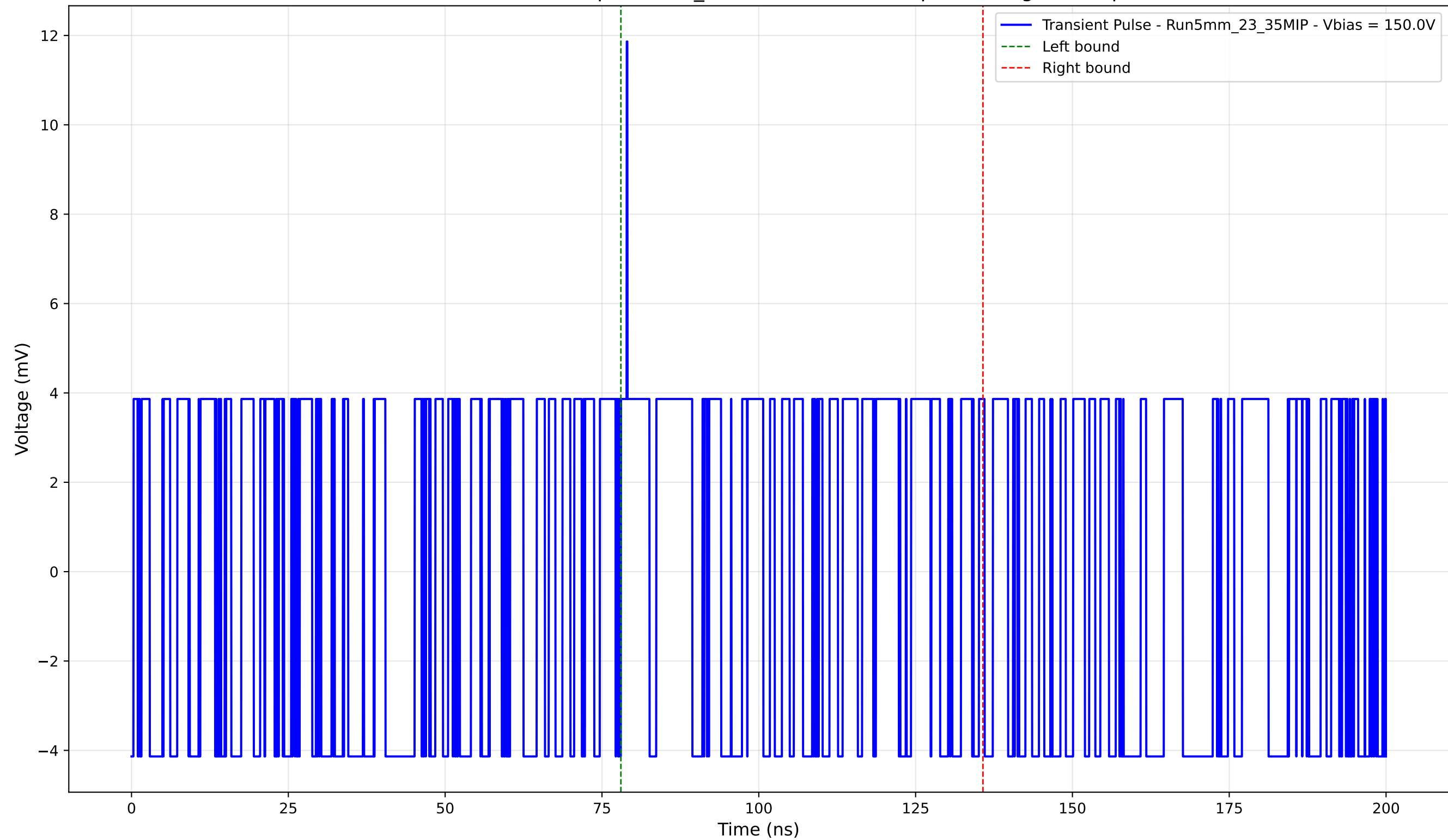
Transient Pulse - Sample: 5mm_23 - Position: 5240.0 \mu\text{m} - Charge: 1.30 pC
