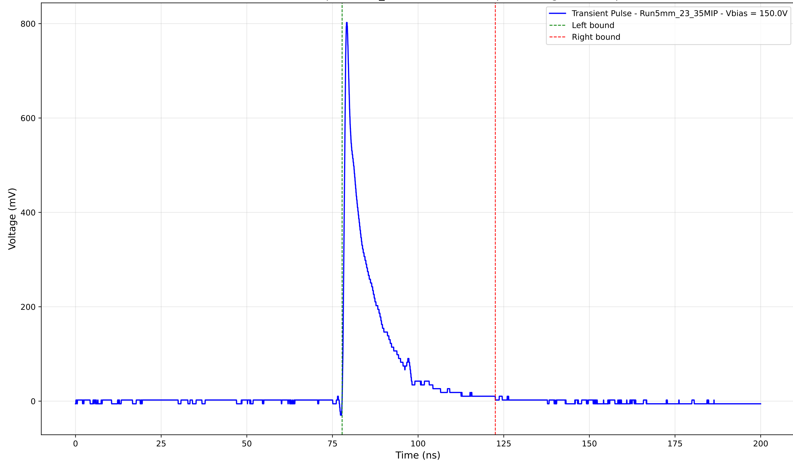
Transient Pulse - Sample: 5mm_23 - Position: 460.0 \mu\text{m} - Charge: 113.96 pC
