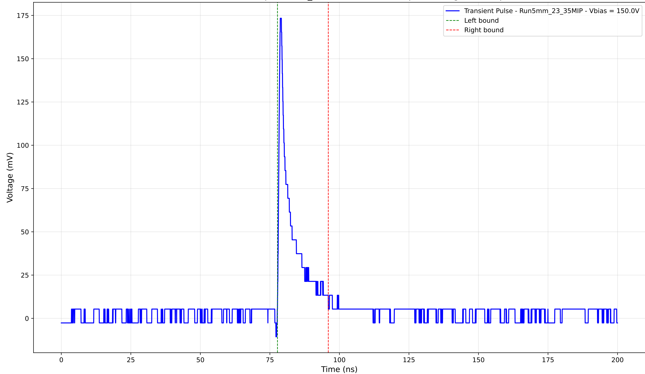
Transient Pulse - Sample: 5mm_23 - Position: 5095.0 \mu\text{m} - Charge: 16.55 pC
