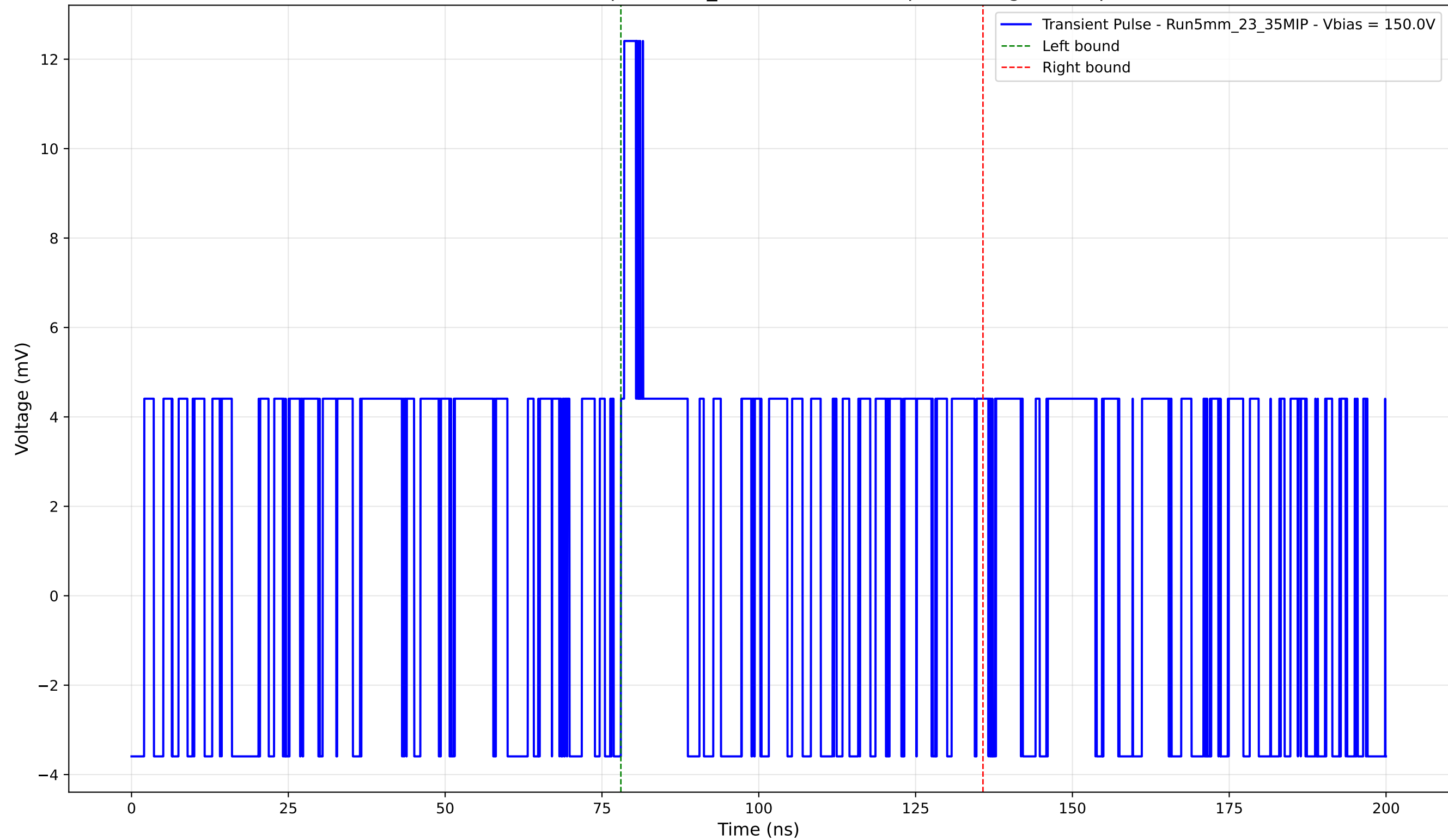
Transient Pulse - Sample: 5mm_23 - Position: 55.0 \mu\text{m} - Charge: 2.53 pC
