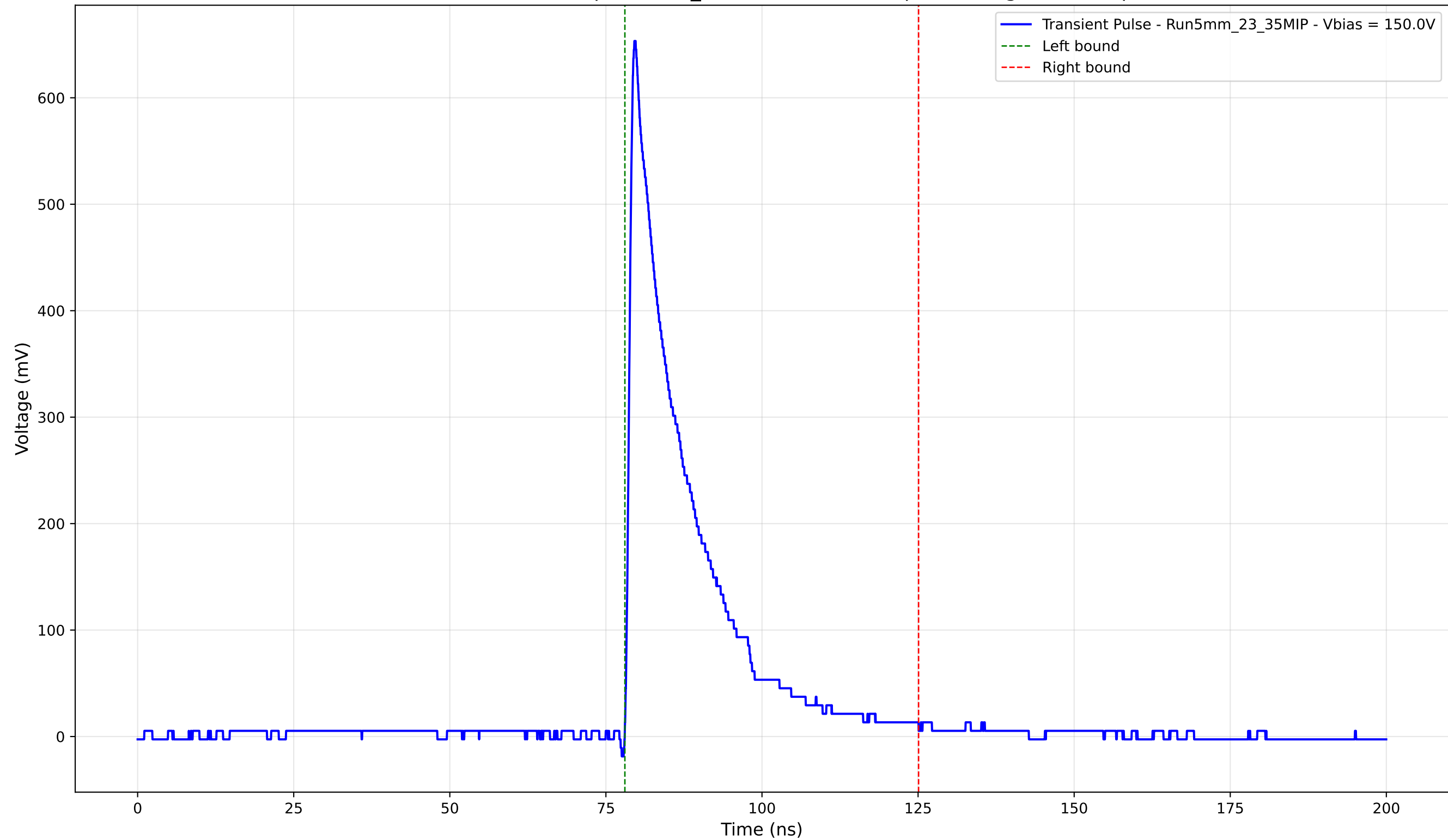
Transient Pulse - Sample: 5mm_23 - Position: 970.0 \mu\text{m} - Charge: 124.51 pC
