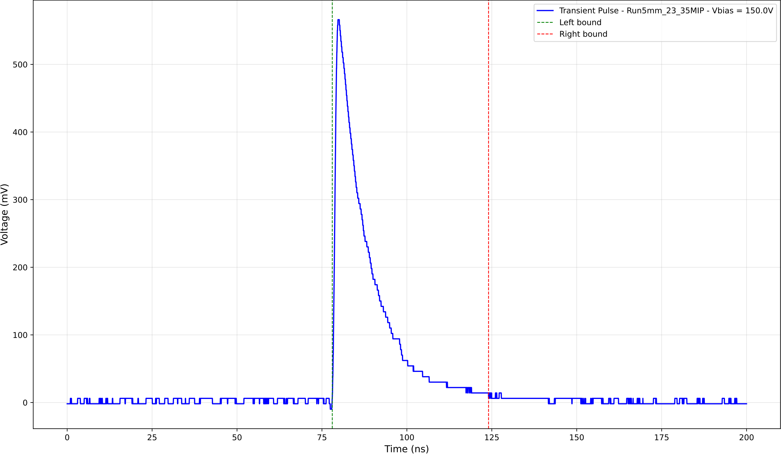
Transient Pulse - Sample: 5mm_23 - Position: 4005.0 \mu\text{m} - Charge: 120.42 pC
