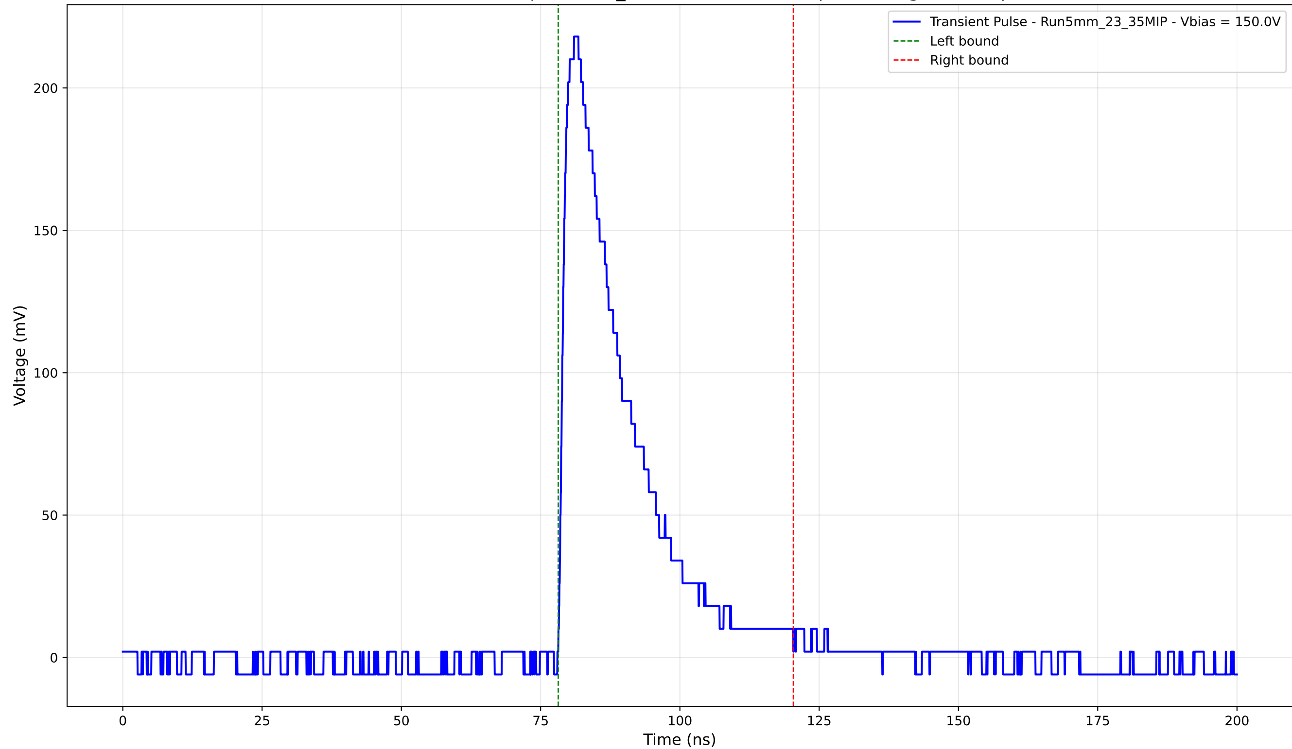
Transient Pulse - Sample: 5mm_23 - Position: 3110.0 \mu\text{m} - Charge: 54.47 pC
