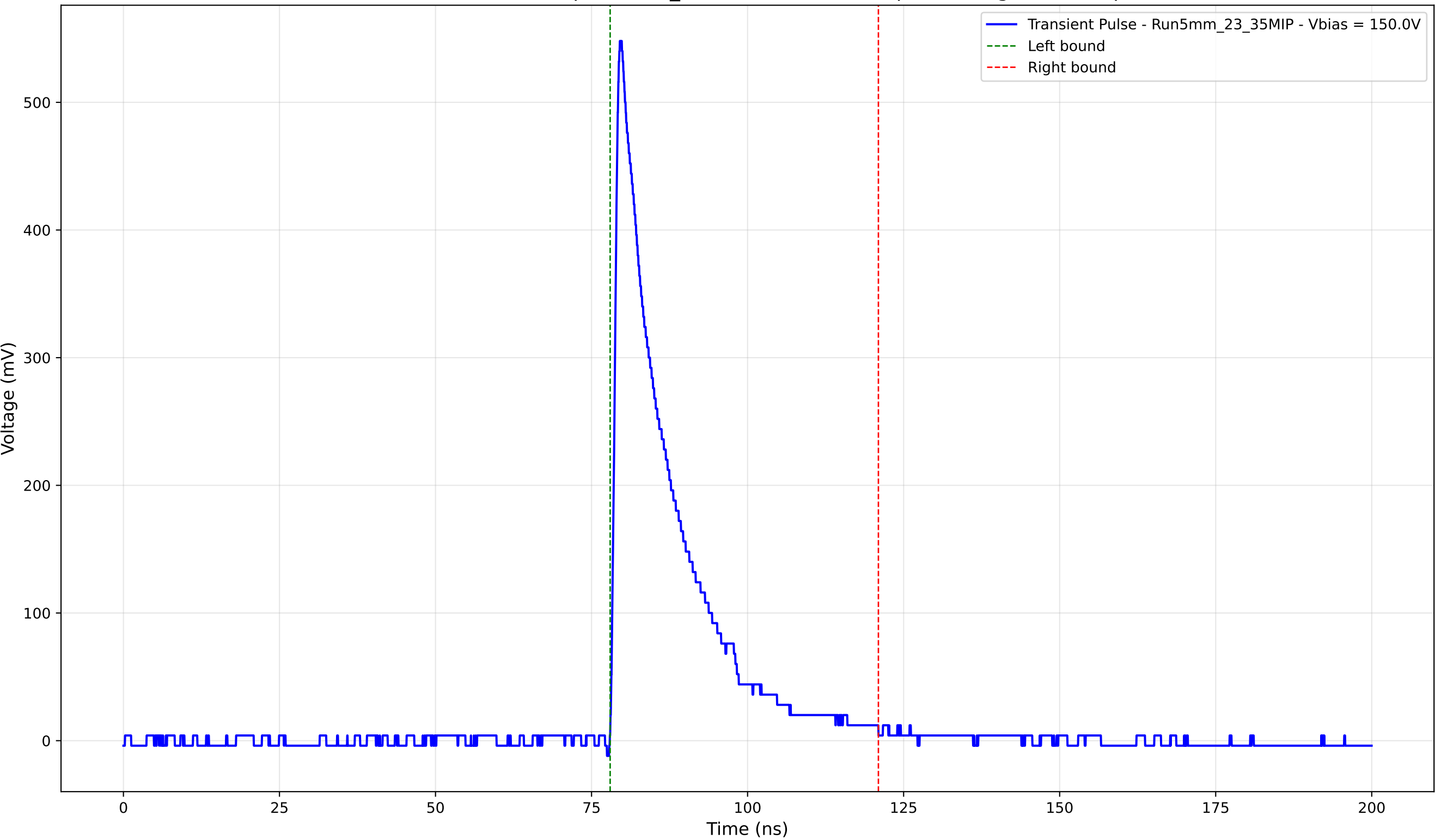
Transient Pulse - Sample: 5mm_23 - Position: 4245.0 \mu\text{m} - Charge: 101.76 pC
