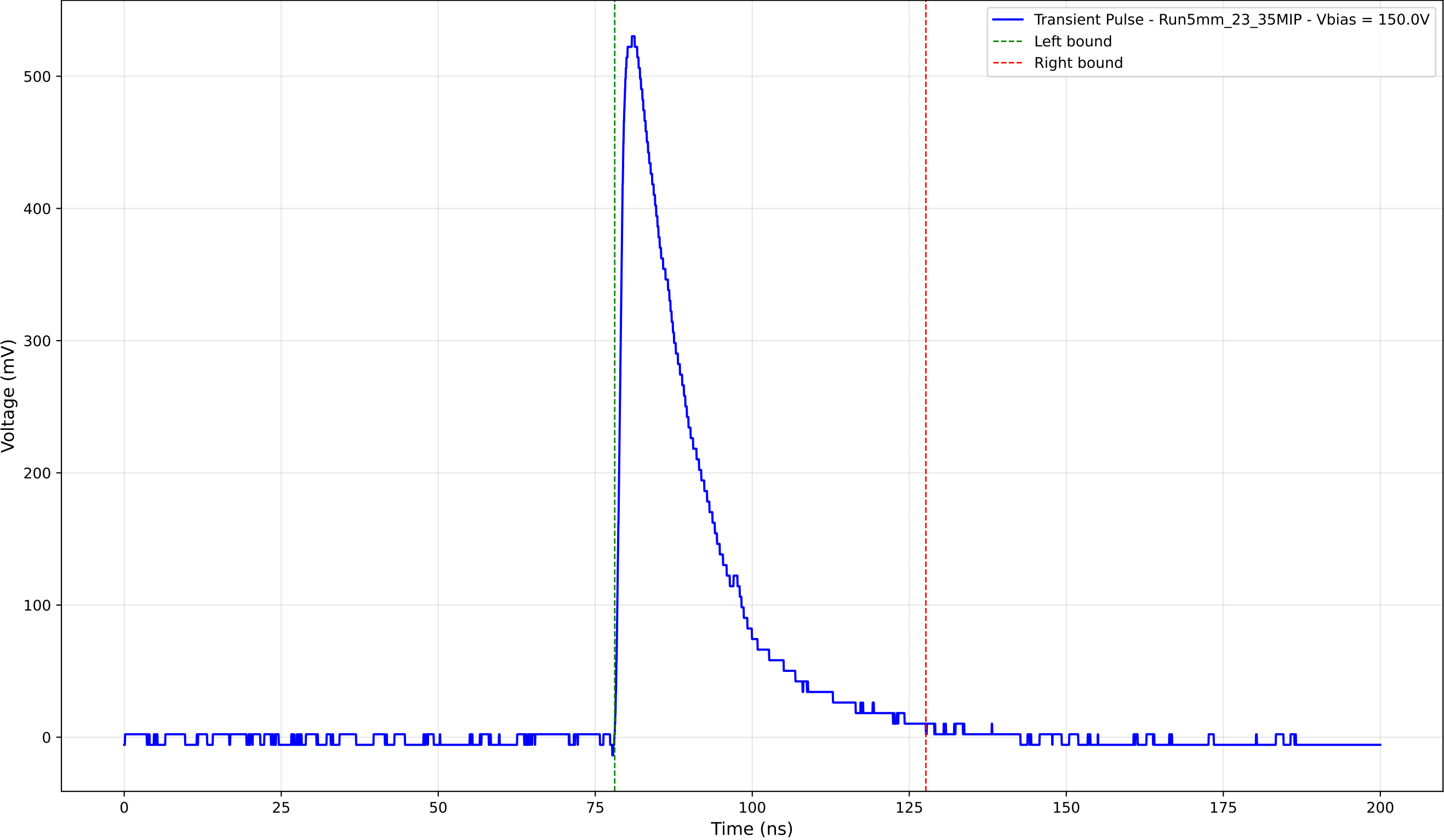
Transient Pulse - Sample: 5mm_23 - Position: 1895.0 \mu\text{m} - Charge: 136.94 pC
