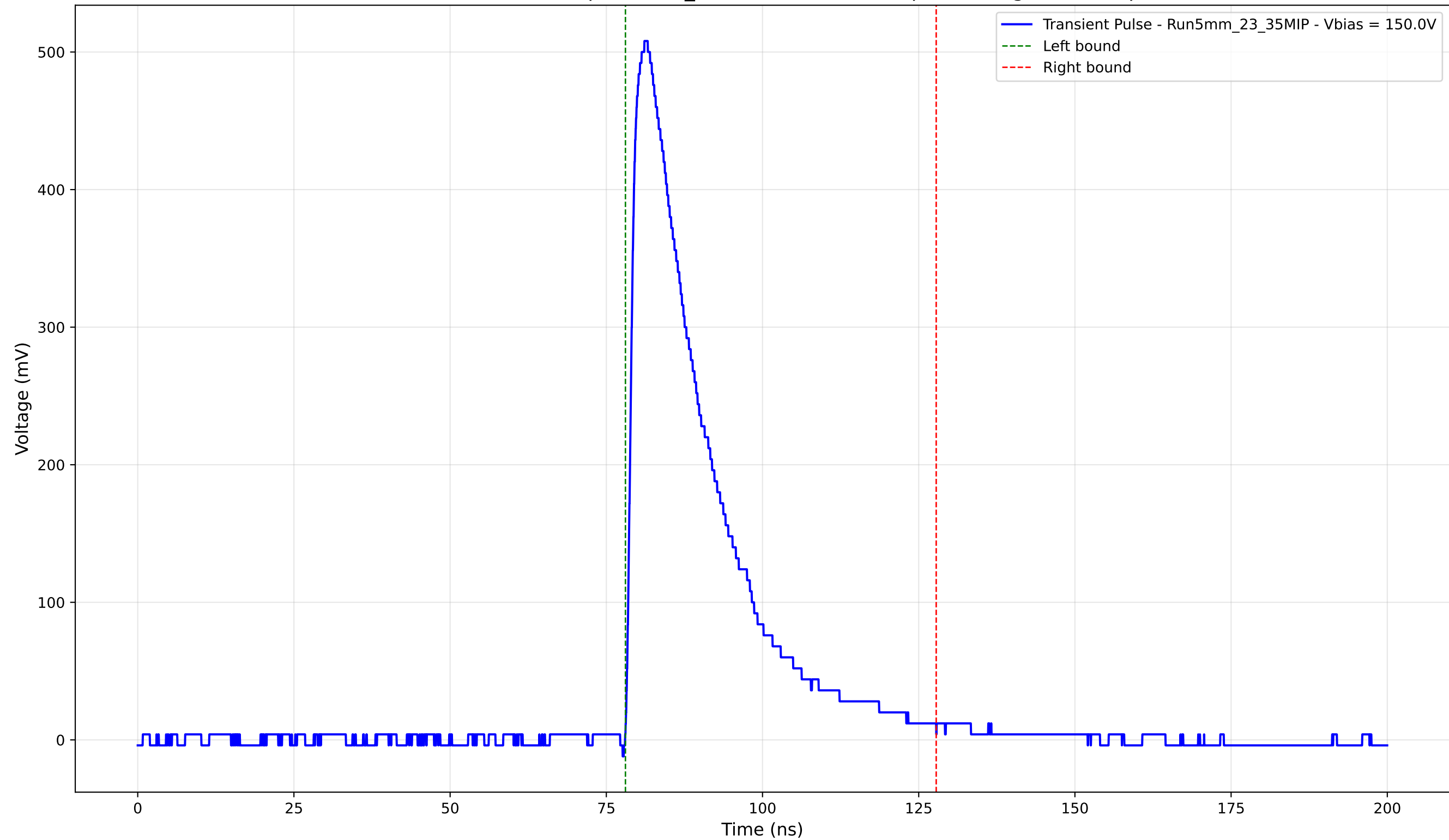
Transient Pulse - Sample: 5mm_23 - Position: 2520.0 \mu\text{m} - Charge: 137.49 pC
