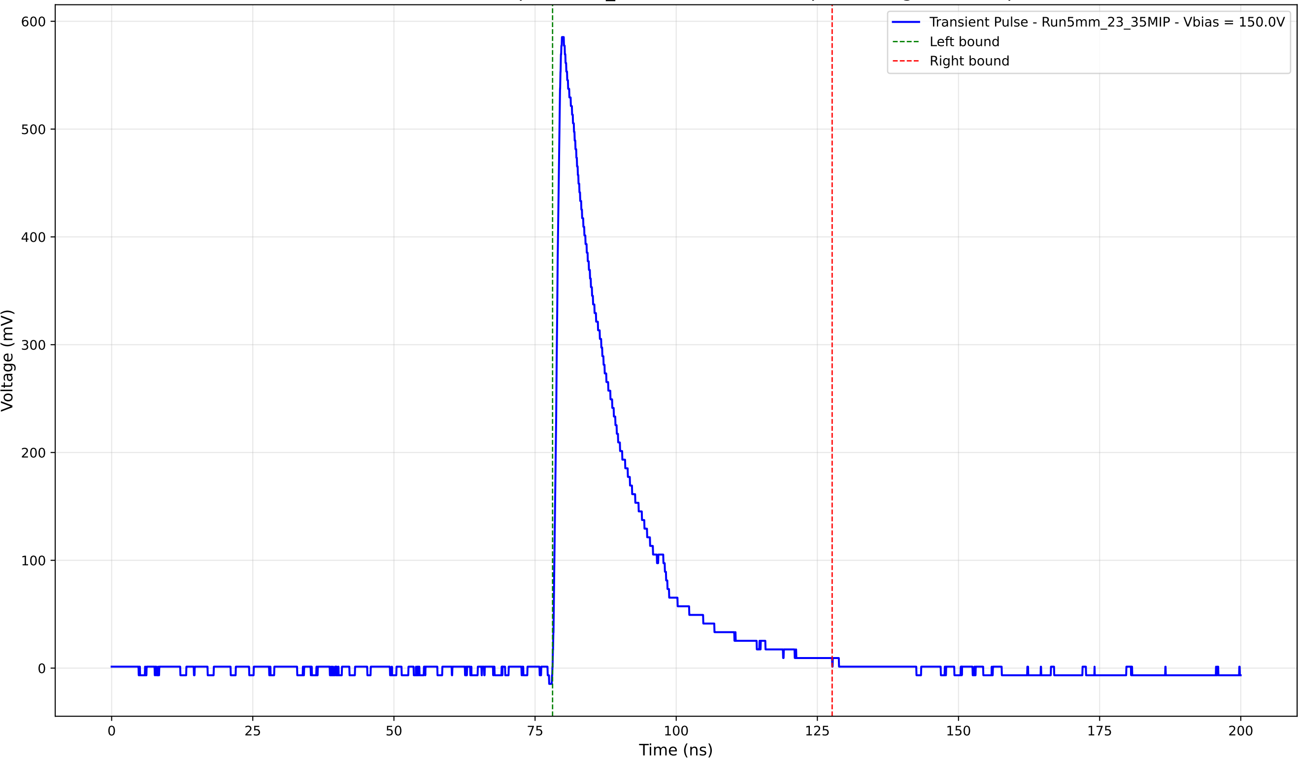
Transient Pulse - Sample: 5mm_23 - Position: 1300.0 \mu\text{m} - Charge: 128.03 pC
