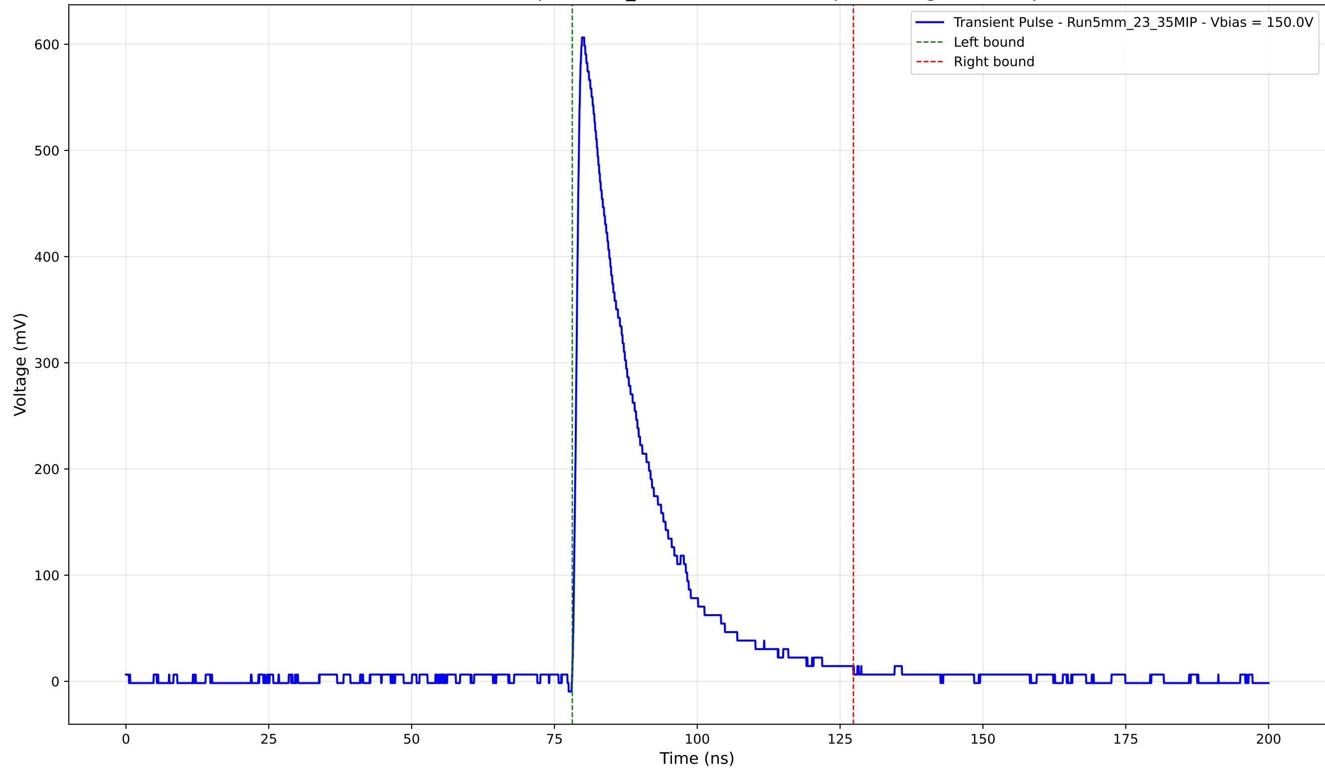
Transient Pulse - Sample: 5mm_23 - Position: 1375.0 \mu\text{m} - Charge: 140.60 pC
