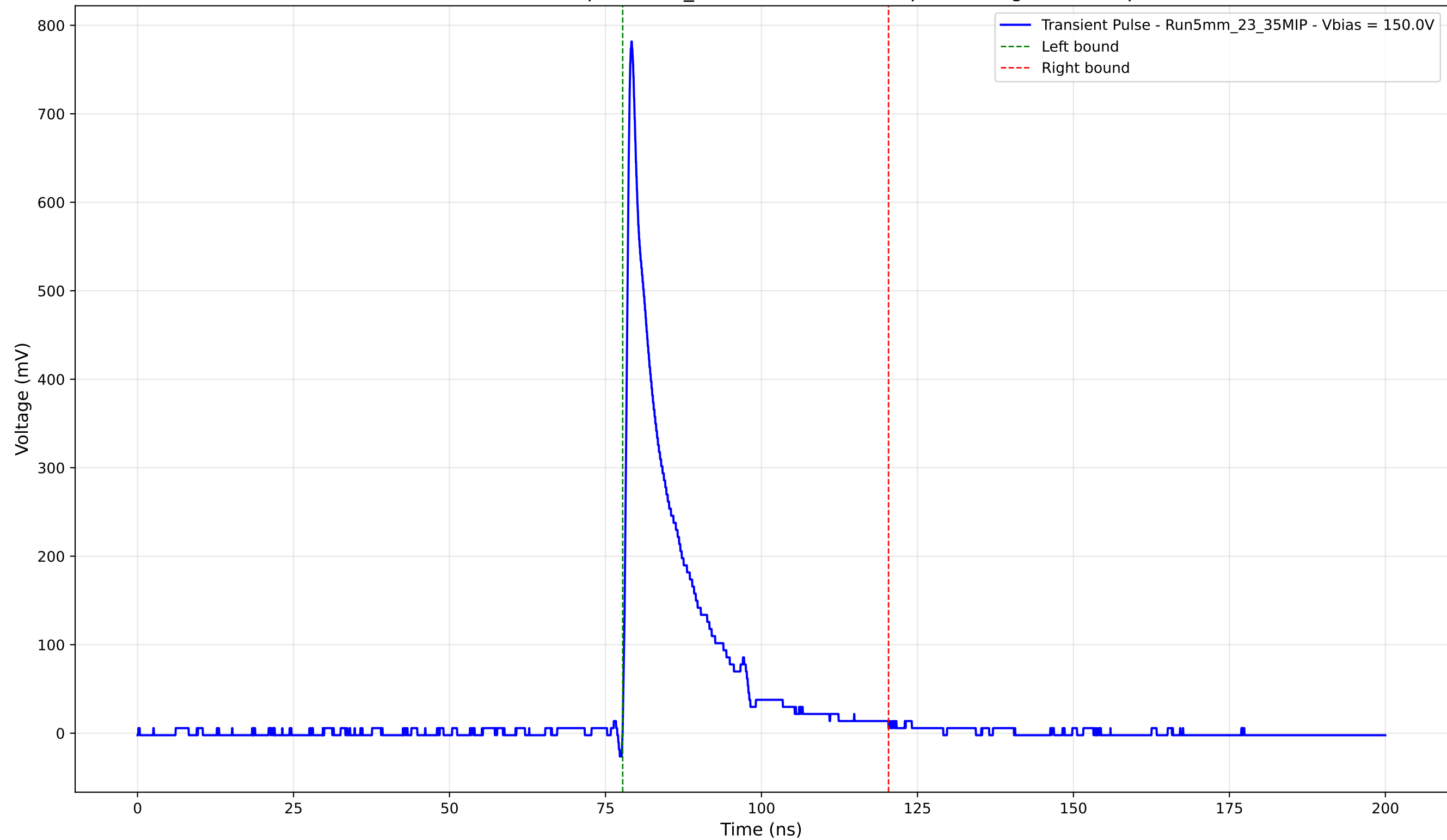
Transient Pulse - Sample: 5mm_23 - Position: 4765.0 \mu\text{m} - Charge: 110.15 pC
