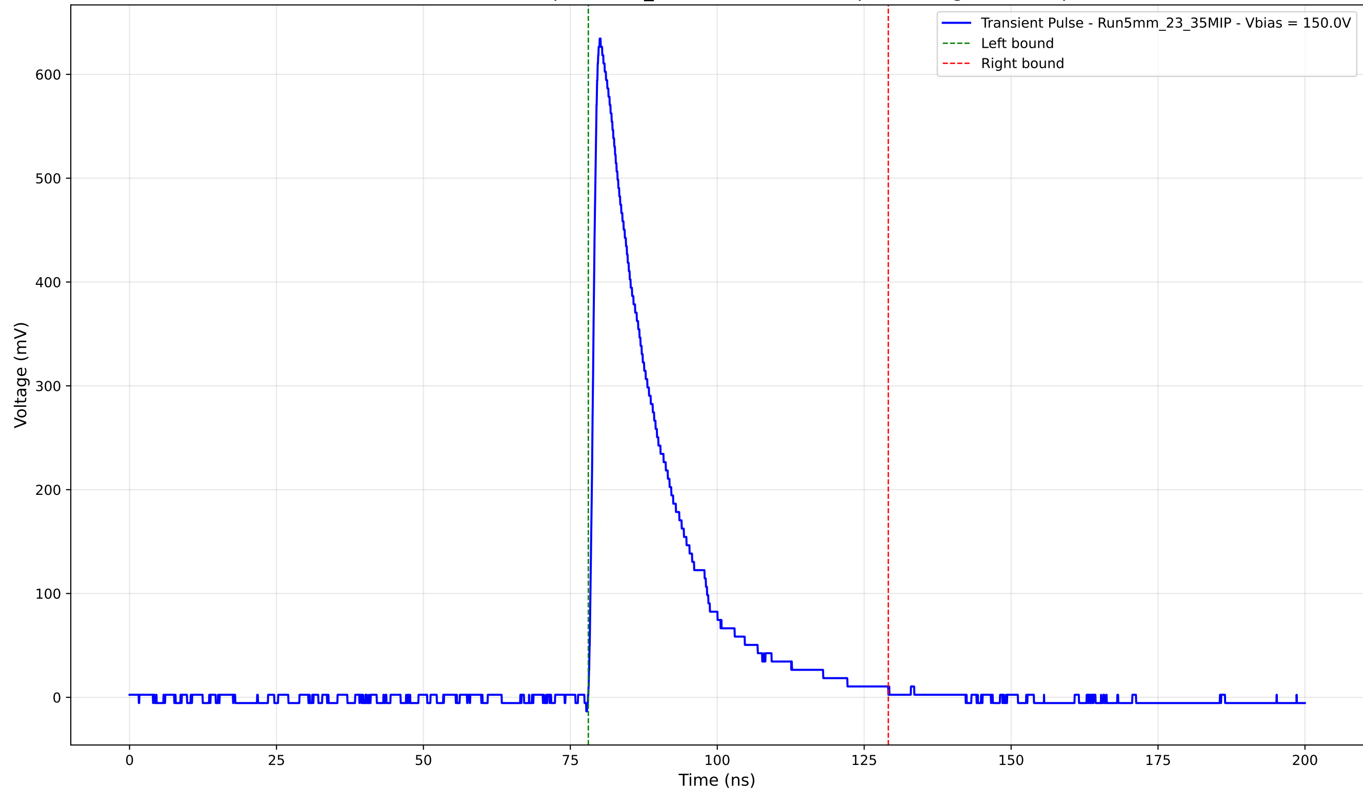
Transient Pulse - Sample: 5mm_23 - Position: 1475.0 \mu\text{m} - Charge: 148.34 pC
