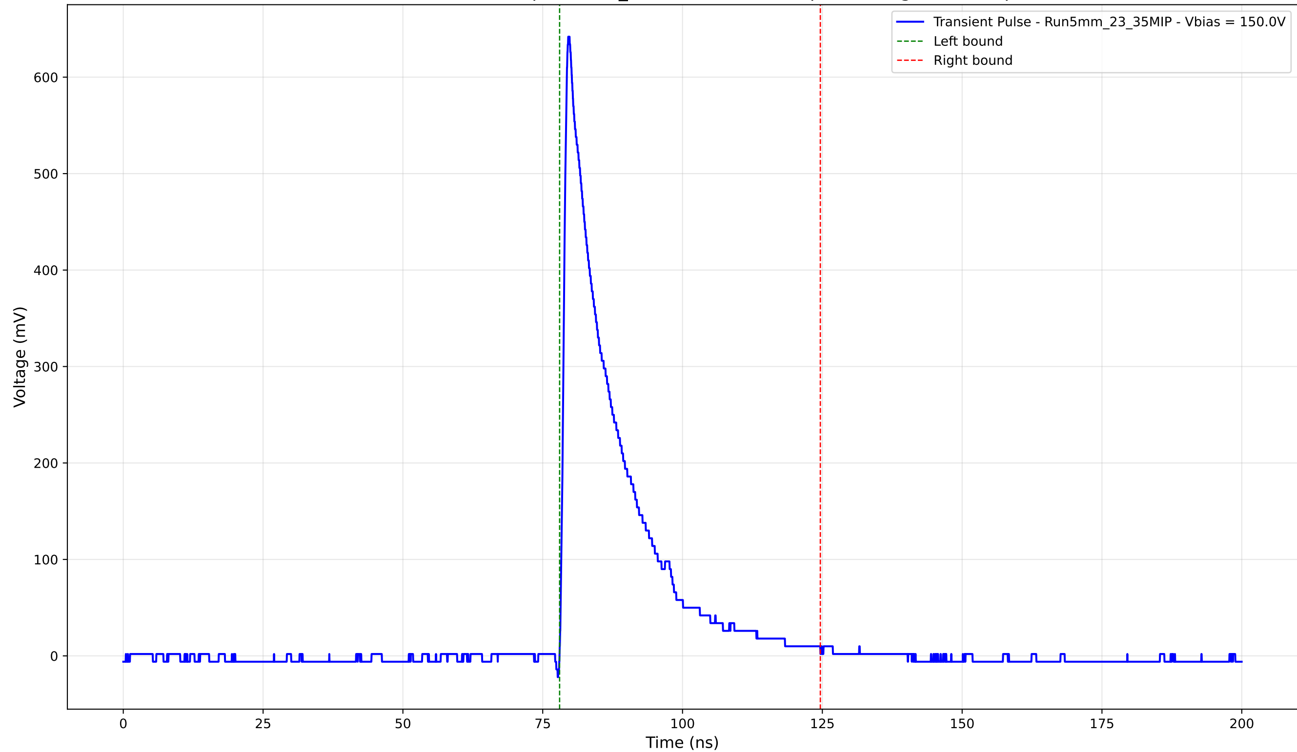
Transient Pulse - Sample: 5mm_23 - Position: 995.0 \mu\text{m} - Charge: 123.21 pC
