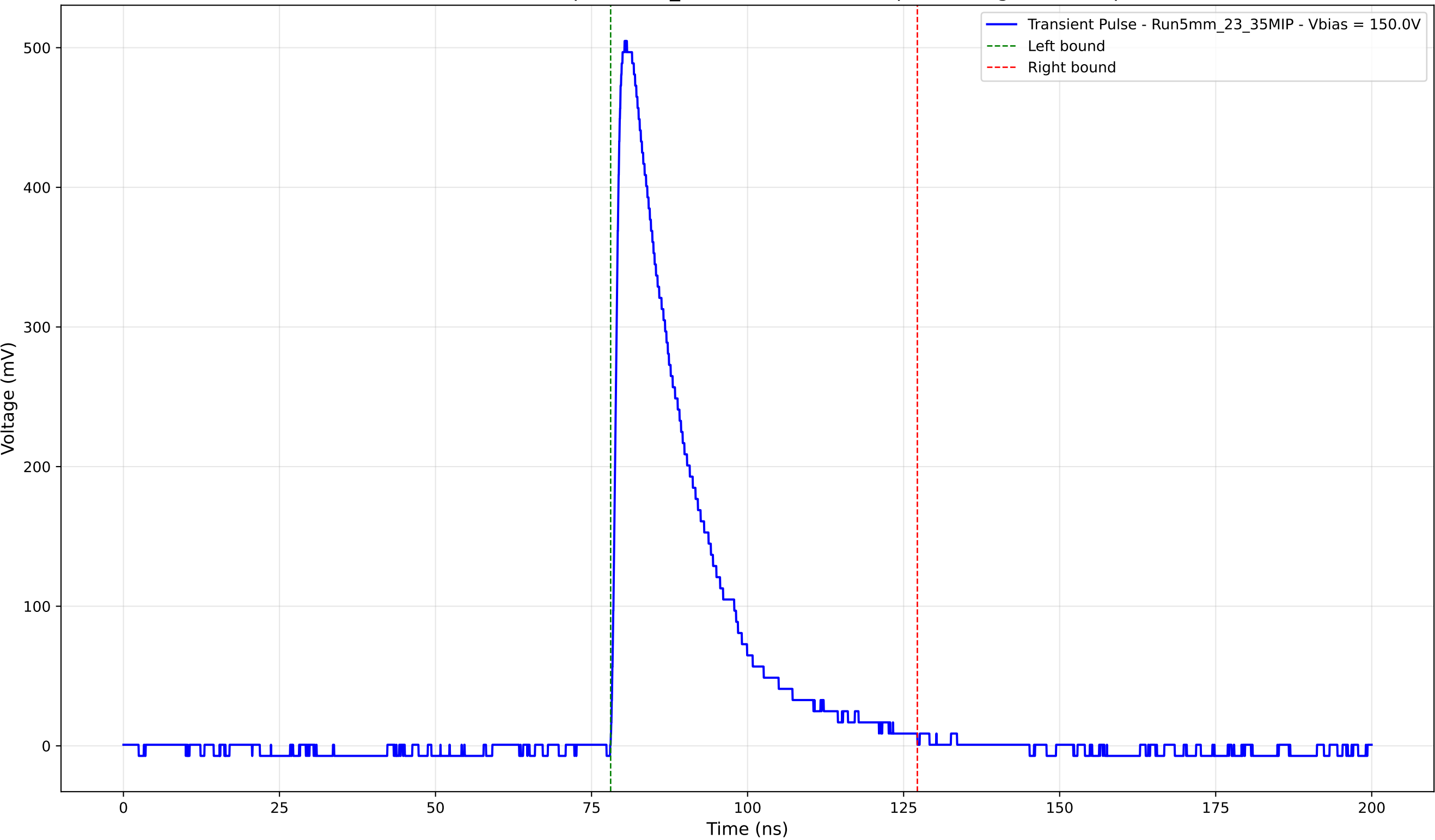
Transient Pulse - Sample: 5mm_23 - Position: 3485.0 \mu\text{m} - Charge: 124.91 pC
