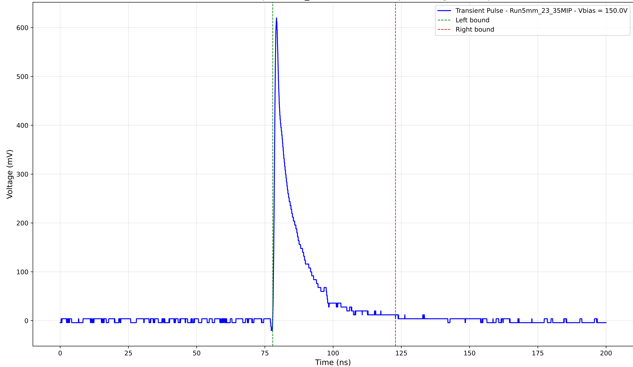
Transient Pulse - Sample: 5mm_23 - Position: 555.0 \mu\text{m} - Charge: 89.42 pC
