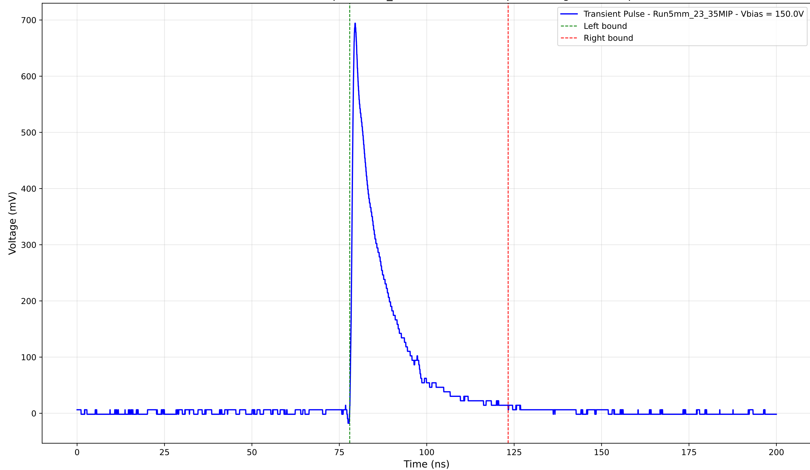
Transient Pulse - Sample: 5mm_23 - Position: 830.0 \mu\text{m} - Charge: 124.84 pC
