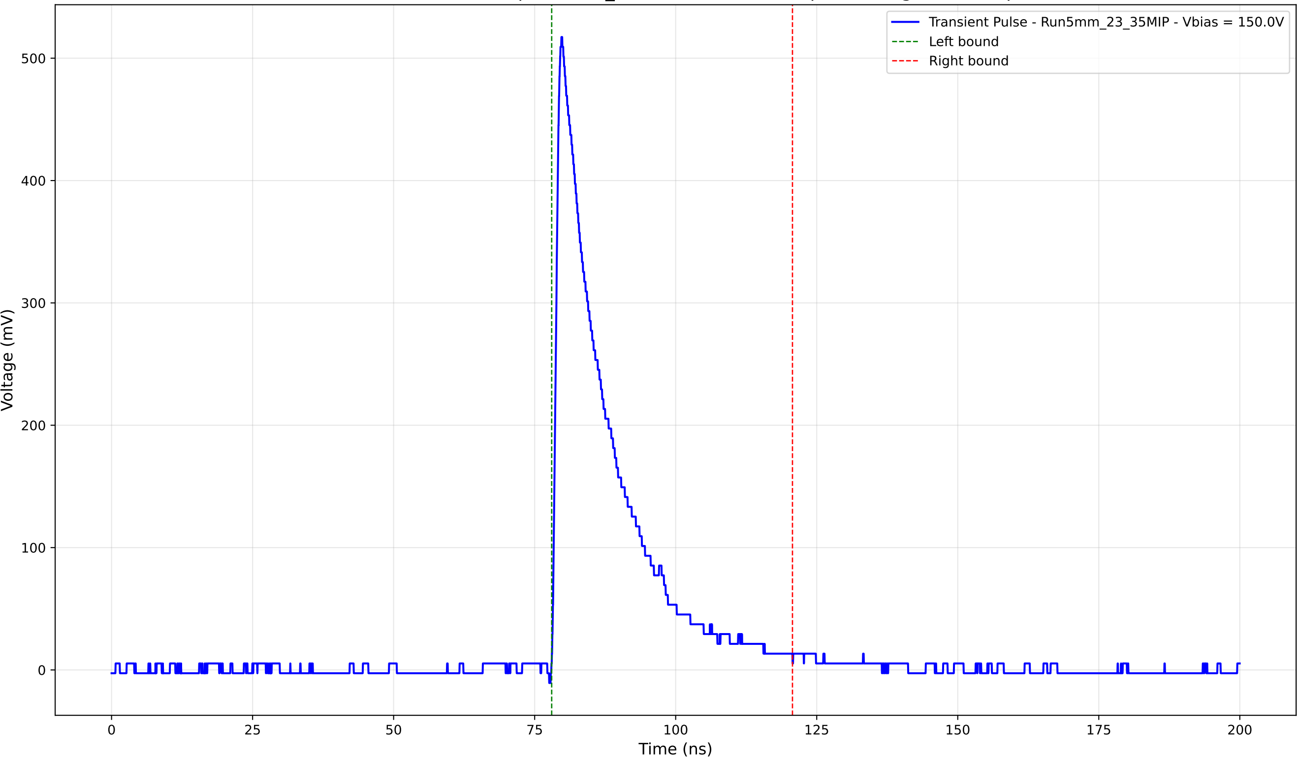
Transient Pulse - Sample: 5mm_23 - Position: 4080.0 \mu\text{m} - Charge: 103.21 pC
