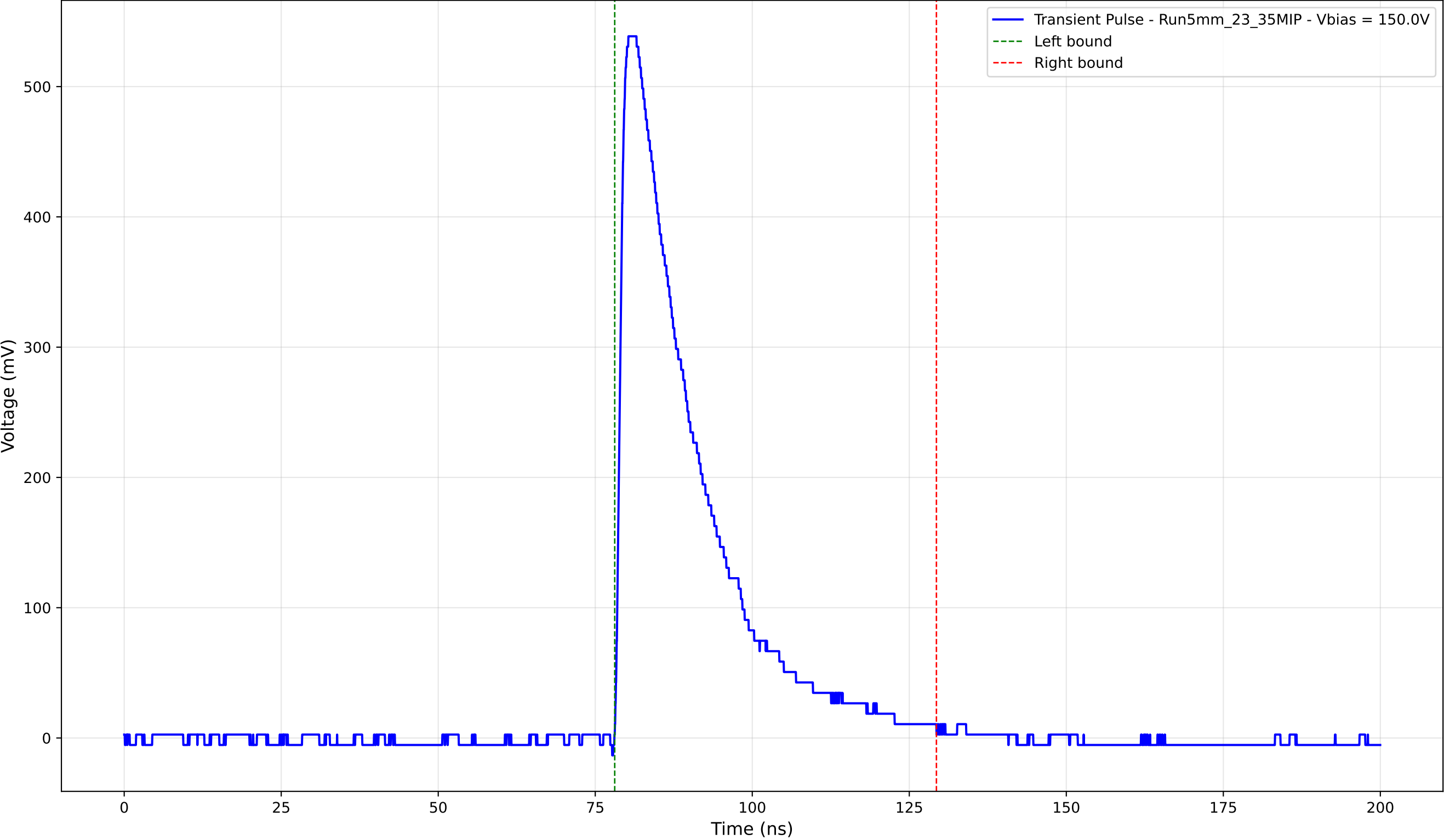
Transient Pulse - Sample: 5mm_23 - Position: 1960.0 \mu\text{m} - Charge: 142.67 pC
