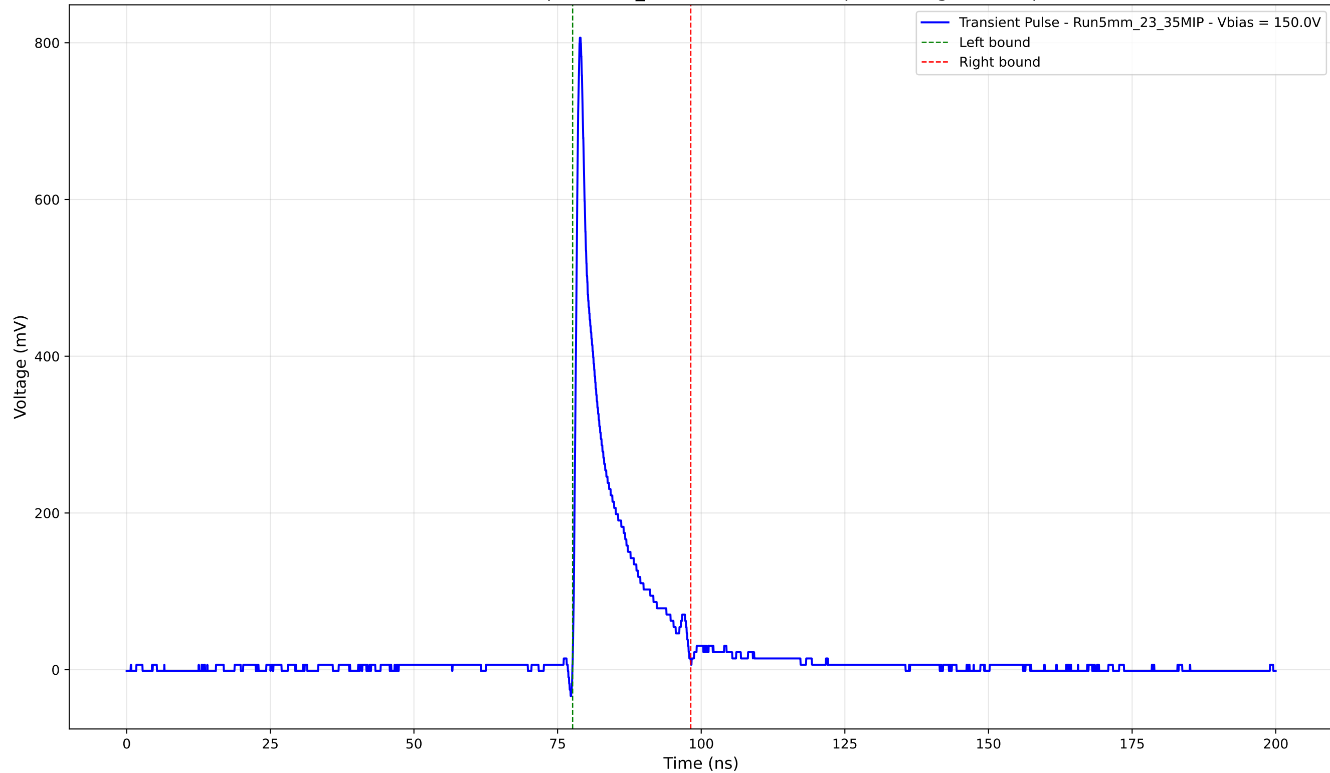
Transient Pulse - Sample: 5mm_23 - Position: 5035.0 \mu\text{m} - Charge: 85.29 pC
