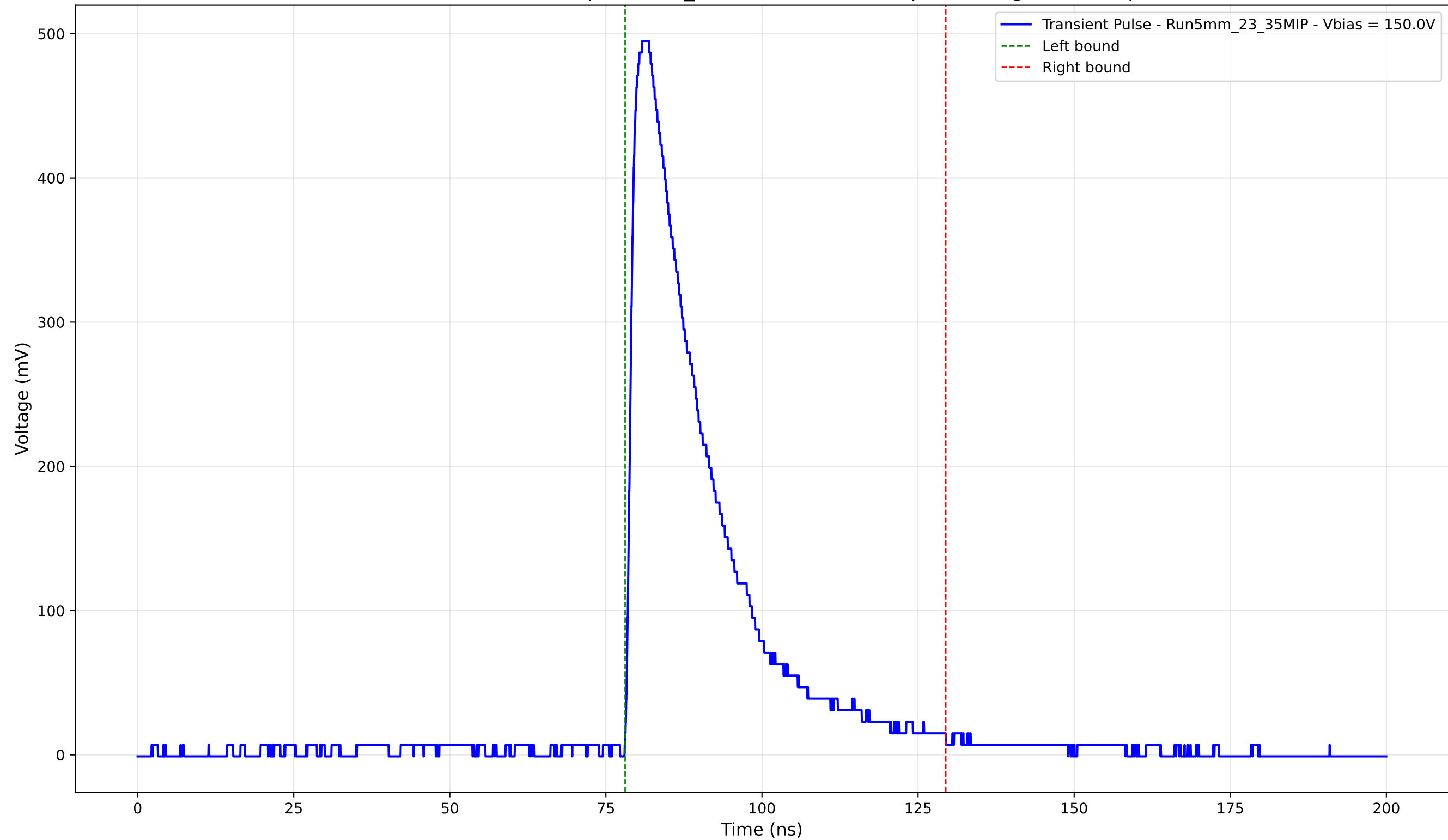
Transient Pulse - Sample: 5mm_23 - Position: 2990.0 \mu\text{m} - Charge: 135.11 pC
