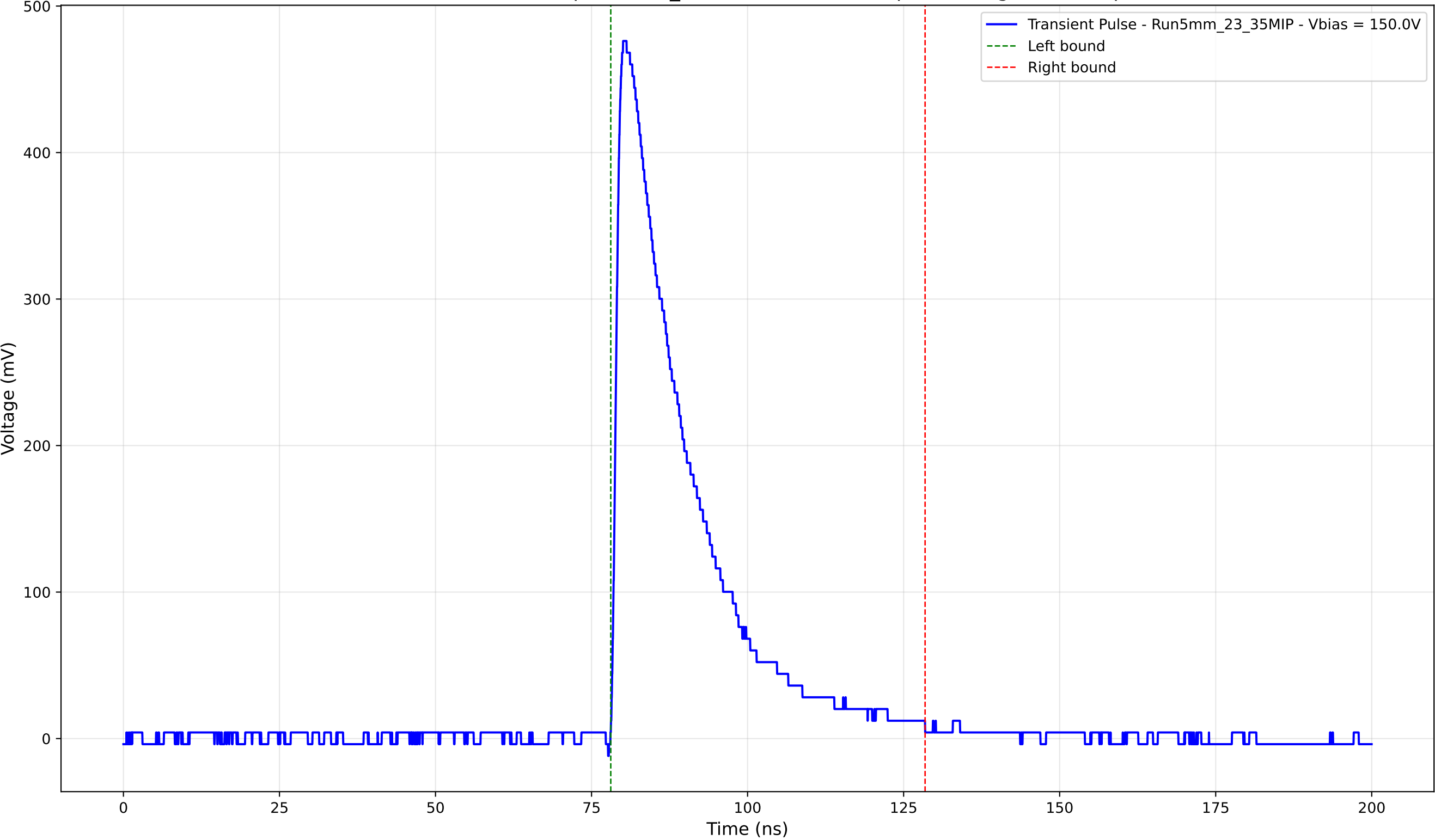
Transient Pulse - Sample: 5mm_23 - Position: 1710.0 \mu\text{m} - Charge: 119.26 pC
