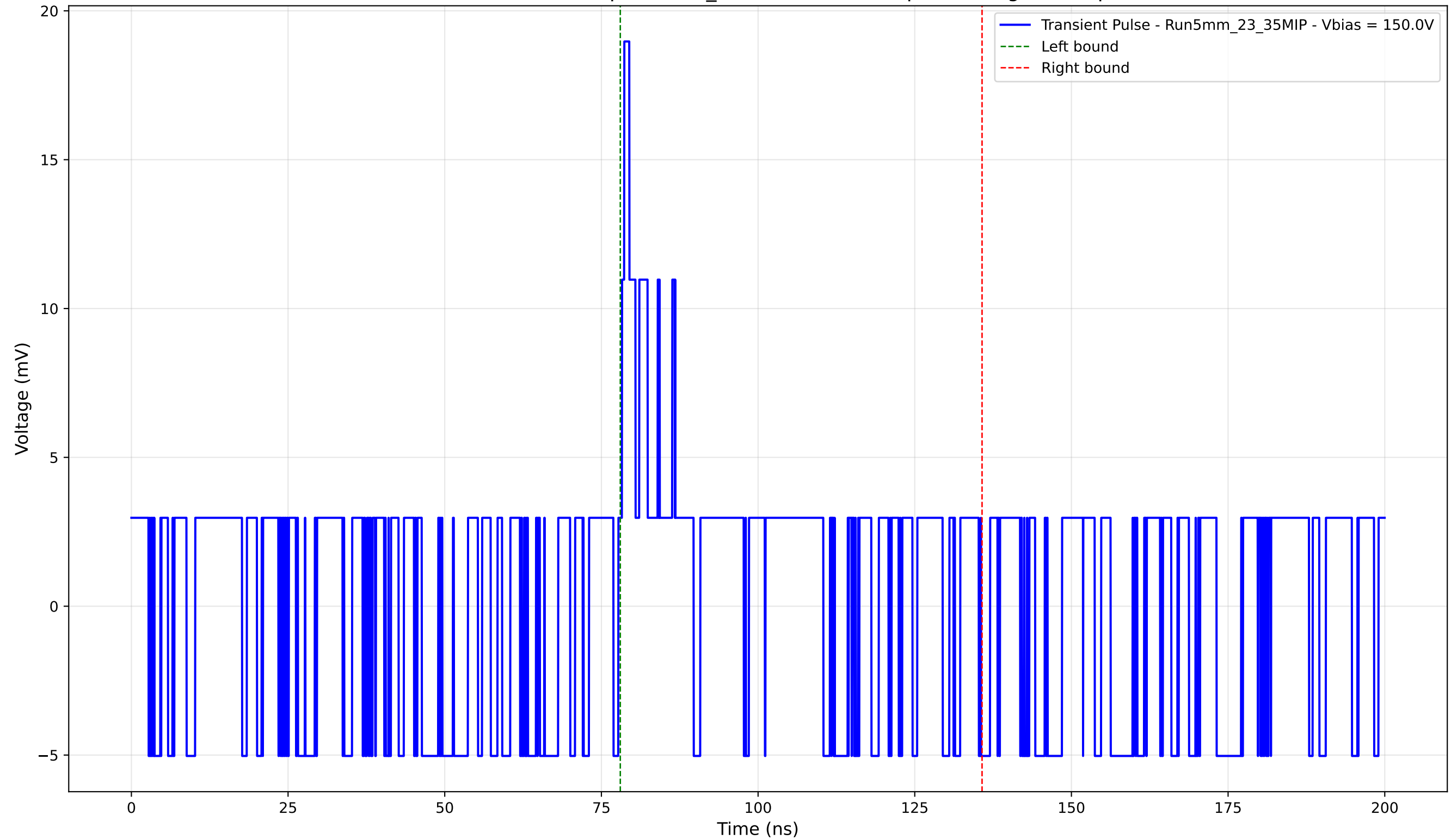
Transient Pulse - Sample: 5mm_23 - Position: 35.0 \mu\text{m} - Charge: 2.43 pC
