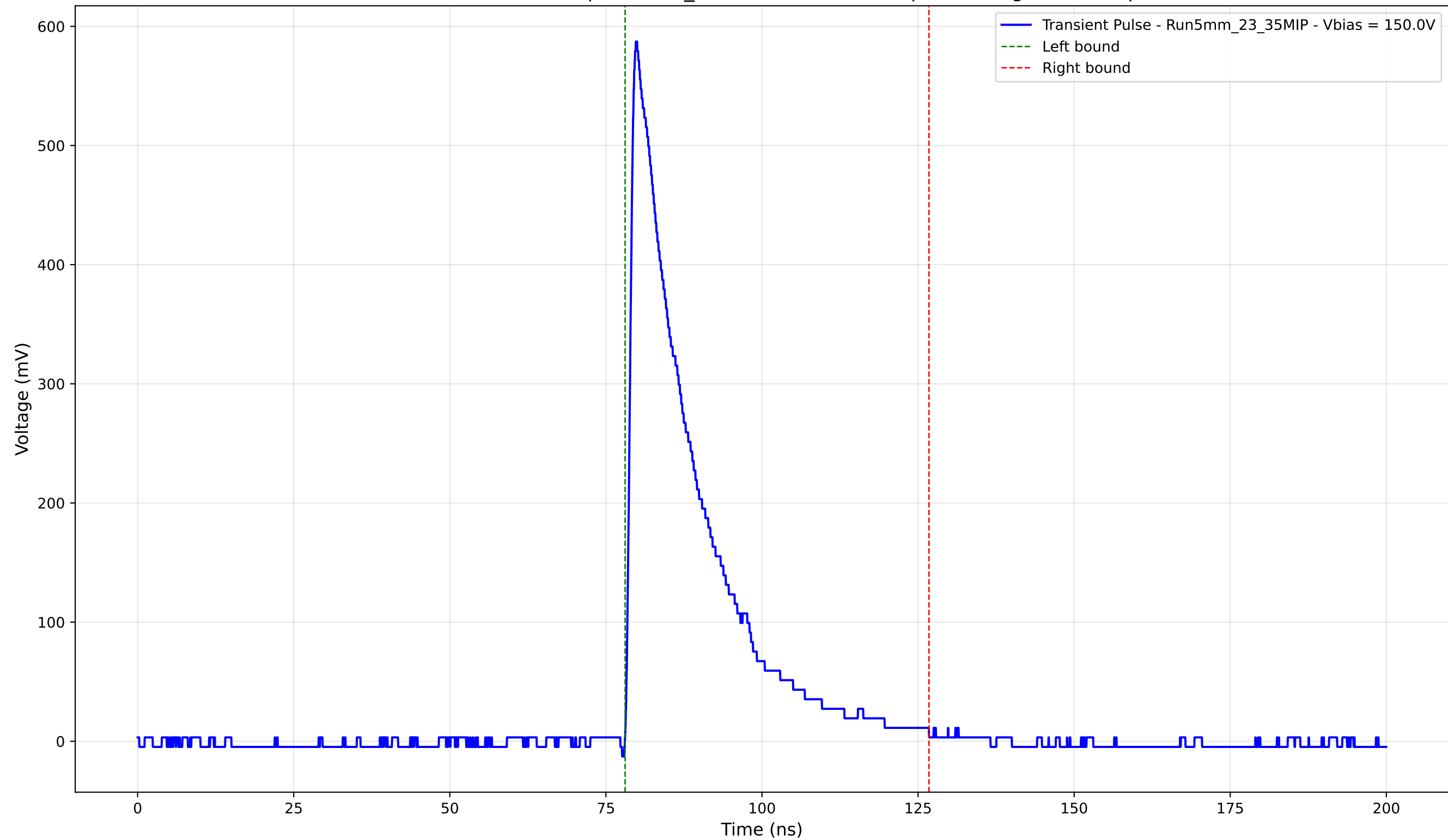
Transient Pulse - Sample: 5mm_23 - Position: 1290.0 \mu\text{m} - Charge: 128.66 pC
