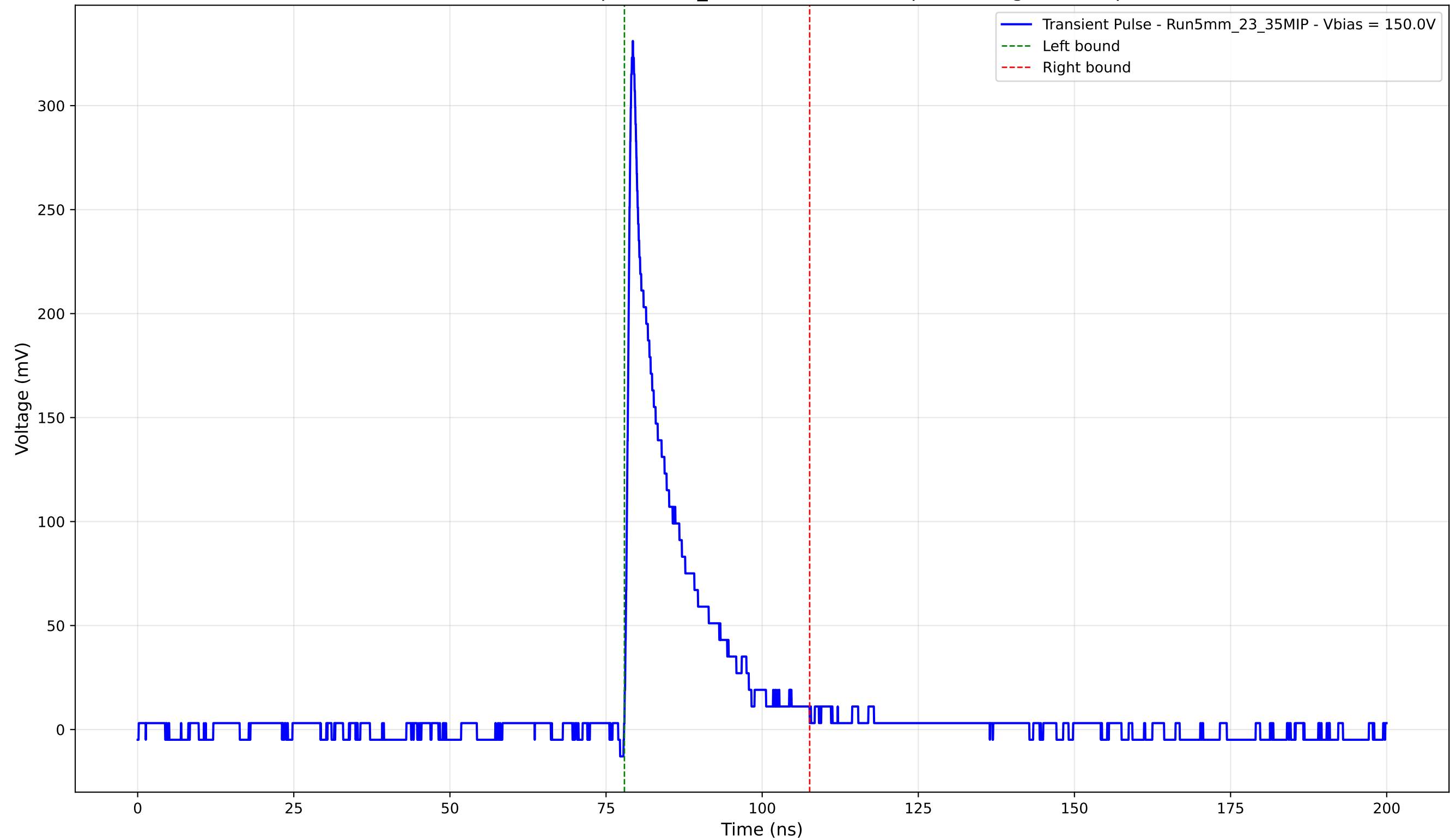
Transient Pulse - Sample: 5mm_23 - Position: 585.0 \mu\text{m} - Charge: 44.14 pC
