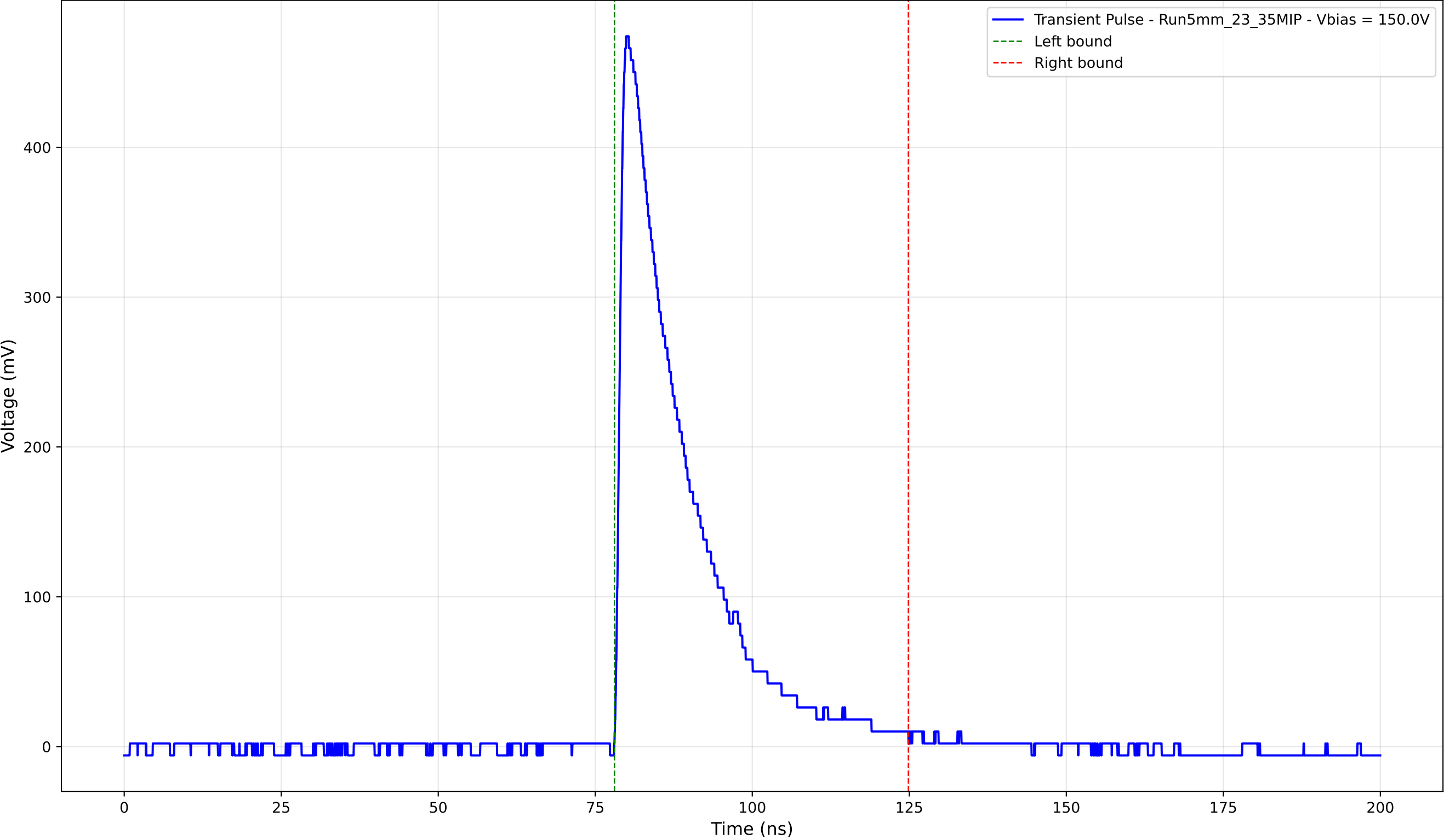
Transient Pulse - Sample: 5mm_23 - Position: 3730.0 \mu\text{m} - Charge: 107.84 pC
