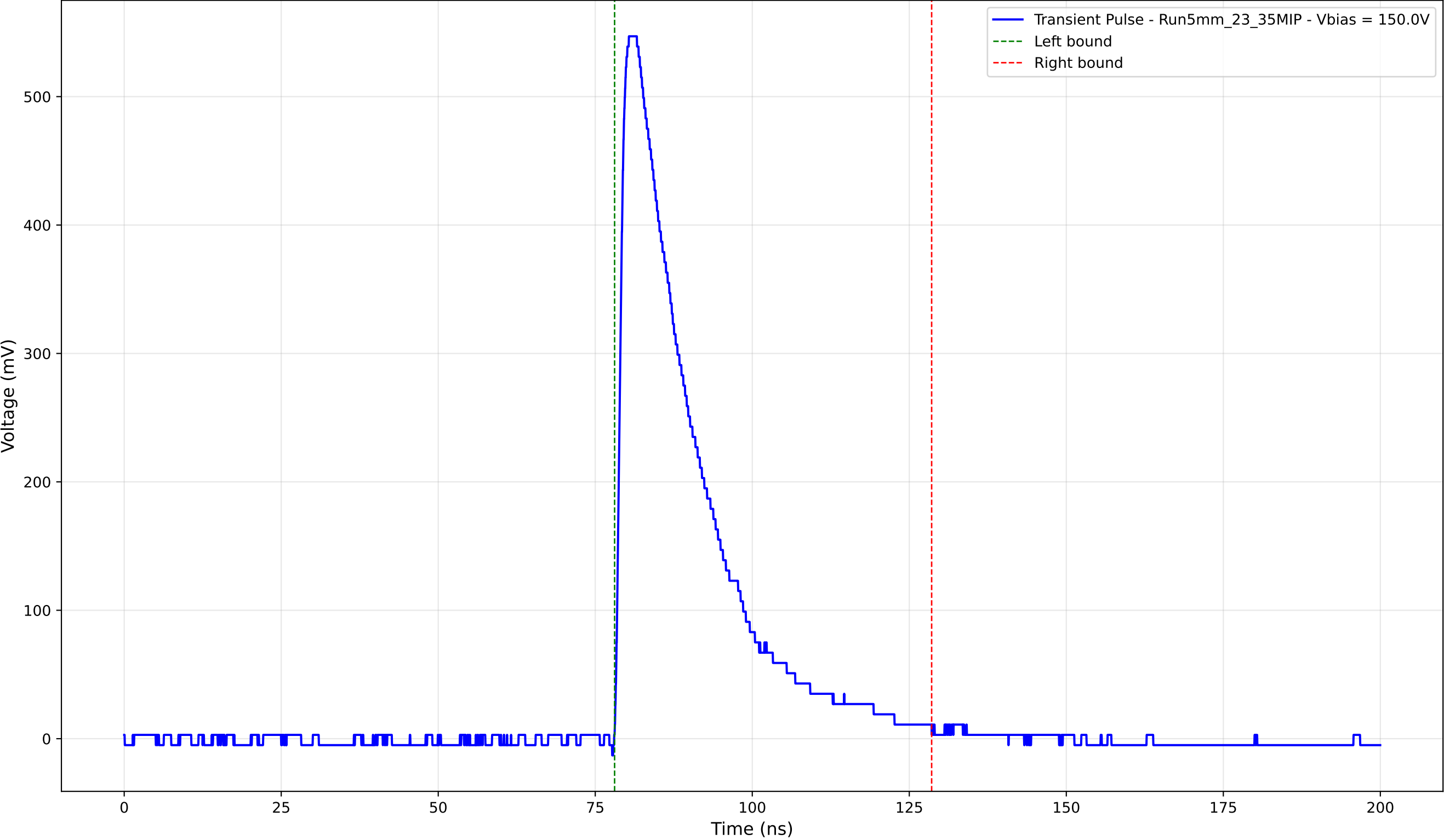
Transient Pulse - Sample: 5mm_23 - Position: 1995.0 \mu\text{m} - Charge: 144.44 pC
