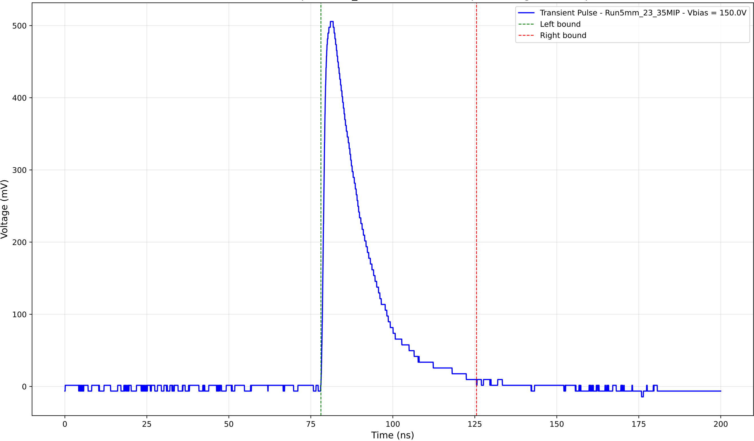
Transient Pulse - Sample: 5mm_23 - Position: 2295.0 \mu\text{m} - Charge: 133.90 pC
