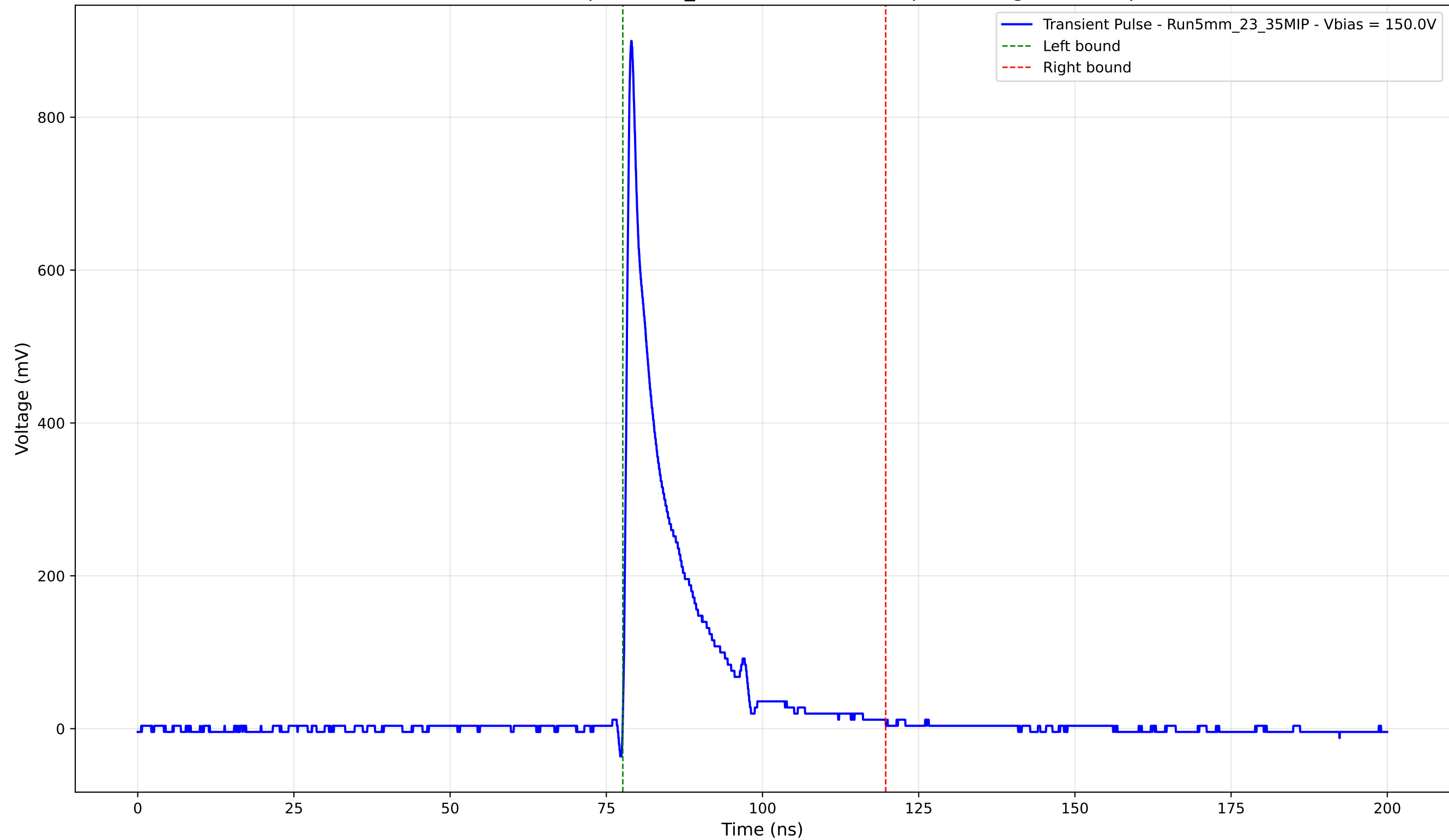
Transient Pulse - Sample: 5mm_23 - Position: 4950.0 \mu\text{m} - Charge: 118.48 pC
