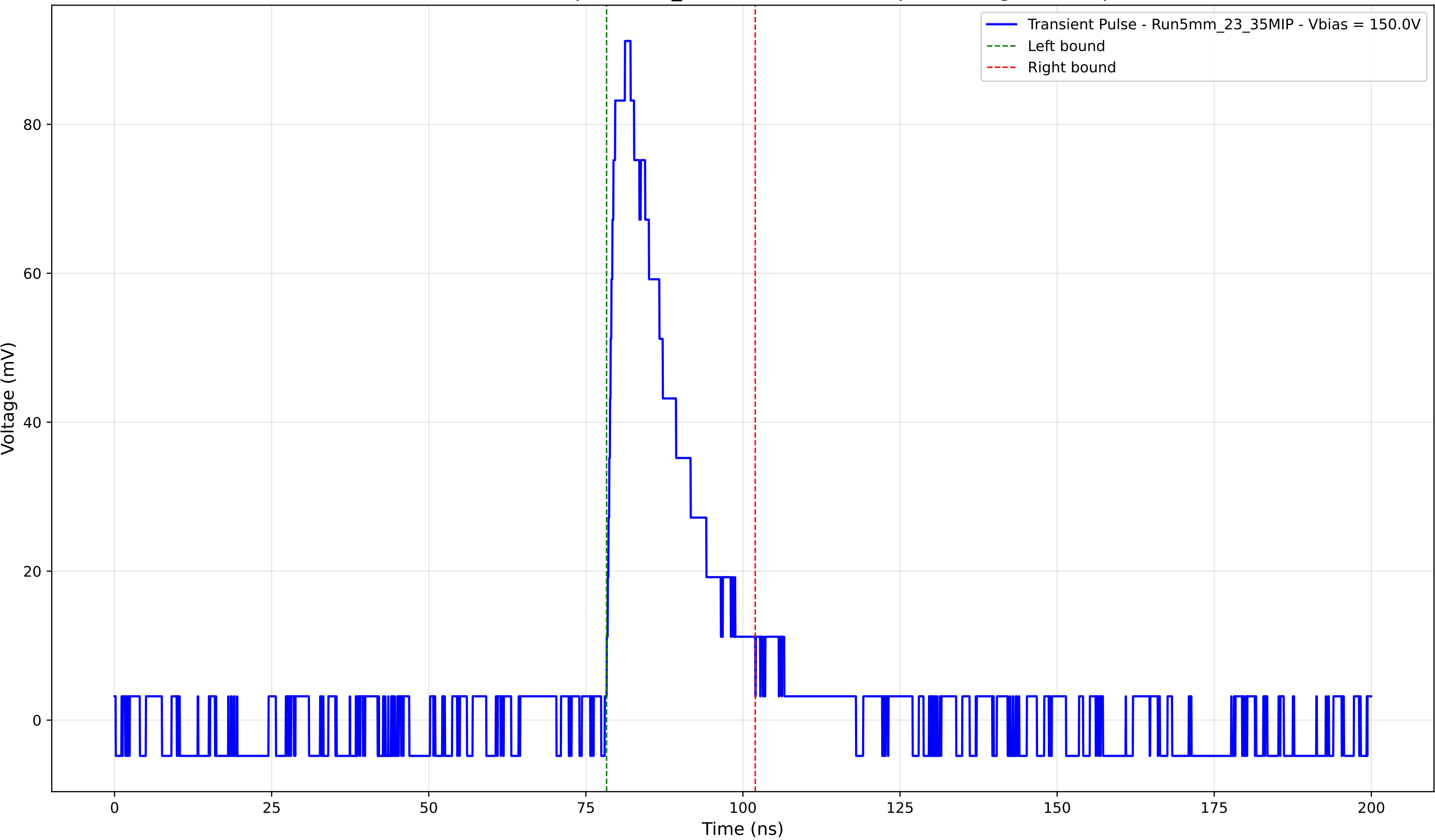
Transient Pulse - Sample: 5mm_23 - Position: 3660.0 \mu\text{m} - Charge: 19.55 pC
