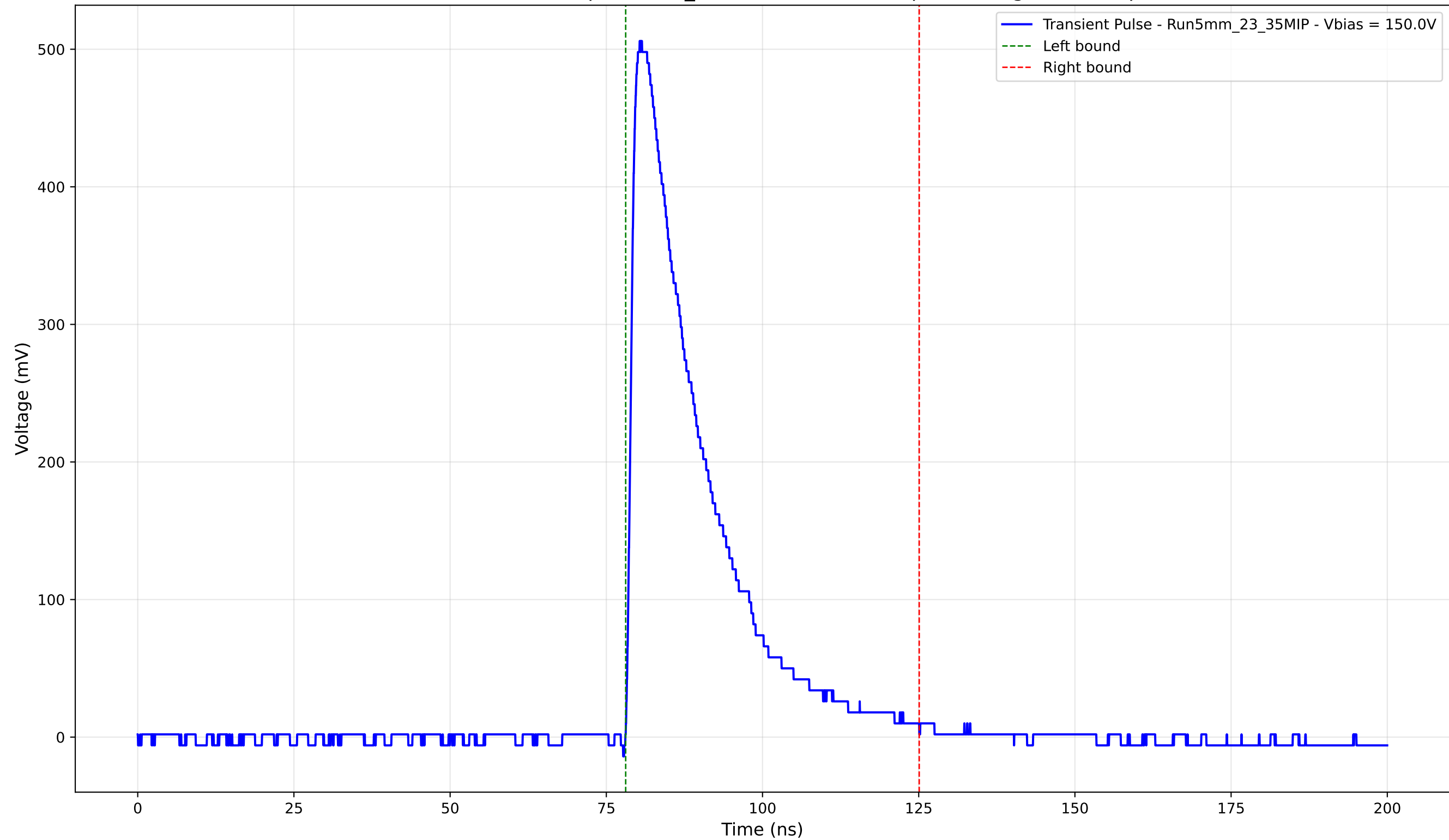
Transient Pulse - Sample: 5mm_23 - Position: 3405.0 \mu\text{m} - Charge: 125.82 pC
