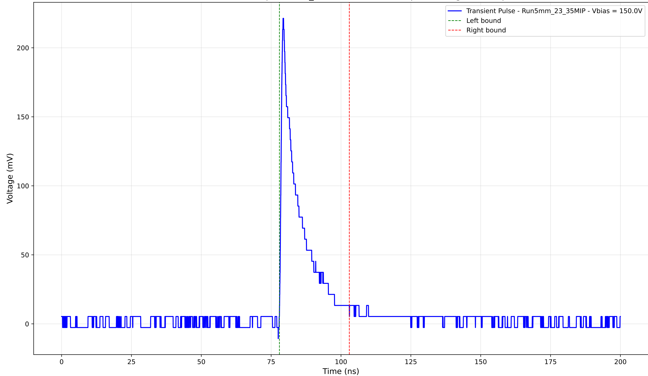
Transient Pulse - Sample: 5mm_23 - Position: 4645.0 \mu\text{m} - Charge: 30.87 pC
