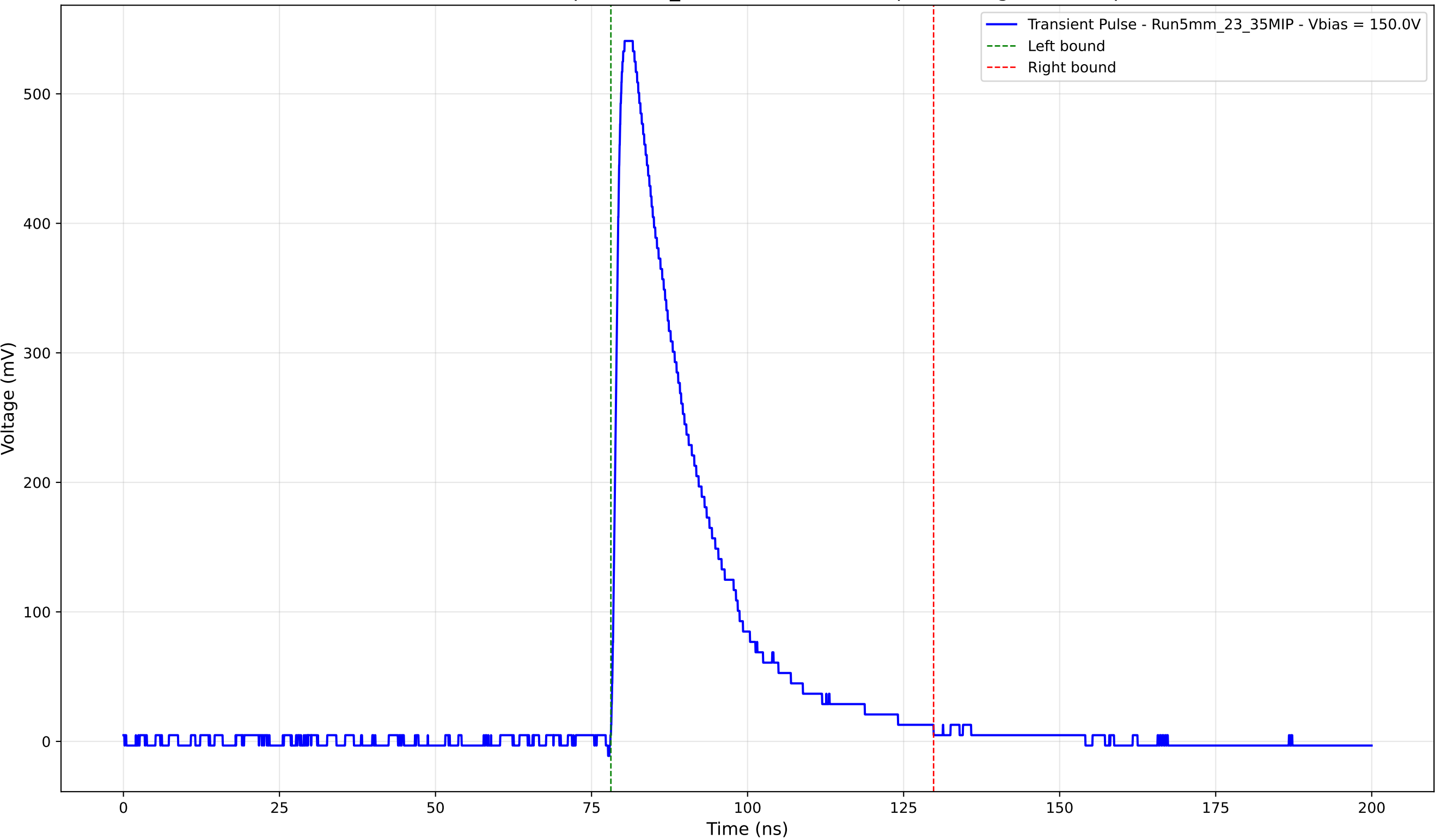
Transient Pulse - Sample: 5mm_23 - Position: 1965.0 \mu\text{m} - Charge: 144.25 pC
