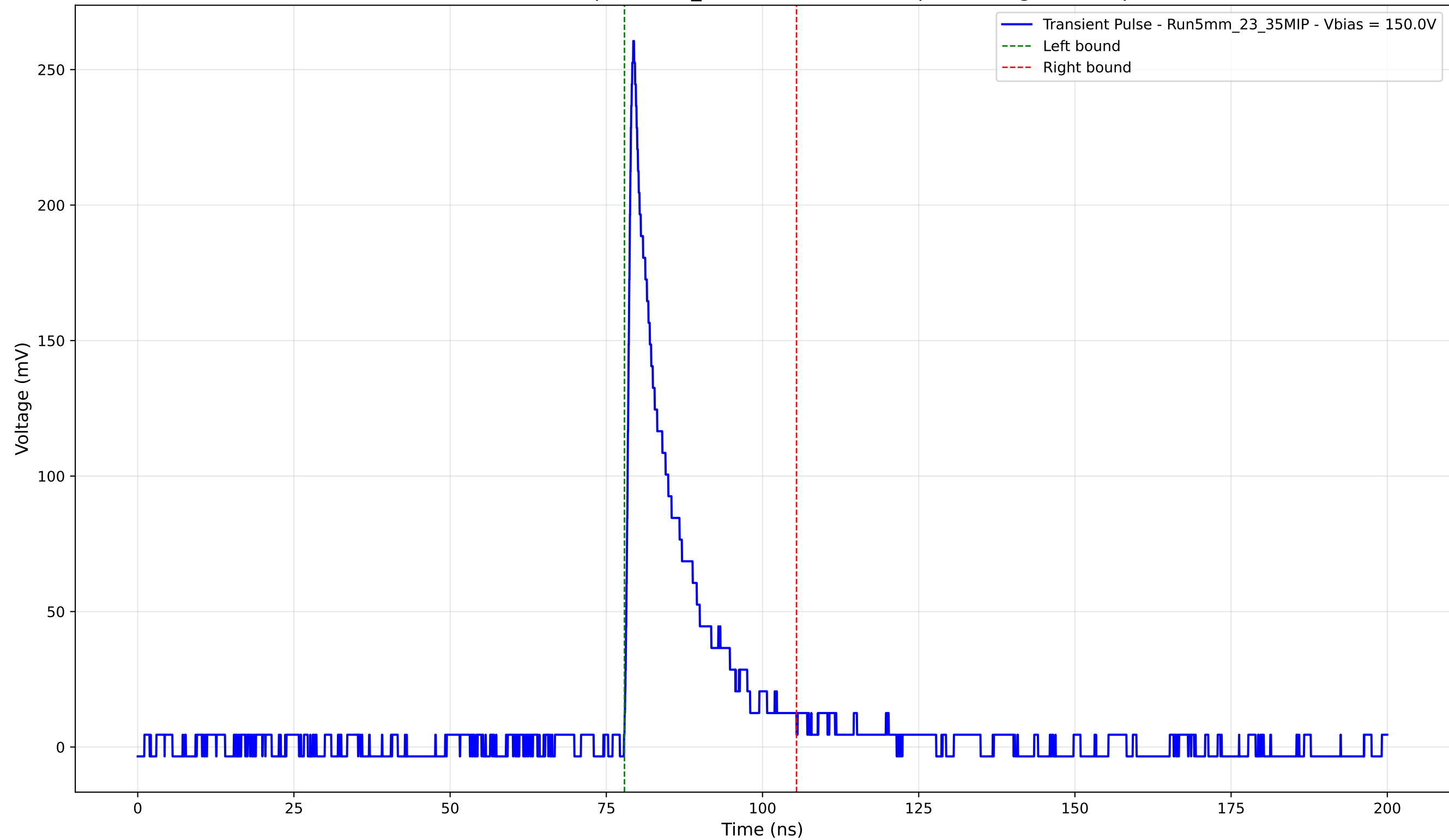
Transient Pulse - Sample: 5mm_23 - Position: 4640.0 \mu\text{m} - Charge: 36.62 pC
