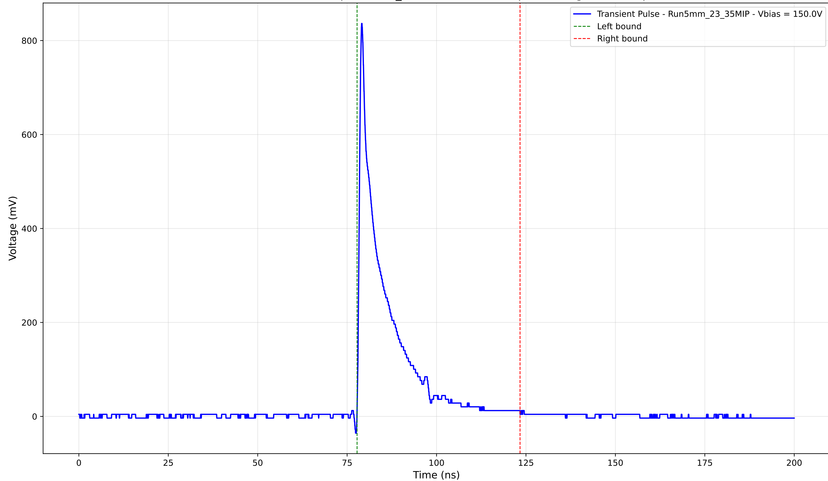
Transient Pulse - Sample: 5mm_23 - Position: 390.0 \mu\text{m} - Charge: 115.58 pC
