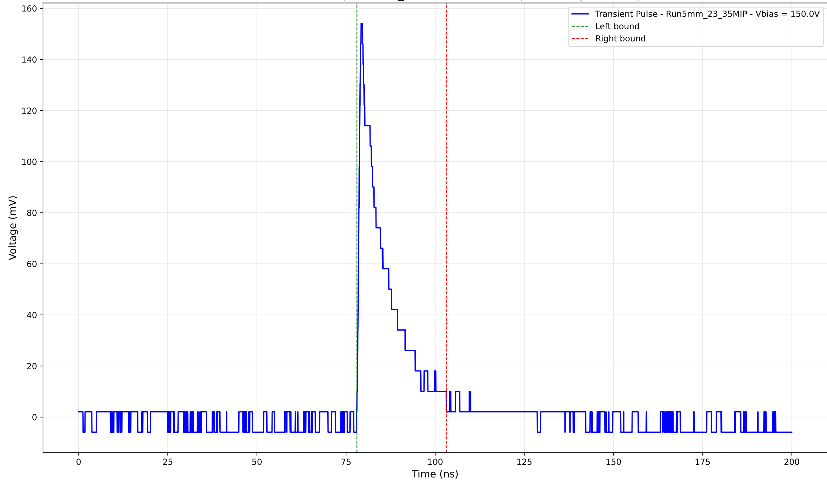
Transient Pulse - Sample: 5mm_23 - Position: 635.0 \mu\text{m} - Charge: 23.32 pC
