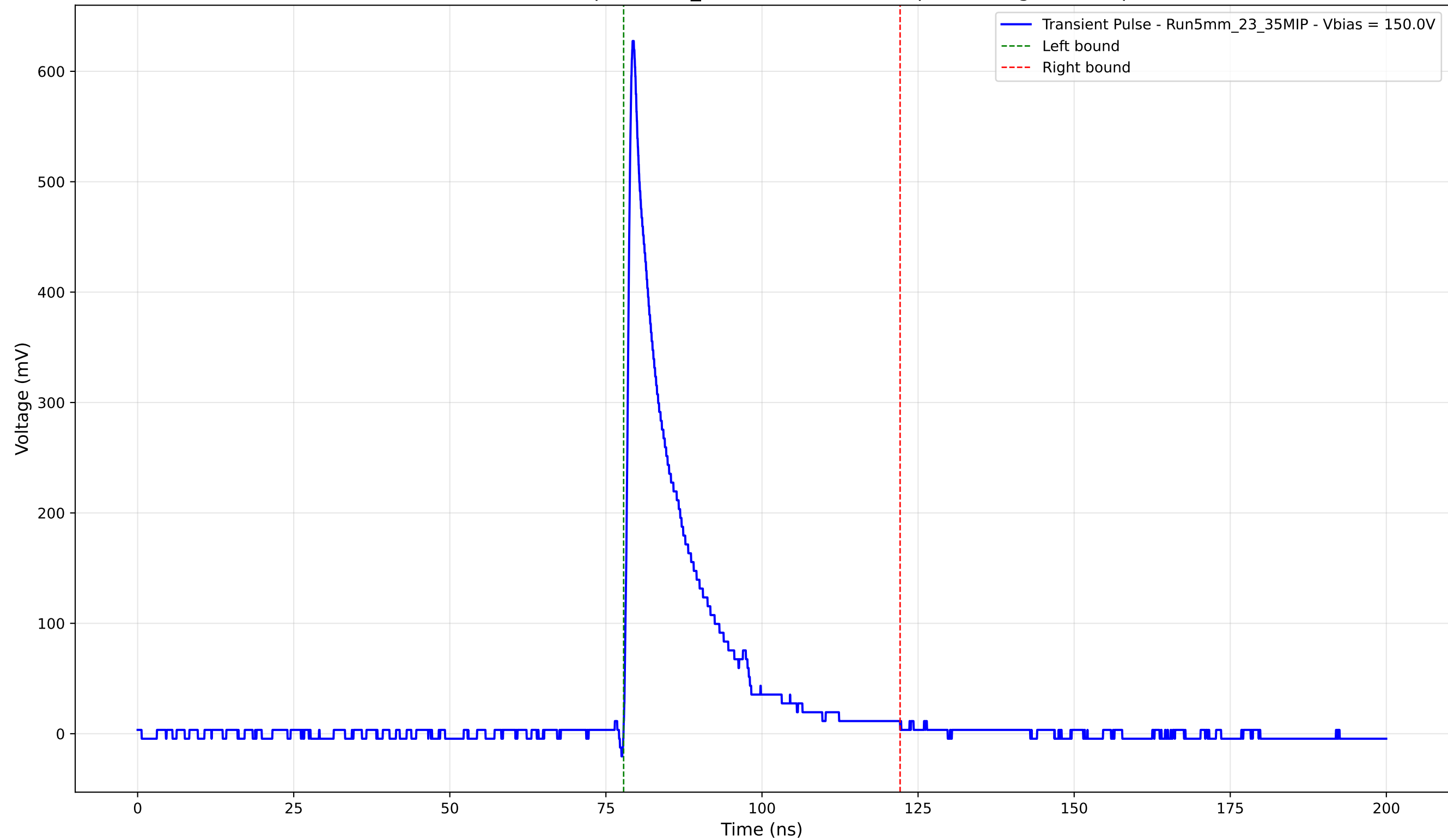
Transient Pulse - Sample: 5mm_23 - Position: 4585.0 \mu\text{m} - Charge: 97.44 pC
