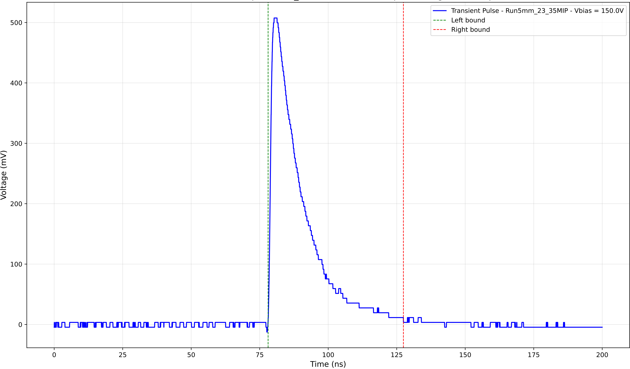
Transient Pulse - Sample: 5mm_23 - Position: 3380.0 \mu\text{m} - Charge: 129.70 pC
