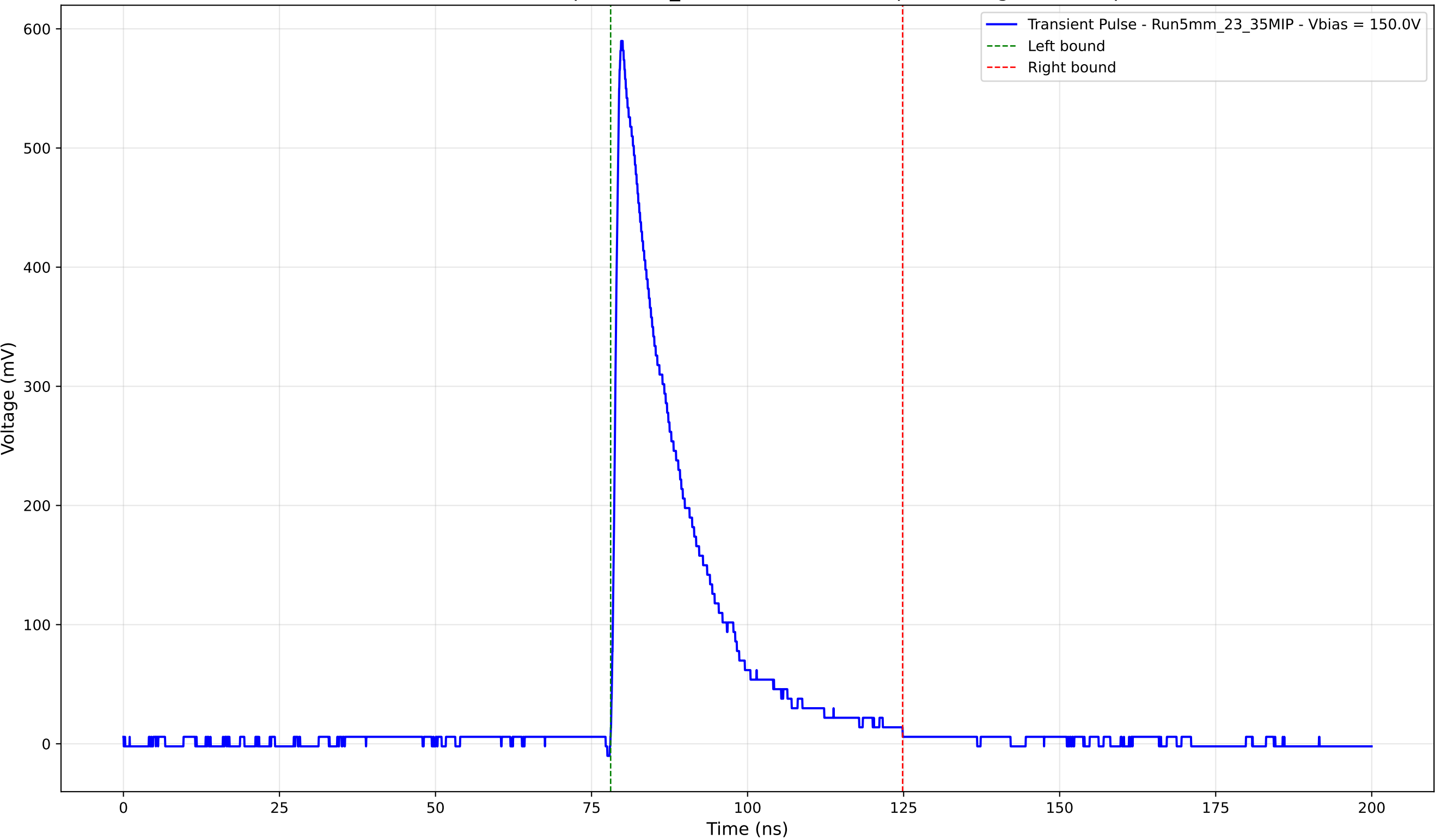
Transient Pulse - Sample: 5mm_23 - Position: 1240.0 \mu\text{m} - Charge: 126.83 pC
