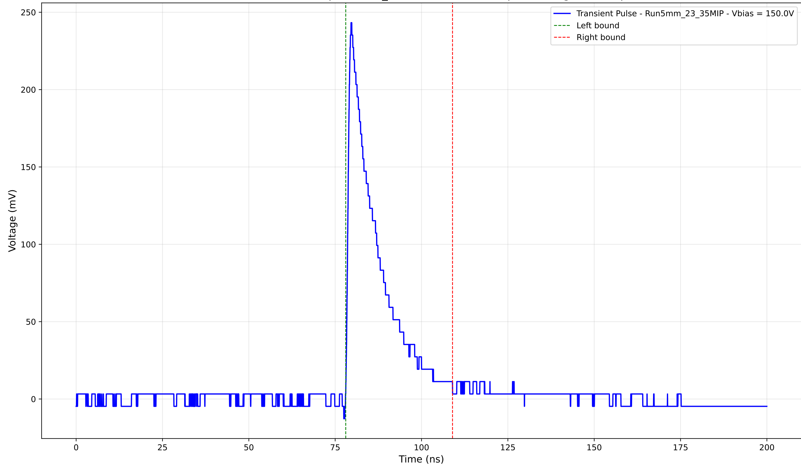
Transient Pulse - Sample: 5mm_23 - Position: 4480.0 \mu\text{m} - Charge: 44.20 pC
