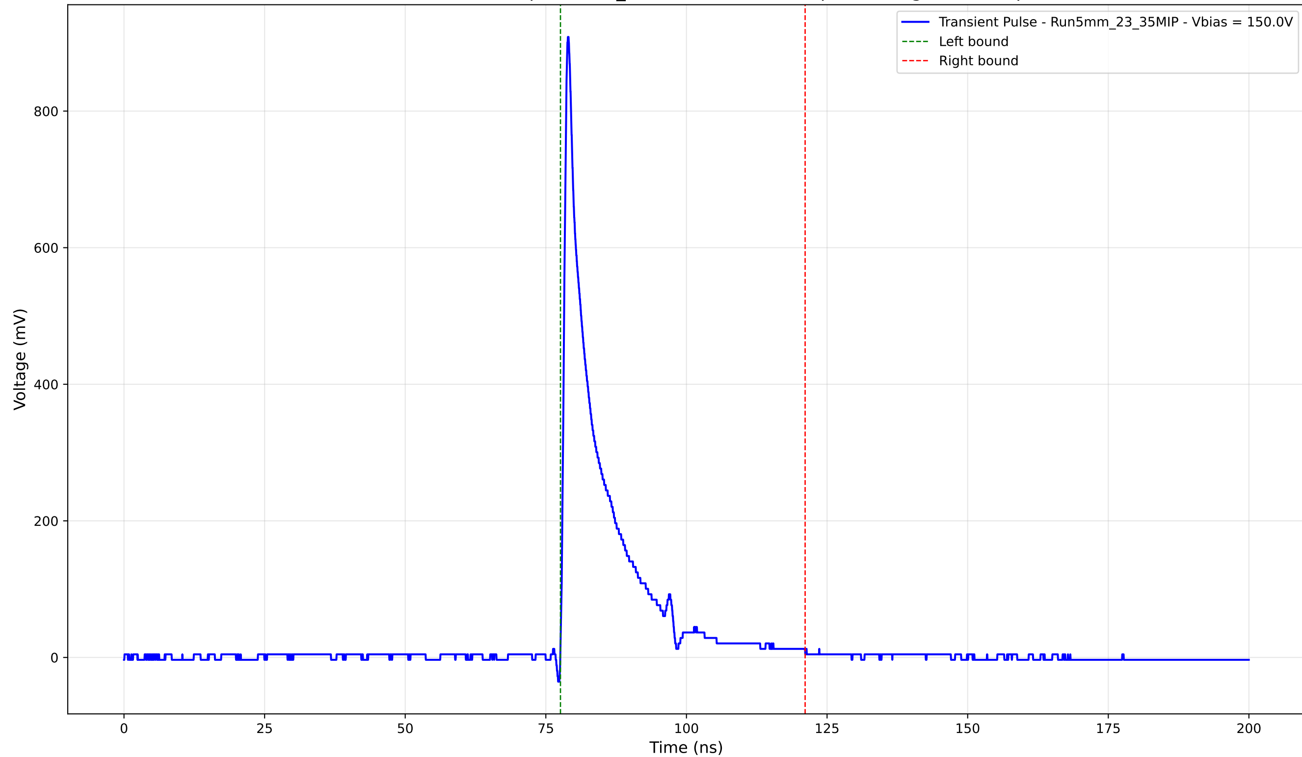
Transient Pulse - Sample: 5mm_23 - Position: 5000.0 \mu\text{m} - Charge: 116.46 pC
