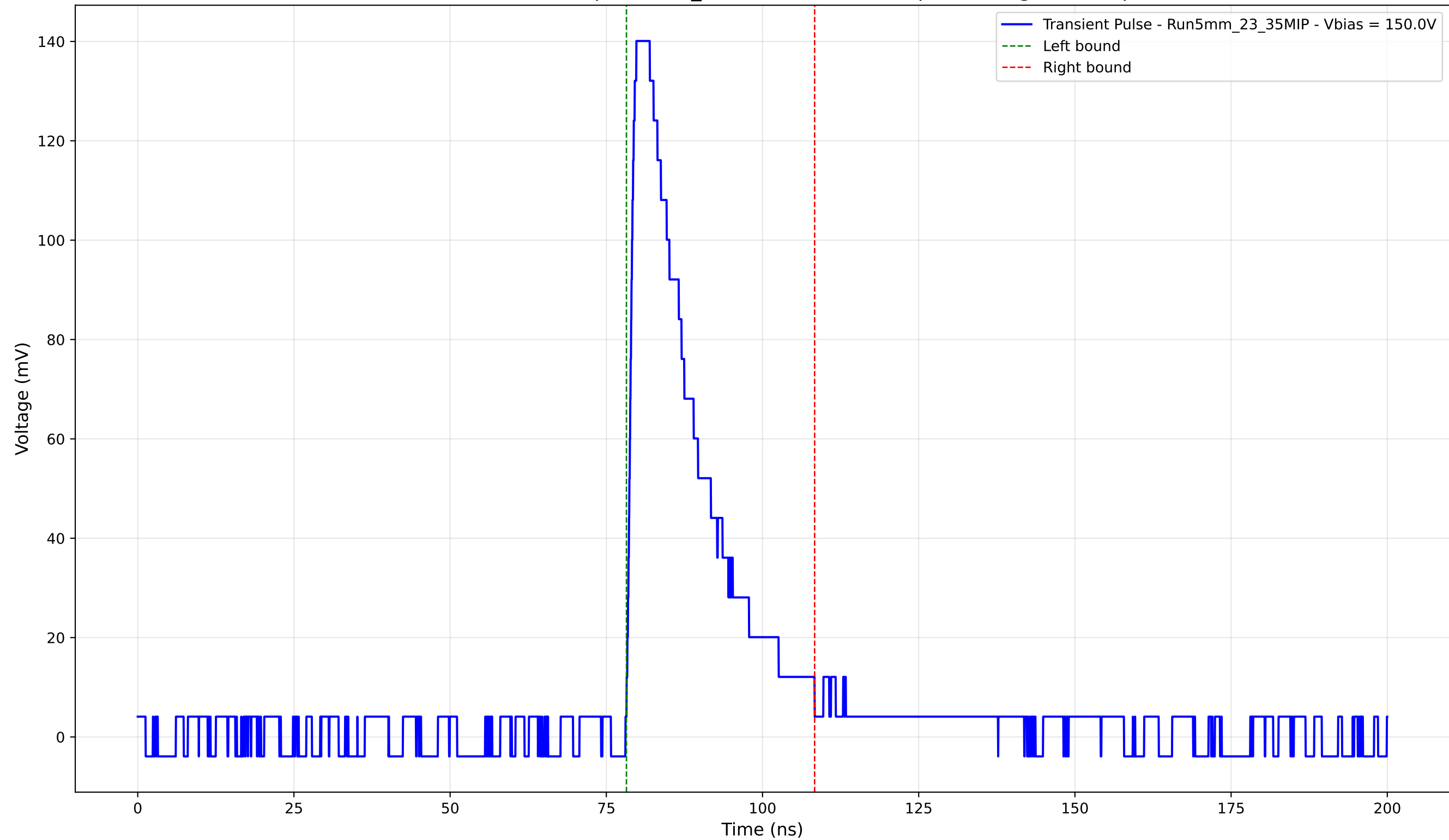
Transient Pulse - Sample: 5mm_23 - Position: 3675.0 \mu\text{m} - Charge: 32.61 pC
