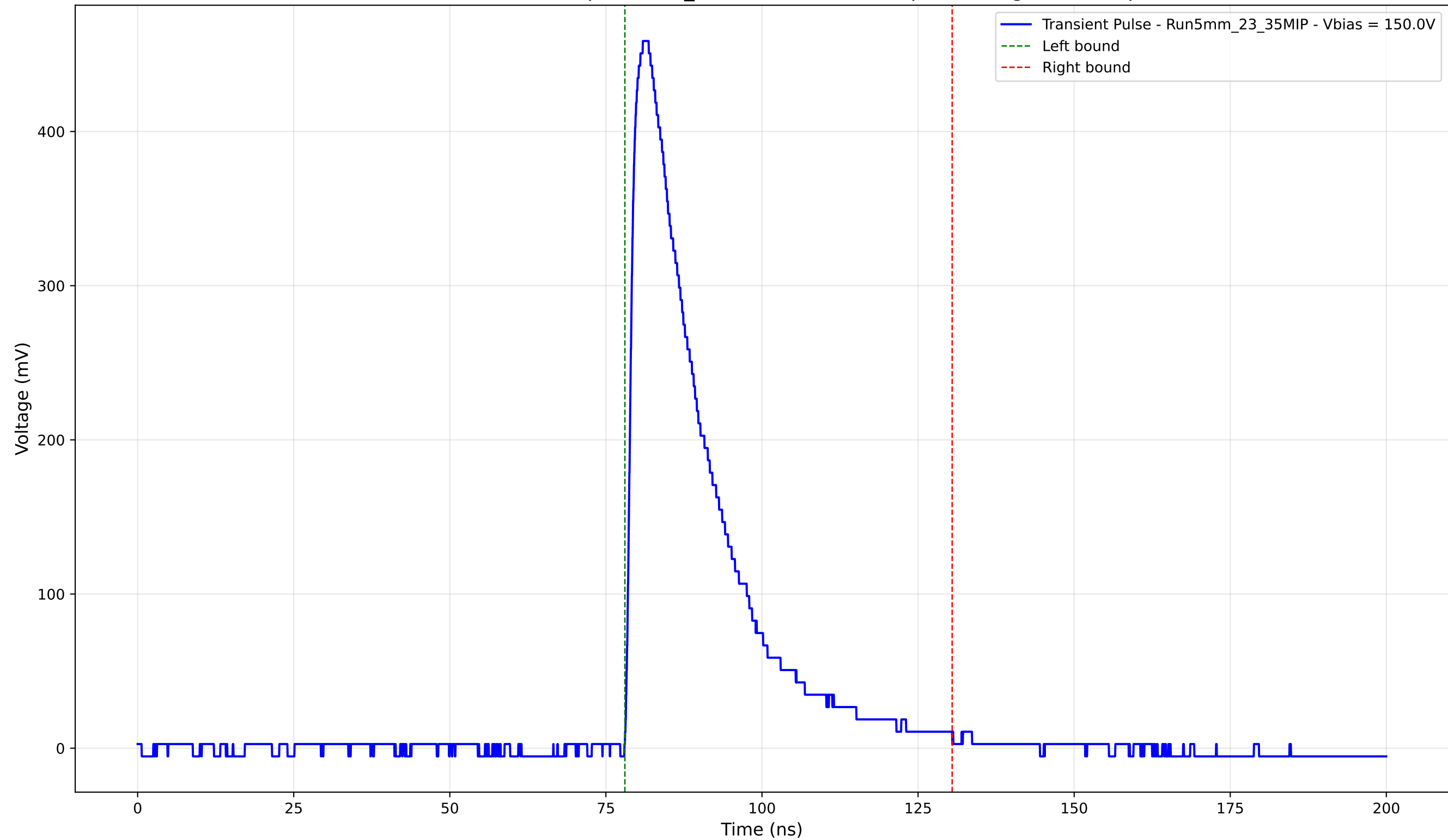
Transient Pulse - Sample: 5mm_23 - Position: 2735.0 \mu\text{m} - Charge: 123.17 pC
