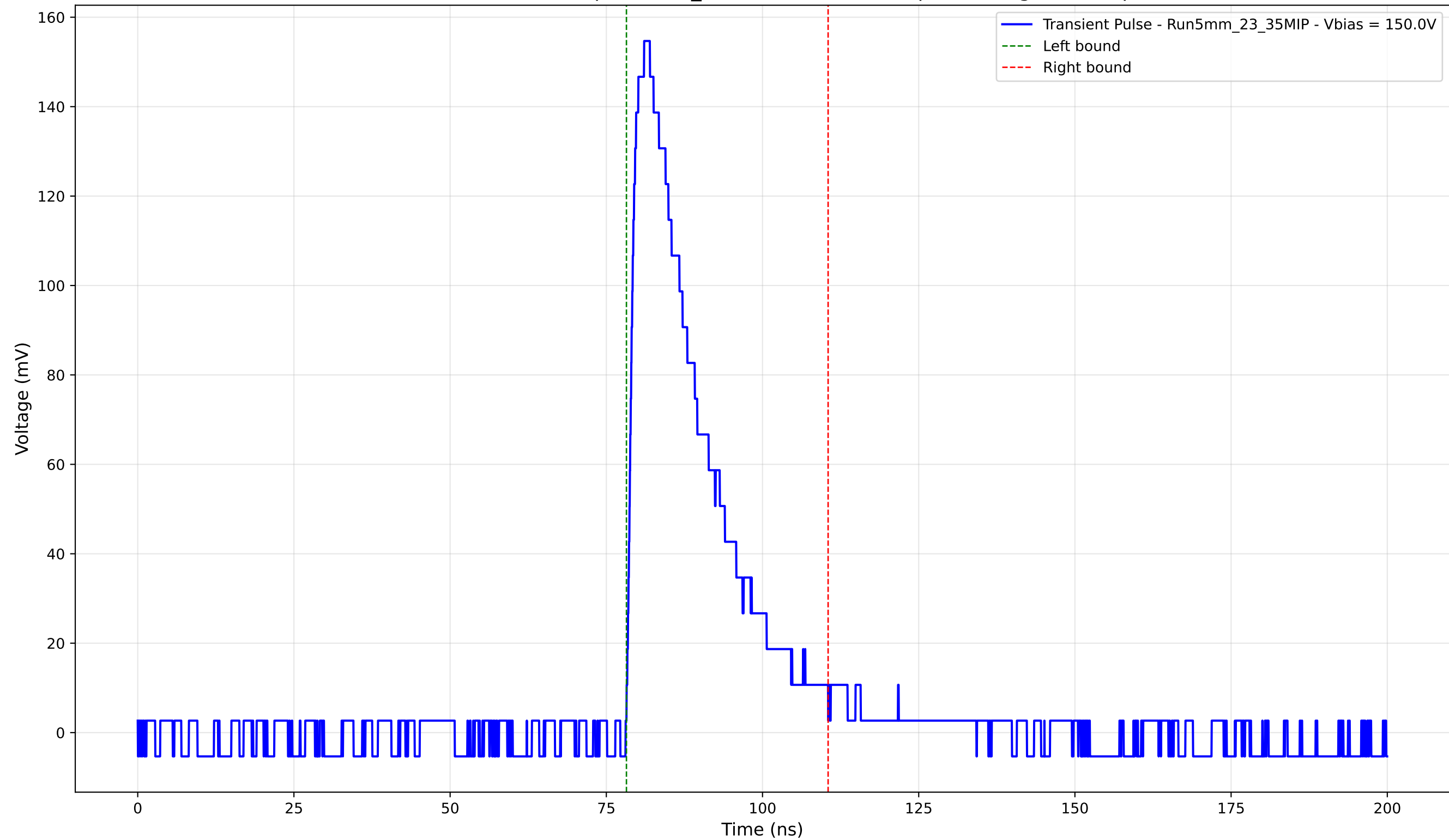
Transient Pulse - Sample: 5mm_23 - Position: 2620.0 \mu\text{m} - Charge: 38.30 pC
