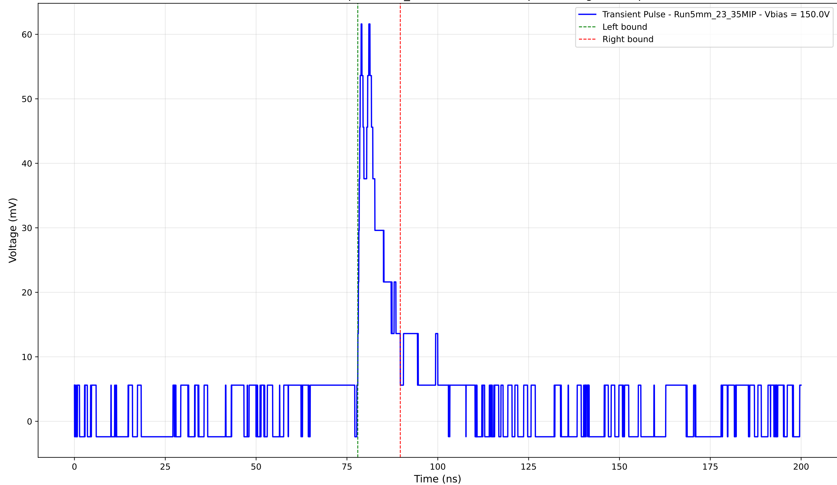
Transient Pulse - Sample: 5mm_23 - Position: 165.0 \mu\text{m} - Charge: 7.33 pC
