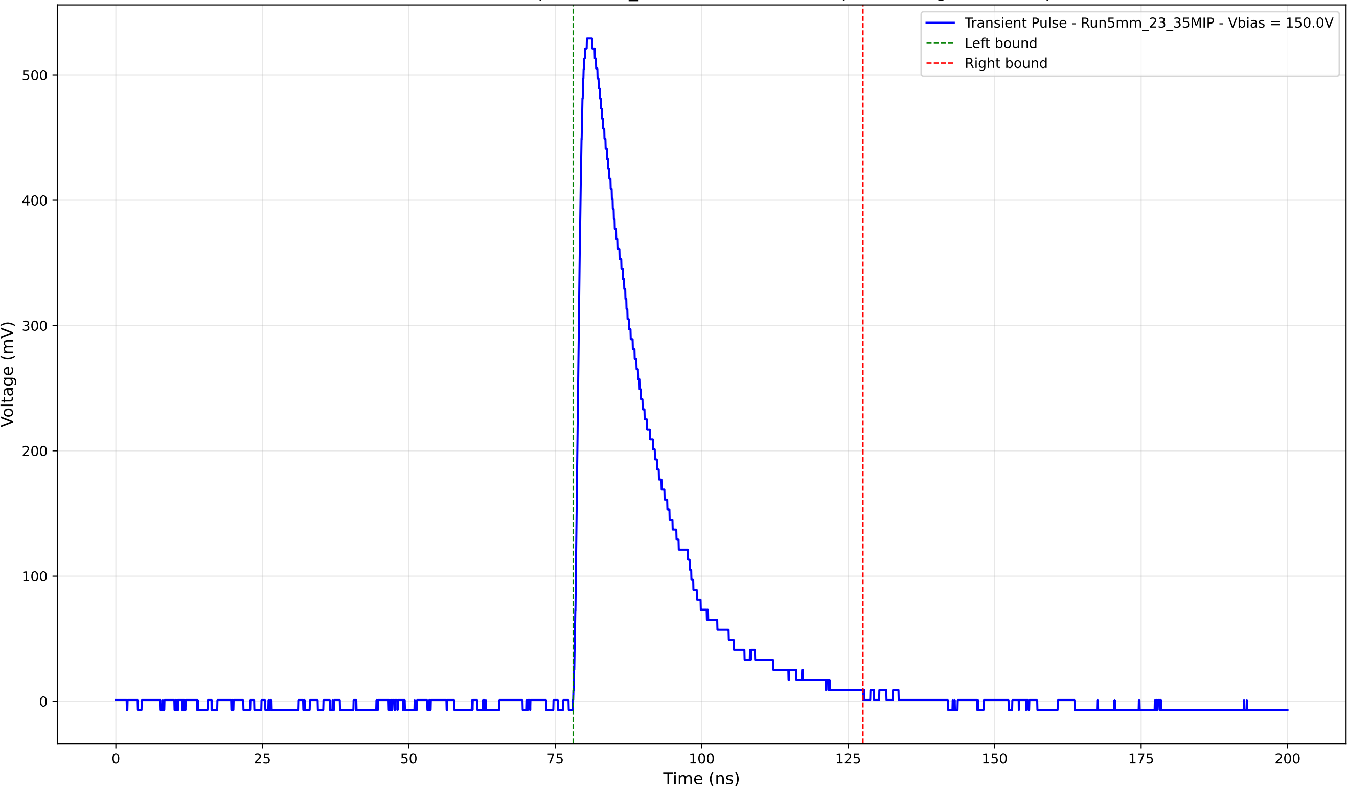
Transient Pulse - Sample: 5mm_23 - Position: 1915.0 \mu\text{m} - Charge: 135.76 pC
