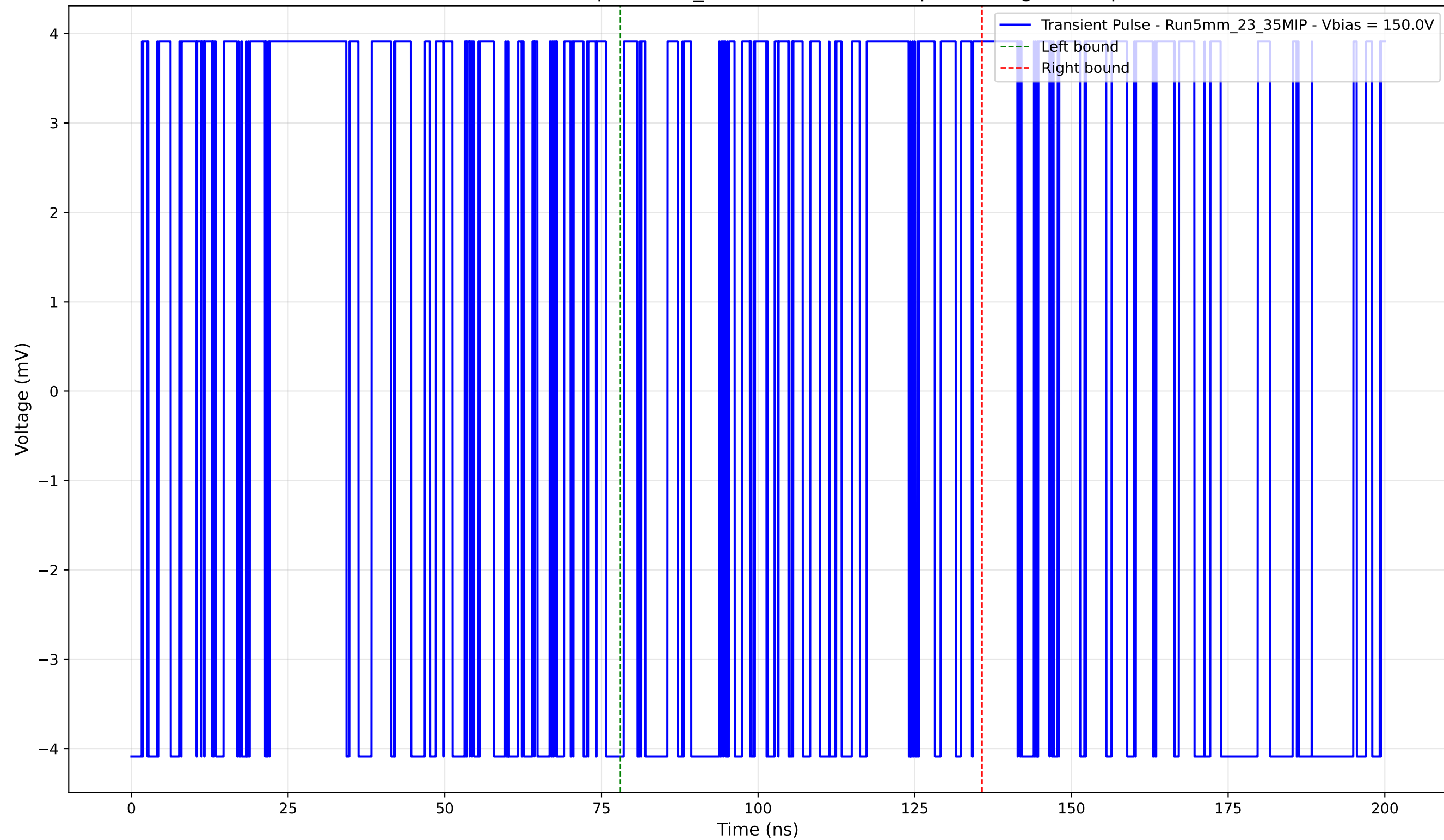
Transient Pulse - Sample: 5mm_23 - Position: 5290.0 \mu\text{m} - Charge: 0.70 pC
