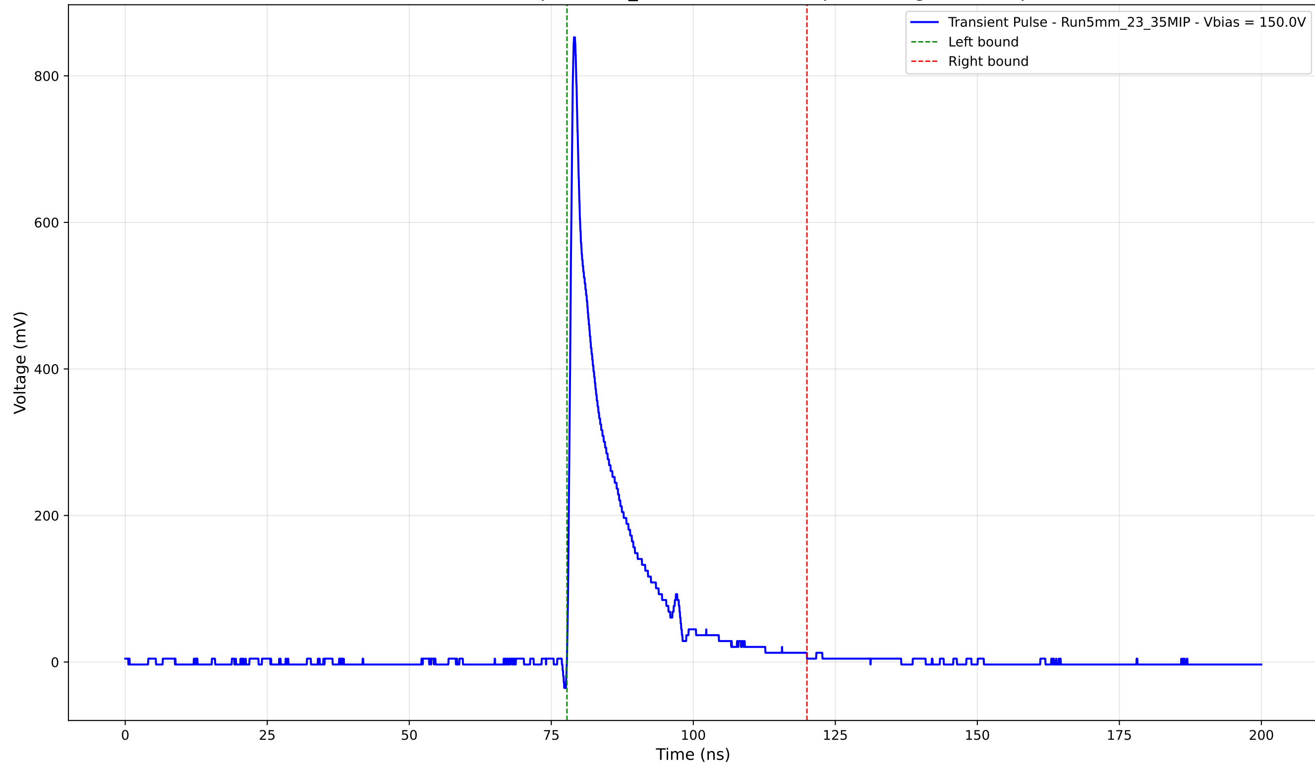
Transient Pulse - Sample: 5mm_23 - Position: 345.0 \mu\text{m} - Charge: 114.90 pC
