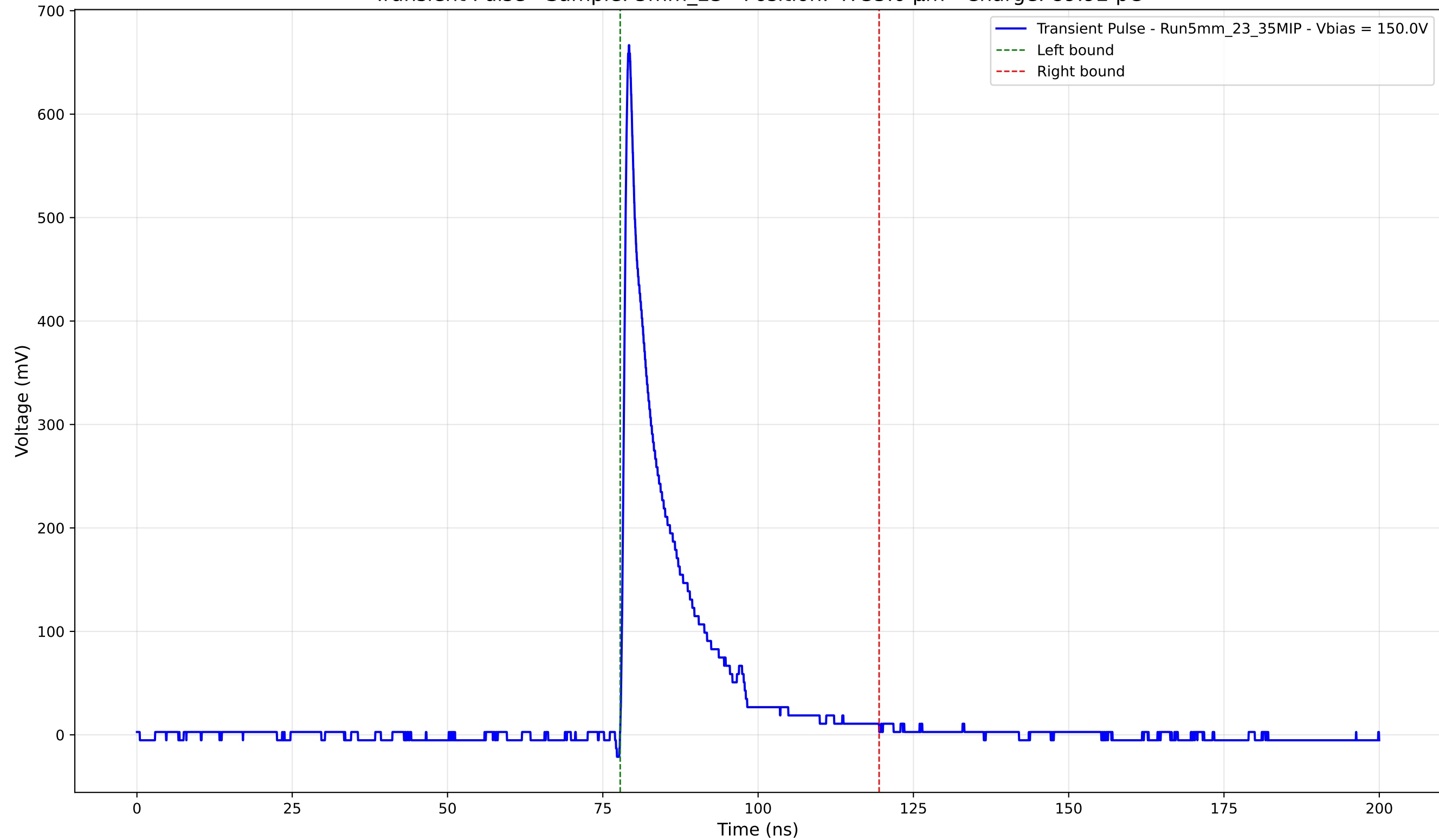
Transient Pulse - Sample: 5mm_23 - Position: 4735.0 \mu\text{m} - Charge: 89.92 pC
