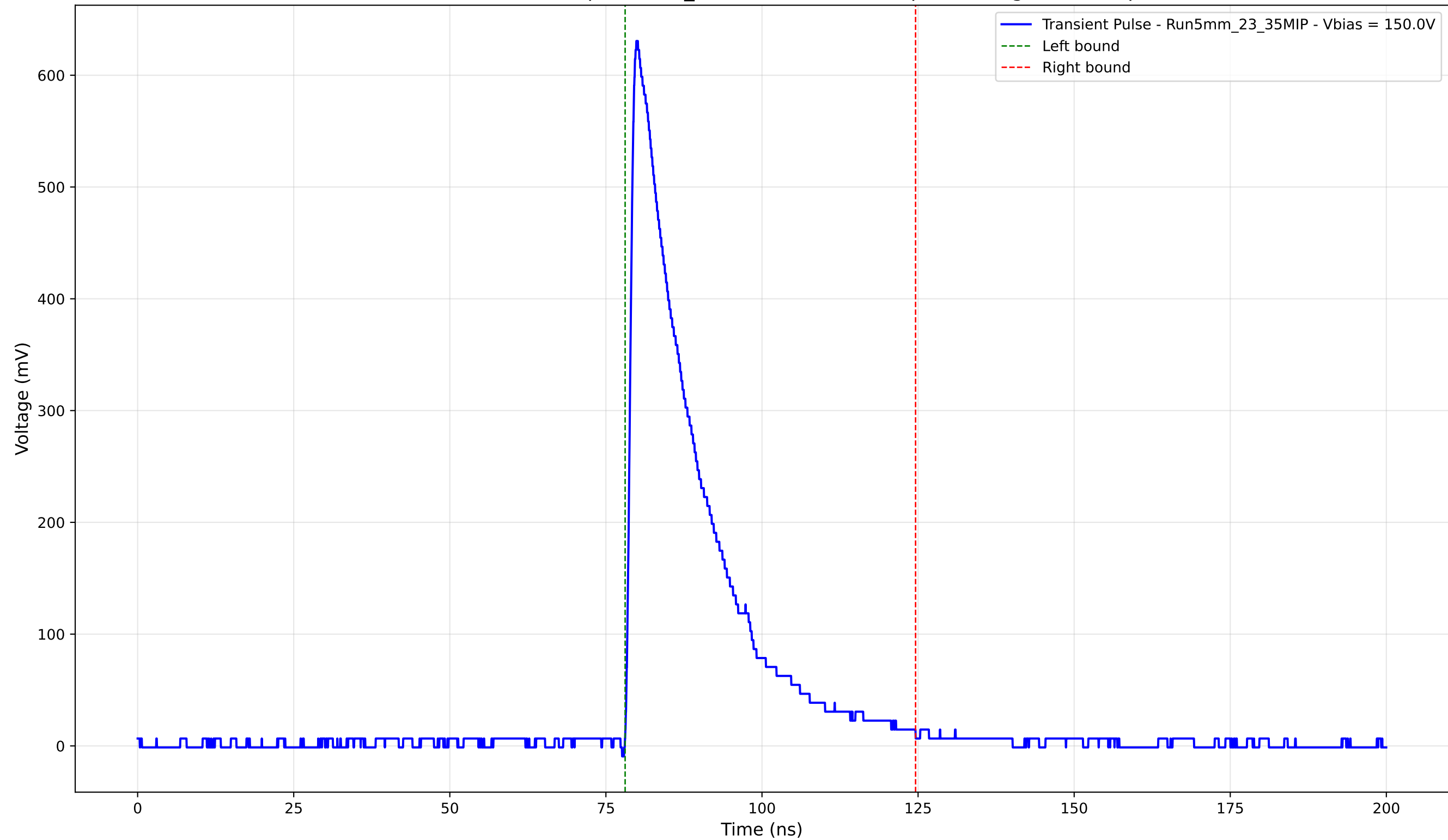
Transient Pulse - Sample: 5mm_23 - Position: 1400.0 \mu\text{m} - Charge: 146.05 pC
