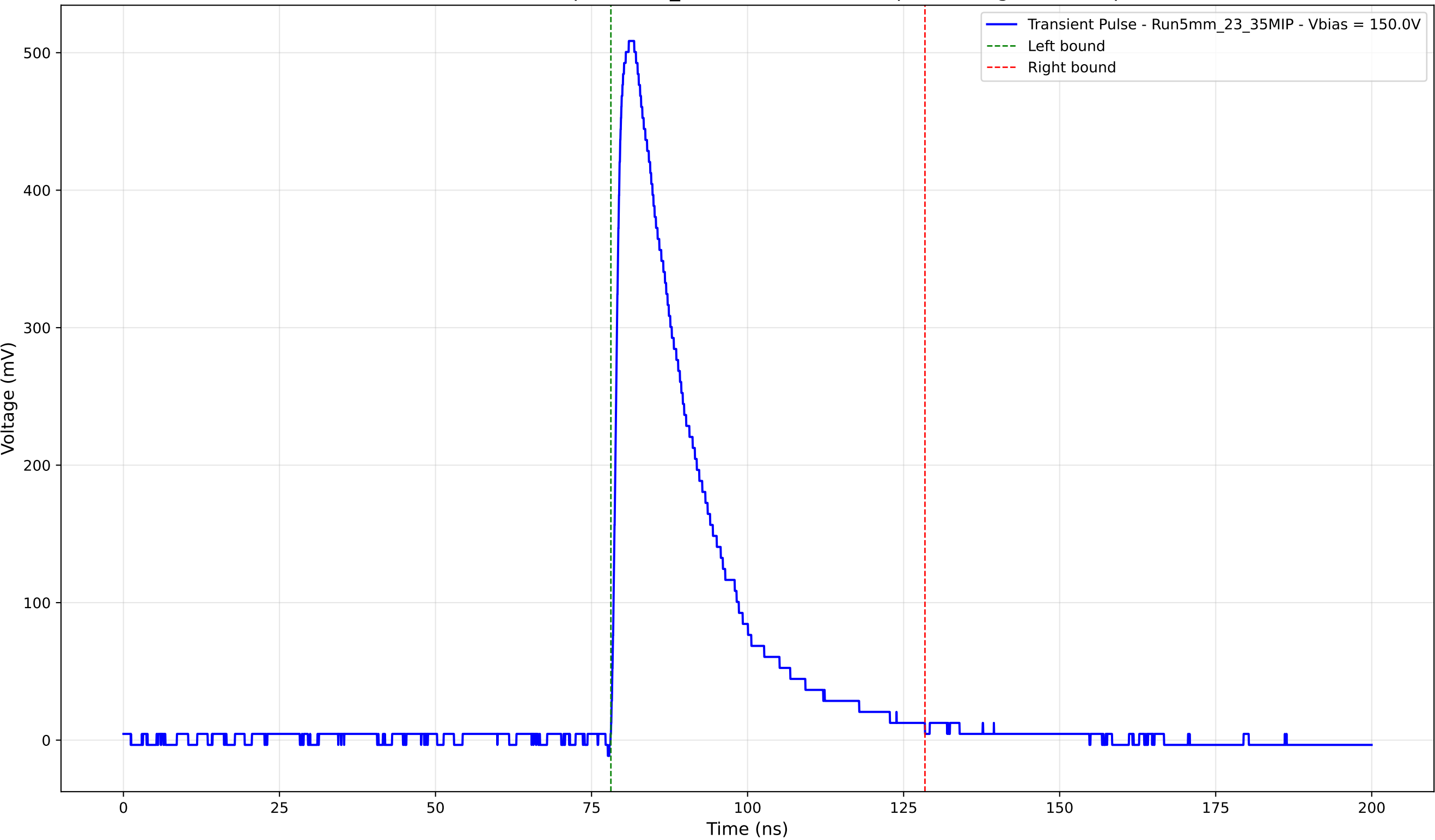
Transient Pulse - Sample: 5mm_23 - Position: 2315.0 \mu\text{m} - Charge: 137.79 pC
