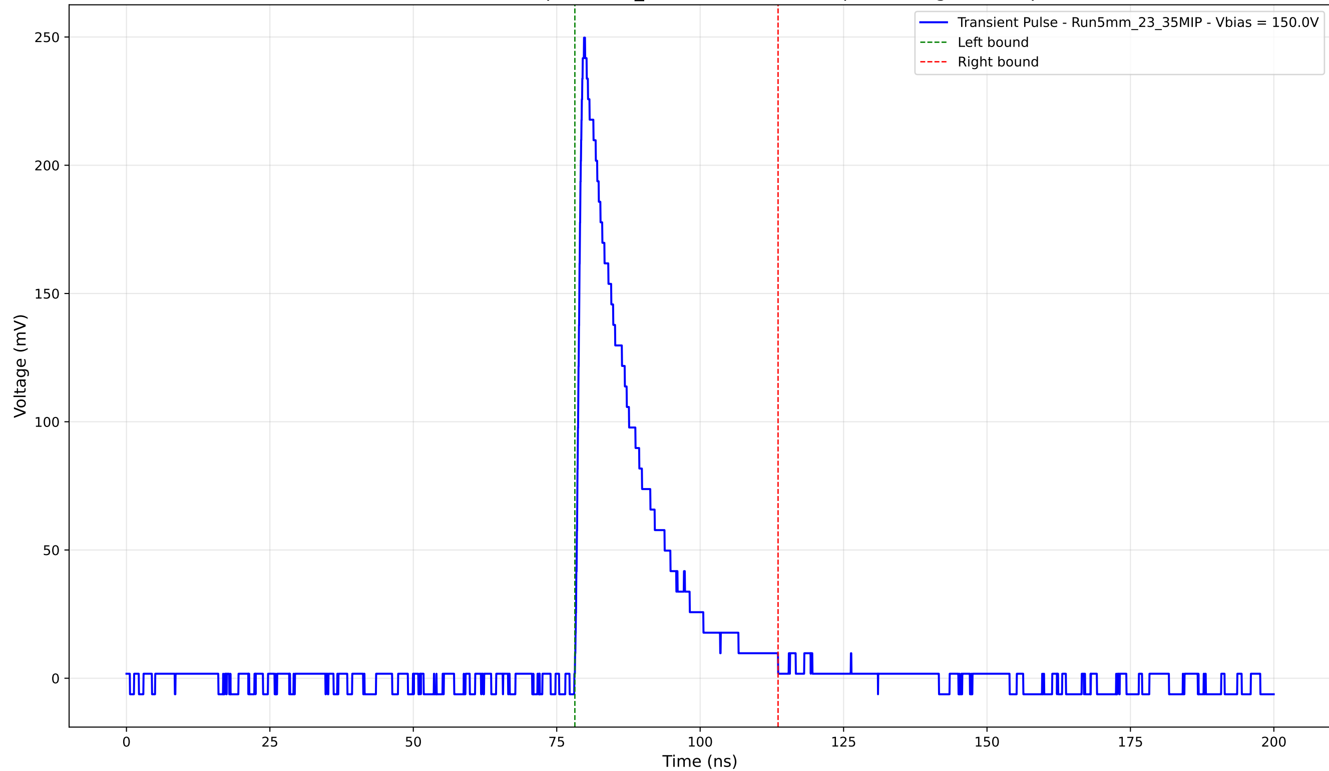
Transient Pulse - Sample: 5mm_23 - Position: 1160.0 \mu\text{m} - Charge: 48.39 pC
