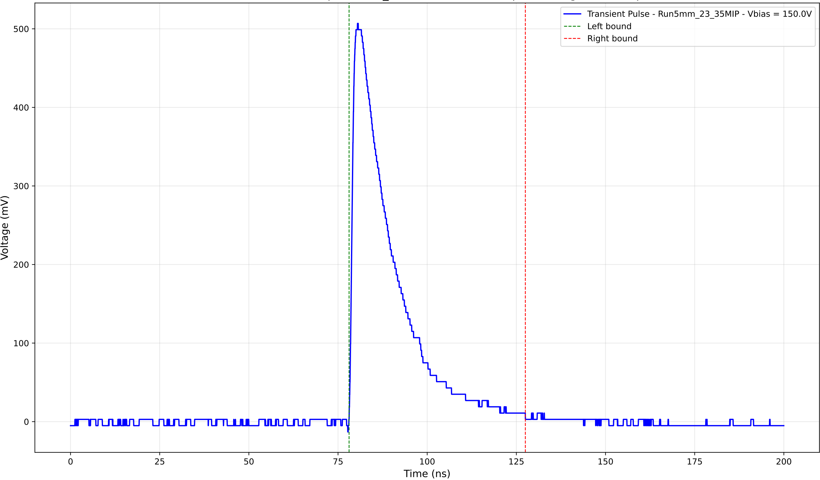
Transient Pulse - Sample: 5mm_23 - Position: 3430.0 \mu\text{m} - Charge: 127.26 pC
