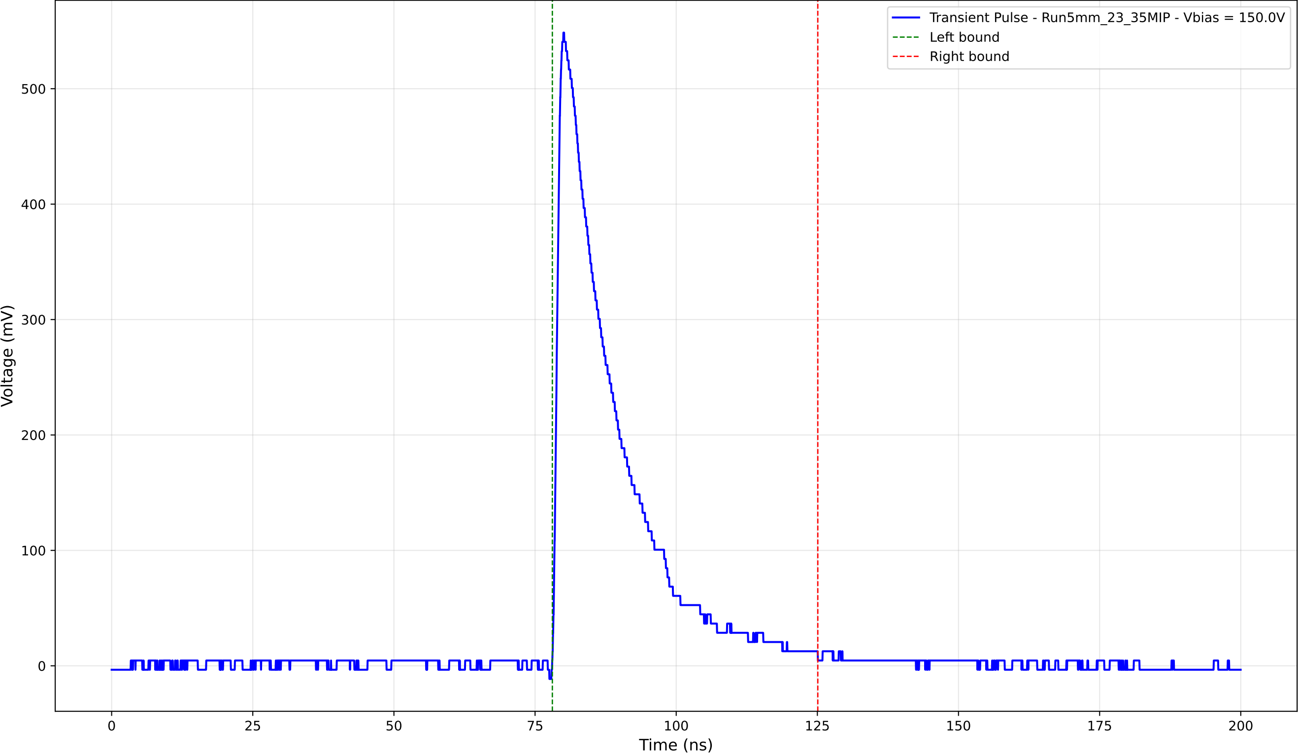
Transient Pulse - Sample: 5mm_23 - Position: 3795.0 \mu\text{m} - Charge: 123.84 pC
