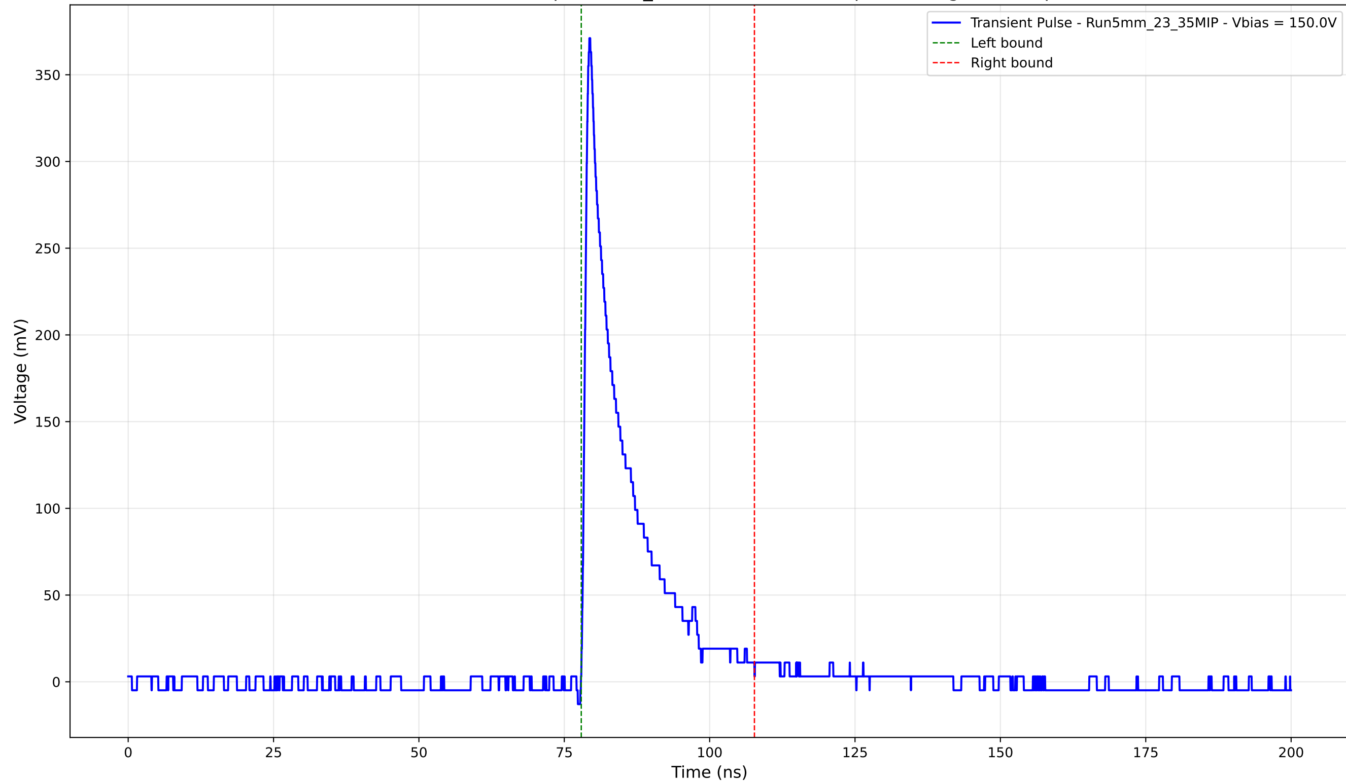
Transient Pulse - Sample: 5mm_23 - Position: 4550.0 \mu\text{m} - Charge: 52.48 pC
