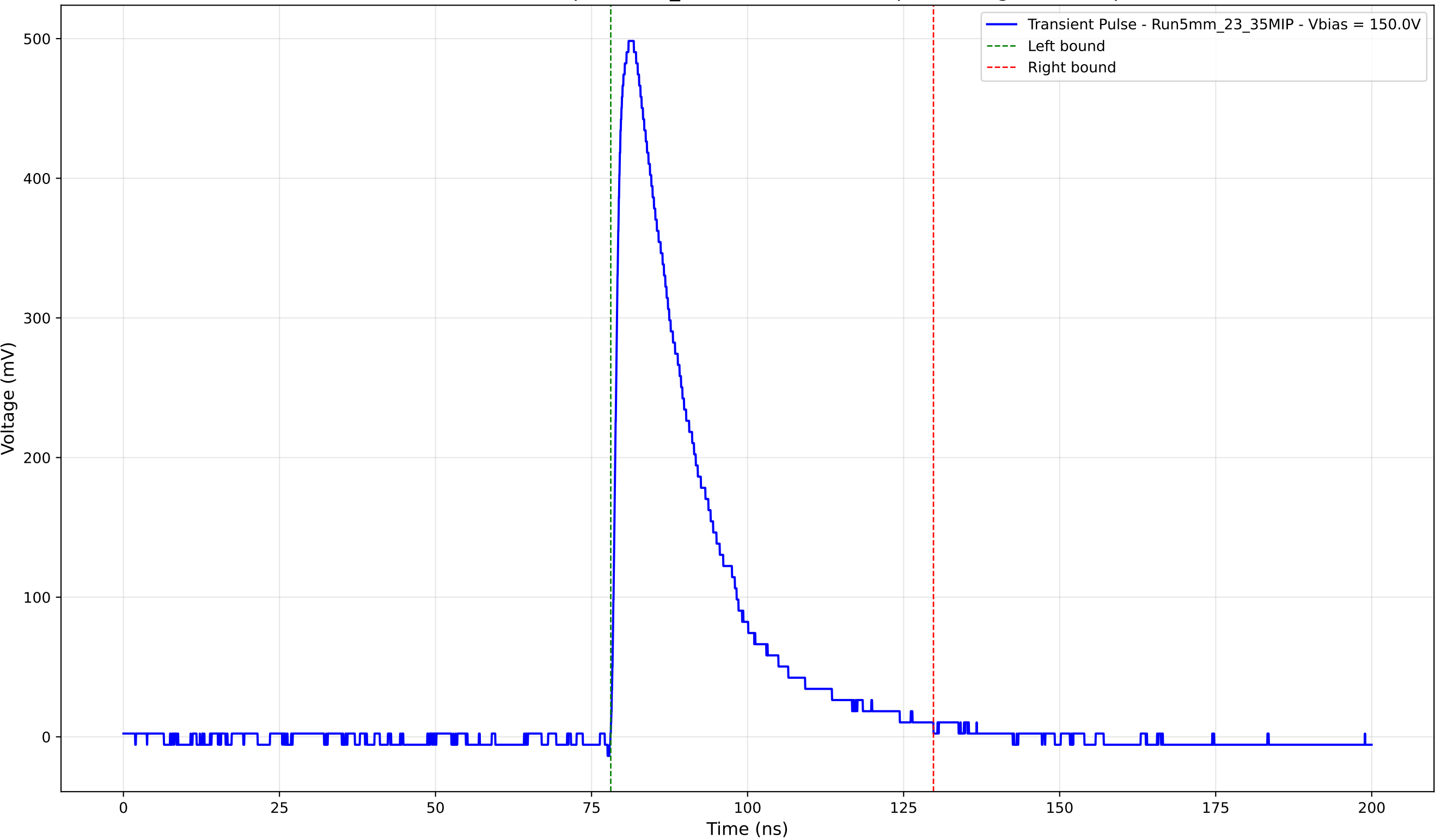
Transient Pulse - Sample: 5mm_23 - Position: 2530.0 \mu\text{m} - Charge: 135.36 pC
