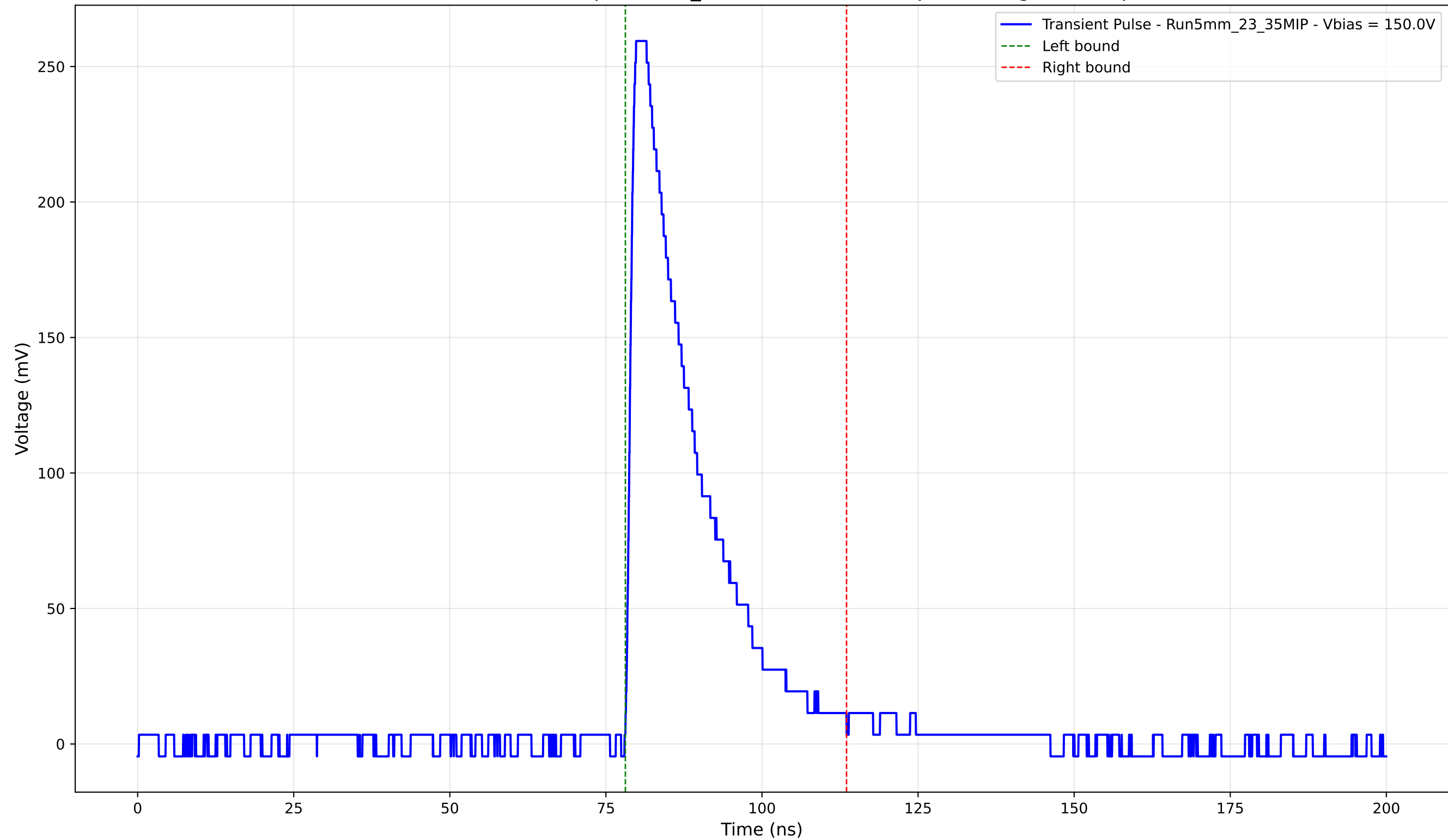
Transient Pulse - Sample: 5mm_23 - Position: 3610.0 \mu\text{m} - Charge: 59.92 pC
