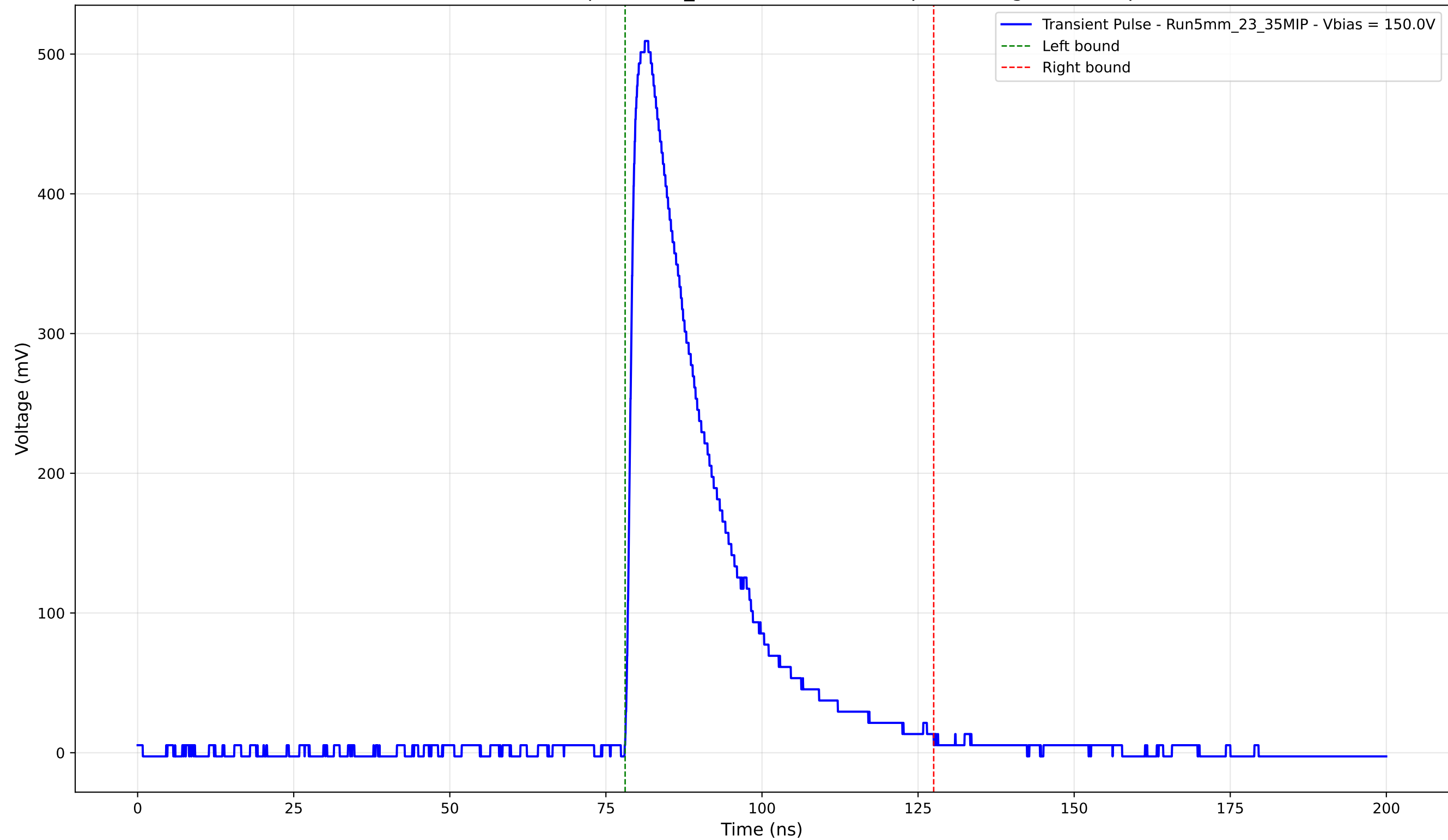
Transient Pulse - Sample: 5mm_23 - Position: 2450.0 \mu\text{m} - Charge: 138.59 pC
