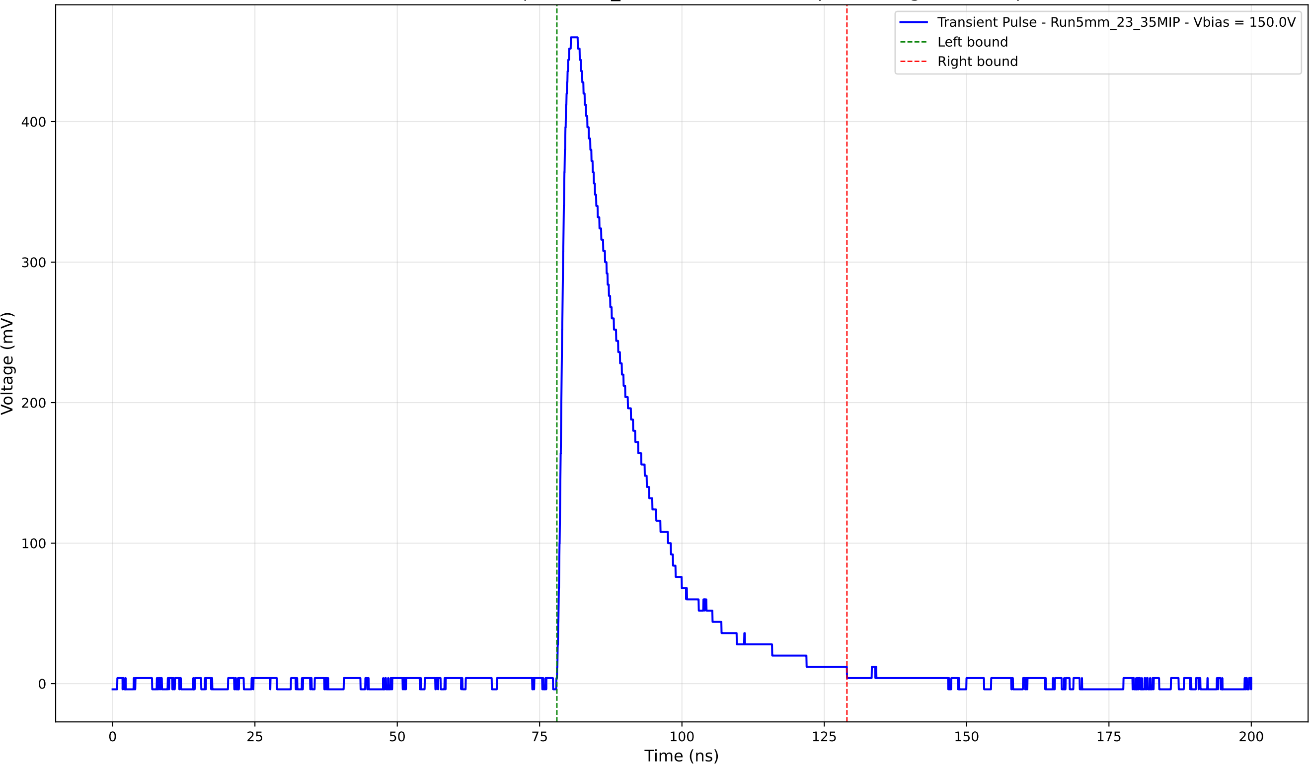
Transient Pulse - Sample: 5mm_23 - Position: 3065.0 \mu\text{m} - Charge: 122.70 pC
