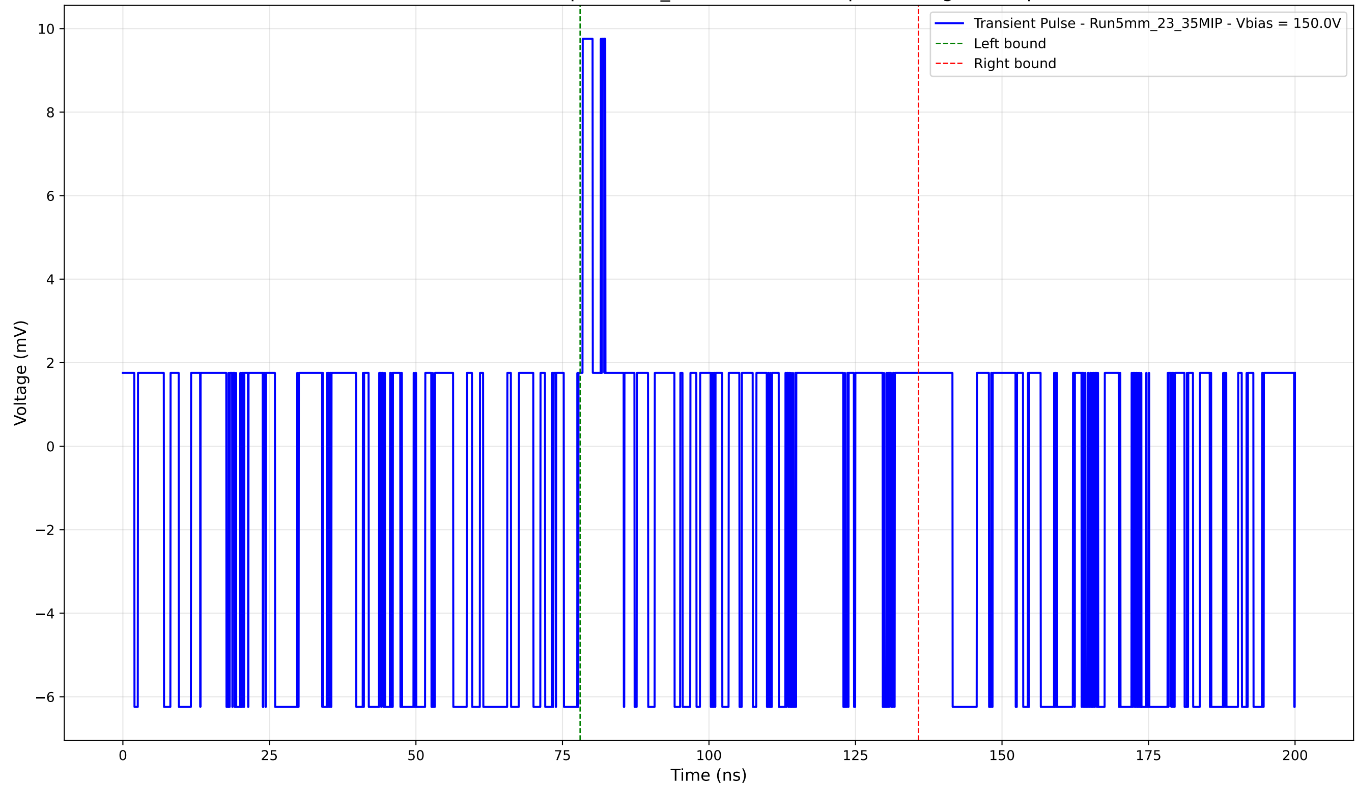
Transient Pulse - Sample: 5mm_23 - Position: 50.0 \mu\text{m} - Charge: 0.45 pC
