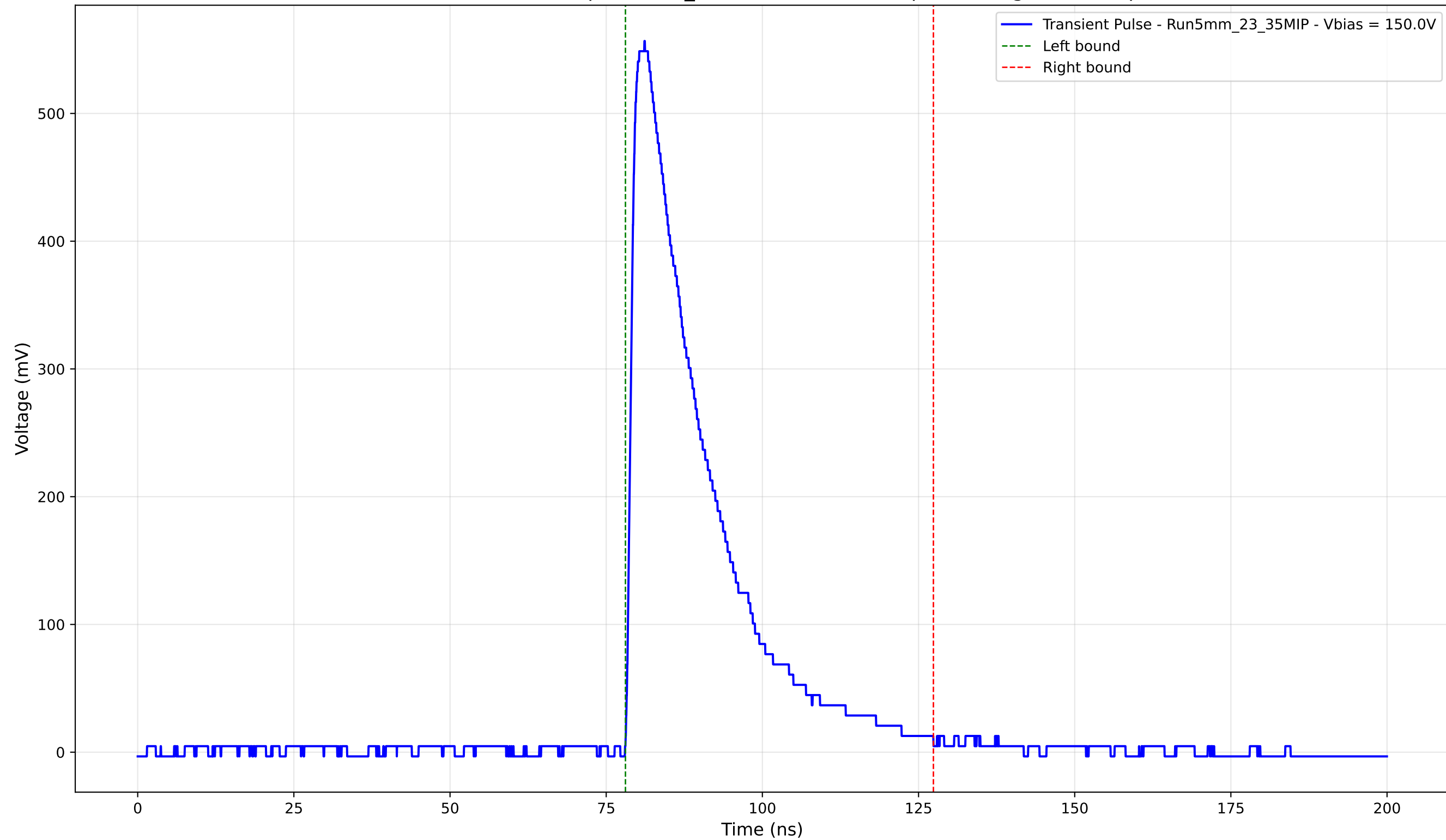
Transient Pulse - Sample: 5mm_23 - Position: 2000.0 \mu\text{m} - Charge: 145.82 pC
