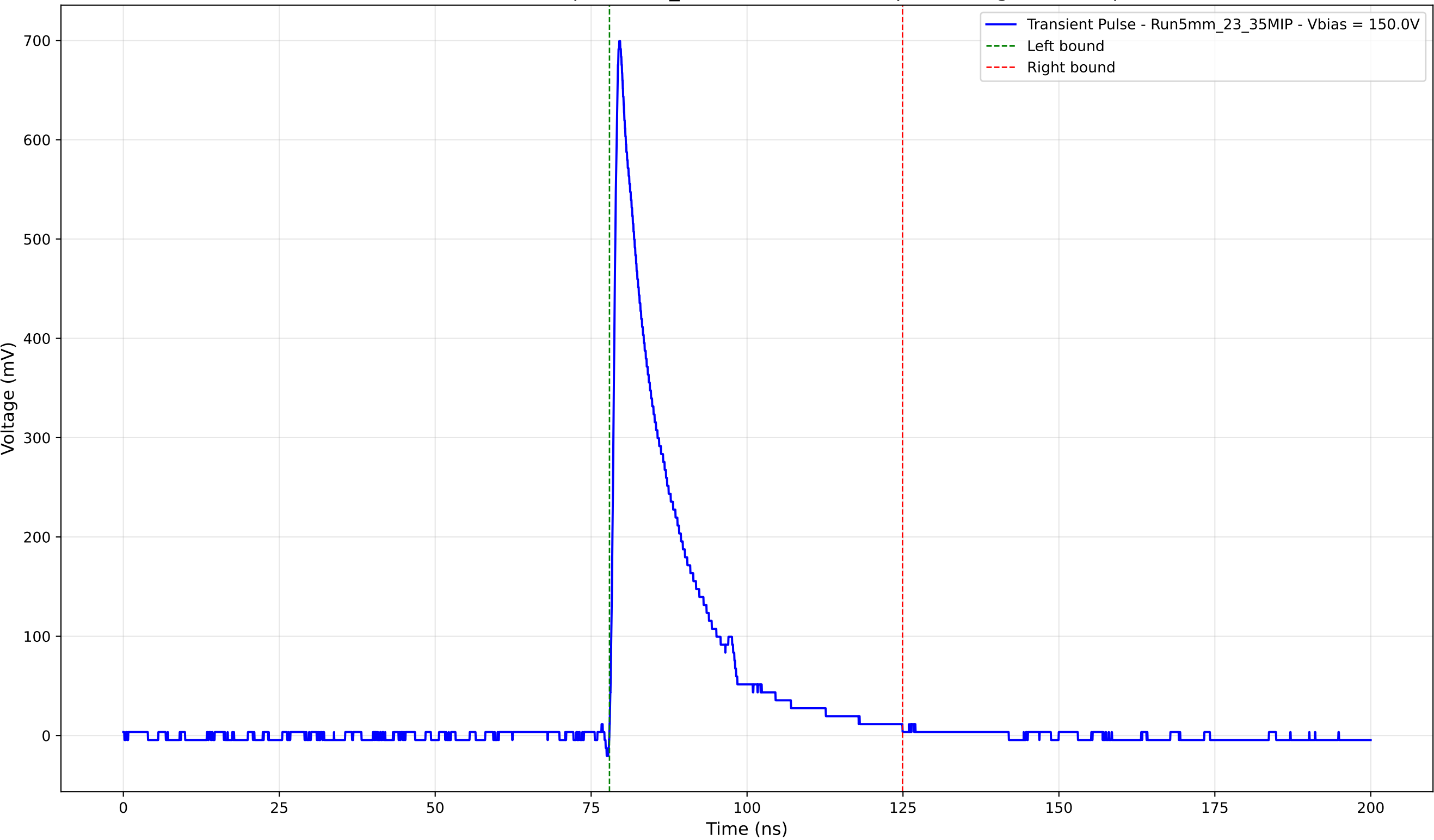
Transient Pulse - Sample: 5mm_23 - Position: 4375.0 \mu\text{m} - Charge: 125.46 pC
