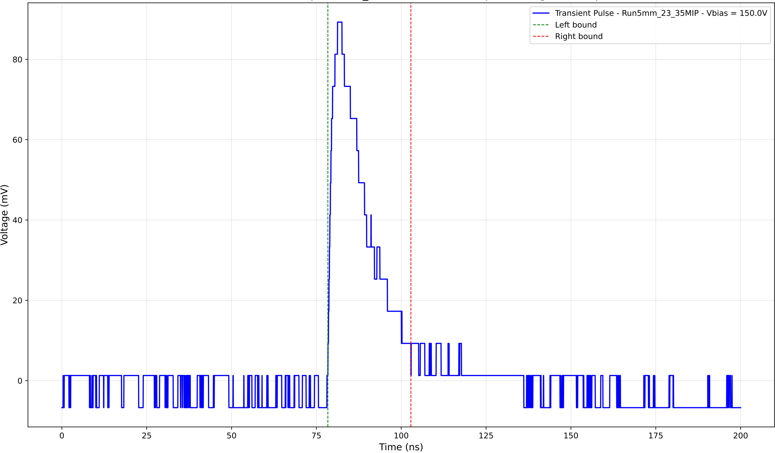
Transient Pulse - Sample: 5mm_23 - Position: 2145.0 \mu\text{m} - Charge: 20.34 pC
