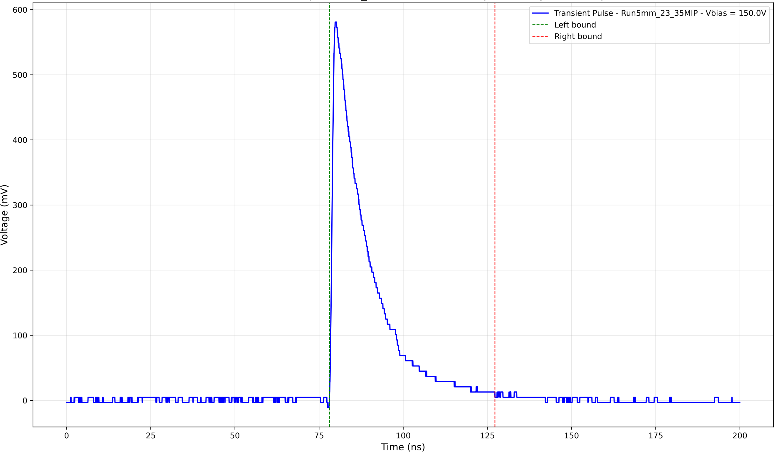
Transient Pulse - Sample: 5mm_23 - Position: 1340.0 \mu\text{m} - Charge: 132.20 pC
