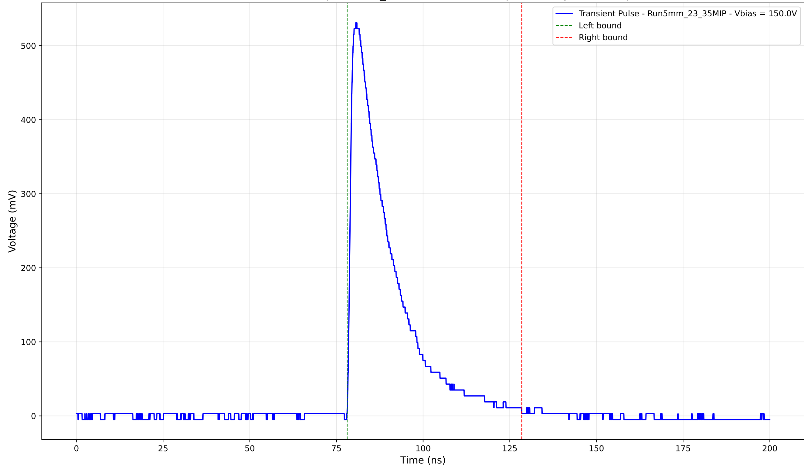
Transient Pulse - Sample: 5mm_23 - Position: 1880.0 \mu\text{m} - Charge: 136.58 pC
