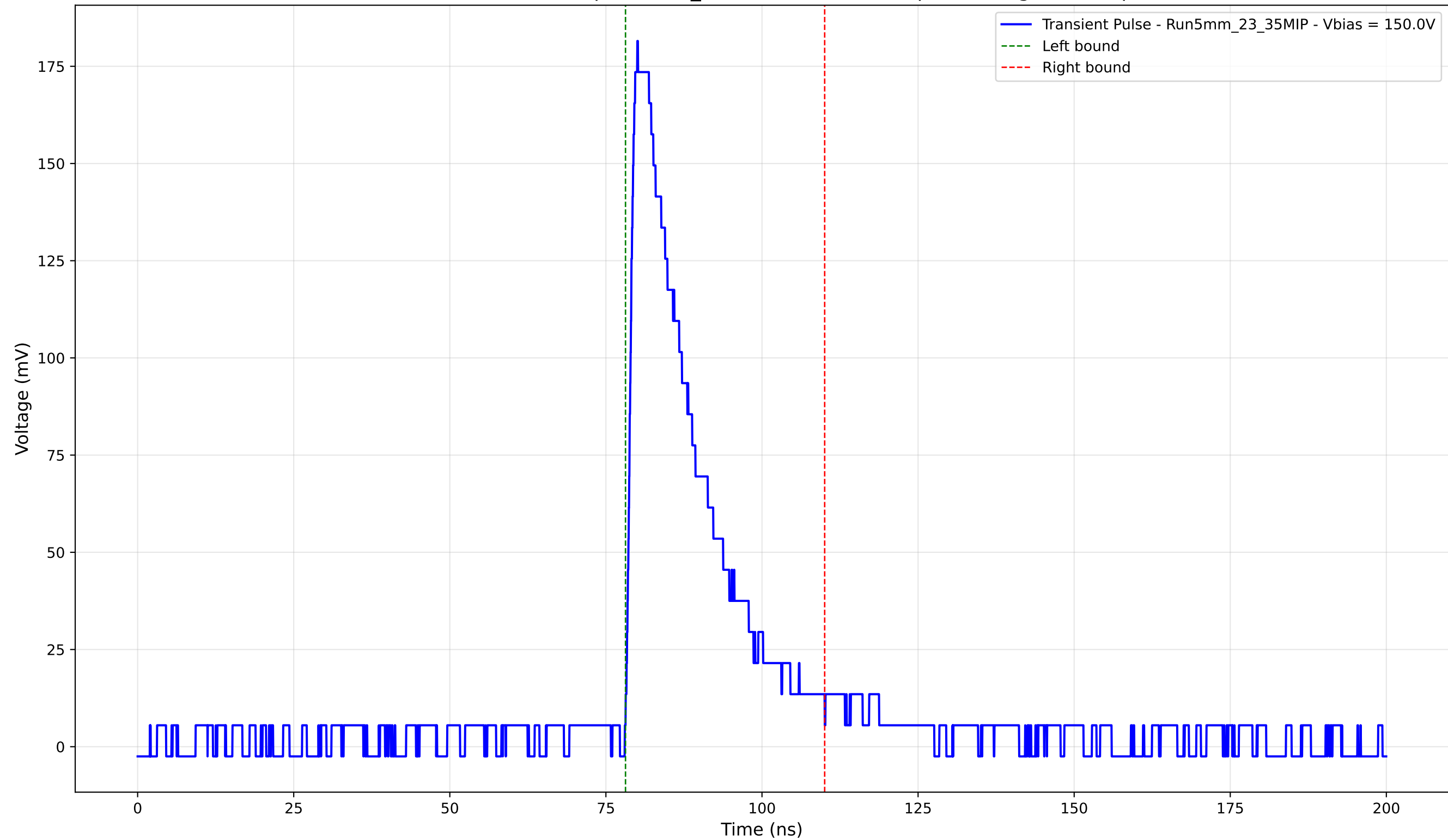
Transient Pulse - Sample: 5mm_23 - Position: 3625.0 \mu\text{m} - Charge: 41.35 pC
