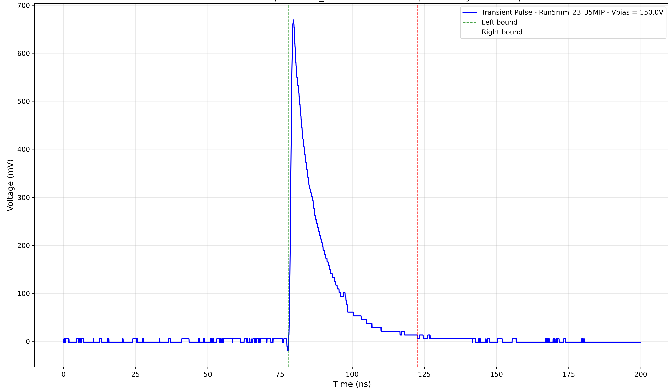
Transient Pulse - Sample: 5mm_23 - Position: 930.0 \mu\text{m} - Charge: 124.92 pC
