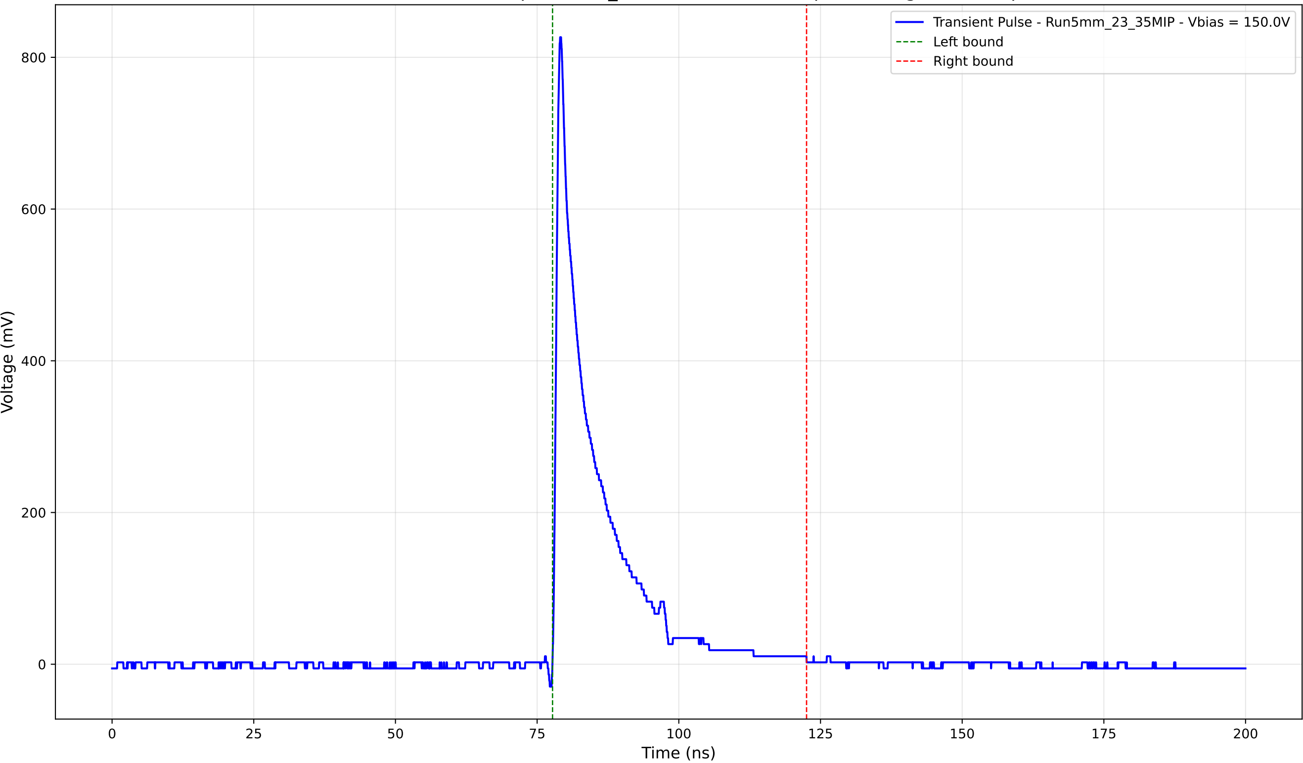
Transient Pulse - Sample: 5mm_23 - Position: 4830.0 \mu\text{m} - Charge: 113.01 pC
