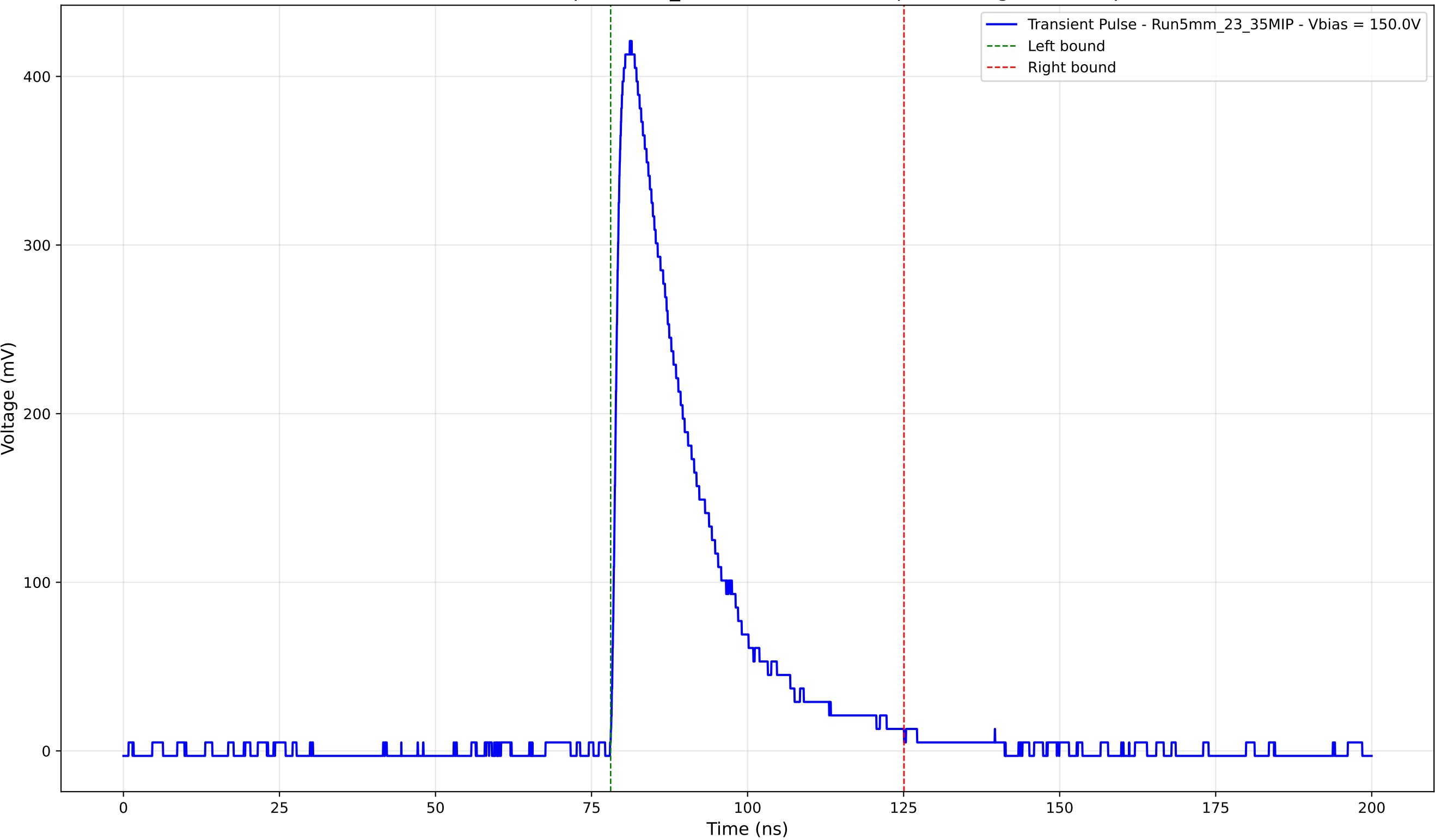
Transient Pulse - Sample: 5mm_23 - Position: 2210.0 \mu\text{m} - Charge: 111.84 pC
