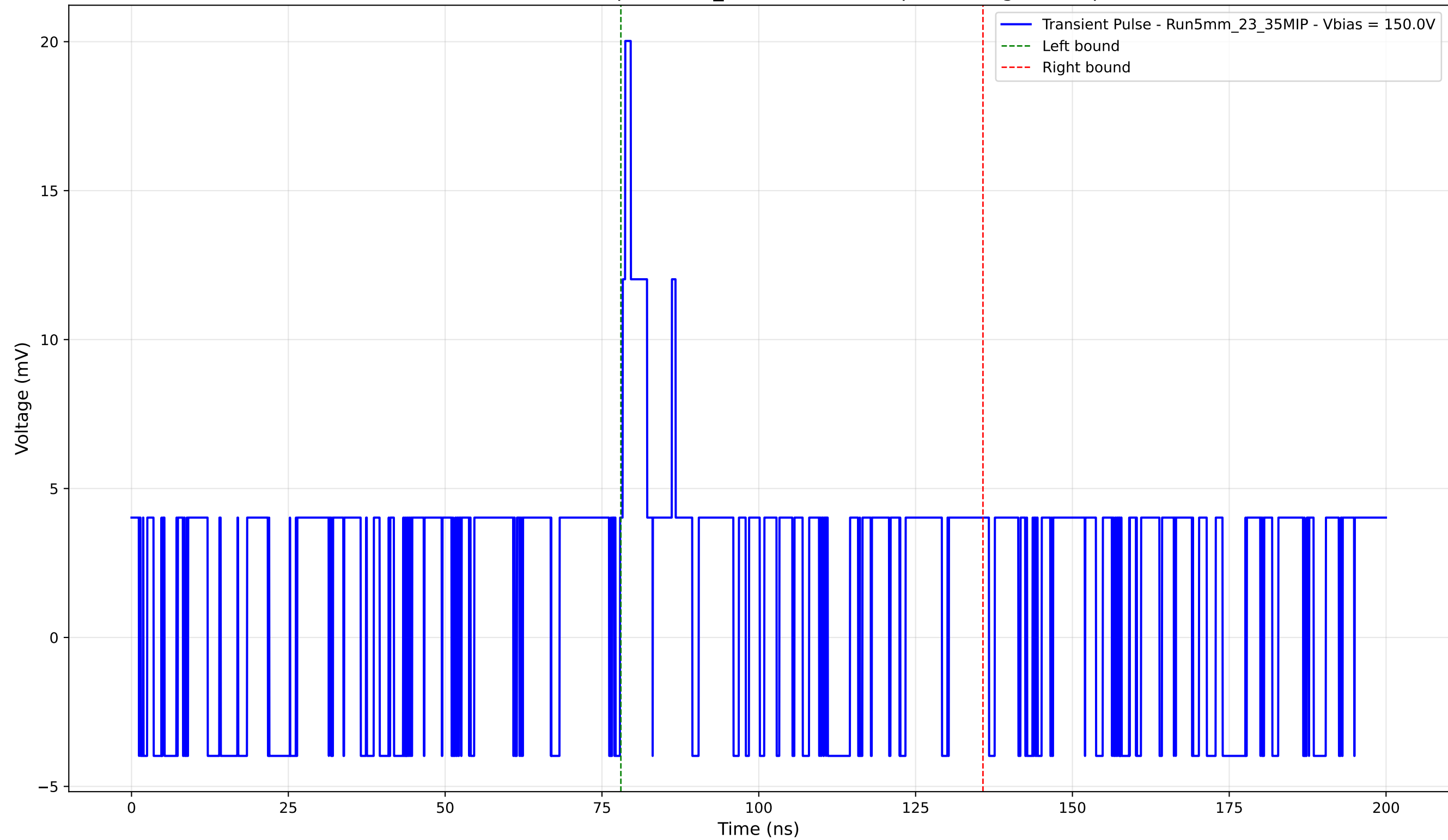
Transient Pulse - Sample: 5mm_23 - Position: 0.0 \mu\text{m} - Charge: 3.65 pC
