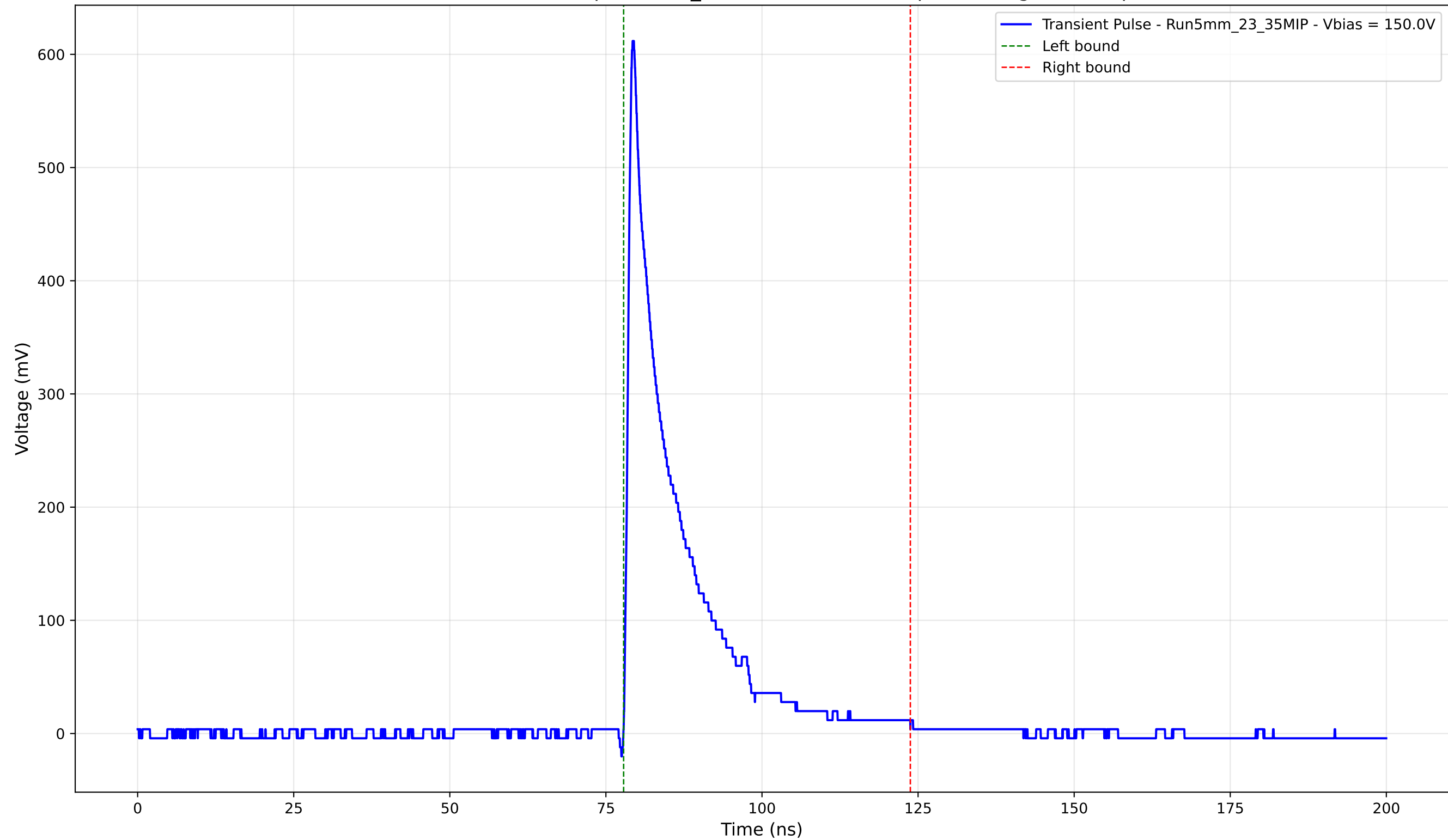
Transient Pulse - Sample: 5mm_23 - Position: 4595.0 \mu\text{m} - Charge: 94.58 pC
