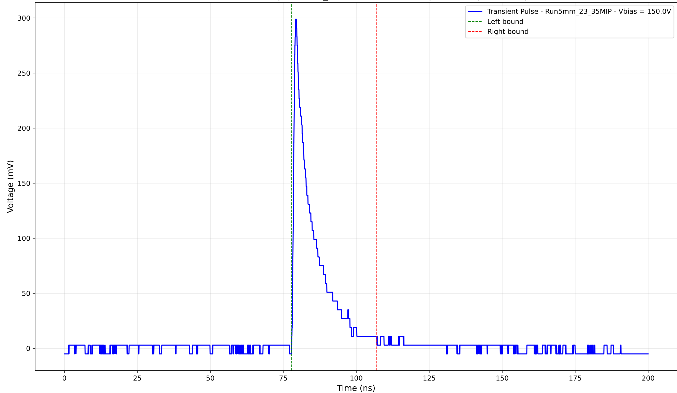
Transient Pulse - Sample: 5mm_23 - Position: 4635.0 \mu\text{m} - Charge: 41.74 pC
