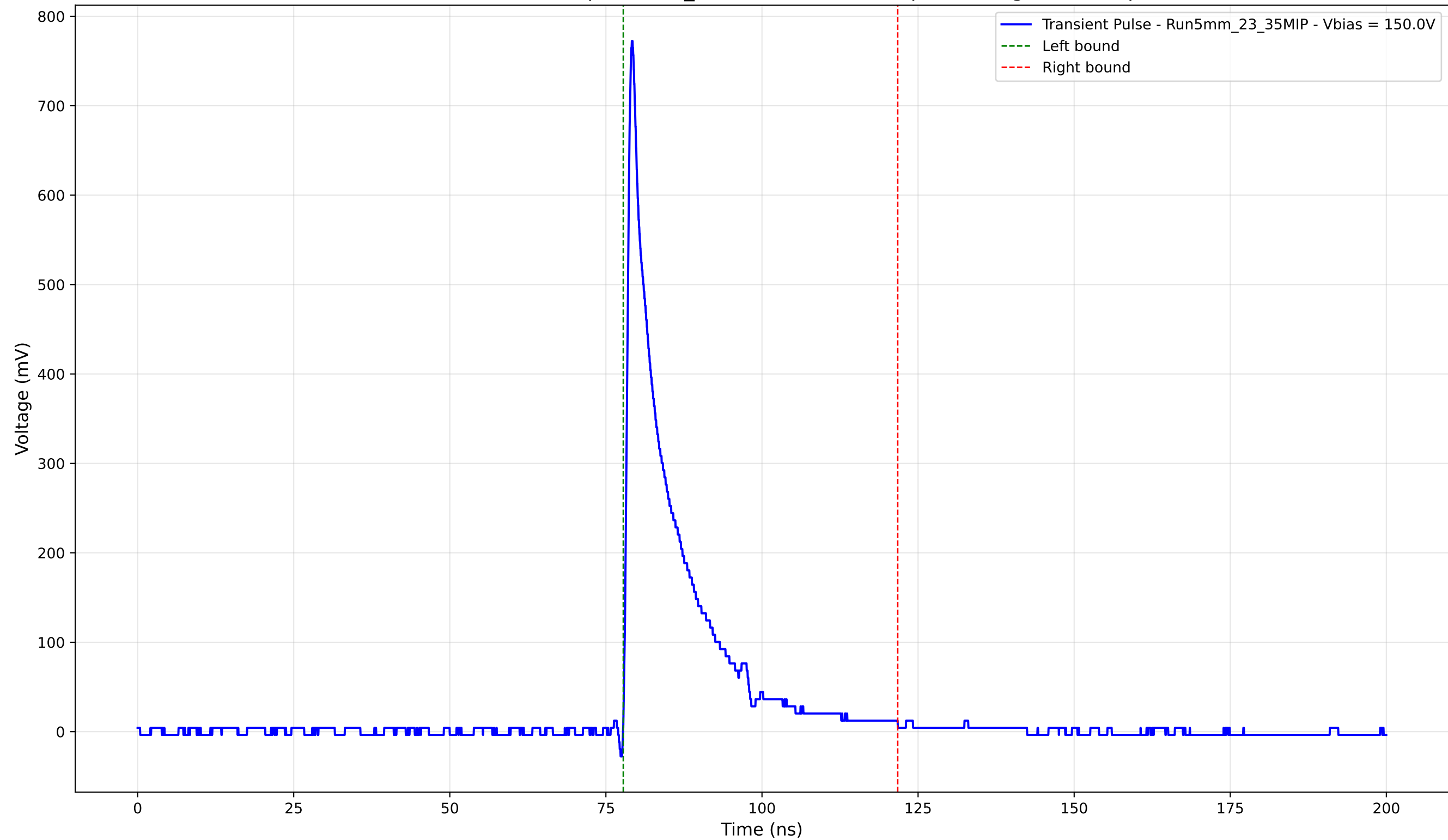
Transient Pulse - Sample: 5mm_23 - Position: 4760.0 \mu\text{m} - Charge: 108.55 pC
