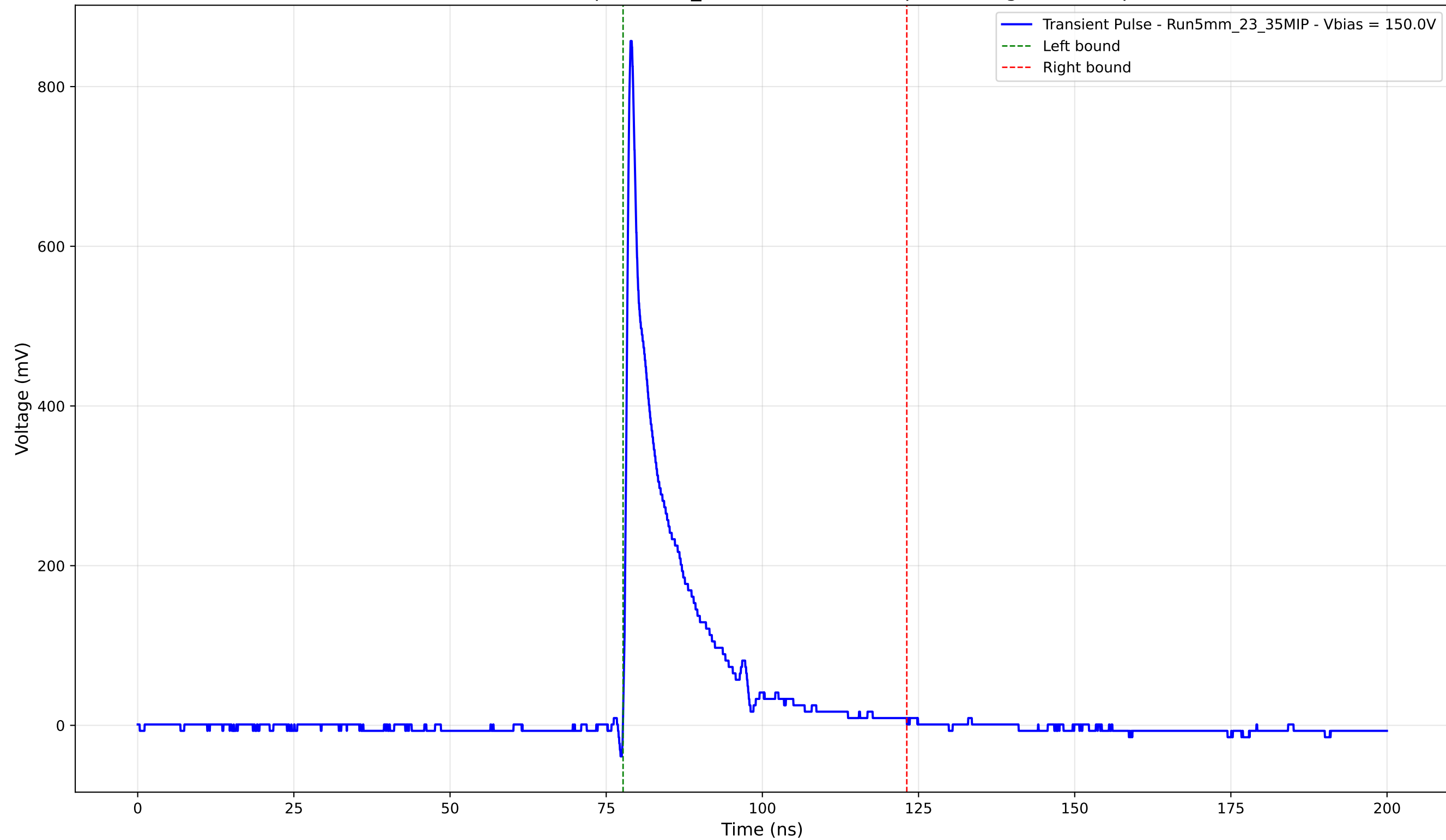
Transient Pulse - Sample: 5mm_23 - Position: 260.0 \mu\text{m} - Charge: 107.27 pC
