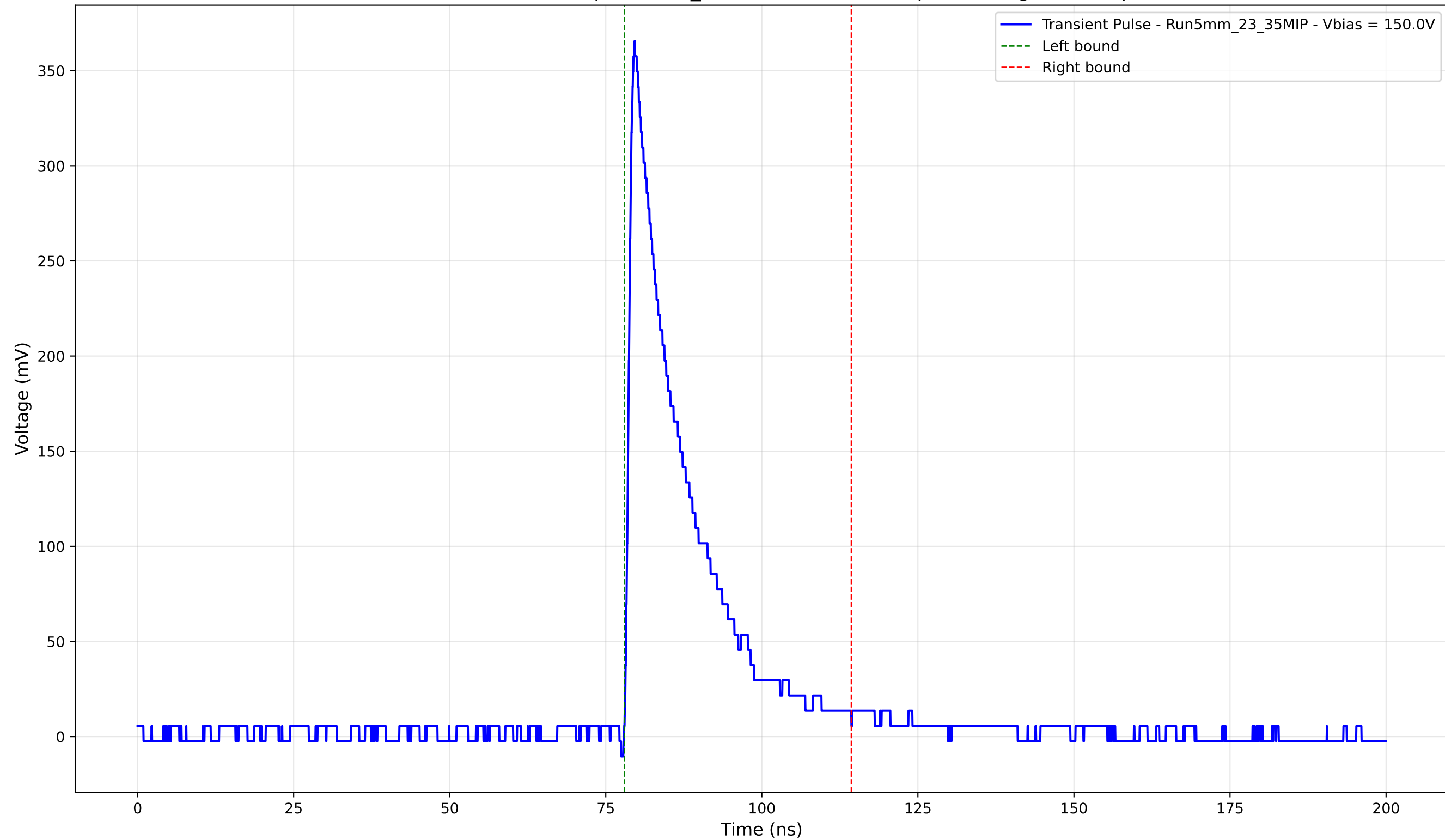
Transient Pulse - Sample: 5mm_23 - Position: 4470.0 \mu\text{m} - Charge: 68.58 pC
