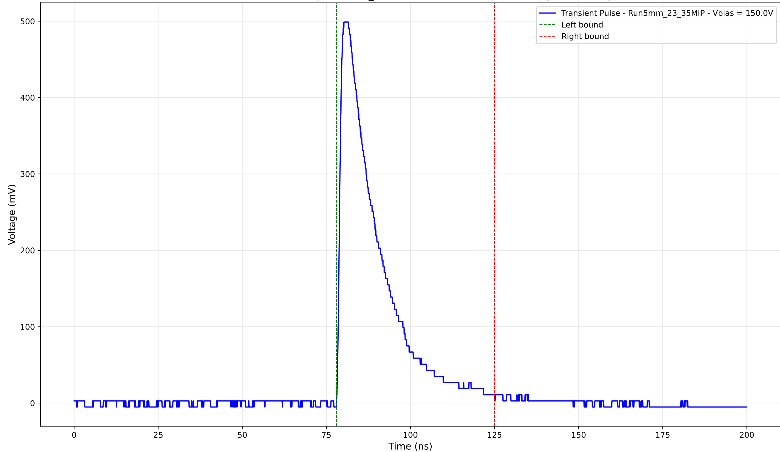
Transient Pulse - Sample: 5mm_23 - Position: 3385.0 \mu\text{m} - Charge: 126.34 pC
