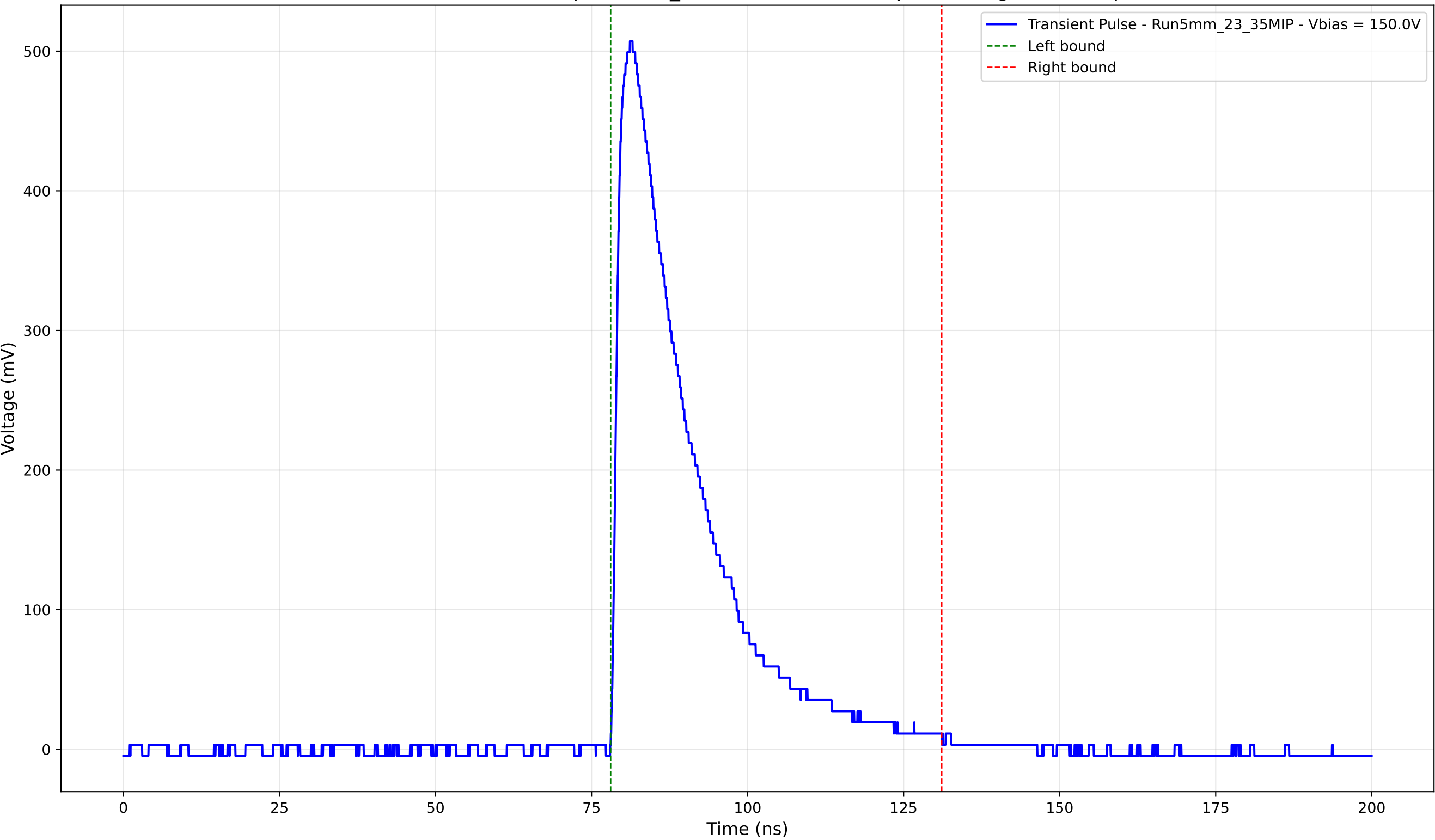
Transient Pulse - Sample: 5mm_23 - Position: 2435.0 \mu\text{m} - Charge: 137.25 pC
