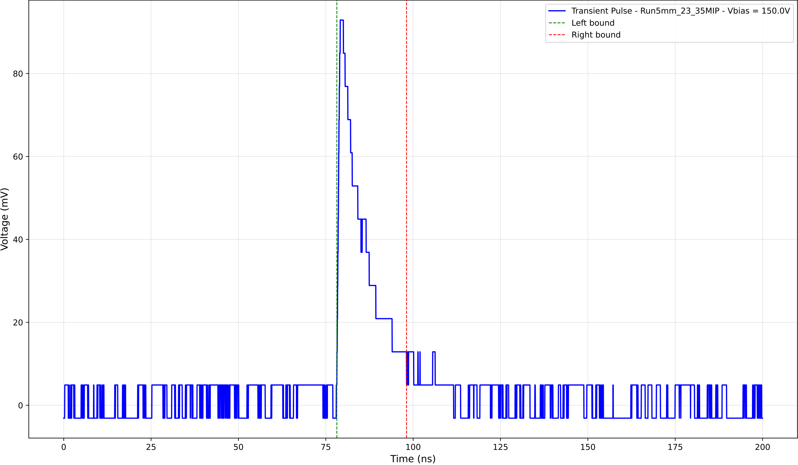
Transient Pulse - Sample: 5mm_23 - Position: 4505.0 \mu\text{m} - Charge: 14.92 pC
