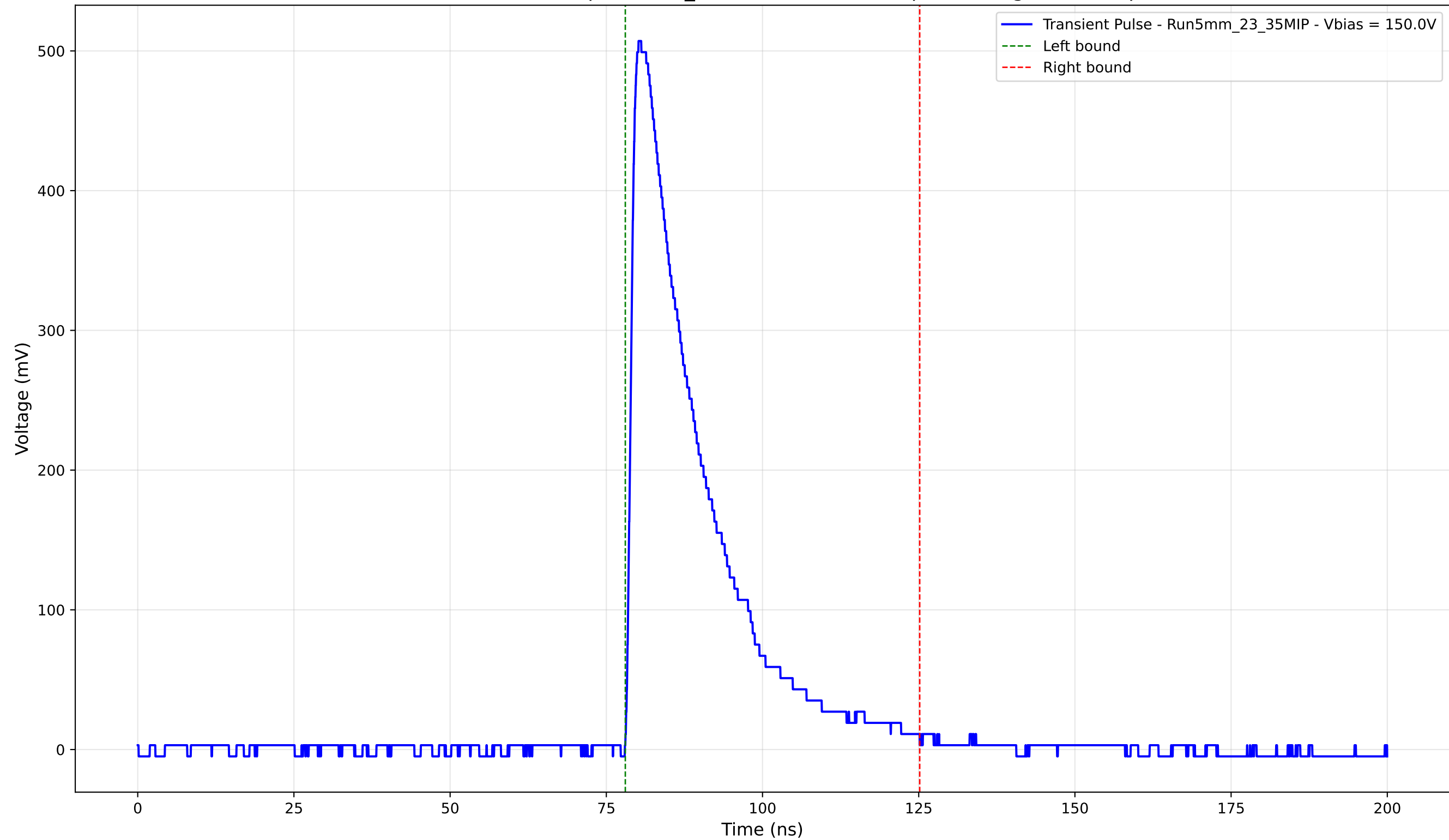
Transient Pulse - Sample: 5mm_23 - Position: 3510.0 \mu\text{m} - Charge: 124.81 pC
