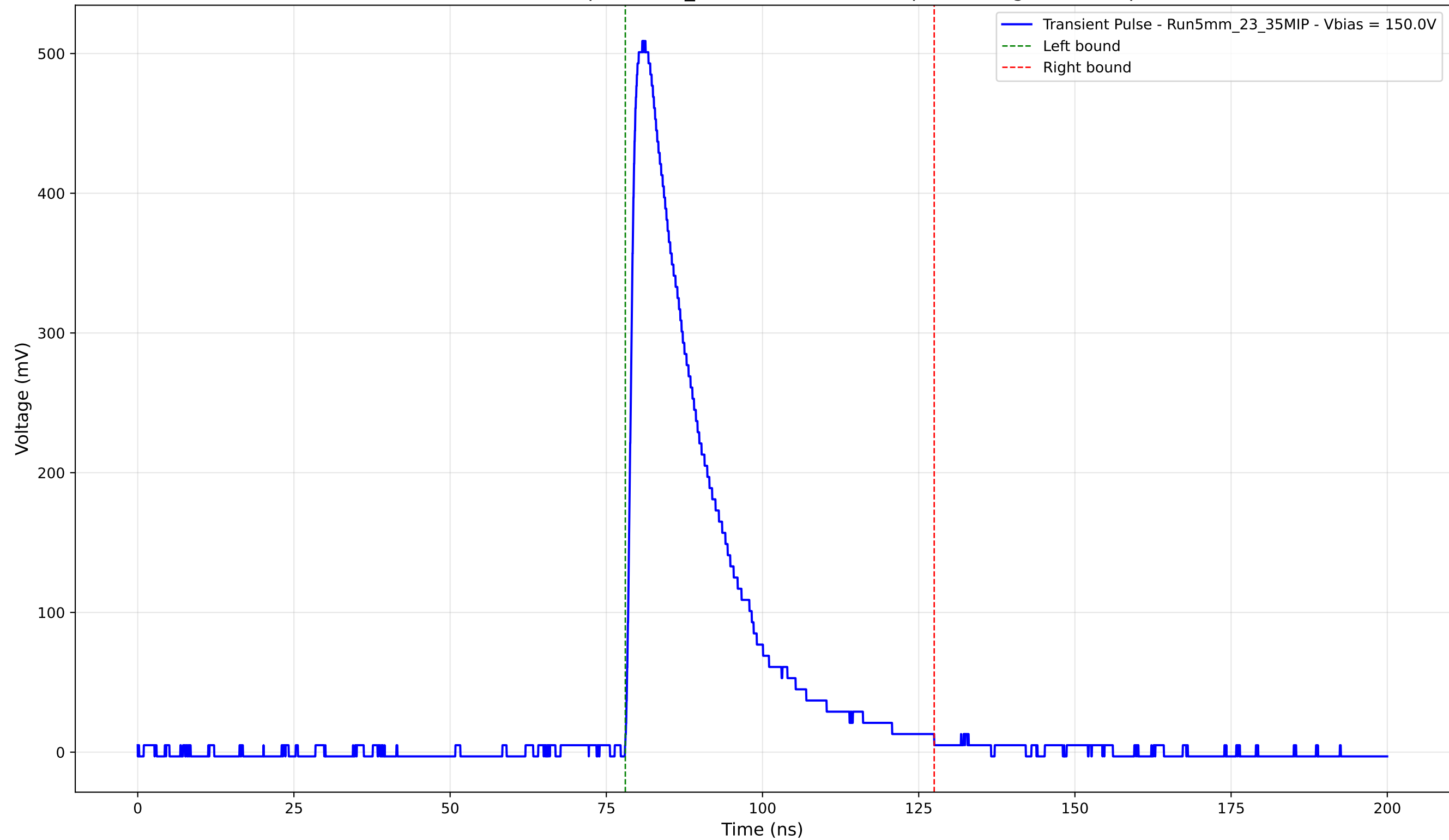
Transient Pulse - Sample: 5mm_23 - Position: 3300.0 \mu\text{m} - Charge: 131.19 pC
