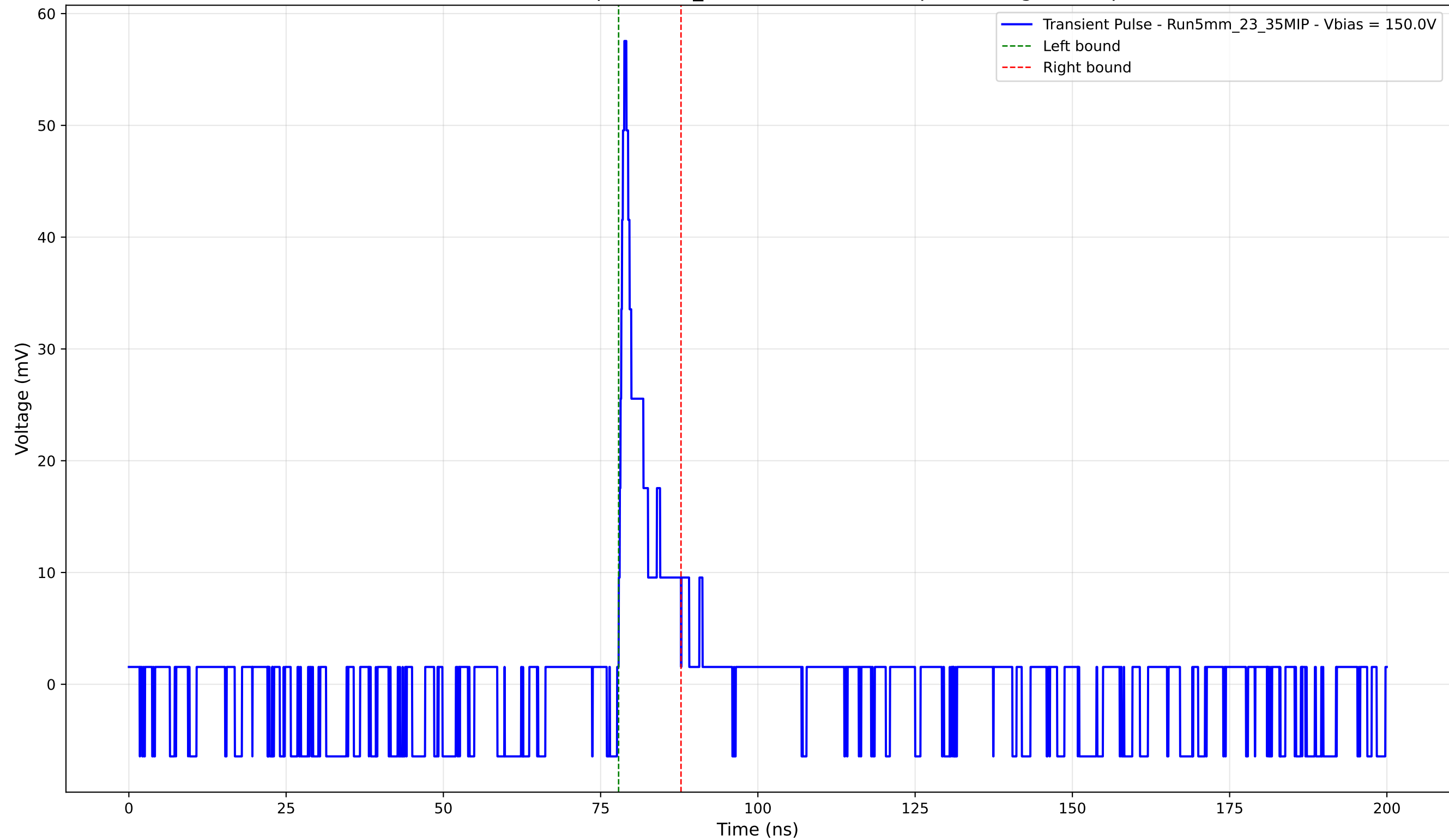
Transient Pulse - Sample: 5mm_23 - Position: 5125.0 \mu\text{m} - Charge: 3.91 pC
