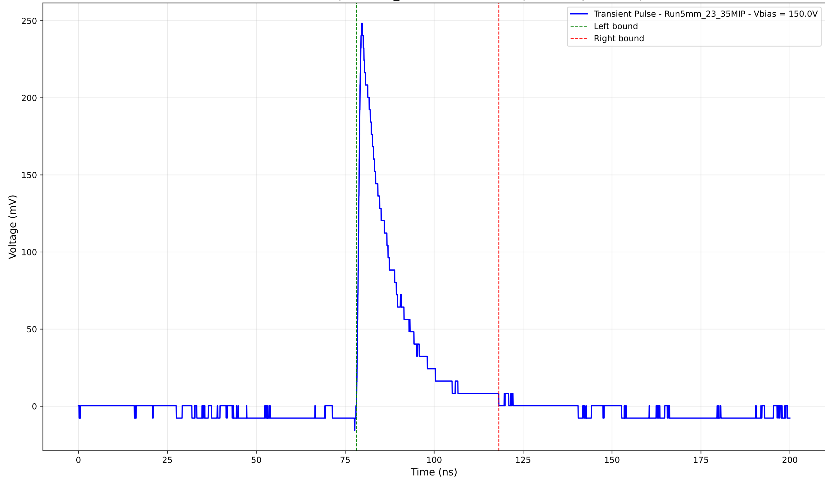
Transient Pulse - Sample: 5mm_23 - Position: 1090.0 \mu\text{m} - Charge: 45.71 pC
