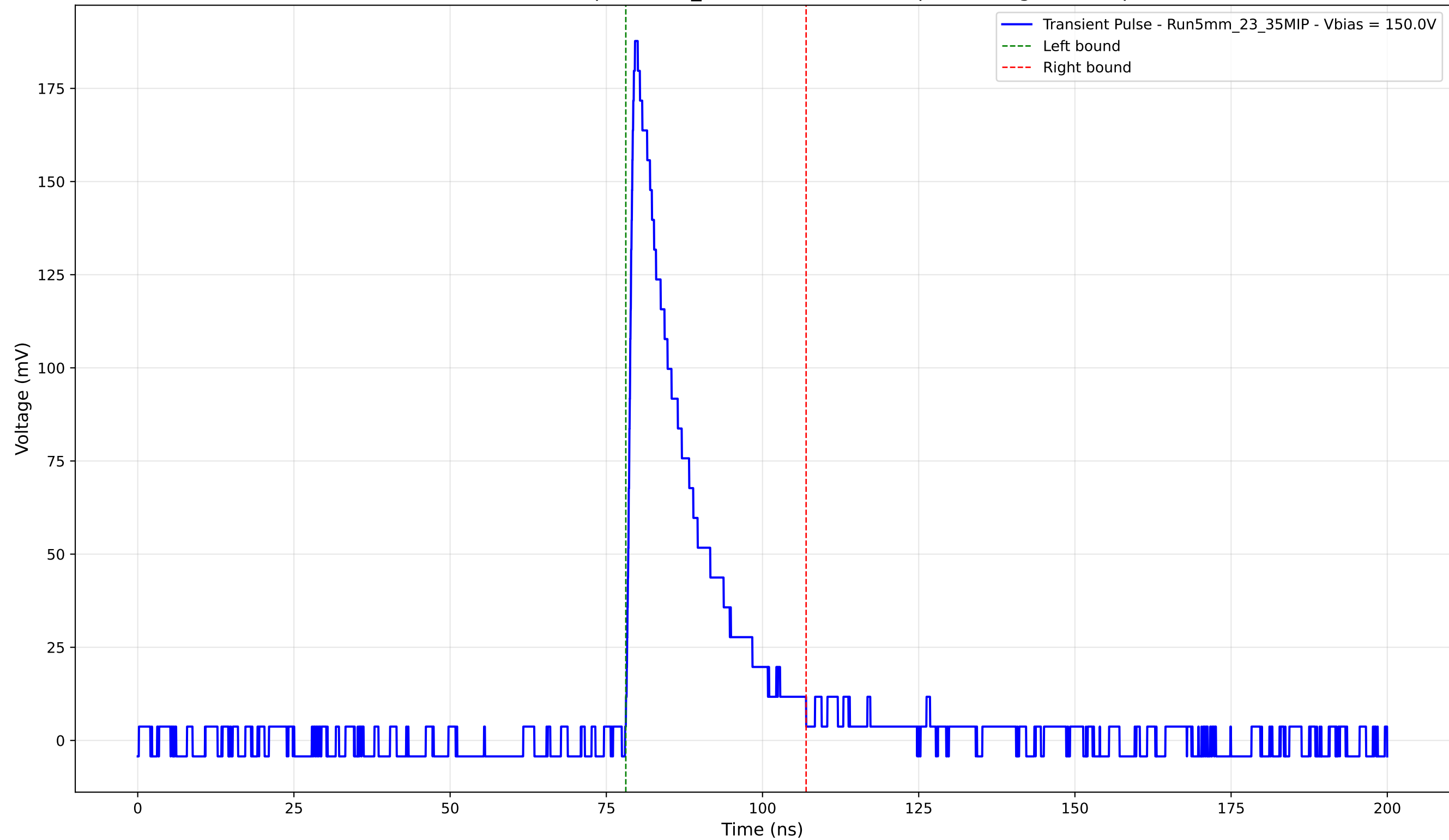
Transient Pulse - Sample: 5mm_23 - Position: 4130.0 \mu\text{m} - Charge: 35.08 pC
