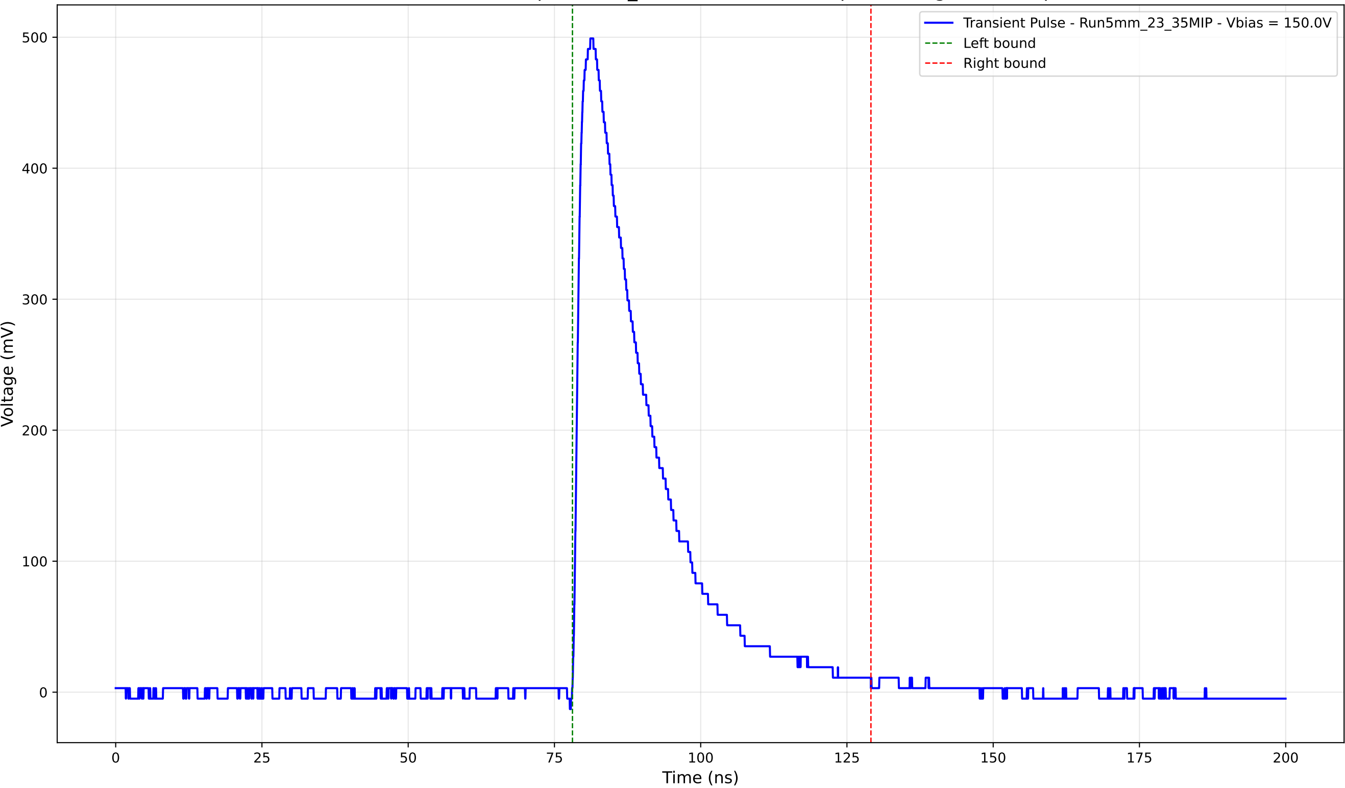
Transient Pulse - Sample: 5mm_23 - Position: 2840.0 \mu\text{m} - Charge: 134.30 pC
