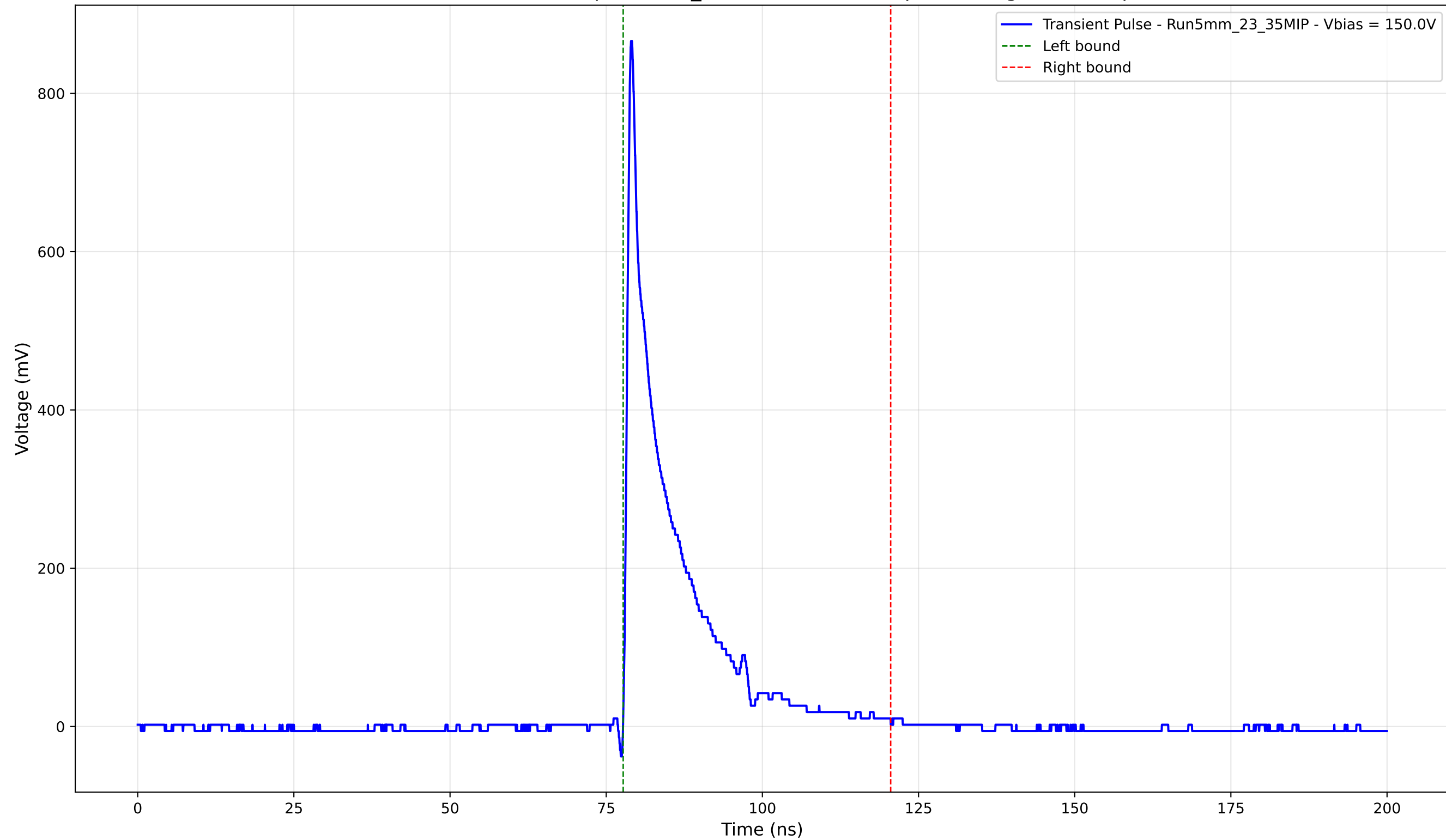
Transient Pulse - Sample: 5mm_23 - Position: 315.0 \mu\text{m} - Charge: 114.65 pC
