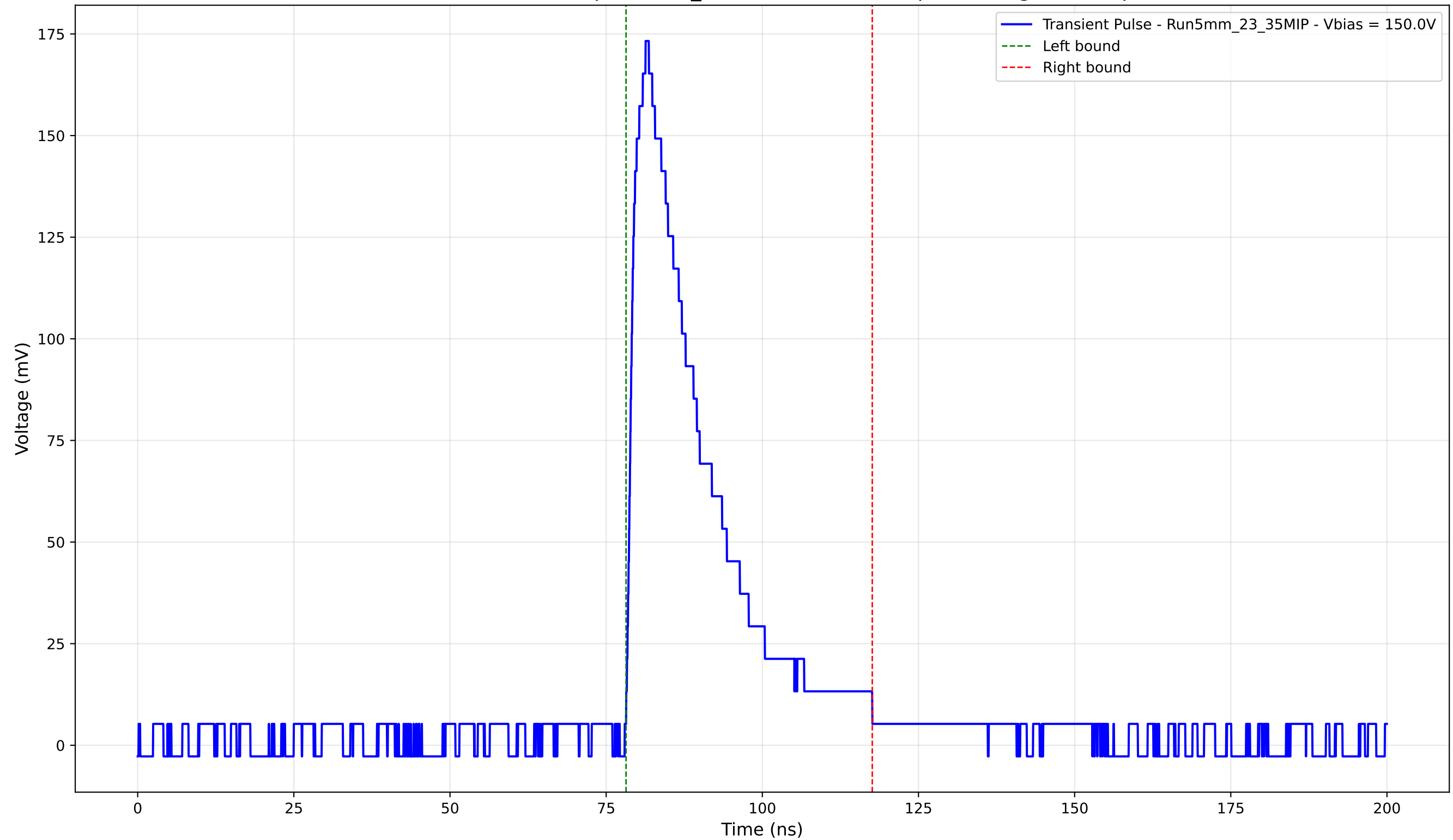
Transient Pulse - Sample: 5mm_23 - Position: 2675.0 \mu\text{m} - Charge: 44.35 pC
