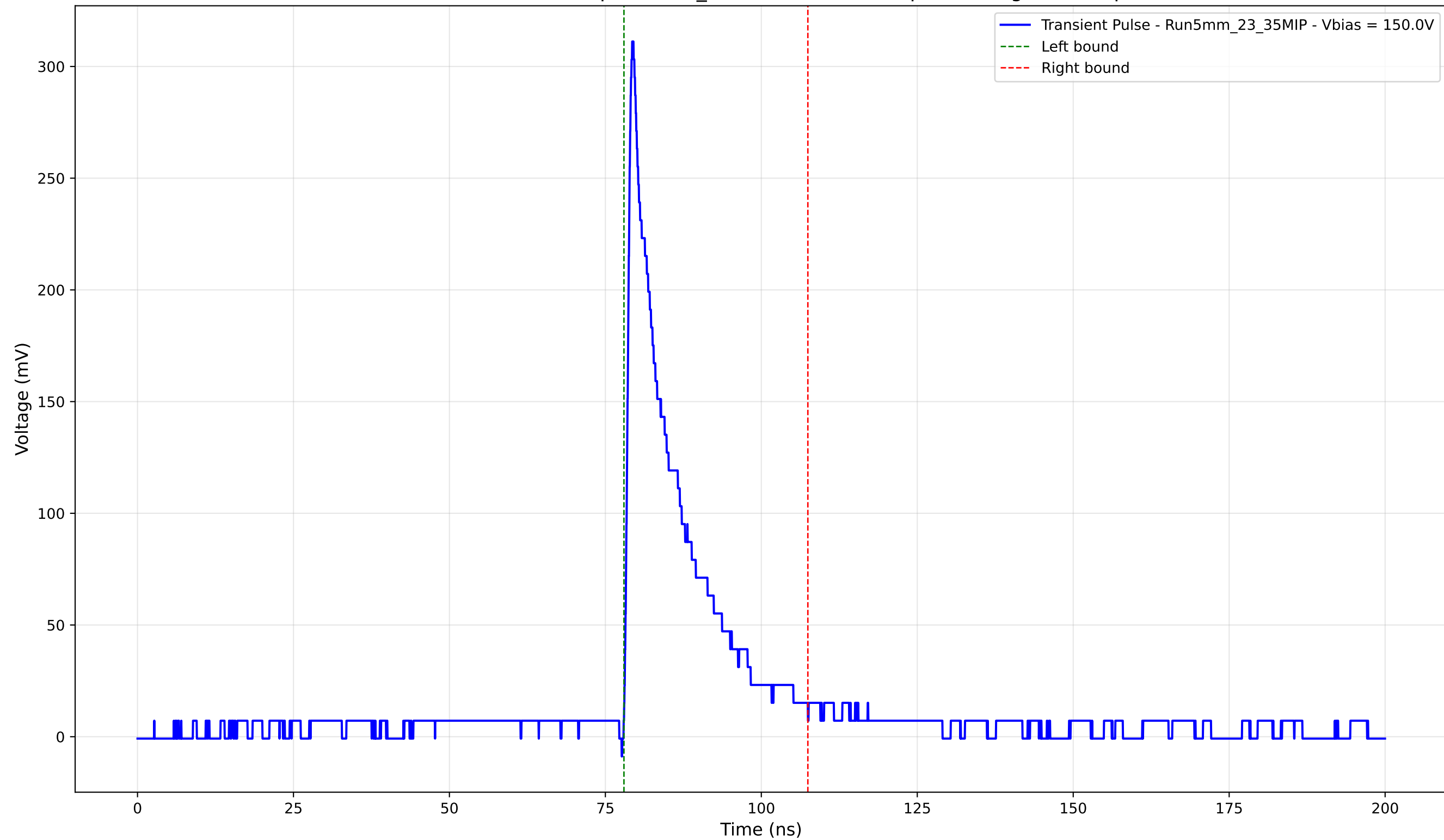
Transient Pulse - Sample: 5mm_23 - Position: 655.0 \mu\text{m} - Charge: 49.19 pC
