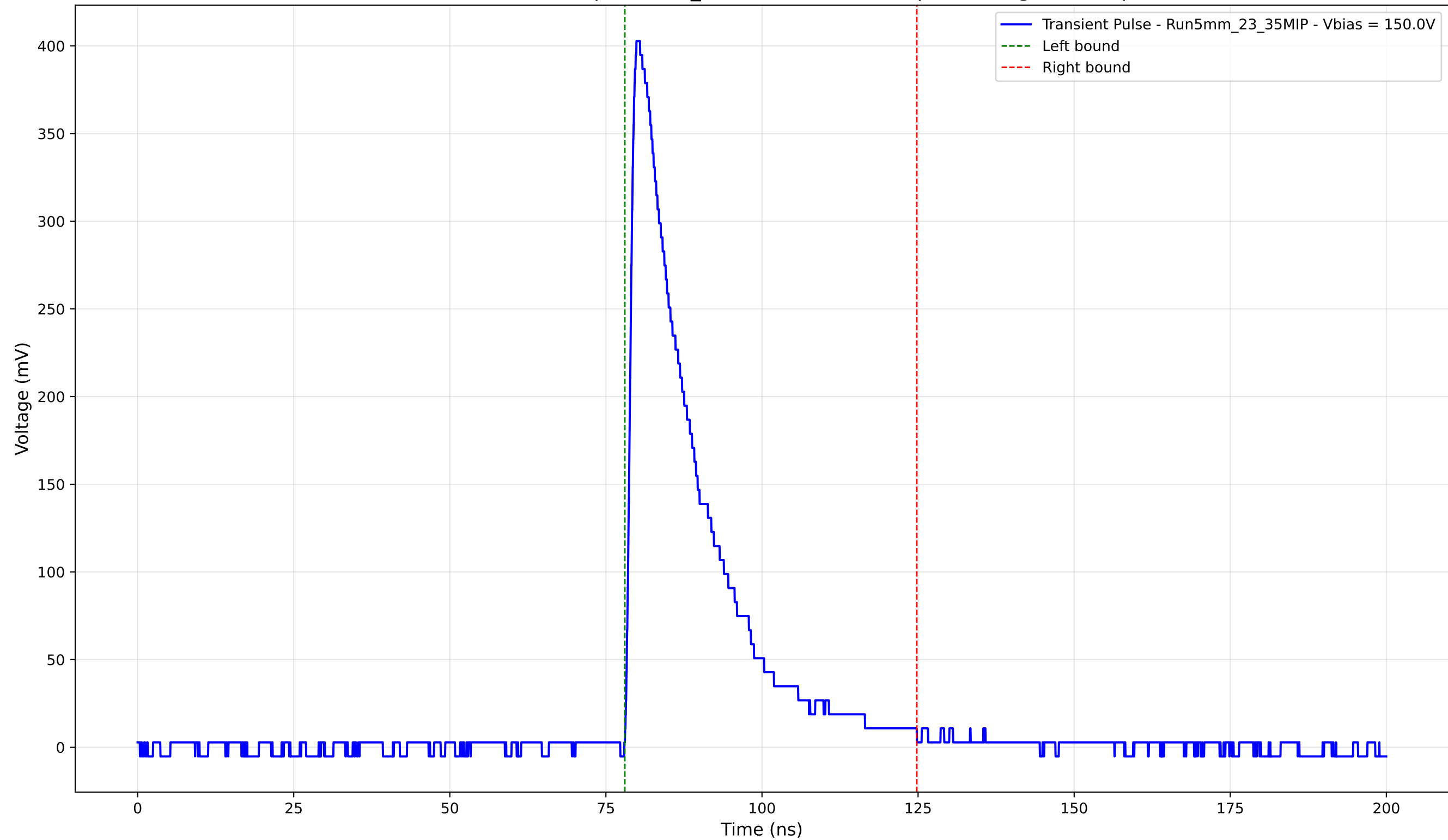
Transient Pulse - Sample: 5mm_23 - Position: 3715.0 \mu\text{m} - Charge: 92.49 pC
