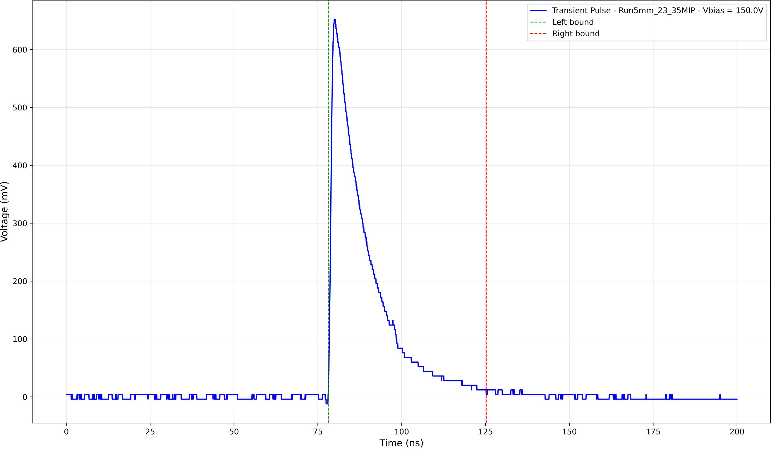
Transient Pulse - Sample: 5mm_23 - Position: 1440.0 \mu\text{m} - Charge: 151.46 pC
