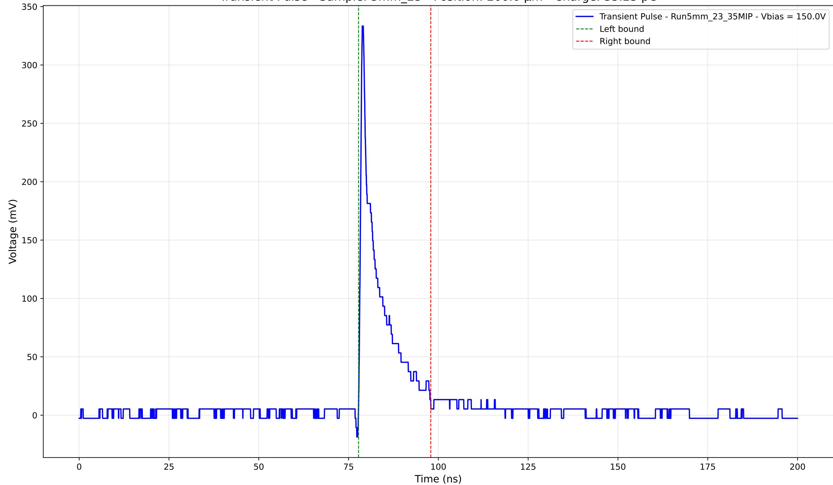
Transient Pulse - Sample: 5mm_23 - Position: 200.0 \mu\text{m} - Charge: 35.23 pC
