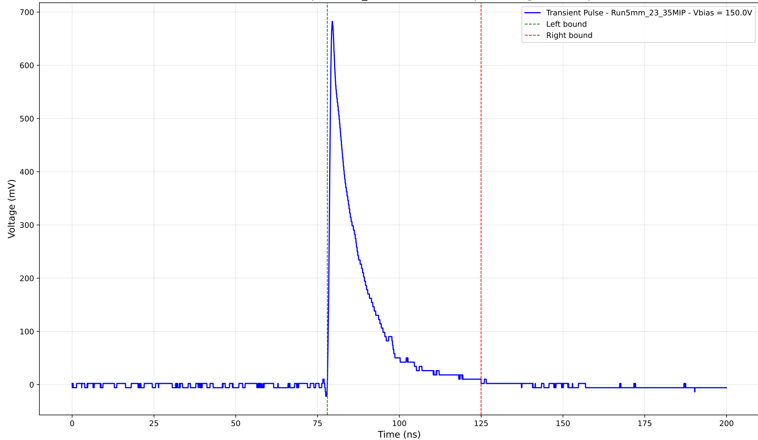
Transient Pulse - Sample: 5mm_23 - Position: 840.0 \mu\text{m} - Charge: 120.91 pC
