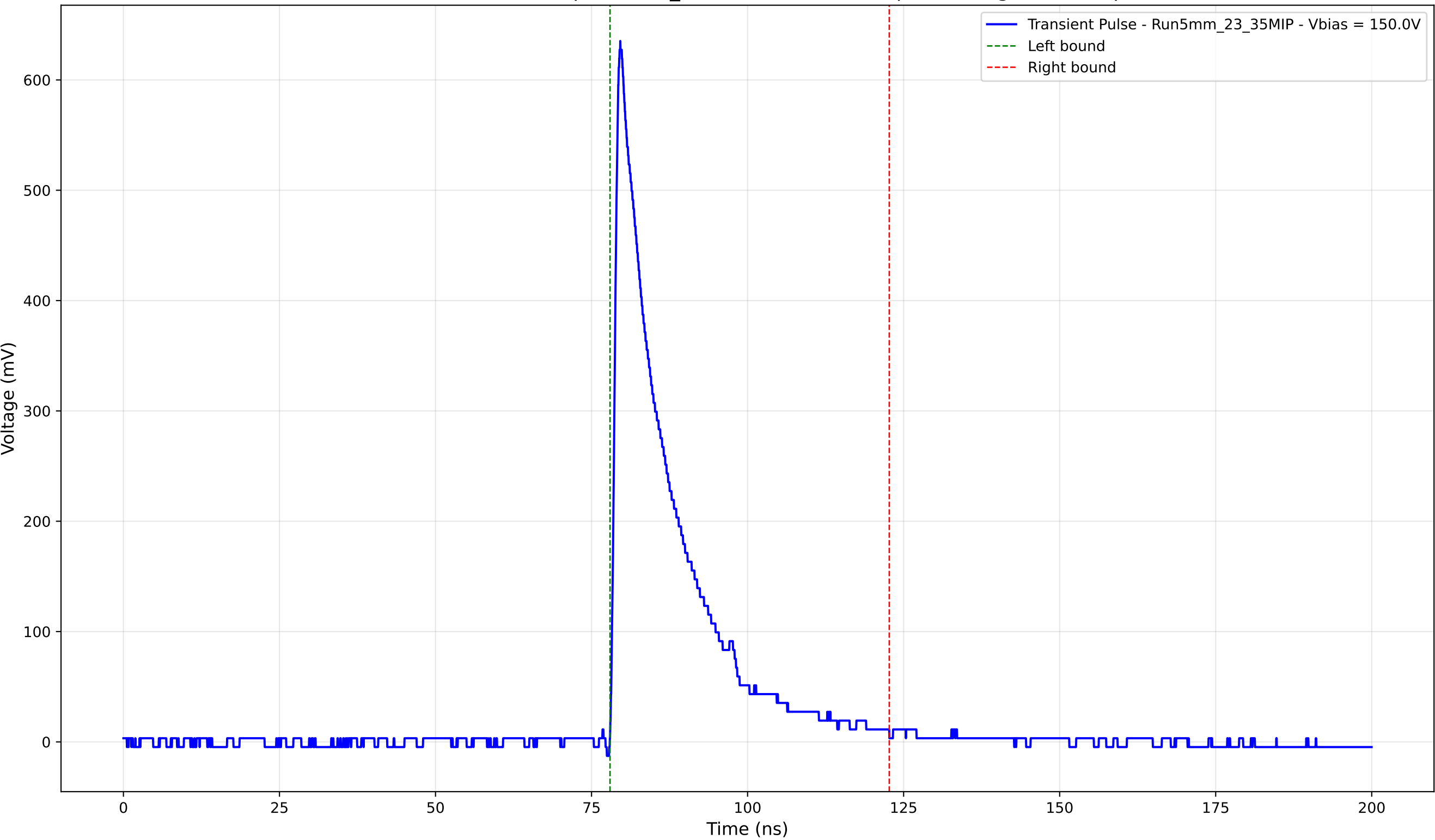
Transient Pulse - Sample: 5mm_23 - Position: 4290.0 \mu\text{m} - Charge: 116.86 pC
