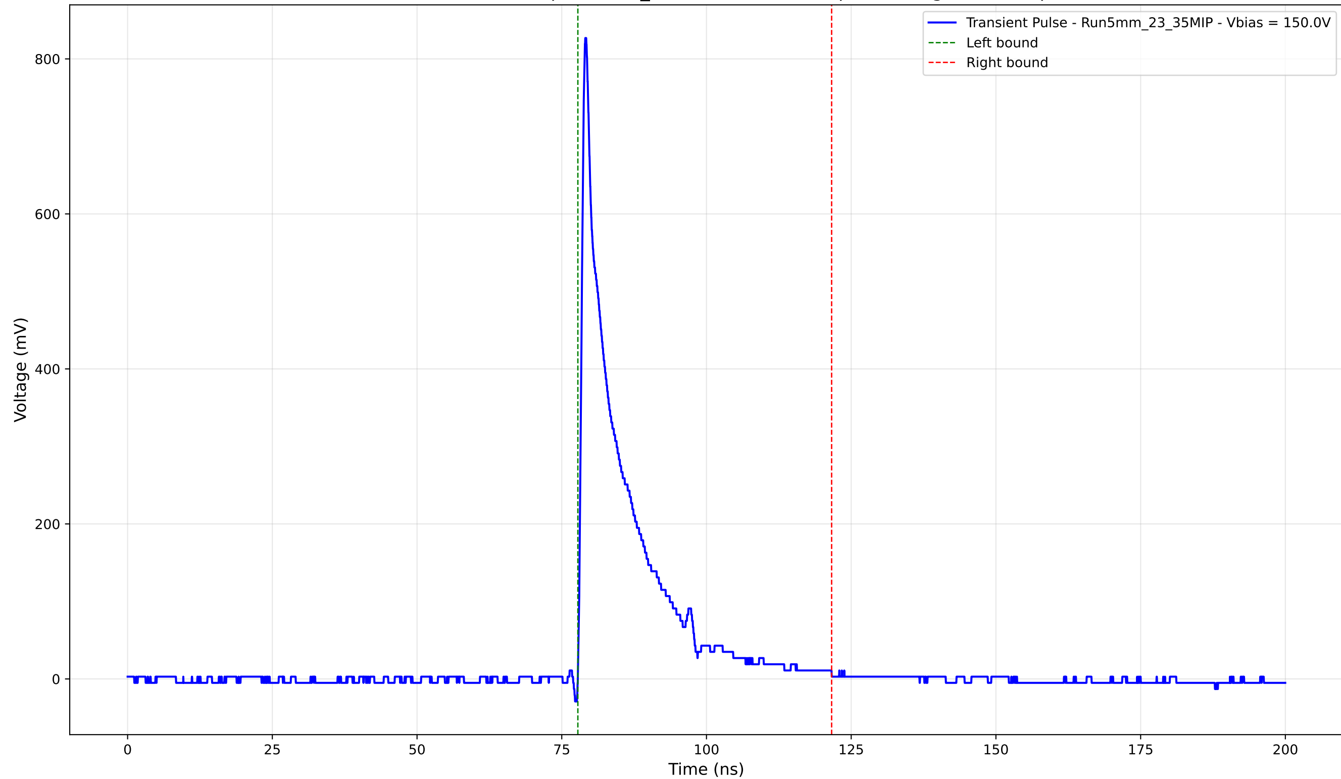
Transient Pulse - Sample: 5mm_23 - Position: 405.0 \mu\text{m} - Charge: 115.02 pC
