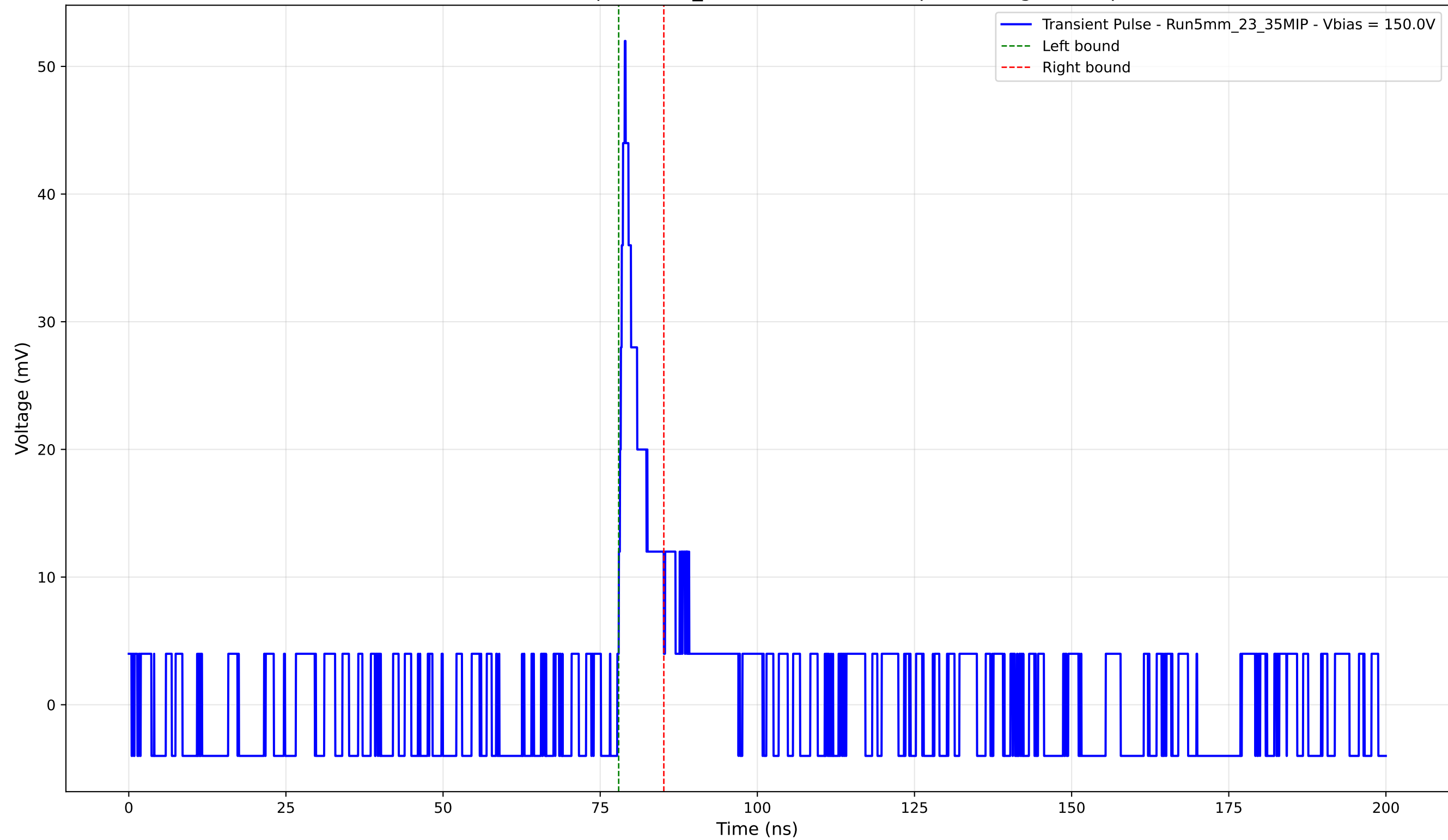
Transient Pulse - Sample: 5mm_23 - Position: 5130.0 \mu\text{m} - Charge: 3.22 pC
