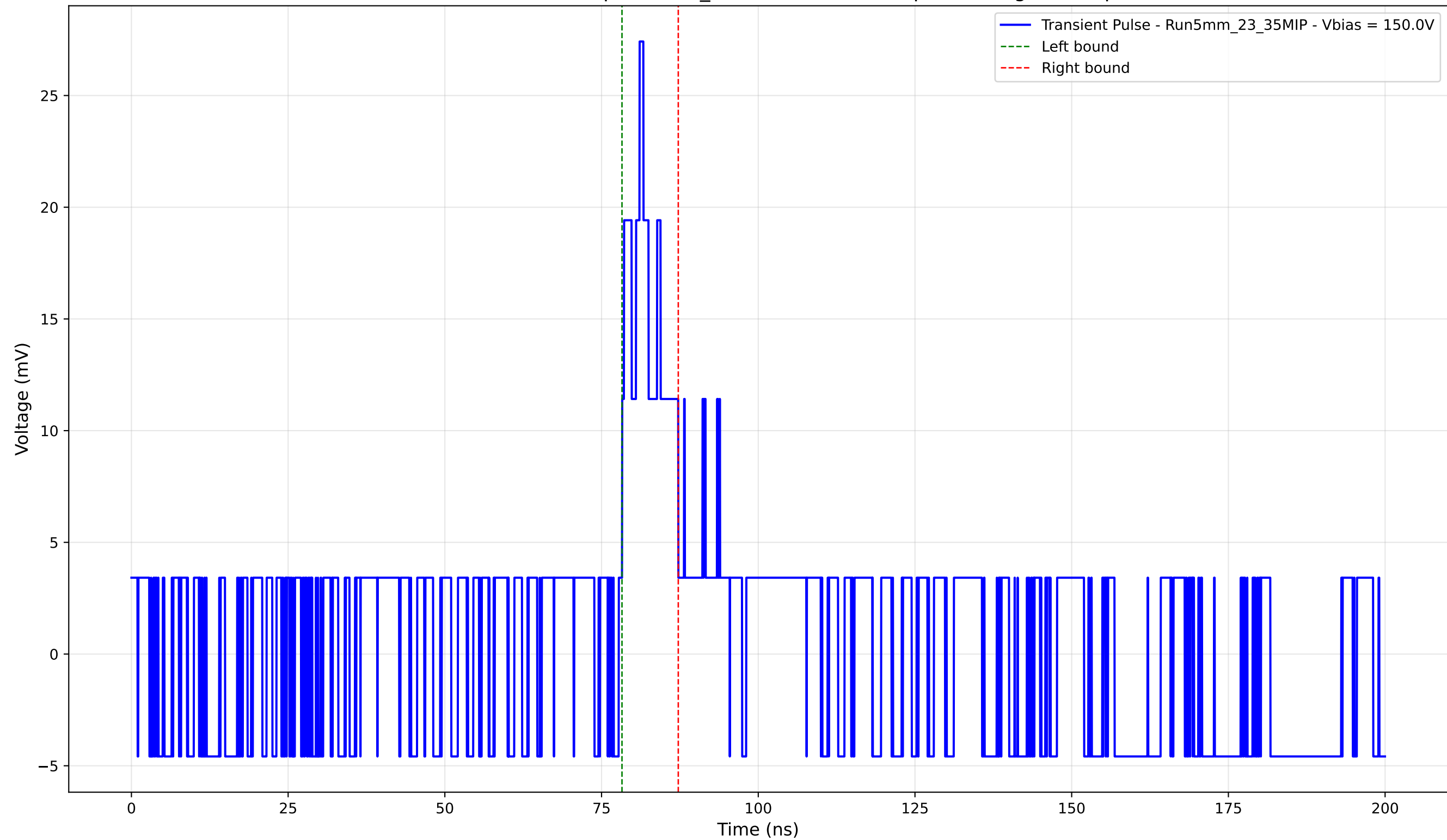
Transient Pulse - Sample: 5mm_23 - Position: 140.0 \mu\text{m} - Charge: 2.75 pC
