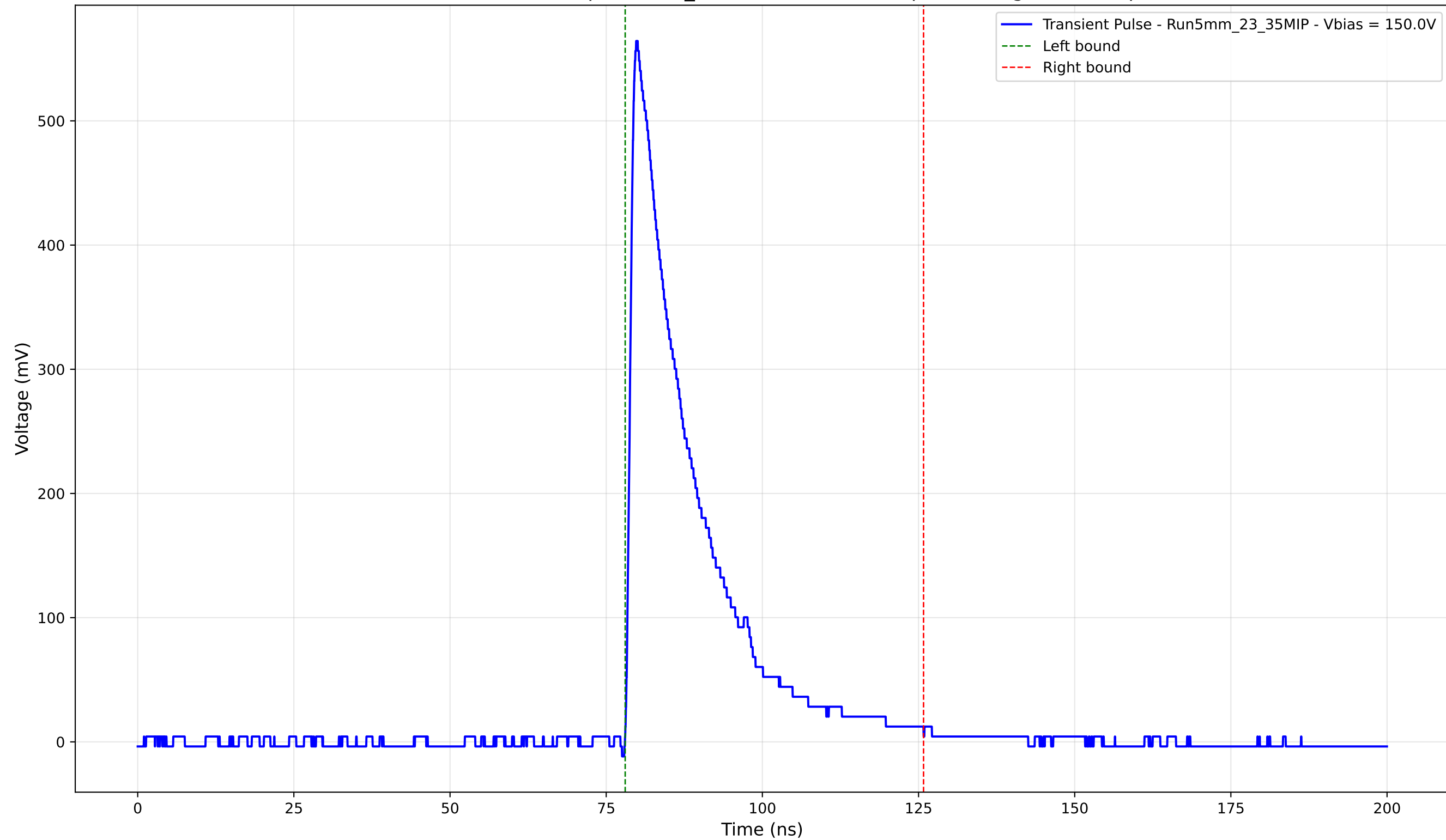
Transient Pulse - Sample: 5mm_23 - Position: 3975.0 \mu\text{m} - Charge: 120.72 pC
