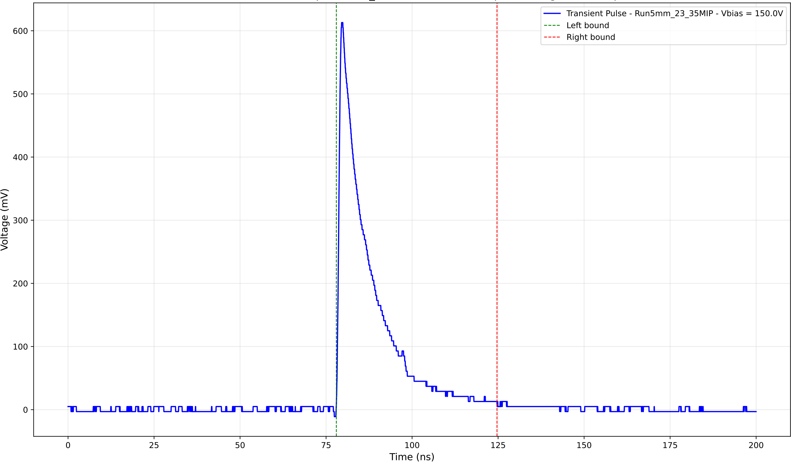
Transient Pulse - Sample: 5mm_23 - Position: 4270.0 \mu\text{m} - Charge: 116.43 pC
