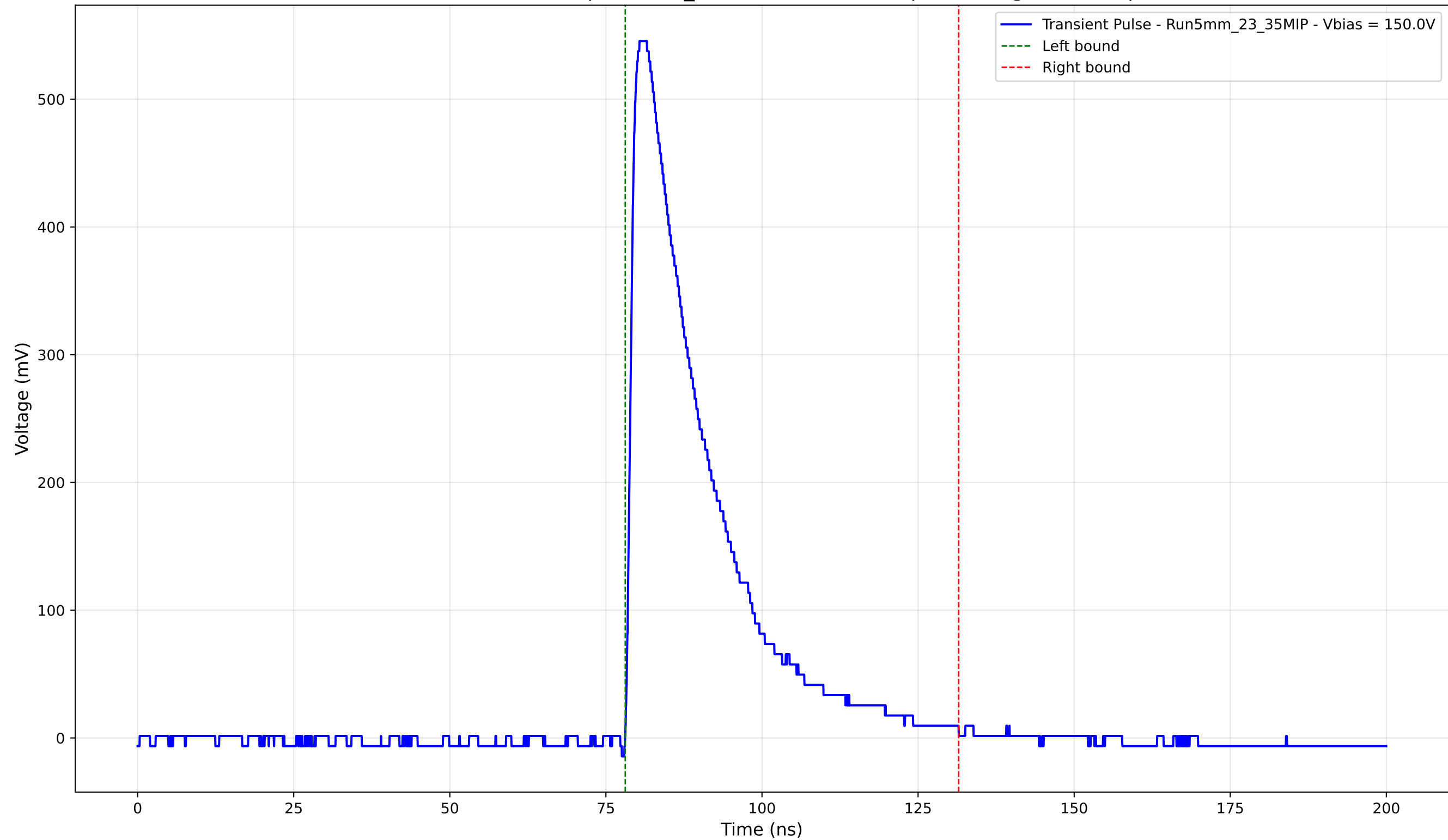
Transient Pulse - Sample: 5mm_23 - Position: 2005.0 \mu\text{m} - Charge: 143.99 pC
