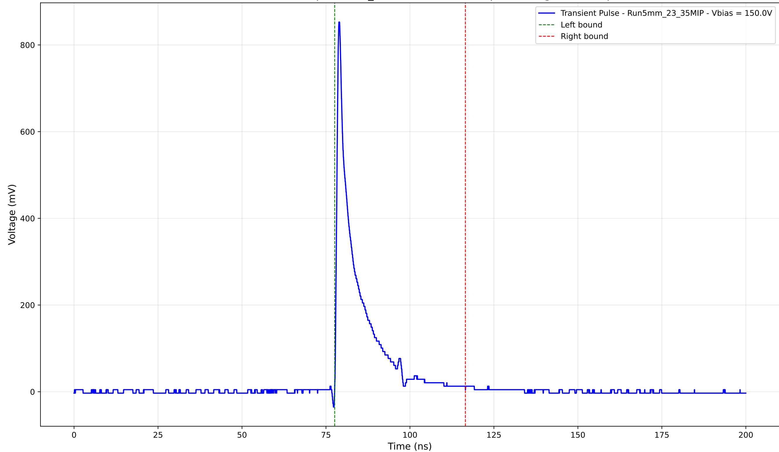
Transient Pulse - Sample: 5mm_23 - Position: 5025.0 \mu\text{m} - Charge: 101.31 pC
