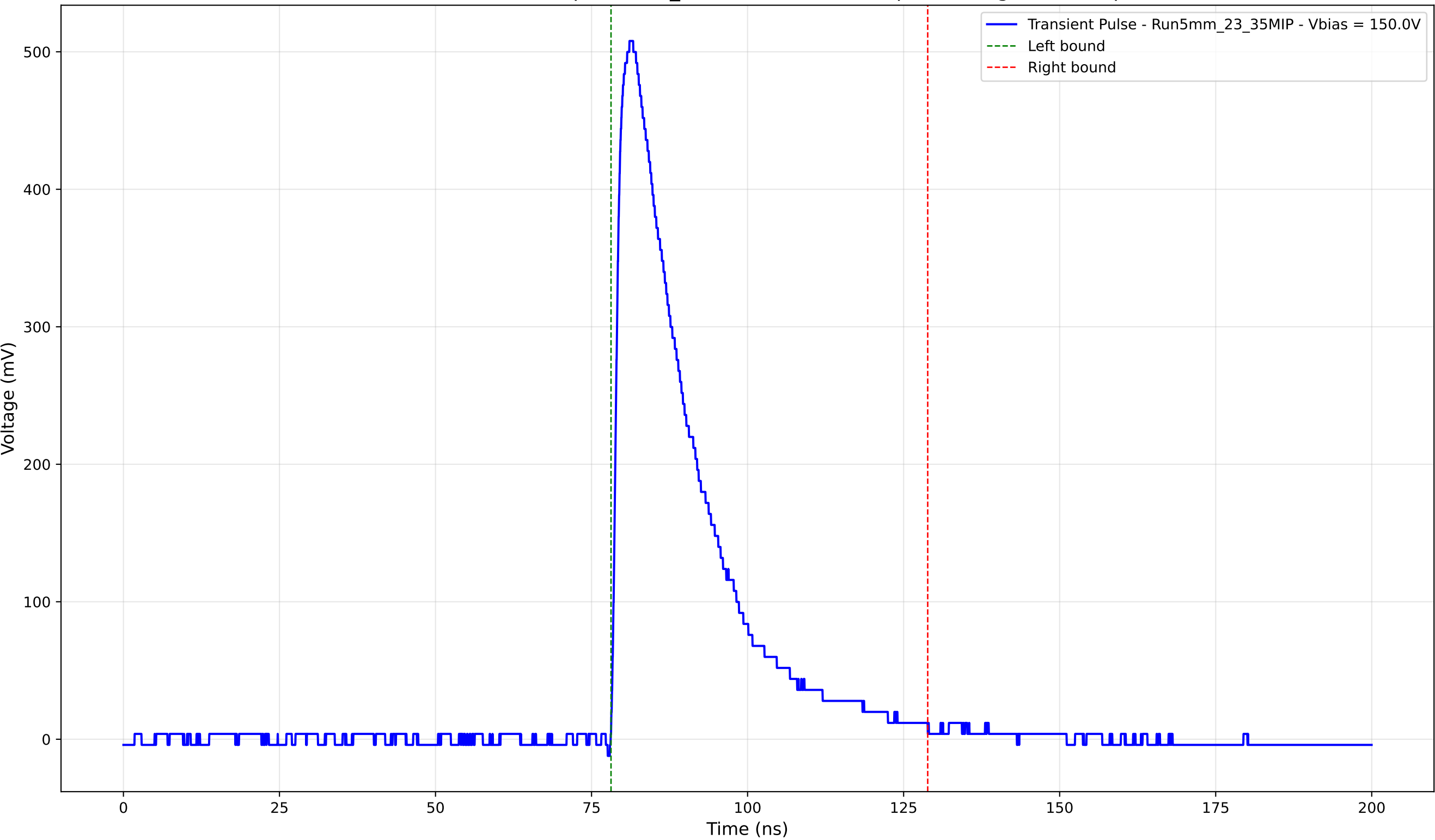
Transient Pulse - Sample: 5mm_23 - Position: 2395.0 \mu\text{m} - Charge: 137.20 pC
