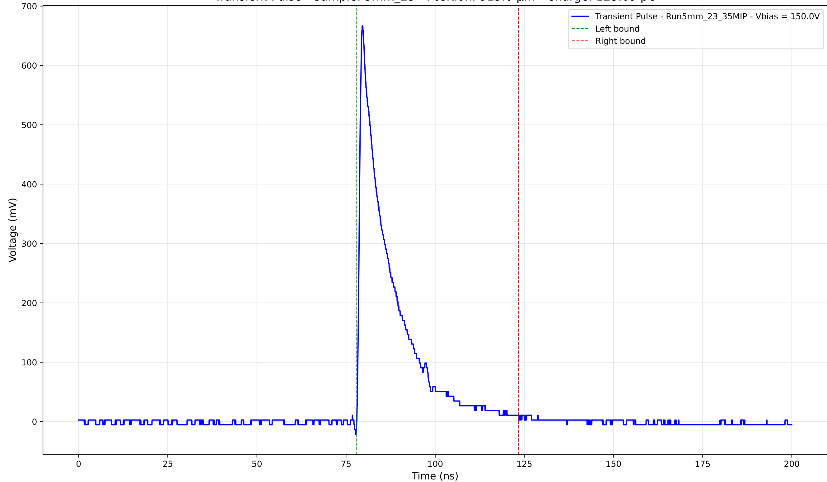
Transient Pulse - Sample: 5mm_23 - Position: 915.0 \mu\text{m} - Charge: 123.09 pC
