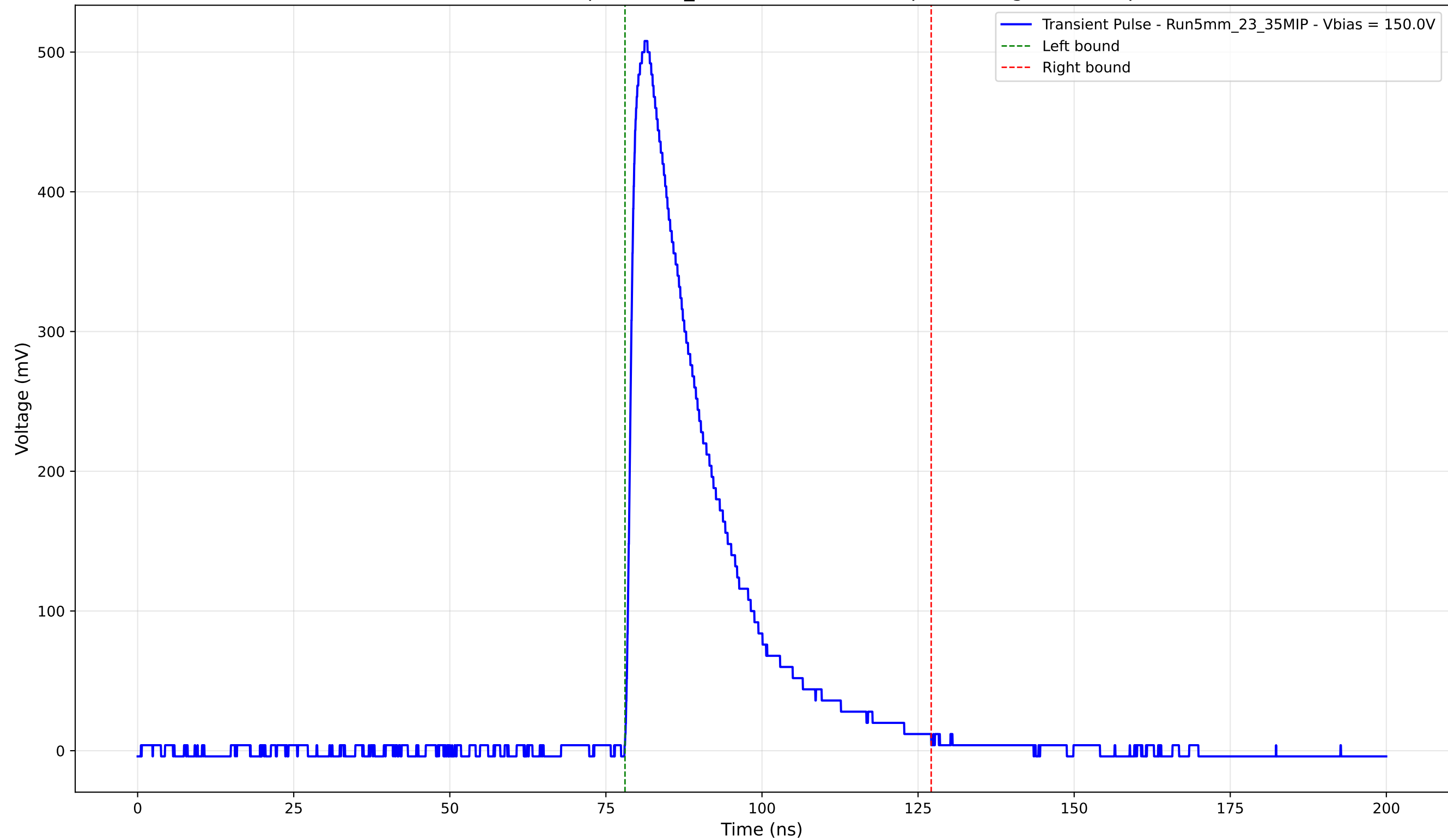
Transient Pulse - Sample: 5mm_23 - Position: 2405.0 \mu\text{m} - Charge: 136.36 pC
