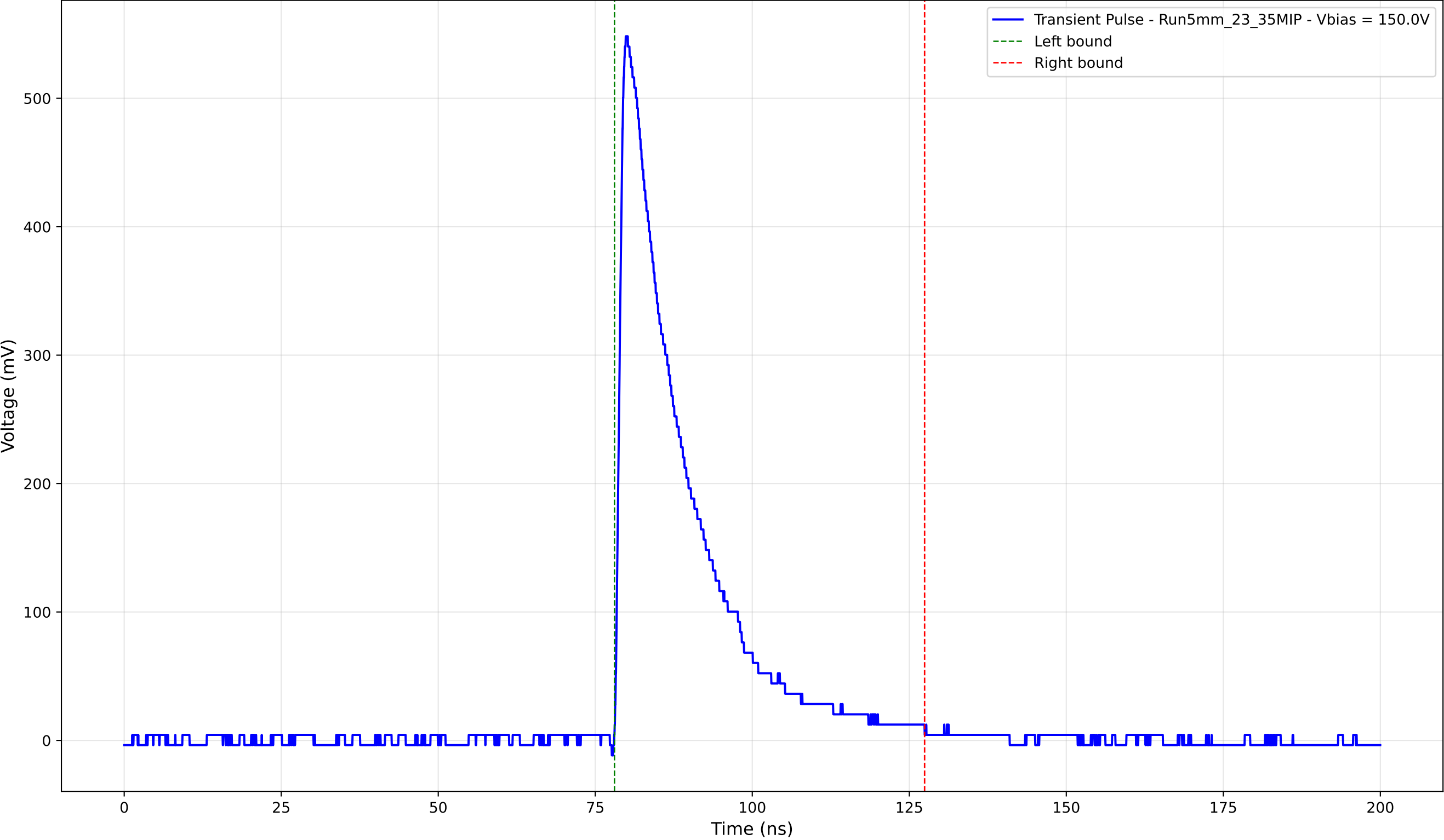
Transient Pulse - Sample: 5mm_23 - Position: 3865.0 \mu\text{m} - Charge: 123.16 pC
