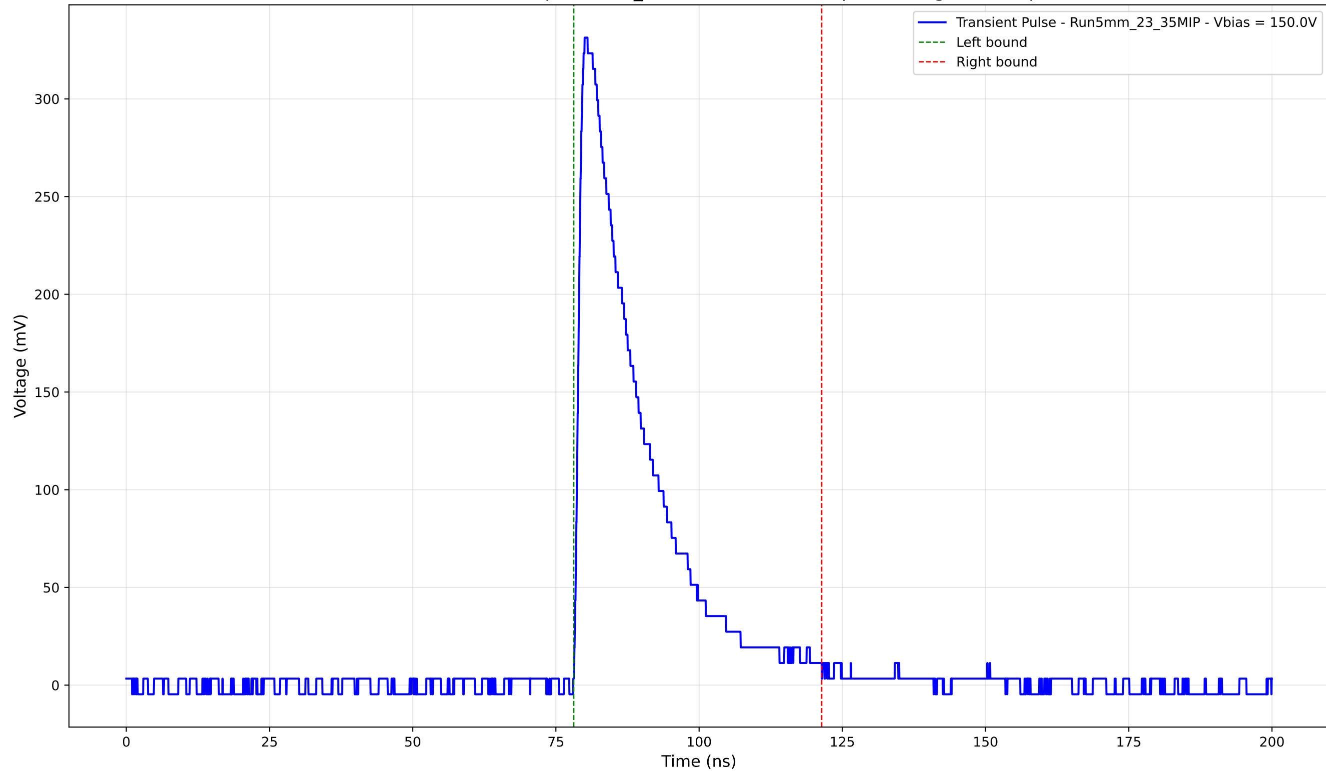
Transient Pulse - Sample: 5mm_23 - Position: 1680.0 \mu\text{m} - Charge: 80.23 pC
