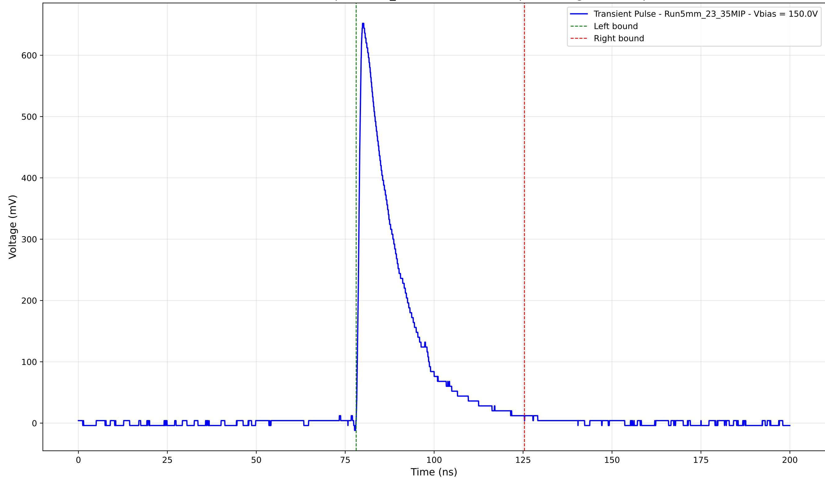
Transient Pulse - Sample: 5mm_23 - Position: 1450.0 \mu\text{m} - Charge: 152.36 pC
