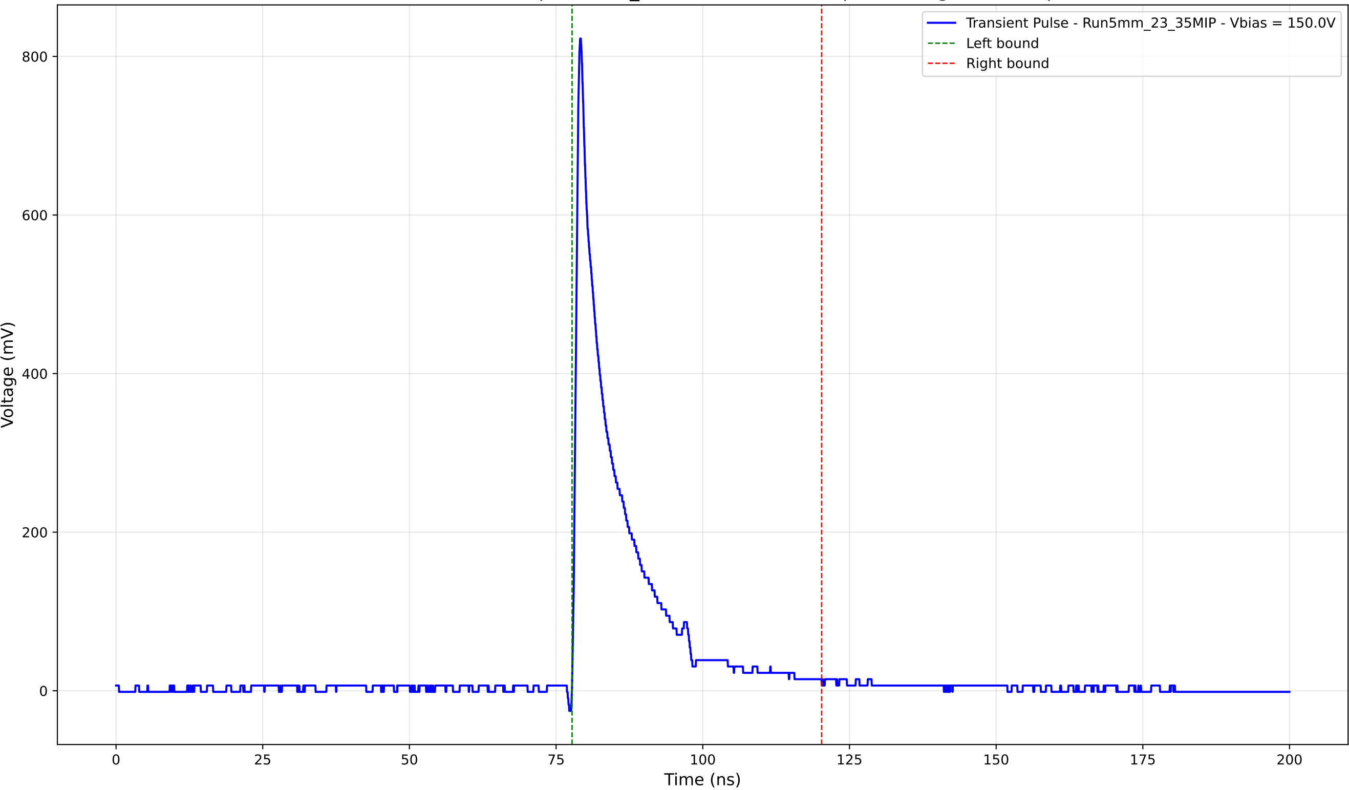
Transient Pulse - Sample: 5mm_23 - Position: 4815.0 \mu\text{m} - Charge: 115.64 pC
