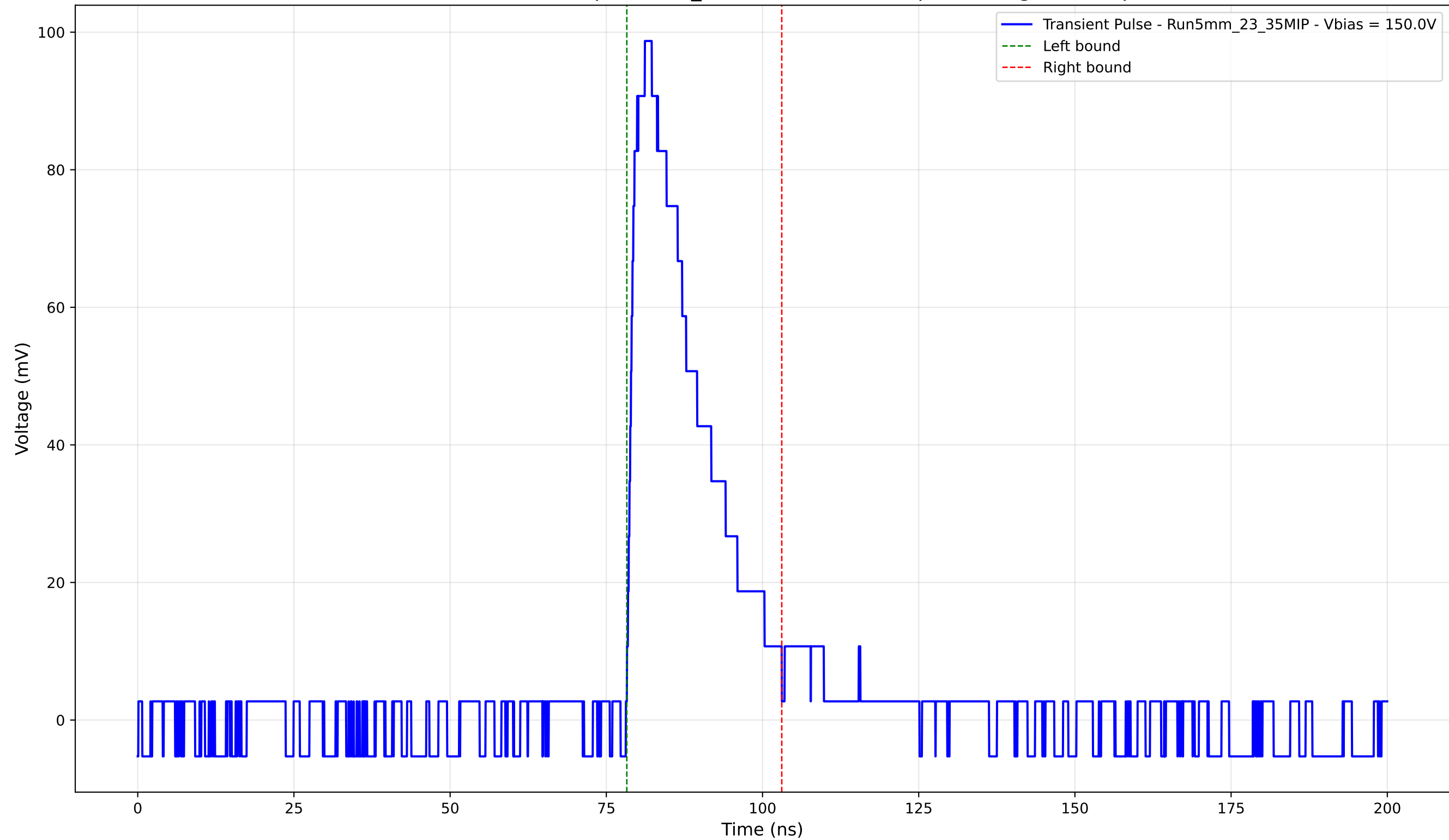
Transient Pulse - Sample: 5mm_23 - Position: 3135.0 \mu\text{m} - Charge: 23.16 pC
