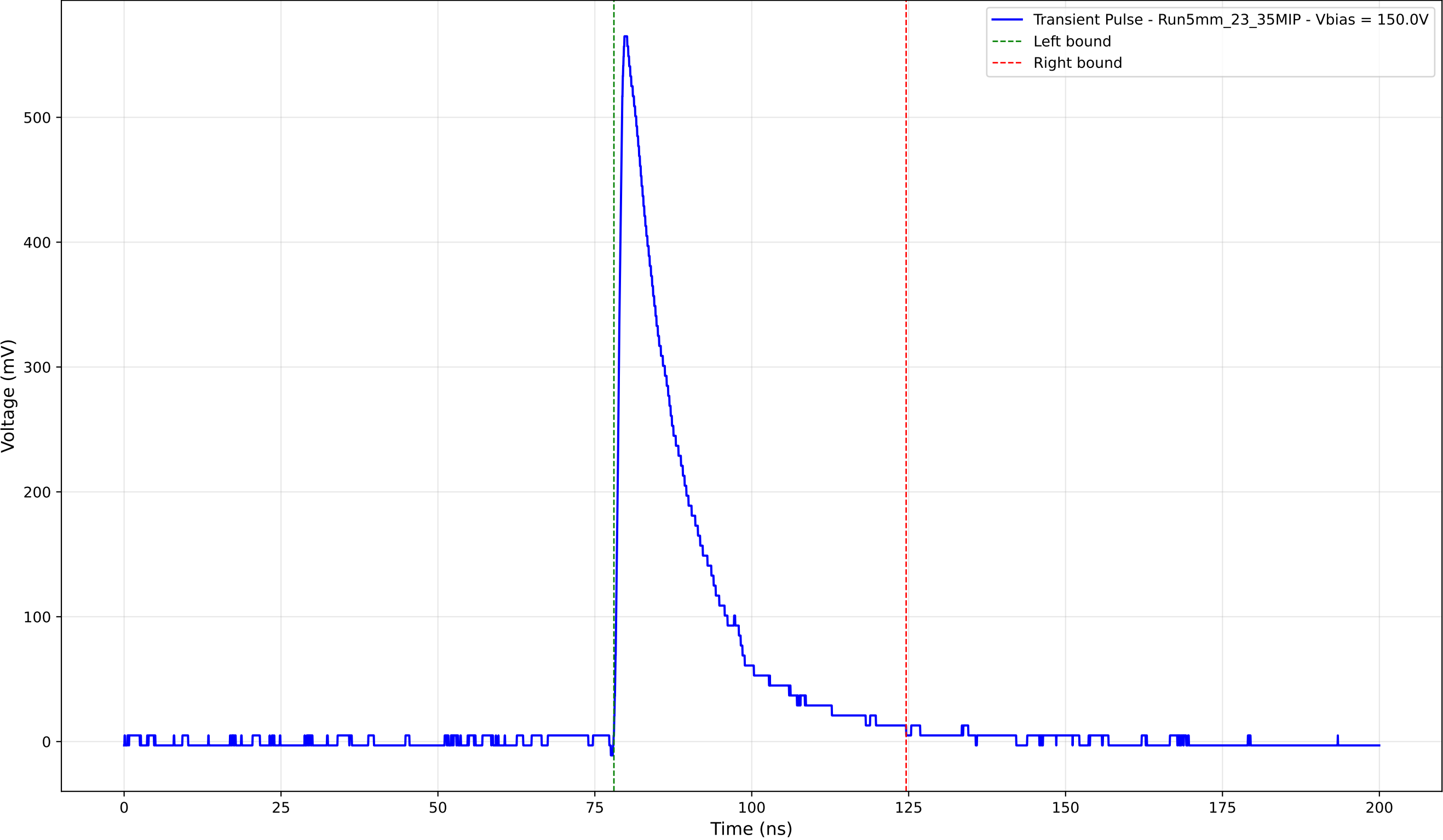
Transient Pulse - Sample: 5mm_23 - Position: 3990.0 \mu\text{m} - Charge: 121.73 pC
