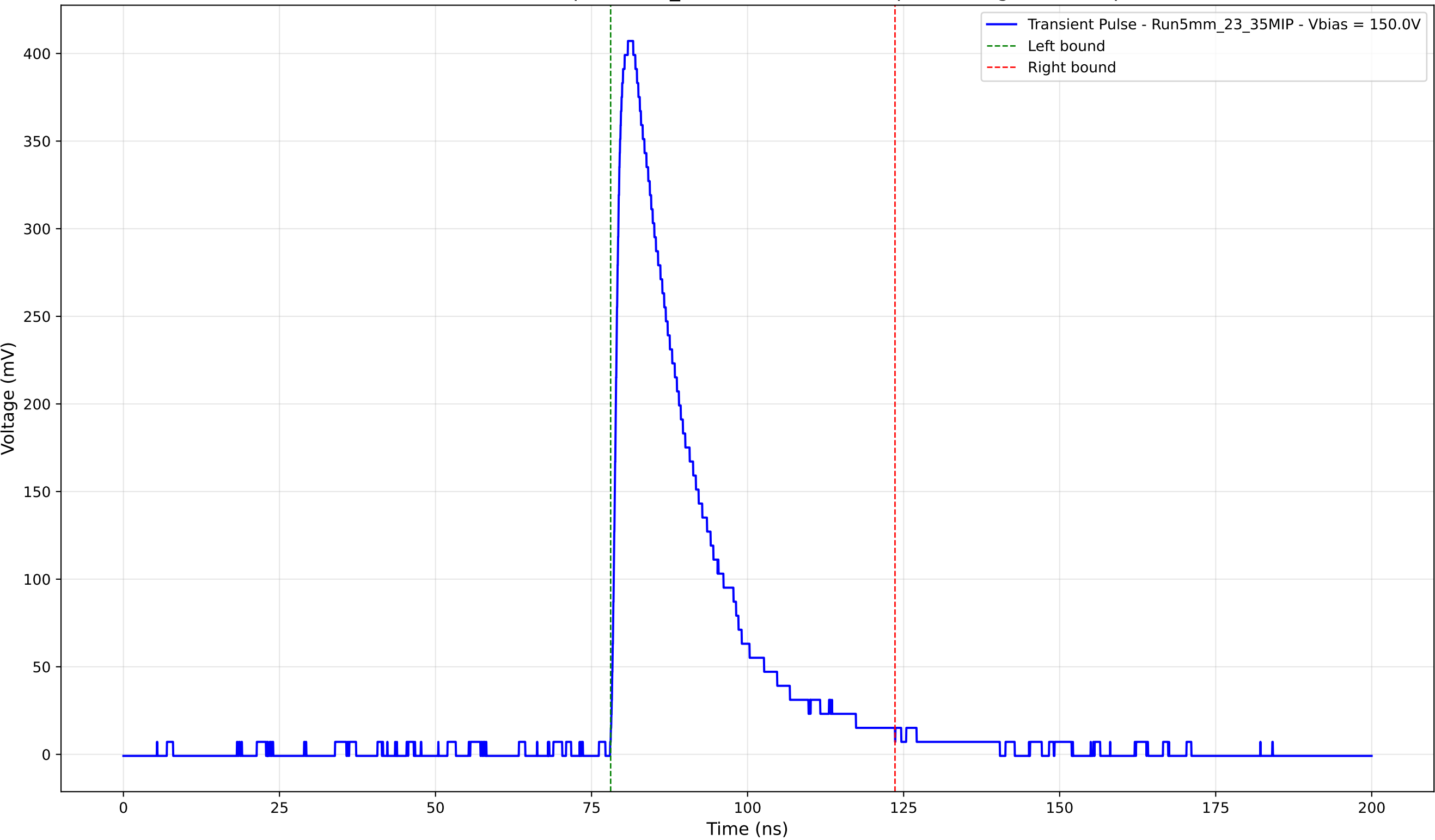
Transient Pulse - Sample: 5mm_23 - Position: 3080.0 \mu\text{m} - Charge: 106.43 pC
