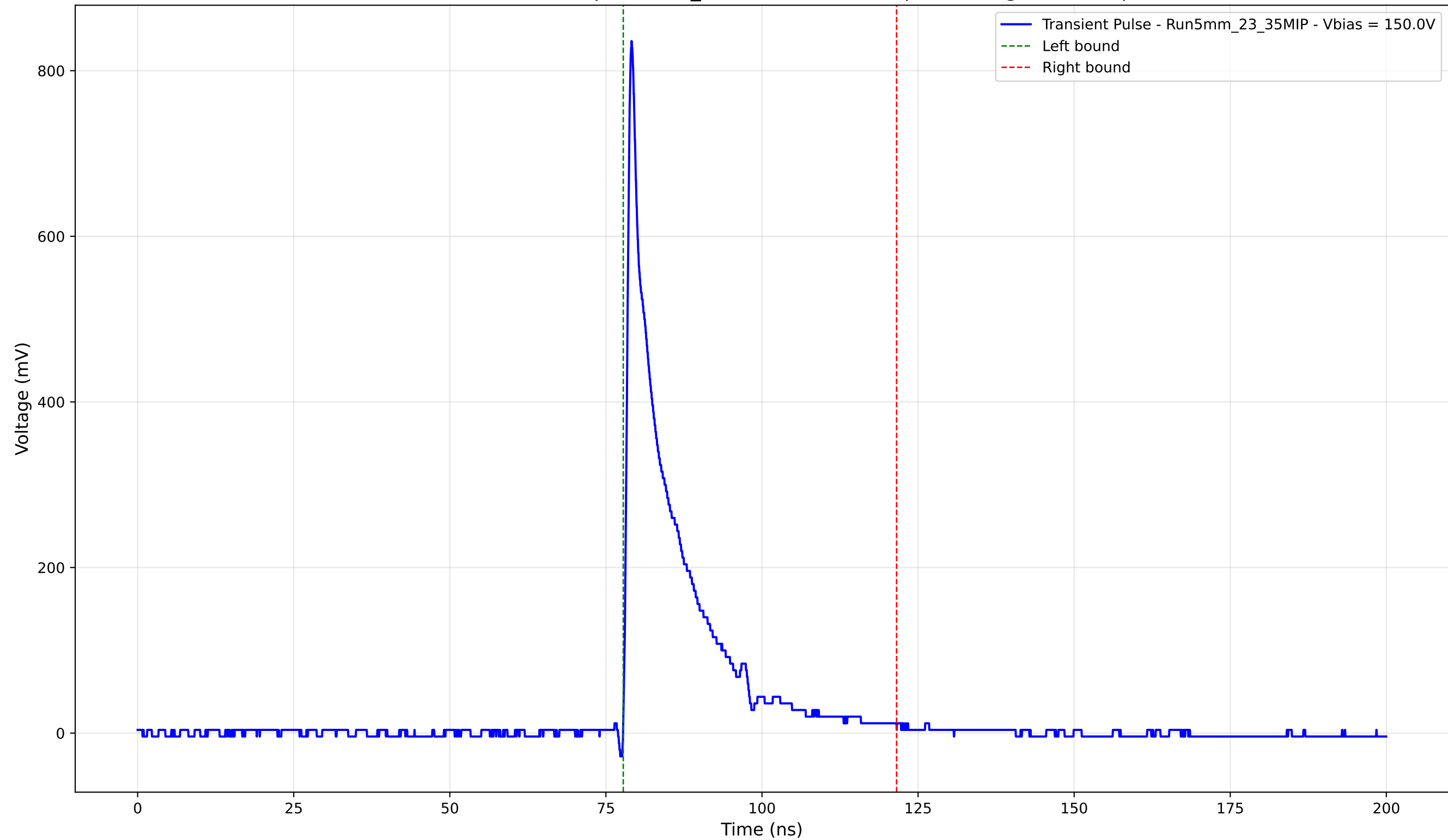
Transient Pulse - Sample: 5mm_23 - Position: 395.0 \mu\text{m} - Charge: 115.41 pC
