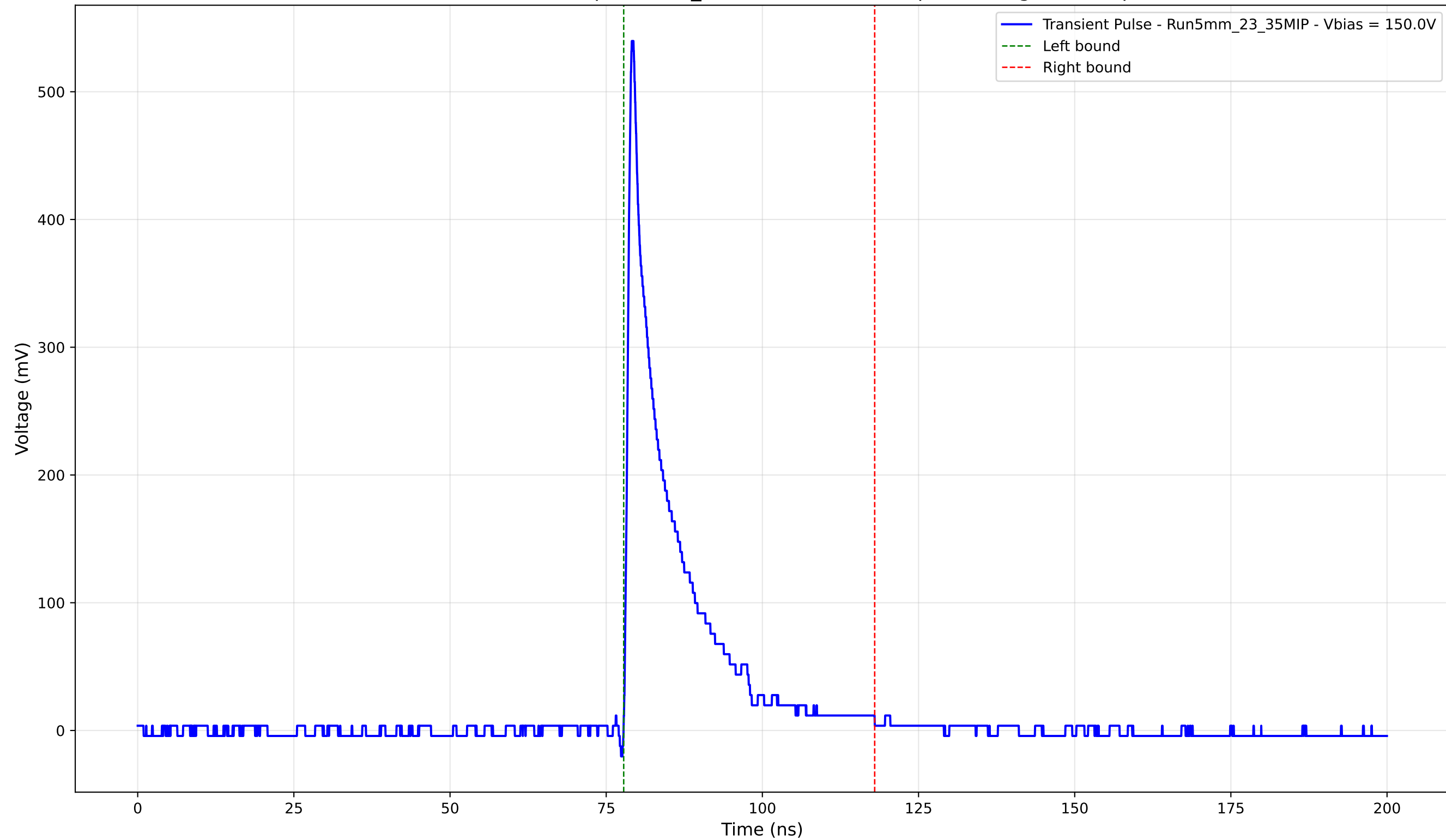
Transient Pulse - Sample: 5mm_23 - Position: 4720.0 \mu\text{m} - Charge: 73.13 pC
