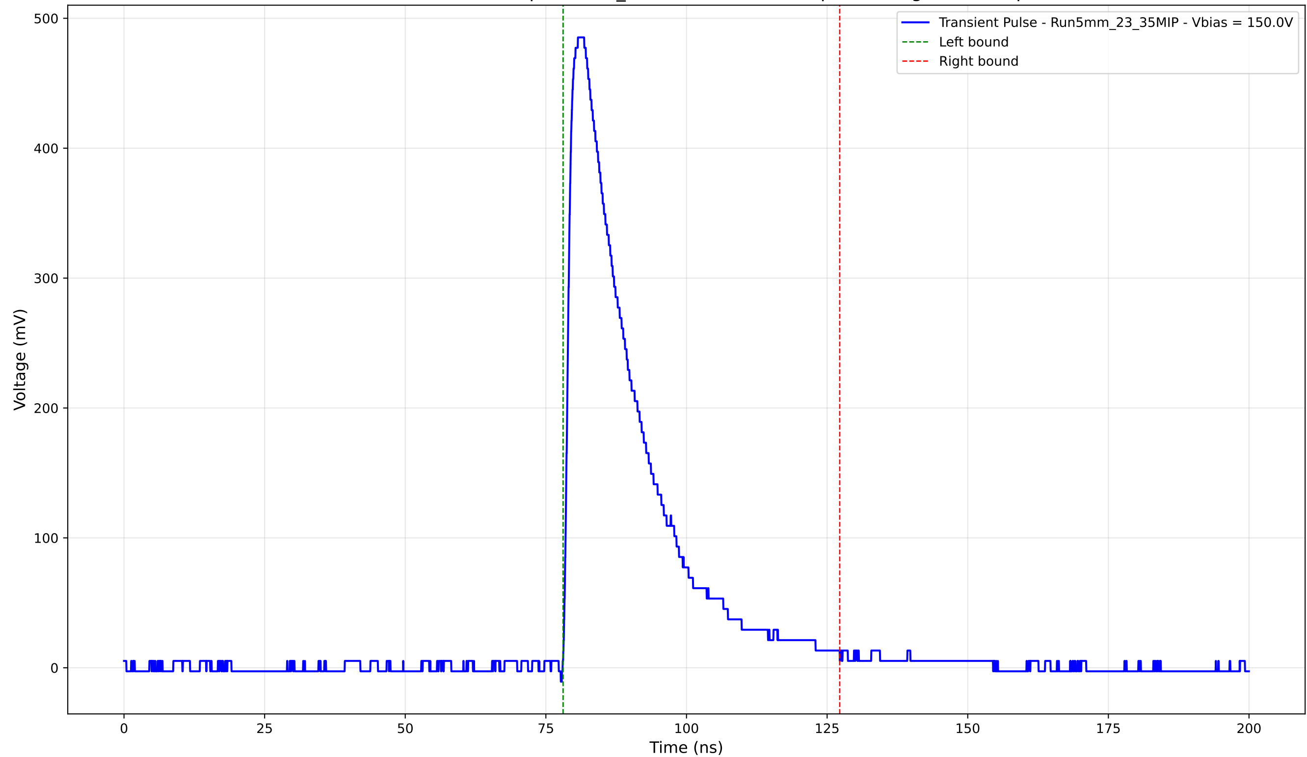
Transient Pulse - Sample: 5mm_23 - Position: 3050.0 \mu\text{m} - Charge: 129.82 pC
