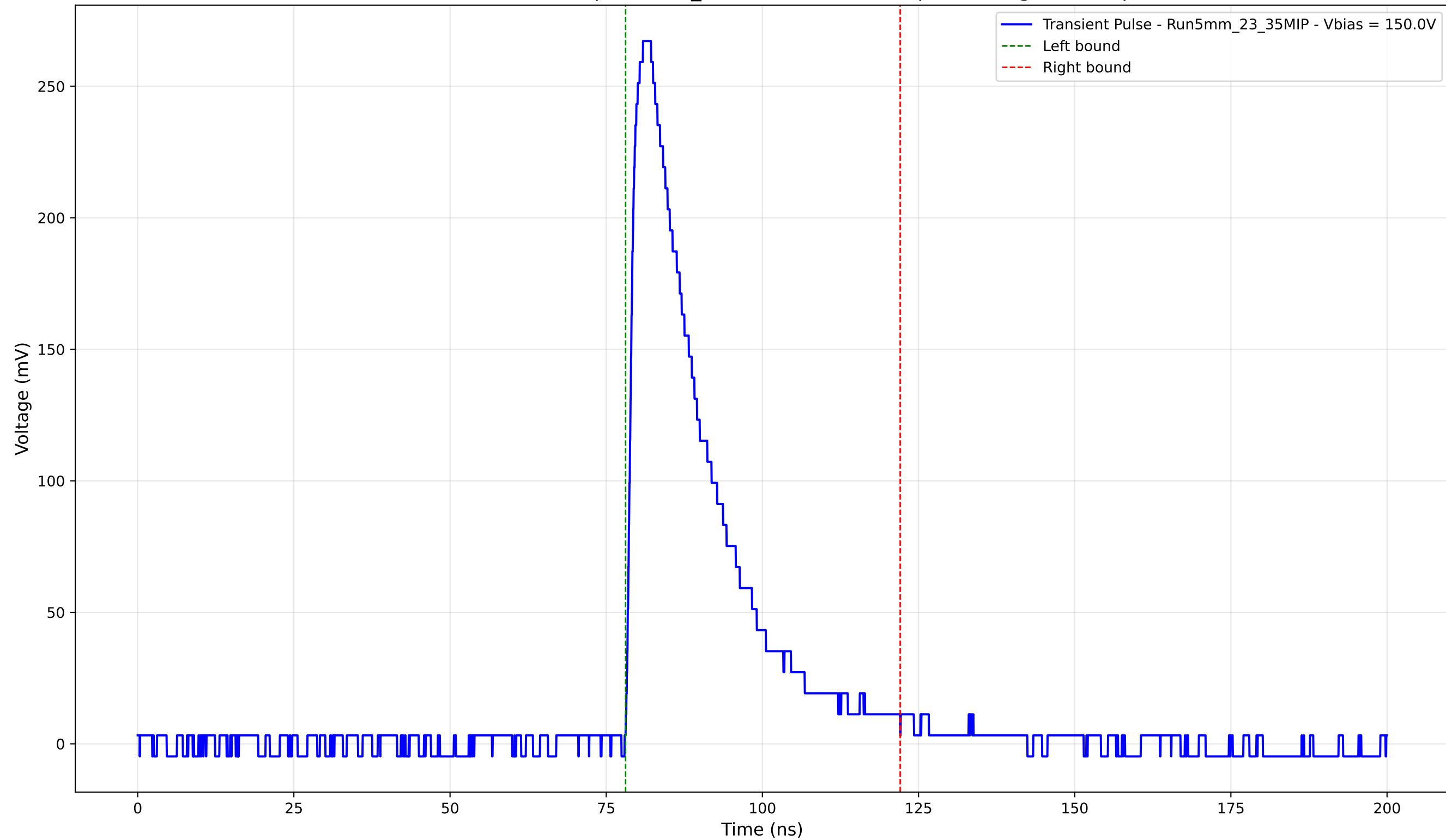
Transient Pulse - Sample: 5mm_23 - Position: 2600.0 \mu\text{m} - Charge: 70.78 pC
