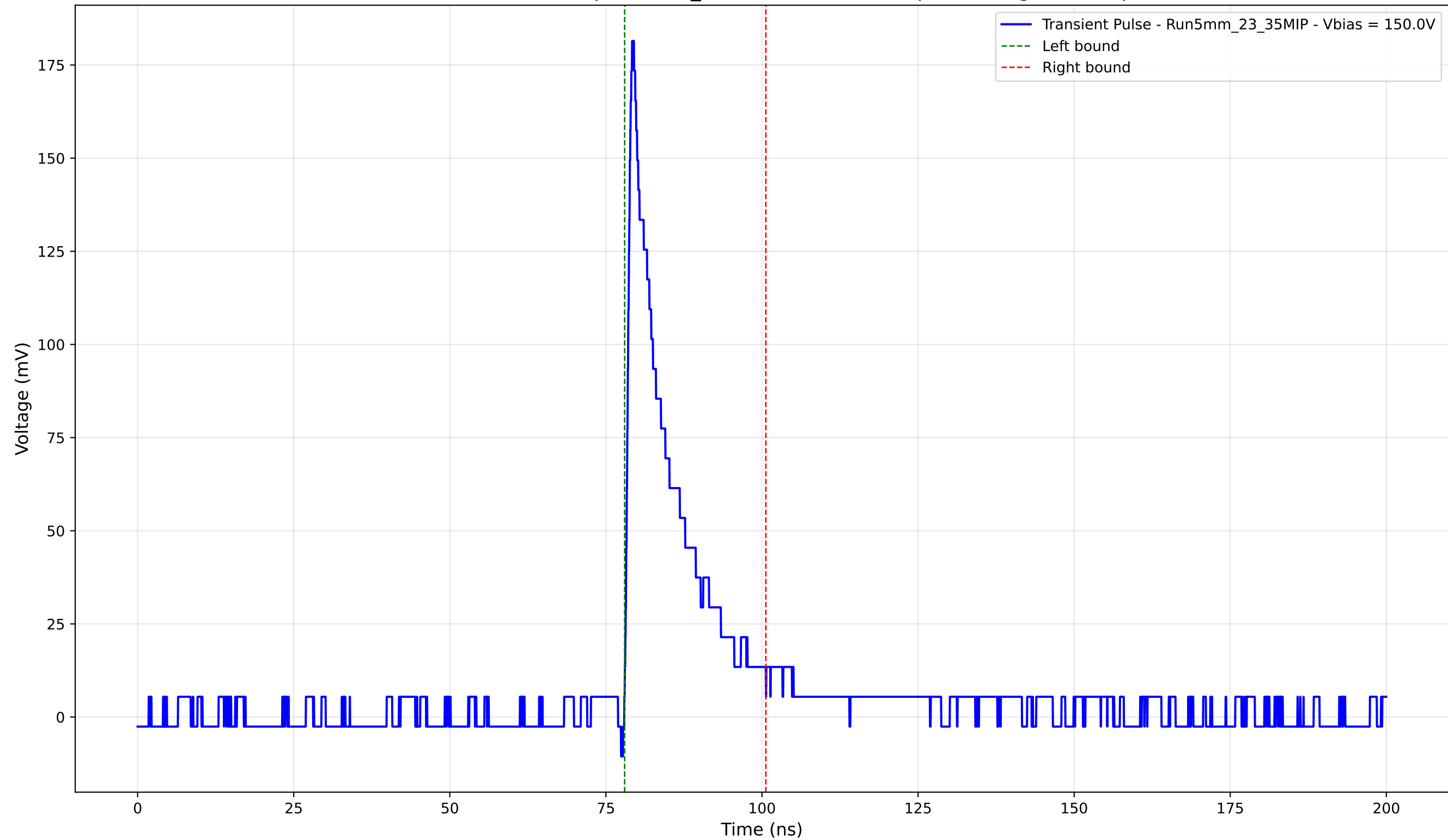
Transient Pulse - Sample: 5mm_23 - Position: 4650.0 \mu\text{m} - Charge: 25.34 pC
