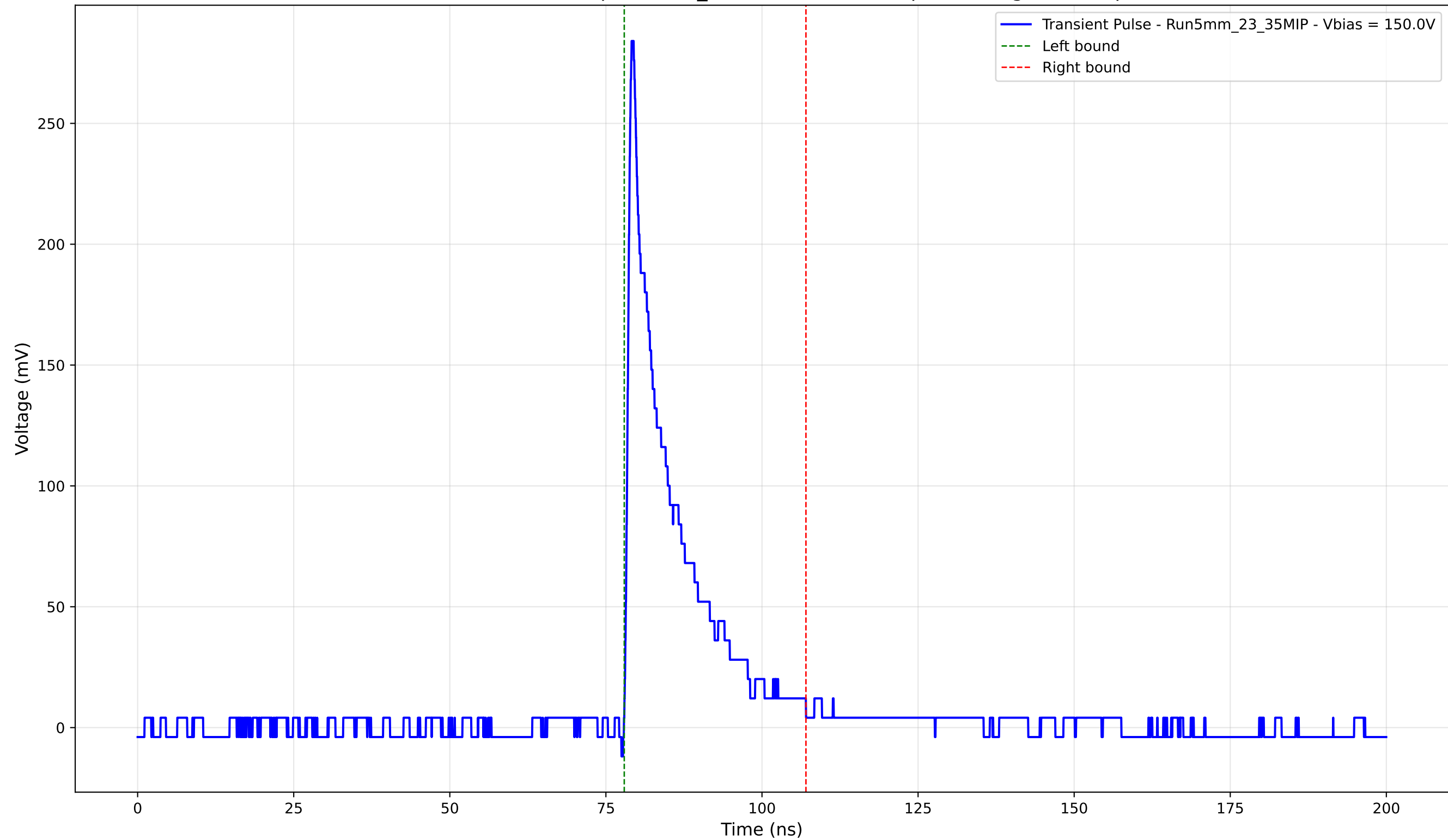
Transient Pulse - Sample: 5mm_23 - Position: 590.0 \mu\text{m} - Charge: 39.43 pC
