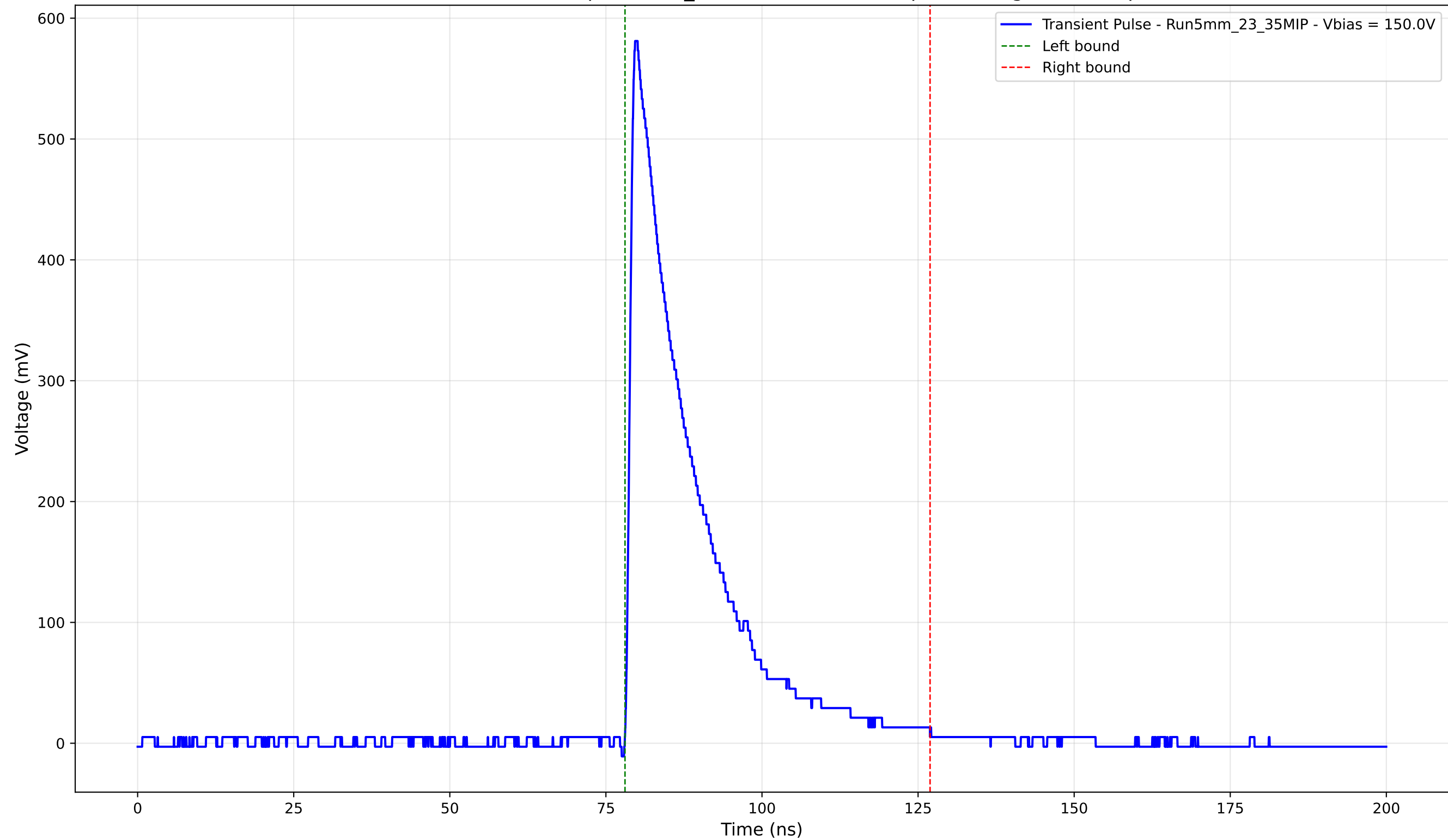
Transient Pulse - Sample: 5mm_23 - Position: 1235.0 \mu\text{m} - Charge: 126.45 pC
