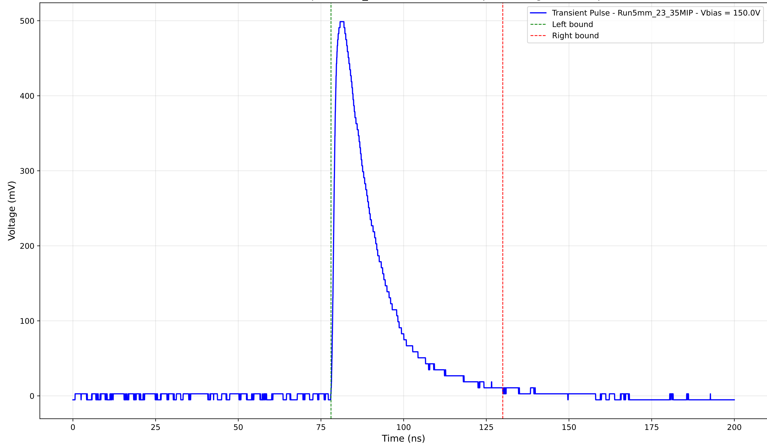
Transient Pulse - Sample: 5mm_23 - Position: 2480.0 \mu\text{m} - Charge: 136.24 pC
