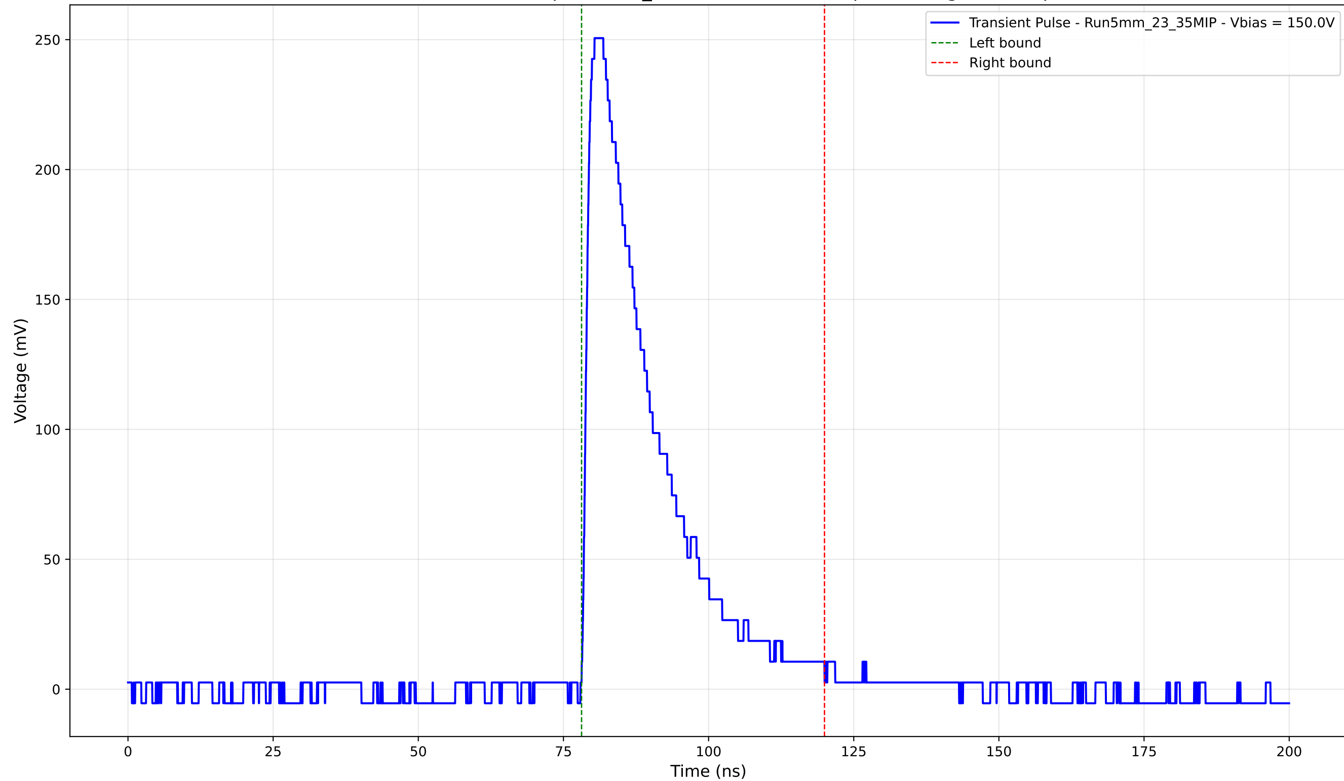
Transient Pulse - Sample: 5mm_23 - Position: 2095.0 \mu\text{m} - Charge: 64.19 pC
