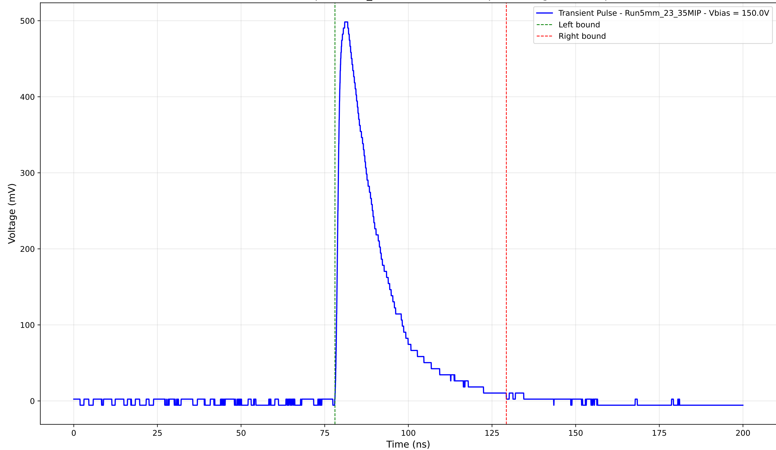
Transient Pulse - Sample: 5mm_23 - Position: 2920.0 \mu\text{m} - Charge: 133.75 pC
