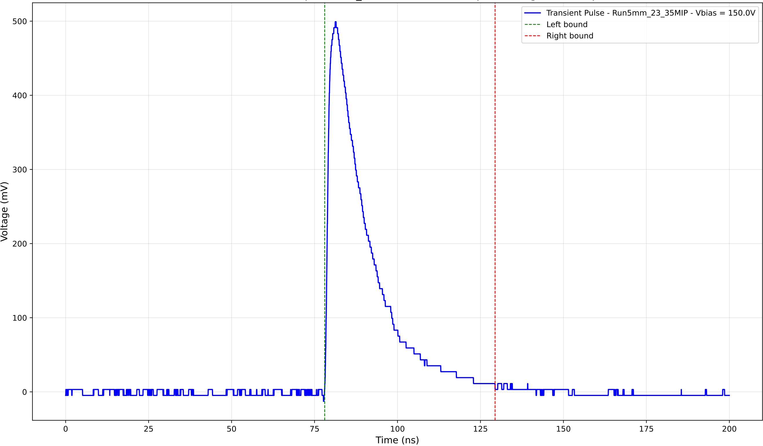
Transient Pulse - Sample: 5mm_23 - Position: 2545.0 \mu\text{m} - Charge: 133.95 pC
