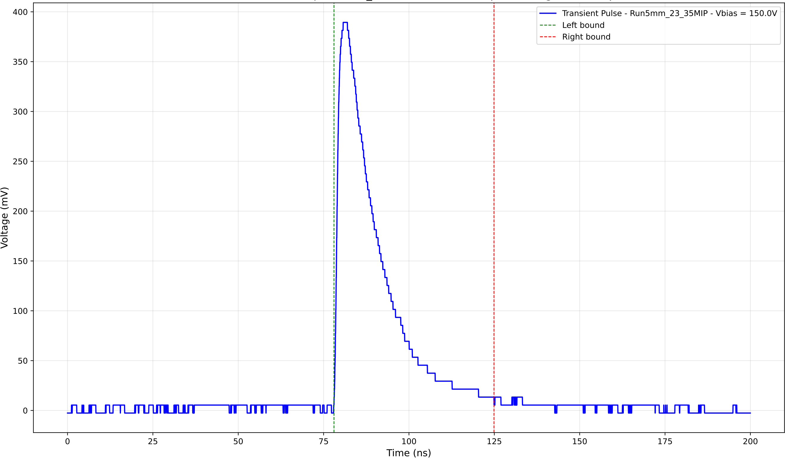
Transient Pulse - Sample: 5mm_23 - Position: 2715.0 \mu\text{m} - Charge: 105.55 pC
