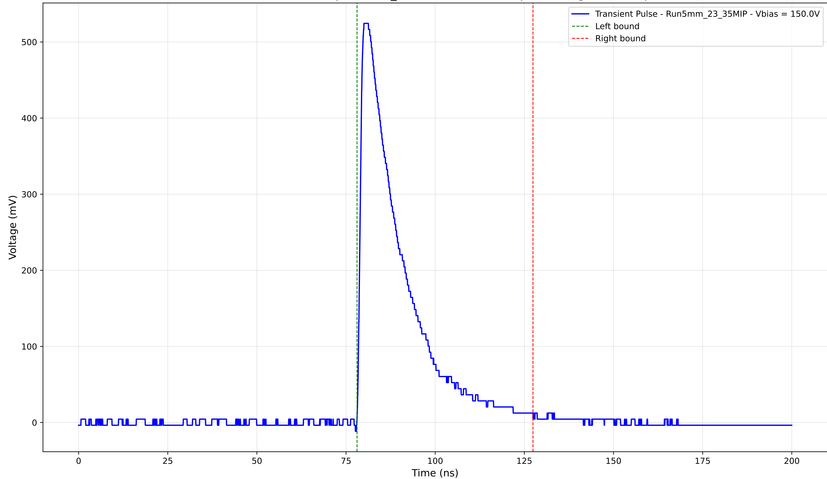
Transient Pulse - Sample: 5mm_23 - Position: 1770.0 \mu\text{m} - Charge: 134.75 pC
