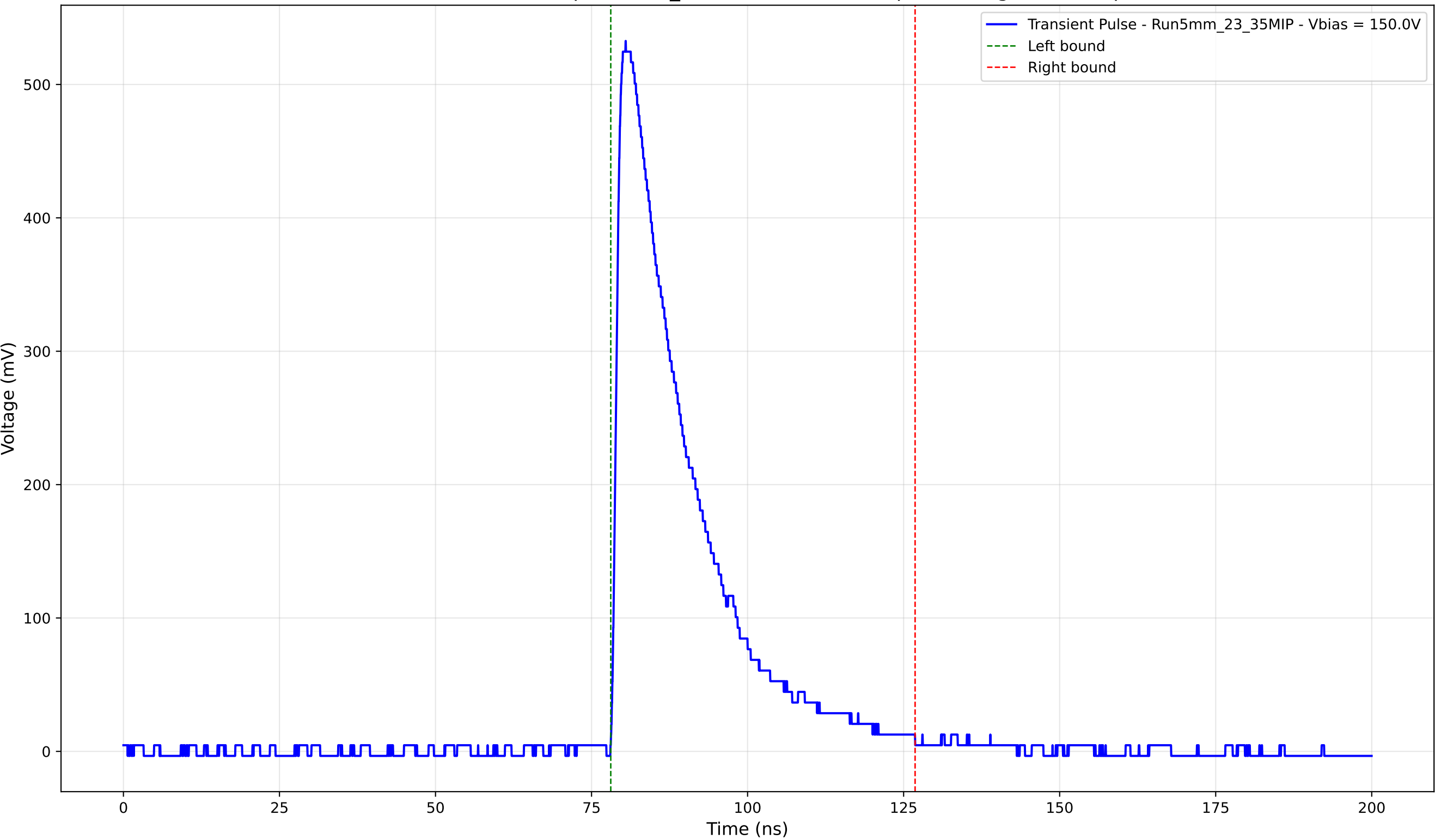
Transient Pulse - Sample: 5mm_23 - Position: 1815.0 \mu\text{m} - Charge: 135.23 pC
