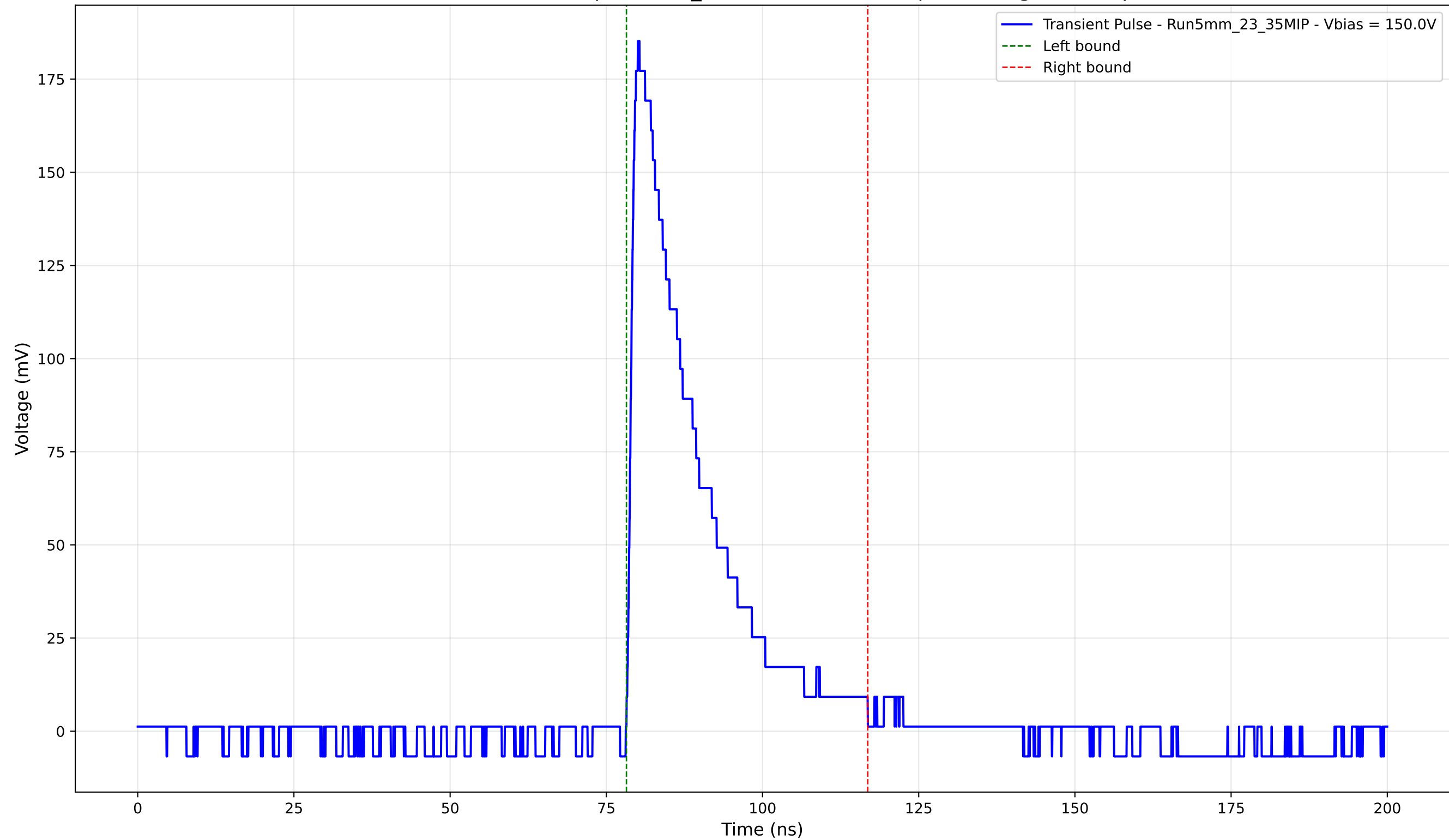
Transient Pulse - Sample: 5mm_23 - Position: 1590.0 \mu\text{m} - Charge: 41.79 pC
