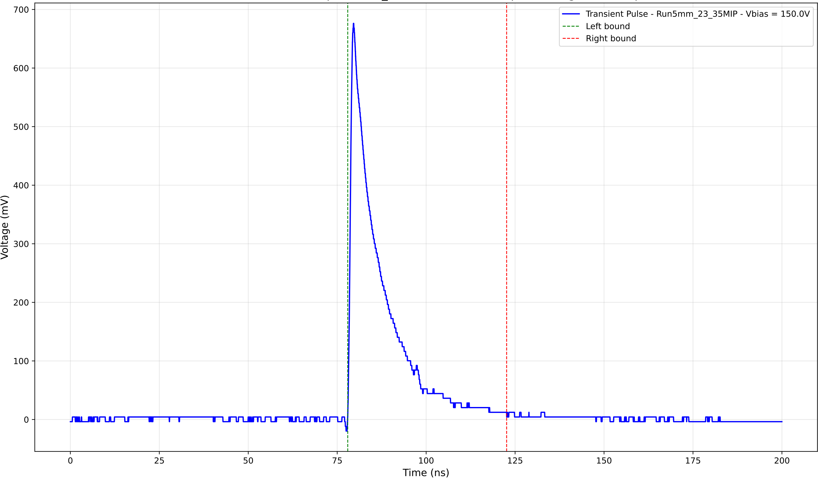
Transient Pulse - Sample: 5mm_23 - Position: 4360.0 \mu\text{m} - Charge: 120.97 pC
