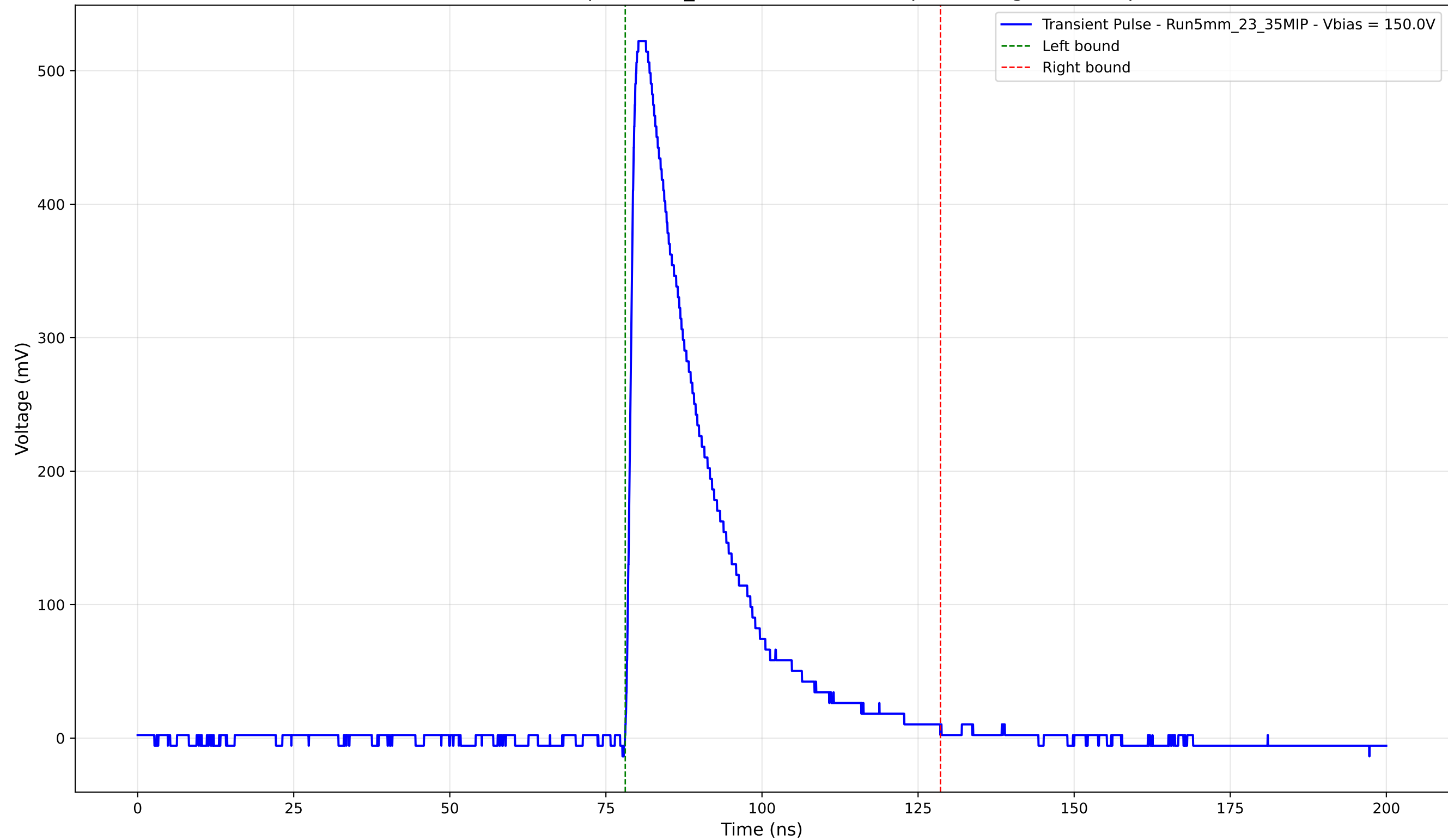
Transient Pulse - Sample: 5mm_23 - Position: 1865.0 \mu\text{m} - Charge: 134.16 pC
