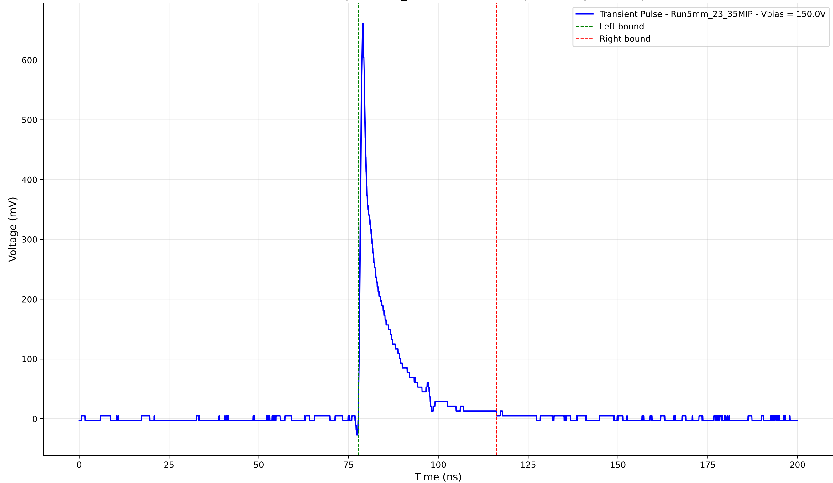
Transient Pulse - Sample: 5mm_23 - Position: 225.0 \mu\text{m} - Charge: 75.09 pC
