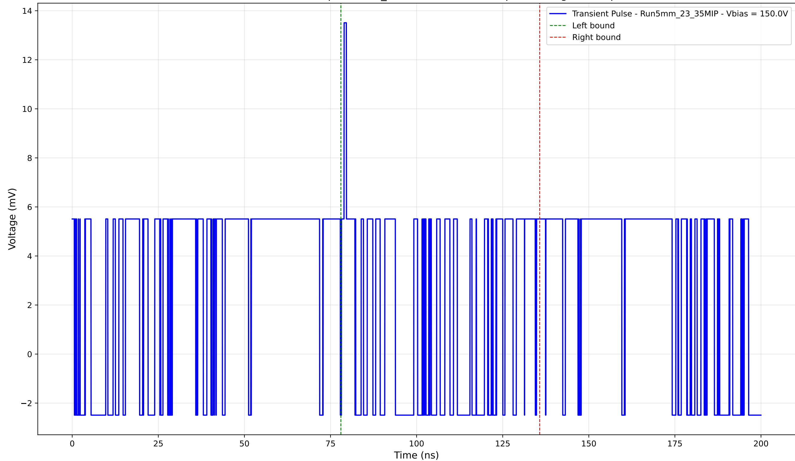
Transient Pulse - Sample: 5mm_23 - Position: 5225.0 \mu\text{m} - Charge: 1.96 pC
