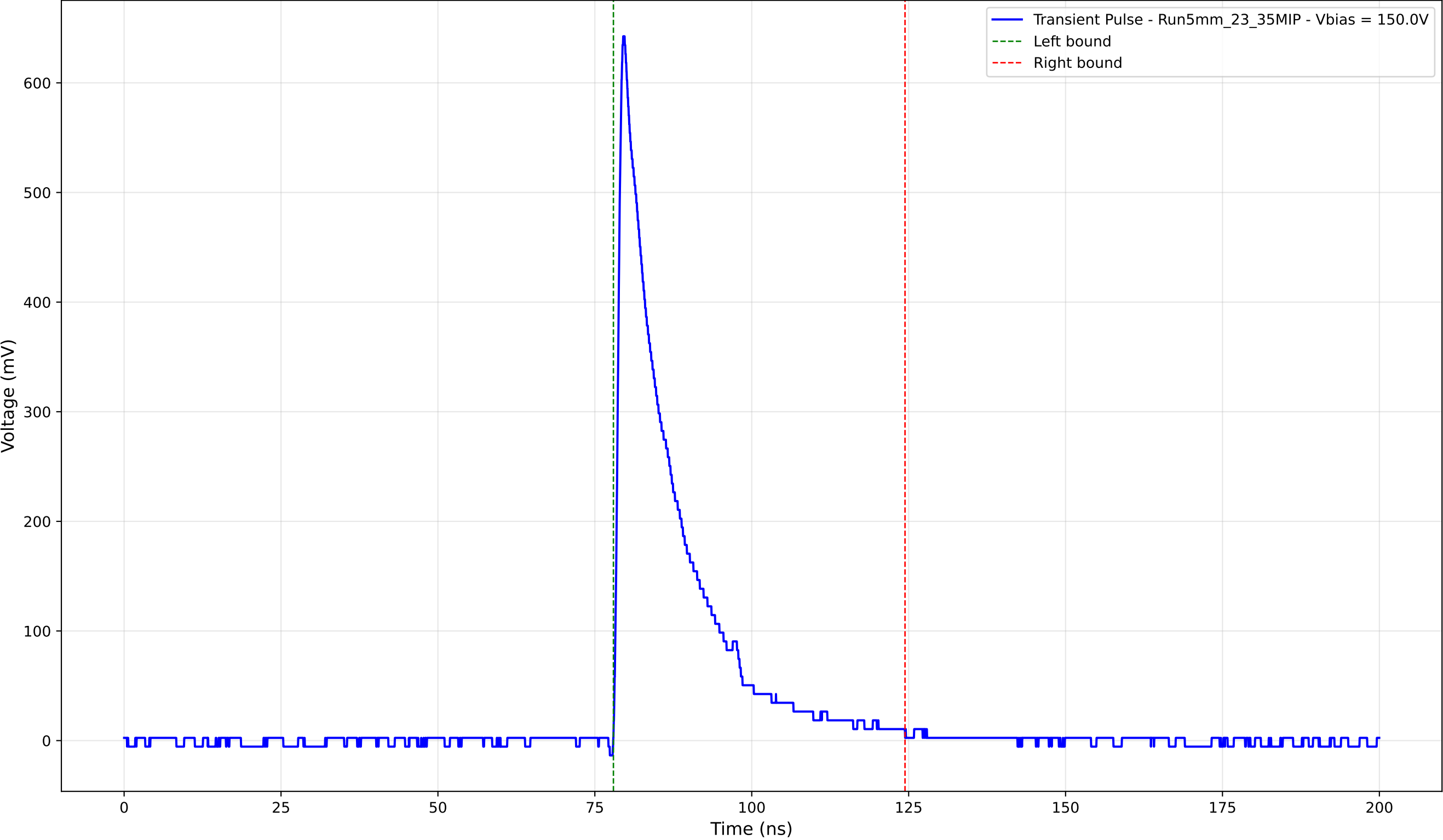
Transient Pulse - Sample: 5mm_23 - Position: 4330.0 \mu\text{m} - Charge: 116.27 pC
