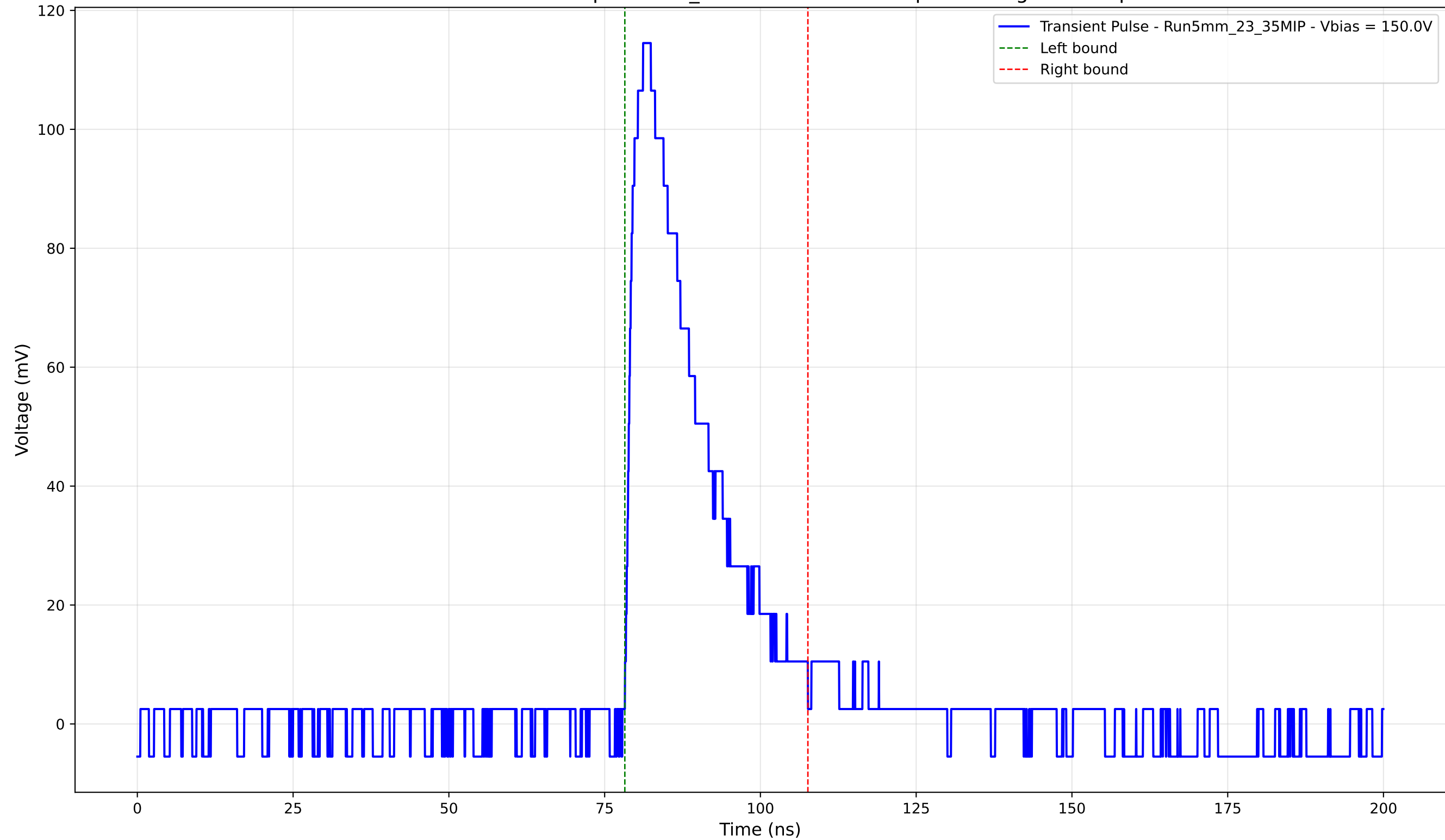
Transient Pulse - Sample: 5mm_23 - Position: 2630.0 \mu\text{m} - Charge: 28.26 pC
