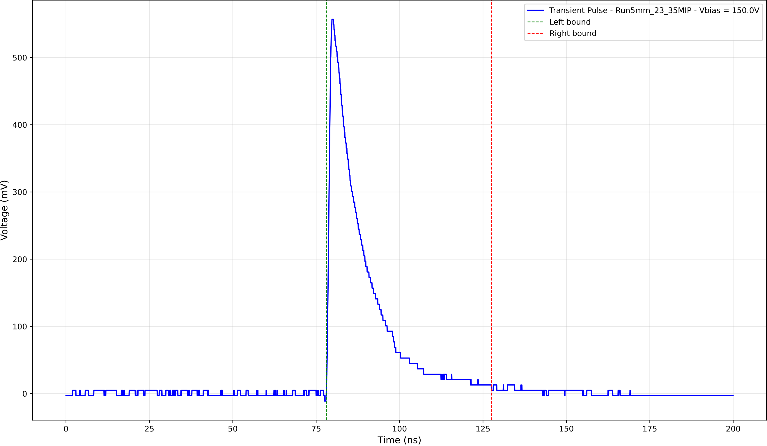
Transient Pulse - Sample: 5mm_23 - Position: 3960.0 \mu\text{m} - Charge: 121.51 pC
