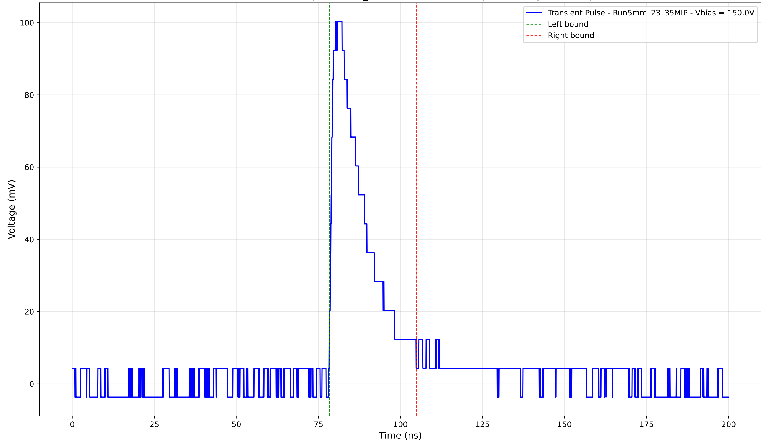
Transient Pulse - Sample: 5mm_23 - Position: 3665.0 \mu\text{m} - Charge: 22.73 pC
