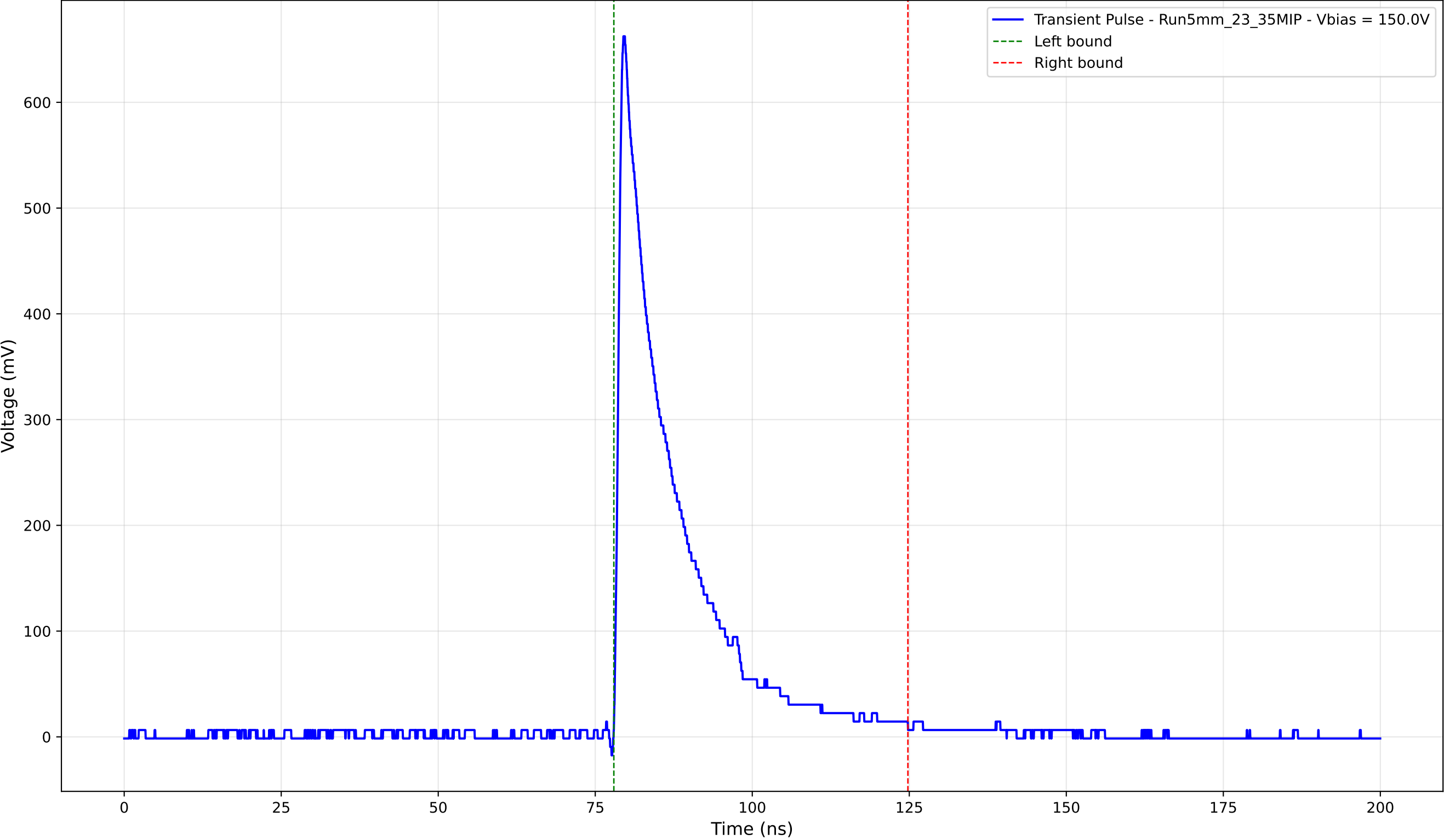
Transient Pulse - Sample: 5mm_23 - Position: 4350.0 \mu\text{m} - Charge: 122.10 pC
