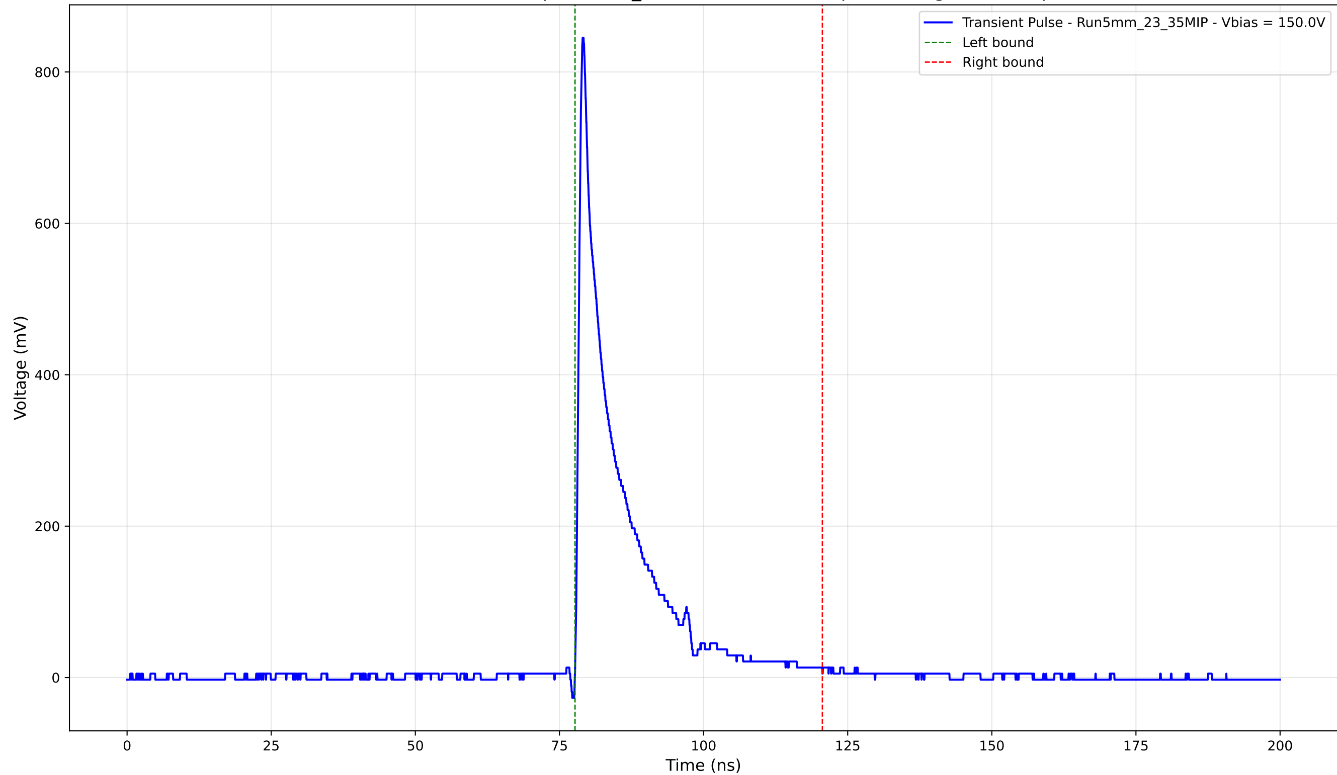
Transient Pulse - Sample: 5mm_23 - Position: 4860.0 \mu\text{m} - Charge: 117.14 pC
