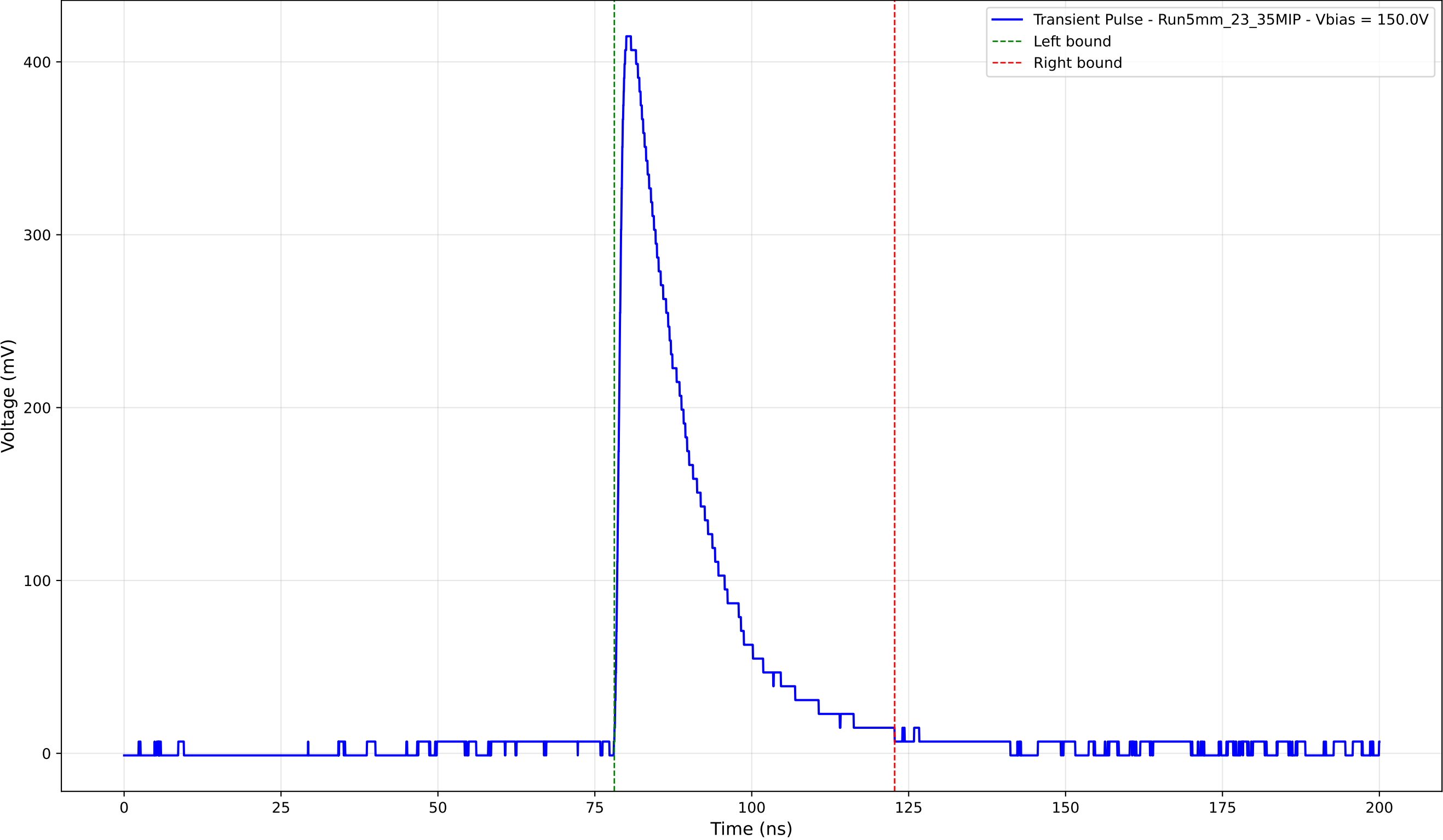
Transient Pulse - Sample: 5mm_23 - Position: 1695.0 \mu\text{m} - Charge: 103.63 pC
