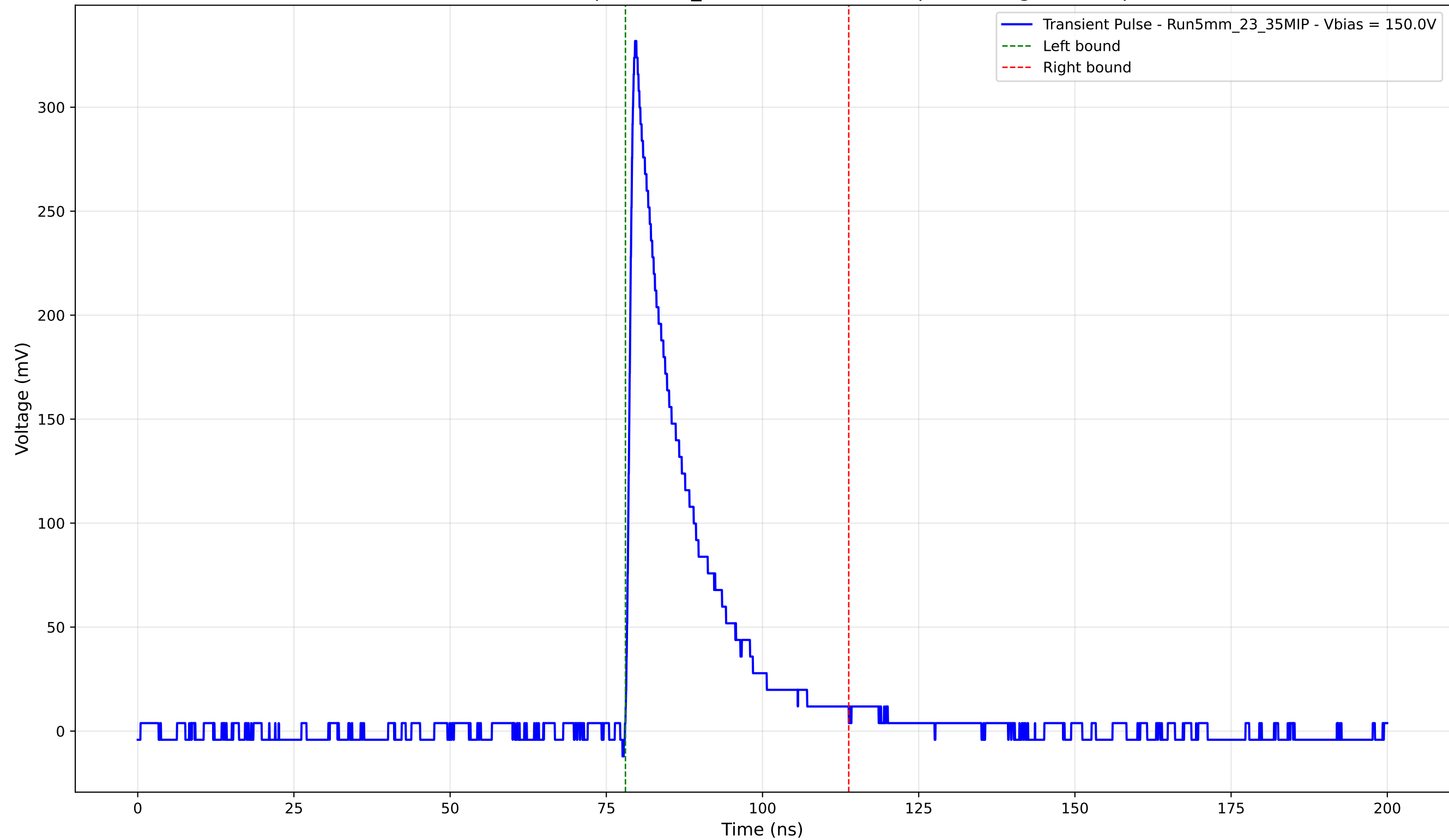
Transient Pulse - Sample: 5mm_23 - Position: 4205.0 \mu\text{m} - Charge: 59.06 pC
