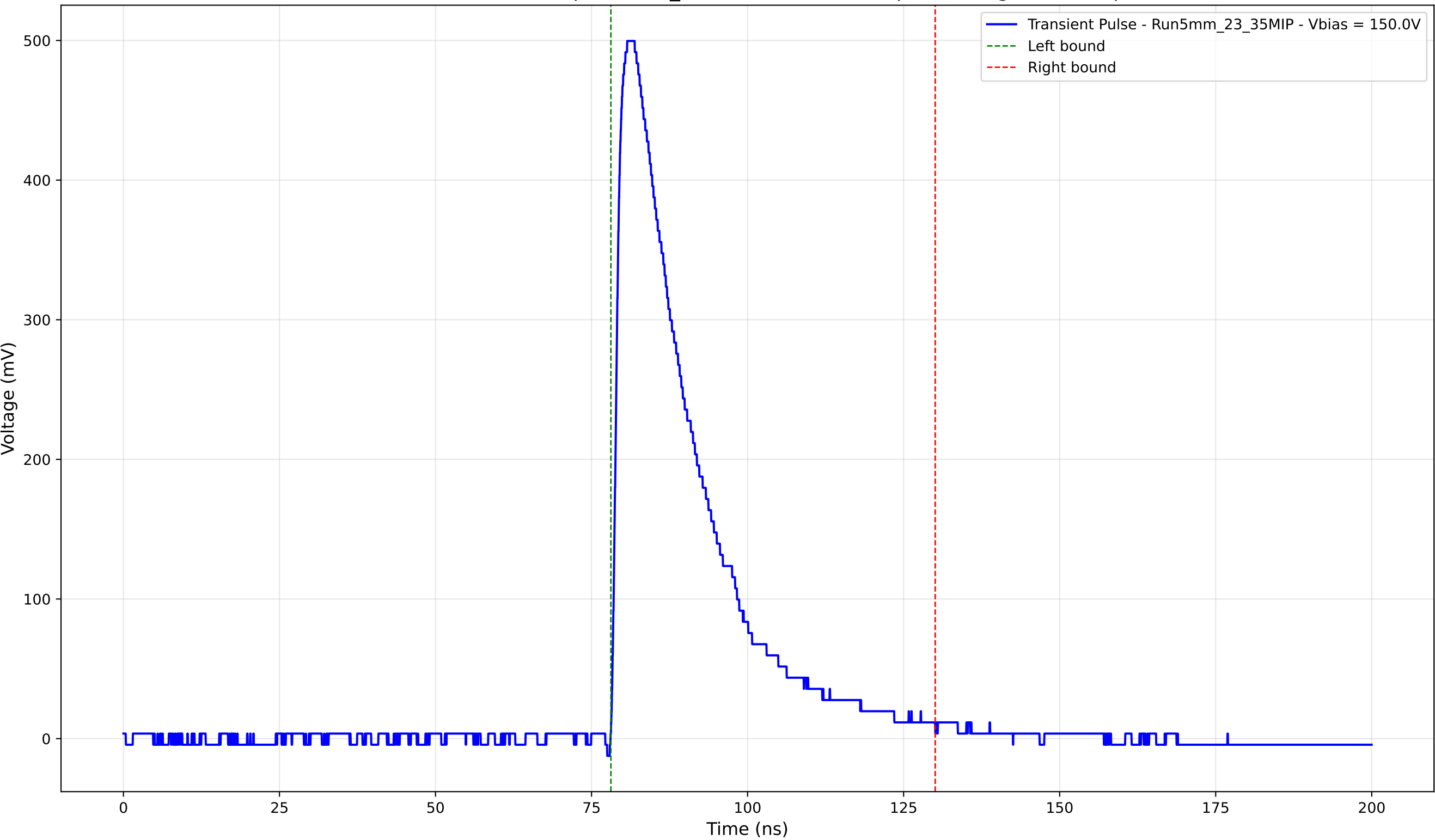
Transient Pulse - Sample: 5mm_23 - Position: 2430.0 \mu\text{m} - Charge: 137.14 pC
