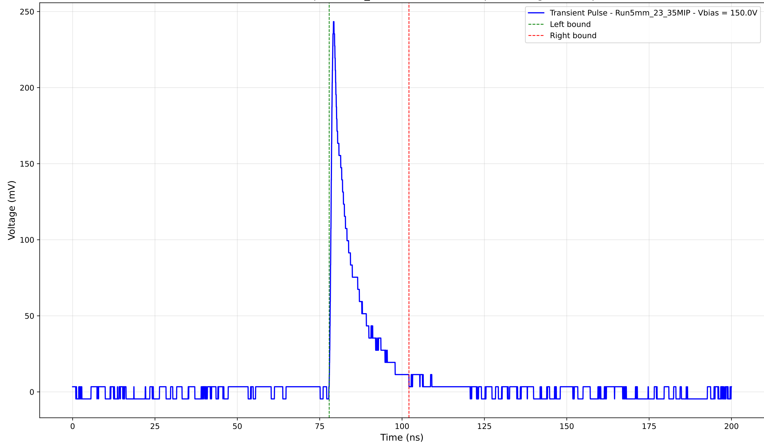
Transient Pulse - Sample: 5mm_23 - Position: 4690.0 \mu\text{m} - Charge: 30.91 pC
