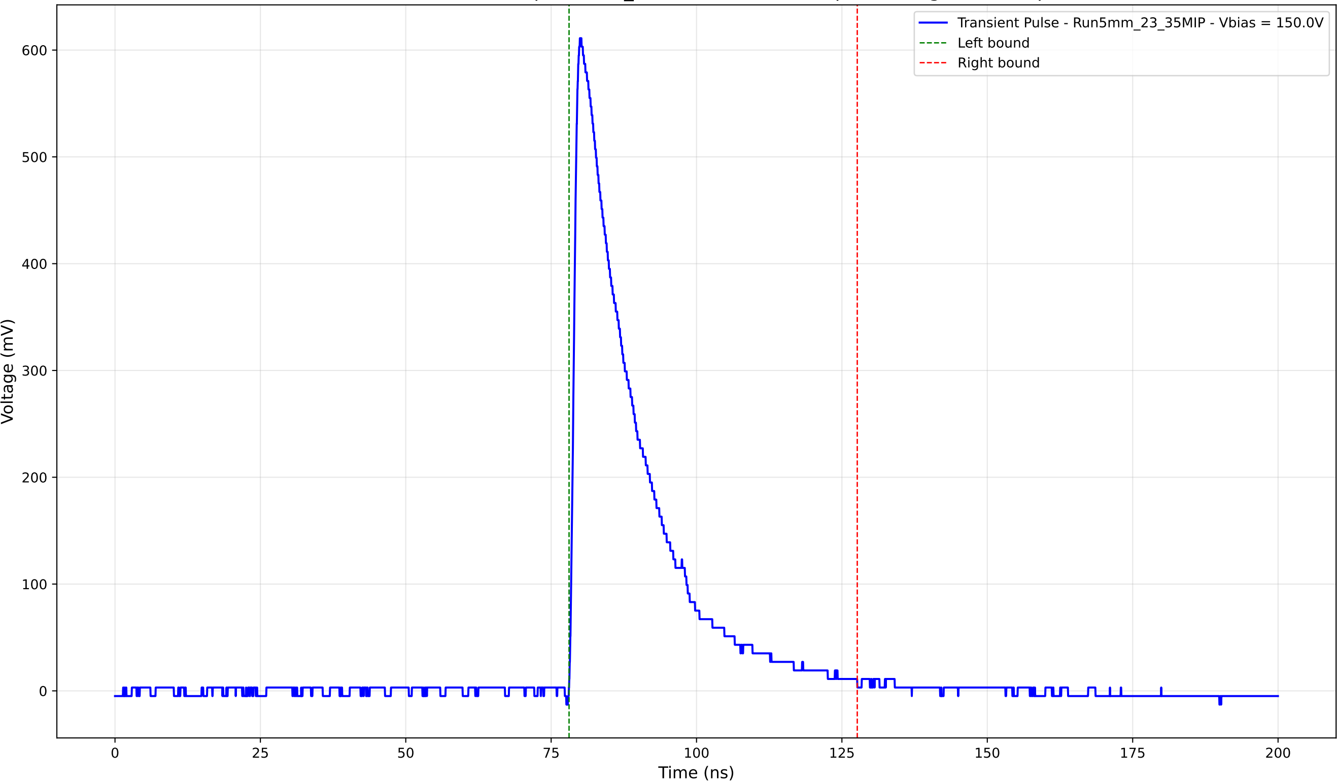
Transient Pulse - Sample: 5mm_23 - Position: 1495.0 \mu\text{m} - Charge: 143.85 pC
