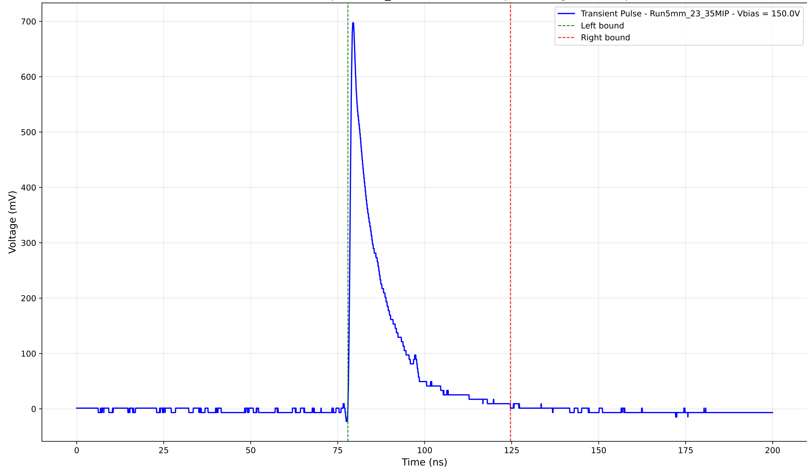
Transient Pulse - Sample: 5mm_23 - Position: 735.0 \mu\text{m} - Charge: 117.87 pC
