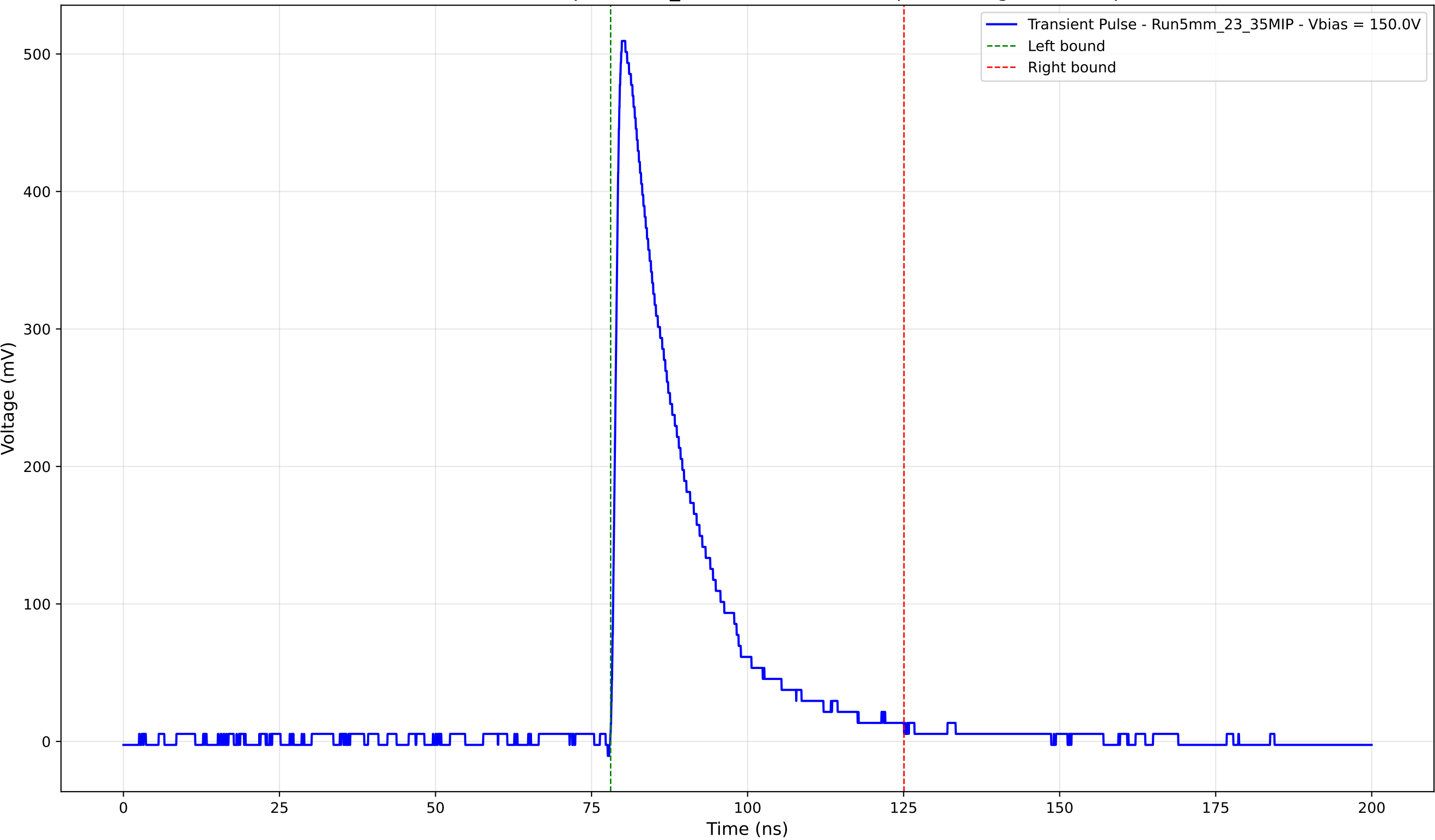
Transient Pulse - Sample: 5mm_23 - Position: 3740.0 \mu\text{m} - Charge: 117.96 pC
