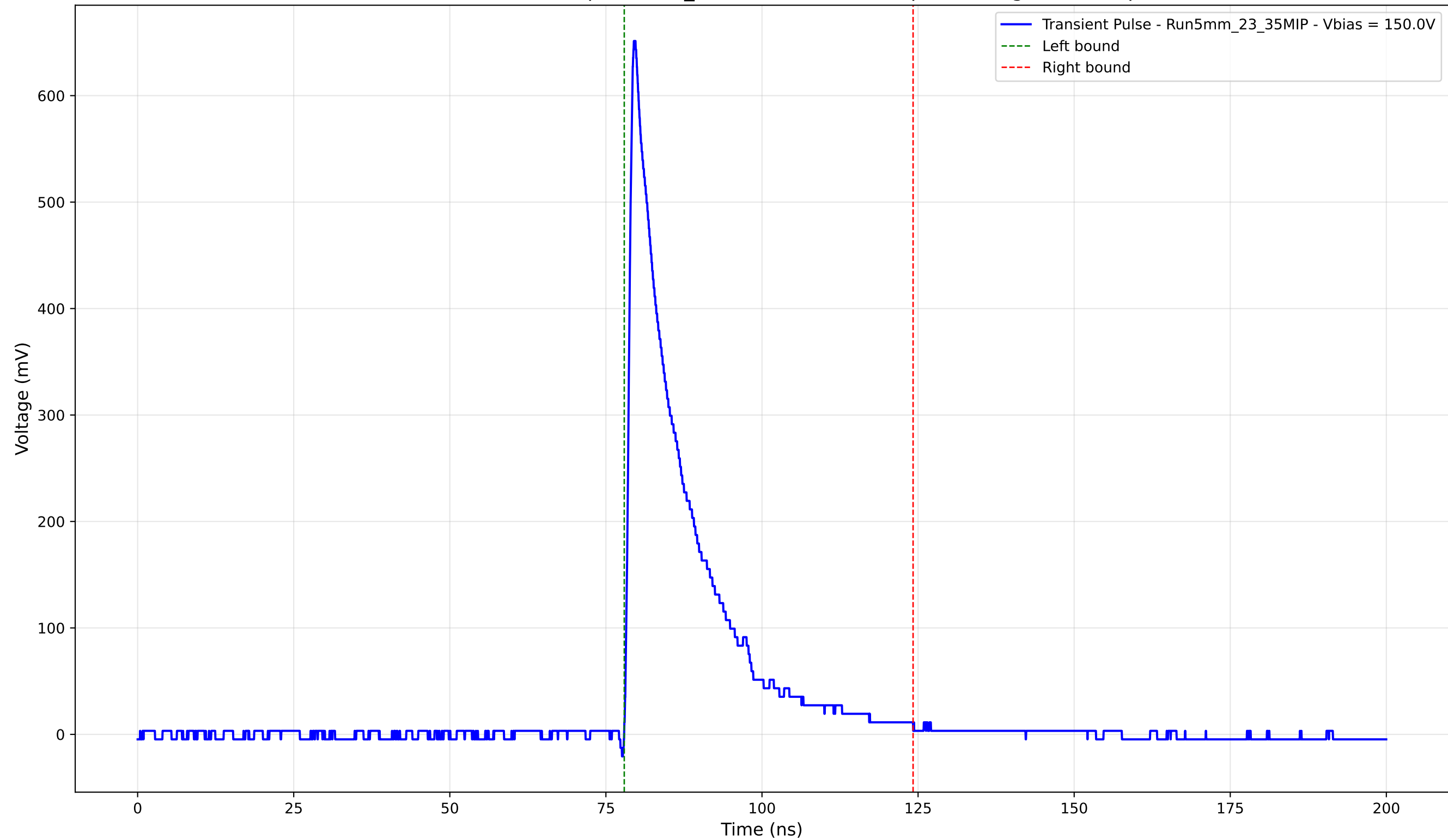
Transient Pulse - Sample: 5mm_23 - Position: 4345.0 \mu\text{m} - Charge: 118.82 pC
