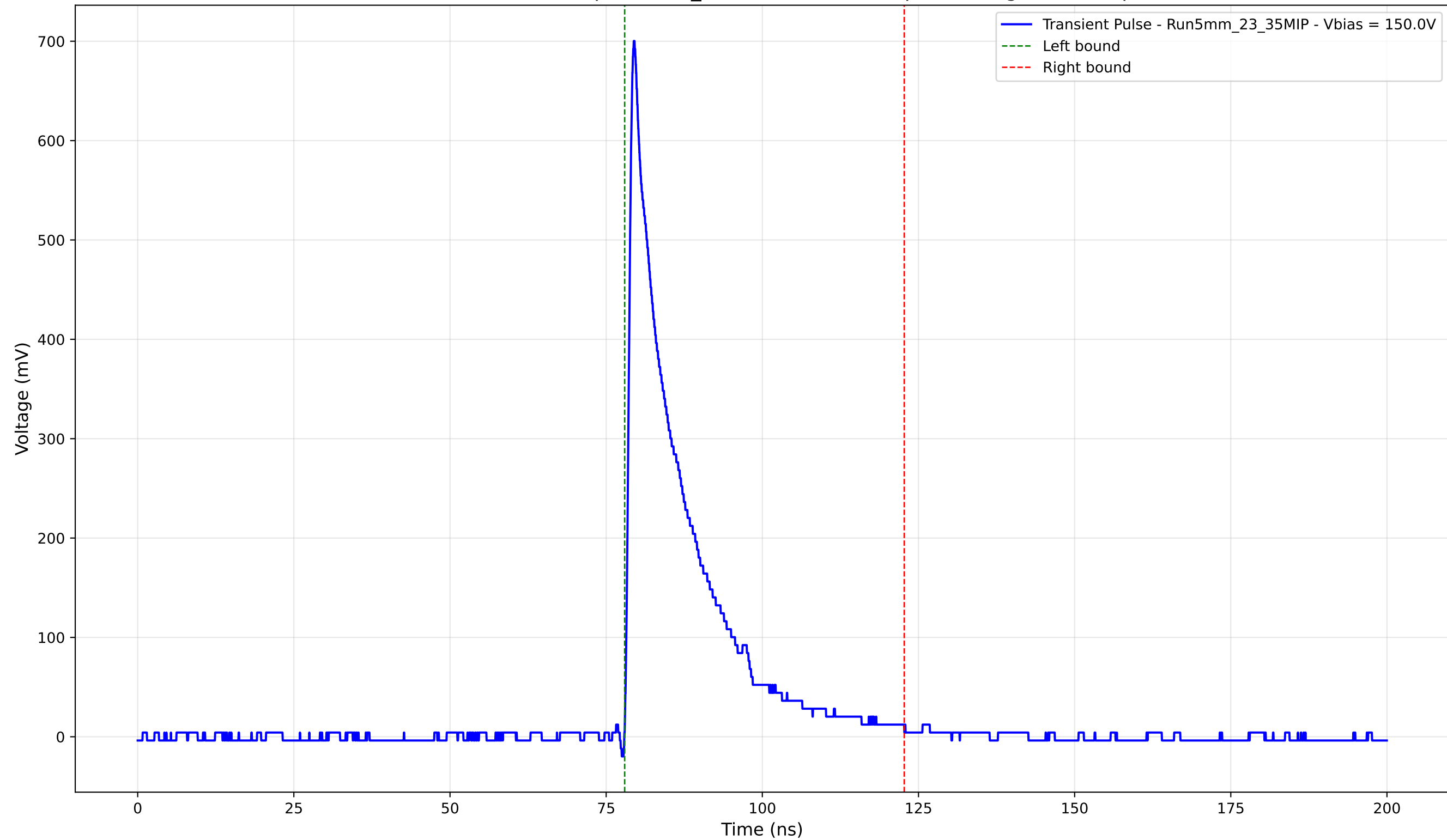
Transient Pulse - Sample: 5mm_23 - Position: 770.0 \mu\text{m} - Charge: 120.65 pC
