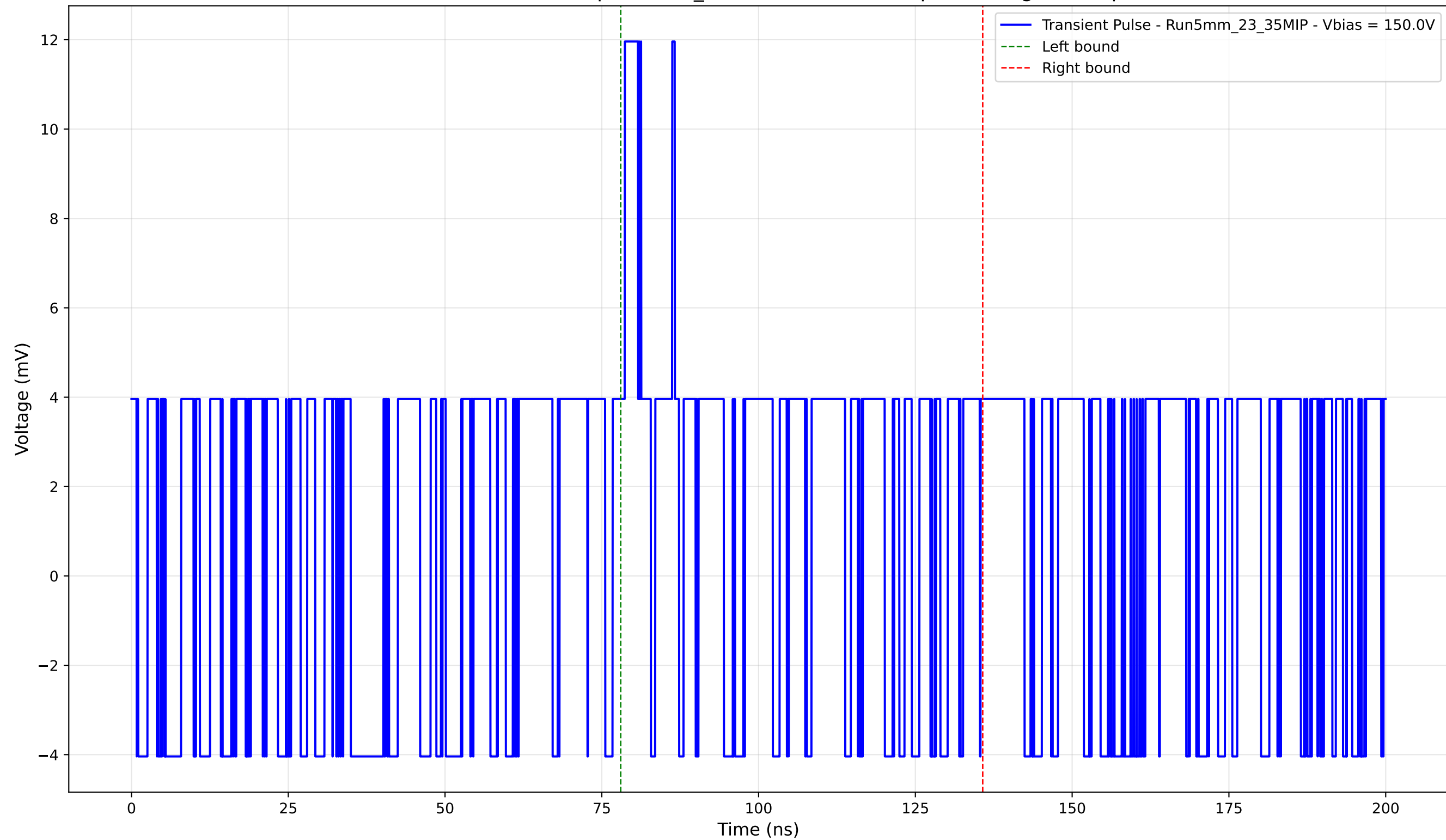
Transient Pulse - Sample: 5mm_23 - Position: 5195.0 \mu\text{m} - Charge: 2.67 pC
