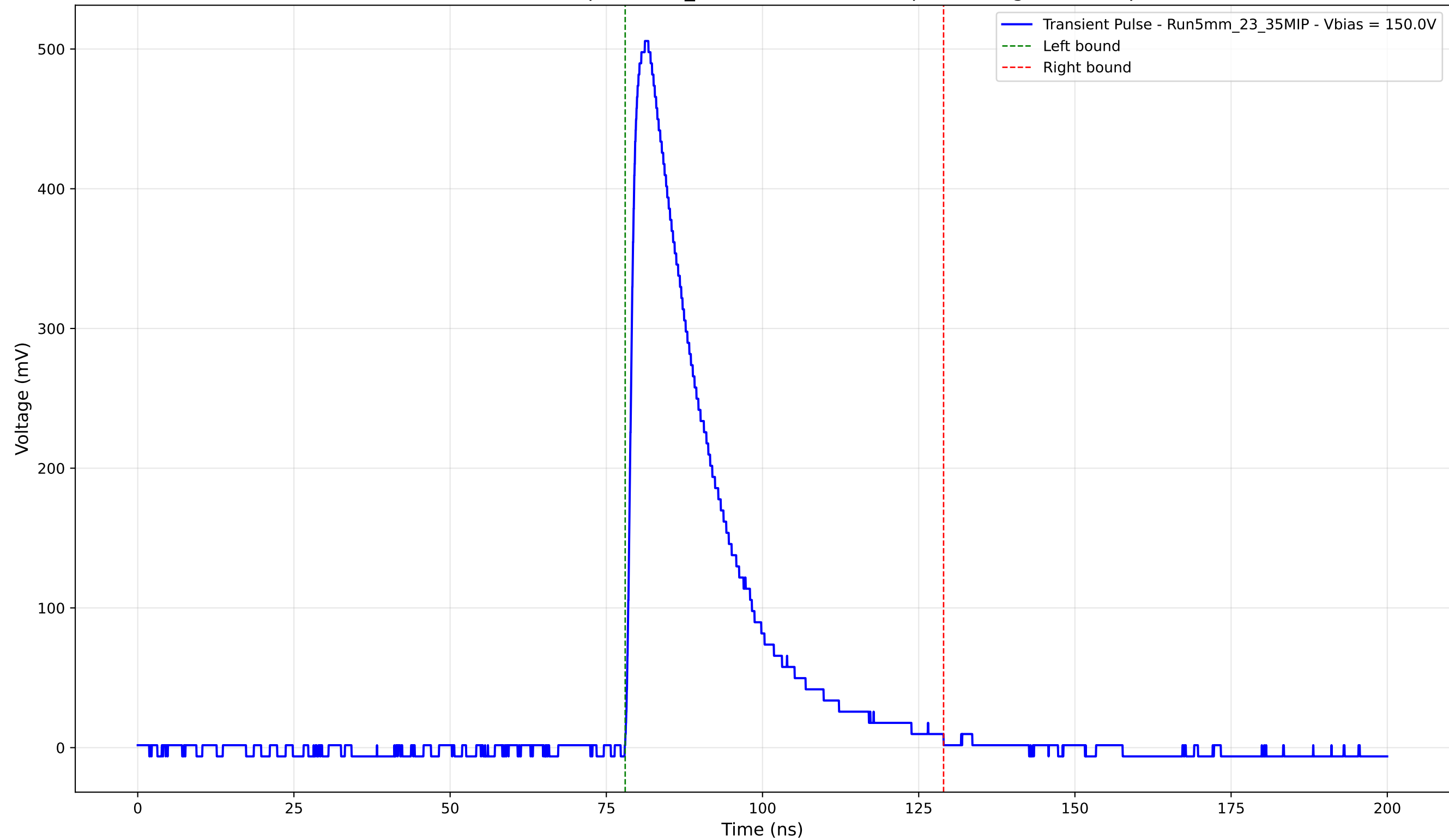
Transient Pulse - Sample: 5mm_23 - Position: 2510.0 \mu\text{m} - Charge: 136.31 pC
