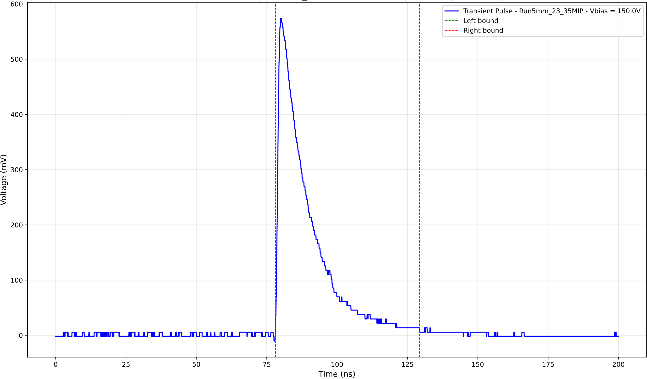
Transient Pulse - Sample: 5mm_23 - Position: 1520.0 \mu\text{m} - Charge: 137.18 pC
