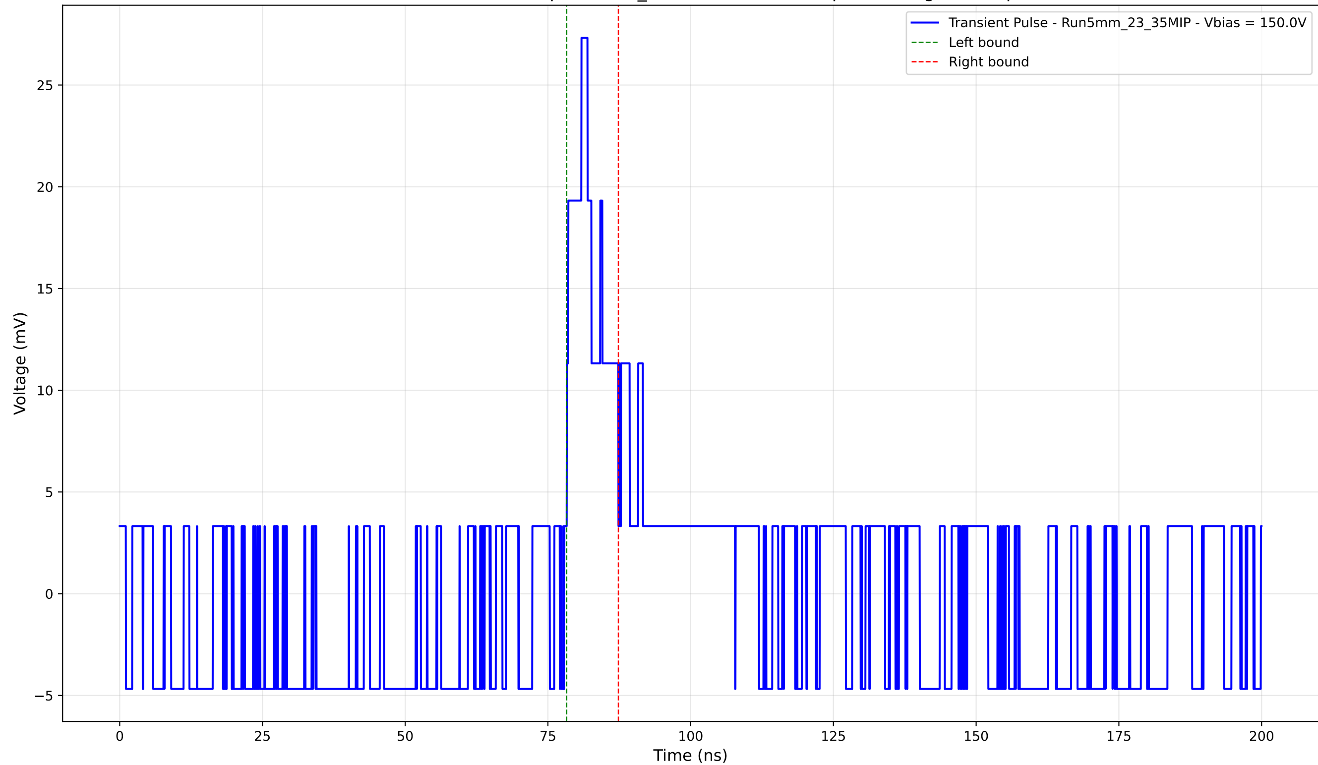
Transient Pulse - Sample: 5mm_23 - Position: 145.0 \mu\text{m} - Charge: 2.93 pC
