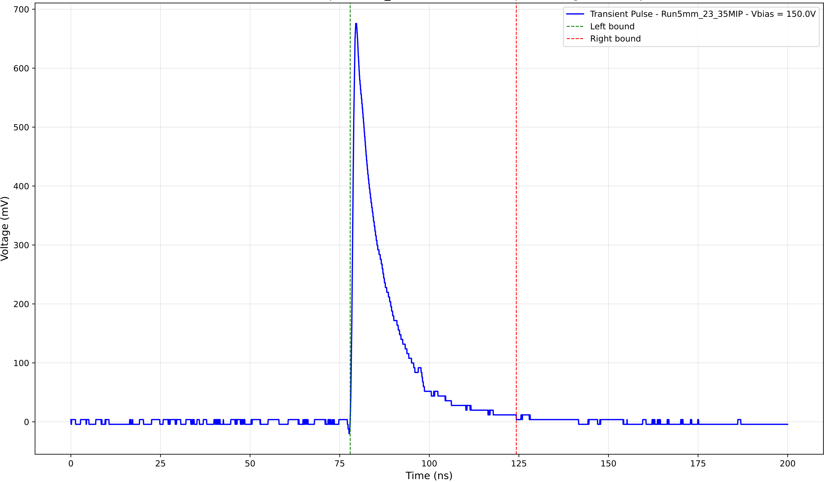
Transient Pulse - Sample: 5mm_23 - Position: 4365.0 \mu\text{m} - Charge: 122.19 pC
