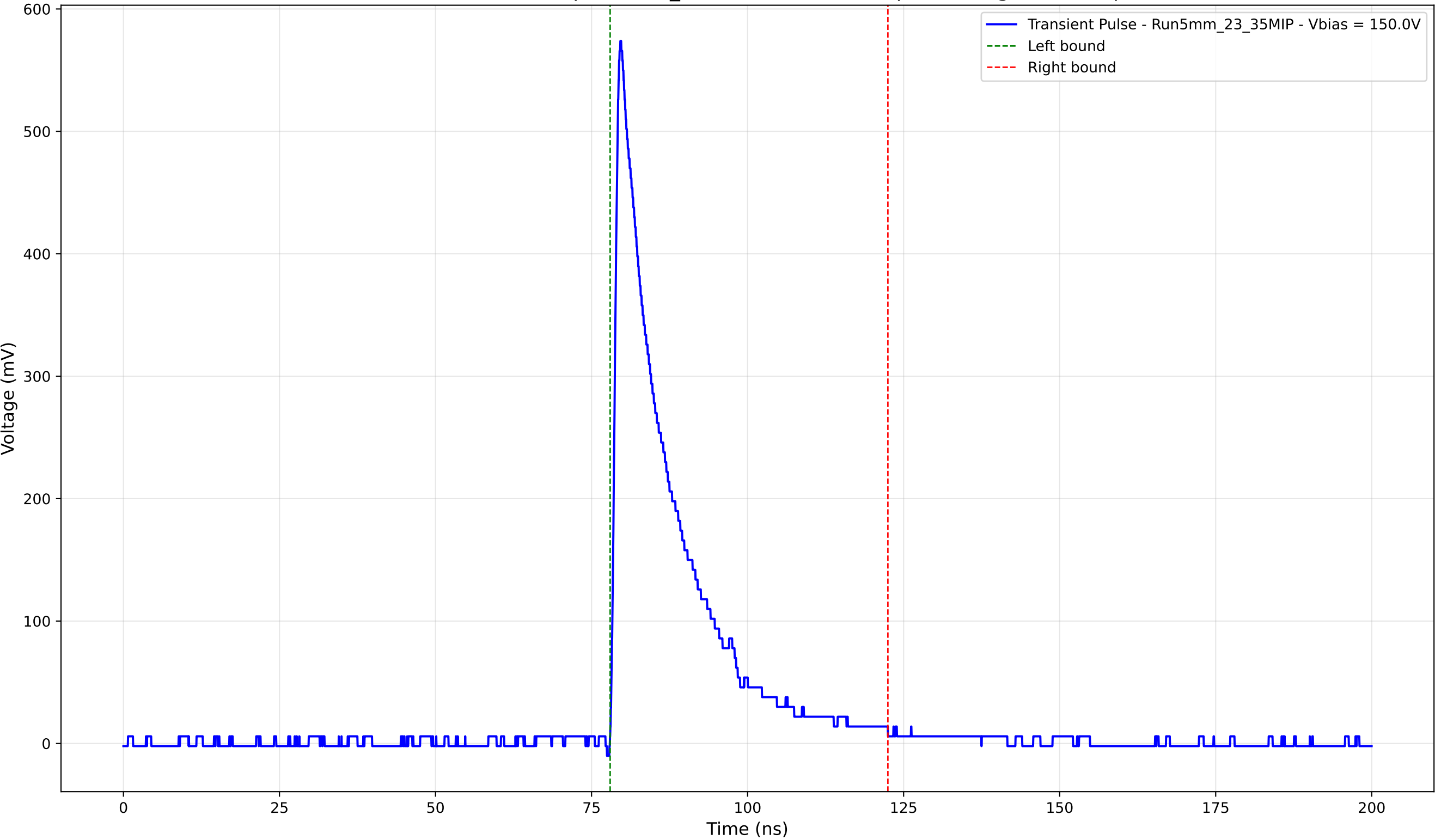
Transient Pulse - Sample: 5mm_23 - Position: 4250.0 \mu\text{m} - Charge: 106.91 pC
