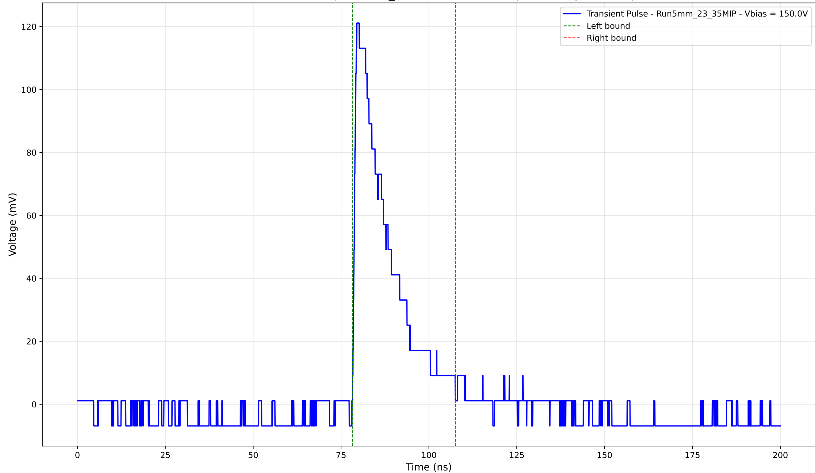
Transient Pulse - Sample: 5mm_23 - Position: 1140.0 \mu\text{m} - Charge: 25.07 pC
