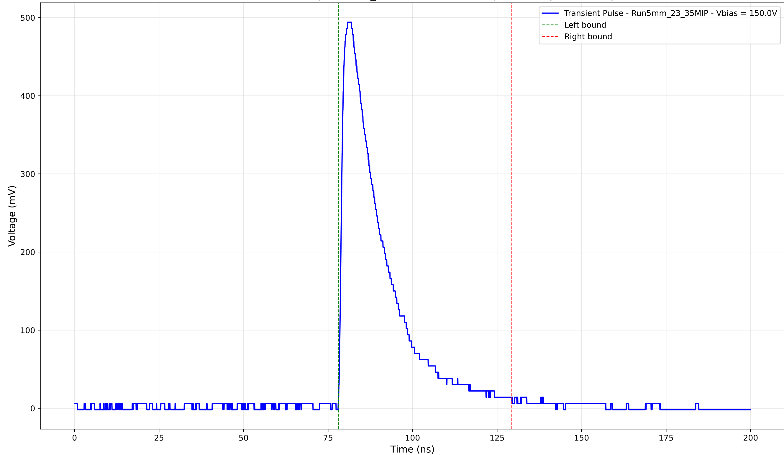
Transient Pulse - Sample: 5mm_23 - Position: 2905.0 \mu\text{m} - Charge: 135.83 pC
