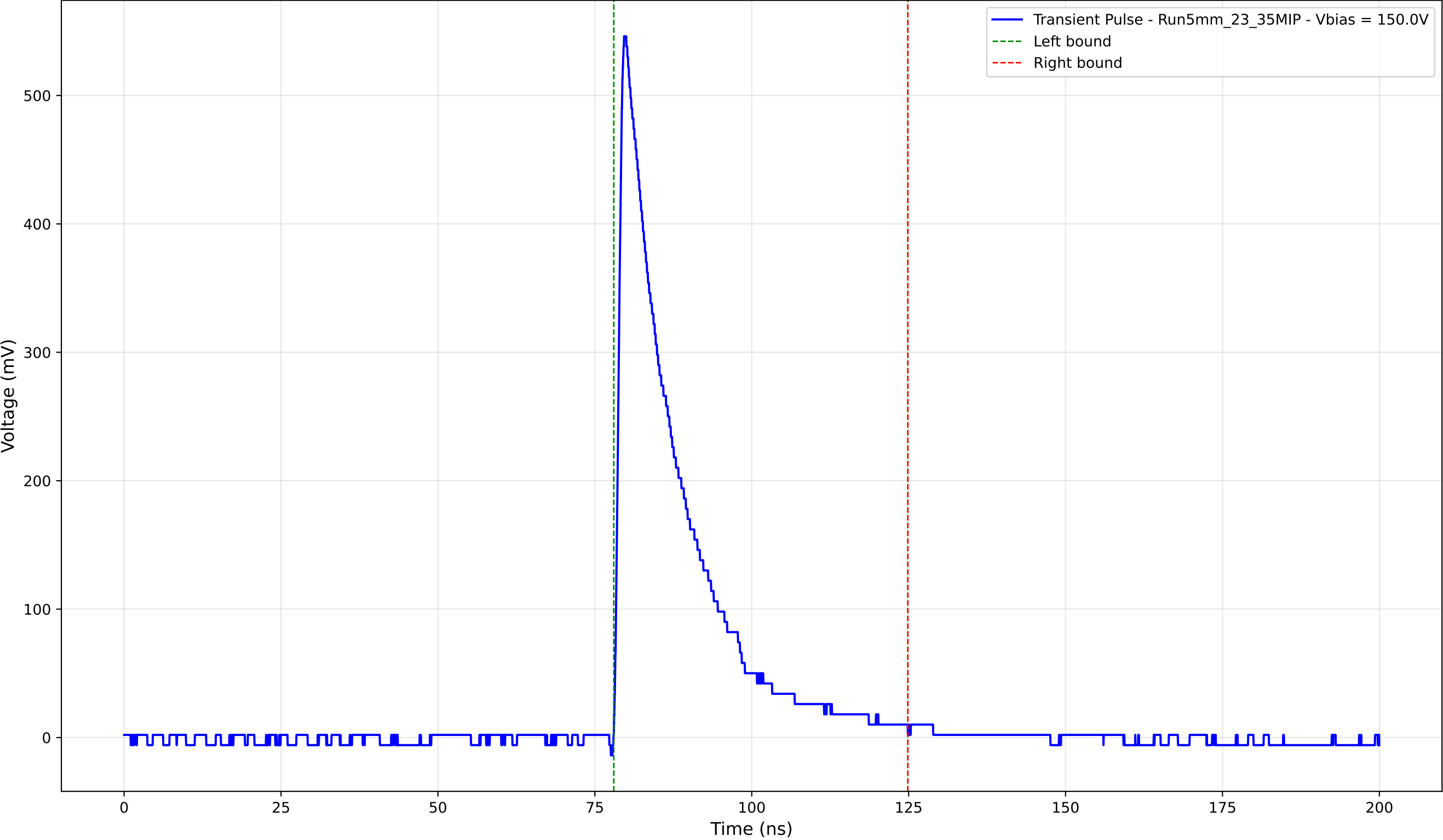
Transient Pulse - Sample: 5mm_23 - Position: 4070.0 \mu\text{m} - Charge: 109.87 pC
