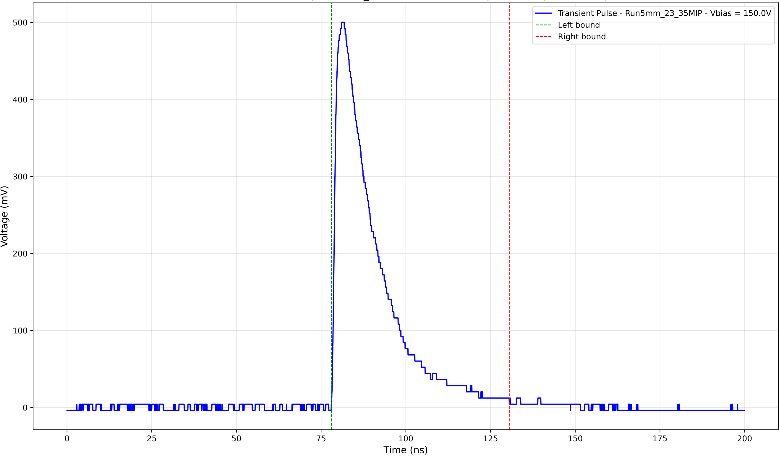
Transient Pulse - Sample: 5mm_23 - Position: 2835.0 \mu\text{m} - Charge: 135.50 pC
