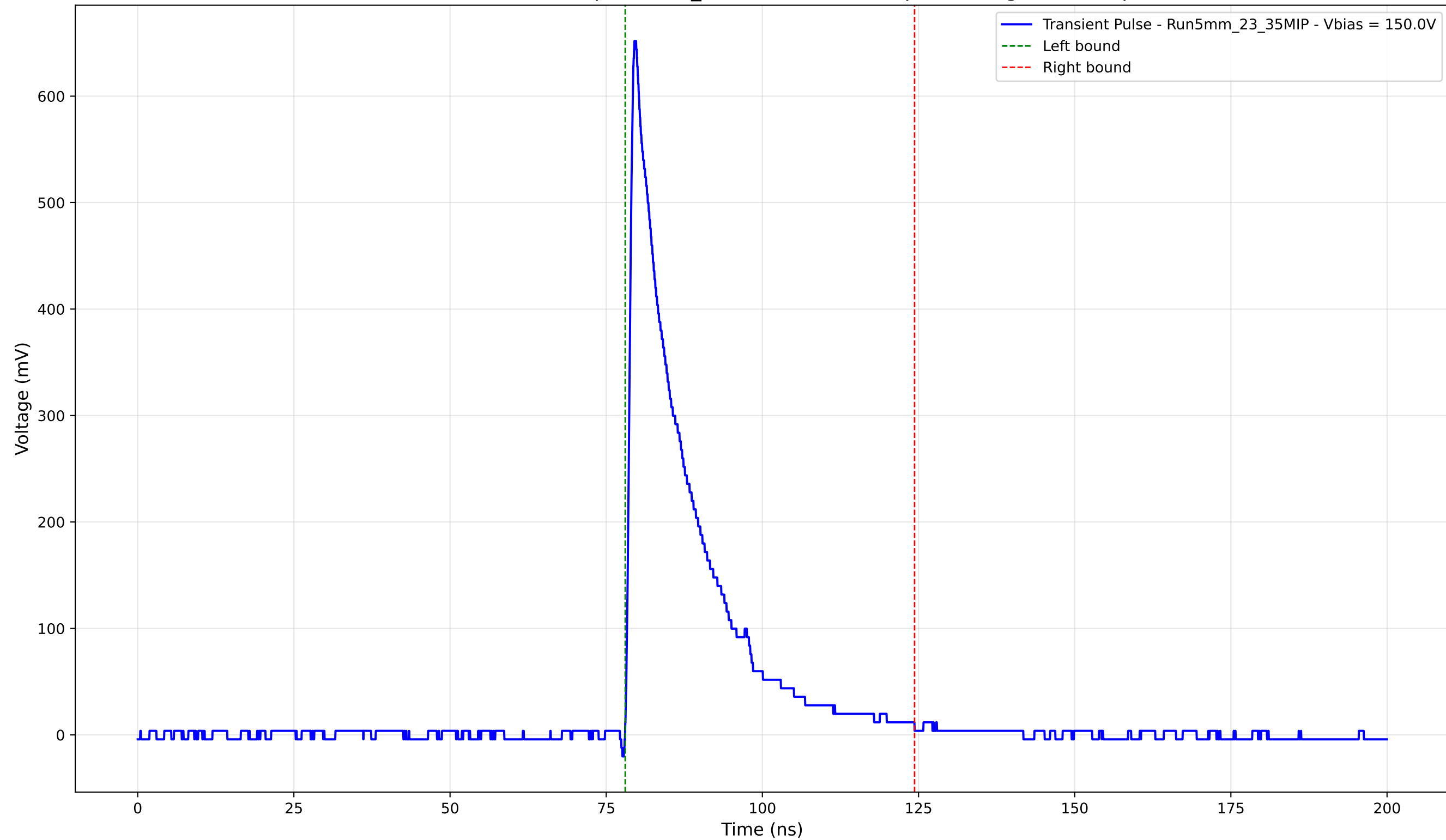
Transient Pulse - Sample: 5mm_23 - Position: 950.0 \mu\text{m} - Charge: 123.57 pC
