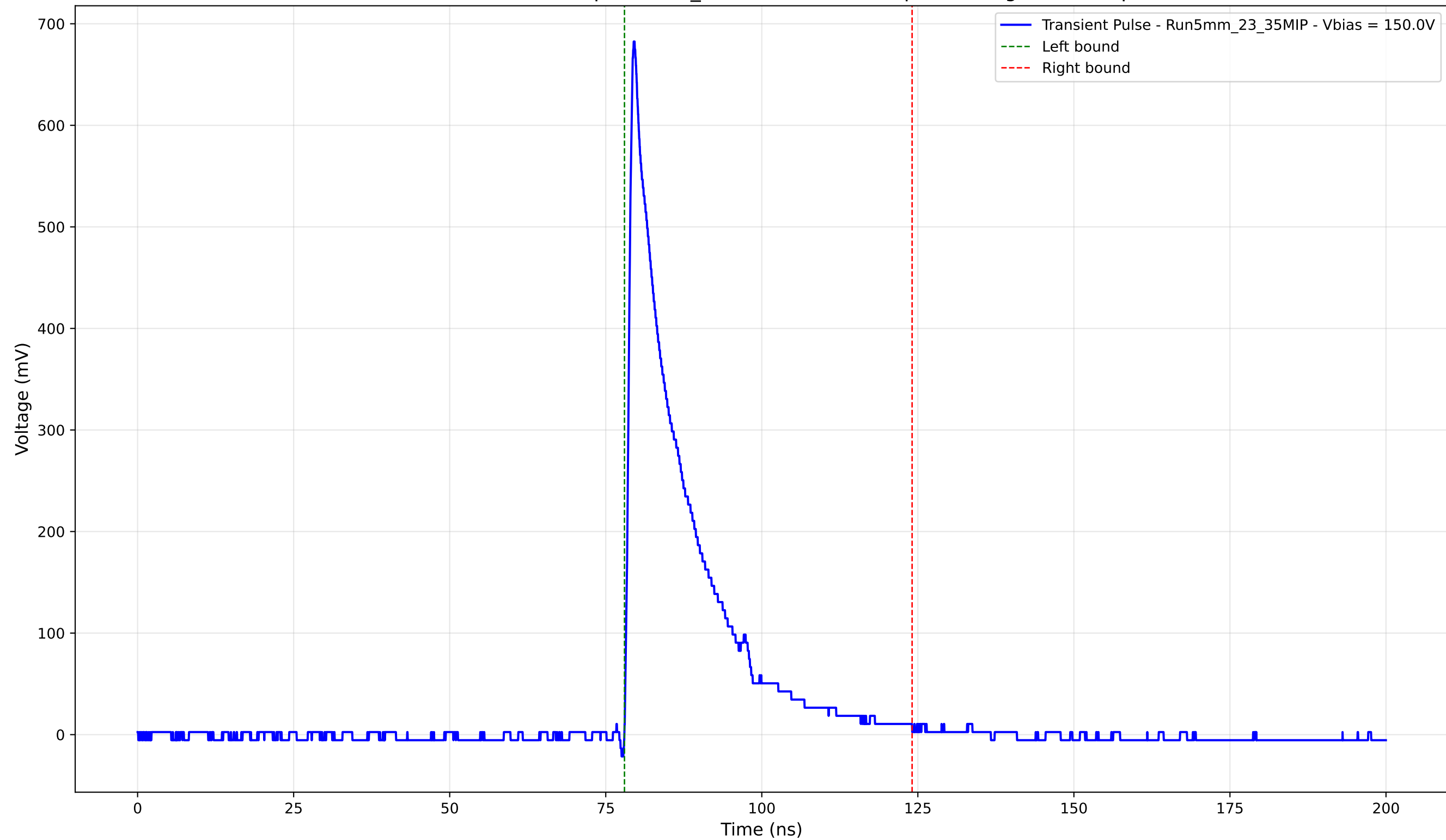
Transient Pulse - Sample: 5mm_23 - Position: 855.0 \mu\text{m} - Charge: 121.97 pC
