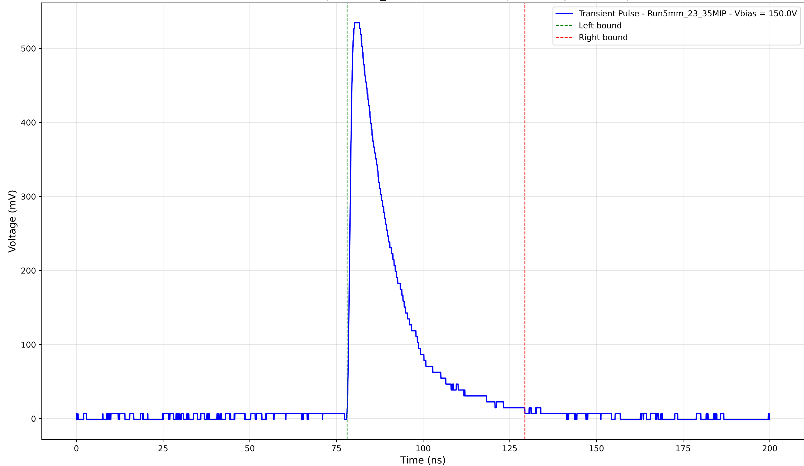
Transient Pulse - Sample: 5mm_23 - Position: 1925.0 \mu\text{m} - Charge: 143.22 pC
