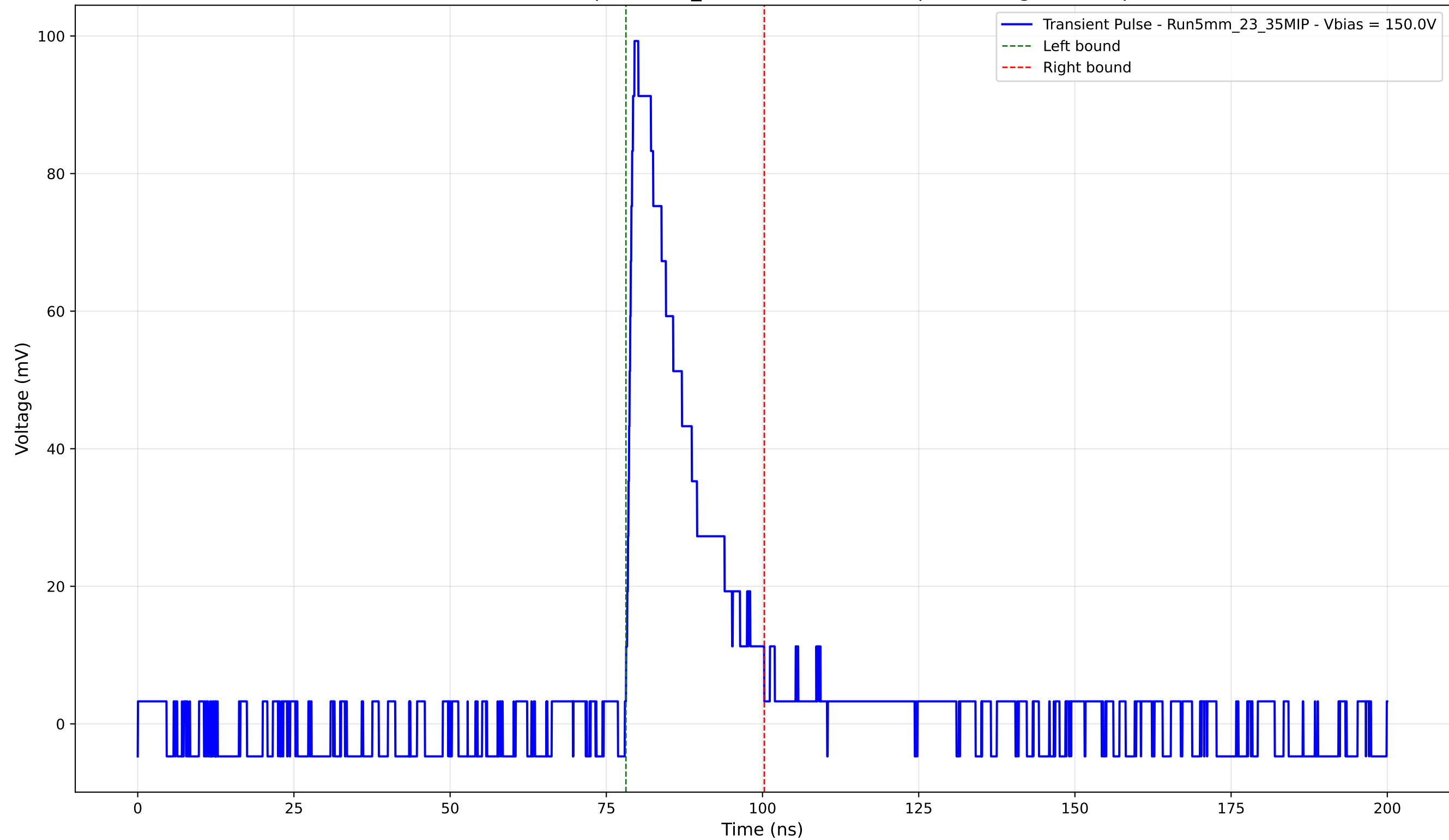
Transient Pulse - Sample: 5mm_23 - Position: 4150.0 \mu\text{m} - Charge: 18.98 pC
