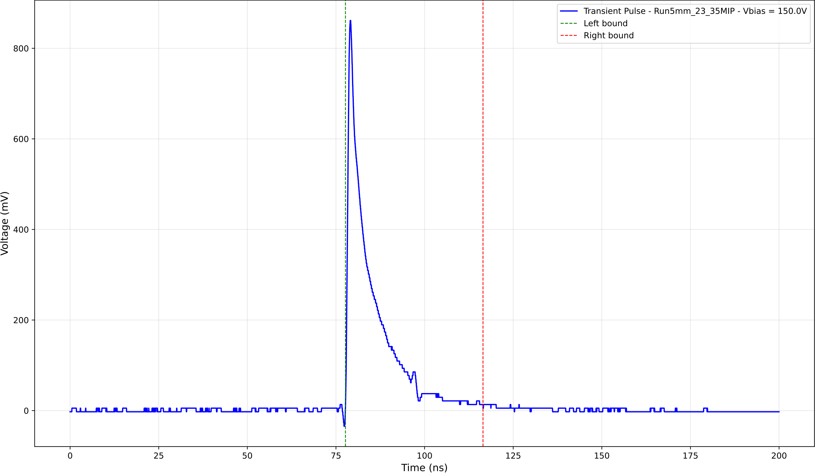
Transient Pulse - Sample: 5mm_23 - Position: 4890.0 \mu\text{m} - Charge: 114.90 pC
