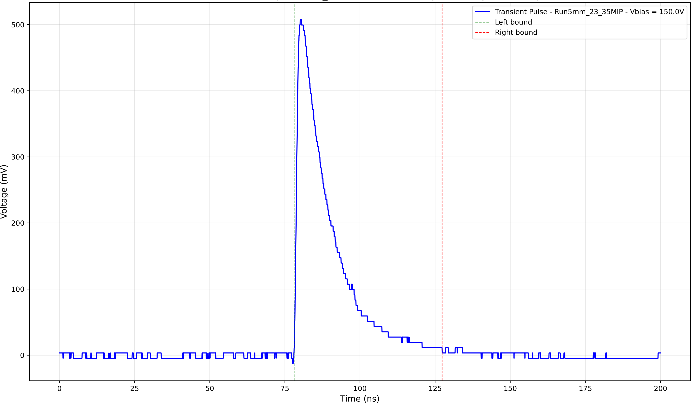
Transient Pulse - Sample: 5mm_23 - Position: 3545.0 \mu\text{m} - Charge: 123.91 pC
