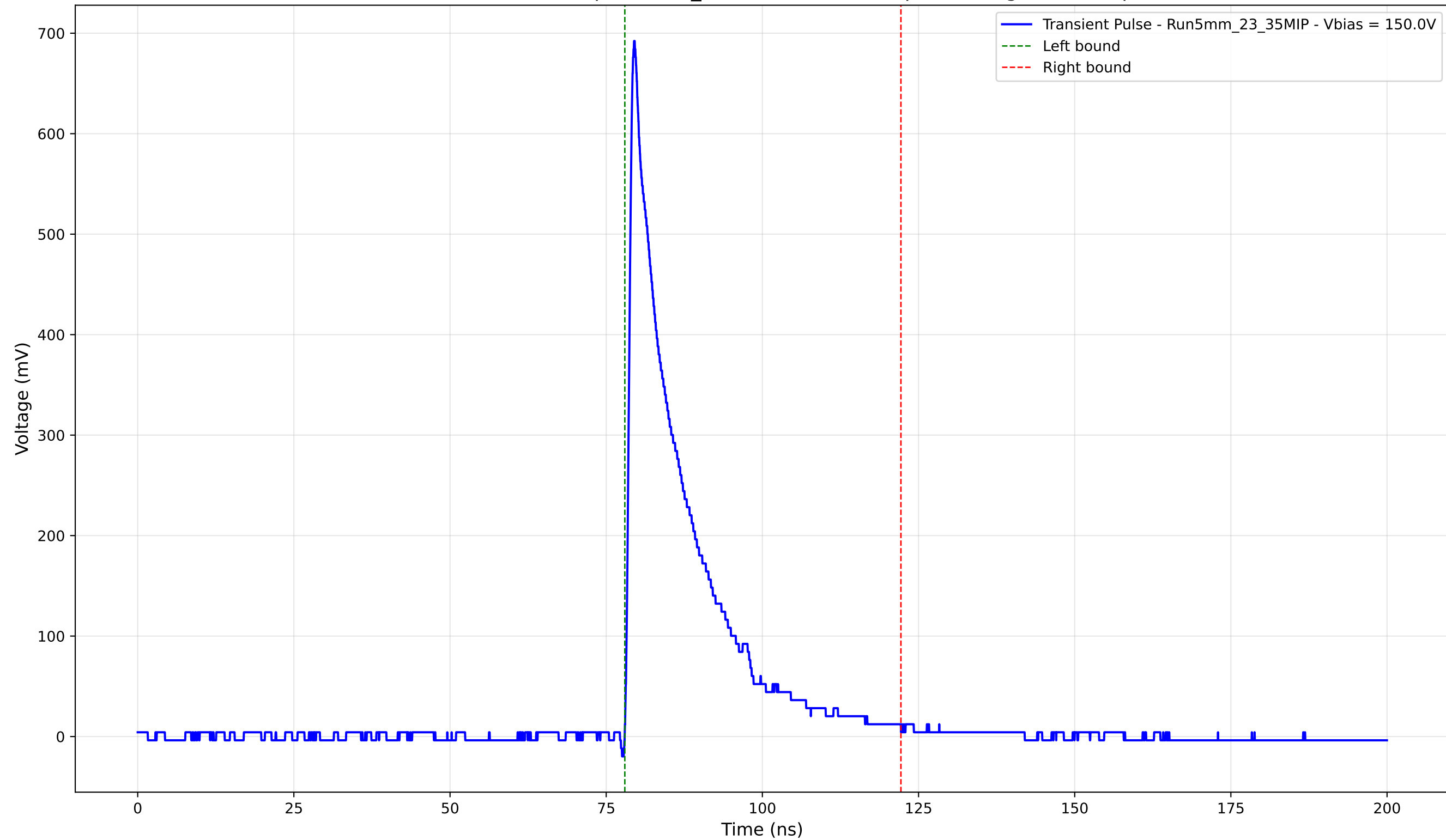
Transient Pulse - Sample: 5mm_23 - Position: 815.0 \mu\text{m} - Charge: 121.56 pC
