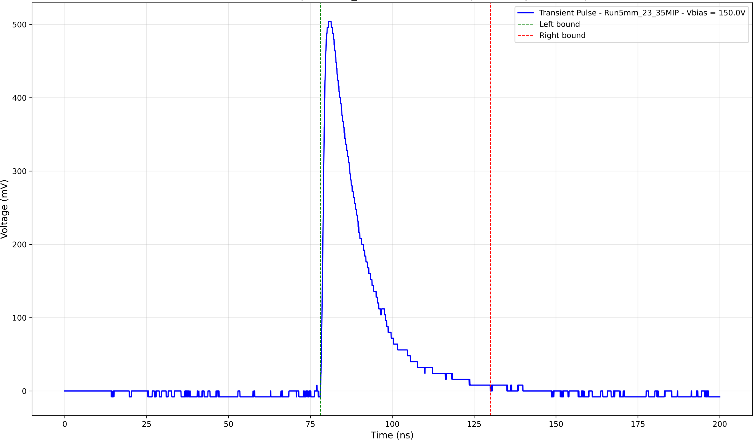
Transient Pulse - Sample: 5mm_23 - Position: 3325.0 \mu\text{m} - Charge: 128.34 pC
