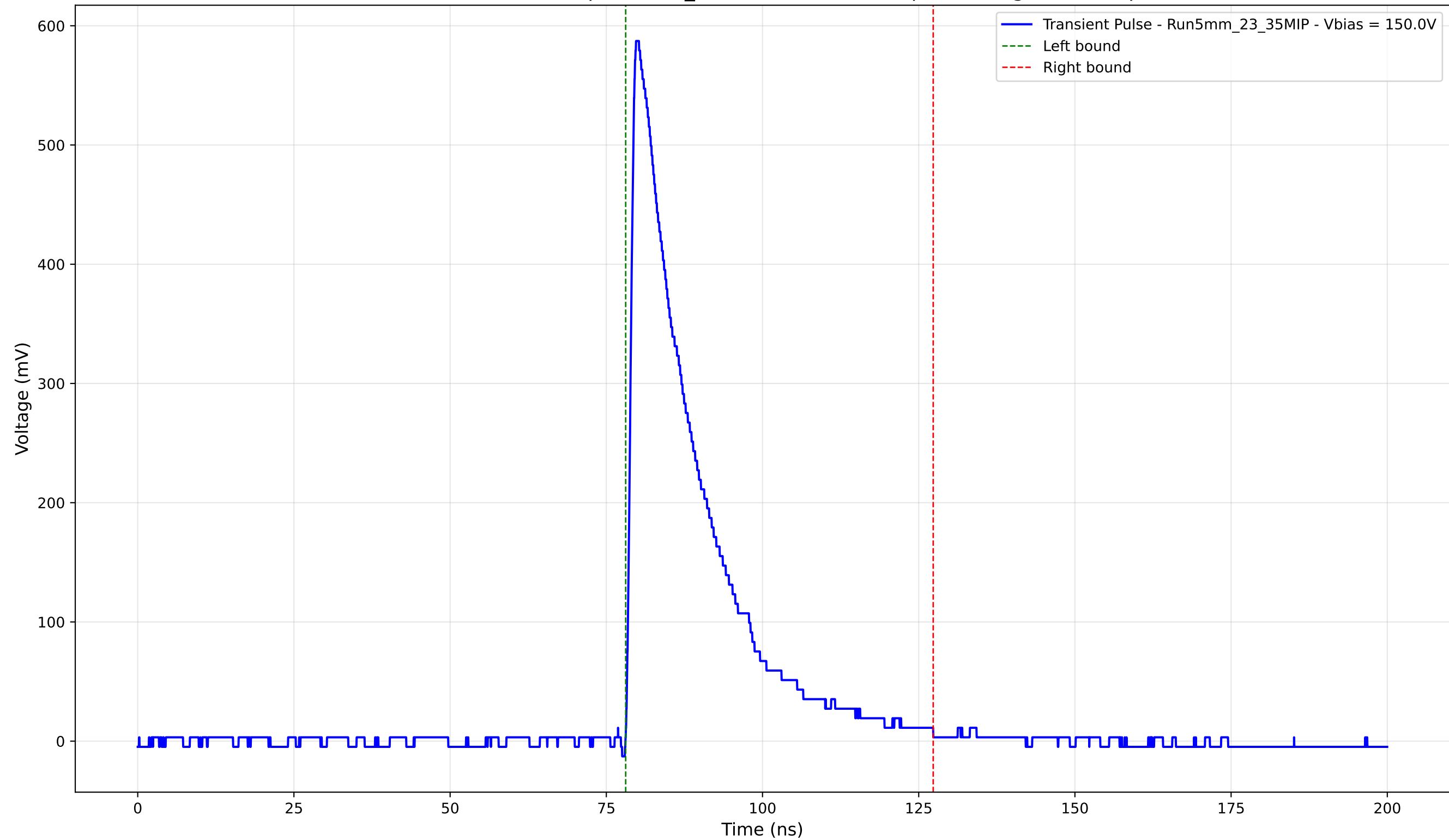
Transient Pulse - Sample: 5mm_23 - Position: 1350.0 \mu\text{m} - Charge: 133.29 pC
