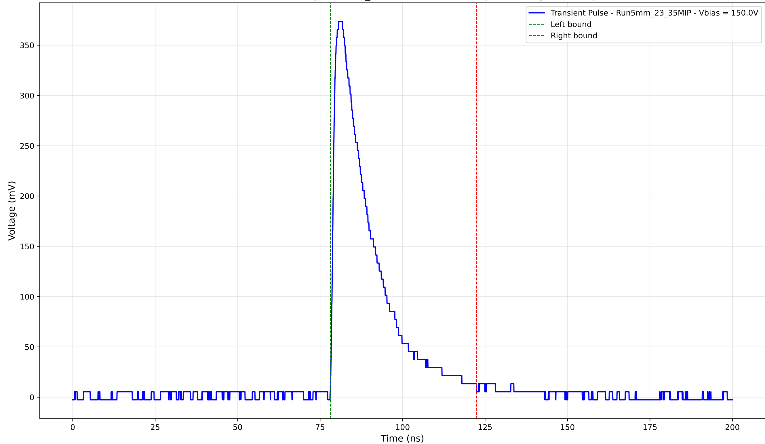
Transient Pulse - Sample: 5mm_23 - Position: 3085.0 \mu\text{m} - Charge: 98.05 pC
