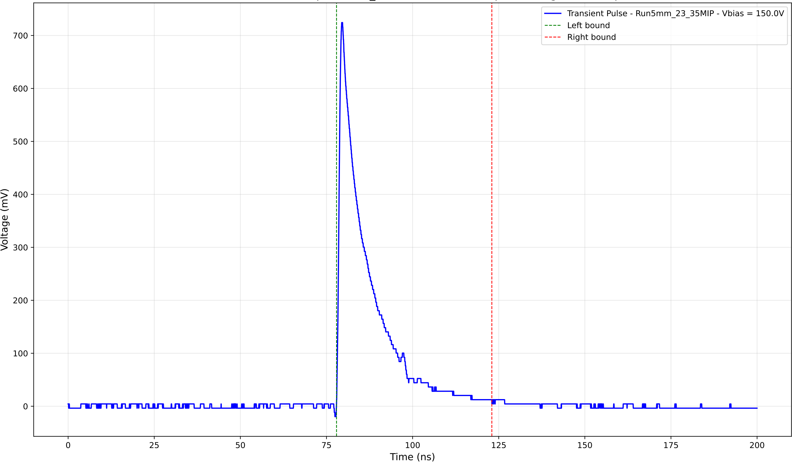
Transient Pulse - Sample: 5mm_23 - Position: 4440.0 \mu\text{m} - Charge: 126.60 pC
