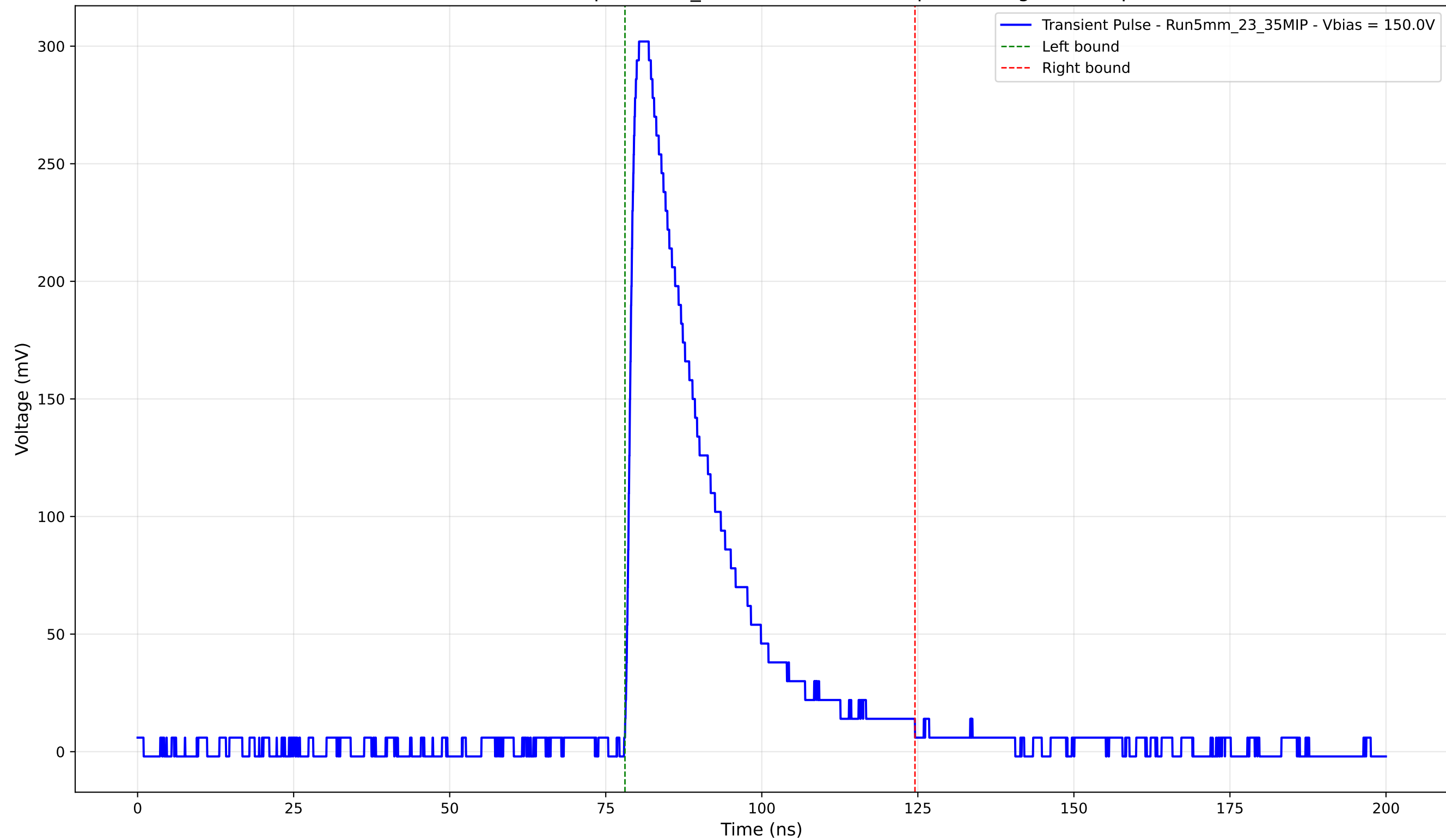
Transient Pulse - Sample: 5mm_23 - Position: 3195.0 \mu\text{m} - Charge: 79.89 pC
