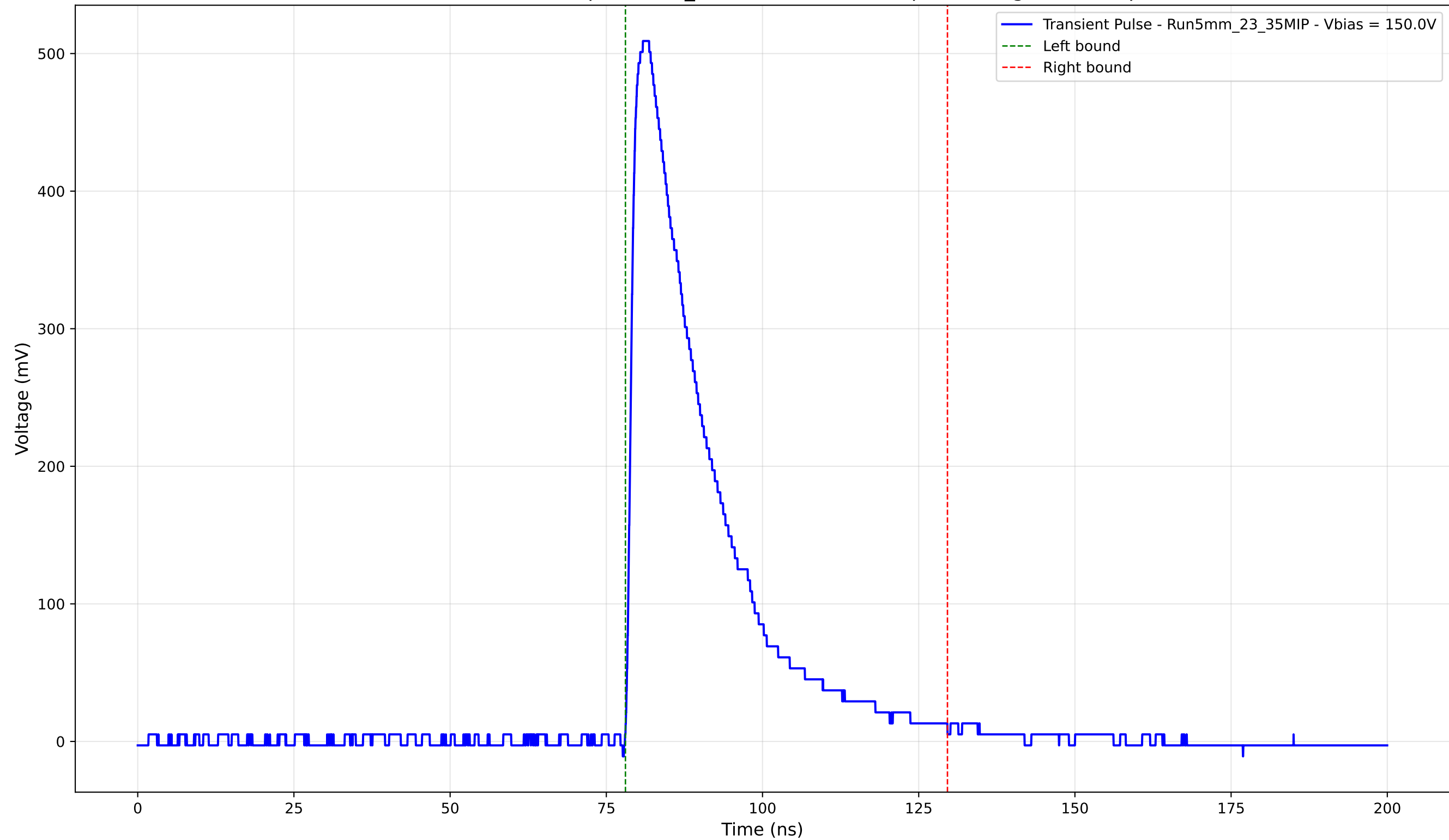
Transient Pulse - Sample: 5mm_23 - Position: 2285.0 \mu\text{m} - Charge: 139.30 pC
