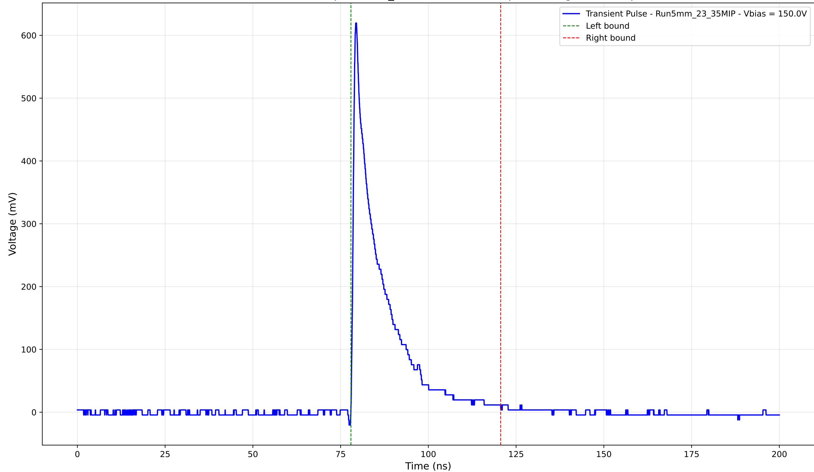
Transient Pulse - Sample: 5mm_23 - Position: 695.0 \mu\text{m} - Charge: 100.46 pC
