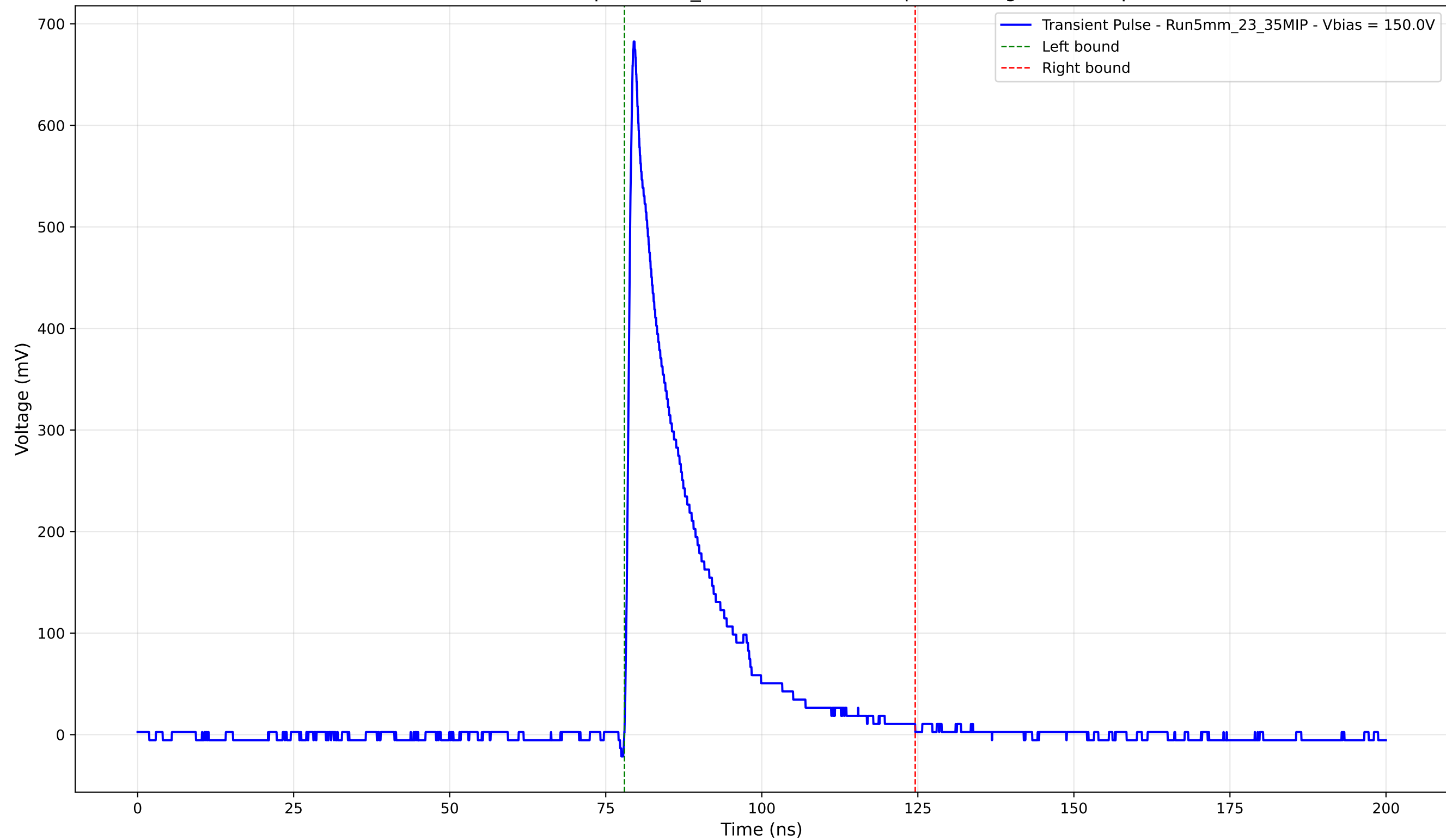
Transient Pulse - Sample: 5mm_23 - Position: 850.0 \mu\text{m} - Charge: 122.75 pC
