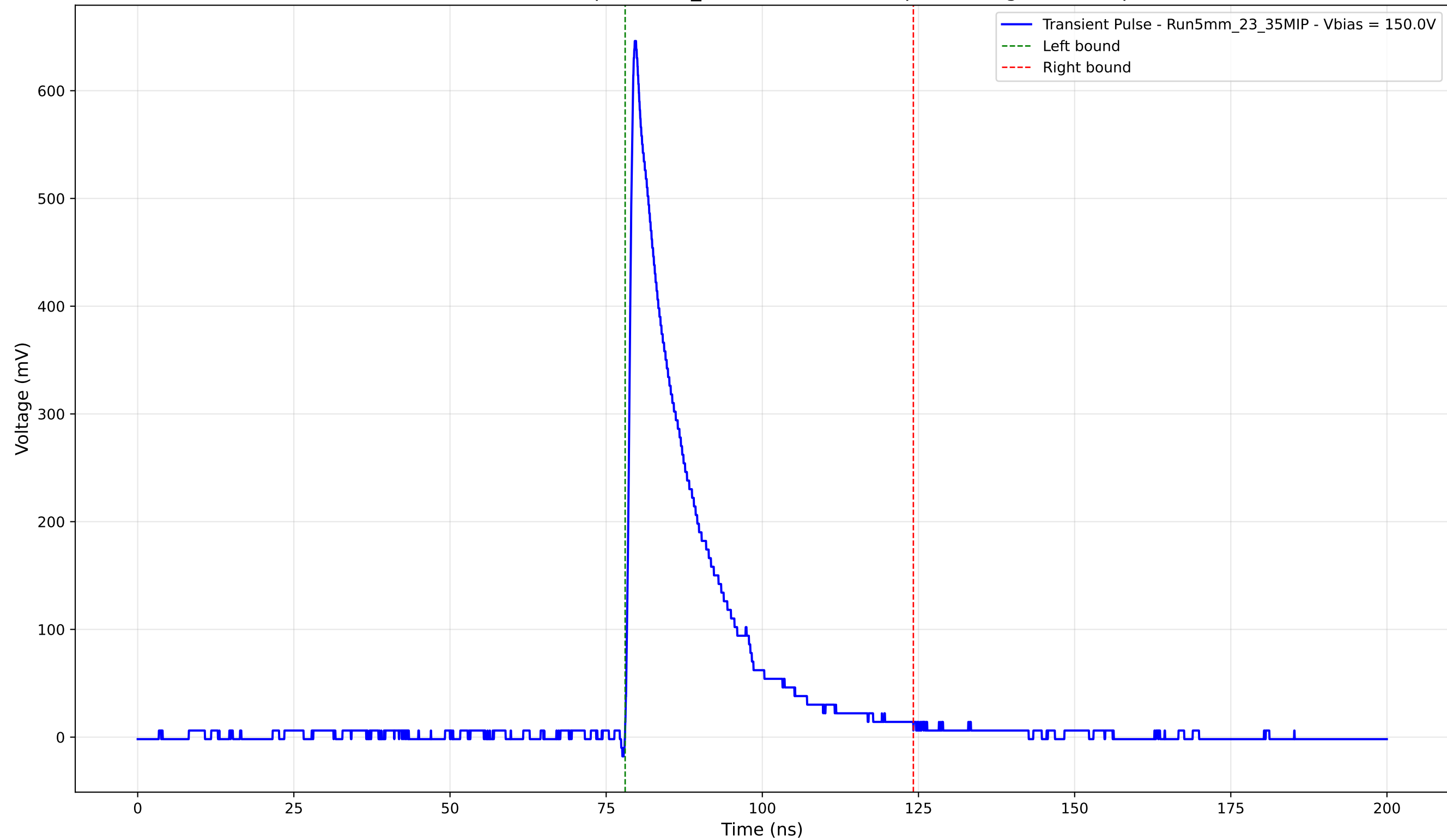
Transient Pulse - Sample: 5mm_23 - Position: 990.0 \mu\text{m} - Charge: 125.62 pC
