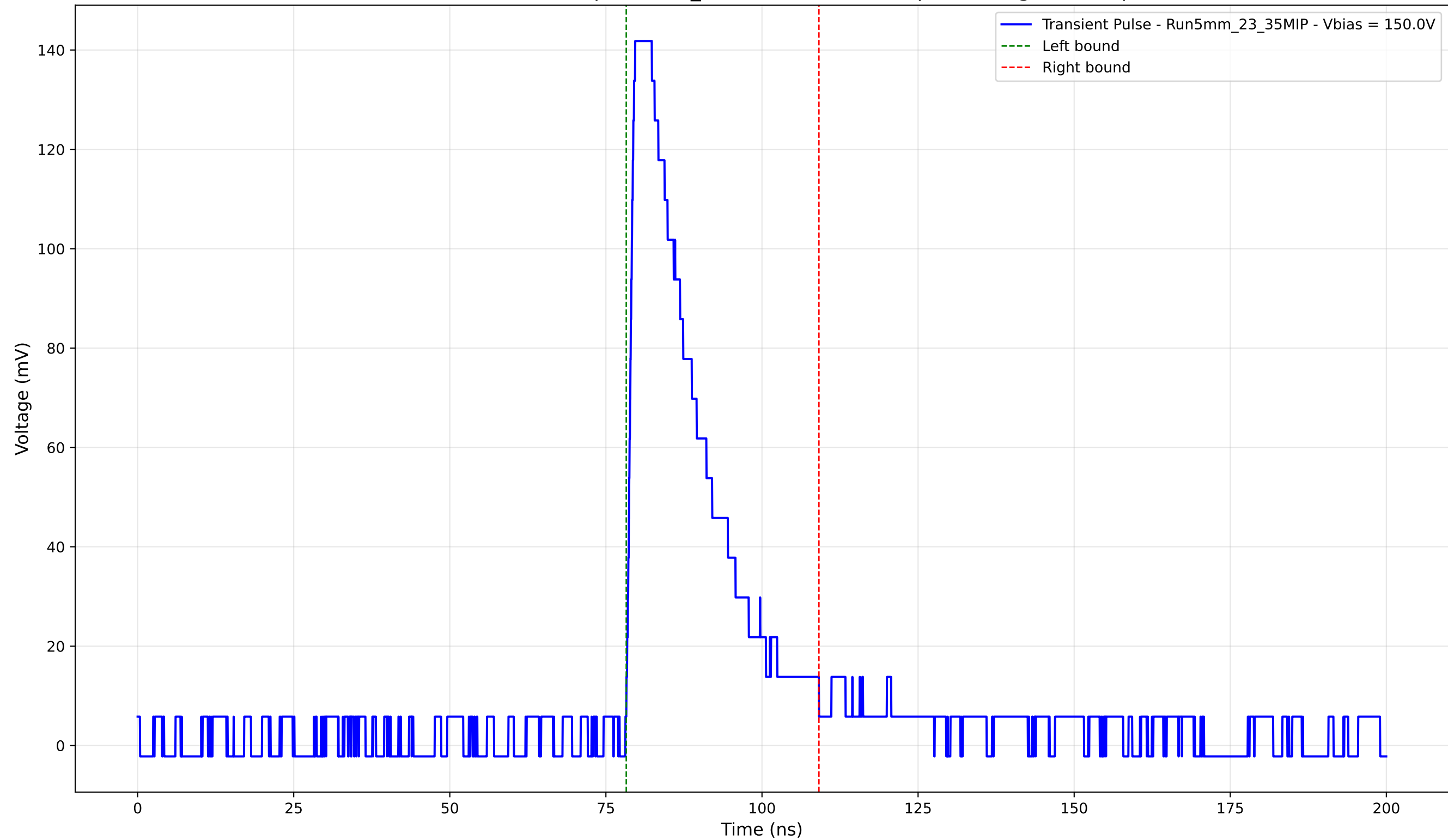
Transient Pulse - Sample: 5mm_23 - Position: 1645.0 \mu\text{m} - Charge: 35.03 pC
