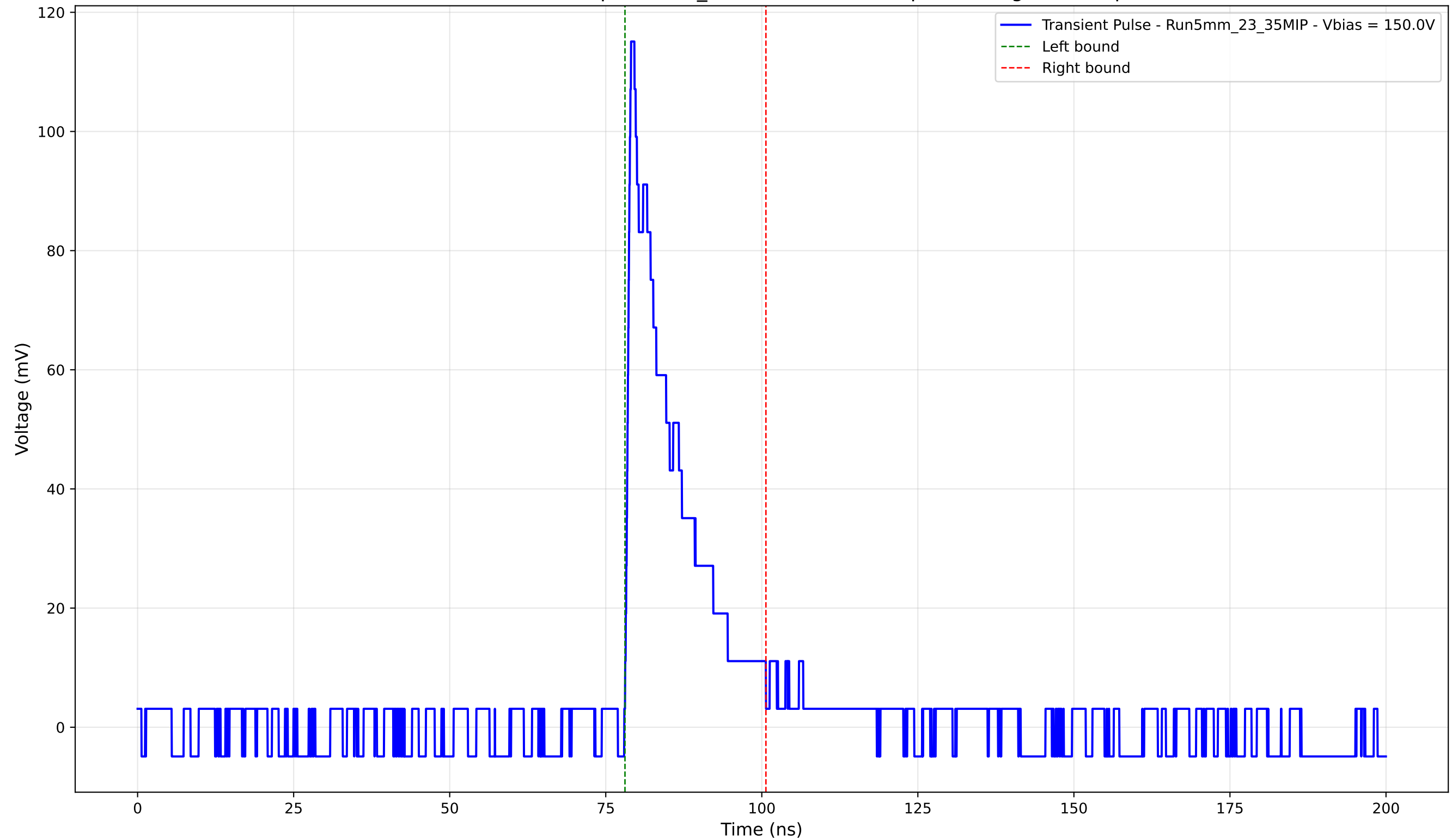
Transient Pulse - Sample: 5mm_23 - Position: 620.0 \mu\text{m} - Charge: 17.88 pC
