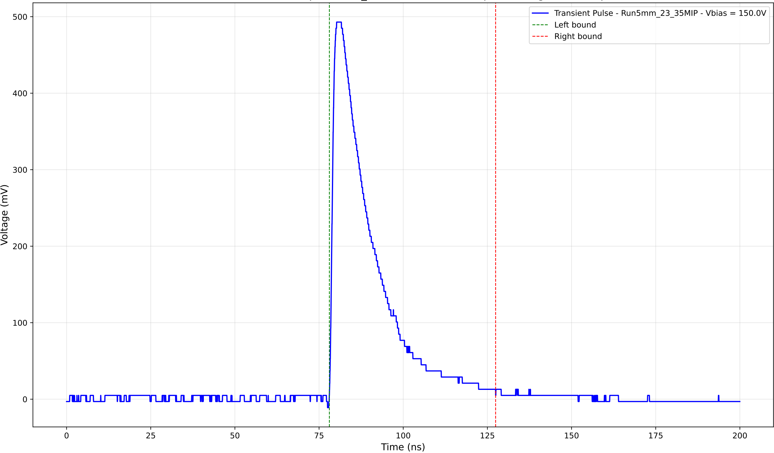
Transient Pulse - Sample: 5mm_23 - Position: 3255.0 \mu\text{m} - Charge: 130.15 pC
