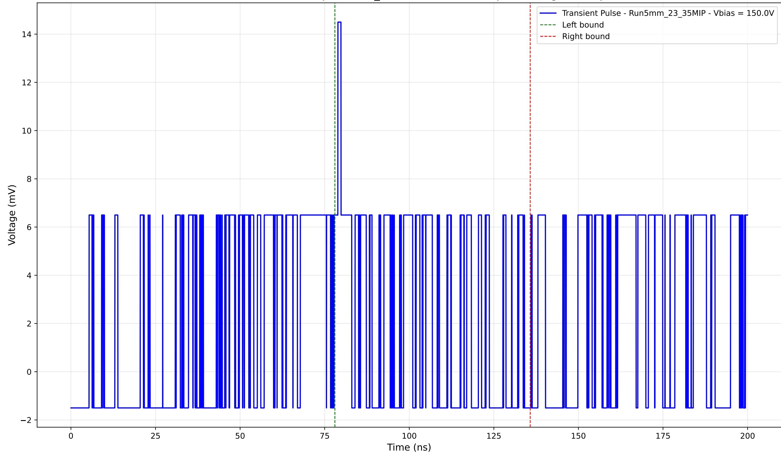
Transient Pulse - Sample: 5mm_23 - Position: 5235.0 \mu\text{m} - Charge: 2.68 pC
