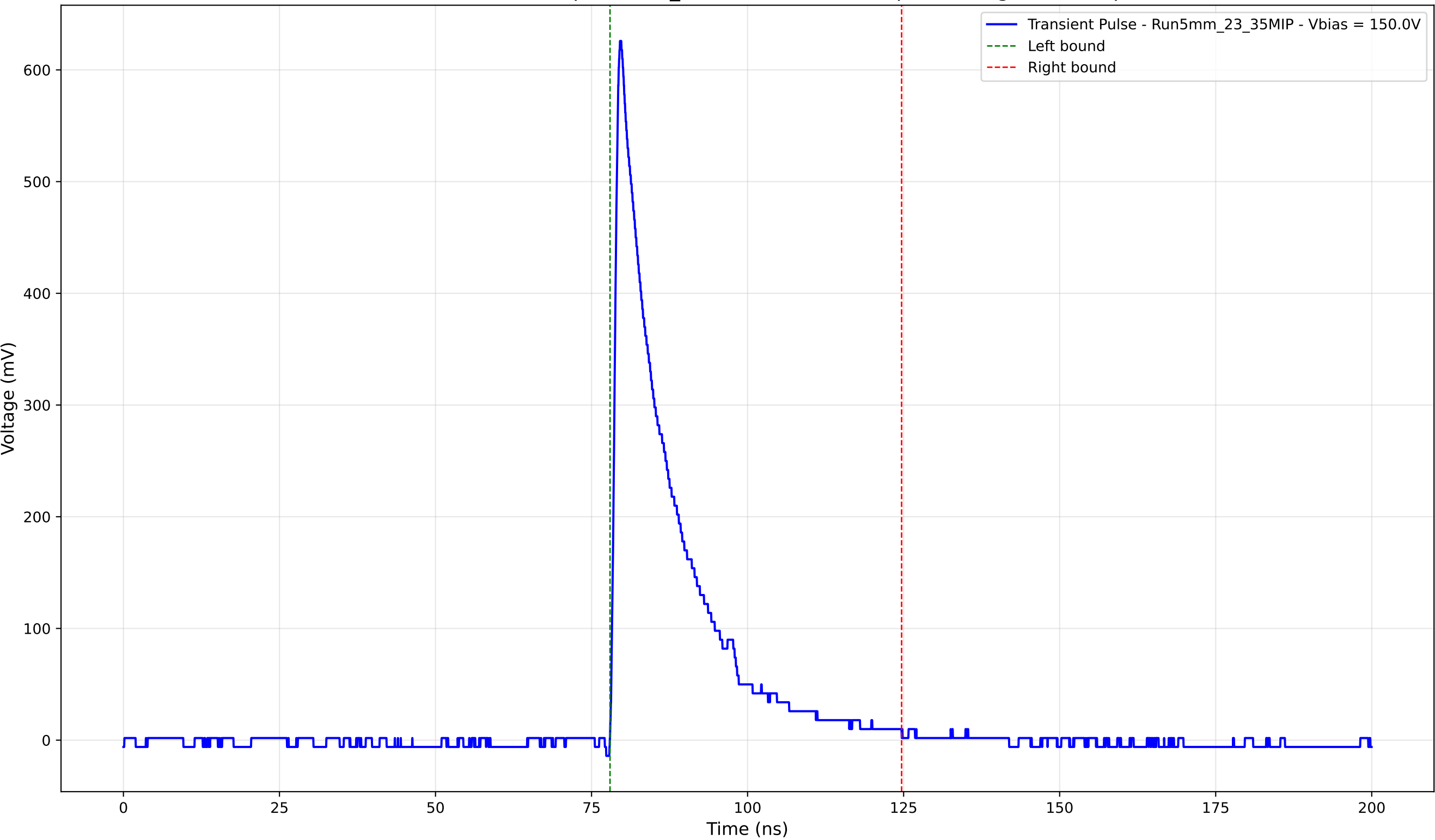
Transient Pulse - Sample: 5mm_23 - Position: 4280.0 \mu\text{m} - Charge: 115.45 pC
