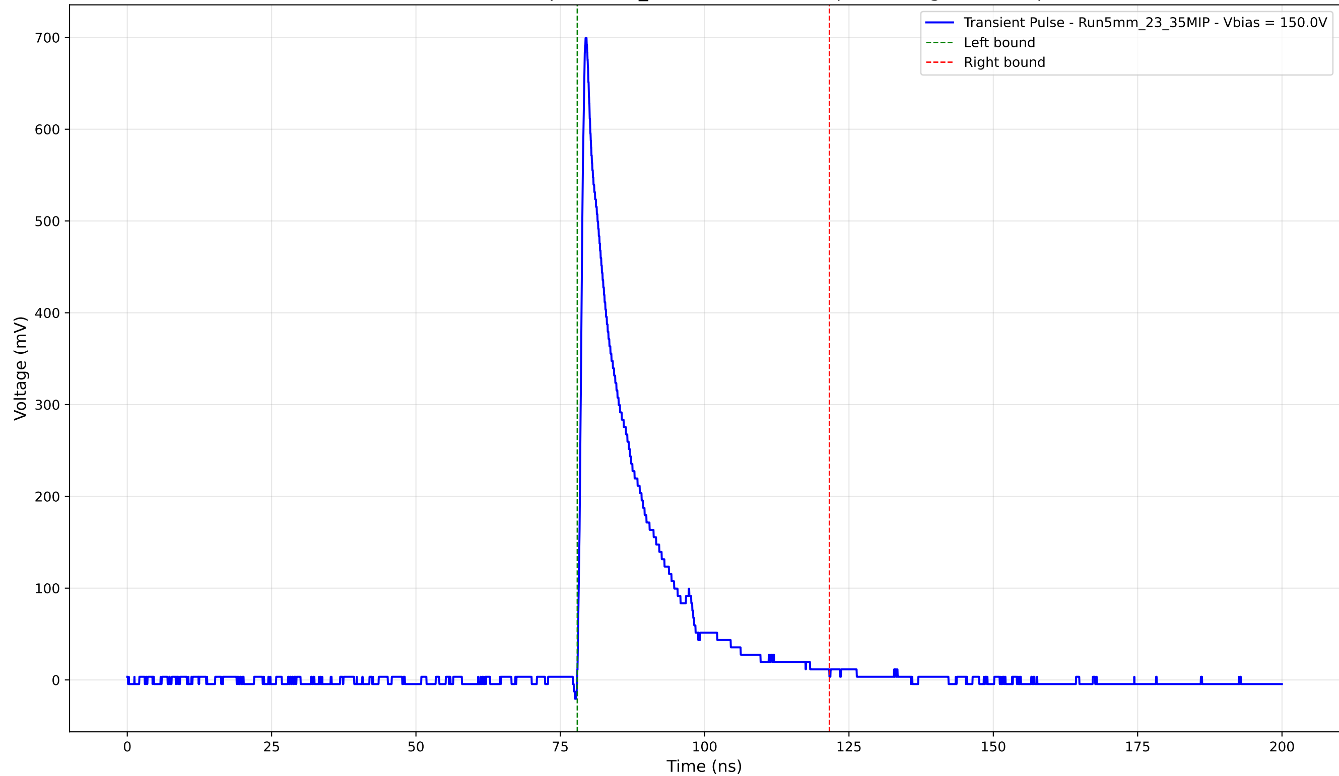
Transient Pulse - Sample: 5mm_23 - Position: 755.0 \mu\text{m} - Charge: 119.48 pC
