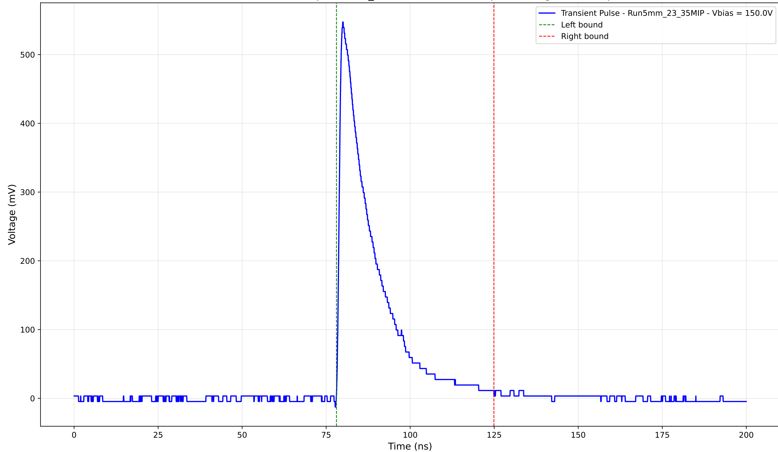
Transient Pulse - Sample: 5mm_23 - Position: 3855.0 \mu\text{m} - Charge: 120.58 pC
