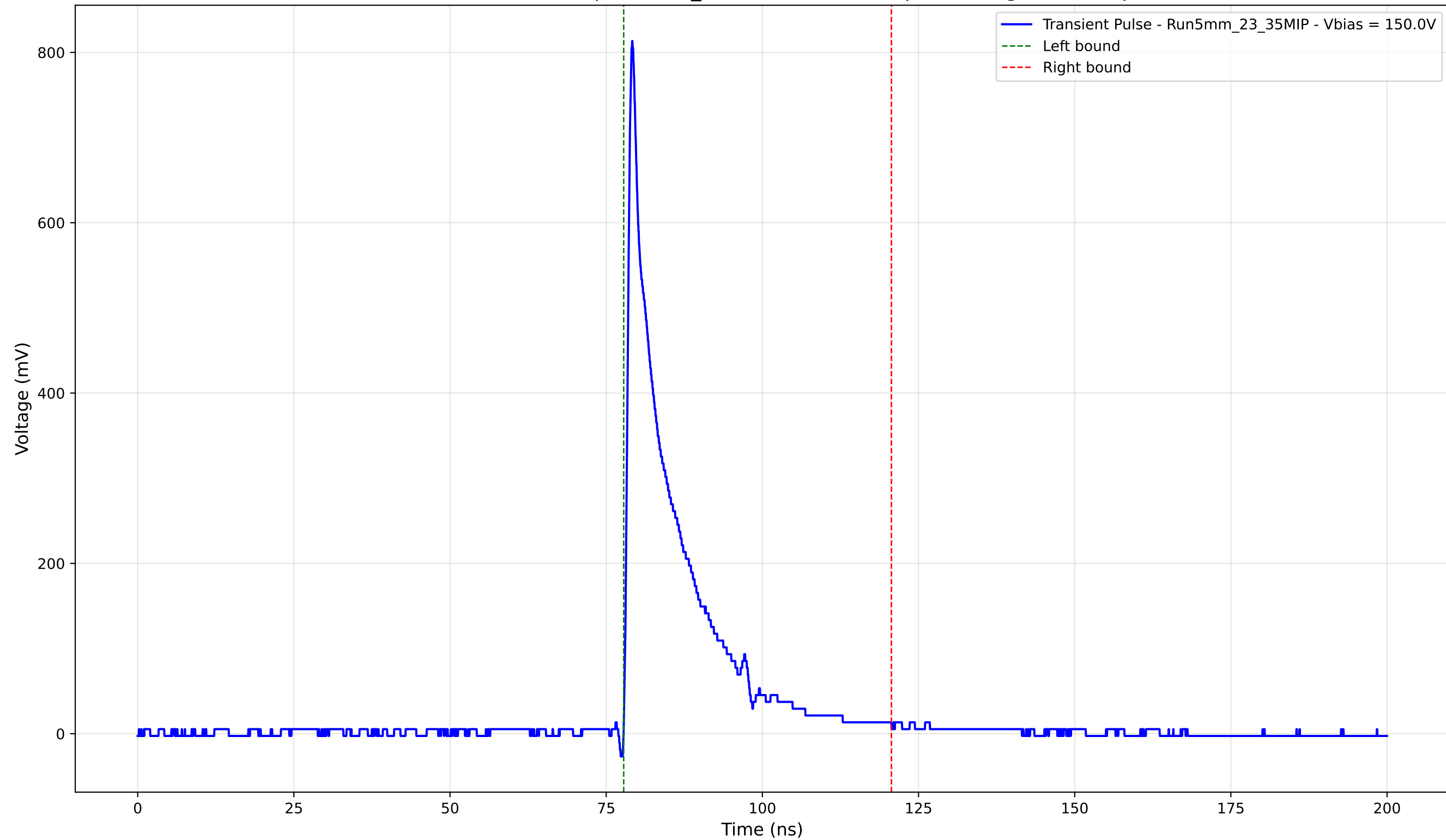
Transient Pulse - Sample: 5mm_23 - Position: 450.0 \mu\text{m} - Charge: 115.88 pC
