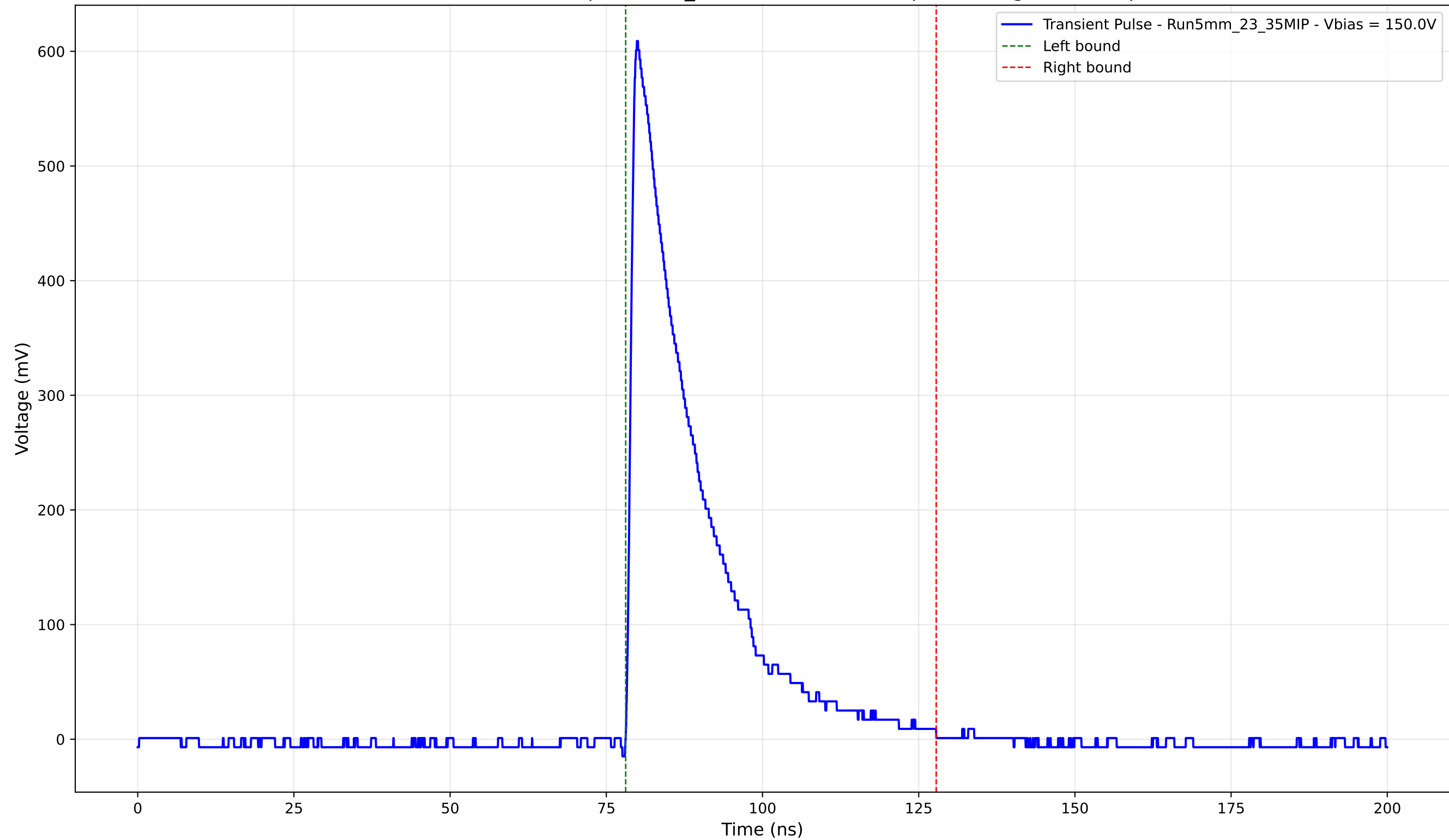
Transient Pulse - Sample: 5mm_23 - Position: 1380.0 \mu\text{m} - Charge: 137.43 pC
