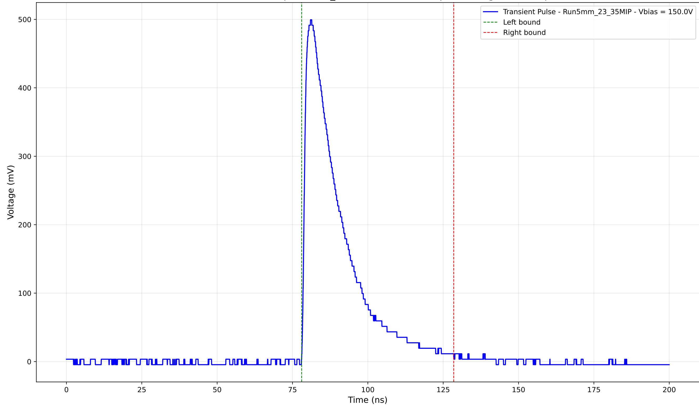
Transient Pulse - Sample: 5mm_23 - Position: 2245.0 \mu\text{m} - Charge: 133.95 pC
