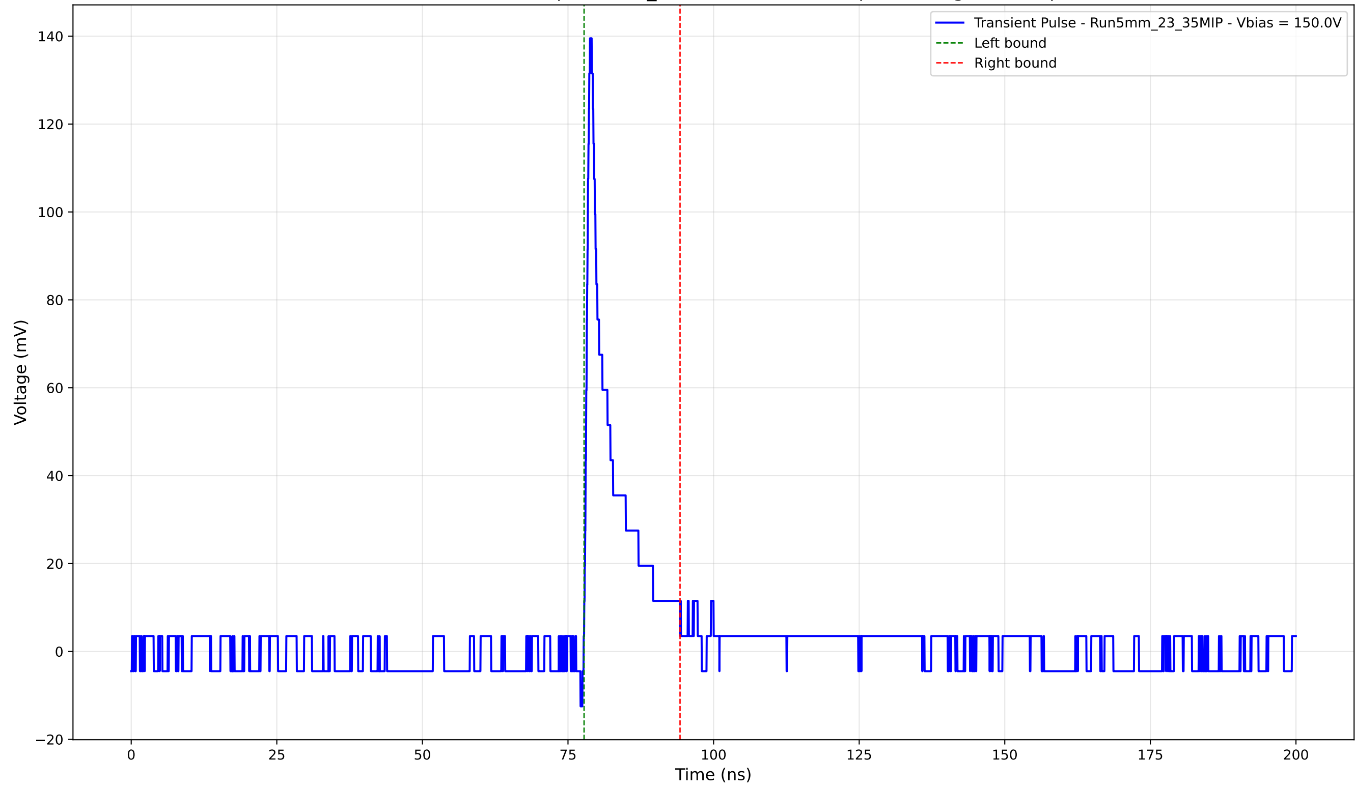
Transient Pulse - Sample: 5mm_23 -Position: 5100.0 \mu\text{m} - Charge: 12.37 pC
