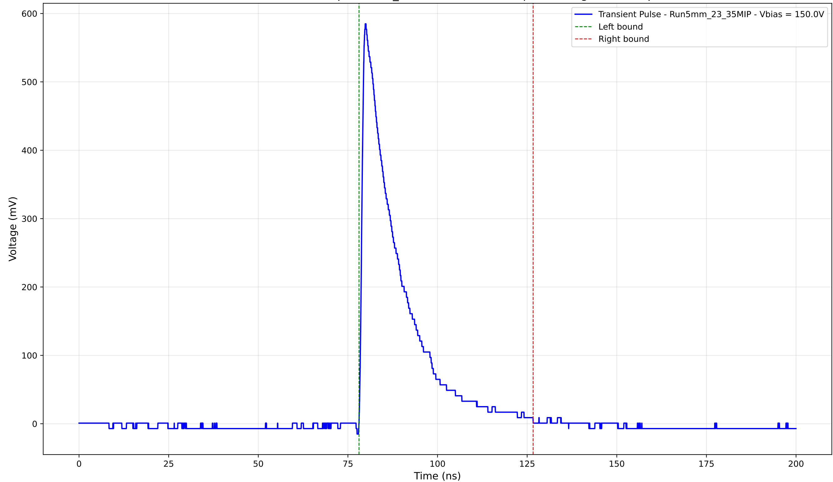
Transient Pulse - Sample: 5mm_23 - Position: 1325.0 \mu\text{m} - Charge: 129.23 pC
