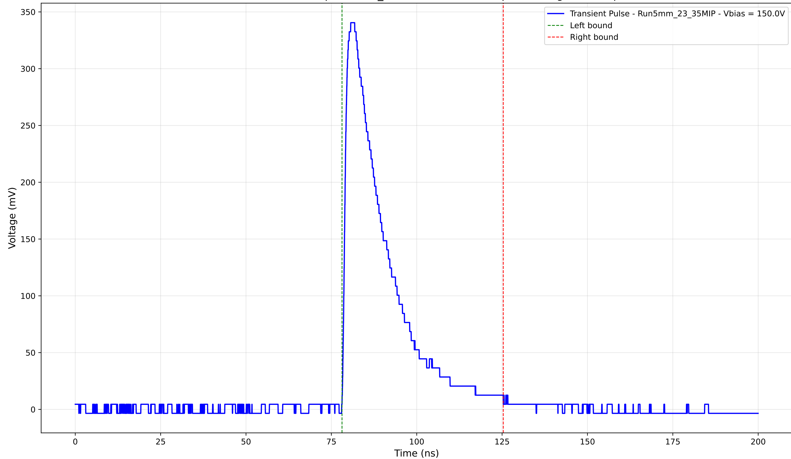
Transient Pulse - Sample: 5mm_23 - Position: 2195.0 \mu\text{m} - Charge: 90.90 pC
