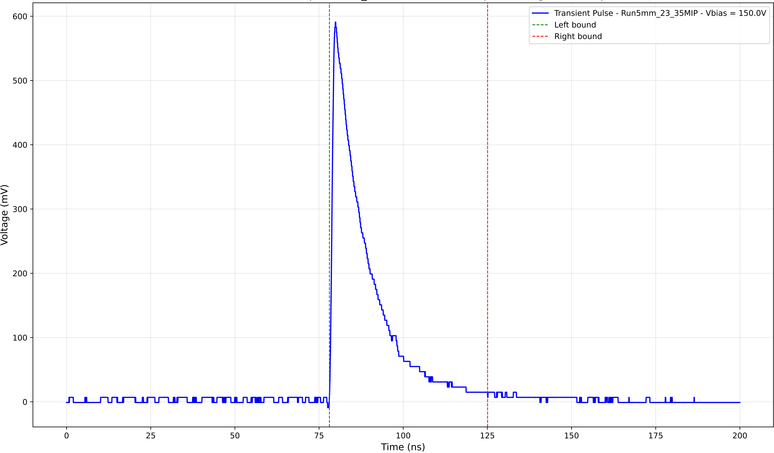
Transient Pulse - Sample: 5mm_23 - Position: 1280.0 \mu\text{m} - Charge: 129.82 pC
