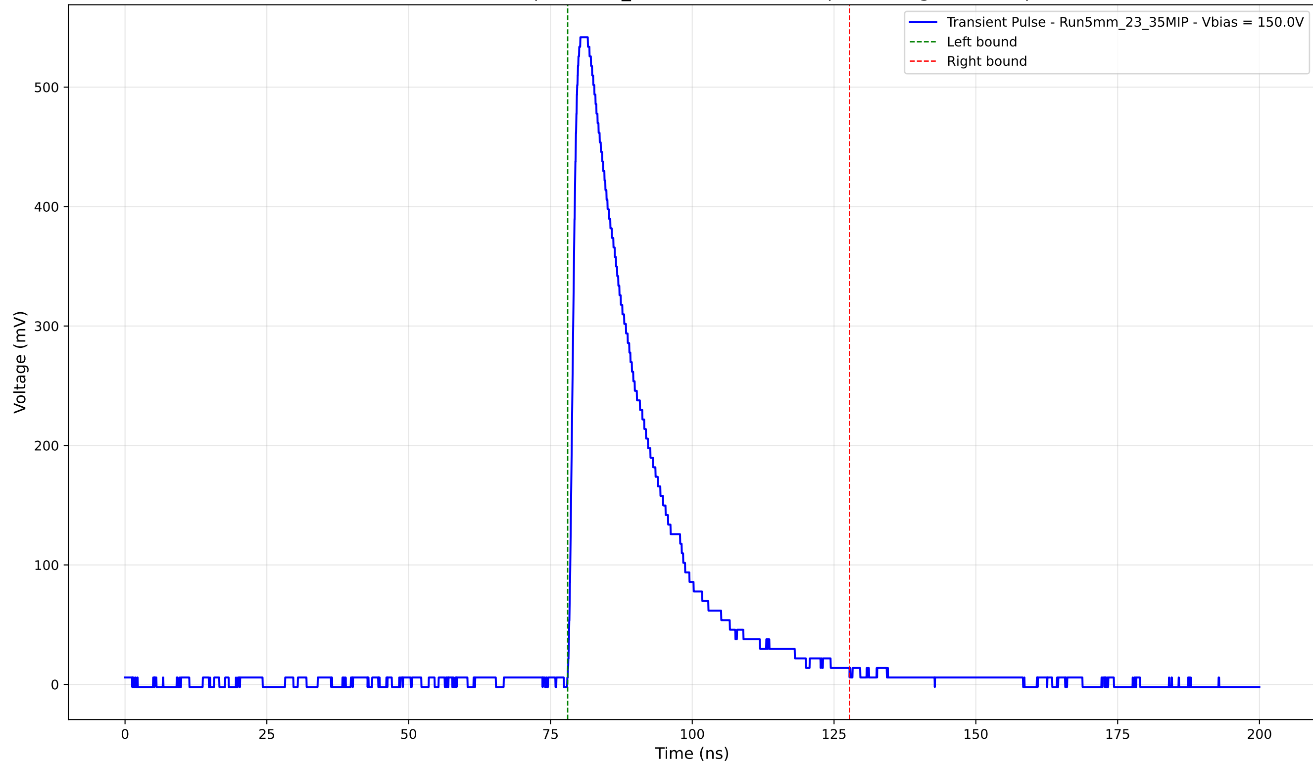
Transient Pulse - Sample: 5mm_23 - Position: 1970.0 \mu\text{m} - Charge: 144.82 pC
