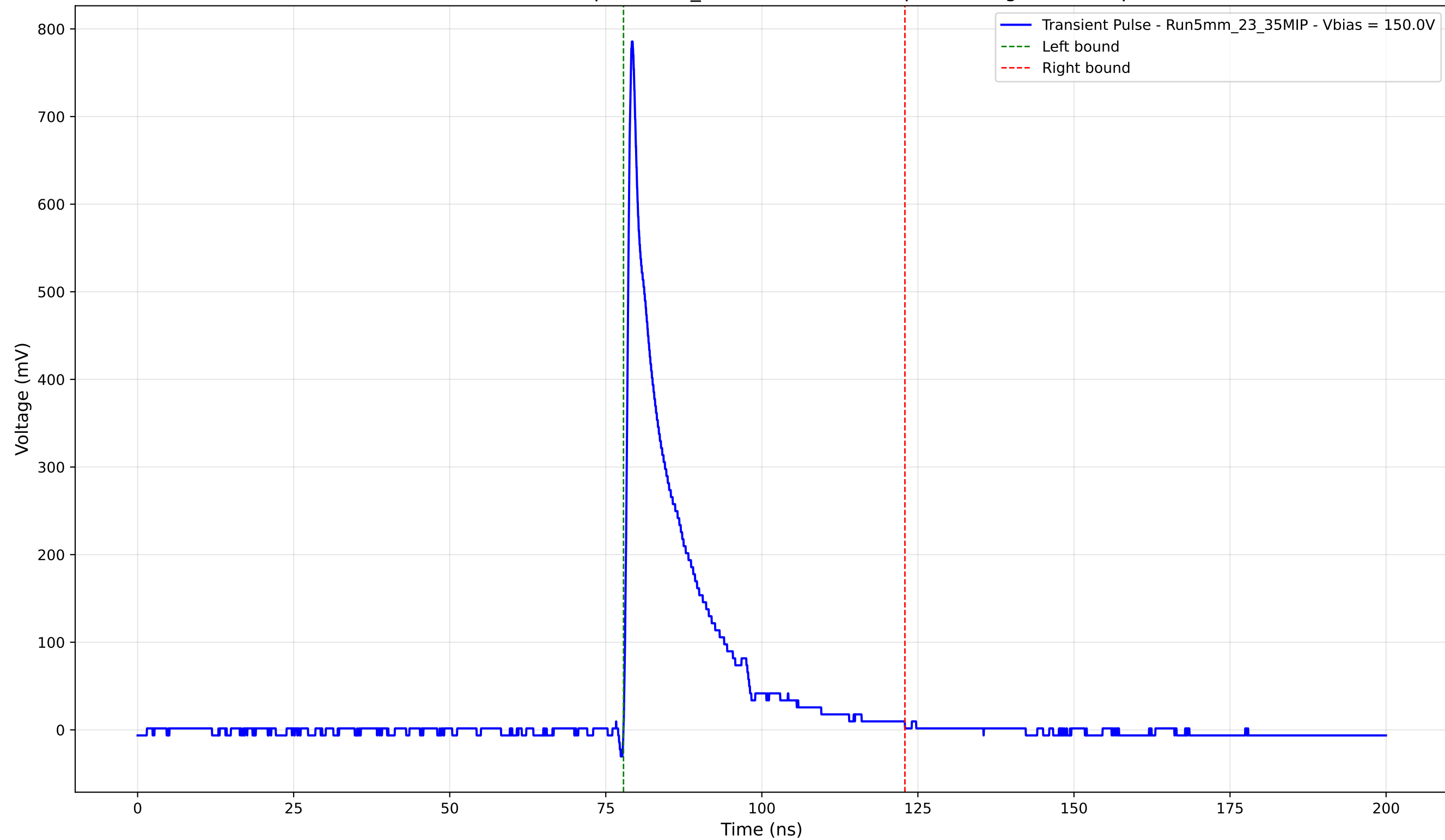
Transient Pulse - Sample: 5mm_23 - Position: 505.0 \mu\text{m} - Charge: 114.10 pC
