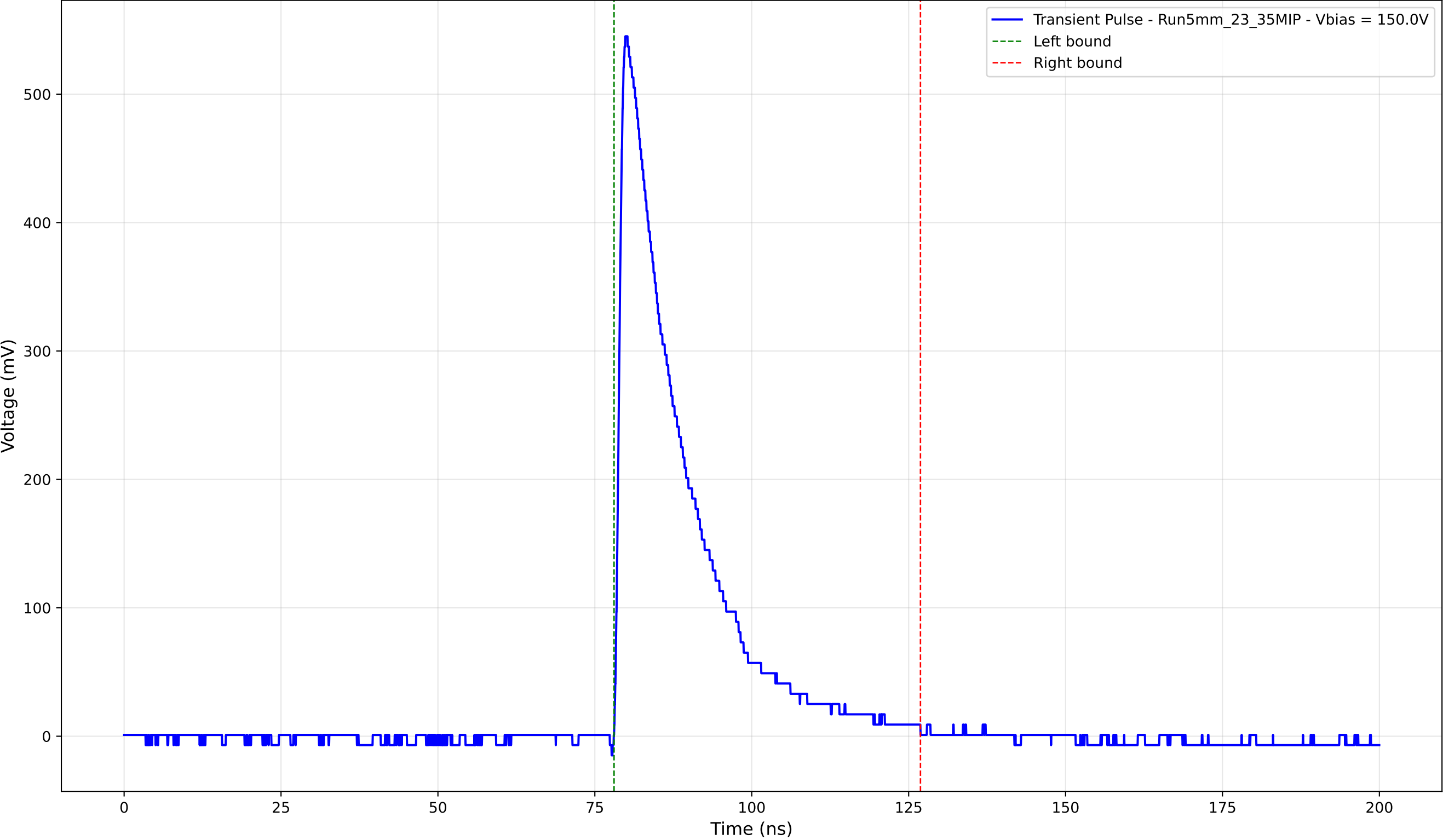
Transient Pulse - Sample: 5mm_23 - Position: 3845.0 \mu\text{m} - Charge: 120.62 pC
