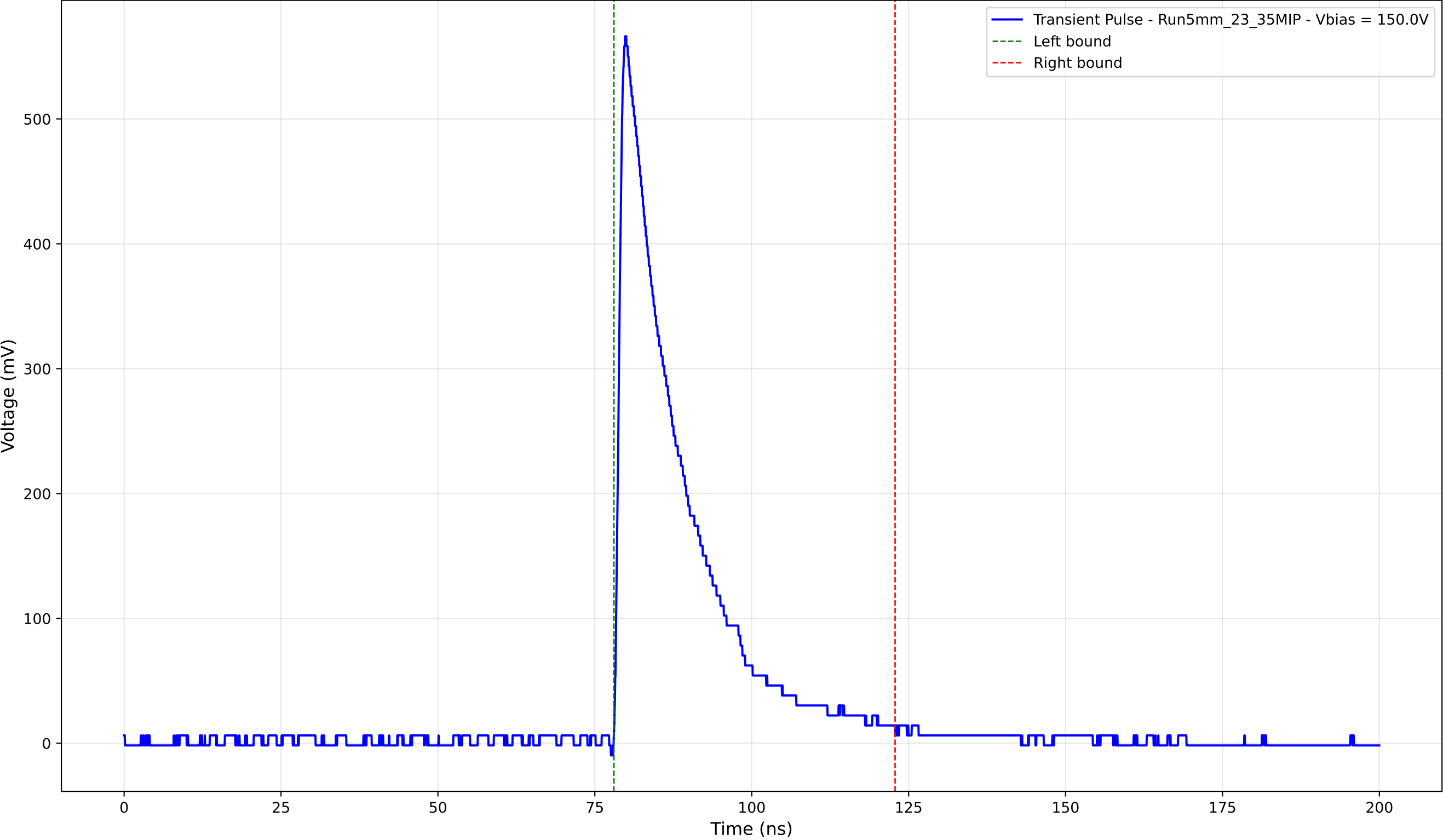
Transient Pulse - Sample: 5mm_23 - Position: 3980.0 \mu\text{m} - Charge: 120.96 pC
