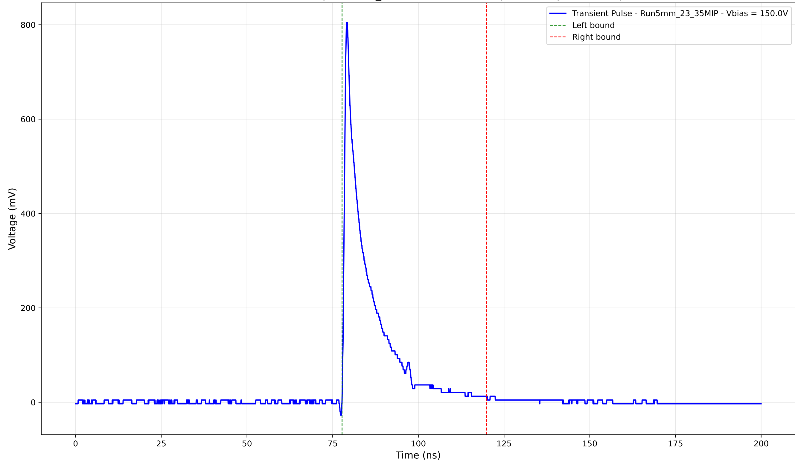
Transient Pulse - Sample: 5mm_23 - Position: 4795.0 \mu\text{m} - Charge: 113.06 pC
