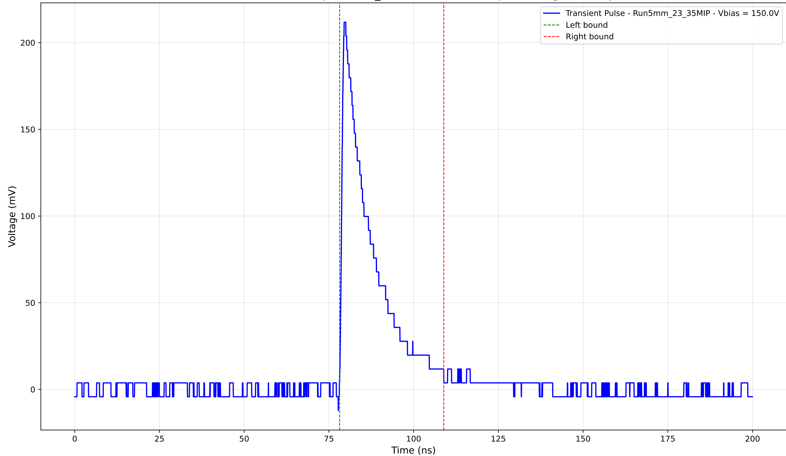
Transient Pulse - Sample: 5mm_23 - Position: 1095.0 \mu\text{m} - Charge: 39.57 pC
