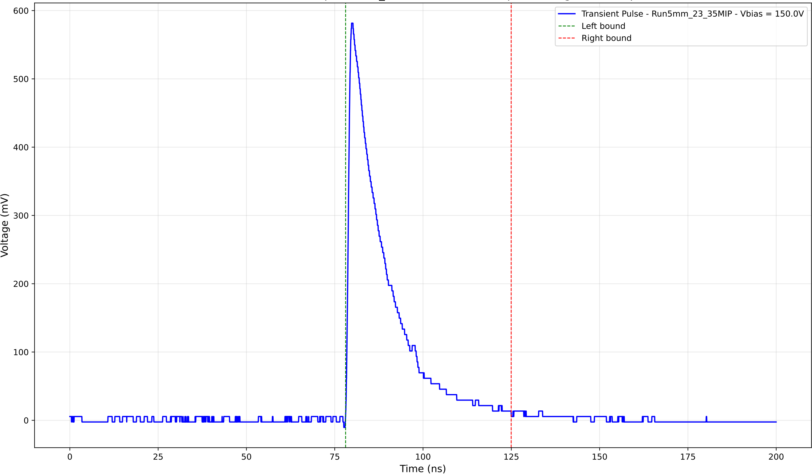
Transient Pulse - Sample: 5mm_23 - Position: 1310.0 \mu\text{m} - Charge: 130.45 pC
