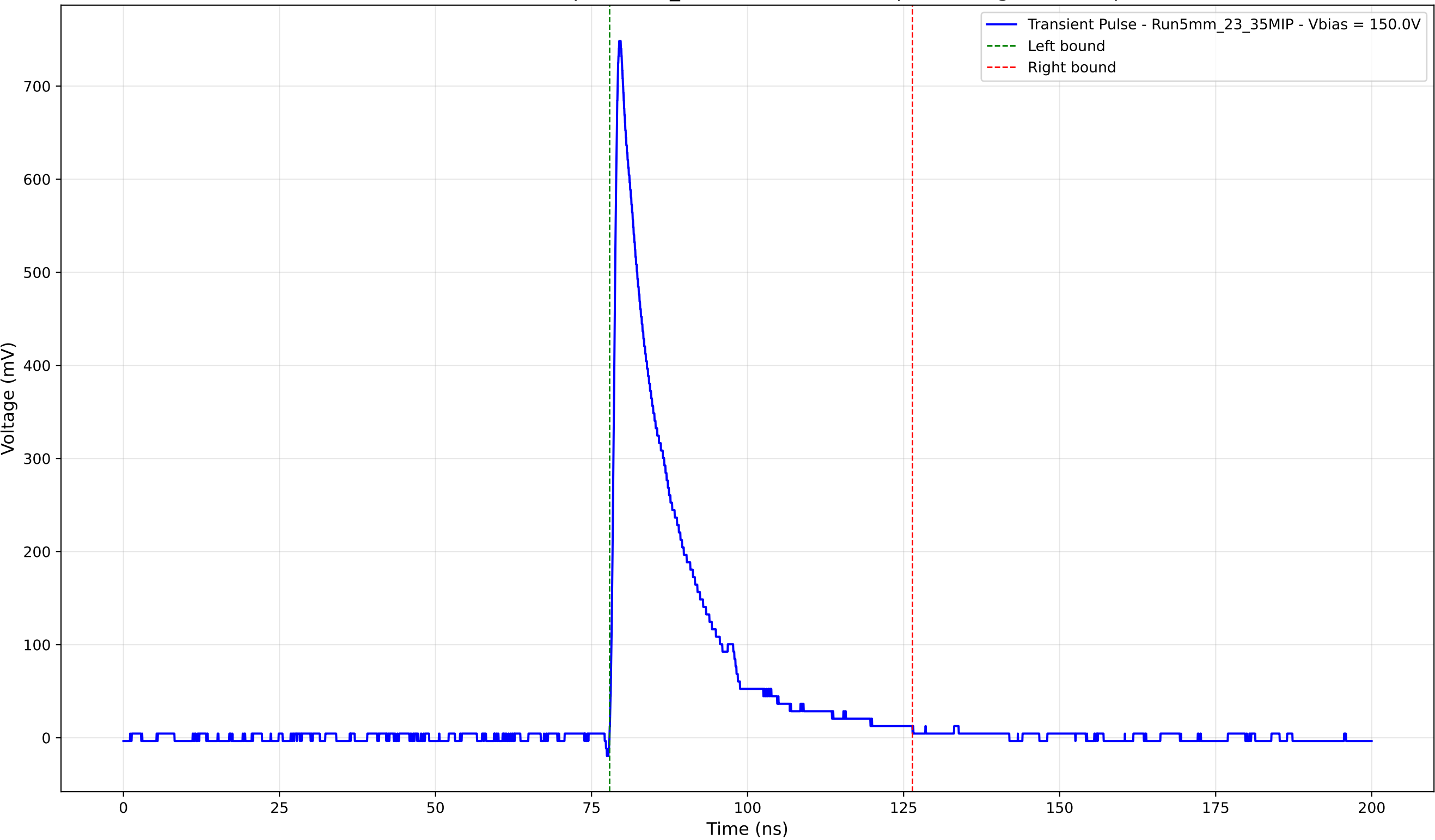
Transient Pulse - Sample: 5mm_23 - Position: 4420.0 \mu\text{m} - Charge: 134.99 pC
