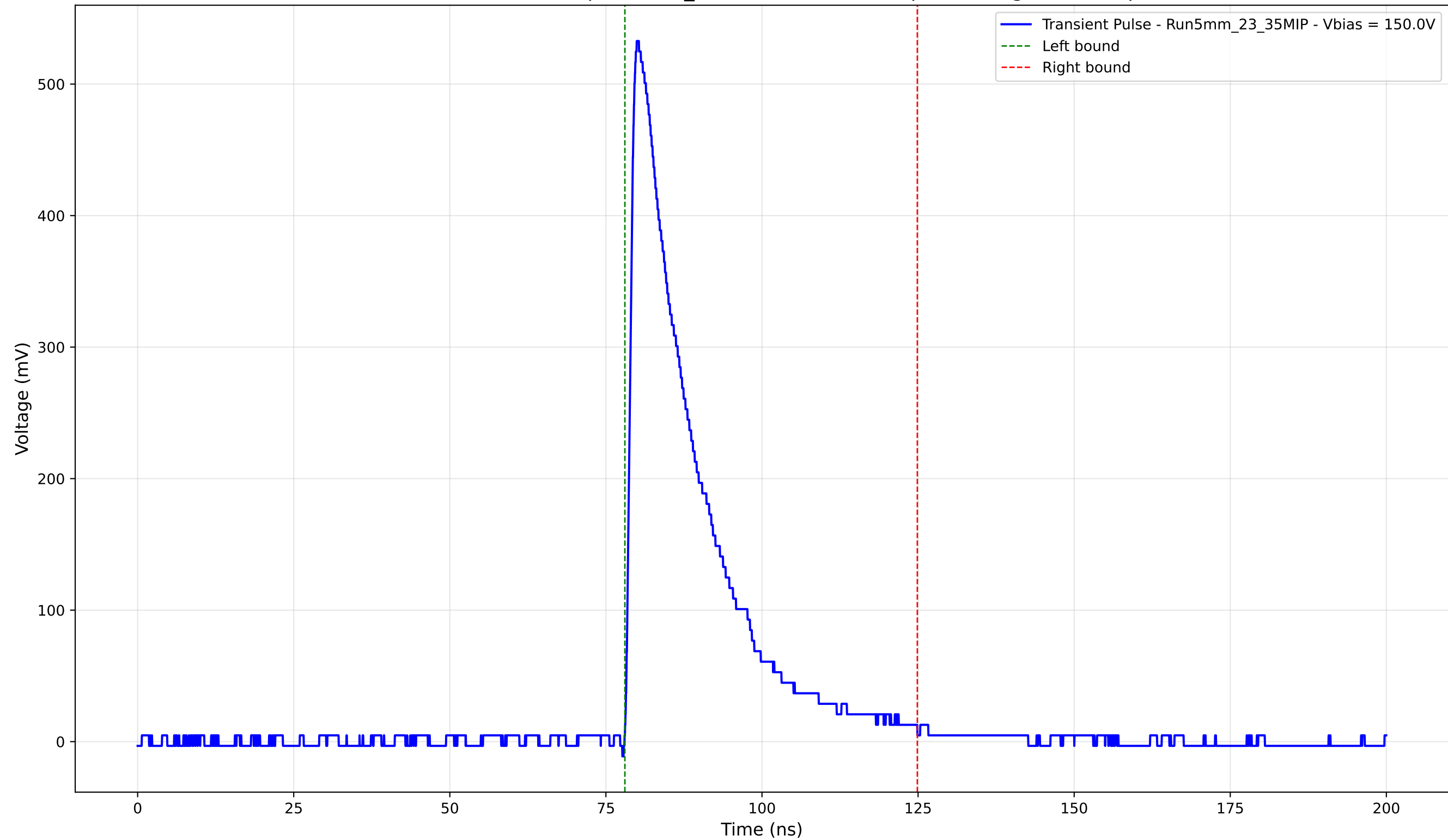
Transient Pulse - Sample: 5mm_23 - Position: 3755.0 \mu\text{m} - Charge: 122.58 pC
