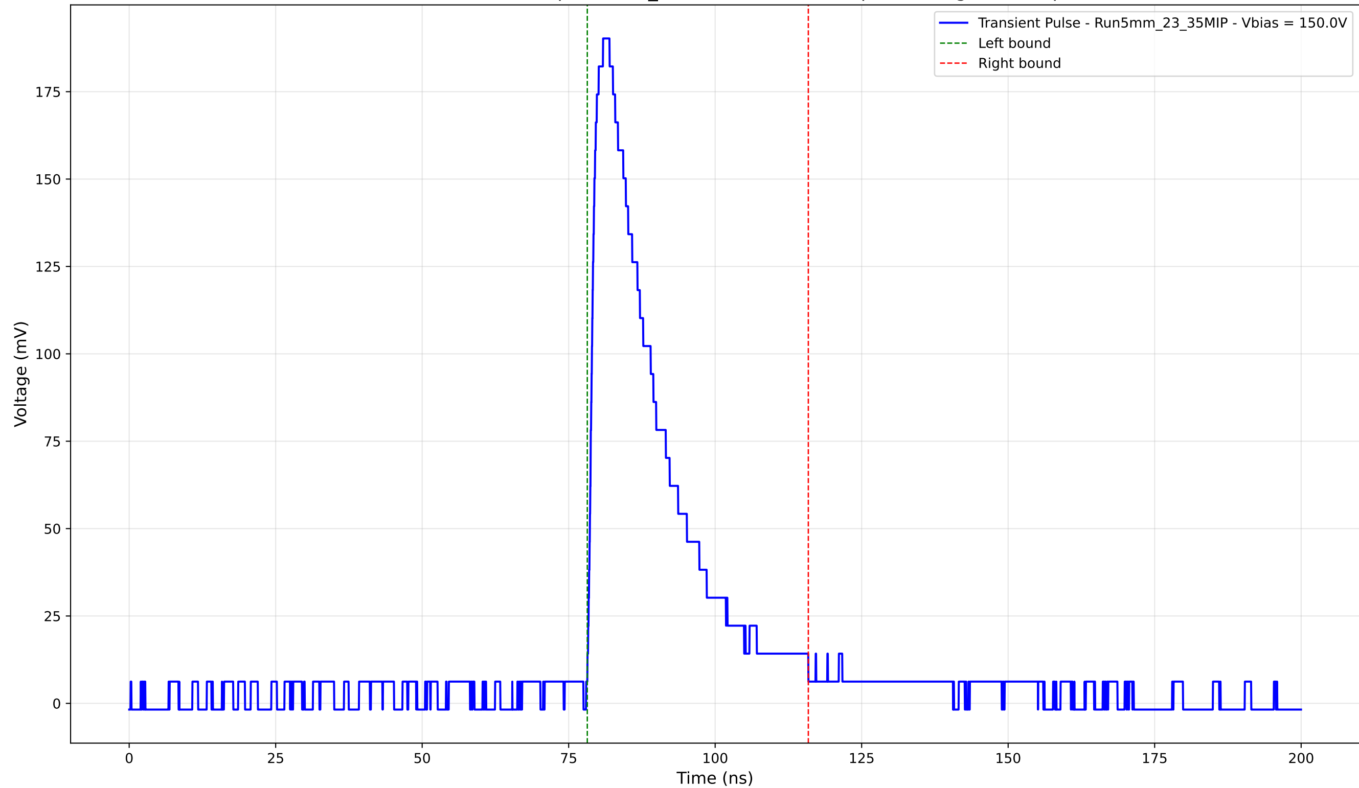
Transient Pulse - Sample: 5mm_23 - Position: 3115.0 \mu\text{m} - Charge: 48.75 pC
