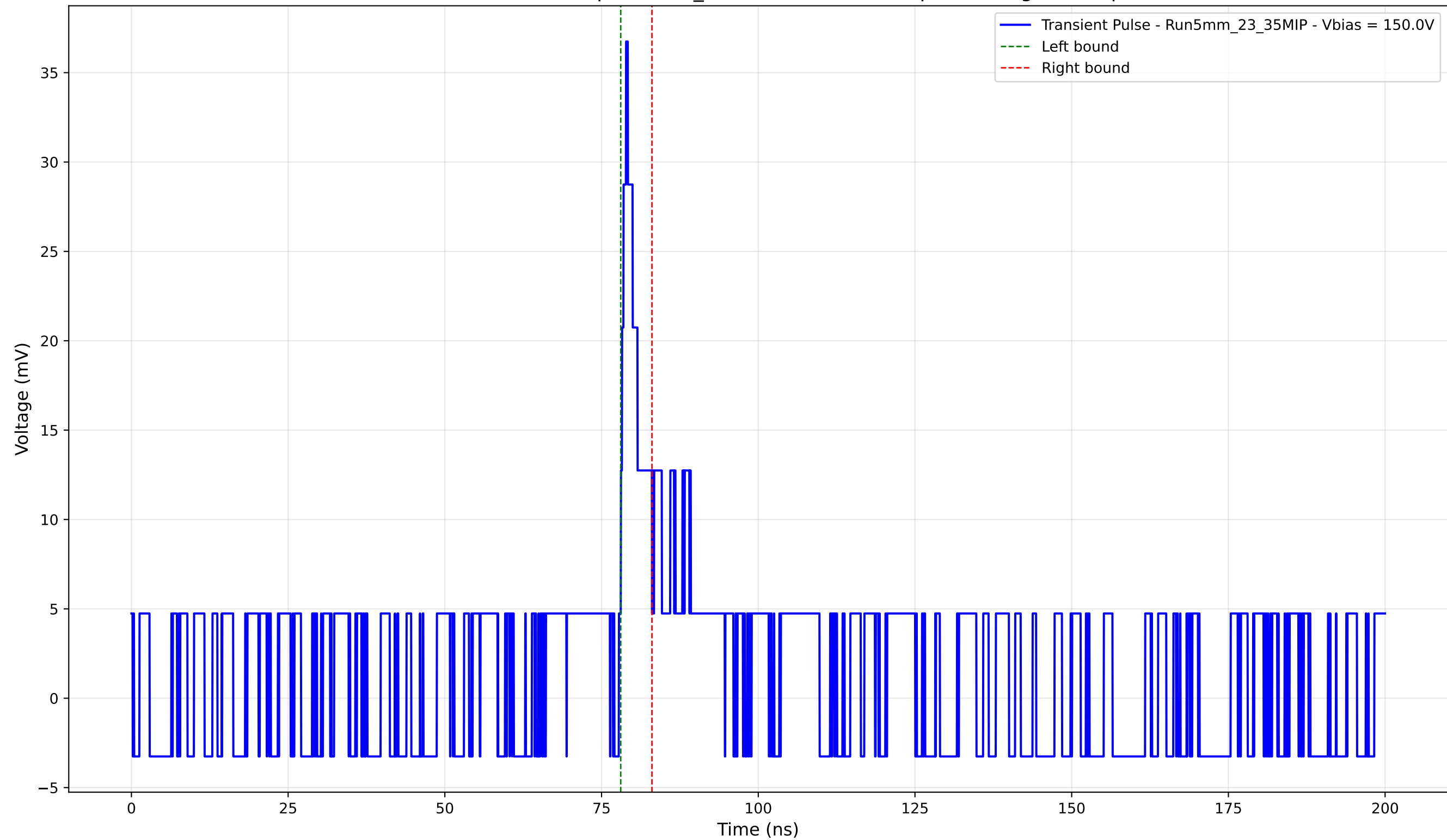
Transient Pulse - Sample: 5mm_23 - Position: 5145.0 \mu\text{m} - Charge: 1.94 pC
