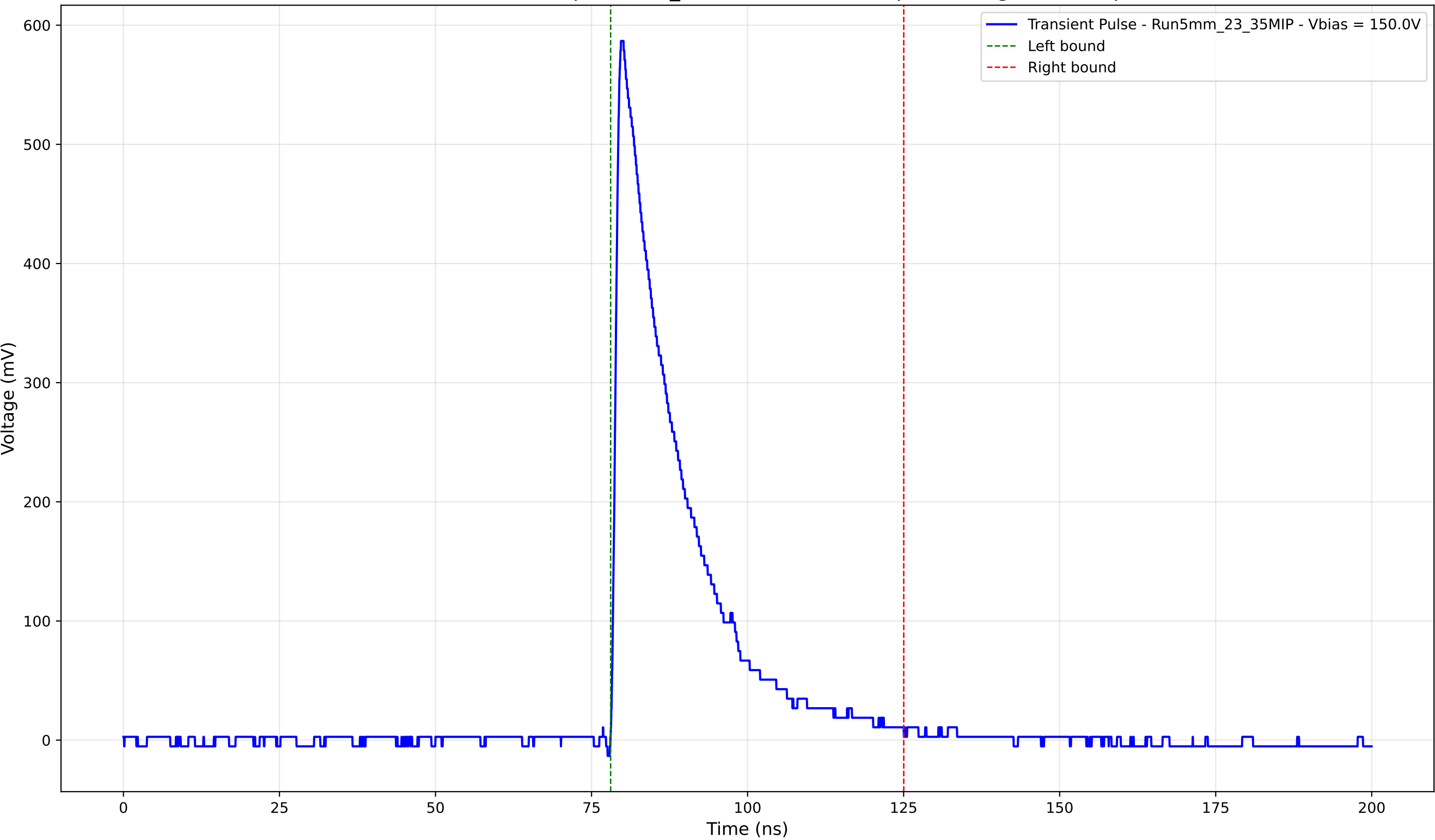
Transient Pulse - Sample: 5mm_23 - Position: 1275.0 \mu\text{m} - Charge: 127.89 pC
