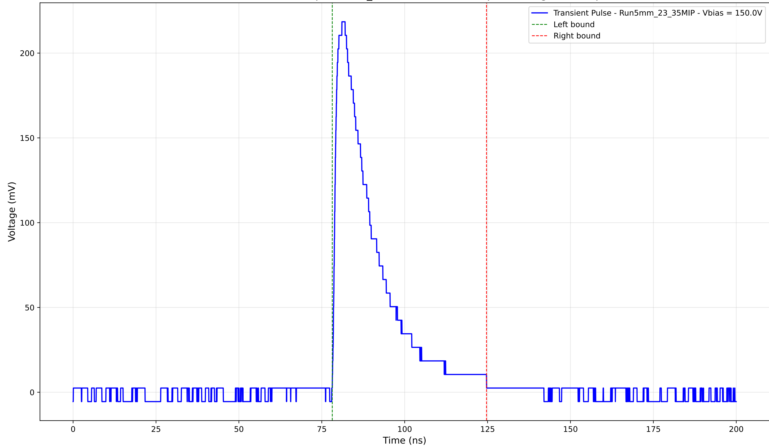
Transient Pulse - Sample: 5mm_23 - Position: 2175.0 \mu\text{m} - Charge: 57.72 pC
