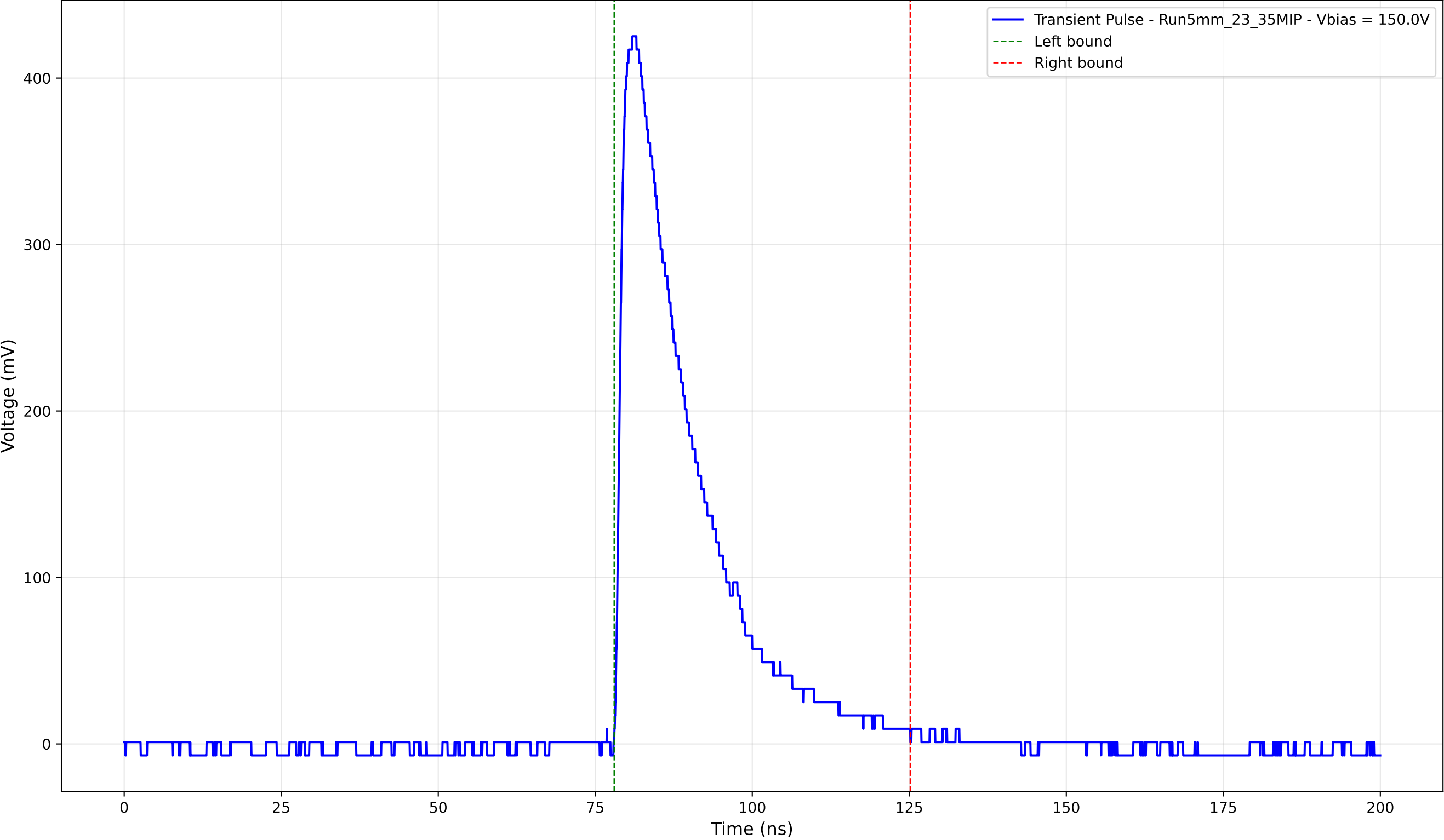
Transient Pulse - Sample: 5mm_23 - Position: 3075.0 \mu\text{m} - Charge: 109.30 pC
