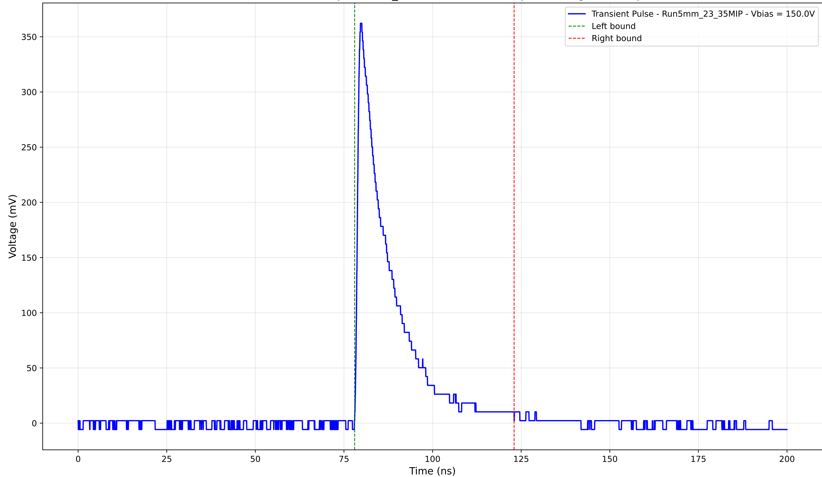
Transient Pulse - Sample: 5mm_23 - Position: 4105.0 \mu\text{m} - Charge: 71.26 pC
