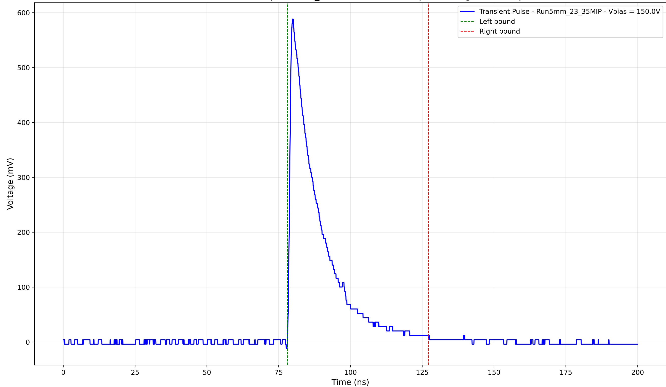
Transient Pulse - Sample: 5mm_23 - Position: 1255.0 \mu\text{m} - Charge: 128.41 pC
