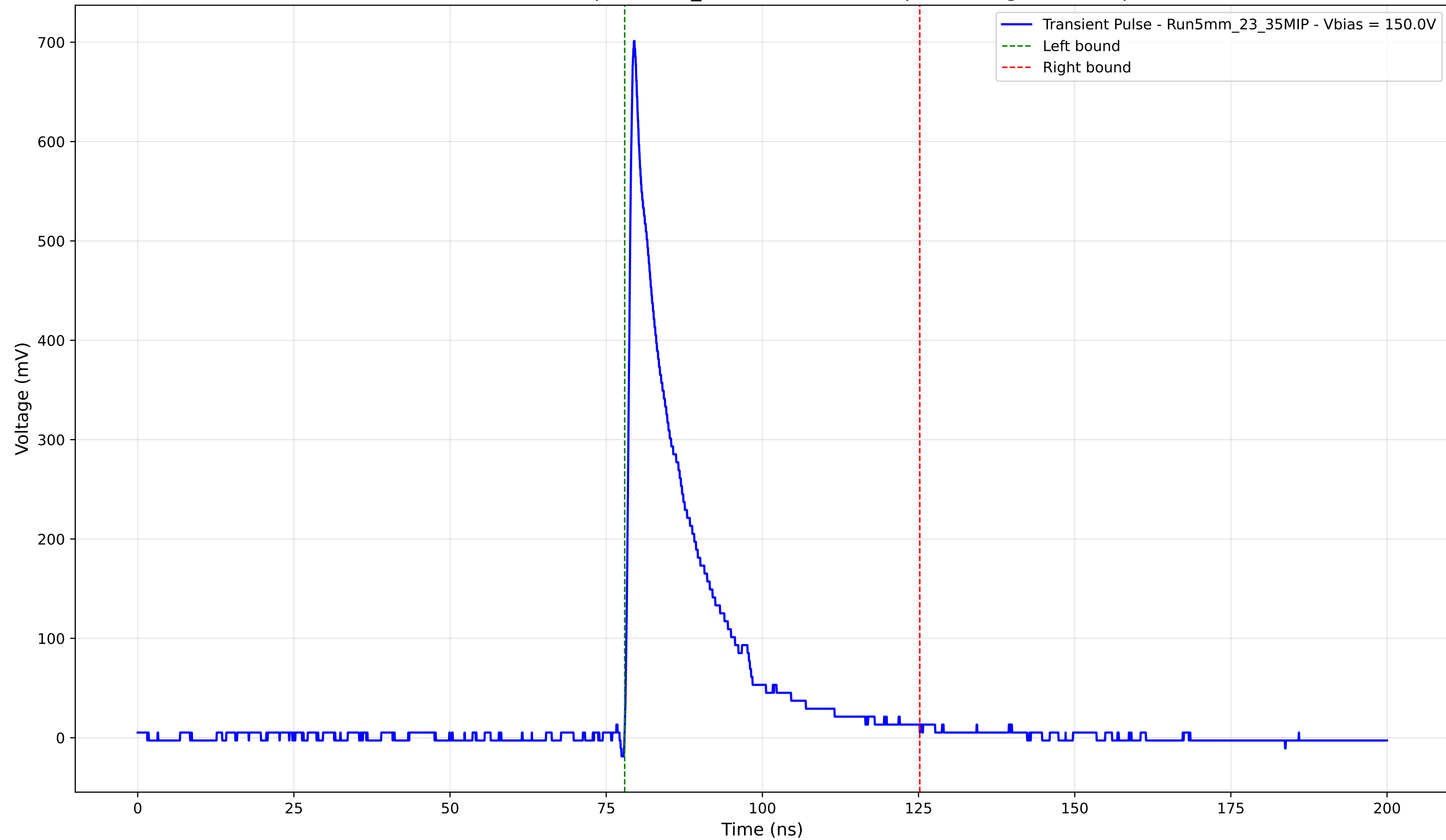
Transient Pulse - Sample: 5mm_23 - Position: 775.0 \mu\text{m} - Charge: 122.61 pC
