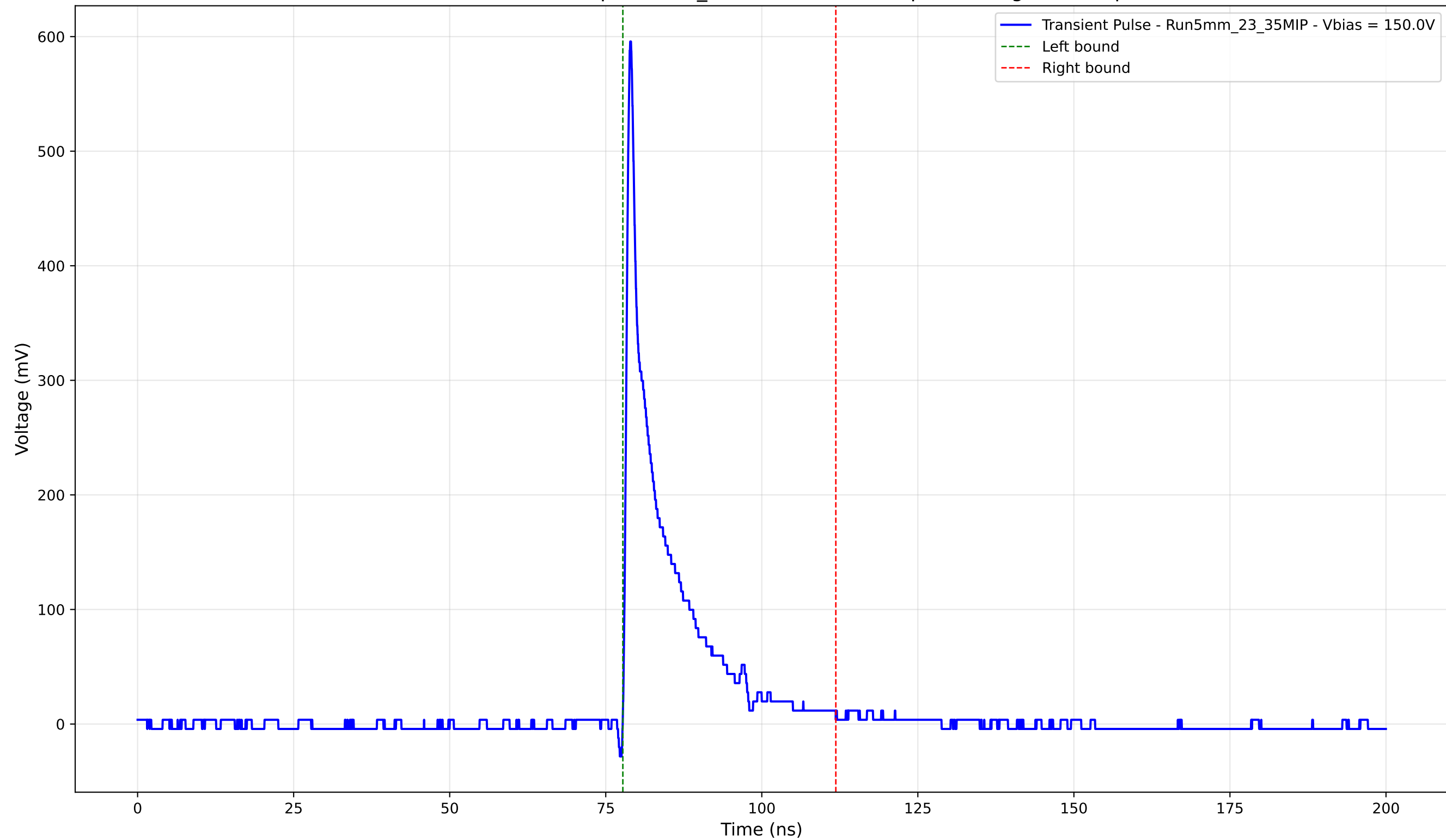
Transient Pulse - Sample: 5mm_23 - Position: 220.0 \mu\text{m} - Charge: 65.27 pC
