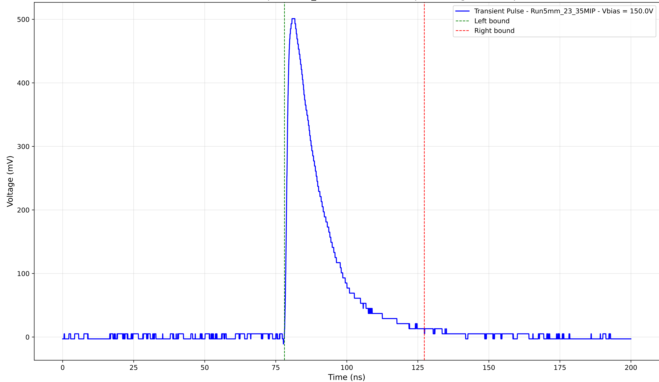
Transient Pulse - Sample: 5mm_23 - Position: 2255.0 \mu\text{m} - Charge: 136.21 pC
