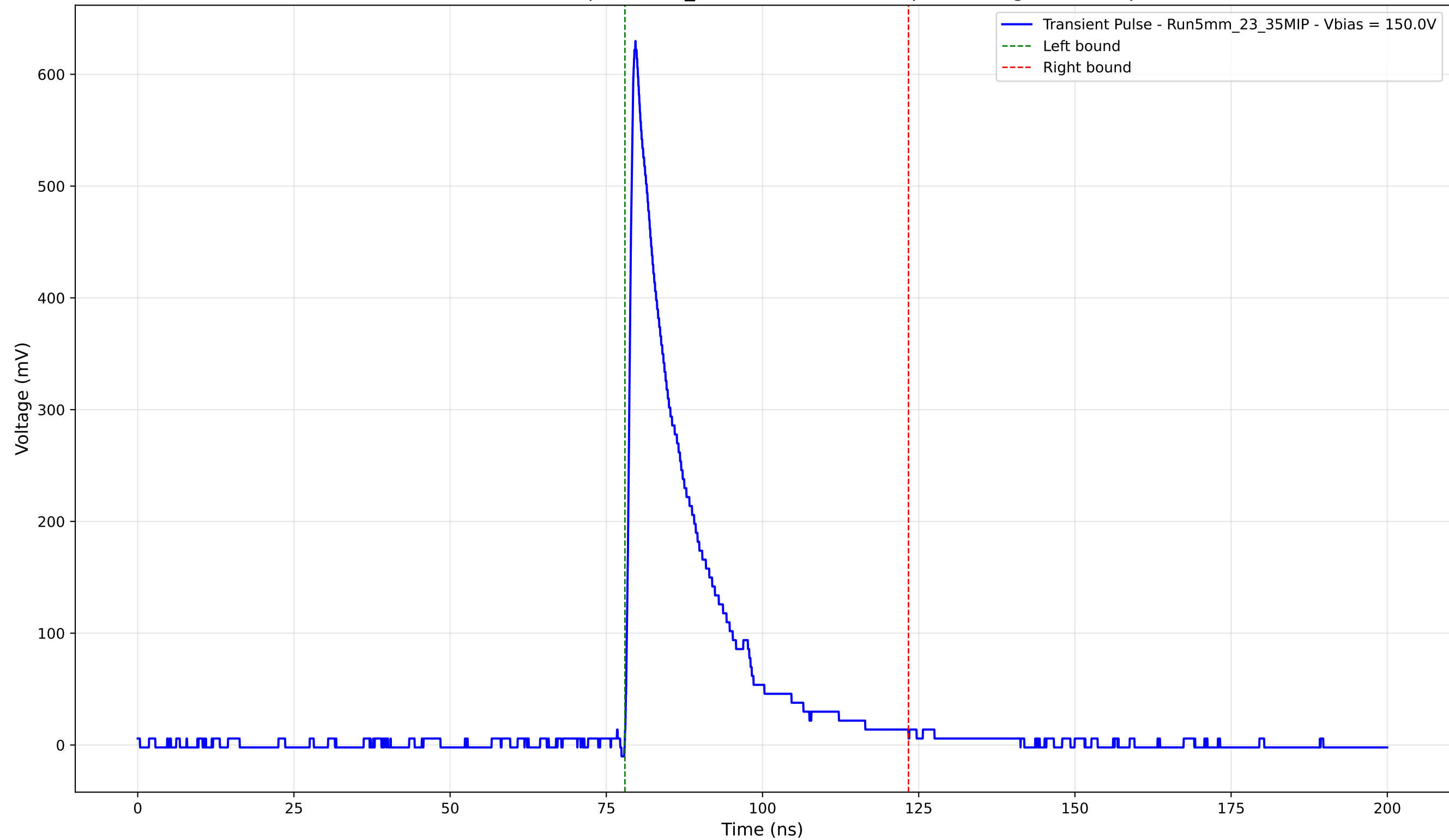
Transient Pulse - Sample: 5mm_23 - Position: 4275.0 \mu\text{m} - Charge: 118.11 pC
