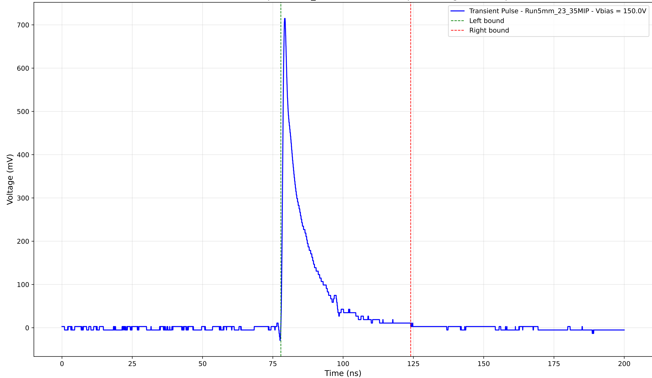
Transient Pulse - Sample: 5mm_23 - Position: 540.0 \mu\text{m} - Charge: 103.20 pC
