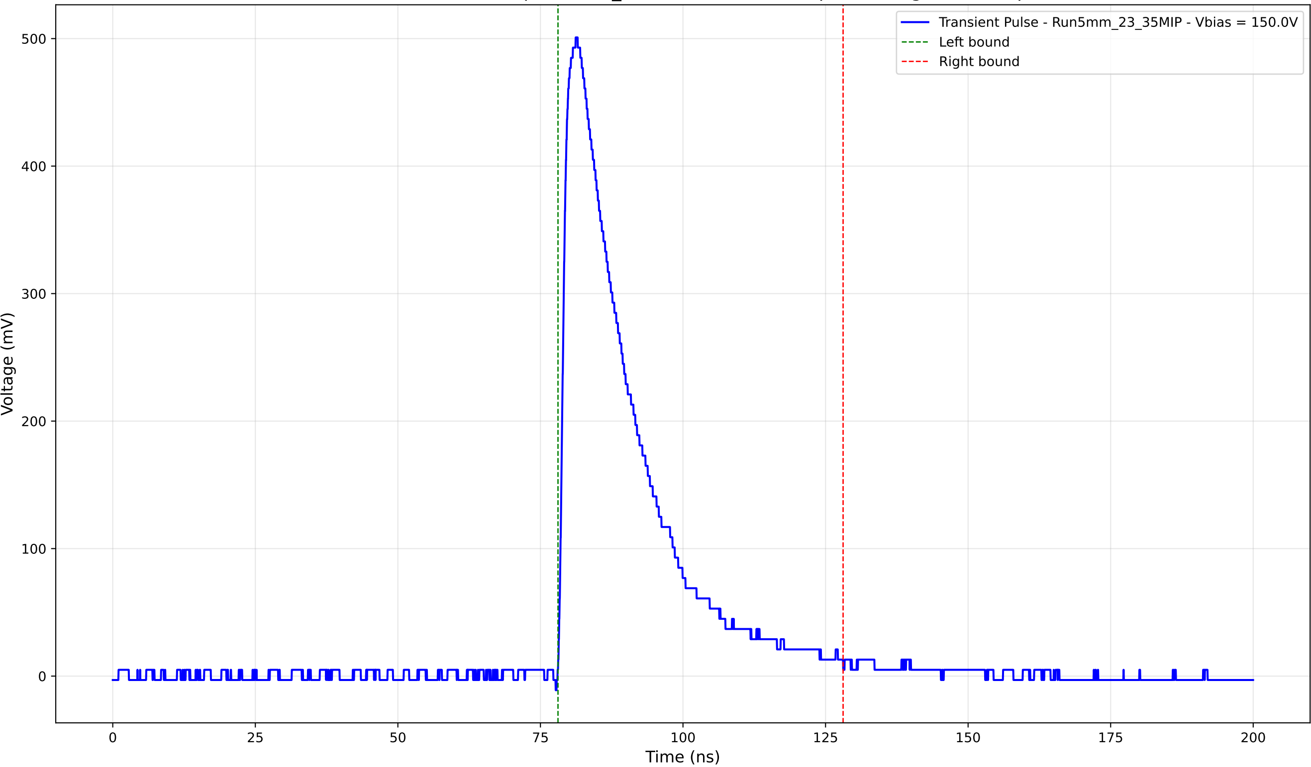
Transient Pulse - Sample: 5mm_23 - Position: 2930.0 \mu\text{m} - Charge: 134.75 pC
