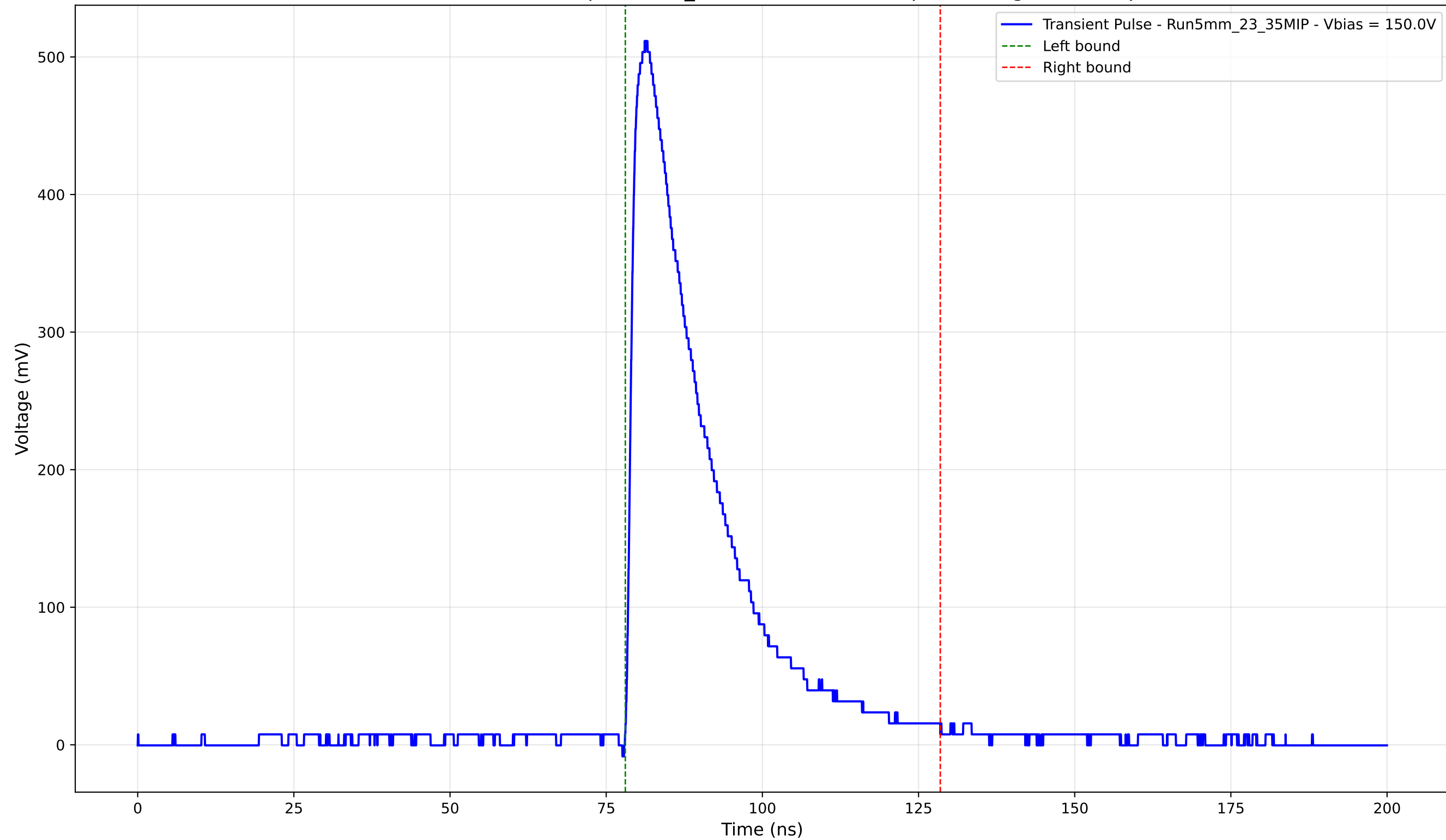
Transient Pulse - Sample: 5mm_23 - Position: 2470.0 \mu\text{m} - Charge: 139.37 pC
