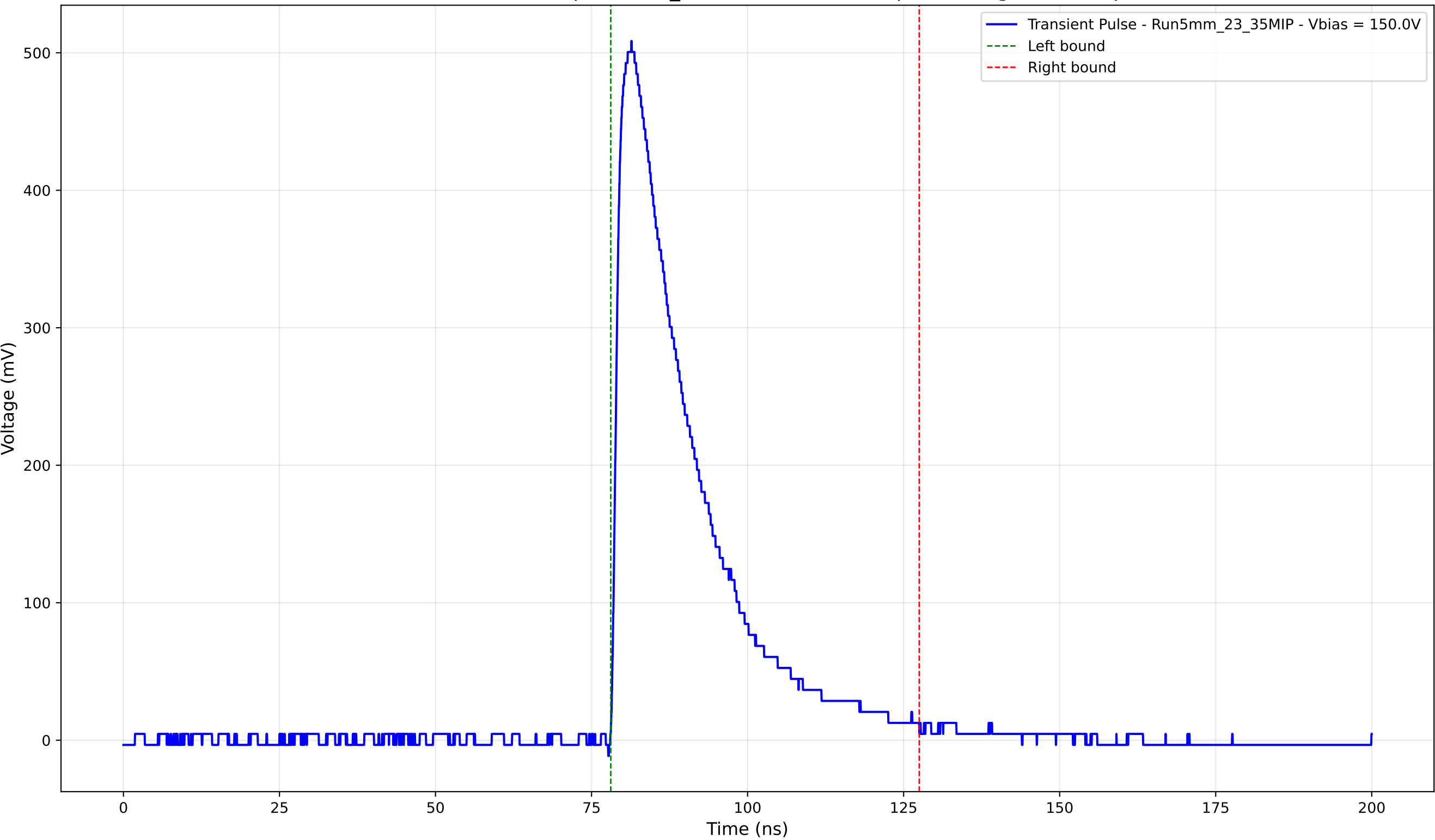
Transient Pulse - Sample: 5mm_23 - Position: 2460.0 \mu\text{m} - Charge: 137.11 pC
