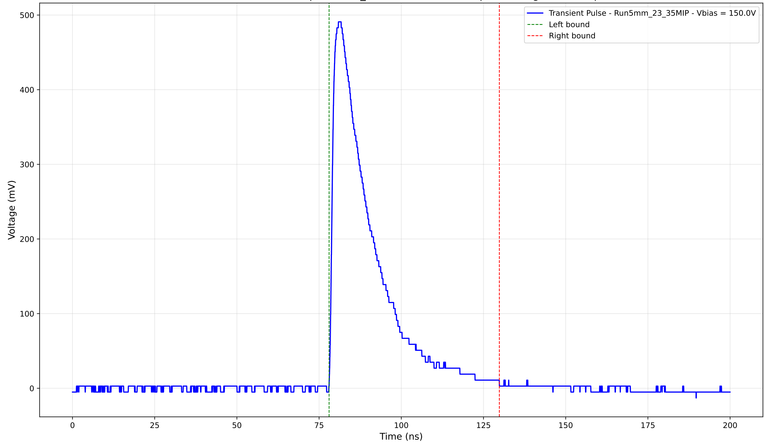
Transient Pulse - Sample: 5mm_23 - Position: 3000.0 \mu\text{m} - Charge: 131.28 pC
