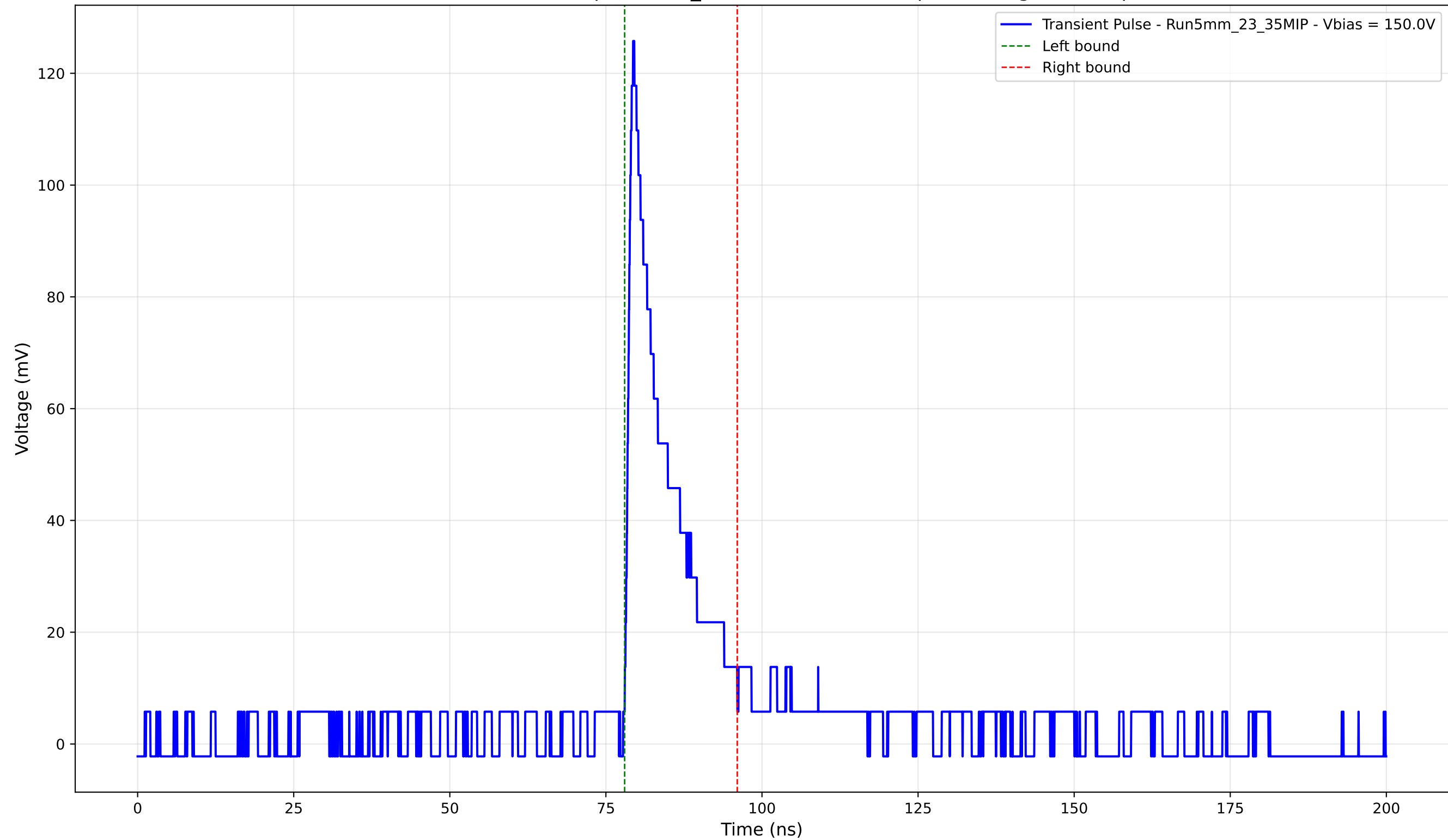
Transient Pulse - Sample: 5mm_23 - Position: 4525.0 \mu\text{m} - Charge: 16.70 pC
