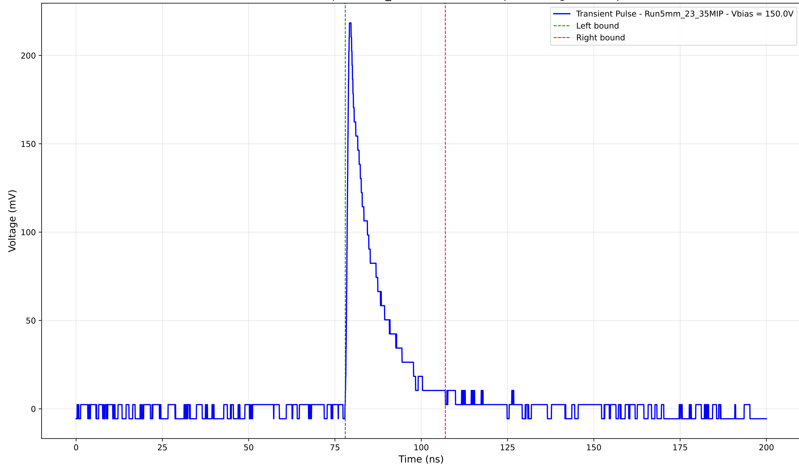
Transient Pulse - Sample: 5mm_23 - Position: 645.0 \mu\text{m} - Charge: 33.90 pC
