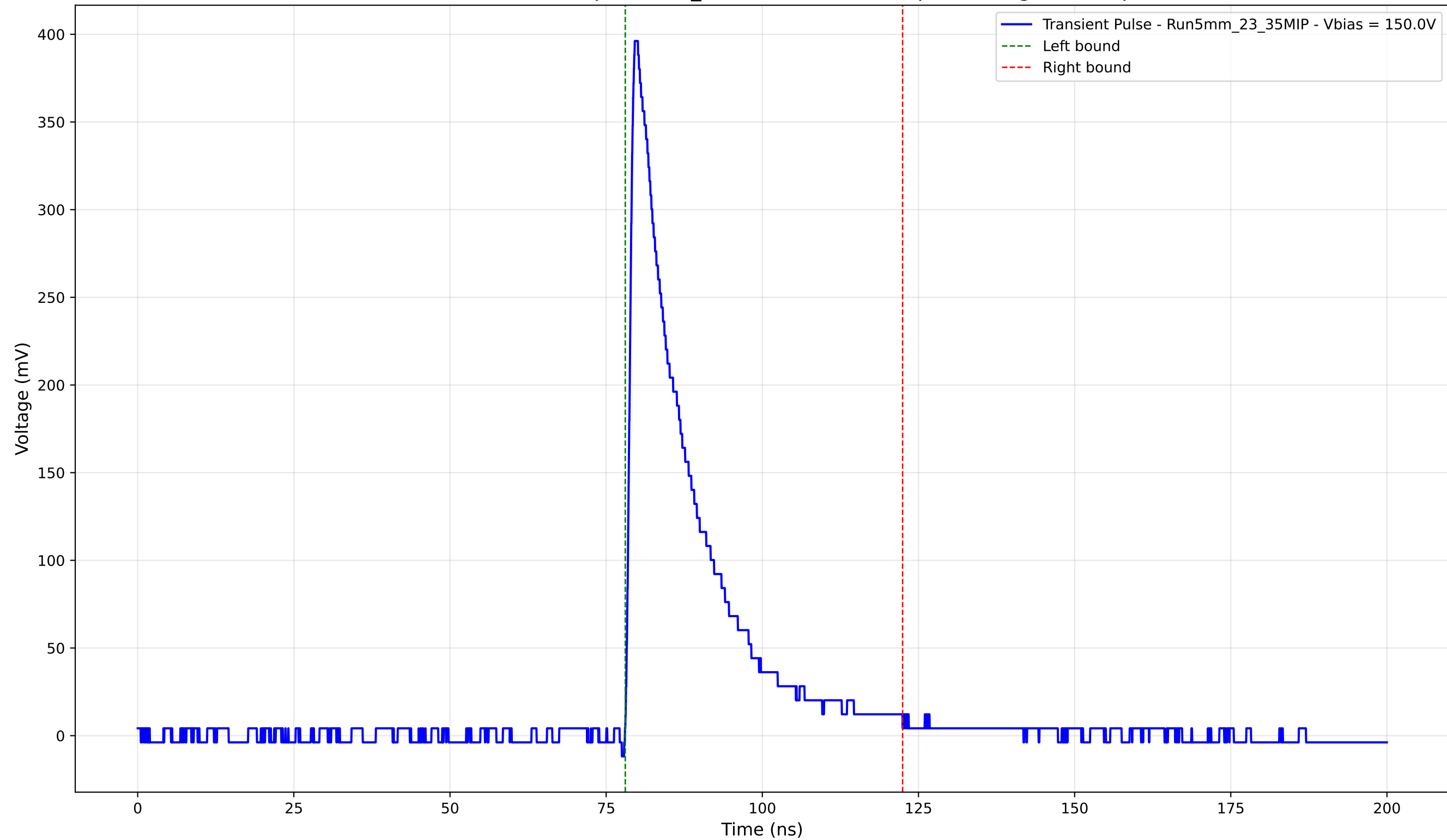
Transient Pulse - Sample: 5mm_23 - Position: 4100.0 \mu\text{m} - Charge: 80.14 pC
