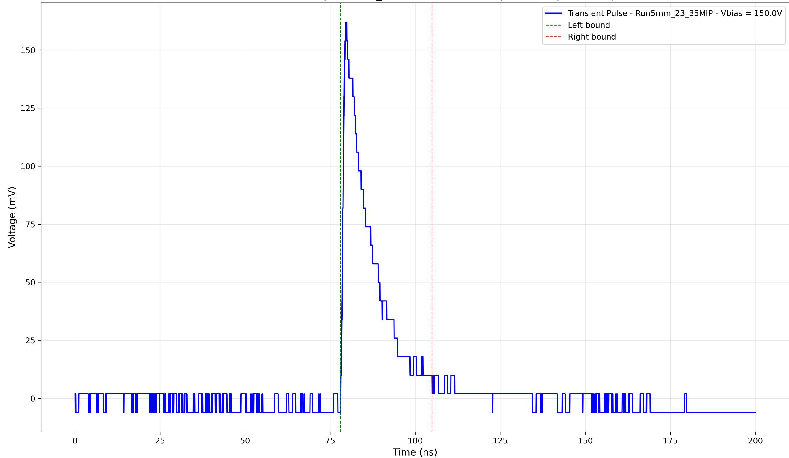
Transient Pulse - Sample: 5mm_23 - Position: 4180.0 \mu\text{m} - Charge: 28.17 pC
