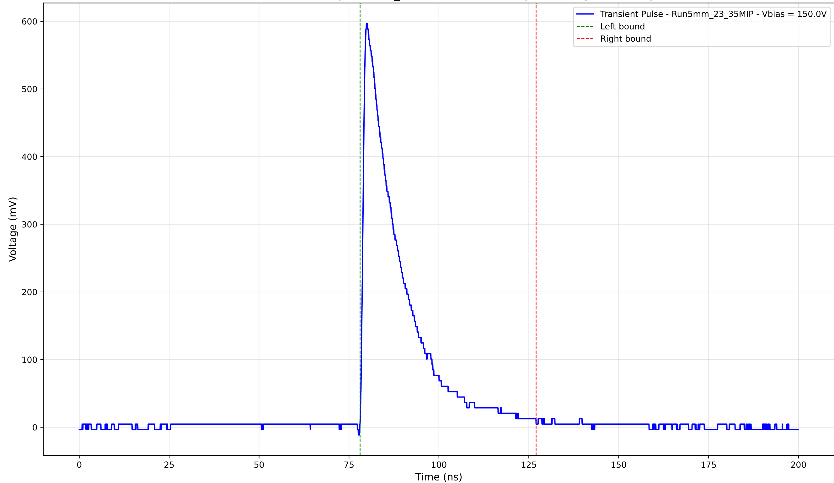
Transient Pulse - Sample: 5mm_23 - Position: 1365.0 \mu\text{m} - Charge: 135.80 pC
