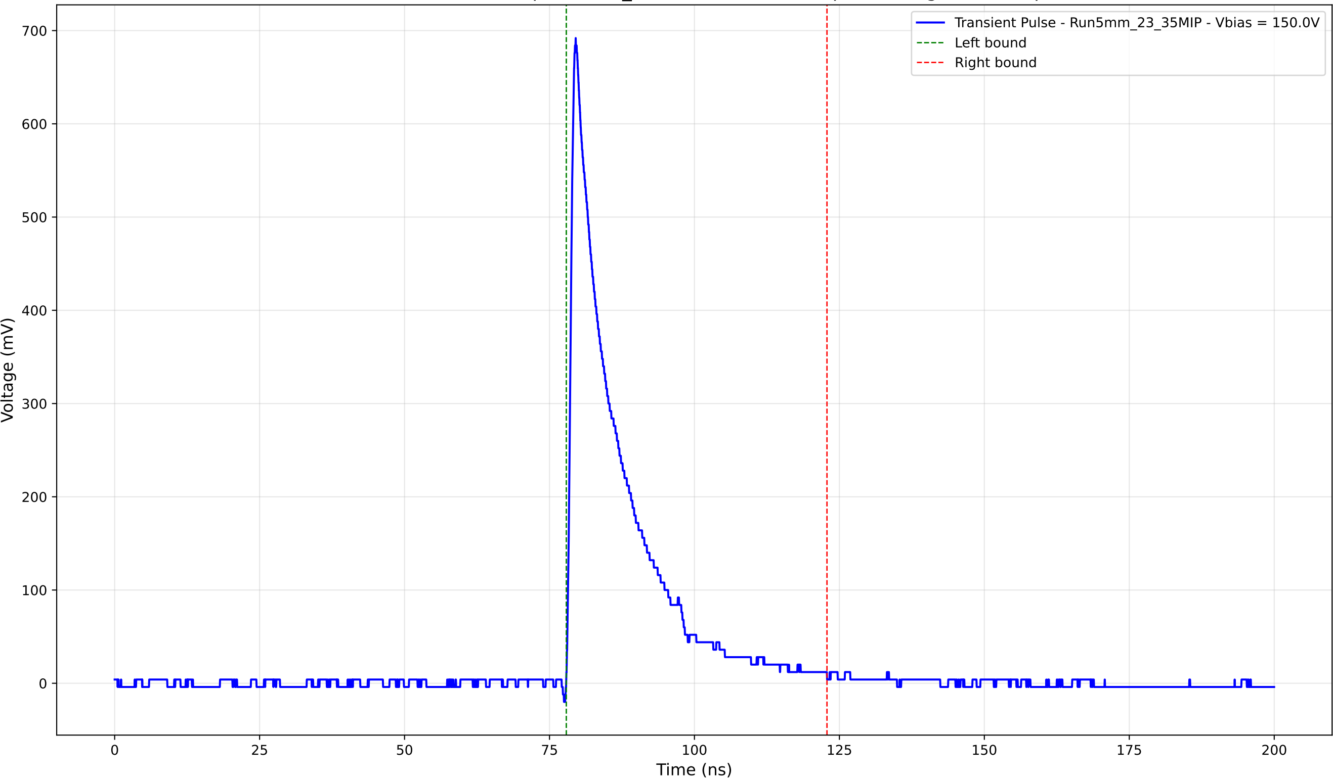
Transient Pulse - Sample: 5mm_23 - Position: 4445.0 \mu\text{m} - Charge: 119.86 pC
