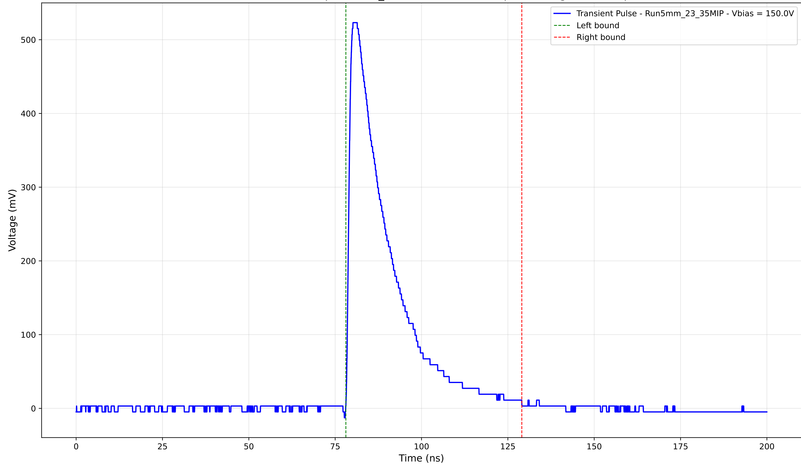
Transient Pulse - Sample: 5mm_23 - Position: 1835.0 \mu\text{m} - Charge: 135.30 pC
