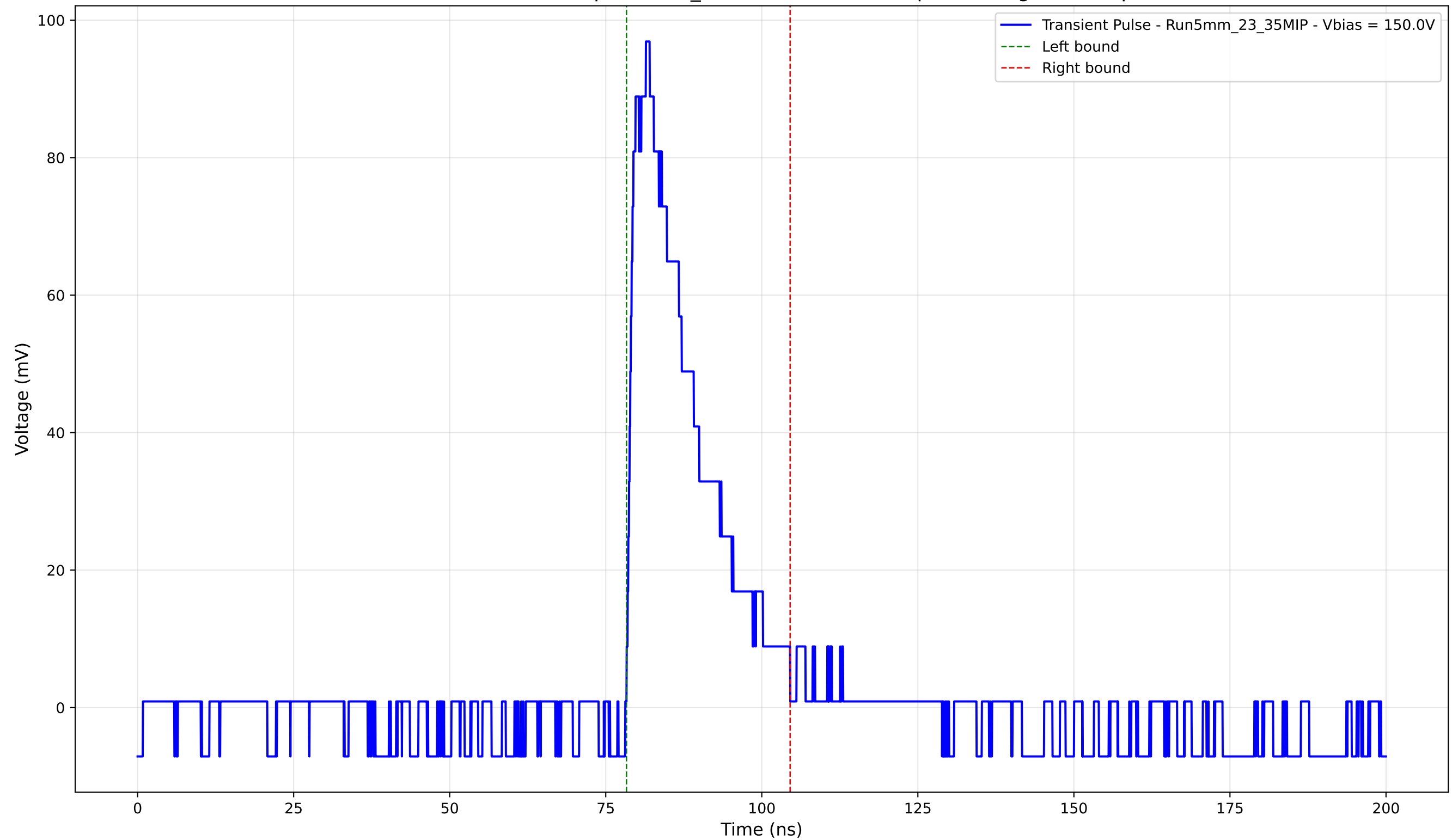
Transient Pulse - Sample: 5mm_23 - Position: 1630.0 \mu\text{m} - Charge: 21.14 pC
