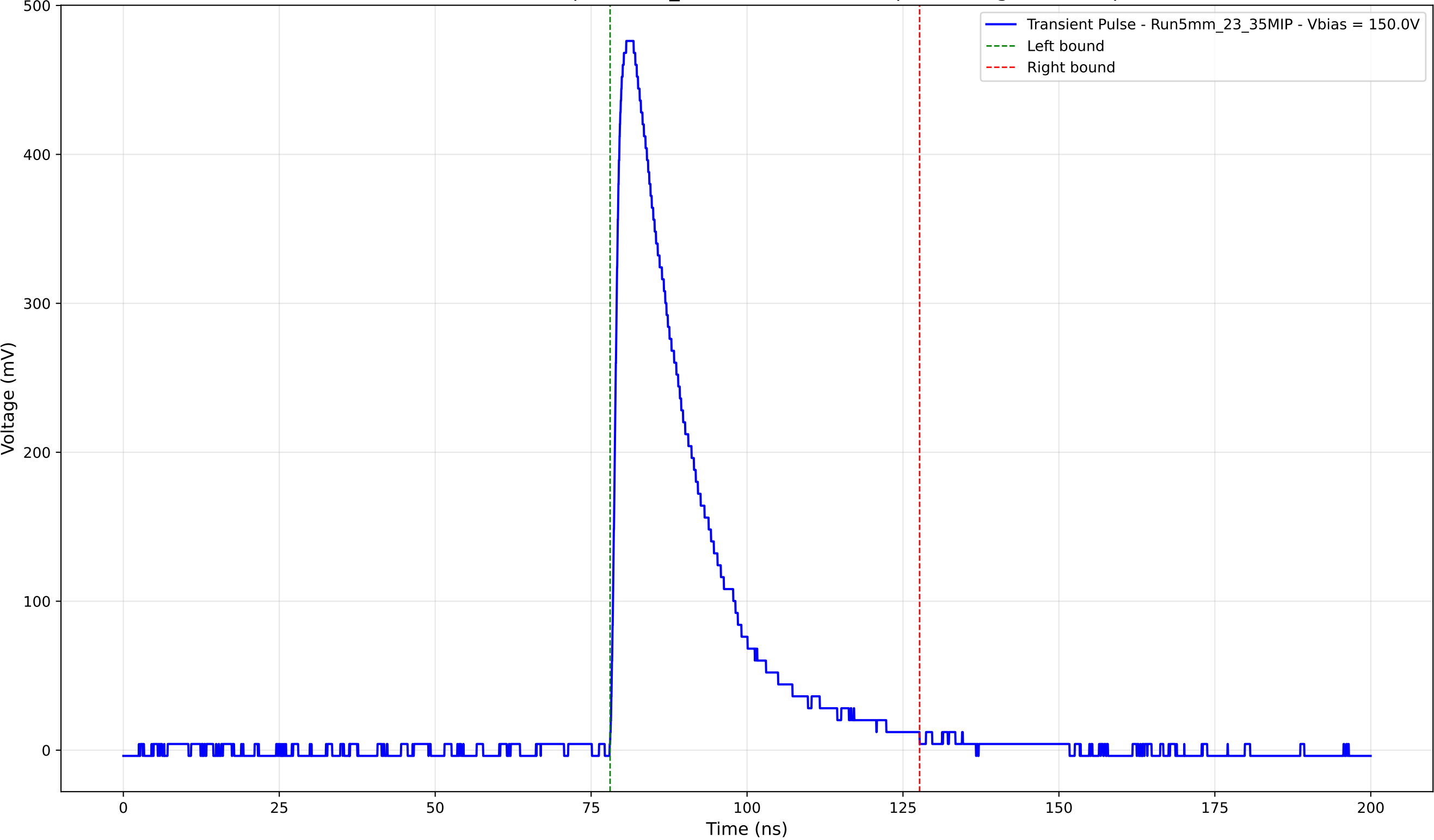
Transient Pulse - Sample: 5mm_23 - Position: 3055.0 \mu\text{m} - Charge: 127.01 pC
