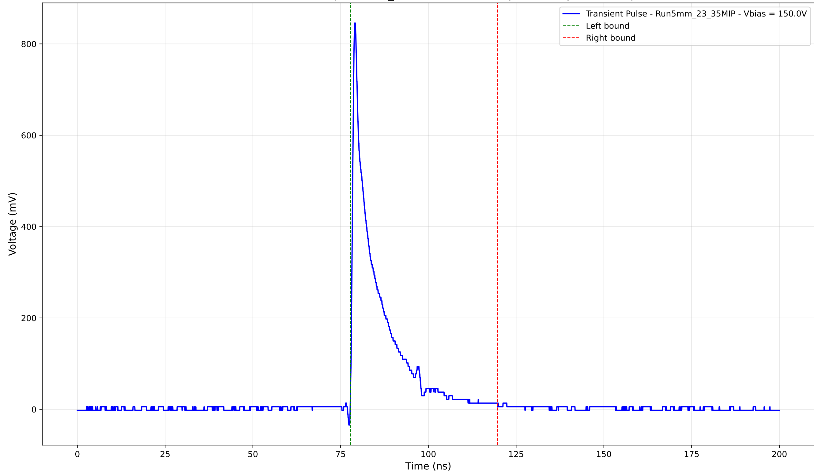
Transient Pulse - Sample: 5mm_23 - Position: 360.0 \mu\text{m} - Charge: 115.52 pC
