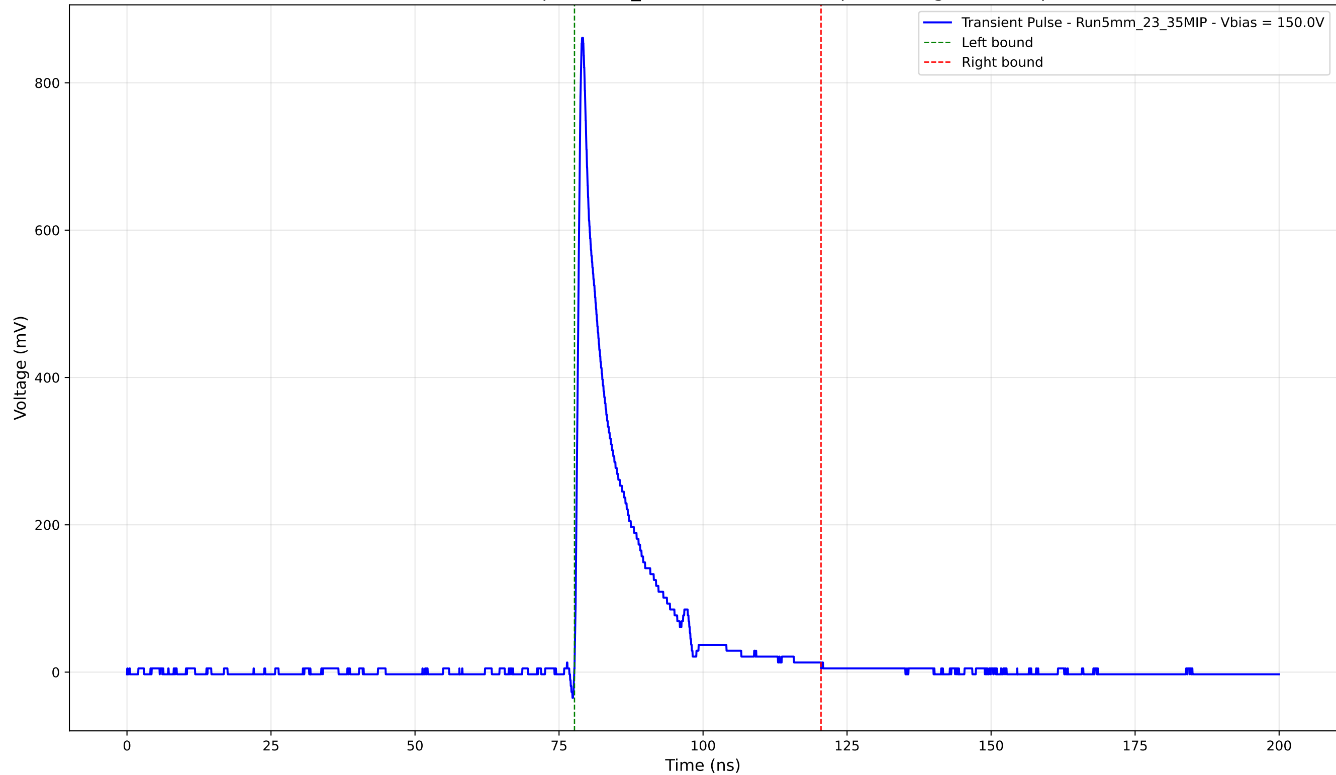
Transient Pulse - Sample: 5mm_23 - Position: 4895.0 \mu\text{m} - Charge: 116.76 pC
