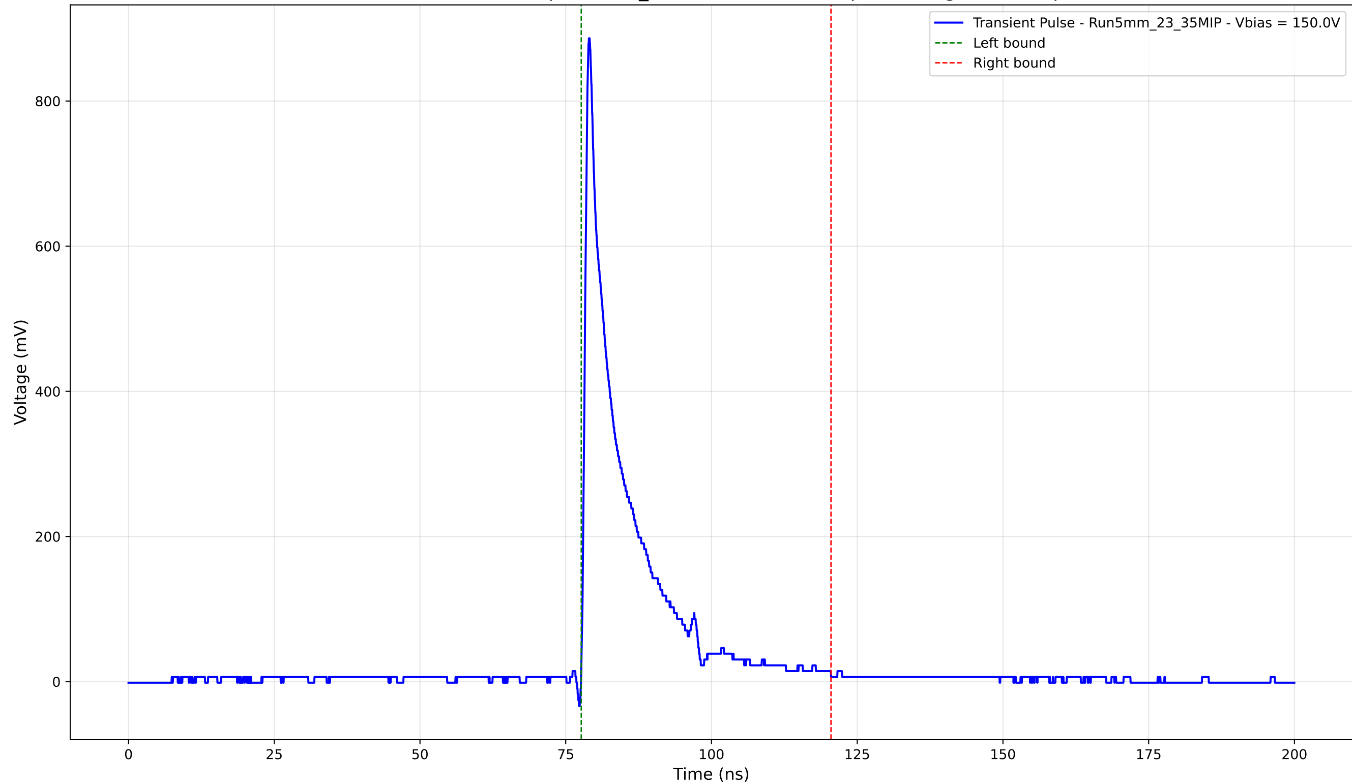
Transient Pulse - Sample: 5mm_23 - Position: 4930.0 \mu\text{m} - Charge: 118.83 pC
