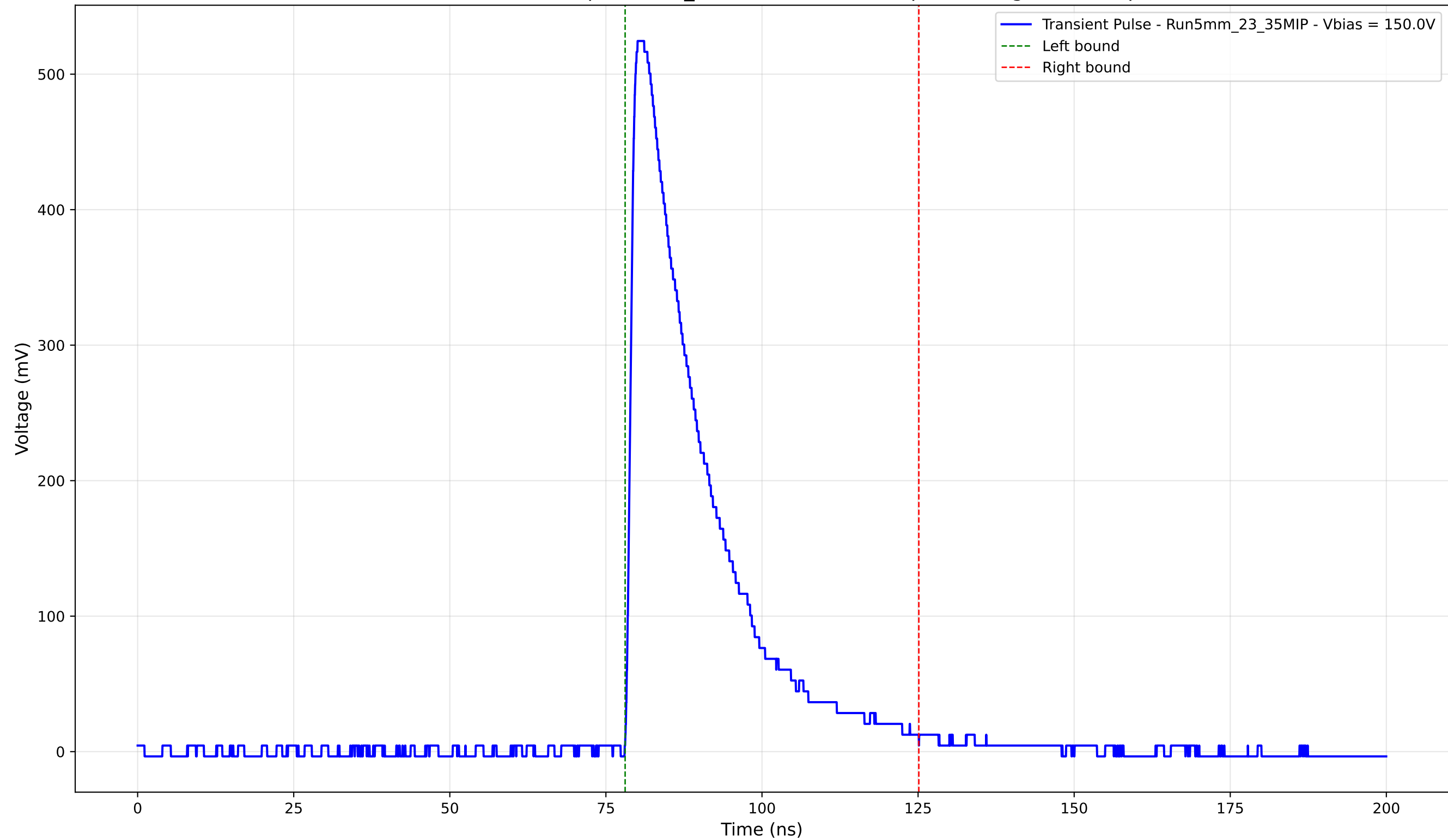
Transient Pulse - Sample: 5mm_23 - Position: 1790.0 \mu\text{m} - Charge: 135.32 pC
