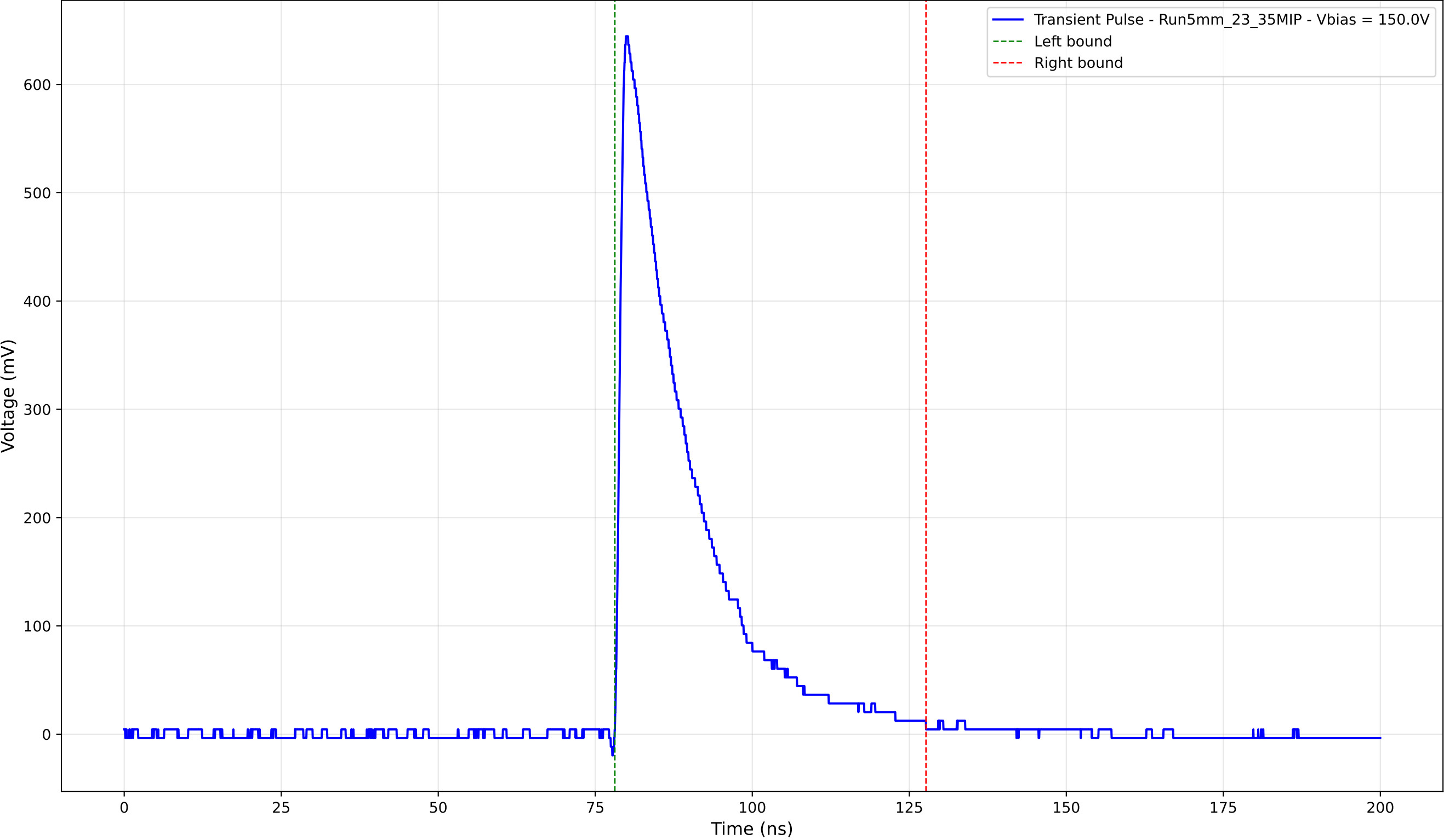
Transient Pulse - Sample: 5mm_23 - Position: 1460.0 \mu\text{m} - Charge: 151.90 pC
