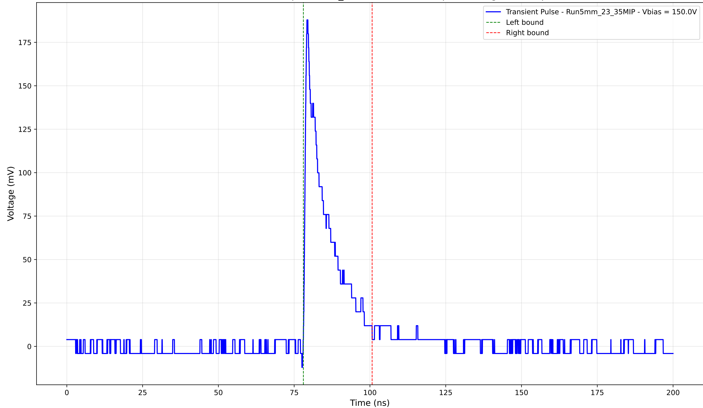
Transient Pulse - Sample: 5mm_23 - Position: 640.0 \mu\text{m} - Charge: 28.08 pC
