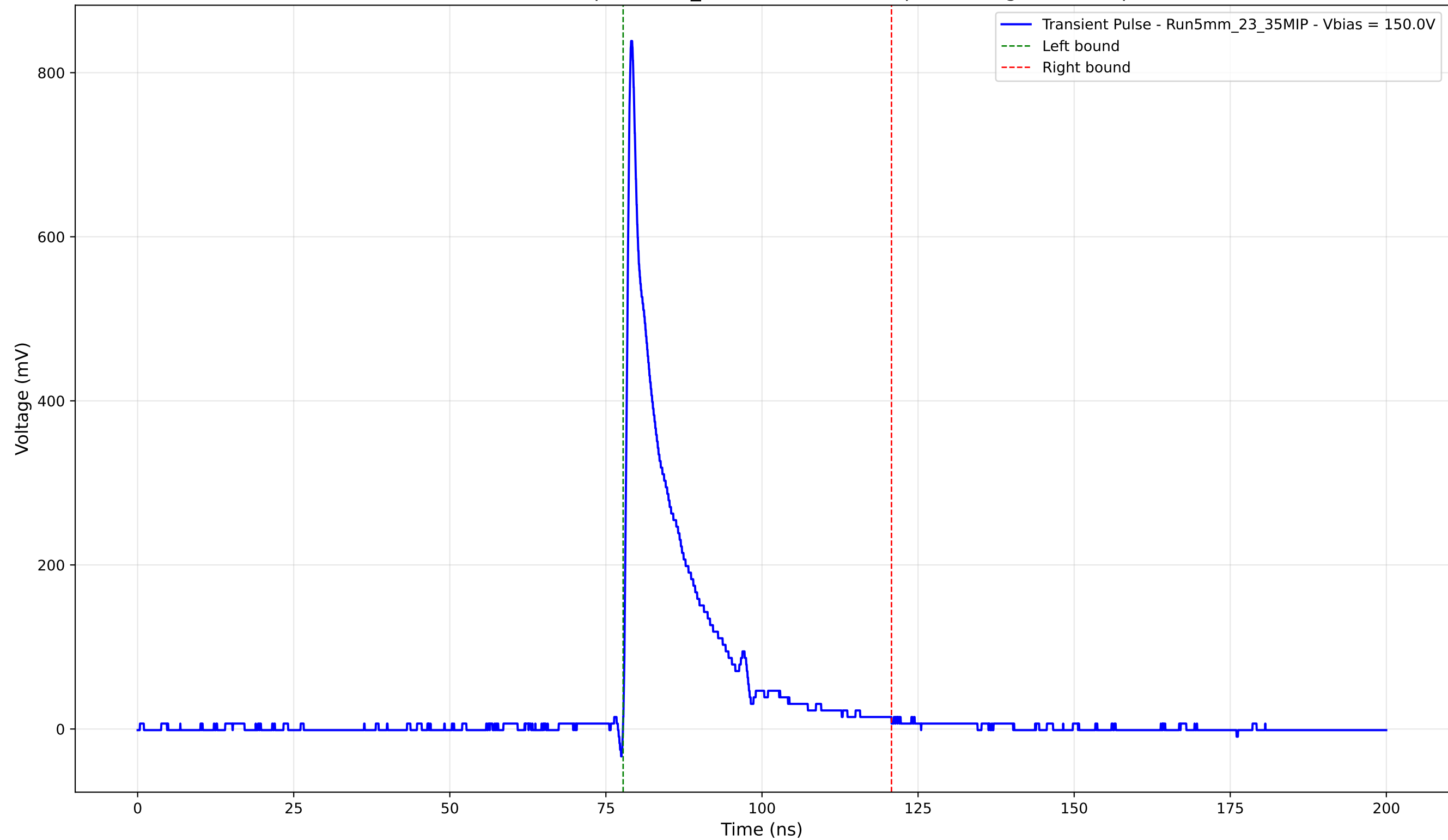
Transient Pulse - Sample: 5mm_23 - Position: 380.0 \mu\text{m} - Charge: 117.44 pC
