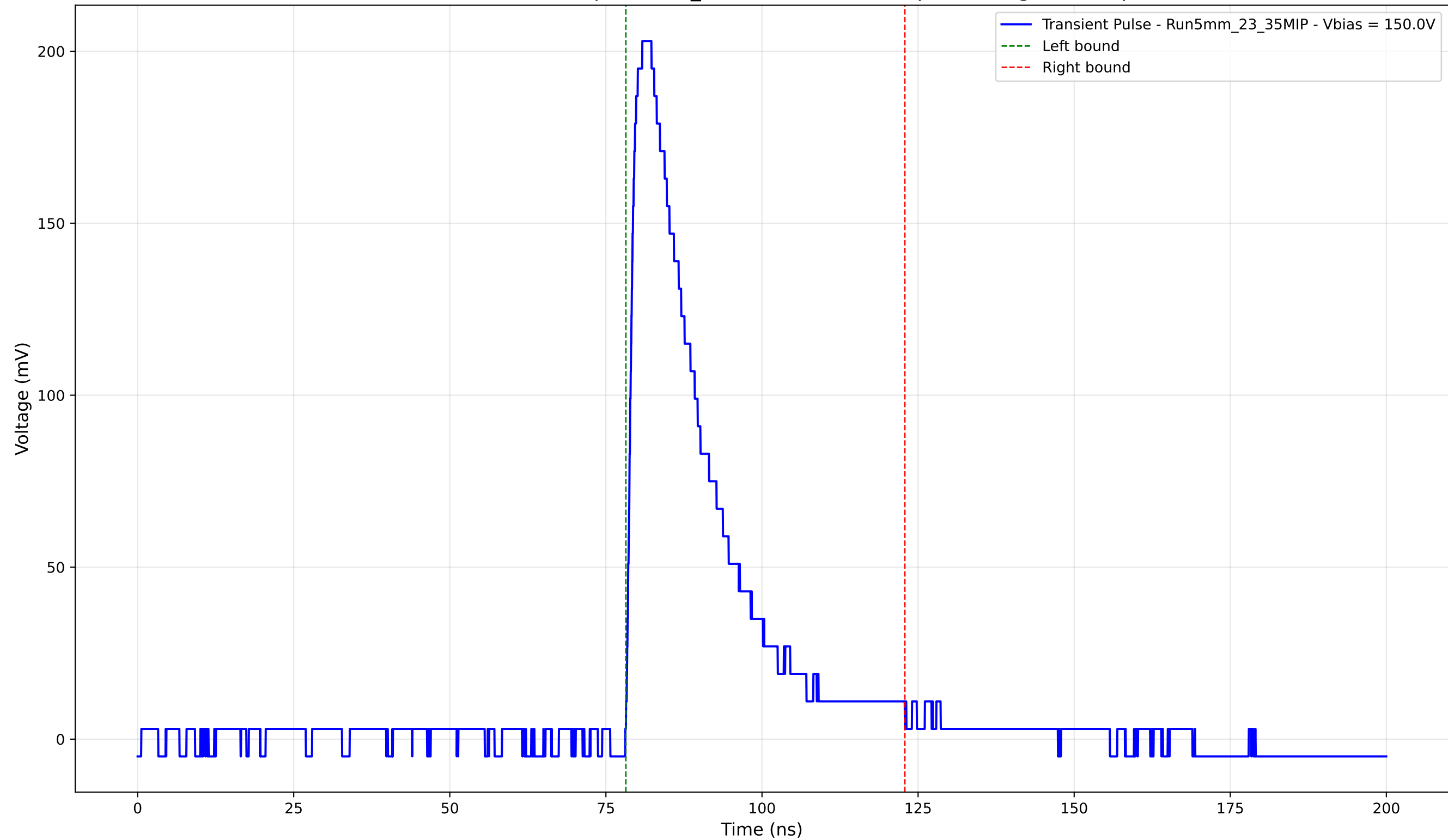
Transient Pulse - Sample: 5mm_23 - Position: 2610.0 \mu\text{m} - Charge: 53.25 pC
