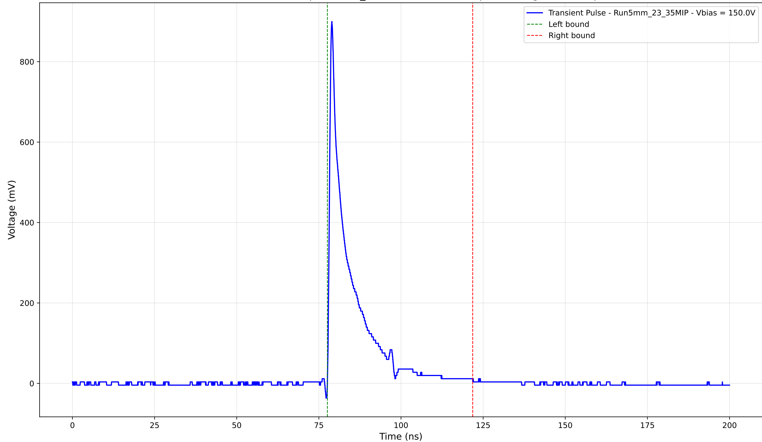
Transient Pulse - Sample: 5mm_23 - Position: 5010.0 \mu\text{m} - Charge: 112.17 pC
