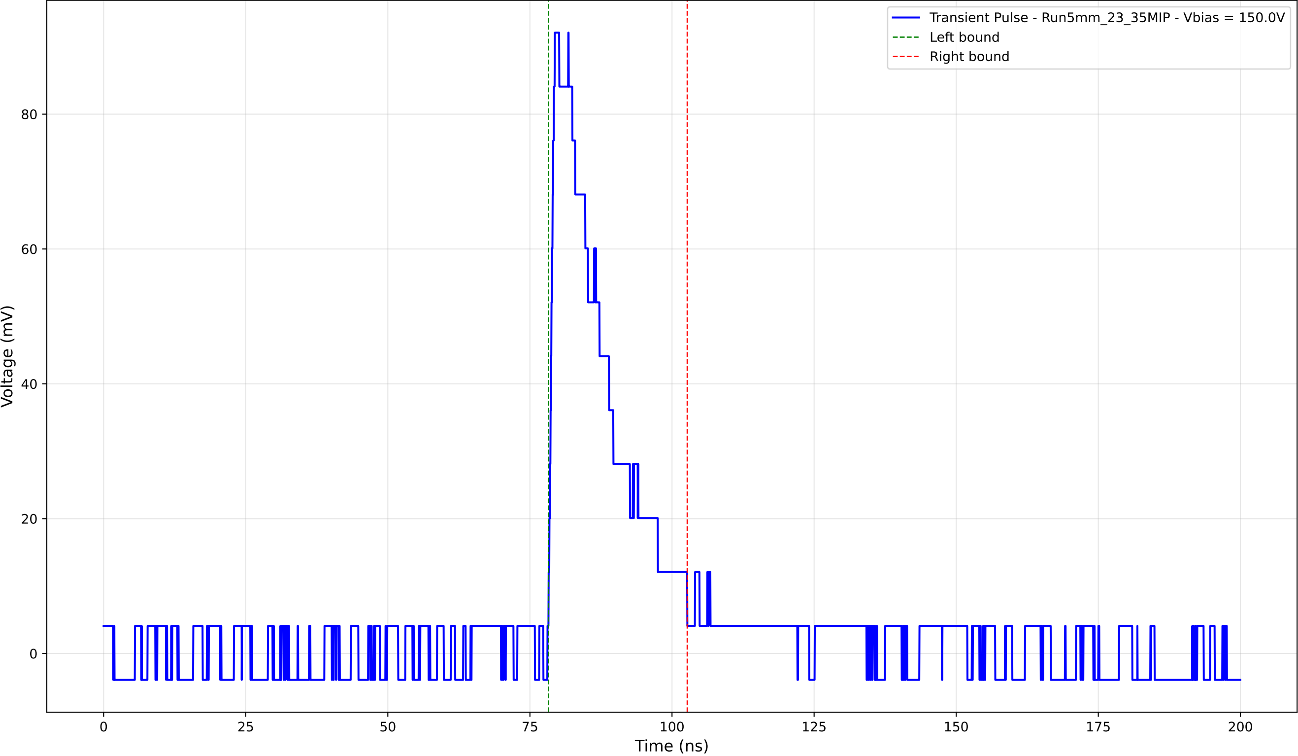
Transient Pulse - Sample: 5mm_23 - Position: 1125.0 \mu\text{m} - Charge: 19.36 pC
