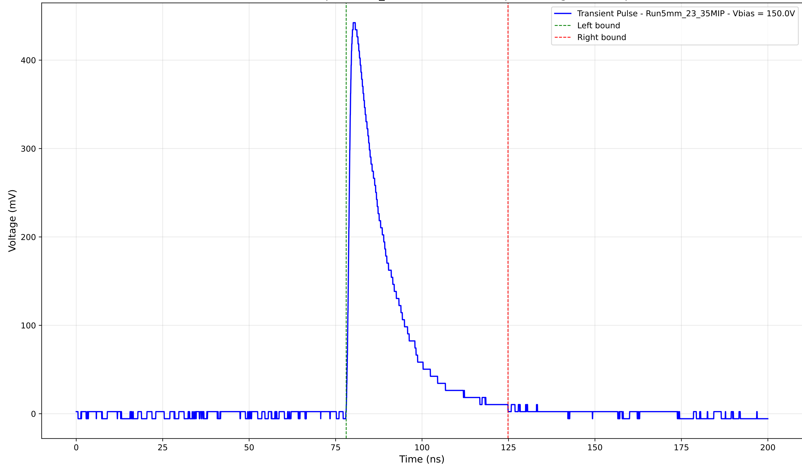
Transient Pulse - Sample: 5mm_23 - Position: 3580.0 \mu\text{m} - Charge: 104.17 pC
