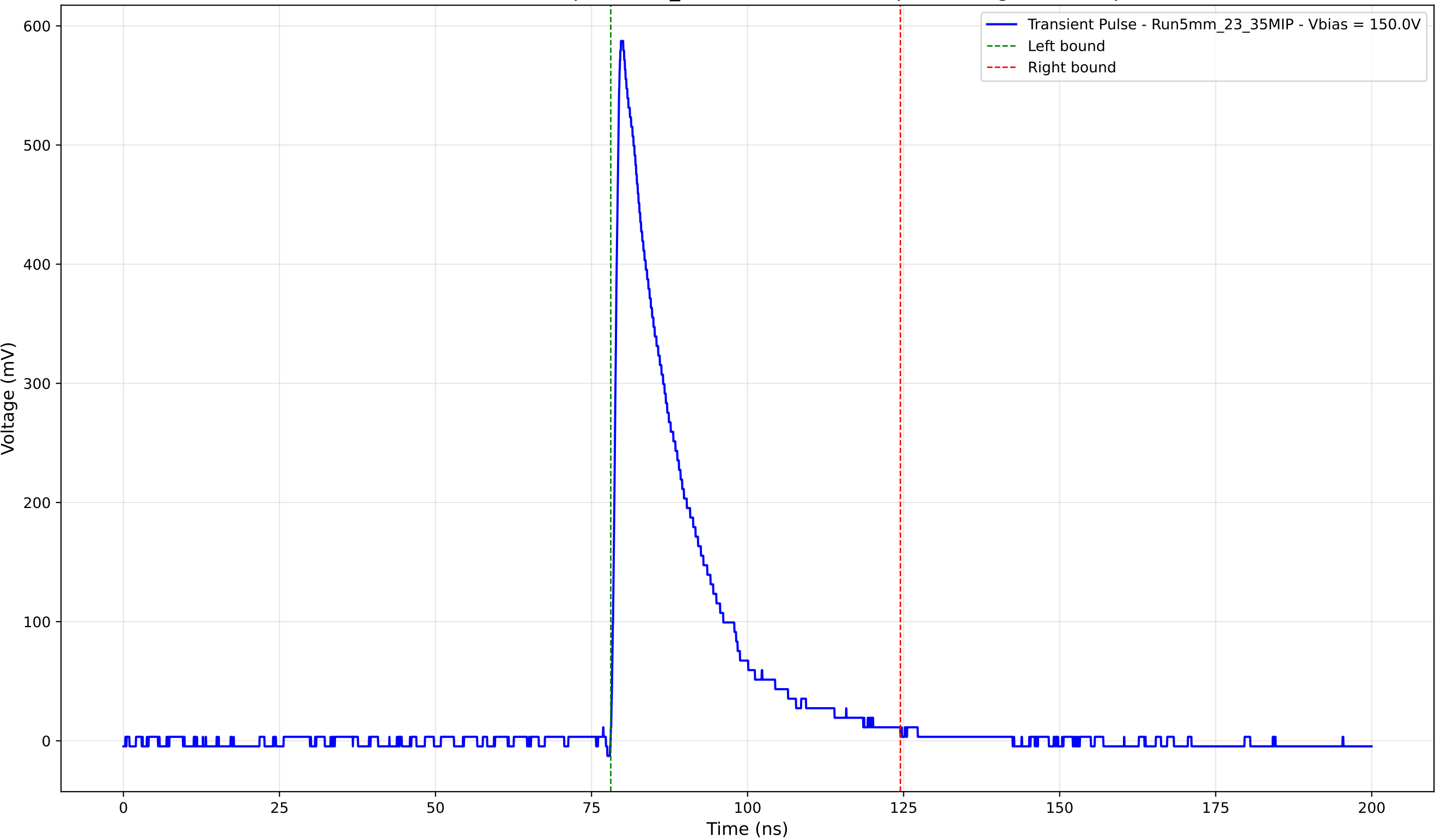
Transient Pulse - Sample: 5mm_23 - Position: 1250.0 \mu\text{m} - Charge: 126.35 pC
