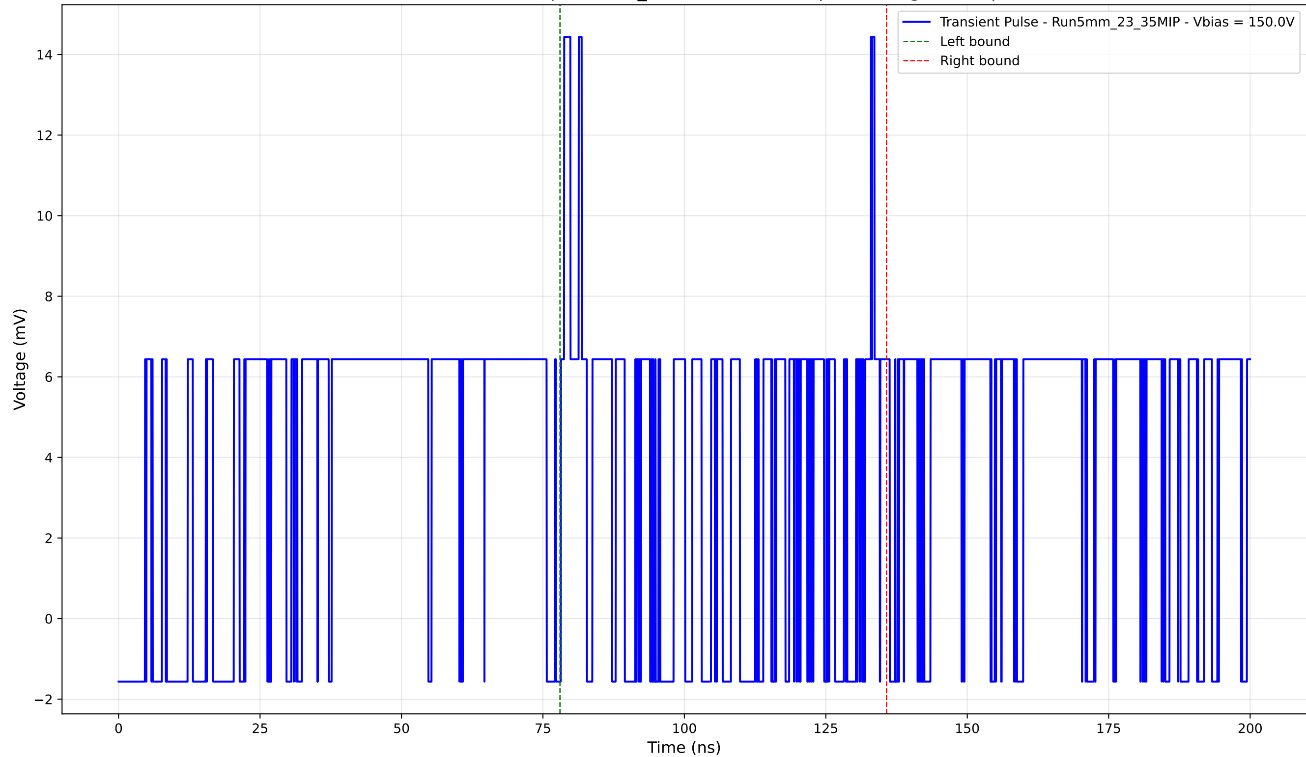
Transient Pulse - Sample: 5mm_23 - Position: 75.0 \mu\text{m} - Charge: 4.15 pC
