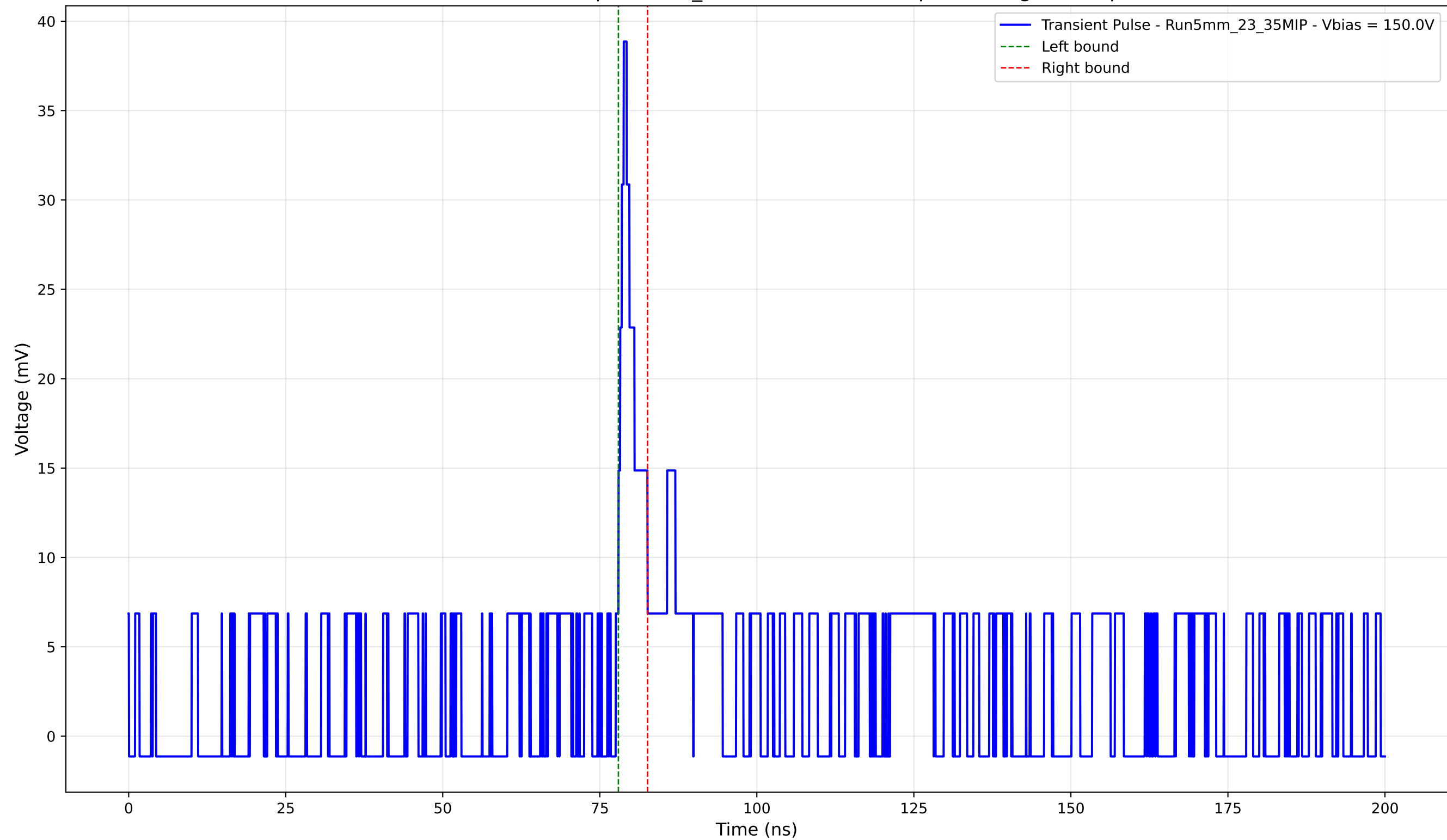
Transient Pulse - Sample: 5mm_23 - Position: 5150.0 \mu\text{m} - Charge: 2.01 pC
