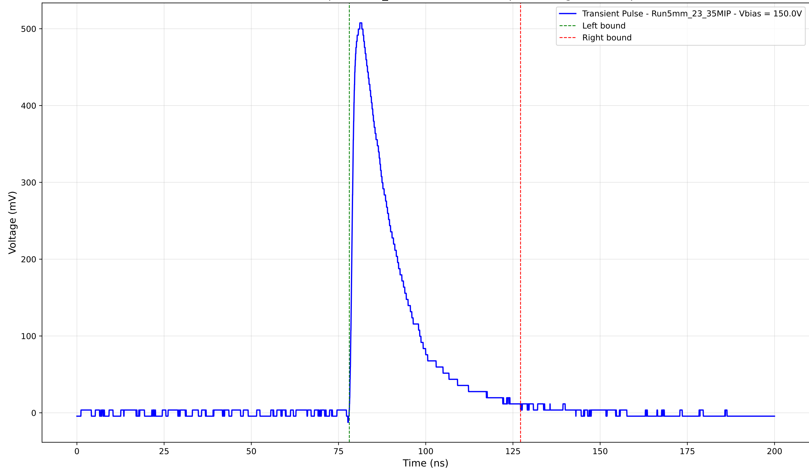
Transient Pulse - Sample: 5mm_23 - Position: 2290.0 \mu\text{m} - Charge: 135.75 pC
