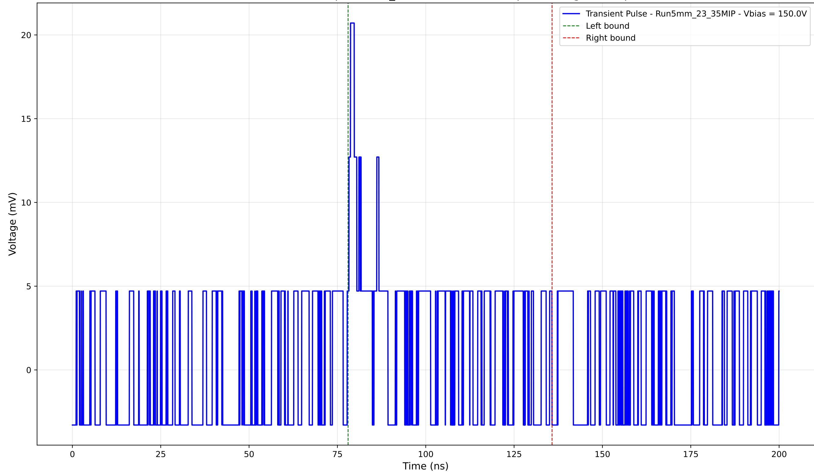
Transient Pulse - Sample: 5mm_23 - Position: 5175.0 \mu\text{m} - Charge: 3.01 pC
