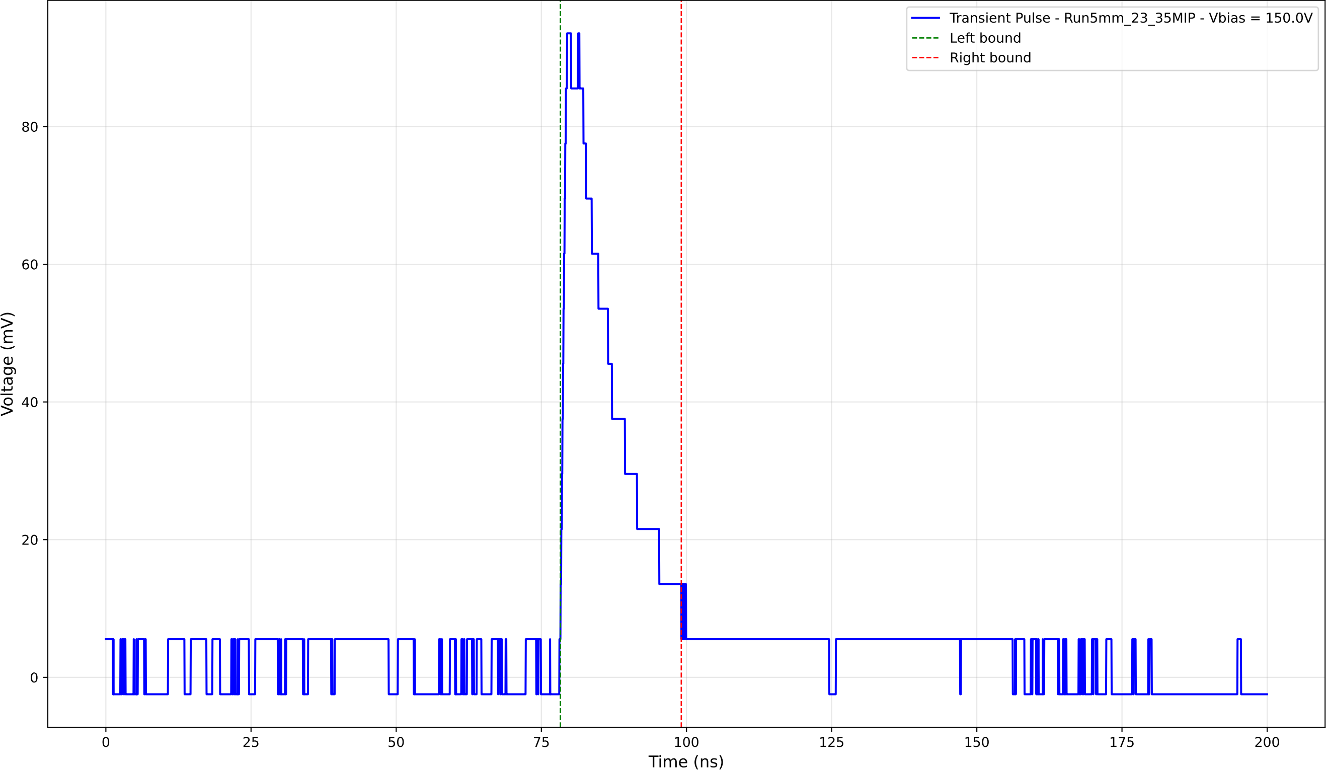
Transient Pulse - Sample: 5mm_23 - Position: 4155.0 \mu\text{m} - Charge: 17.62 pC
