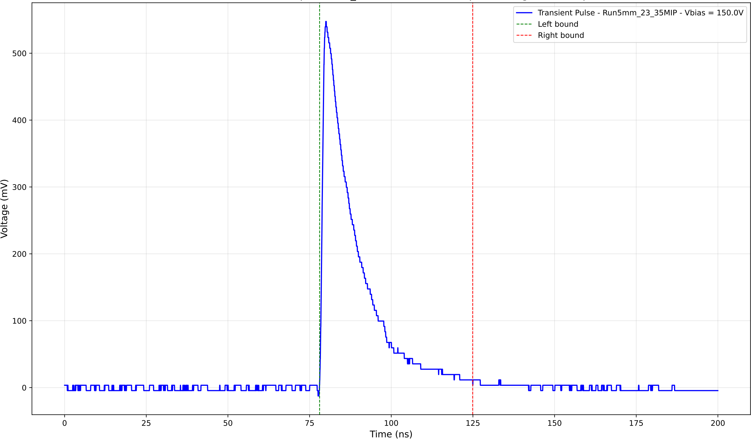
Transient Pulse - Sample: 5mm_23 - Position: 3825.0 \mu\text{m} - Charge: 123.22 pC
