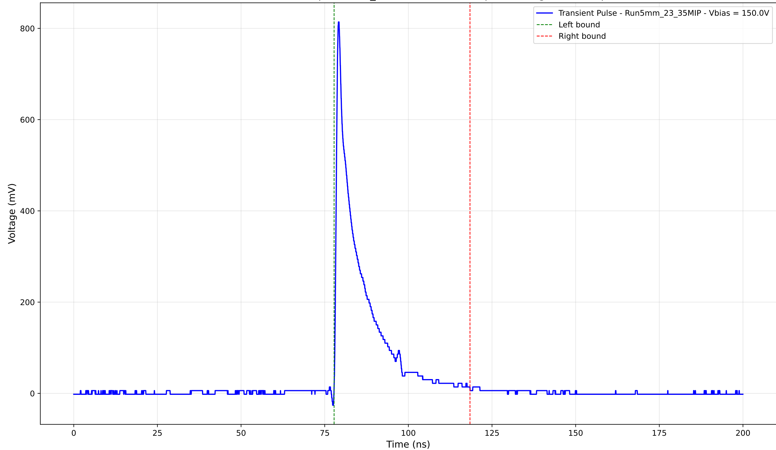
Transient Pulse - Sample: 5mm_23 - Position: 445.0 \mu\text{m} - Charge: 117.21 pC
