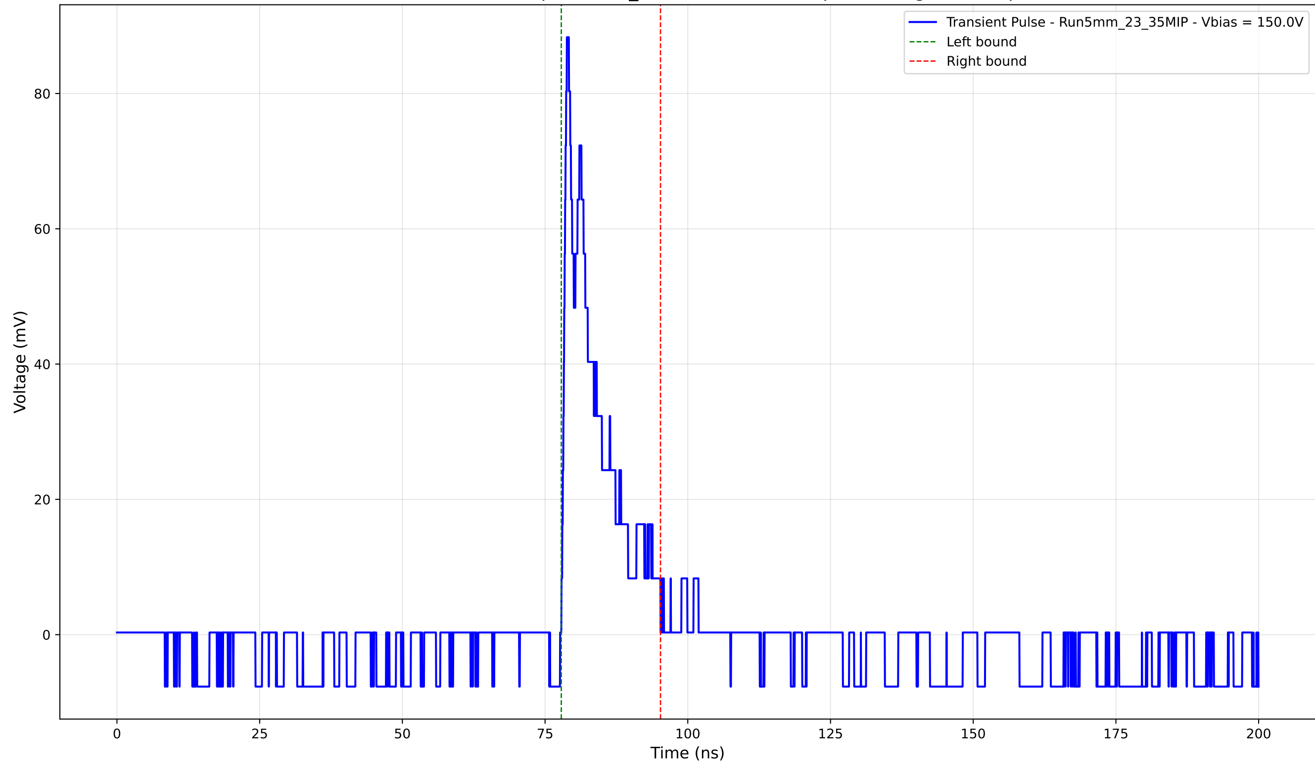
Transient Pulse - Sample: 5mm_23 - Position: 175.0 \mu\text{m} - Charge: 10.52 pC
