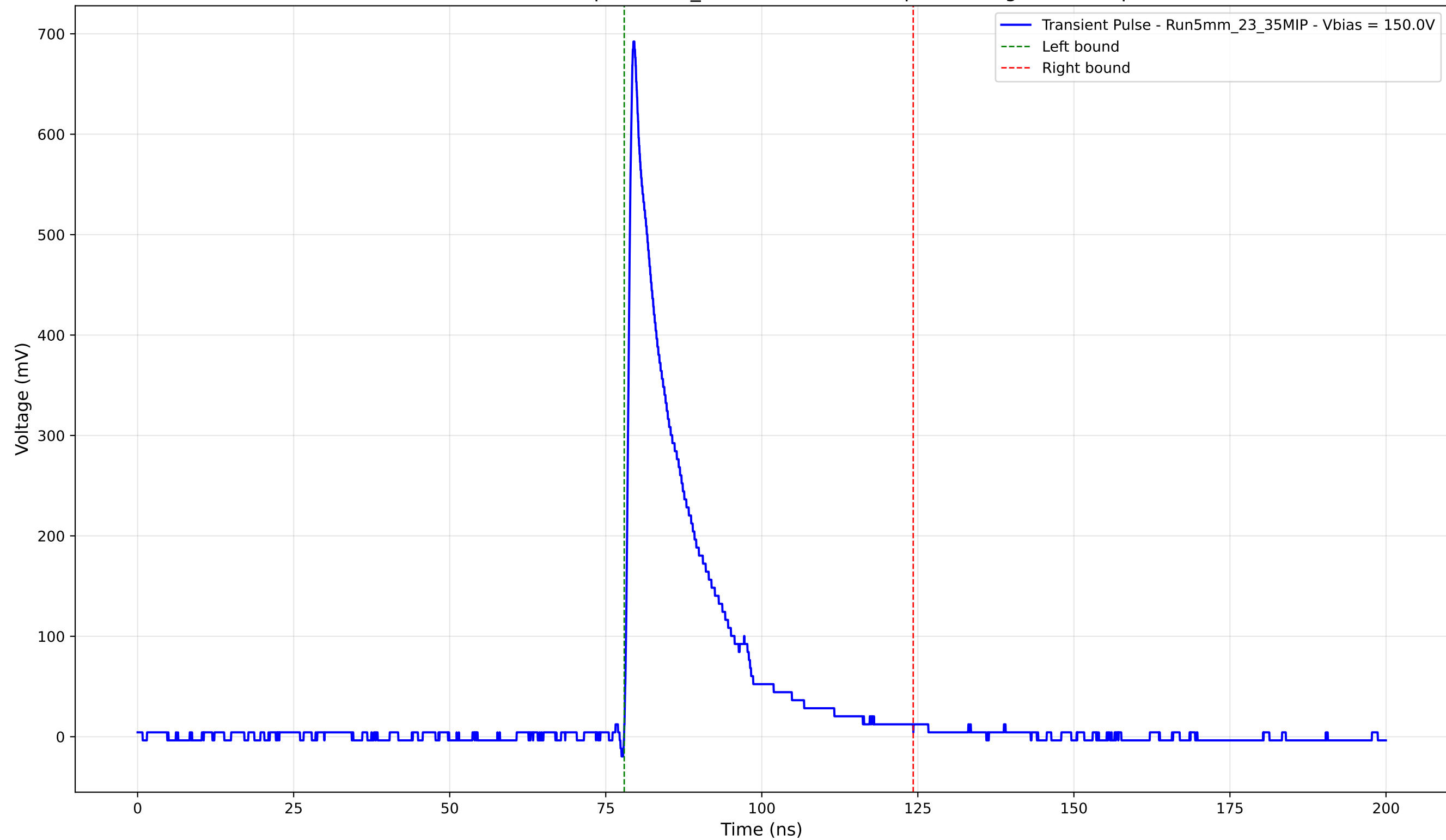
Transient Pulse - Sample: 5mm_23 - Position: 810.0 \mu\text{m} - Charge: 123.14 pC
