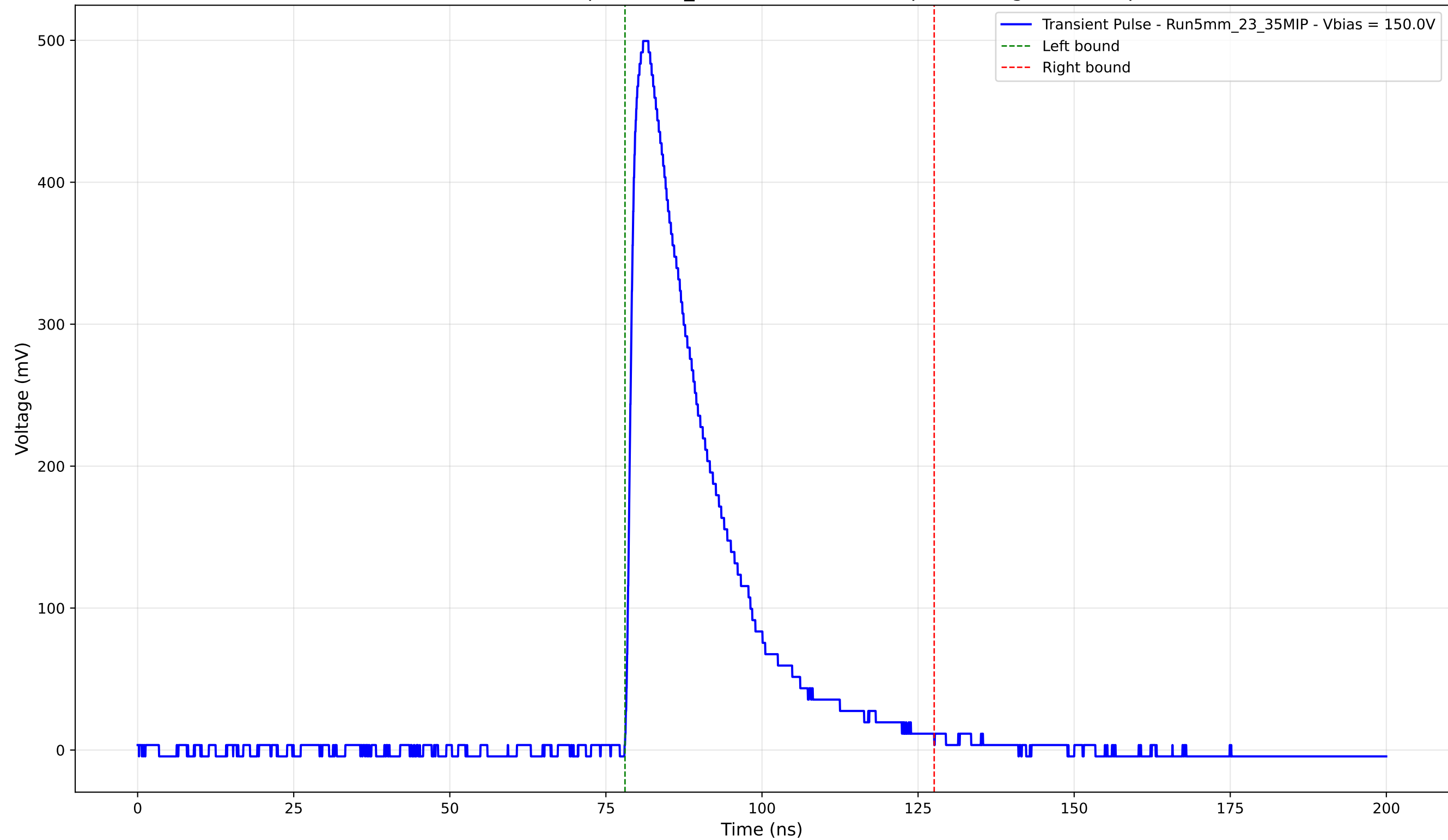
Transient Pulse - Sample: 5mm_23 - Position: 2830.0 \mu\text{m} - Charge: 134.29 pC
