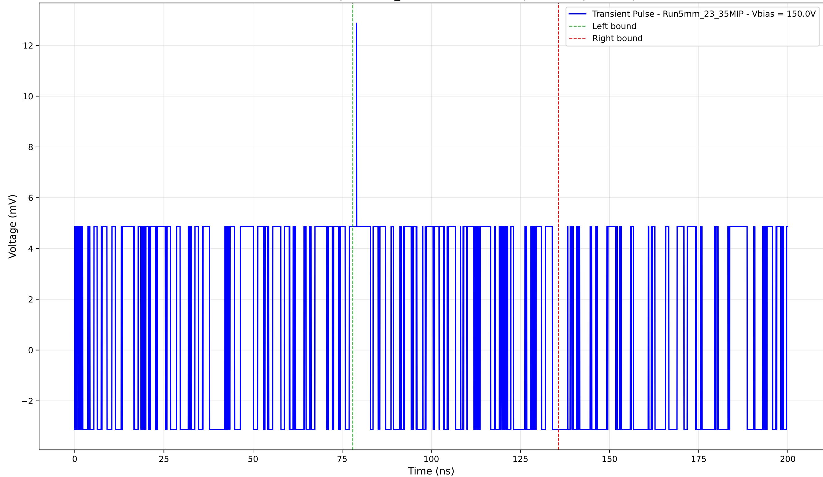
Transient Pulse - Sample: 5mm_23 - Position: 5250.0 \mu\text{m} - Charge: 1.67 pC
