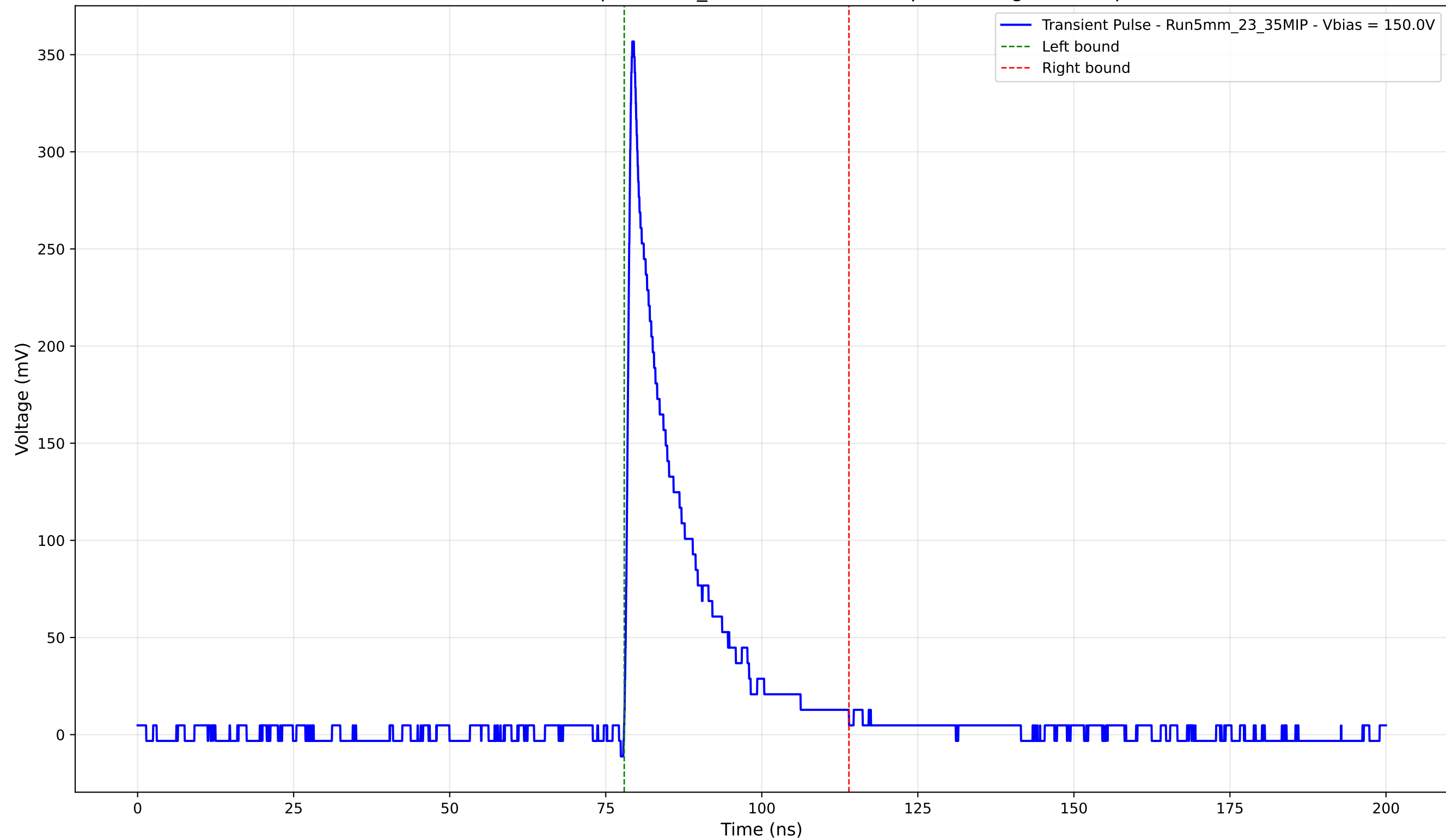
Transient Pulse - Sample: 5mm_23 - Position: 660.0 \mu\text{m} - Charge: 56.01 pC
