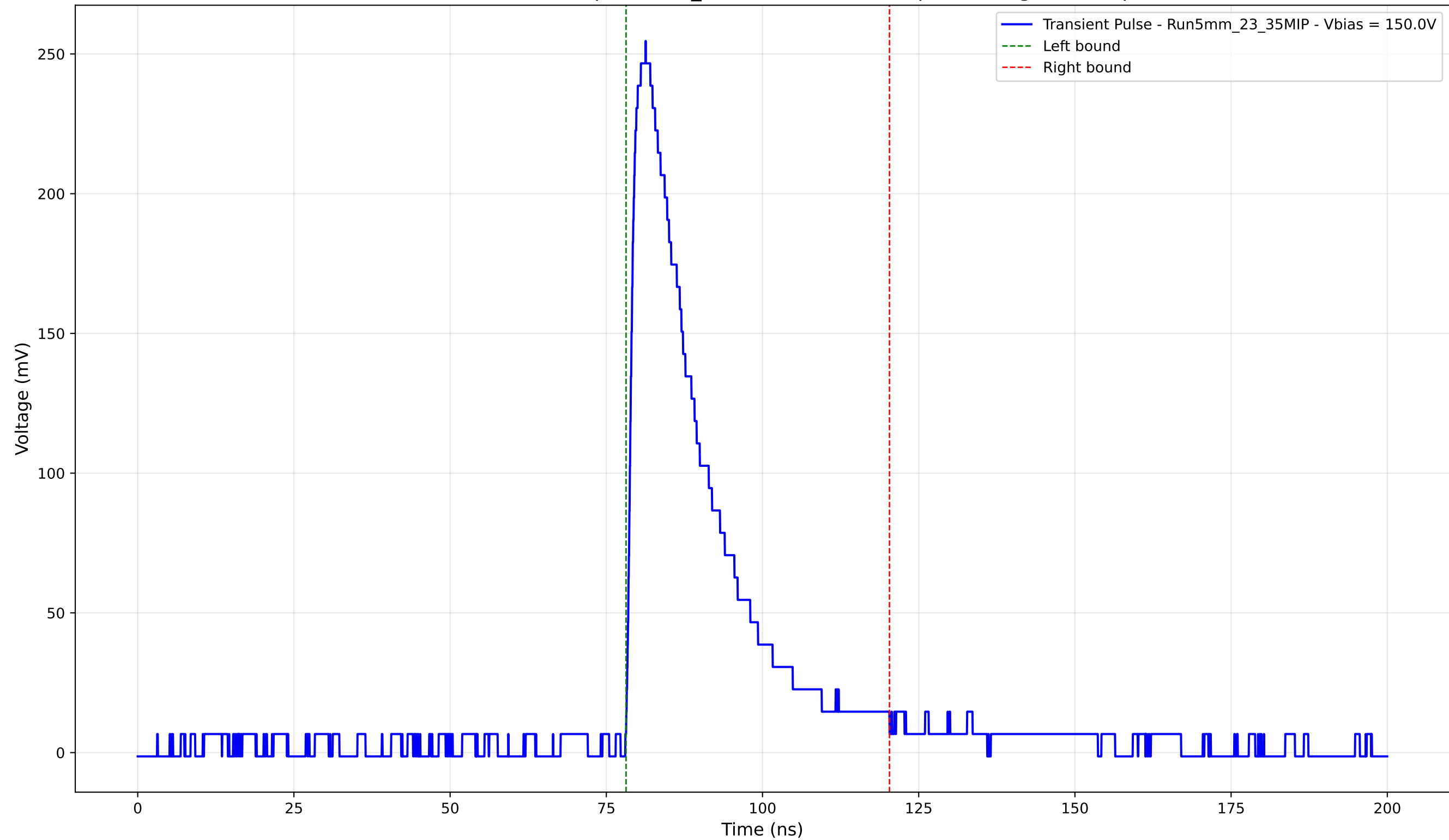
Transient Pulse - Sample: 5mm_23 - Position: 3105.0 \mu\text{m} - Charge: 65.05 pC
