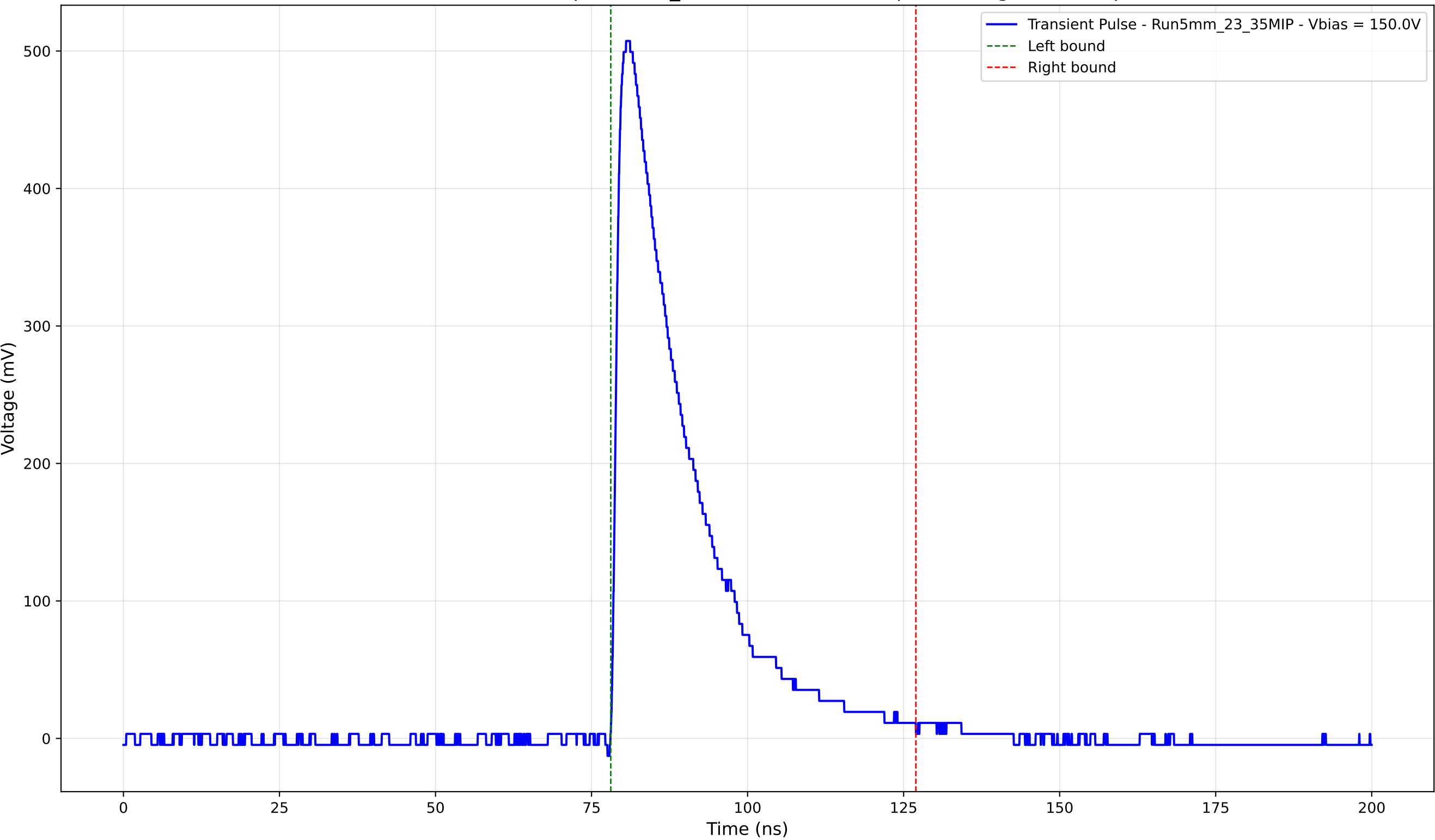
Transient Pulse - Sample: 5mm_23 - Position: 3350.0 \mu\text{m} - Charge: 129.55 pC
