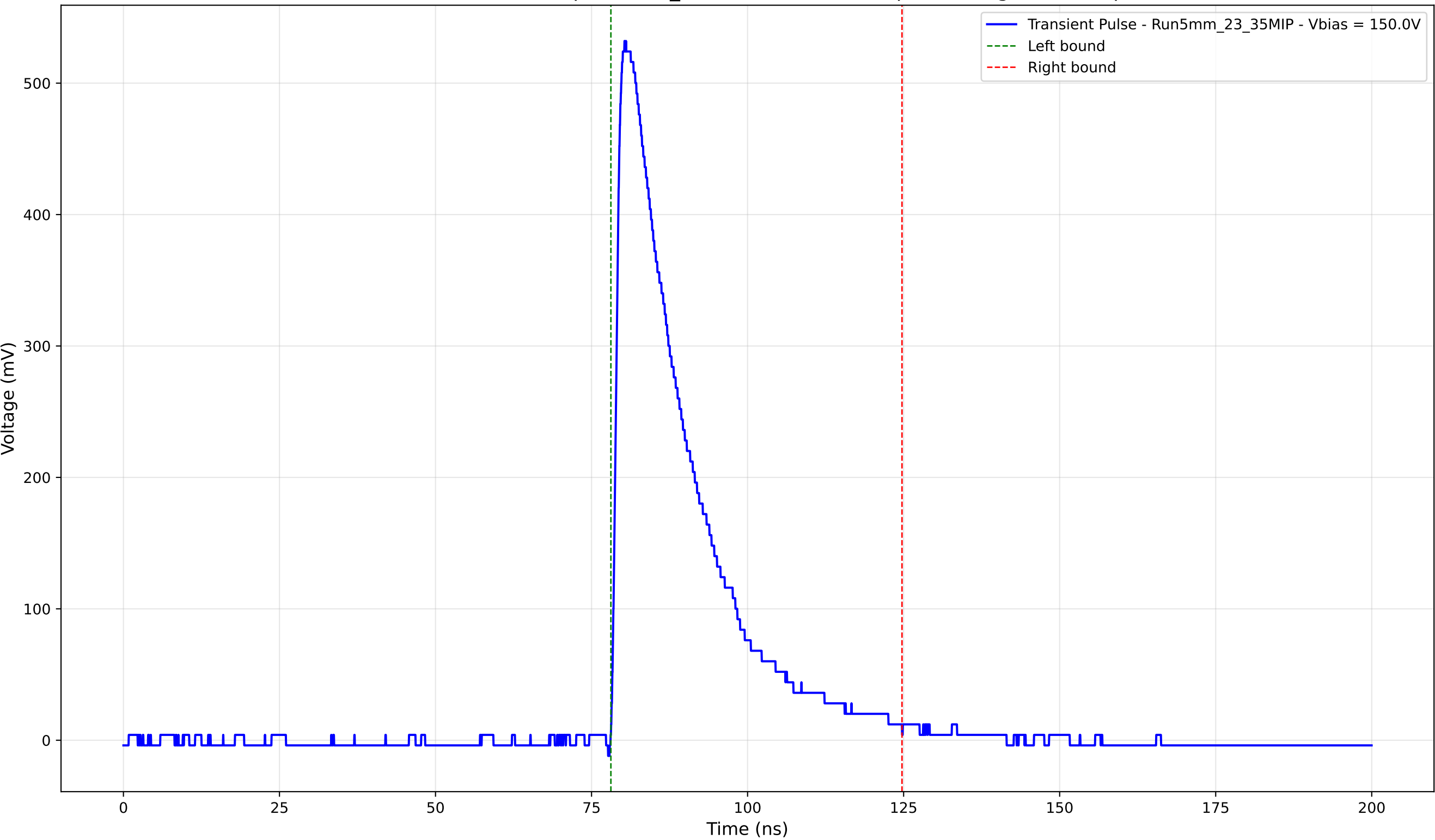
Transient Pulse - Sample: 5mm_23 - Position: 1810.0 \mu\text{m} - Charge: 134.97 pC
