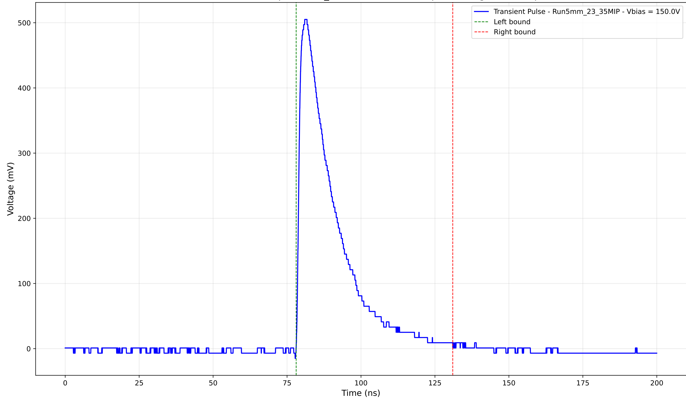
Transient Pulse - Sample: 5mm_23 - Position: 2355.0 \mu\text{m} - Charge: 134.98 pC
