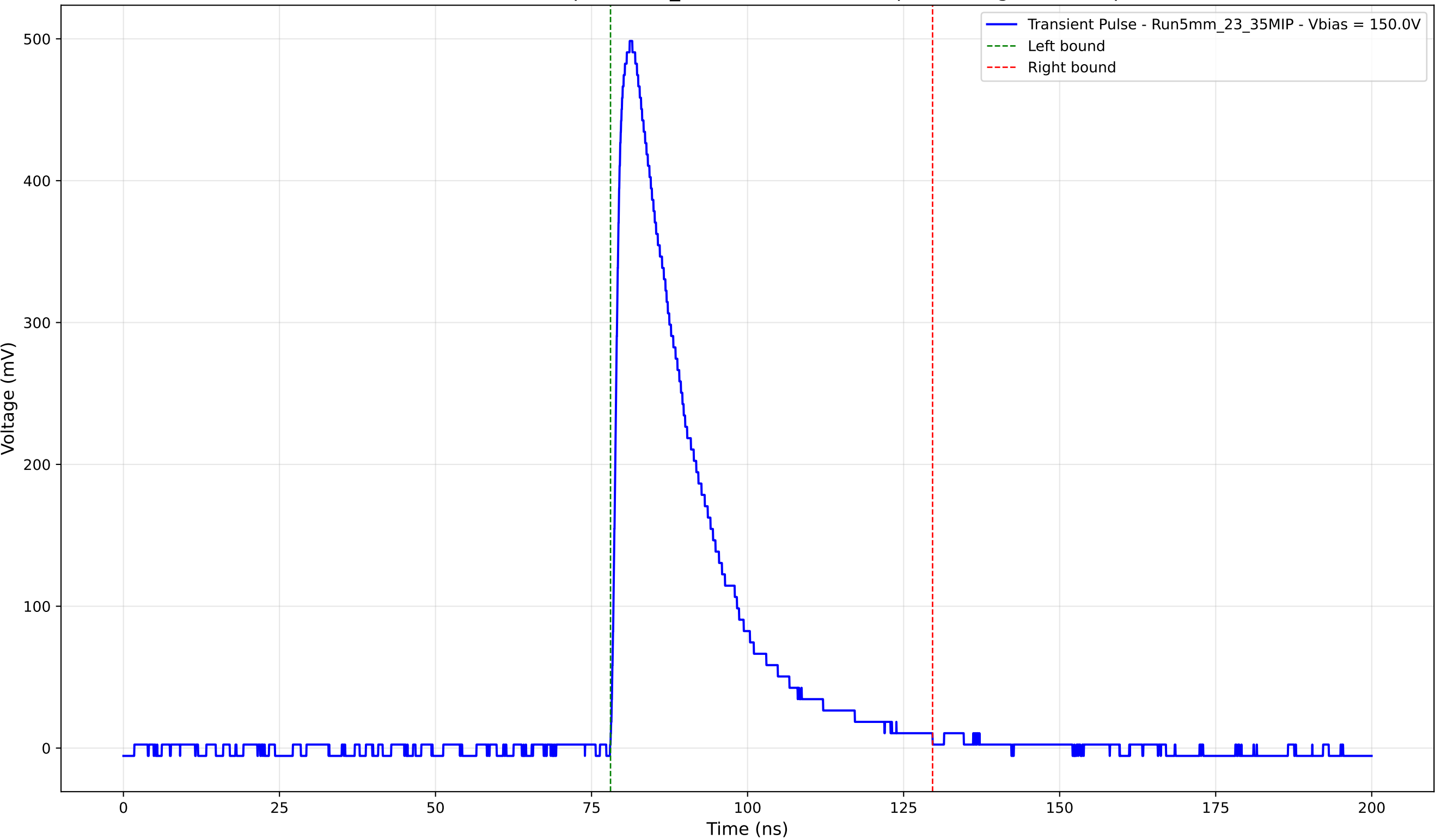
Transient Pulse - Sample: 5mm_23 - Position: 2540.0 \mu\text{m} - Charge: 134.02 pC
