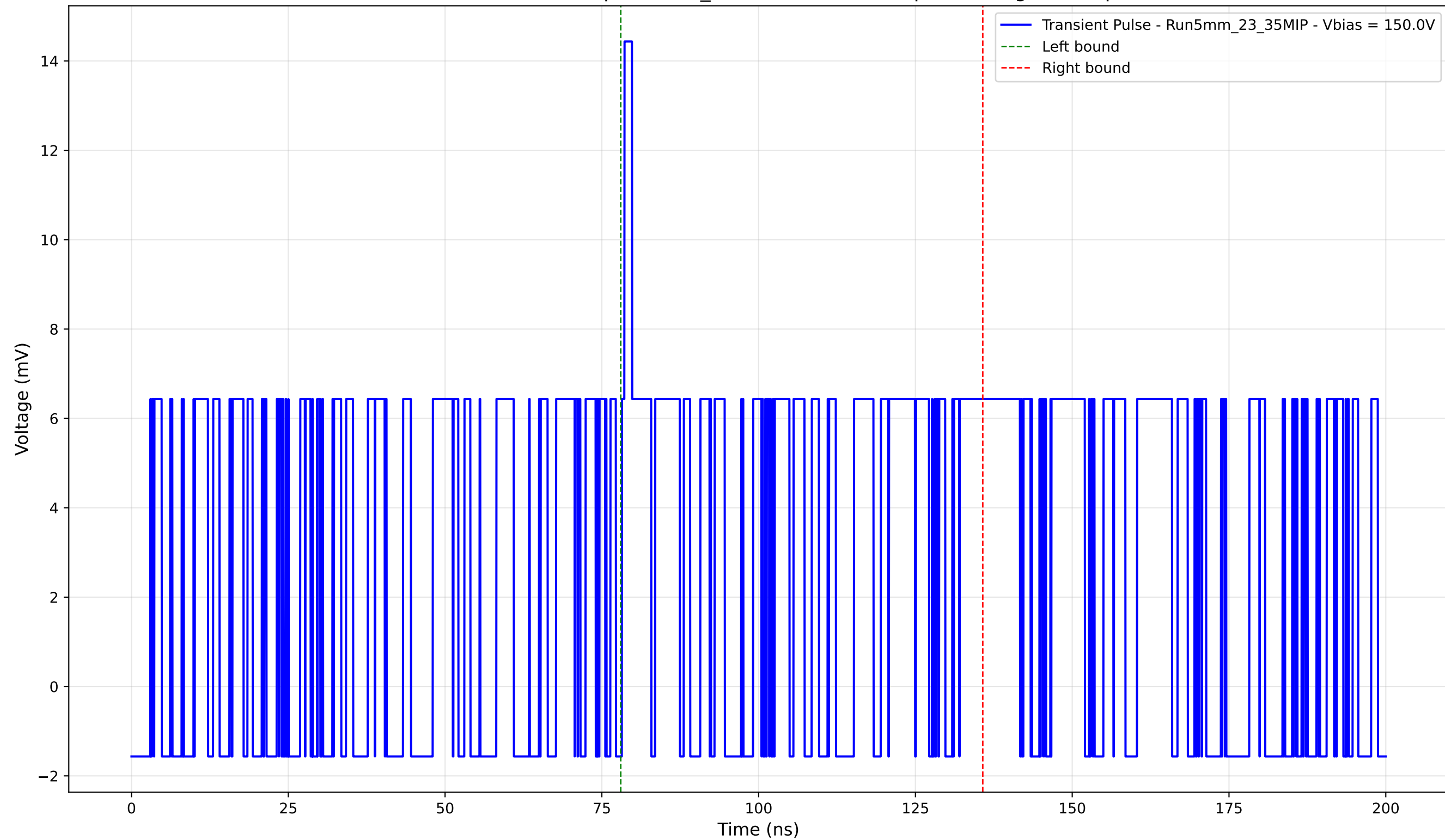
Transient Pulse - Sample: 5mm_23 - Position: 100.0 \mu\text{m} - Charge: 4.57 pC
