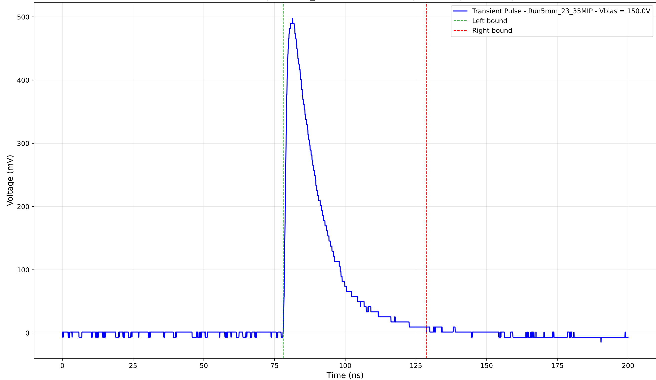
Transient Pulse - Sample: 5mm_23 - Position: 2960.0 \mu\text{m} - Charge: 130.82 pC
