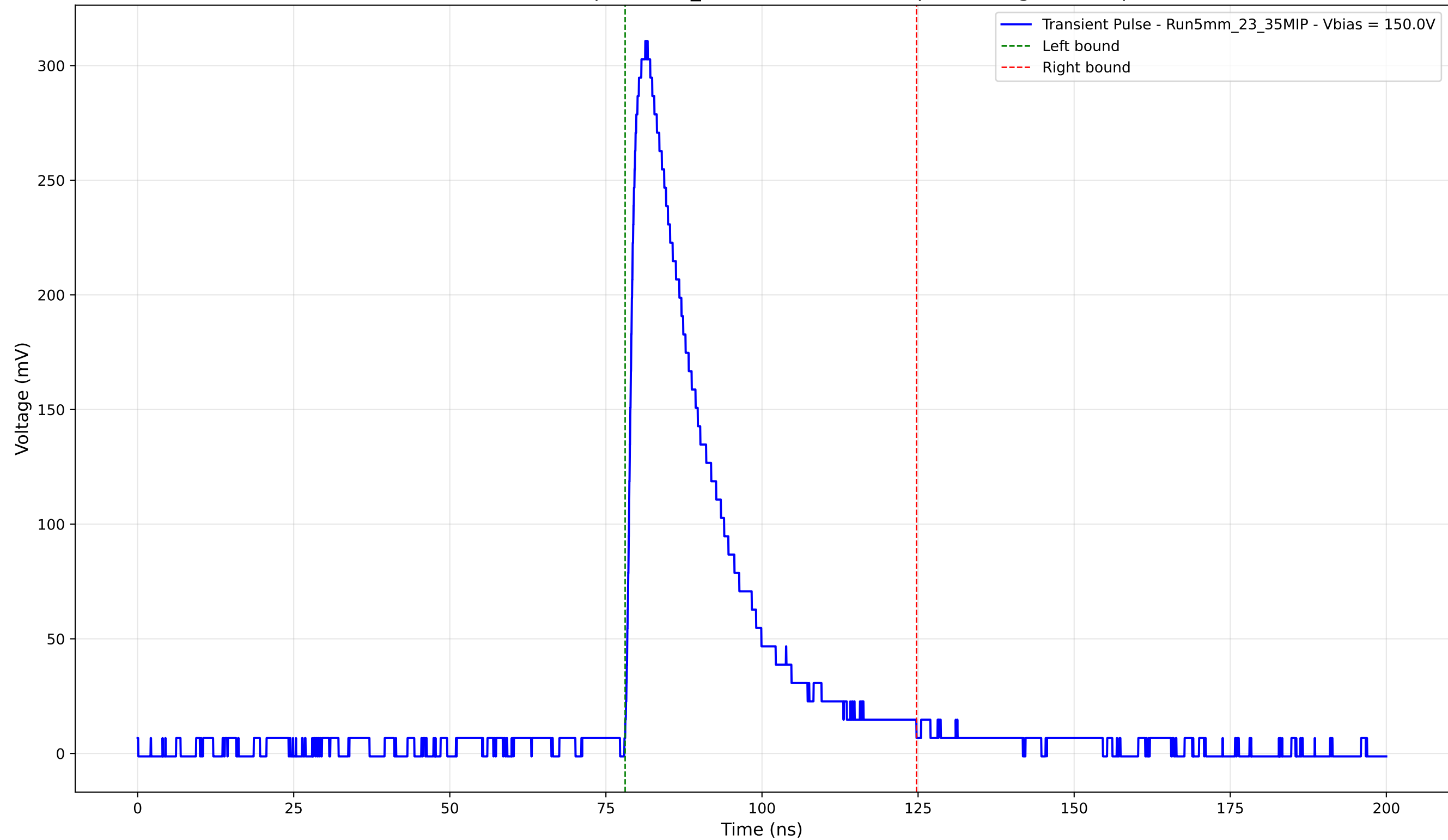
Transient Pulse - Sample: 5mm_23 - Position: 2595.0 \mu\text{m} - Charge: 83.30 pC
