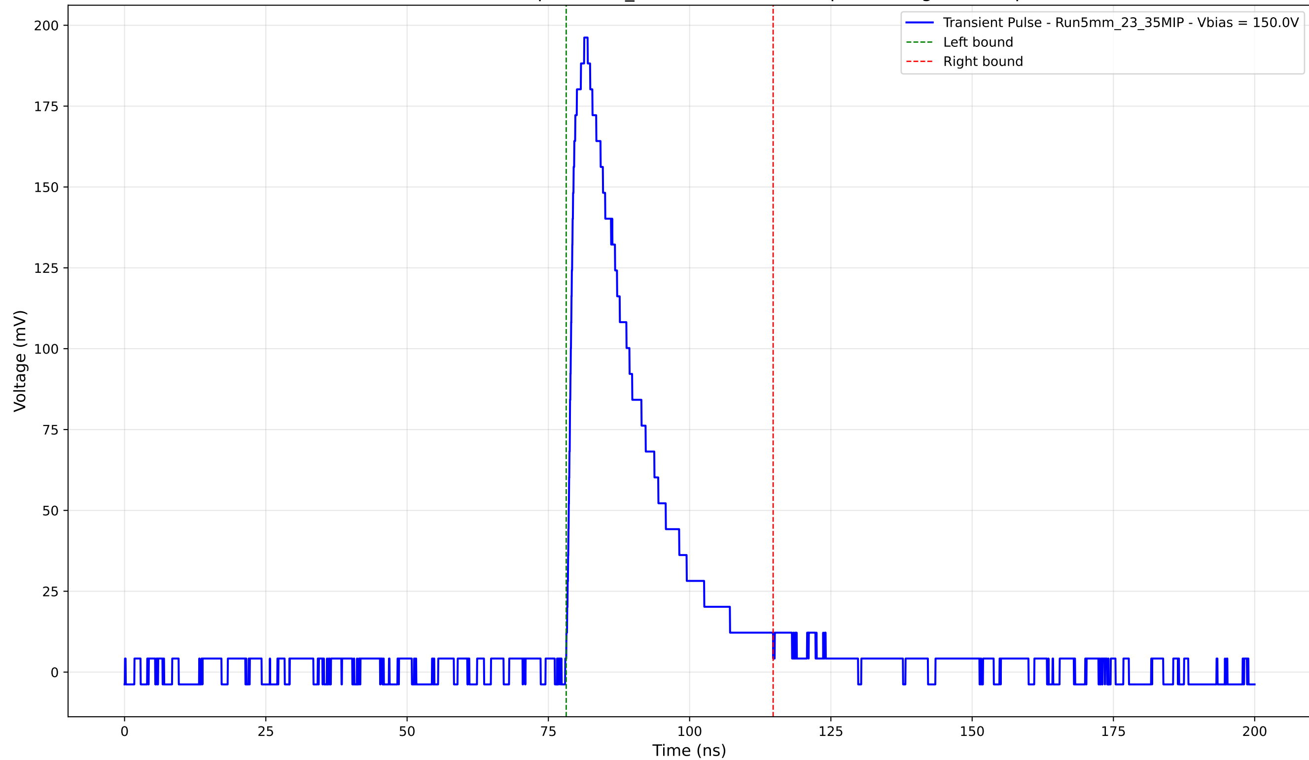
Transient Pulse - Sample: 5mm_23 - Position: 2680.0 \mu\text{m} - Charge: 49.60 pC
