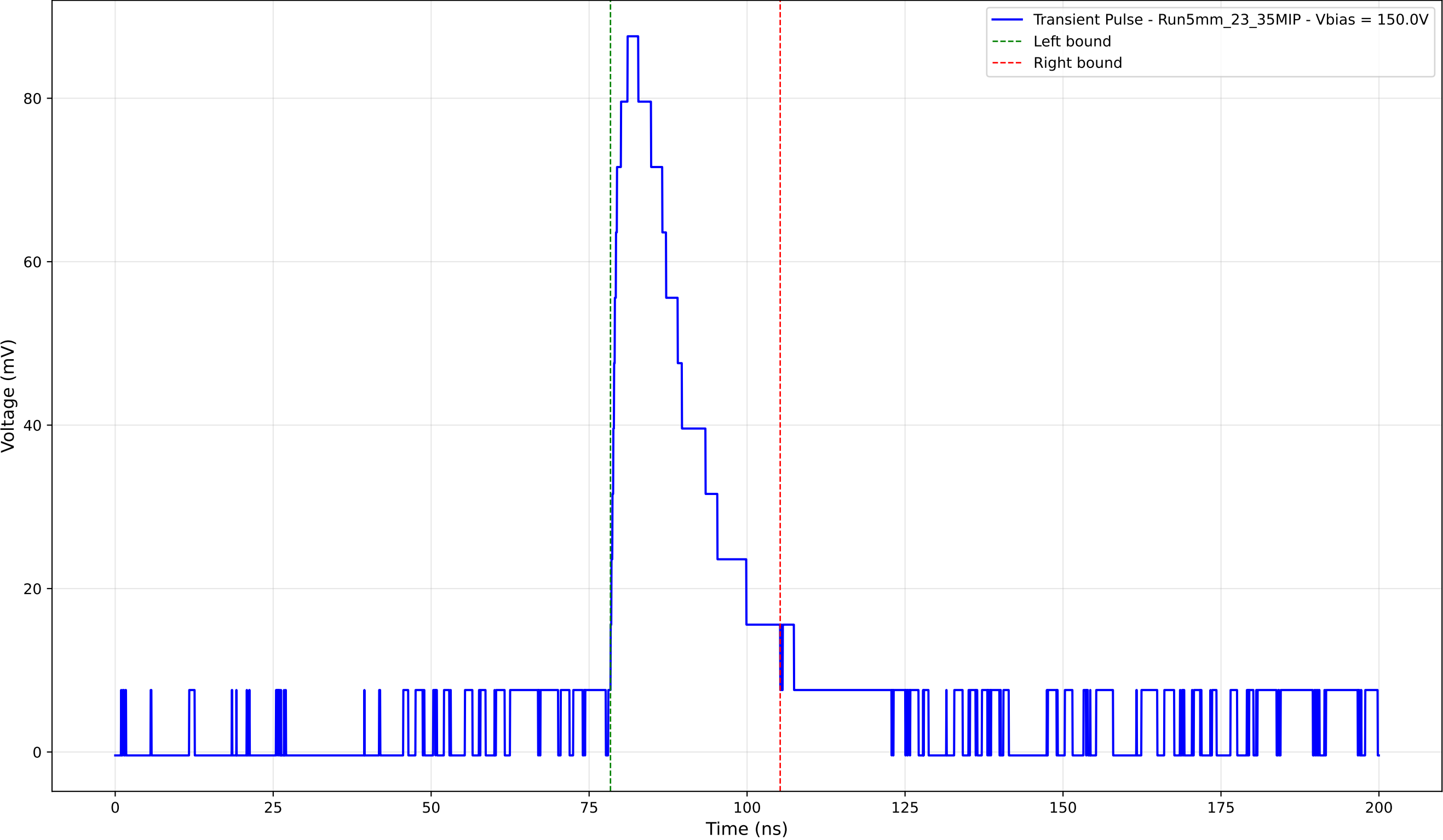
Transient Pulse - Sample: 5mm_23 - Position: 2645.0 \mu\text{m} - Charge: 23.55 pC
