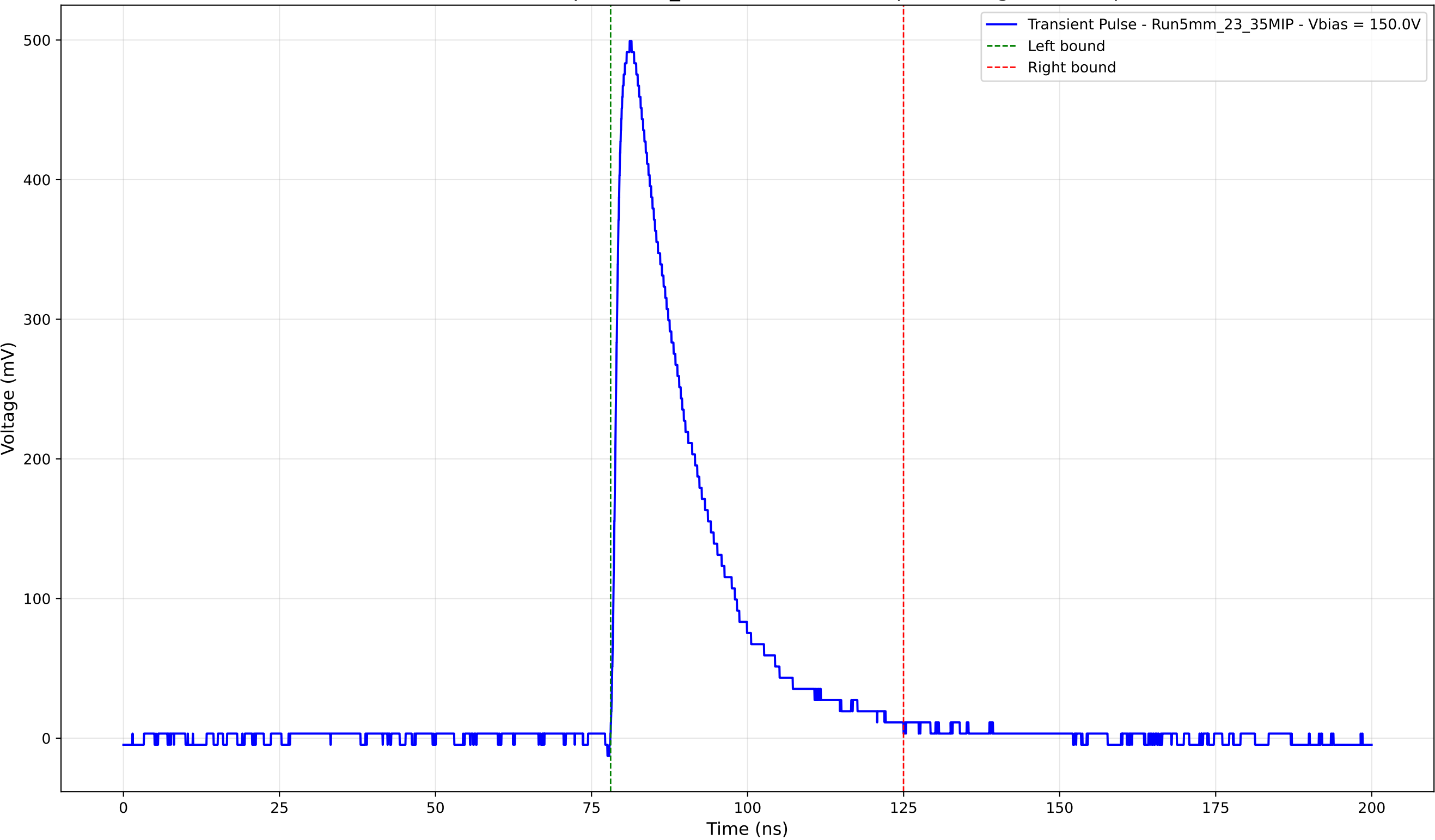
Transient Pulse - Sample: 5mm_23 - Position: 2995.0 \mu\text{m} - Charge: 130.53 pC
