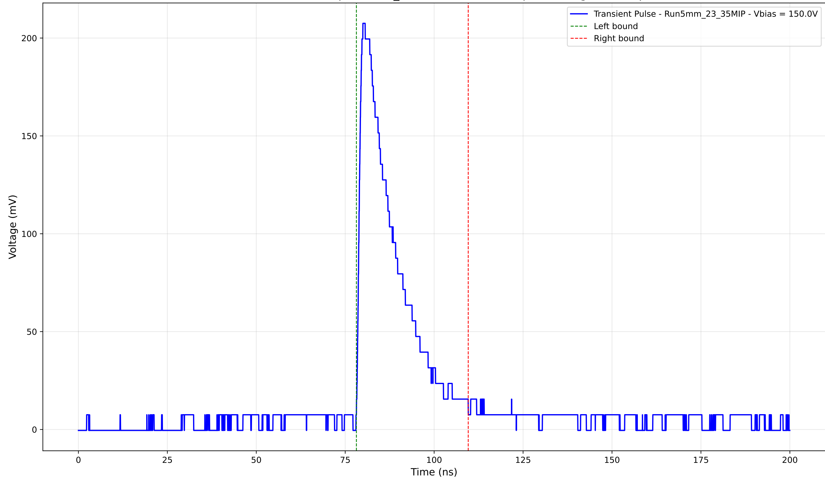
Transient Pulse - Sample: 5mm_23 - Position: 3620.0 \mu\text{m} - Charge: 47.51 pC
