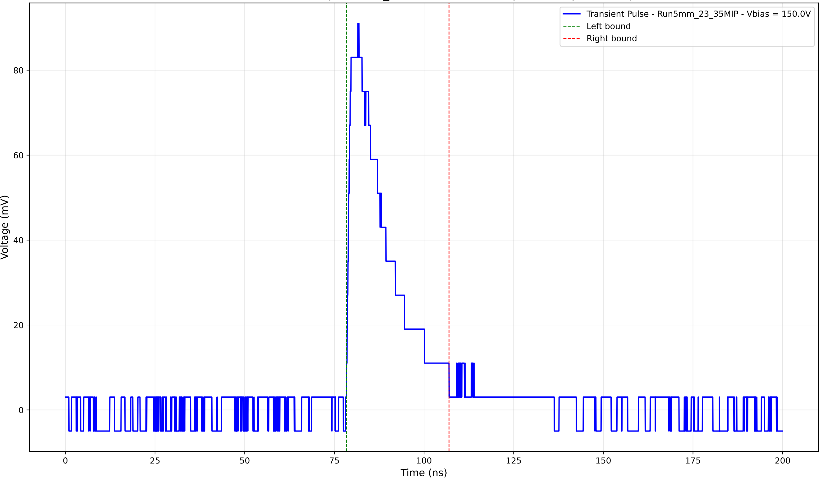
Transient Pulse - Sample: 5mm_23 - Position: 1625.0 \mu\text{m} - Charge: 21.05 pC
