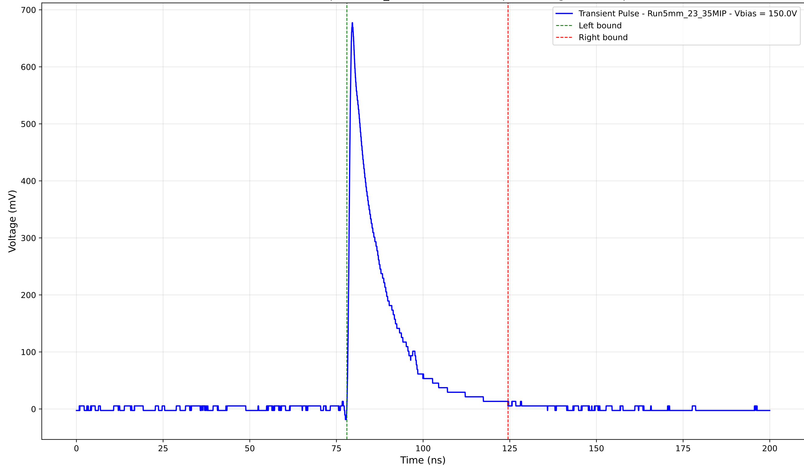
Transient Pulse - Sample: 5mm_23 - Position: 900.0 \mu\text{m} - Charge: 125.84 pC
