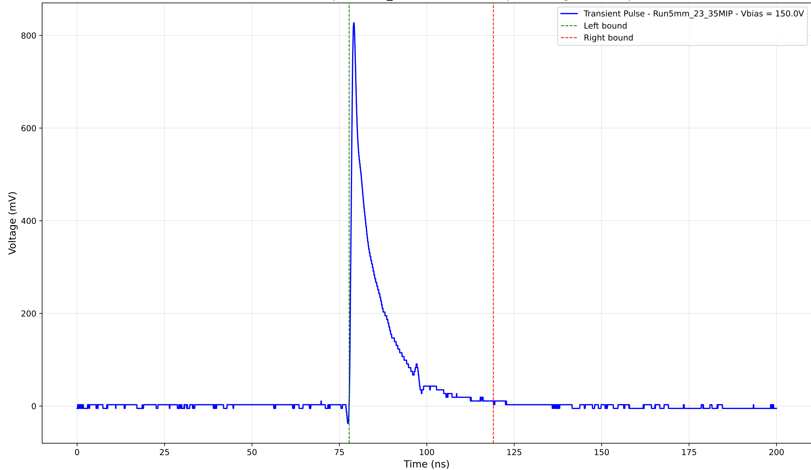
Transient Pulse - Sample: 5mm_23 - Position: 410.0 \mu\text{m} - Charge: 114.18 pC
