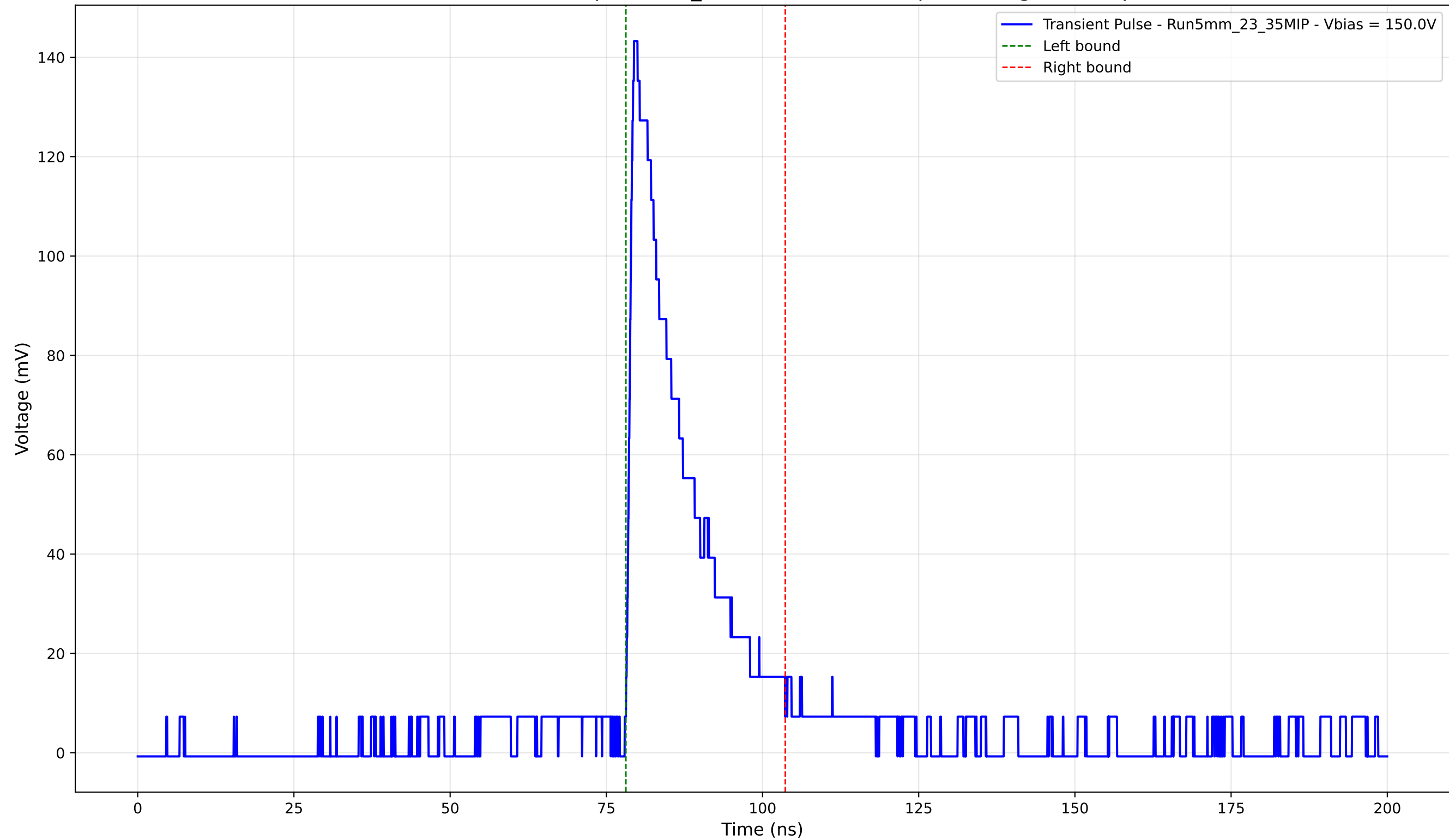
Transient Pulse - Sample: 5mm_23 - Position: 4175.0 \mu\text{m} - Charge: 27.23 pC
