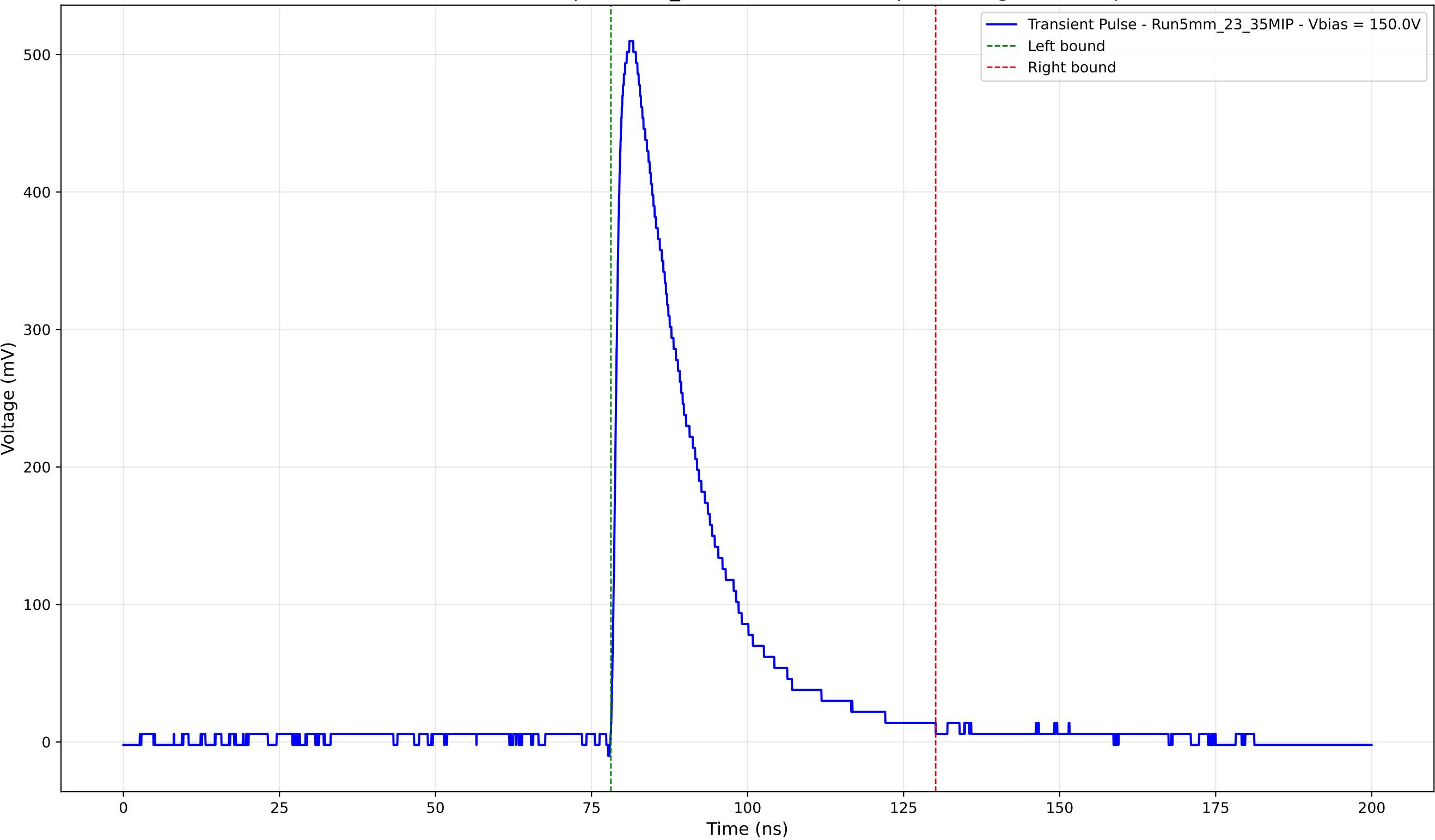
Transient Pulse - Sample: 5mm_23 - Position: 2495.0 \mu\text{m} - Charge: 138.14 pC
