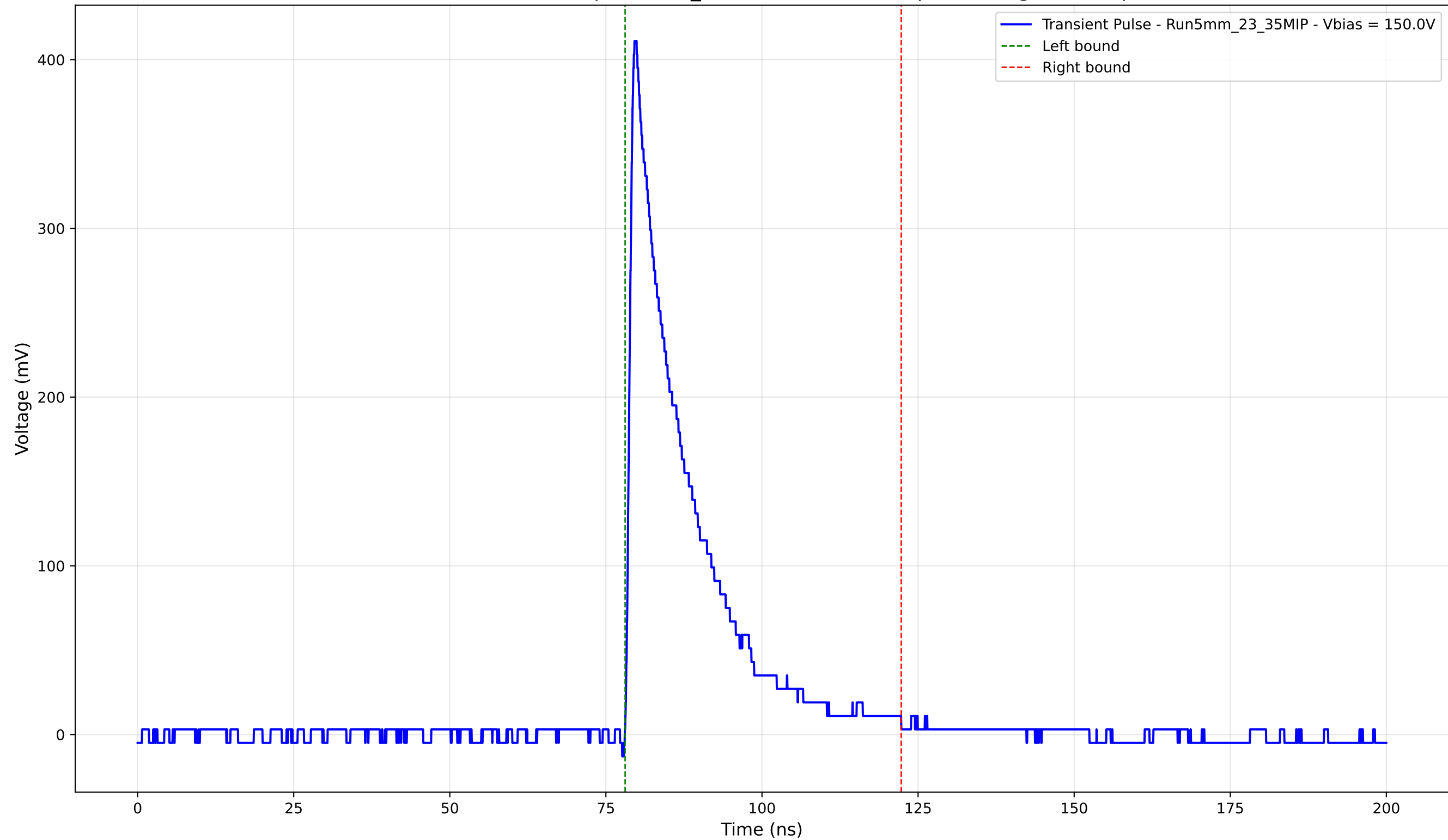
Transient Pulse - Sample: 5mm_23 - Position: 1070.0 \mu\text{m} - Charge: 78.73 pC
