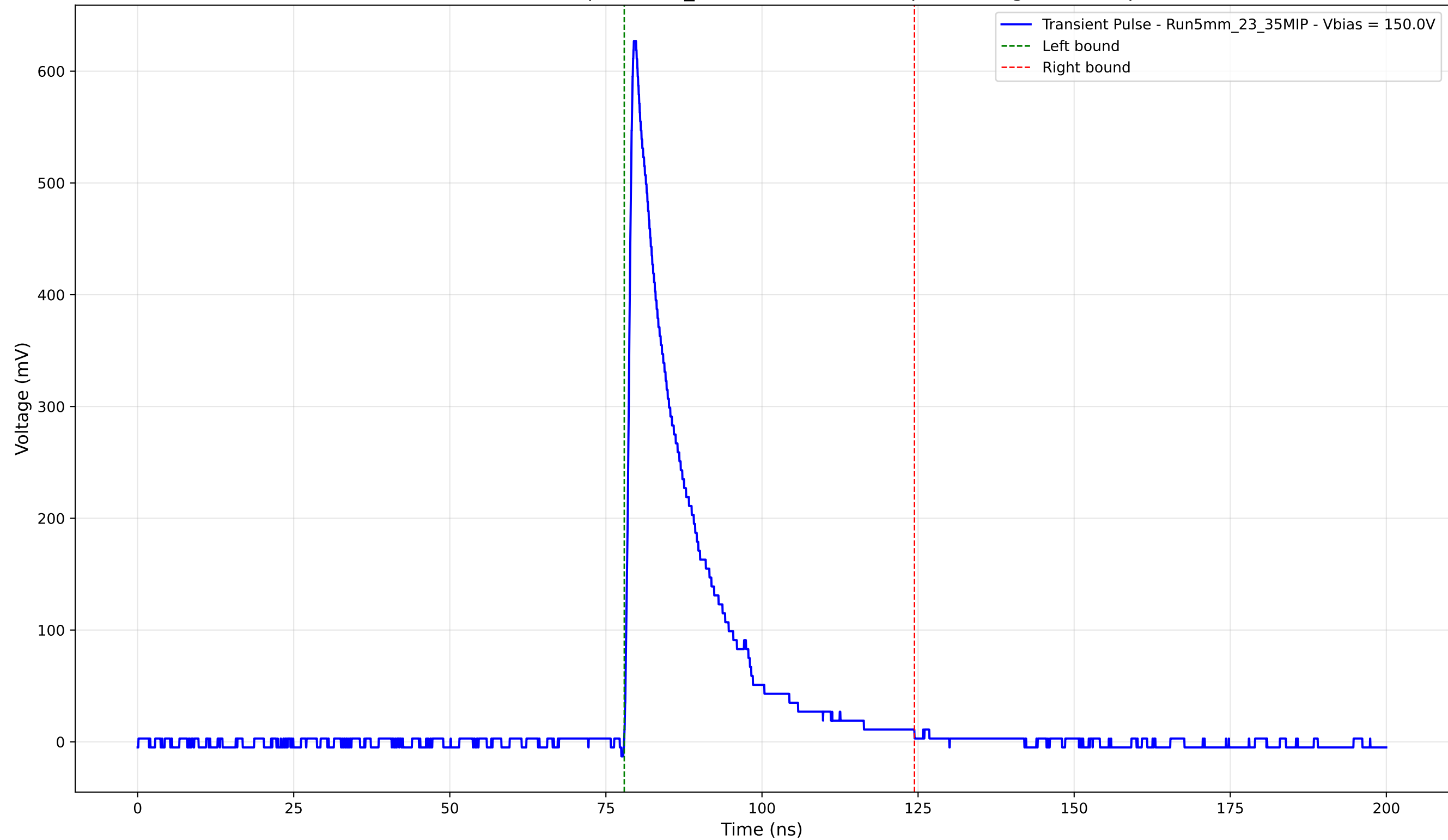
Transient Pulse - Sample: 5mm_23 - Position: 4305.0 \mu\text{m} - Charge: 115.97 pC
