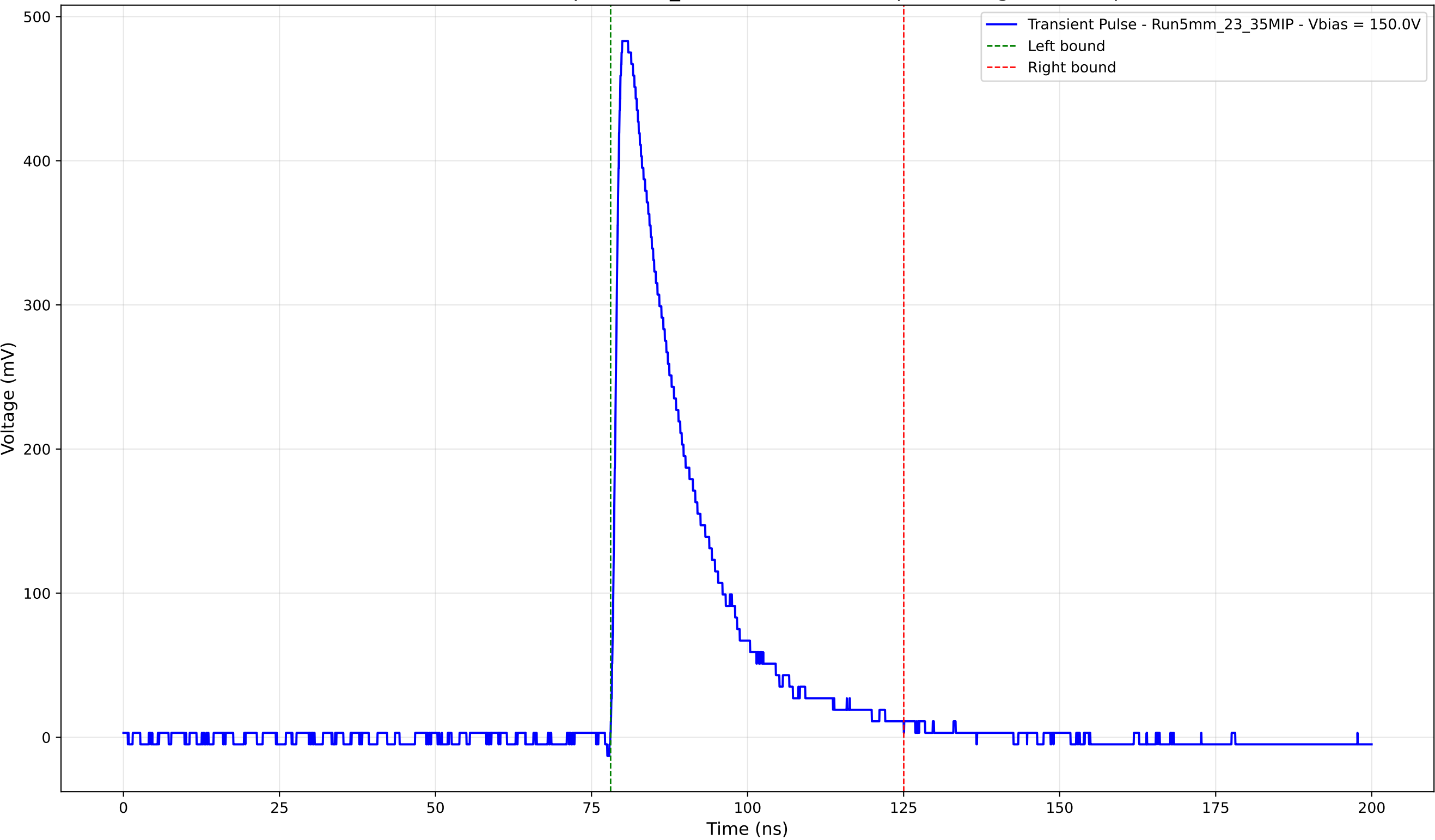
Transient Pulse - Sample: 5mm_23 - Position: 3565.0 \mu\text{m} - Charge: 117.43 pC
