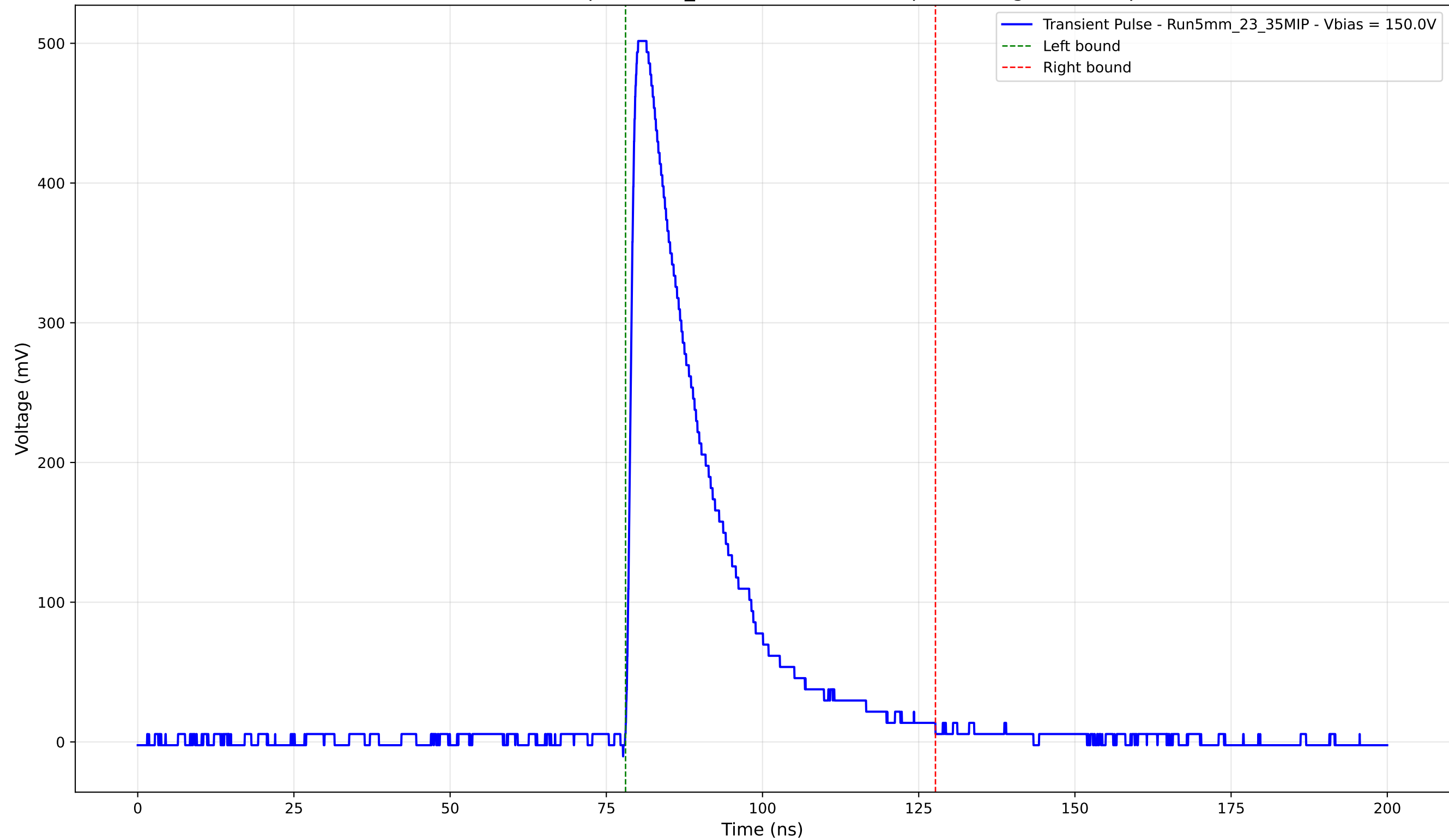
Transient Pulse - Sample: 5mm_23 - Position: 3440.0 \mu\text{m} - Charge: 129.67 pC
