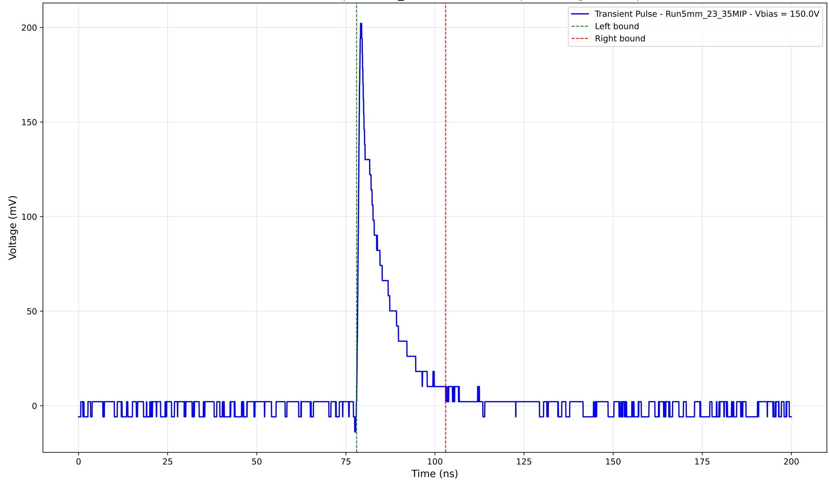
Transient Pulse - Sample: 5mm_23 - Position: 600.0 \mu\text{m} - Charge: 26.89 pC
