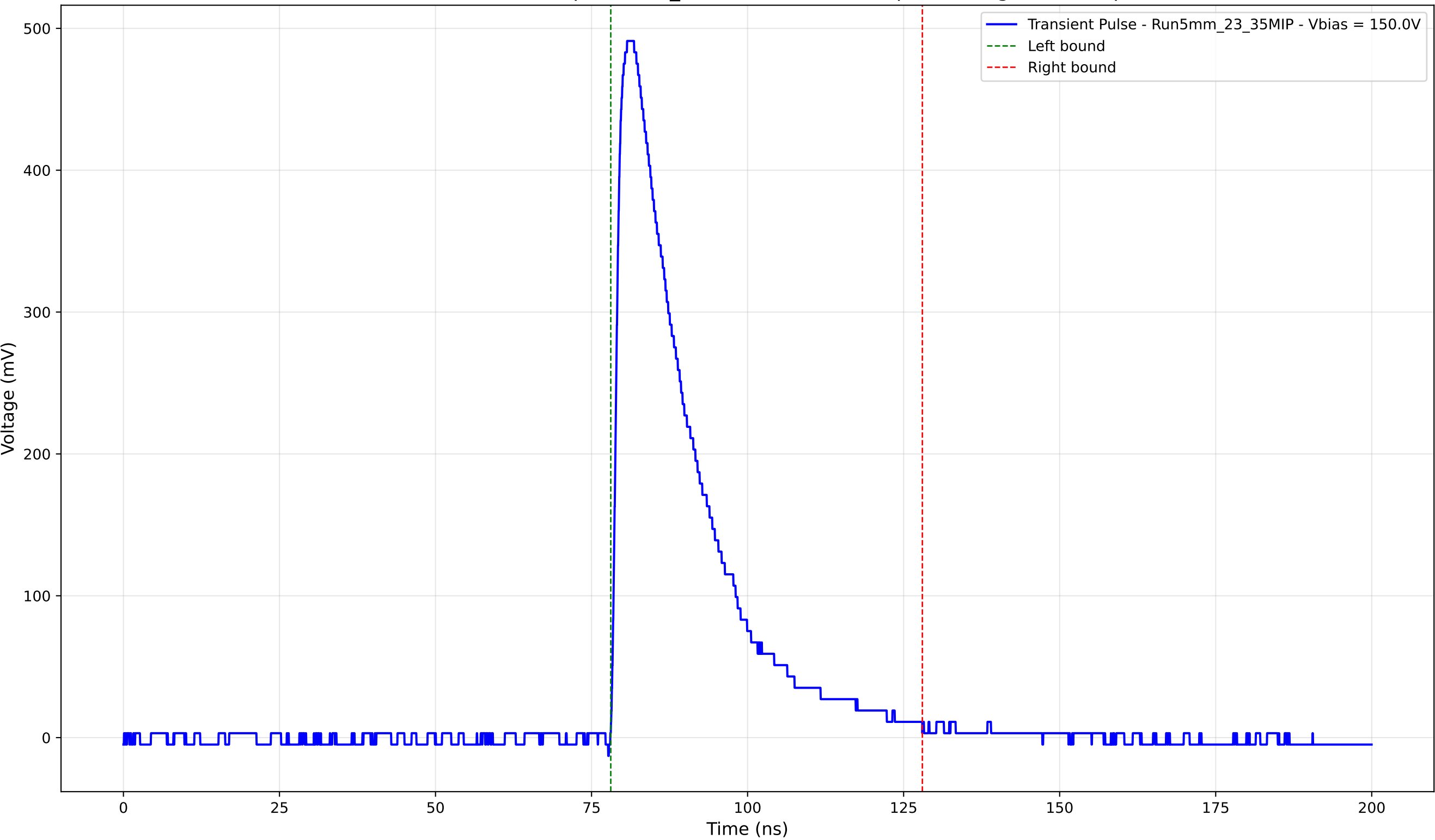
Transient Pulse - Sample: 5mm_23 - Position: 2950.0 \mu\text{m} - Charge: 132.11 pC
