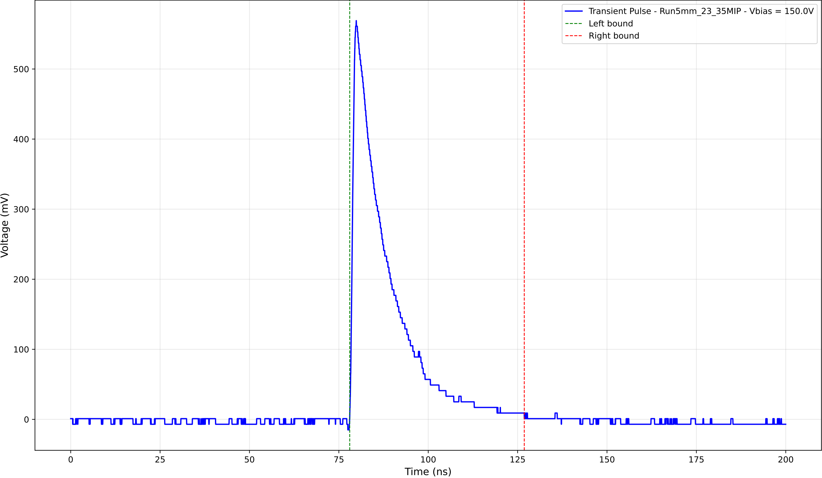
Transient Pulse - Sample: 5mm_23 - Position: 3995.0 \mu\text{m} - Charge: 118.12 pC
