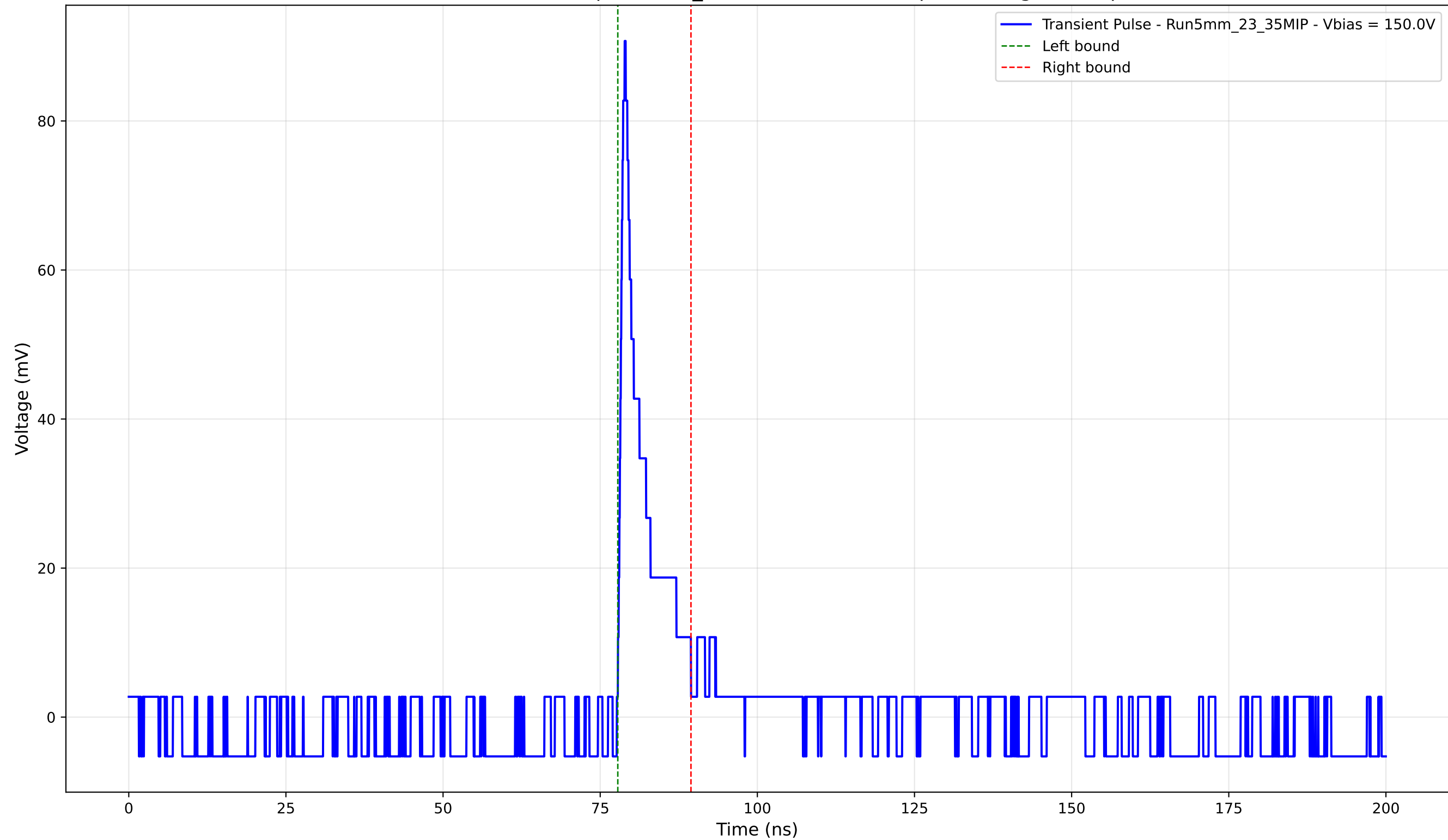
Transient Pulse - Sample: 5mm_23 - Position: 5110.0 \mu\text{m} - Charge: 6.98 pC
