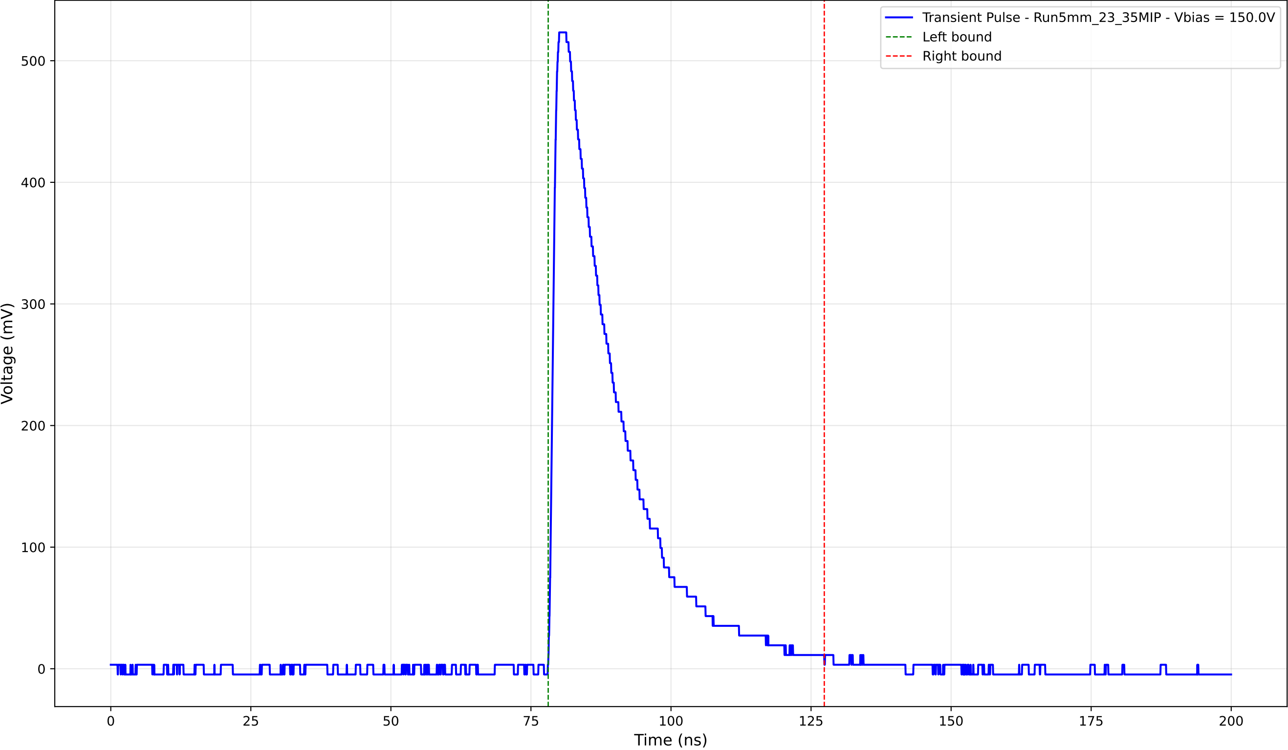
Transient Pulse - Sample: 5mm_23 - Position: 1805.0 \mu\text{m} - Charge: 134.36 pC
