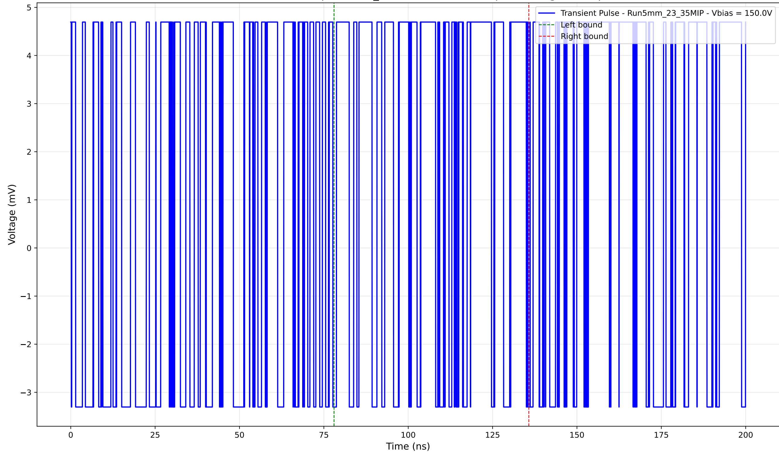
Transient Pulse - Sample: 5mm_23 - Position: 5300.0 \mu\text{m} - Charge: 2.76 pC
