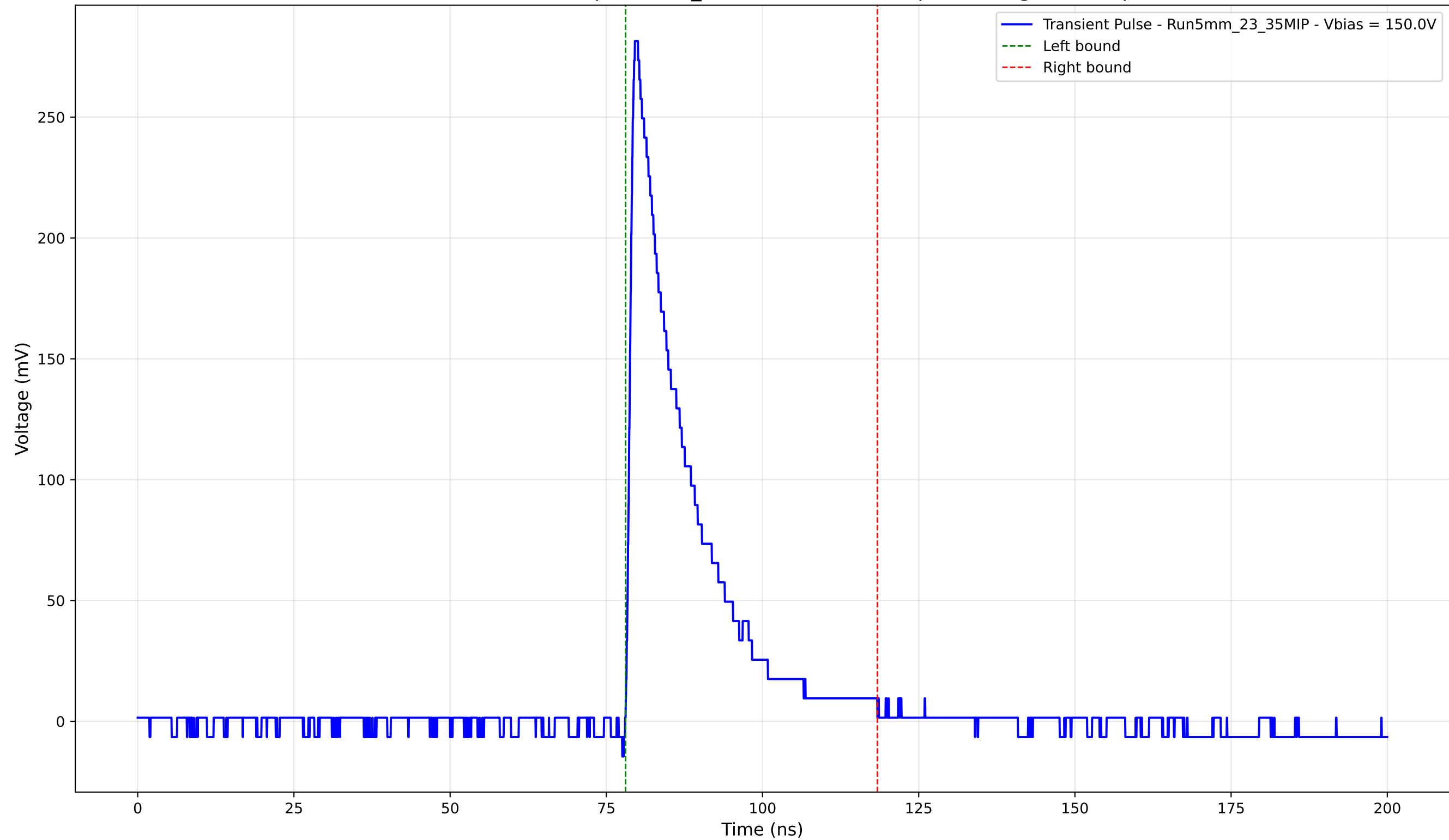
Transient Pulse - Sample: 5mm_23 - Position: 4115.0 \mu\text{m} - Charge: 53.67 pC
