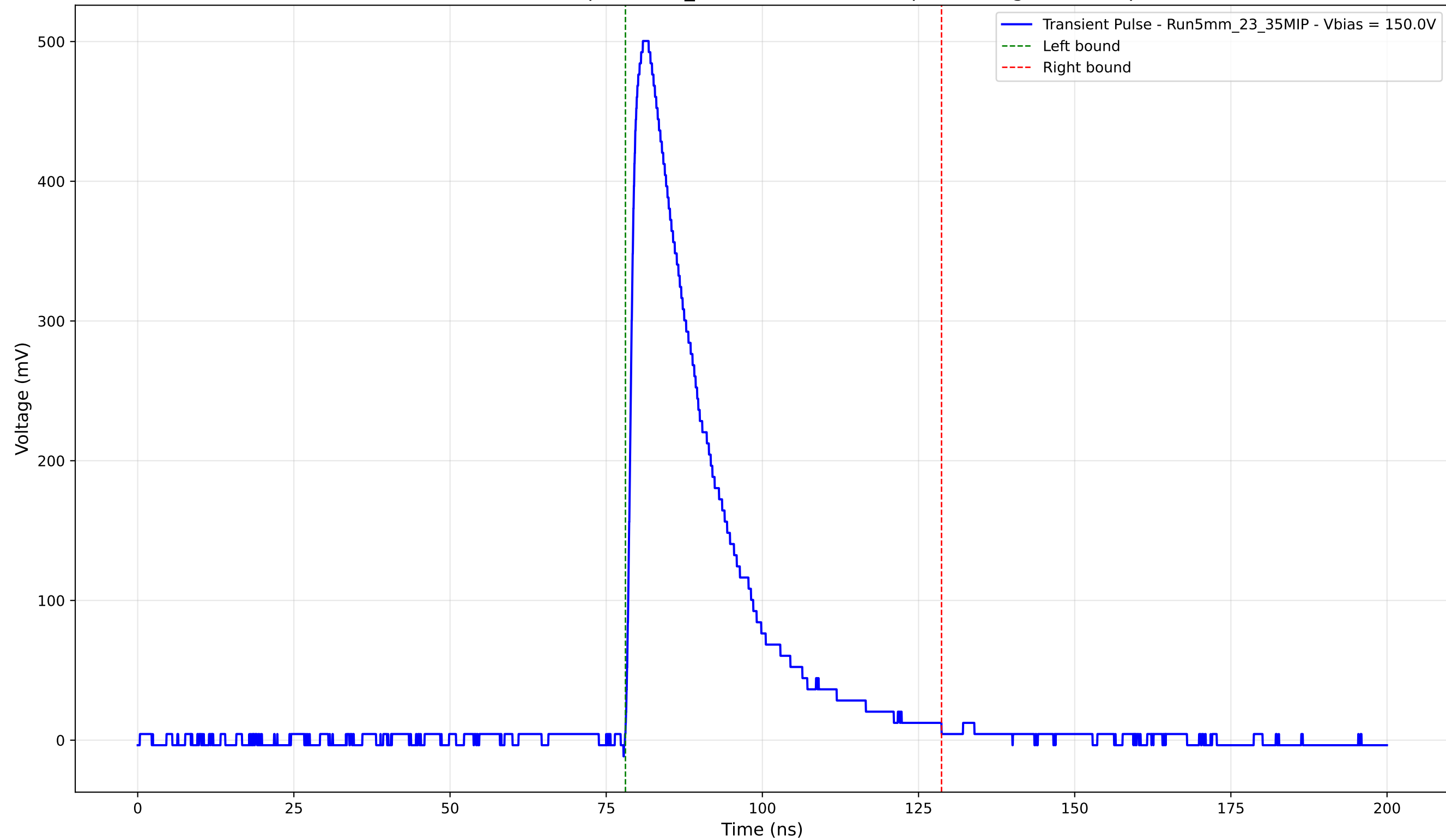
Transient Pulse - Sample: 5mm_23 - Position: 2850.0 \mu\text{m} - Charge: 135.04 pC
