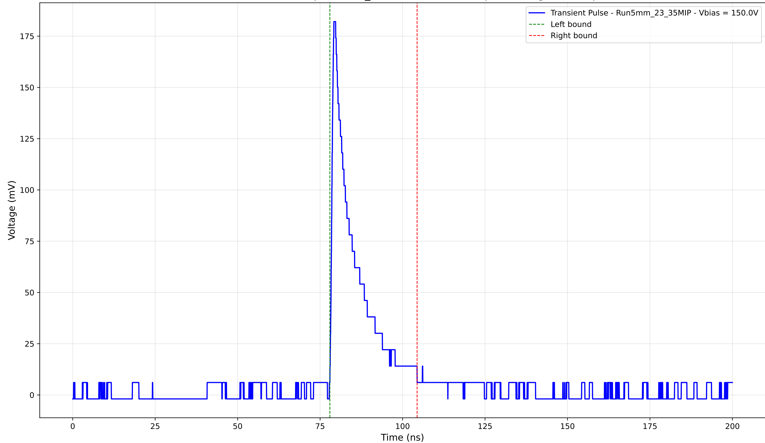
Transient Pulse - Sample: 5mm_23 - Position: 4535.0 \mu\text{m} - Charge: 27.44 pC
