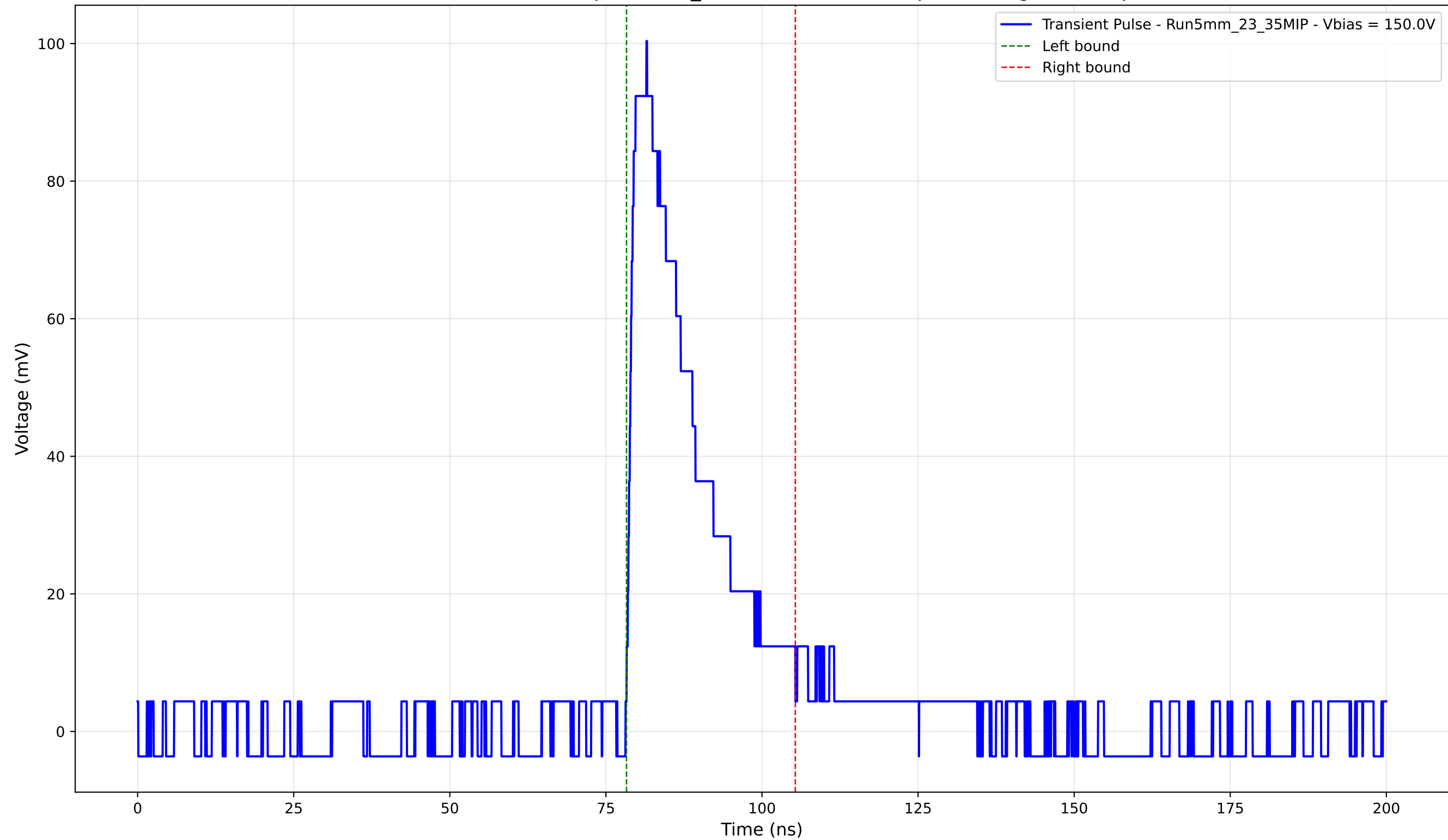
Transient Pulse - Sample: 5mm_23 - Position: 3645.0 \mu\text{m} - Charge: 22.40 pC
