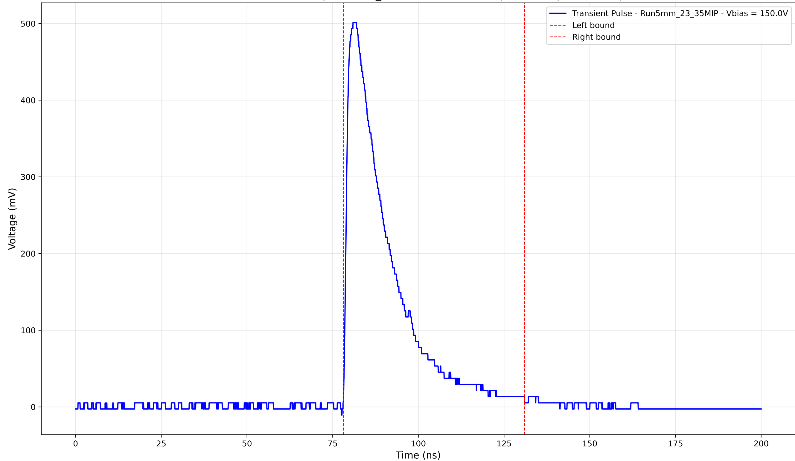
Transient Pulse - Sample: 5mm_23 - Position: 2380.0 \mu\text{m} - Charge: 137.41 pC
