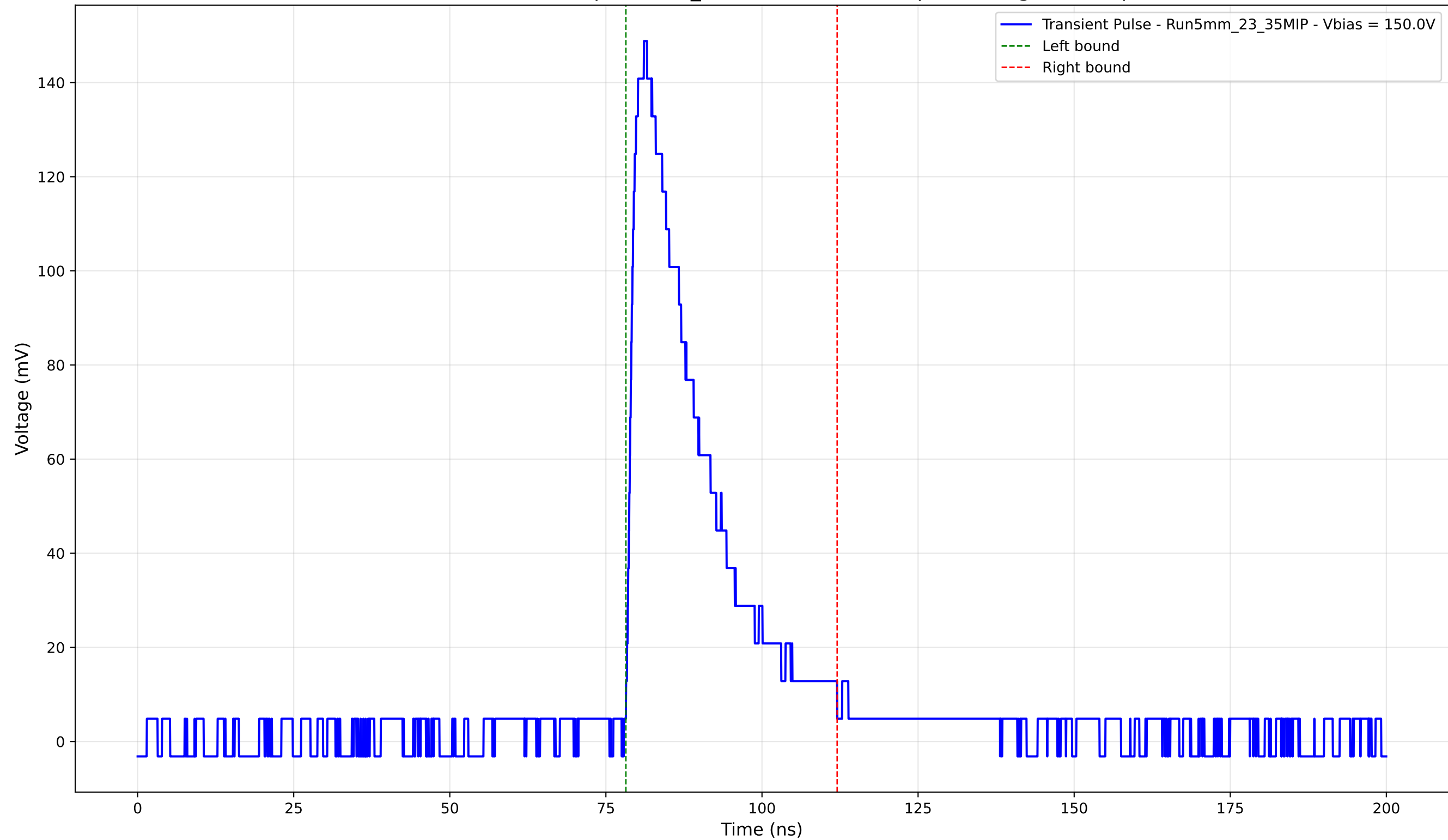
Transient Pulse - Sample: 5mm_23 - Position: 2115.0 \mu\text{m} - Charge: 36.35 pC
