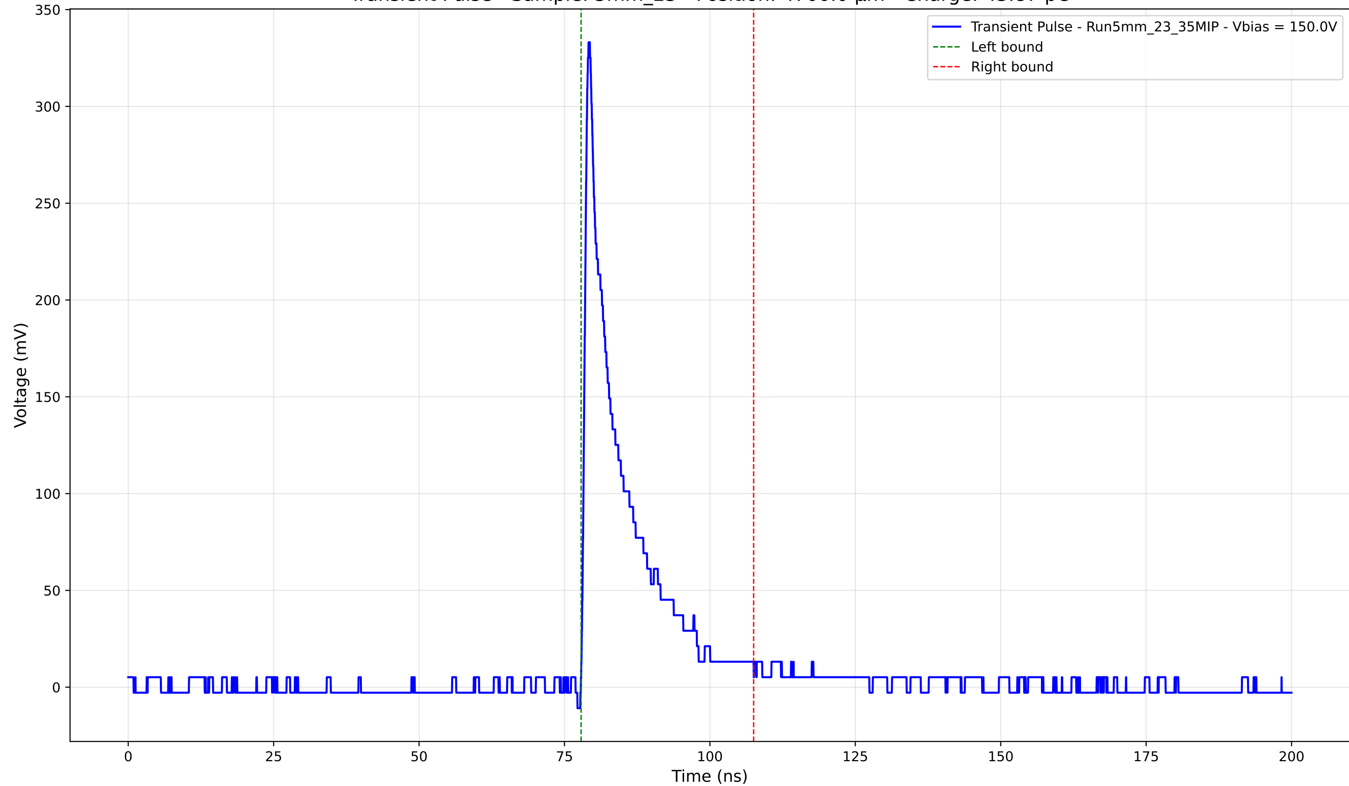
Transient Pulse - Sample: 5mm_23 - Position: 4700.0 \mu\text{m} - Charge: 43.87 pC
