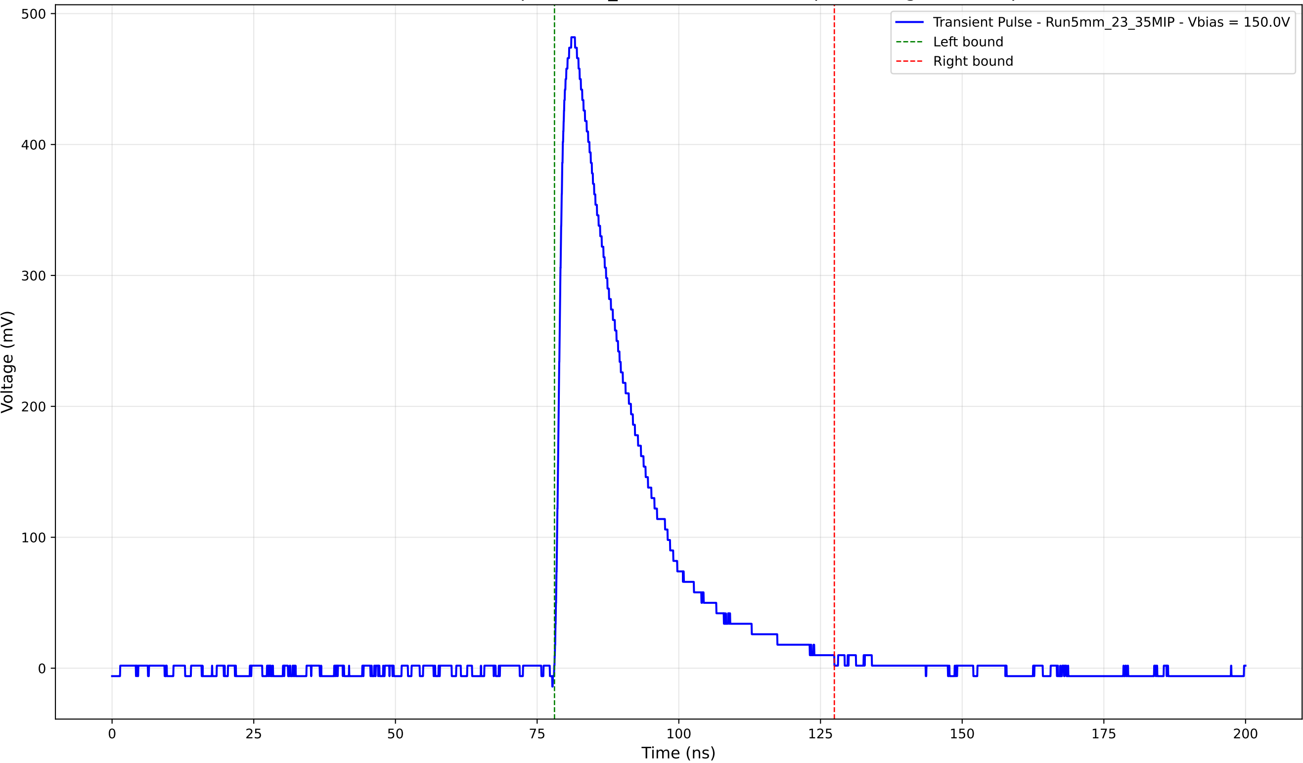
Transient Pulse - Sample: 5mm_23 - Position: 2745.0 \mu\text{m} - Charge: 129.44 pC
