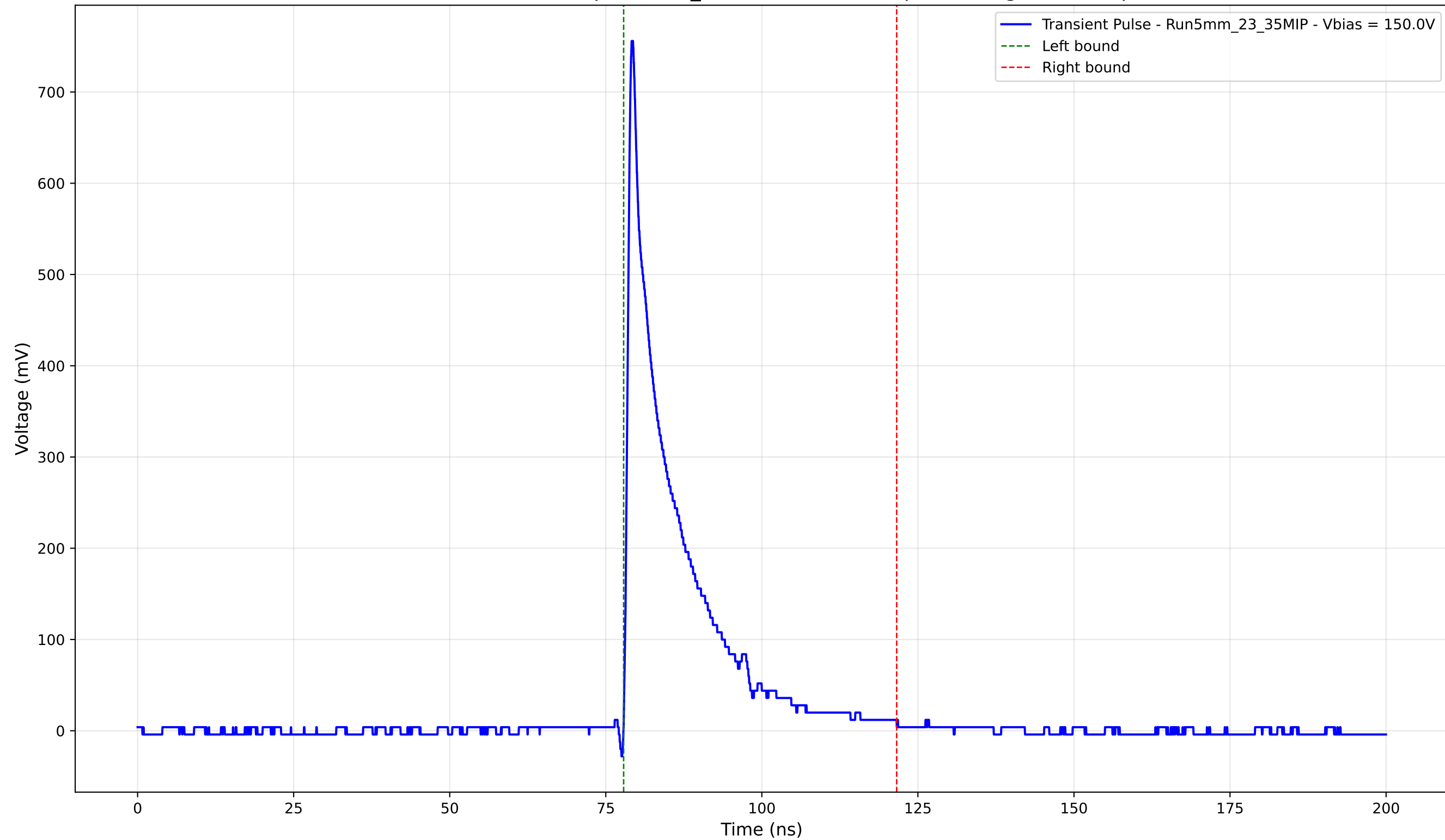
Transient Pulse - Sample: 5mm_23 - Position: 530.0 \mu\text{m} - Charge: 111.56 pC
