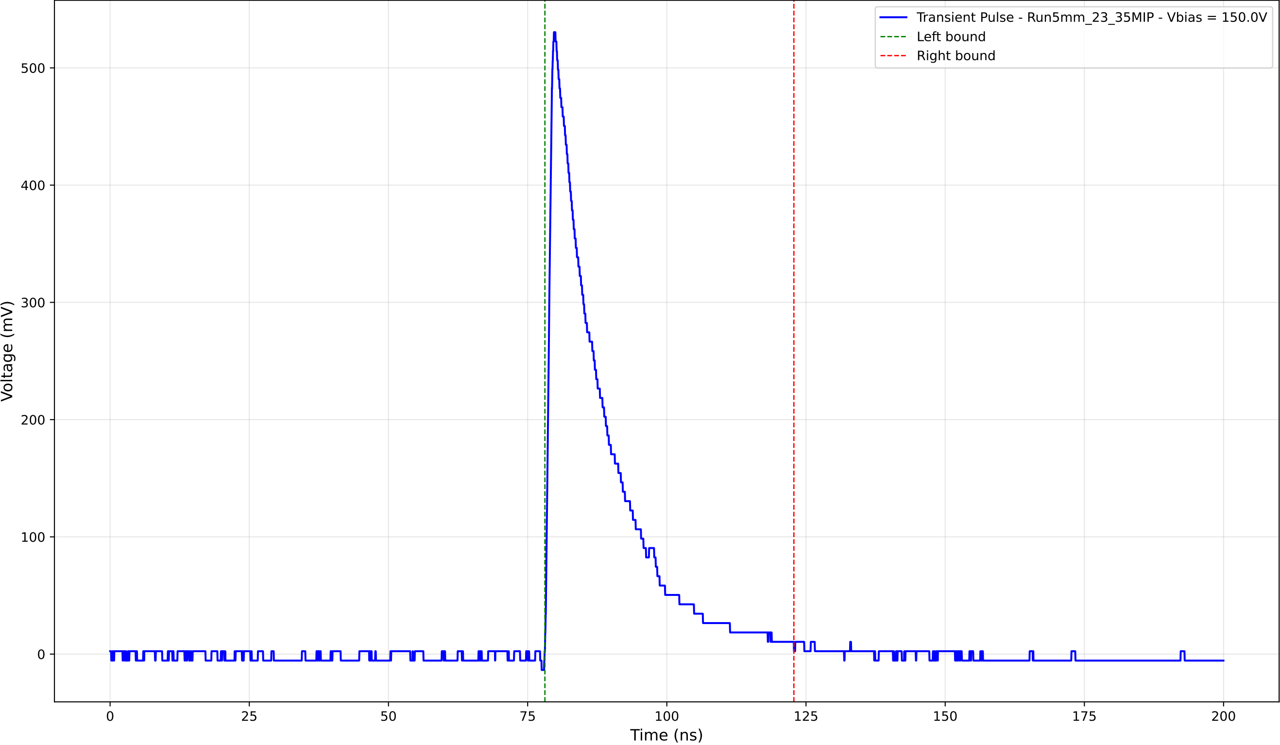
Transient Pulse - Sample: 5mm_23 - Position: 1205.0 \mu\text{m} - Charge: 110.11 pC
