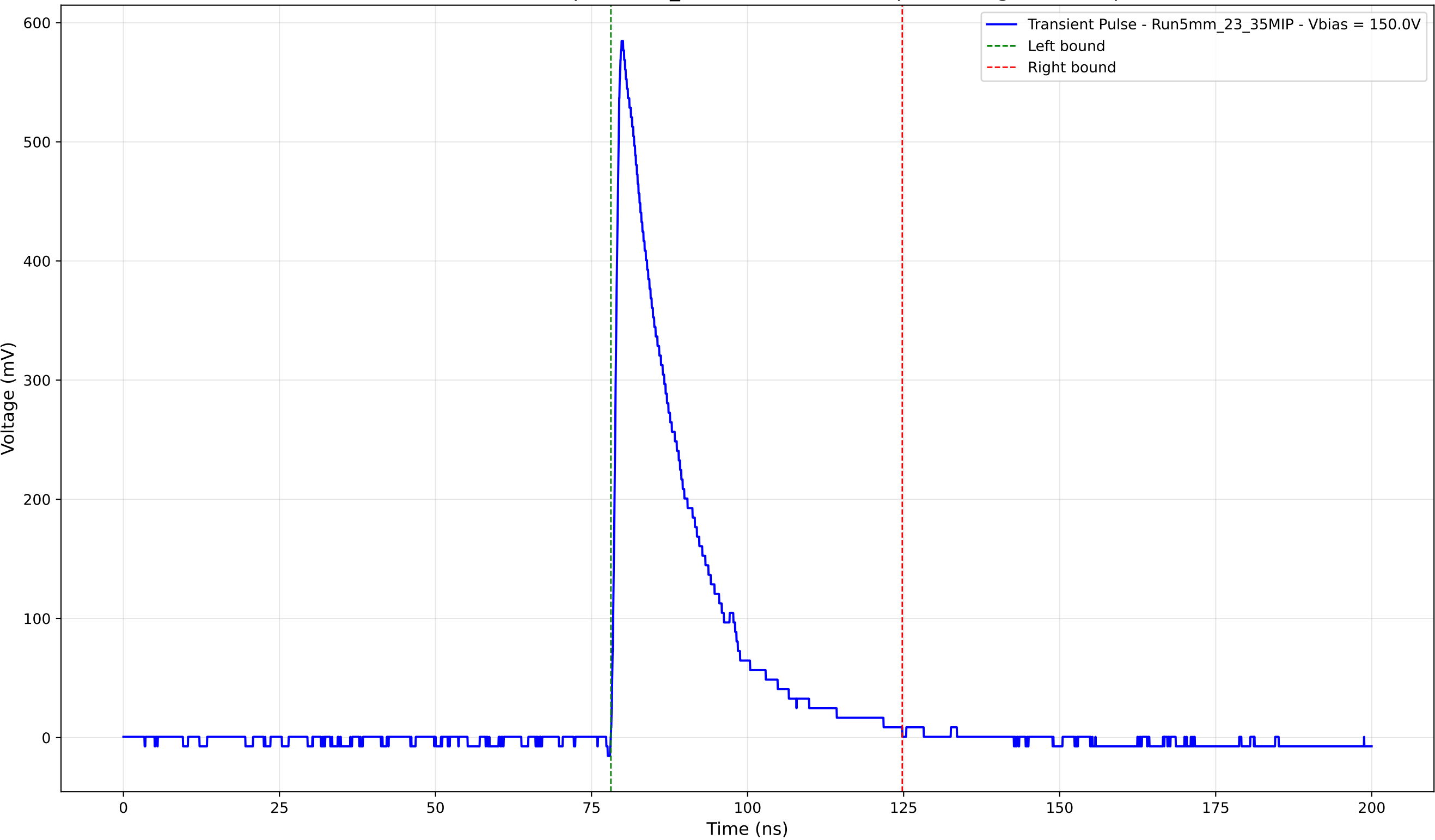
Transient Pulse - Sample: 5mm_23 - Position: 1305.0 \mu\text{m} - Charge: 126.28 pC
