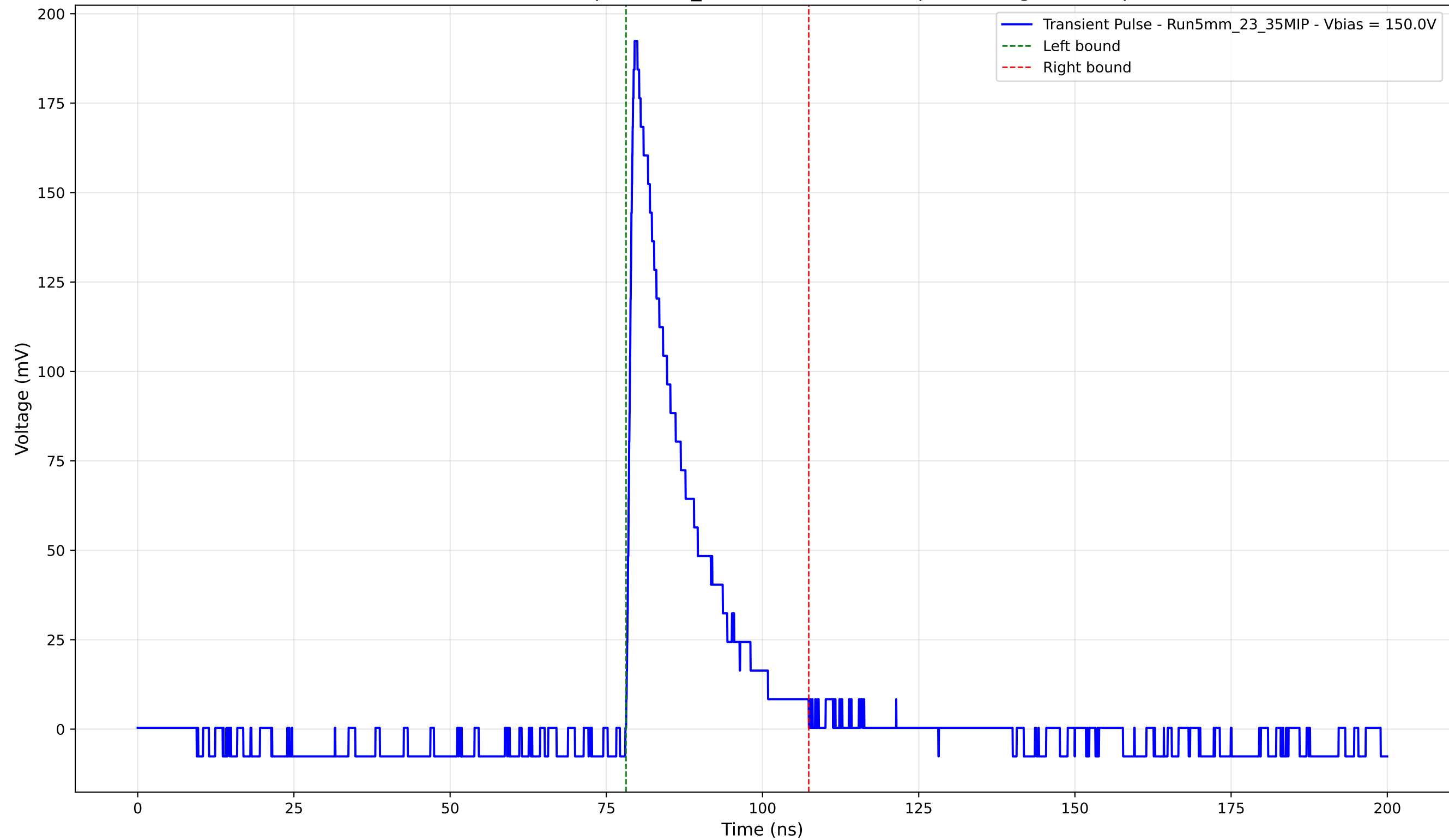
Transient Pulse - Sample: 5mm_23 - Position: 4185.0 \mu\text{m} - Charge: 33.15 pC
