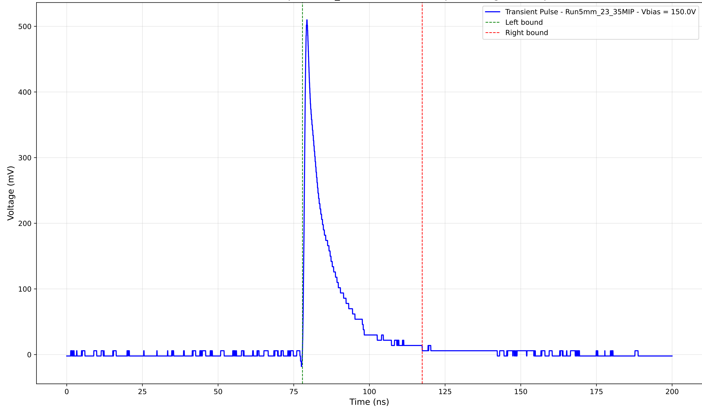
Transient Pulse - Sample: 5mm_23 - Position: 4615.0 \mu\text{m} - Charge: 76.77 pC
