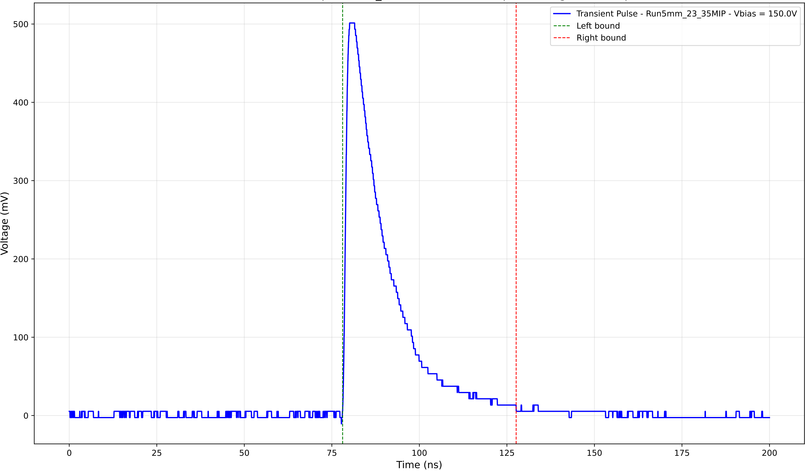
Transient Pulse - Sample: 5mm_23 - Position: 3410.0 \mu\text{m} - Charge: 129.47 pC
