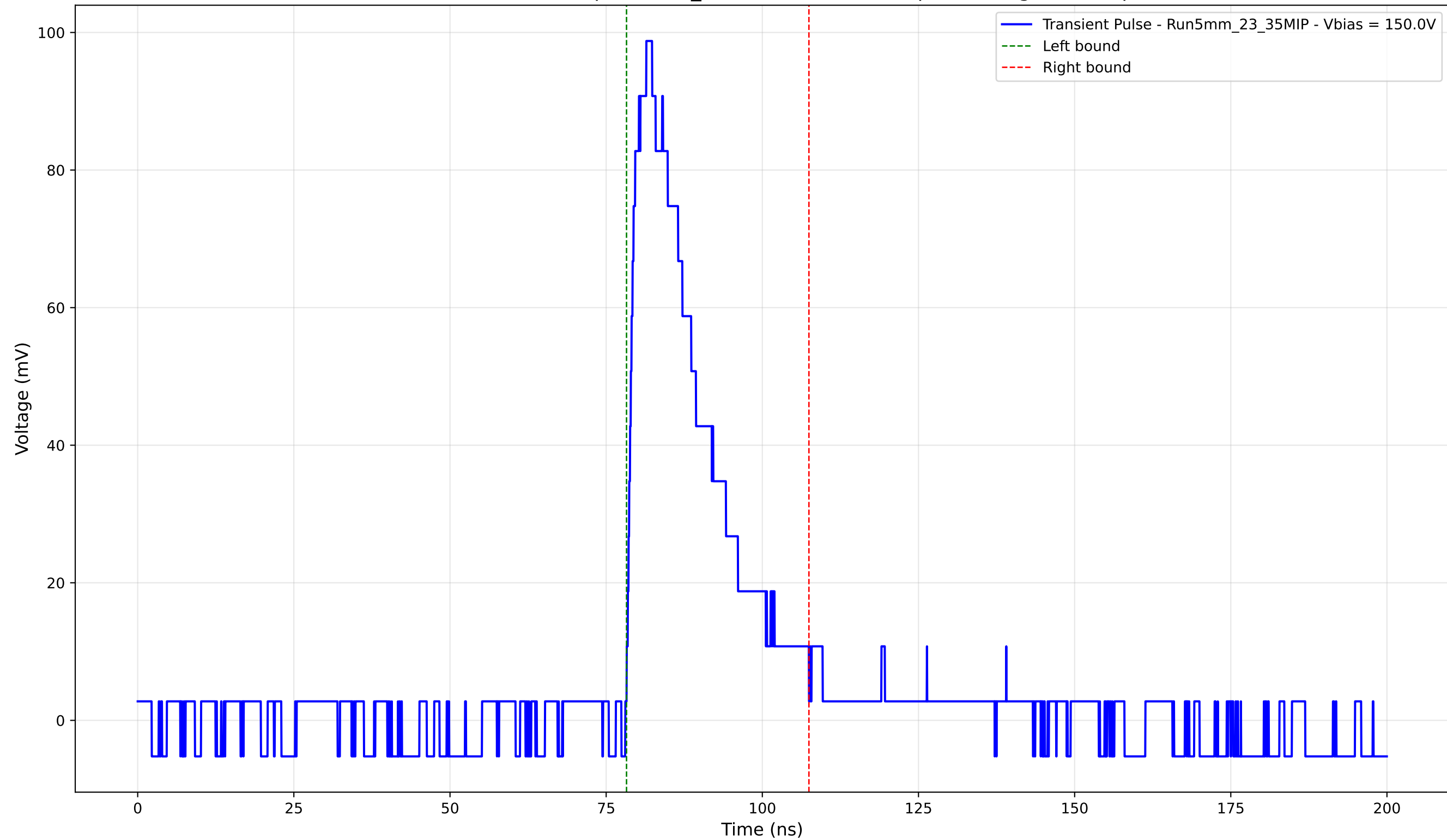
Transient Pulse - Sample: 5mm_23 - Position: 2150.0 \mu\text{m} - Charge: 24.37 pC
