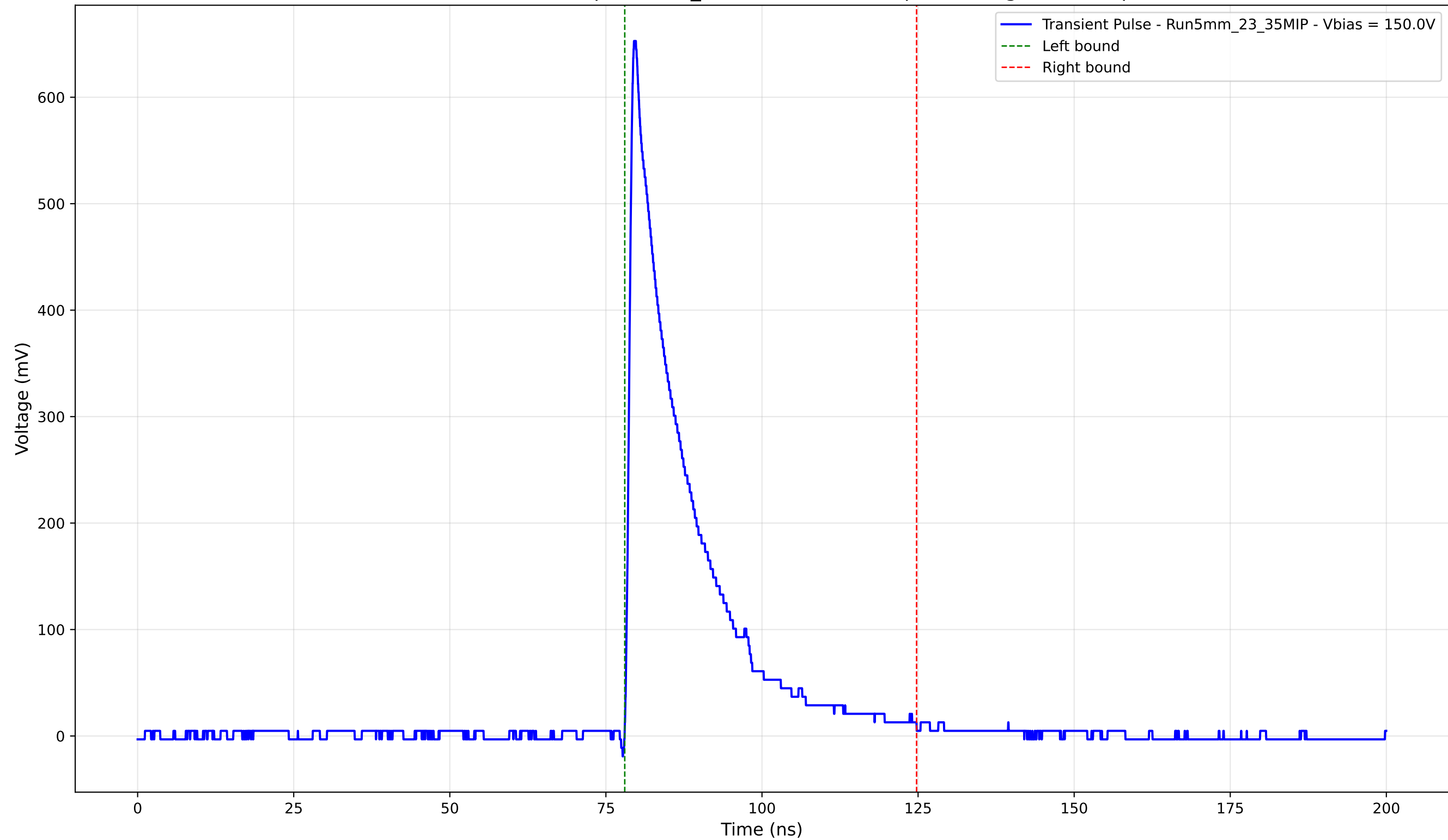
Transient Pulse - Sample: 5mm_23 - Position: 960.0 \mu\text{m} - Charge: 125.47 pC
