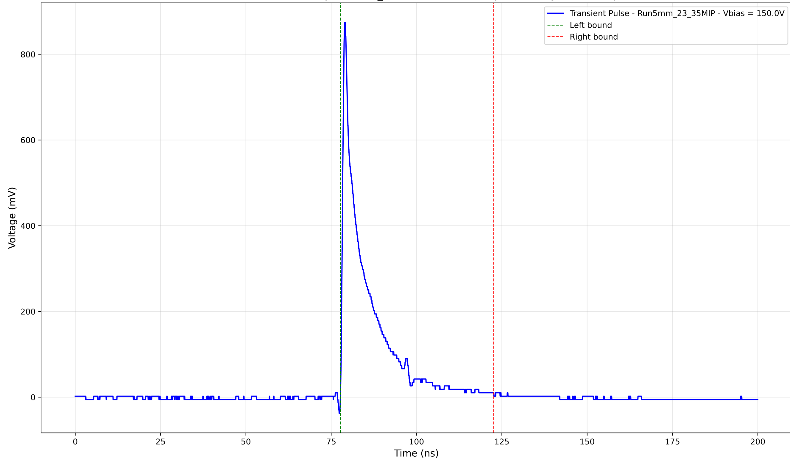
Transient Pulse - Sample: 5mm_23 - Position: 295.0 \mu\text{m} - Charge: 115.37 pC
