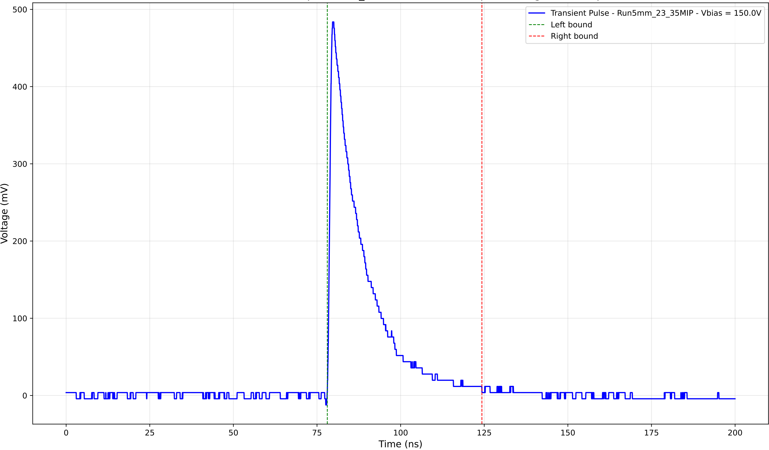
Transient Pulse - Sample: 5mm_23 - Position: 1195.0 \mu\text{m} - Charge: 101.23 pC
