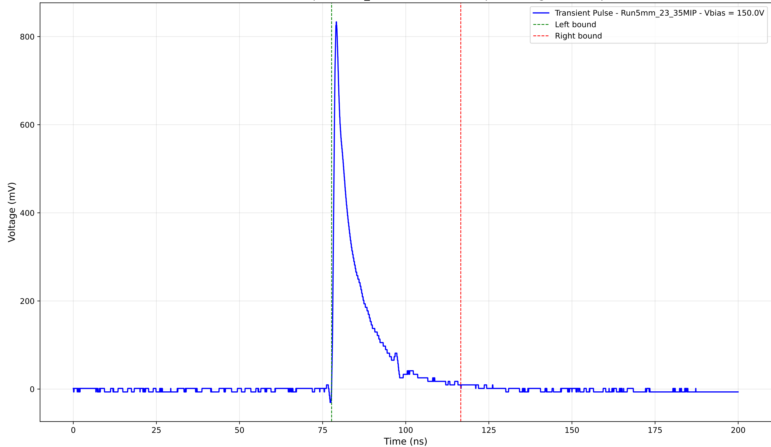
Transient Pulse - Sample: 5mm_23 - Position: 4835.0 \mu\text{m} - Charge: 111.60 pC
