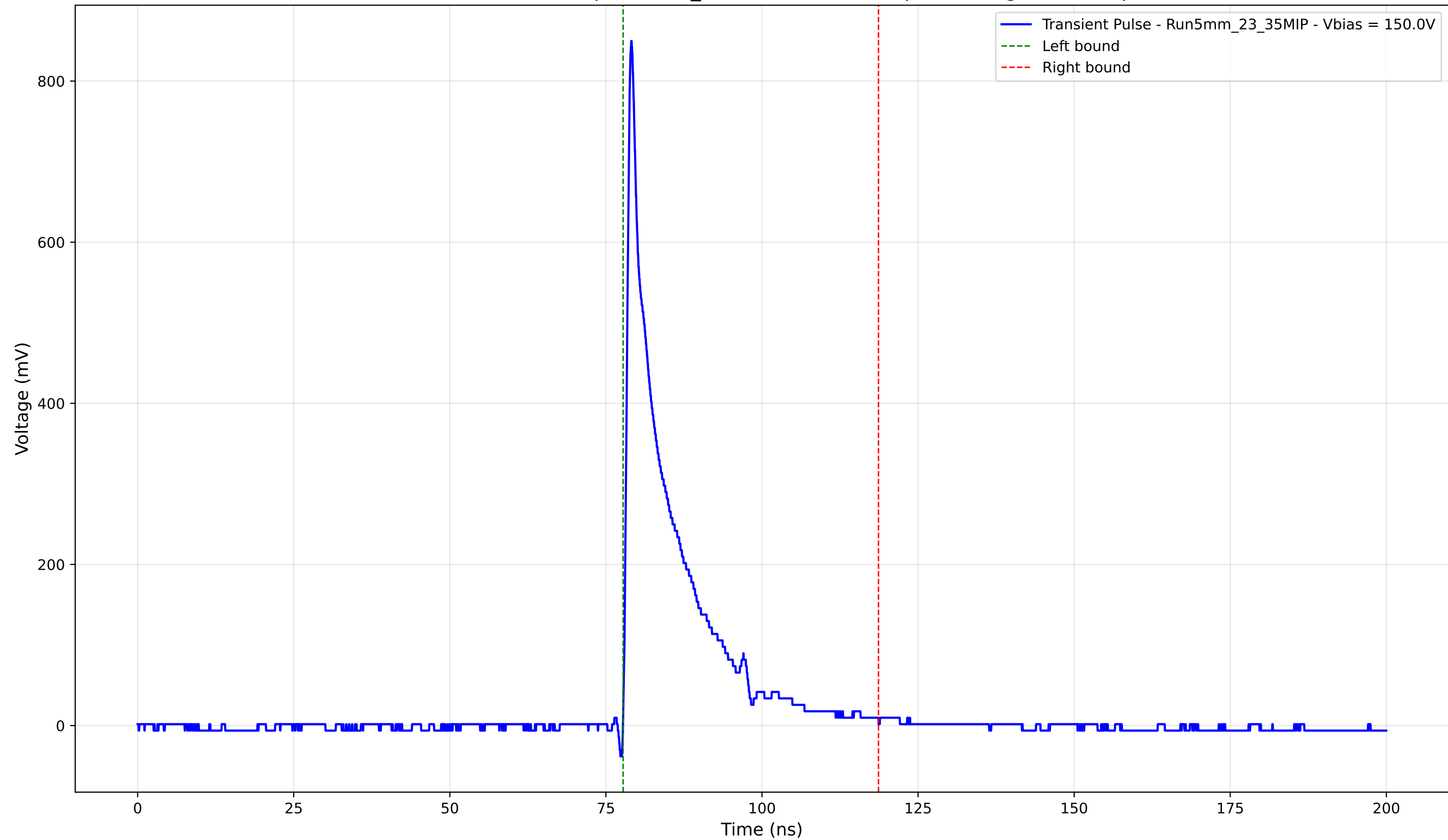
Transient Pulse - Sample: 5mm_23 - Position: 355.0 \mu\text{m} - Charge: 112.46 pC
