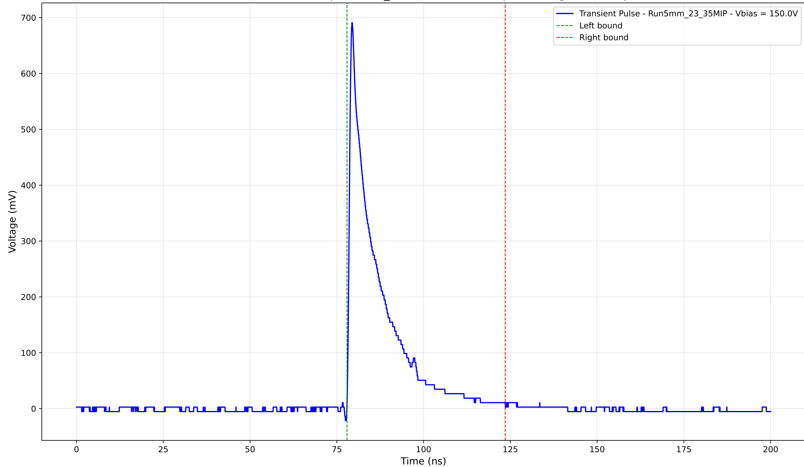
Transient Pulse - Sample: 5mm_23 - Position: 715.0 \mu\text{m} - Charge: 114.66 pC
