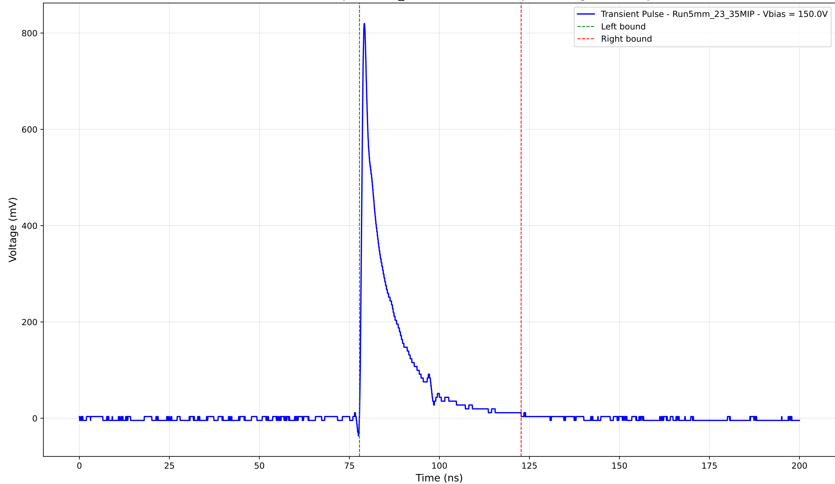
Transient Pulse - Sample: 5mm_23 - Position: 425.0 \mu\text{m} - Charge: 115.86 pC
