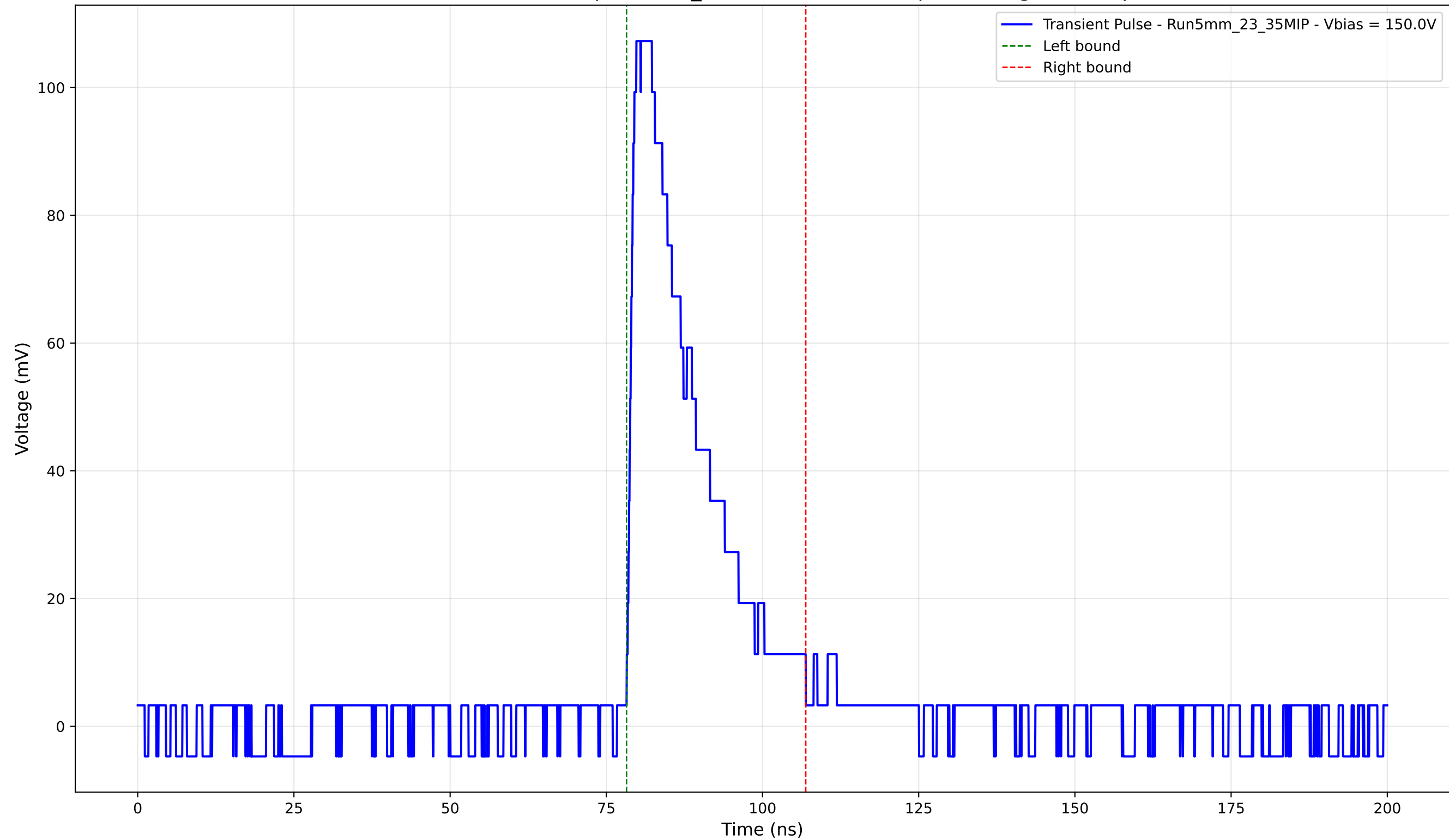
Transient Pulse - Sample: 5mm_23 - Position: 3640.0 \mu\text{m} - Charge: 25.22 pC
