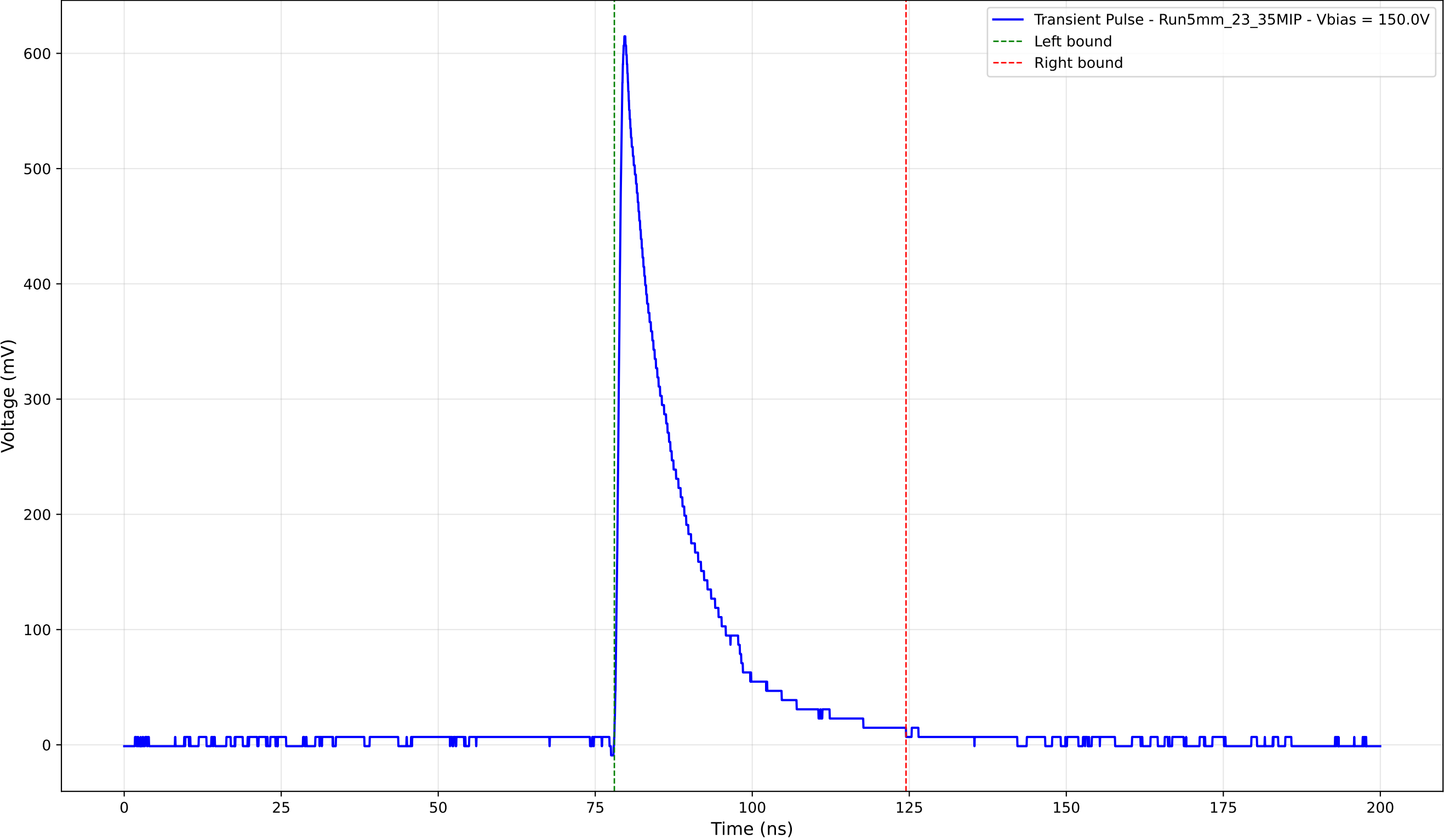
Transient Pulse - Sample: 5mm_23 - Position: 1035.0 \mu\text{m} - Charge: 120.64 pC
