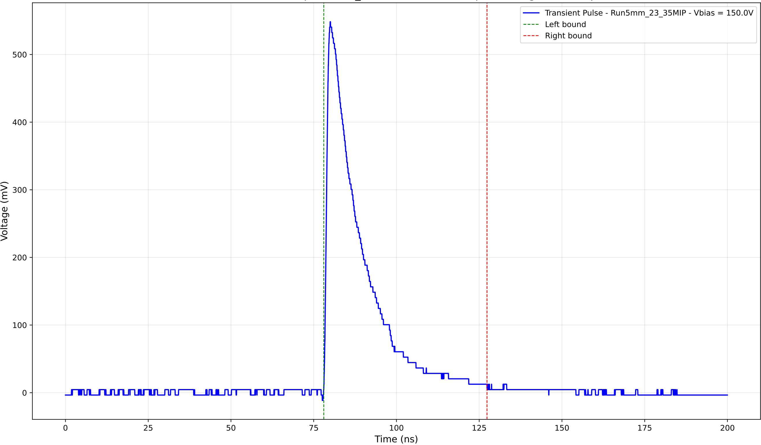
Transient Pulse - Sample: 5mm_23 - Position: 3790.0 \mu\text{m} - Charge: 125.62 pC
