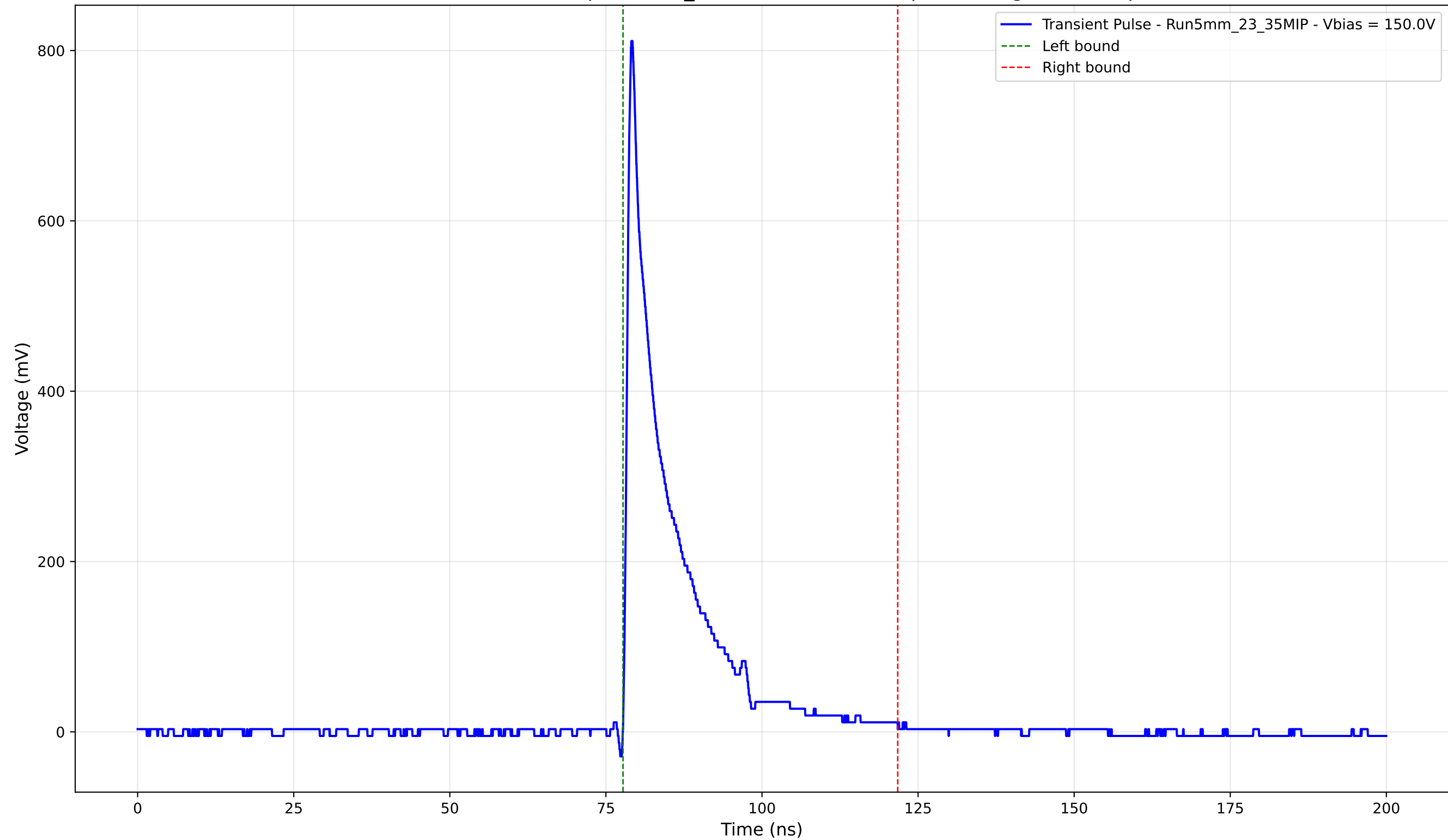
Transient Pulse - Sample: 5mm_23 - Position: 4805.0 \mu\text{m} - Charge: 113.24 pC
