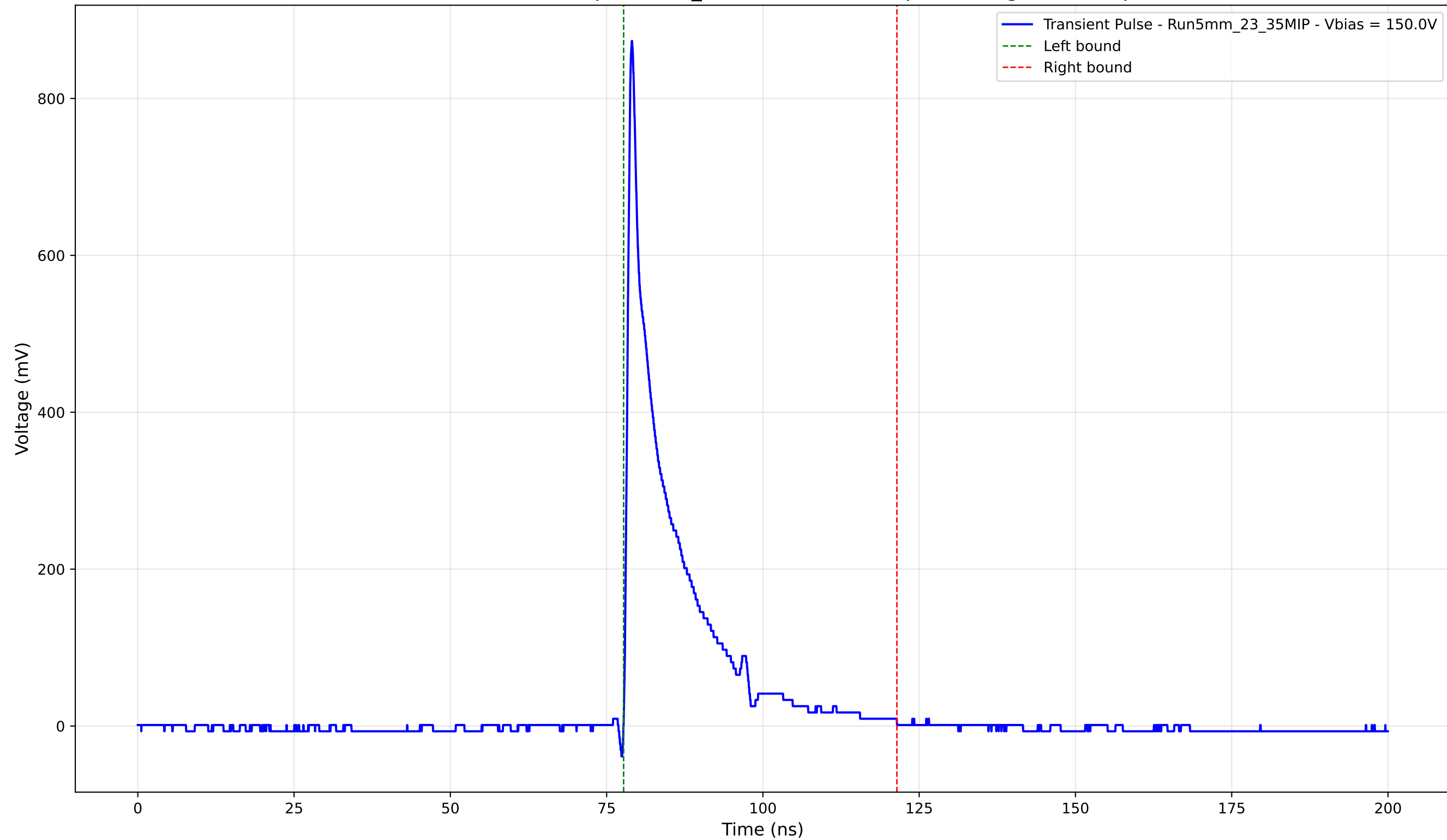
Transient Pulse - Sample: 5mm_23 - Position: 310.0 \mu\text{m} - Charge: 114.56 pC
