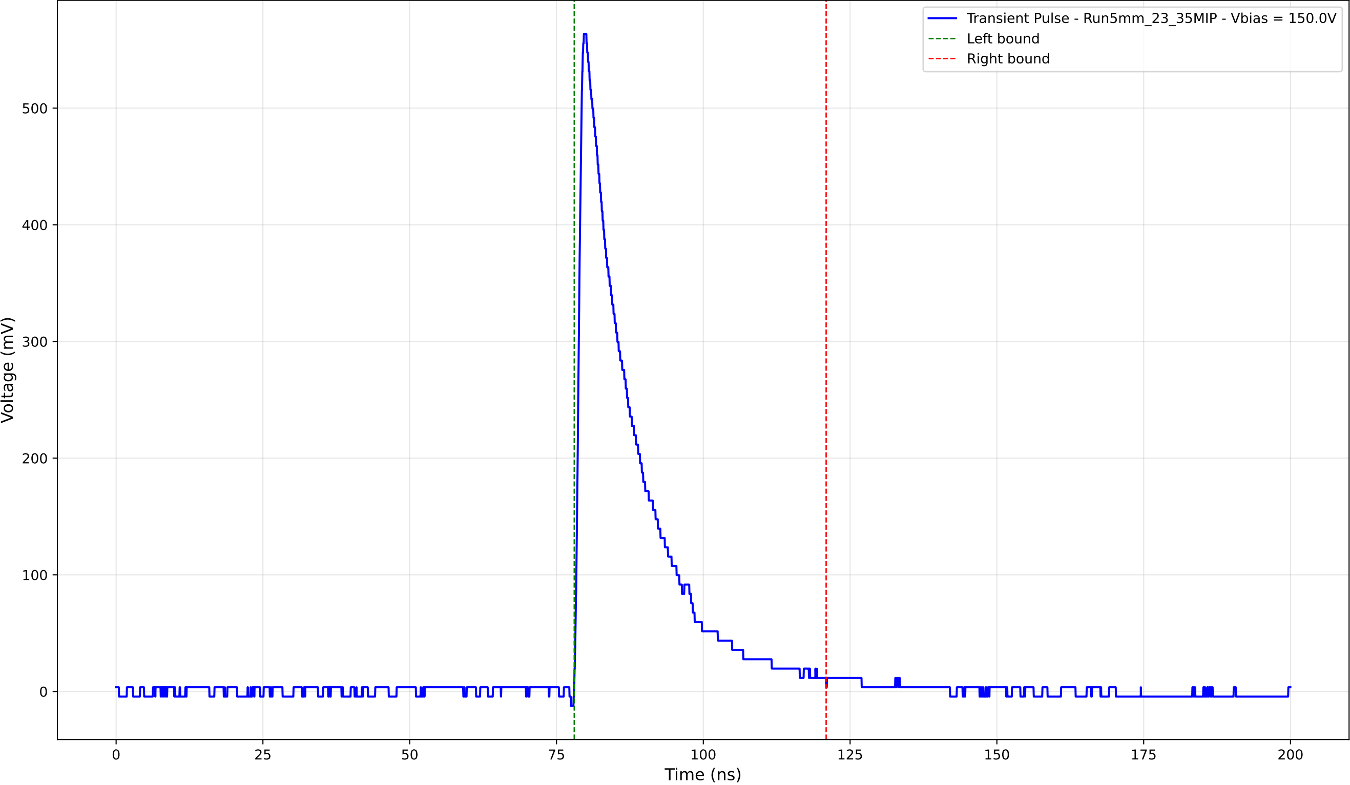
Transient Pulse - Sample: 5mm_23 - Position: 4055.0 \mu\text{m} - Charge: 115.21 pC
