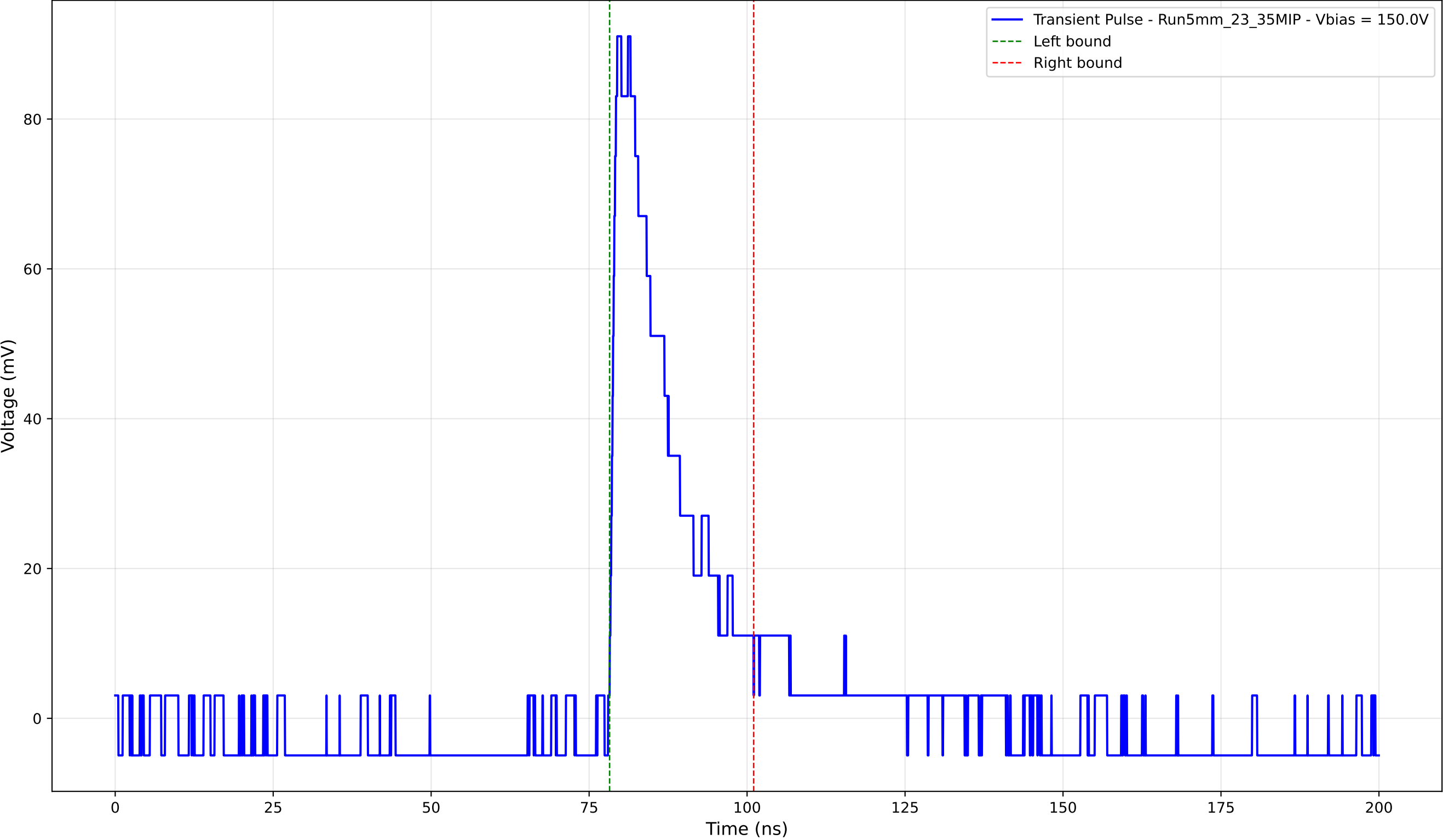
Transient Pulse - Sample: 5mm_23 - Position: 4160.0 \mu\text{m} - Charge: 17.60 pC
