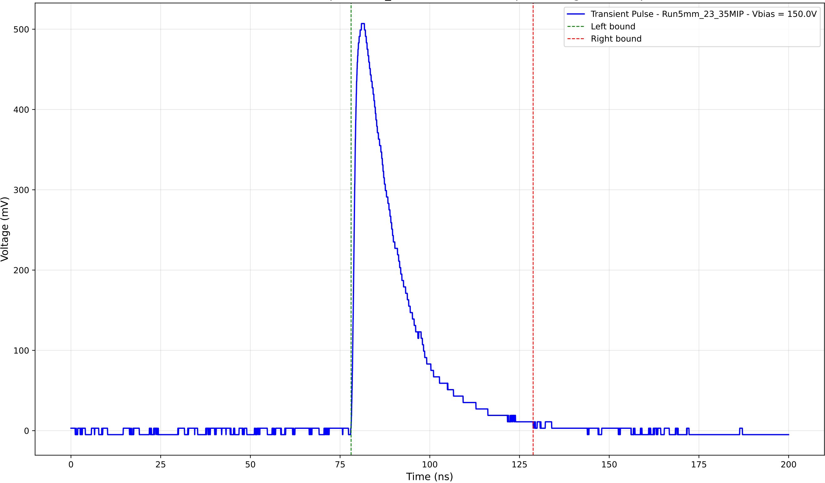
Transient Pulse - Sample: 5mm_23 - Position: 2465.0 \mu\text{m} - Charge: 136.78 pC
