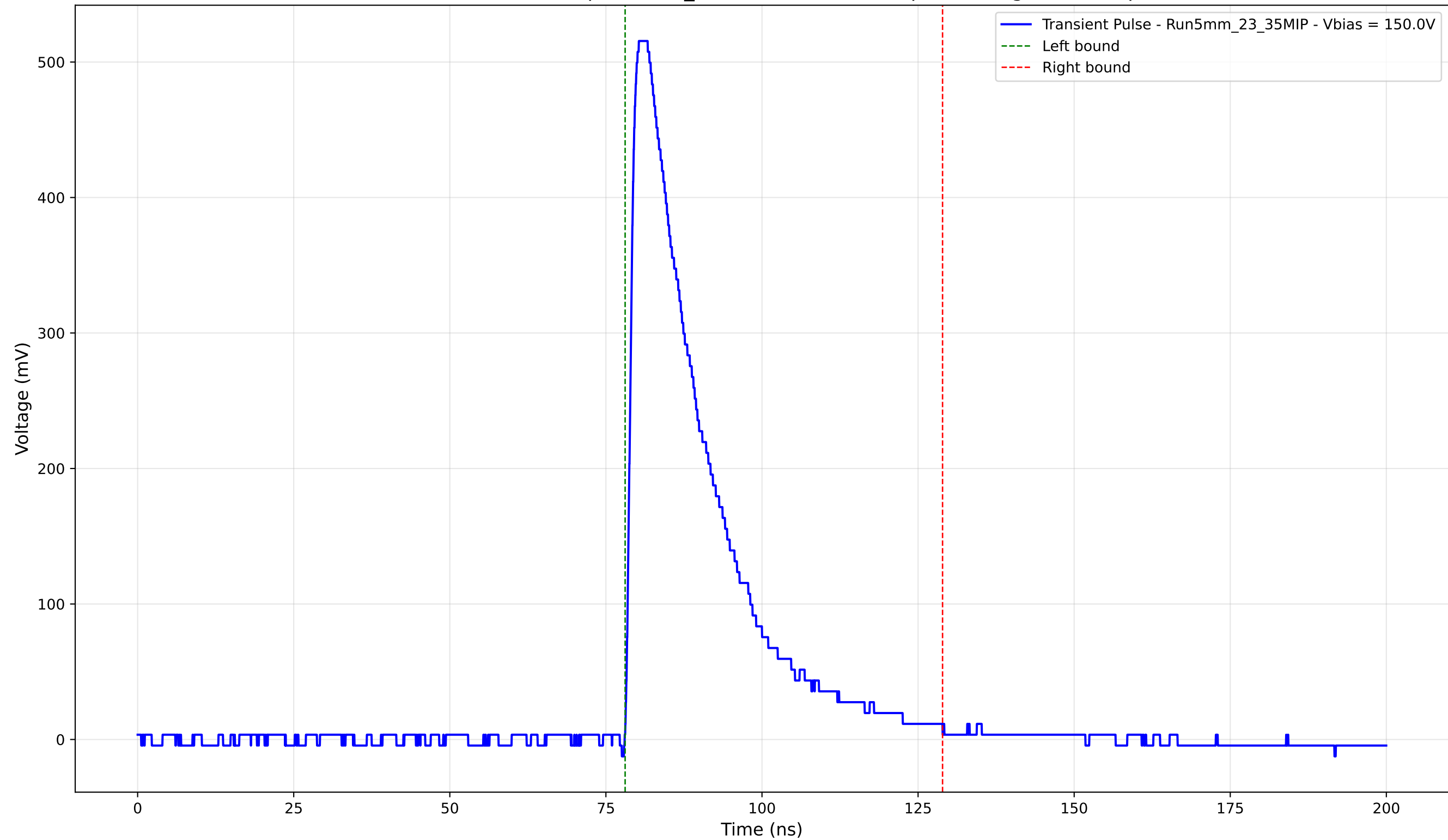
Transient Pulse - Sample: 5mm_23 - Position: 2045.0 \mu\text{m} - Charge: 136.59 pC
