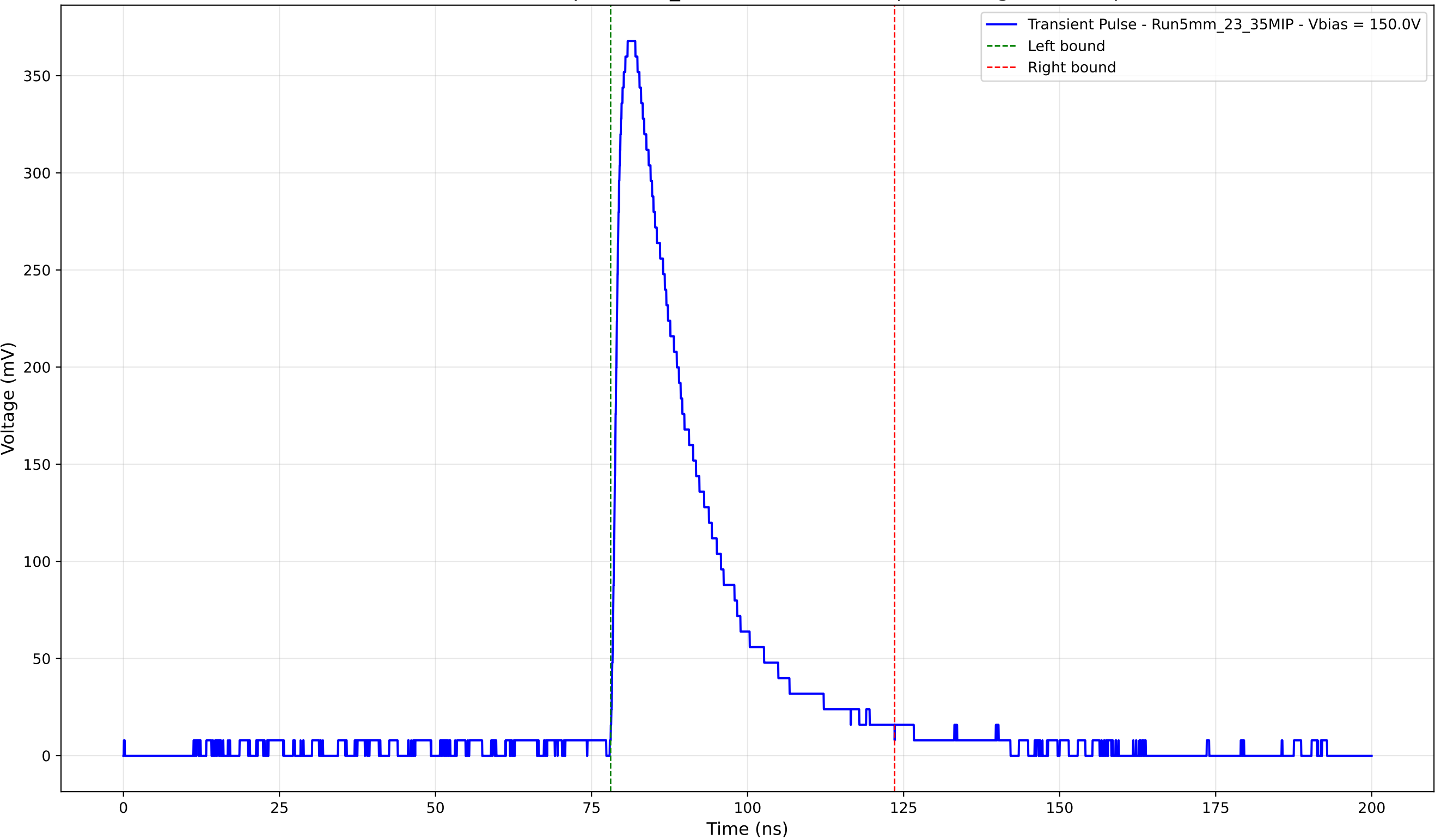
Transient Pulse - Sample: 5mm_23 - Position: 2710.0 \mu\text{m} - Charge: 101.09 pC
