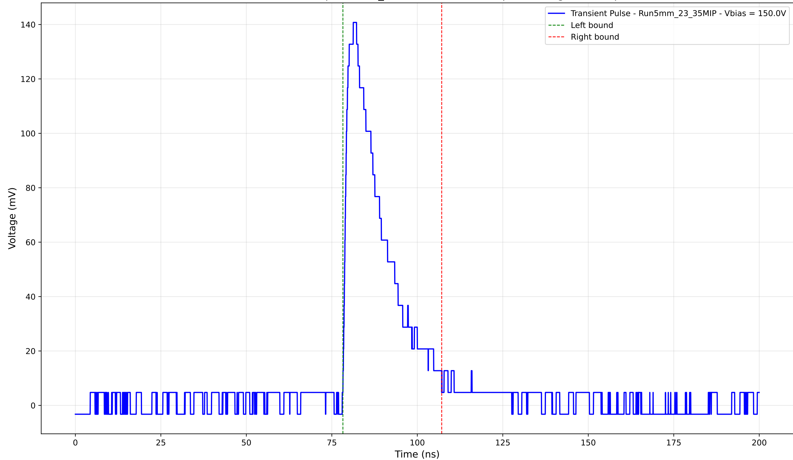
Transient Pulse - Sample: 5mm_23 - Position: 3125.0 \mu\text{m} - Charge: 34.38 pC
