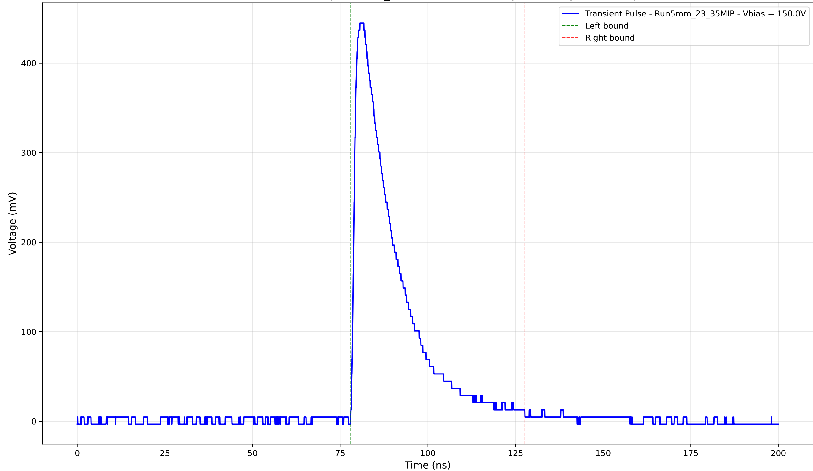
Transient Pulse - Sample: 5mm_23 - Position: 3070.0 \mu\text{m} - Charge: 117.68 pC
