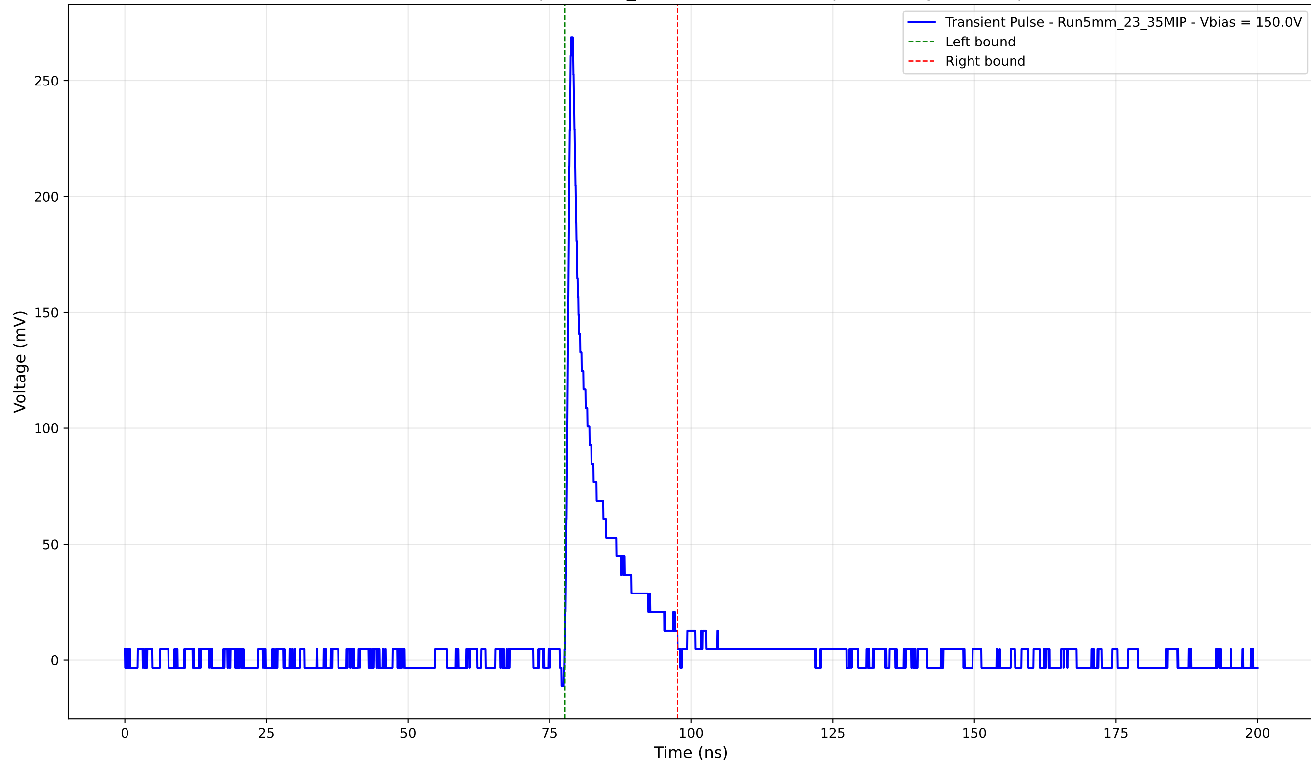
Transient Pulse - Sample: 5mm_23 - Position: 5085.0 \mu\text{m} - Charge: 25.31 pC
