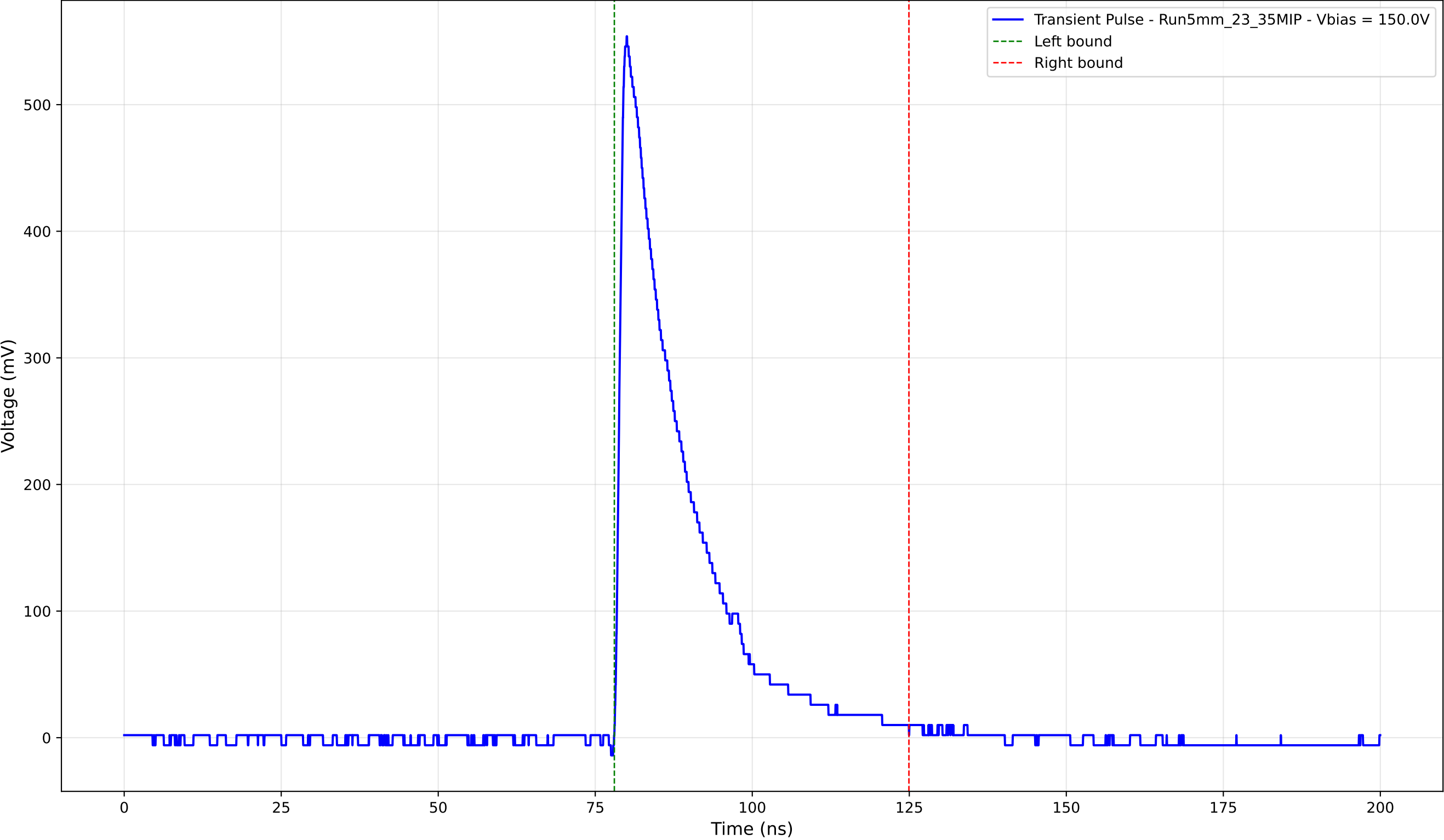
Transient Pulse - Sample: 5mm_23 - Position: 3875.0 \mu\text{m} - Charge: 120.53 pC
