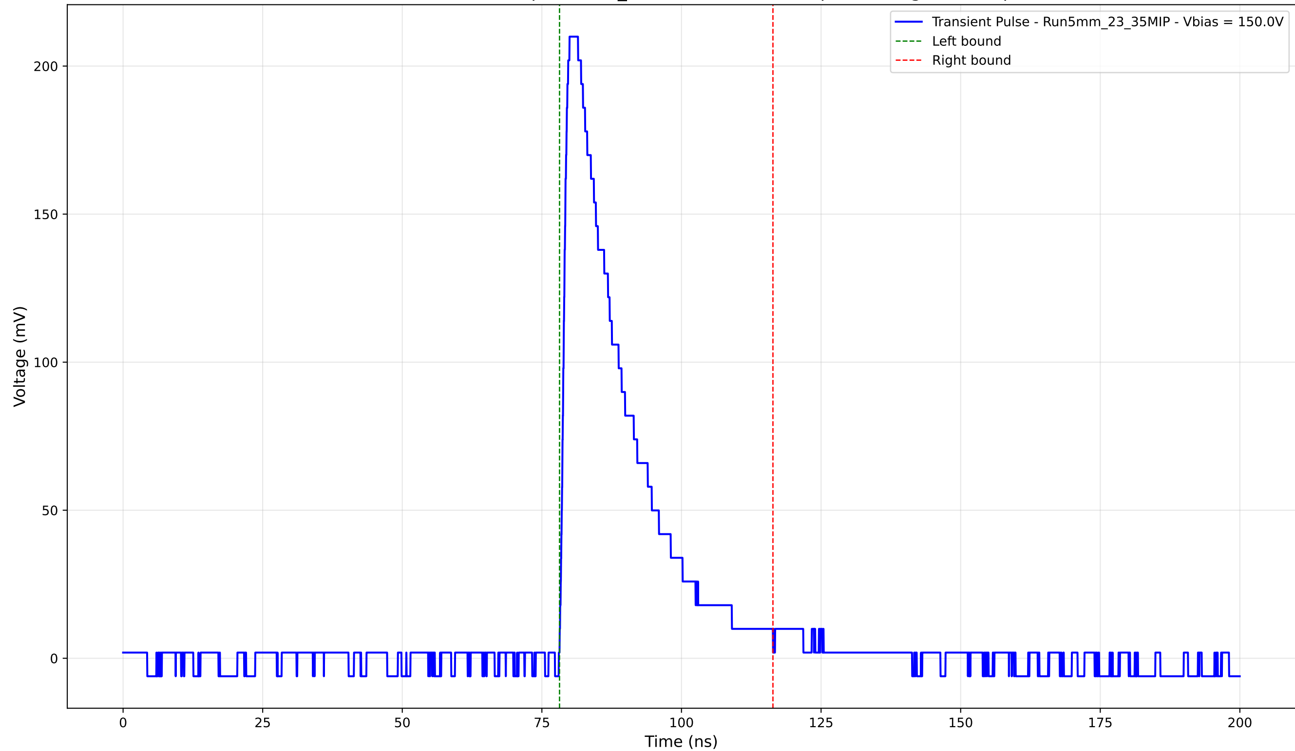
Transient Pulse - Sample: 5mm_23 - Position: 1660.0 \mu\text{m} - Charge: 50.63 pC
