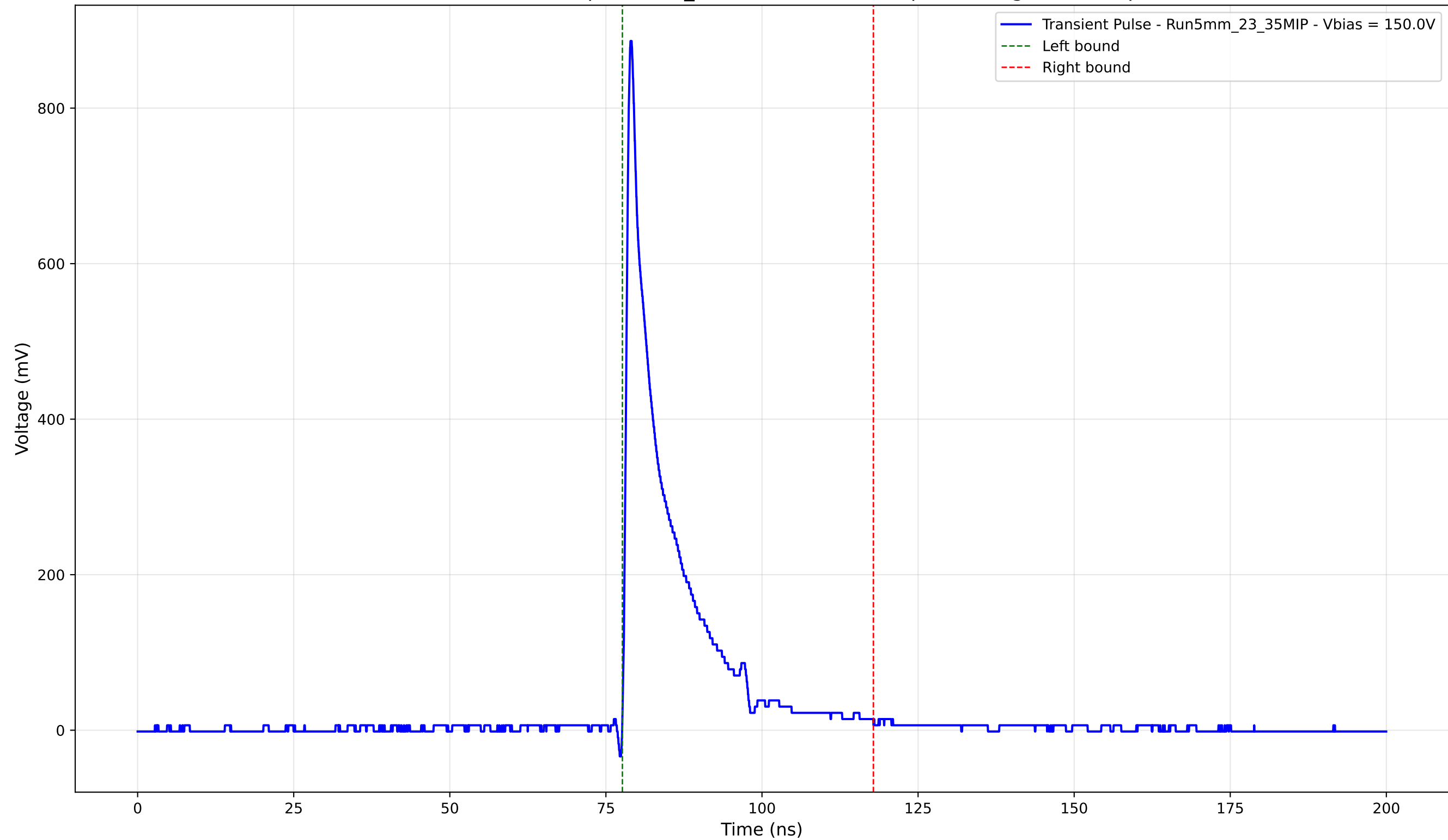
Transient Pulse - Sample: 5mm_23 - Position: 4940.0 \mu\text{m} - Charge: 117.44 pC
