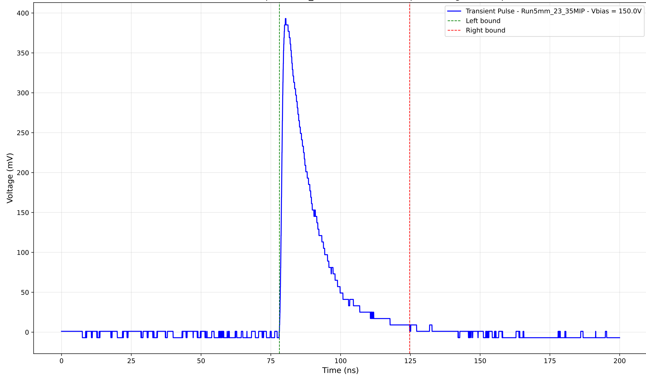
Transient Pulse - Sample: 5mm_23 - Position: 1690.0 \mu\text{m} - Charge: 94.11 pC
