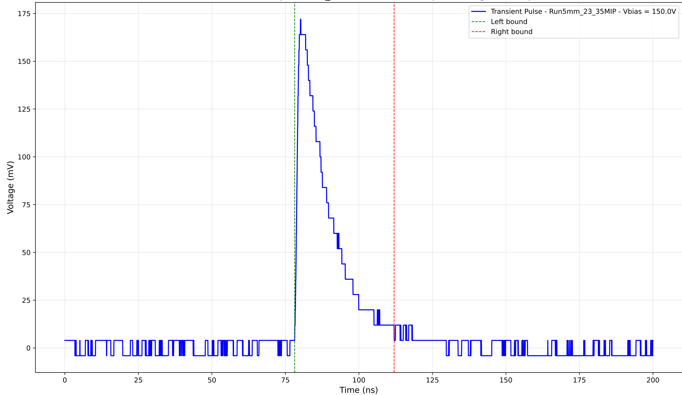
Transient Pulse - Sample: 5mm_23 - Position: 1650.0 \mu\text{m} - Charge: 40.45 pC
