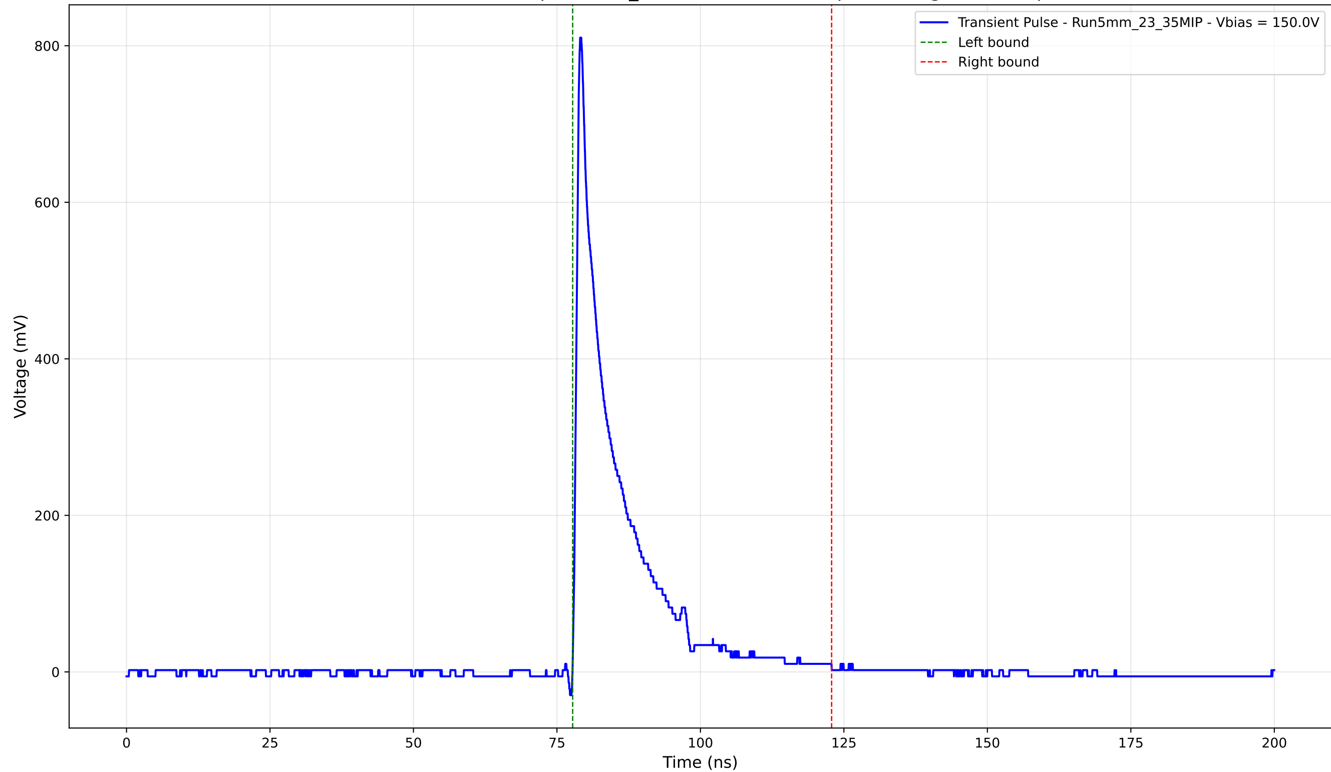
Transient Pulse - Sample: 5mm_23 - Position: 4810.0 \mu\text{m} - Charge: 112.21 pC
