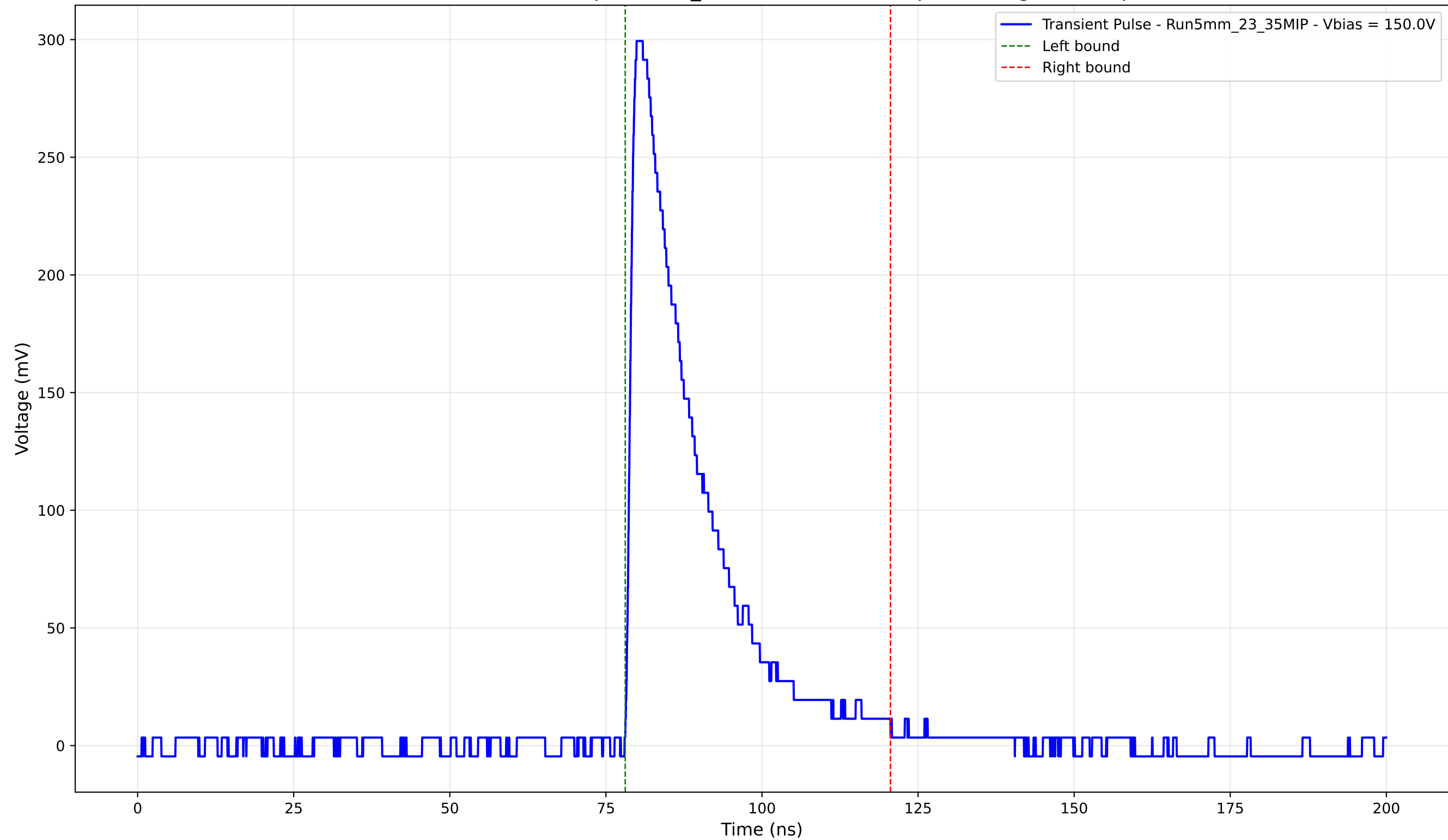
Transient Pulse - Sample: 5mm_23 - Position: 3605.0 \mu\text{m} - Charge: 70.43 pC
