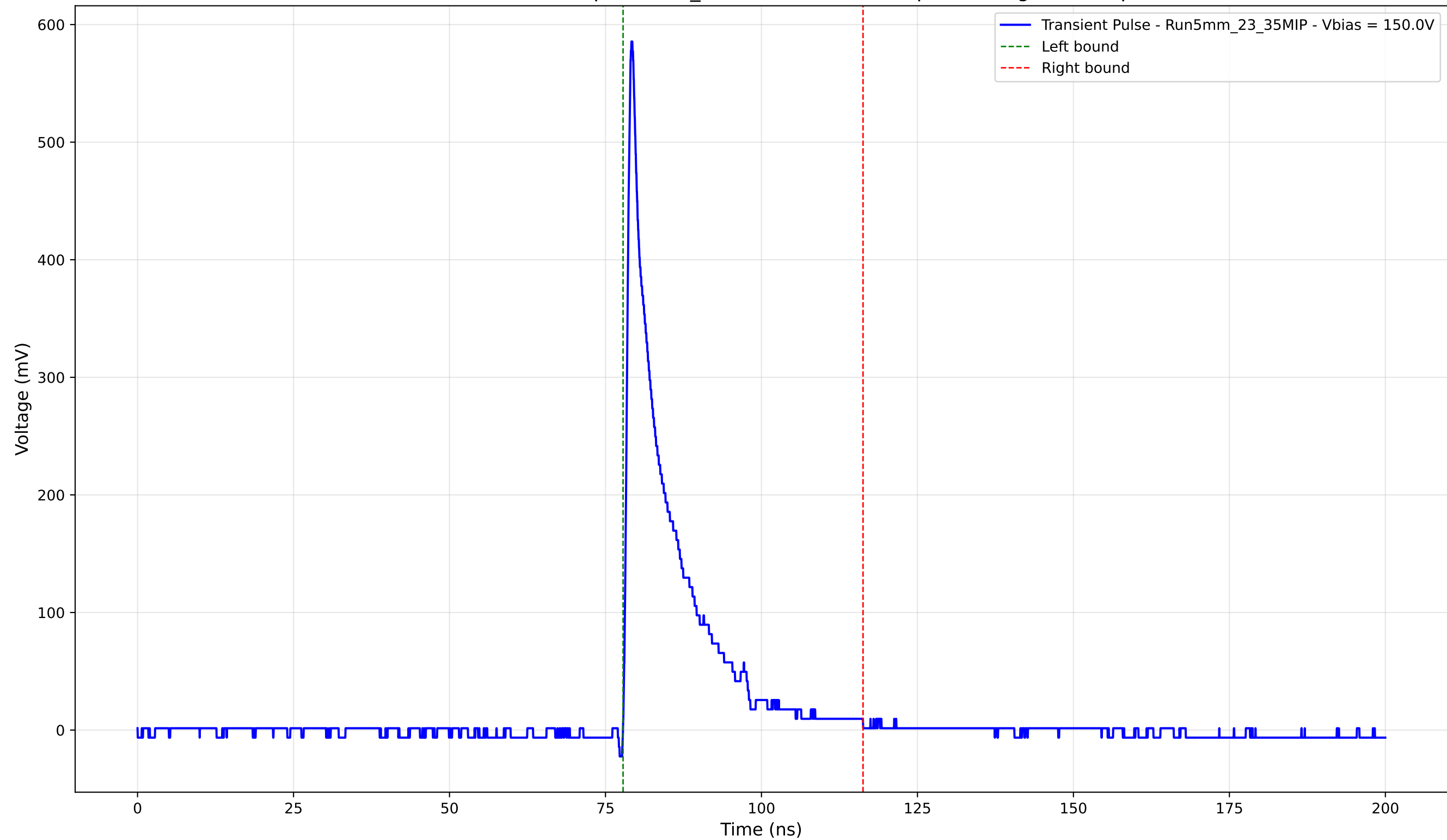
Transient Pulse - Sample: 5mm_23 - Position: 4725.0 \mu\text{m} - Charge: 76.12 pC
