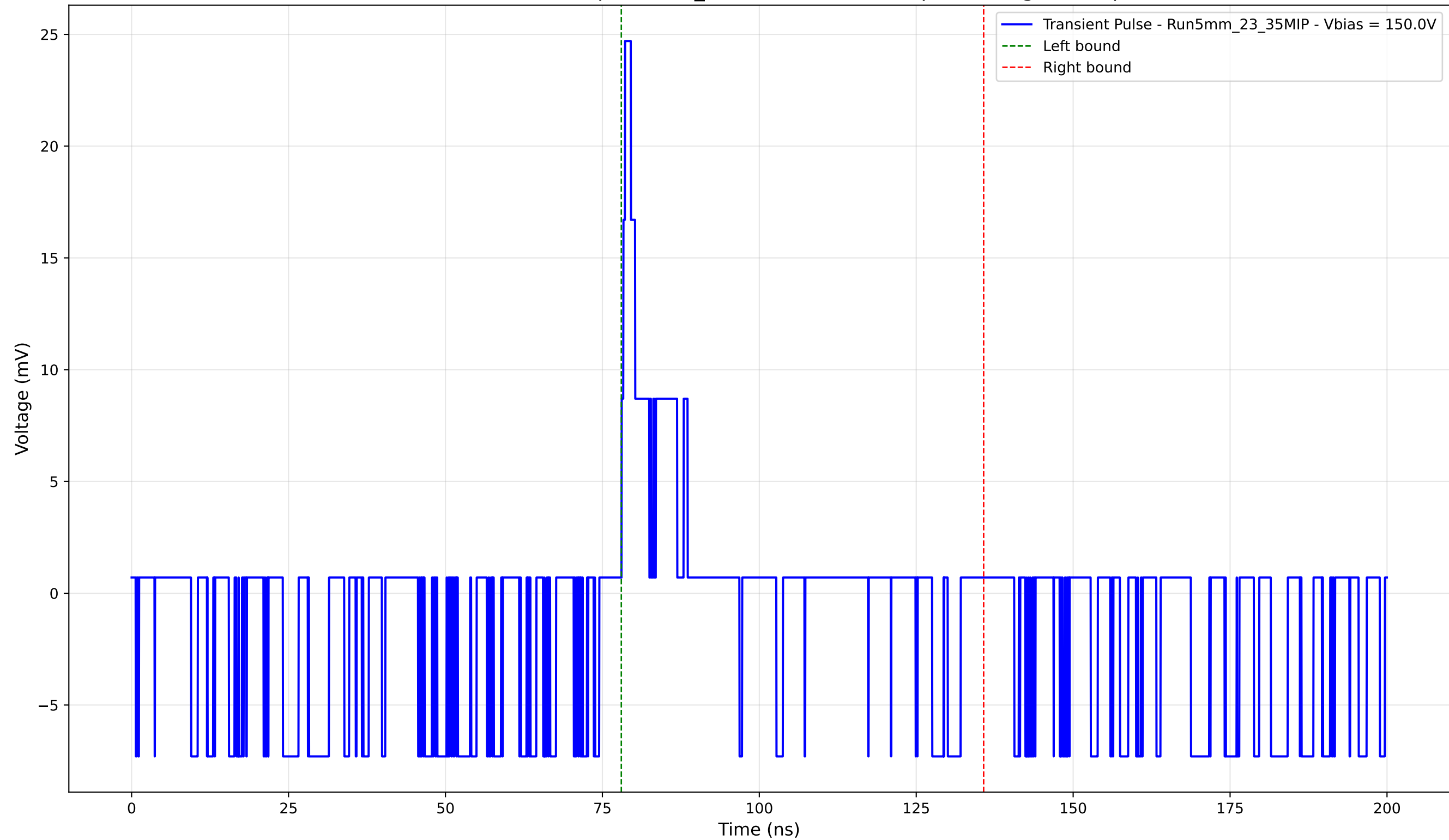
Transient Pulse - Sample: 5mm_23 - Position: 5155.0 \mu\text{m} - Charge: 1.73 pC
