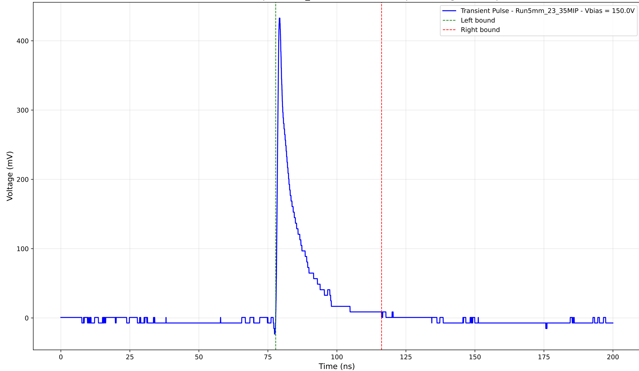
Transient Pulse - Sample: 5mm_23 - Position: 4710.0 \mu\text{m} - Charge: 56.27 pC
