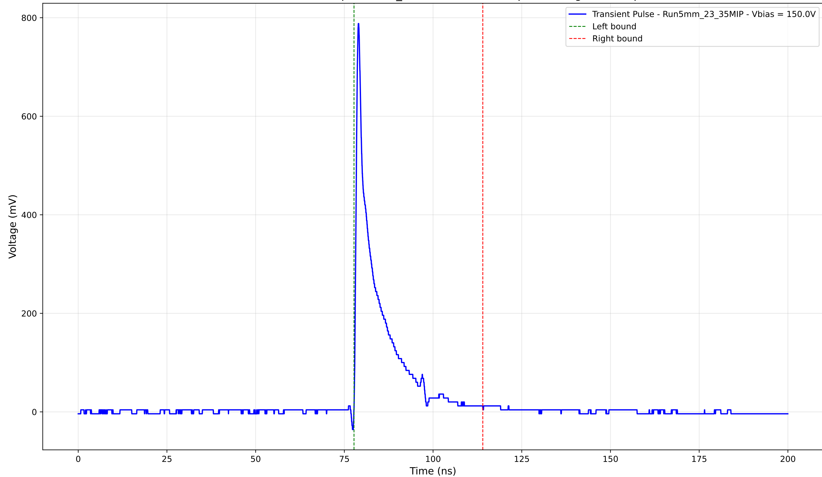
Transient Pulse - Sample: 5mm_23 - Position: 240.0 \mu\text{m} - Charge: 91.51 pC
