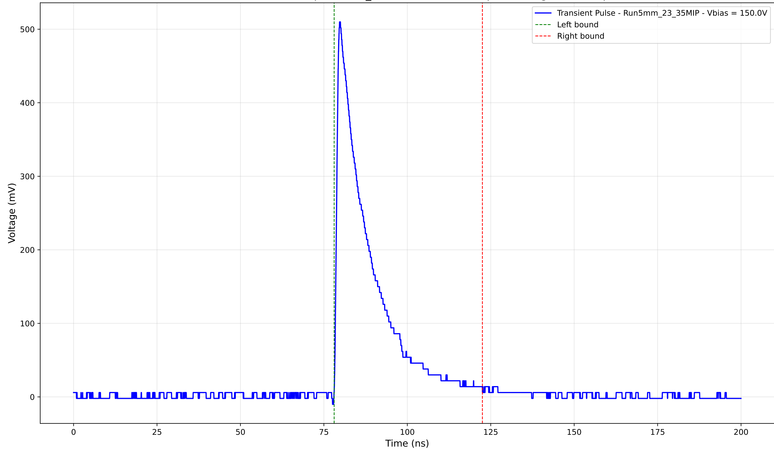
Transient Pulse - Sample: 5mm_23 - Position: 1200.0 \mu\text{m} - Charge: 107.04 pC
