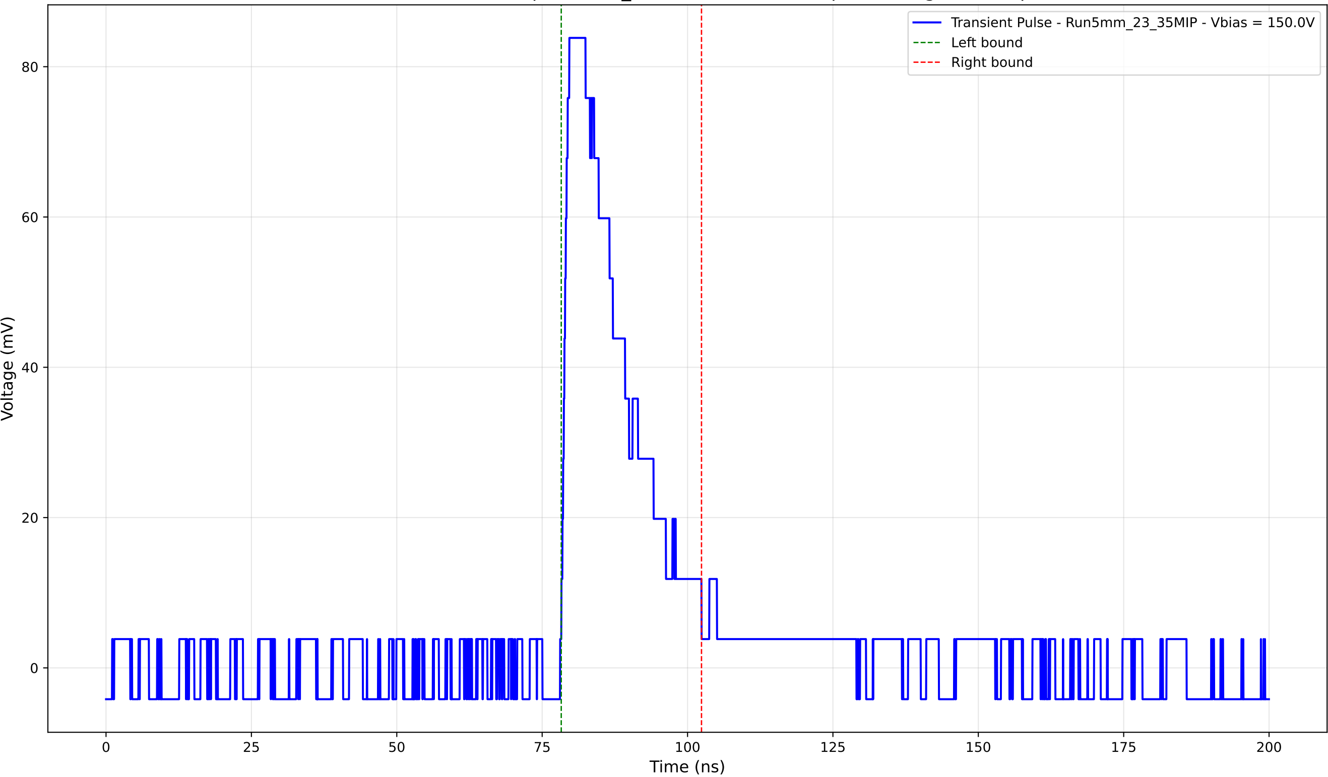
Transient Pulse - Sample: 5mm_23 - Position: 3650.0 \mu\text{m} - Charge: 19.29 pC
