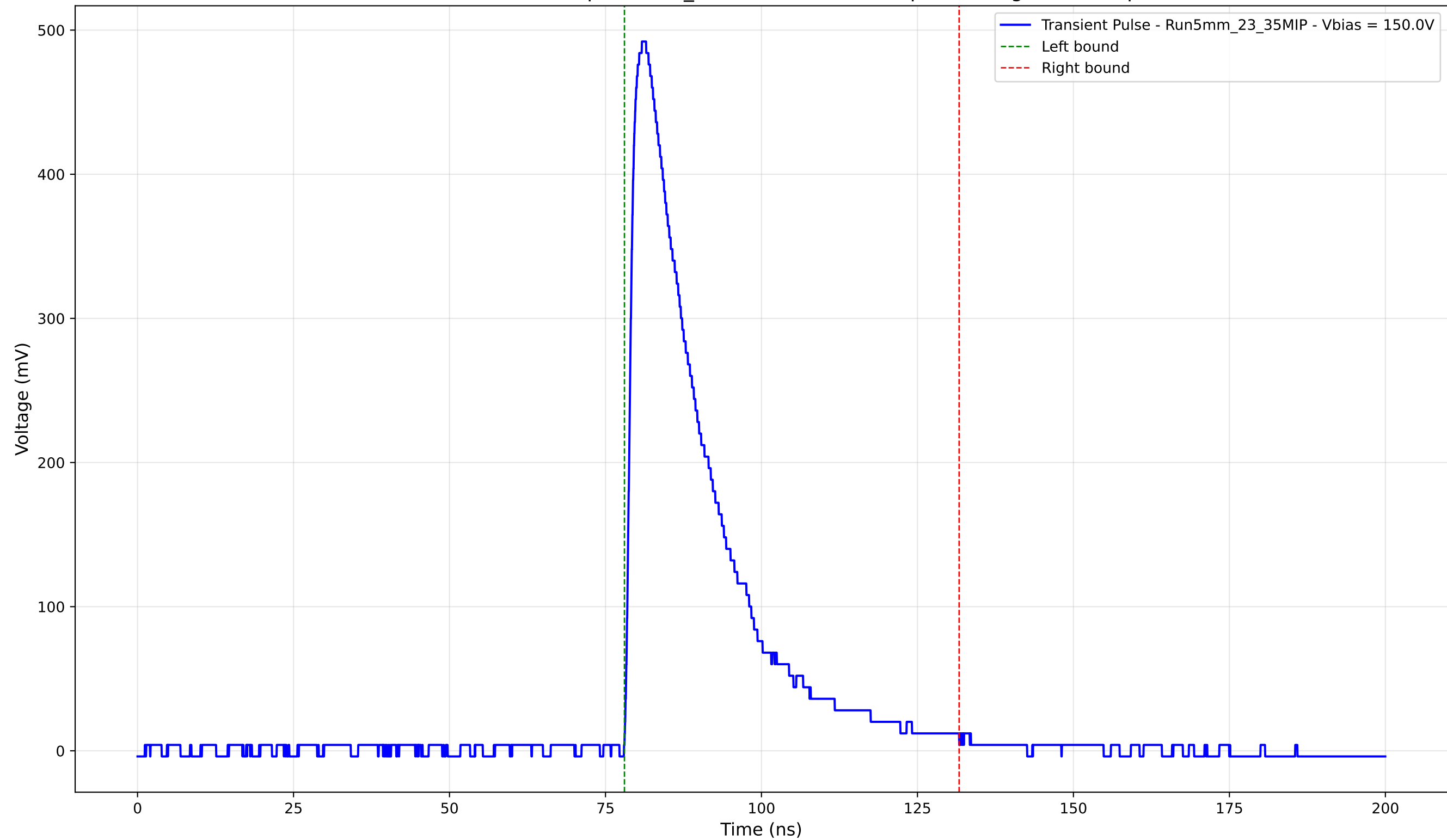
Transient Pulse - Sample: 5mm_23 - Position: 3045.0 \mu\text{m} - Charge: 132.25 pC
