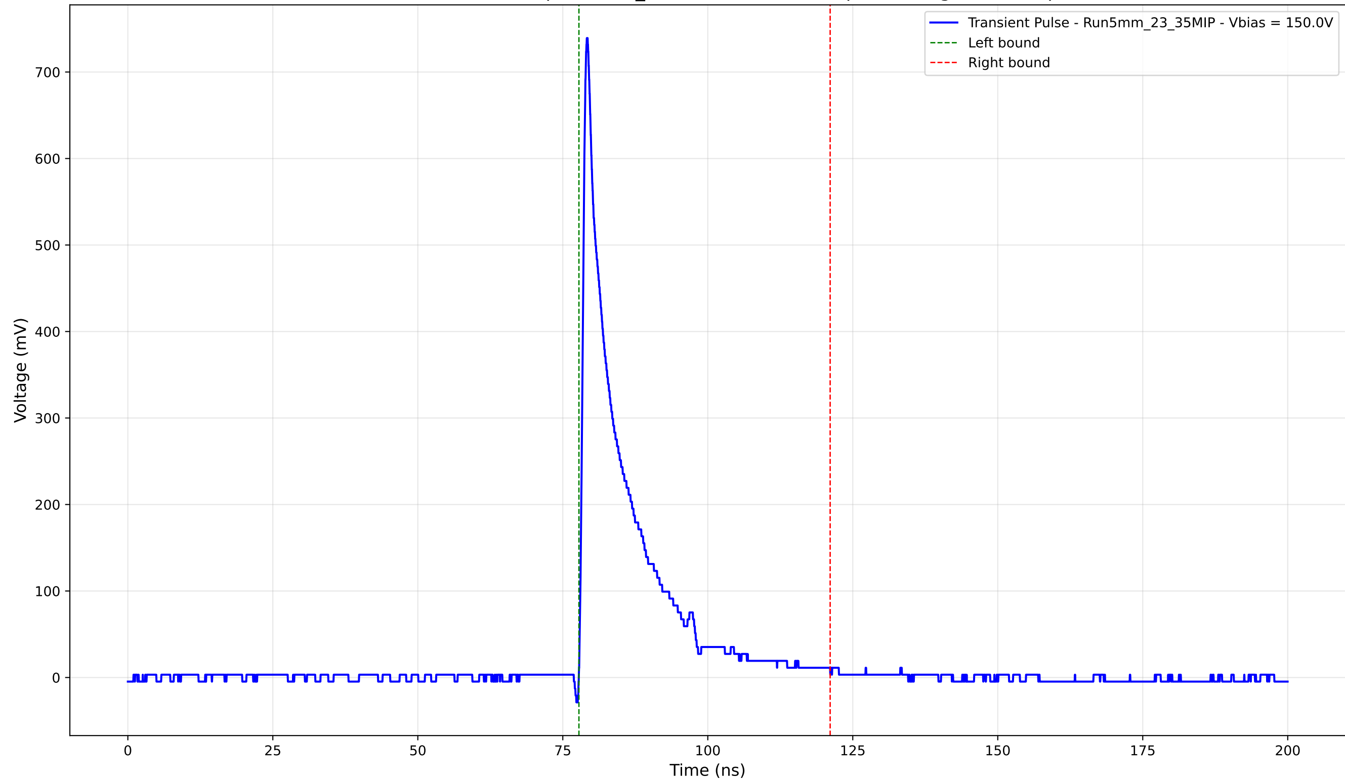
Transient Pulse - Sample: 5mm_23 - Position: 4750.0 \mu\text{m} - Charge: 103.17 pC
