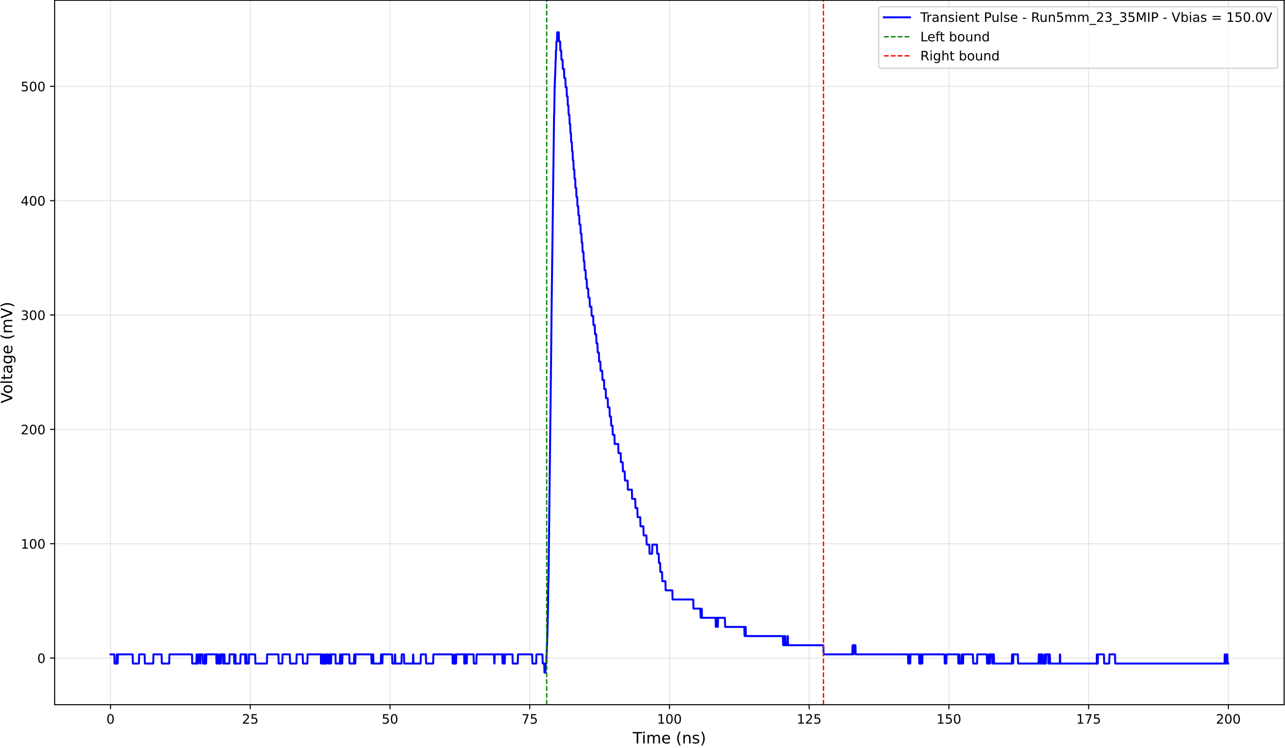
Transient Pulse - Sample: 5mm_23 - Position: 3850.0 \mu\text{m} - Charge: 122.59 pC
