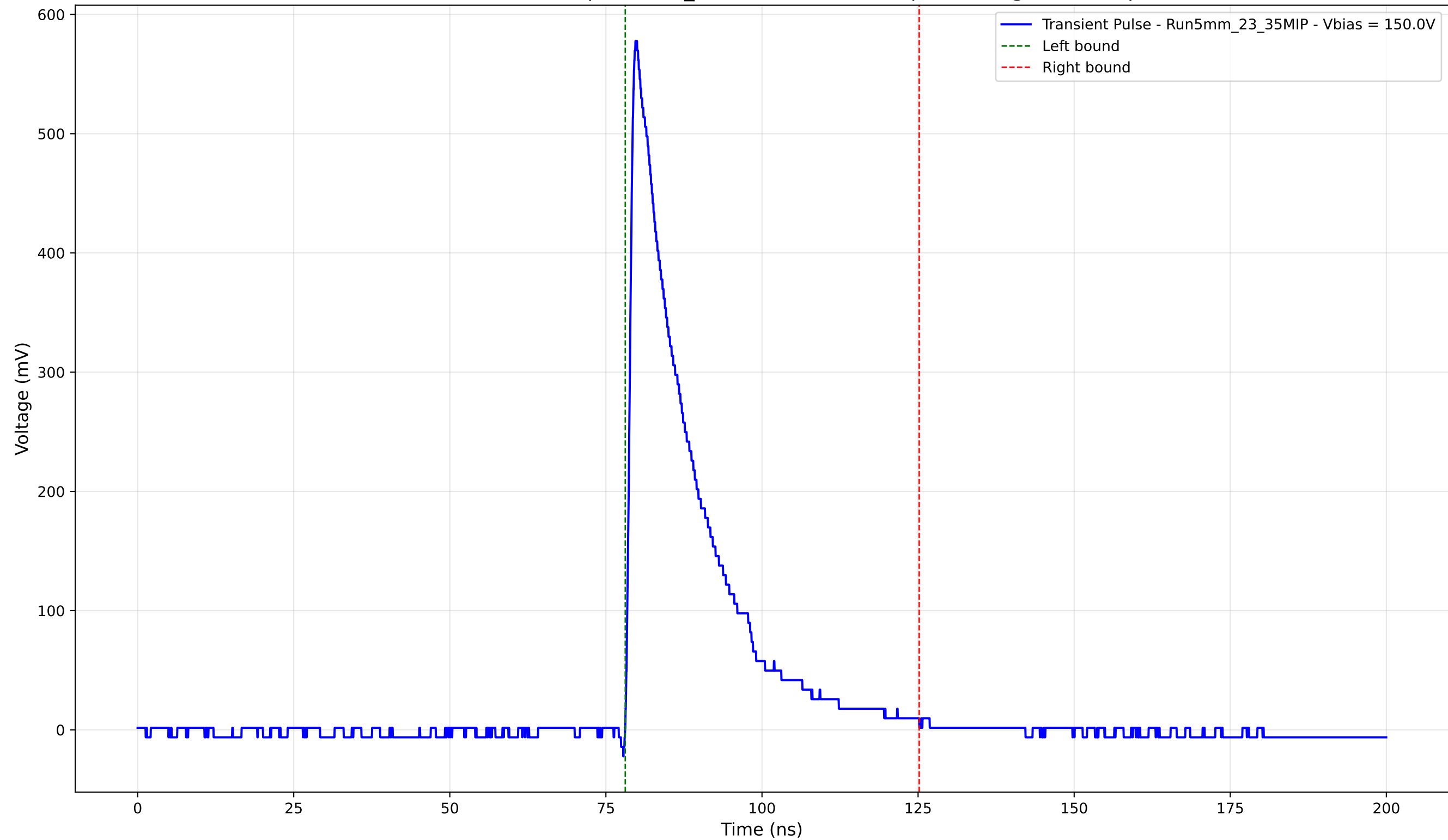
Transient Pulse - Sample: 5mm_23 - Position: 1225.0 \mu\text{m} - Charge: 121.37 pC
