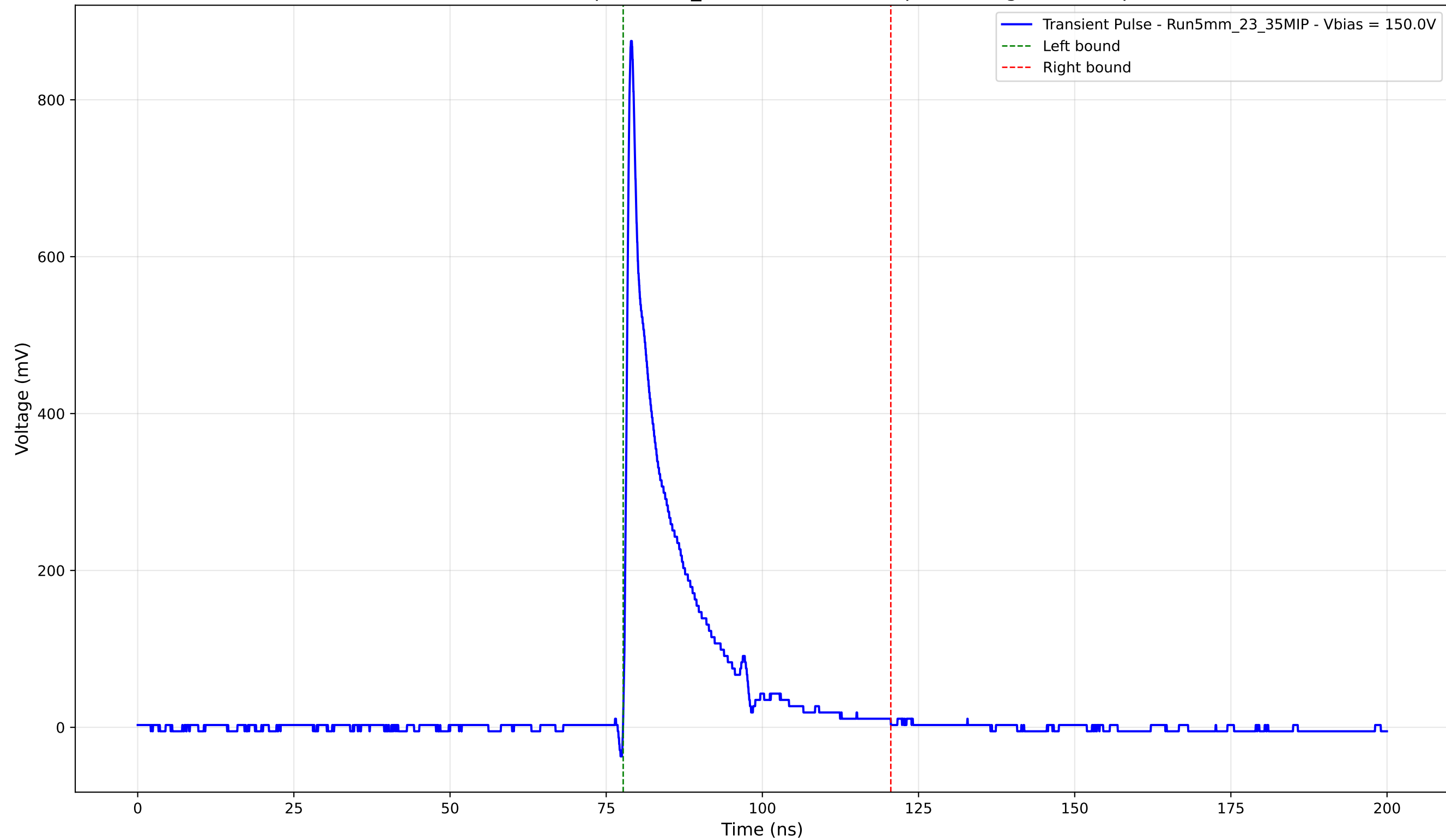
Transient Pulse - Sample: 5mm_23 - Position: 290.0 \mu\text{m} - Charge: 113.87 pC
