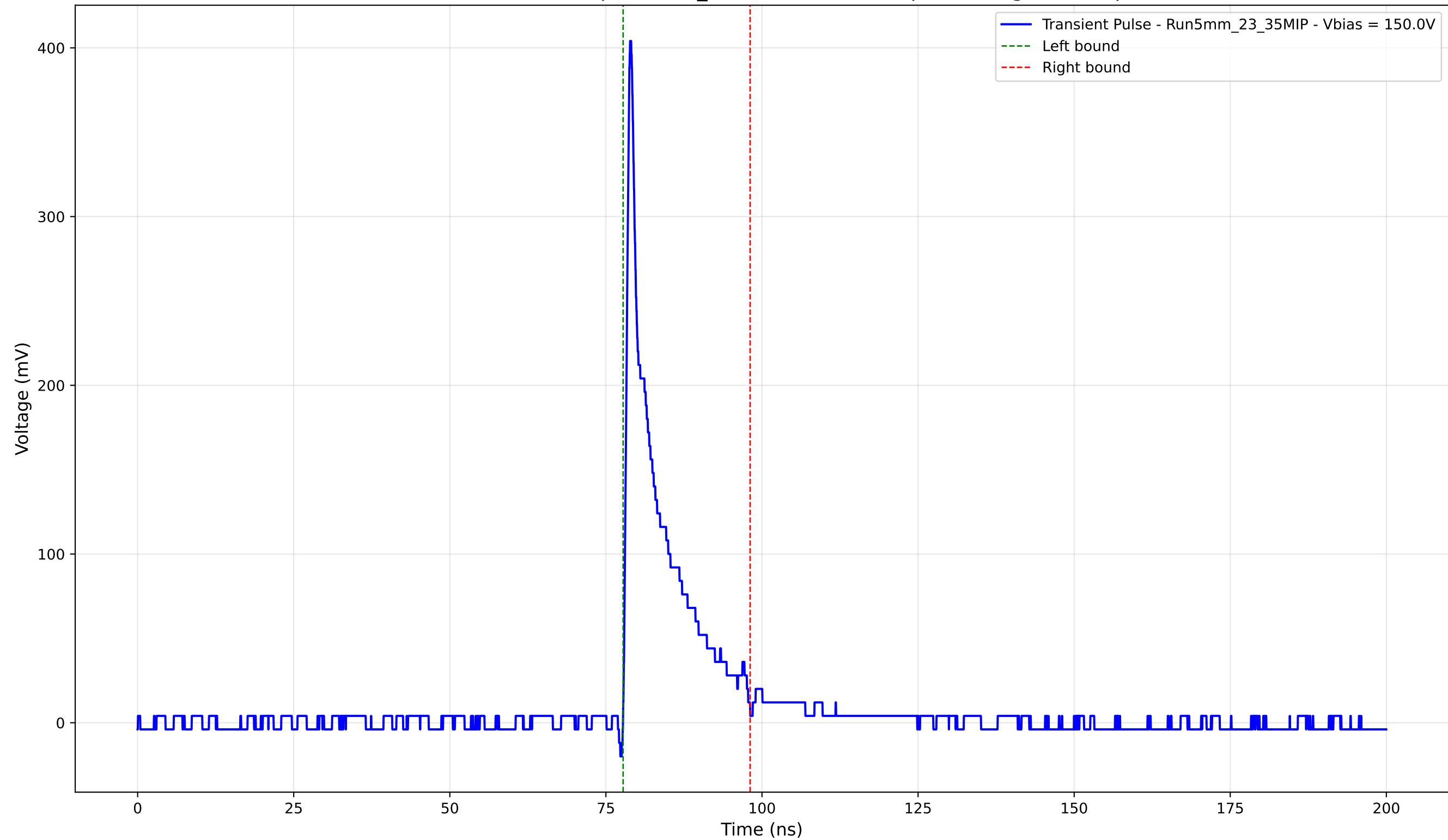
Transient Pulse - Sample: 5mm_23 - Position: 205.0 \mu\text{m} - Charge: 41.29 pC
