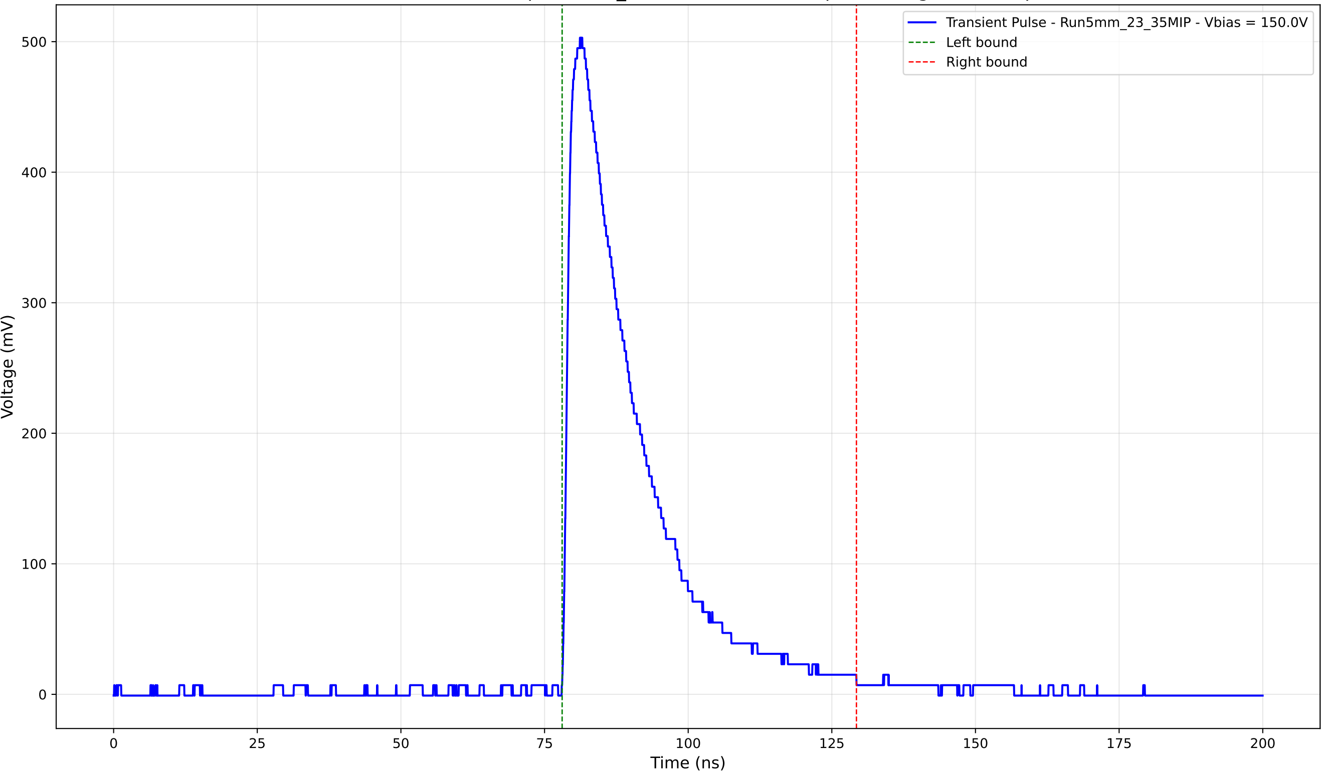
Transient Pulse - Sample: 5mm_23 - Position: 2975.0 \mu\text{m} - Charge: 136.22 pC
