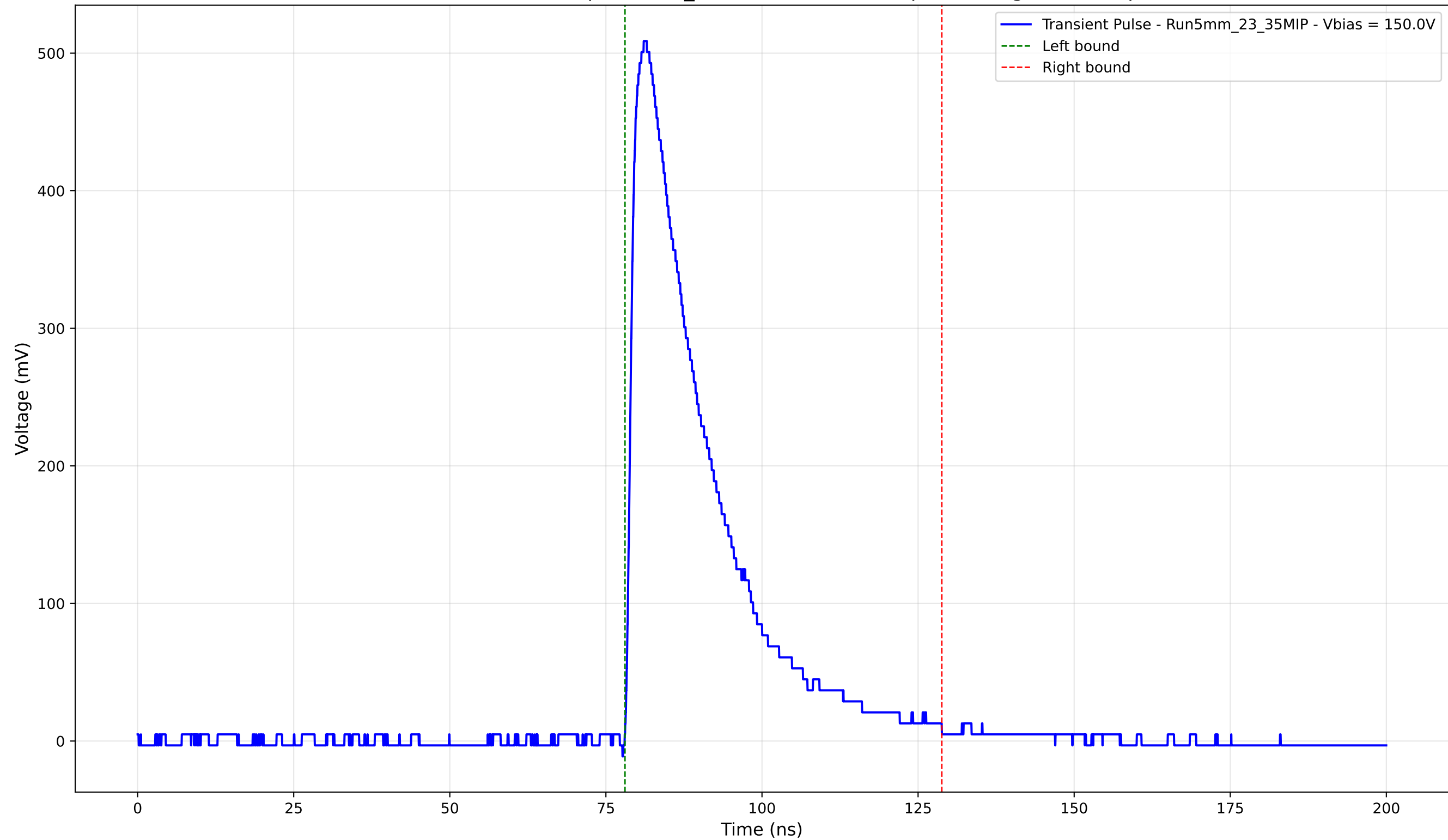
Transient Pulse - Sample: 5mm_23 - Position: 2400.0 \mu\text{m} - Charge: 137.17 pC
