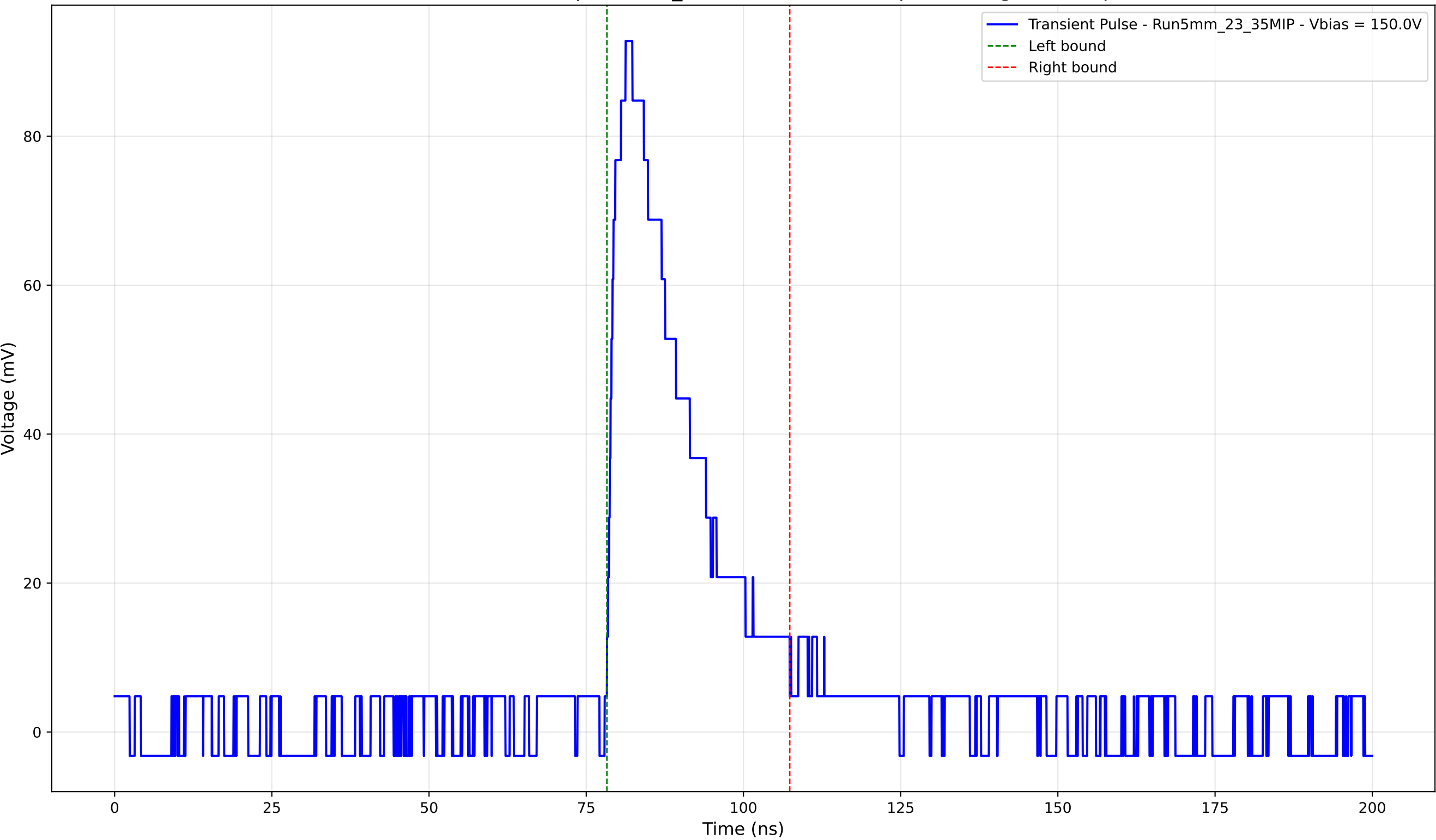
Transient Pulse - Sample: 5mm_23 - Position: 2655.0 \mu\text{m} - Charge: 23.89 pC
