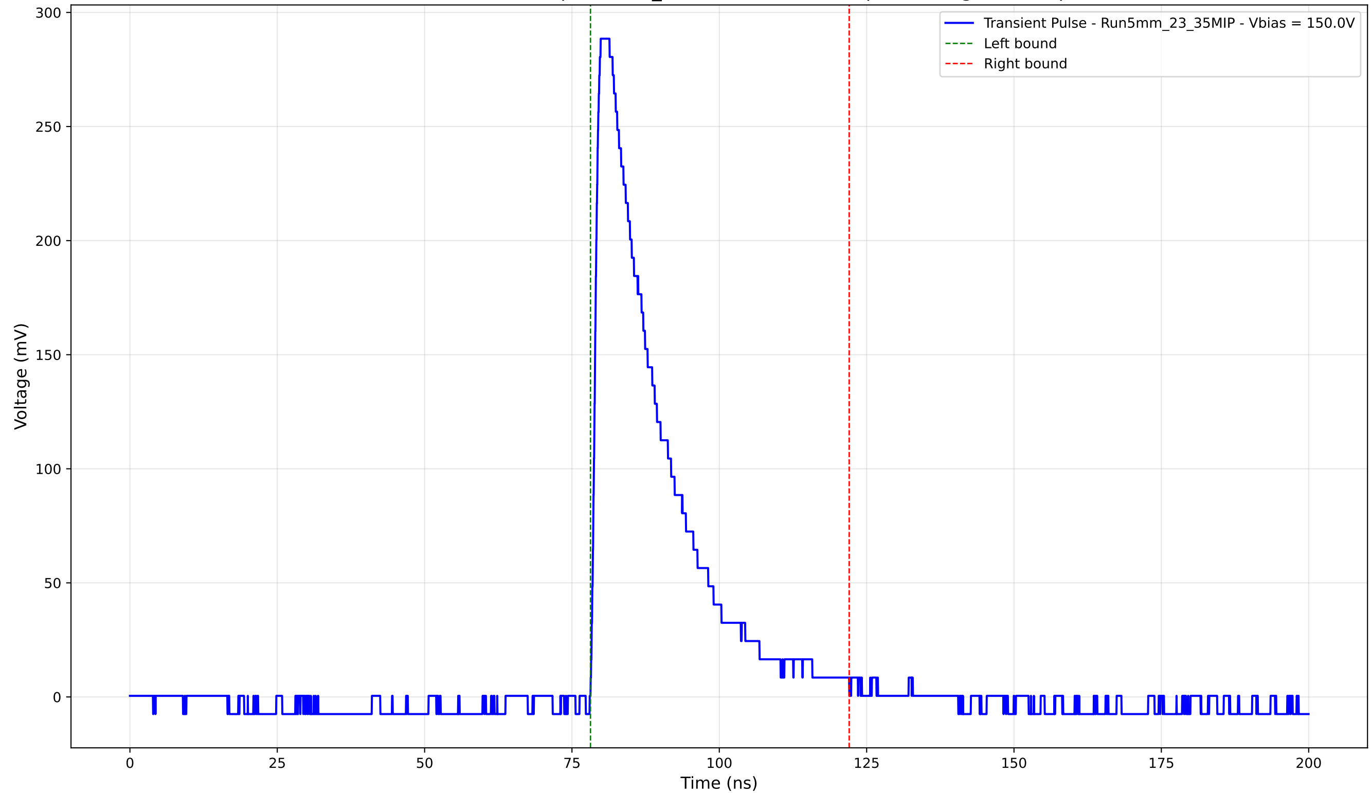
Transient Pulse - Sample: 5mm_23 - Position: 1675.0 \mu\text{m} - Charge: 70.28 pC
