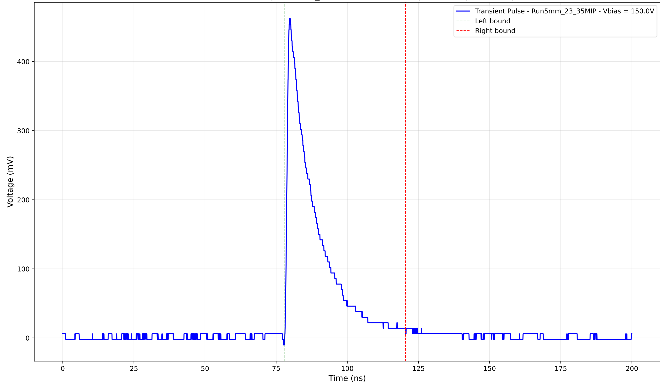
Transient Pulse - Sample: 5mm_23 - Position: 1190.0 \mu\text{m} - Charge: 96.37 pC
