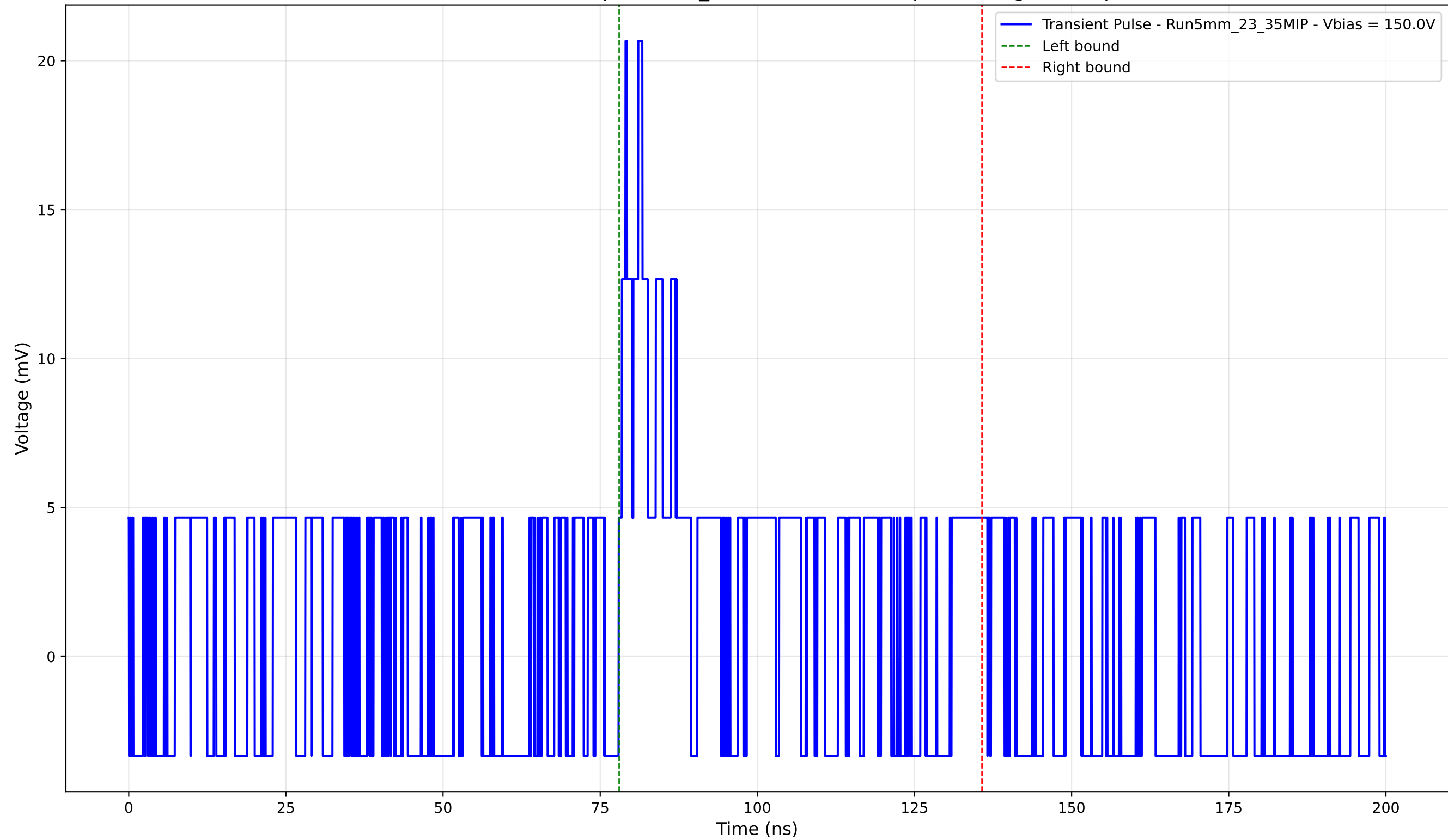
Transient Pulse - Sample: 5mm_23 - Position: 130.0 \mu\text{m} - Charge: 3.97 pC
