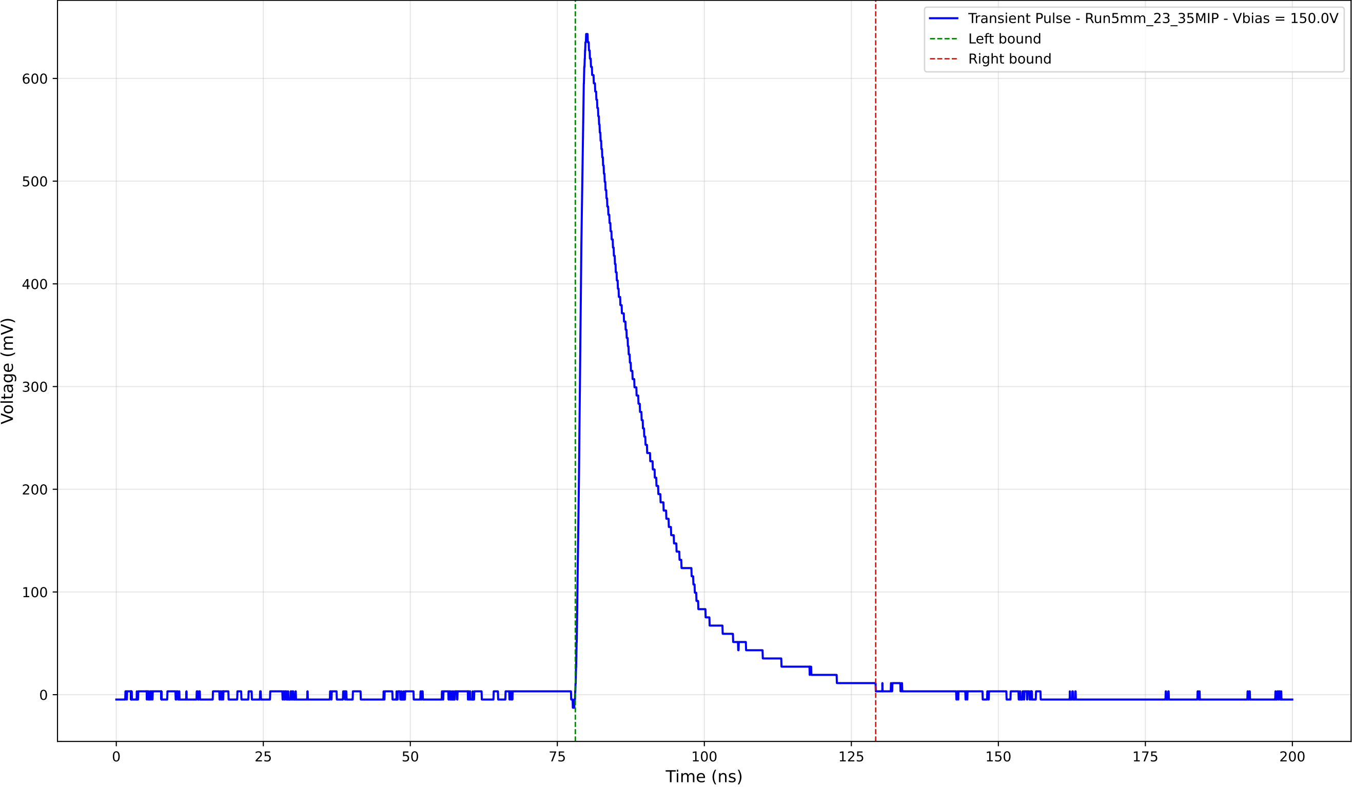
Transient Pulse - Sample: 5mm_23 - Position: 1420.0 \mu\text{m} - Charge: 150.27 pC
