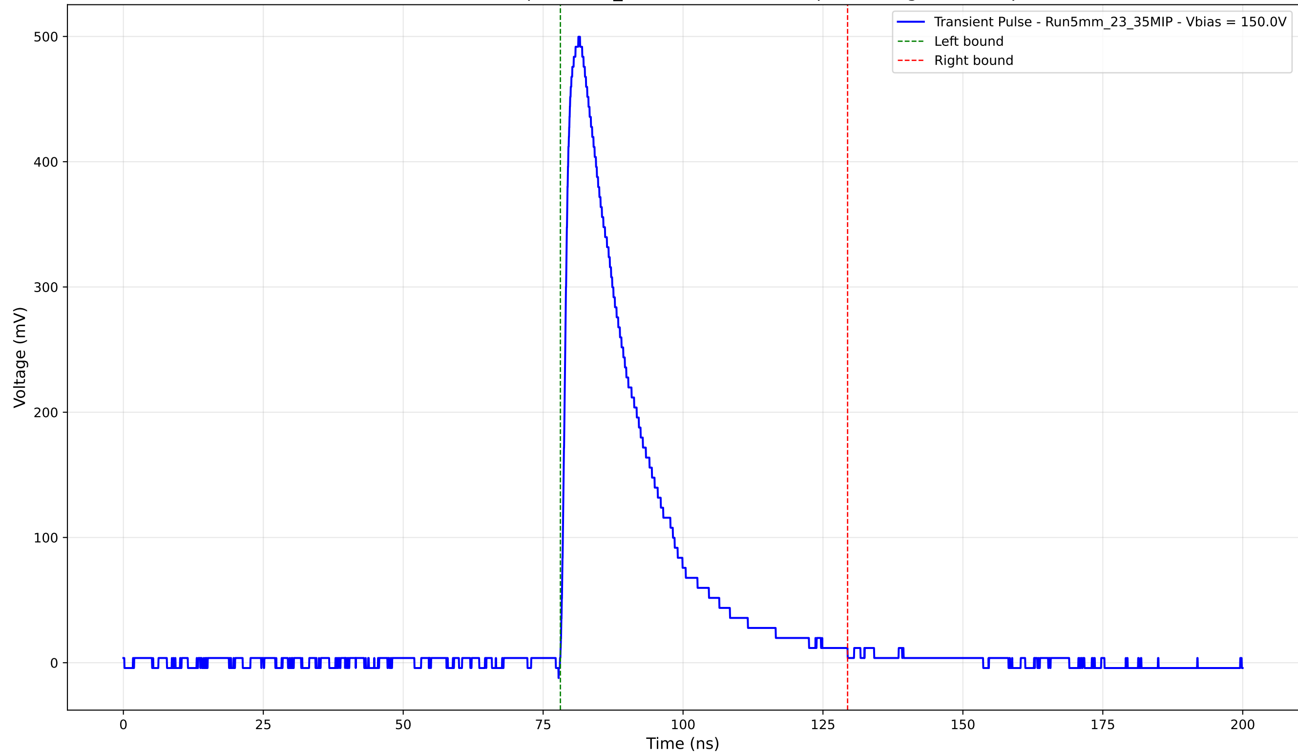
Transient Pulse - Sample: 5mm_23 - Position: 2925.0 \mu\text{m} - Charge: 133.64 pC
