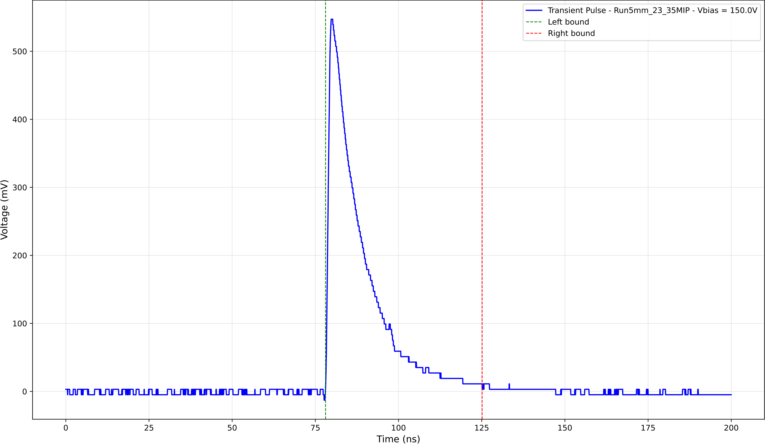
Transient Pulse - Sample: 5mm_23 - Position: 3905.0 \mu\text{m} - Charge: 120.12 pC
