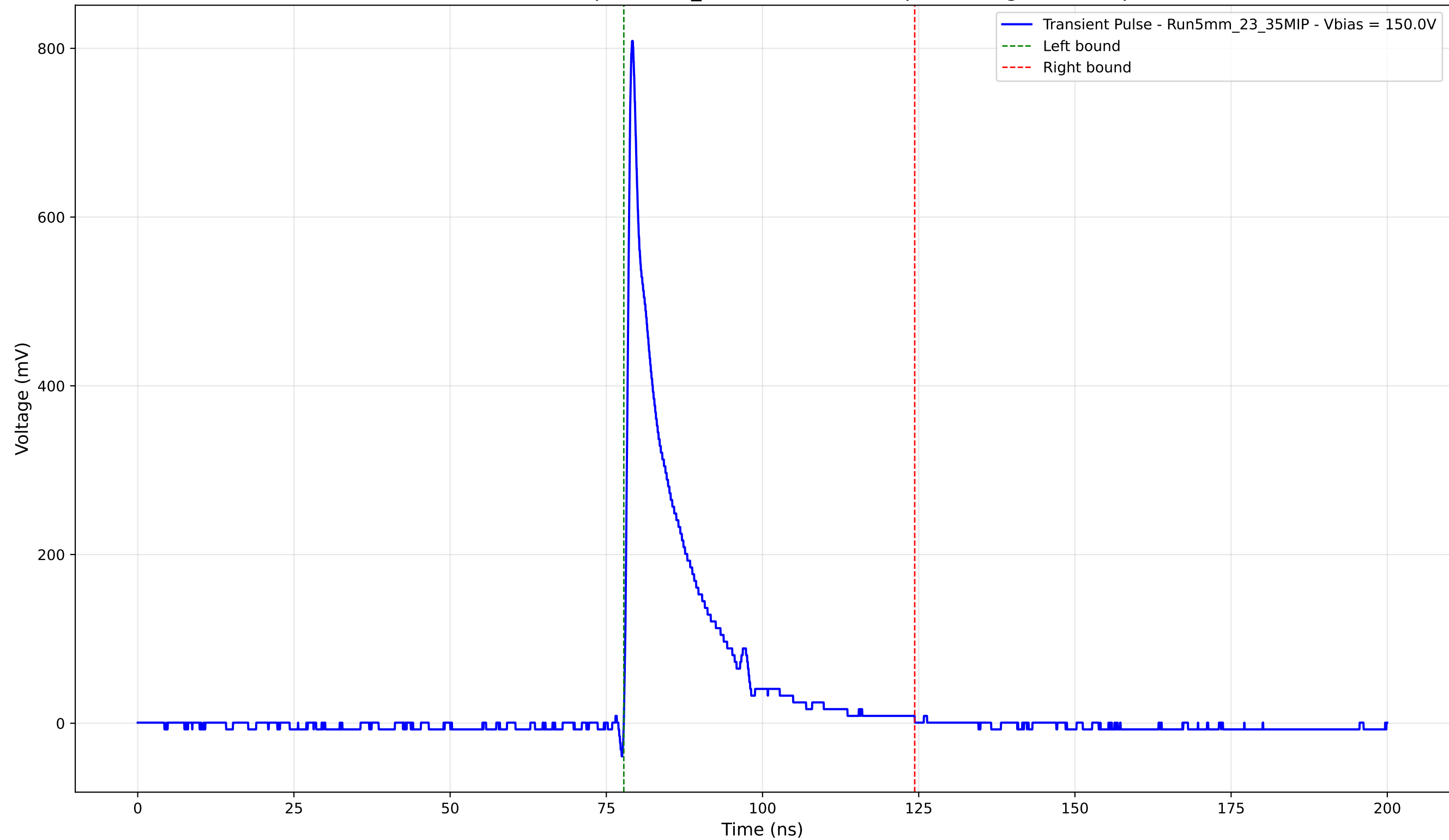
Transient Pulse - Sample: 5mm_23 - Position: 440.0 \mu\text{m} - Charge: 113.24 pC
