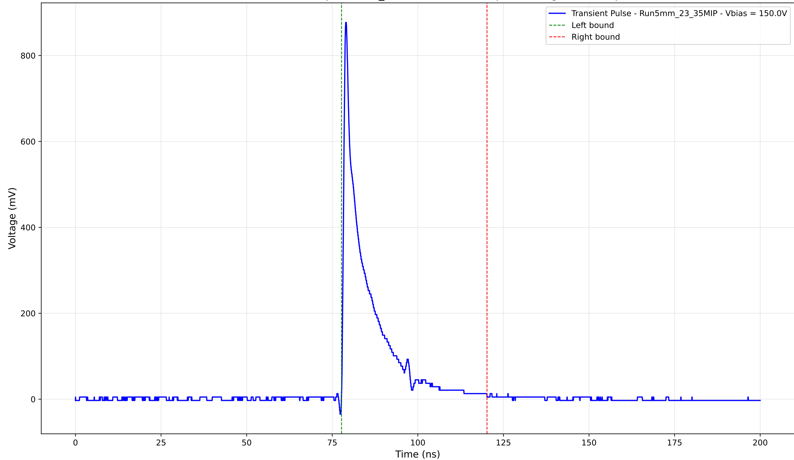
Transient Pulse - Sample: 5mm_23 - Position: 280.0 \mu\text{m} - Charge: 114.95 pC
