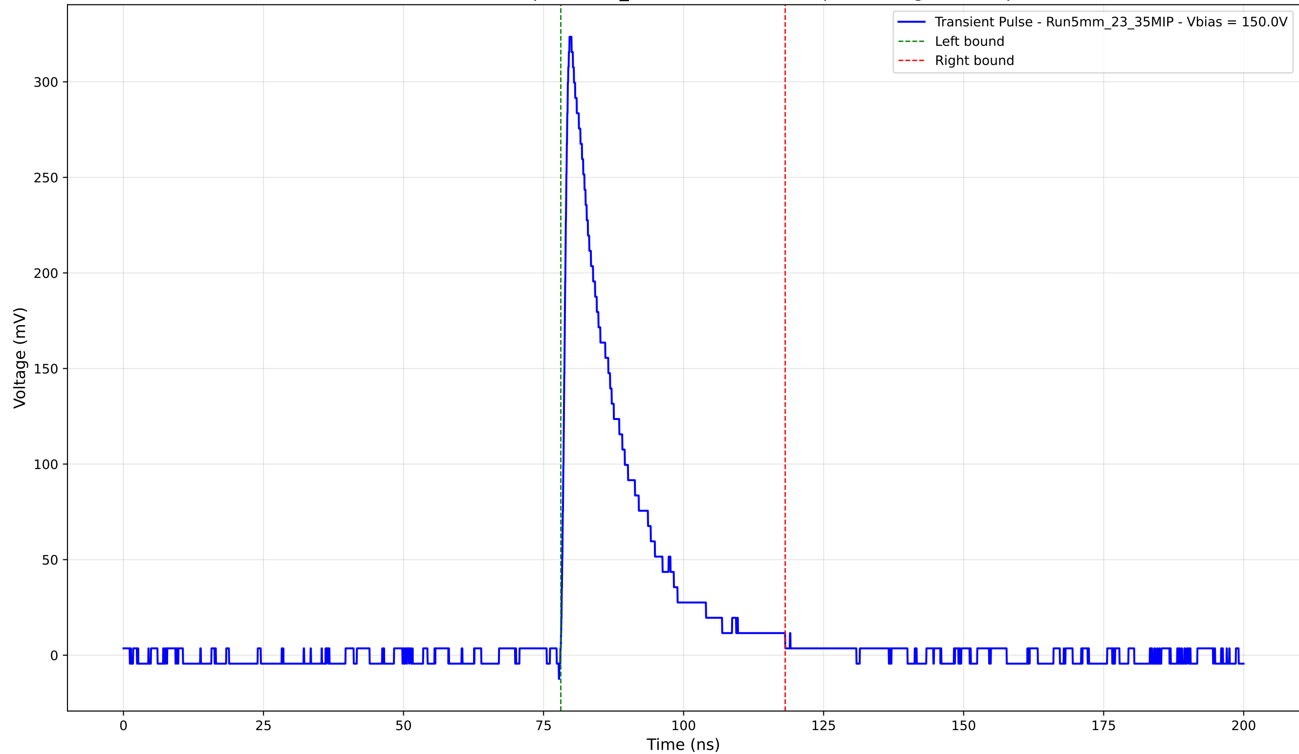
Transient Pulse - Sample: 5mm_23 - Position: 4110.0 \mu\text{m} - Charge: 63.31 pC
