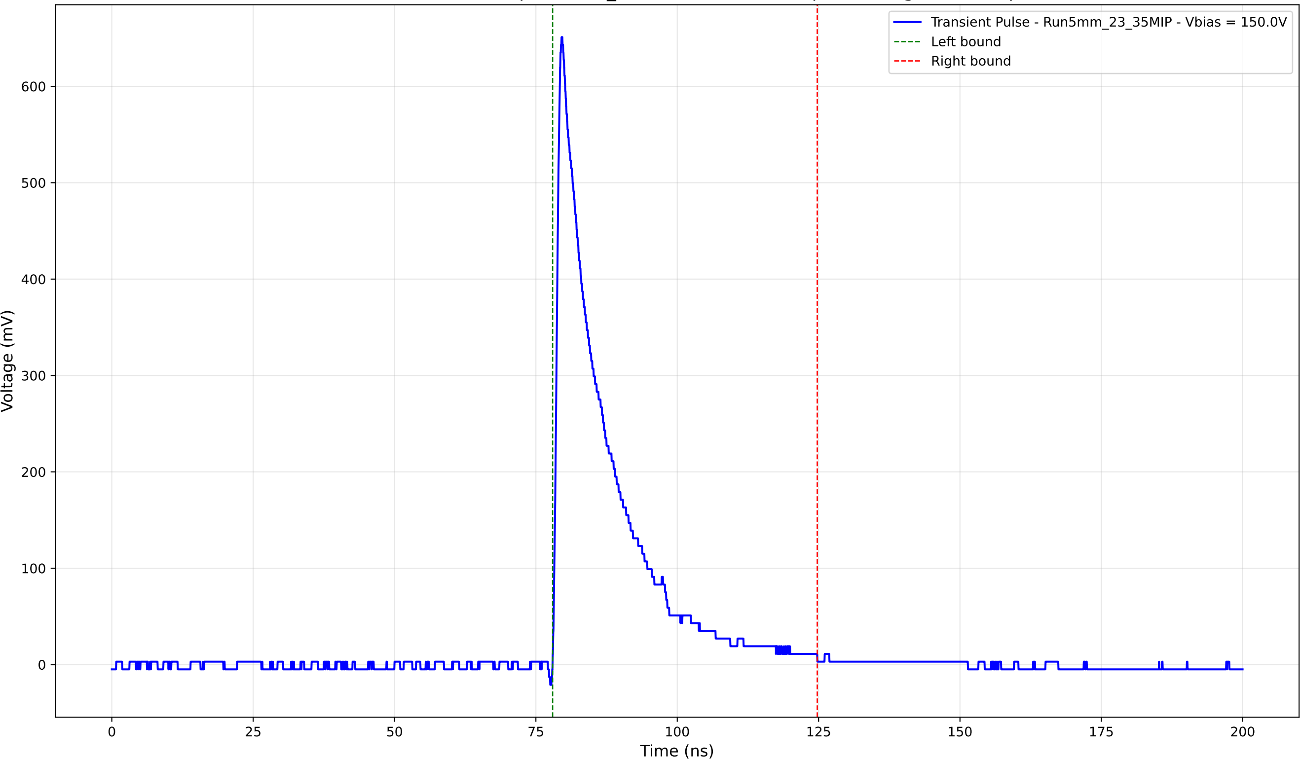
Transient Pulse - Sample: 5mm_23 - Position: 4340.0 \mu\text{m} - Charge: 118.13 pC
