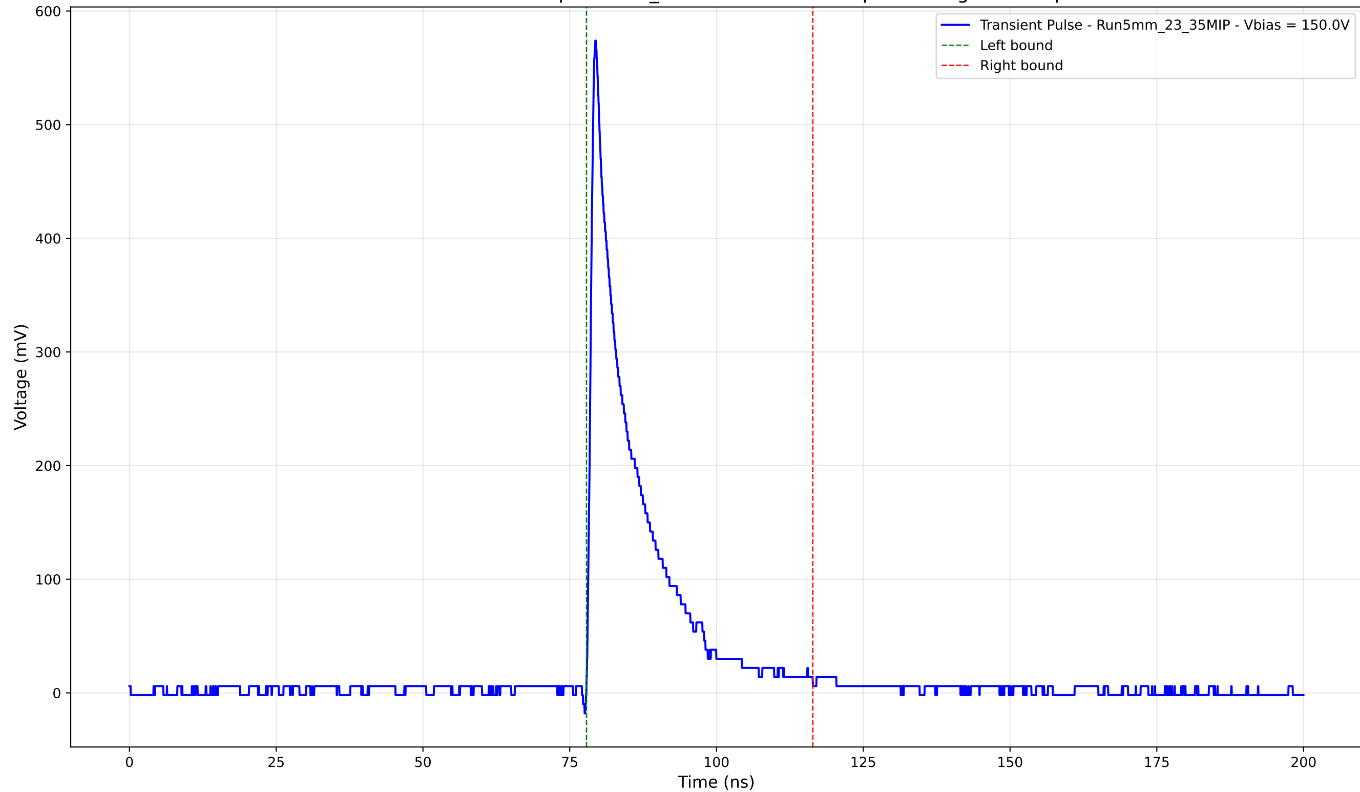
Transient Pulse - Sample: 5mm_23 - Position: 4570.0 \mu\text{m} - Charge: 88.37 pC
