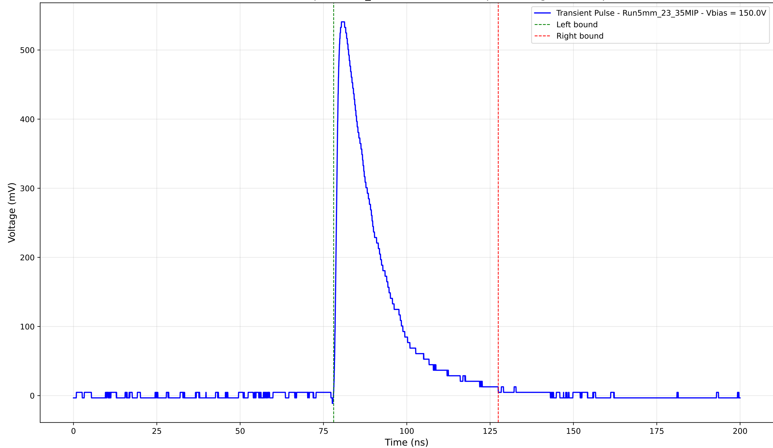
Transient Pulse - Sample: 5mm_23 - Position: 1950.0 \mu\text{m} - Charge: 141.90 pC
