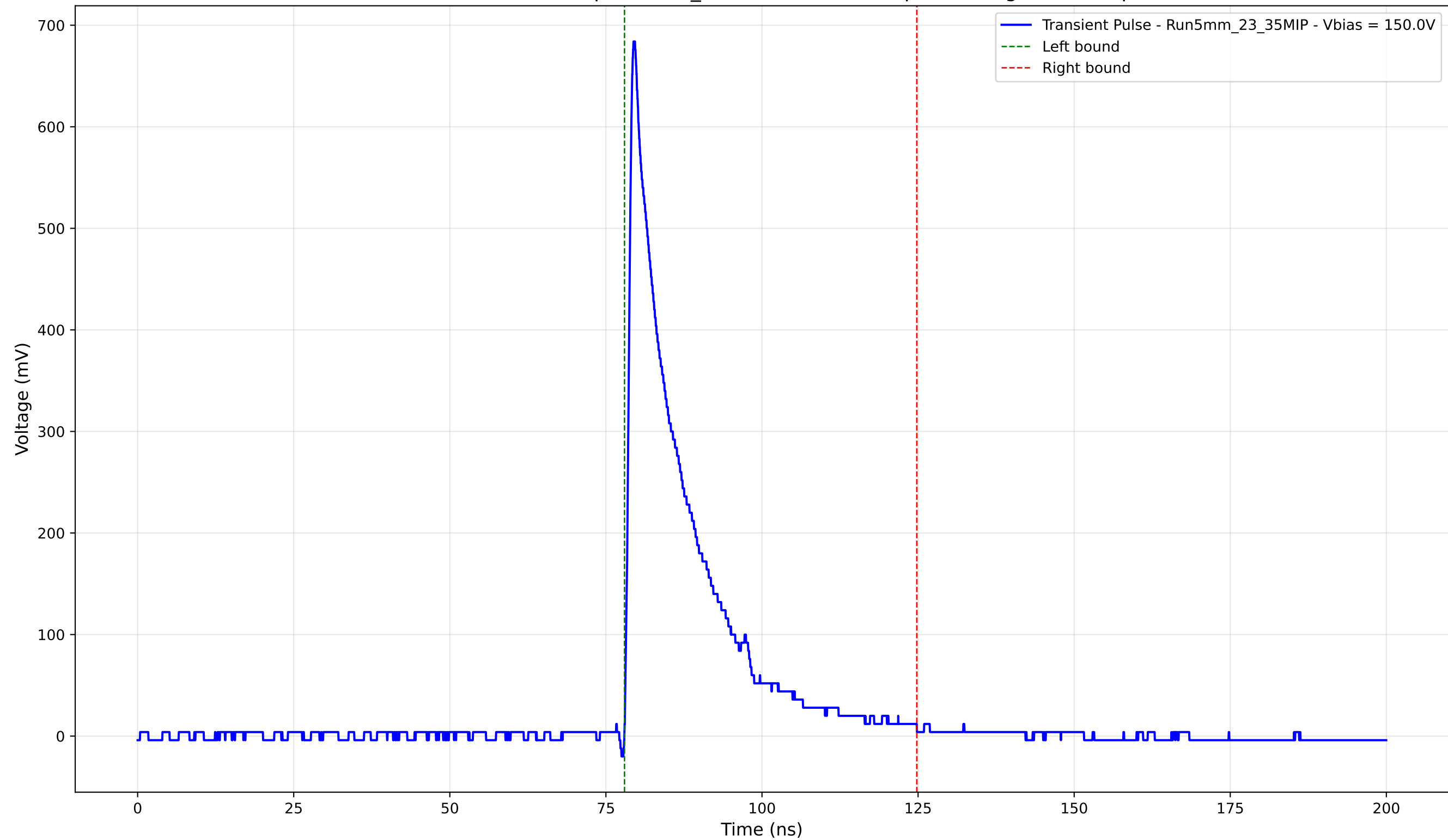
Transient Pulse - Sample: 5mm_23 - Position: 825.0 \mu\text{m} - Charge: 122.95 pC
