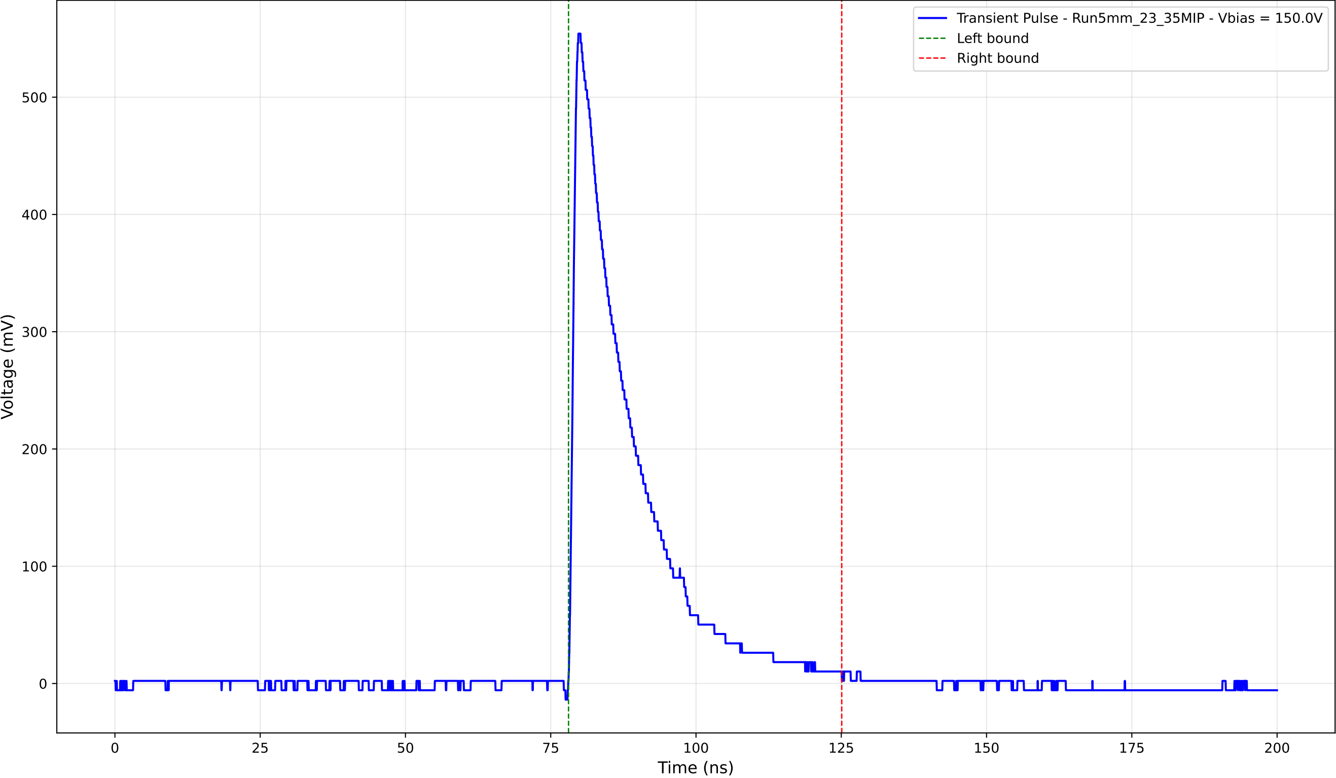
Transient Pulse - Sample: 5mm_23 - Position: 3950.0 \mu\text{m} - Charge: 118.41 pC
