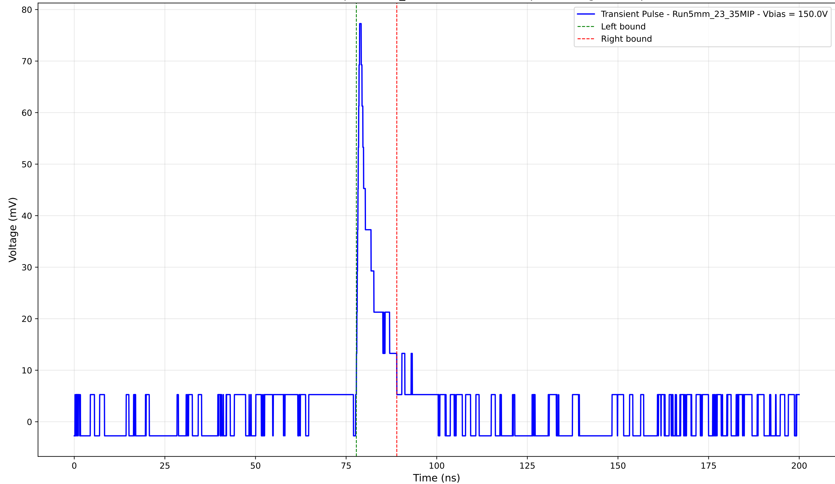
Transient Pulse - Sample: 5mm_23 - Position: 5115.0 \mu\text{m} - Charge: 6.60 pC
