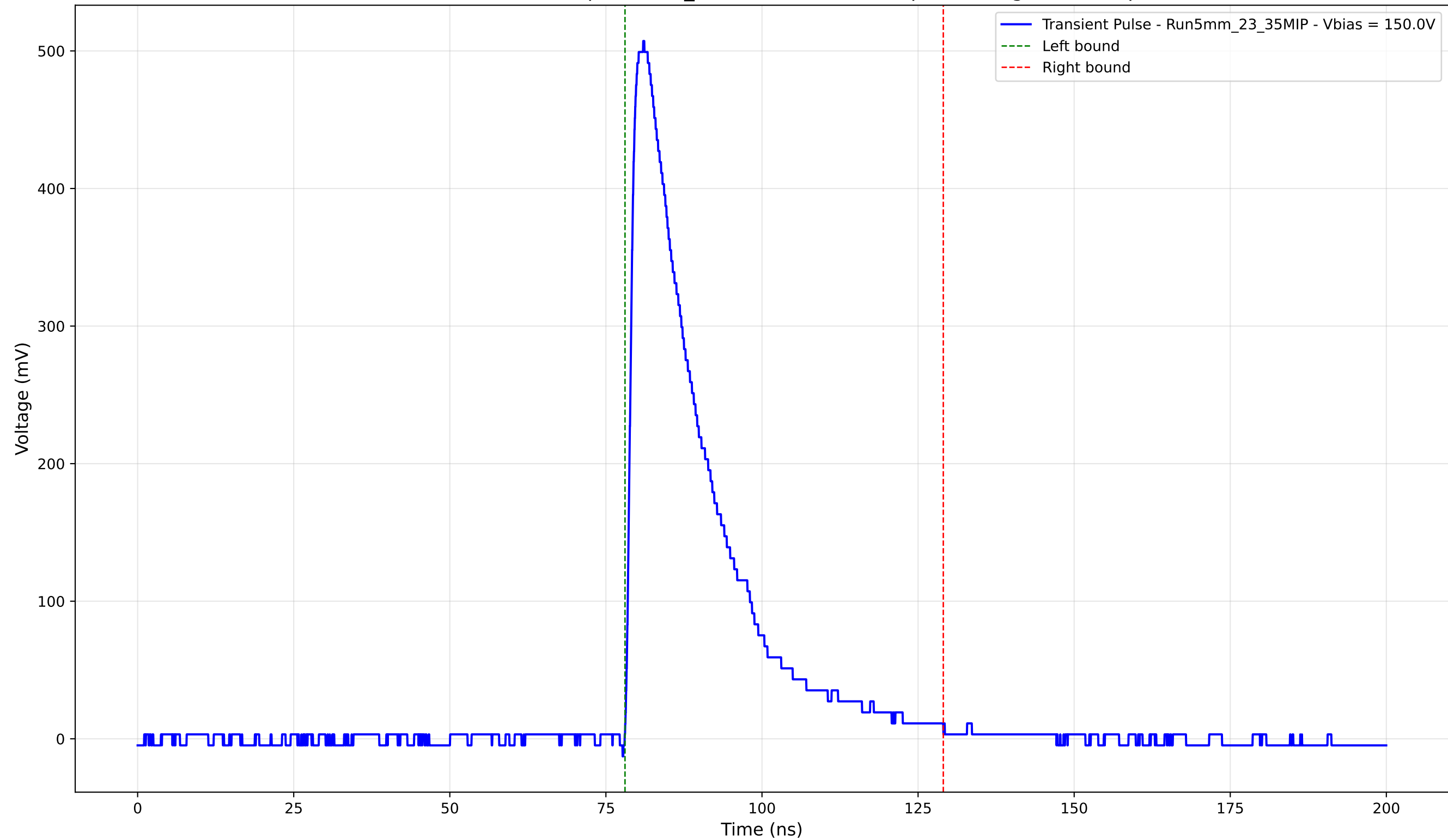
Transient Pulse - Sample: 5mm_23 - Position: 3275.0 \mu\text{m} - Charge: 130.50 pC
