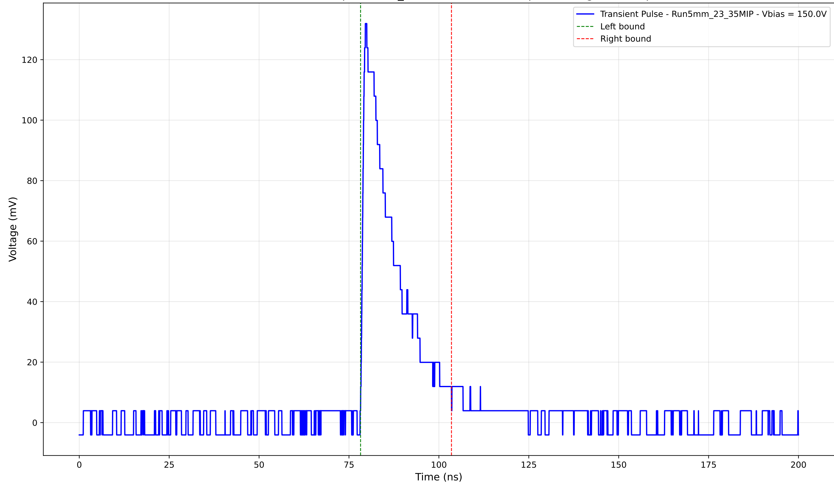
Transient Pulse - Sample: 5mm_23 - Position: 1110.0 \mu\text{m} - Charge: 25.21 pC
