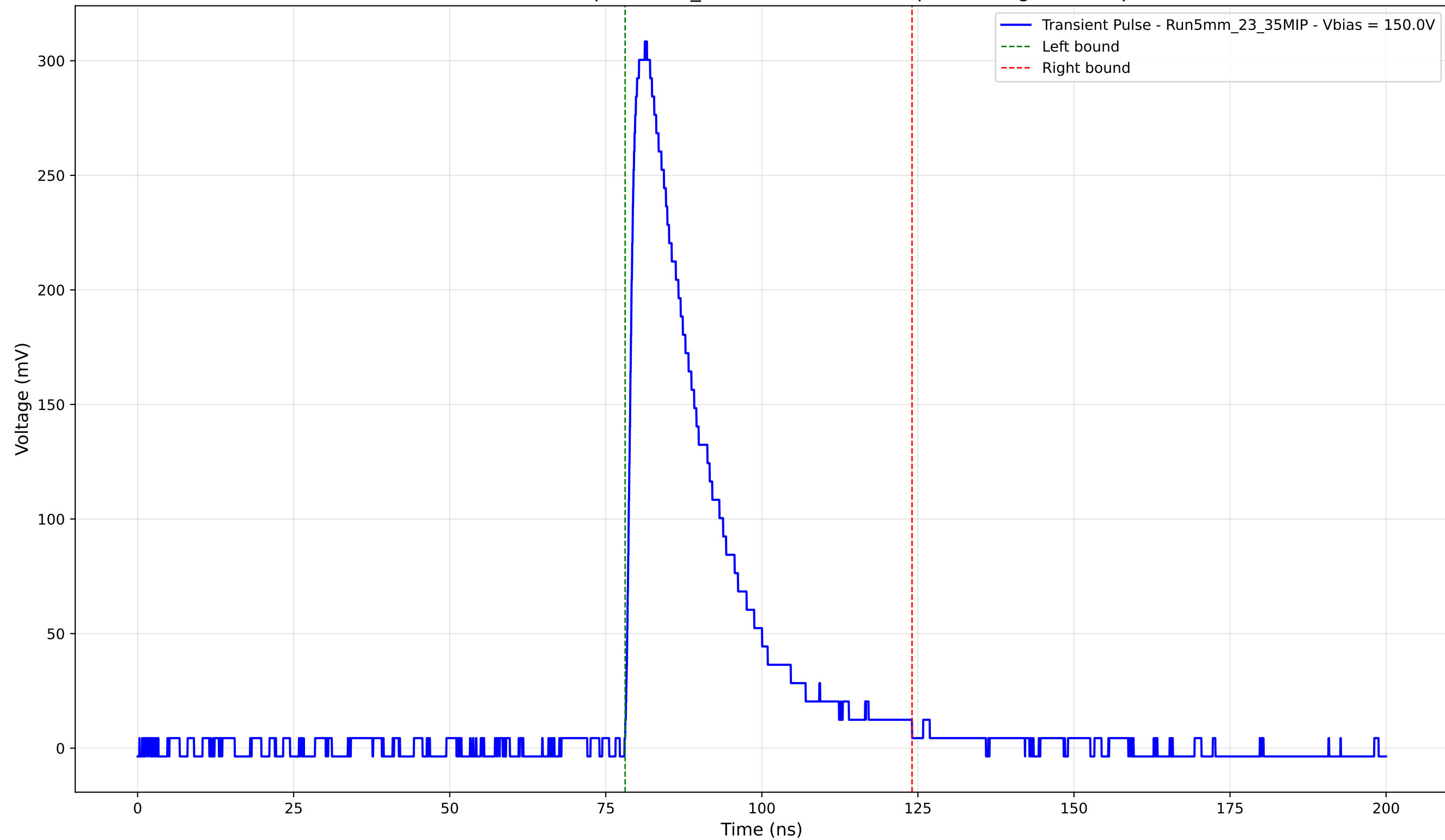
Transient Pulse - Sample: 5mm_23 - Position: 2190.0 \mu\text{m} - Charge: 80.20 pC
