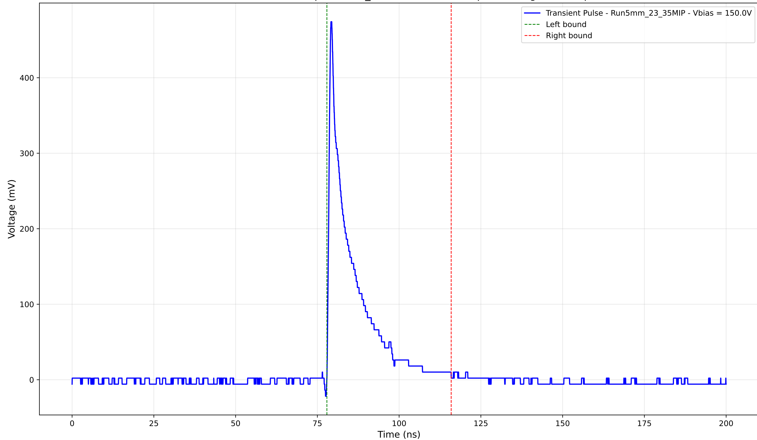
Transient Pulse - Sample: 5mm_23 - Position: 570.0 \mu\text{m} - Charge: 66.05 pC
