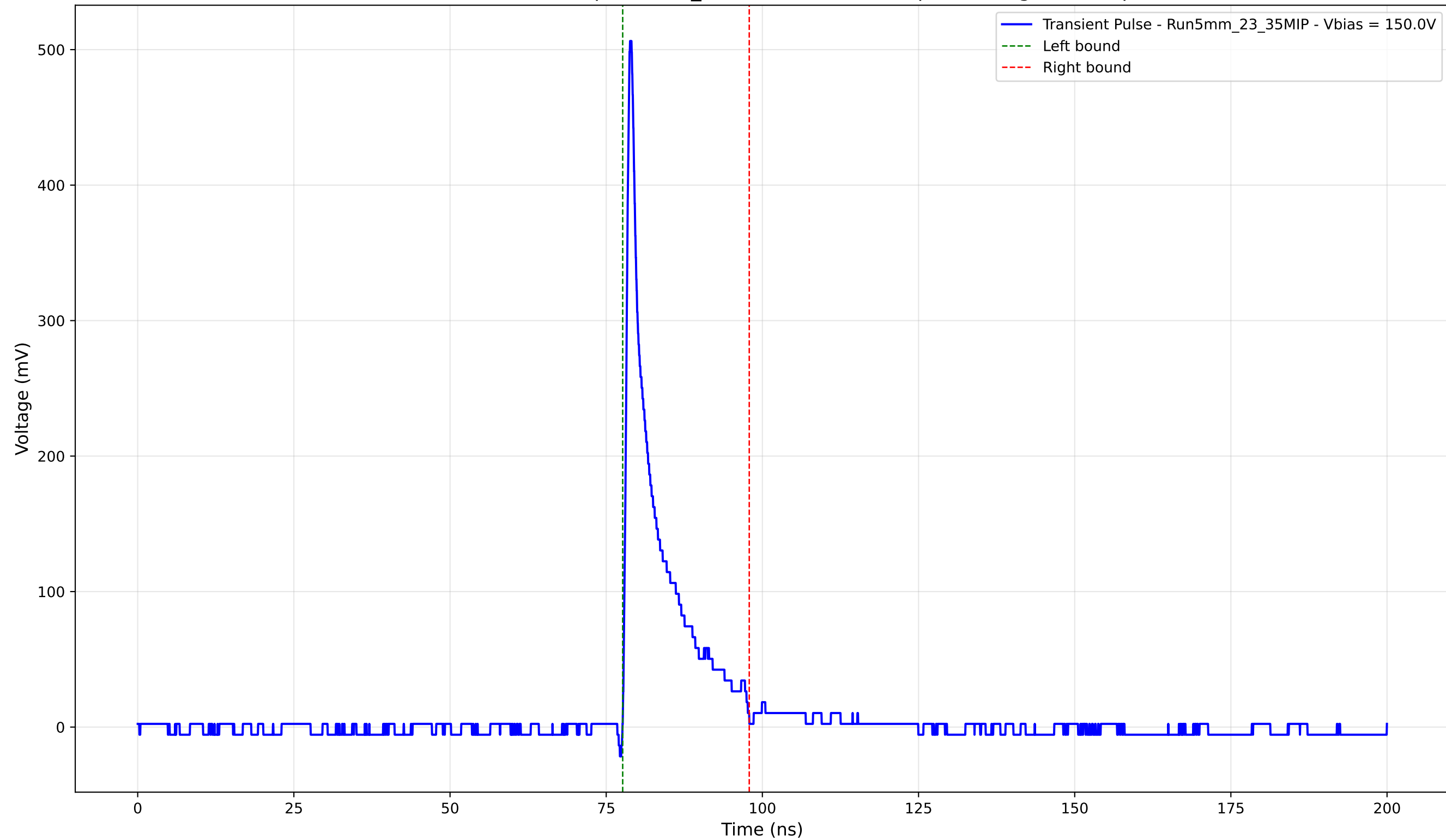
Transient Pulse - Sample: 5mm_23 - Position: 5065.0 \mu\text{m} - Charge: 48.36 pC
