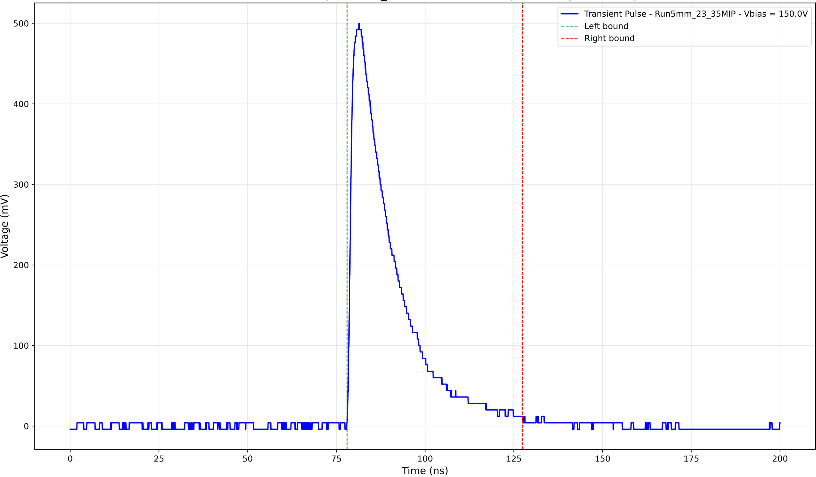
Transient Pulse - Sample: 5mm_23 - Position: 2955.0 \mu\text{m} - Charge: 133.70 pC
