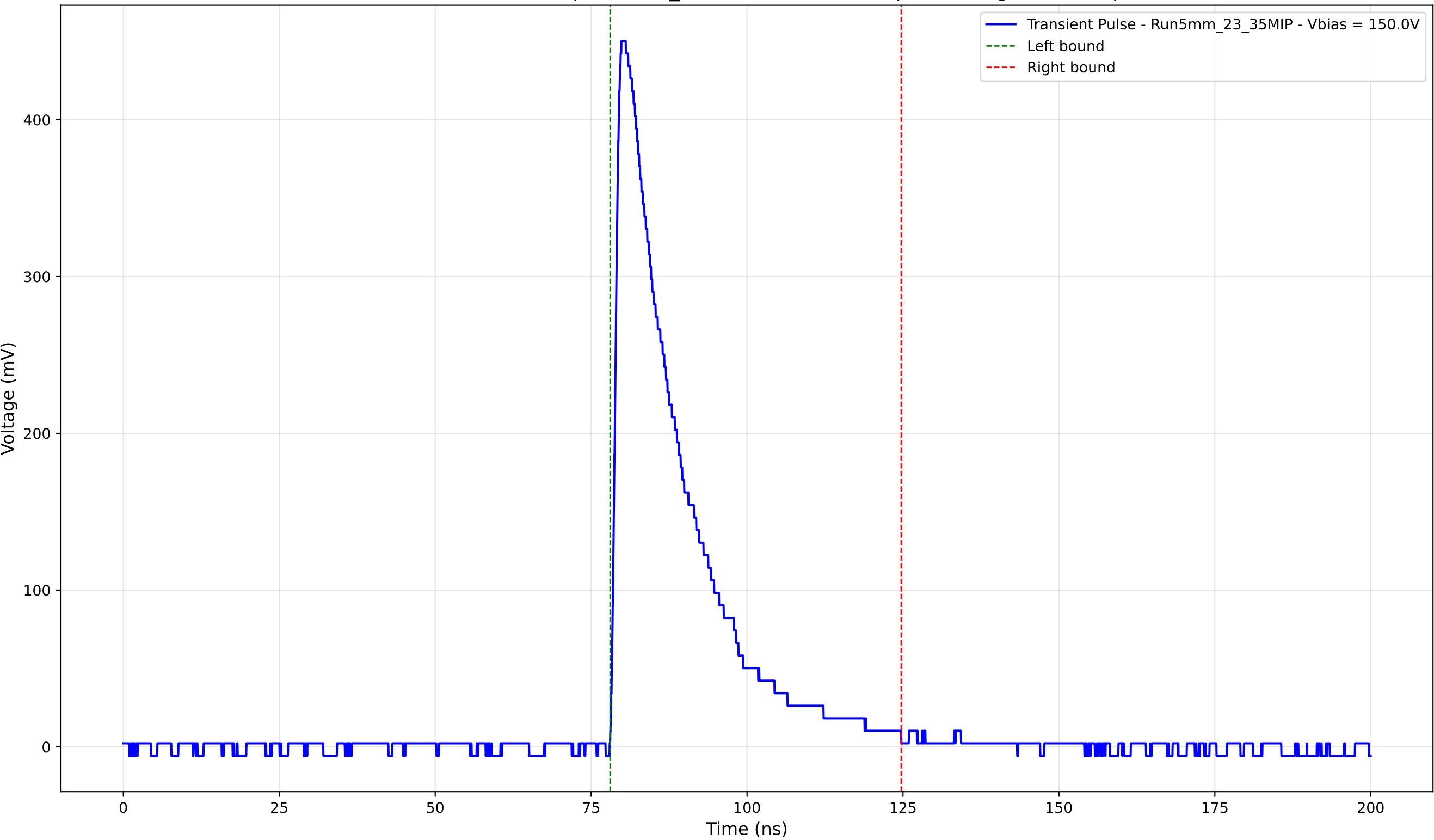
Transient Pulse - Sample: 5mm_23 - Position: 3725.0 \mu\text{m} - Charge: 103.81 pC
