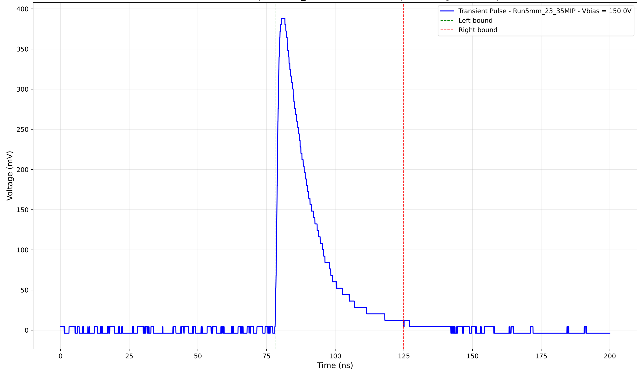
Transient Pulse - Sample: 5mm_23 - Position: 2075.0 \mu\text{m} - Charge: 101.17 pC
