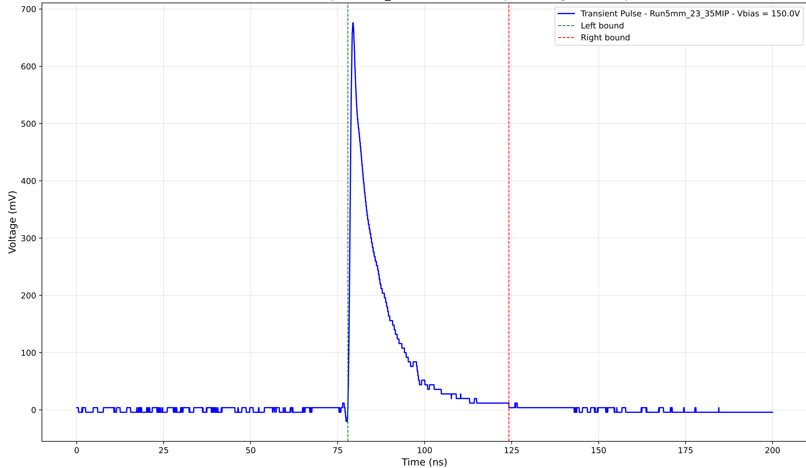
Transient Pulse - Sample: 5mm_23 - Position: 710.0 \mu\text{m} - Charge: 111.46 pC
