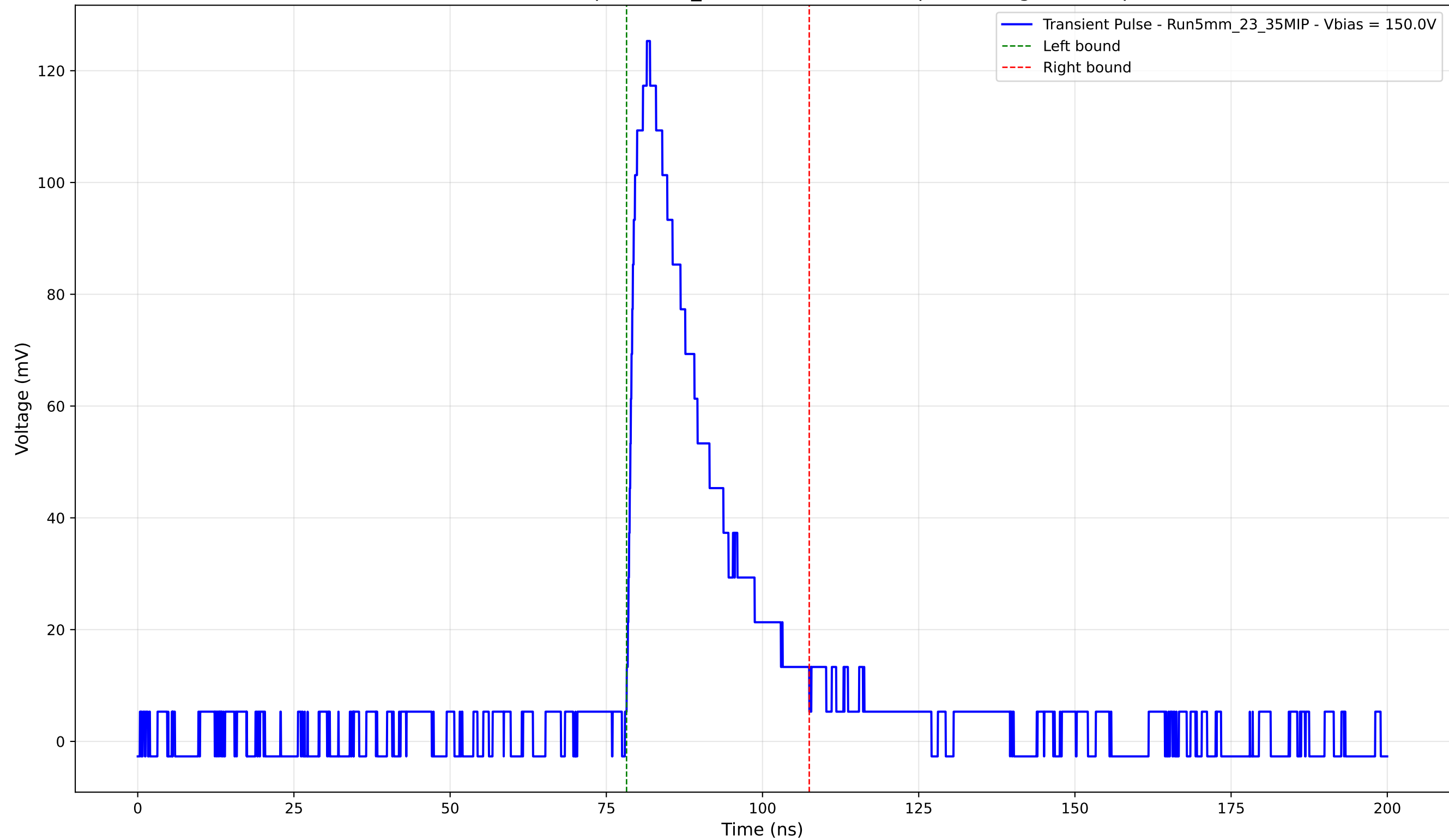
Transient Pulse - Sample: 5mm_23 - Position: 2665.0 \mu\text{m} - Charge: 30.82 pC
