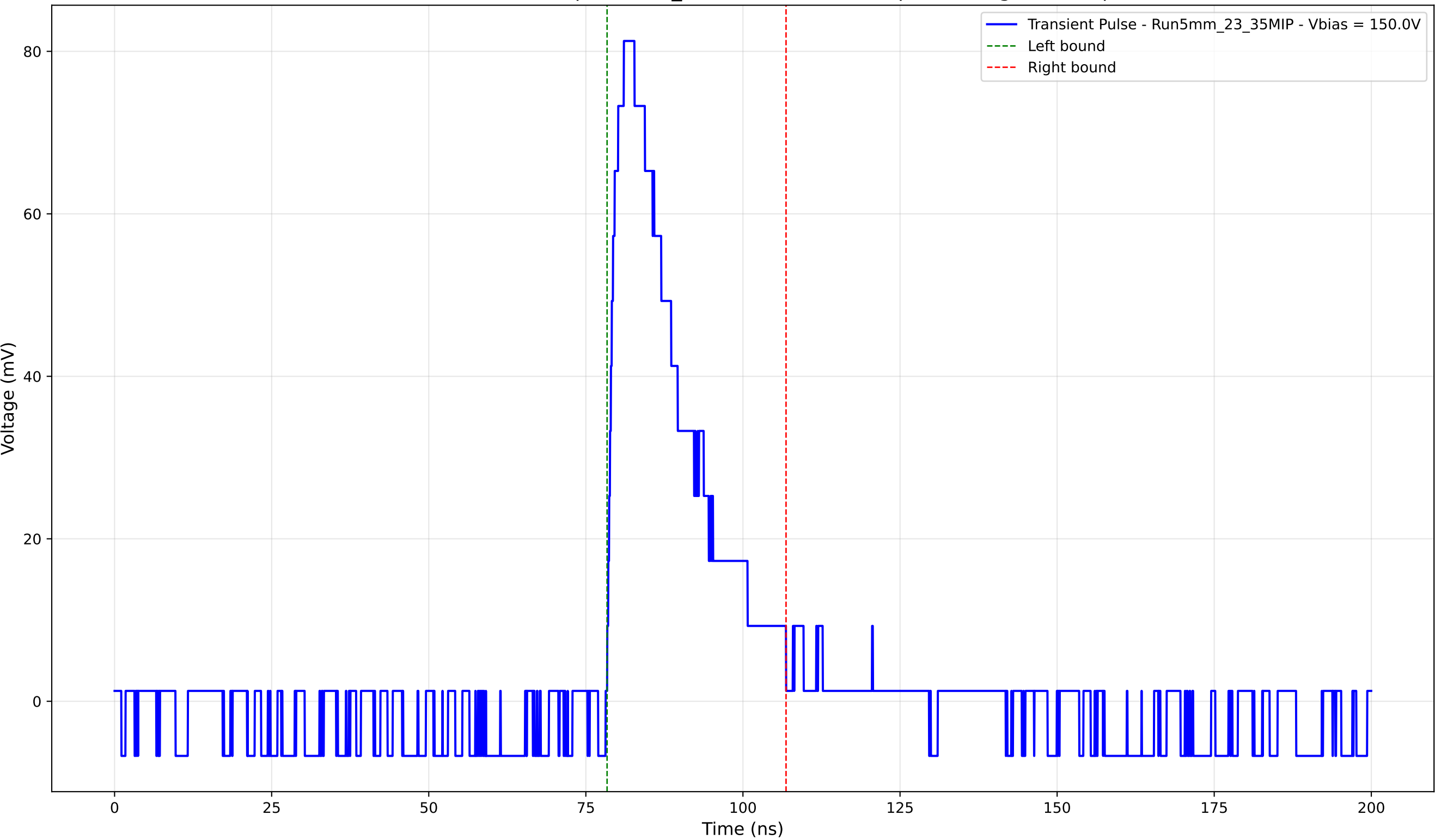
Transient Pulse - Sample: 5mm_23 - Position: 2650.0 \mu\text{m} - Charge: 20.09 pC
