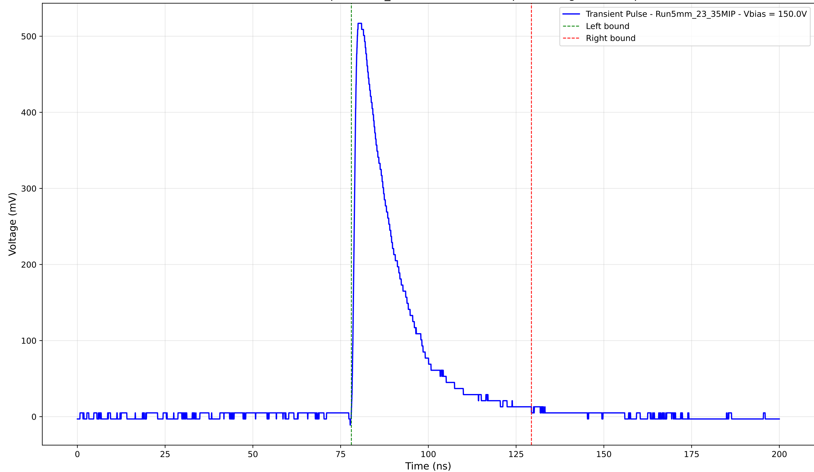
Transient Pulse - Sample: 5mm_23 - Position: 1735.0 \mu\text{m} - Charge: 132.16 pC
