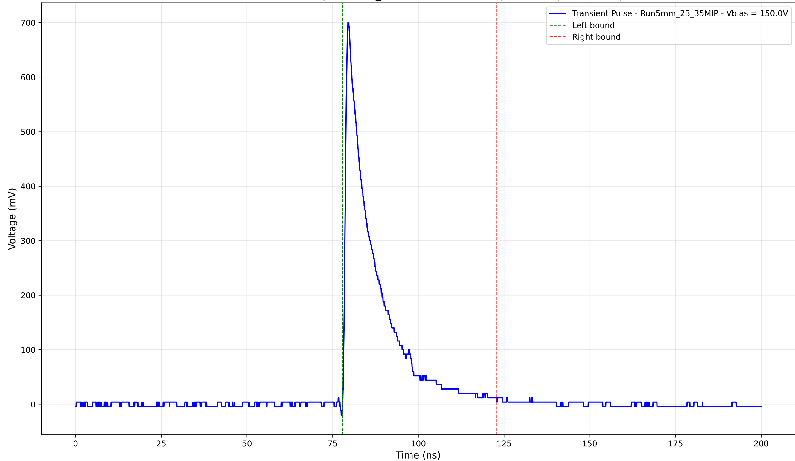
Transient Pulse - Sample: 5mm_23 - Position: 4380.0 \mu\text{m} - Charge: 126.28 pC
