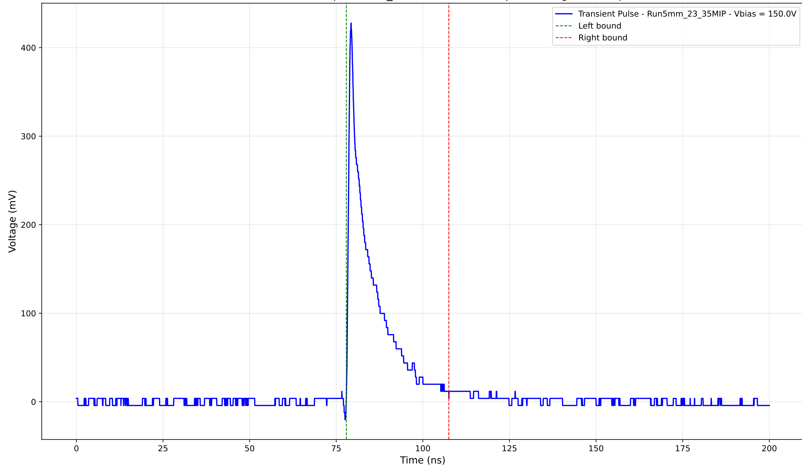
Transient Pulse - Sample: 5mm_23 - Position: 575.0 \mu\text{m} - Charge: 57.33 pC
