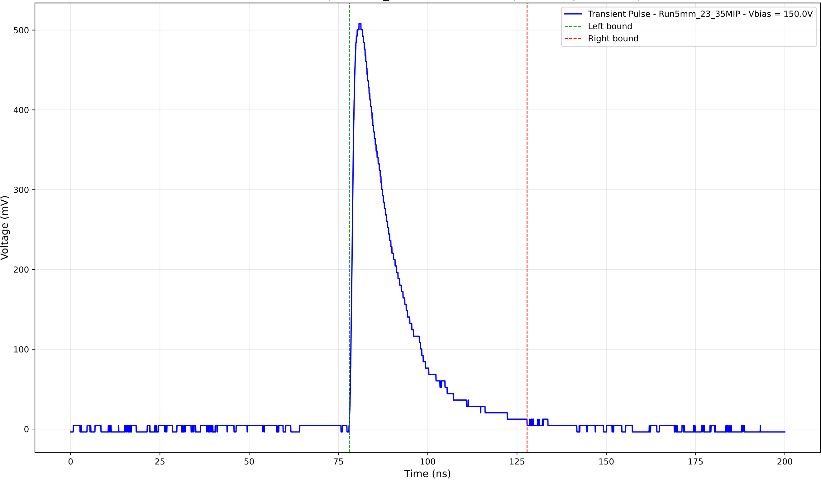
Transient Pulse - Sample: 5mm_23 - Position: 3285.0 \mu\text{m} - Charge: 132.21 pC
