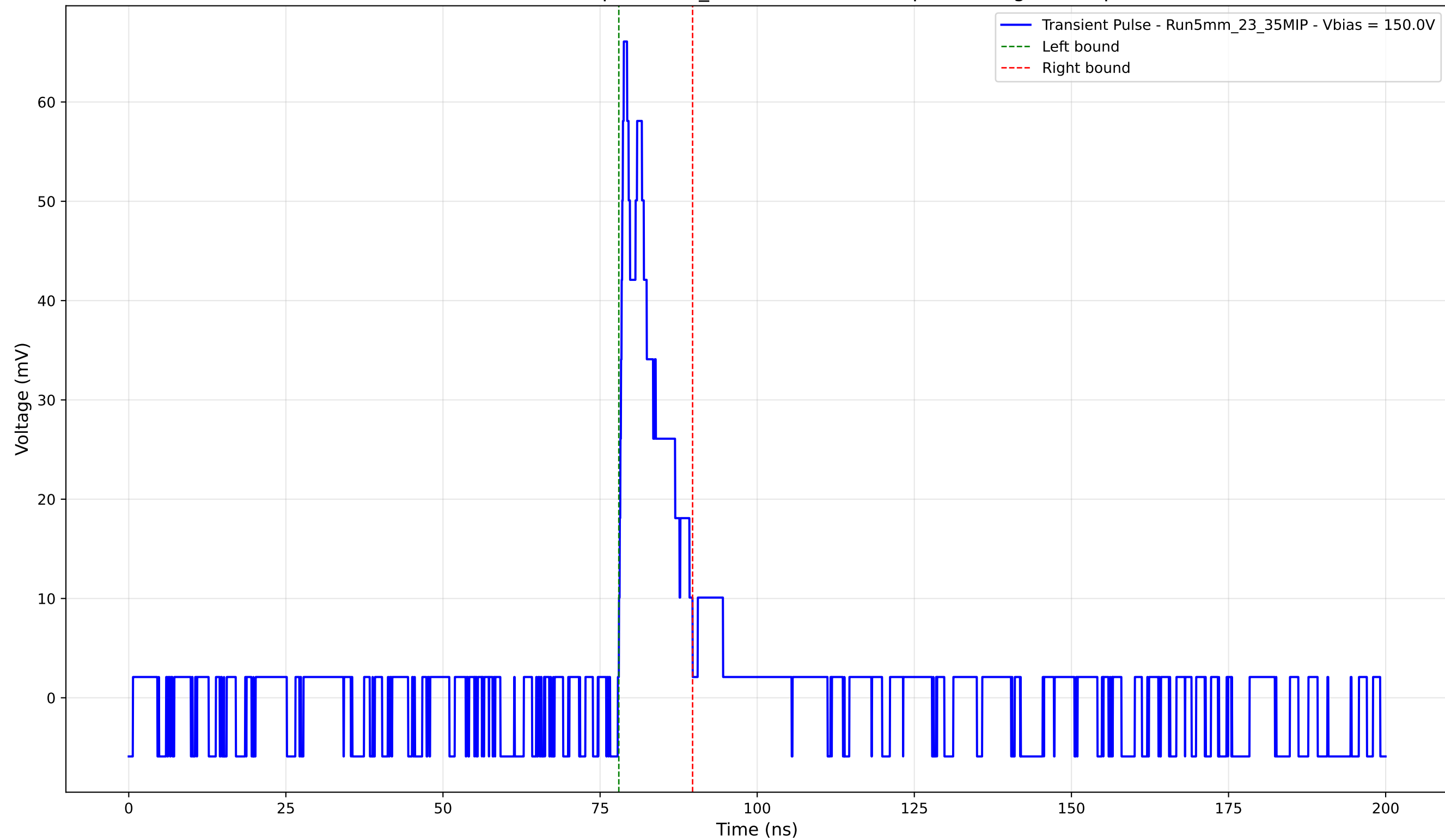
Transient Pulse - Sample: 5mm_23 - Position: 170.0 \mu\text{m} - Charge: 7.77 pC
