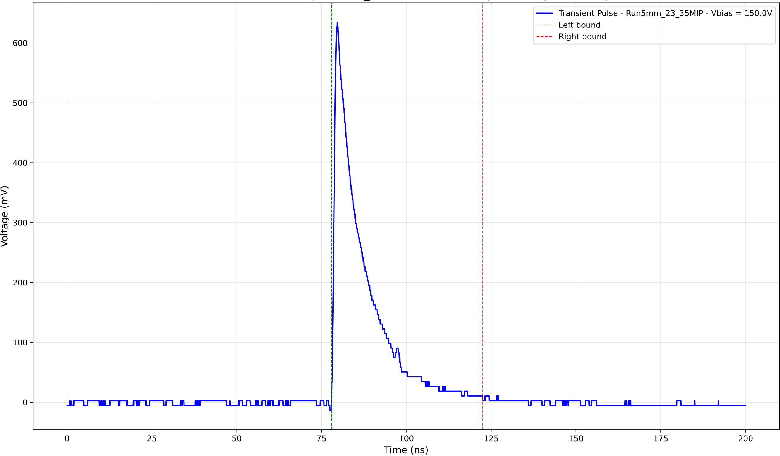
Transient Pulse - Sample: 5mm_23 - Position: 4315.0 \mu\text{m} - Charge: 114.91 pC
