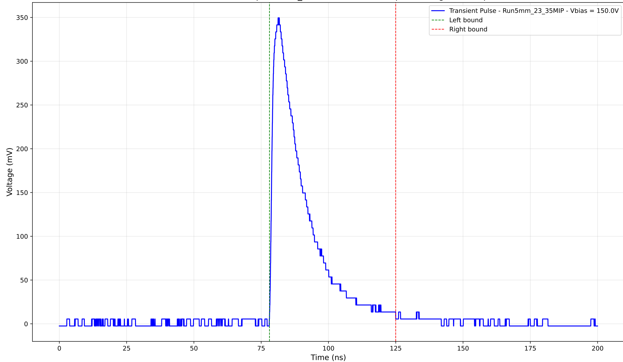
Transient Pulse - Sample: 5mm_23 - Position: 2705.0 \mu\text{m} - Charge: 93.57 pC
