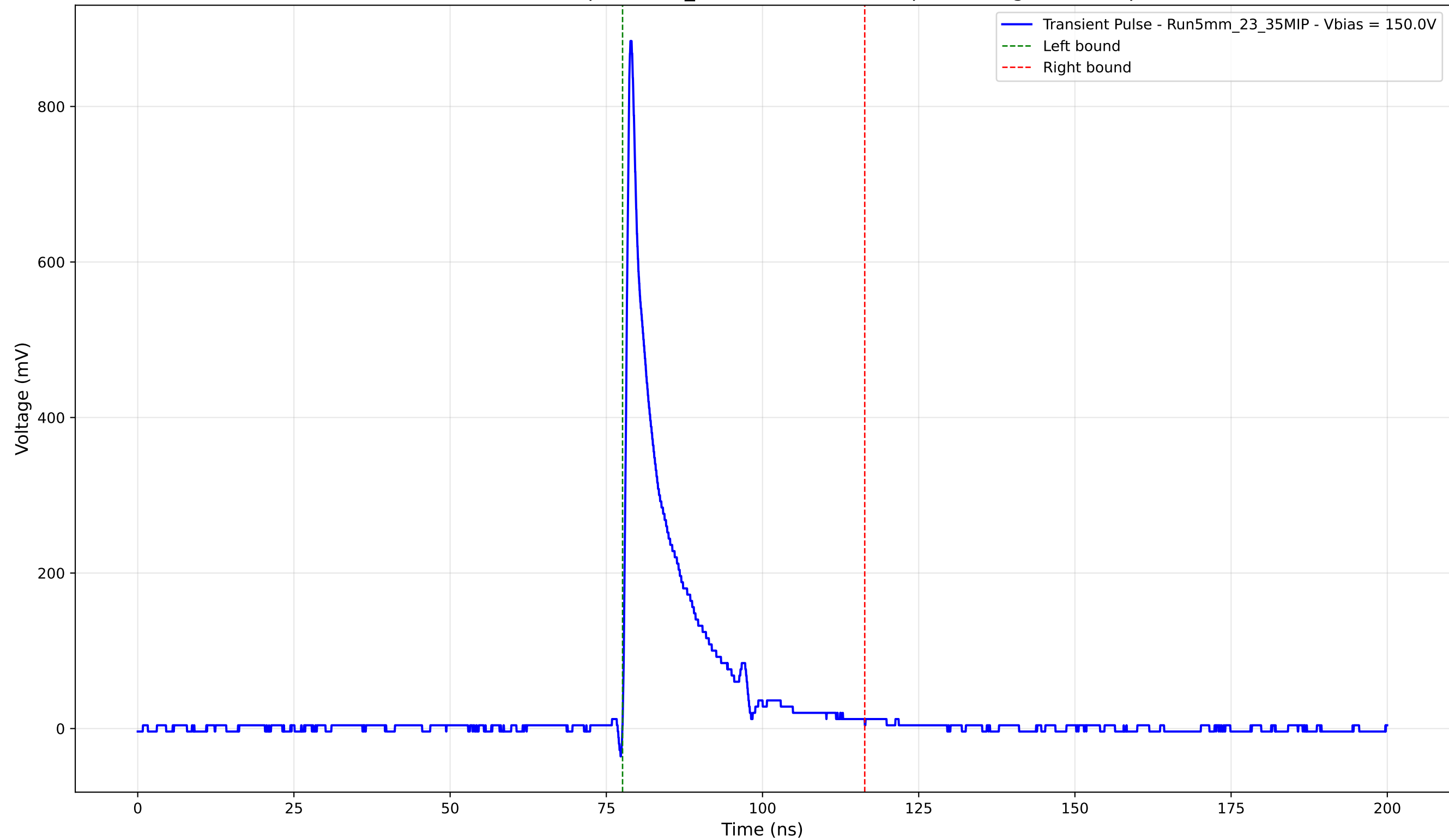
Transient Pulse - Sample: 5mm_23 - Position: 5015.0 \mu\text{m} - Charge: 108.44 pC
