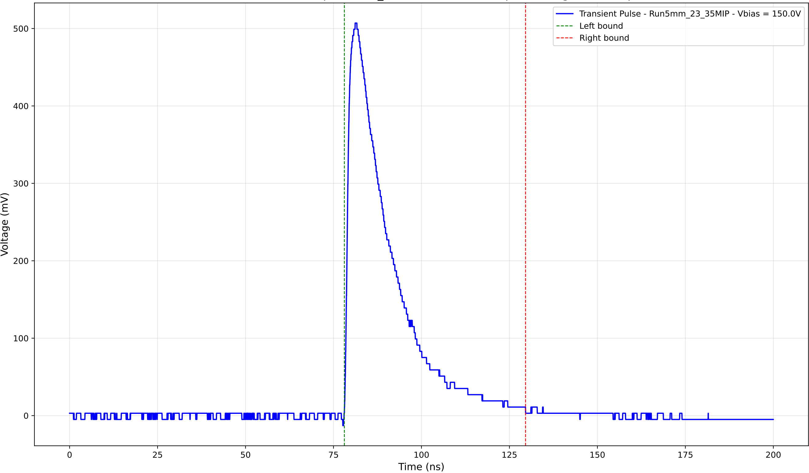
Transient Pulse - Sample: 5mm_23 - Position: 2455.0 \mu\text{m} - Charge: 136.50 pC
