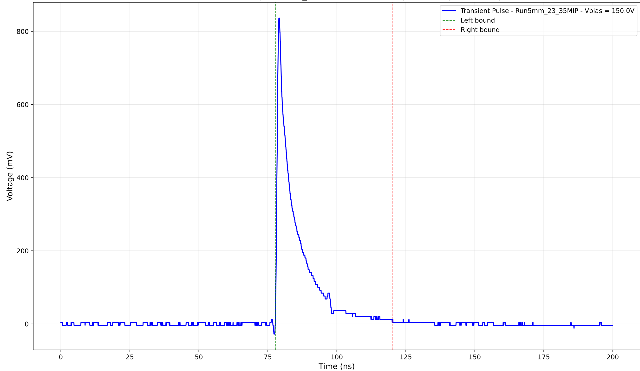
Transient Pulse - Sample: 5mm_23 - Position: 4845.0 \mu\text{m} - Charge: 114.61 pC
