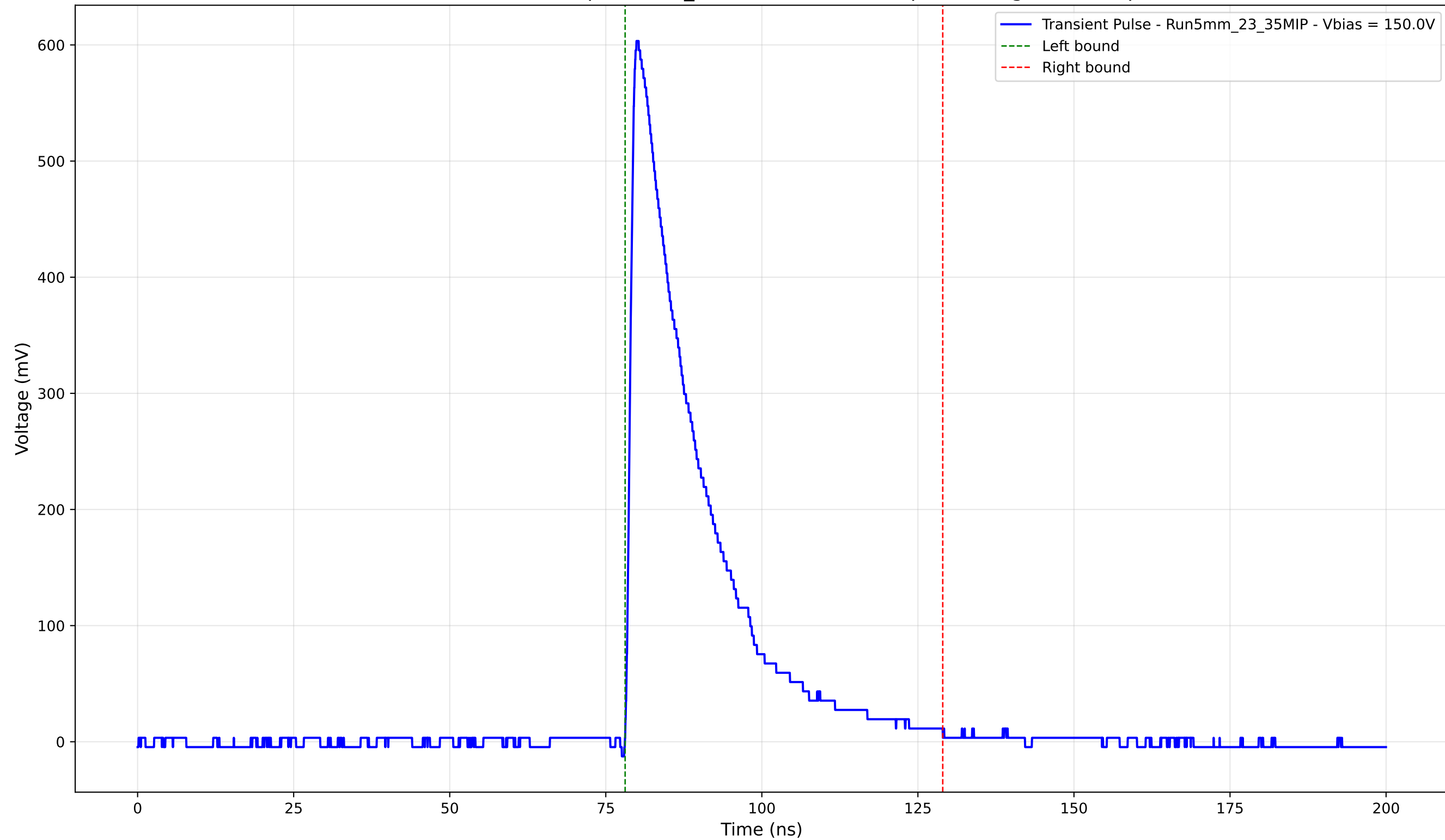
Transient Pulse - Sample: 5mm_23 - Position: 1500.0 \mu\text{m} - Charge: 142.79 pC
