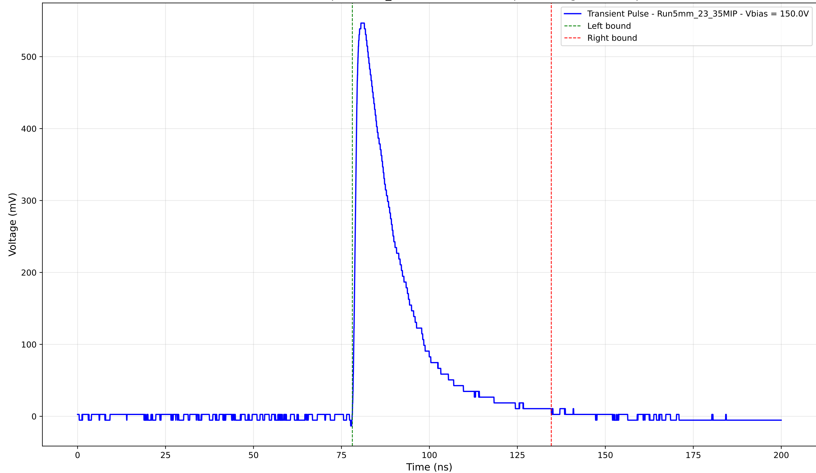
Transient Pulse - Sample: 5mm_23 - Position: 1985.0 \mu\text{m} - Charge: 145.54 pC
