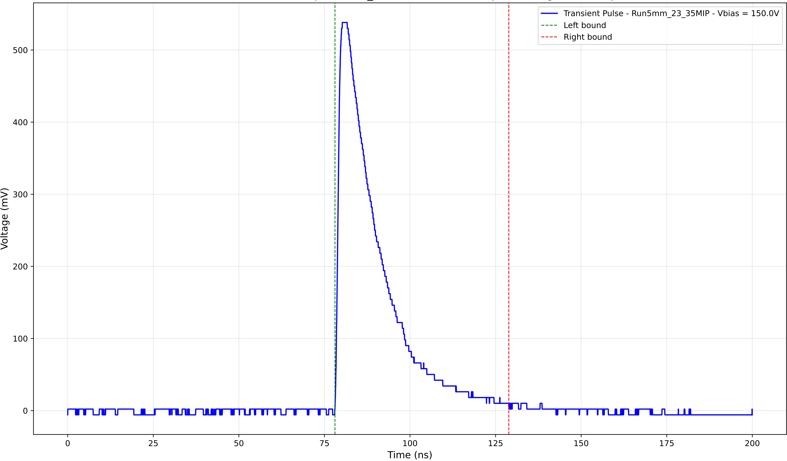
Transient Pulse - Sample: 5mm_23 - Position: 1955.0 \mu\text{m} - Charge: 142.05 pC
