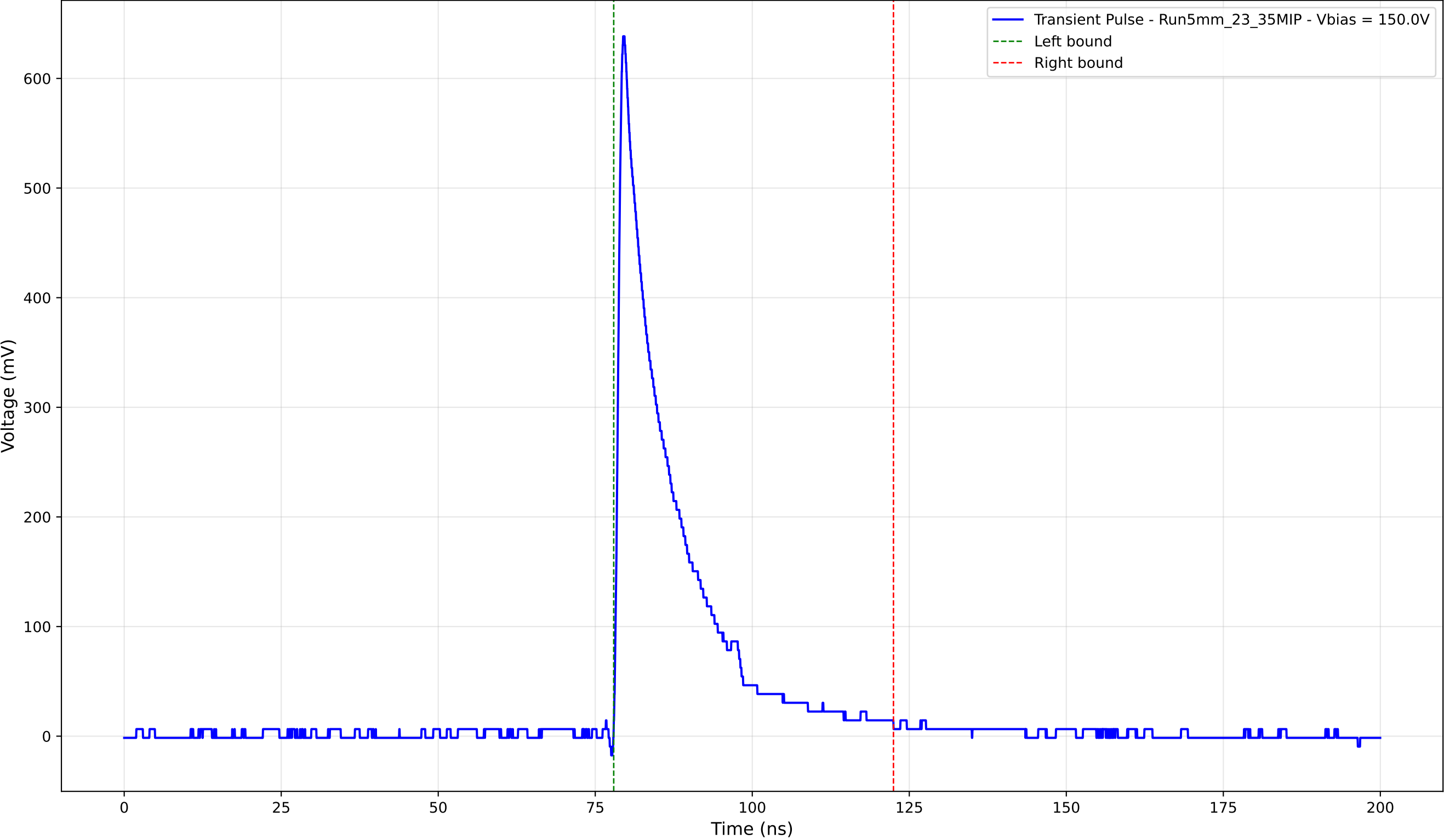
Transient Pulse - Sample: 5mm_23 - Position: 4450.0 \mu\text{m} - Charge: 112.57 pC
