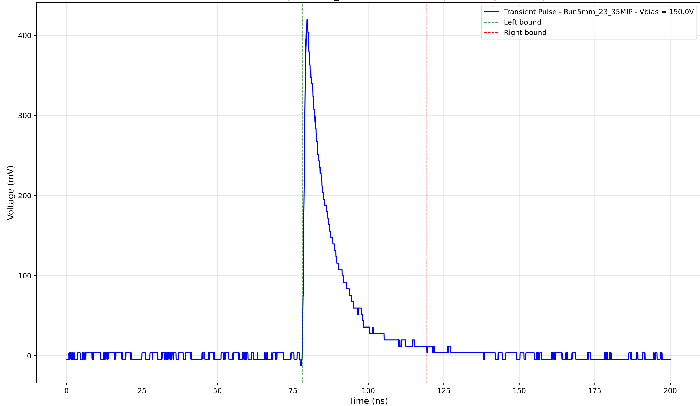
Transient Pulse - Sample: 5mm_23 - Position: 4220.0 \mu\text{m} - Charge: 76.44 pC
