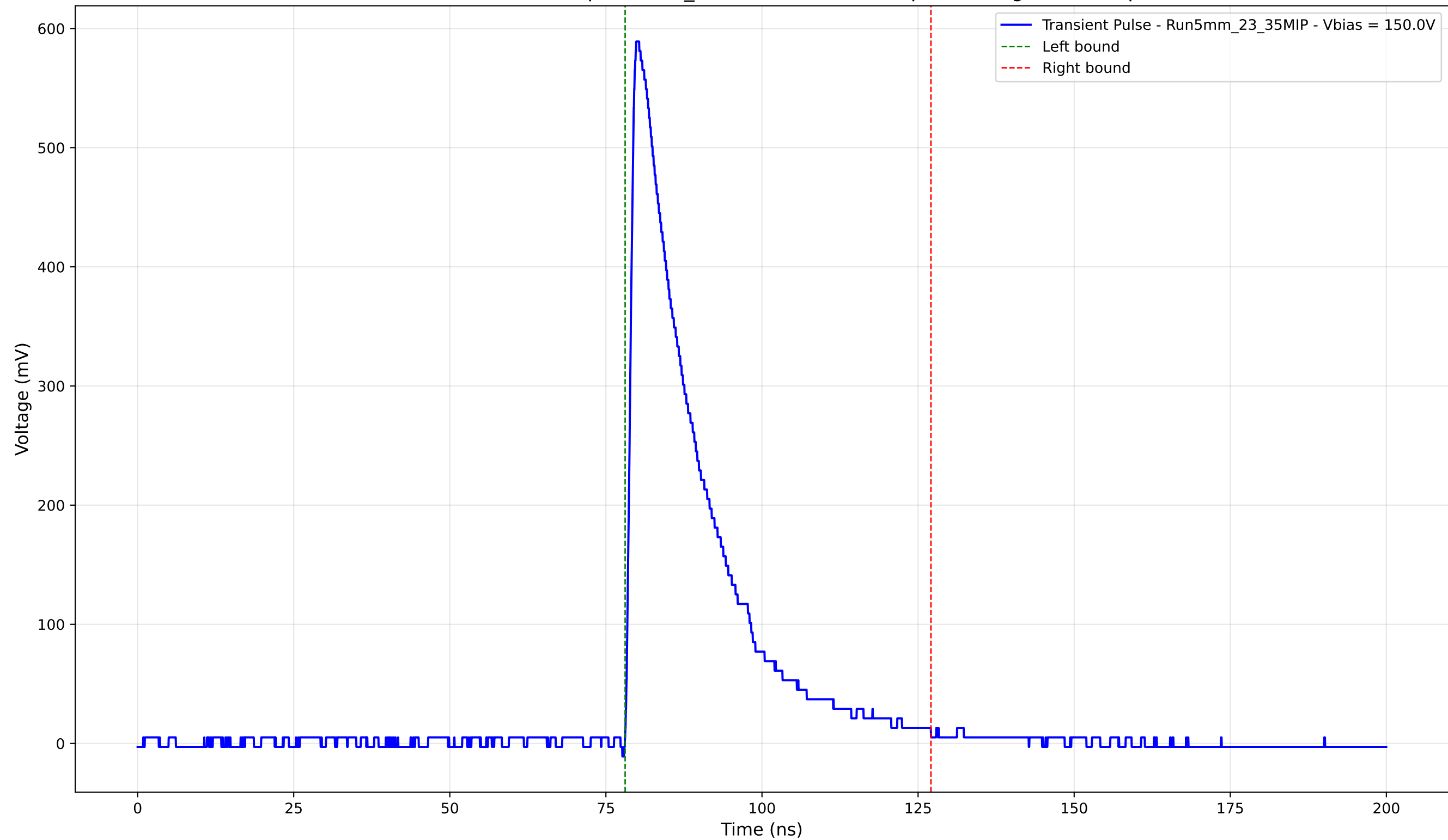
Transient Pulse - Sample: 5mm_23 - Position: 1510.0 \mu\text{m} - Charge: 139.87 pC
