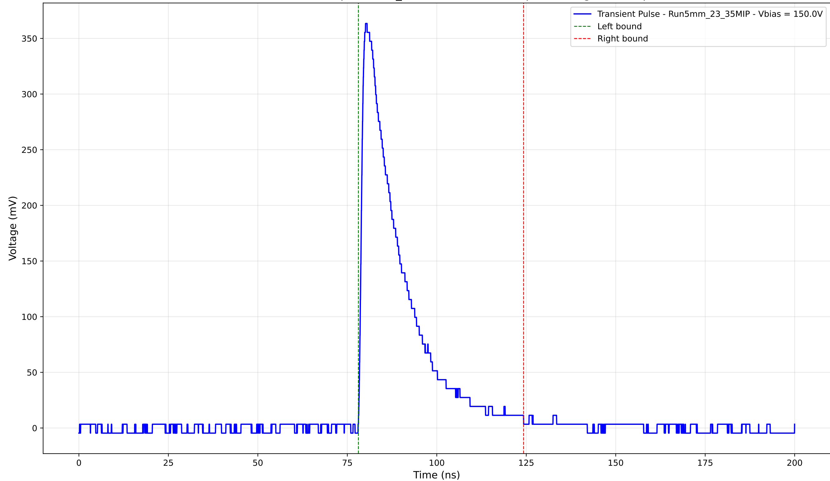
Transient Pulse - Sample: 5mm_23 - Position: 1685.0 \mu\text{m} - Charge: 87.97 pC
