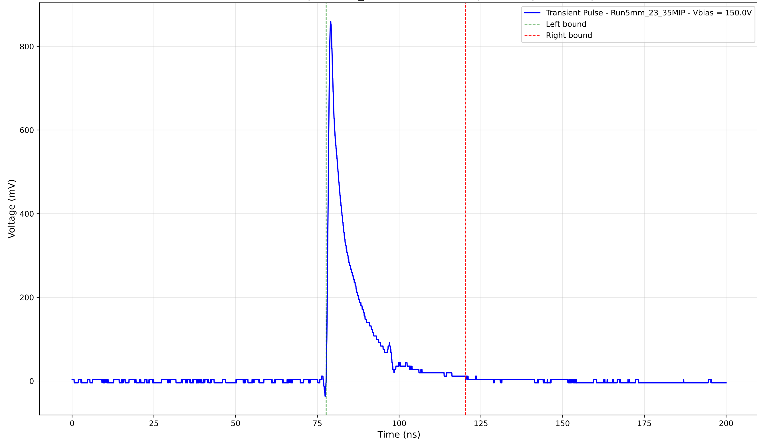
Transient Pulse - Sample: 5mm_23 - Position: 4885.0 \mu\text{m} - Charge: 115.47 pC
