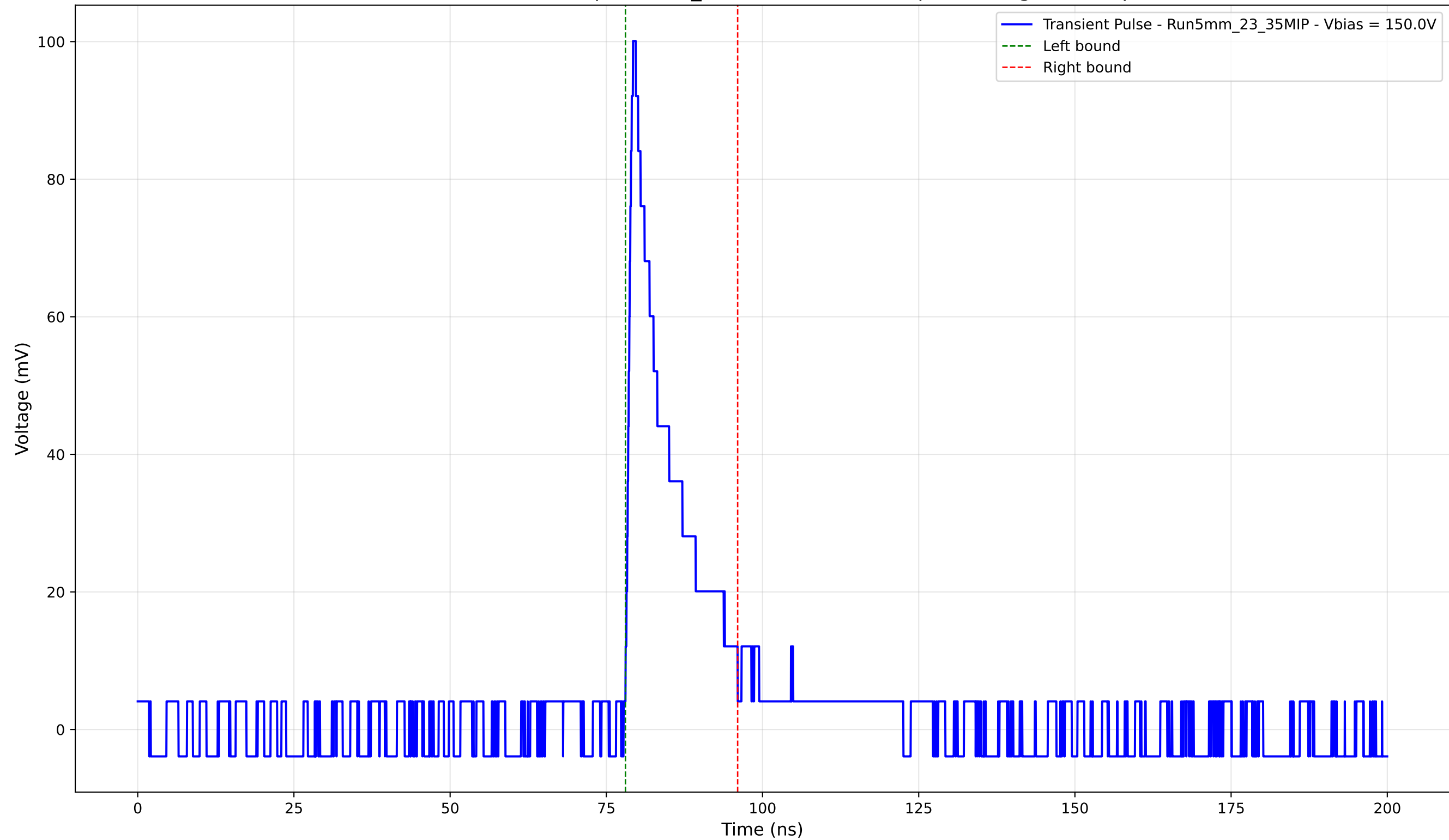
Transient Pulse - Sample: 5mm_23 - Position: 4515.0 \mu\text{m} - Charge: 13.76 pC
