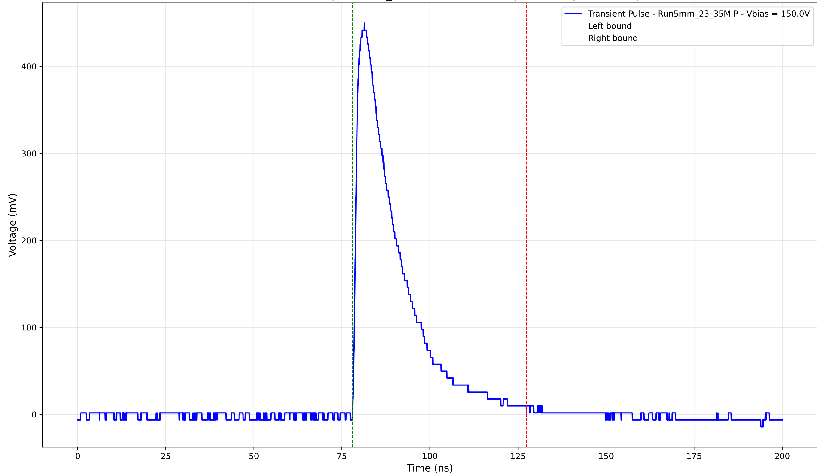
Transient Pulse - Sample: 5mm_23 - Position: 2730.0 \mu\text{m} - Charge: 118.82 pC
