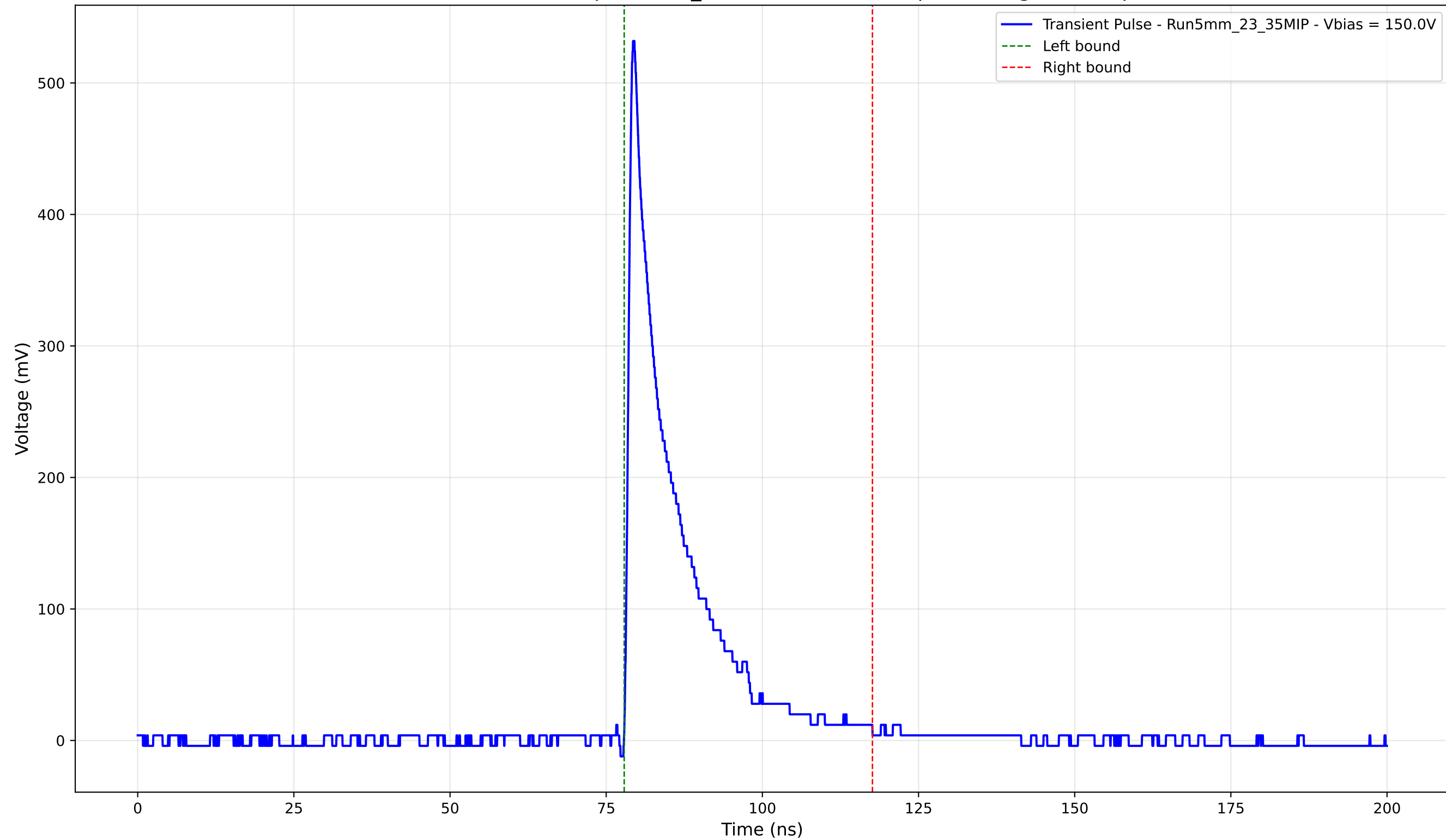
Transient Pulse - Sample: 5mm_23 - Position: 4565.0 \mu\text{m} - Charge: 81.29 pC
