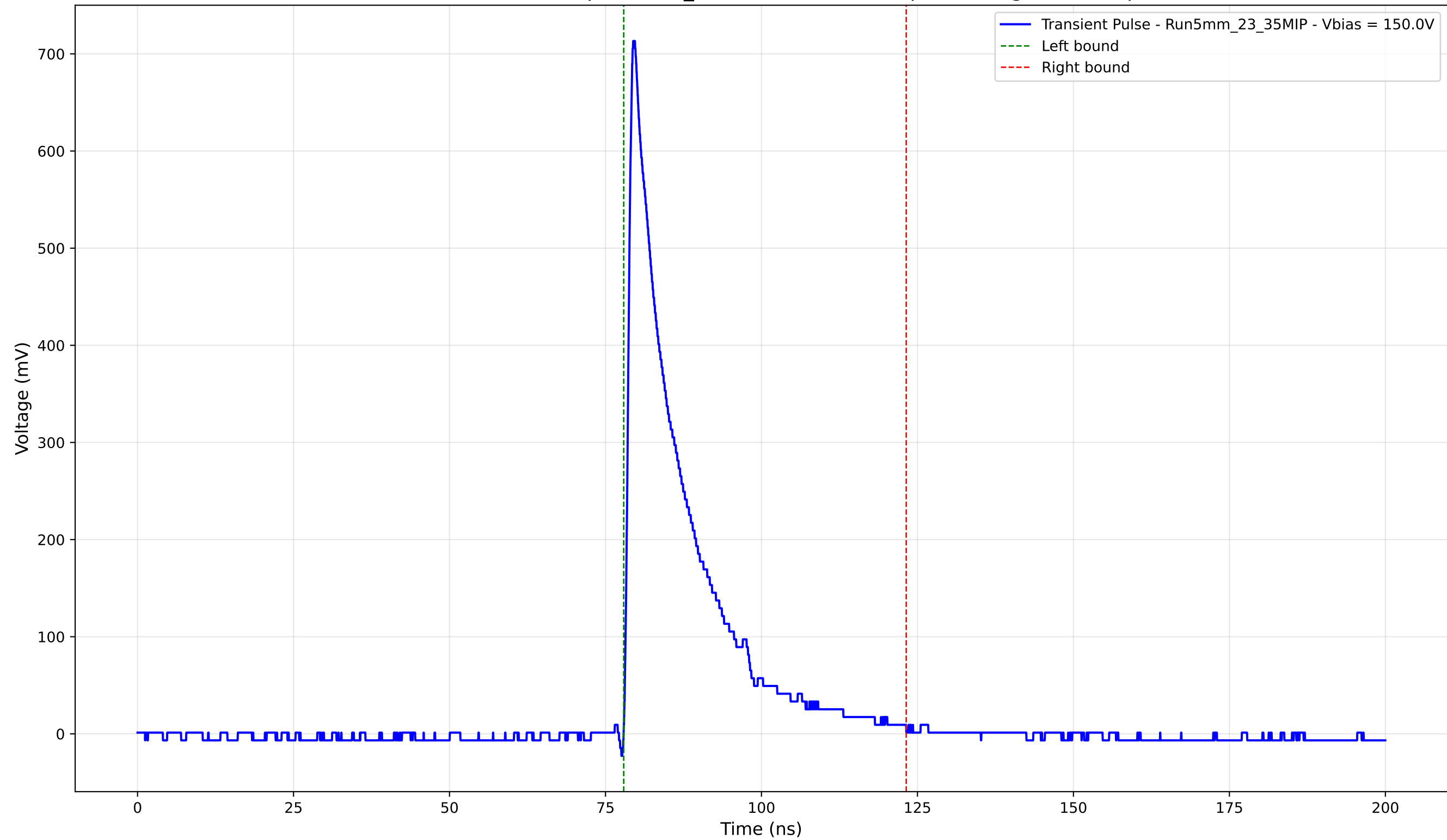
Transient Pulse - Sample: 5mm_23 - Position: 4390.0 \mu\text{m} - Charge: 127.01 pC
