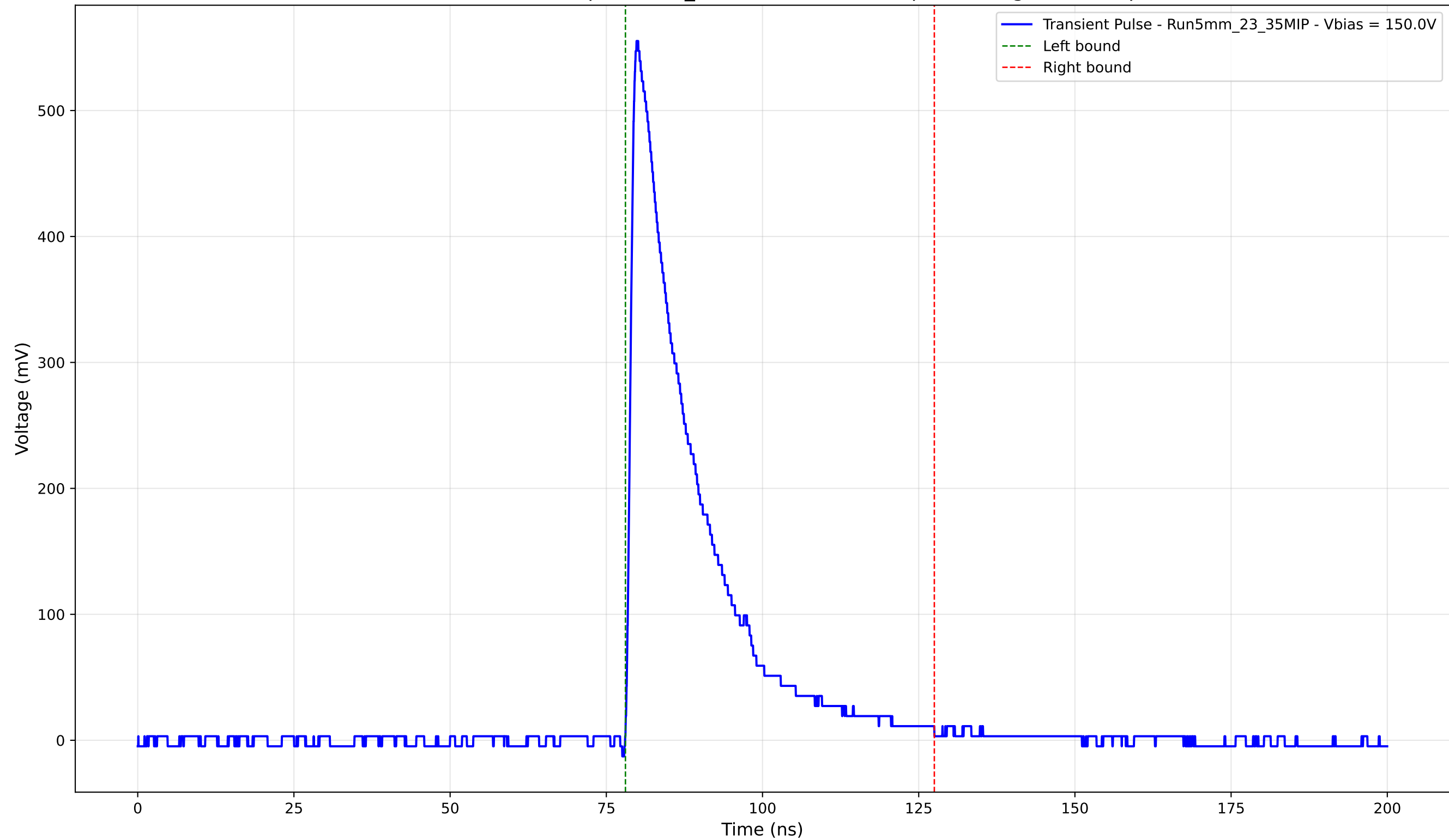
Transient Pulse - Sample: 5mm_23 - Position: 3920.0 \mu\text{m} - Charge: 121.10 pC
