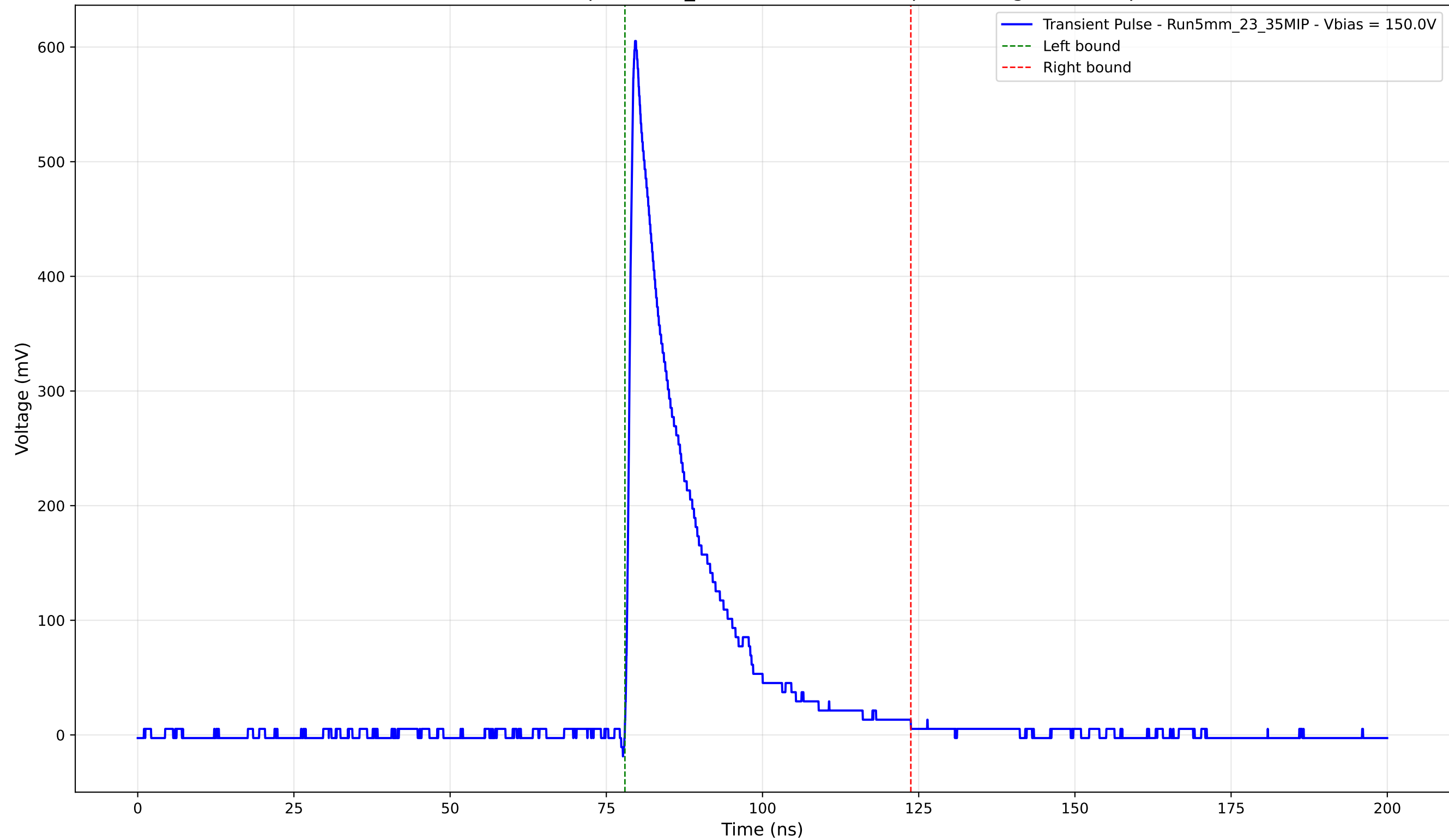
Transient Pulse - Sample: 5mm_23 - Position: 4260.0 \mu\text{m} - Charge: 113.08 pC
