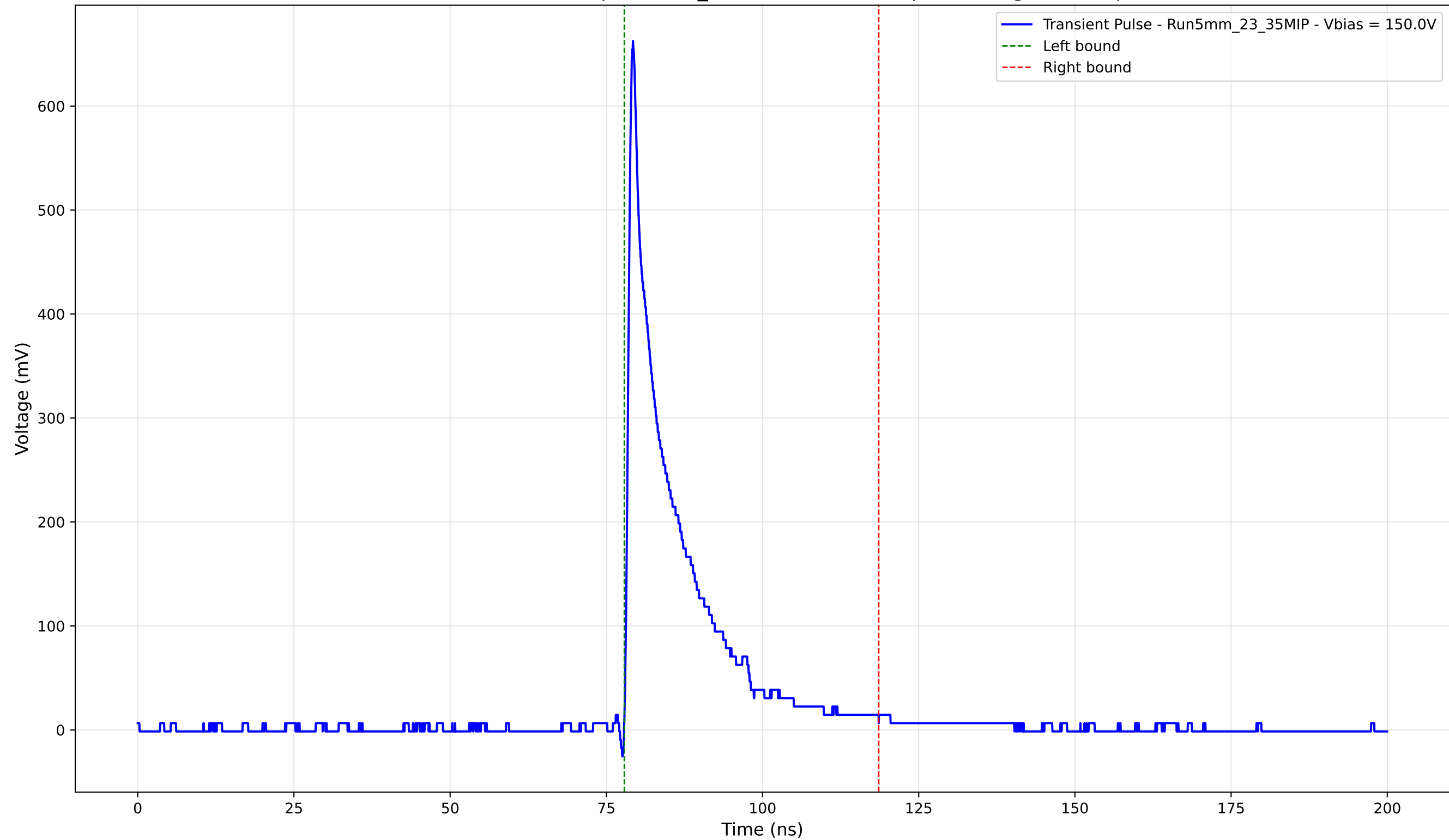
Transient Pulse - Sample: 5mm_23 - Position: 550.0 \mu\text{m} - Charge: 94.85 pC
