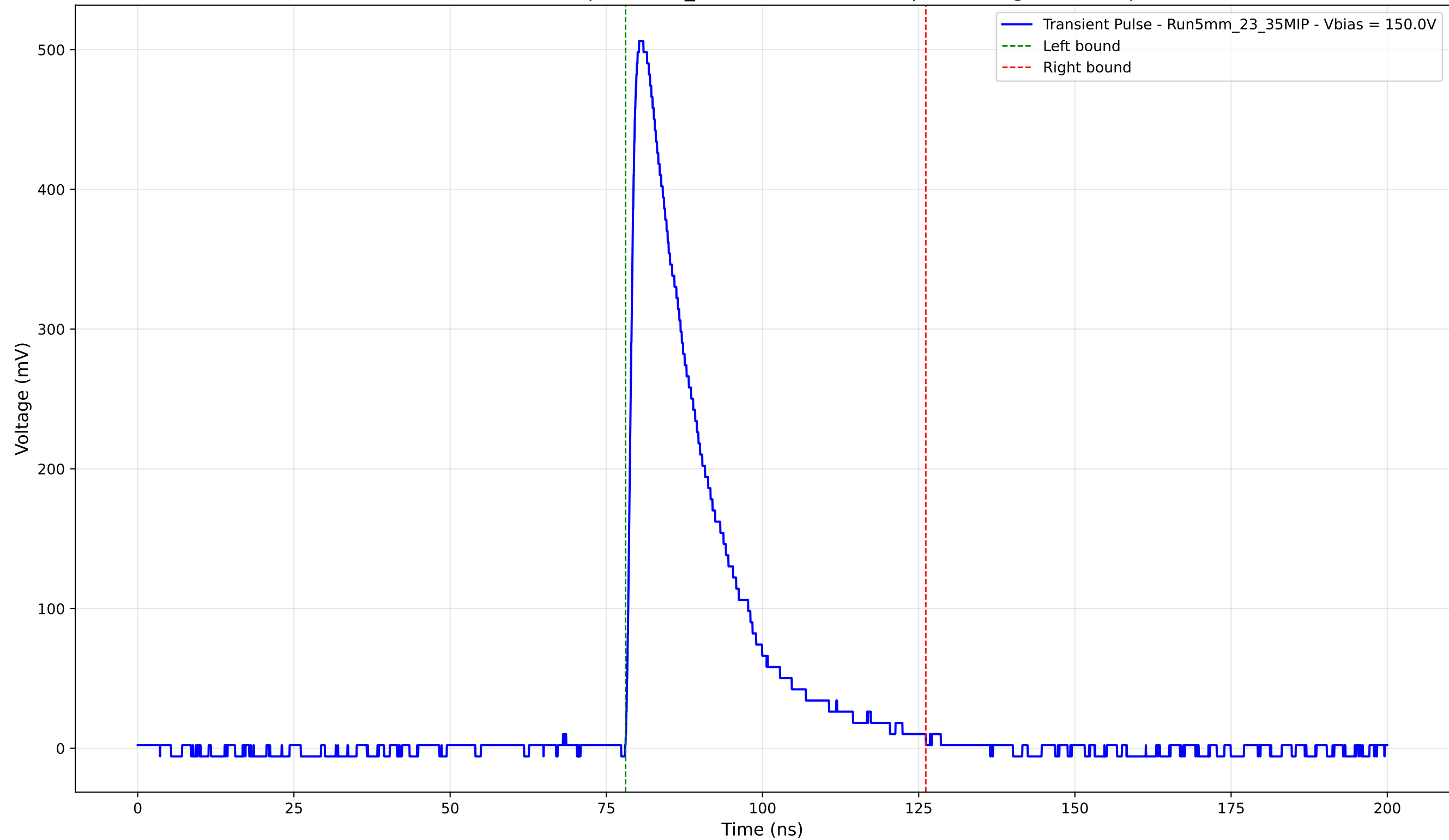
Transient Pulse - Sample: 5mm_23 - Position: 3425.0 \mu\text{m} - Charge: 126.19 pC
