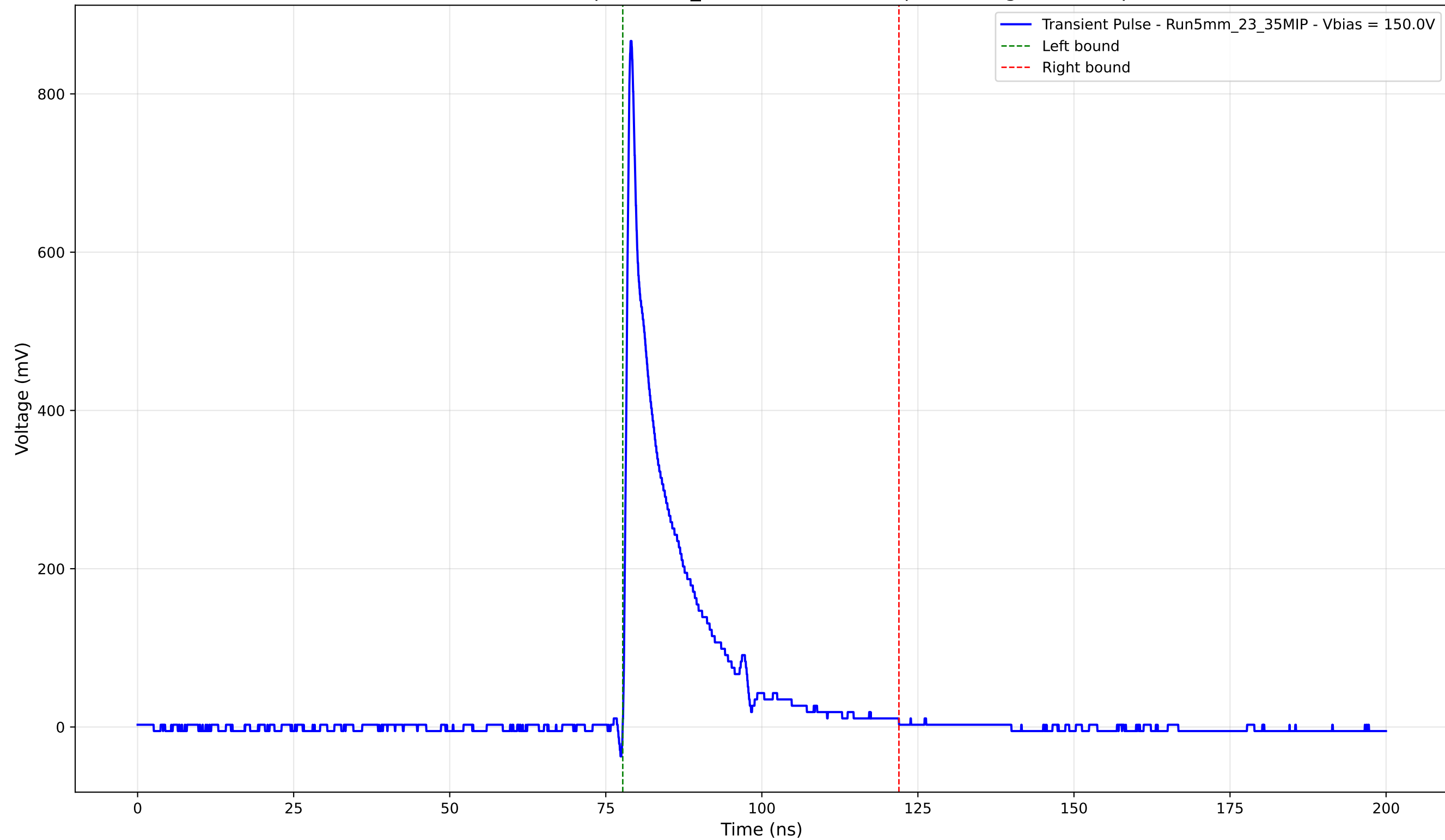
Transient Pulse - Sample: 5mm_23 - Position: 320.0 \mu\text{m} - Charge: 114.72 pC
