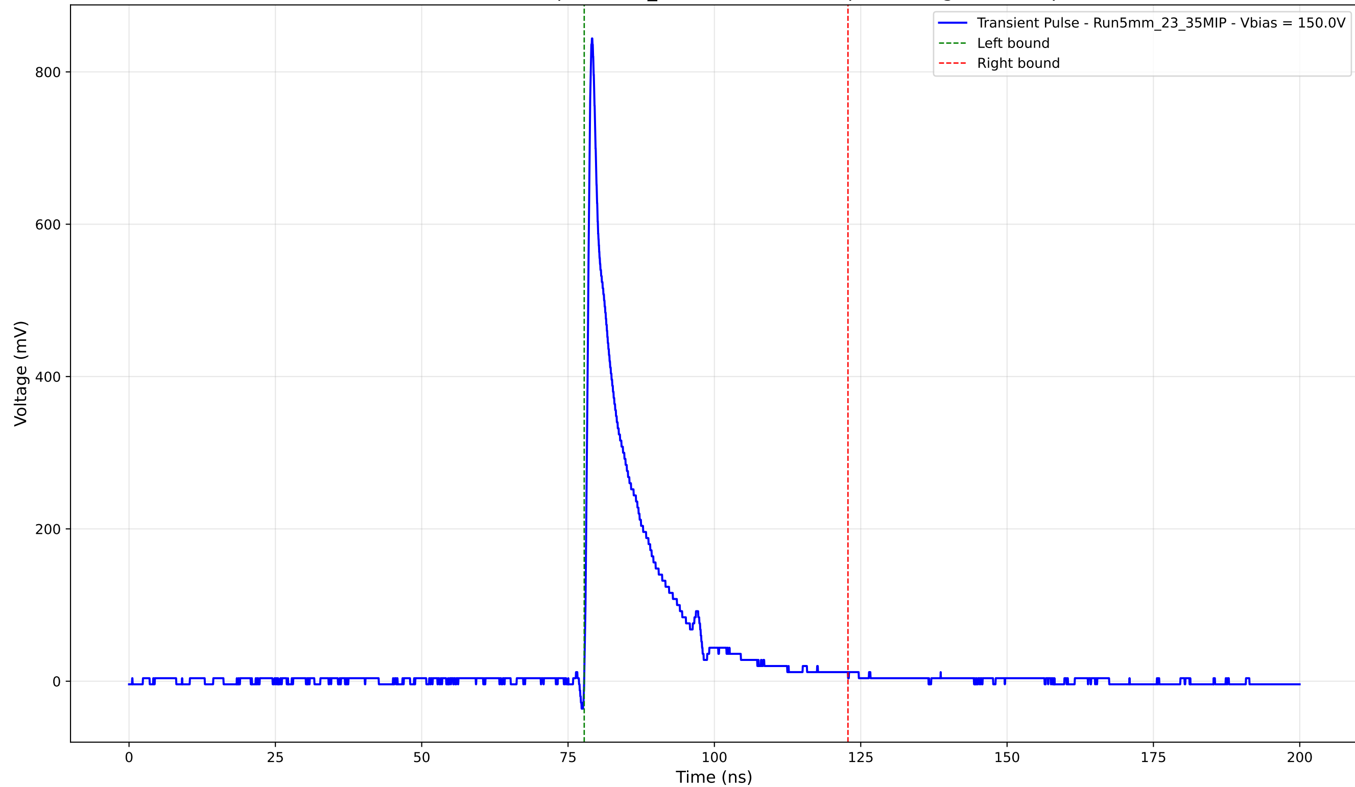
Transient Pulse - Sample: 5mm_23 - Position: 375.0 \mu\text{m} - Charge: 115.71 pC
