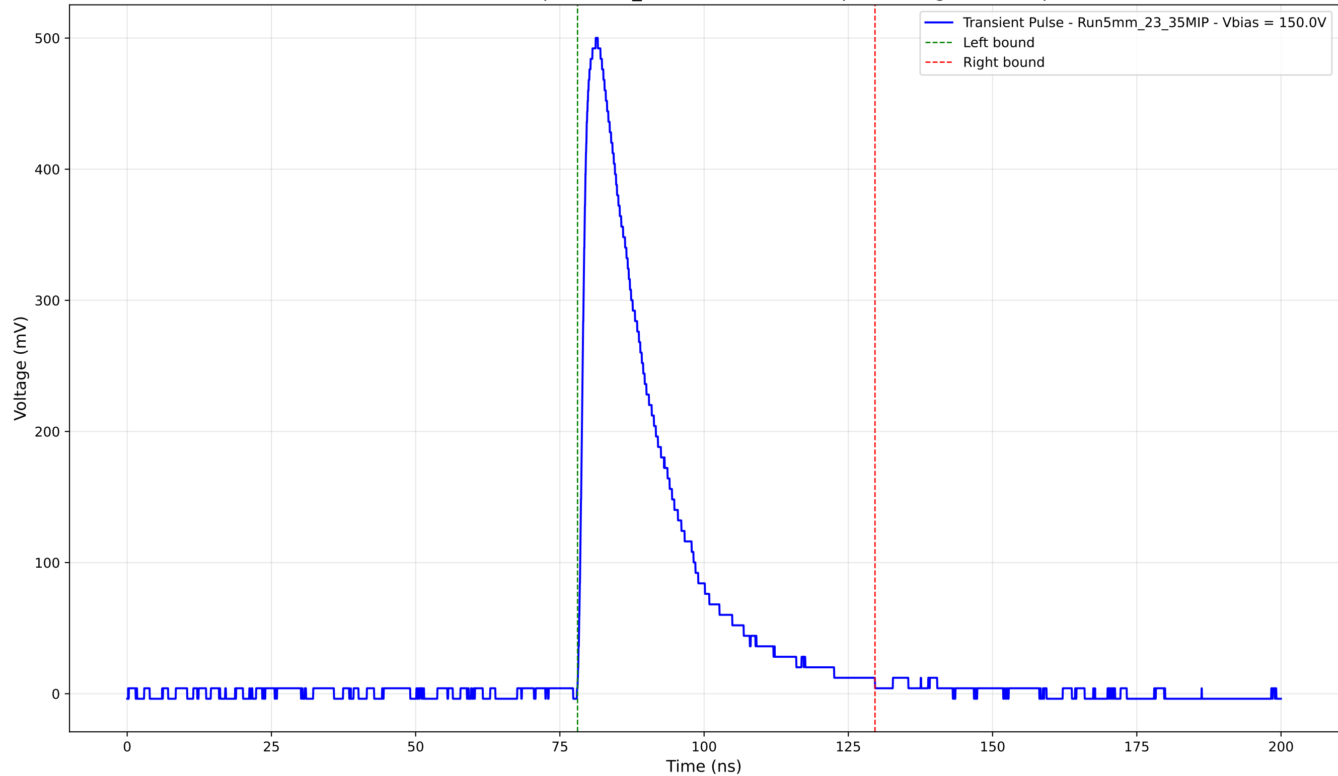
Transient Pulse - Sample: 5mm_23 - Position: 2825.0 \mu\text{m} - Charge: 135.23 pC
