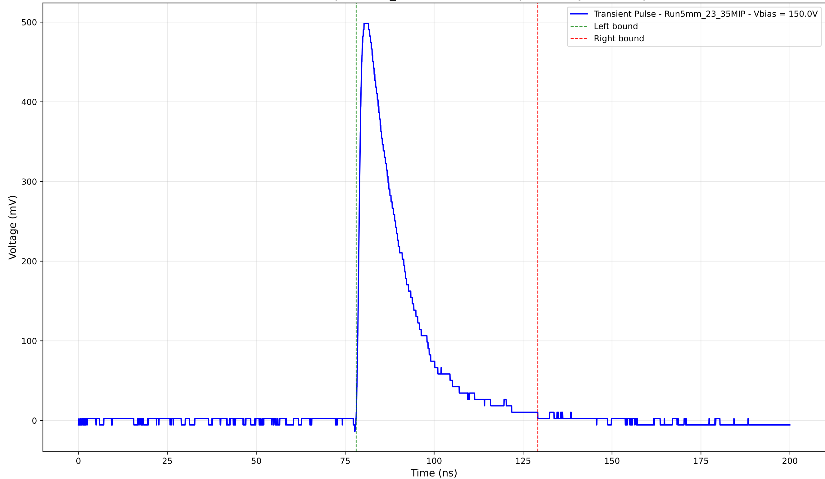
Transient Pulse - Sample: 5mm_23 - Position: 3280.0 \mu\text{m} - Charge: 129.27 pC
