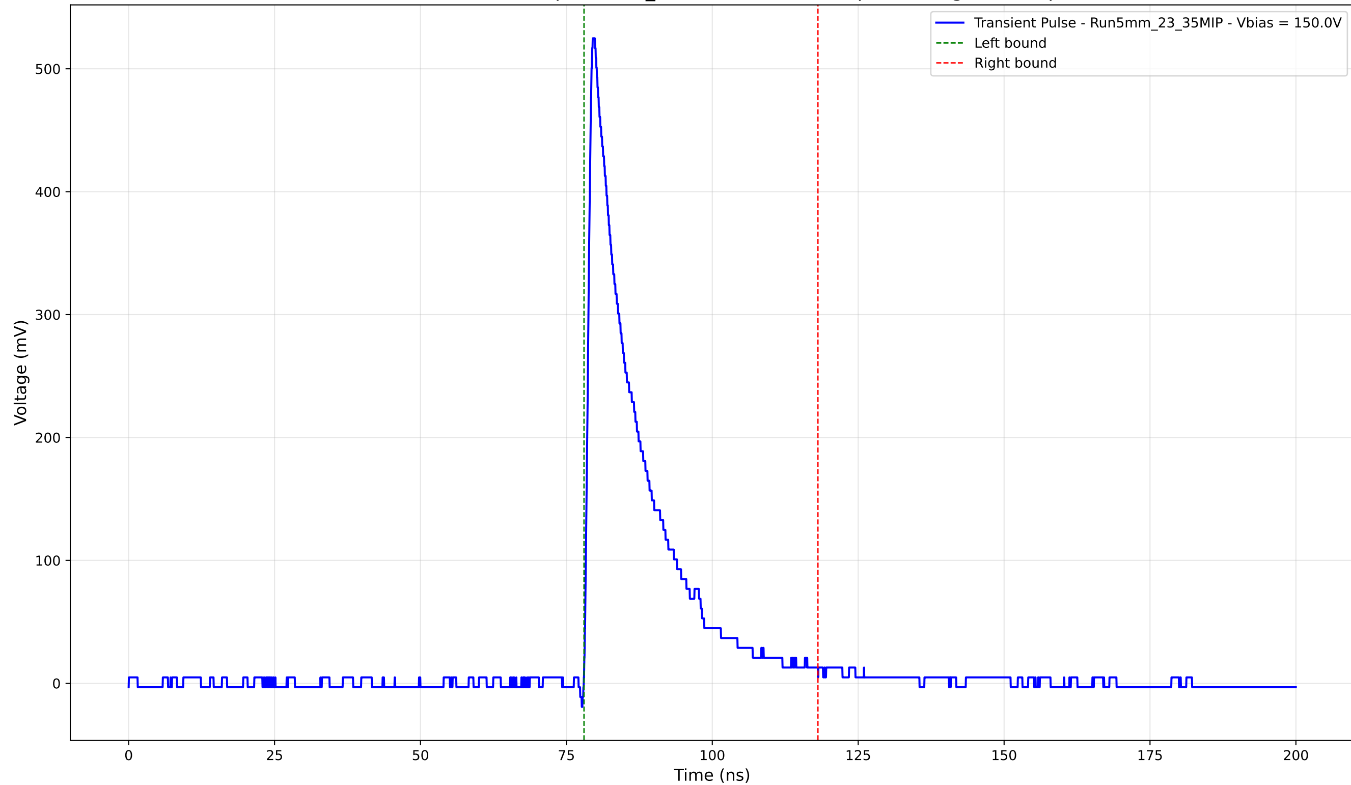
Transient Pulse - Sample: 5mm_23 - Position: 4240.0 \mu\text{m} - Charge: 97.47 pC
