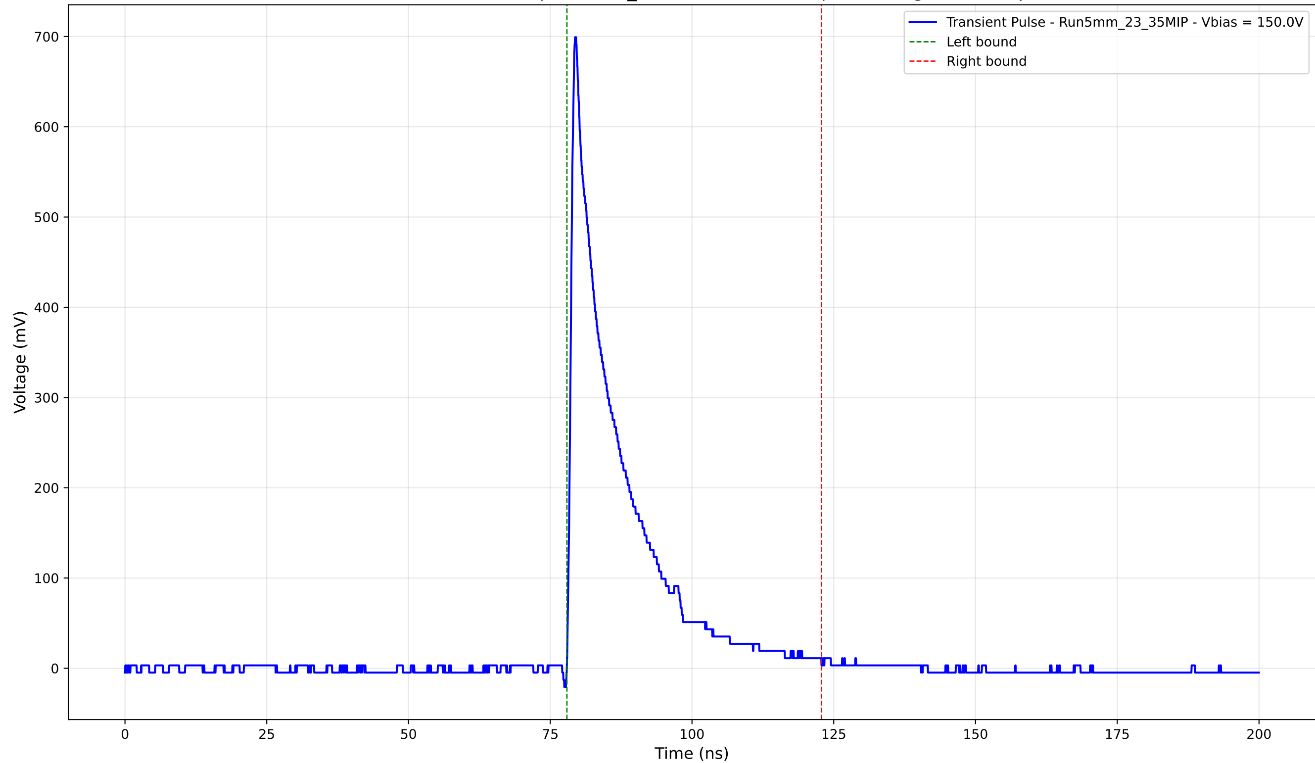
Transient Pulse - Sample: 5mm_23 - Position: 750.0 \mu\text{m} - Charge: 119.57 pC
