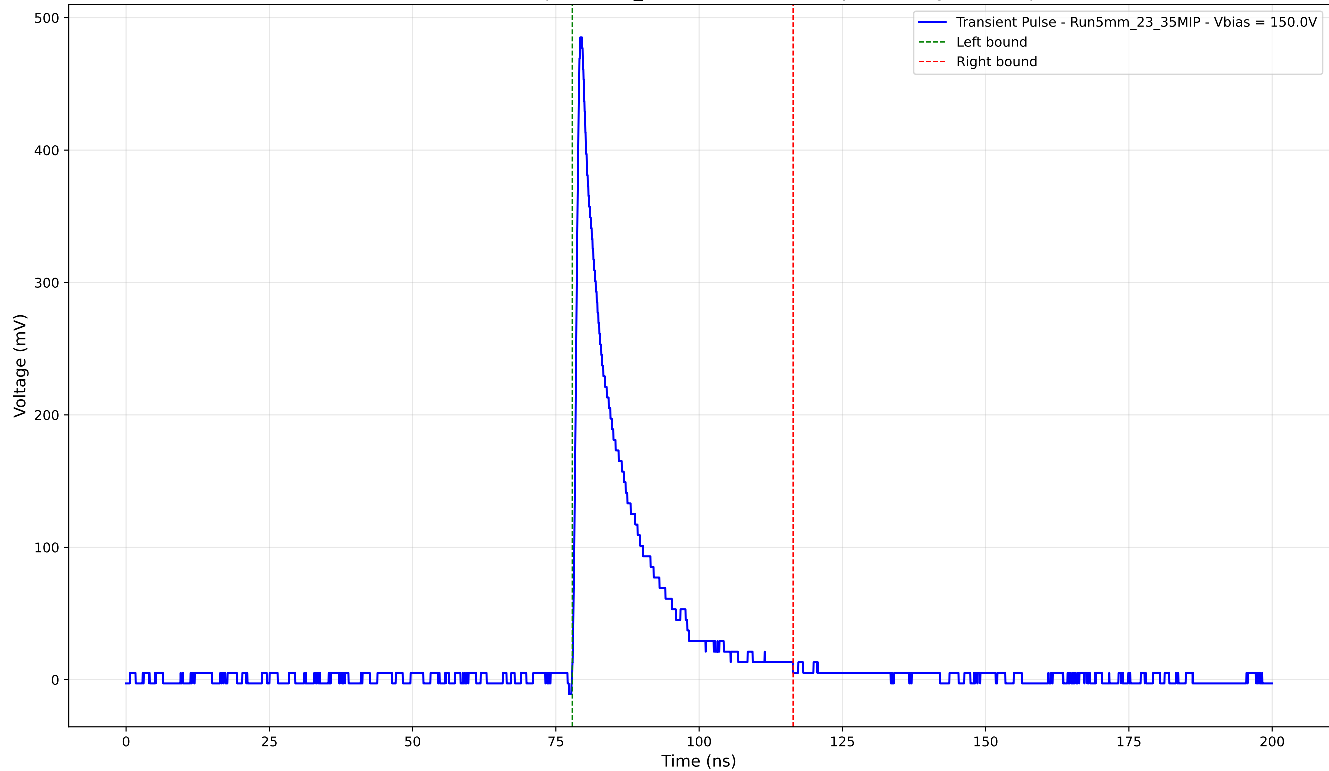
Transient Pulse - Sample: 5mm_23 - Position: 4560.0 \mu\text{m} - Charge: 74.48 pC
