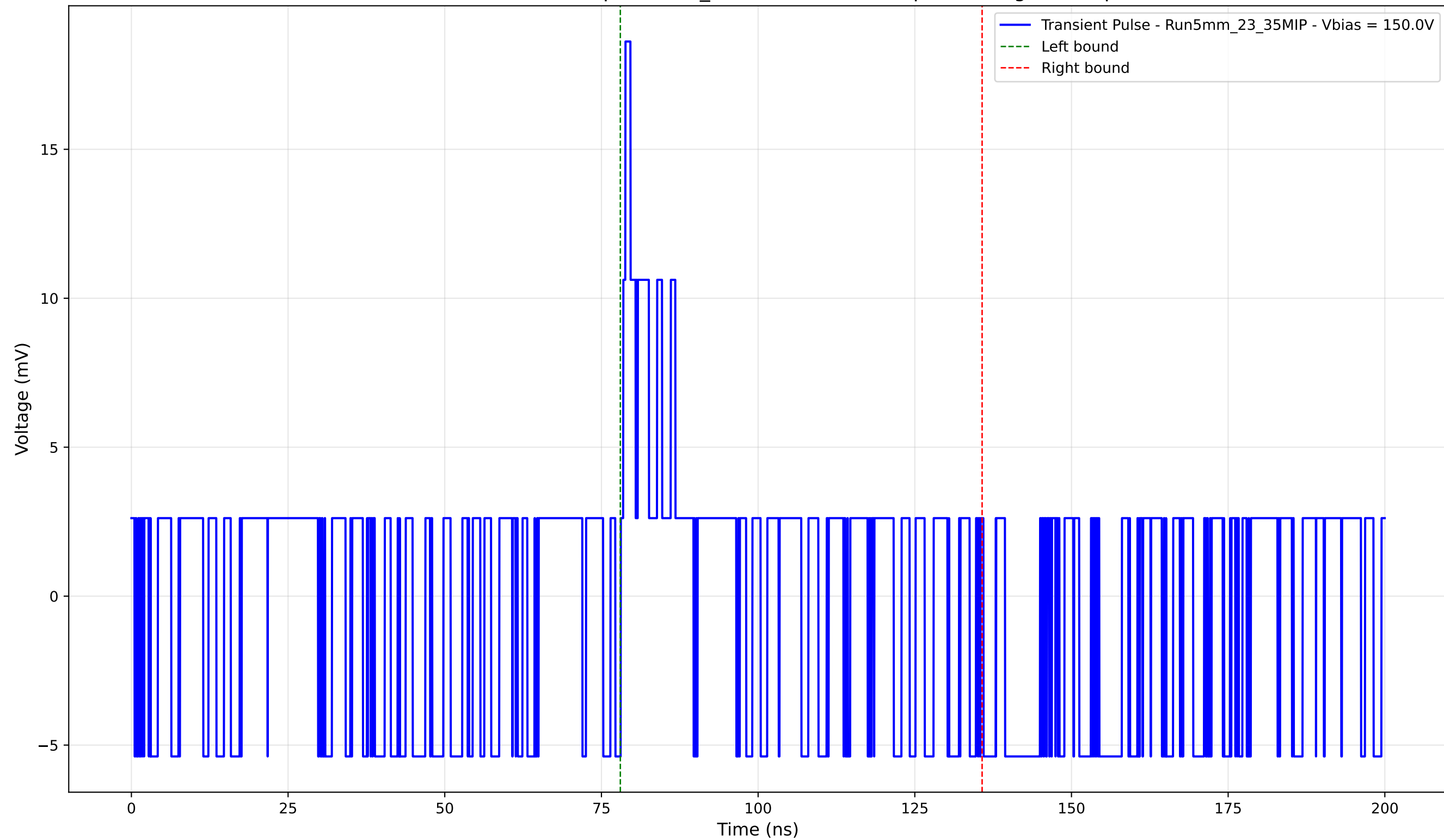
Transient Pulse - Sample: 5mm_23 - Position: 120.0 \mu\text{m} - Charge: 1.83 pC
