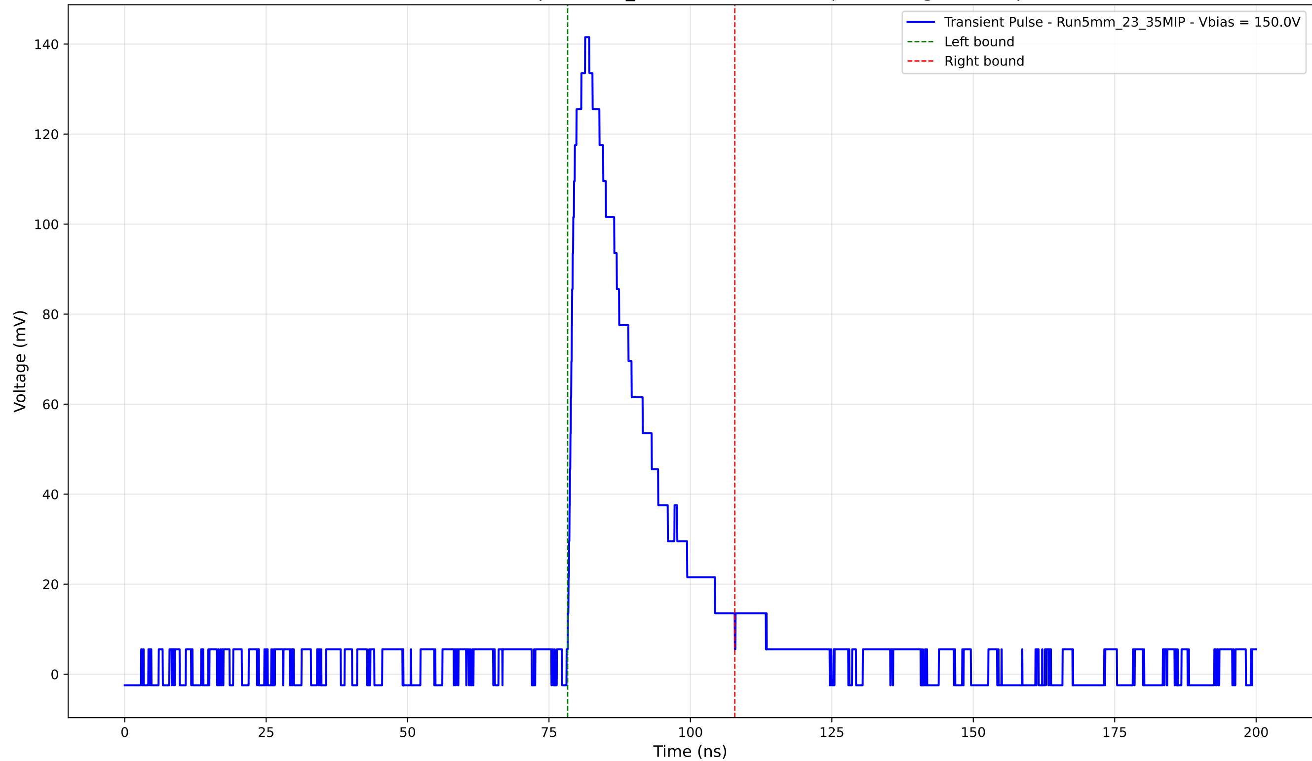
Transient Pulse - Sample: 5mm_23 - Position: 2160.0 \mu\text{m} - Charge: 35.01 pC
