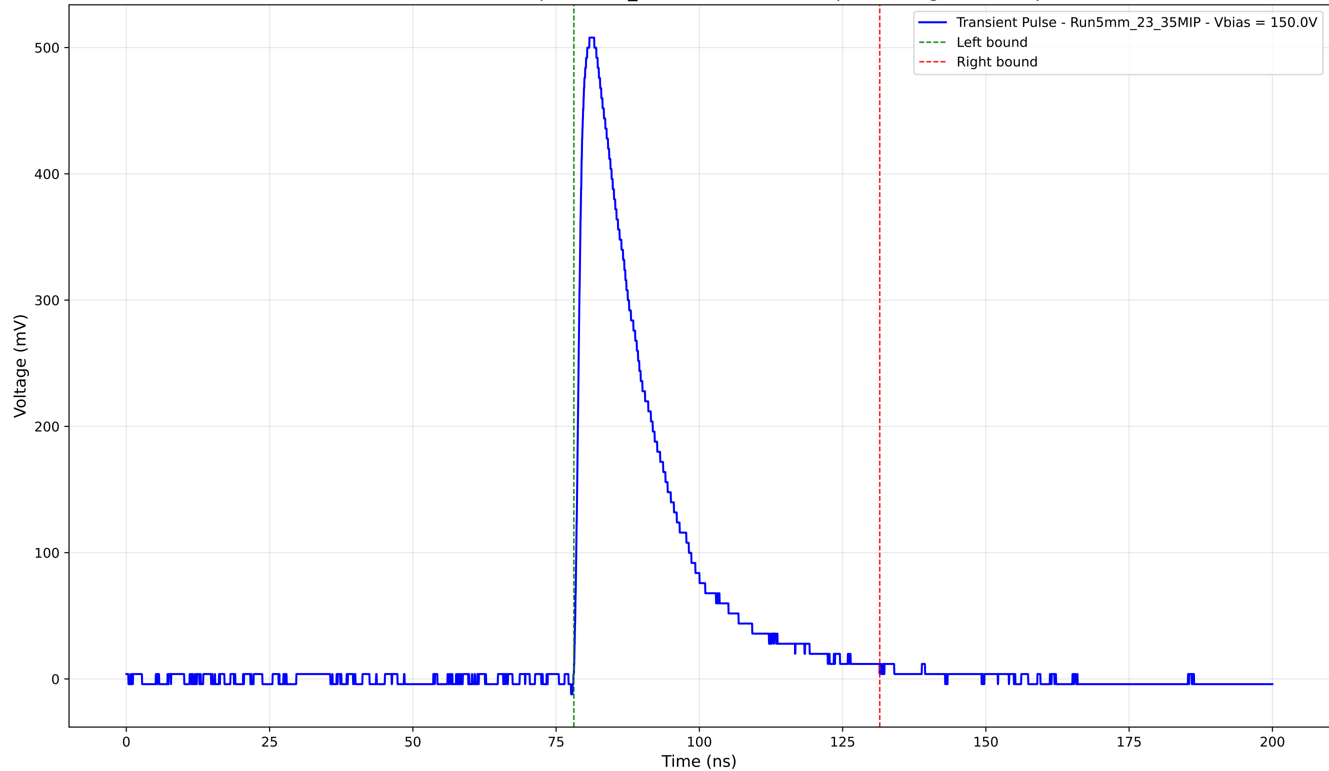
Transient Pulse - Sample: 5mm_23 - Position: 2270.0 \mu\text{m} - Charge: 138.05 pC
