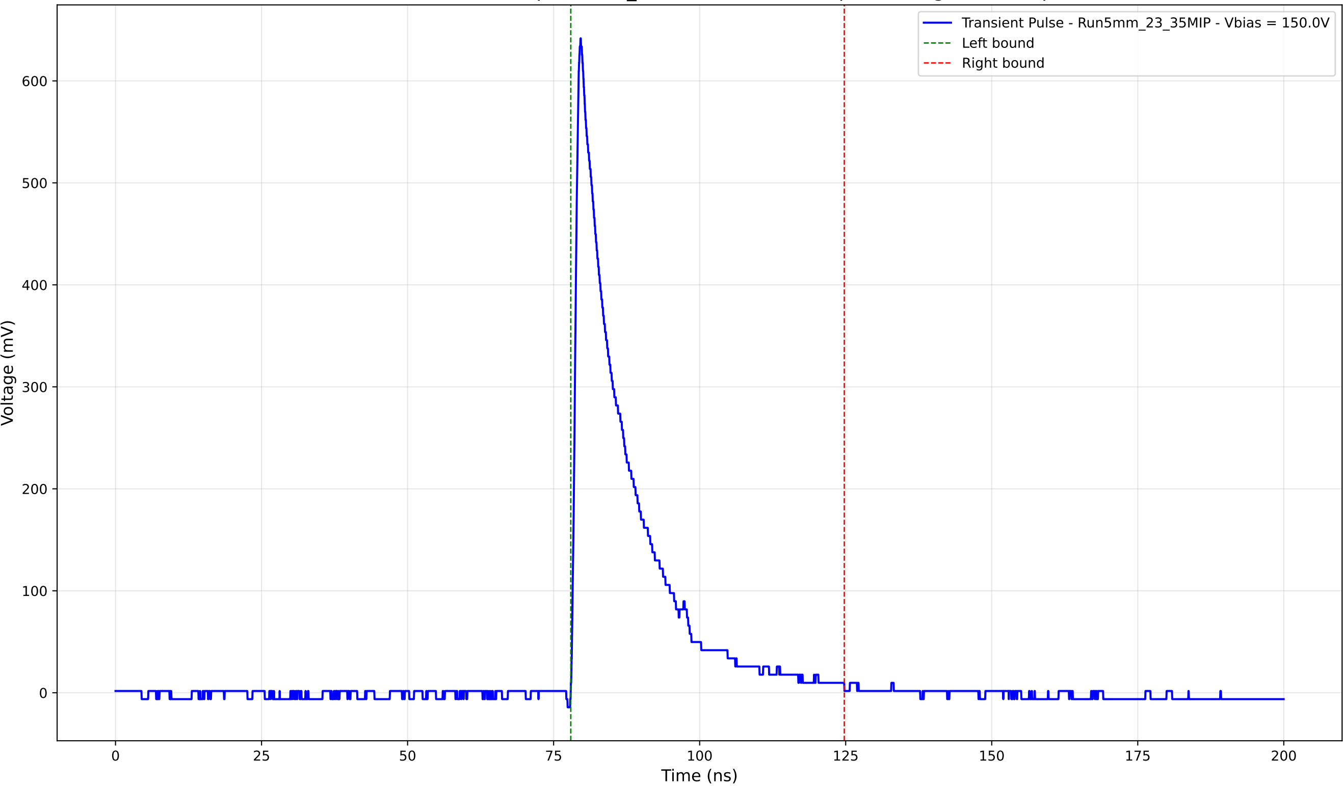
Transient Pulse - Sample: 5mm_23 - Position: 4320.0 \mu\text{m} - Charge: 116.29 pC
