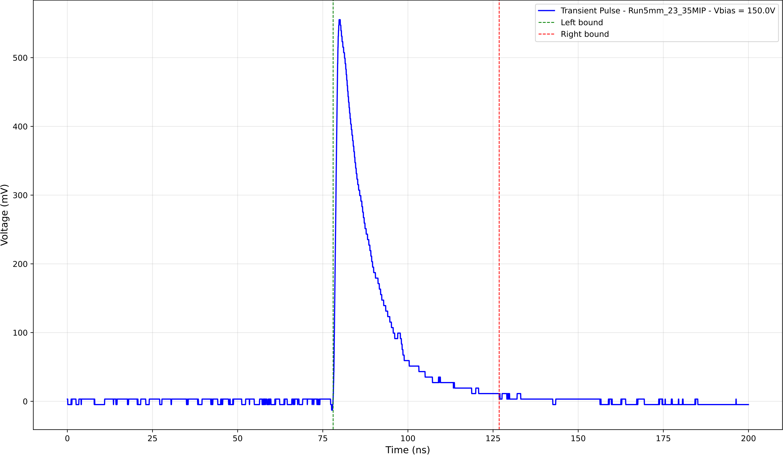
Transient Pulse - Sample: 5mm_23 - Position: 3925.0 \mu\text{m} - Charge: 120.59 pC
