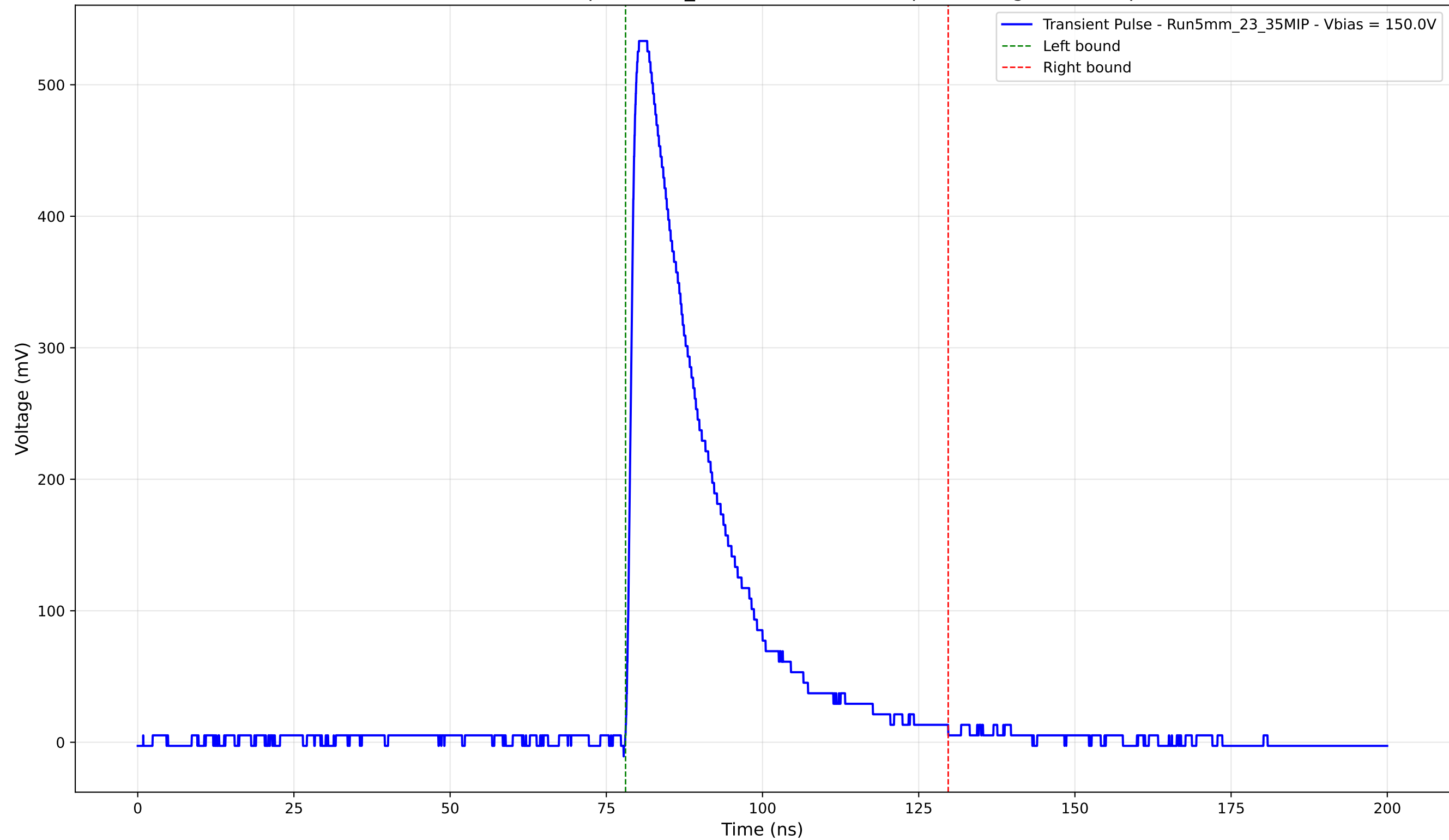
Transient Pulse - Sample: 5mm_23 - Position: 1935.0 \mu\text{m} - Charge: 141.39 pC
