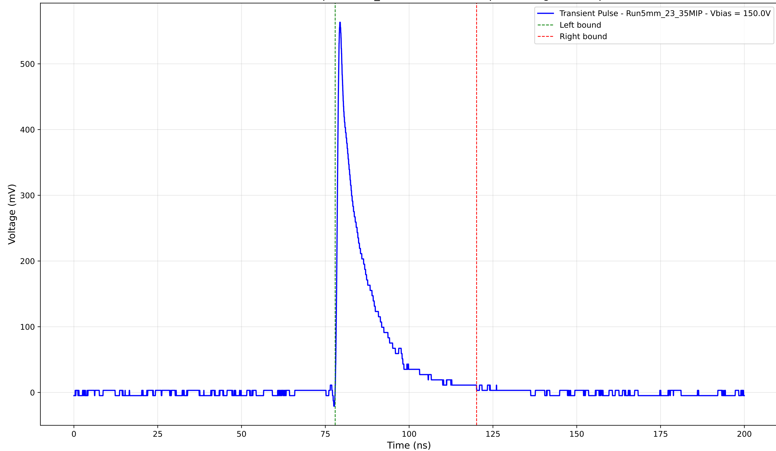
Transient Pulse - Sample: 5mm_23 - Position: 685.0 \mu\text{m} - Charge: 89.23 pC
