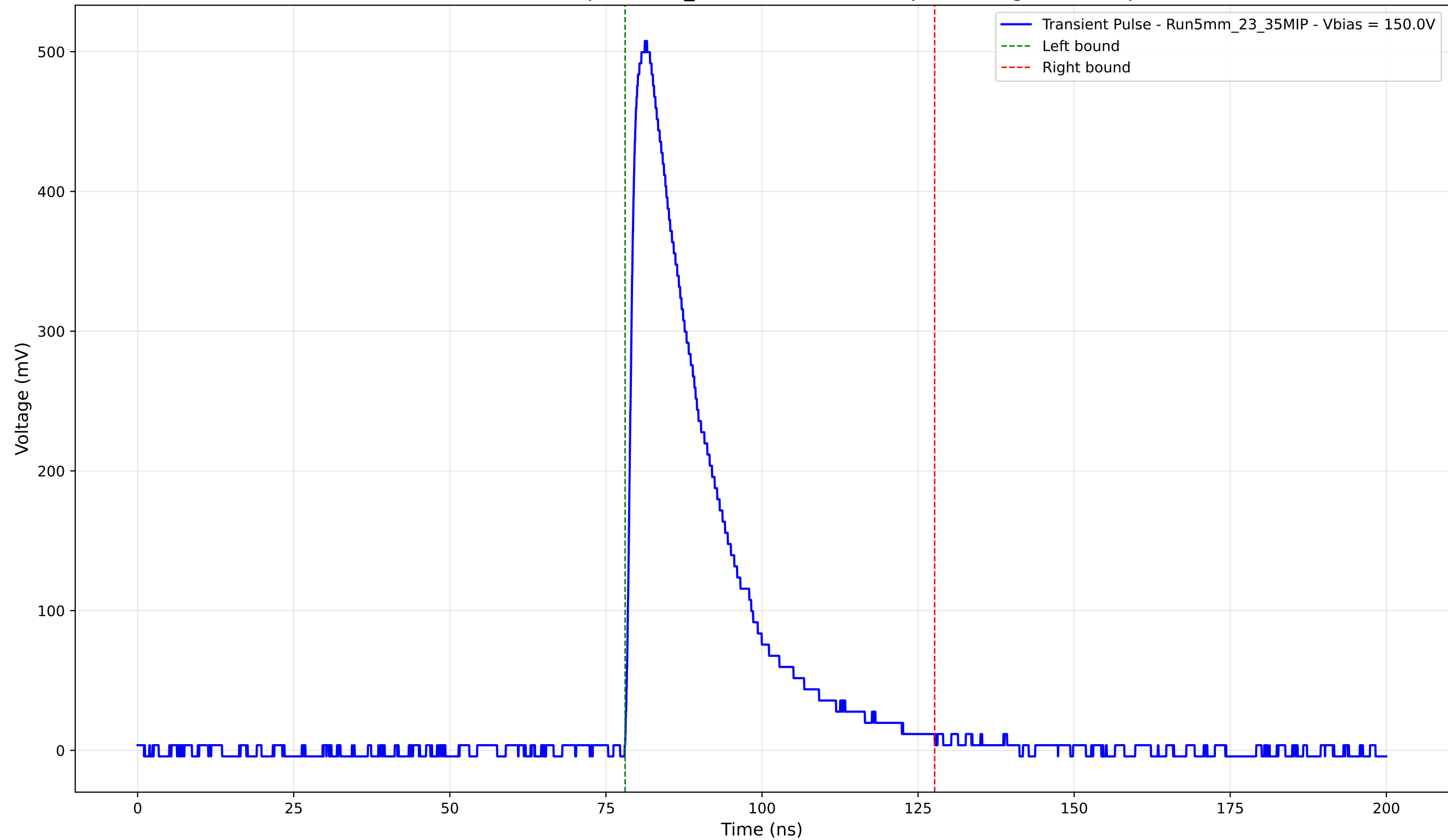
Transient Pulse - Sample: 5mm_23 - Position: 2360.0 \mu\text{m} - Charge: 136.37 pC
