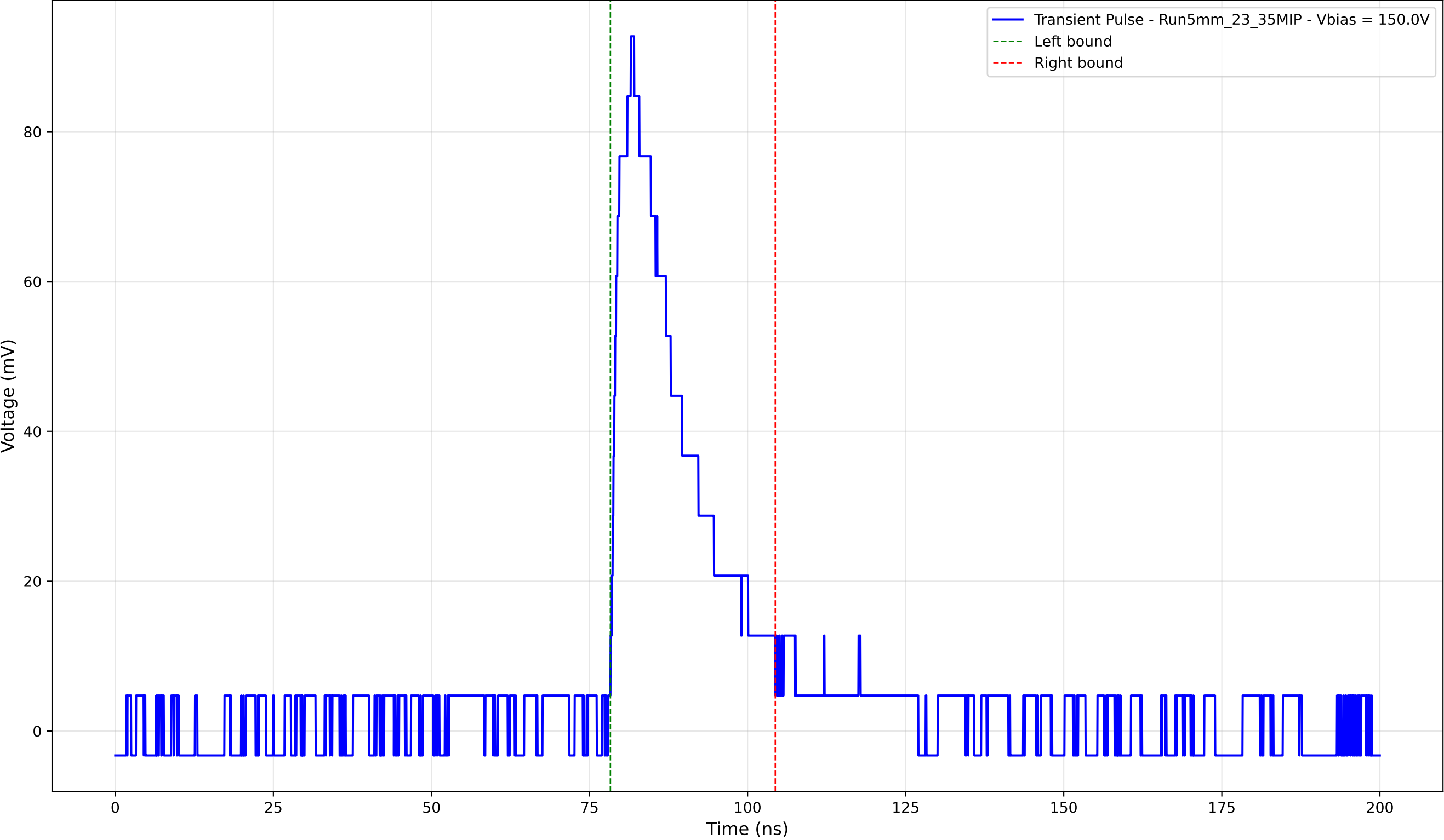
Transient Pulse - Sample: 5mm_23 - Position: 3150.0 \mu\text{m} - Charge: 21.33 pC
