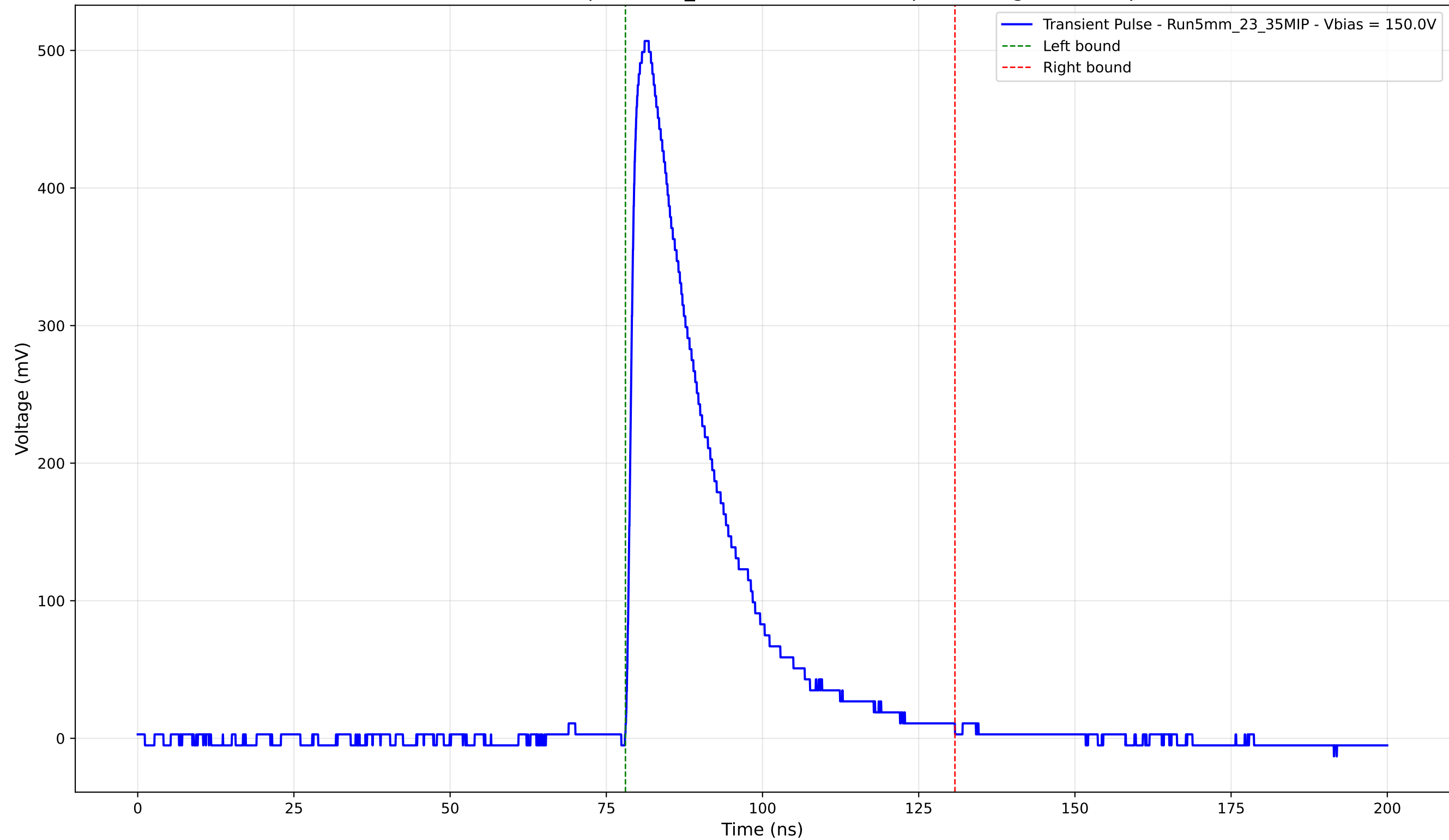
Transient Pulse - Sample: 5mm_23 - Position: 2420.0 \mu\text{m} - Charge: 137.20 pC
