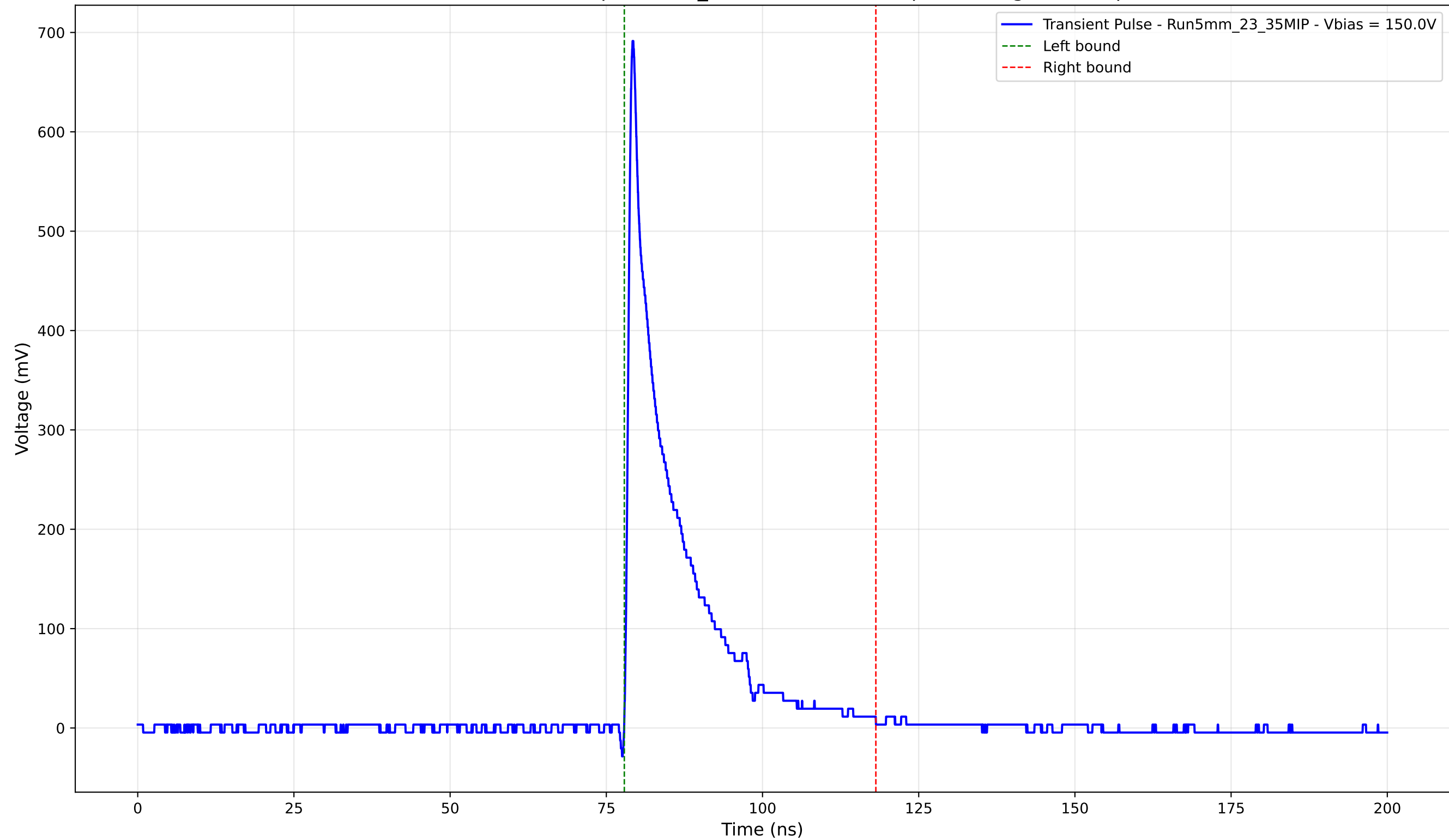
Transient Pulse - Sample: 5mm_23 - Position: 545.0 \mu\text{m} - Charge: 98.55 pC
