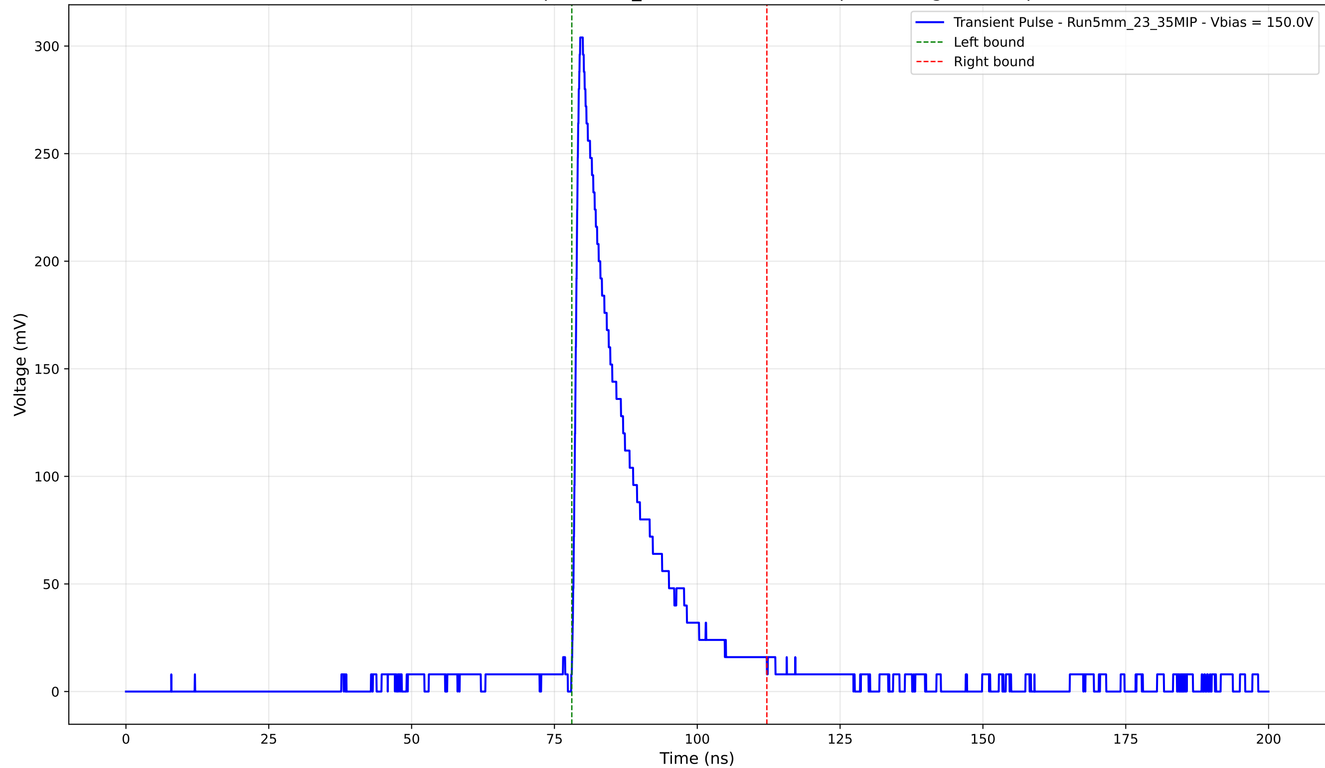
Transient Pulse - Sample: 5mm_23 - Position: 4200.0 \mu\text{m} - Charge: 56.70 pC
