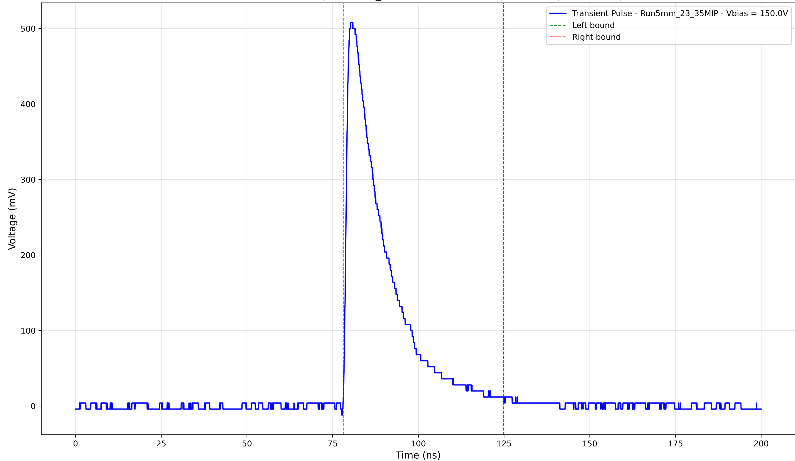
Transient Pulse - Sample: 5mm_23 - Position: 3450.0 \mu\text{m} - Charge: 126.54 pC
