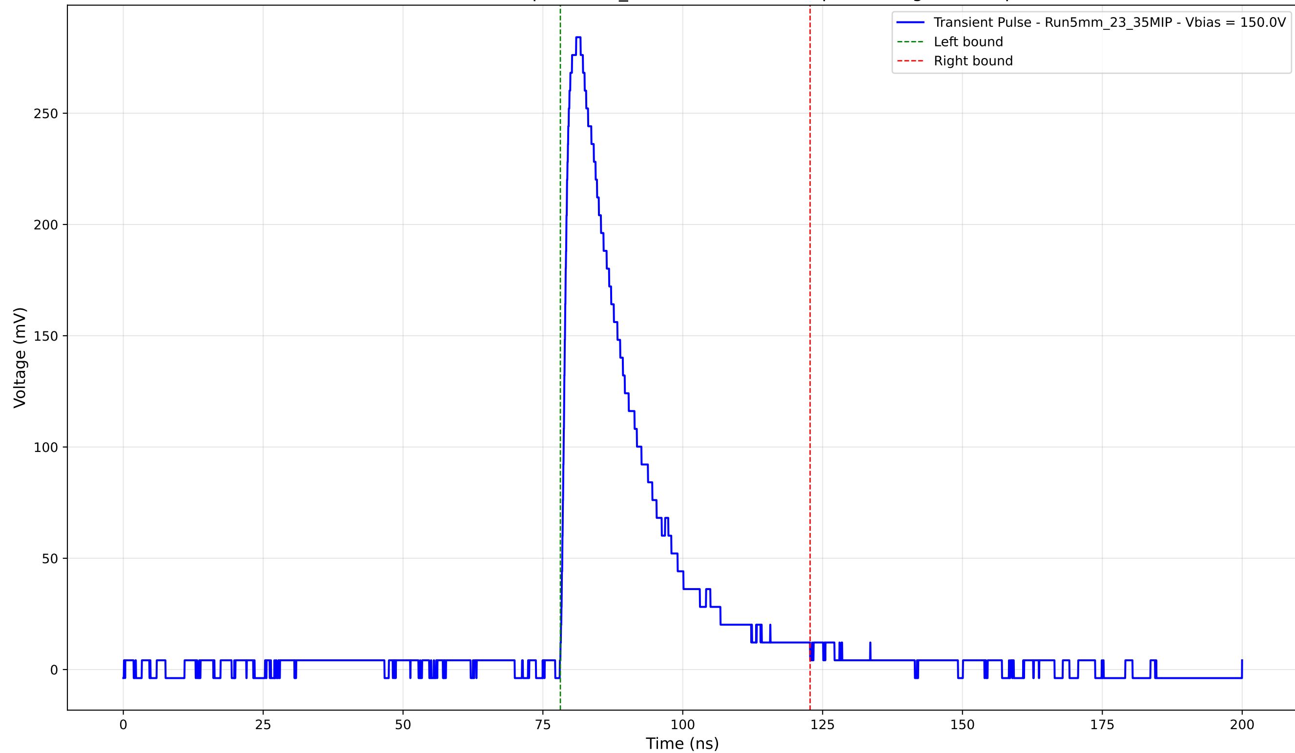
Transient Pulse - Sample: 5mm_23 - Position: 3100.0 \mu\text{m} - Charge: 73.22 pC
