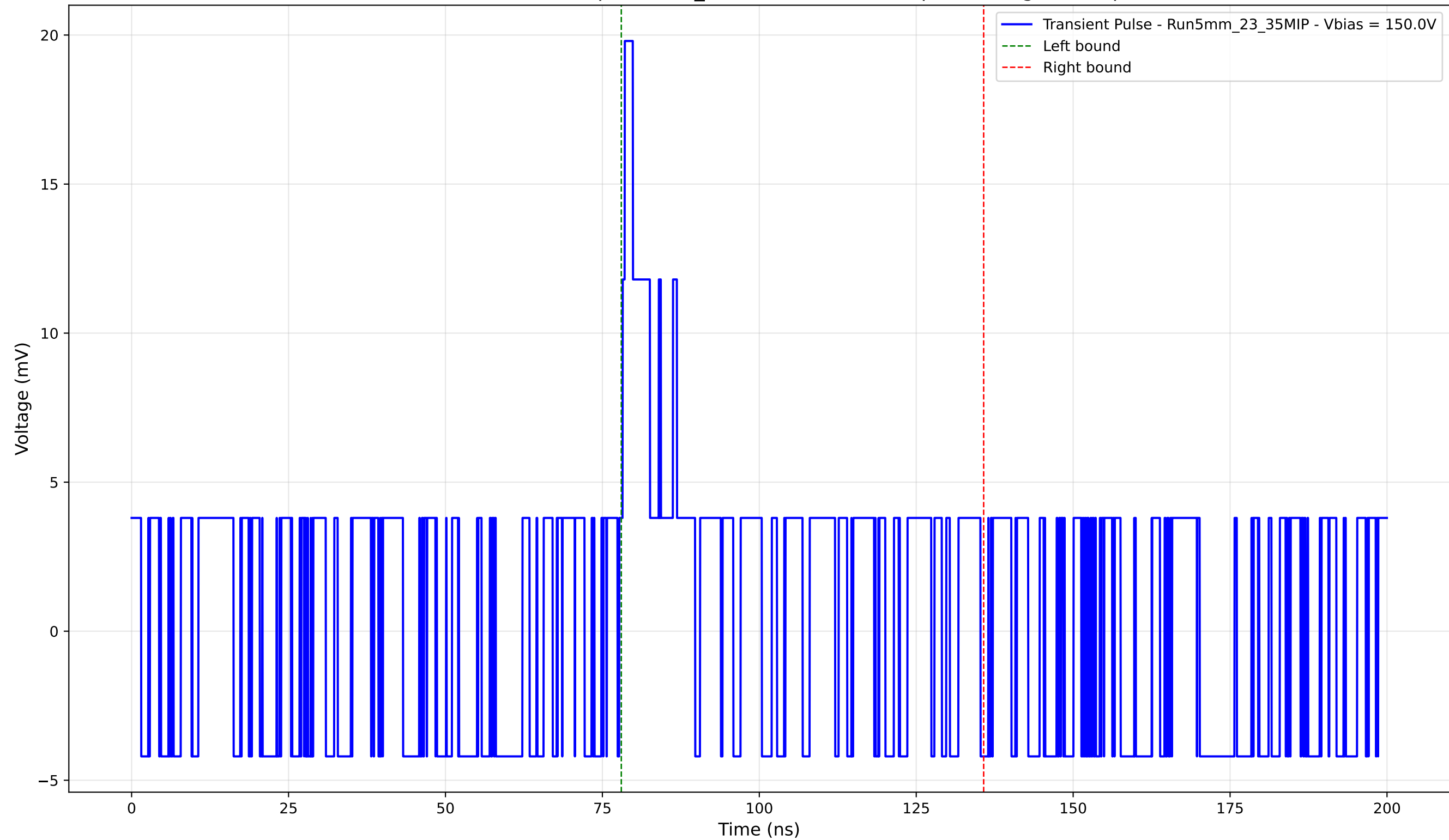
Transient Pulse - Sample: 5mm_23 - Position: 5170.0 \mu\text{m} - Charge: 3.19 pC
