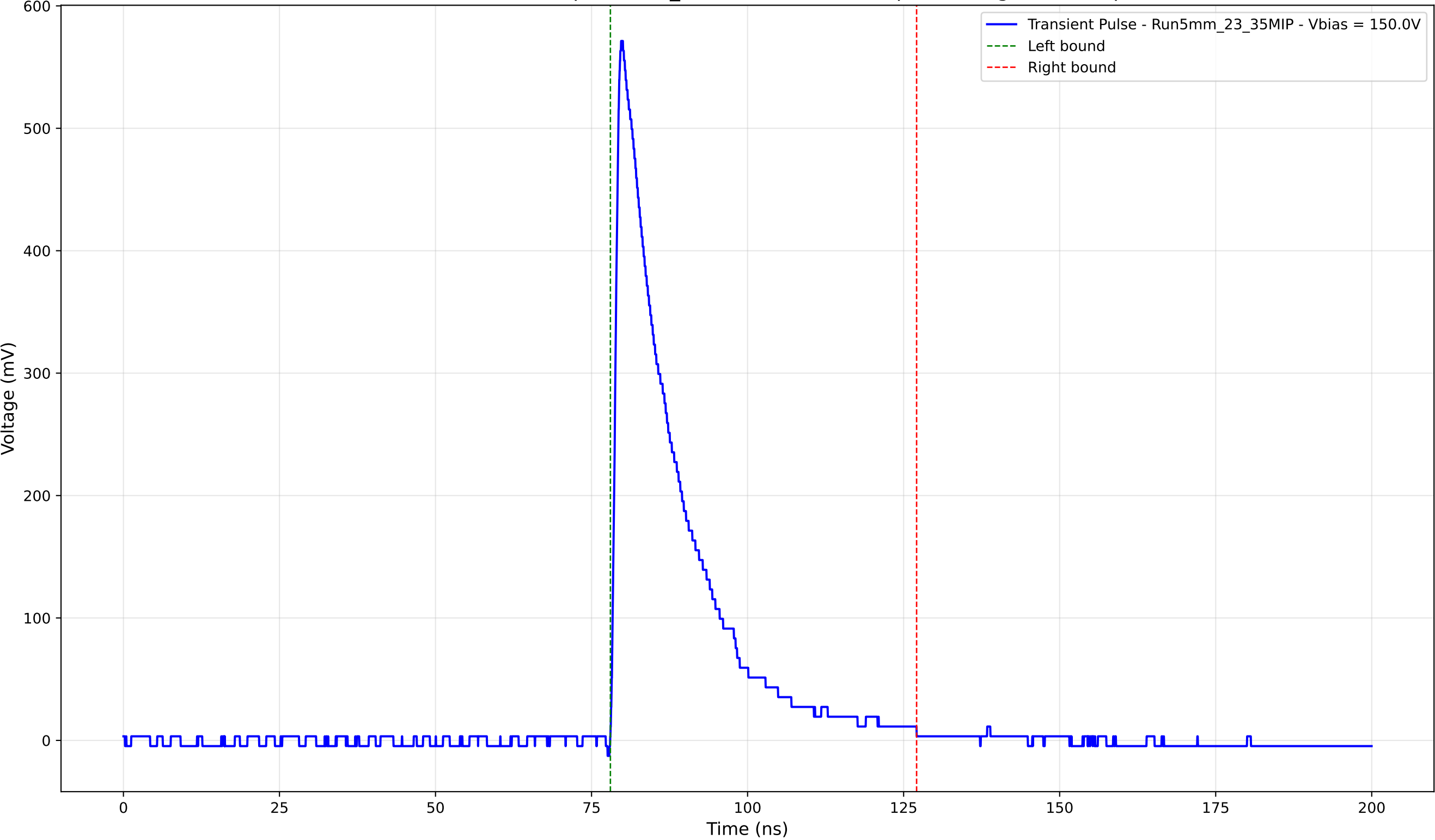
Transient Pulse - Sample: 5mm_23 - Position: 4010.0 \mu\text{m} - Charge: 119.91 pC
