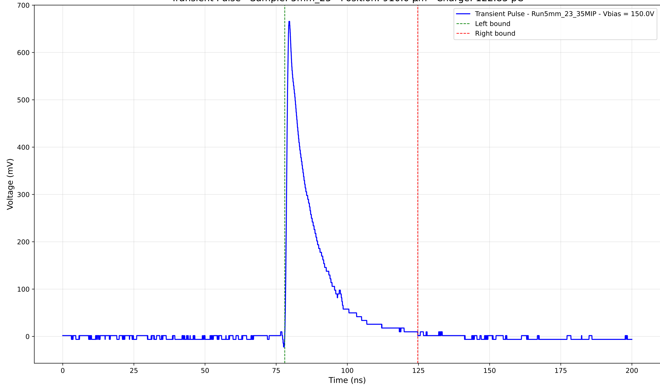
Transient Pulse - Sample: 5mm_23 - Position: 910.0 \mu\text{m} - Charge: 122.83 pC
