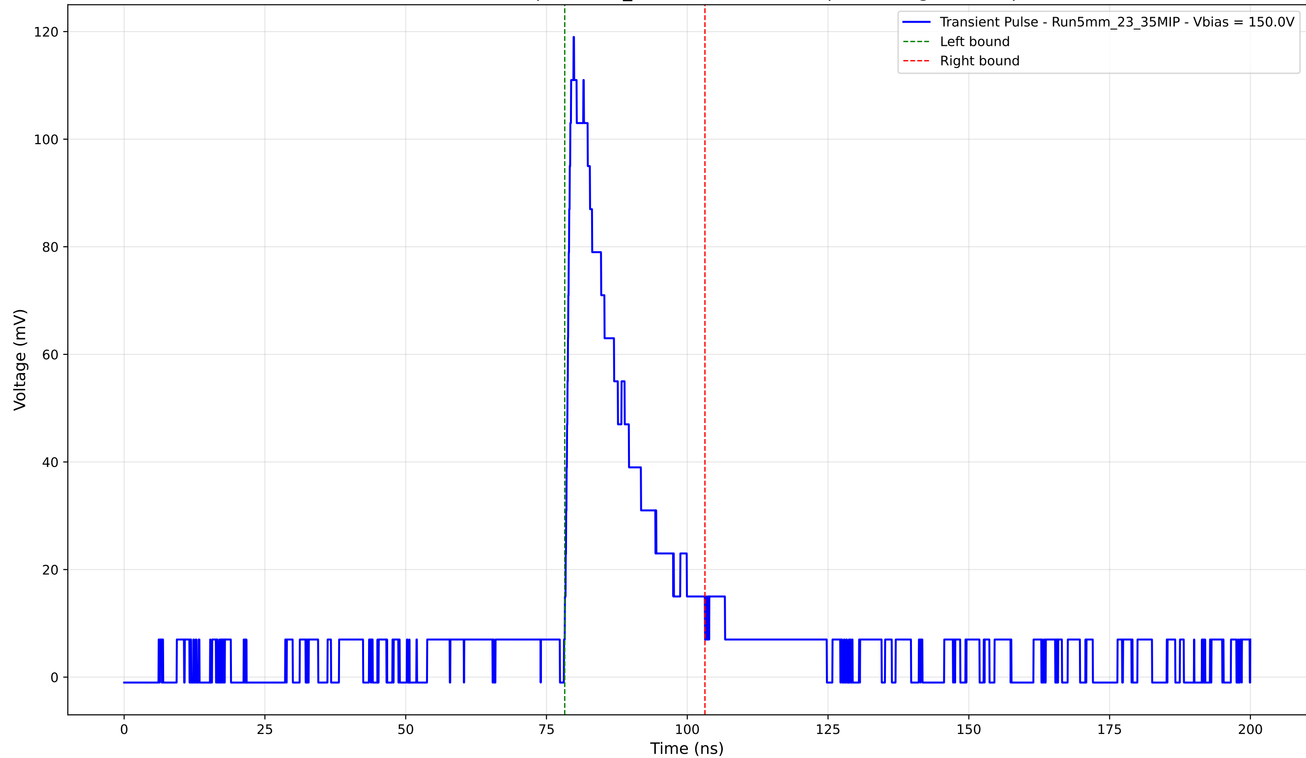
Transient Pulse - Sample: 5mm_23 - Position: 1115.0 \mu\text{m} - Charge: 23.85 pC
