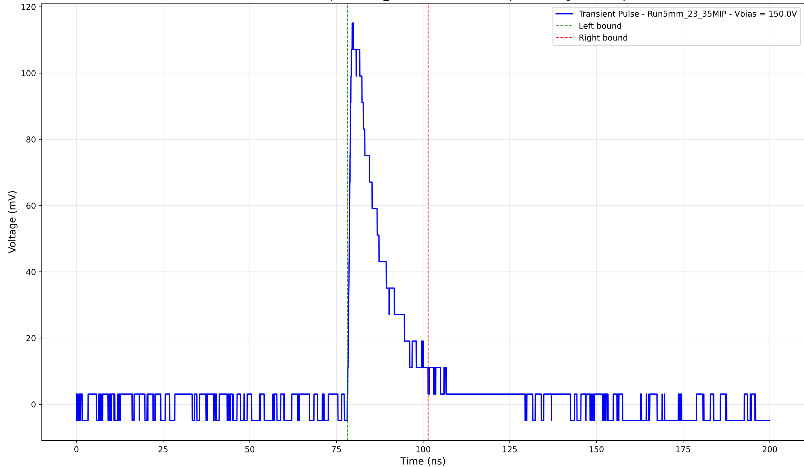
Transient Pulse - Sample: 5mm_23 - Position: 4145.0 \mu\text{m} - Charge: 21.42 pC
