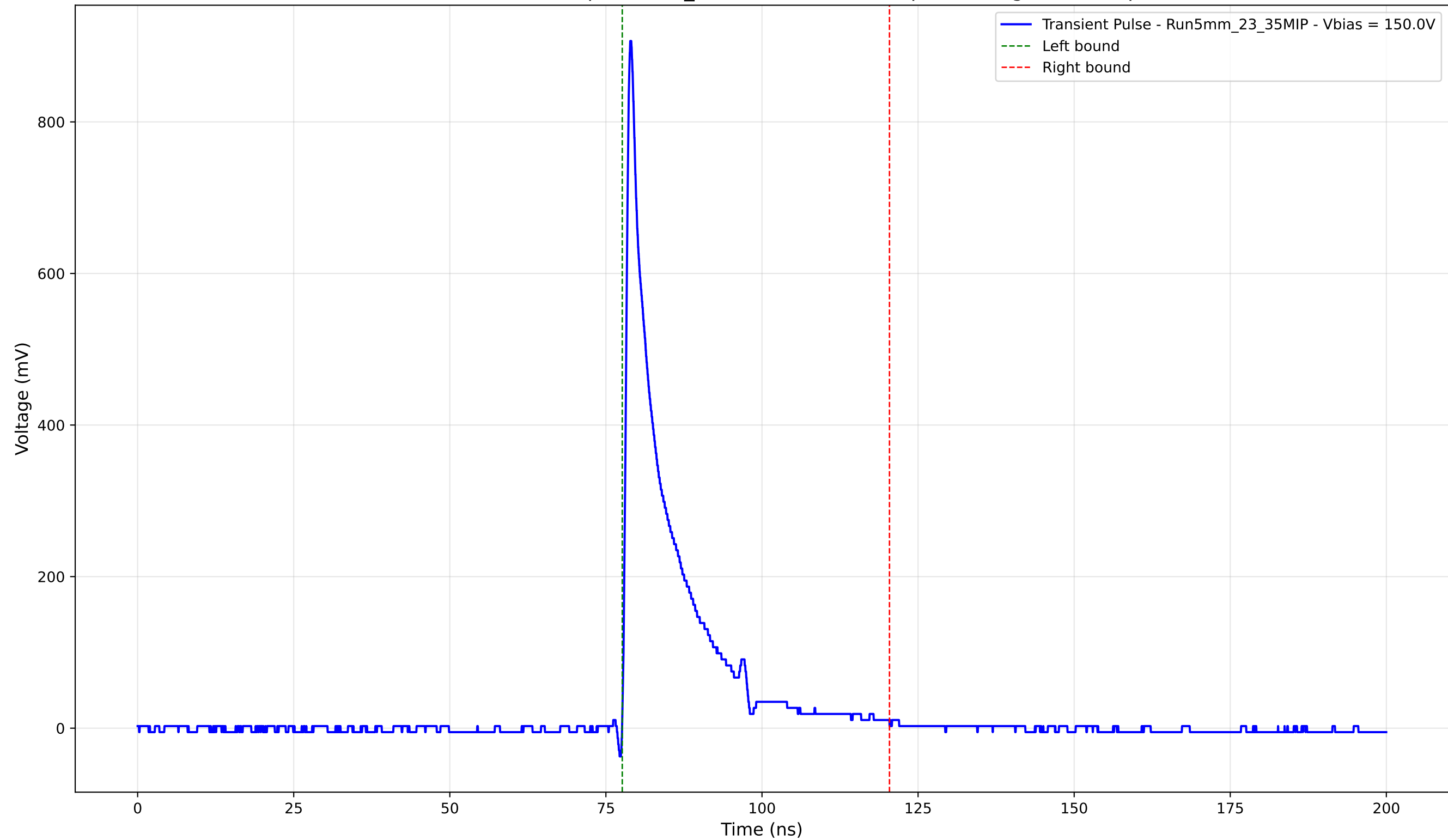
Transient Pulse - Sample: 5mm_23 - Position: 4980.0 \mu\text{m} - Charge: 117.62 pC
