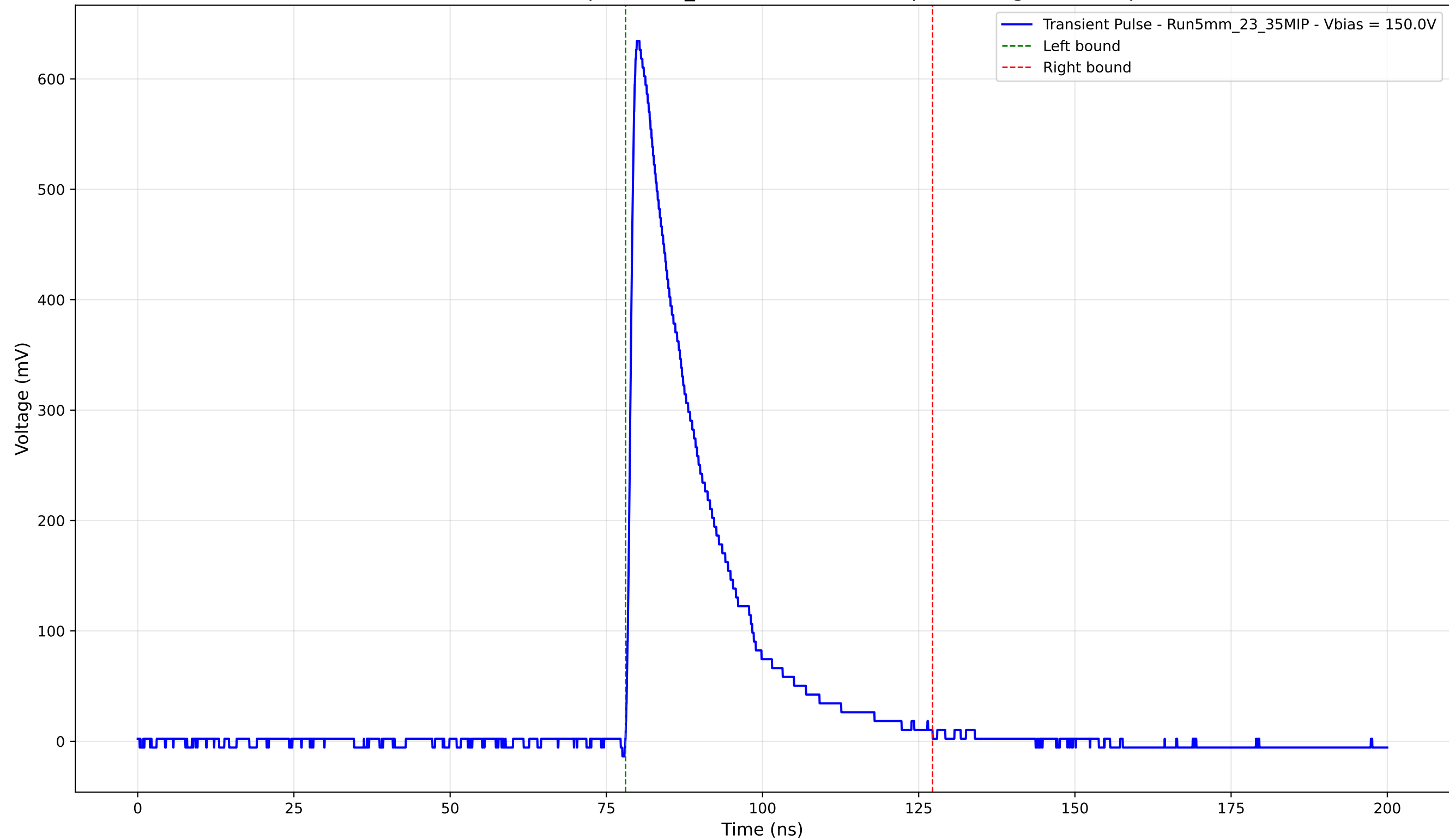
Transient Pulse - Sample: 5mm_23 - Position: 1470.0 \mu\text{m} - Charge: 148.83 pC
