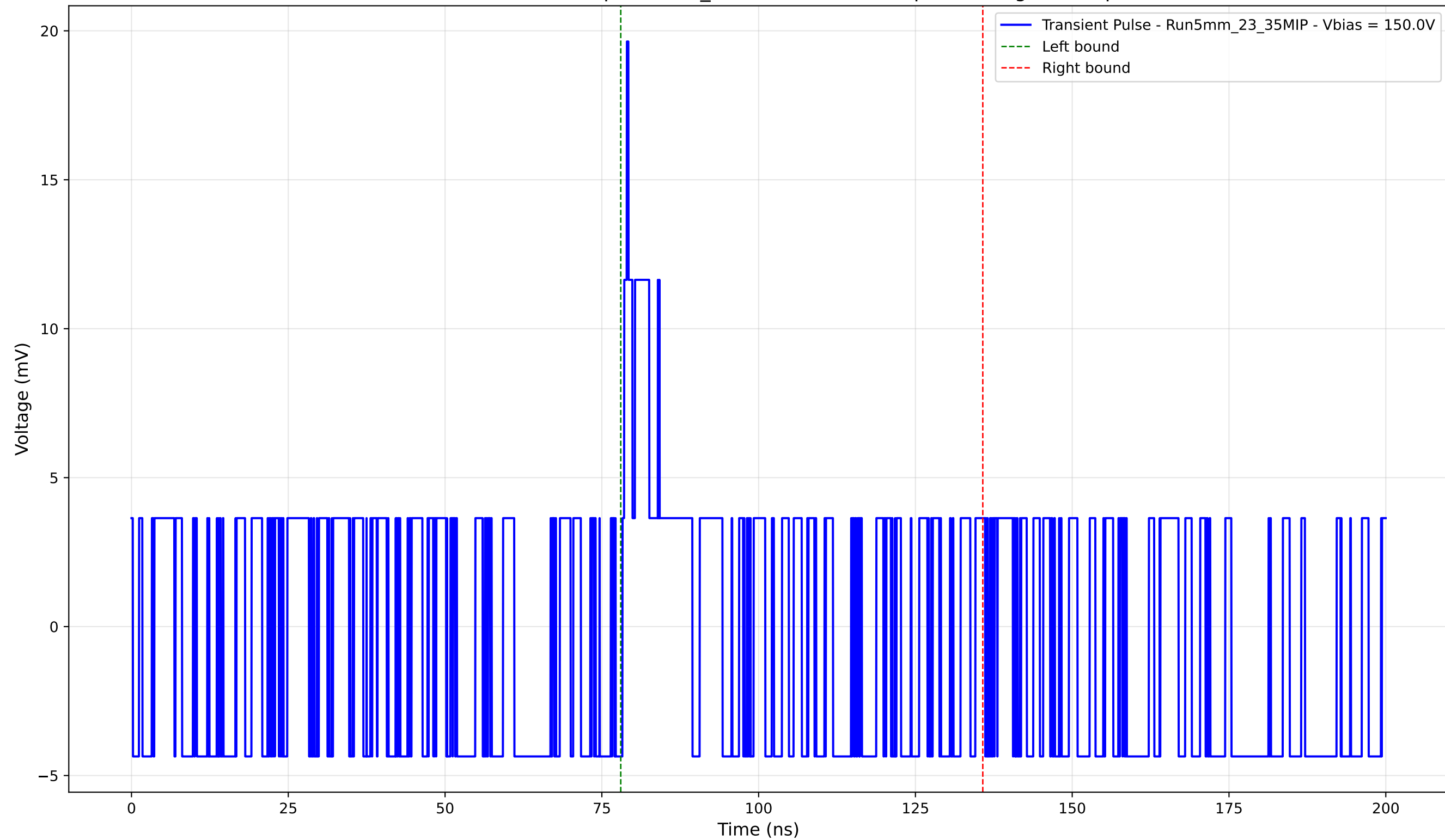
Transient Pulse - Sample: 5mm_23 - Position: 125.0 \mu\text{m} - Charge: 0.90 pC
