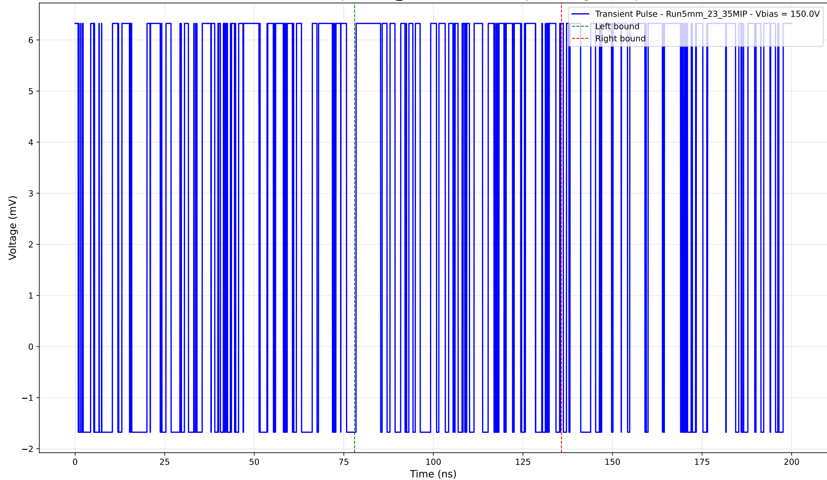
Transient Pulse - Sample: 5mm_23 - Position: 5245.0 \mu\text{m} - Charge: 3.93 pC
