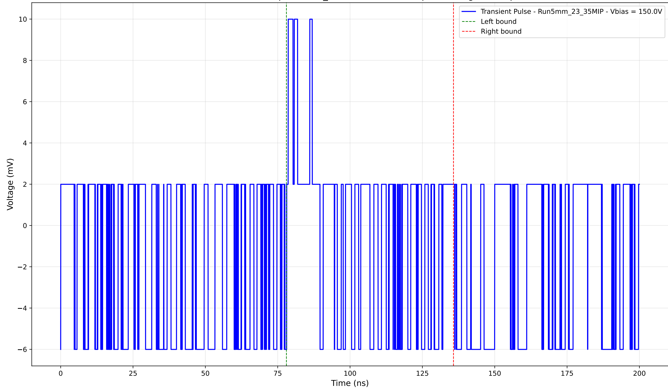
Transient Pulse - Sample: 5mm_23 - Position: 115.0 \mu\text{m} - Charge: 0.28 pC
