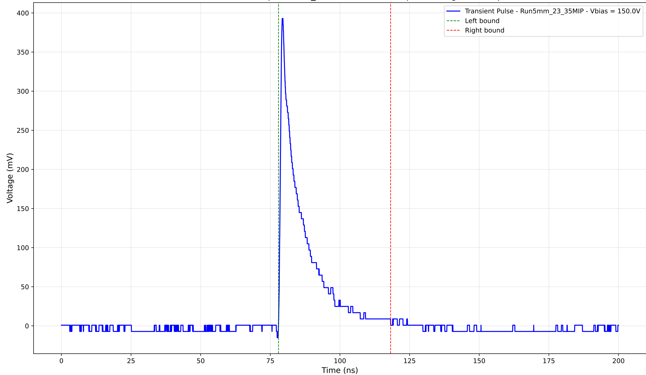
Transient Pulse - Sample: 5mm_23 - Position: 665.0 \mu\text{m} - Charge: 61.43 pC
