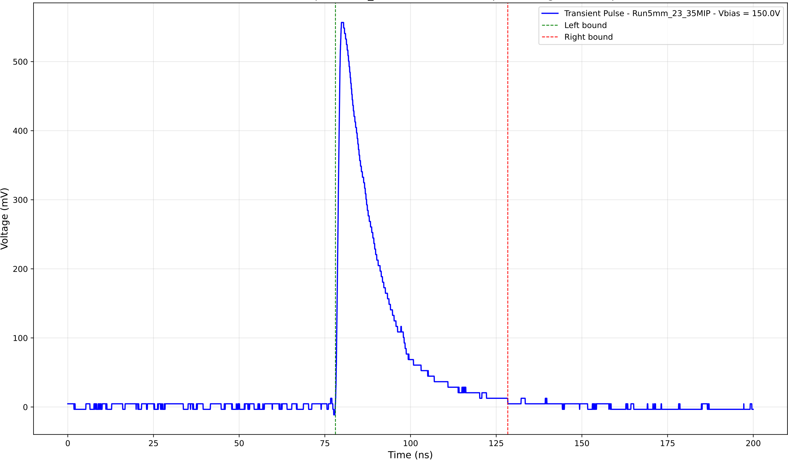
Transient Pulse - Sample: 5mm_23 - Position: 1525.0 \mu\text{m} - Charge: 133.28 pC
