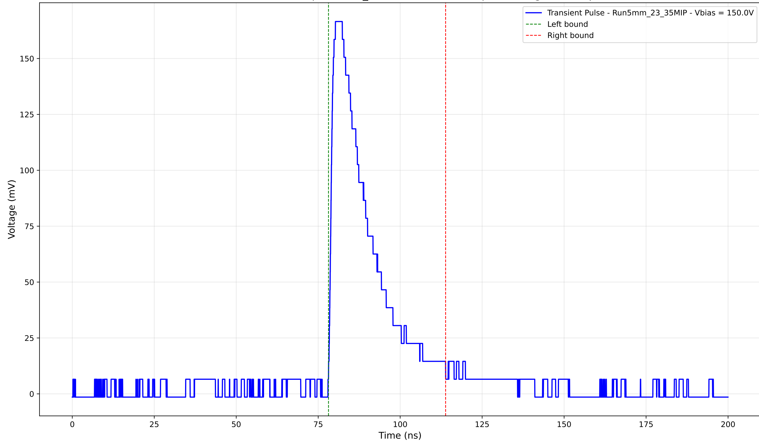
Transient Pulse - Sample: 5mm_23 - Position: 2110.0 \mu\text{m} - Charge: 44.14 pC
