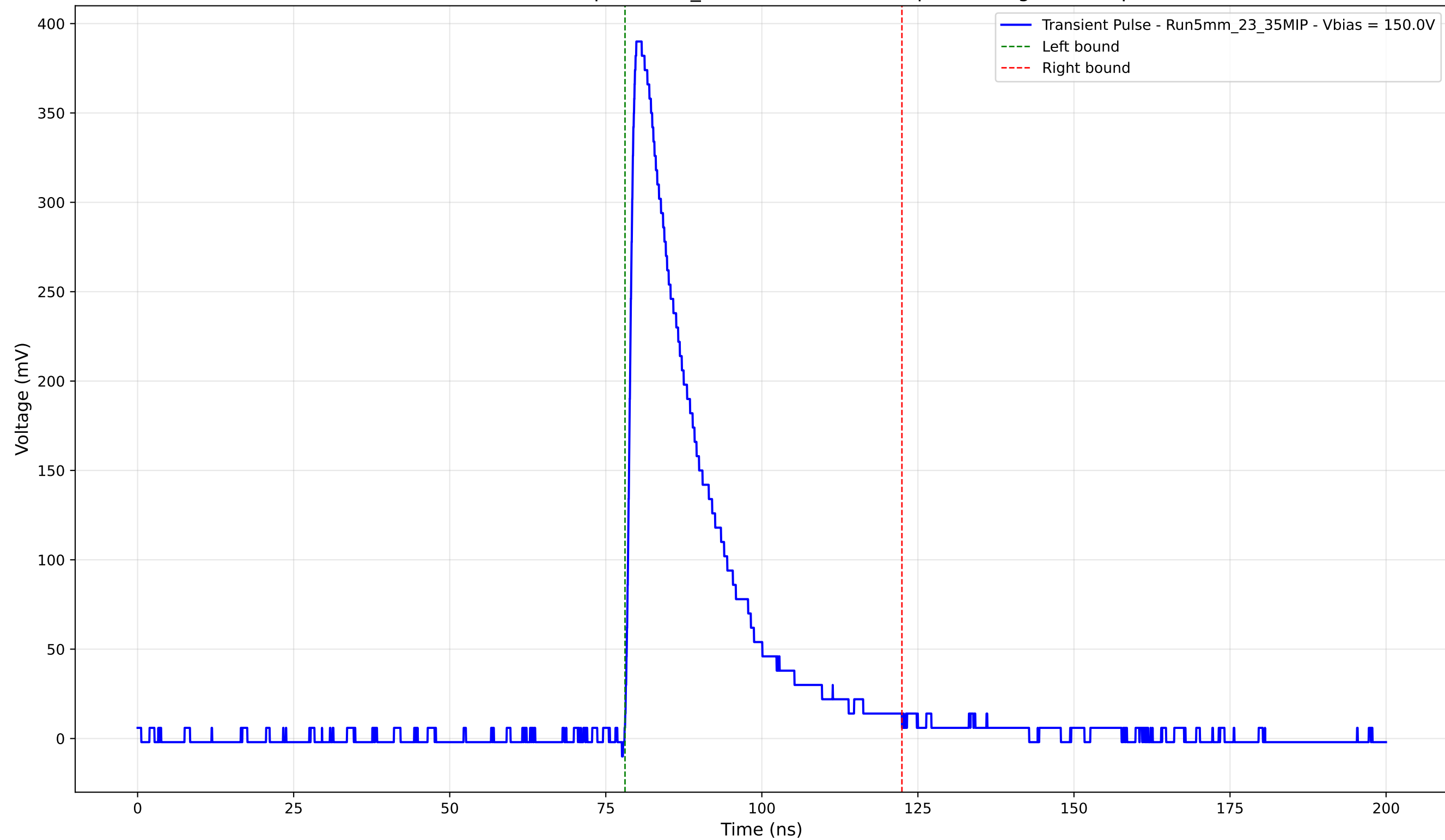
Transient Pulse - Sample: 5mm_23 - Position: 3590.0 \mu\text{m} - Charge: 94.01 pC
