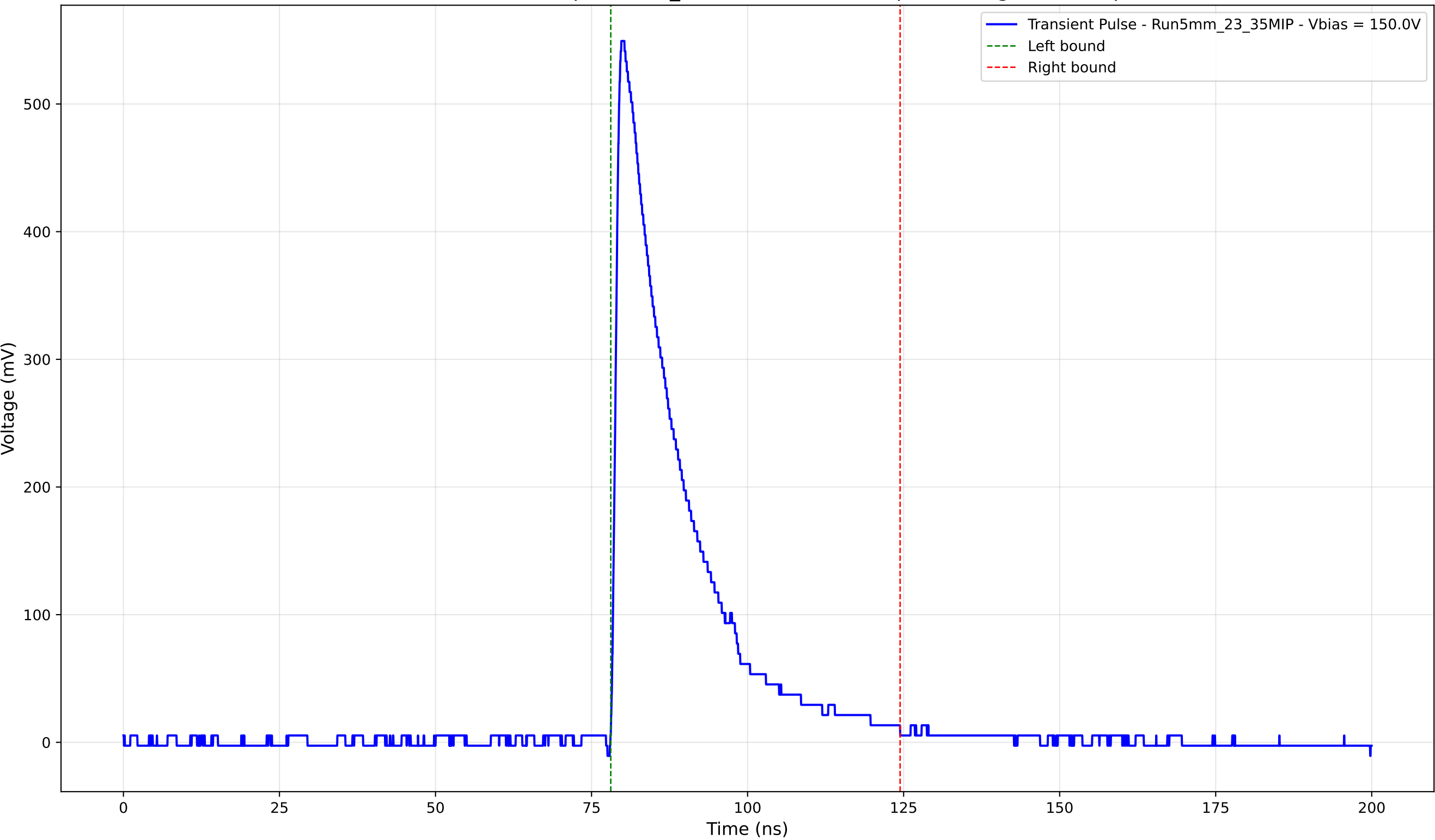
Transient Pulse - Sample: 5mm_23 - Position: 3885.0 \mu\text{m} - Charge: 122.25 pC
