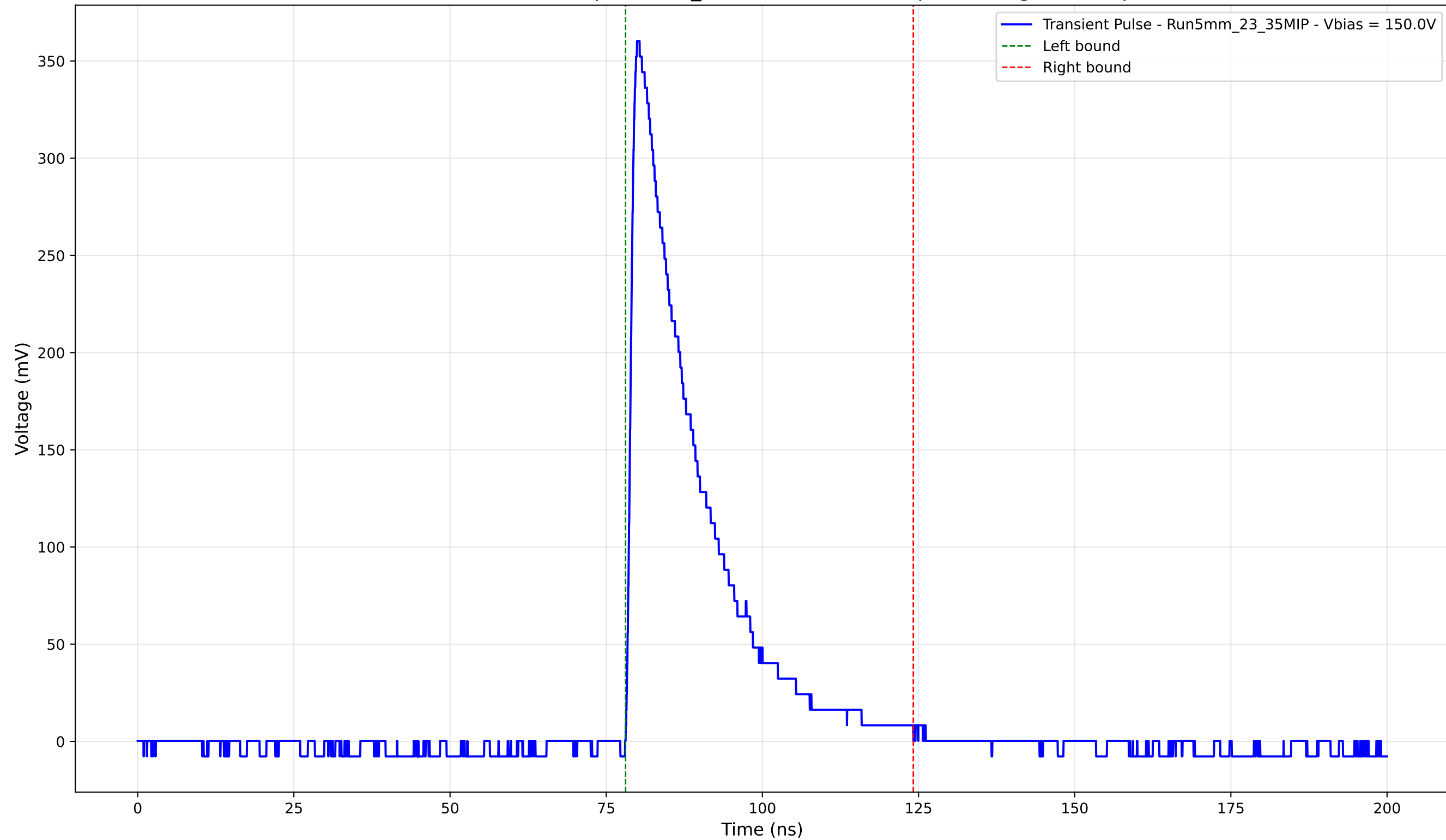
Transient Pulse - Sample: 5mm_23 - Position: 1565.0 \mu\text{m} - Charge: 81.86 pC
