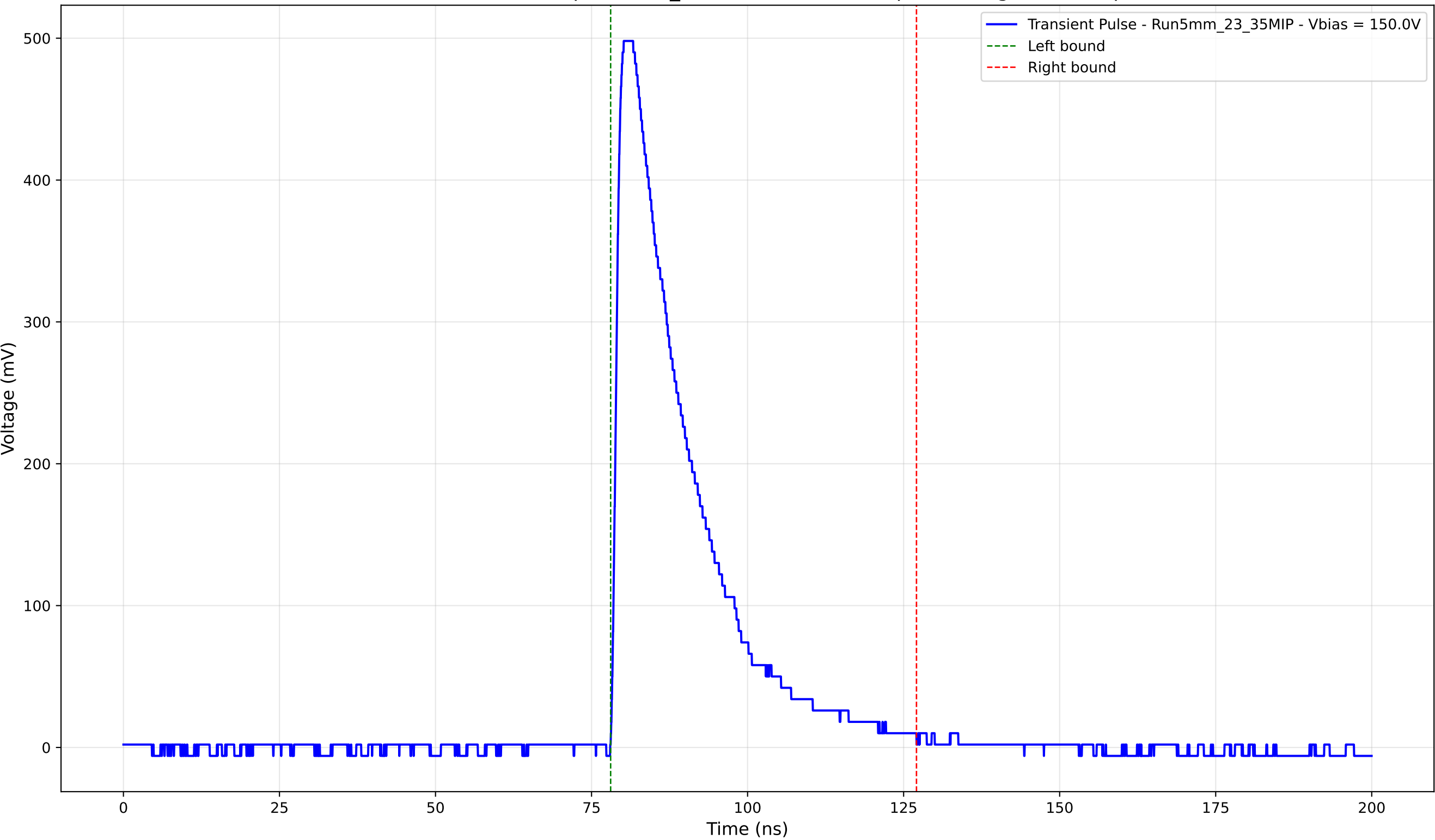
Transient Pulse - Sample: 5mm_23 - Position: 3360.0 \mu\text{m} - Charge: 127.59 pC
