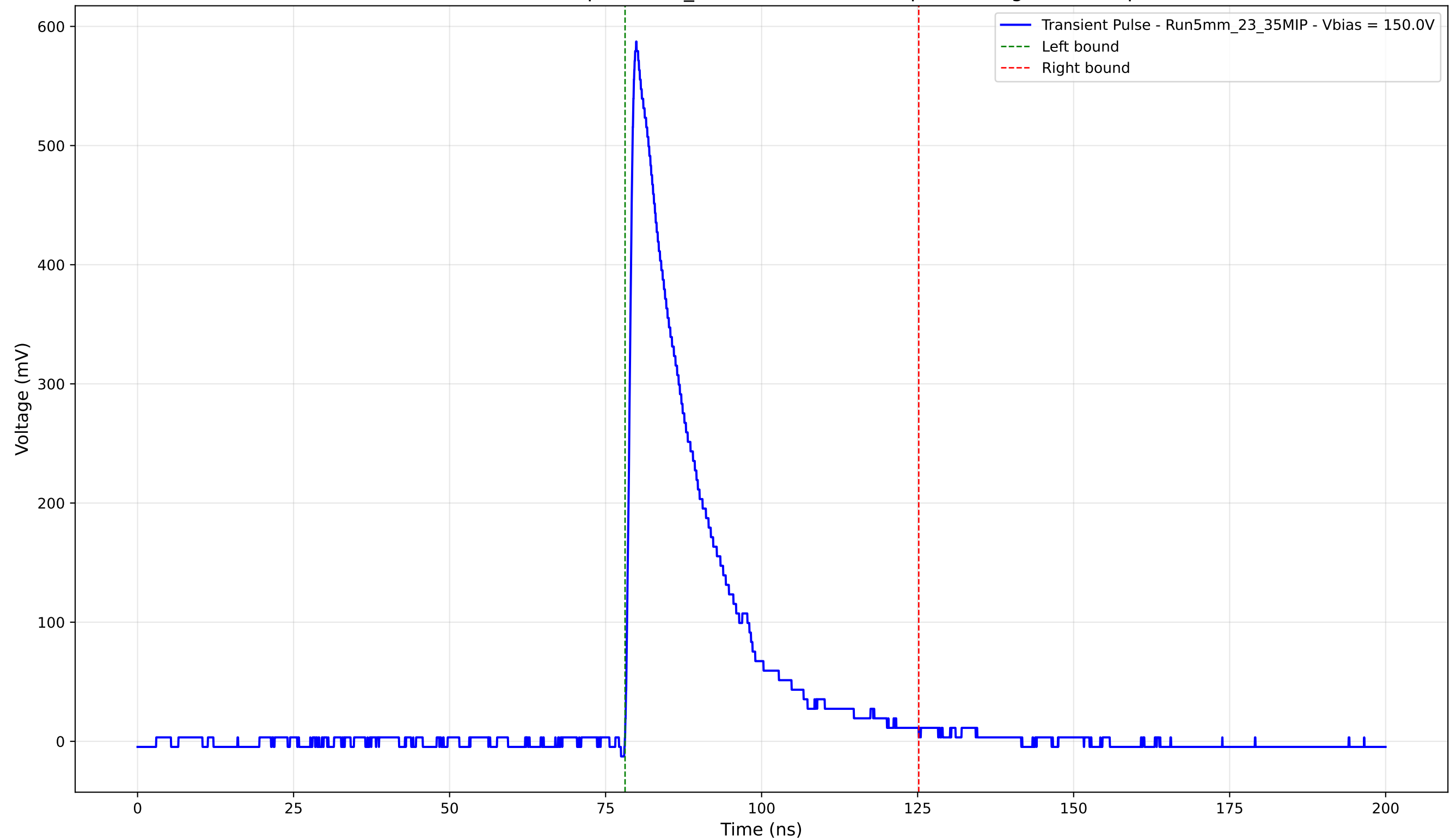
Transient Pulse - Sample: 5mm_23 - Position: 1315.0 \mu\text{m} - Charge: 129.09 pC
