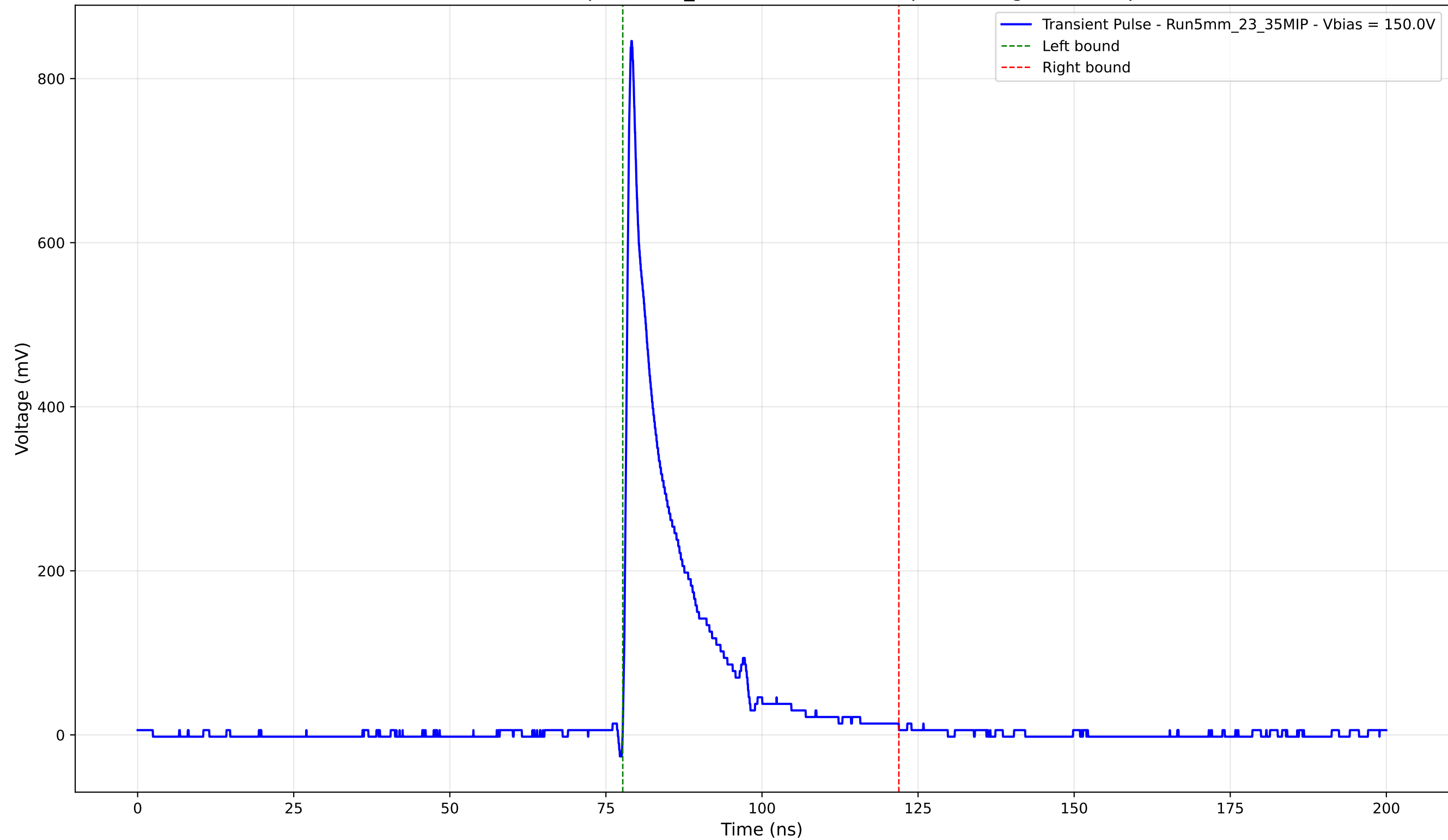
Transient Pulse - Sample: 5mm_23 - Position: 4850.0 \mu\text{m} - Charge: 117.83 pC
