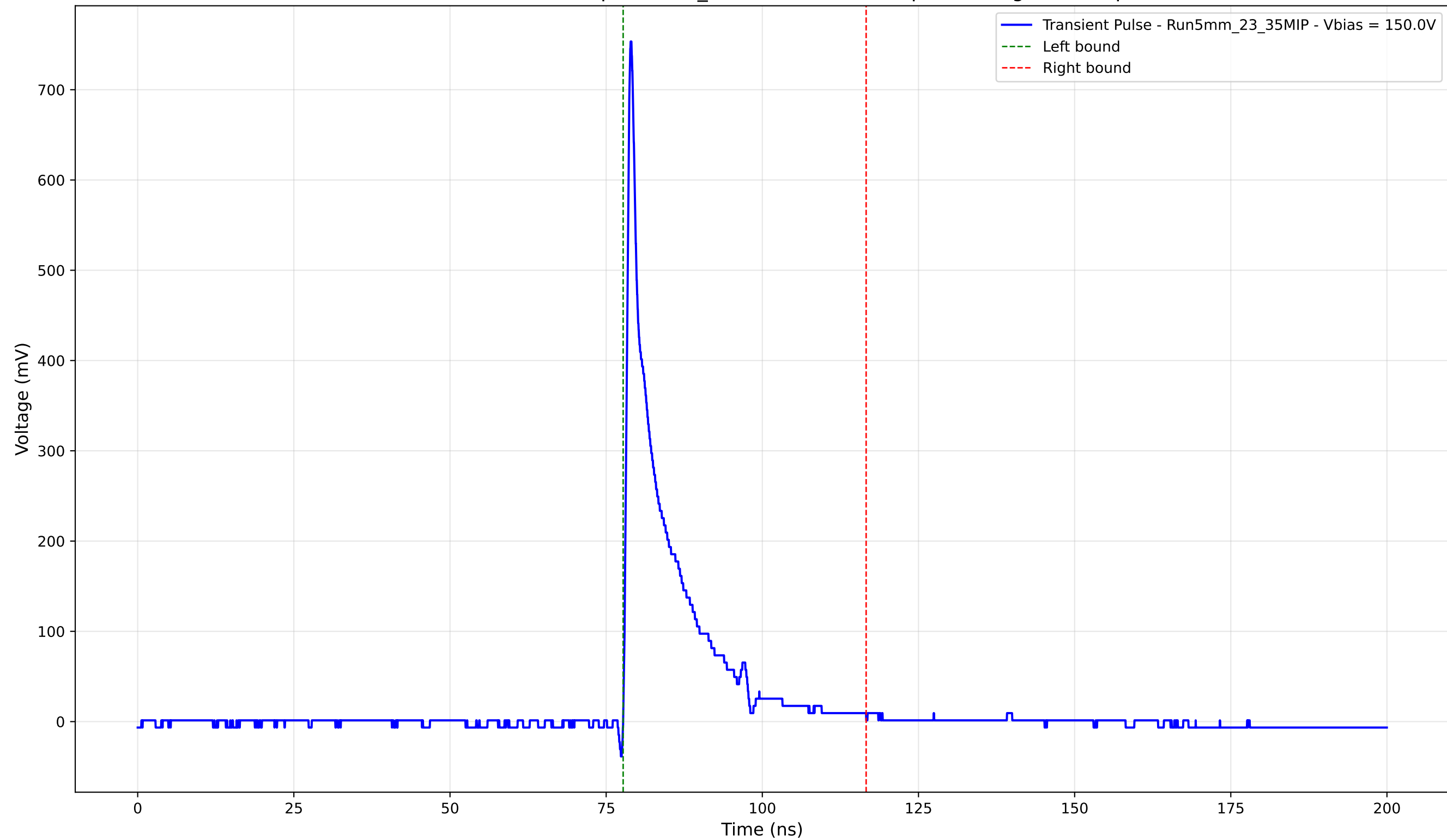
Transient Pulse - Sample: 5mm_23 - Position: 235.0 \mu\text{m} - Charge: 84.84 pC
