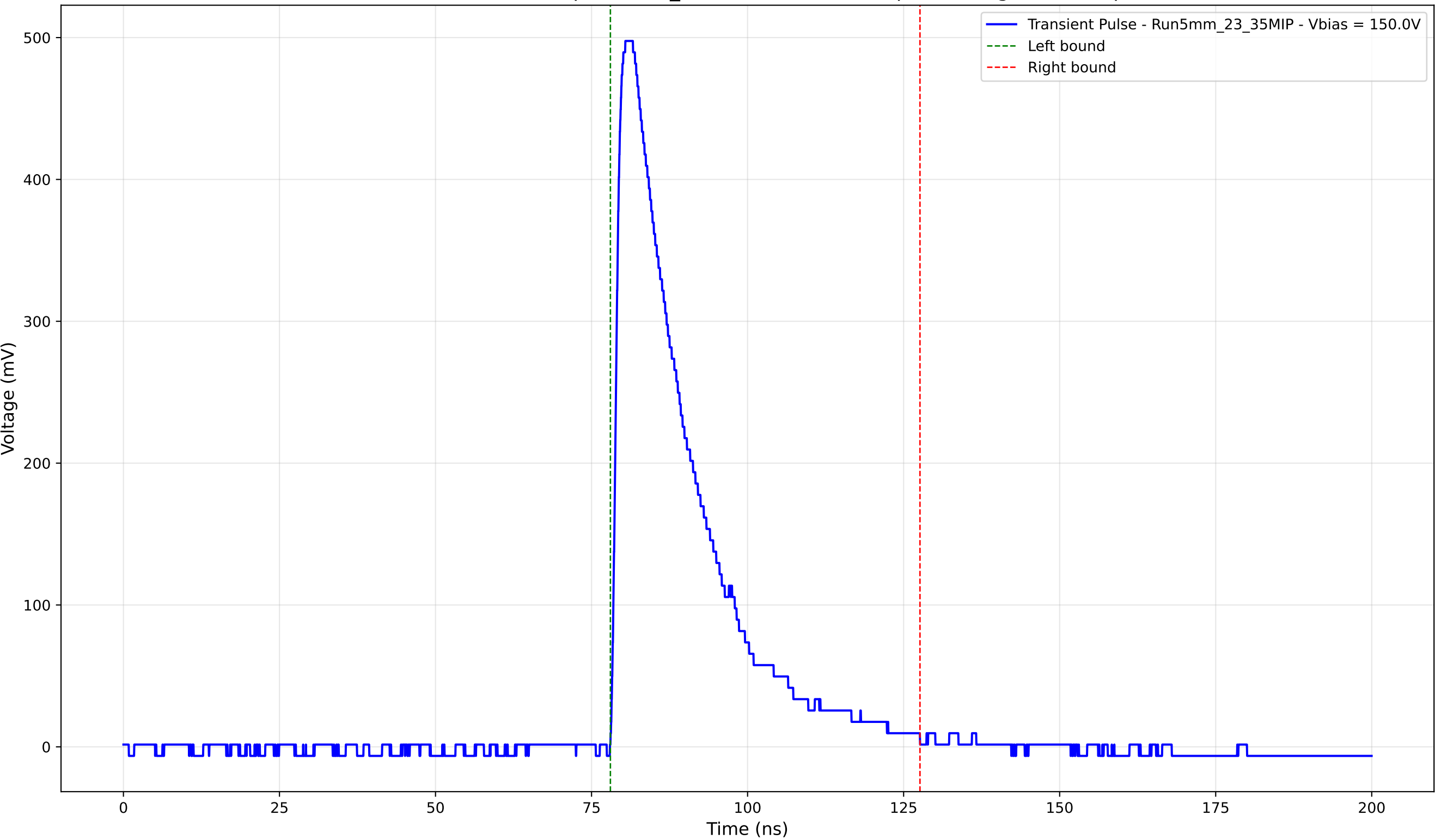
Transient Pulse - Sample: 5mm_23 - Position: 3260.0 \mu\text{m} - Charge: 128.53 pC
