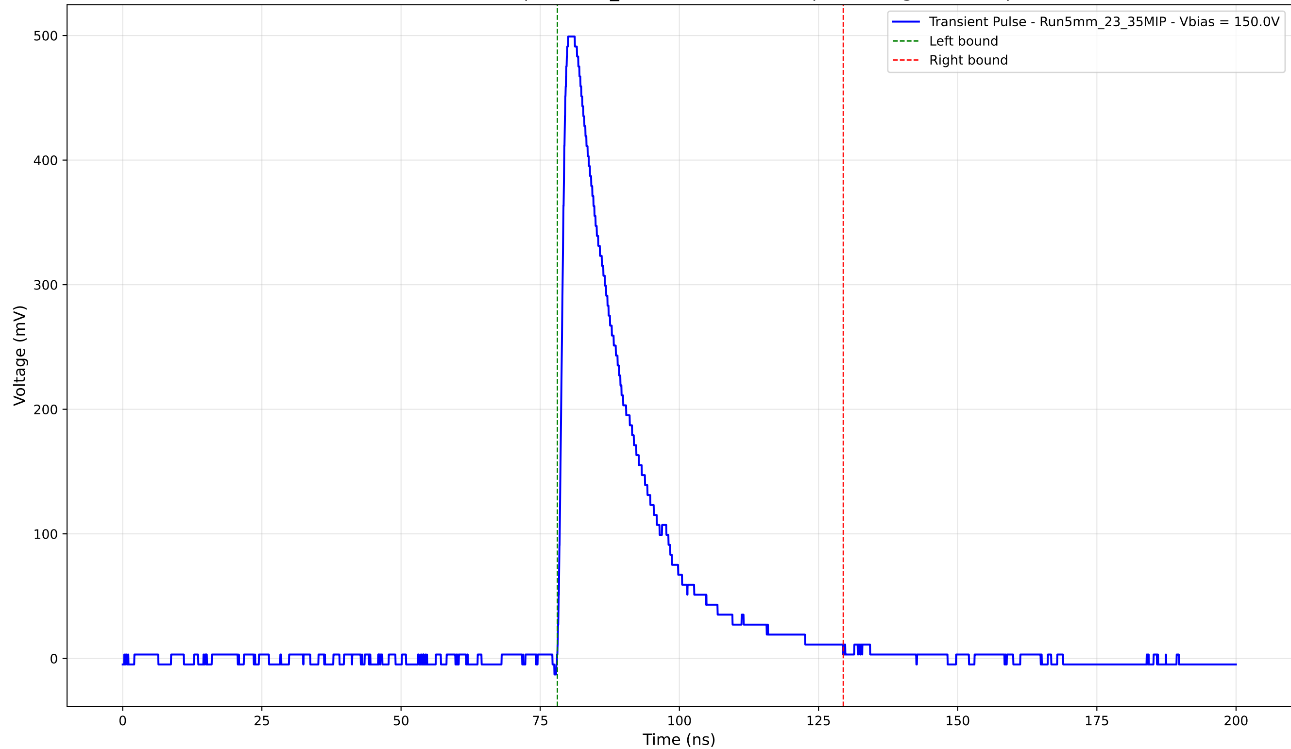
Transient Pulse - Sample: 5mm_23 - Position: 3515.0 \mu\text{m} - Charge: 125.49 pC
