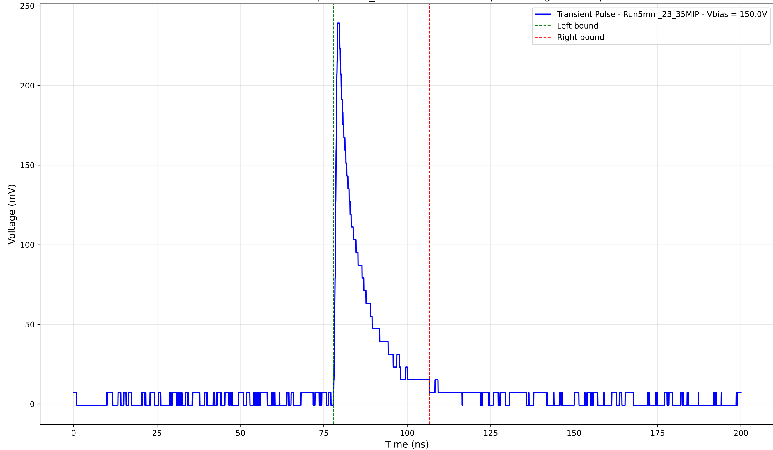
Transient Pulse - Sample: 5mm_23 - Position: 4540.0 \mu\text{m} - Charge: 36.24 pC
