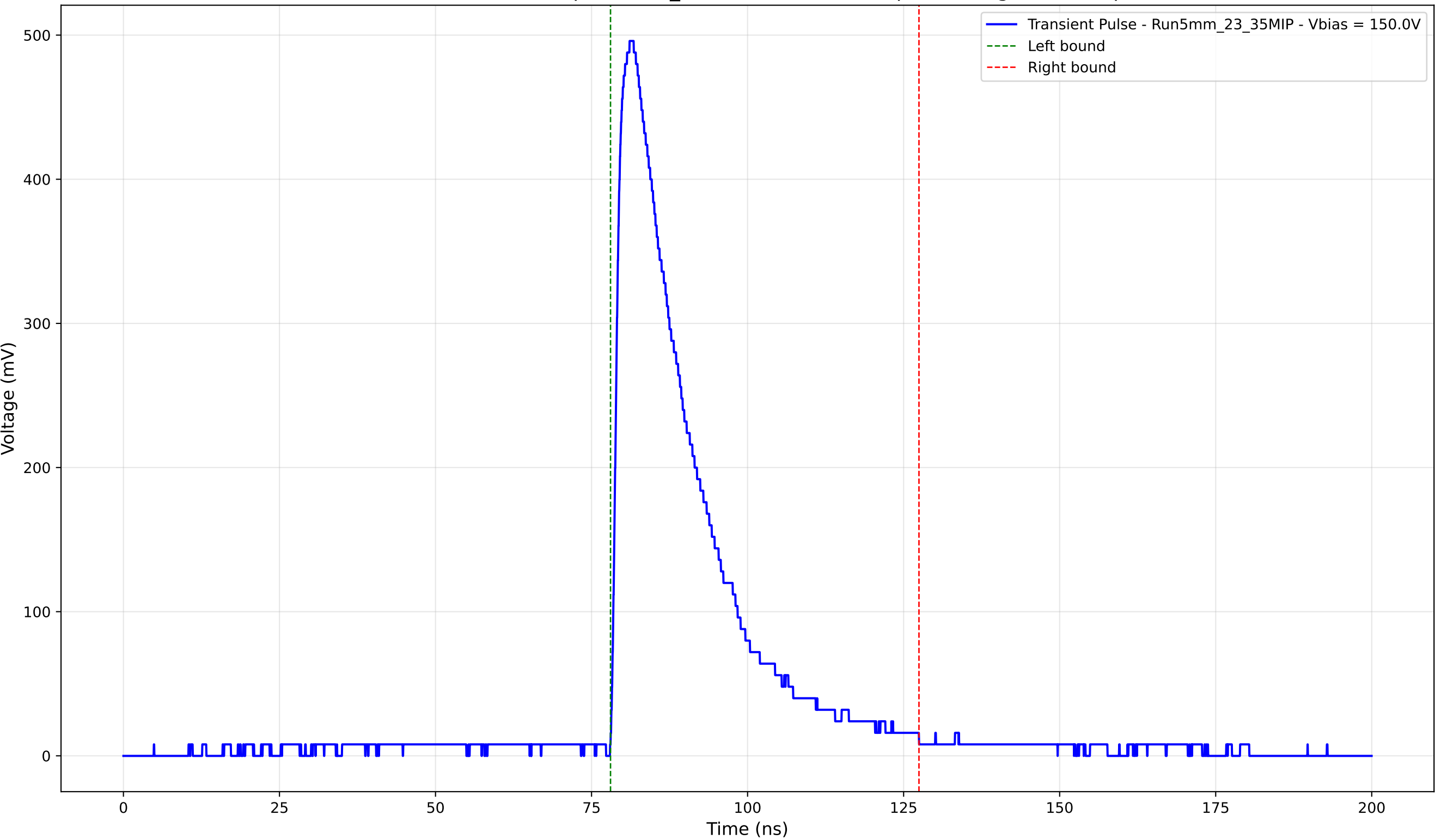
Transient Pulse - Sample: 5mm_23 - Position: 2755.0 \mu\text{m} - Charge: 135.51 pC
