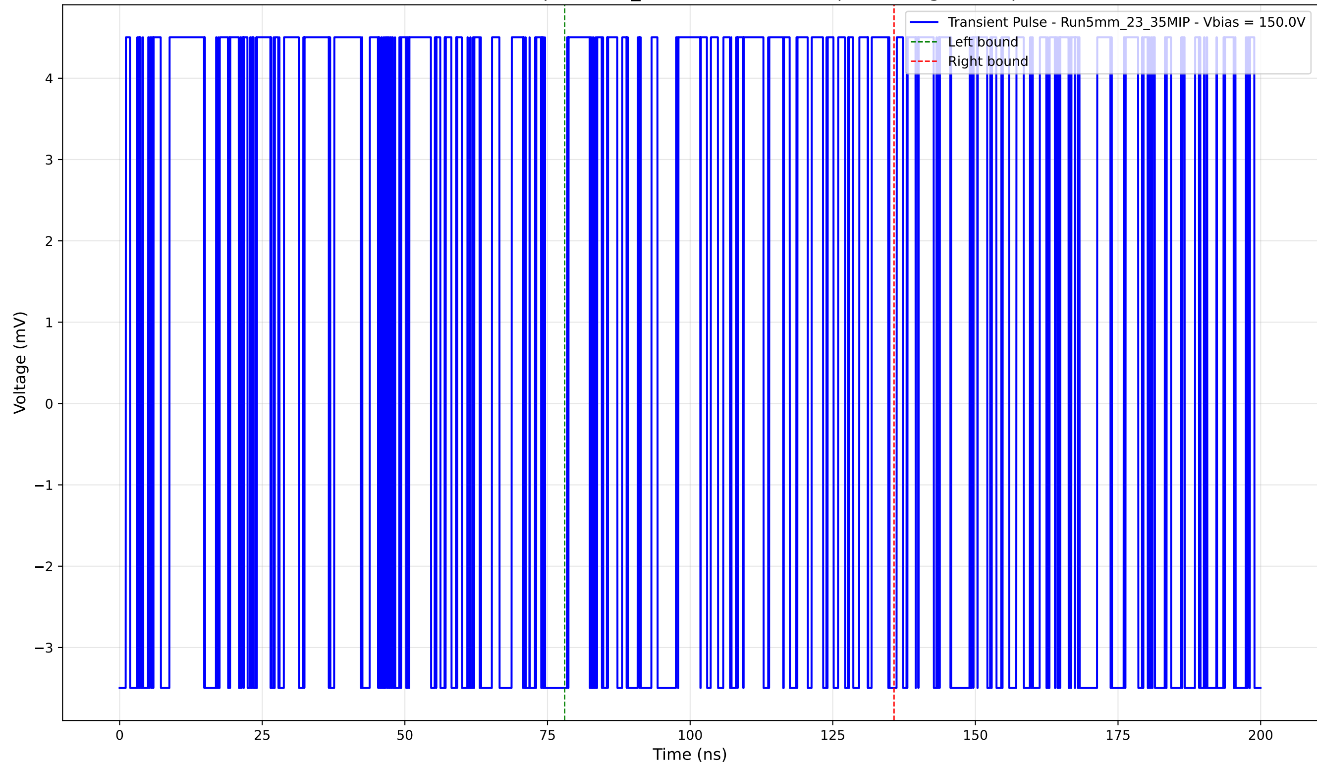
Transient Pulse - Sample: 5mm_23 - Position: 5275.0 \mu\text{m} - Charge: 1.89 pC
