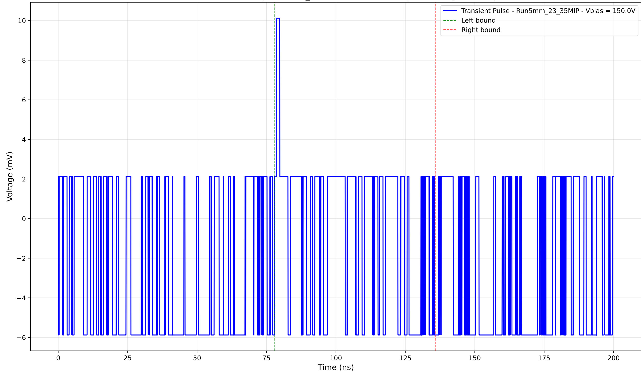
Transient Pulse - Sample: 5mm_23 - Position: 5210.0 \mu\text{m} - Charge: -0.28 pC
