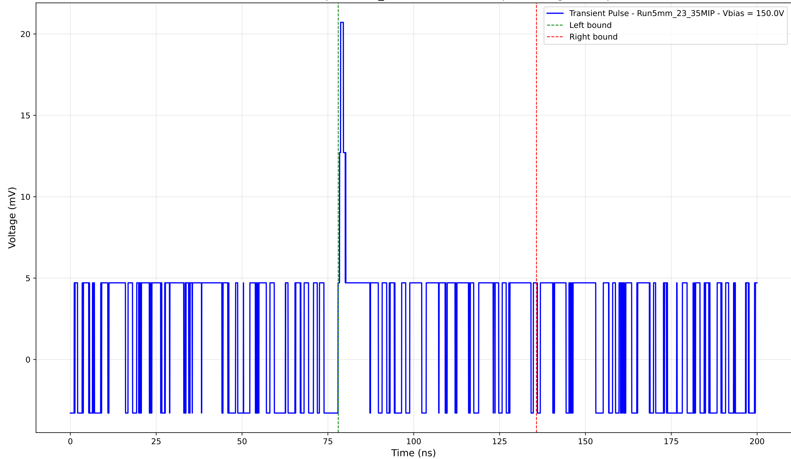
Transient Pulse - Sample: 5mm_23 - Position: 5180.0 \mu\text{m} - Charge: 3.93 pC
