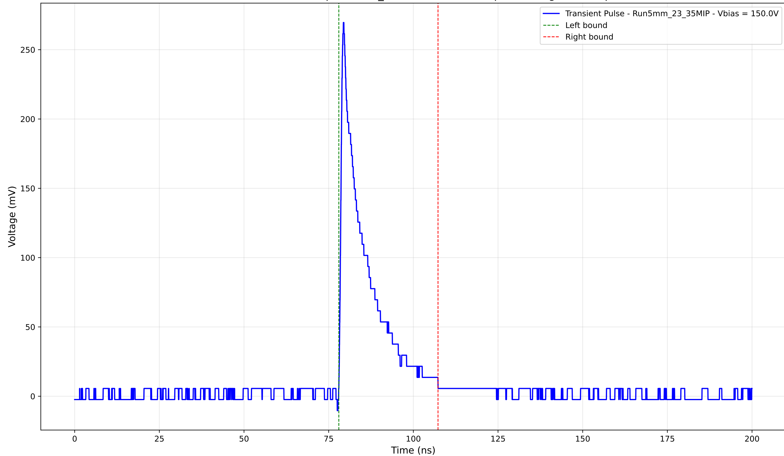
Transient Pulse - Sample: 5mm_23 - Position: 650.0 \mu\text{m} - Charge: 41.52 pC
