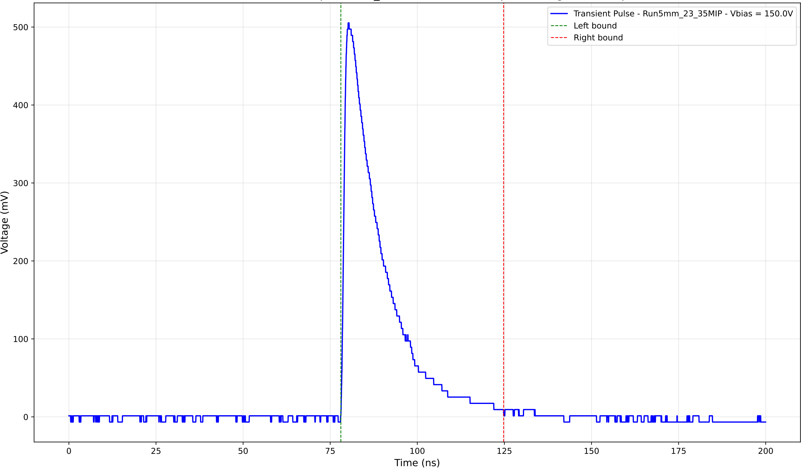
Transient Pulse - Sample: 5mm_23 - Position: 3535.0 \mu\text{m} - Charge: 121.54 pC
