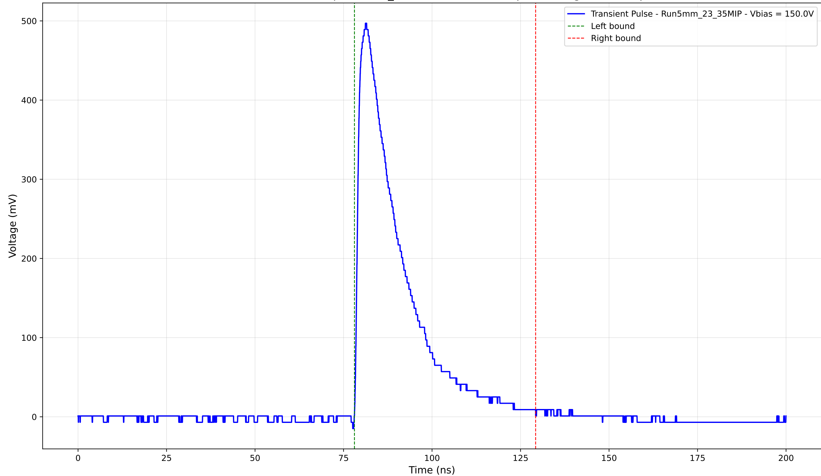
Transient Pulse - Sample: 5mm_23 - Position: 2775.0 \mu\text{m} - Charge: 132.36 pC
