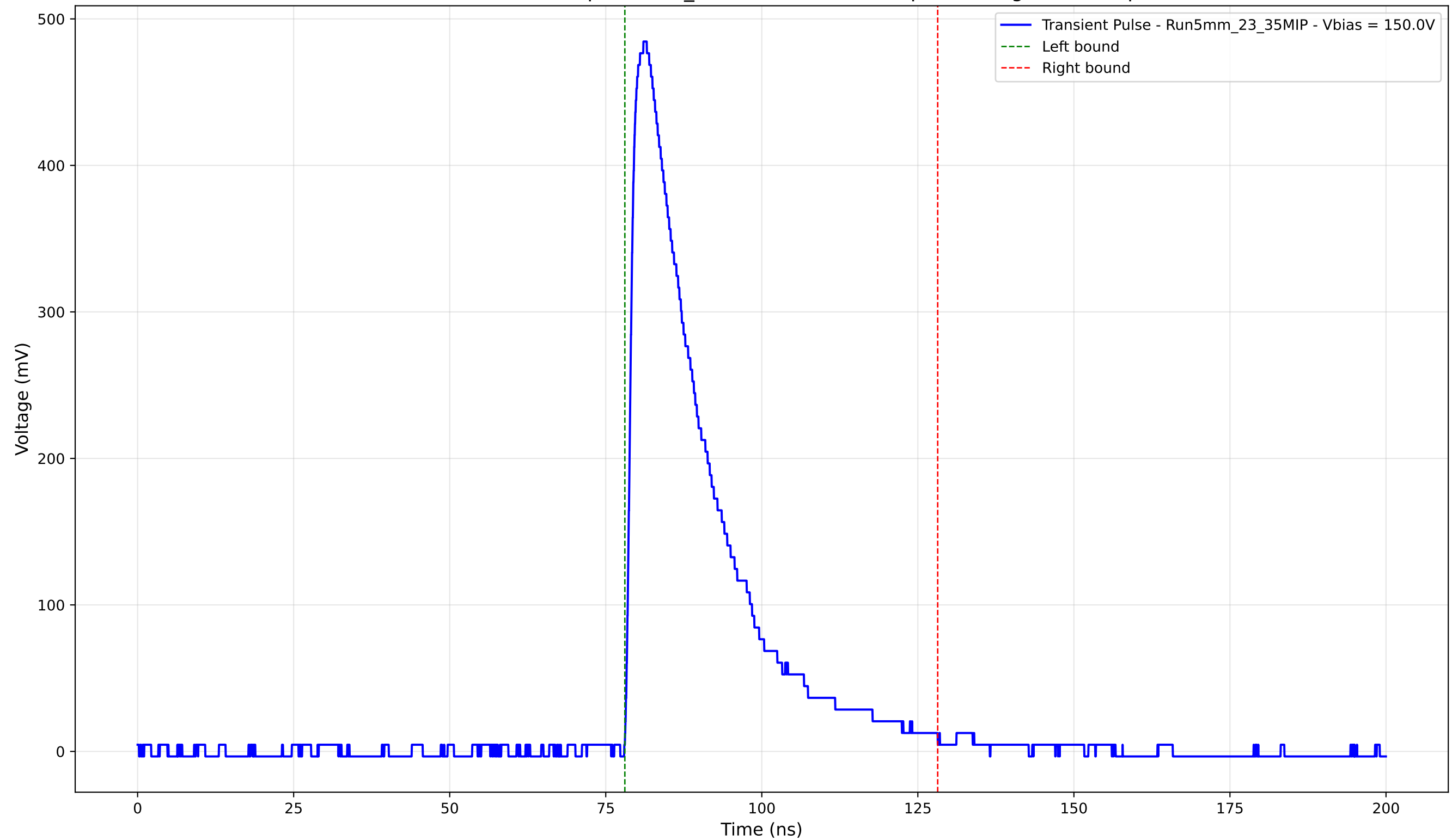
Transient Pulse - Sample: 5mm_23 - Position: 2230.0 \mu\text{m} - Charge: 130.54 pC
