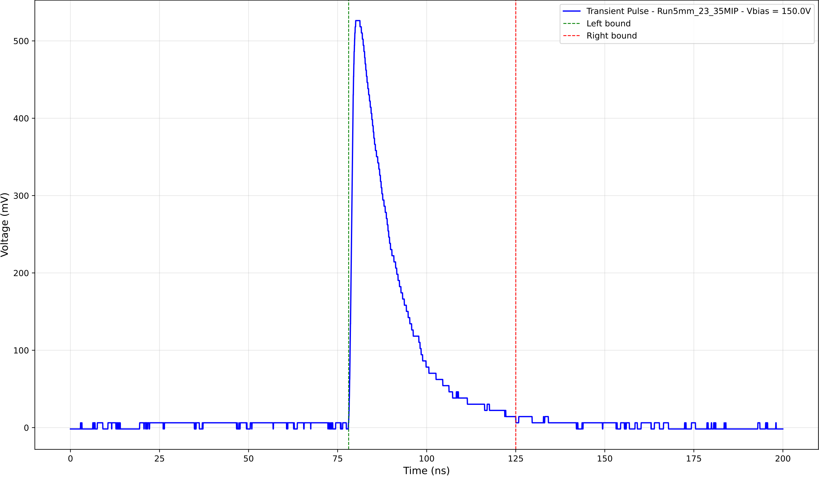
Transient Pulse - Sample: 5mm_23 - Position: 1855.0 \mu\text{m} - Charge: 137.46 pC
