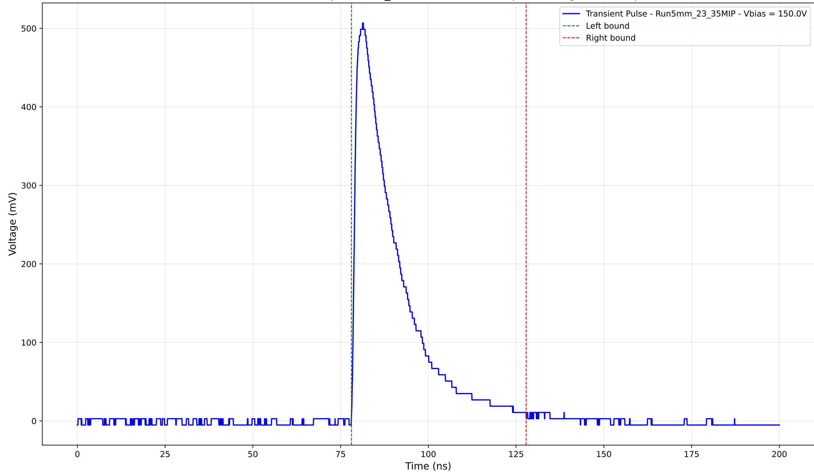
Transient Pulse - Sample: 5mm_23 - Position: 2260.0 \mu\text{m} - Charge: 134.91 pC
