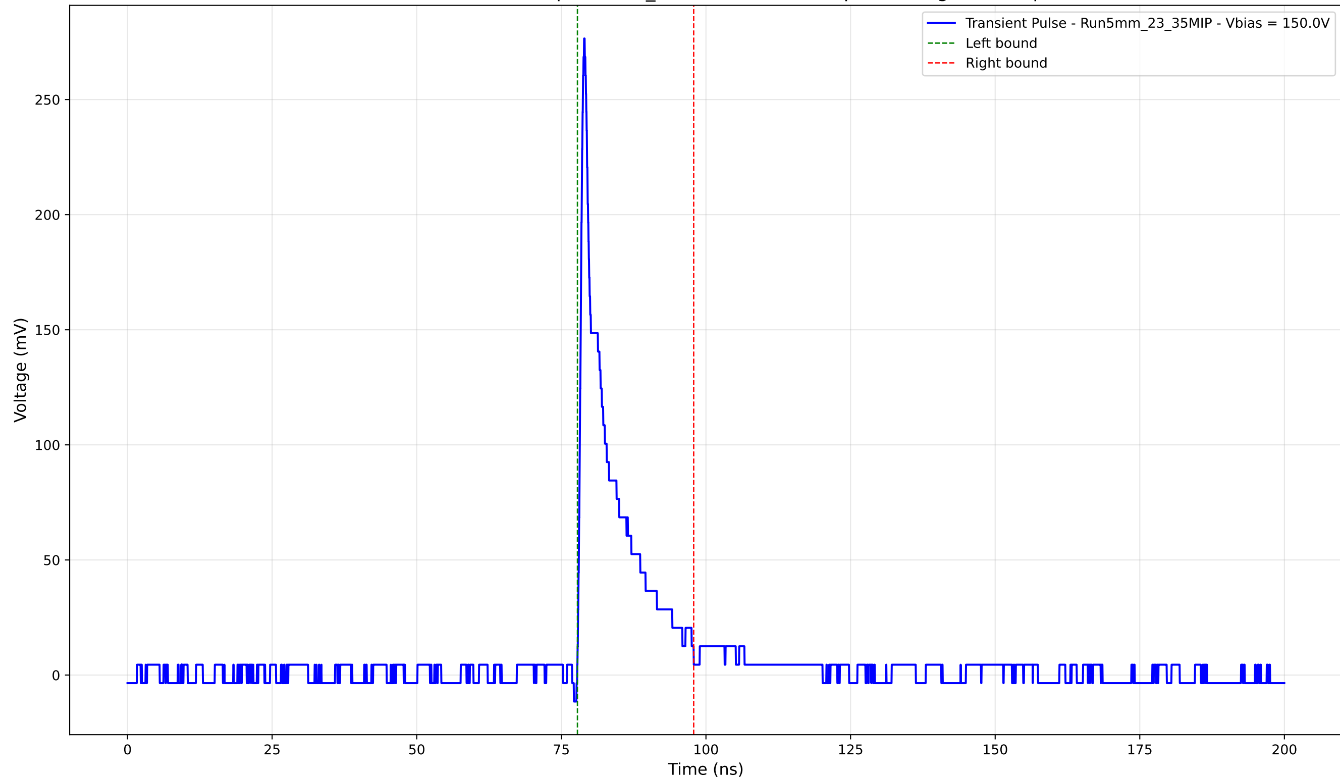
Transient Pulse - Sample: 5mm_23 - Position: 195.0 \mu\text{m} - Charge: 28.85 pC
