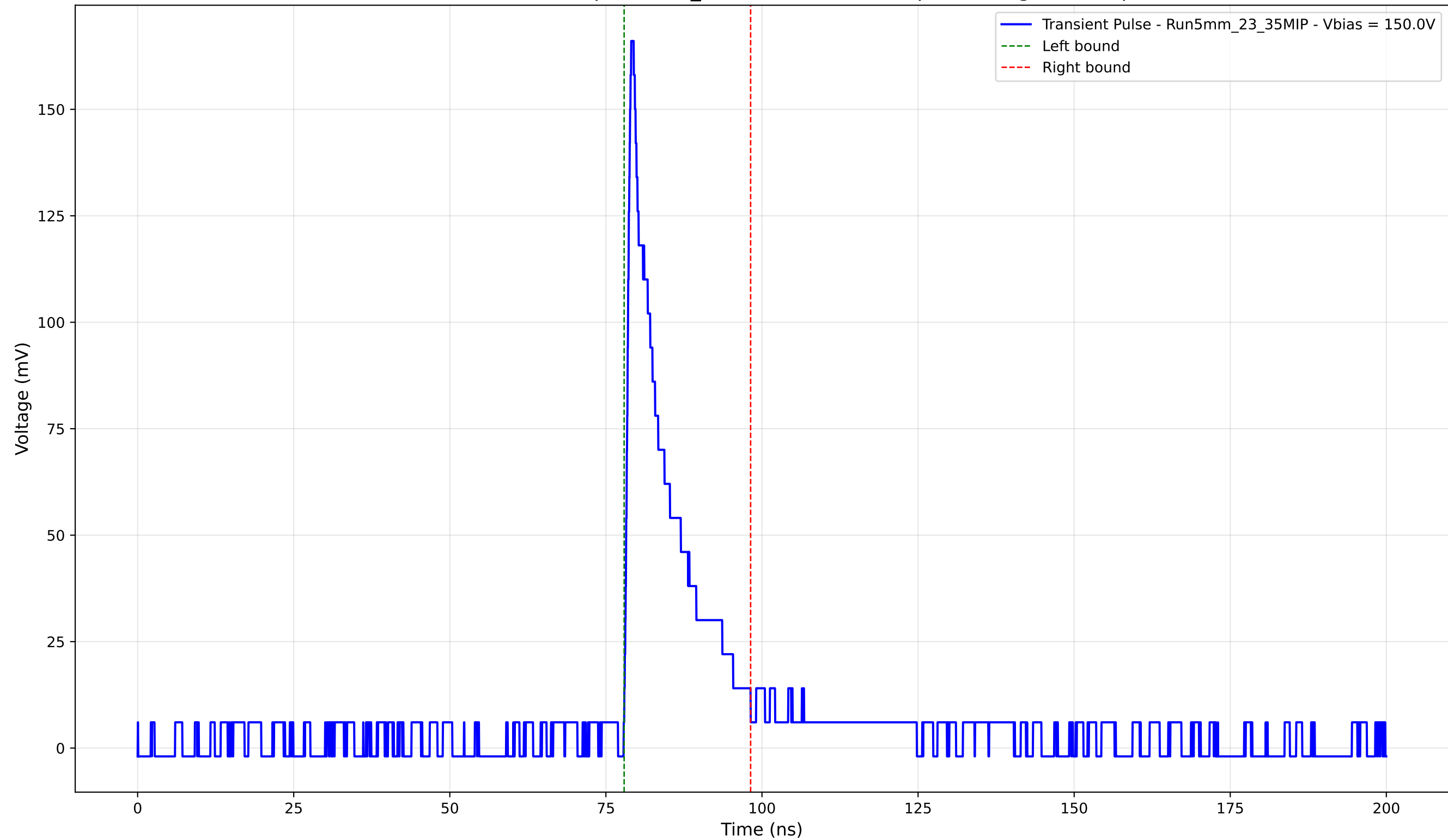
Transient Pulse - Sample: 5mm_23 - Position: 4680.0 \mu\text{m} - Charge: 22.40 pC
