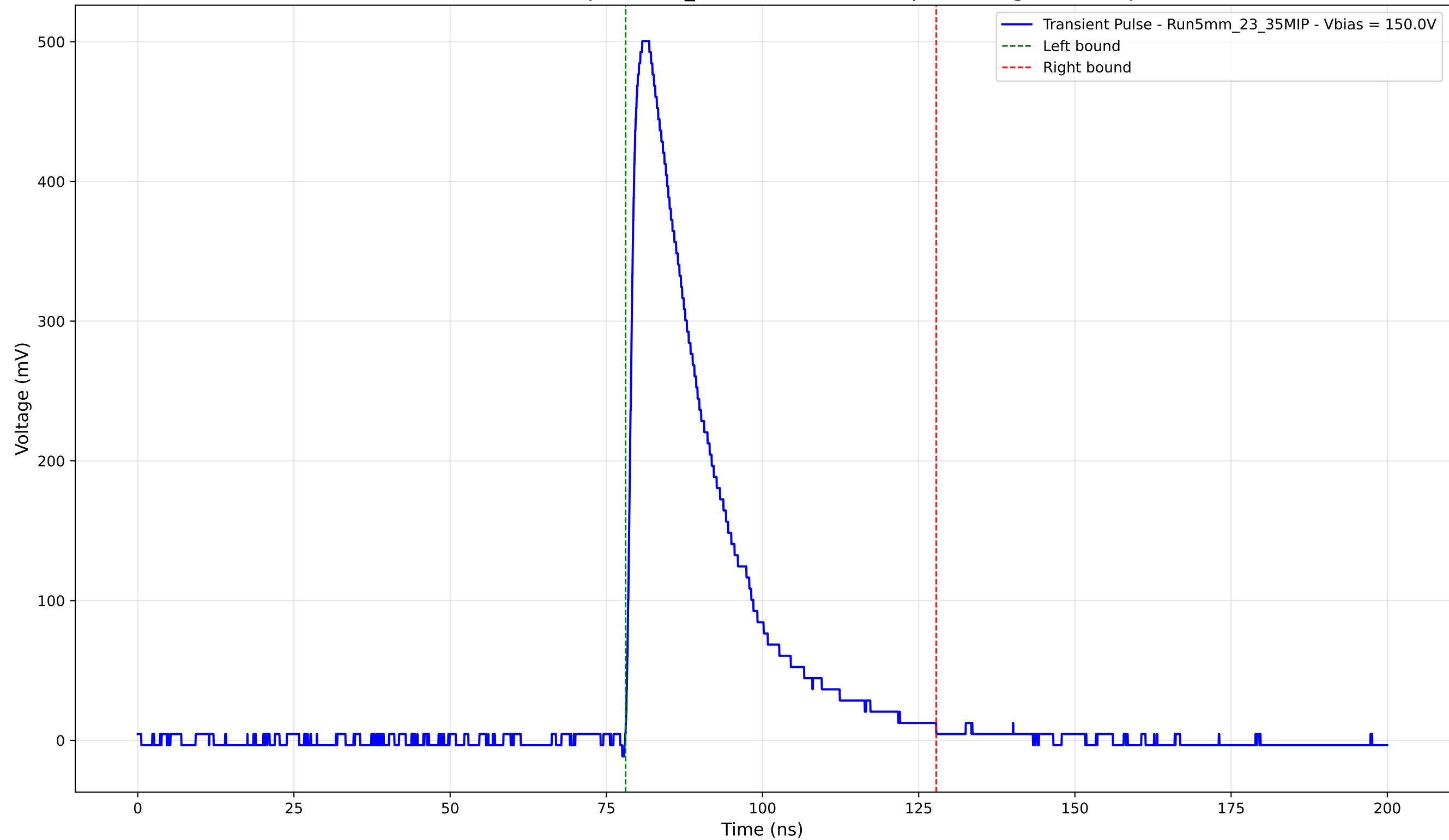
Transient Pulse - Sample: 5mm_23 - Position: 2515.0 \mu\text{m} - Charge: 136.87 pC
