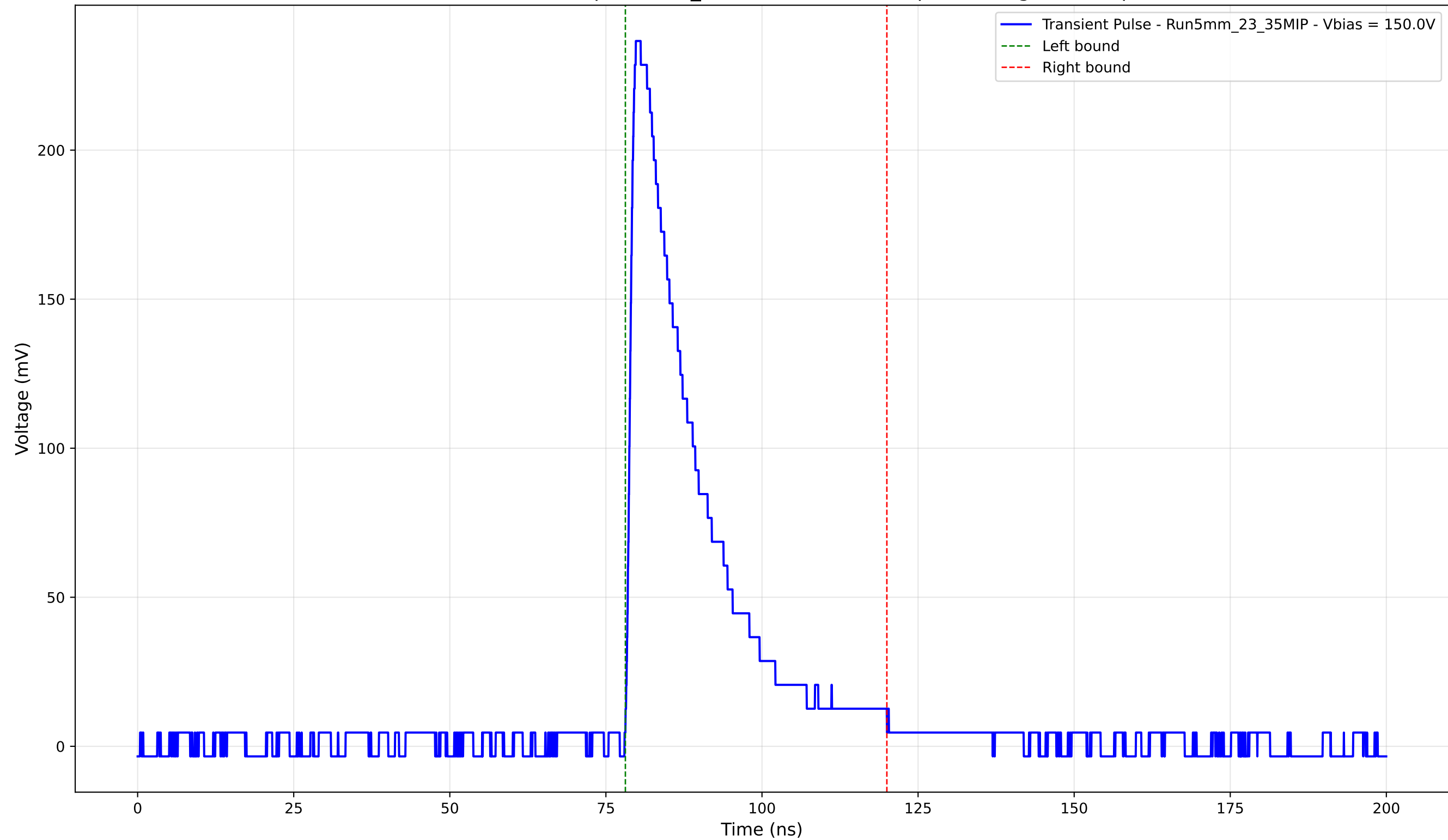
Transient Pulse - Sample: 5mm_23 - Position: 3690.0 \mu\text{m} - Charge: 55.49 pC
