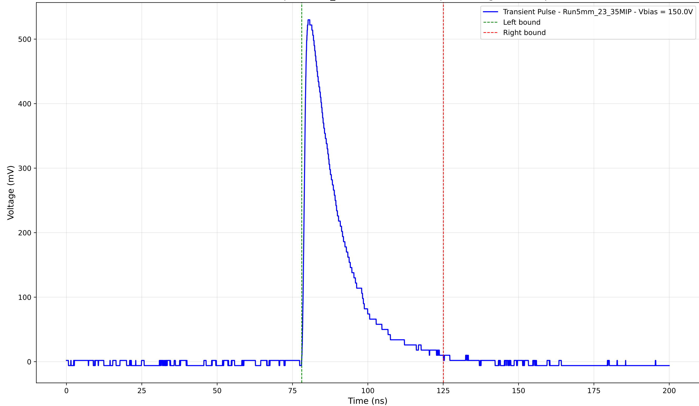
Transient Pulse - Sample: 5mm_23 - Position: 1800.0 \mu\text{m} - Charge: 134.29 pC
