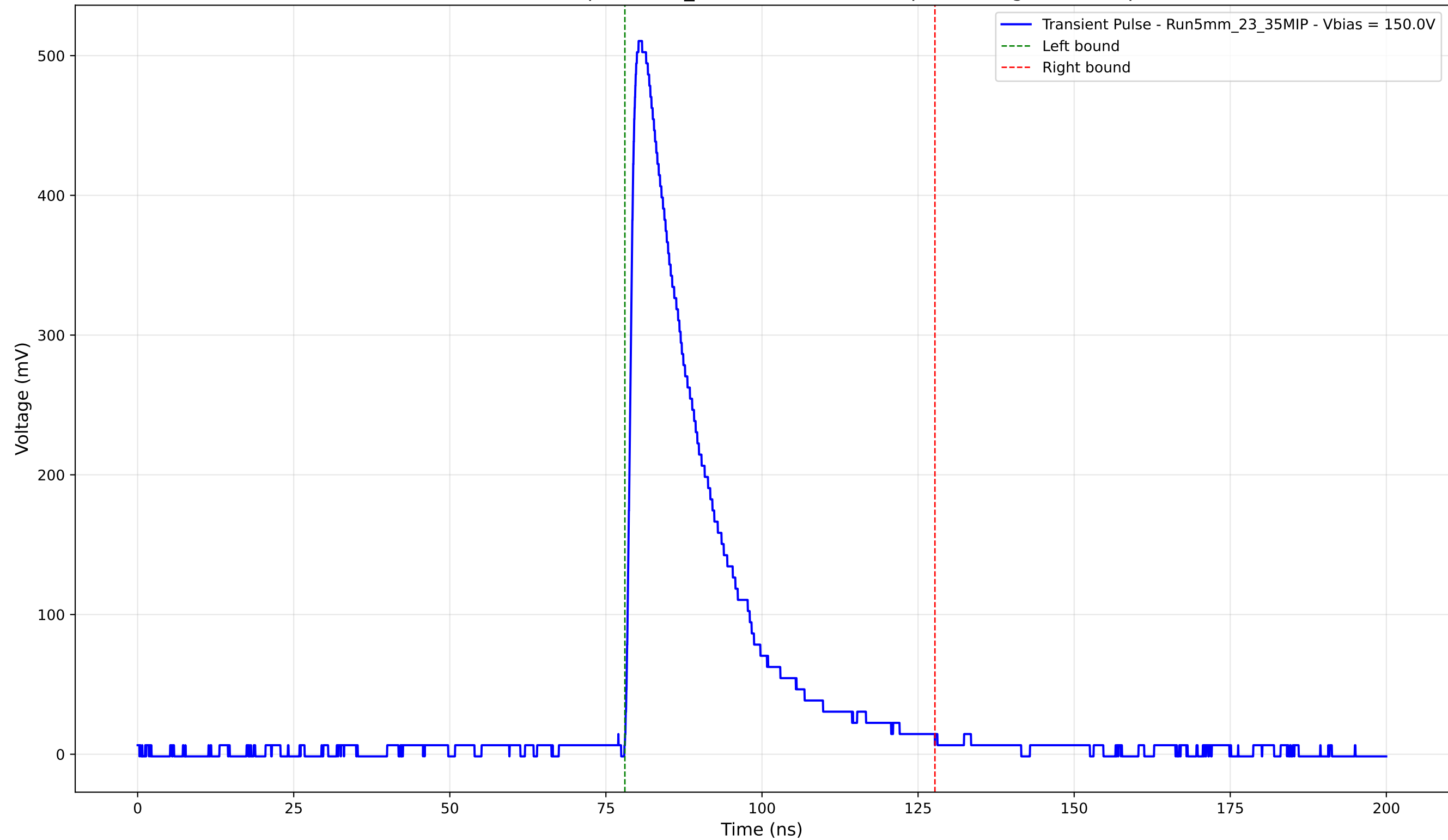
Transient Pulse - Sample: 5mm_23 - Position: 3475.0 \mu\text{m} - Charge: 130.19 pC
