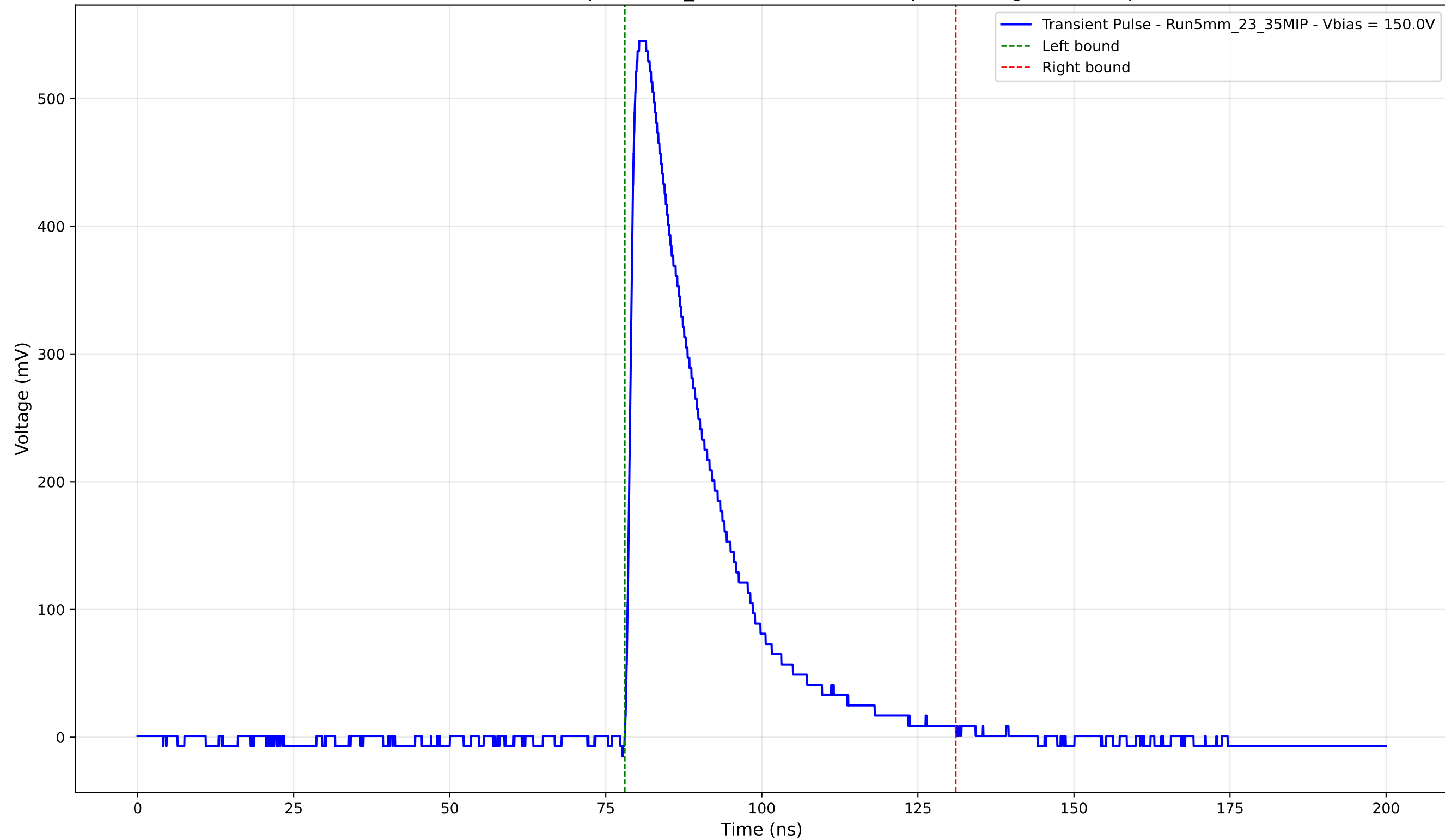
Transient Pulse - Sample: 5mm_23 - Position: 2015.0 \mu\text{m} - Charge: 142.93 pC
