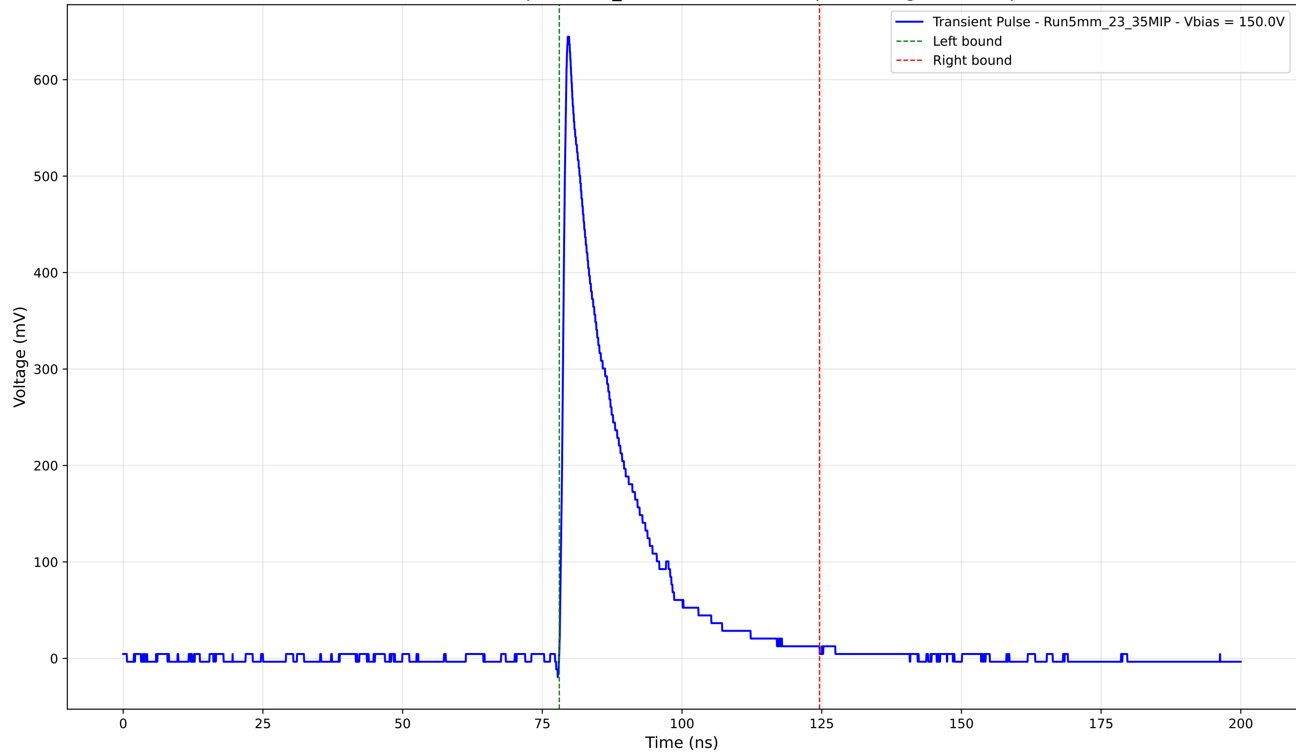
Transient Pulse - Sample: 5mm_23 - Position: 1000.0 \mu\text{m} - Charge: 124.50 pC
