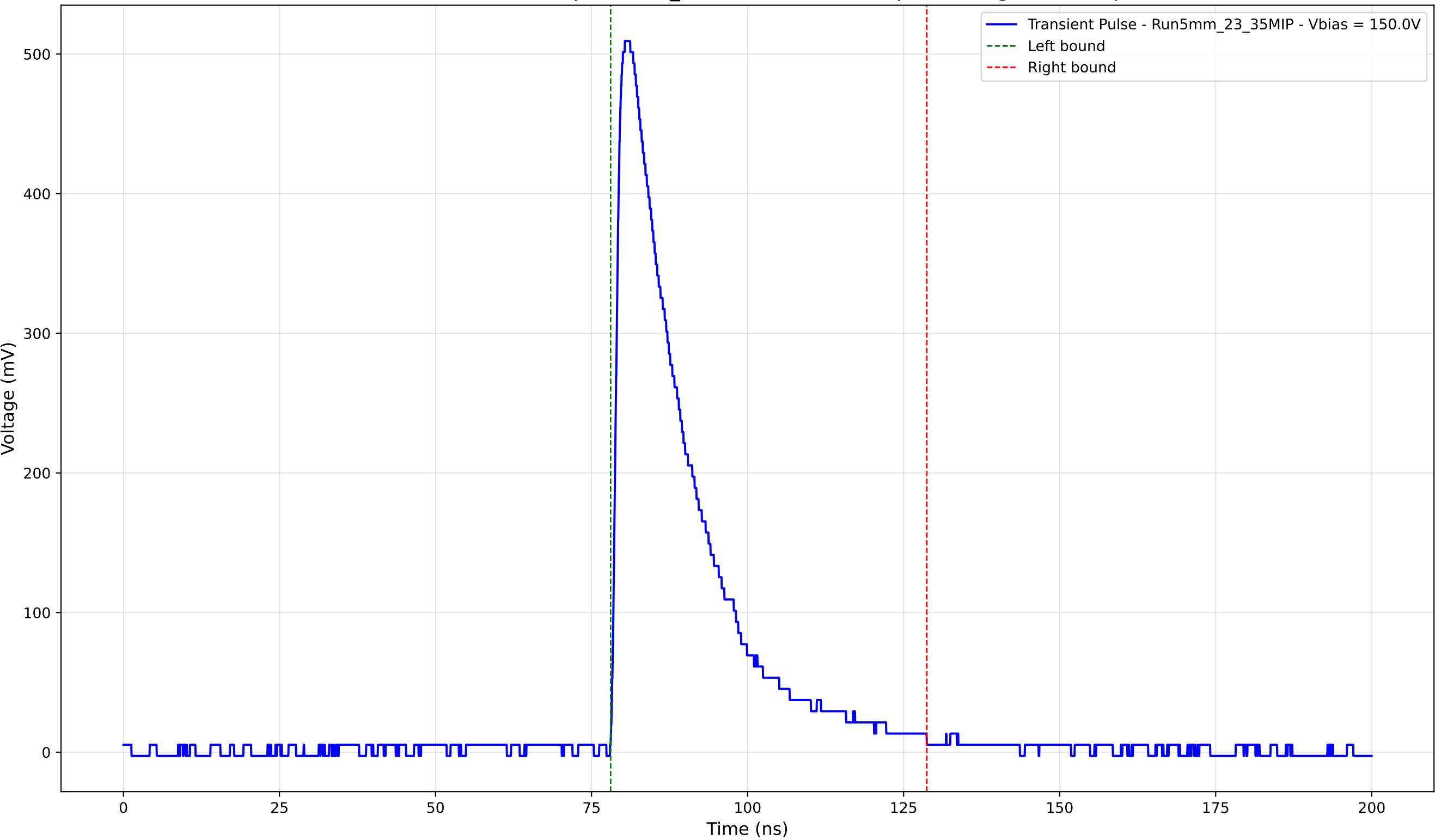
Transient Pulse - Sample: 5mm_23 - Position: 3420.0 \mu\text{m} - Charge: 130.79 pC
