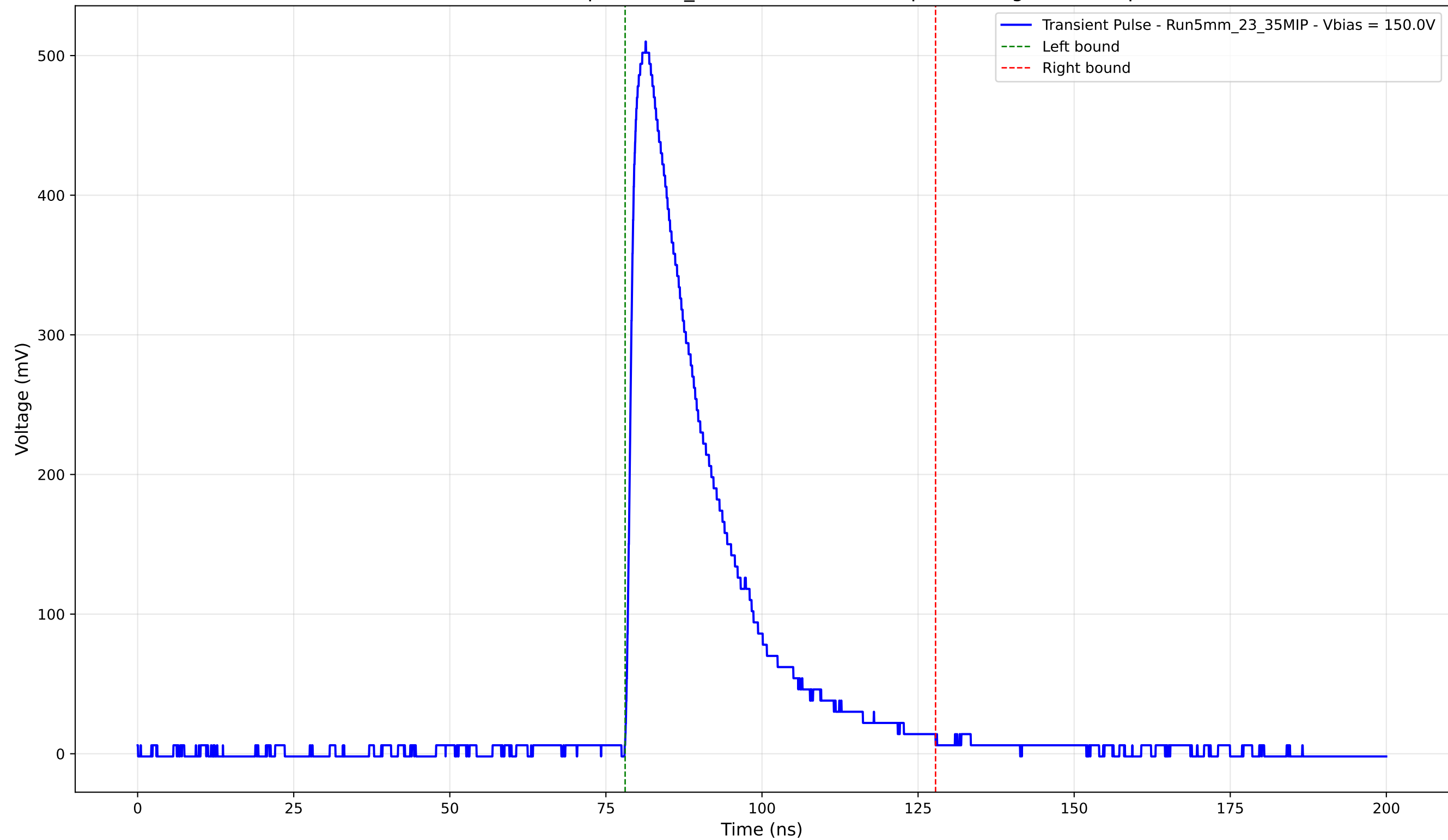
Transient Pulse - Sample: 5mm_23 - Position: 2415.0 \mu\text{m} - Charge: 137.85 pC
