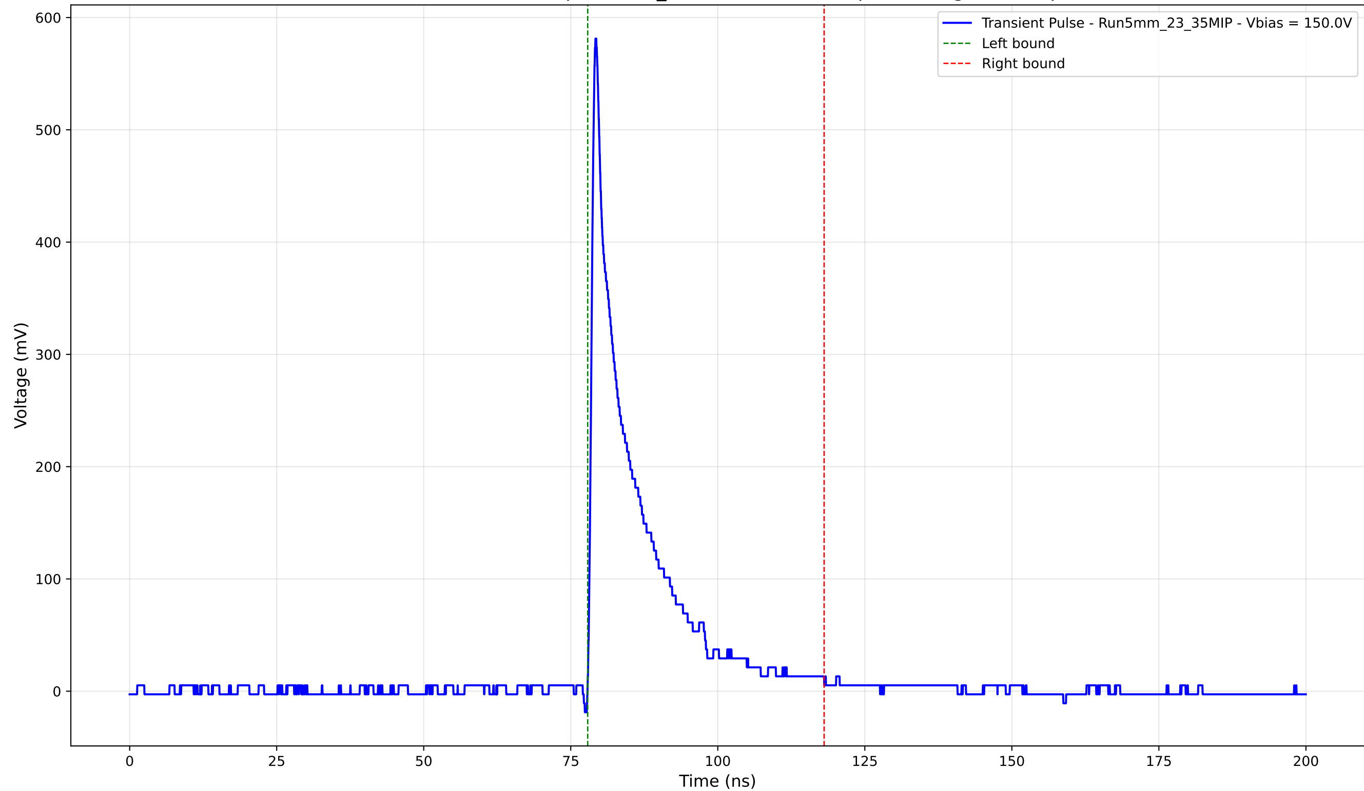
Transient Pulse - Sample: 5mm_23 - Position: 560.0 \mu\text{m} - Charge: 82.83 pC
