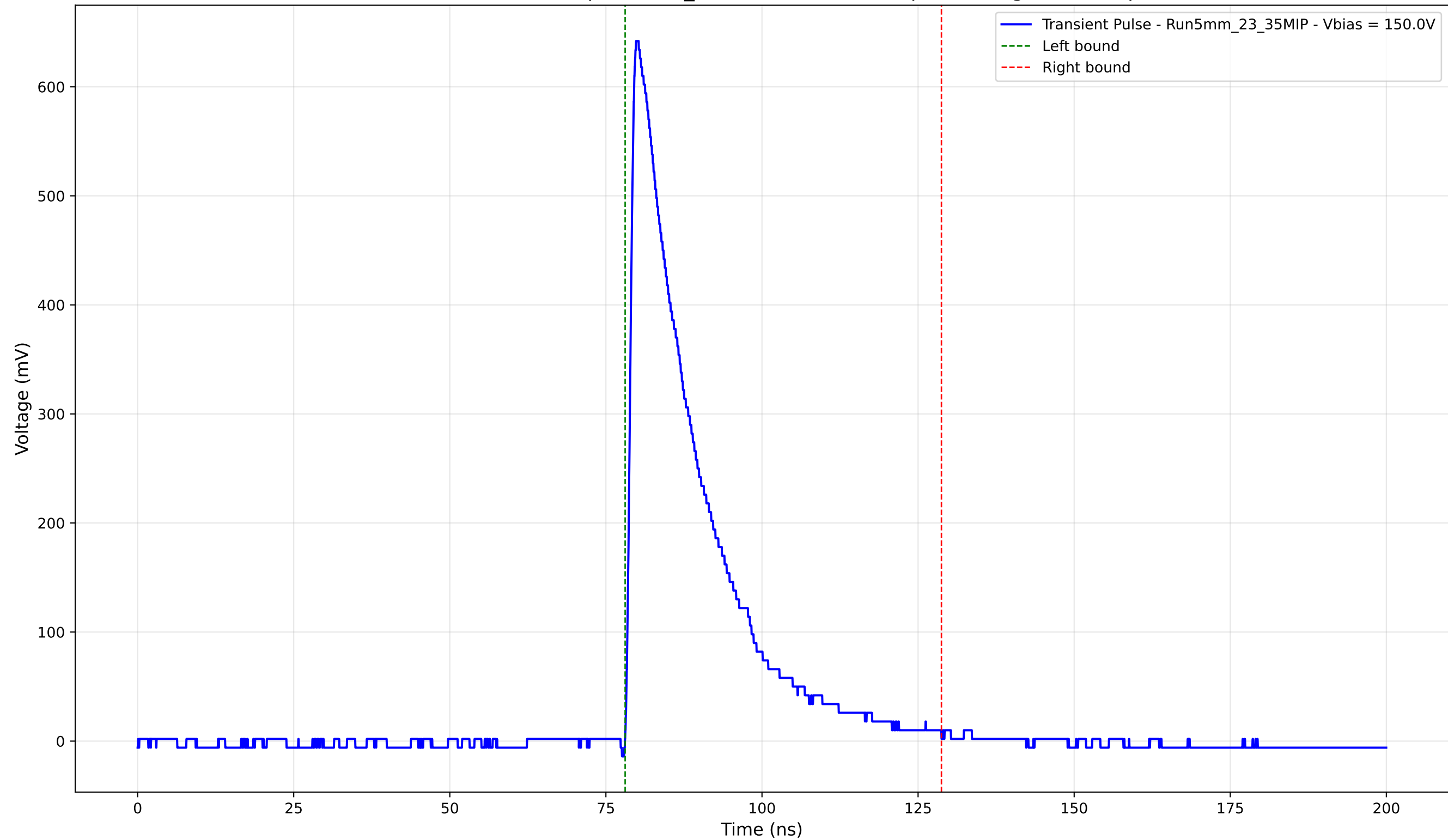
Transient Pulse - Sample: 5mm_23 - Position: 1425.0 \mu\text{m} - Charge: 148.55 pC
