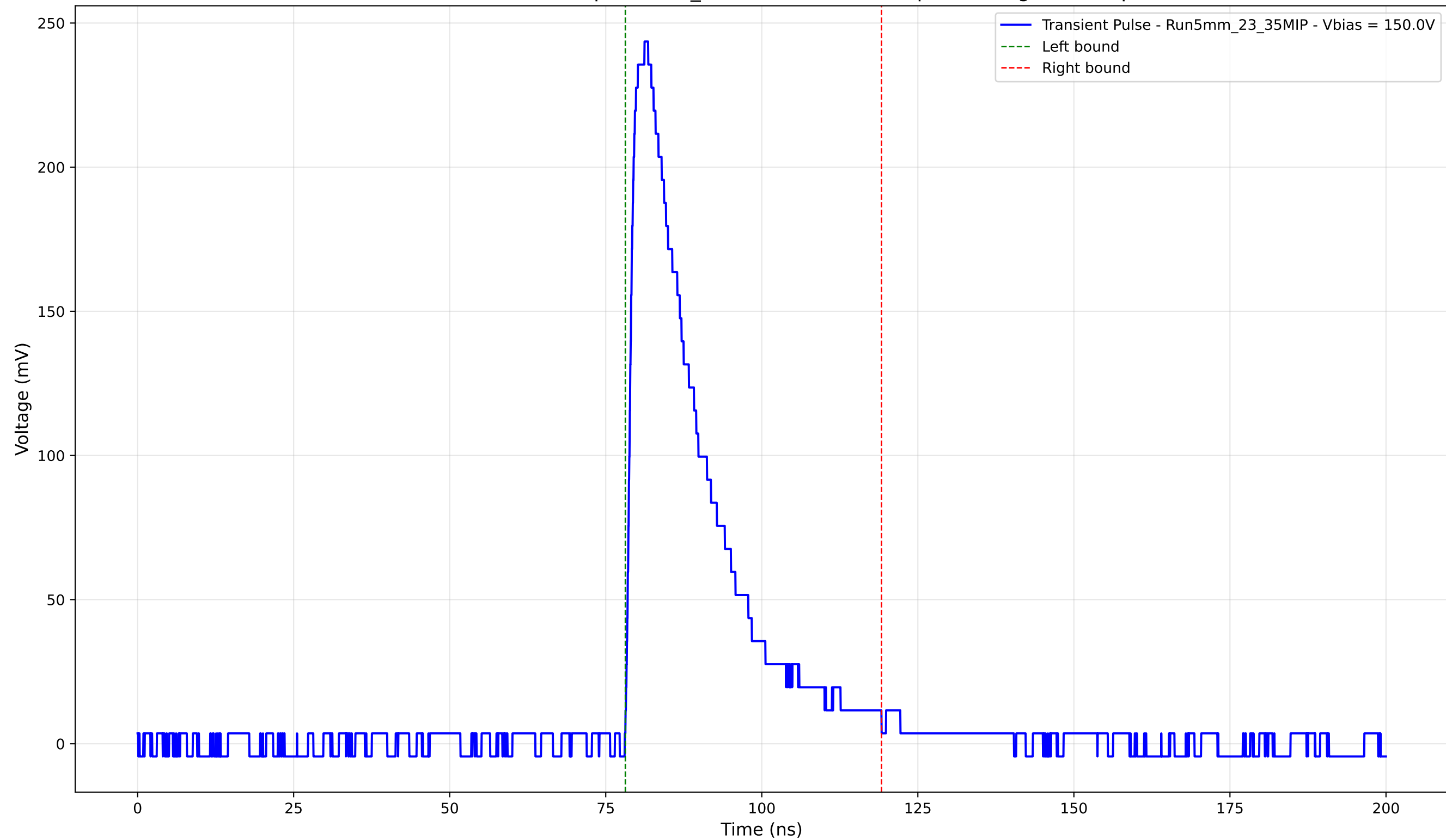
Transient Pulse - Sample: 5mm_23 - Position: 3185.0 \mu\text{m} - Charge: 61.28 pC
