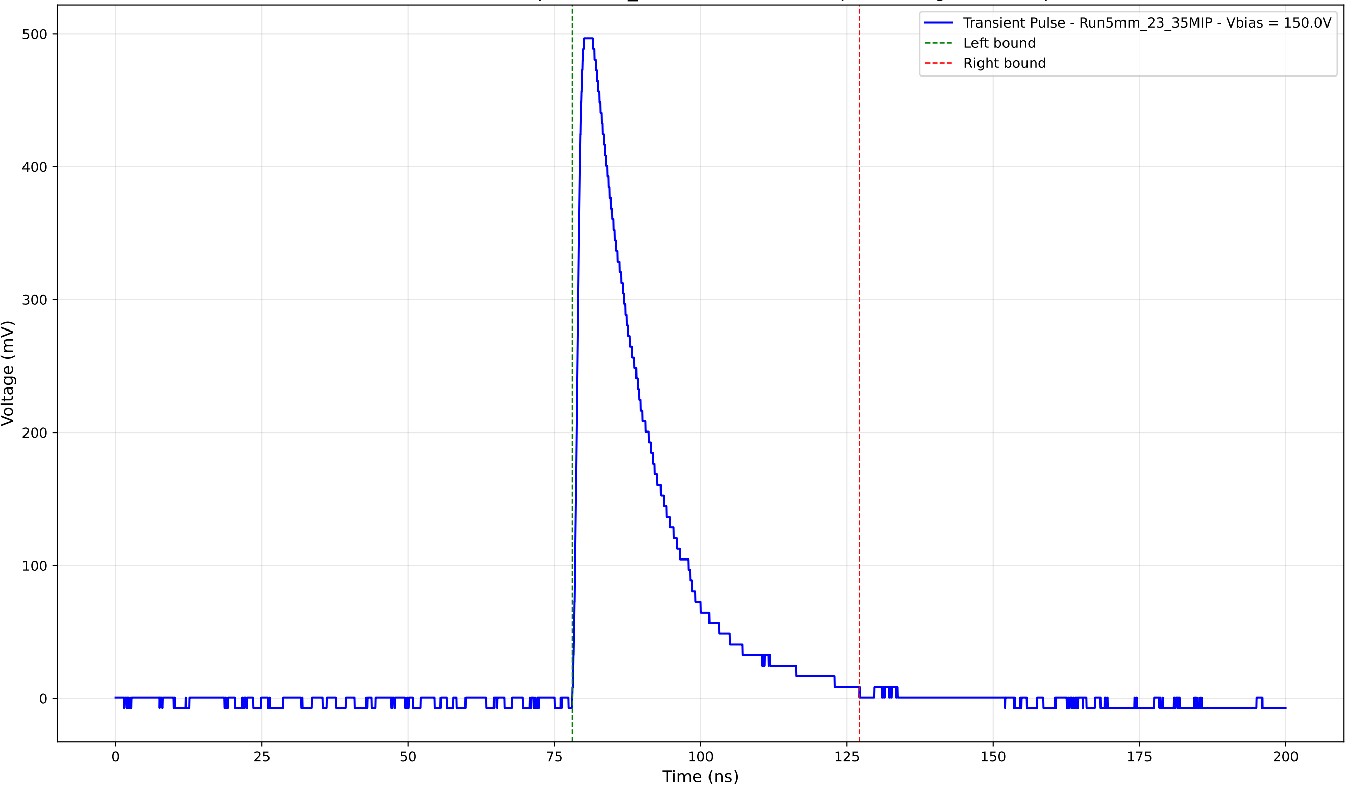
Transient Pulse - Sample: 5mm_23 - Position: 3375.0 \mu\text{m} - Charge: 125.97 pC
