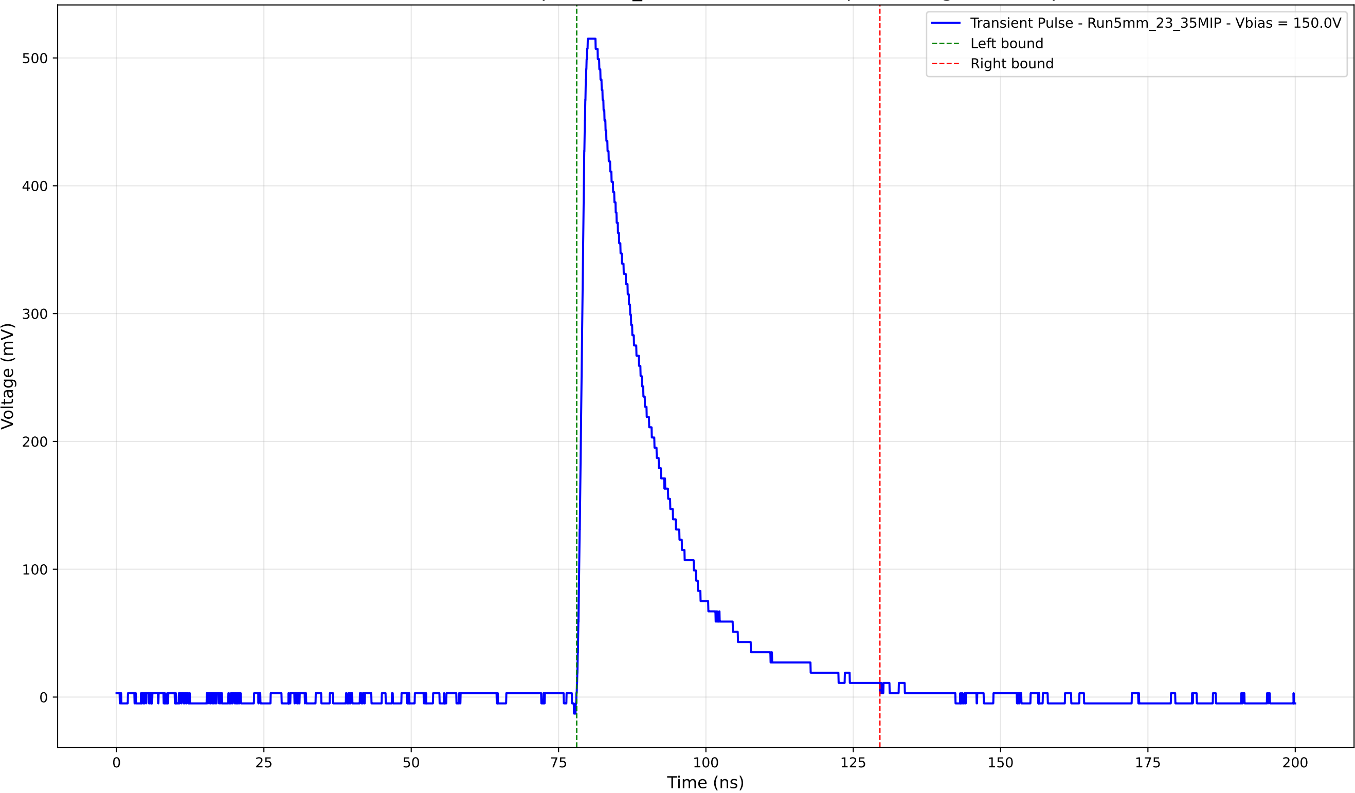
Transient Pulse - Sample: 5mm_23 - Position: 1740.0 \mu\text{m} - Charge: 132.27 pC
