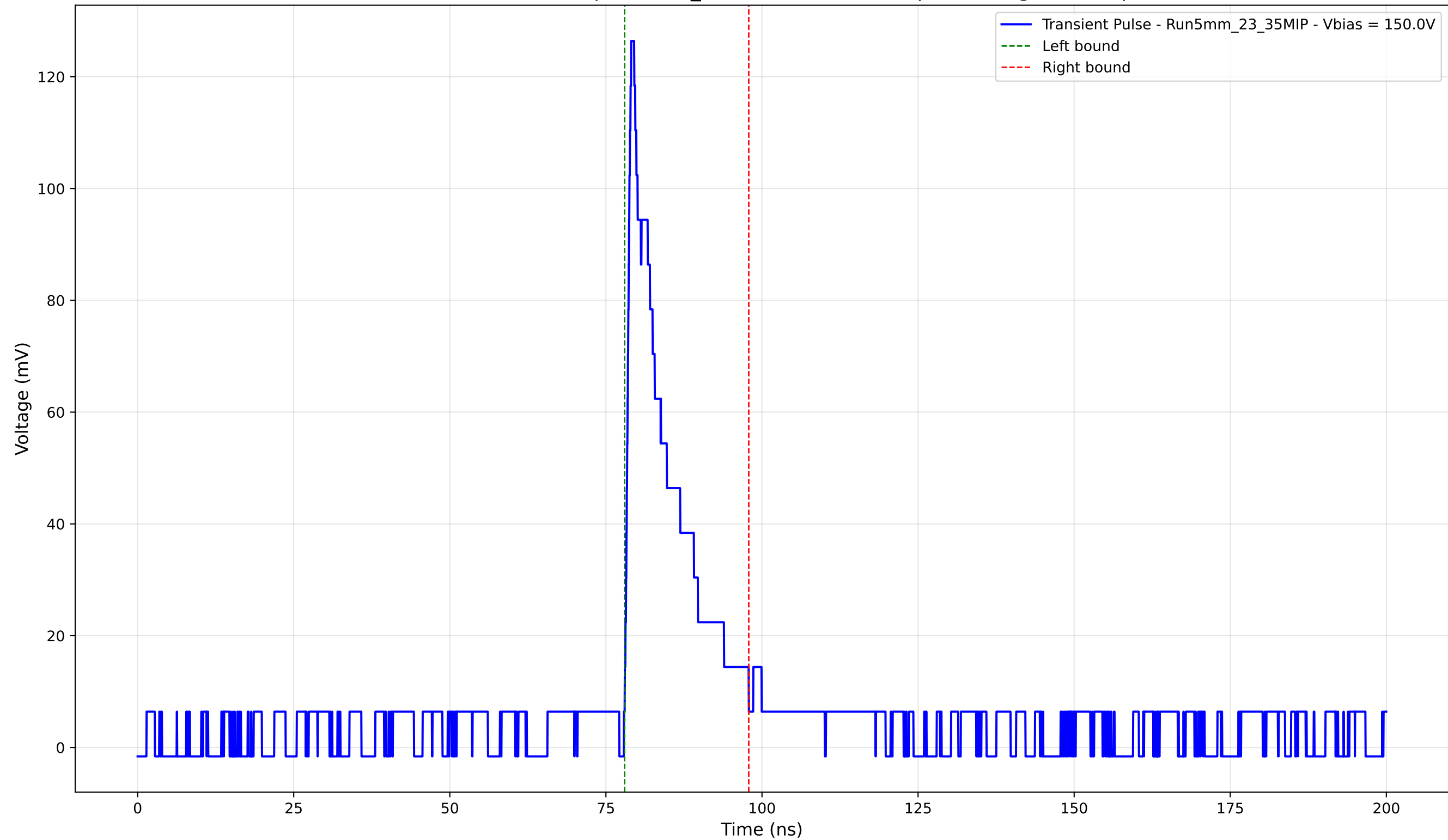
Transient Pulse - Sample: 5mm_23 - Position: 4670.0 \mu\text{m} - Charge: 17.97 pC
