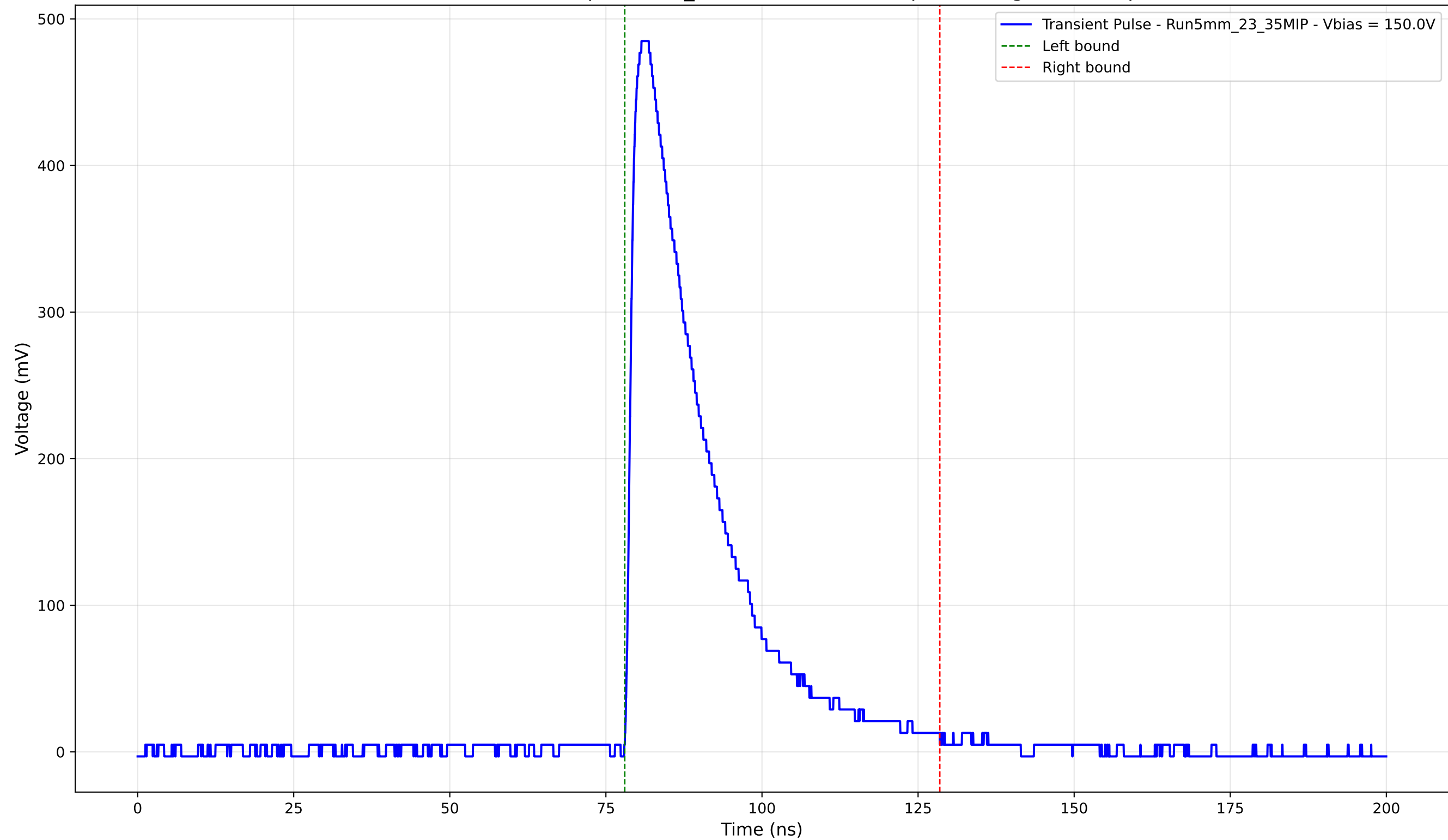
Transient Pulse - Sample: 5mm_23 - Position: 2550.0 \mu\text{m} - Charge: 132.83 pC
