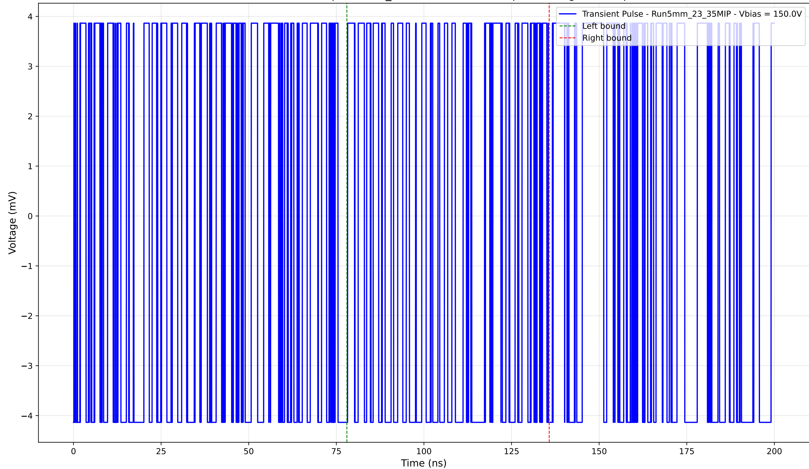
Transient Pulse - Sample: 5mm_23 - Position: 5280.0 \mu\text{m} - Charge: -0.26 pC
