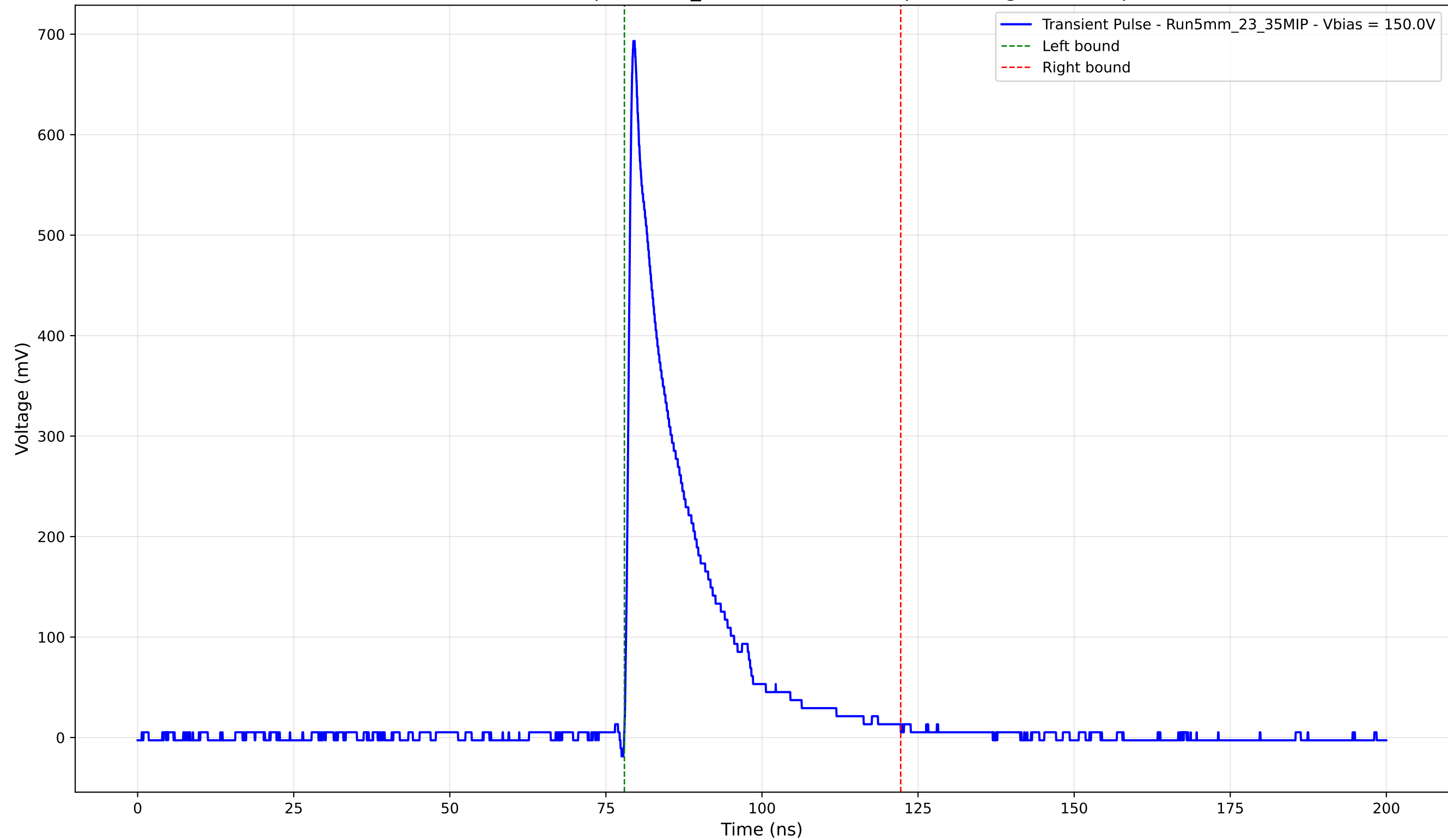
Transient Pulse - Sample: 5mm_23 - Position: 795.0 \mu\text{m} - Charge: 122.48 pC
