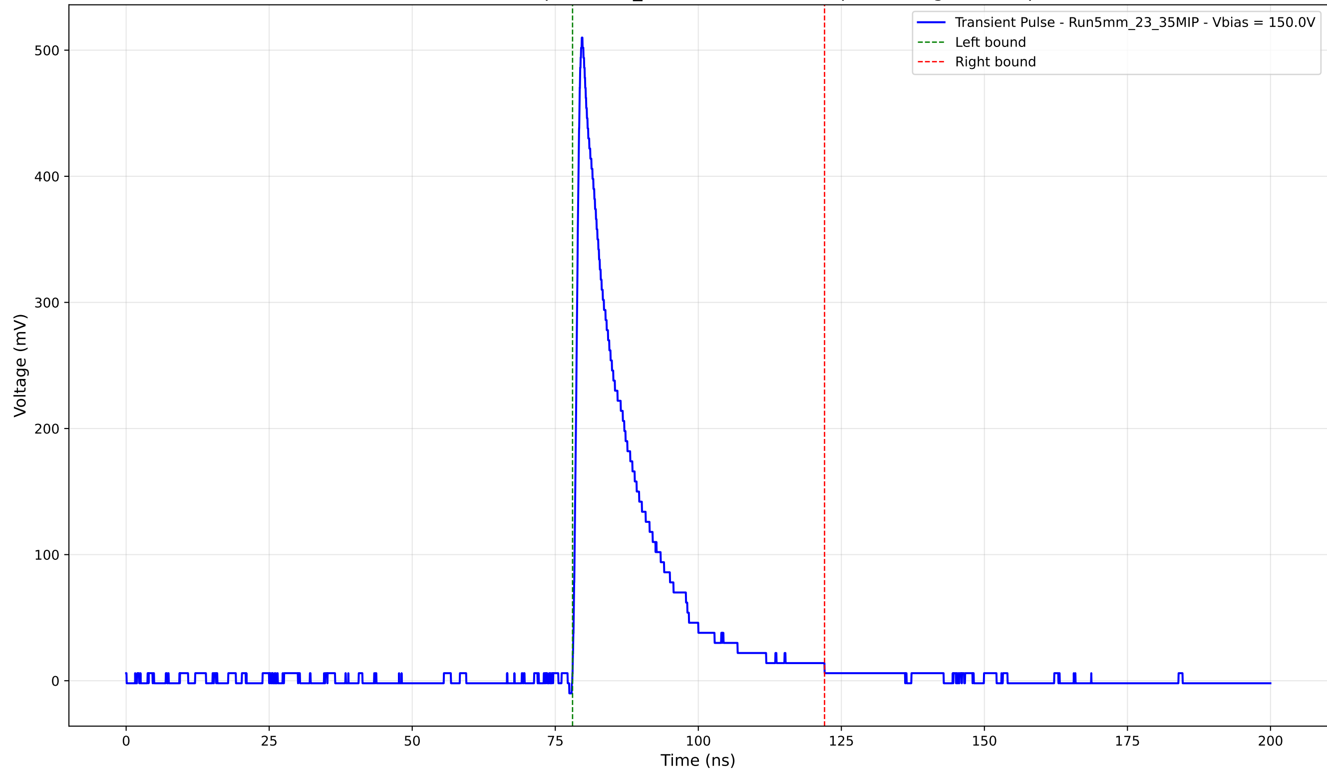
Transient Pulse - Sample: 5mm_23 - Position: 4235.0 \mu\text{m} - Charge: 94.08 pC
