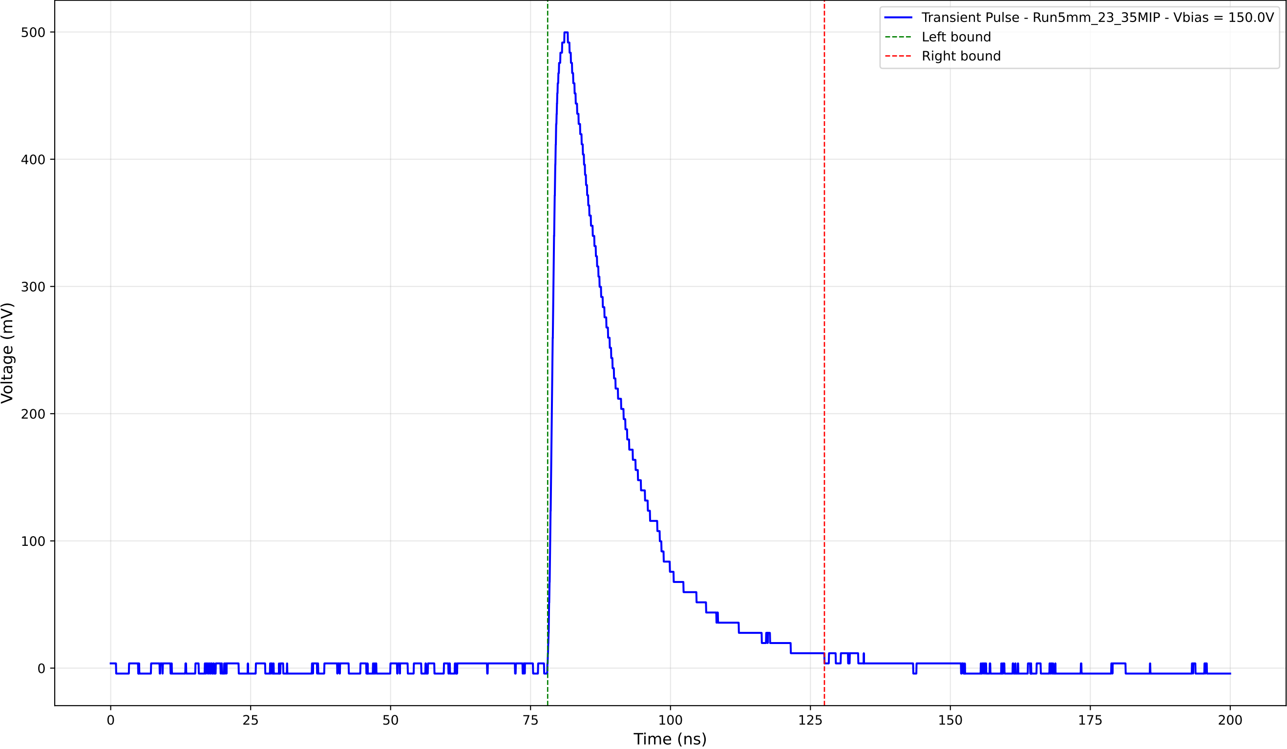
Transient Pulse - Sample: 5mm_23 - Position: 2980.0 \mu\text{m} - Charge: 133.01 pC
