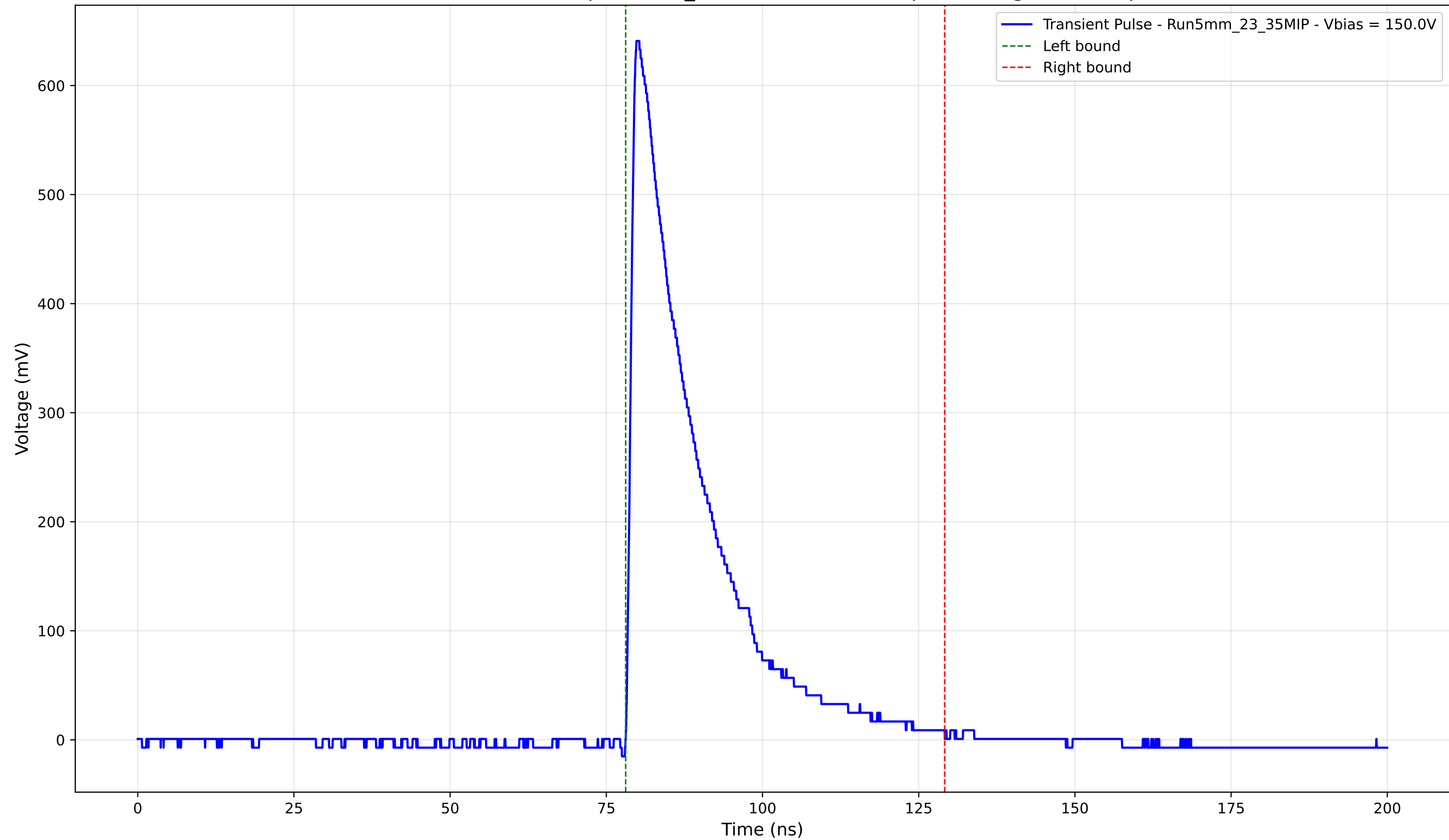
Transient Pulse - Sample: 5mm_23 - Position: 1430.0 \mu\text{m} - Charge: 148.36 pC
