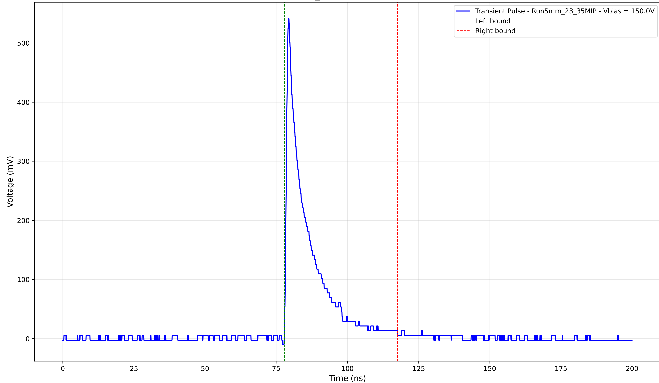
Transient Pulse - Sample: 5mm_23 - Position: 4610.0 \mu\text{m} - Charge: 81.38 pC
