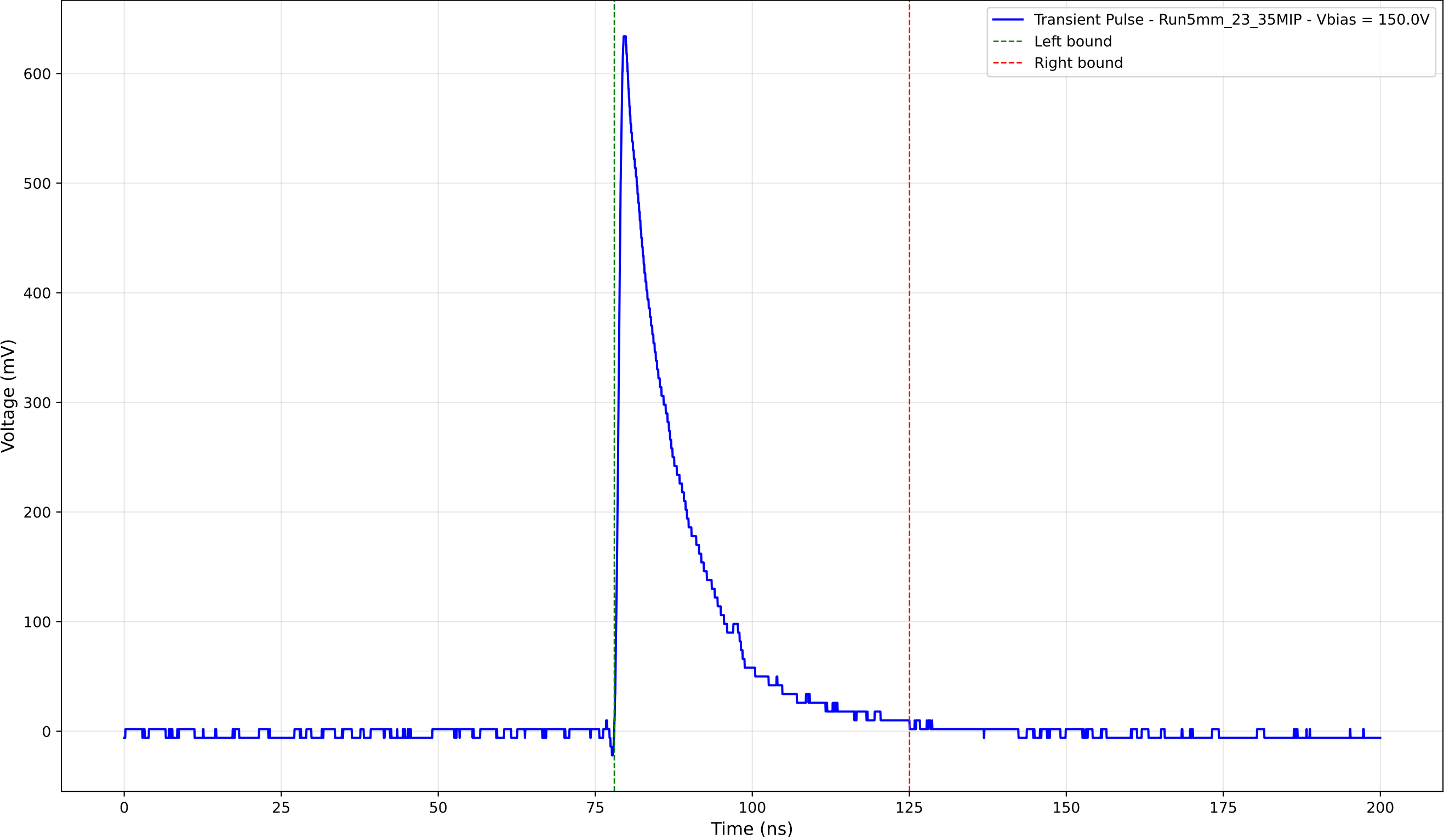
Transient Pulse - Sample: 5mm_23 - Position: 1010.0 \mu\text{m} - Charge: 122.19 pC
