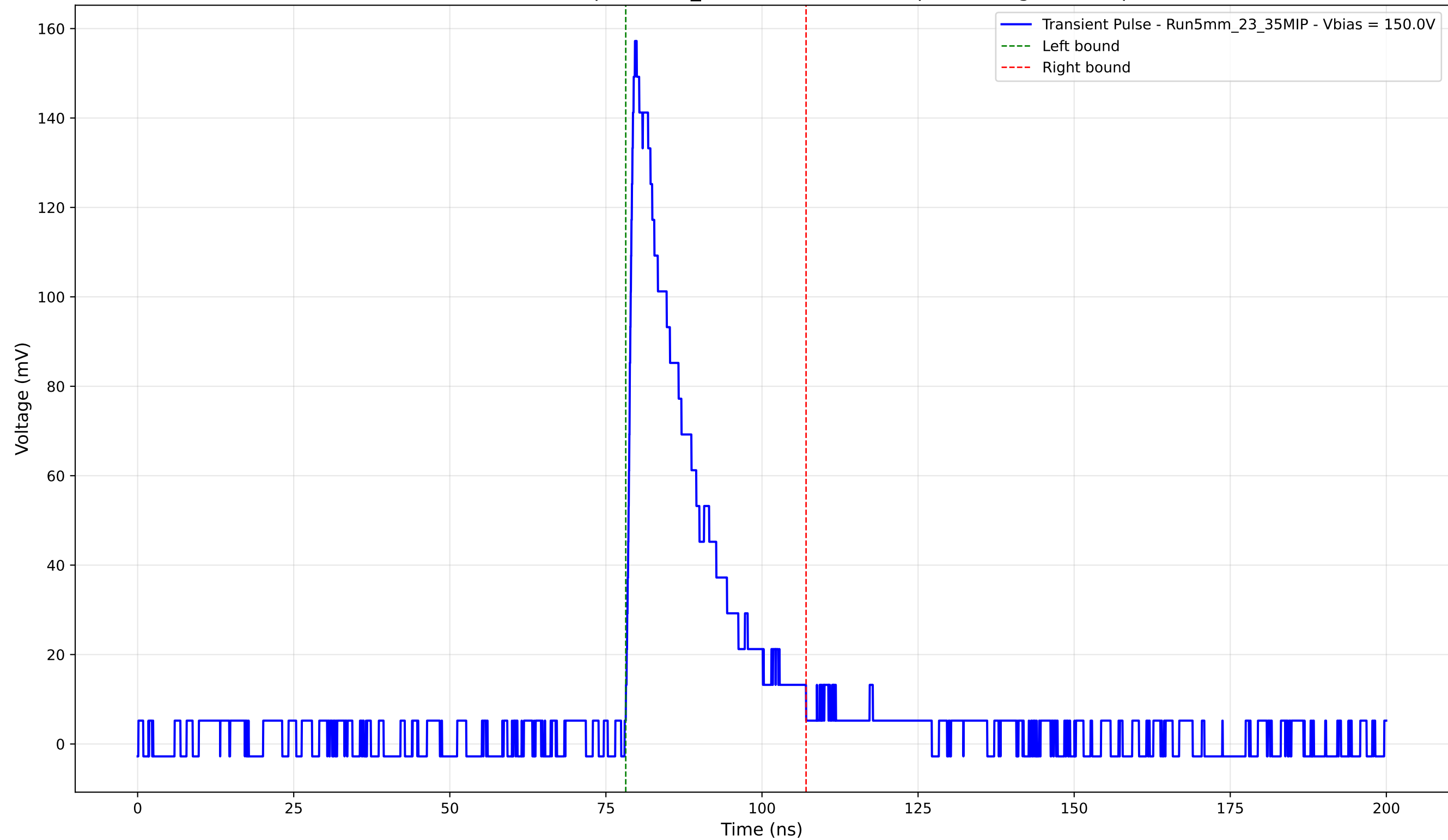
Transient Pulse - Sample: 5mm_23 - Position: 1145.0 \mu\text{m} - Charge: 31.66 pC
