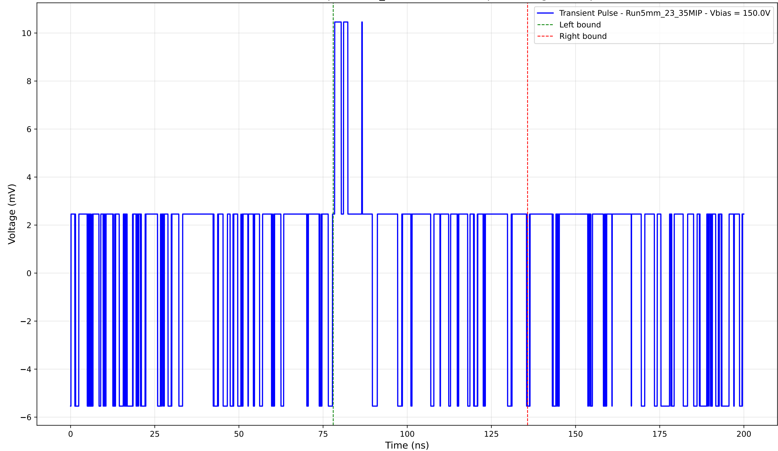
Transient Pulse - Sample: 5mm_23 - Position: 95.0 \mu\text{m} - Charge: 2.05 pC
