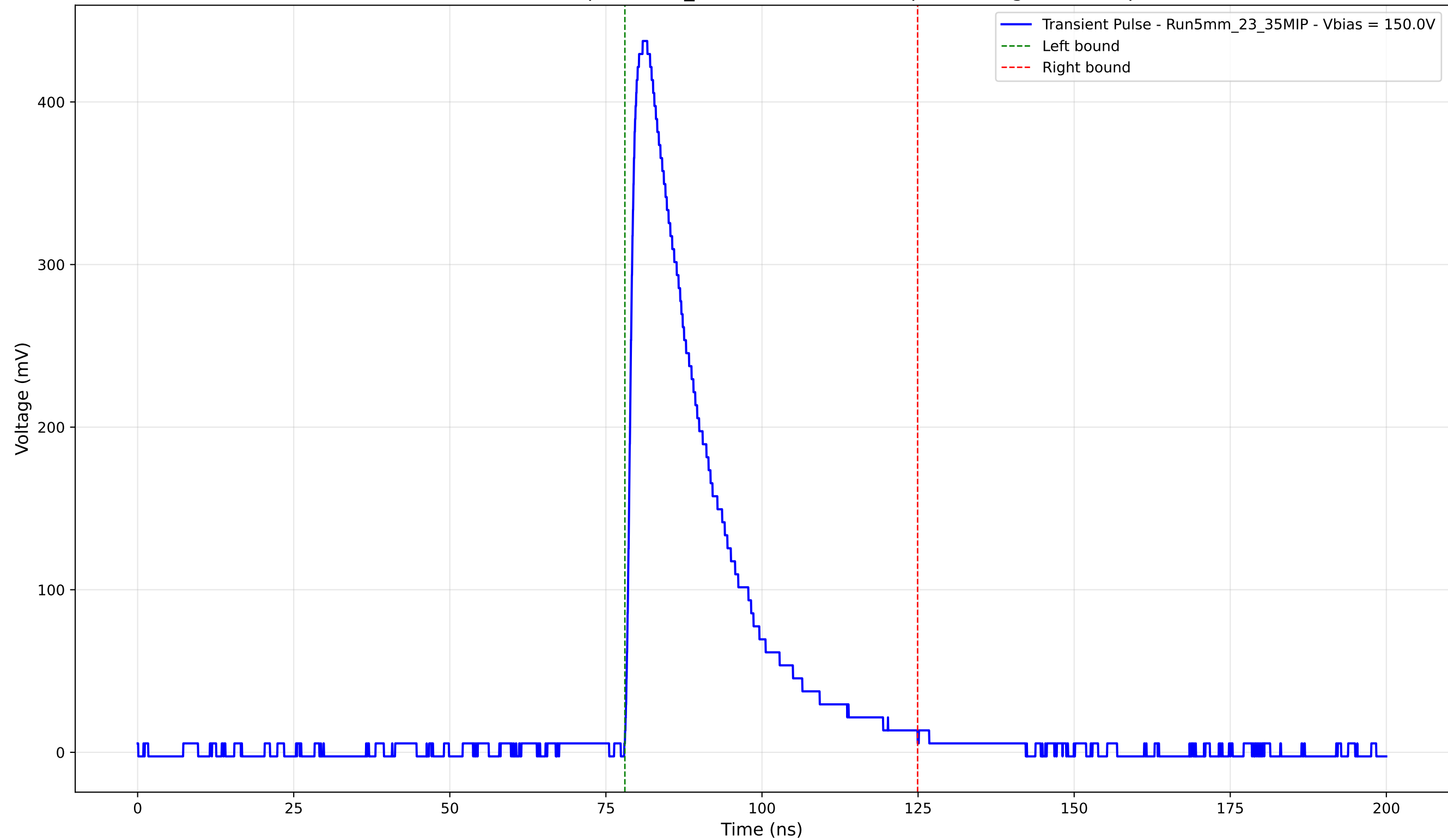
Transient Pulse - Sample: 5mm_23 - Position: 2215.0 \mu\text{m} - Charge: 116.77 pC
