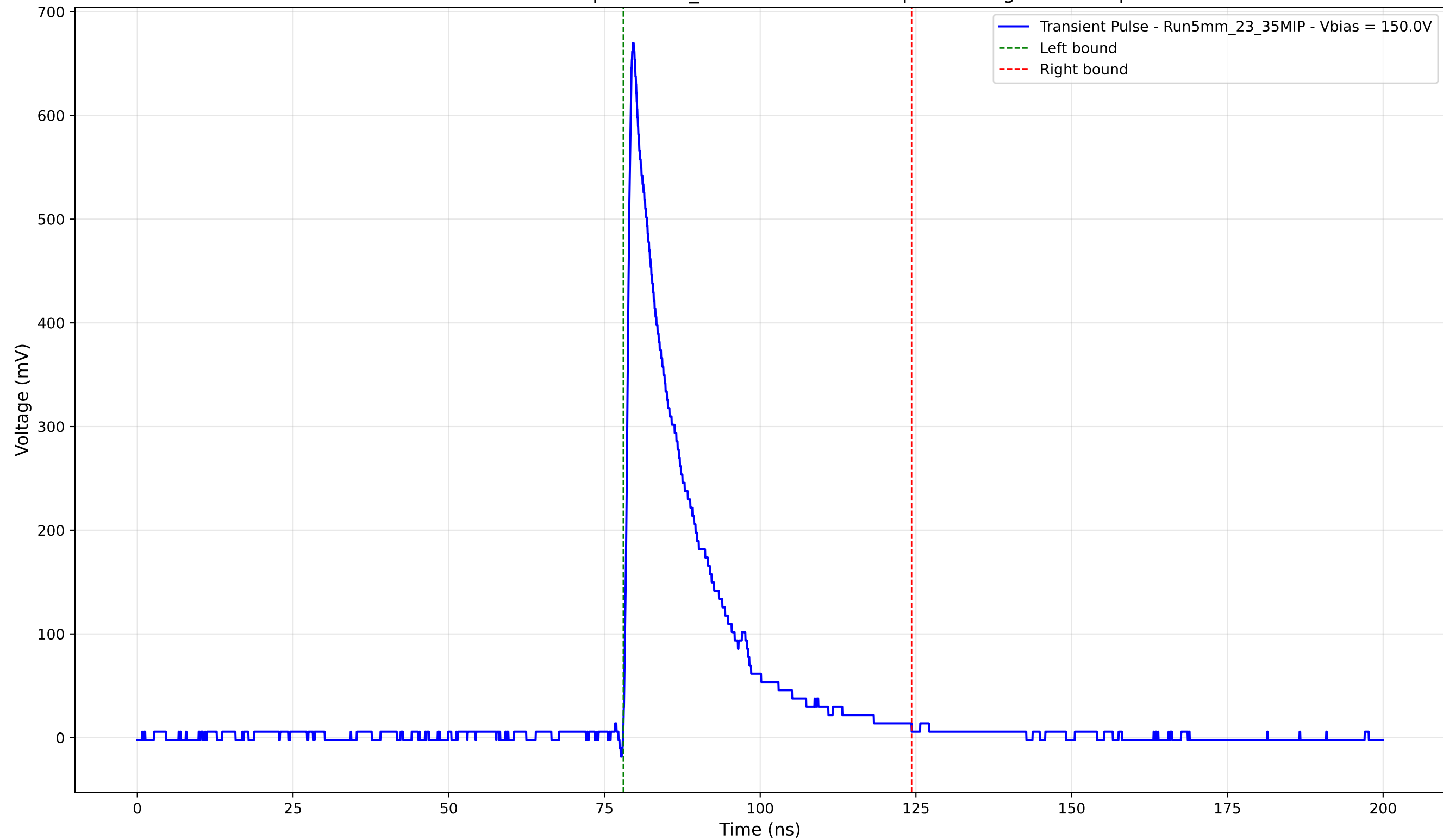
Transient Pulse - Sample: 5mm_23 - Position: 925.0 \mu\text{m} - Charge: 126.55 pC
