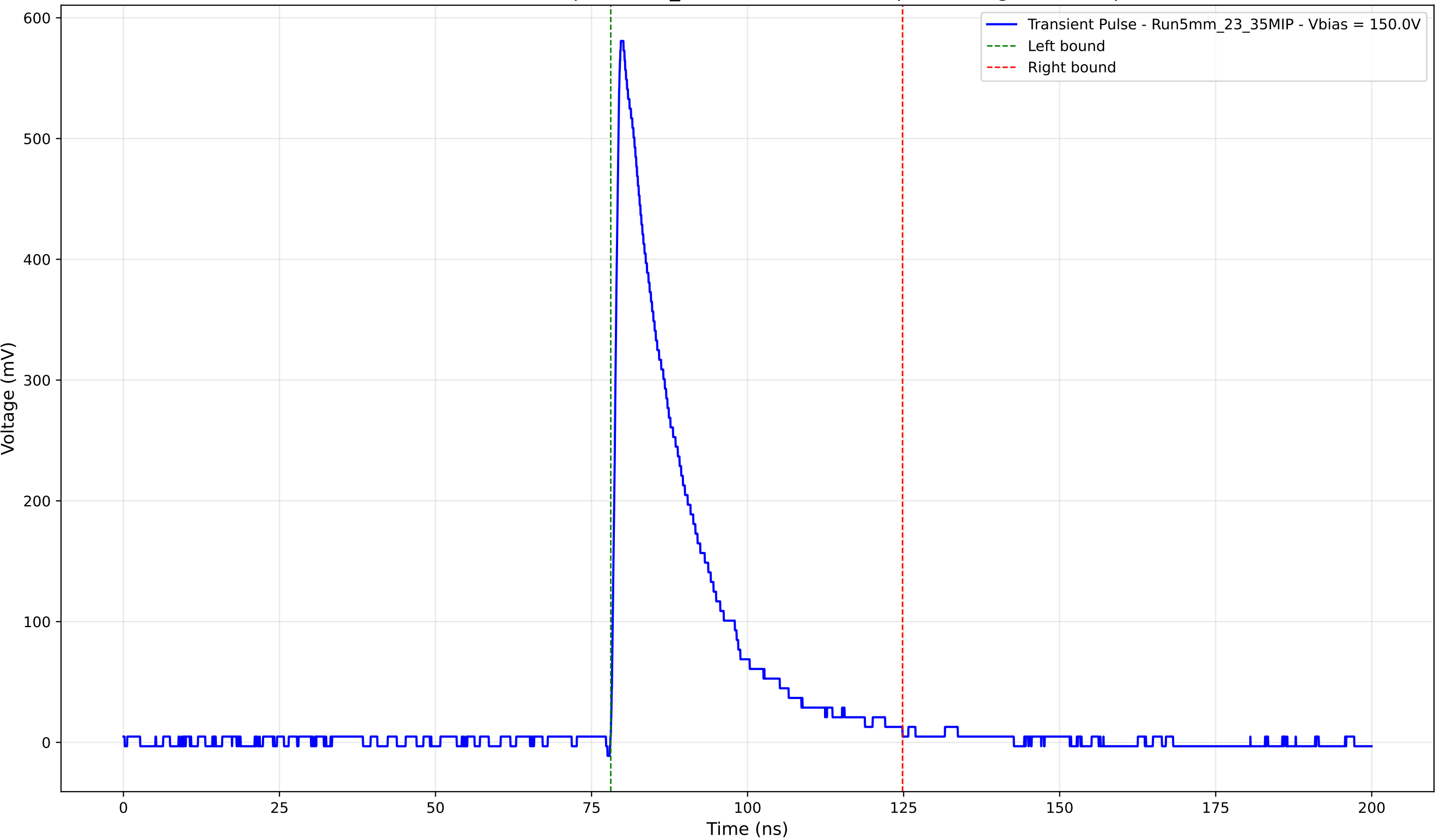
Transient Pulse - Sample: 5mm_23 - Position: 1265.0 \mu\text{m} - Charge: 128.44 pC
