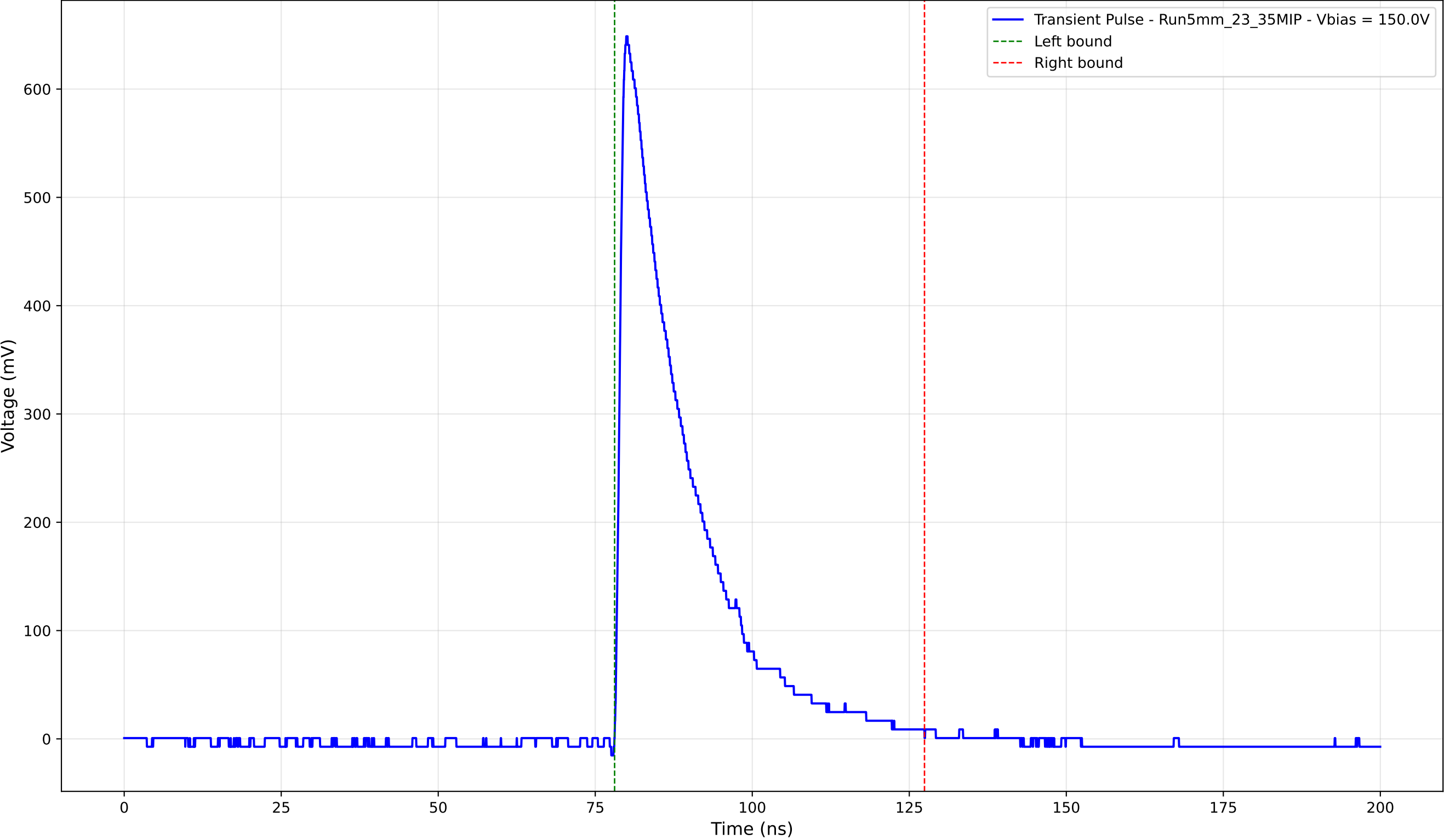
Transient Pulse - Sample: 5mm_23 - Position: 1445.0 \mu\text{m} - Charge: 149.49 pC
