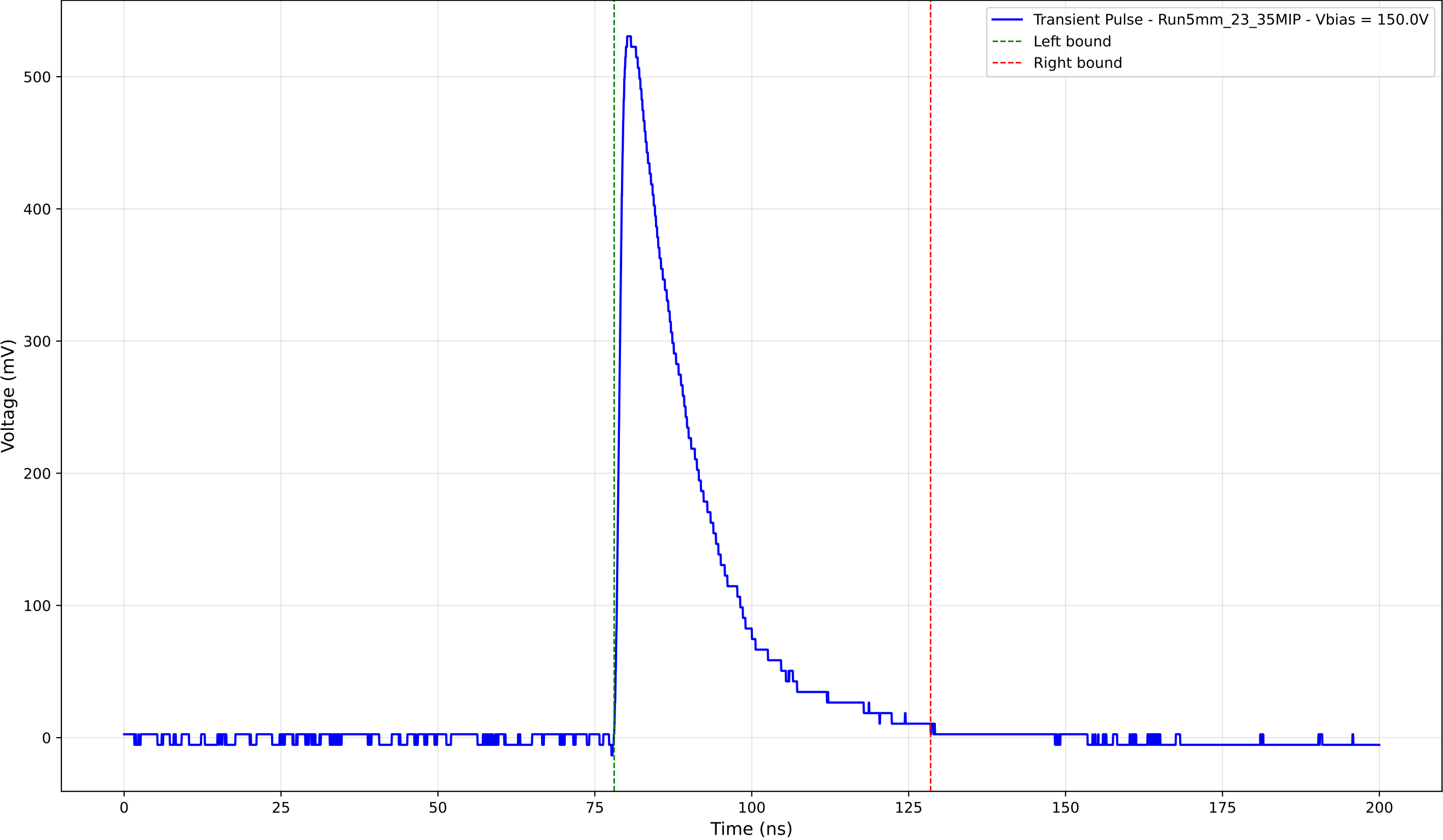
Transient Pulse - Sample: 5mm_23 - Position: 1795.0 \mu\text{m} - Charge: 135.40 pC
