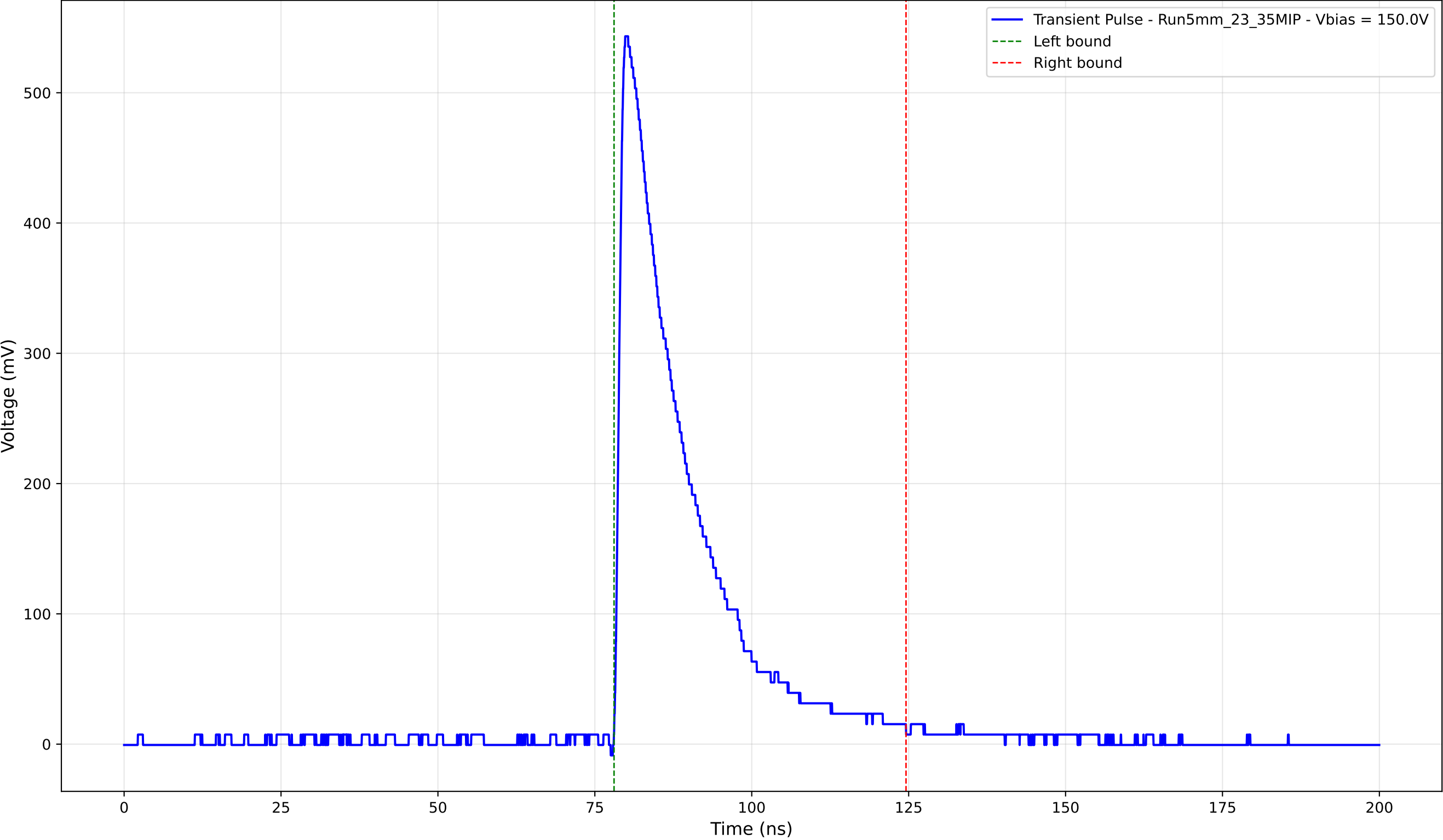
Transient Pulse - Sample: 5mm_23 - Position: 3785.0 \mu\text{m} - Charge: 126.33 pC
