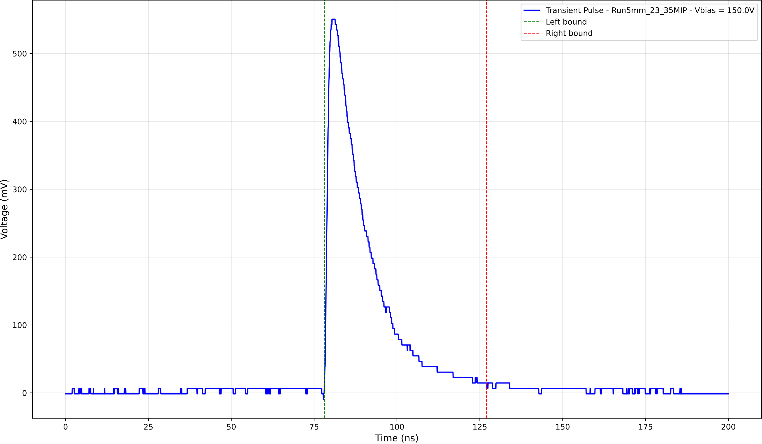
Transient Pulse - Sample: 5mm_23 - Position: 1975.0 \mu\text{m} - Charge: 145.89 pC
