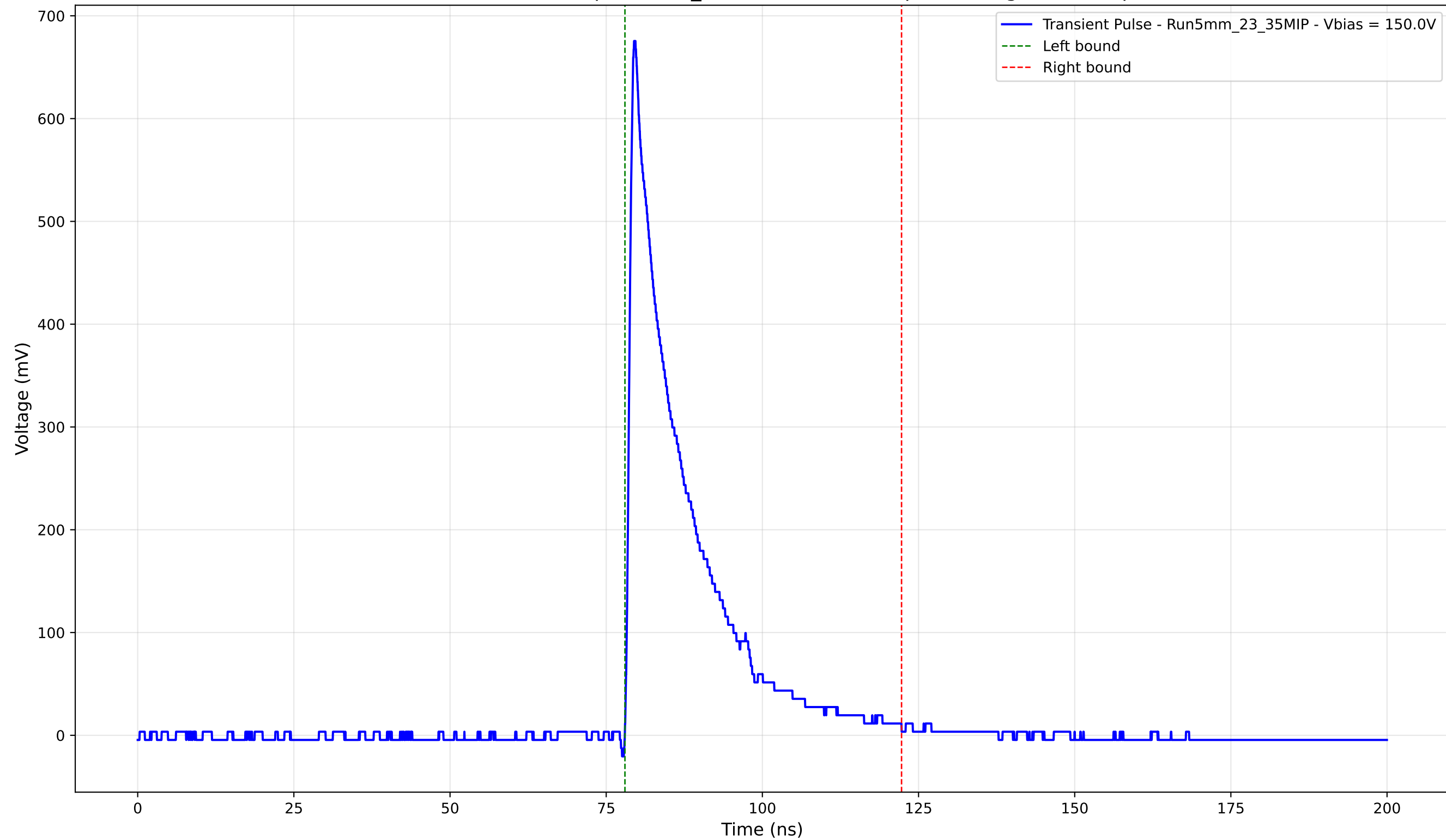
Transient Pulse - Sample: 5mm_23 - Position: 870.0 \mu\text{m} - Charge: 122.35 pC
