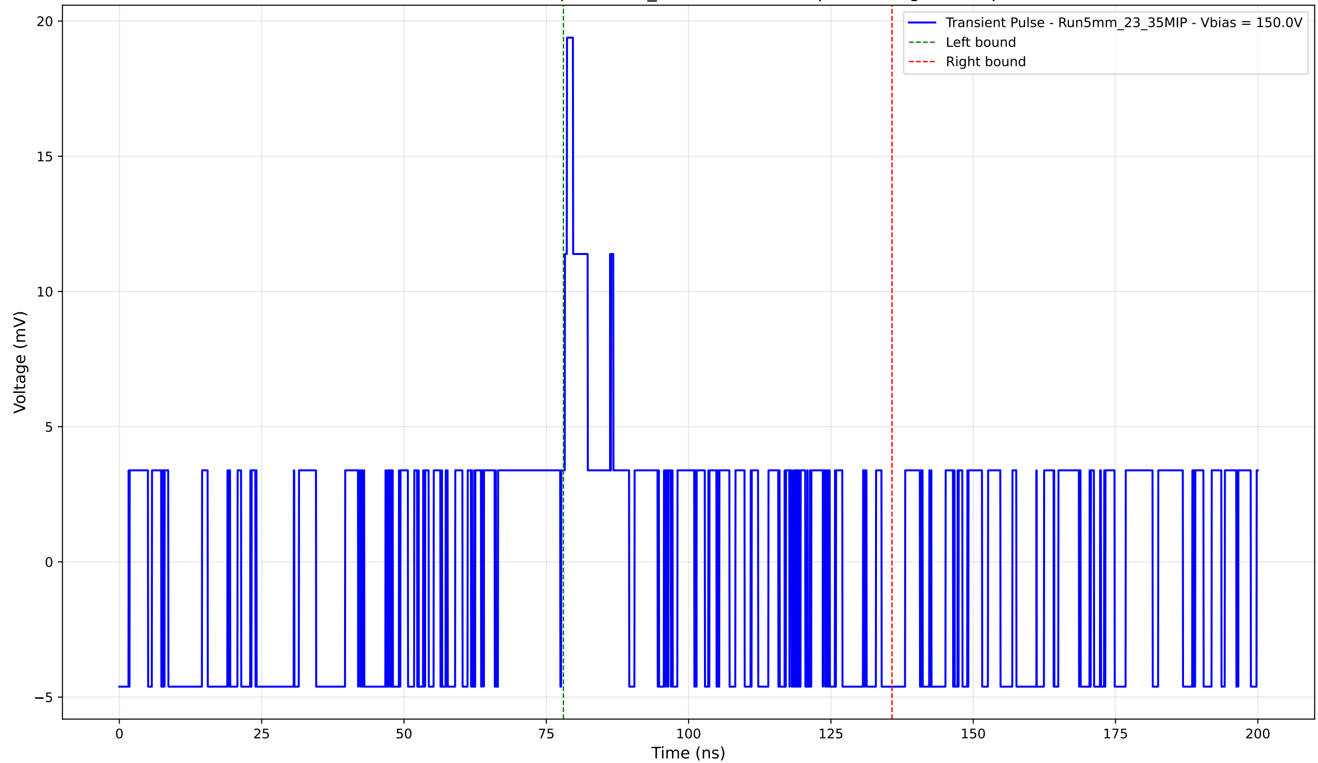
Transient Pulse - Sample: 5mm_23 - Position: 5.0 \mu\text{m} - Charge: 1.59 pC
