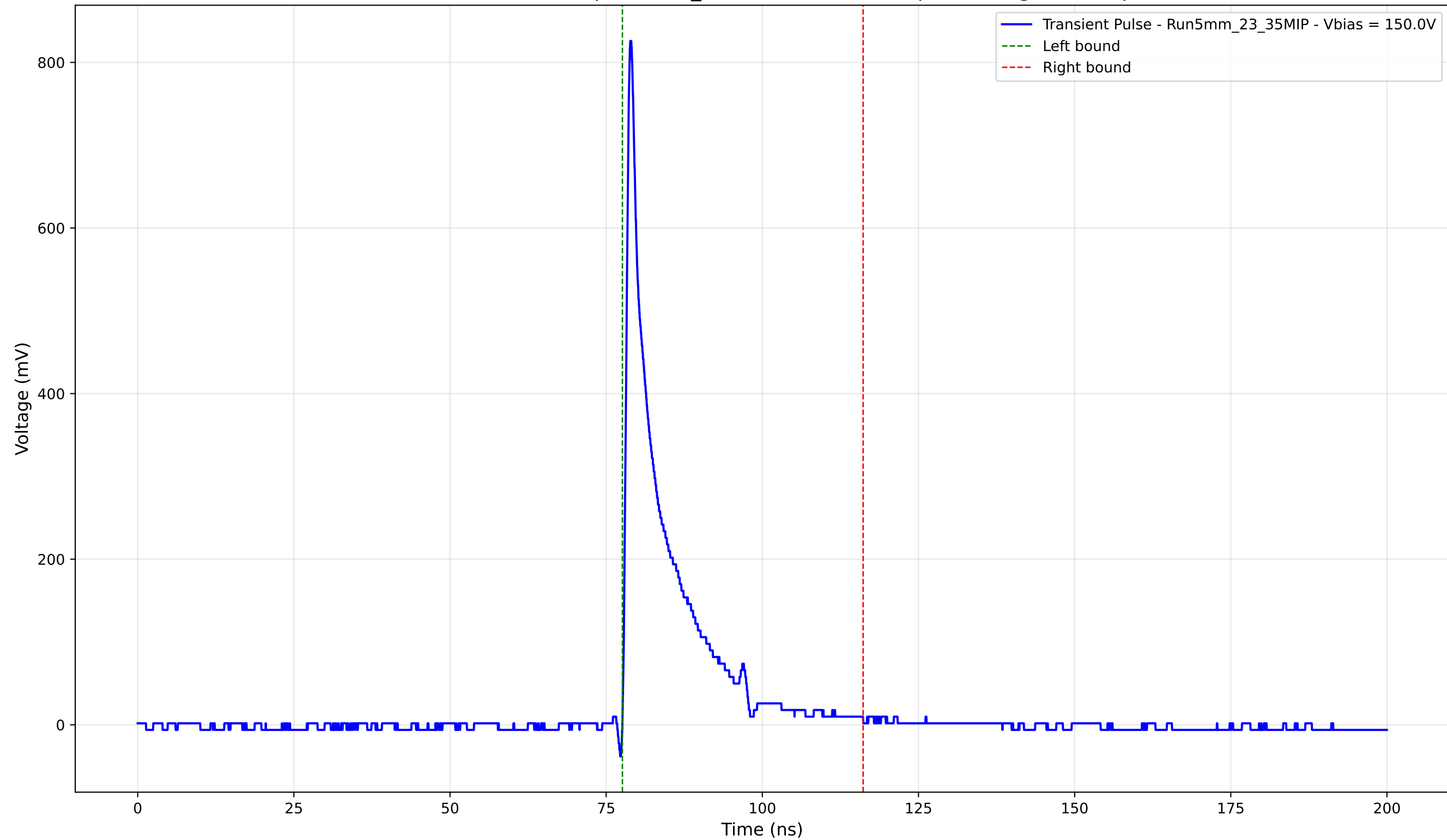
Transient Pulse - Sample: 5mm_23 - Position: 5030.0 \mu\text{m} - Charge: 93.99 pC
