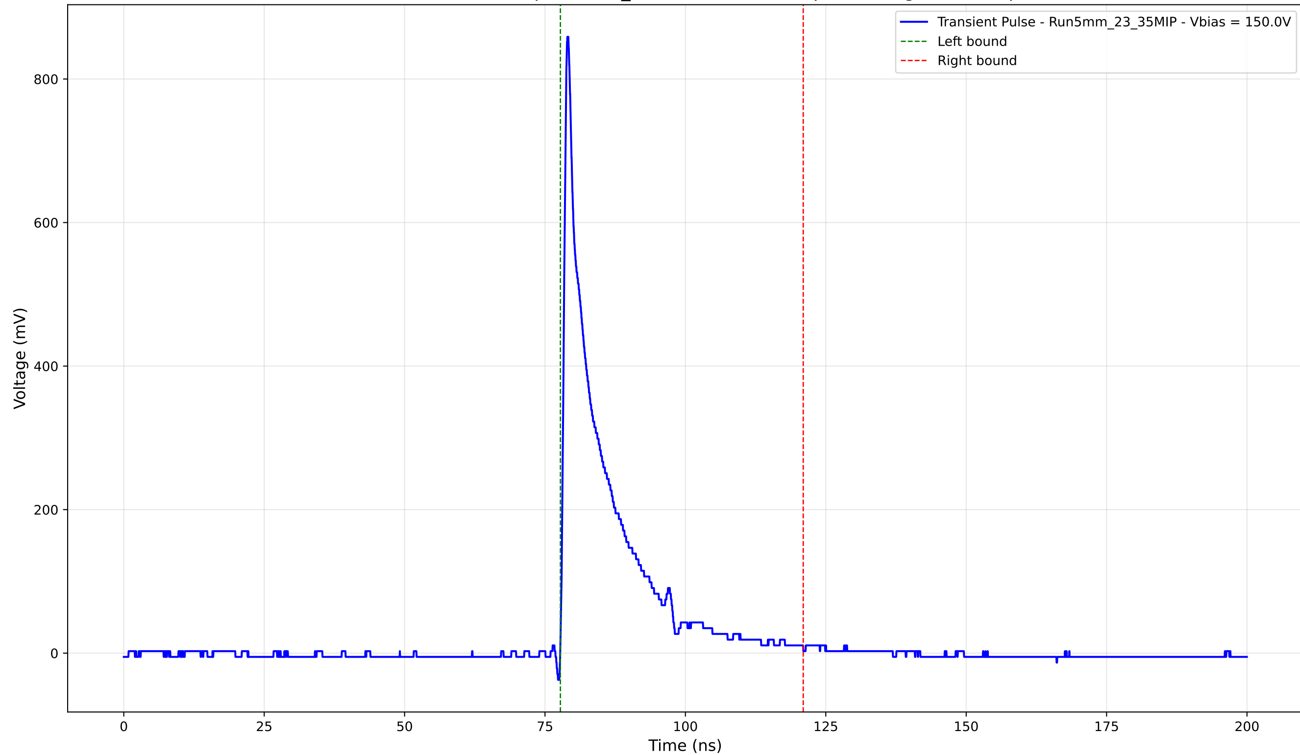
Transient Pulse - Sample: 5mm_23 - Position: 330.0 \mu\text{m} - Charge: 114.91 pC
