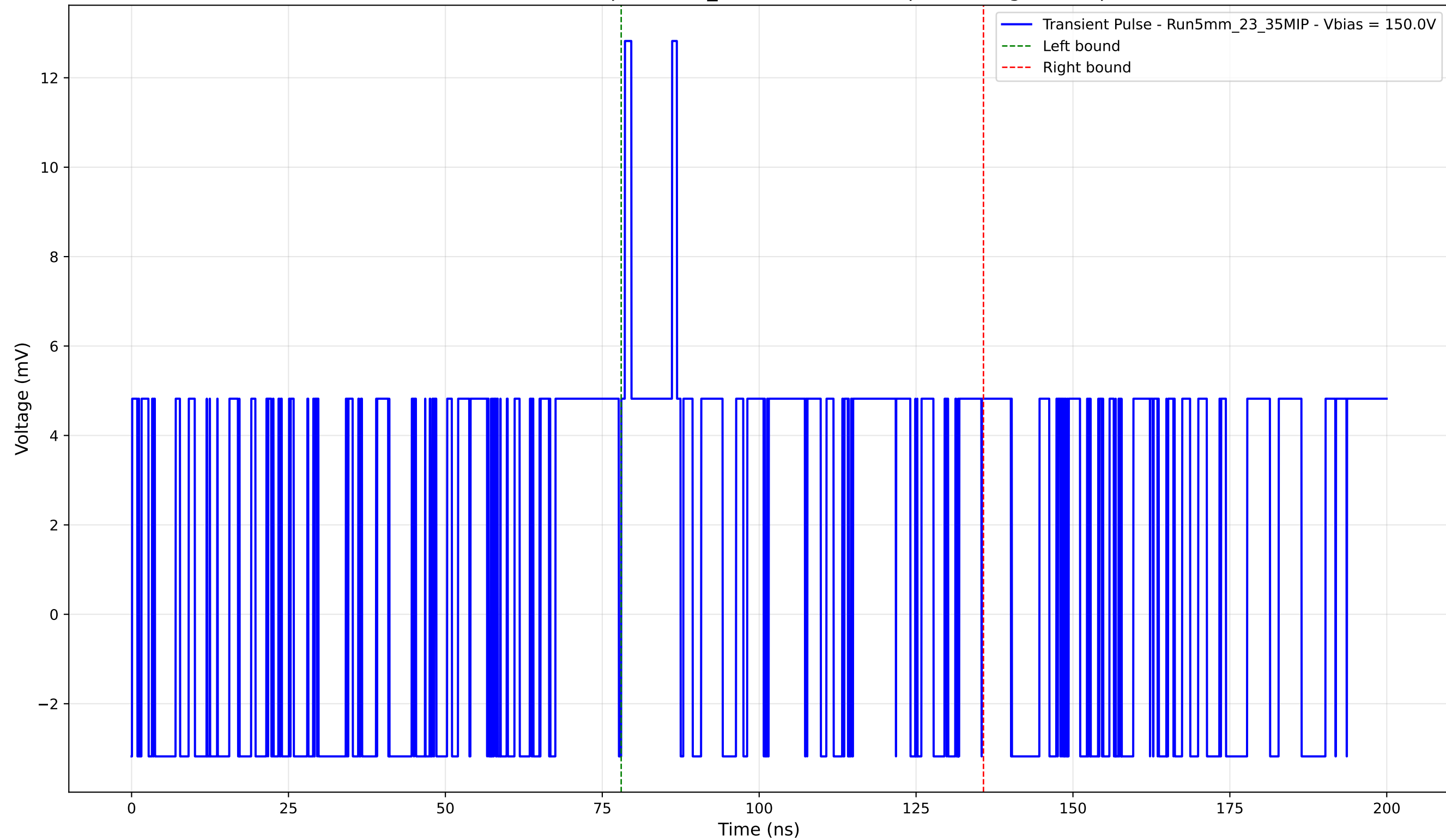
Transient Pulse - Sample: 5mm_23 - Position: 80.0 \mu\text{m} - Charge: 3.69 pC
