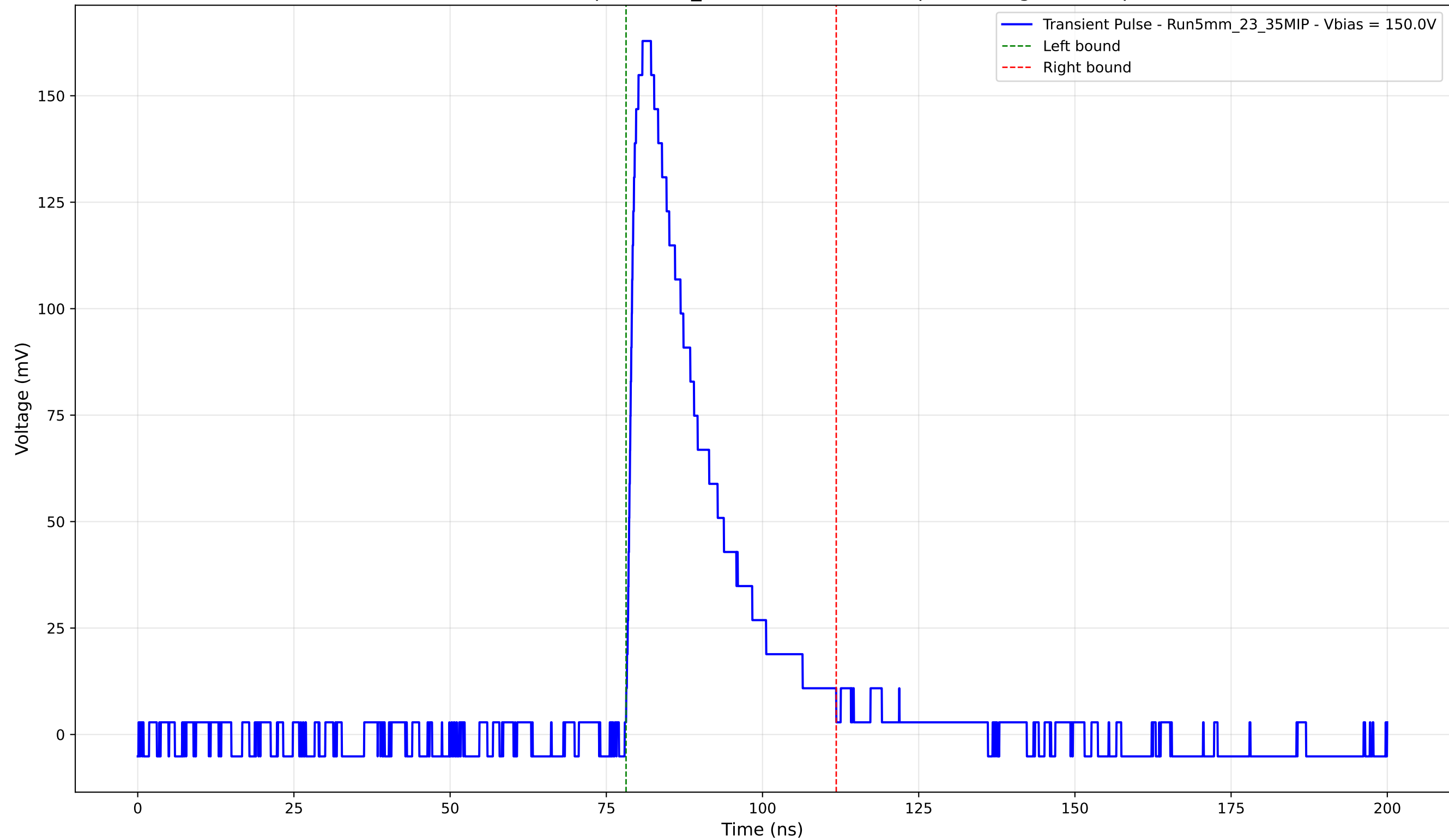
Transient Pulse - Sample: 5mm_23 - Position: 3120.0 \mu\text{m} - Charge: 40.20 pC
