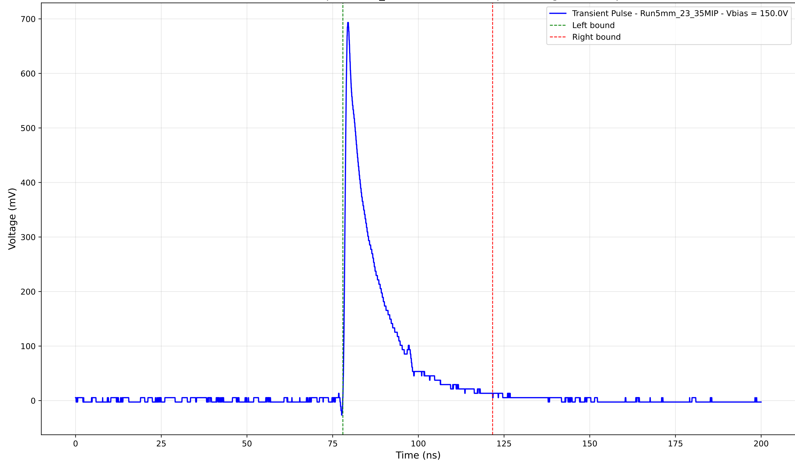
Transient Pulse - Sample: 5mm_23 - Position: 785.0 \mu\text{m} - Charge: 121.25 pC
