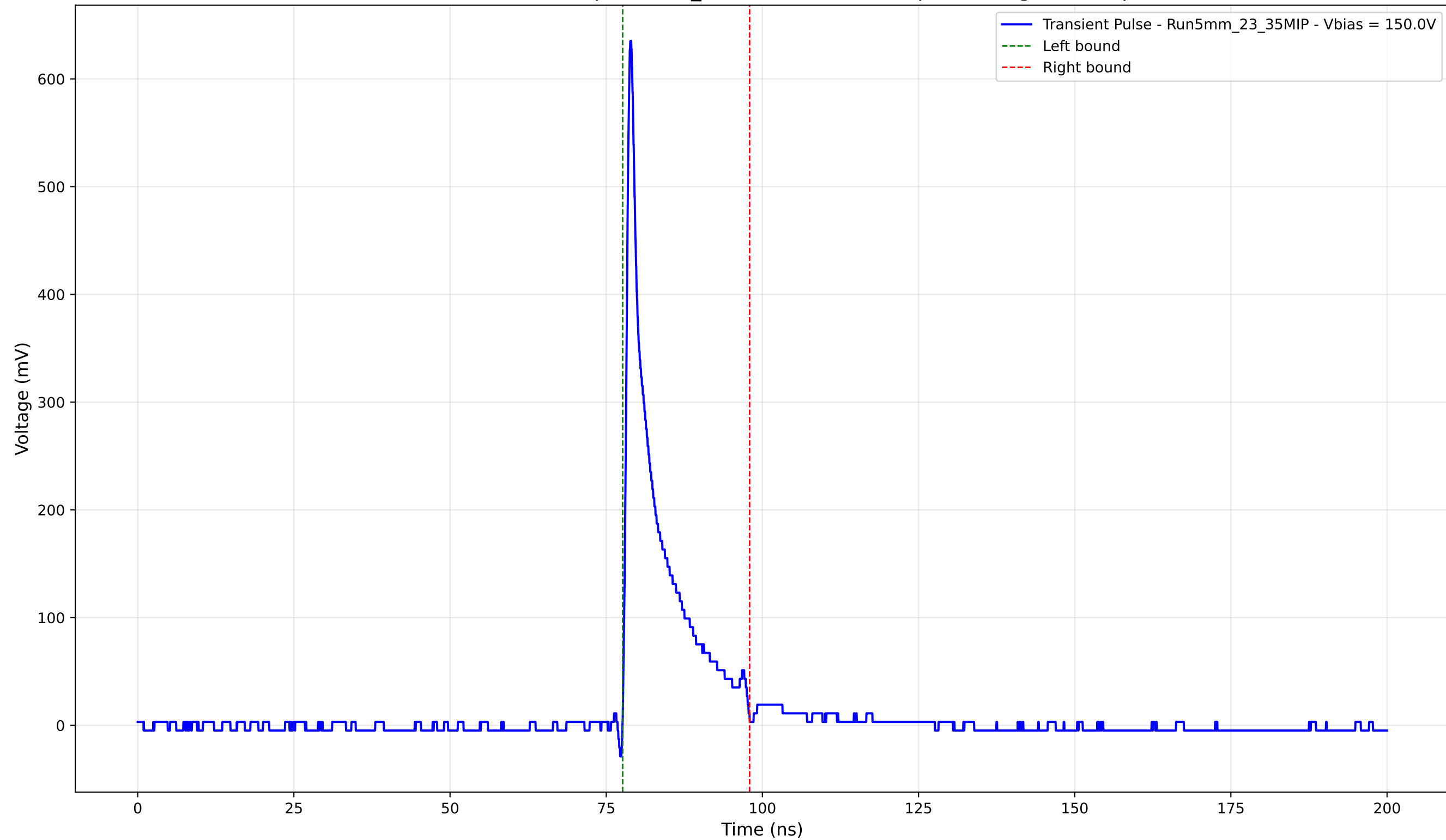
Transient Pulse - Sample: 5mm_23 - Position: 5055.0 \mu\text{m} - Charge: 61.89 pC
