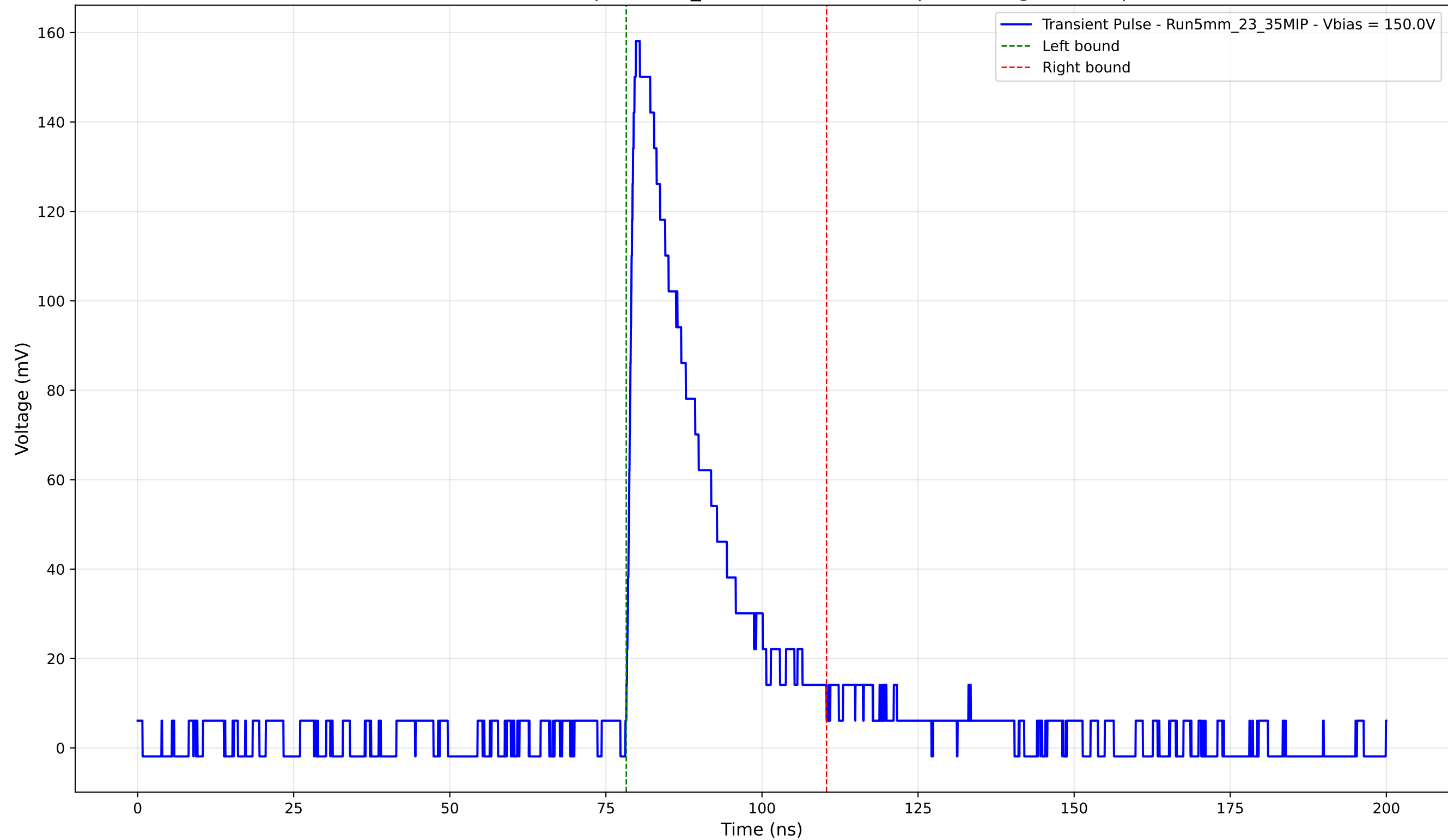
Transient Pulse - Sample: 5mm_23 - Position: 1595.0 \mu\text{m} - Charge: 37.75 pC
