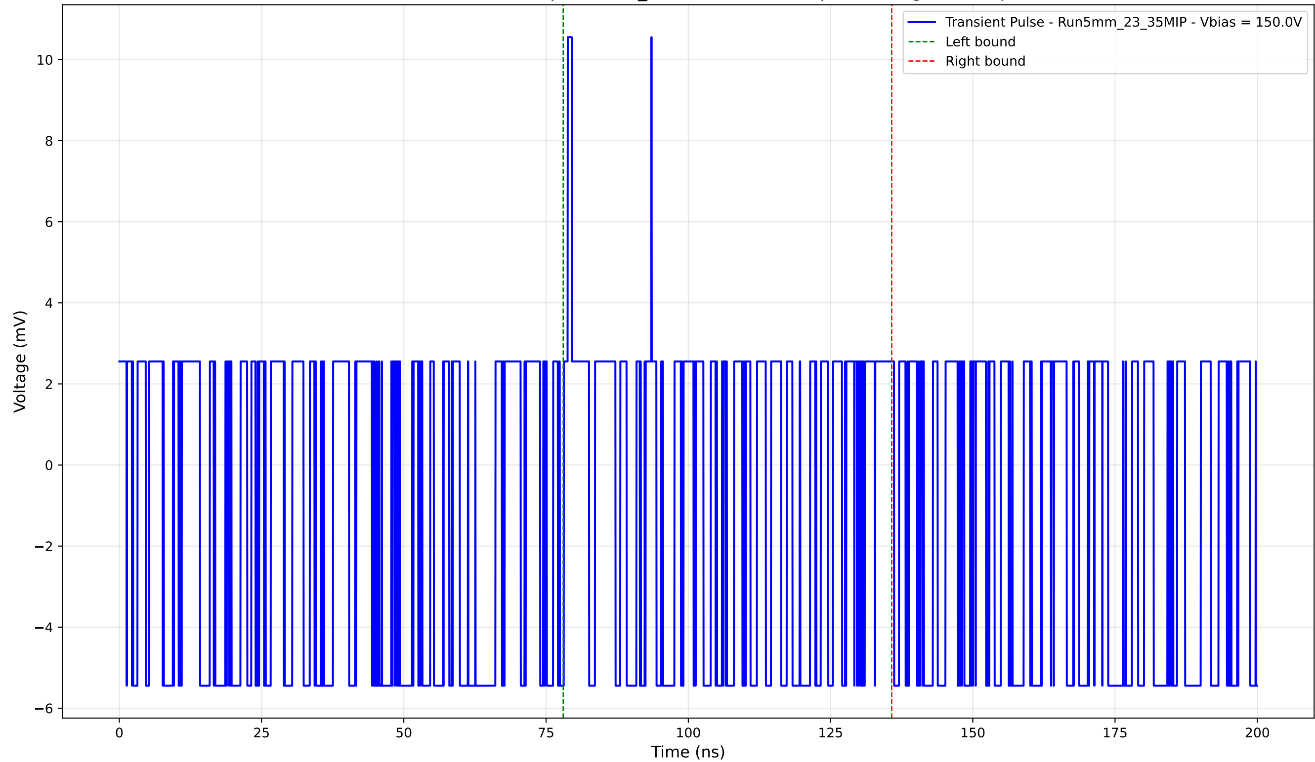
Transient Pulse - Sample: 5mm_23 - Position: 65.0 \mu\text{m} - Charge: -0.33 pC
