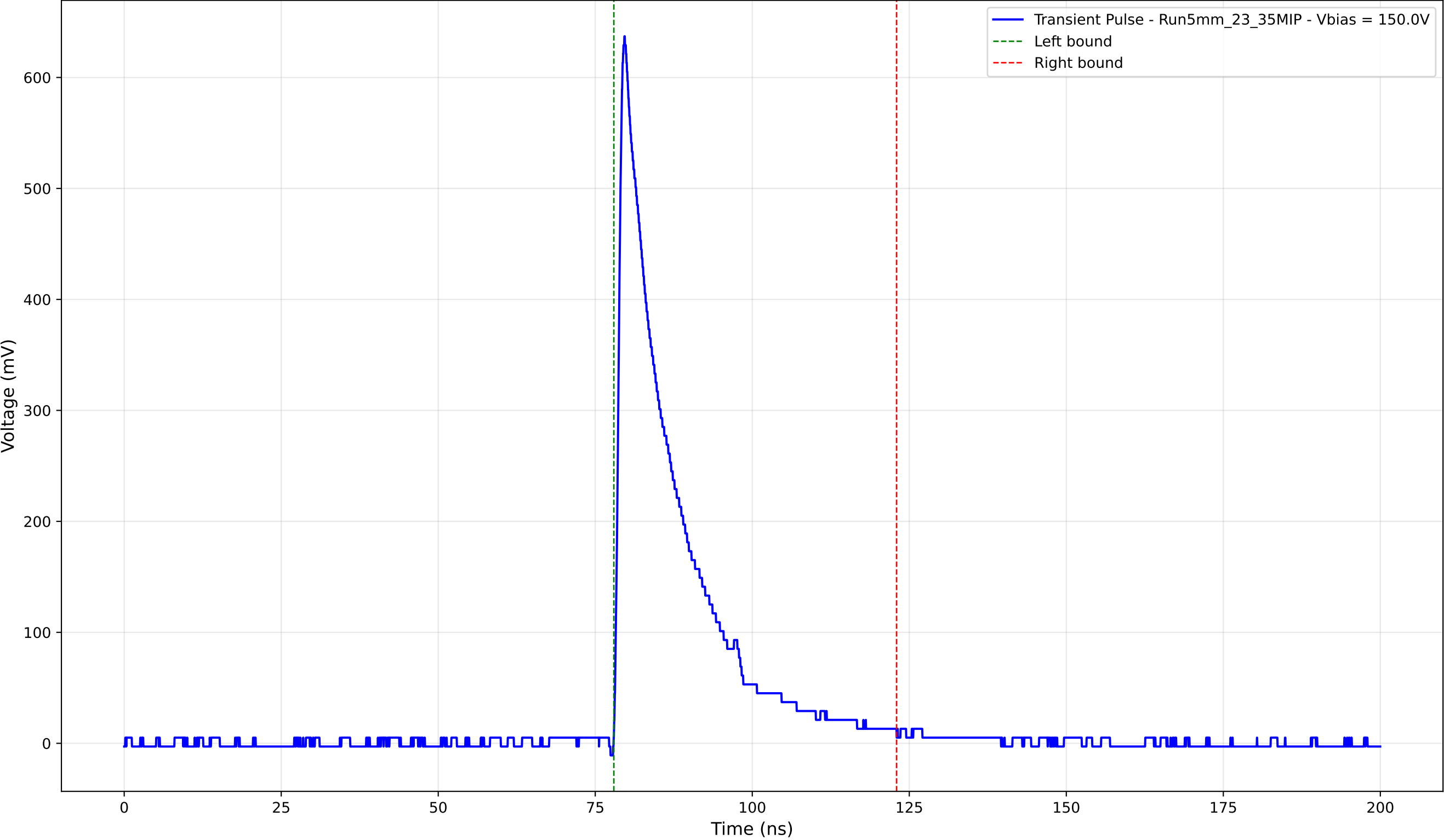
Transient Pulse - Sample: 5mm_23 - Position: 4285.0 \mu\text{m} - Charge: 118.50 pC
