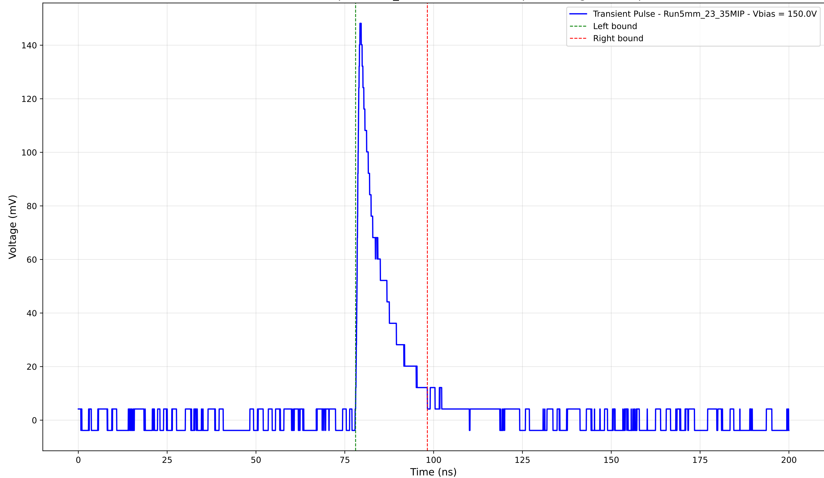
Transient Pulse - Sample: 5mm_23 - Position: 4530.0 \mu\text{m} - Charge: 19.89 pC
