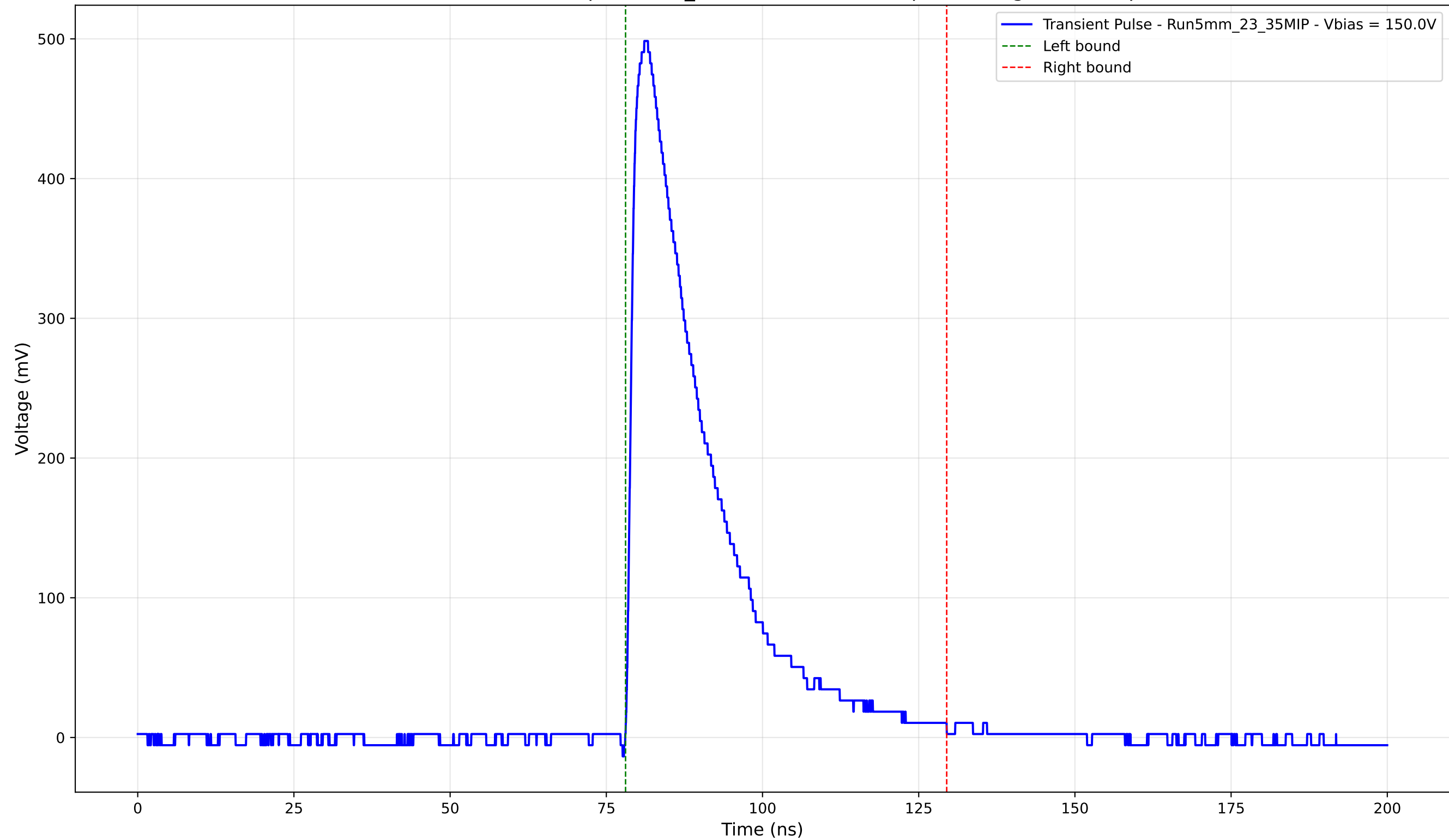
Transient Pulse - Sample: 5mm_23 - Position: 2855.0 \mu\text{m} - Charge: 132.90 pC
