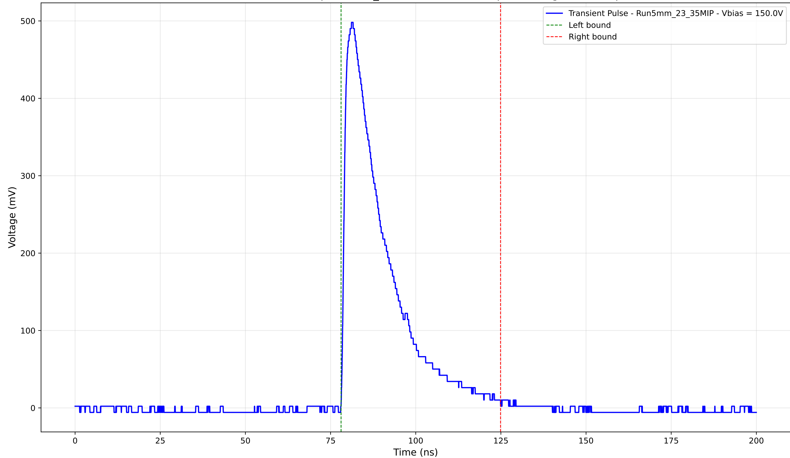
Transient Pulse - Sample: 5mm_23 - Position: 2860.0 \mu\text{m} - Charge: 132.61 pC
