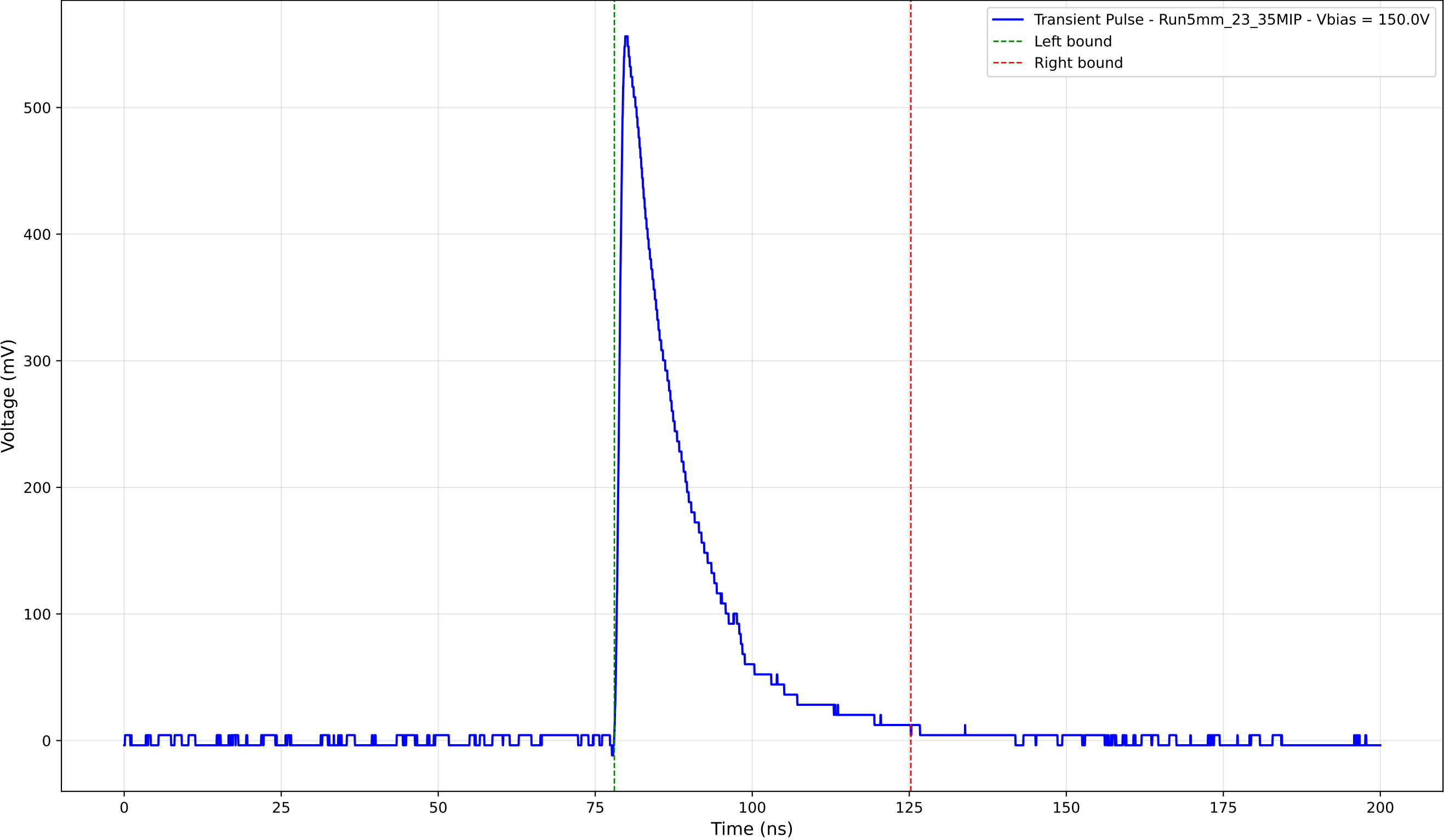
Transient Pulse - Sample: 5mm_23 - Position: 3935.0 \mu\text{m} - Charge: 120.71 pC
