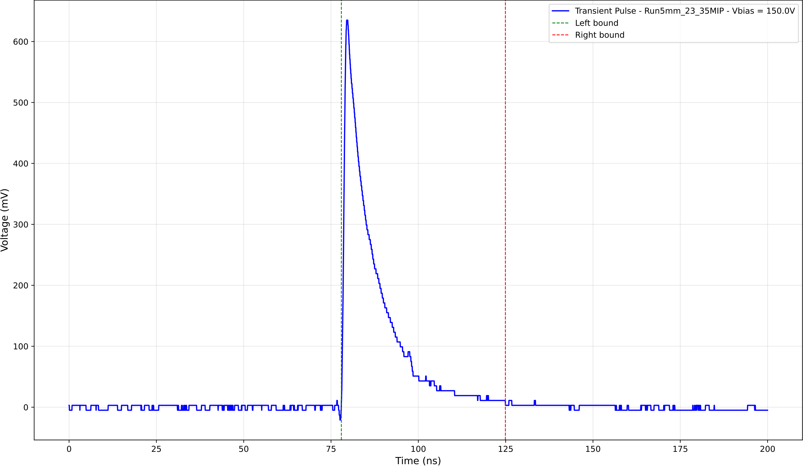
Transient Pulse - Sample: 5mm_23 - Position: 4325.0 \mu\text{m} - Charge: 116.70 pC
