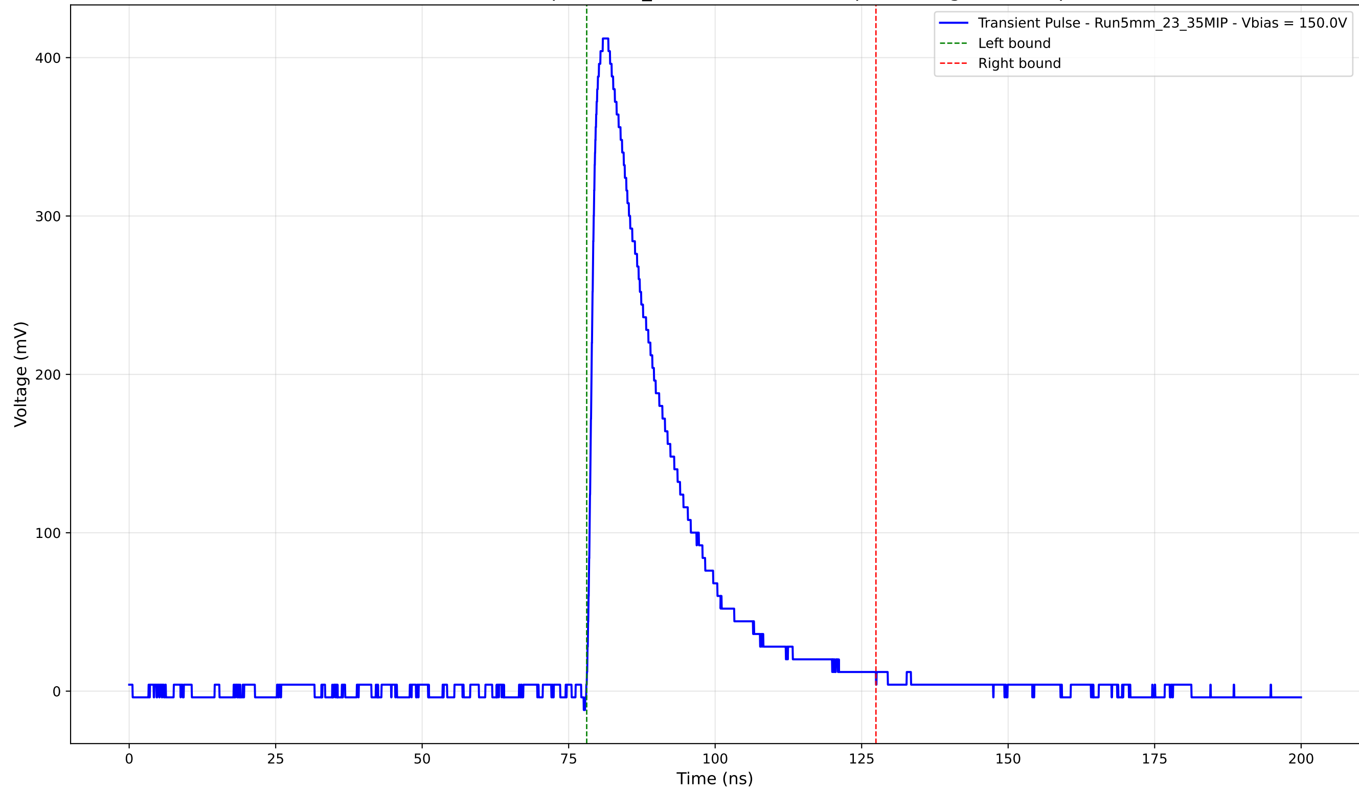
Transient Pulse - Sample: 5mm_23 - Position: 2575.0 \mu\text{m} - Charge: 110.45 pC
