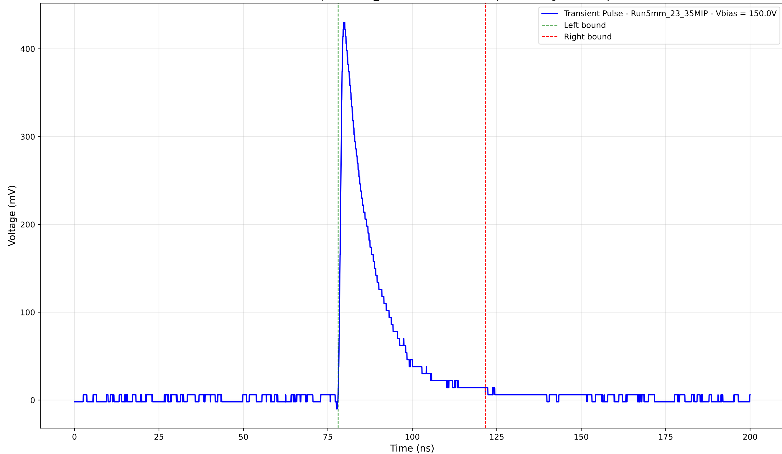
Transient Pulse - Sample: 5mm_23 - Position: 4095.0 \mu\text{m} - Charge: 86.48 pC
