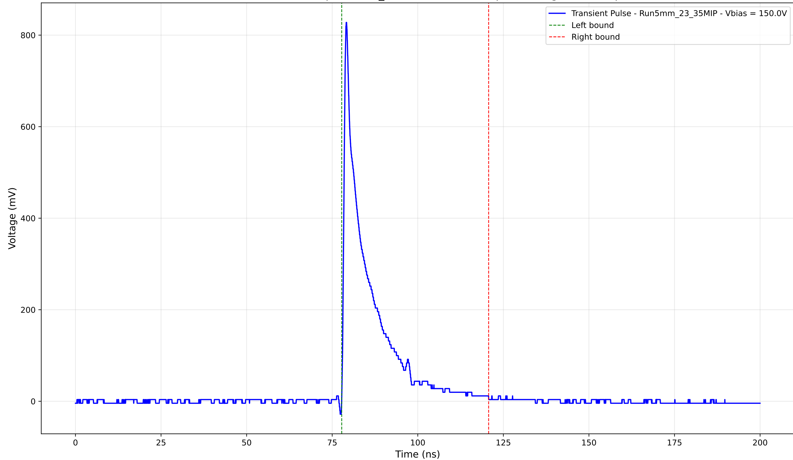
Transient Pulse - Sample: 5mm_23 - Position: 415.0 \mu\text{m} - Charge: 115.89 pC
