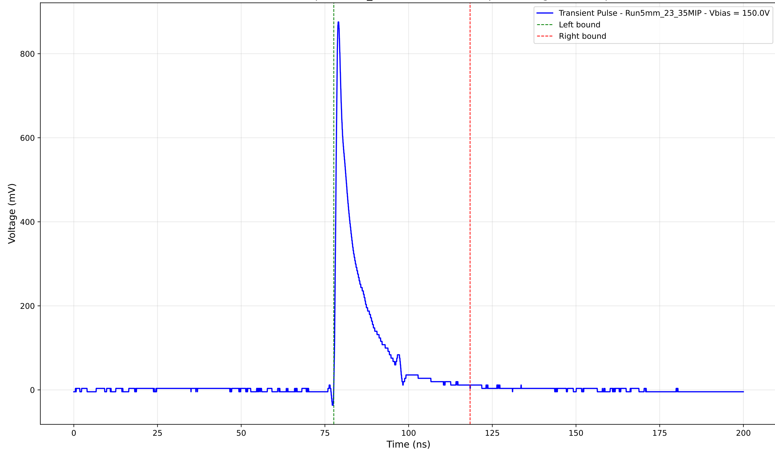
Transient Pulse - Sample: 5mm_23 - Position: 4925.0 \mu\text{m} - Charge: 114.44 pC
