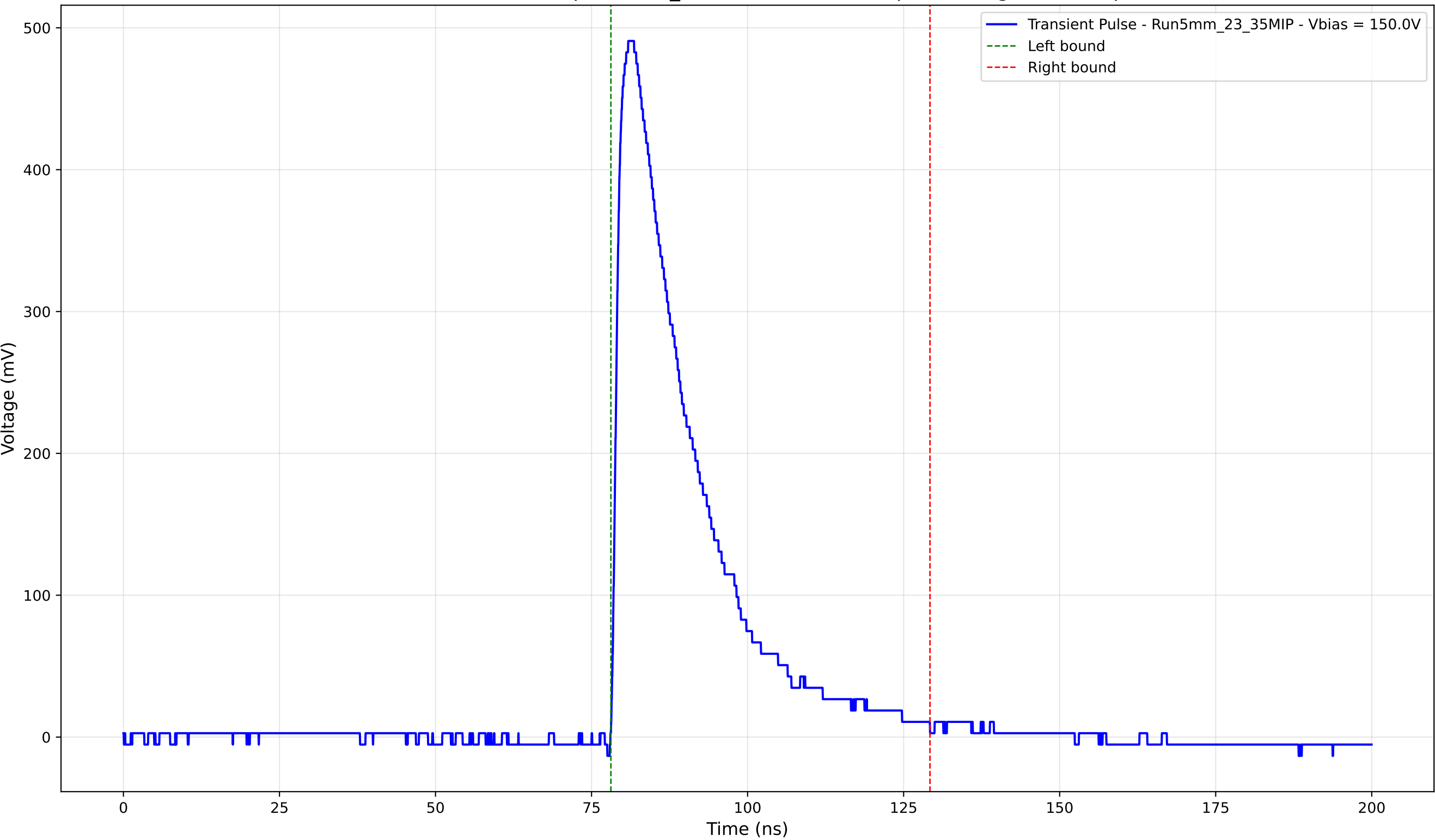
Transient Pulse - Sample: 5mm_23 - Position: 2815.0 \mu\text{m} - Charge: 132.46 pC
