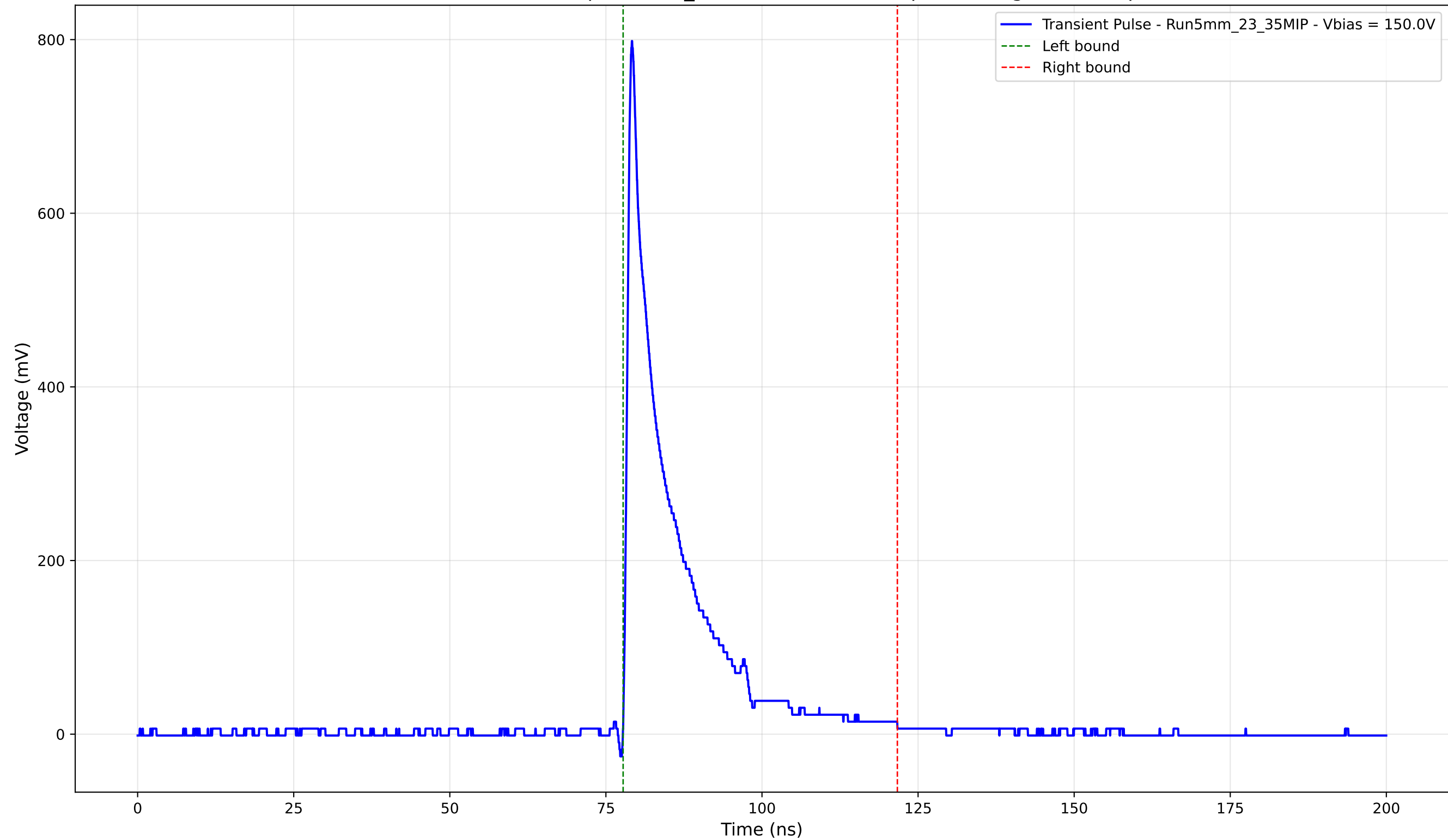
Transient Pulse - Sample: 5mm_23 - Position: 4775.0 \mu\text{m} - Charge: 113.71 pC
