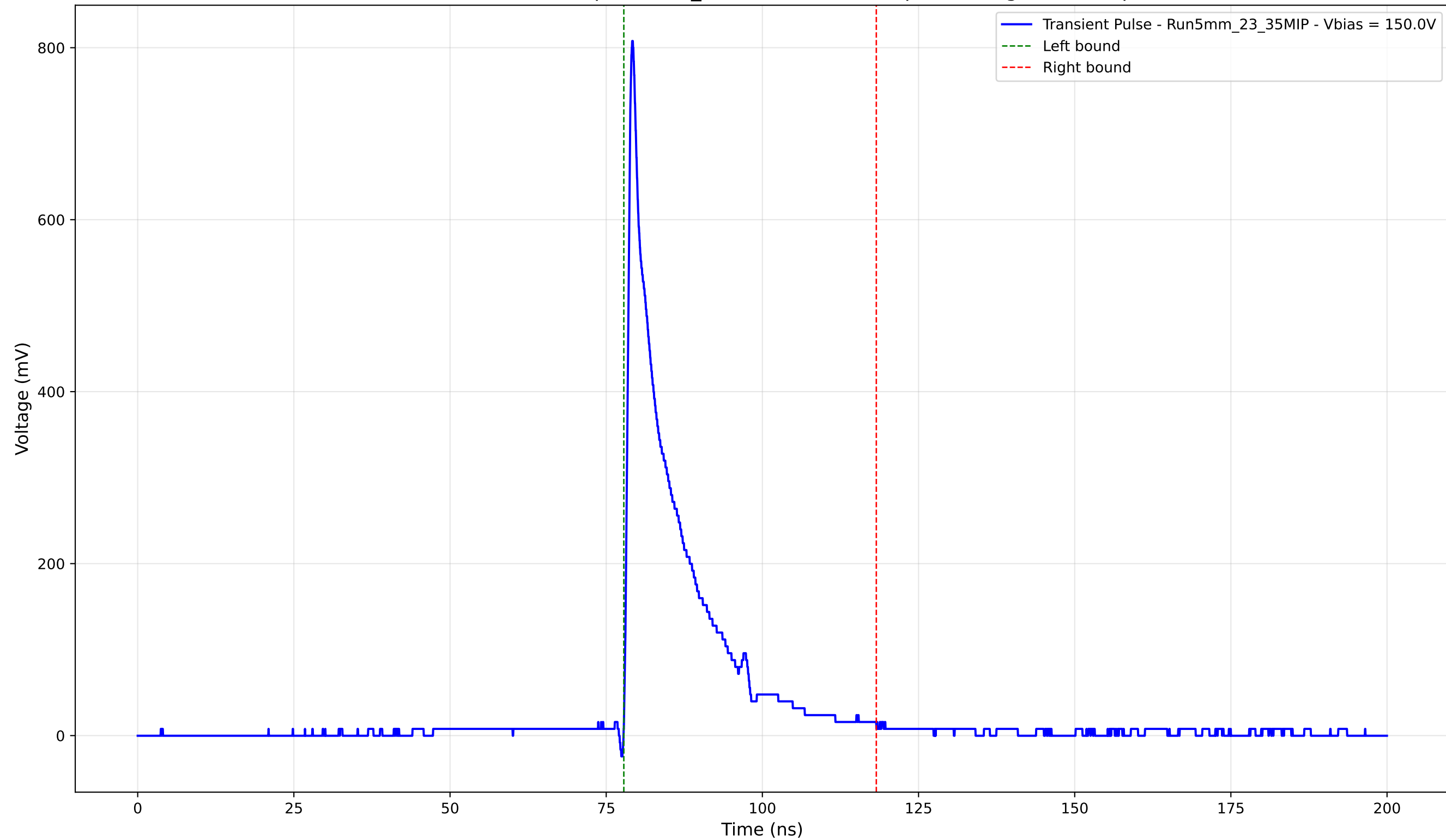
Transient Pulse - Sample: 5mm_23 - Position: 480.0 \mu\text{m} - Charge: 118.45 pC
