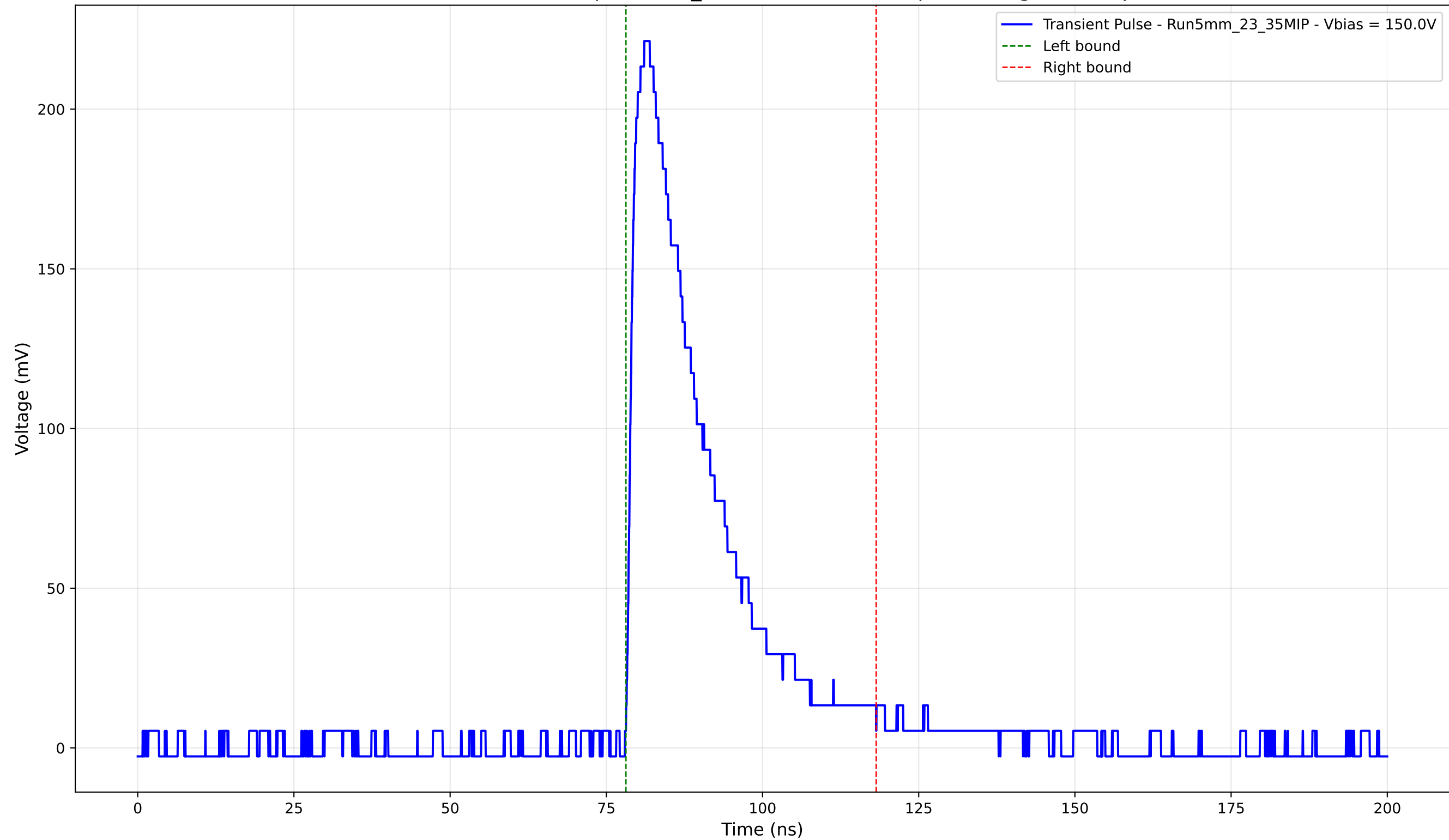
Transient Pulse - Sample: 5mm_23 - Position: 2685.0 \mu\text{m} - Charge: 58.02 pC
