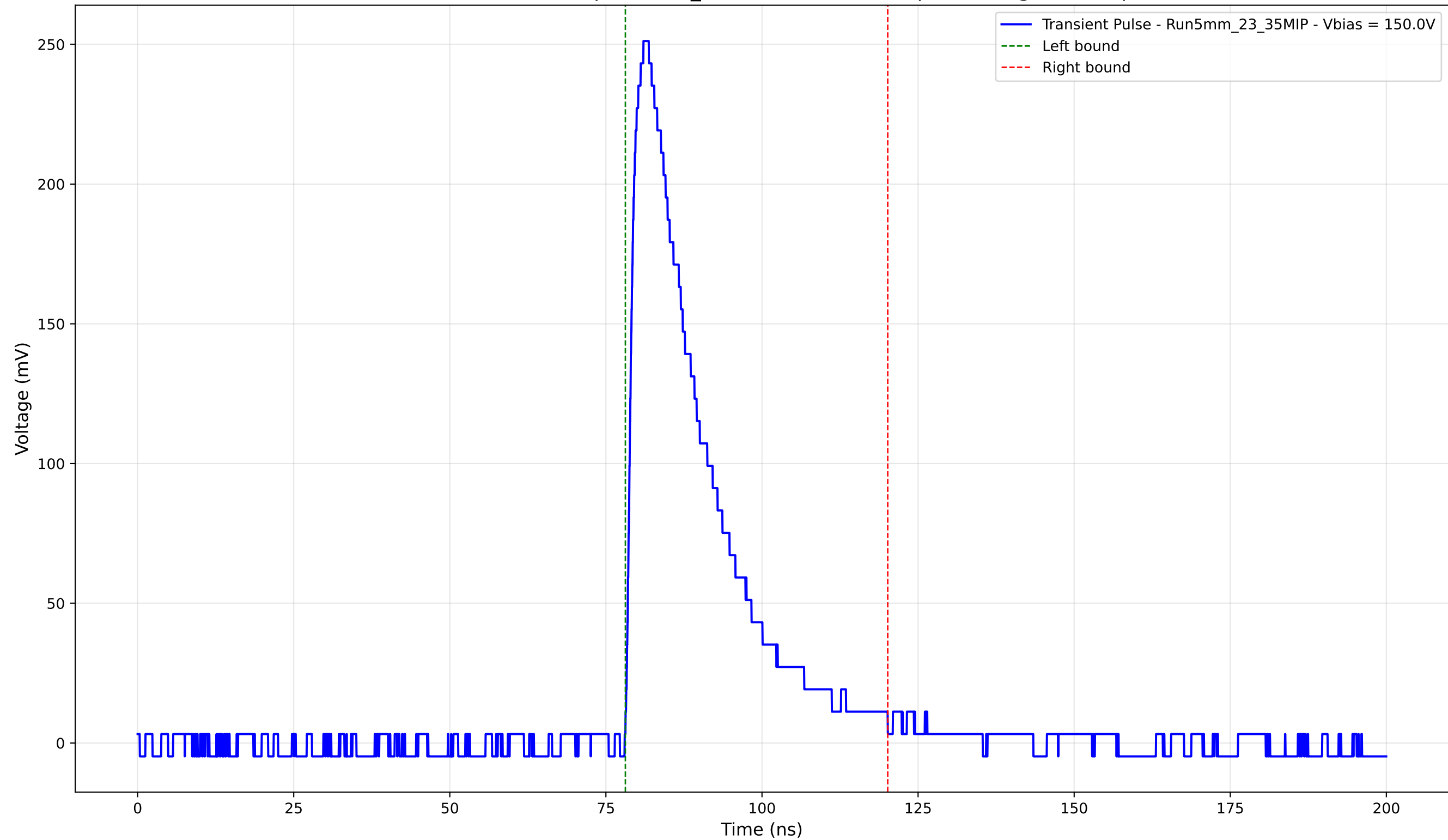
Transient Pulse - Sample: 5mm_23 - Position: 2690.0 \mu\text{m} - Charge: 65.19 pC
