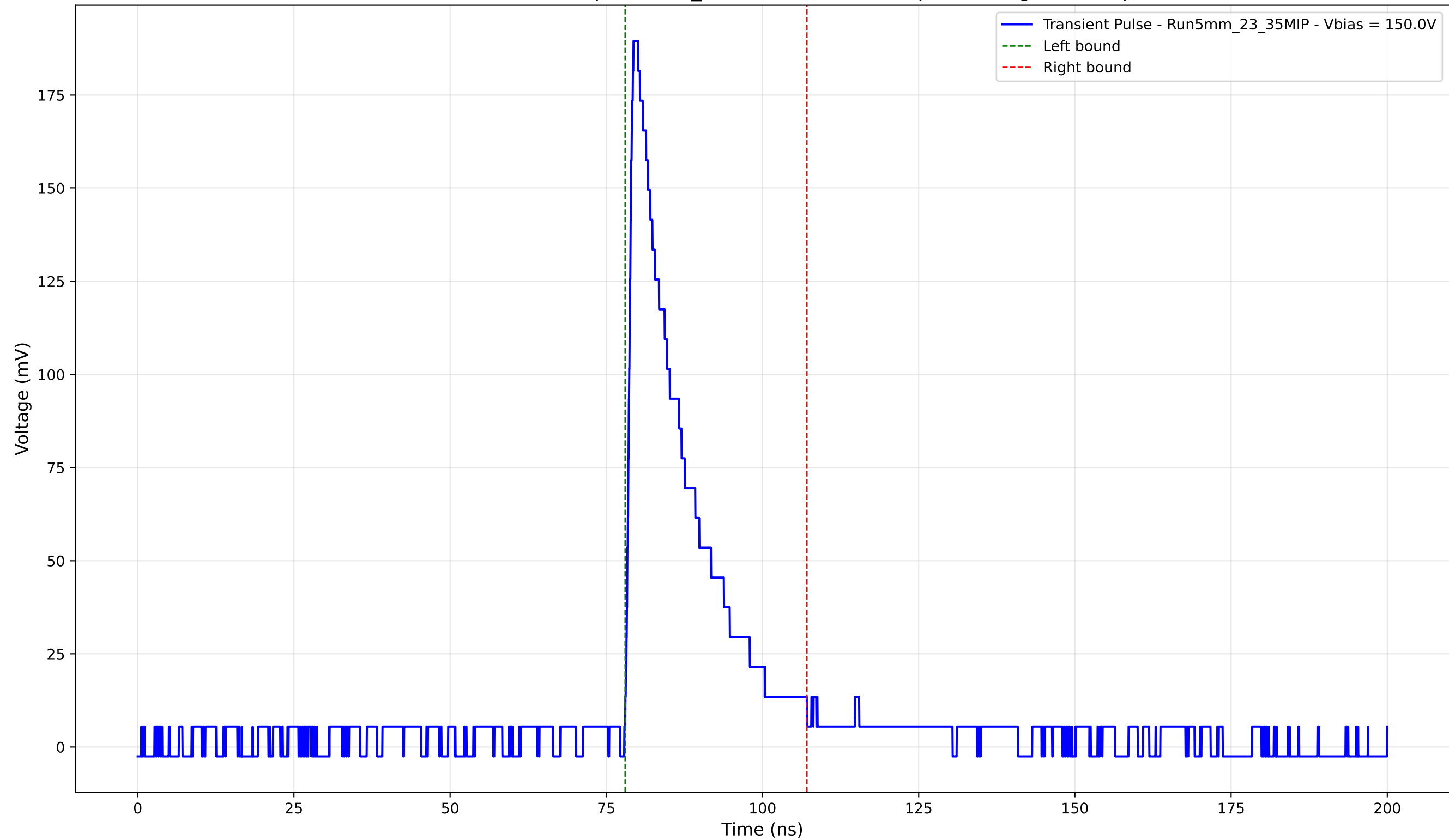
Transient Pulse - Sample: 5mm_23 - Position: 4485.0 \mu\text{m} - Charge: 36.13 pC
