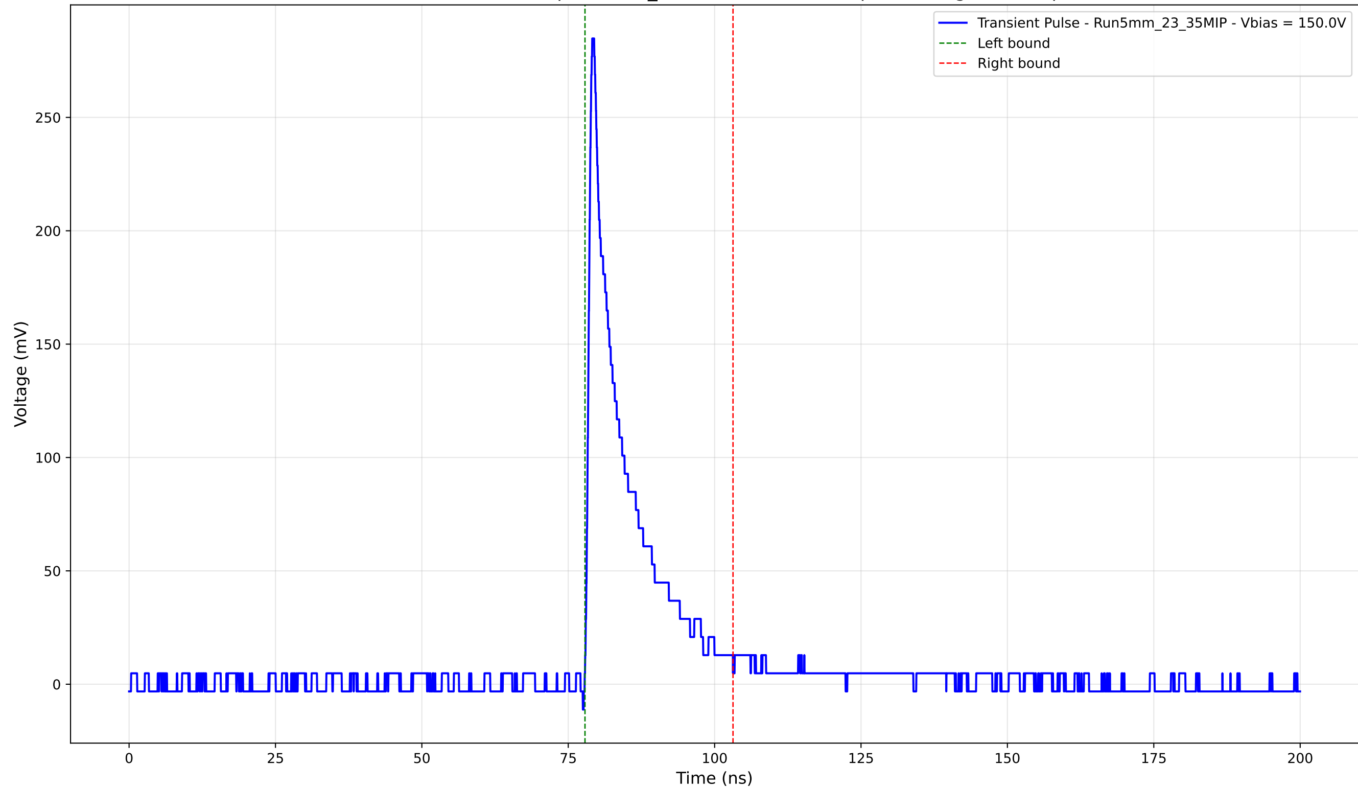
Transient Pulse - Sample: 5mm_23 - Position: 4695.0 \mu\text{m} - Charge: 36.79 pC
