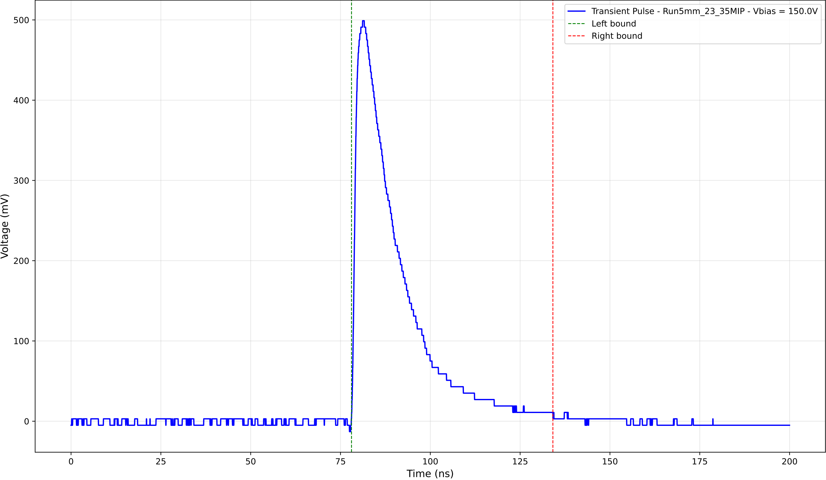
Transient Pulse - Sample: 5mm_23 - Position: 2875.0 \mu\text{m} - Charge: 134.40 pC
