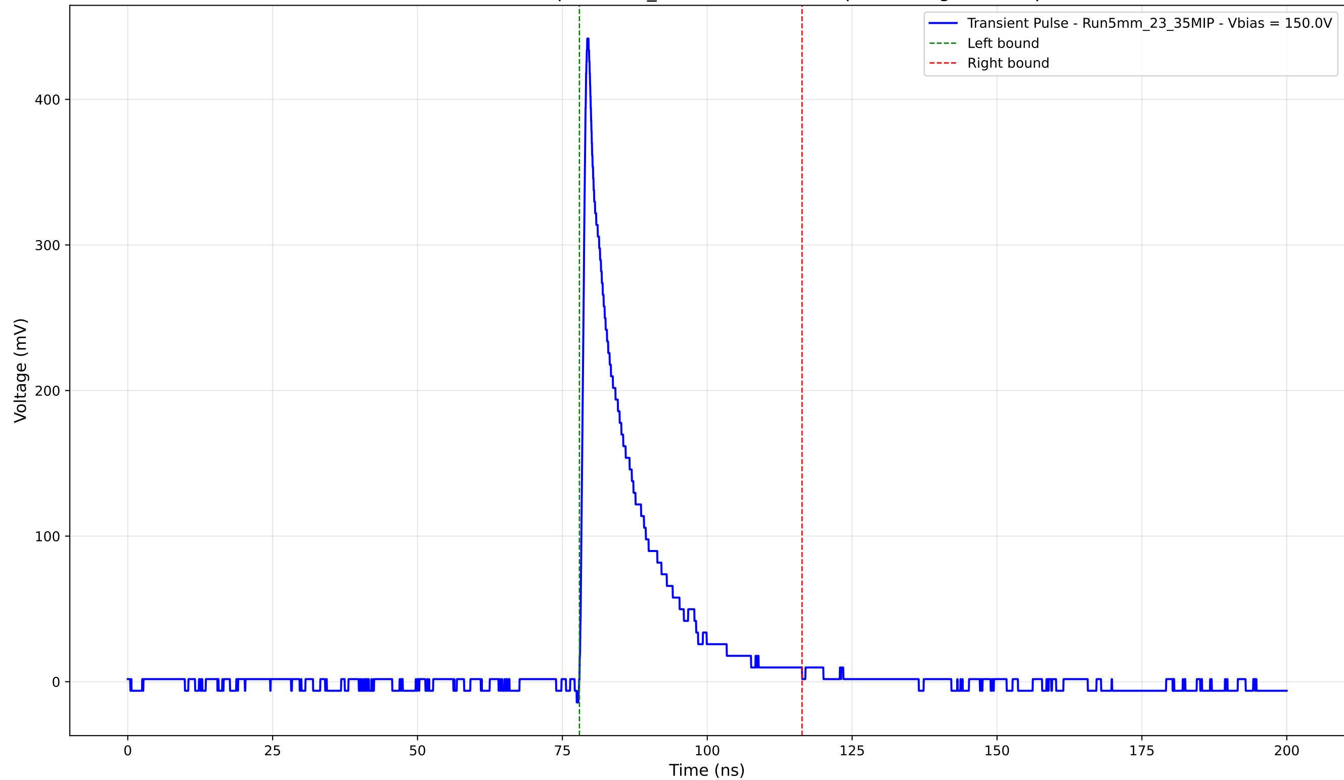
Transient Pulse - Sample: 5mm_23 - Position: 670.0 \mu\text{m} - Charge: 67.57 pC
