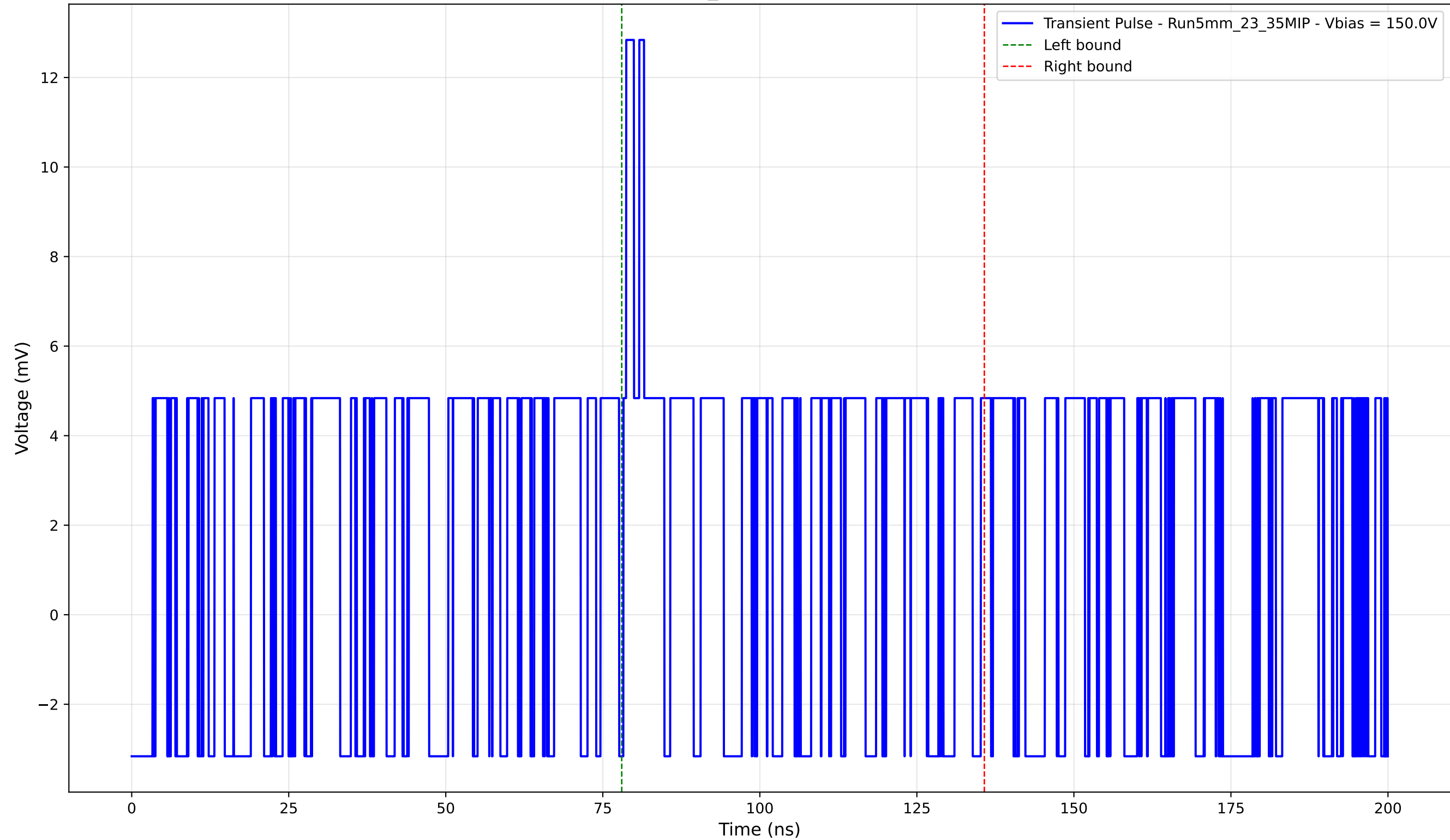
Transient Pulse - Sample: 5mm_23 - Position: 90.0 \mu\text{m} - Charge: 3.06 pC
