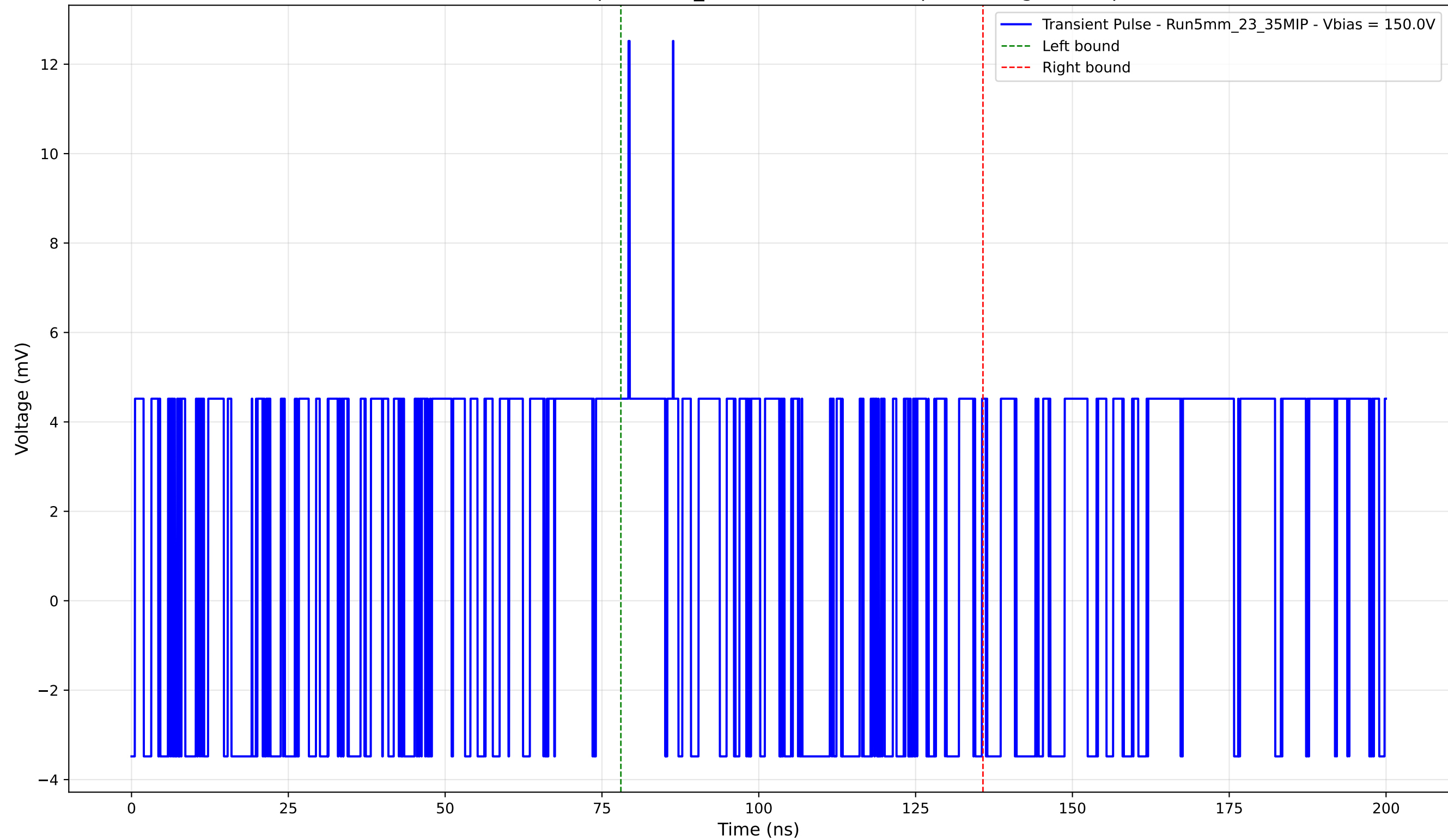
Transient Pulse - Sample: 5mm_23 - Position: 5265.0 \mu\text{m} - Charge: 1.17 pC
