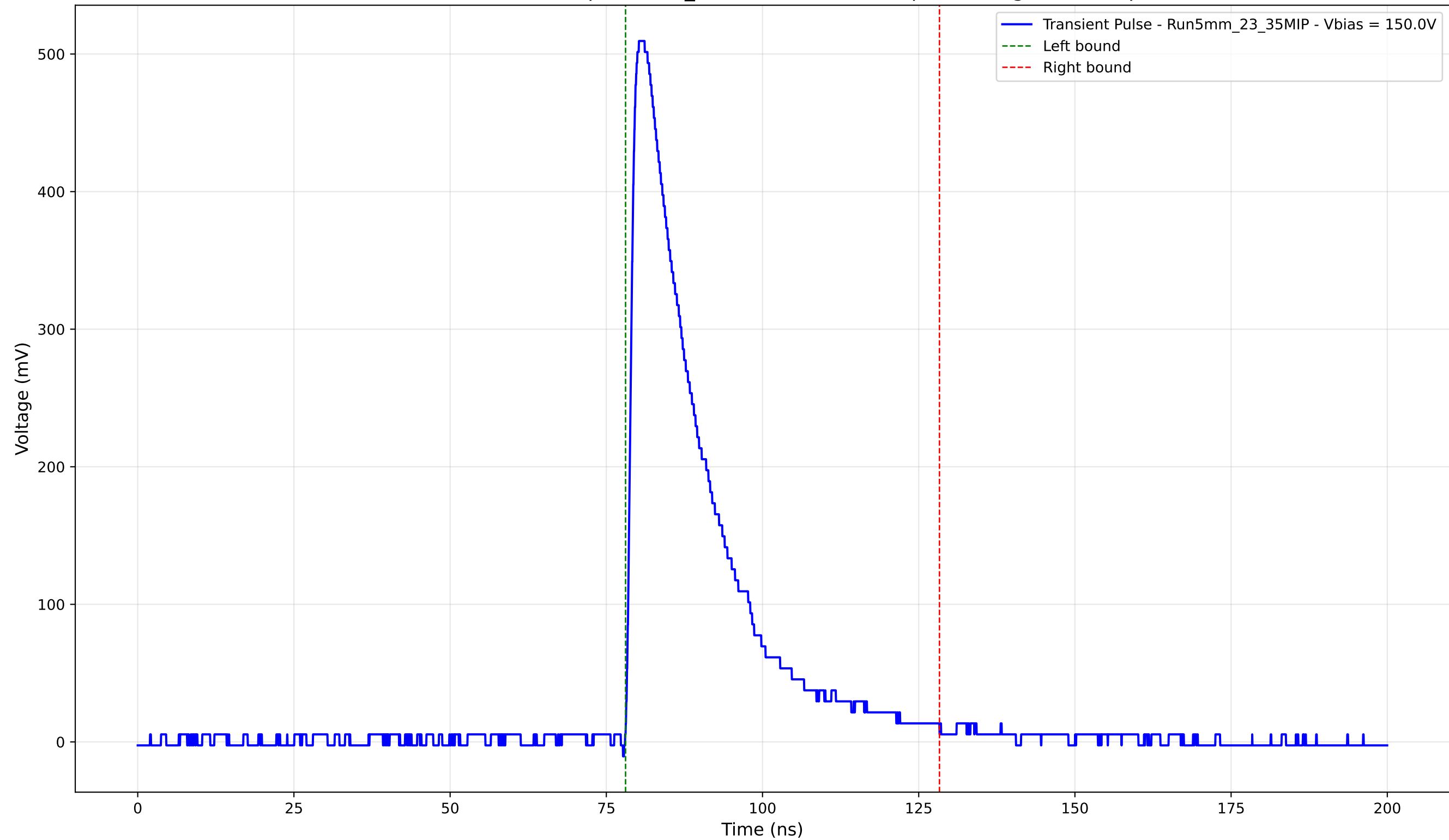
Transient Pulse - Sample: 5mm_23 - Position: 3470.0 \mu\text{m} - Charge: 129.42 pC
