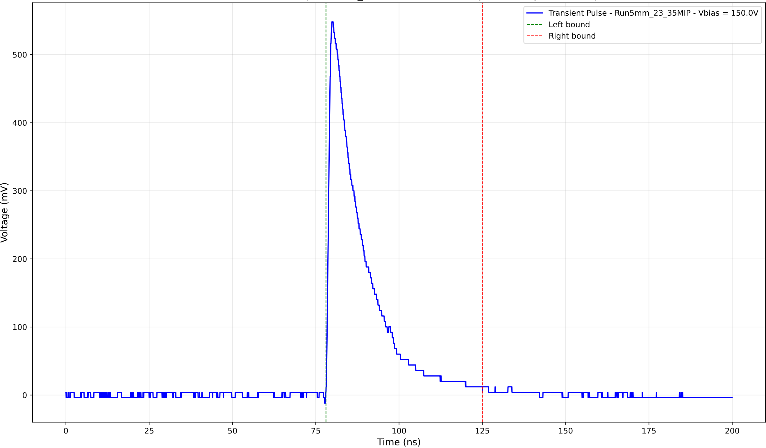
Transient Pulse - Sample: 5mm_23 - Position: 3835.0 \mu\text{m} - Charge: 122.07 pC
