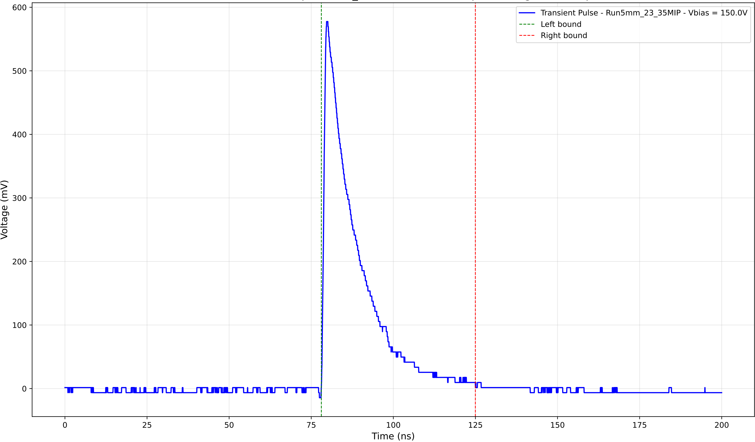
Transient Pulse - Sample: 5mm_23 - Position: 1230.0 \mu\text{m} - Charge: 122.22 pC
