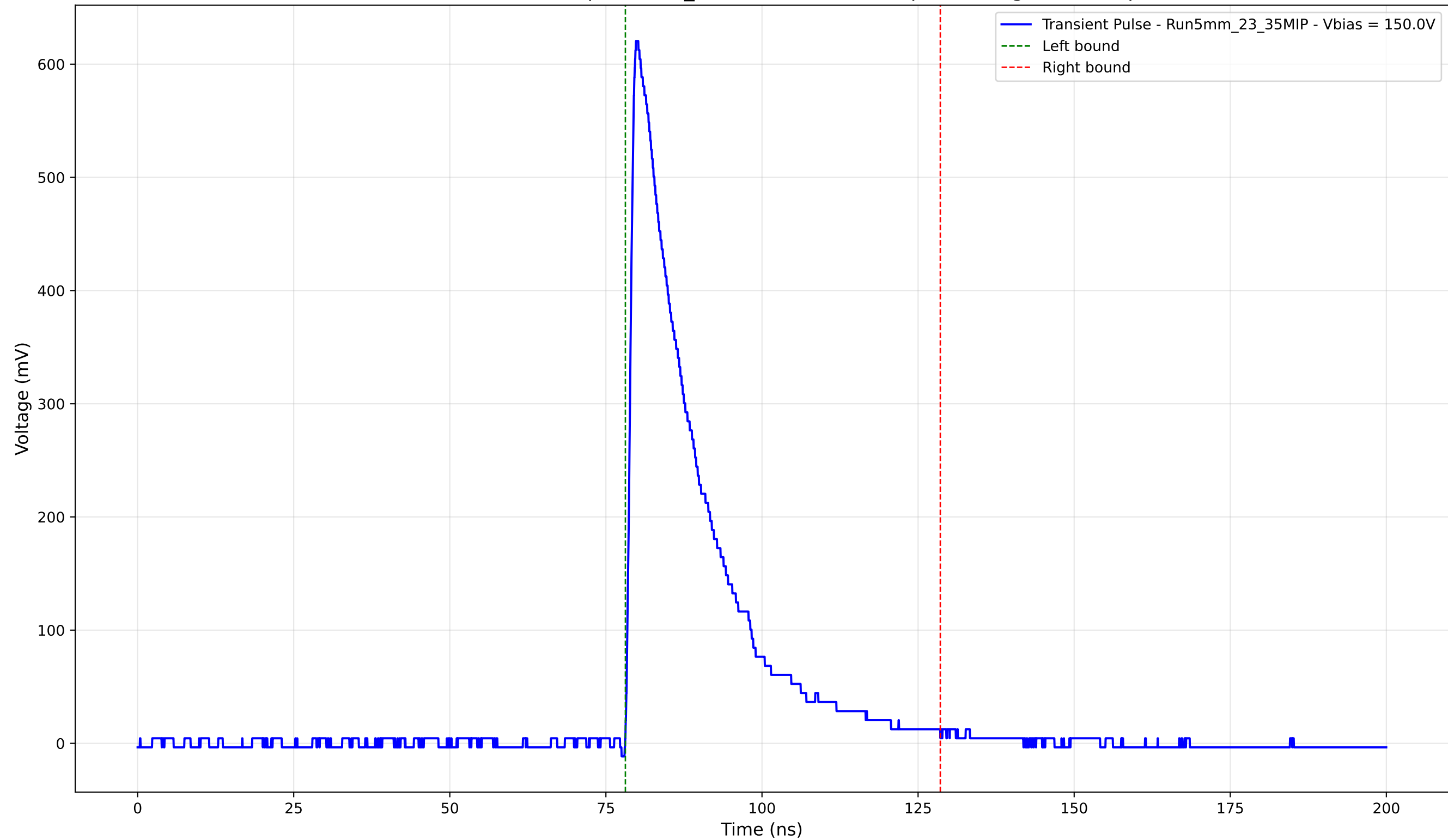
Transient Pulse - Sample: 5mm_23 - Position: 1395.0 \mu\text{m} - Charge: 143.24 pC
