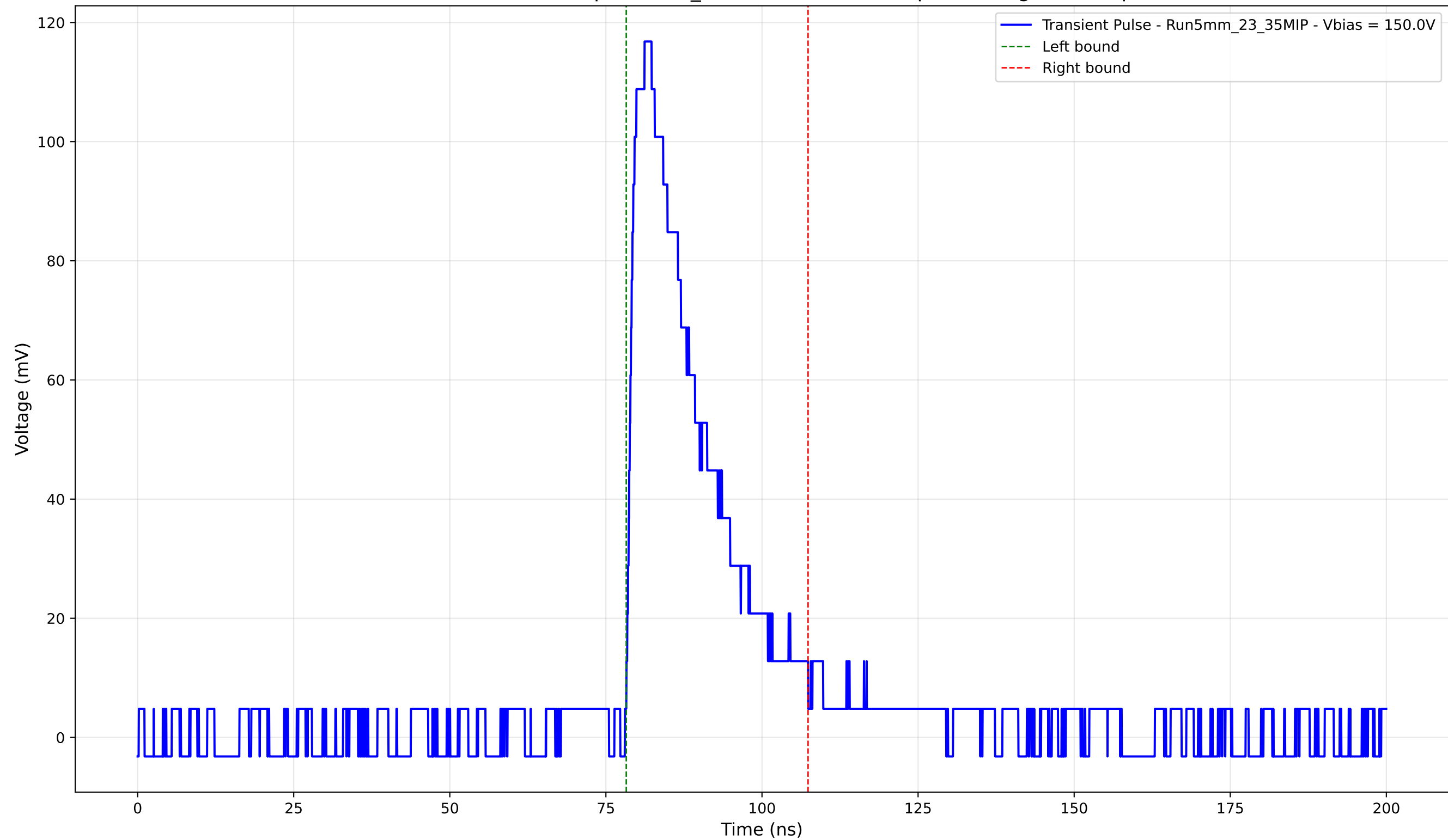
Transient Pulse - Sample: 5mm_23 - Position: 3130.0 \mu\text{m} - Charge: 28.97 pC
