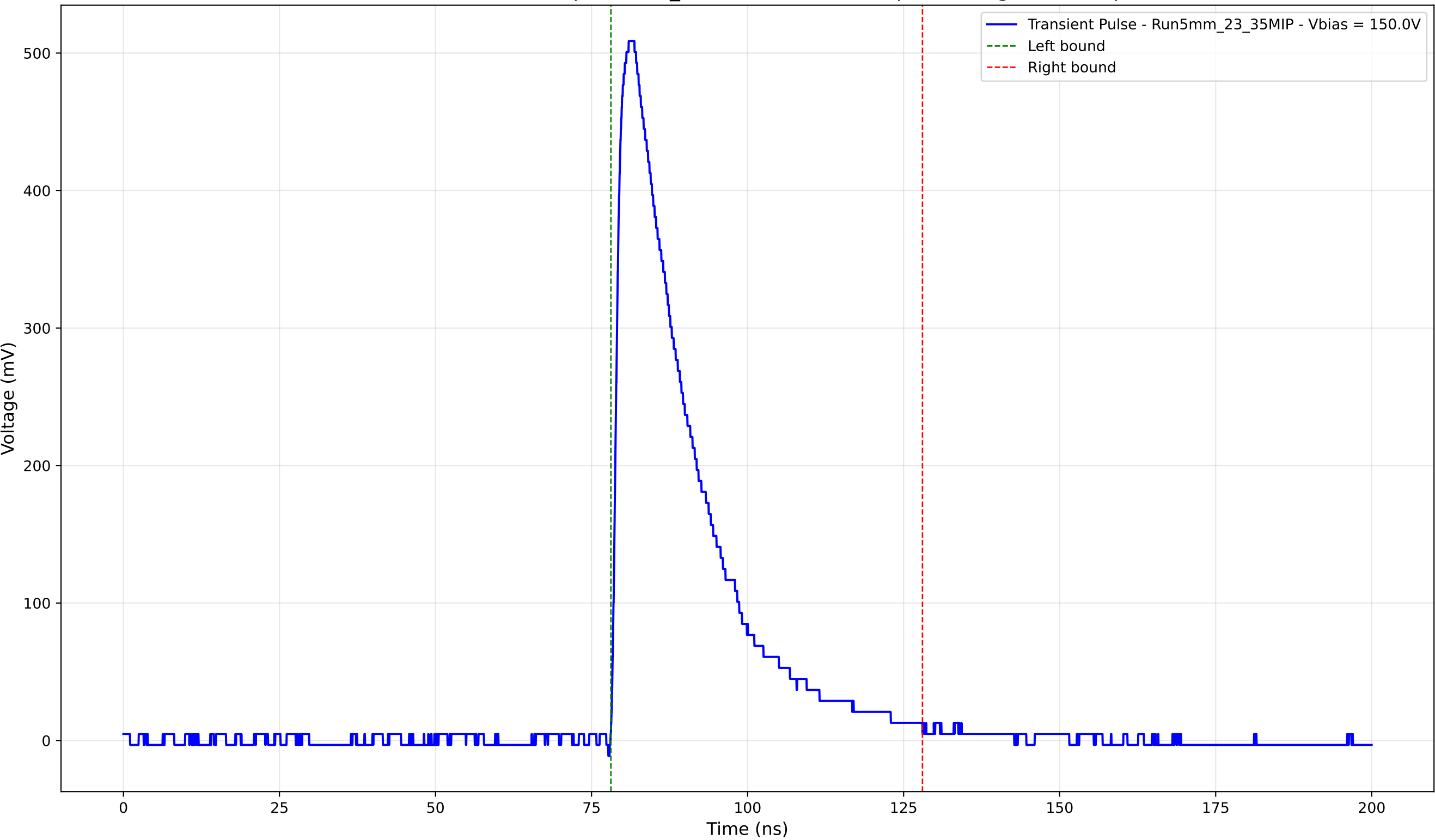
Transient Pulse - Sample: 5mm_23 - Position: 2330.0 \mu\text{m} - Charge: 137.56 pC
