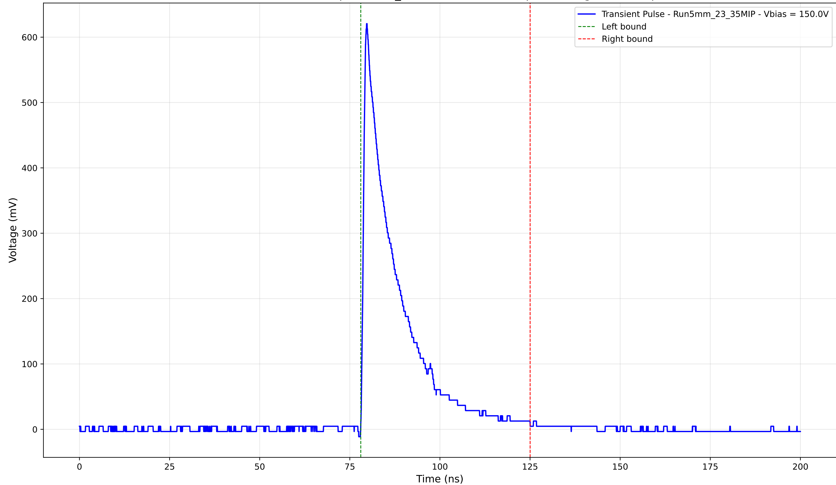
Transient Pulse - Sample: 5mm_23 - Position: 1030.0 \mu\text{m} - Charge: 120.05 pC
