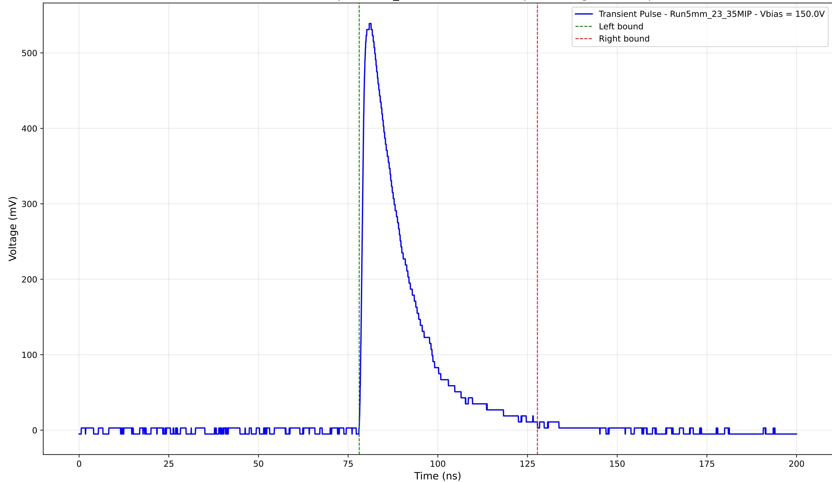
Transient Pulse - Sample: 5mm_23 - Position: 1940.0 \mu\text{m} - Charge: 140.62 pC
