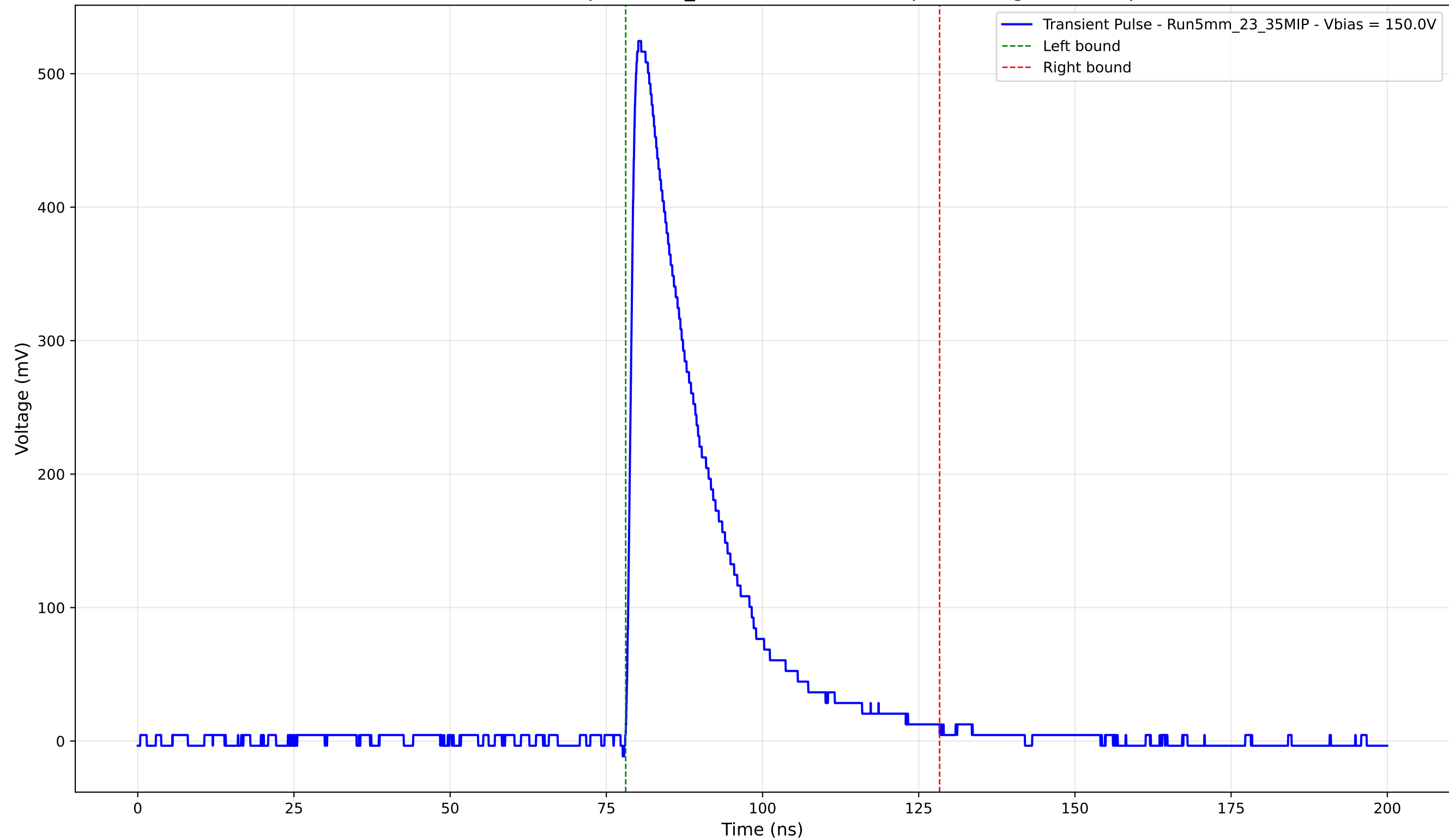
Transient Pulse - Sample: 5mm_23 - Position: 1745.0 \mu\text{m} - Charge: 133.03 pC
