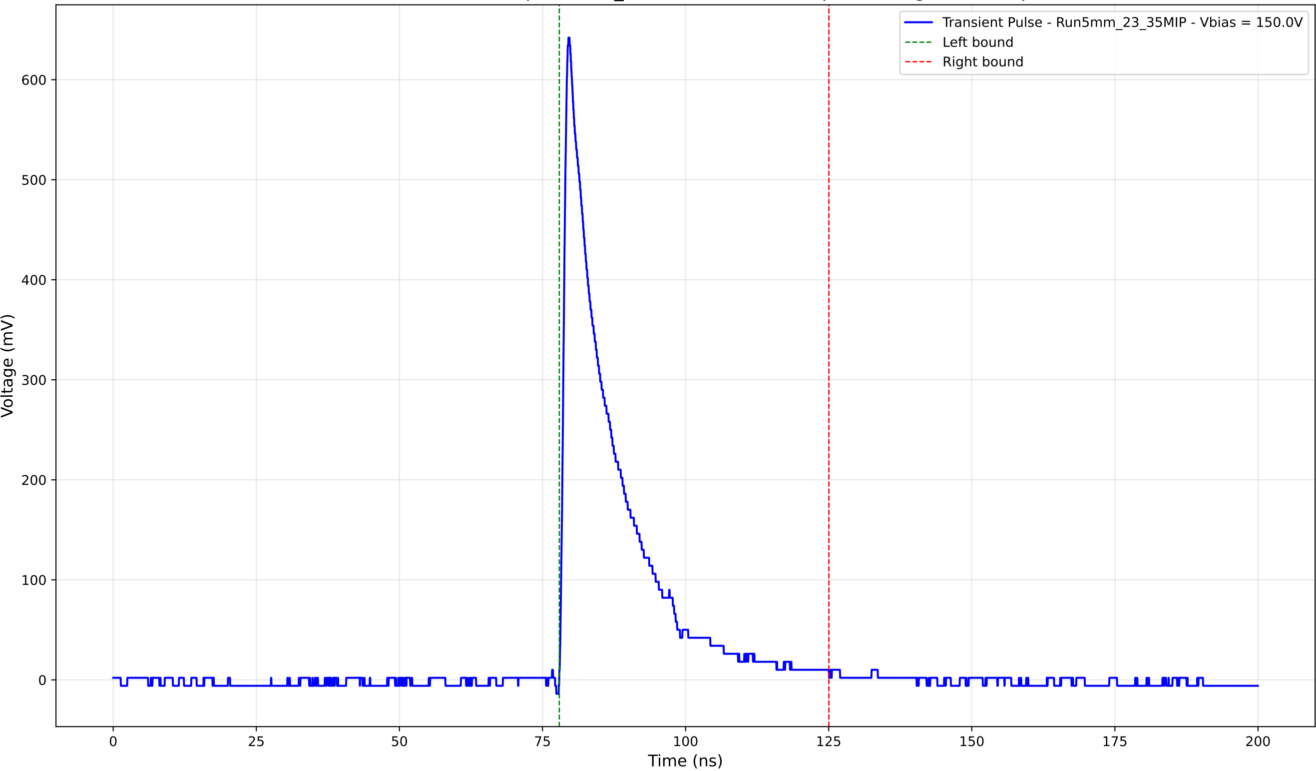
Transient Pulse - Sample: 5mm_23 - Position: 4335.0 \mu\text{m} - Charge: 115.80 pC
