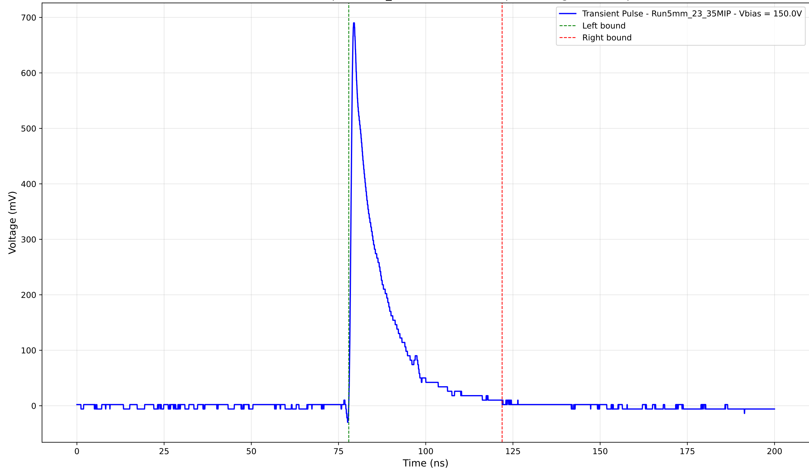
Transient Pulse - Sample: 5mm_23 - Position: 720.0 \mu\text{m} - Charge: 114.53 pC
