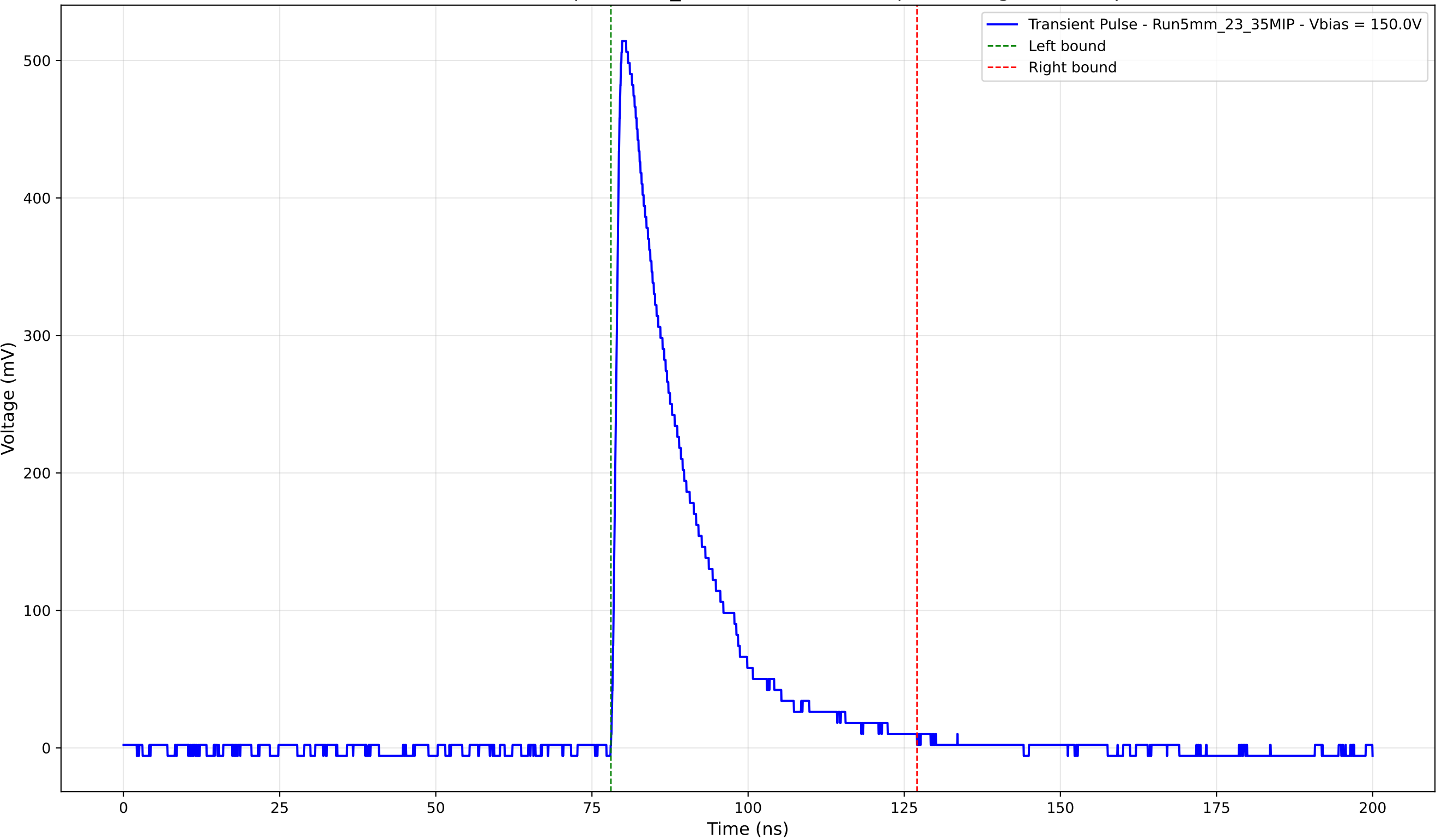
Transient Pulse - Sample: 5mm_23 - Position: 3745.0 \mu\text{m} - Charge: 119.47 pC
