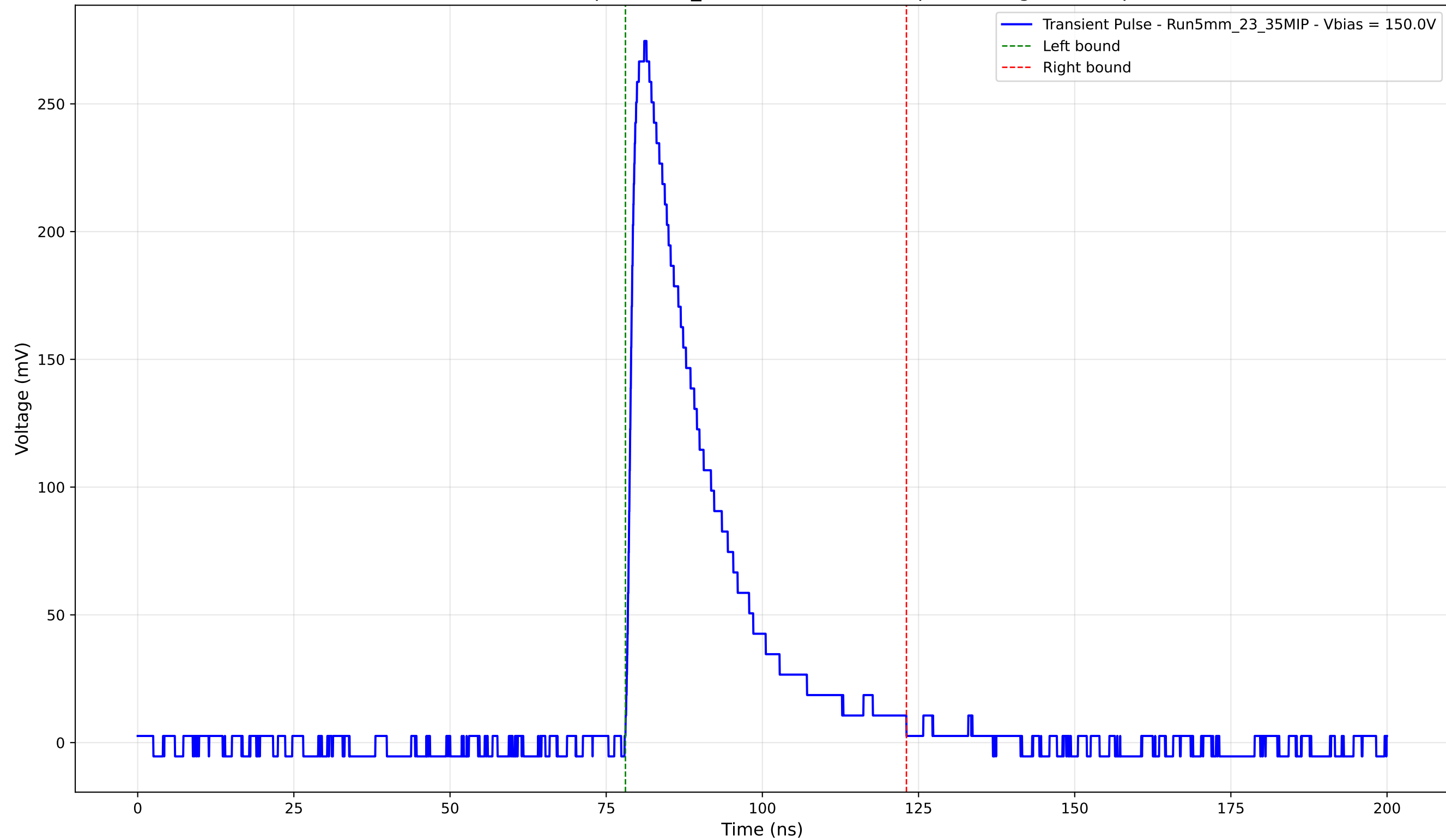
Transient Pulse - Sample: 5mm_23 - Position: 3190.0 \mu\text{m} - Charge: 69.67 pC
