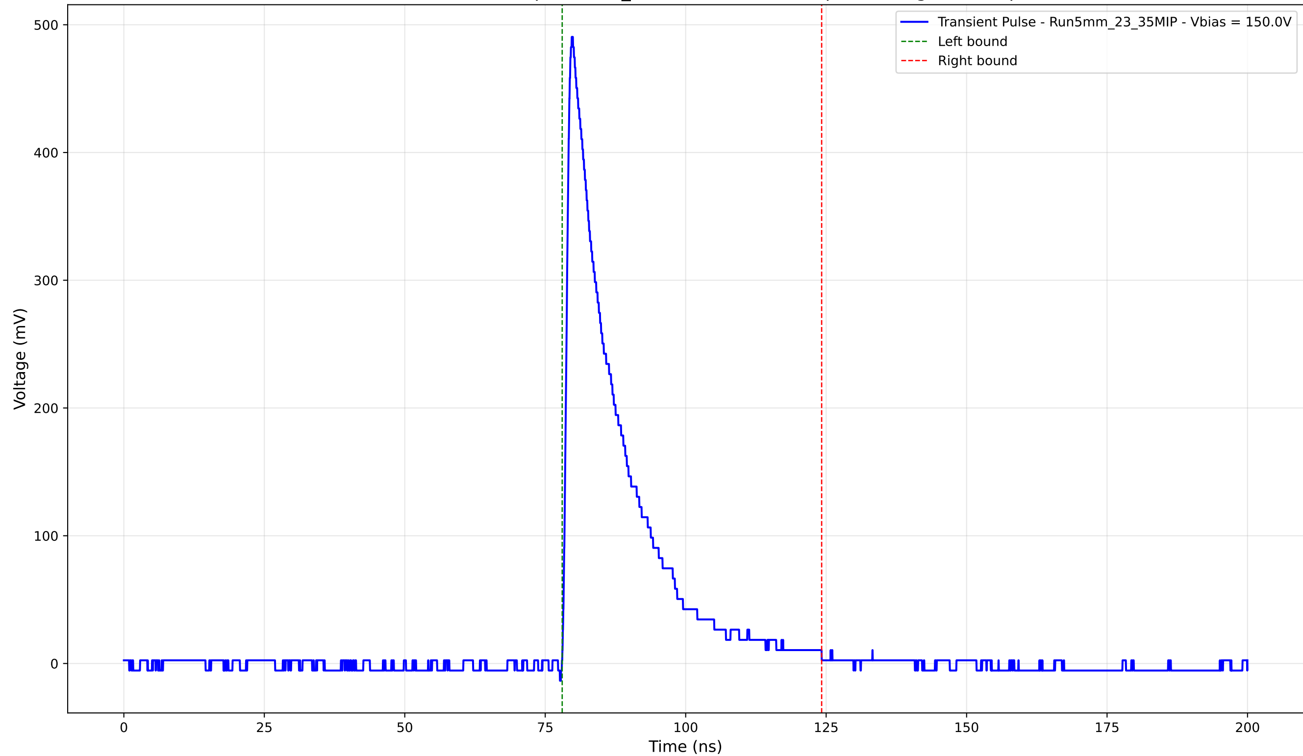
Transient Pulse - Sample: 5mm_23 - Position: 4085.0 \mu\text{m} - Charge: 97.12 pC
