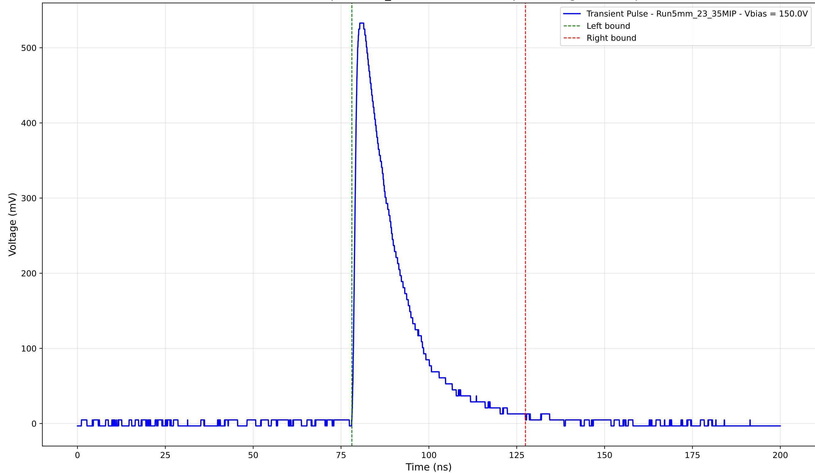
Transient Pulse - Sample: 5mm_23 - Position: 1900.0 \mu\text{m} - Charge: 139.28 pC
