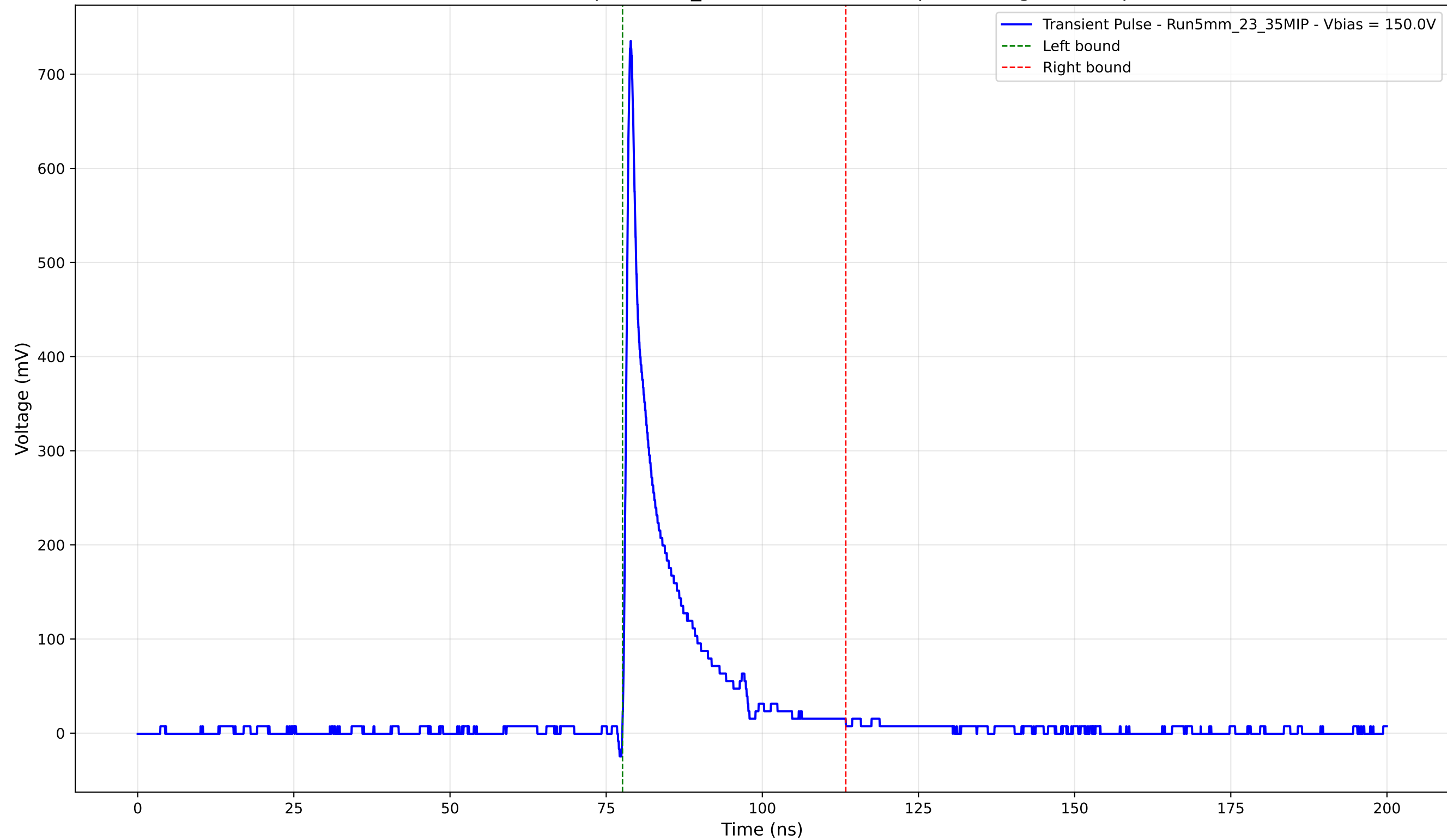
Transient Pulse - Sample: 5mm_23 - Position: 5045.0 \mu\text{m} - Charge: 80.97 pC
