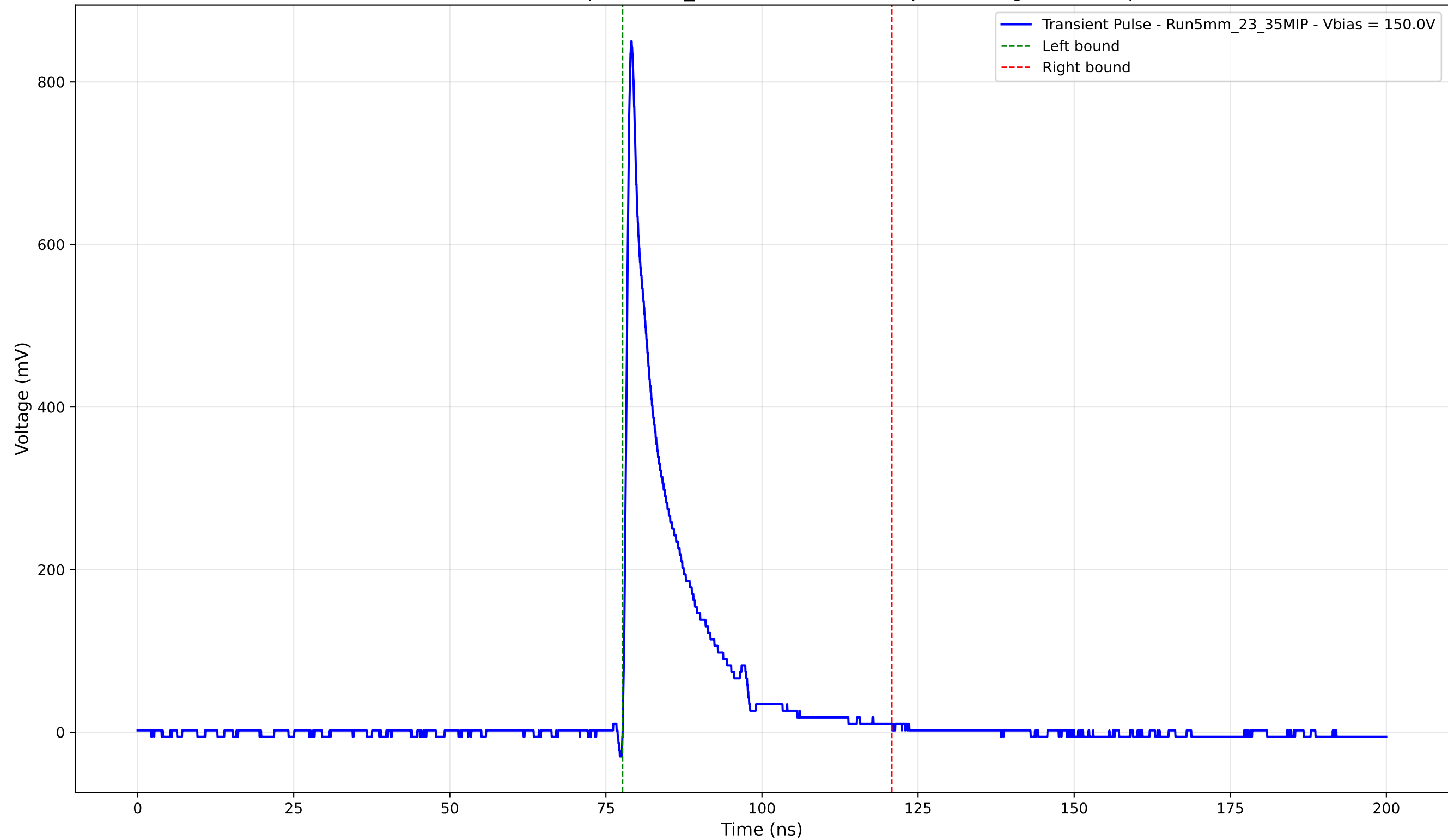
Transient Pulse - Sample: 5mm_23 - Position: 4865.0 \mu\text{m} - Charge: 113.54 pC
