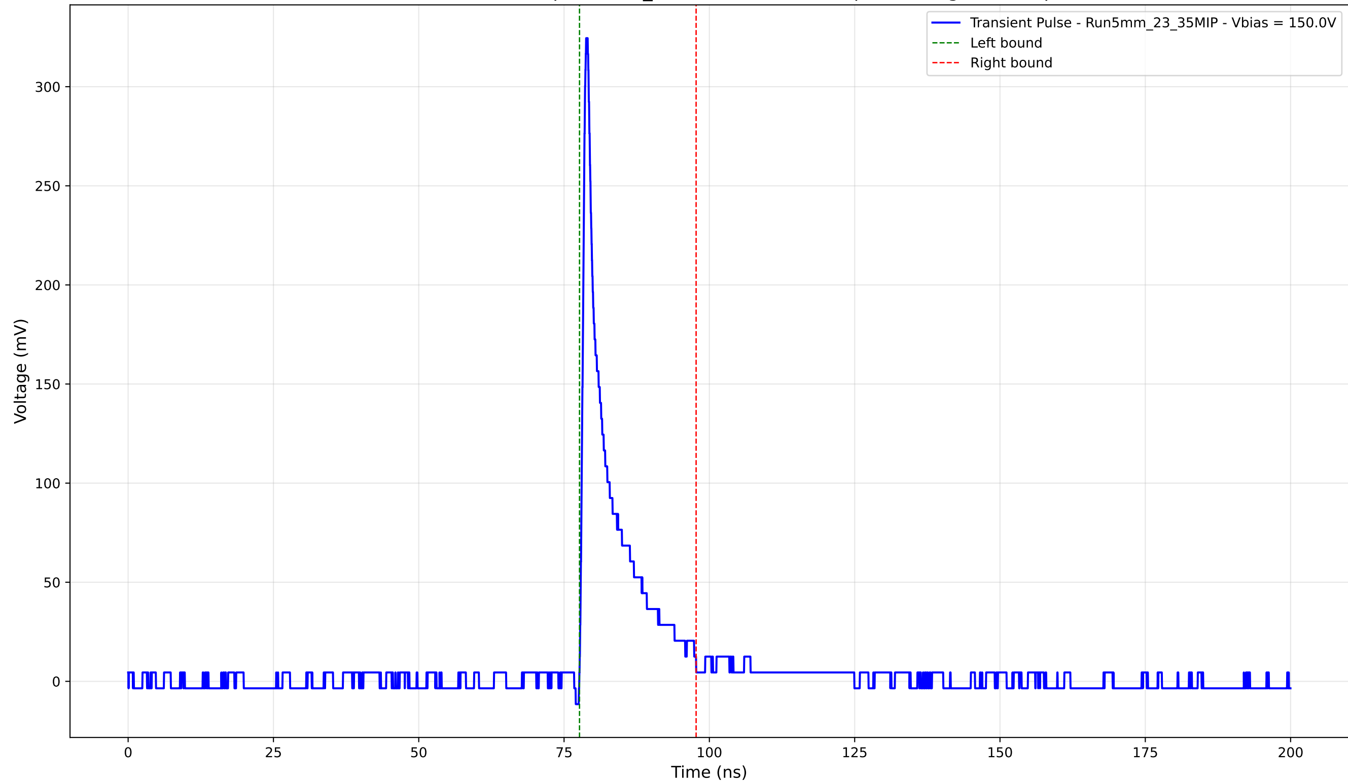
Transient Pulse - Sample: 5mm_23 - Position: 5080.0 \mu\text{m} - Charge: 30.96 pC
