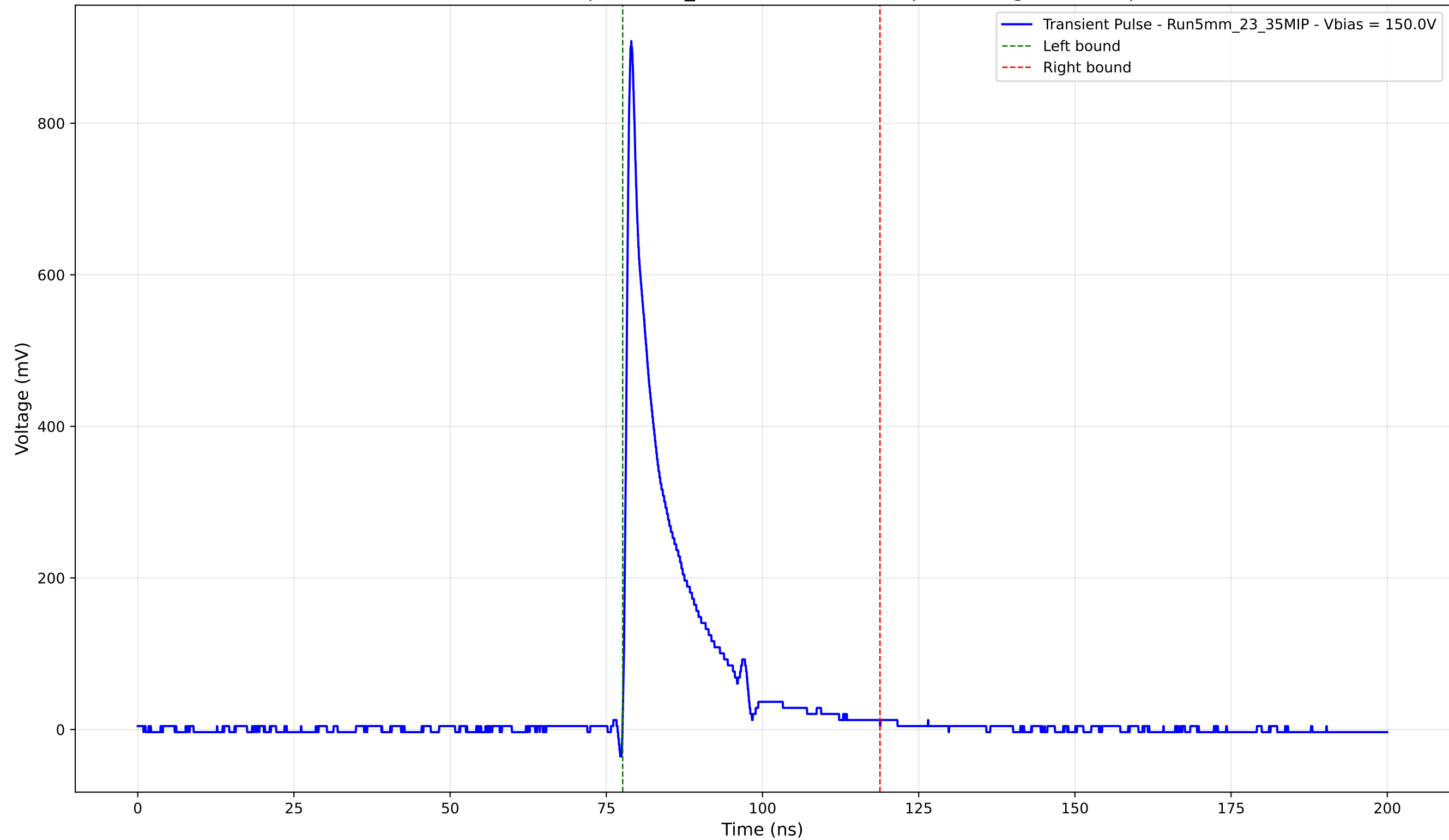
Transient Pulse - Sample: 5mm_23 - Position: 4970.0 \mu\text{m} - Charge: 118.37 pC
