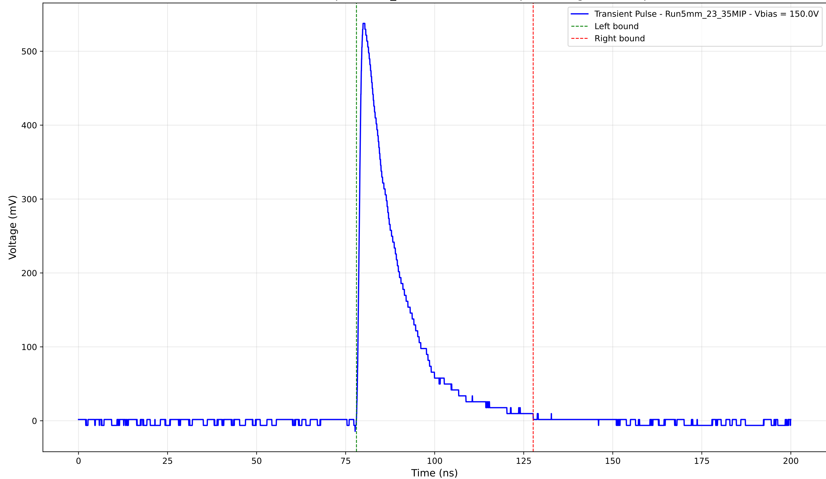
Transient Pulse - Sample: 5mm_23 - Position: 3770.0 \mu\text{m} - Charge: 123.52 pC
