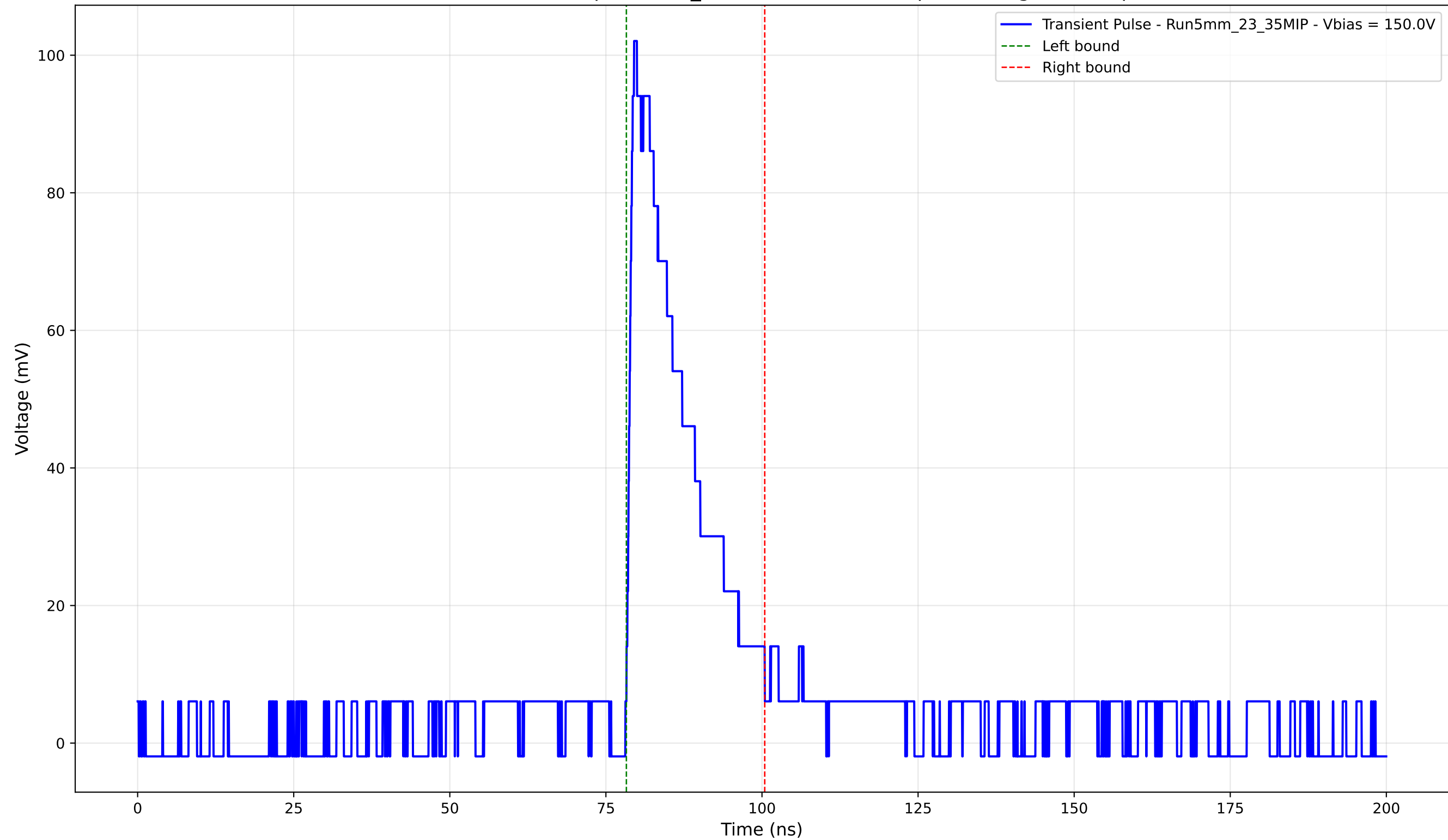
Transient Pulse - Sample: 5mm_23 - Position: 1120.0 \mu\text{m} - Charge: 20.15 pC
