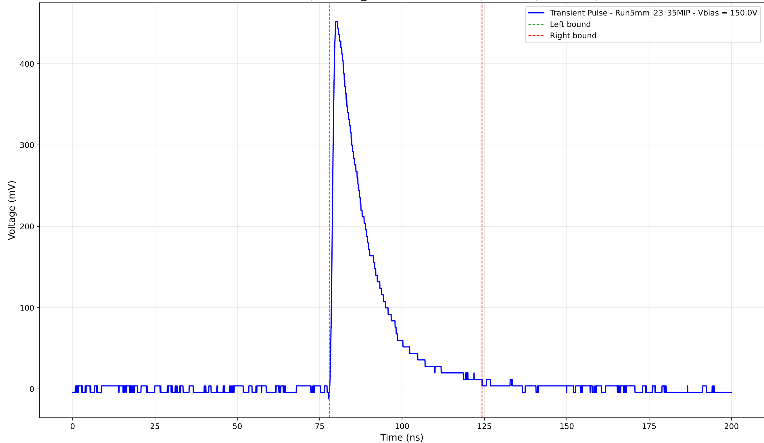
Transient Pulse - Sample: 5mm_23 - Position: 1550.0 \mu\text{m} - Charge: 105.70 pC
