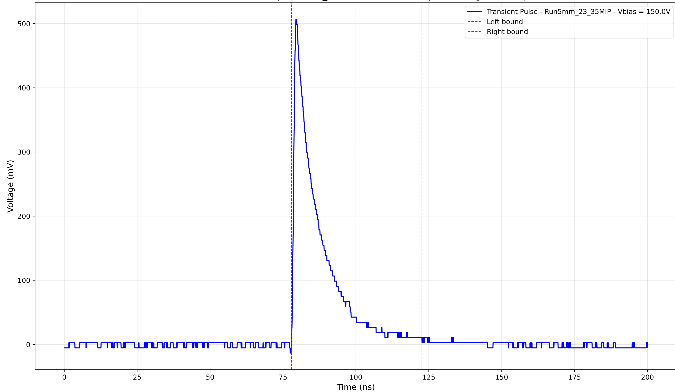
Transient Pulse - Sample: 5mm_23 - Position: 4460.0 \mu\text{m} - Charge: 91.48 pC
