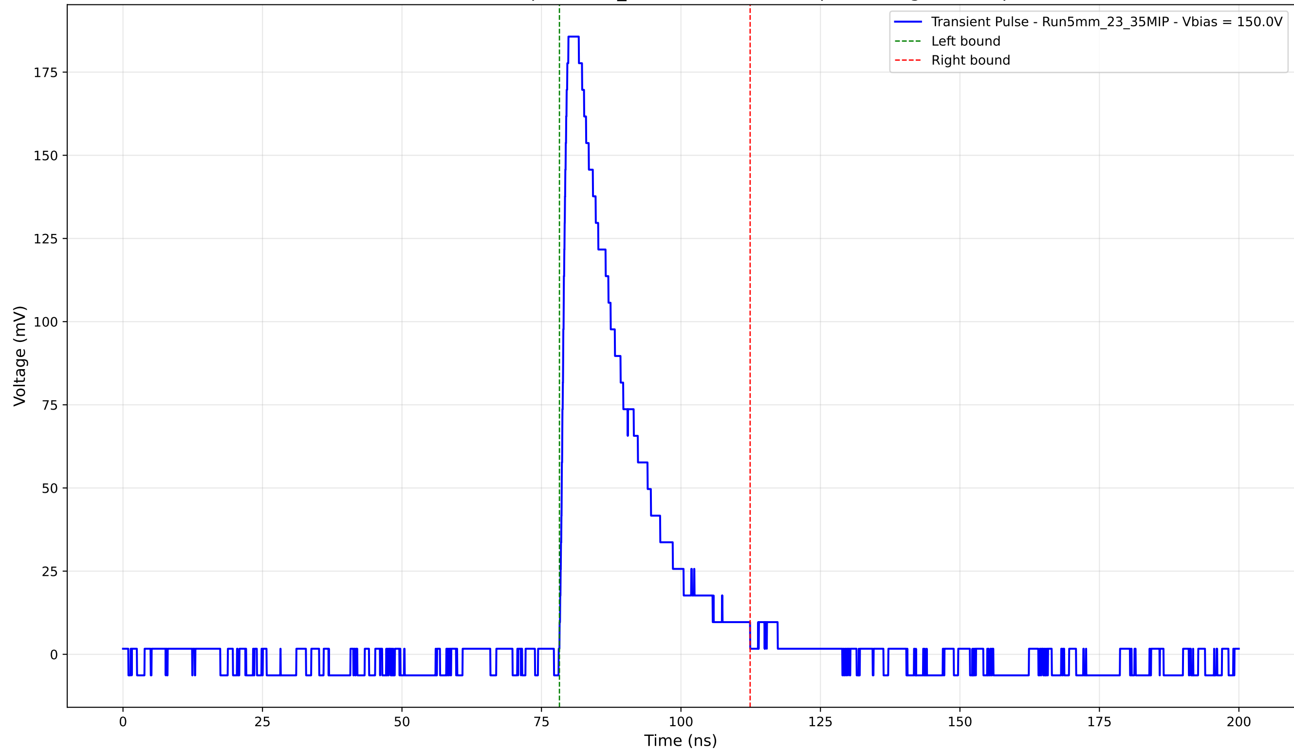
Transient Pulse - Sample: 5mm_23 - Position: 1655.0 \mu\text{m} - Charge: 43.61 pC
