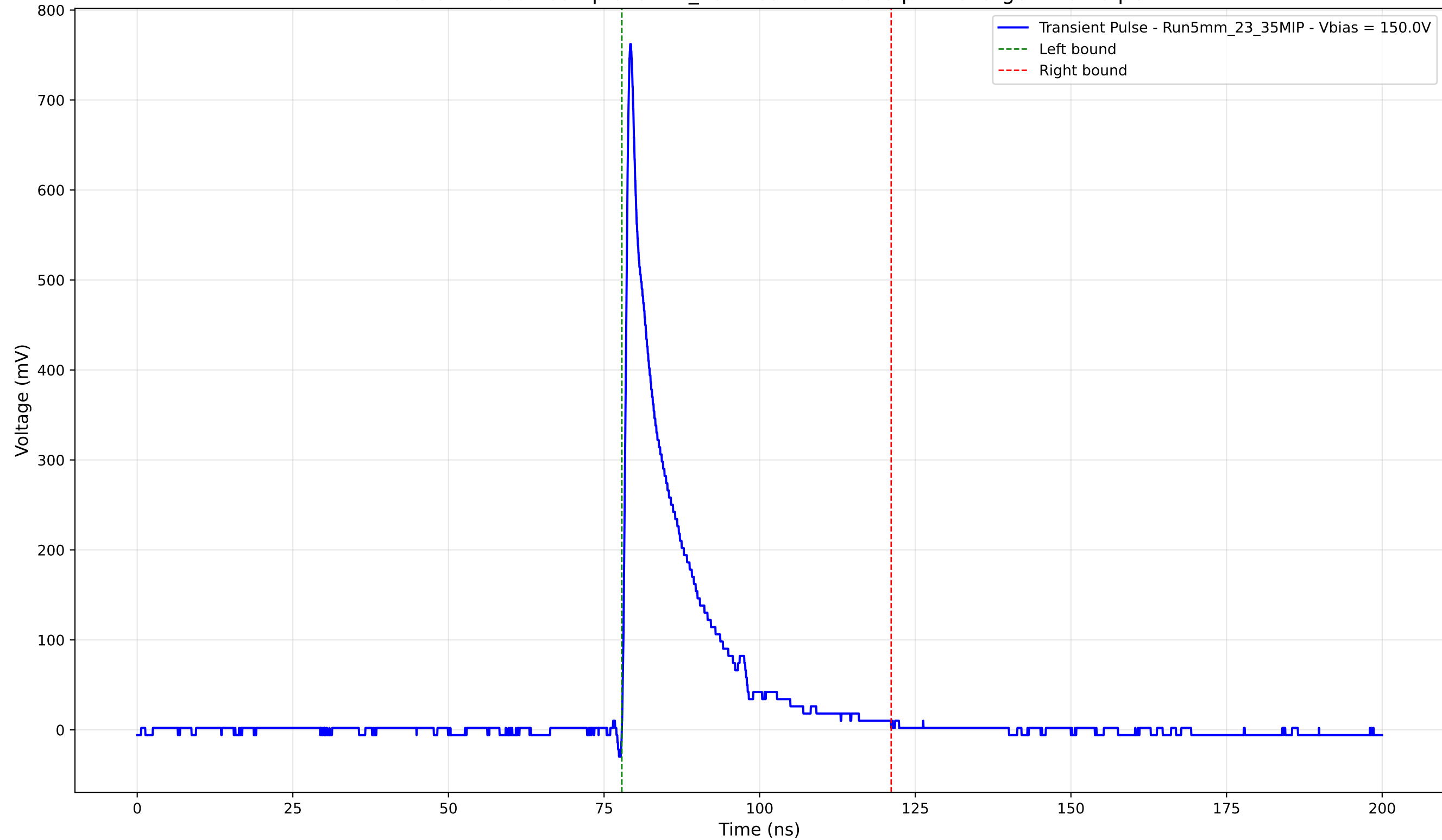
Transient Pulse - Sample: 5mm_23 - Position: 525.0 \mu\text{m} - Charge: 110.28 pC
