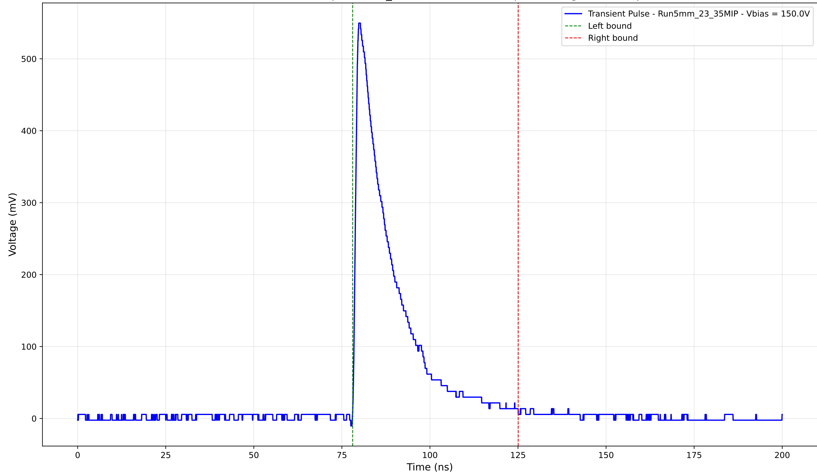
Transient Pulse - Sample: 5mm_23 - Position: 3880.0 \mu\text{m} - Charge: 123.18 pC
