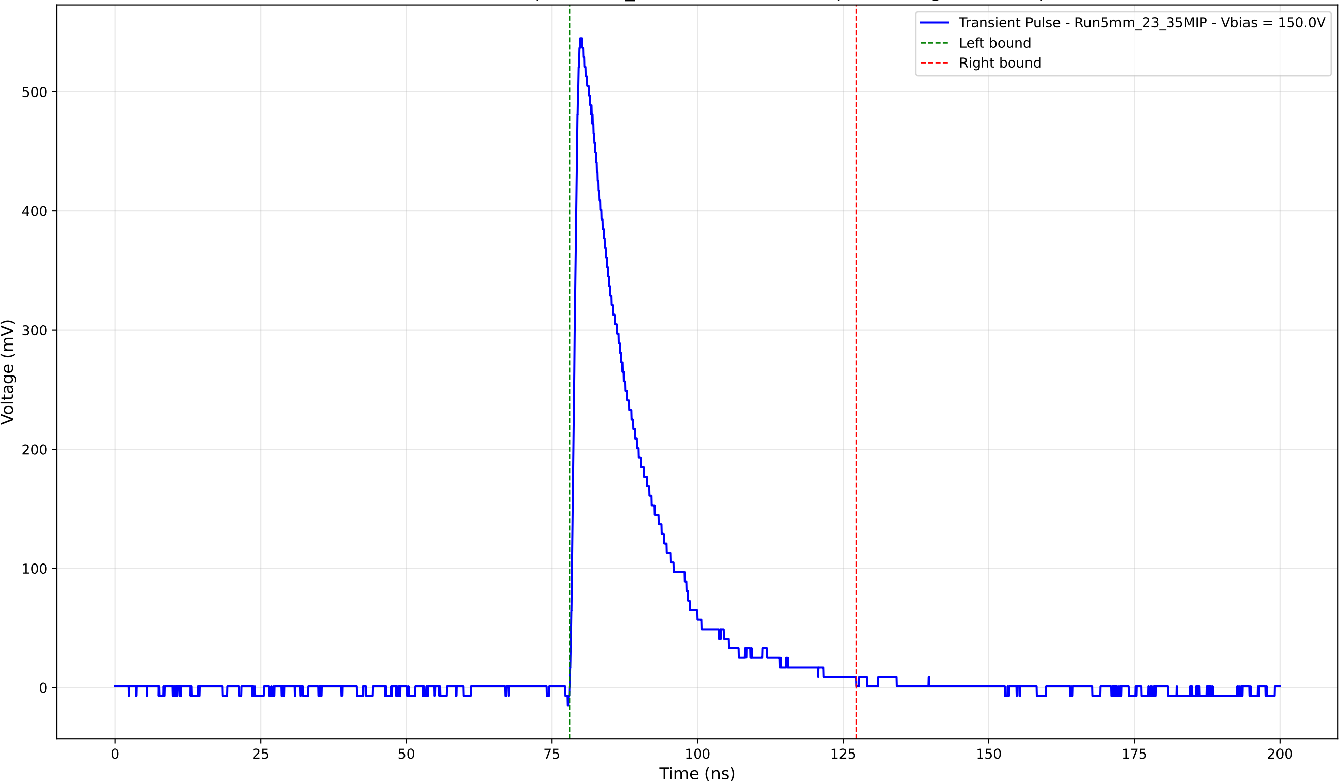
Transient Pulse - Sample: 5mm_23 - Position: 3860.0 \mu\text{m} - Charge: 120.44 pC
