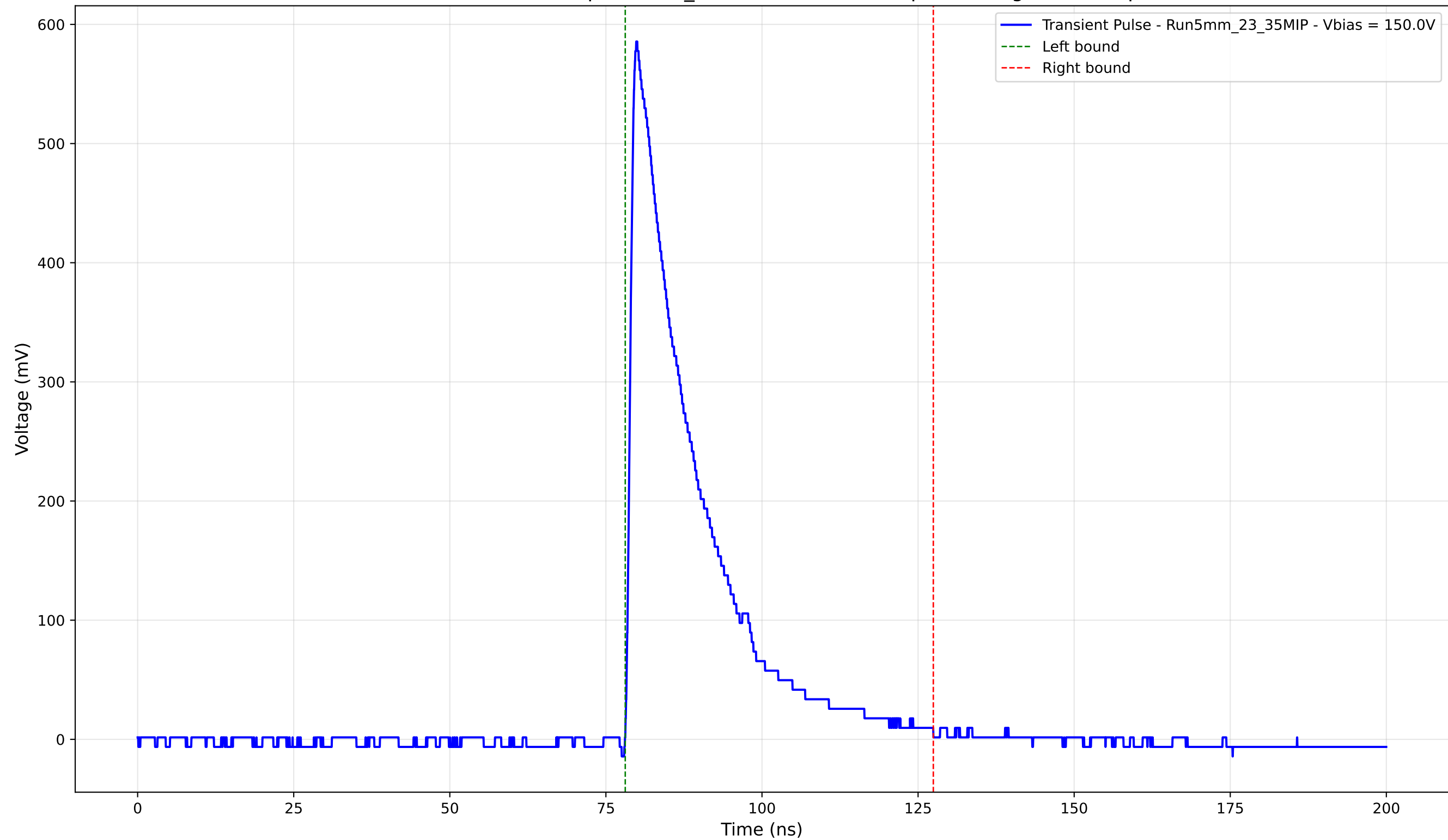
Transient Pulse - Sample: 5mm_23 - Position: 1330.0 \mu\text{m} - Charge: 129.69 pC
