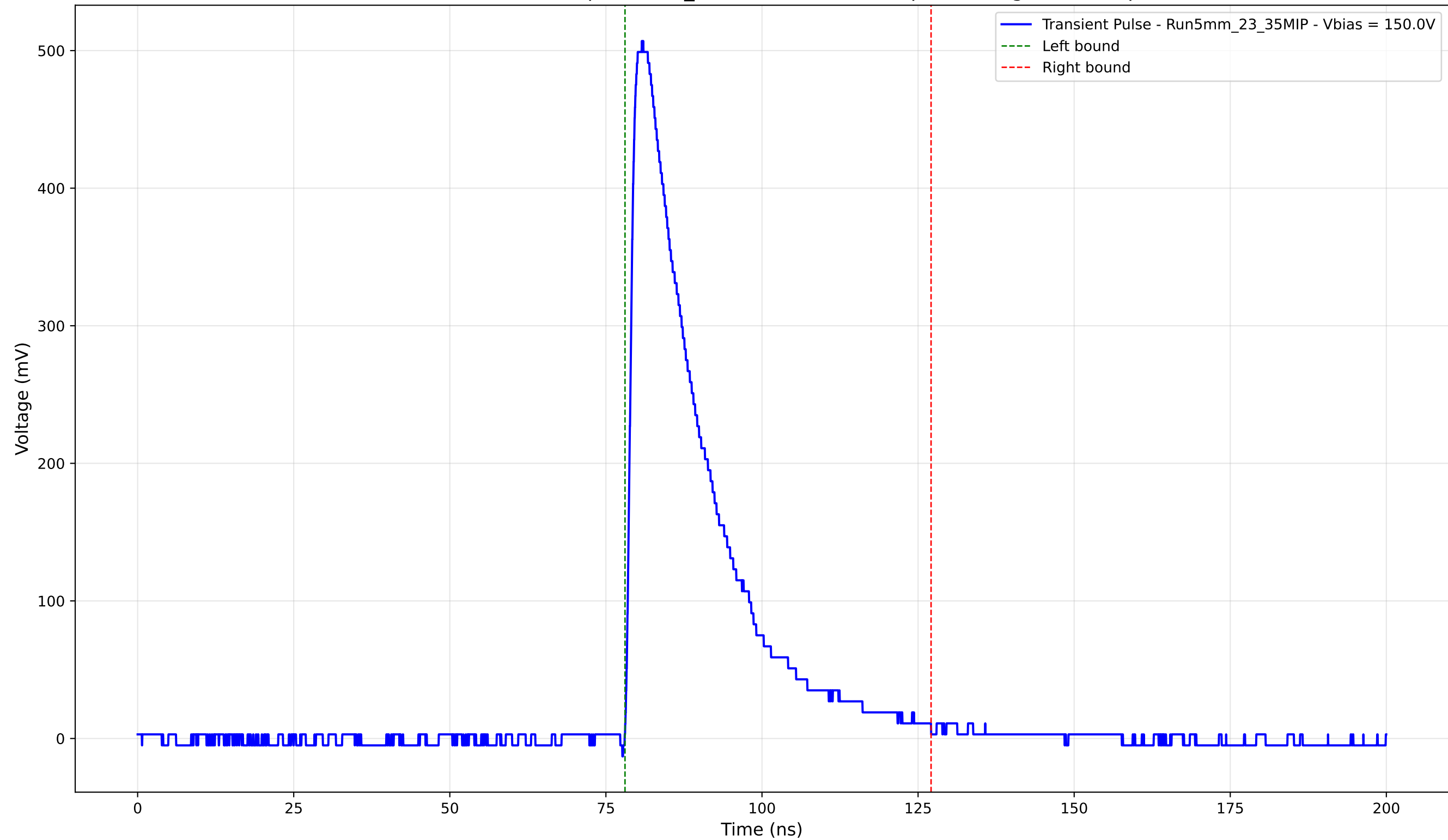
Transient Pulse - Sample: 5mm_23 - Position: 3335.0 \mu\text{m} - Charge: 129.95 pC
