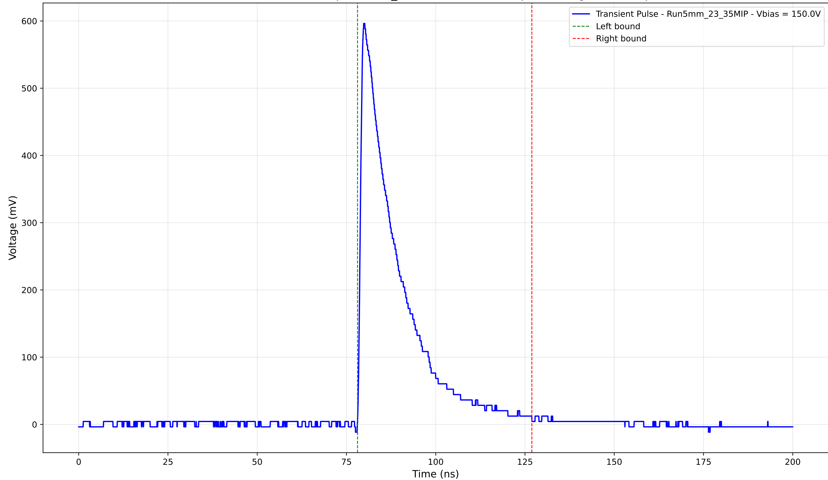
Transient Pulse - Sample: 5mm_23 - Position: 1370.0 \mu\text{m} - Charge: 136.28 pC
