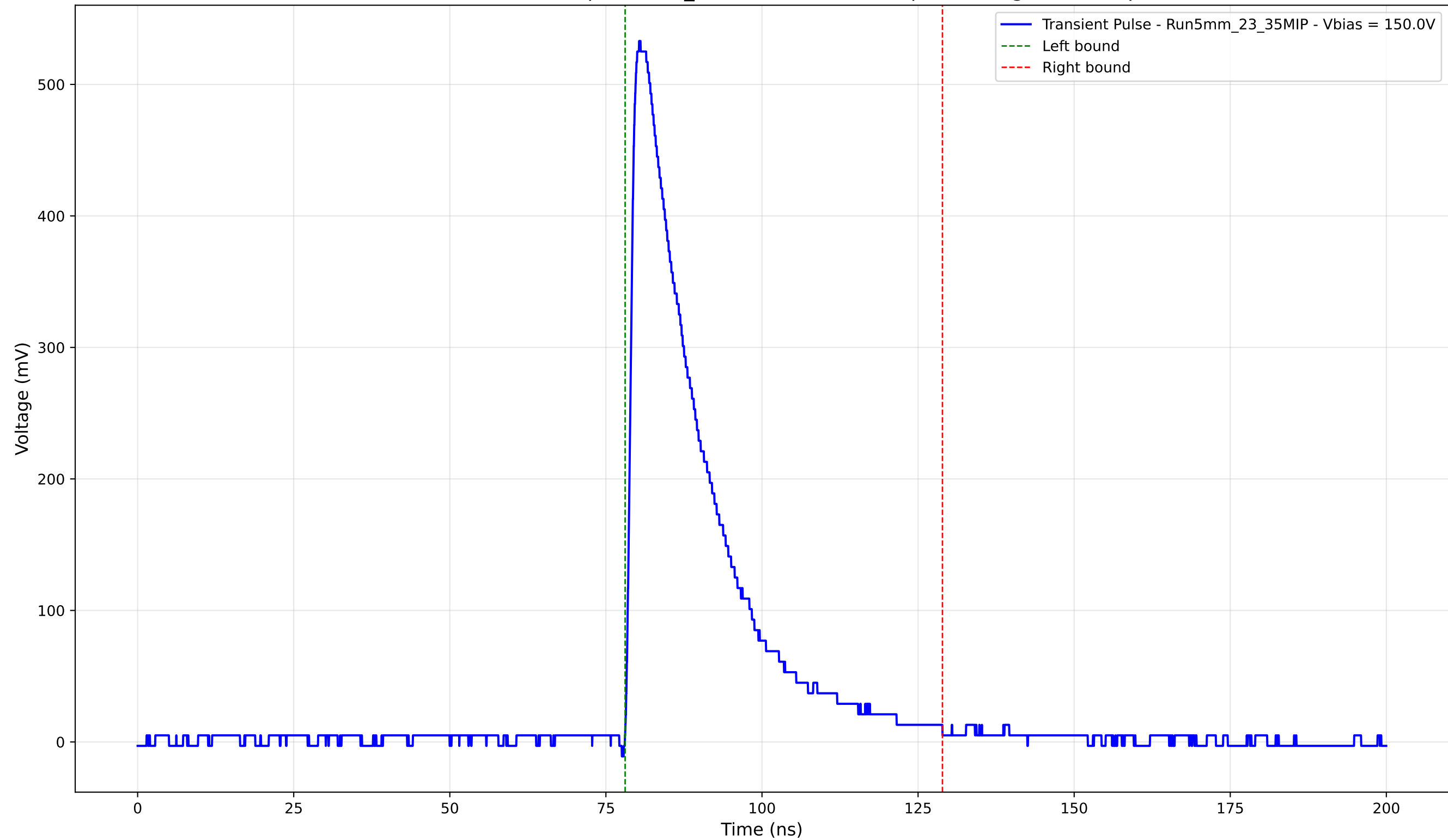
Transient Pulse - Sample: 5mm_23 - Position: 1780.0 \mu\text{m} - Charge: 136.02 pC
