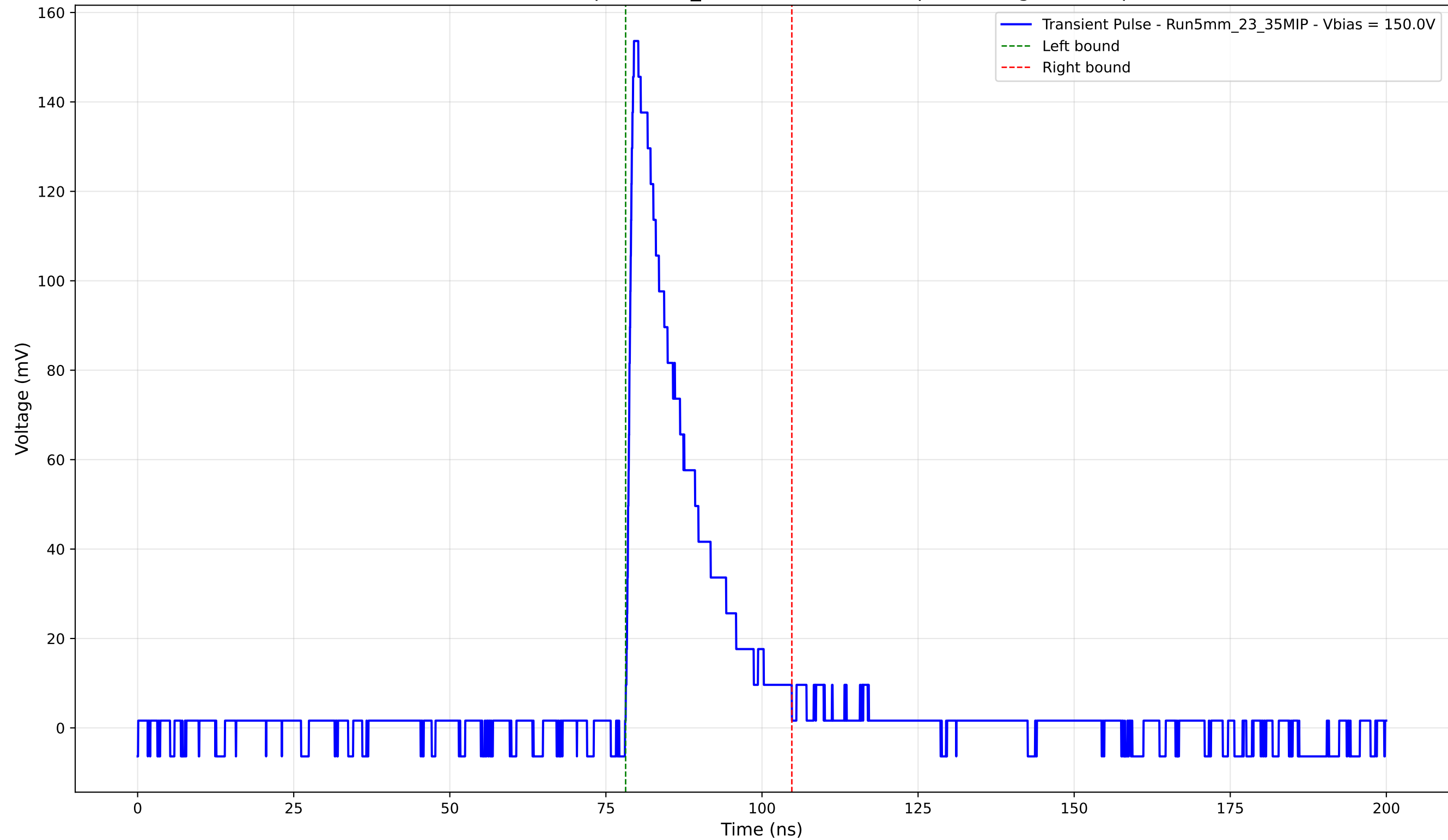
Transient Pulse - Sample: 5mm_23 - Position: 4135.0 \mu\text{m} - Charge: 28.29 pC
