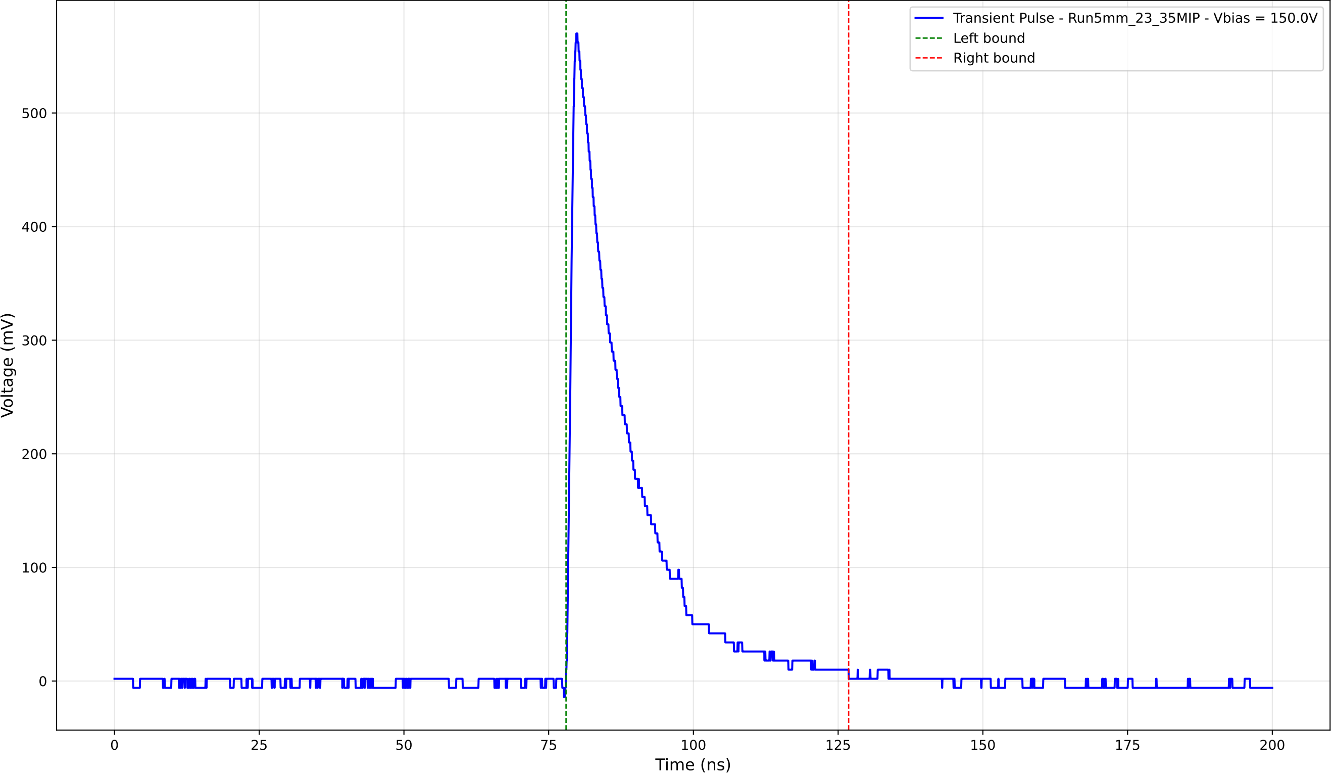
Transient Pulse - Sample: 5mm_23 - Position: 4020.0 \mu\text{m} - Charge: 117.98 pC
