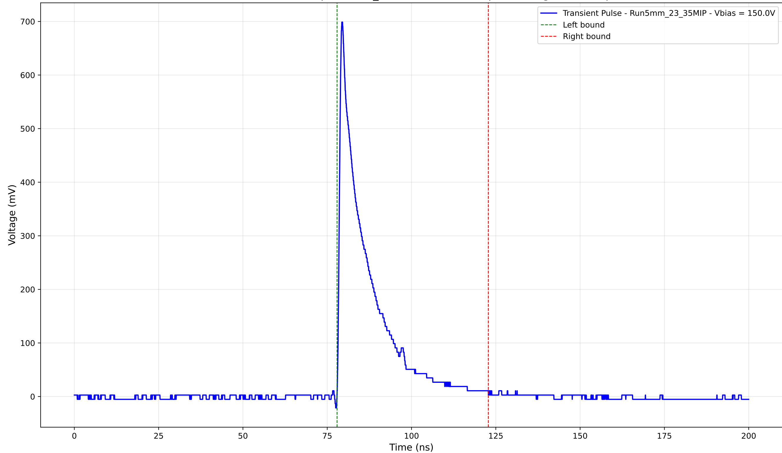
Transient Pulse - Sample: 5mm_23 - Position: 730.0 \mu\text{m} - Charge: 117.75 pC
