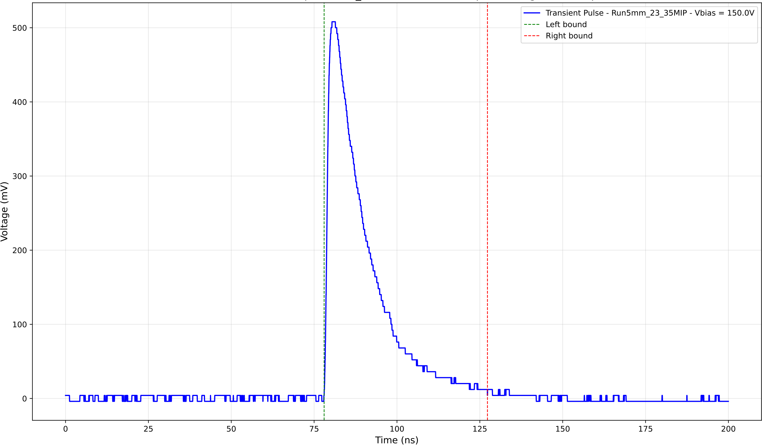
Transient Pulse - Sample: 5mm_23 - Position: 2050.0 \mu\text{m} - Charge: 134.62 pC
