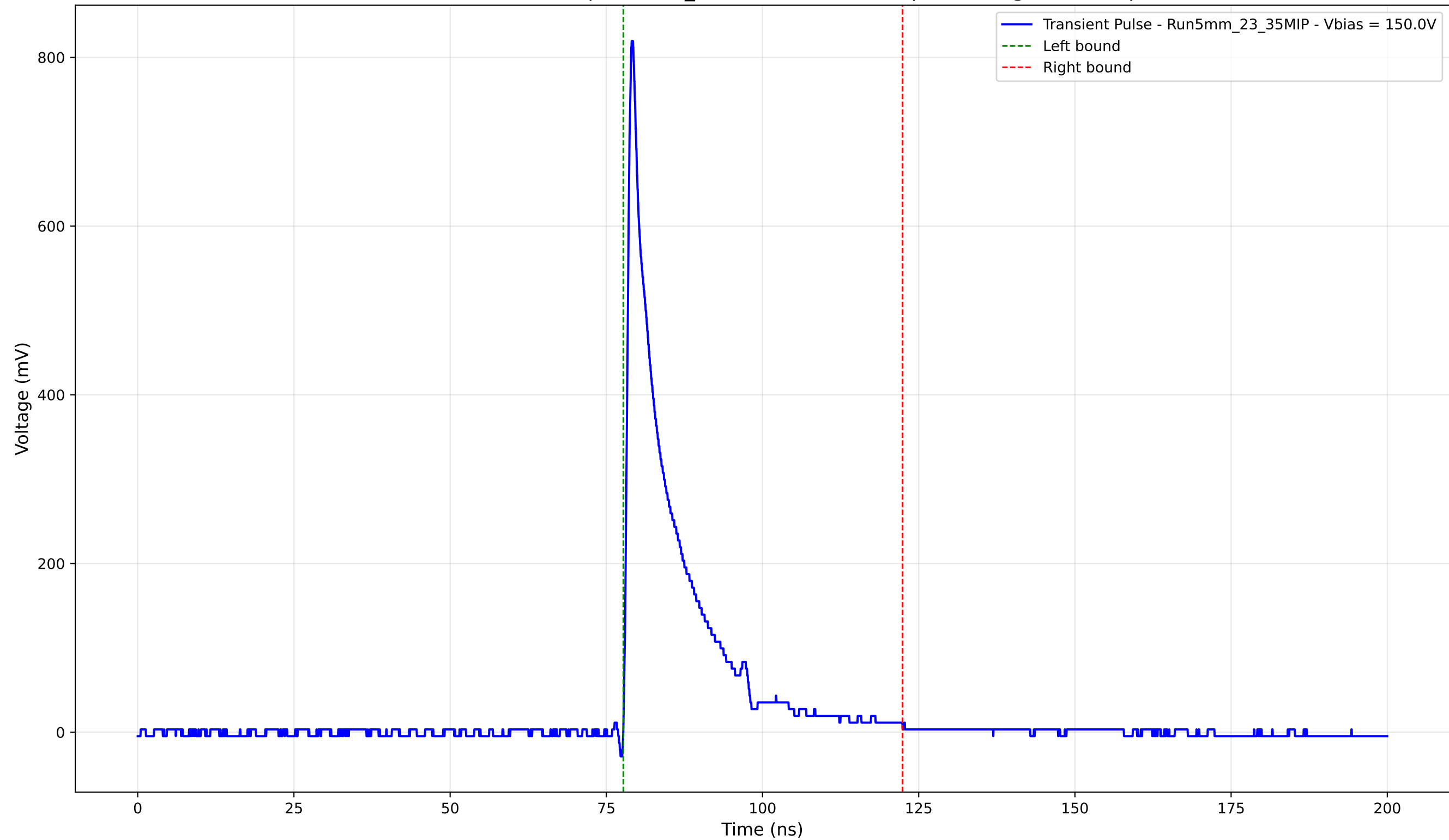
Transient Pulse - Sample: 5mm_23 - Position: 4820.0 \mu\text{m} - Charge: 113.75 pC
