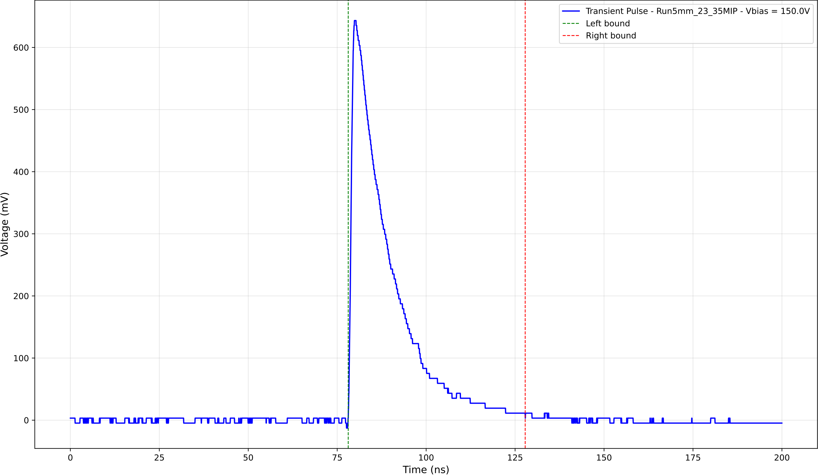
Transient Pulse - Sample: 5mm_23 - Position: 1455.0 \mu\text{m} - Charge: 150.81 pC
