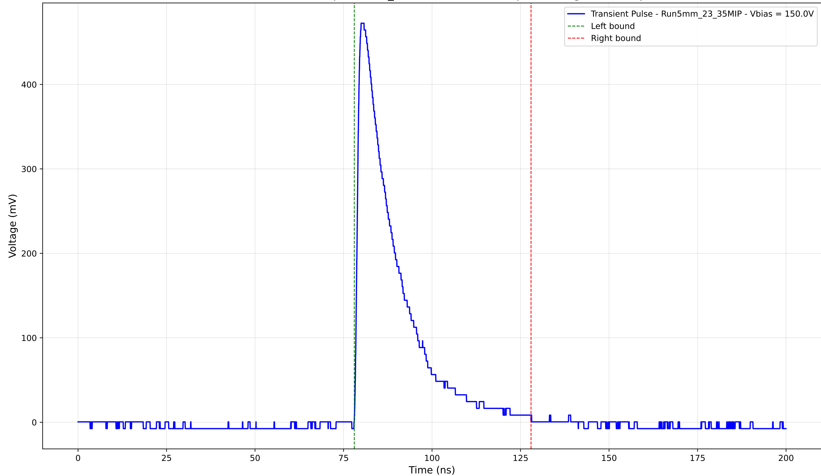
Transient Pulse - Sample: 5mm_23 - Position: 3570.0 \mu\text{m} - Charge: 113.81 pC
