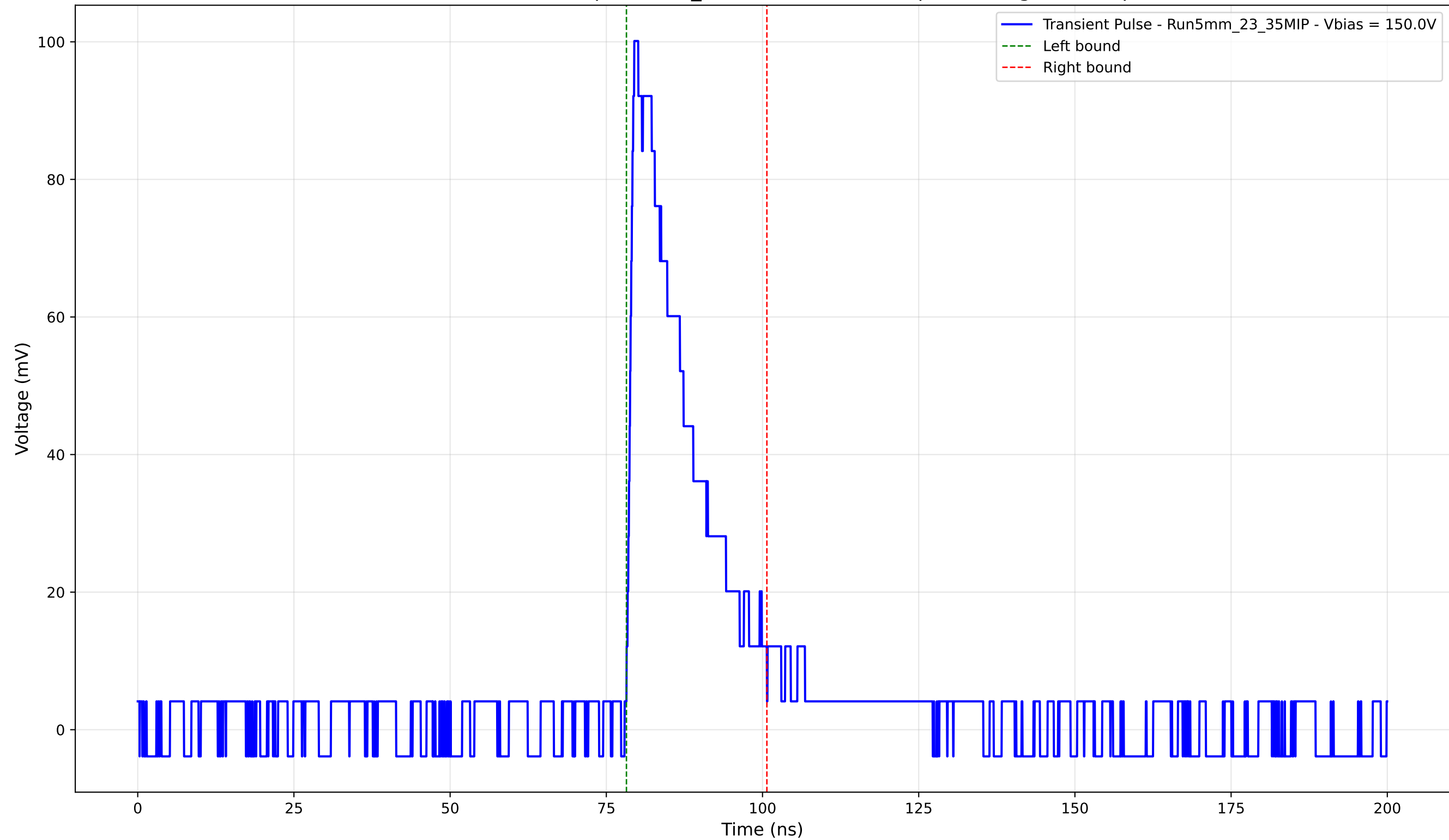
Transient Pulse - Sample: 5mm_23 - Position: 1130.0 \mu\text{m} - Charge: 20.05 pC
