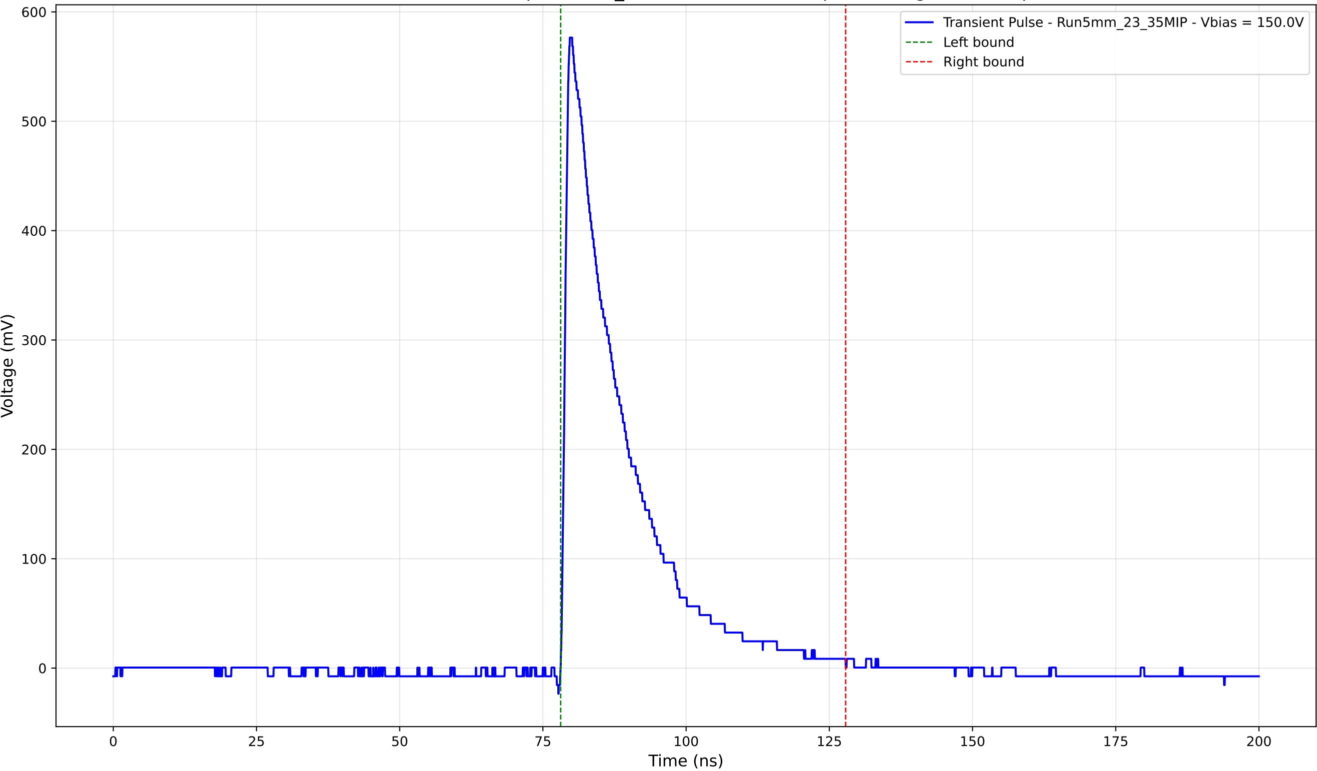
Transient Pulse - Sample: 5mm_23 - Position: 1260.0 \mu\text{m} - Charge: 124.51 pC
