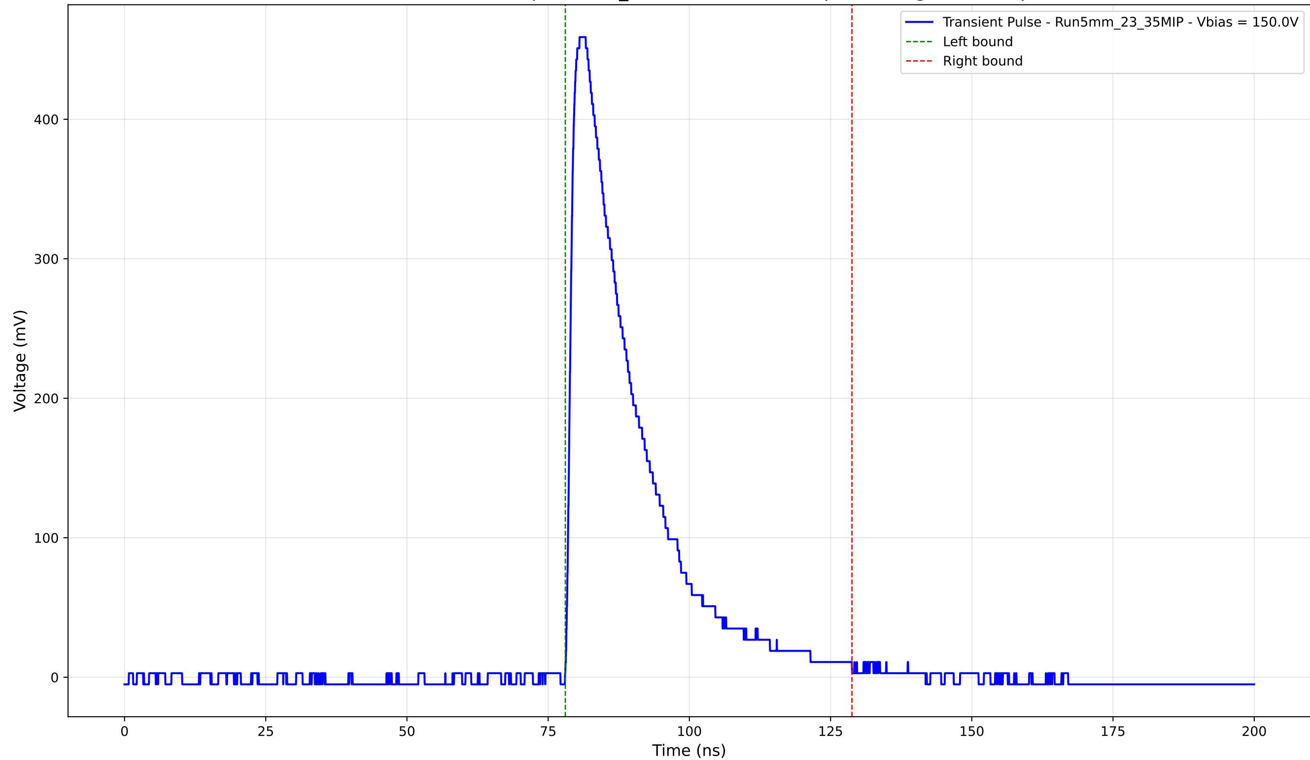
Transient Pulse - Sample: 5mm_23 - Position: 3230.0 \mu\text{m} - Charge: 118.93 pC
