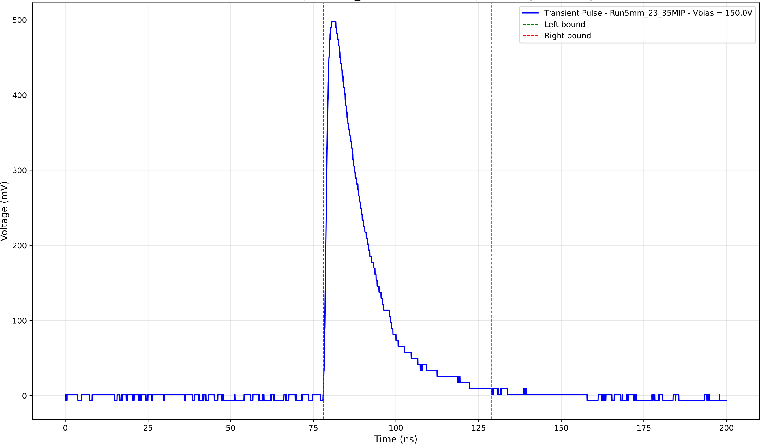
Transient Pulse - Sample: 5mm_23 - Position: 2265.0 \mu\text{m} - Charge: 133.81 pC
