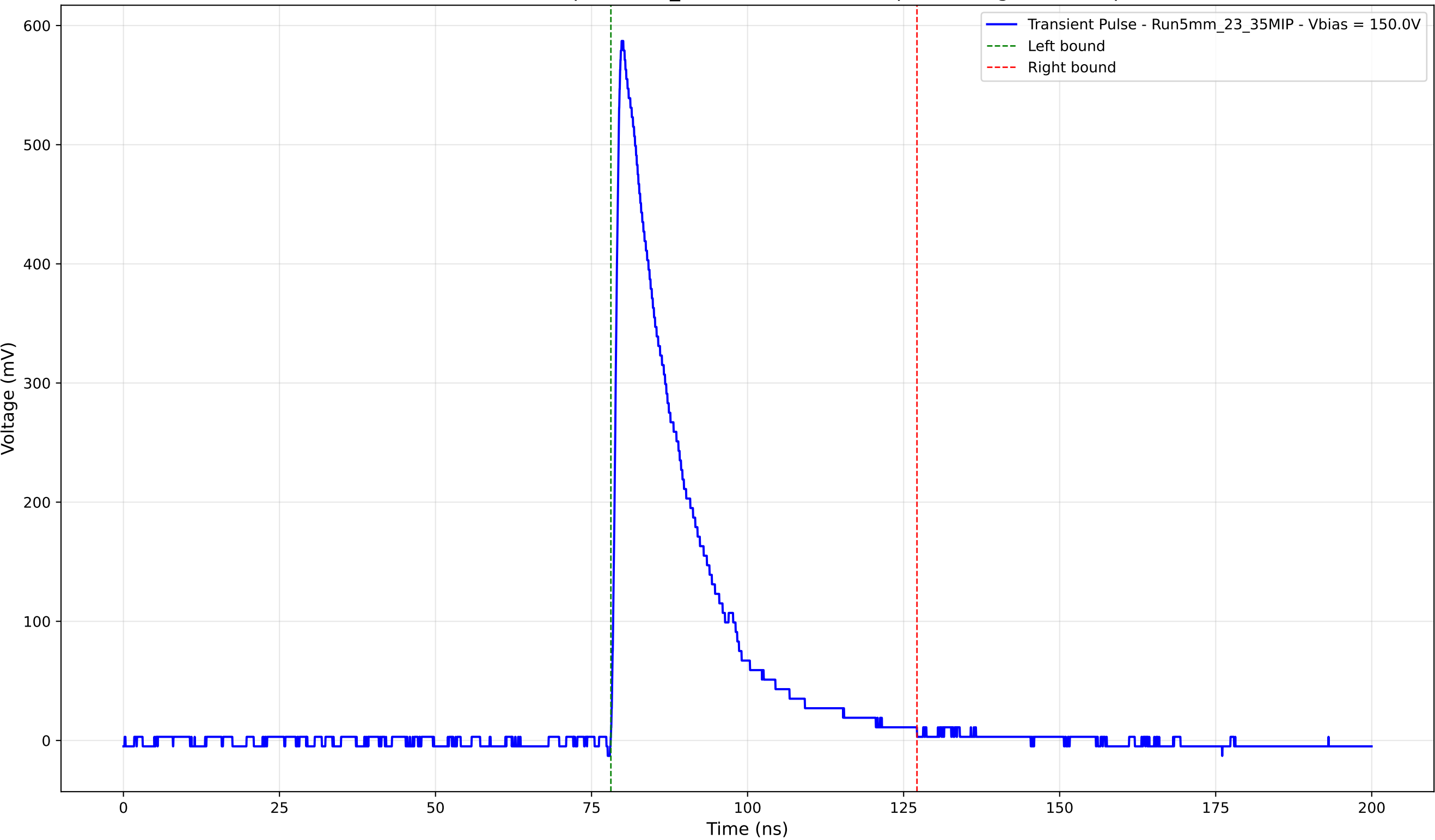
Transient Pulse - Sample: 5mm_23 - Position: 1335.0 \mu\text{m} - Charge: 130.40 pC
