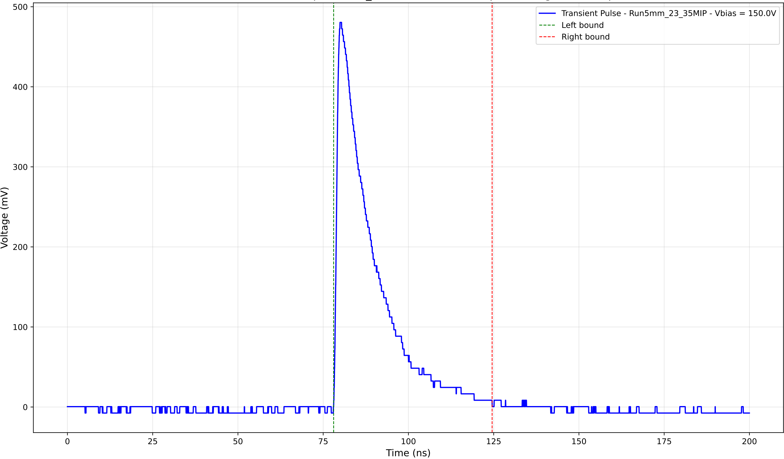
Transient Pulse - Sample: 5mm_23 - Position: 1545.0 \mu\text{m} - Charge: 110.91 pC
