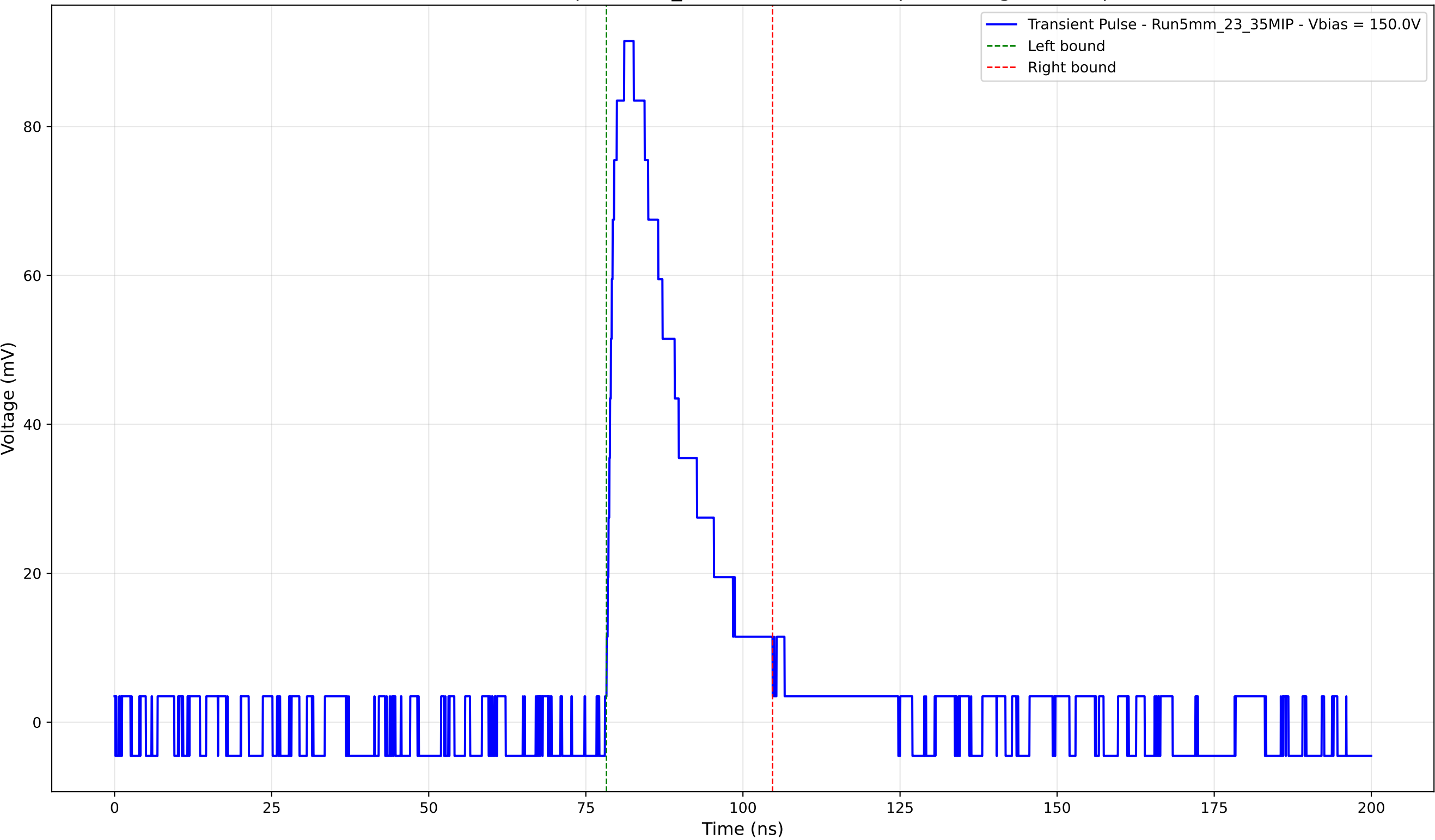
Transient Pulse - Sample: 5mm_23 - Position: 3155.0 \mu\text{m} - Charge: 21.86 pC
