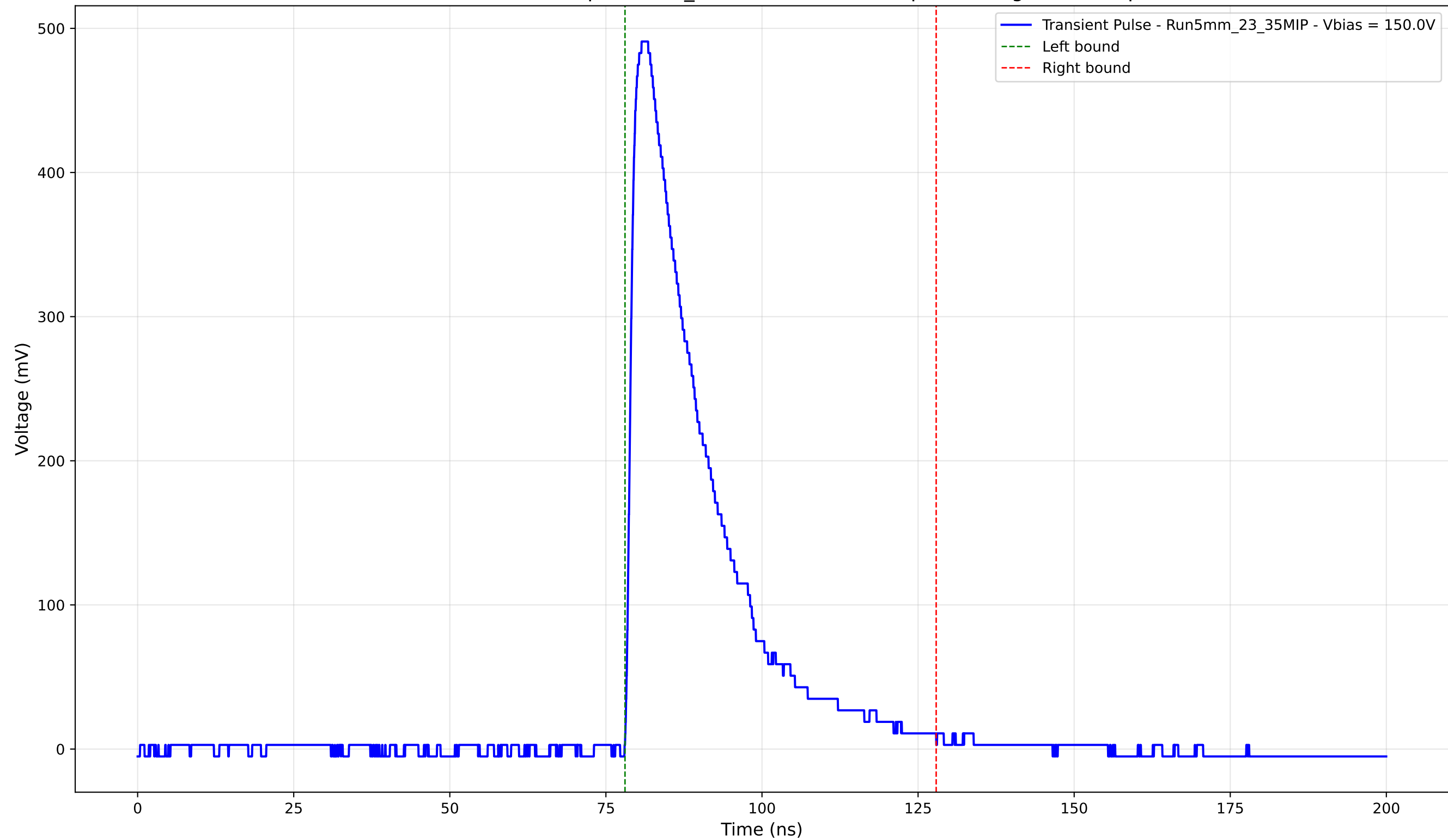
Transient Pulse - Sample: 5mm_23 - Position: 3030.0 \mu\text{m} - Charge: 129.92 pC
