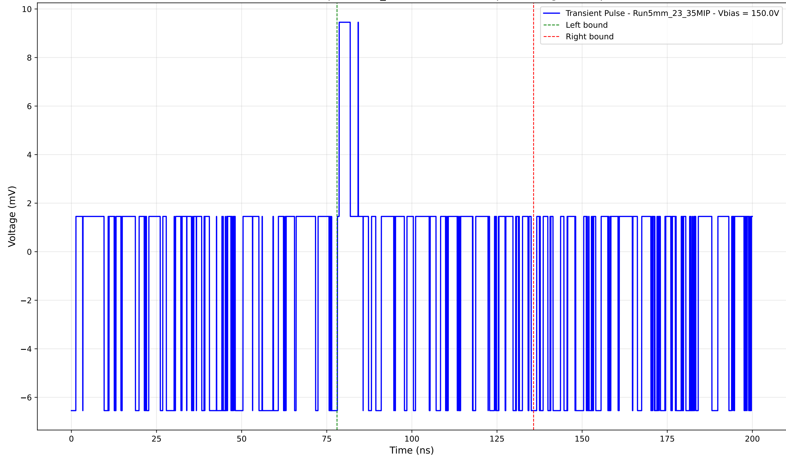
Transient Pulse - Sample: 5mm_23 - Position: 105.0 \mu\text{m} - Charge: 0.11 pC
