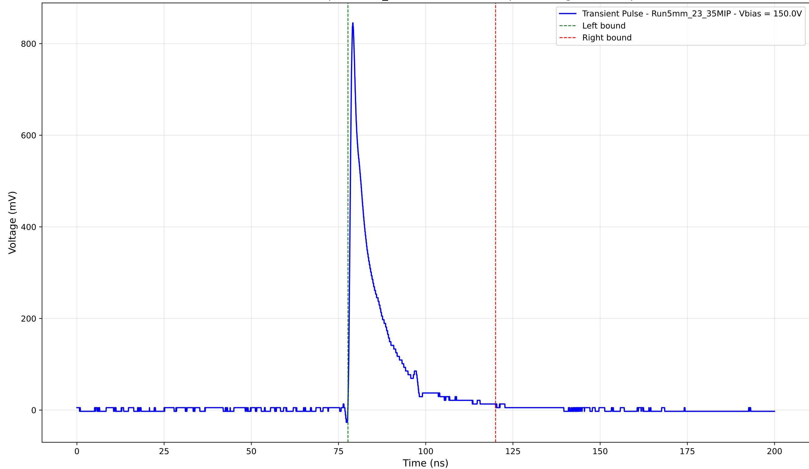
Transient Pulse - Sample: 5mm_23 - Position: 4855.0 \mu\text{m} - Charge: 115.89 pC
