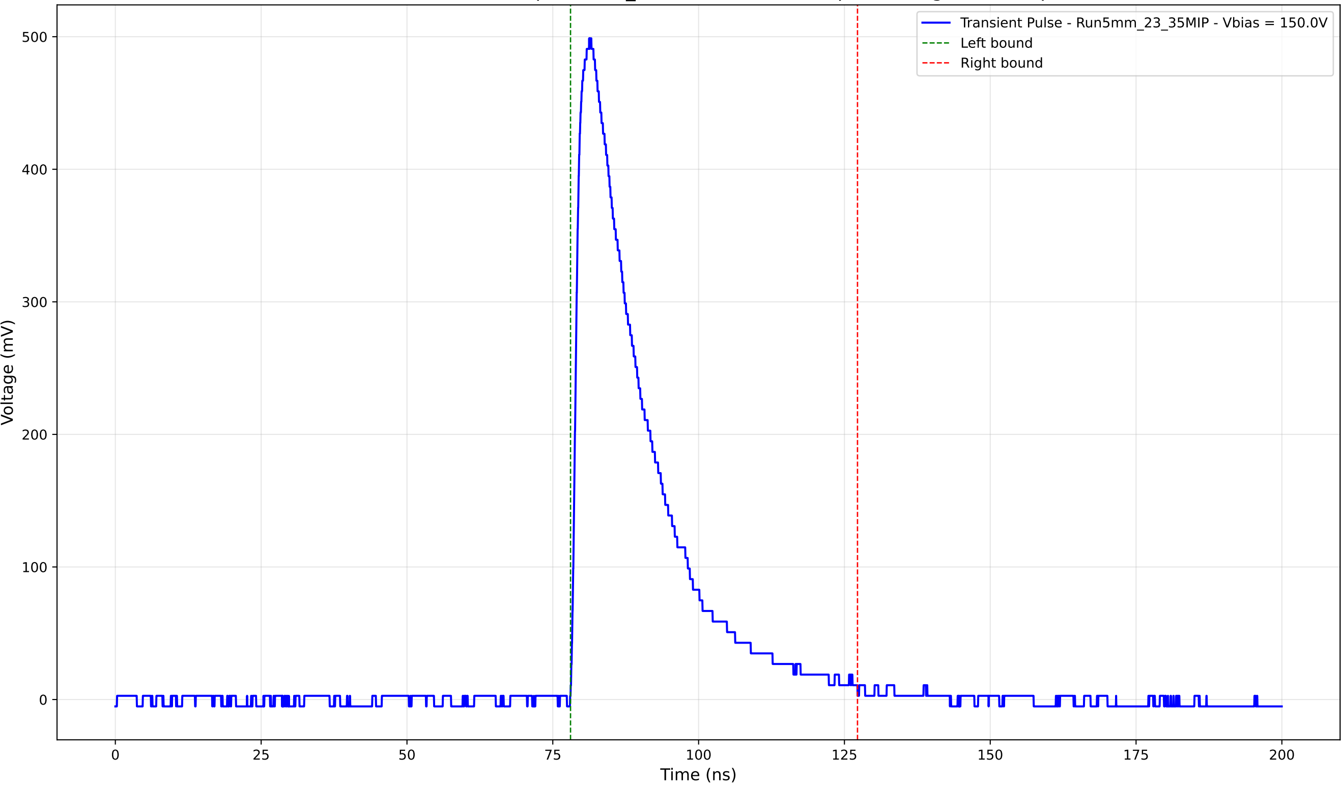
Transient Pulse - Sample: 5mm_23 - Position: 2780.0 \mu\text{m} - Charge: 132.95 pC
