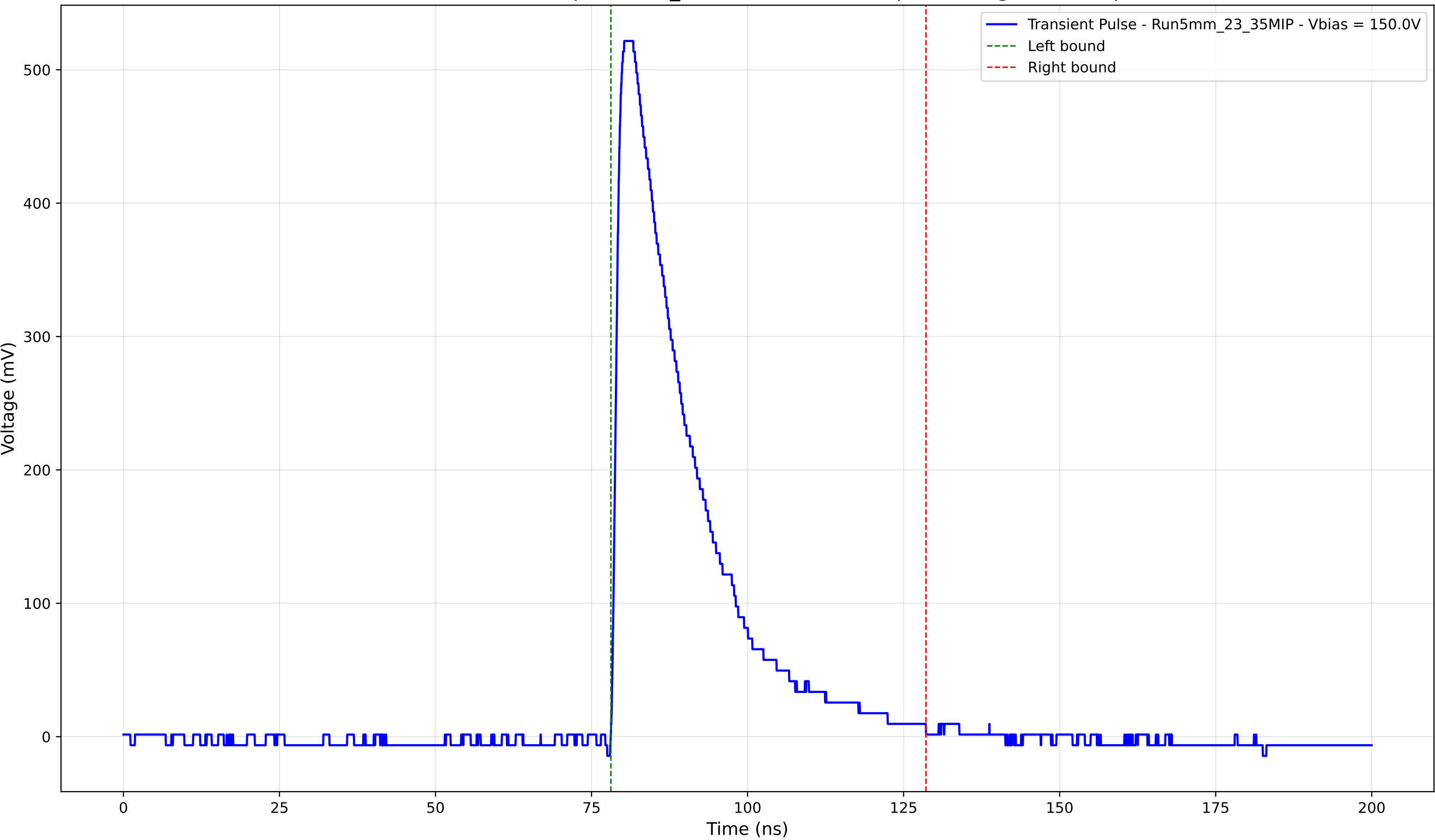
Transient Pulse - Sample: 5mm_23 - Position: 2040.0 \mu\text{m} - Charge: 136.91 pC
