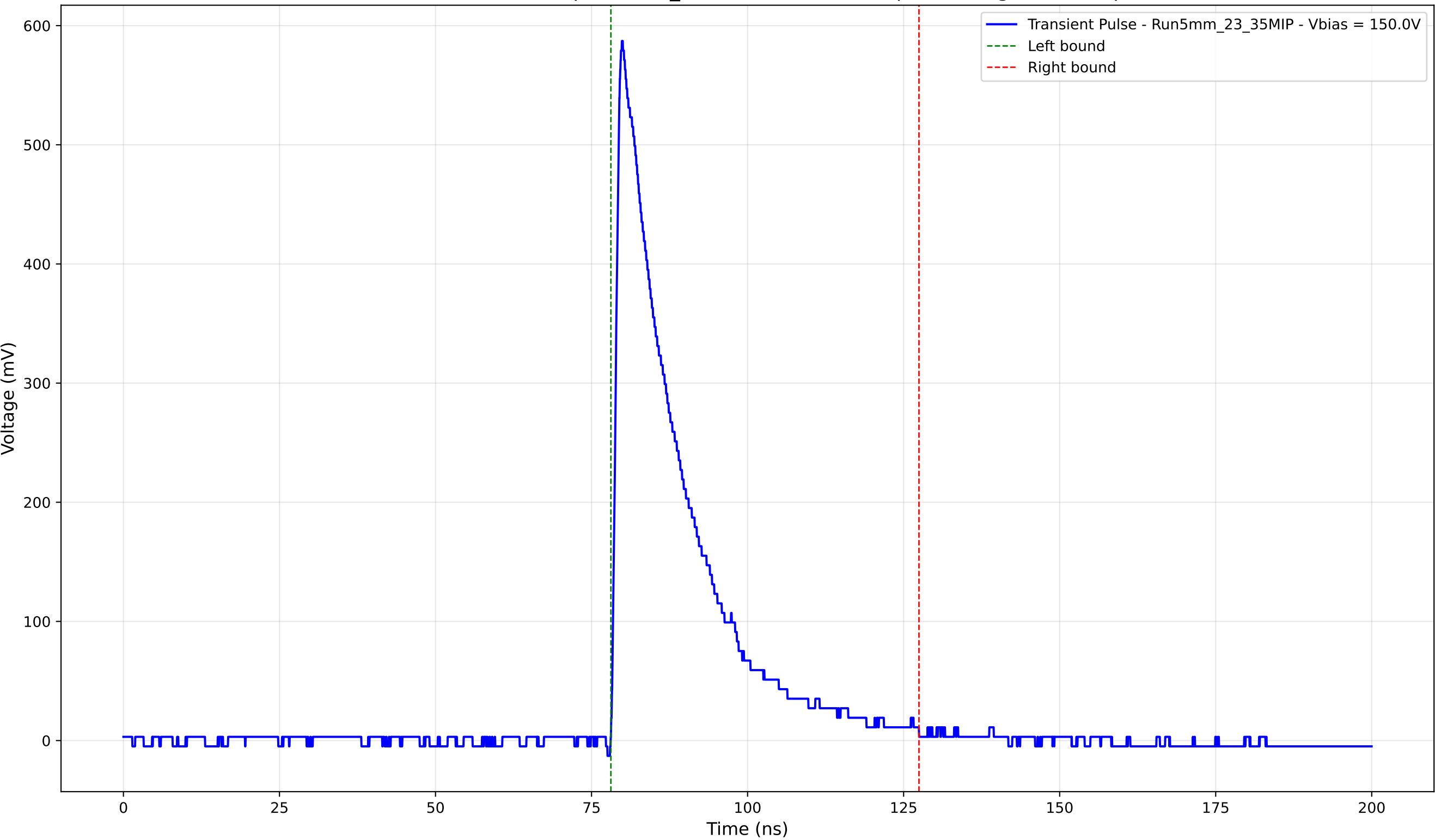
Transient Pulse - Sample: 5mm_23 - Position: 1320.0 \mu\text{m} - Charge: 129.41 pC
