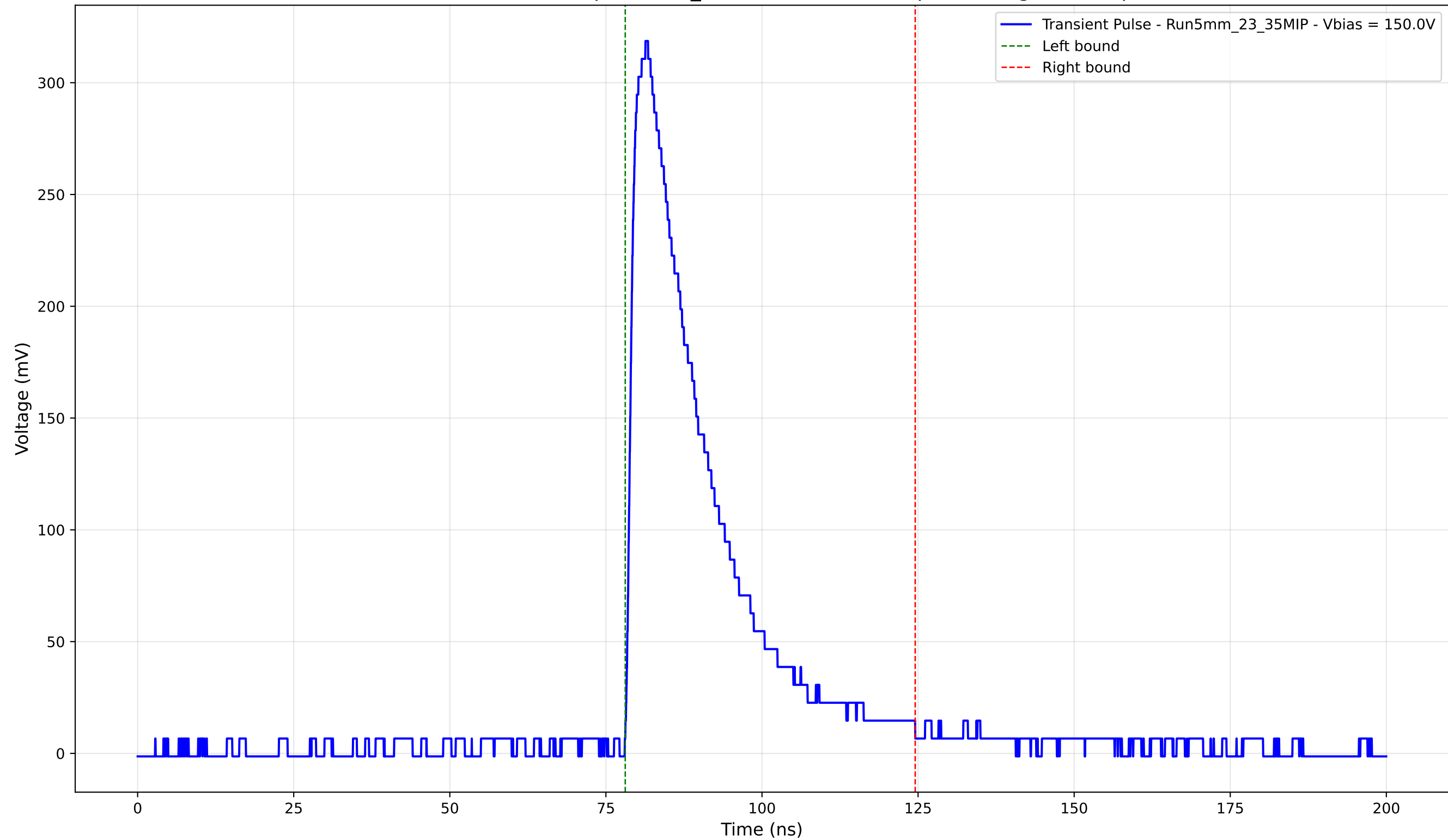
Transient Pulse - Sample: 5mm_23 - Position: 2700.0 \mu\text{m} - Charge: 85.02 pC
