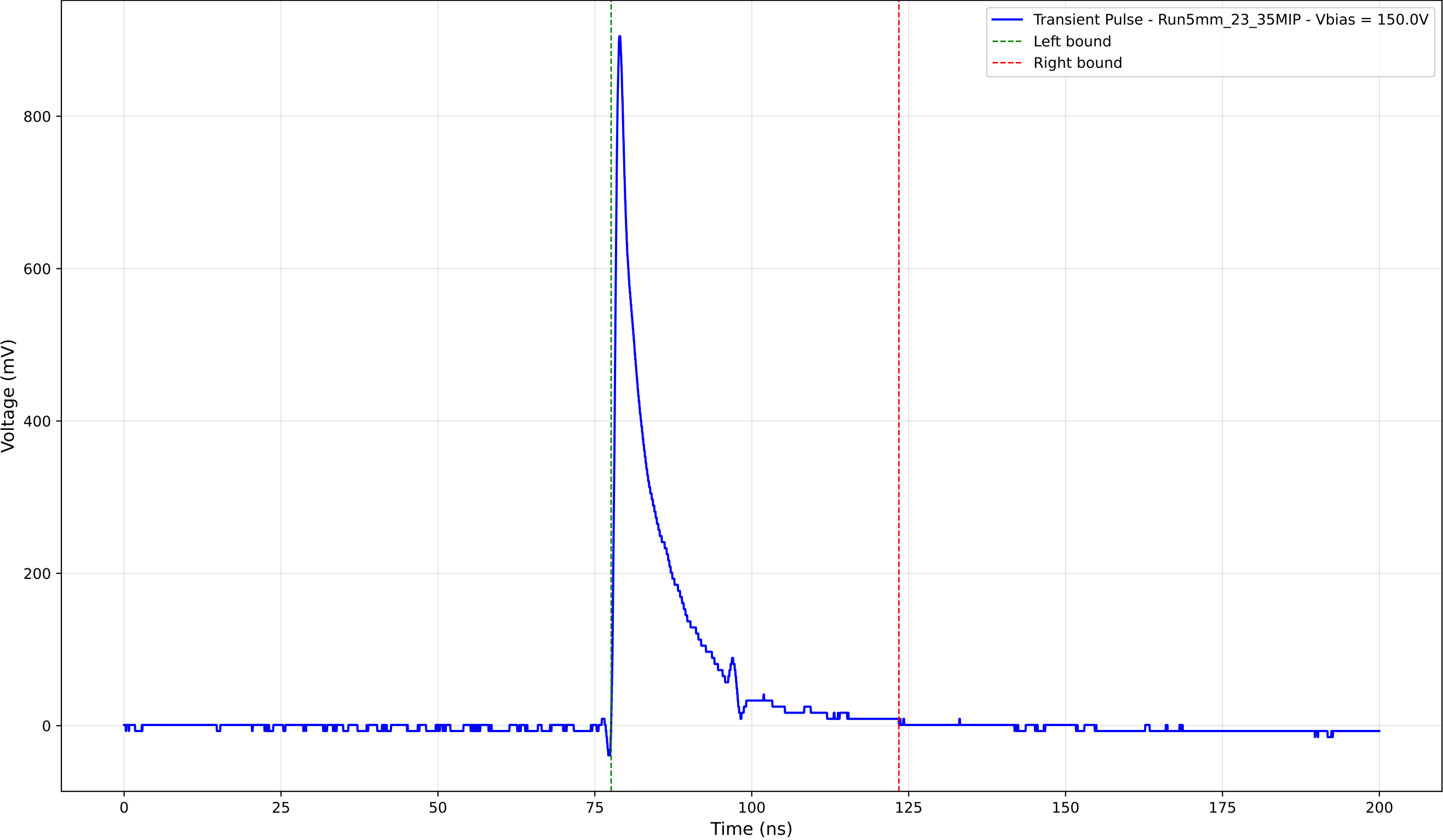
Transient Pulse - Sample: 5mm_23 - Position: 4995.0 \mu\text{m} - Charge: 114.29 pC
