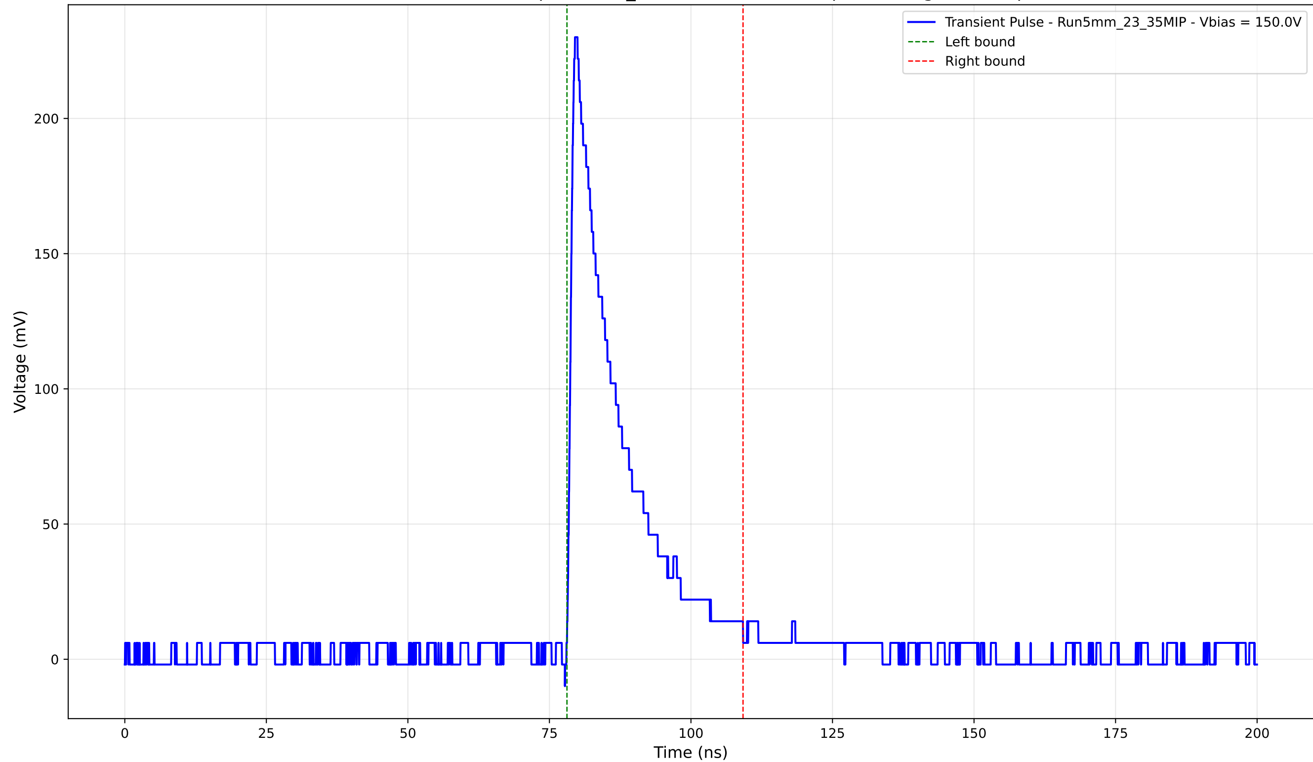
Transient Pulse - Sample: 5mm_23 - Position: 4190.0 \mu\text{m} - Charge: 42.25 pC
