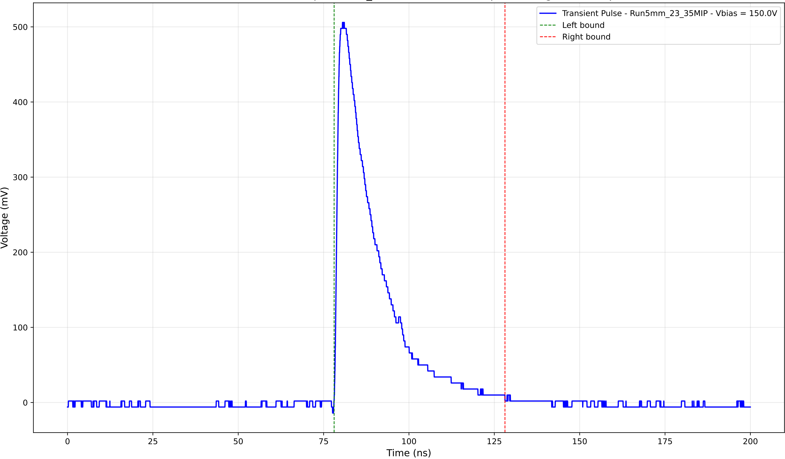
Transient Pulse - Sample: 5mm_23 - Position: 3415.0 \mu\text{m} - Charge: 127.41 pC
