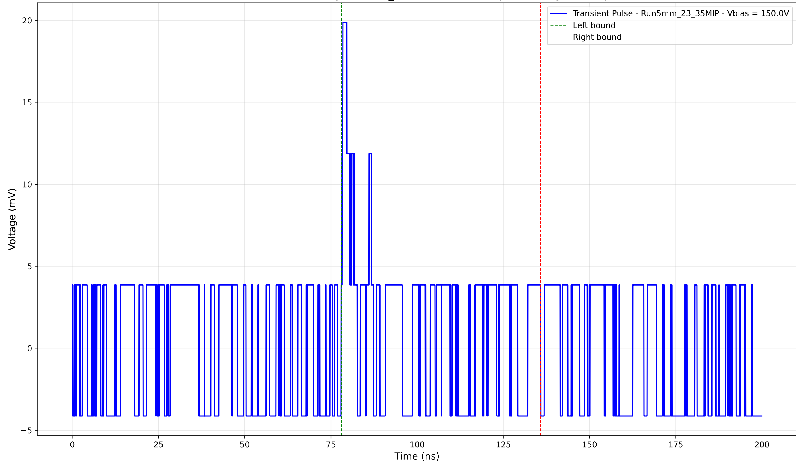
Transient Pulse - Sample: 5mm_23 - Position: 15.0 \mu\text{m} - Charge: 2.34 pC
