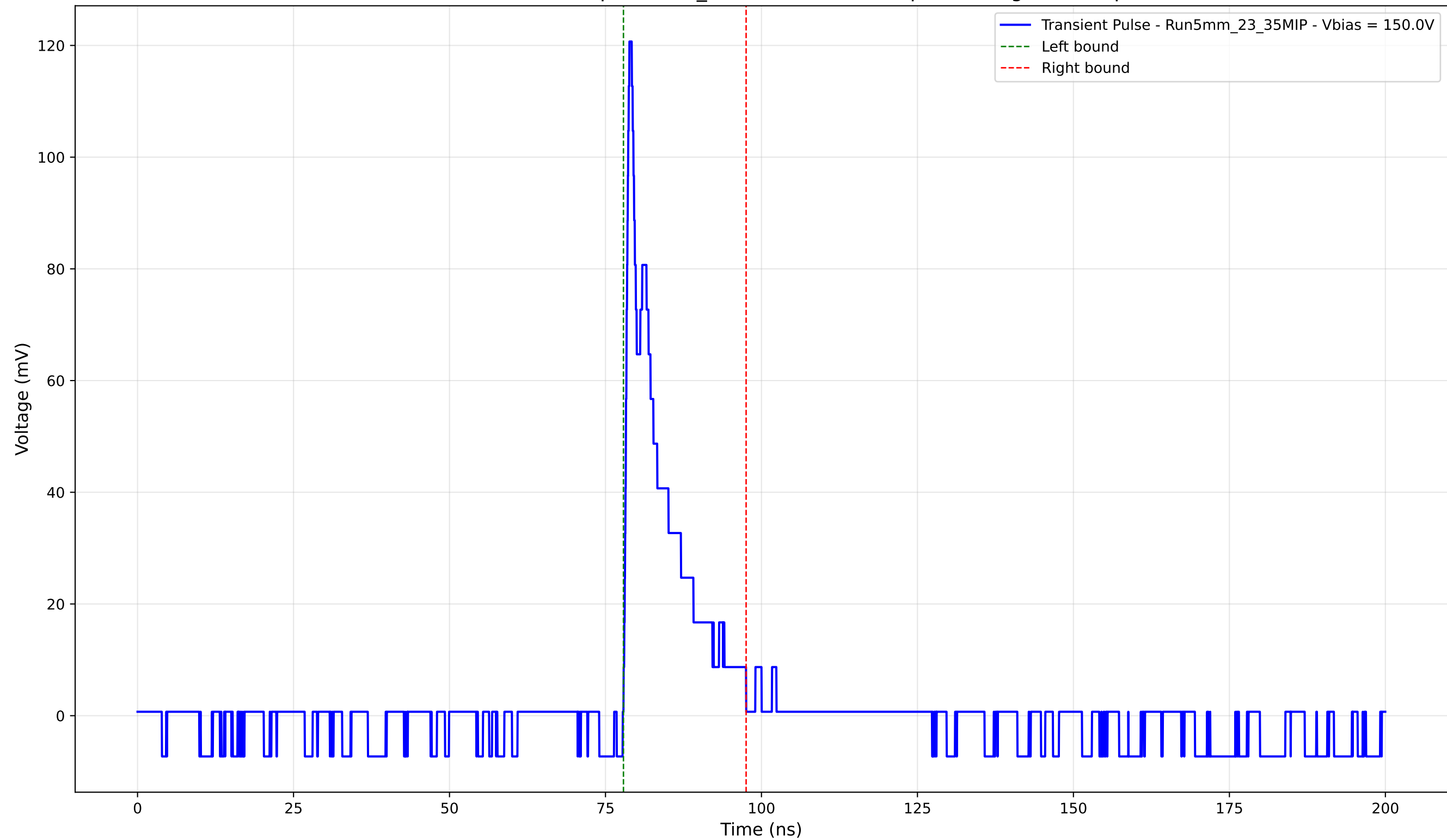
Transient Pulse - Sample: 5mm_23 - Position: 180.0 \mu\text{m} - Charge: 13.69 pC
