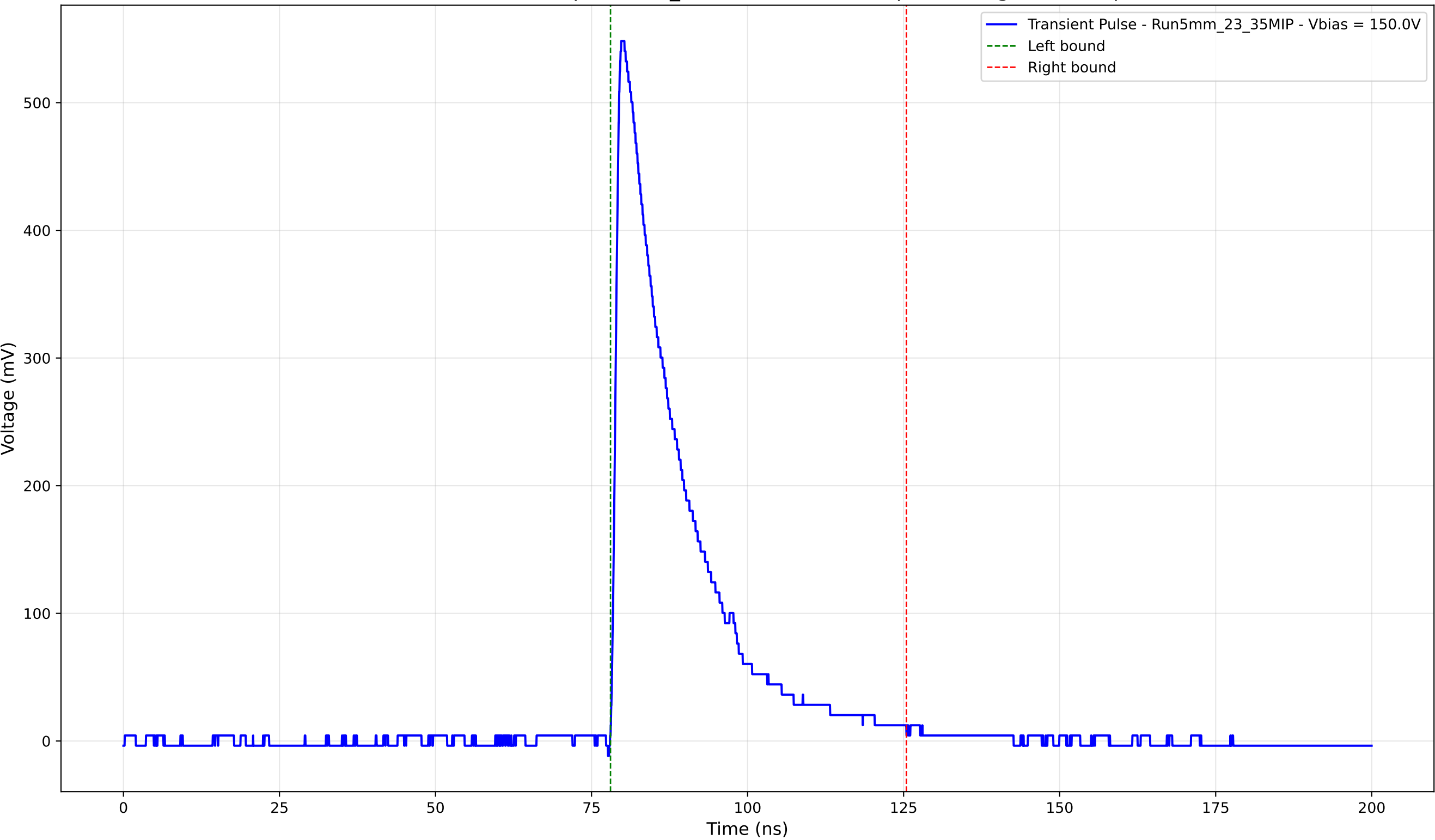
Transient Pulse - Sample: 5mm_23 - Position: 3890.0 \mu\text{m} - Charge: 122.48 pC
