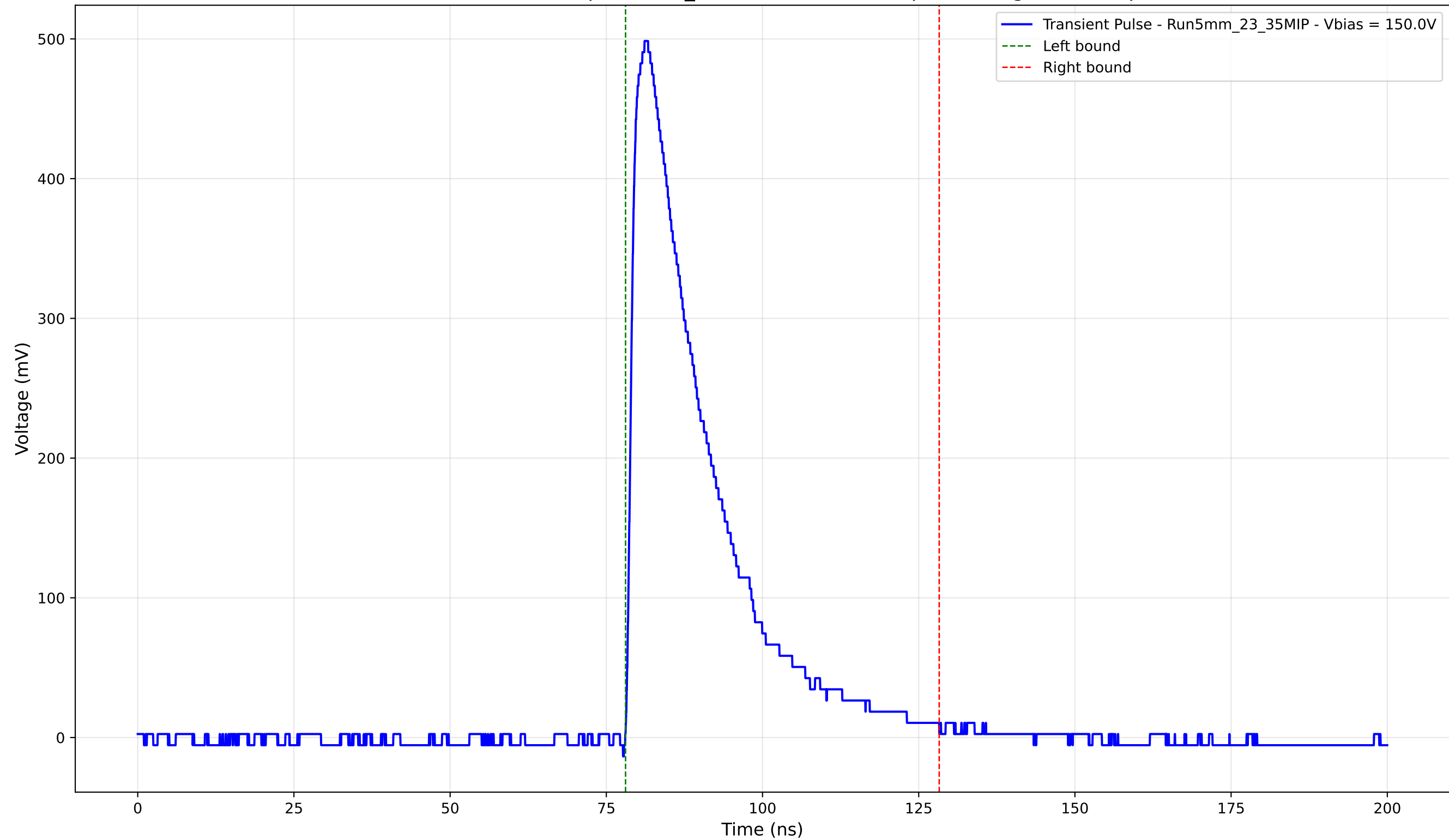
Transient Pulse - Sample: 5mm_23 - Position: 2820.0 \mu\text{m} - Charge: 133.49 pC
