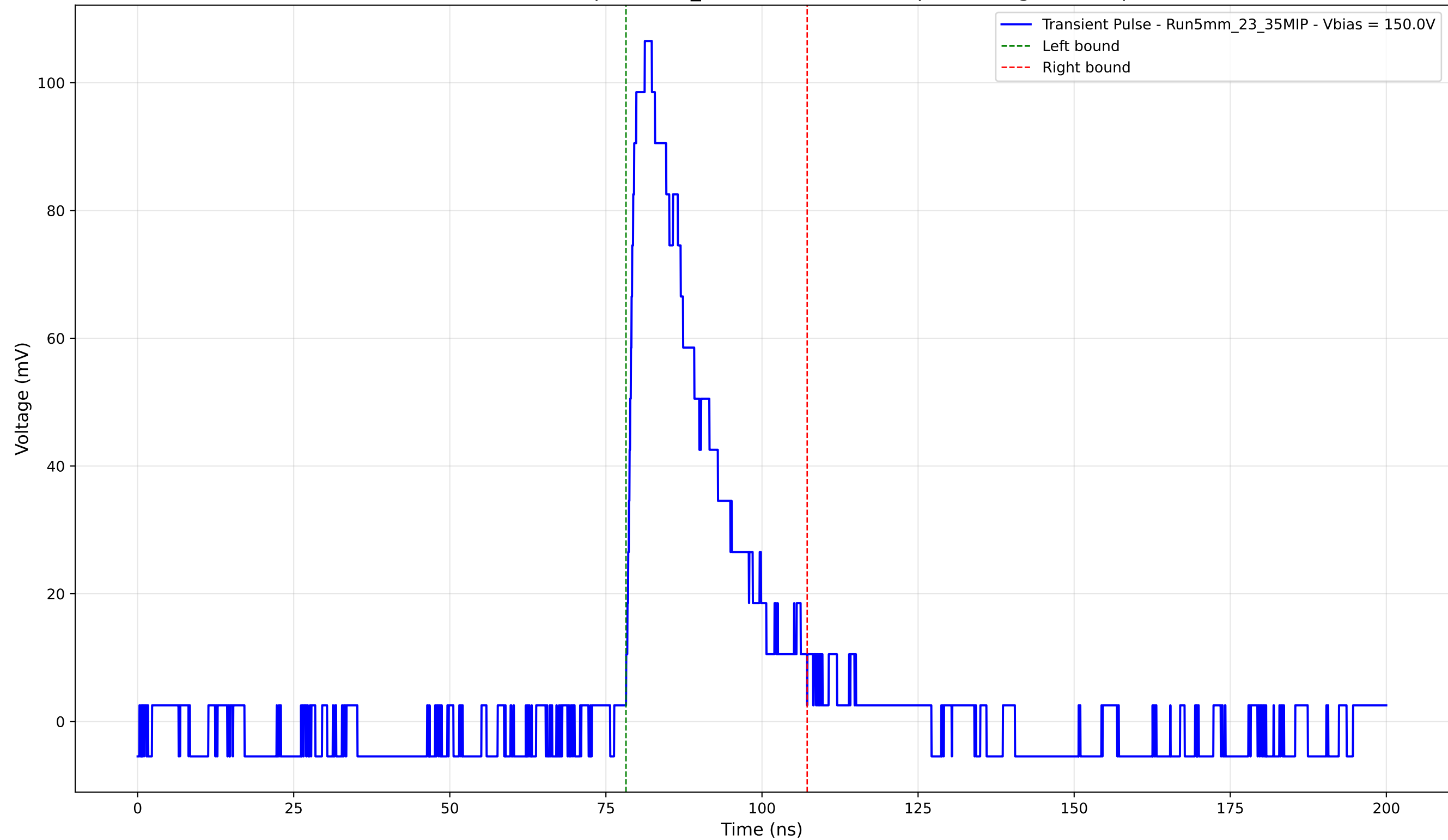
Transient Pulse - Sample: 5mm_23 - Position: 2125.0 \mu\text{m} - Charge: 26.68 pC
