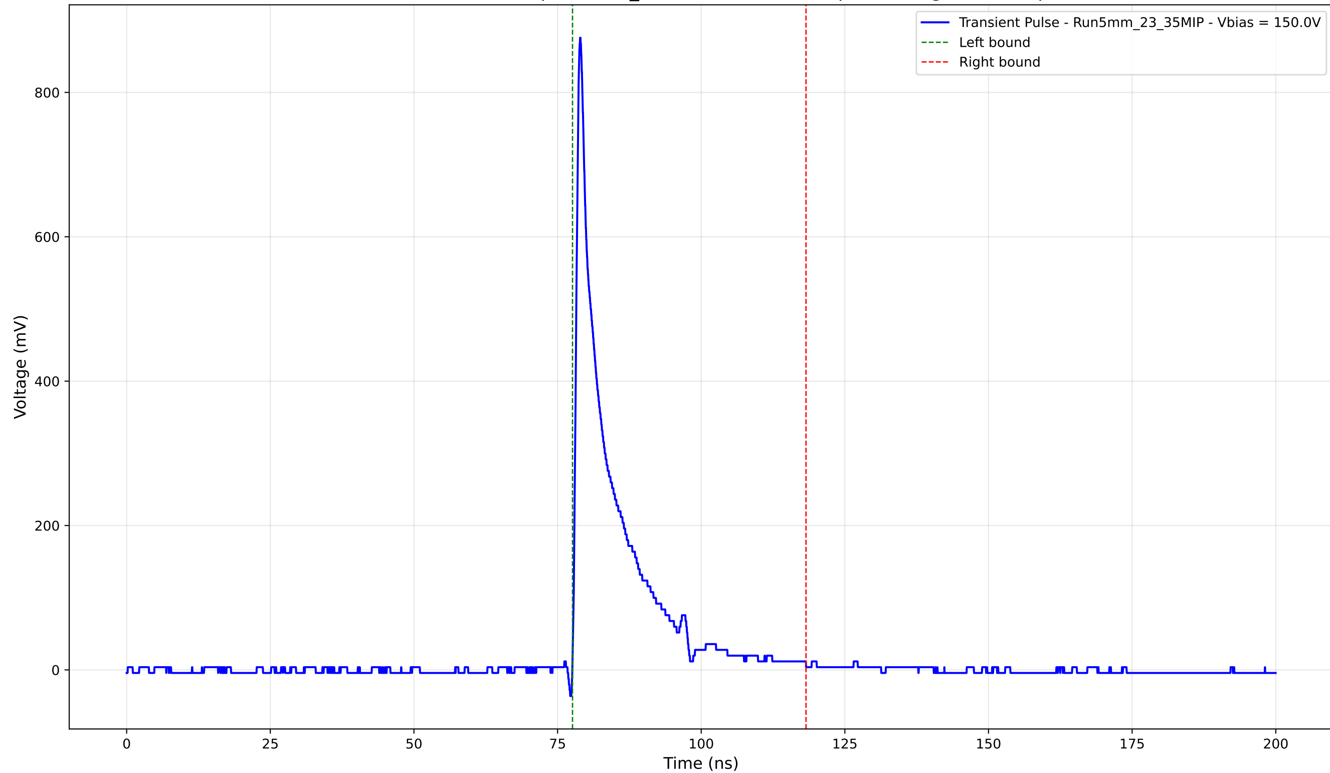
Transient Pulse - Sample: 5mm_23 - Position: 5020.0 \mu\text{m} - Charge: 104.61 pC
