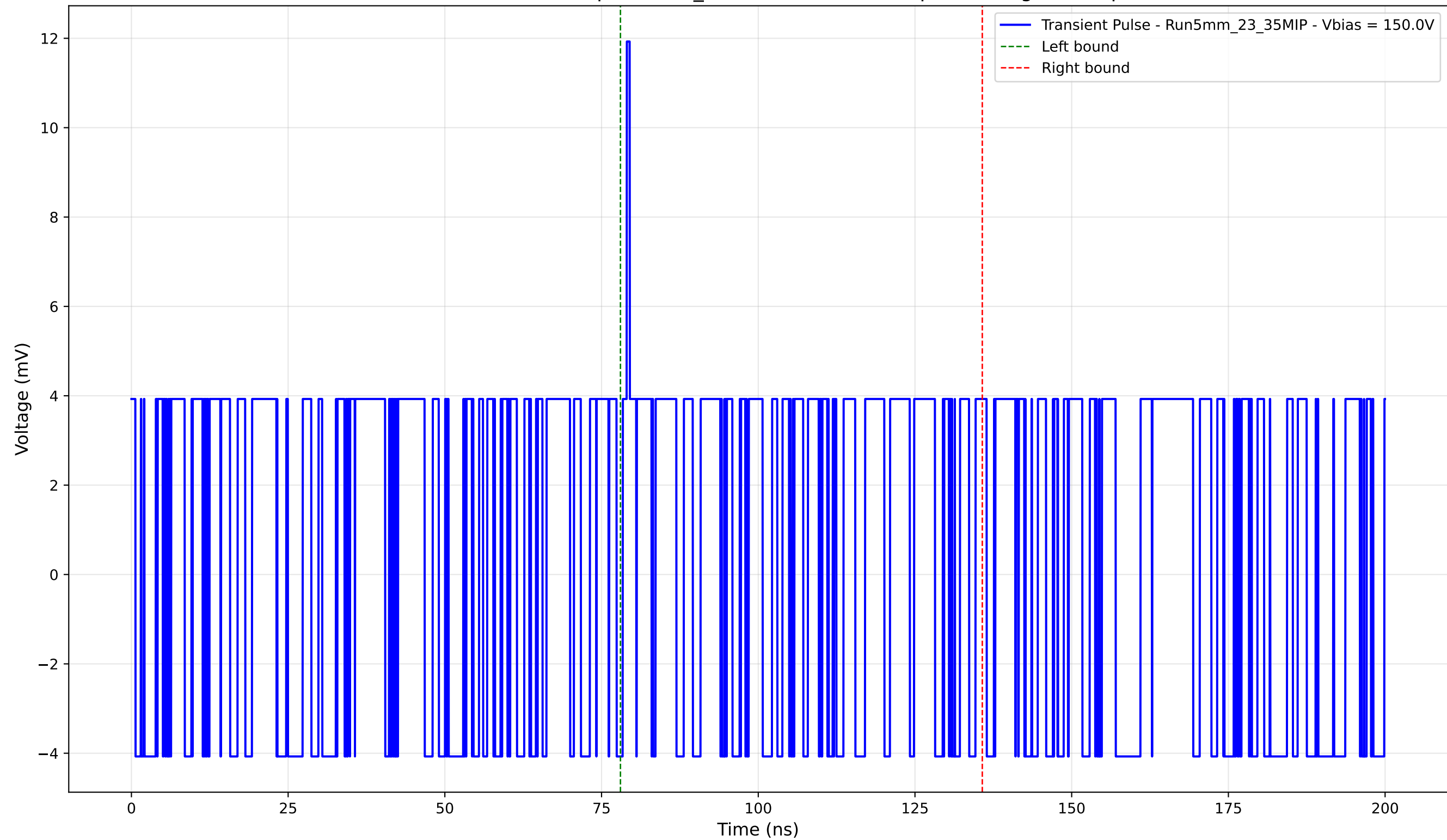
Transient Pulse - Sample: 5mm_23 - Position: 5220.0 \mu\text{m} - Charge: 1.66 pC
