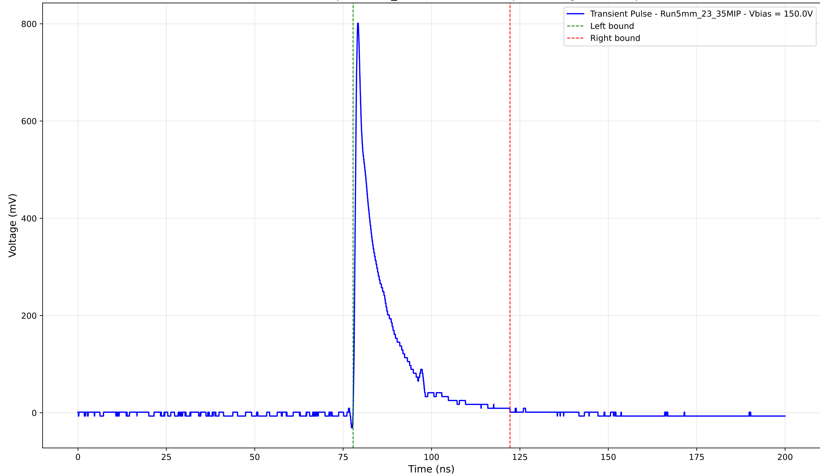
Transient Pulse - Sample: 5mm_23 - Position: 470.0 \mu\text{m} - Charge: 114.01 pC
