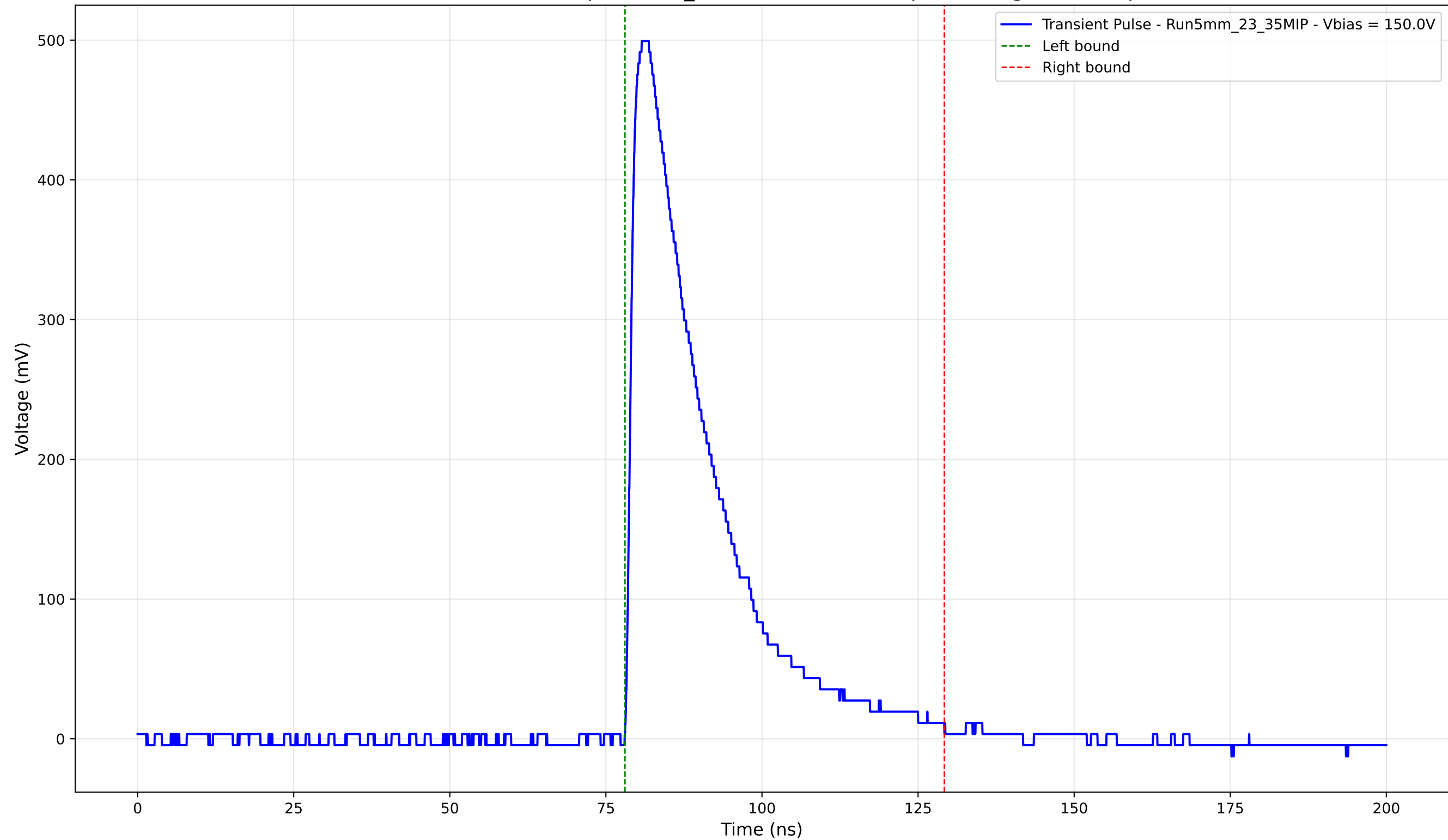
Transient Pulse - Sample: 5mm_23 - Position: 2365.0 \mu\text{m} - Charge: 136.53 pC
