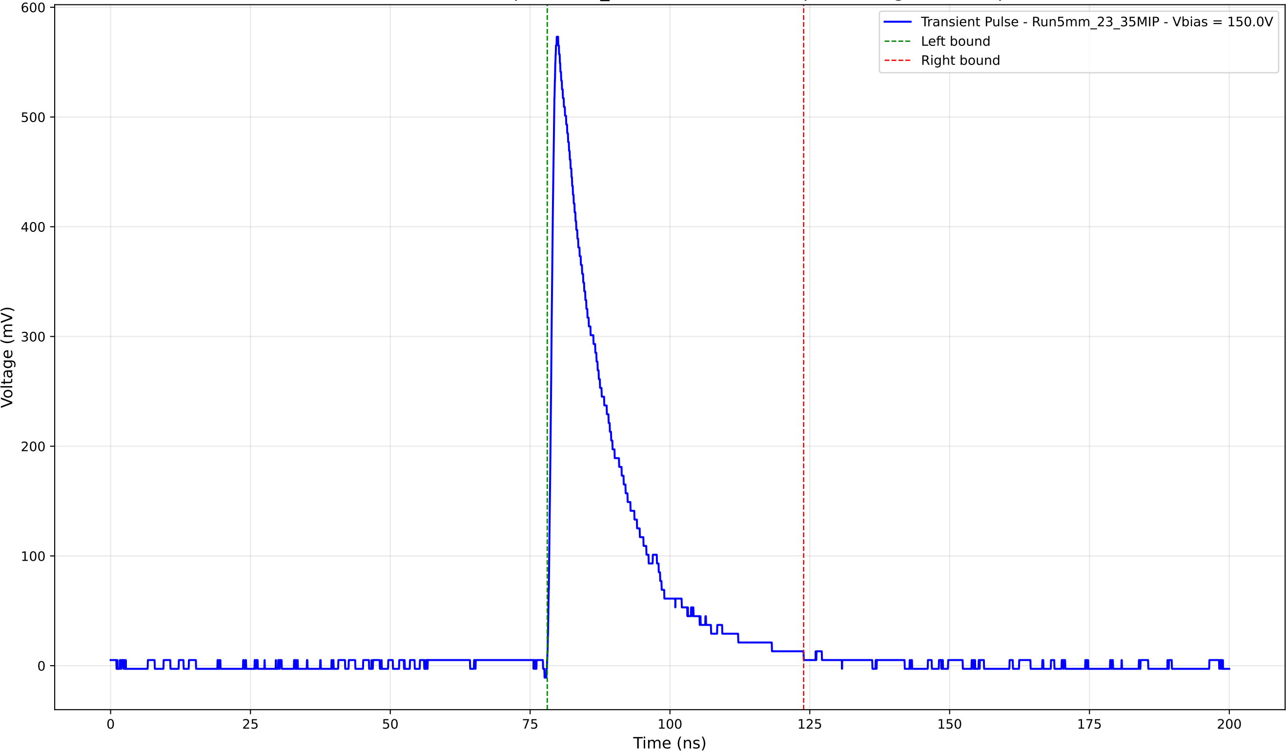
Transient Pulse - Sample: 5mm_23 - Position: 1220.0 \mu\text{m} - Charge: 122.54 pC
