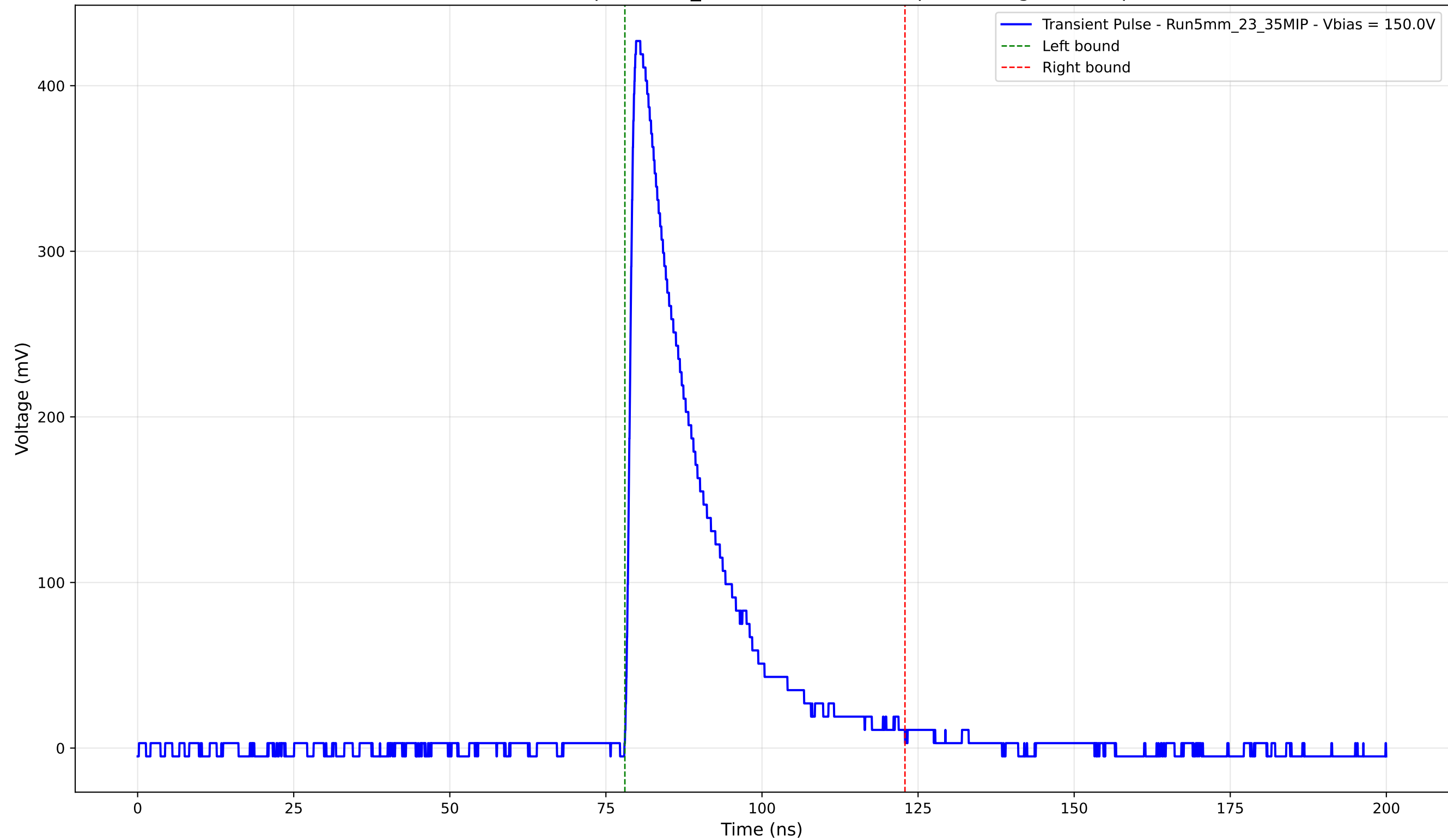
Transient Pulse - Sample: 5mm_23 - Position: 3720.0 \mu\text{m} - Charge: 98.79 pC
