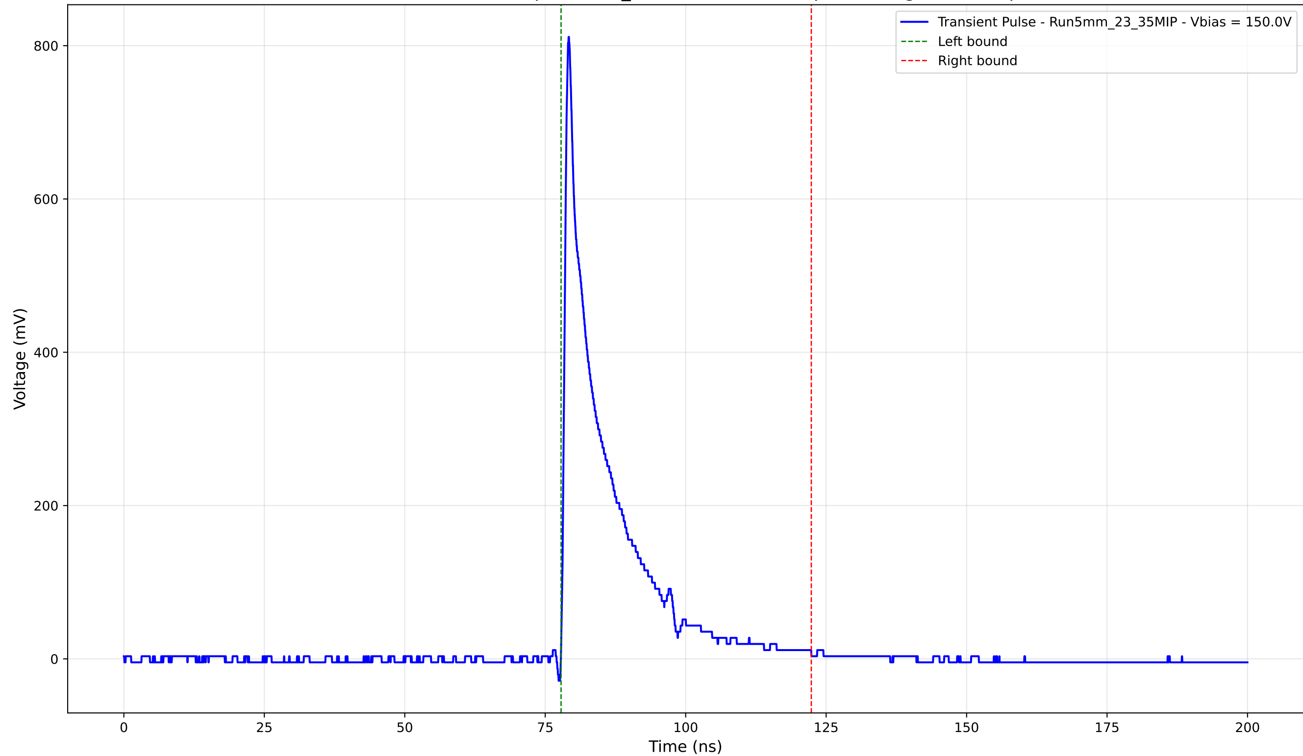
Transient Pulse - Sample: 5mm_23 - Position: 455.0 \mu\text{m} - Charge: 116.25 pC
