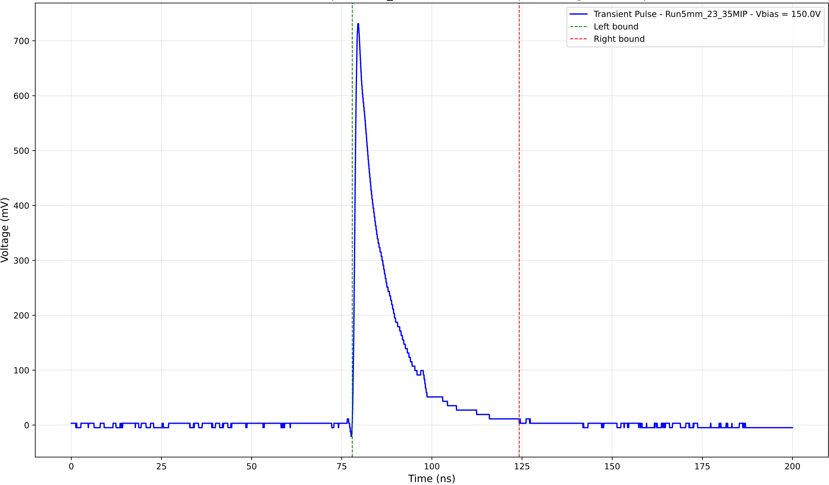
Transient Pulse - Sample: 5mm_23 - Position: 4400.0 \mu\text{m} - Charge: 129.46 pC
