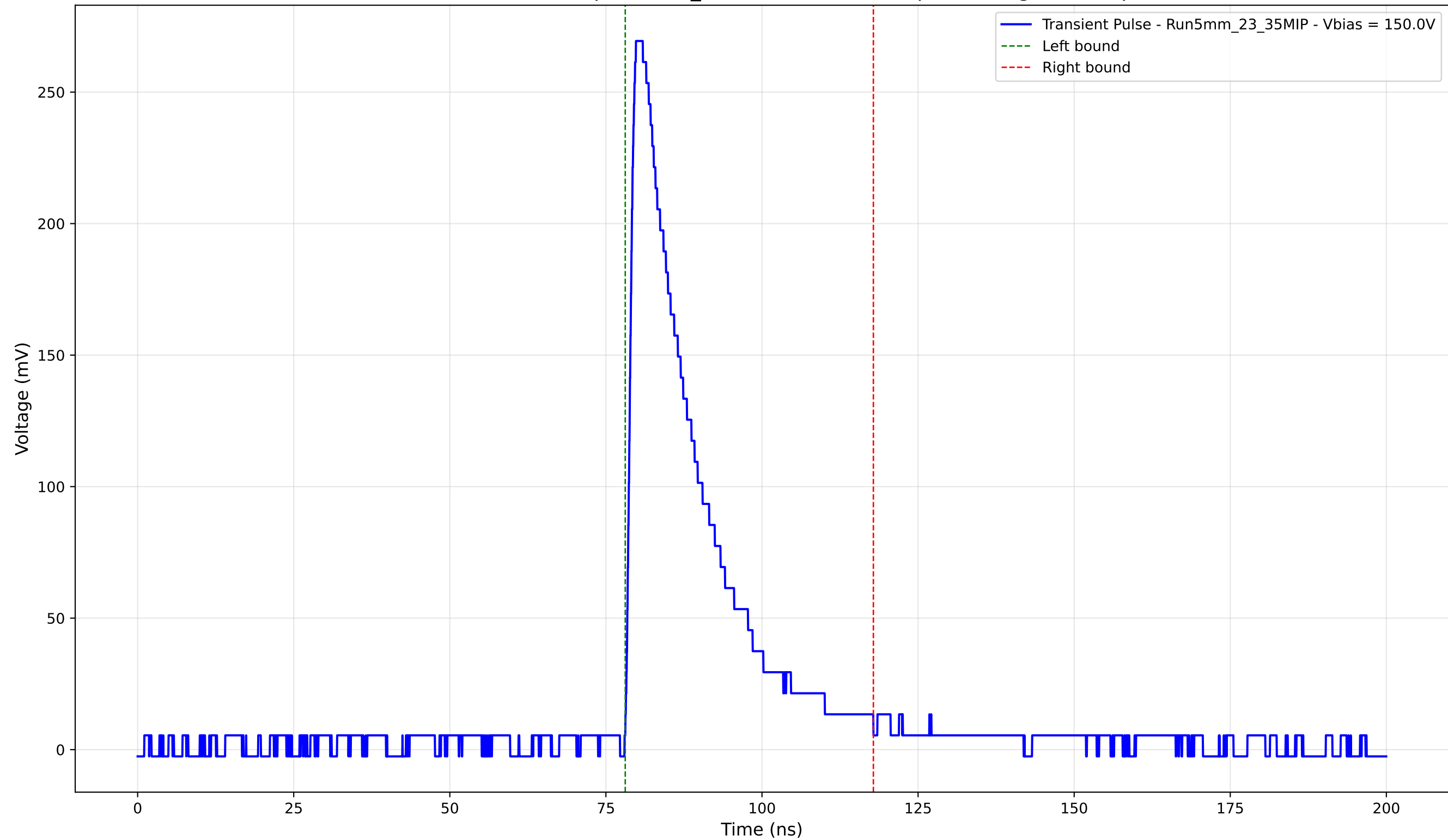
Transient Pulse - Sample: 5mm_23 - Position: 3695.0 \mu\text{m} - Charge: 62.84 pC
