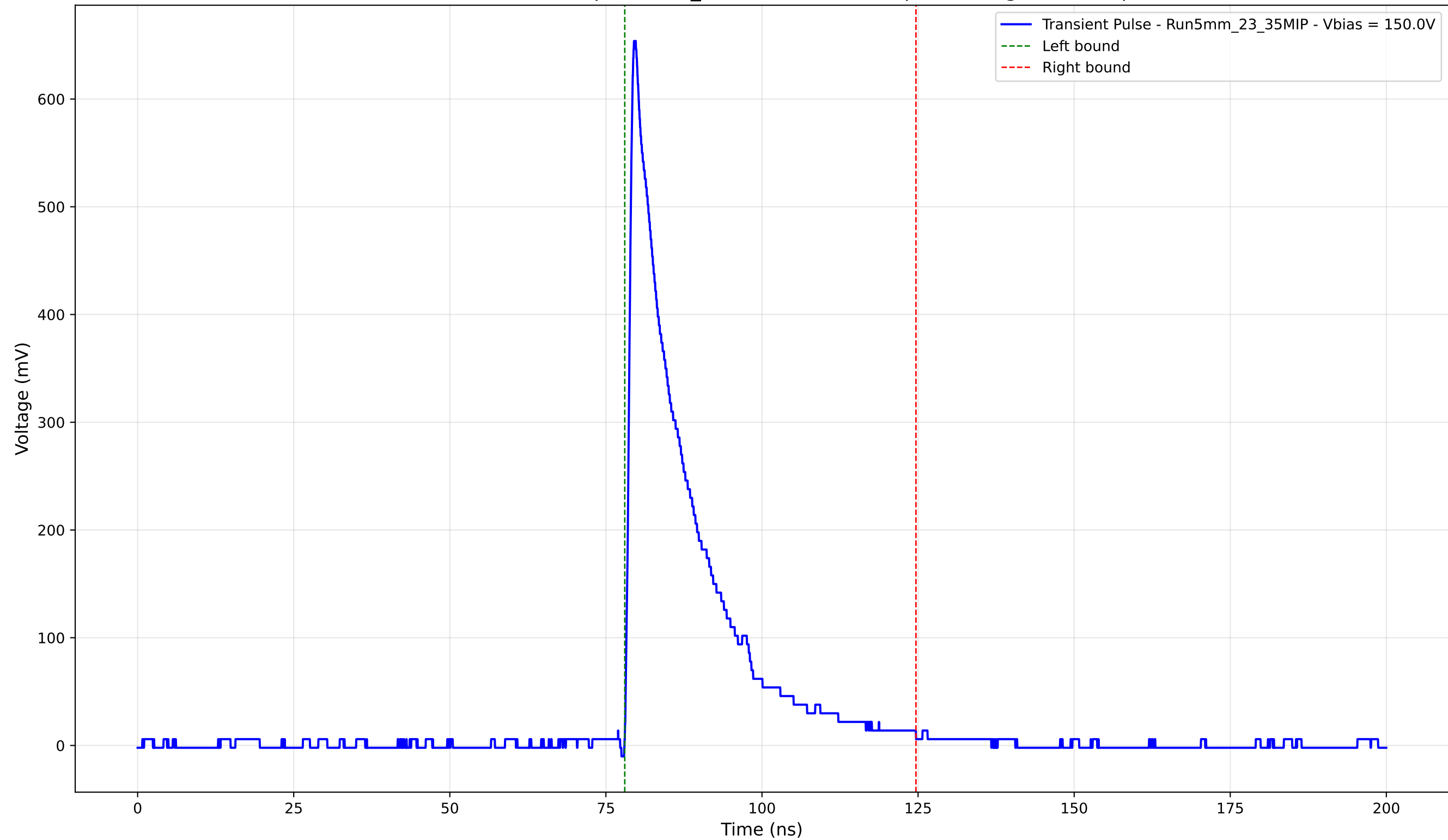
Transient Pulse - Sample: 5mm_23 - Position: 955.0 \mu\text{m} - Charge: 126.44 pC
