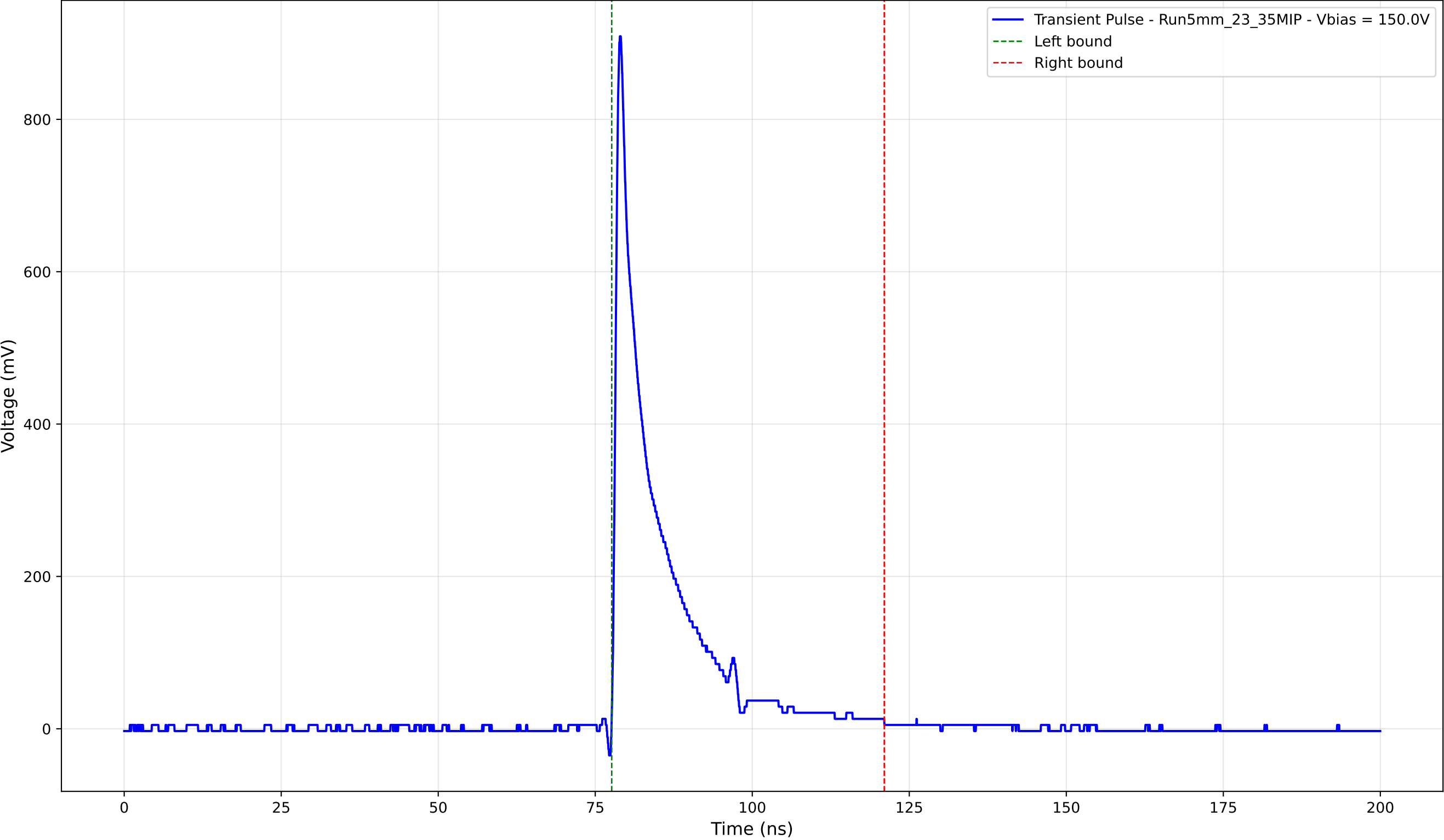
Transient Pulse - Sample: 5mm_23 - Position: 4990.0 \mu\text{m} - Charge: 118.25 pC
