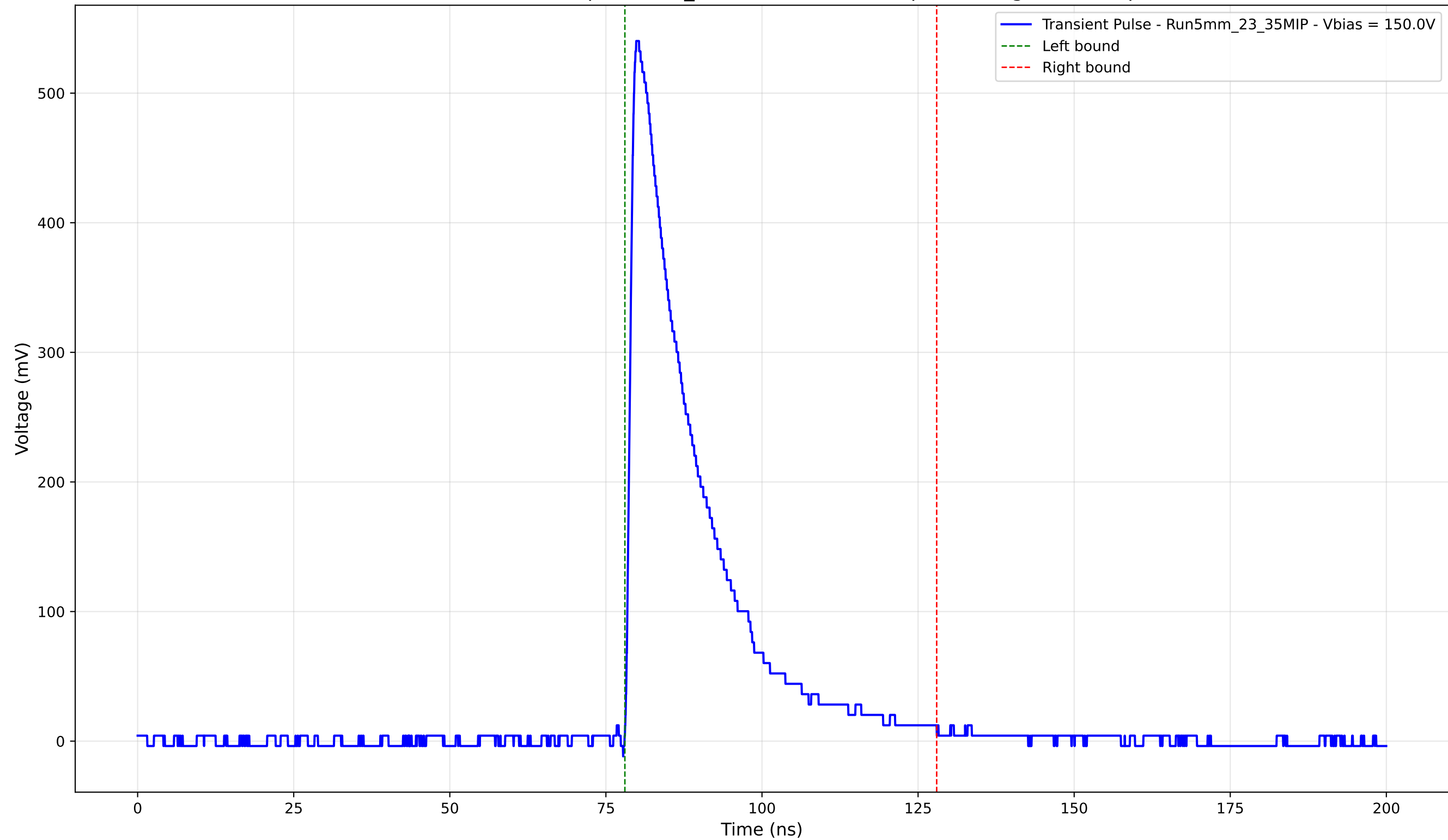
Transient Pulse - Sample: 5mm_23 - Position: 3765.0 \mu\text{m} - Charge: 124.99 pC
