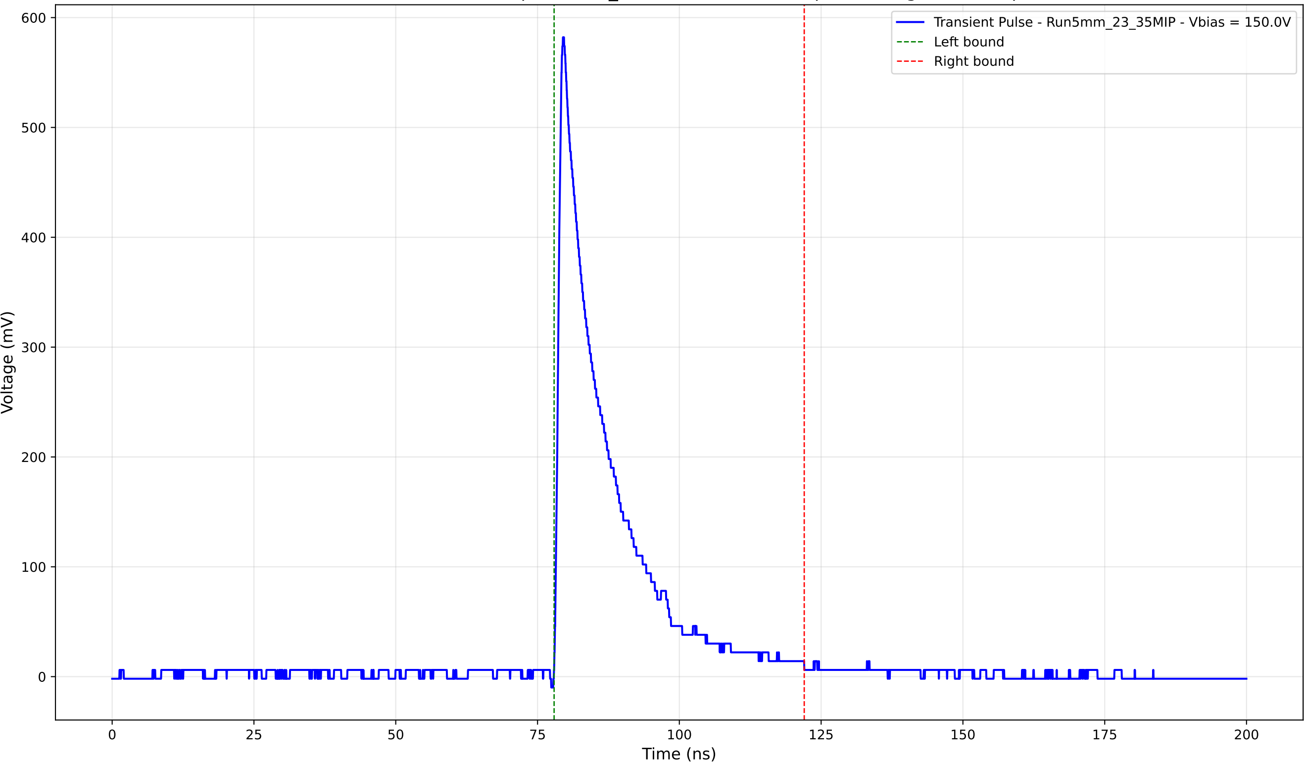
Transient Pulse - Sample: 5mm_23 - Position: 4455.0 \mu\text{m} - Charge: 104.29 pC
