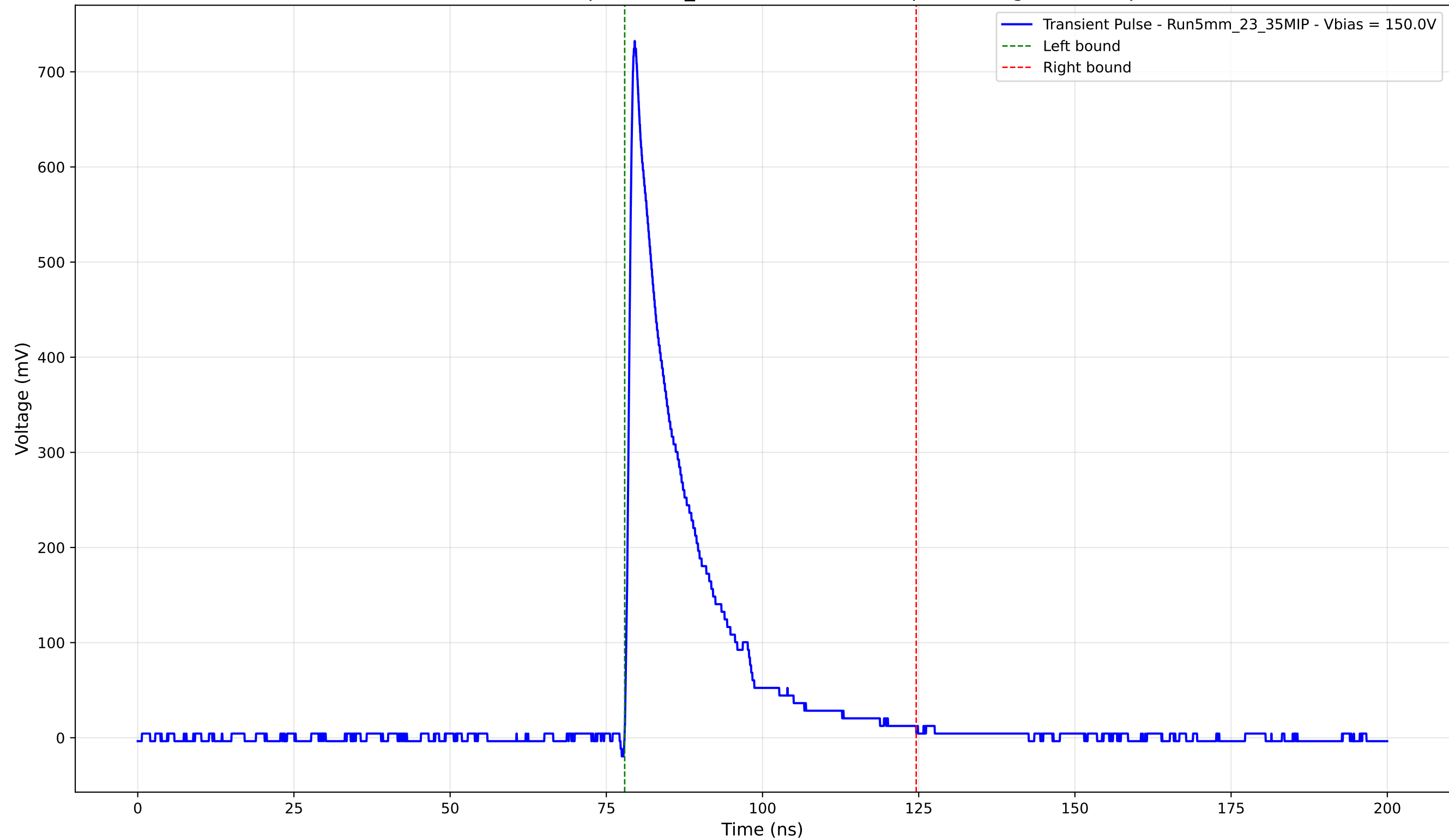
Transient Pulse - Sample: 5mm_23 - Position: 4395.0 \mu\text{m} - Charge: 131.22 pC
