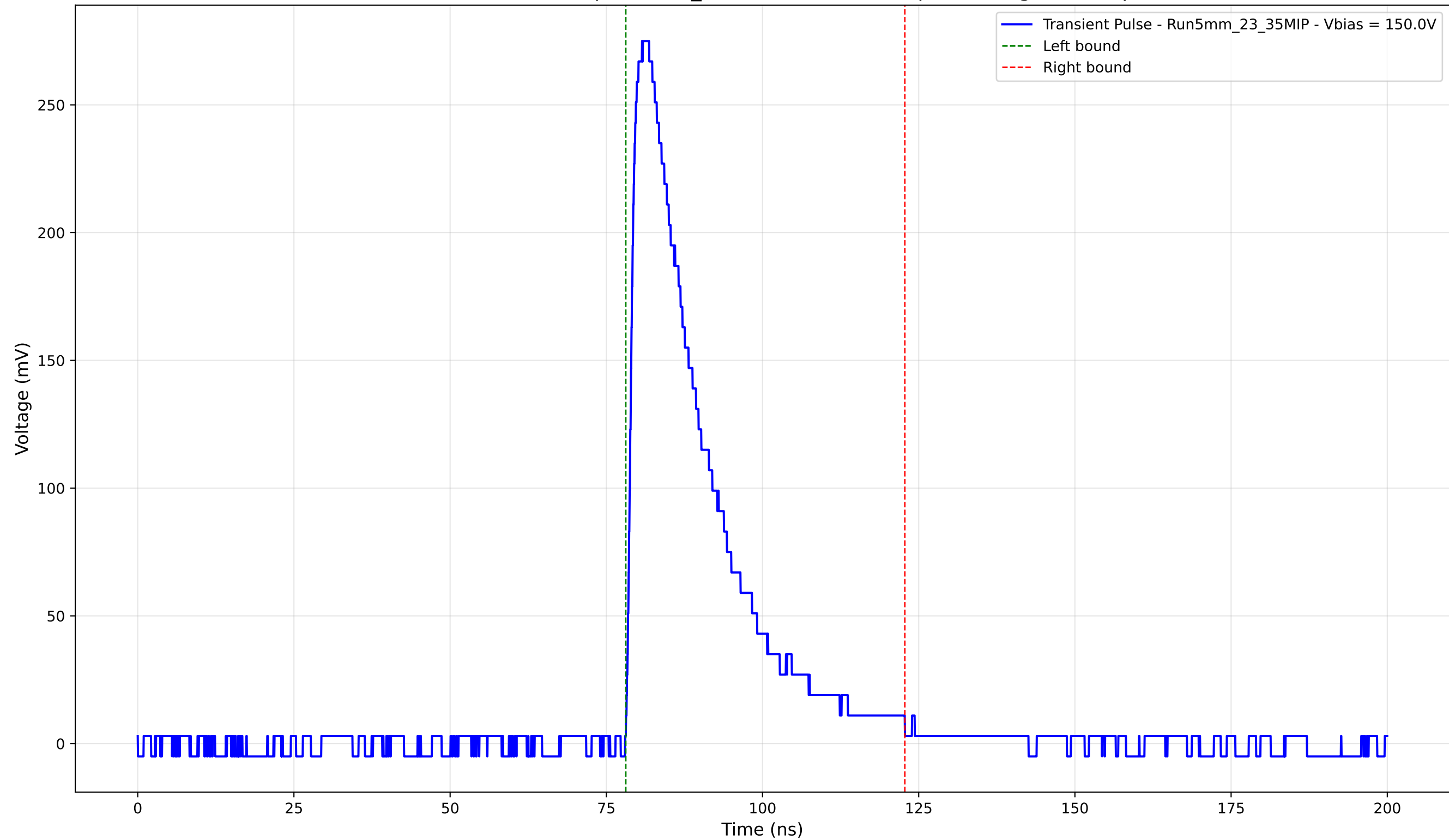
Transient Pulse - Sample: 5mm_23 - Position: 2185.0 \mu\text{m} - Charge: 71.74 pC
