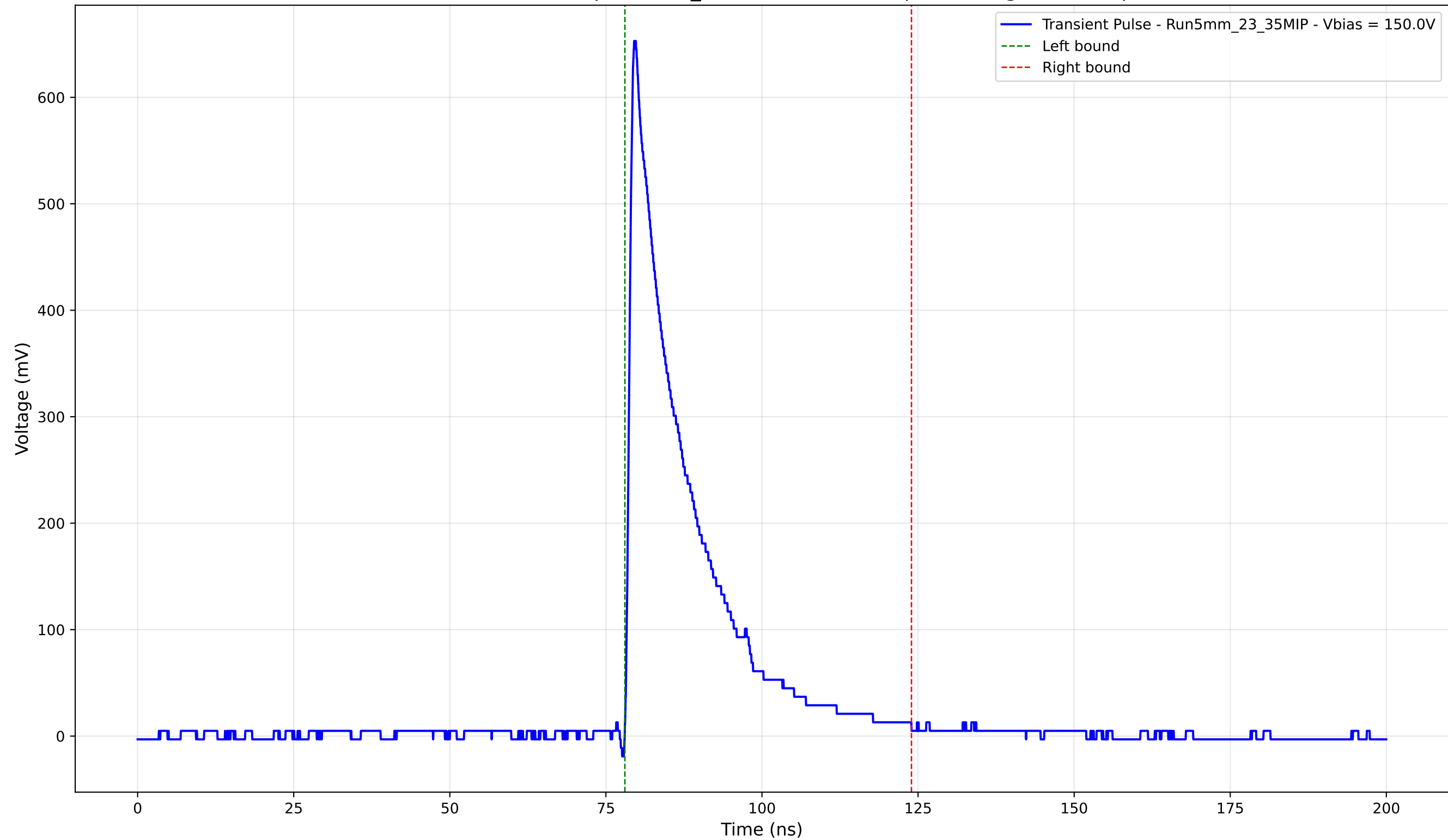
Transient Pulse - Sample: 5mm_23 - Position: 975.0 \mu\text{m} - Charge: 125.49 pC
