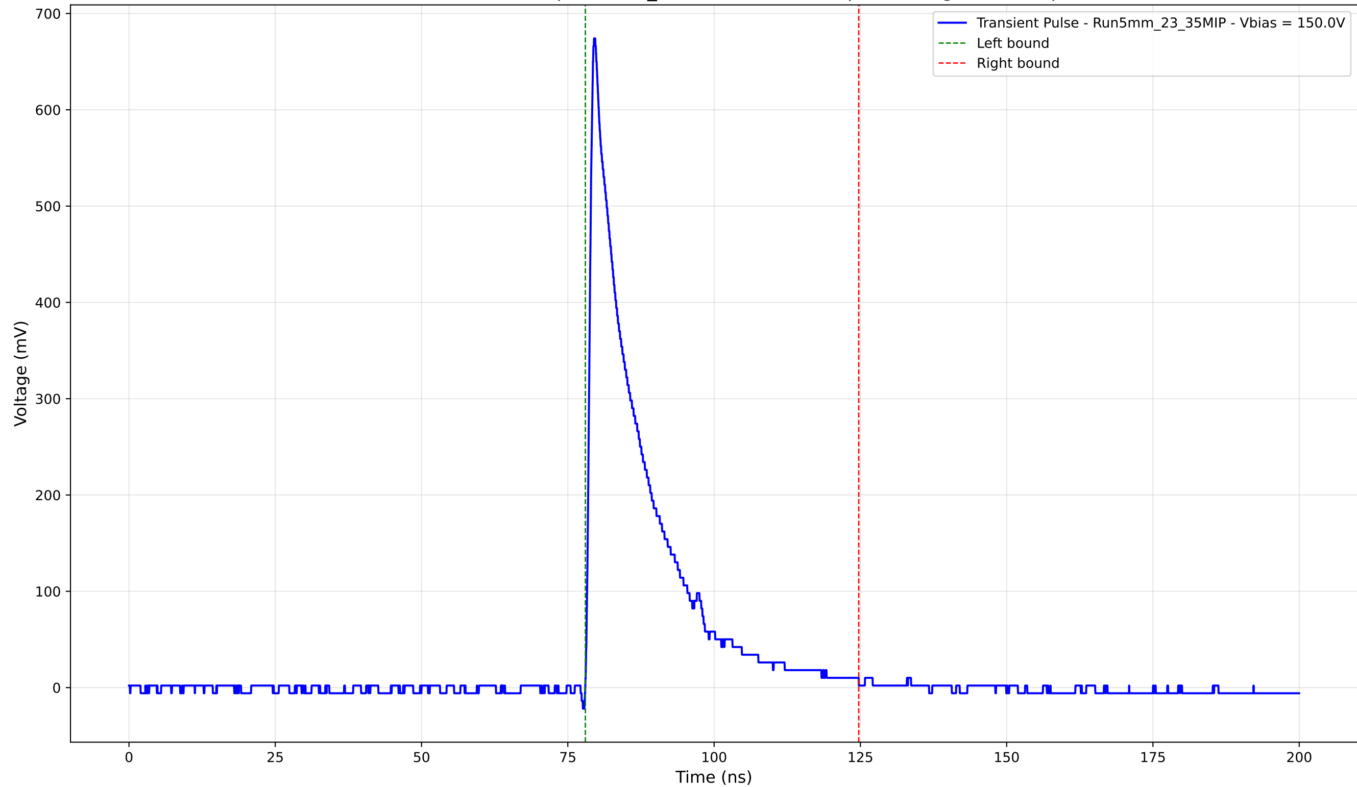
Transient Pulse - Sample: 5mm_23 - Position: 875.0 \mu\text{m} - Charge: 122.67 pC
