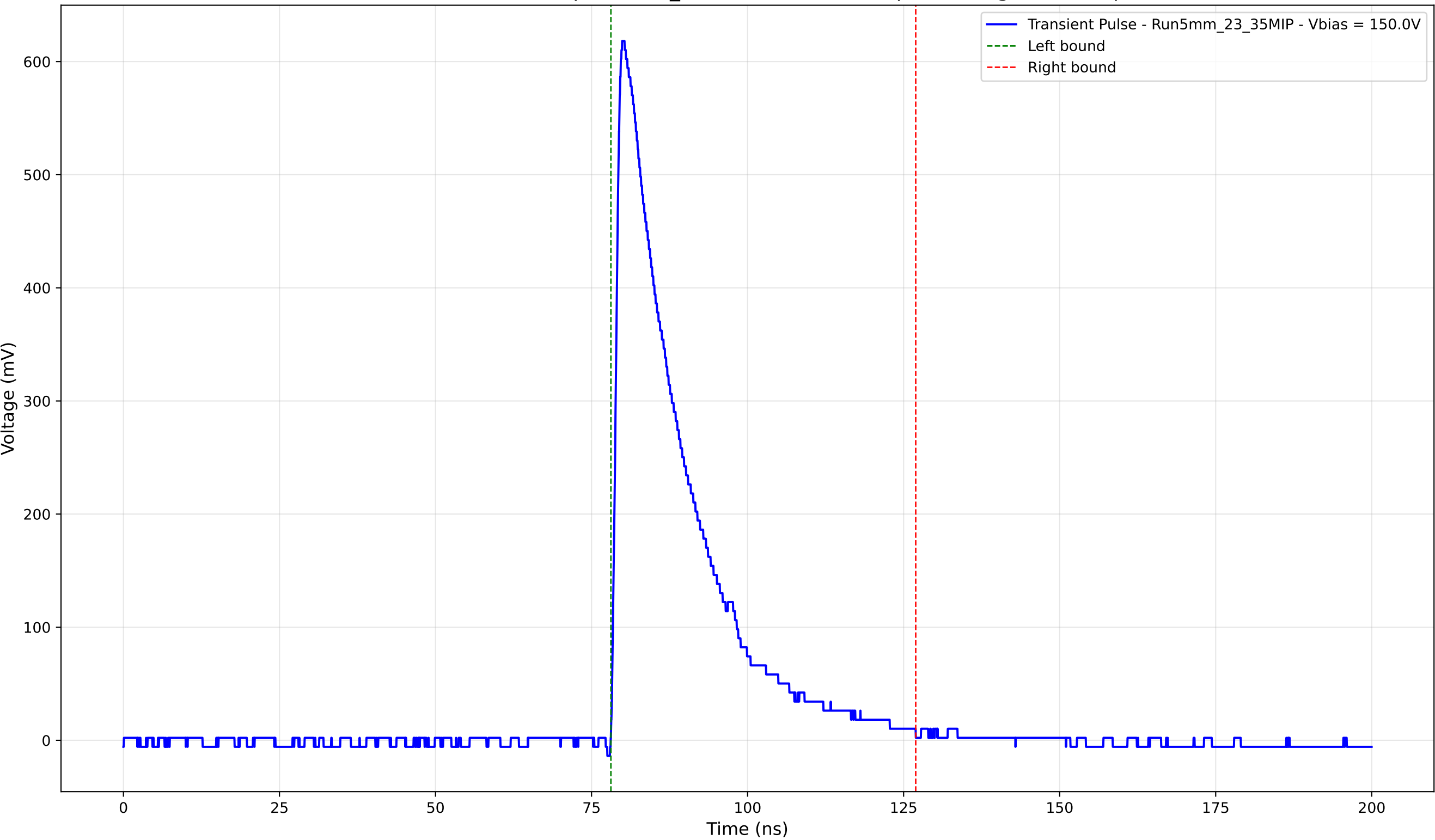
Transient Pulse - Sample: 5mm_23 - Position: 1485.0 \mu\text{m} - Charge: 144.63 pC
