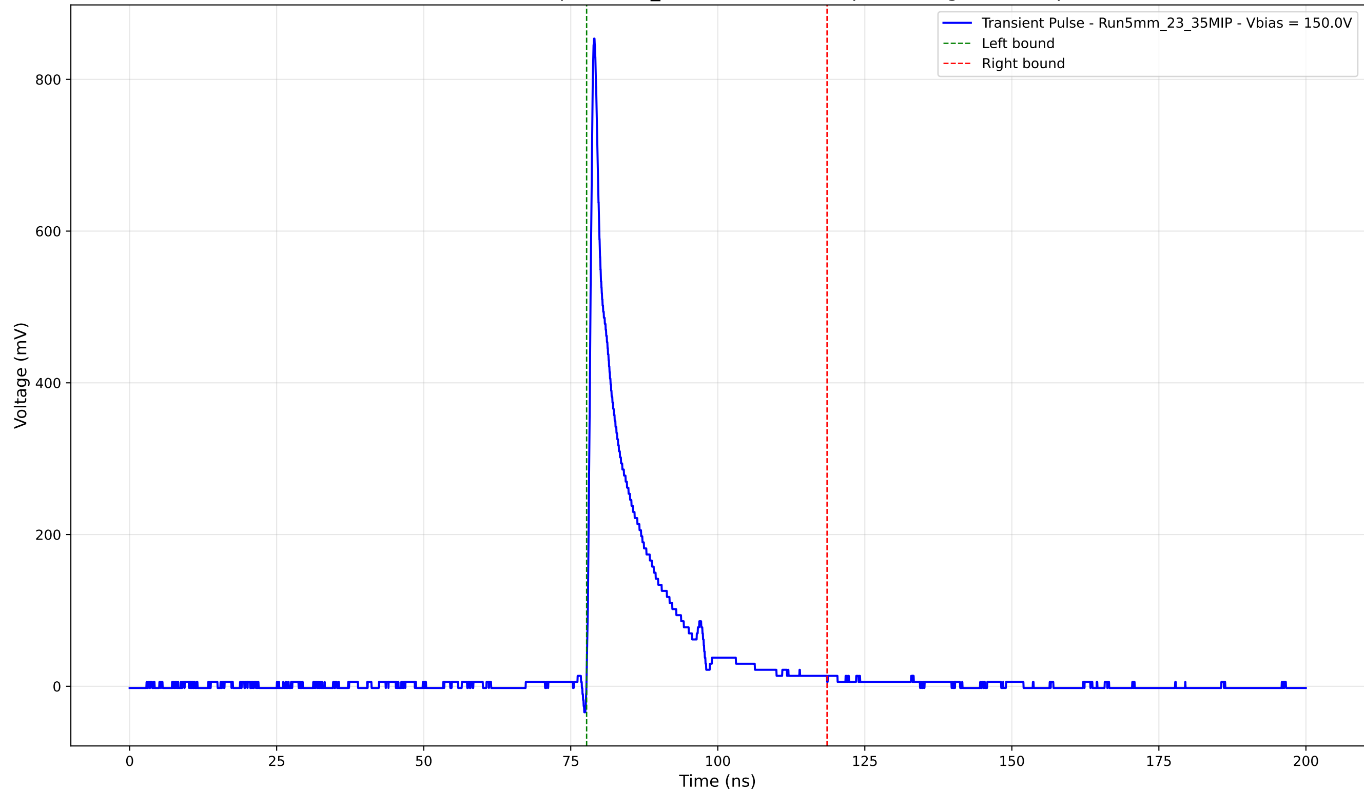
Transient Pulse - Sample: 5mm_23 - Position: 255.0 \mu\text{m} - Charge: 106.53 pC
