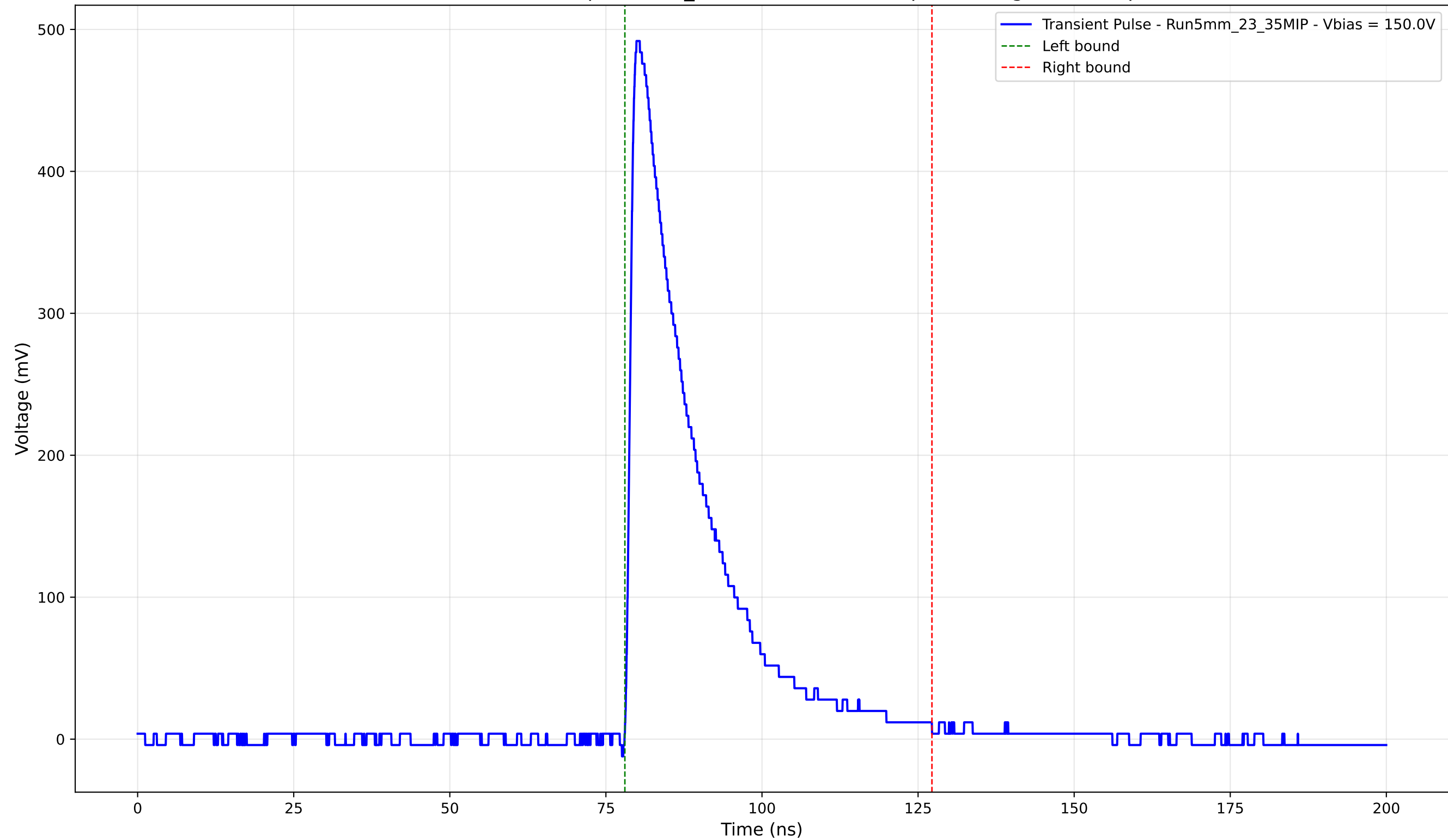
Transient Pulse - Sample: 5mm_23 - Position: 3735.0 \mu\text{m} - Charge: 114.48 pC
