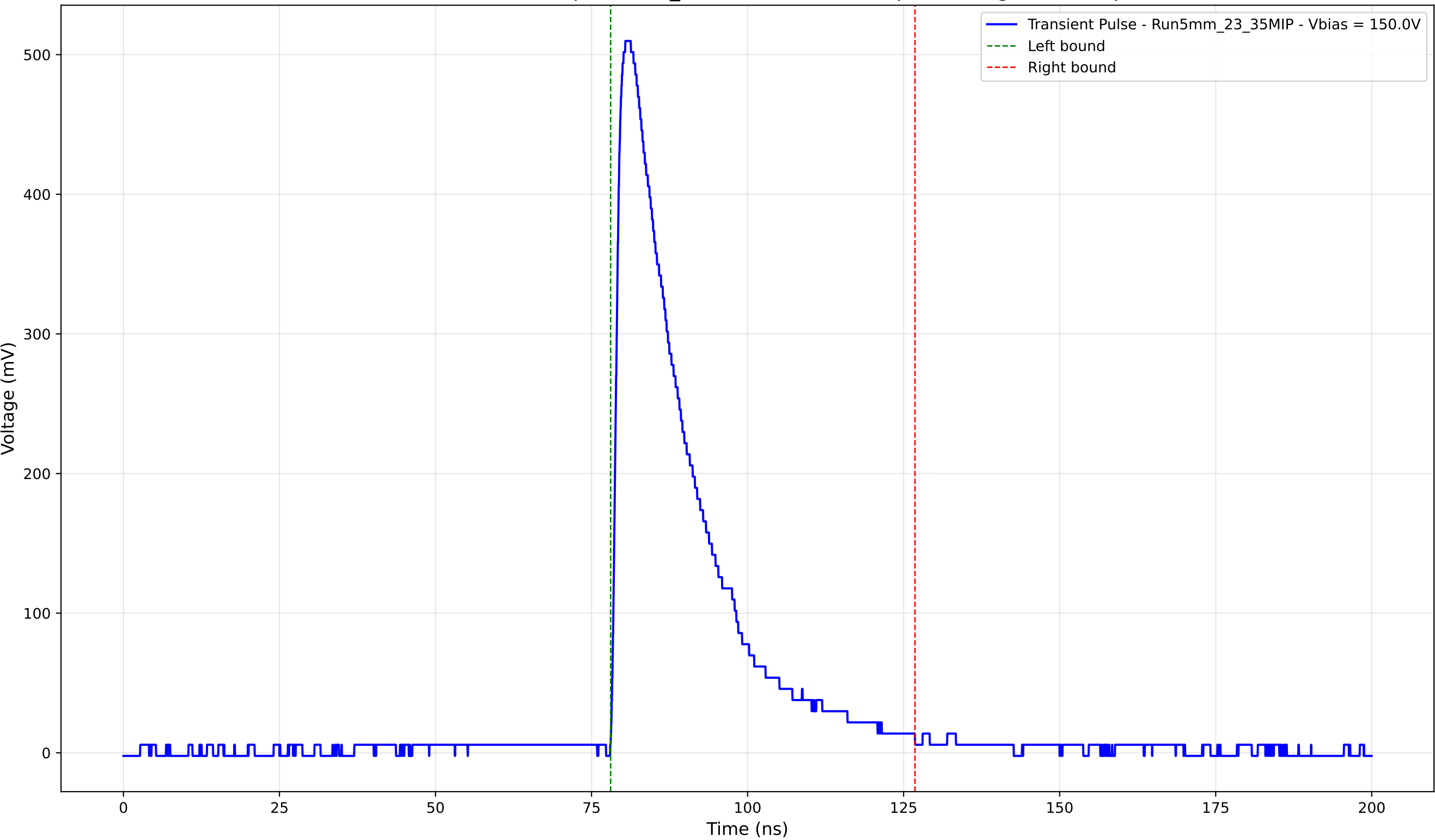
Transient Pulse - Sample: 5mm_23 - Position: 3320.0 \mu\text{m} - Charge: 132.17 pC
