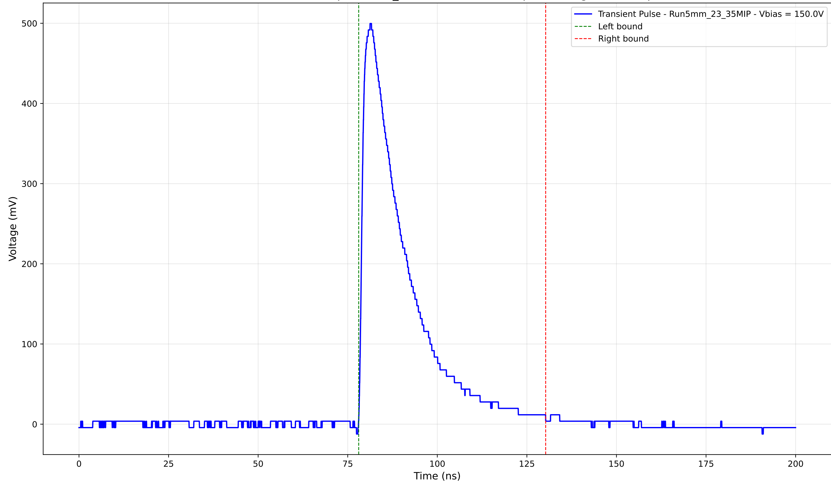
Transient Pulse - Sample: 5mm_23 - Position: 2940.0 \mu\text{m} - Charge: 133.96 pC
