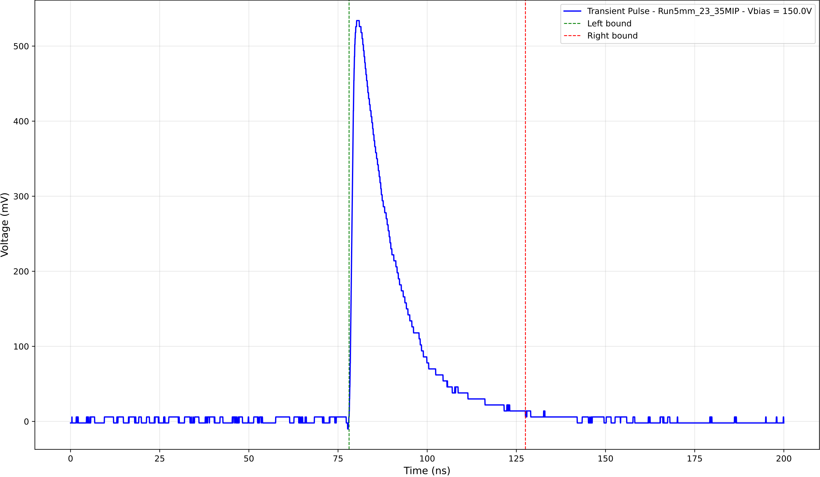
Transient Pulse - Sample: 5mm_23 - Position: 1775.0 \mu\text{m} - Charge: 137.04 pC
