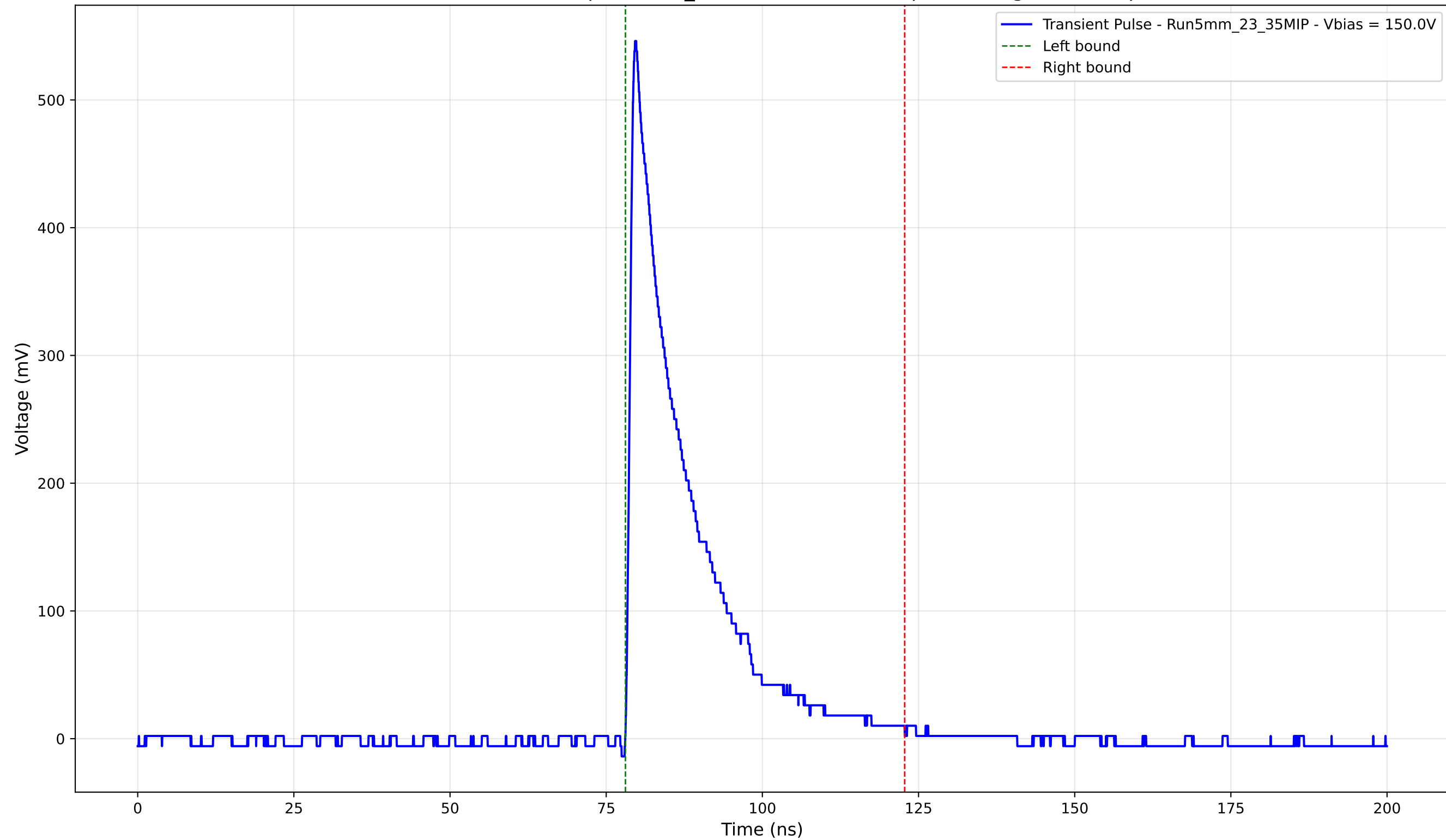
Transient Pulse - Sample: 5mm_23 - Position: 1050.0 \mu\text{m} - Charge: 103.88 pC
