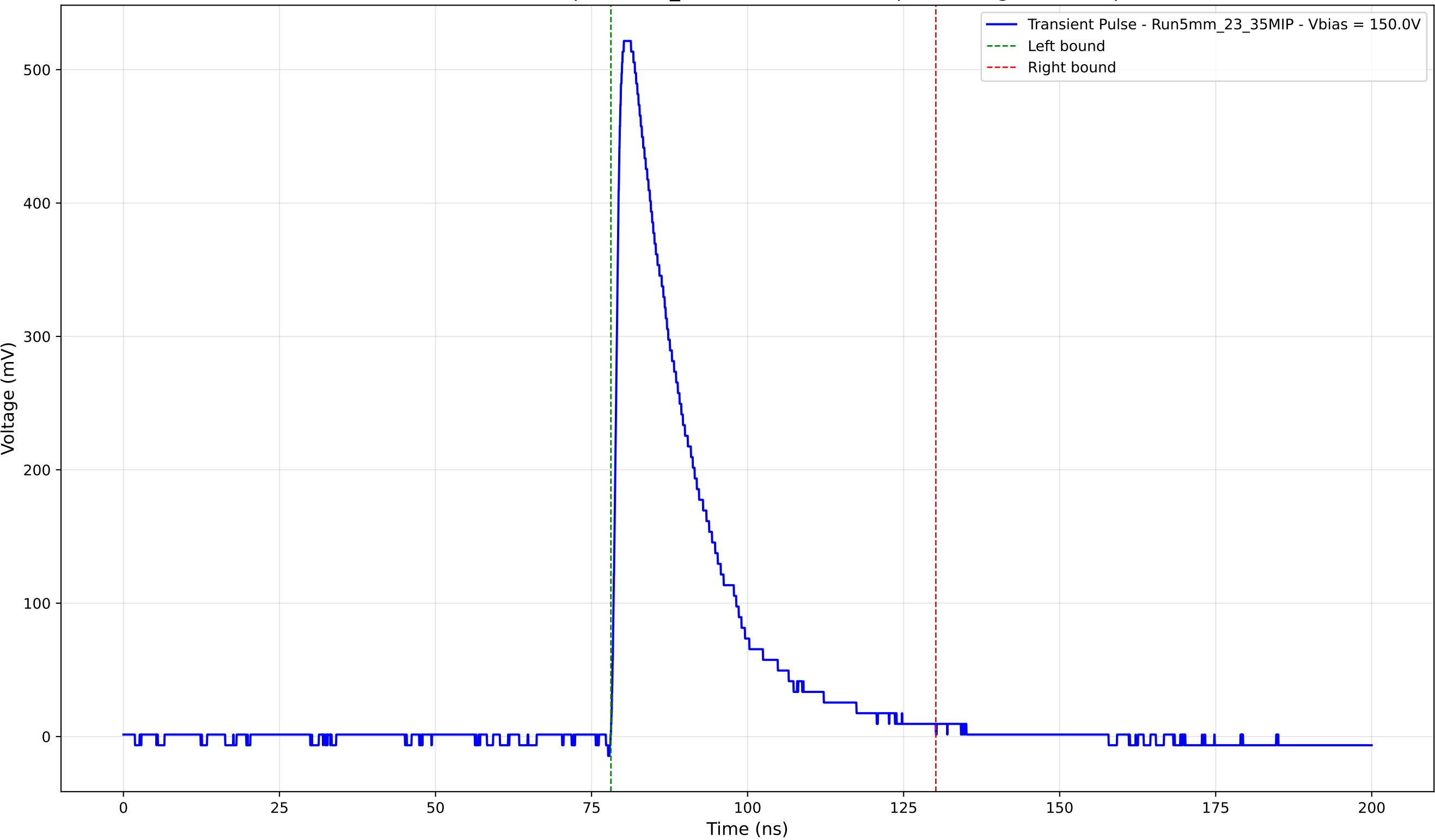
Transient Pulse - Sample: 5mm_23 - Position: 1845.0 \mu\text{m} - Charge: 134.12 pC
