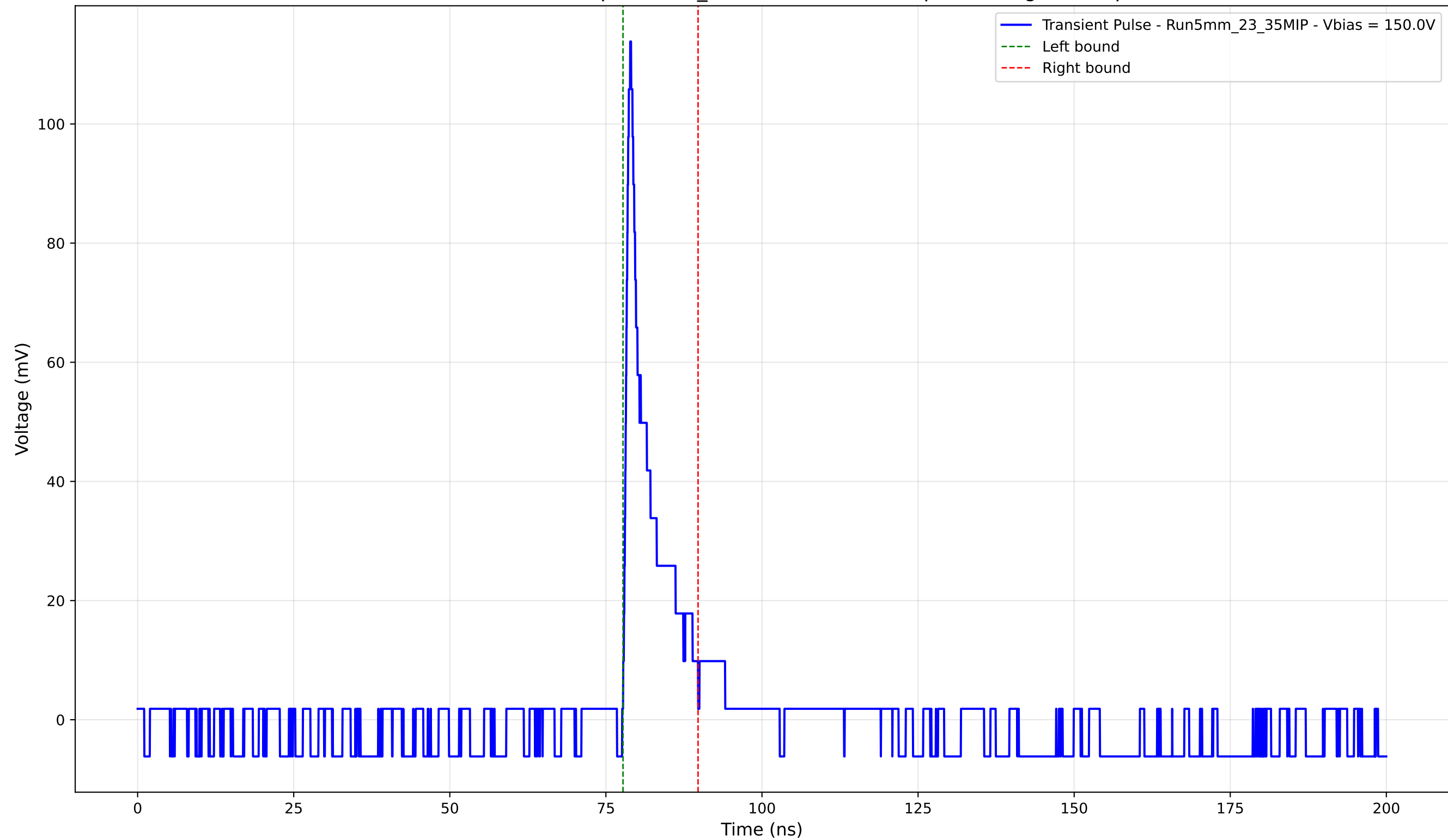
Transient Pulse - Sample: 5mm_23 - Position: 5105.0 \mu\text{m} - Charge: 8.92 pC
