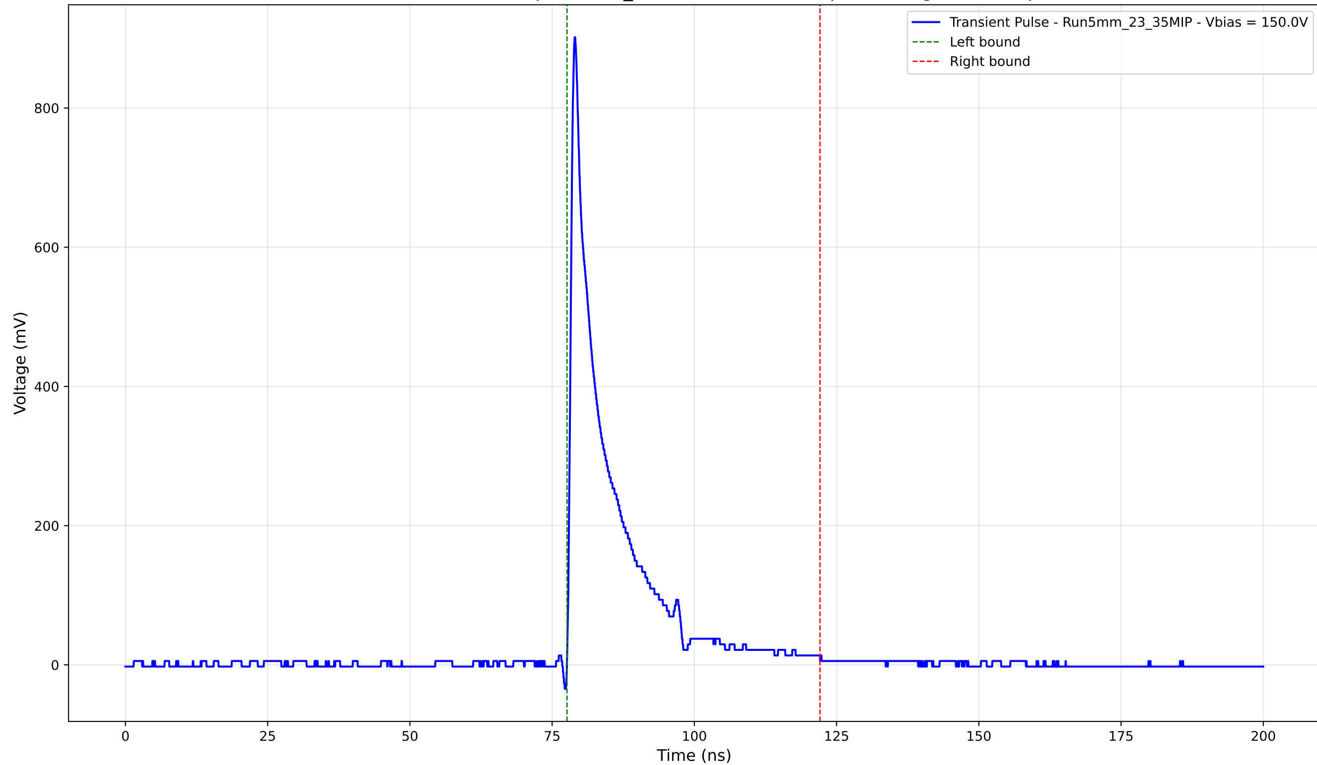
Transient Pulse - Sample: 5mm_23 - Position: 4960.0 \mu\text{m} - Charge: 120.07 pC
