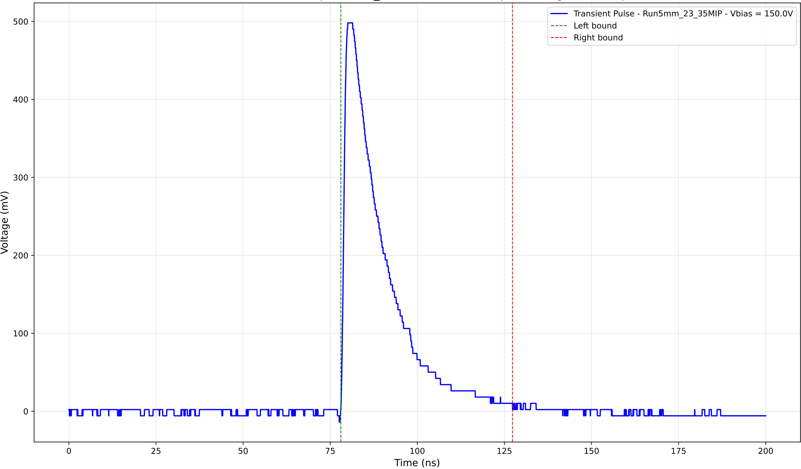
Transient Pulse - Sample: 5mm_23 - Position: 3460.0 \mu\text{m} - Charge: 125.44 pC
