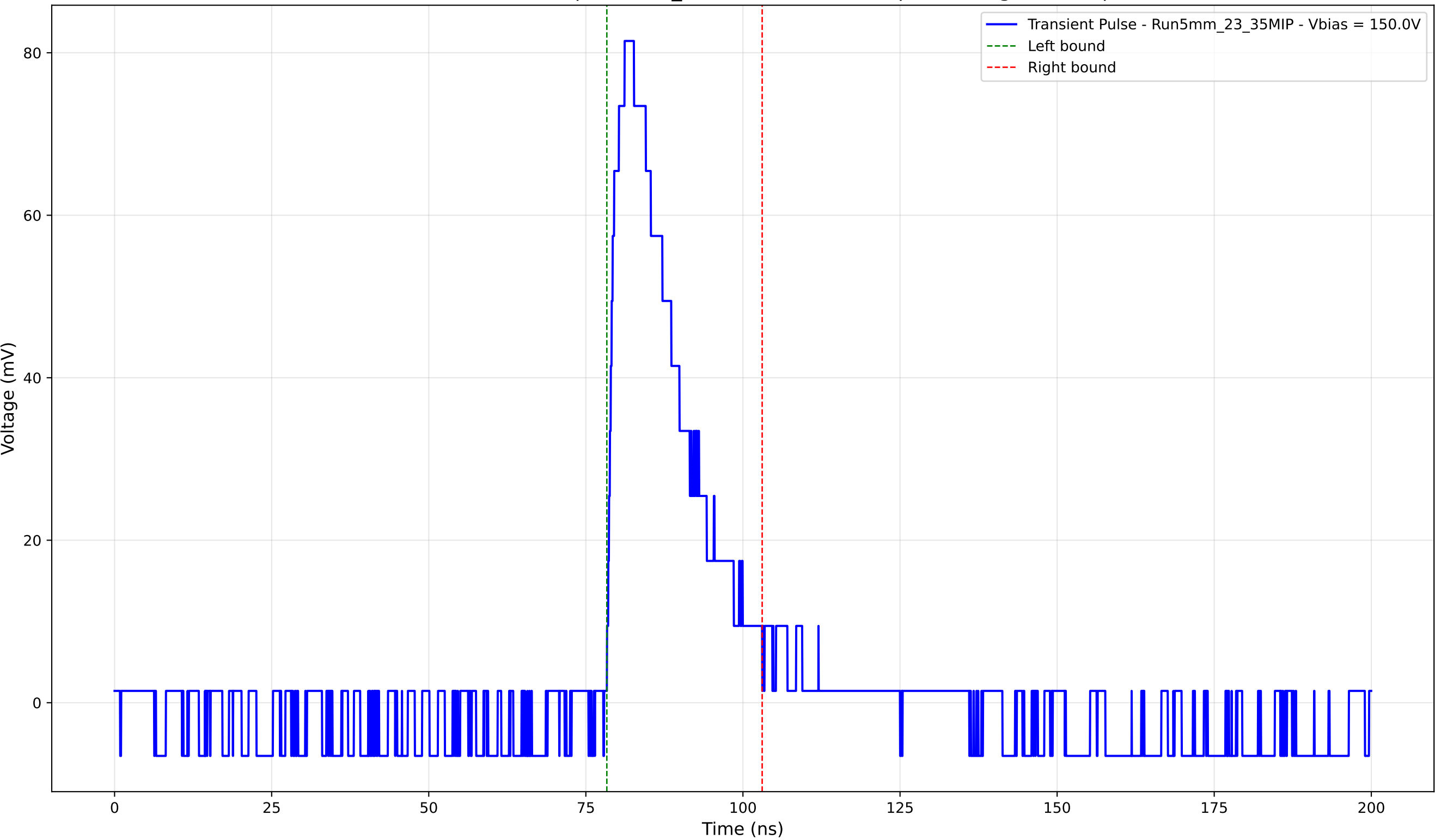
Transient Pulse - Sample: 5mm_23 - Position: 2140.0 \mu\text{m} - Charge: 18.98 pC
