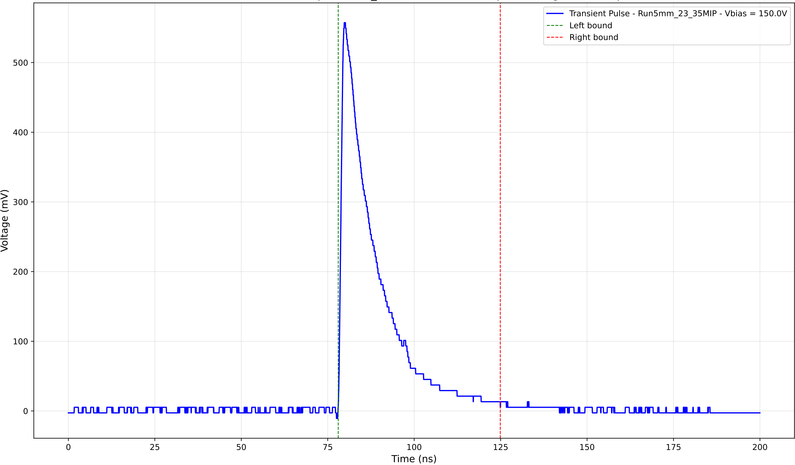
Transient Pulse - Sample: 5mm_23 - Position: 3945.0 \mu\text{m} - Charge: 121.31 pC
