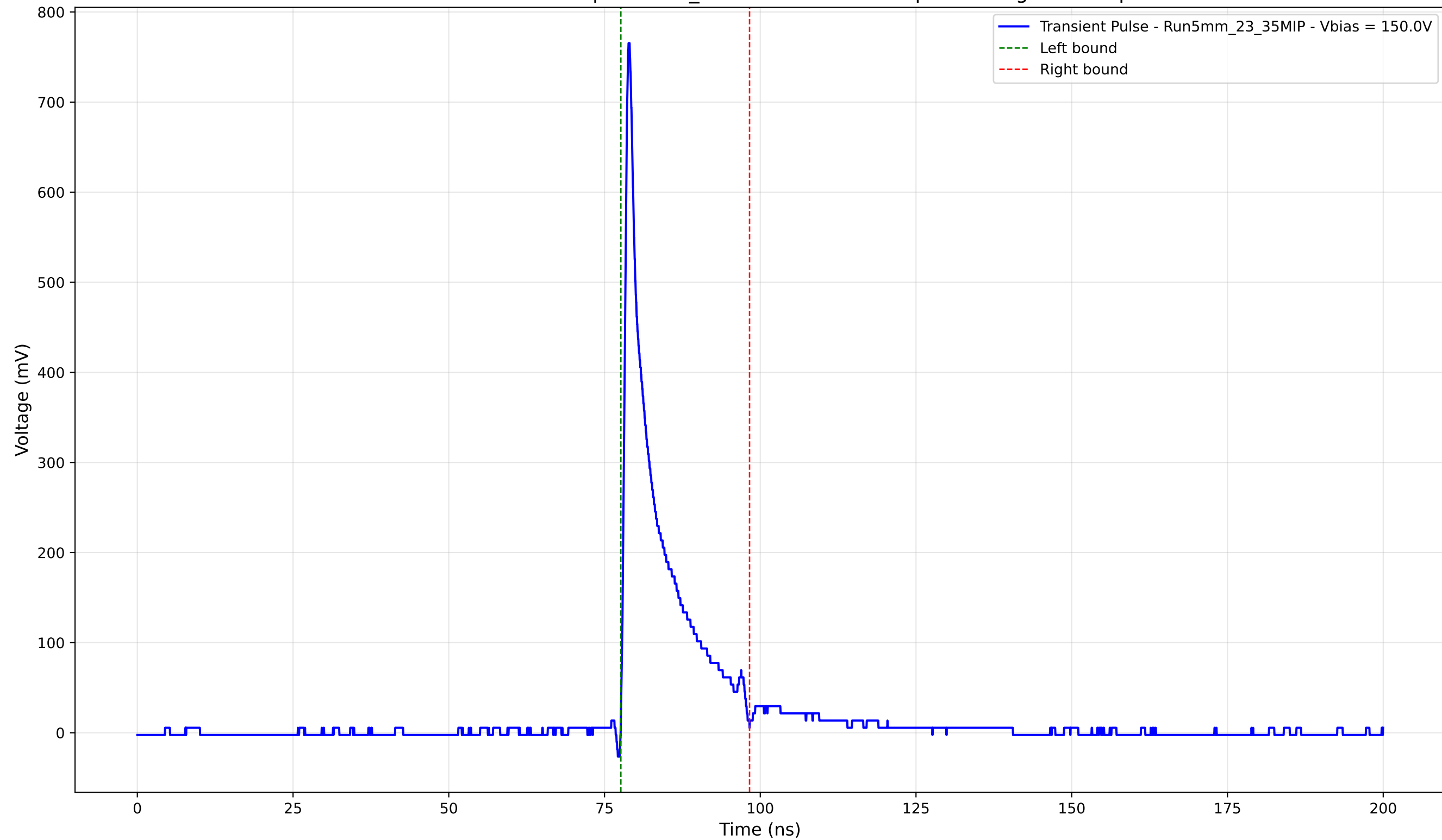
Transient Pulse - Sample: 5mm_23 - Position: 5040.0 \mu\text{m} - Charge: 80.17 pC
