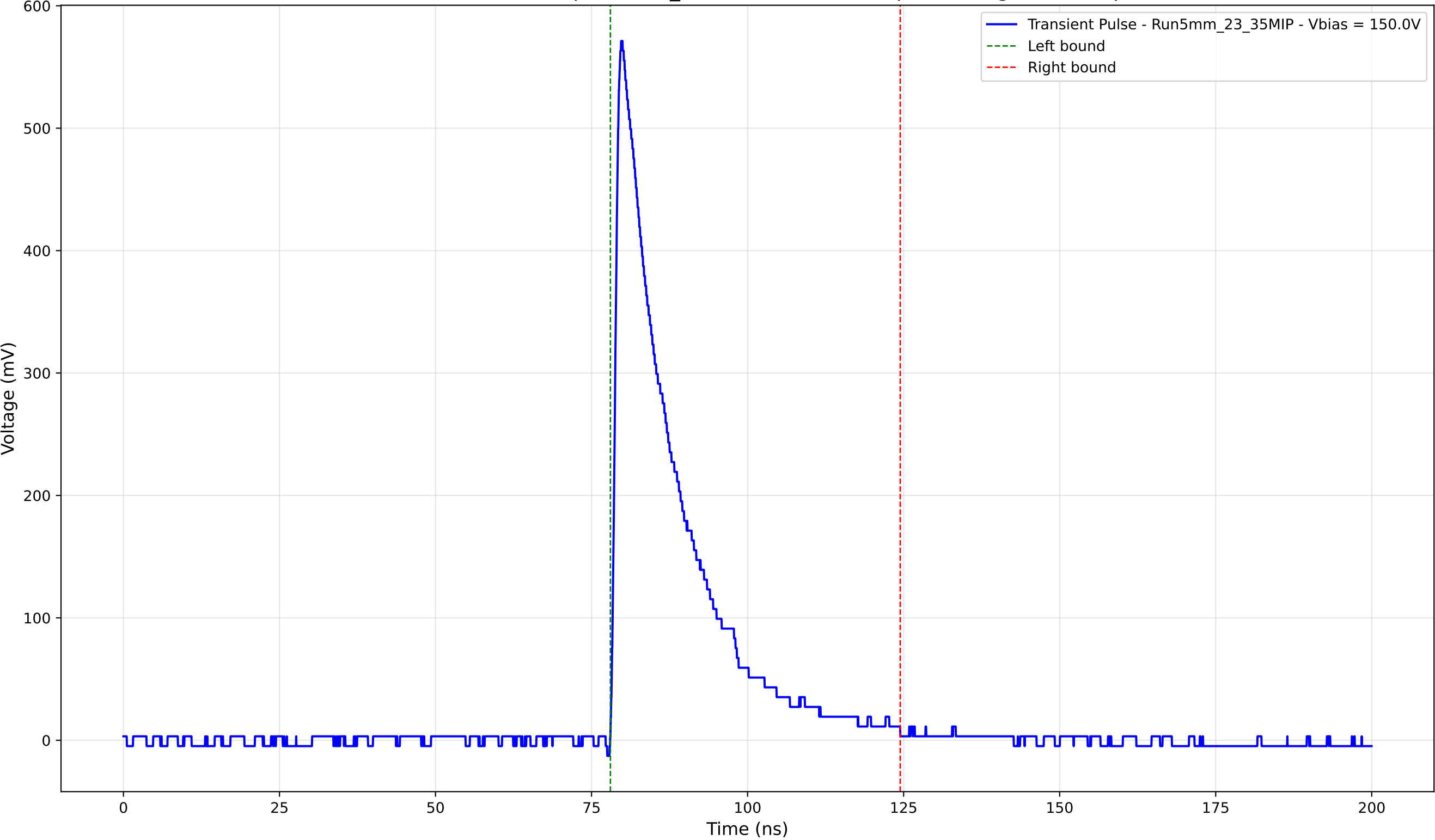
Transient Pulse - Sample: 5mm_23 - Position: 4050.0 \mu\text{m} - Charge: 116.99 pC
