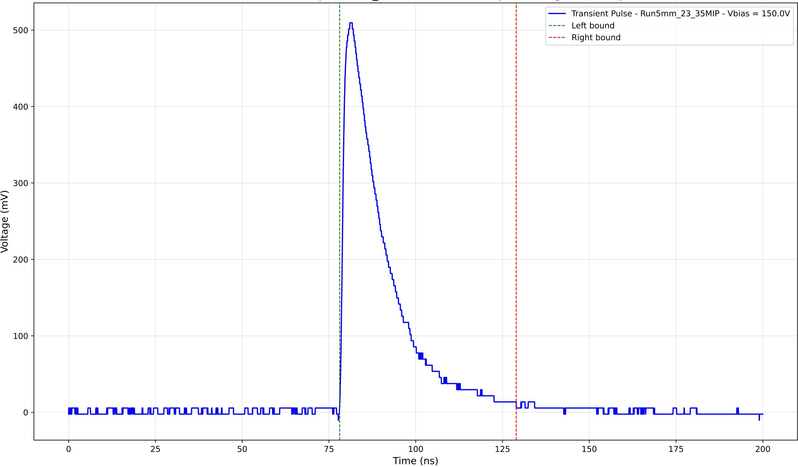
Transient Pulse - Sample: 5mm_23 - Position: 2335.0 \mu\text{m} - Charge: 138.63 pC
