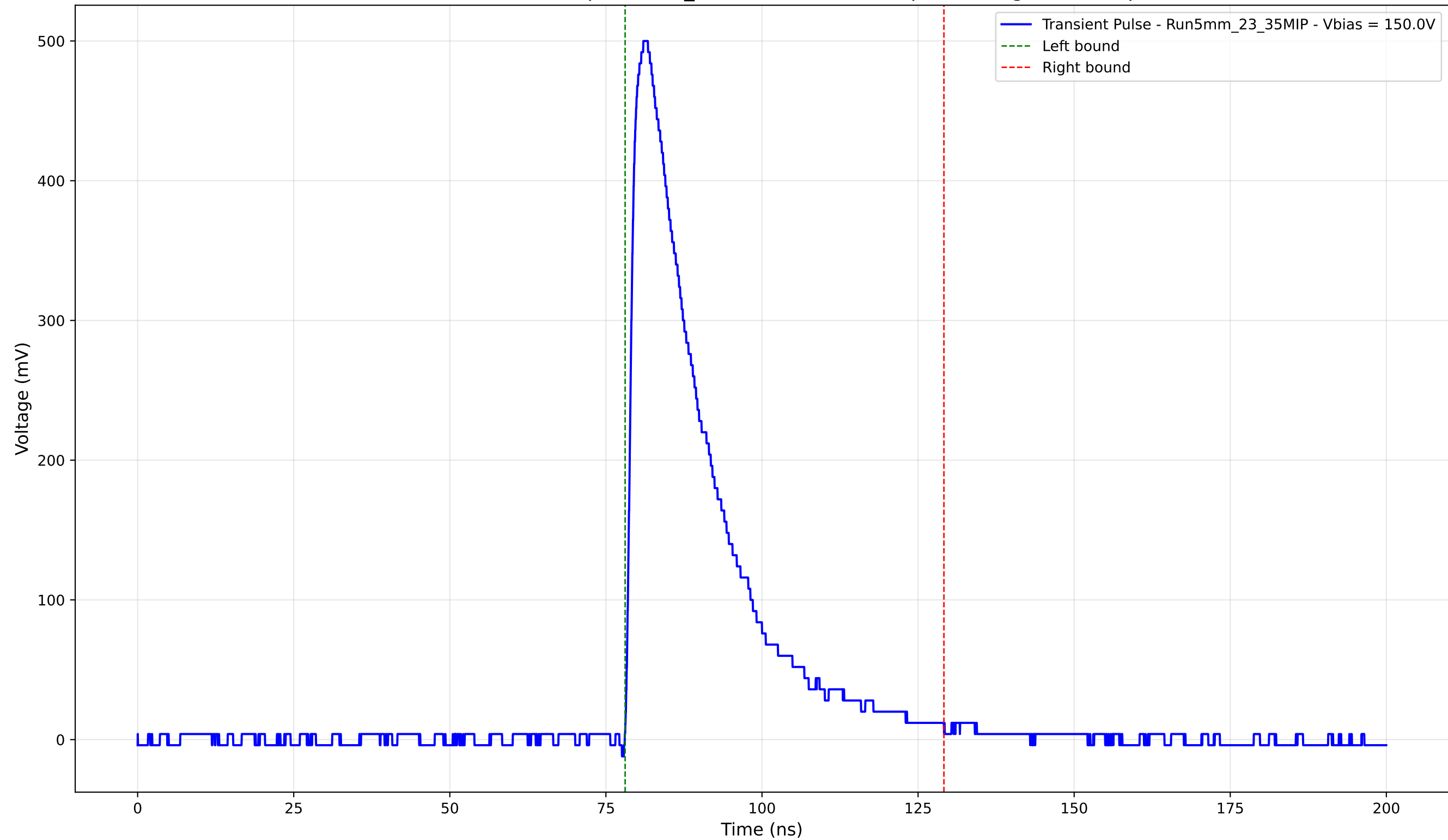
Transient Pulse - Sample: 5mm_23 - Position: 2900.0 \mu\text{m} - Charge: 134.73 pC
