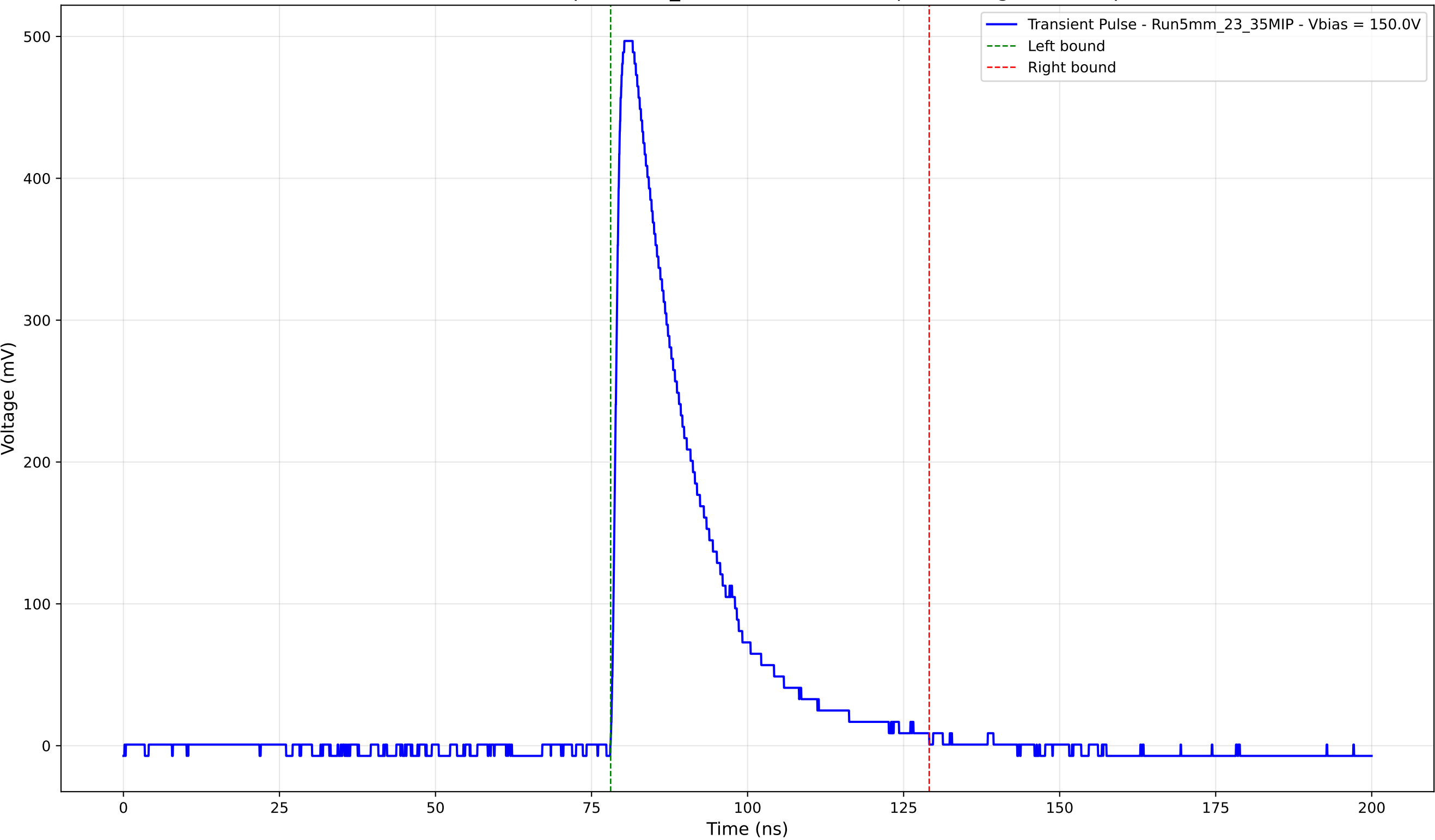
Transient Pulse - Sample: 5mm_23 - Position: 3315.0 \mu\text{m} - Charge: 128.46 pC
