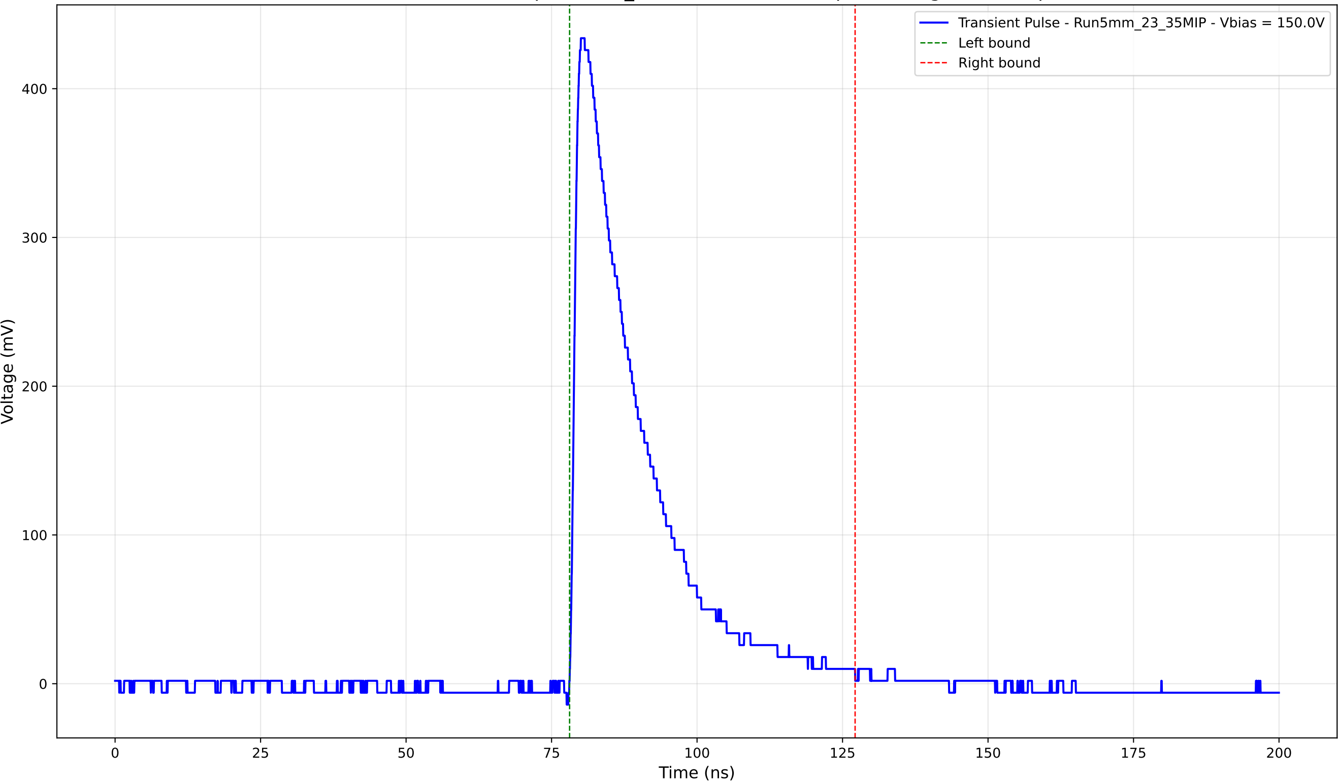
Transient Pulse - Sample: 5mm_23 - Position: 1700.0 \mu\text{m} - Charge: 107.18 pC
