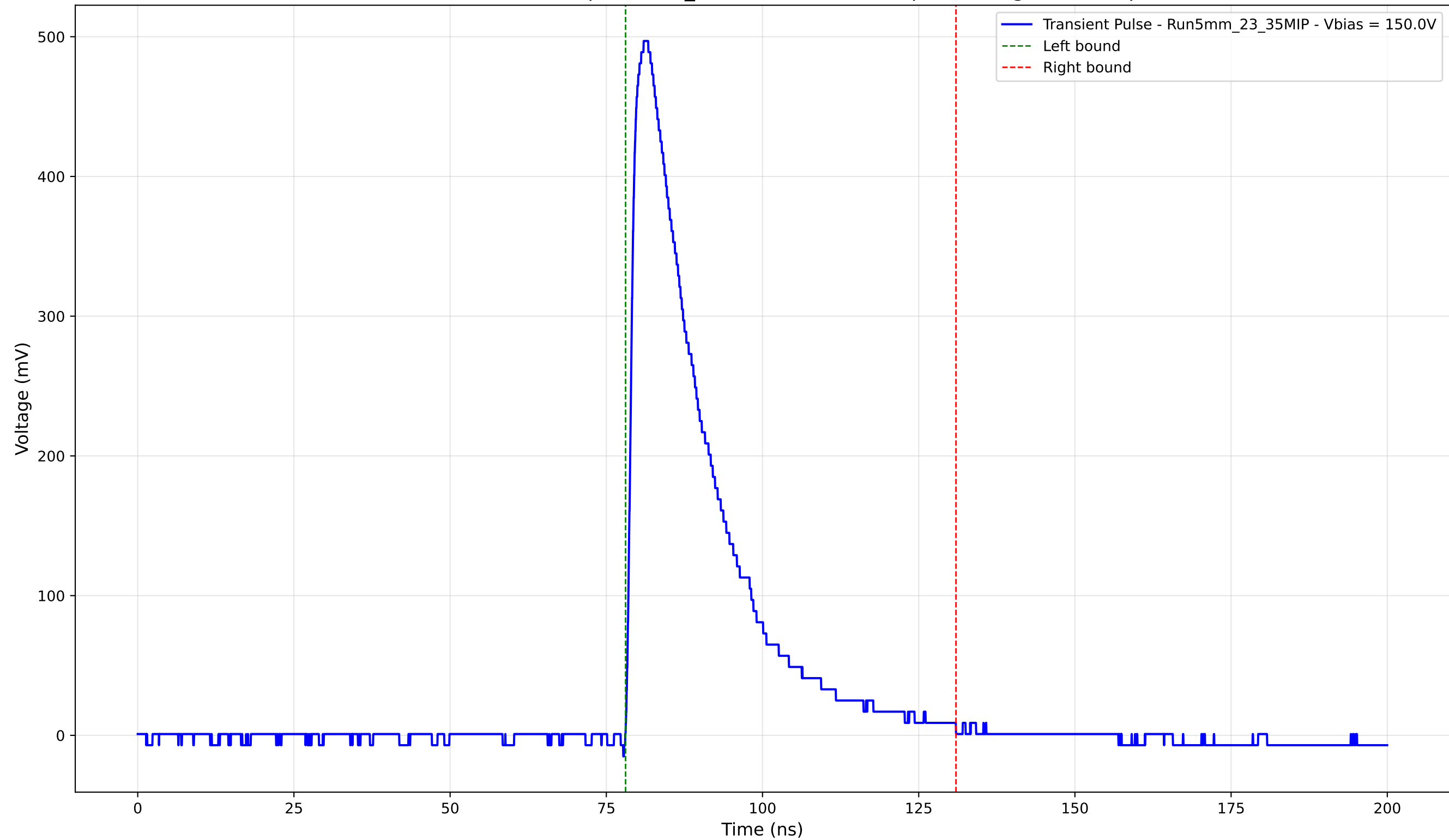
Transient Pulse - Sample: 5mm_23 - Position: 2965.0 \mu\text{m} - Charge: 131.98 pC
