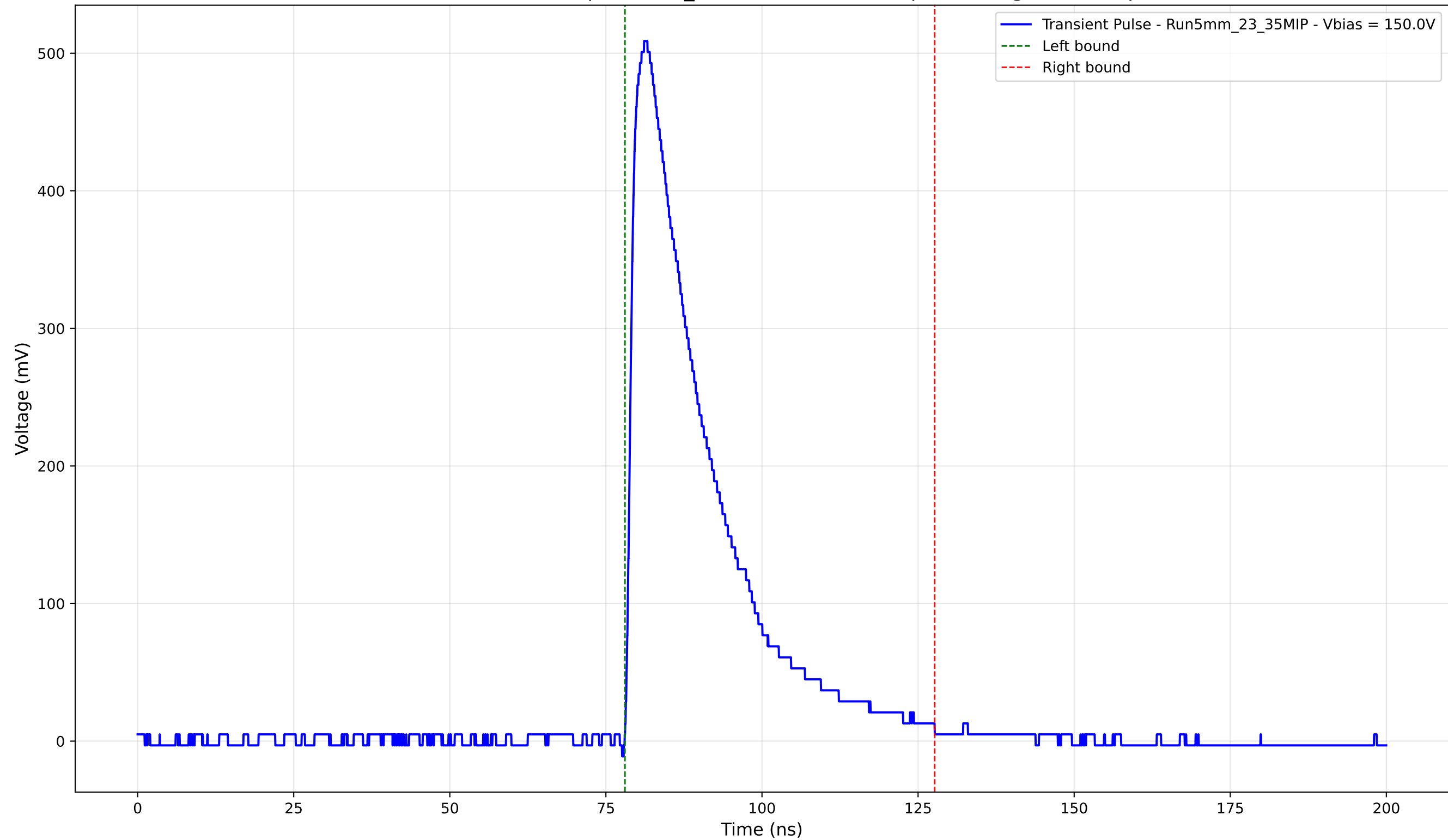
Transient Pulse - Sample: 5mm_23 - Position: 2500.0 \mu\text{m} - Charge: 138.16 pC
