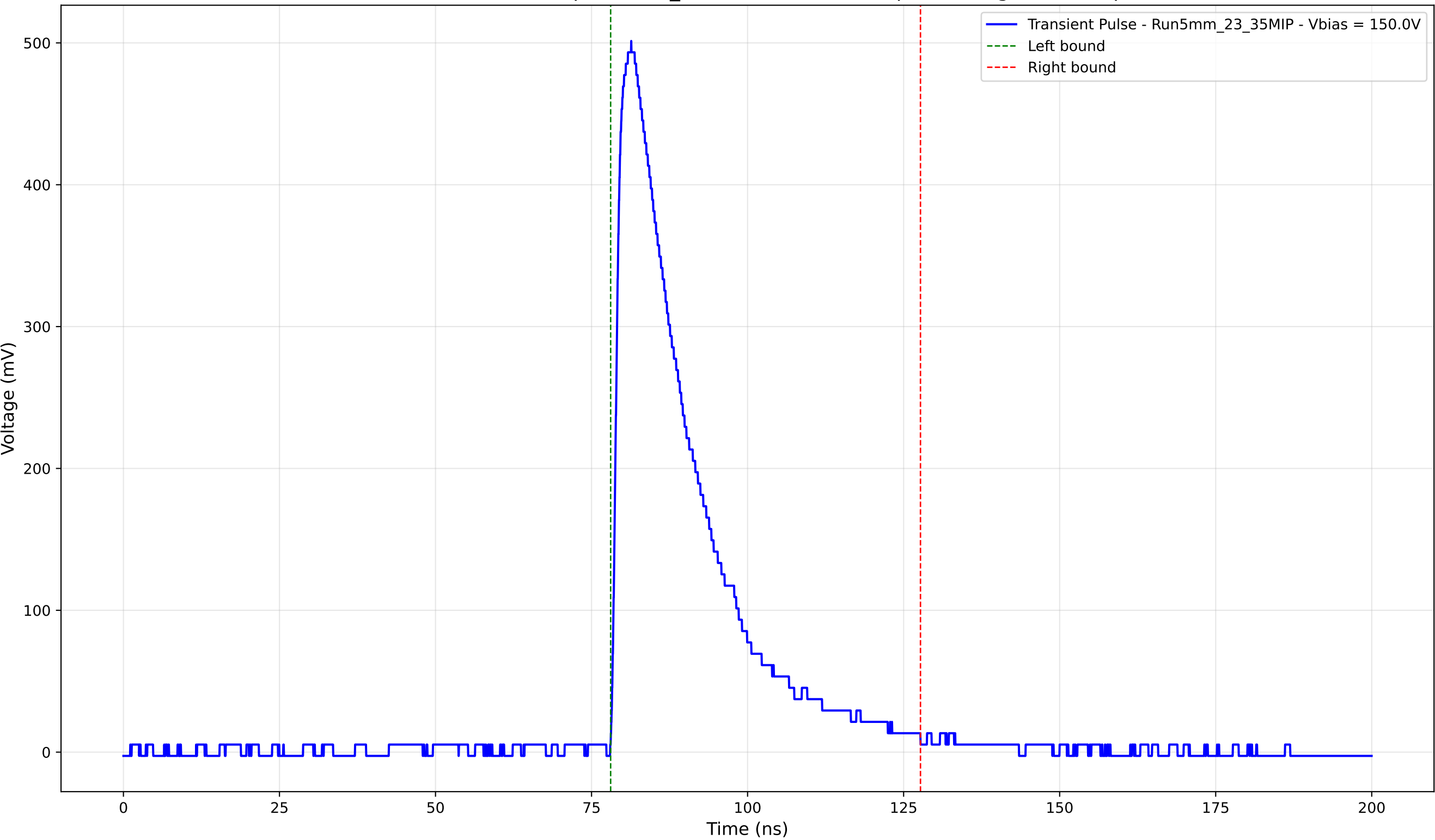
Transient Pulse - Sample: 5mm_23 - Position: 2915.0 \mu\text{m} - Charge: 134.63 pC
