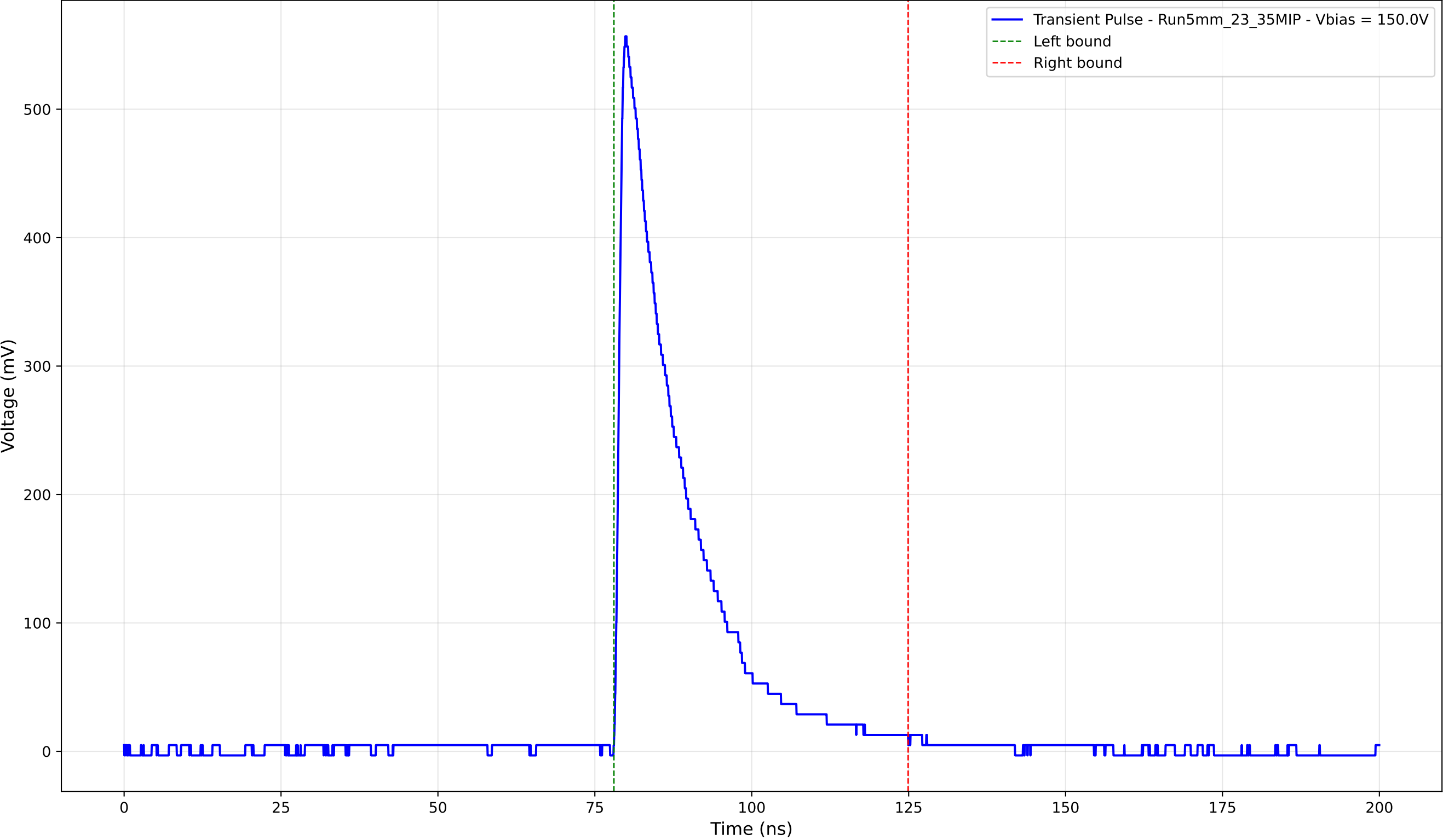
Transient Pulse - Sample: 5mm_23 - Position: 3930.0 \mu\text{m} - Charge: 120.20 pC
