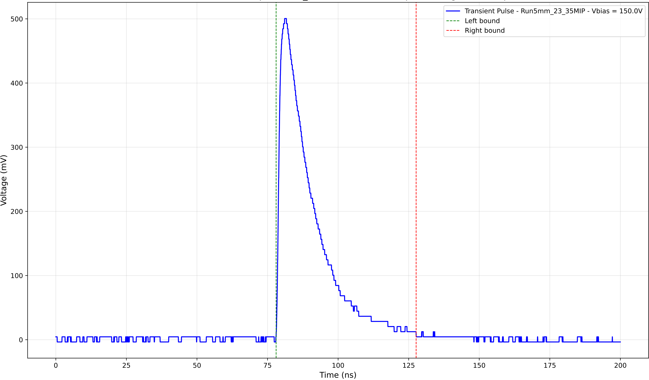
Transient Pulse - Sample: 5mm_23 - Position: 2885.0 \mu\text{m} - Charge: 134.19 pC
