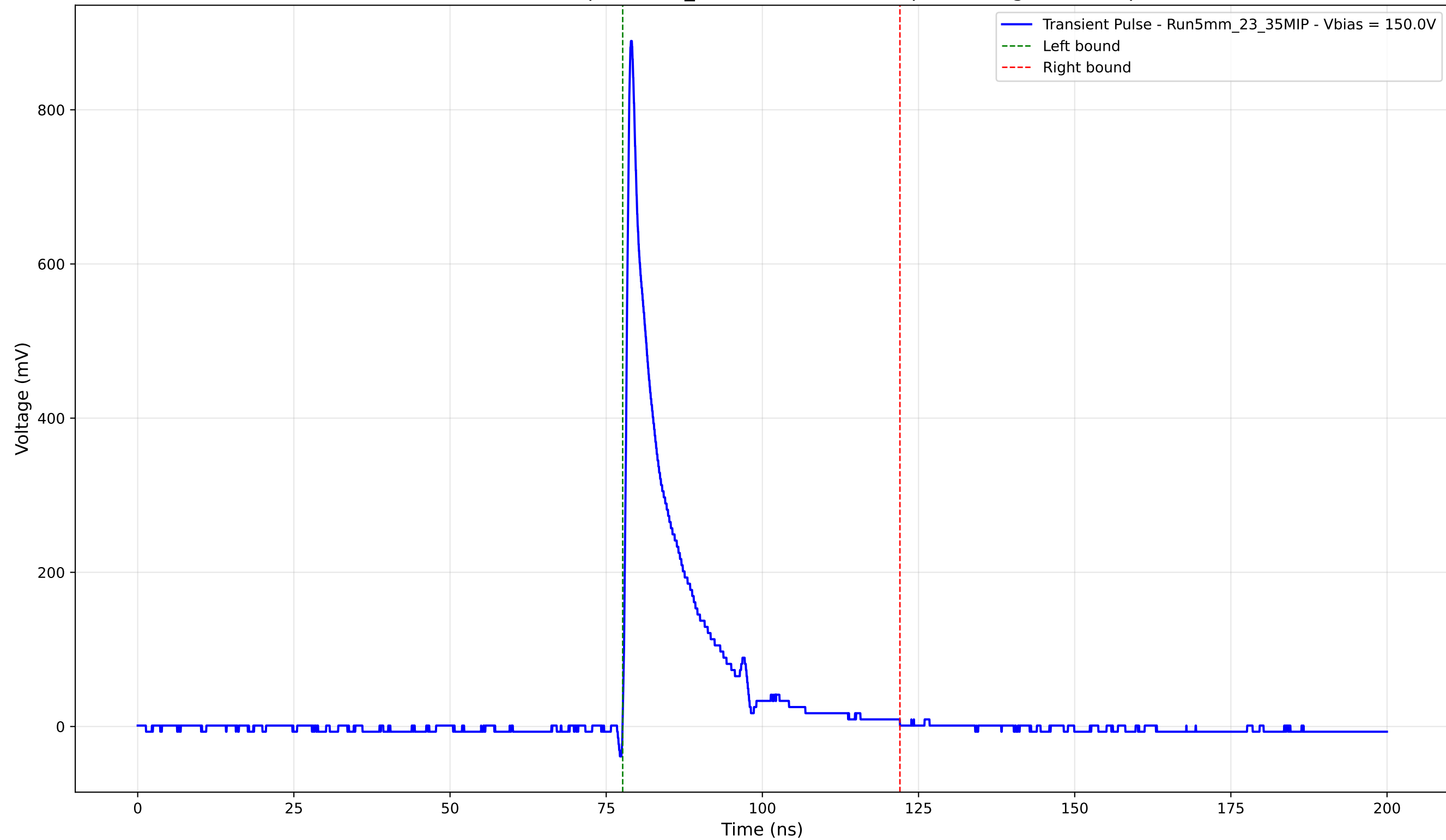
Transient Pulse - Sample: 5mm_23 - Position: 4945.0 \mu\text{m} - Charge: 116.00 pC
