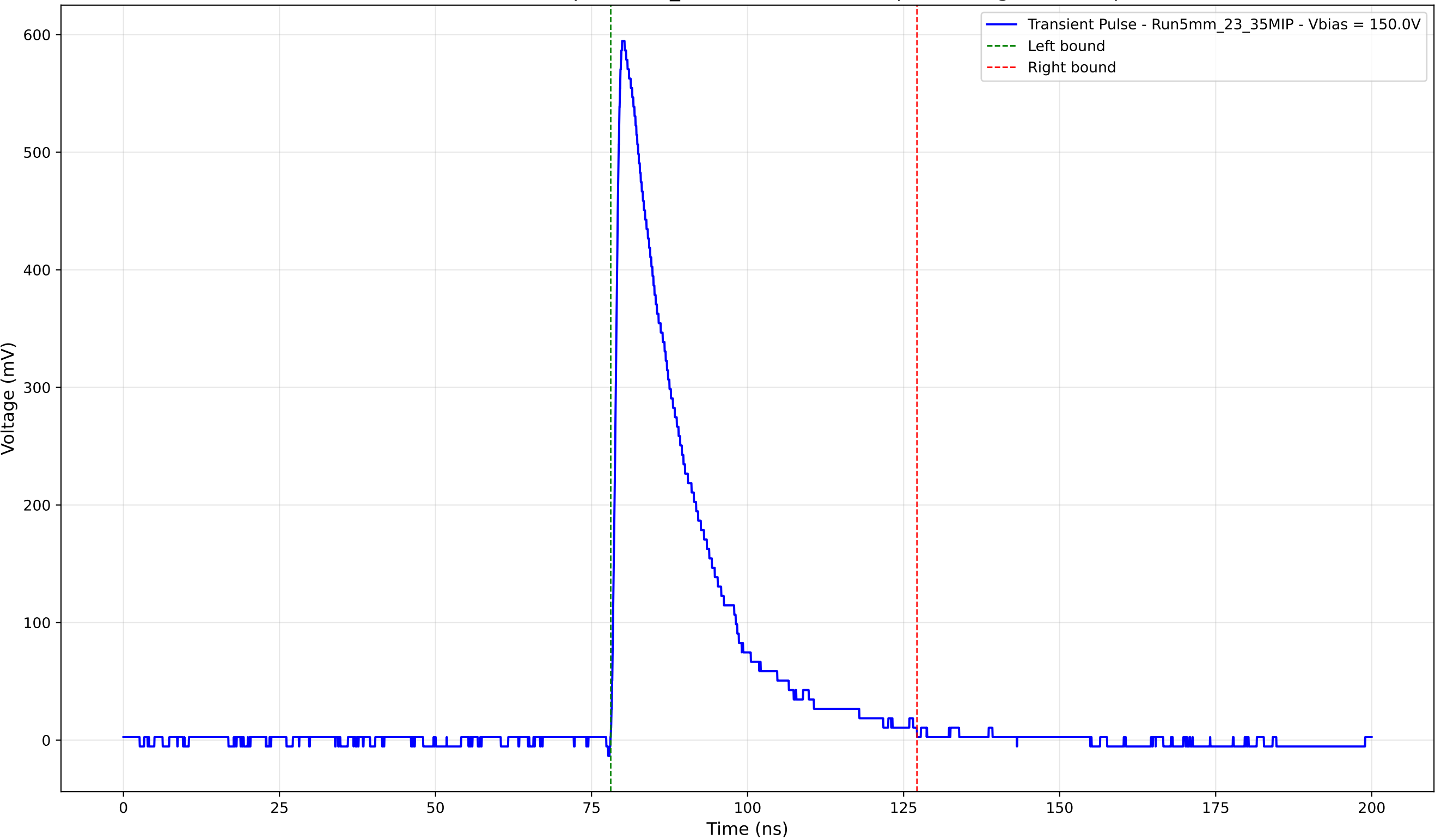
Transient Pulse - Sample: 5mm_23 - Position: 1505.0 \mu\text{m} - Charge: 140.04 pC
