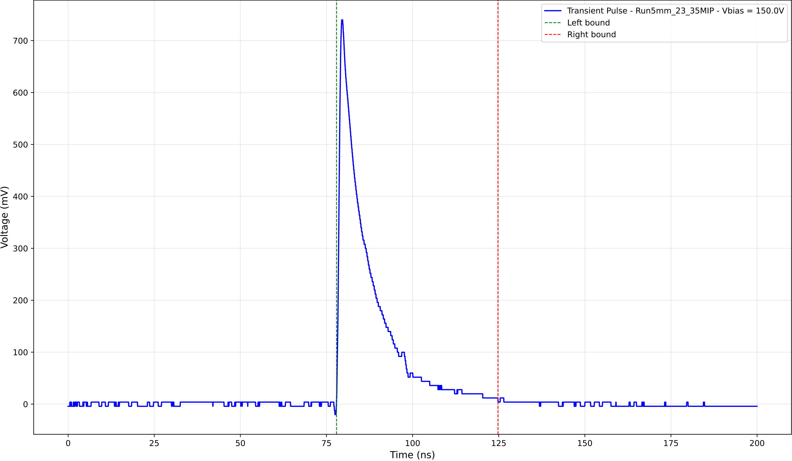
Transient Pulse - Sample: 5mm_23 - Position: 4410.0 \mu\text{m} - Charge: 133.21 pC
