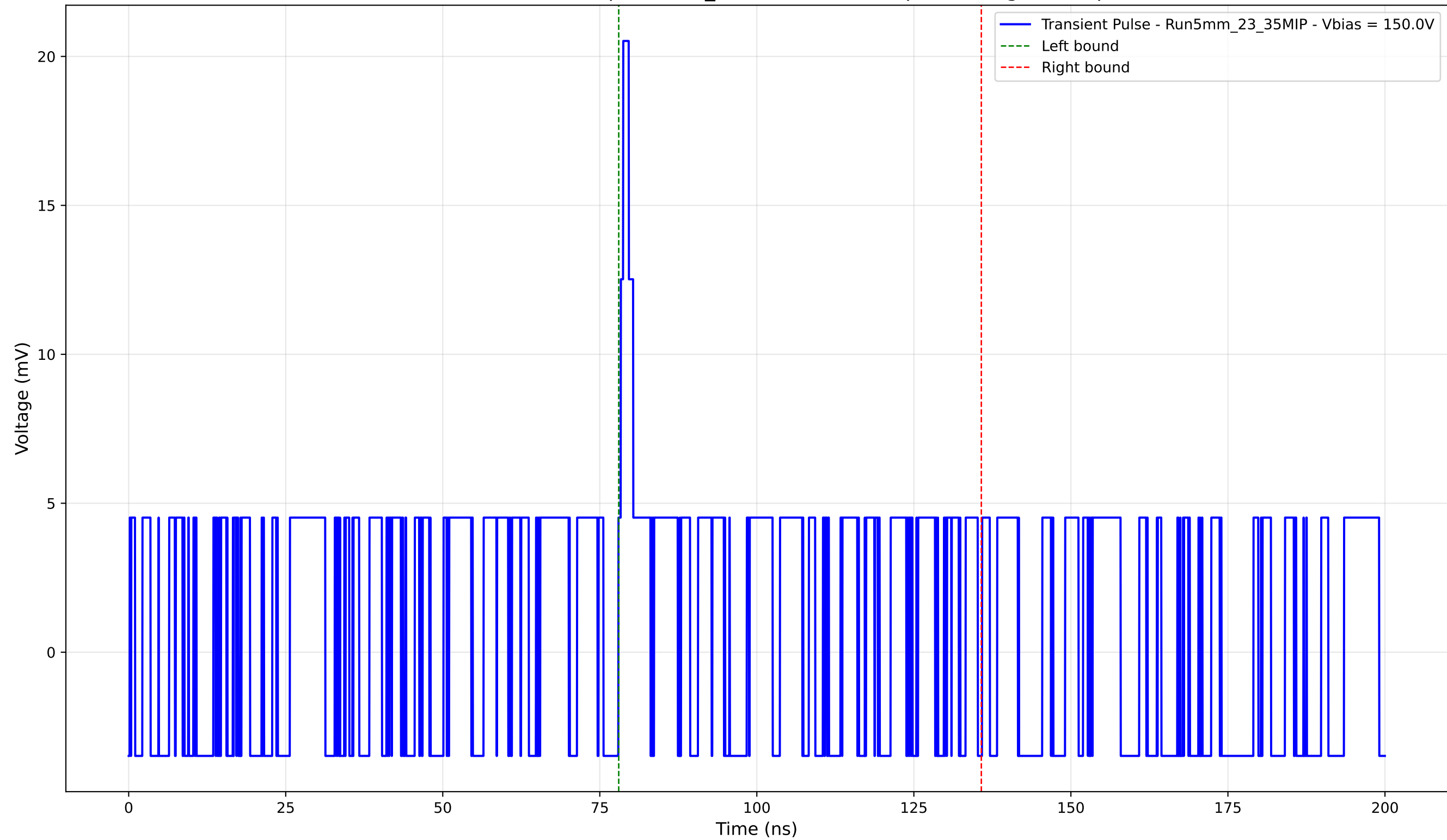
Transient Pulse - Sample: 5mm_23 - Position: 30.0 \mu\text{m} - Charge: 2.68 pC
