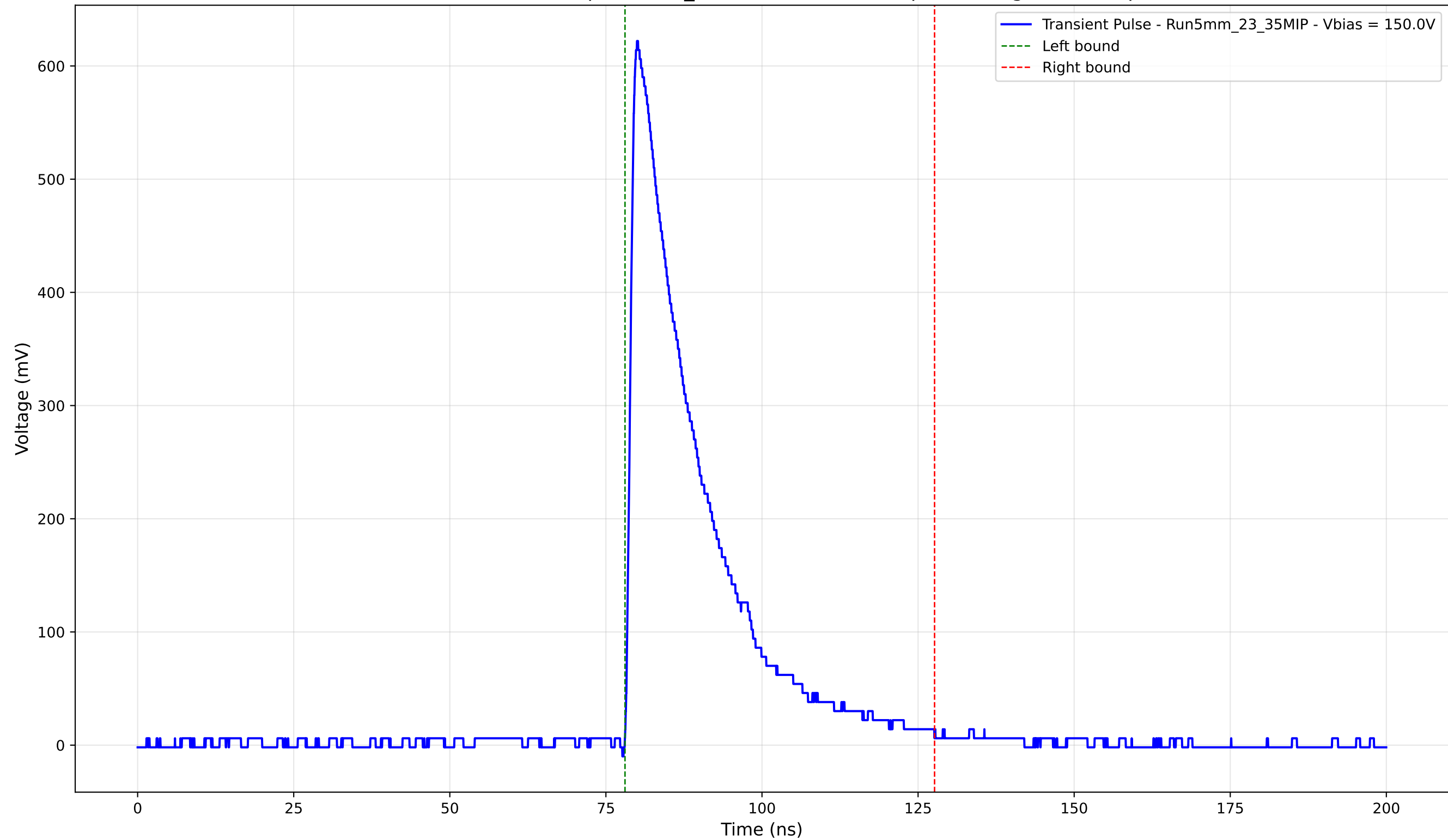
Transient Pulse - Sample: 5mm_23 - Position: 1490.0 \mu\text{m} - Charge: 148.06 pC
