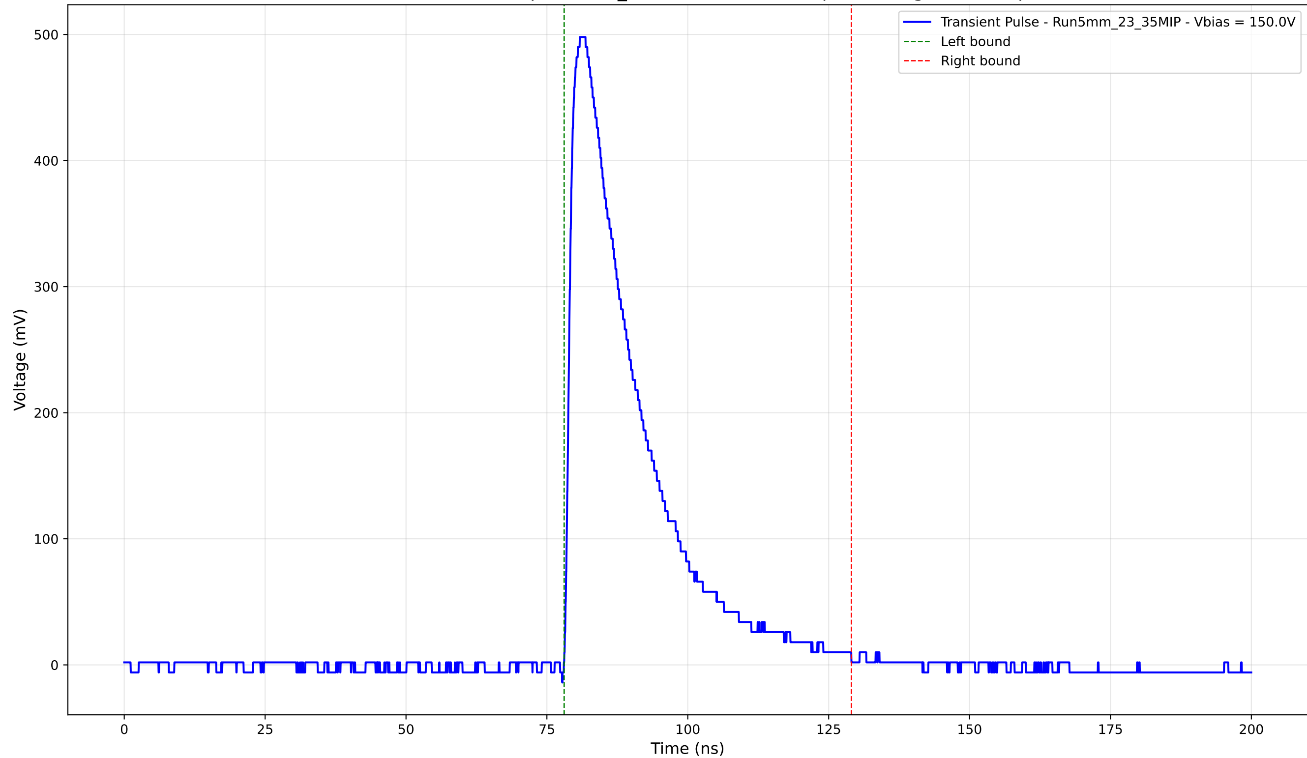
Transient Pulse - Sample: 5mm_23 - Position: 2525.0 \mu\text{m} - Charge: 134.66 pC
