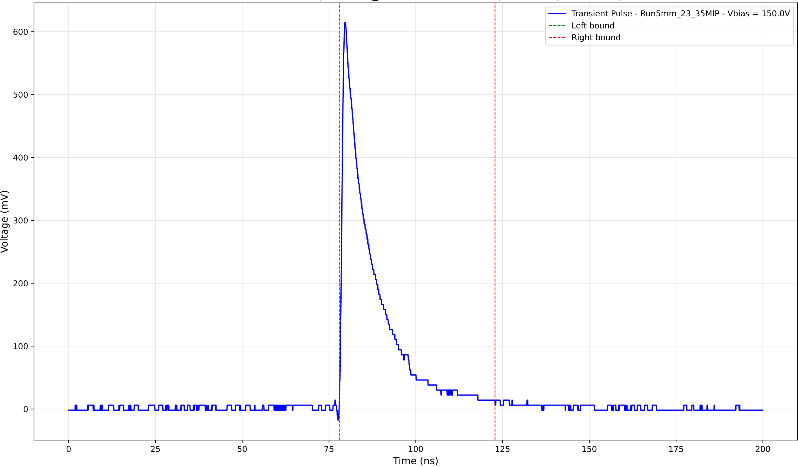
Transient Pulse - Sample: 5mm_23 - Position: 4265.0 \mu\text{m} - Charge: 115.41 pC
