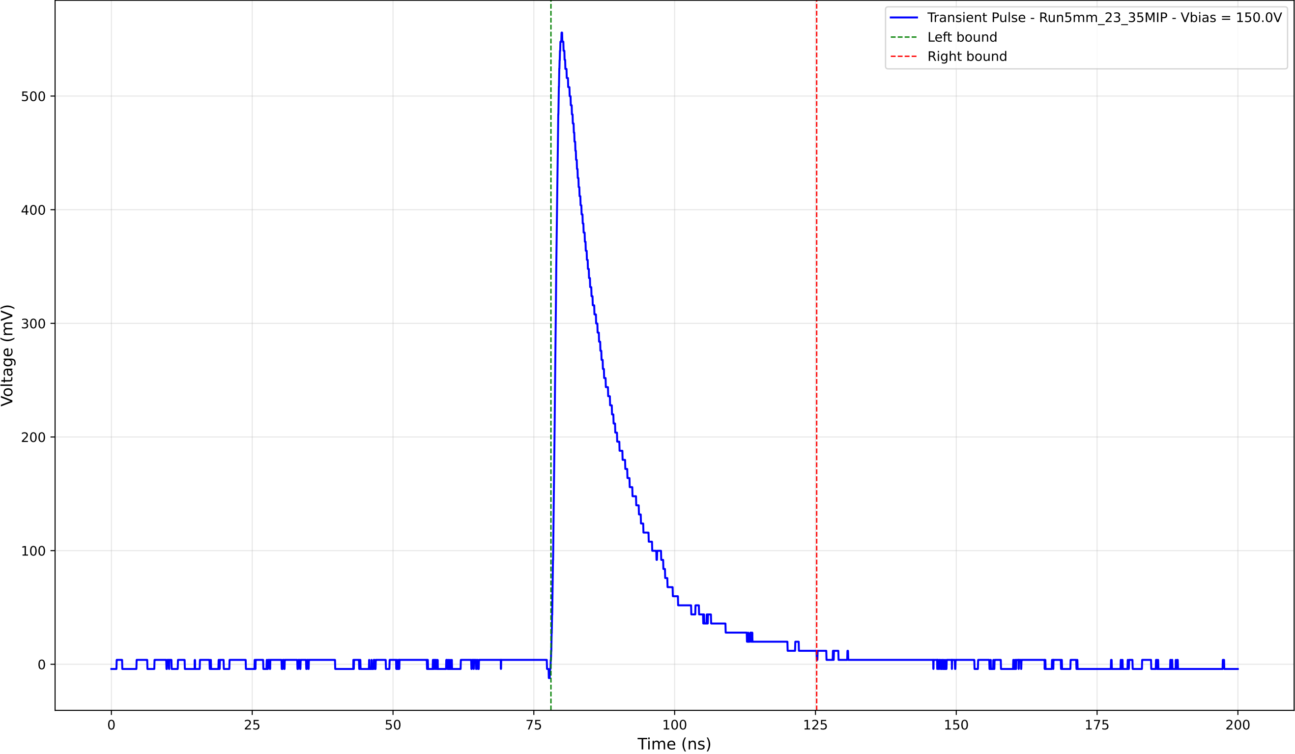
Transient Pulse - Sample: 5mm_23 - Position: 3900.0 \mu\text{m} - Charge: 122.12 pC
