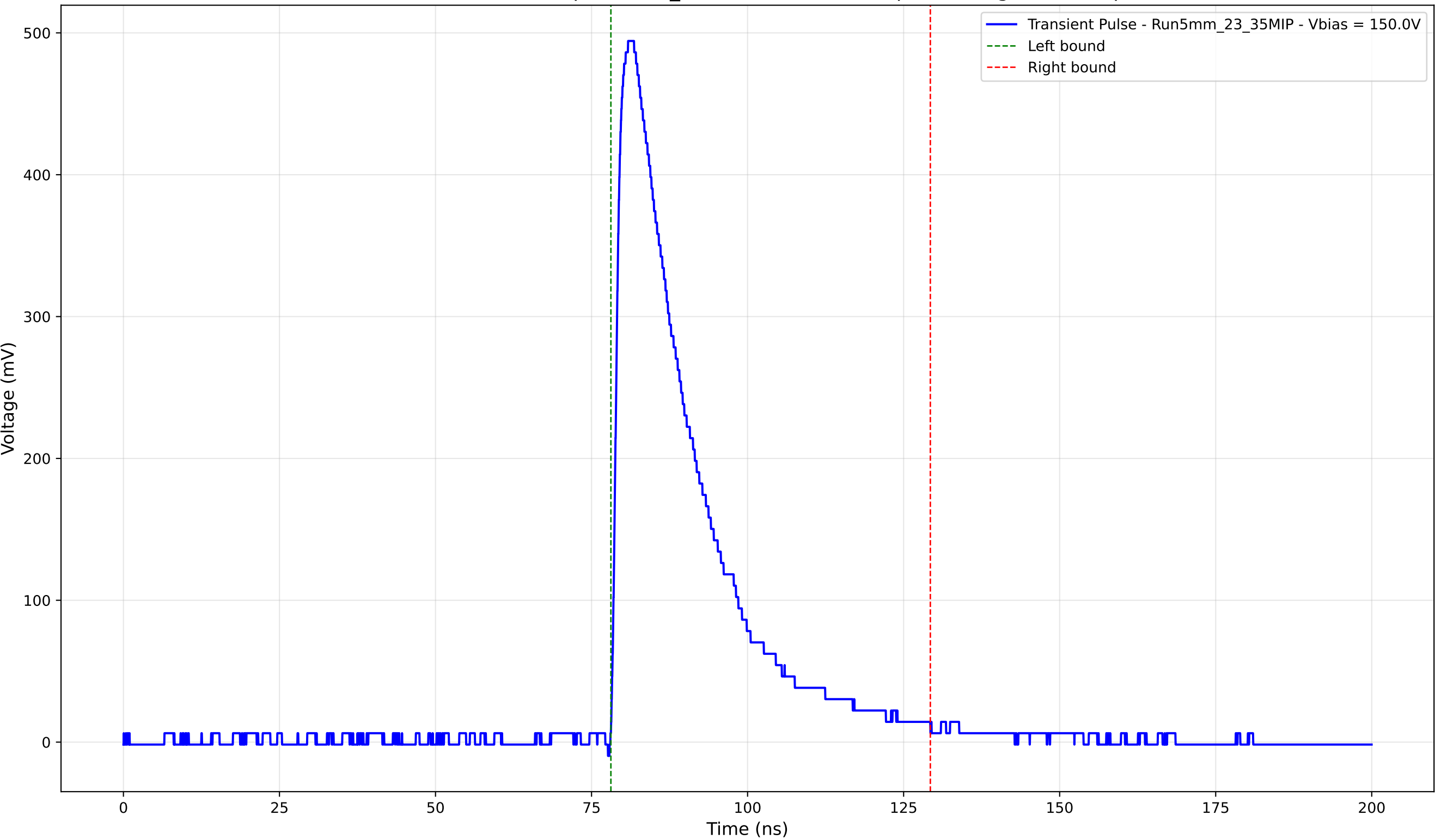
Transient Pulse - Sample: 5mm_23 - Position: 2910.0 \mu\text{m} - Charge: 135.24 pC
