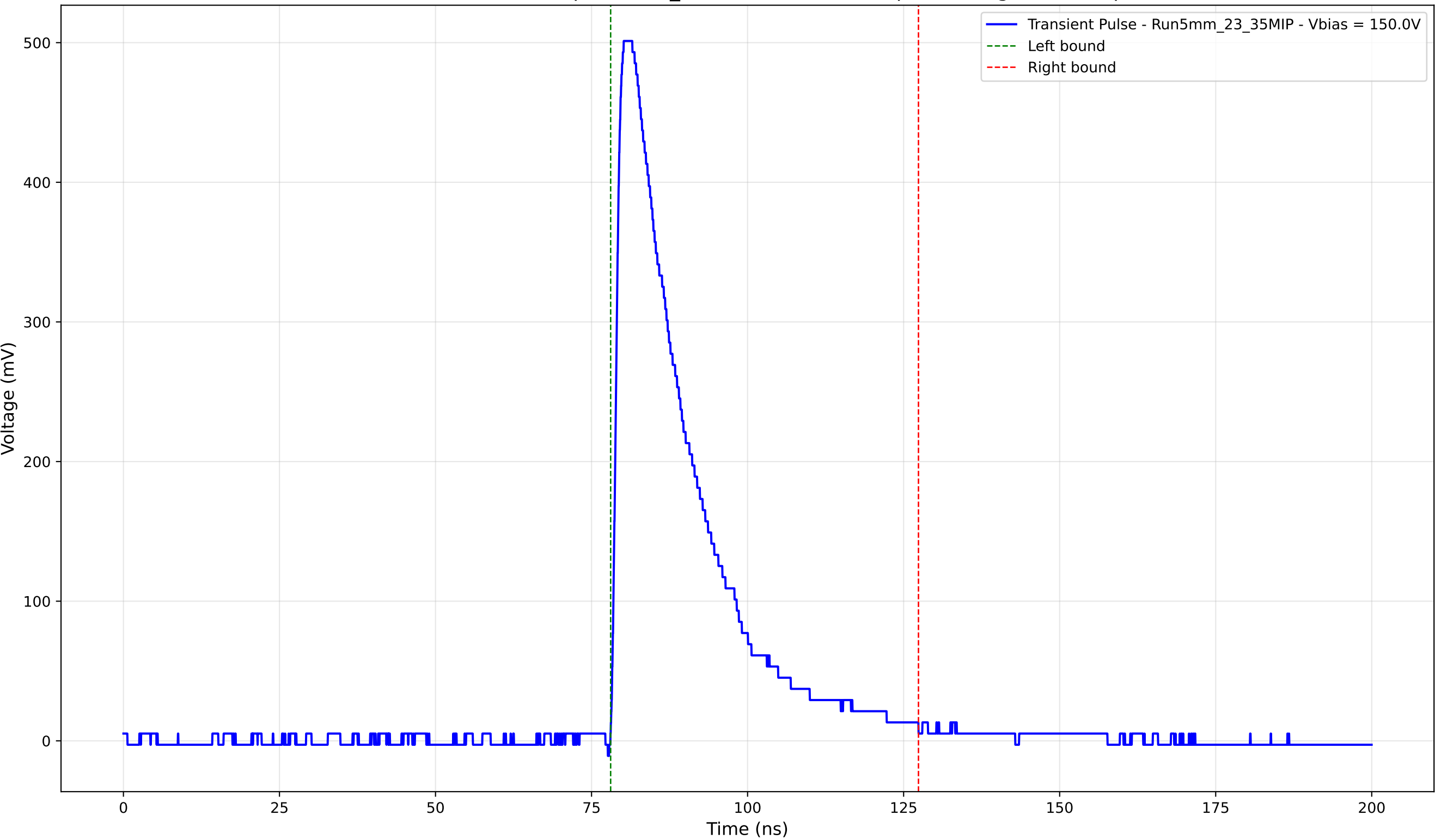
Transient Pulse - Sample: 5mm_23 - Position: 3330.0 \mu\text{m} - Charge: 130.49 pC
