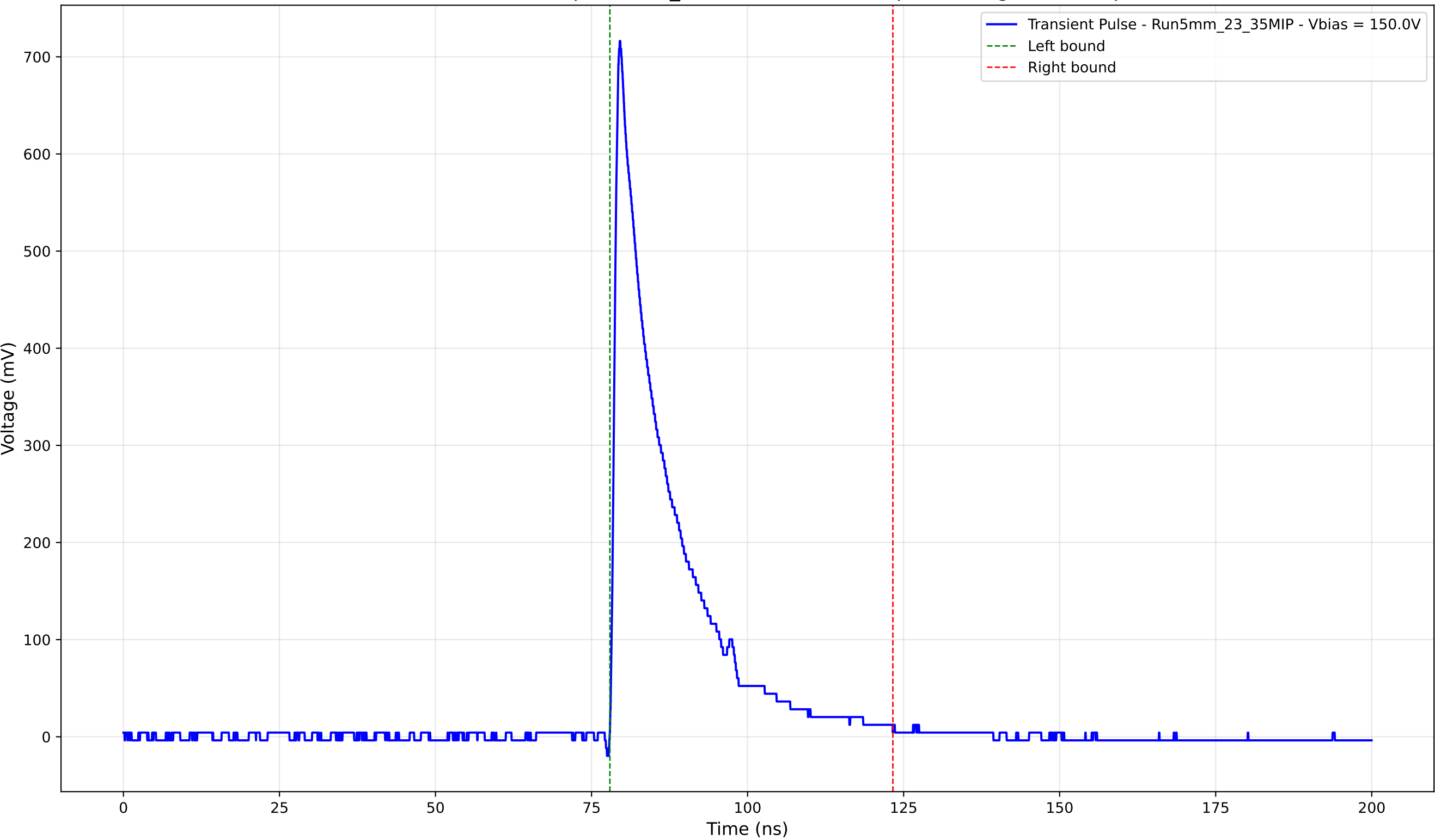
Transient Pulse - Sample: 5mm_23 - Position: 4385.0 \mu\text{m} - Charge: 127.75 pC
