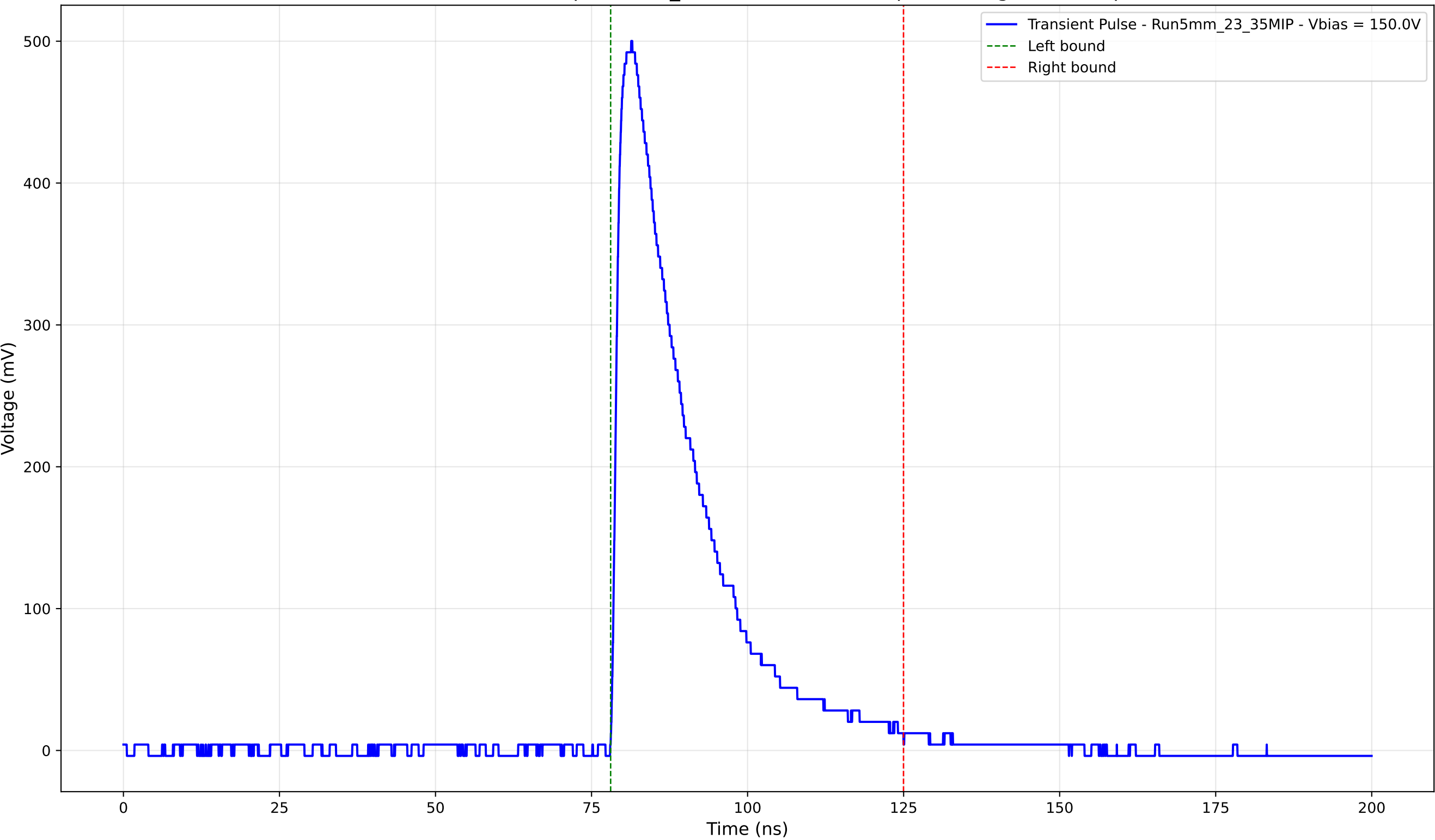
Transient Pulse - Sample: 5mm_23 - Position: 3005.0 \mu\text{m} - Charge: 132.48 pC
