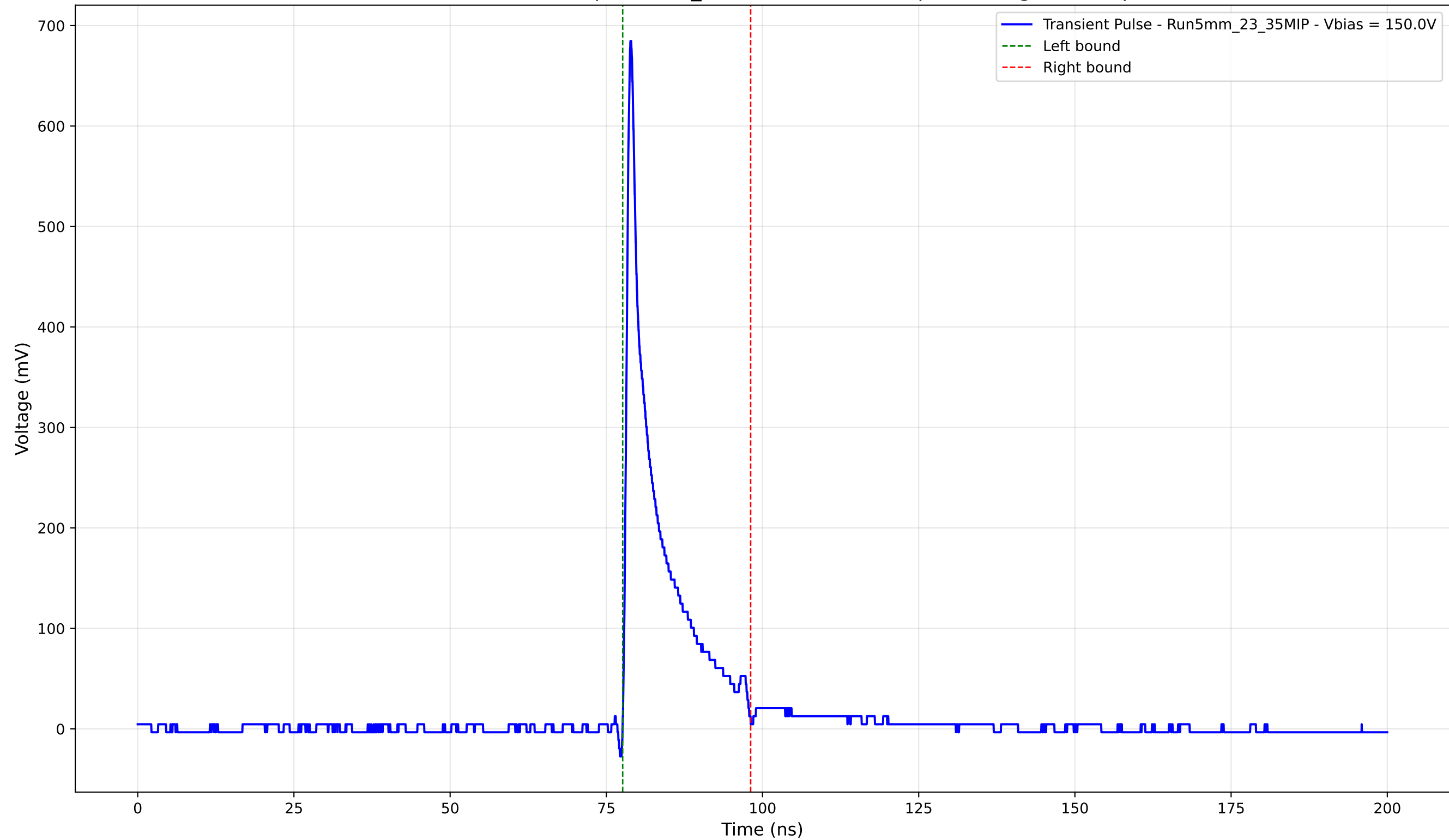
Transient Pulse - Sample: 5mm_23 - Position: 5050.0 \mu\text{m} - Charge: 68.24 pC
