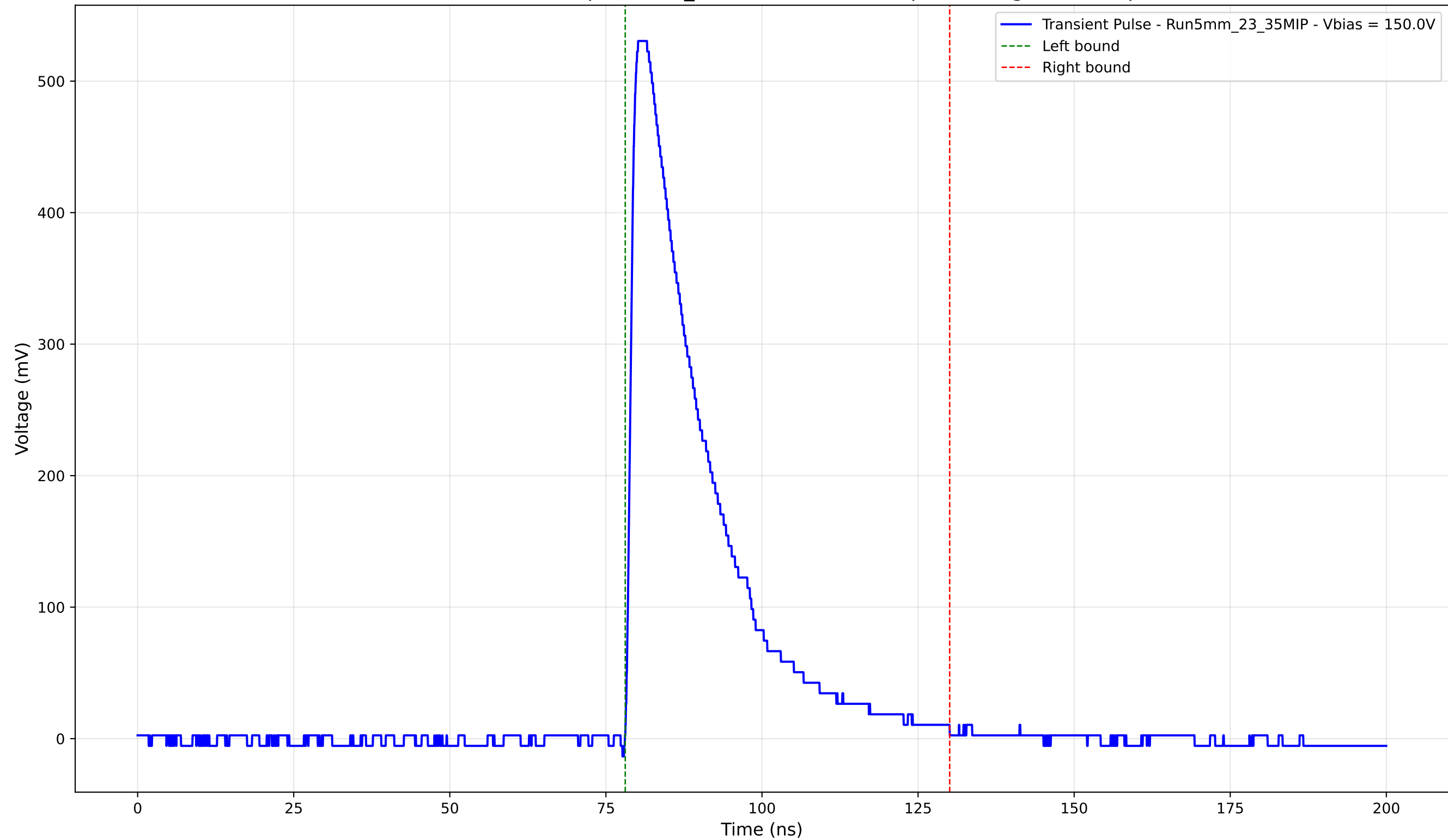
Transient Pulse - Sample: 5mm_23 - Position: 1930.0 \mu\text{m} - Charge: 139.96 pC
