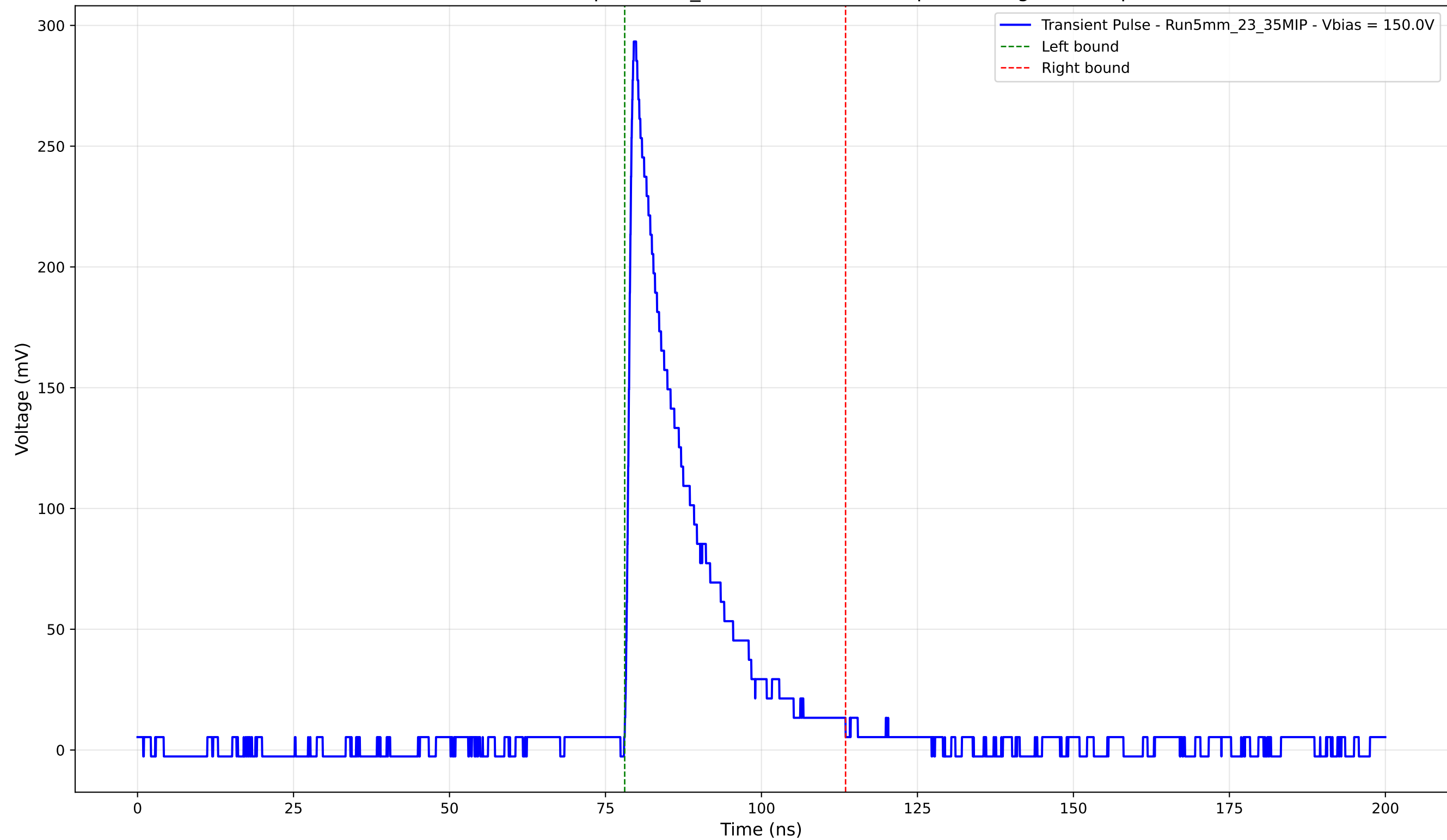
Transient Pulse - Sample: 5mm_23 - Position: 1085.0 \mu\text{m} - Charge: 55.66 pC
