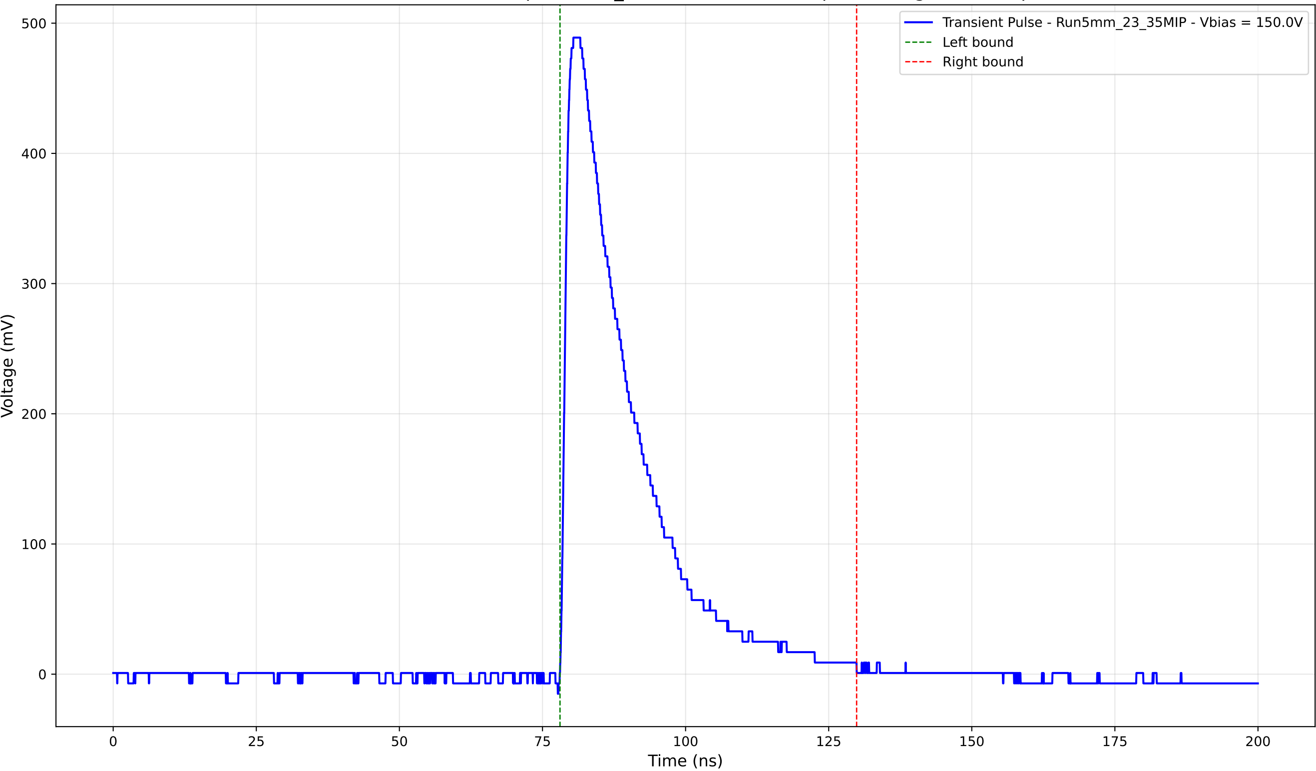
Transient Pulse - Sample: 5mm_23 - Position: 3250.0 \mu\text{m} - Charge: 126.30 pC
