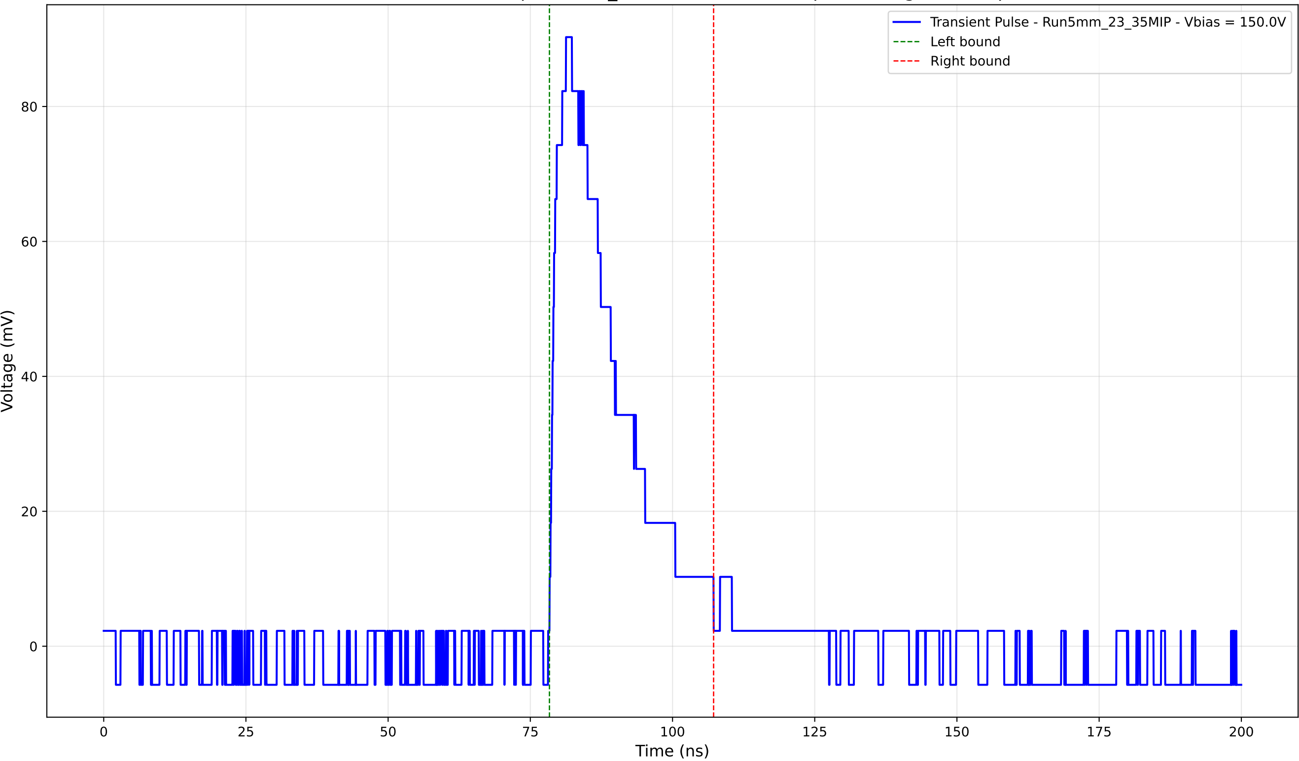
Transient Pulse - Sample: 5mm_23 - Position: 2640.0 \mu\text{m} - Charge: 21.92 pC
