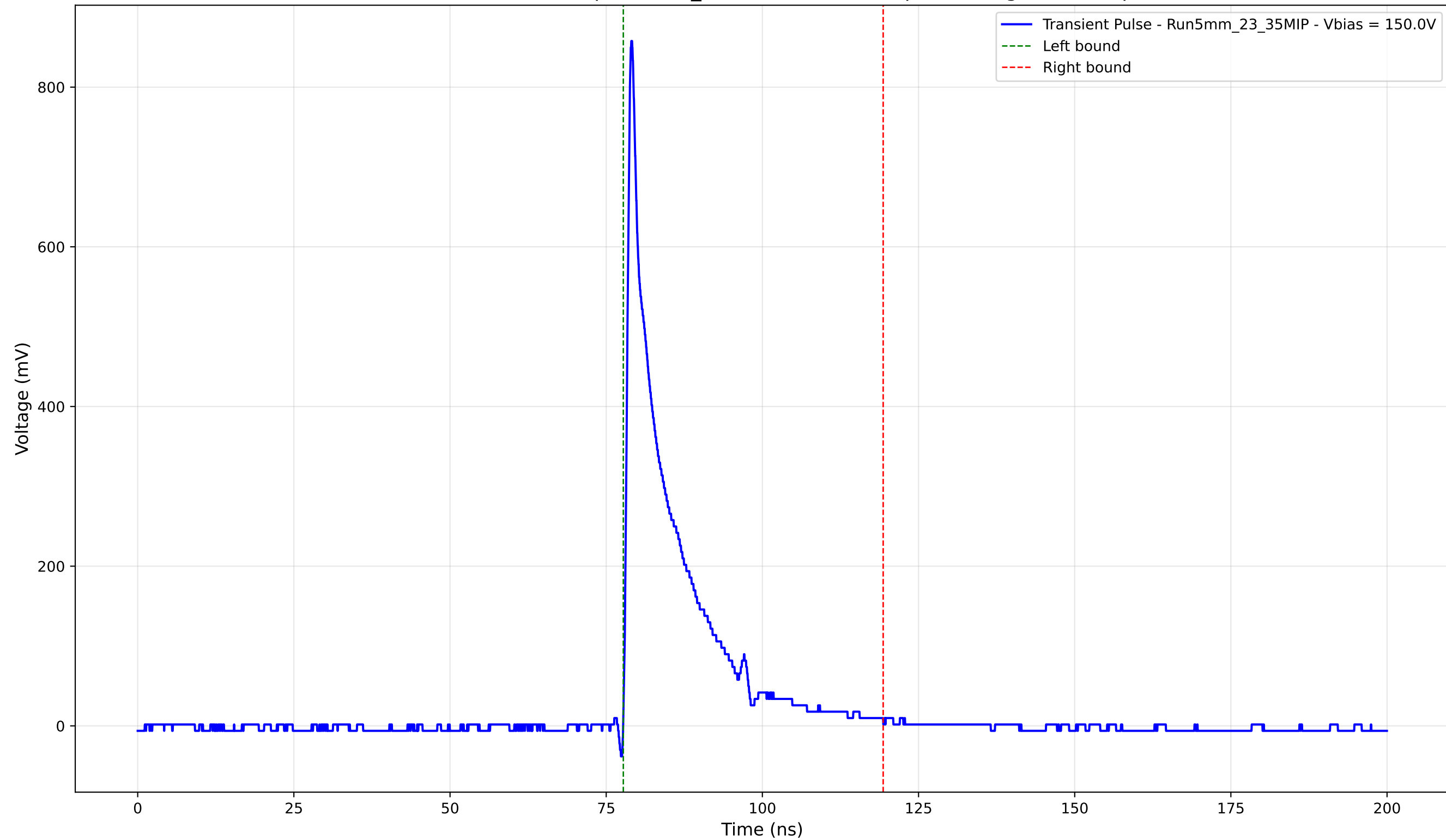
Transient Pulse - Sample: 5mm_23 - Position: 335.0 \mu\text{m} - Charge: 113.12 pC
