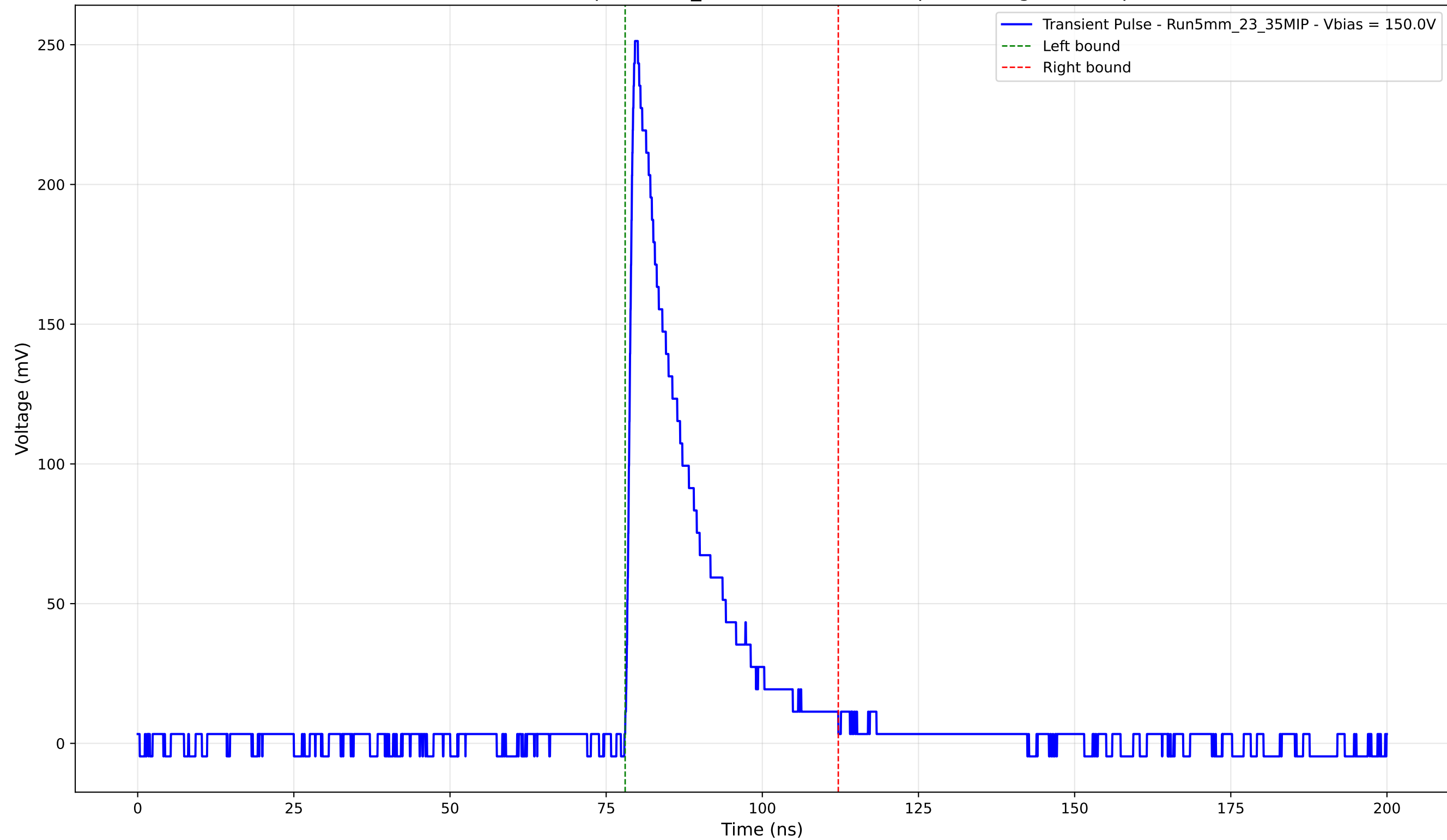
Transient Pulse - Sample: 5mm_23 - Position: 4120.0 \mu\text{m} - Charge: 47.98 pC
