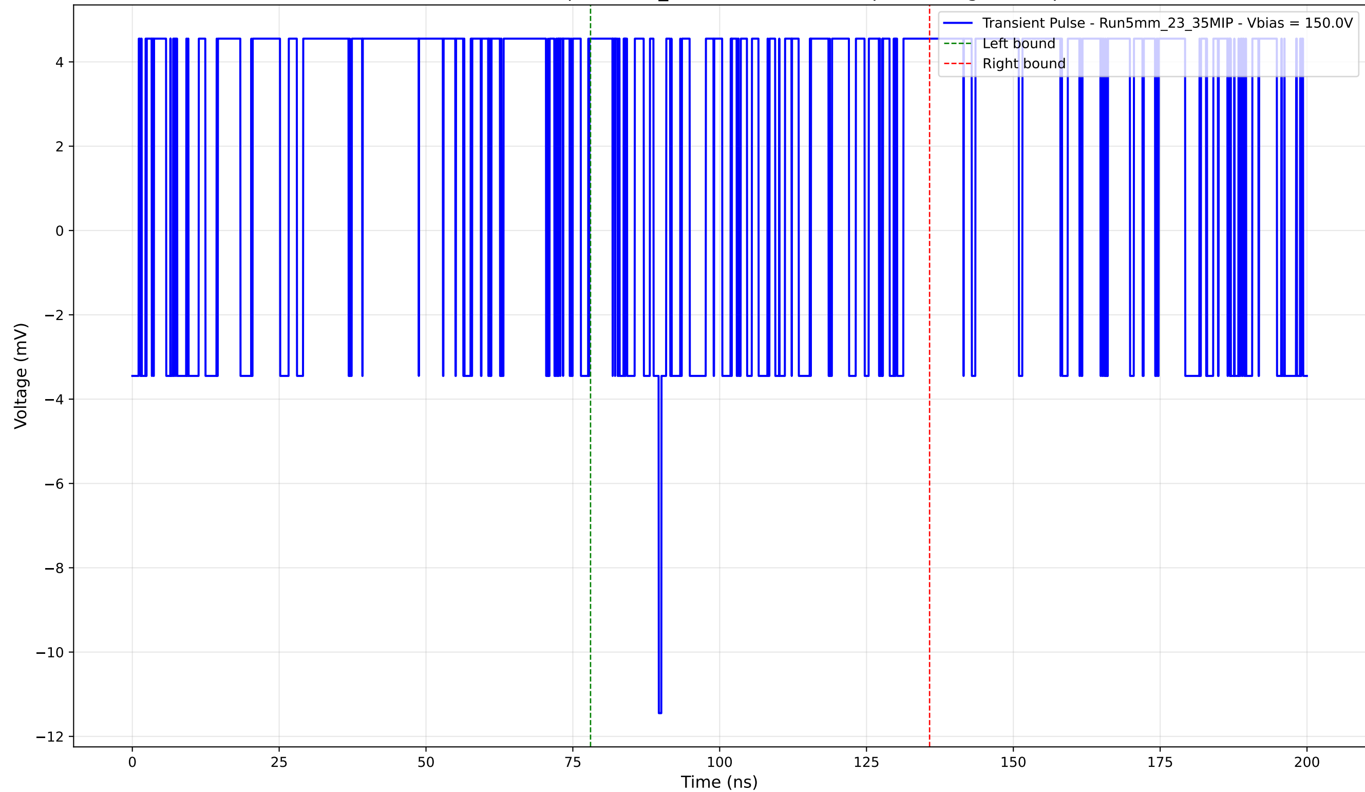
Transient Pulse - Sample: 5mm_23 - Position: 5285.0 \mu\text{m} - Charge: 1.47 pC
