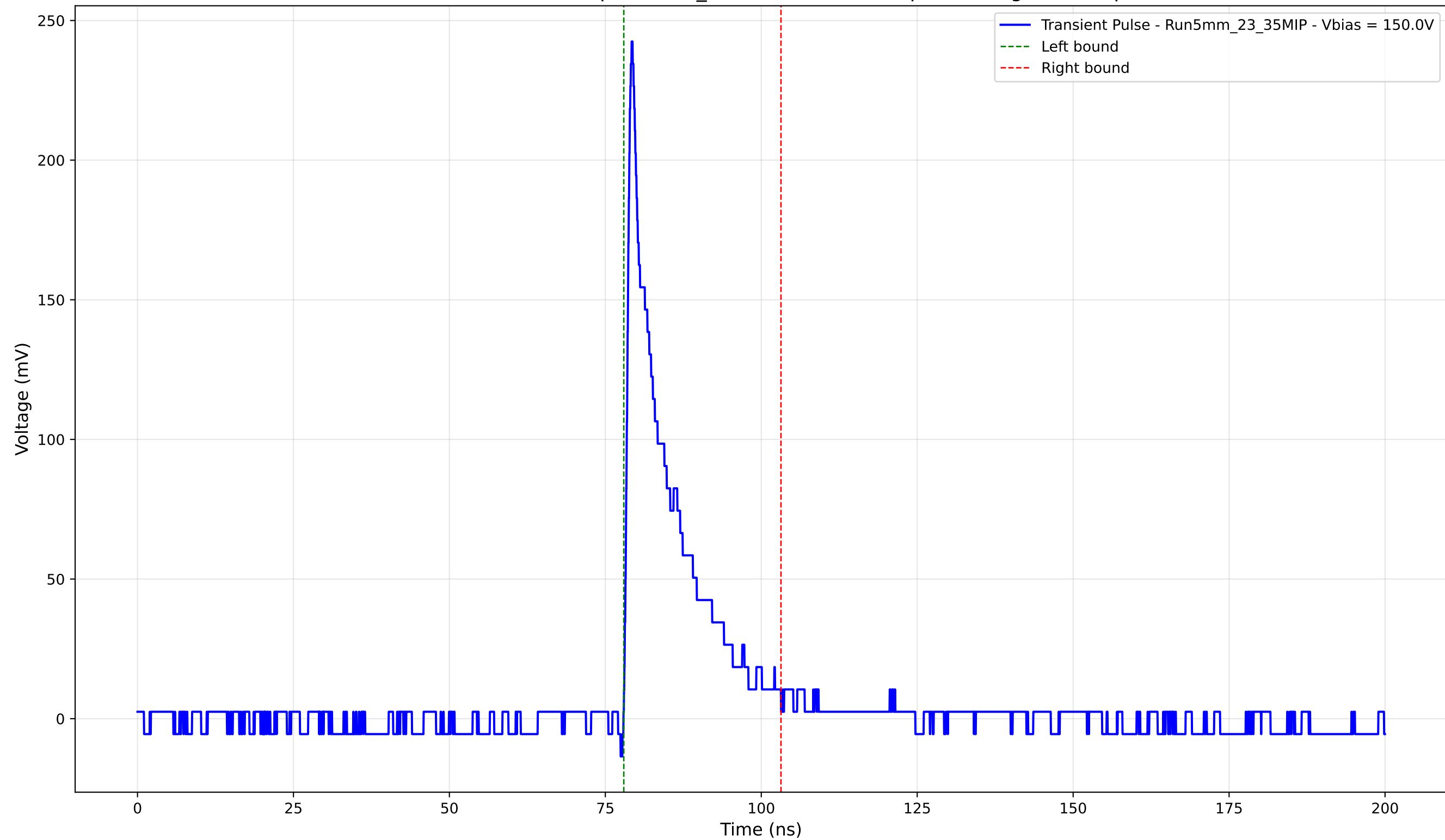
Transient Pulse - Sample: 5mm_23 - Position: 595.0 \mu\text{m} - Charge: 31.91 pC
