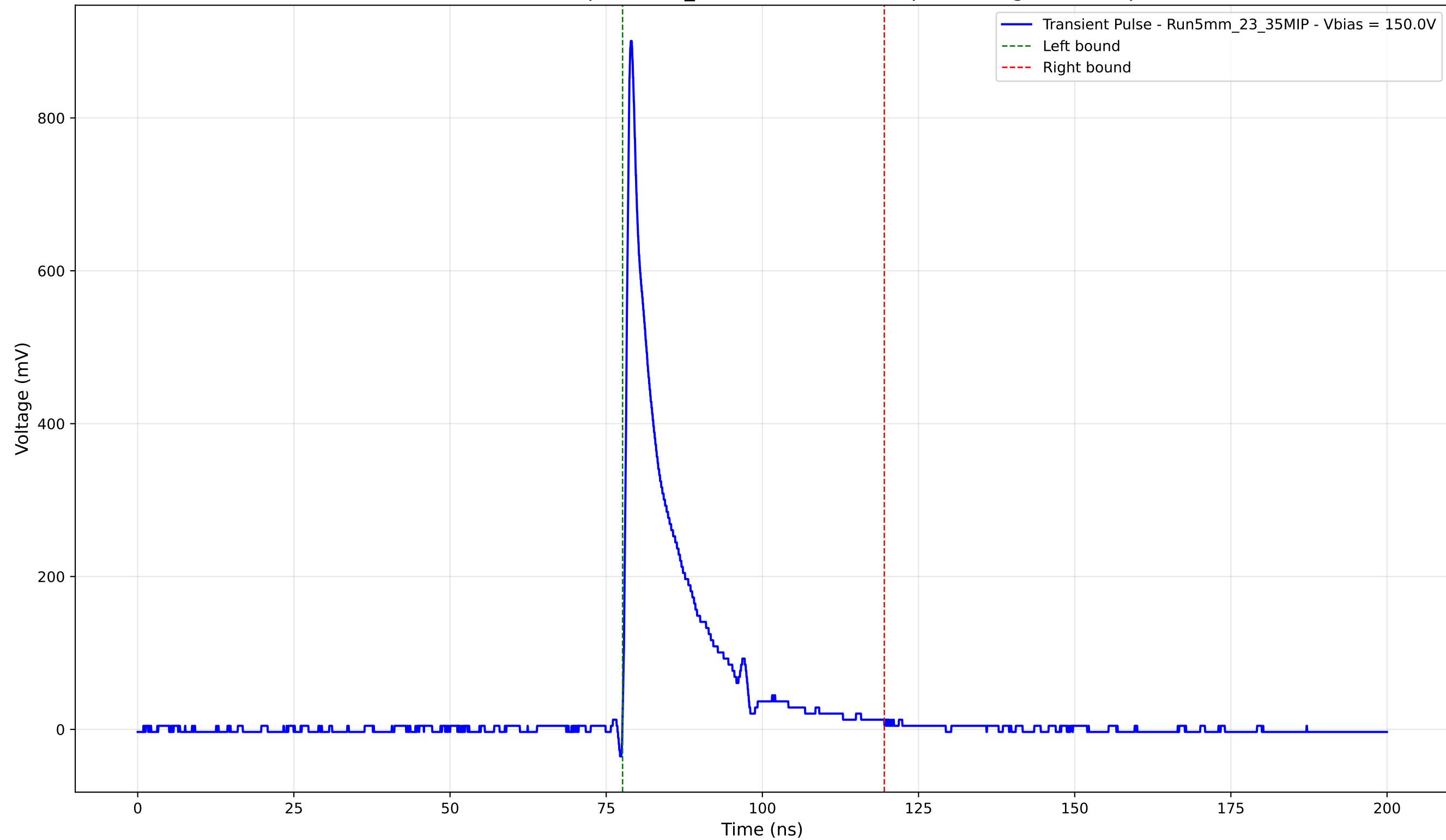
Transient Pulse - Sample: 5mm_23 - Position: 4965.0 \mu\text{m} - Charge: 118.79 pC
