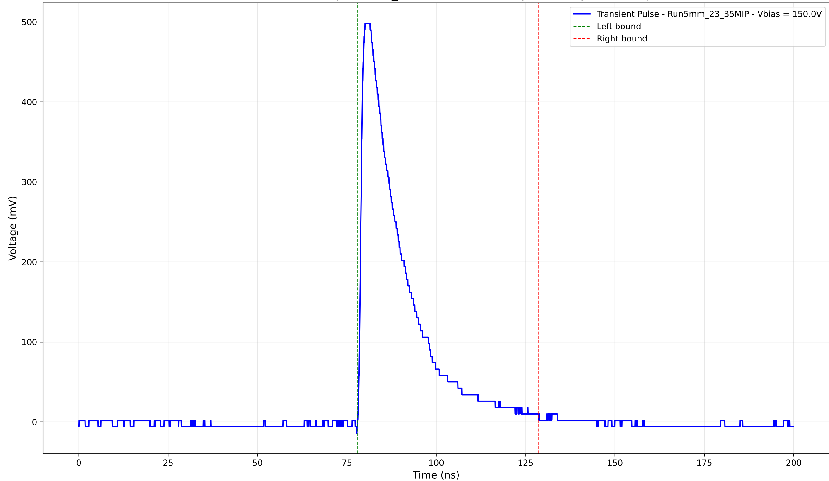
Transient Pulse - Sample: 5mm_23 - Position: 3455.0 \mu\text{m} - Charge: 126.62 pC
