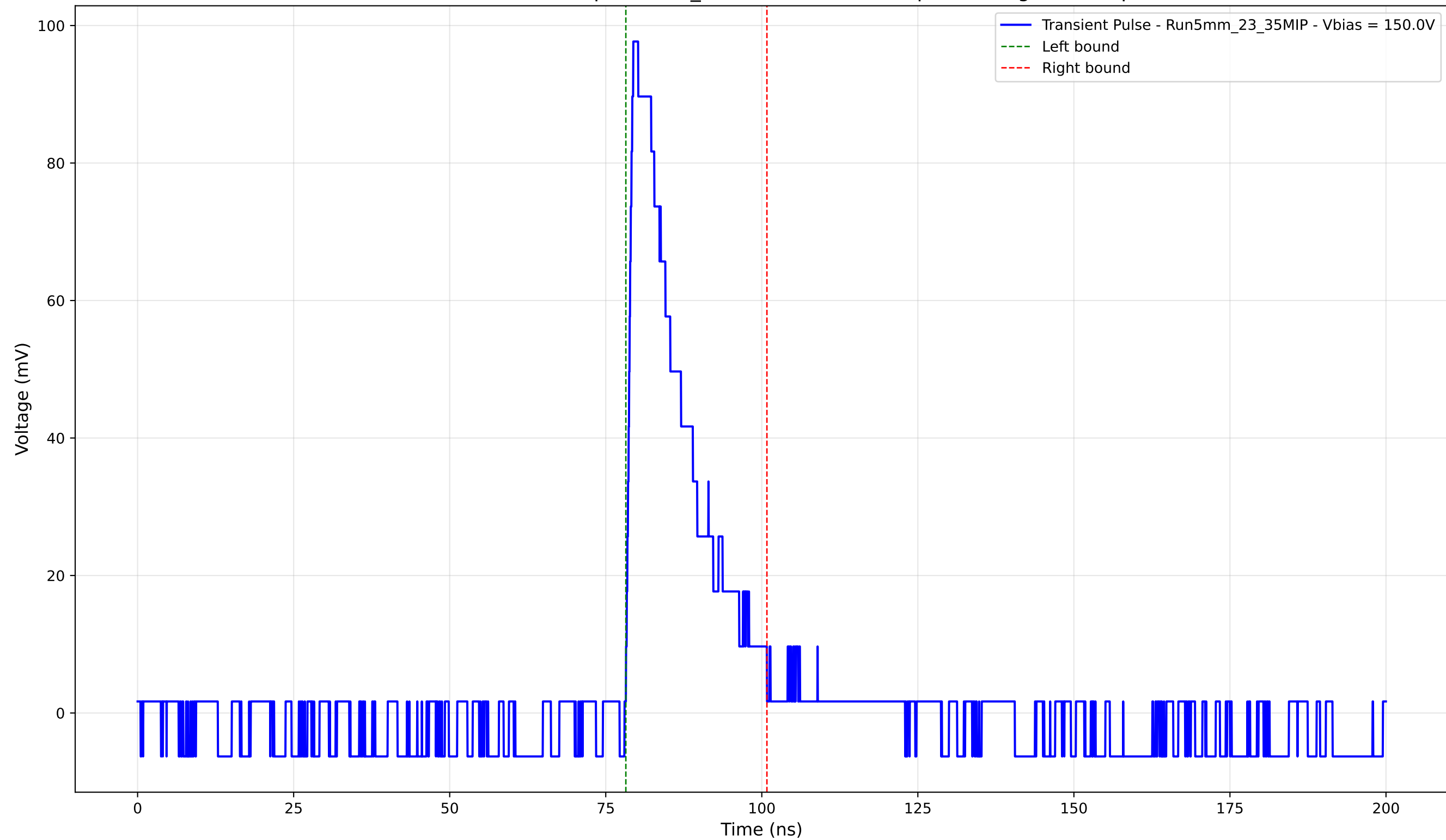
Transient Pulse - Sample: 5mm_23 - Position: 4165.0 \mu\text{m} - Charge: 18.35 pC
