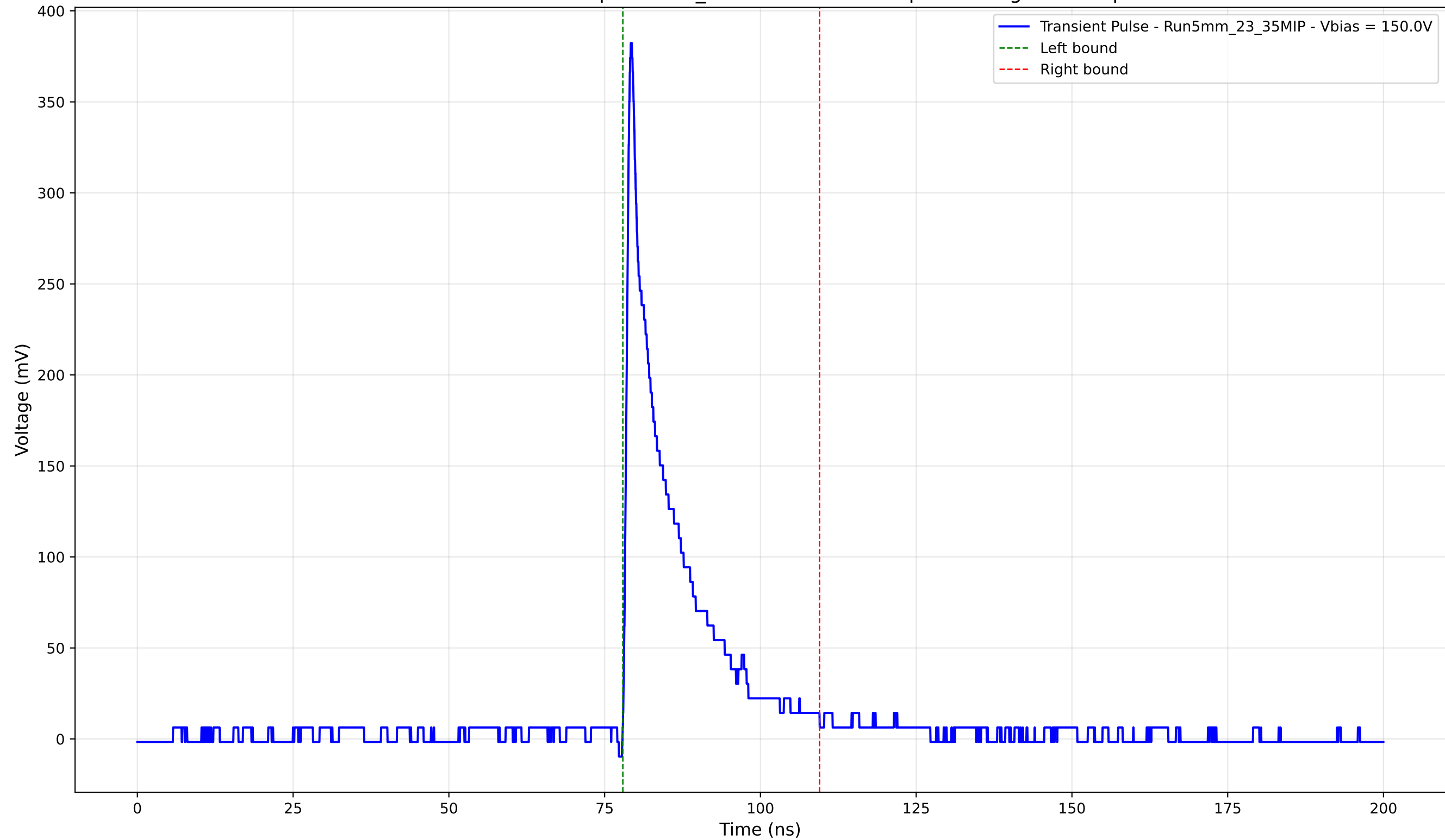
Transient Pulse - Sample: 5mm_23 - Position: 580.0 \mu\text{m} - Charge: 53.38 pC
