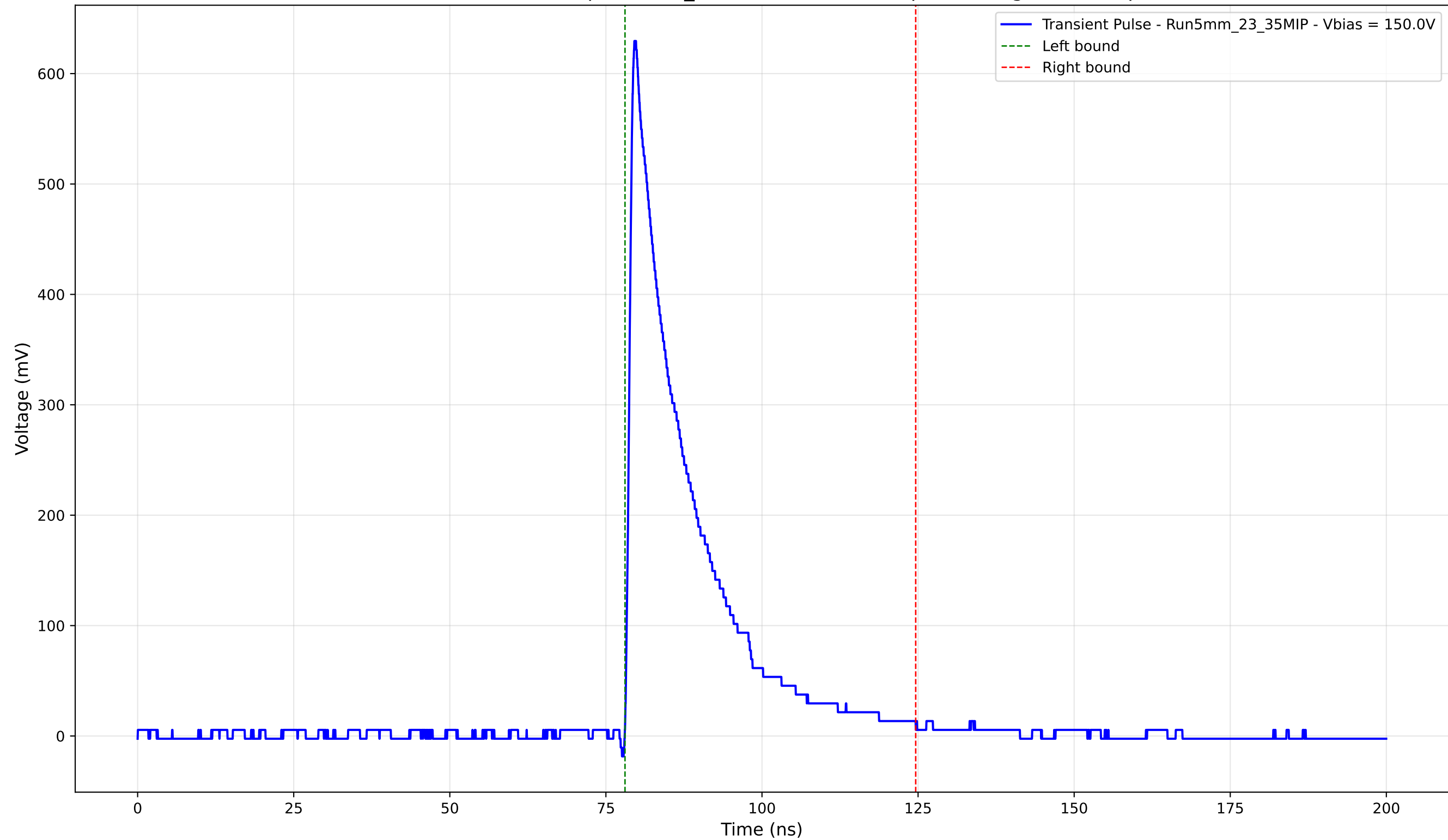
Transient Pulse - Sample: 5mm_23 - Position: 1020.0 \mu\text{m} - Charge: 123.52 pC
