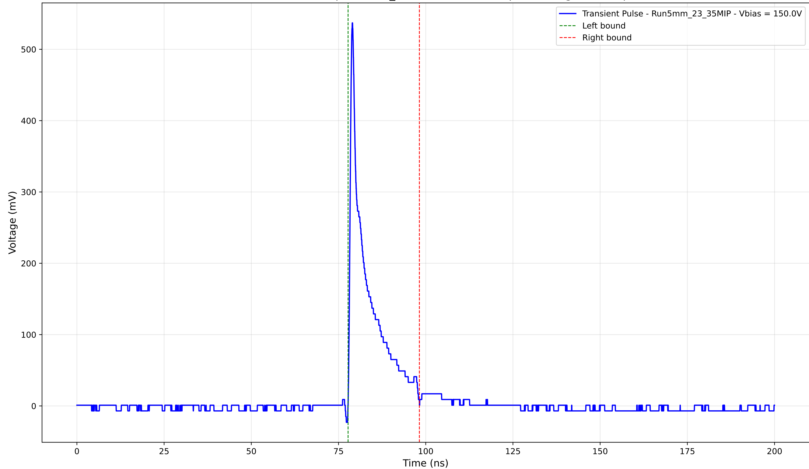
Transient Pulse - Sample: 5mm_23 - Position: 215.0 \mu\text{m} - Charge: 53.76 pC
