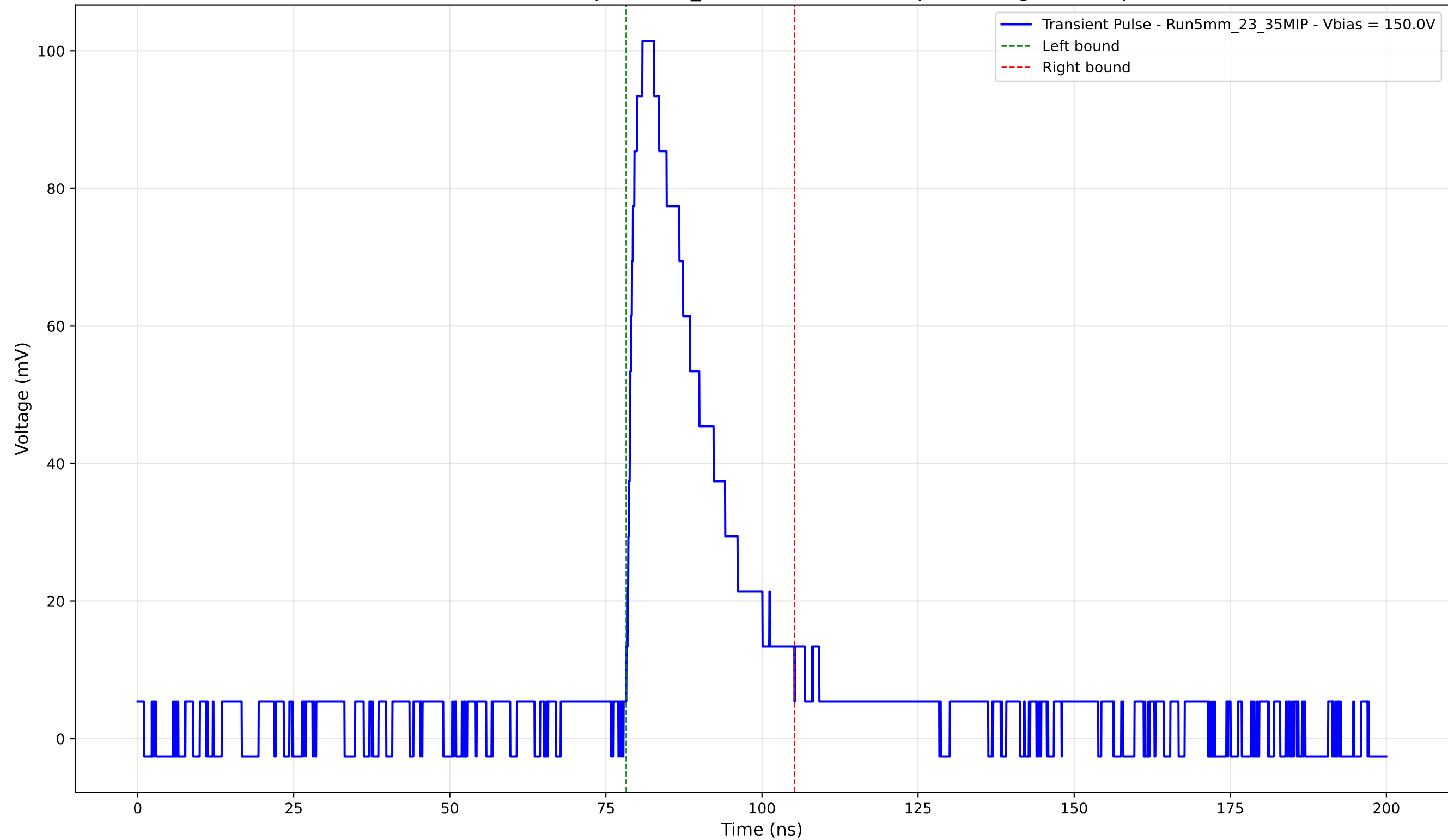
Transient Pulse - Sample: 5mm_23 - Position: 2660.0 \mu\text{m} - Charge: 25.59 pC
