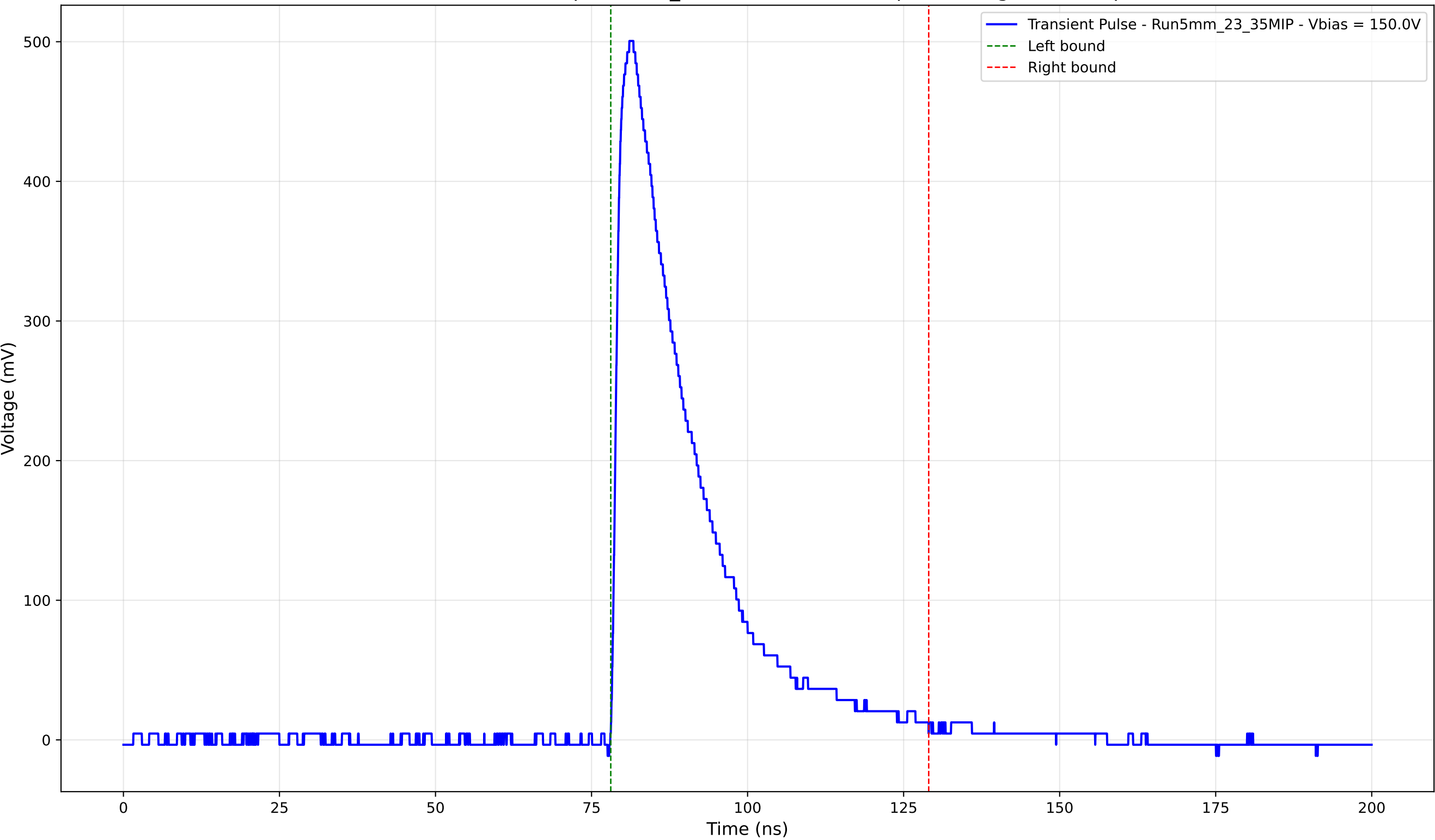
Transient Pulse - Sample: 5mm_23 - Position: 2790.0 \mu\text{m} - Charge: 136.22 pC
