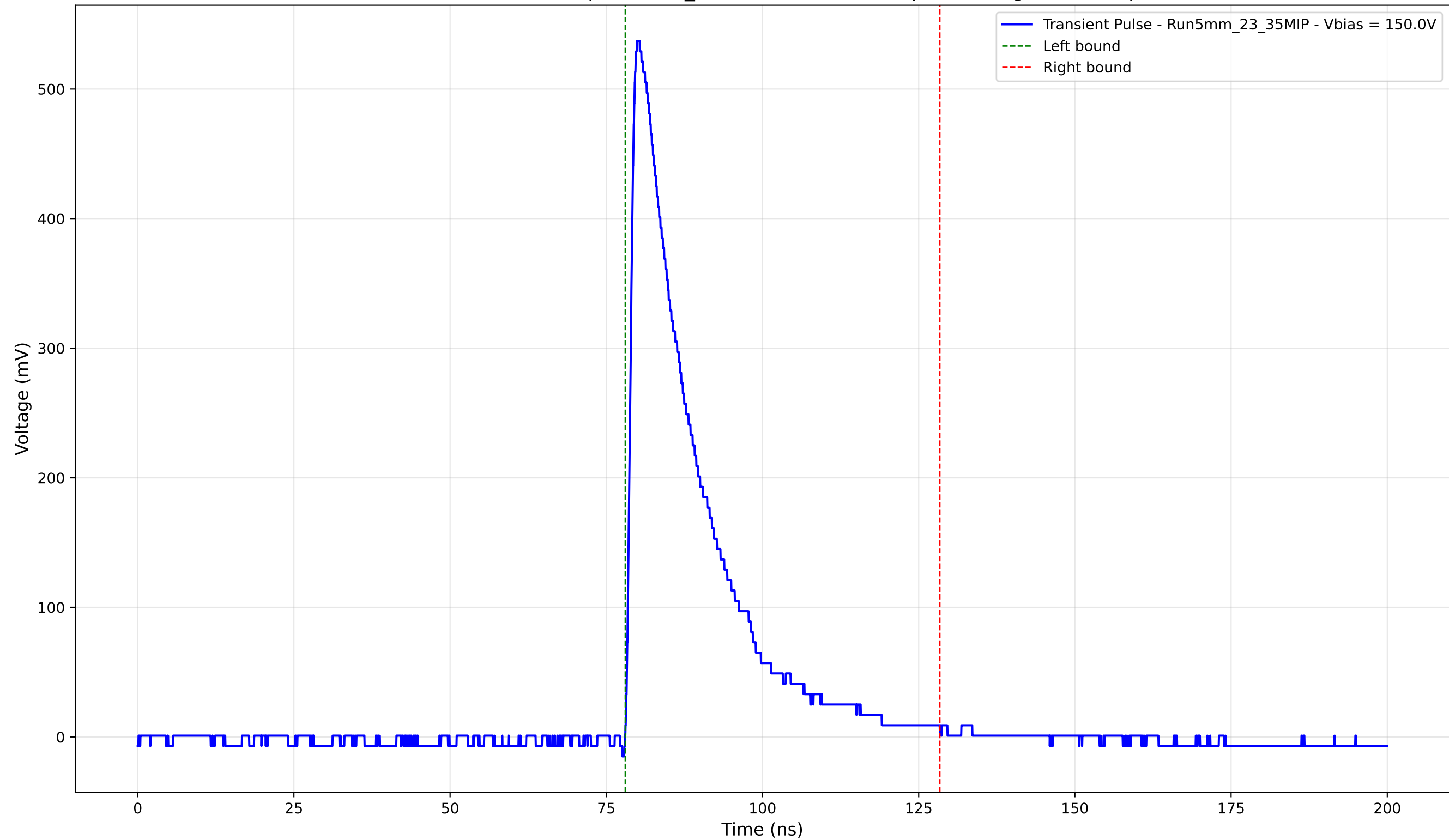
Transient Pulse - Sample: 5mm_23 - Position: 3775.0 \mu\text{m} - Charge: 121.91 pC
