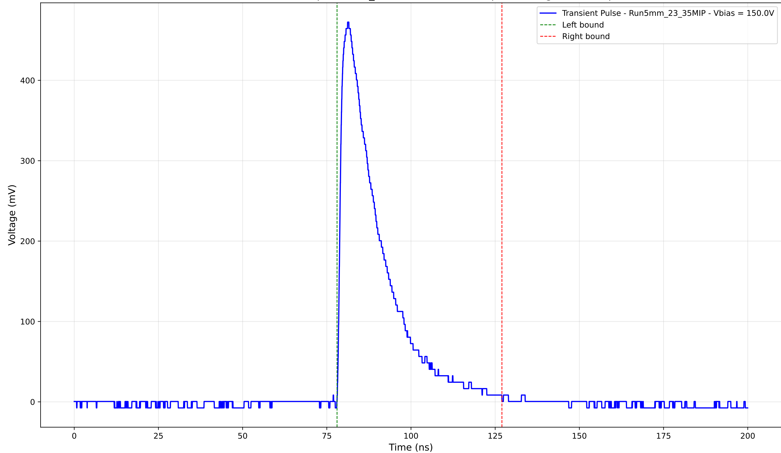
Transient Pulse - Sample: 5mm_23 - Position: 2740.0 \mu\text{m} - Charge: 124.53 pC
