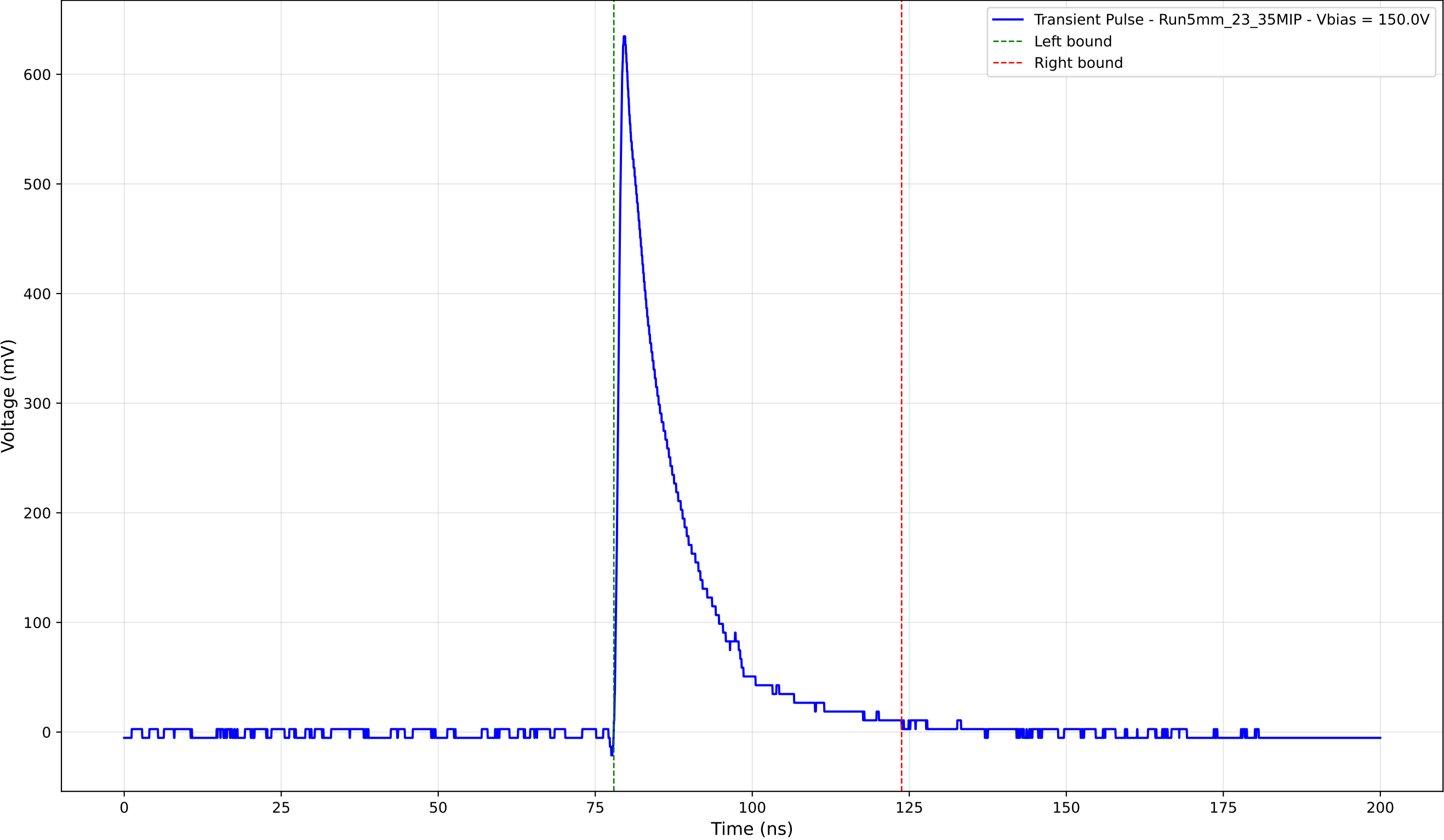
Transient Pulse - Sample: 5mm_23 - Position: 4310.0 \mu\text{m} - Charge: 115.77 pC
