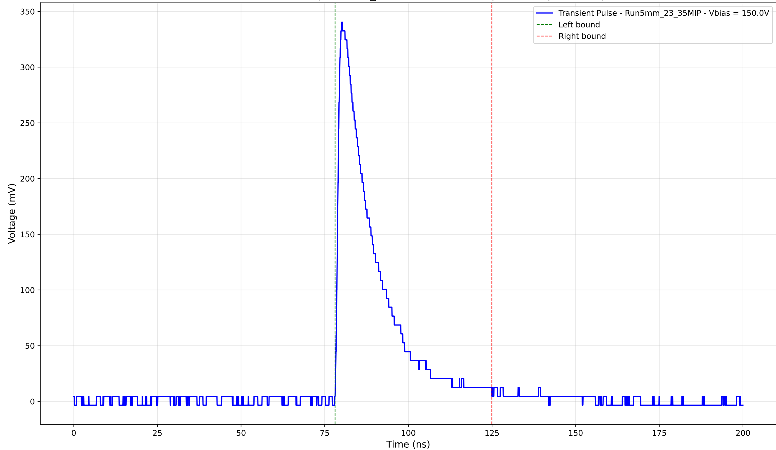
Transient Pulse - Sample: 5mm_23 - Position: 3600.0 \mu\text{m} - Charge: 81.06 pC
