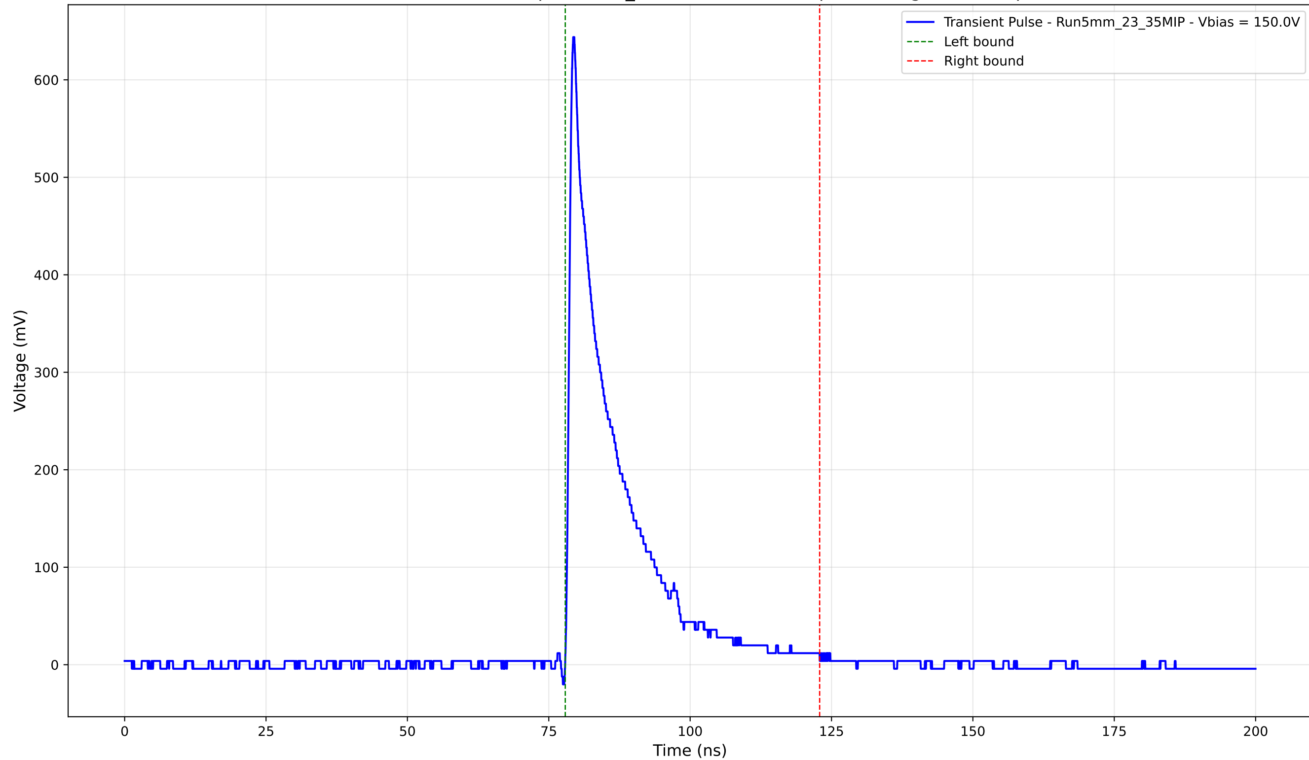
Transient Pulse - Sample: 5mm_23 - Position: 700.0 \mu\text{m} - Charge: 105.35 pC
