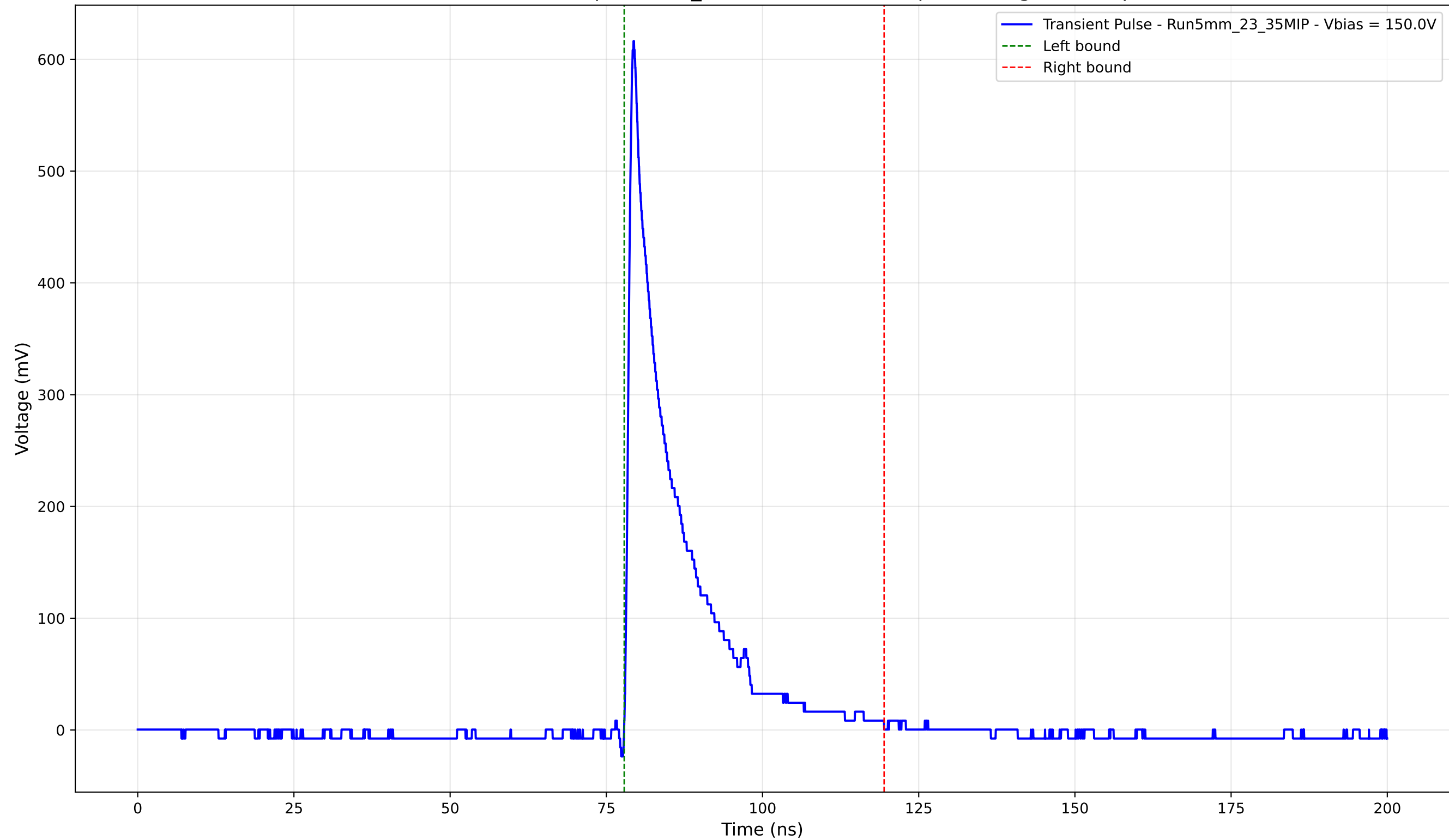
Transient Pulse - Sample: 5mm_23 - Position: 4580.0 \mu\text{m} - Charge: 93.22 pC
