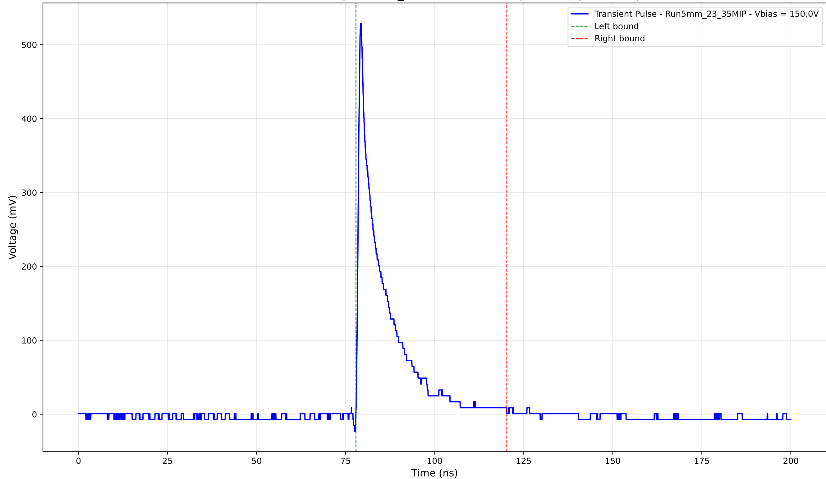
Transient Pulse - Sample: 5mm_23 - Position: 565.0 \mu\text{m} - Charge: 73.57 pC
