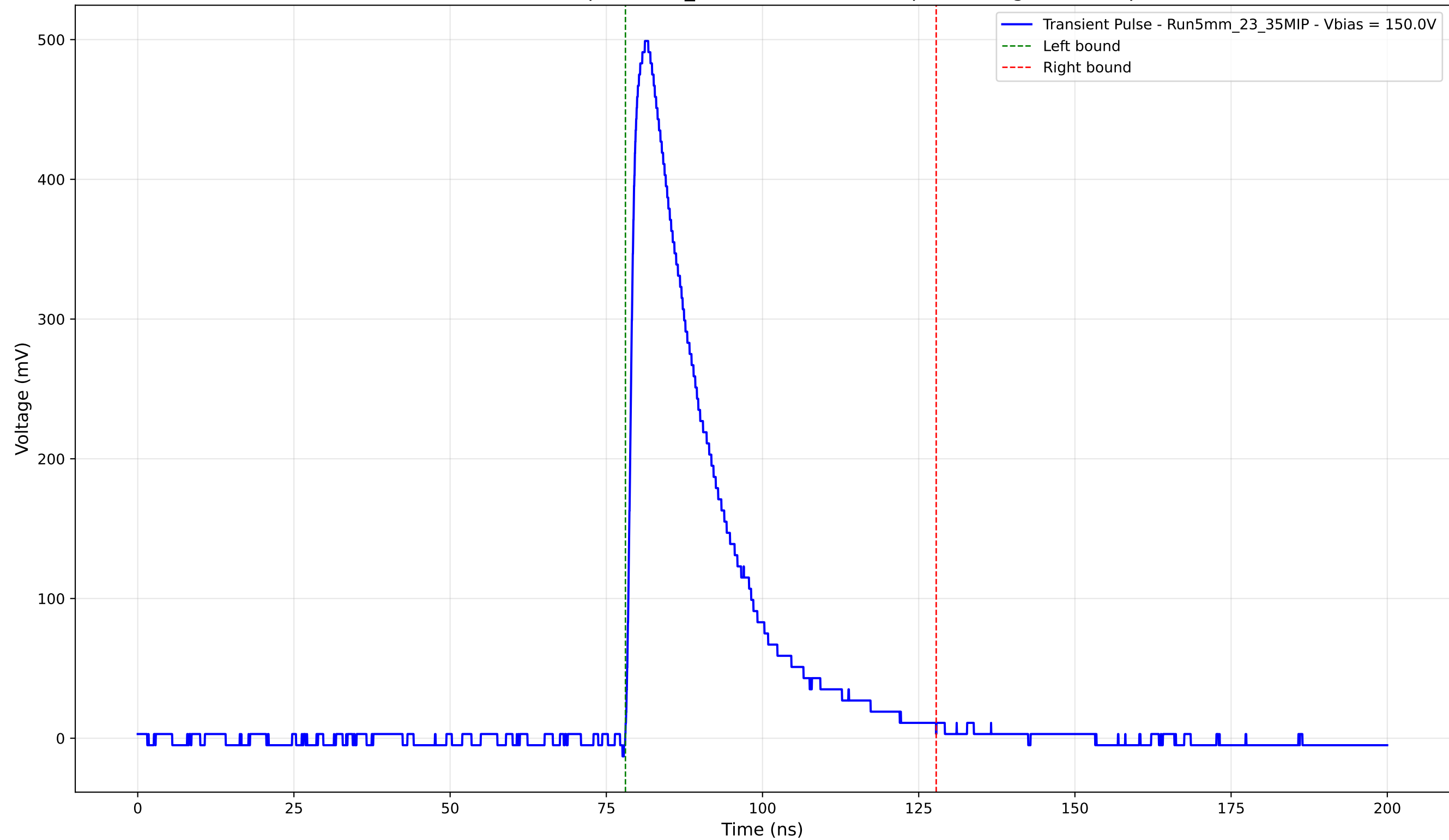
Transient Pulse - Sample: 5mm_23 - Position: 2795.0 \mu\text{m} - Charge: 133.71 pC
