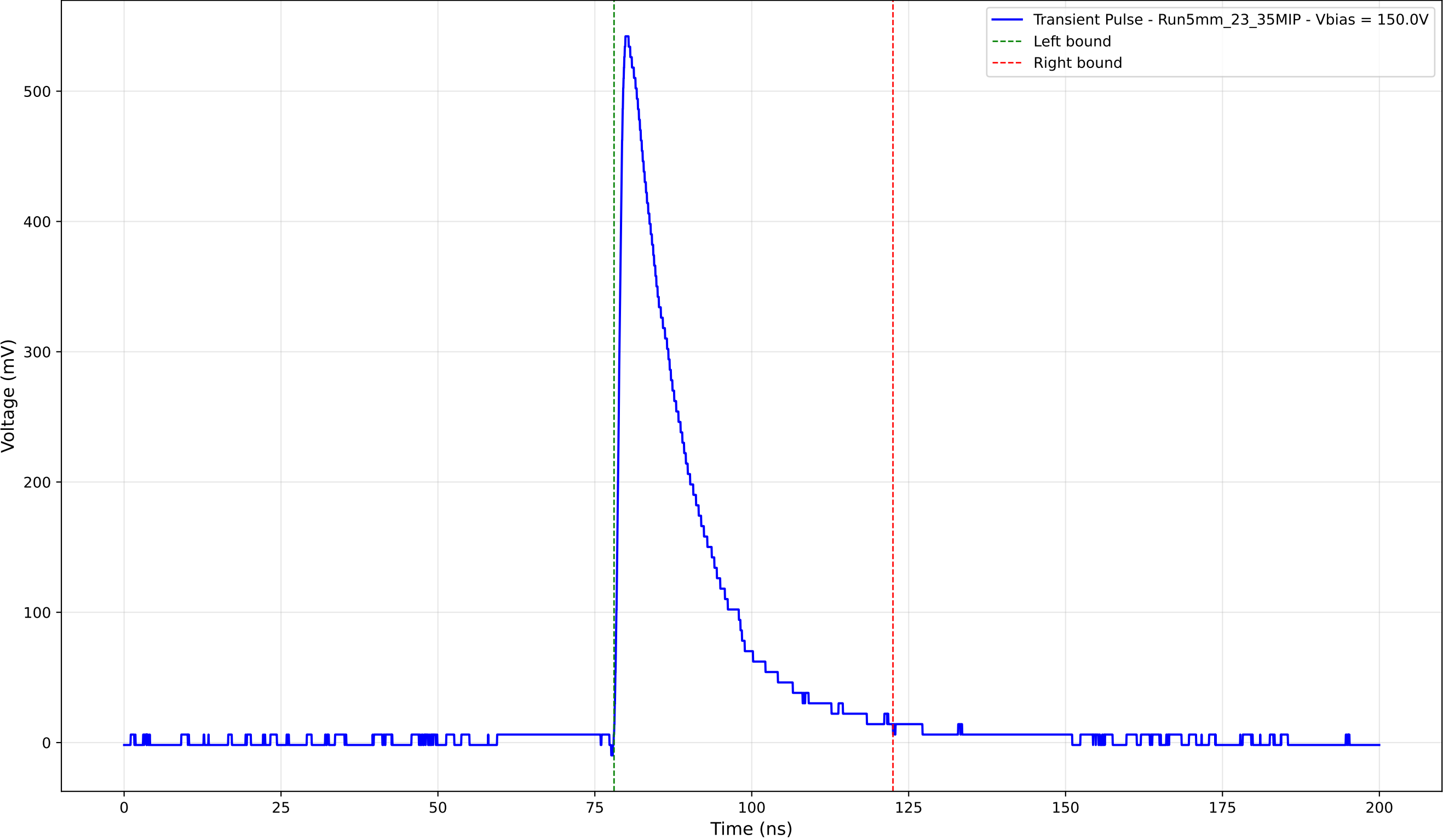
Transient Pulse - Sample: 5mm_23 - Position: 3760.0 \mu\text{m} - Charge: 125.83 pC
