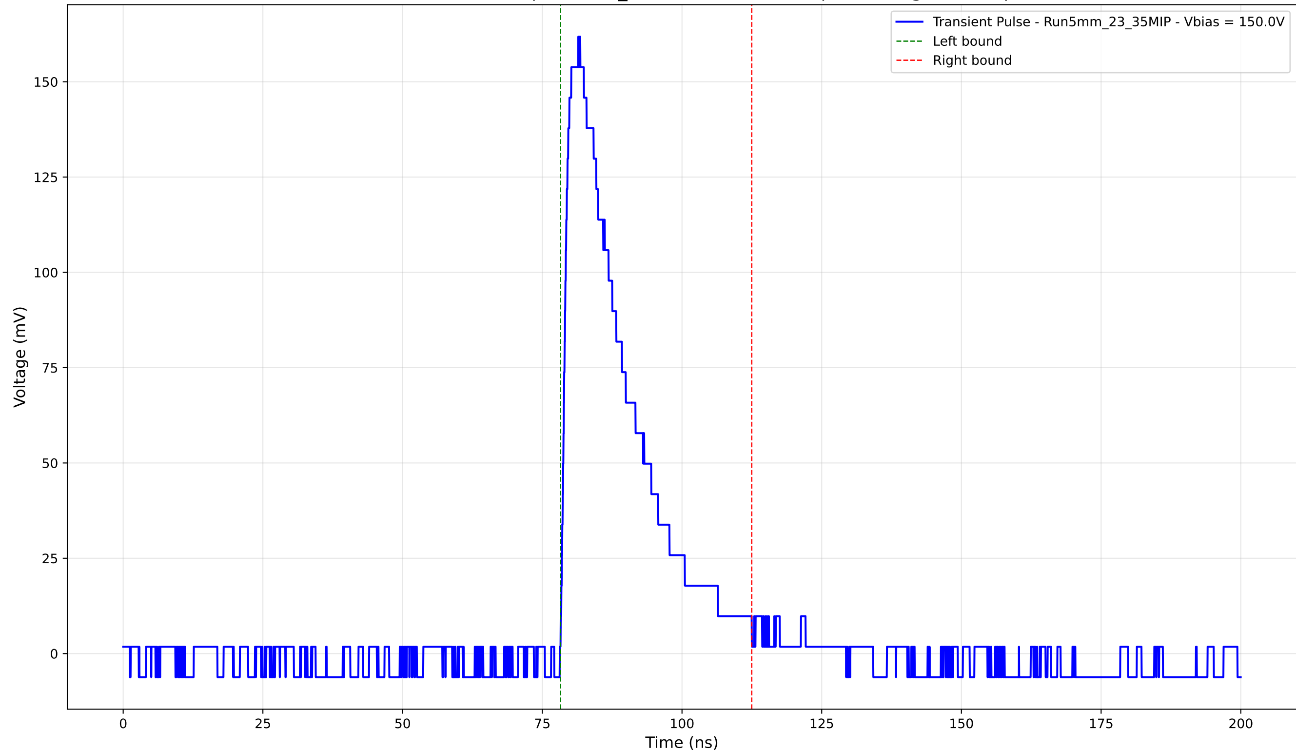
Transient Pulse - Sample: 5mm_23 - Position: 2165.0 \mu\text{m} - Charge: 39.29 pC
