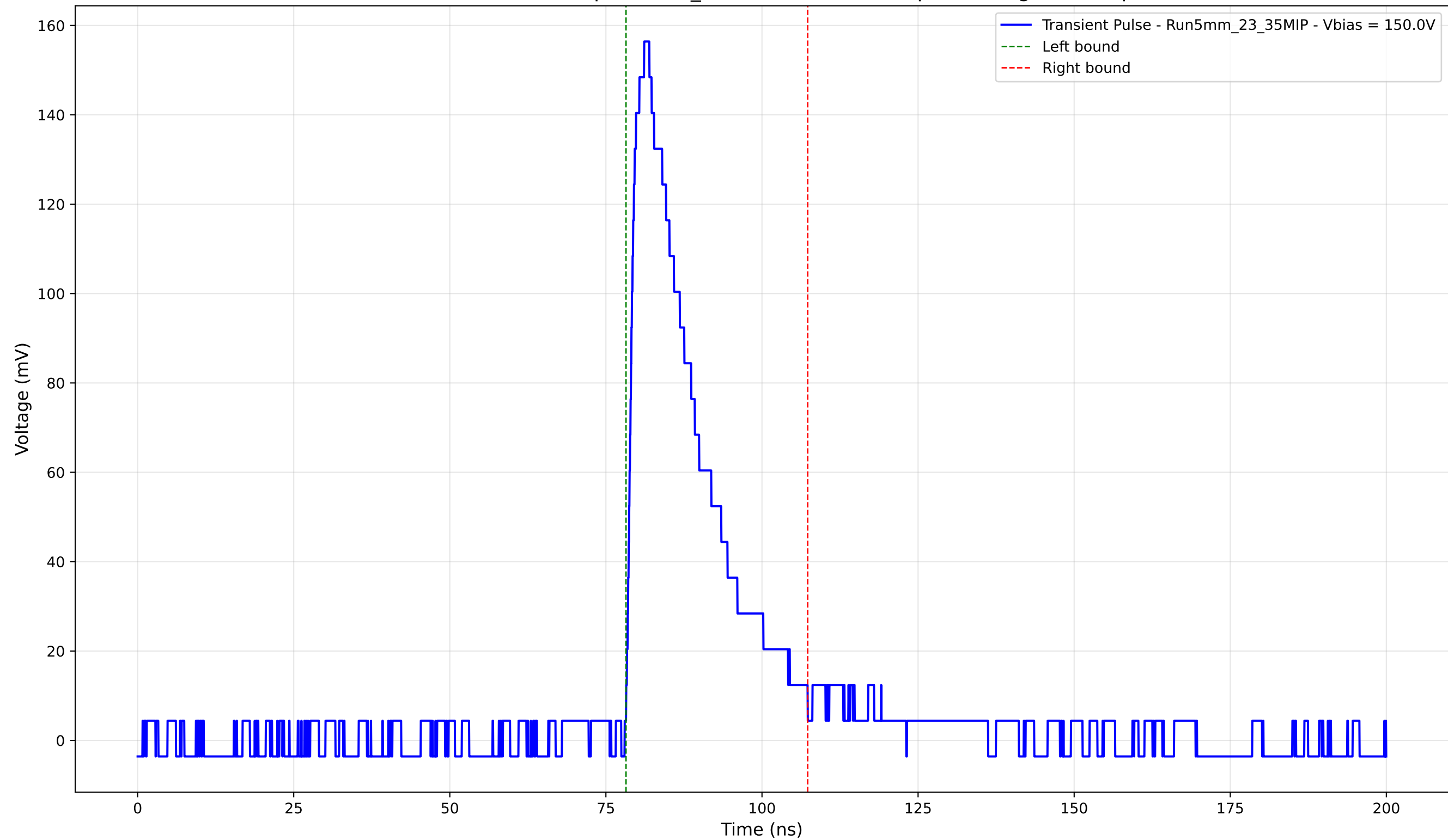
Transient Pulse - Sample: 5mm_23 - Position: 3170.0 \mu\text{m} - Charge: 36.63 pC
