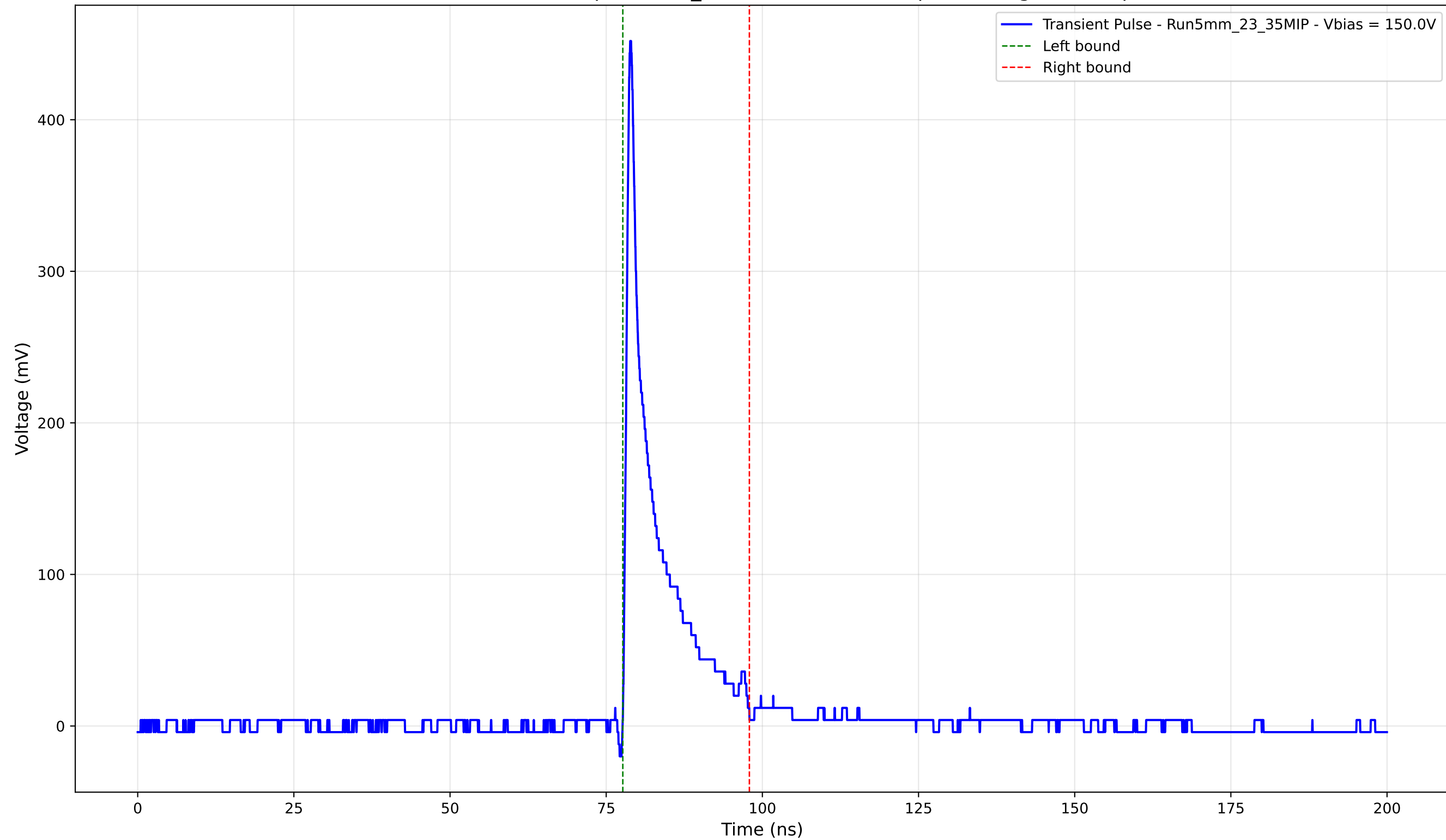
Transient Pulse - Sample: 5mm_23 - Position: 5070.0 \mu\text{m} - Charge: 42.54 pC
