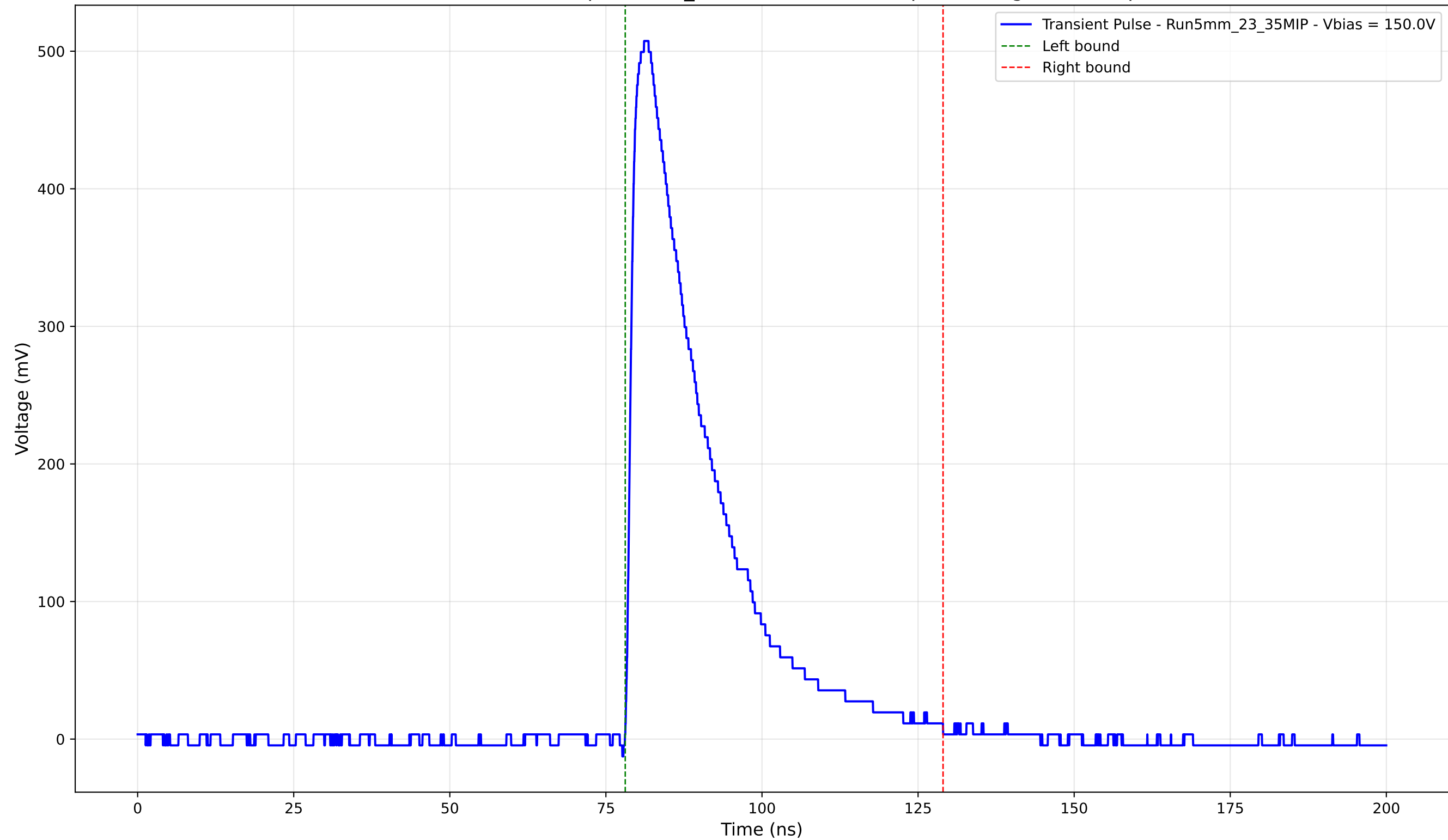
Transient Pulse - Sample: 5mm_23 - Position: 2440.0 \mu\text{m} - Charge: 138.01 pC
