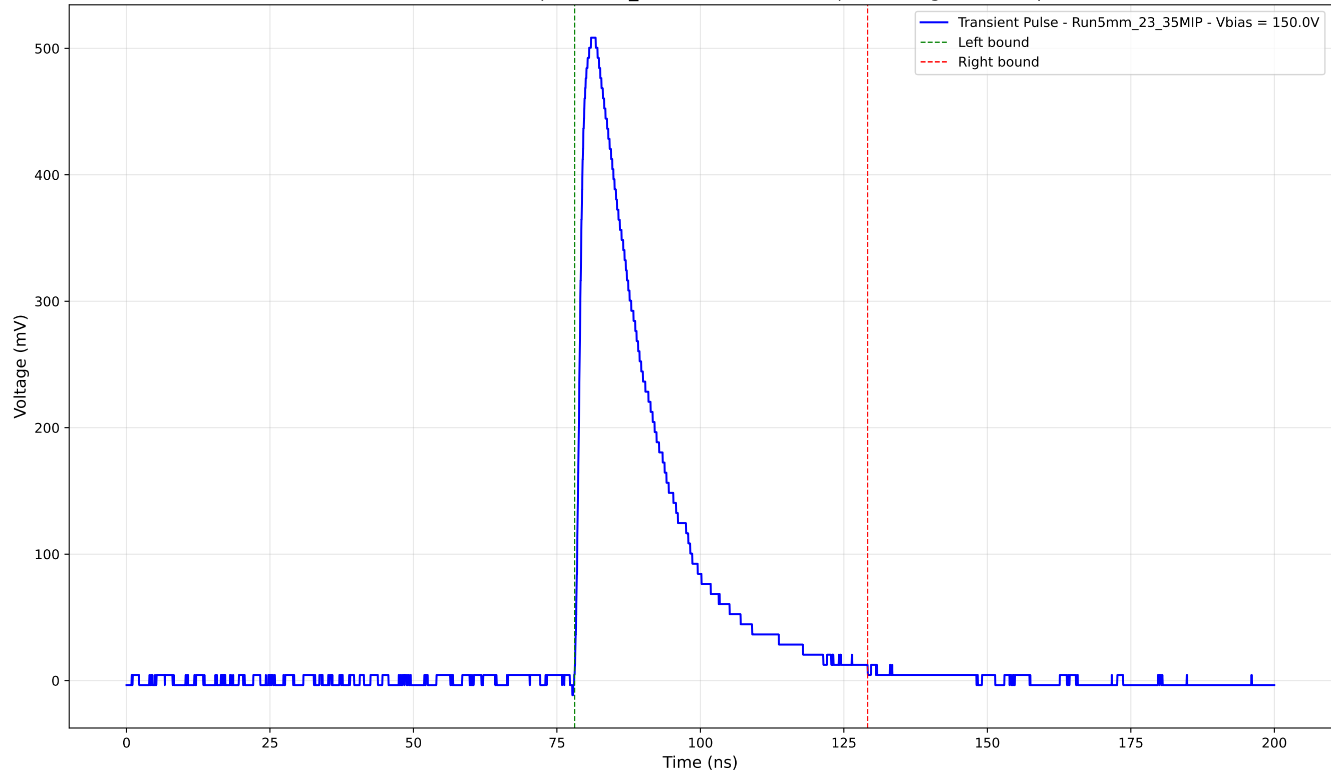
Transient Pulse - Sample: 5mm_23 - Position: 2445.0 \mu\text{m} - Charge: 139.07 pC
