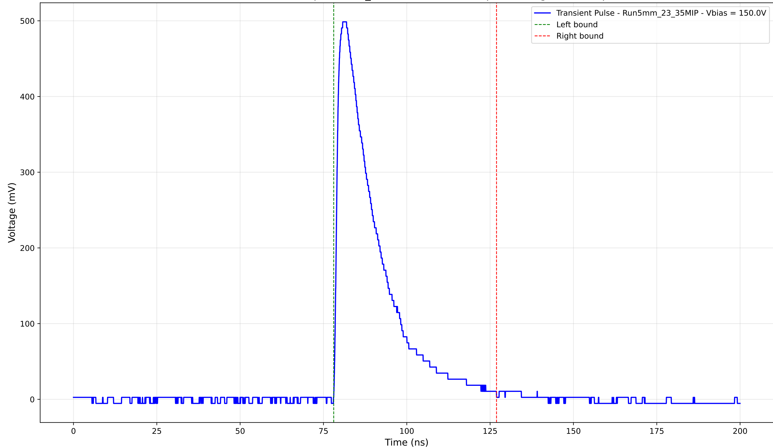
Transient Pulse - Sample: 5mm_23 - Position: 2425.0 \mu\text{m} - Charge: 135.03 pC
