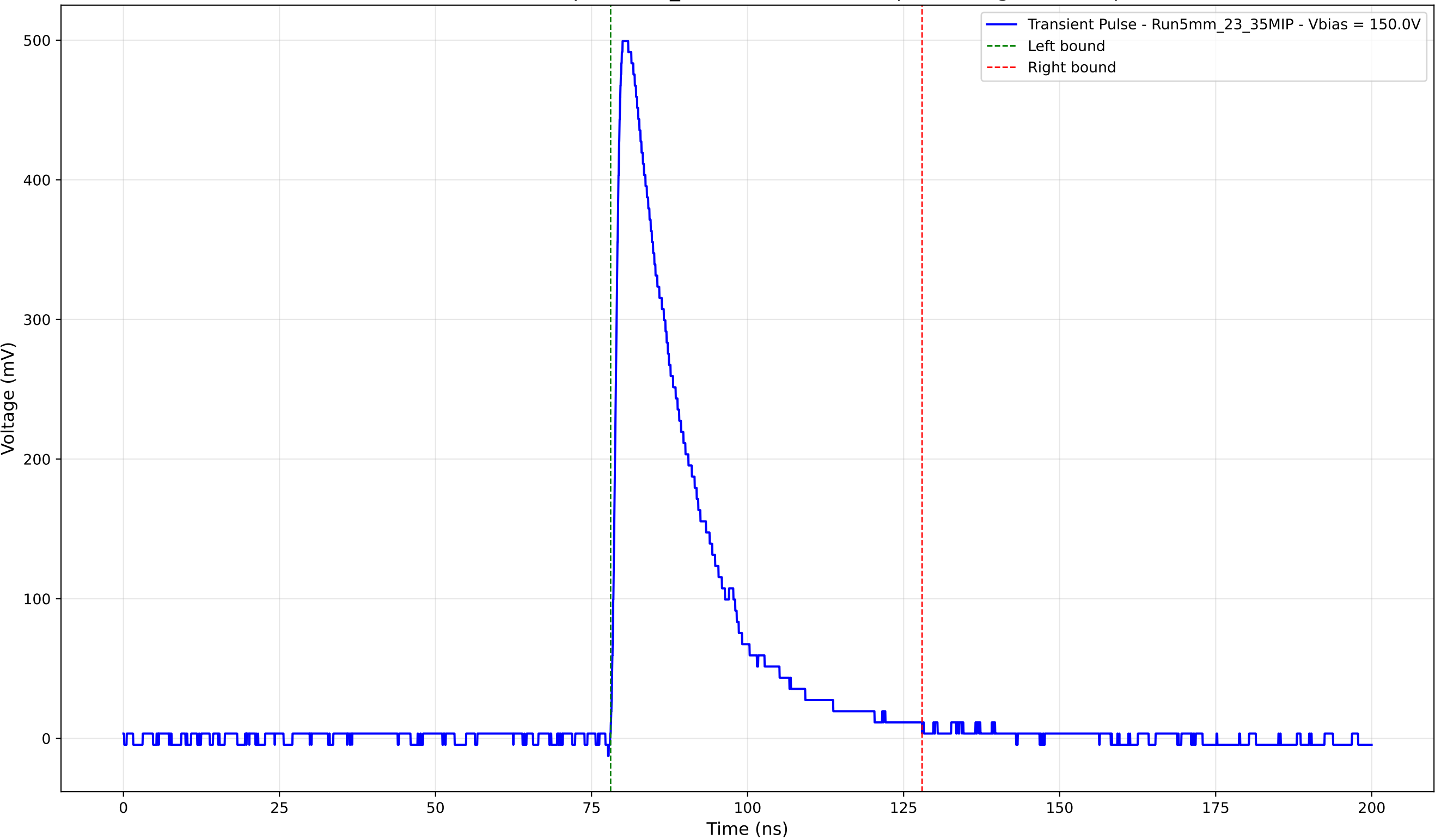
Transient Pulse - Sample: 5mm_23 - Position: 3525.0 \mu\text{m} - Charge: 123.97 pC
