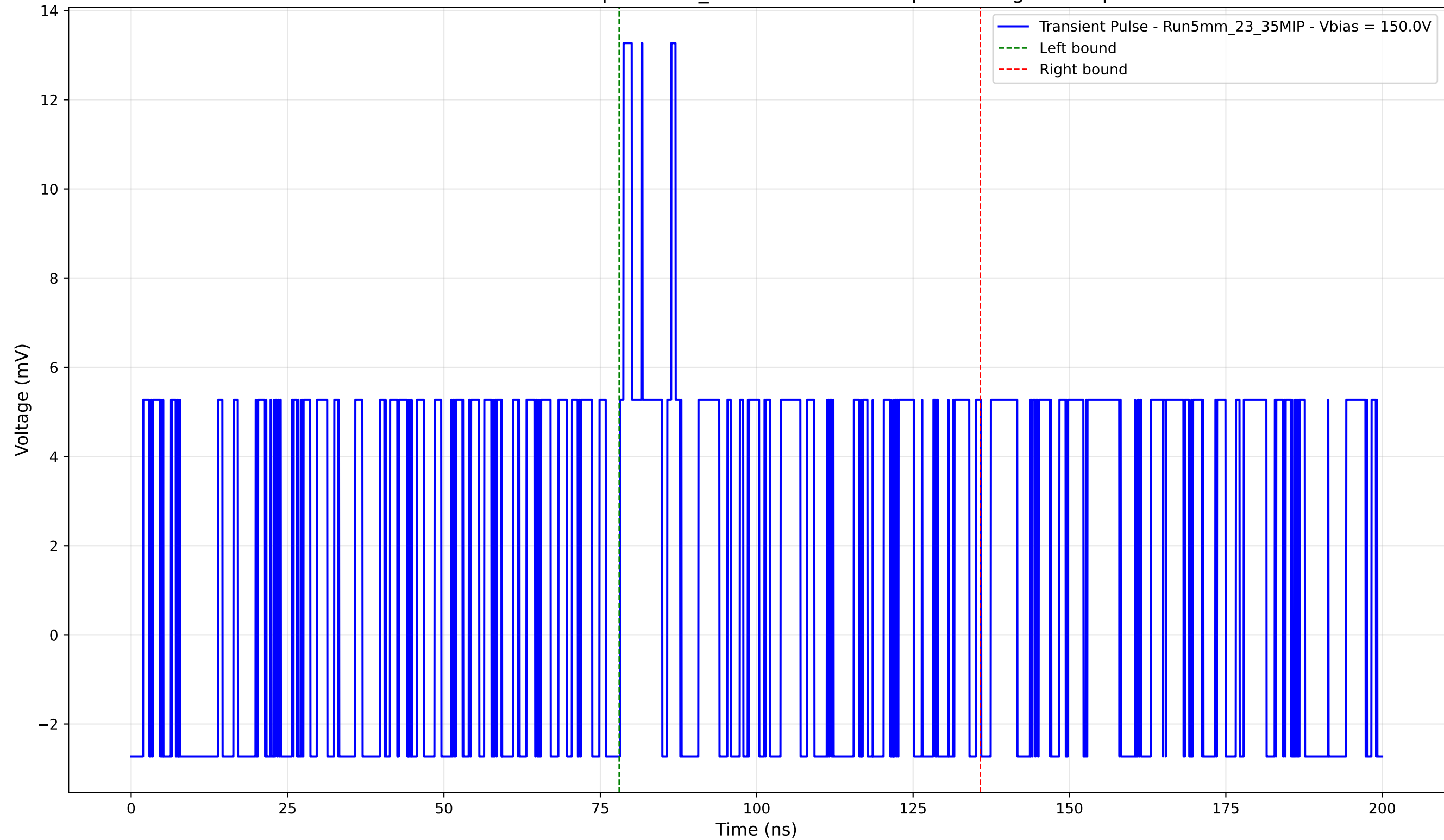
Transient Pulse - Sample: 5mm_23 - Position: 110.0 \mu\text{m} - Charge: 2.05 pC
