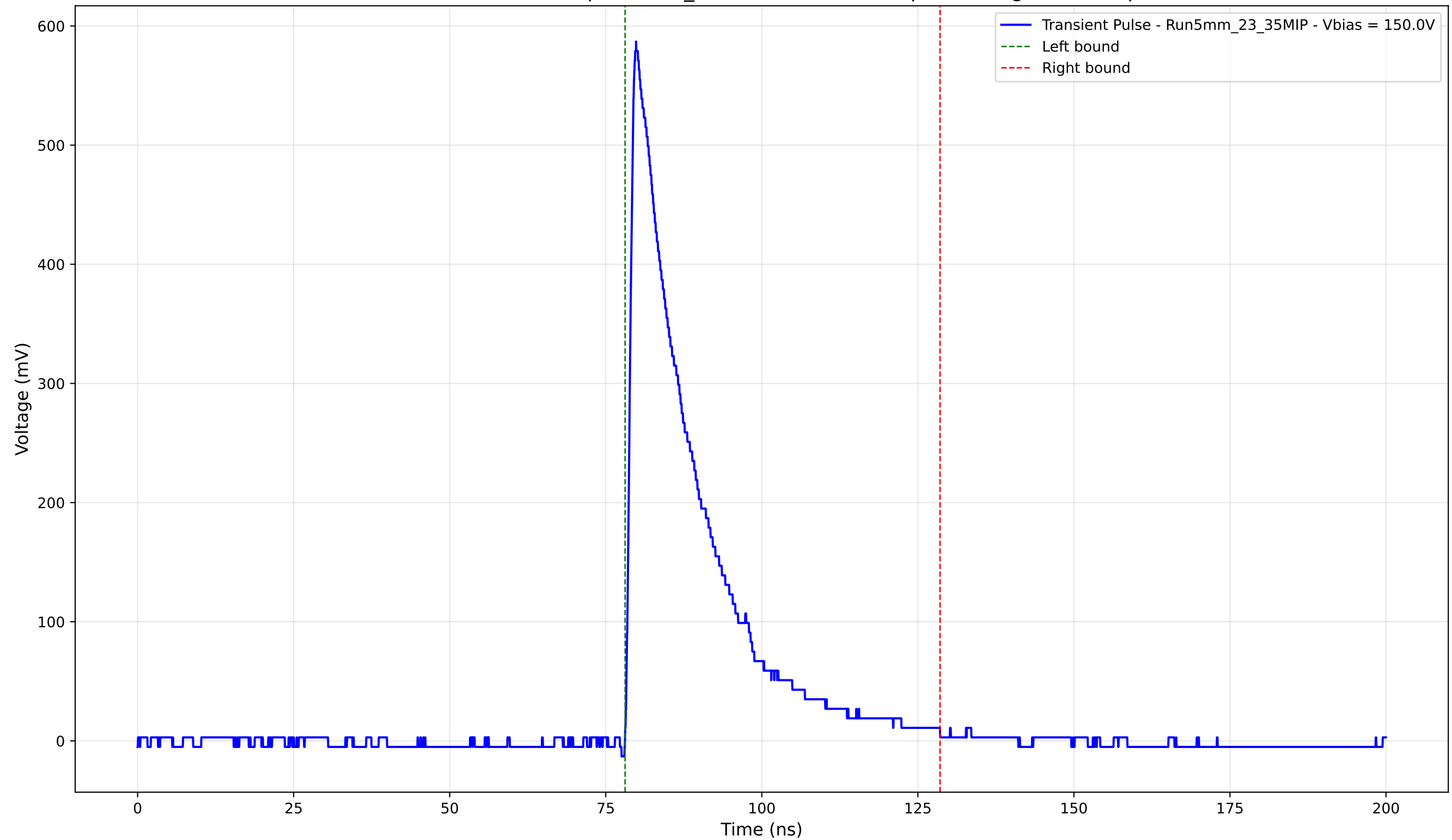
Transient Pulse - Sample: 5mm_23 - Position: 1285.0 \mu\text{m} - Charge: 128.22 pC
