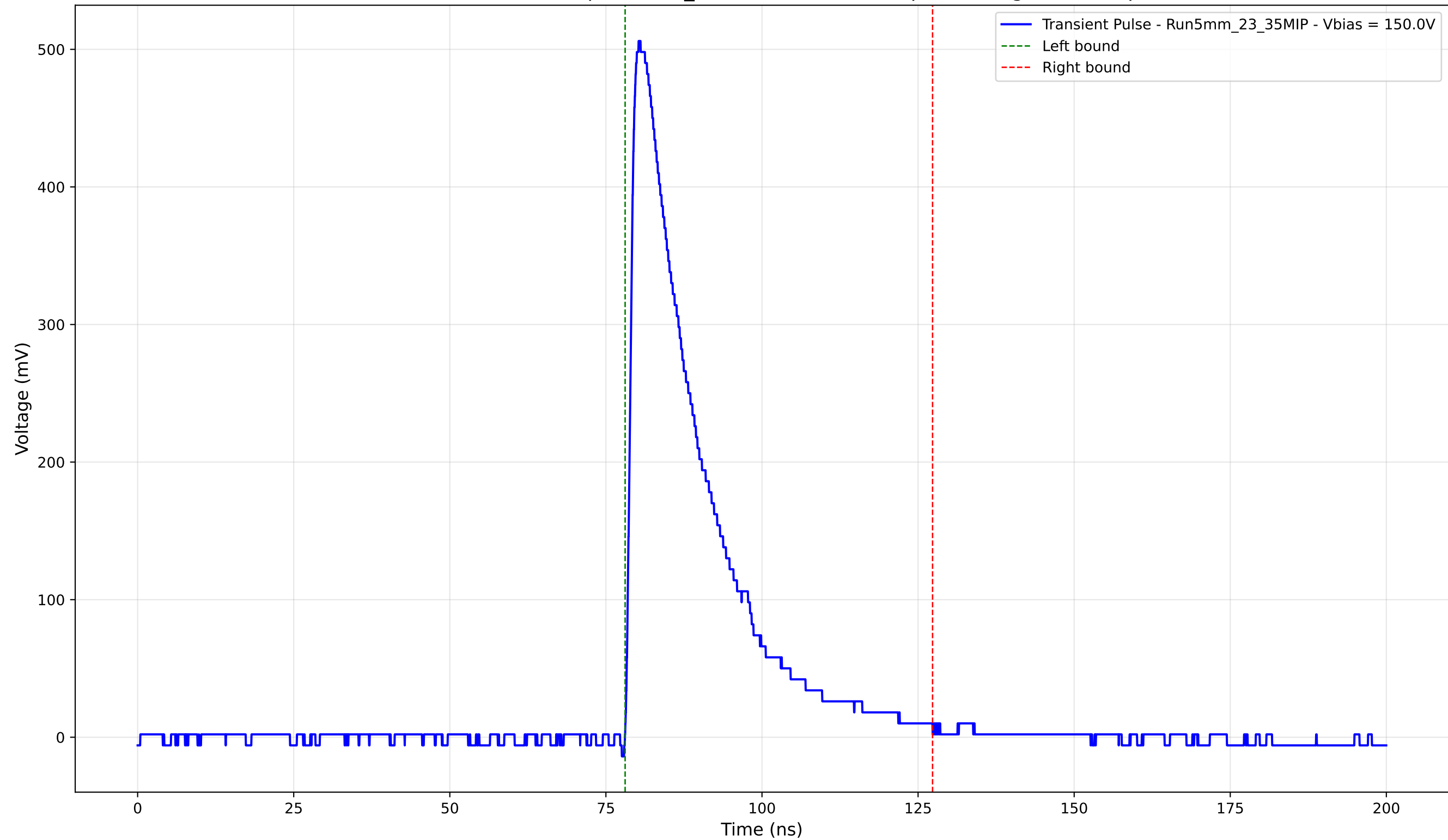
Transient Pulse - Sample: 5mm_23 - Position: 3520.0 \mu\text{m} - Charge: 124.06 pC
