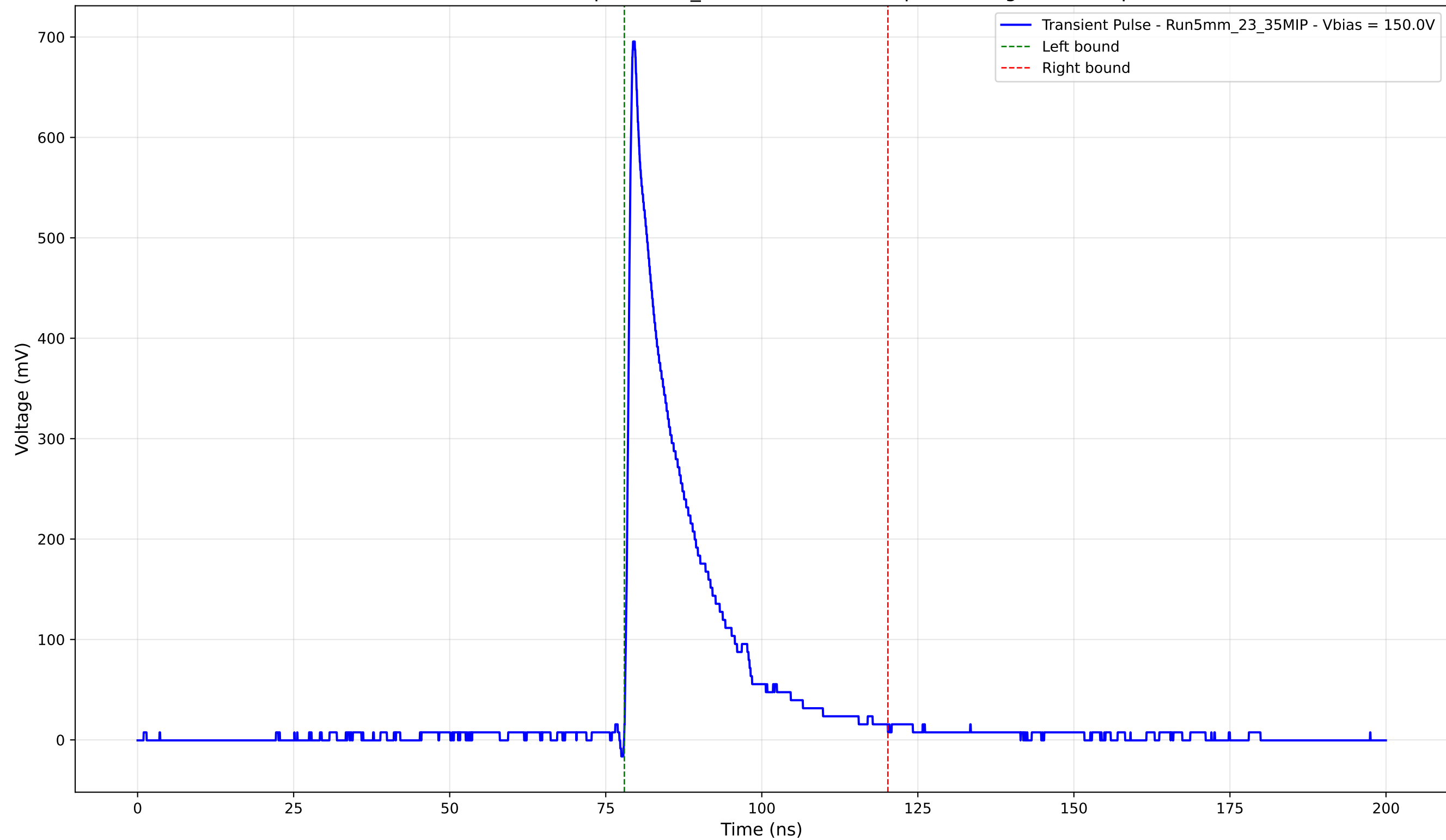
Transient Pulse - Sample: 5mm_23 - Position: 800.0 \mu\text{m} - Charge: 123.32 pC
