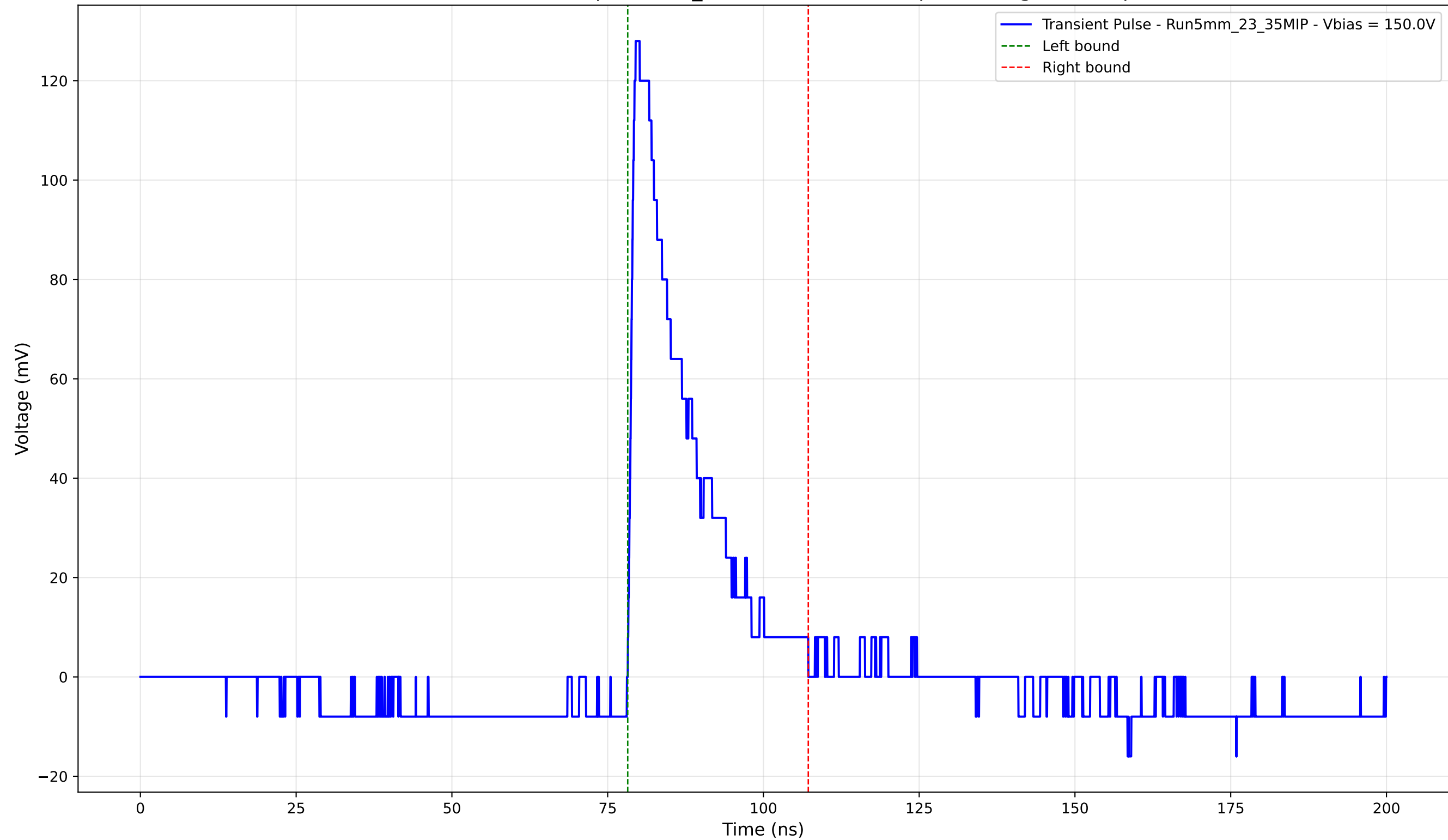
Transient Pulse - Sample: 5mm_23 -Position: 4140.0 \mu\text{m} - Charge: 24.44 pC
