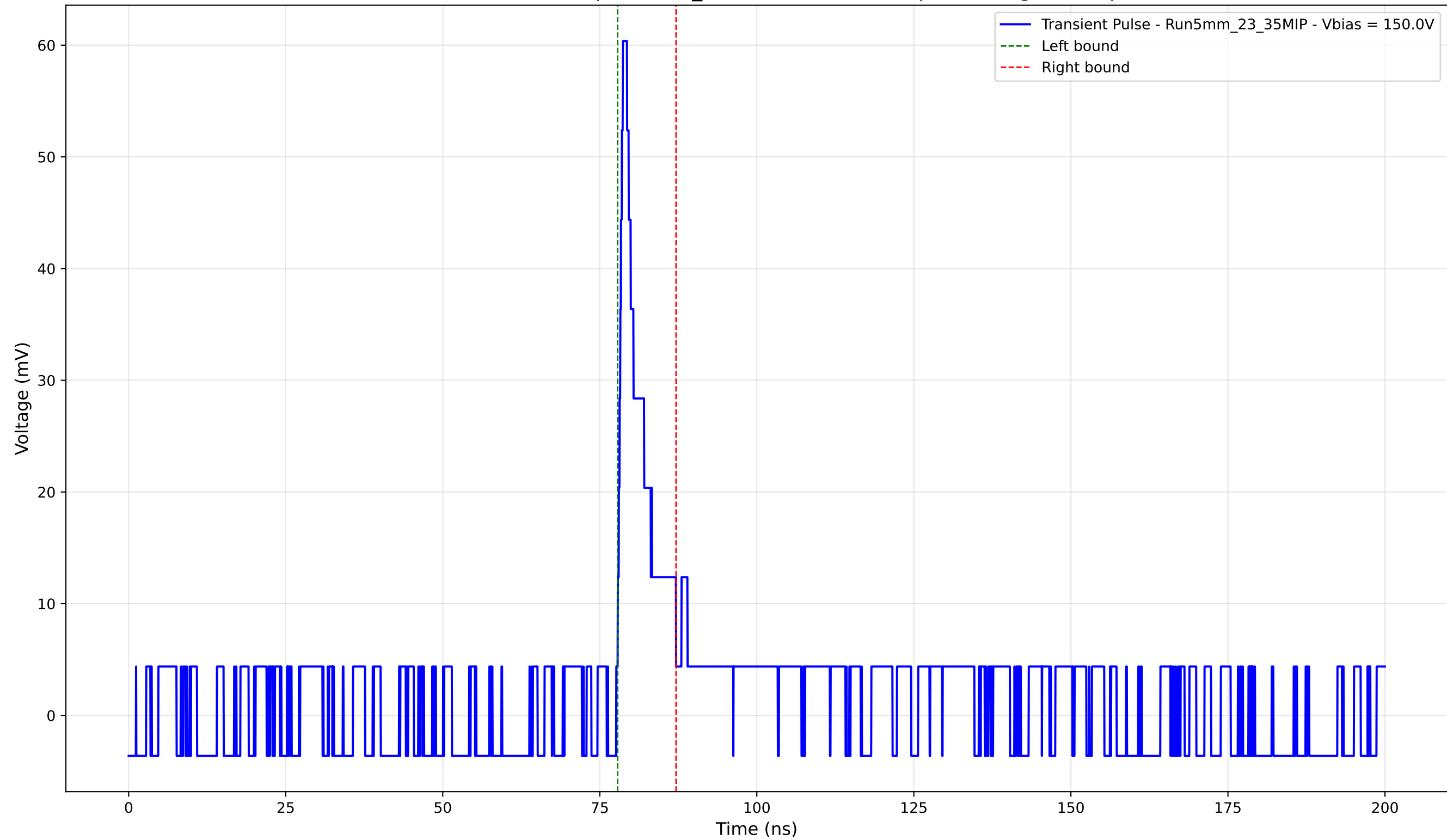
Transient Pulse - Sample: 5mm_23 - Position: 5120.0 \mu\text{m} - Charge: 4.62 pC
