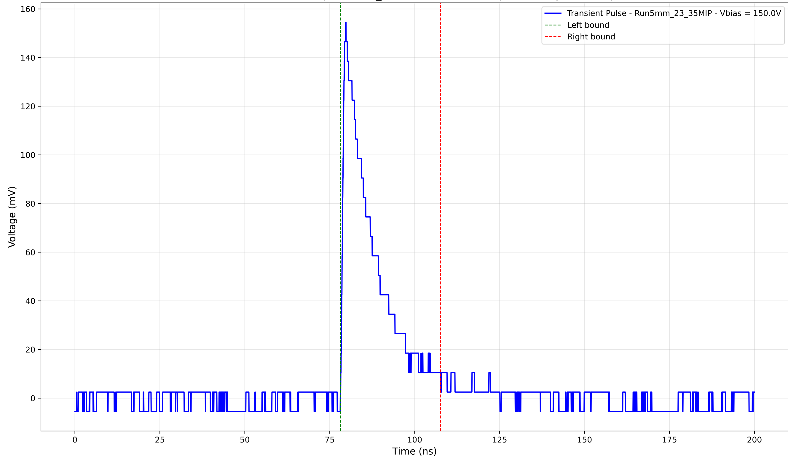
Transient Pulse - Sample: 5mm_23 - Position: 1105.0 \mu\text{m} - Charge: 29.22 pC
