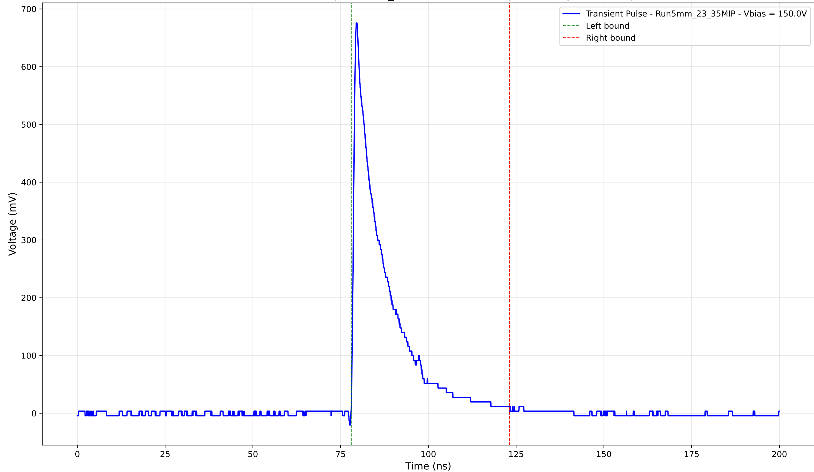
Transient Pulse - Sample: 5mm_23 - Position: 865.0 \mu\text{m} - Charge: 123.15 pC
