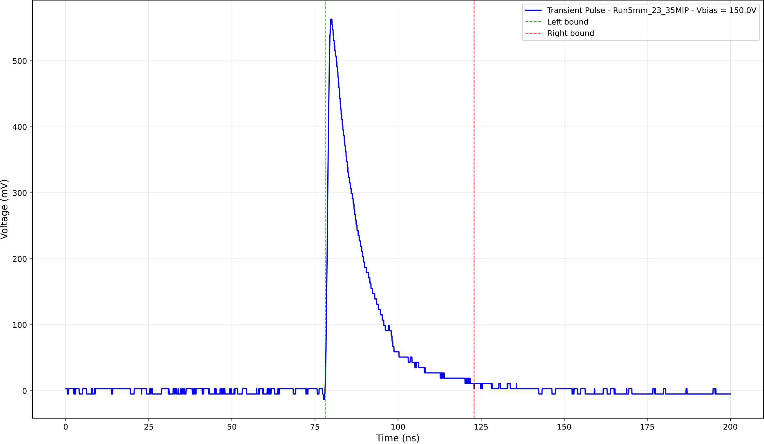
Transient Pulse - Sample: 5mm_23 - Position: 3955.0 \mu\text{m} - Charge: 120.39 pC
