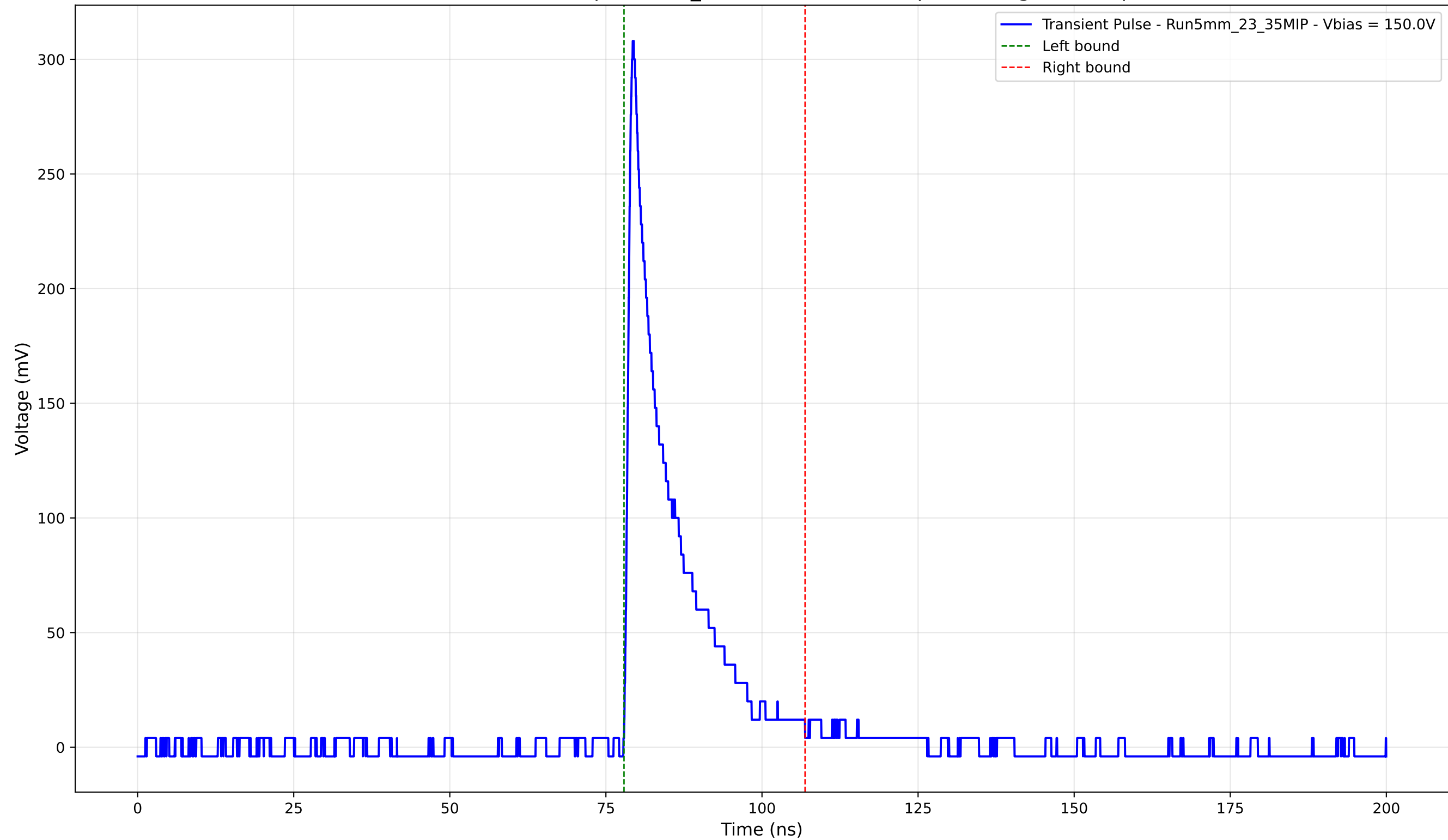
Transient Pulse - Sample: 5mm_23 - Position: 4545.0 \mu\text{m} - Charge: 43.26 pC
