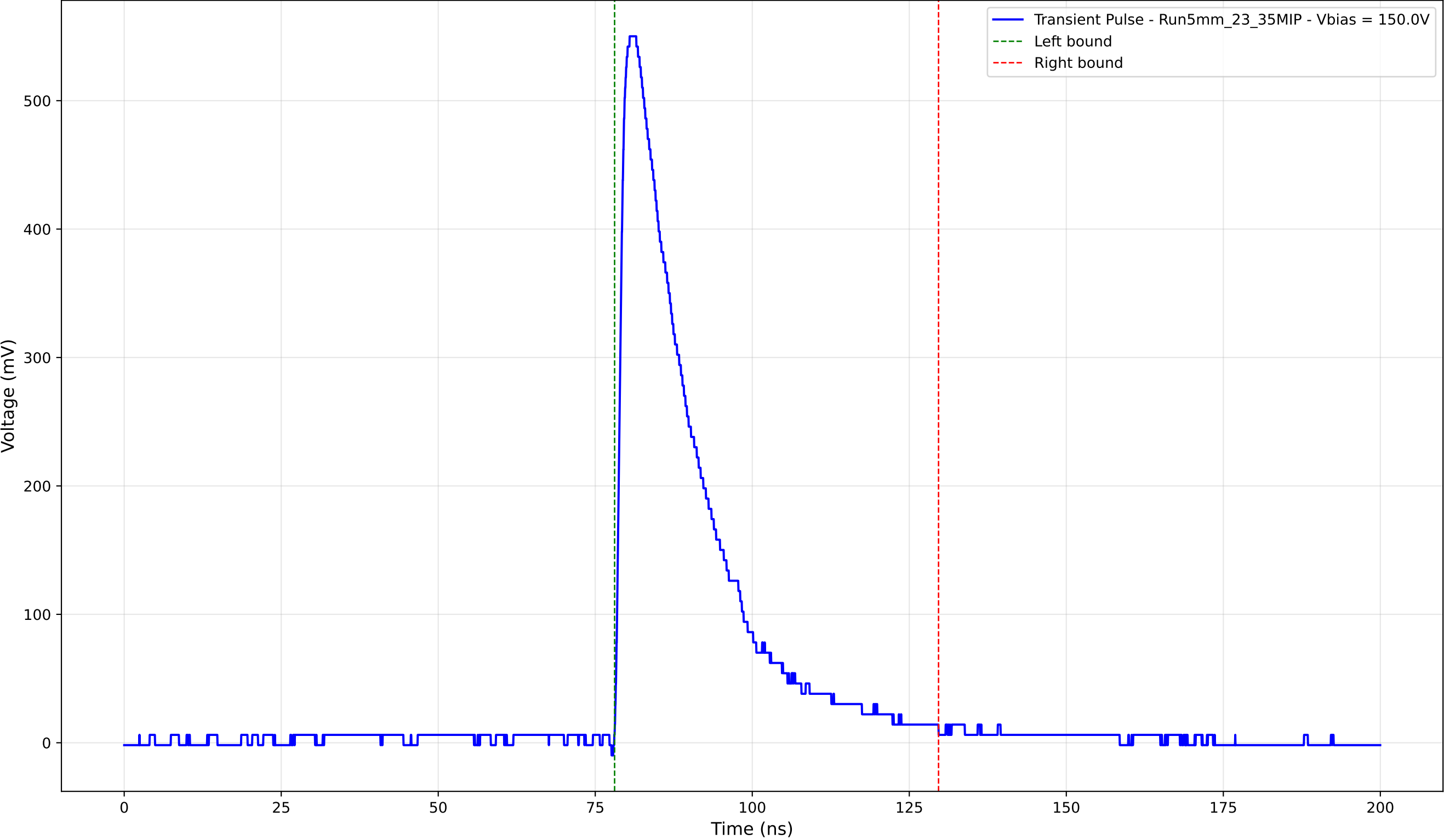
Transient Pulse - Sample: 5mm_23 - Position: 2010.0 \mu\text{m} - Charge: 145.96 pC
