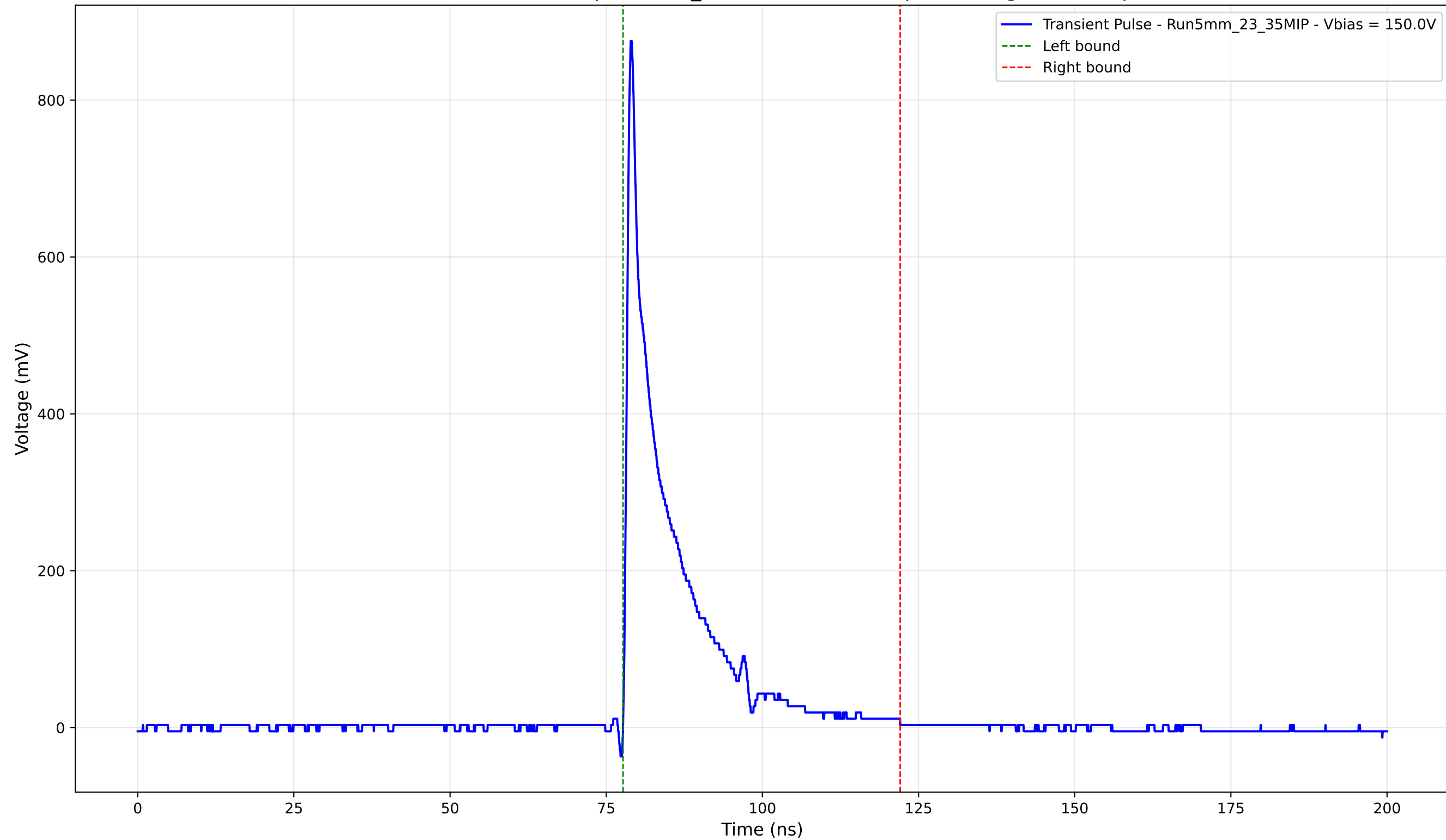
Transient Pulse - Sample: 5mm_23 - Position: 275.0 \mu\text{m} - Charge: 113.07 pC
