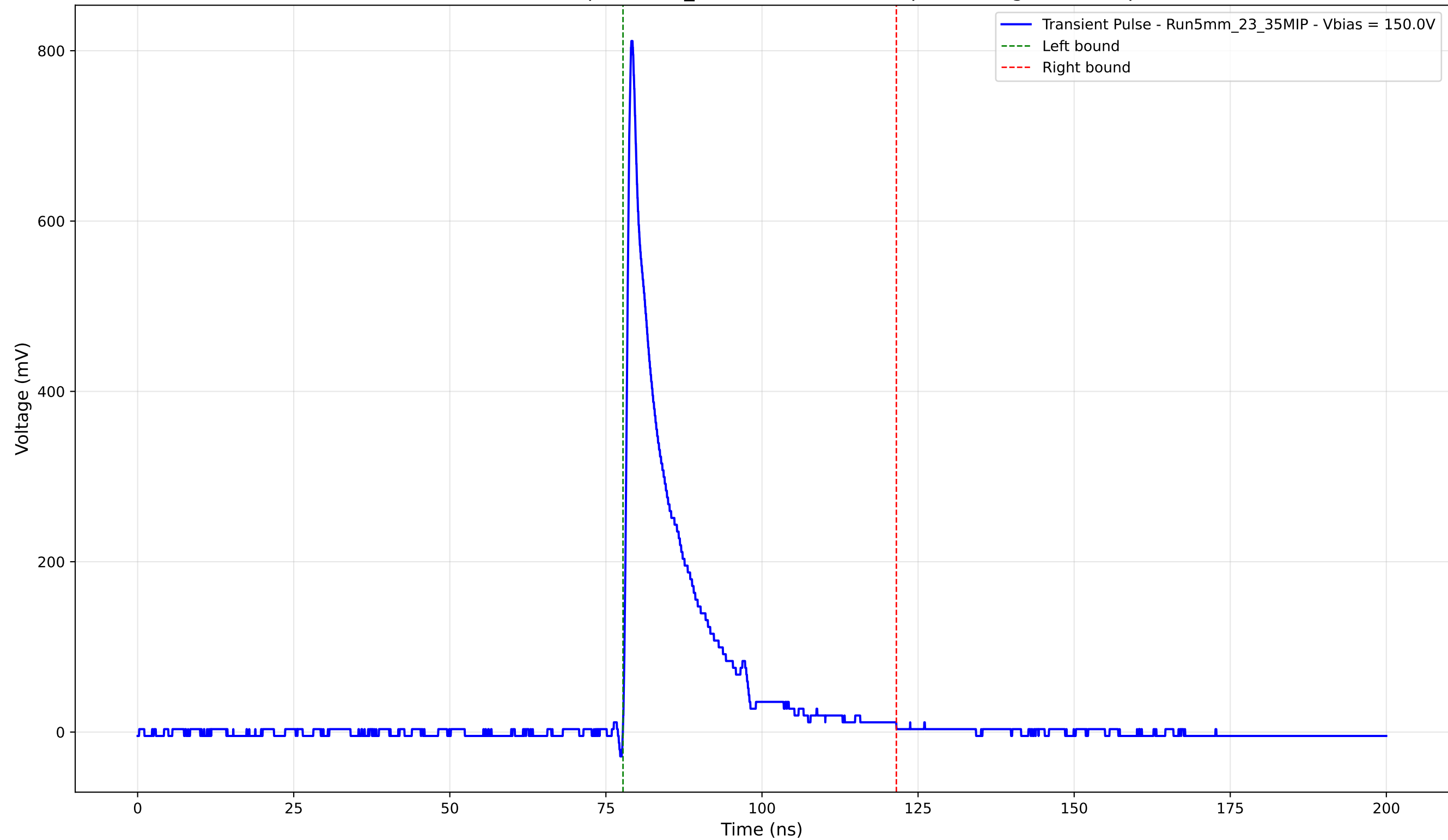
Transient Pulse - Sample: 5mm_23 - Position: 4800.0 \mu\text{m} - Charge: 112.82 pC
