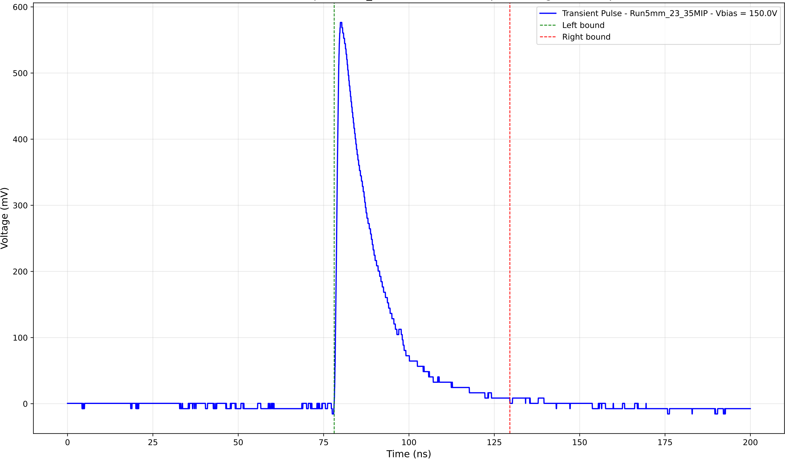
Transient Pulse - Sample: 5mm_23 - Position: 1515.0 \mu\text{m} - Charge: 135.01 pC
