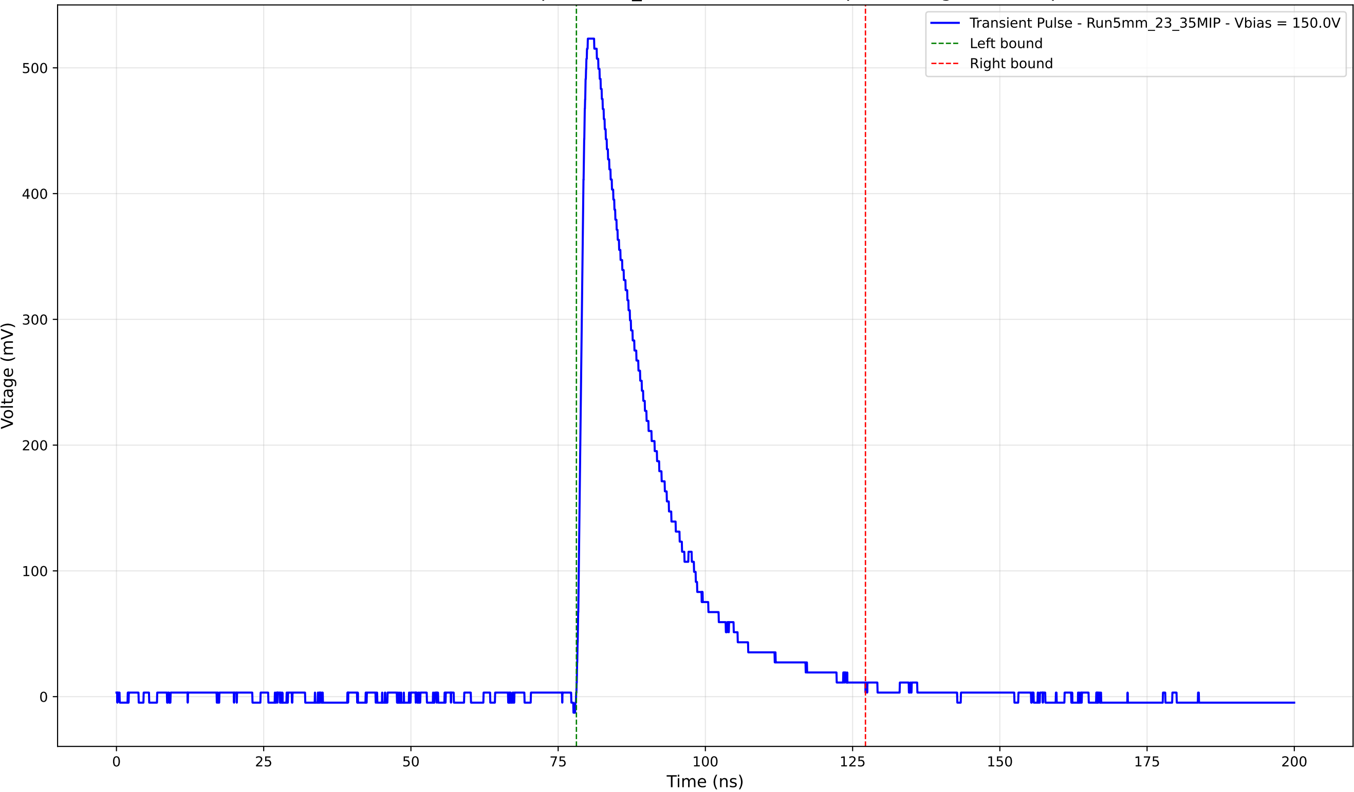
Transient Pulse - Sample: 5mm_23 - Position: 1755.0 \mu\text{m} - Charge: 132.85 pC
