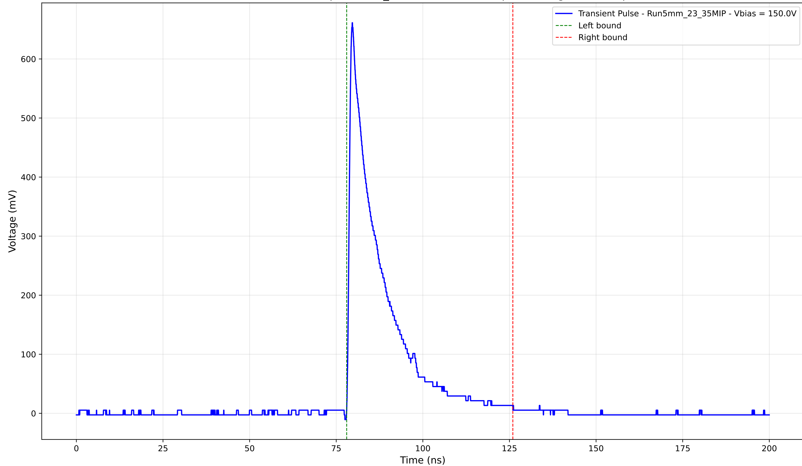
Transient Pulse - Sample: 5mm_23 - Position: 945.0 \mu\text{m} - Charge: 126.72 pC
