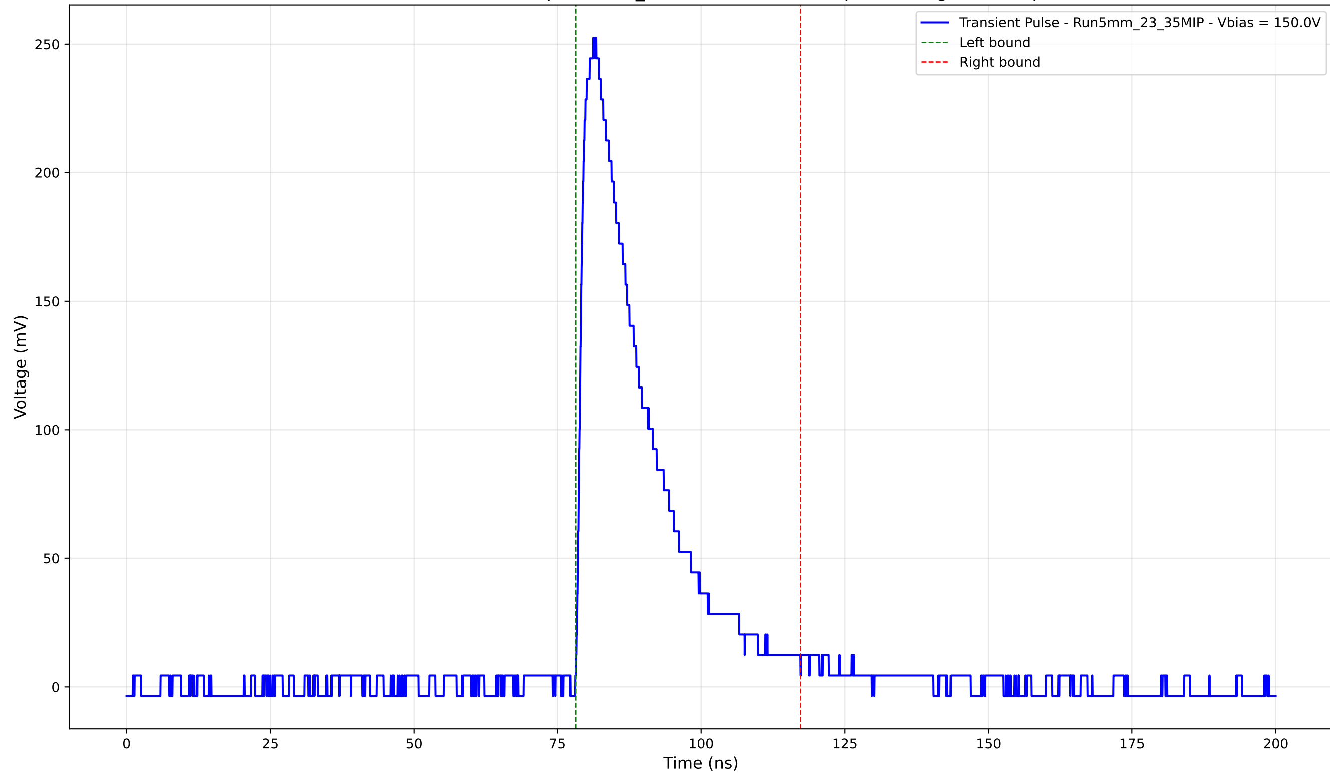
Transient Pulse - Sample: 5mm_23 - Position: 2180.0 \mu\text{m} - Charge: 63.56 pC
