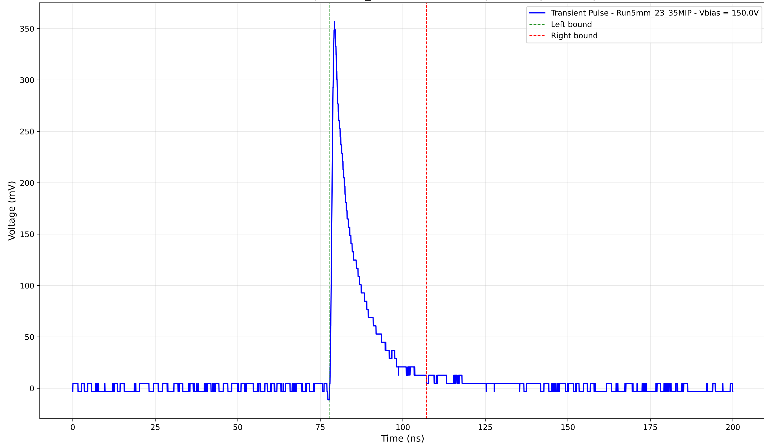
Transient Pulse - Sample: 5mm_23 - Position: 4630.0 \mu\text{m} - Charge: 50.54 pC
