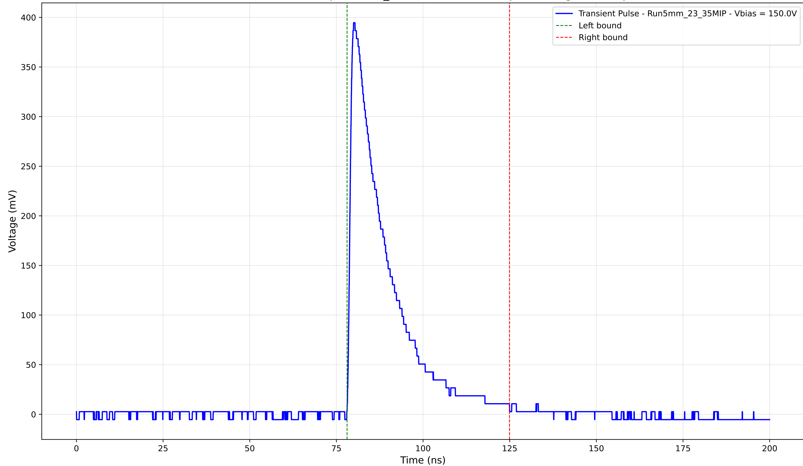
Transient Pulse - Sample: 5mm_23 - Position: 1560.0 \mu\text{m} - Charge: 91.44 pC
