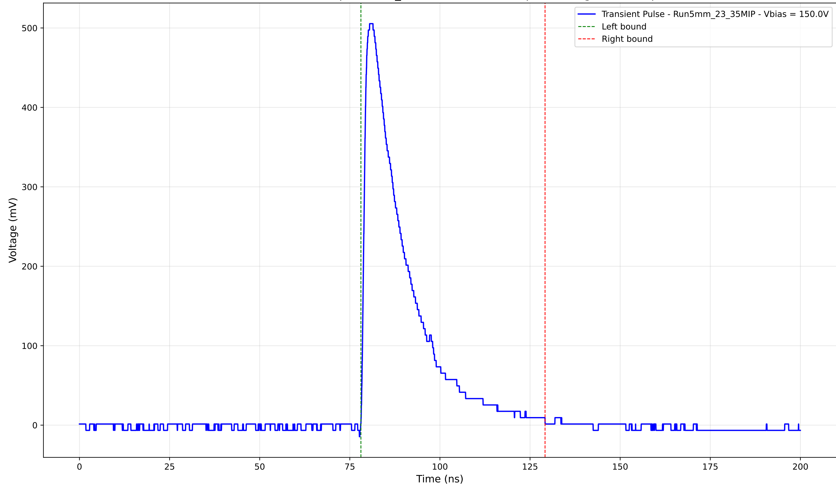
Transient Pulse - Sample: 5mm_23 - Position: 3365.0 \mu\text{m} - Charge: 128.29 pC
