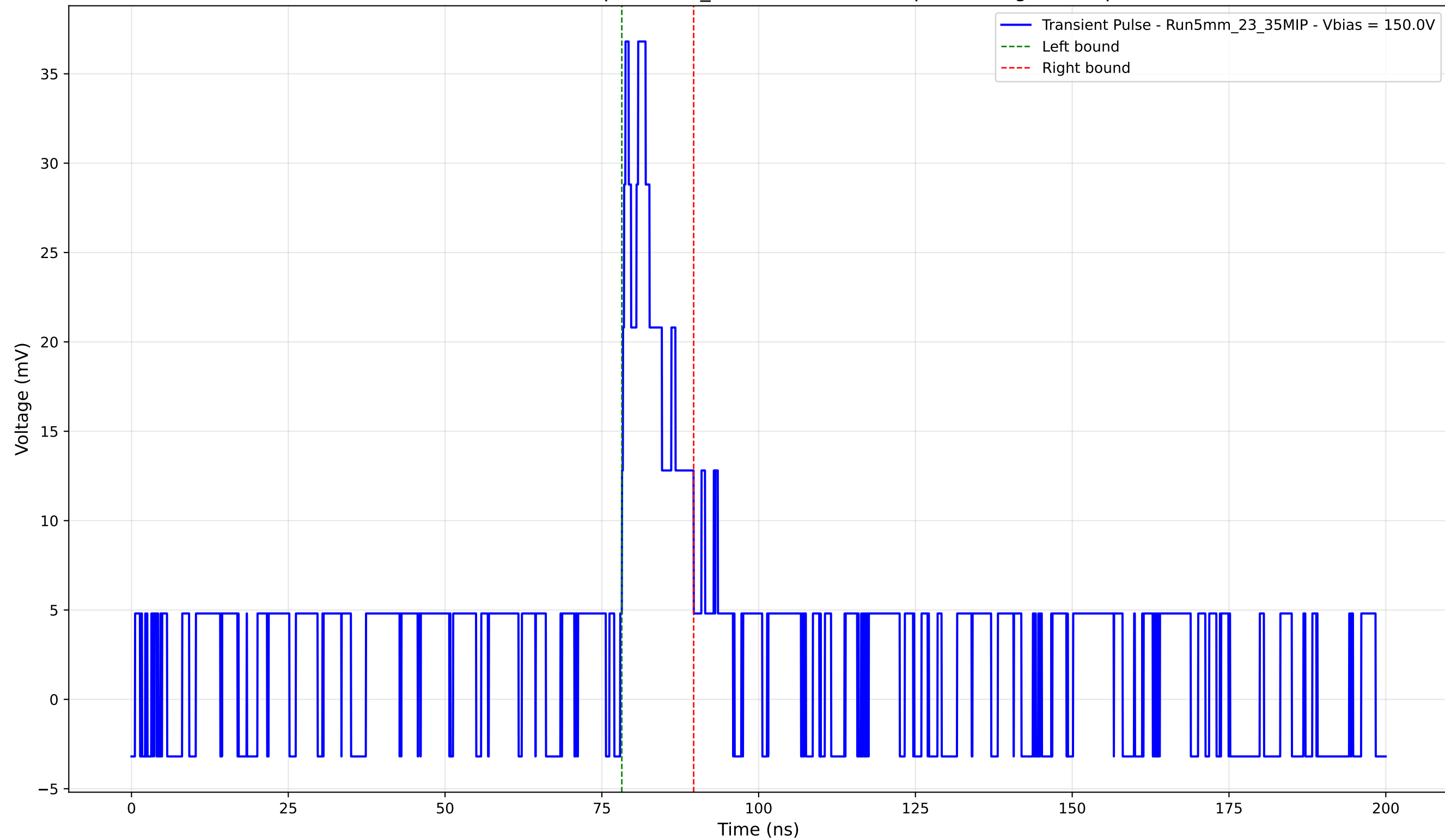
Transient Pulse - Sample: 5mm_23 - Position: 155.0 \mu\text{m} - Charge: 4.82 pC
