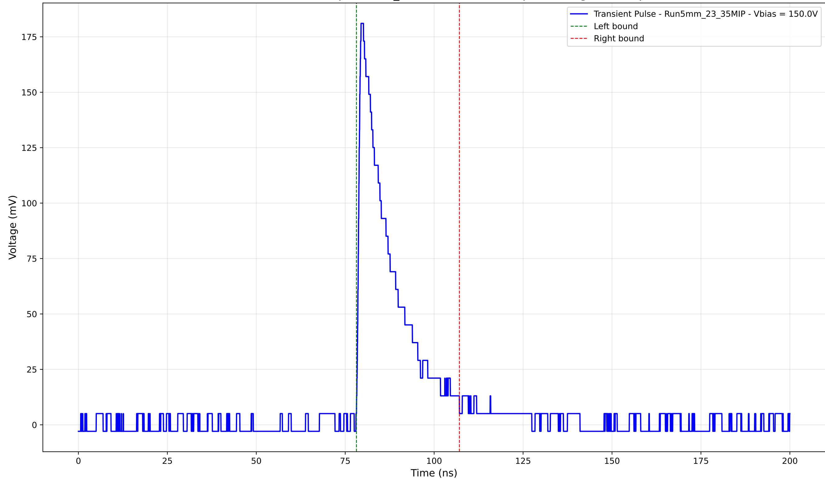
Transient Pulse - Sample: 5mm_23 - Position: 1100.0 \mu\text{m} - Charge: 35.34 pC
