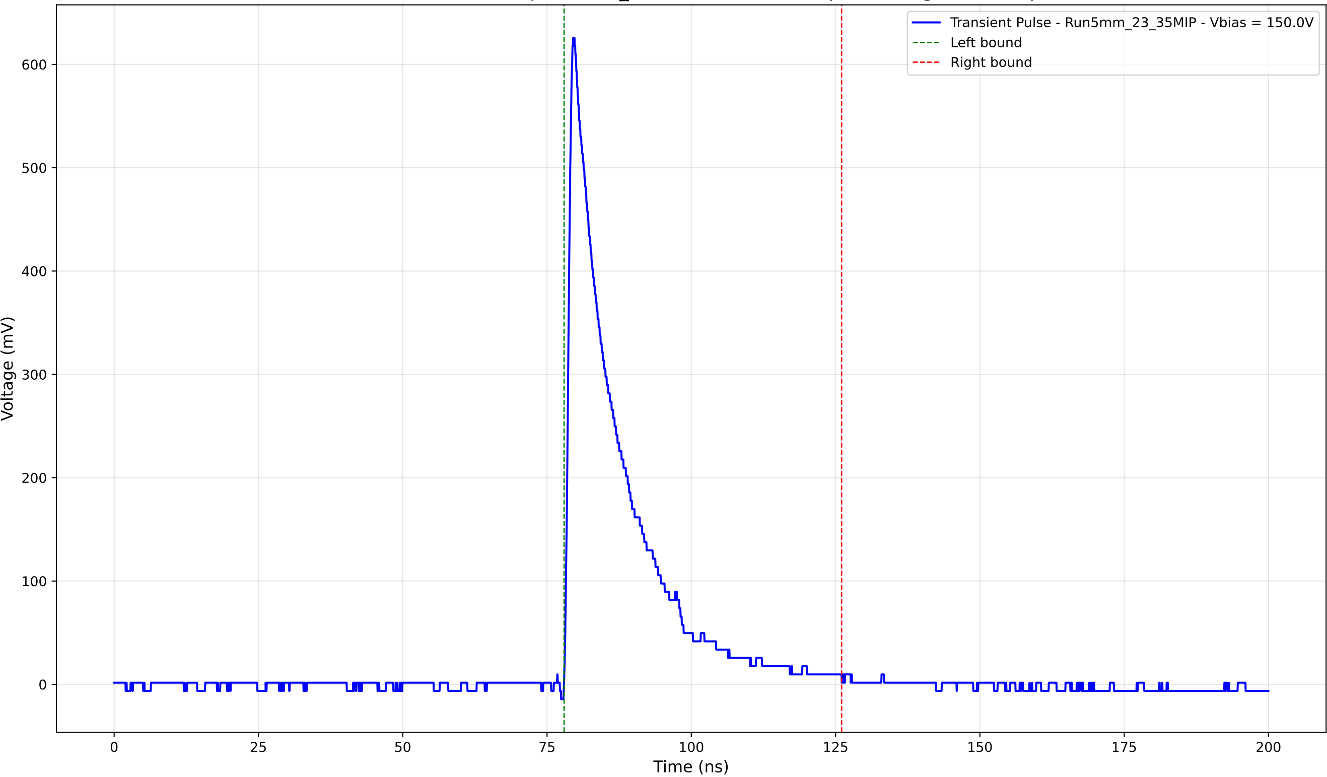
Transient Pulse - Sample: 5mm_23 - Position: 4295.0 \mu\text{m} - Charge: 115.36 pC
