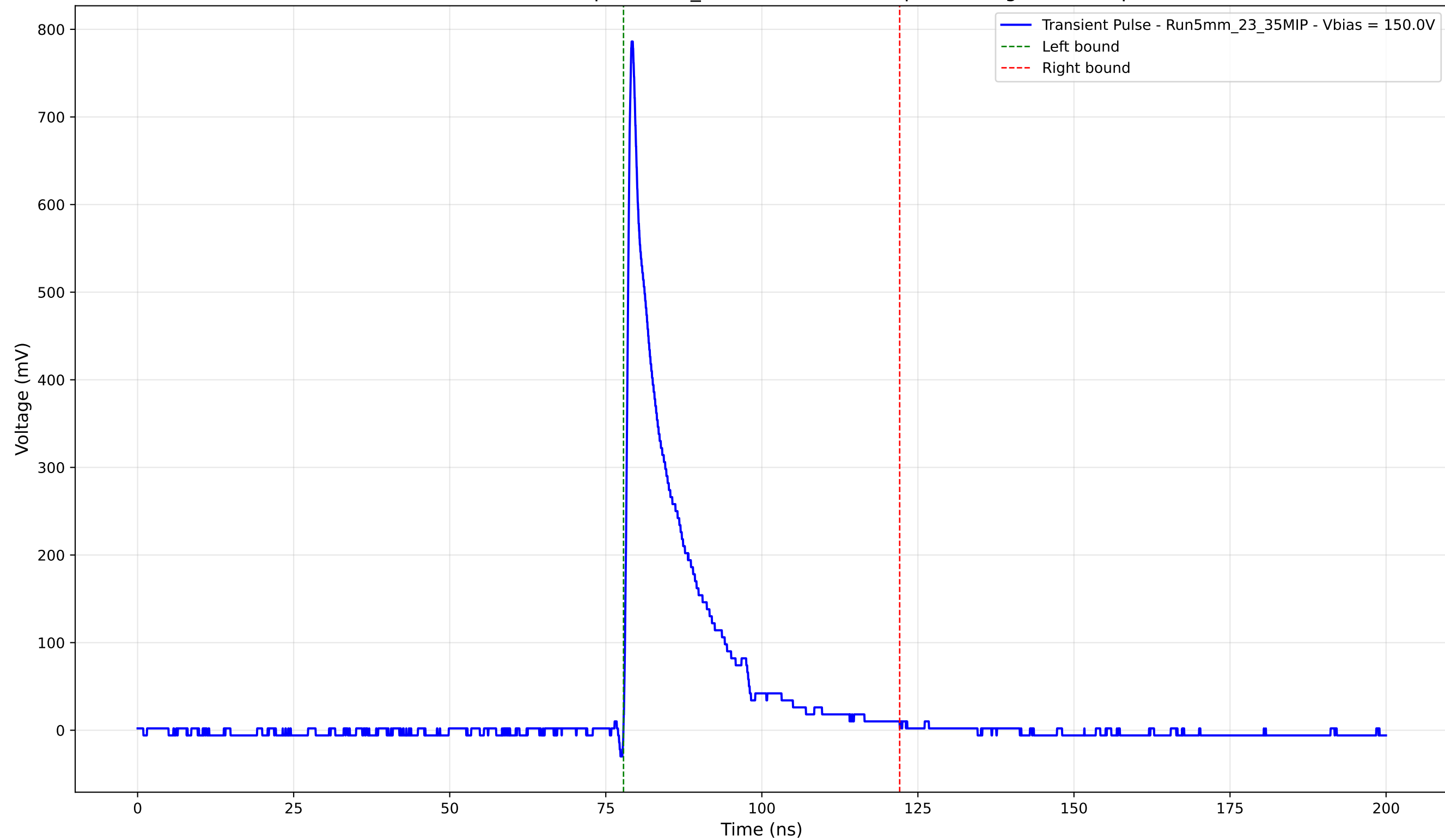
Transient Pulse - Sample: 5mm_23 - Position: 500.0 \mu\text{m} - Charge: 114.48 pC
