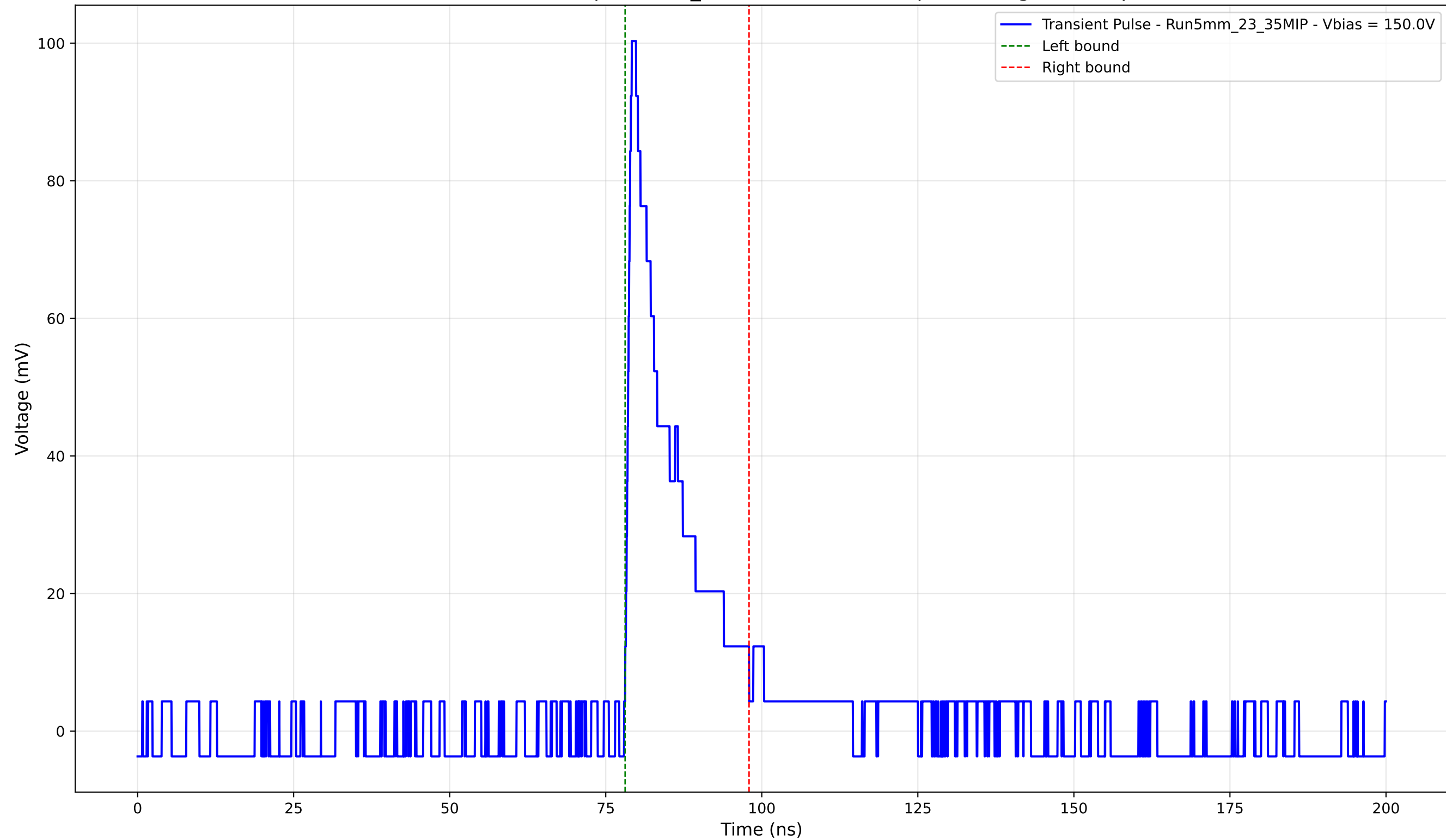
Transient Pulse - Sample: 5mm_23 - Position: 4520.0 \mu\text{m} - Charge: 14.69 pC
