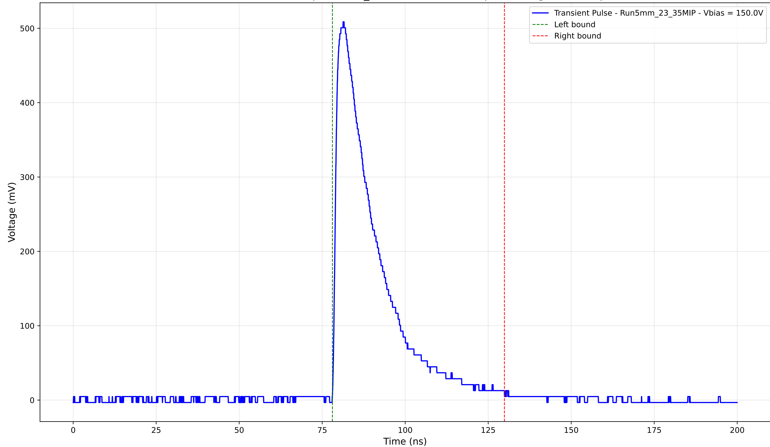
Transient Pulse - Sample: 5mm_23 - Position: 2385.0 \mu\text{m} - Charge: 138.00 pC
