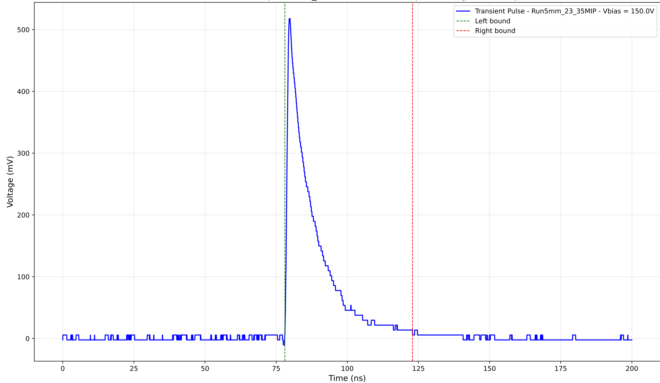
Transient Pulse - Sample: 5mm_23 - Position: 1055.0 \mu\text{m} - Charge: 101.25 pC
