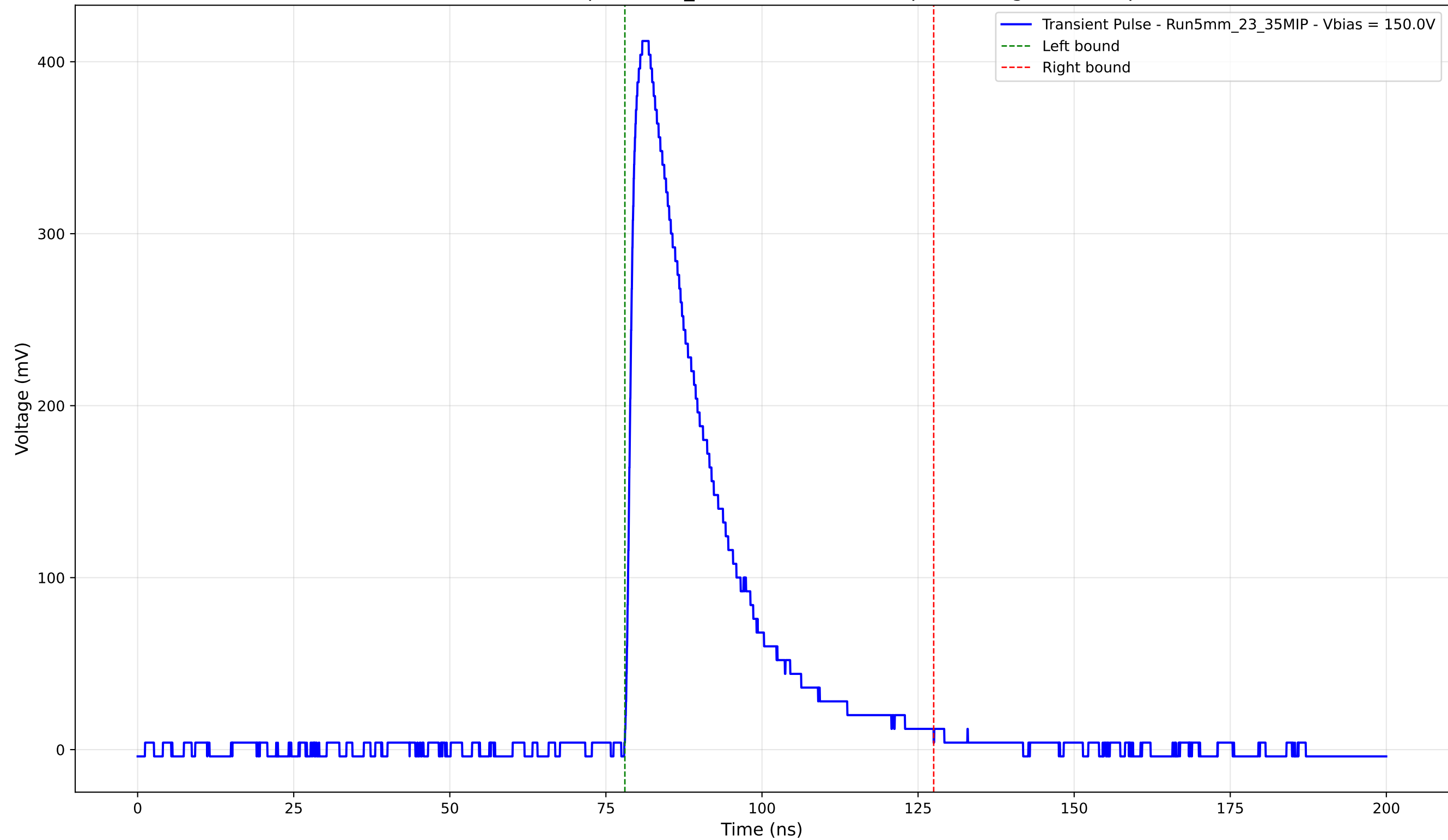
Transient Pulse - Sample: 5mm_23 - Position: 2720.0 \mu\text{m} - Charge: 111.75 pC
