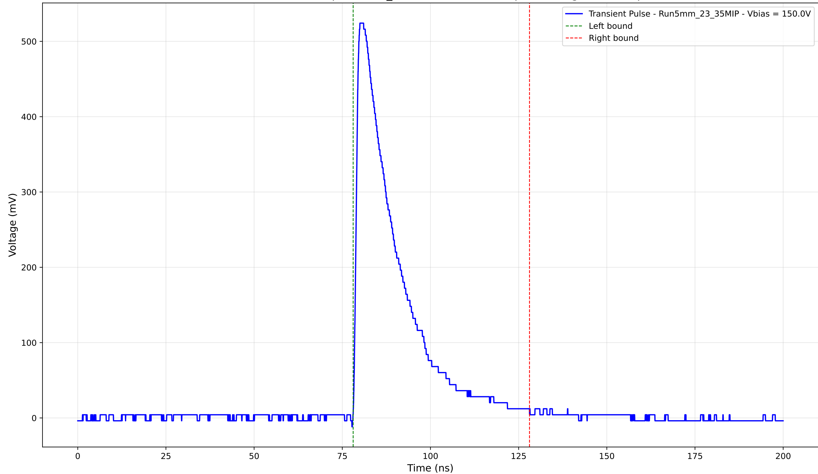
Transient Pulse - Sample: 5mm_23 - Position: 1760.0 \mu\text{m} - Charge: 134.54 pC
