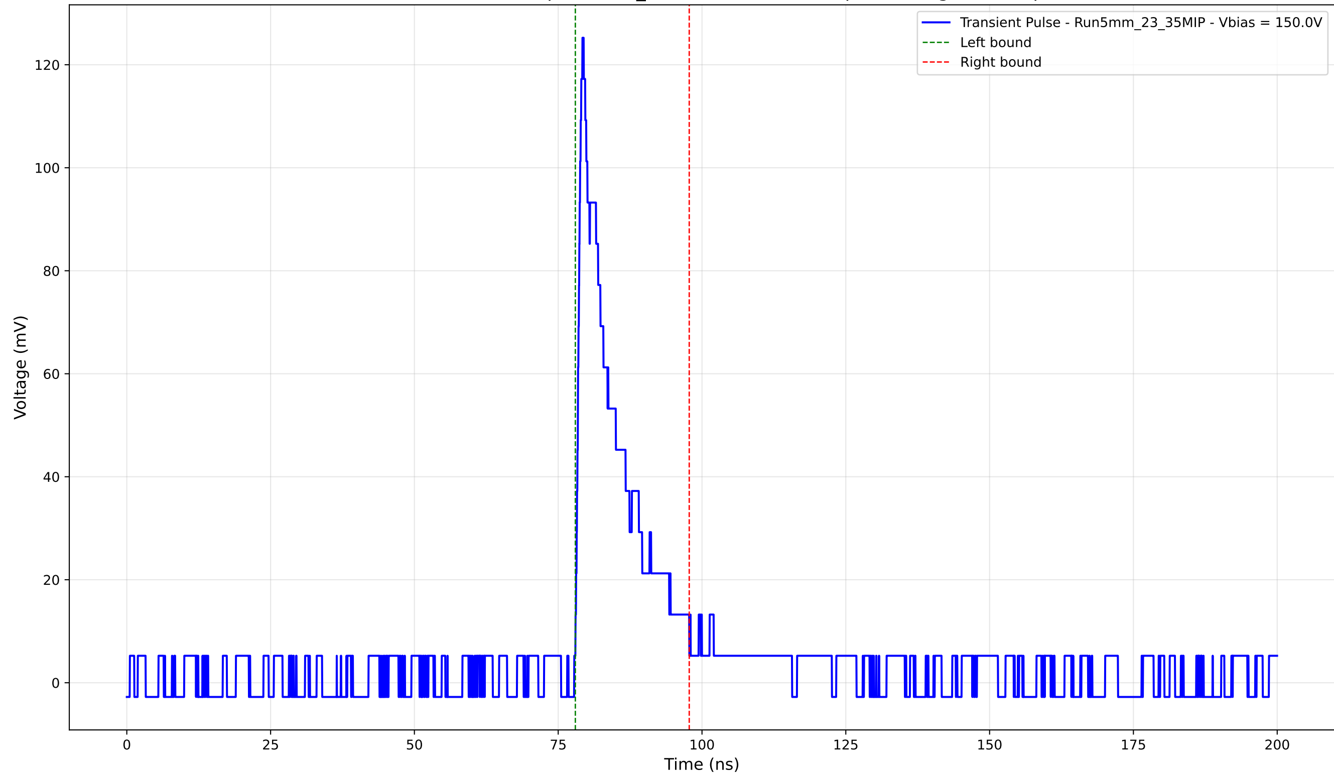
Transient Pulse - Sample: 5mm_23 - Position: 4665.0 \mu\text{m} - Charge: 17.38 pC
