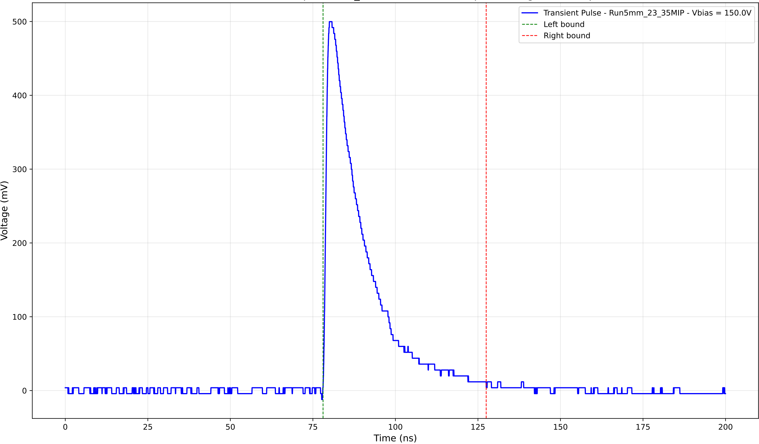
Transient Pulse - Sample: 5mm_23 - Position: 1720.0 \mu\text{m} - Charge: 126.08 pC
