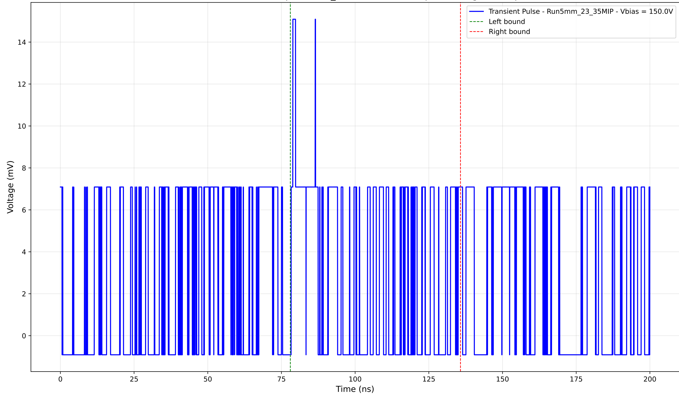
Transient Pulse - Sample: 5mm_23 - Position: 70.0 \mu\text{m} - Charge: 3.63 pC
