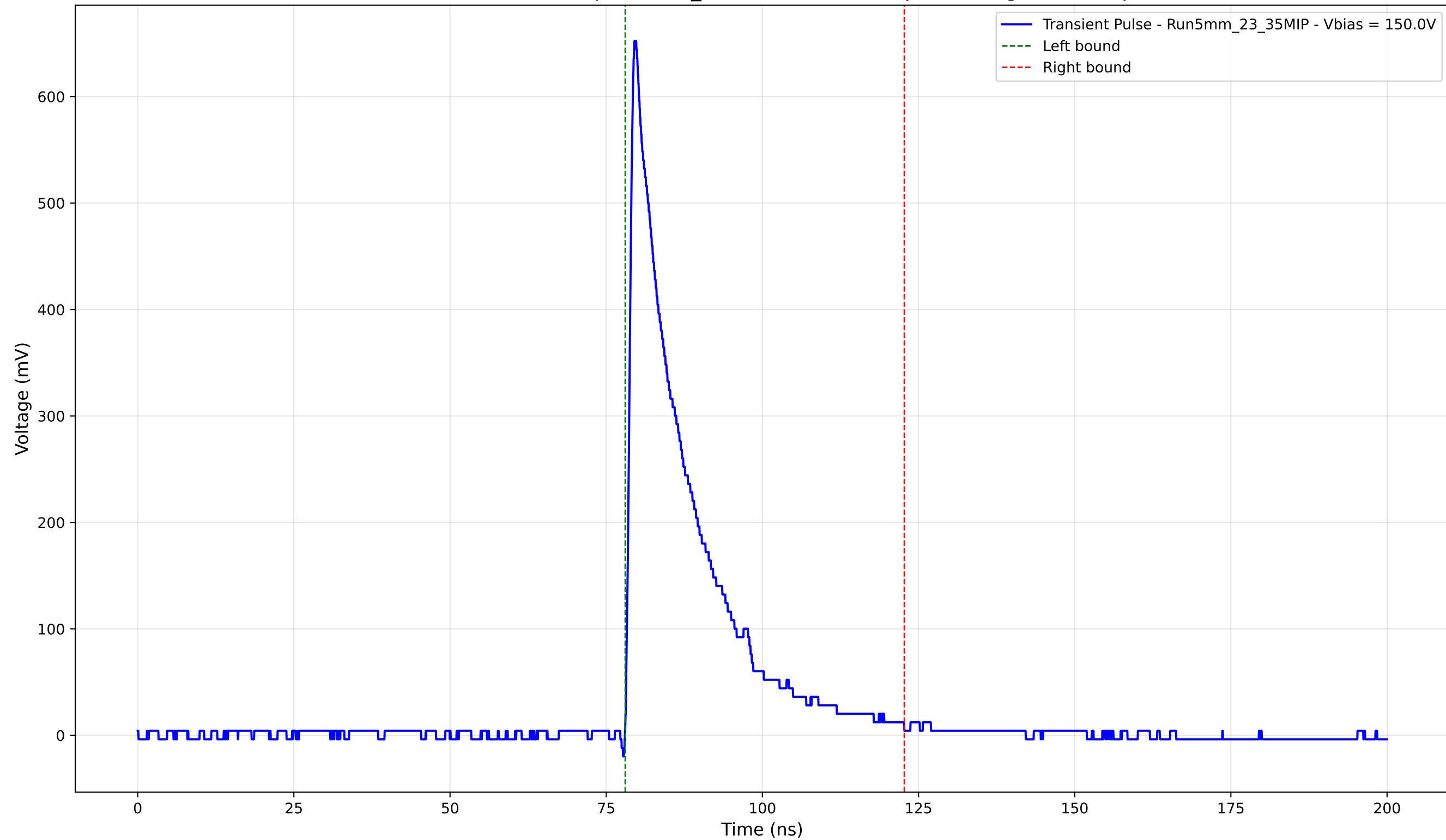
Transient Pulse - Sample: 5mm_23 - Position: 965.0 \mu\text{m} - Charge: 124.42 pC
