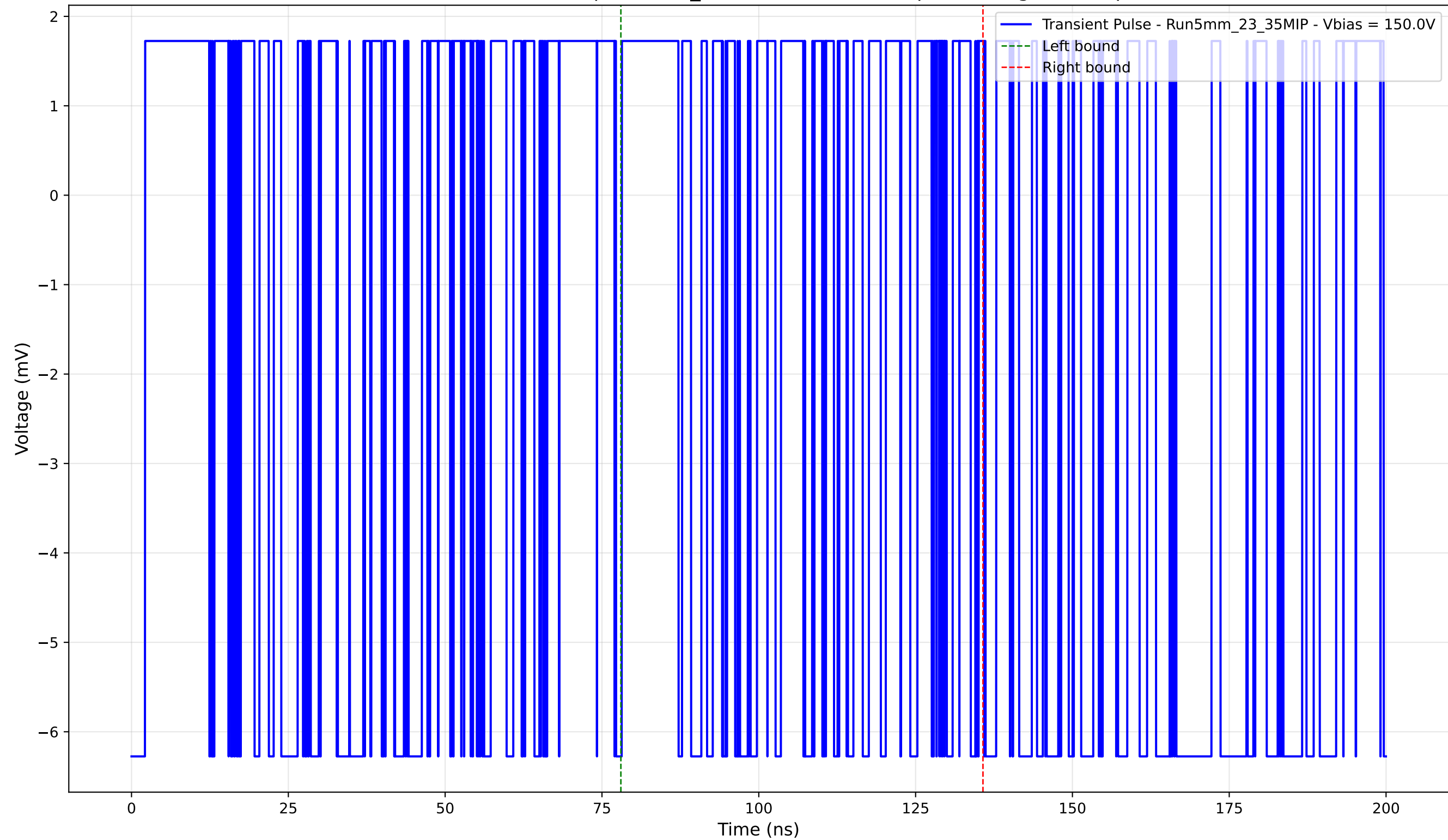
Transient Pulse - Sample: 5mm_23 - Position: 5230.0 \mu\text{m} - Charge: -0.75 pC
