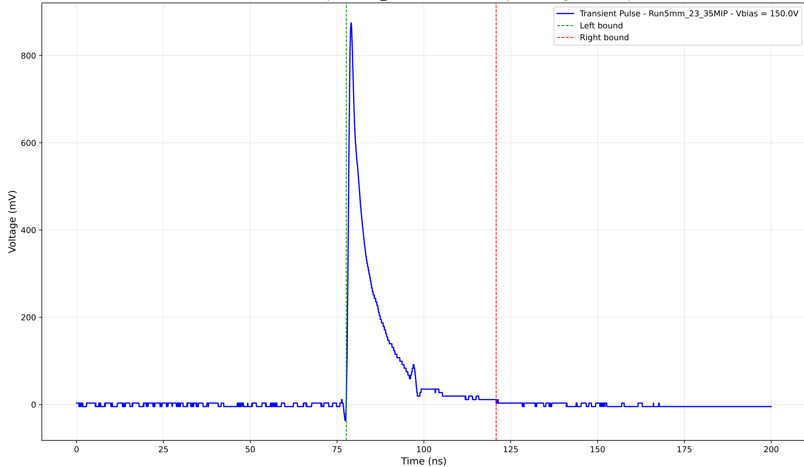
Transient Pulse - Sample: 5mm_23 - Position: 4920.0 \mu\text{m} - Charge: 114.95 pC
