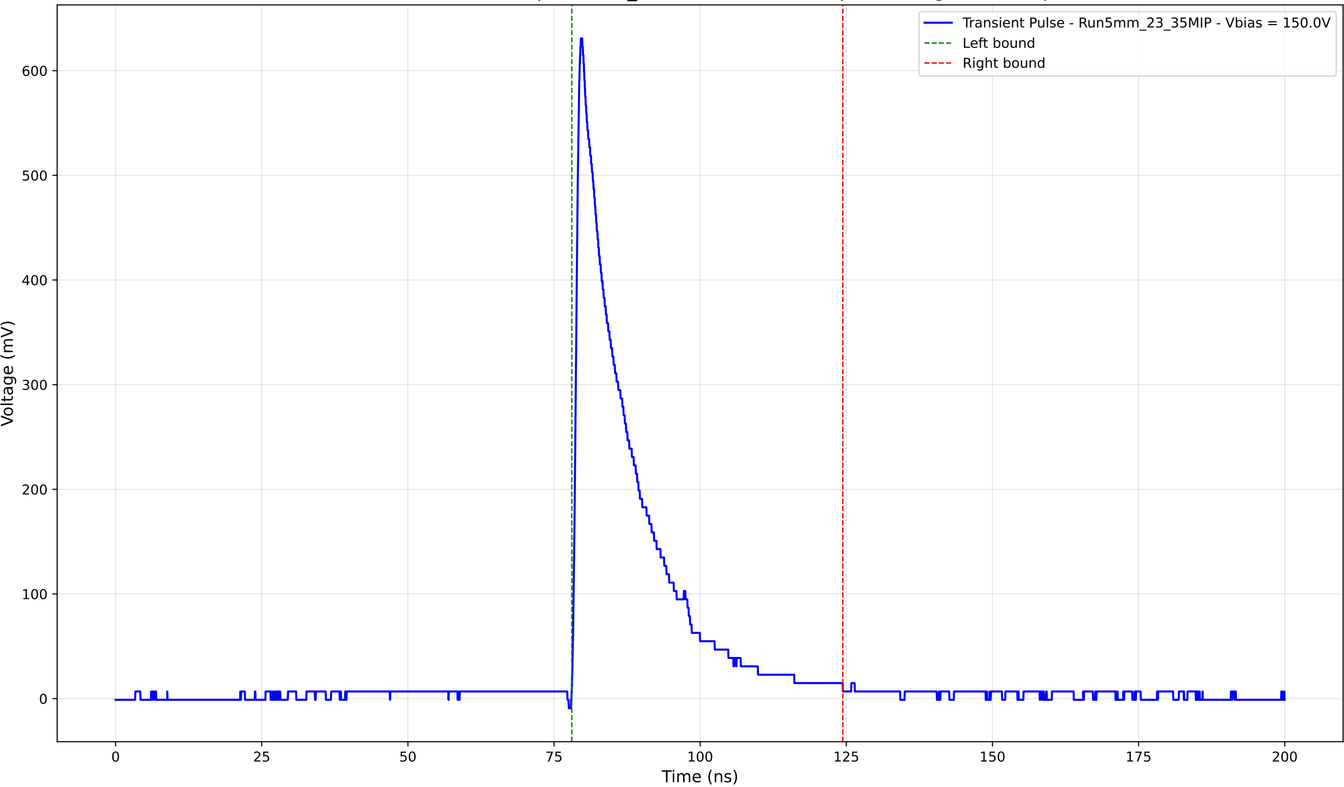
Transient Pulse - Sample: 5mm_23 - Position: 1025.0 \mu\text{m} - Charge: 123.35 pC
