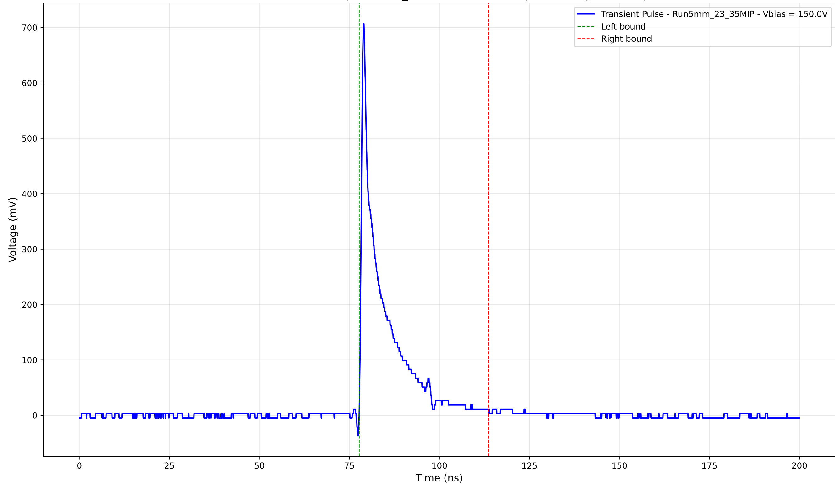
Transient Pulse - Sample: 5mm_23 - Position: 230.0 \mu\text{m} - Charge: 79.81 pC
