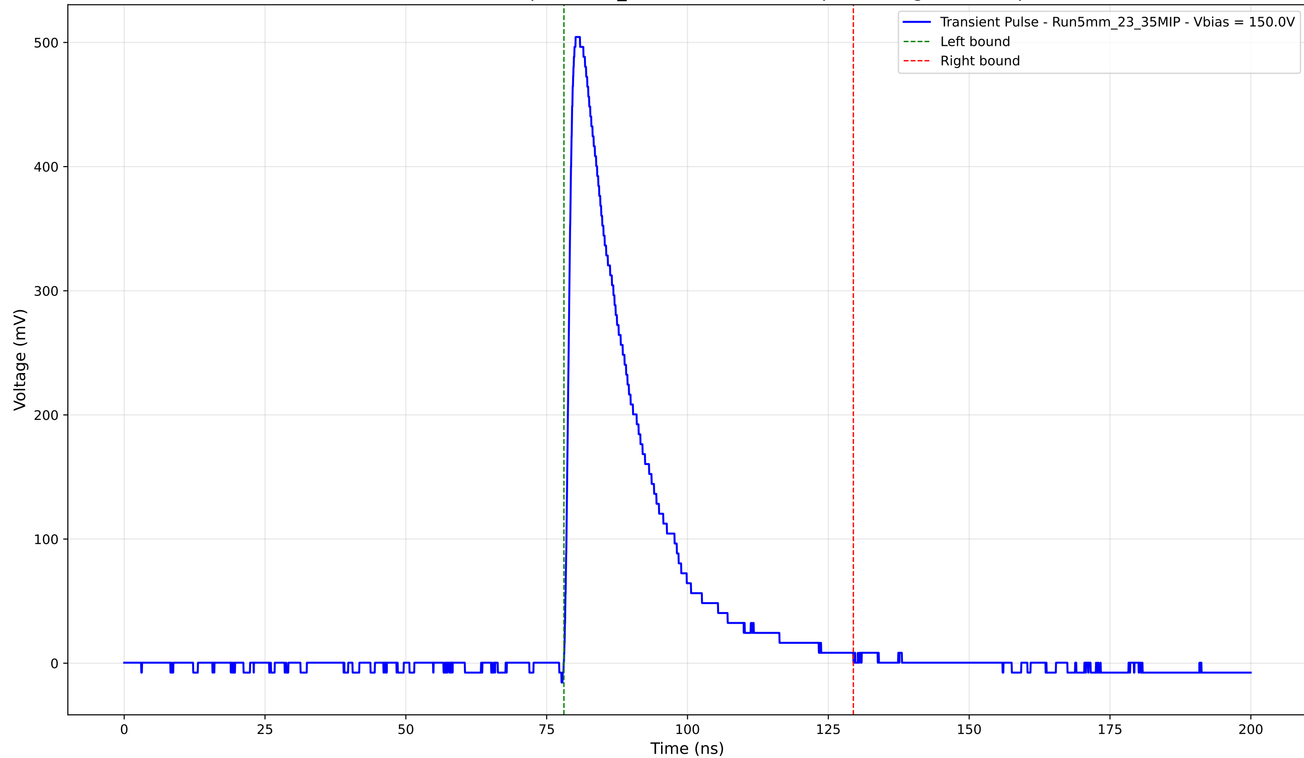
Transient Pulse - Sample: 5mm_23 - Position: 3480.0 \mu\text{m} - Charge: 125.19 pC
