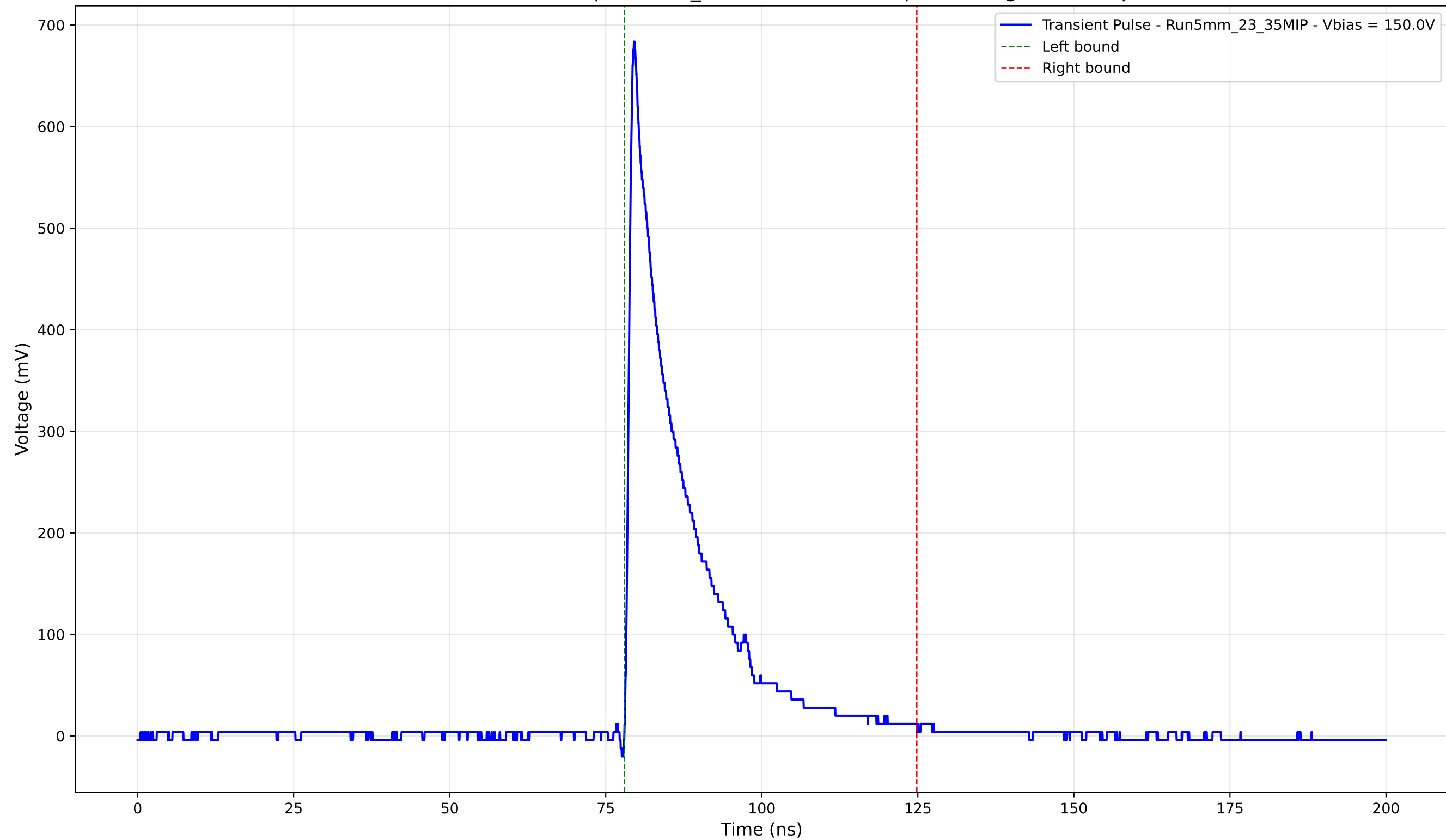
Transient Pulse - Sample: 5mm_23 - Position: 860.0 \mu\text{m} - Charge: 123.48 pC
