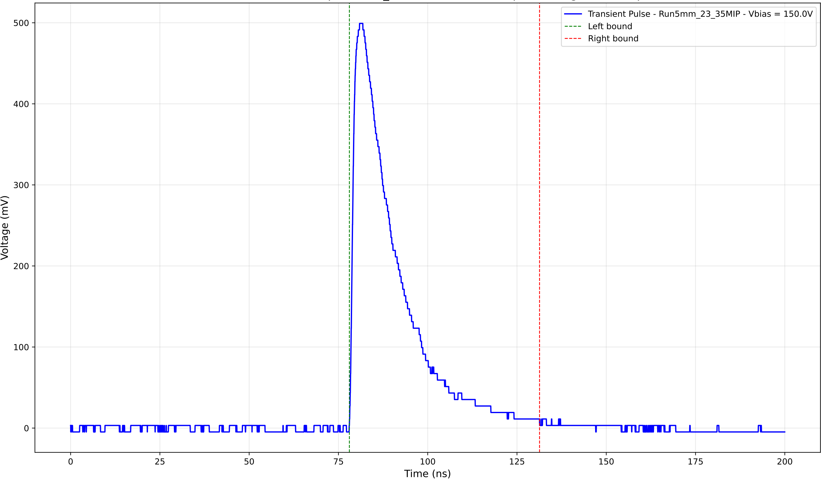
Transient Pulse - Sample: 5mm_23 - Position: 2800.0 \mu\text{m} - Charge: 135.80 pC
