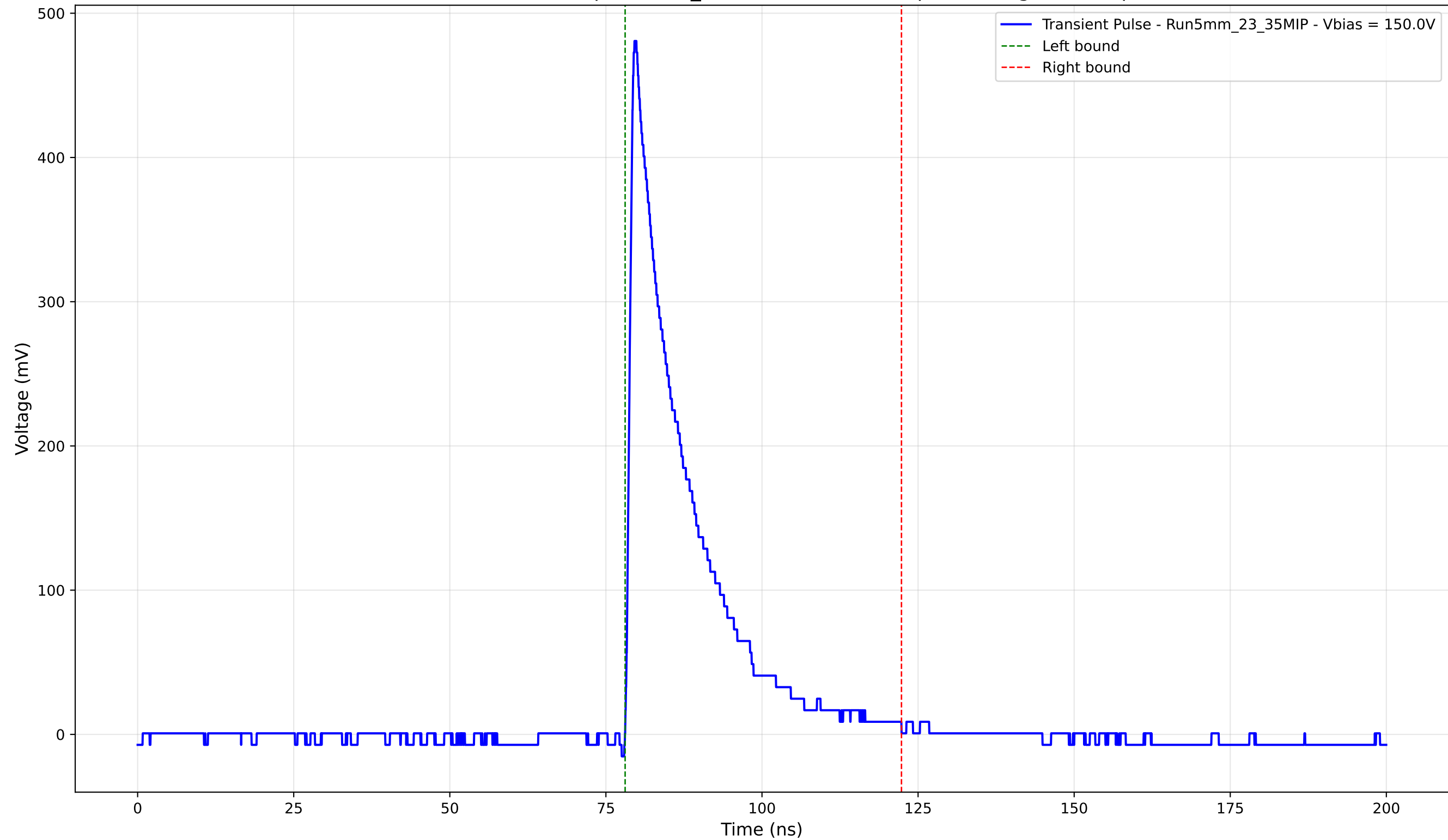
Transient Pulse - Sample: 5mm_23 - Position: 1060.0 \mu\text{m} - Charge: 90.37 pC
