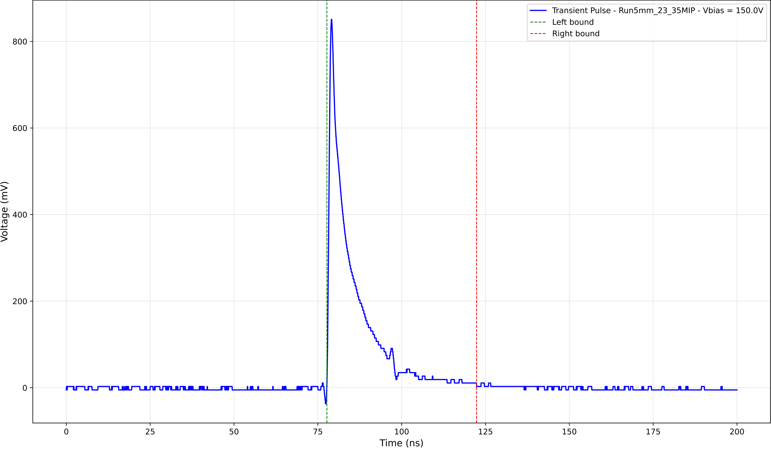
Transient Pulse - Sample: 5mm_23 - Position: 4875.0 \mu\text{m} - Charge: 114.94 pC
