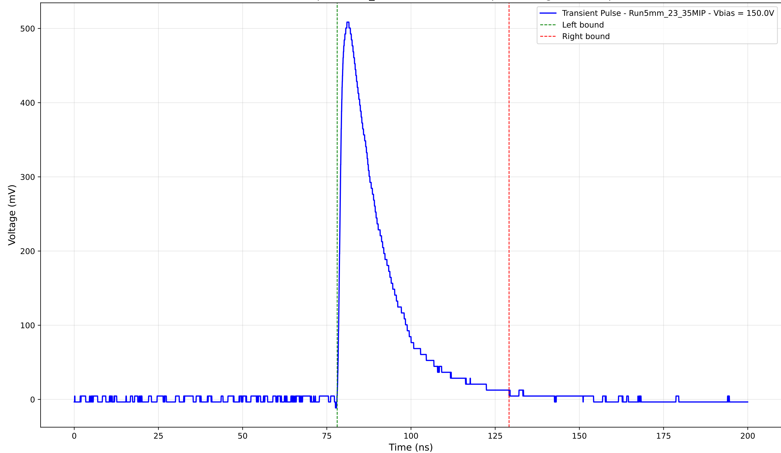
Transient Pulse - Sample: 5mm_23 - Position: 2505.0 \mu\text{m} - Charge: 137.72 pC
