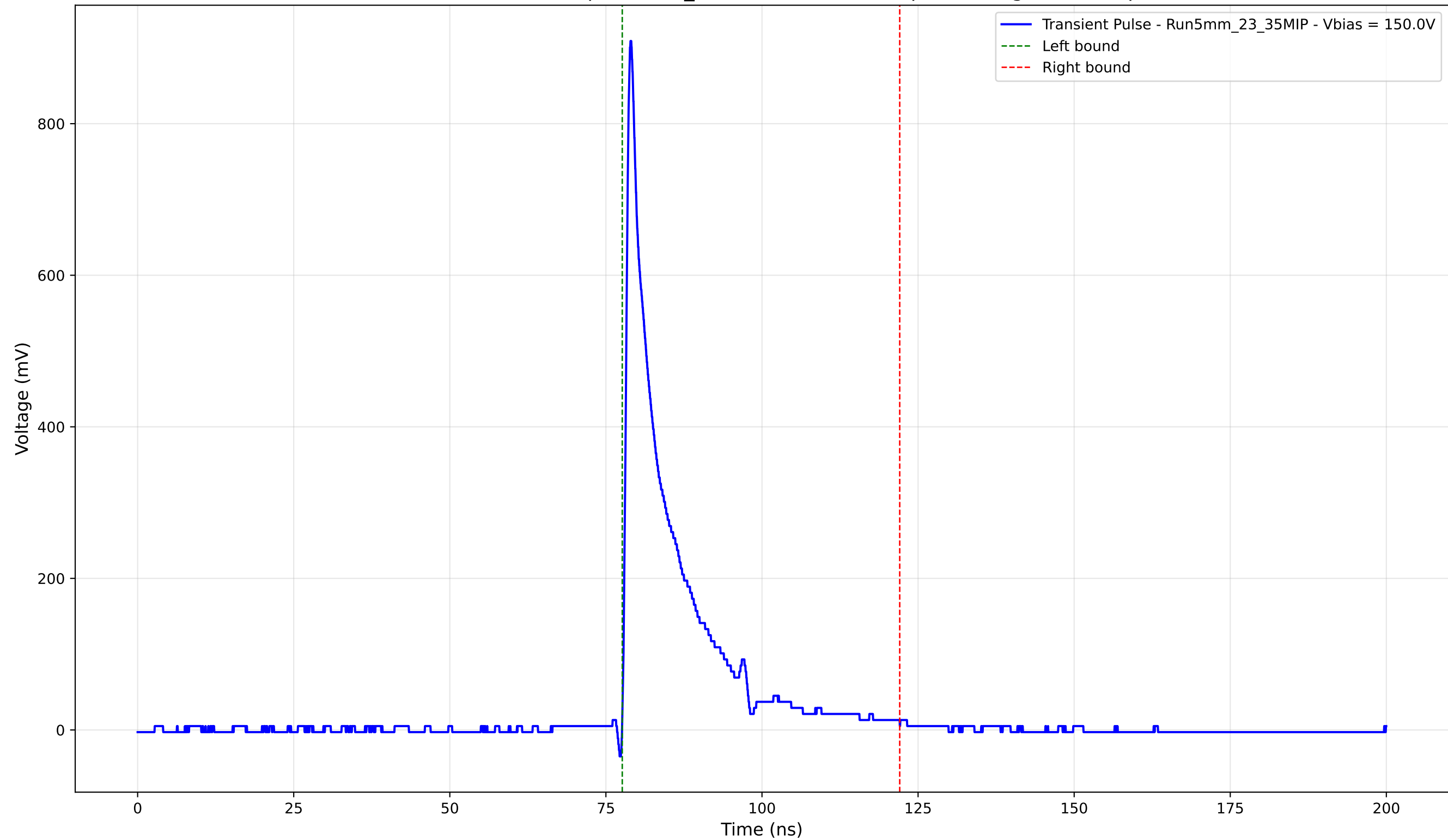
Transient Pulse - Sample: 5mm_23 - Position: 4975.0 \mu\text{m} - Charge: 121.07 pC
