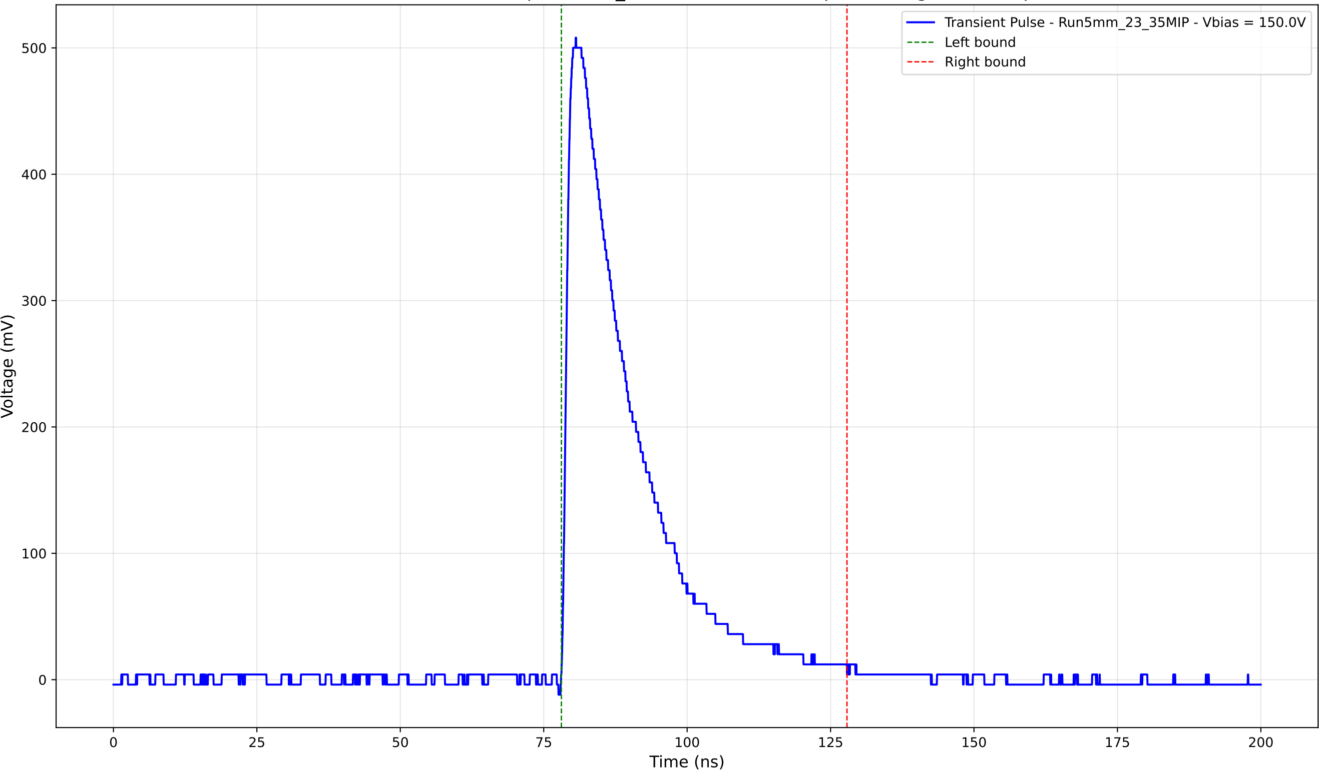
Transient Pulse - Sample: 5mm_23 - Position: 3345.0 \mu\text{m} - Charge: 129.32 pC
