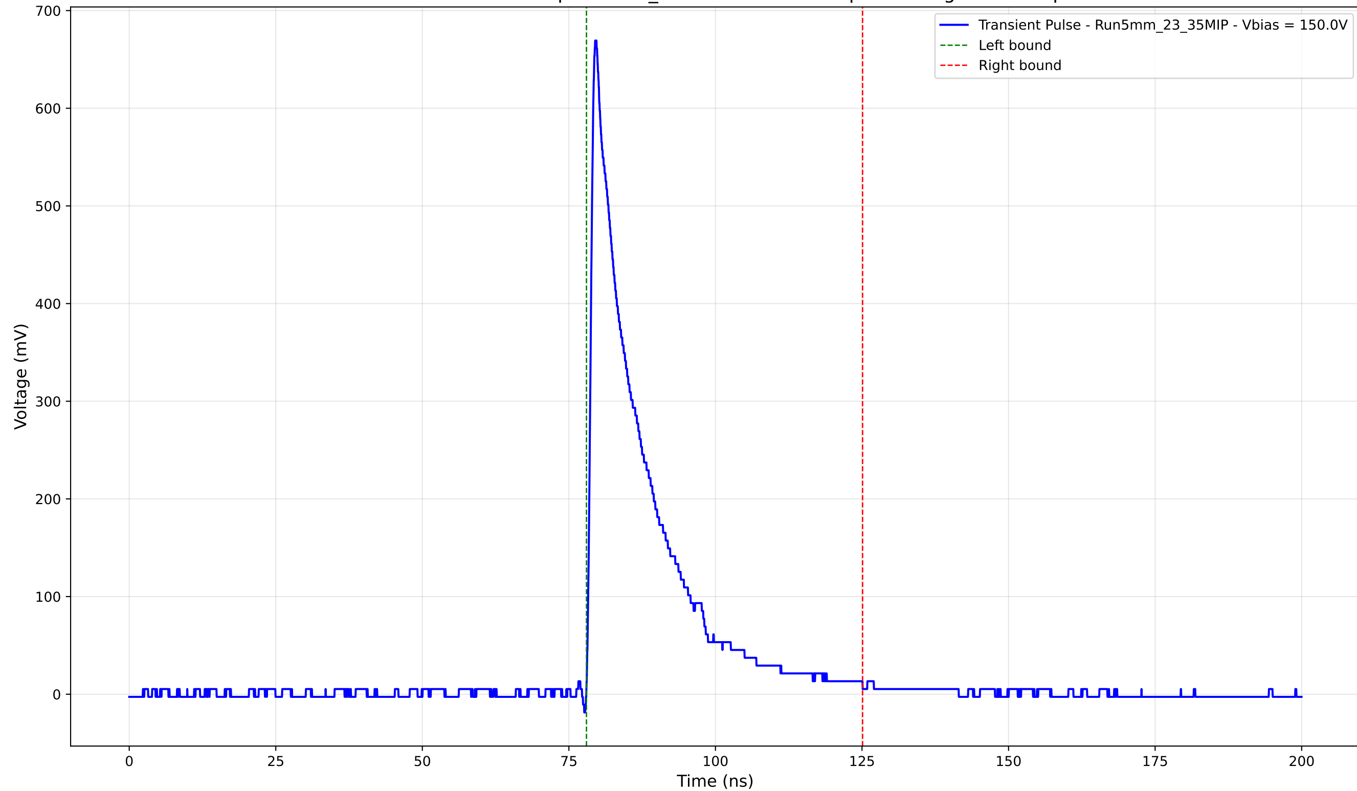
Transient Pulse - Sample: 5mm_23 - Position: 890.0 \mu\text{m} - Charge: 124.43 pC
