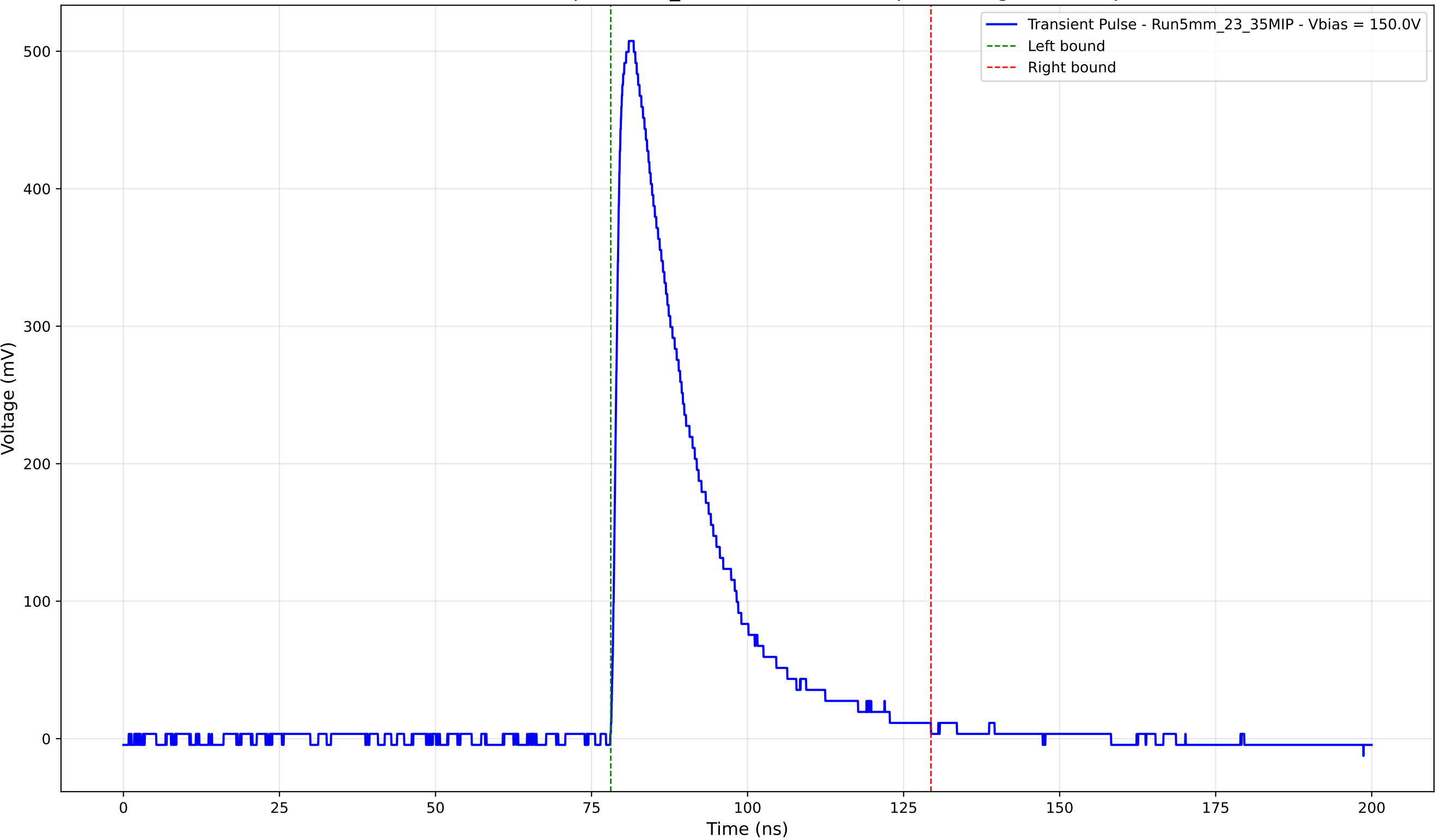
Transient Pulse - Sample: 5mm_23 - Position: 2320.0 \mu\text{m} - Charge: 136.96 pC
