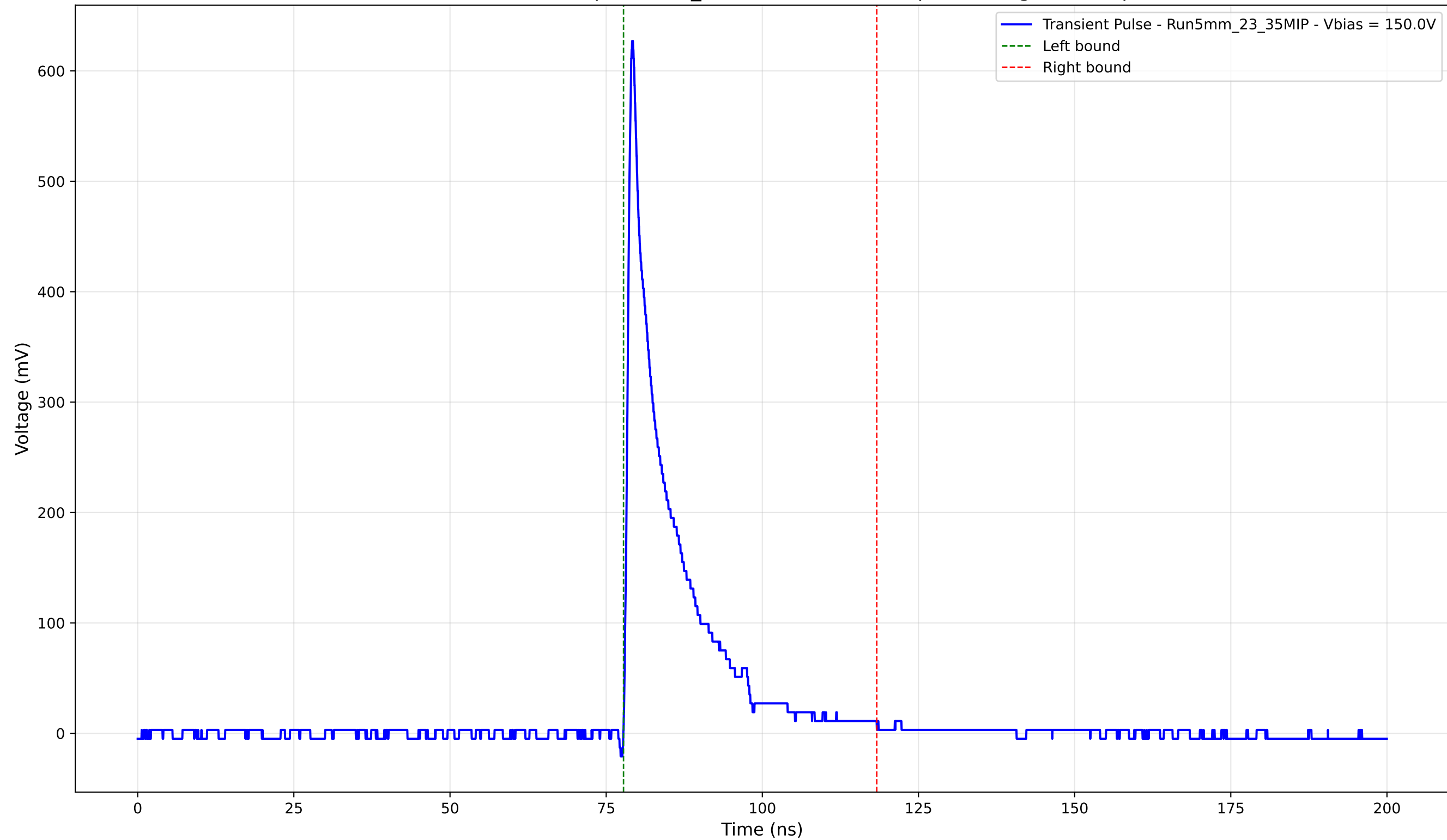
Transient Pulse - Sample: 5mm_23 - Position: 4730.0 \mu\text{m} - Charge: 84.57 pC
