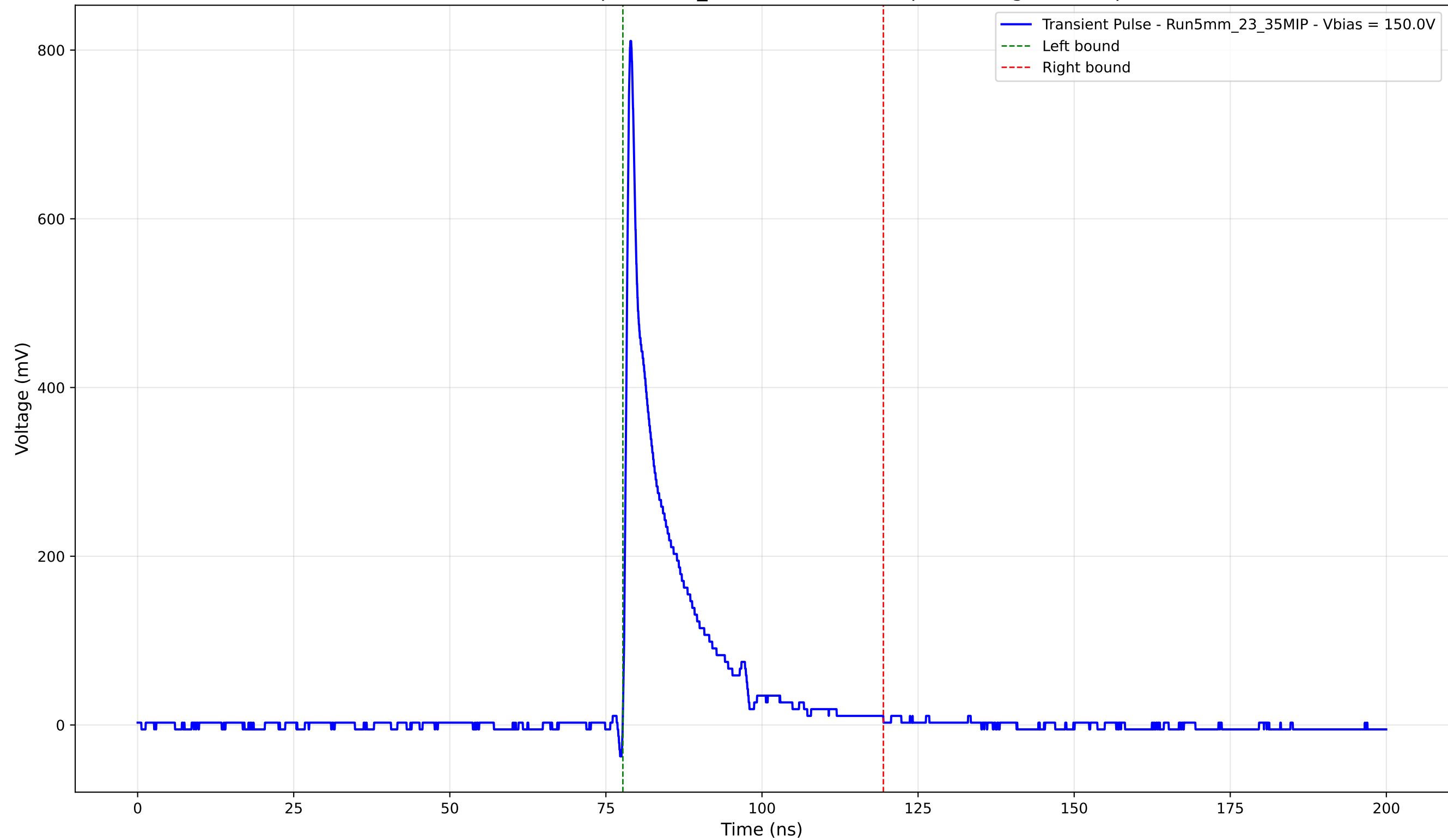
Transient Pulse - Sample: 5mm_23 - Position: 245.0 \mu\text{m} - Charge: 97.19 pC
