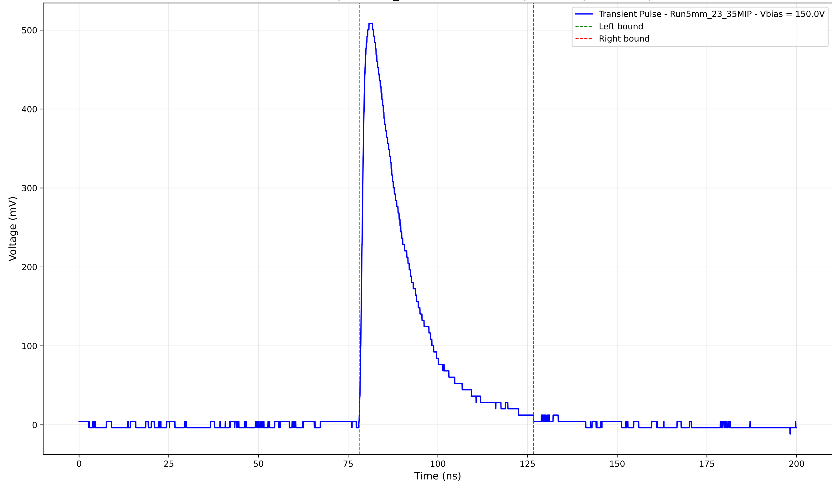
Transient Pulse - Sample: 5mm_23 - Position: 2345.0 \mu\text{m} - Charge: 138.05 pC
