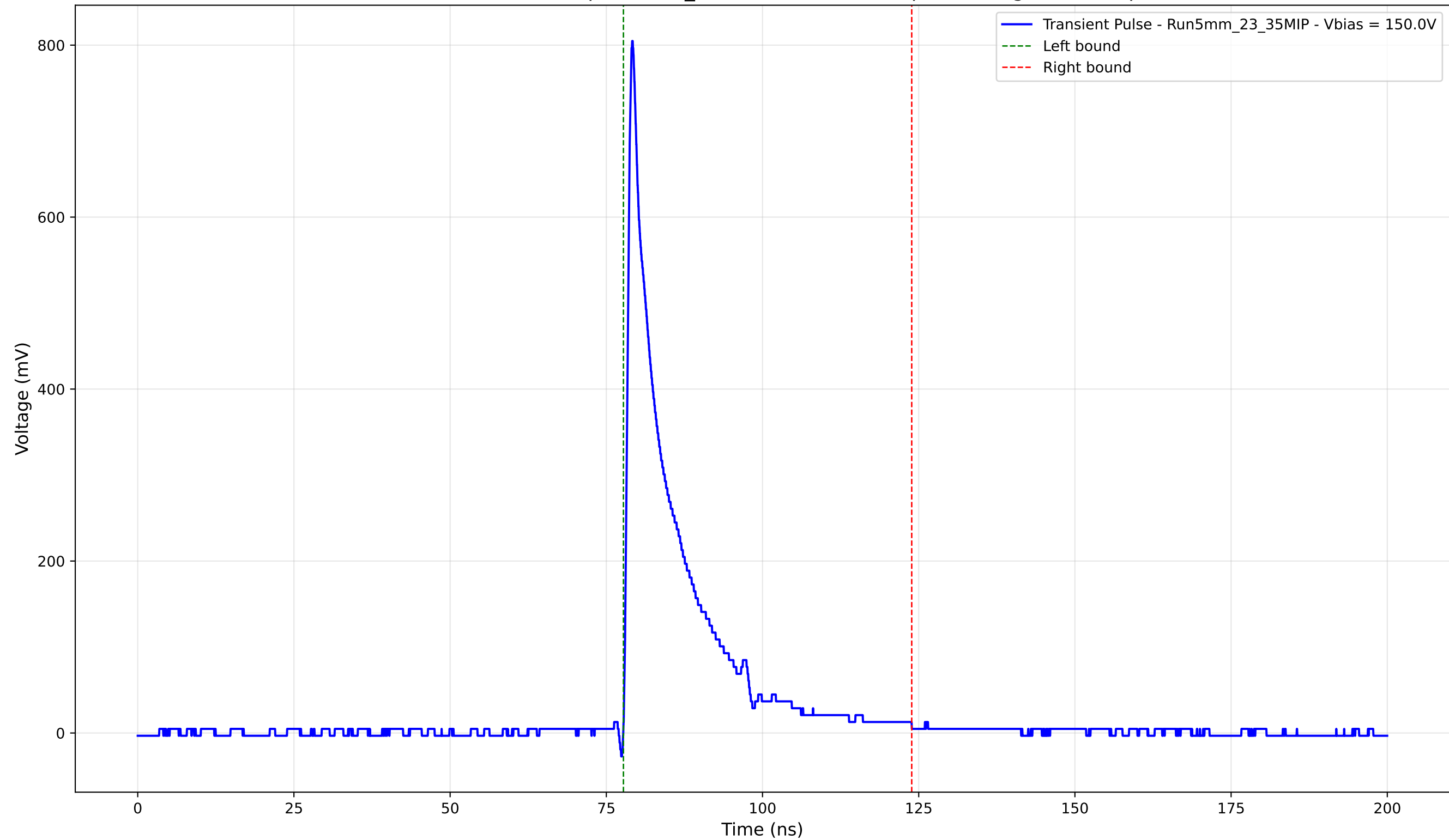
Transient Pulse - Sample: 5mm_23 - Position: 4785.0 \mu\text{m} - Charge: 114.82 pC
