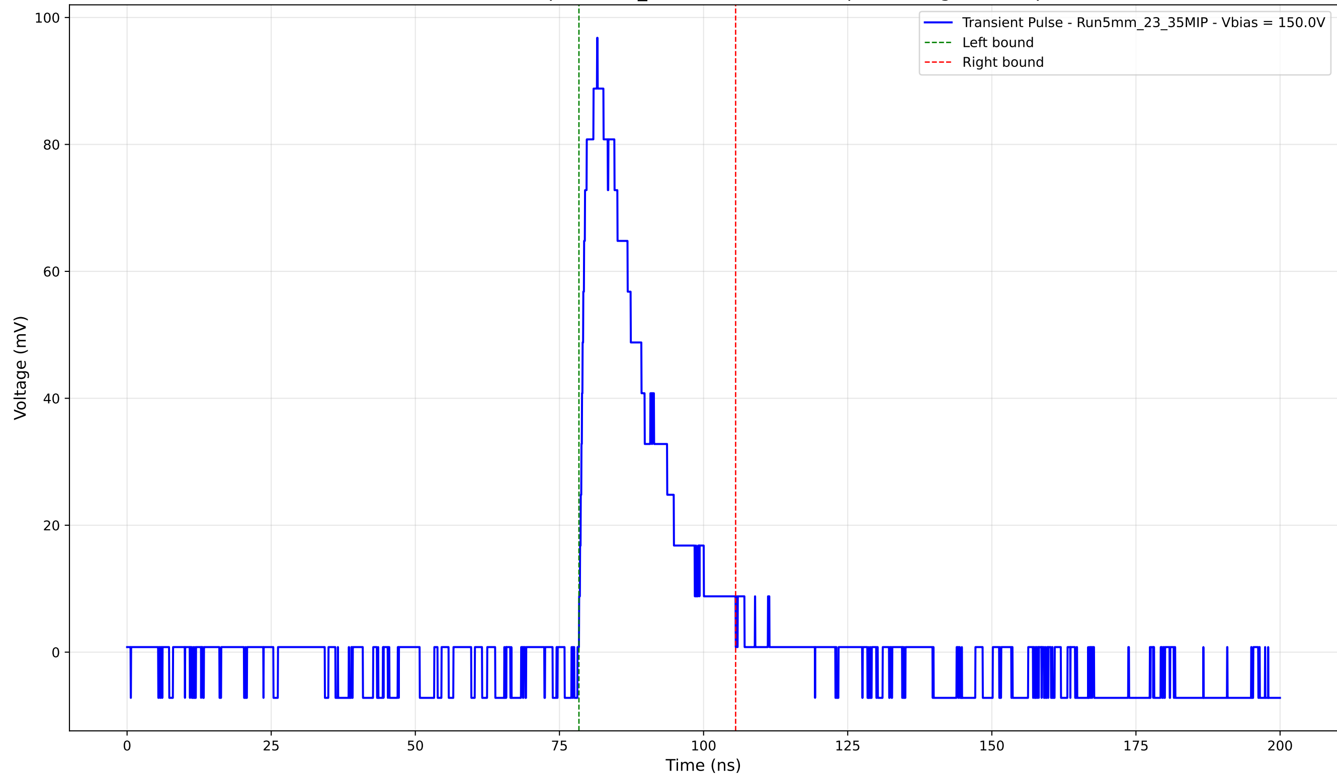
Transient Pulse - Sample: 5mm_23 - Position: 2130.0 \mu\text{m} - Charge: 21.04 pC
