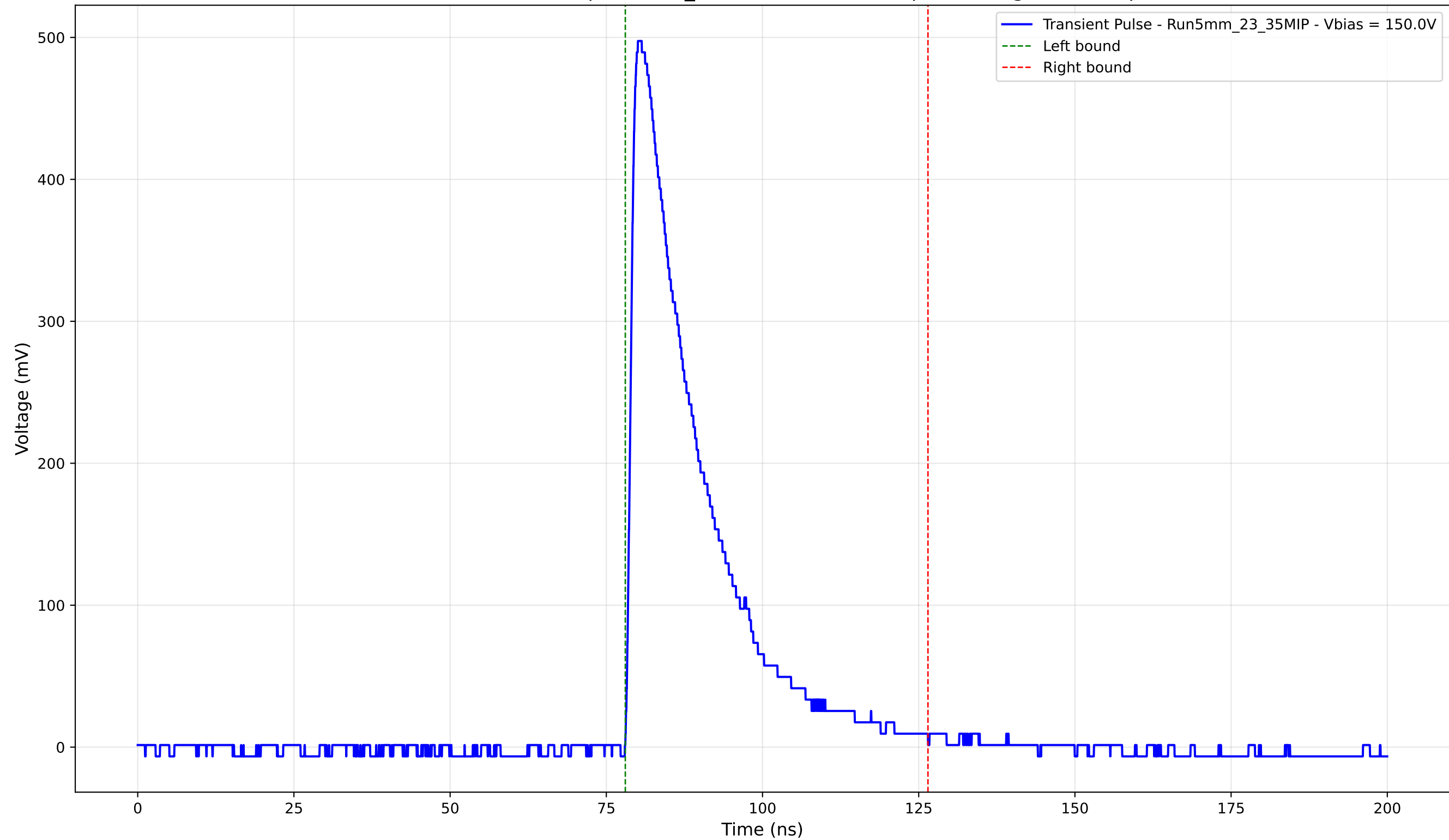
Transient Pulse - Sample: 5mm_23 - Position: 3555.0 \mu\text{m} - Charge: 120.21 pC
