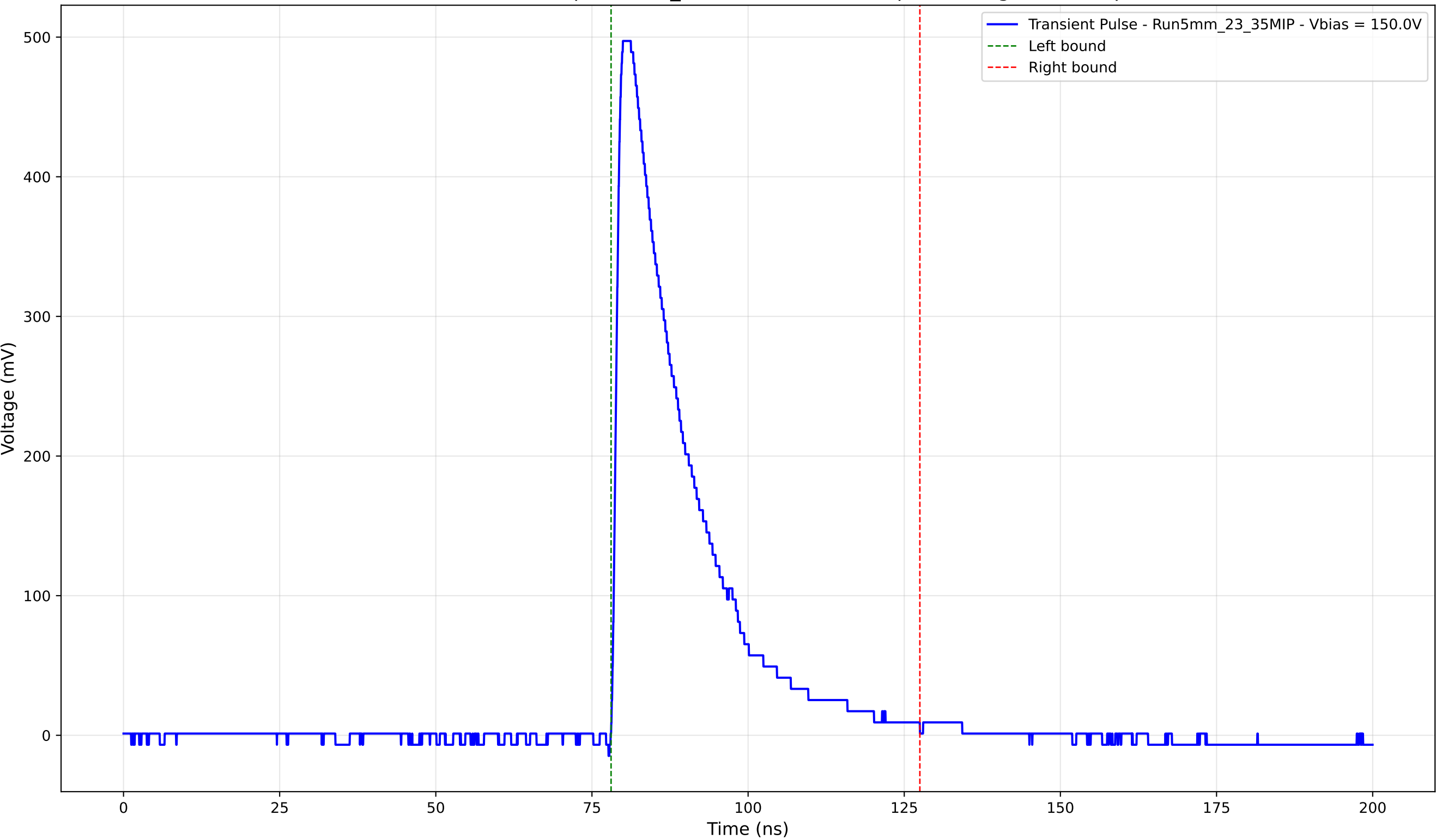
Transient Pulse - Sample: 5mm_23 - Position: 3530.0 \mu\text{m} - Charge: 122.35 pC
