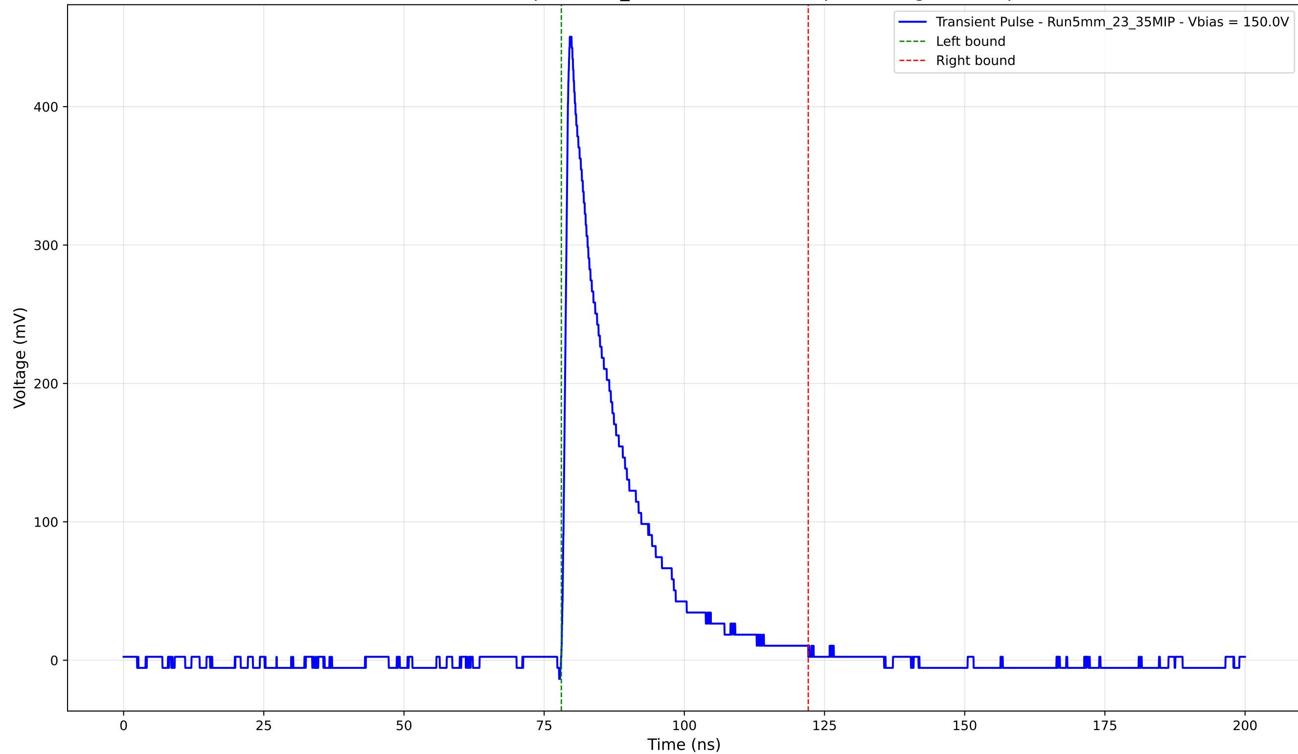
Transient Pulse - Sample: 5mm_23 - Position: 1065.0 \mu\text{m} - Charge: 85.70 pC
