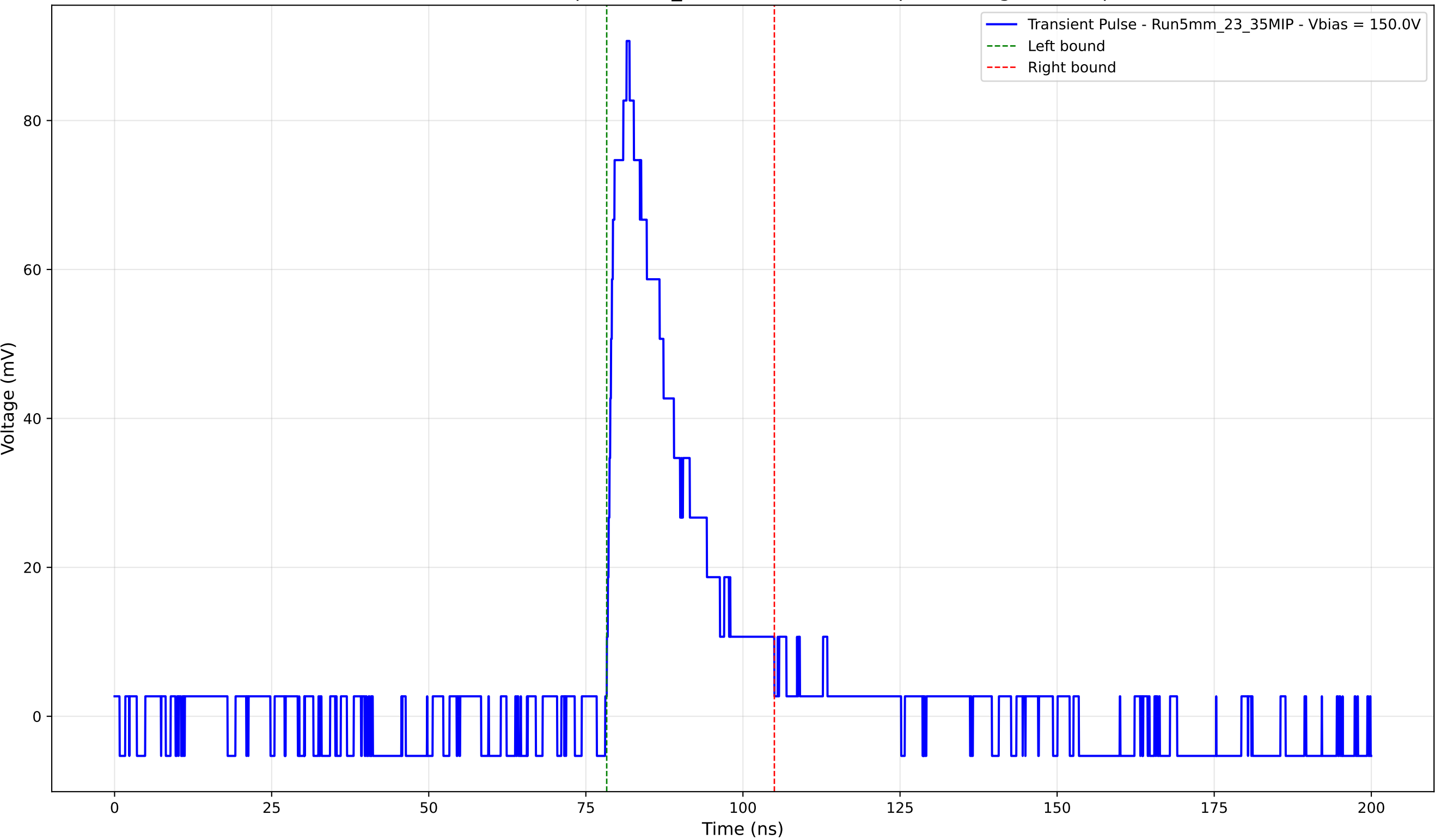
Transient Pulse - Sample: 5mm_23 - Position: 3655.0 \mu\text{m} - Charge: 19.23 pC
