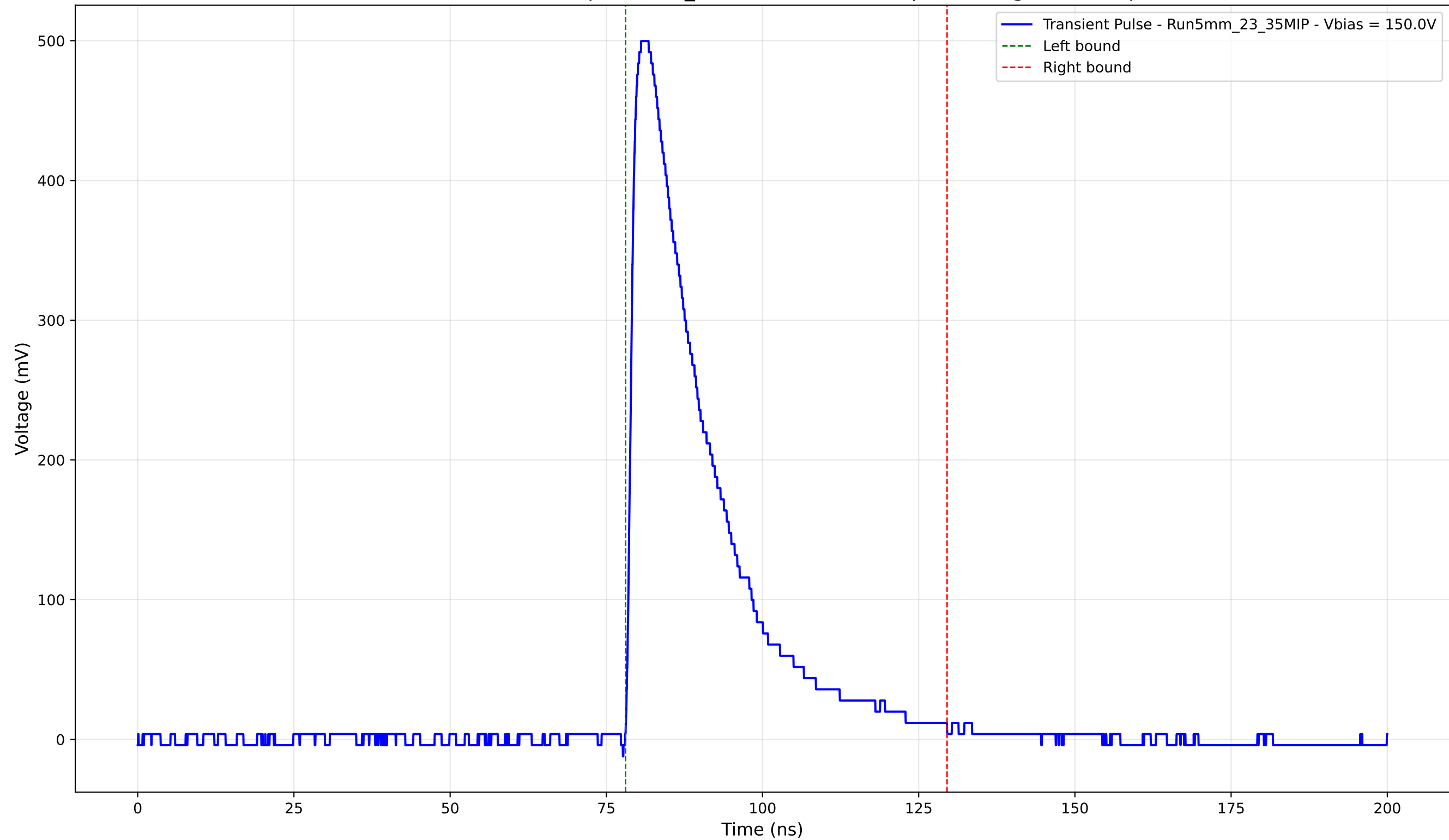
Transient Pulse - Sample: 5mm_23 - Position: 2280.0 \mu\text{m} - Charge: 136.73 pC
