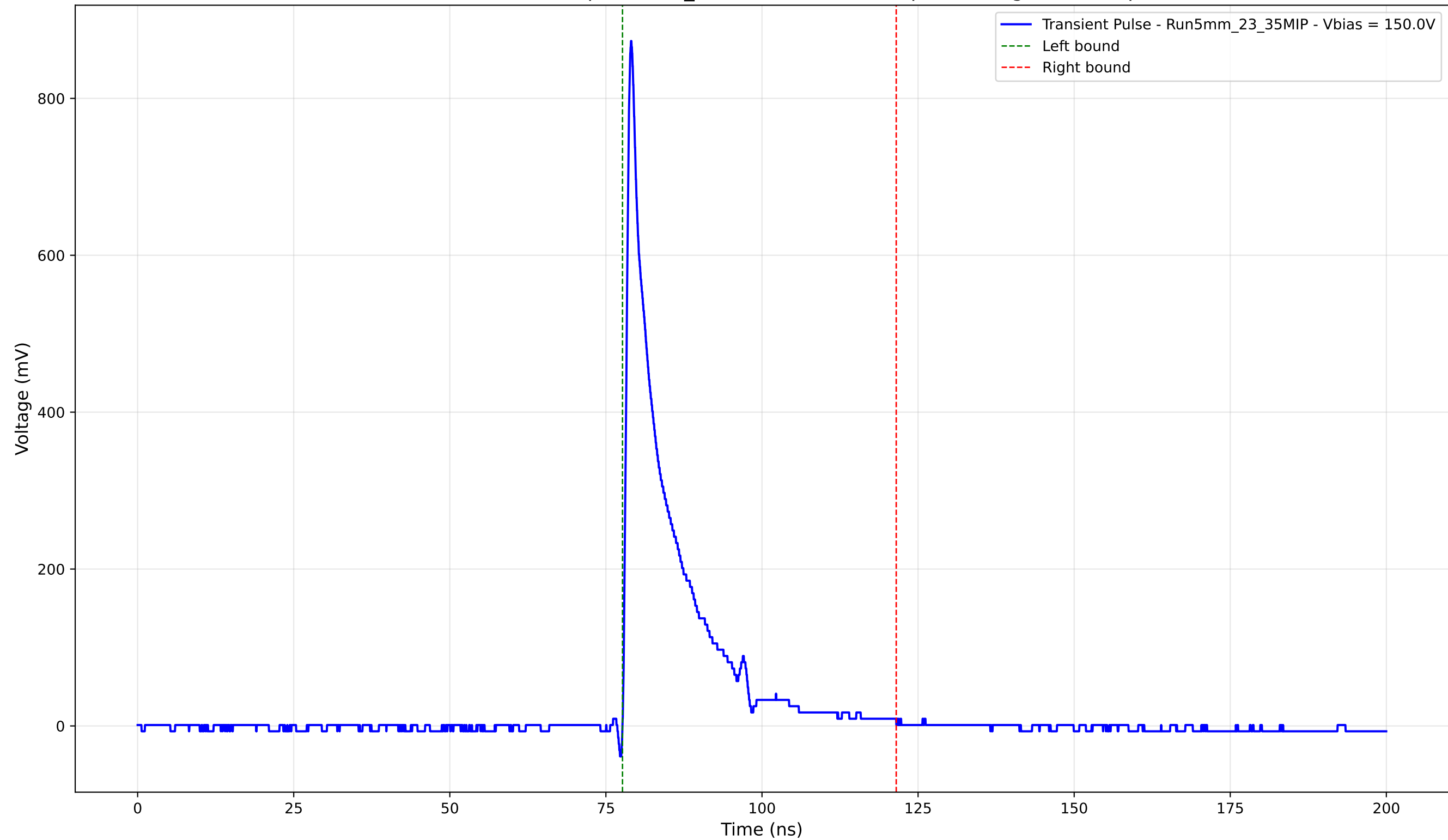
Transient Pulse - Sample: 5mm_23 - Position: 4915.0 \mu\text{m} - Charge: 114.01 pC
