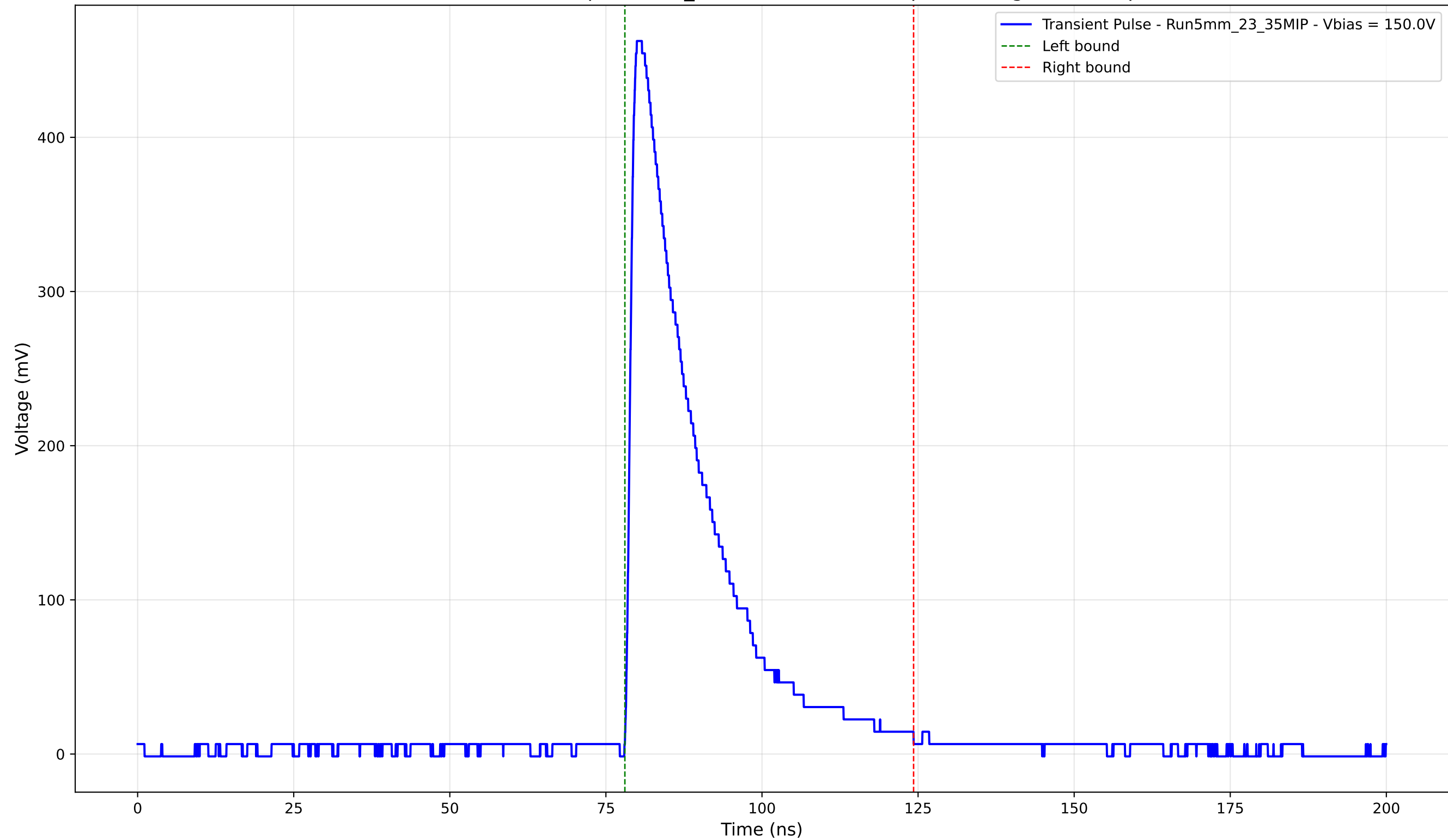
Transient Pulse - Sample: 5mm_23 - Position: 3575.0 \mu\text{m} - Charge: 112.61 pC
