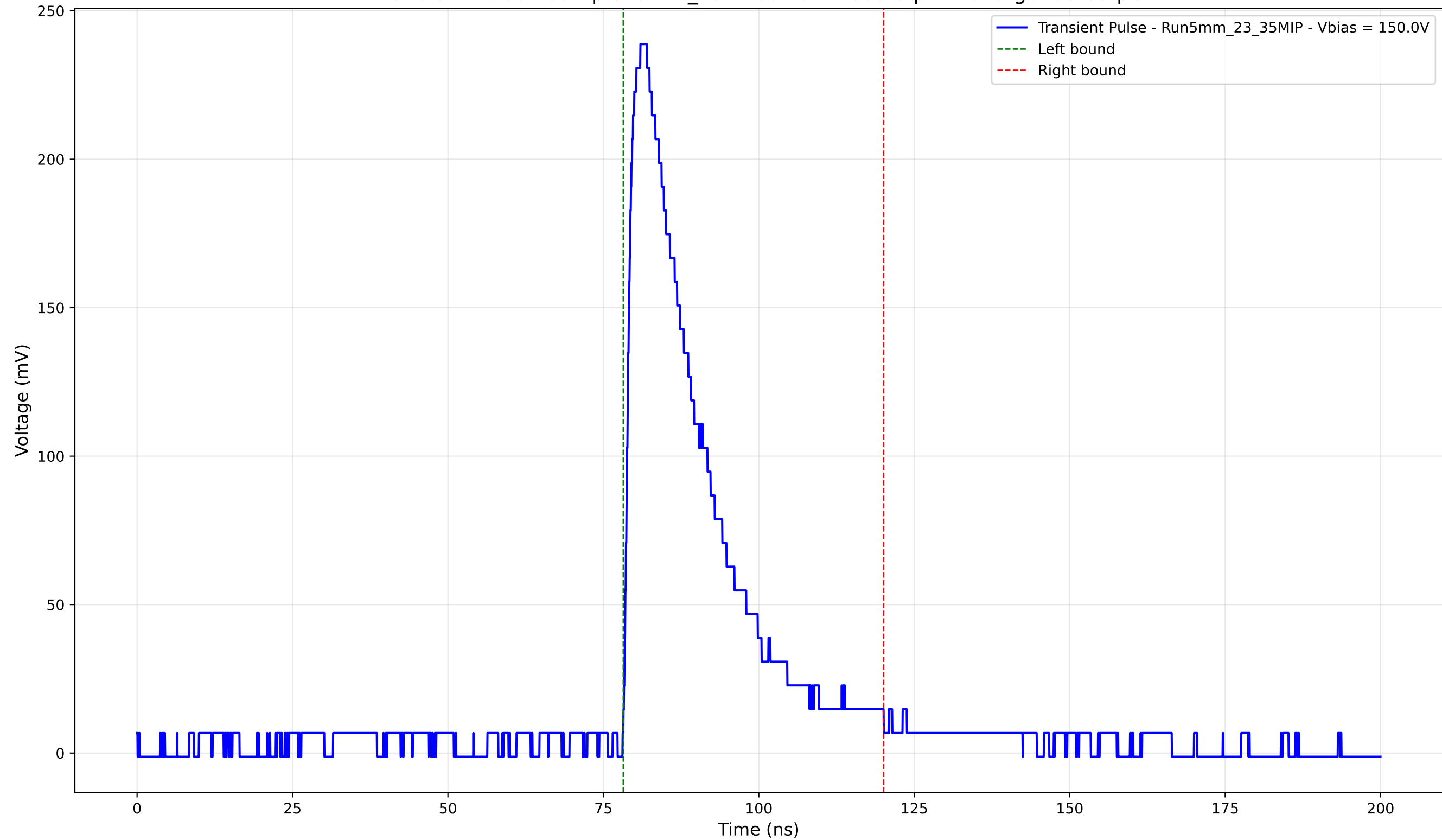
Transient Pulse - Sample: 5mm_23 - Position: 2605.0 \mu\text{m} - Charge: 63.65 pC
