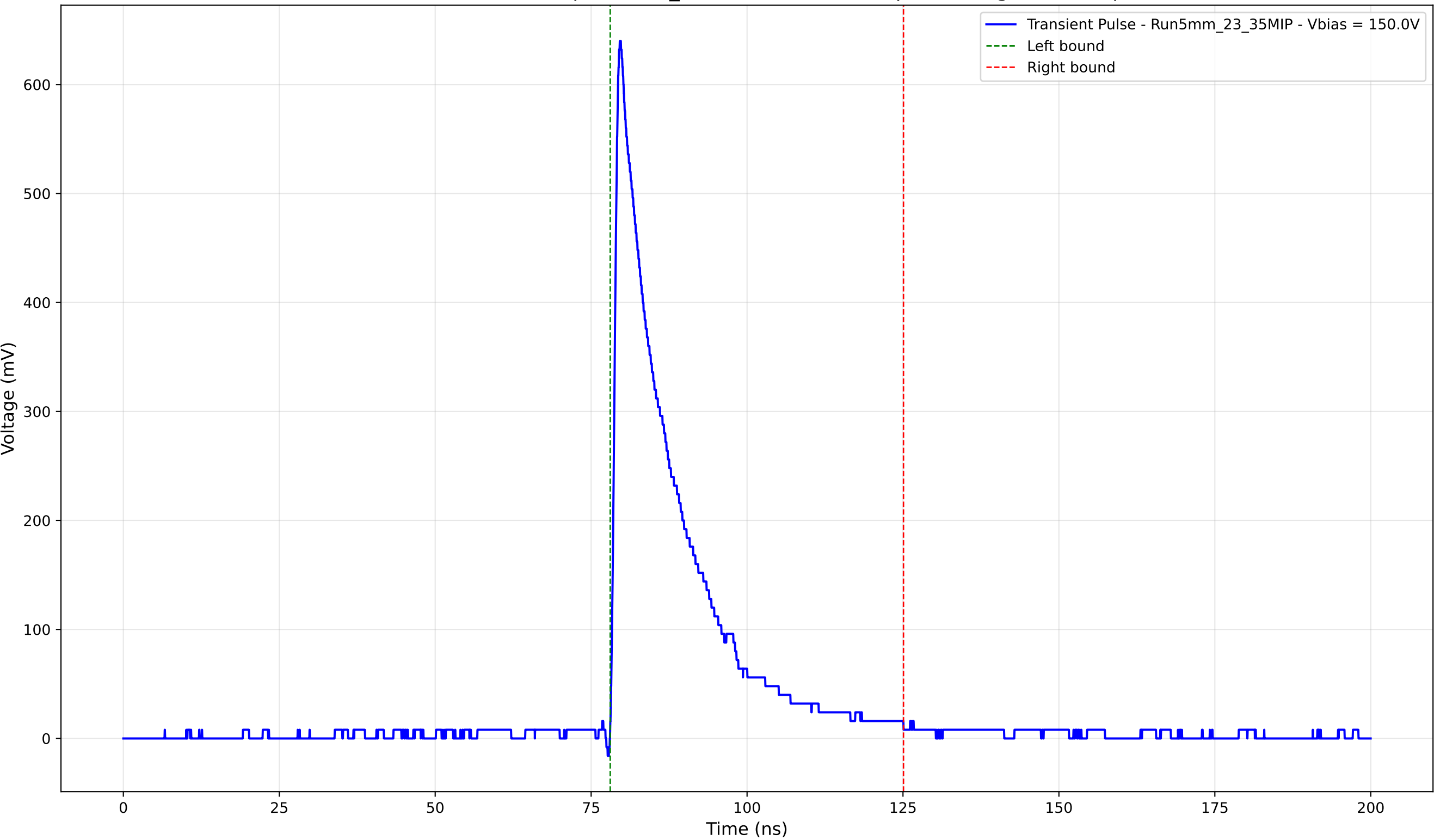
Transient Pulse - Sample: 5mm_23 - Position: 1015.0 \mu\text{m} - Charge: 126.06 pC
