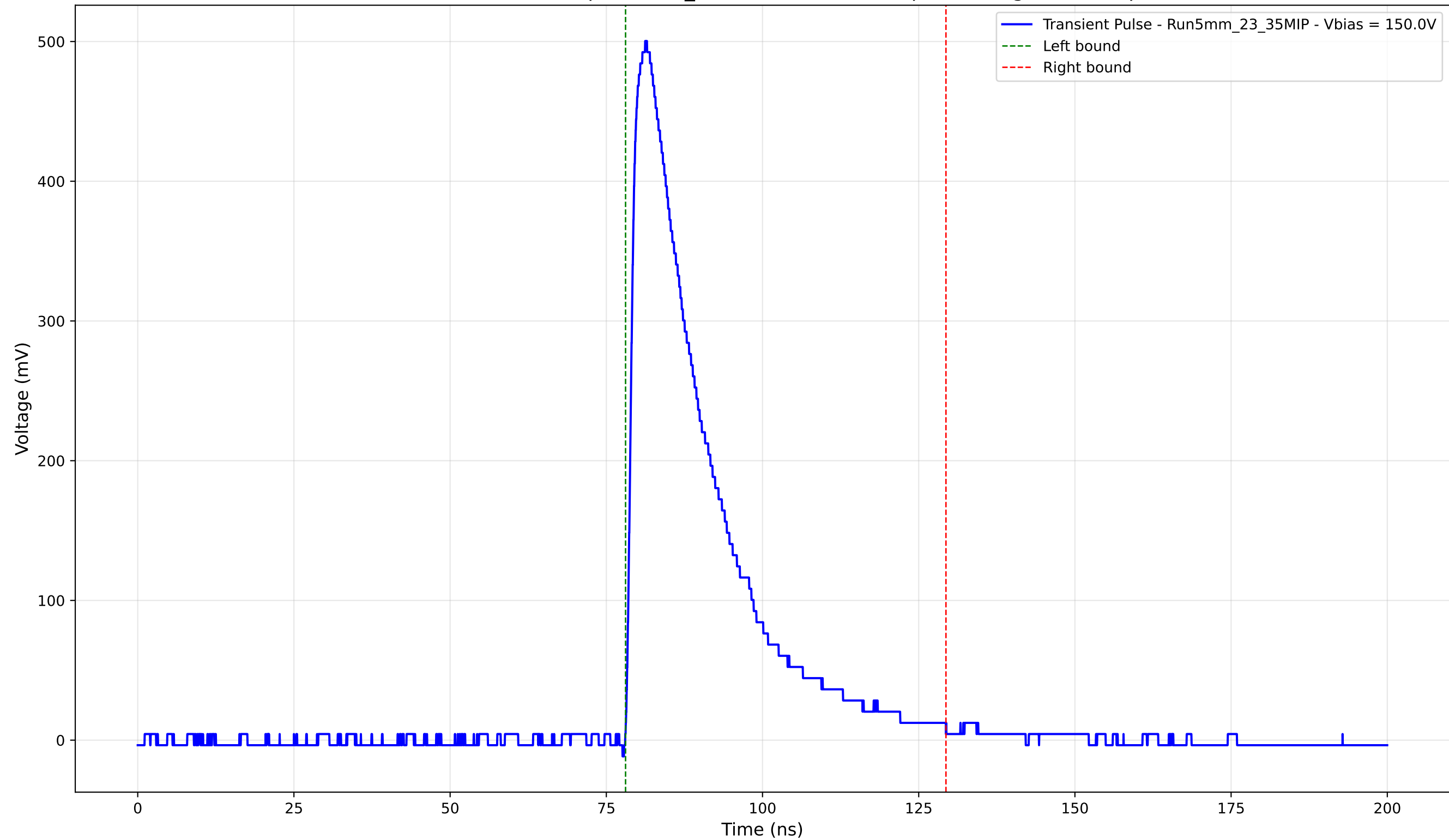
Transient Pulse - Sample: 5mm_23 - Position: 2890.0 \mu\text{m} - Charge: 134.62 pC
