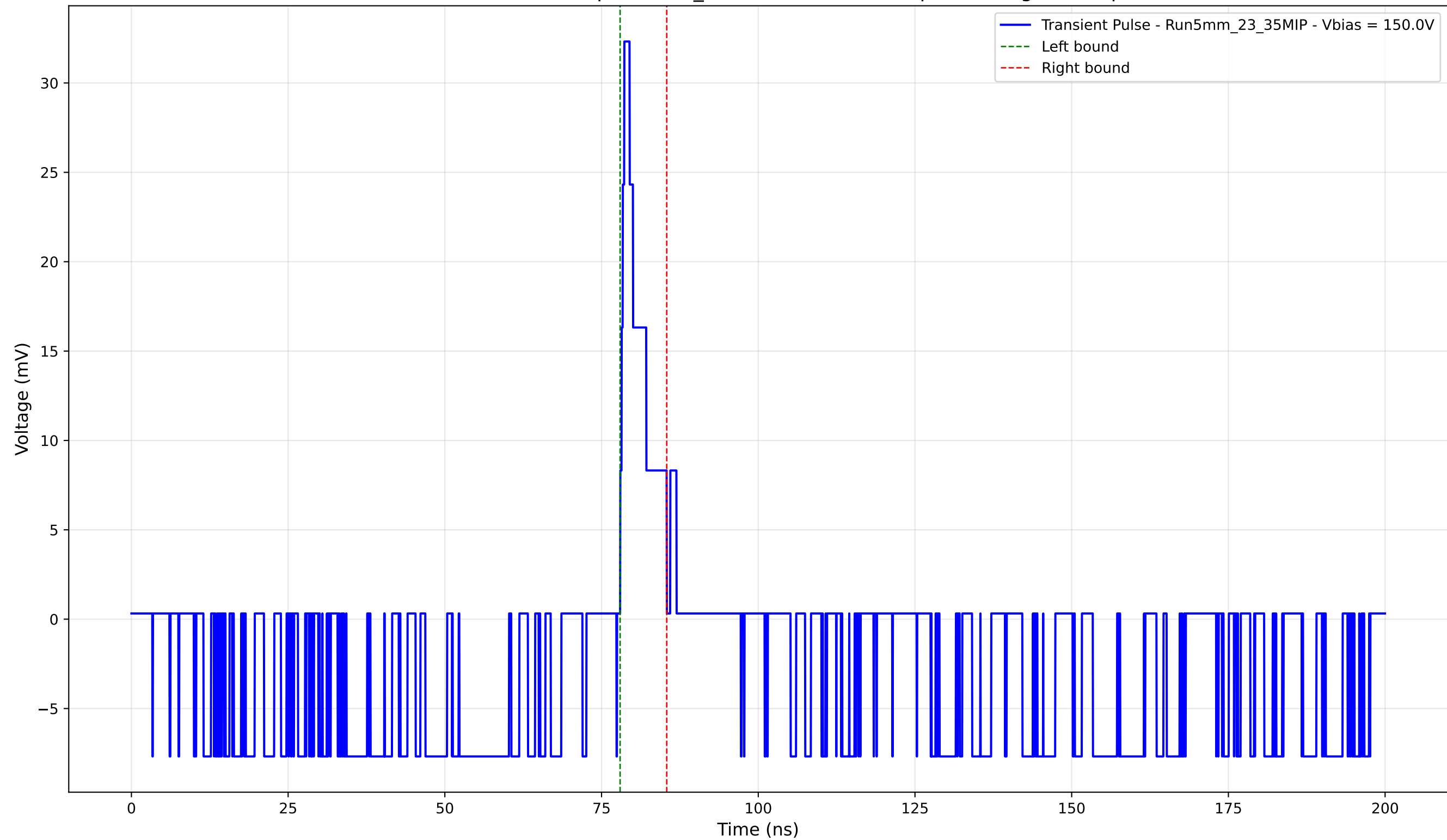
Transient Pulse - Sample: 5mm_23 - Position: 5140.0 \mu\text{m} - Charge: 2.27 pC
