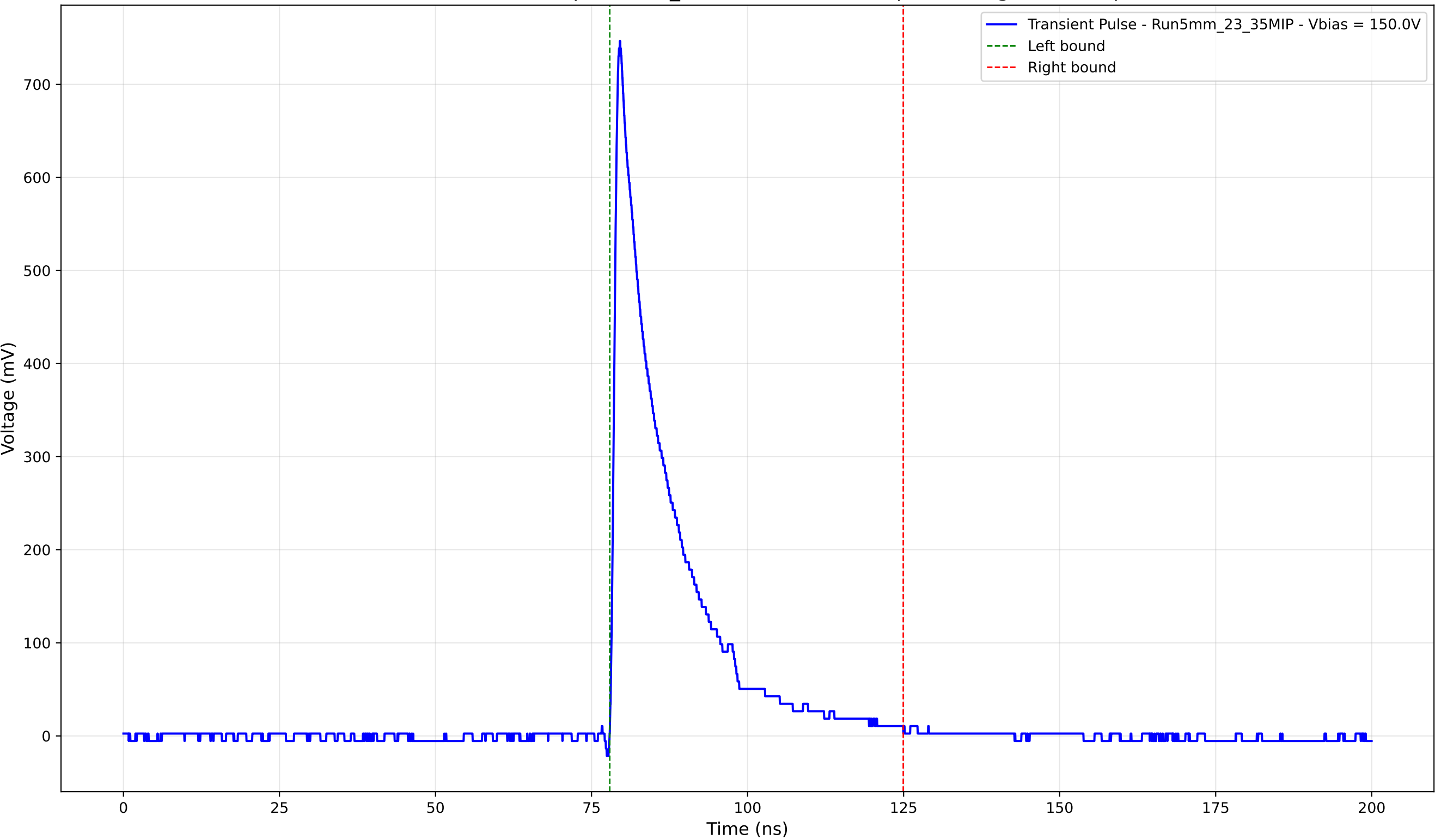
Transient Pulse - Sample: 5mm_23 - Position: 4415.0 \mu\text{m} - Charge: 131.78 pC
