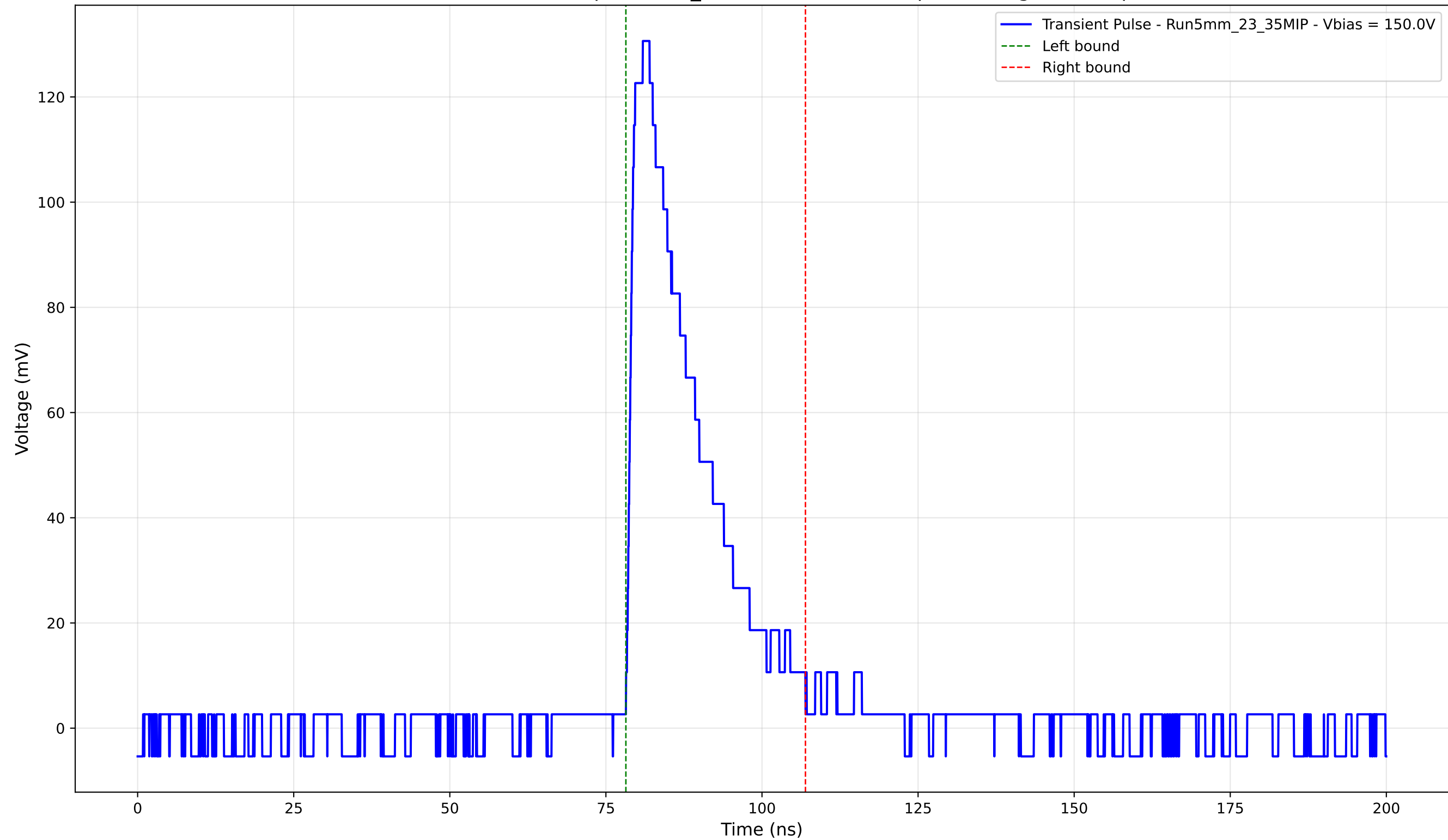
Transient Pulse - Sample: 5mm_23 - Position: 1640.0 \mu\text{m} - Charge: 30.40 pC
