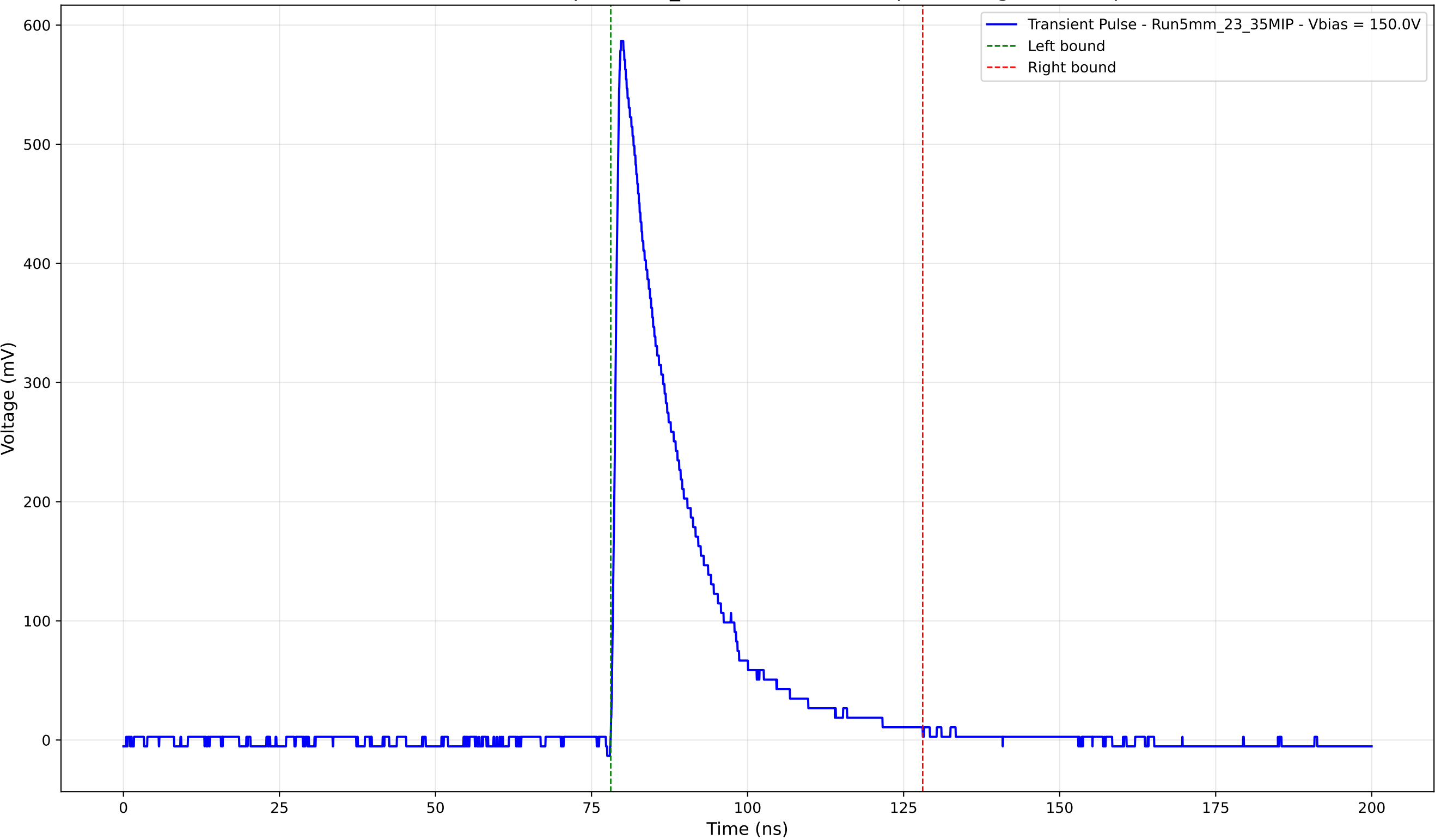
Transient Pulse - Sample: 5mm_23 - Position: 1245.0 \mu\text{m} - Charge: 127.68 pC
