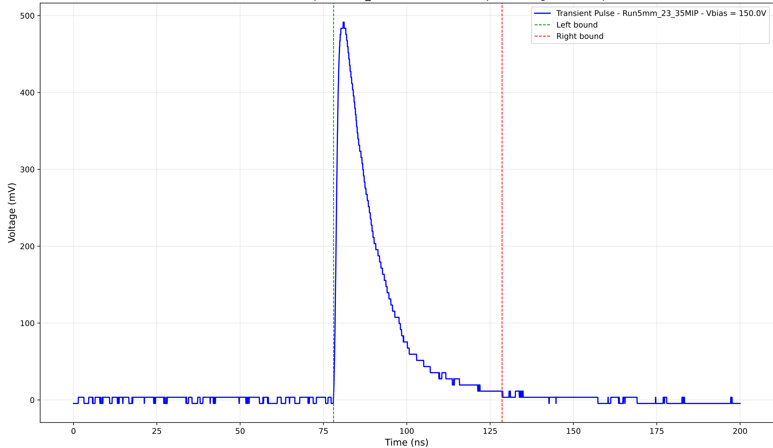
Transient Pulse - Sample: 5mm_23 - Position: 3245.0 \mu\text{m} - Charge: 126.58 pC
