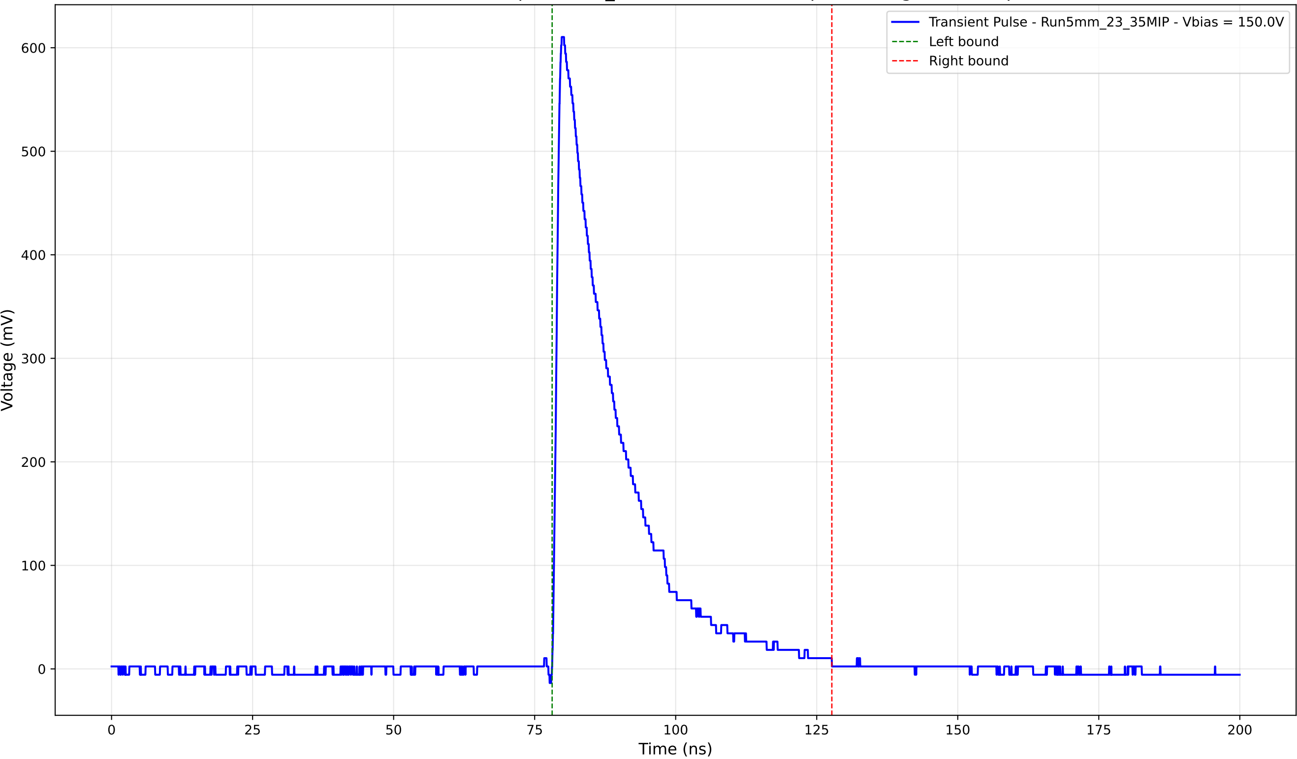
Transient Pulse - Sample: 5mm_23 - Position: 1385.0 \mu\text{m} - Charge: 140.54 pC
