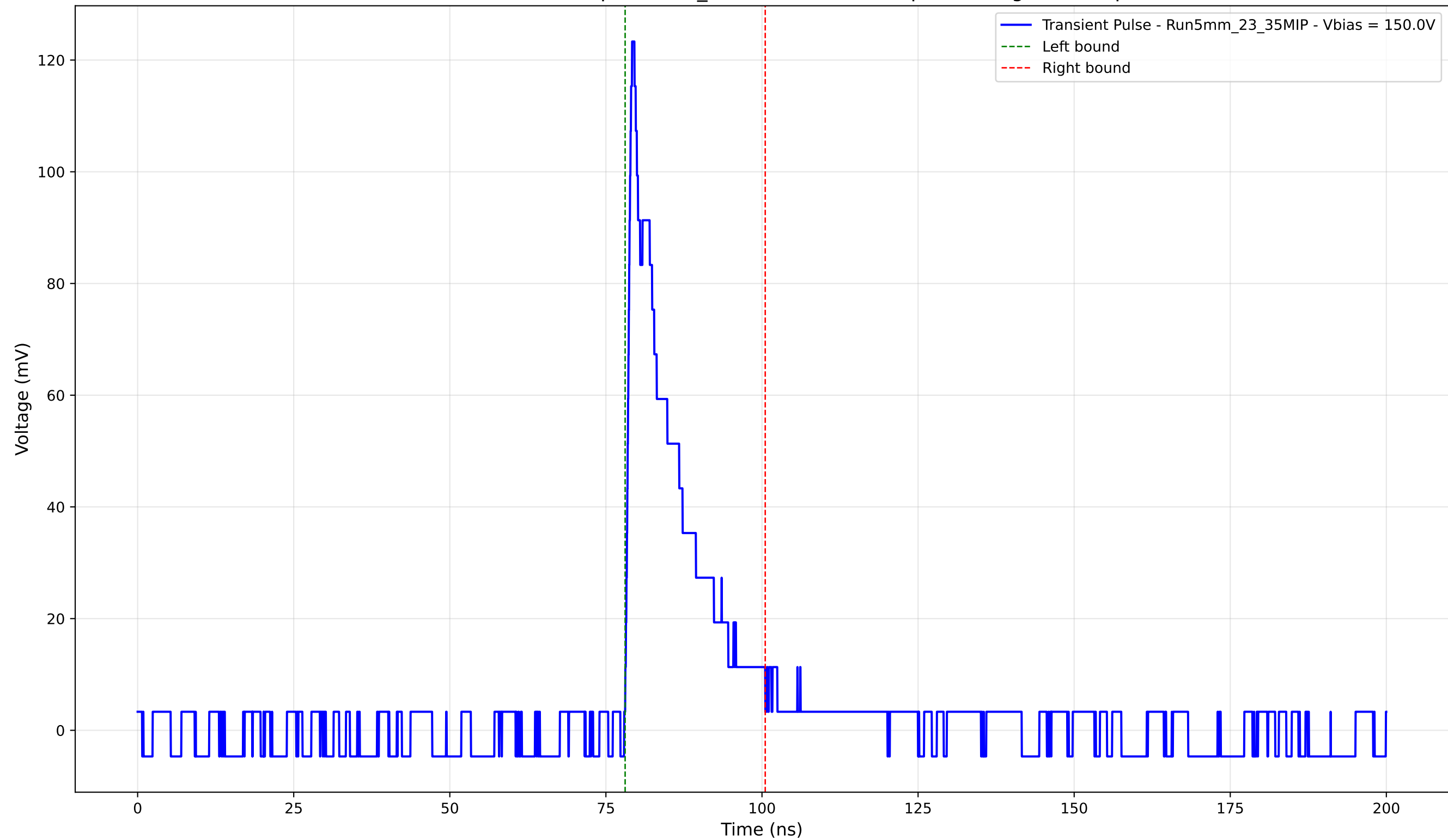
Transient Pulse - Sample: 5mm_23 - Position: 625.0 \mu\text{m} - Charge: 18.50 pC
