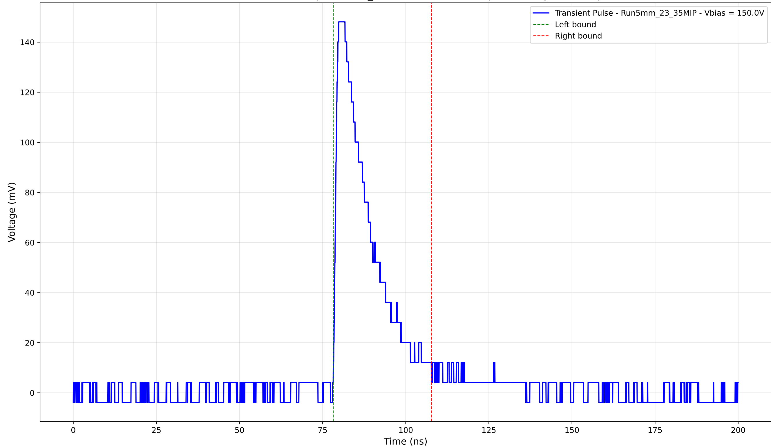
Transient Pulse - Sample: 5mm_23 - Position: 3630.0 \mu\text{m} - Charge: 34.08 pC
