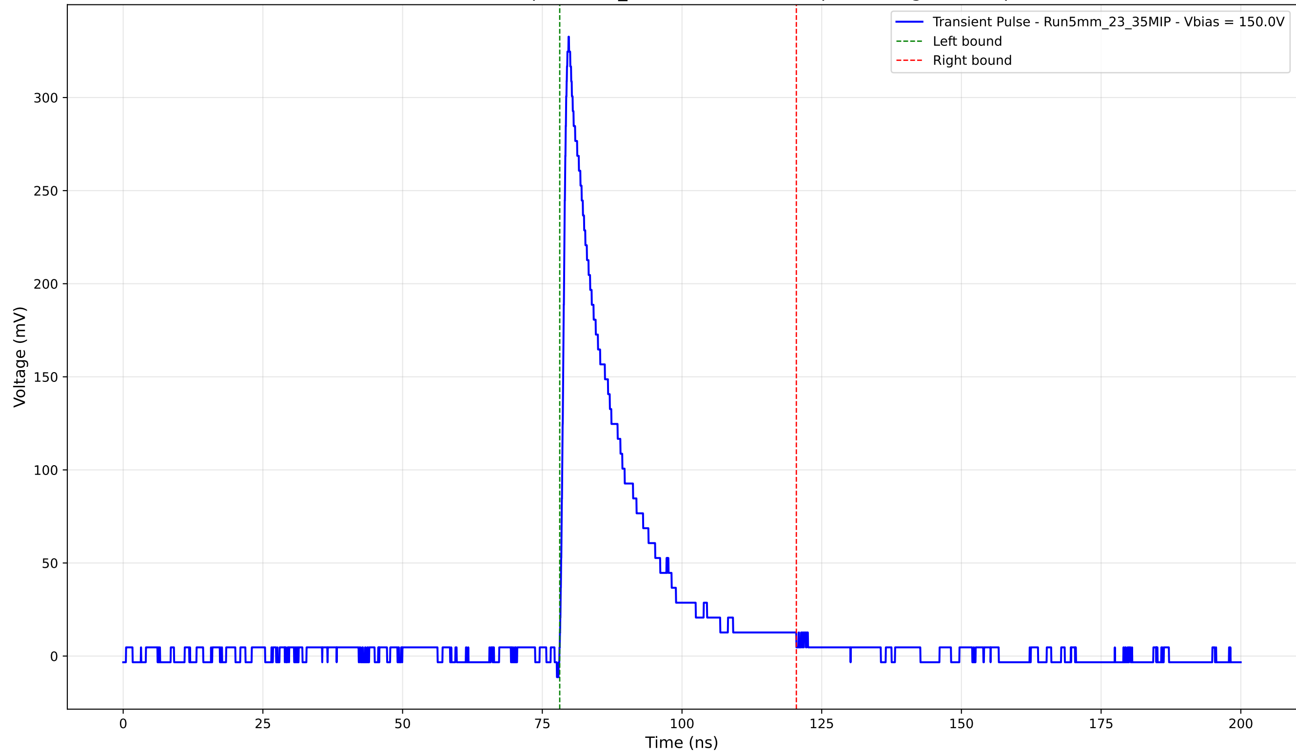
Transient Pulse - Sample: 5mm_23 - Position: 1080.0 \mu\text{m} - Charge: 63.45 pC
