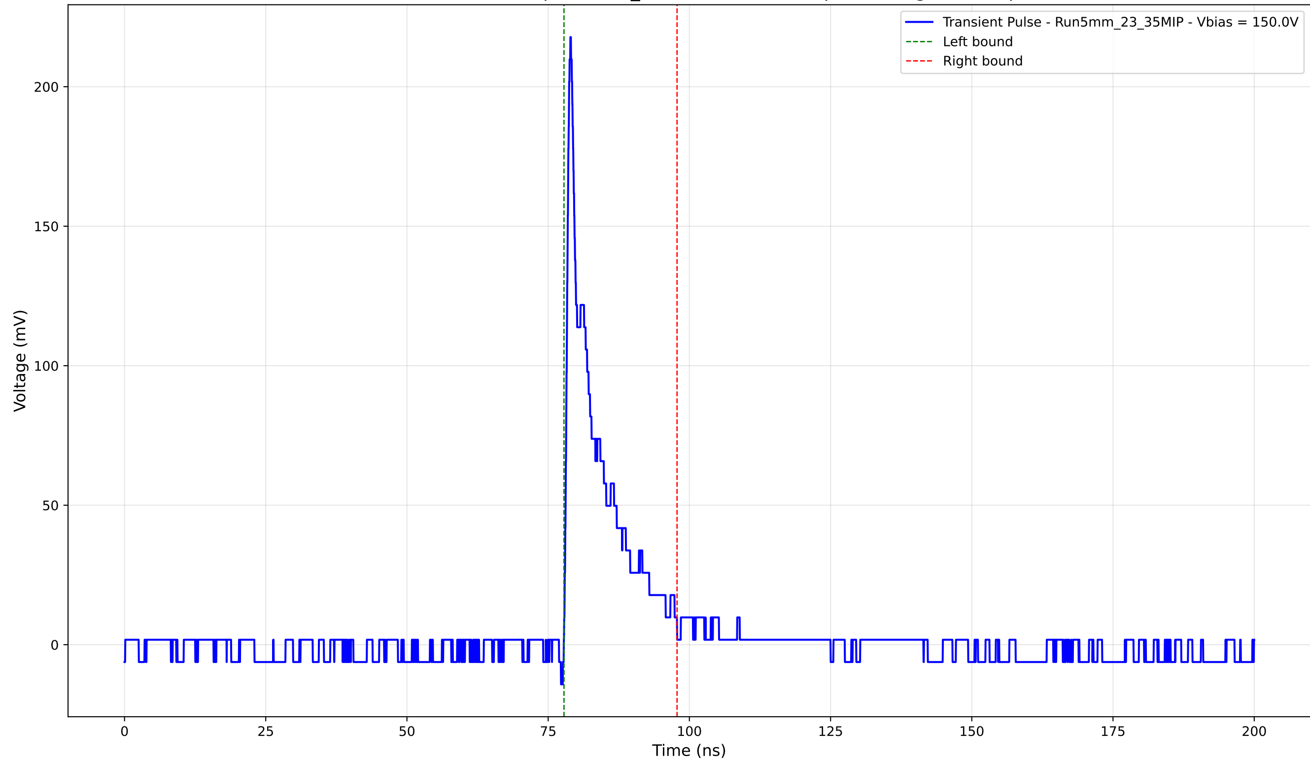
Transient Pulse - Sample: 5mm_23 - Position: 190.0 \mu\text{m} - Charge: 22.87 pC
