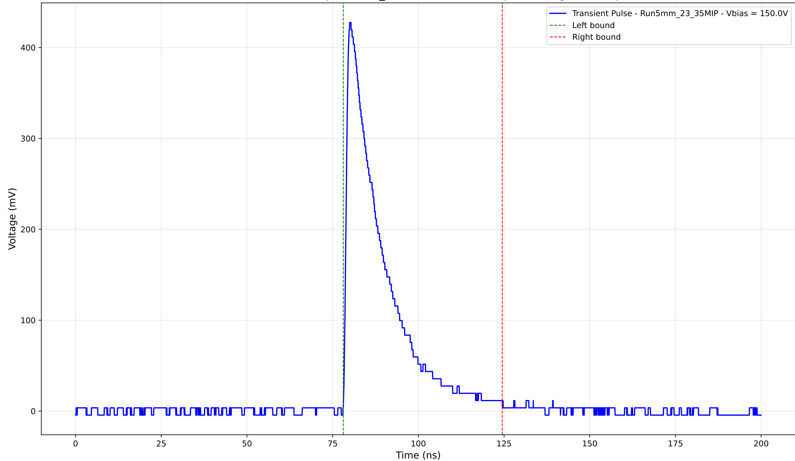
Transient Pulse - Sample: 5mm_23 - Position: 1555.0 \mu\text{m} - Charge: 99.45 pC
