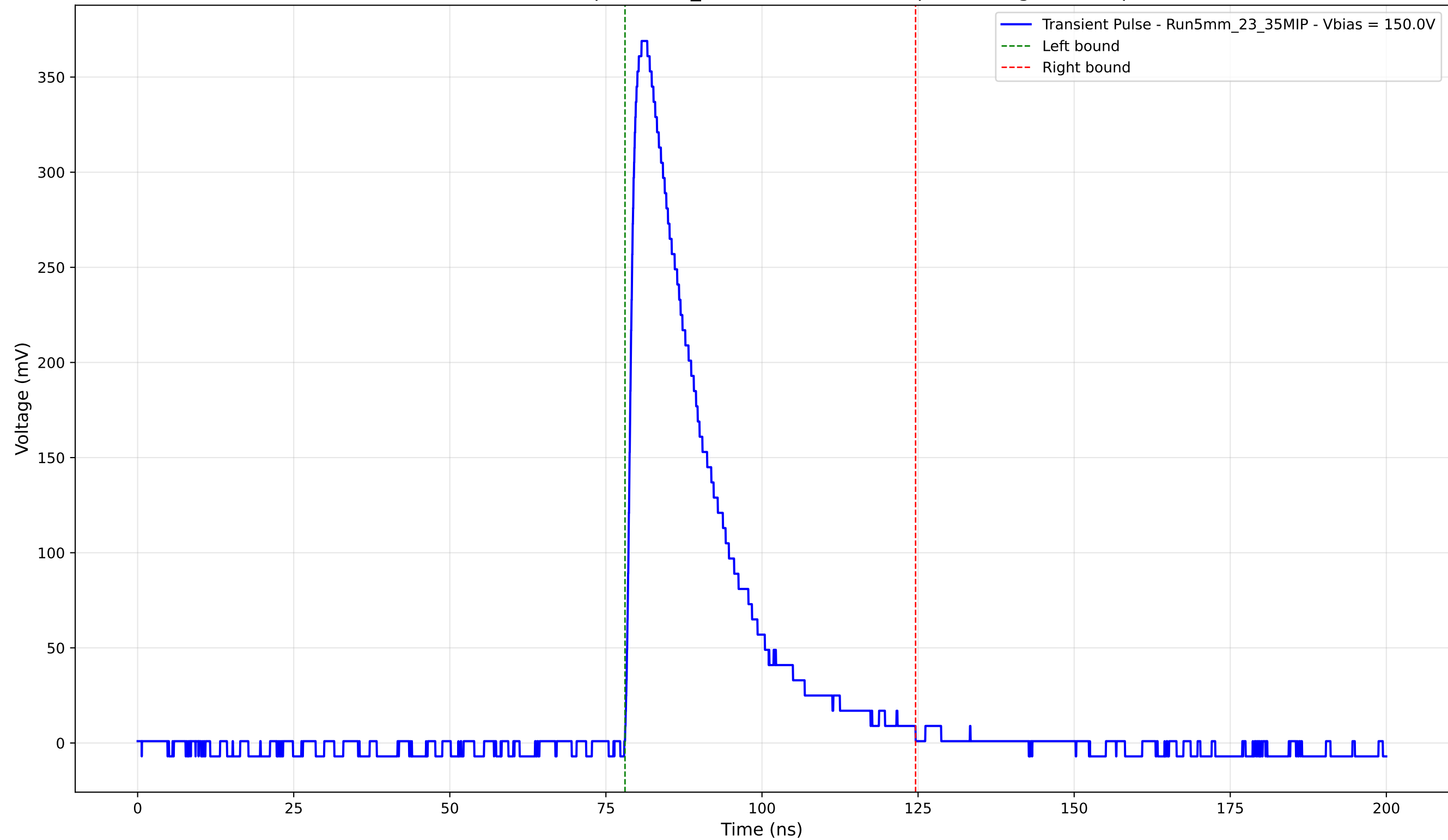
Transient Pulse - Sample: 5mm_23 - Position: 2200.0 \mu\text{m} - Charge: 95.37 pC
