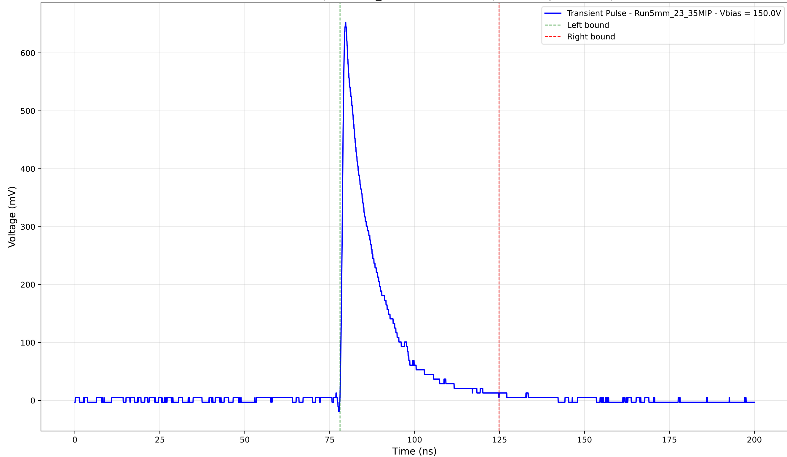
Transient Pulse - Sample: 5mm_23 - Position: 985.0 \mu\text{m} - Charge: 125.59 pC
