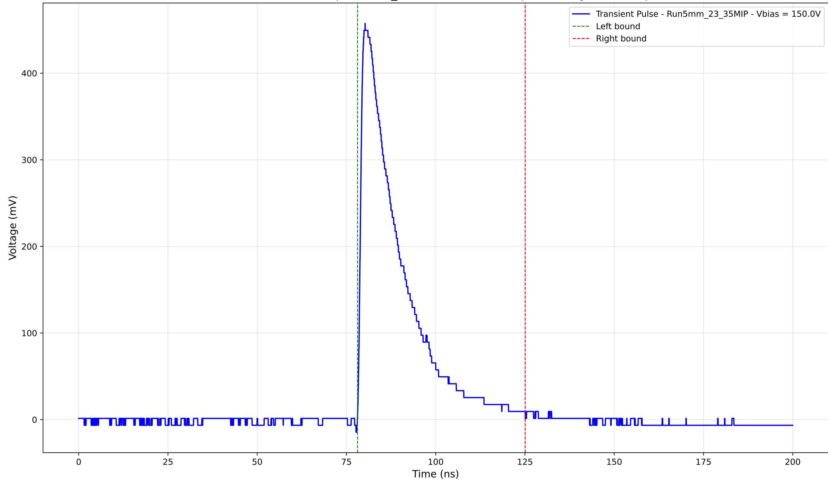
Transient Pulse - Sample: 5mm_23 - Position: 1705.0 \mu\text{m} - Charge: 110.80 pC
