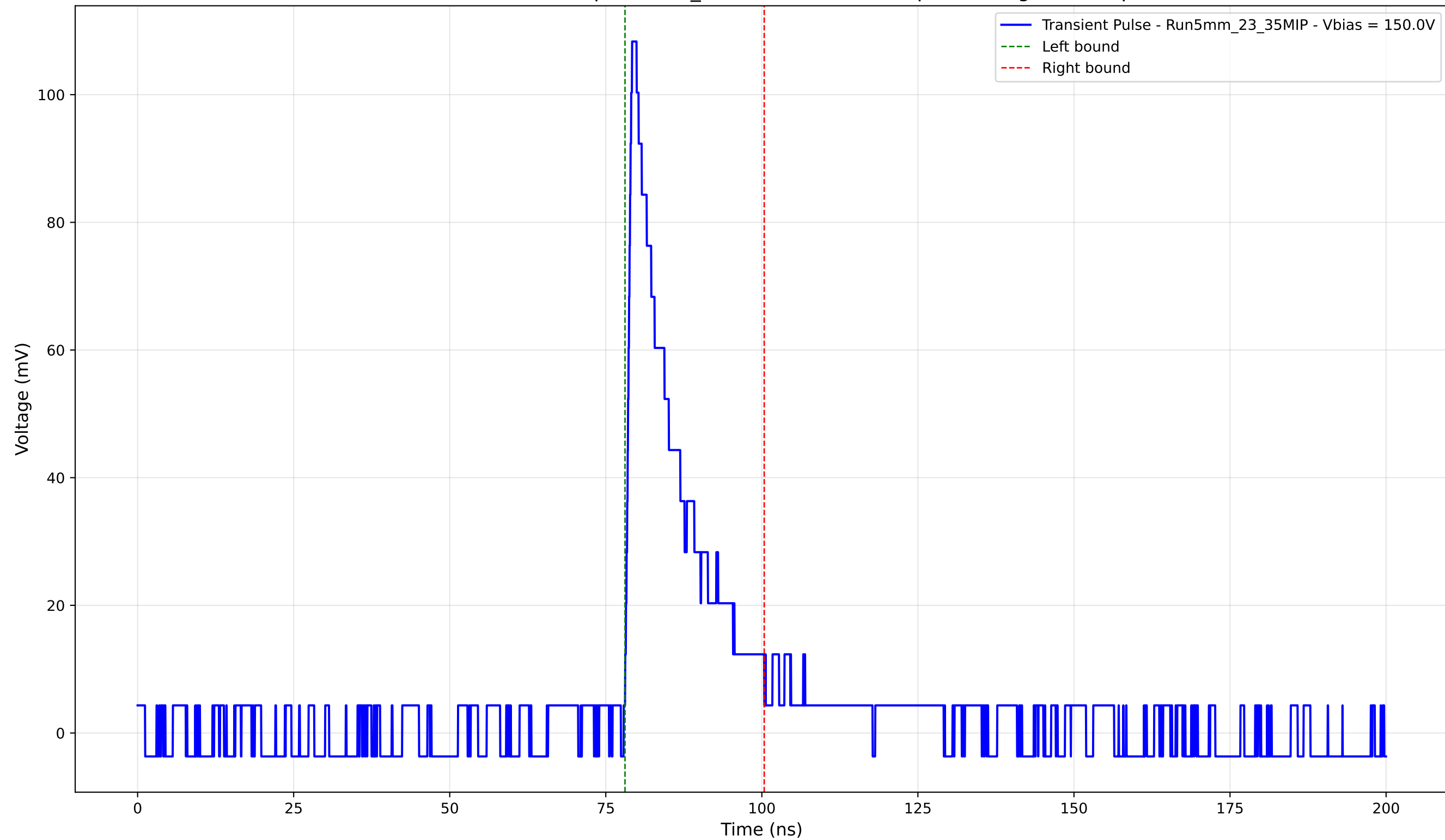
Transient Pulse - Sample: 5mm_23 - Position: 4500.0 \mu\text{m} - Charge: 17.59 pC
