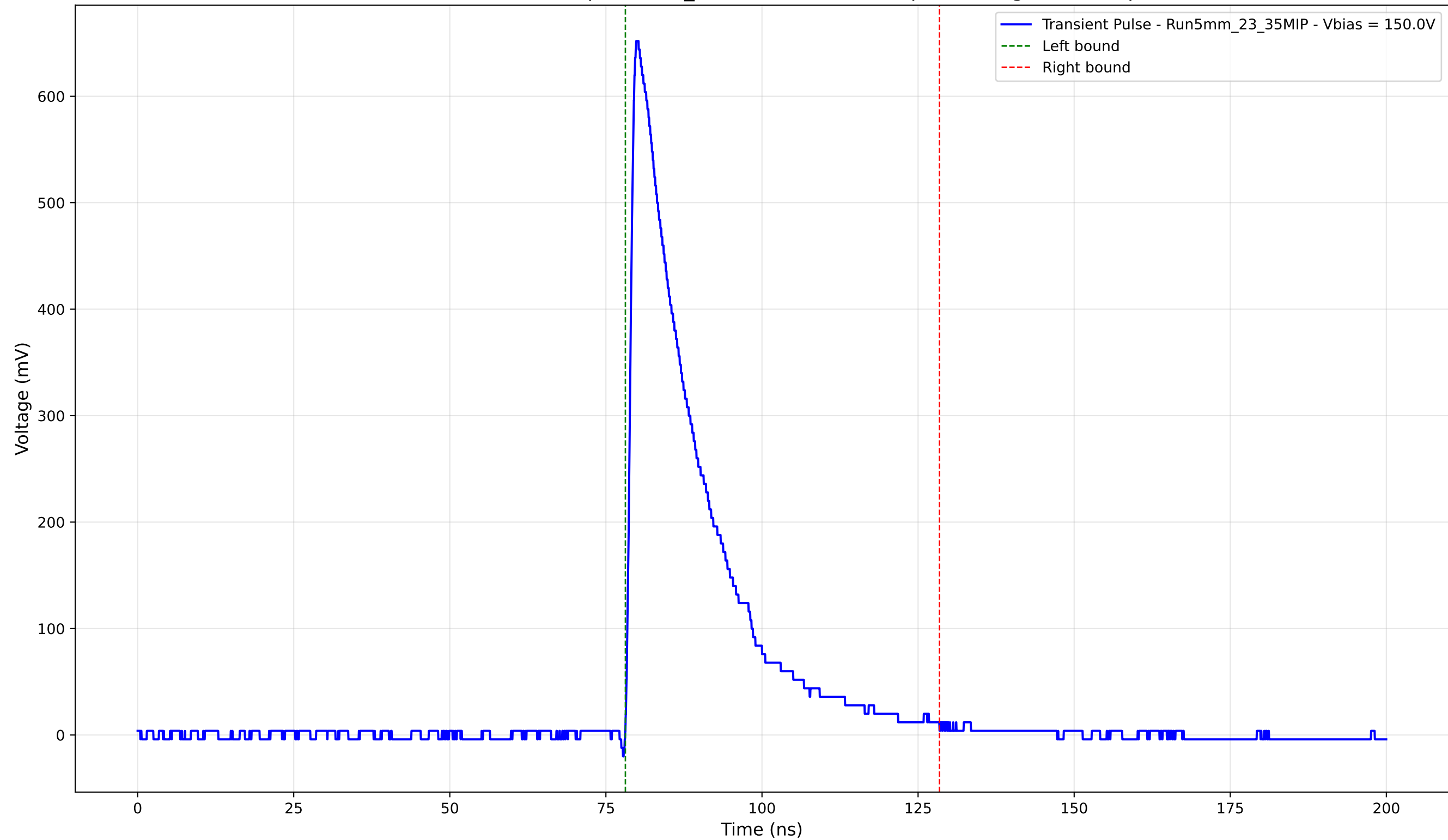
Transient Pulse - Sample: 5mm_23 - Position: 1435.0 \mu\text{m} - Charge: 152.13 pC
