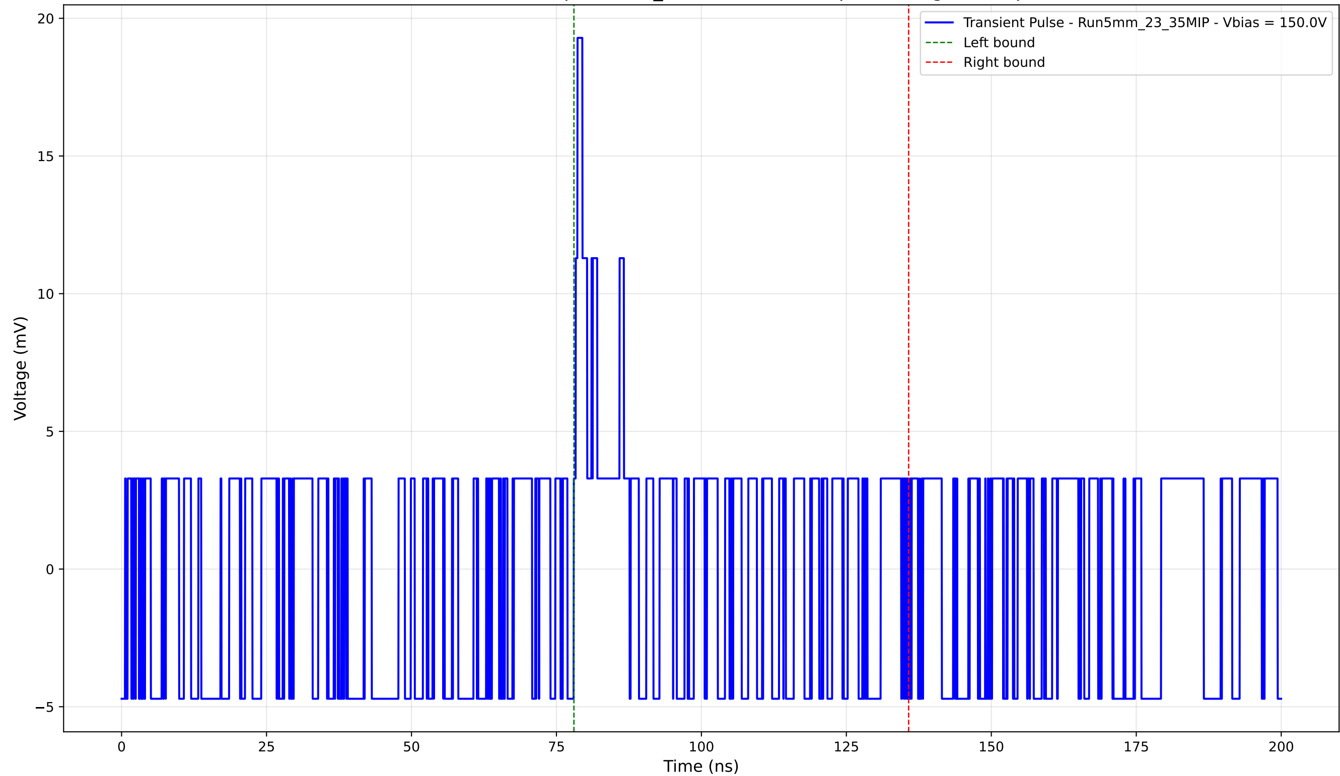
Transient Pulse - Sample: 5mm_23 - Position: 10.0 \mu\text{m} - Charge: 1.52 pC
