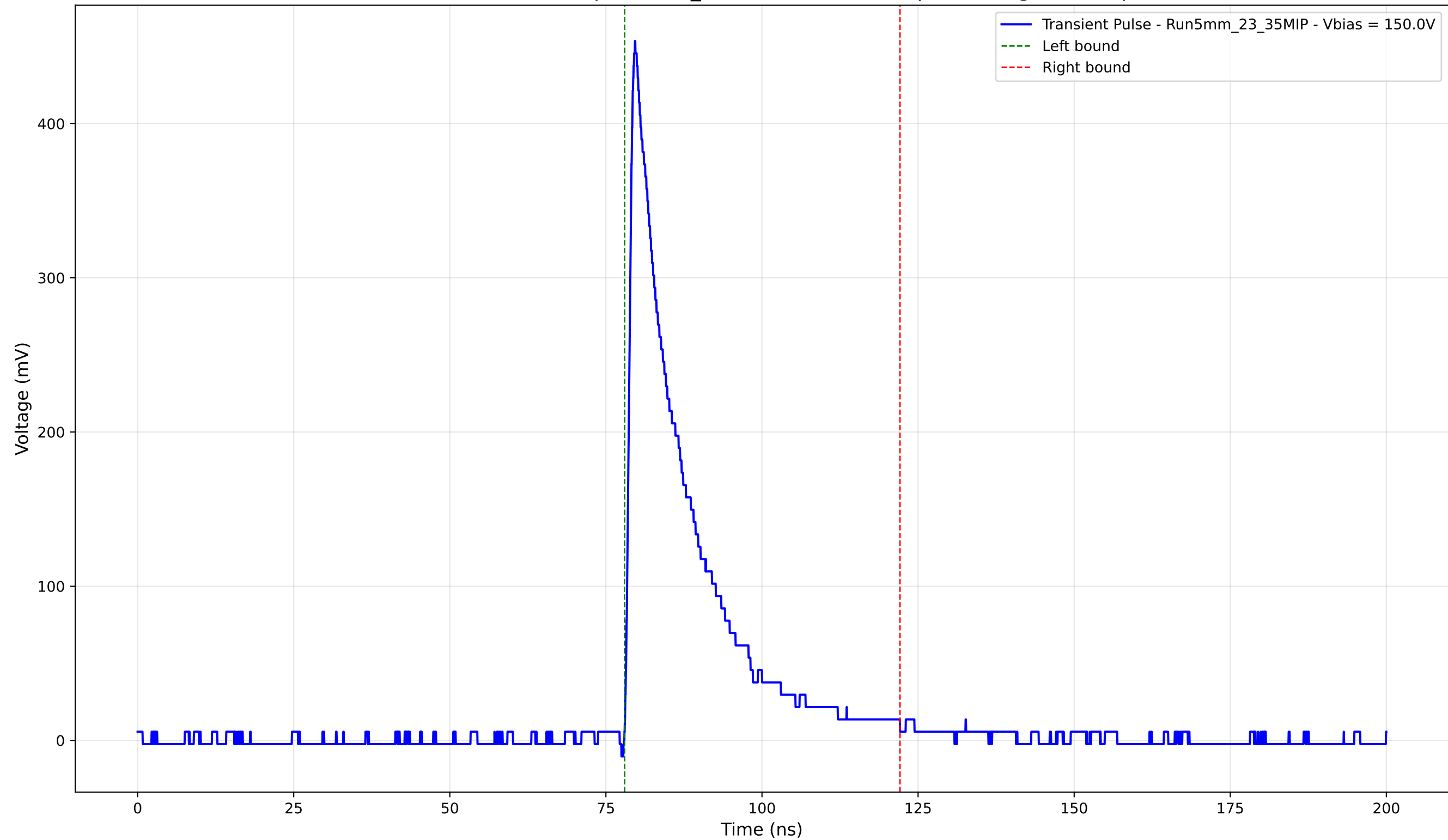
Transient Pulse - Sample: 5mm_23 - Position: 4225.0 \mu\text{m} - Charge: 85.08 pC
