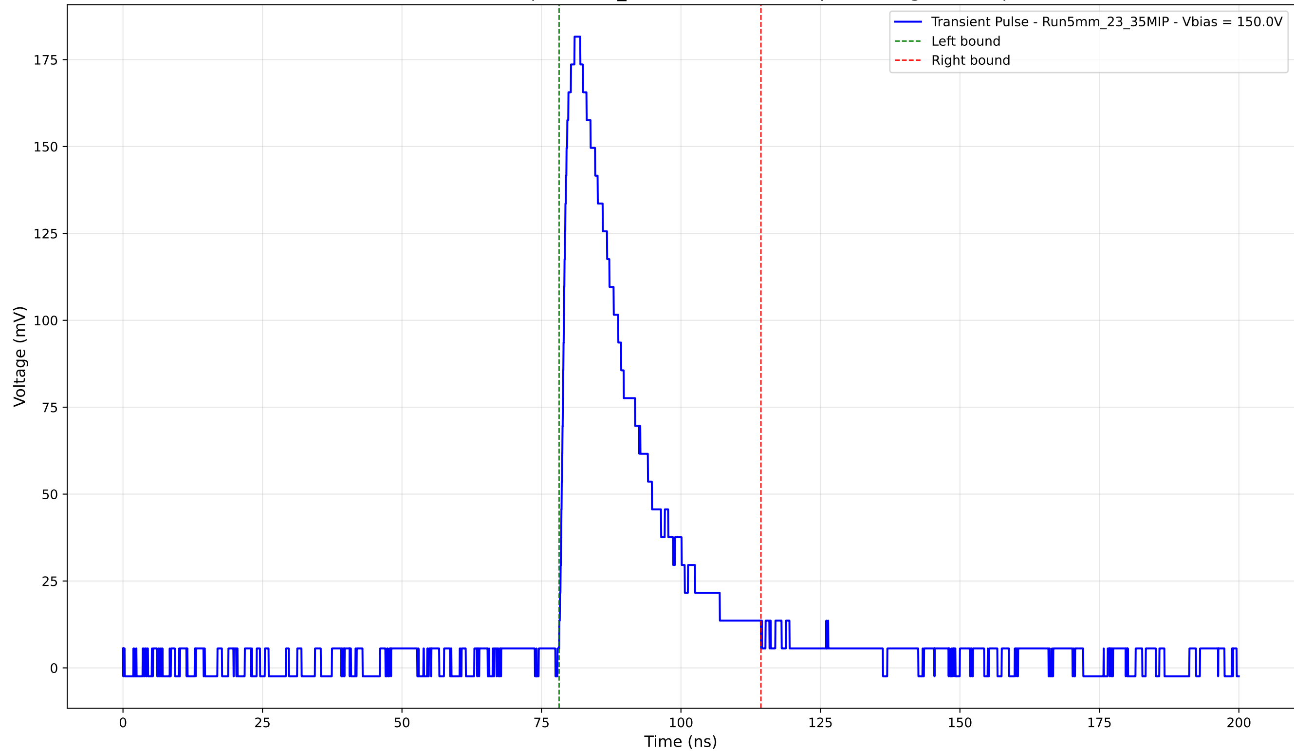
Transient Pulse - Sample: 5mm_23 - Position: 2615.0 \mu\text{m} - Charge: 47.29 pC
