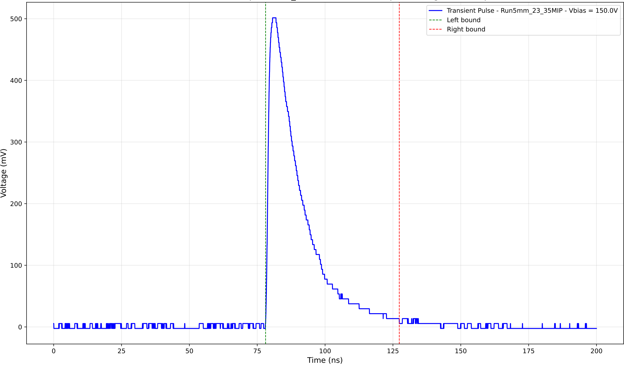
Transient Pulse - Sample: 5mm_23 - Position: 2375.0 \mu\text{m} - Charge: 137.09 pC
