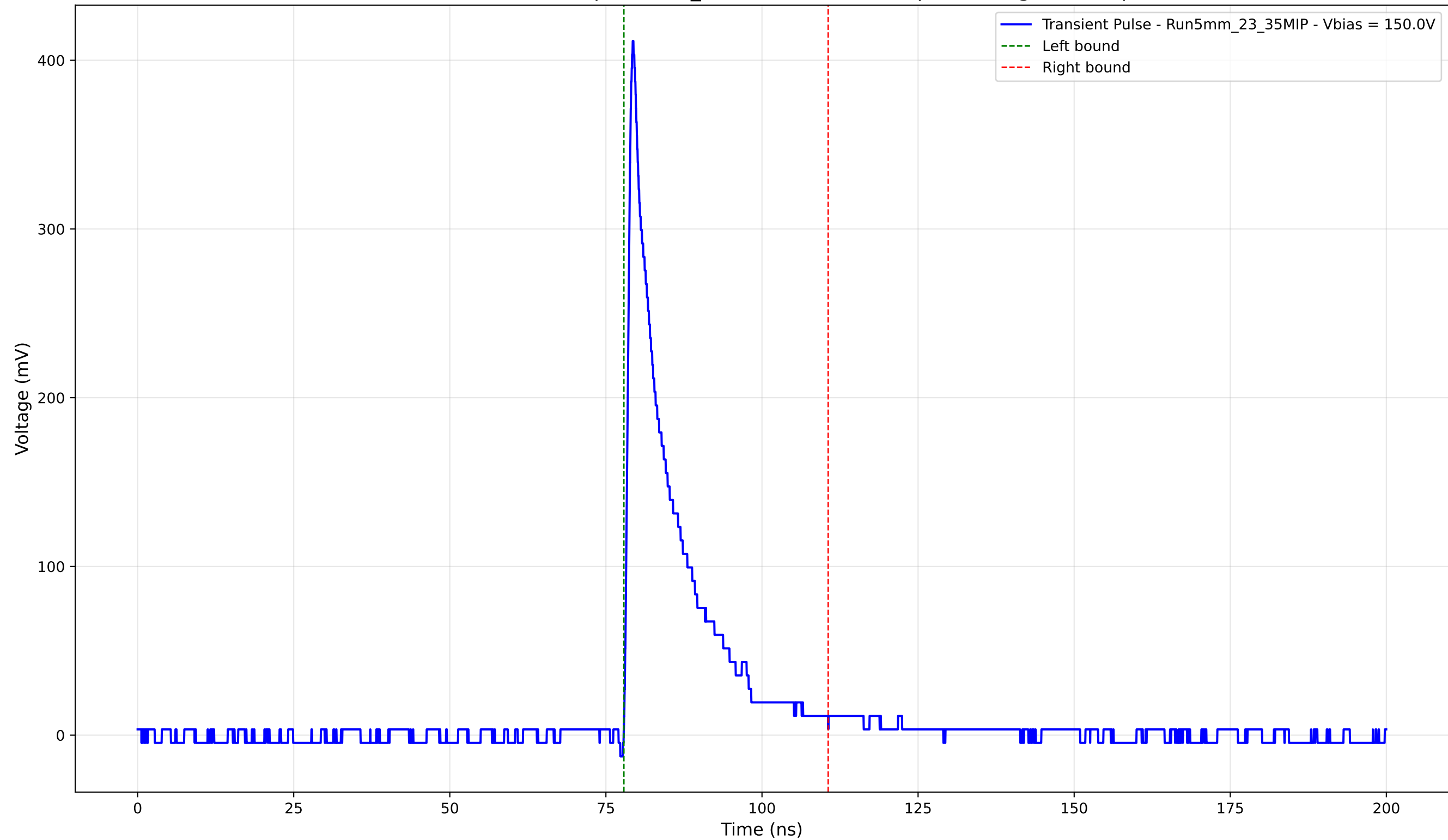
Transient Pulse - Sample: 5mm_23 - Position: 4625.0 \mu\text{m} - Charge: 58.57 pC
