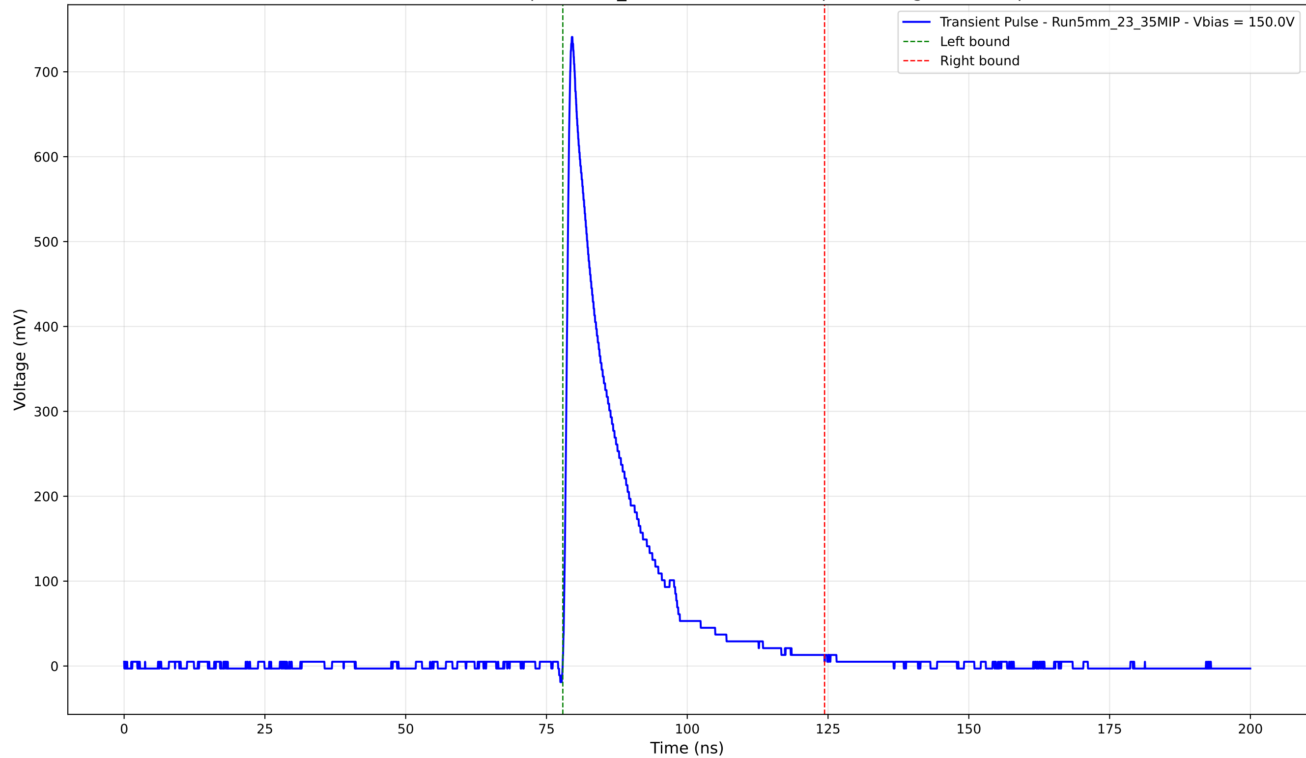
Transient Pulse - Sample: 5mm_23 - Position: 4405.0 \mu\text{m} - Charge: 132.67 pC
