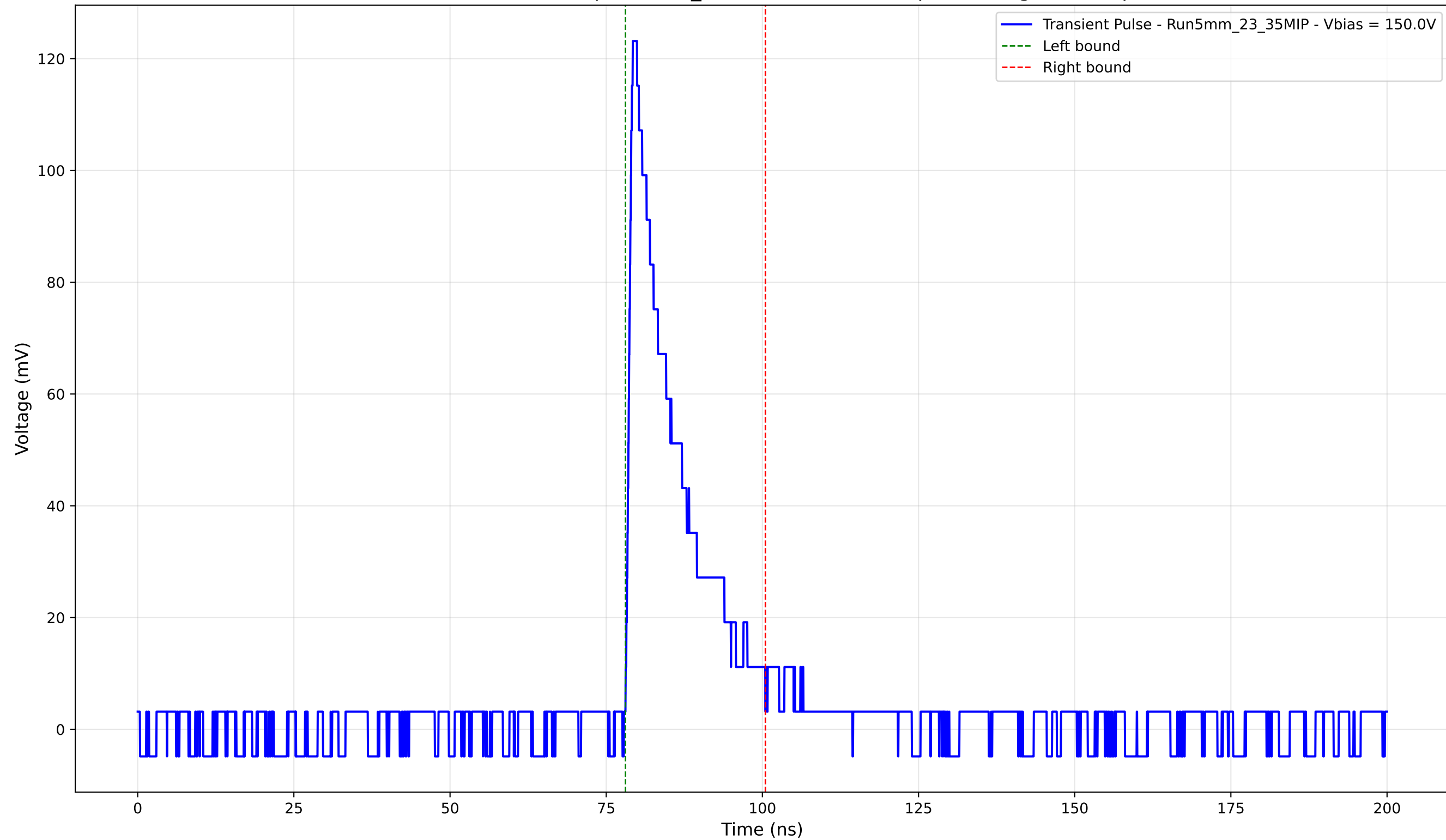
Transient Pulse - Sample: 5mm_23 - Position: 4495.0 \mu\text{m} - Charge: 19.92 pC
