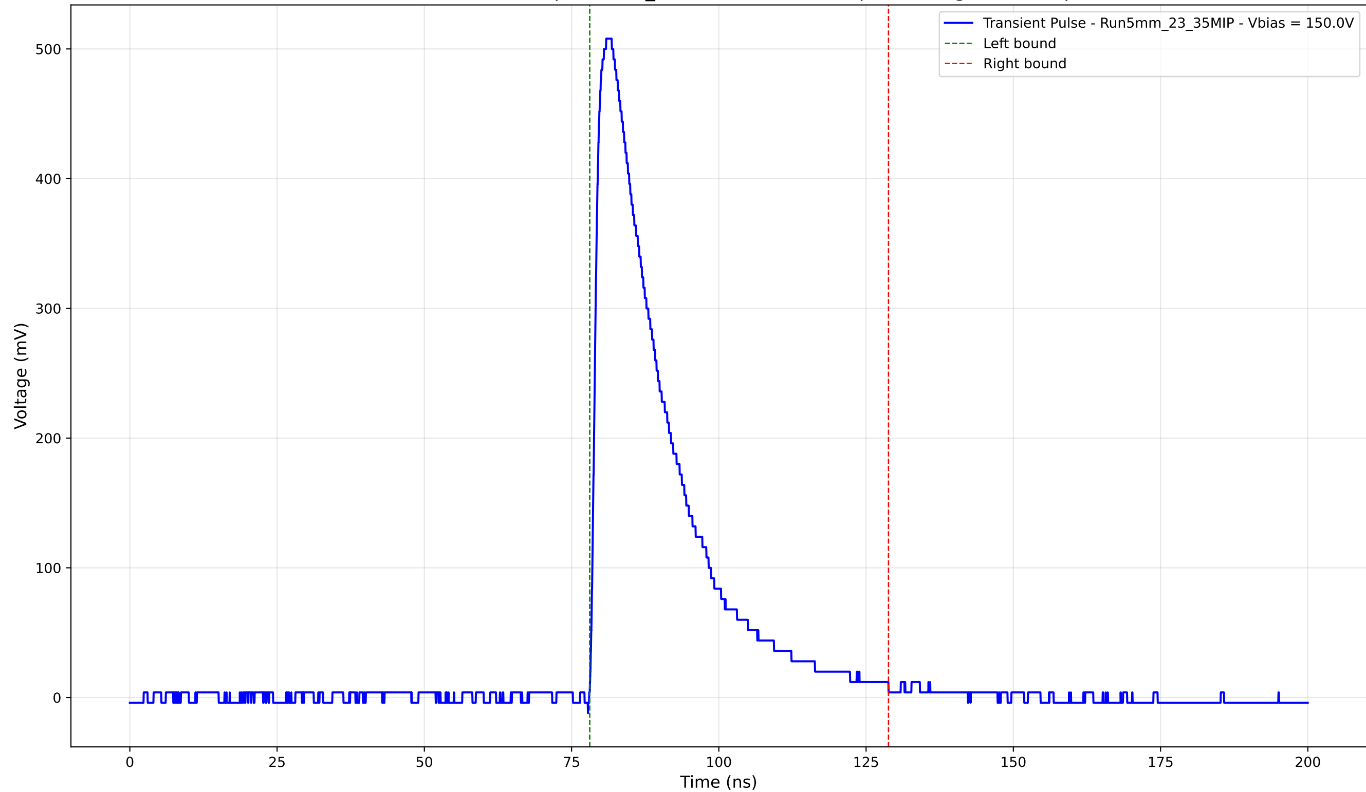
Transient Pulse - Sample: 5mm_23 - Position: 2325.0 \mu\text{m} - Charge: 137.61 pC
