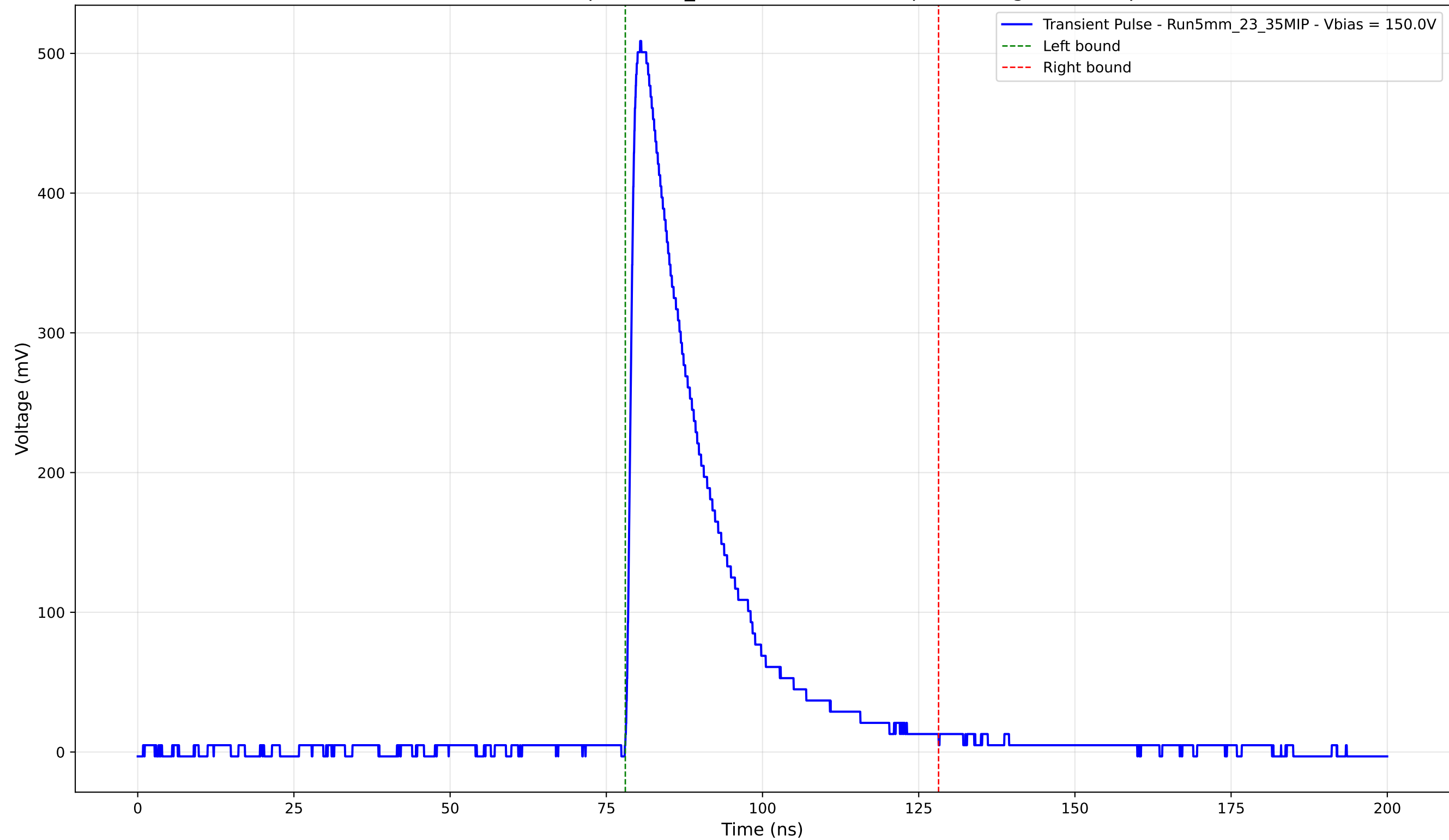
Transient Pulse - Sample: 5mm_23 - Position: 3490.0 \mu\text{m} - Charge: 128.02 pC
