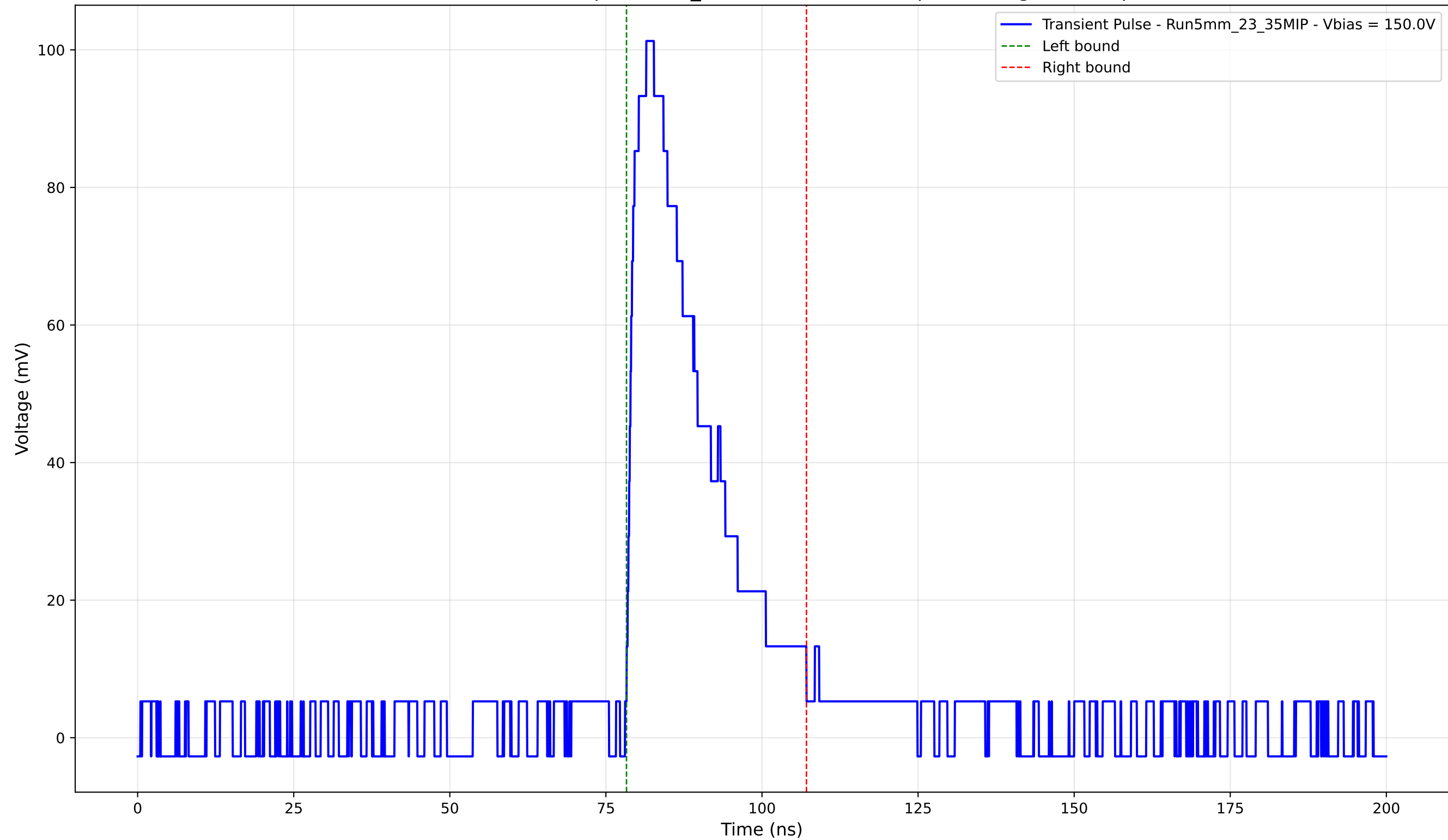
Transient Pulse - Sample: 5mm_23 - Position: 2635.0 \mu\text{m} - Charge: 26.03 pC
