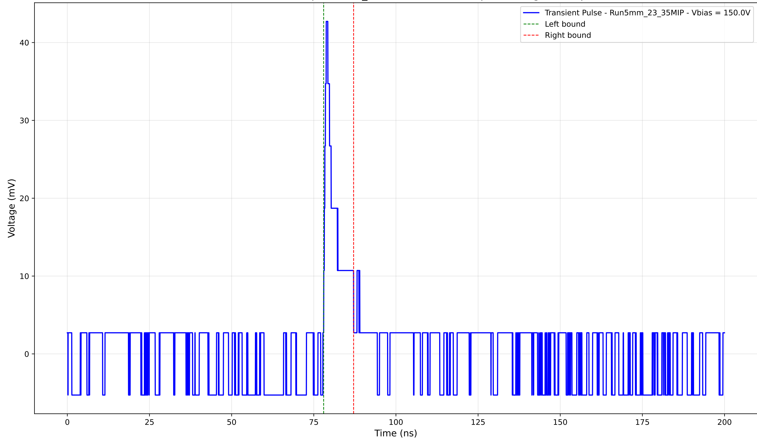
Transient Pulse - Sample: 5mm_23 - Position: 5135.0 \mu\text{m} - Charge: 3.18 pC
