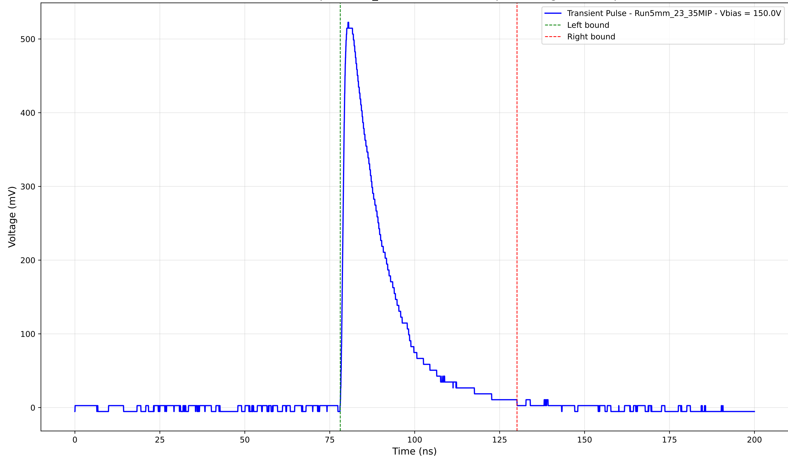
Transient Pulse - Sample: 5mm_23 - Position: 1870.0 \mu\text{m} - Charge: 135.45 pC
