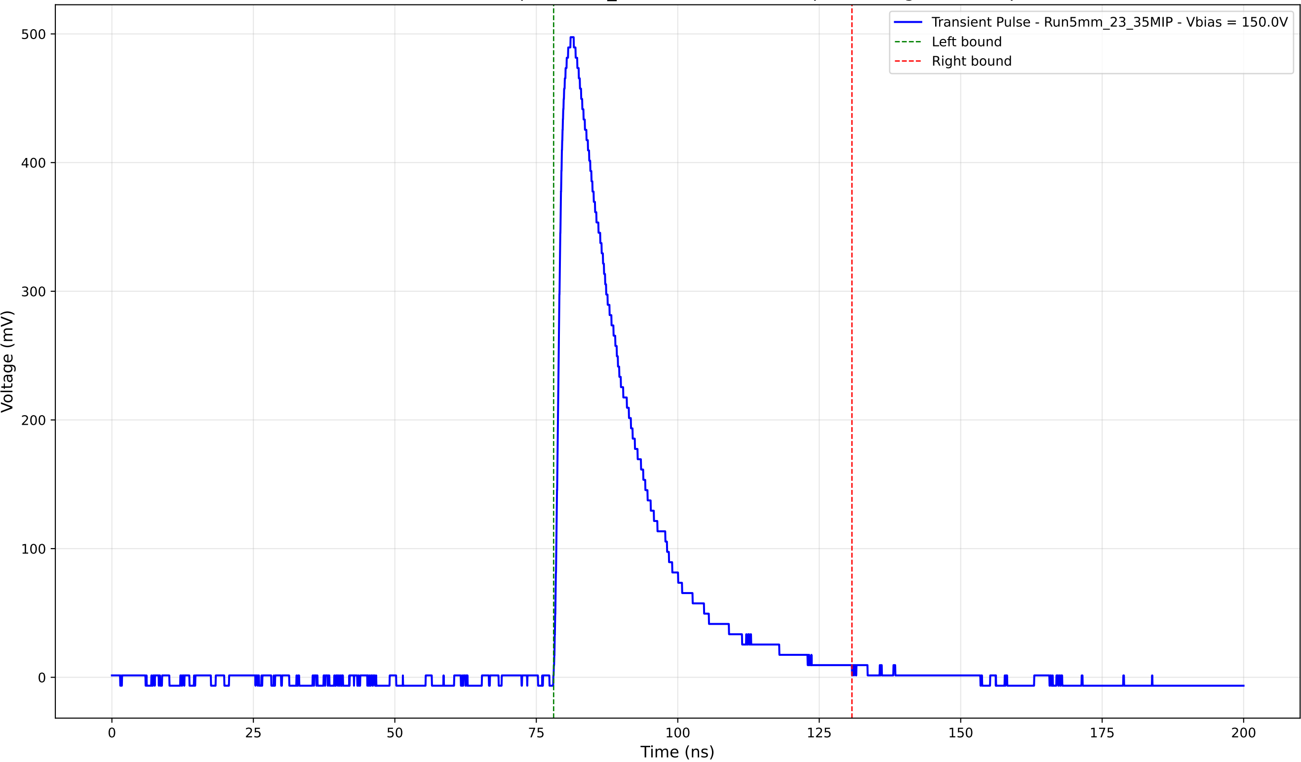
Transient Pulse - Sample: 5mm_23 - Position: 2870.0 \mu\text{m} - Charge: 132.28 pC
