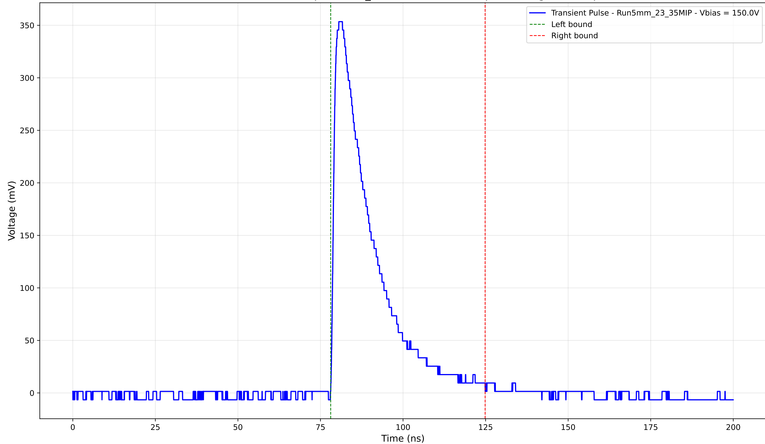
Transient Pulse - Sample: 5mm_23 - Position: 2080.0 \mu\text{m} - Charge: 90.96 pC
