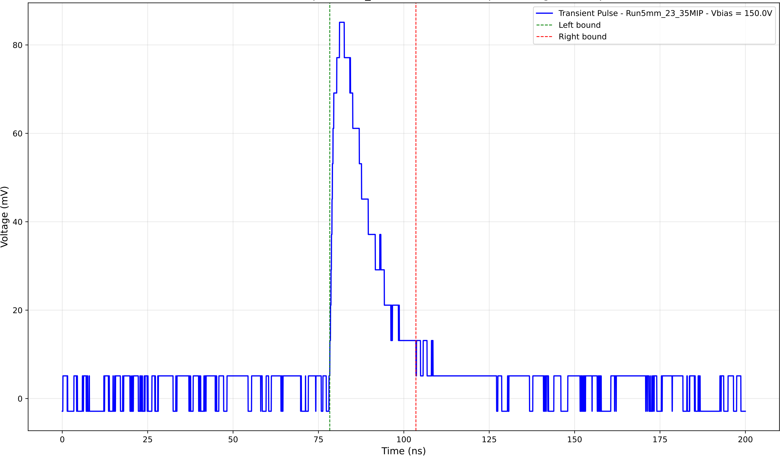
Transient Pulse - Sample: 5mm_23 - Position: 3145.0 \mu\text{m} - Charge: 20.40 pC
