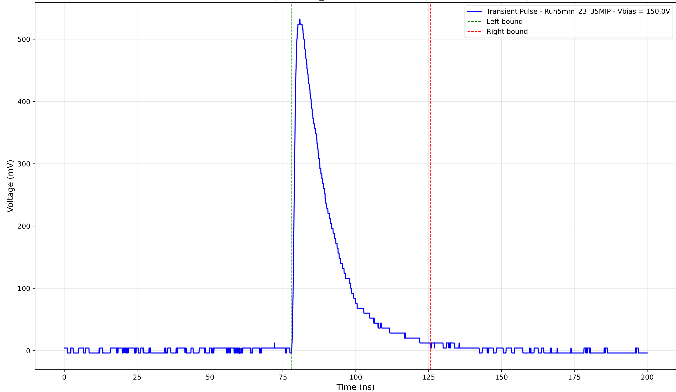
Transient Pulse - Sample: 5mm_23 - Position: 1885.0 \mu\text{m} - Charge: 137.13 pC
