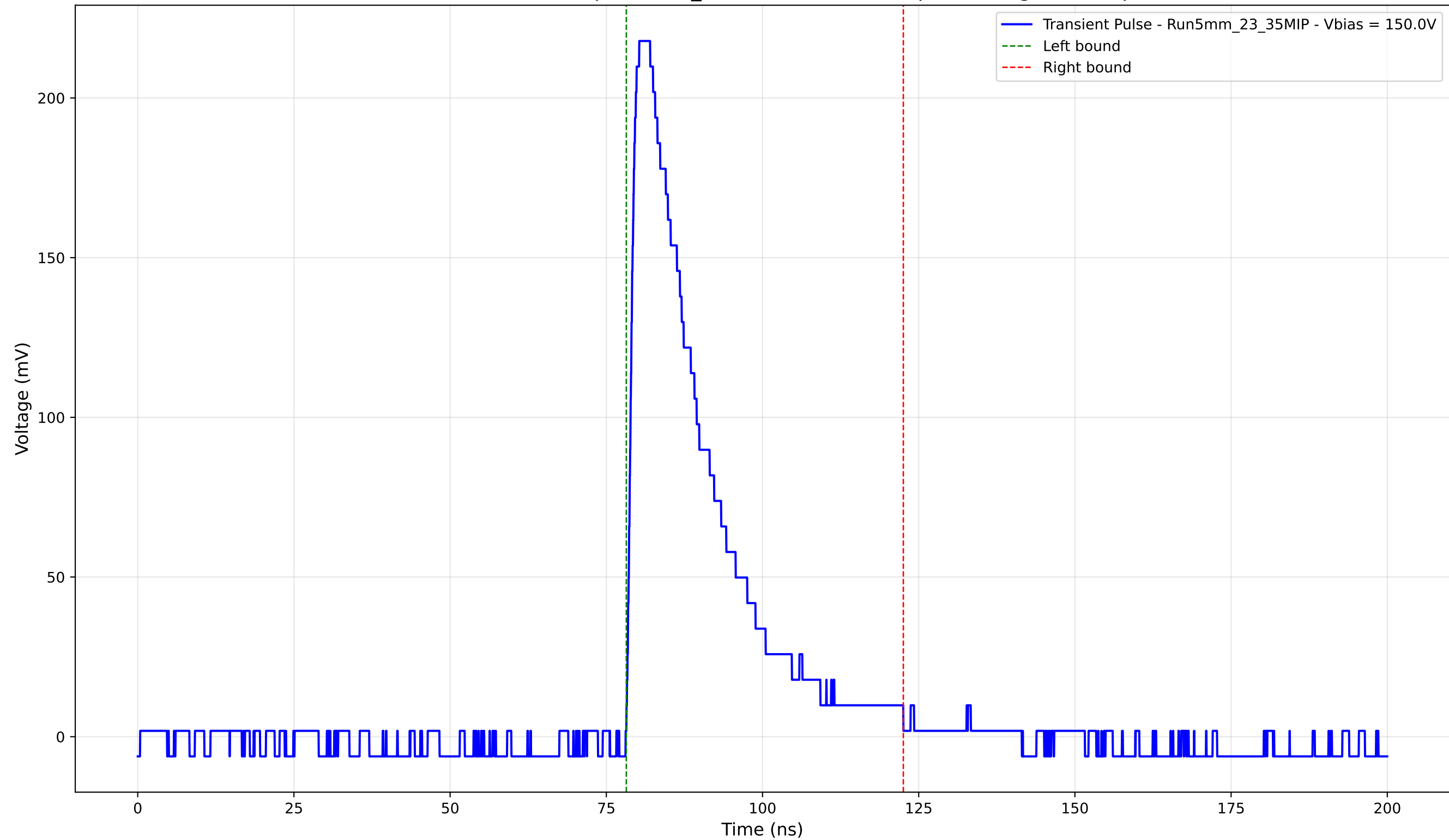
Transient Pulse - Sample: 5mm_23 - Position: 2100.0 \mu\text{m} - Charge: 56.27 pC
