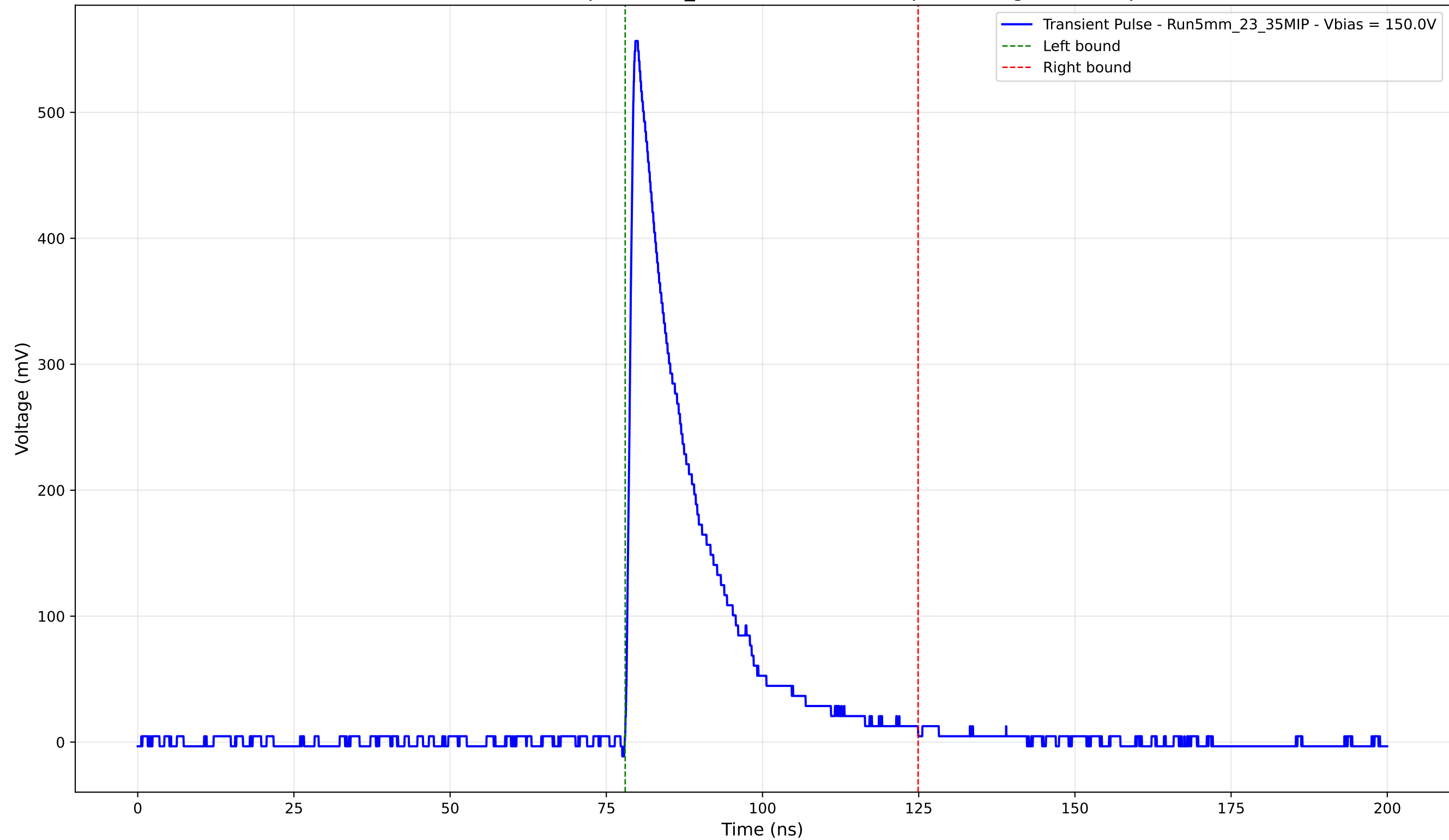
Transient Pulse - Sample: 5mm_23 - Position: 4065.0 \mu\text{m} - Charge: 114.26 pC
