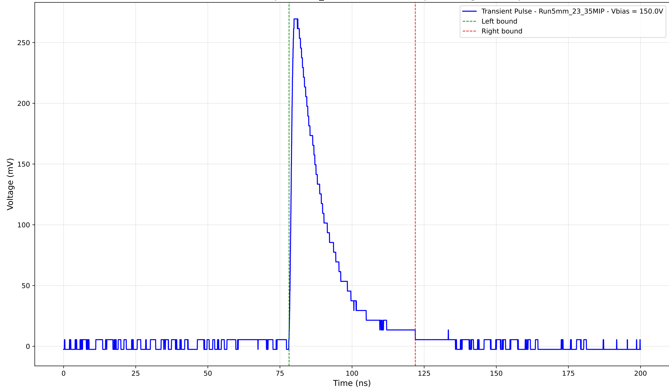
Transient Pulse - Sample: 5mm_23 - Position: 1670.0 \mu\text{m} - Charge: 67.04 pC
