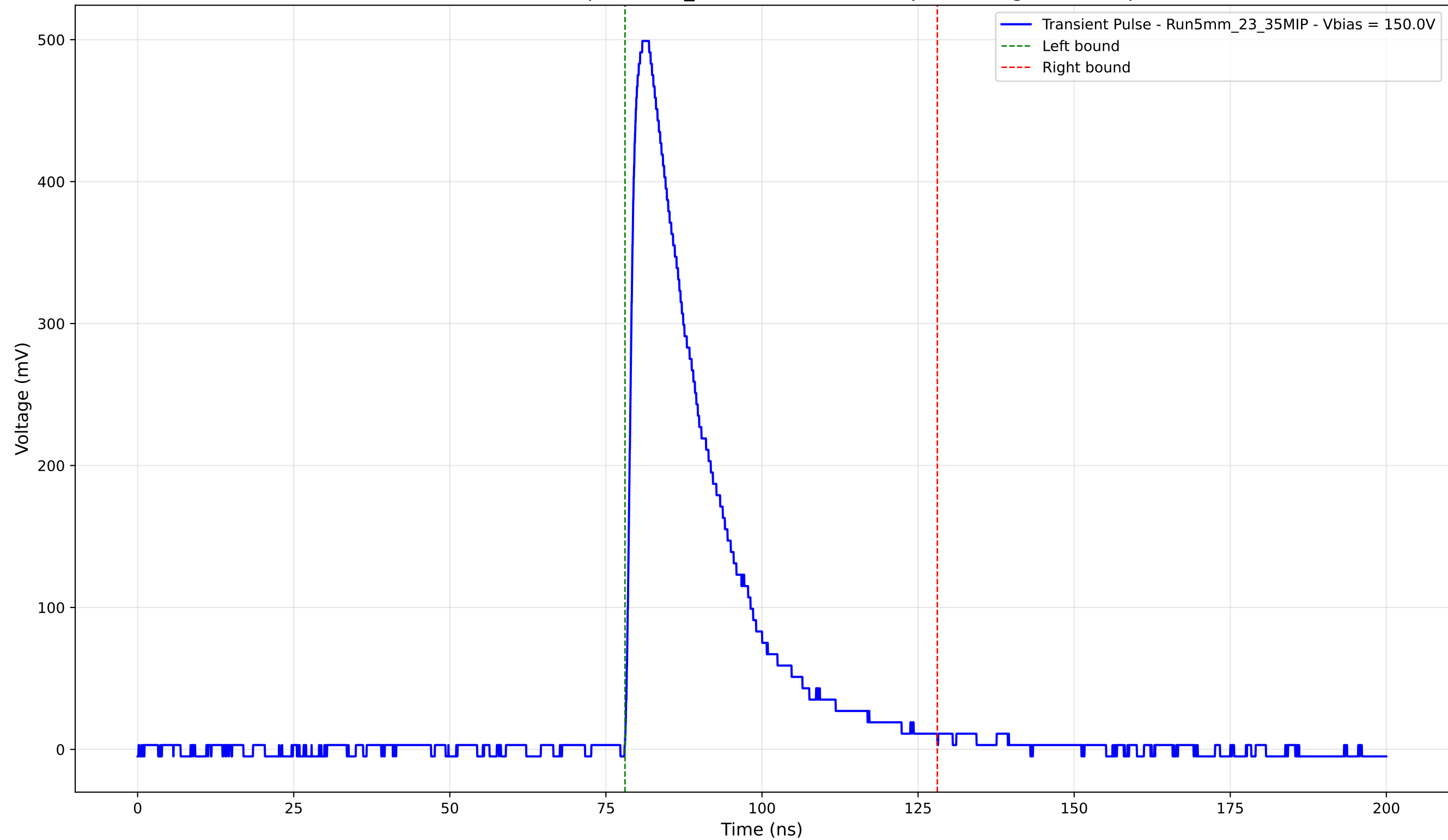
Transient Pulse - Sample: 5mm_23 - Position: 2845.0 \mu\text{m} - Charge: 134.29 pC
