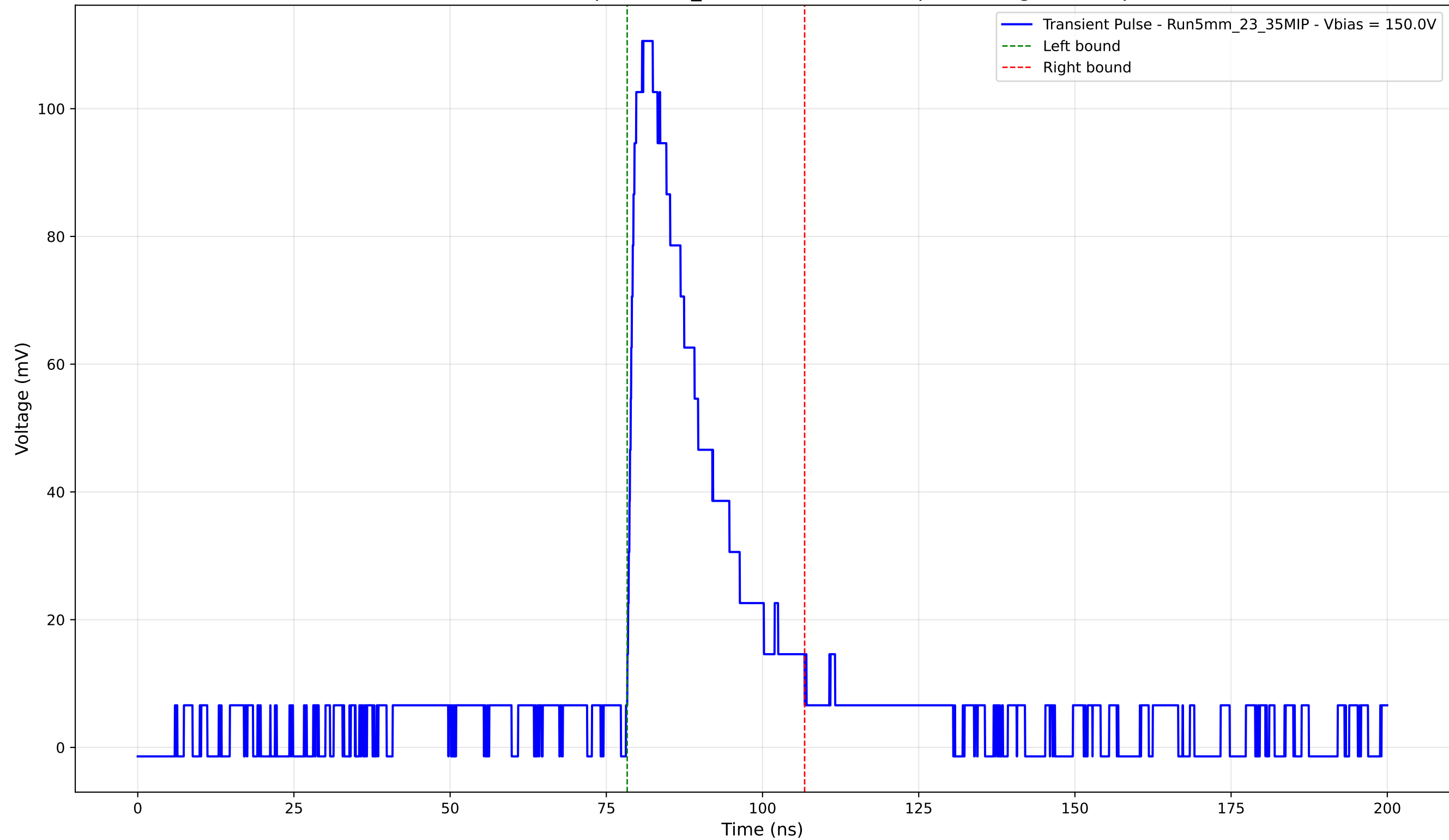
Transient Pulse - Sample: 5mm_23 - Position: 3160.0 \mu\text{m} - Charge: 27.89 pC
