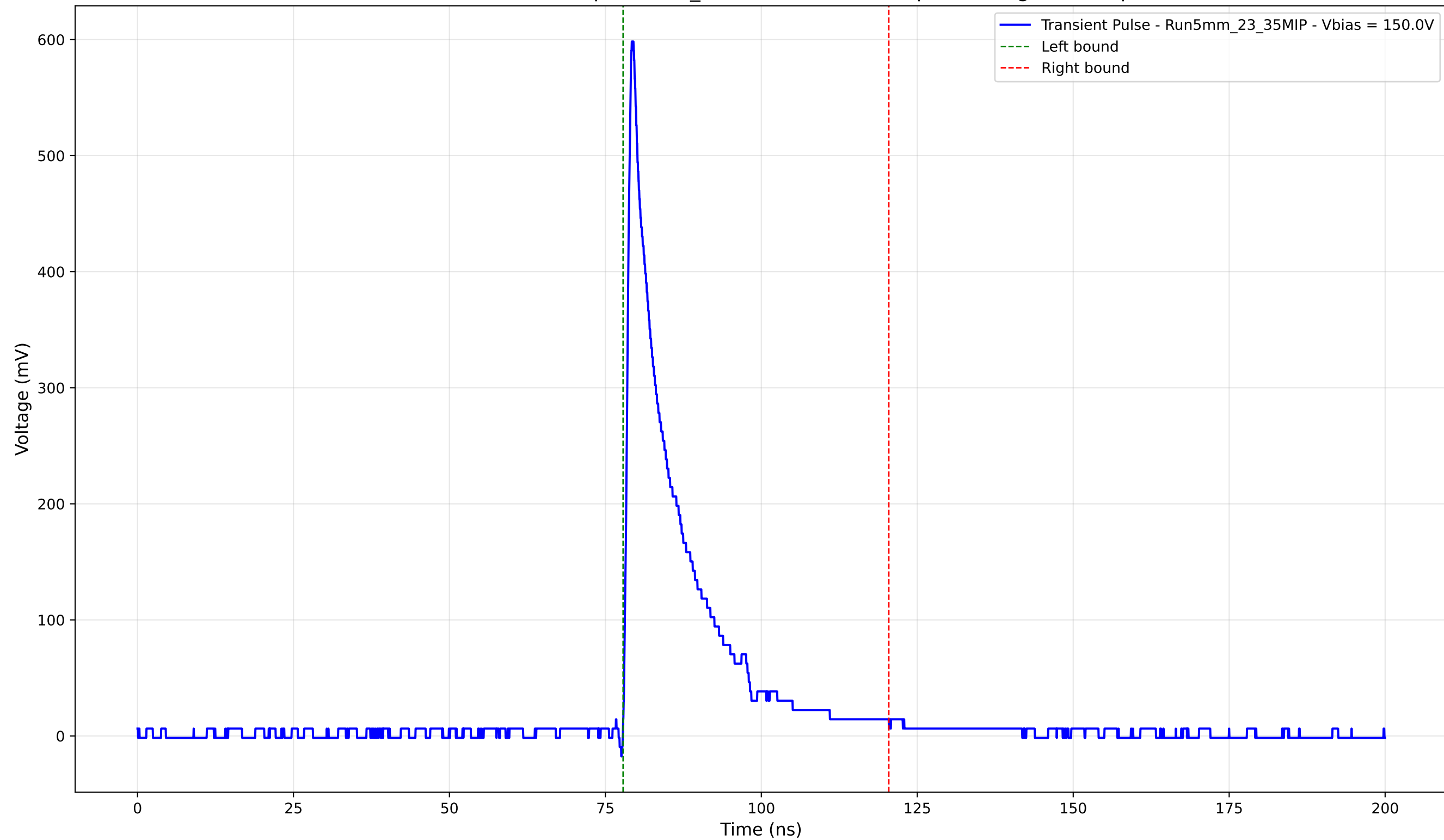
Transient Pulse - Sample: 5mm_23 - Position: 4600.0 \mu\text{m} - Charge: 93.39 pC
