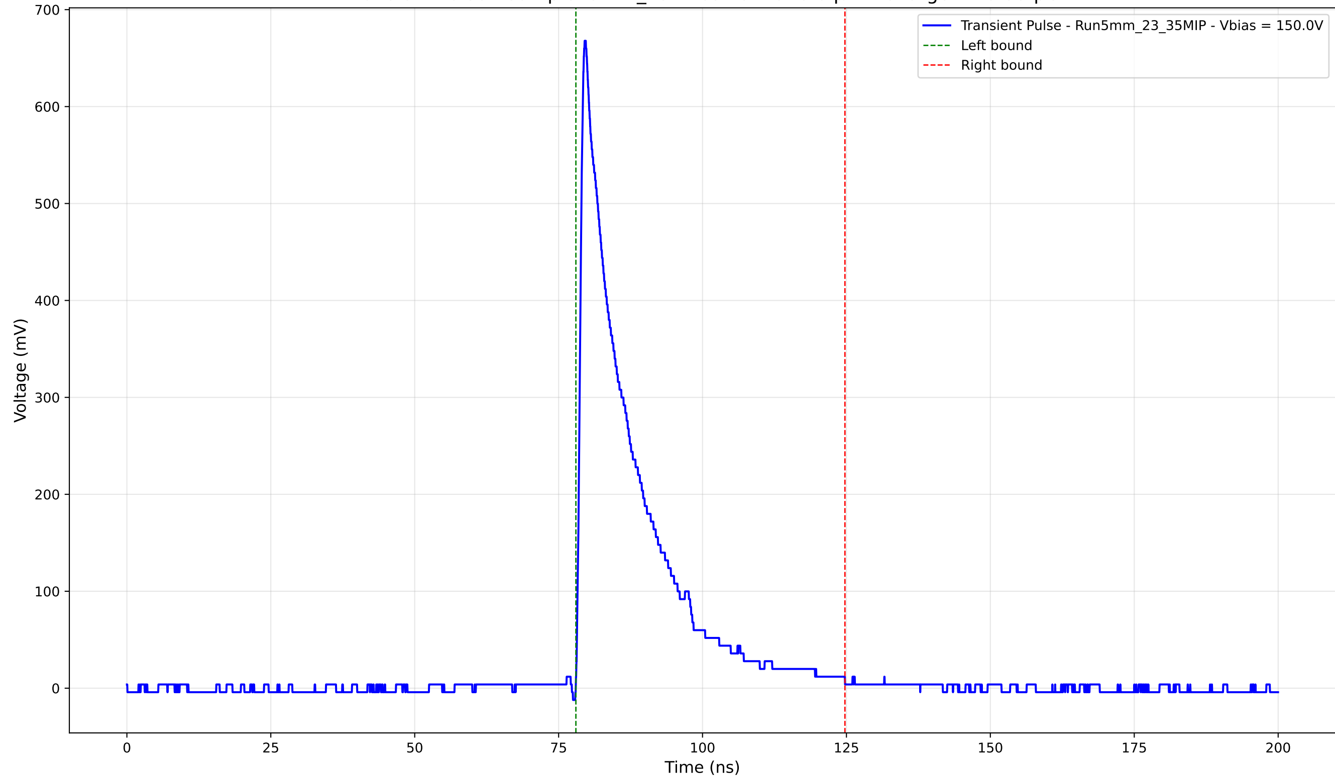
Transient Pulse - Sample: 5mm_23 - Position: 920.0 \mu\text{m} - Charge: 125.55 pC
