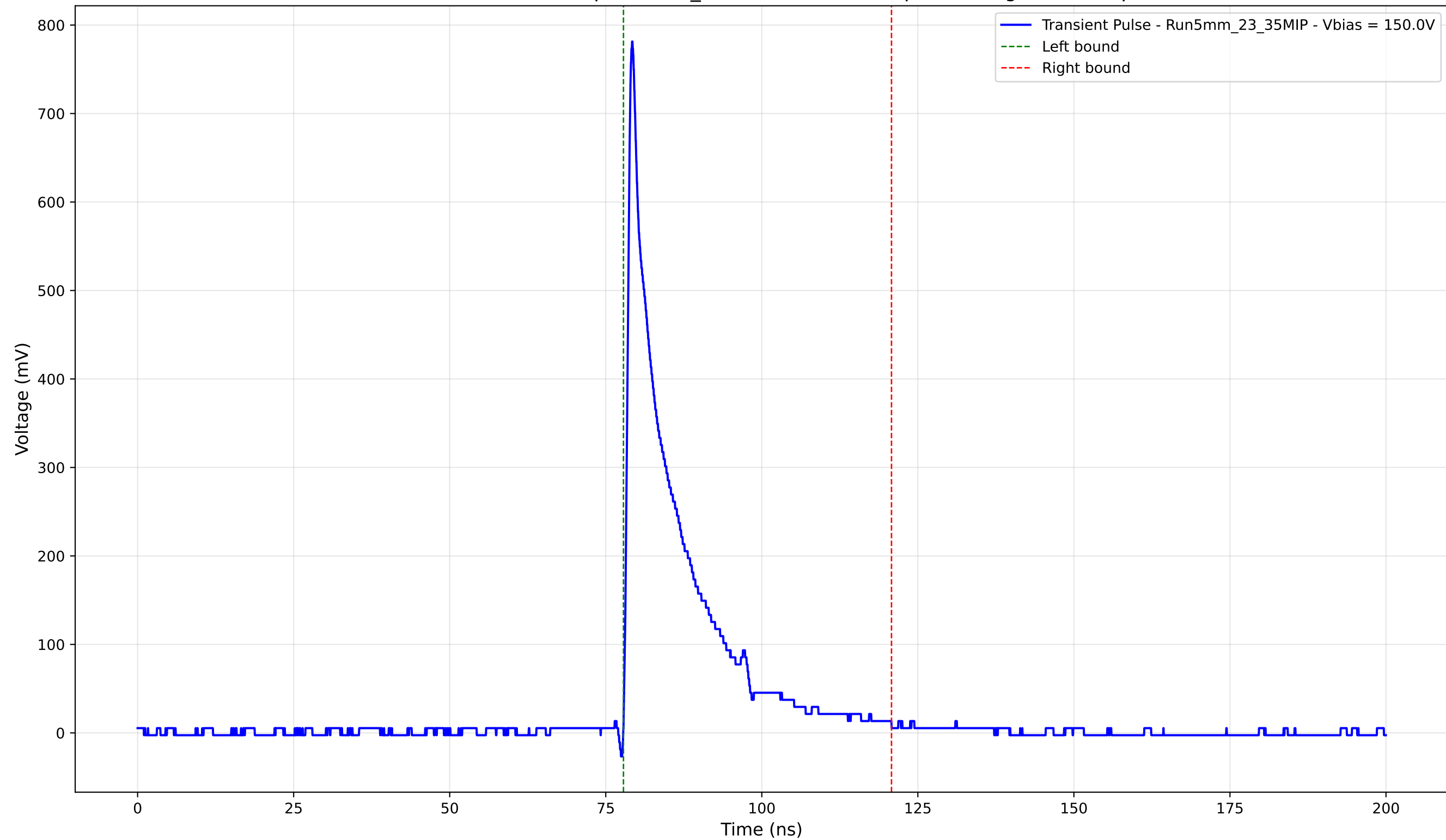
Transient Pulse - Sample: 5mm_23 - Position: 515.0 \mu\text{m} - Charge: 115.76 pC
