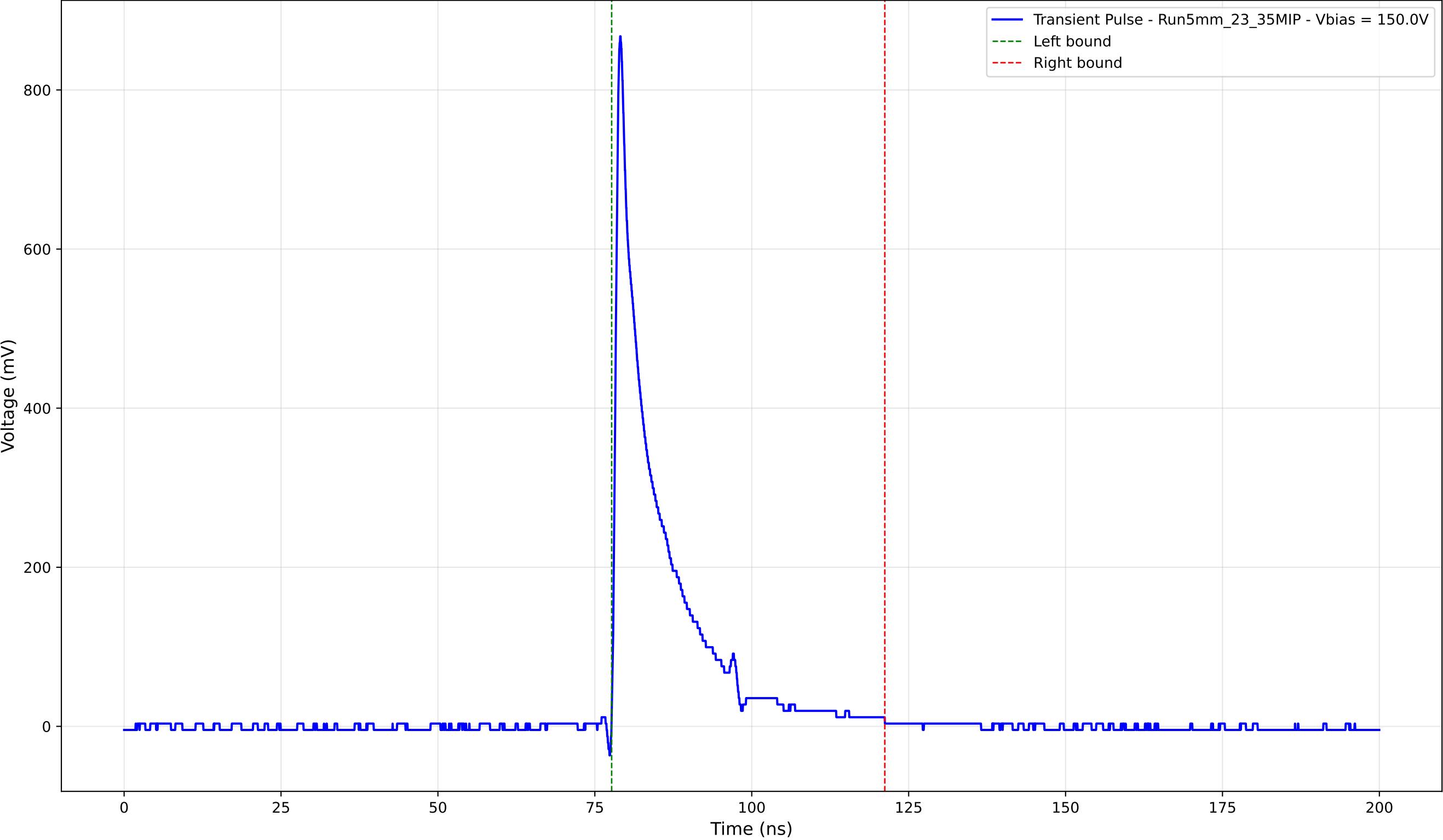
Transient Pulse - Sample: 5mm_23 - Position: 4900.0 \mu\text{m} - Charge: 115.56 pC
