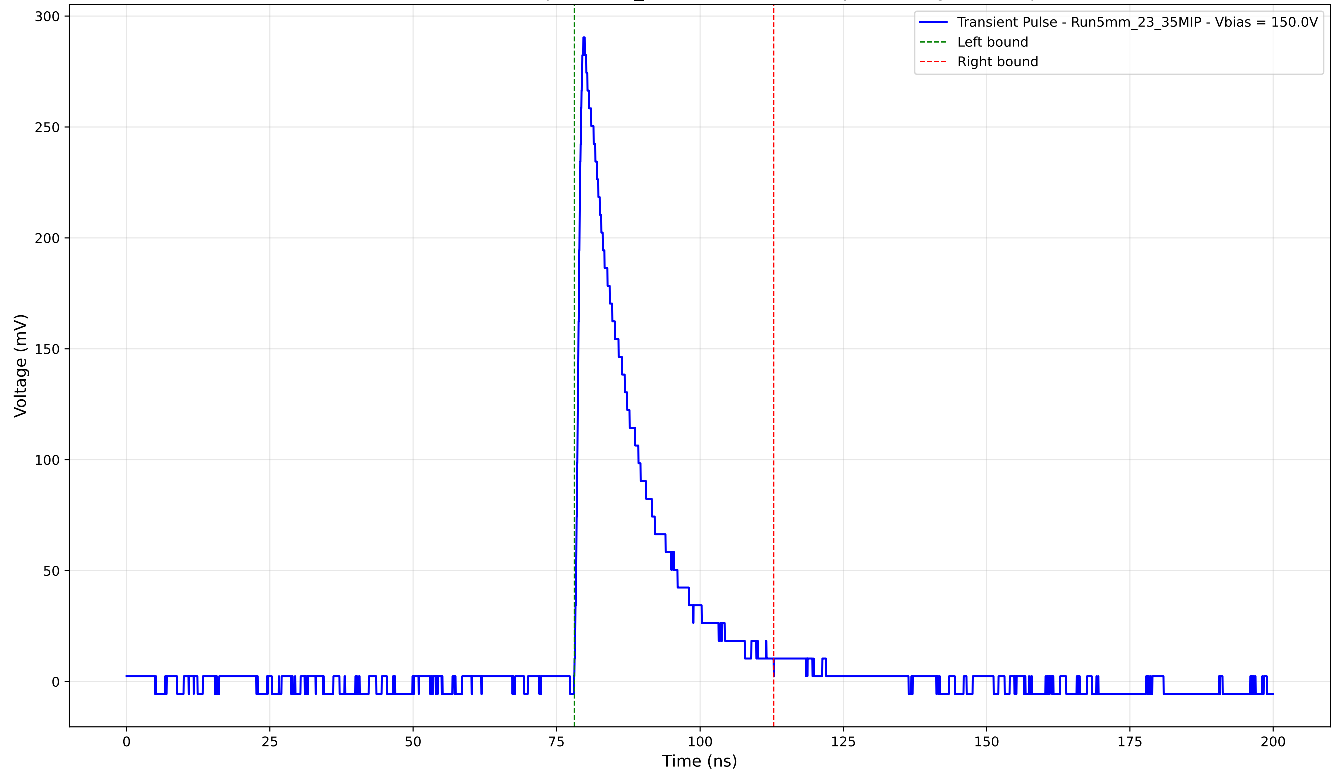
Transient Pulse - Sample: 5mm_23 - Position: 1165.0 \mu\text{m} - Charge: 57.22 pC
