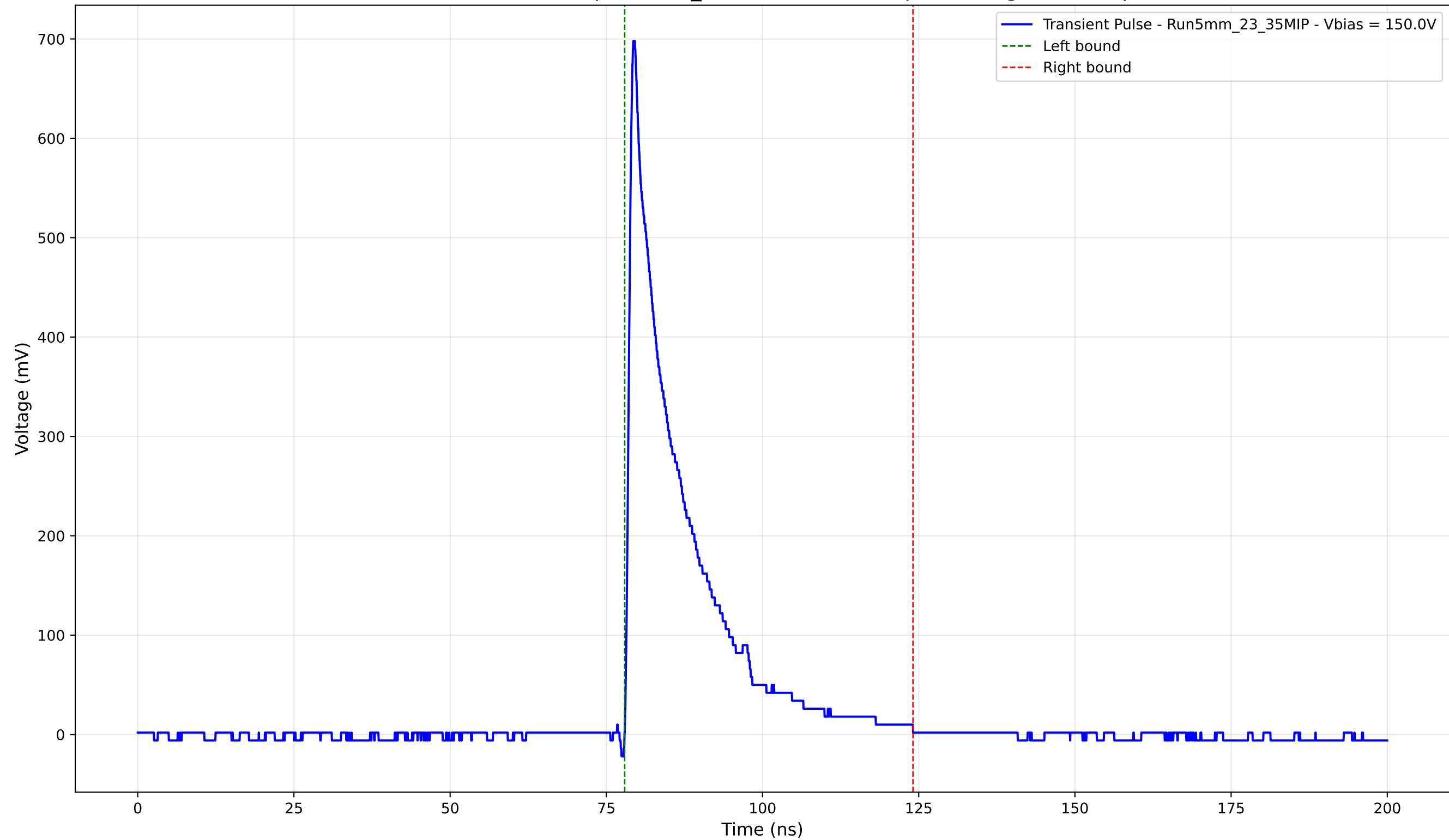
Transient Pulse - Sample: 5mm_23 - Position: 740.0 \mu\text{m} - Charge: 118.24 pC
