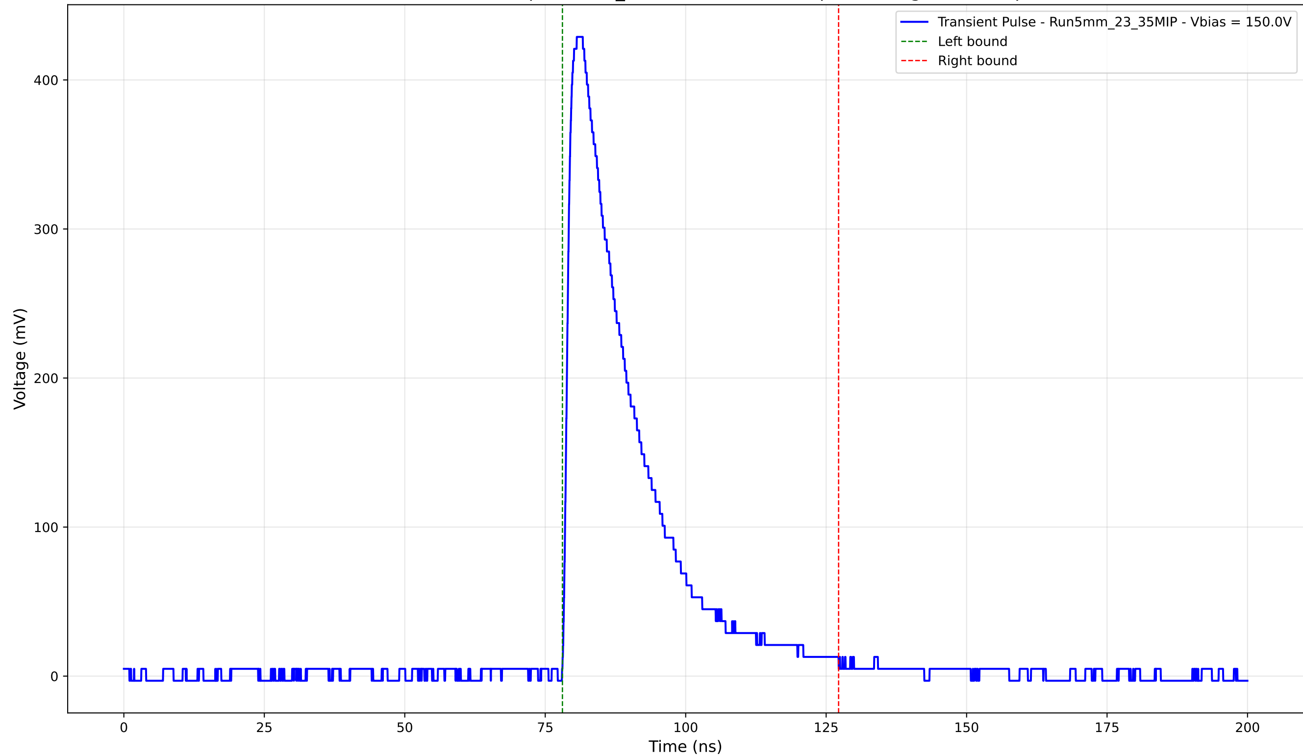
Transient Pulse - Sample: 5mm_23 - Position: 3220.0 \mu\text{m} - Charge: 112.00 pC
