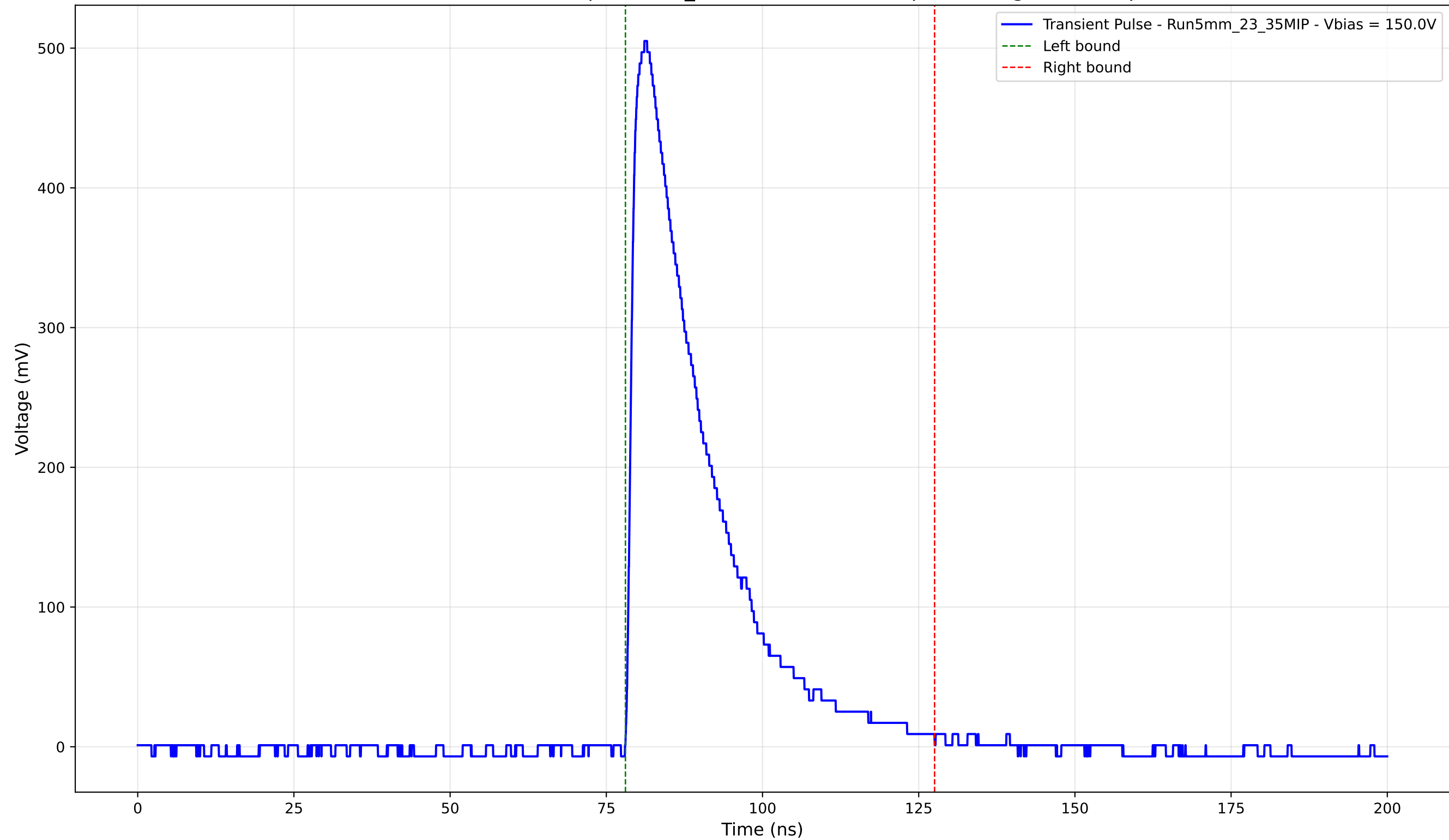
Transient Pulse - Sample: 5mm_23 - Position: 2275.0 \mu\text{m} - Charge: 133.51 pC
