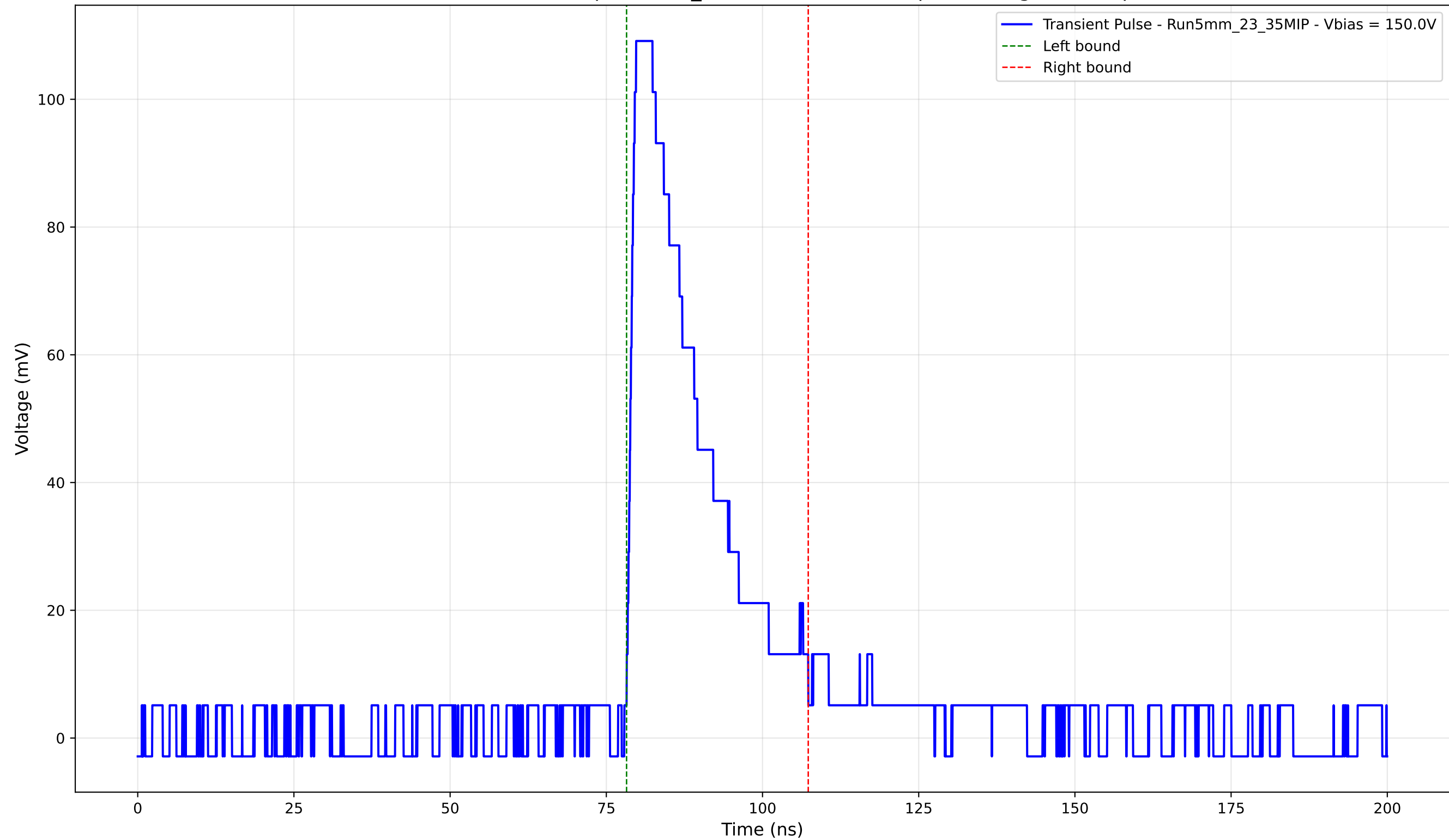
Transient Pulse - Sample: 5mm_23 - Position: 1635.0 \mu\text{m} - Charge: 27.32 pC
