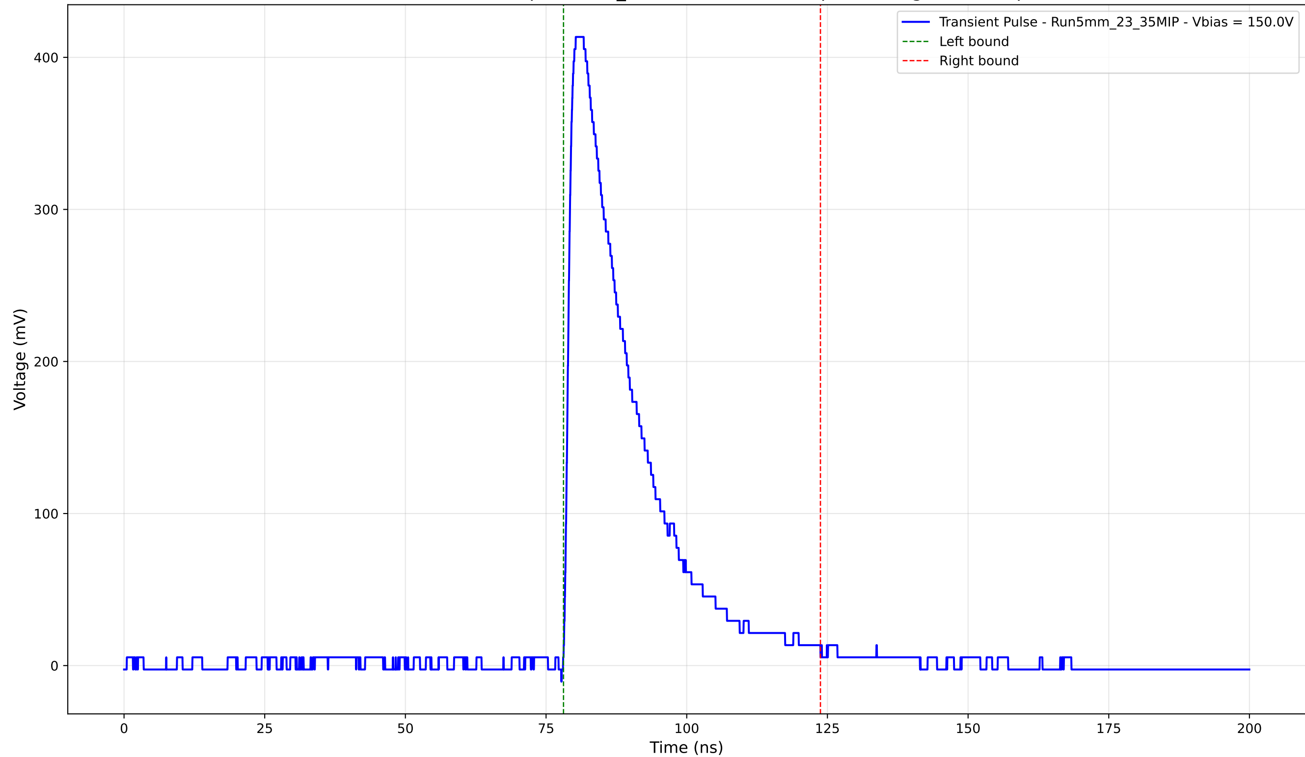
Transient Pulse - Sample: 5mm_23 - Position: 2070.0 \mu\text{m} - Charge: 107.23 pC
