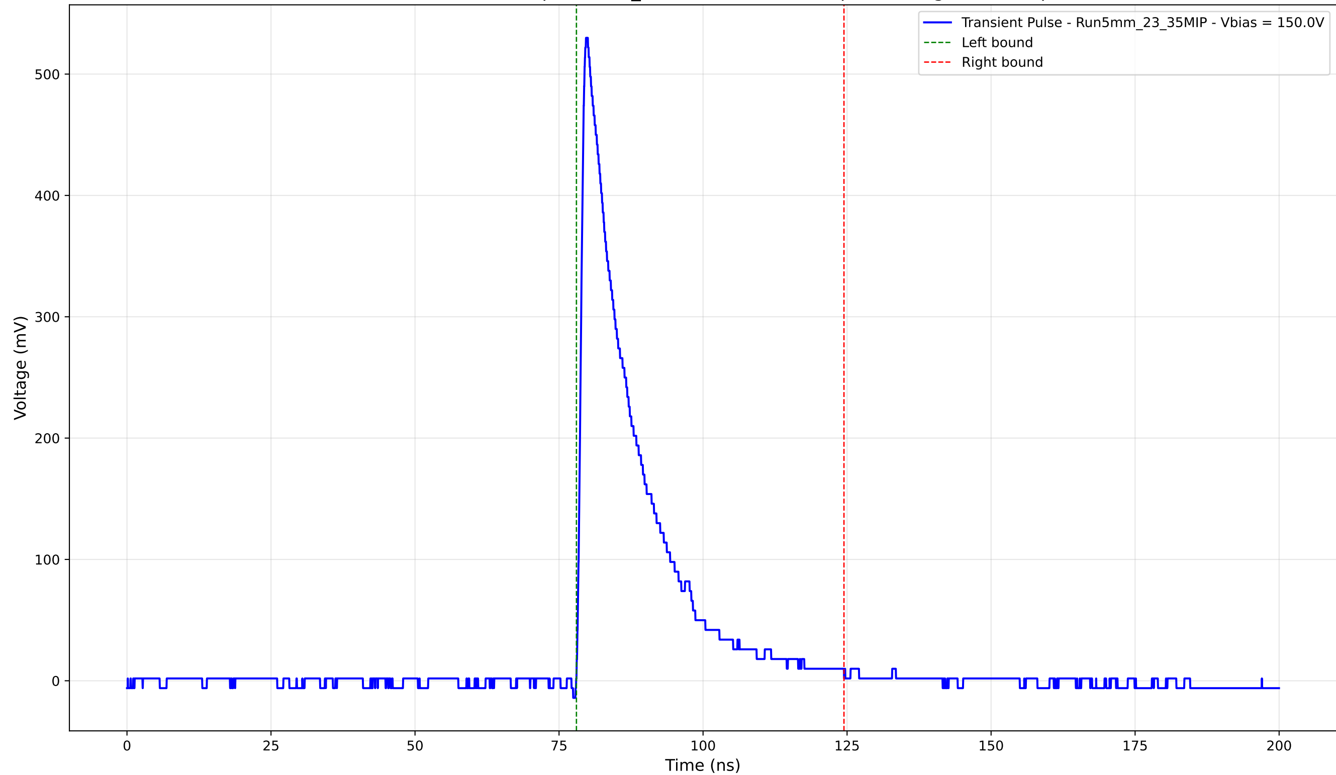
Transient Pulse - Sample: 5mm_23 - Position: 4075.0 \mu\text{m} - Charge: 105.25 pC
