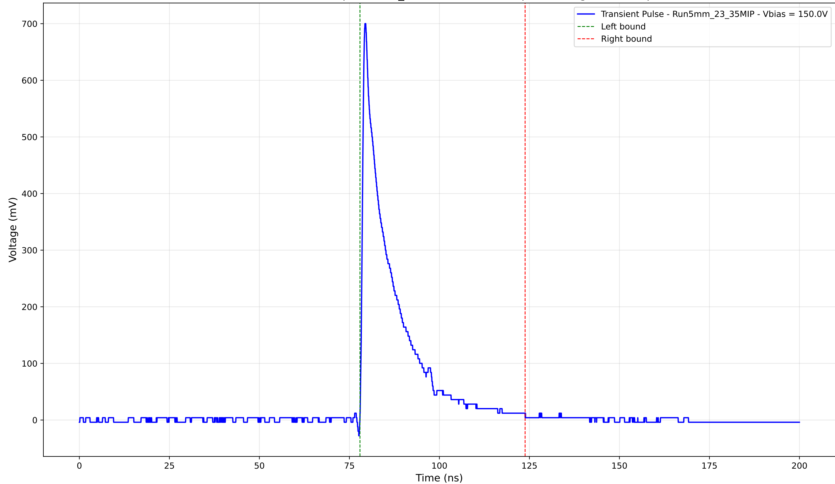
Transient Pulse - Sample: 5mm_23 - Position: 725.0 \mu\text{m} - Charge: 118.06 pC
