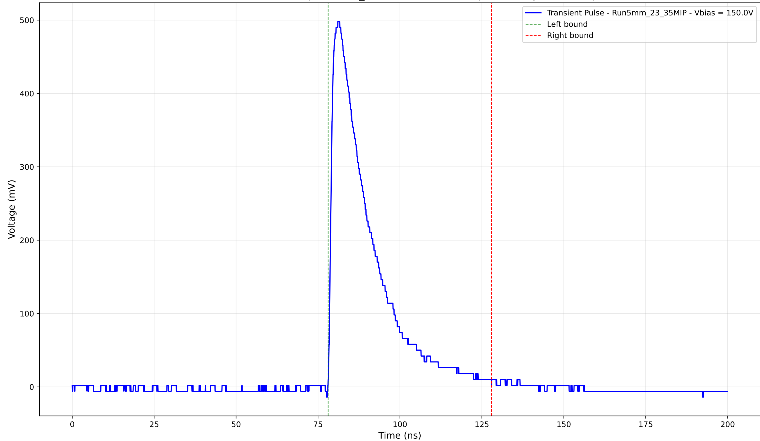
Transient Pulse - Sample: 5mm_23 - Position: 2250.0 \mu\text{m} - Charge: 132.45 pC
