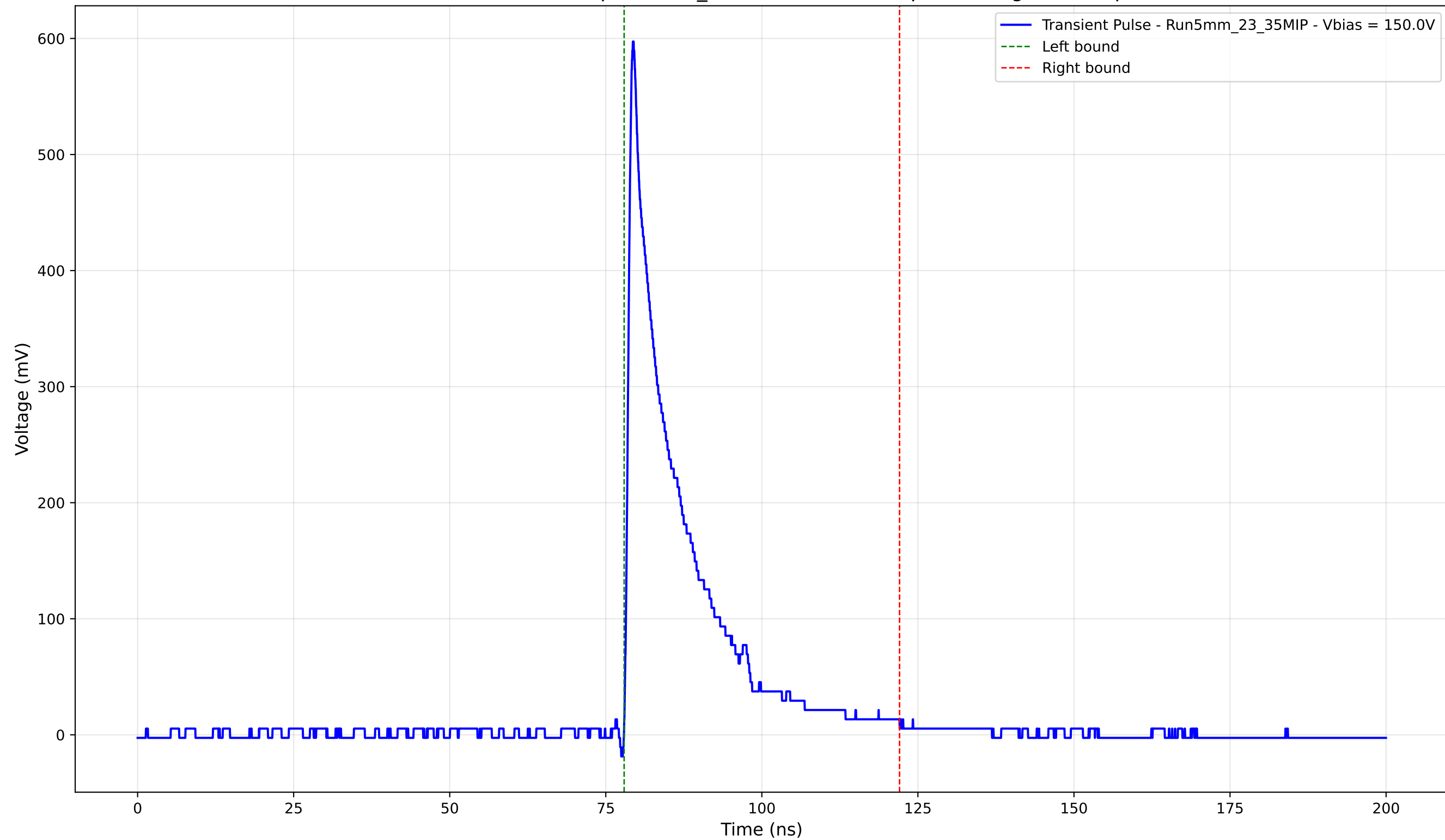
Transient Pulse - Sample: 5mm_23 - Position: 690.0 \mu\text{m} - Charge: 97.45 pC
