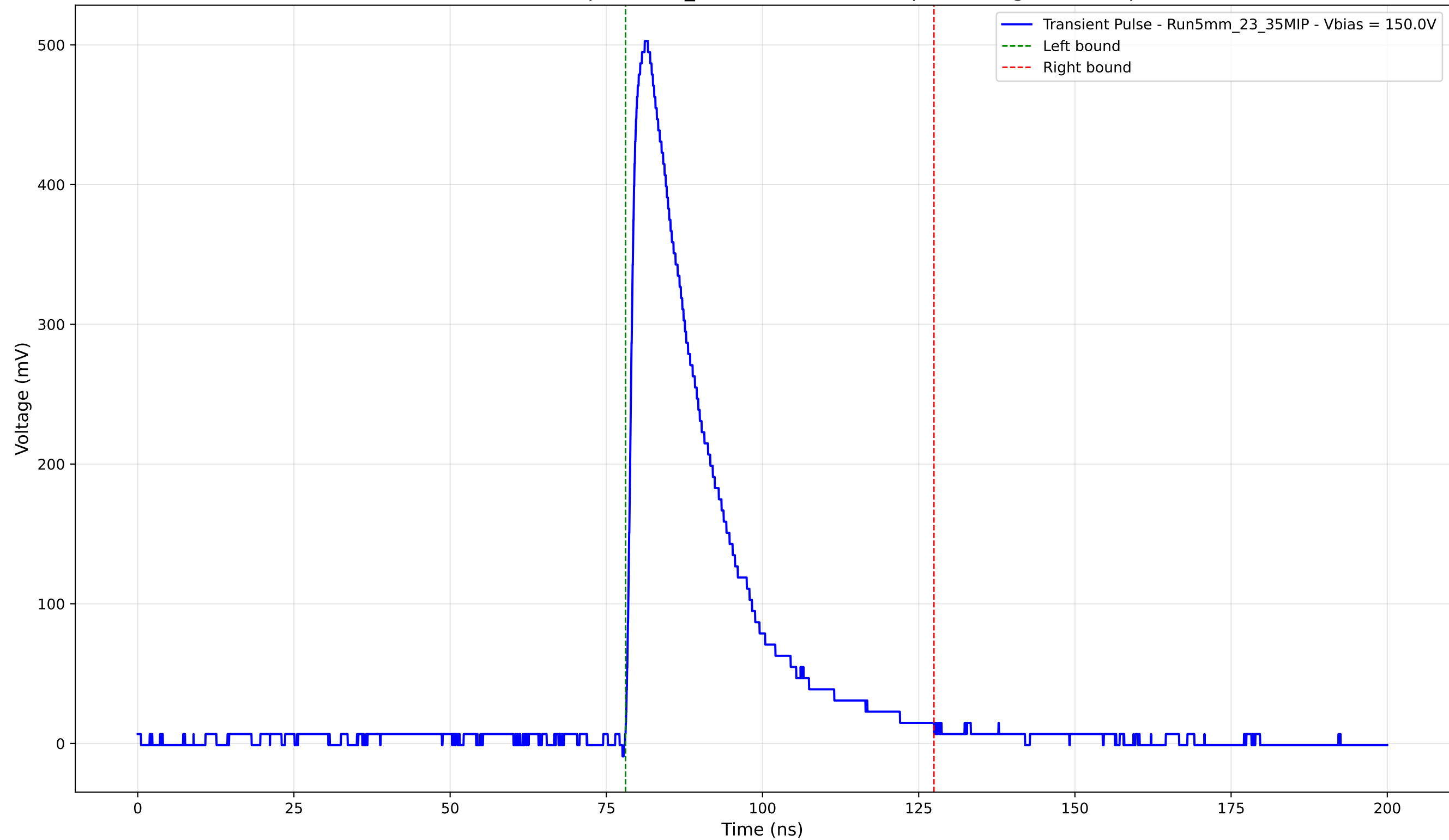
Transient Pulse - Sample: 5mm_23 - Position: 2880.0 \mu\text{m} - Charge: 135.25 pC
