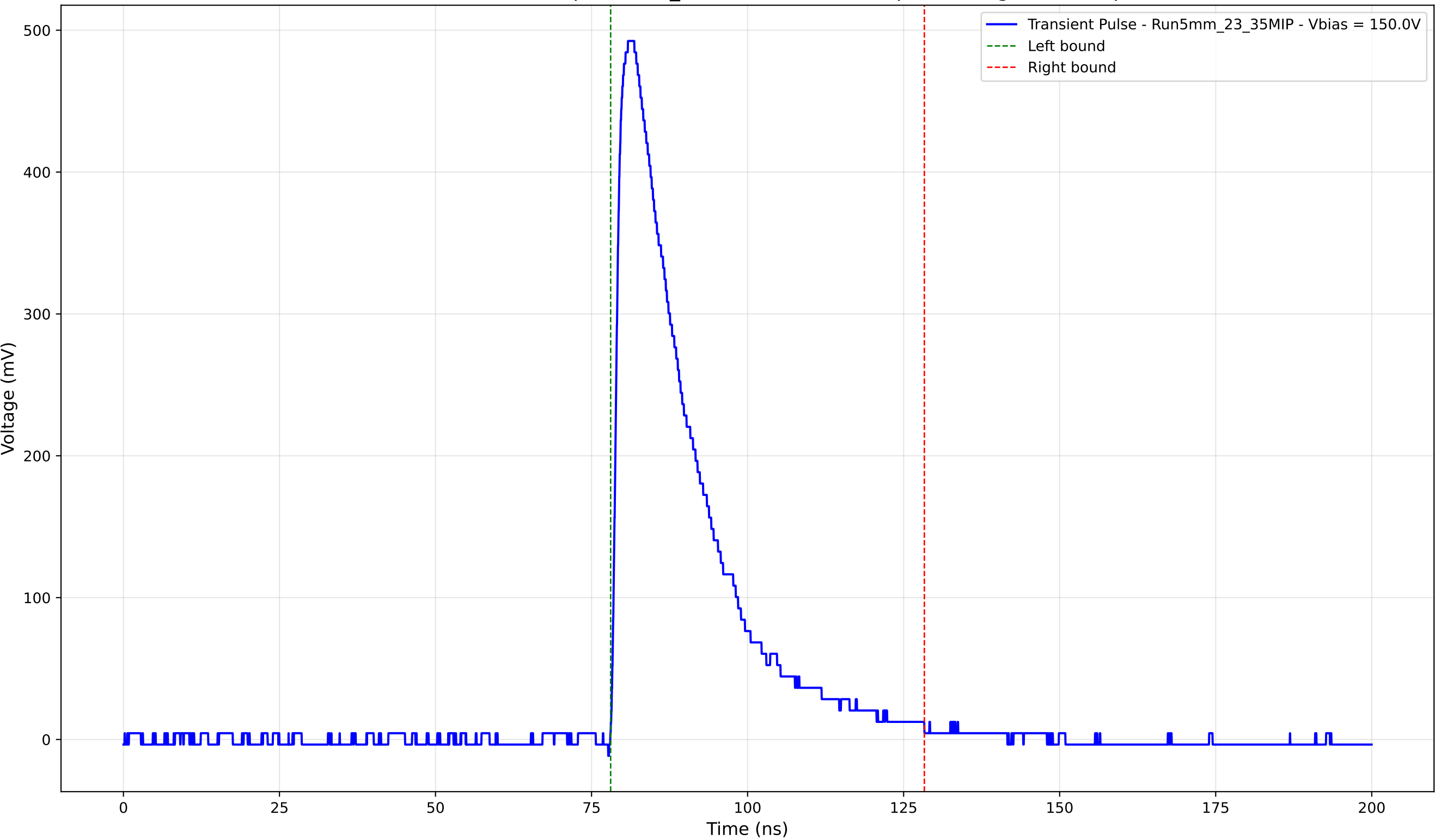
Transient Pulse - Sample: 5mm_23 - Position: 2945.0 \mu\text{m} - Charge: 132.86 pC
