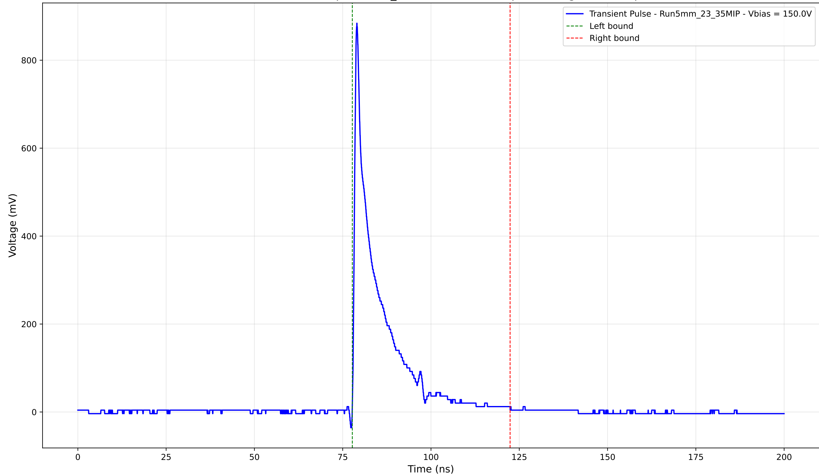
Transient Pulse - Sample: 5mm_23 - Position: 285.0 \mu\text{m} - Charge: 115.44 pC
