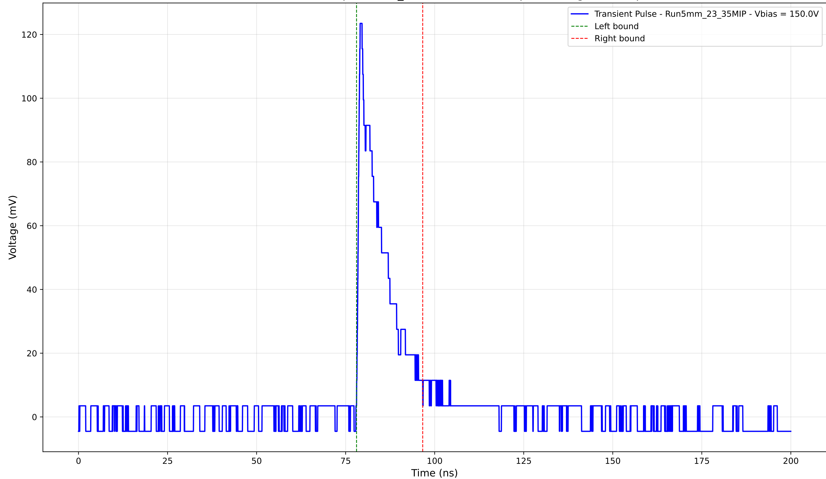
Transient Pulse - Sample: 5mm_23 - Position: 615.0 \mu\text{m} - Charge: 17.86 pC
