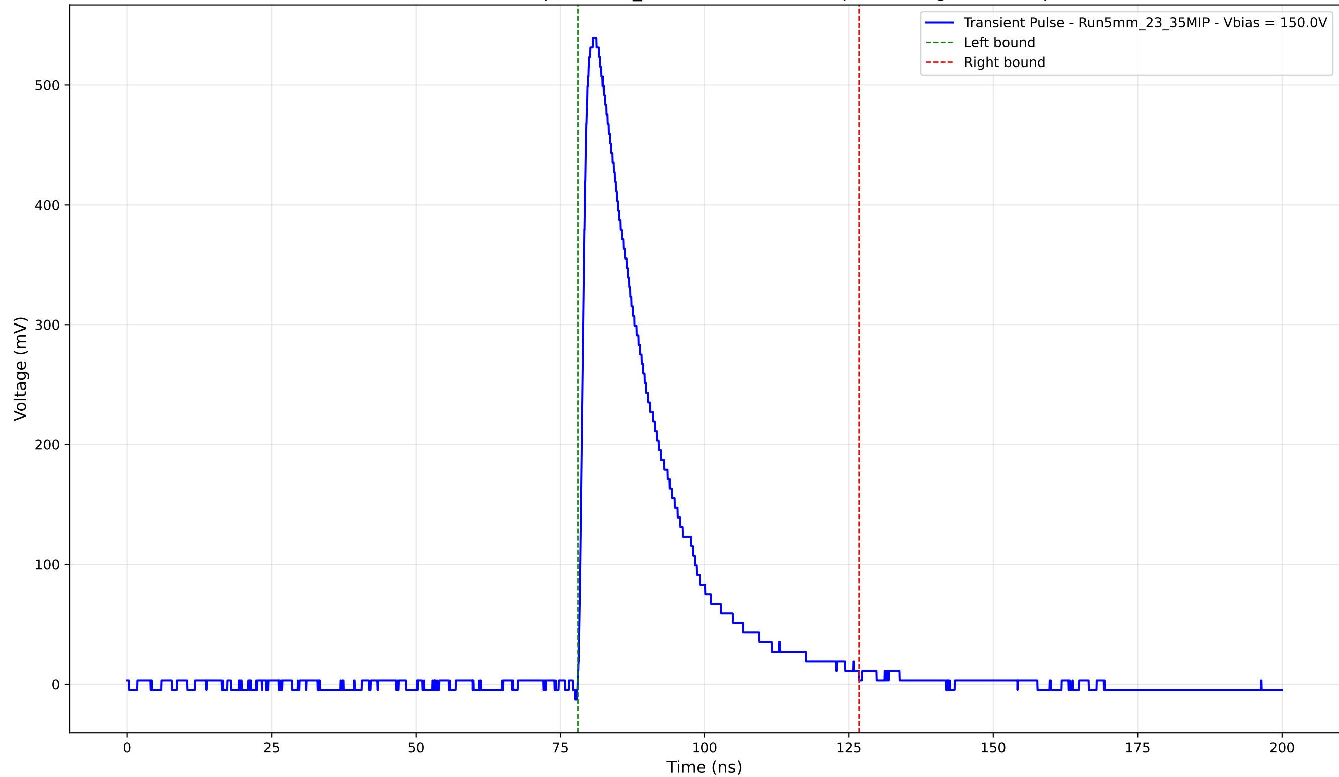
Transient Pulse - Sample: 5mm_23 - Position: 2030.0 \mu\text{m} - Charge: 140.95 pC
