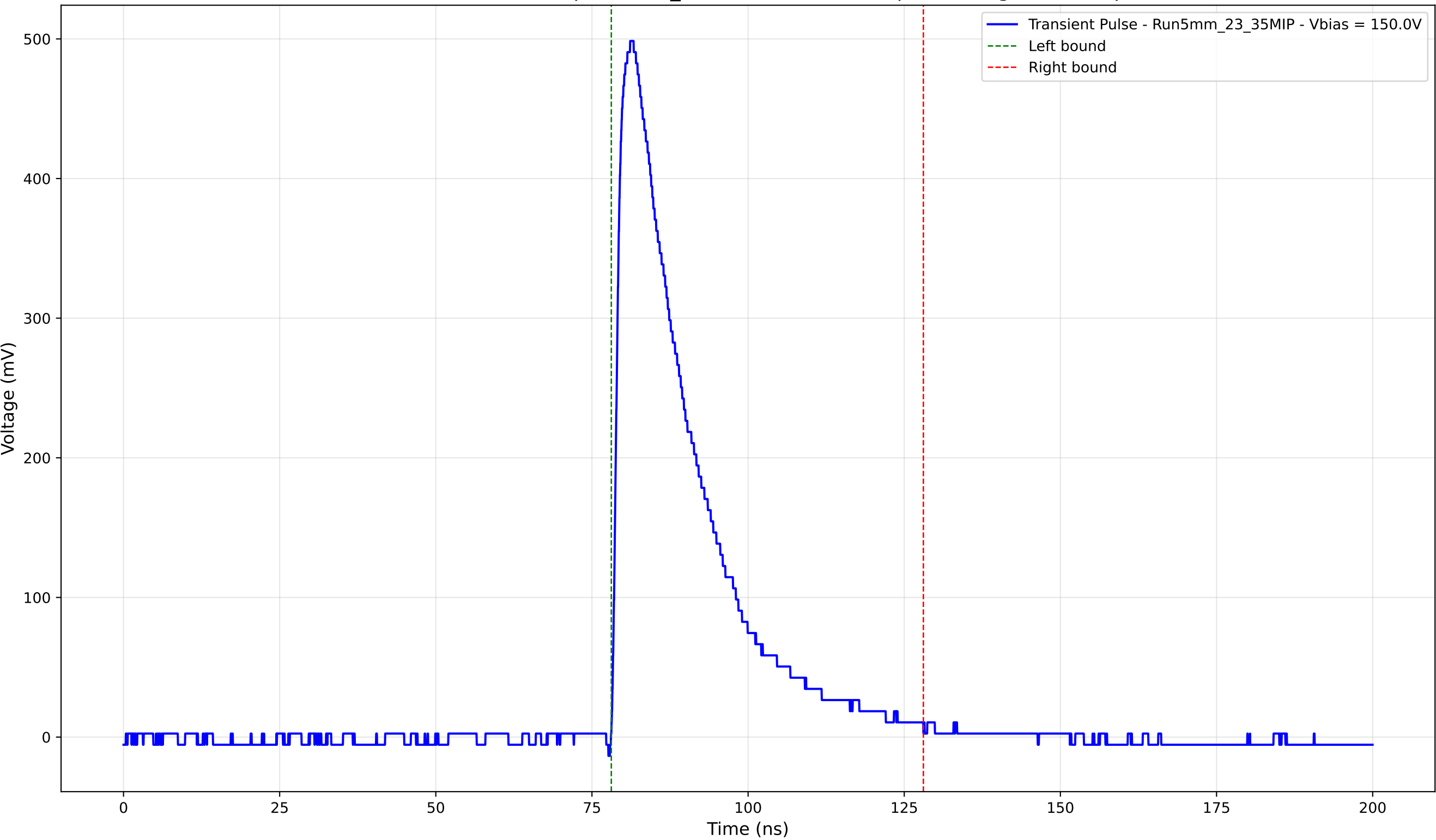
Transient Pulse - Sample: 5mm_23 - Position: 2935.0 \mu\text{m} - Charge: 132.89 pC
