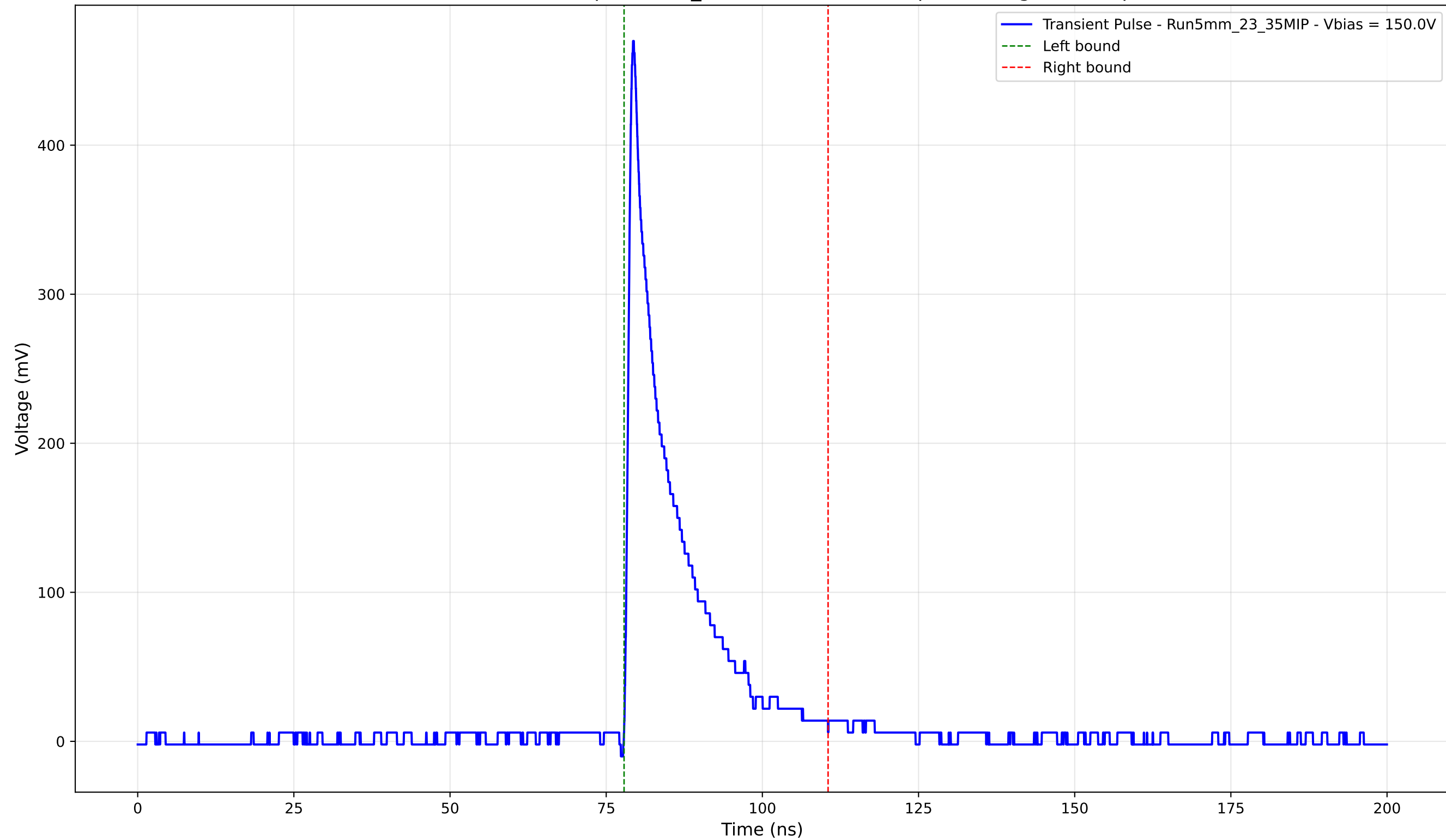
Transient Pulse - Sample: 5mm_23 - Position: 4620.0 \mu\text{m} - Charge: 68.73 pC
