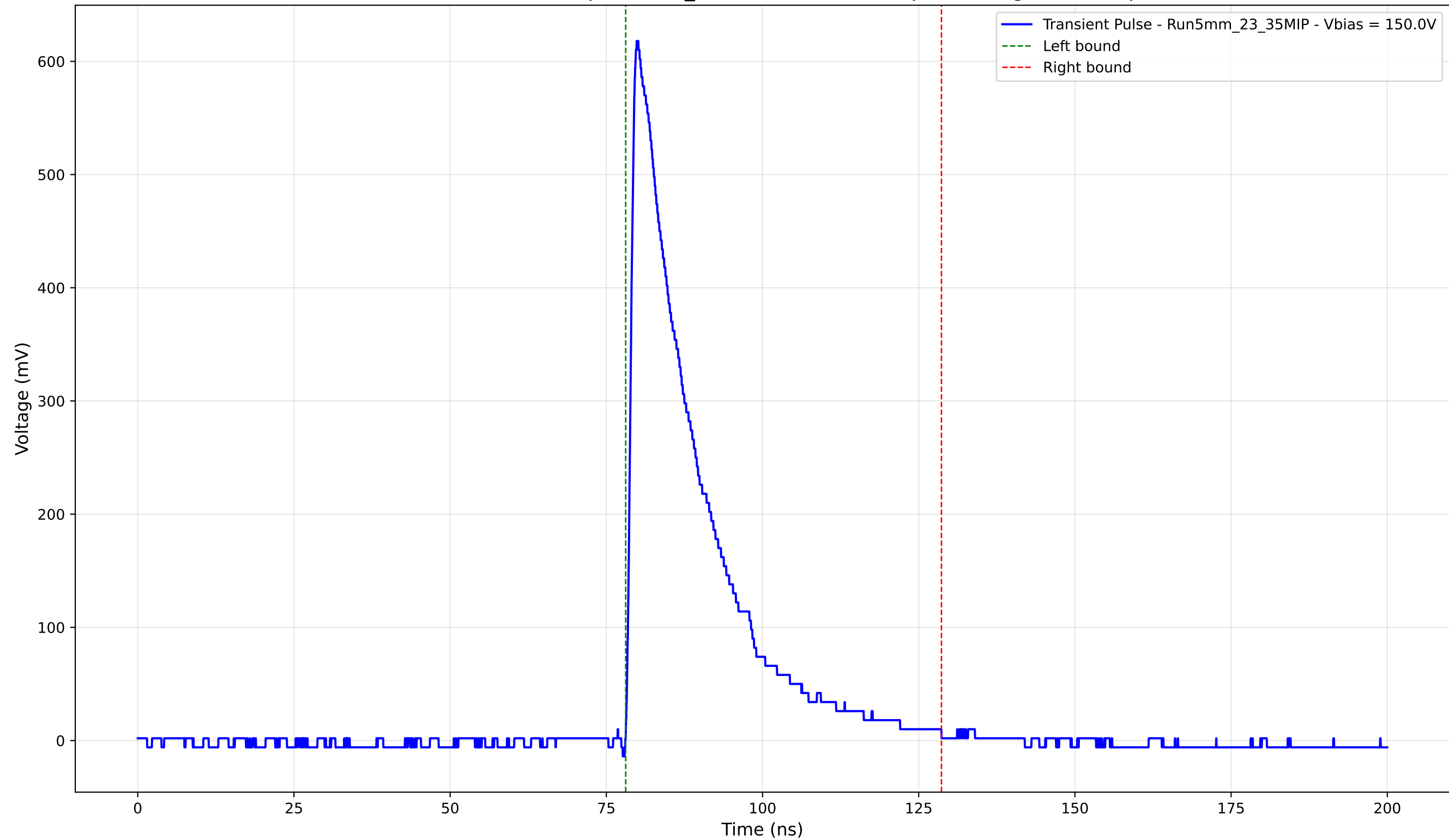
Transient Pulse - Sample: 5mm_23 - Position: 1390.0 \mu\text{m} - Charge: 140.93 pC
