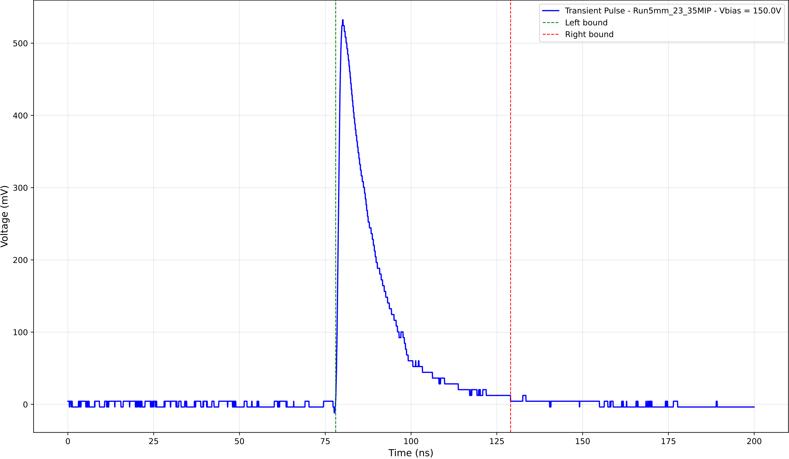
Transient Pulse - Sample: 5mm_23 - Position: 3750.0 \mu\text{m} - Charge: 122.54 pC
