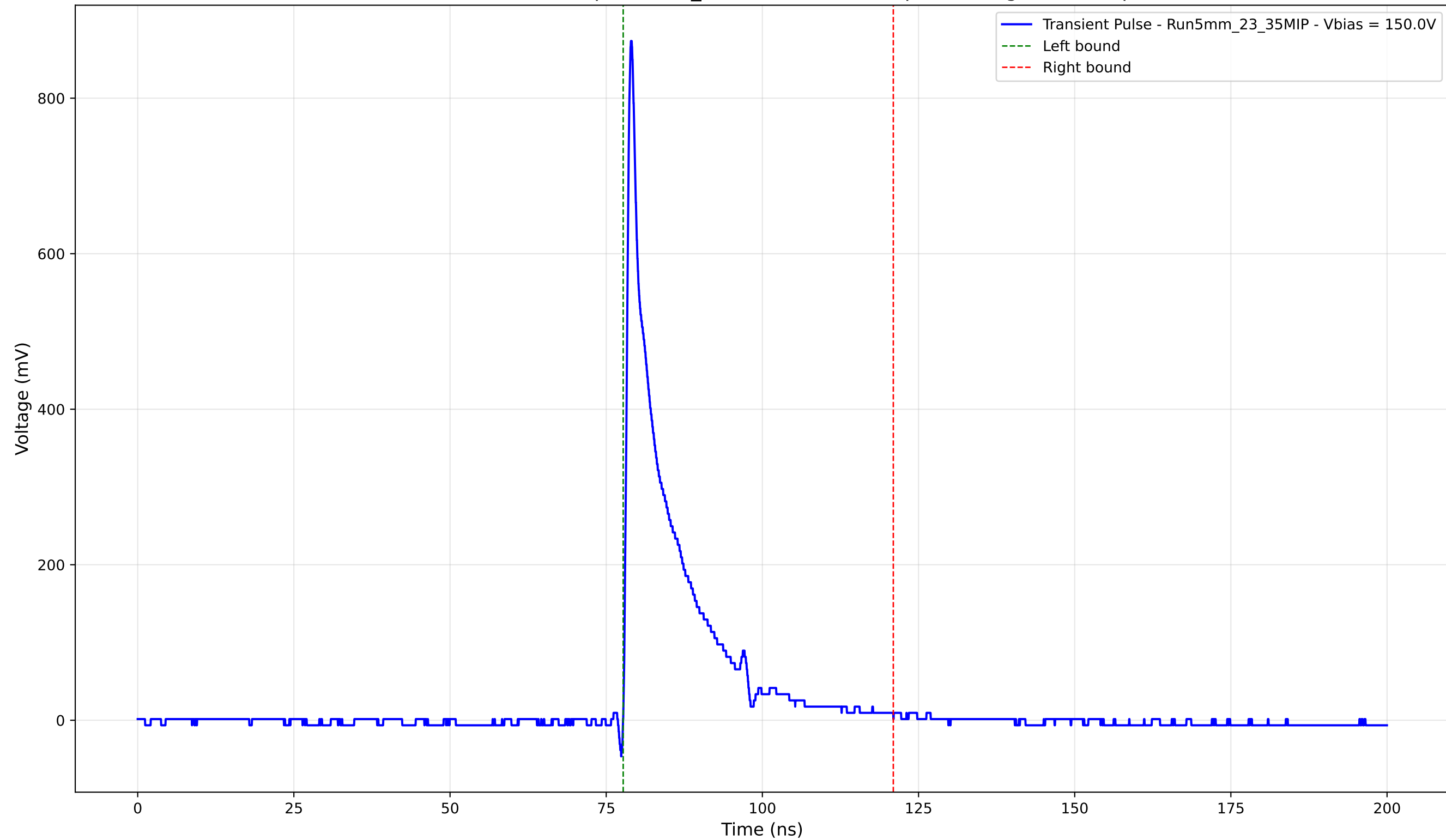
Transient Pulse - Sample: 5mm_23 - Position: 270.0 \mu\text{m} - Charge: 110.57 pC
