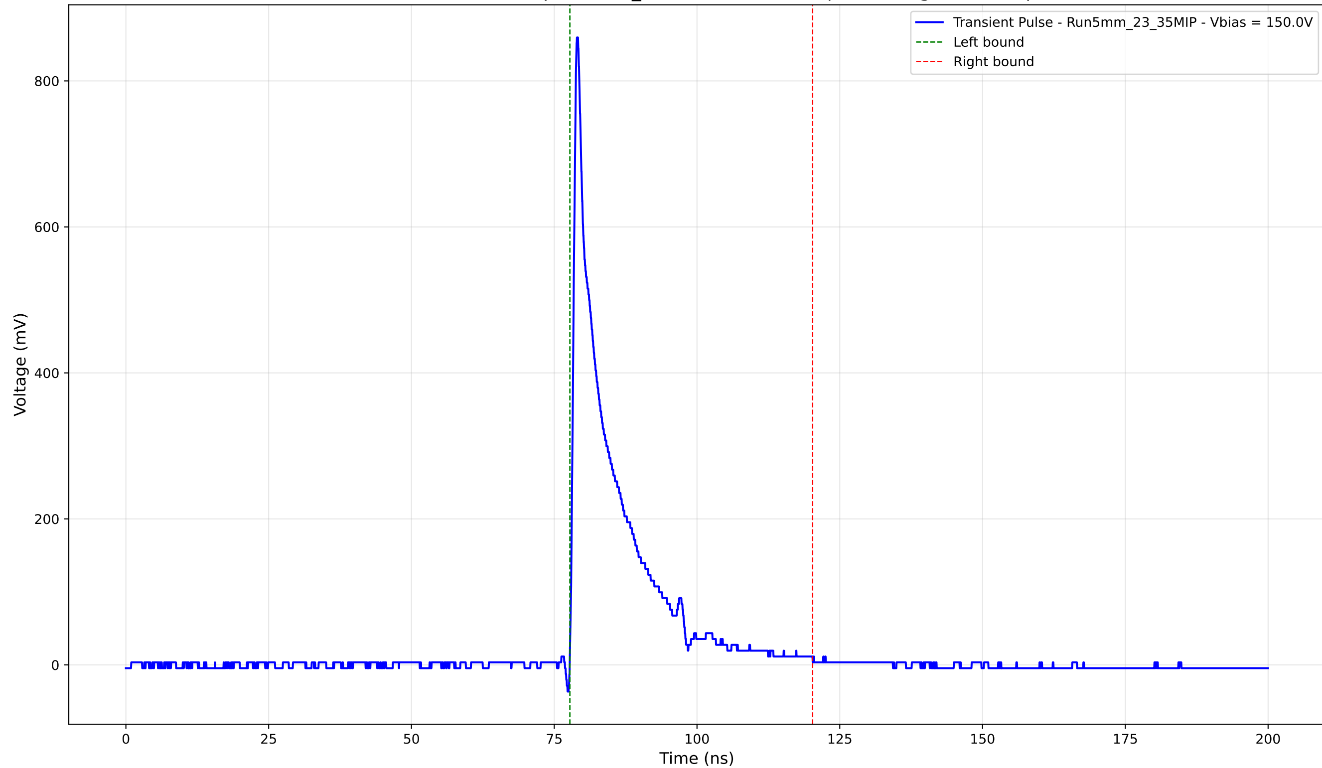
Transient Pulse - Sample: 5mm_23 - Position: 325.0 \mu\text{m} - Charge: 113.69 pC
