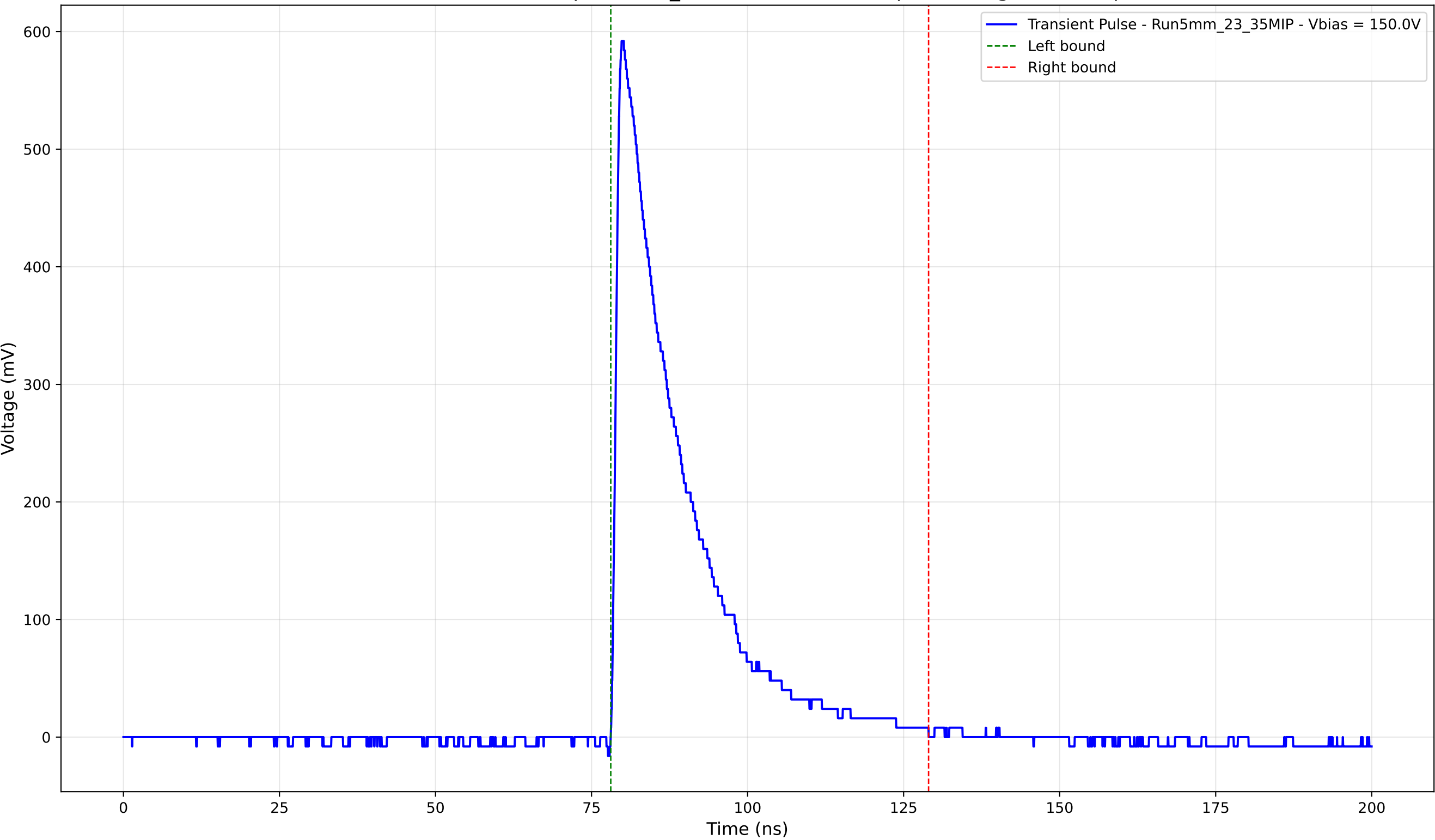
Transient Pulse - Sample: 5mm_23 - Position: 1360.0 \mu\text{m} - Charge: 132.65 pC
