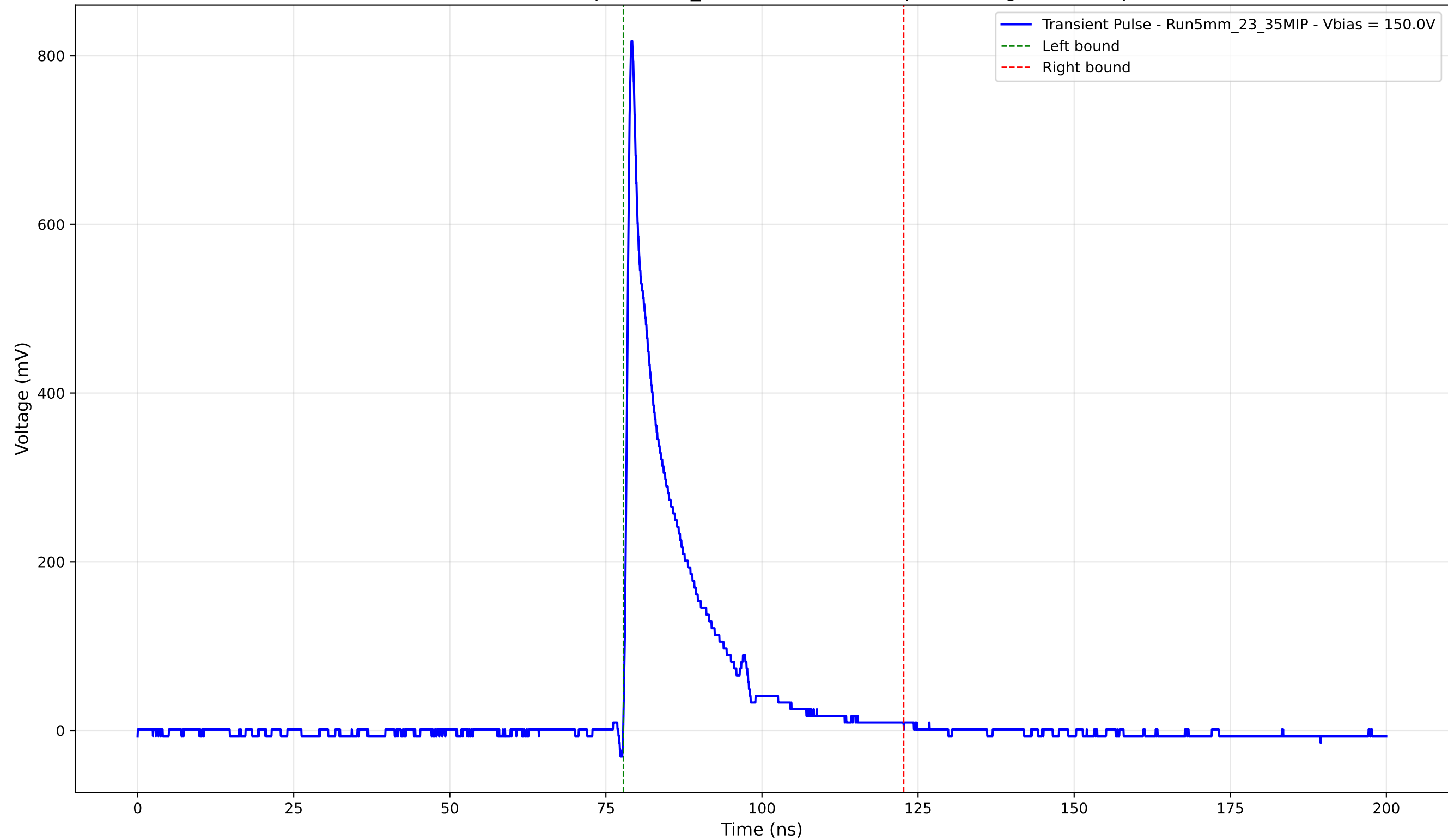
Transient Pulse - Sample: 5mm_23 - Position: 430.0 \mu\text{m} - Charge: 114.00 pC
