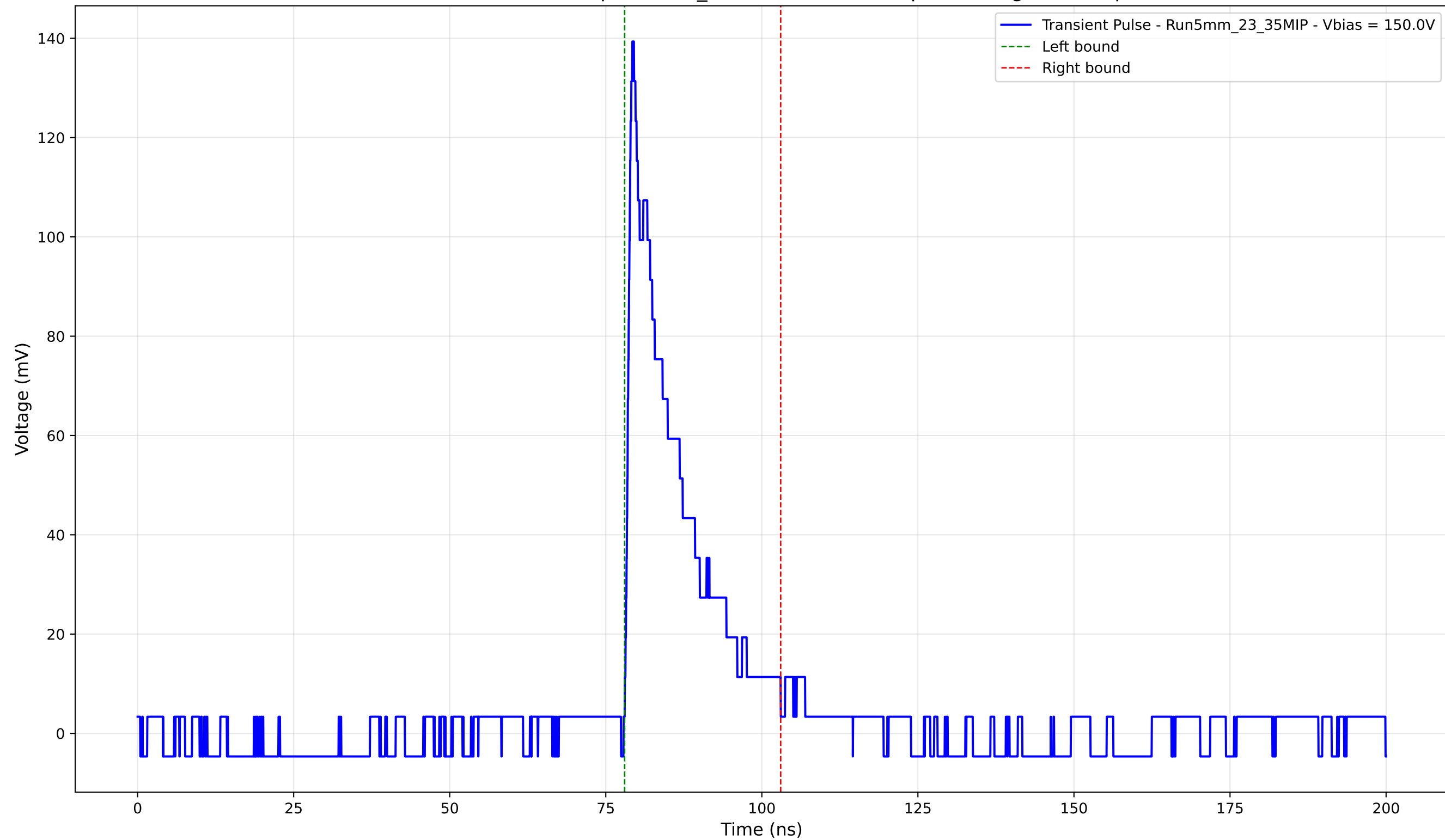
Transient Pulse - Sample: 5mm_23 - Position: 630.0 \mu\text{m} - Charge: 22.21 pC
