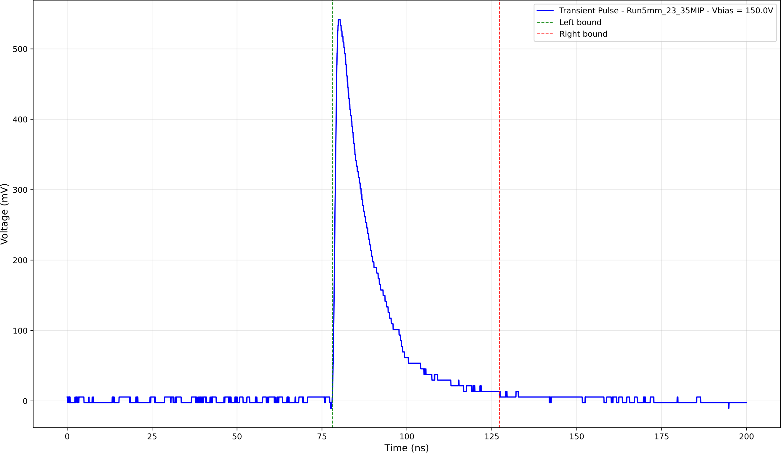
Transient Pulse - Sample: 5mm_23 - Position: 3800.0 \mu\text{m} - Charge: 124.93 pC
