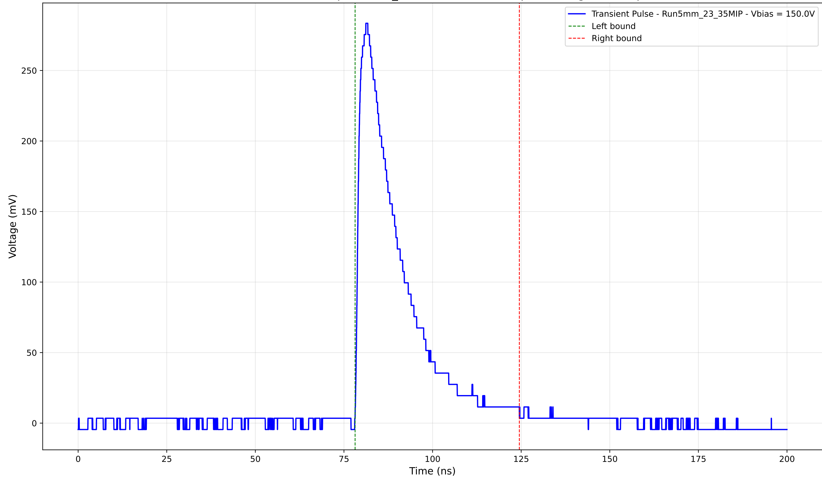
Transient Pulse - Sample: 5mm_23 - Position: 2695.0 \mu\text{m} - Charge: 73.95 pC
