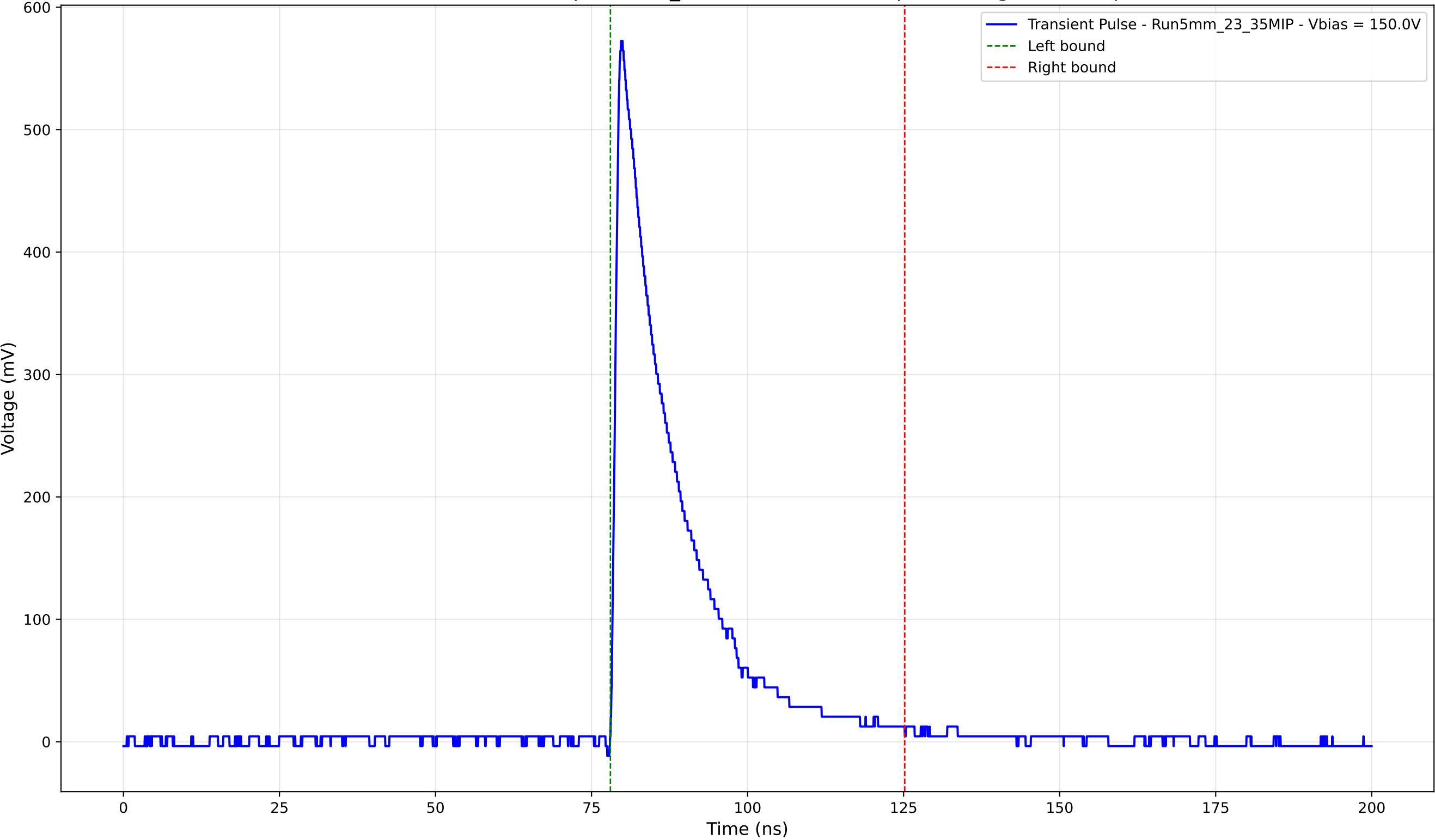
Transient Pulse - Sample: 5mm_23 - Position: 4045.0 \mu\text{m} - Charge: 117.90 pC
