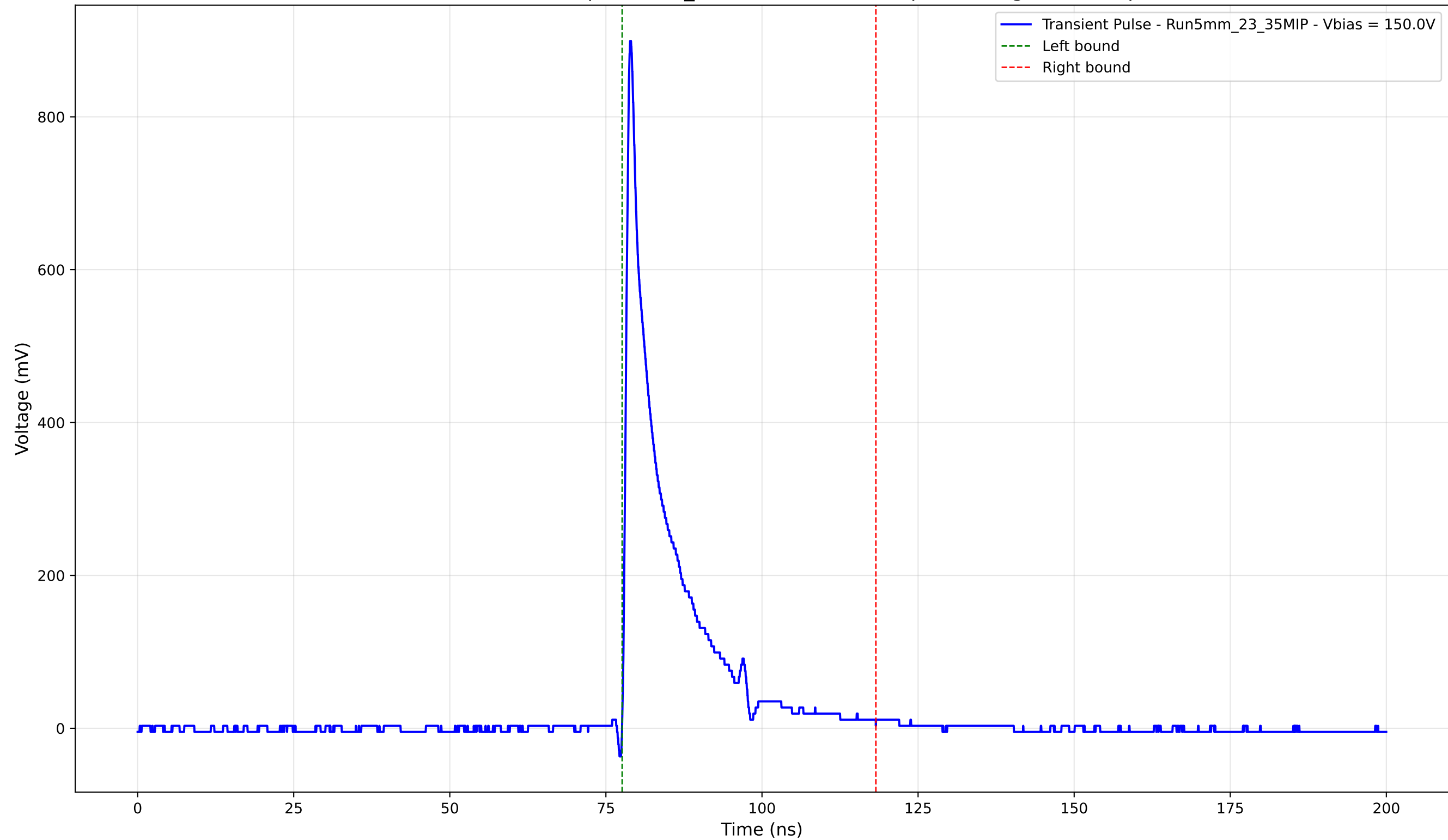
Transient Pulse - Sample: 5mm_23 - Position: 5005.0 \mu\text{m} - Charge: 112.37 pC
