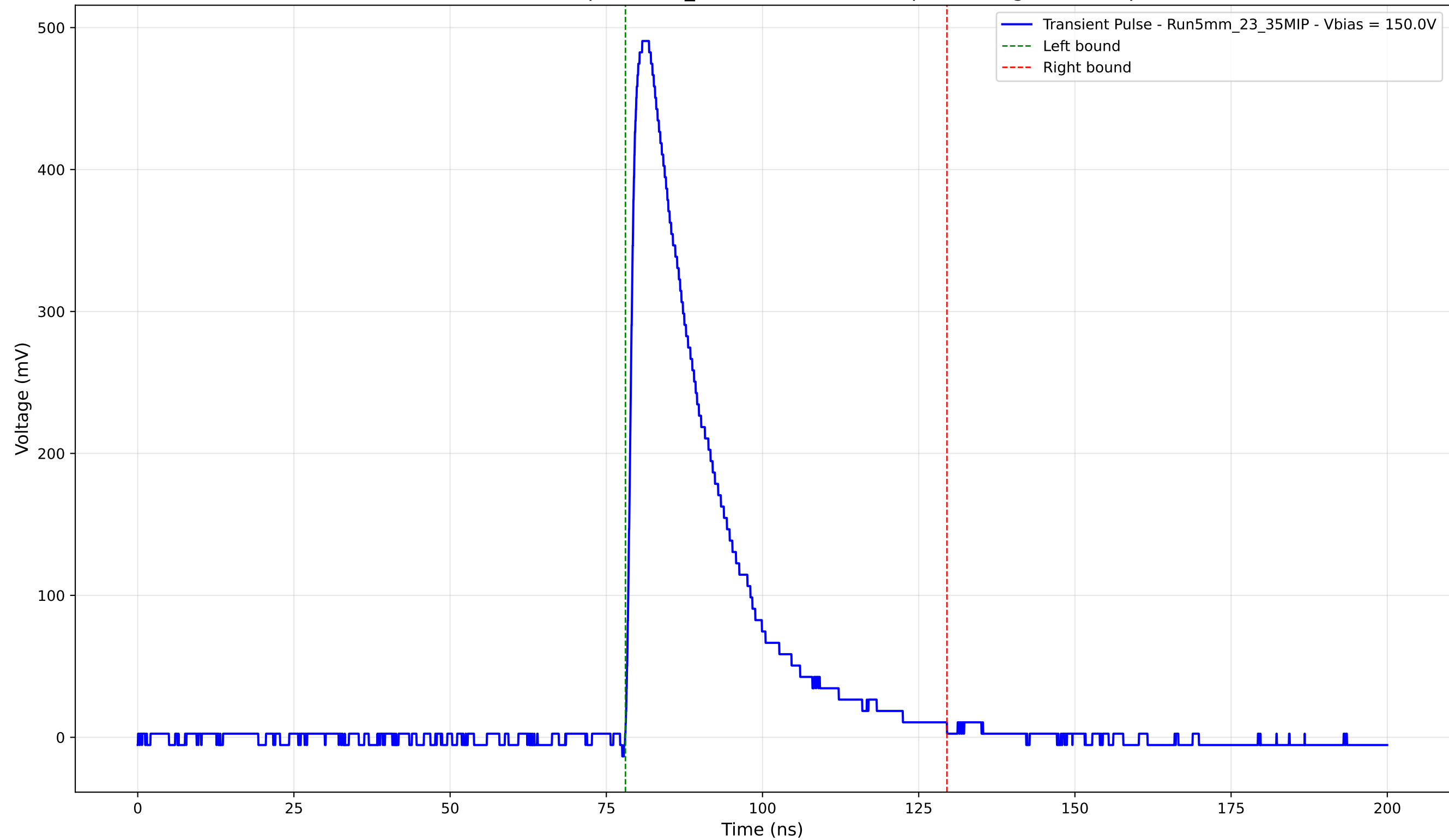
Transient Pulse - Sample: 5mm_23 - Position: 2240.0 \mu\text{m} - Charge: 132.01 pC
