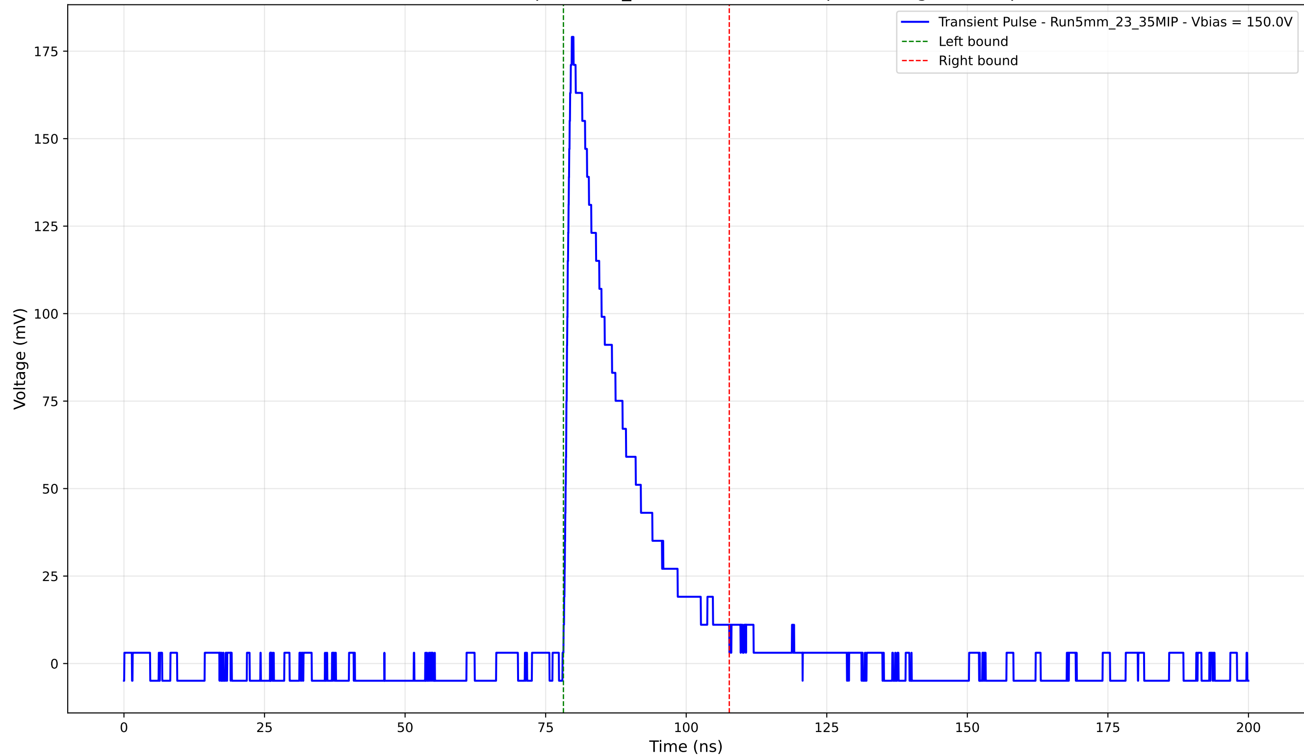
Transient Pulse - Sample: 5mm_23 - Position: 1150.0 \mu\text{m} - Charge: 35.60 pC
