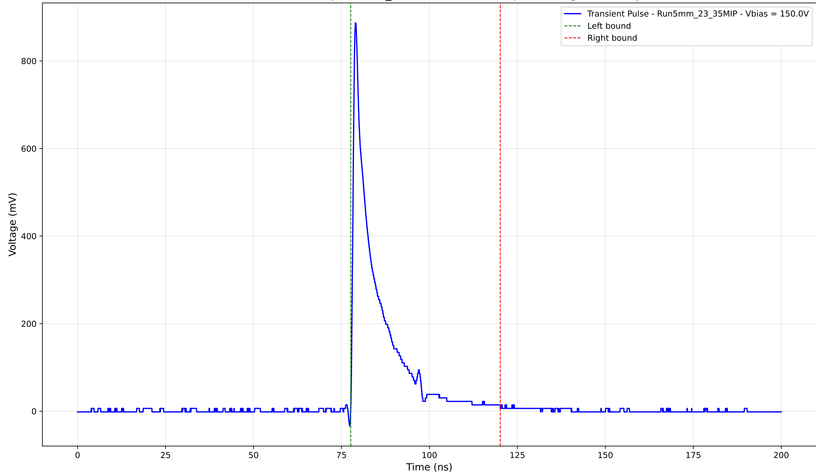
Transient Pulse - Sample: 5mm_23 - Position: 4935.0 \mu\text{m} - Charge: 118.23 pC
