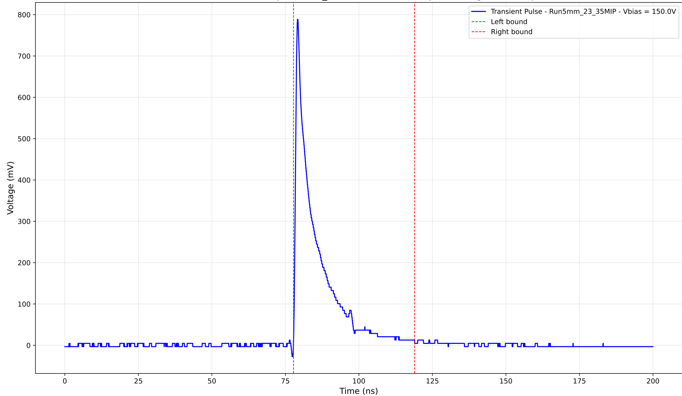
Transient Pulse - Sample: 5mm_23 - Position: 4770.0 \mu\text{m} - Charge: 110.62 pC
