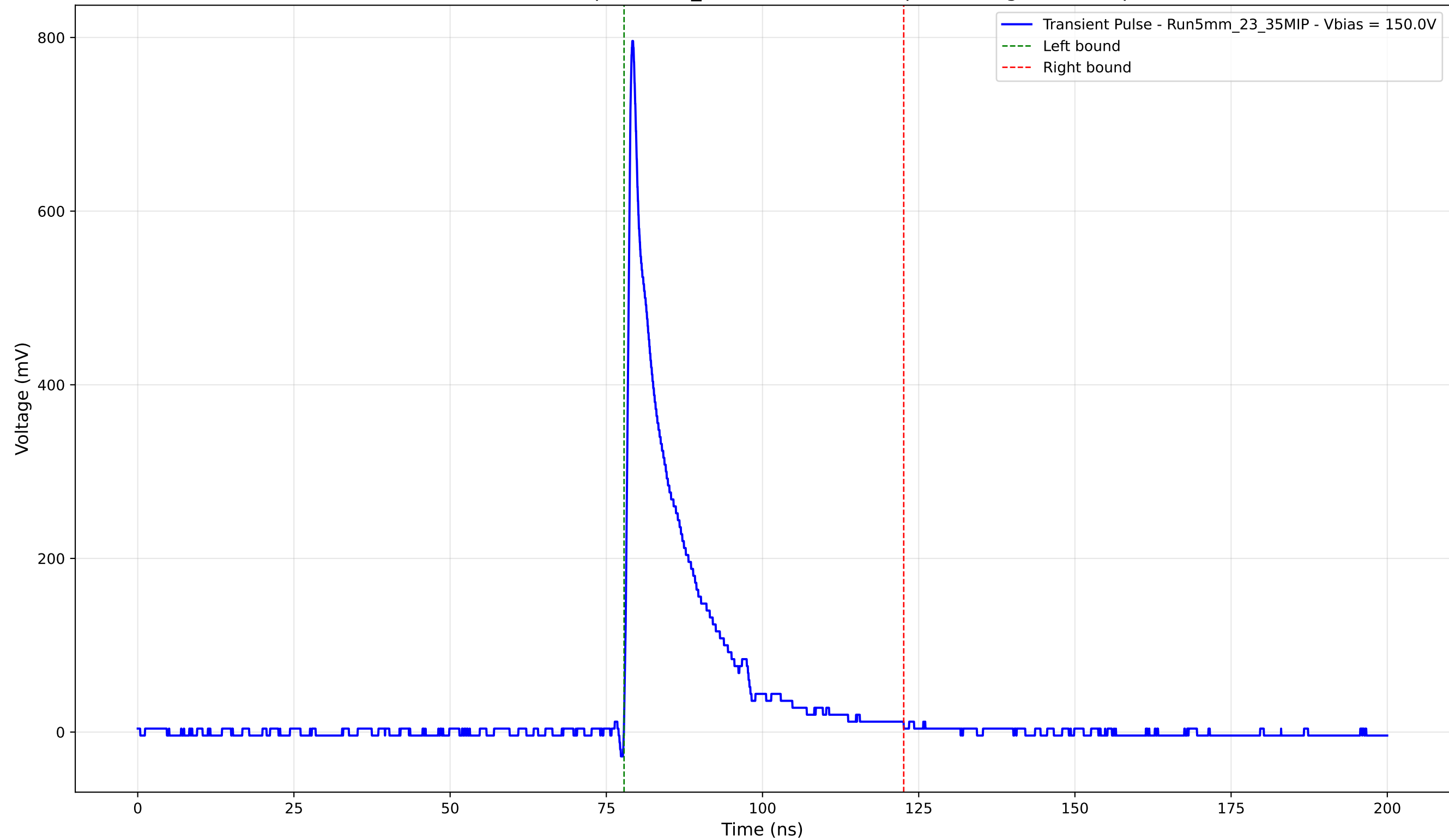
Transient Pulse - Sample: 5mm_23 - Position: 485.0 \mu\text{m} - Charge: 115.68 pC
