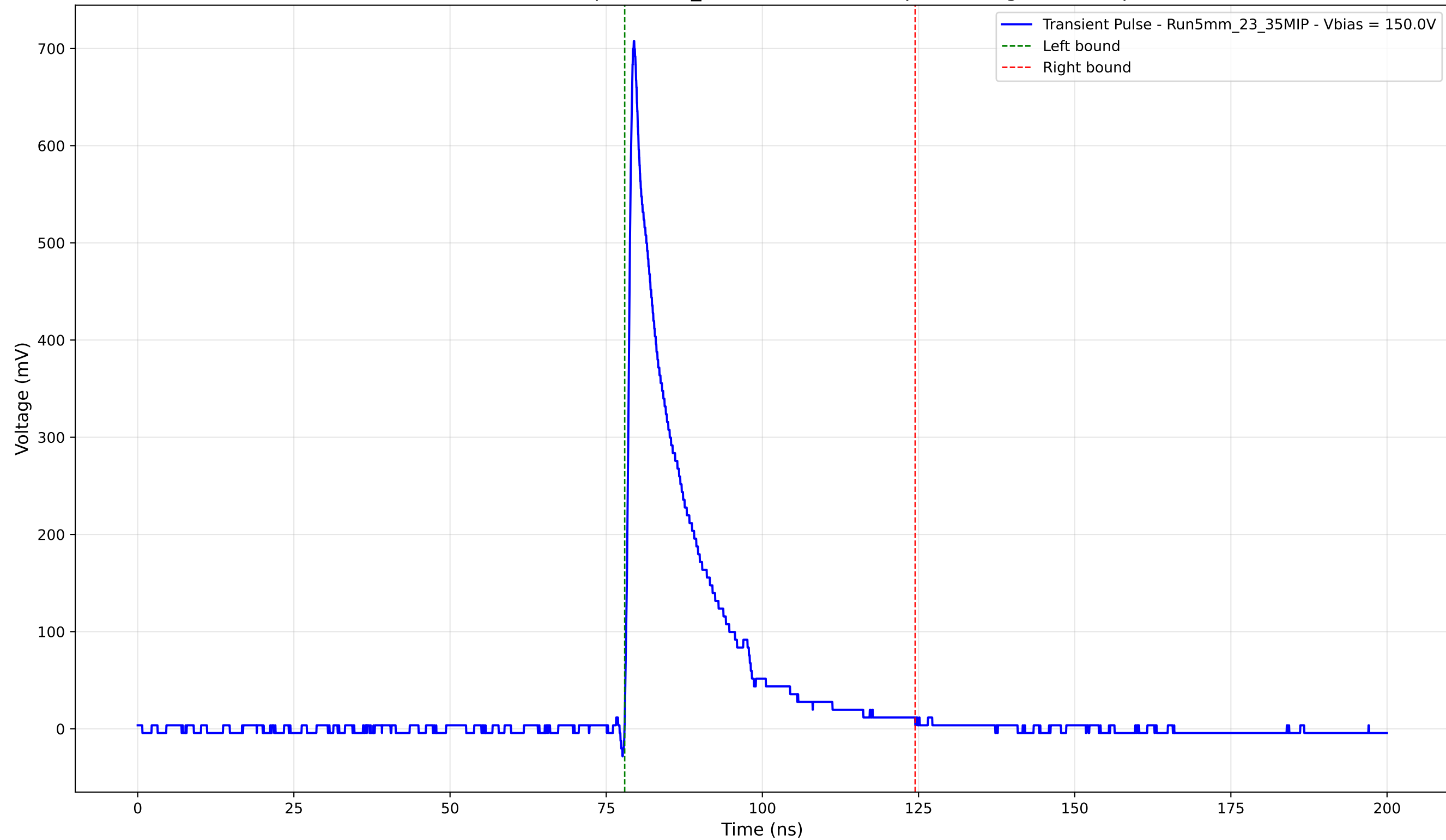
Transient Pulse - Sample: 5mm_23 - Position: 745.0 \mu\text{m} - Charge: 119.91 pC
