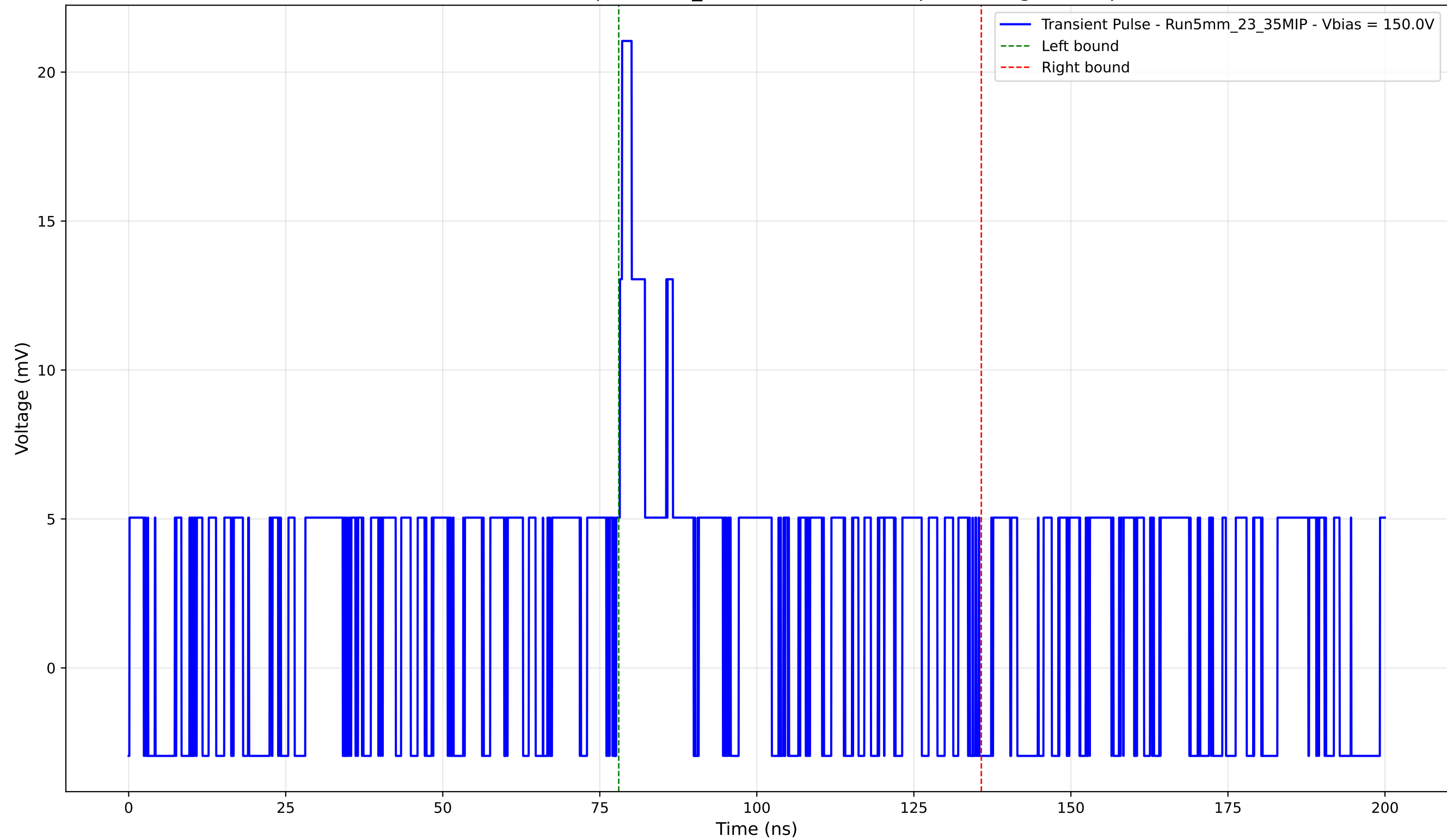
Transient Pulse - Sample: 5mm_23 - Position: 5165.0 \mu\text{m} - Charge: 4.07 pC
