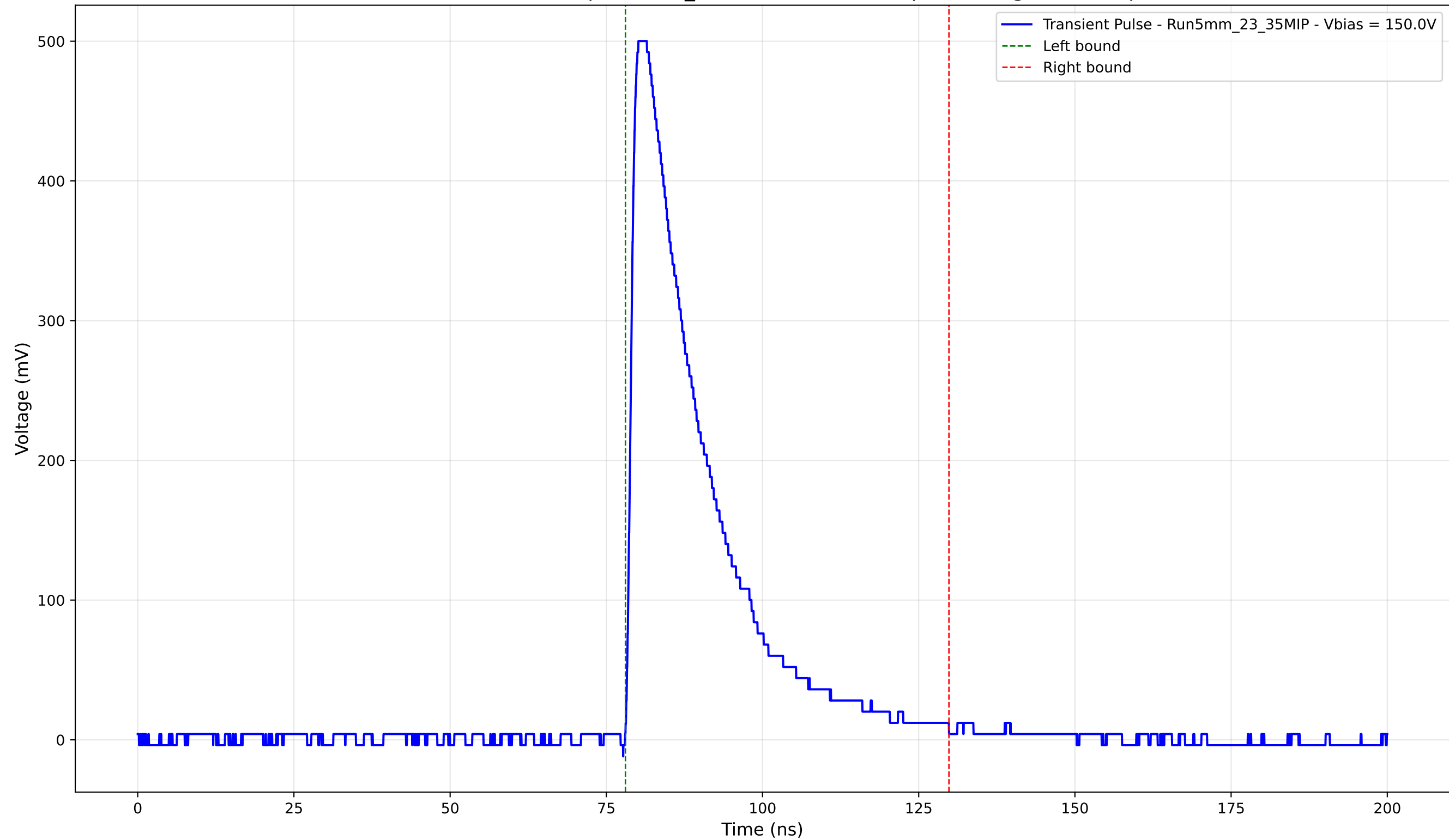
Transient Pulse - Sample: 5mm_23 - Position: 3370.0 \mu\text{m} - Charge: 129.77 pC
