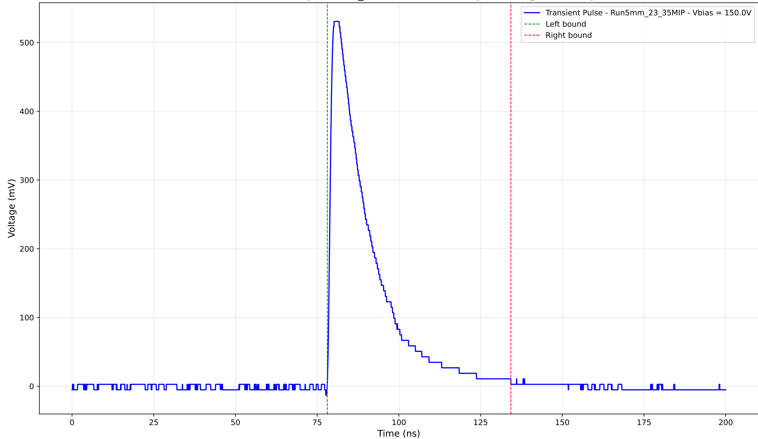
Transient Pulse - Sample: 5mm_23 - Position: 1945.0 \mu\text{m} - Charge: 142.08 pC
