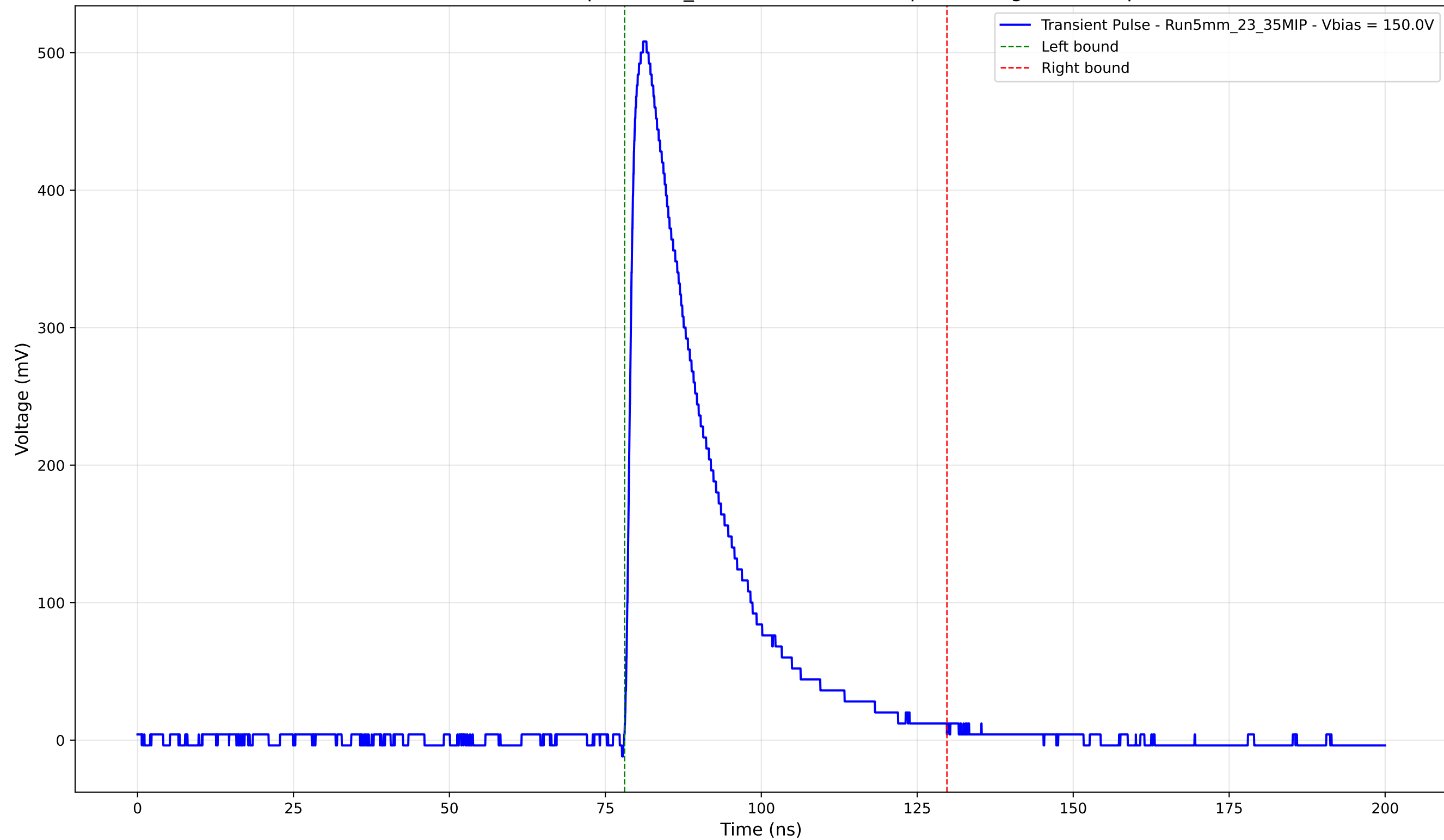
Transient Pulse - Sample: 5mm_23 - Position: 2350.0 \mu\text{m} - Charge: 137.92 pC
