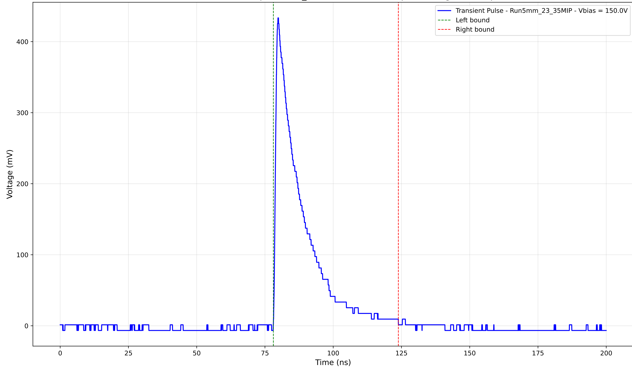
Transient Pulse - Sample: 5mm_23 - Position: 1185.0 \mu\text{m} - Charge: 87.86 pC
