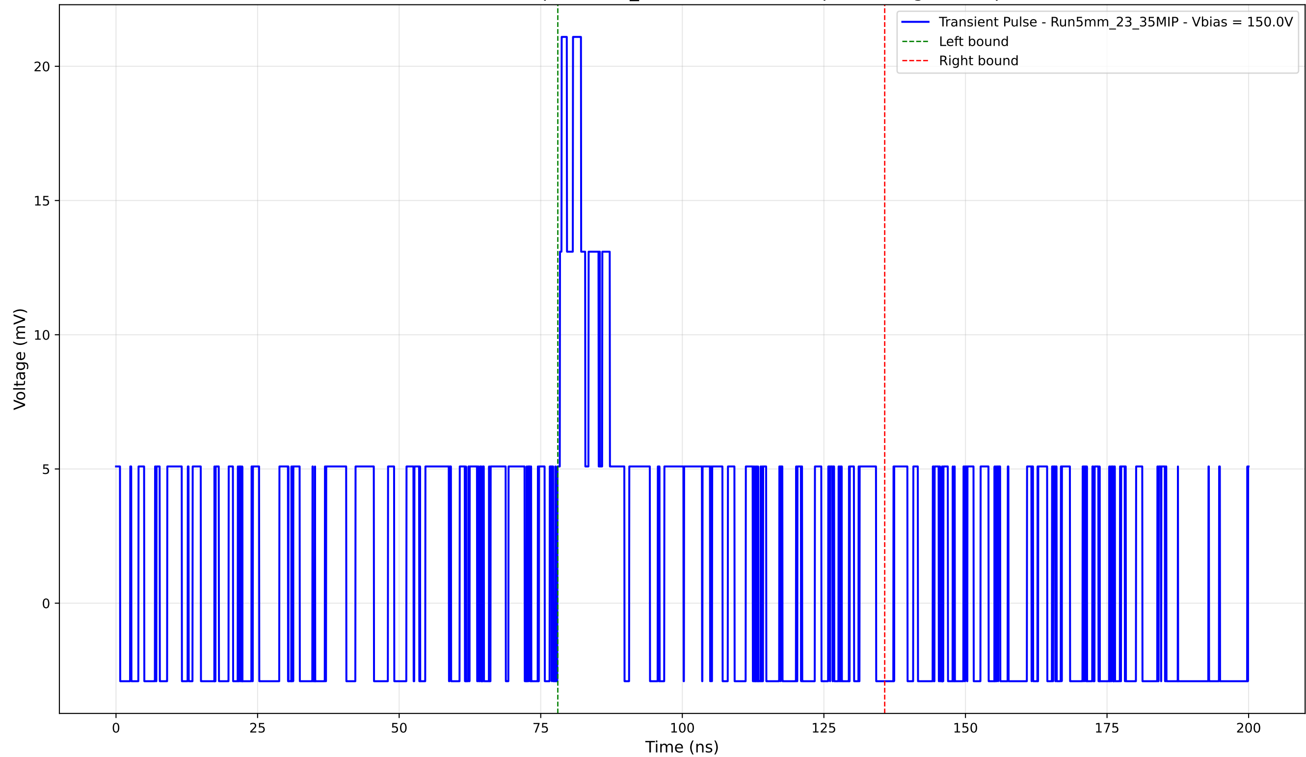
Transient Pulse - Sample: 5mm_23 - Position: 135.0 \mu\text{m} - Charge: 4.12 pC
