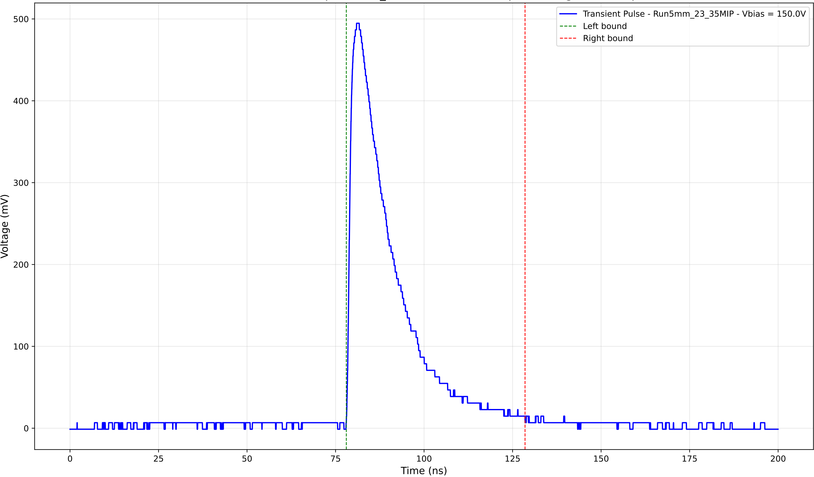
Transient Pulse - Sample: 5mm_23 - Position: 2760.0 \mu\text{m} - Charge: 135.64 pC
