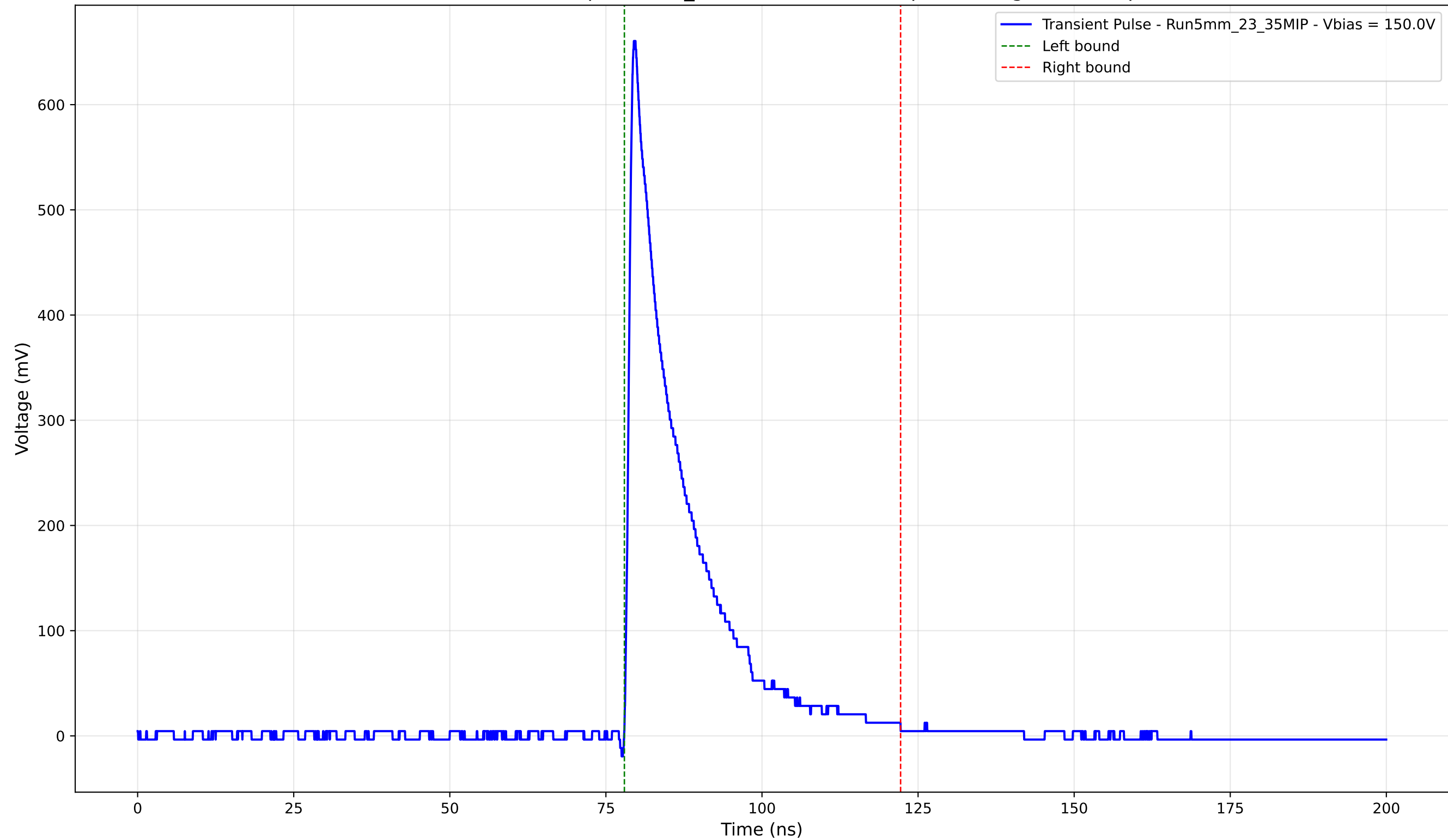
Transient Pulse - Sample: 5mm_23 - Position: 4355.0 \mu\text{m} - Charge: 119.10 pC
