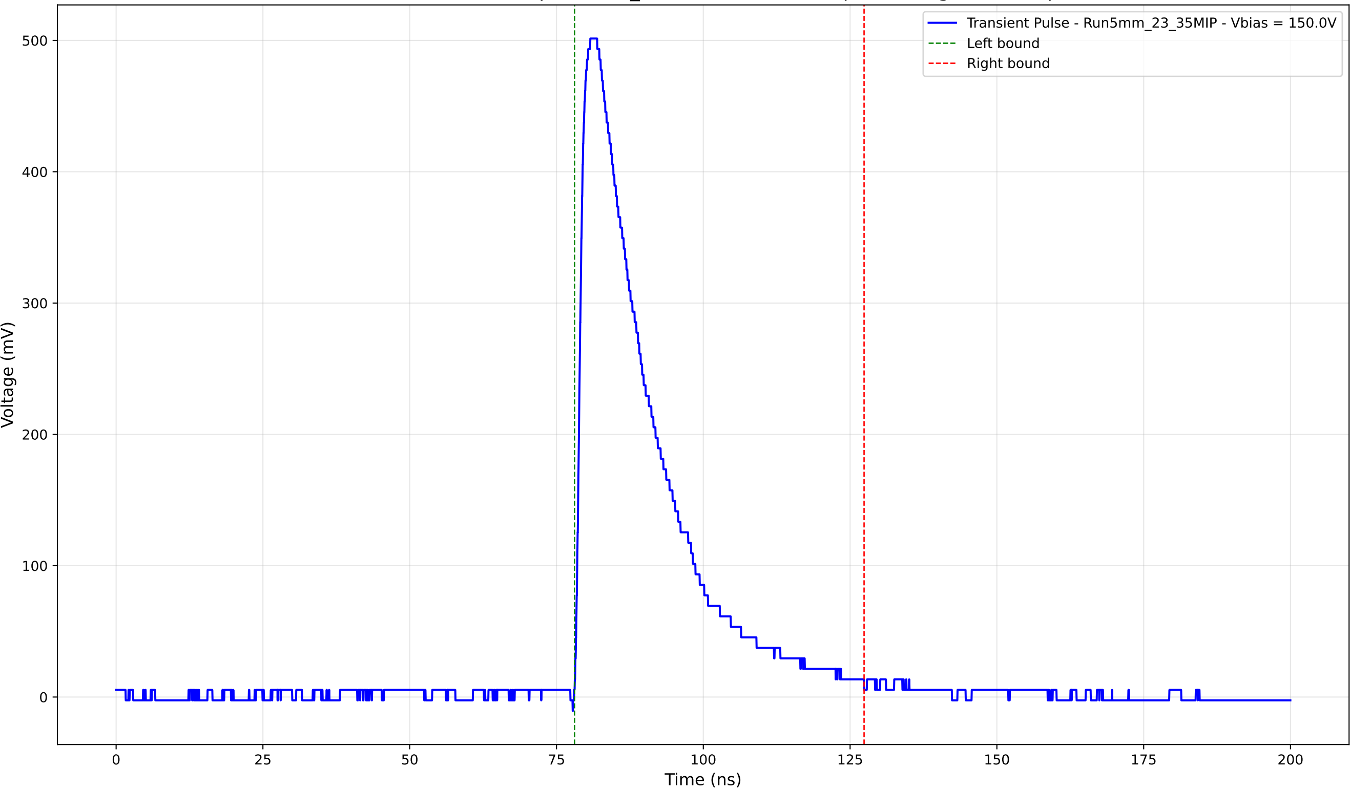
Transient Pulse - Sample: 5mm_23 - Position: 2390.0 \mu\text{m} - Charge: 138.03 pC
