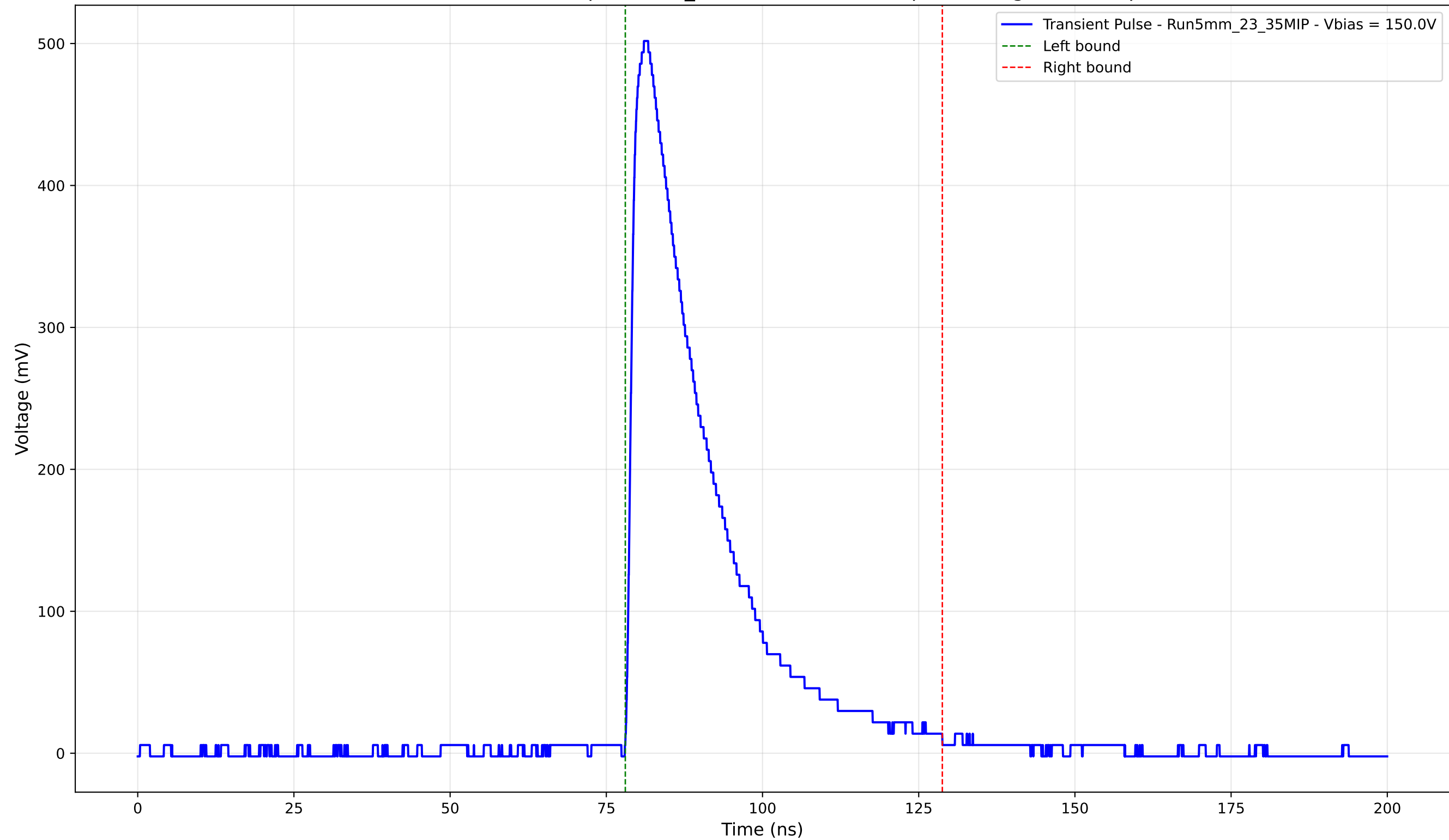
Transient Pulse - Sample: 5mm_23 - Position: 2865.0 \mu\text{m} - Charge: 137.10 pC
