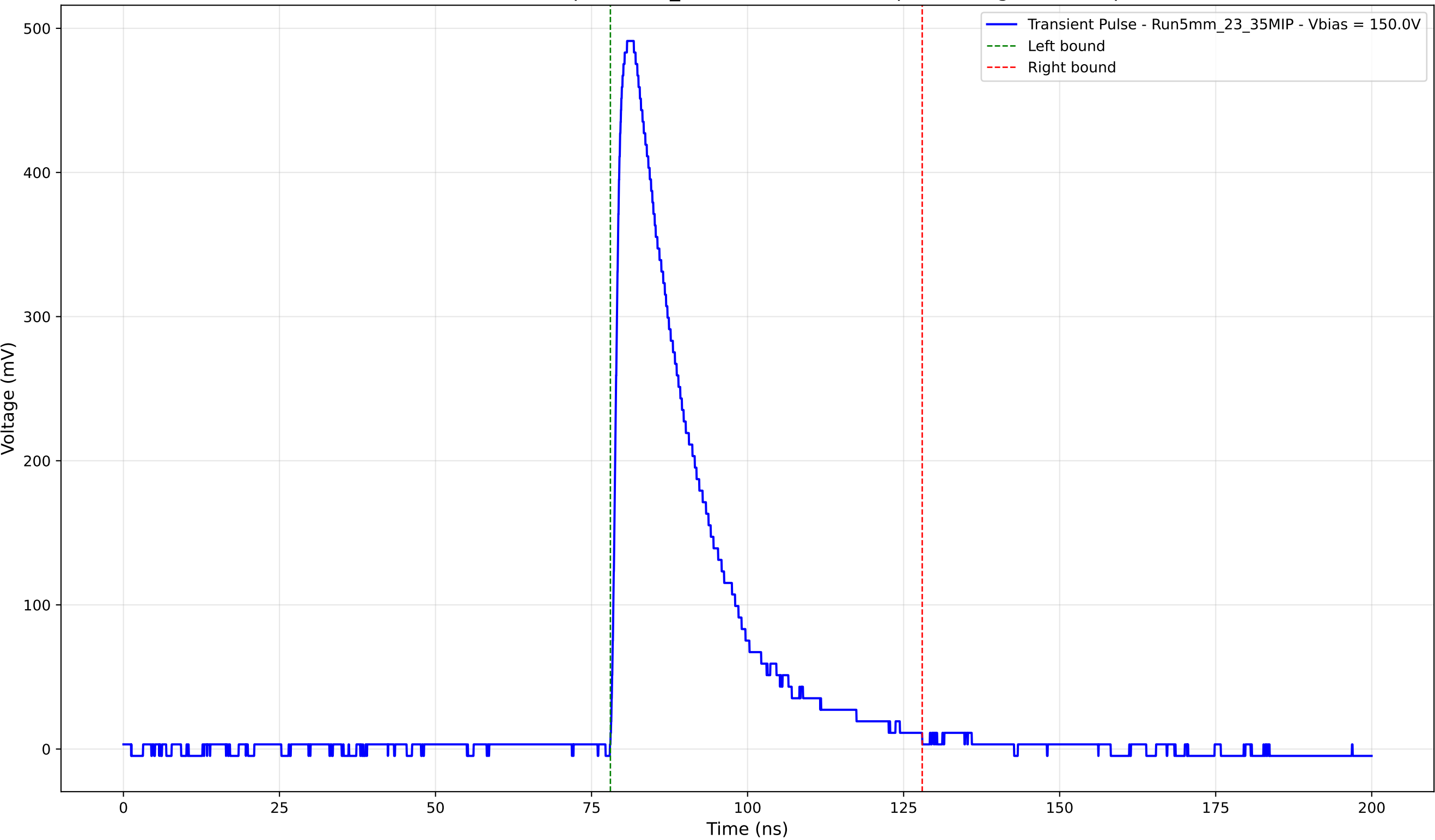
Transient Pulse - Sample: 5mm_23 - Position: 3035.0 \mu\text{m} - Charge: 131.62 pC
