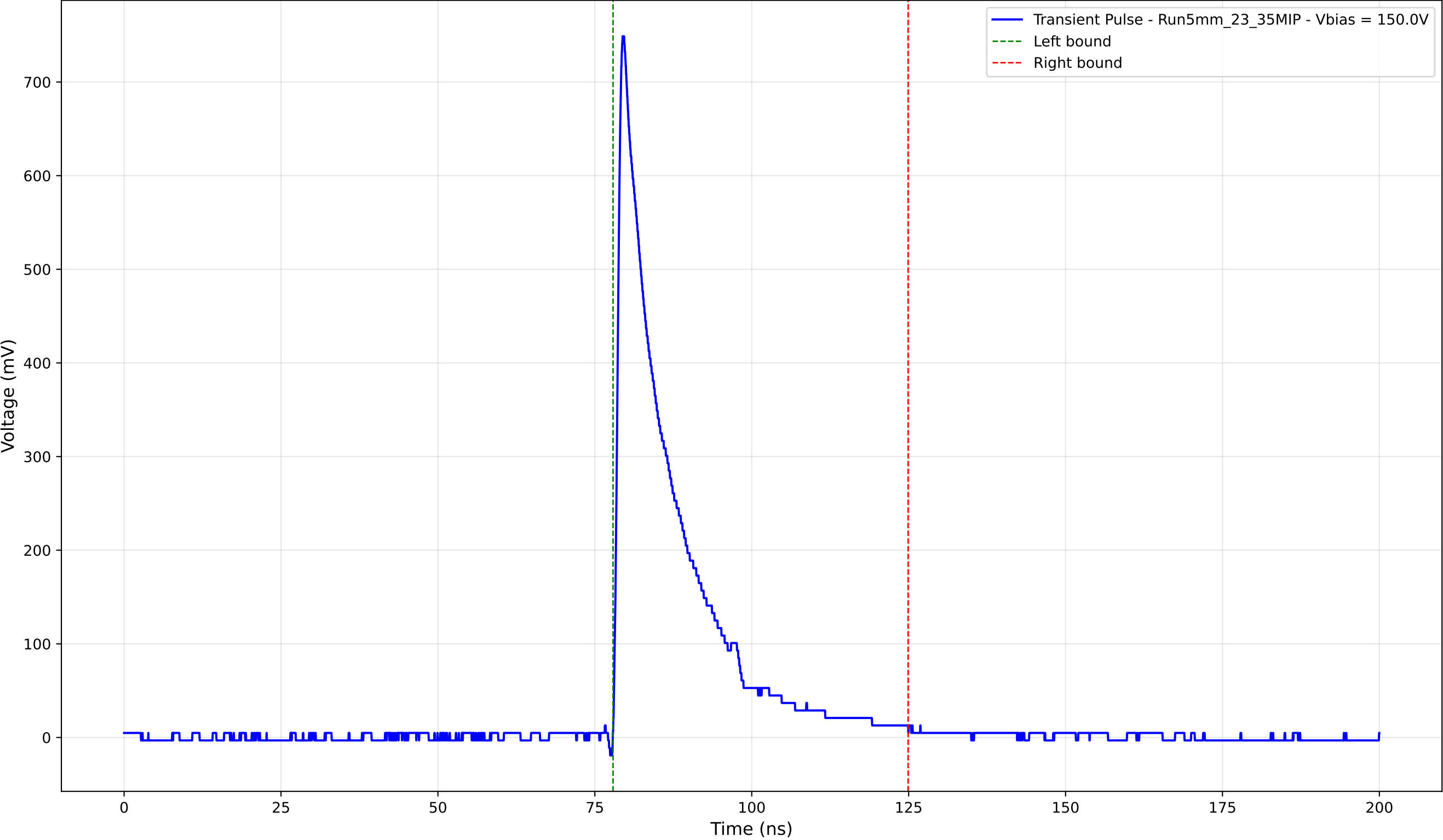
Transient Pulse - Sample: 5mm_23 - Position: 4425.0 \mu\text{m} - Charge: 134.35 pC
