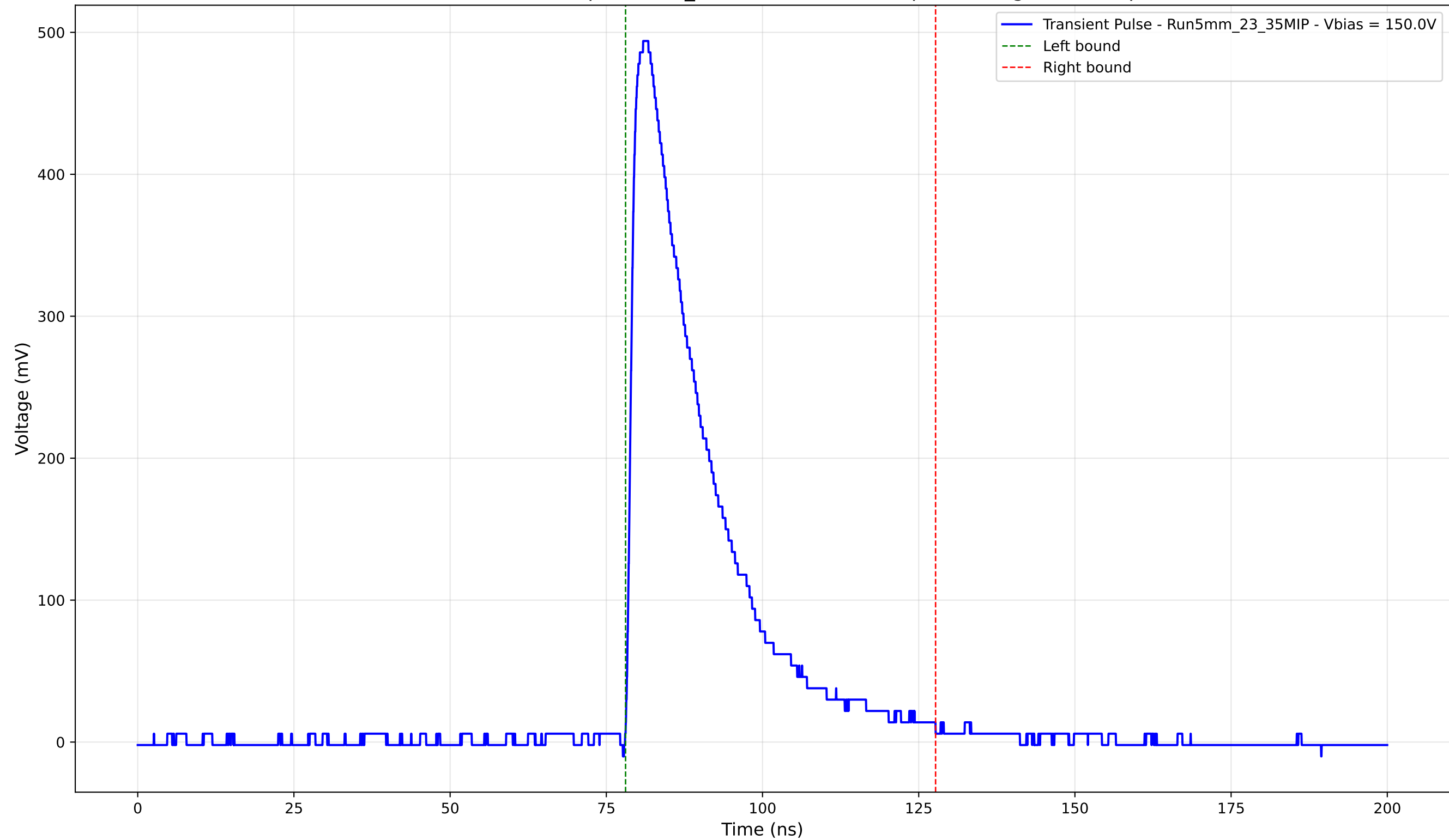
Transient Pulse - Sample: 5mm_23 - Position: 3015.0 \mu\text{m} - Charge: 132.68 pC
