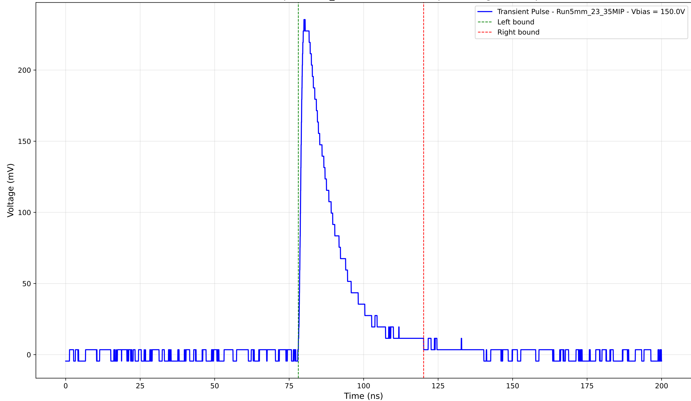
Transient Pulse - Sample: 5mm_23 - Position: 3615.0 \mu\text{m} - Charge: 55.68 pC
