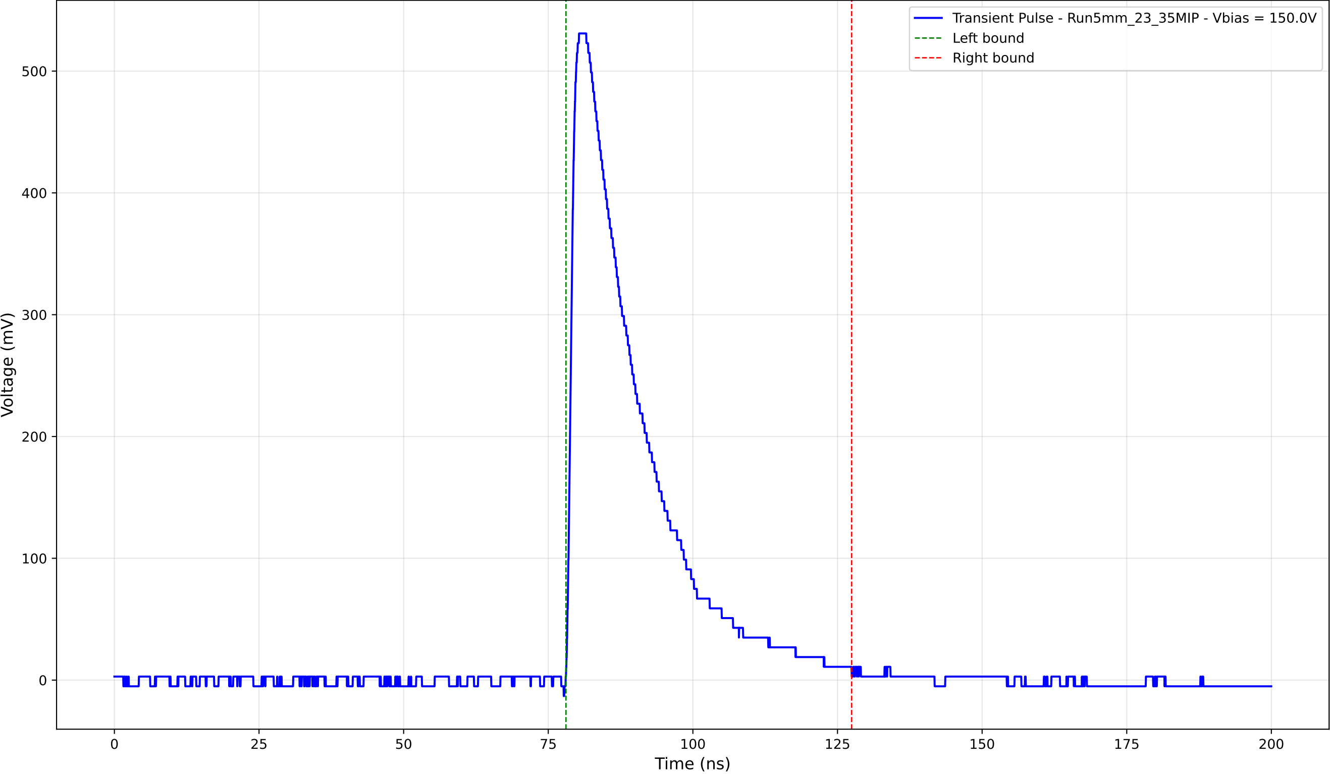
Transient Pulse - Sample: 5mm_23 - Position: 2035.0 \mu\text{m} - Charge: 139.93 pC
