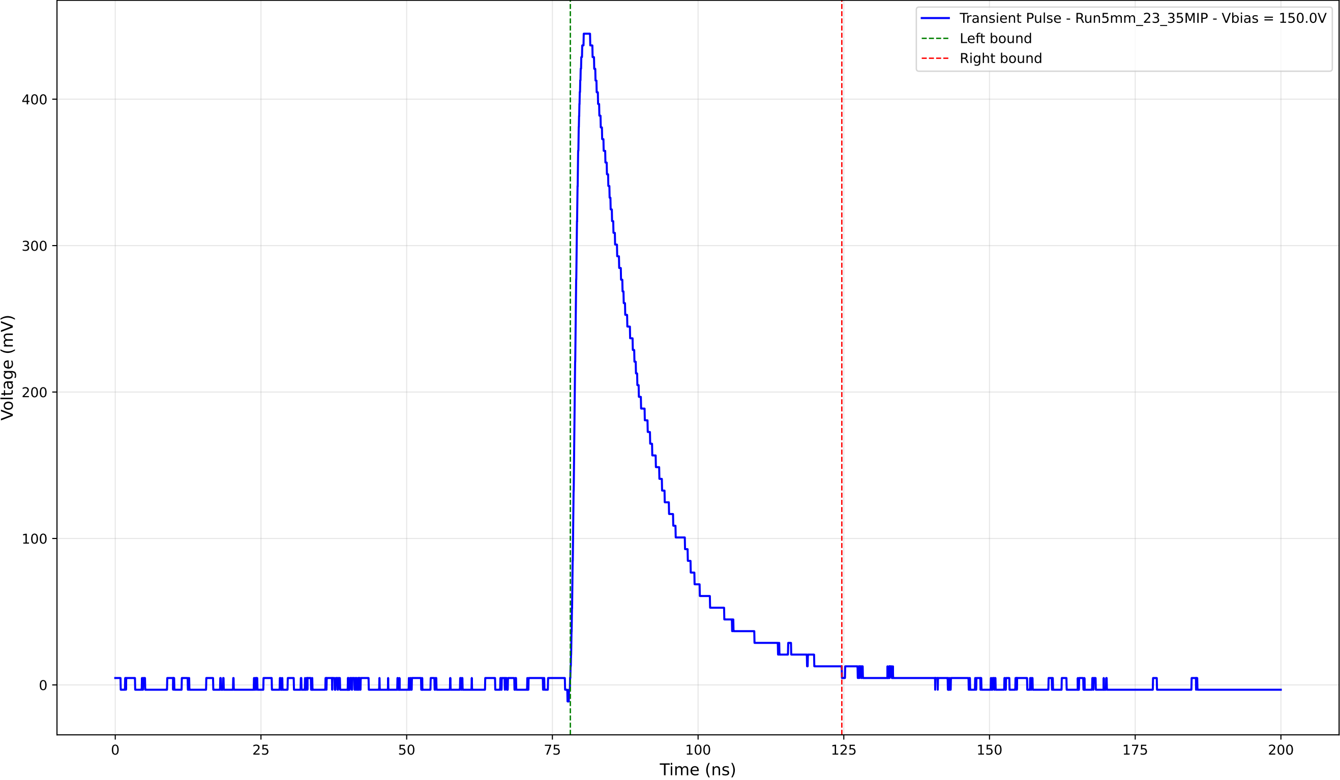
Transient Pulse - Sample: 5mm_23 - Position: 2065.0 \mu\text{m} - Charge: 116.08 pC
