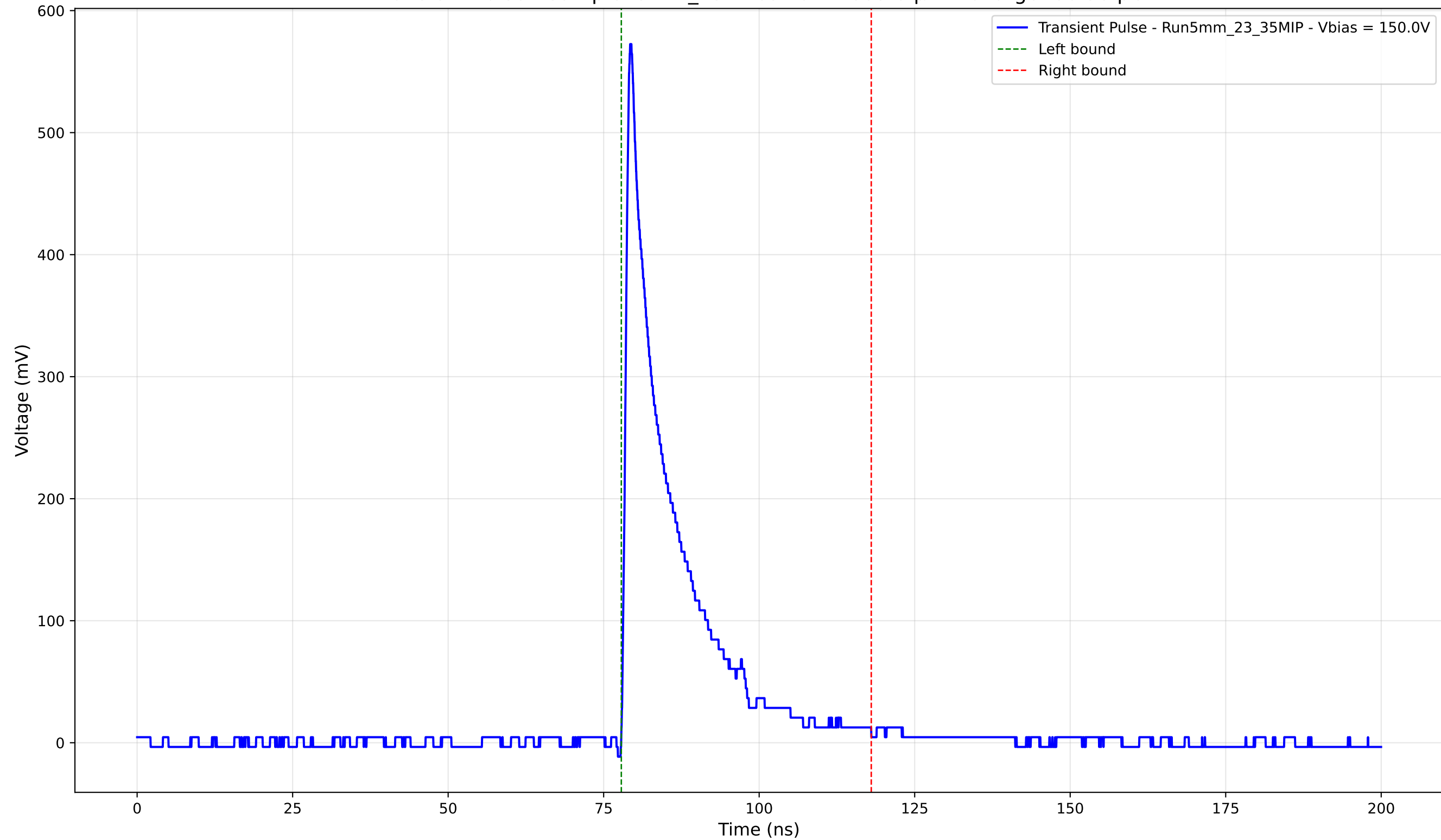
Transient Pulse - Sample: 5mm_23 - Position: 4605.0 \mu\text{m} - Charge: 86.30 pC
