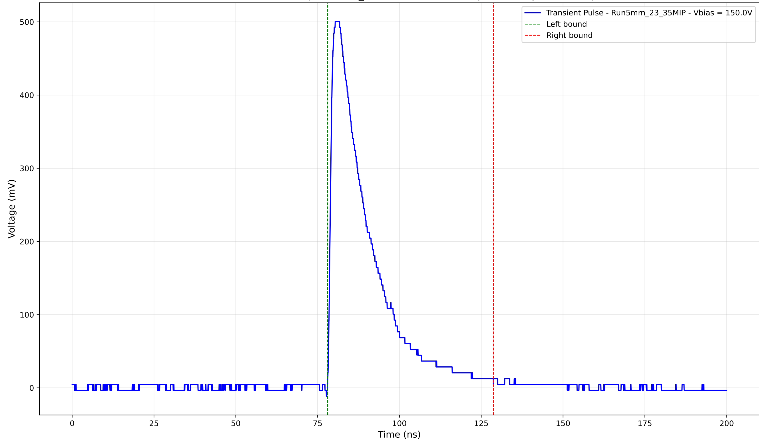
Transient Pulse - Sample: 5mm_23 - Position: 3295.0 \mu\text{m} - Charge: 131.60 pC
