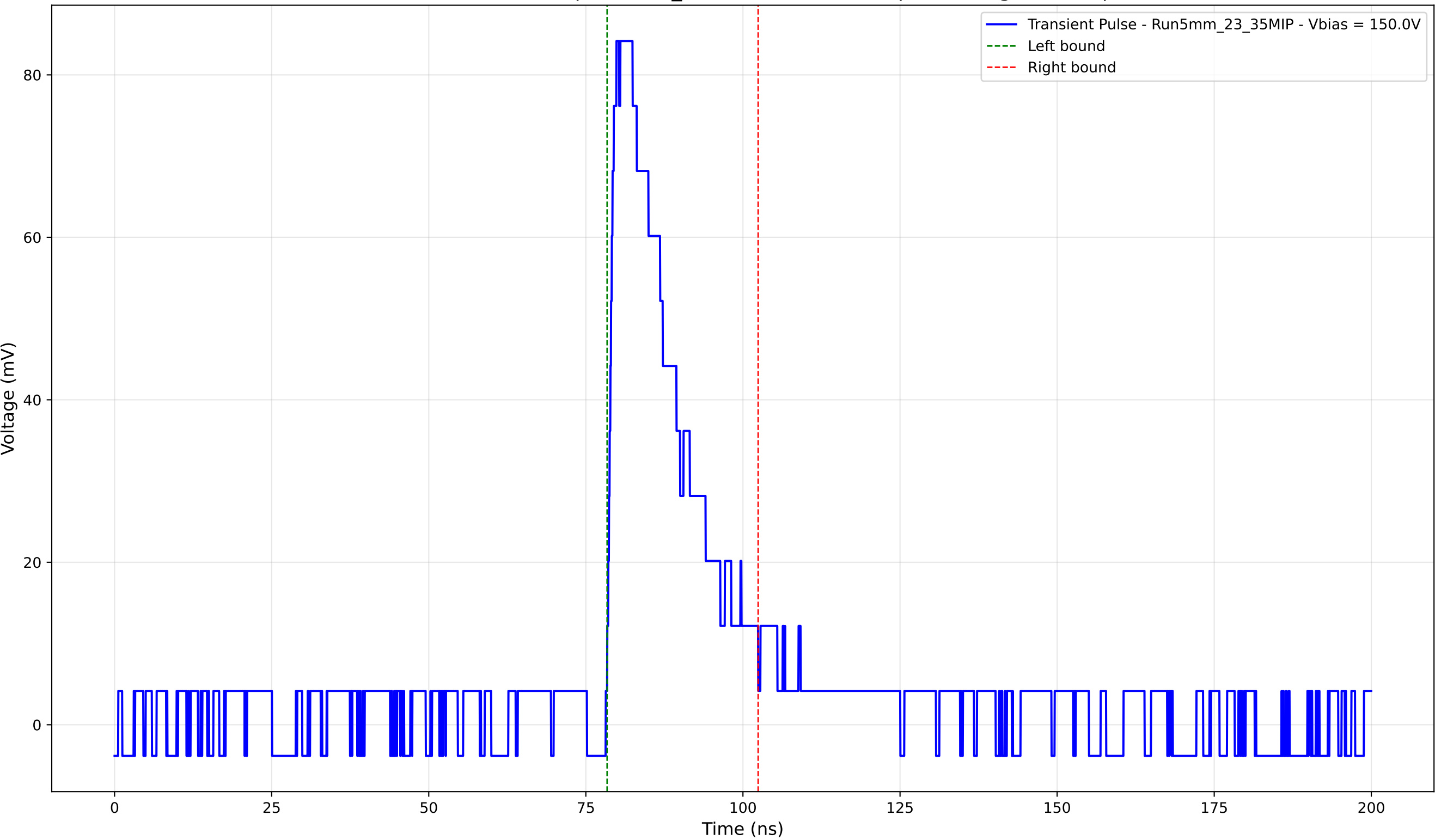
Transient Pulse - Sample: 5mm_23 - Position: 1620.0 \mu\text{m} - Charge: 19.42 pC
