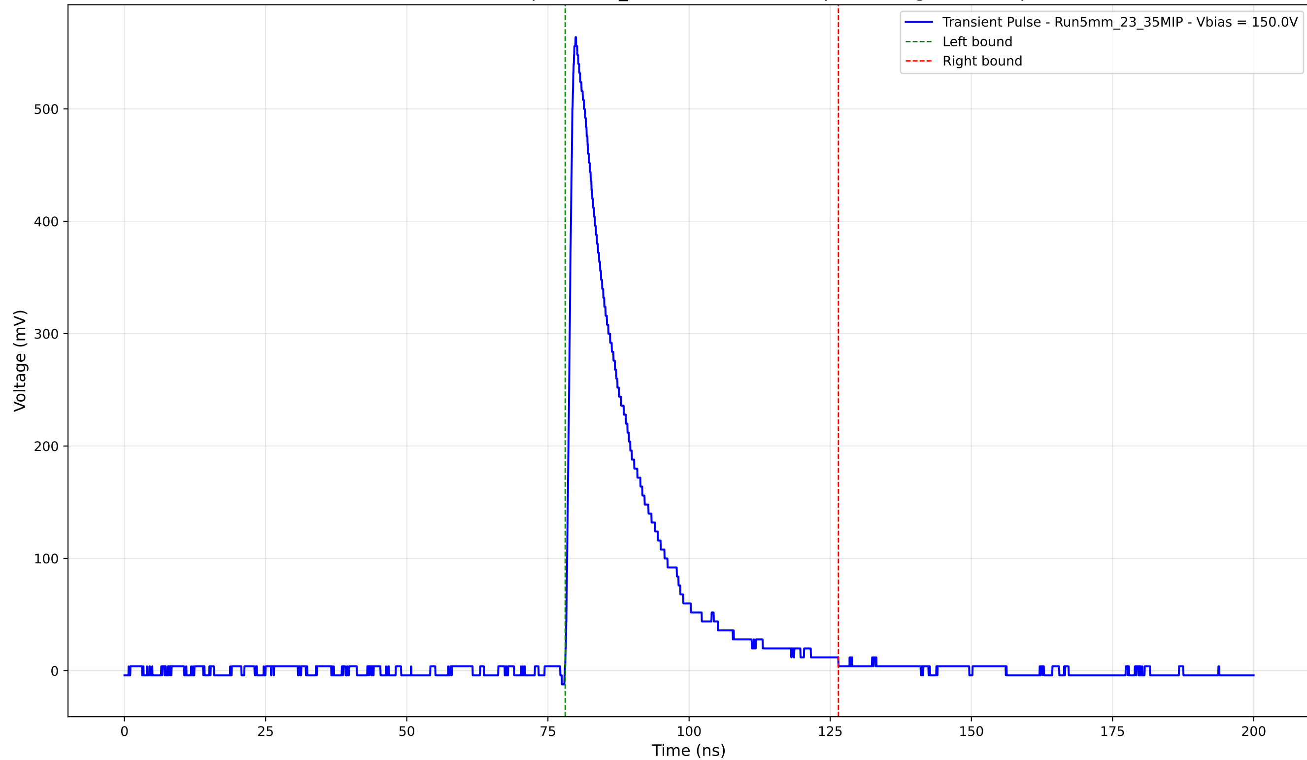
Transient Pulse - Sample: 5mm_23 - Position: 3970.0 \mu\text{m} - Charge: 120.46 pC
