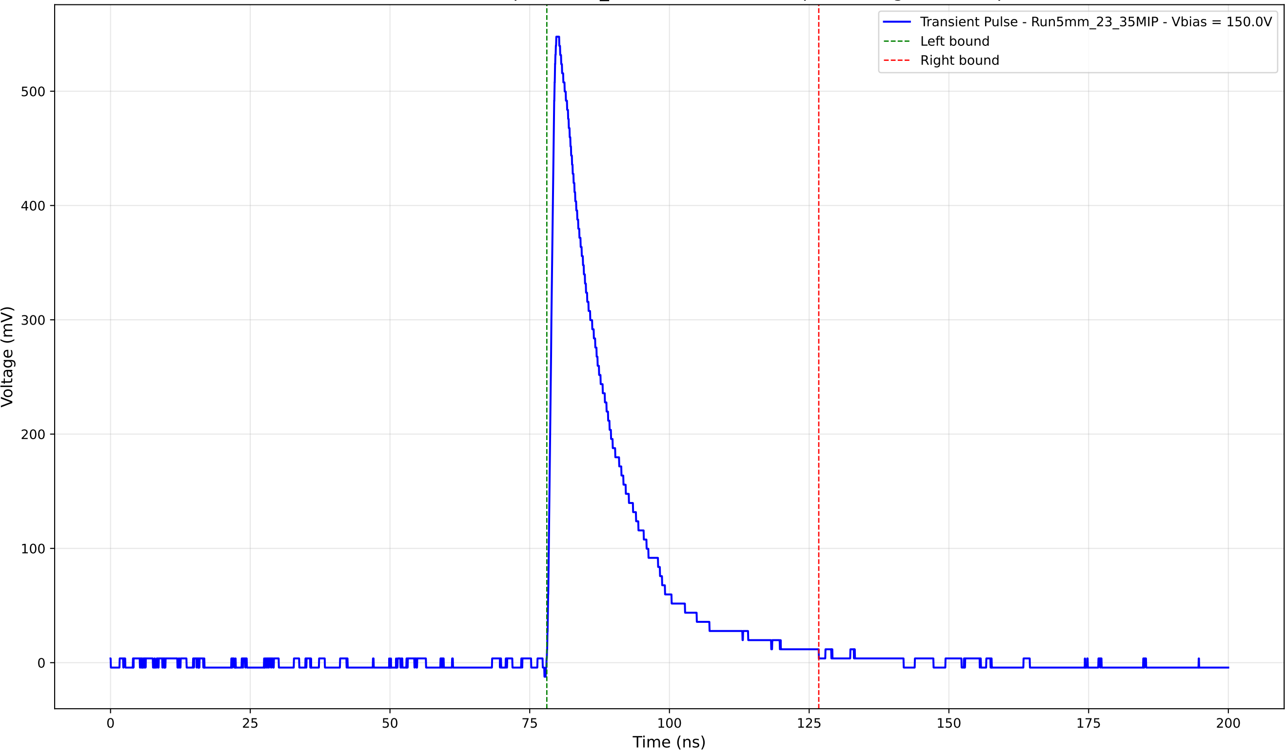
Transient Pulse - Sample: 5mm_23 - Position: 3915.0 \mu\text{m} - Charge: 120.23 pC
