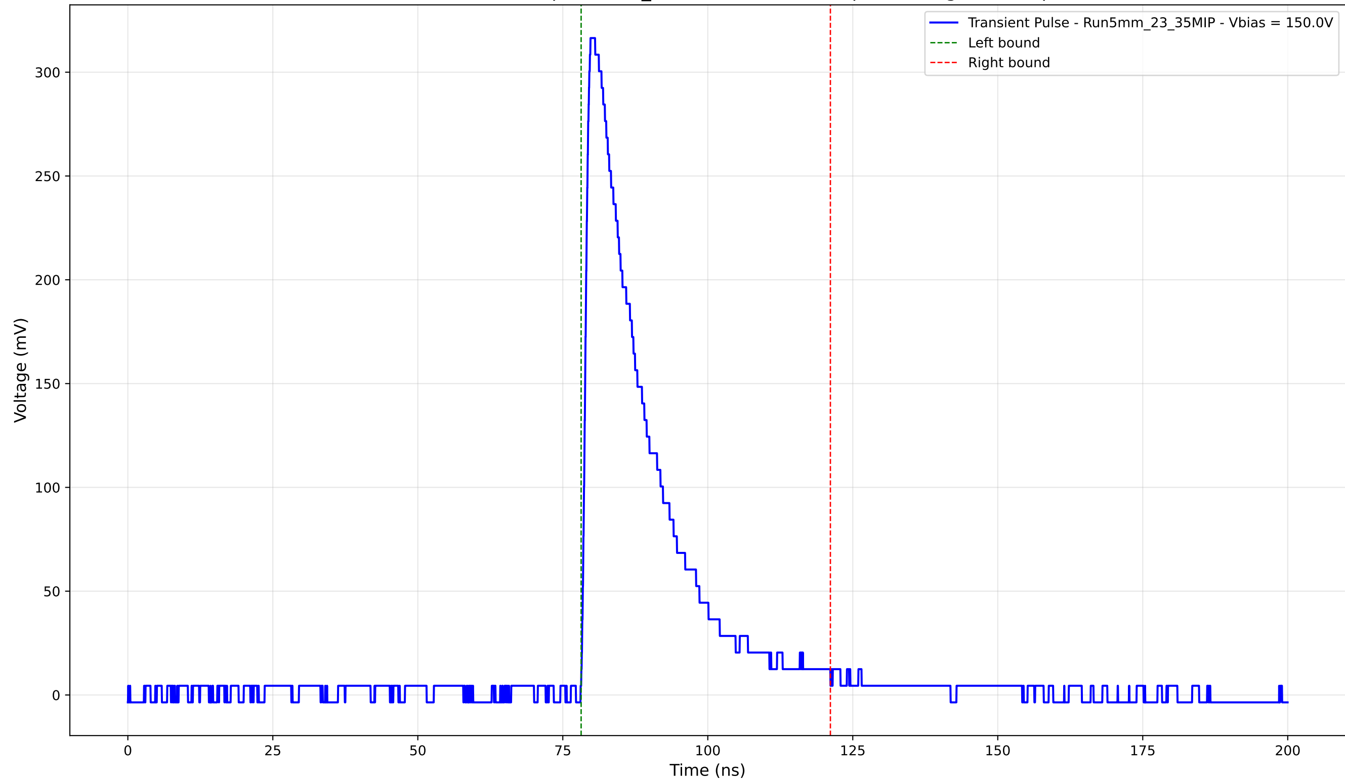
Transient Pulse - Sample: 5mm_23 - Position: 1570.0 \mu\text{m} - Charge: 74.16 pC
