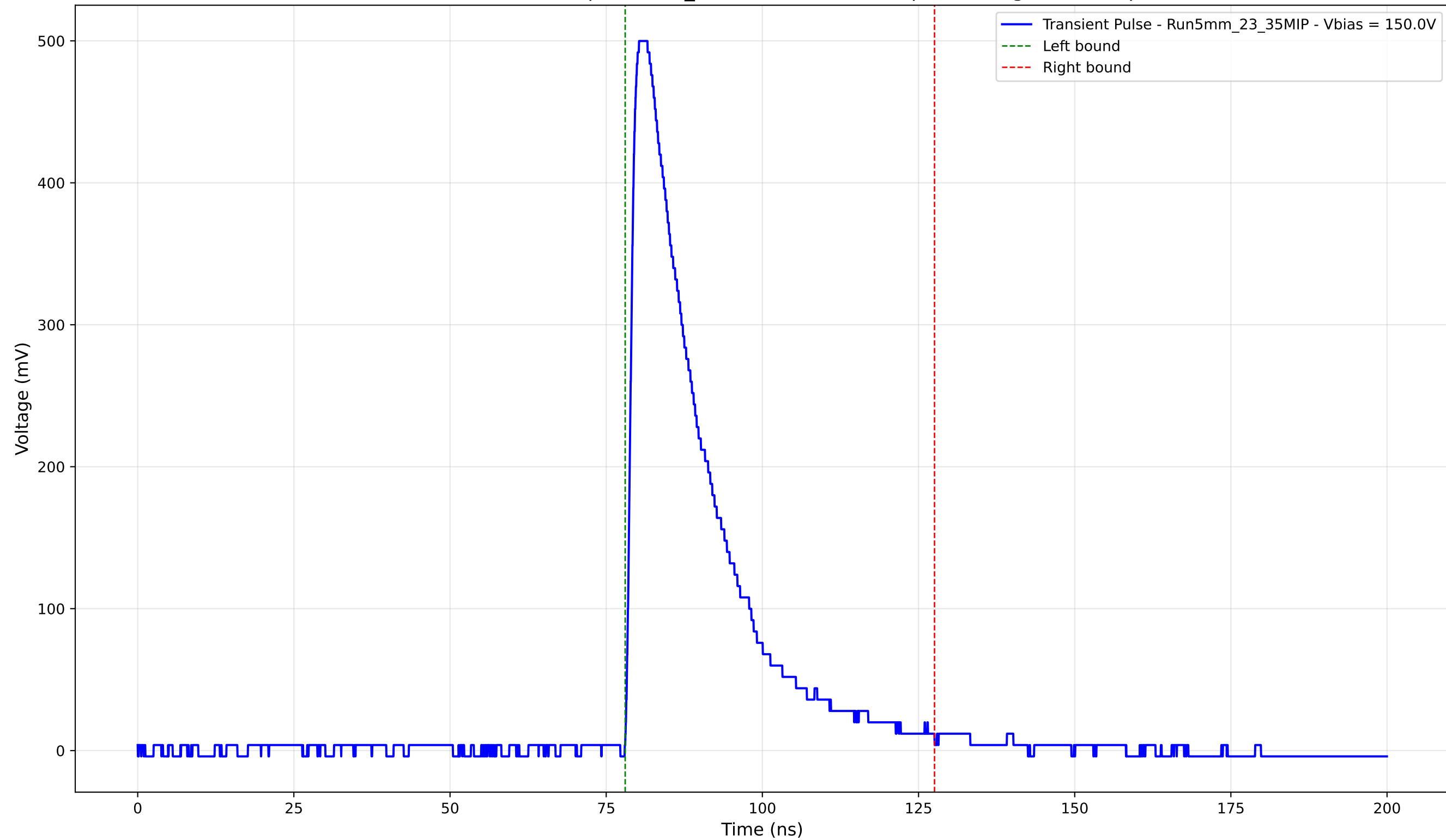
Transient Pulse - Sample: 5mm_23 - Position: 3305.0 \mu\text{m} - Charge: 130.36 pC
