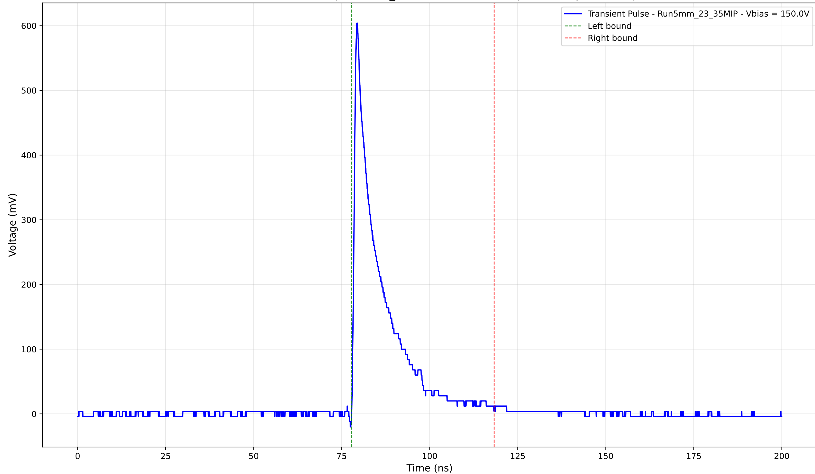
Transient Pulse - Sample: 5mm_23 - Position: 4575.0 \mu\text{m} - Charge: 93.25 pC
