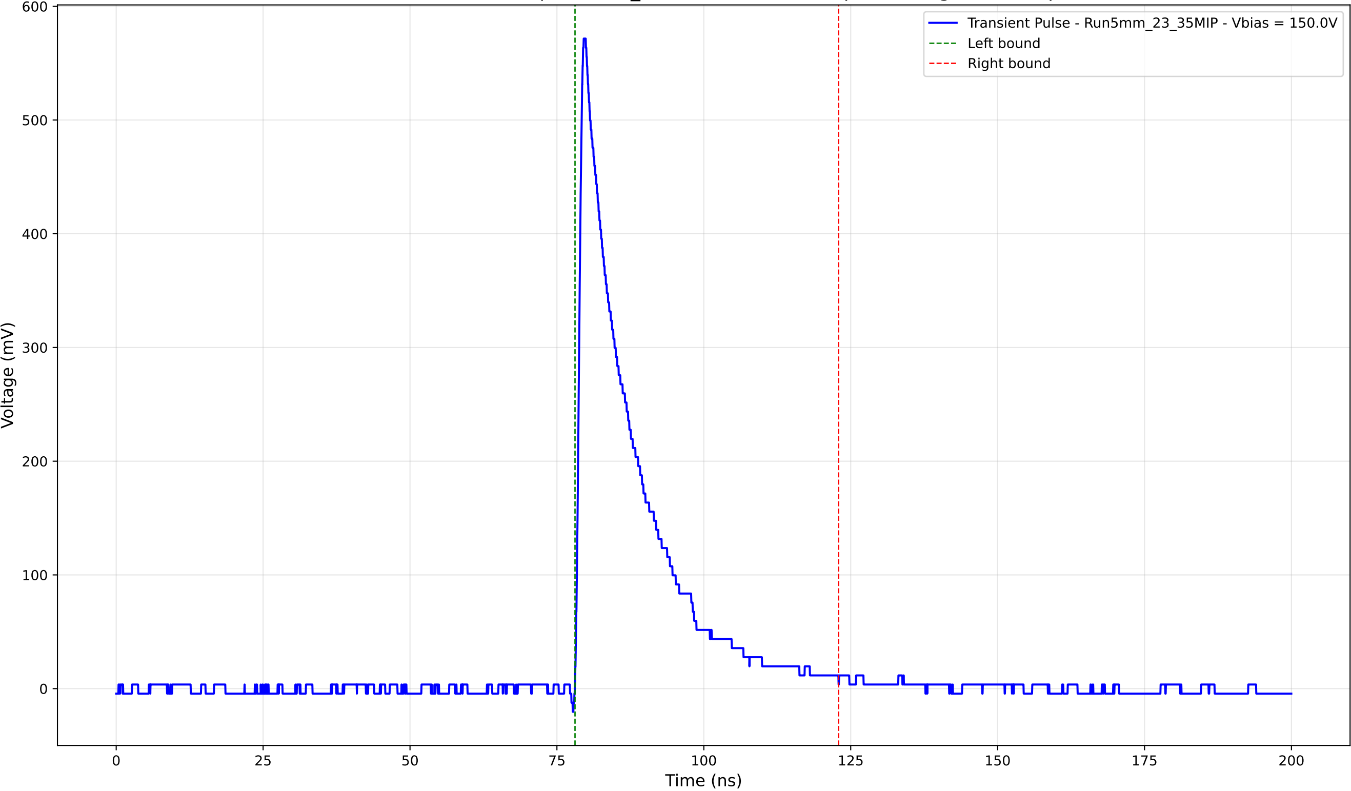
Transient Pulse - Sample: 5mm_23 - Position: 1045.0 \mu\text{m} - Charge: 110.41 pC
