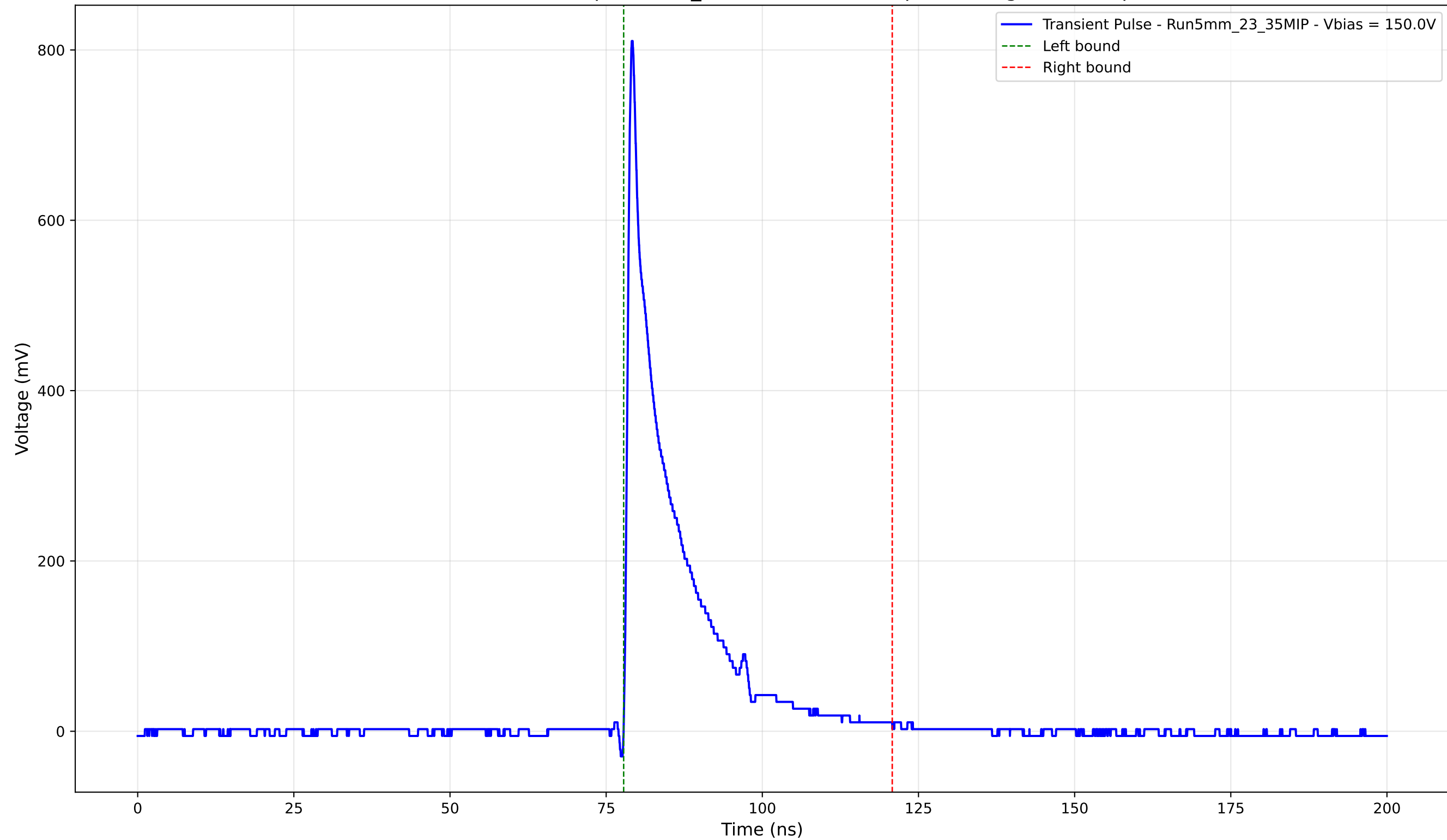
Transient Pulse - Sample: 5mm_23 - Position: 435.0 \mu\text{m} - Charge: 113.74 pC
