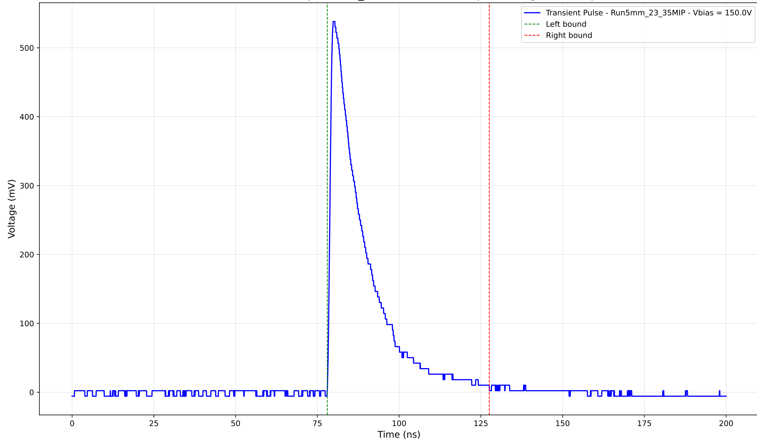
Transient Pulse - Sample: 5mm_23 - Position: 3780.0 \mu\text{m} - Charge: 124.61 pC
