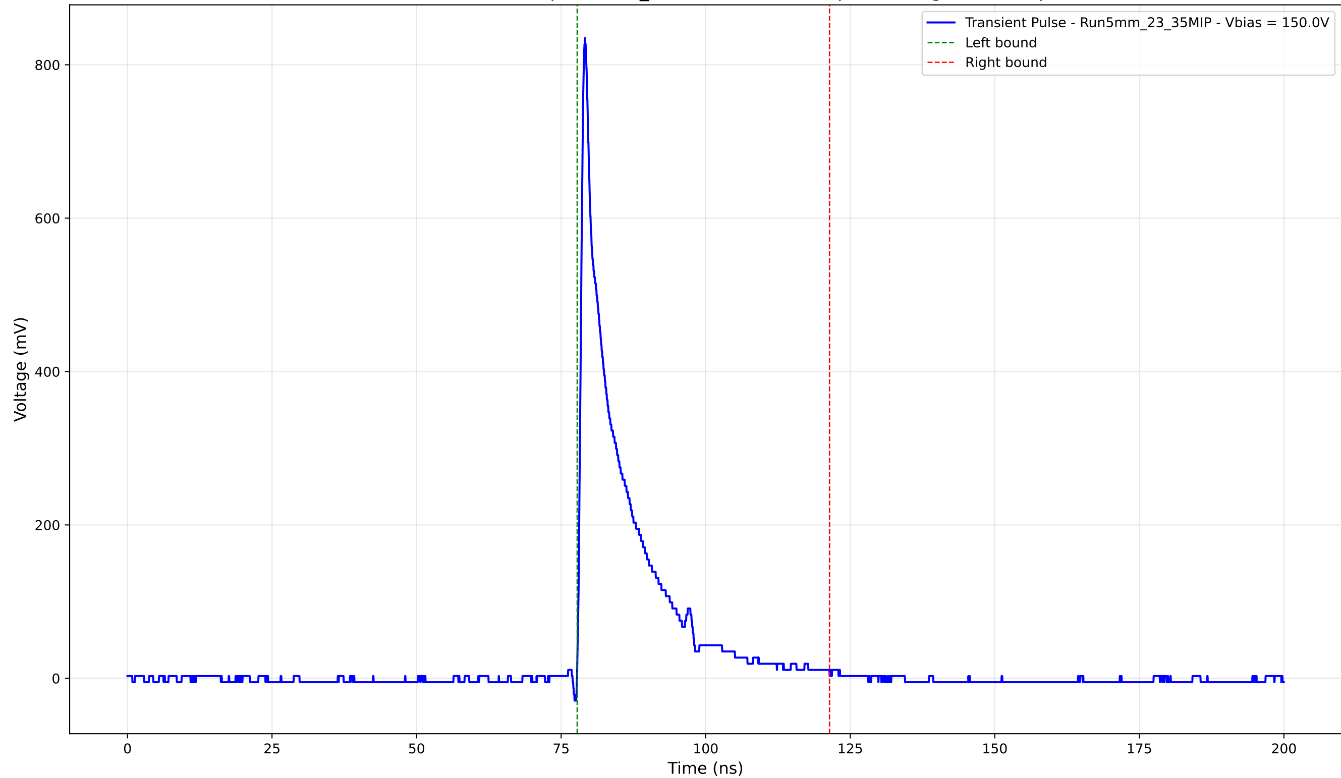
Transient Pulse - Sample: 5mm_23 - Position: 400.0 \mu\text{m} - Charge: 115.54 pC
