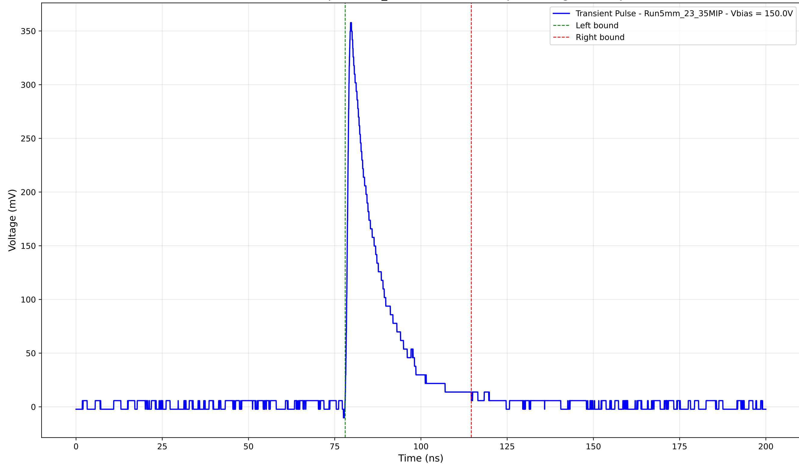
Transient Pulse - Sample: 5mm_23 - Position: 4210.0 \mu\text{m} - Charge: 65.18 pC
