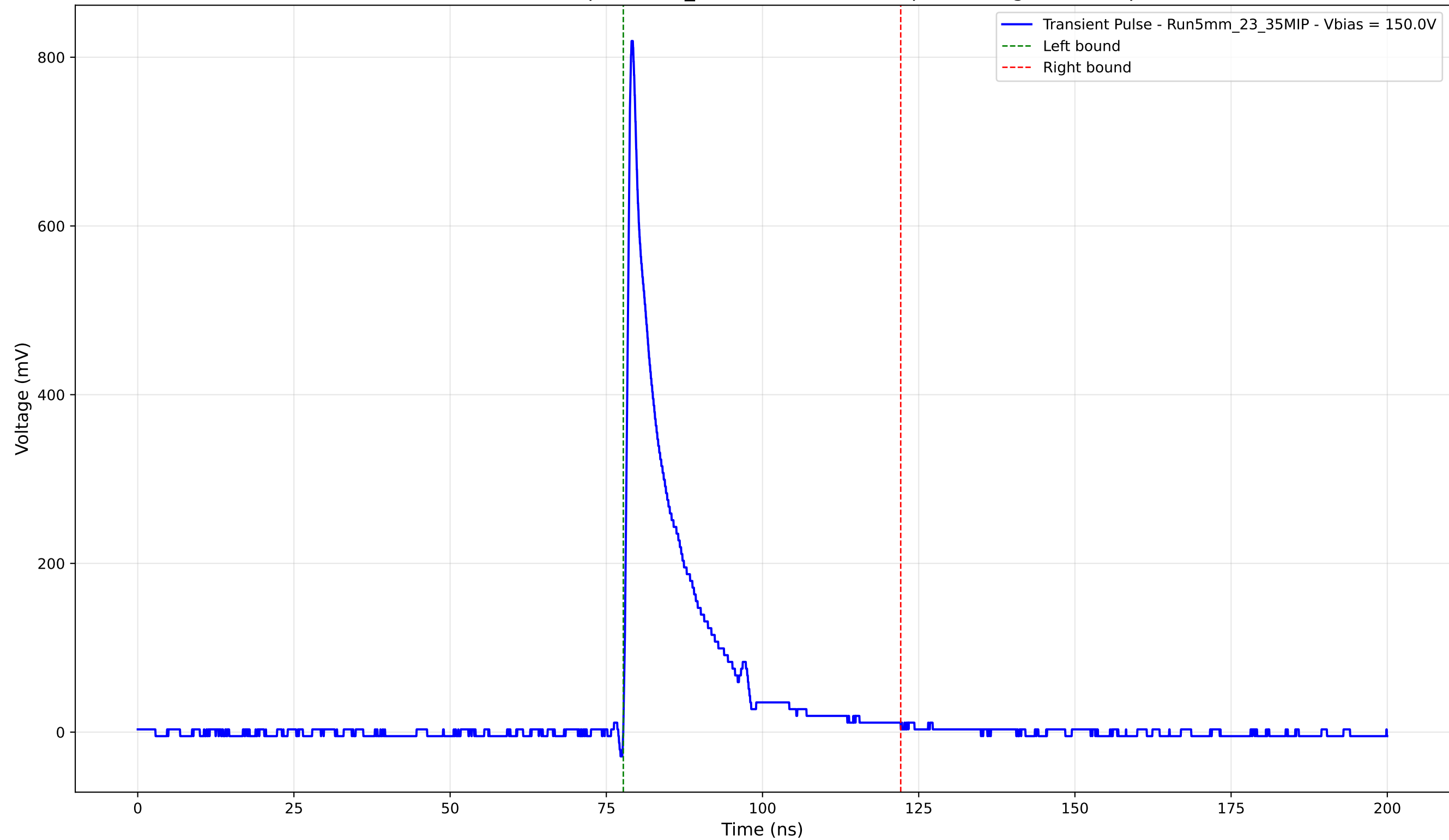
Transient Pulse - Sample: 5mm_23 - Position: 4825.0 \mu\text{m} - Charge: 113.16 pC
