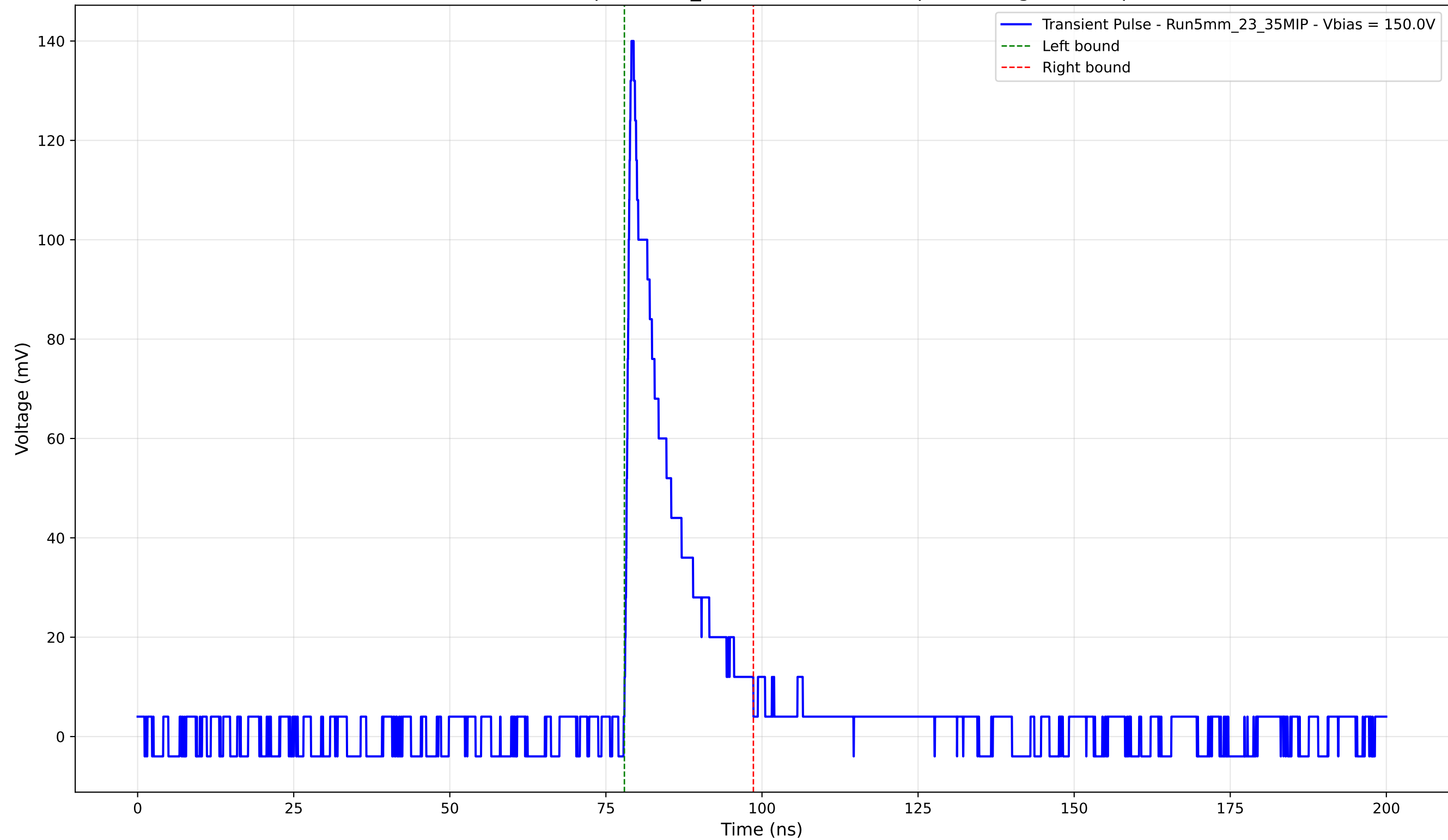
Transient Pulse - Sample: 5mm_23 - Position: 4675.0 \mu\text{m} - Charge: 18.97 pC
