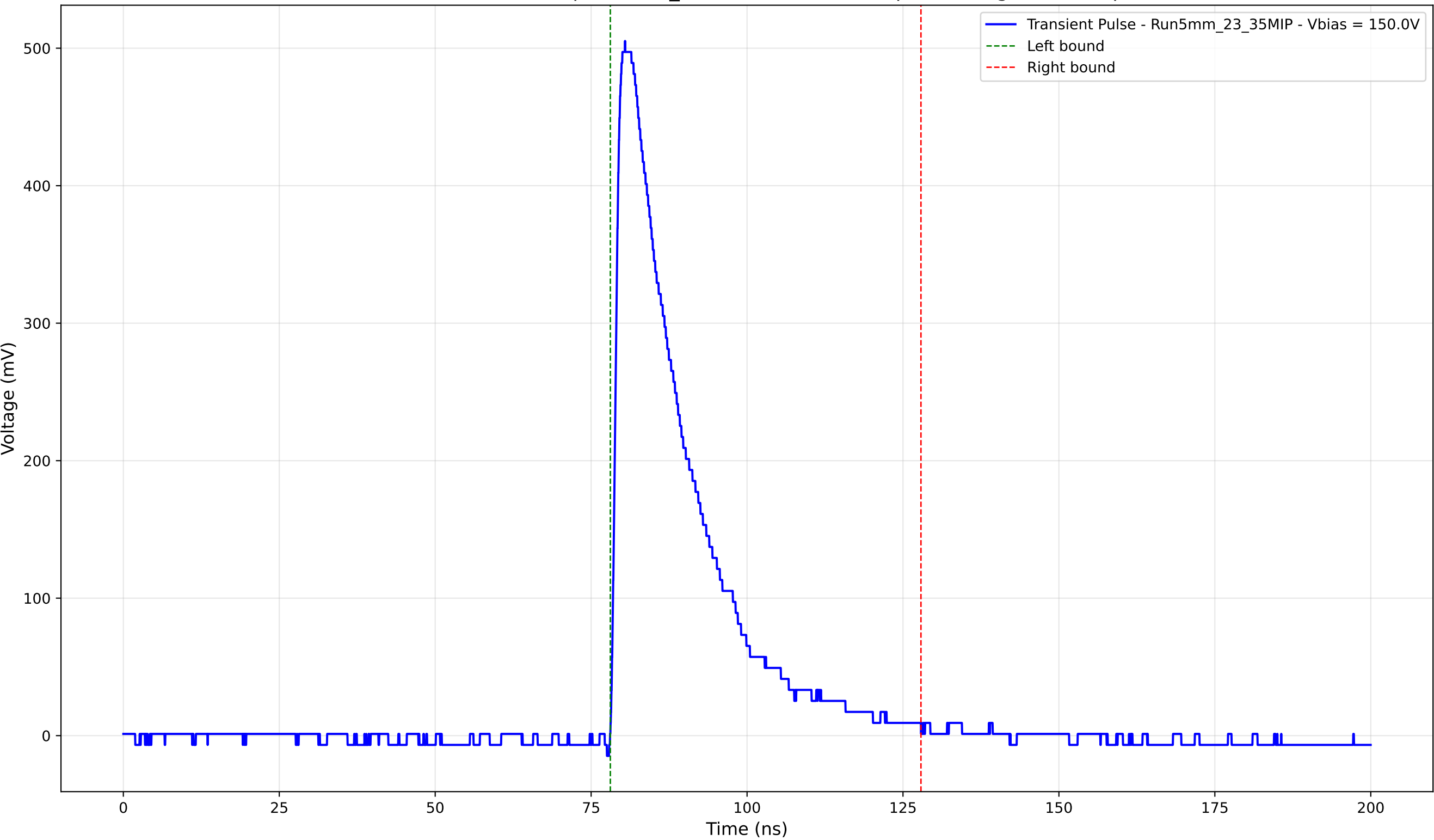
Transient Pulse - Sample: 5mm_23 - Position: 3465.0 \mu\text{m} - Charge: 124.73 pC
