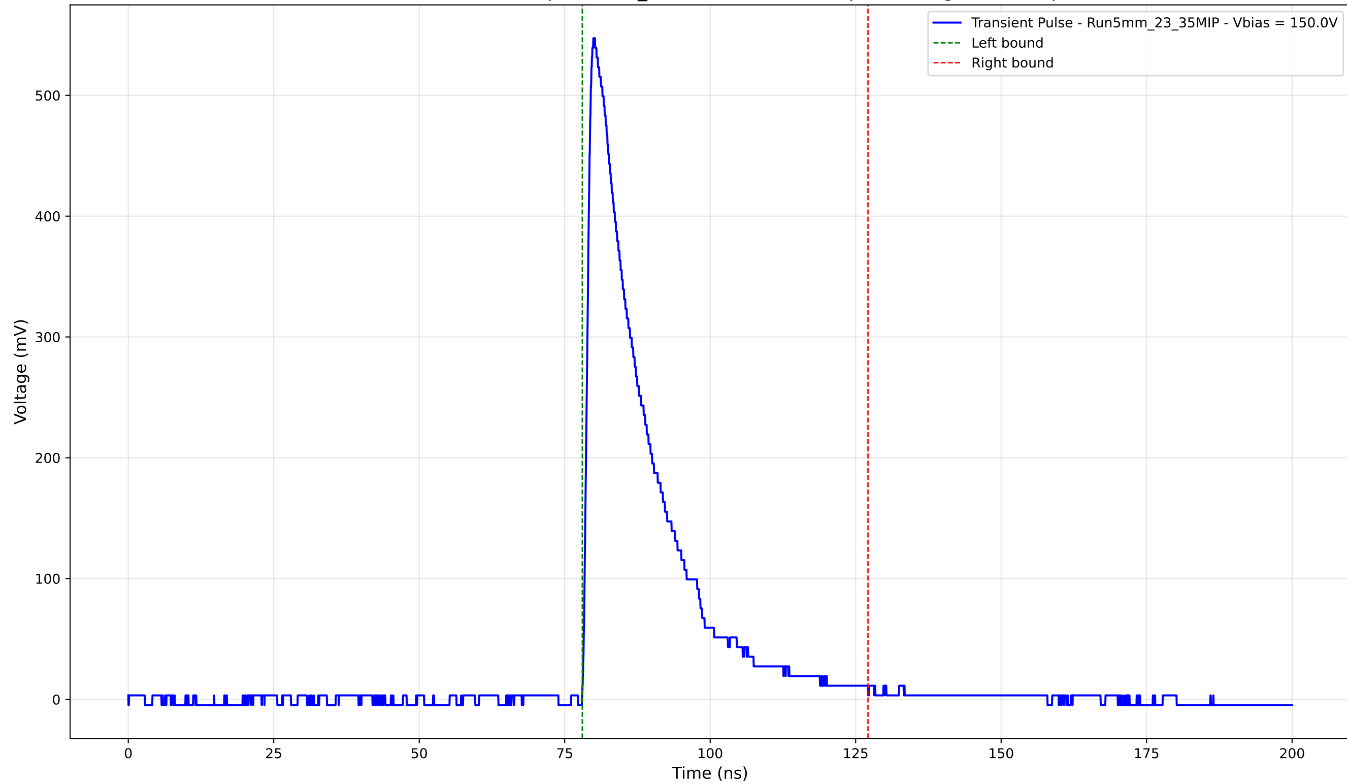
Transient Pulse - Sample: 5mm_23 - Position: 3805.0 \mu\text{m} - Charge: 123.16 pC
