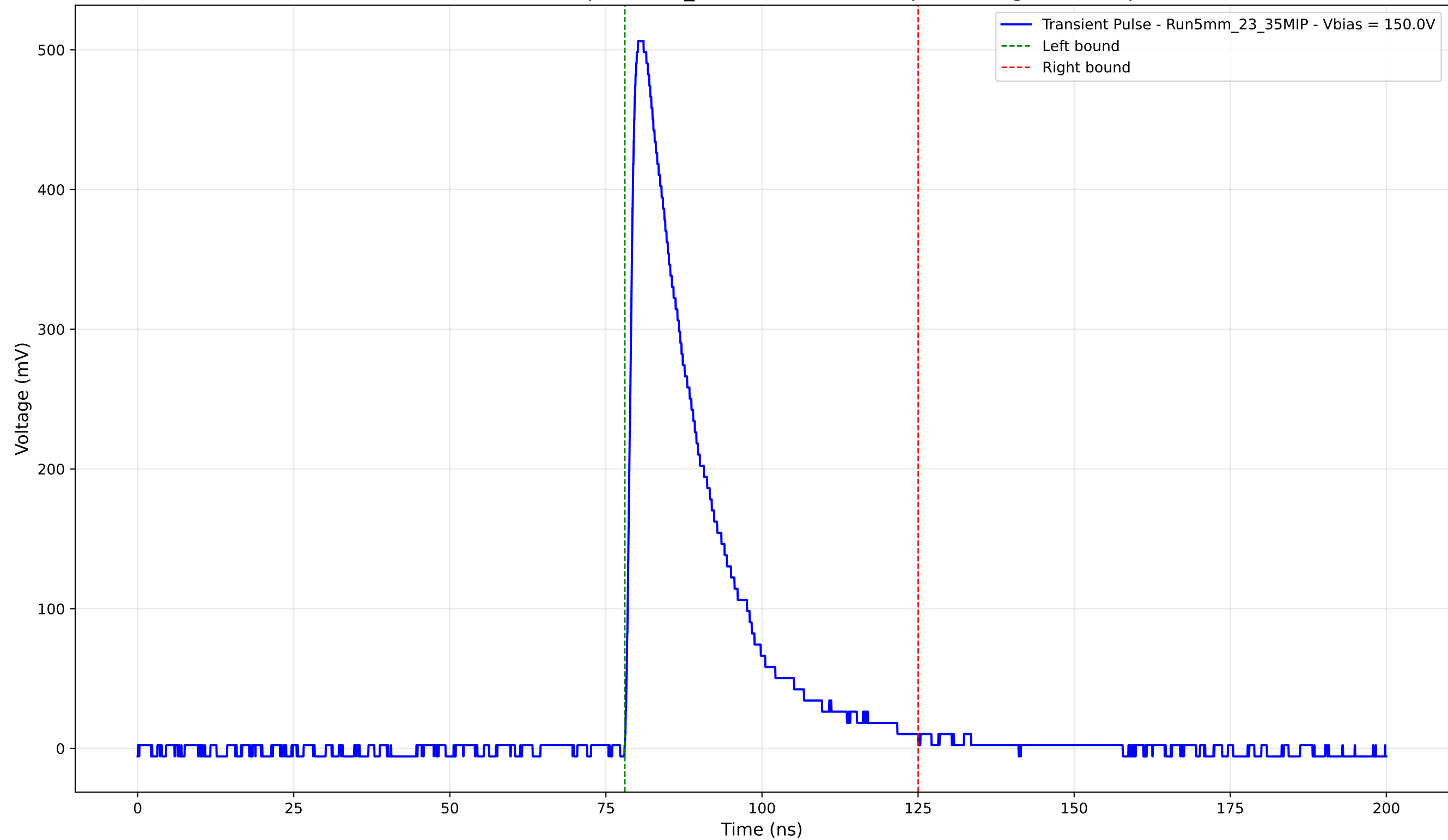
Transient Pulse - Sample: 5mm_23 - Position: 3500.0 \mu\text{m} - Charge: 124.72 pC
