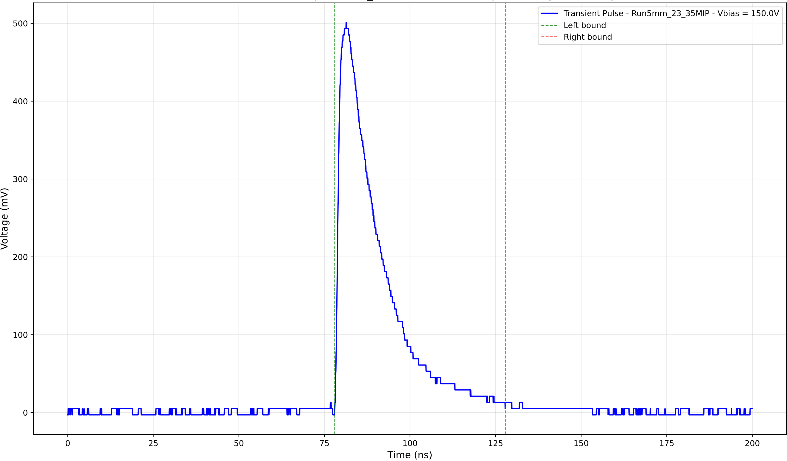
Transient Pulse - Sample: 5mm_23 - Position: 2785.0 \mu\text{m} - Charge: 136.02 pC
