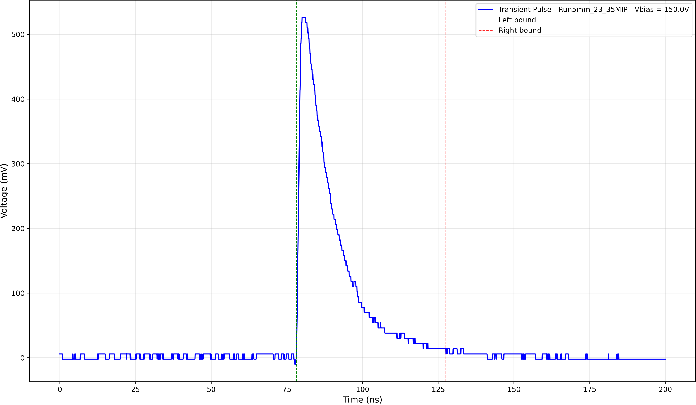
Transient Pulse - Sample: 5mm_23 - Position: 1765.0 \mu\text{m} - Charge: 136.48 pC
