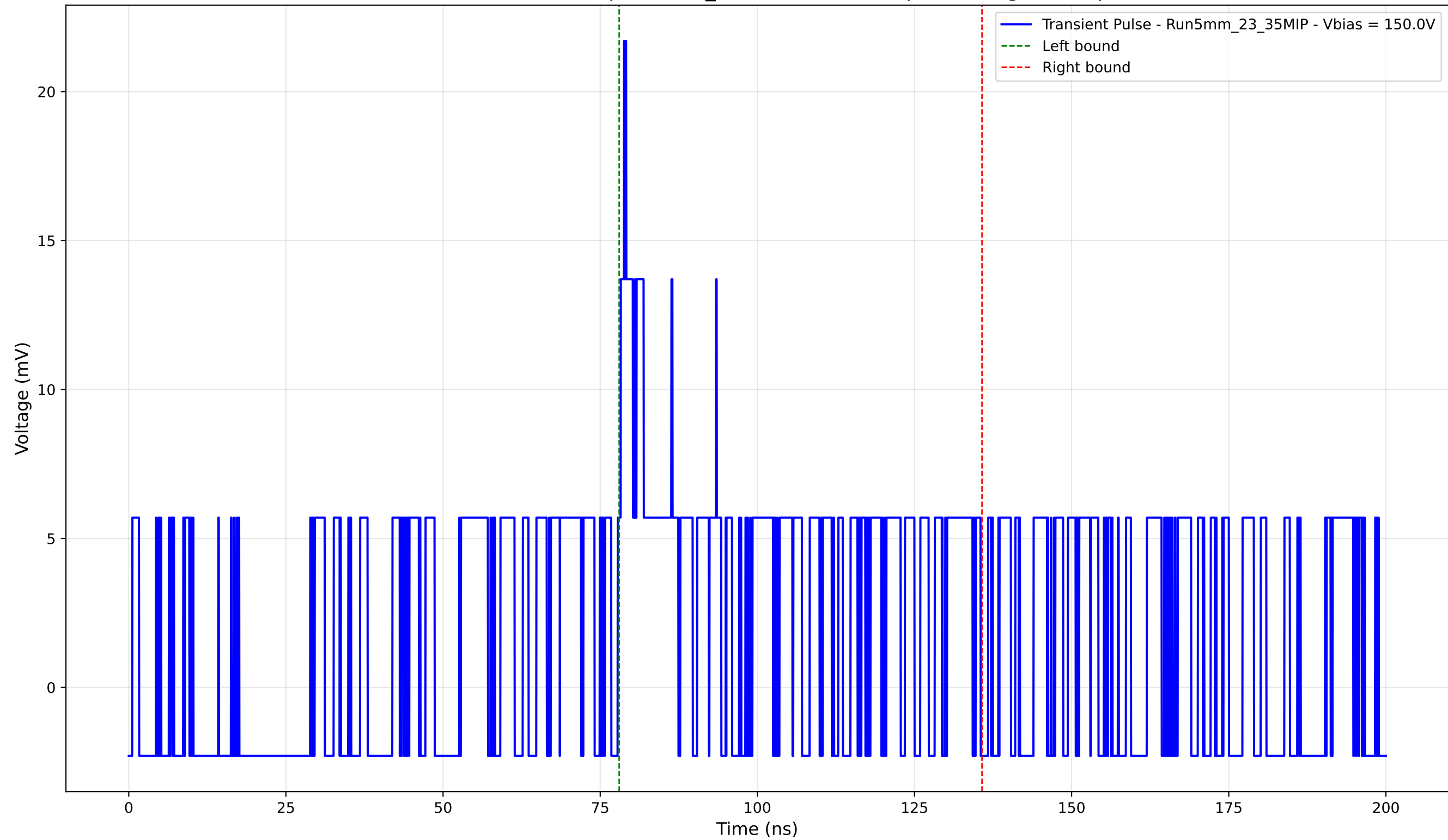
Transient Pulse - Sample: 5mm_23 - Position: 40.0 \mu\text{m} - Charge: 4.88 pC
