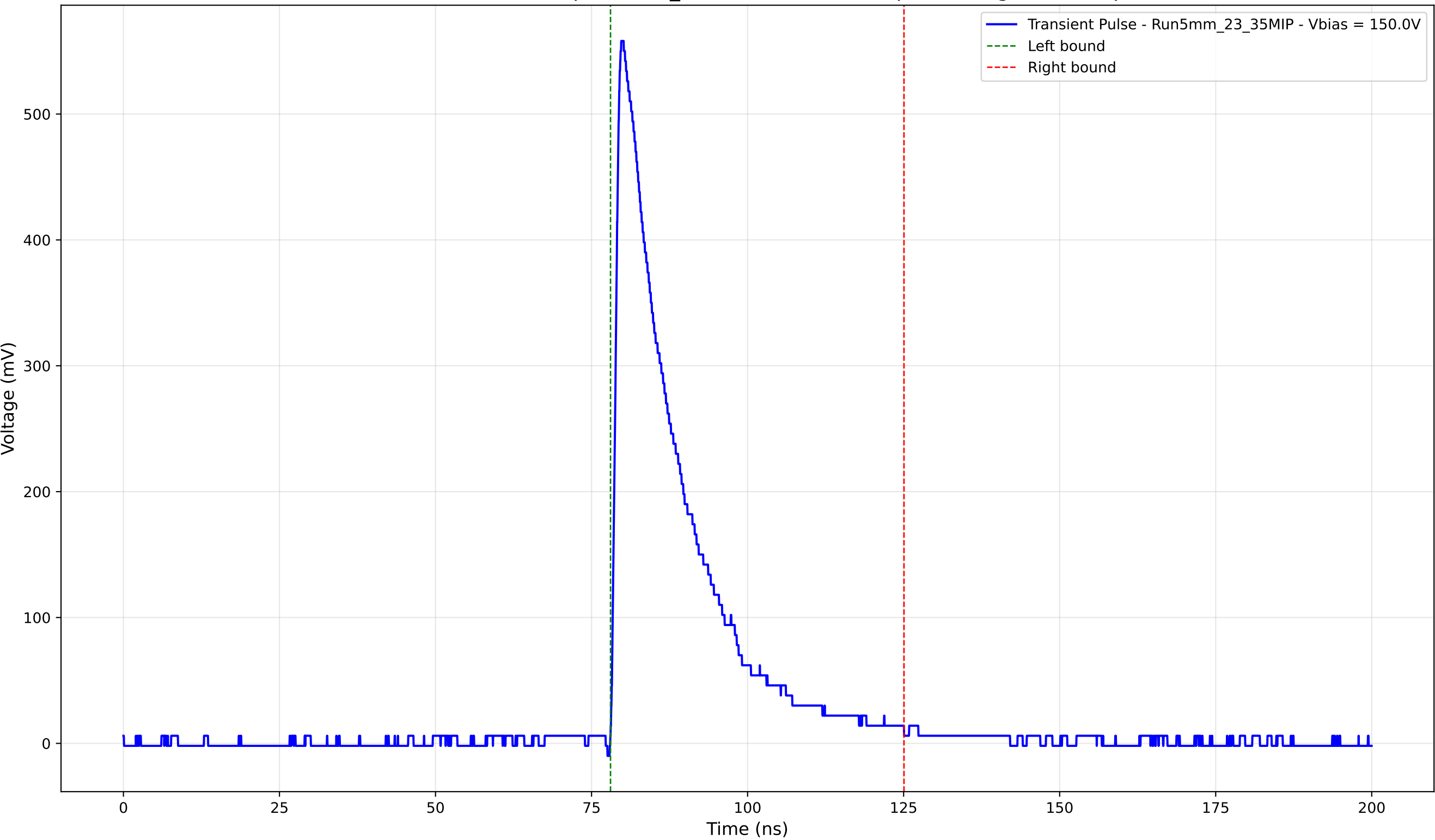
Transient Pulse - Sample: 5mm_23 - Position: 3940.0 \mu\text{m} - Charge: 122.68 pC
