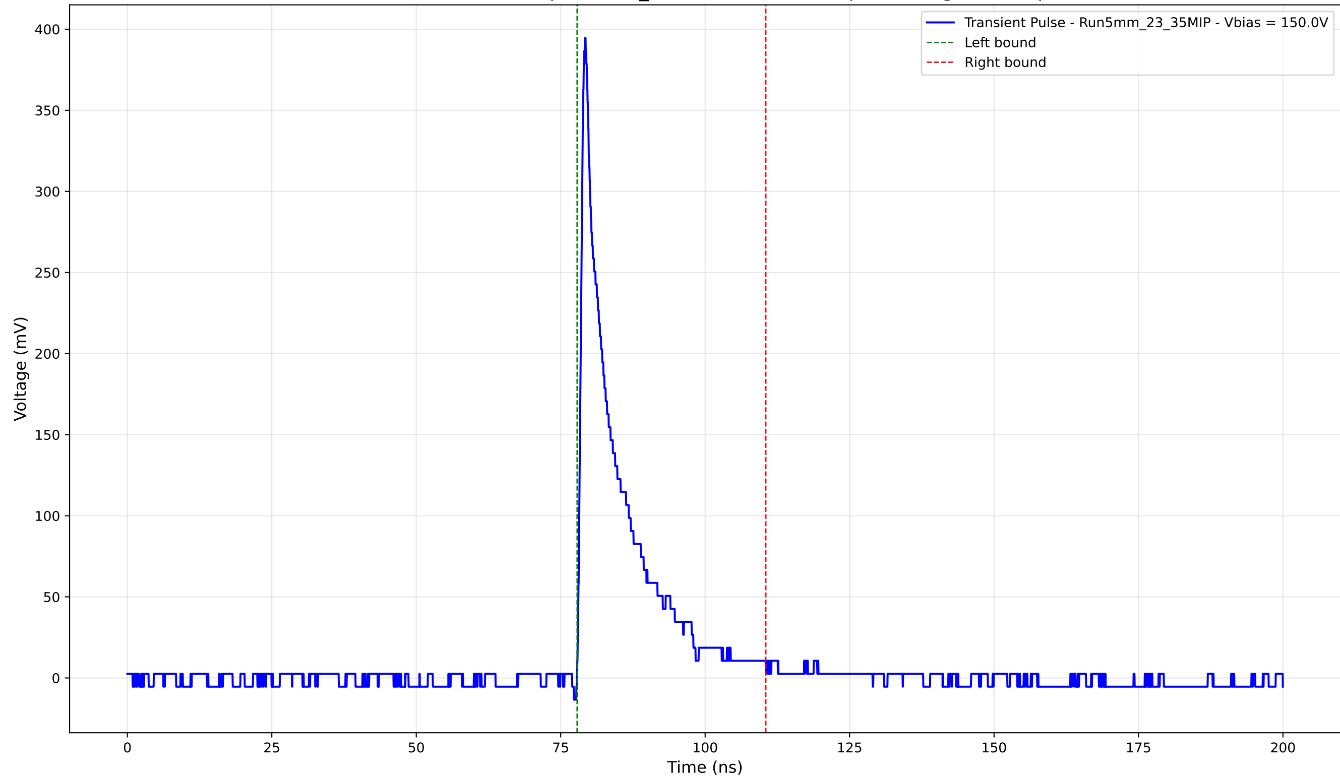
Transient Pulse - Sample: 5mm_23 - Position: 4705.0 \mu\text{m} - Charge: 50.68 pC
