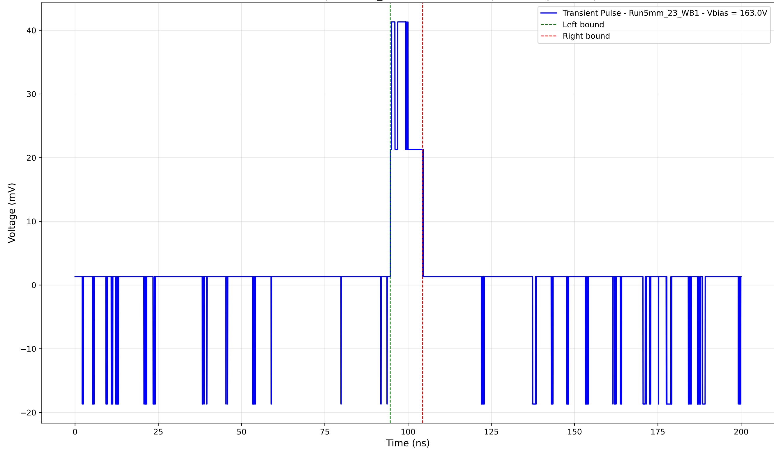
Transient Pulse - Sample: 5mm_23 - Position: 250.0 \mu\text{m} - Charge: 5.58 pC
