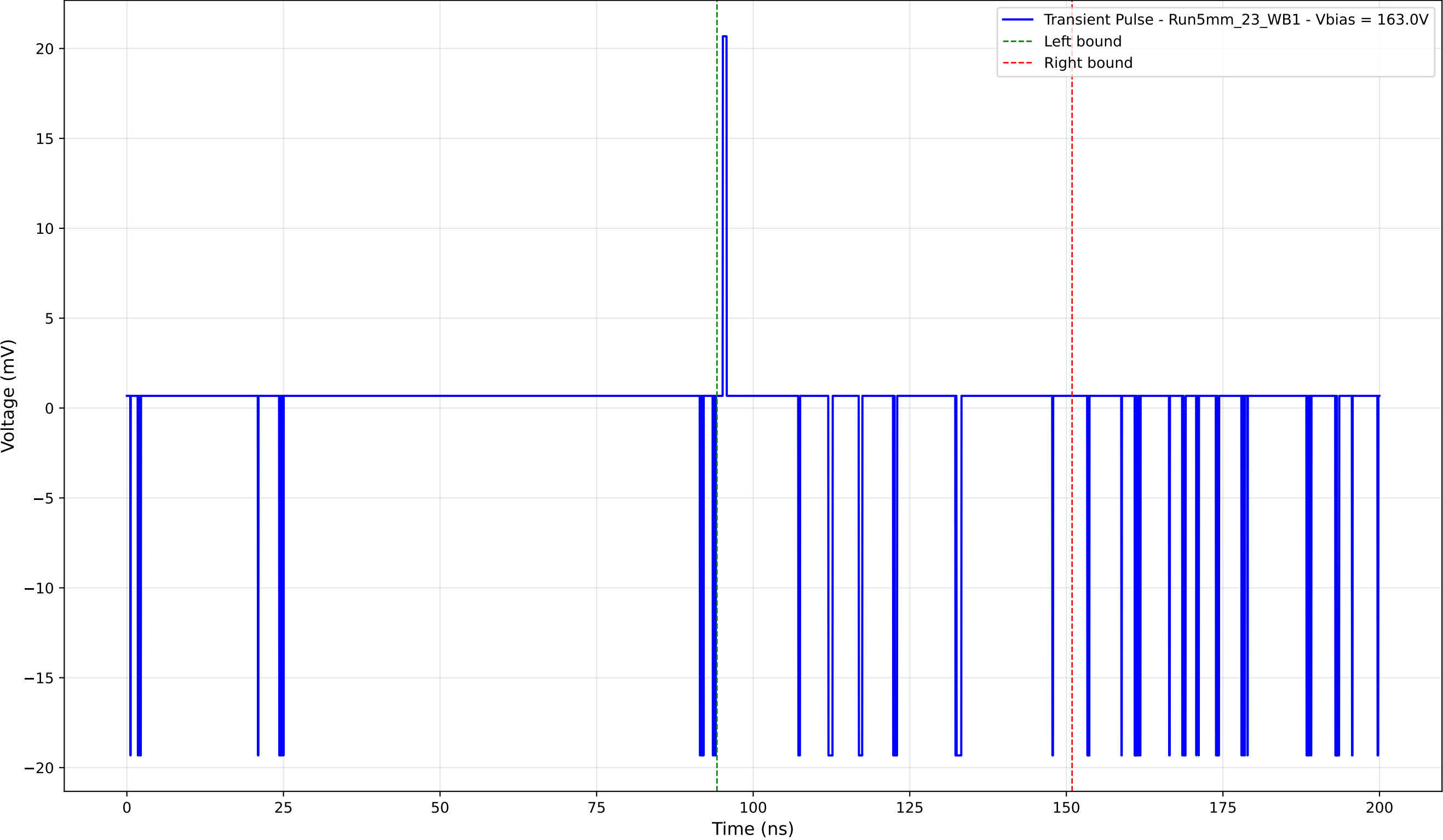
Transient Pulse - Sample: 5mm_23 - Position: 170.0 \mu\text{m} - Charge: -0.18 pC
