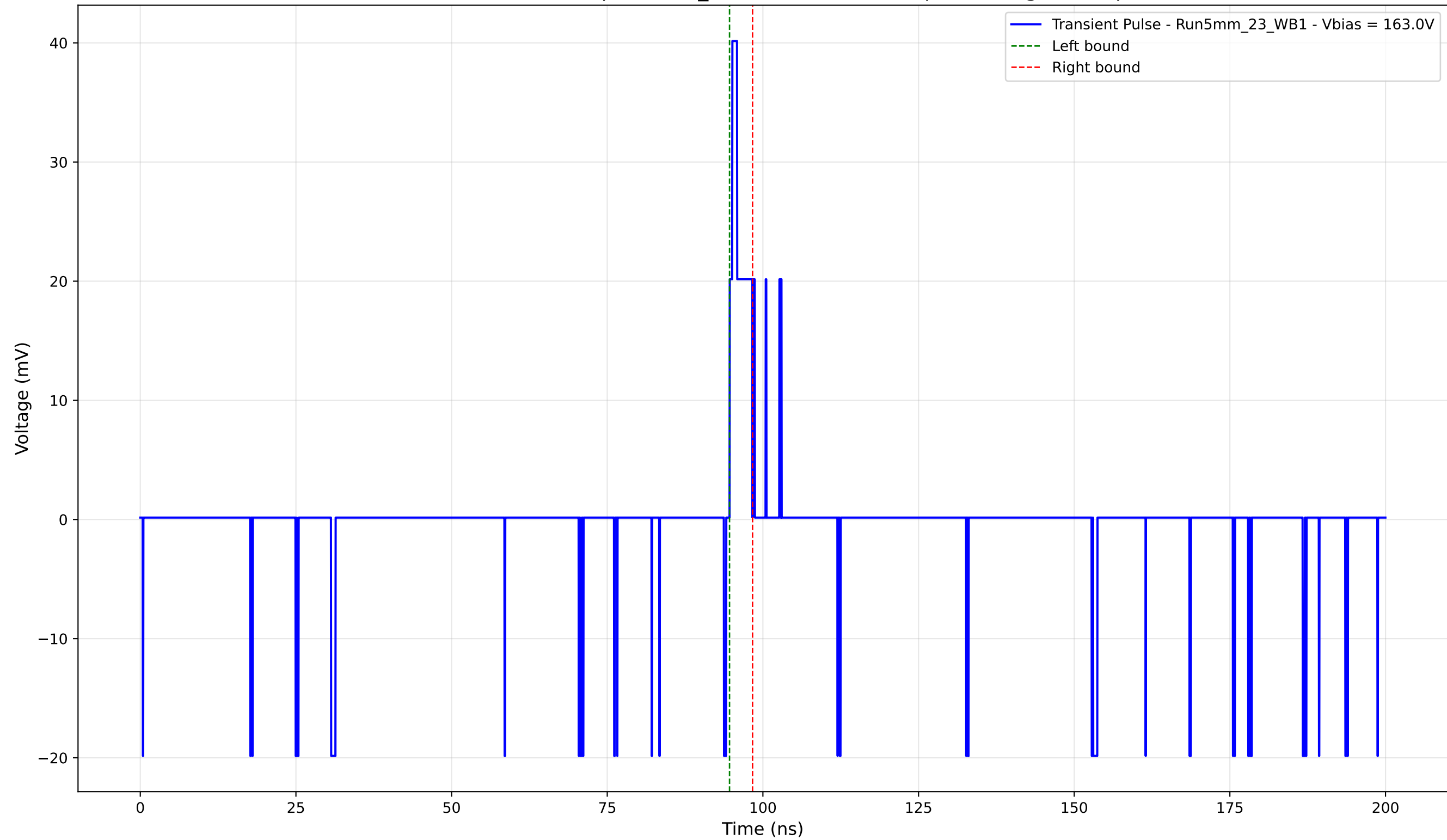
Transient Pulse - Sample: 5mm_23 - Position: 5245.0 \mu\text{m} - Charge: 1.80 pC
