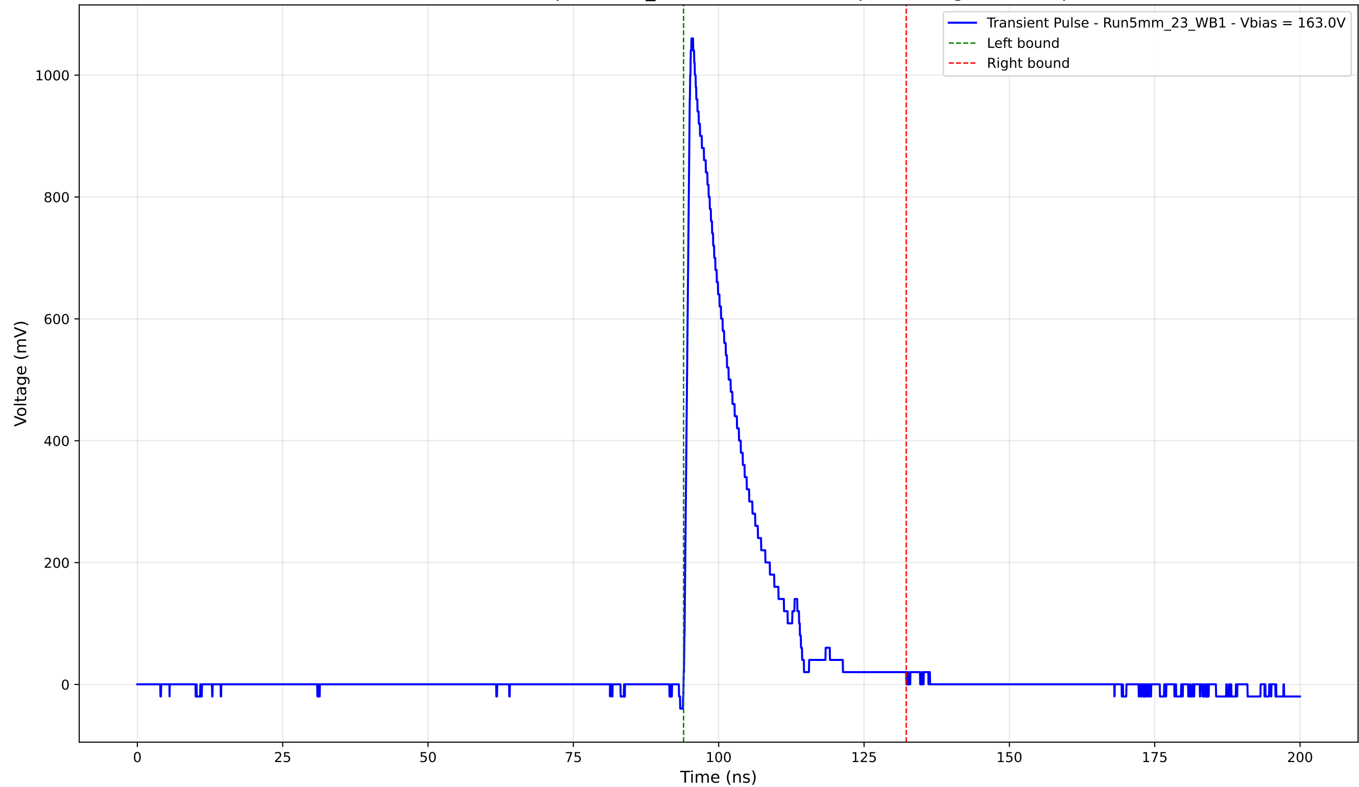
Transient Pulse - Sample: 5mm_23 - Position: 5070.0 \mu\text{m} - Charge: 185.81 pC
