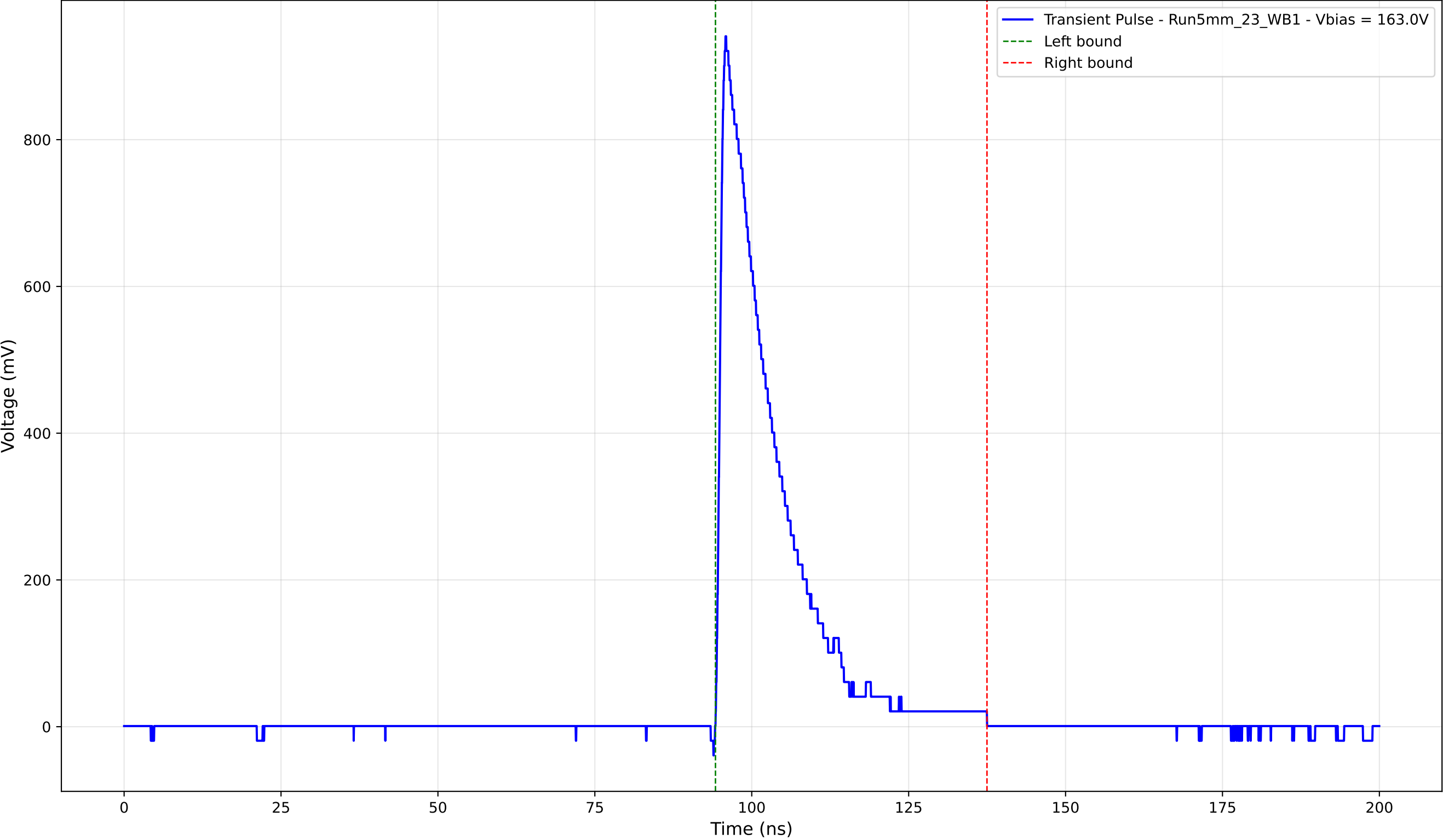
Transient Pulse - Sample: 5mm_23 - Position: 4625.0 \mu\text{m} - Charge: 175.70 pC
