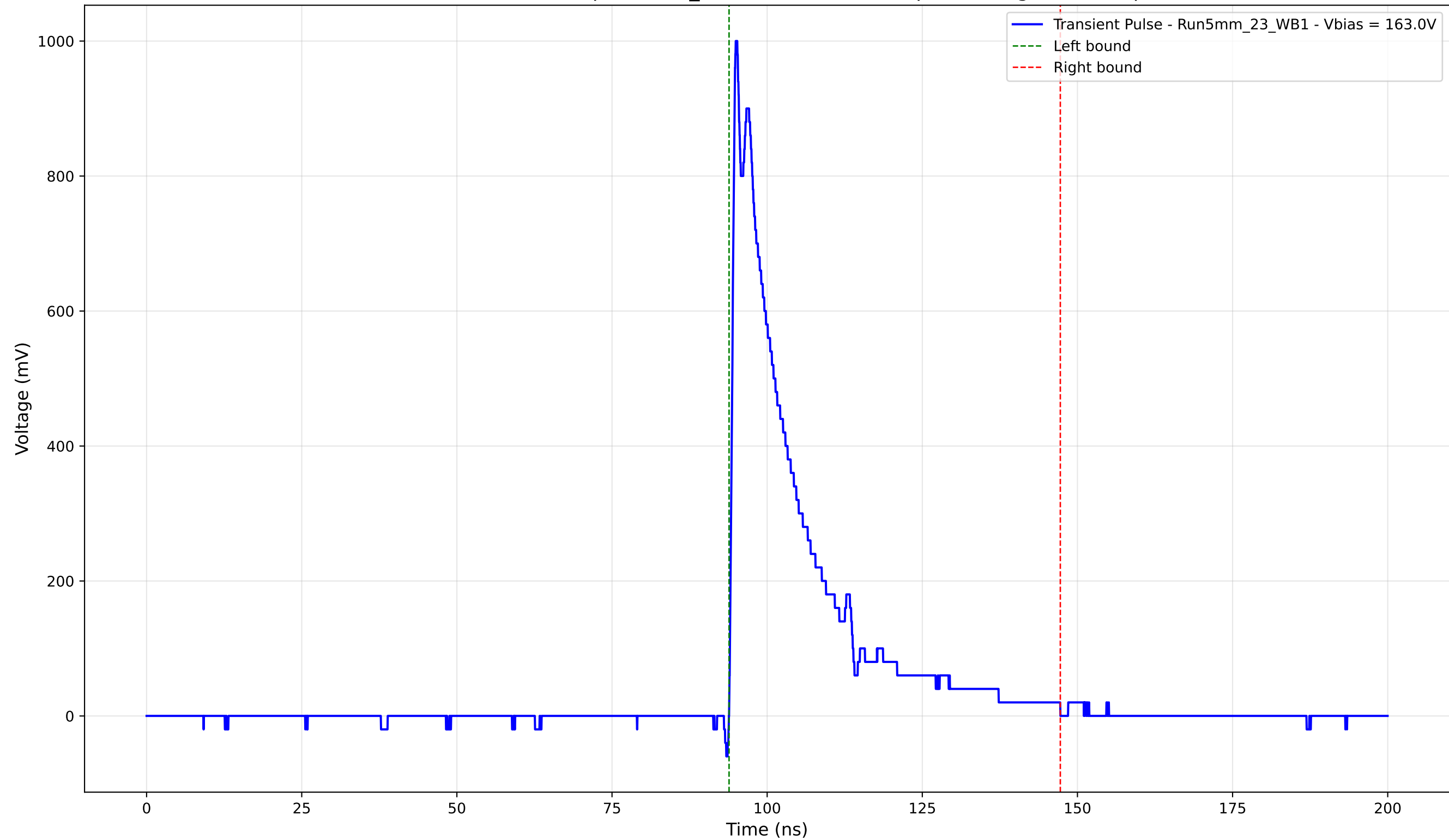
Transient Pulse - Sample: 5mm_23 - Position: 2820.0 \mu\text{m} - Charge: 202.17 pC
