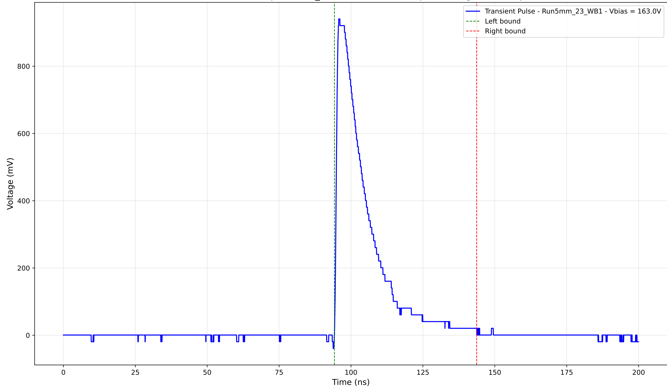
Transient Pulse - Sample: 5mm_23 - Position: 3560.0 \mu\text{m} - Charge: 219.39 pC
