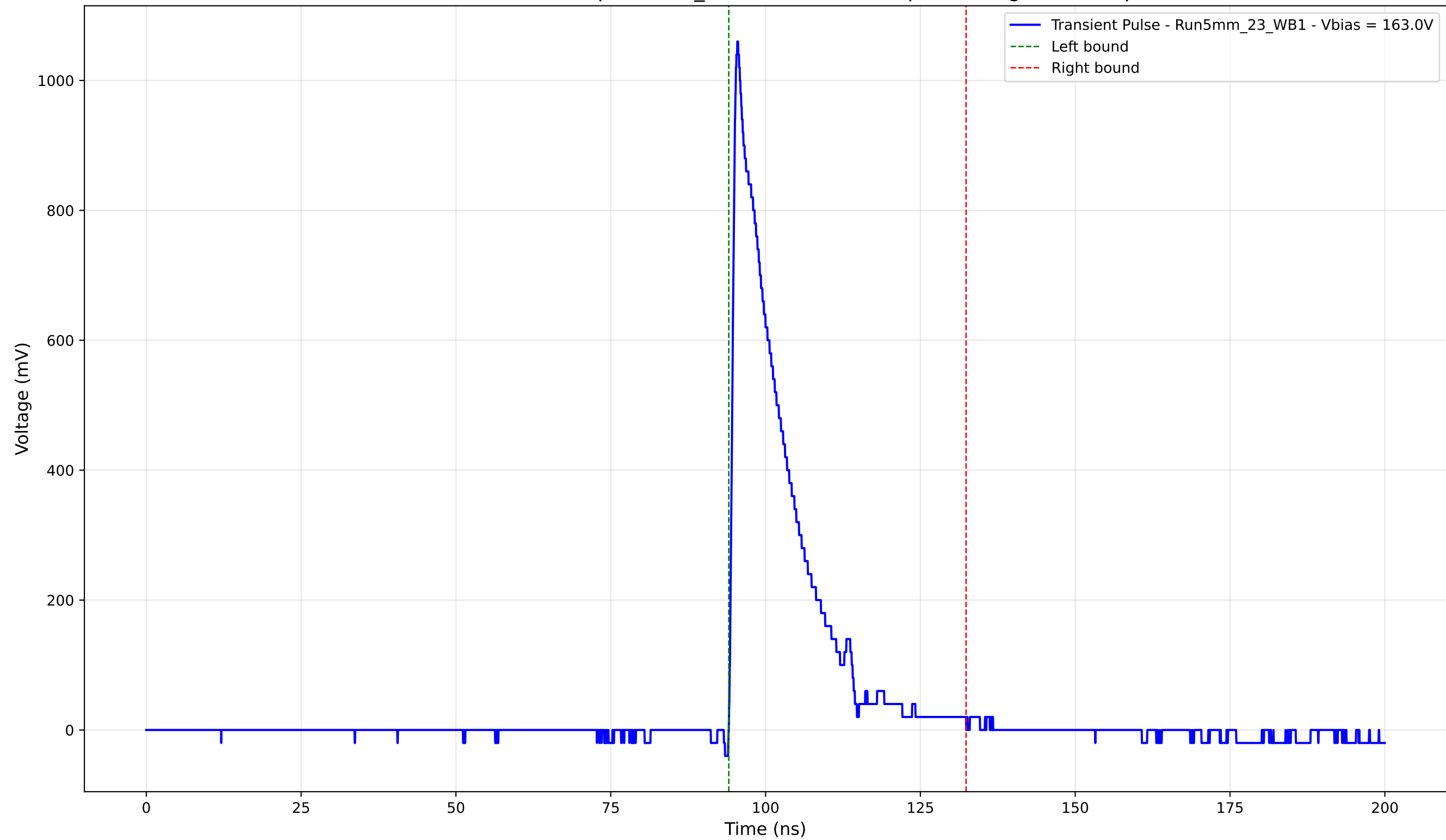
Transient Pulse - Sample: 5mm_23 - Position: 365.0 \mu\text{m} - Charge: 184.02 pC
