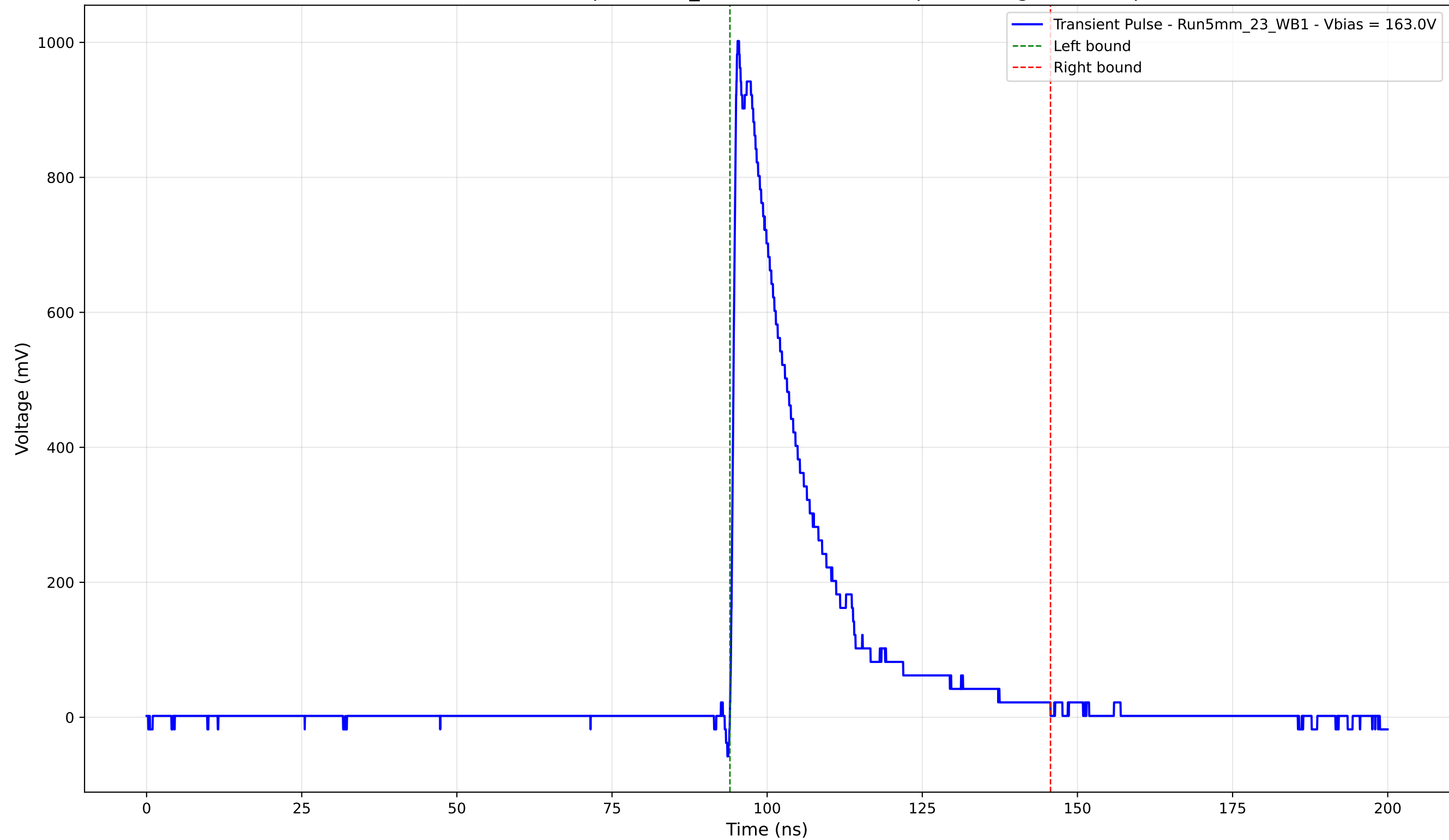
Transient Pulse - Sample: 5mm_23 - Position: 2375.0 \mu\text{m} - Charge: 227.66 pC
