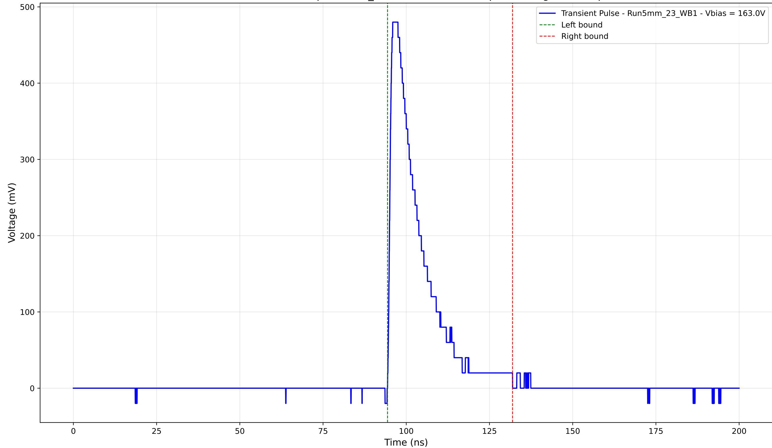
Transient Pulse - Sample: 5mm_23 - Position: 1765.0 \mu\text{m} - Charge: 97.34 pC
