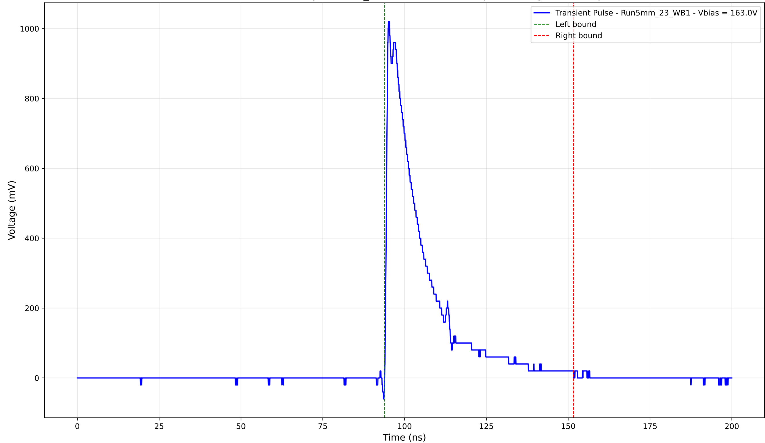
Transient Pulse - Sample: 5mm_23 - Position: 2510.0 \mu\text{m} - Charge: 235.23 pC
