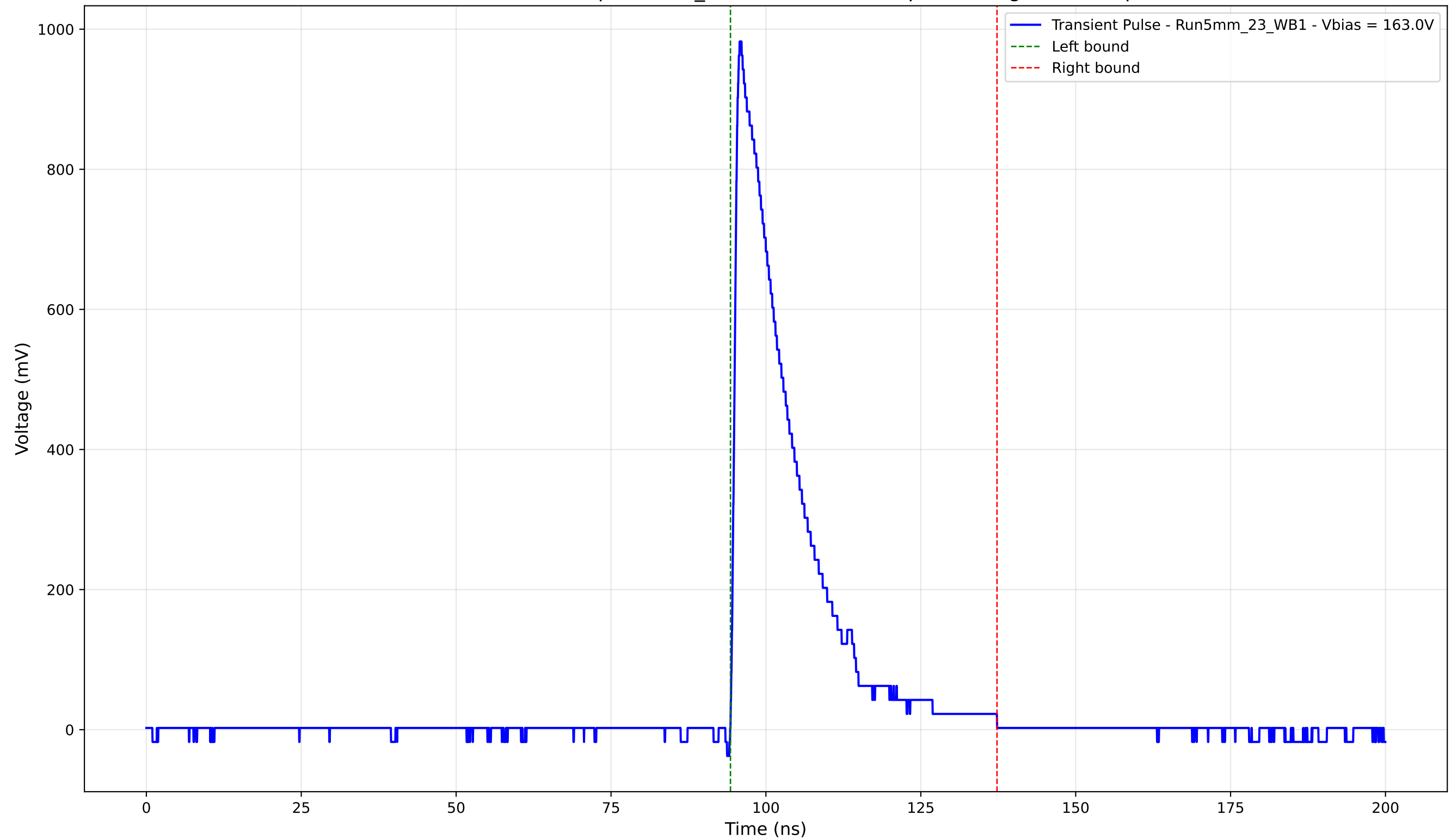
Transient Pulse - Sample: 5mm_23 - Position: 805.0 \mu\text{m} - Charge: 196.61 pC
