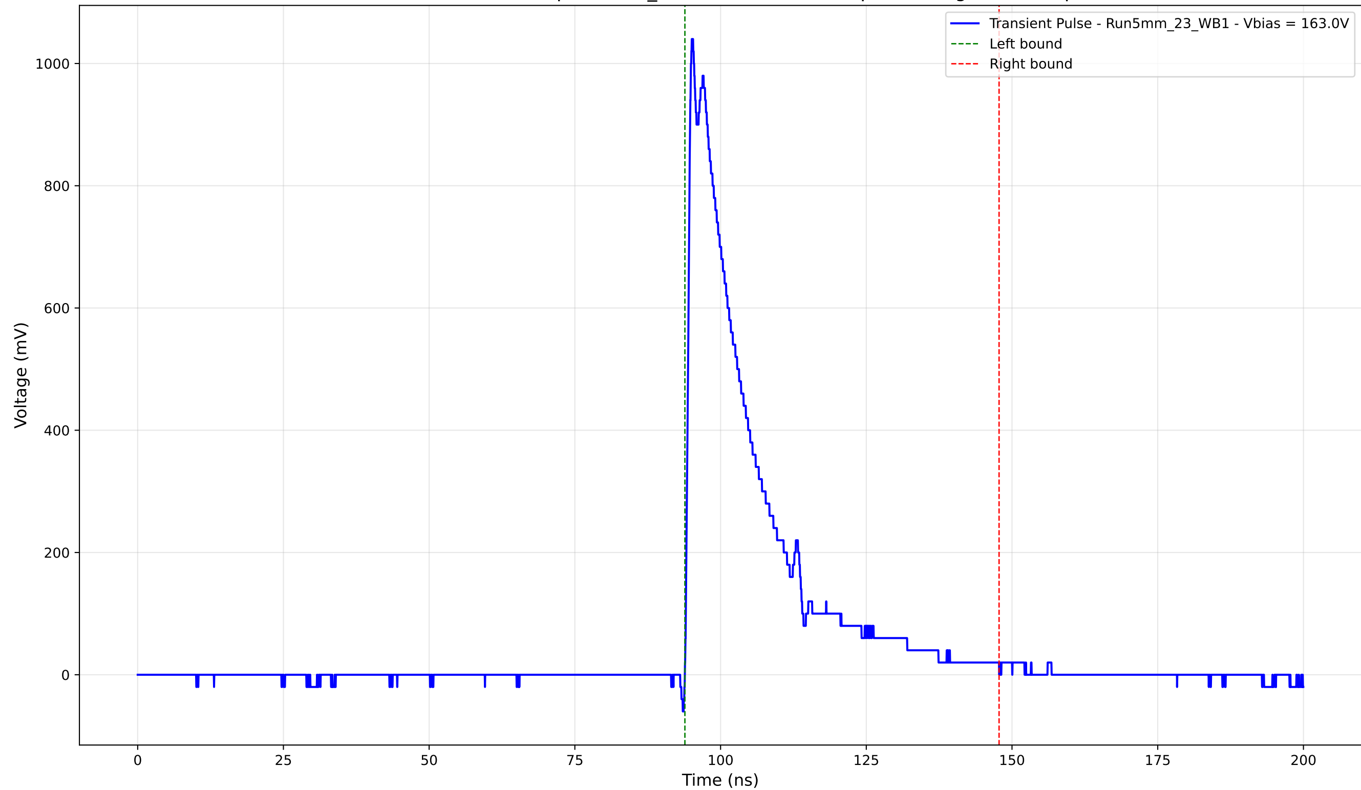
Transient Pulse - Sample: 5mm_23 - Position: 2935.0 \mu\text{m} - Charge: 235.70 pC
