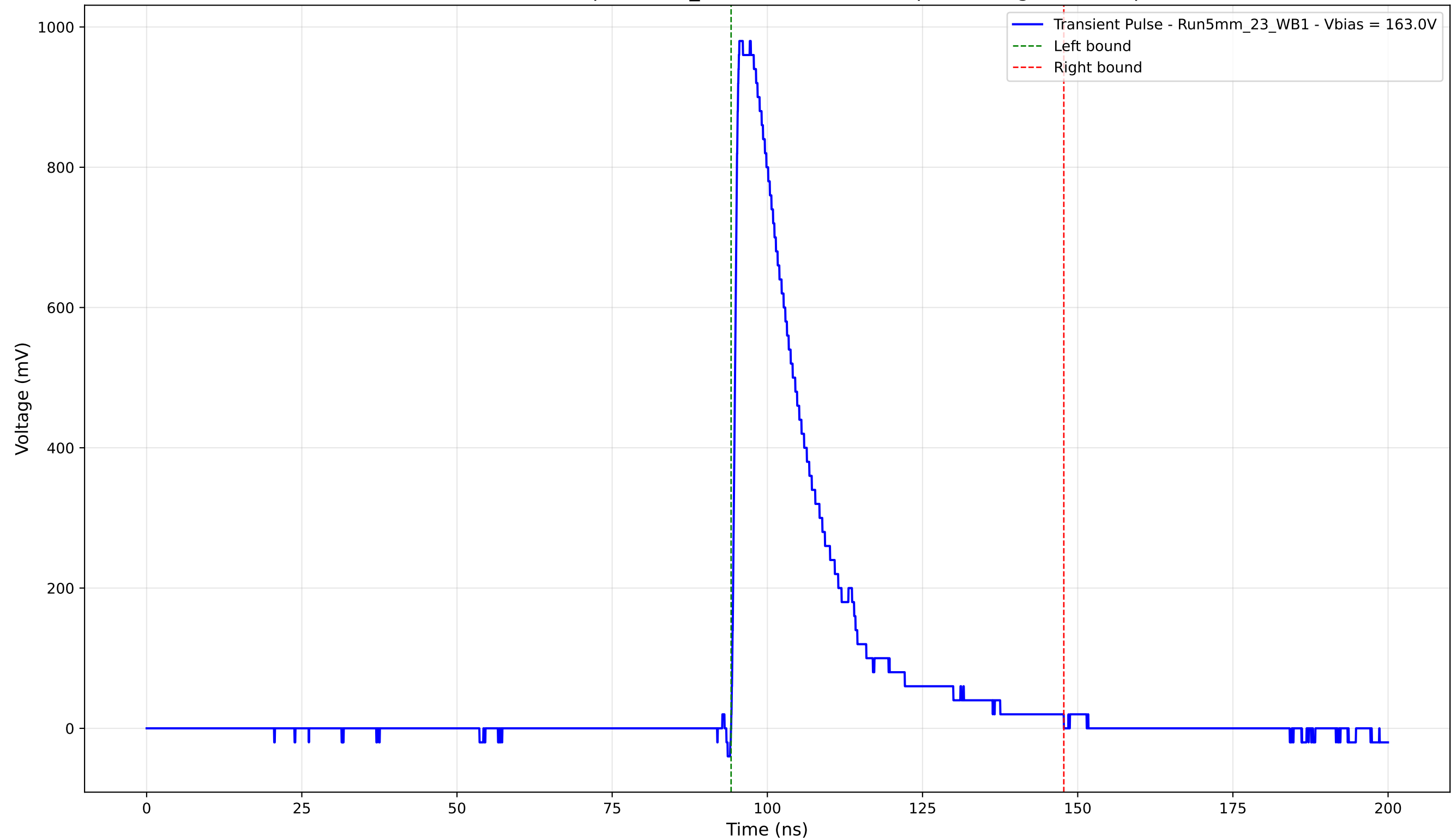
Transient Pulse - Sample: 5mm_23 - Position: 2045.0 \mu\text{m} - Charge: 245.44 pC
