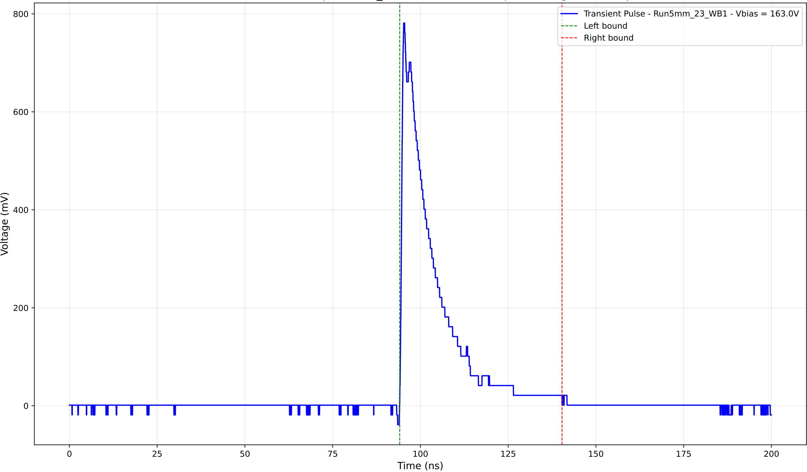
Transient Pulse - Sample: 5mm_23 - Position: 3190.0 \mu\text{m} - Charge: 149.20 pC
