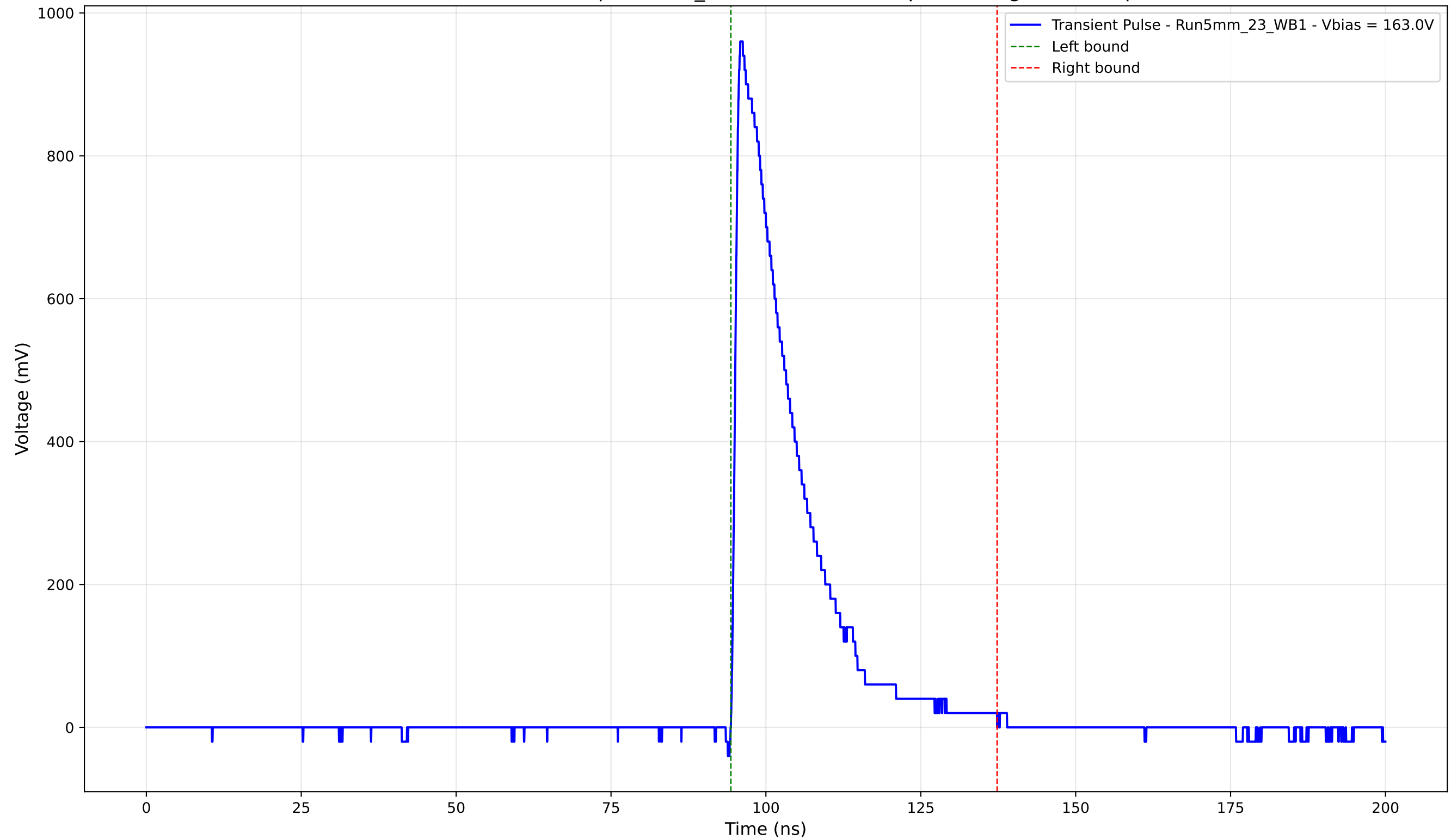
Transient Pulse - Sample: 5mm_23 - Position: 975.0 \mu\text{m} - Charge: 200.06 pC
