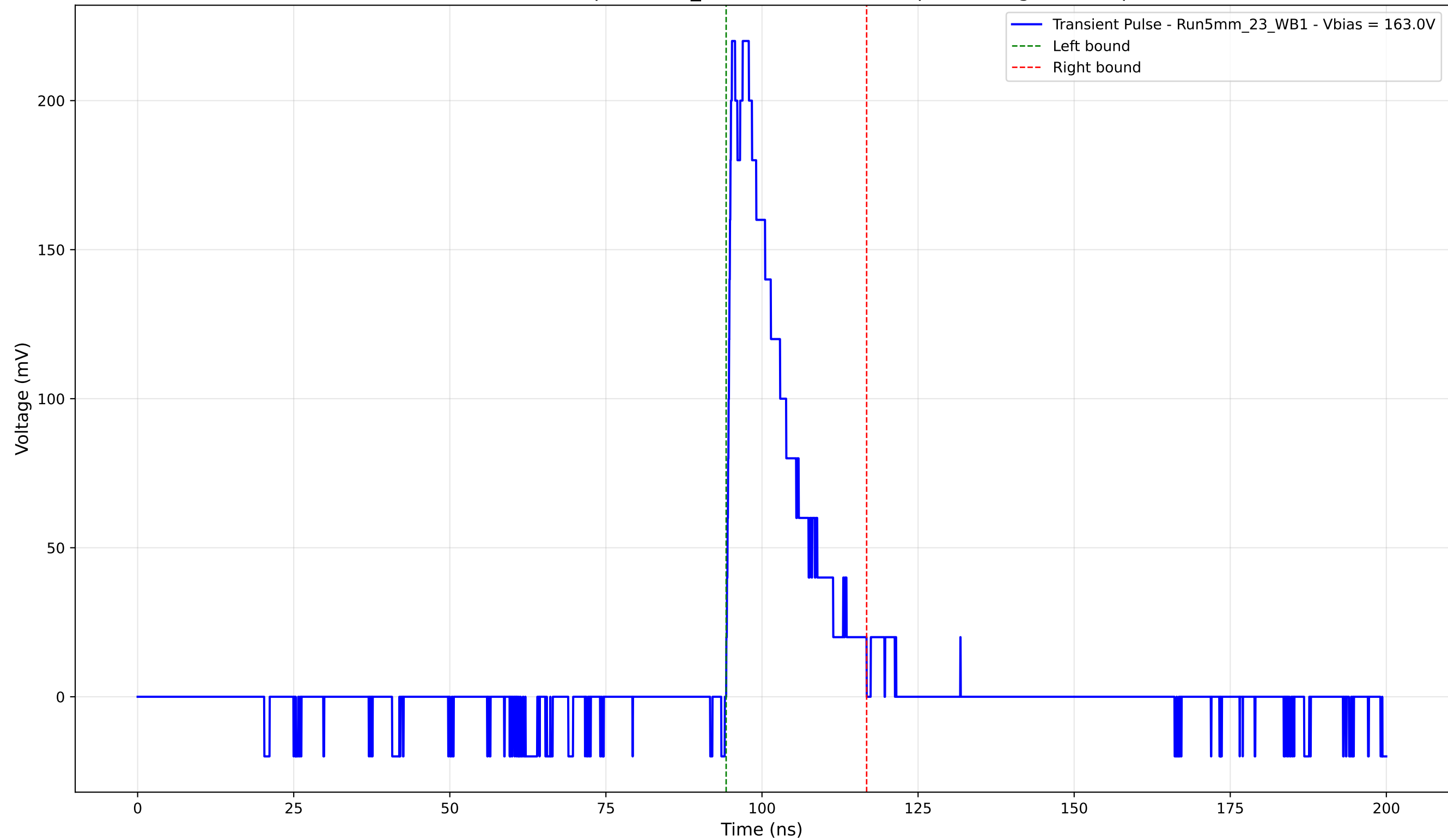
Transient Pulse - Sample: 5mm_23 - Position: 2245.0 \mu\text{m} - Charge: 41.34 pC
