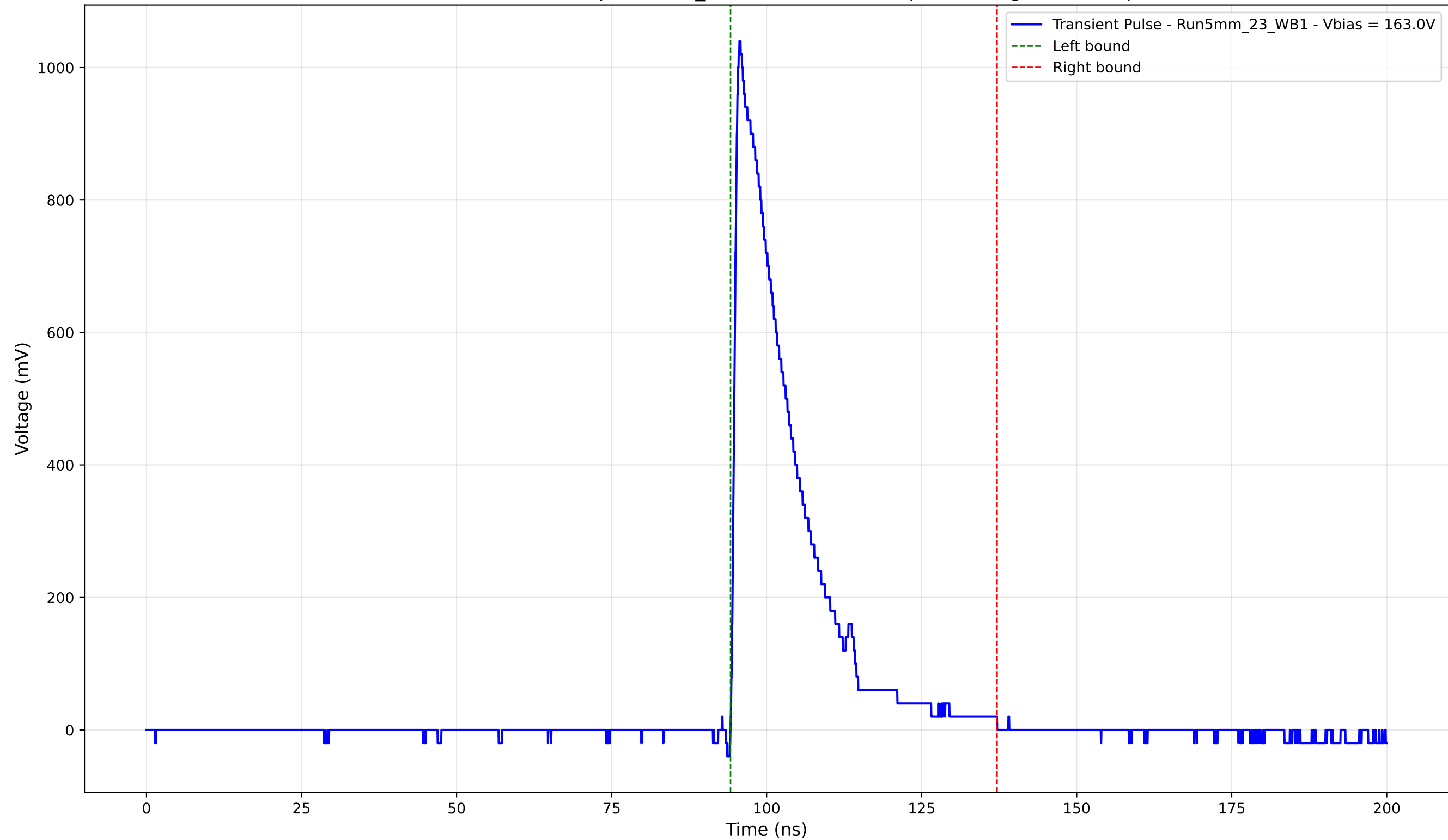
Transient Pulse - Sample: 5mm_23 - Position: 625.0 \mu\text{m} - Charge: 207.16 pC
