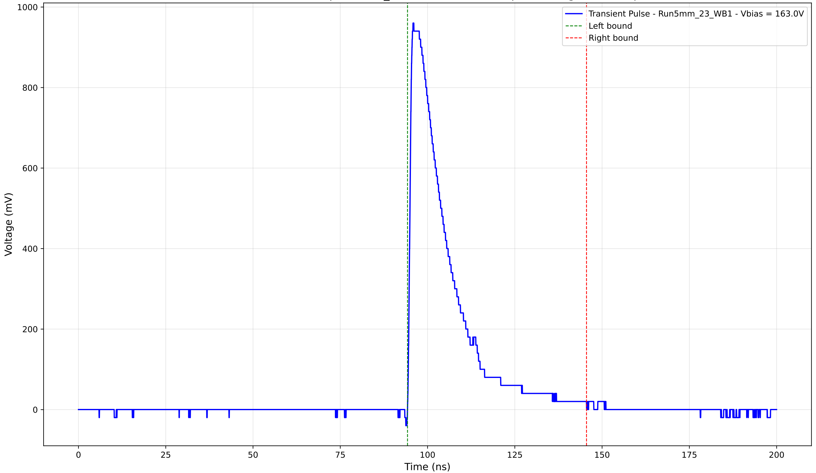
Transient Pulse - Sample: 5mm_23 - Position: 1855.0 \mu\text{m} - Charge: 229.84 pC
