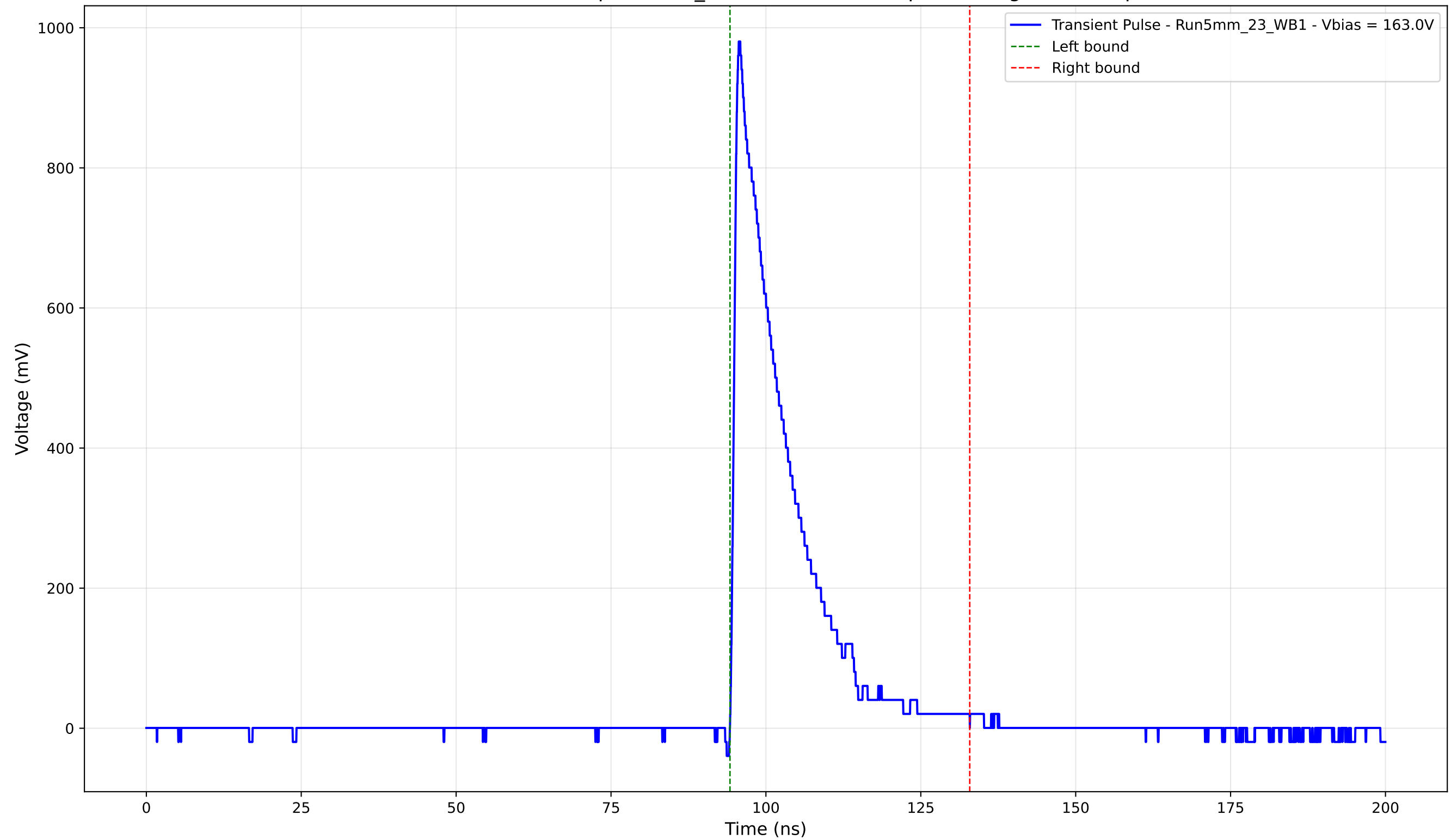
Transient Pulse - Sample: 5mm_23 - Position: 650.0 \mu\text{m} - Charge: 174.88 pC
