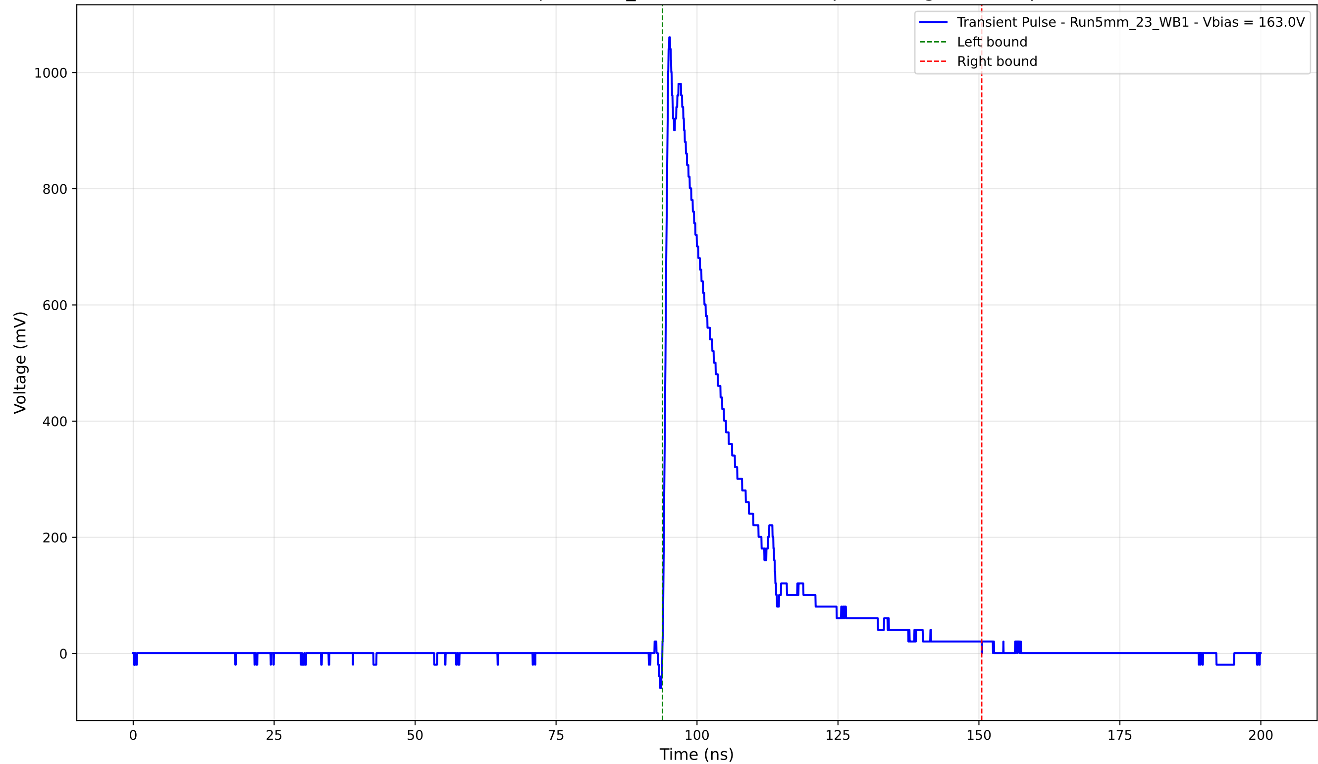
Transient Pulse - Sample: 5mm_23 - Position: 2580.0 \mu\text{m} - Charge: 242.37 pC
