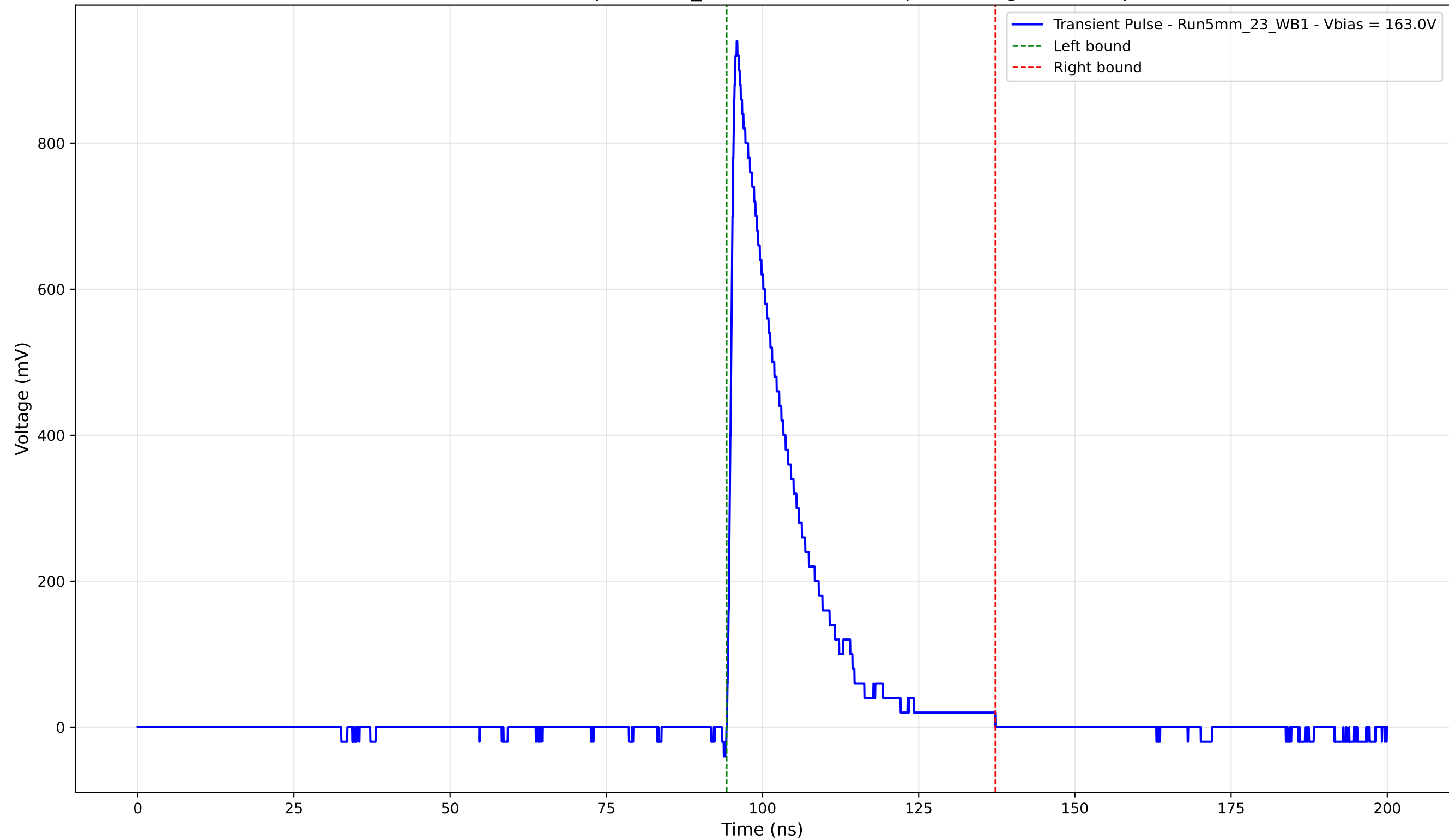
Transient Pulse - Sample: 5mm_23 - Position: 790.0 \mu\text{m} - Charge: 175.56 pC
