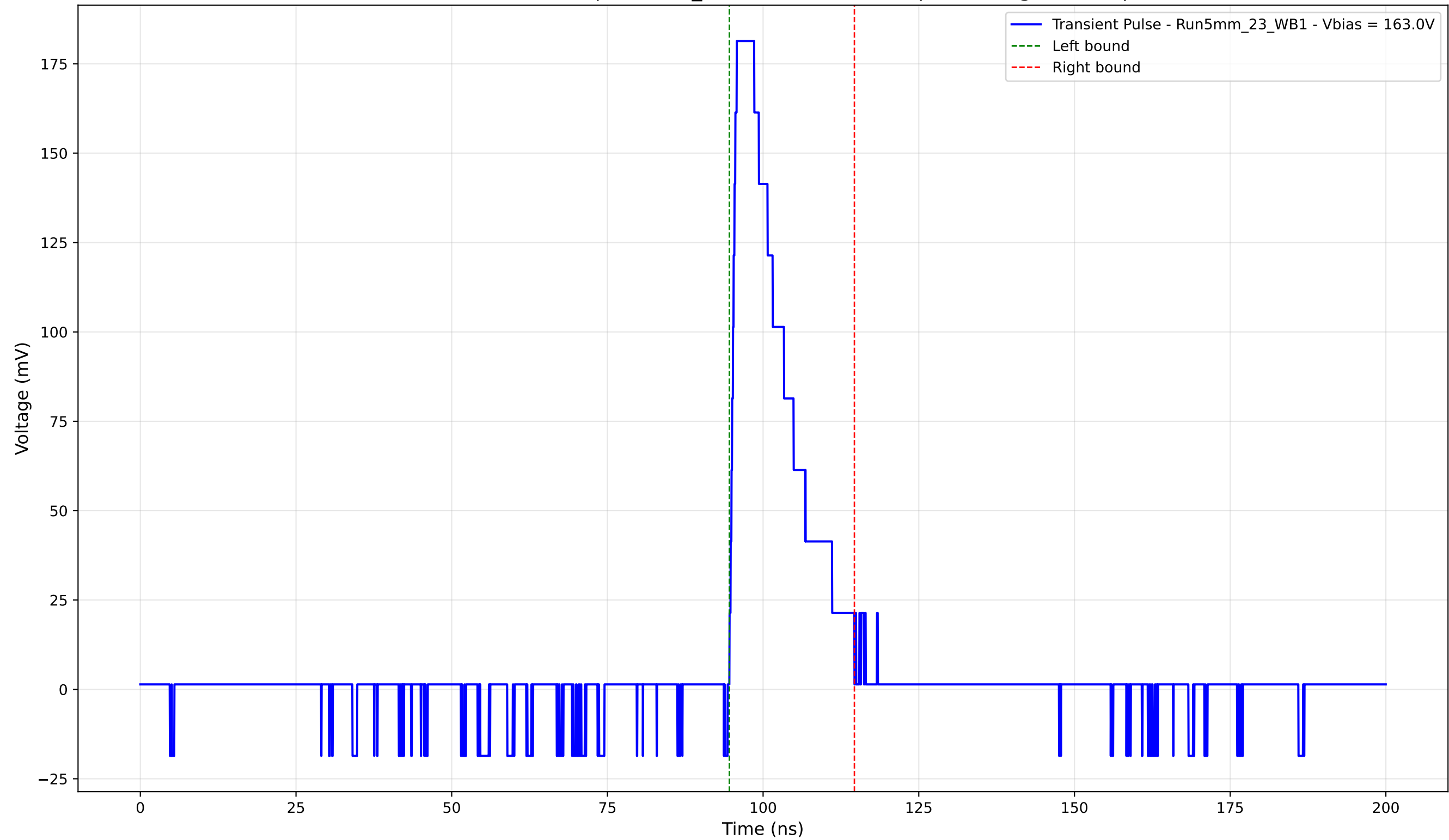
Transient Pulse - Sample: 5mm_23 -Position: 4255.0 \mu\text{m} - Charge: 34.37 pC
