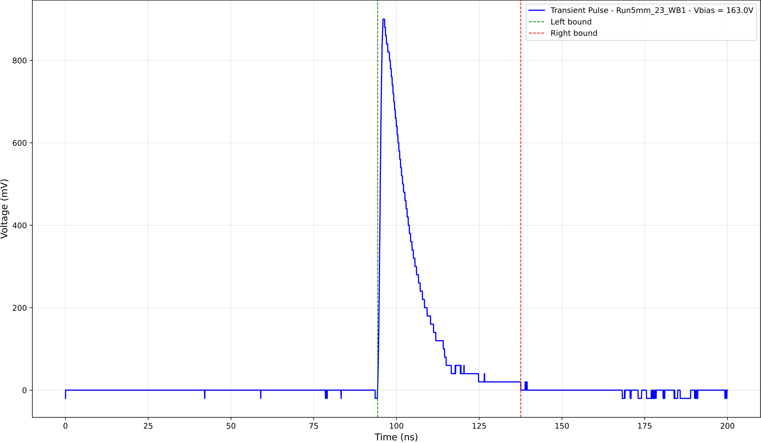
Transient Pulse - Sample: 5mm_23 - Position: 4375.0 \mu\text{m} - Charge: 178.92 pC
