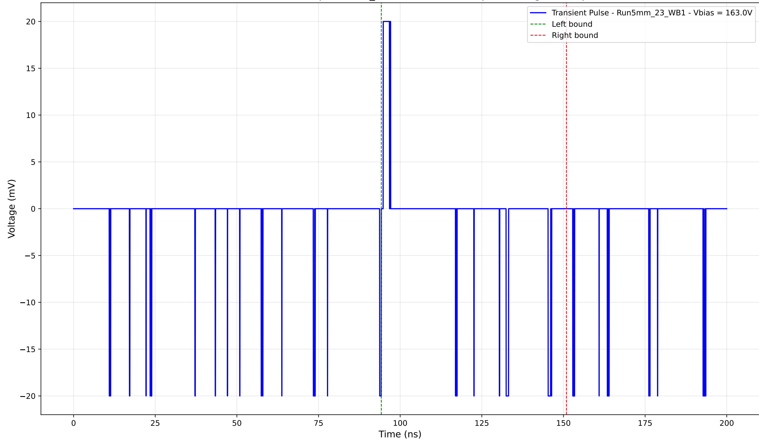
Transient Pulse - Sample: 5mm_23 - Position: 115.0 \mu\text{m} - Charge: 0.04 pC
