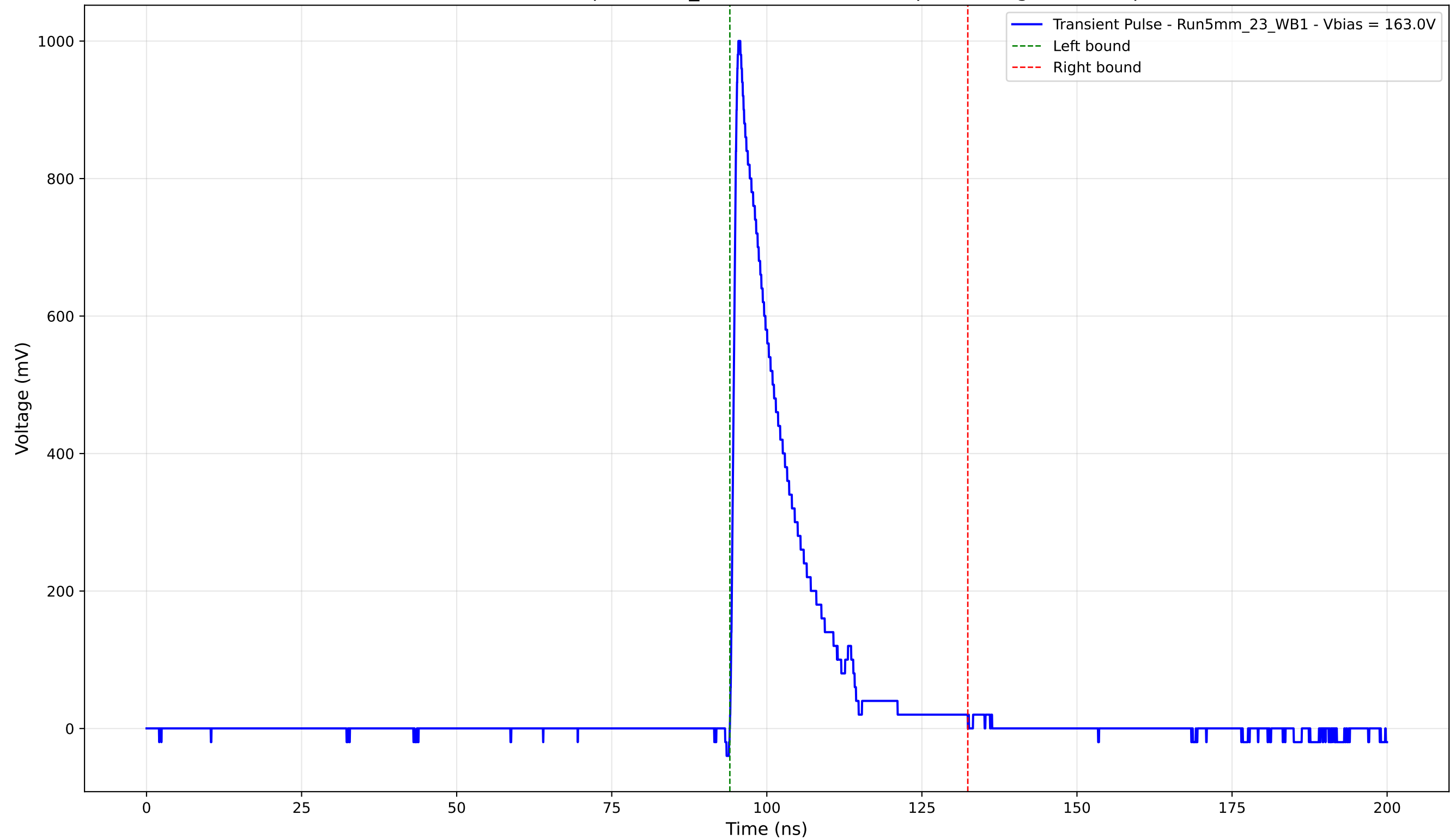
Transient Pulse - Sample: 5mm_23 - Position: 4980.0 \mu\text{m} - Charge: 167.29 pC
