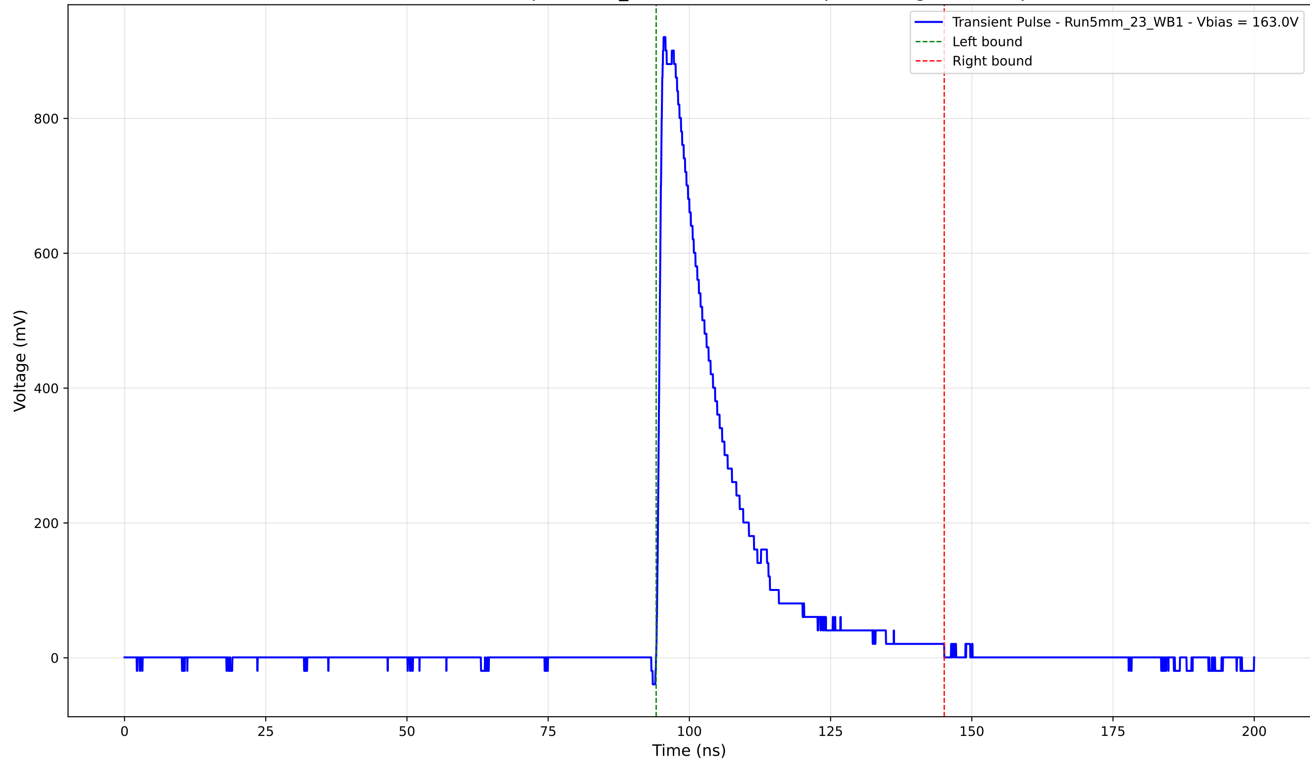
Transient Pulse - Sample: 5mm_23 - Position: 2160.0 \mu\text{m} - Charge: 208.08 pC
