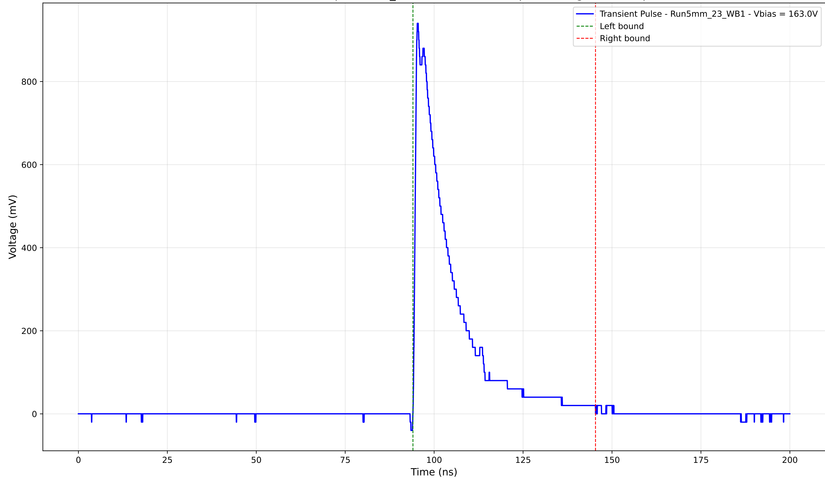
Transient Pulse - Sample: 5mm_23 - Position: 3165.0 \mu\text{m} - Charge: 200.25 pC
