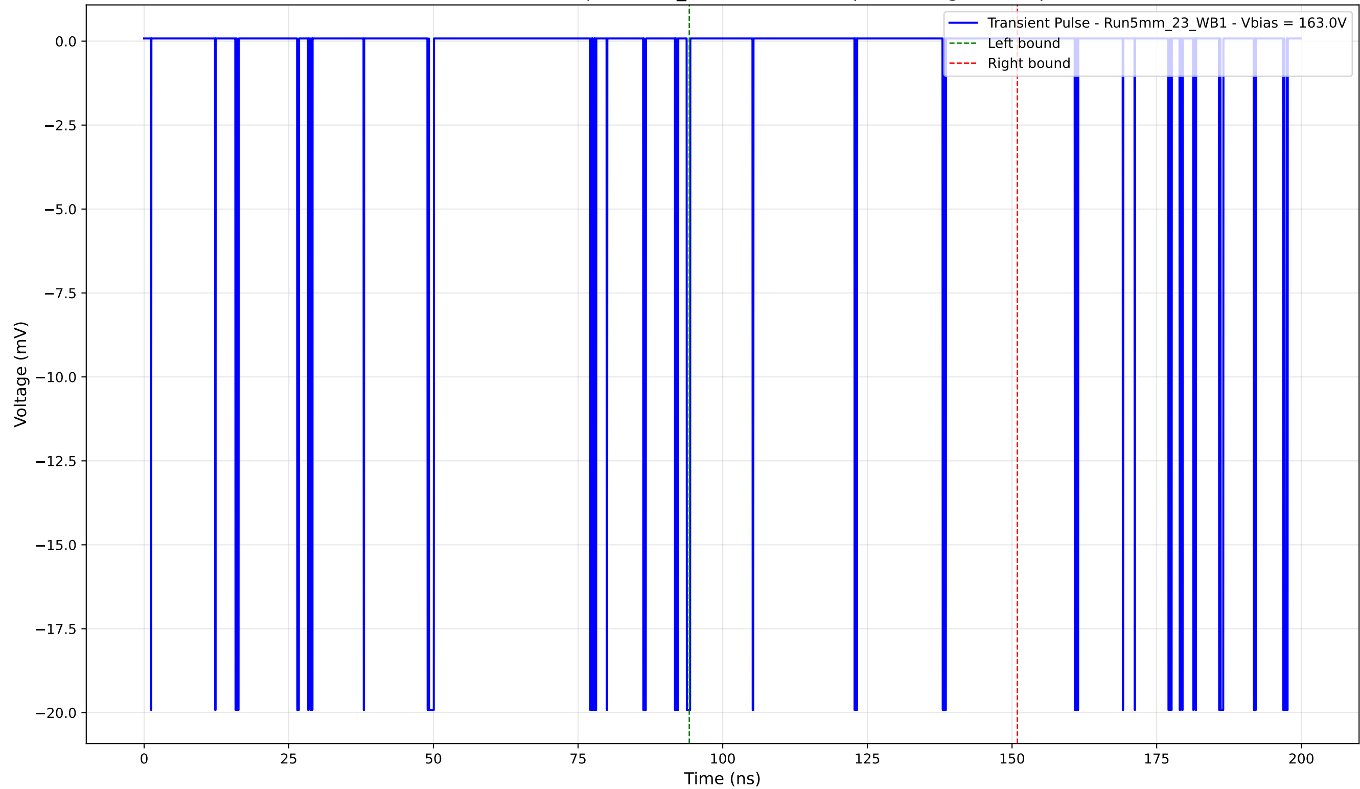
Transient Pulse - Sample: 5mm_23 - Position: 0.0 \mu\text{m} - Charge: -0.31 pC
