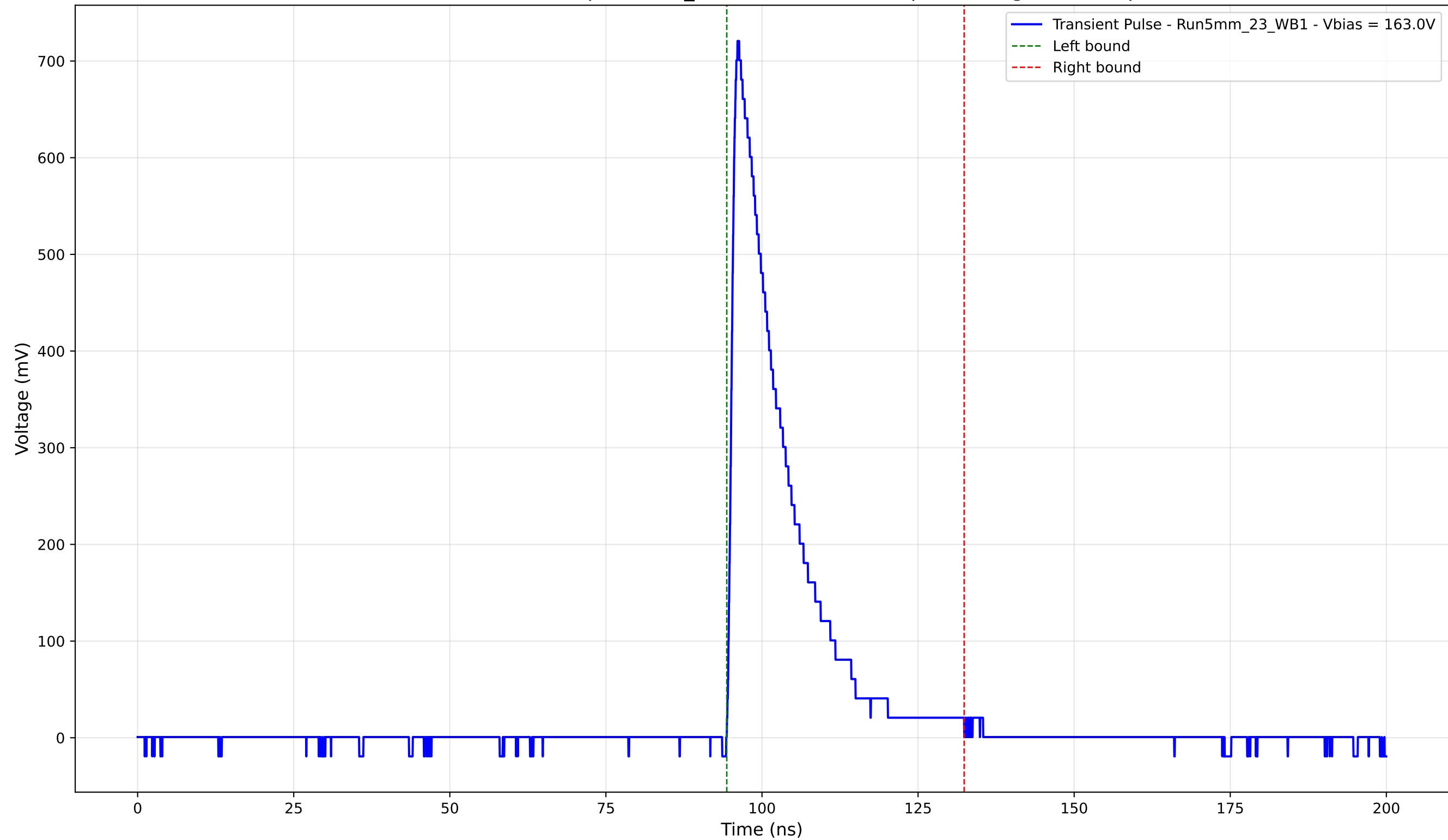
Transient Pulse - Sample: 5mm_23 - Position: 4325.0 \mu\text{m} - Charge: 131.35 pC
