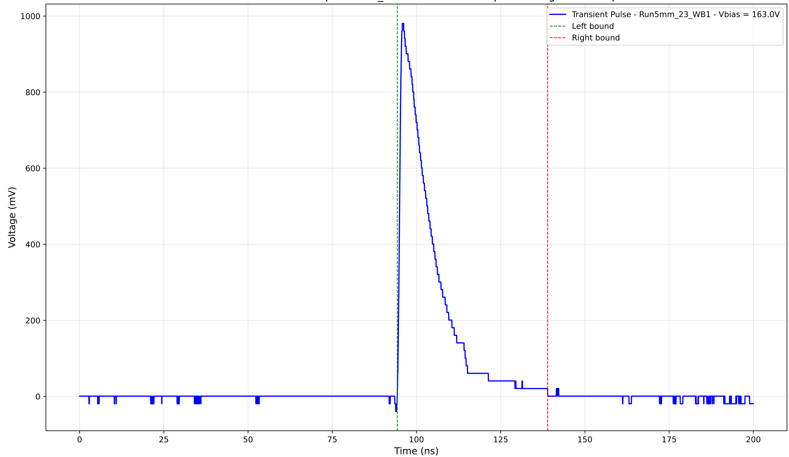
Transient Pulse - Sample: 5mm_23 - Position: 885.0 \mu\text{m} - Charge: 205.11 pC
