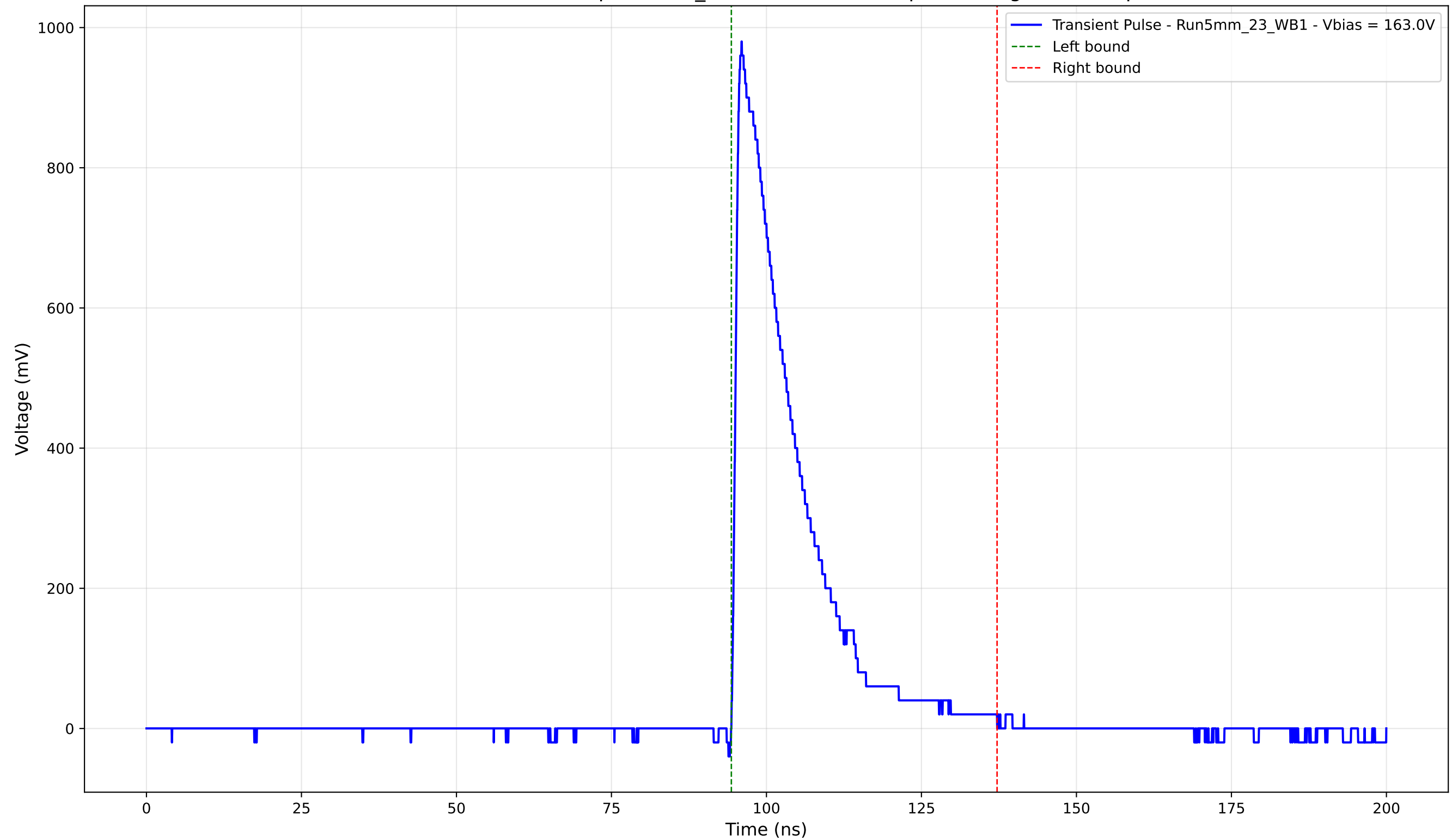
Transient Pulse - Sample: 5mm_23 - Position: 920.0 \mu\text{m} - Charge: 201.30 pC
