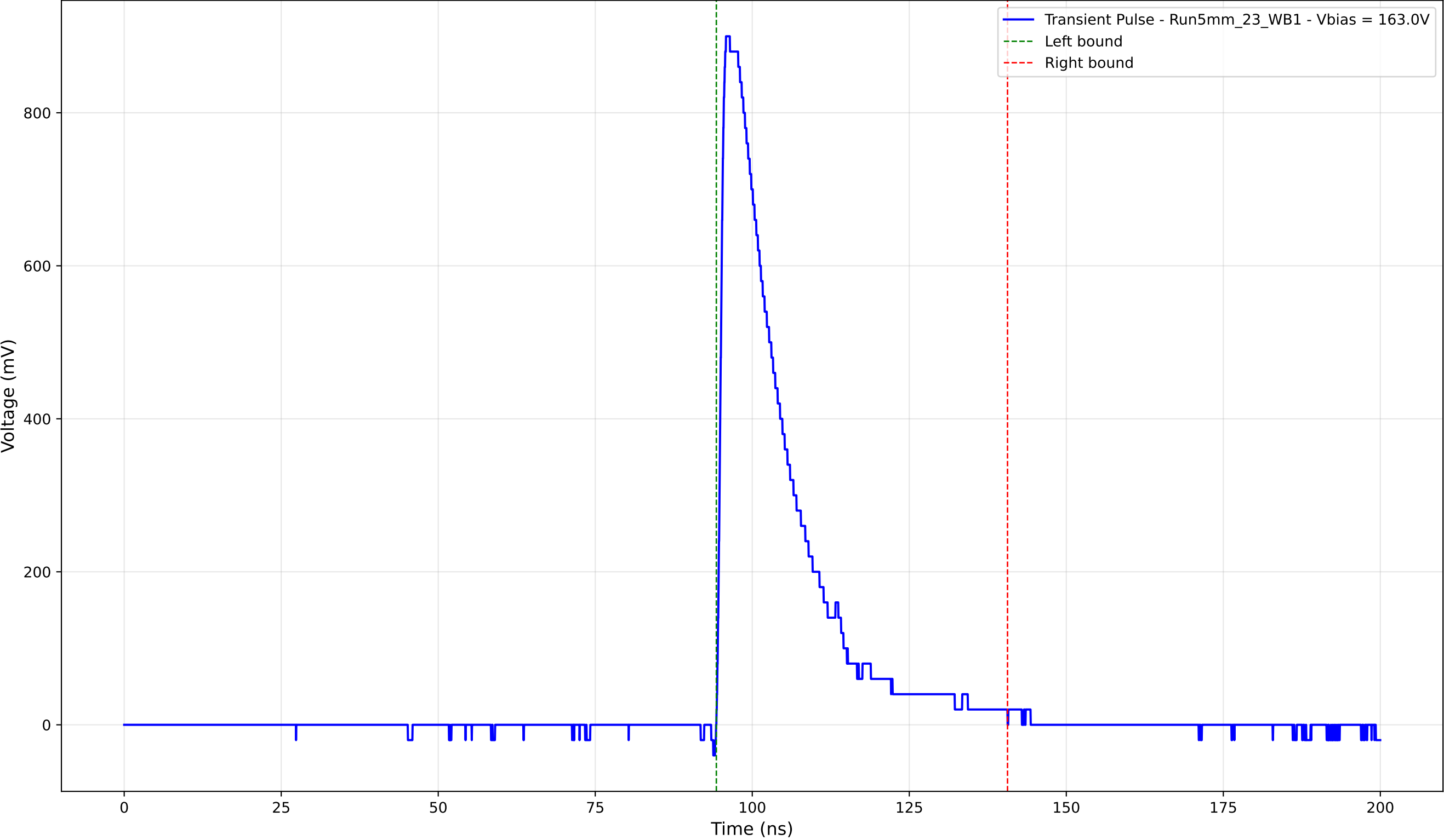
Transient Pulse - Sample: 5mm_23 - Position: 3640.0 \mu\text{m} - Charge: 202.30 pC
