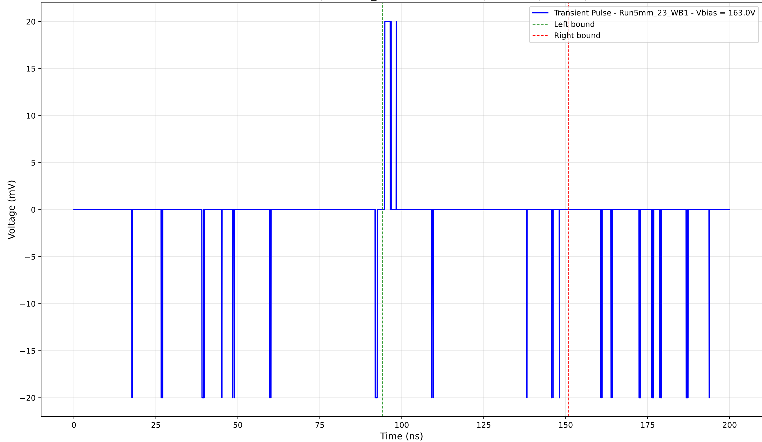
Transient Pulse - Sample: 5mm_23 - Position: 140.0 \mu\text{m} - Charge: 0.58 pC
