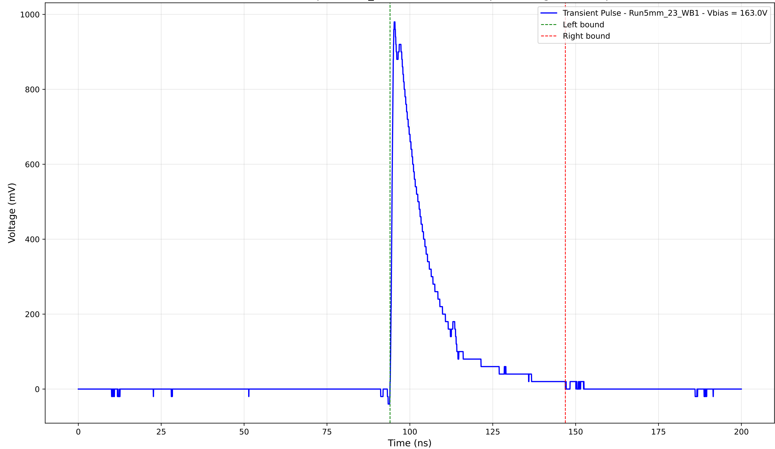
Transient Pulse - Sample: 5mm_23 - Position: 3145.0 \mu\text{m} - Charge: 216.07 pC
