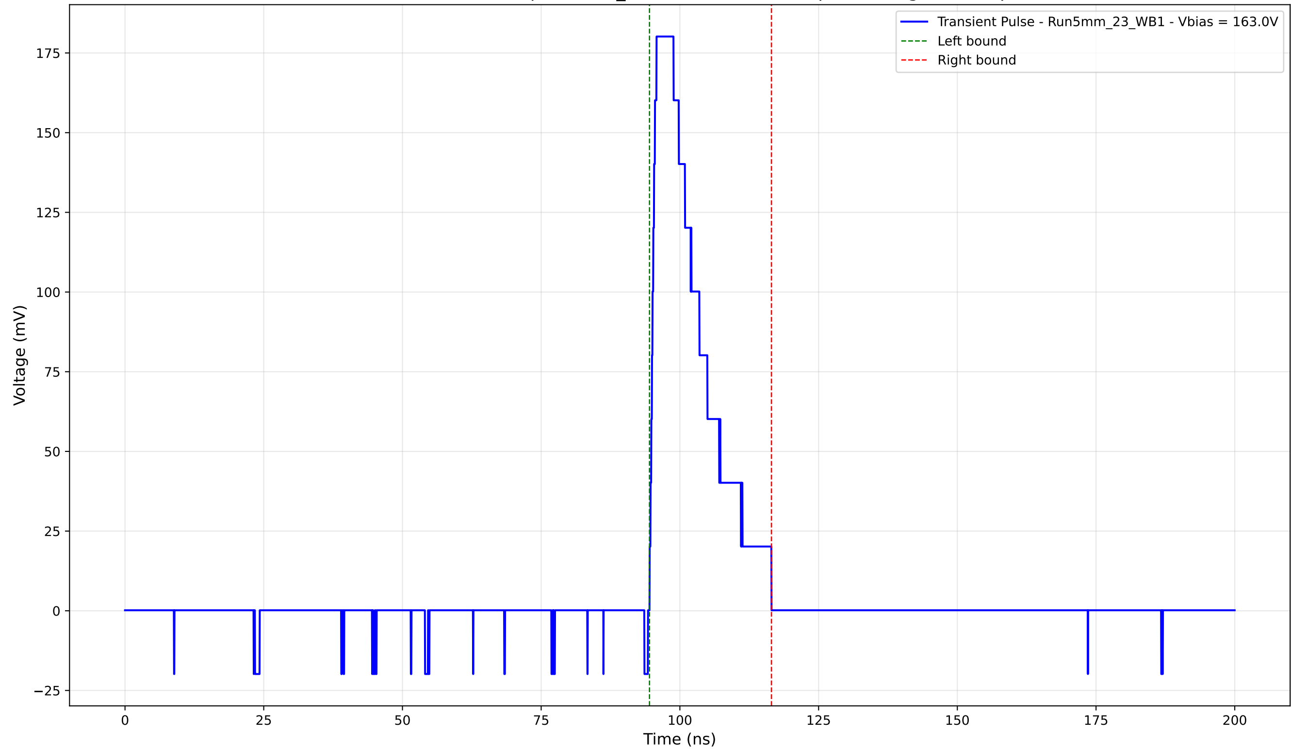
Transient Pulse - Sample: 5mm_23 -Position: 3750.0 \mu\text{m} - Charge: 35.69 pC
