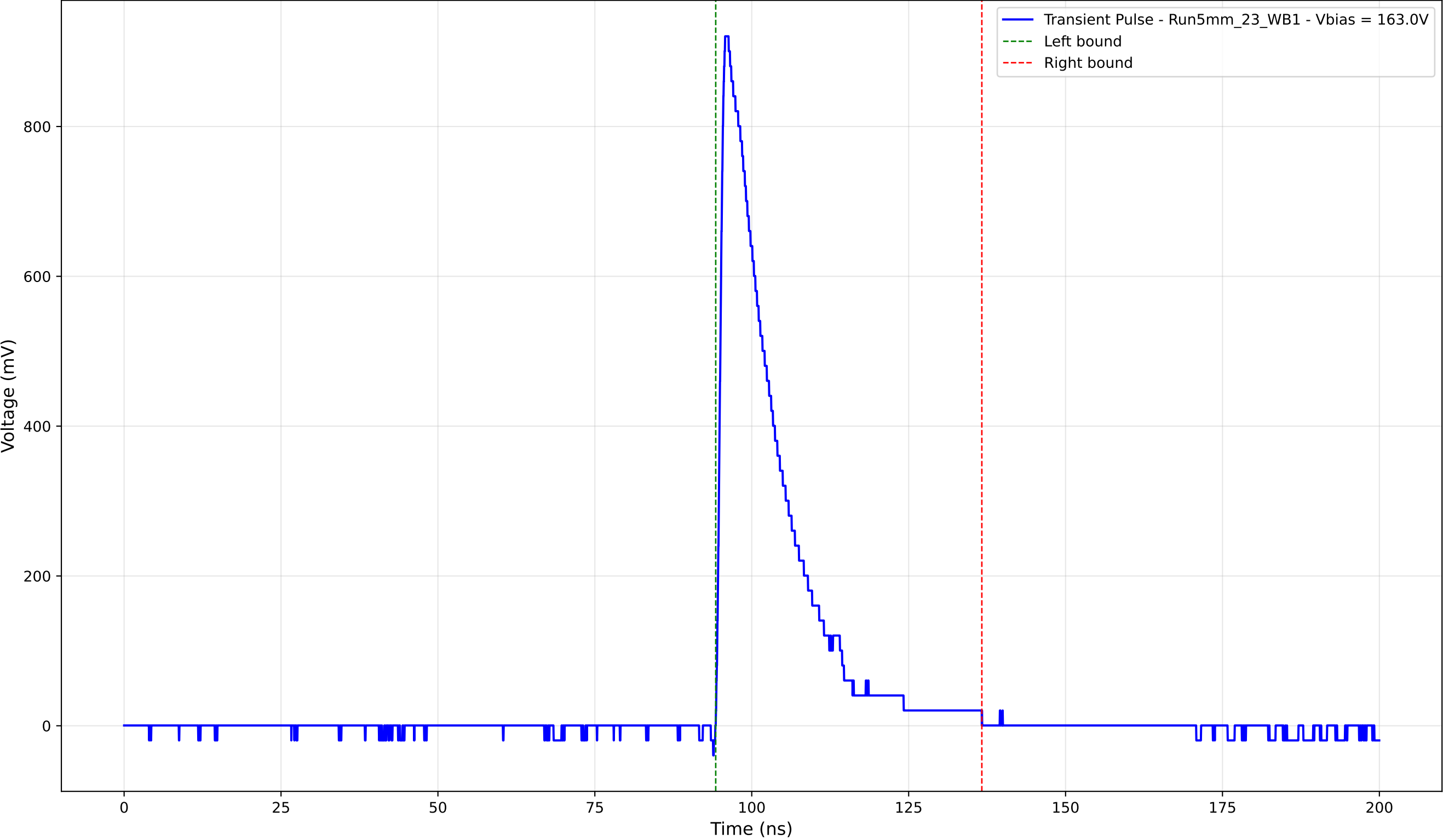
Transient Pulse - Sample: 5mm_23 - Position: 4565.0 \mu\text{m} - Charge: 177.66 pC
