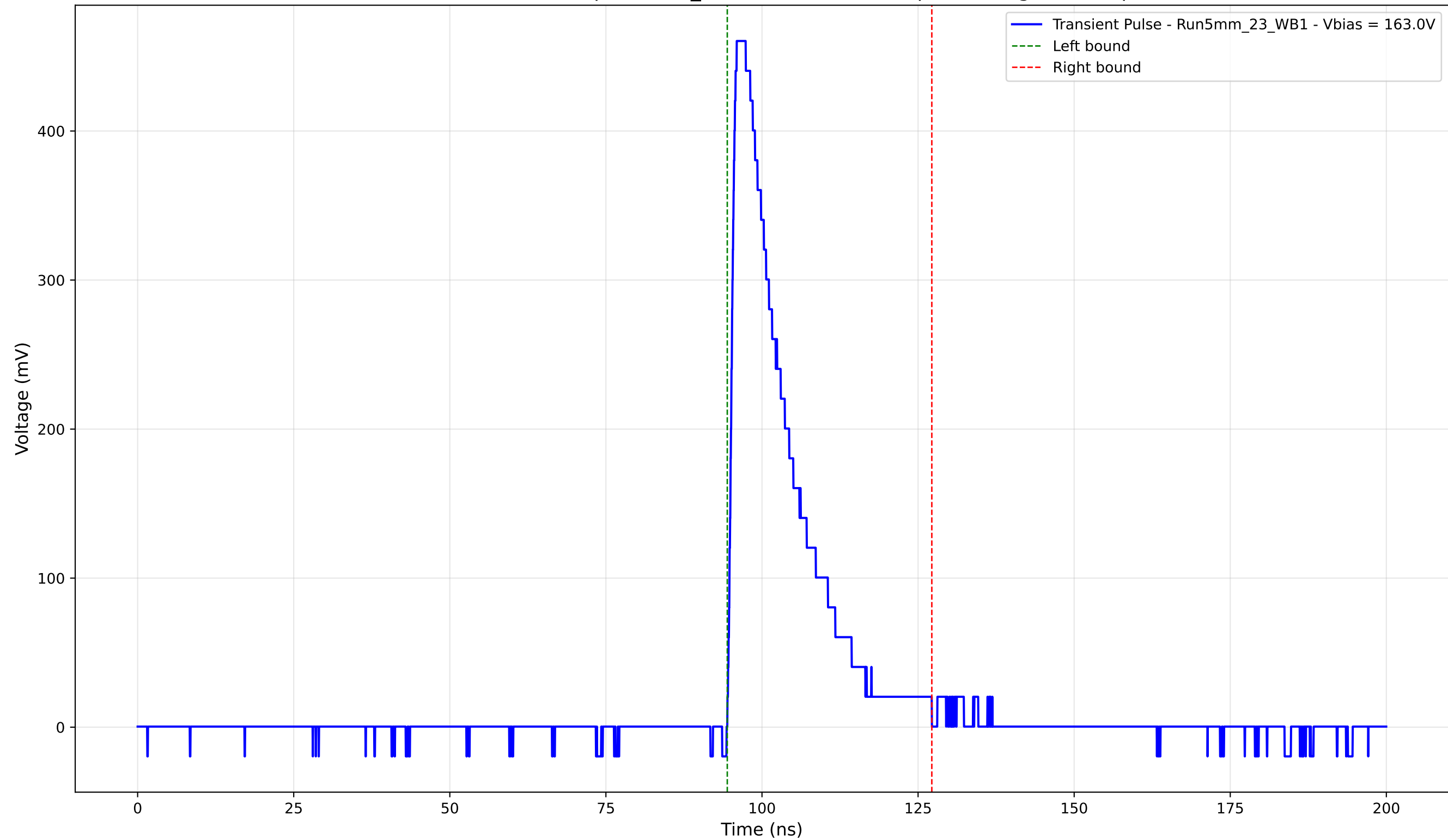
Transient Pulse - Sample: 5mm_23 - Position: 1690.0 \mu\text{m} - Charge: 91.62 pC
