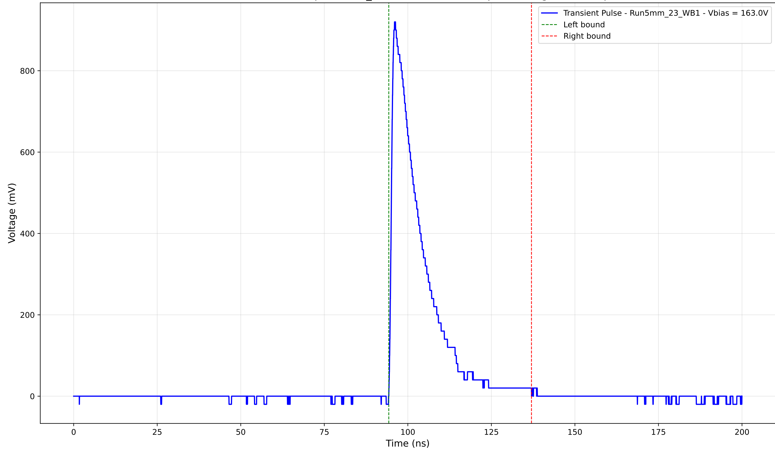
Transient Pulse - Sample: 5mm_23 - Position: 4425.0 \mu\text{m} - Charge: 179.75 pC
