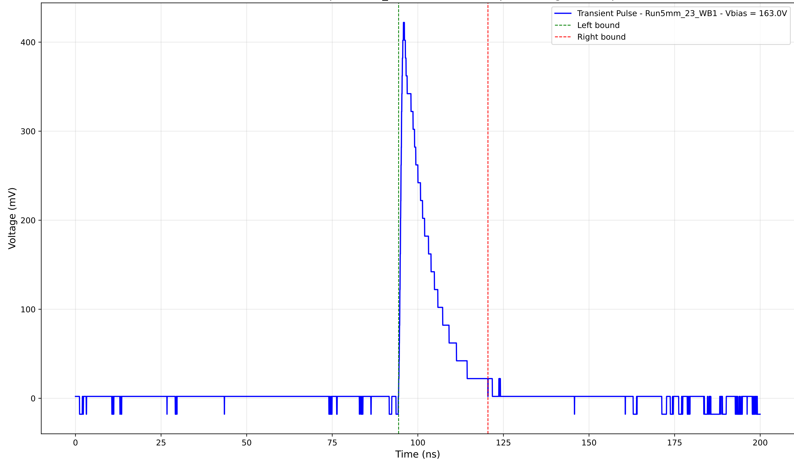
Transient Pulse - Sample: 5mm_23 - Position: 745.0 \mu\text{m} - Charge: 69.00 pC
