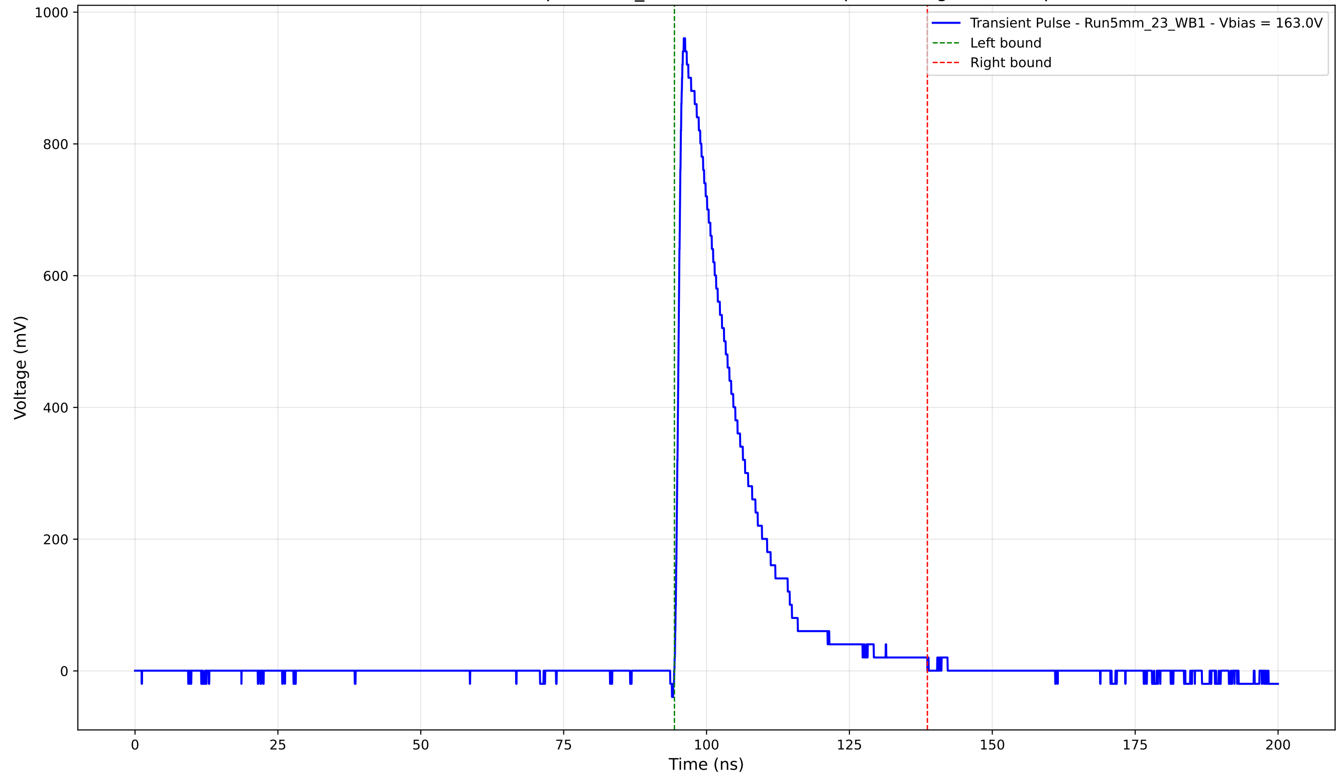
Transient Pulse - Sample: 5mm_23 - Position: 1100.0 \mu\text{m} - Charge: 201.89 pC
