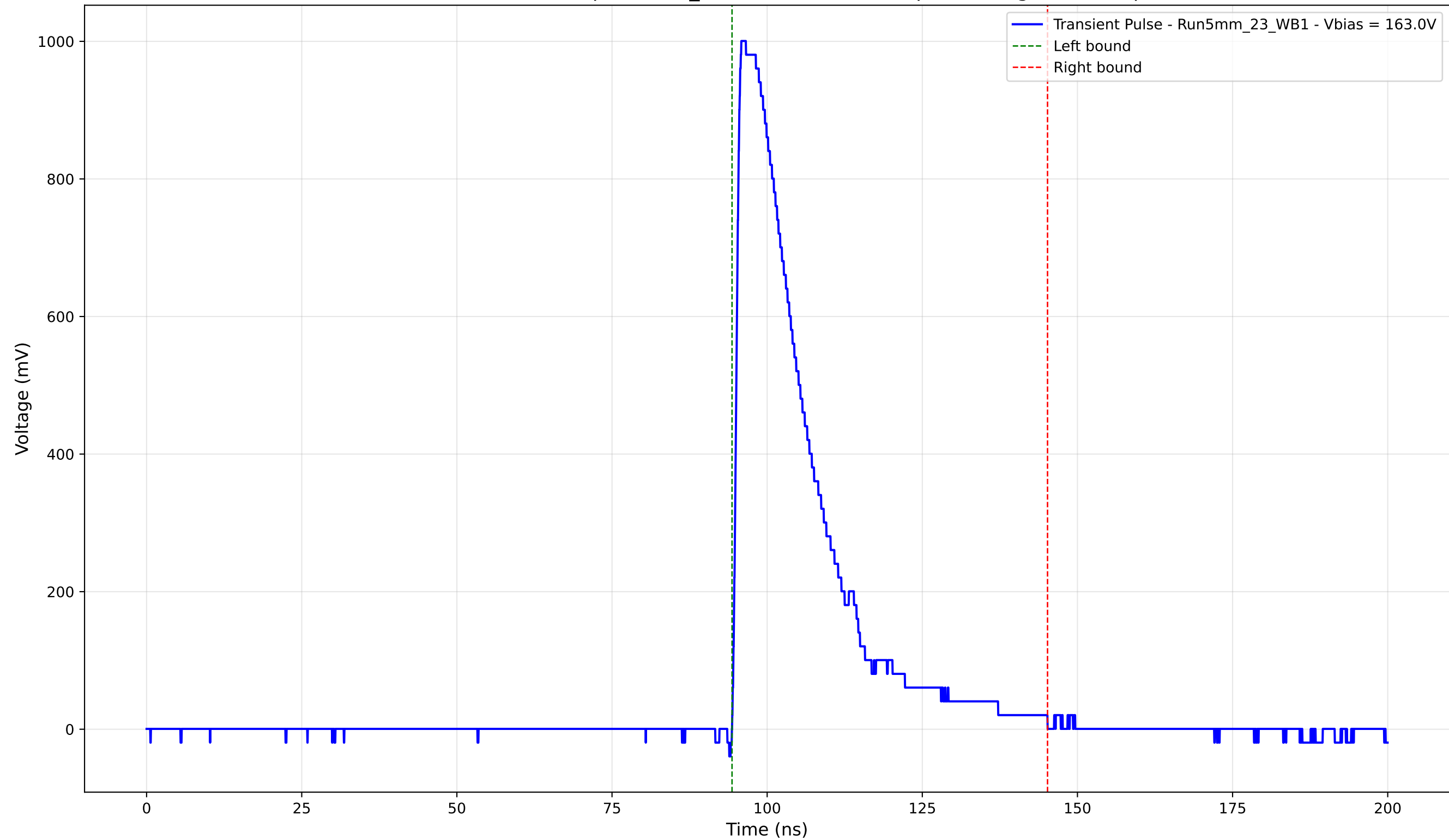
Transient Pulse - Sample: 5mm_23 - Position: 1565.0 \mu\text{m} - Charge: 254.90 pC
