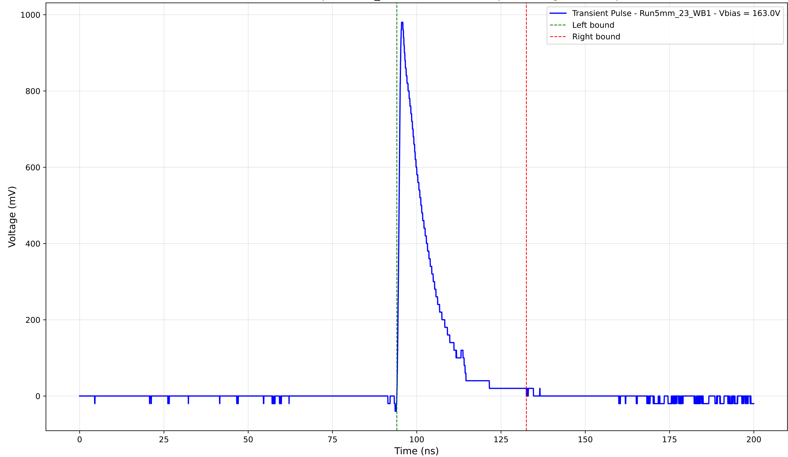
Transient Pulse - Sample: 5mm_23 - Position: 4875.0 \mu\text{m} - Charge: 170.85 pC
