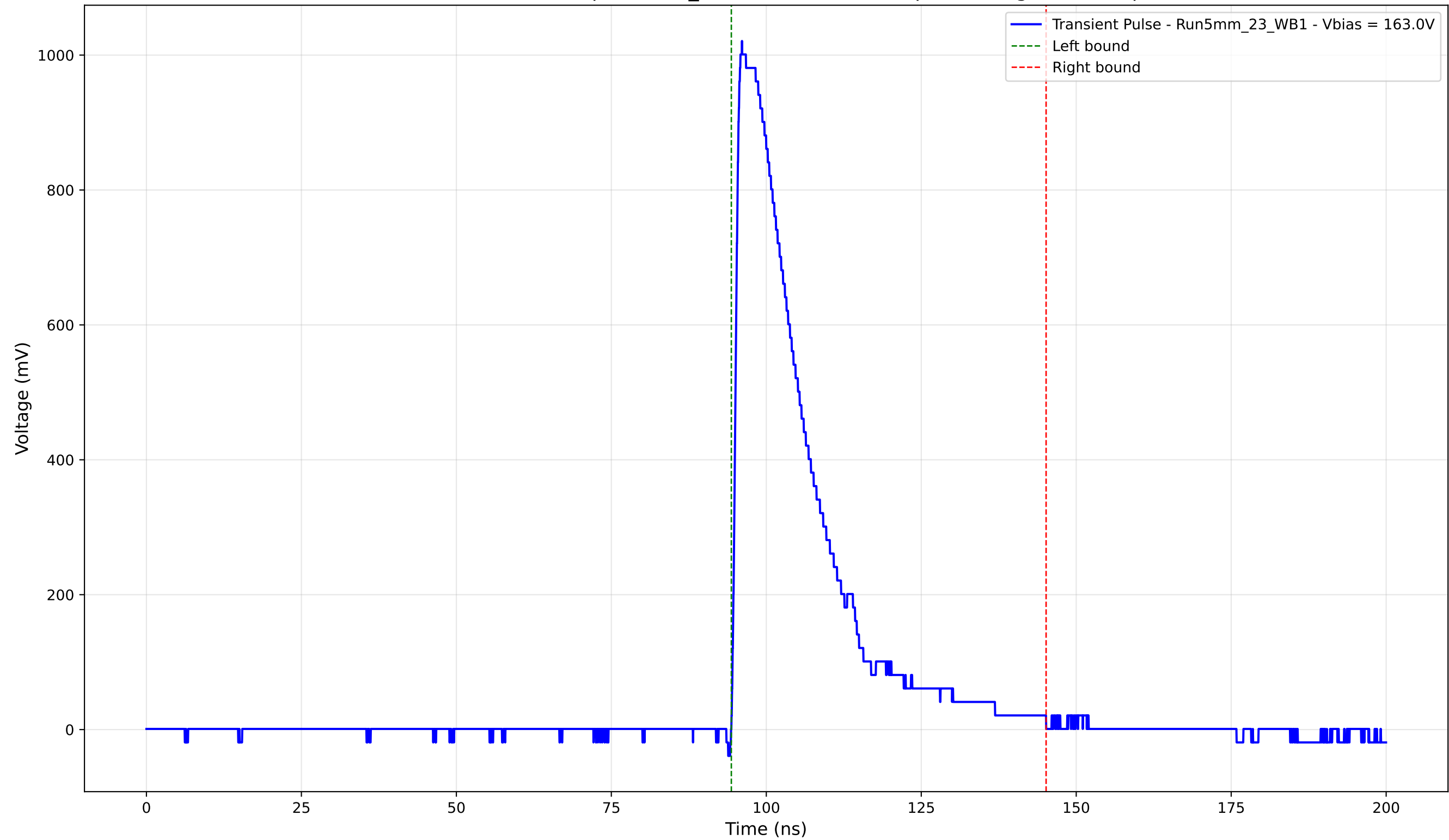
Transient Pulse - Sample: 5mm_23 - Position: 1560.0 \mu\text{m} - Charge: 255.99 pC
