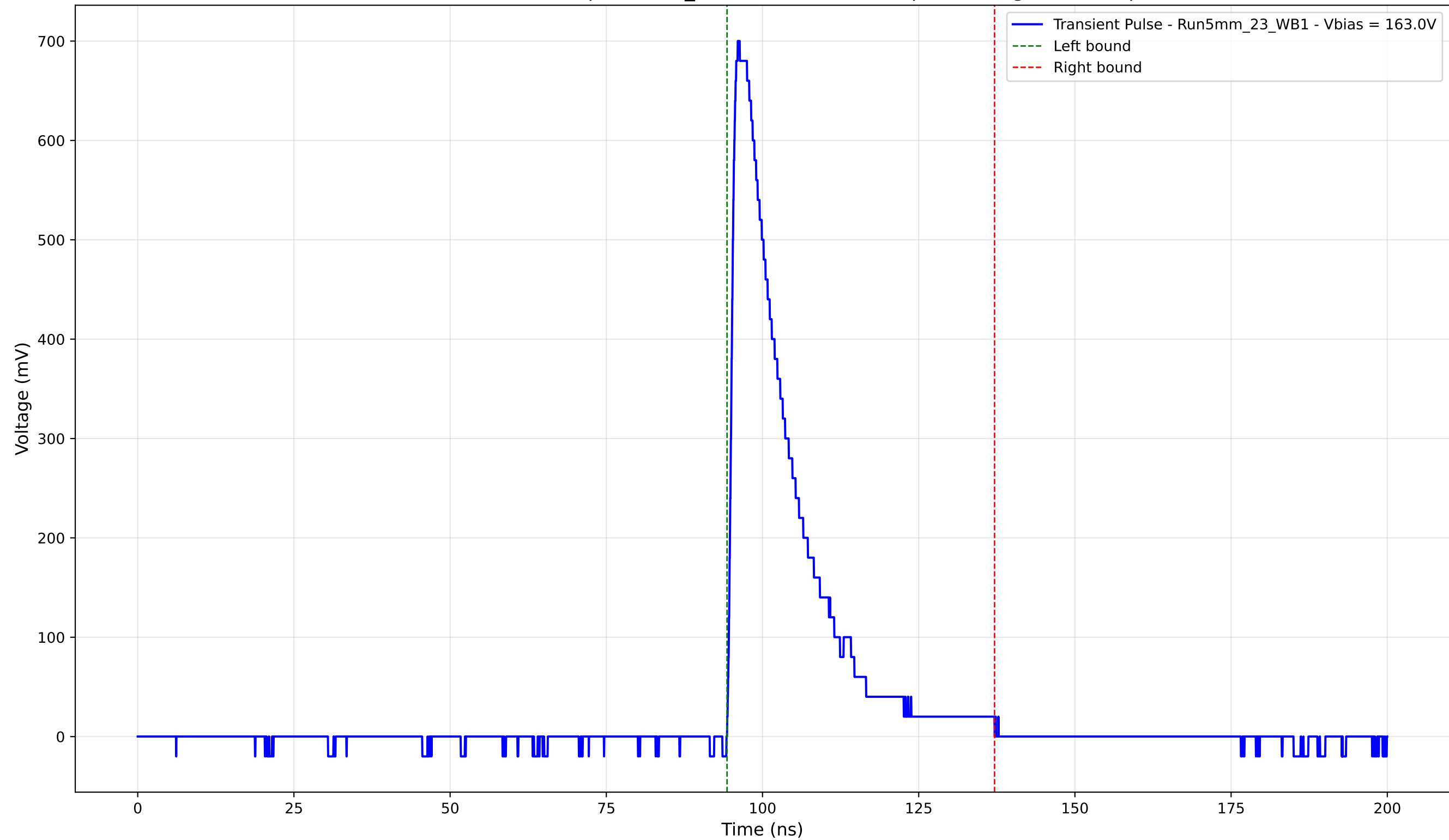
Transient Pulse - Sample: 5mm_23 - Position: 3695.0 \mu\text{m} - Charge: 141.72 pC
