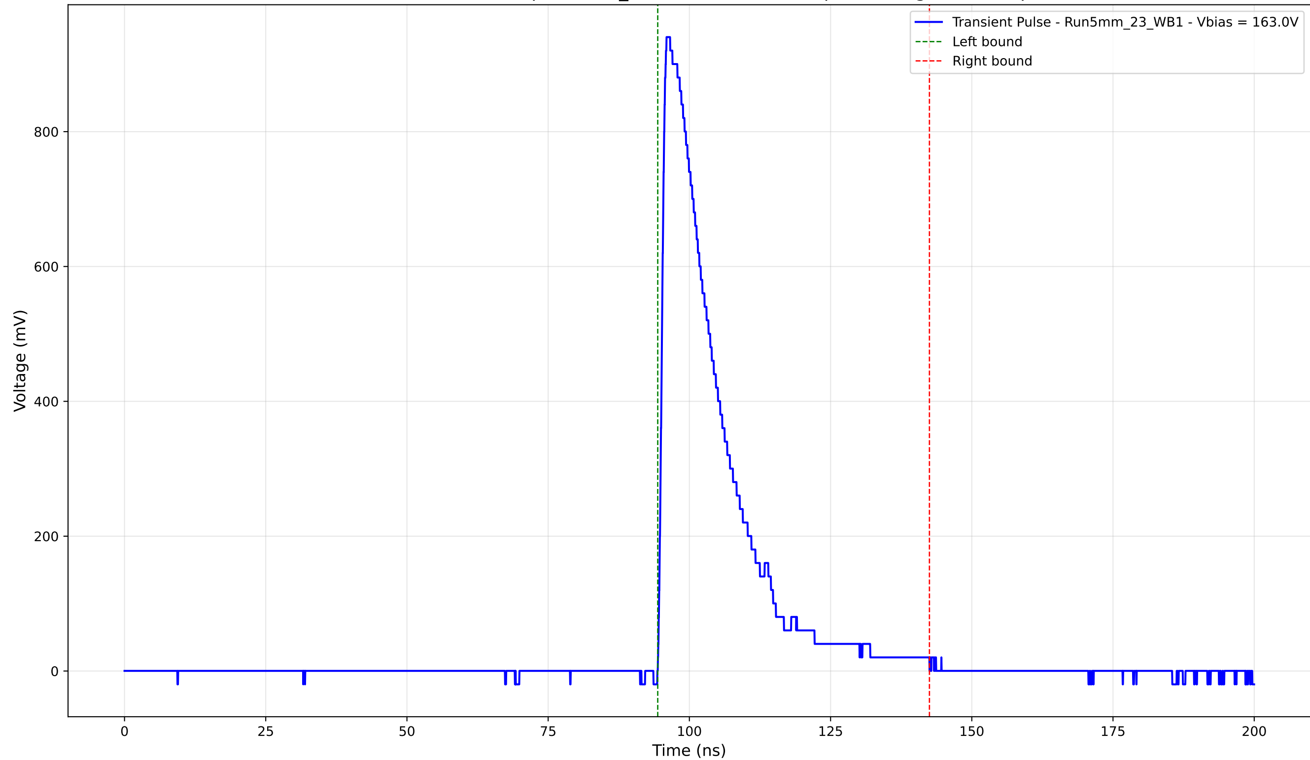
Transient Pulse - Sample: 5mm_23 - Position: 1325.0 \mu\text{m} - Charge: 210.99 pC
