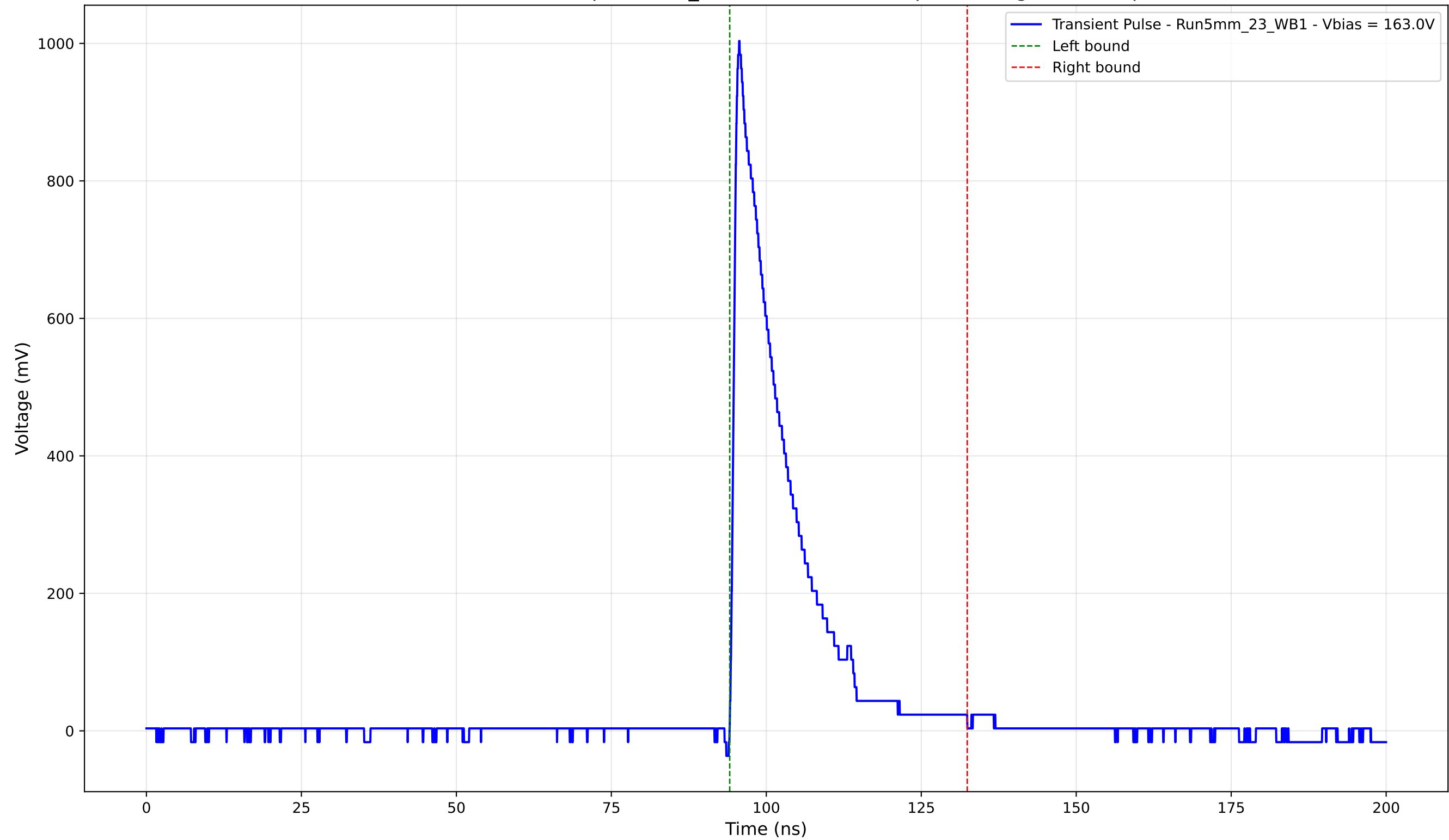
Transient Pulse - Sample: 5mm_23 - Position: 4890.0 \mu\text{m} - Charge: 173.32 pC
