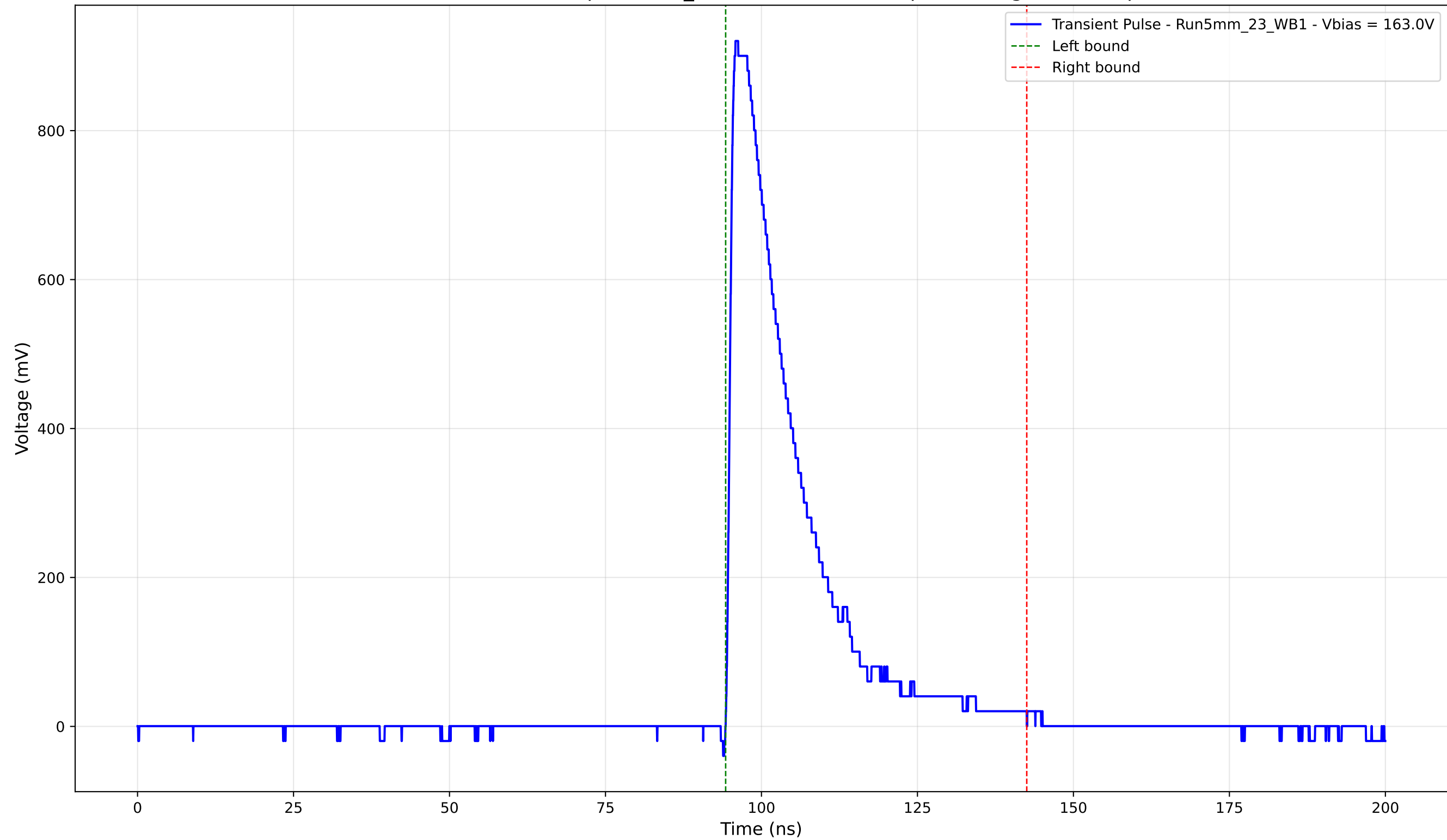
Transient Pulse - Sample: 5mm_23 - Position: 3605.0 \mu\text{m} - Charge: 209.39 pC
