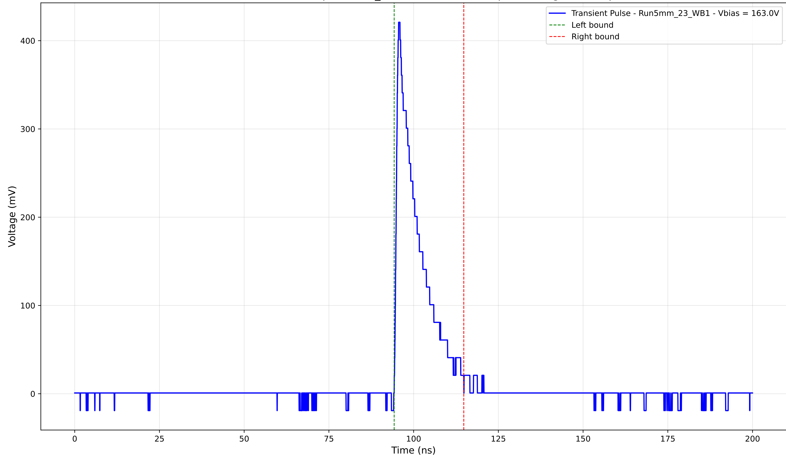
Transient Pulse - Sample: 5mm_23 - Position: 4795.0 \mu\text{m} - Charge: 60.02 pC
