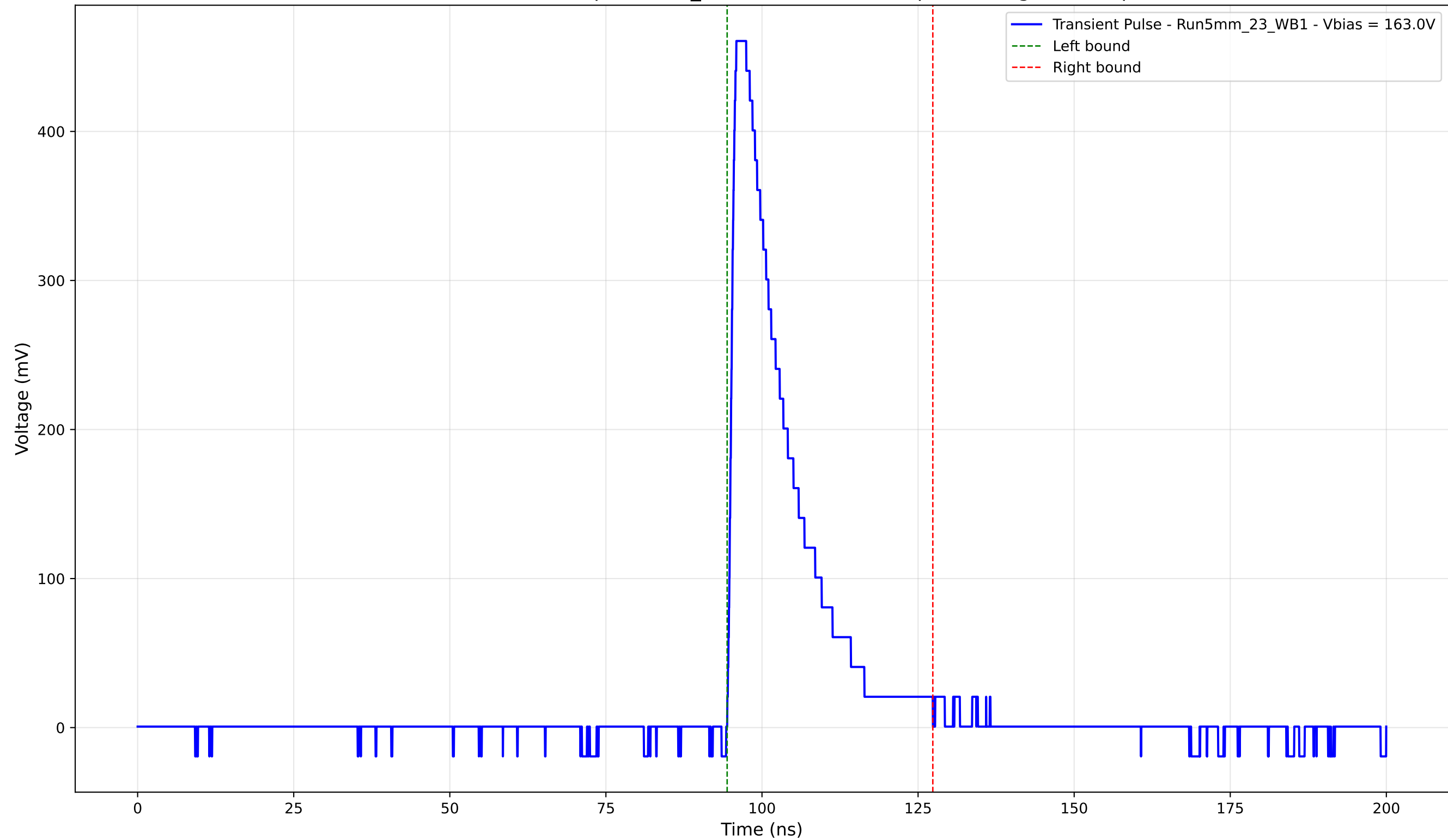
Transient Pulse - Sample: 5mm_23 - Position: 3795.0 \mu\text{m} - Charge: 90.48 pC
