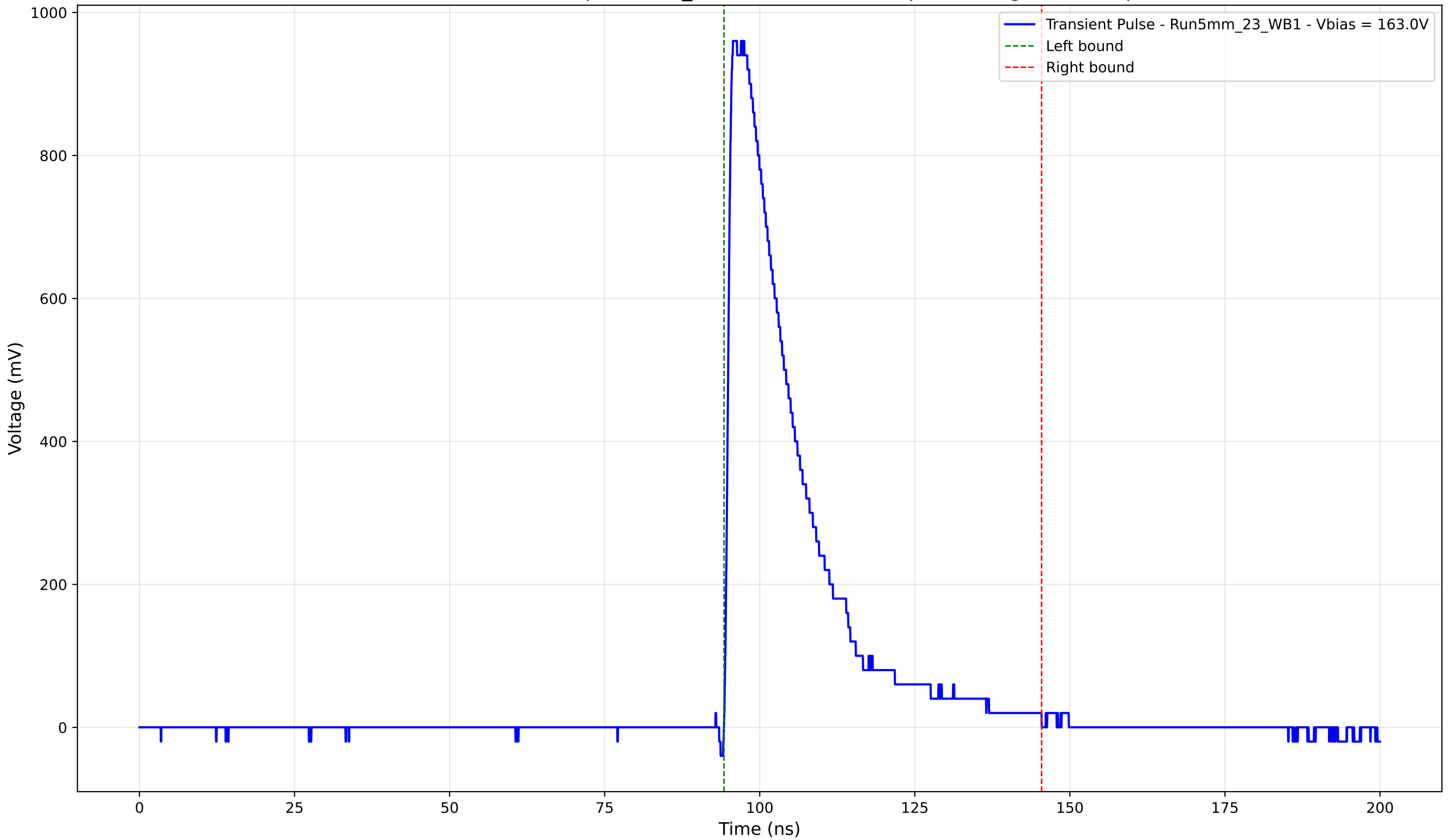
Transient Pulse - Sample: 5mm_23 - Position: 1915.0 \mu\text{m} - Charge: 235.88 pC
