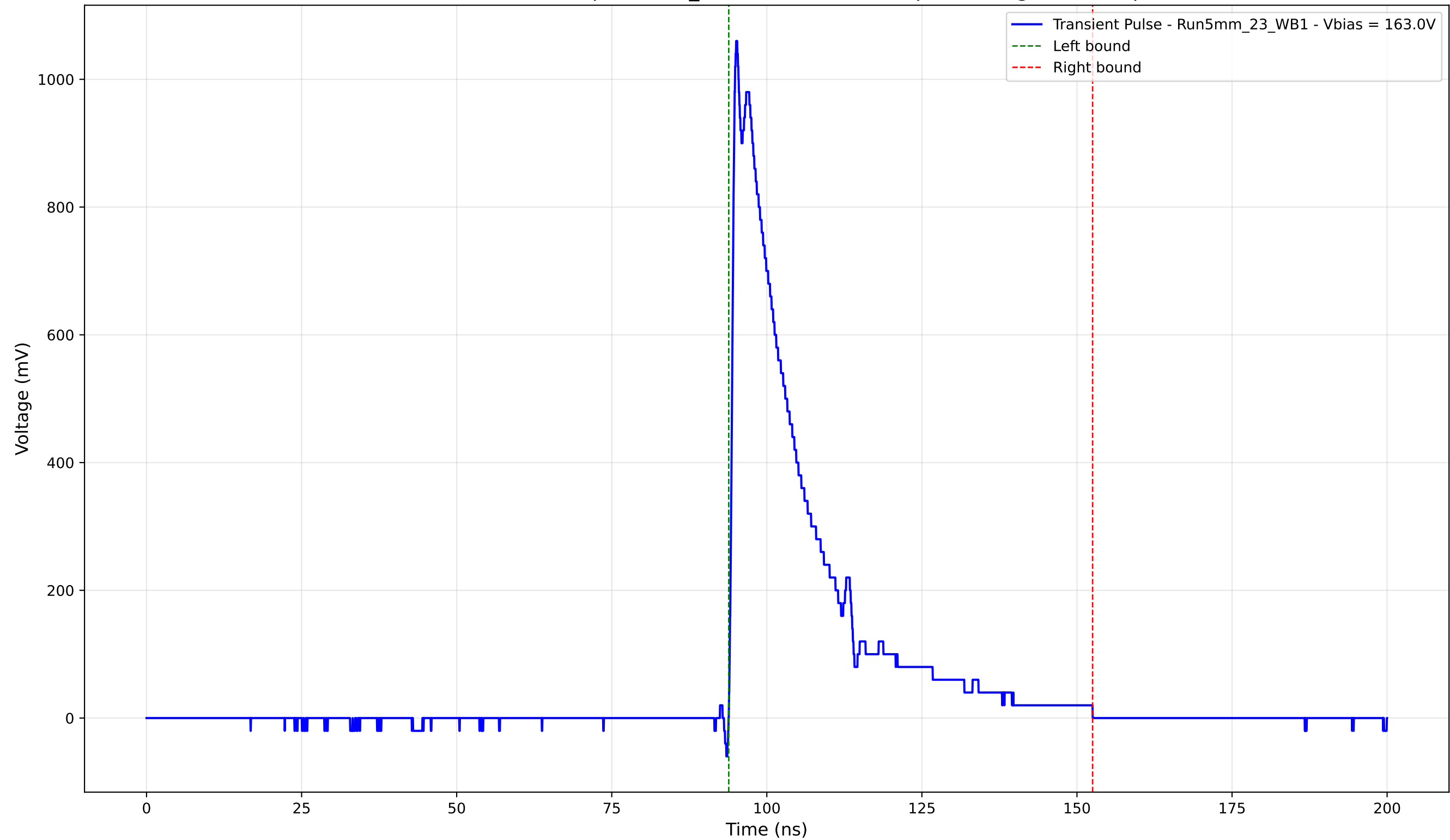
Transient Pulse - Sample: 5mm_23 - Position: 2895.0 \mu\text{m} - Charge: 242.59 pC
