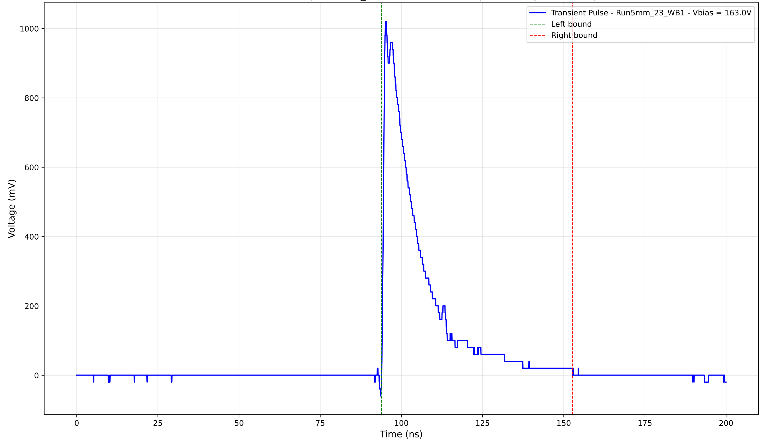
Transient Pulse - Sample: 5mm_23 - Position: 2490.0 \mu\text{m} - Charge: 234.62 pC
