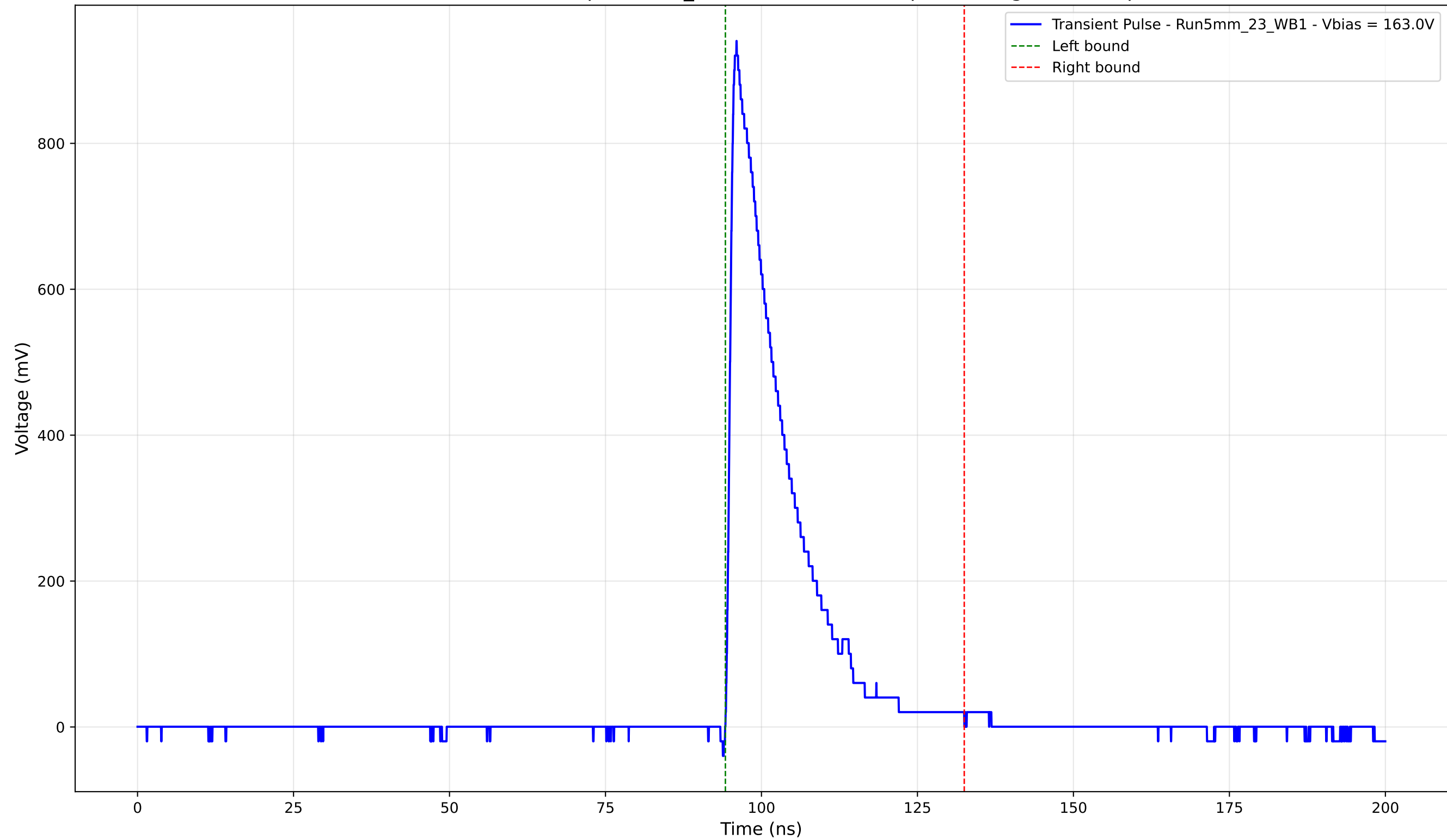
Transient Pulse - Sample: 5mm_23 - Position: 4600.0 \mu\text{m} - Charge: 174.00 pC
