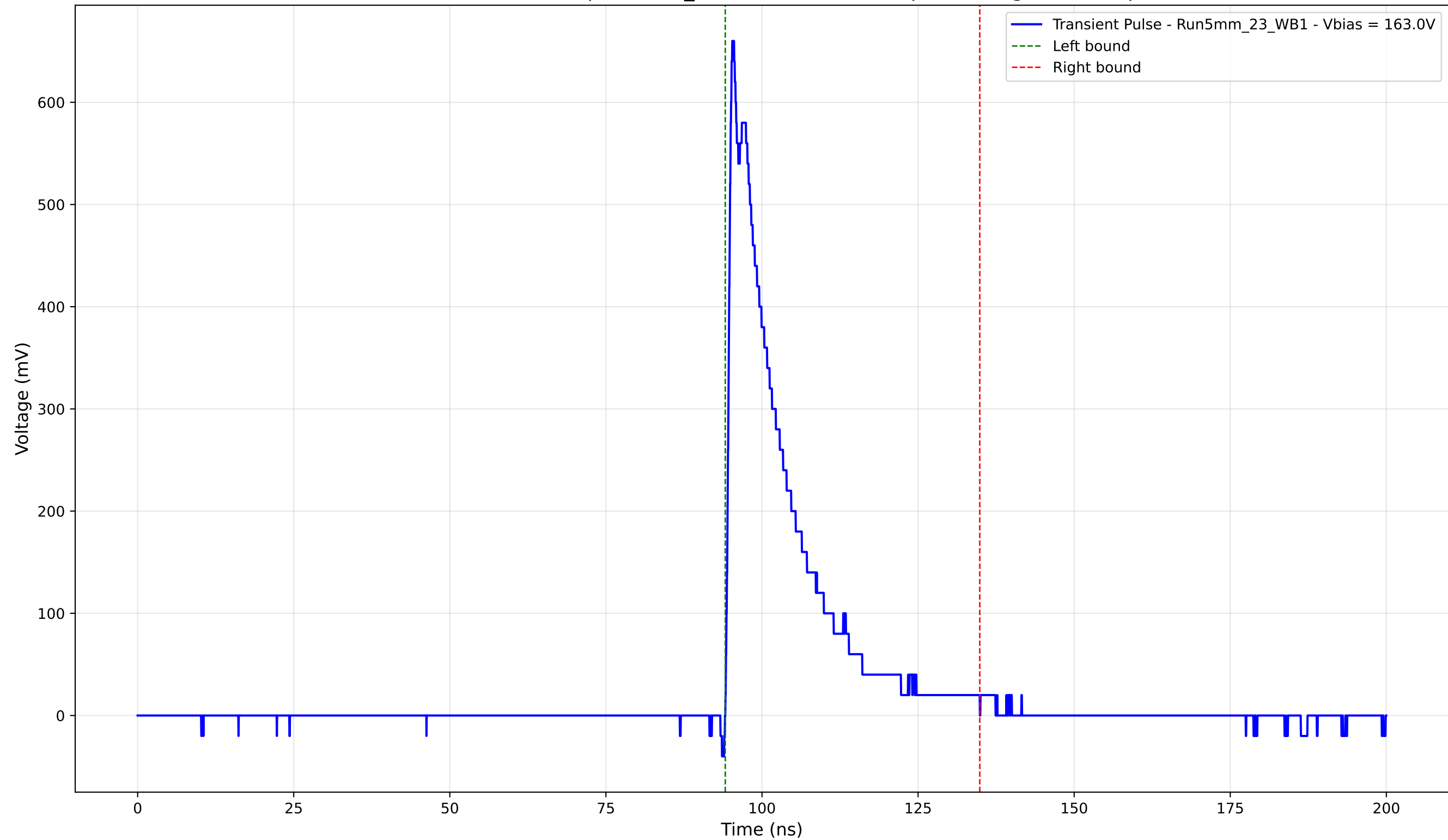
Transient Pulse - Sample: 5mm_23 - Position: 3200.0 \mu\text{m} - Charge: 120.64 pC
