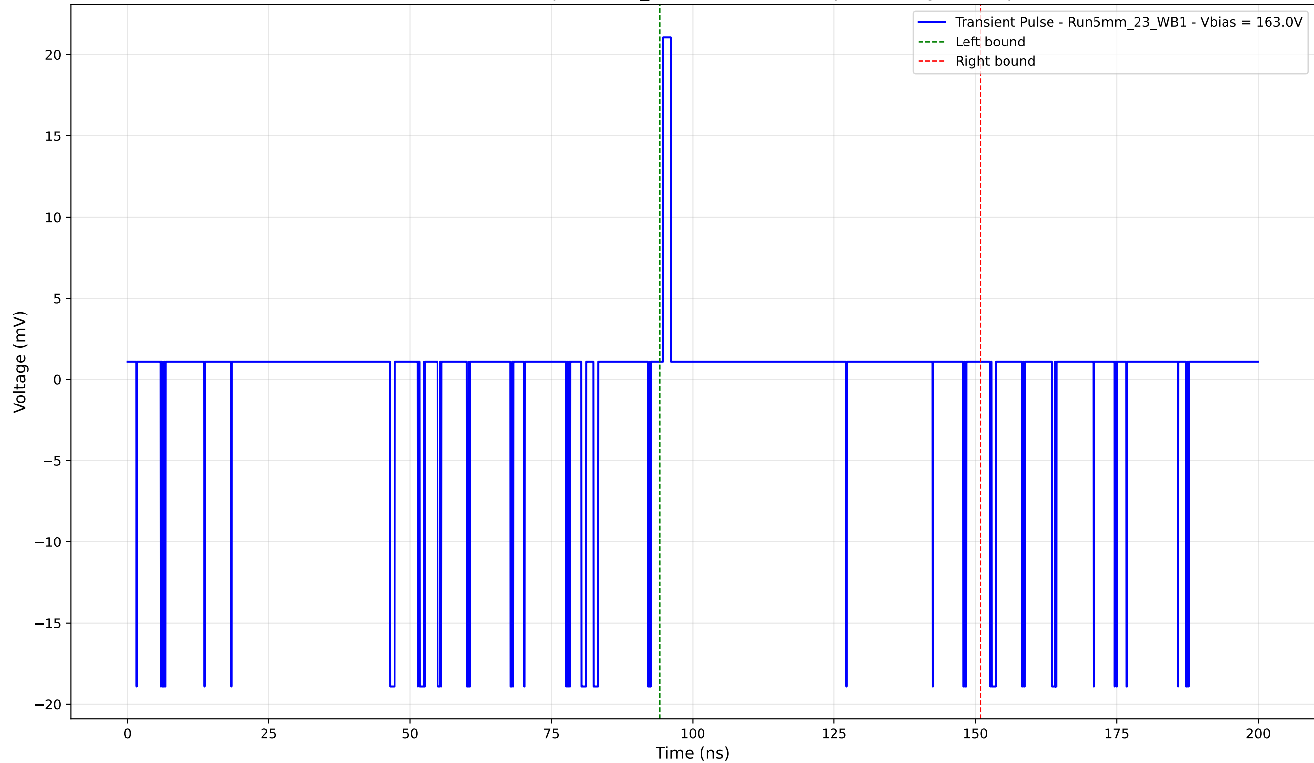
Transient Pulse - Sample: 5mm_23 - Position: 130.0 \mu\text{m} - Charge: 1.51 pC
