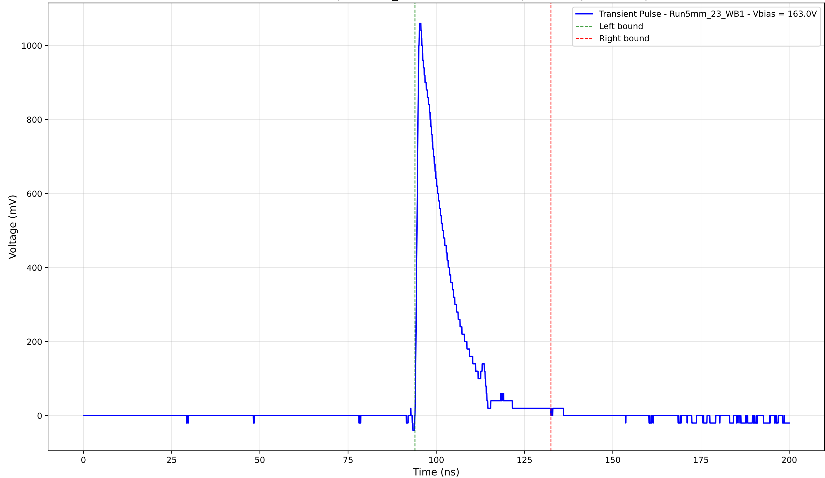
Transient Pulse - Sample: 5mm_23 - Position: 5090.0 \mu\text{m} - Charge: 185.78 pC
