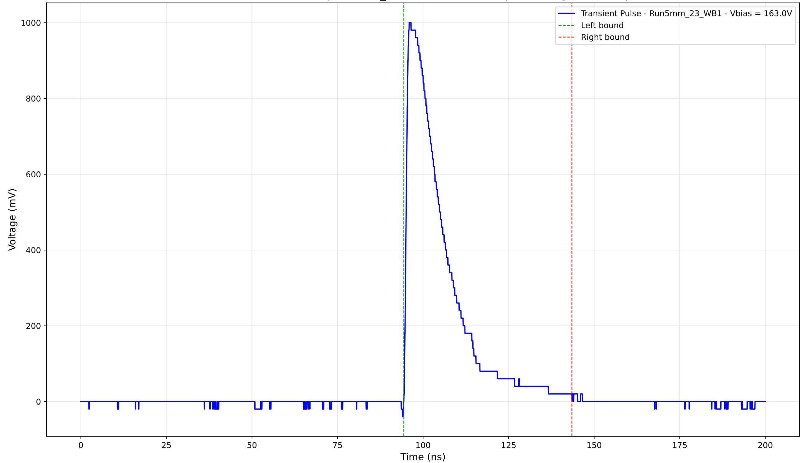
Transient Pulse - Sample: 5mm_23 - Position: 1475.0 \mu\text{m} - Charge: 245.92 pC
