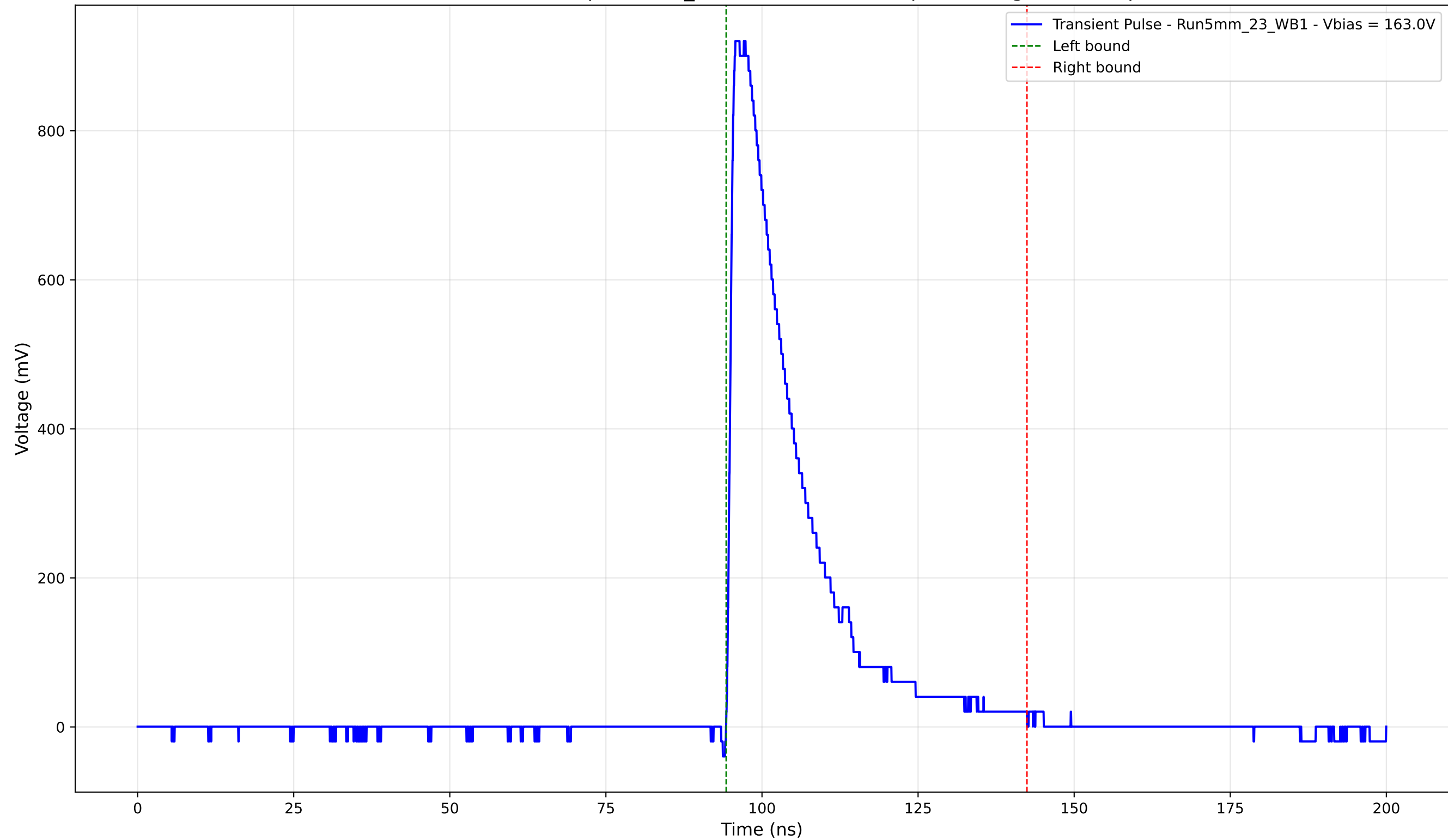
Transient Pulse - Sample: 5mm_23 - Position: 3590.0 \mu\text{m} - Charge: 213.20 pC
