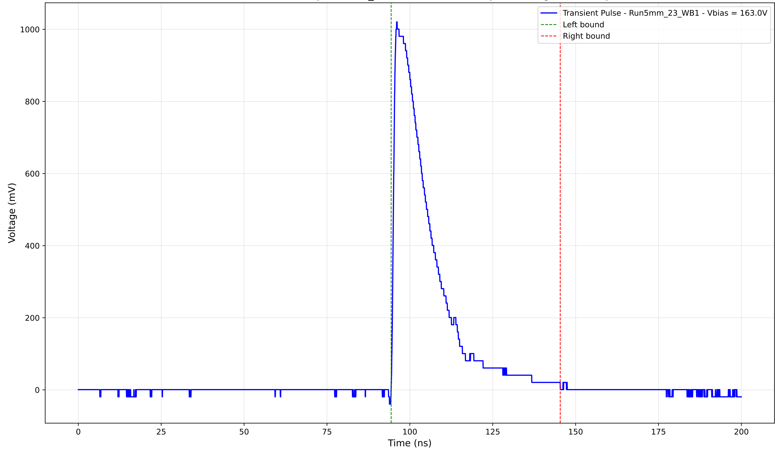
Transient Pulse - Sample: 5mm_23 - Position: 1520.0 \mu\text{m} - Charge: 253.89 pC
