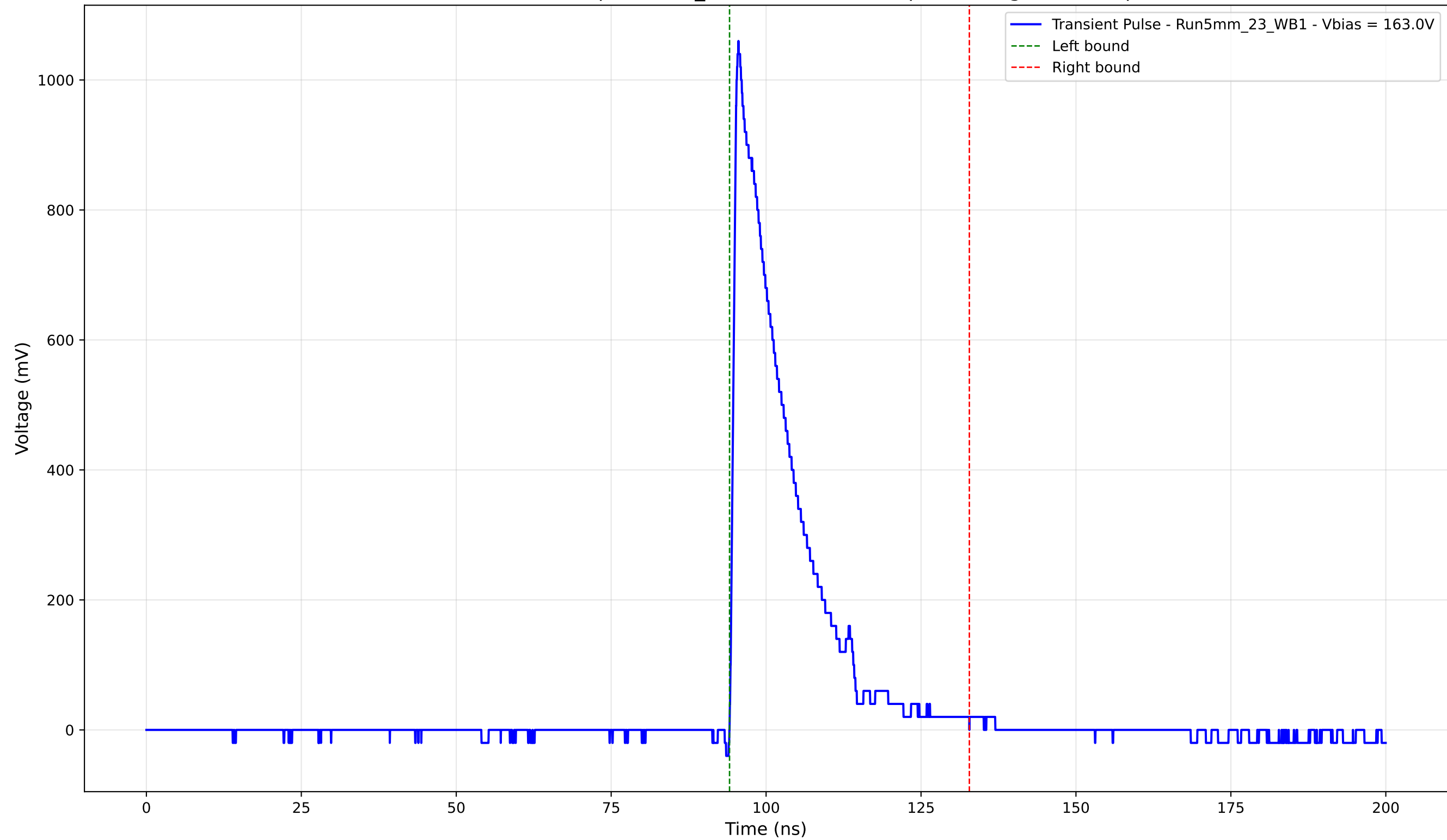
Transient Pulse - Sample: 5mm_23 - Position: 460.0 \mu\text{m} - Charge: 195.69 pC
