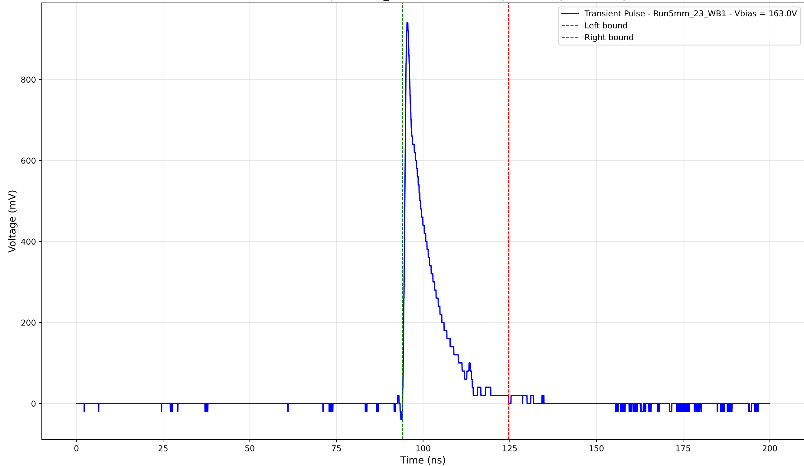
Transient Pulse - Sample: 5mm_23 - Position: 330.0 \mu\text{m} - Charge: 132.97 pC
