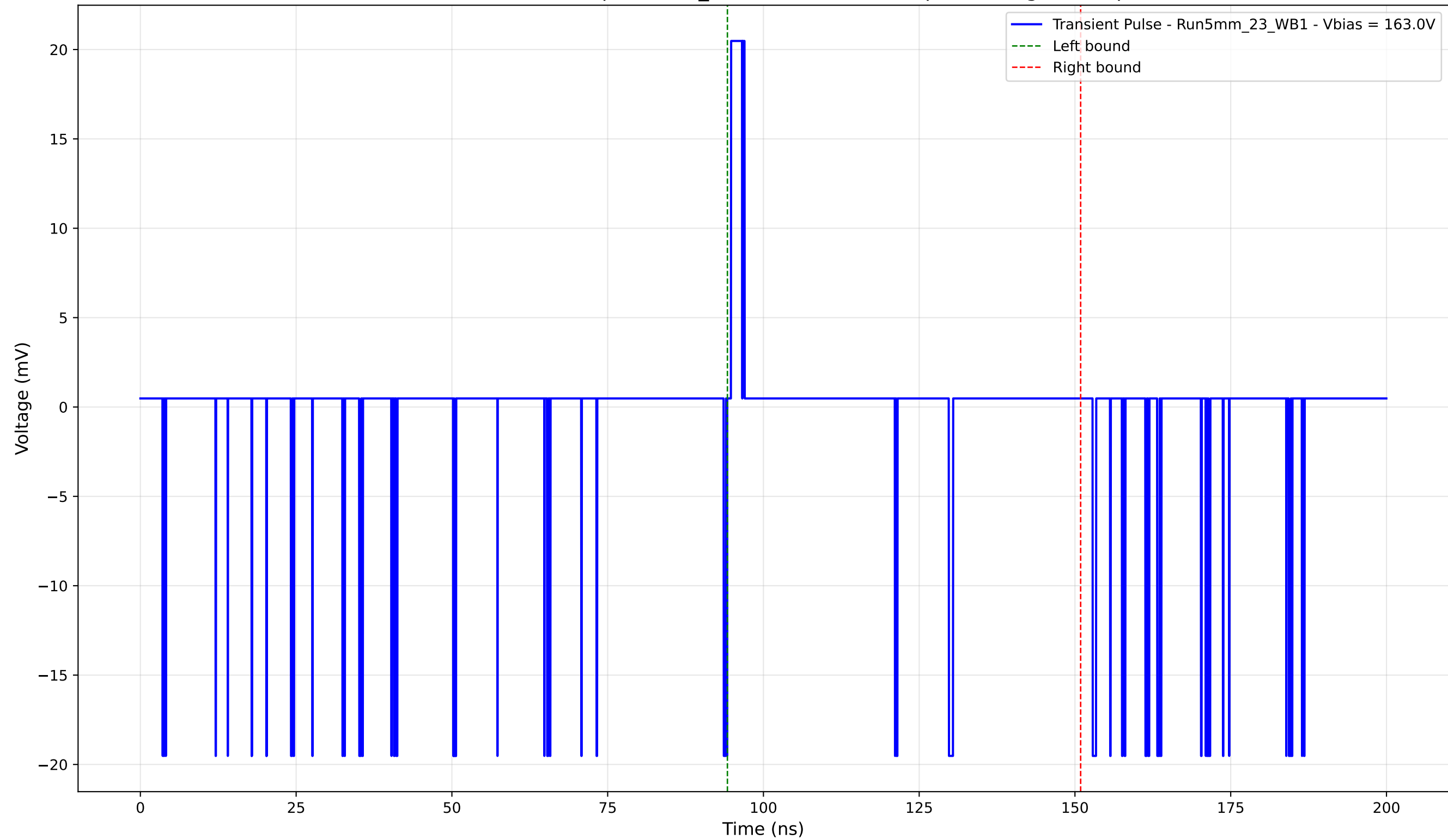
Transient Pulse - Sample: 5mm_23 - Position: 5270.0 \mu\text{m} - Charge: 1.02 pC
