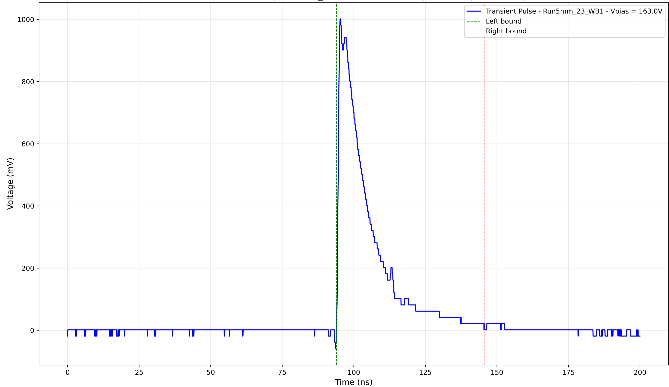
Transient Pulse - Sample: 5mm_23 - Position: 3085.0 \mu\text{m} - Charge: 226.68 pC
