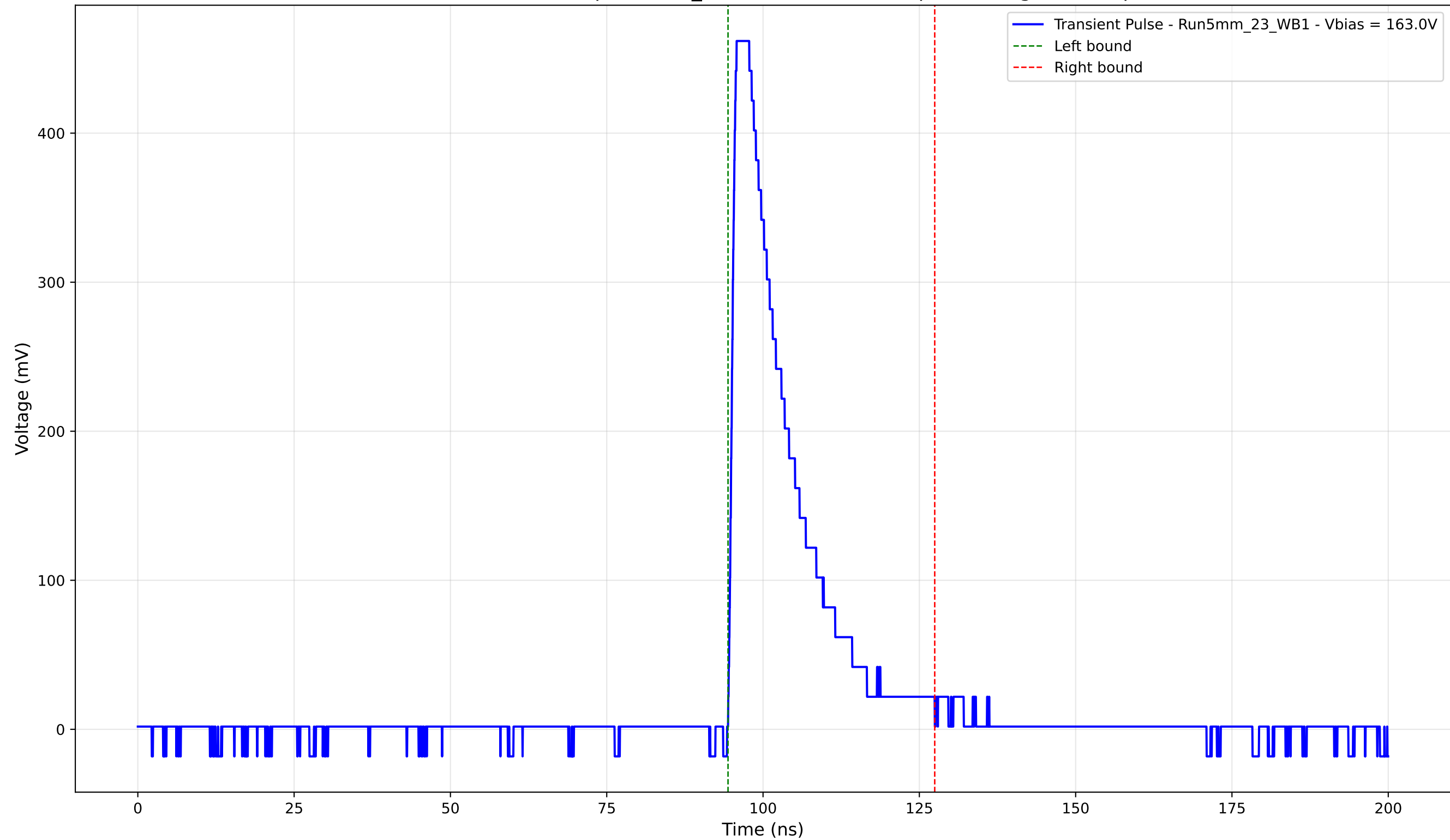
Transient Pulse - Sample: 5mm_23 - Position: 3715.0 \mu\text{m} - Charge: 92.55 pC
