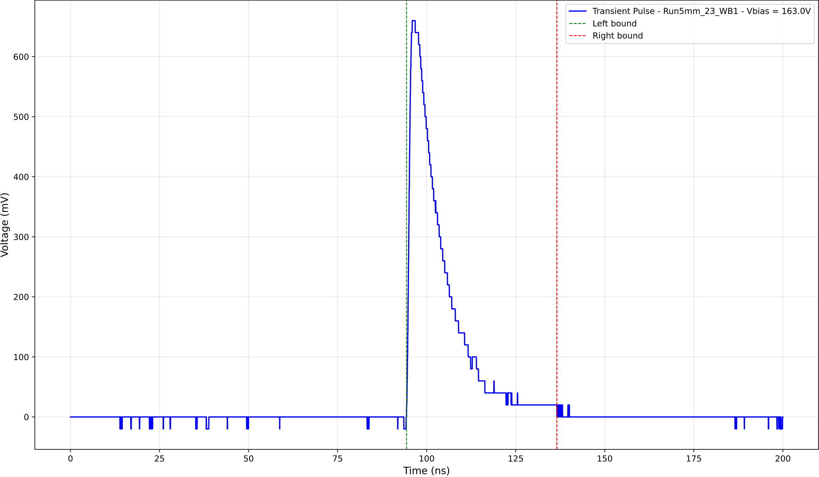
Transient Pulse - Sample: 5mm_23 - Position: 1780.0 \mu\text{m} - Charge: 136.77 pC
