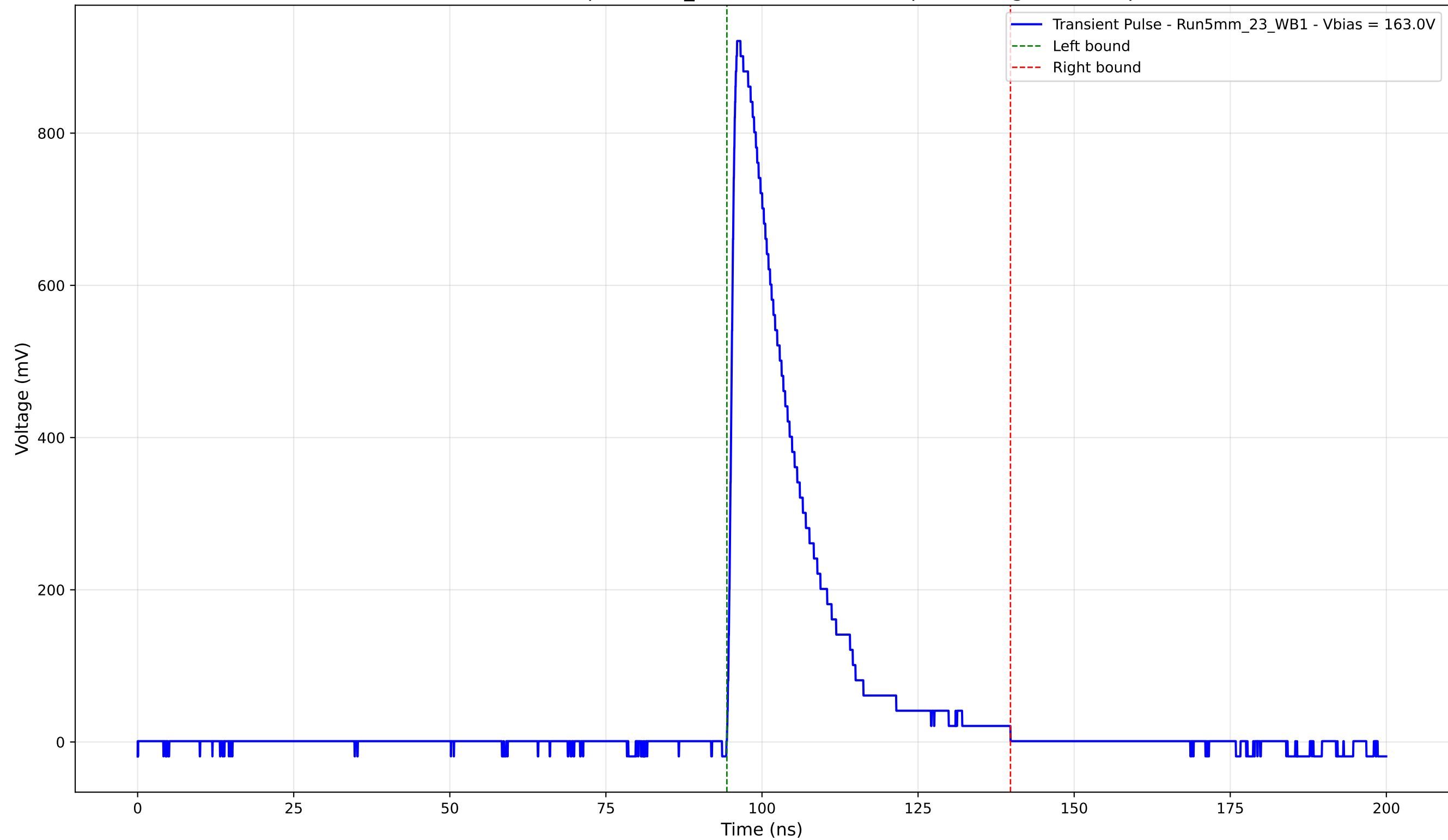
Transient Pulse - Sample: 5mm_23 - Position: 4040.0 \mu\text{m} - Charge: 199.37 pC
