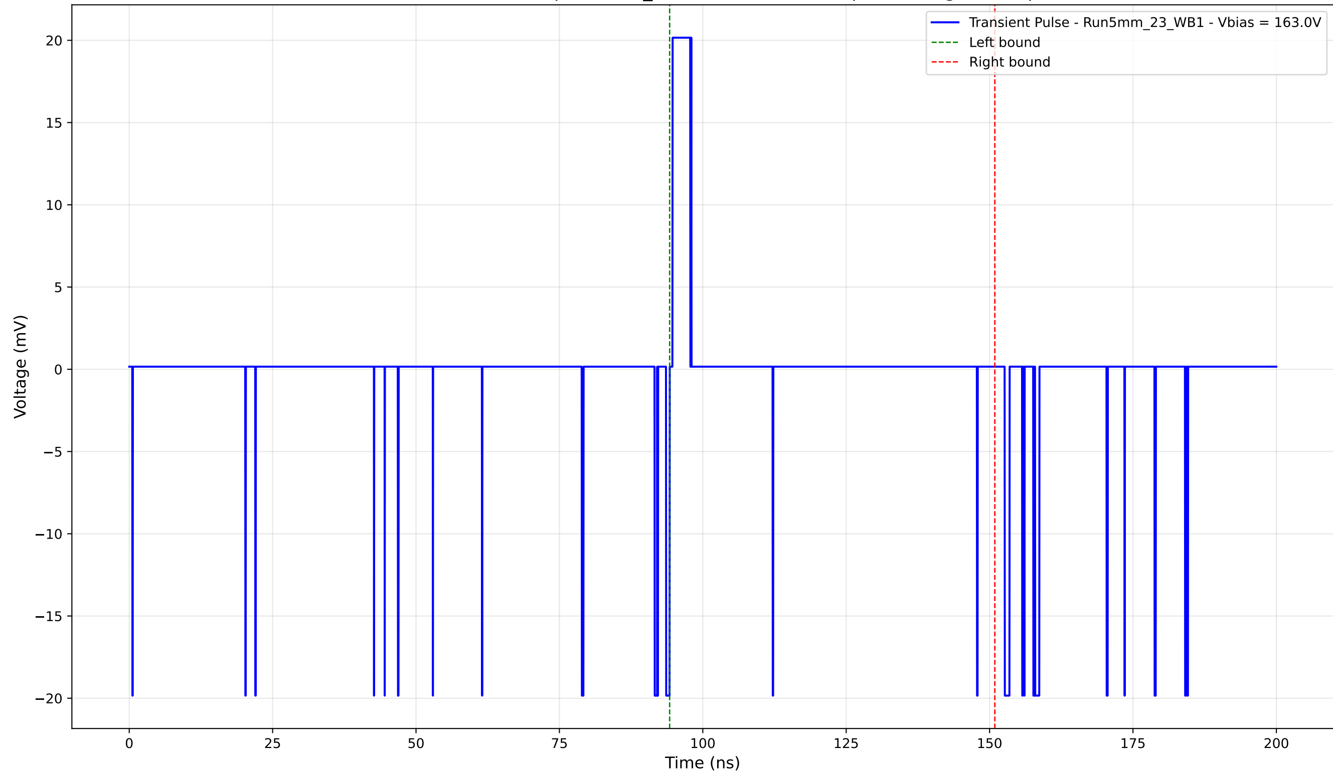
Transient Pulse - Sample: 5mm_23 - Position: 5265.0 \mu\text{m} - Charge: 1.36 pC
