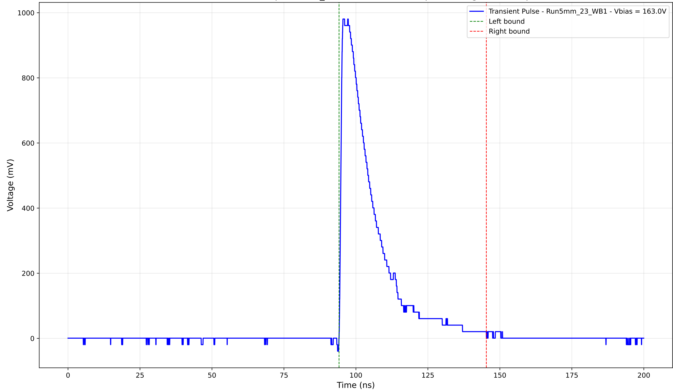
Transient Pulse - Sample: 5mm_23 - Position: 2055.0 \mu\text{m} - Charge: 245.10 pC
