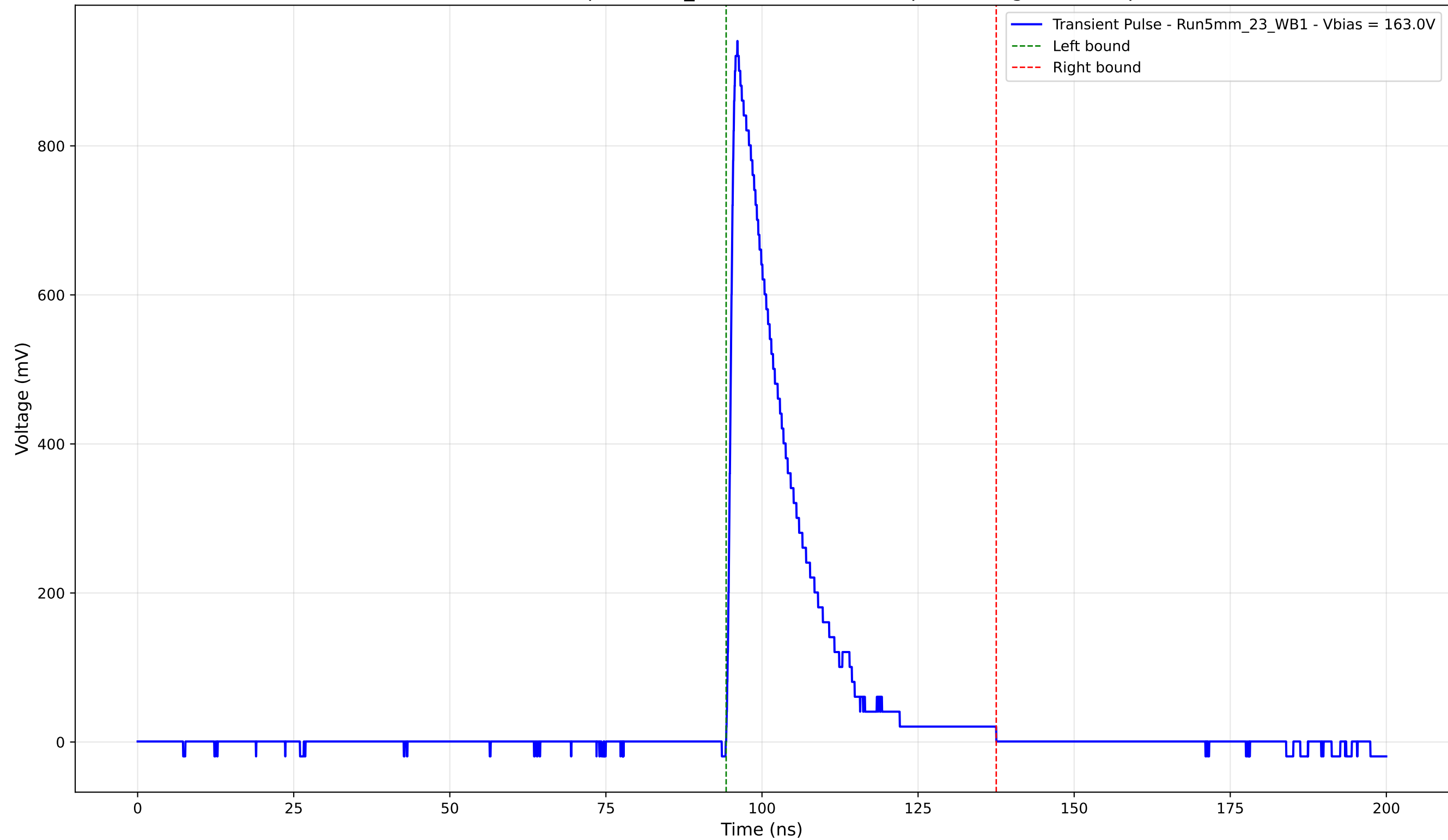
Transient Pulse - Sample: 5mm_23 - Position: 4545.0 \mu\text{m} - Charge: 178.66 pC
