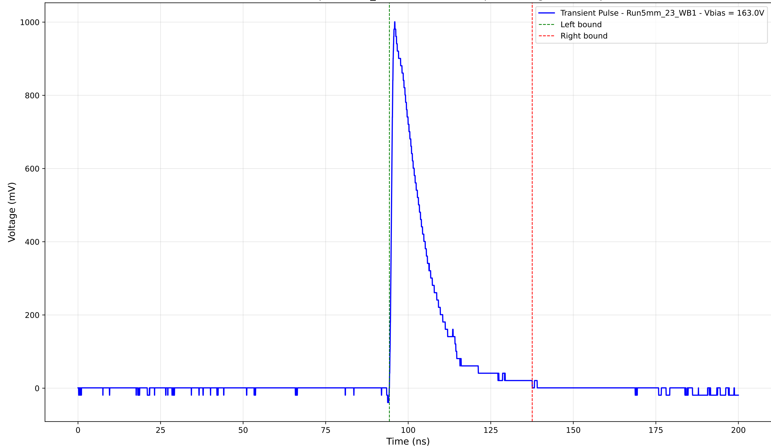
Transient Pulse - Sample: 5mm_23 - Position: 855.0 \mu\text{m} - Charge: 206.23 pC
