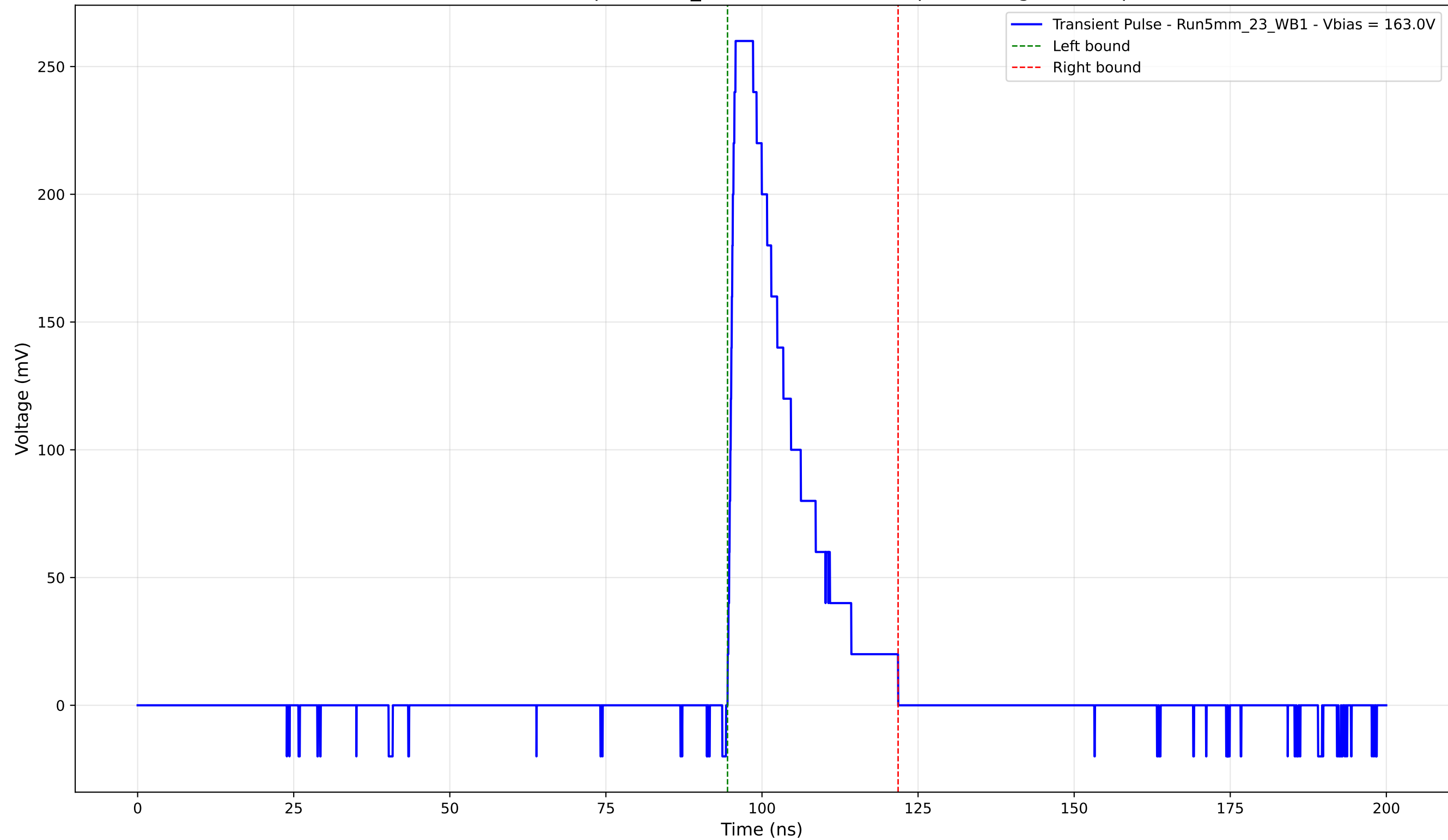
Transient Pulse - Sample: 5mm_23 - Position: 1745.0 \mu\text{m} - Charge: 54.42 pC
