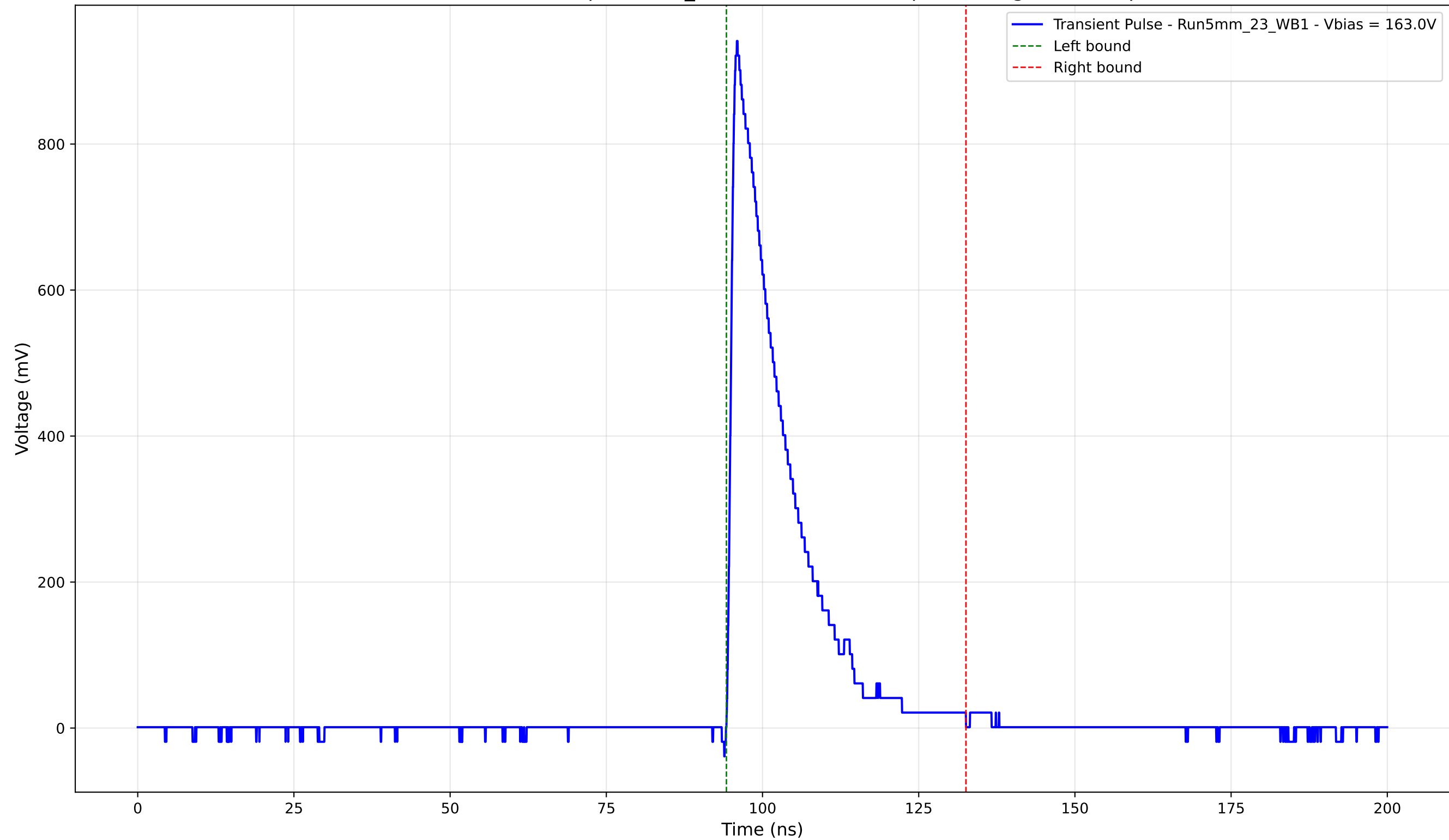
Transient Pulse - Sample: 5mm_23 - Position: 4610.0 \mu\text{m} - Charge: 174.60 pC
