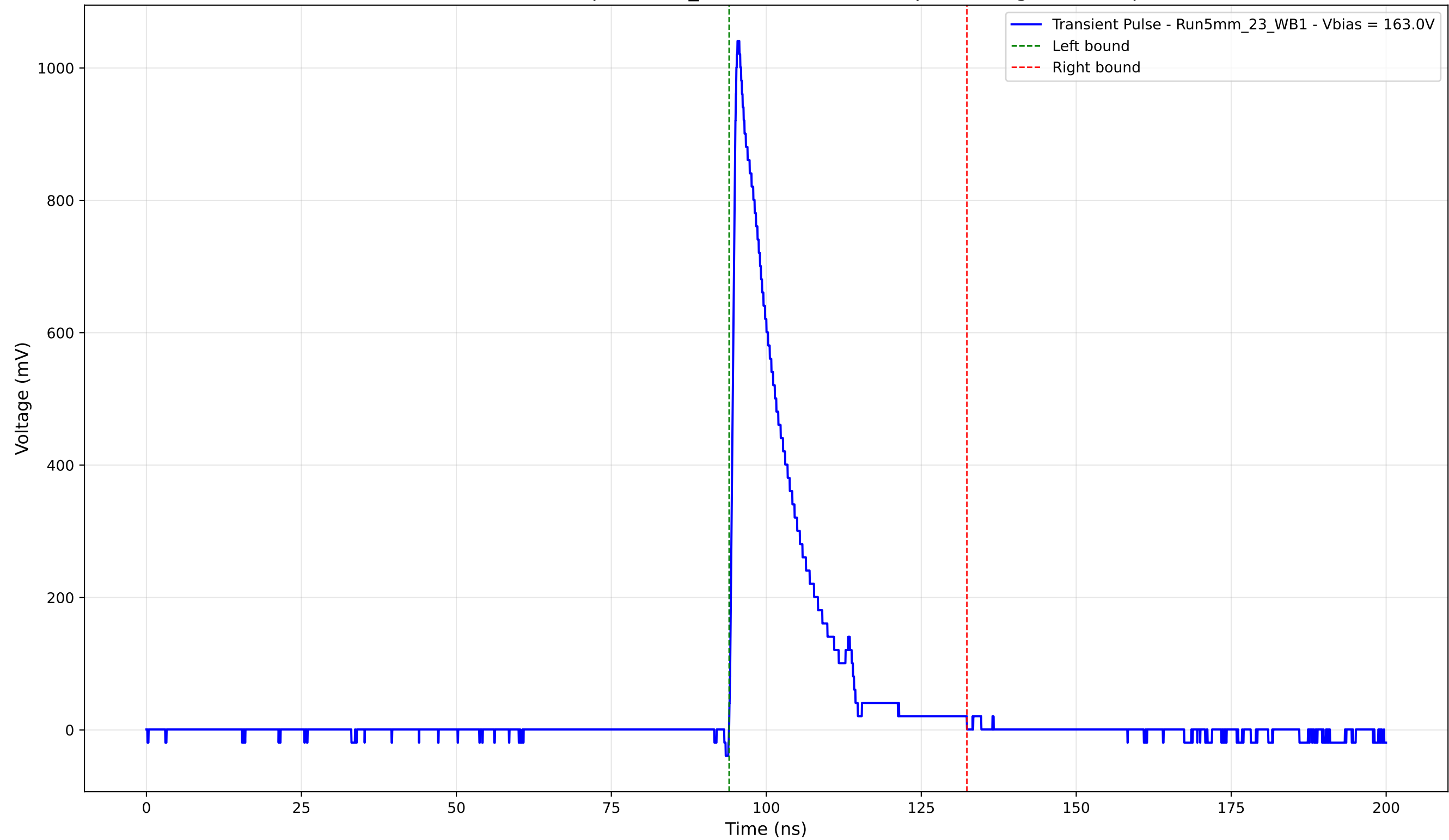
Transient Pulse - Sample: 5mm_23 - Position: 5040.0 \mu\text{m} - Charge: 178.47 pC
