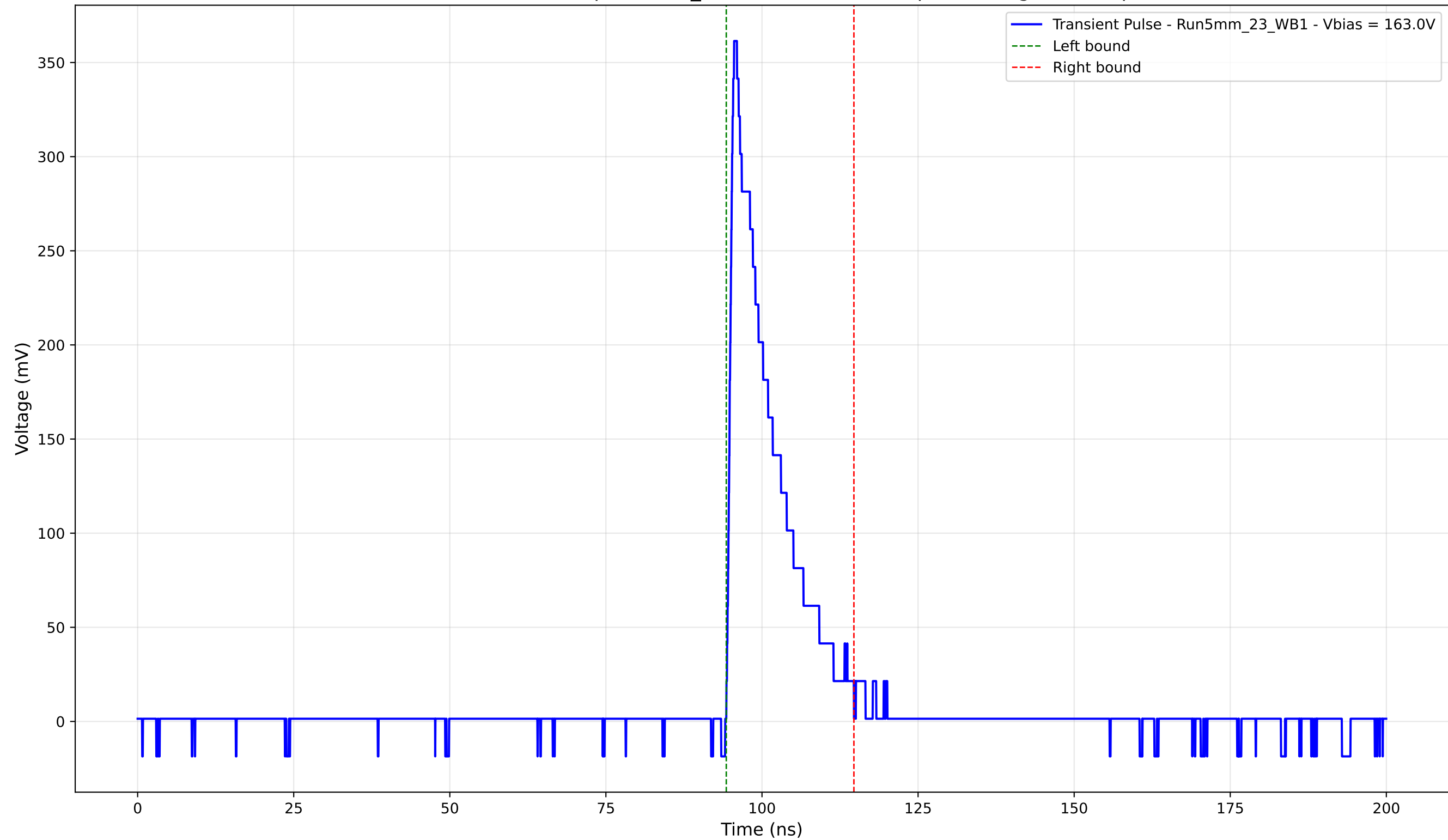
Transient Pulse - Sample: 5mm_23 - Position: 4790.0 \mu\text{m} - Charge: 52.47 pC
