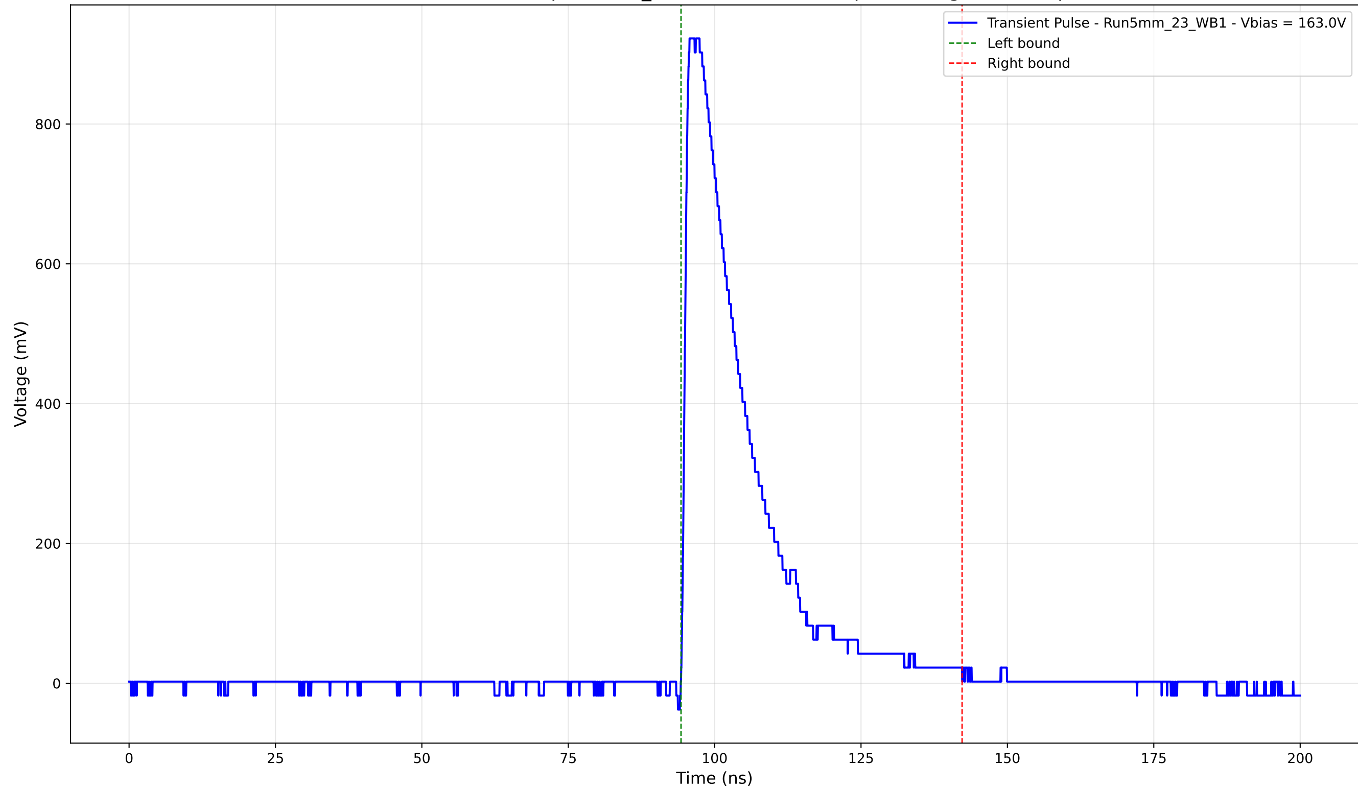
Transient Pulse - Sample: 5mm_23 - Position: 3580.0 \mu\text{m} - Charge: 215.21 pC
