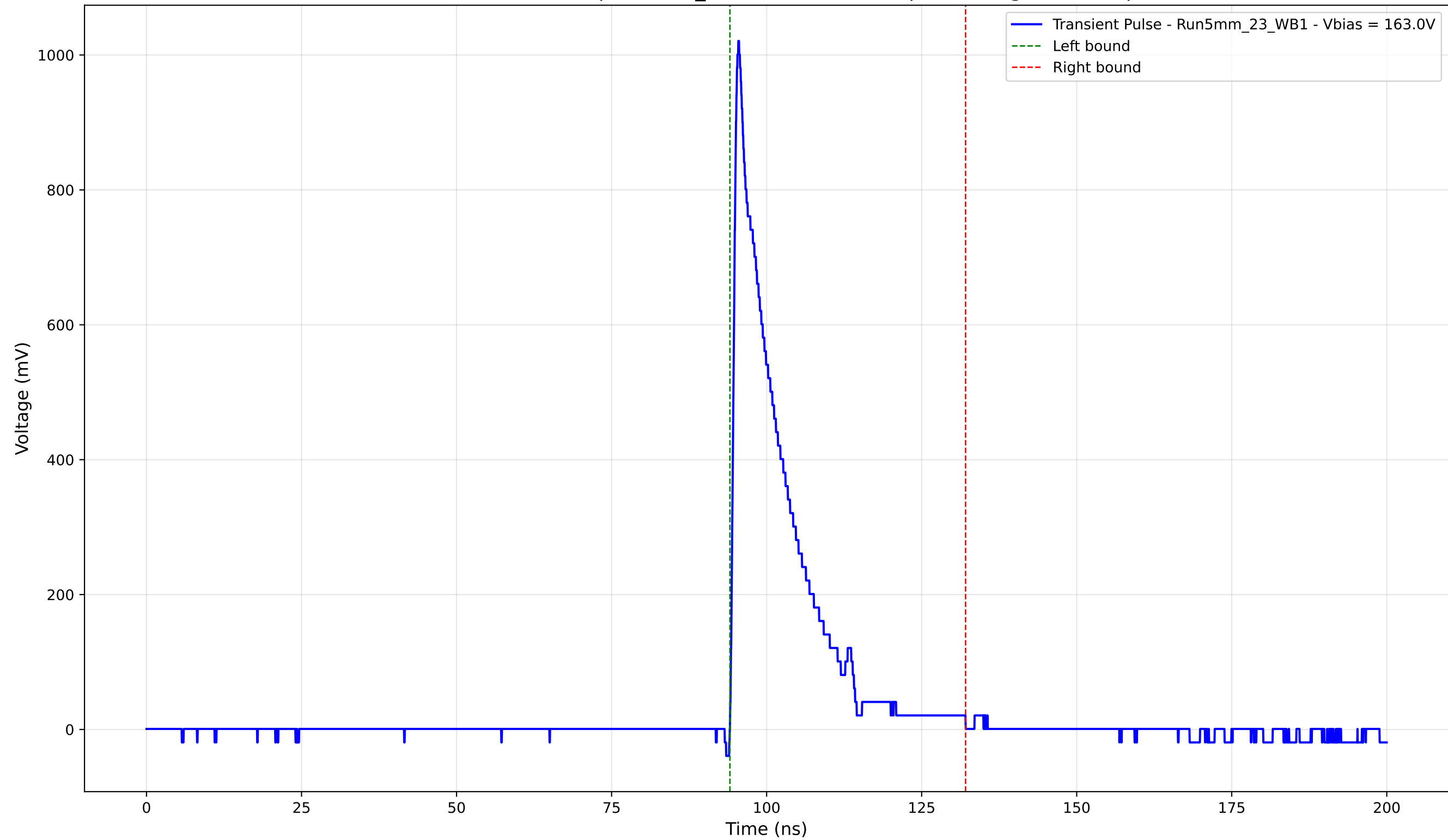
Transient Pulse - Sample: 5mm_23 - Position: 345.0 \mu\text{m} - Charge: 161.69 pC
