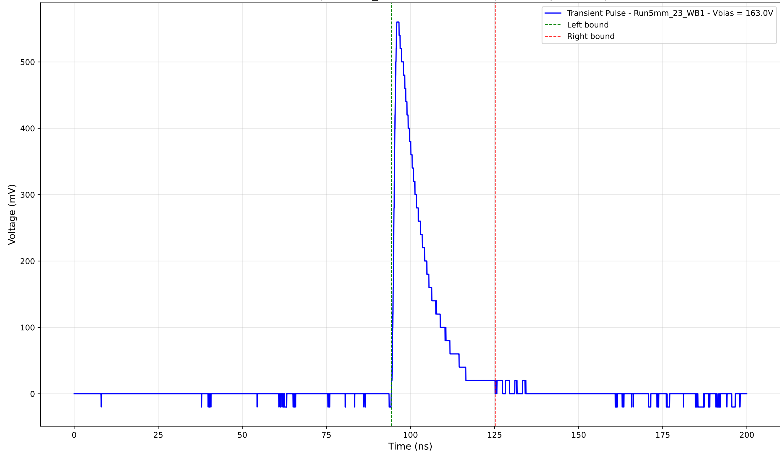
Transient Pulse - Sample: 5mm_23 - Position: 4310.0 \mu\text{m} - Charge: 99.61 pC
