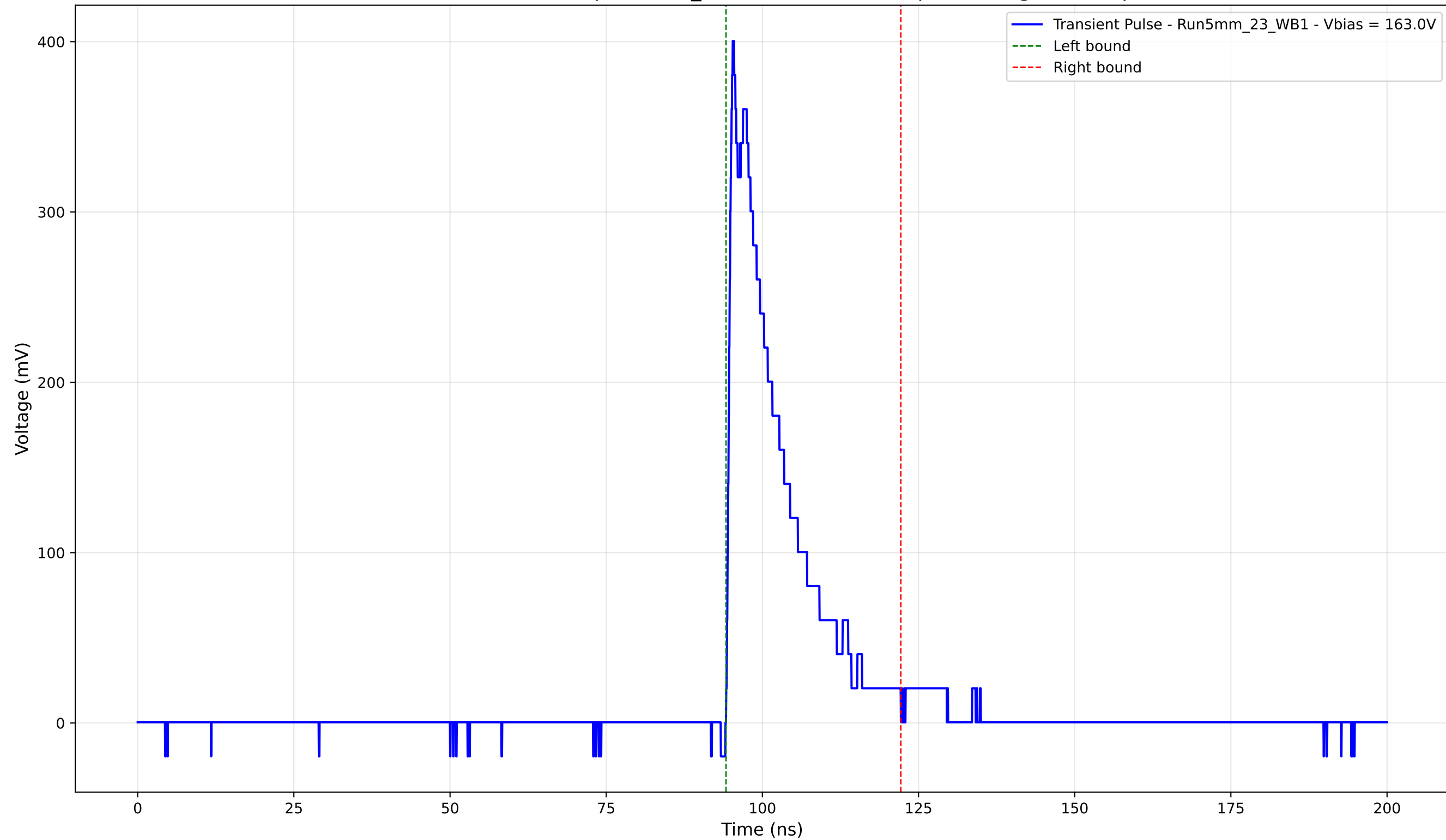
Transient Pulse - Sample: 5mm_23 - Position: 2265.0 \mu\text{m} - Charge: 68.91 pC
