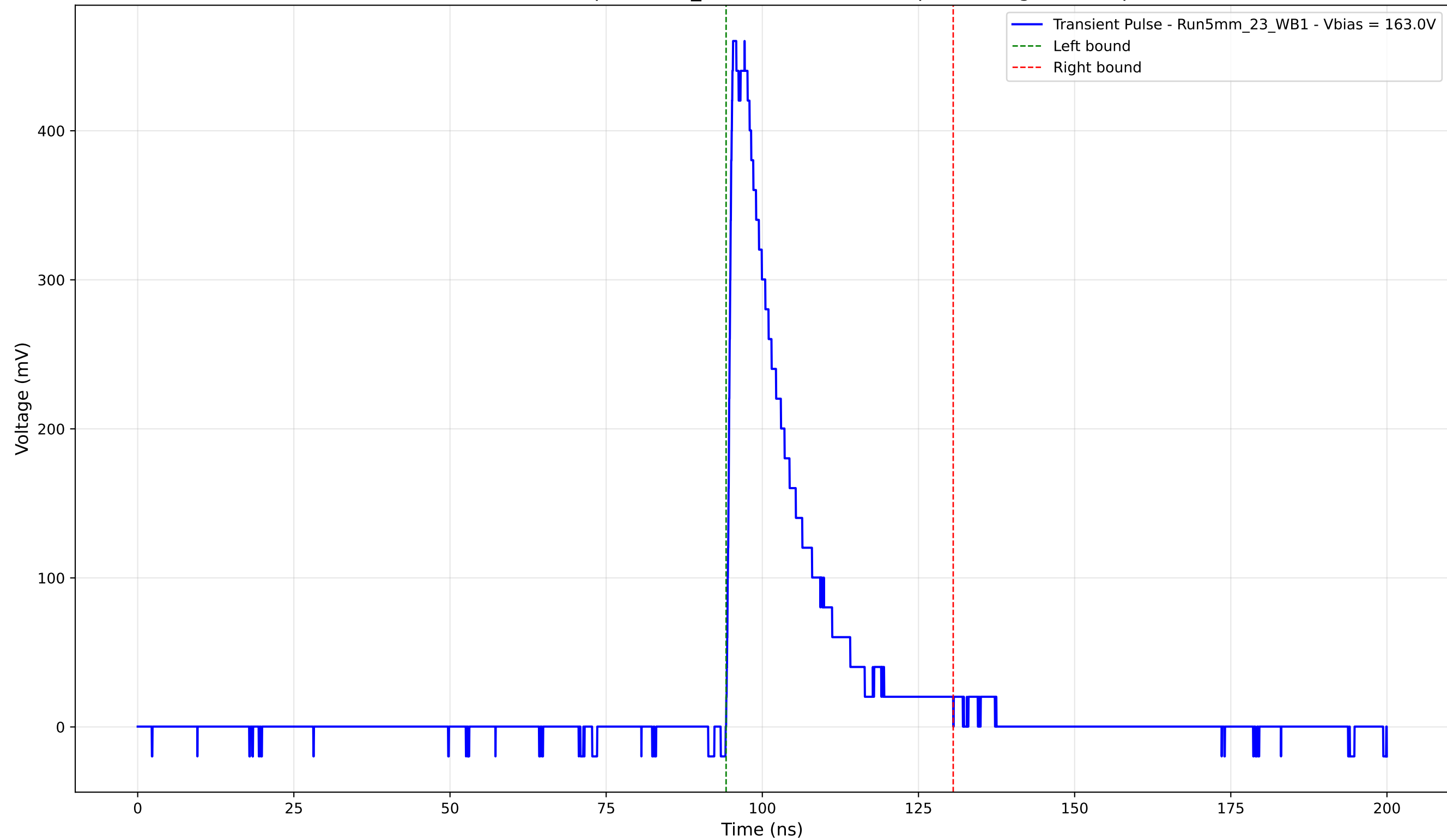
Transient Pulse - Sample: 5mm_23 - Position: 2205.0 \mu\text{m} - Charge: 90.61 pC
