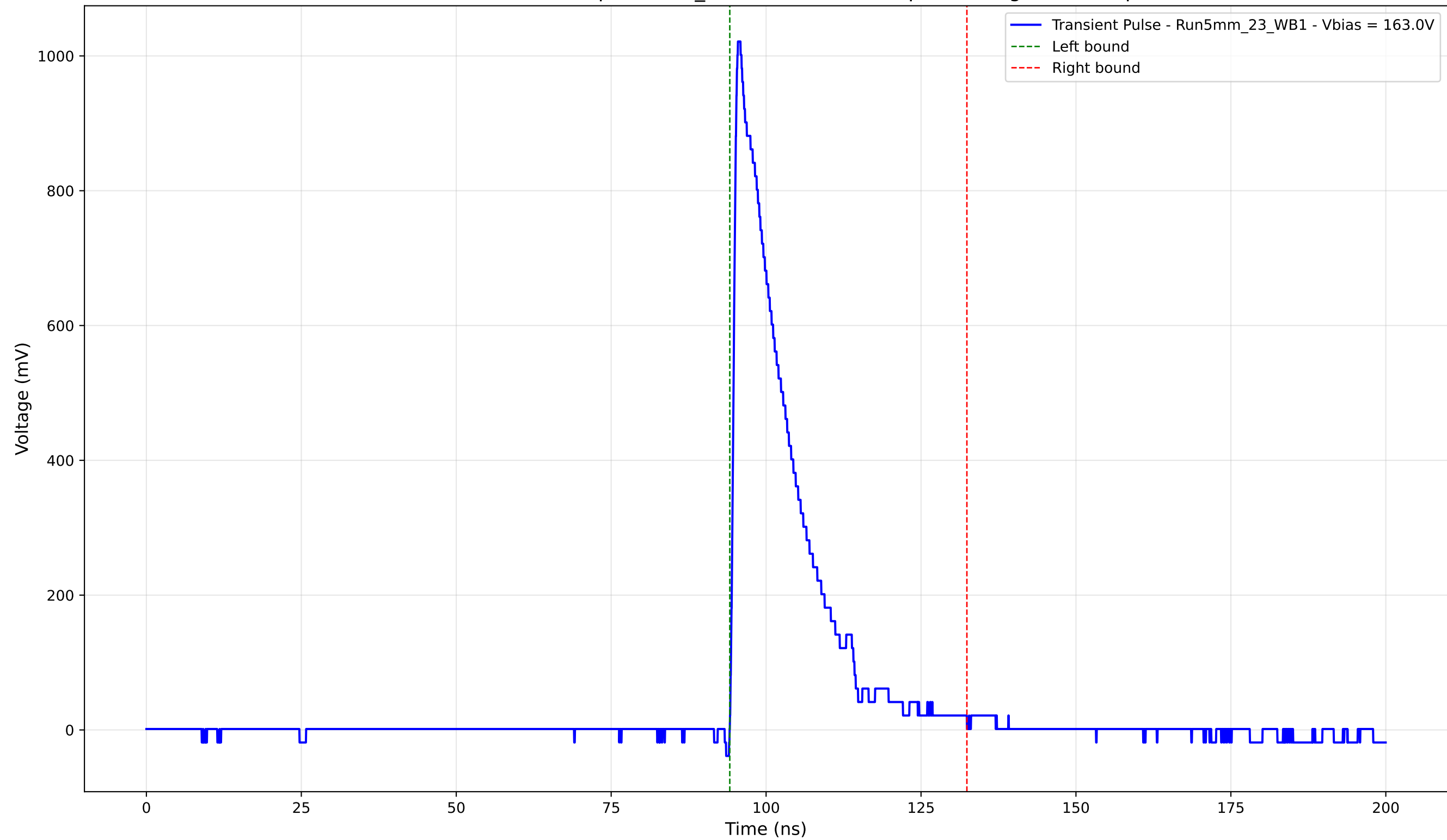
Transient Pulse - Sample: 5mm_23 - Position: 530.0 \mu\text{m} - Charge: 193.65 pC
