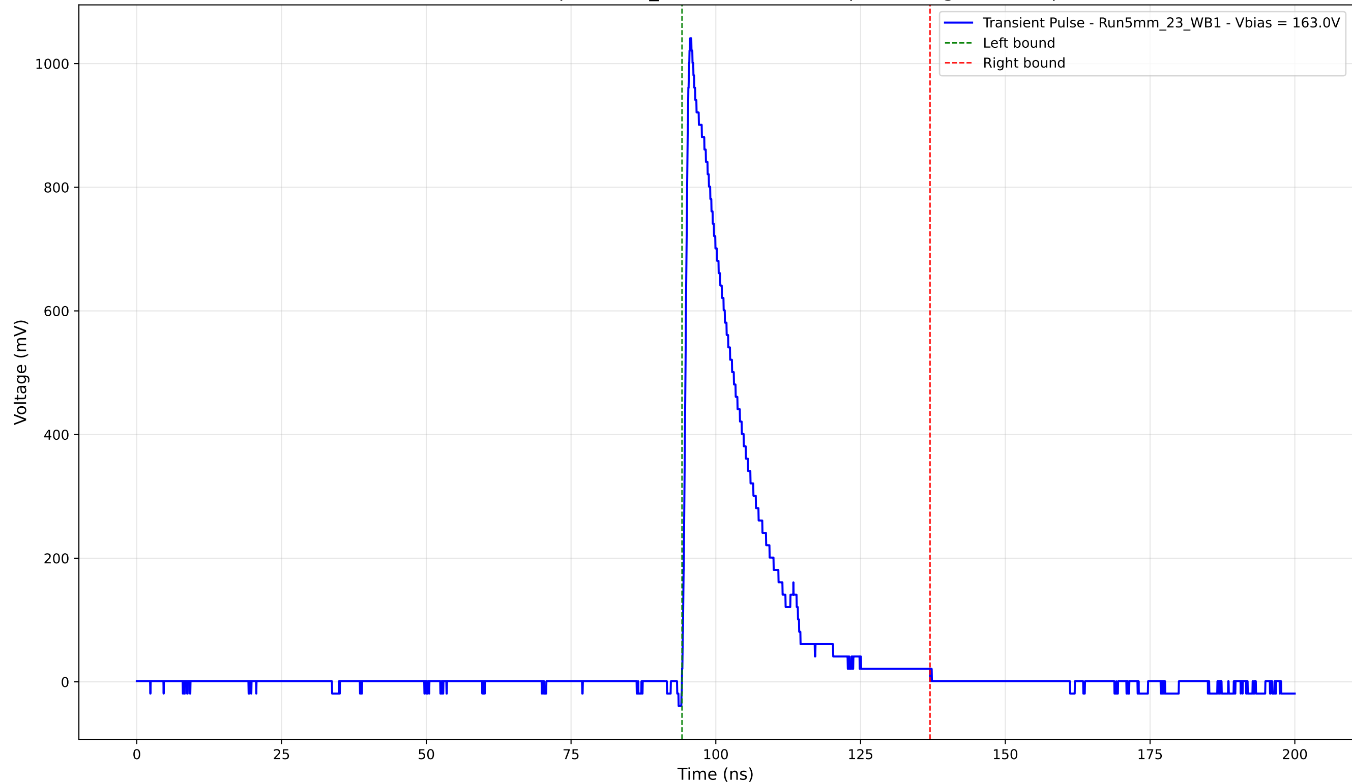
Transient Pulse - Sample: 5mm_23 - Position: 570.0 \mu\text{m} - Charge: 203.08 pC
