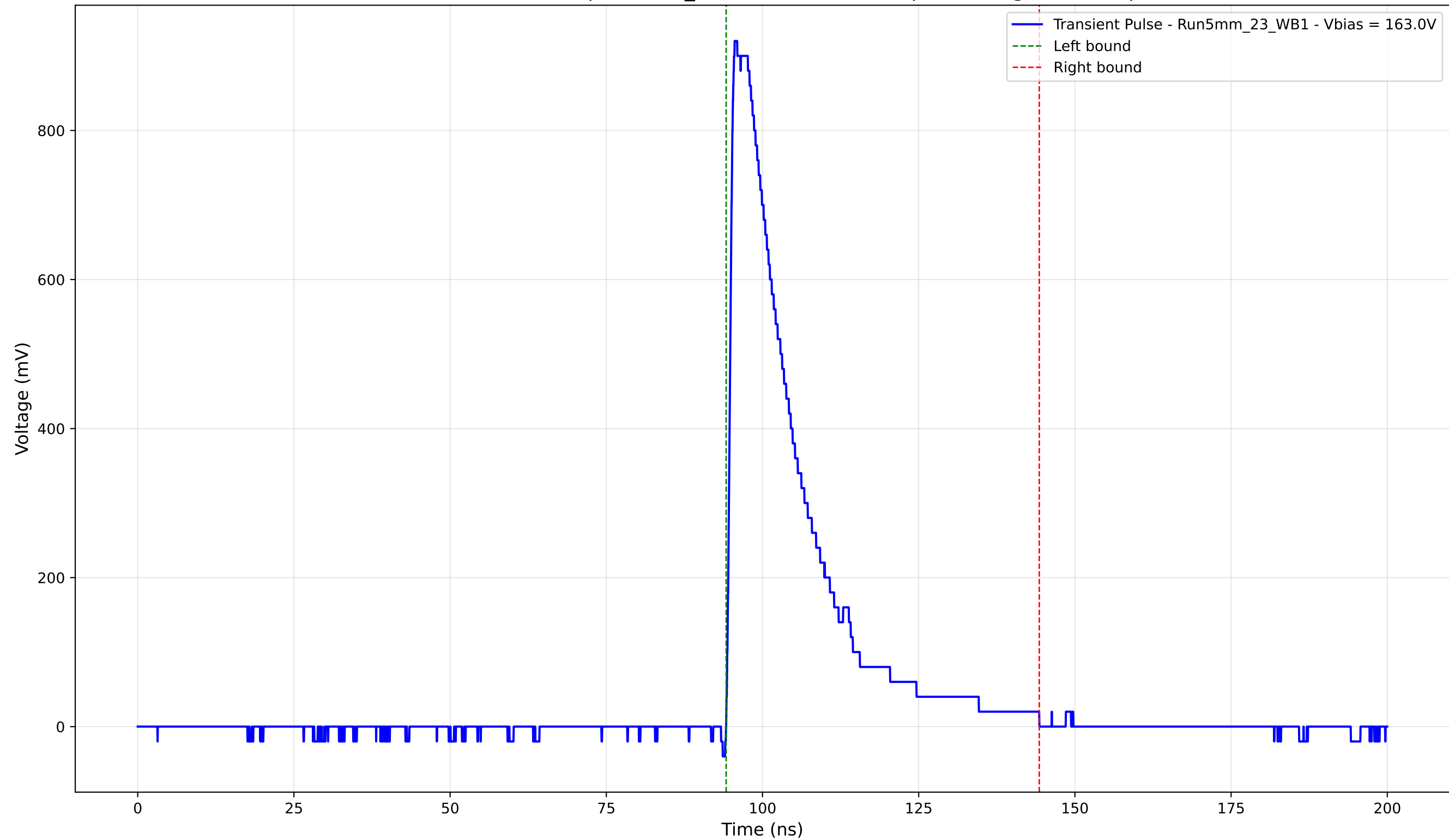
Transient Pulse - Sample: 5mm_23 - Position: 3420.0 \mu\text{m} - Charge: 212.28 pC
