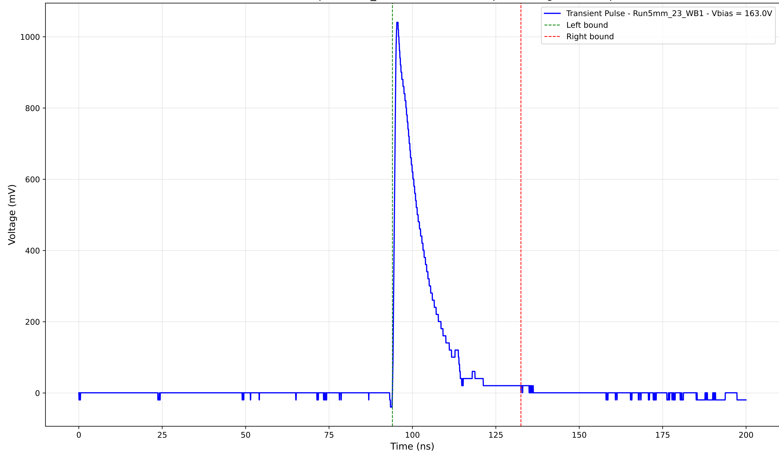
Transient Pulse - Sample: 5mm_23 - Position: 5045.0 \mu\text{m} - Charge: 180.64 pC
