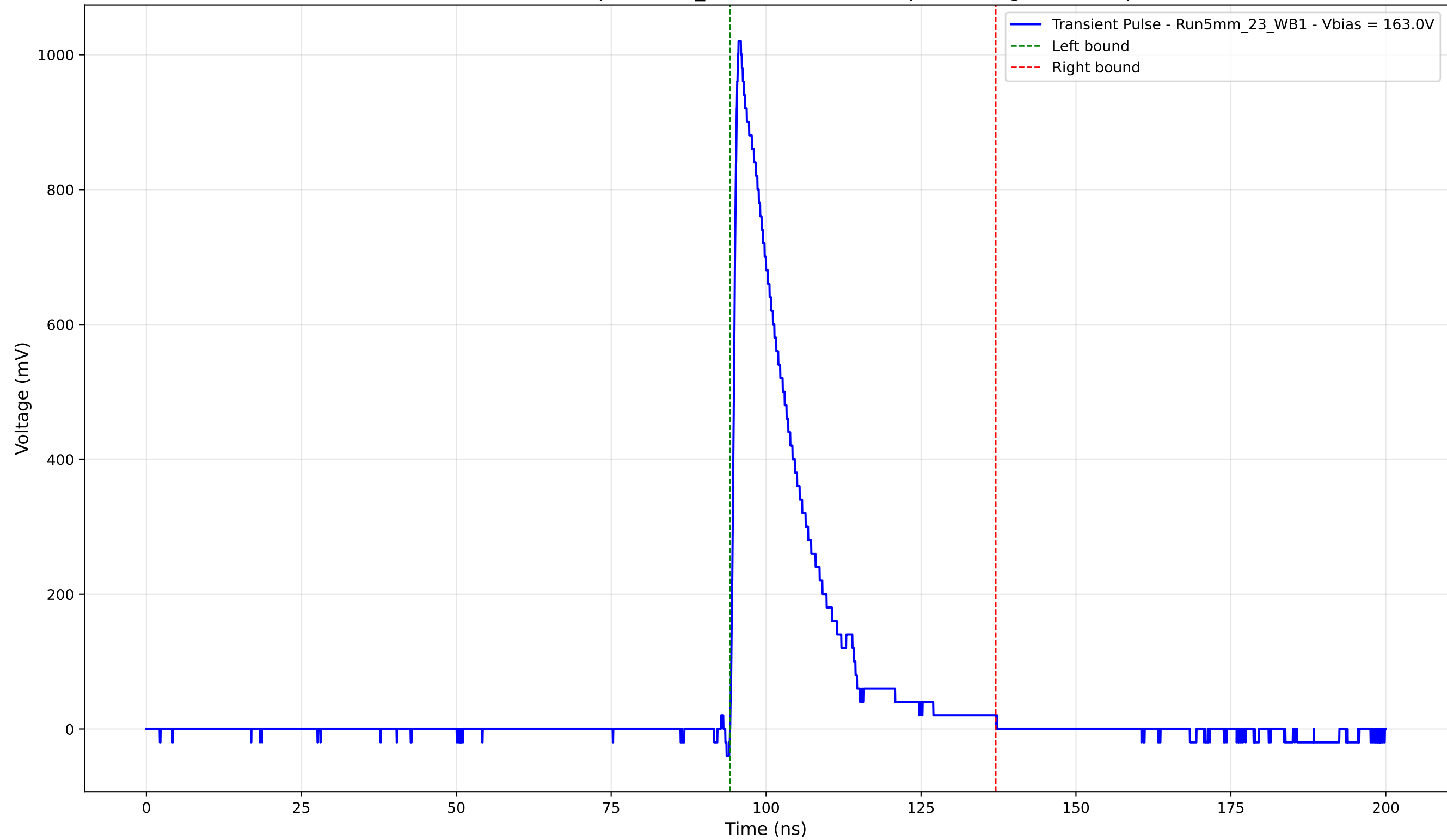
Transient Pulse - Sample: 5mm_23 - Position: 635.0 \mu\text{m} - Charge: 199.62 pC
