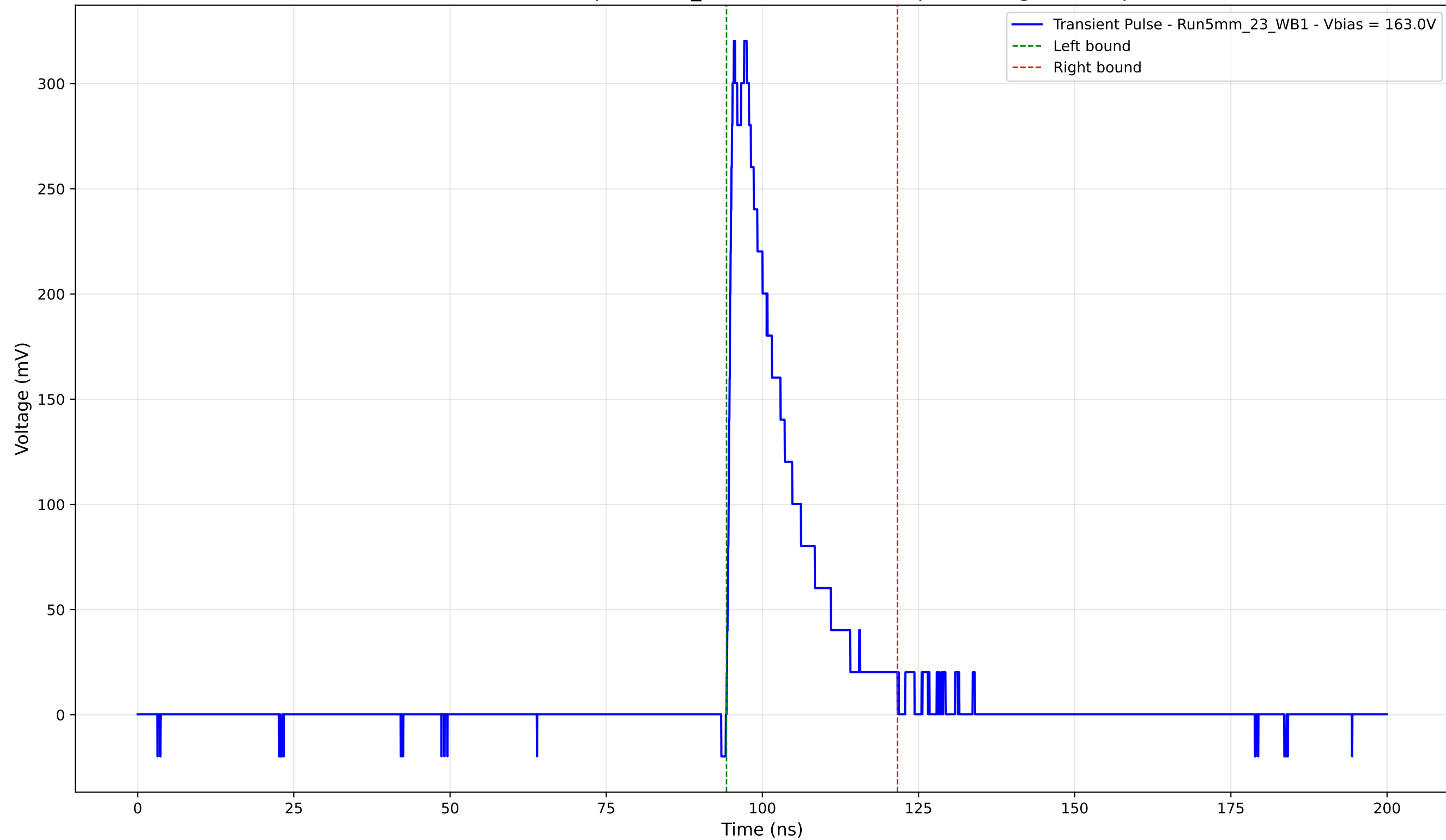
Transient Pulse - Sample: 5mm_23 - Position: 2220.0 \mu\text{m} - Charge: 59.24 pC
