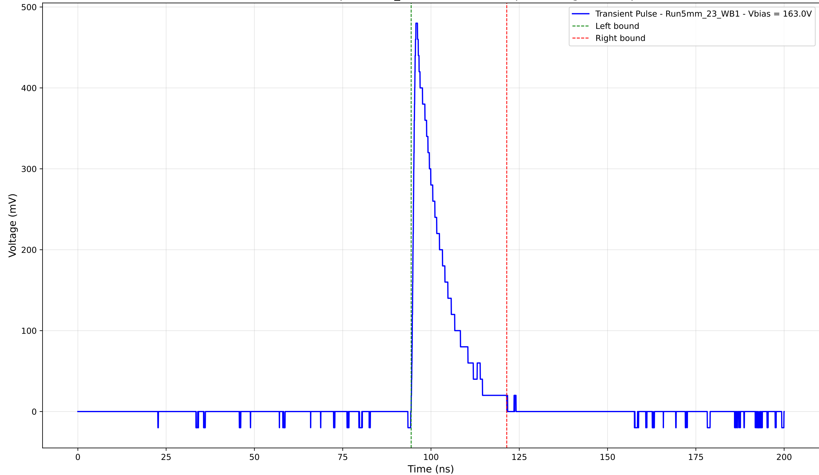
Transient Pulse - Sample: 5mm_23 - Position: 750.0 \mu\text{m} - Charge: 78.60 pC
