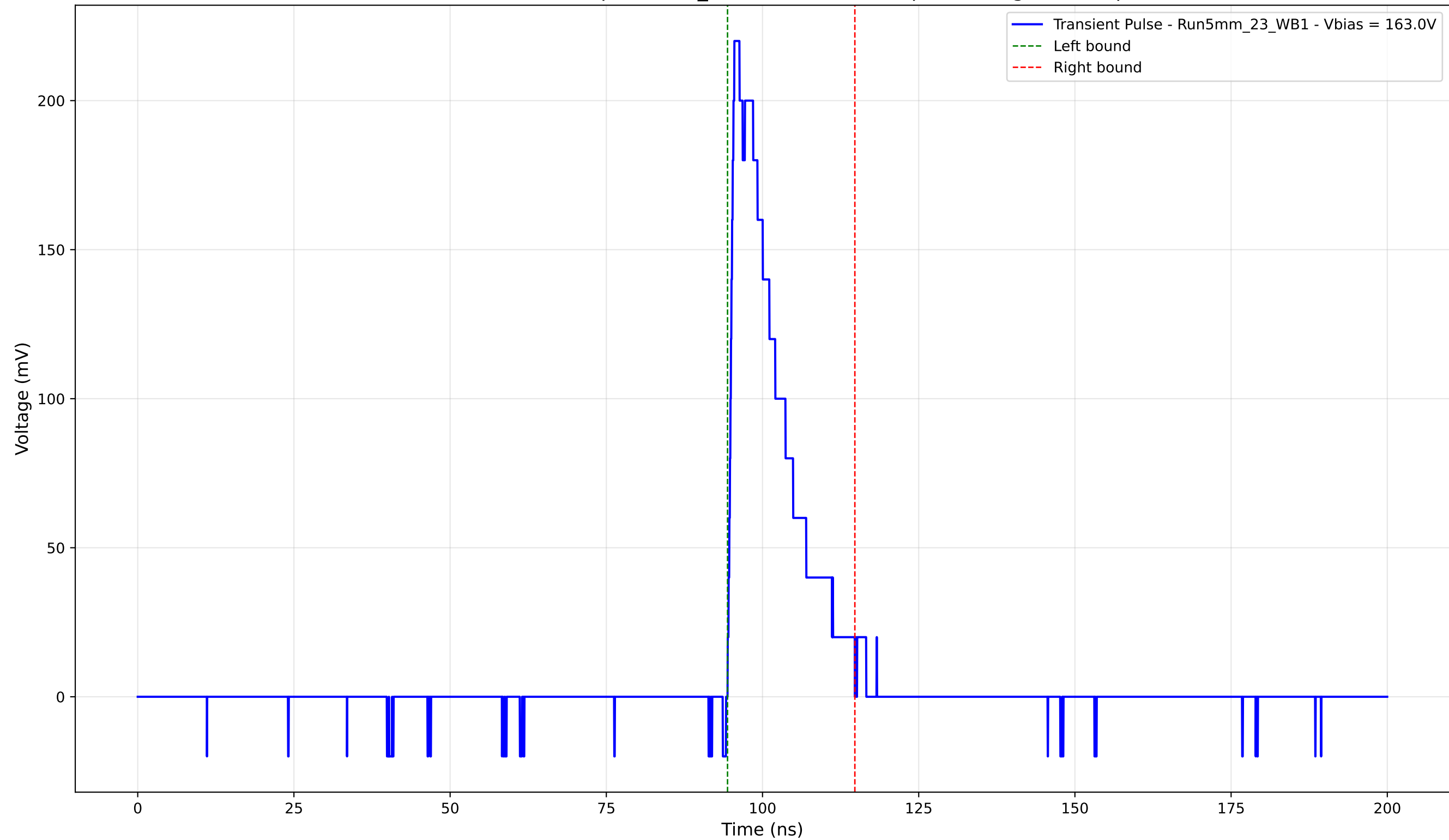
Transient Pulse - Sample: 5mm_23 - Position: 720.0 \mu\text{m} - Charge: 37.61 pC
