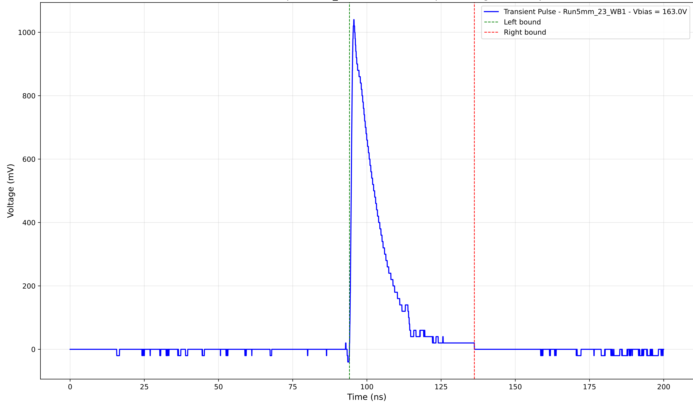
Transient Pulse - Sample: 5mm_23 - Position: 505.0 \mu\text{m} - Charge: 191.90 pC
