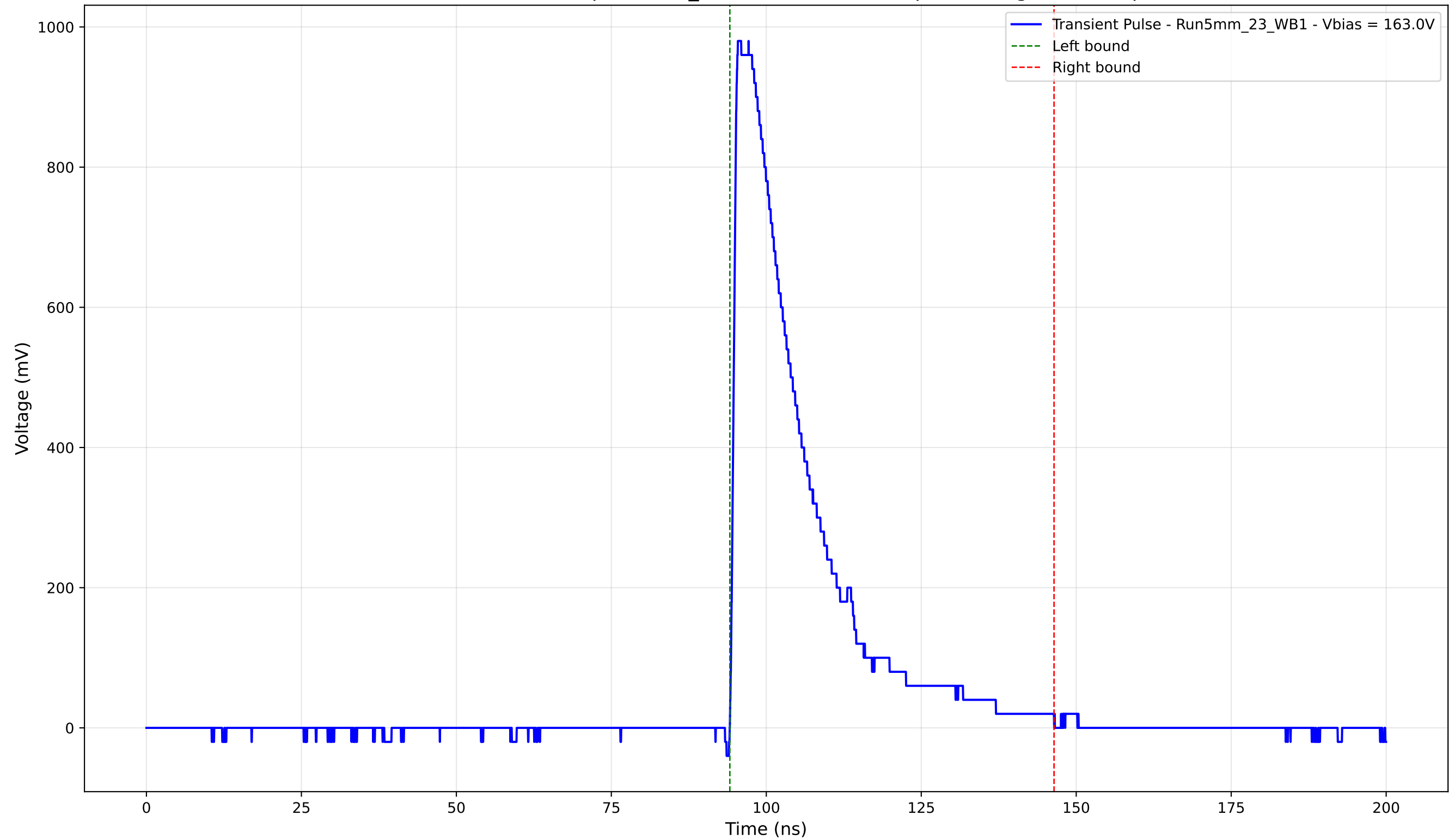
Transient Pulse - Sample: 5mm_23 - Position: 2115.0 \mu\text{m} - Charge: 243.78 pC
