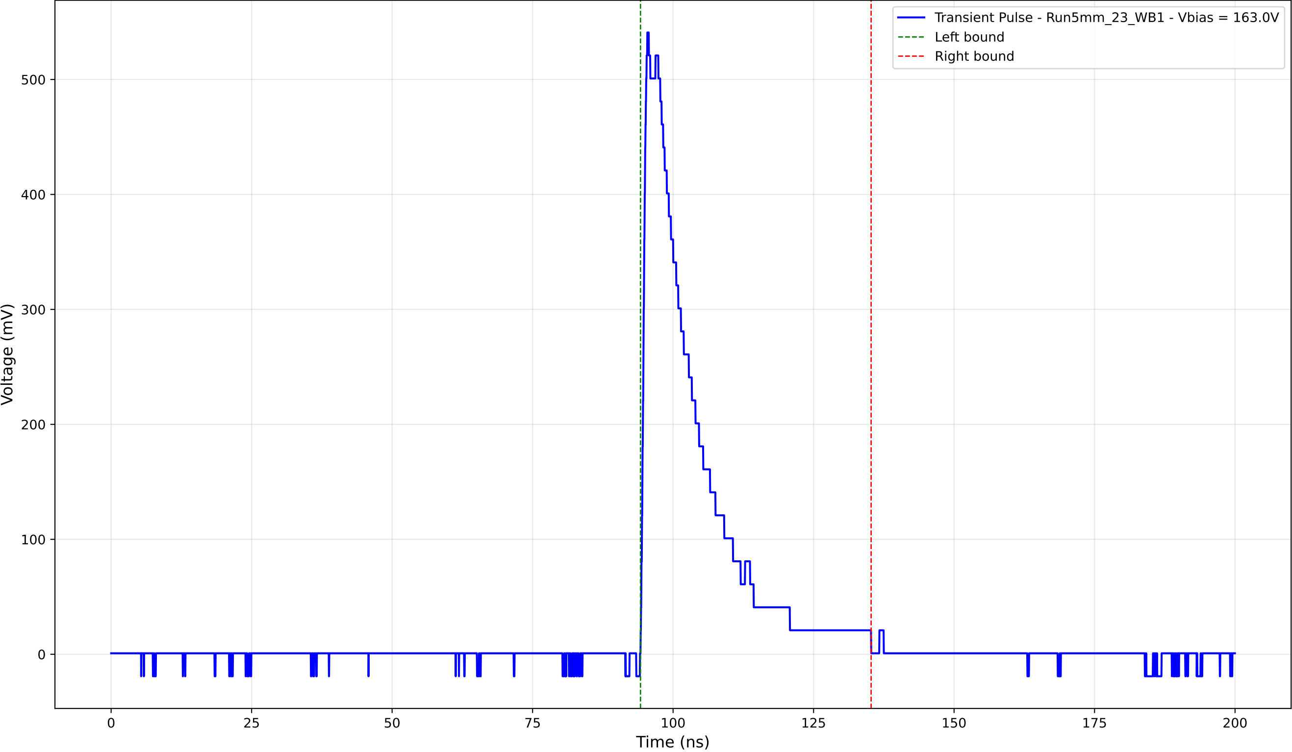
Transient Pulse - Sample: 5mm_23 - Position: 2200.0 \mu\text{m} - Charge: 107.02 pC
