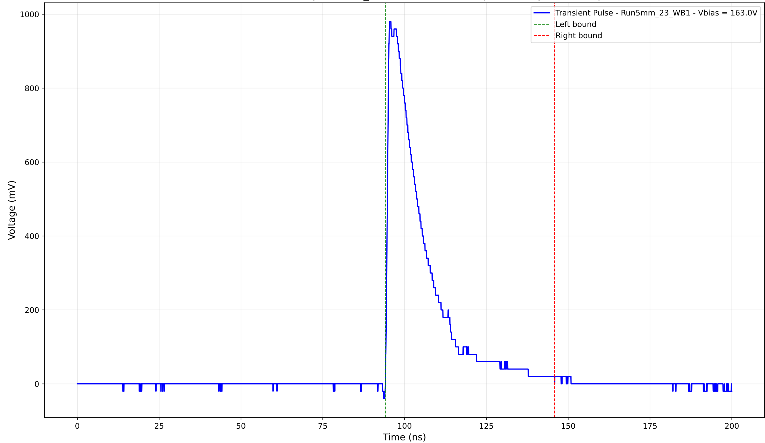
Transient Pulse - Sample: 5mm_23 - Position: 2130.0 \mu\text{m} - Charge: 237.54 pC
