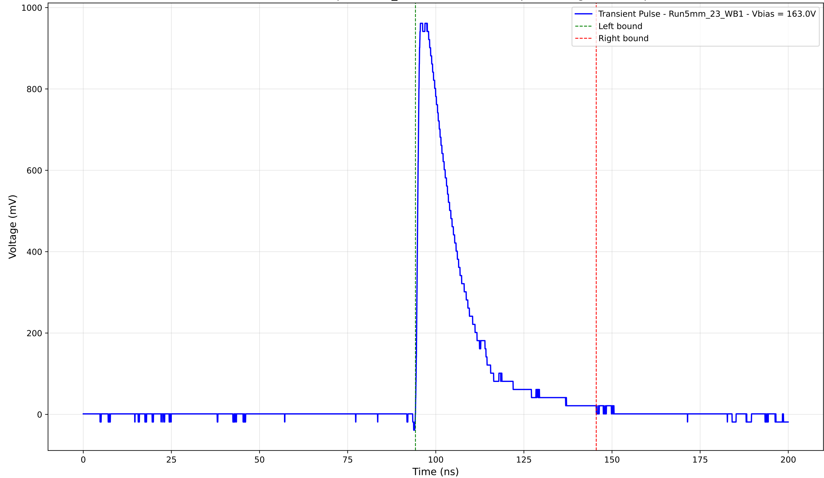
Transient Pulse - Sample: 5mm_23 - Position: 1940.0 \mu\text{m} - Charge: 237.28 pC
