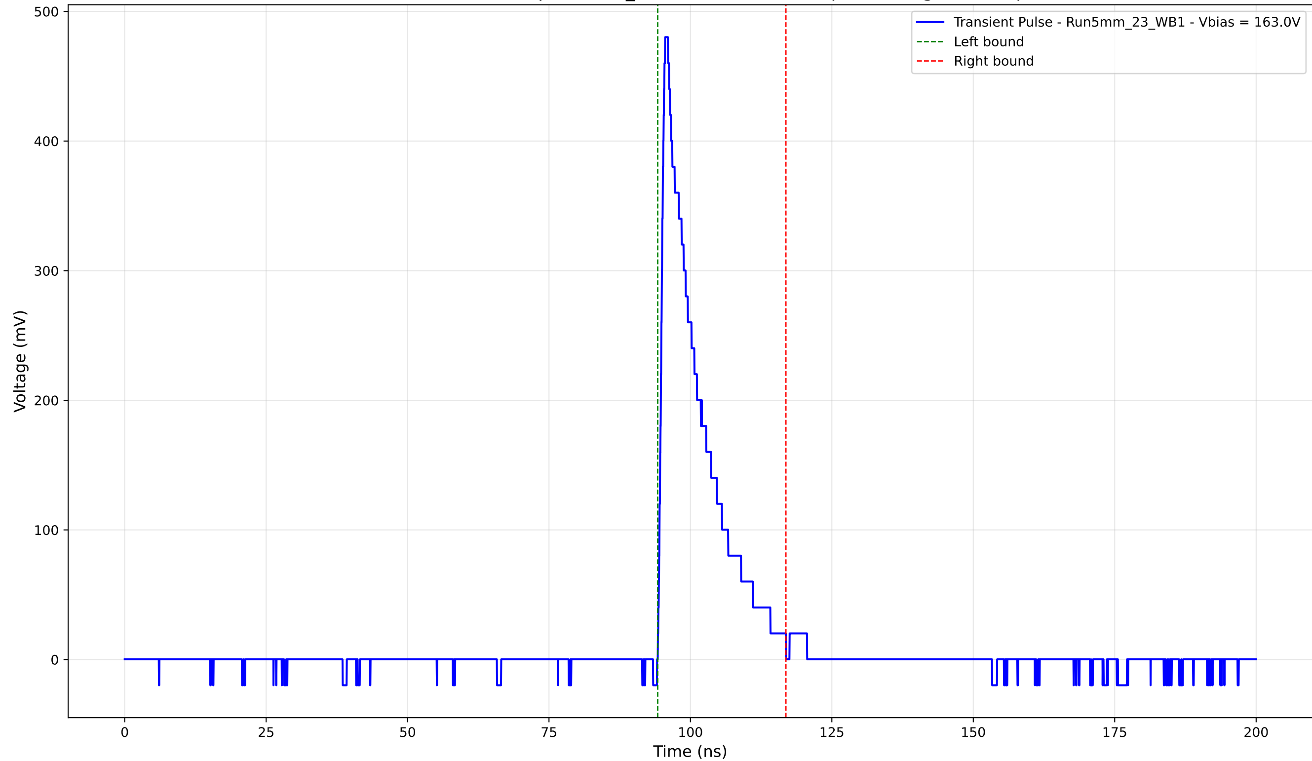
Transient Pulse - Sample: 5mm_23 - Position: 4800.0 \mu\text{m} - Charge: 70.02 pC
