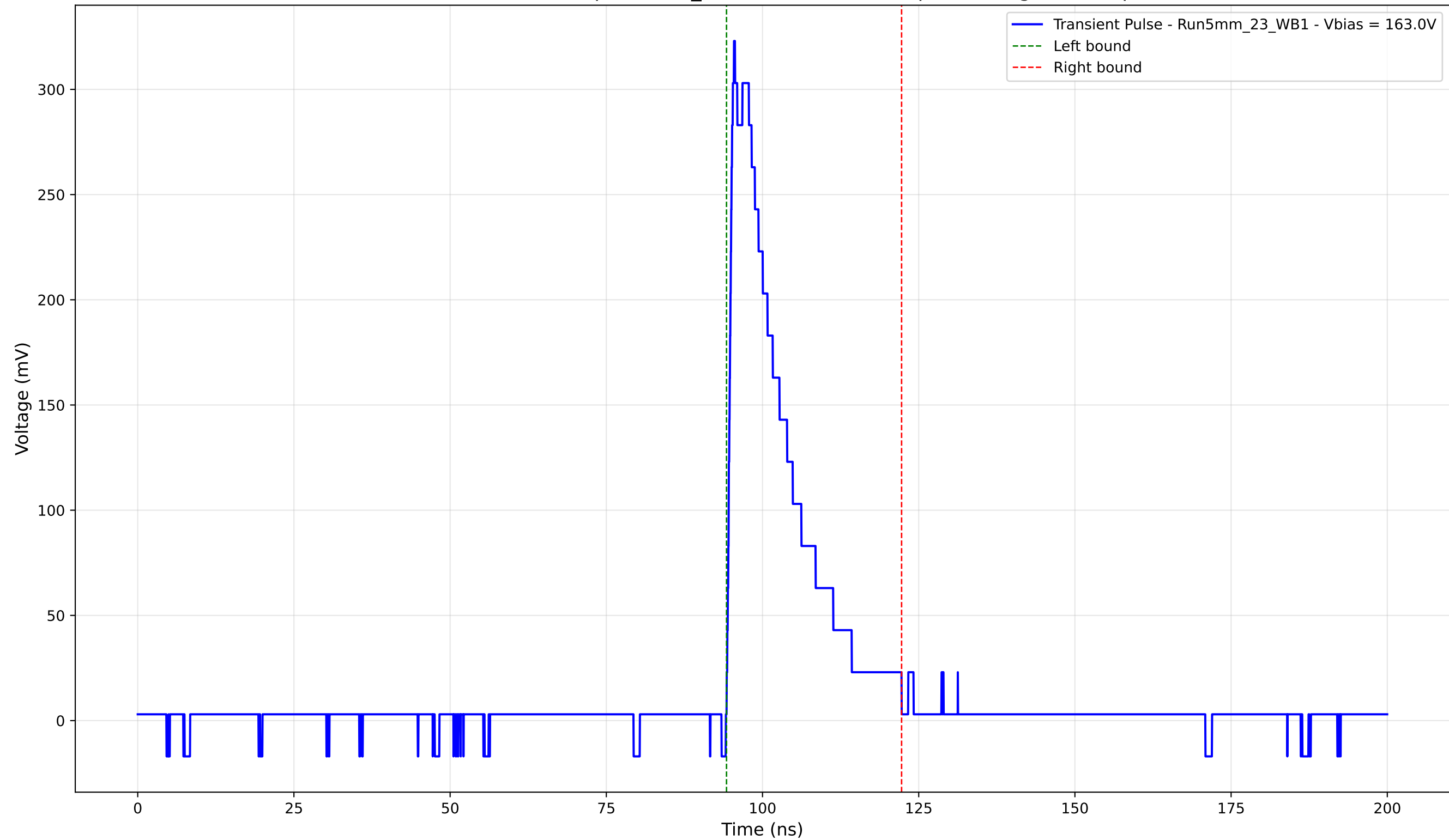
Transient Pulse - Sample: 5mm_23 - Position: 3270.0 \mu\text{m} - Charge: 61.27 pC
