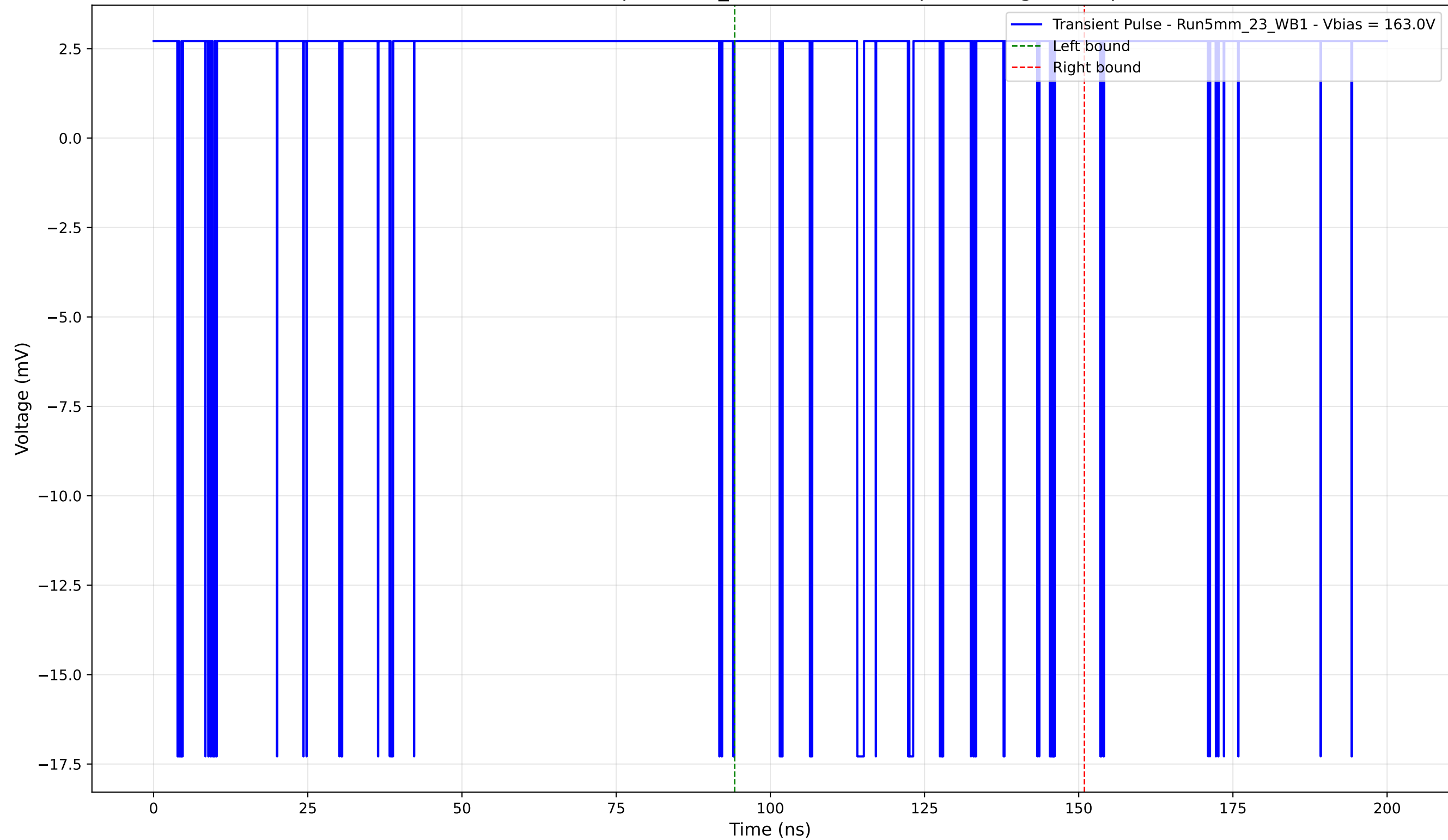
Transient Pulse - Sample: 5mm_23 - Position: 35.0 \mu\text{m} - Charge: 1.33 pC
