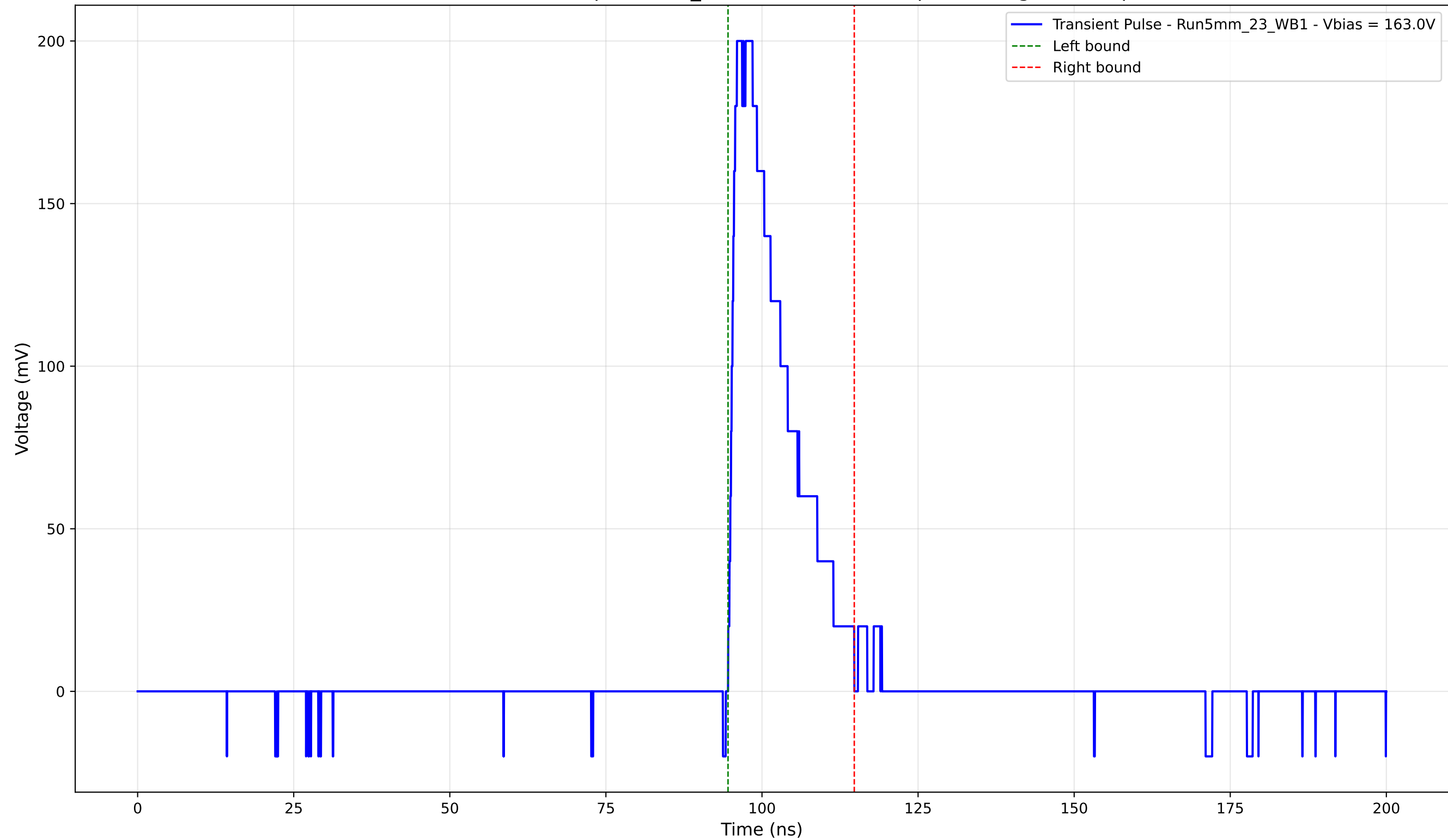
Transient Pulse - Sample: 5mm_23 - Position: 1230.0 \mu\text{m} - Charge: 37.80 pC
