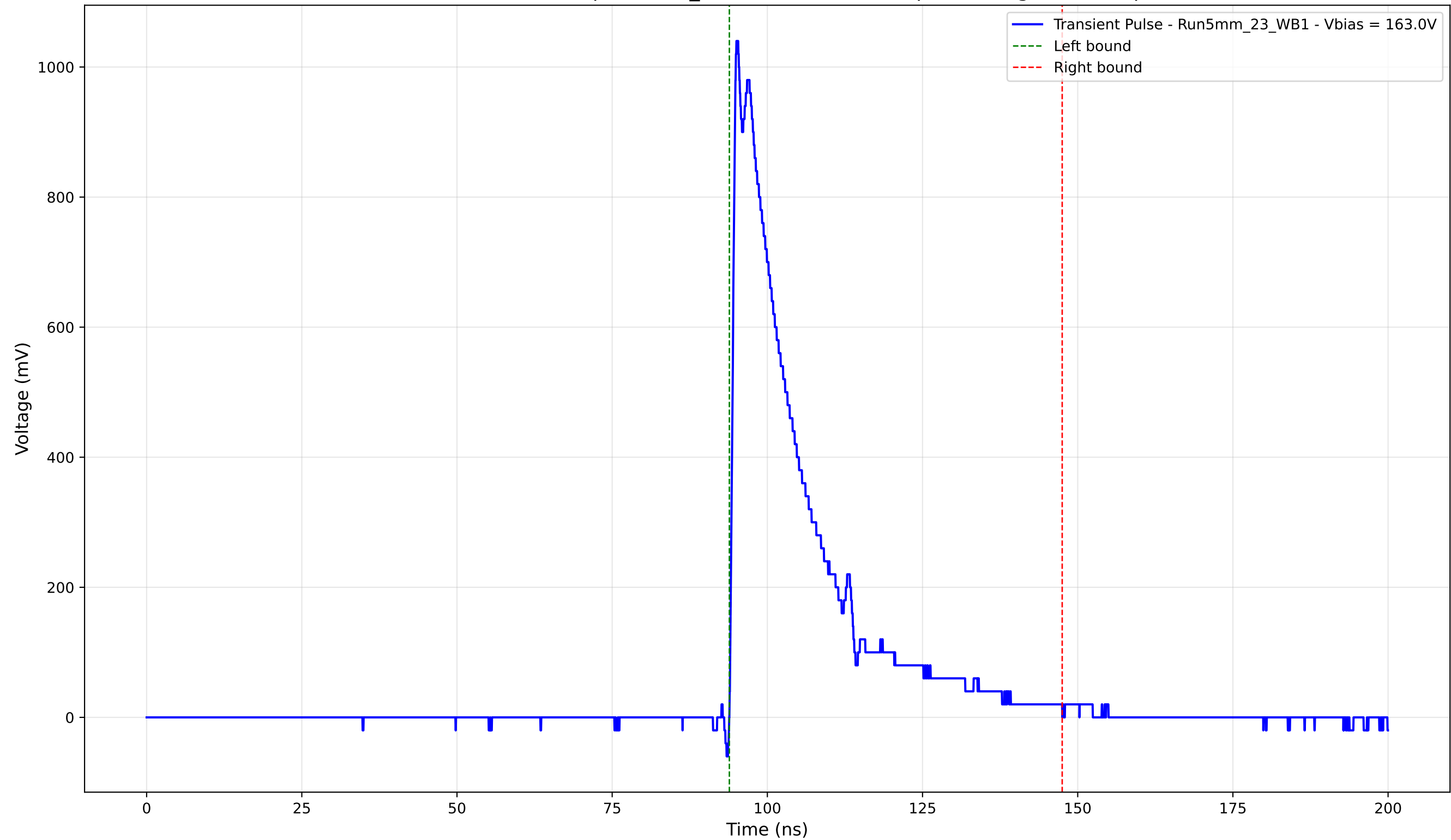
Transient Pulse - Sample: 5mm_23 - Position: 2565.0 \mu\text{m} - Charge: 238.02 pC
