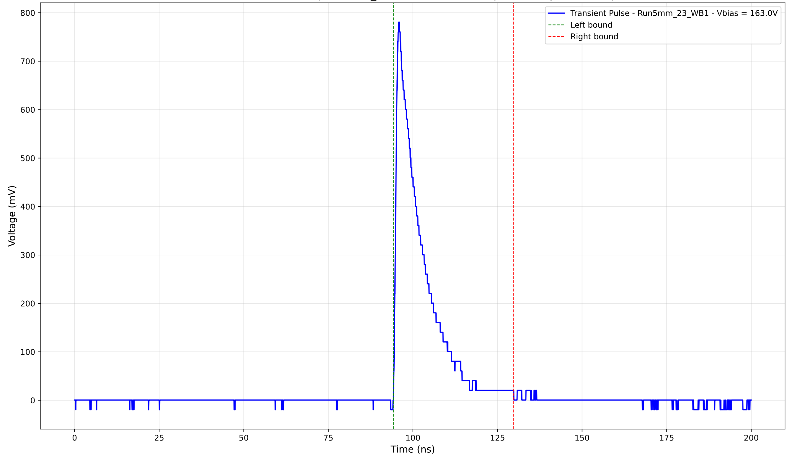
Transient Pulse - Sample: 5mm_23 - Position: 4705.0 \mu\text{m} - Charge: 128.69 pC
