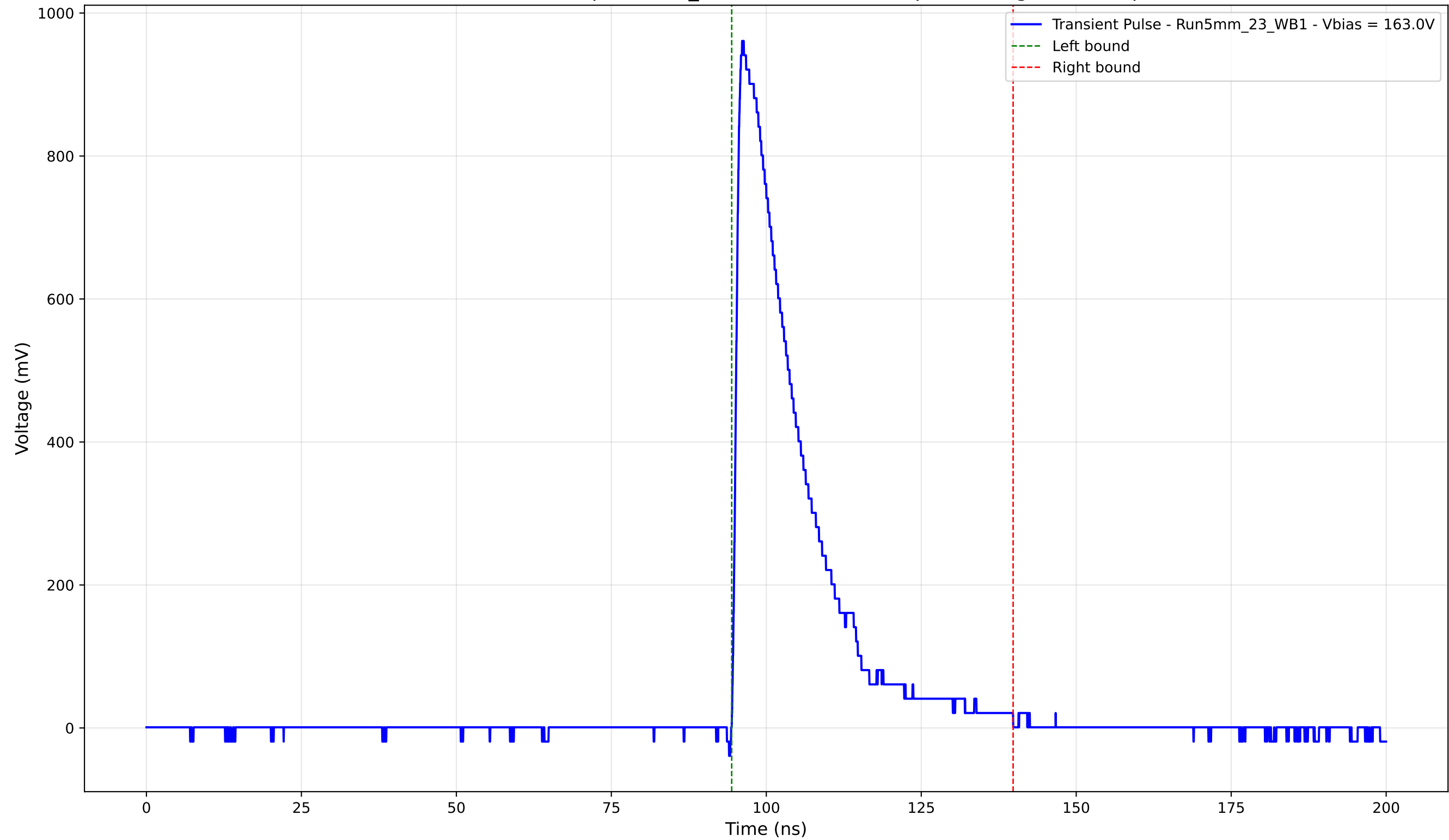
Transient Pulse - Sample: 5mm_23 - Position: 1330.0 \mu\text{m} - Charge: 213.13 pC
