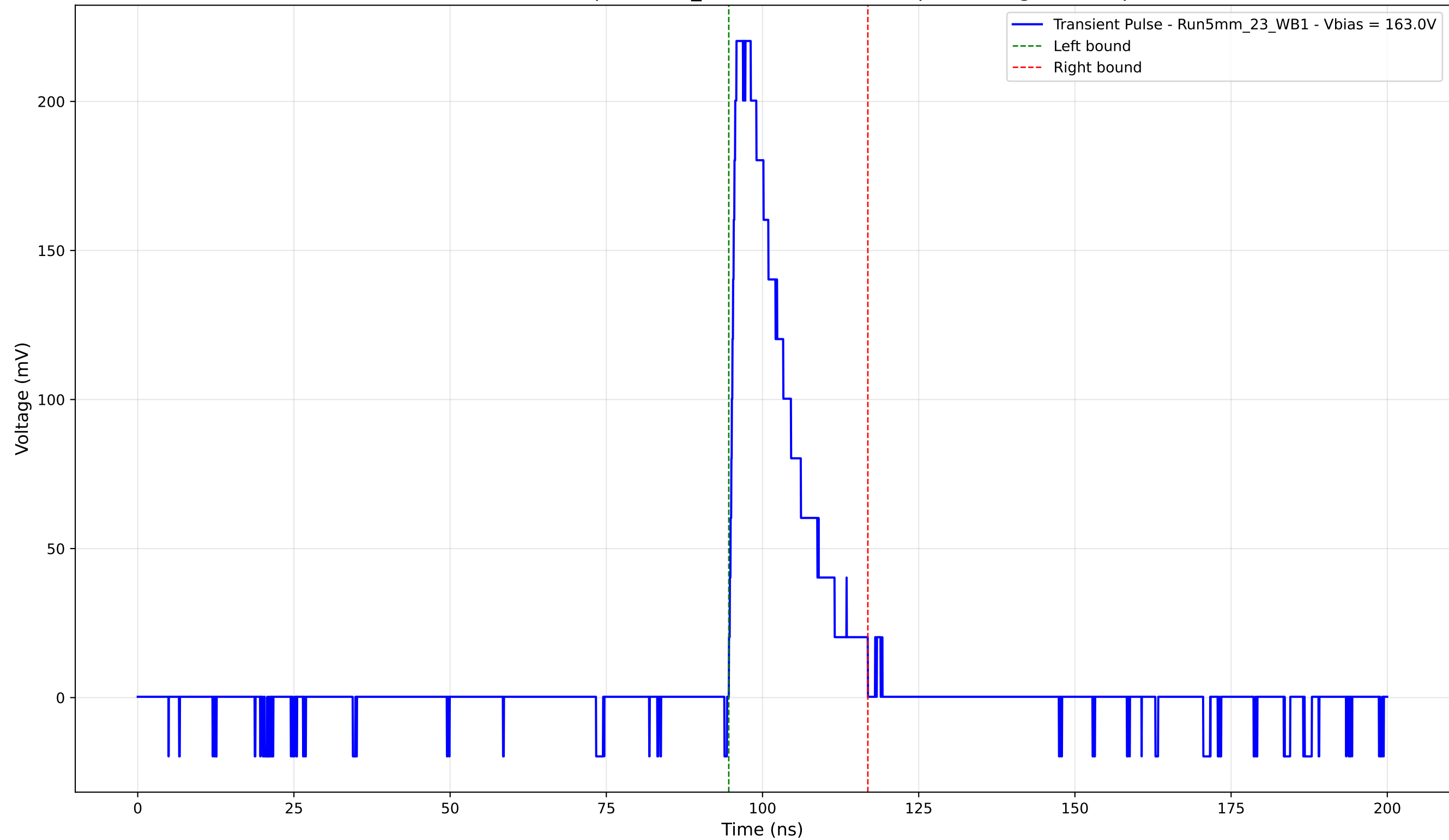
Transient Pulse - Sample: 5mm_23 - Position: 1215.0 \mu\text{m} - Charge: 41.88 pC
