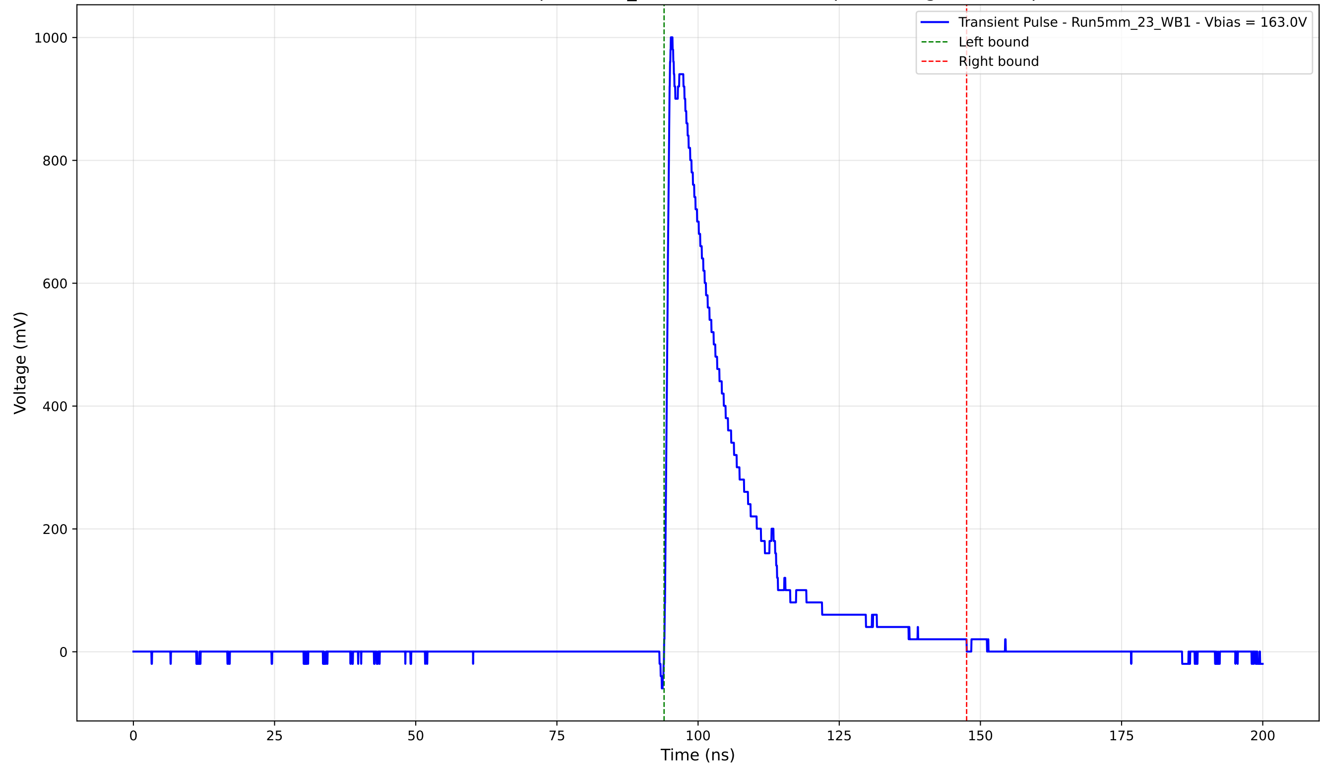
Transient Pulse - Sample: 5mm_23 - Position: 3075.0 \mu\text{m} - Charge: 227.43 pC
