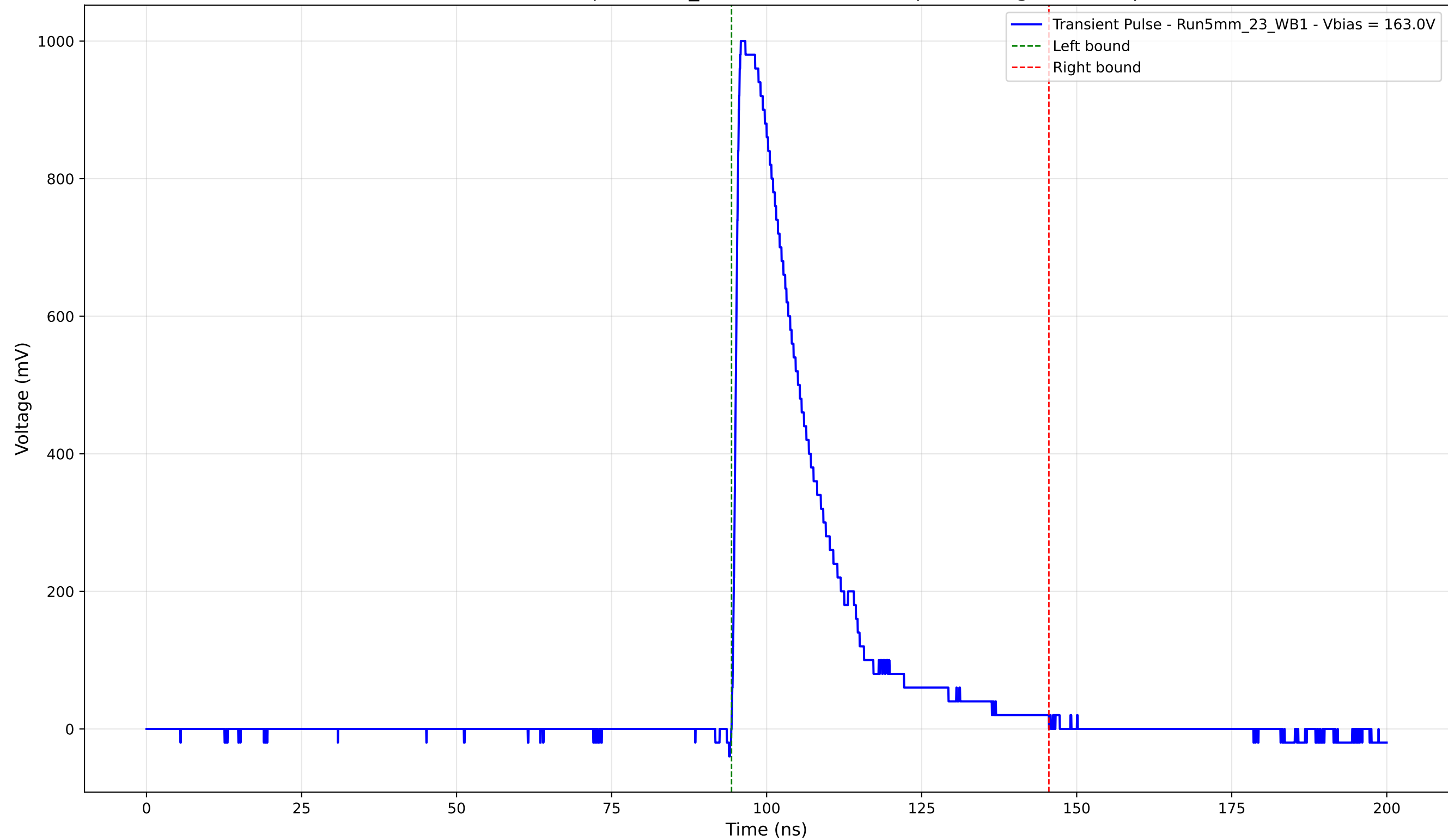
Transient Pulse - Sample: 5mm_23 - Position: 1570.0 \mu\text{m} - Charge: 254.40 pC
