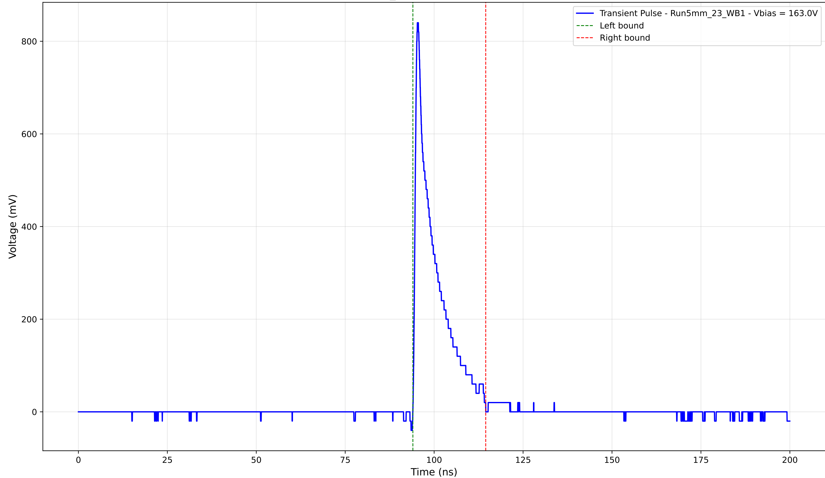
Transient Pulse - Sample: 5mm_23 - Position: 5150.0 \mu\text{m} - Charge: 101.08 pC
