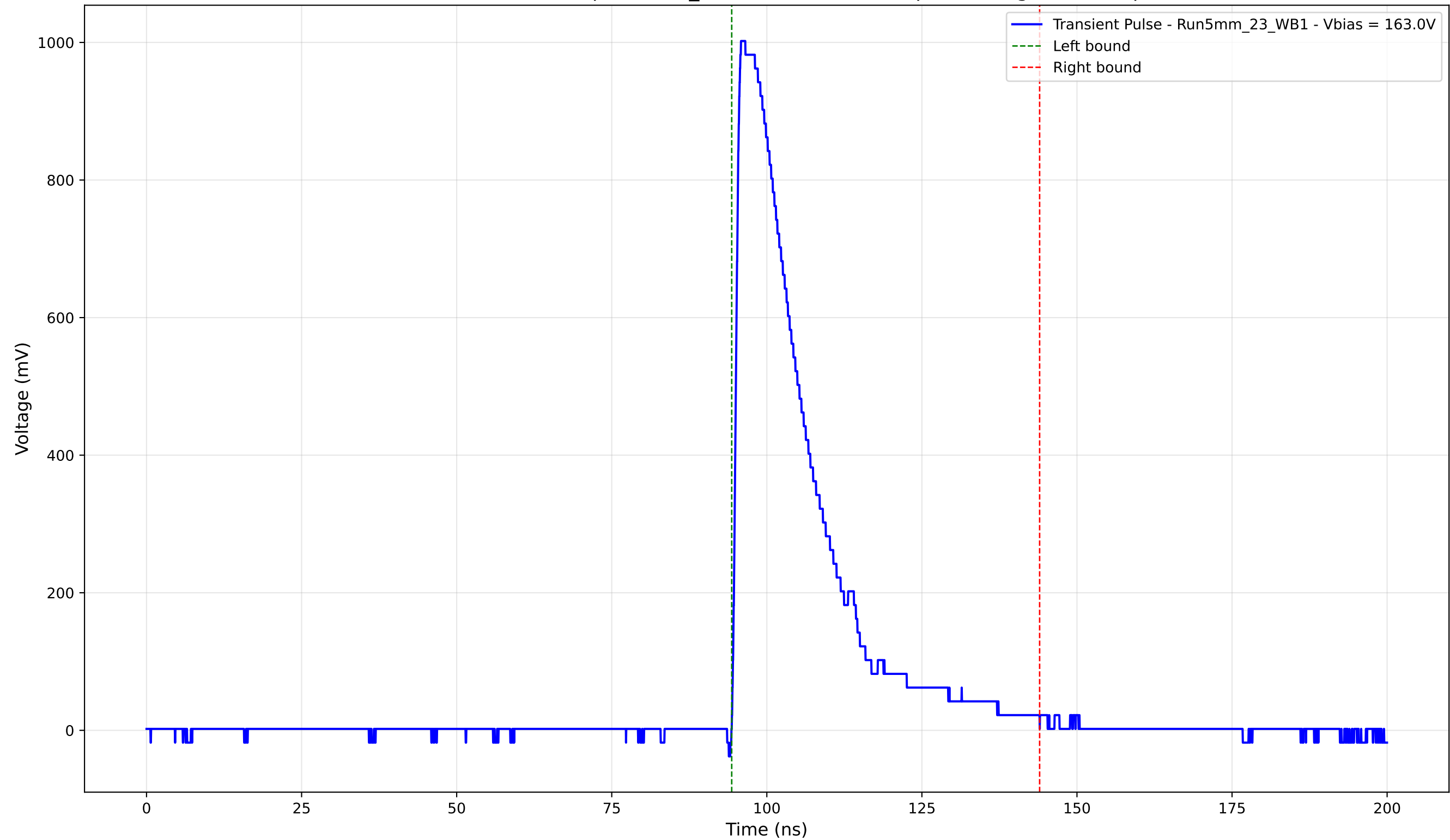
Transient Pulse - Sample: 5mm_23 - Position: 1600.0 \mu\text{m} - Charge: 254.41 pC
