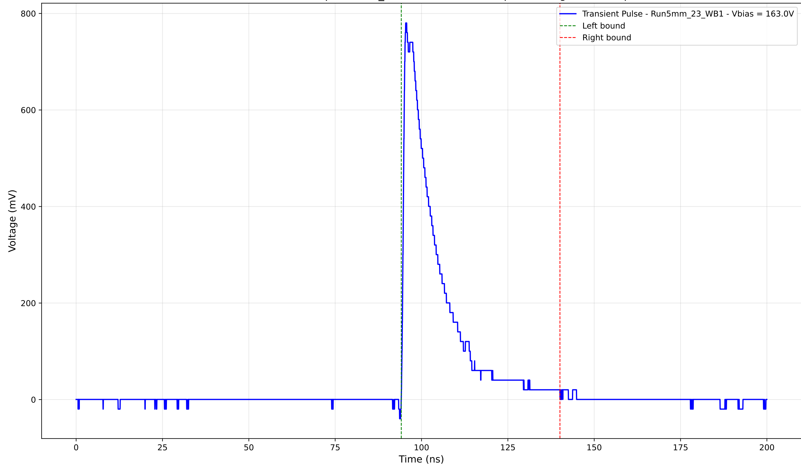
Transient Pulse - Sample: 5mm_23 - Position: 2180.0 \mu\text{m} - Charge: 162.66 pC
