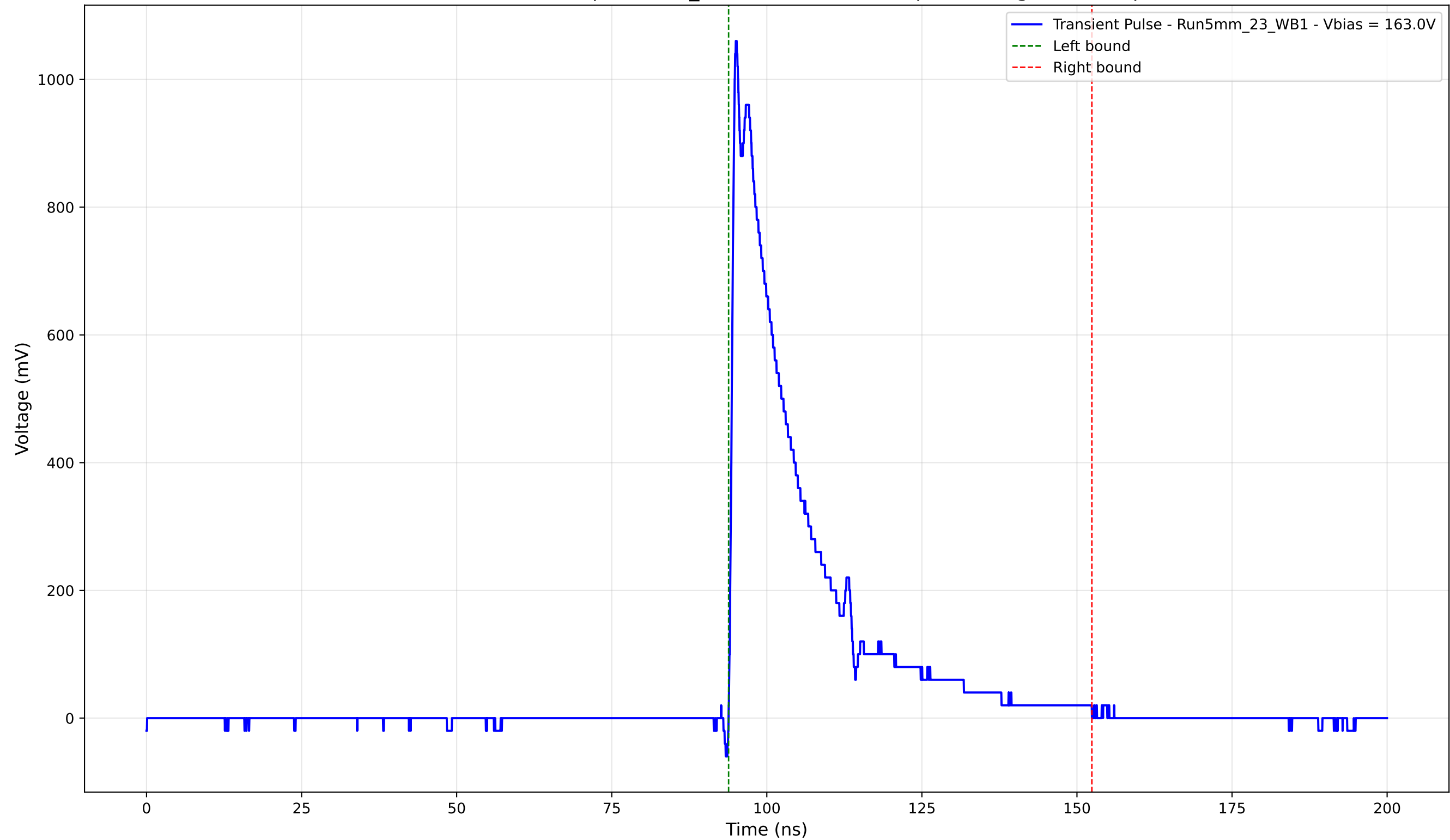
Transient Pulse - Sample: 5mm_23 - Position: 2655.0 \mu\text{m} - Charge: 231.74 pC
