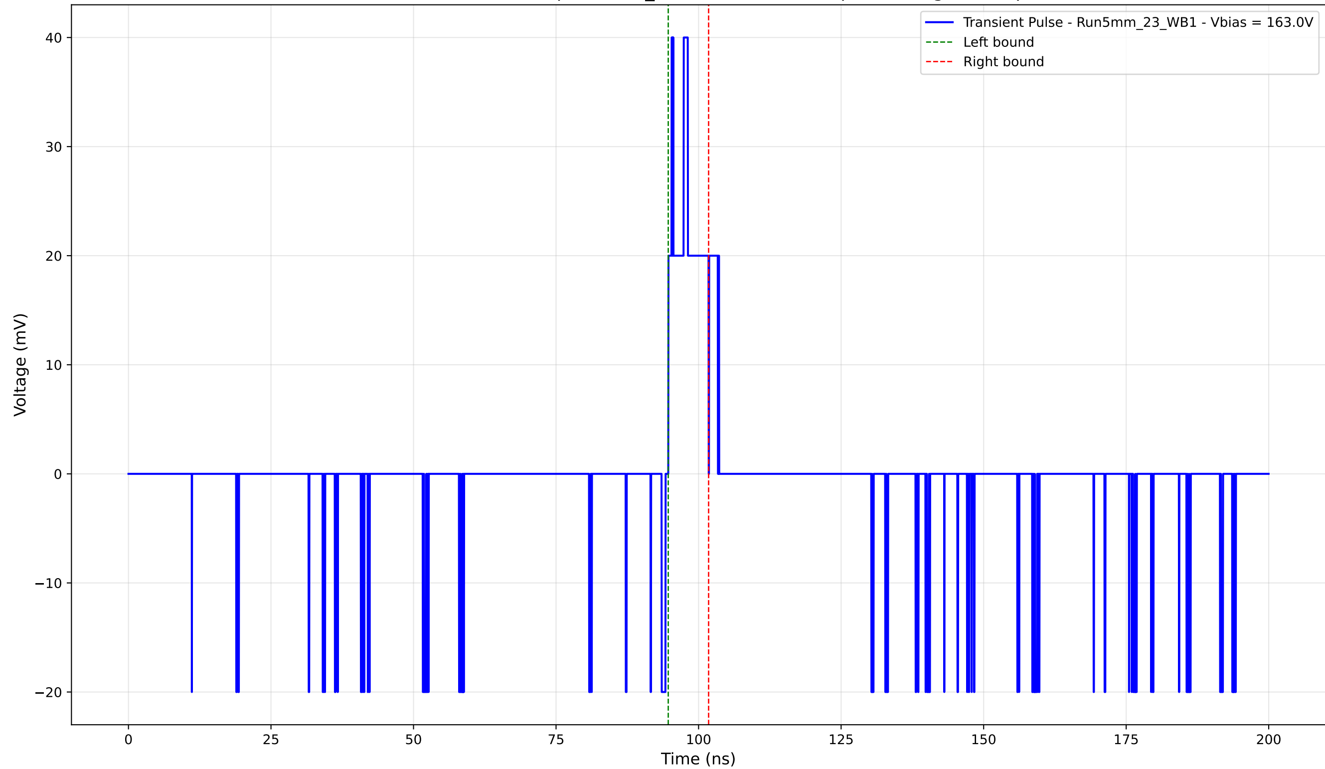
Transient Pulse - Sample: 5mm_23 - Position: 240.0 \mu\text{m} - Charge: 3.20 pC
