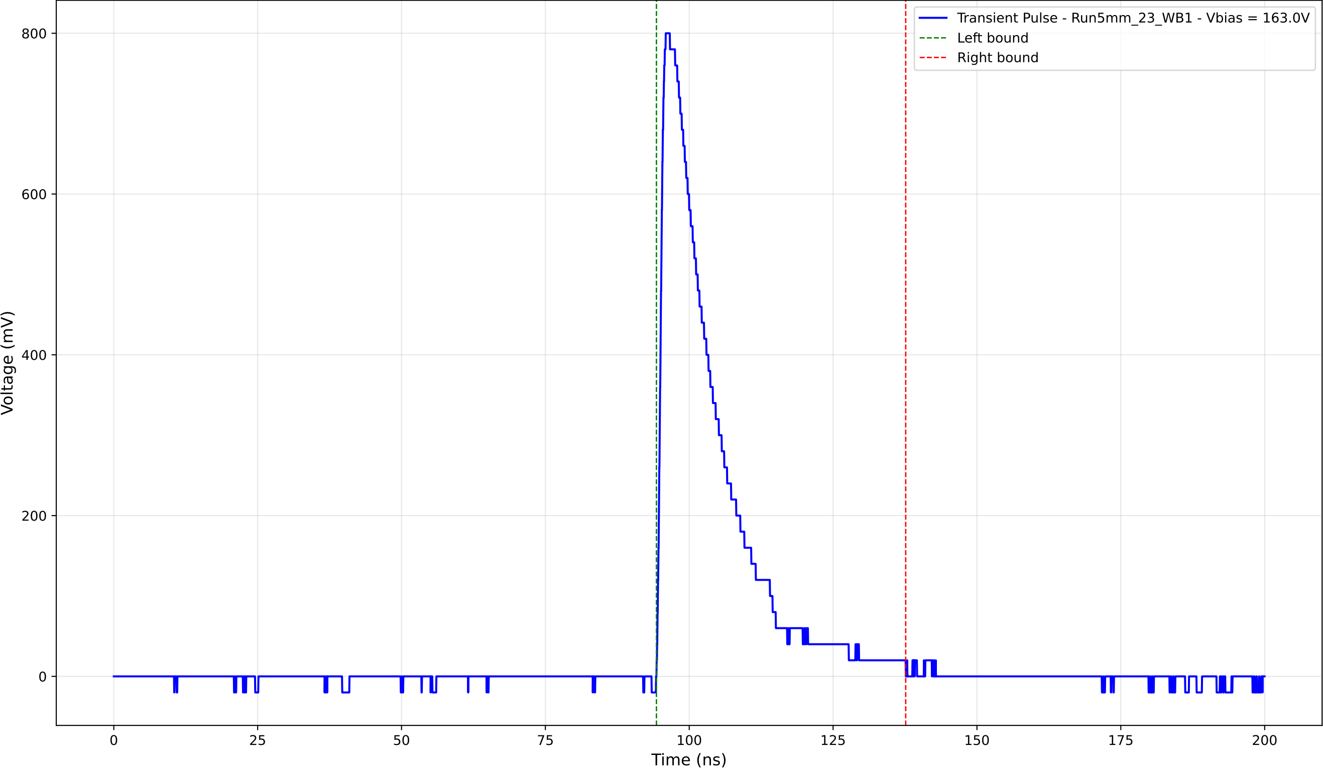
Transient Pulse - Sample: 5mm_23 - Position: 3680.0 \mu\text{m} - Charge: 168.90 pC
