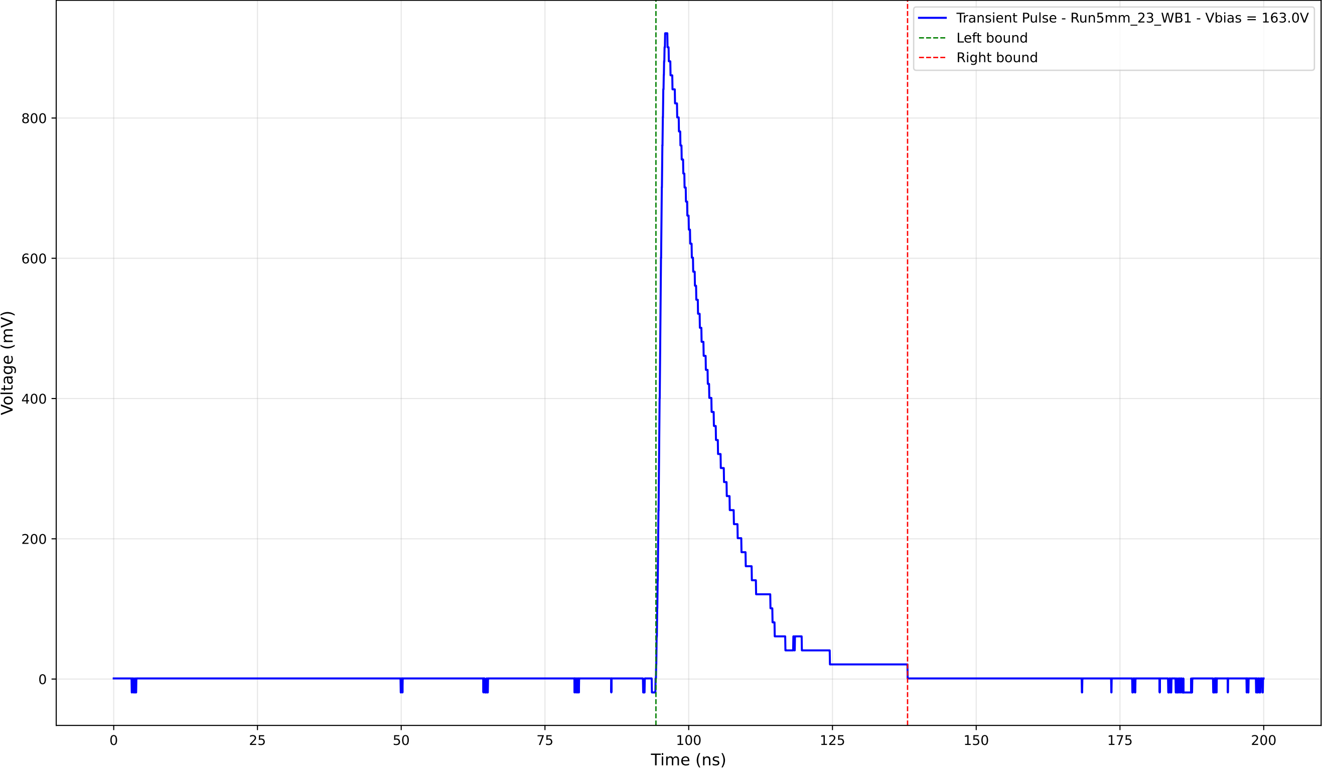
Transient Pulse - Sample: 5mm_23 - Position: 4455.0 \mu\text{m} - Charge: 181.38 pC
