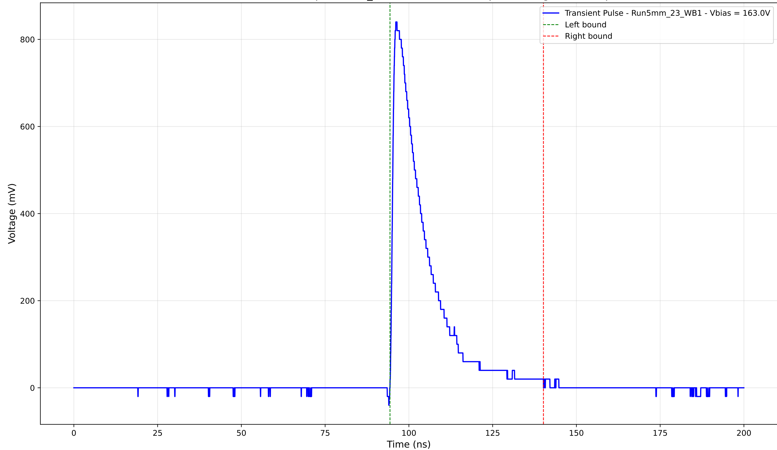
Transient Pulse - Sample: 5mm_23 - Position: 1660.0 \mu\text{m} - Charge: 179.10 pC
