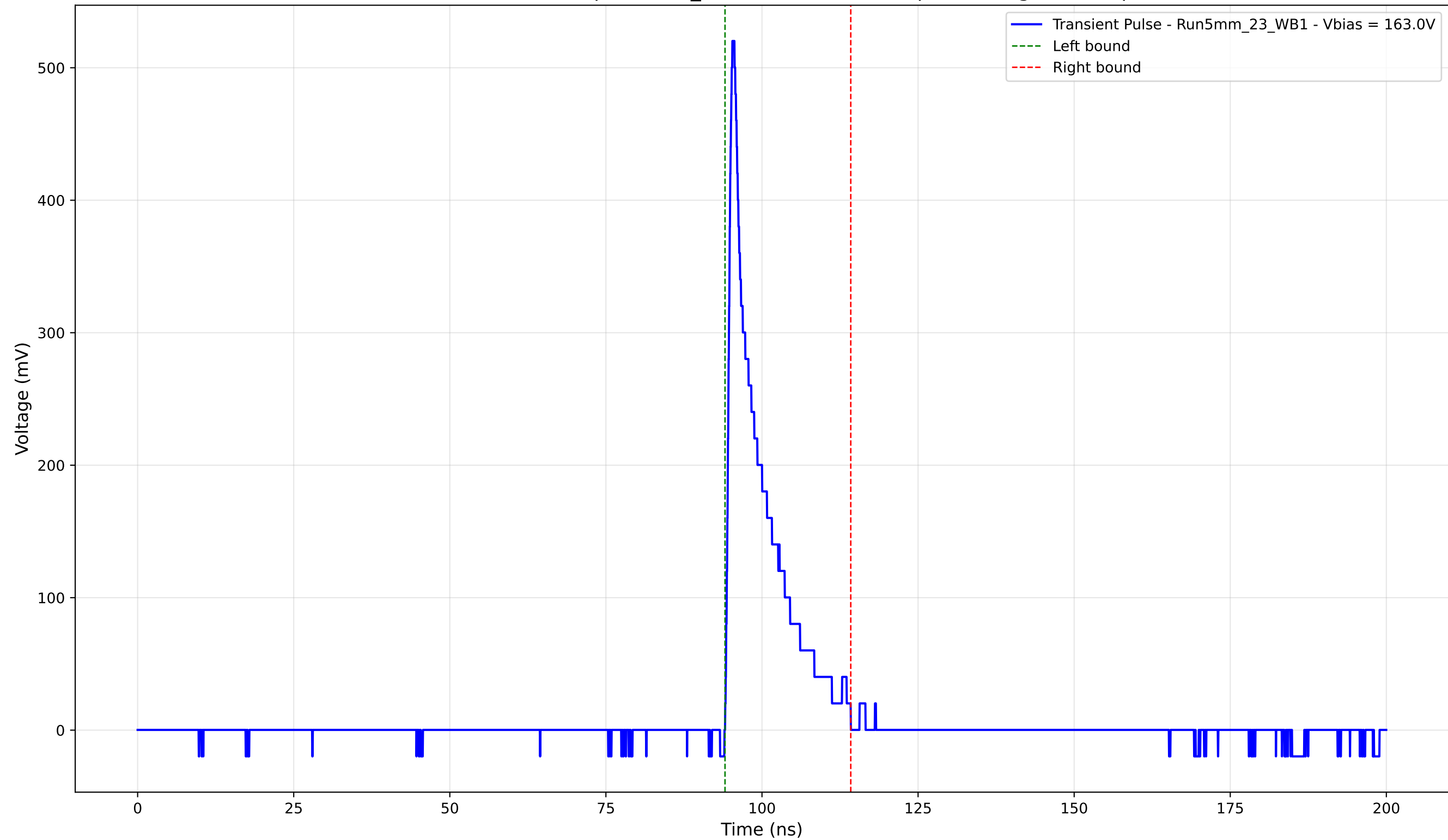
Transient Pulse - Sample: 5mm_23 - Position: 5170.0 \mu\text{m} - Charge: 56.98 pC
