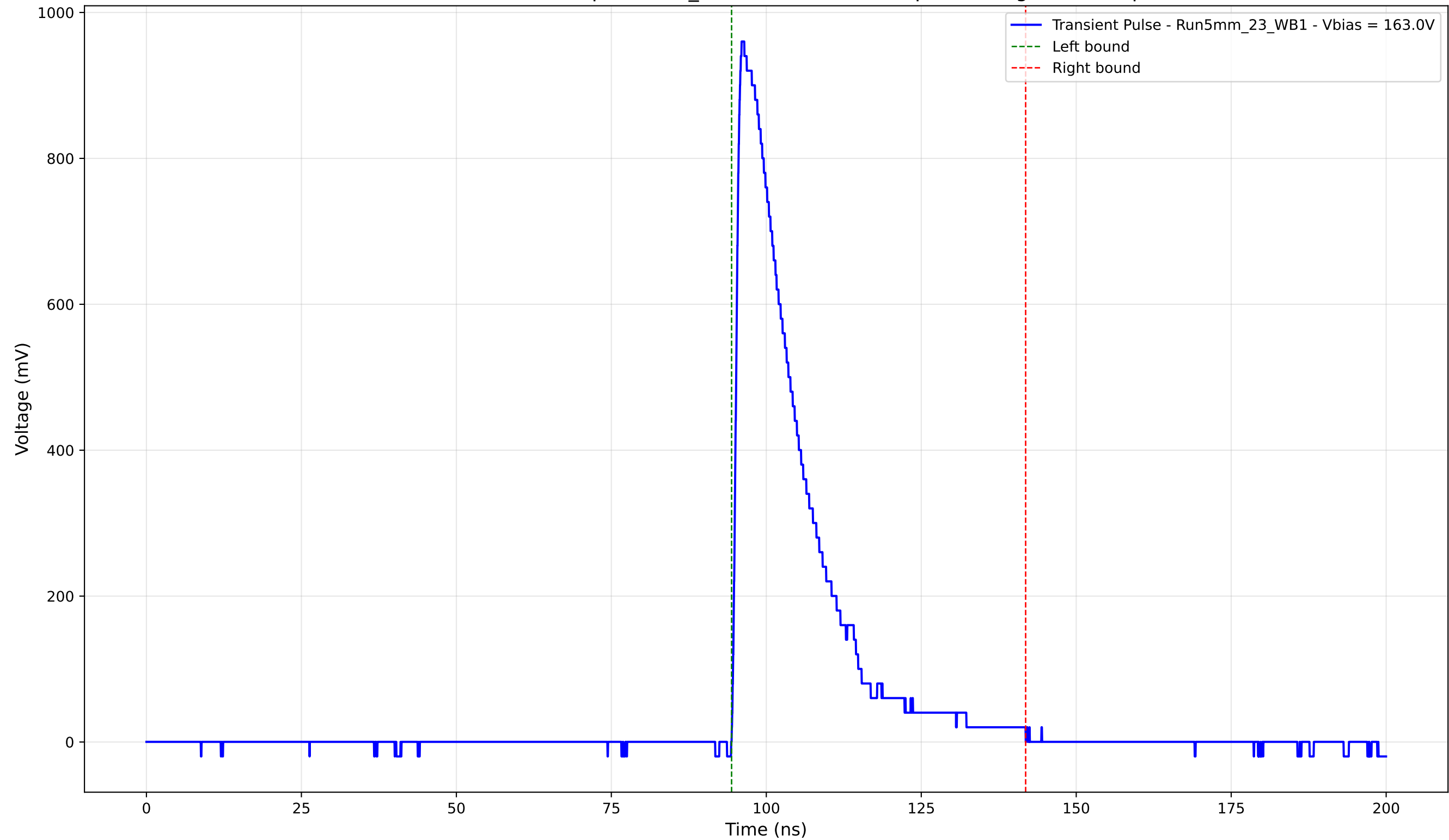
Transient Pulse - Sample: 5mm_23 - Position: 1335.0 \mu\text{m} - Charge: 215.47 pC
