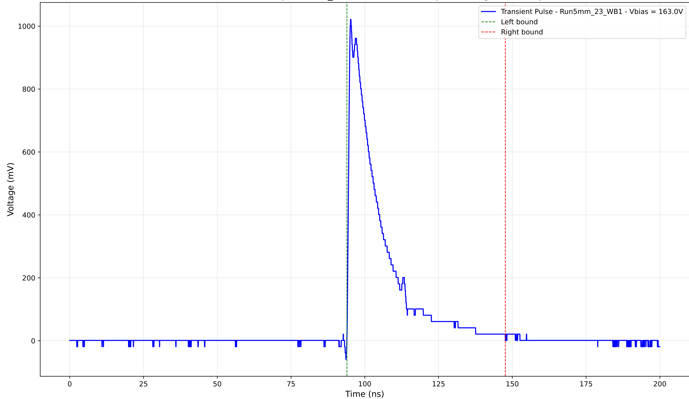
Transient Pulse - Sample: 5mm_23 - Position: 2455.0 \mu\text{m} - Charge: 231.85 pC
