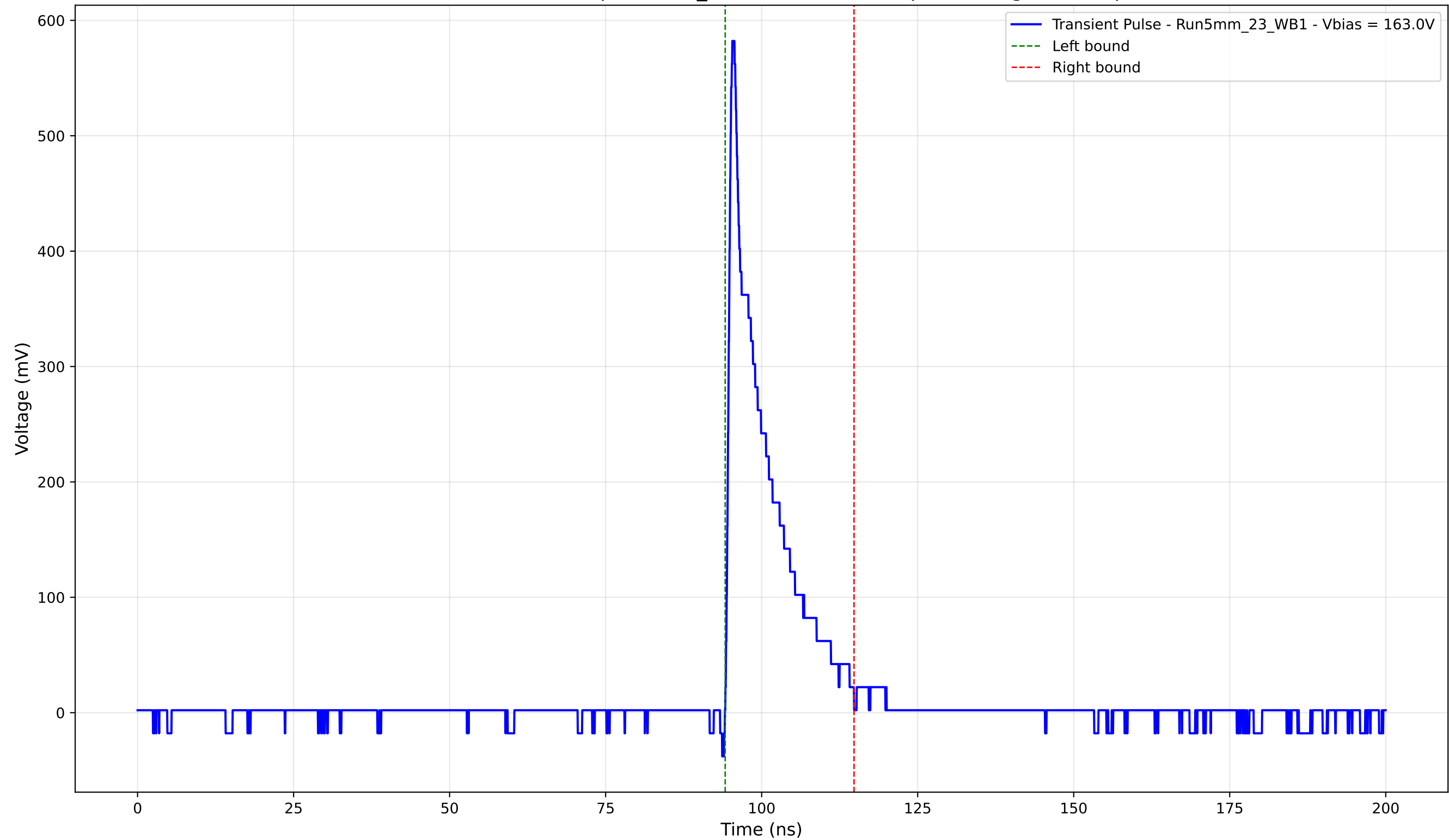
Transient Pulse - Sample: 5mm_23 - Position: 305.0 \mu\text{m} - Charge: 72.48 pC
