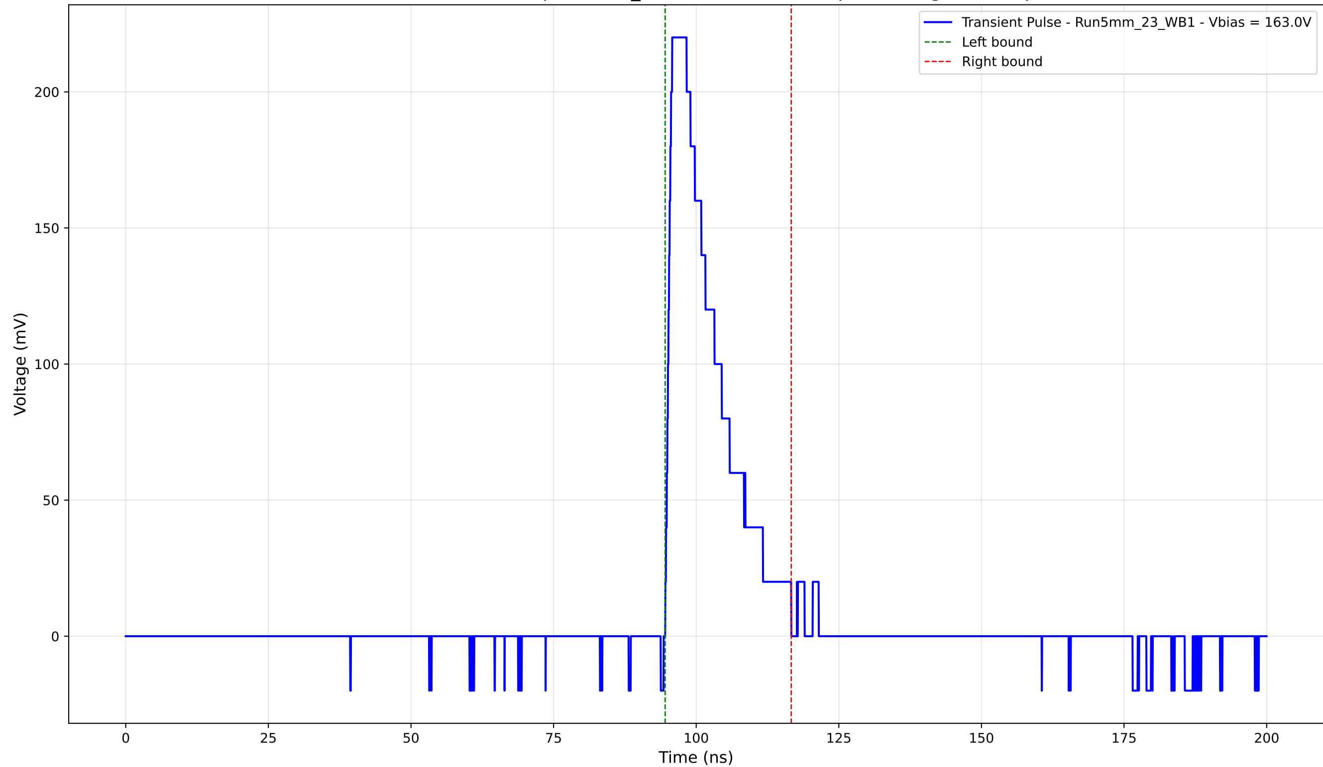
Transient Pulse - Sample: 5mm_23 - Position: 4245.0 \mu\text{m} - Charge: 41.36 pC
