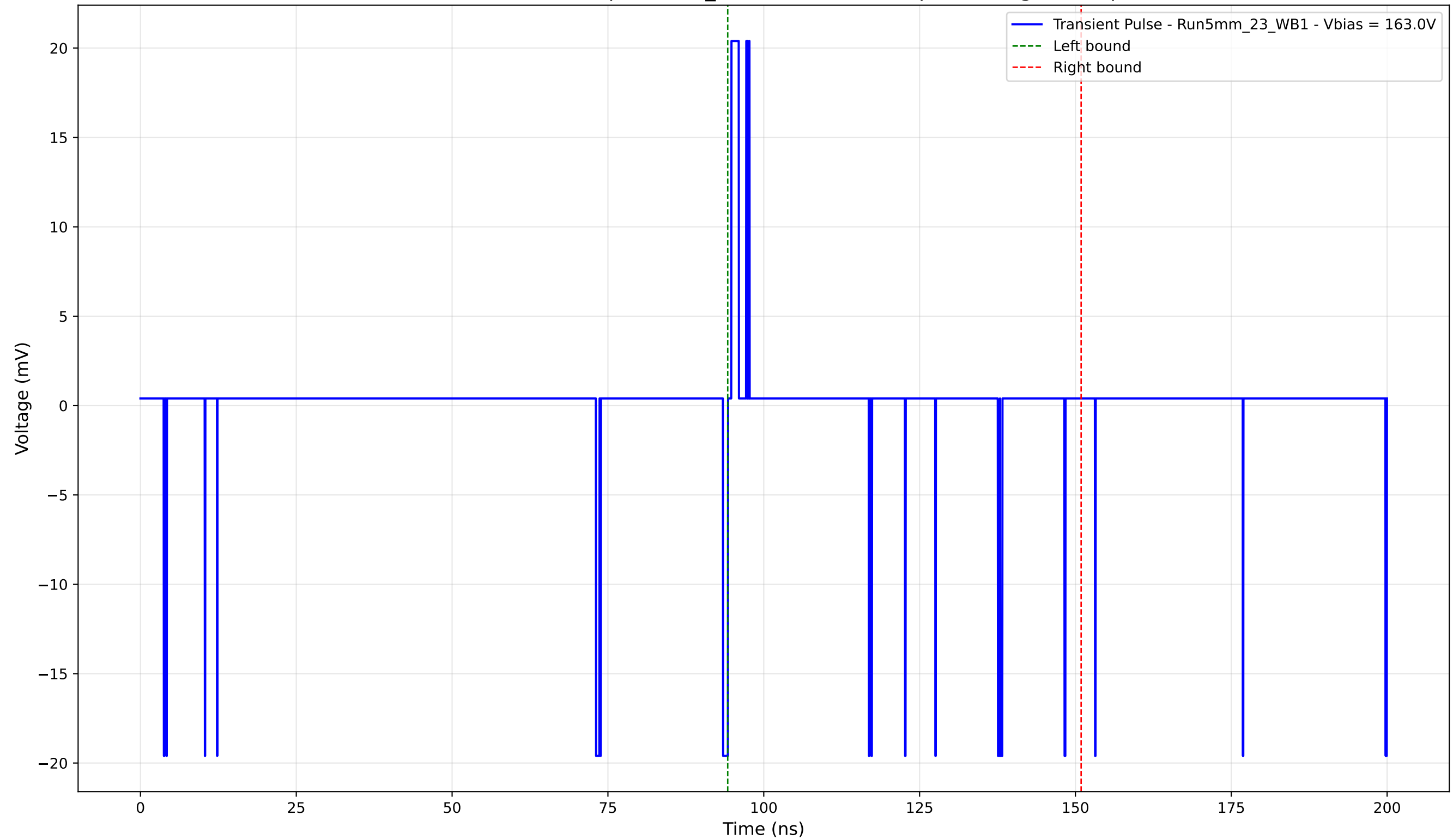
Transient Pulse - Sample: 5mm_23 - Position: 100.0 \mu\text{m} - Charge: 0.54 pC
