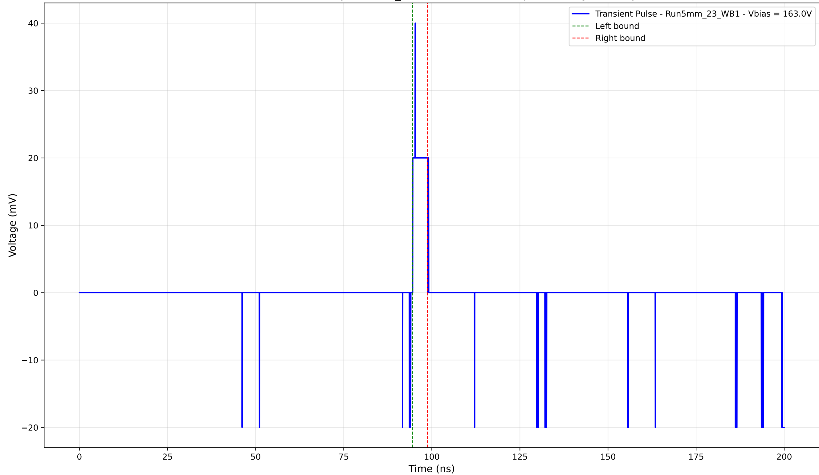
Transient Pulse - Sample: 5mm_23 - Position: 5255.0 \mu\text{m} - Charge: 1.73 pC
