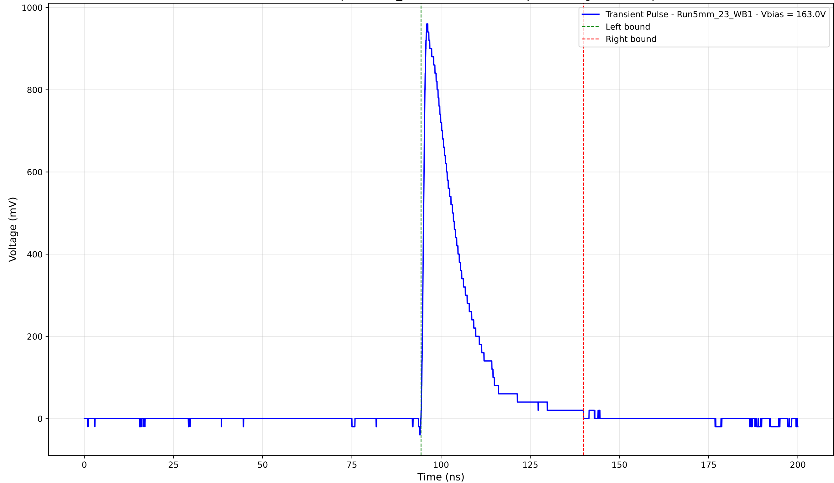
Transient Pulse - Sample: 5mm_23 - Position: 1095.0 \mu\text{m} - Charge: 203.43 pC
