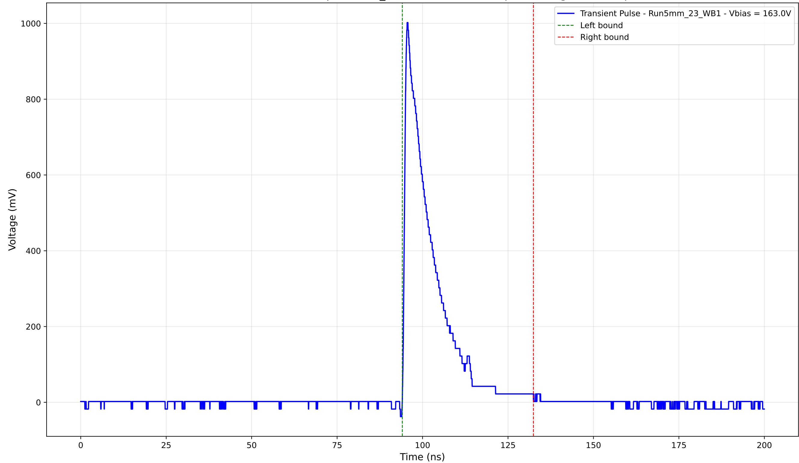
Transient Pulse - Sample: 5mm_23 - Position: 4925.0 \mu\text{m} - Charge: 171.10 pC
