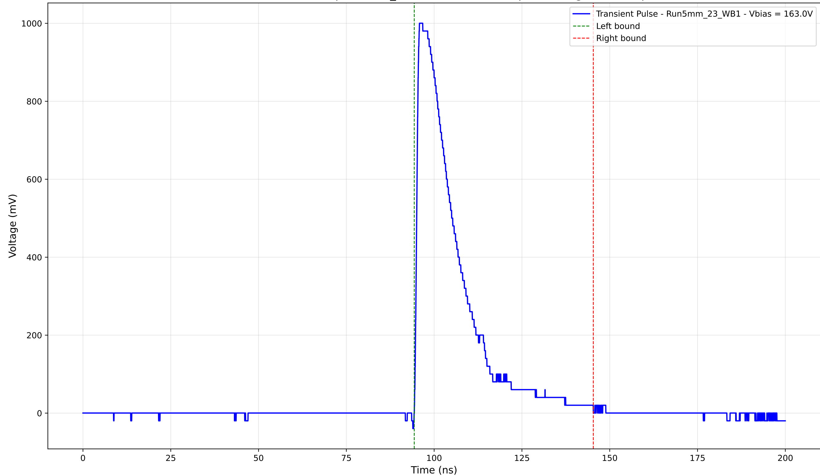
Transient Pulse - Sample: 5mm_23 - Position: 1575.0 \mu\text{m} - Charge: 254.30 pC
