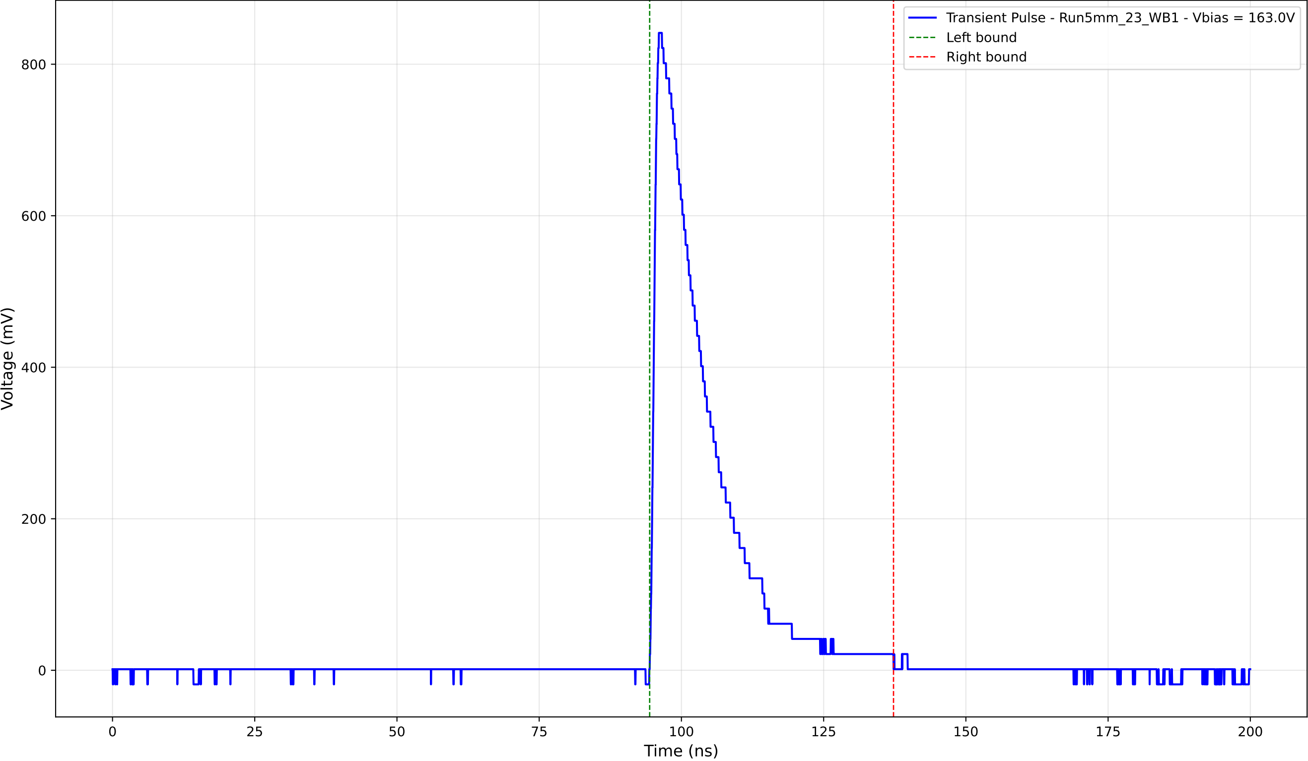
Transient Pulse - Sample: 5mm_23 - Position: 1295.0 \mu\text{m} - Charge: 173.62 pC
