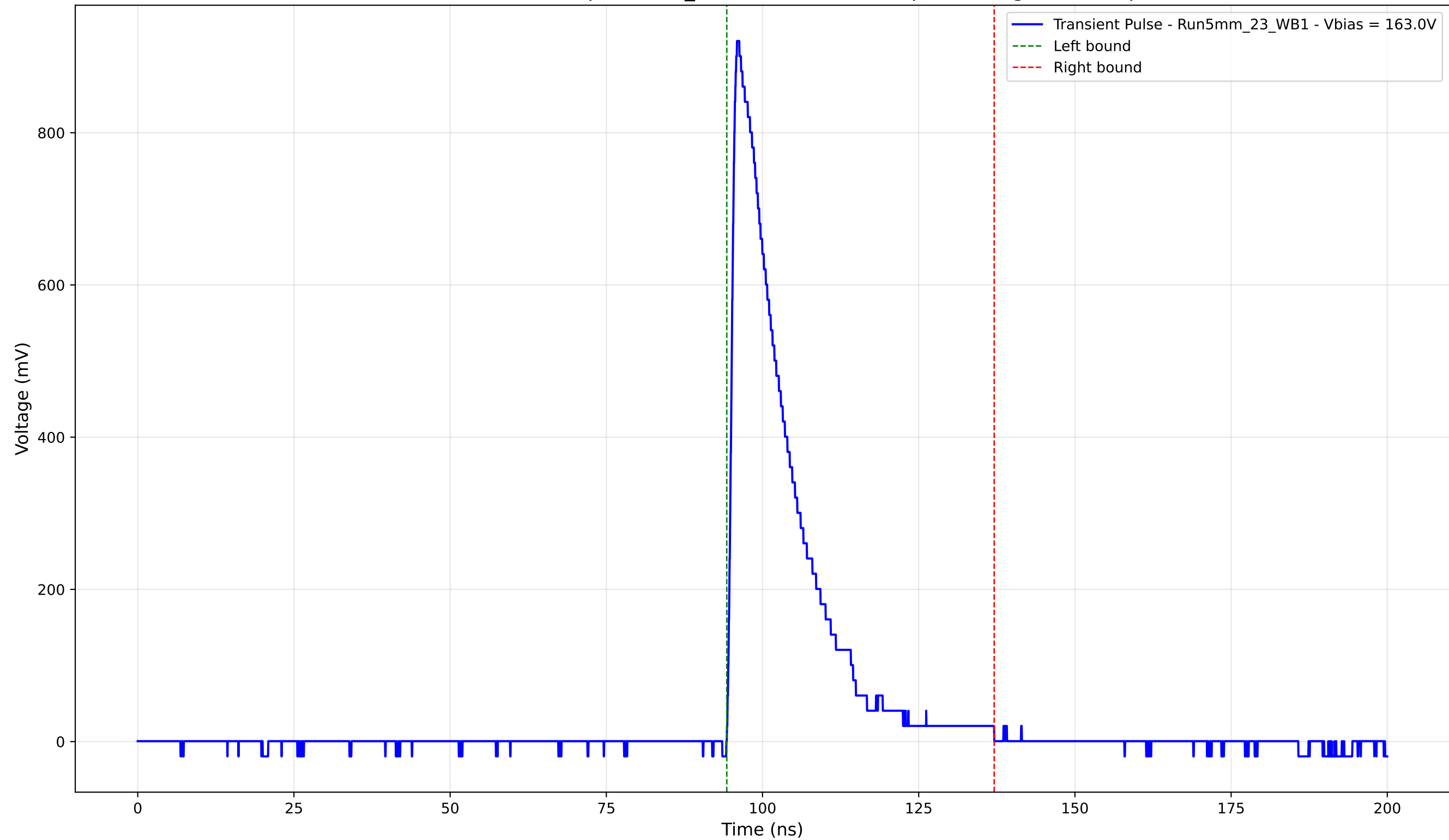
Transient Pulse - Sample: 5mm_23 - Position: 4460.0 \mu\text{m} - Charge: 179.99 pC
