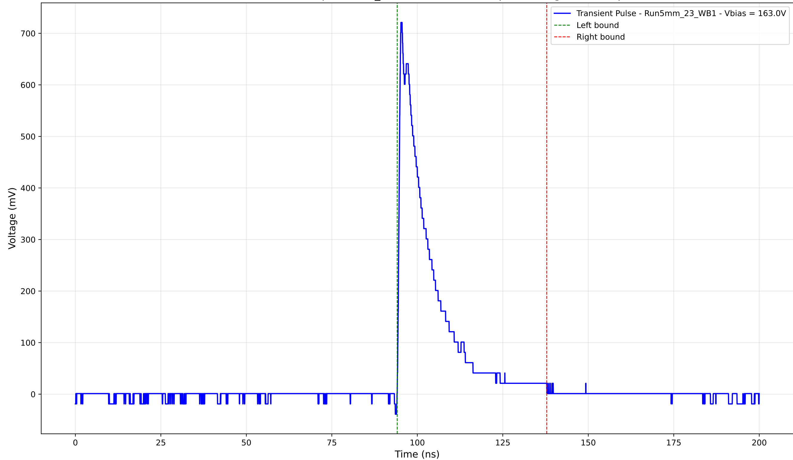
Transient Pulse - Sample: 5mm_23 - Position: 3195.0 \mu\text{m} - Charge: 134.13 pC
