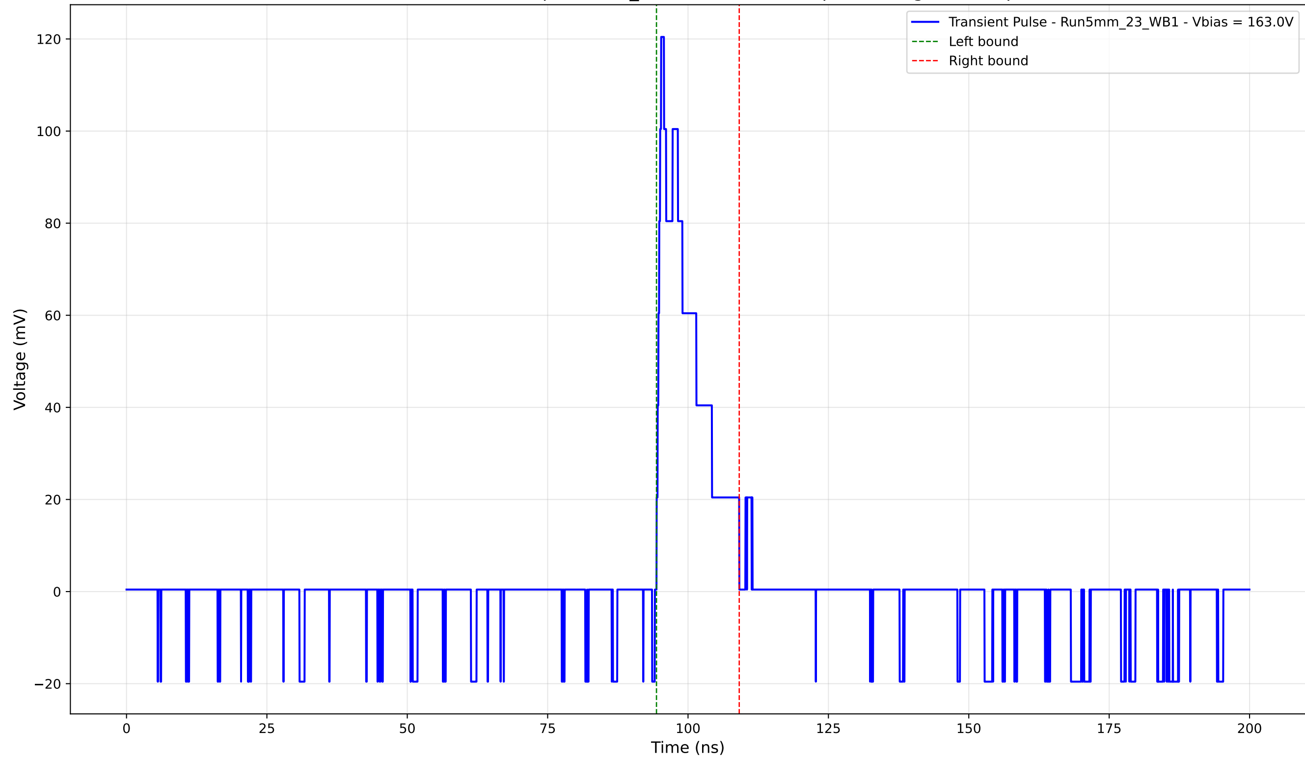
Transient Pulse - Sample: 5mm_23 - Position: 270.0 \mu\text{m} - Charge: 15.27 pC
