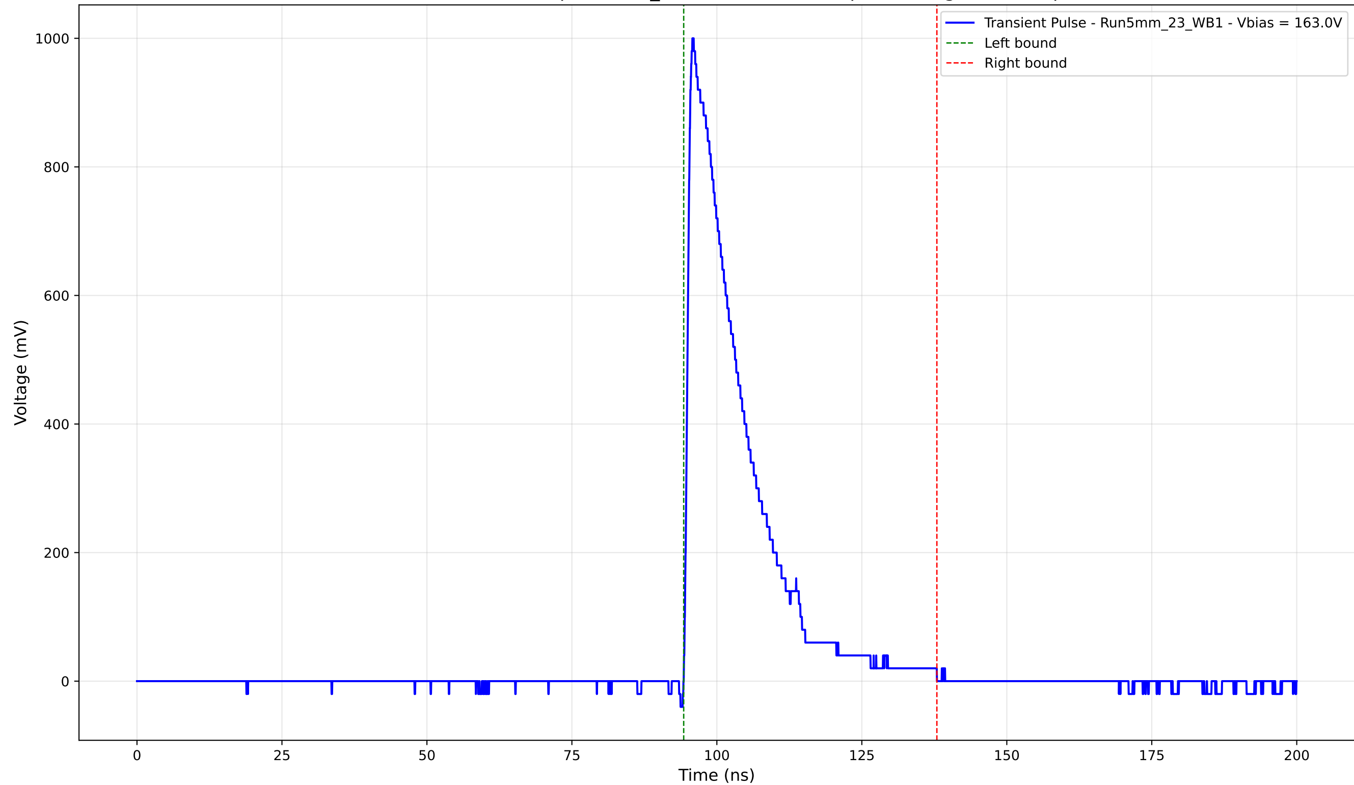
Transient Pulse - Sample: 5mm_23 - Position: 825.0 \mu\text{m} - Charge: 204.83 pC
