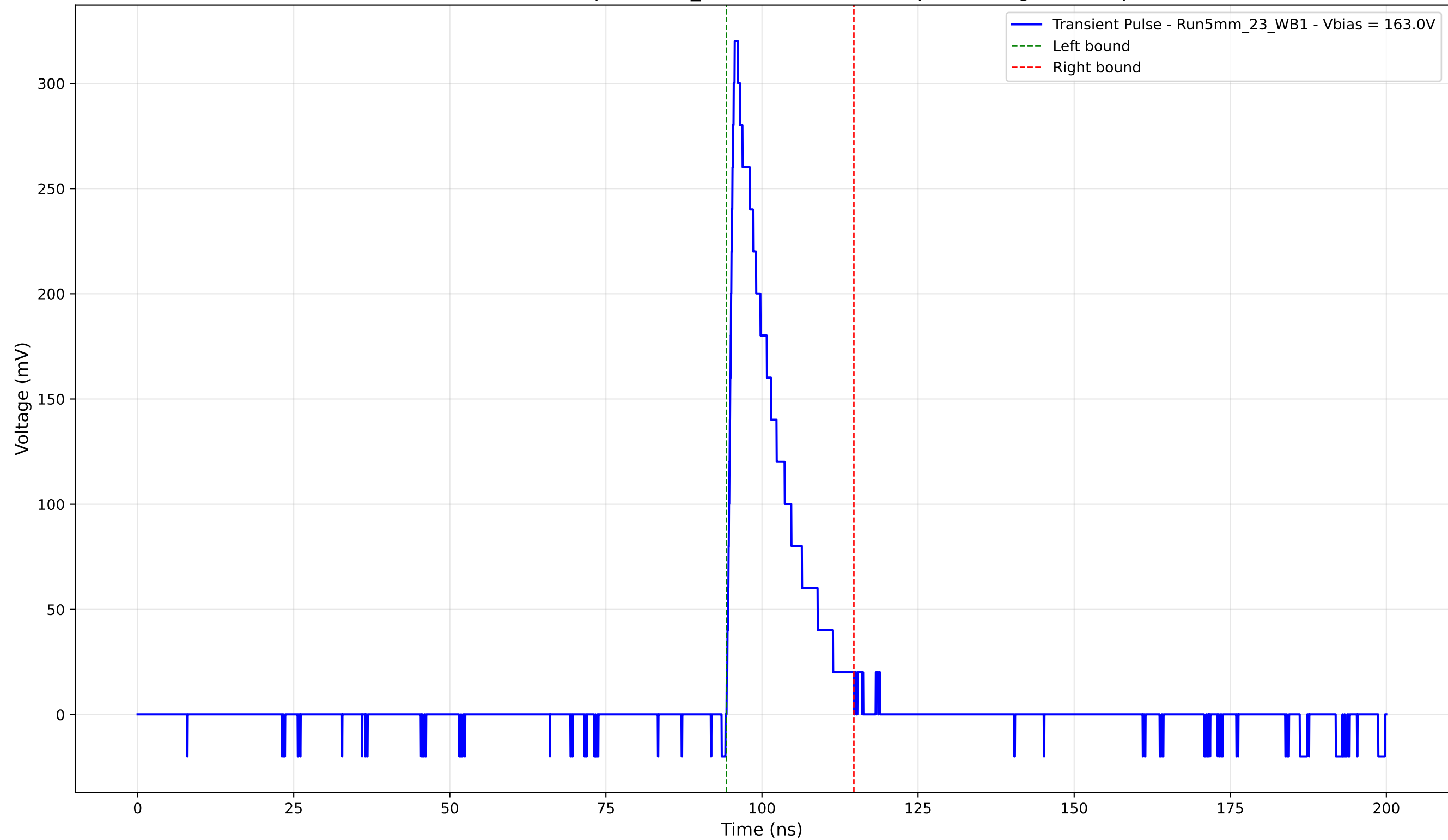
Transient Pulse - Sample: 5mm_23 - Position: 4745.0 \mu\text{m} - Charge: 48.10 pC
