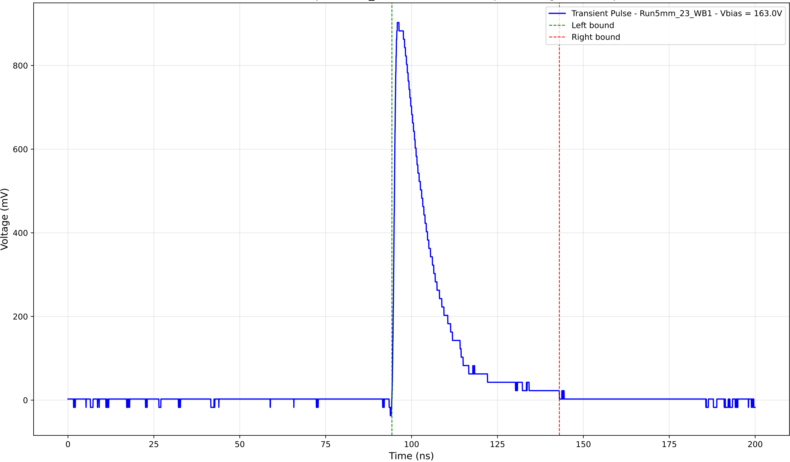
Transient Pulse - Sample: 5mm_23 - Position: 3645.0 \mu\text{m} - Charge: 202.94 pC
