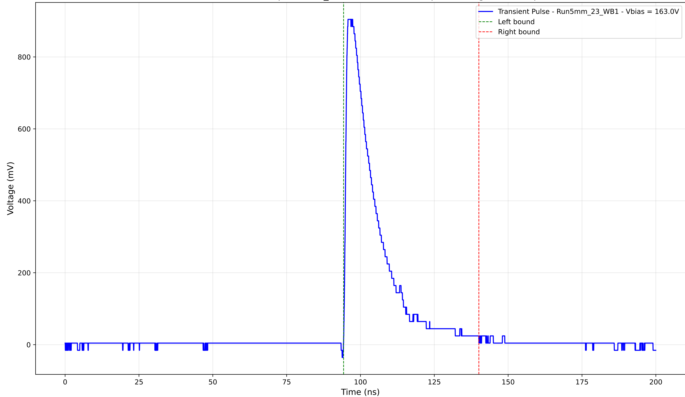
Transient Pulse - Sample: 5mm_23 - Position: 3630.0 \mu\text{m} - Charge: 207.29 pC
