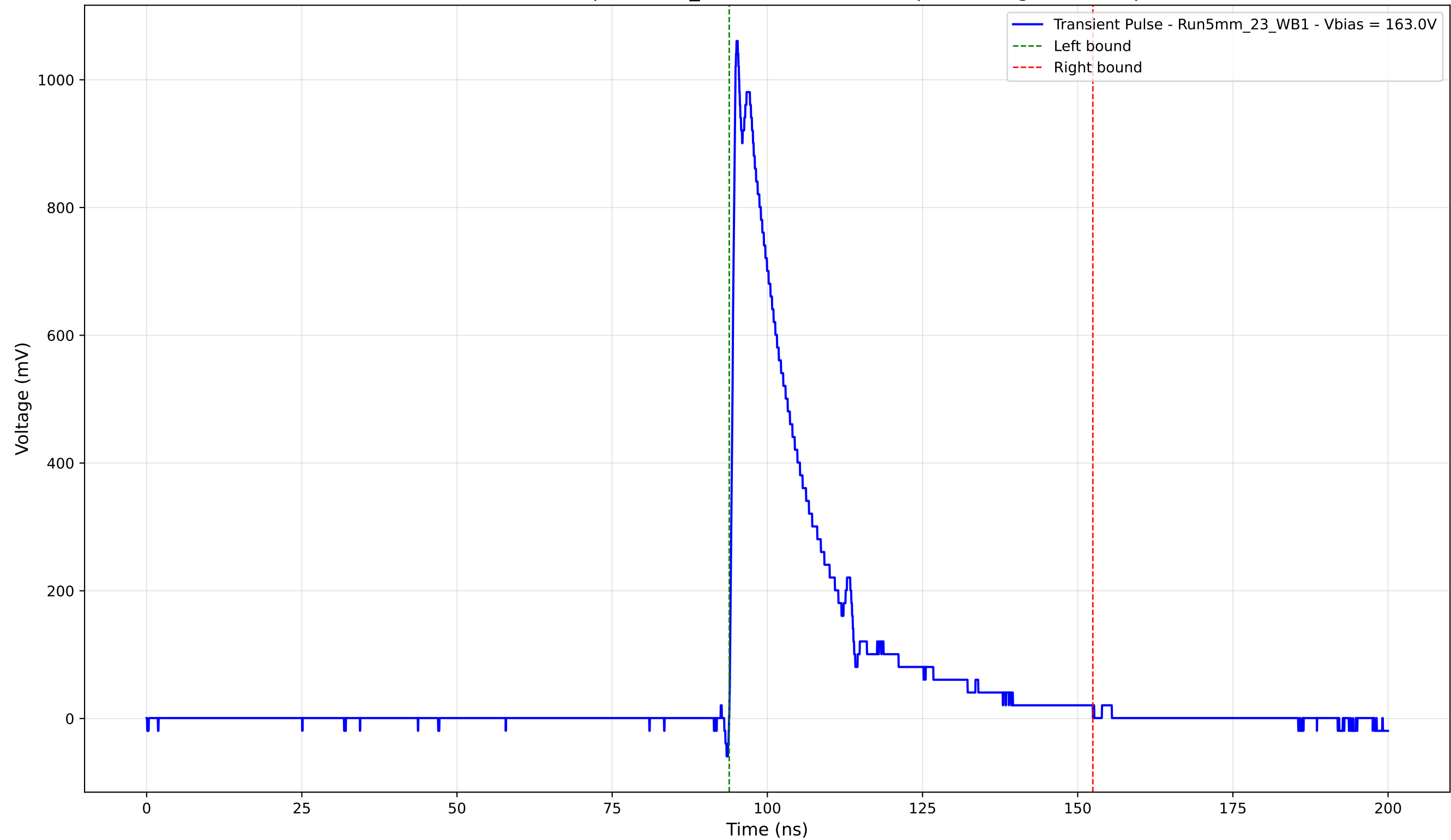
Transient Pulse - Sample: 5mm_23 - Position: 2600.0 \mu\text{m} - Charge: 243.86 pC
