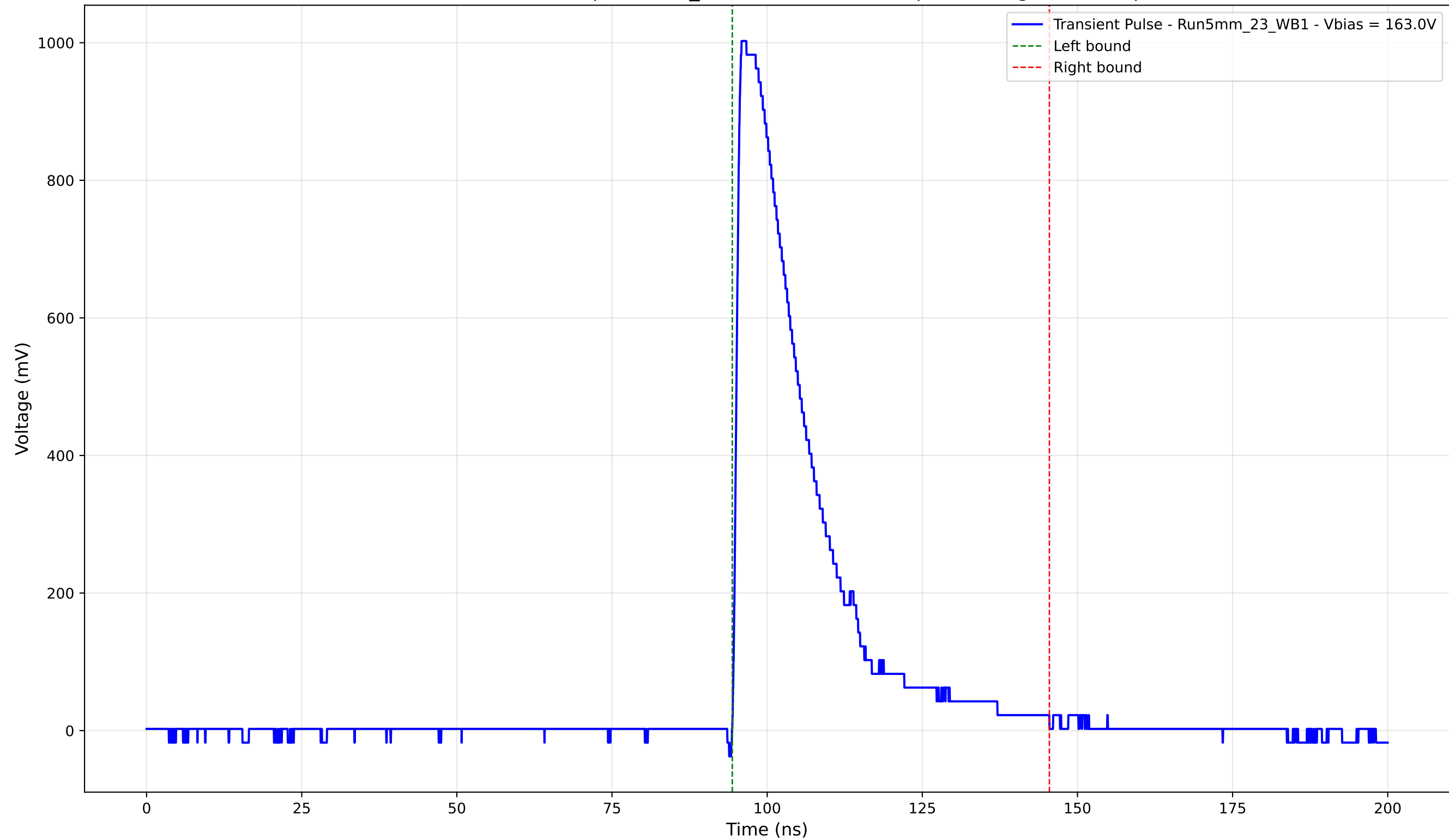
Transient Pulse - Sample: 5mm_23 - Position: 1500.0 \mu\text{m} - Charge: 253.92 pC
