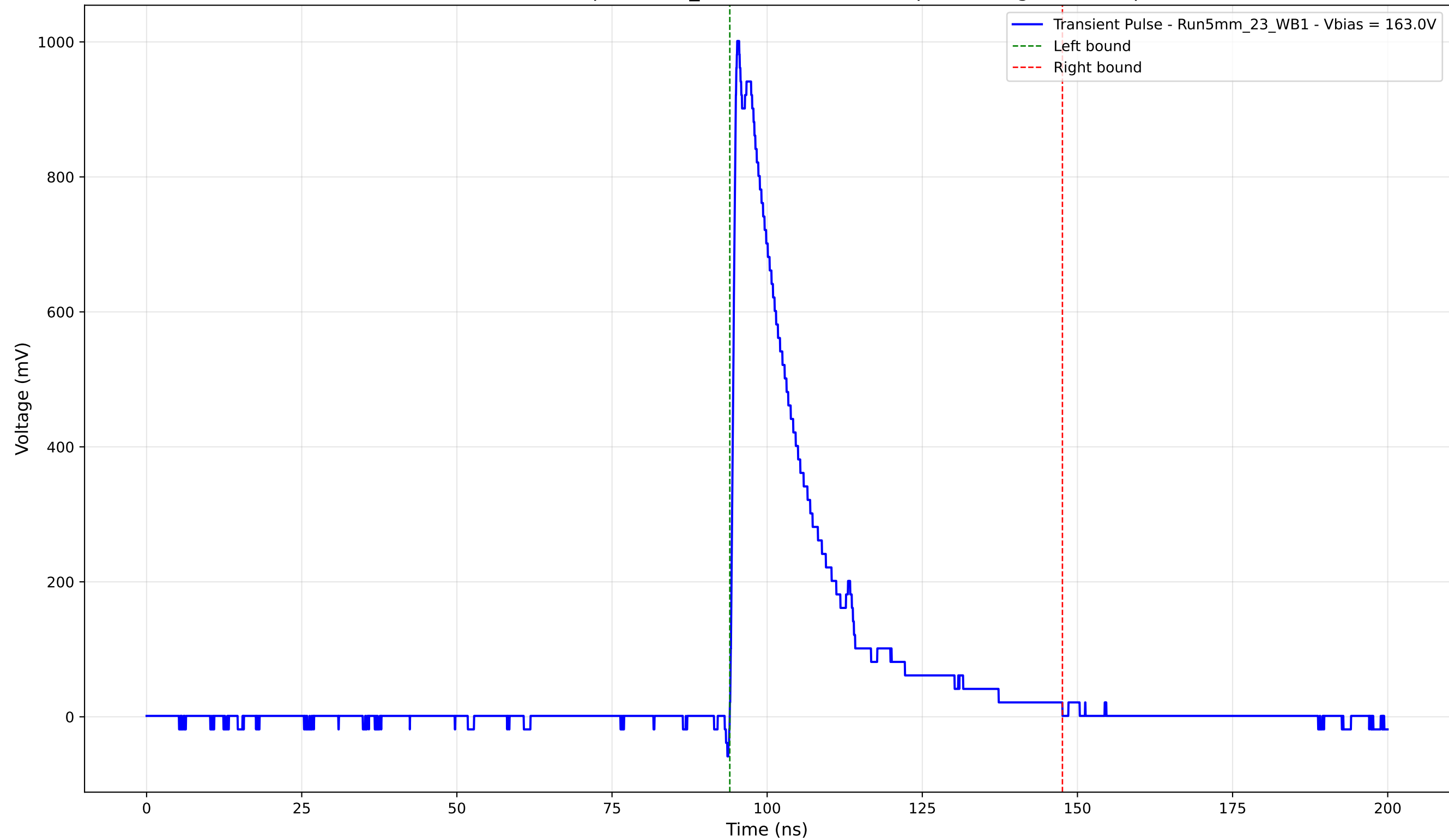
Transient Pulse - Sample: 5mm_23 - Position: 3080.0 \mu\text{m} - Charge: 229.48 pC
