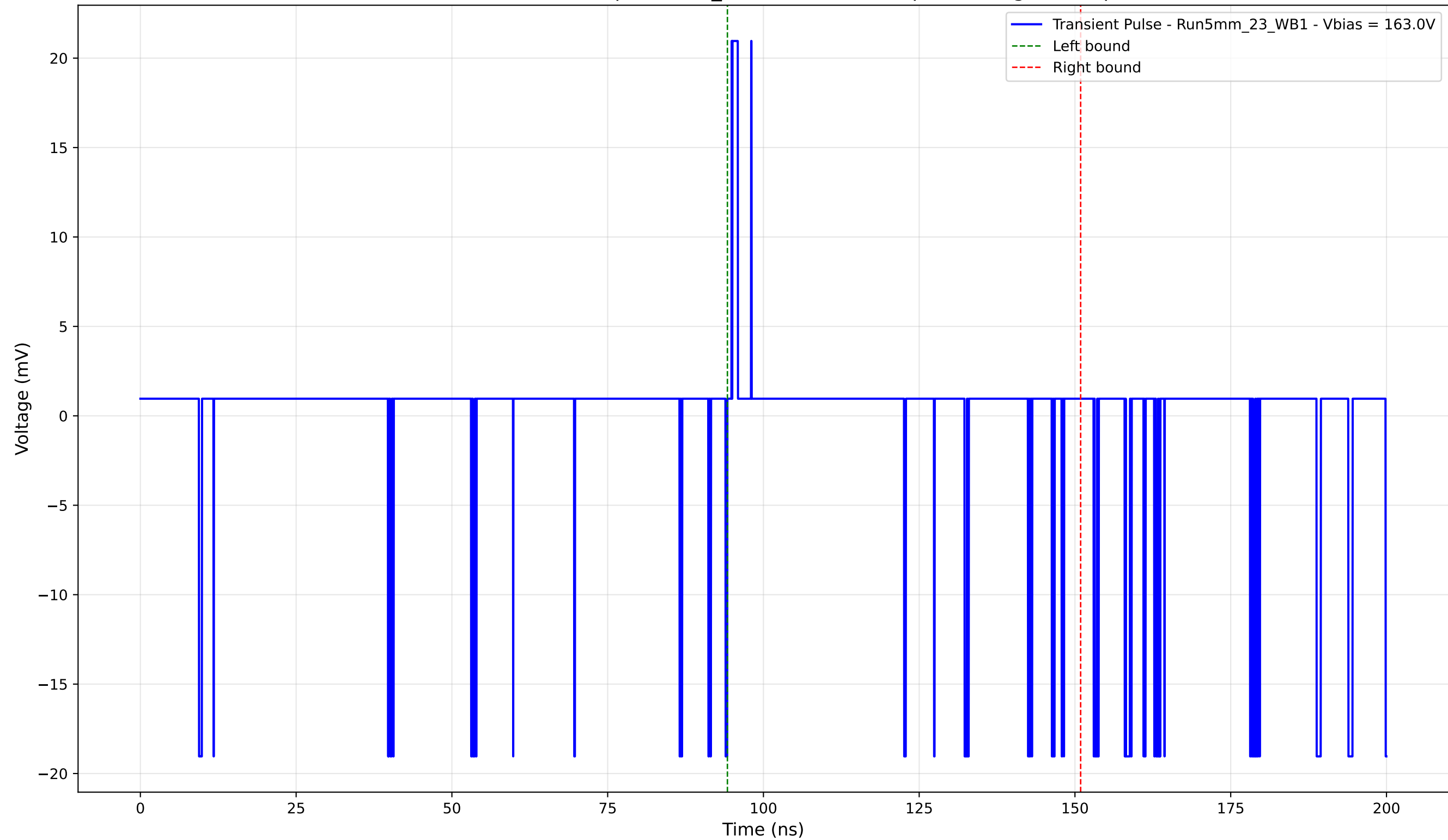
Transient Pulse - Sample: 5mm_23 - Position: 85.0 \mu\text{m} - Charge: 0.77 pC
