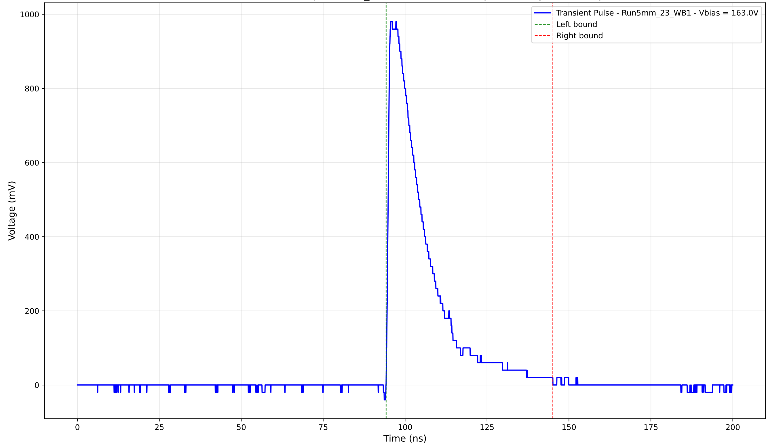
Transient Pulse - Sample: 5mm_23 - Position: 2020.0 \mu\text{m} - Charge: 243.71 pC
