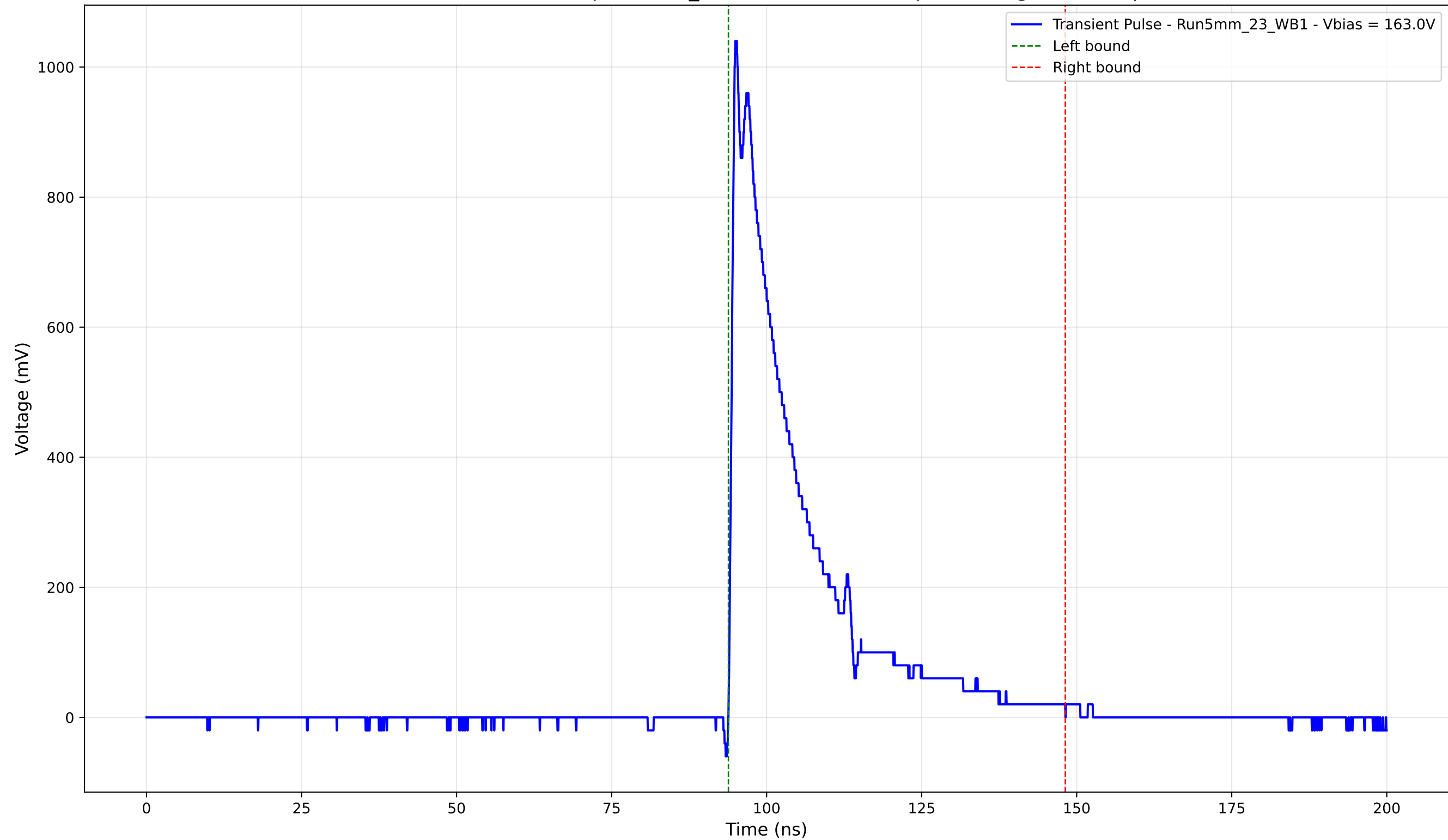
Transient Pulse - Sample: 5mm_23 - Position: 2835.0 \mu\text{m} - Charge: 225.38 pC
