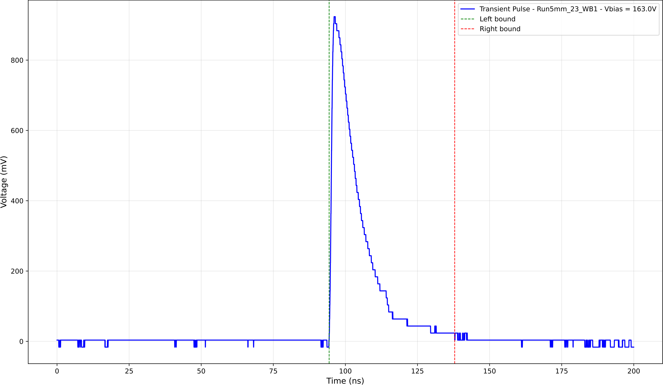
Transient Pulse - Sample: 5mm_23 - Position: 4010.0 \mu\text{m} - Charge: 200.67 pC
