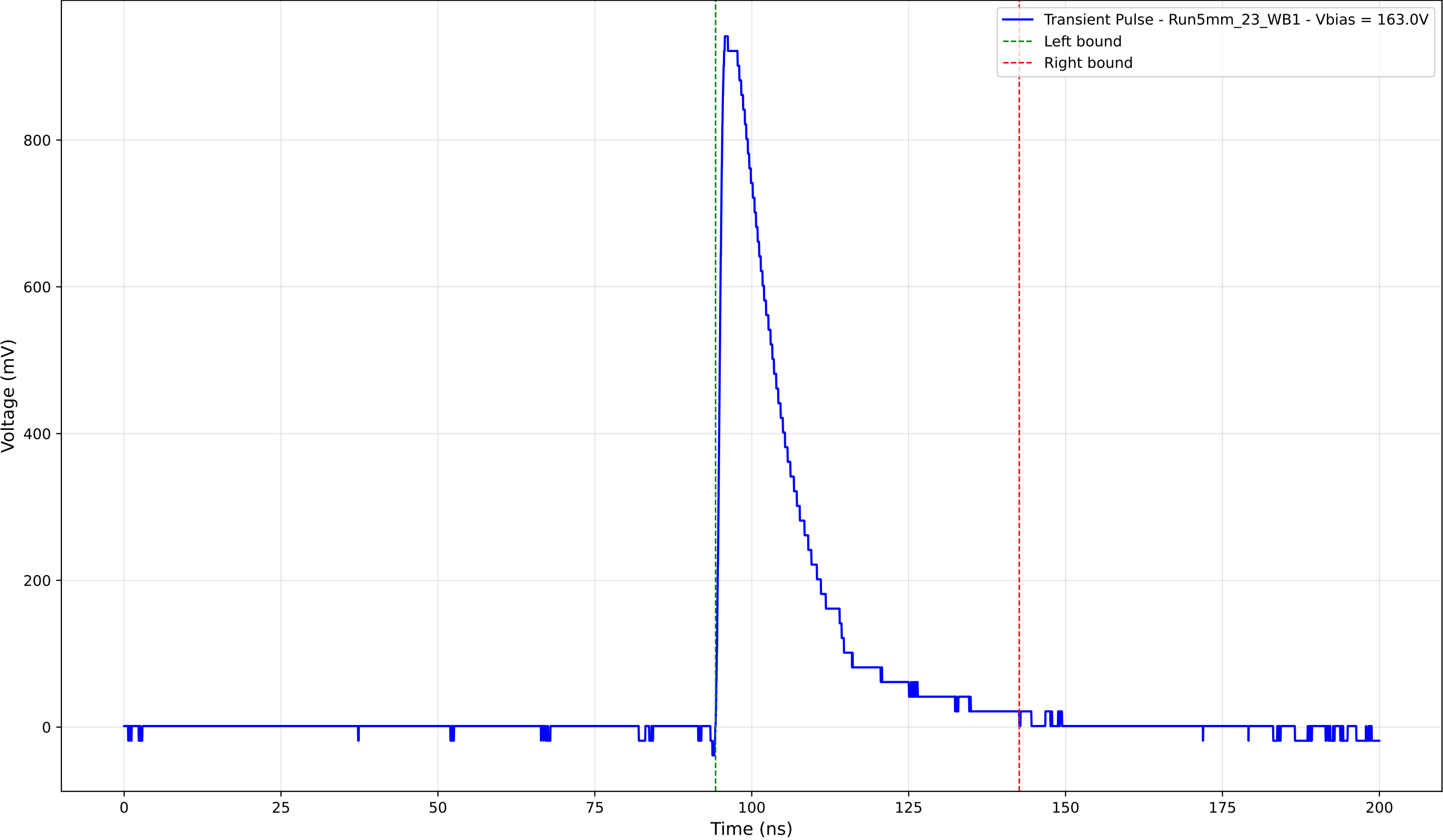
Transient Pulse - Sample: 5mm_23 - Position: 3550.0 \mu\text{m} - Charge: 220.18 pC
