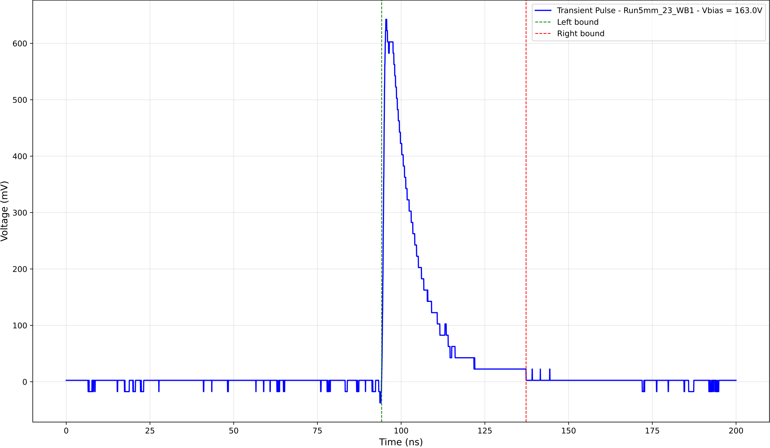
Transient Pulse - Sample: 5mm_23 - Position: 3300.0 \mu\text{m} - Charge: 128.38 pC
