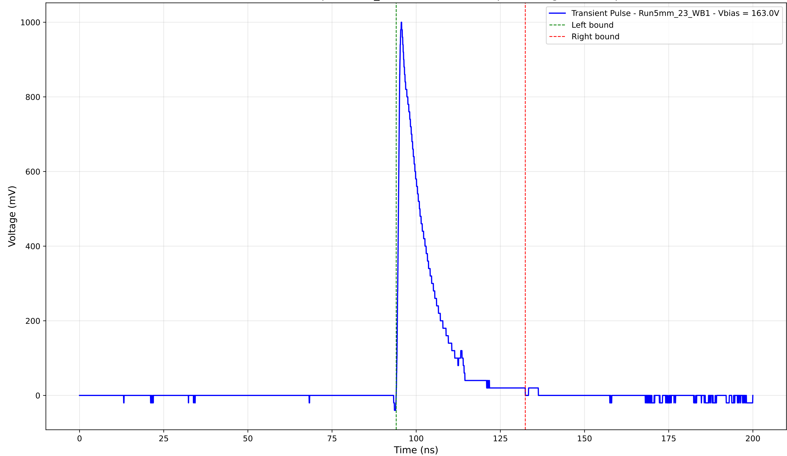
Transient Pulse - Sample: 5mm_23 - Position: 4940.0 \mu\text{m} - Charge: 167.26 pC
