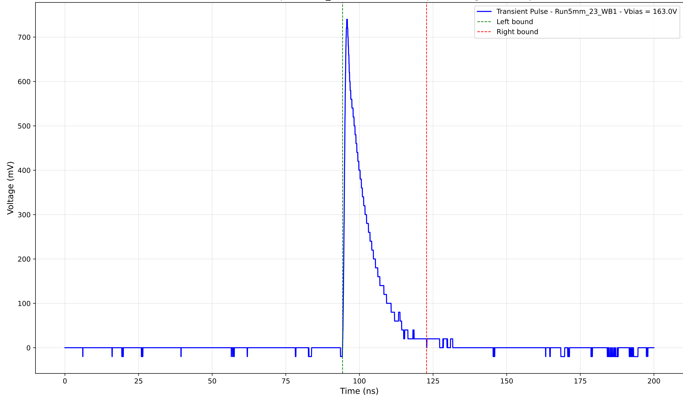
Transient Pulse - Sample: 5mm_23 - Position: 675.0 \mu\text{m} - Charge: 112.41 pC
