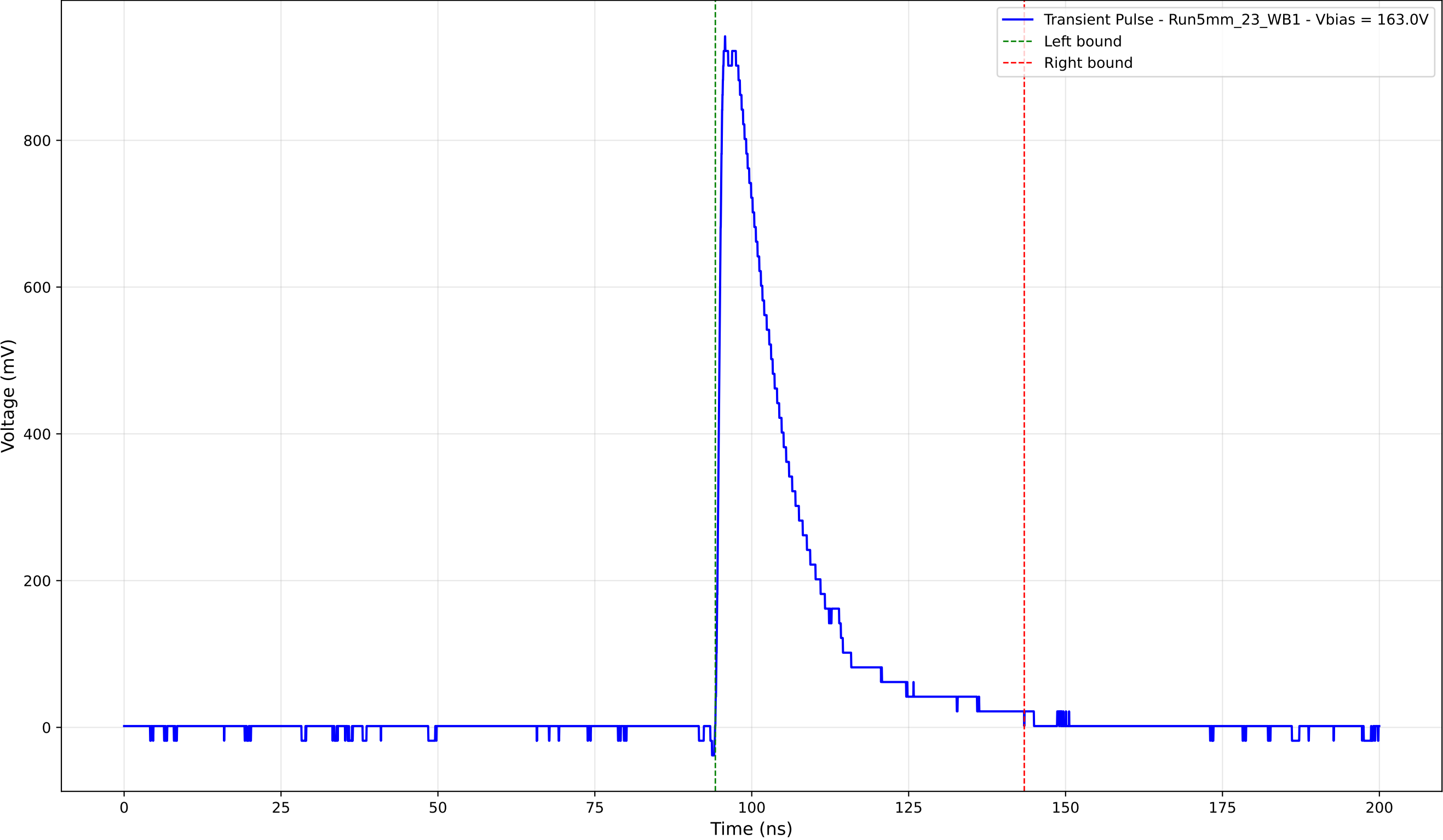
Transient Pulse - Sample: 5mm_23 - Position: 3455.0 \mu\text{m} - Charge: 218.02 pC
