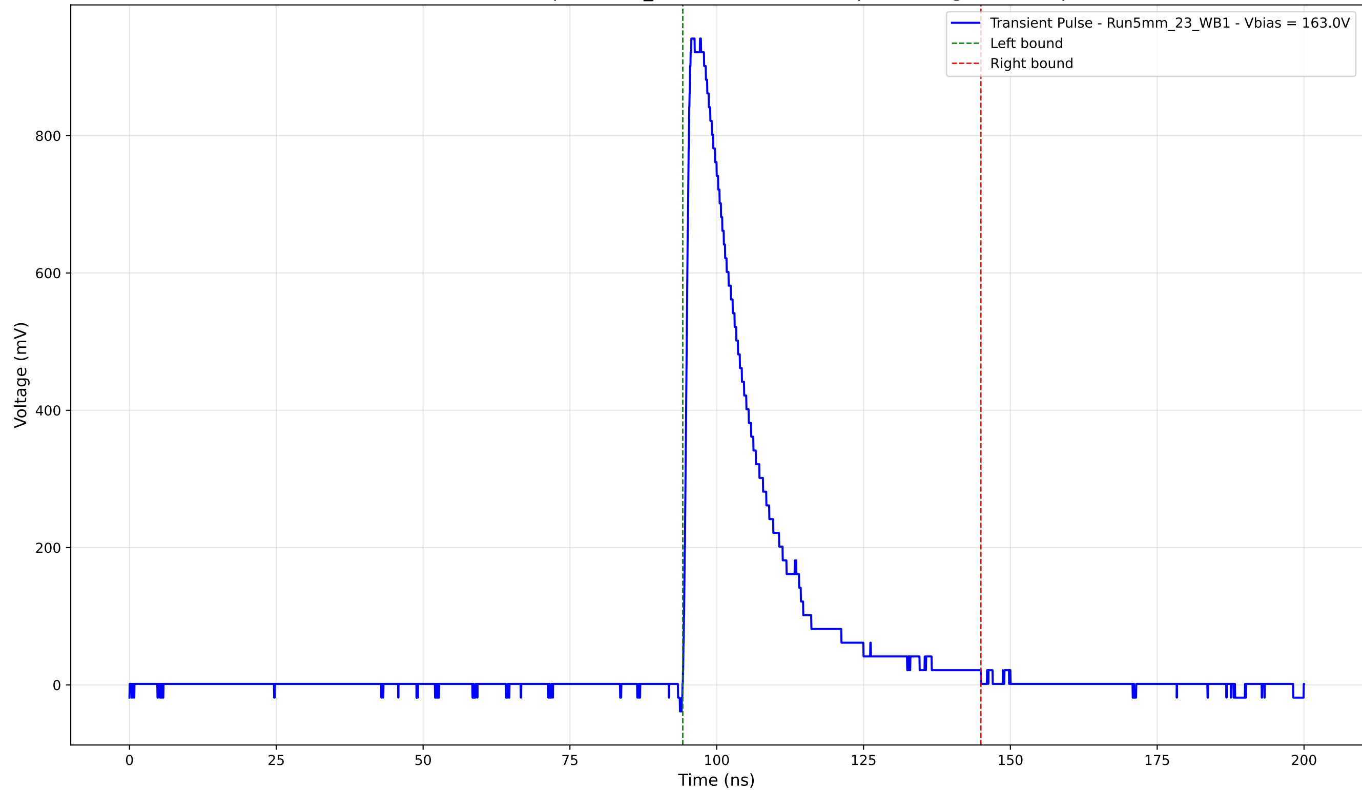
Transient Pulse - Sample: 5mm_23 - Position: 3530.0 \mu\text{m} - Charge: 223.25 pC
