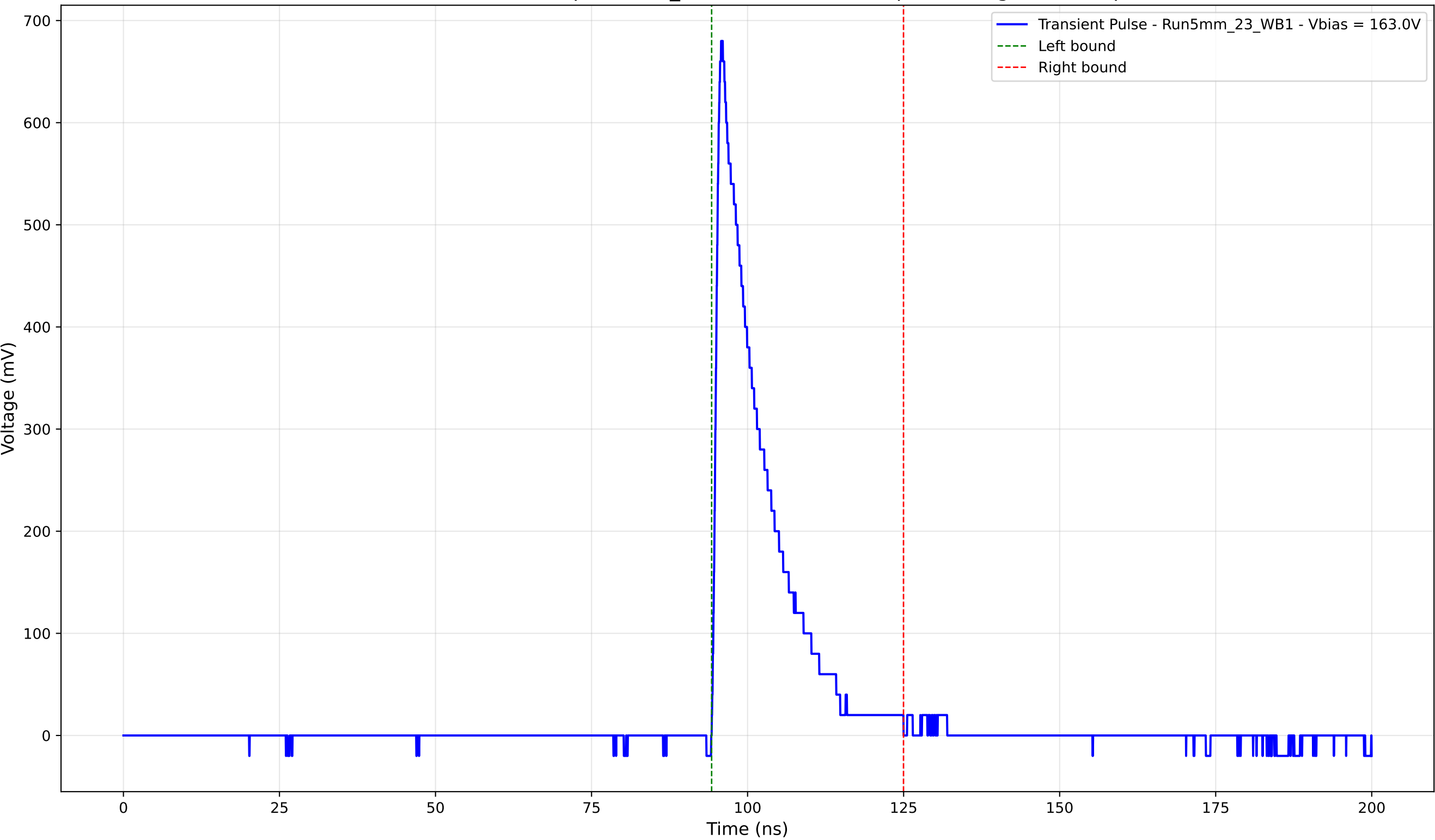
Transient Pulse - Sample: 5mm_23 - Position: 4715.0 \mu\text{m} - Charge: 107.38 pC
