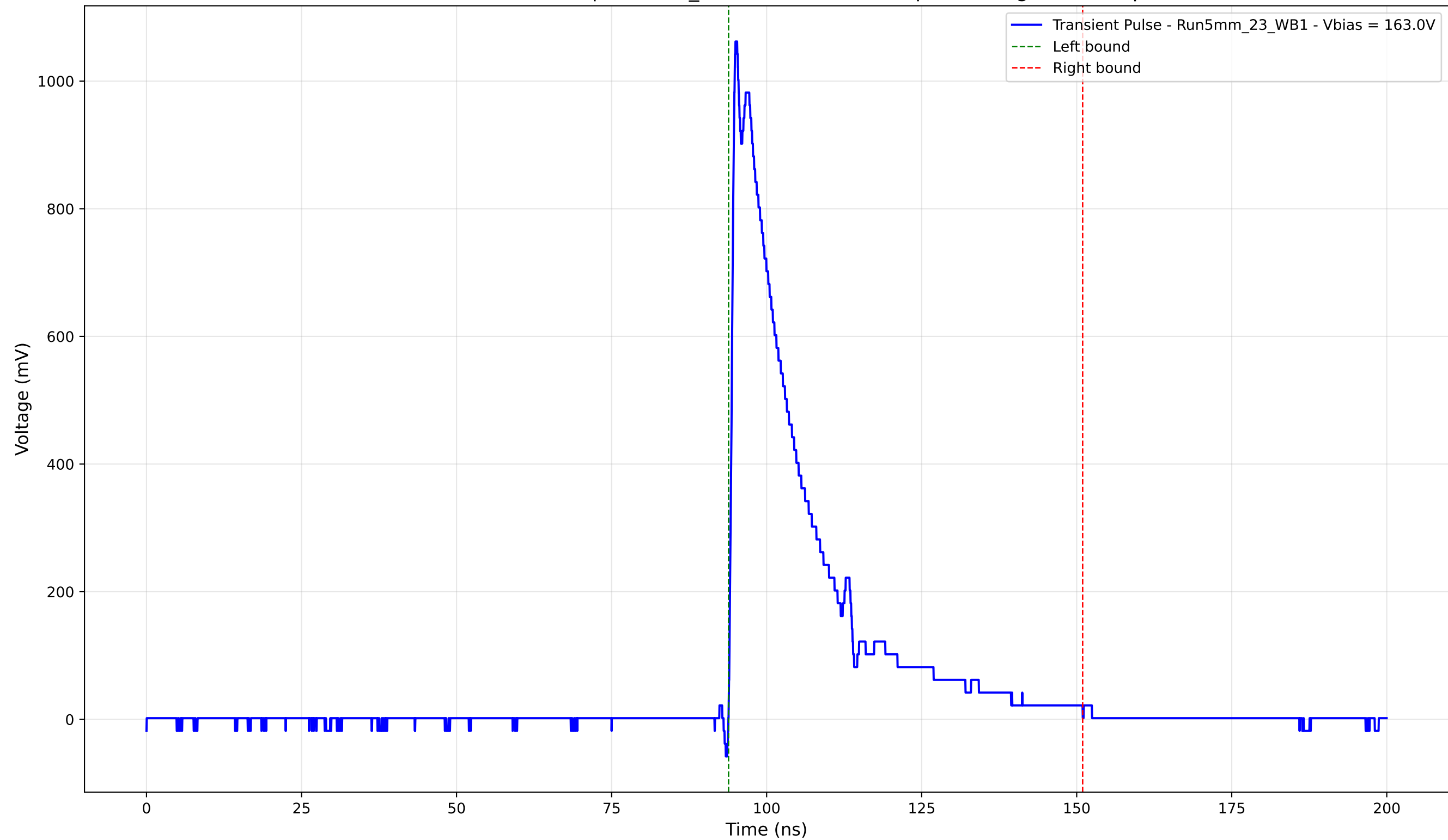
Transient Pulse - Sample: 5mm_23 - Position: 2870.0 \mu\text{m} - Charge: 245.75 pC
