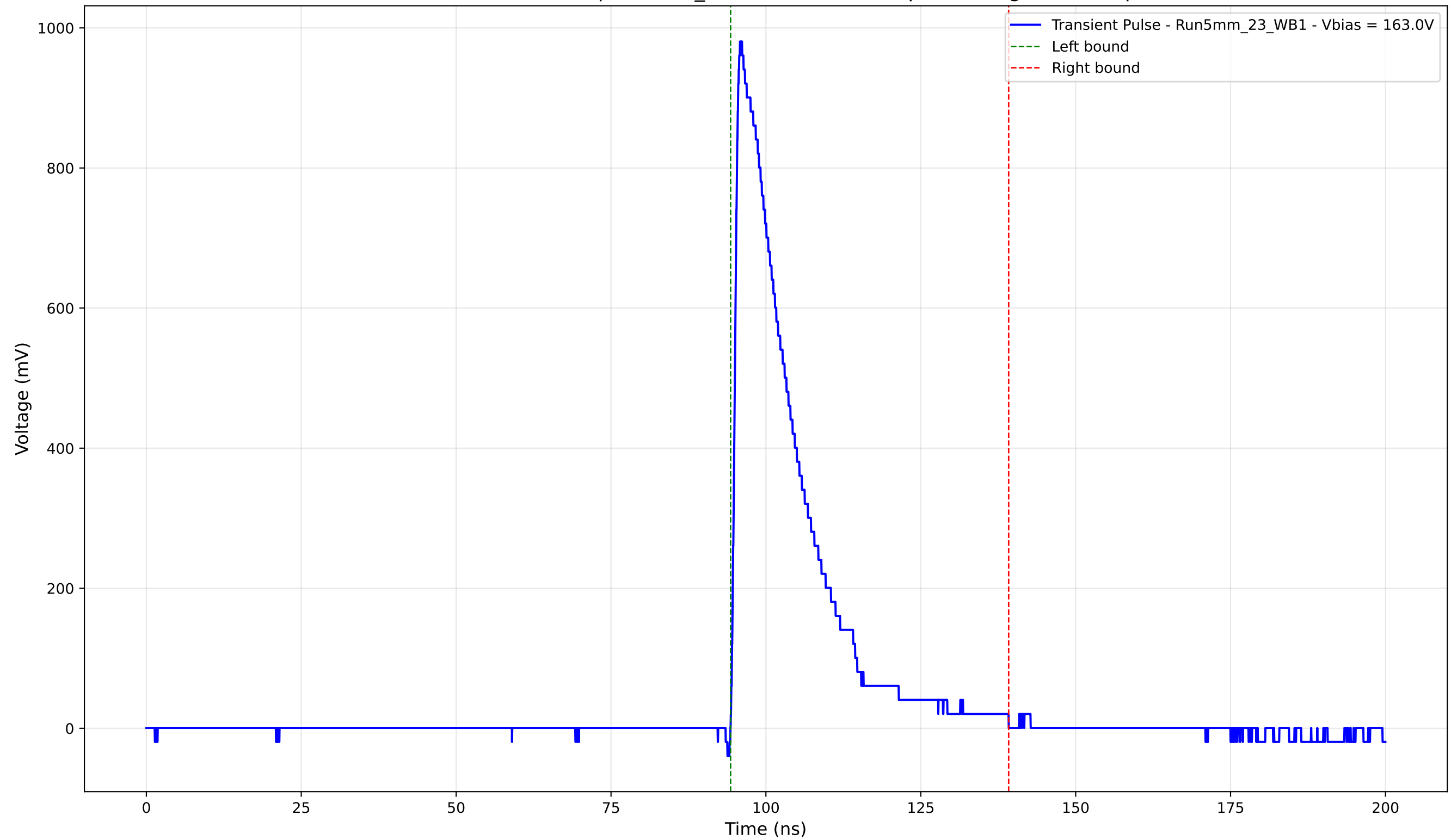
Transient Pulse - Sample: 5mm_23 - Position: 890.0 \mu\text{m} - Charge: 204.94 pC
