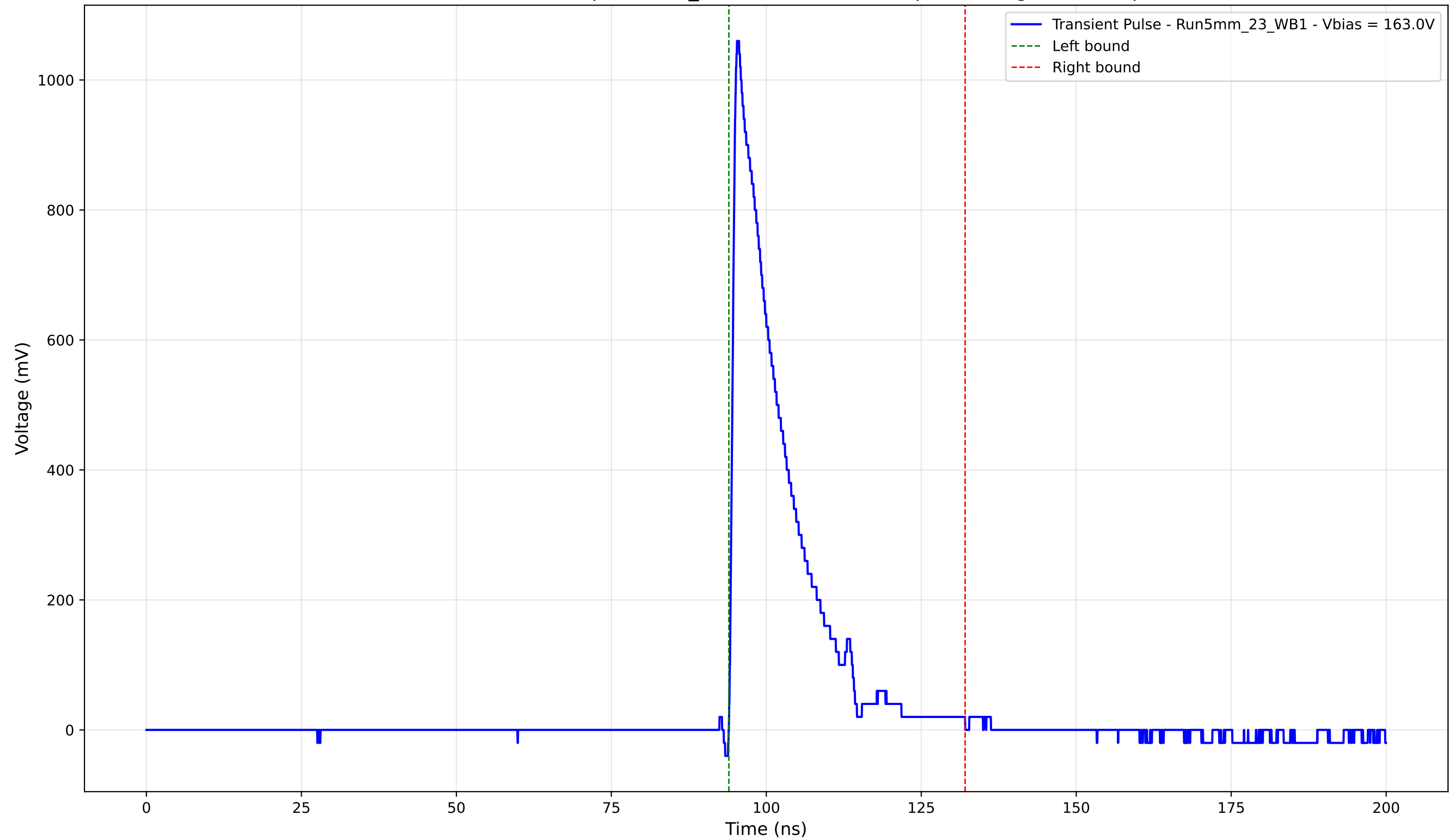
Transient Pulse - Sample: 5mm_23 - Position: 5095.0 \mu\text{m} - Charge: 185.08 pC
