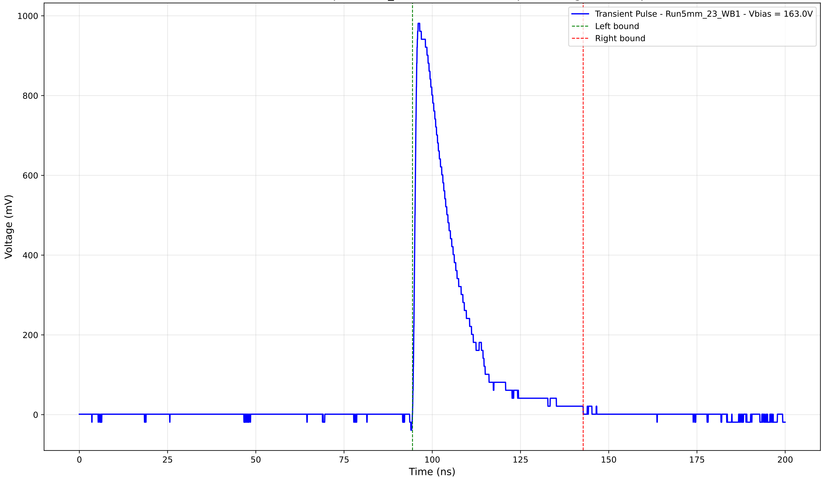
Transient Pulse - Sample: 5mm_23 - Position: 1400.0 \mu\text{m} - Charge: 230.80 pC
