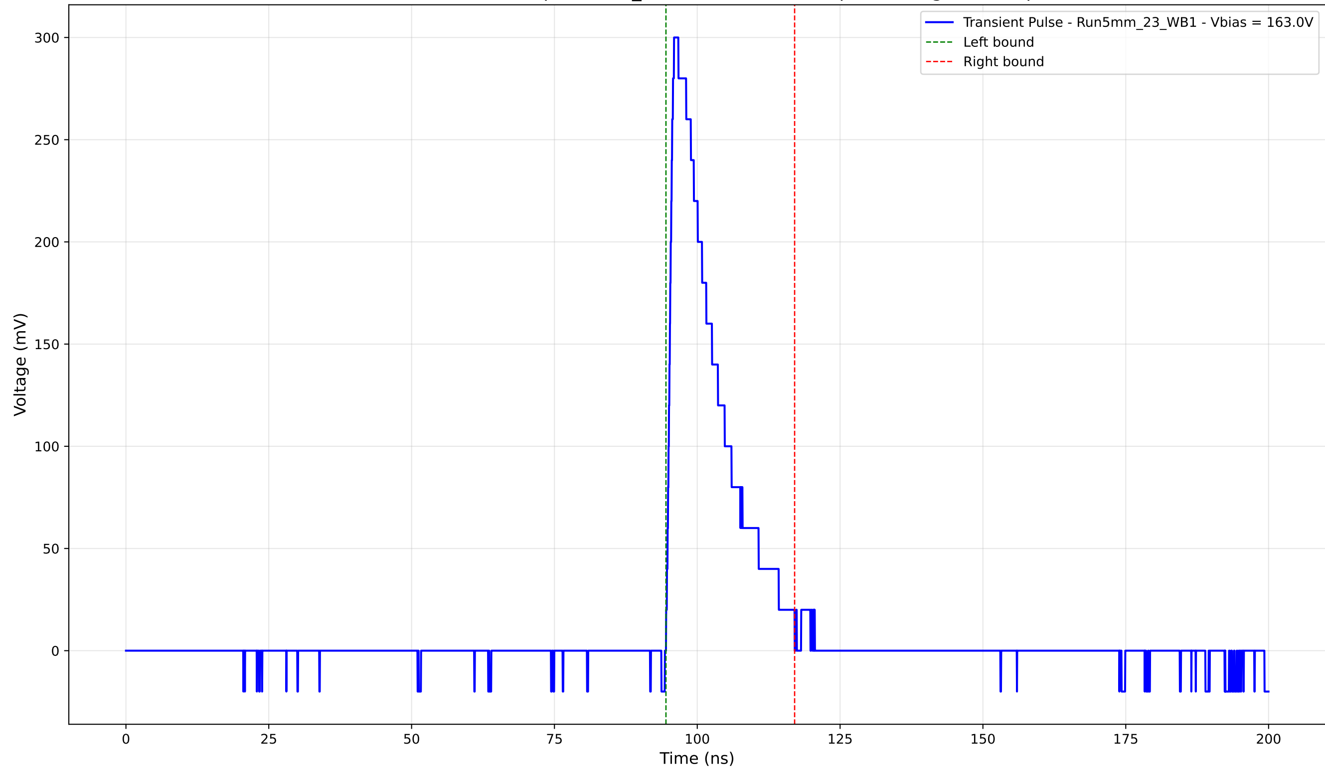
Transient Pulse - Sample: 5mm_23 - Position: 1205.0 \mu\text{m} - Charge: 53.72 pC
