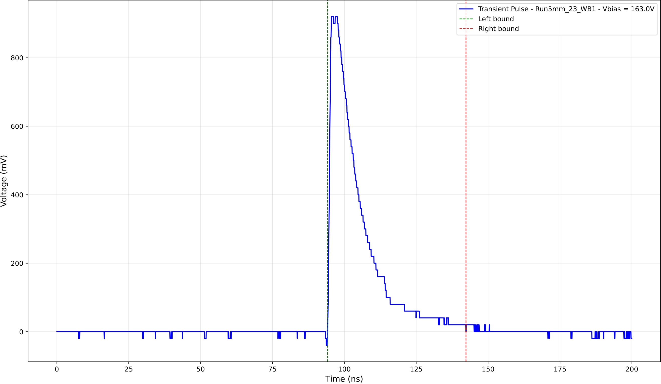
Transient Pulse - Sample: 5mm_23 - Position: 3450.0 \mu\text{m} - Charge: 216.29 pC
