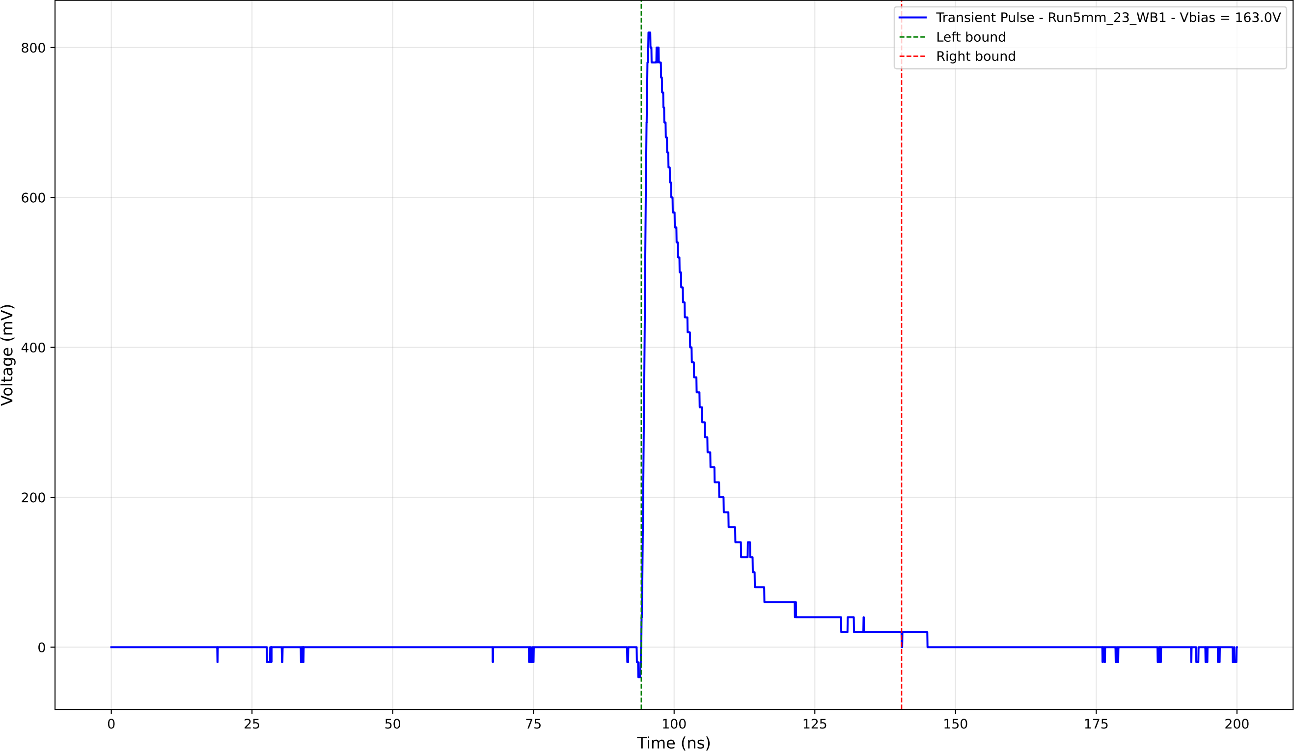
Transient Pulse - Sample: 5mm_23 - Position: 3325.0 \mu\text{m} - Charge: 174.91 pC
