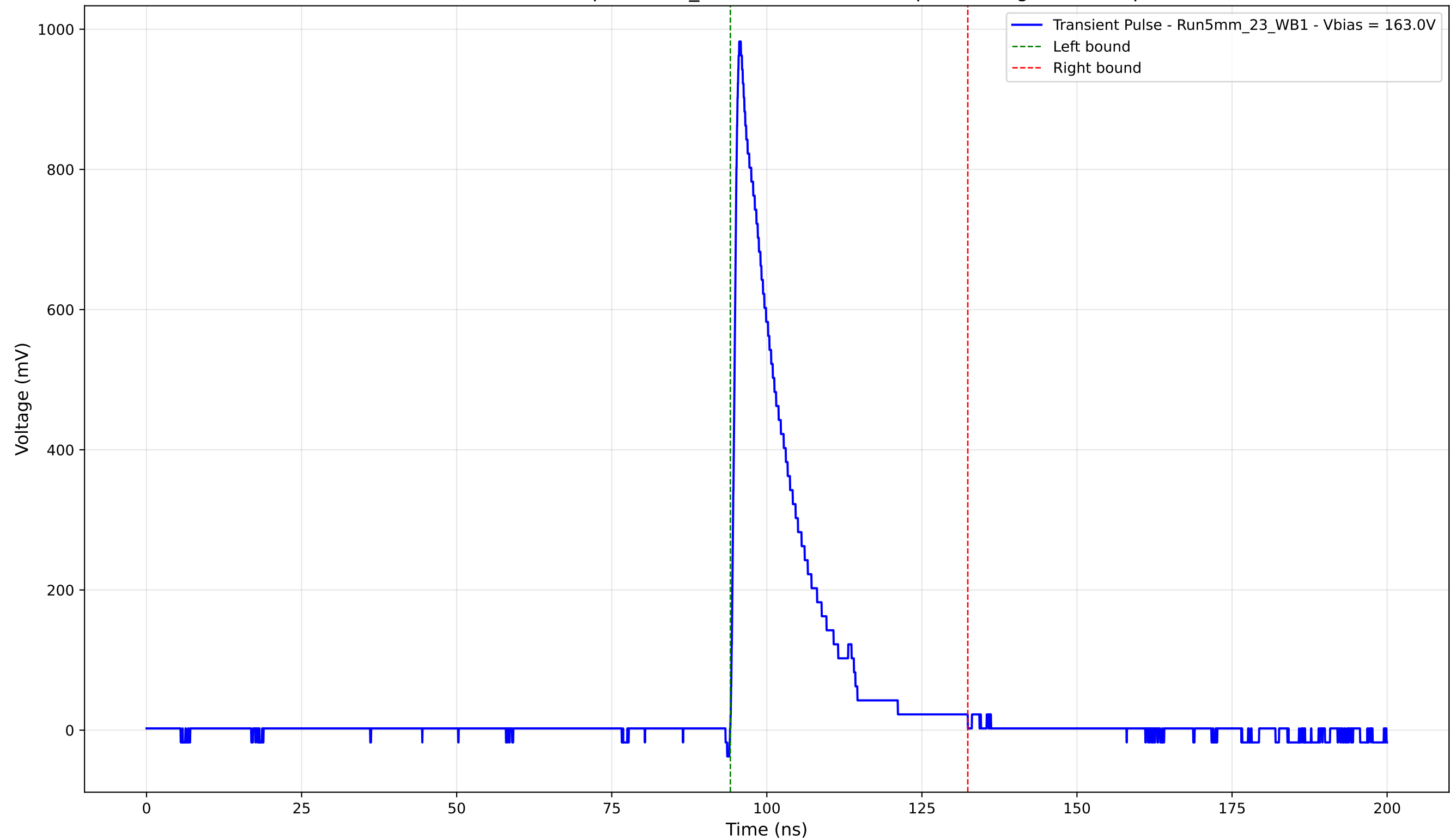
Transient Pulse - Sample: 5mm_23 - Position: 4860.0 \mu\text{m} - Charge: 168.51 pC
