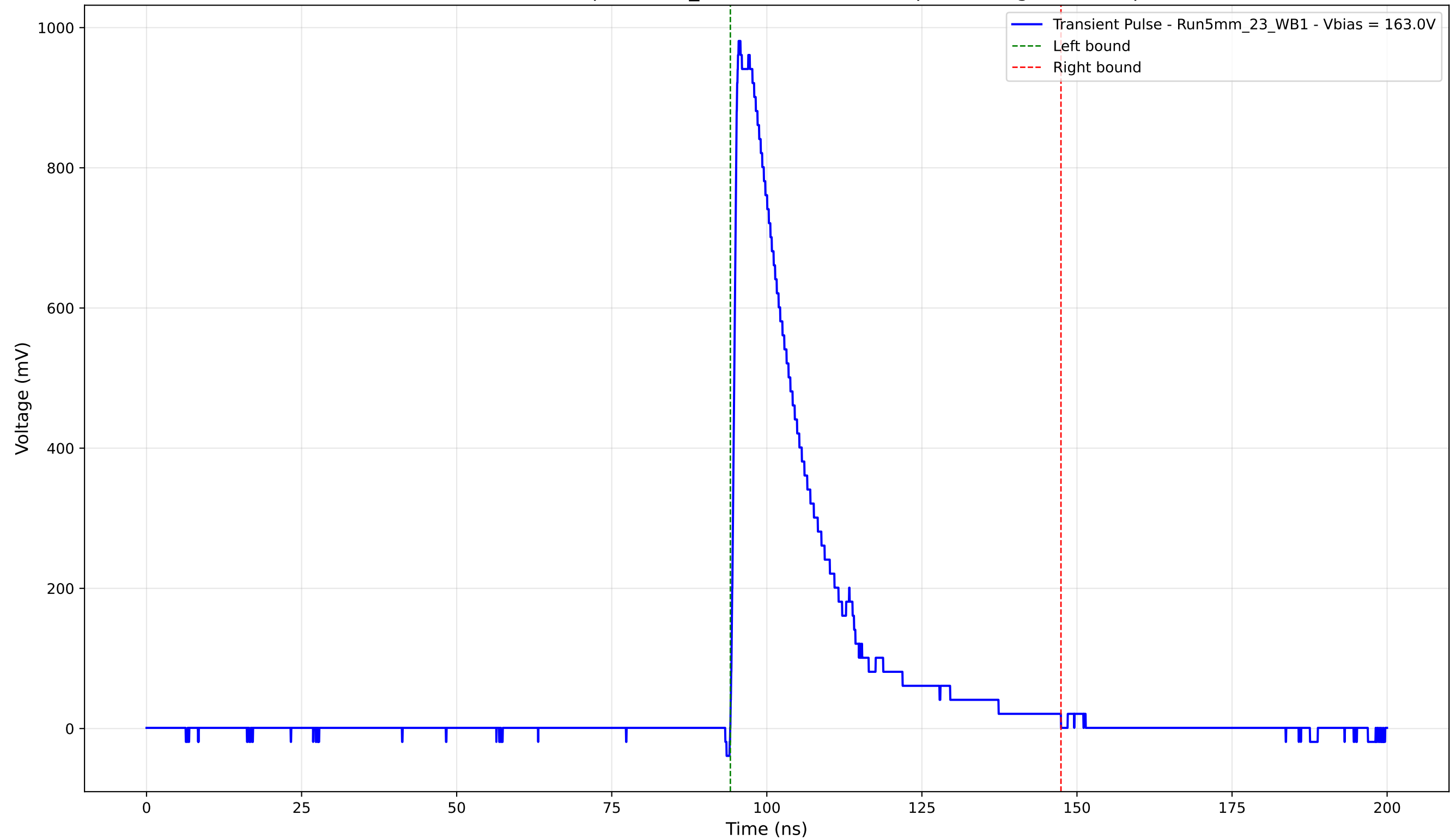
Transient Pulse - Sample: 5mm_23 - Position: 2140.0 \mu\text{m} - Charge: 235.20 pC
