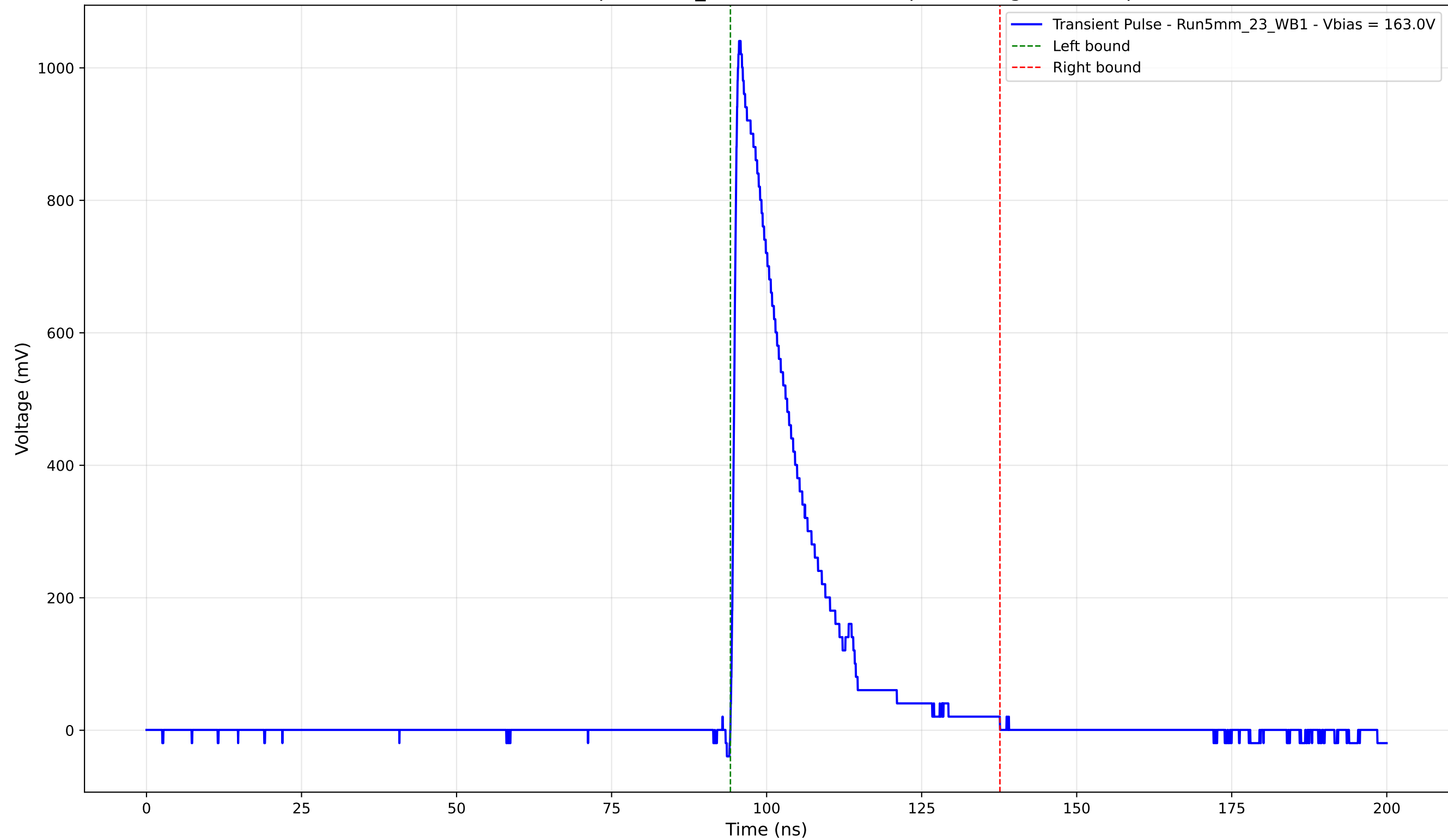
Transient Pulse - Sample: 5mm_23 - Position: 585.0 \mu\text{m} - Charge: 208.09 pC
