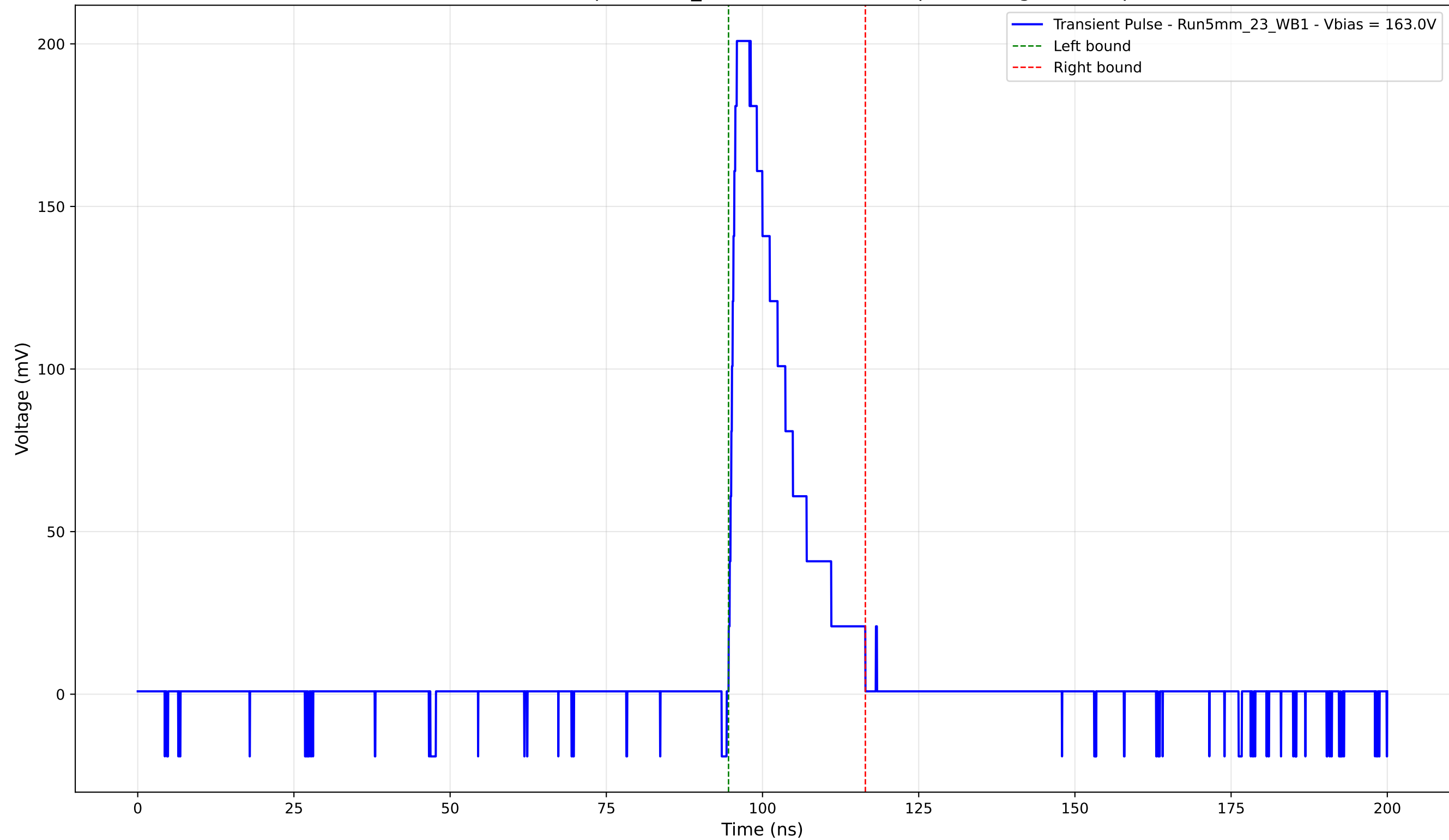
Transient Pulse - Sample: 5mm_23 - Position: 4250.0 \mu\text{m} - Charge: 37.12 pC
