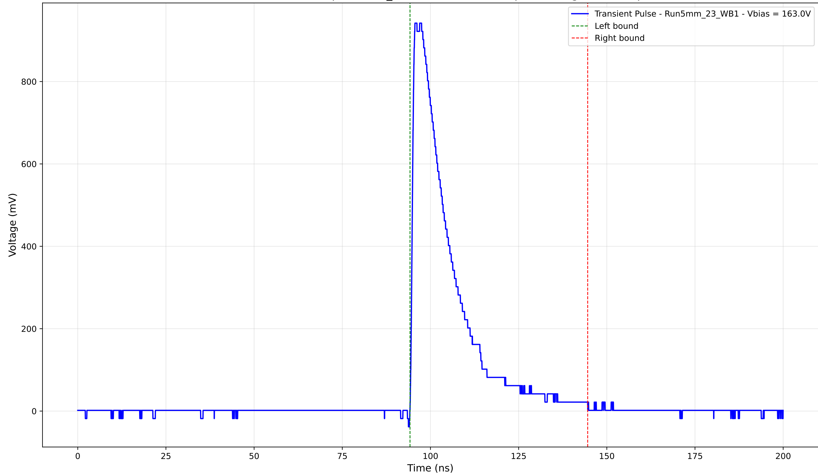
Transient Pulse - Sample: 5mm_23 - Position: 3510.0 \mu\text{m} - Charge: 224.57 pC
