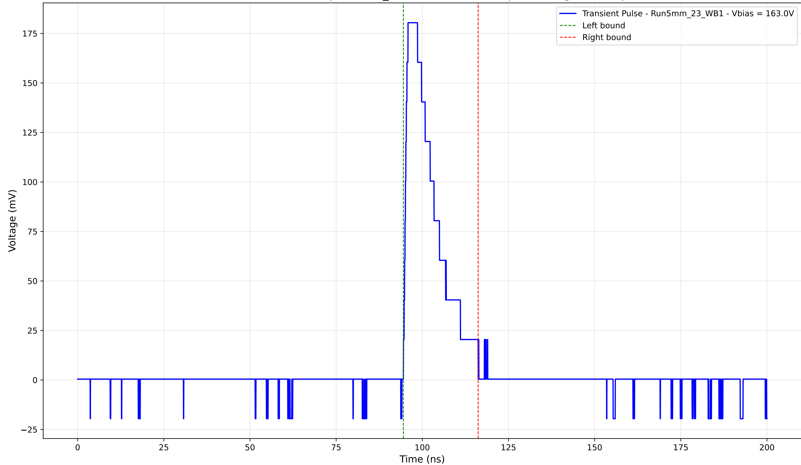
Transient Pulse - Sample: 5mm_23 -Position: 3760.0 \mu\text{m} - Charge: 35.33 pC
