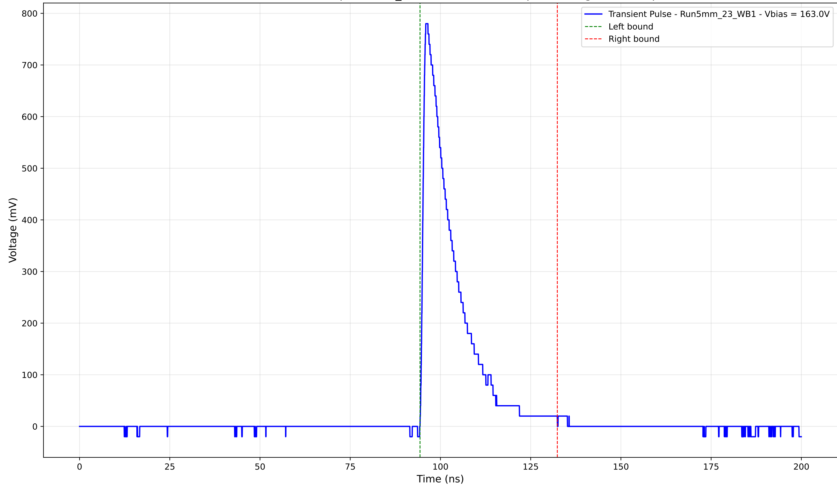
Transient Pulse - Sample: 5mm_23 - Position: 4335.0 \mu\text{m} - Charge: 146.46 pC
