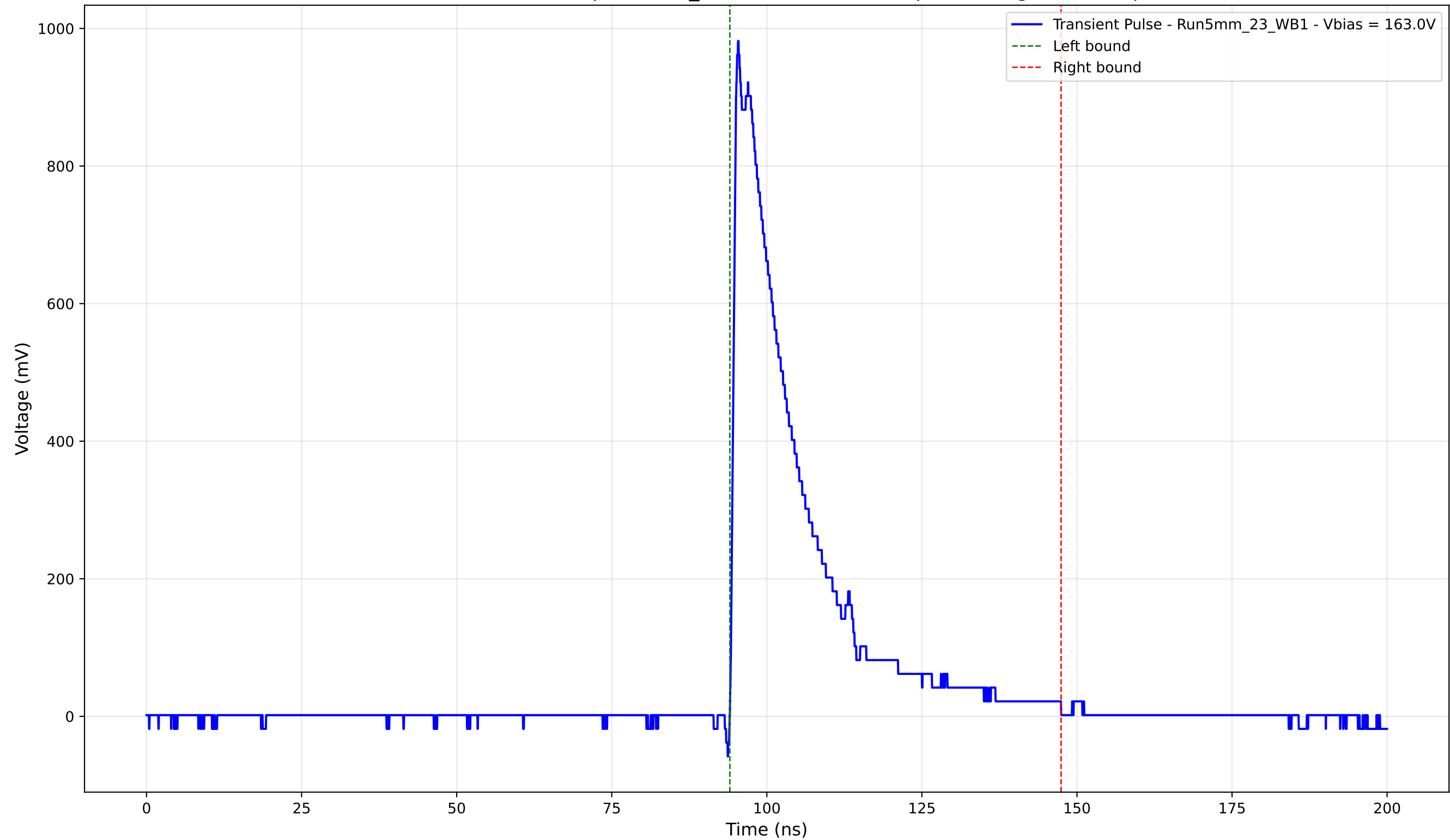
Transient Pulse - Sample: 5mm_23 - Position: 3150.0 \mu\text{m} - Charge: 214.44 pC
