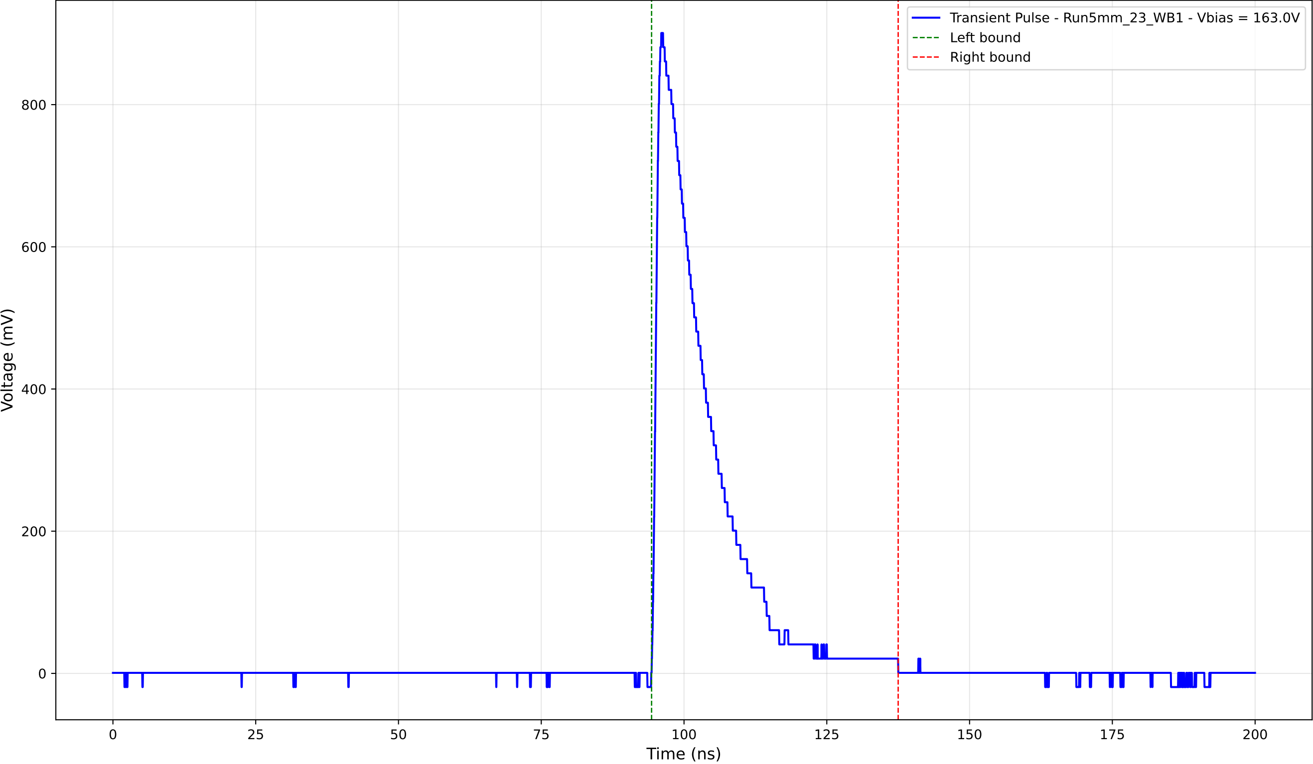
Transient Pulse - Sample: 5mm_23 - Position: 4370.0 \mu\text{m} - Charge: 177.18 pC
