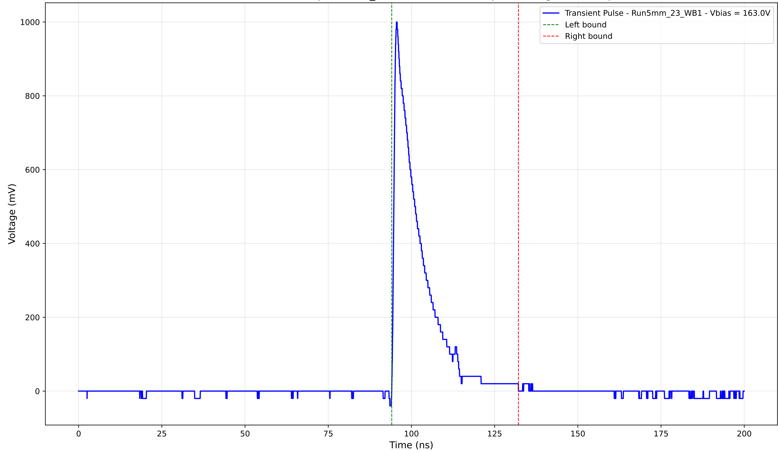
Transient Pulse - Sample: 5mm_23 - Position: 4945.0 \mu\text{m} - Charge: 166.74 pC
