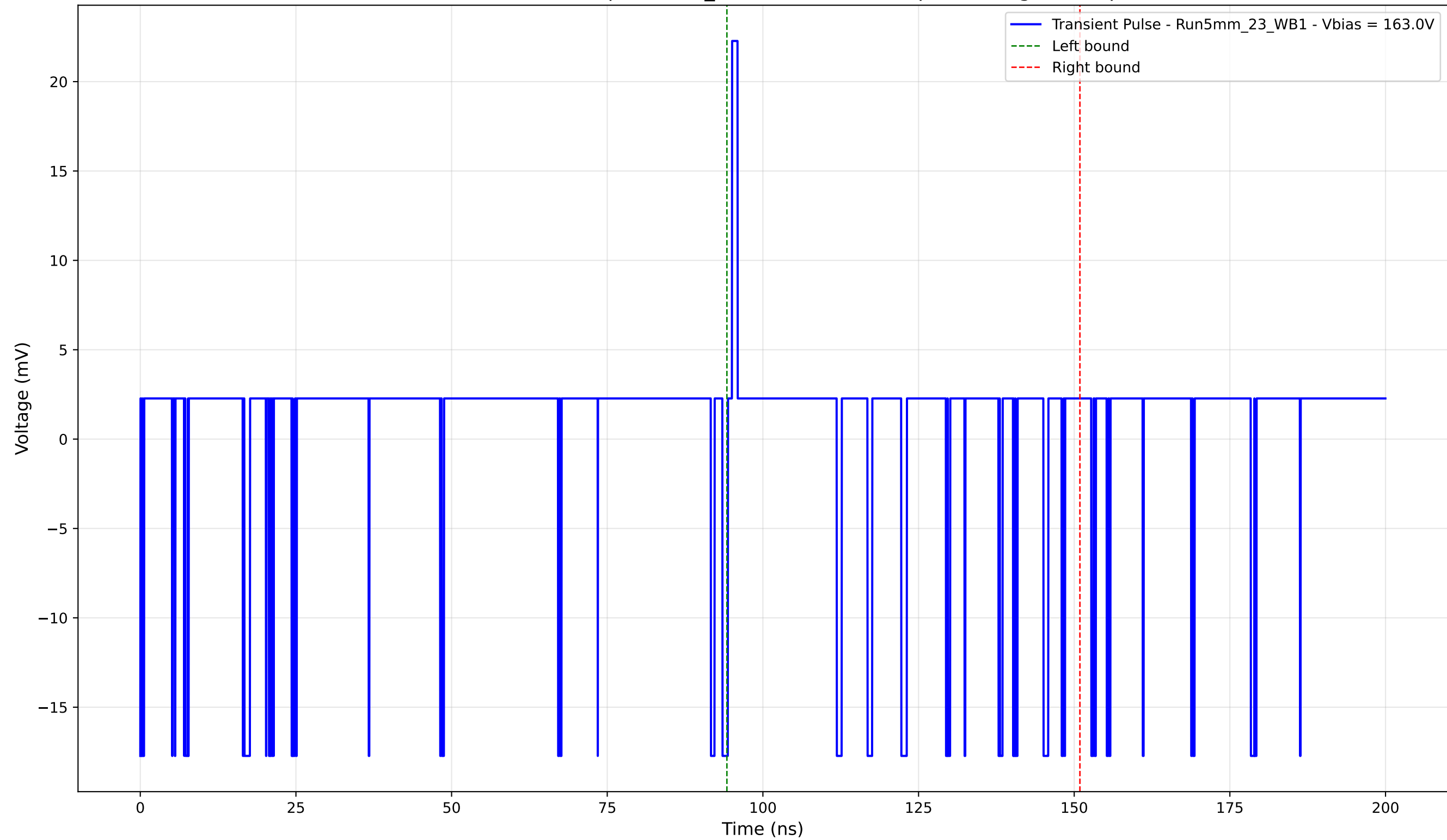
Transient Pulse - Sample: 5mm_23 - Position: 200.0 \mu\text{m} - Charge: 0.64 pC
