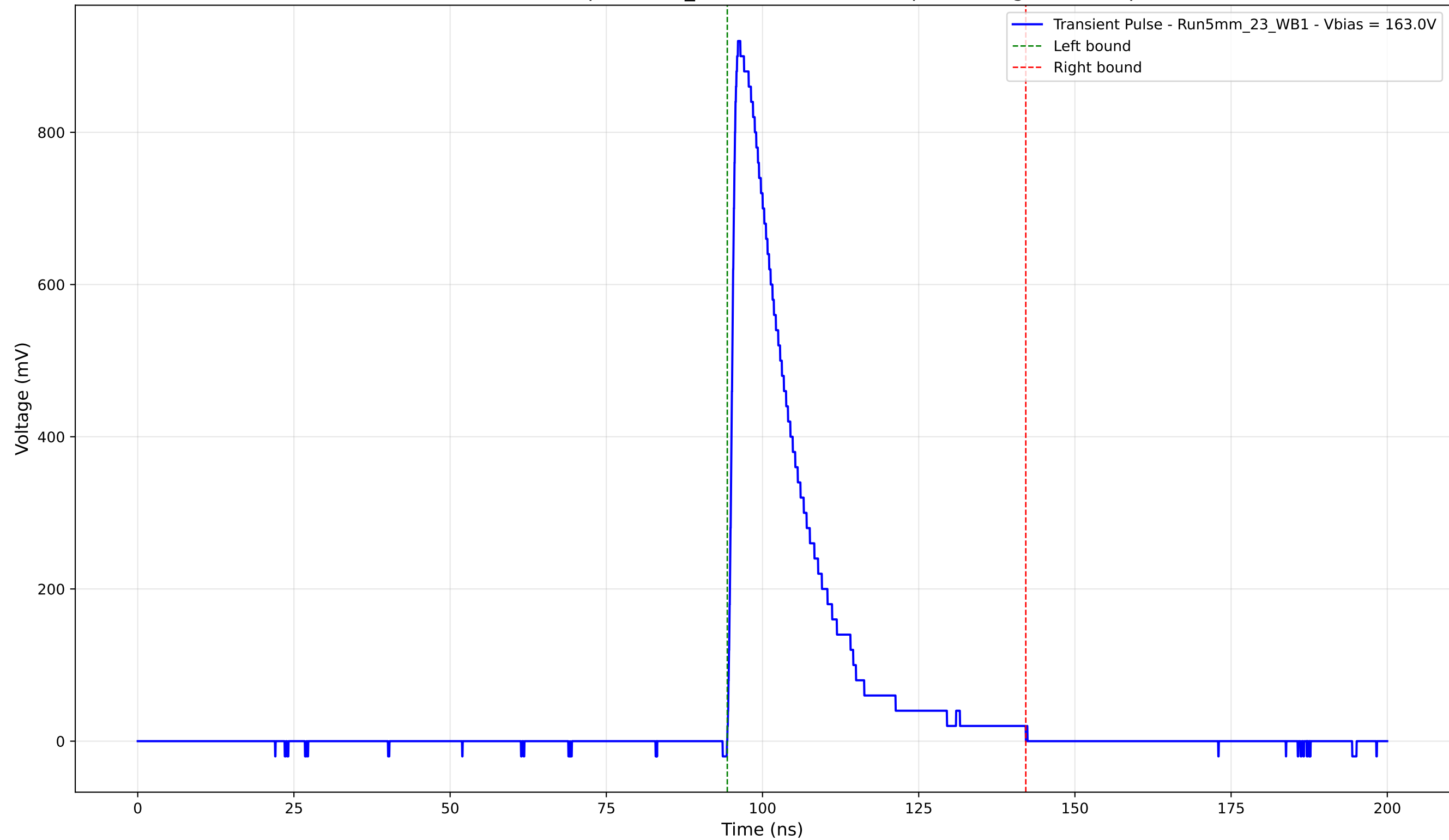
Transient Pulse - Sample: 5mm_23 - Position: 3990.0 \mu\text{m} - Charge: 199.26 pC
