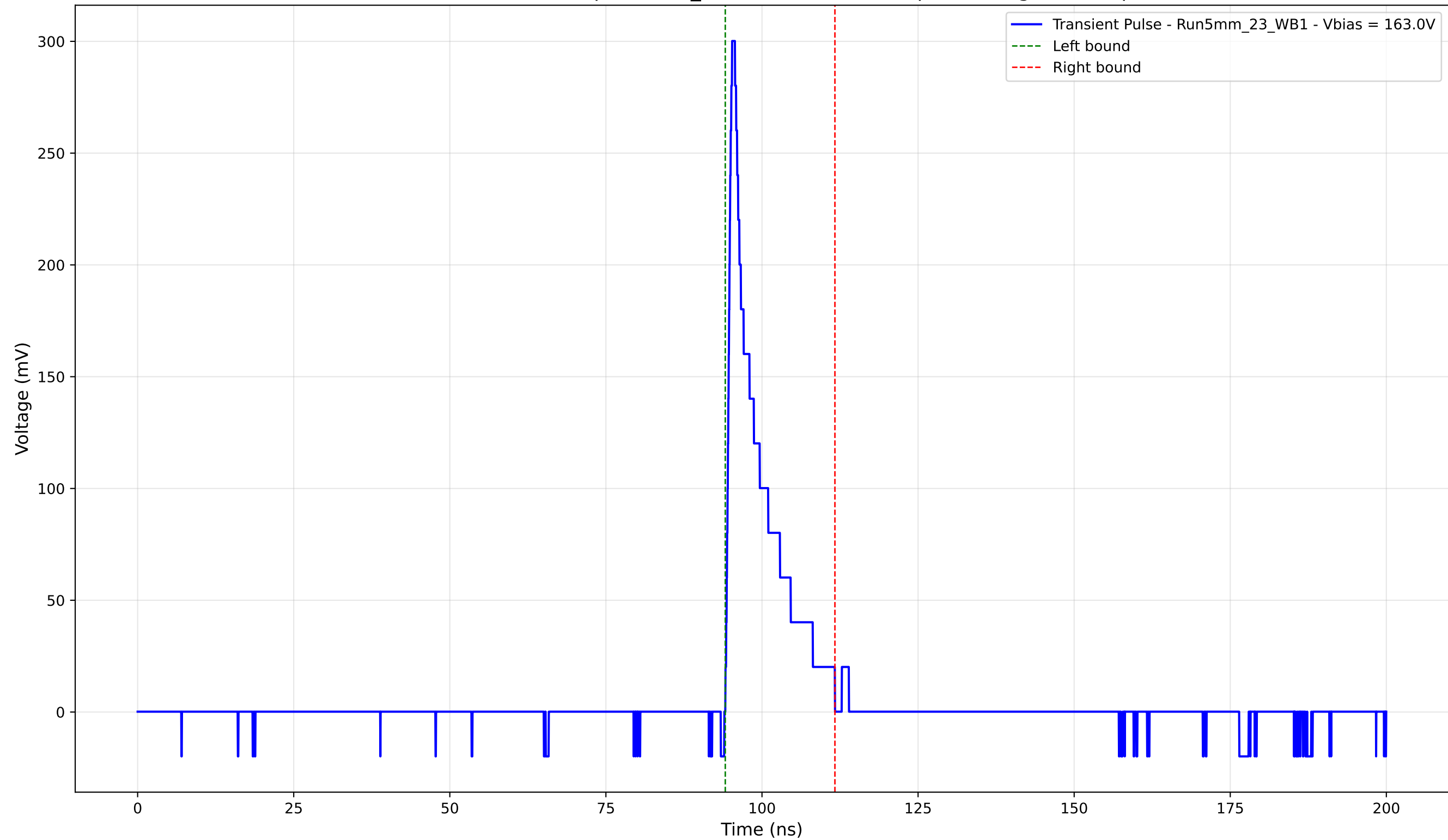
Transient Pulse - Sample: 5mm_23 - Position: 5185.0 \mu\text{m} - Charge: 31.46 pC
