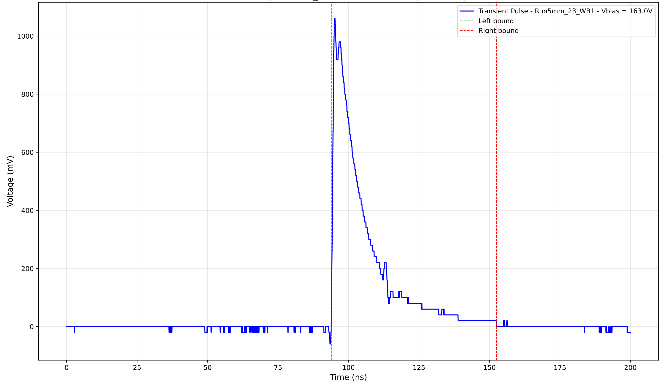
Transient Pulse - Sample: 5mm_23 - Position: 2590.0 \mu\text{m} - Charge: 242.43 pC
