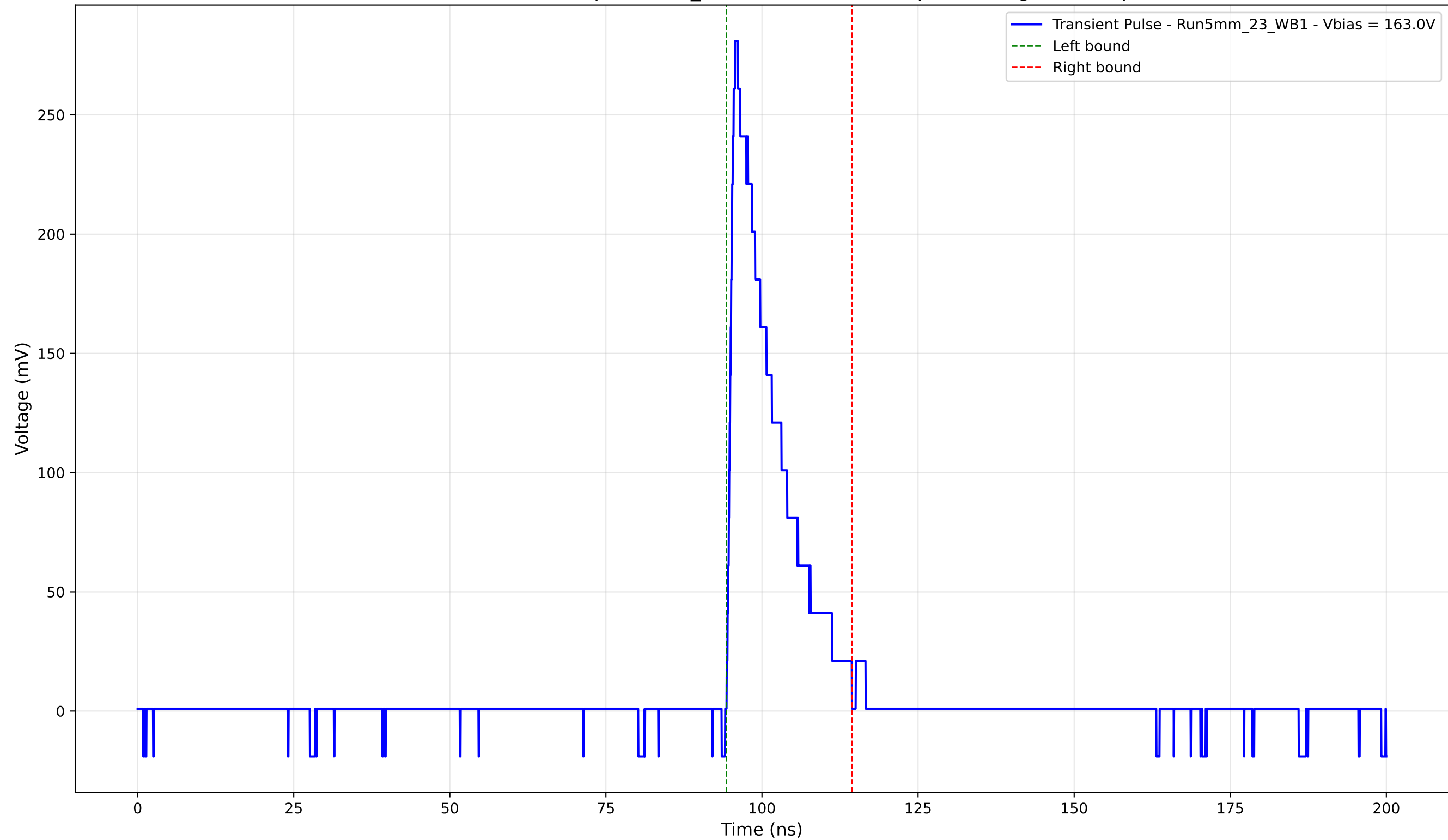
Transient Pulse - Sample: 5mm_23 - Position: 4750.0 \mu\text{m} - Charge: 42.98 pC
