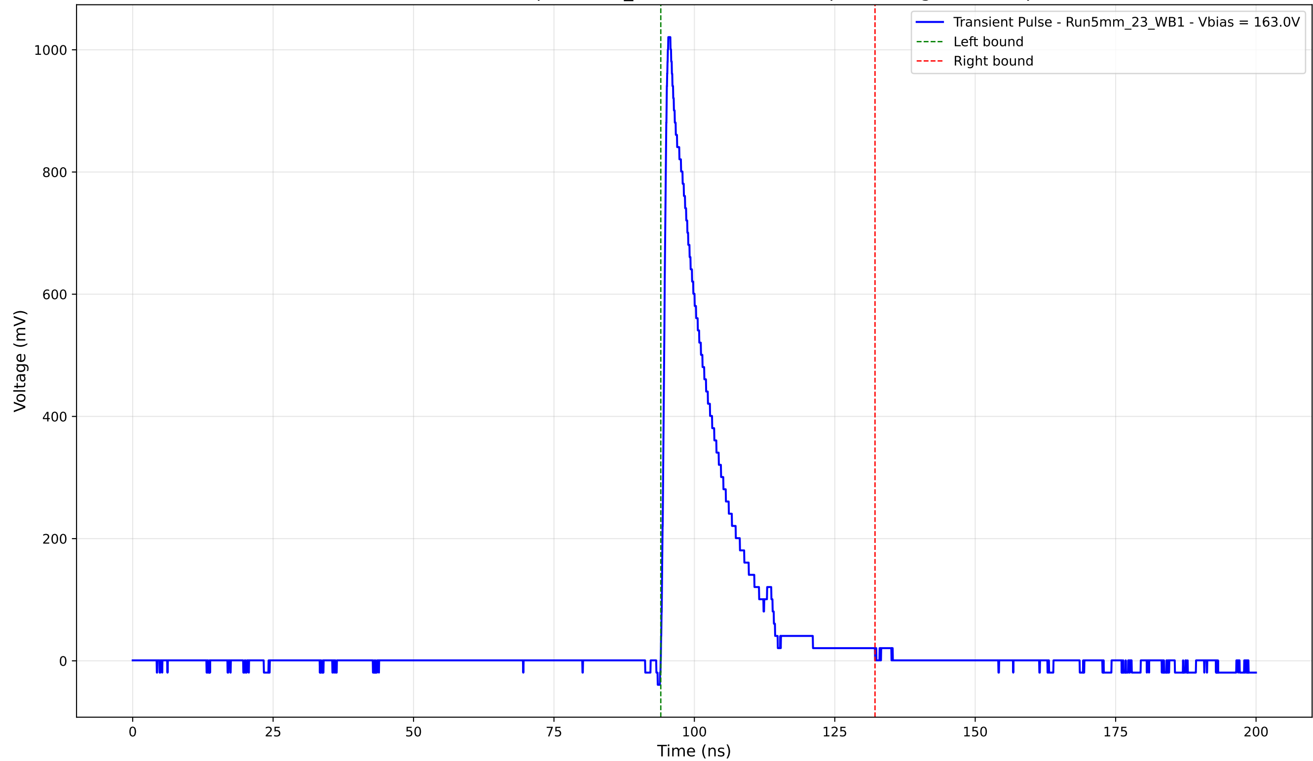
Transient Pulse - Sample: 5mm_23 - Position: 5020.0 \mu\text{m} - Charge: 173.19 pC
