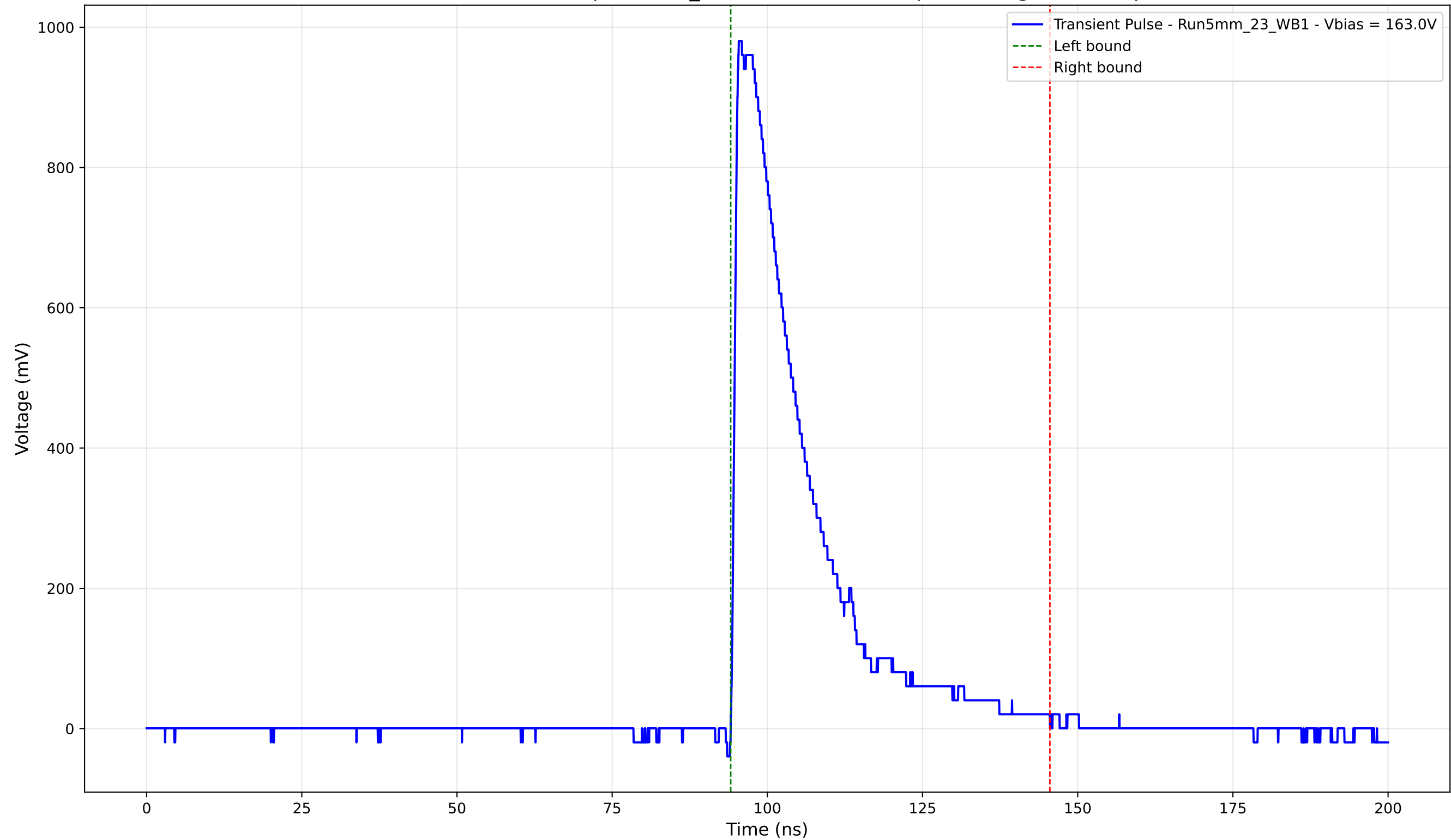
Transient Pulse - Sample: 5mm_23 - Position: 2120.0 \mu\text{m} - Charge: 241.20 pC
