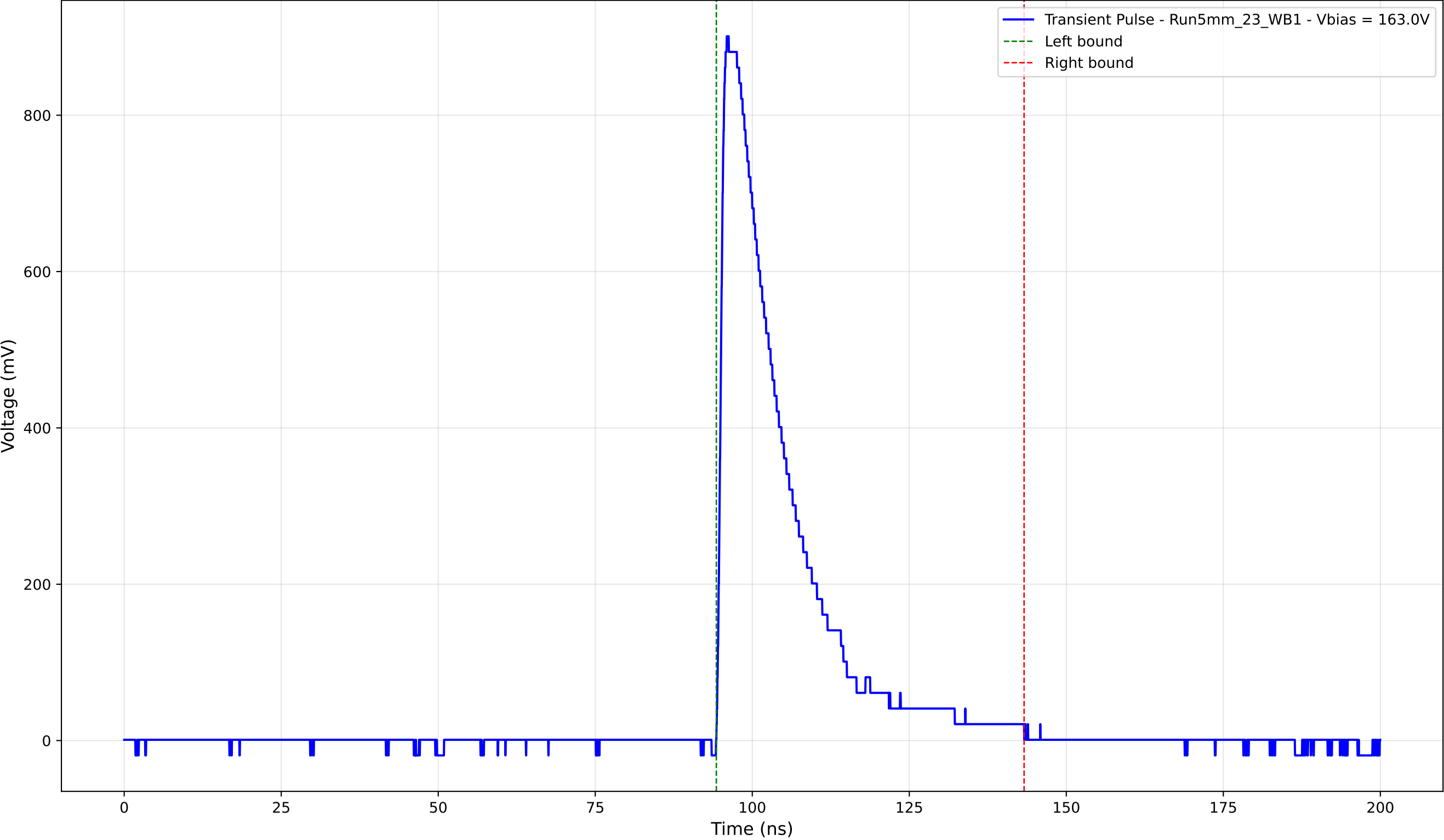
Transient Pulse - Sample: 5mm_23 - Position: 3650.0 \mu\text{m} - Charge: 200.66 pC
