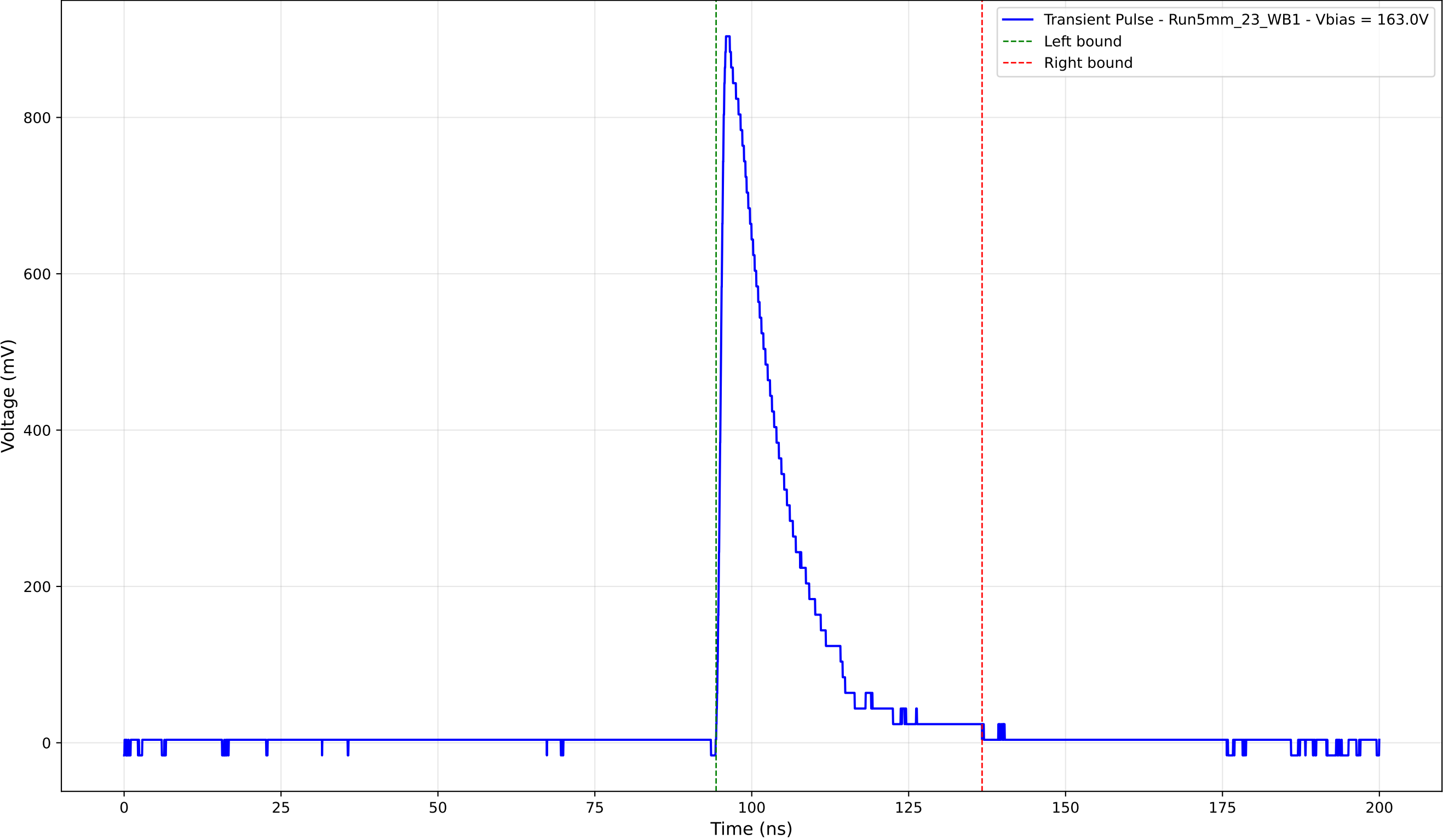
Transient Pulse - Sample: 5mm_23 - Position: 4385.0 \mu\text{m} - Charge: 180.99 pC
