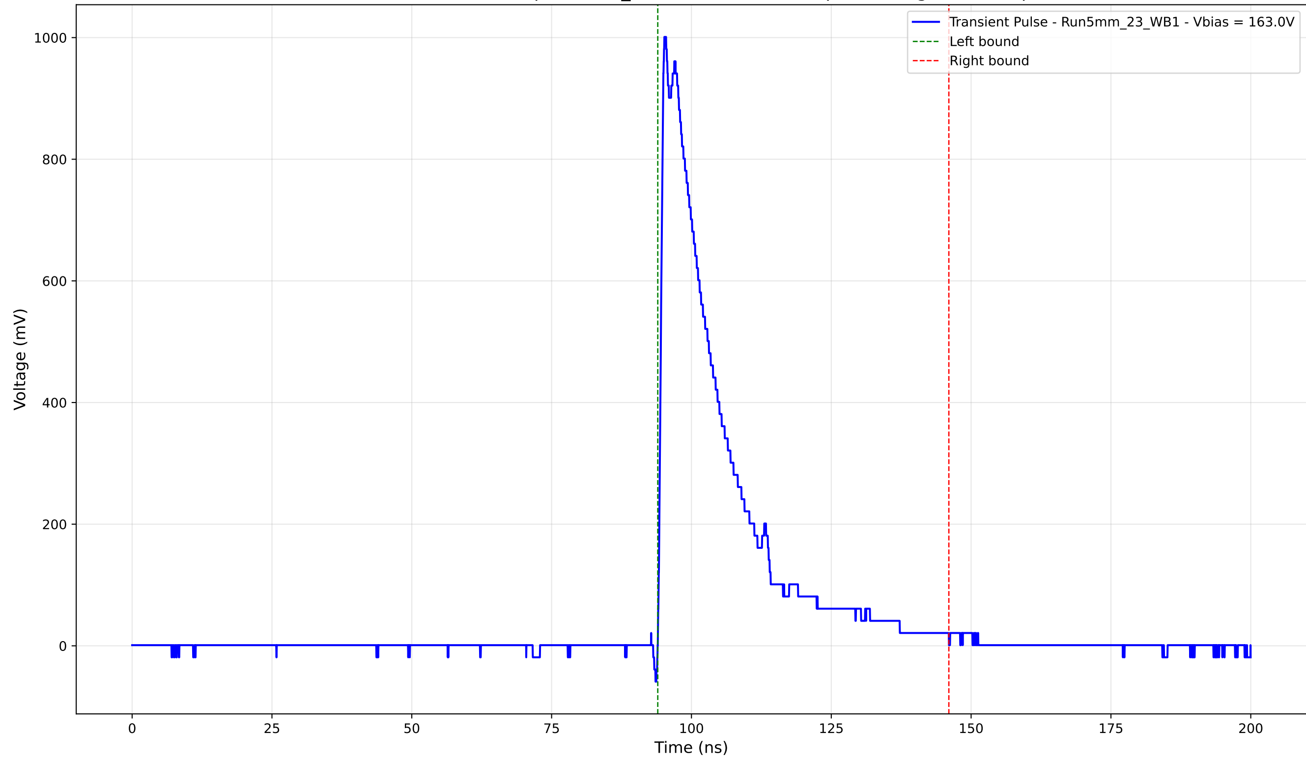
Transient Pulse - Sample: 5mm_23 - Position: 2420.0 \mu\text{m} - Charge: 229.10 pC
