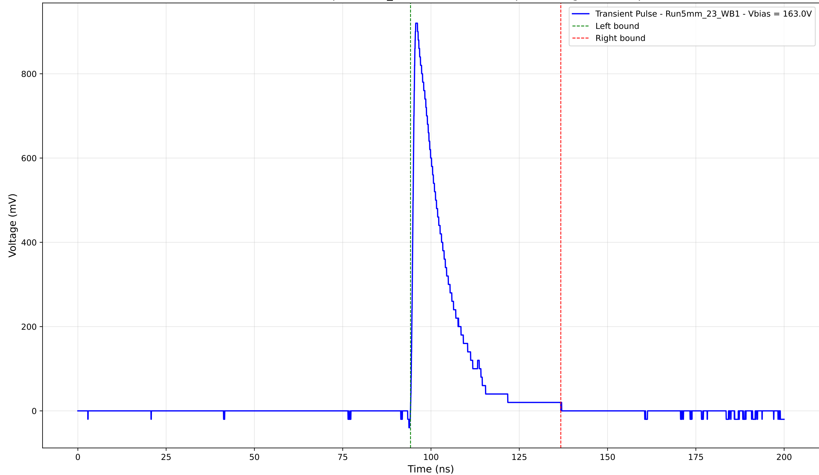
Transient Pulse - Sample: 5mm_23 - Position: 4660.0 \mu\text{m} - Charge: 169.94 pC
