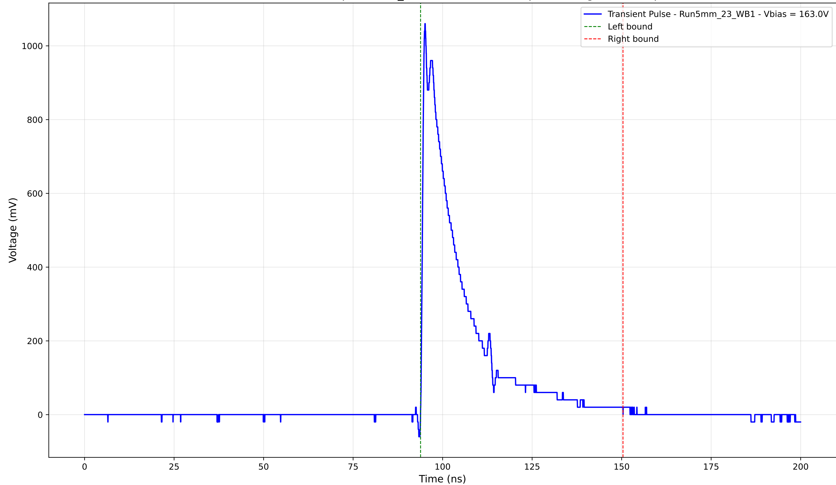
Transient Pulse - Sample: 5mm_23 - Position: 2840.0 \mu\text{m} - Charge: 230.82 pC
