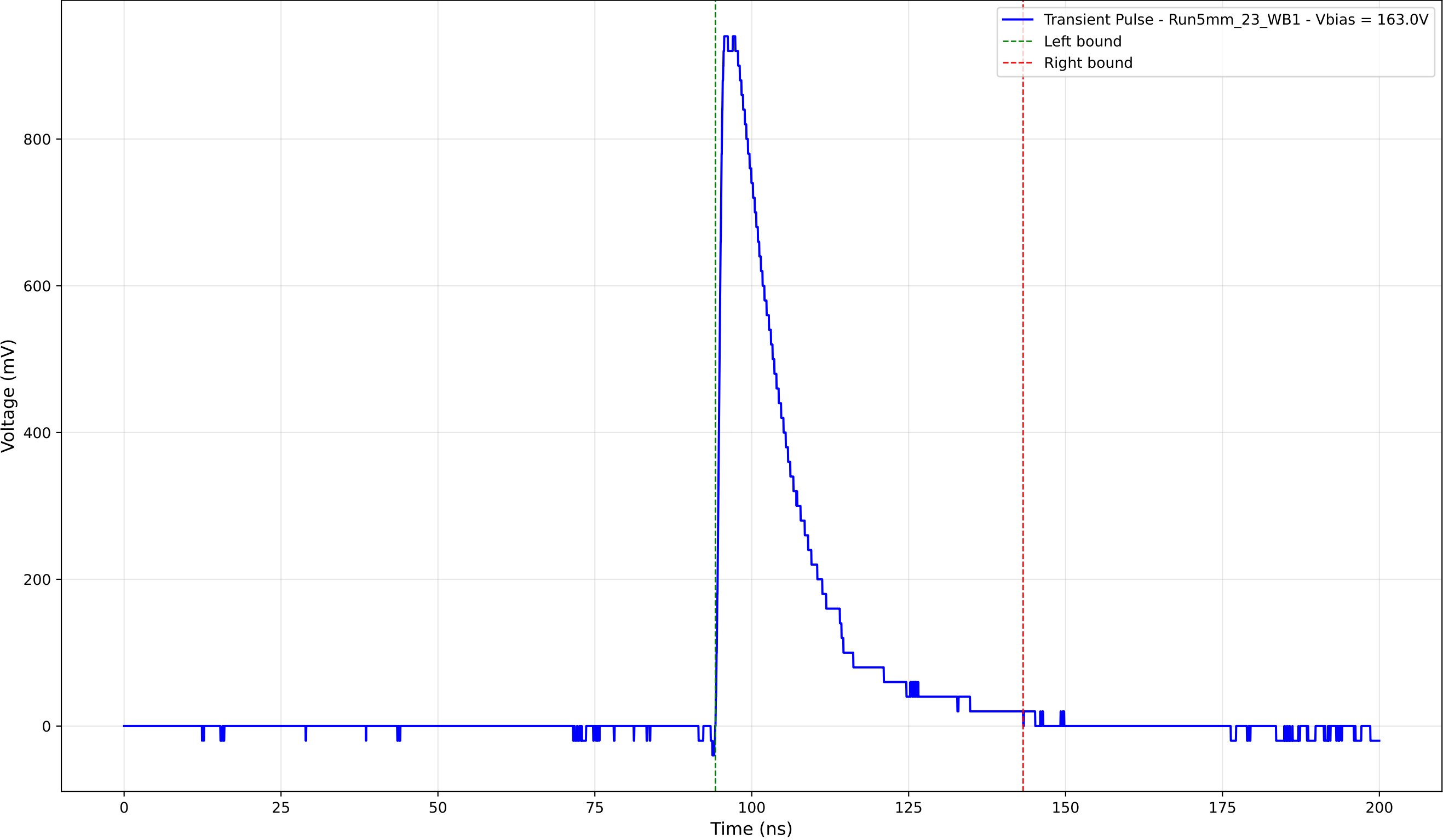
Transient Pulse - Sample: 5mm_23 - Position: 3505.0 \mu\text{m} - Charge: 221.04 pC
