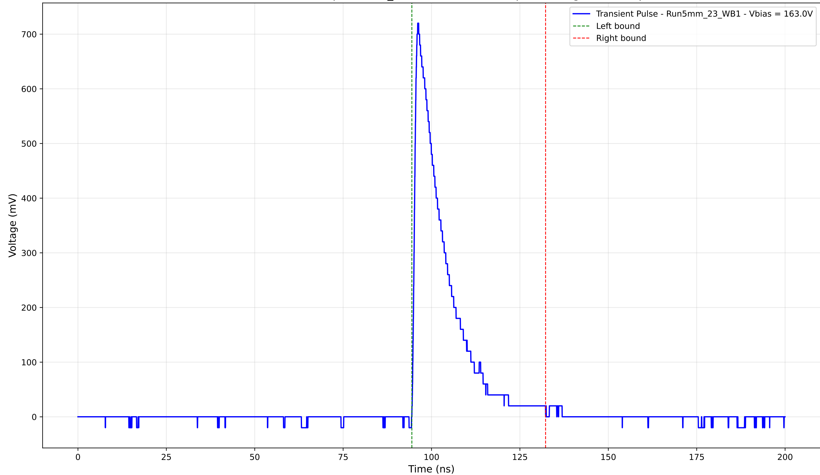
Transient Pulse - Sample: 5mm_23 - Position: 1170.0 \mu\text{m} - Charge: 134.16 pC
