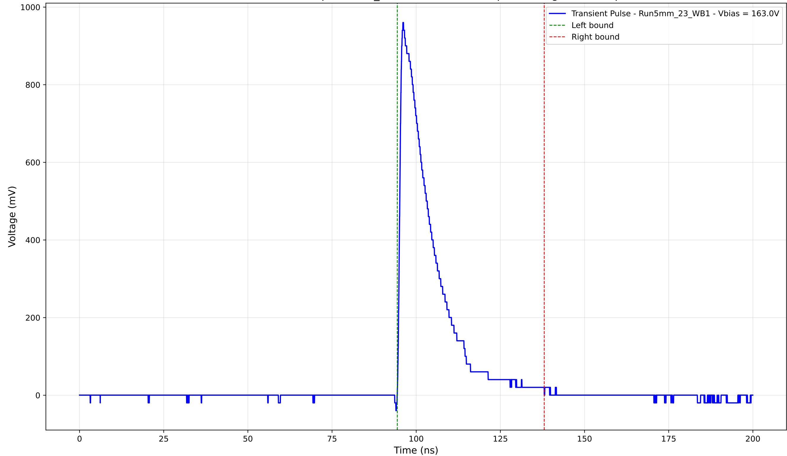
Transient Pulse - Sample: 5mm_23 - Position: 1105.0 \mu\text{m} - Charge: 201.32 pC
