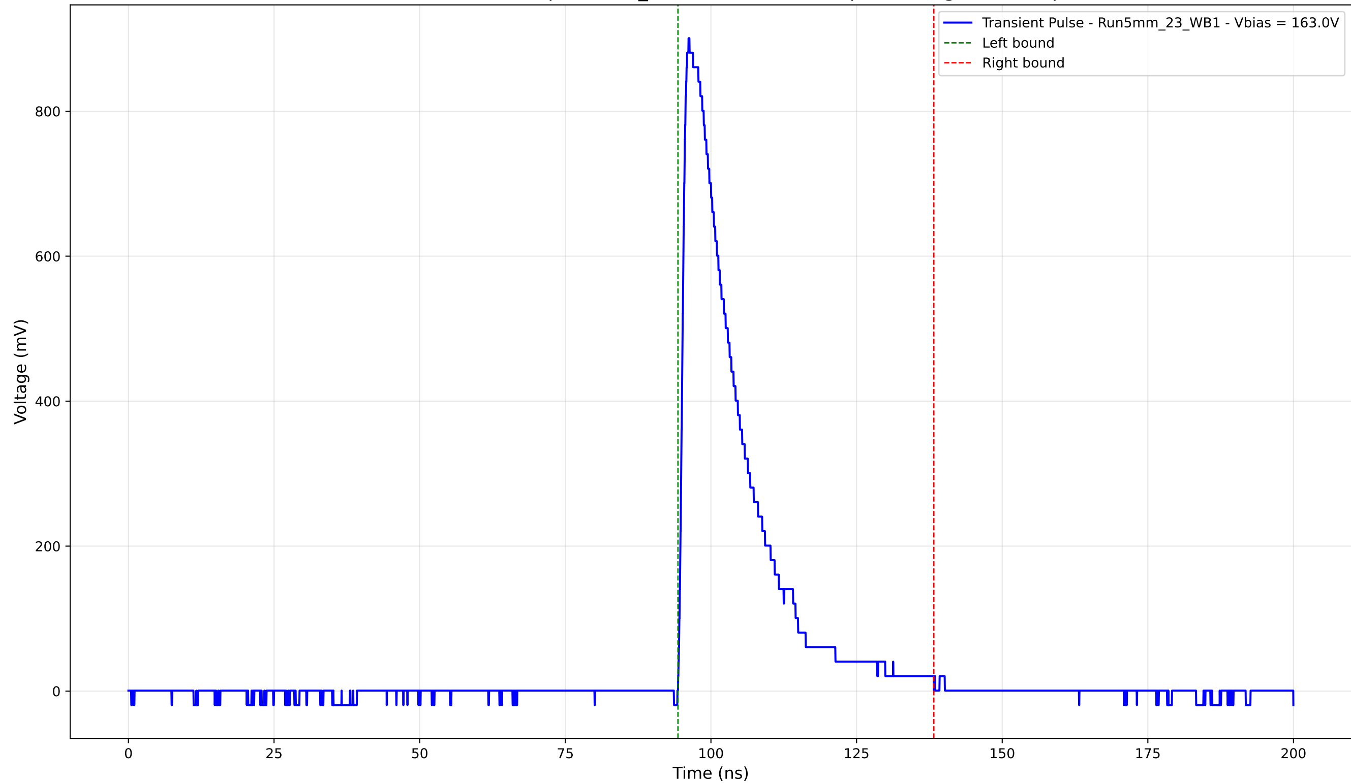
Transient Pulse - Sample: 5mm_23 - Position: 3870.0 \mu\text{m} - Charge: 193.67 pC
