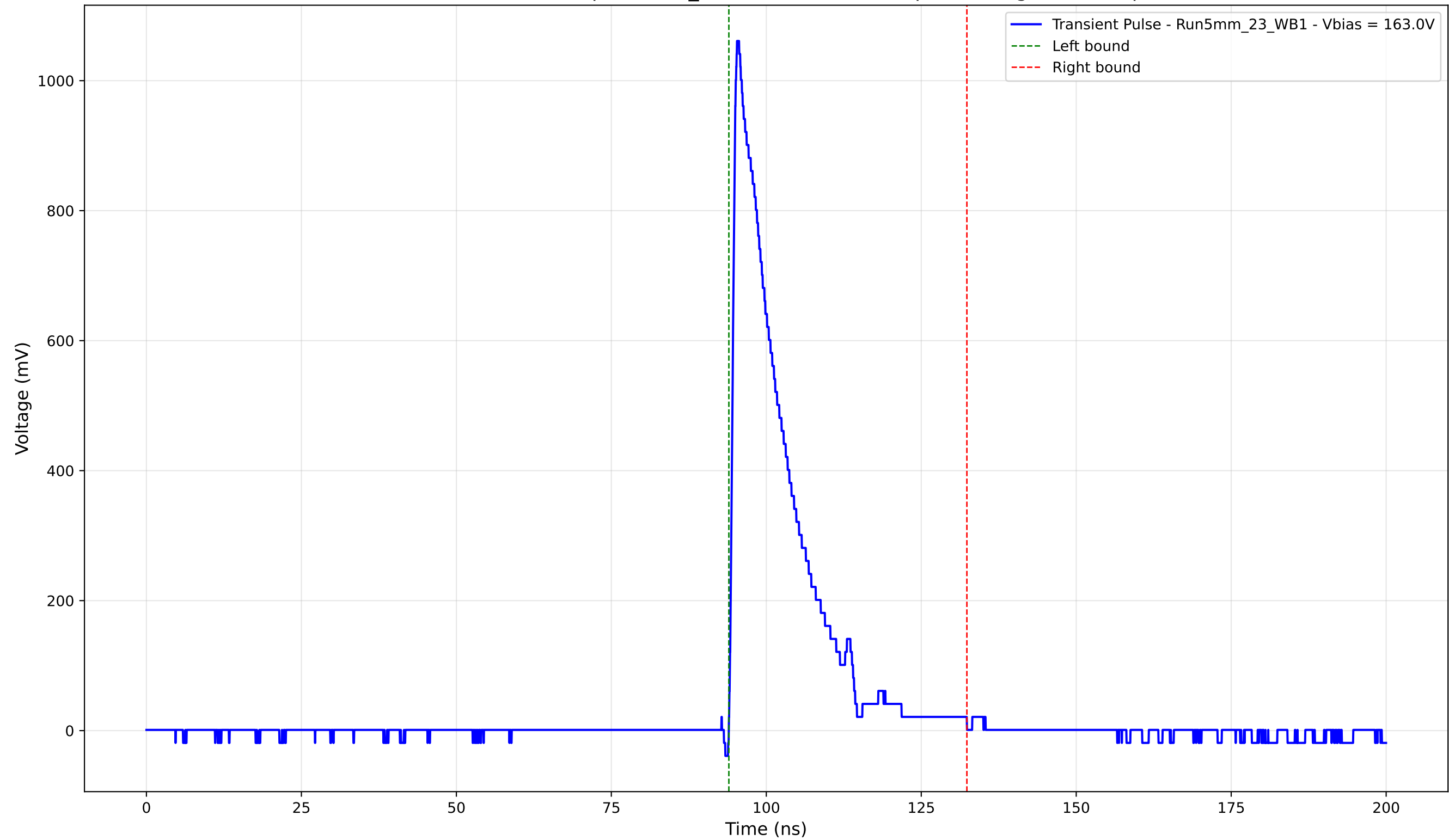
Transient Pulse - Sample: 5mm_23 - Position: 5080.0 \mu\text{m} - Charge: 187.18 pC
