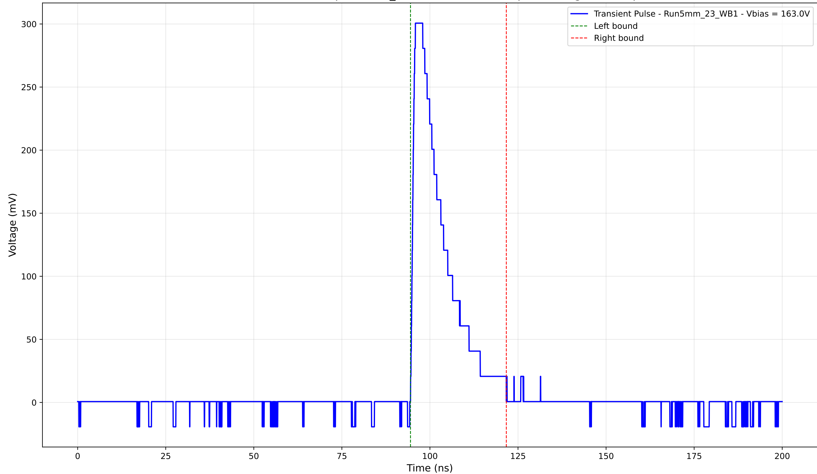
Transient Pulse - Sample: 5mm_23 - Position: 3780.0 \mu\text{m} - Charge: 58.93 pC
