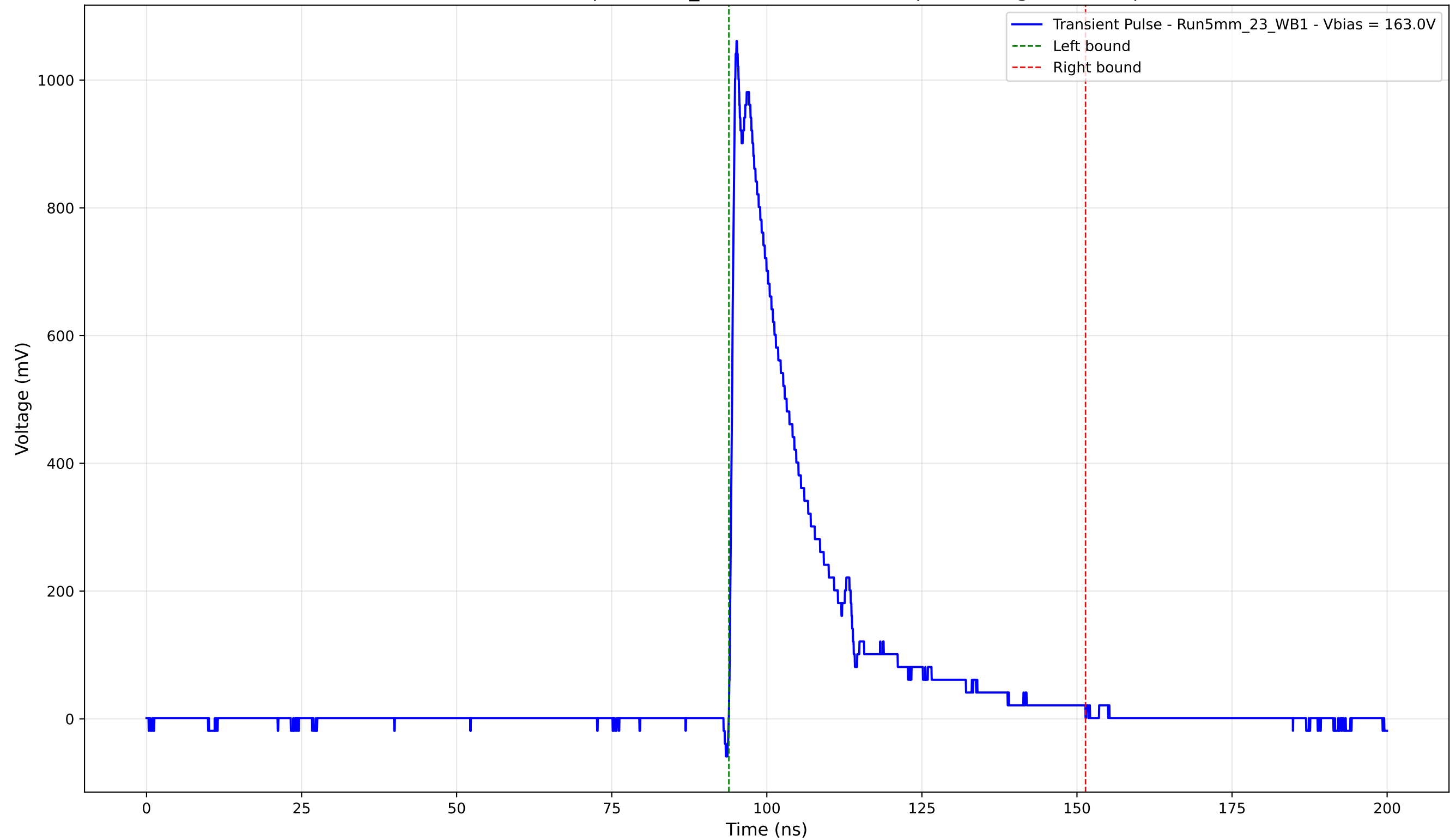
Transient Pulse - Sample: 5mm_23 - Position: 2570.0 \mu\text{m} - Charge: 241.87 pC
