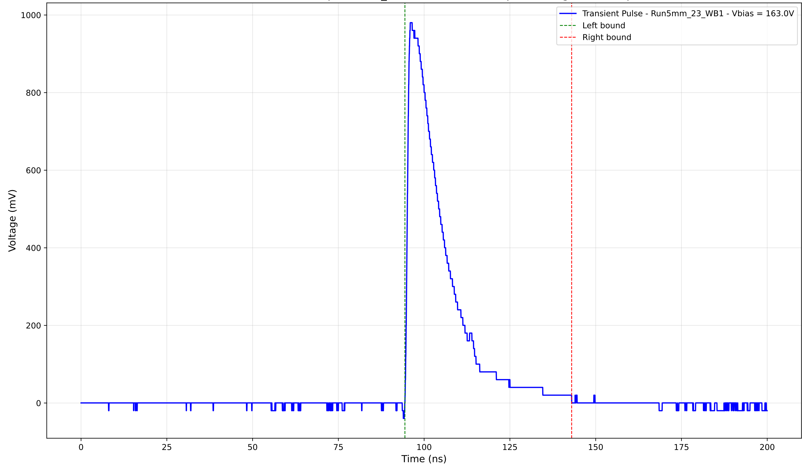
Transient Pulse - Sample: 5mm_23 - Position: 1410.0 \mu\text{m} - Charge: 232.40 pC
