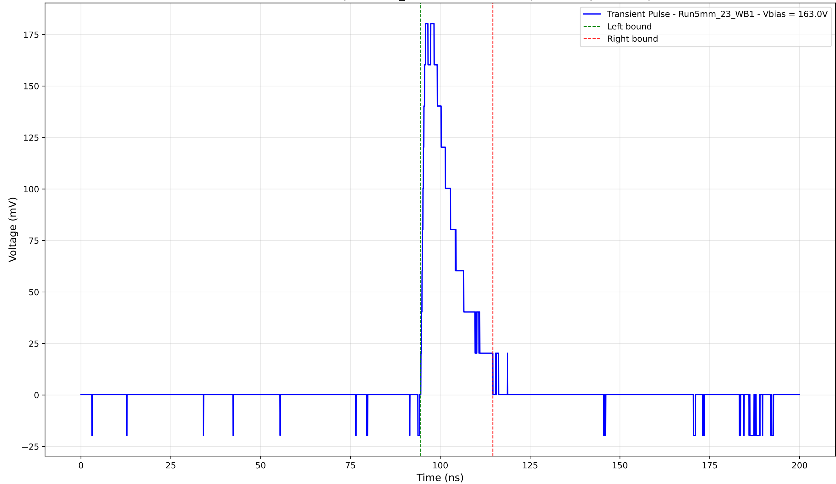
Transient Pulse - Sample: 5mm_23 -Position: 4265.0 \mu\text{m} - Charge: 32.33 pC
