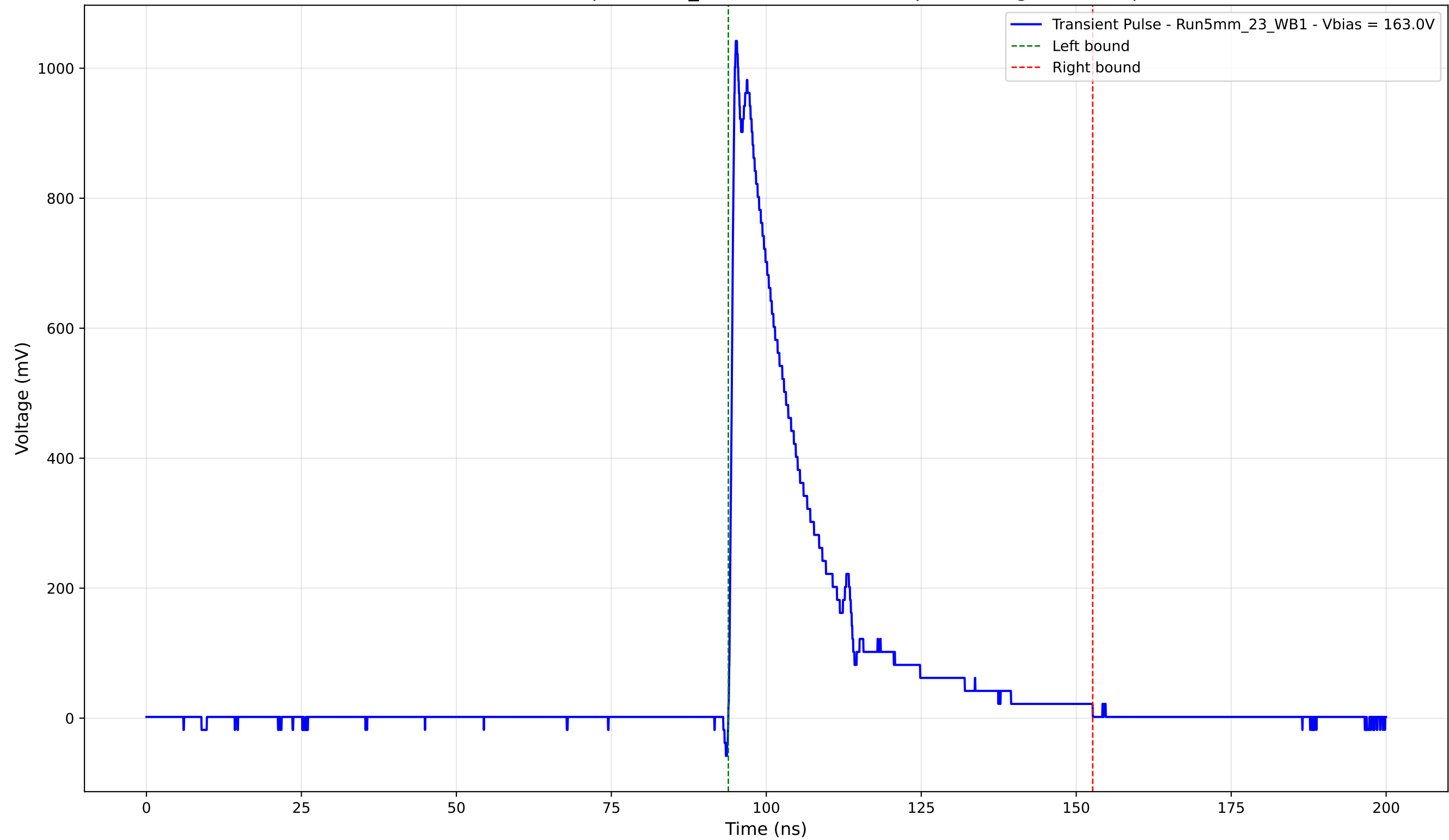
Transient Pulse - Sample: 5mm_23 - Position: 2540.0 \mu\text{m} - Charge: 240.49 pC
