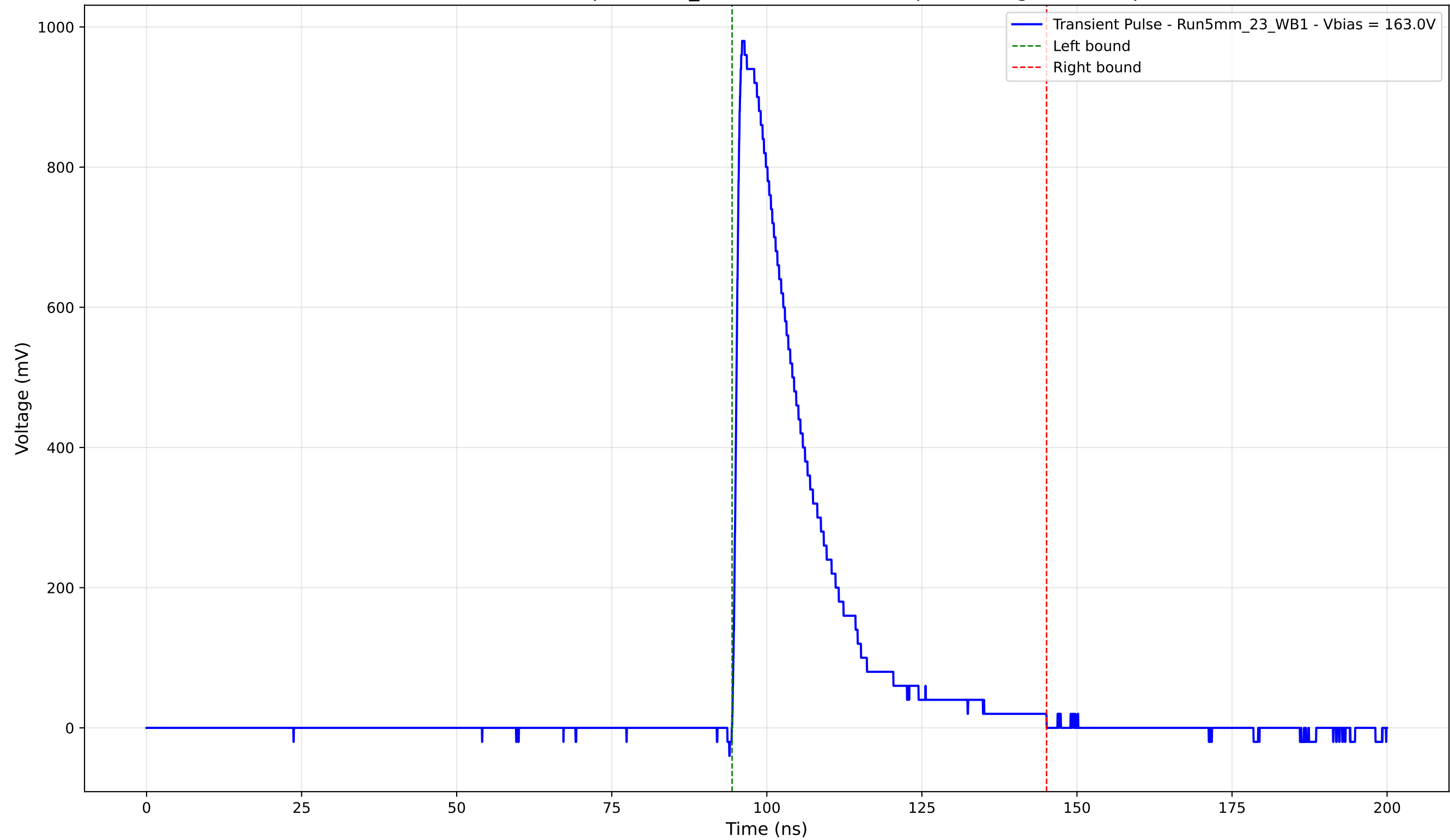
Transient Pulse - Sample: 5mm_23 - Position: 1395.0 \mu\text{m} - Charge: 229.70 pC
