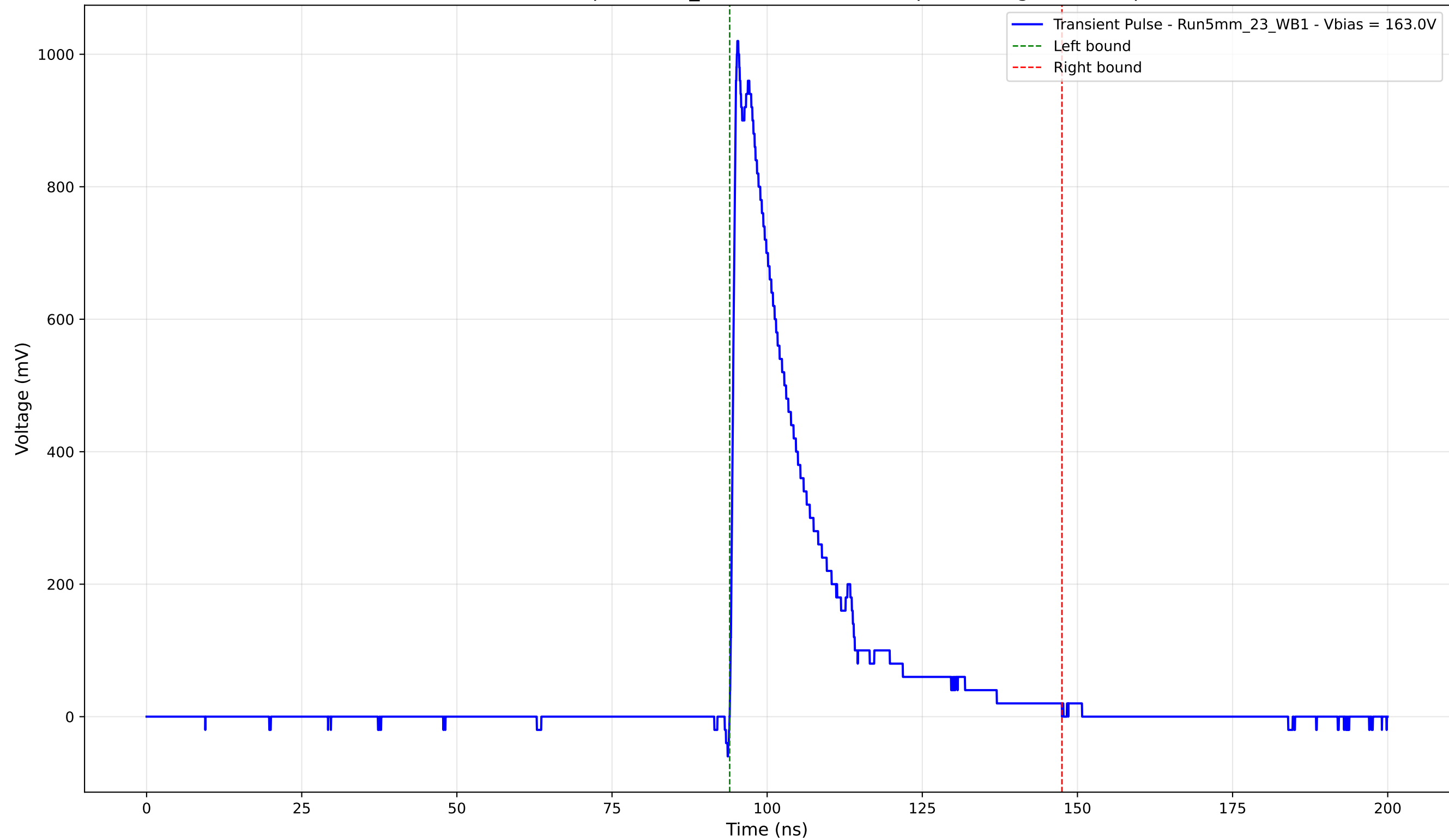
Transient Pulse - Sample: 5mm_23 - Position: 3040.0 \mu\text{m} - Charge: 229.11 pC
