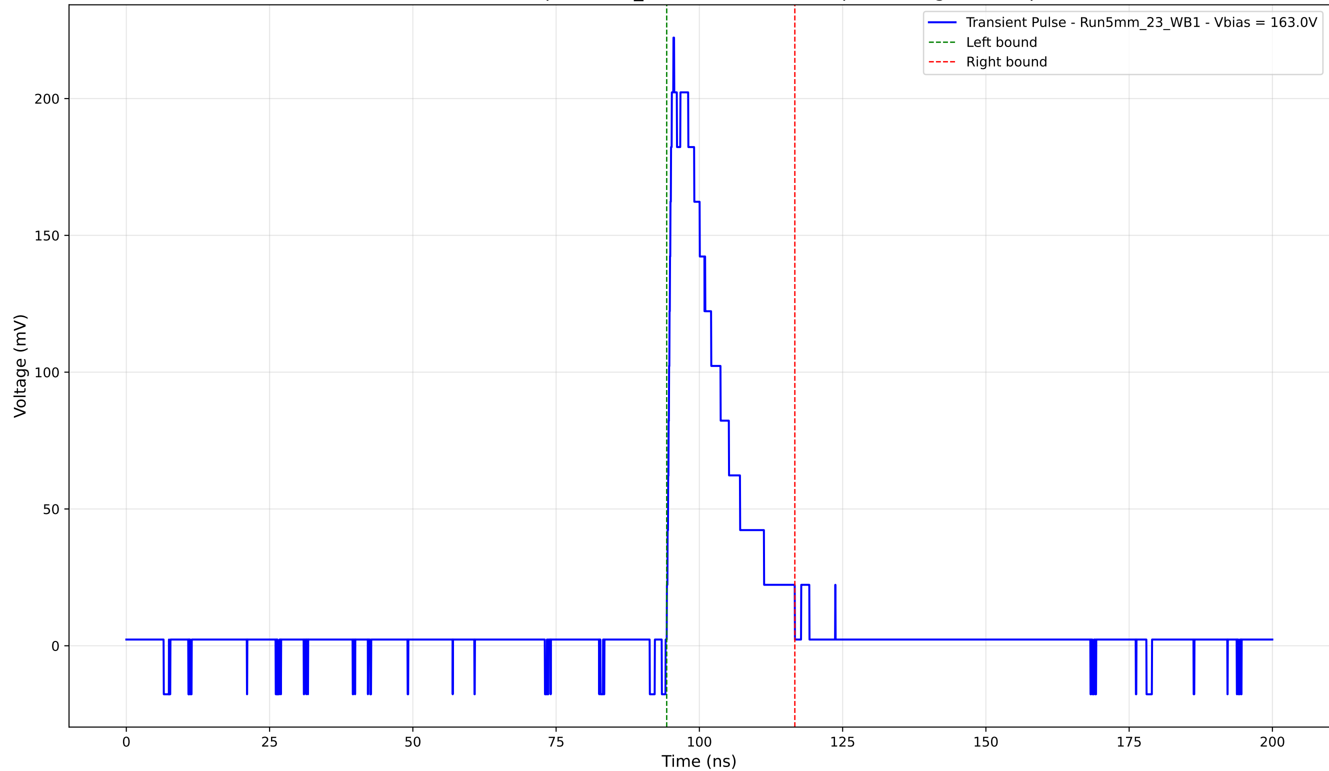
Transient Pulse - Sample: 5mm_23 - Position: 3255.0 \mu\text{m} - Charge: 39.54 pC
