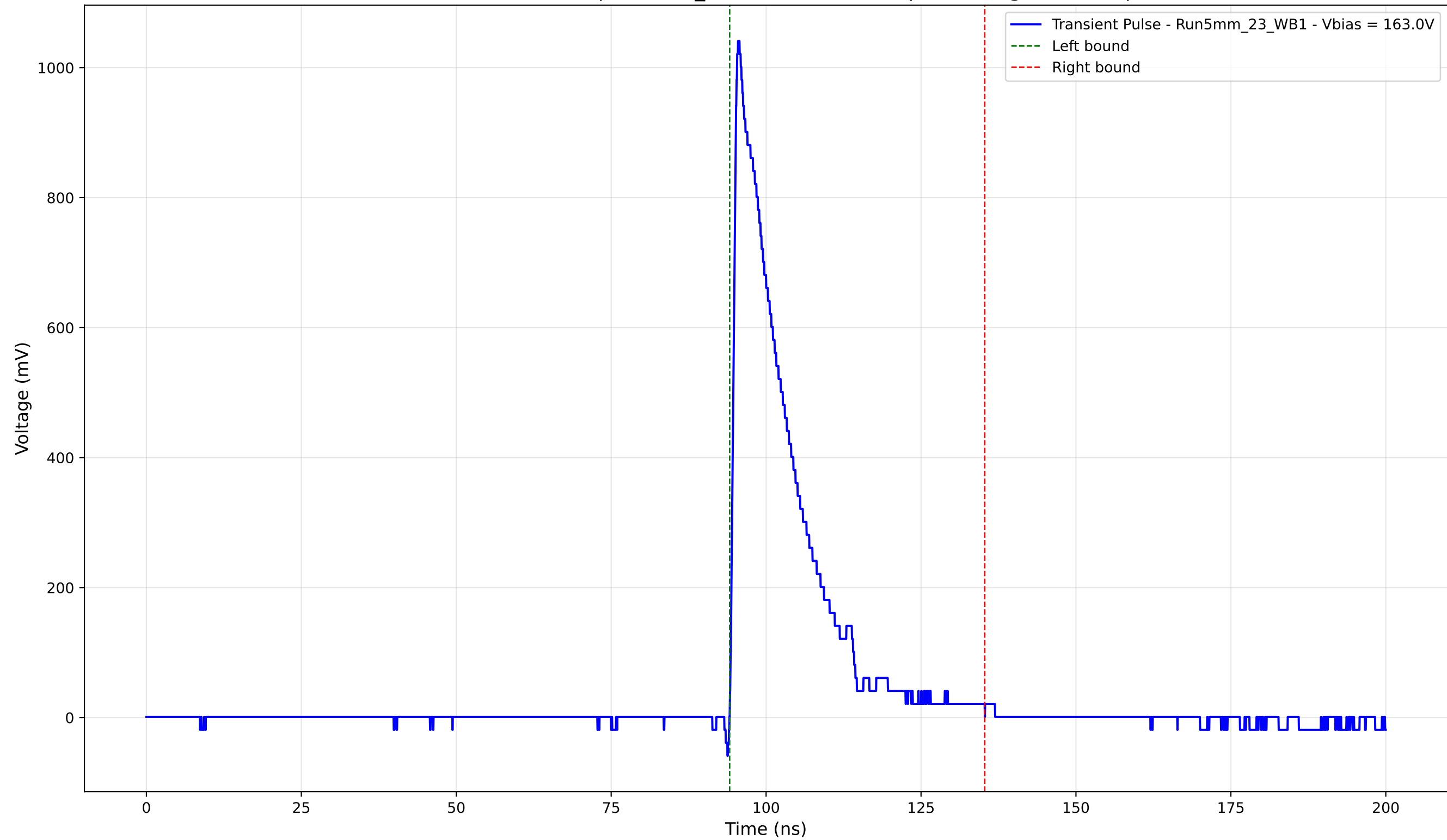
Transient Pulse - Sample: 5mm_23 - Position: 485.0 \mu\text{m} - Charge: 194.86 pC
