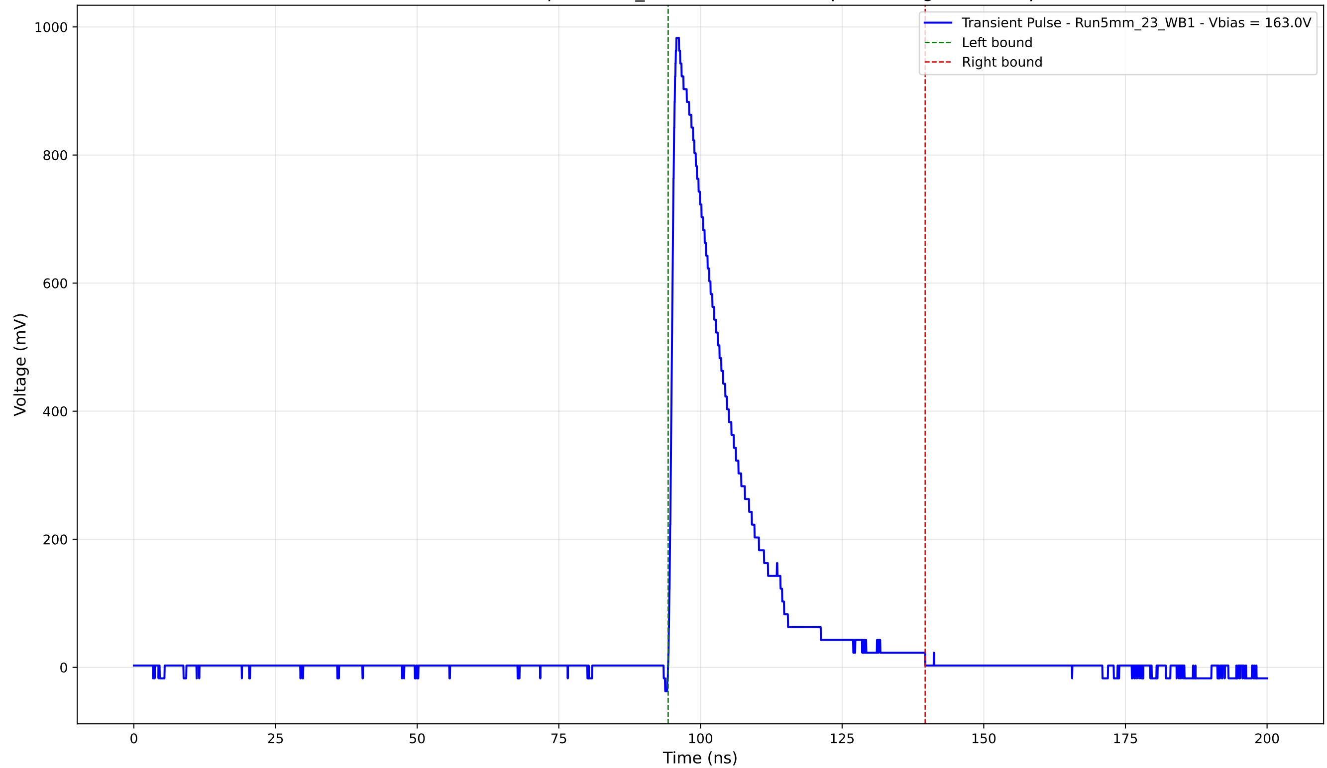
Transient Pulse - Sample: 5mm_23 - Position: 870.0 \mu\text{m} - Charge: 207.91 pC
