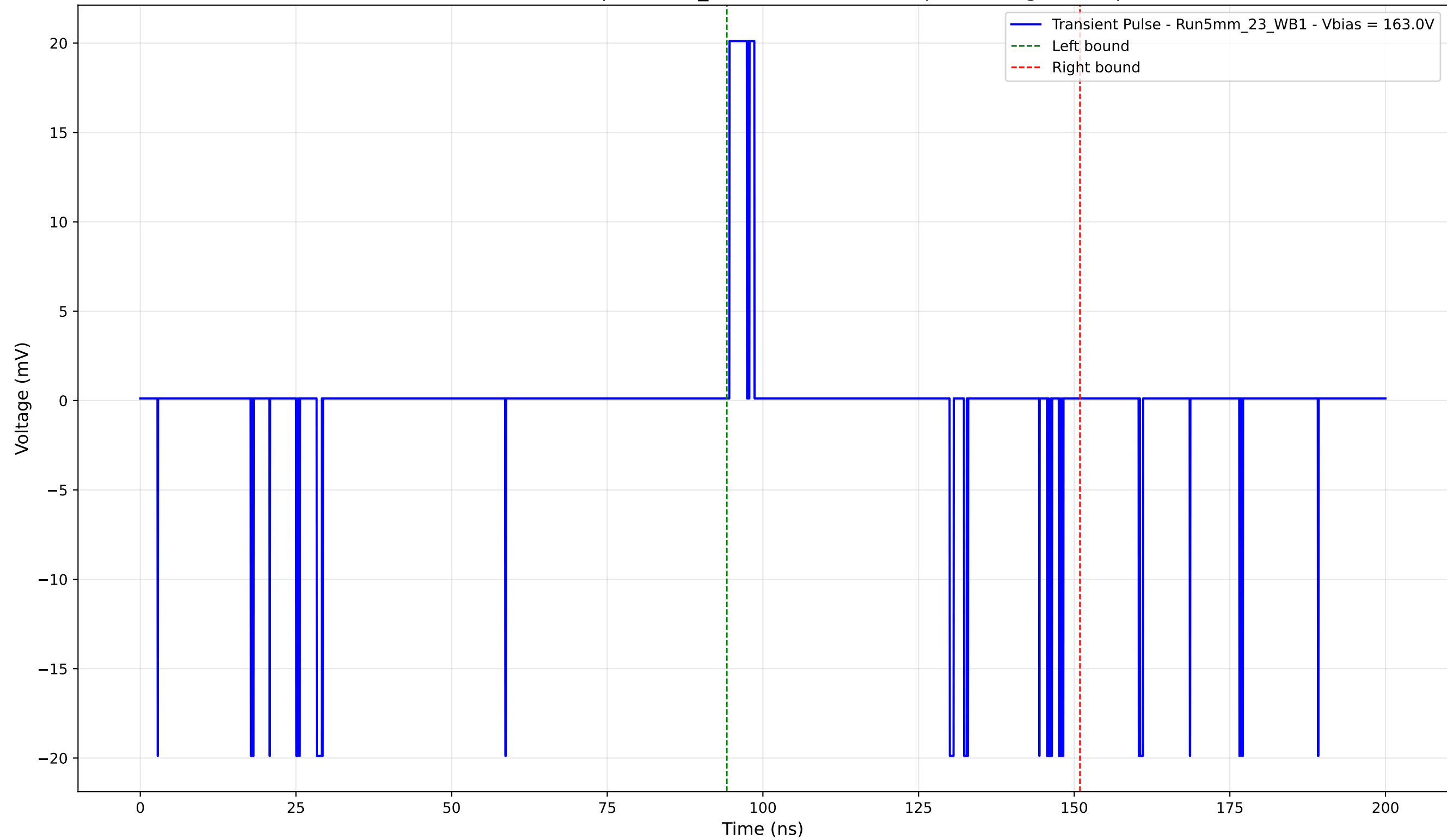
Transient Pulse - Sample: 5mm_23 - Position: 5260.0 \mu\text{m} - Charge: 0.70 pC
