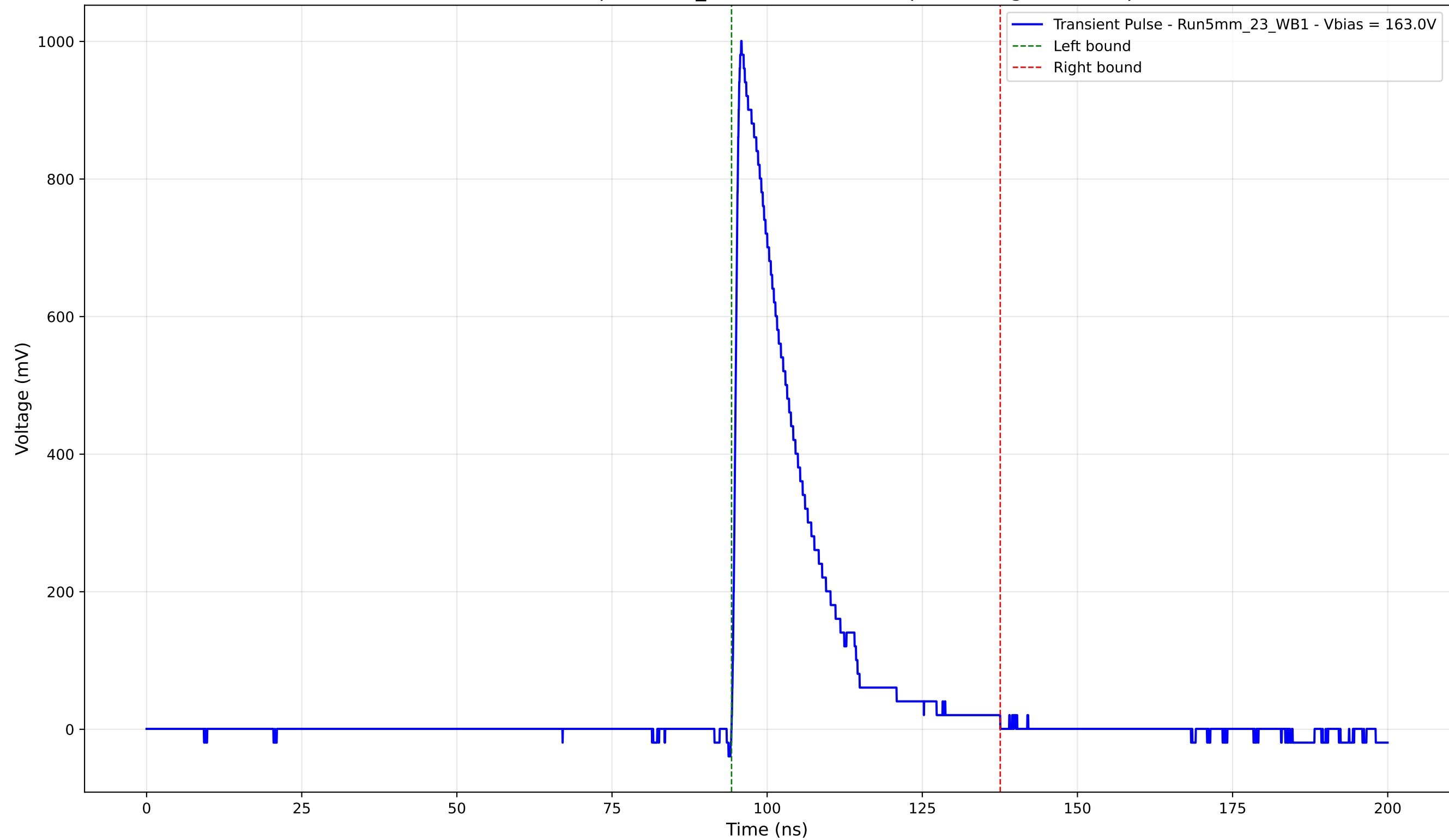
Transient Pulse - Sample: 5mm_23 - Position: 815.0 \mu\text{m} - Charge: 202.34 pC
