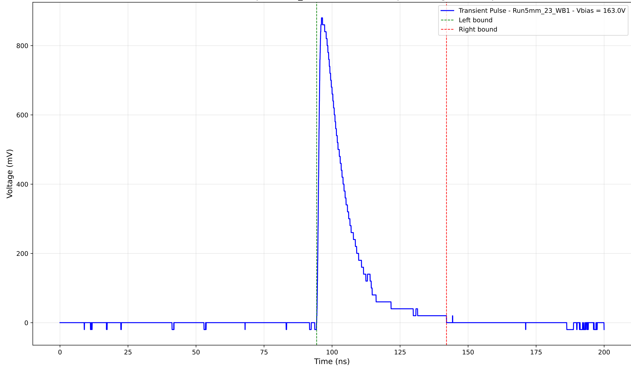
Transient Pulse - Sample: 5mm_23 - Position: 3855.0 \mu\text{m} - Charge: 190.70 pC
