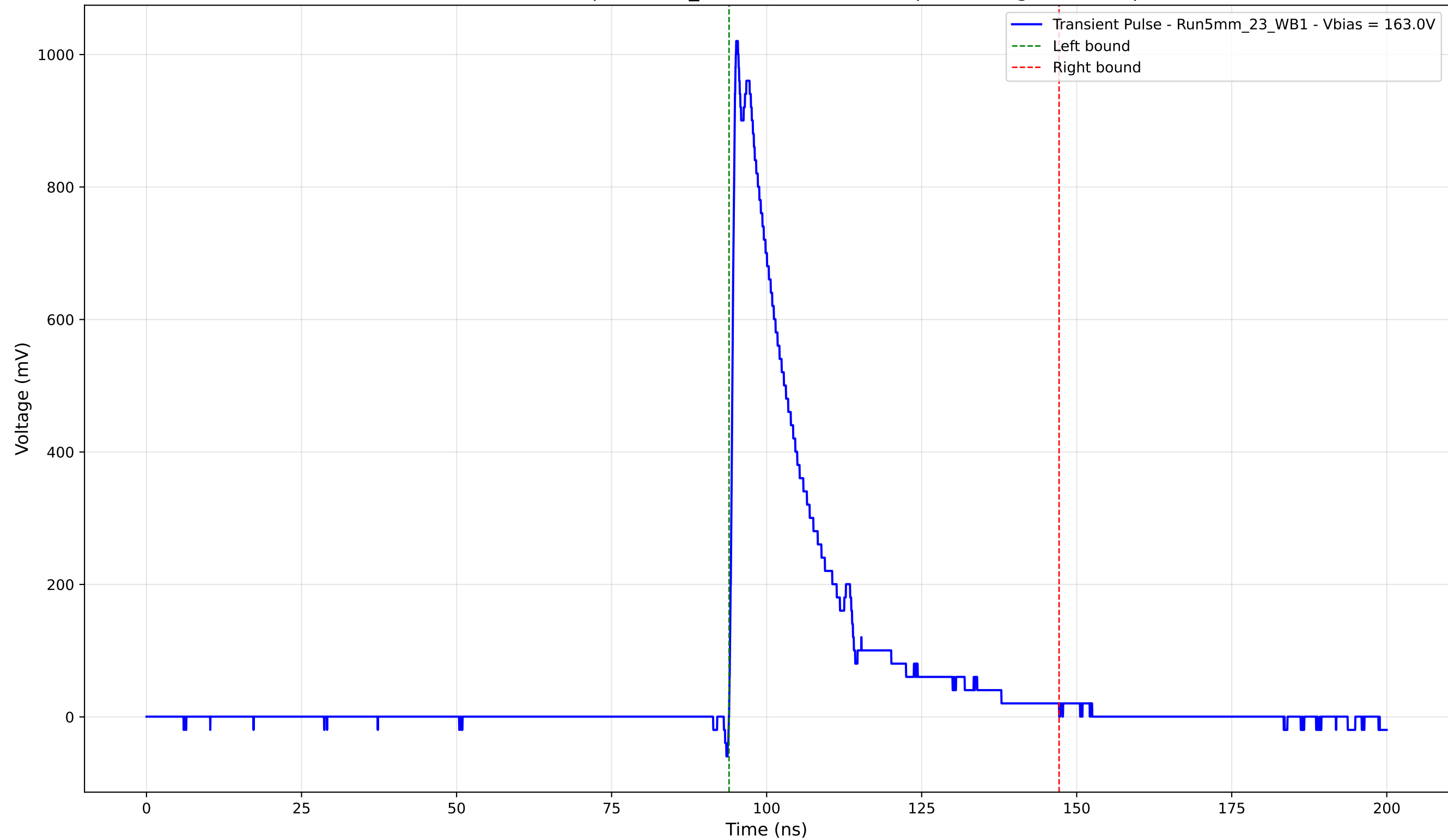
Transient Pulse - Sample: 5mm_23 - Position: 2990.0 \mu\text{m} - Charge: 231.78 pC
