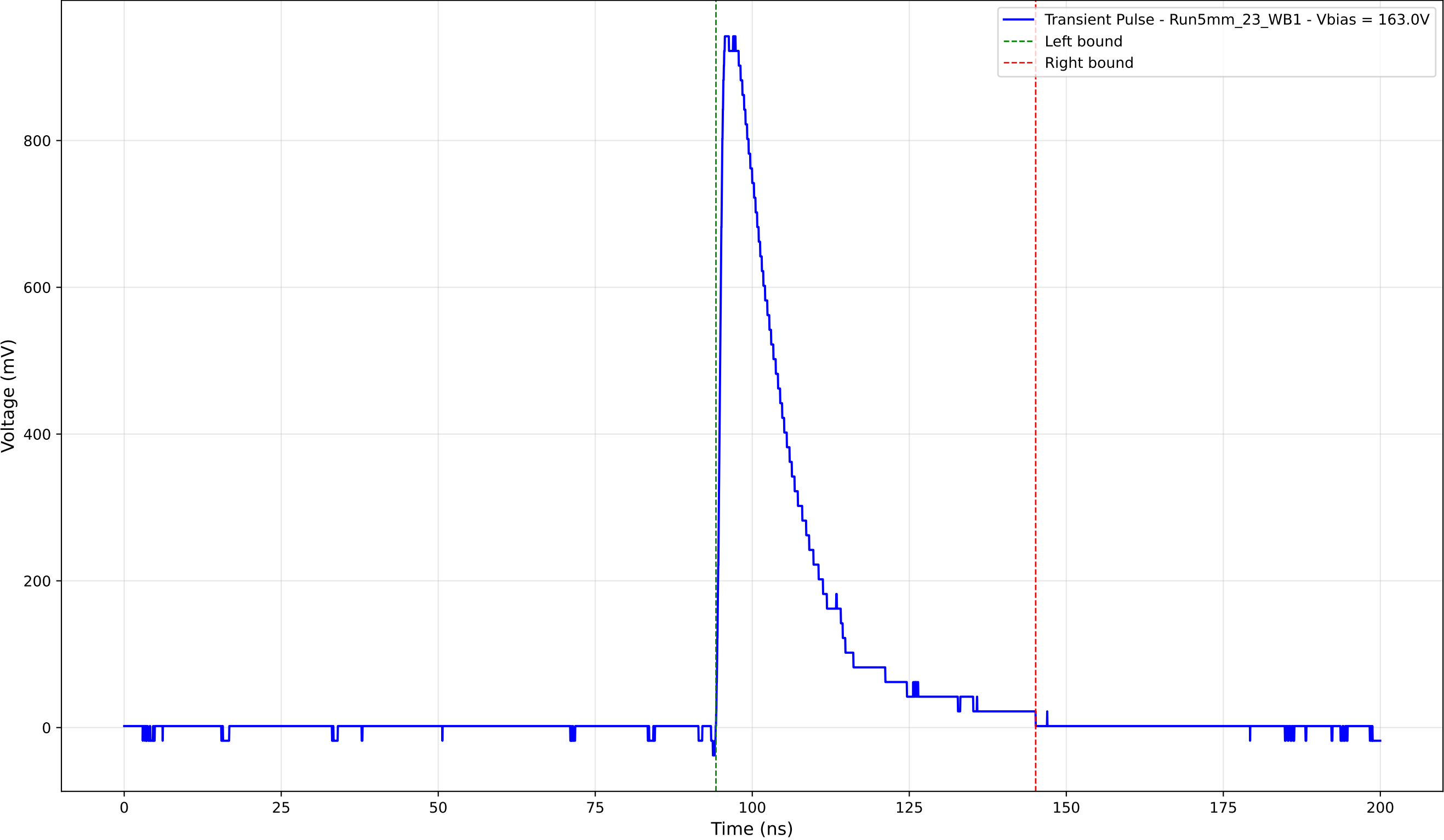
Transient Pulse - Sample: 5mm_23 - Position: 3525.0 \mu\text{m} - Charge: 224.80 pC
