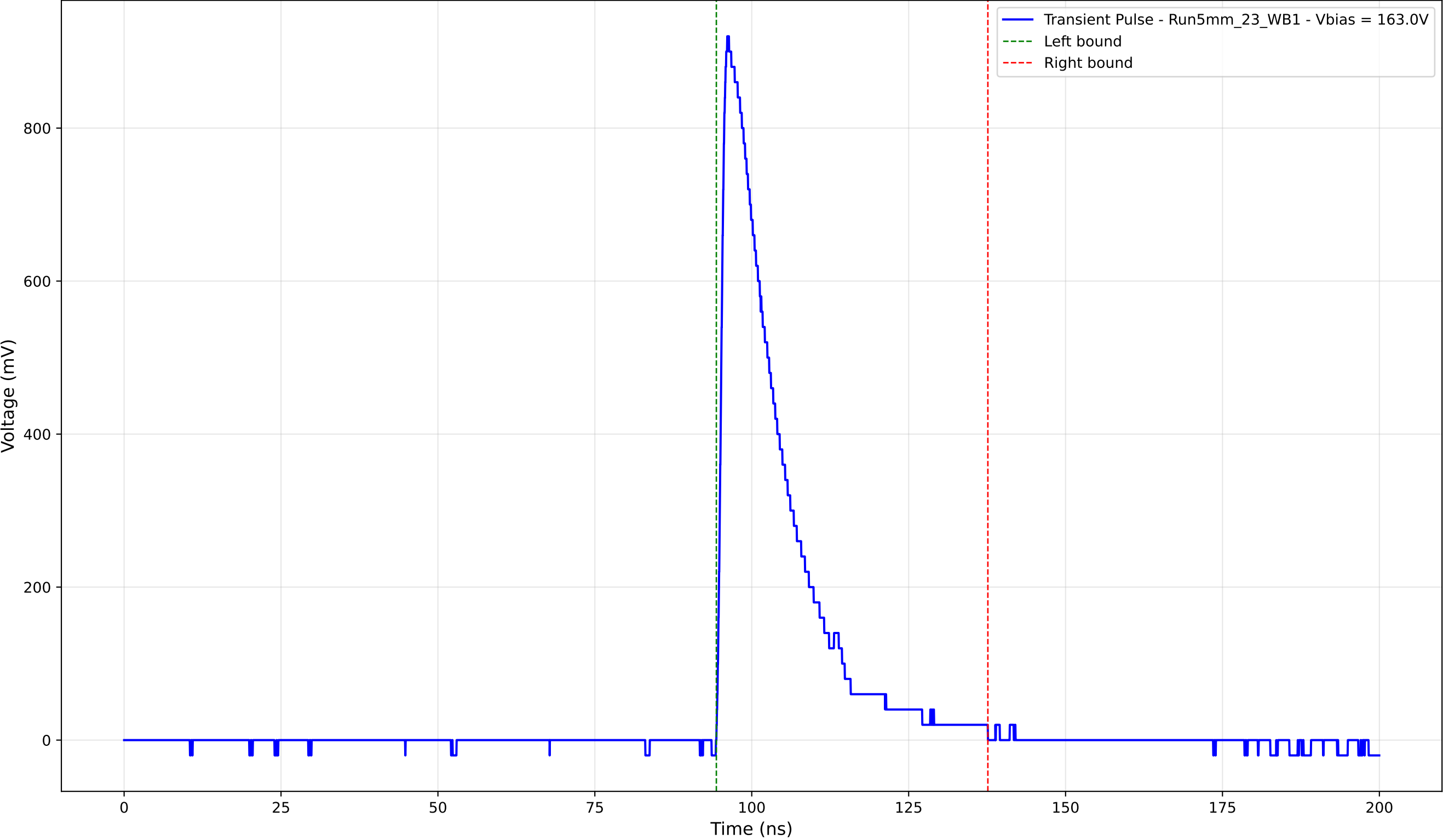
Transient Pulse - Sample: 5mm_23 - Position: 4150.0 \mu\text{m} - Charge: 190.05 pC
