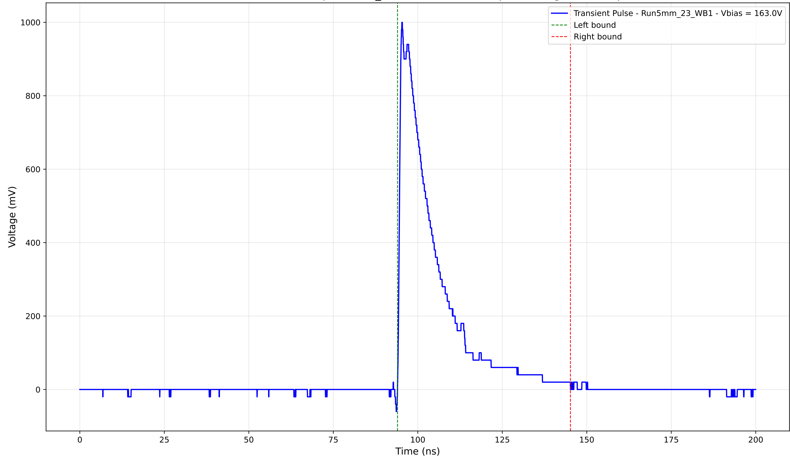
Transient Pulse - Sample: 5mm_23 - Position: 3110.0 \mu\text{m} - Charge: 222.44 pC
