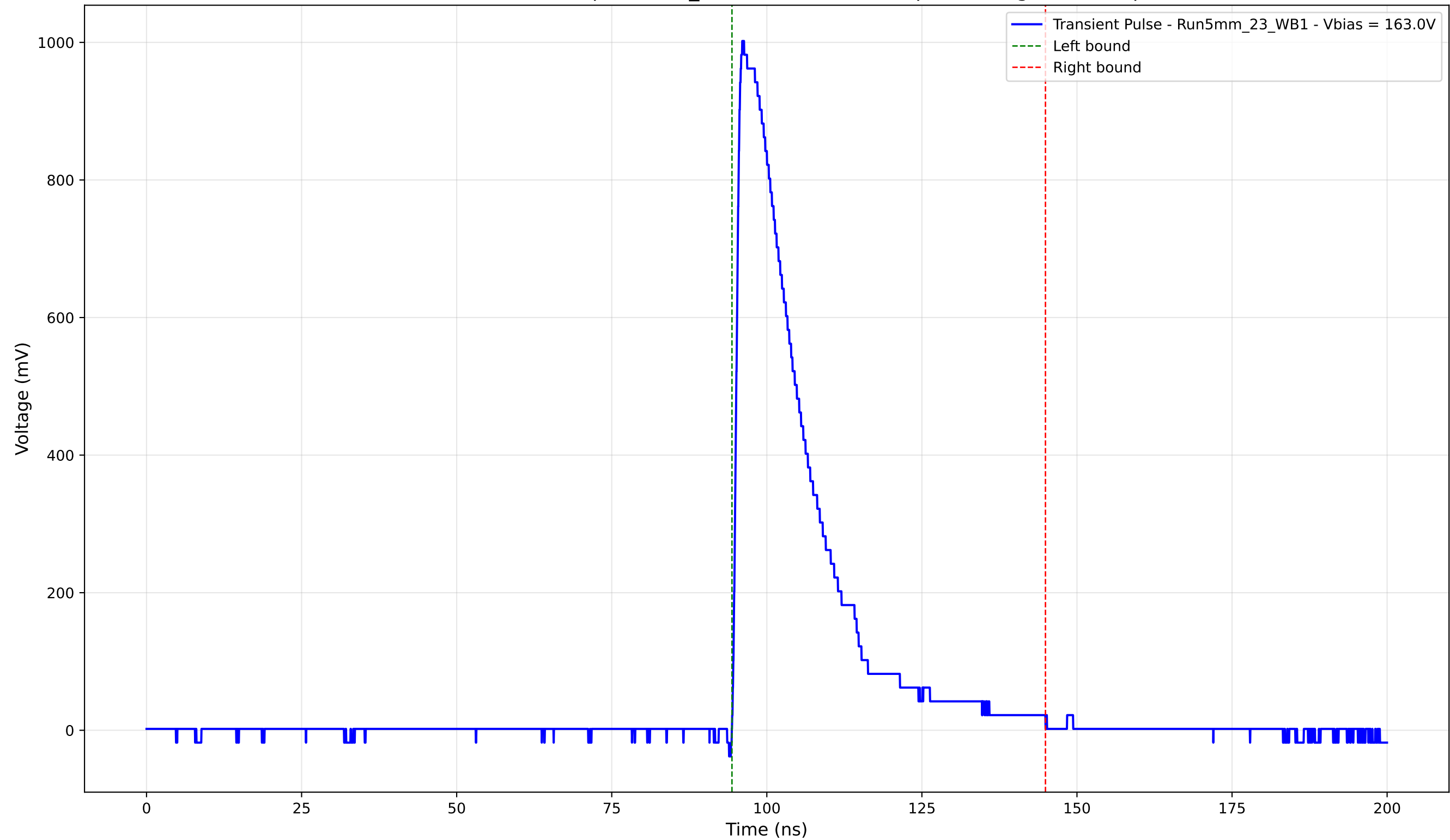
Transient Pulse - Sample: 5mm_23 - Position: 1450.0 \mu\text{m} - Charge: 242.02 pC
