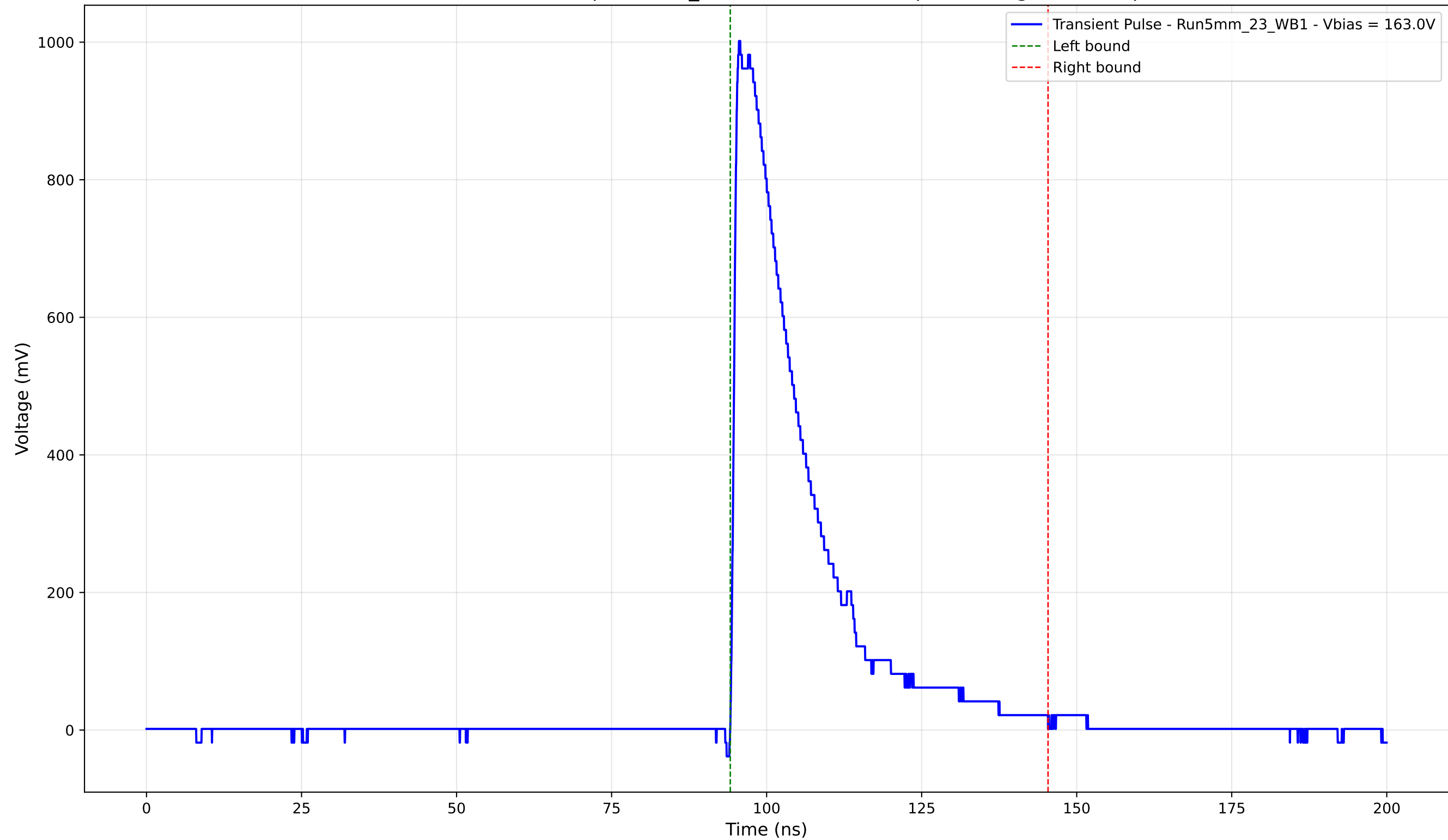
Transient Pulse - Sample: 5mm_23 - Position: 2100.0 \mu\text{m} - Charge: 247.54 pC
