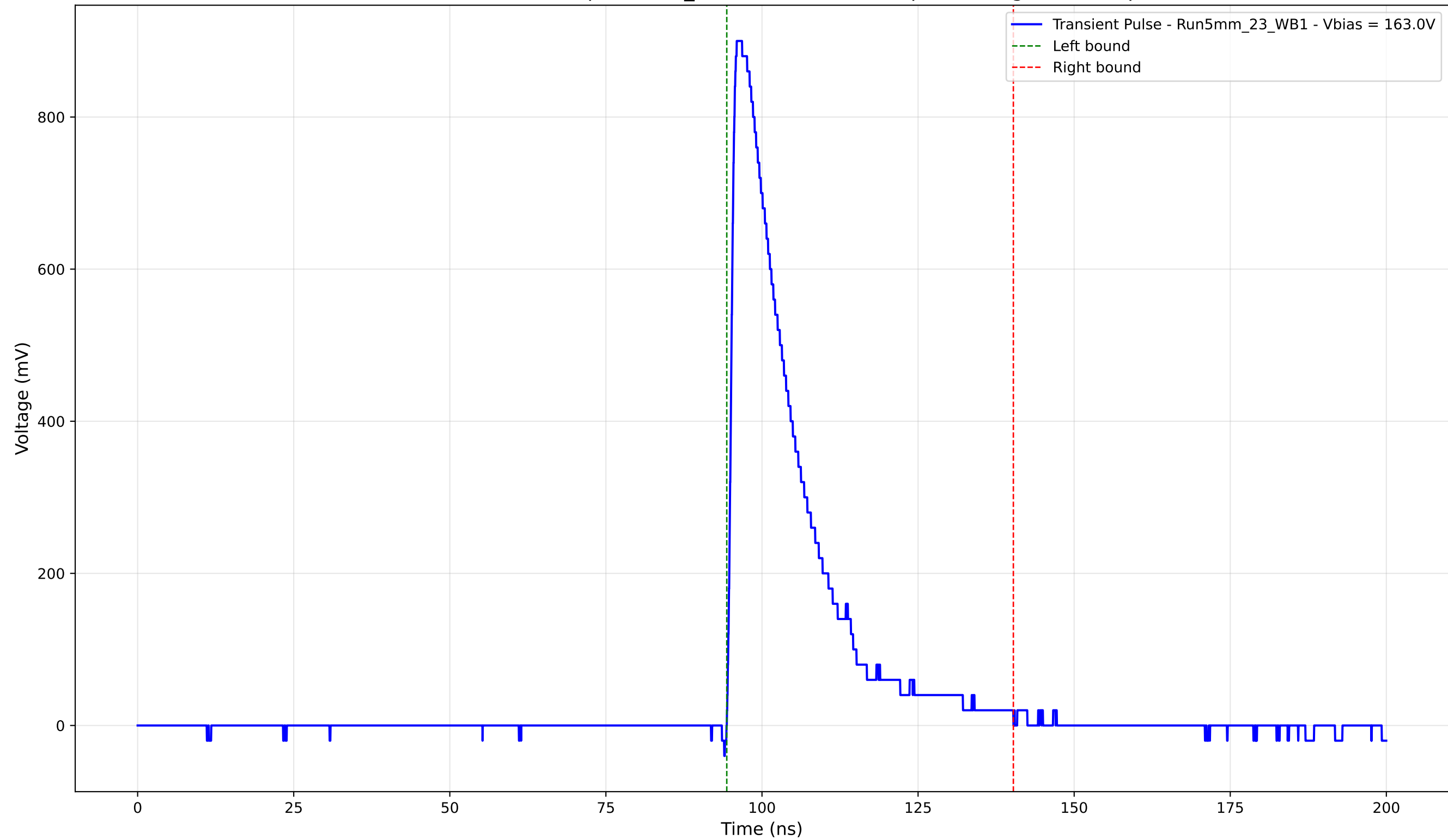
Transient Pulse - Sample: 5mm_23 - Position: 1650.0 \mu\text{m} - Charge: 201.32 pC
