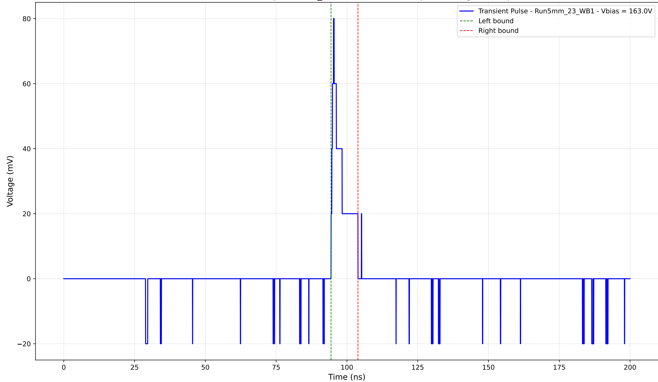
Transient Pulse - Sample: 5mm_23 - Position: 5220.0 \mu\text{m} - Charge: 5.90 pC
