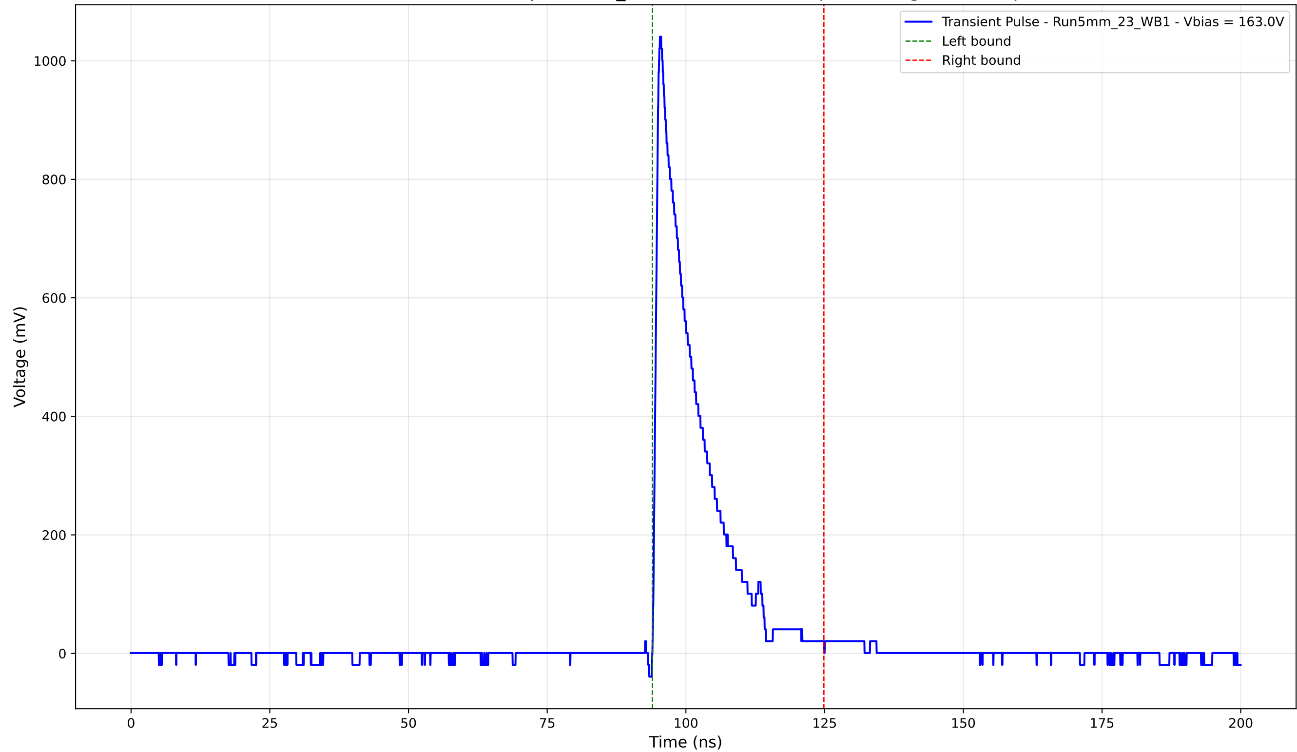
Transient Pulse - Sample: 5mm_23 - Position: 5120.0 \mu\text{m} - Charge: 163.23 pC
