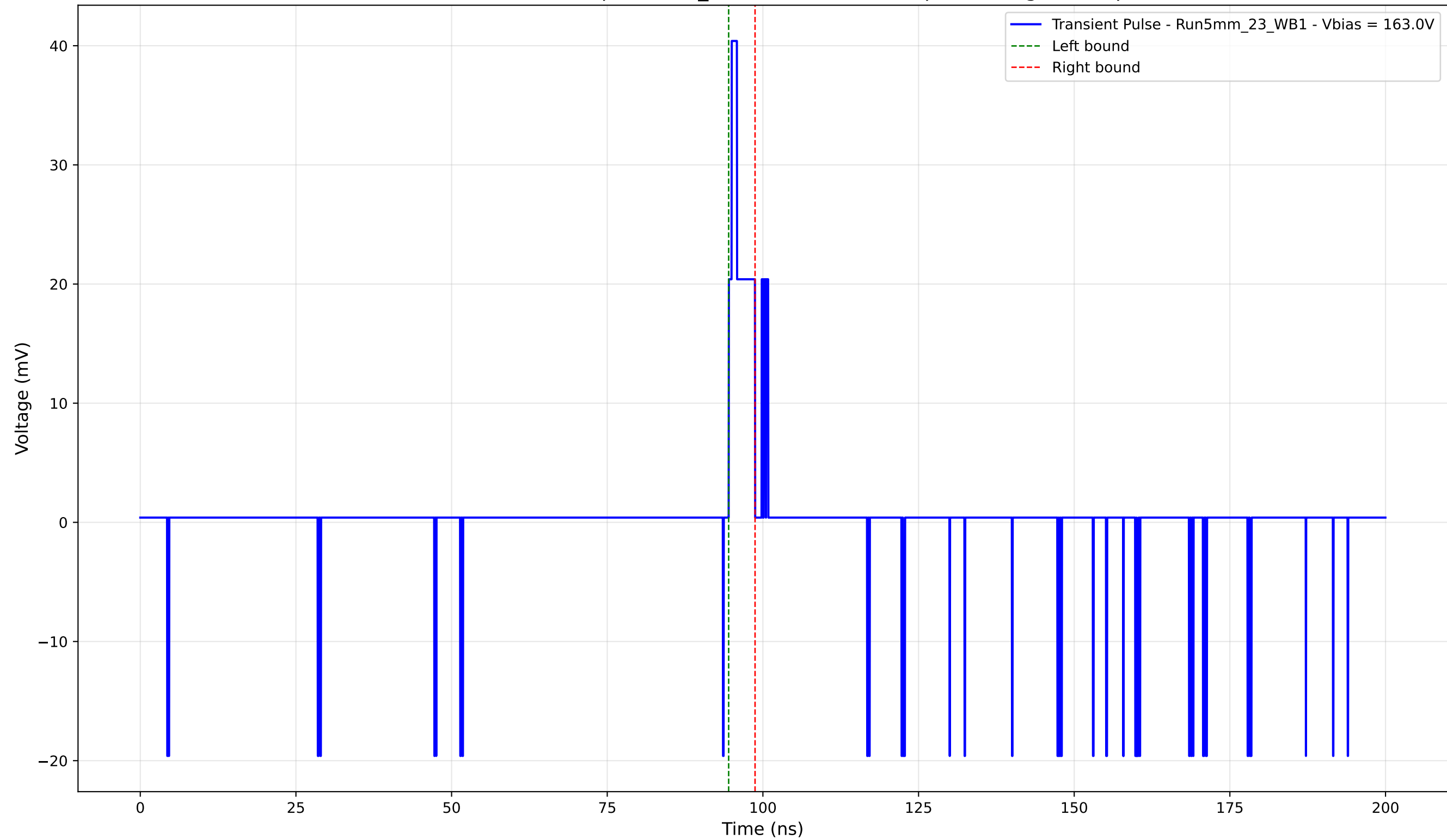
Transient Pulse - Sample: 5mm_23 - Position: 5250.0 \mu\text{m} - Charge: 2.07 pC
