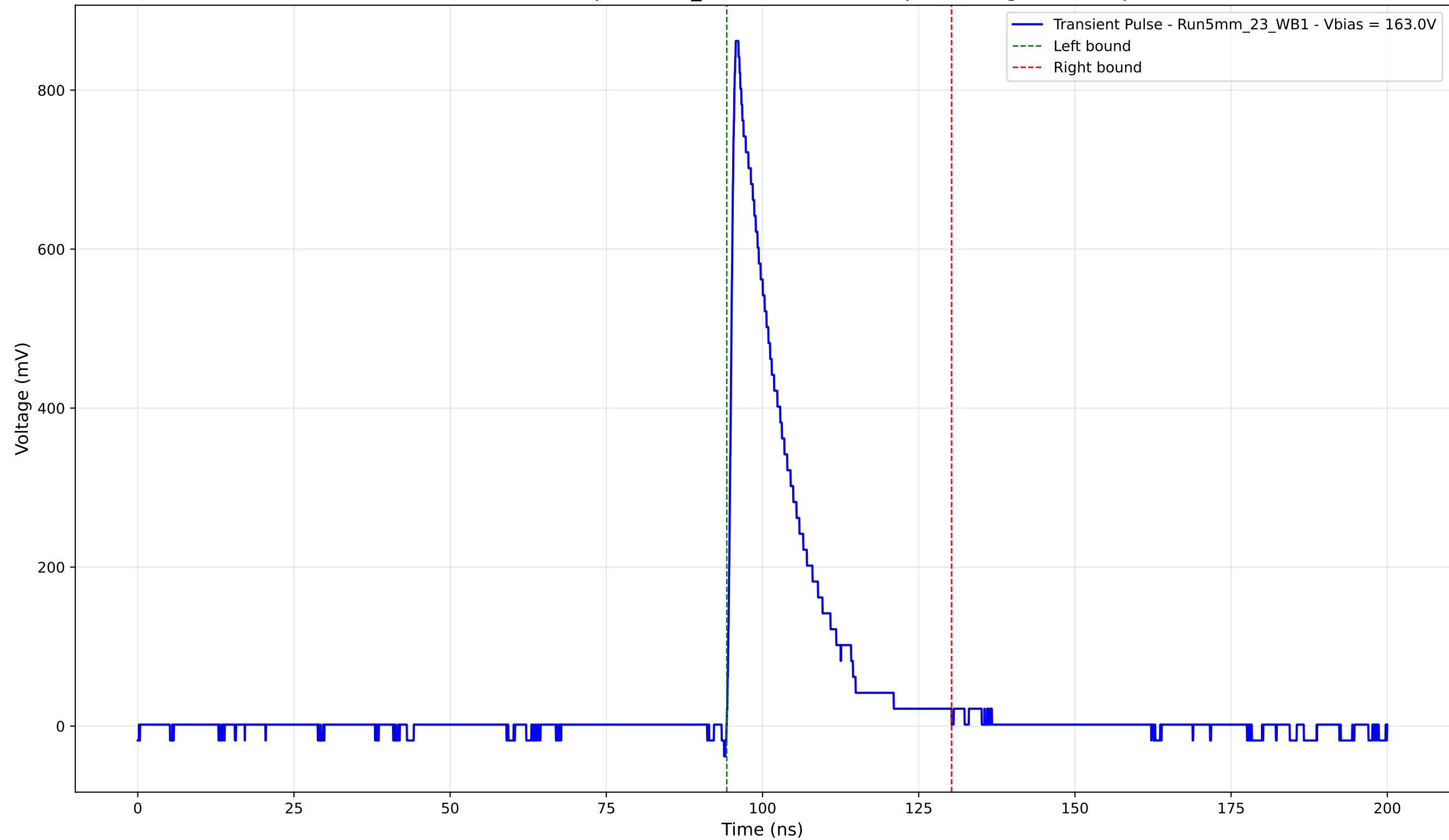
Transient Pulse - Sample: 5mm_23 - Position: 780.0 \mu\text{m} - Charge: 154.78 pC
