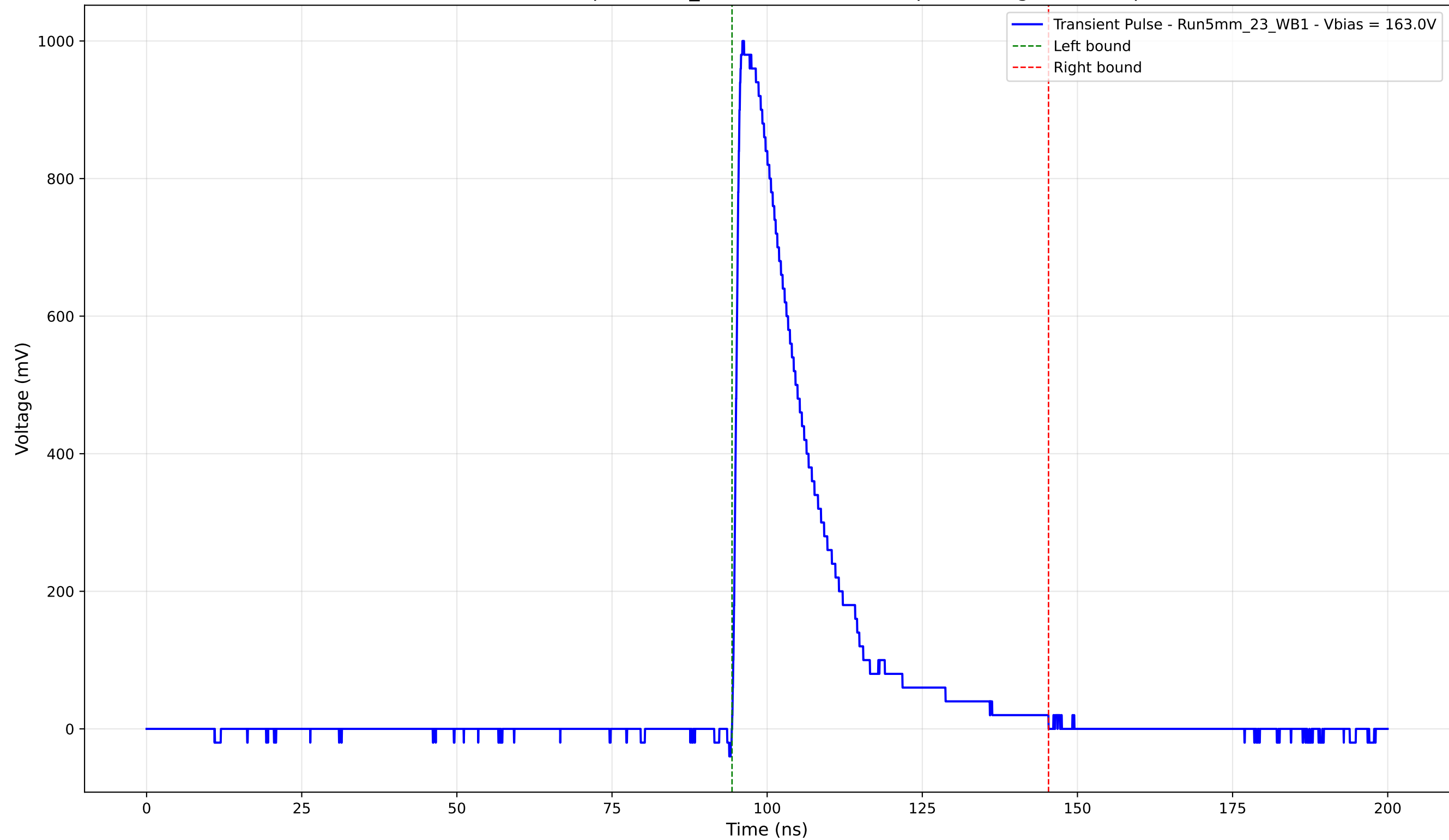
Transient Pulse - Sample: 5mm_23 - Position: 1620.0 \mu\text{m} - Charge: 245.11 pC
