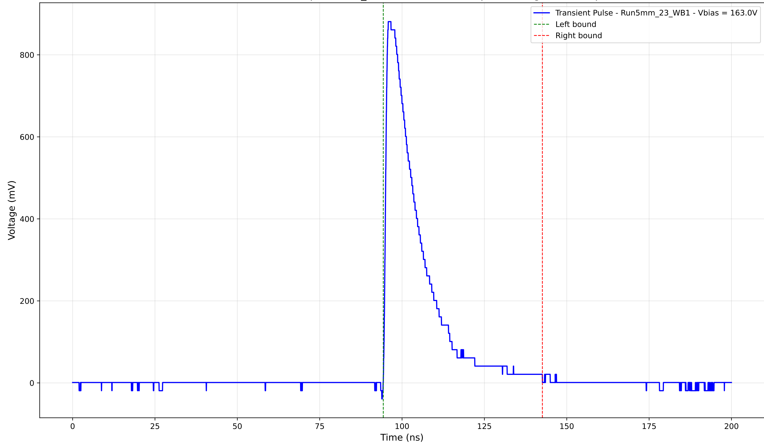
Transient Pulse - Sample: 5mm_23 - Position: 1810.0 \mu\text{m} - Charge: 200.10 pC
