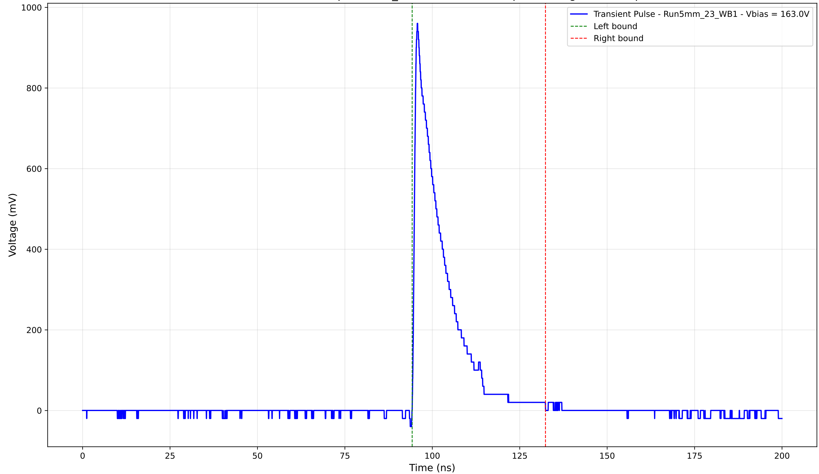
Transient Pulse - Sample: 5mm_23 - Position: 655.0 \mu\text{m} - Charge: 164.91 pC
