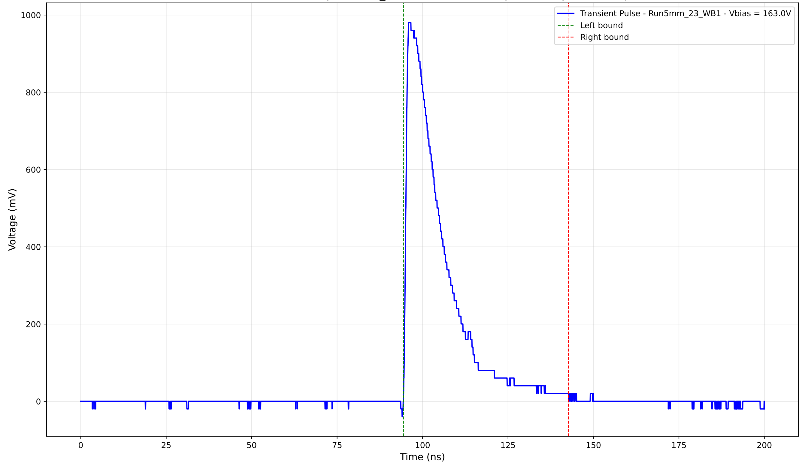
Transient Pulse - Sample: 5mm_23 - Position: 1415.0 \mu\text{m} - Charge: 234.19 pC
