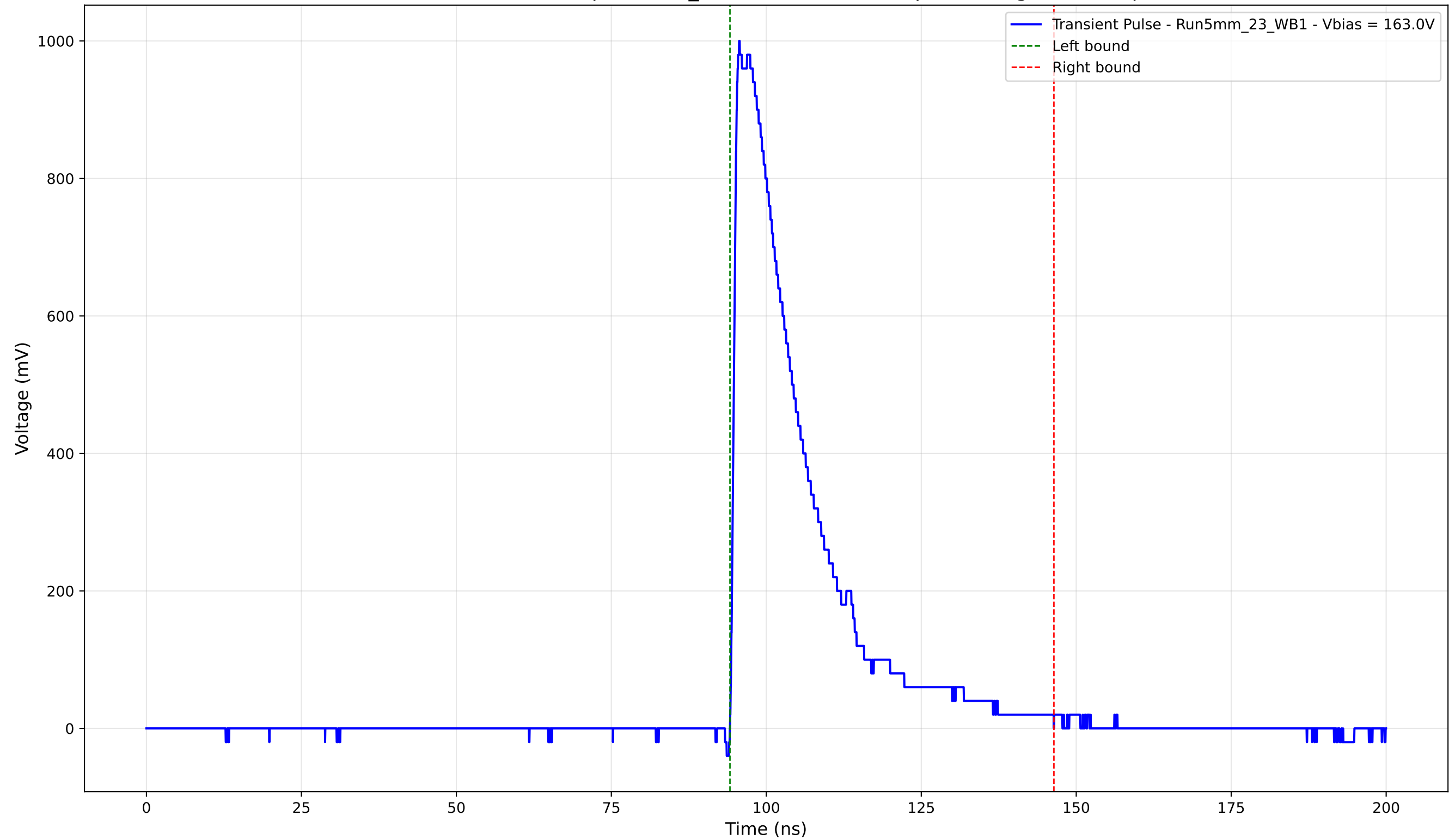
Transient Pulse - Sample: 5mm_23 - Position: 2075.0 \mu\text{m} - Charge: 246.22 pC
