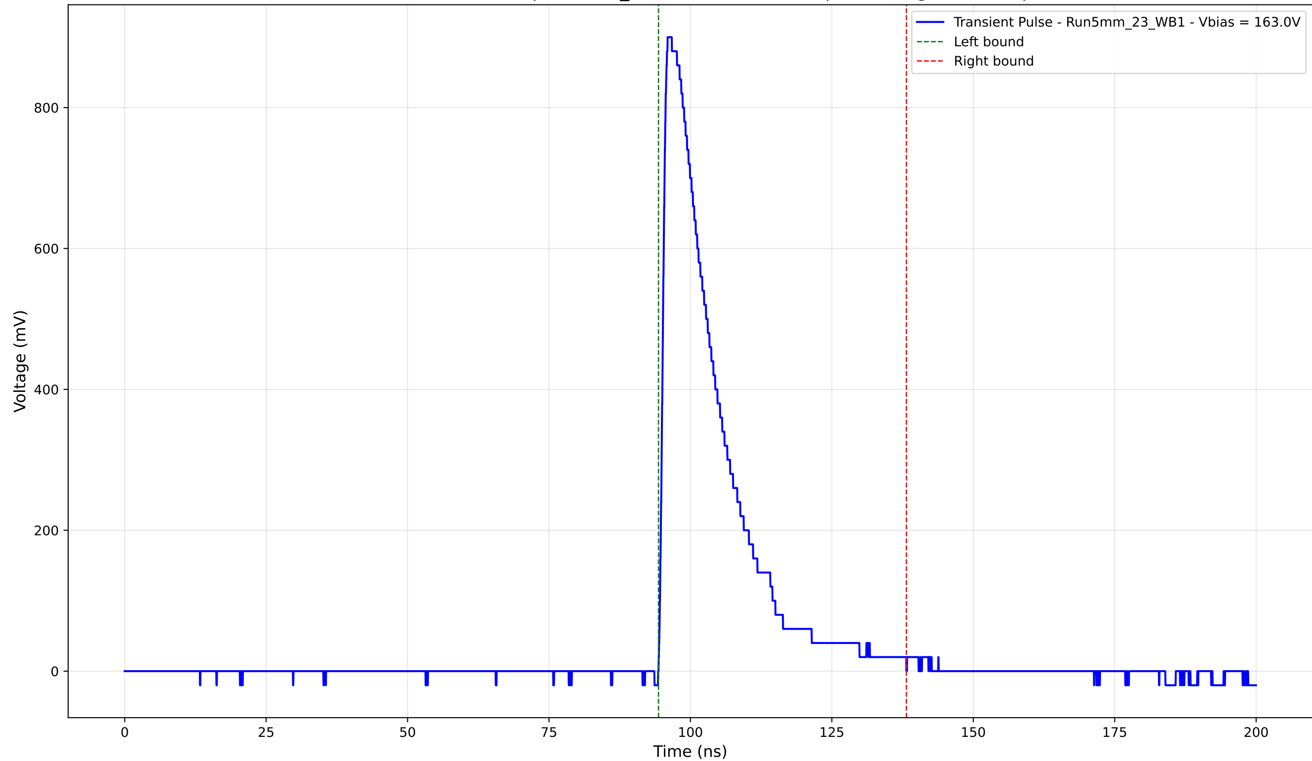
Transient Pulse - Sample: 5mm_23 - Position: 3935.0 \mu\text{m} - Charge: 196.49 pC
