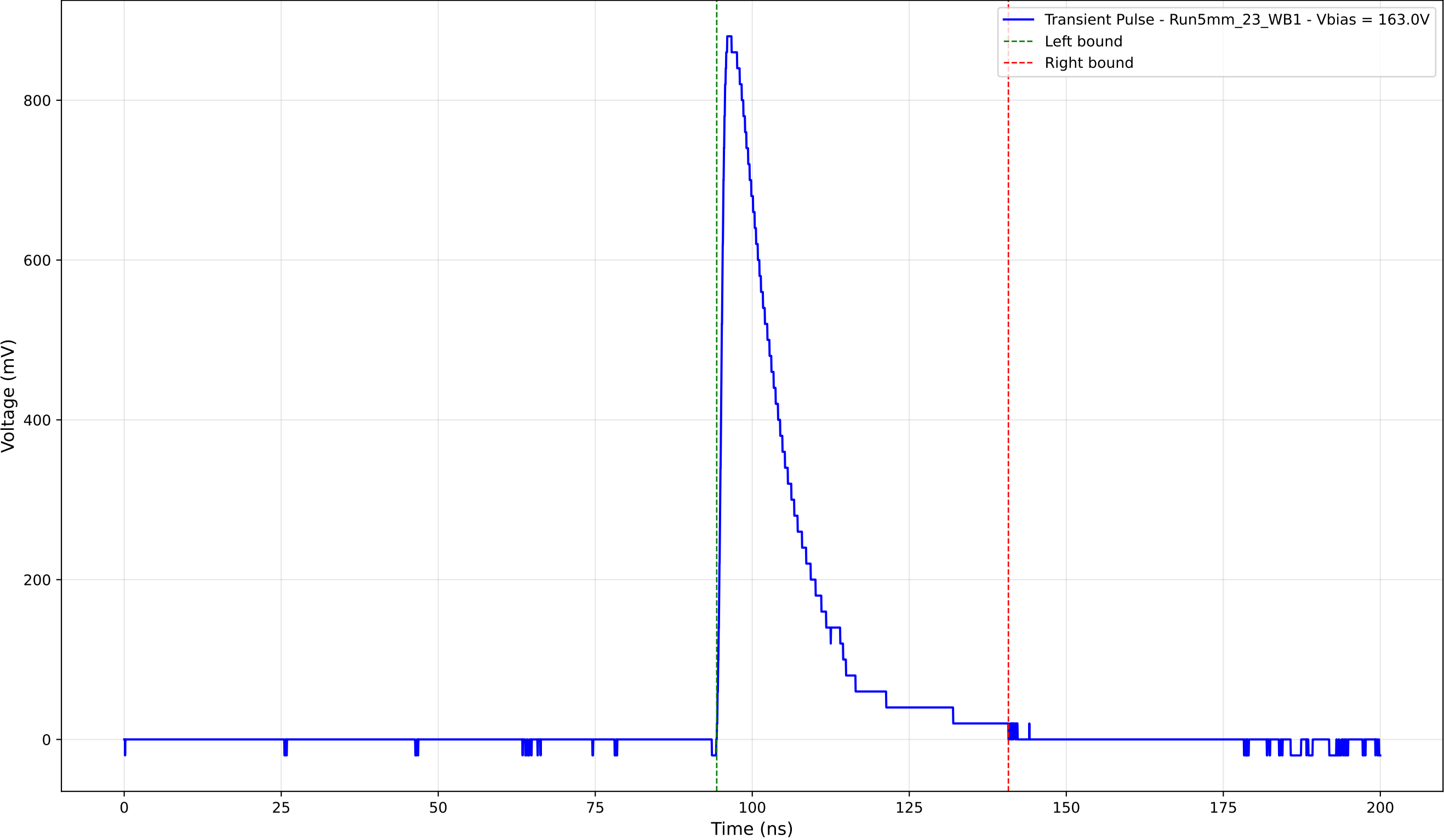
Transient Pulse - Sample: 5mm_23 - Position: 3860.0 \mu\text{m} - Charge: 192.78 pC
