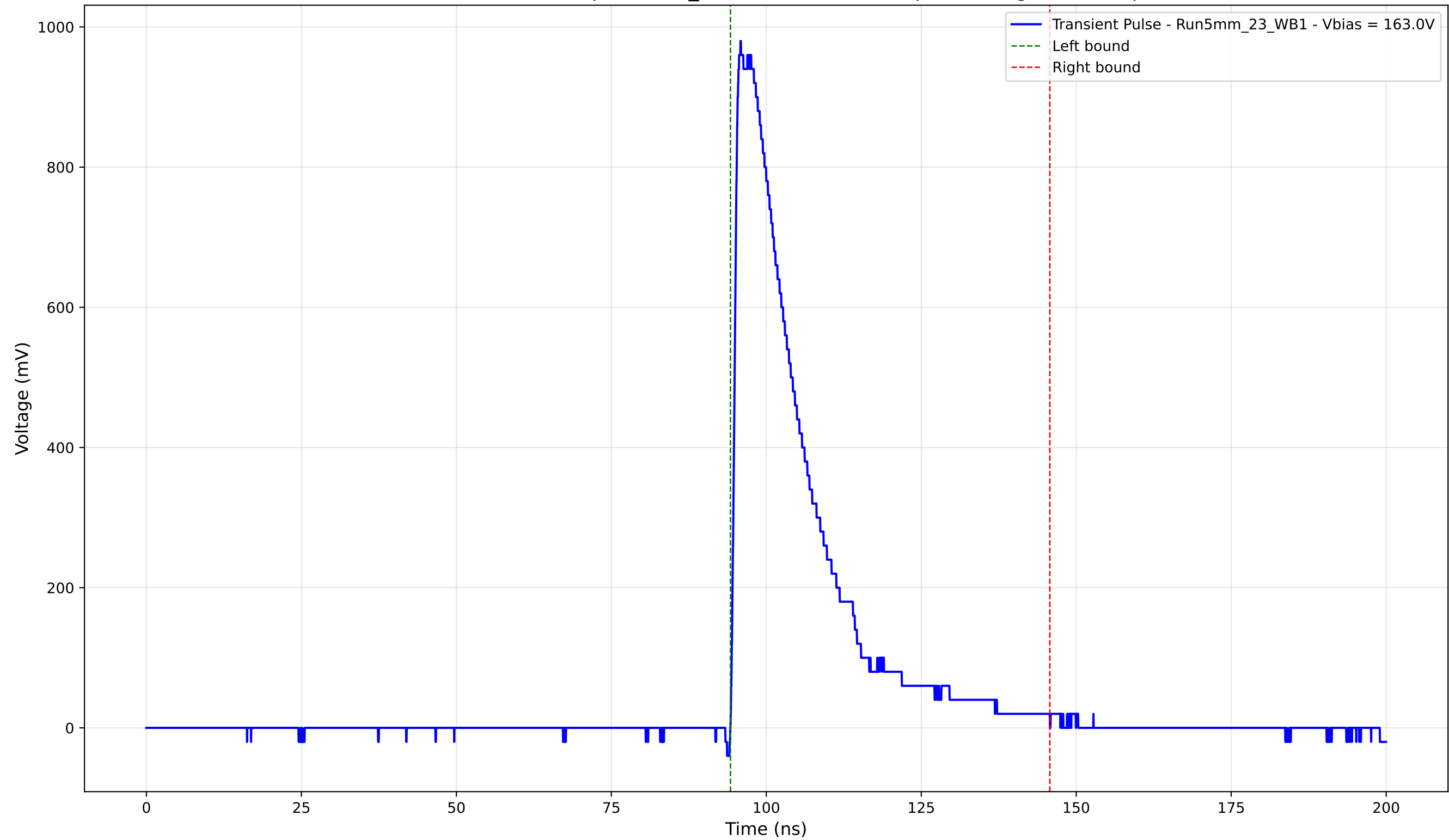
Transient Pulse - Sample: 5mm_23 - Position: 1950.0 \mu\text{m} - Charge: 237.69 pC
