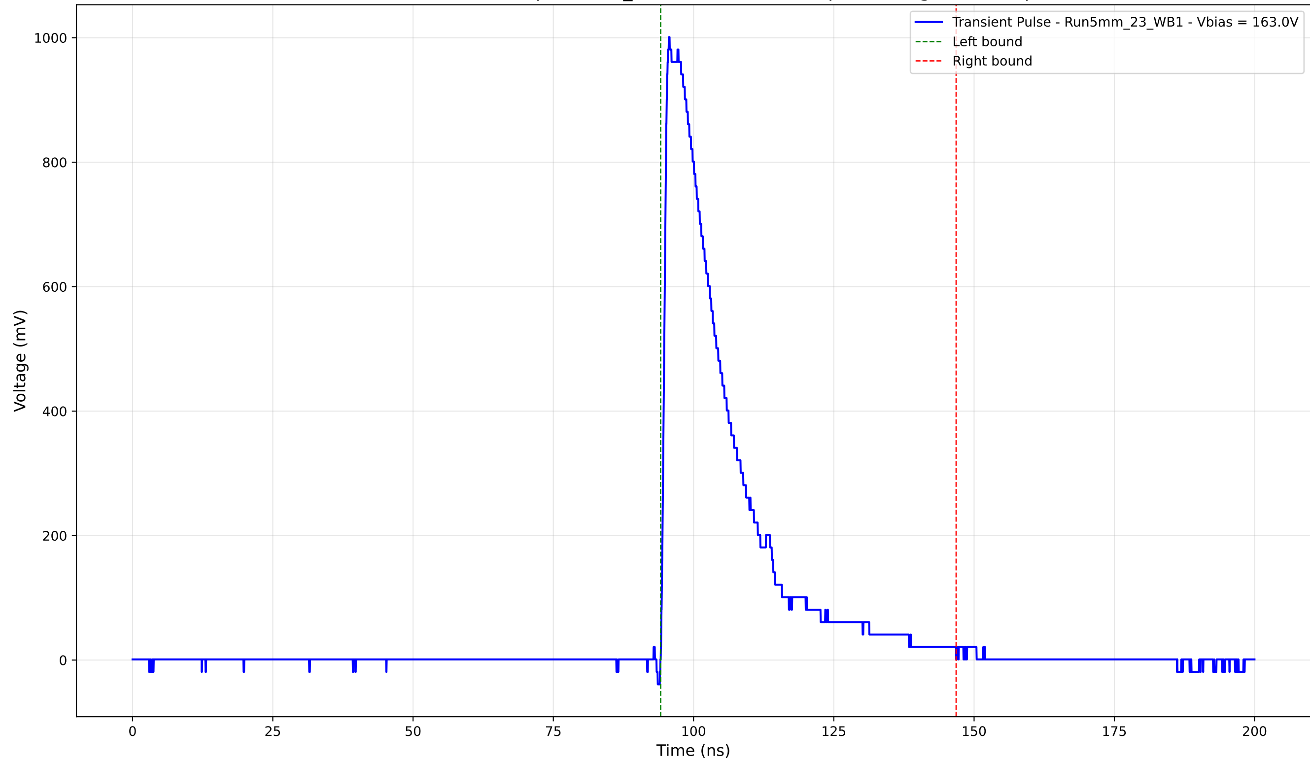
Transient Pulse - Sample: 5mm_23 - Position: 2080.0 \mu\text{m} - Charge: 247.58 pC
