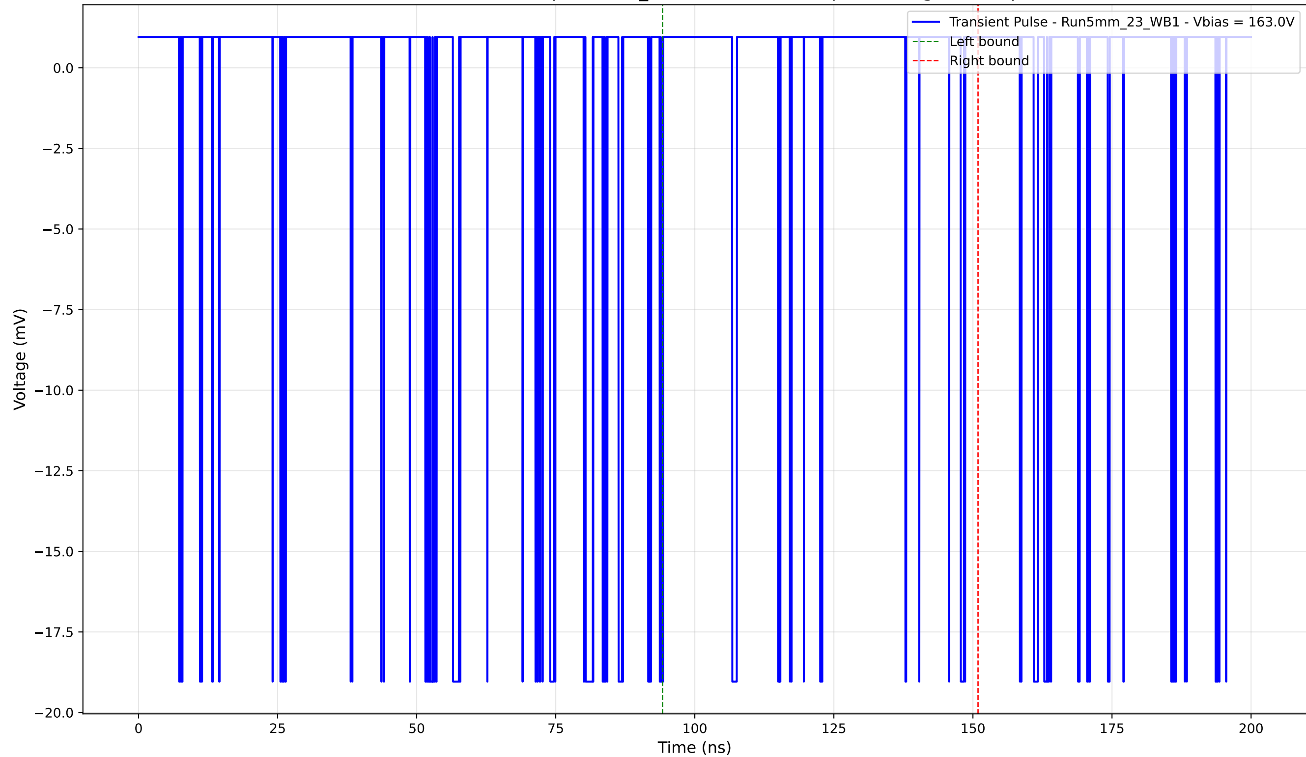
Transient Pulse - Sample: 5mm_23 - Position: 185.0 \mu\text{m} - Charge: -0.03 pC
