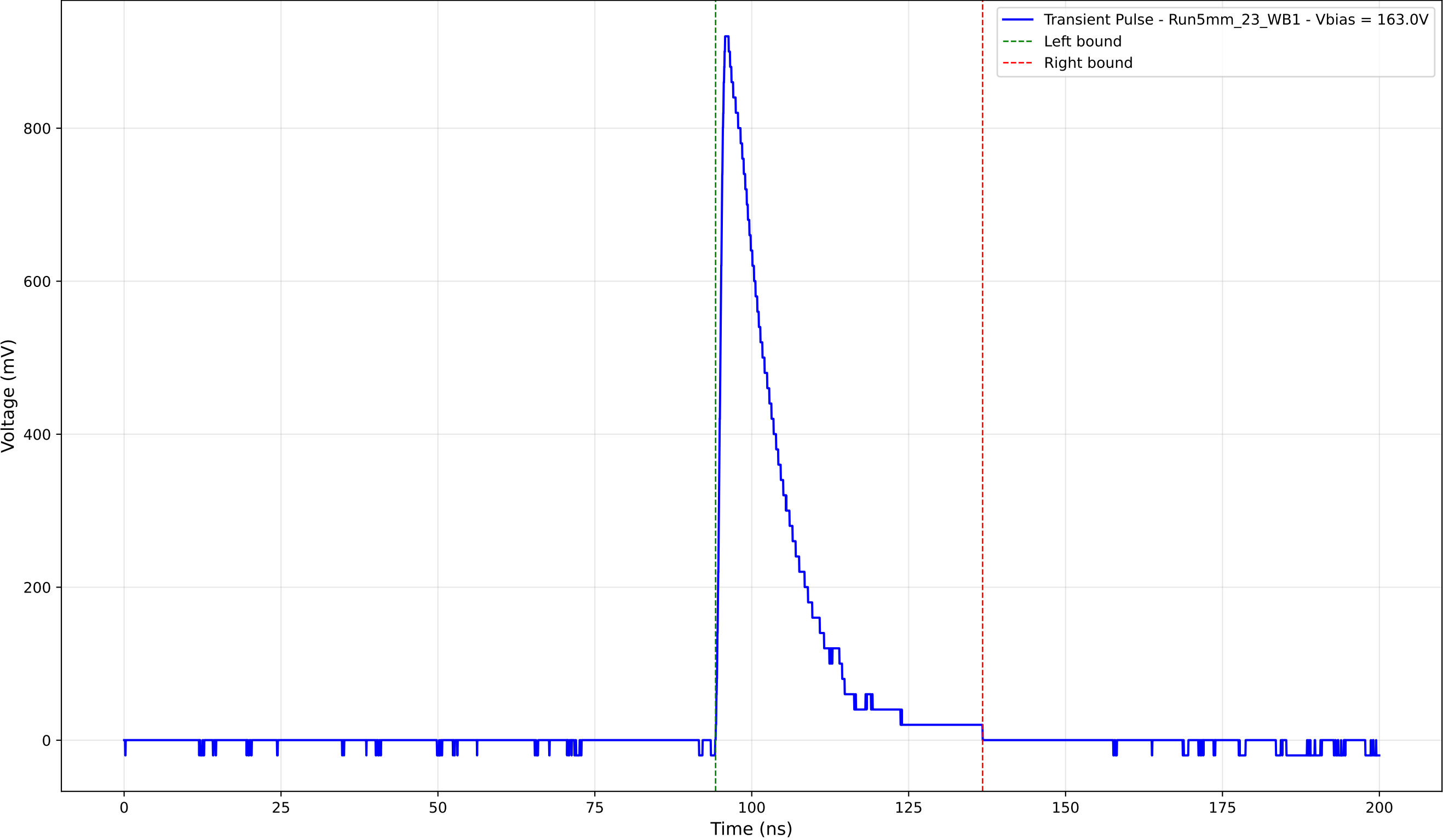
Transient Pulse - Sample: 5mm_23 - Position: 4550.0 \mu\text{m} - Charge: 178.54 pC
