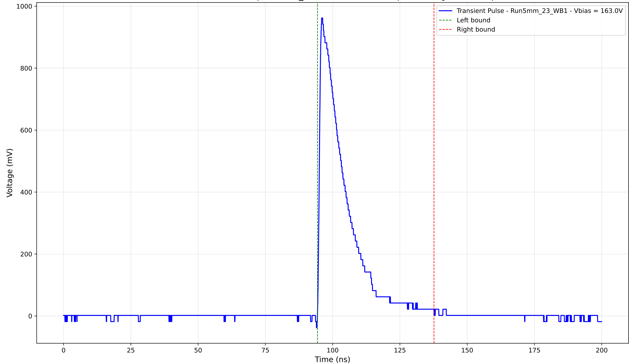
Transient Pulse - Sample: 5mm_23 - Position: 1010.0 \mu\text{m} - Charge: 202.71 pC
