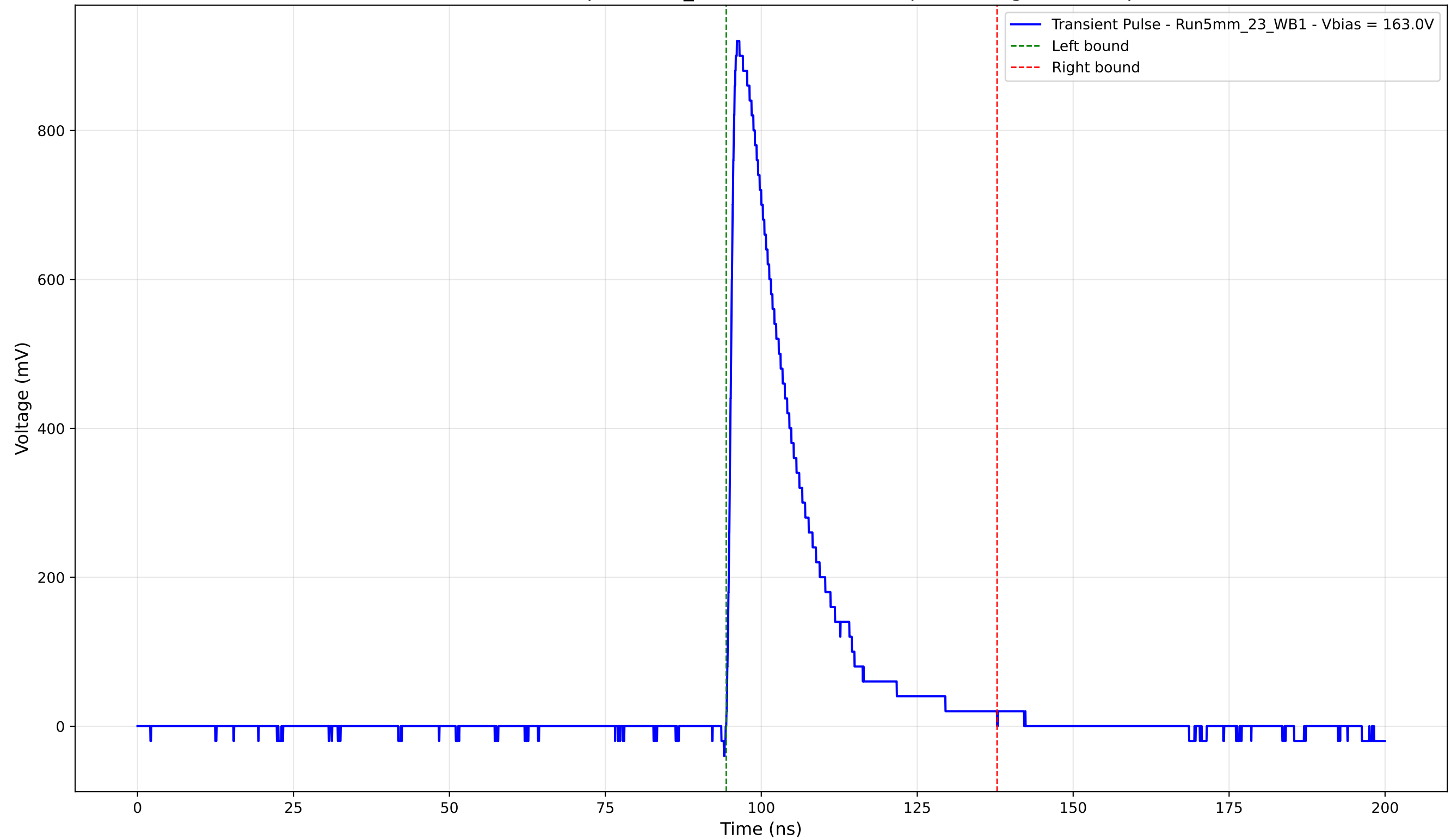
Transient Pulse - Sample: 5mm_23 - Position: 4015.0 \mu\text{m} - Charge: 197.19 pC
