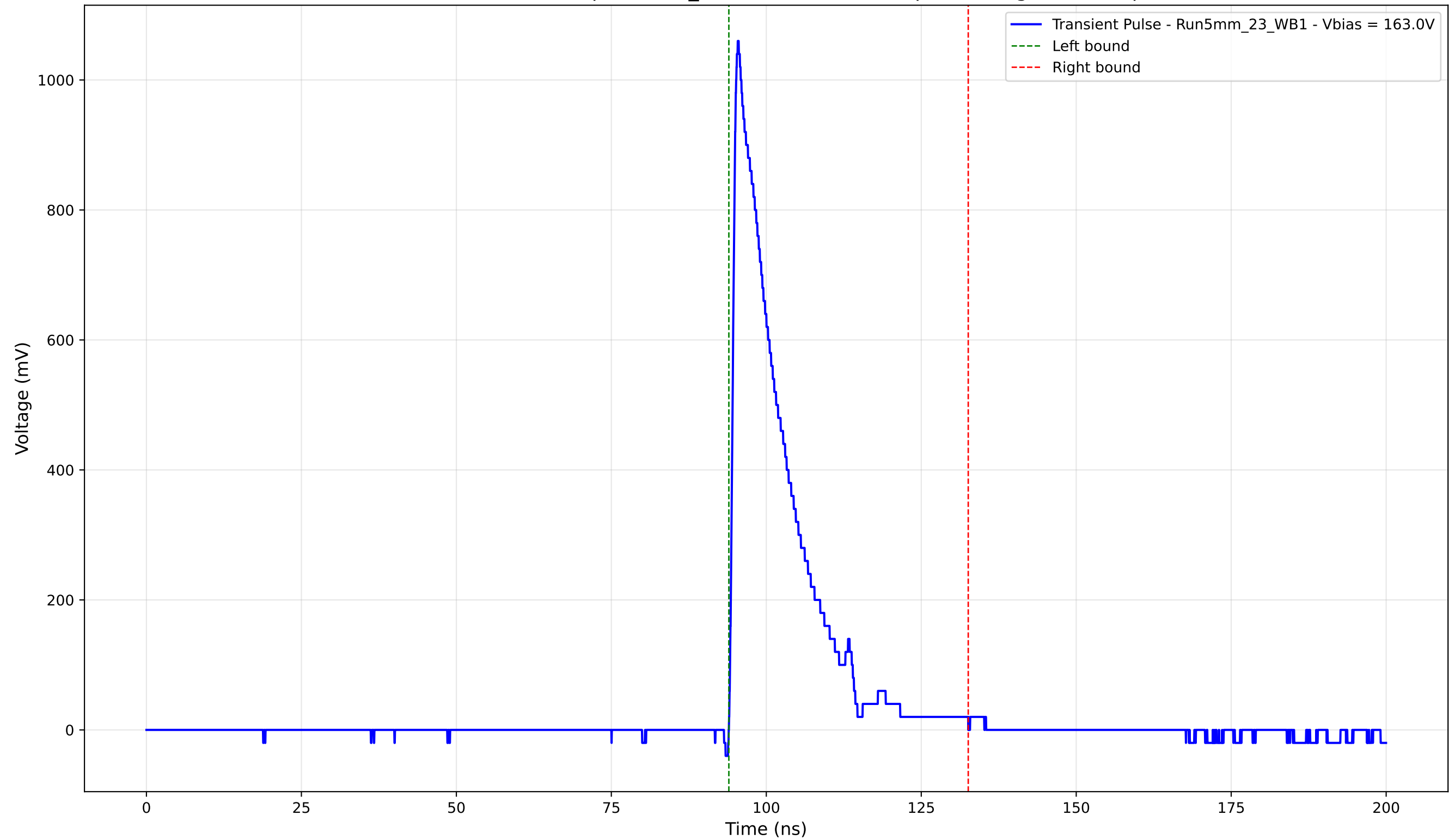
Transient Pulse - Sample: 5mm_23 - Position: 5060.0 \mu\text{m} - Charge: 183.58 pC
