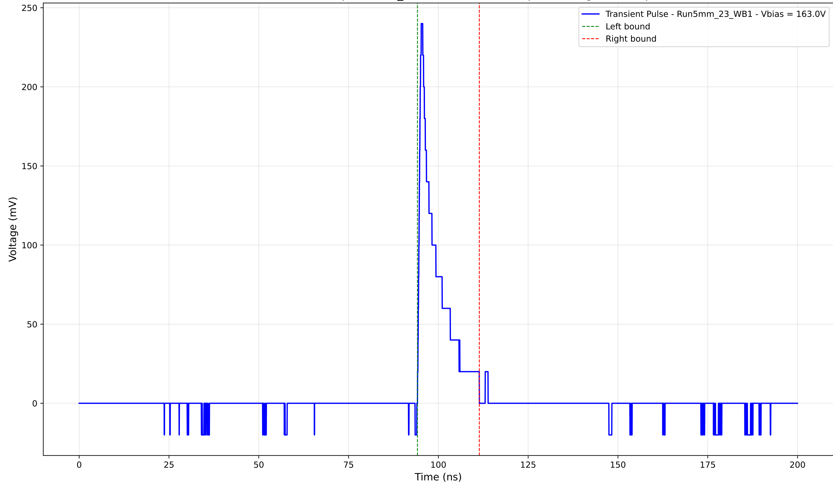
Transient Pulse - Sample: 5mm_23 - Position: 5190.0 \mu\text{m} - Charge: 24.44 pC
