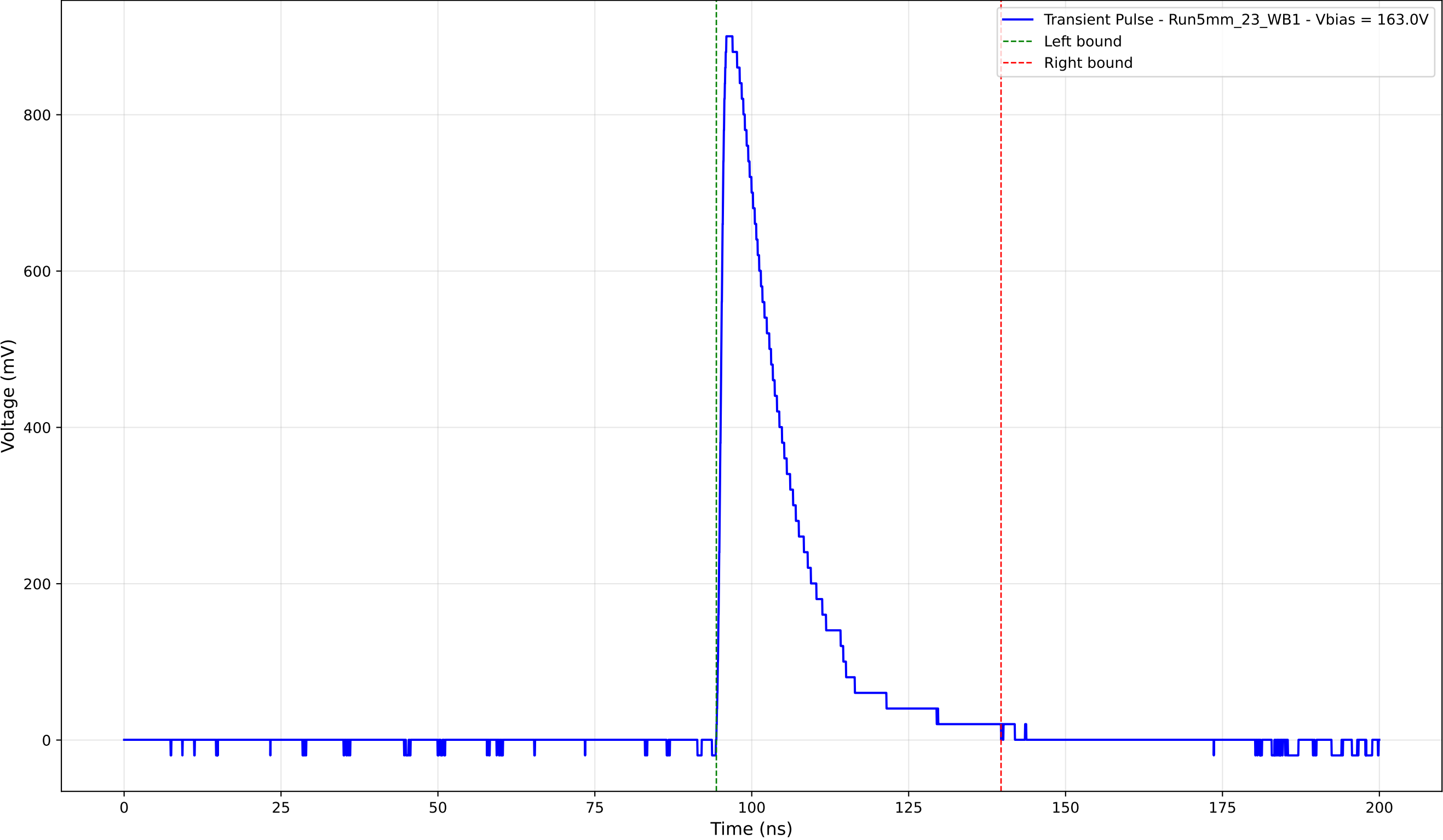
Transient Pulse - Sample: 5mm_23 - Position: 3950.0 \mu\text{m} - Charge: 197.46 pC
