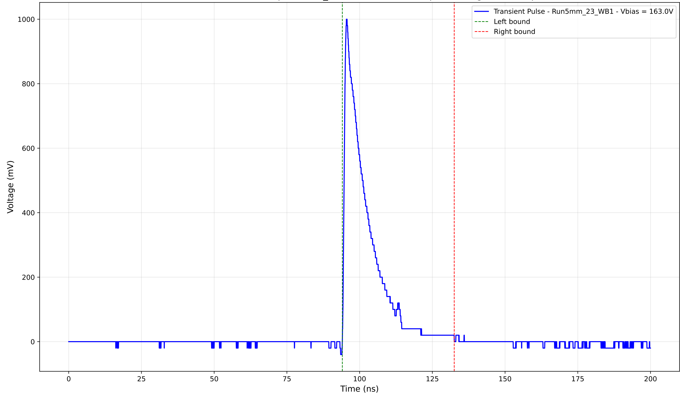
Transient Pulse - Sample: 5mm_23 - Position: 4970.0 \mu\text{m} - Charge: 166.22 pC
