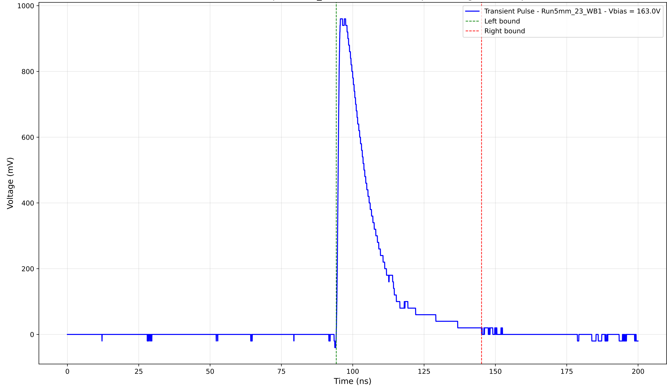
Transient Pulse - Sample: 5mm_23 - Position: 1930.0 \mu\text{m} - Charge: 236.75 pC
