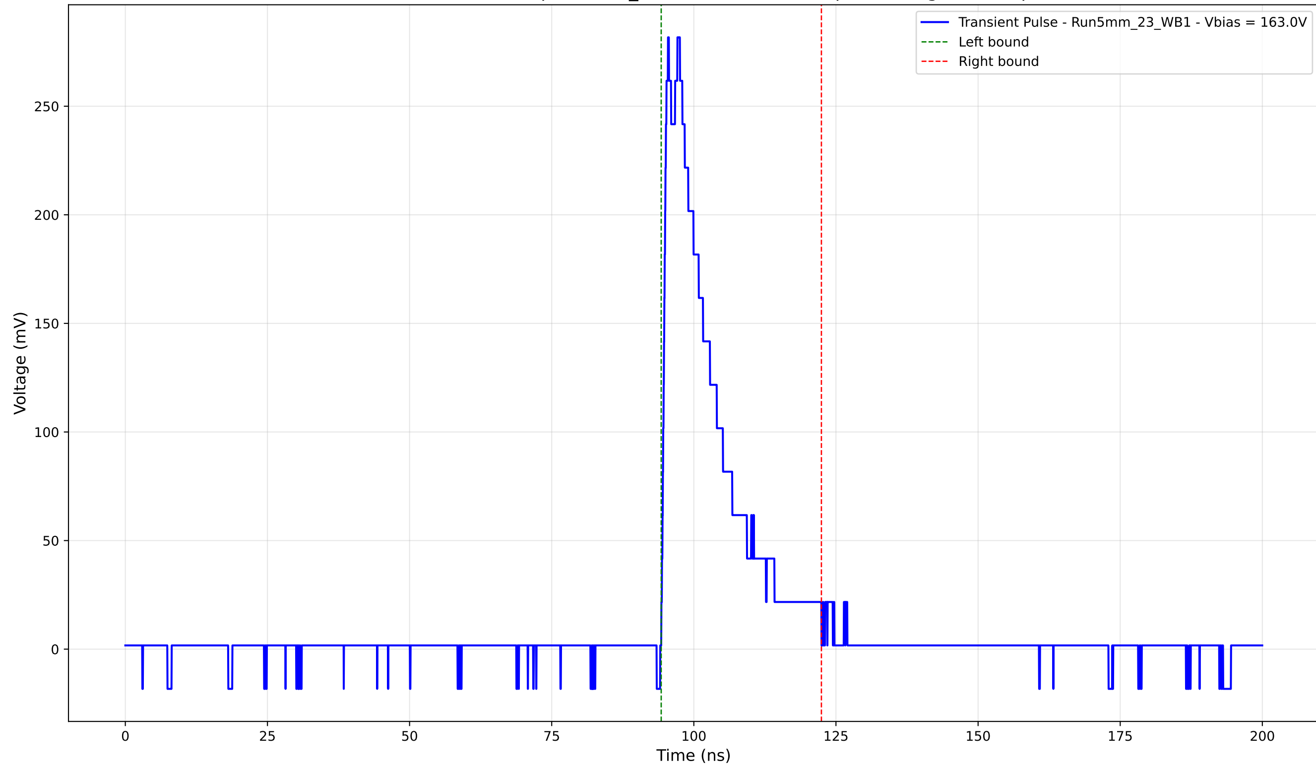
Transient Pulse - Sample: 5mm_23 - Position: 2225.0 \mu\text{m} - Charge: 53.37 pC
