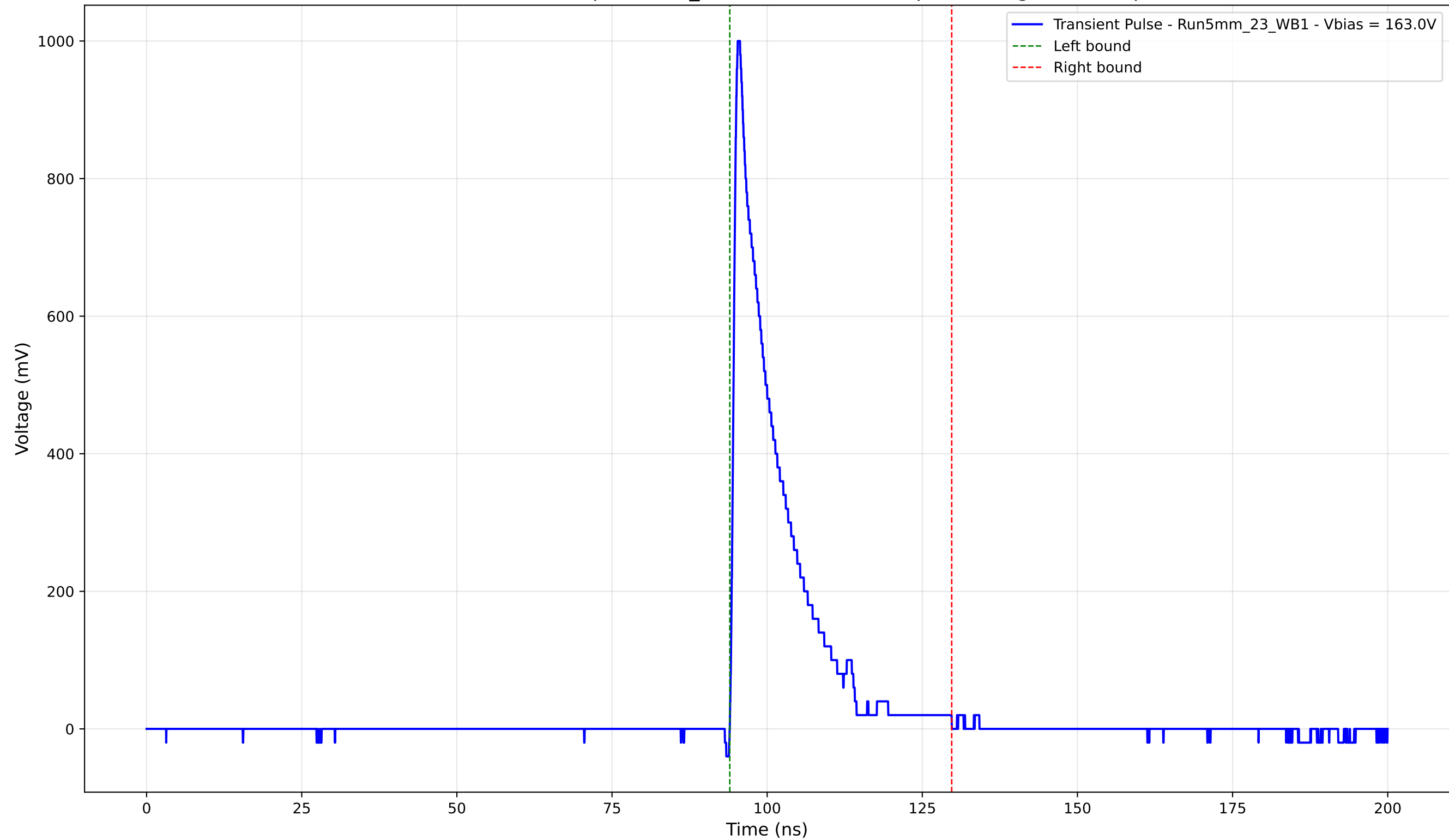
Transient Pulse - Sample: 5mm_23 - Position: 5130.0 \mu\text{m} - Charge: 148.67 pC
