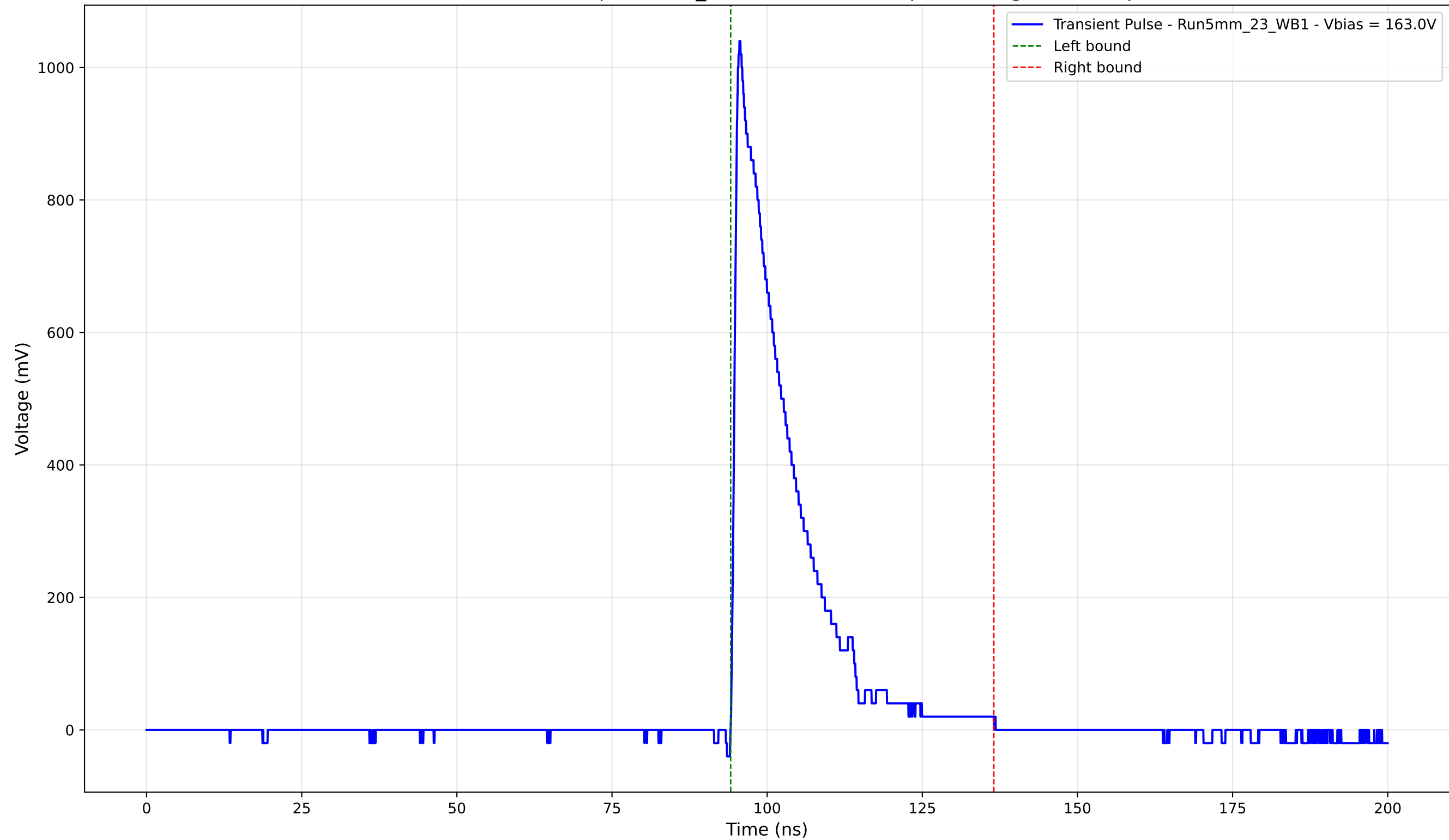
Transient Pulse - Sample: 5mm_23 - Position: 495.0 \mu\text{m} - Charge: 193.30 pC
