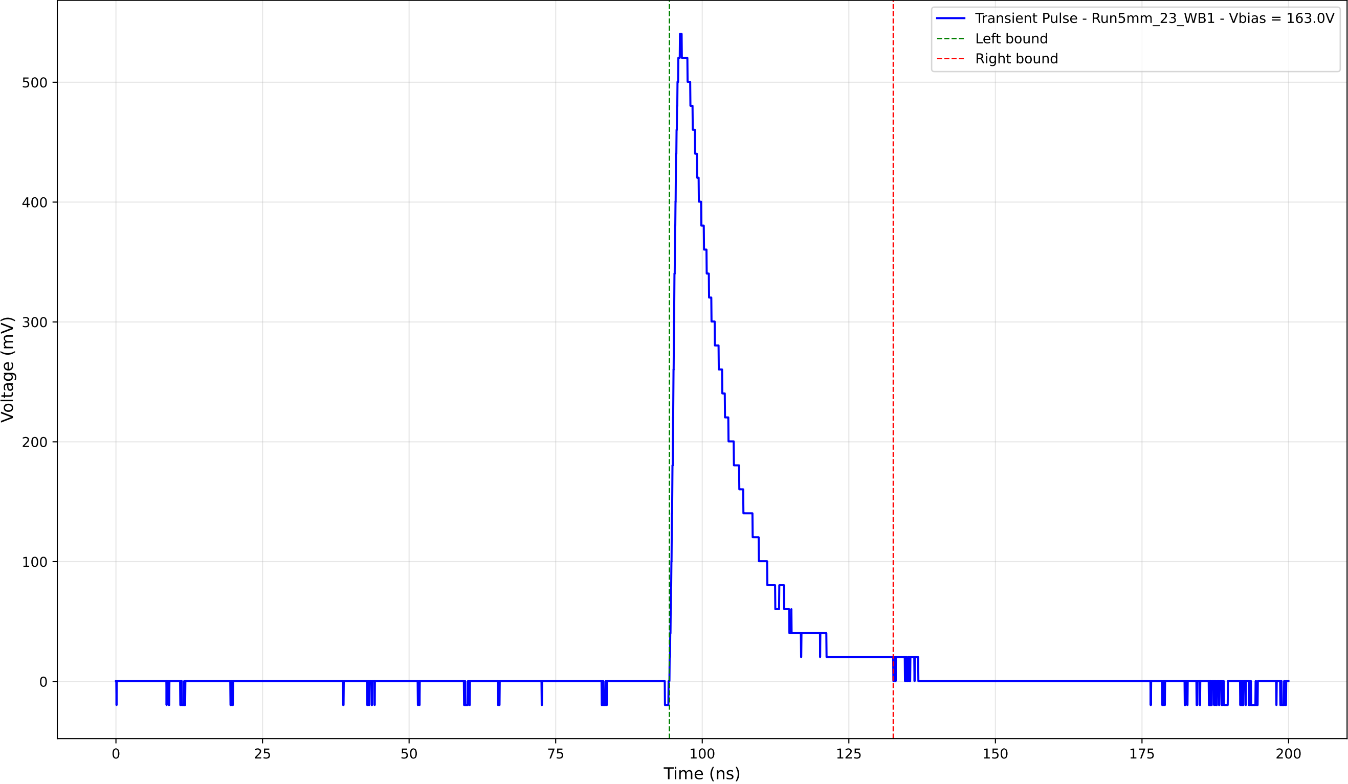
Transient Pulse - Sample: 5mm_23 - Position: 1685.0 \mu\text{m} - Charge: 107.51 pC
