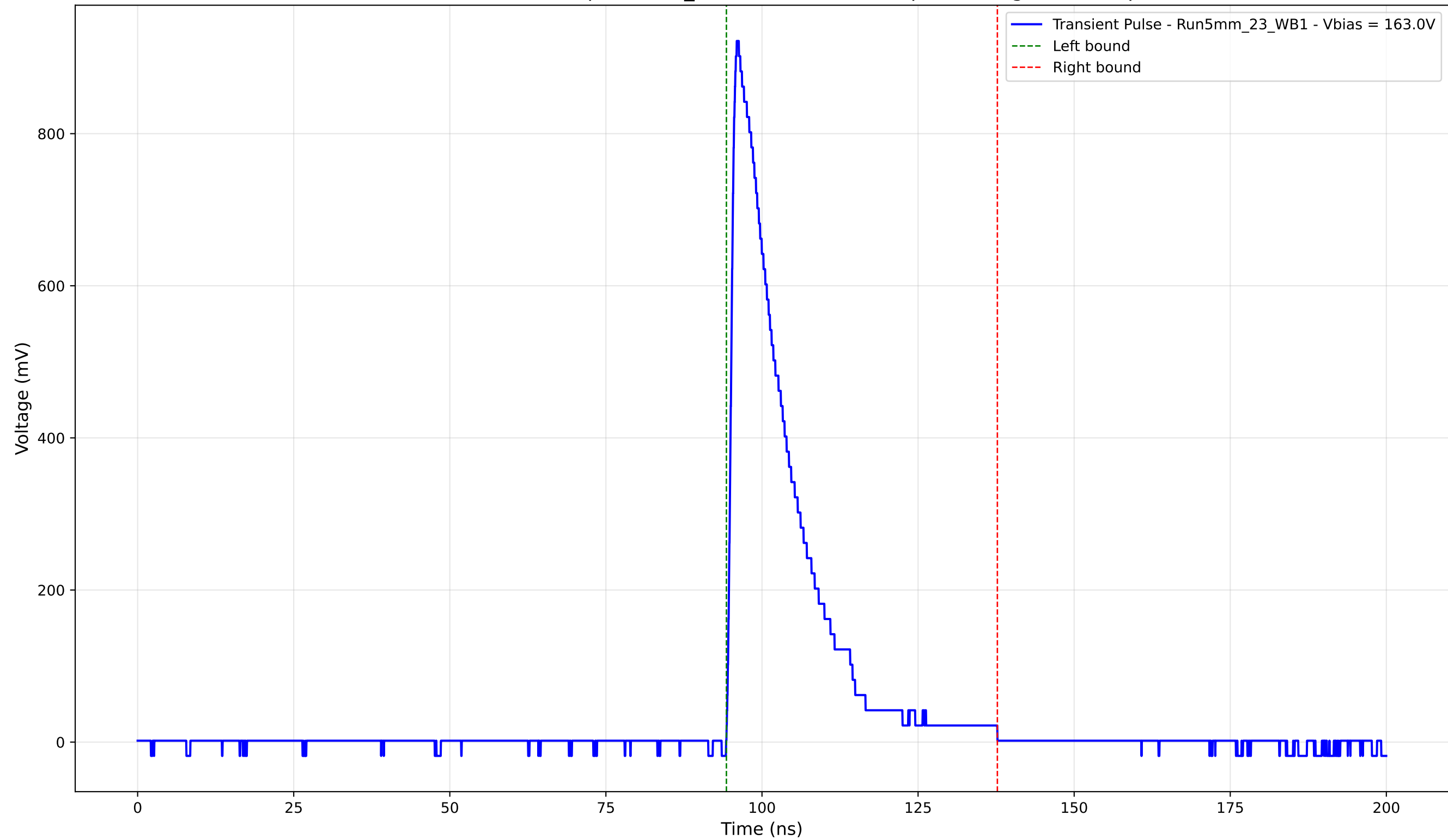
Transient Pulse - Sample: 5mm_23 - Position: 4445.0 \mu\text{m} - Charge: 181.00 pC
