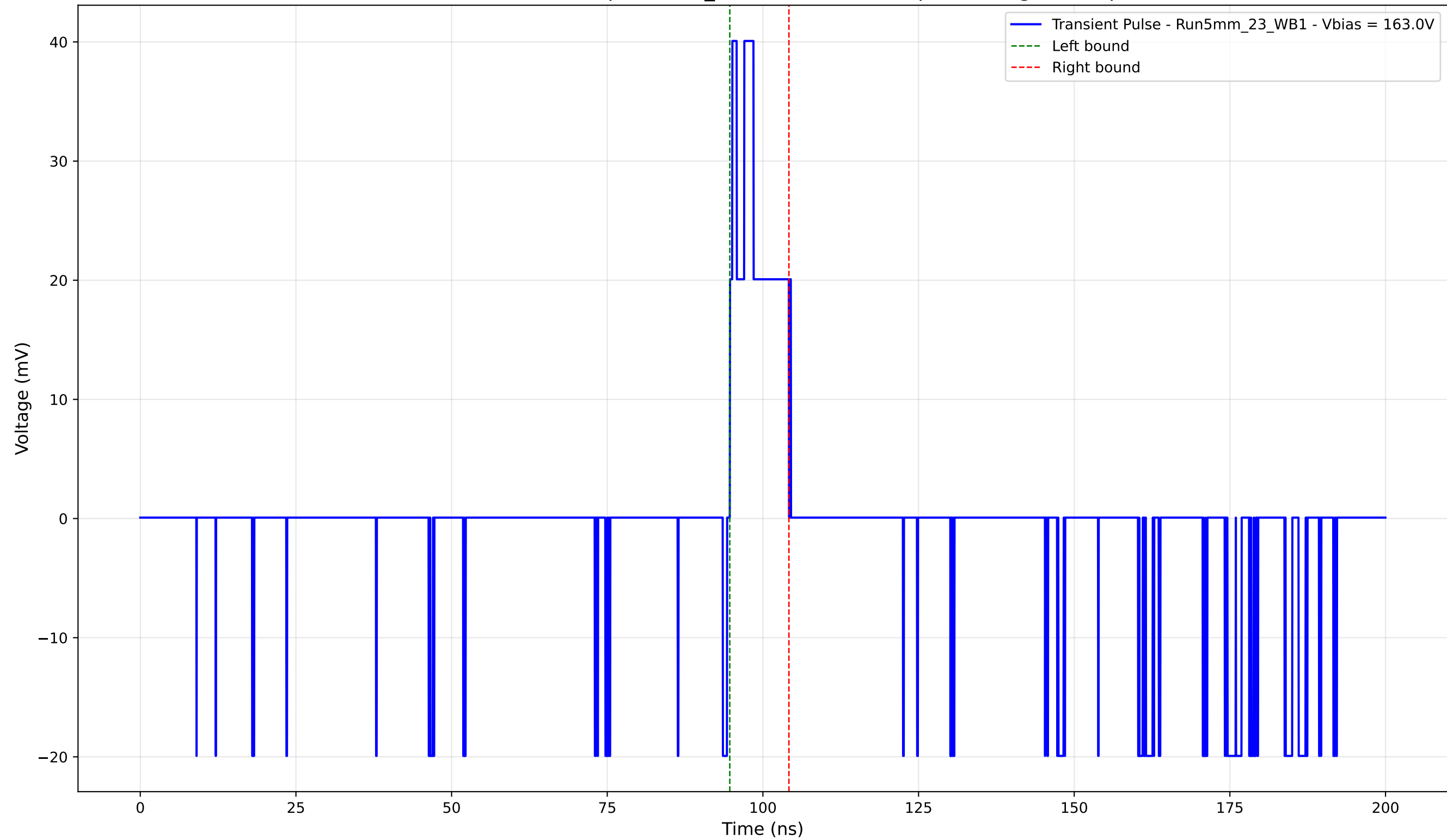
Transient Pulse - Sample: 5mm_23 - Position: 245.0 \mu\text{m} - Charge: 4.70 pC
