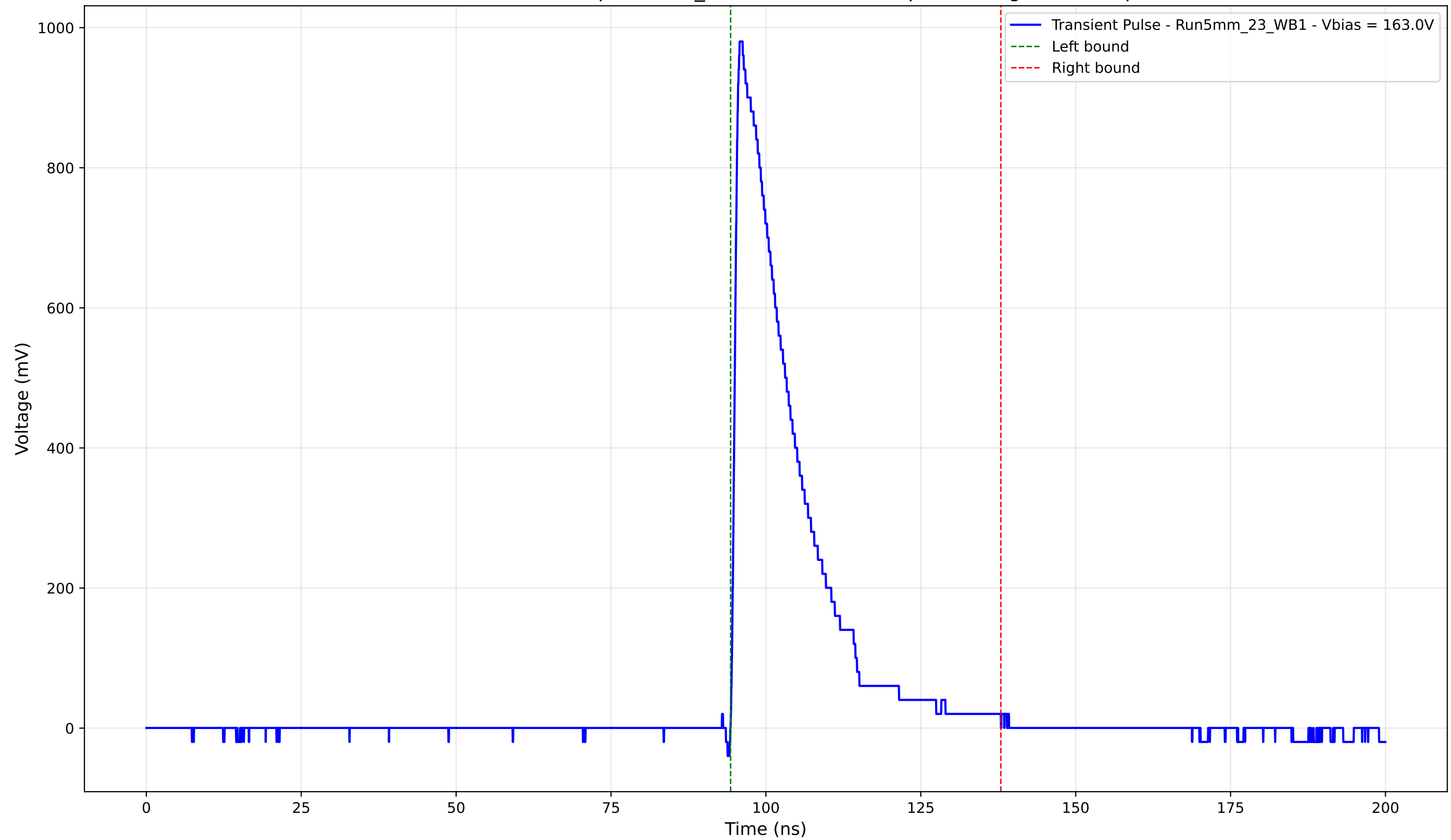
Transient Pulse - Sample: 5mm_23 - Position: 875.0 \mu\text{m} - Charge: 204.37 pC
