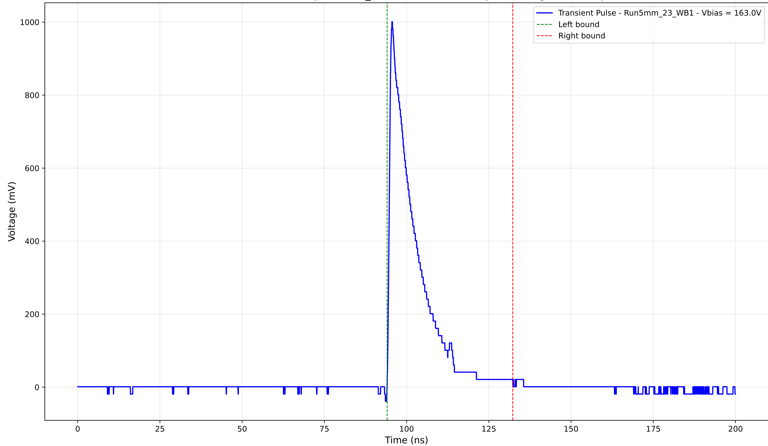
Transient Pulse - Sample: 5mm_23 - Position: 4930.0 \mu\text{m} - Charge: 169.06 pC
