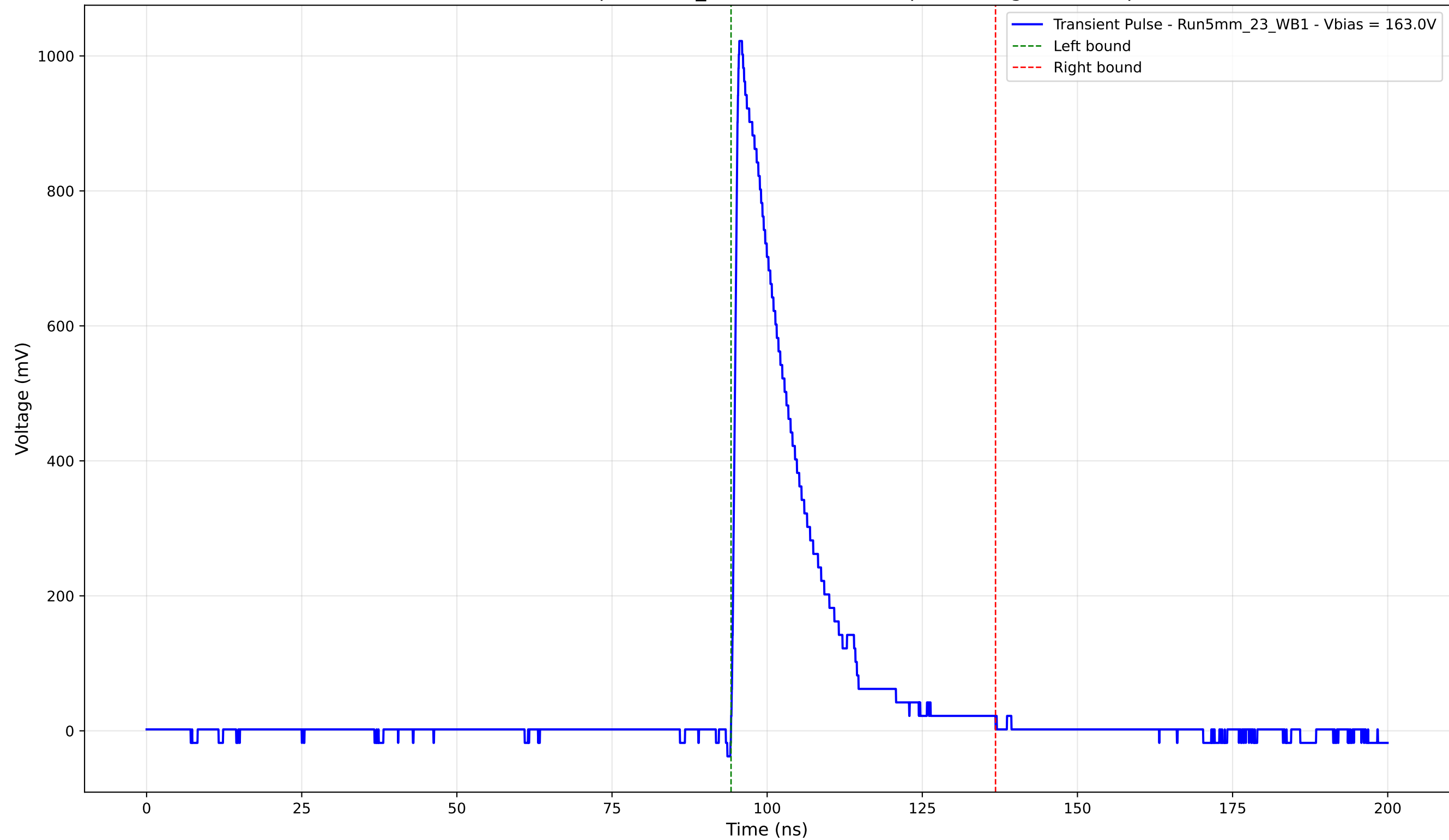
Transient Pulse - Sample: 5mm_23 - Position: 630.0 \mu\text{m} - Charge: 203.76 pC
