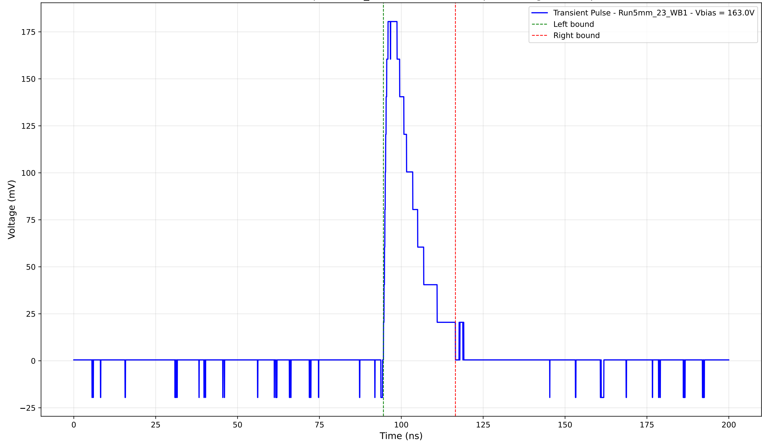
Transient Pulse - Sample: 5mm_23 -Position: 3755.0 \mu\text{m} - Charge: 35.02 pC
