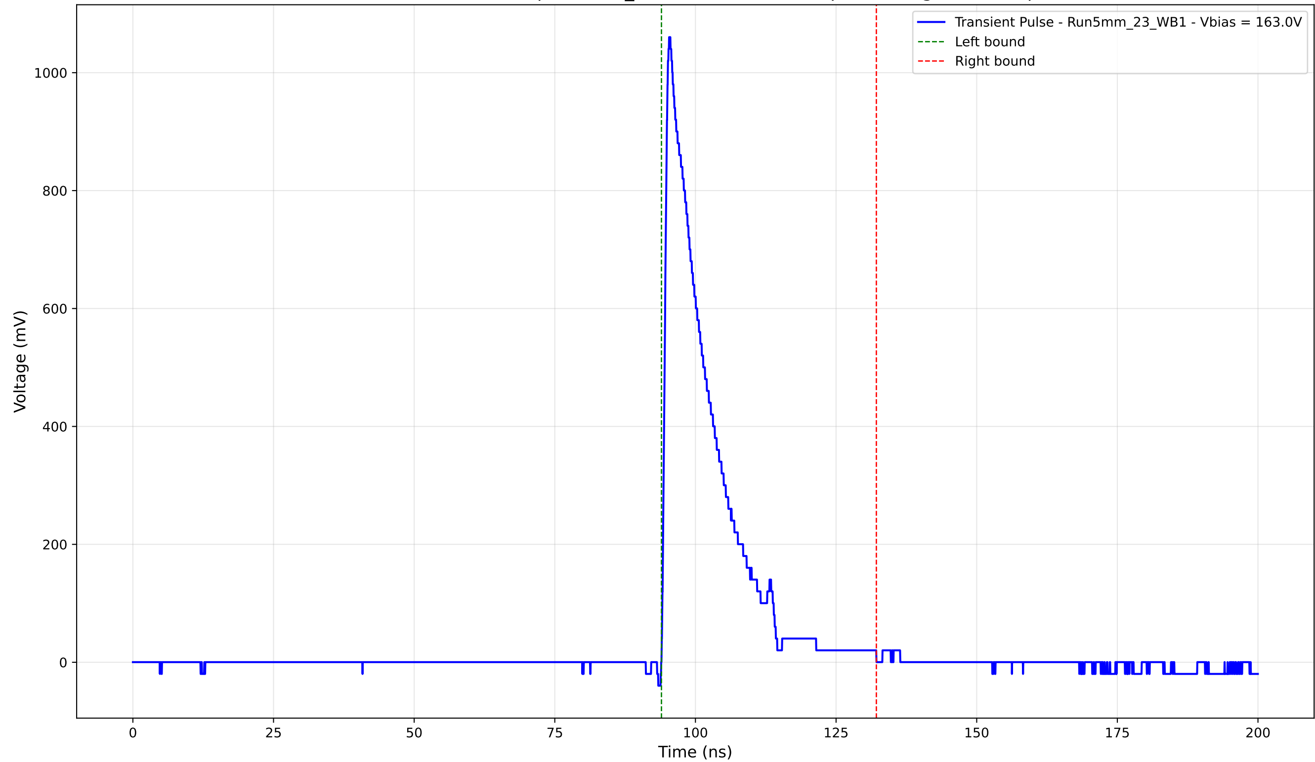
Transient Pulse - Sample: 5mm_23 - Position: 5105.0 \mu\text{m} - Charge: 180.00 pC
