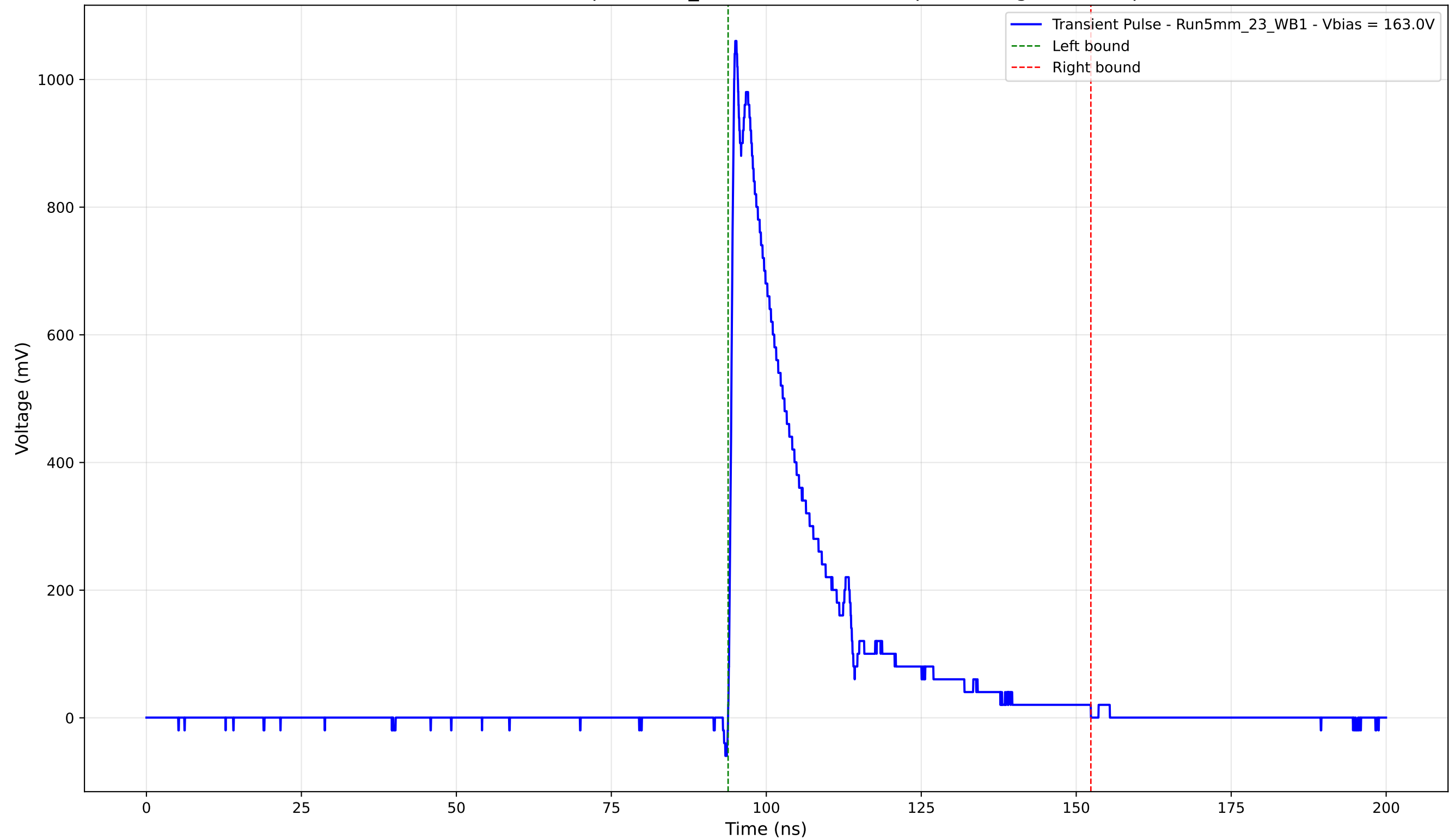
Transient Pulse - Sample: 5mm_23 - Position: 2850.0 \mu\text{m} - Charge: 238.35 pC
