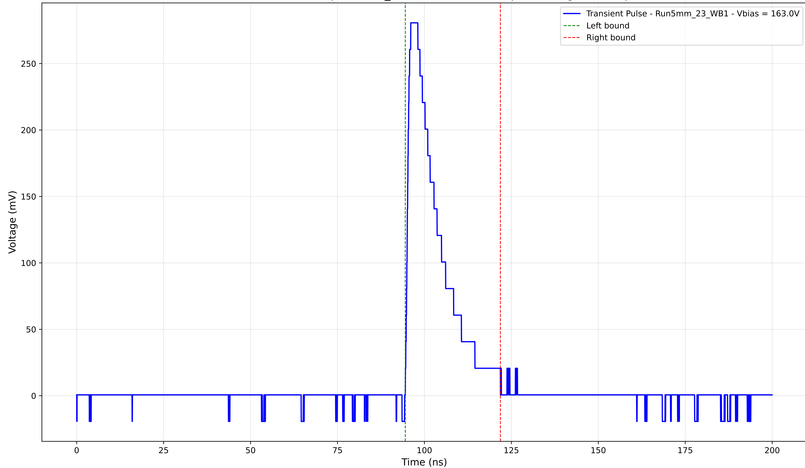
Transient Pulse - Sample: 5mm_23 - Position: 1710.0 \mu\text{m} - Charge: 56.14 pC
