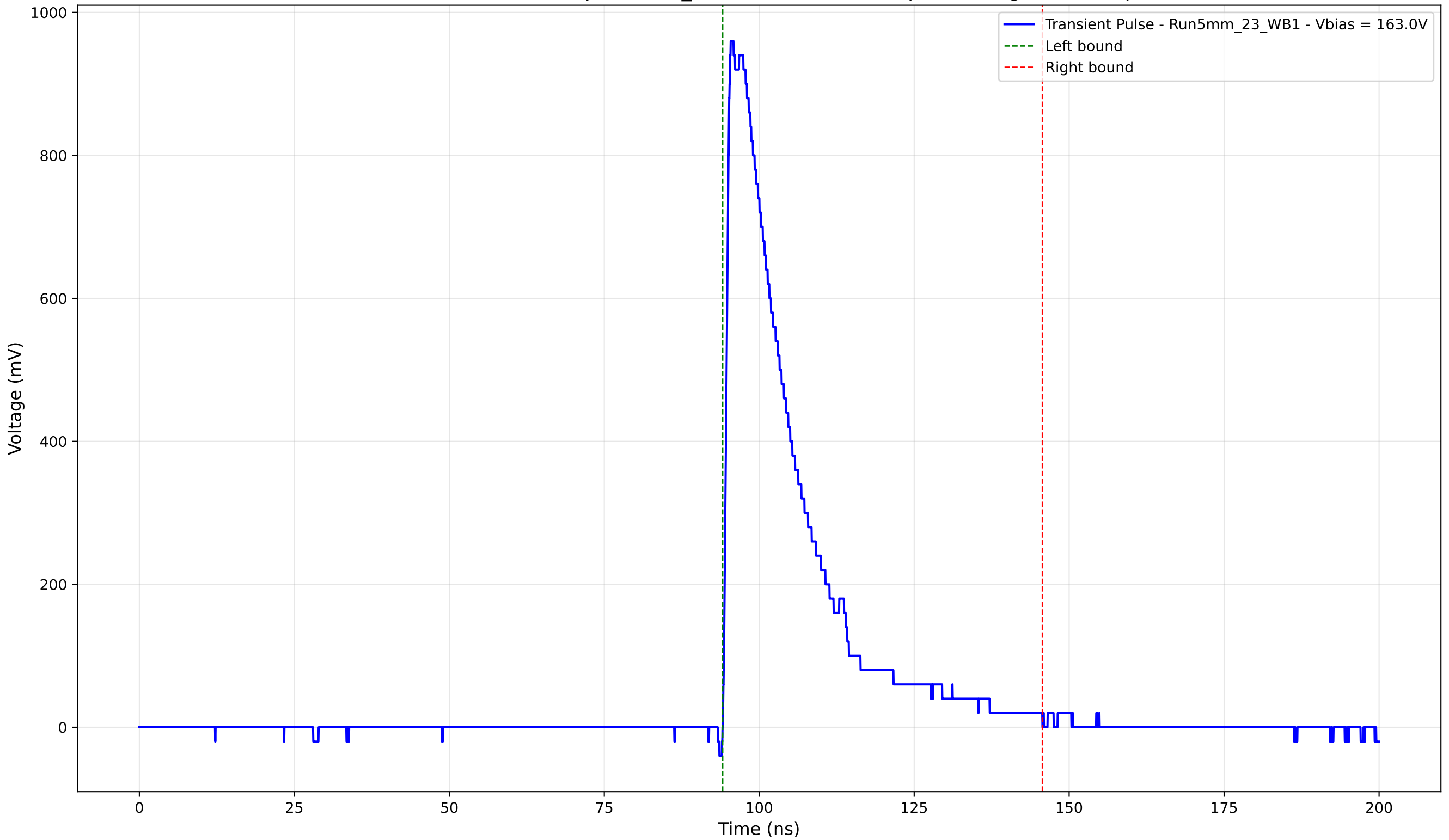
Transient Pulse - Sample: 5mm_23 - Position: 2145.0 \mu\text{m} - Charge: 227.97 pC
