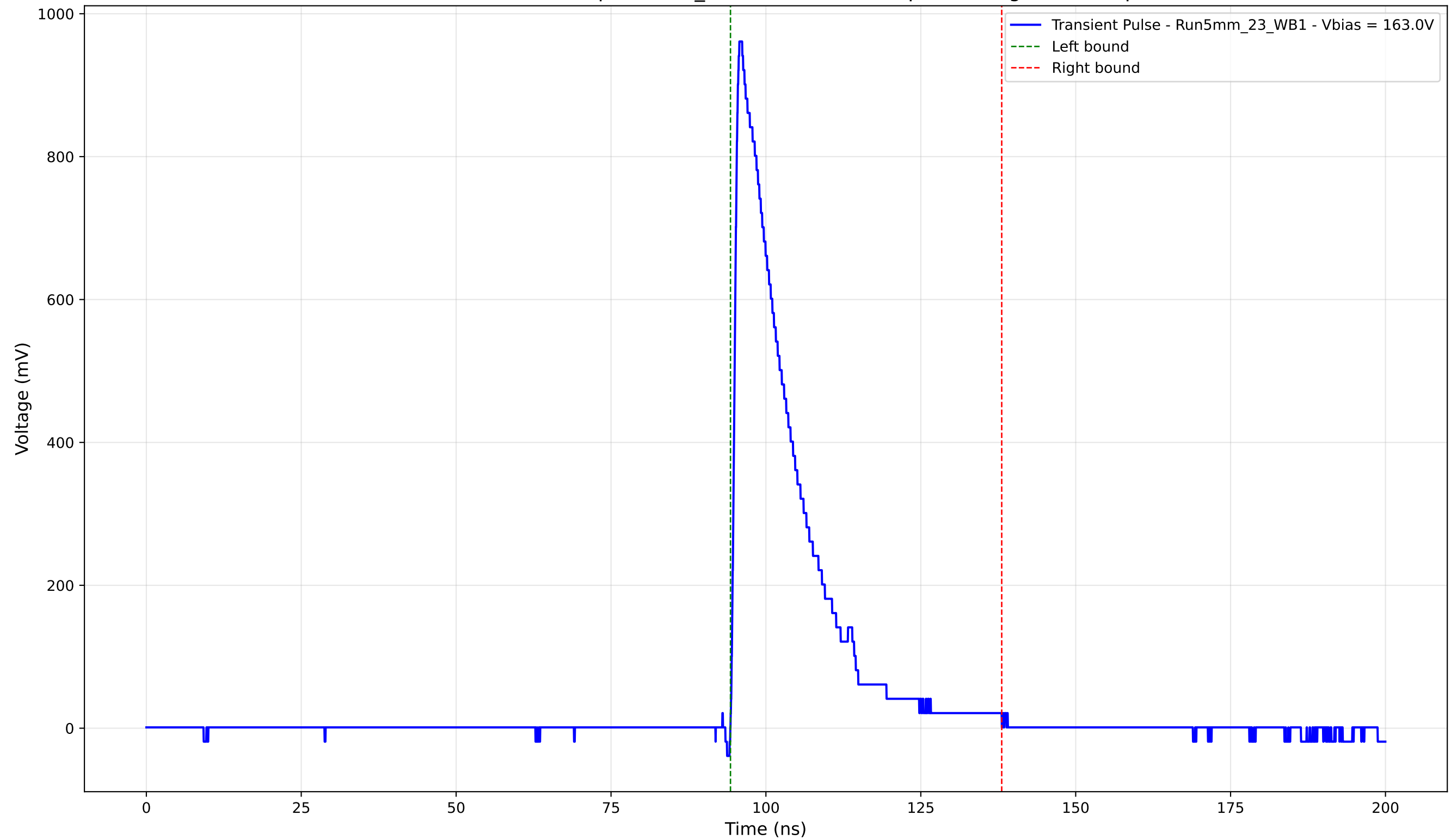
Transient Pulse - Sample: 5mm_23 - Position: 800.0 \mu\text{m} - Charge: 190.71 pC
