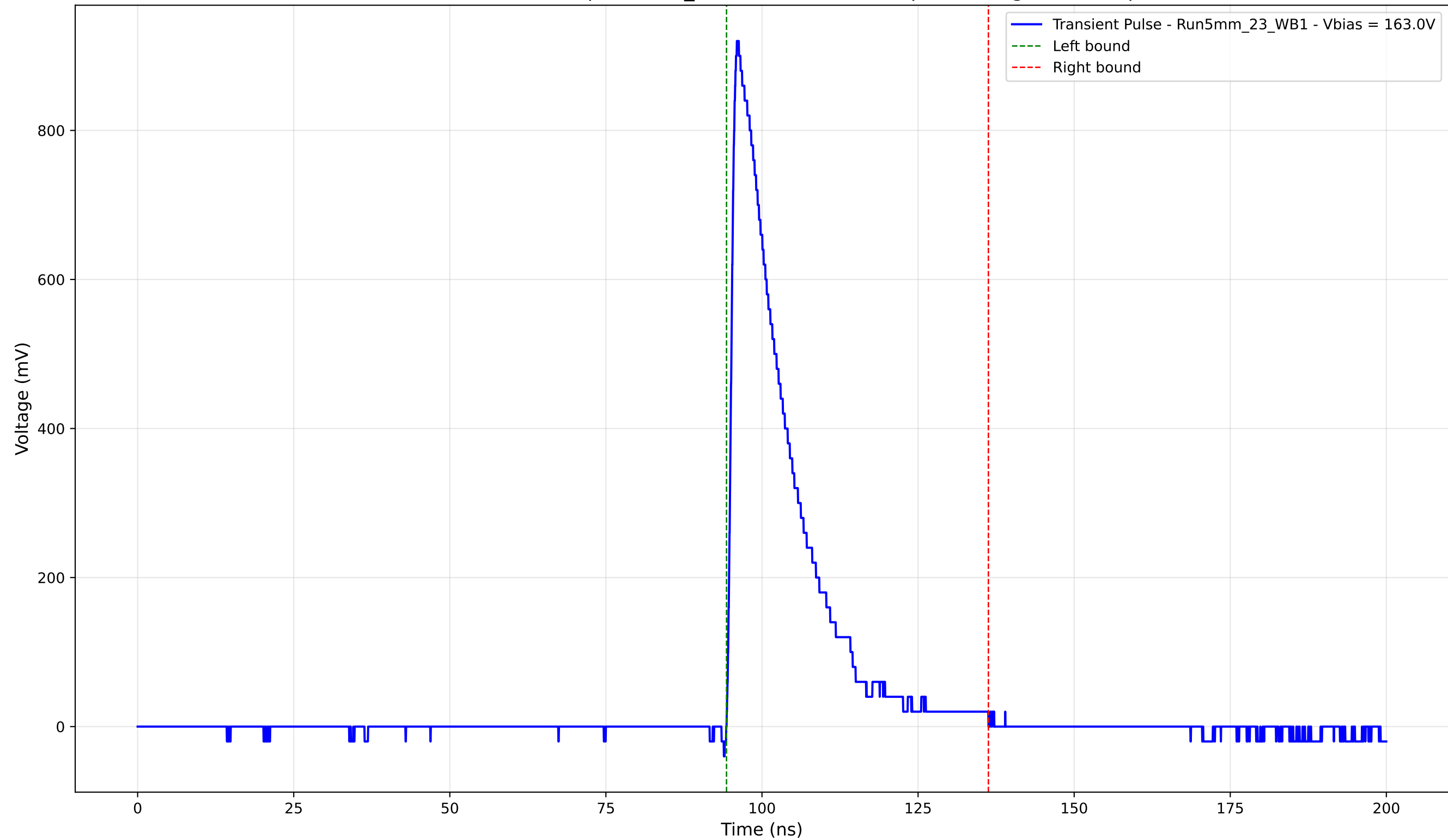
Transient Pulse - Sample: 5mm_23 - Position: 4410.0 \mu\text{m} - Charge: 180.30 pC
