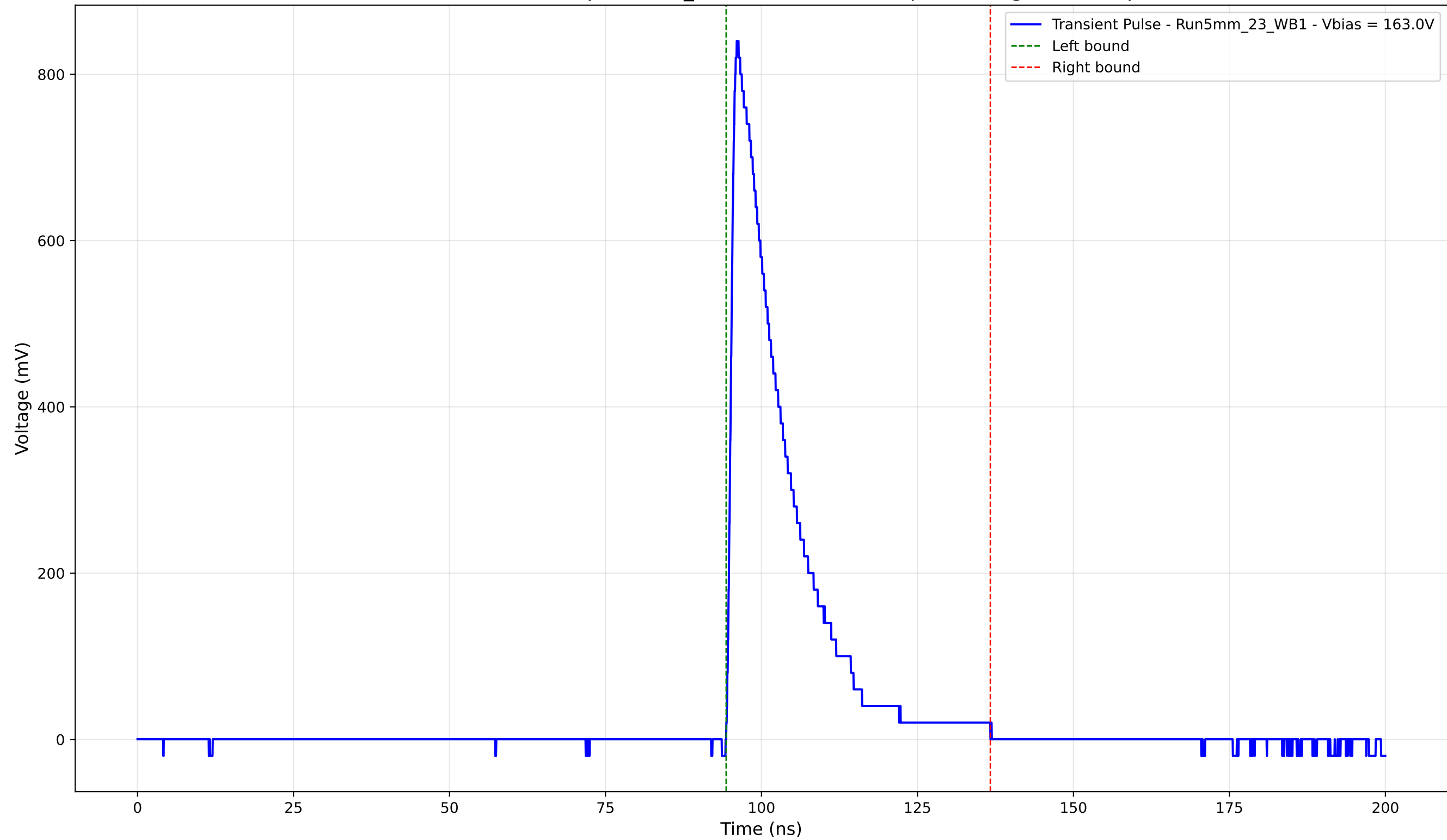
Transient Pulse - Sample: 5mm_23 - Position: 4345.0 \mu\text{m} - Charge: 159.45 pC
