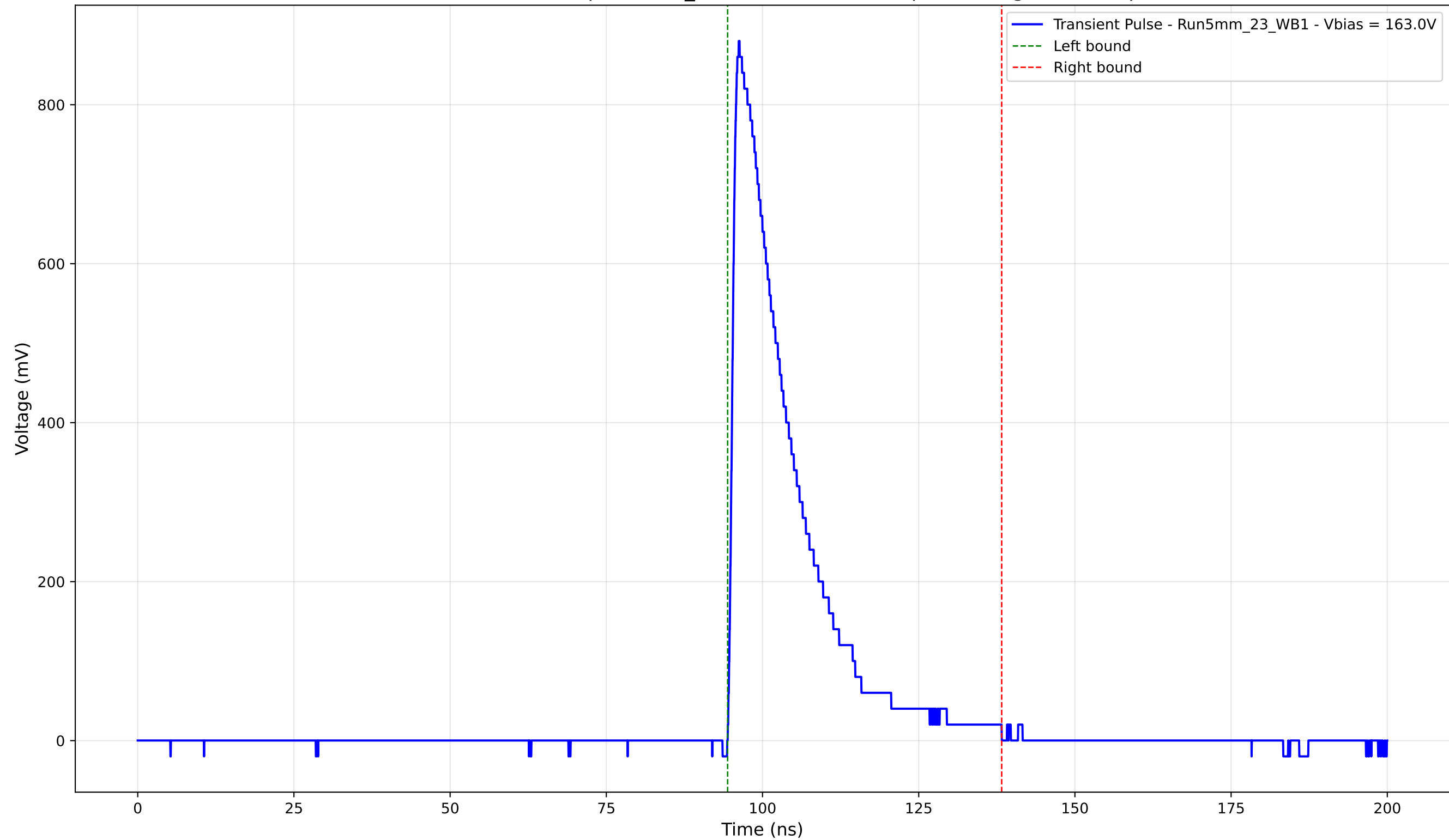
Transient Pulse - Sample: 5mm_23 - Position: 1300.0 \mu\text{m} - Charge: 182.02 pC
