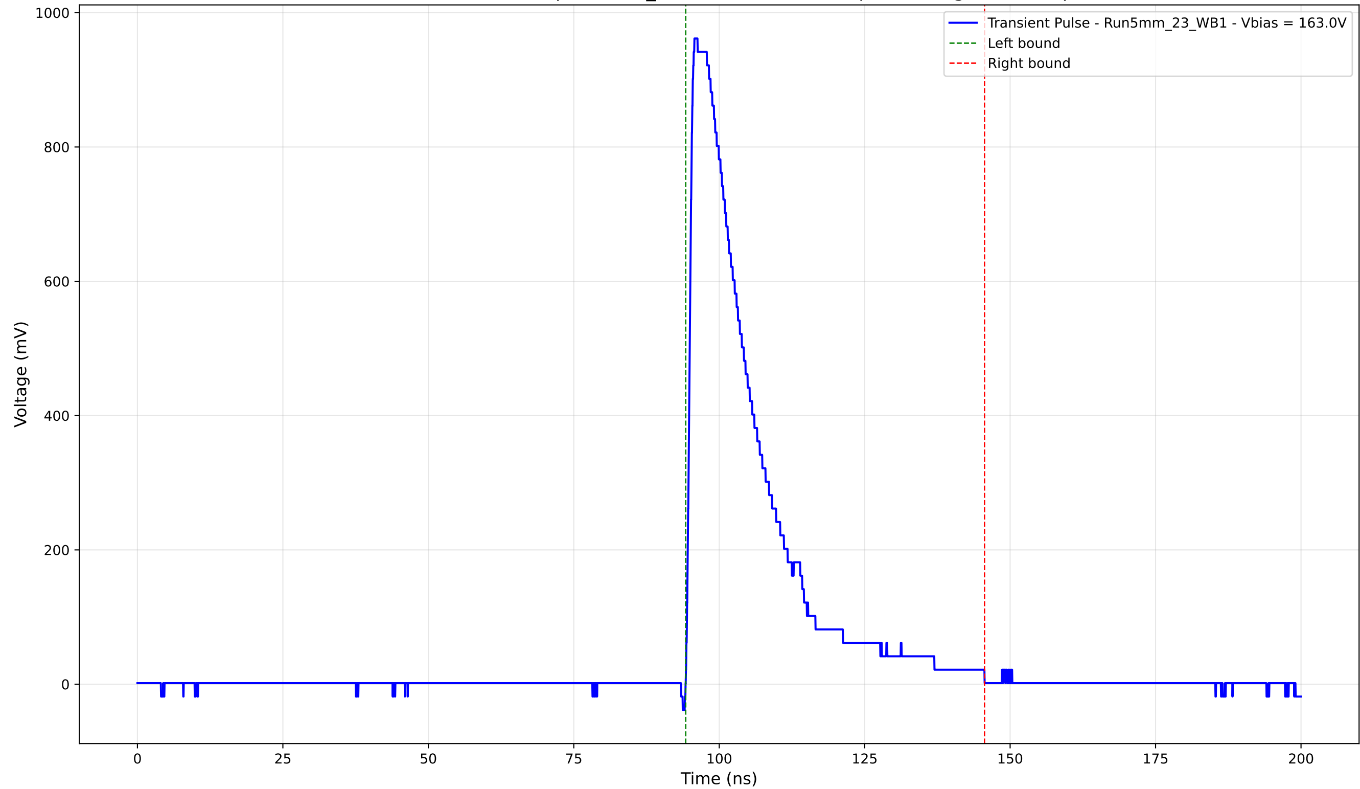
Transient Pulse - Sample: 5mm_23 - Position: 1895.0 \mu\text{m} - Charge: 235.48 pC
