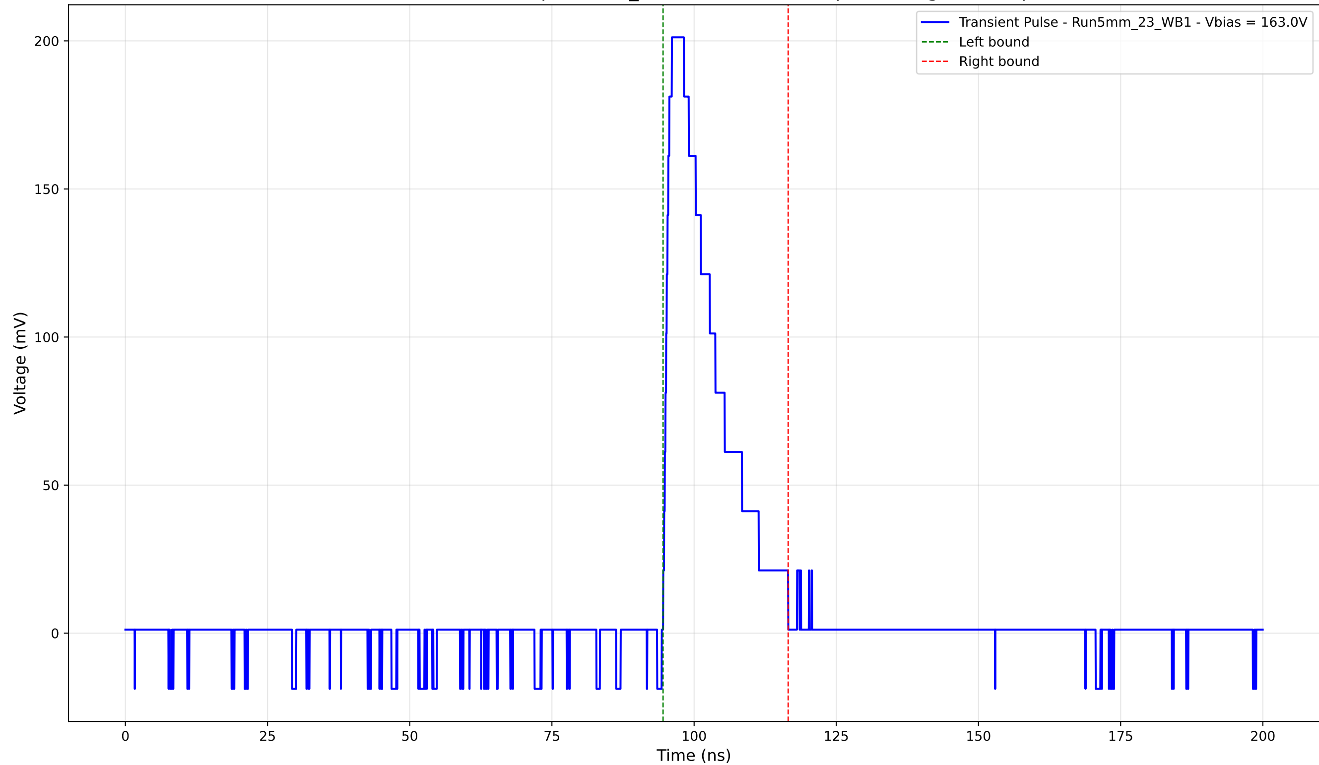
Transient Pulse - Sample: 5mm_23 - Position: 3765.0 \mu\text{m} - Charge: 38.57 pC
