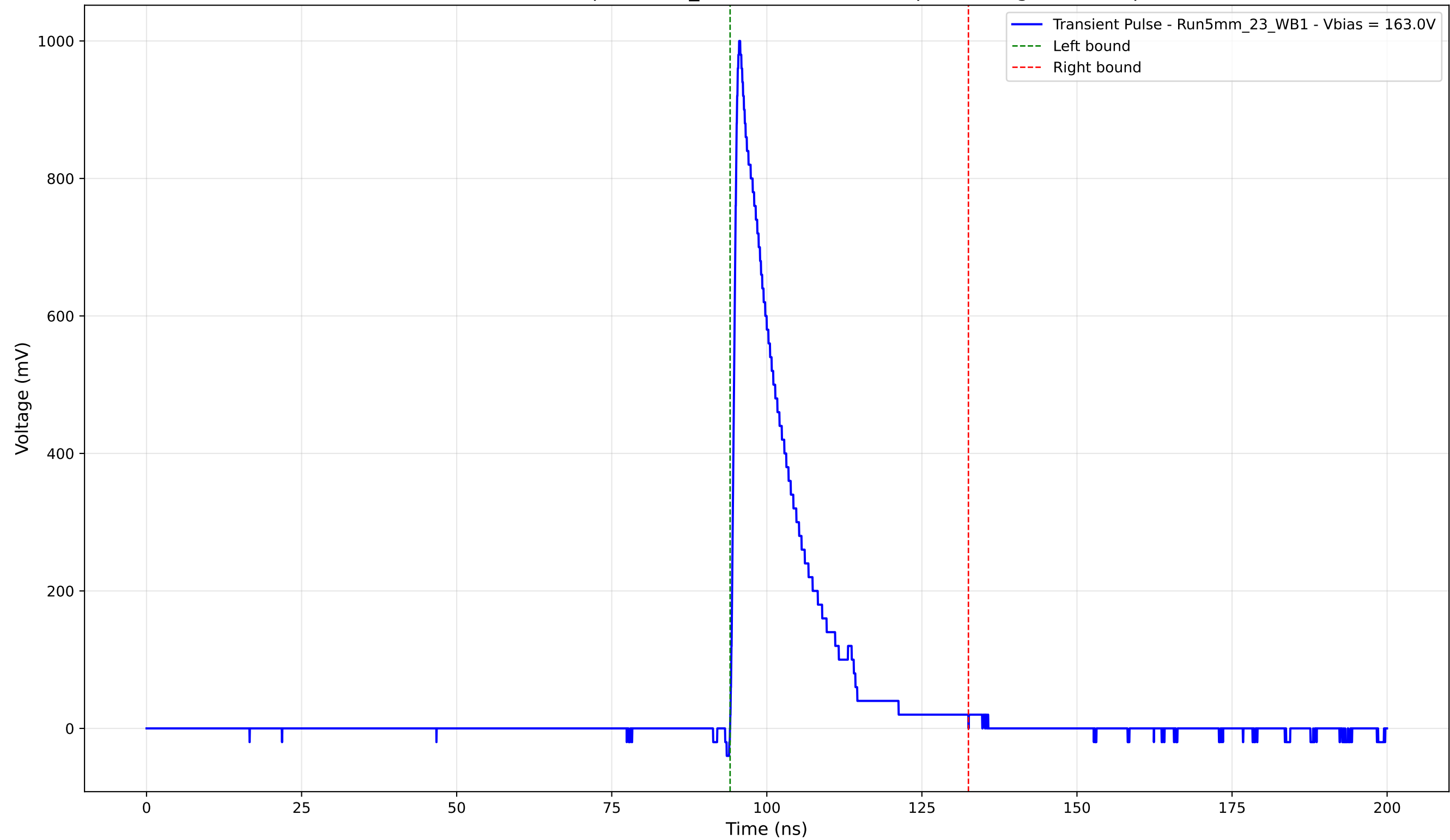
Transient Pulse - Sample: 5mm_23 - Position: 4915.0 \mu\text{m} - Charge: 169.96 pC
