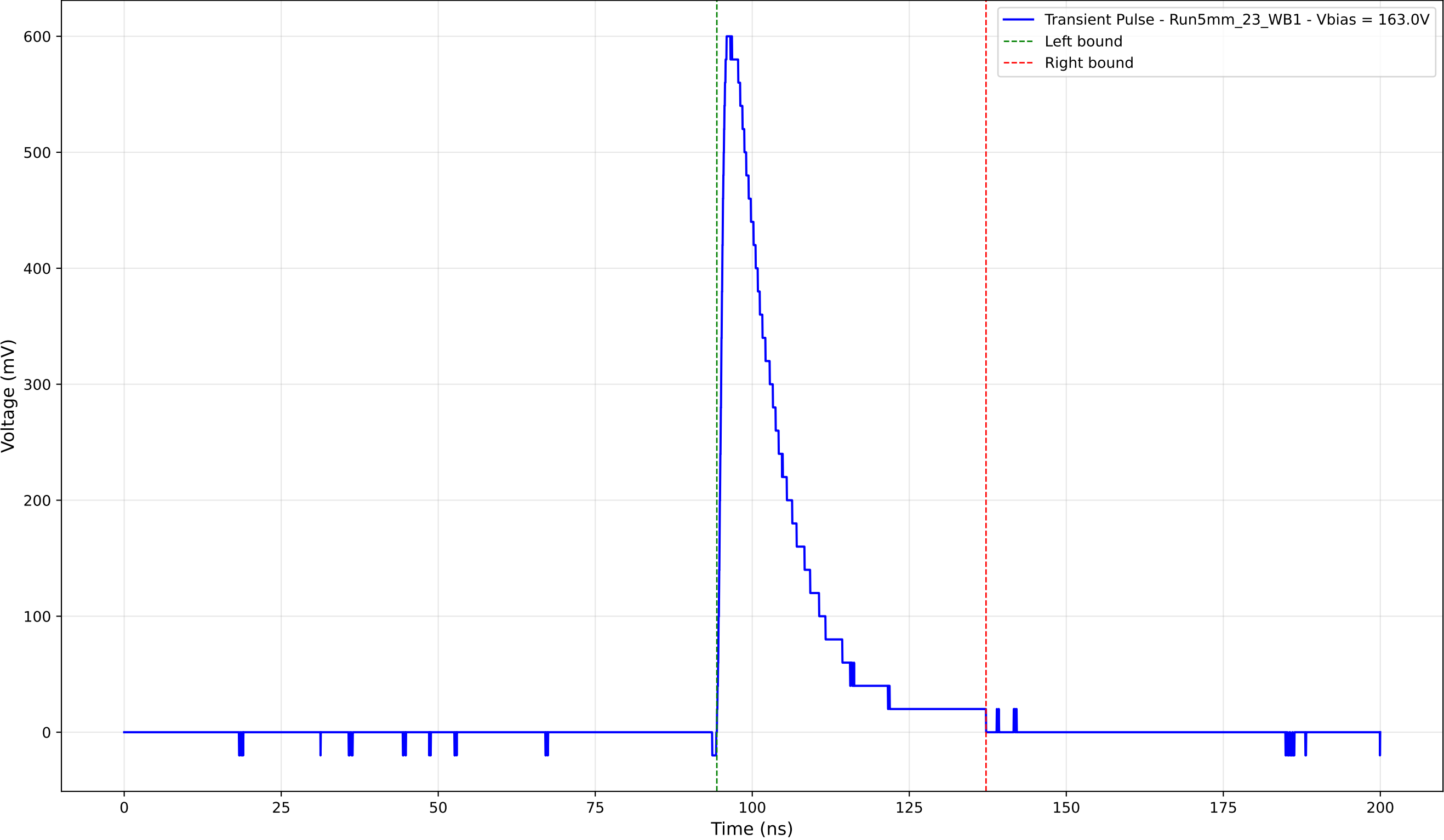
Transient Pulse - Sample: 5mm_23 - Position: 1775.0 \mu\text{m} - Charge: 123.68 pC
