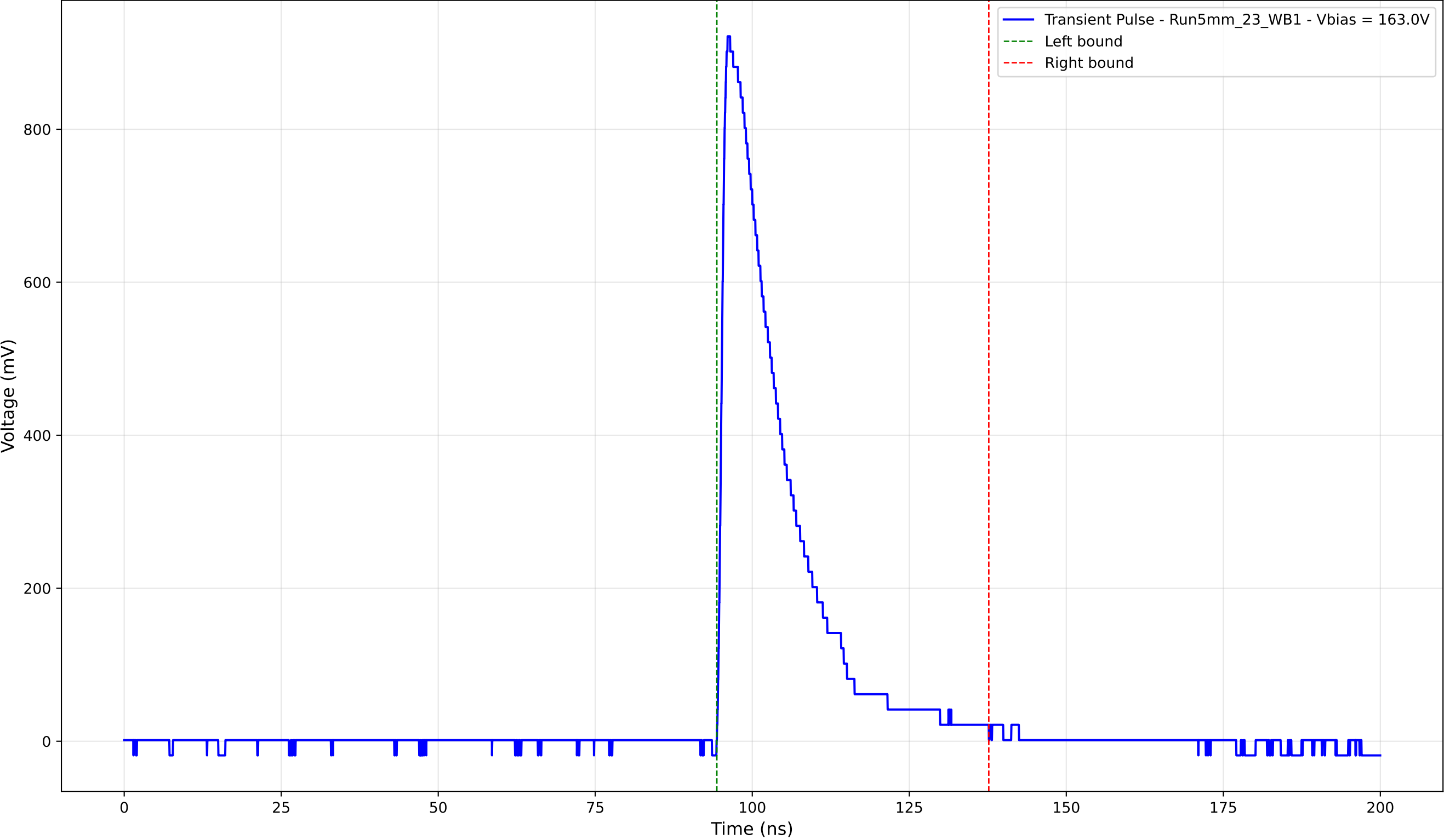
Transient Pulse - Sample: 5mm_23 - Position: 3985.0 \mu\text{m} - Charge: 198.59 pC
