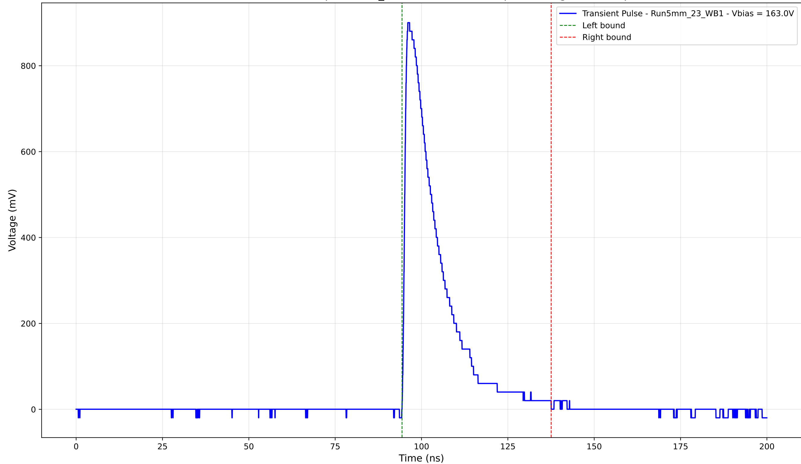
Transient Pulse - Sample: 5mm_23 - Position: 3895.0 \mu\text{m} - Charge: 194.10 pC
