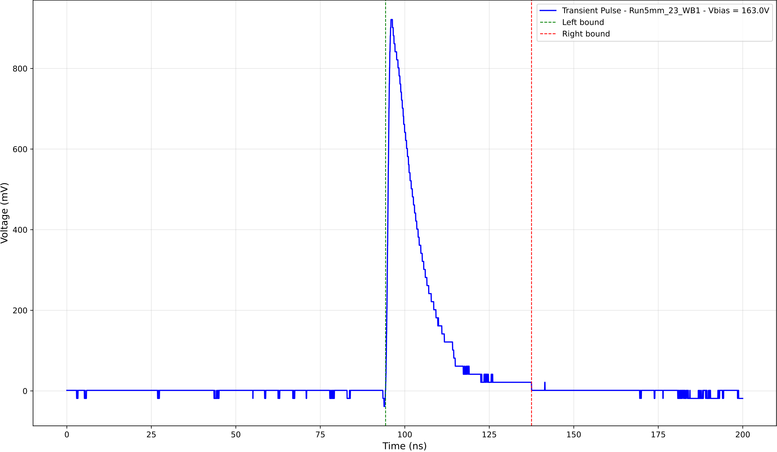
Transient Pulse - Sample: 5mm_23 - Position: 4450.0 \mu\text{m} - Charge: 180.83 pC
