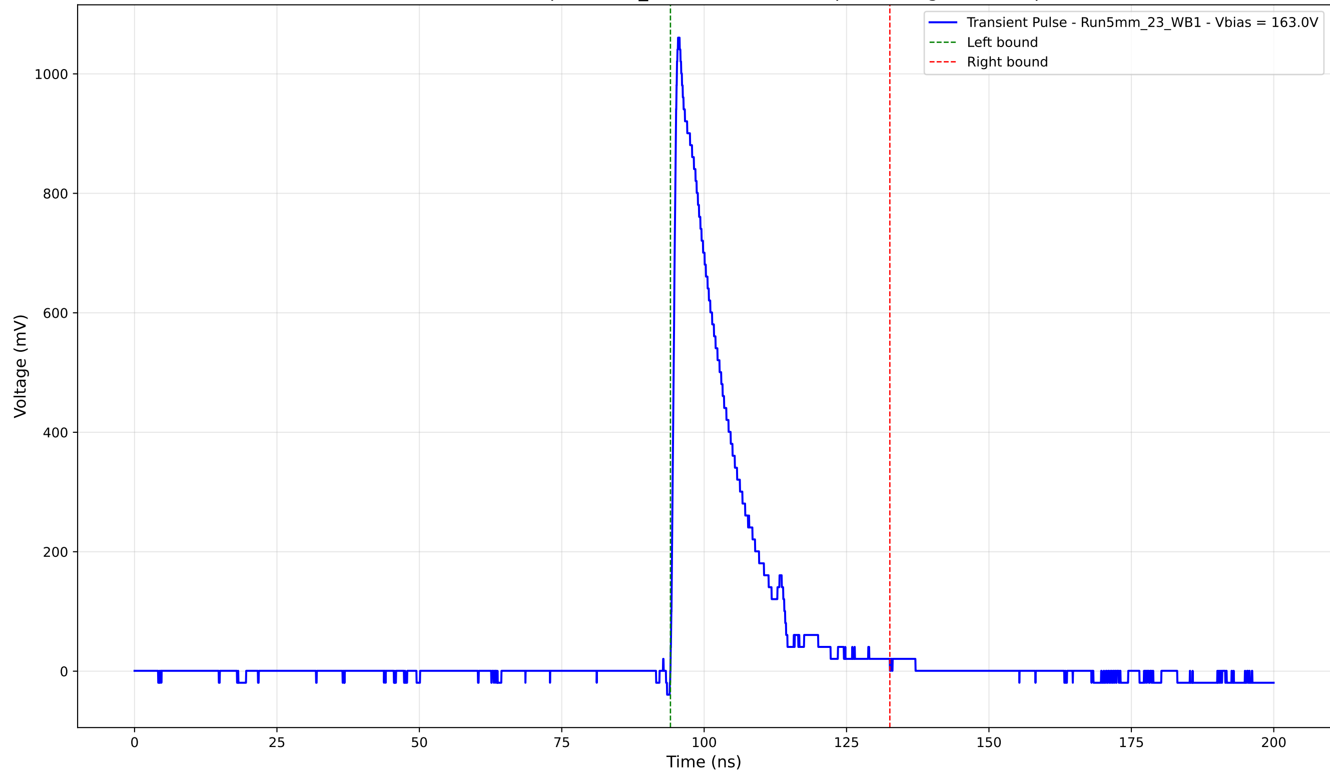
Transient Pulse - Sample: 5mm_23 - Position: 425.0 \mu\text{m} - Charge: 199.40 pC
