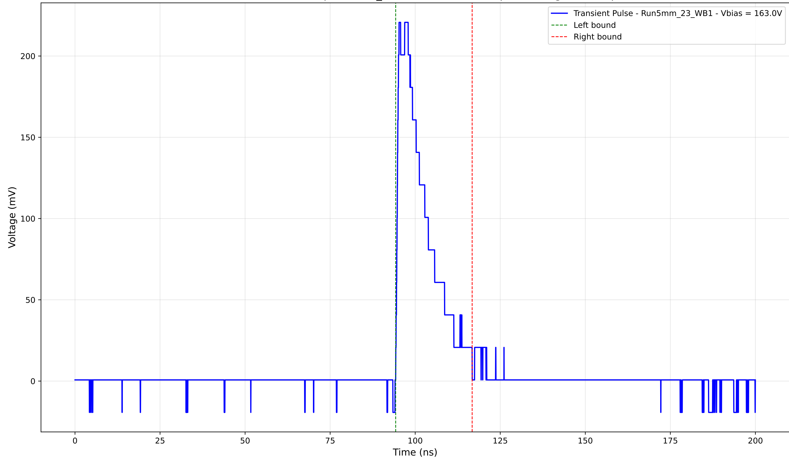
Transient Pulse - Sample: 5mm_23 - Position: 2235.0 \mu\text{m} - Charge: 41.64 pC
