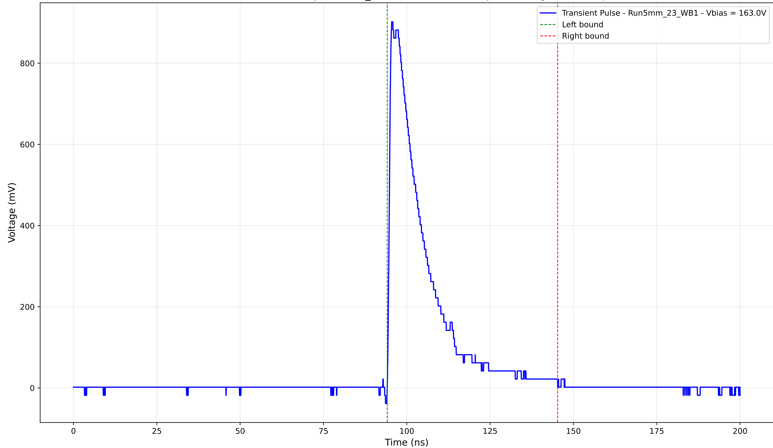
Transient Pulse - Sample: 5mm_23 - Position: 3355.0 \mu\text{m} - Charge: 205.26 pC
