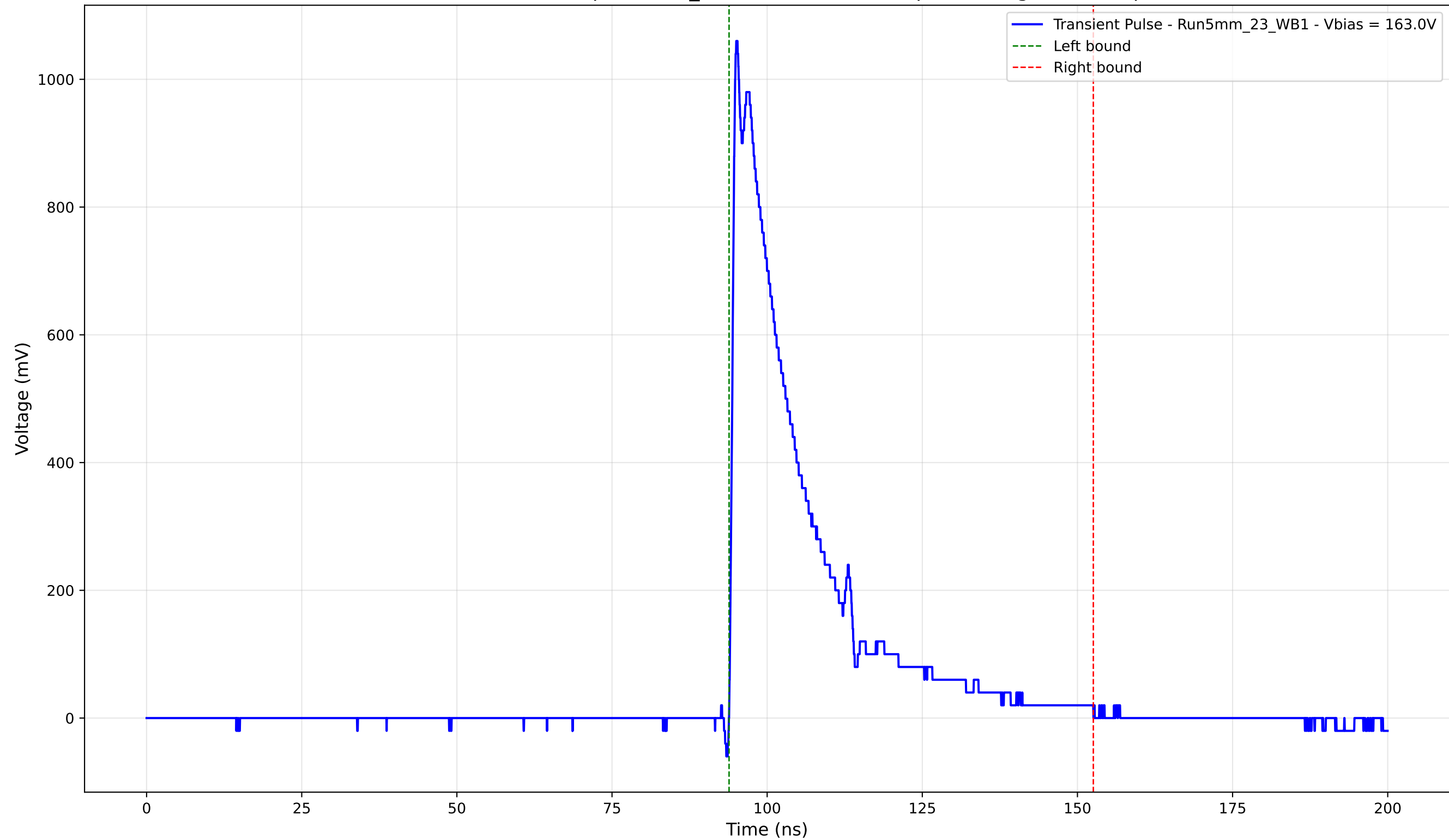
Transient Pulse - Sample: 5mm_23 - Position: 2880.0 \mu\text{m} - Charge: 243.46 pC
