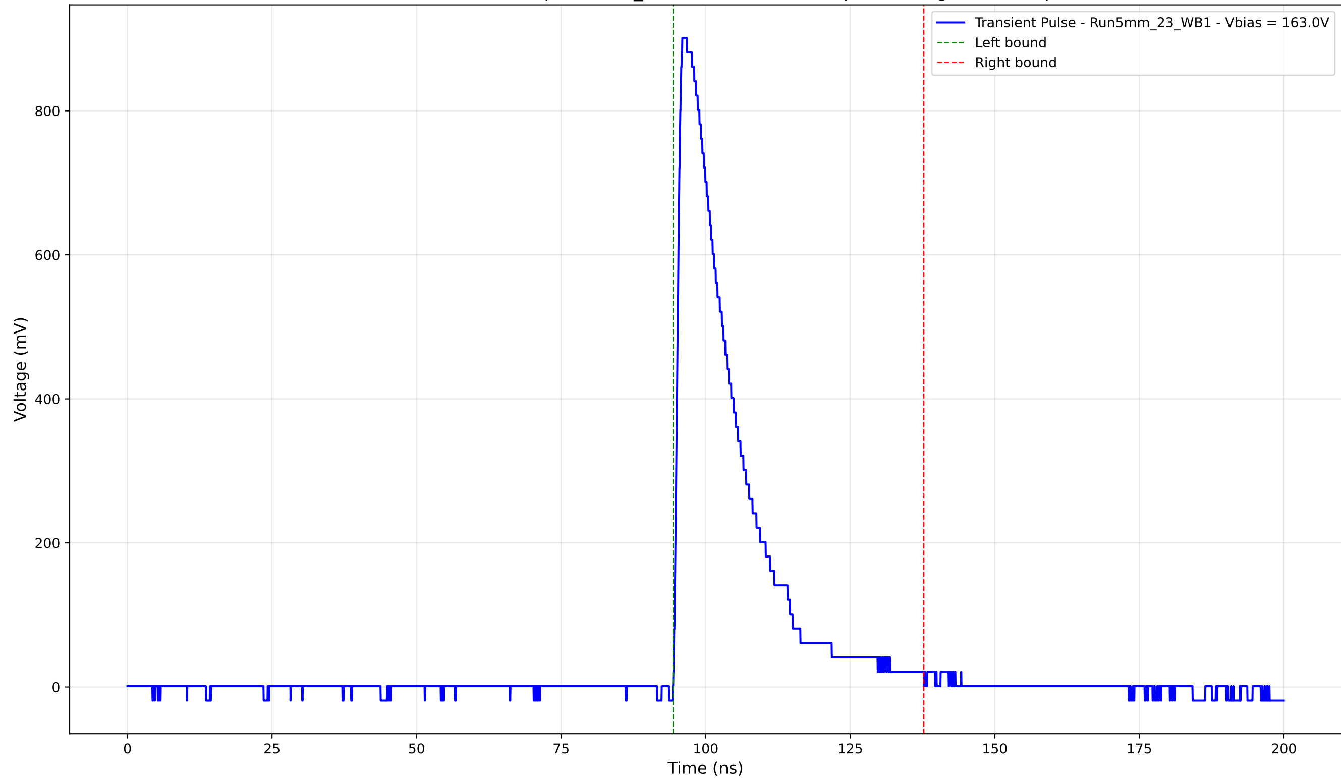
Transient Pulse - Sample: 5mm_23 - Position: 3960.0 \mu\text{m} - Charge: 197.64 pC
