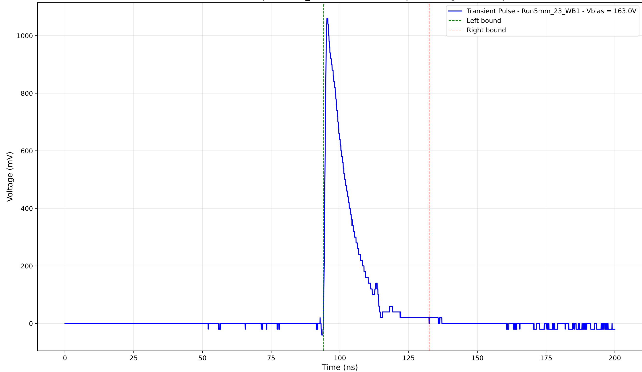
Transient Pulse - Sample: 5mm_23 - Position: 5075.0 \mu\text{m} - Charge: 186.33 pC
