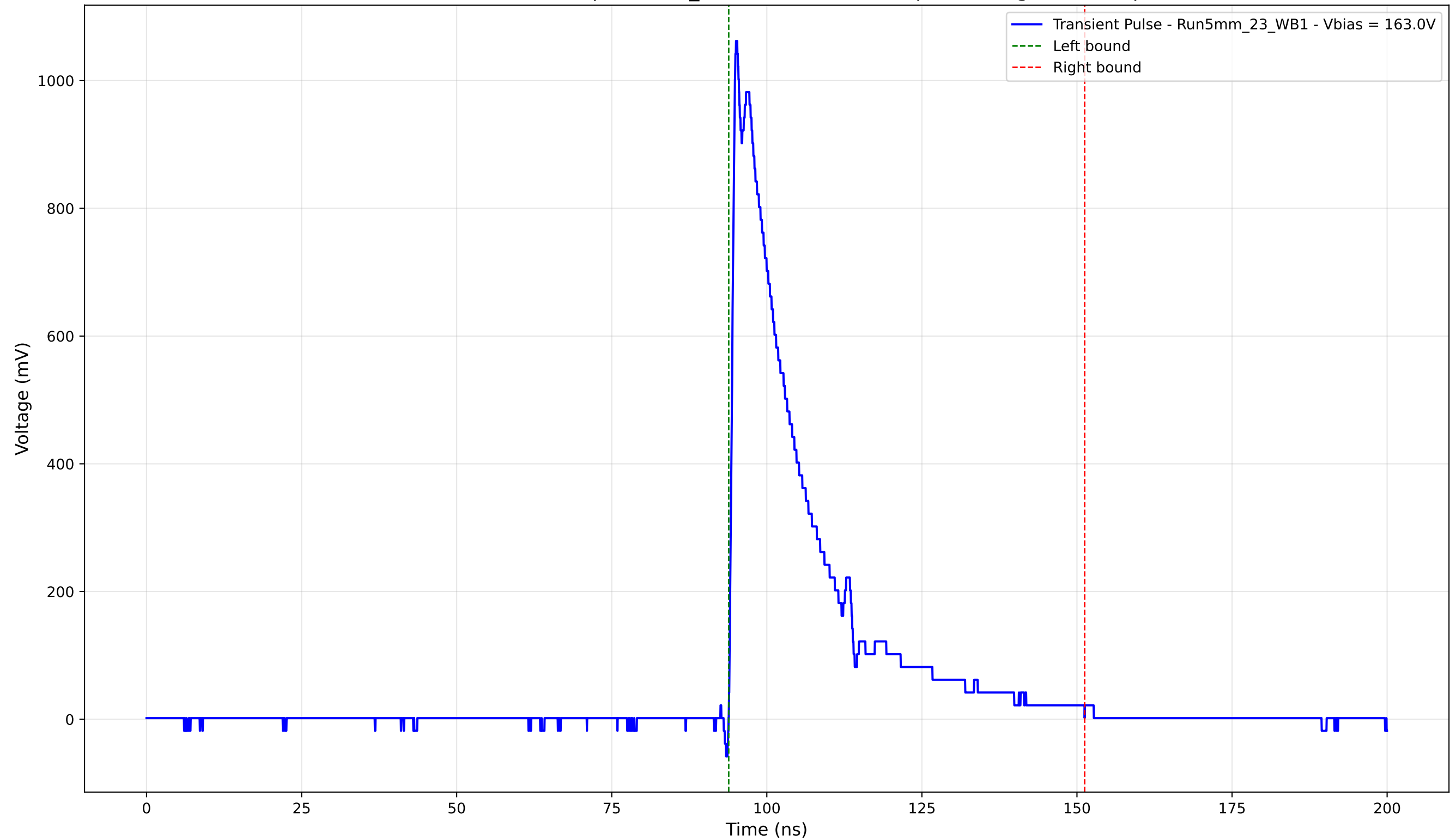
Transient Pulse - Sample: 5mm_23 - Position: 2595.0 \mu\text{m} - Charge: 246.21 pC
