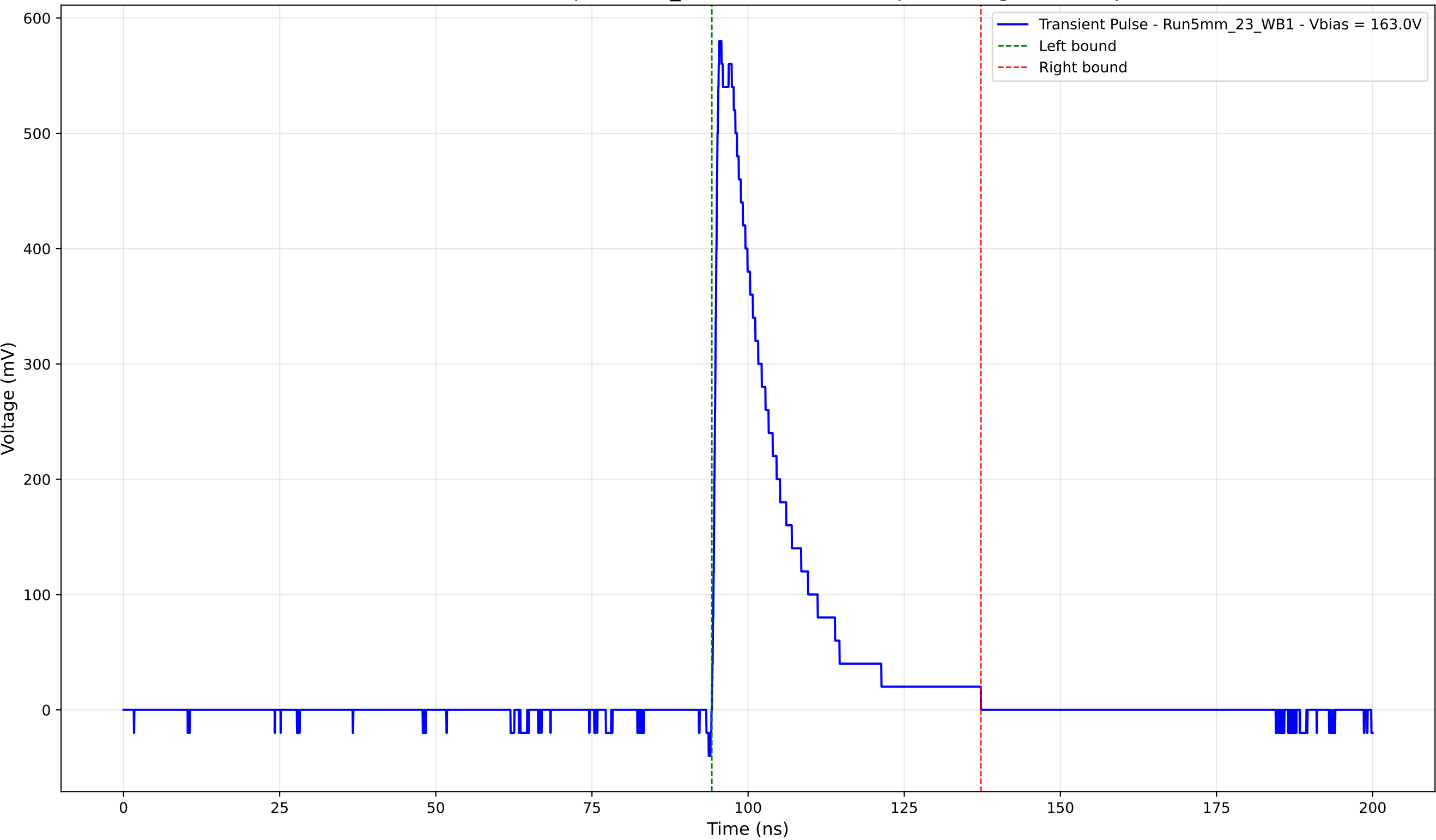
Transient Pulse - Sample: 5mm_23 - Position: 3295.0 \mu\text{m} - Charge: 115.67 pC
