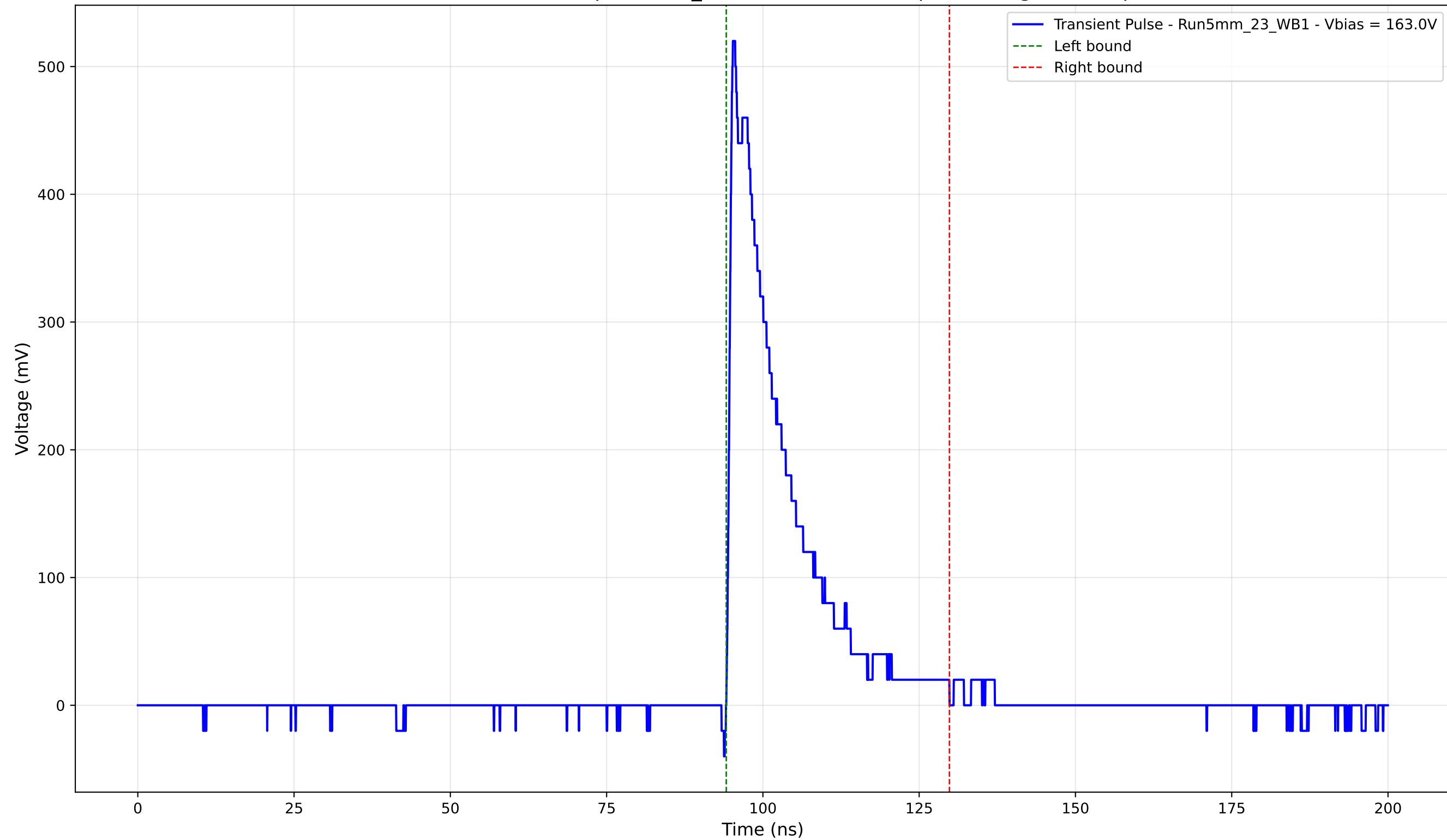
Transient Pulse - Sample: 5mm_23 - Position: 2275.0 \mu\text{m} - Charge: 94.07 pC
