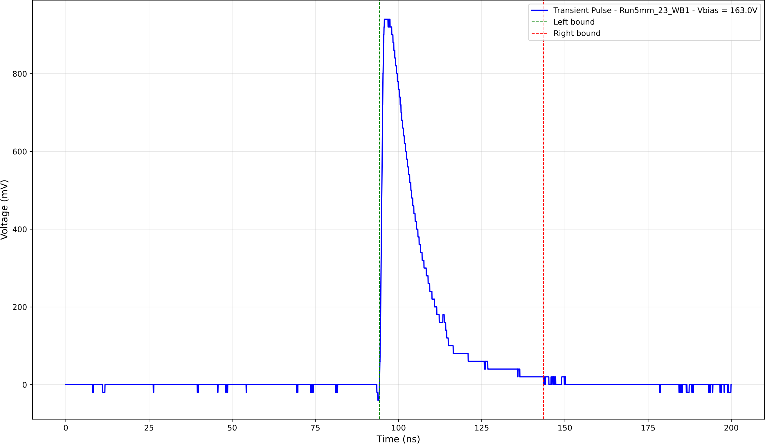
Transient Pulse - Sample: 5mm_23 - Position: 1840.0 \mu\text{m} - Charge: 226.34 pC
