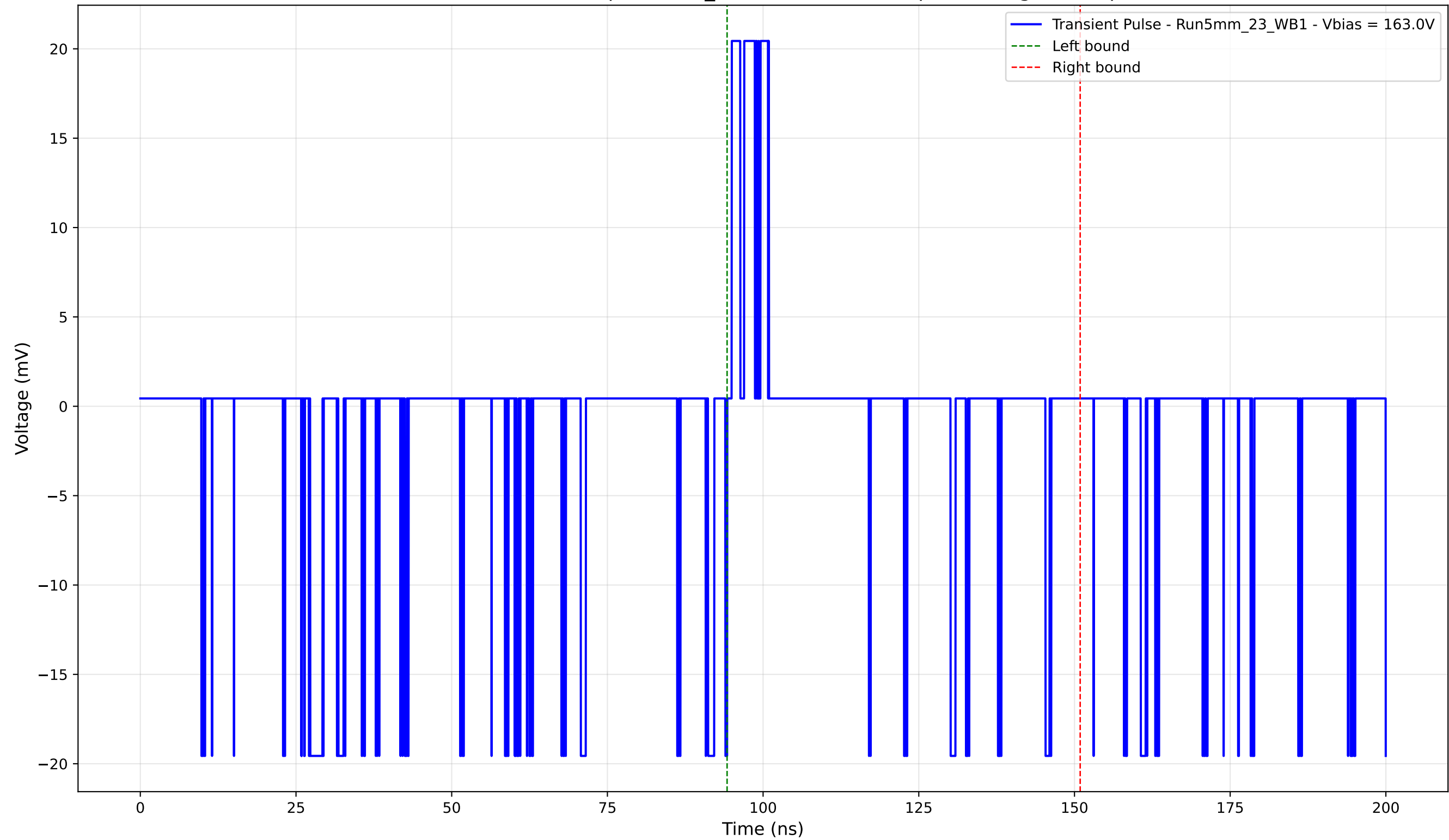
Transient Pulse - Sample: 5mm_23 - Position: 225.0 \mu\text{m} - Charge: 1.21 pC
