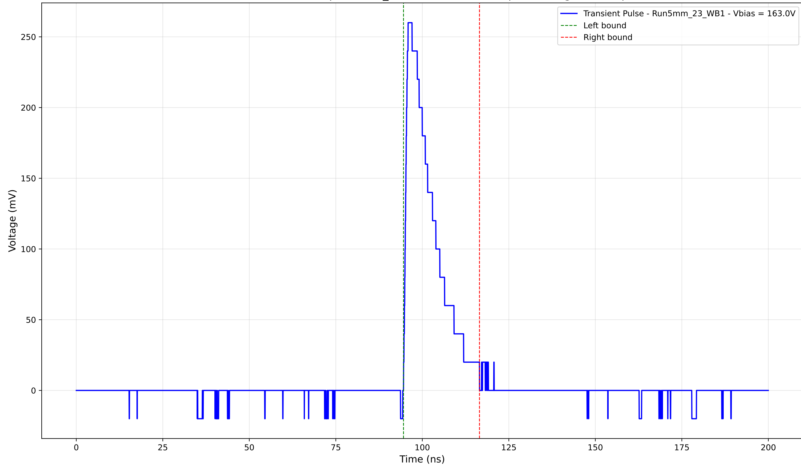
Transient Pulse - Sample: 5mm_23 - Position: 4240.0 \mu\text{m} - Charge: 46.23 pC
