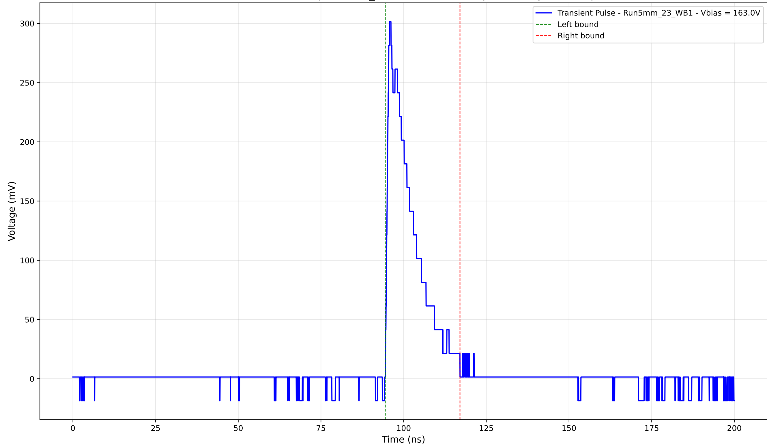
Transient Pulse - Sample: 5mm_23 - Position: 735.0 \mu\text{m} - Charge: 50.08 pC
