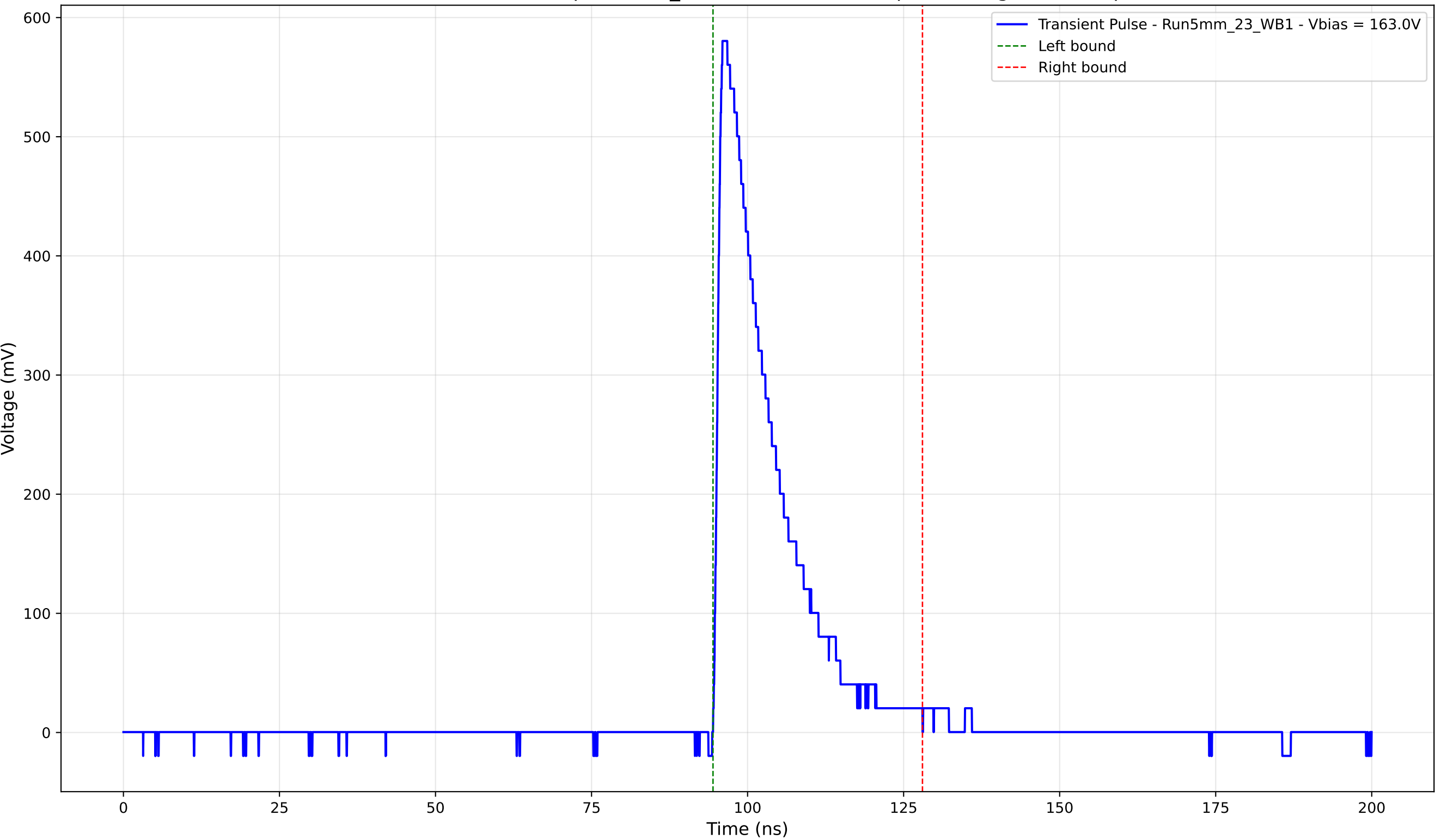
Transient Pulse - Sample: 5mm_23 - Position: 1270.0 \mu\text{m} - Charge: 112.35 pC
