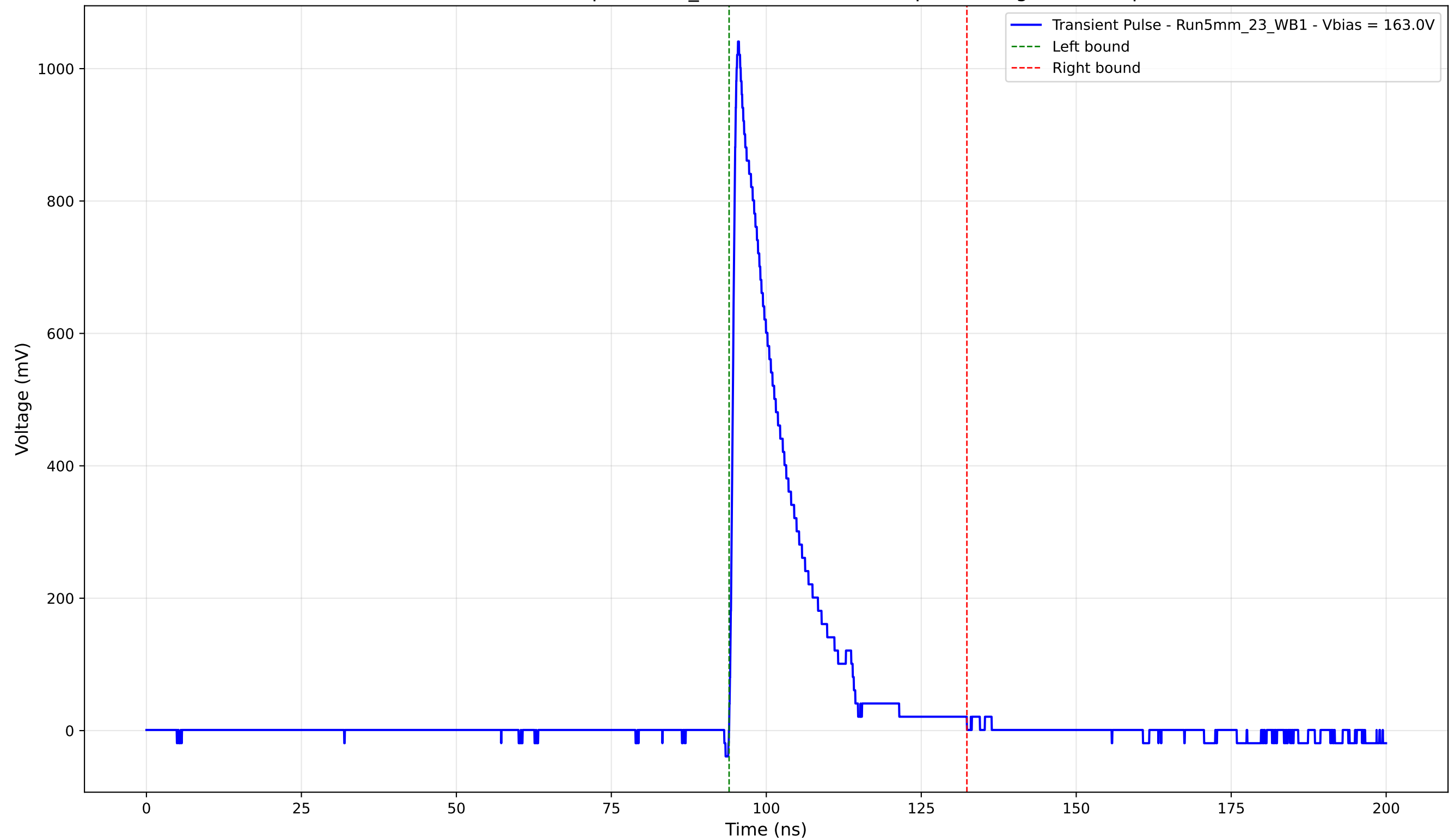
Transient Pulse - Sample: 5mm_23 - Position: 5030.0 \mu\text{m} - Charge: 176.49 pC
