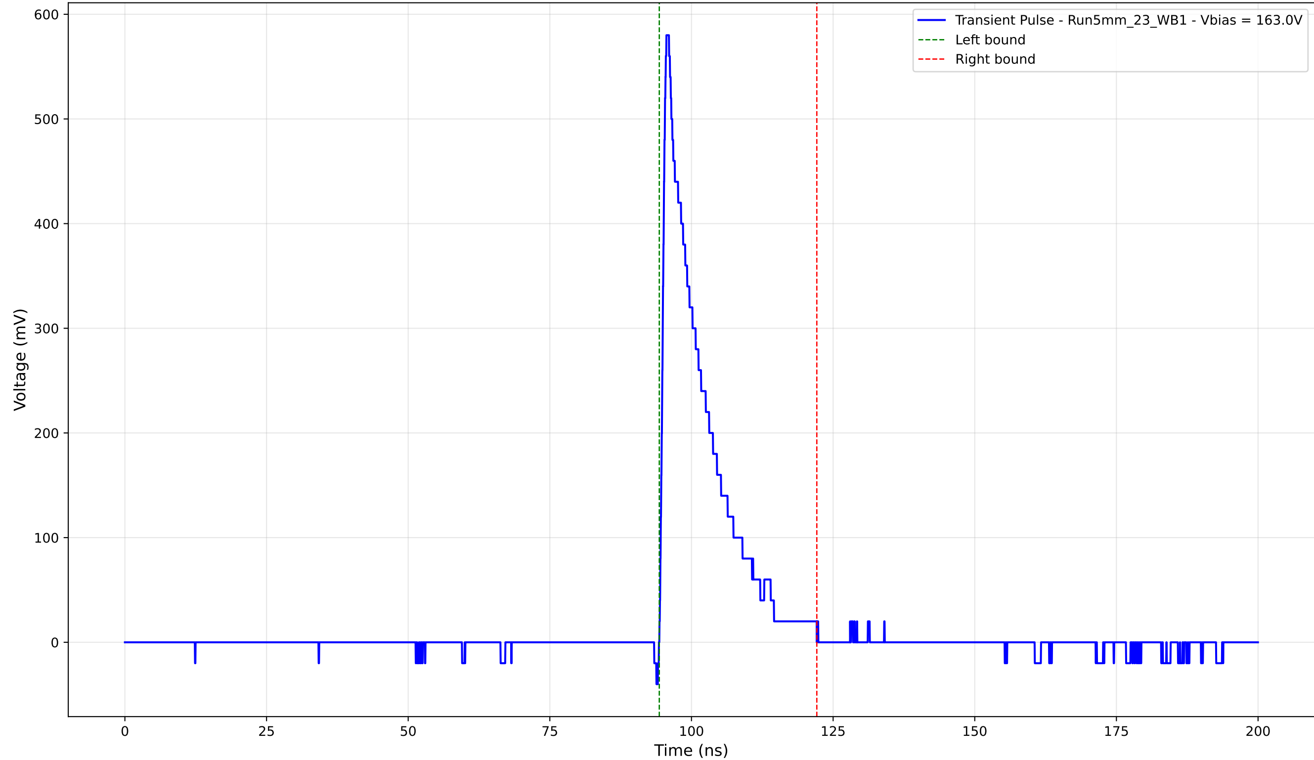
Transient Pulse - Sample: 5mm_23 - Position: 685.0 \mu\text{m} - Charge: 88.47 pC
