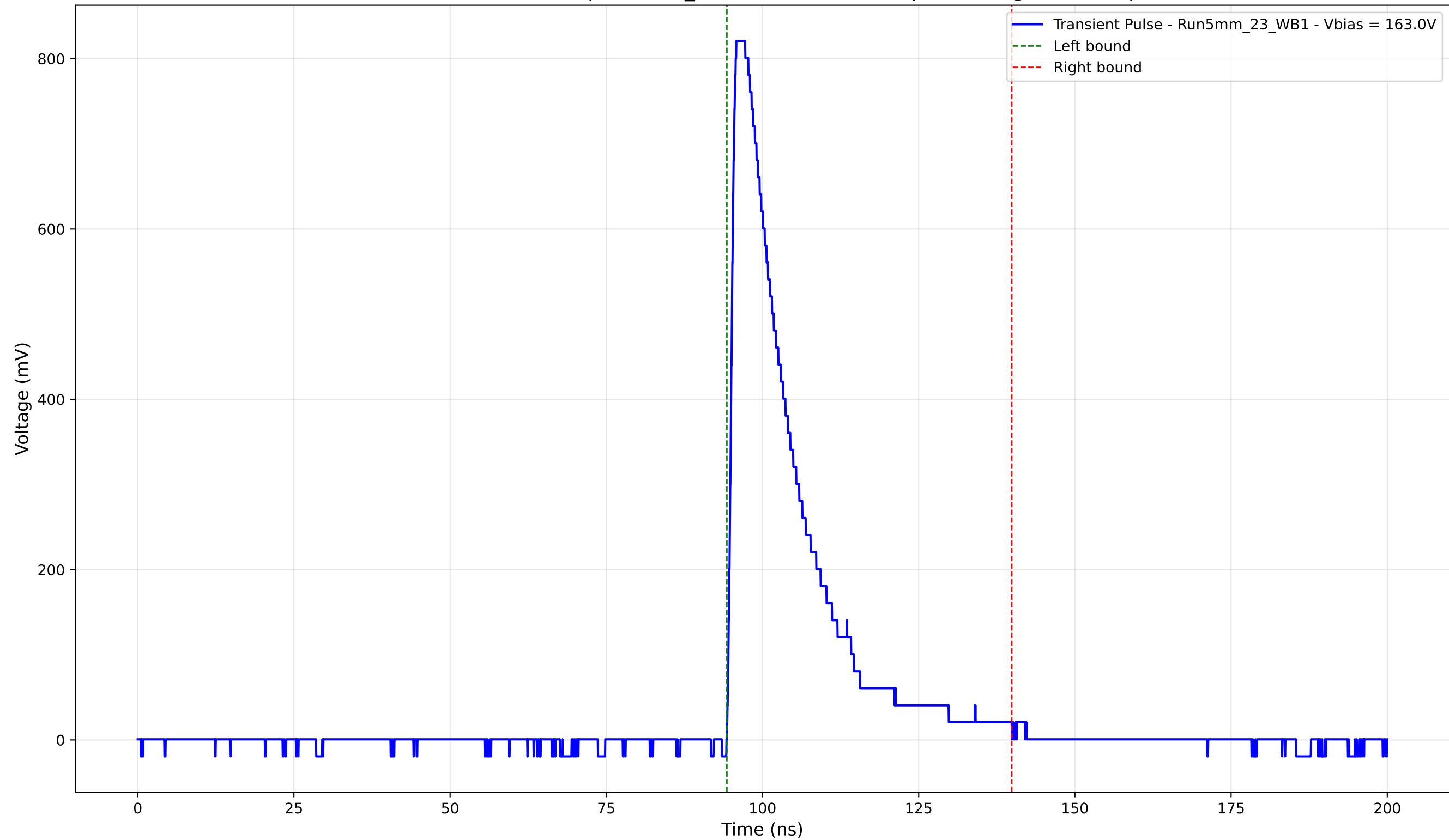
Transient Pulse - Sample: 5mm_23 - Position: 3675.0 \mu\text{m} - Charge: 178.33 pC
