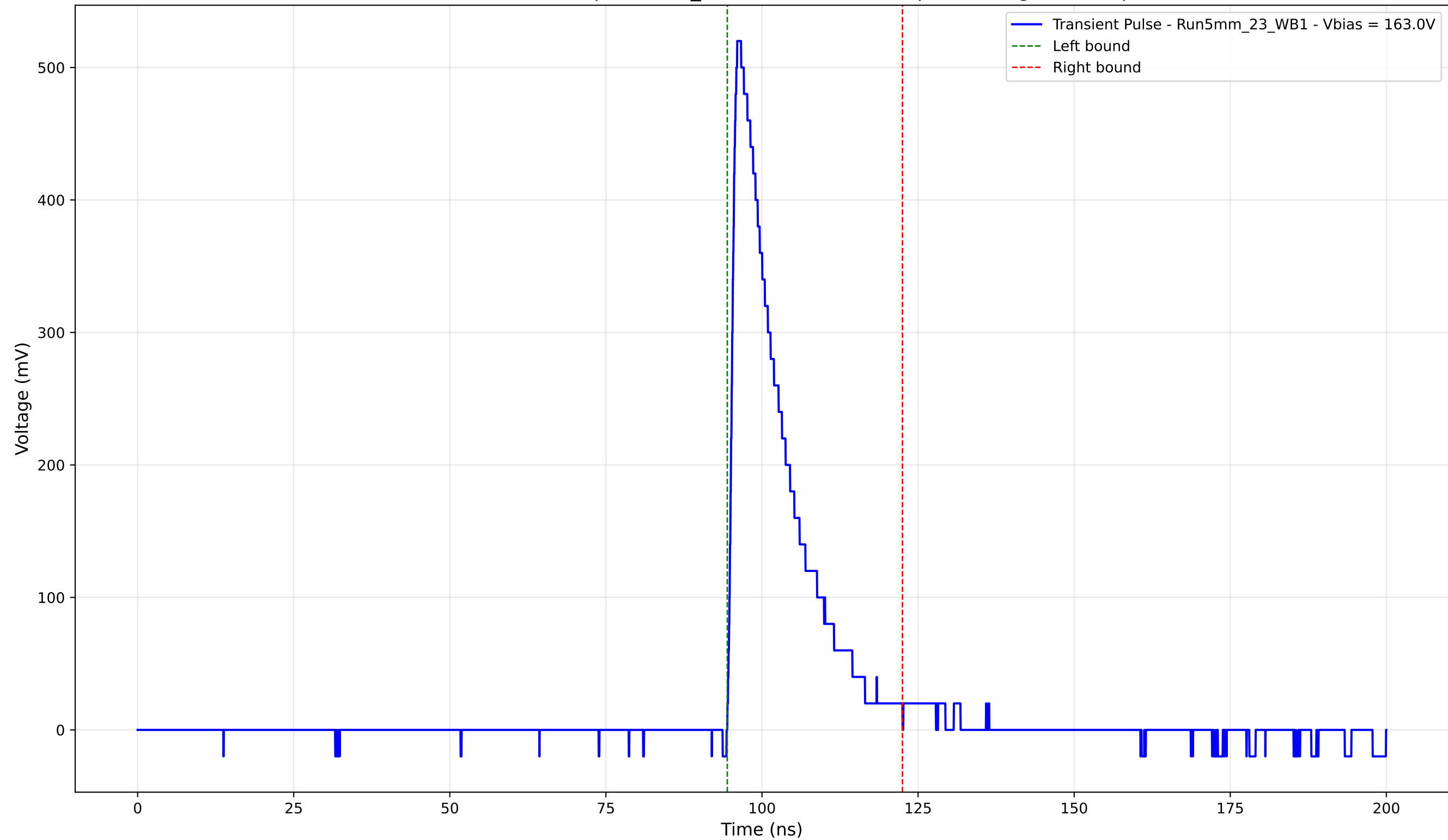
Transient Pulse - Sample: 5mm_23 - Position: 4215.0 \mu\text{m} - Charge: 92.78 pC
