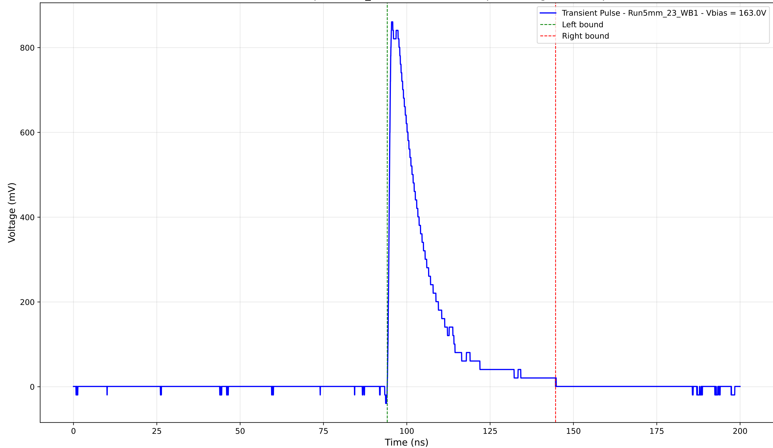
Transient Pulse - Sample: 5mm_23 - Position: 3335.0 \mu\text{m} - Charge: 189.45 pC
