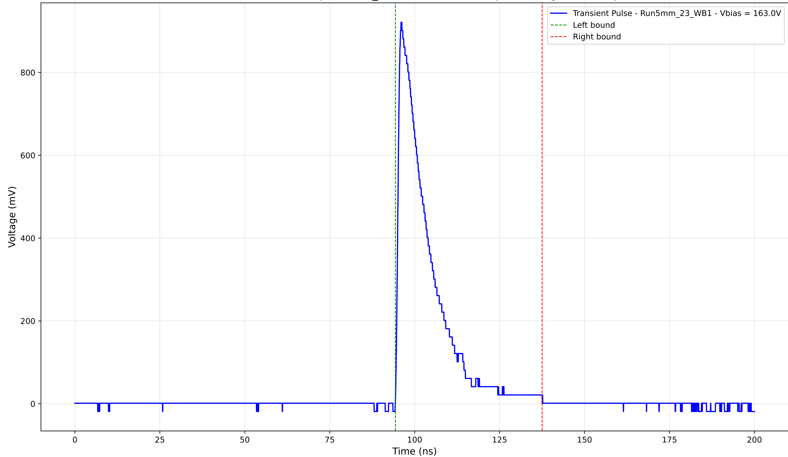
Transient Pulse - Sample: 5mm_23 - Position: 4415.0 \mu\text{m} - Charge: 181.37 pC
