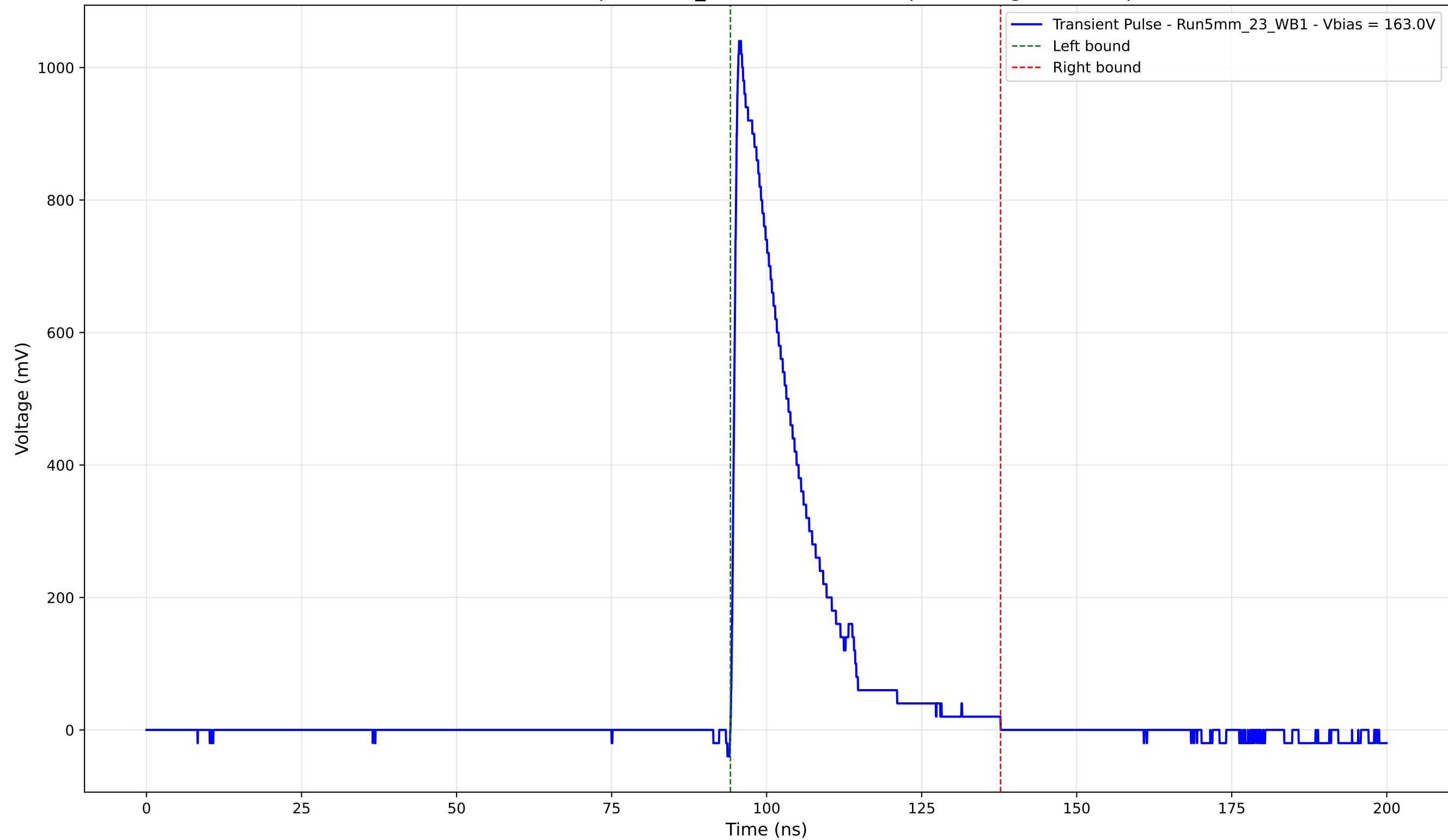
Transient Pulse - Sample: 5mm_23 - Position: 610.0 \mu\text{m} - Charge: 211.36 pC
