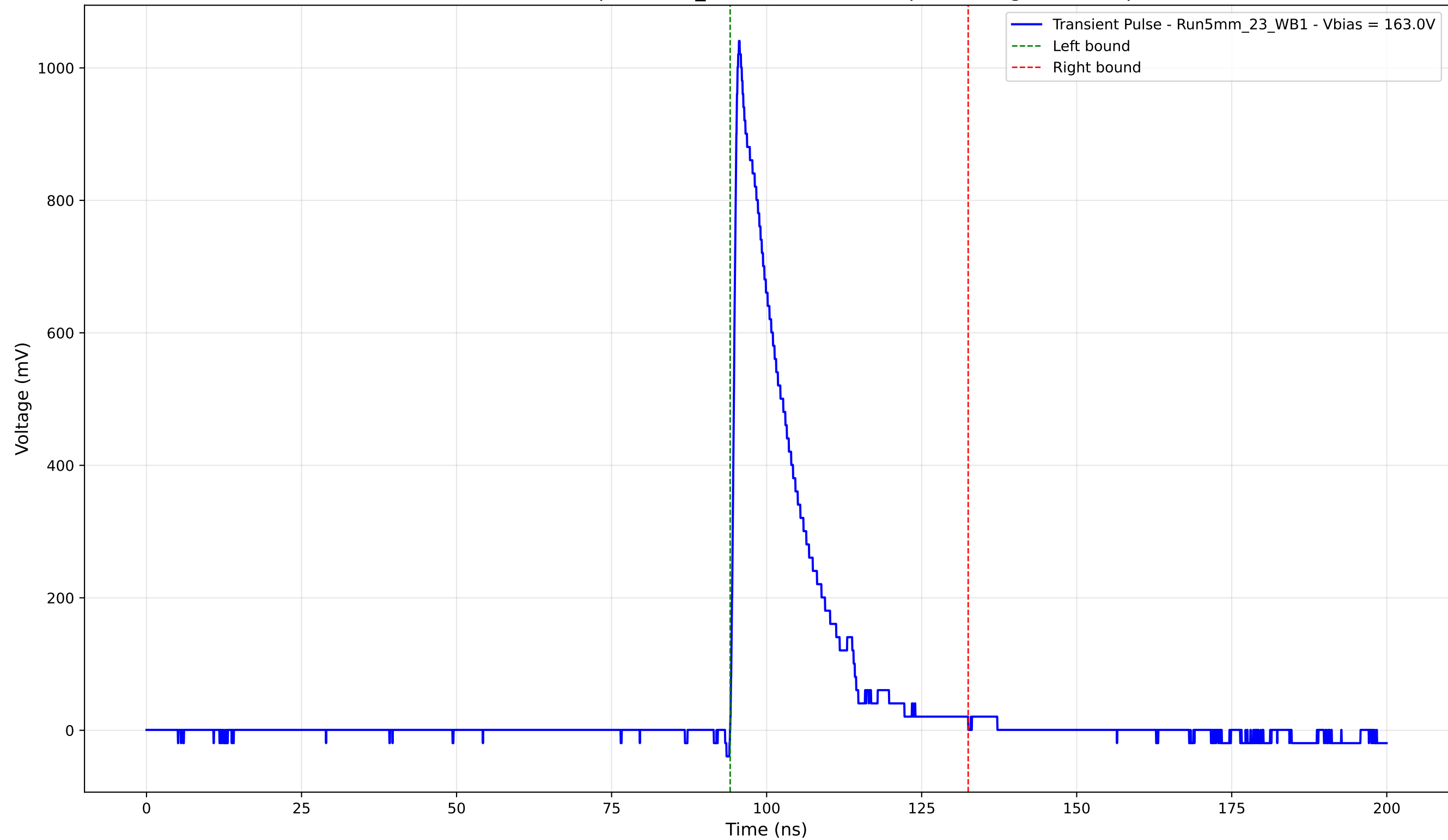
Transient Pulse - Sample: 5mm_23 - Position: 500.0 \mu\text{m} - Charge: 190.80 pC
