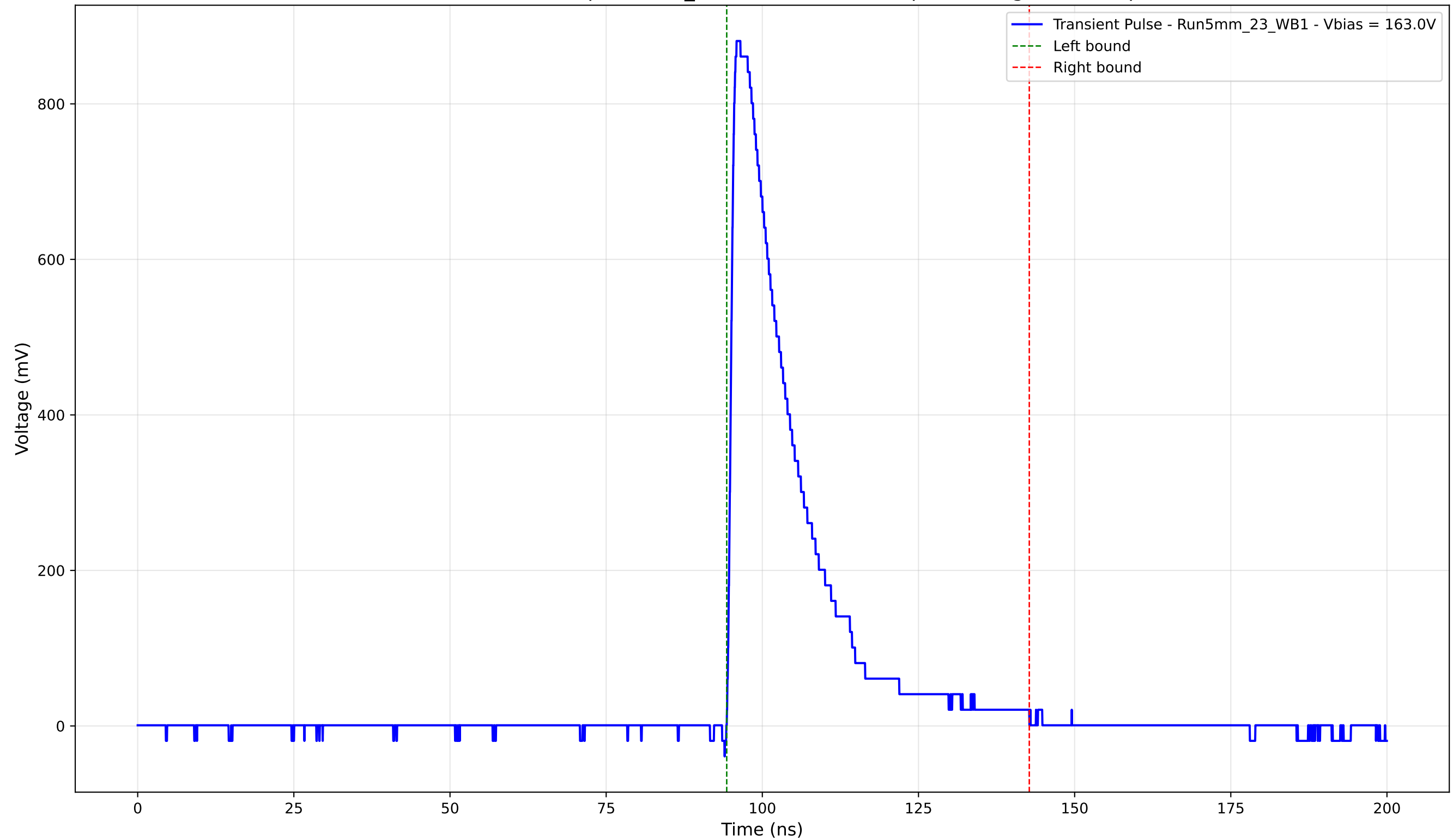
Transient Pulse - Sample: 5mm_23 - Position: 3660.0 \mu\text{m} - Charge: 195.25 pC
