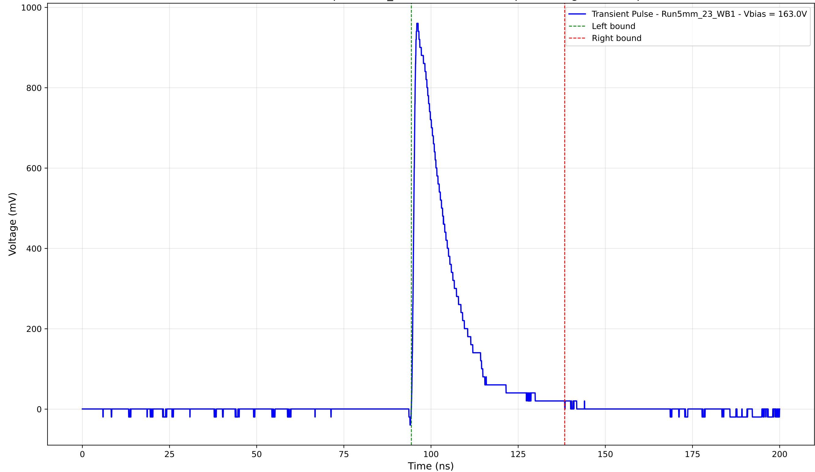
Transient Pulse - Sample: 5mm_23 - Position: 1030.0 \mu\text{m} - Charge: 201.94 pC
