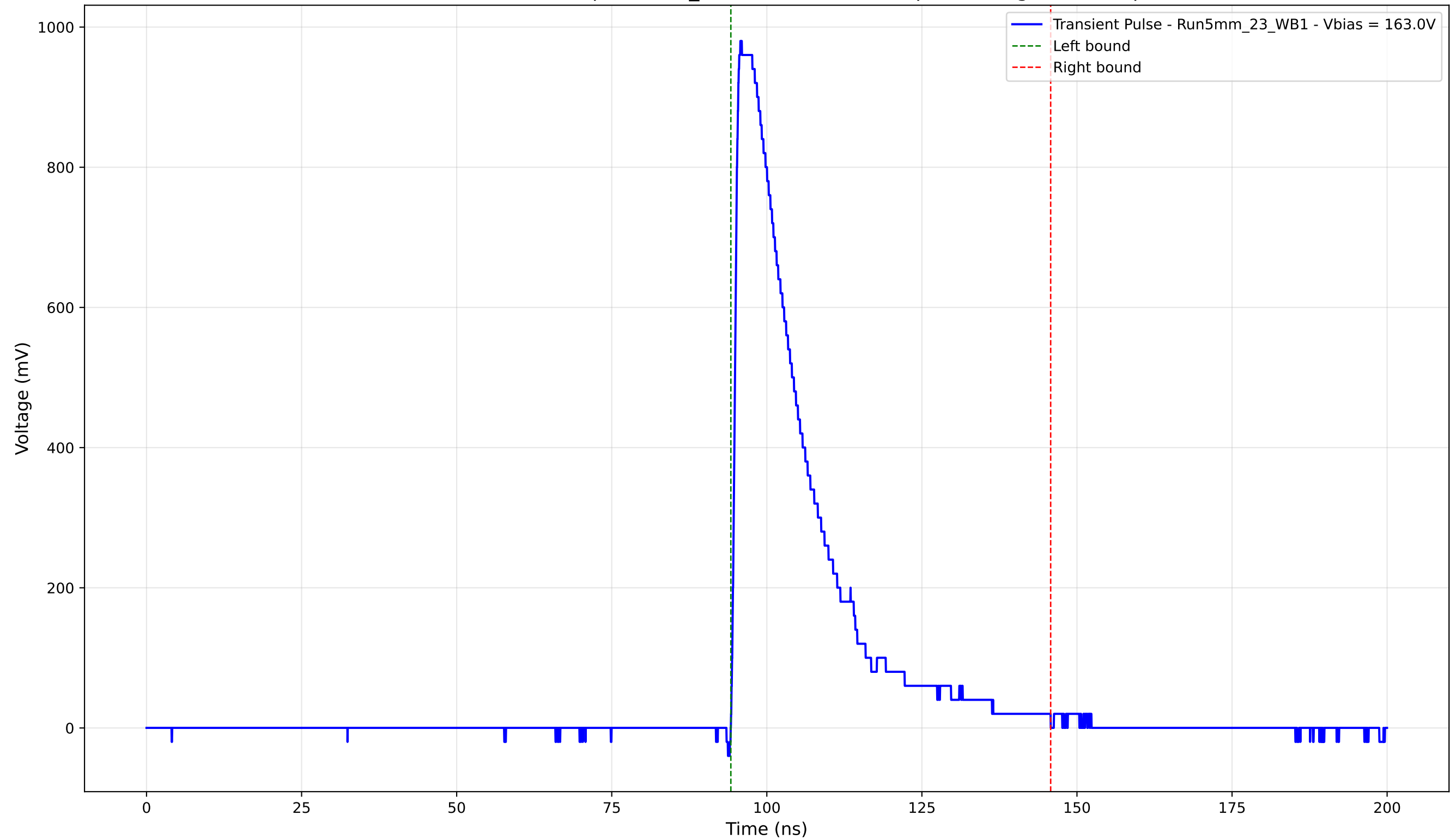
Transient Pulse - Sample: 5mm_23 - Position: 1965.0 \mu\text{m} - Charge: 240.45 pC
