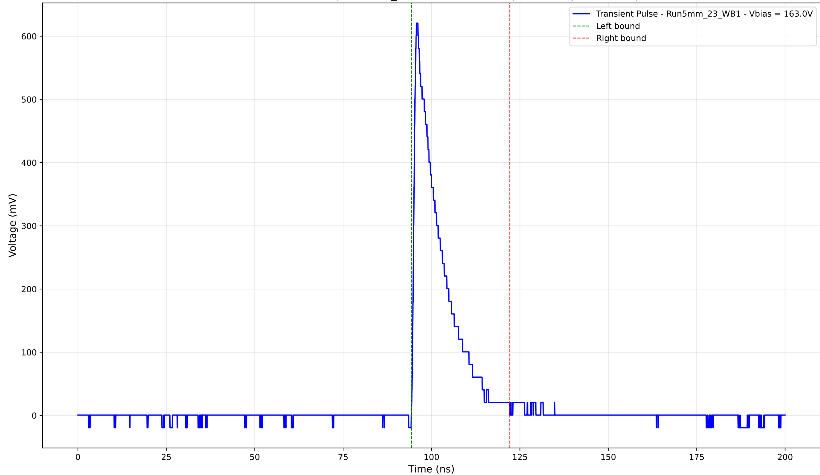
Transient Pulse - Sample: 5mm_23 - Position: 760.0 \mu\text{m} - Charge: 101.74 pC
