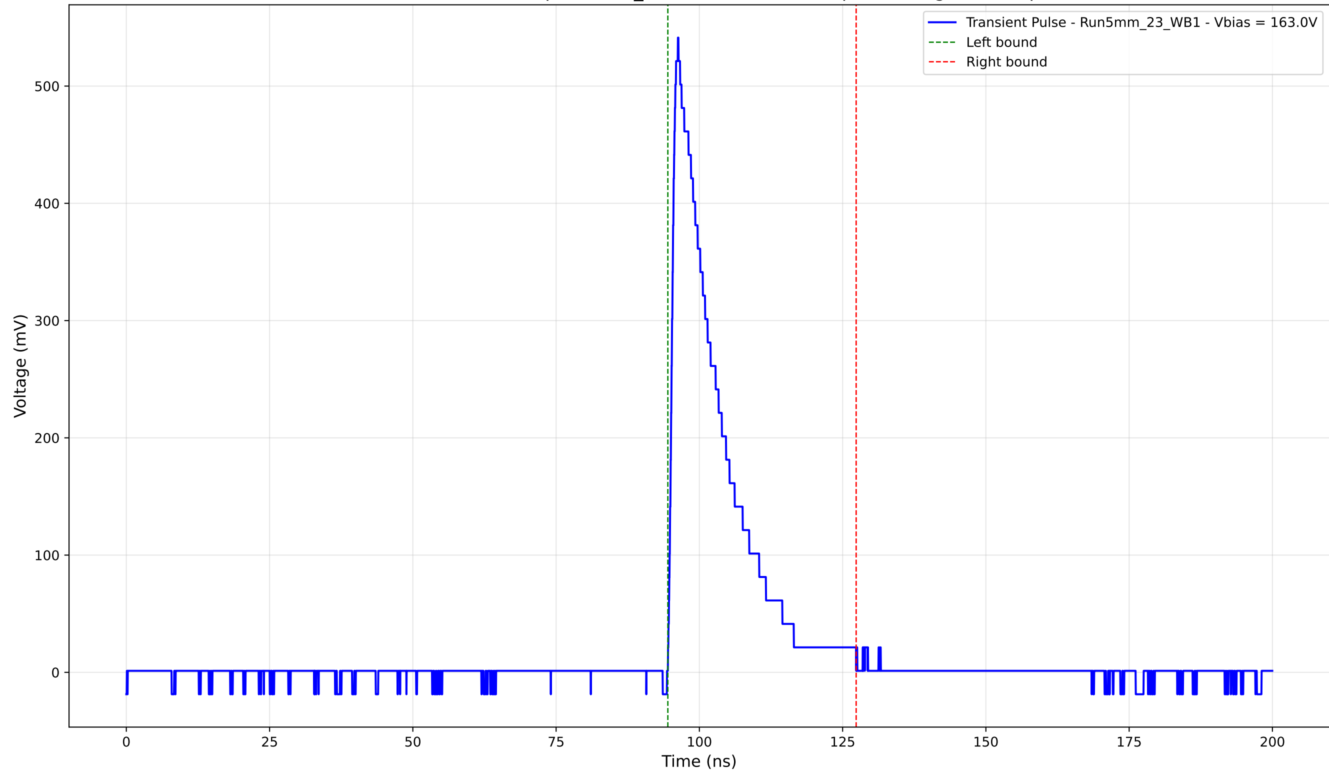
Transient Pulse - Sample: 5mm_23 - Position: 1185.0 \mu\text{m} - Charge: 96.28 pC
