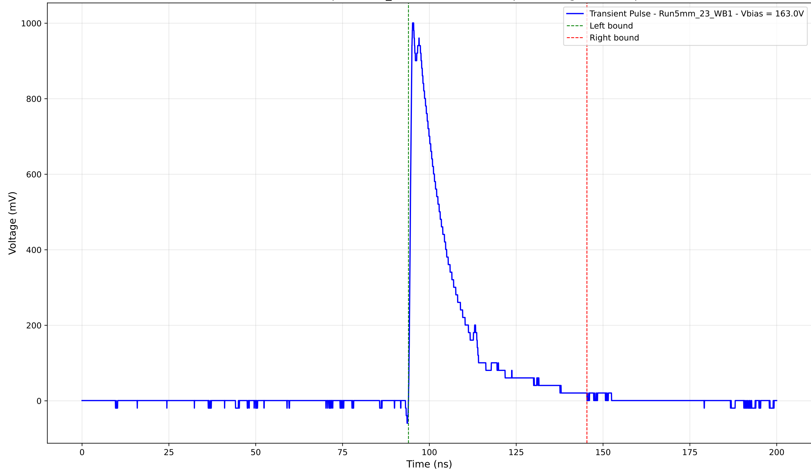
Transient Pulse - Sample: 5mm_23 - Position: 2415.0 \mu\text{m} - Charge: 228.18 pC
