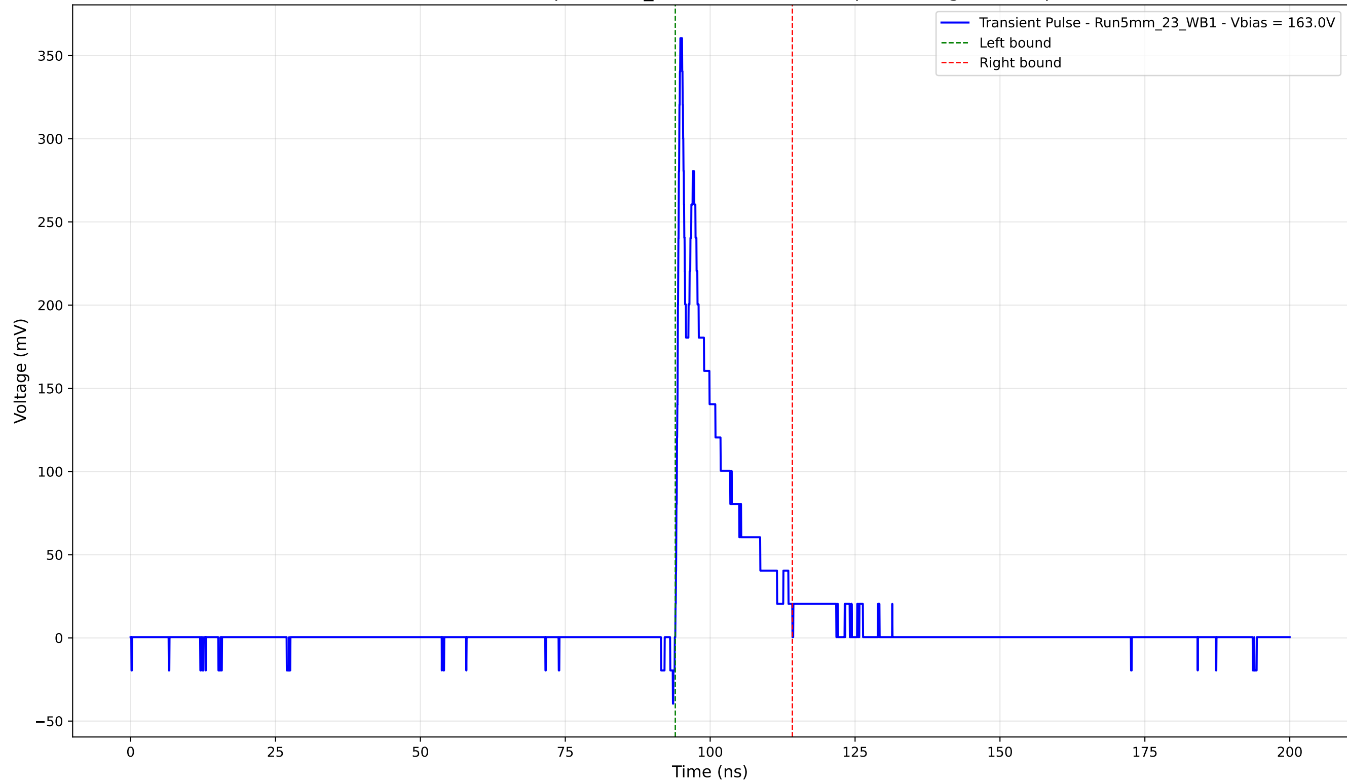
Transient Pulse - Sample: 5mm_23 -Position: 2740.0 \mu\text{m} - Charge: 44.20 pC
