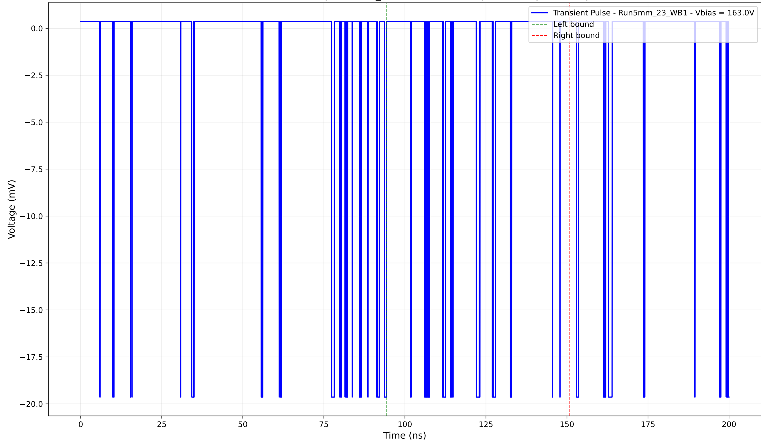
Transient Pulse - Sample: 5mm_23- Position: 45.0 \mu\text{m} - Charge: -1.55 pC
