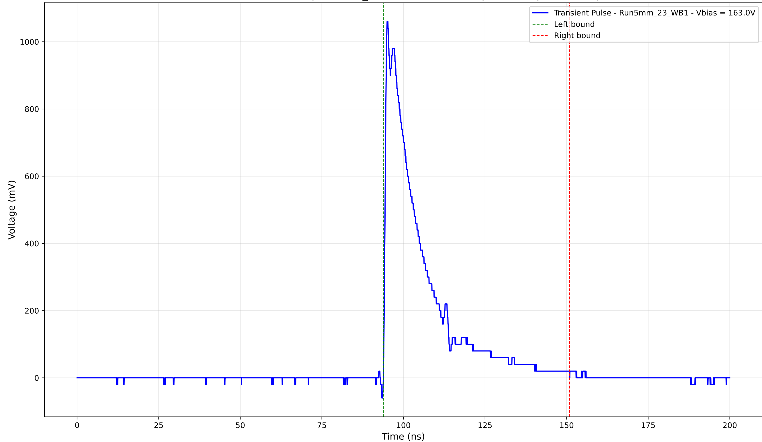
Transient Pulse - Sample: 5mm_23 - Position: 2615.0 \mu\text{m} - Charge: 244.26 pC
