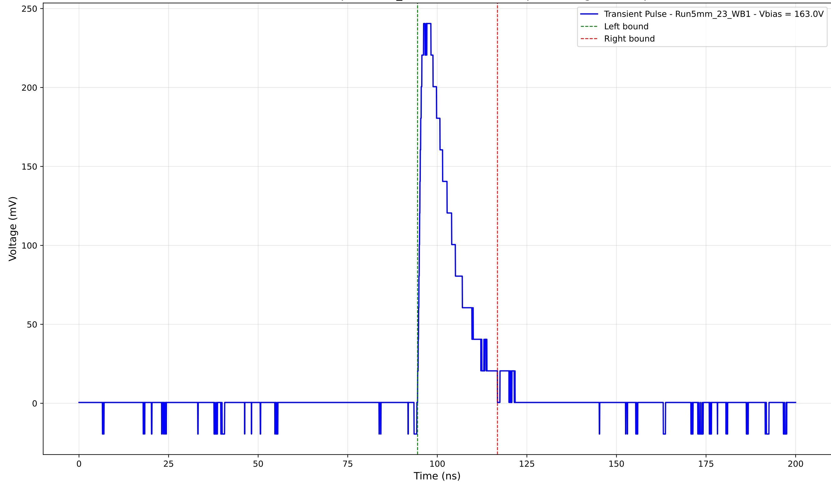
Transient Pulse - Sample: 5mm_23 - Position: 1740.0 \mu\text{m} - Charge: 46.22 pC
