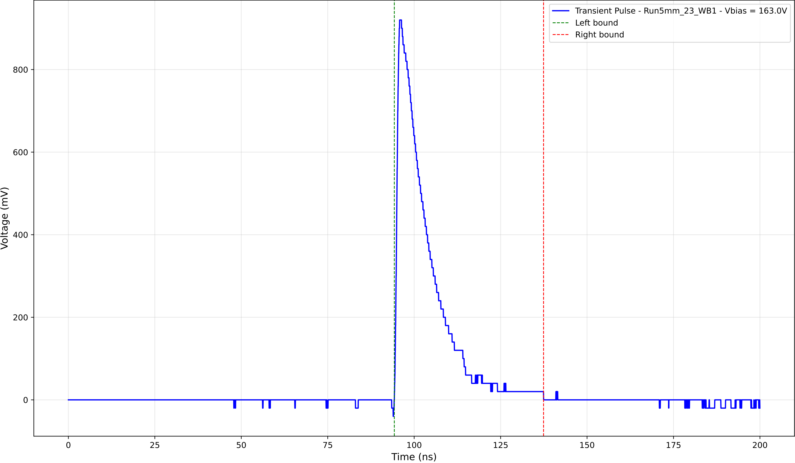
Transient Pulse - Sample: 5mm_23 - Position: 4530.0 \mu\text{m} - Charge: 179.92 pC
