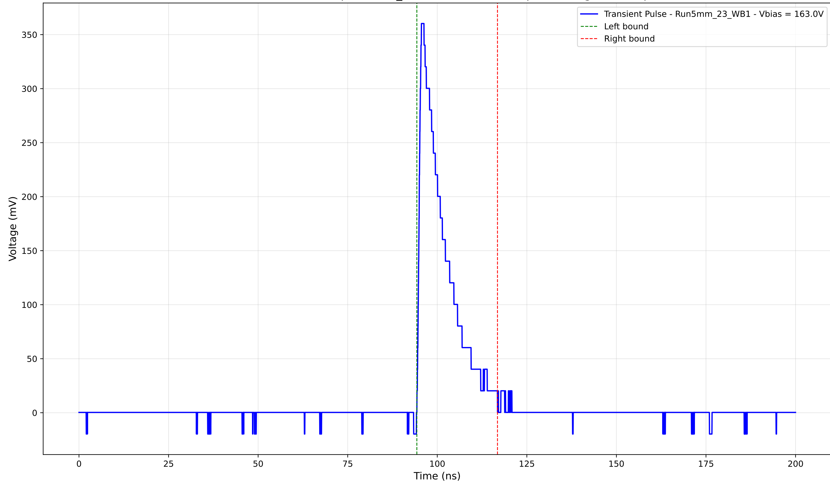
Transient Pulse - Sample: 5mm_23 - Position: 4740.0 \mu\text{m} - Charge: 56.22 pC
