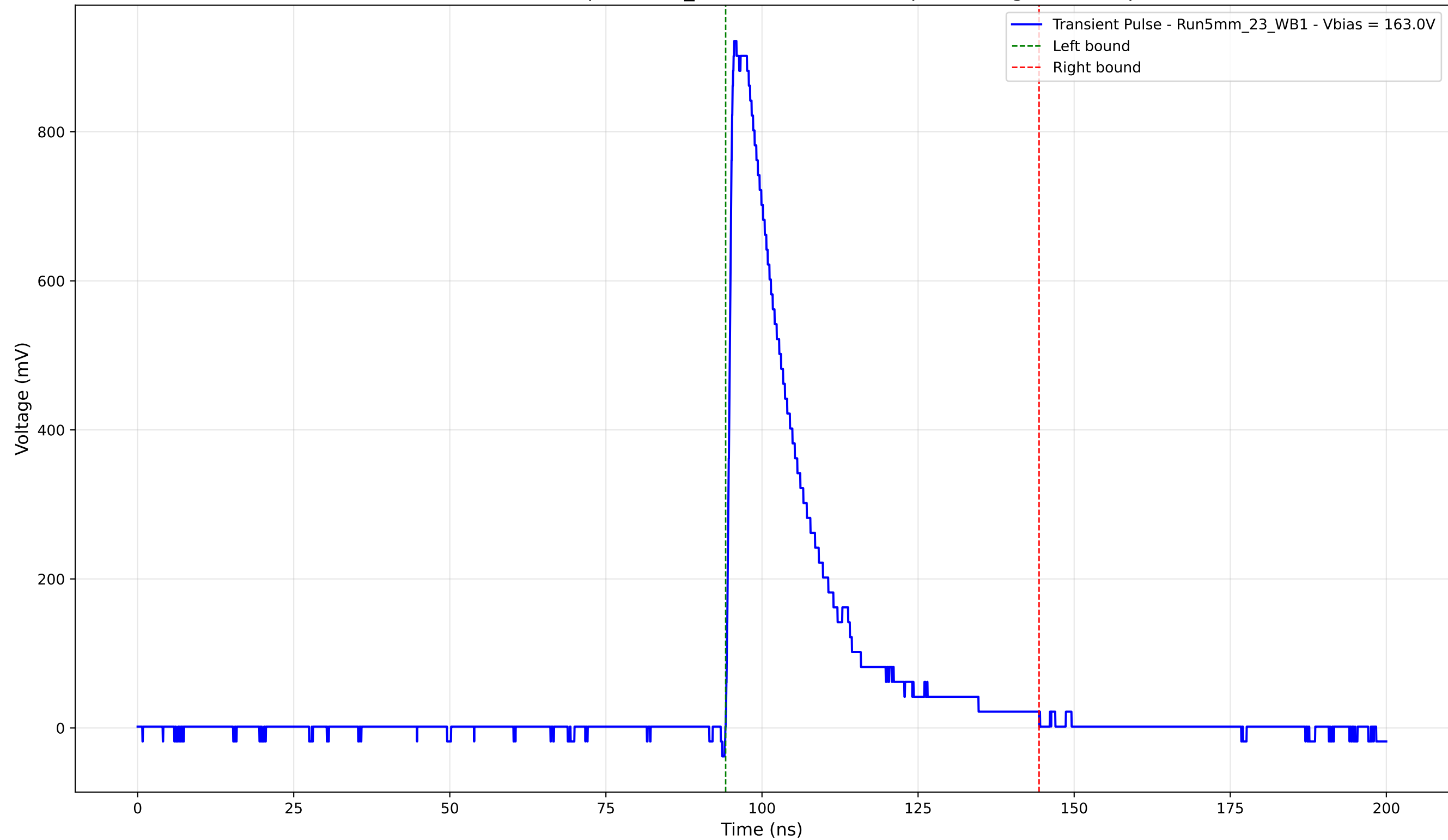
Transient Pulse - Sample: 5mm_23 - Position: 3415.0 \mu\text{m} - Charge: 213.22 pC
