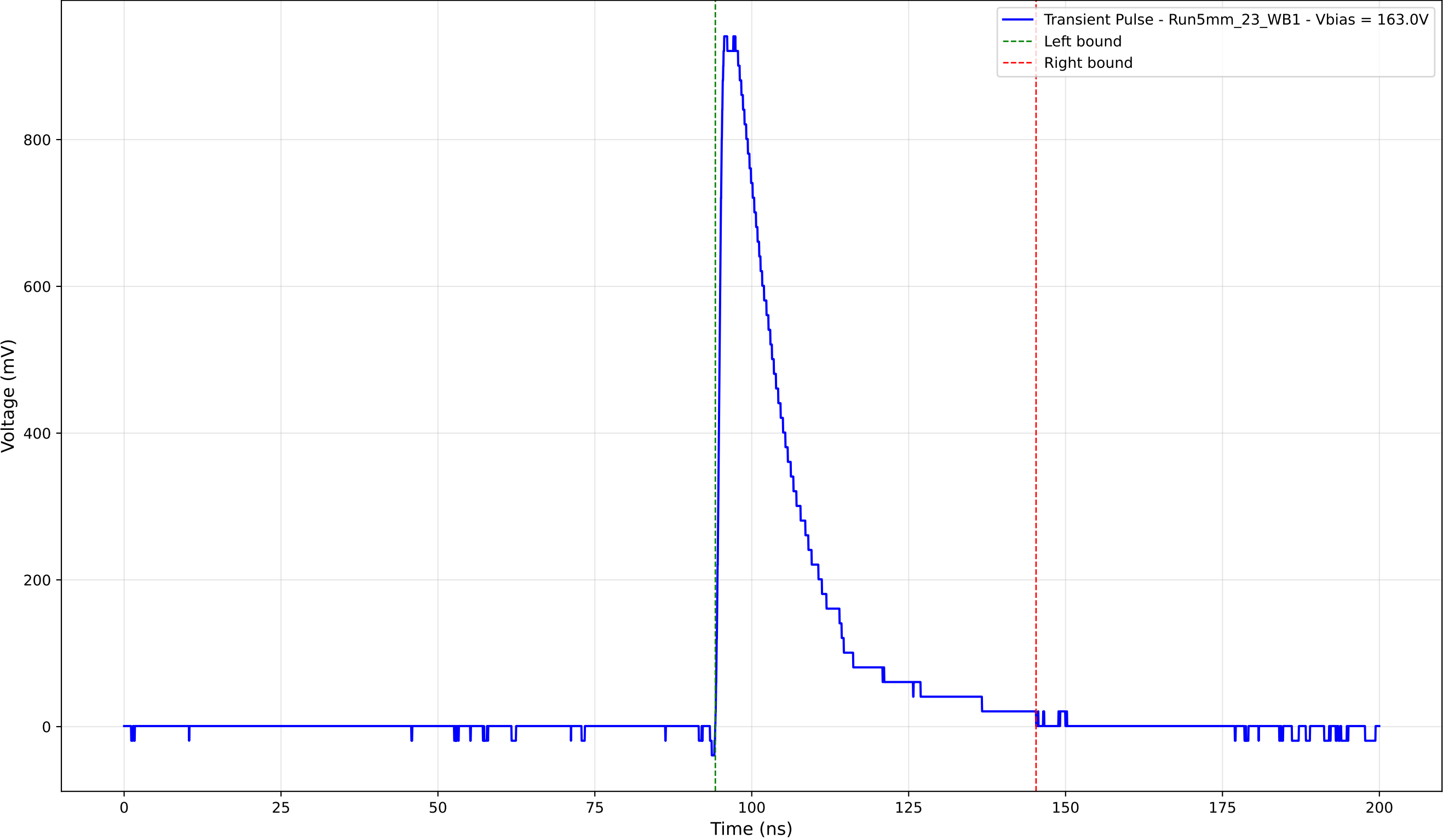
Transient Pulse - Sample: 5mm_23 - Position: 3495.0 \mu\text{m} - Charge: 223.63 pC
