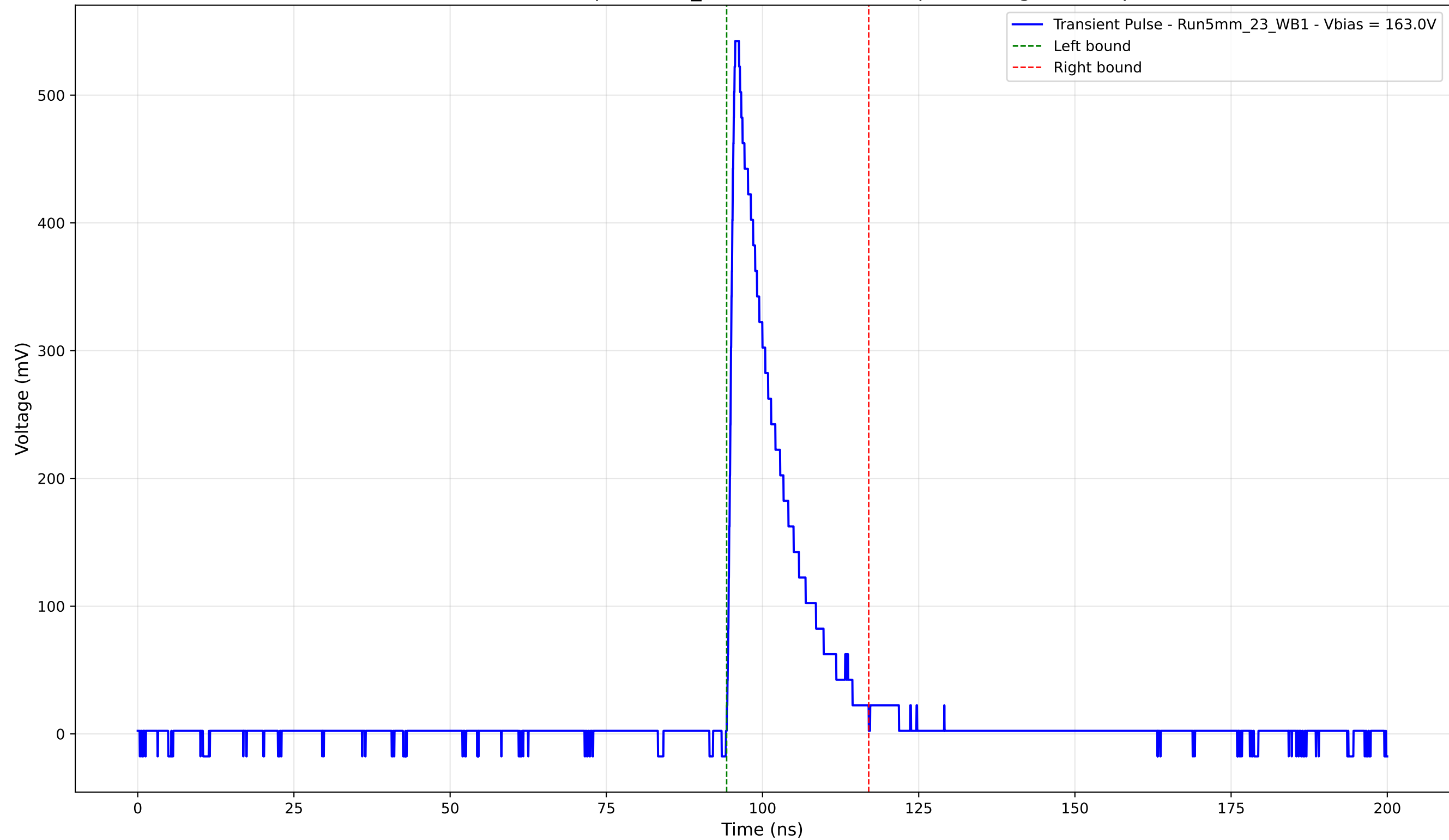
Transient Pulse - Sample: 5mm_23 - Position: 4725.0 \mu\text{m} - Charge: 83.60 pC
