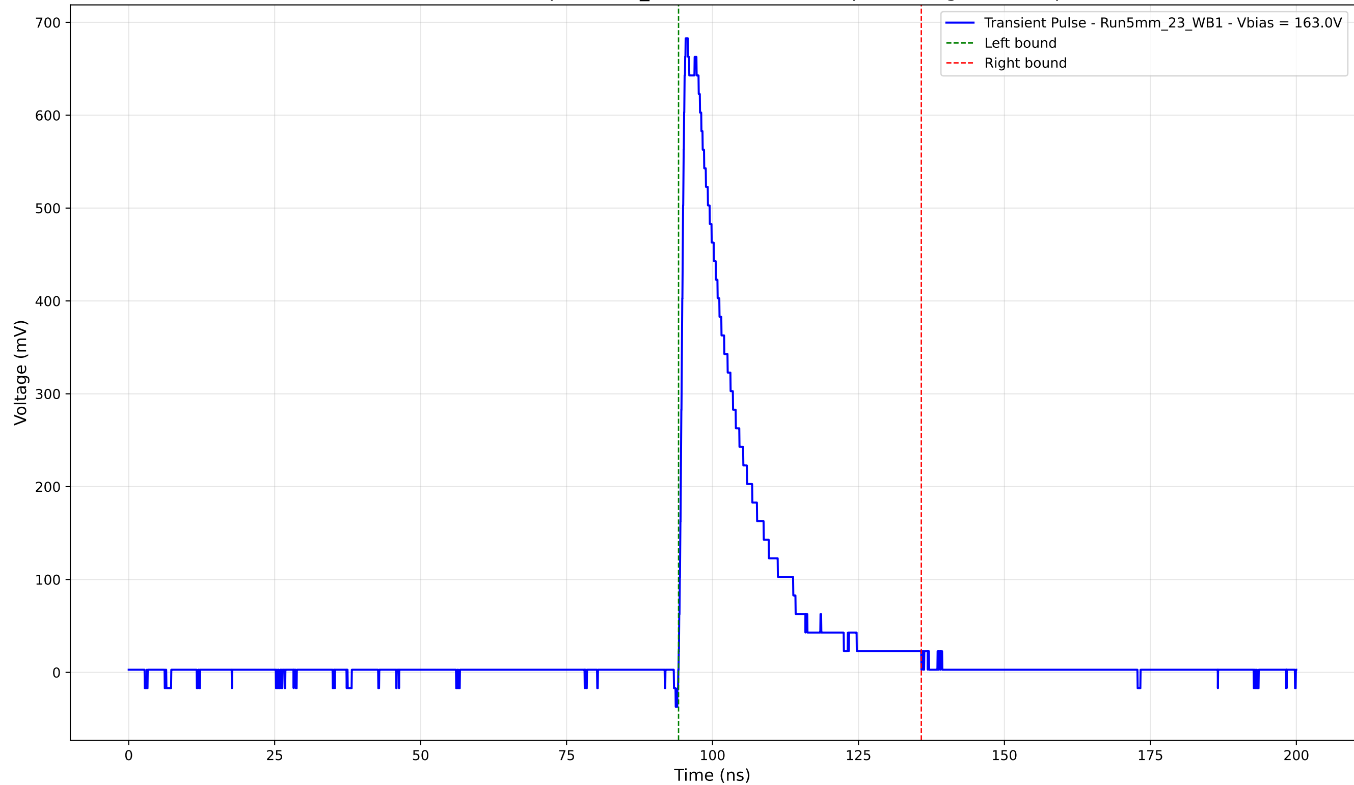
Transient Pulse - Sample: 5mm_23 - Position: 3305.0 \mu\text{m} - Charge: 138.87 pC
