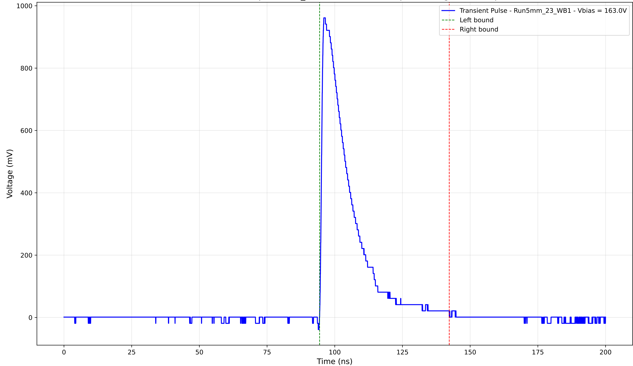
Transient Pulse - Sample: 5mm_23 - Position: 1350.0 \mu\text{m} - Charge: 221.88 pC
