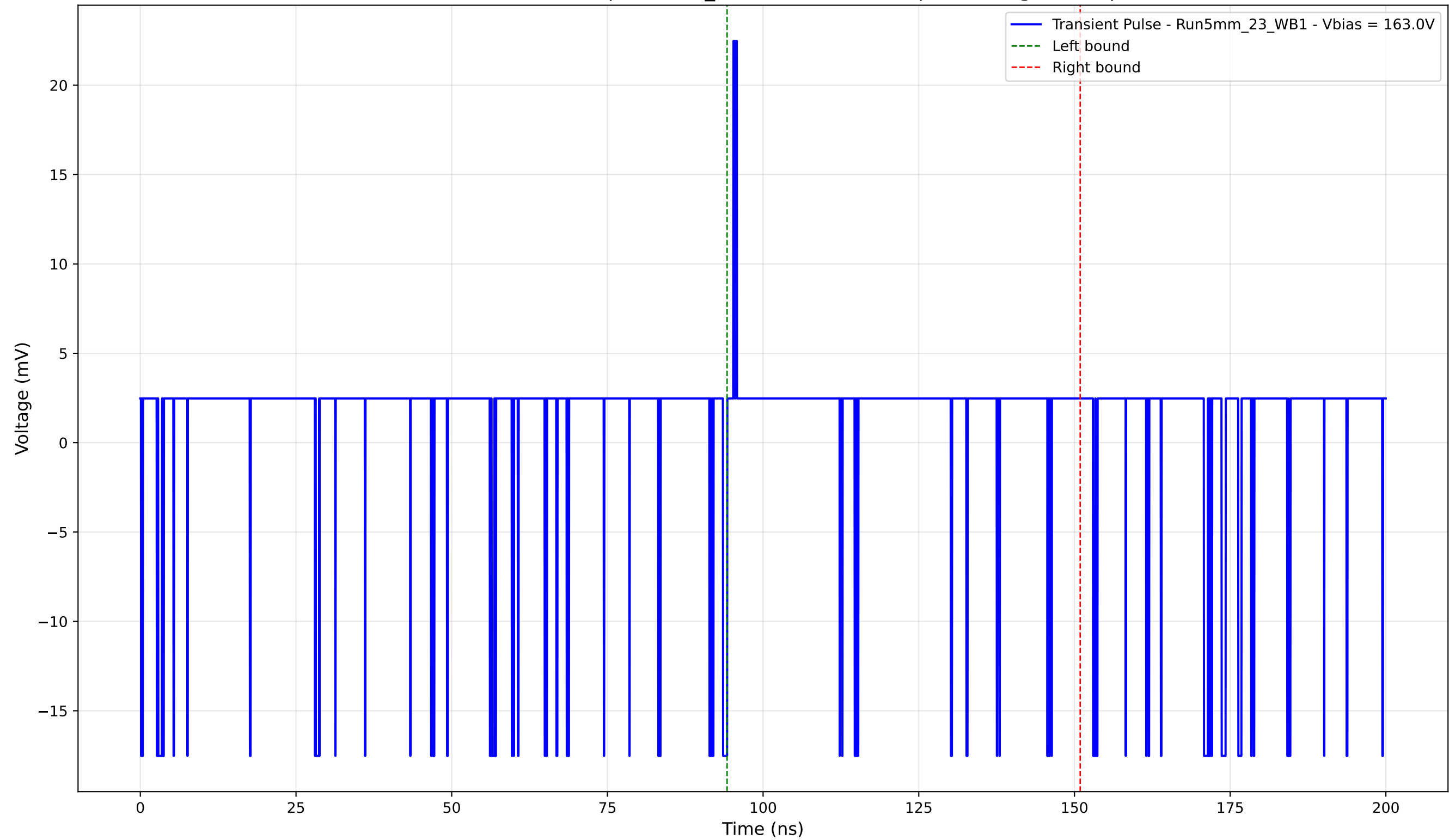
Transient Pulse - Sample: 5mm_23 - Position: 195.0 \mu\text{m} - Charge: 2.48 pC
