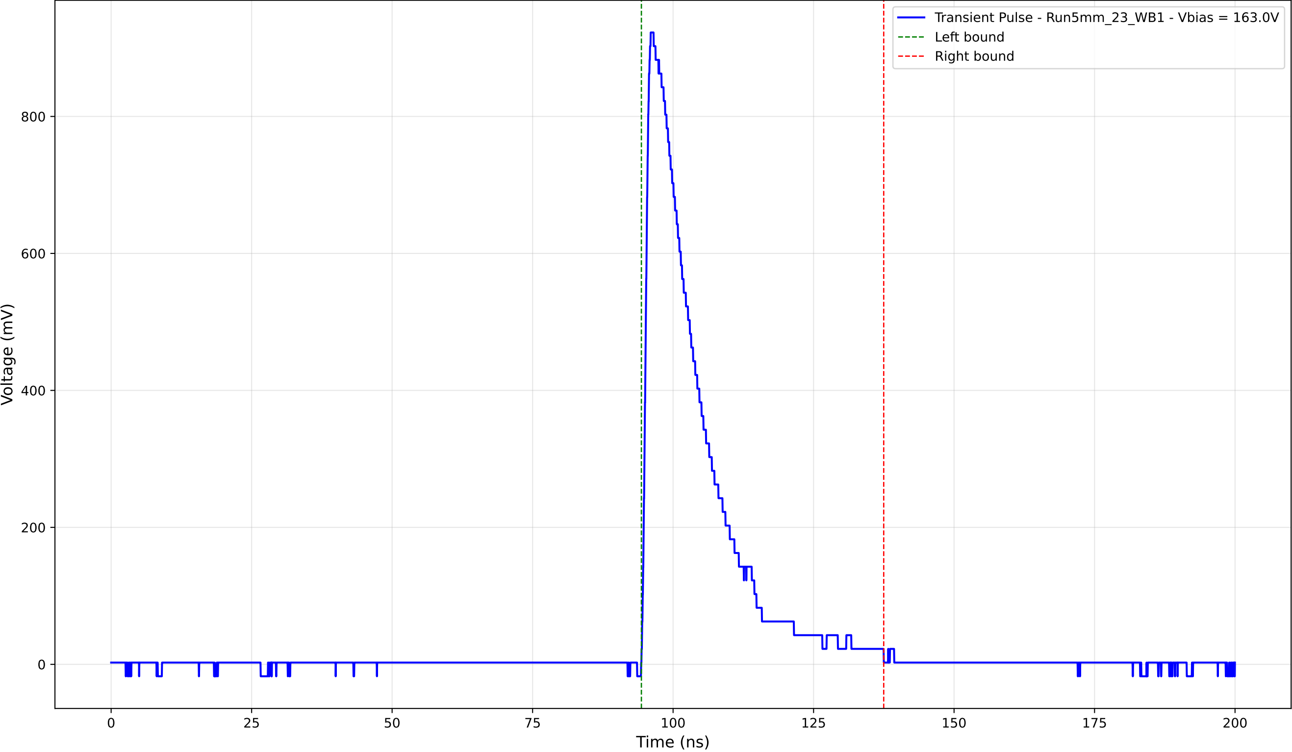
Transient Pulse - Sample: 5mm_23 - Position: 4130.0 \mu\text{m} - Charge: 196.34 pC
