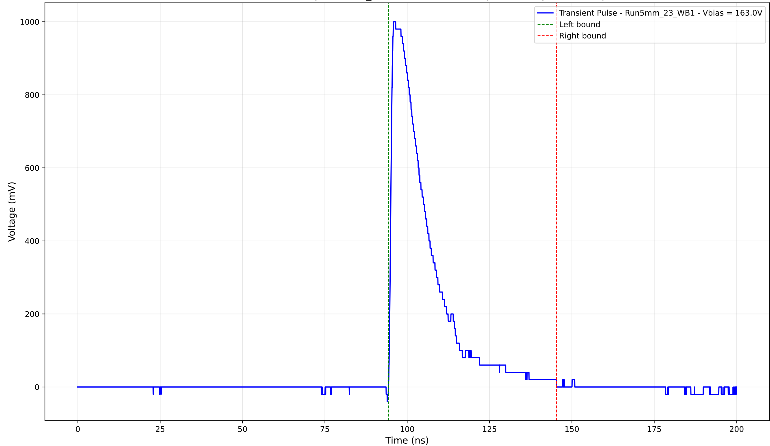
Transient Pulse - Sample: 5mm_23 - Position: 1605.0 \mu\text{m} - Charge: 251.25 pC
