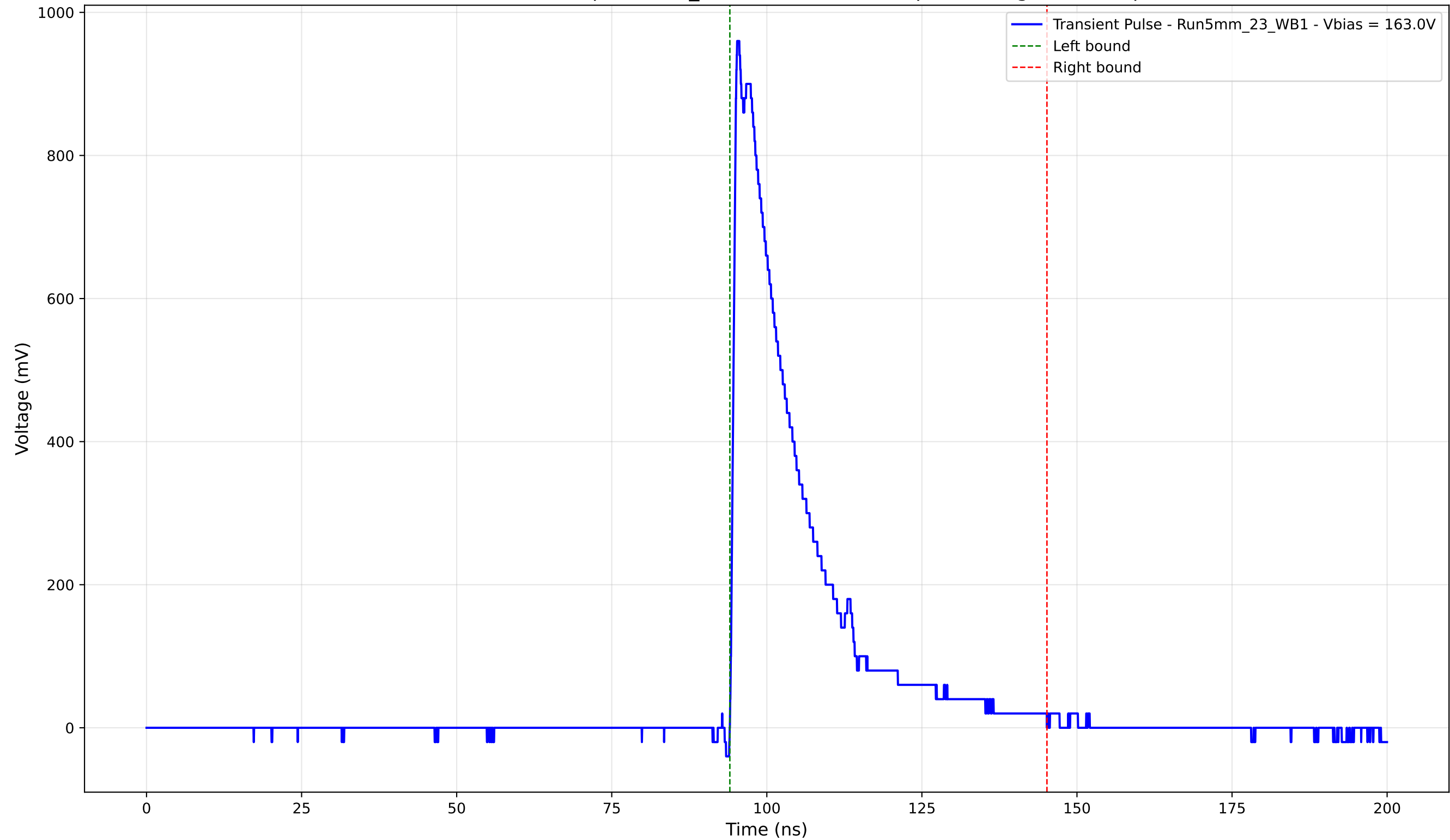
Transient Pulse - Sample: 5mm_23 - Position: 2330.0 \mu\text{m} - Charge: 211.83 pC
