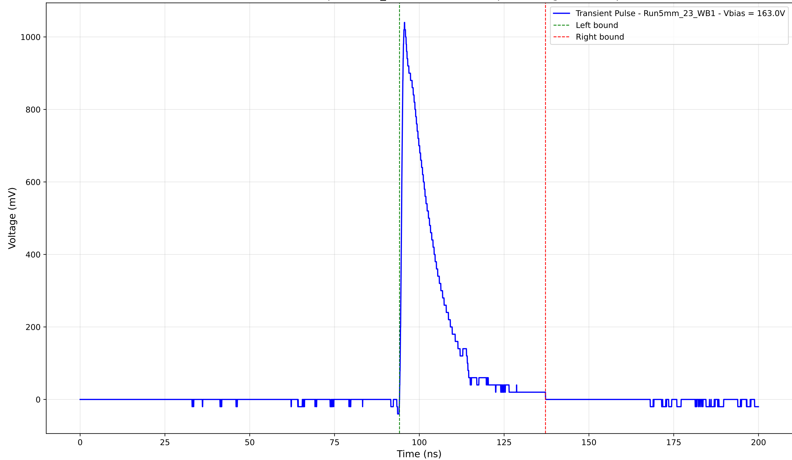
Transient Pulse - Sample: 5mm_23 - Position: 560.0 \mu\text{m} - Charge: 200.30 pC
