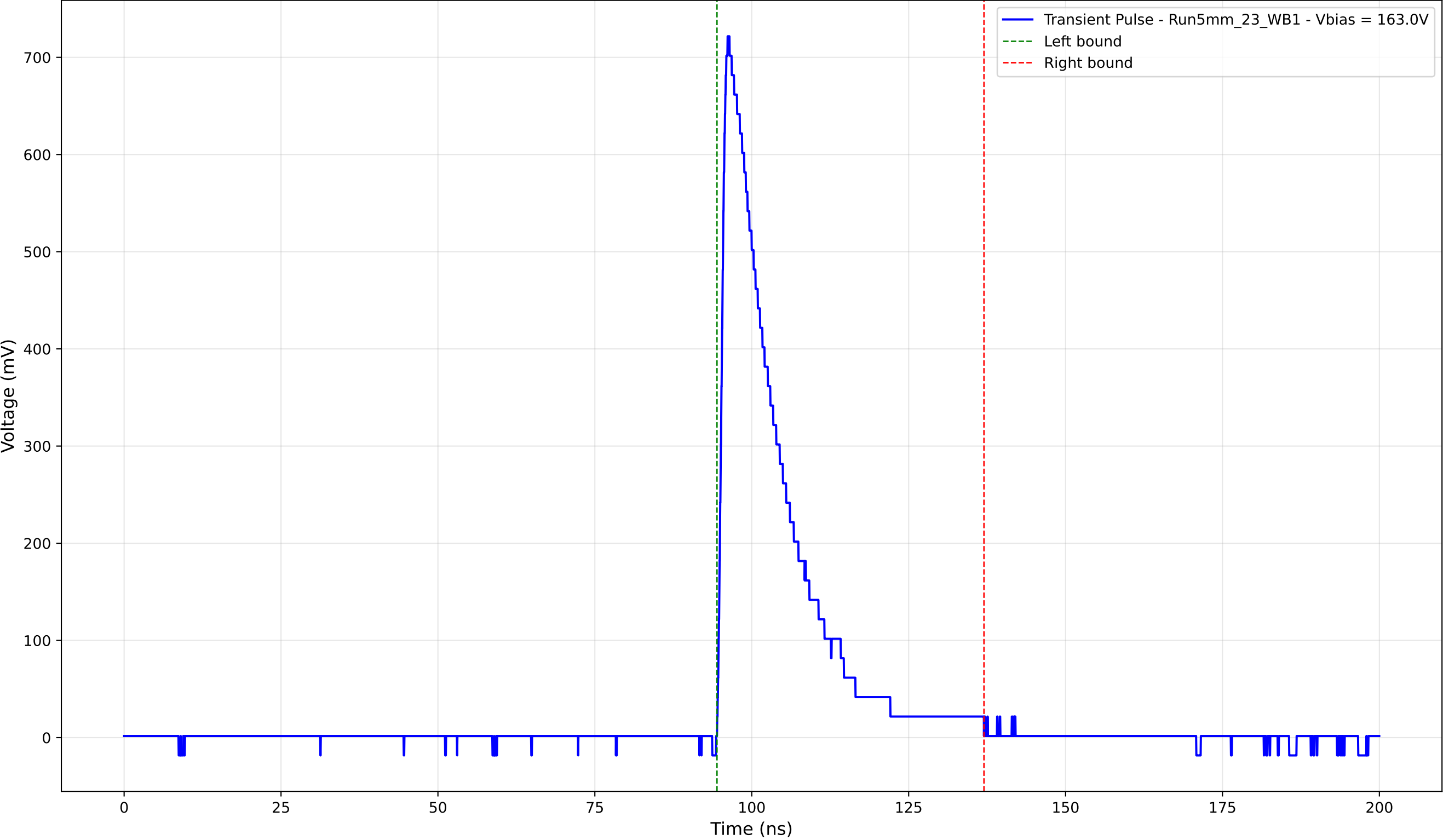
Transient Pulse - Sample: 5mm_23 - Position: 1280.0 \mu\text{m} - Charge: 142.59 pC
