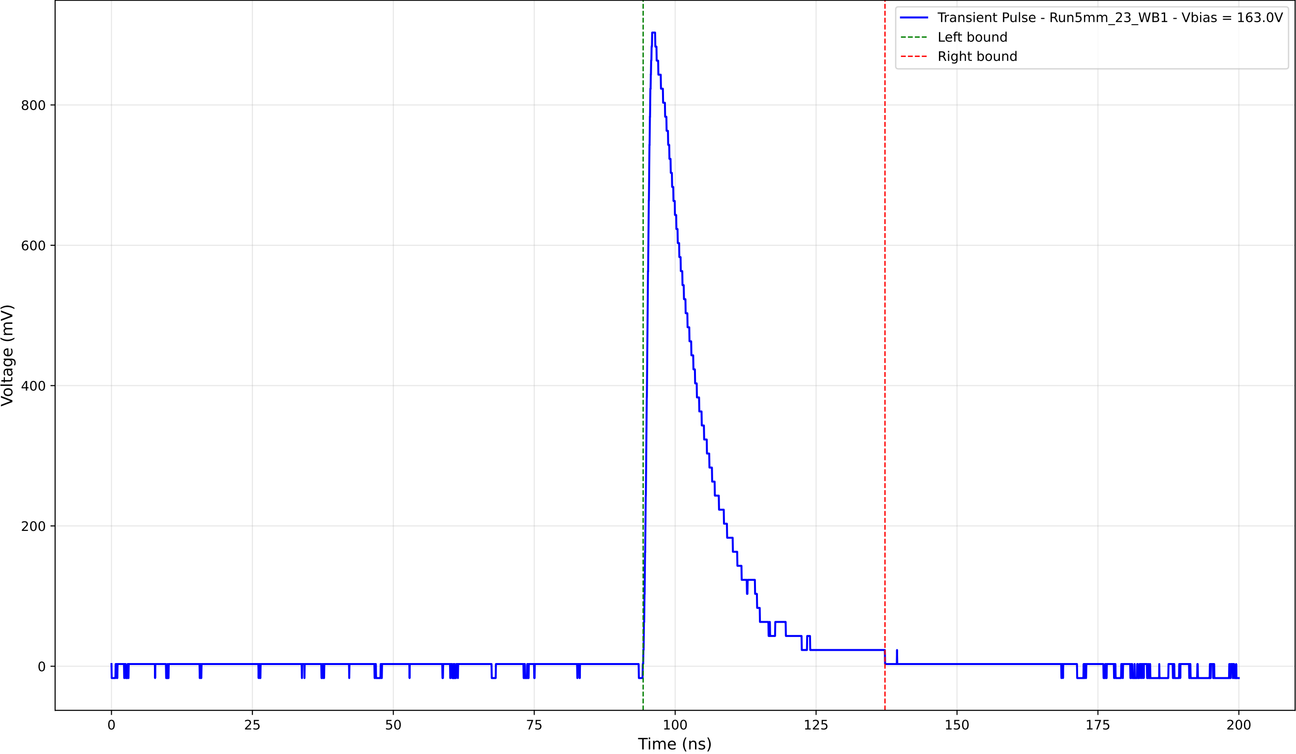
Transient Pulse - Sample: 5mm_23 - Position: 4380.0 \mu\text{m} - Charge: 180.74 pC
