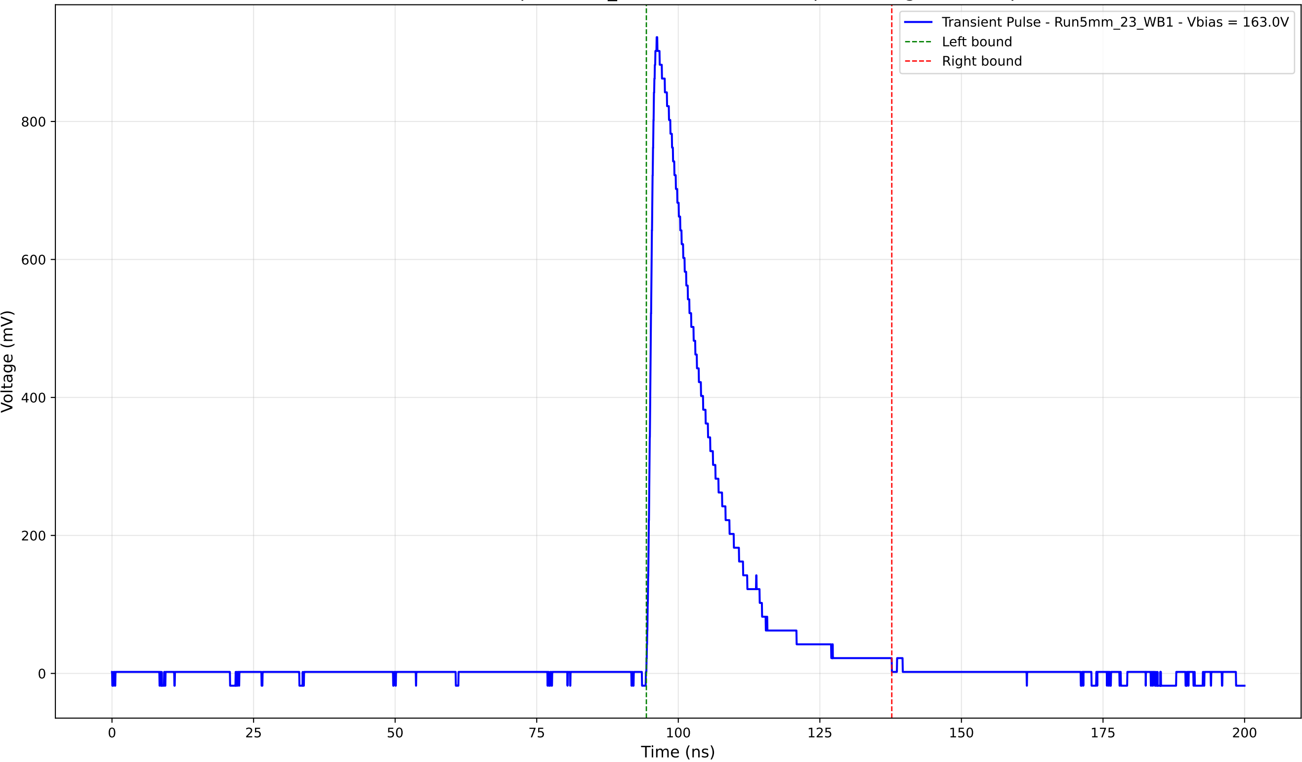
Transient Pulse - Sample: 5mm_23 - Position: 4155.0 \mu\text{m} - Charge: 189.50 pC
