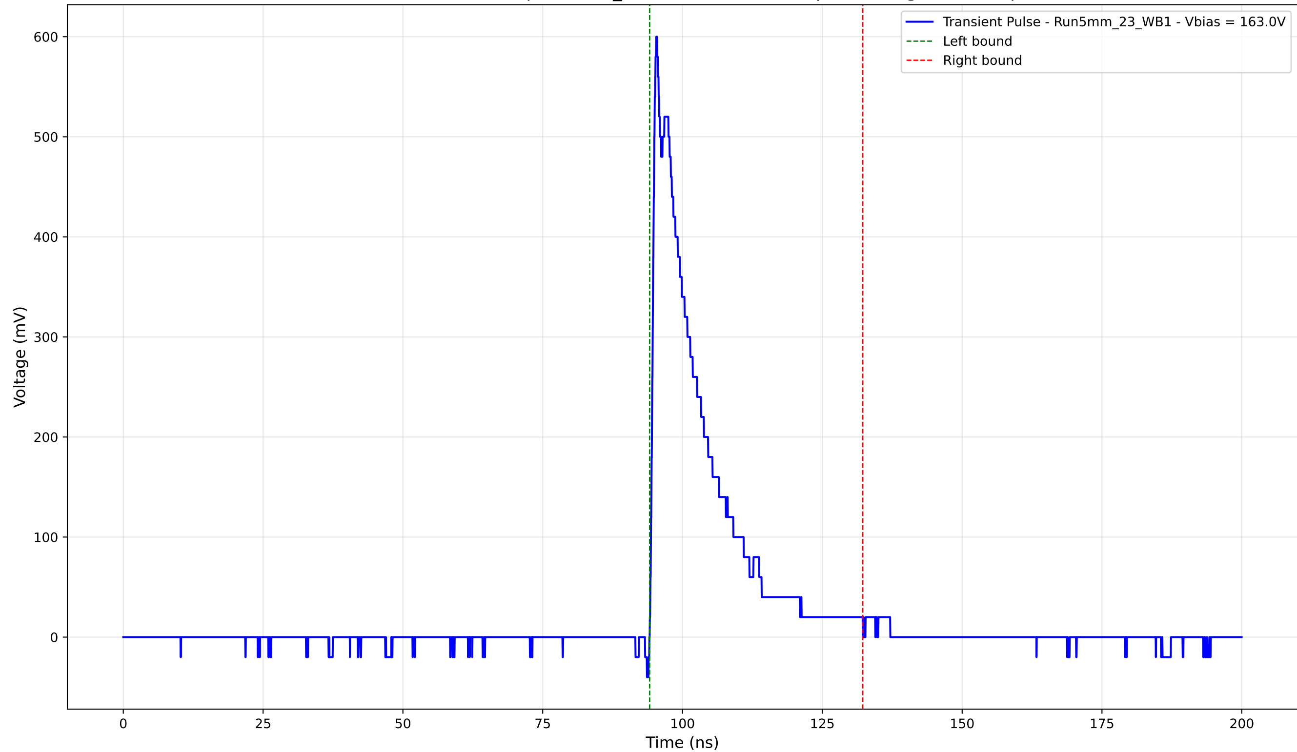
Transient Pulse - Sample: 5mm_23 - Position: 2280.0 \mu\text{m} - Charge: 106.74 pC
