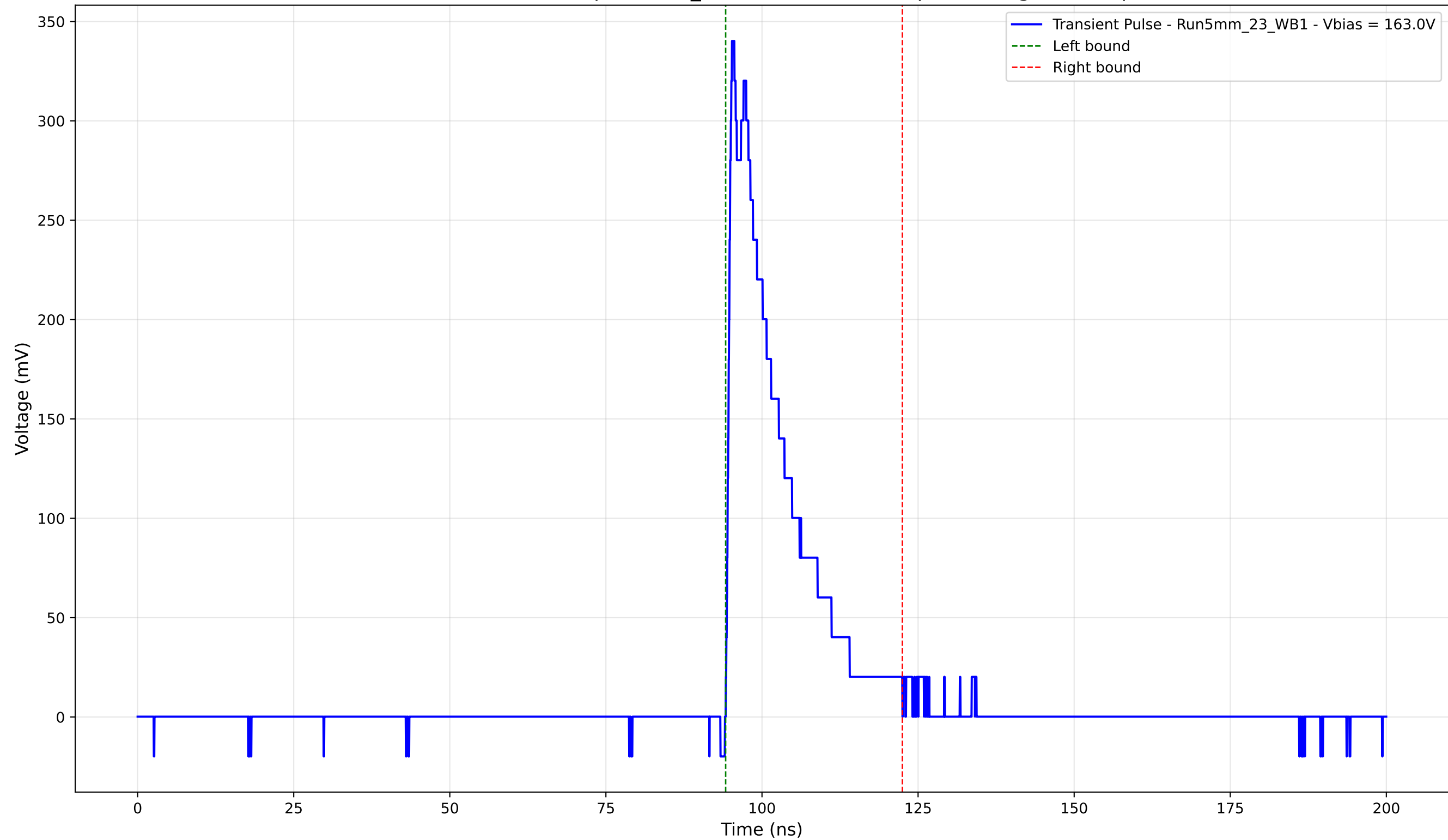
Transient Pulse - Sample: 5mm_23 - Position: 2260.0 \mu\text{m} - Charge: 60.64 pC
