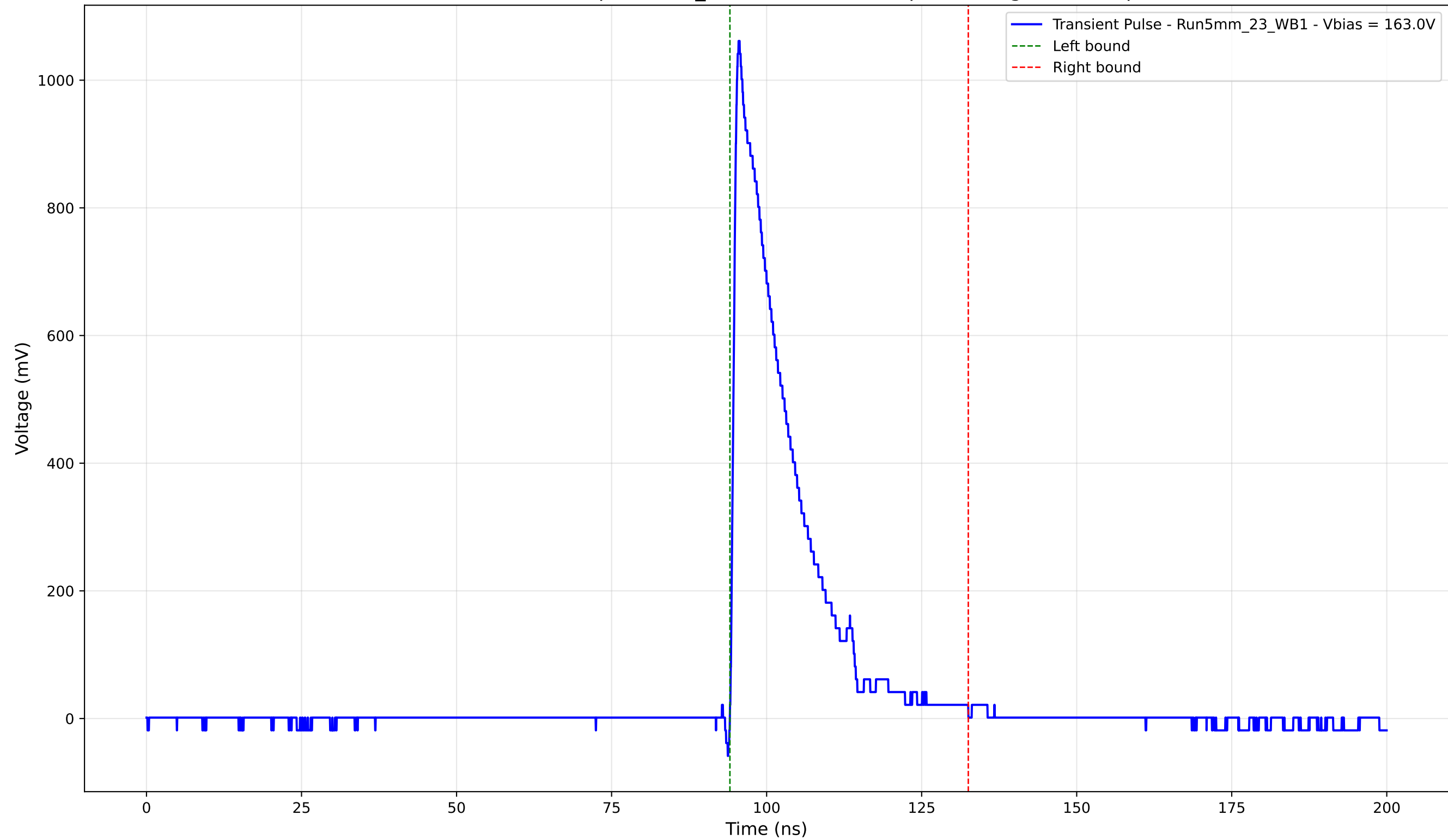
Transient Pulse - Sample: 5mm_23 - Position: 440.0 \mu\text{m} - Charge: 197.81 pC
