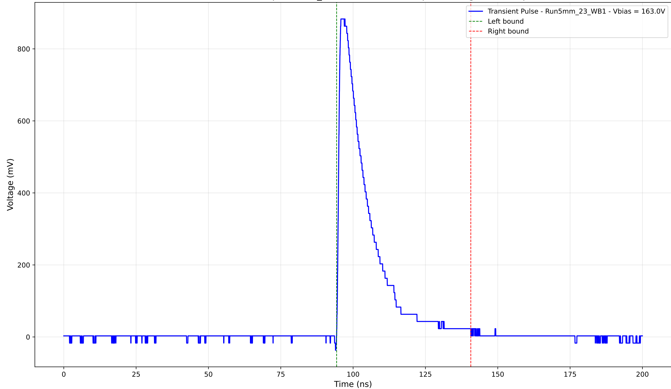
Transient Pulse - Sample: 5mm_23 - Position: 3655.0 \mu\text{m} - Charge: 197.86 pC
