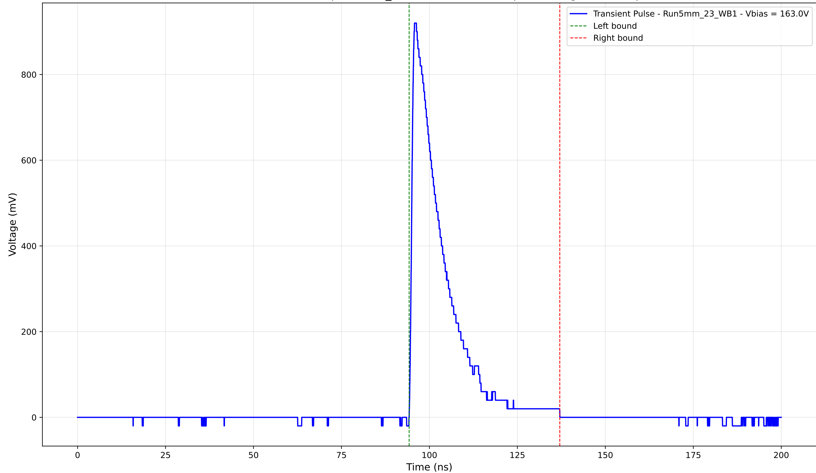
Transient Pulse - Sample: 5mm_23 - Position: 4575.0 \mu\text{m} - Charge: 177.06 pC
