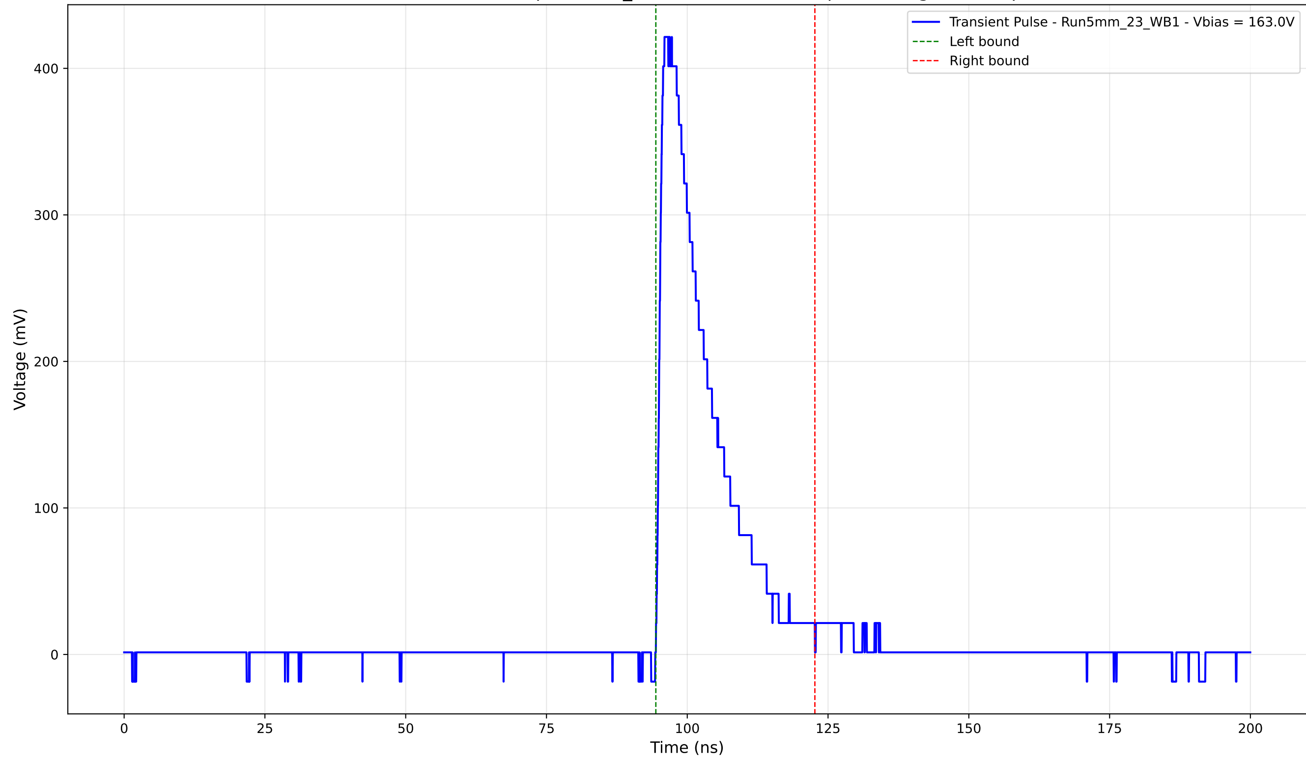
Transient Pulse - Sample: 5mm_23 - Position: 1760.0 \mu\text{m} - Charge: 82.36 pC
