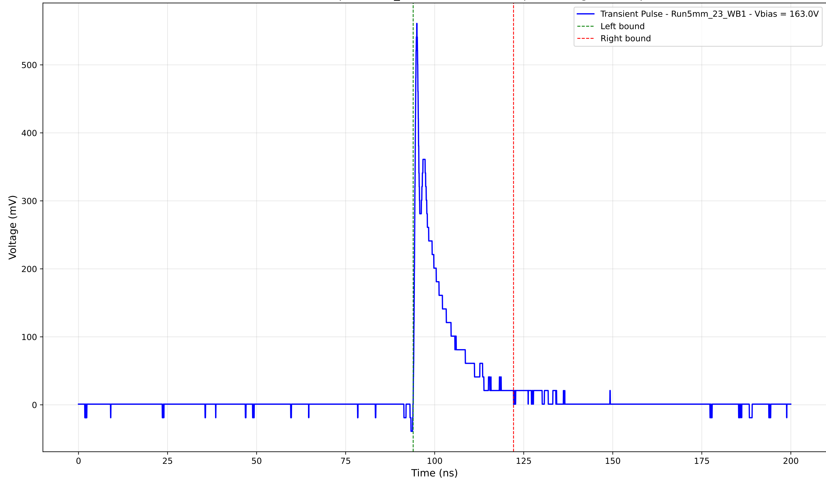
Transient Pulse - Sample: 5mm_23 - Position: 2725.0 \mu\text{m} - Charge: 67.05 pC
