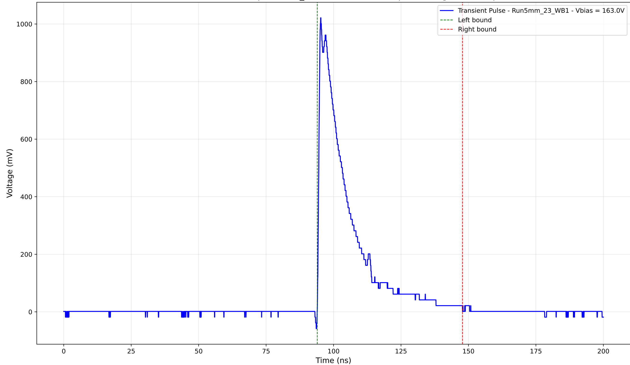
Transient Pulse - Sample: 5mm_23 - Position: 2440.0 \mu\text{m} - Charge: 231.99 pC
