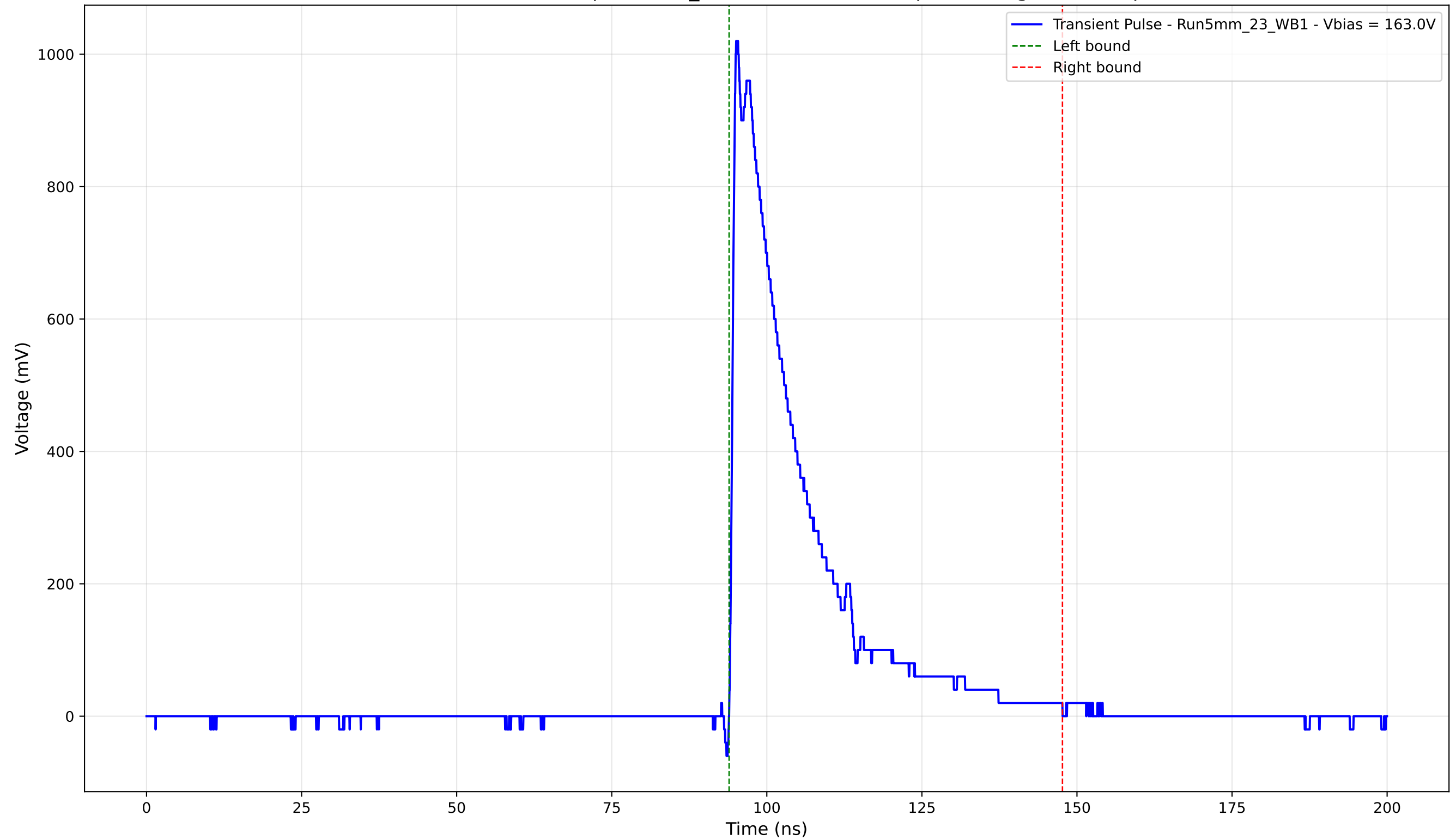
Transient Pulse - Sample: 5mm_23 - Position: 2505.0 \mu\text{m} - Charge: 231.94 pC
