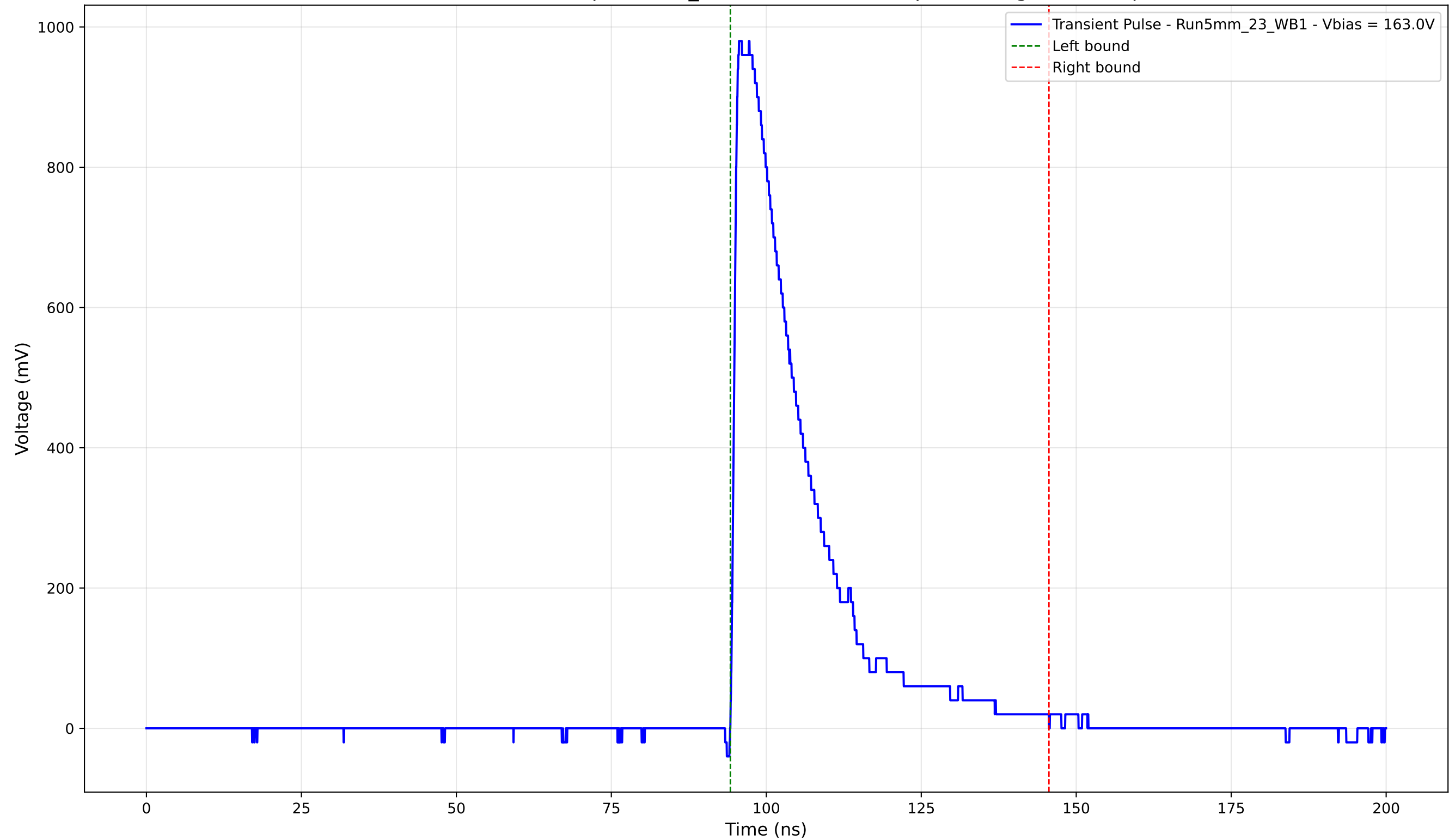
Transient Pulse - Sample: 5mm_23 - Position: 2000.0 \mu\text{m} - Charge: 243.31 pC
