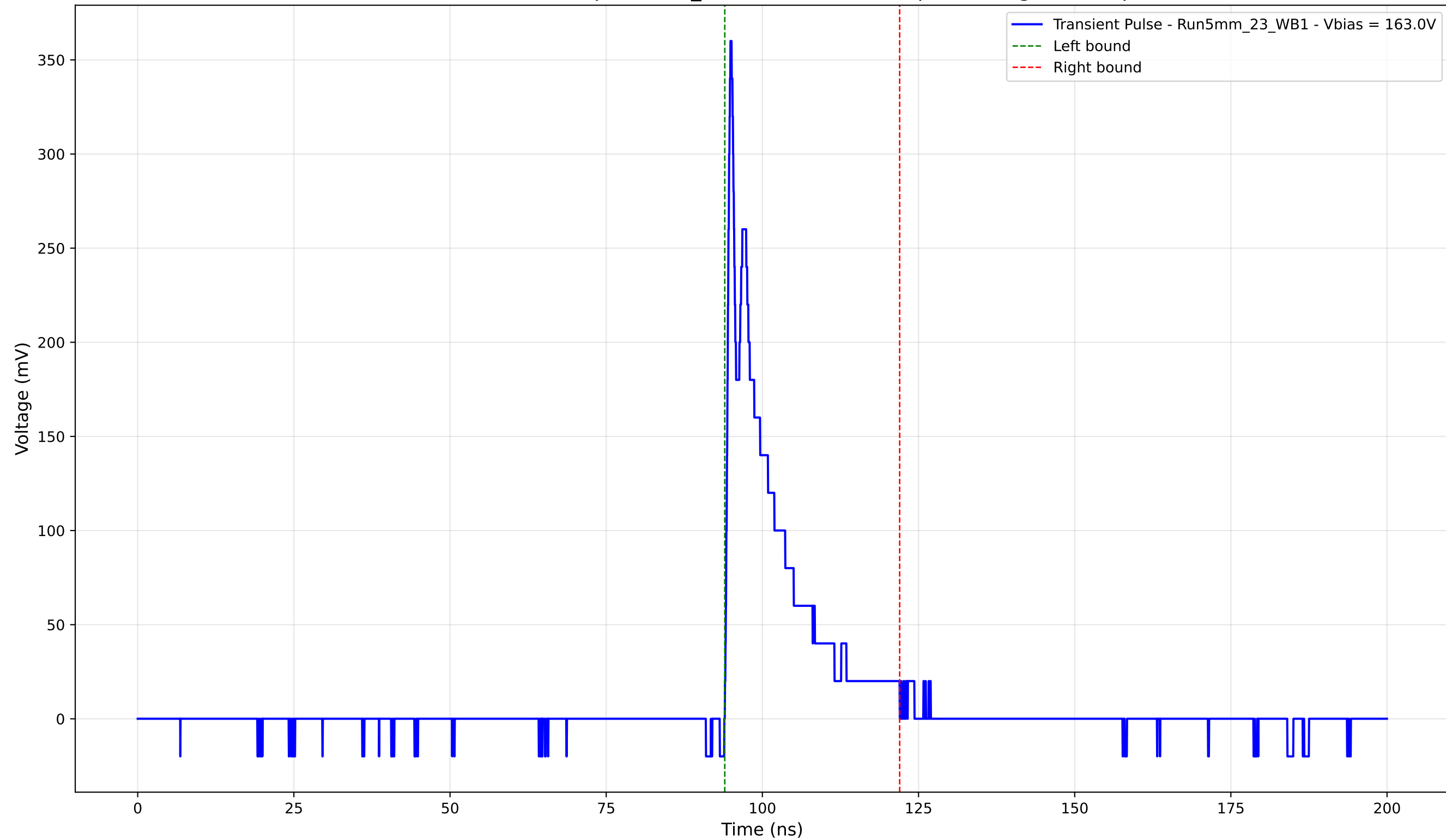
Transient Pulse - Sample: 5mm_23 - Position: 2755.0 \mu\text{m} - Charge: 46.47 pC
