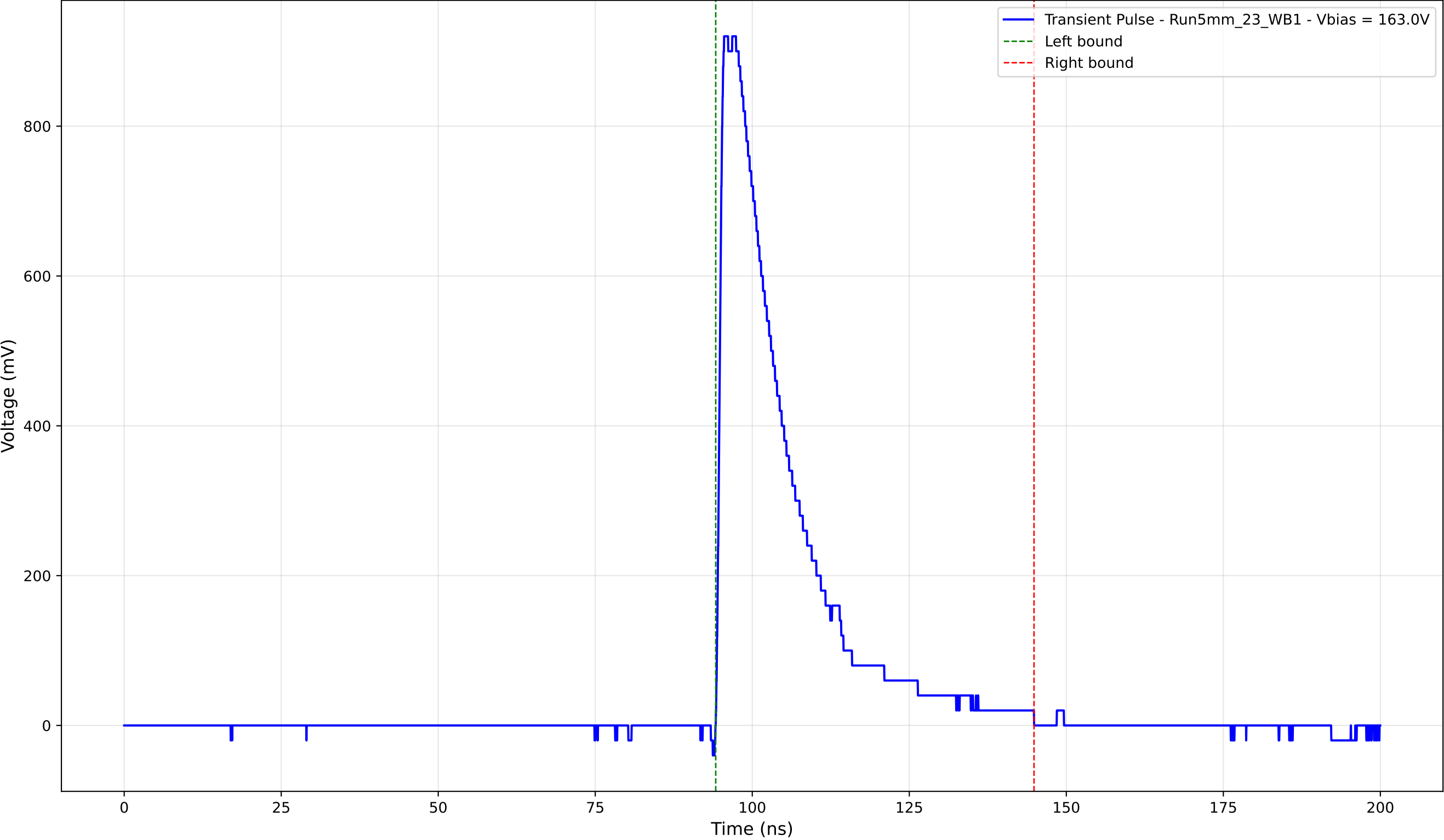
Transient Pulse - Sample: 5mm_23 - Position: 3445.0 \mu\text{m} - Charge: 216.94 pC
