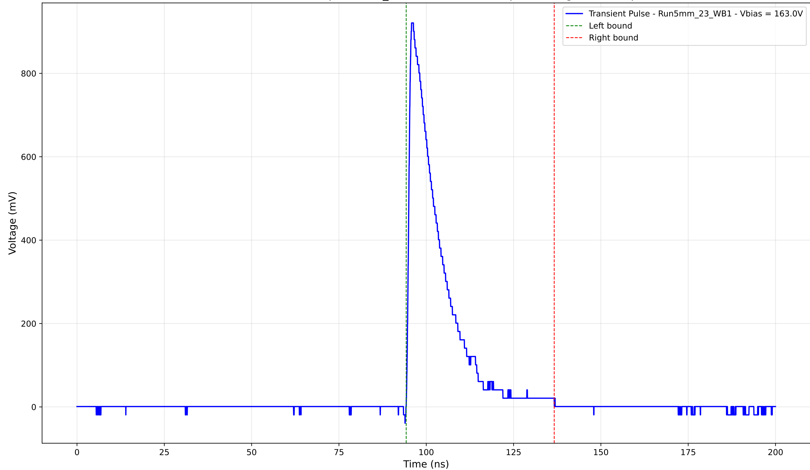
Transient Pulse - Sample: 5mm_23 - Position: 4535.0 \mu\text{m} - Charge: 178.87 pC
