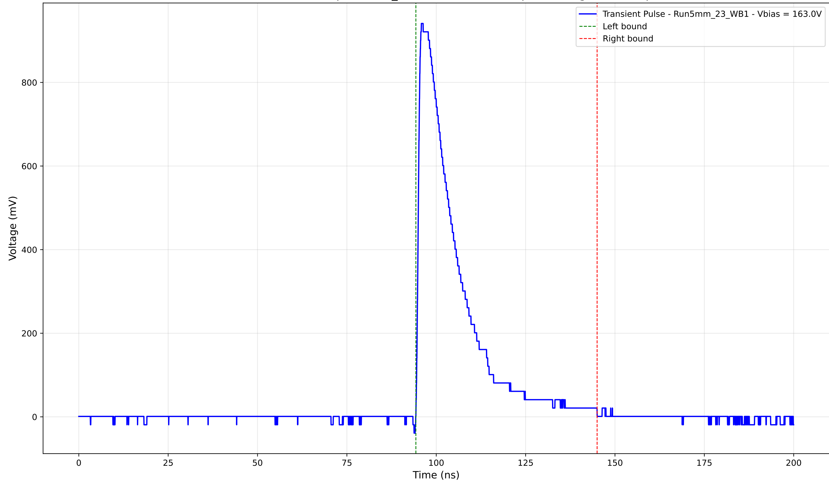
Transient Pulse - Sample: 5mm_23 - Position: 1830.0 \mu\text{m} - Charge: 221.96 pC
