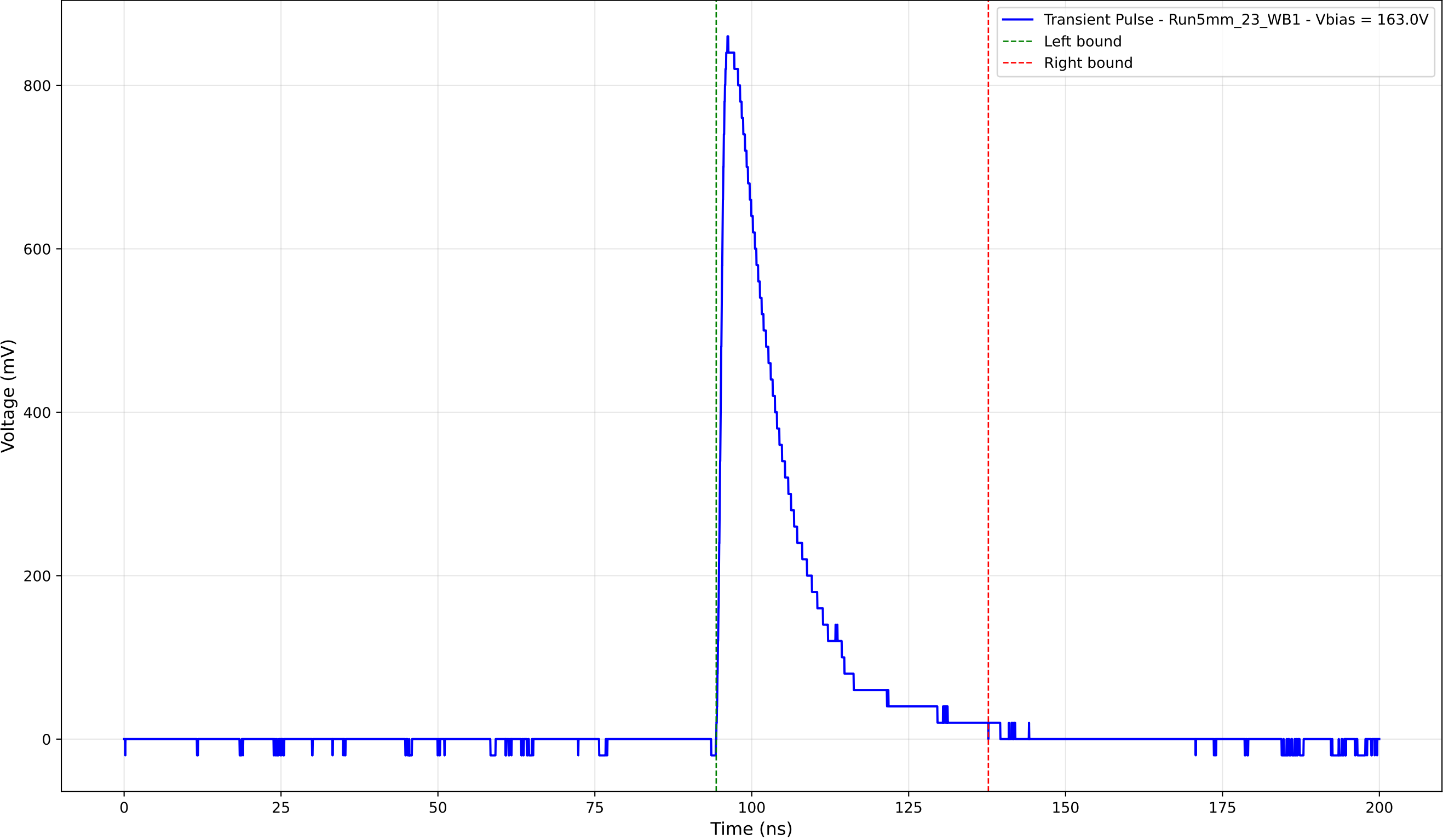
Transient Pulse - Sample: 5mm_23 - Position: 3845.0 \mu\text{m} - Charge: 182.31 pC
