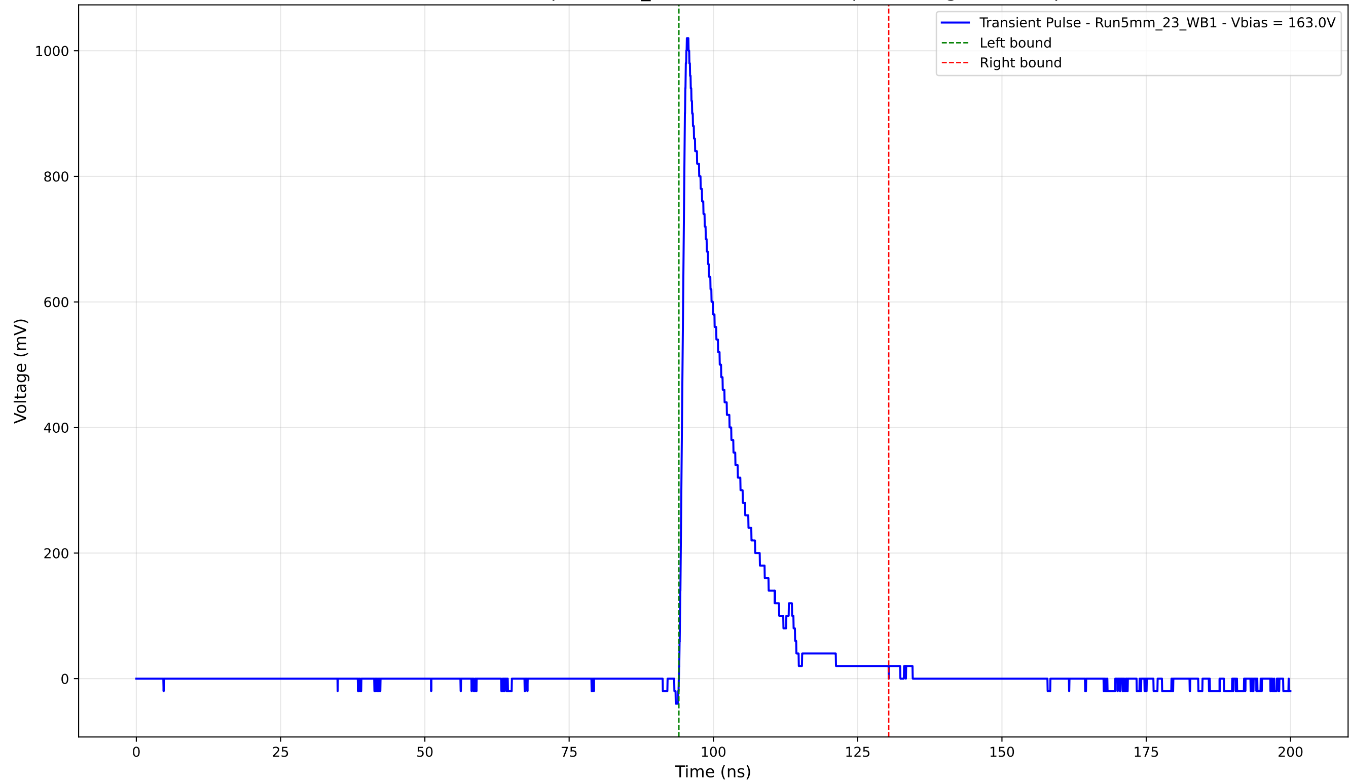
Transient Pulse - Sample: 5mm_23 - Position: 5010.0 \mu\text{m} - Charge: 169.86 pC
