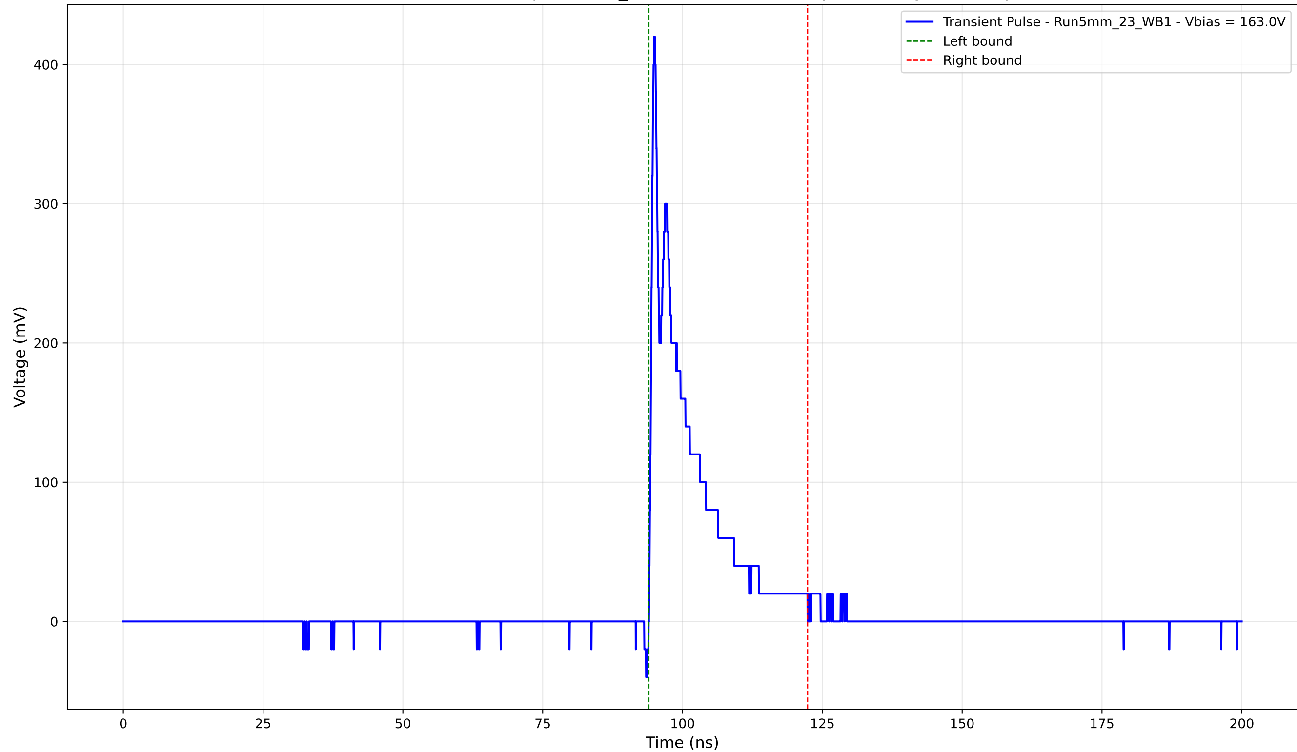
Transient Pulse - Sample: 5mm_23 - Position: 2735.0 \mu\text{m} - Charge: 52.50 pC
