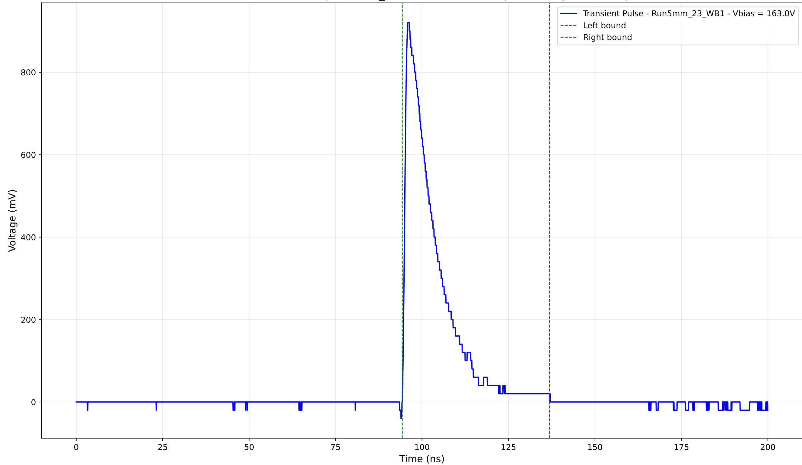
Transient Pulse - Sample: 5mm_23 - Position: 4525.0 \mu\text{m} - Charge: 177.71 pC
