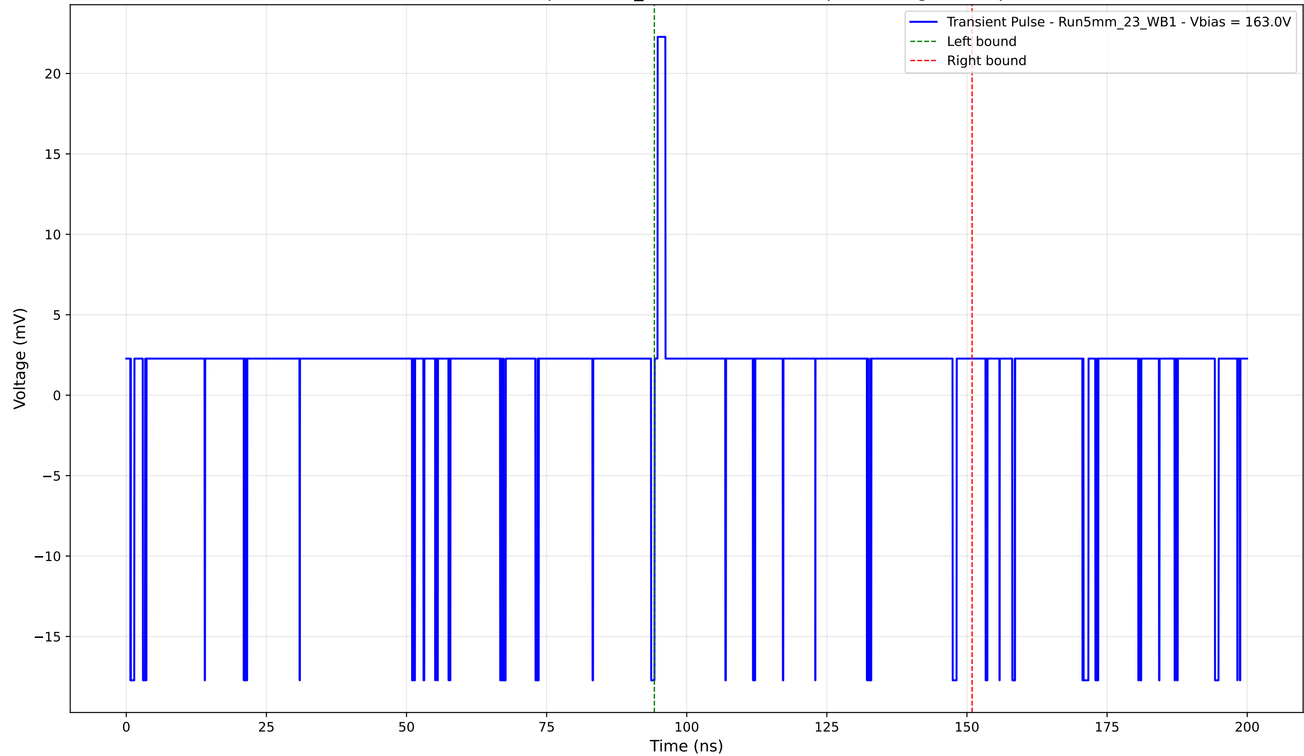
Transient Pulse - Sample: 5mm_23 - Position: 125.0 \mu\text{m} - Charge: 2.42 pC
