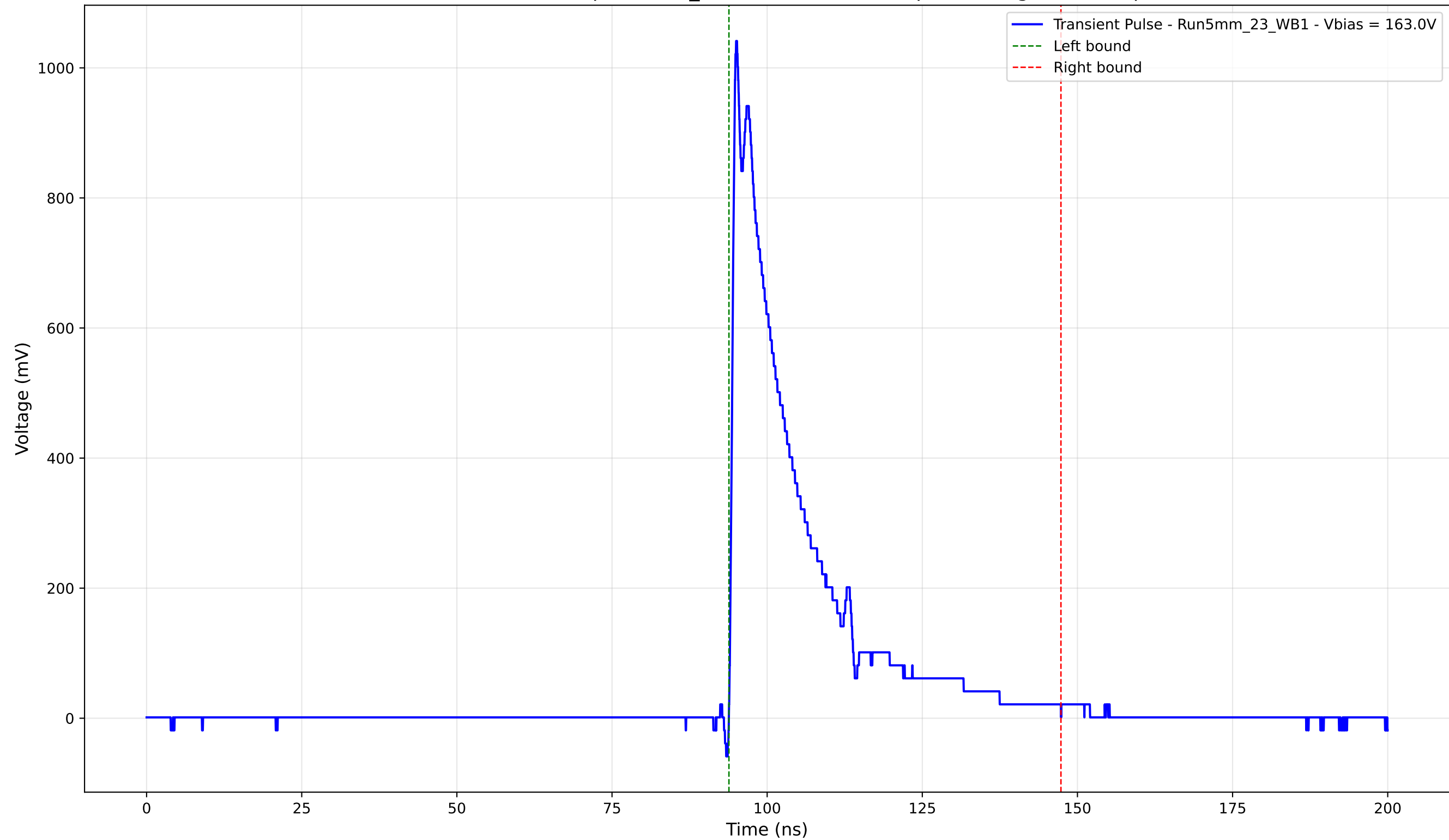
Transient Pulse - Sample: 5mm_23 - Position: 2665.0 \mu\text{m} - Charge: 218.11 pC
