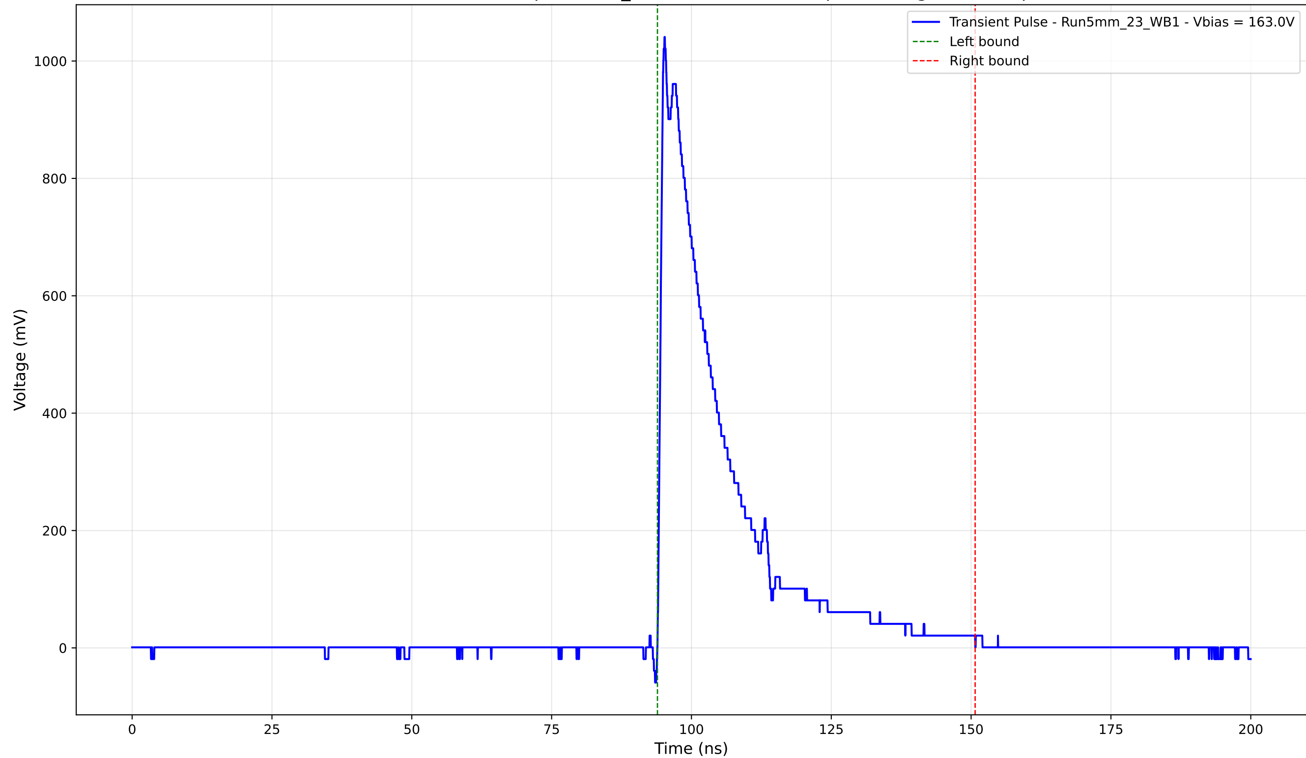
Transient Pulse - Sample: 5mm_23 - Position: 2530.0 \mu\text{m} - Charge: 236.27 pC
