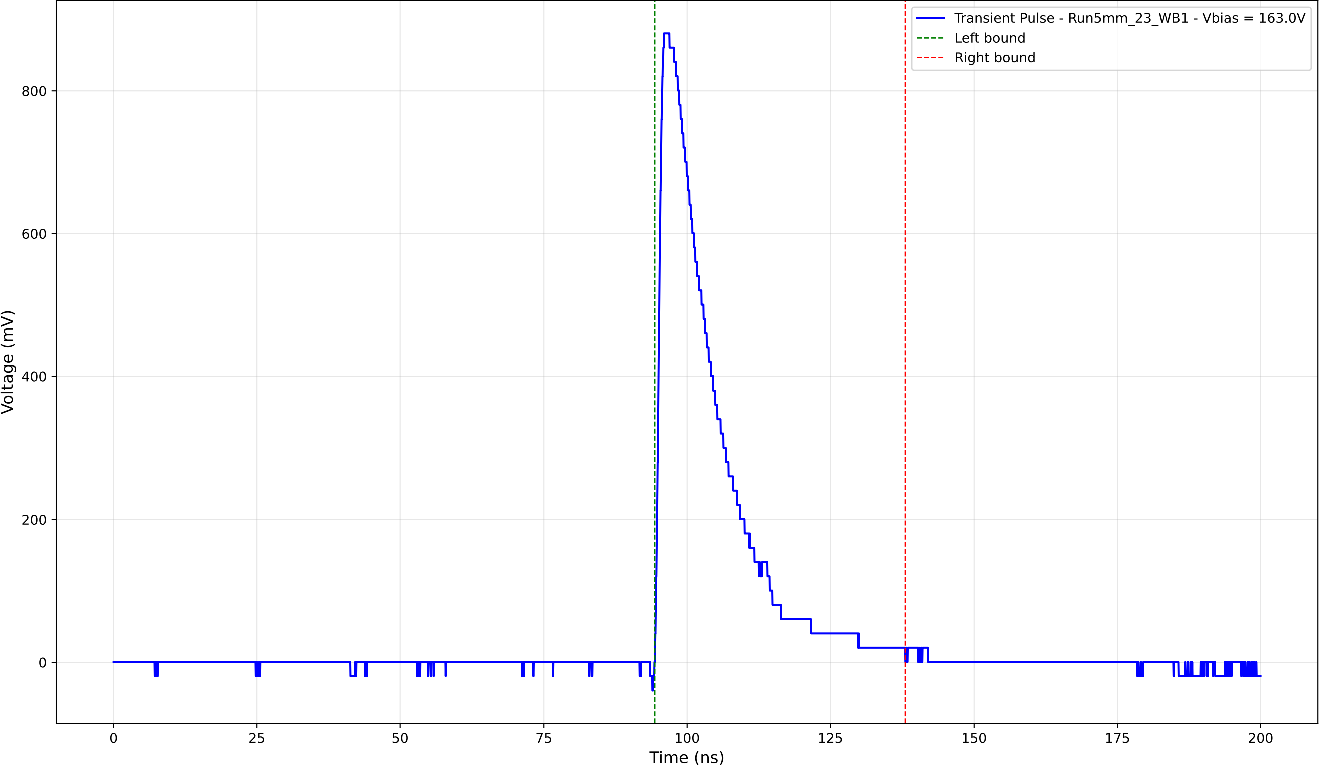
Transient Pulse - Sample: 5mm_23 - Position: 3865.0 \mu\text{m} - Charge: 191.96 pC
