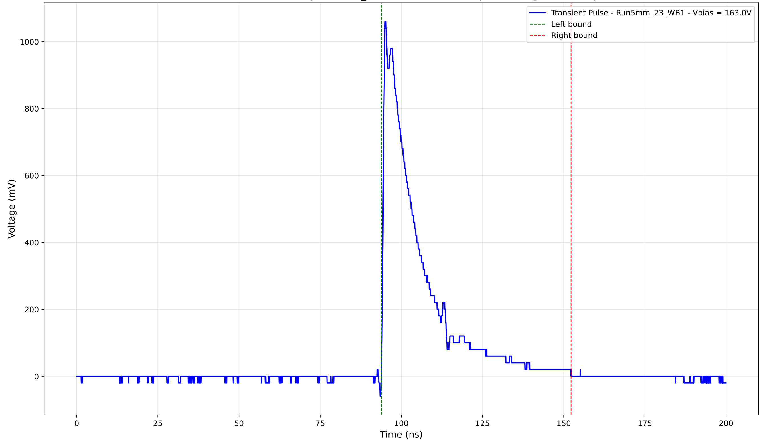
Transient Pulse - Sample: 5mm_23 - Position: 2610.0 \mu\text{m} - Charge: 243.53 pC
