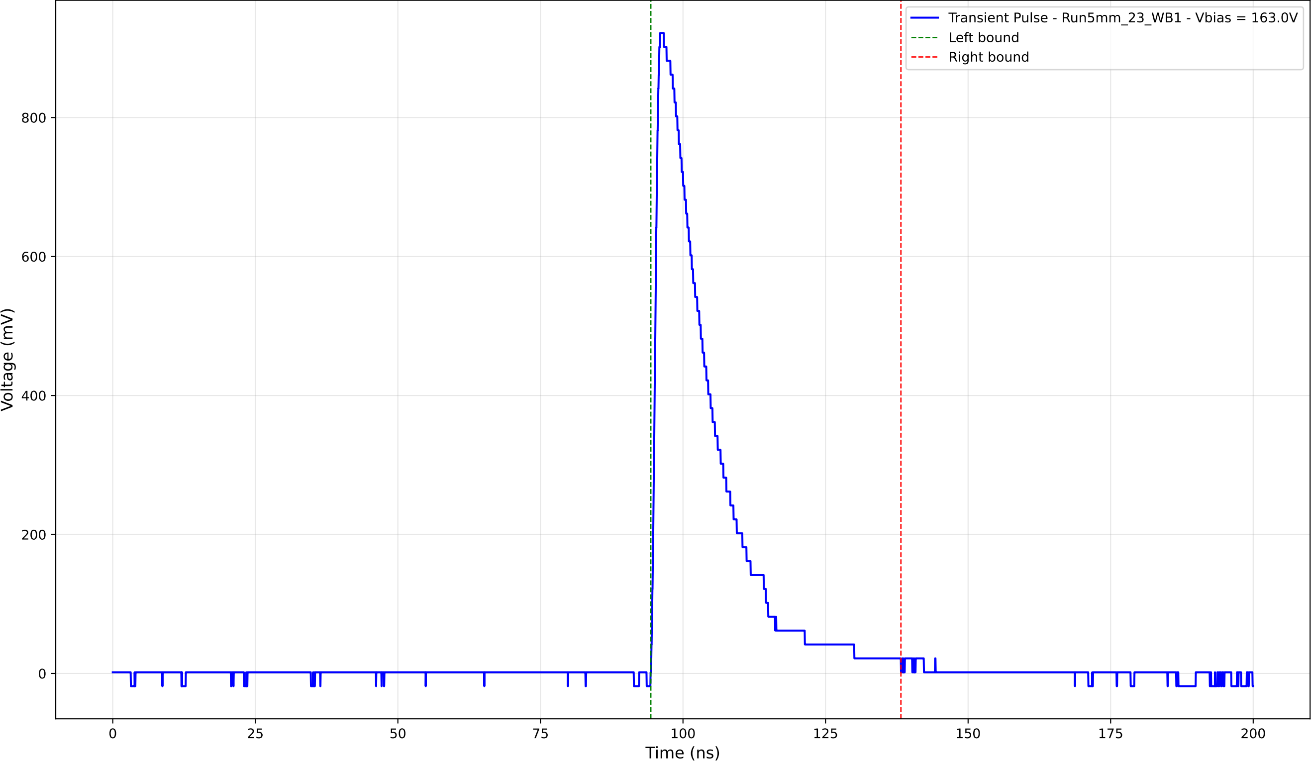
Transient Pulse - Sample: 5mm_23 - Position: 4075.0 \mu\text{m} - Charge: 199.40 pC
