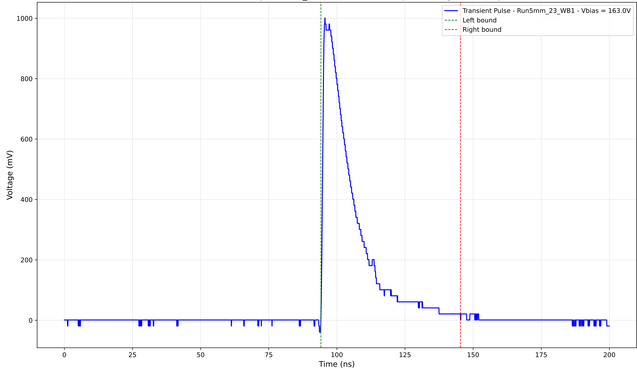
Transient Pulse - Sample: 5mm_23 - Position: 2090.0 \mu\text{m} - Charge: 245.02 pC
