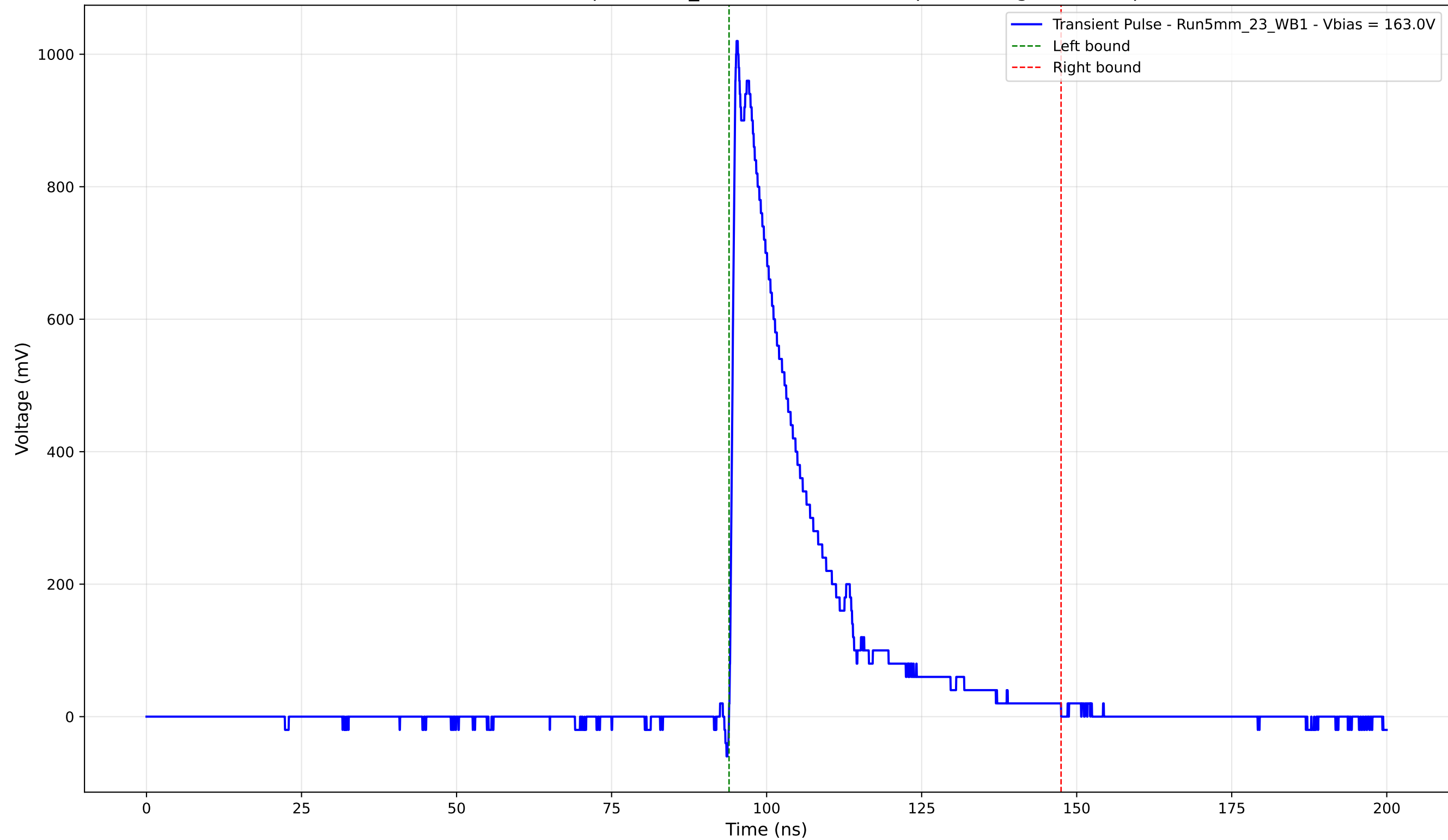
Transient Pulse - Sample: 5mm_23 - Position: 2470.0 \mu\text{m} - Charge: 229.95 pC
