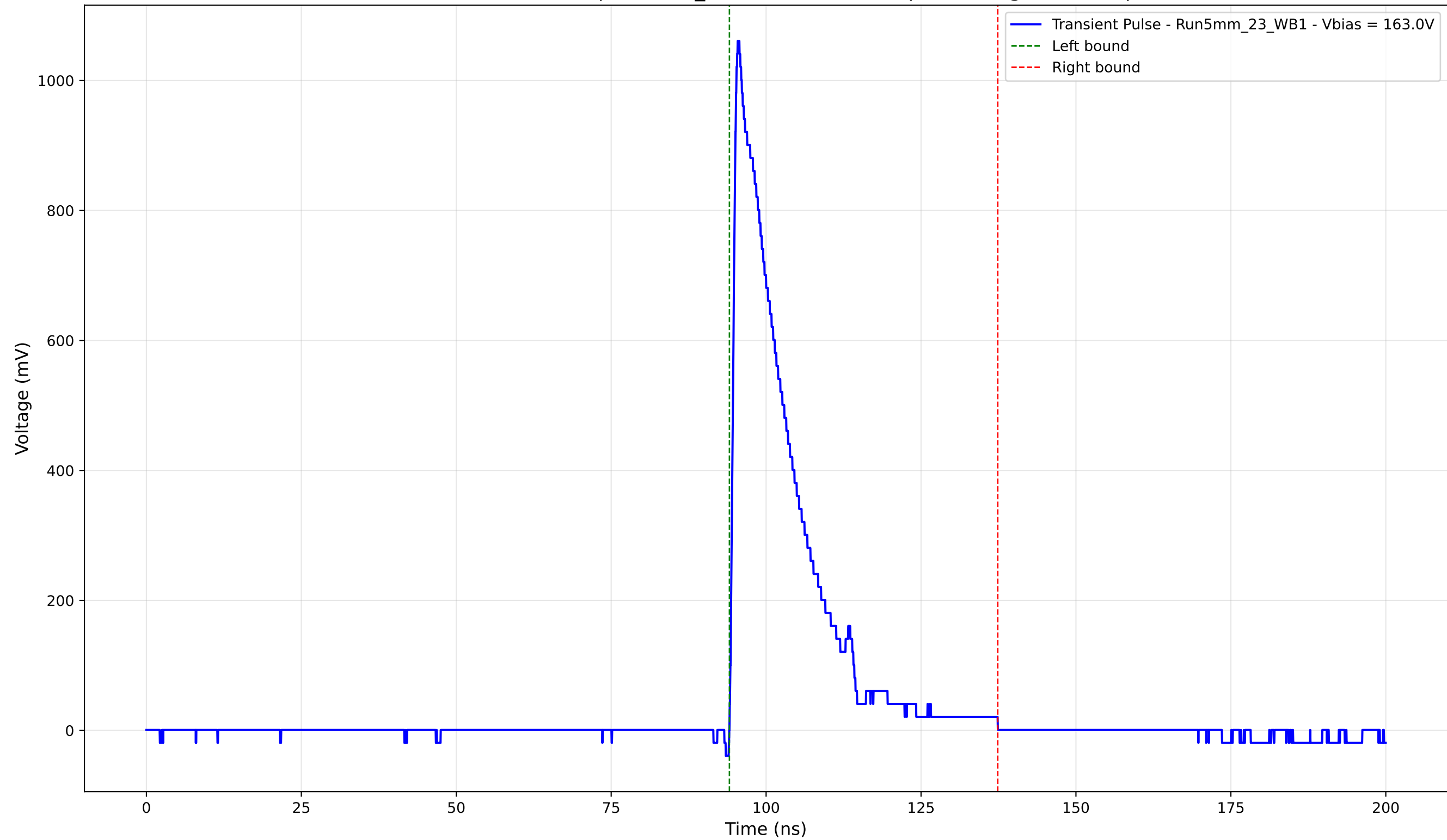
Transient Pulse - Sample: 5mm_23 - Position: 430.0 \mu\text{m} - Charge: 201.27 pC
