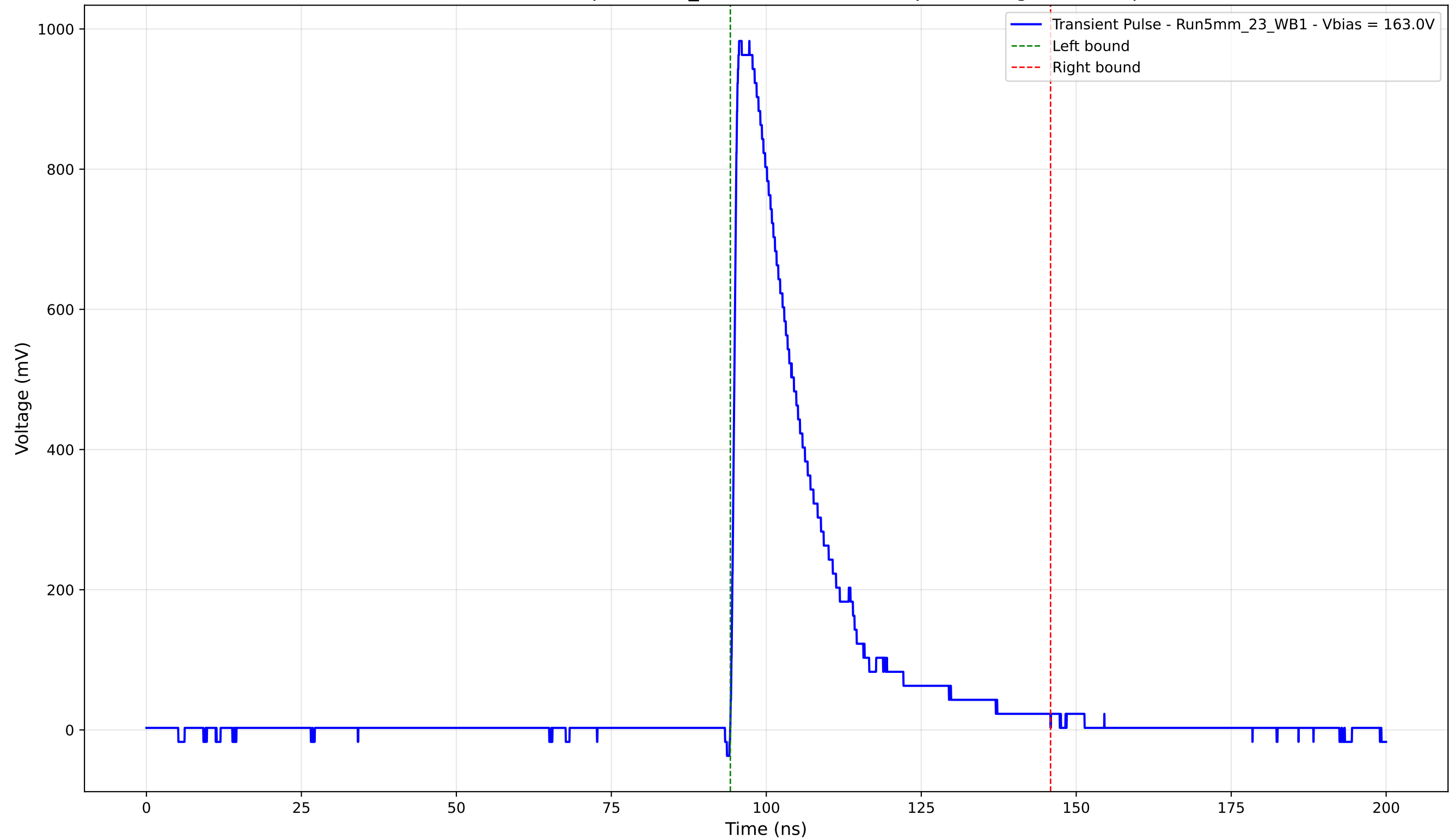
Transient Pulse - Sample: 5mm_23 - Position: 1995.0 \mu\text{m} - Charge: 245.06 pC
