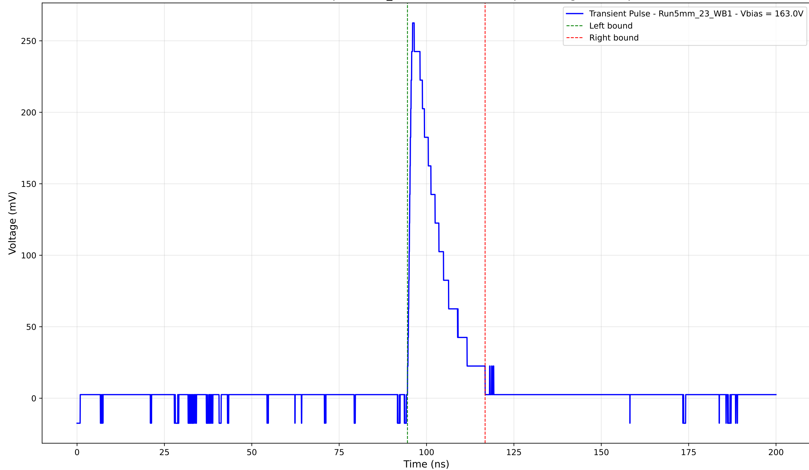
Transient Pulse - Sample: 5mm_23 - Position: 4280.0 \mu\text{m} - Charge: 45.64 pC
