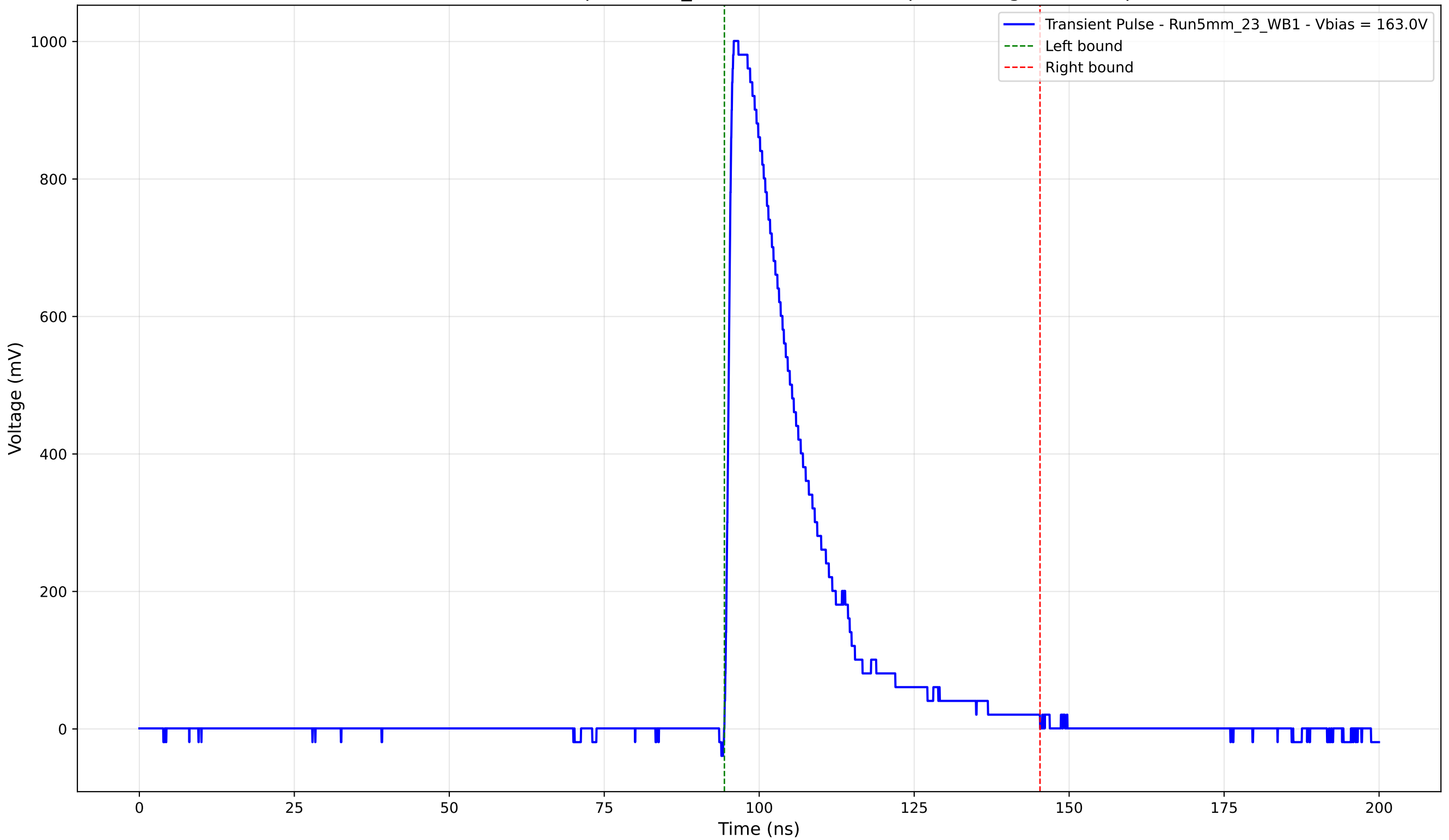
Transient Pulse - Sample: 5mm_23 - Position: 1495.0 \mu\text{m} - Charge: 251.38 pC
