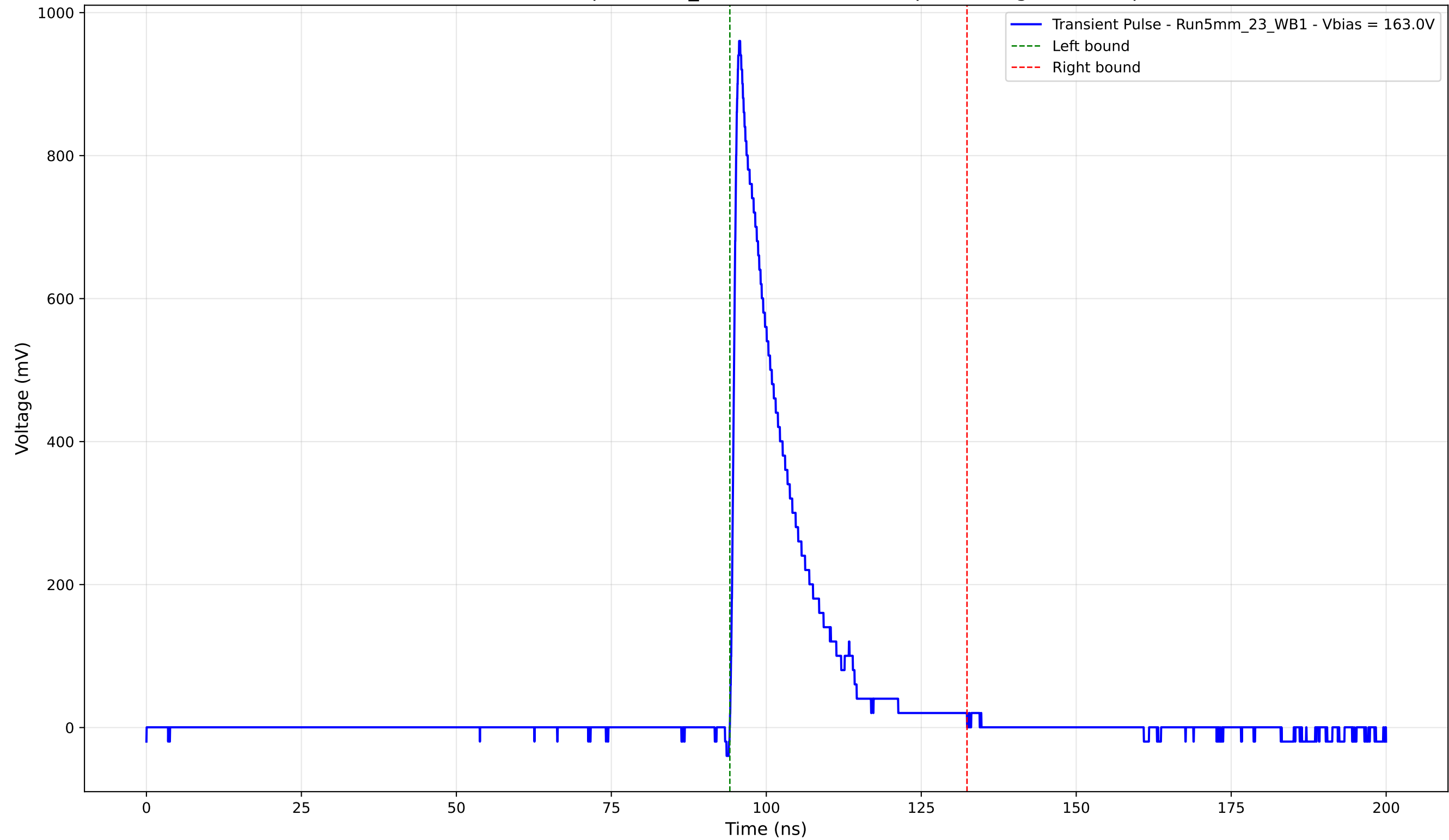
Transient Pulse - Sample: 5mm_23 - Position: 4850.0 \mu\text{m} - Charge: 159.98 pC
