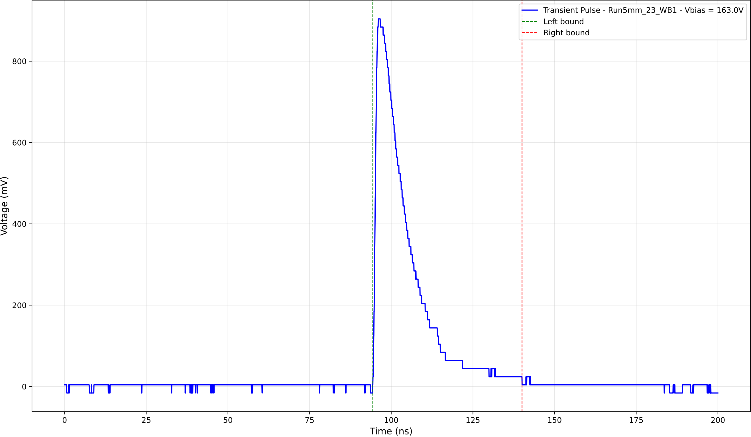
Transient Pulse - Sample: 5mm_23 - Position: 3920.0 \mu\text{m} - Charge: 200.30 pC
