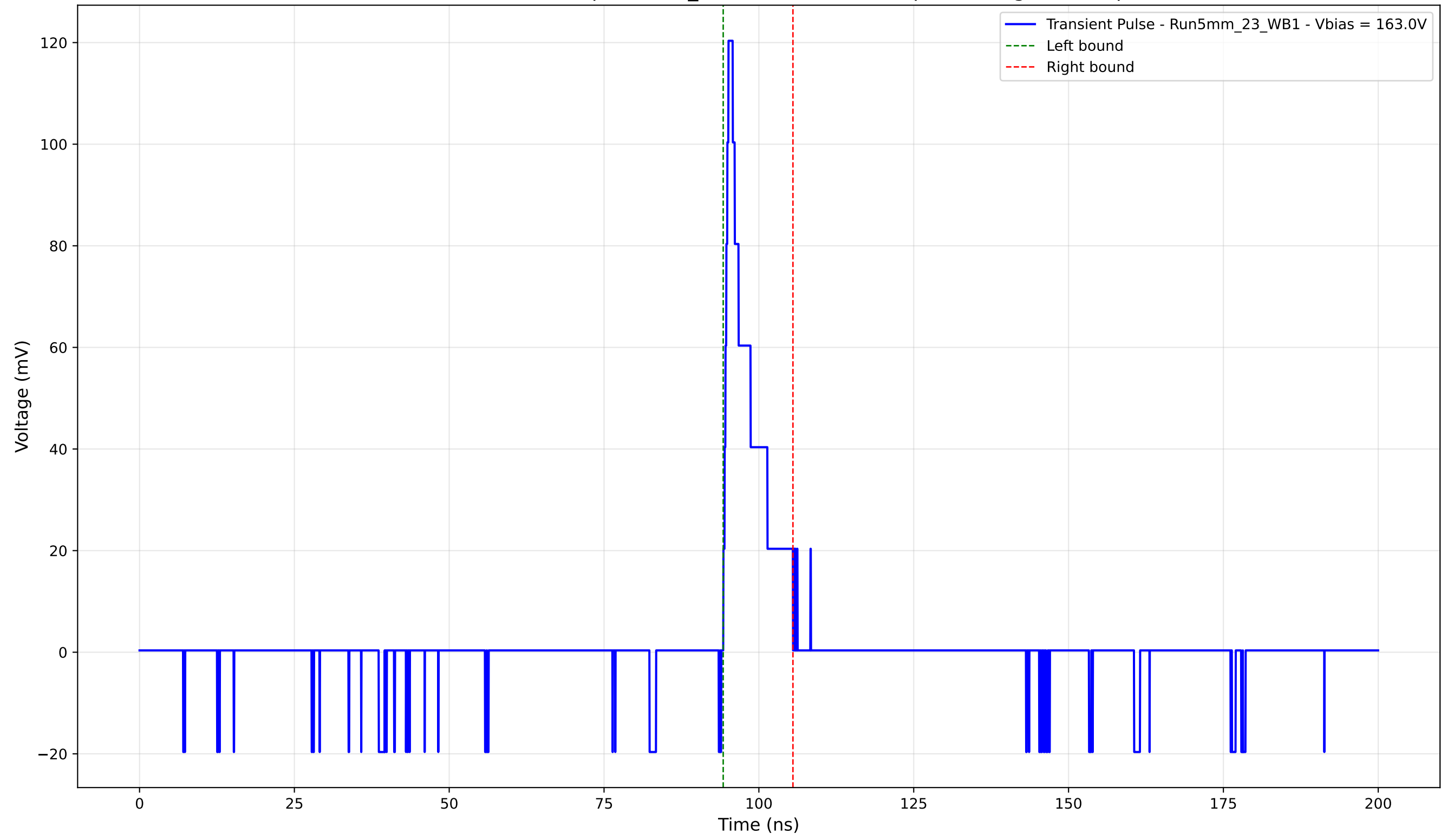
Transient Pulse - Sample: 5mm_23 -Position: 5205.0 \mu\text{m} - Charge: 10.52 pC
