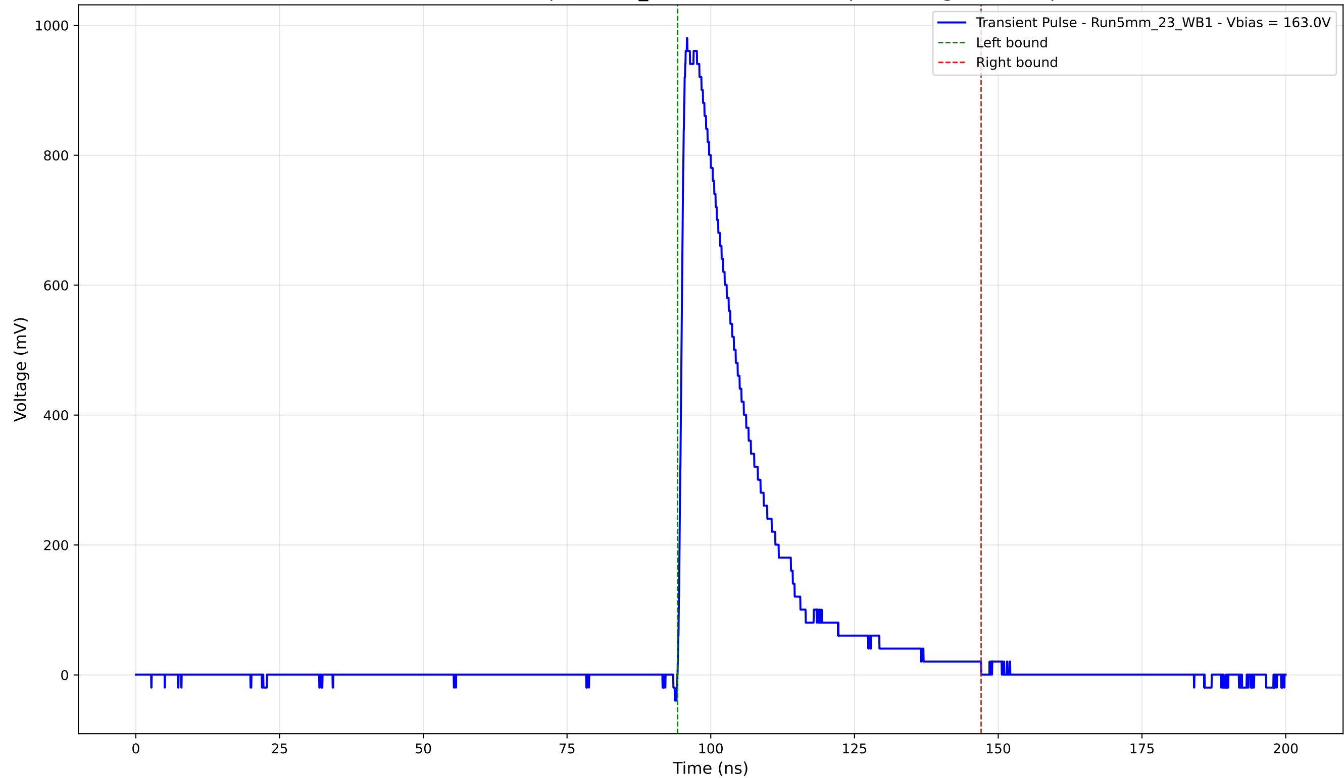
Transient Pulse - Sample: 5mm_23 - Position: 1925.0 \mu\text{m} - Charge: 239.12 pC
