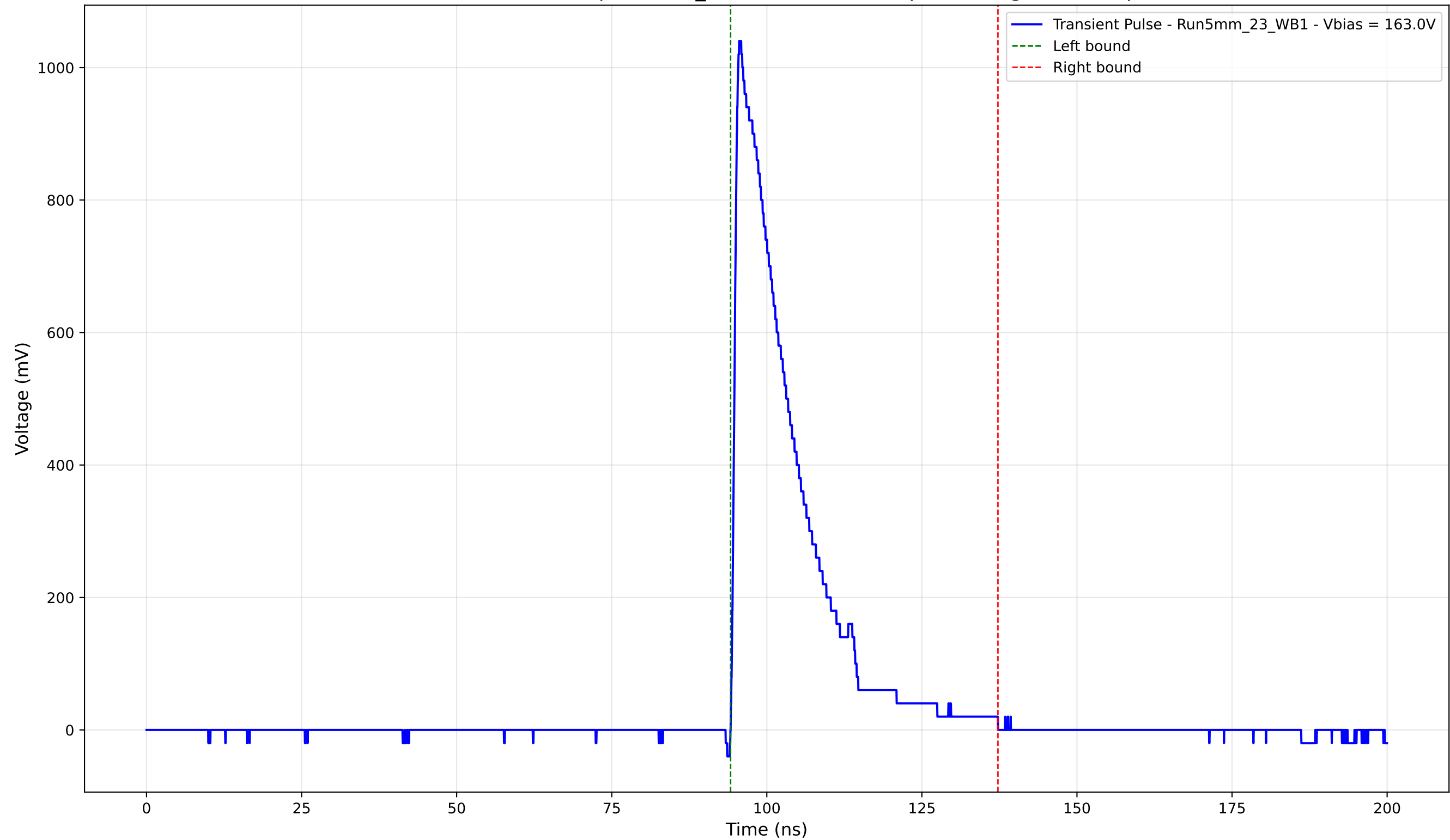
Transient Pulse - Sample: 5mm_23 - Position: 600.0 \mu\text{m} - Charge: 210.81 pC
