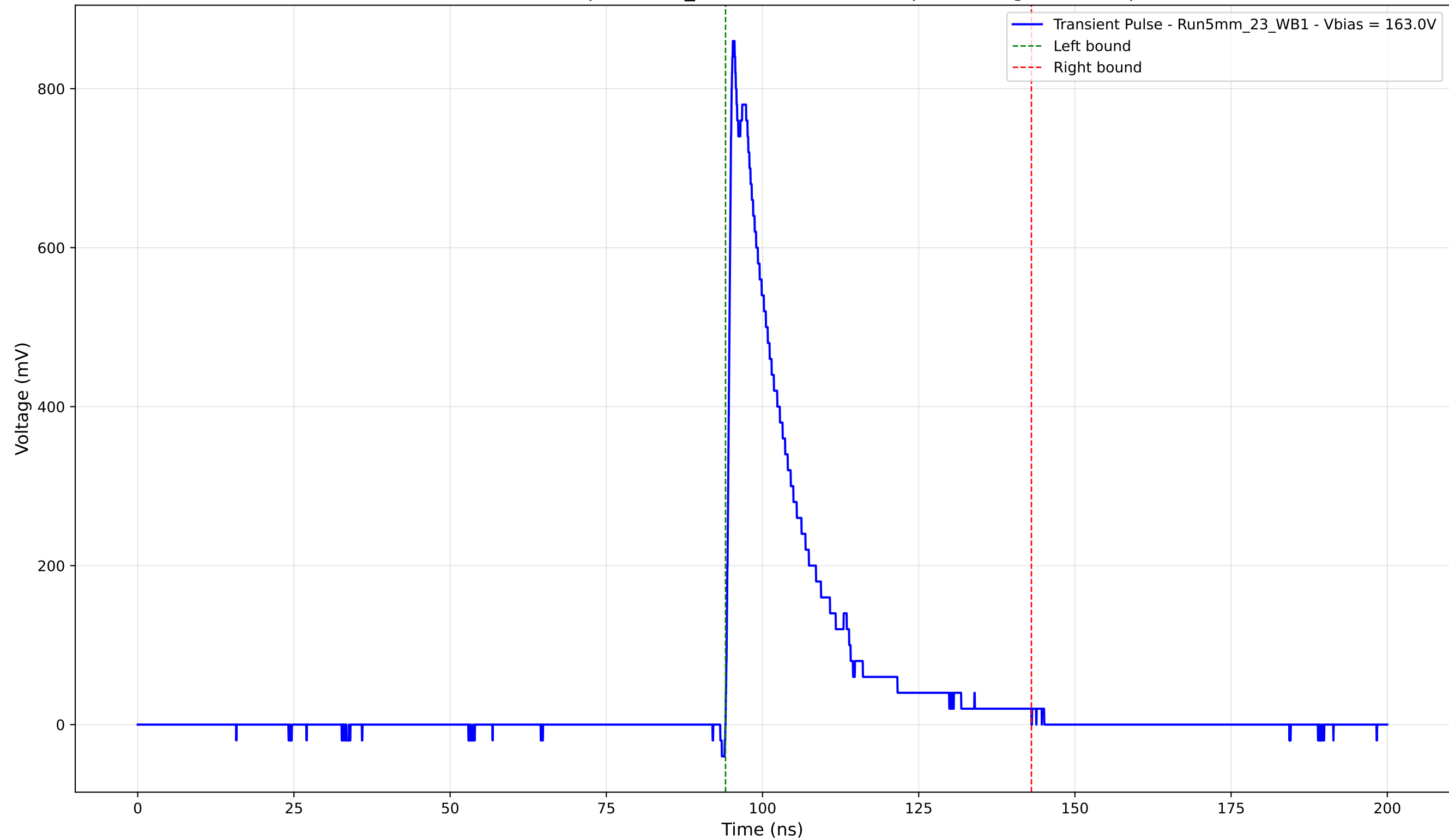
Transient Pulse - Sample: 5mm_23 - Position: 2305.0 \mu\text{m} - Charge: 172.80 pC
