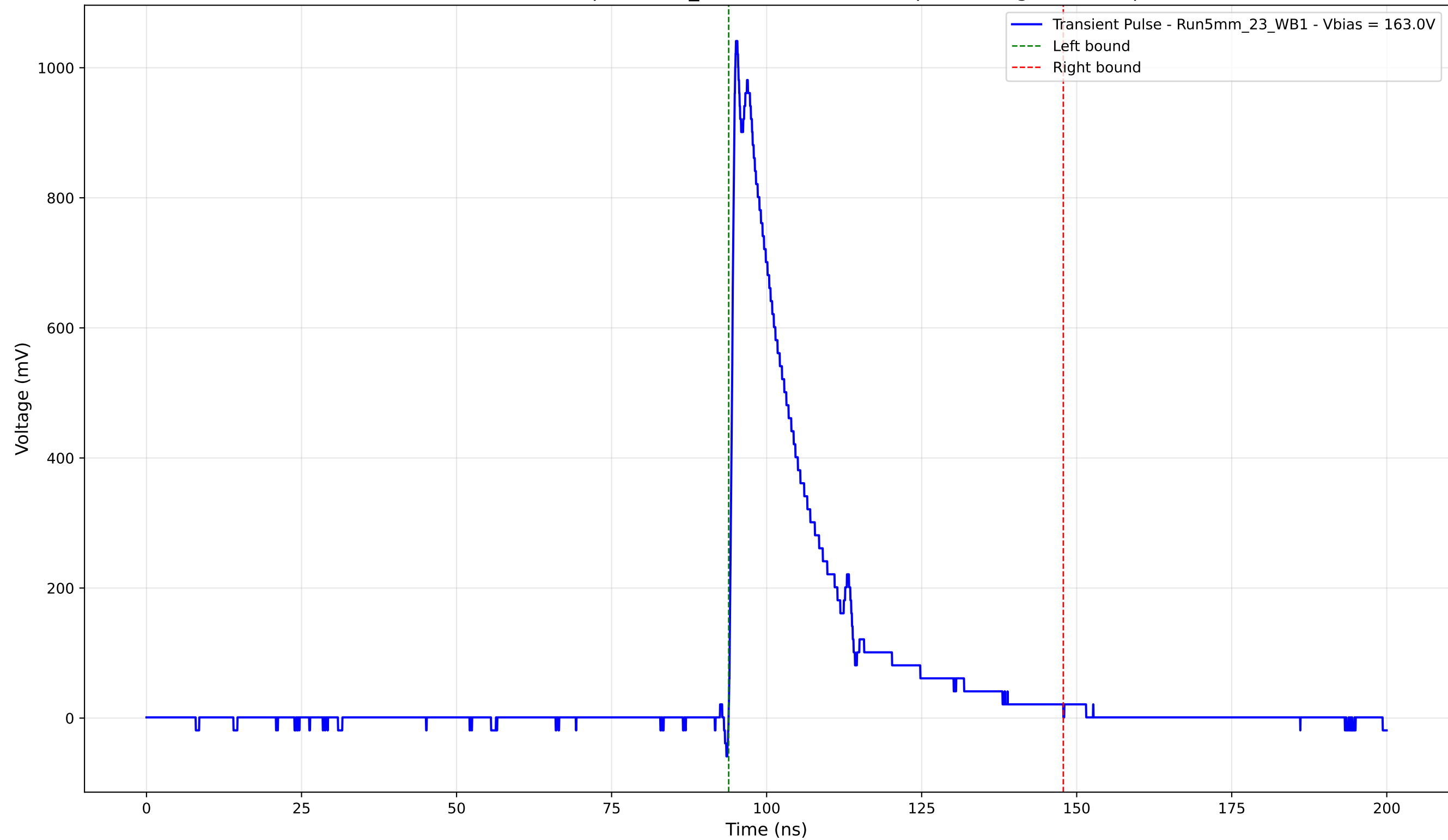
Transient Pulse - Sample: 5mm_23 - Position: 2545.0 \mu\text{m} - Charge: 236.58 pC
