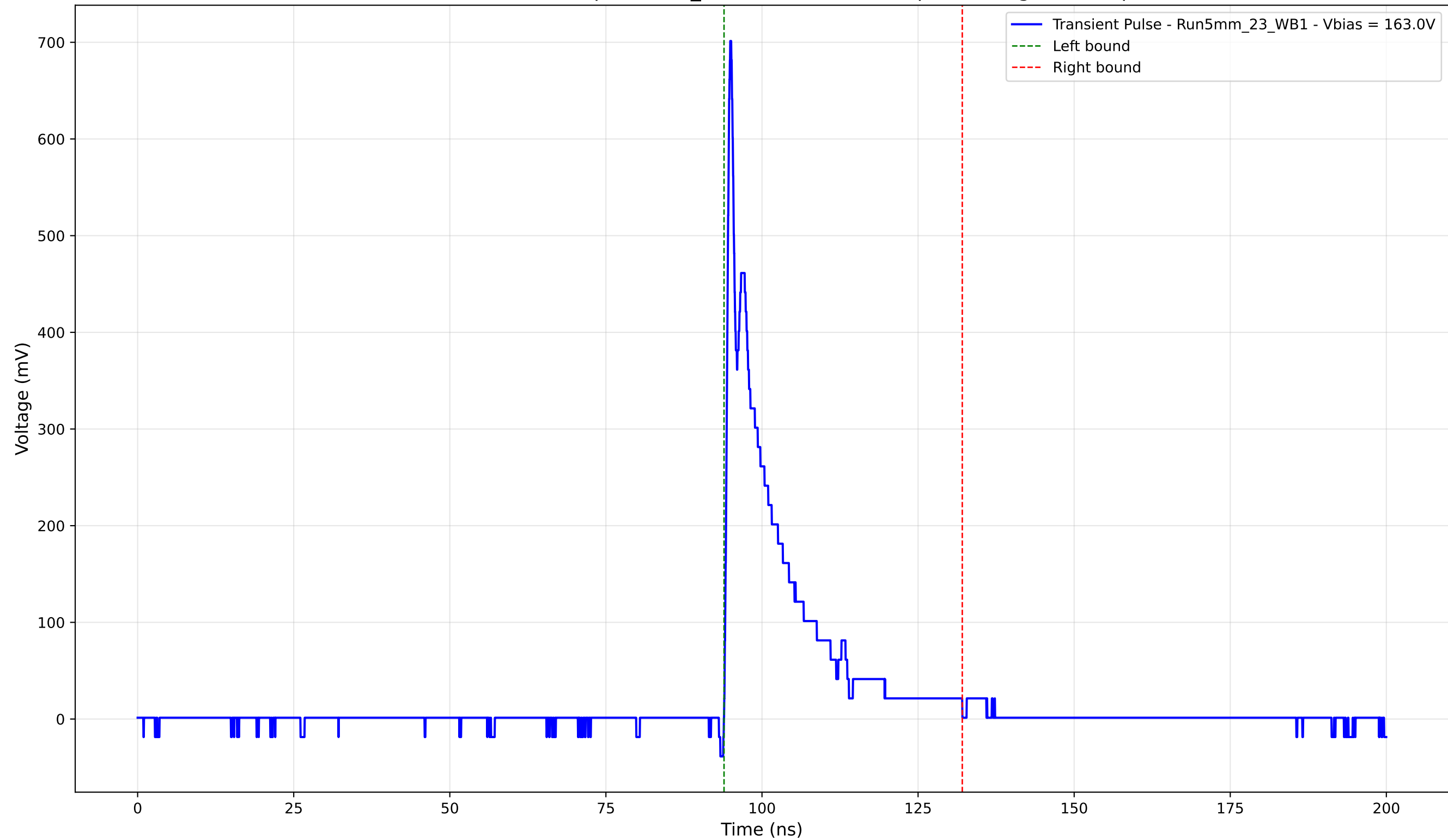
Transient Pulse - Sample: 5mm_23 - Position: 2715.0 \mu\text{m} - Charge: 92.30 pC
