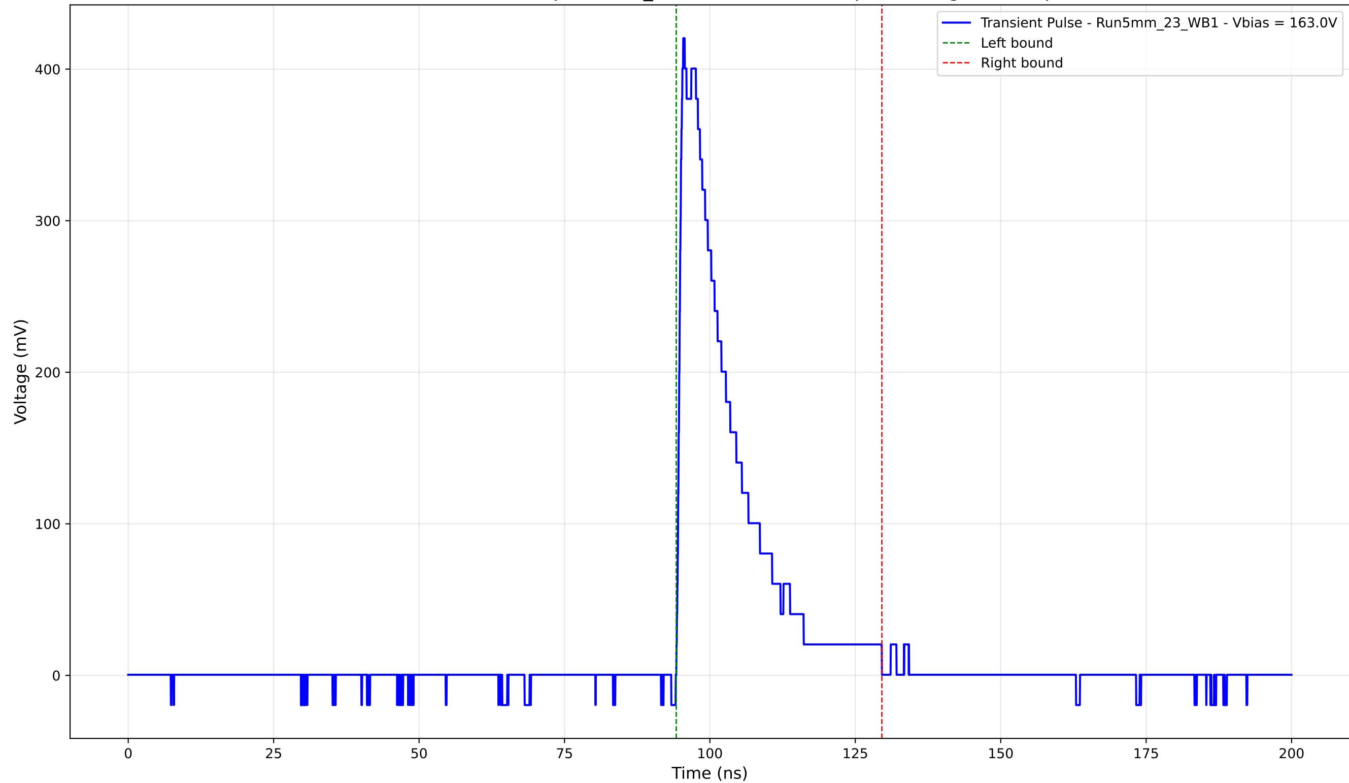
Transient Pulse - Sample: 5mm_23 - Position: 3280.0 \mu\text{m} - Charge: 80.79 pC
