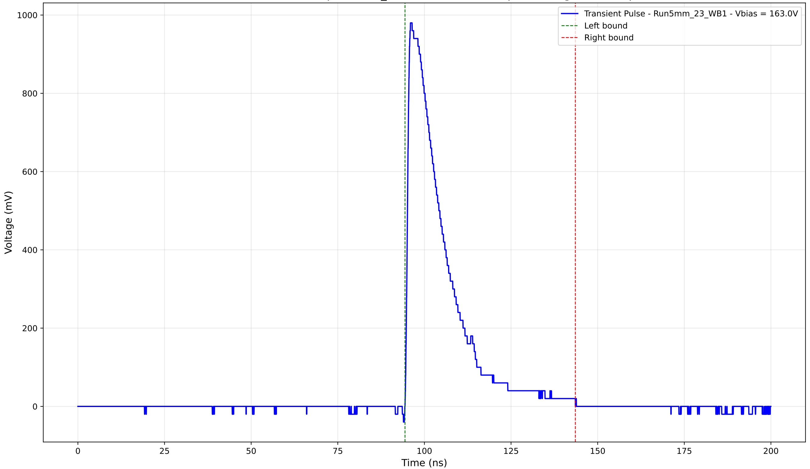
Transient Pulse - Sample: 5mm_23 - Position: 1405.0 \mu\text{m} - Charge: 229.95 pC
