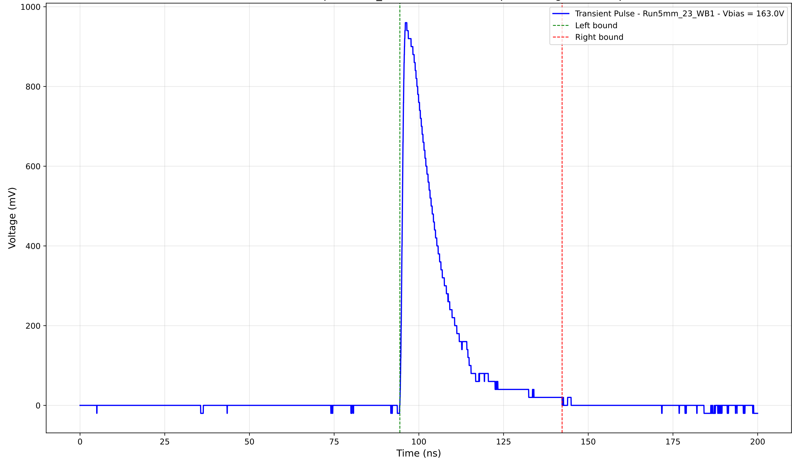
Transient Pulse - Sample: 5mm_23 - Position: 1340.0 \mu\text{m} - Charge: 217.28 pC
