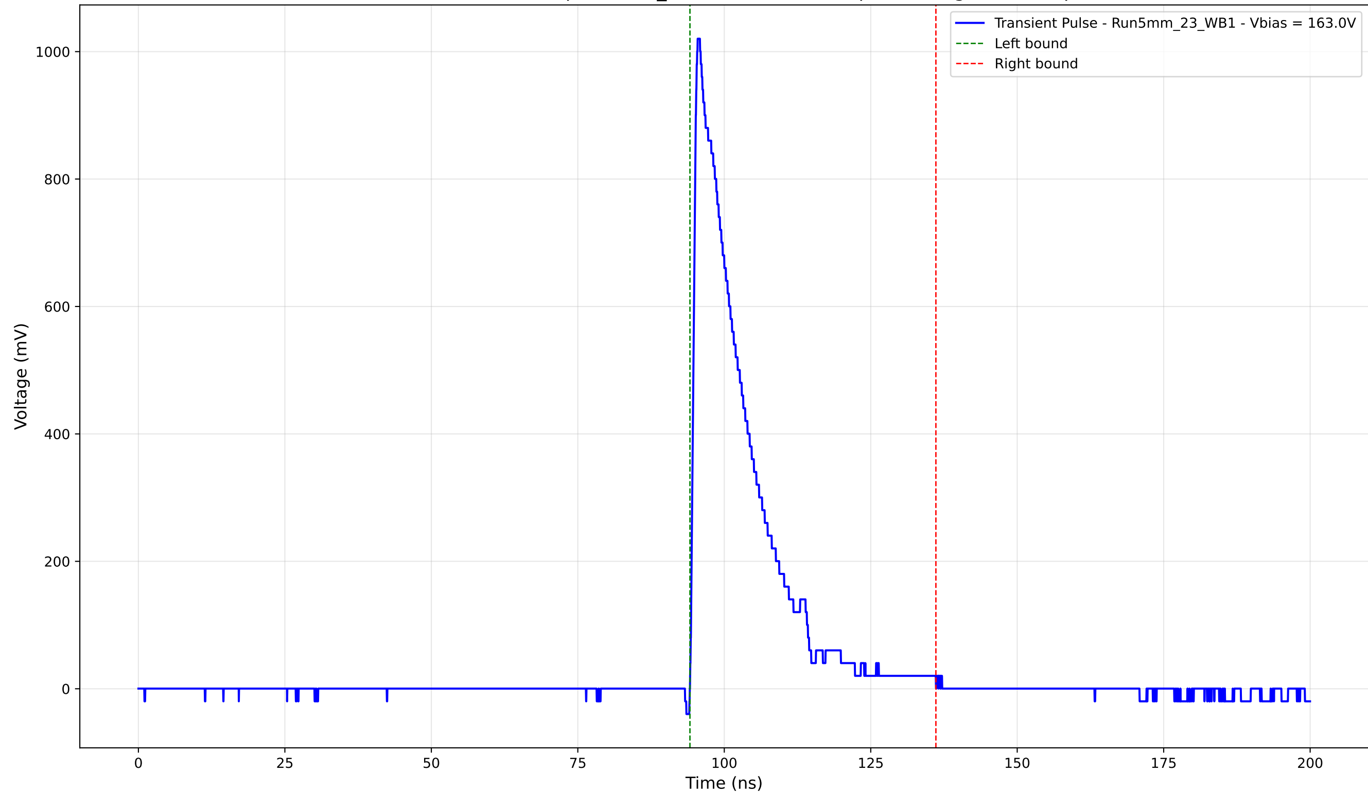
Transient Pulse - Sample: 5mm_23 - Position: 520.0 \mu\text{m} - Charge: 192.87 pC
