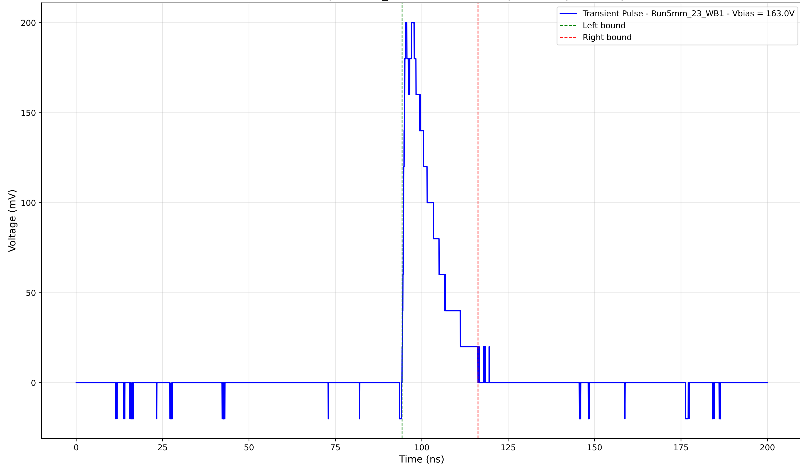
Transient Pulse - Sample: 5mm_23 - Position: 3245.0 \mu\text{m} - Charge: 36.41 pC
