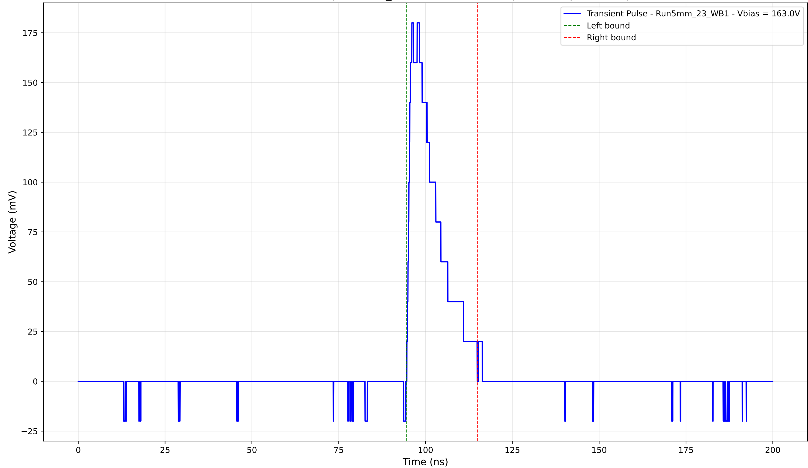
Transient Pulse - Sample: 5mm_23 -Position: 4260.0 \mu\text{m} - Charge: 32.09 pC
