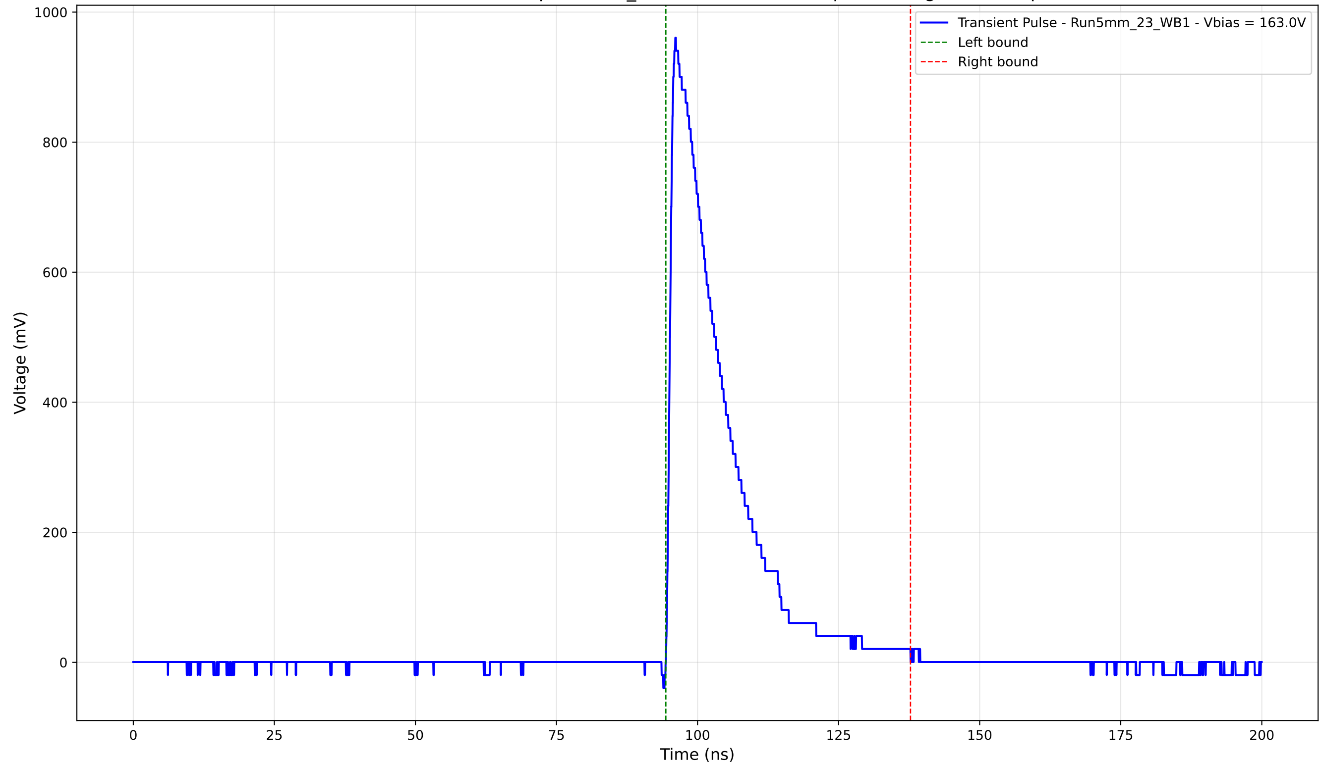
Transient Pulse - Sample: 5mm_23 - Position: 1110.0 \mu\text{m} - Charge: 200.48 pC
