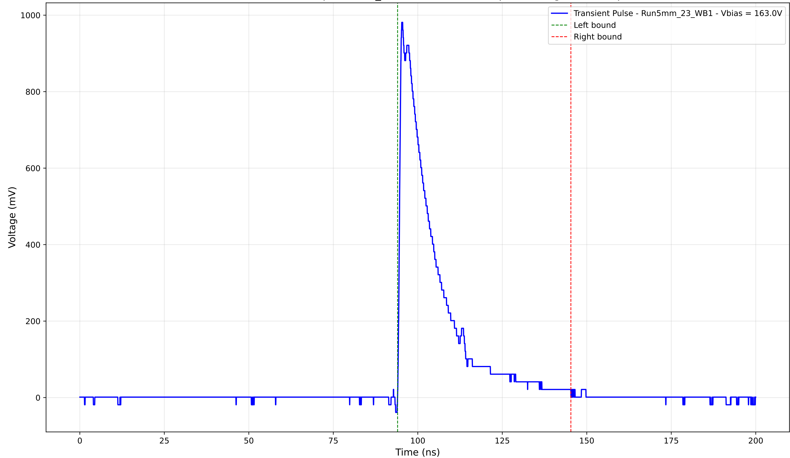
Transient Pulse - Sample: 5mm_23 - Position: 3140.0 \mu\text{m} - Charge: 218.11 pC
