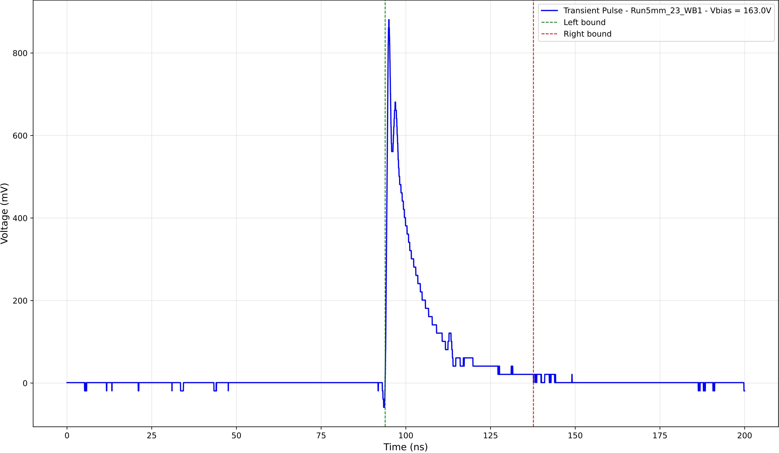
Transient Pulse - Sample: 5mm_23 - Position: 2795.0 \mu\text{m} - Charge: 136.16 pC
