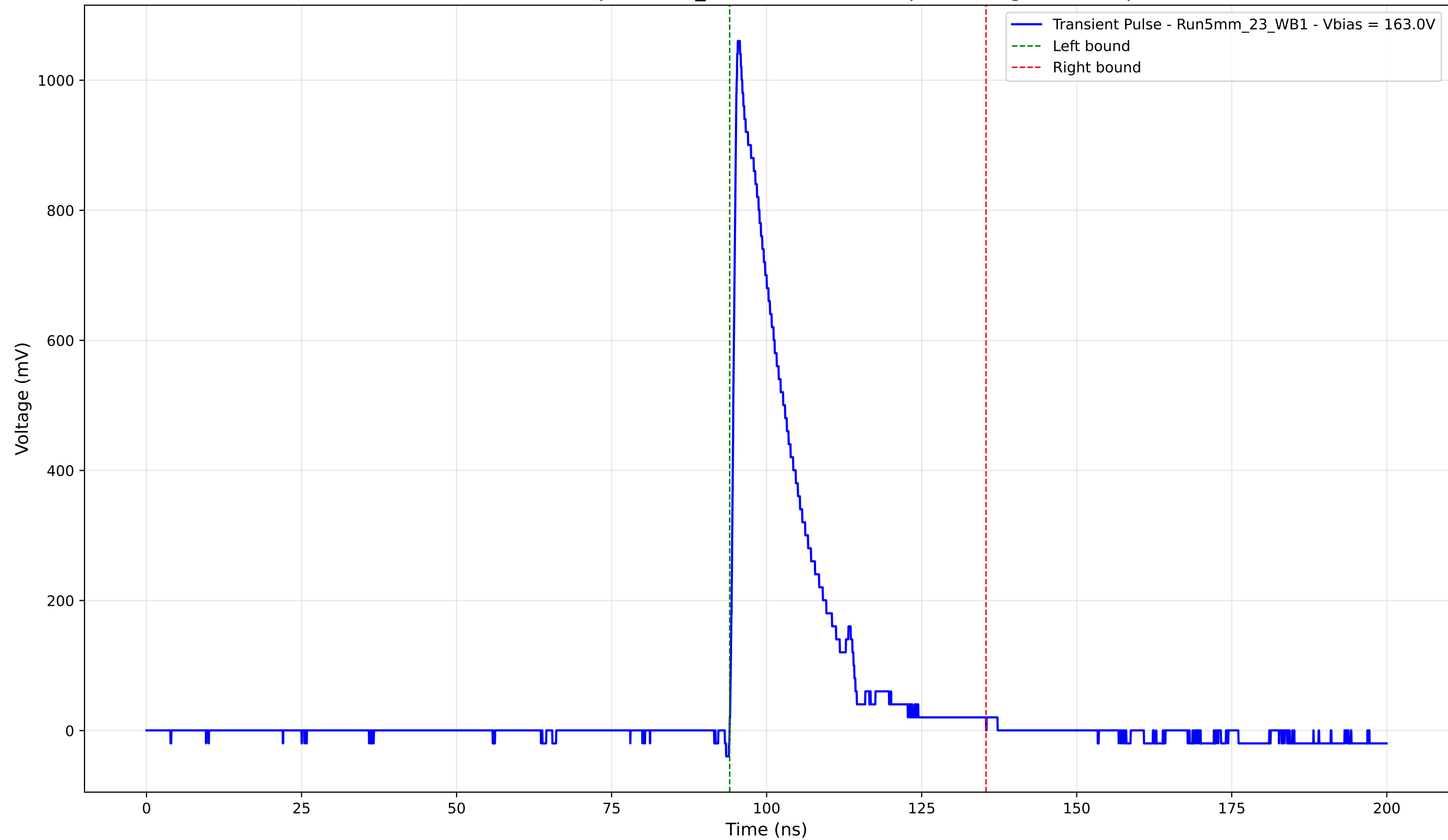
Transient Pulse - Sample: 5mm_23 - Position: 405.0 \mu\text{m} - Charge: 200.29 pC
