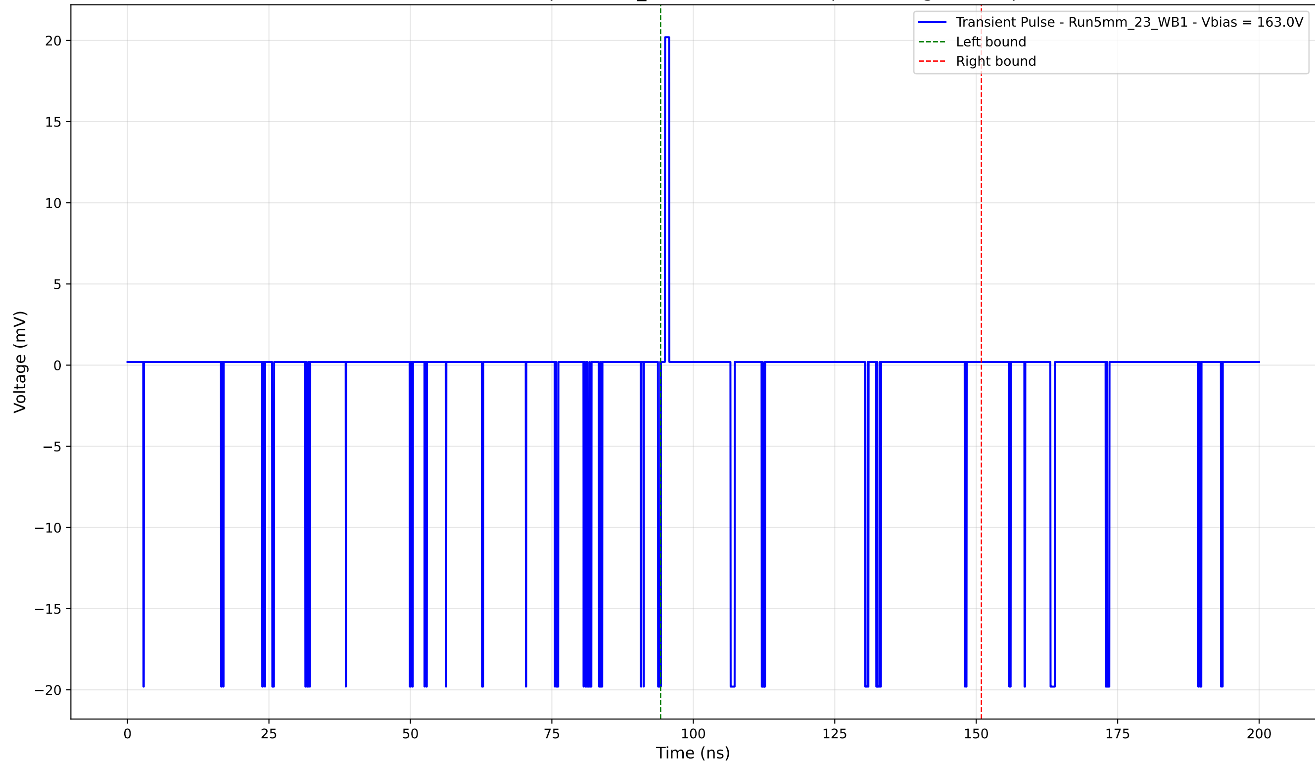
Transient Pulse - Sample: 5mm_23 - Position: 165.0 \mu\text{m} - Charge: -0.55 pC
