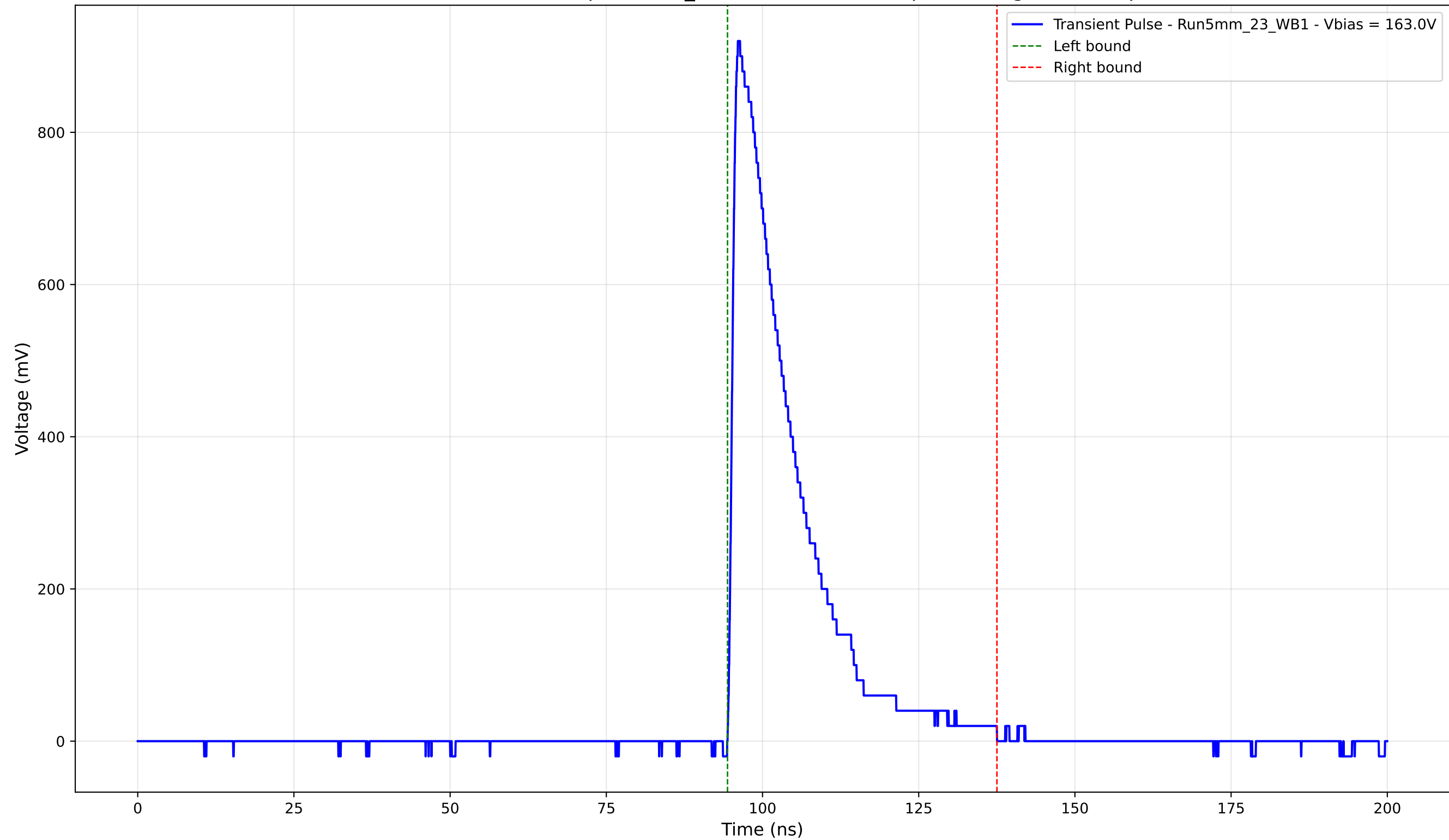
Transient Pulse - Sample: 5mm_23 - Position: 1310.0 \mu\text{m} - Charge: 195.21 pC
