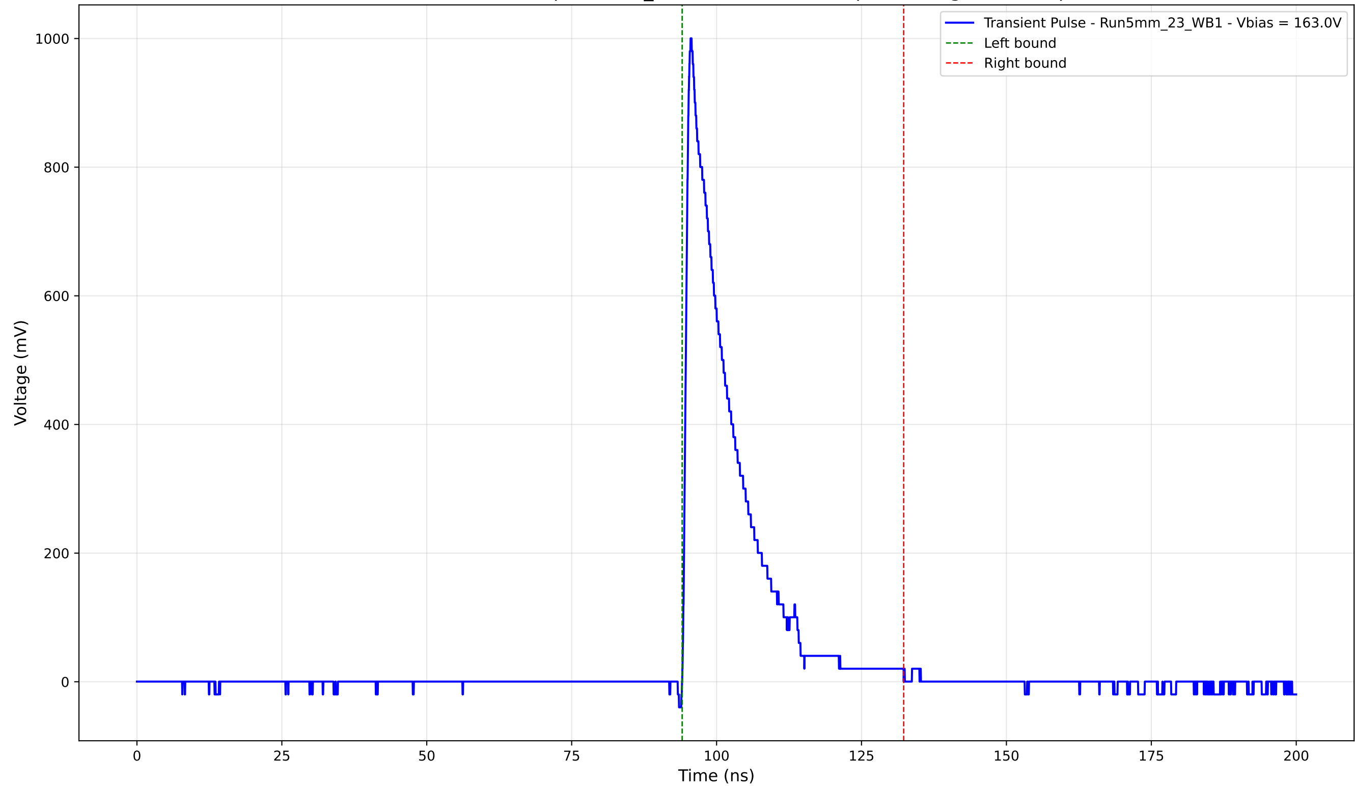
Transient Pulse - Sample: 5mm_23 - Position: 4950.0 \mu\text{m} - Charge: 166.78 pC
