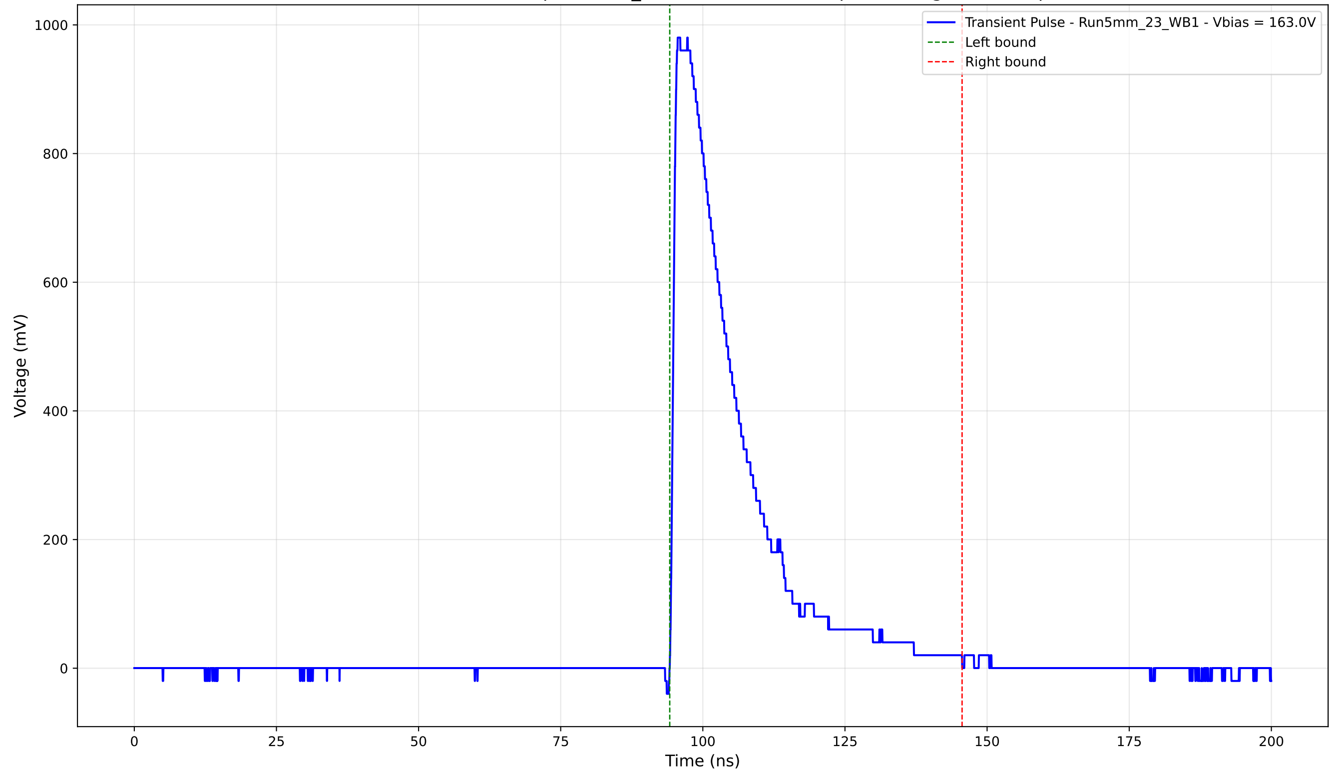
Transient Pulse - Sample: 5mm_23 - Position: 2015.0 \mu\text{m} - Charge: 243.69 pC
