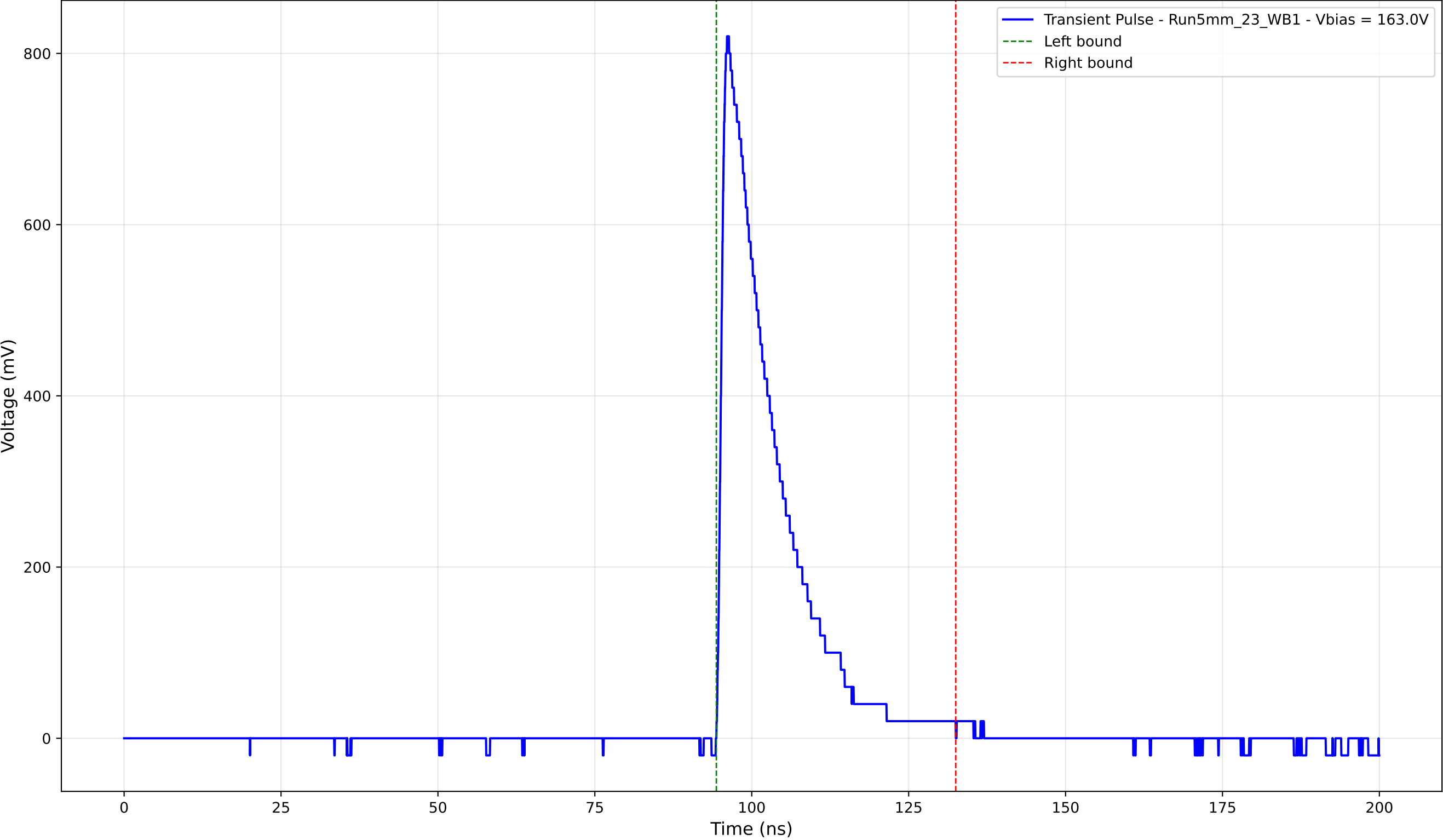
Transient Pulse - Sample: 5mm_23 - Position: 4340.0 \mu\text{m} - Charge: 152.98 pC
