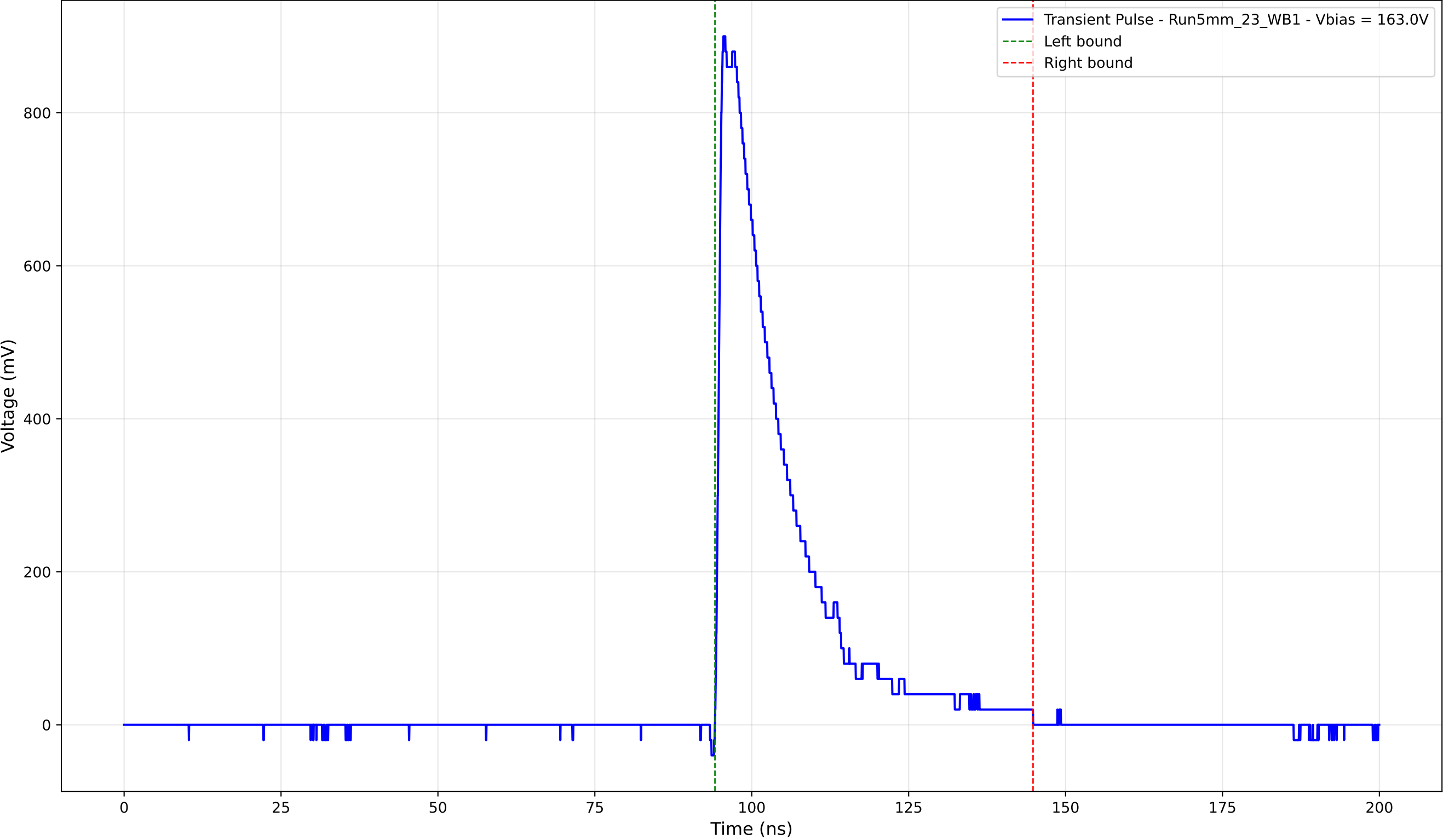
Transient Pulse - Sample: 5mm_23 - Position: 3350.0 \mu\text{m} - Charge: 200.98 pC
