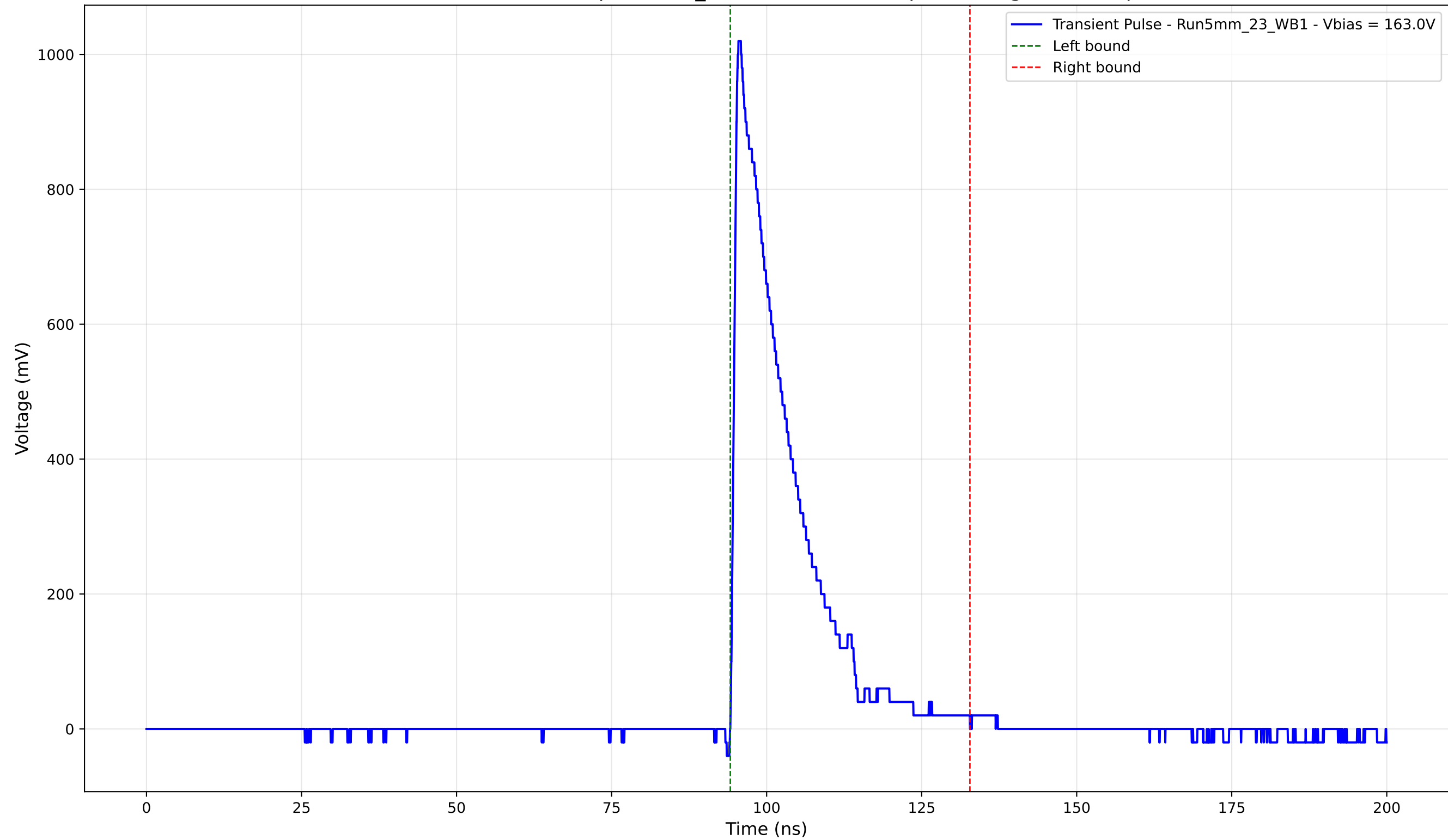
Transient Pulse - Sample: 5mm_23 - Position: 515.0 \mu\text{m} - Charge: 190.10 pC
