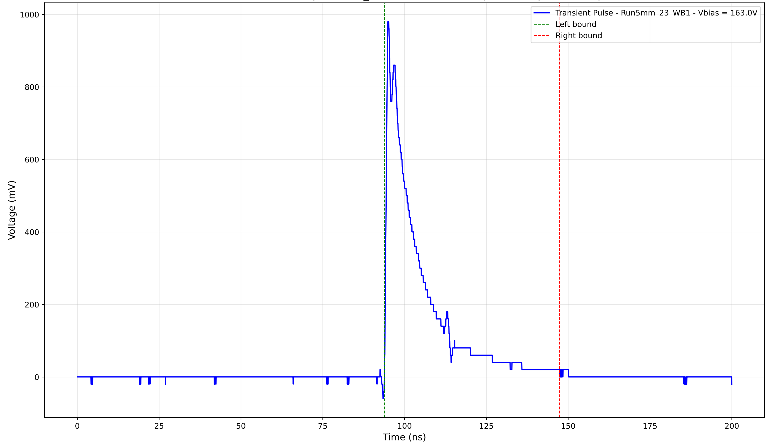
Transient Pulse - Sample: 5mm_23 - Position: 2680.0 \mu\text{m} - Charge: 189.29 pC
