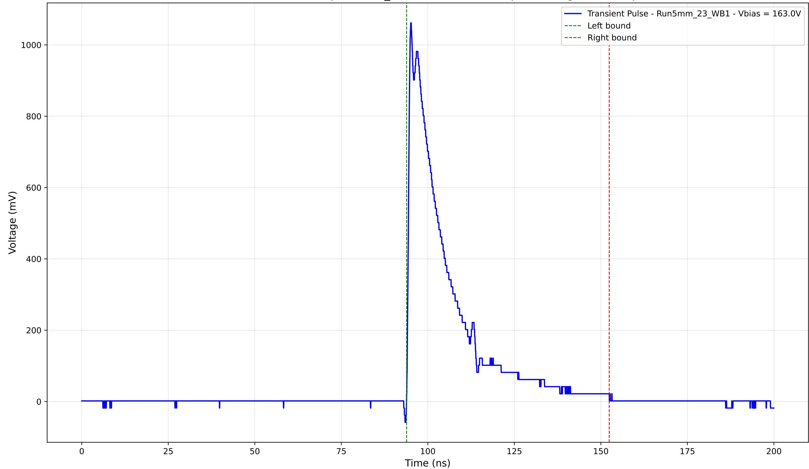
Transient Pulse - Sample: 5mm_23 - Position: 2900.0 \mu\text{m} - Charge: 244.14 pC
