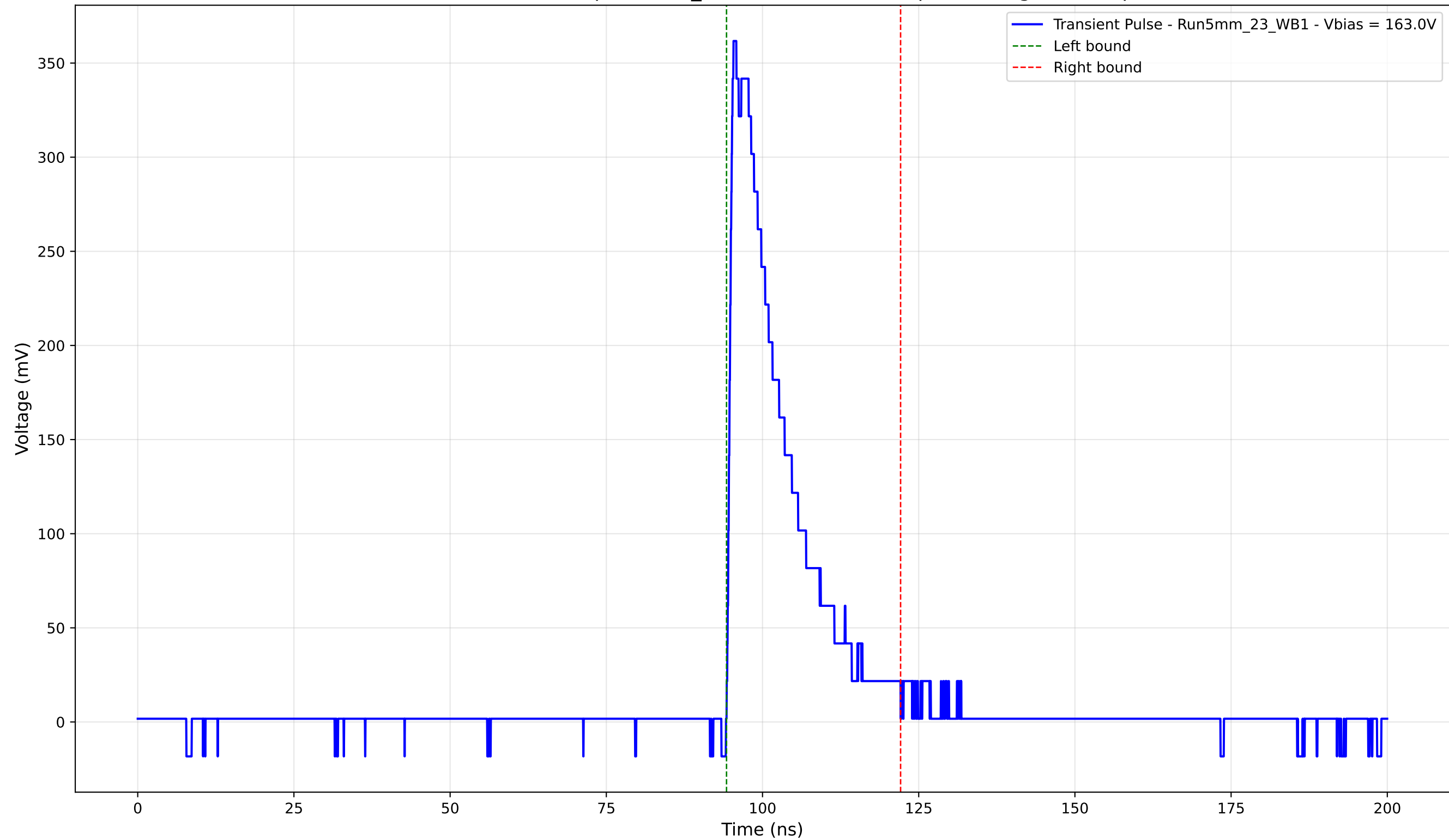
Transient Pulse - Sample: 5mm_23 - Position: 3275.0 \mu\text{m} - Charge: 67.96 pC
