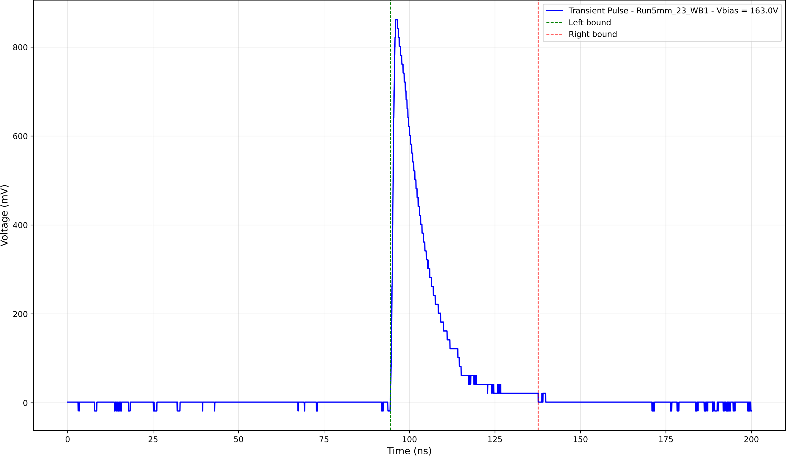
Transient Pulse - Sample: 5mm_23 - Position: 1150.0 \mu\text{m} - Charge: 173.12 pC
