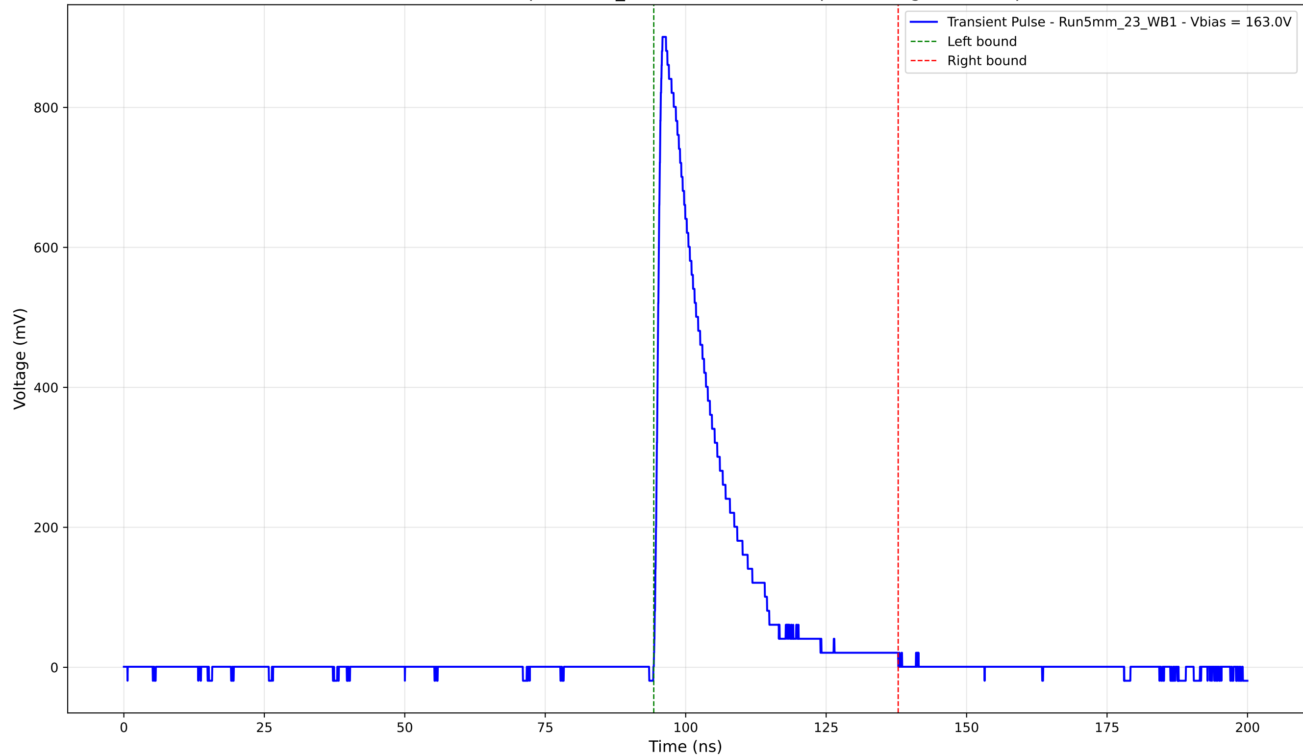
Transient Pulse - Sample: 5mm_23 - Position: 4395.0 \mu\text{m} - Charge: 179.80 pC
