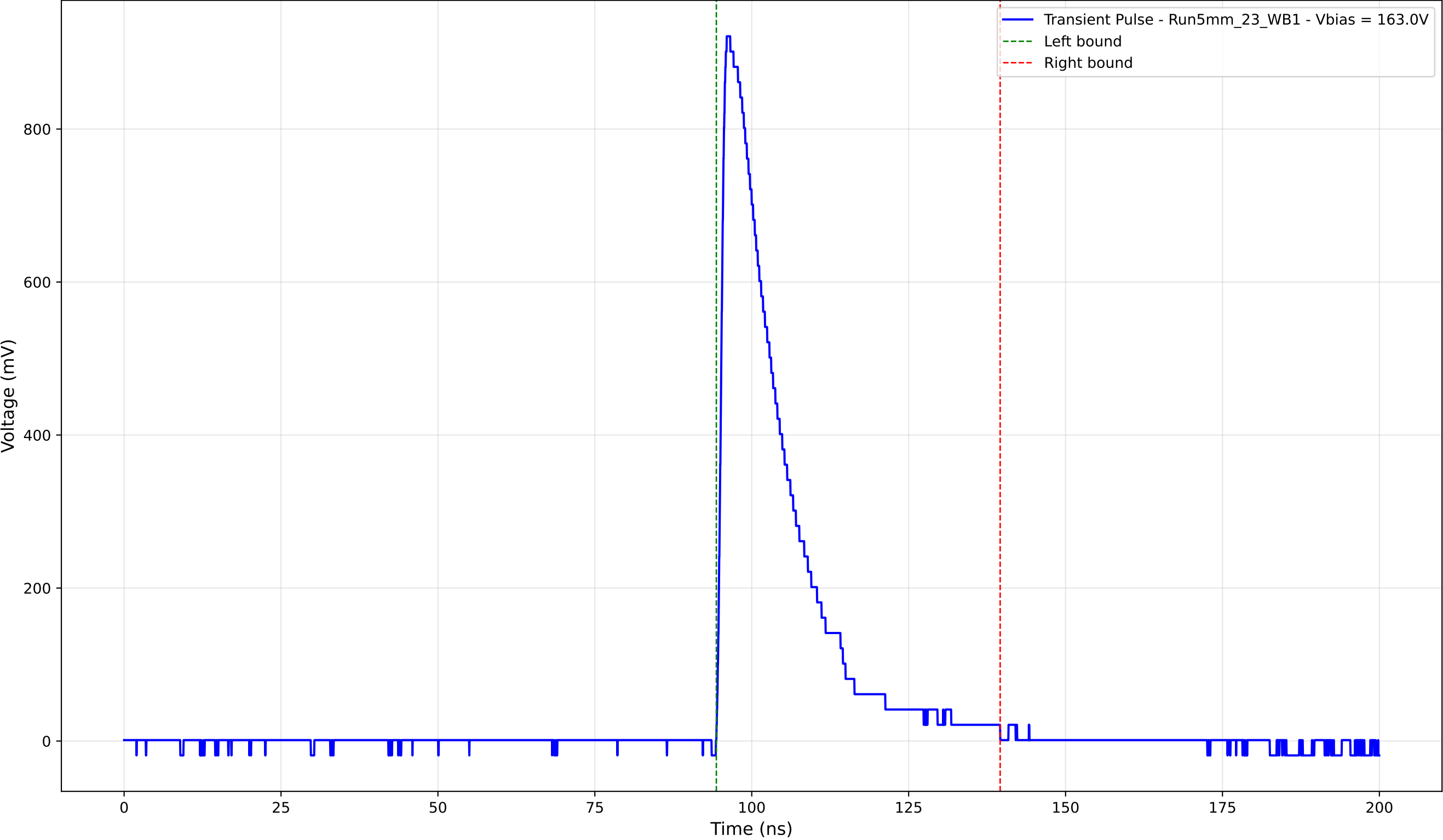
Transient Pulse - Sample: 5mm_23 - Position: 4090.0 \mu\text{m} - Charge: 199.29 pC
