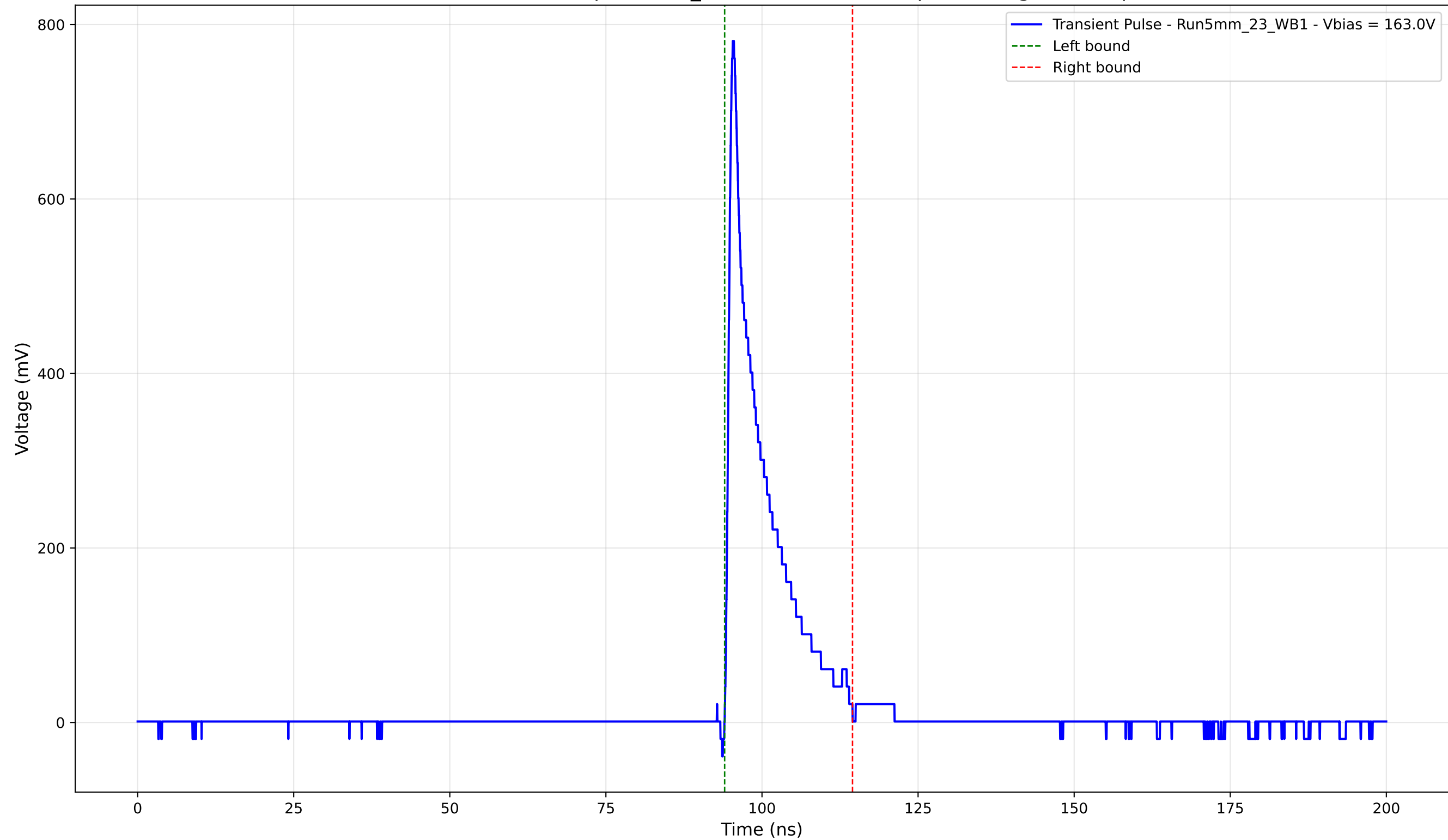
Transient Pulse - Sample: 5mm_23 - Position: 5155.0 \mu\text{m} - Charge: 90.44 pC
