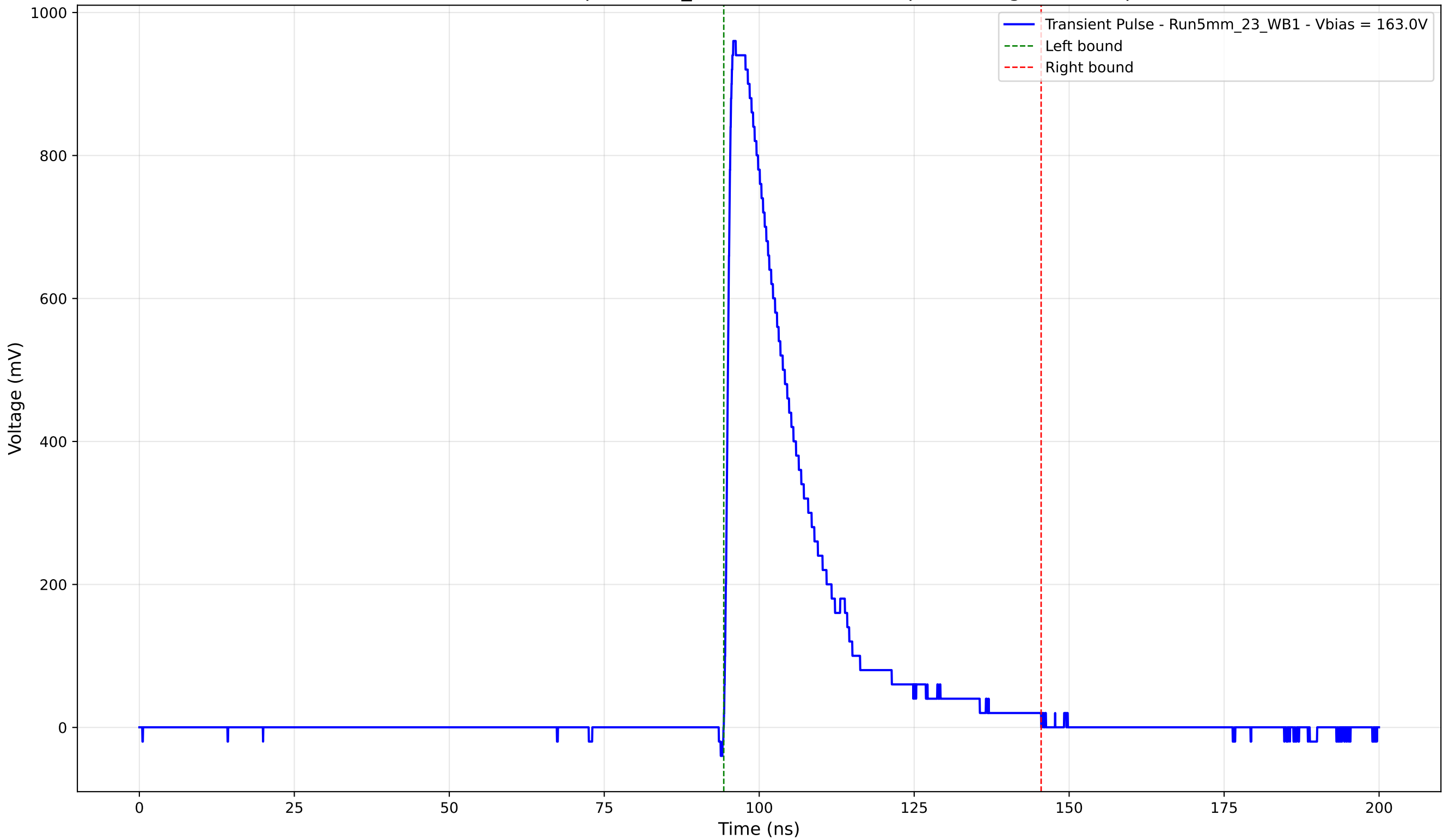
Transient Pulse - Sample: 5mm_23 - Position: 1850.0 \mu\text{m} - Charge: 230.47 pC
