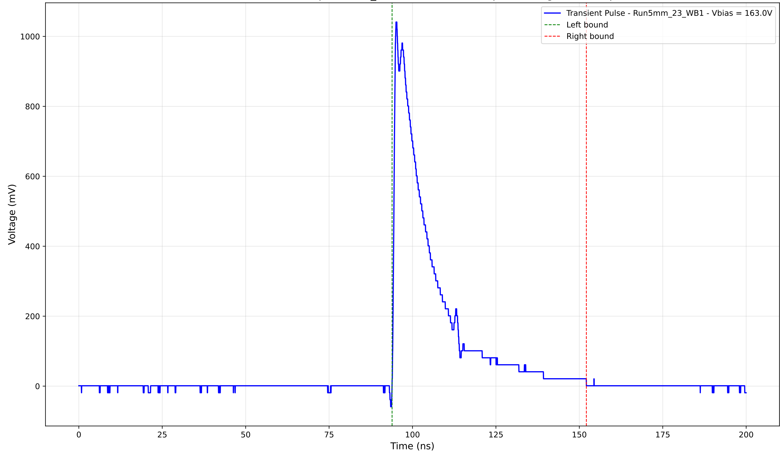
Transient Pulse - Sample: 5mm_23 - Position: 2930.0 \mu\text{m} - Charge: 238.36 pC
