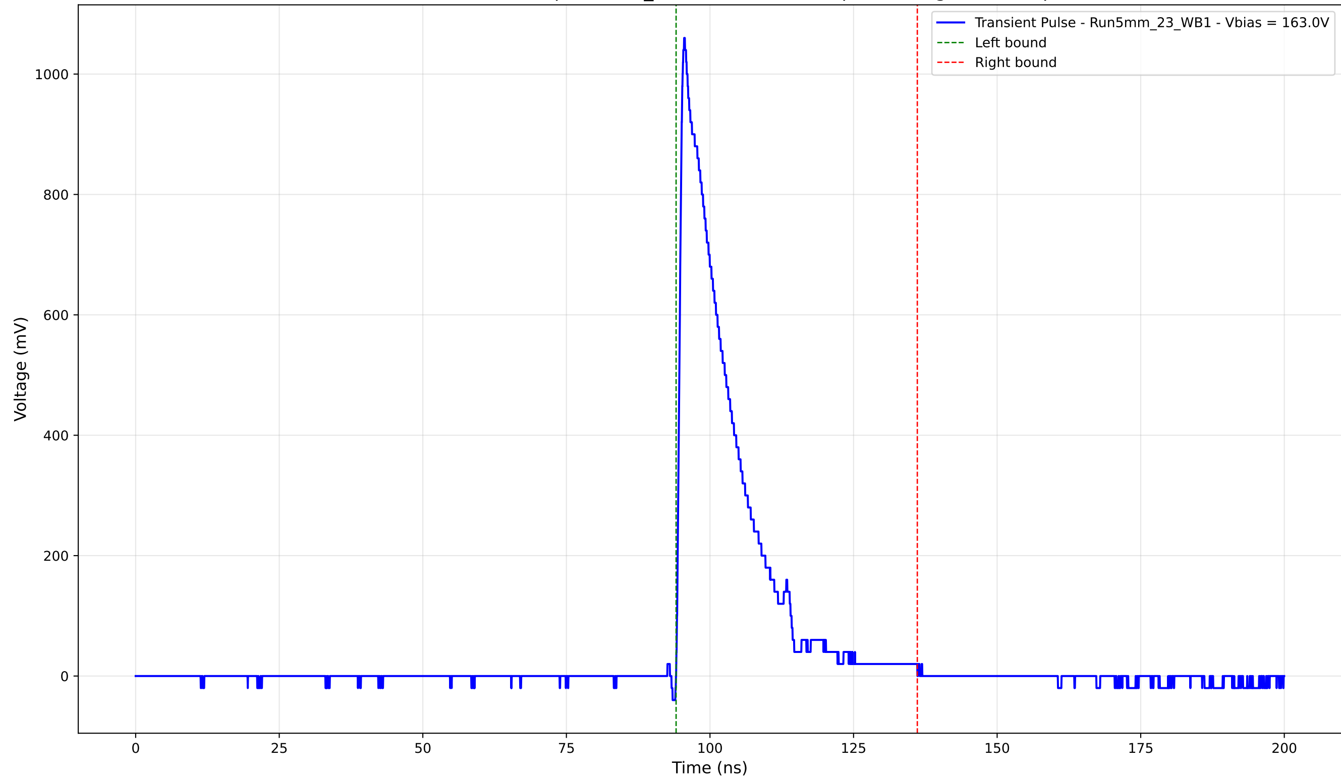
Transient Pulse - Sample: 5mm_23 - Position: 450.0 \mu\text{m} - Charge: 198.34 pC
