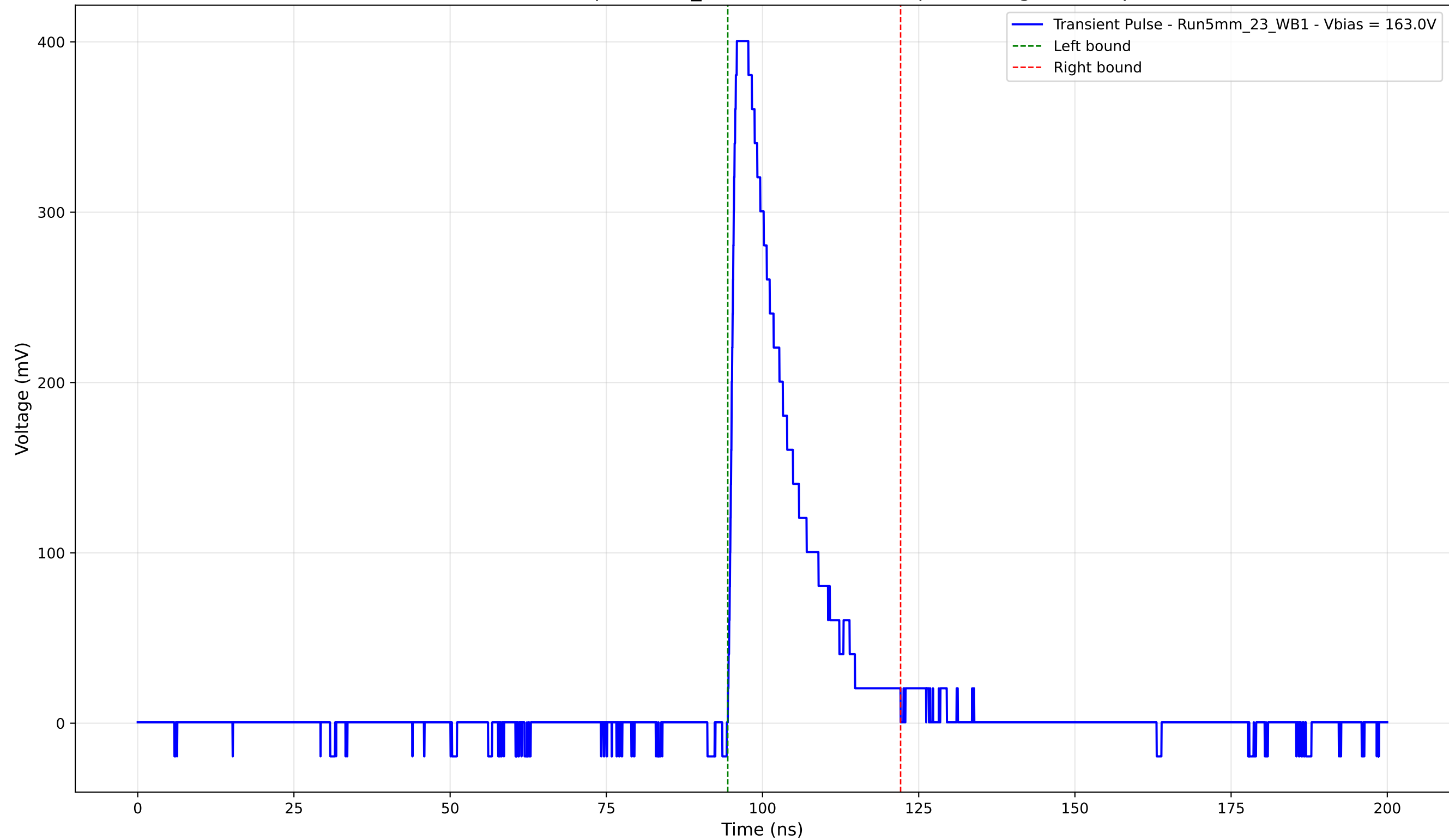
Transient Pulse - Sample: 5mm_23 - Position: 3790.0 \mu\text{m} - Charge: 77.25 pC
