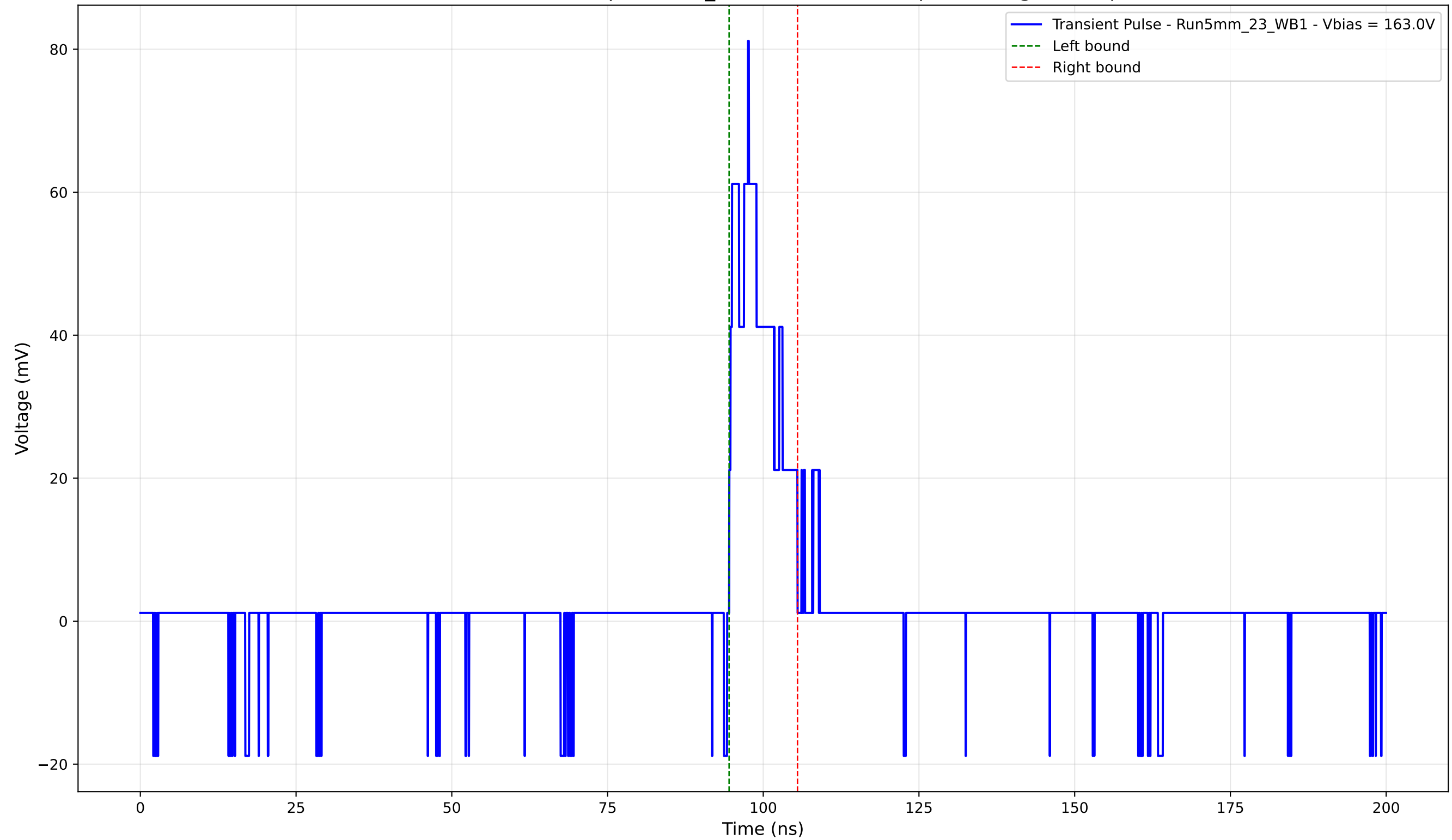
Transient Pulse - Sample: 5mm_23 - Position: 260.0 \mu\text{m} - Charge: 8.99 pC
