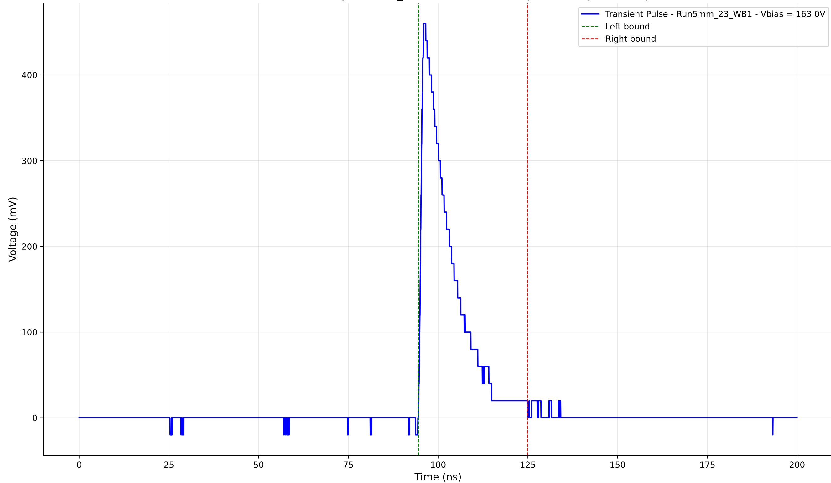
Transient Pulse - Sample: 5mm_23 - Position: 1190.0 \mu\text{m} - Charge: 82.69 pC
