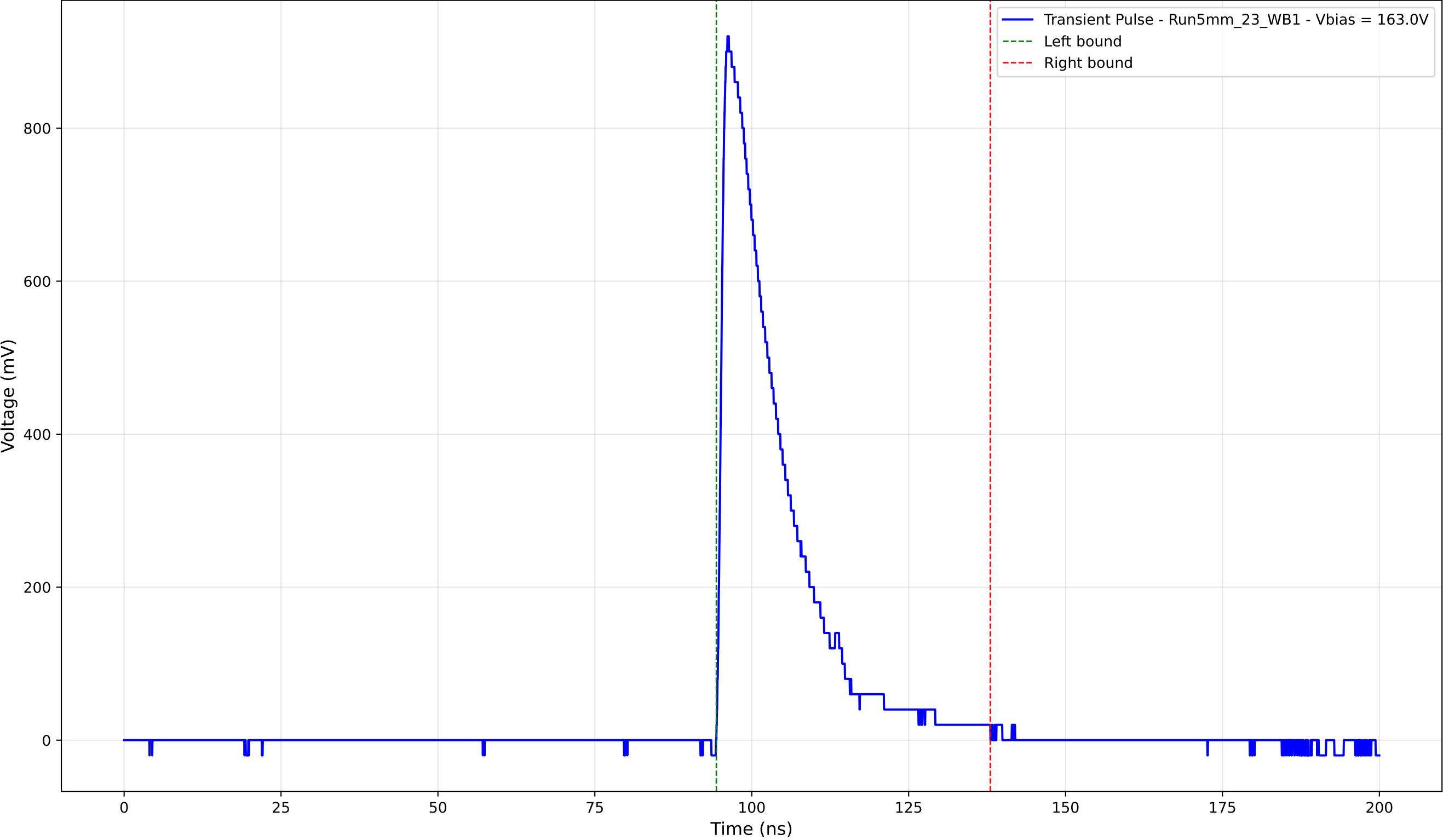
Transient Pulse - Sample: 5mm_23 - Position: 4145.0 \mu\text{m} - Charge: 191.41 pC
