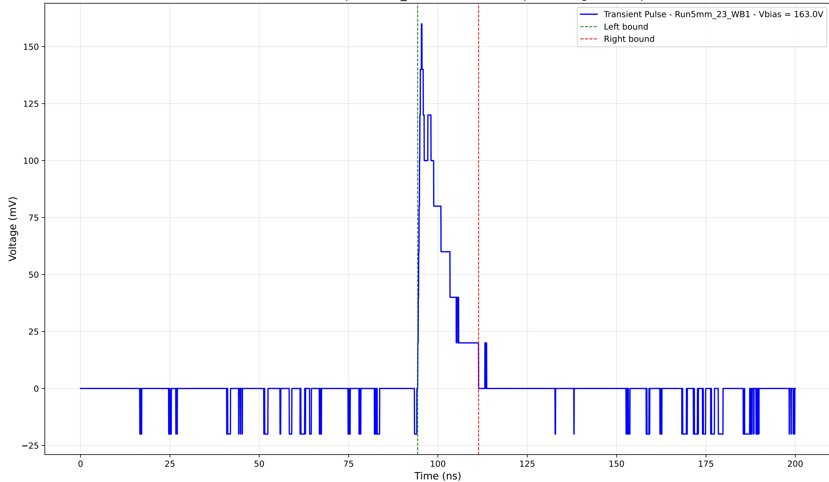
Transient Pulse - Sample: 5mm_23 - Position: 275.0 \mu\text{m} - Charge: 20.06 pC
