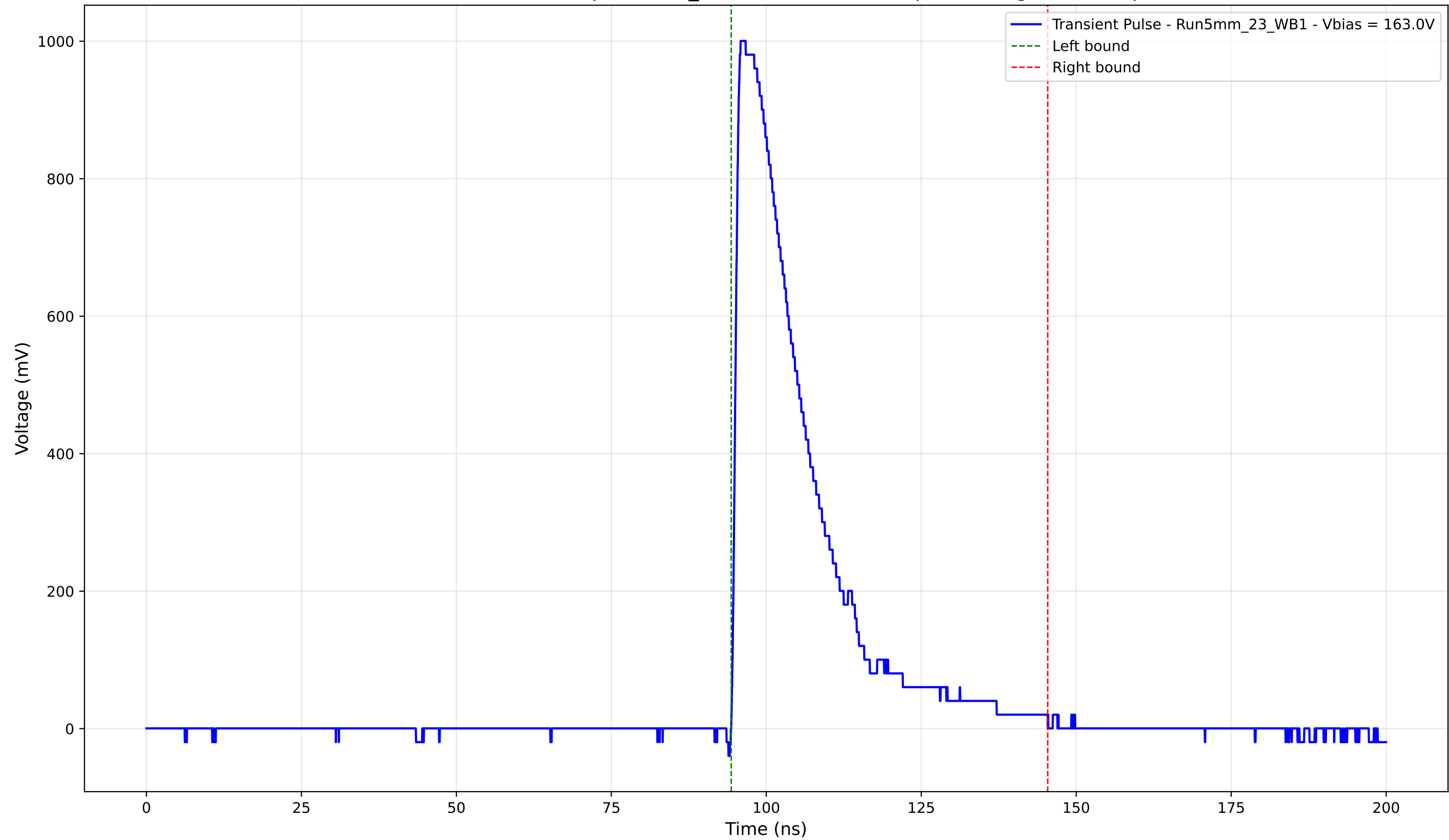
Transient Pulse - Sample: 5mm_23 - Position: 1590.0 \mu\text{m} - Charge: 253.10 pC
