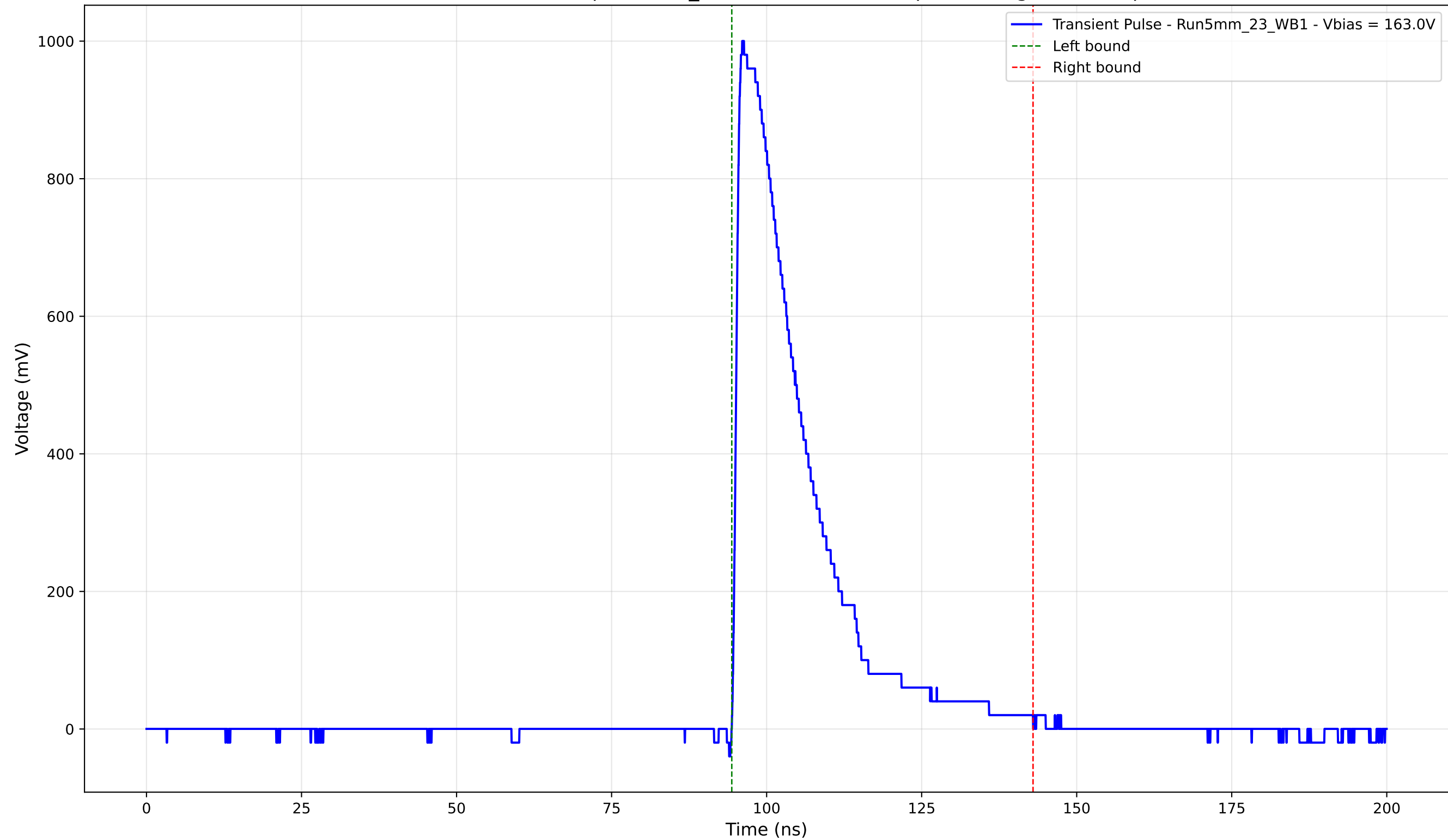
Transient Pulse - Sample: 5mm_23 - Position: 1455.0 \mu\text{m} - Charge: 241.11 pC
