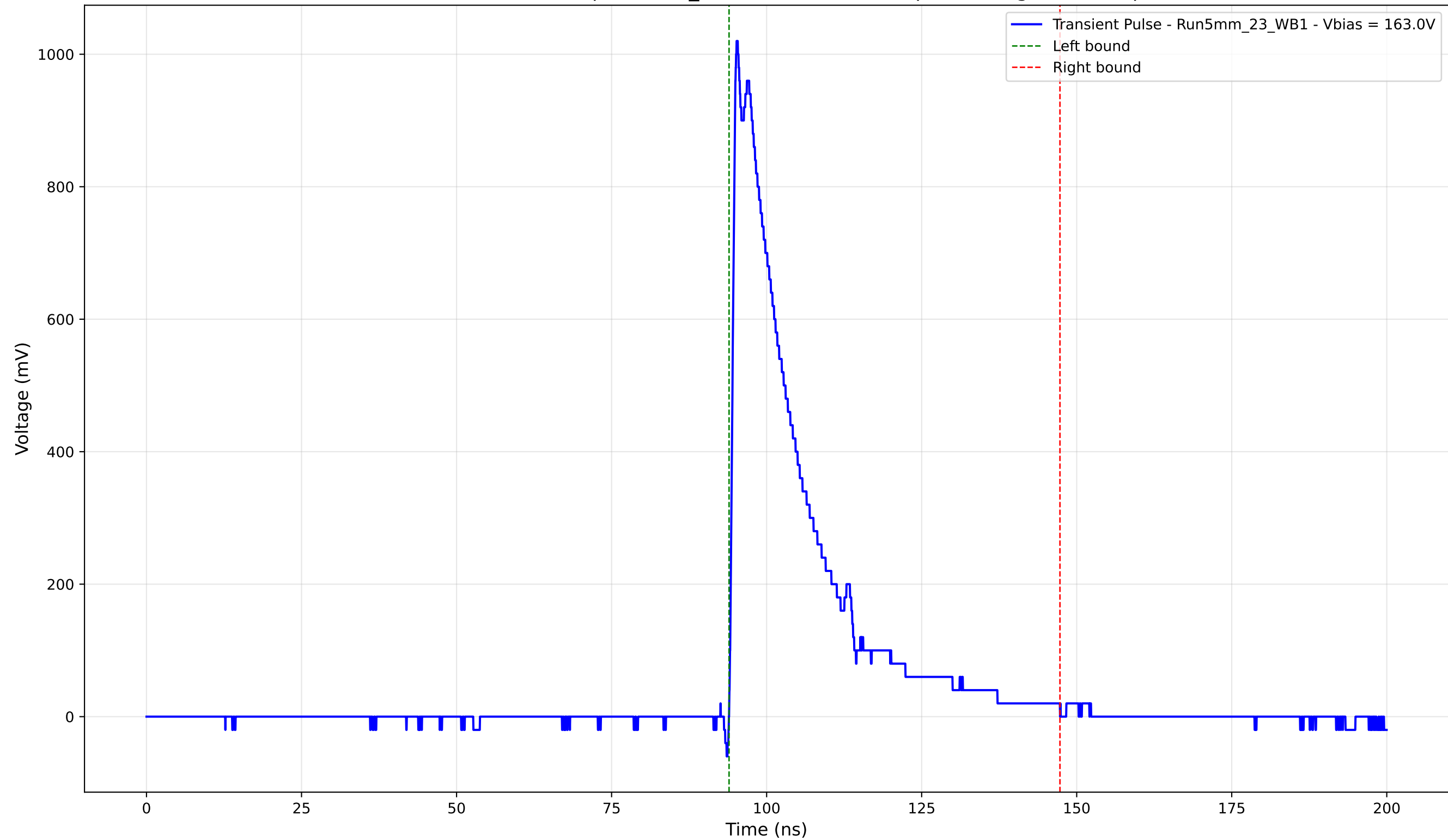
Transient Pulse - Sample: 5mm_23 - Position: 2460.0 \mu\text{m} - Charge: 229.72 pC
