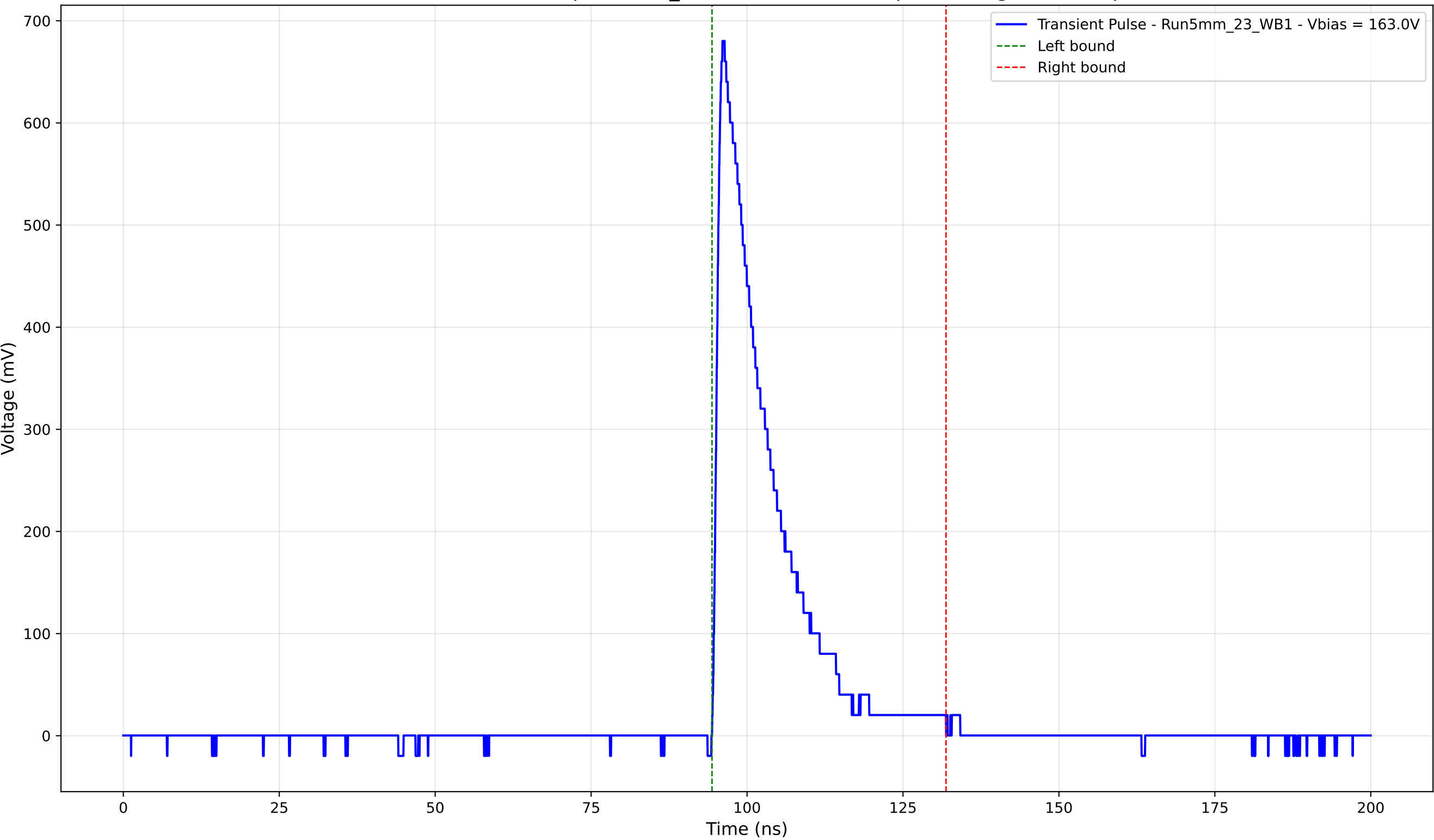
Transient Pulse - Sample: 5mm_23 - Position: 4320.0 \mu\text{m} - Charge: 122.59 pC
