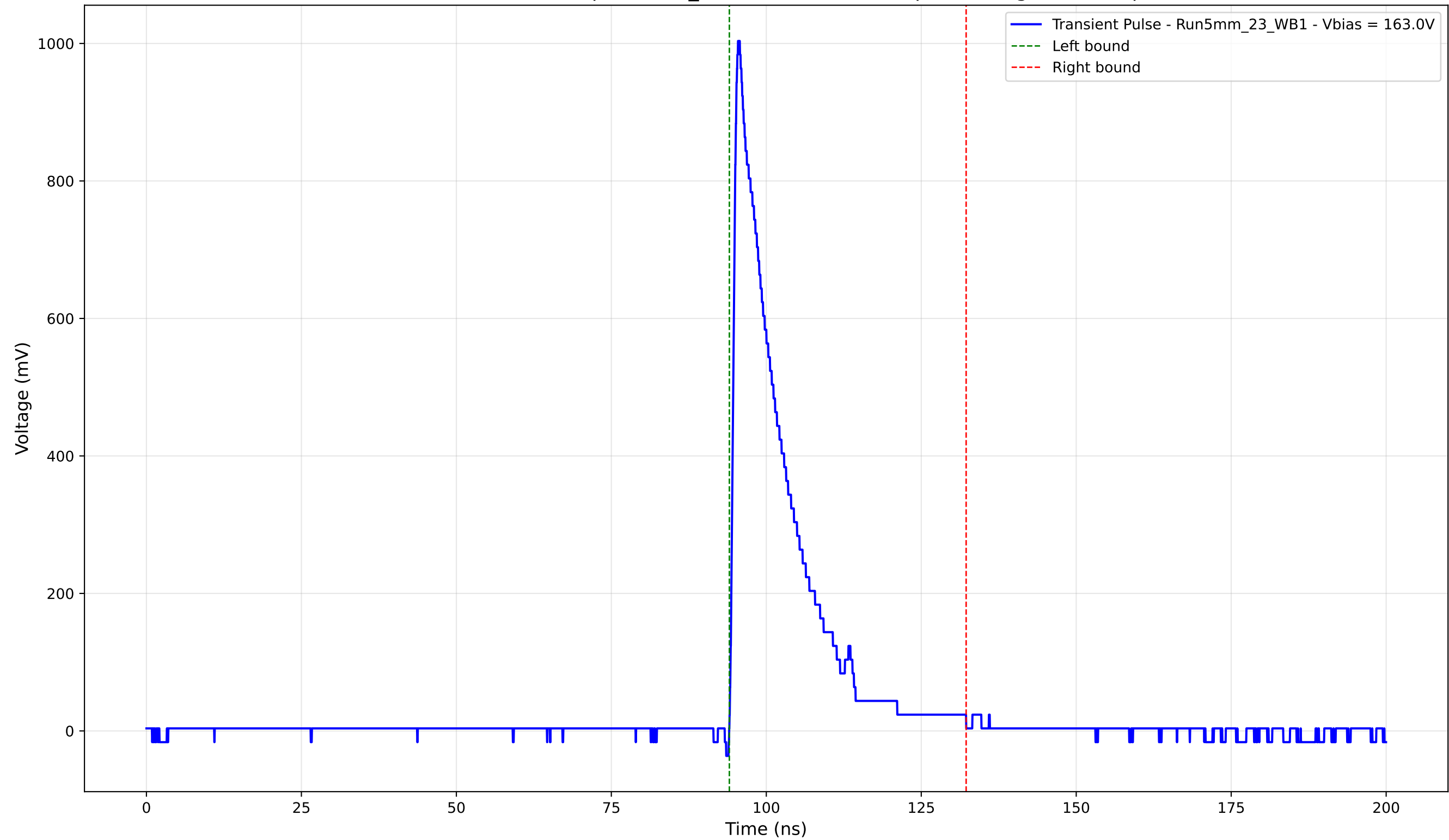
Transient Pulse - Sample: 5mm_23 - Position: 4975.0 \mu\text{m} - Charge: 168.91 pC
