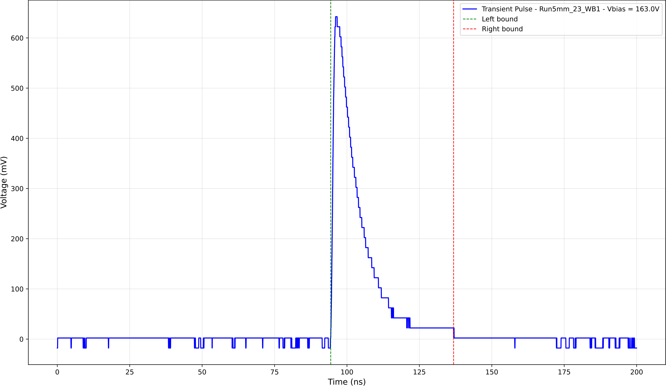
Transient Pulse - Sample: 5mm_23 - Position: 3810.0 \mu\text{m} - Charge: 129.78 pC
