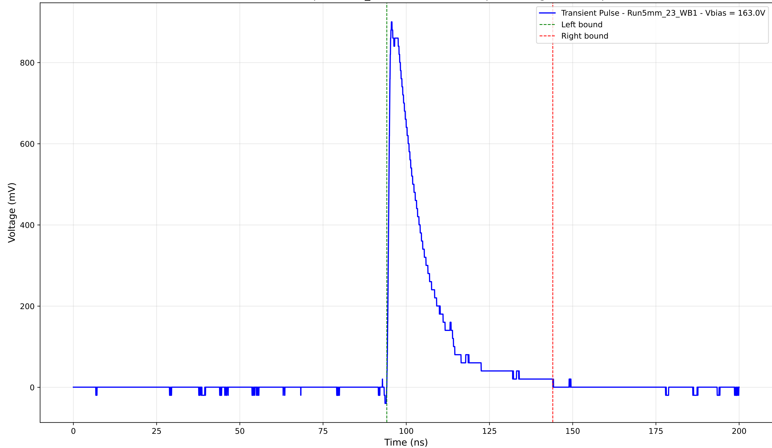
Transient Pulse - Sample: 5mm_23 - Position: 3345.0 \mu\text{m} - Charge: 197.25 pC
