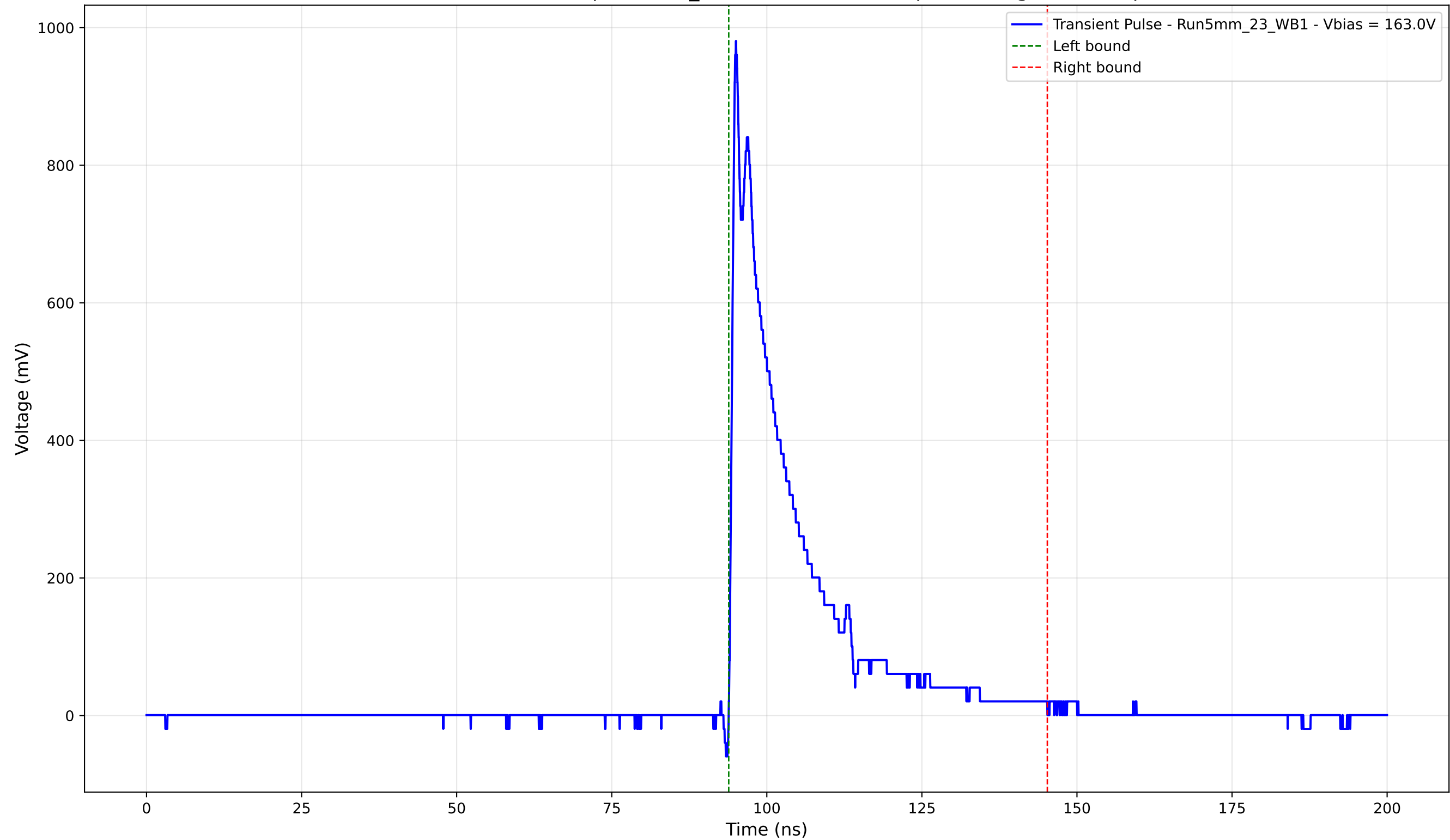
Transient Pulse - Sample: 5mm_23 - Position: 2810.0 \mu\text{m} - Charge: 180.00 pC
