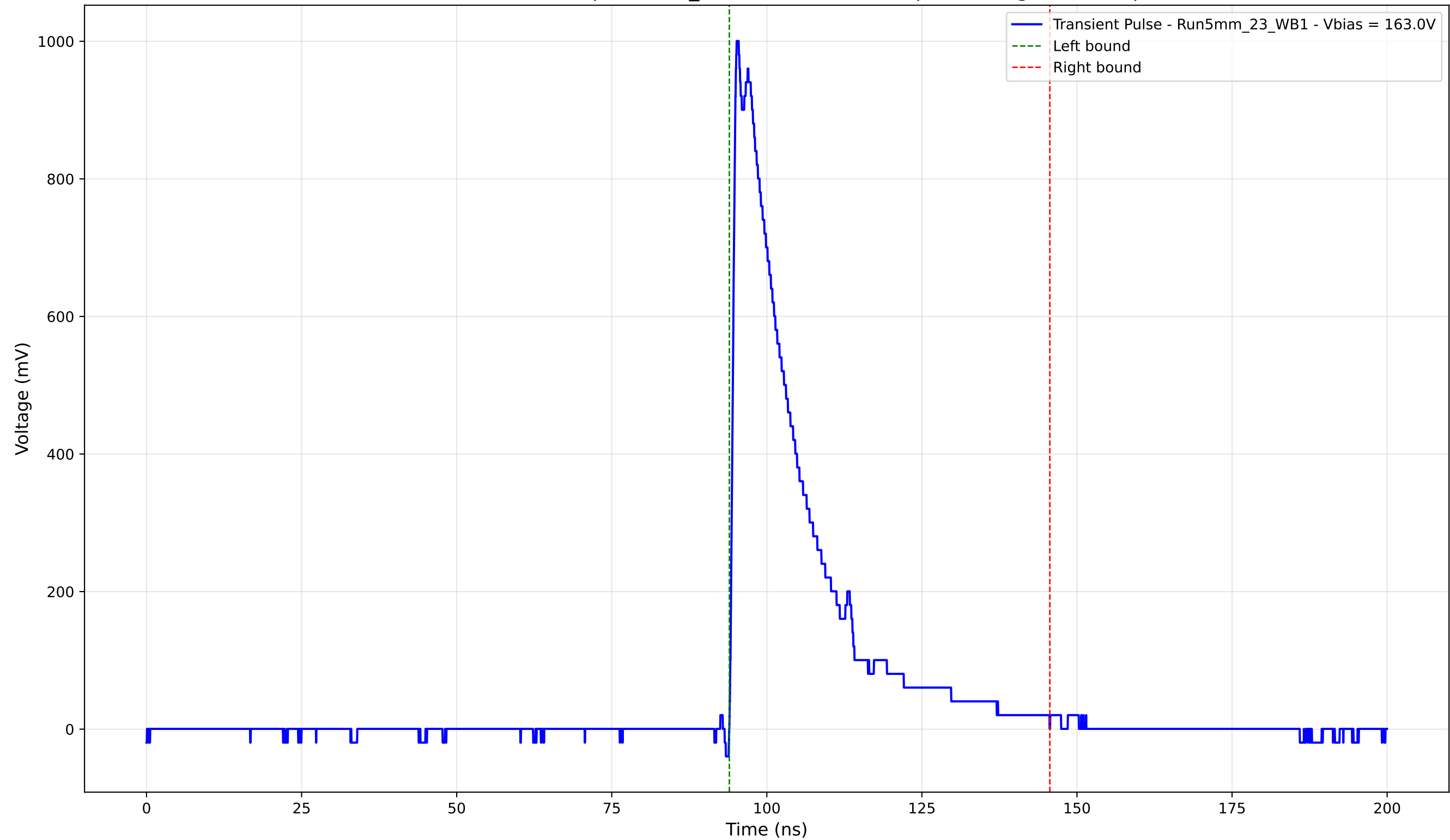
Transient Pulse - Sample: 5mm_23 - Position: 3055.0 \mu\text{m} - Charge: 227.12 pC
