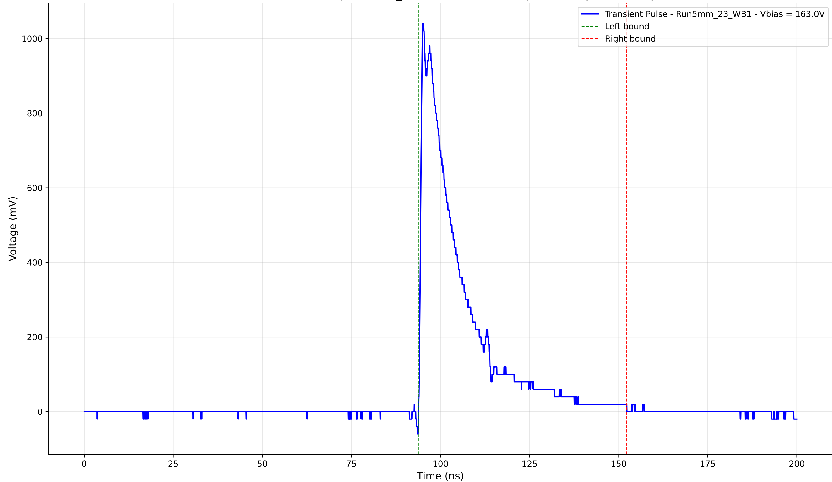
Transient Pulse - Sample: 5mm_23 - Position: 2555.0 \mu\text{m} - Charge: 238.84 pC
