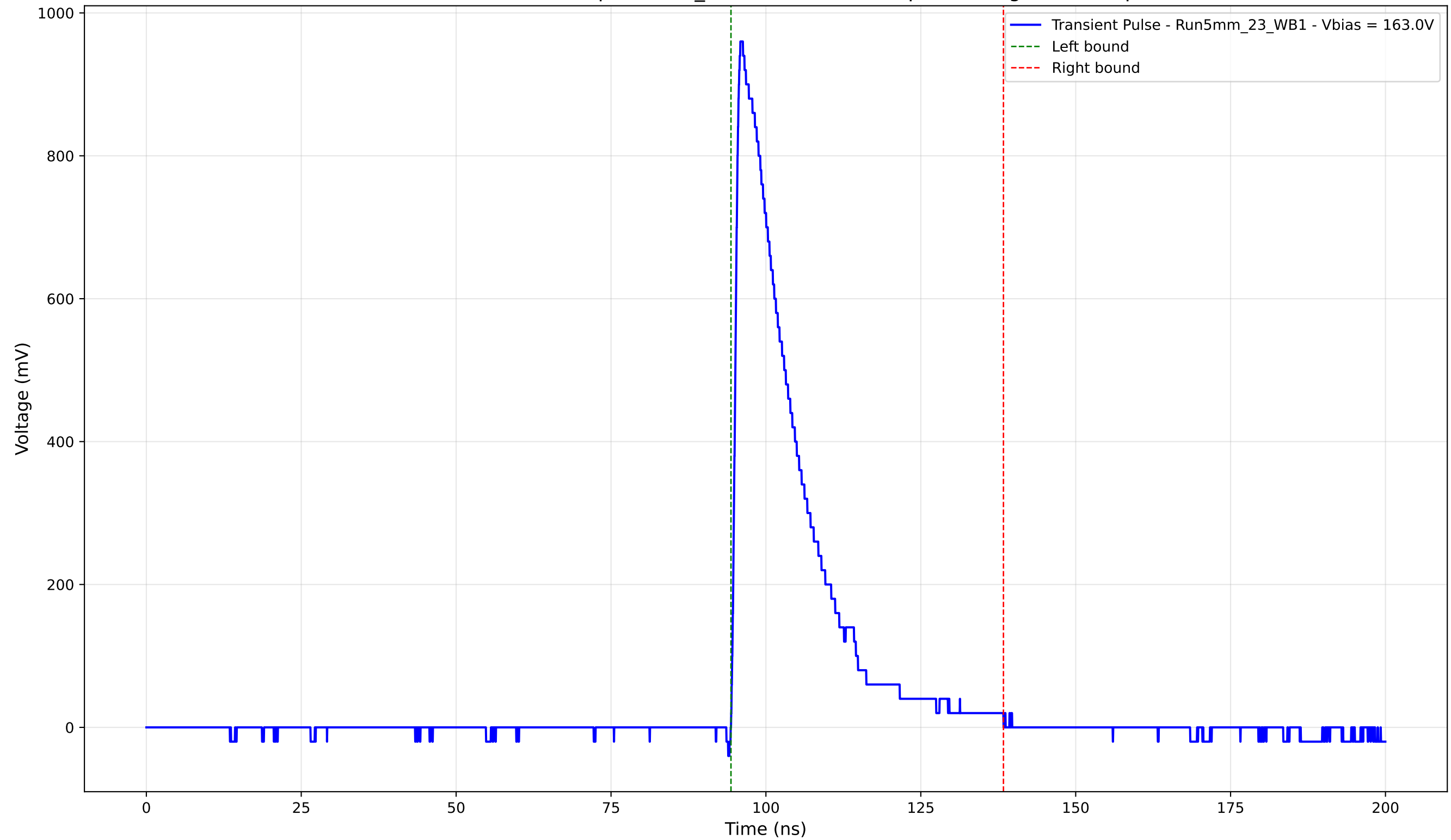
Transient Pulse - Sample: 5mm_23 - Position: 990.0 \mu\text{m} - Charge: 201.24 pC
