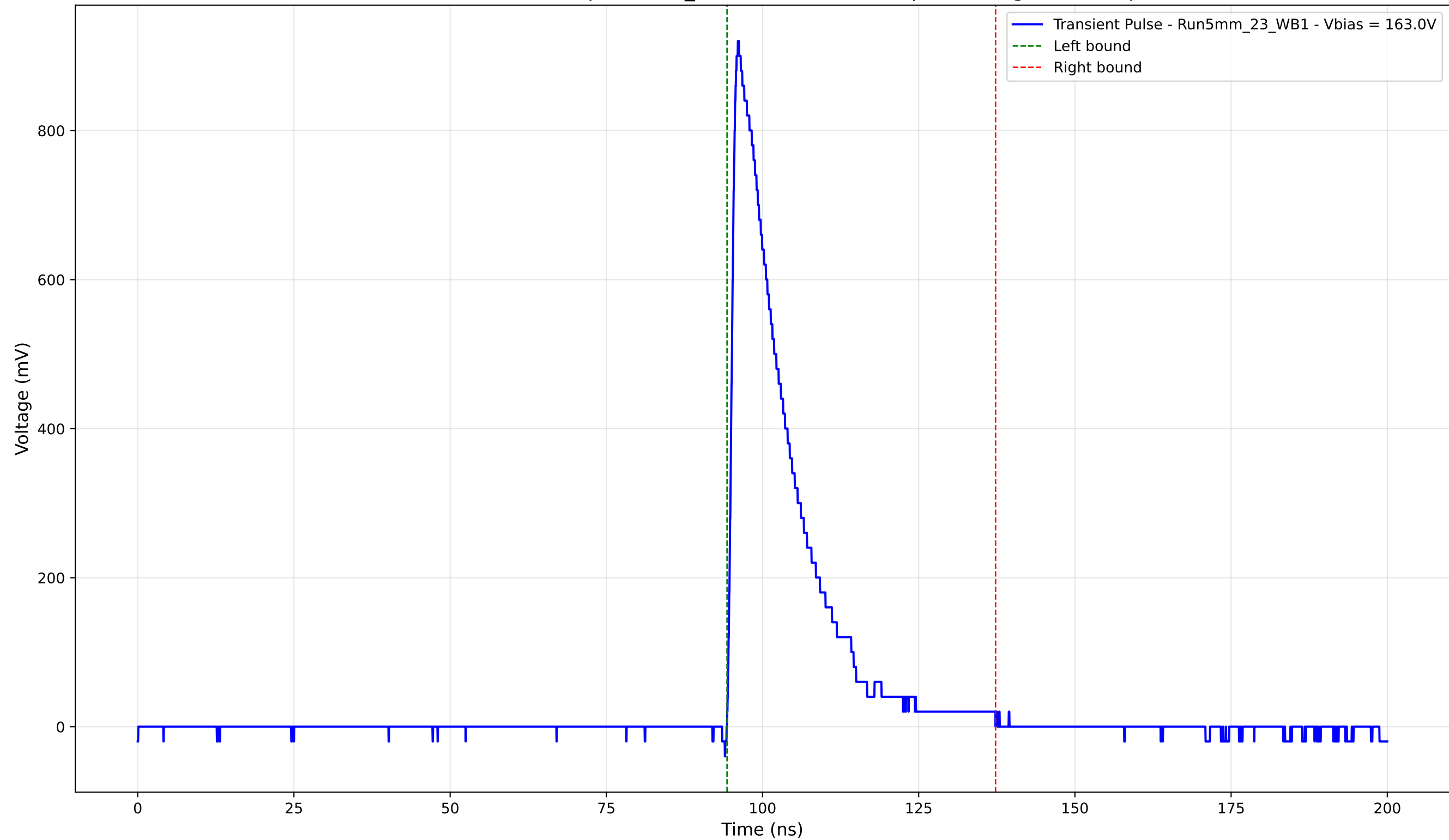
Transient Pulse - Sample: 5mm_23 - Position: 4405.0 \mu\text{m} - Charge: 179.82 pC
