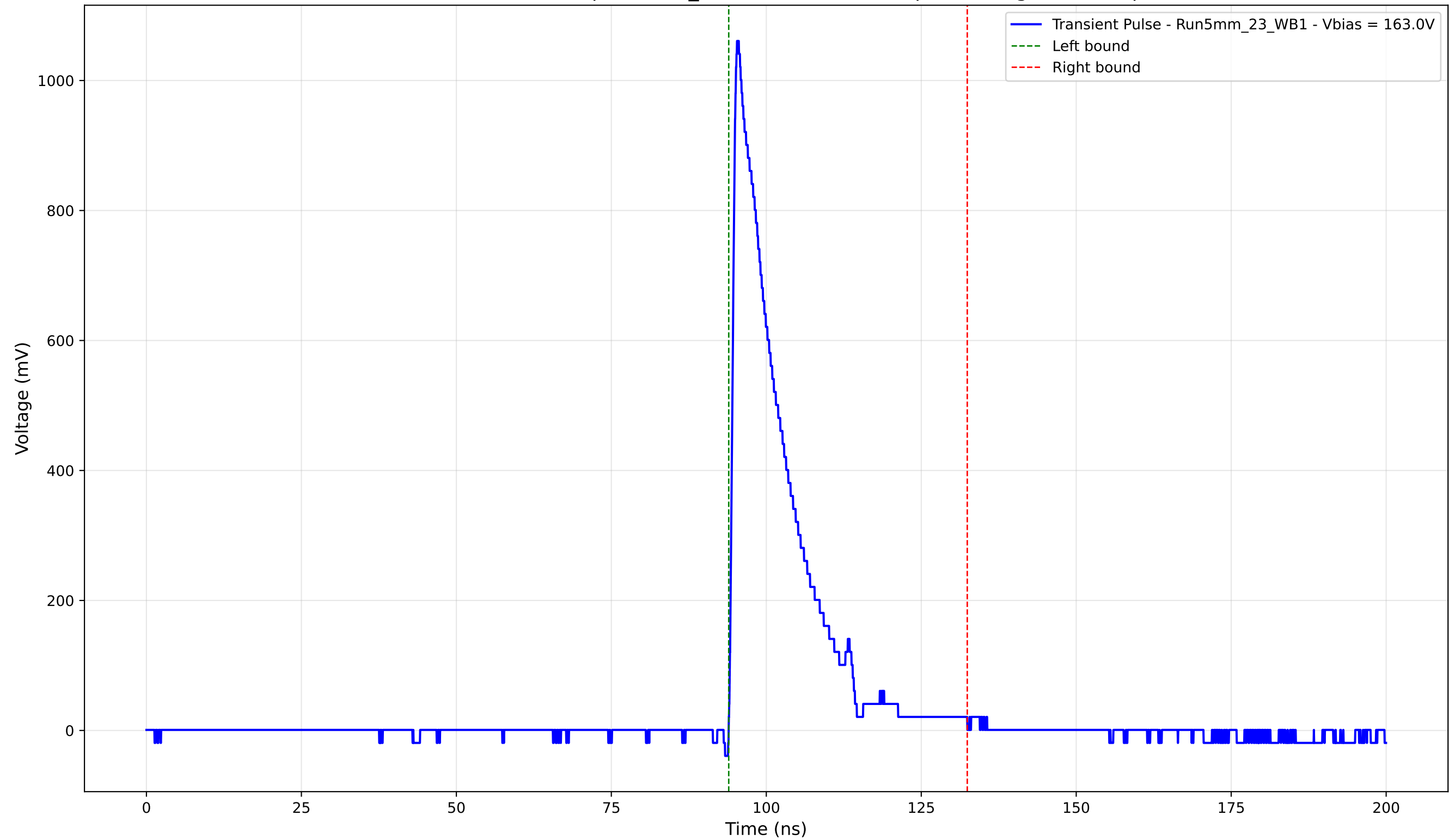
Transient Pulse - Sample: 5mm_23 - Position: 5100.0 \mu\text{m} - Charge: 183.29 pC
