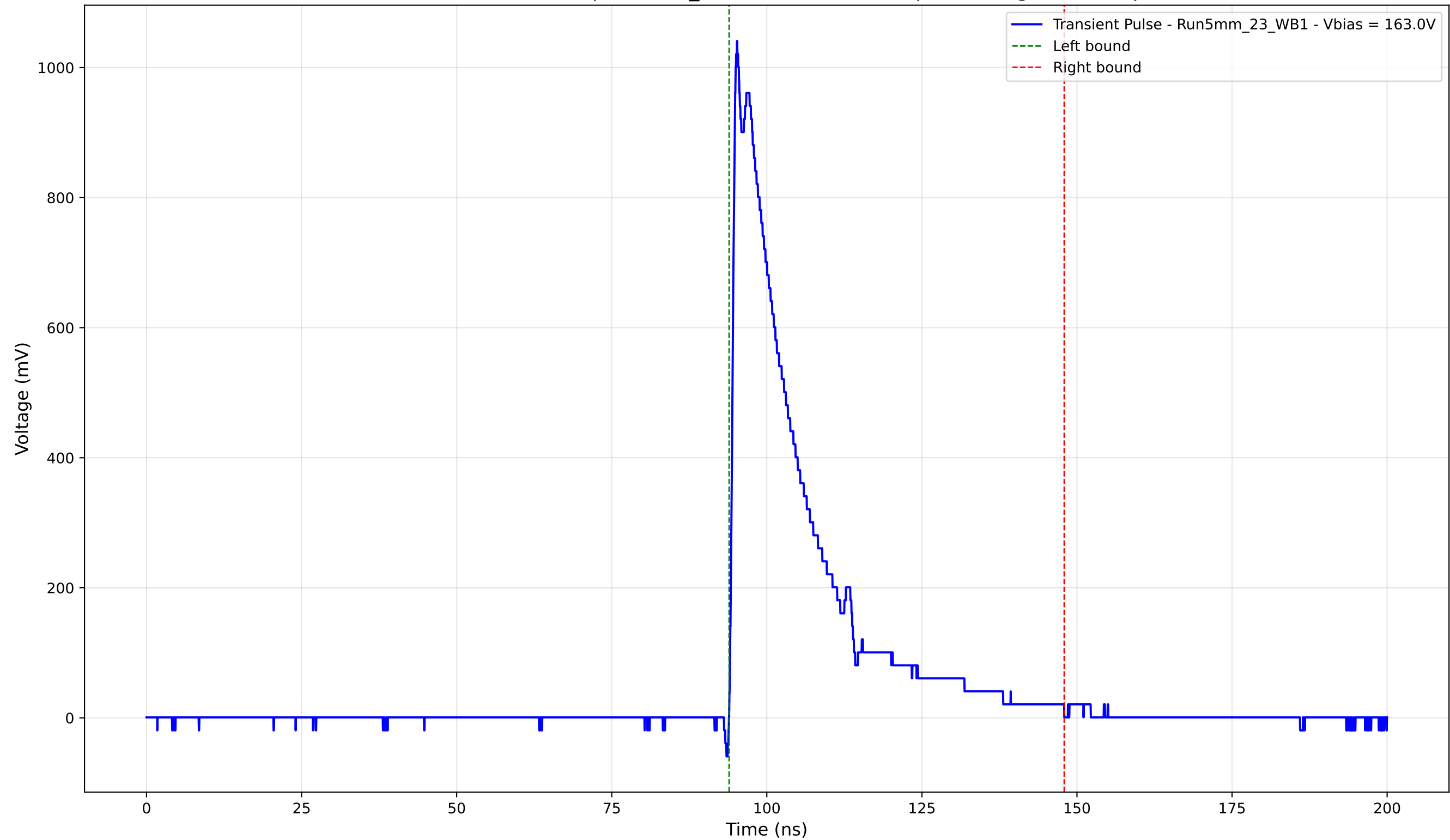
Transient Pulse - Sample: 5mm_23 - Position: 2970.0 \mu\text{m} - Charge: 233.34 pC
