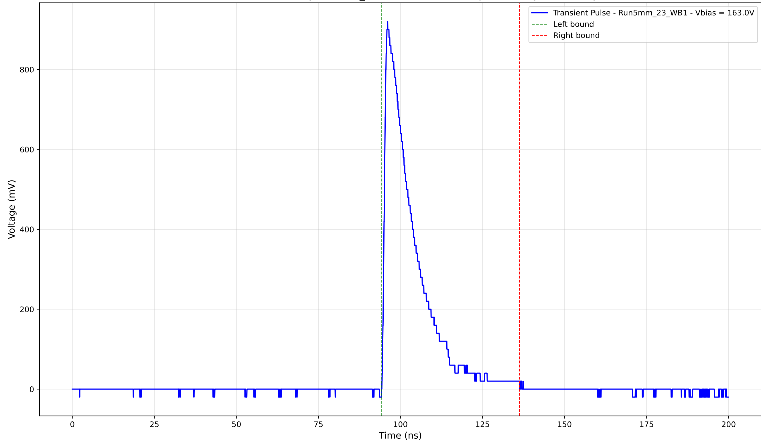
Transient Pulse - Sample: 5mm_23 - Position: 4390.0 \mu\text{m} - Charge: 179.84 pC
