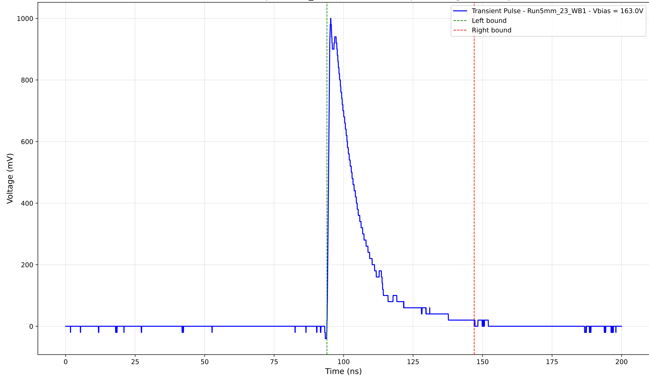
Transient Pulse - Sample: 5mm_23 - Position: 2350.0 \mu\text{m} - Charge: 224.66 pC
