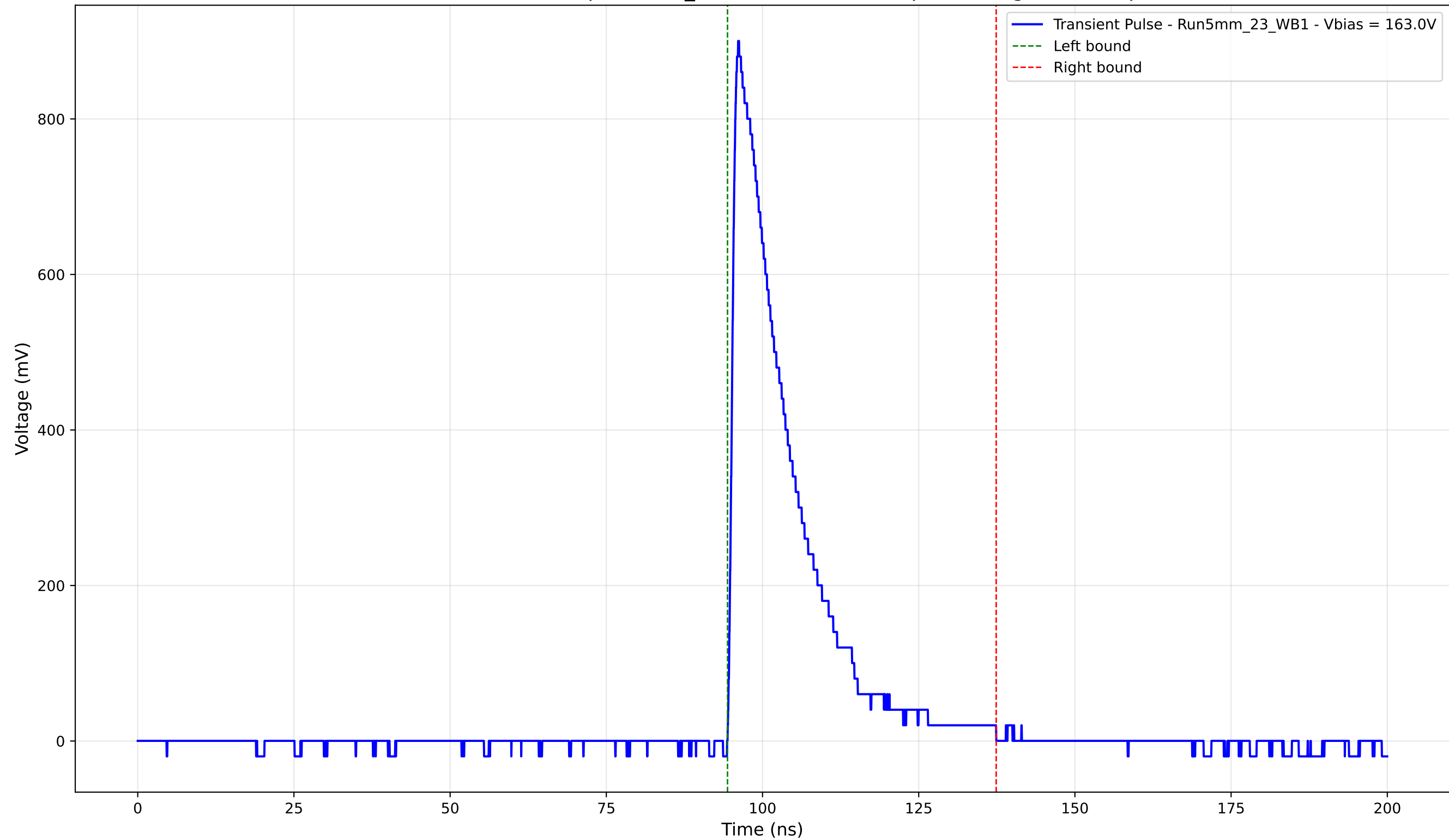
Transient Pulse - Sample: 5mm_23 - Position: 1145.0 \mu\text{m} - Charge: 179.75 pC
