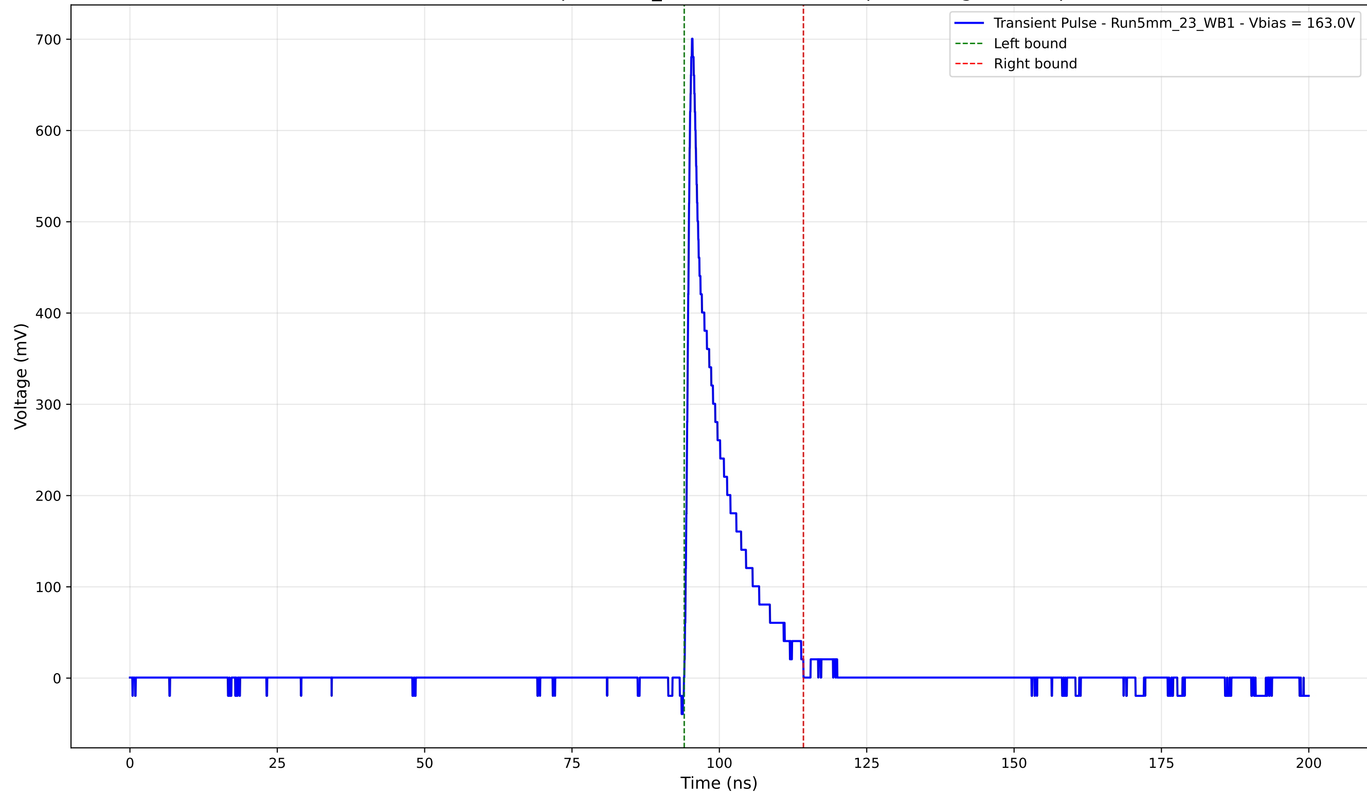
Transient Pulse - Sample: 5mm_23 - Position: 5160.0 \mu\text{m} - Charge: 78.14 pC
