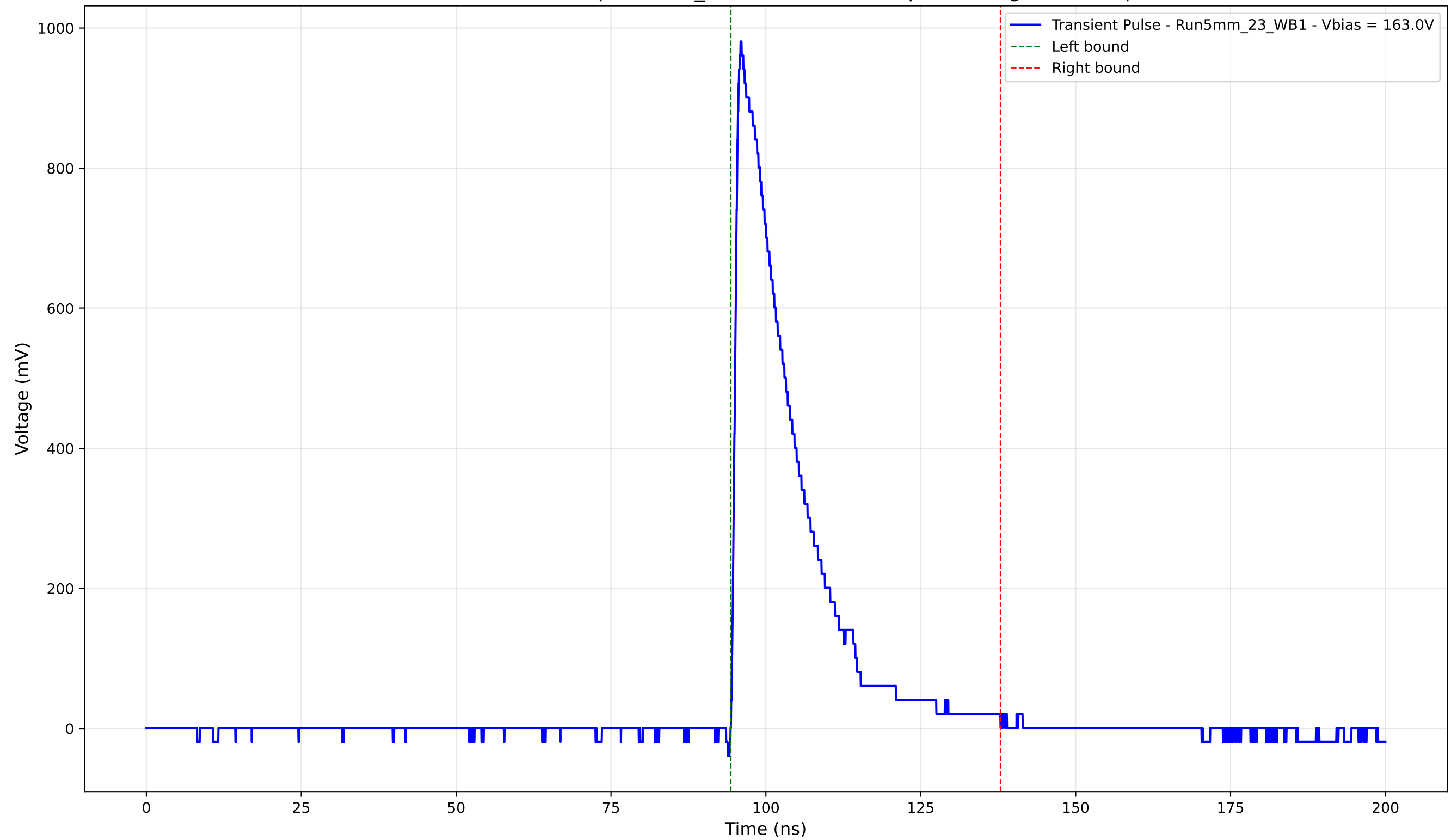
Transient Pulse - Sample: 5mm_23 - Position: 925.0 \mu\text{m} - Charge: 201.52 pC
