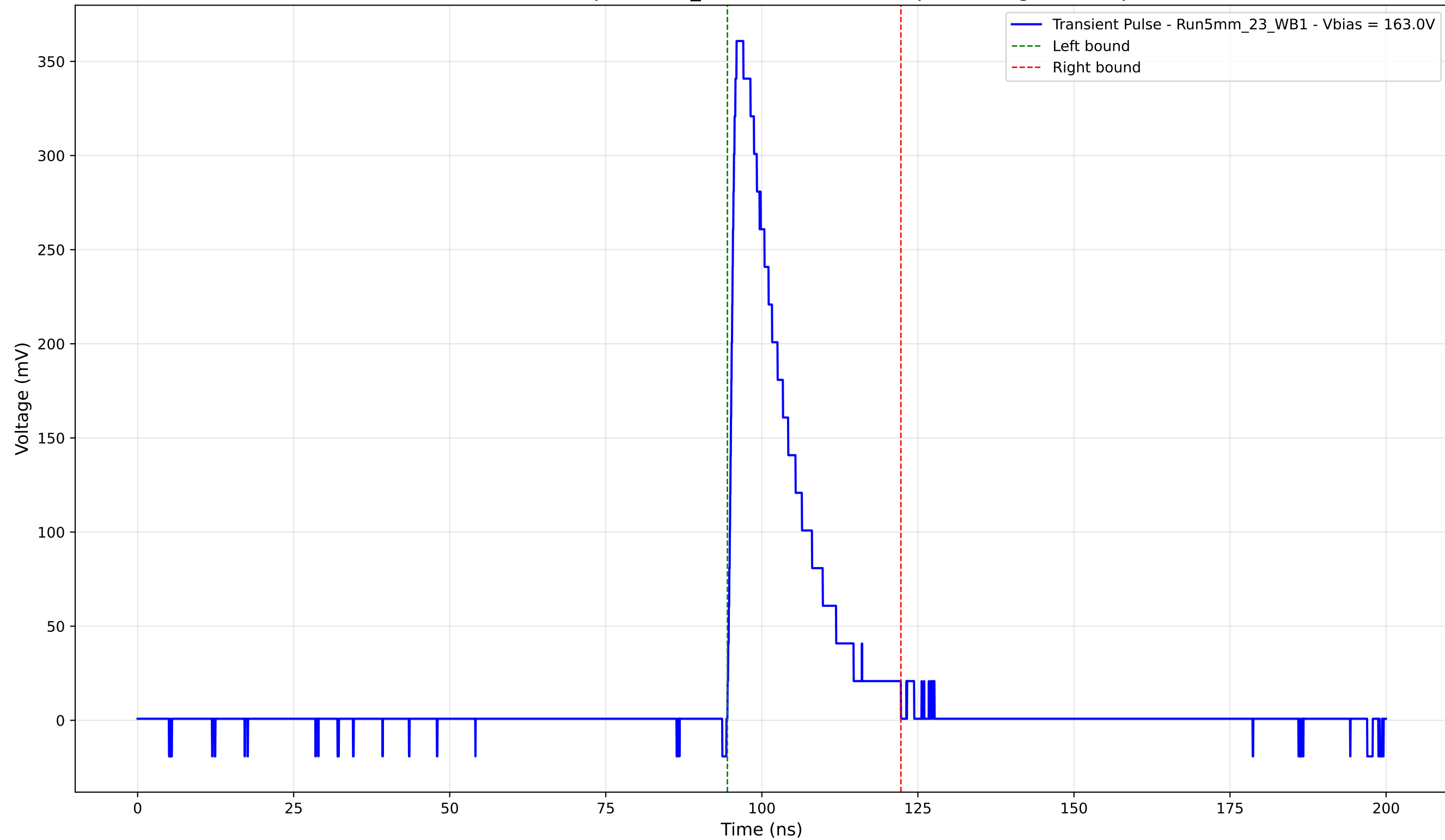
Transient Pulse - Sample: 5mm_23 - Position: 1700.0 \mu\text{m} - Charge: 69.23 pC
