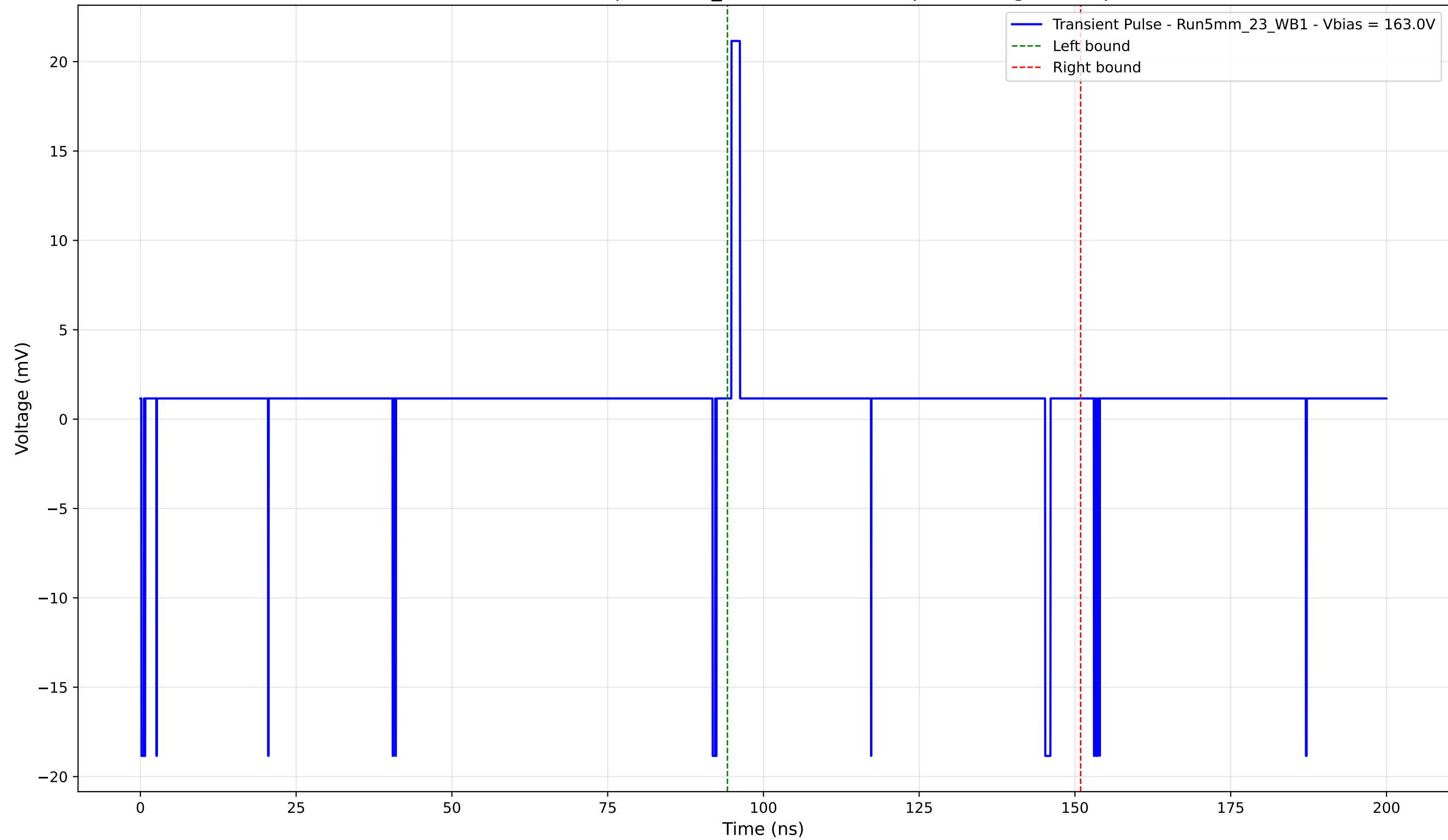
Transient Pulse - Sample: 5mm_23 - Position: 90.0 \mu\text{m} - Charge: 1.50 pC
