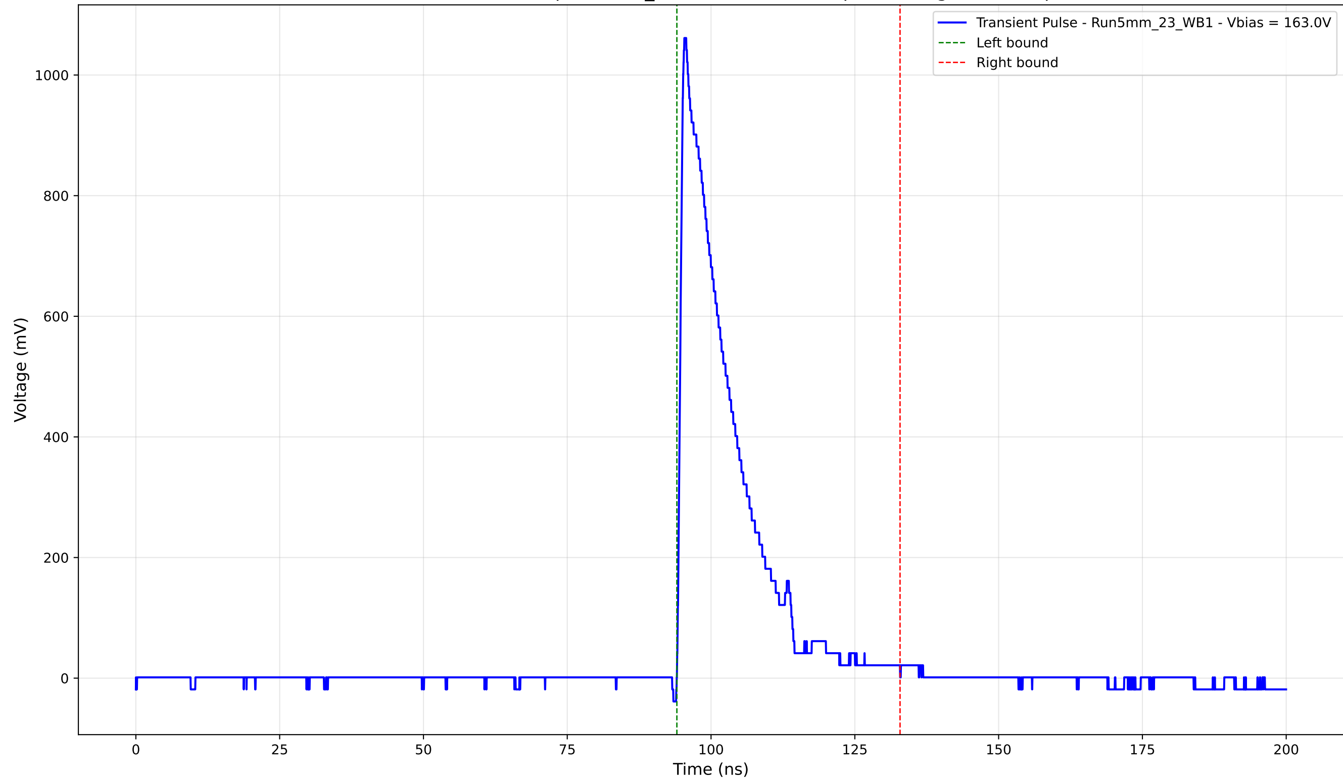
Transient Pulse - Sample: 5mm_23 - Position: 395.0 \mu\text{m} - Charge: 198.63 pC
