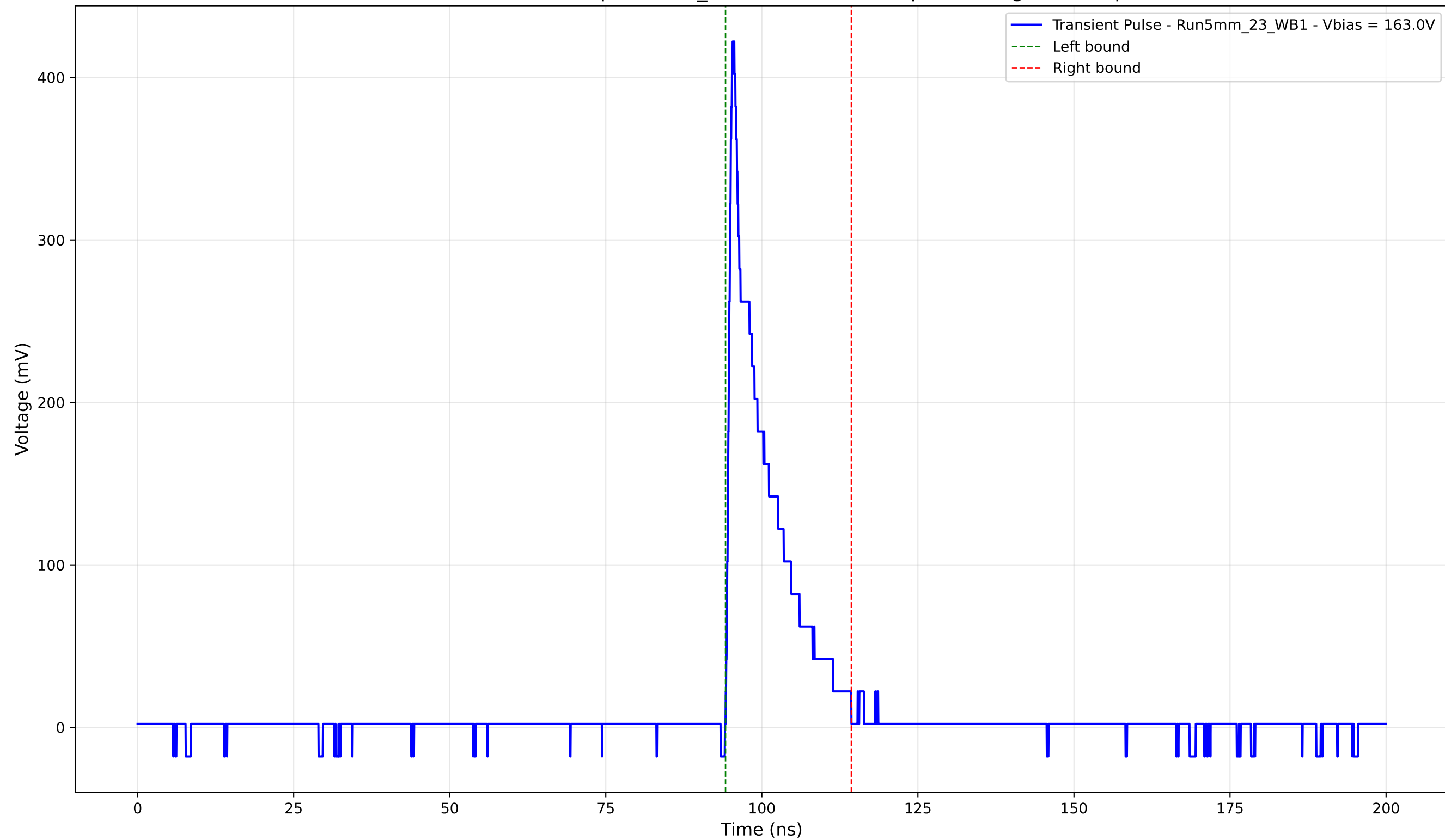
Transient Pulse - Sample: 5mm_23 - Position: 295.0 \mu\text{m} - Charge: 51.26 pC
