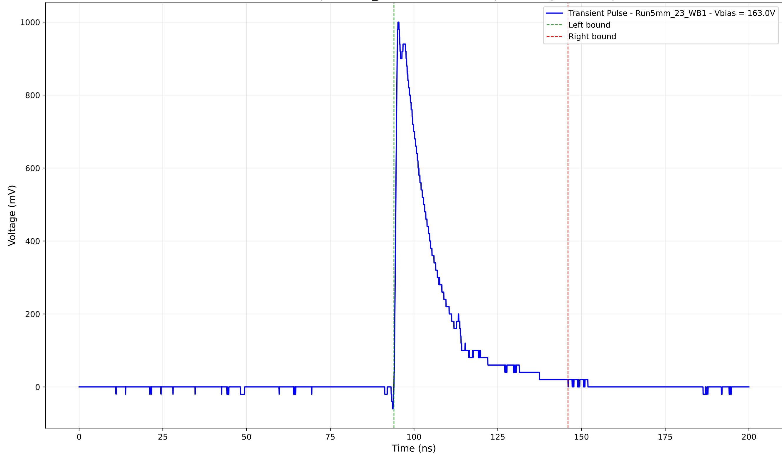
Transient Pulse - Sample: 5mm_23 - Position: 2385.0 \mu\text{m} - Charge: 227.40 pC
