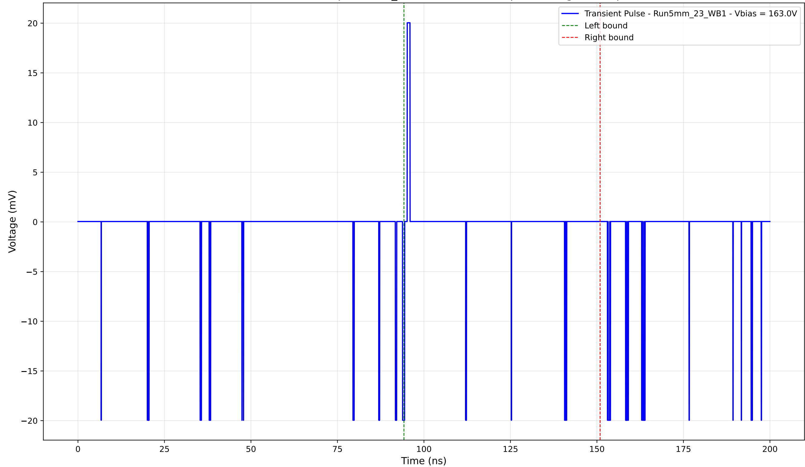
Transient Pulse - Sample: 5mm_23 - Position: 205.0 \mu\text{m} - Charge: 0.10 pC
