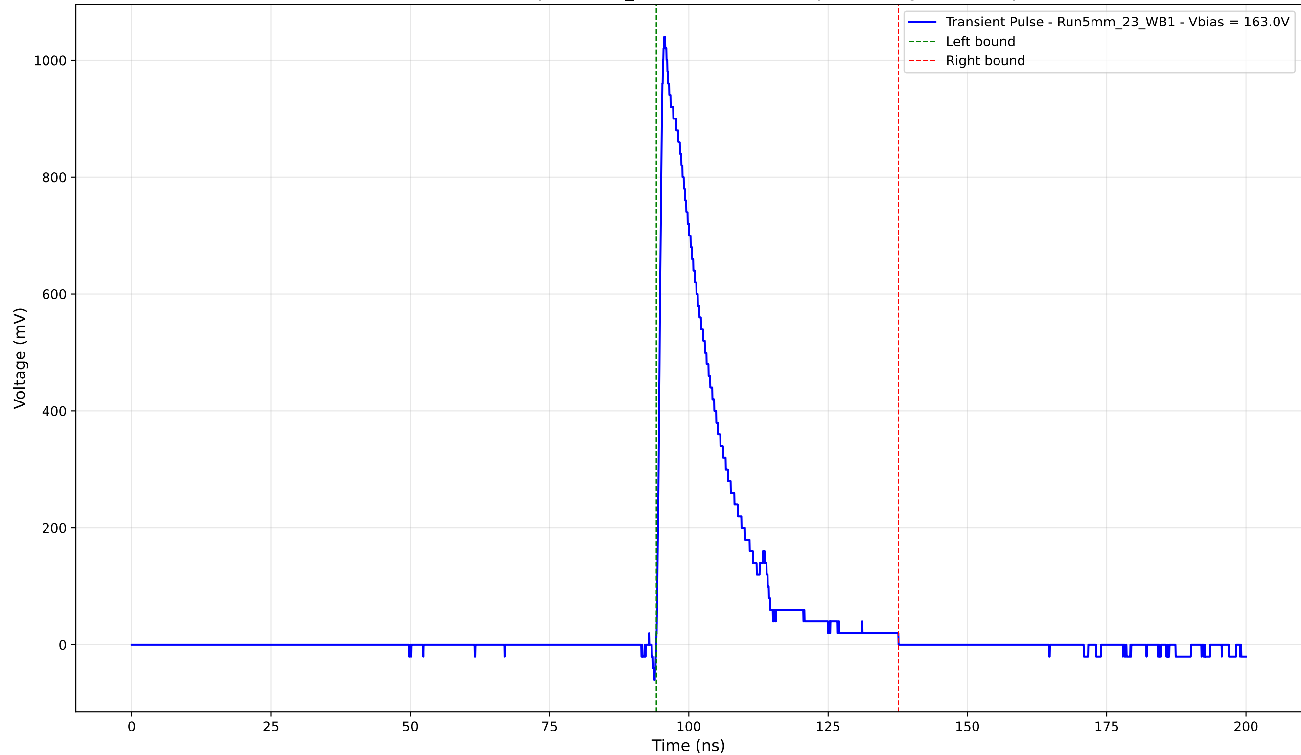
Transient Pulse - Sample: 5mm_23 - Position: 575.0 \mu\text{m} - Charge: 205.19 pC
