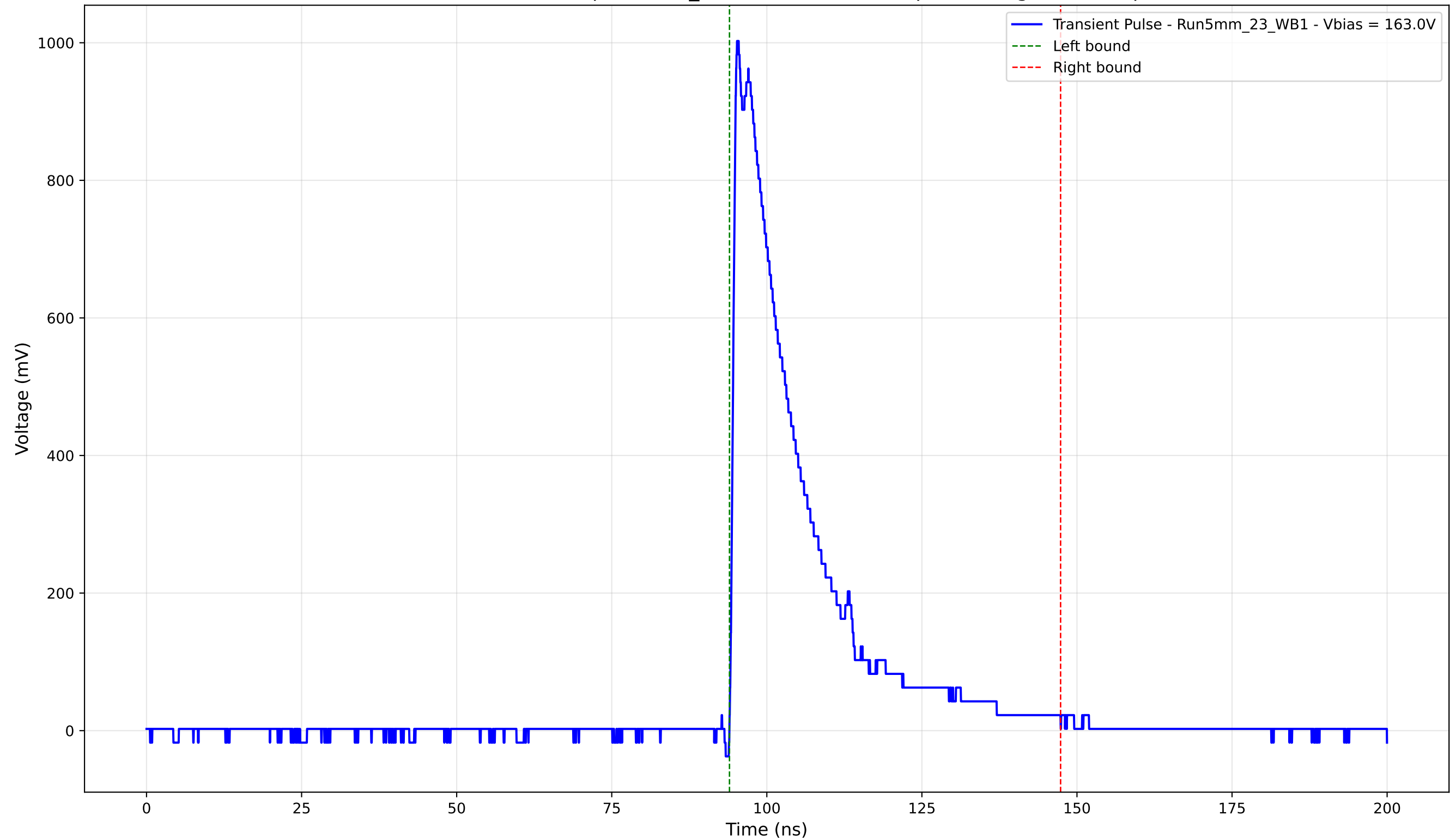
Transient Pulse - Sample: 5mm_23 - Position: 2390.0 \mu\text{m} - Charge: 230.63 pC
