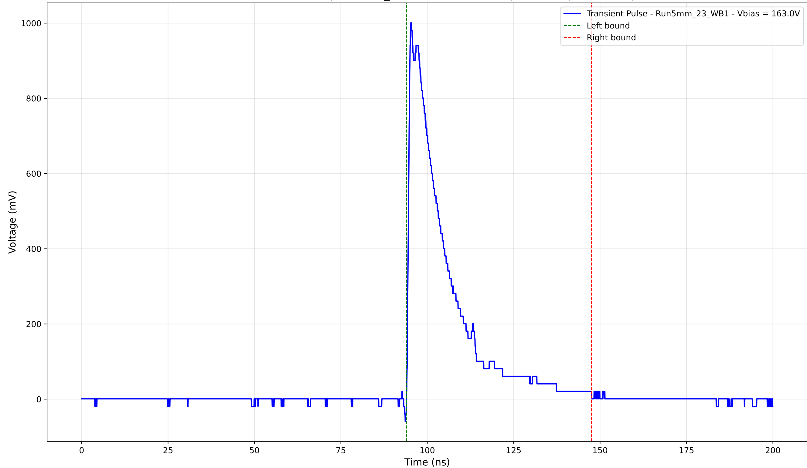
Transient Pulse - Sample: 5mm_23 - Position: 2370.0 \mu\text{m} - Charge: 228.47 pC
