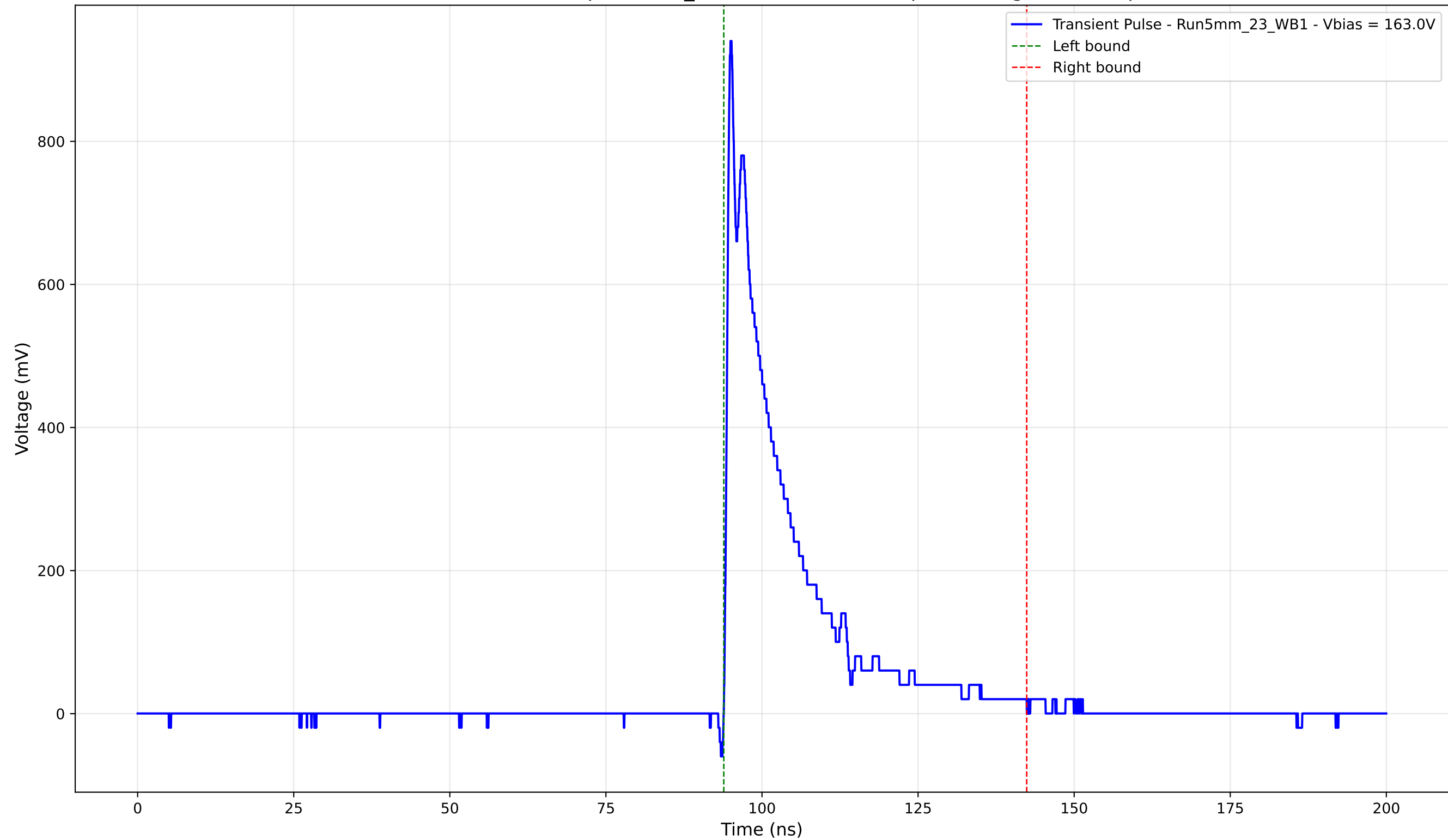
Transient Pulse - Sample: 5mm_23 - Position: 2805.0 \mu\text{m} - Charge: 165.51 pC
