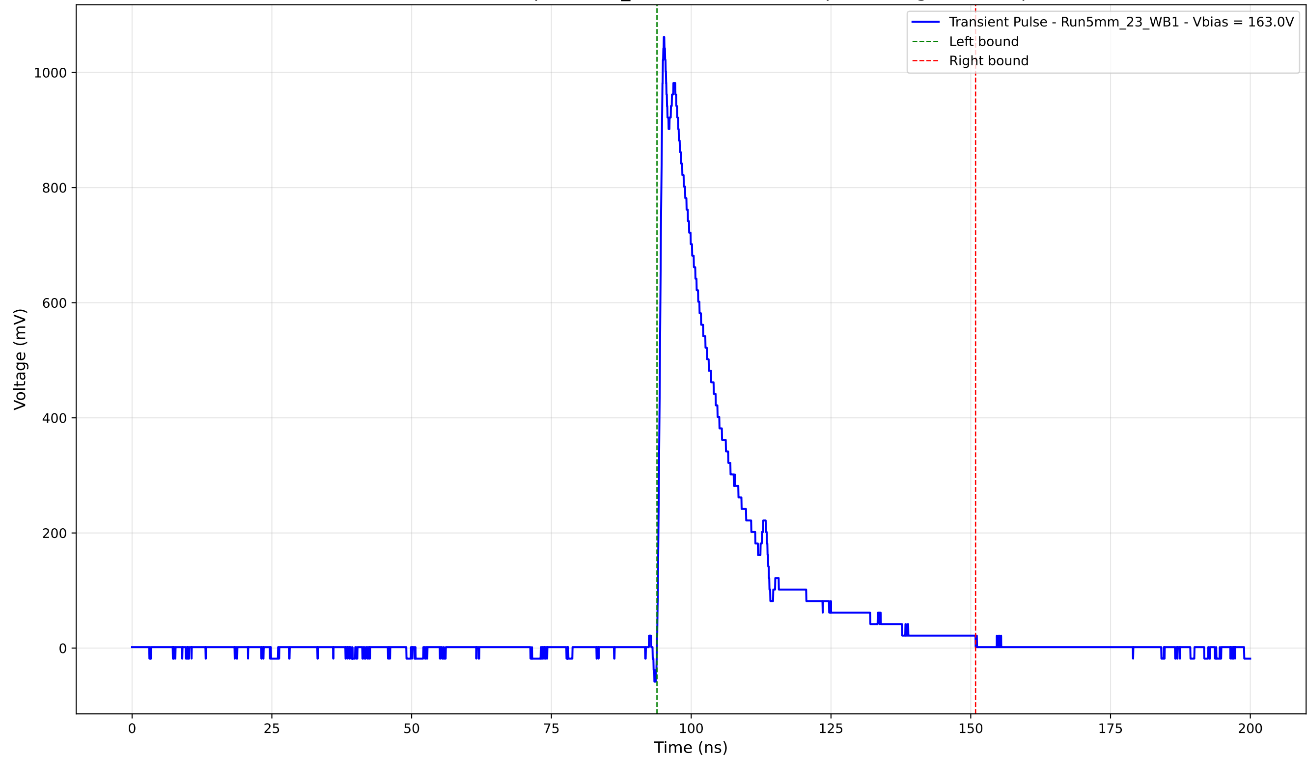
Transient Pulse - Sample: 5mm_23 - Position: 2915.0 \mu\text{m} - Charge: 239.94 pC
