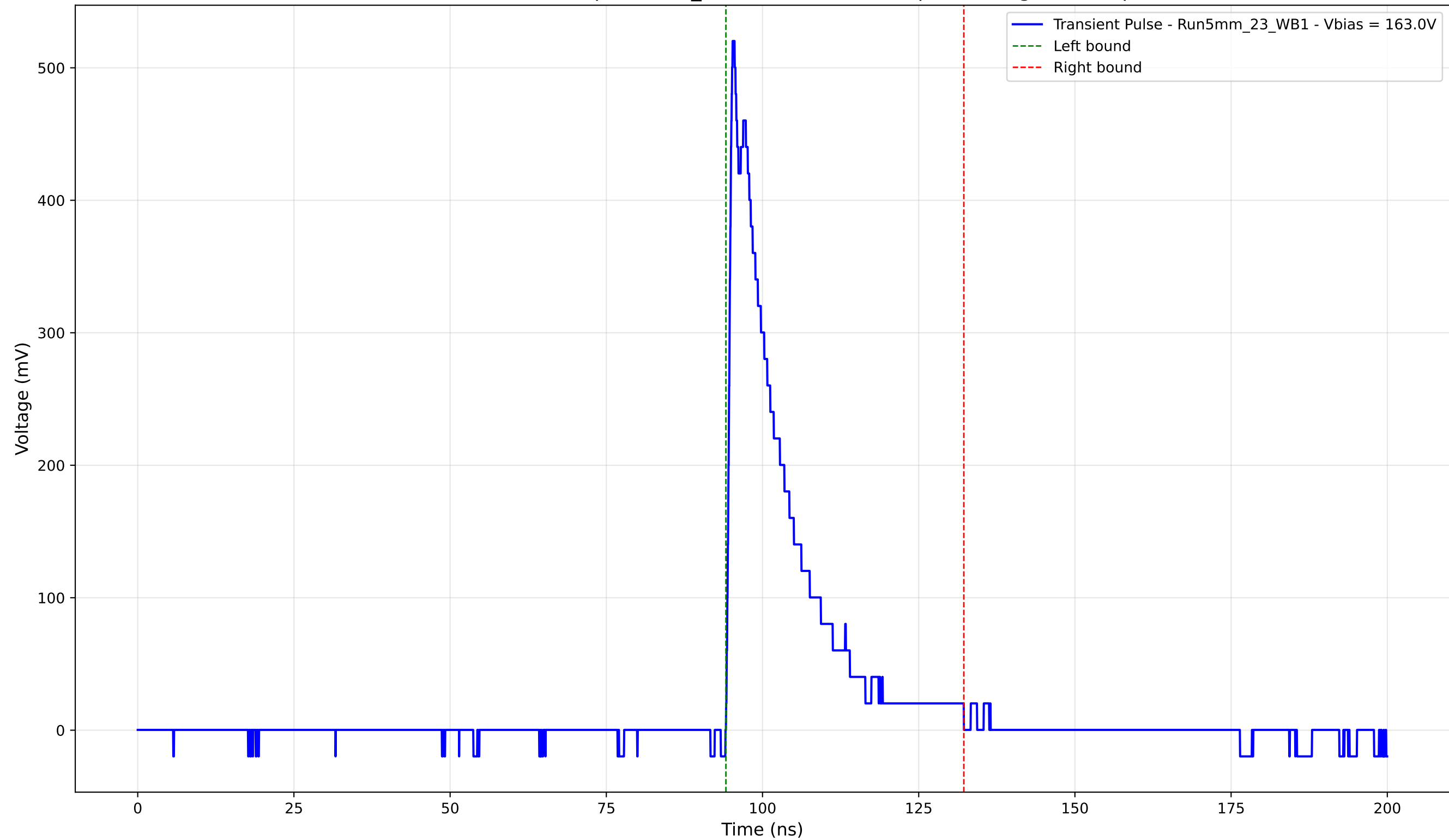
Transient Pulse - Sample: 5mm_23 - Position: 3210.0 \mu\text{m} - Charge: 92.03 pC
