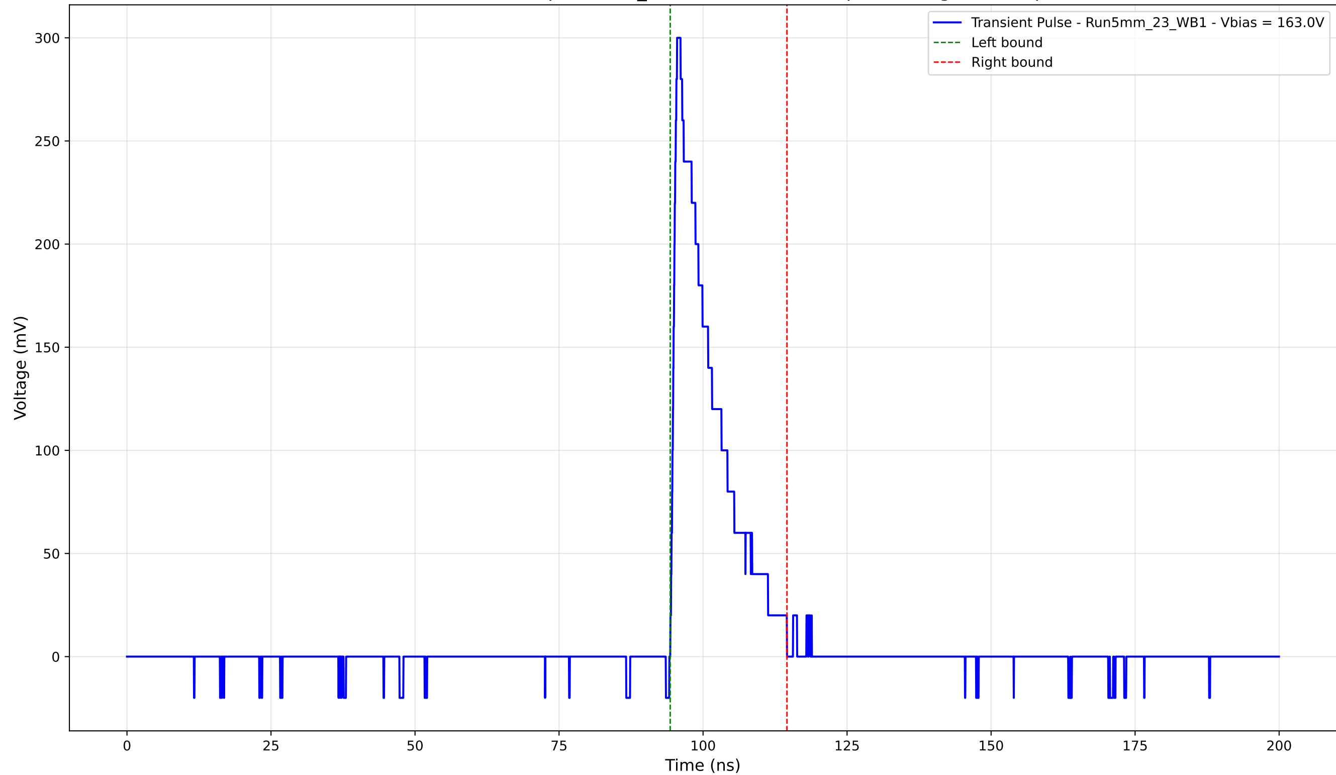
Transient Pulse - Sample: 5mm_23 - Position: 4785.0 \mu\text{m} - Charge: 44.46 pC
