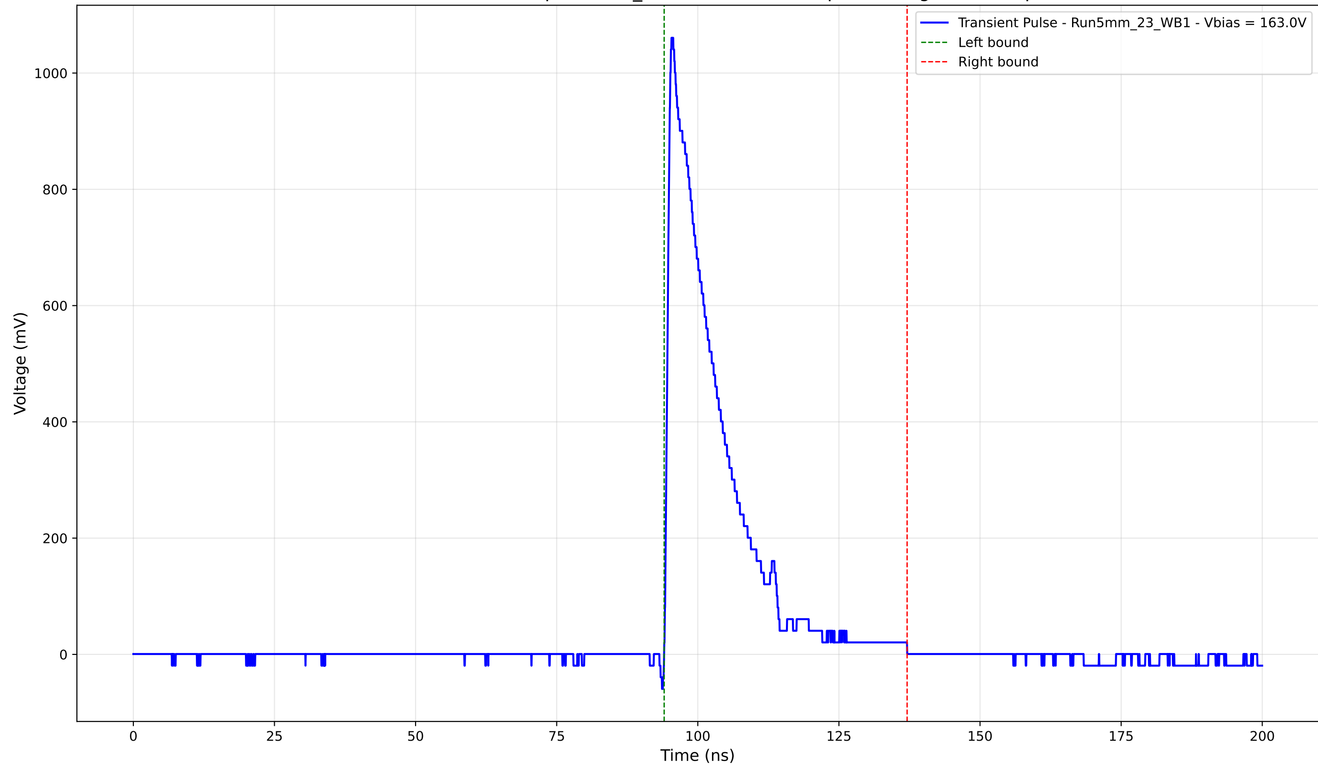
Transient Pulse - Sample: 5mm_23 - Position: 385.0 \mu\text{m} - Charge: 198.59 pC
