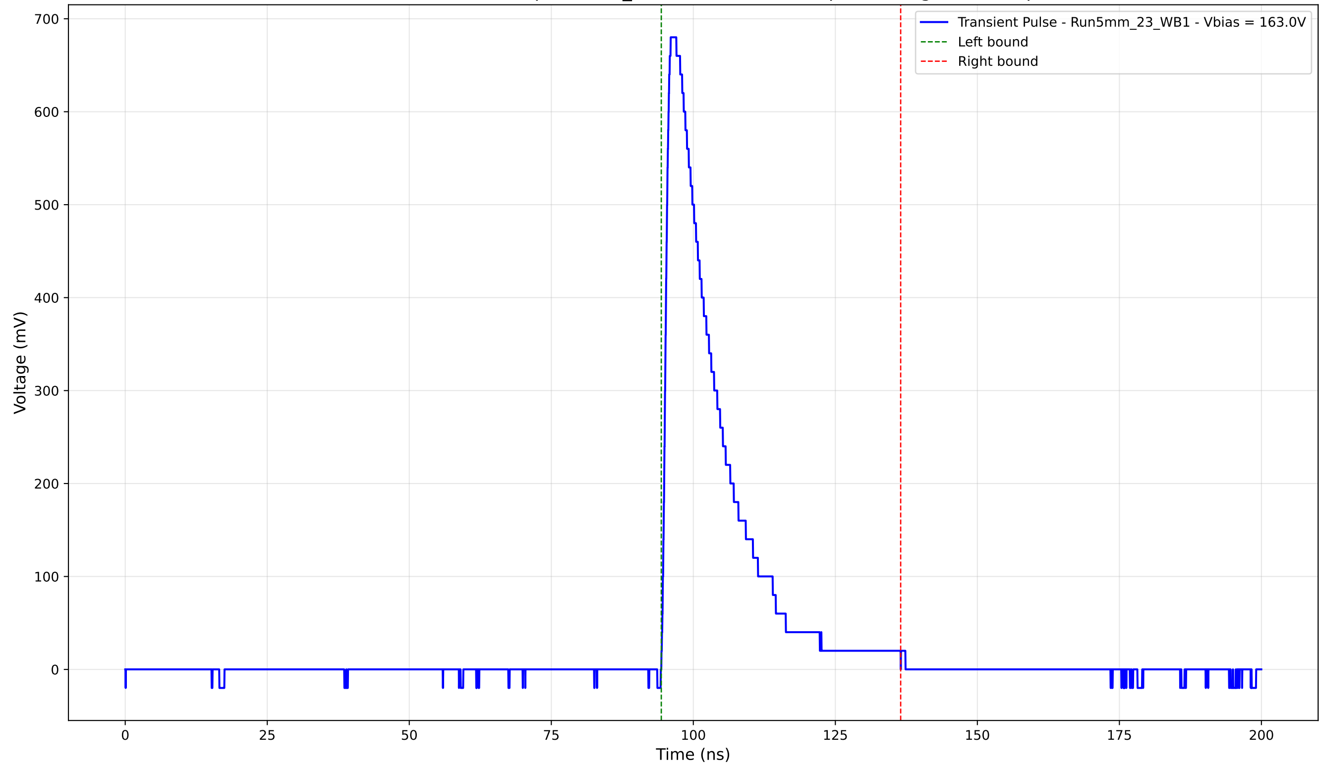
Transient Pulse - Sample: 5mm_23 - Position: 3815.0 \mu\text{m} - Charge: 138.74 pC
