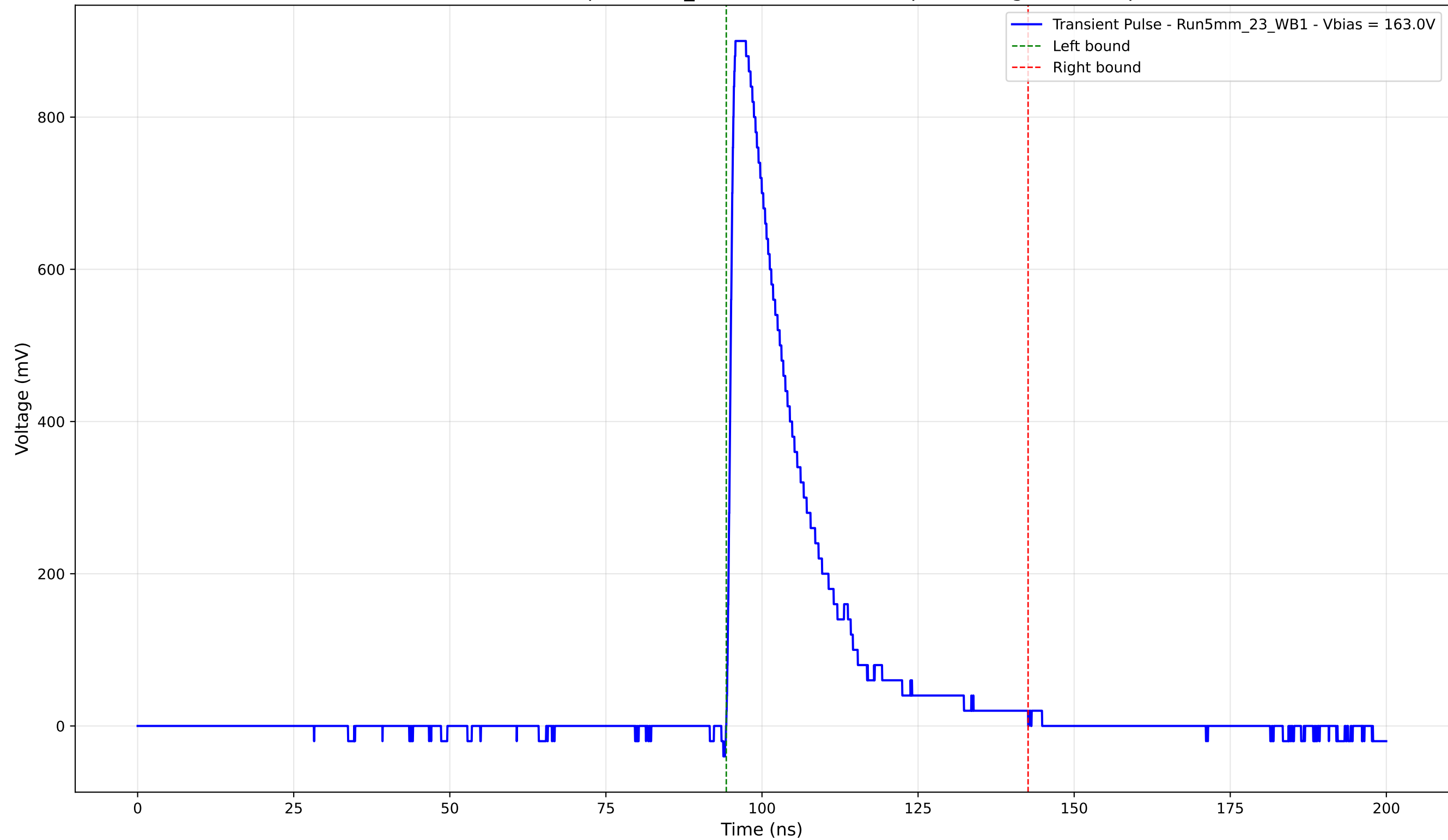
Transient Pulse - Sample: 5mm_23 - Position: 3625.0 \mu\text{m} - Charge: 205.19 pC
