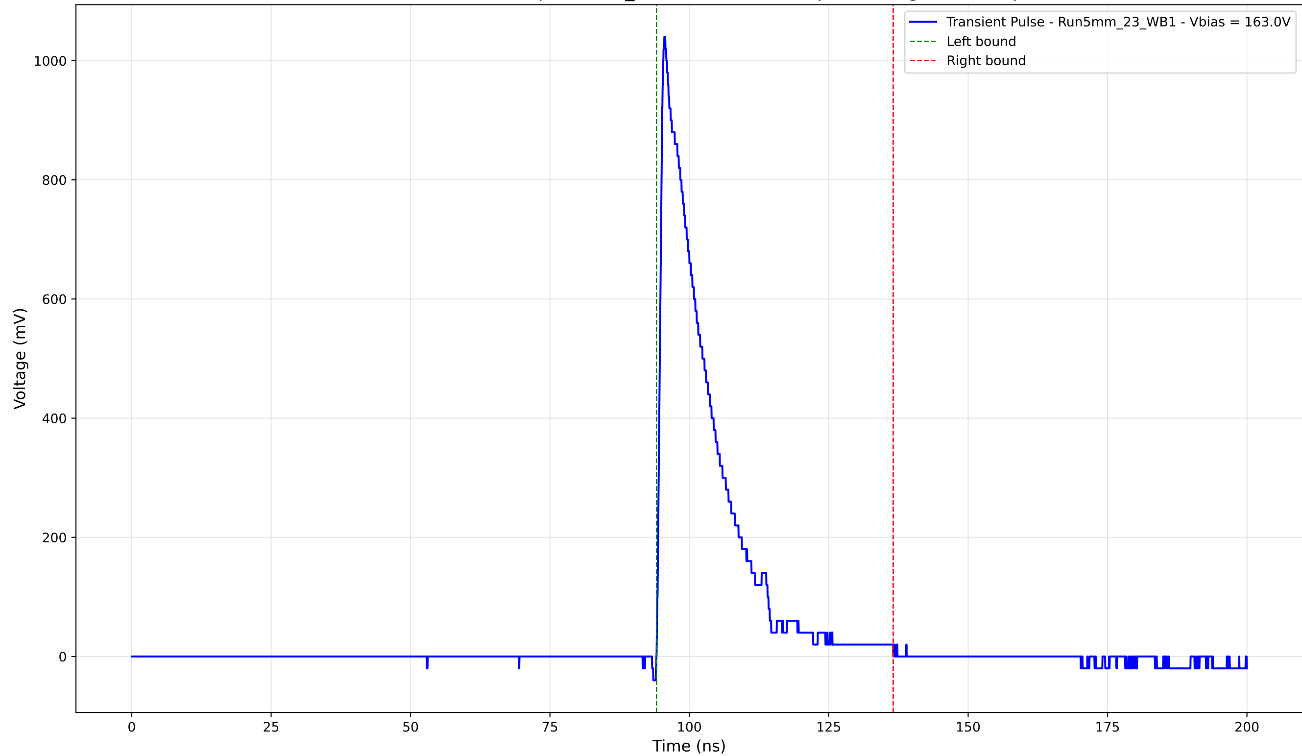
Transient Pulse - Sample: 5mm_23 - Position: 490.0 \mu\text{m} - Charge: 193.90 pC
