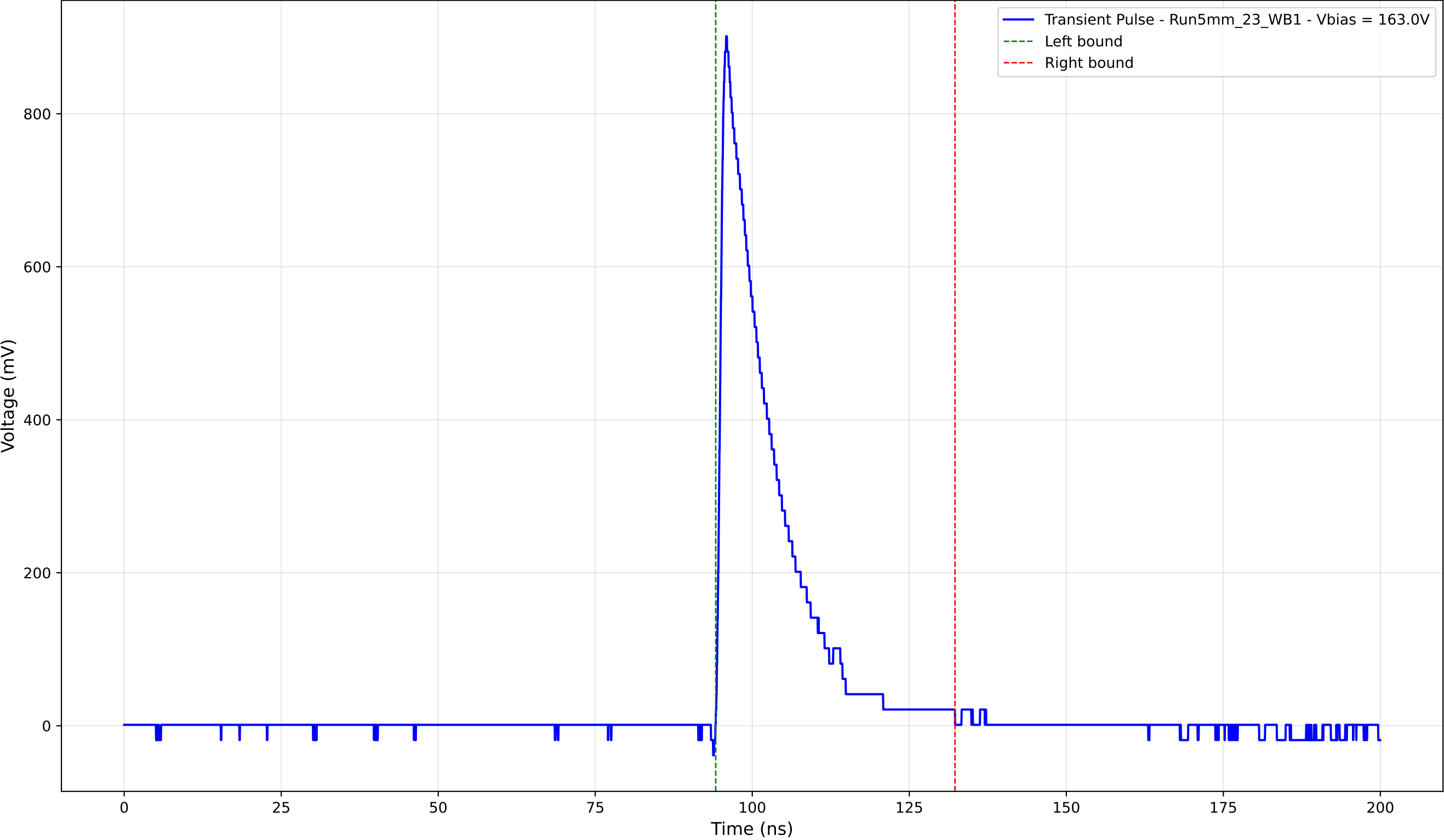
Transient Pulse - Sample: 5mm_23 - Position: 4685.0 \mu\text{m} - Charge: 156.88 pC
