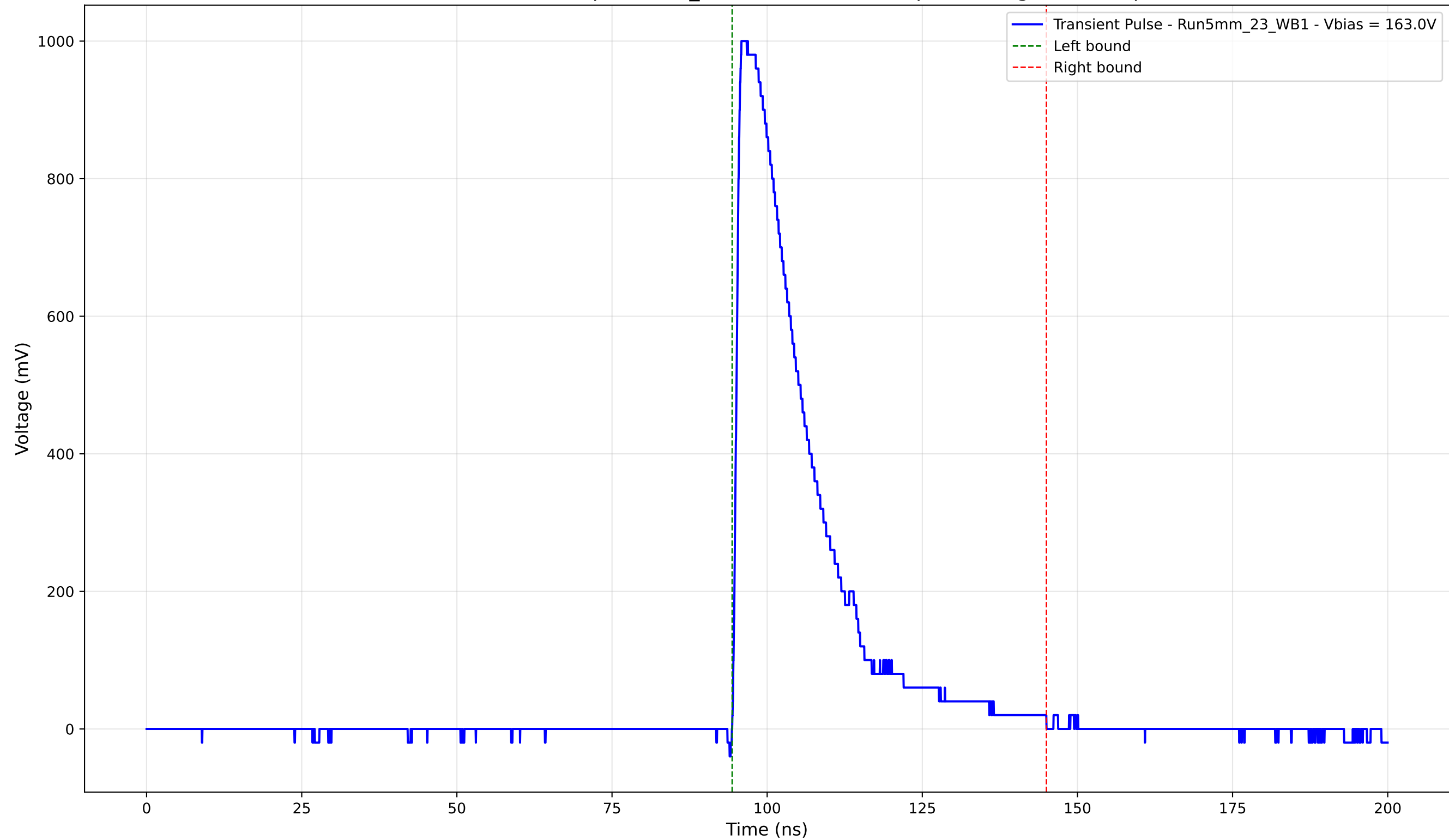
Transient Pulse - Sample: 5mm_23 - Position: 1515.0 \mu\text{m} - Charge: 252.06 pC
