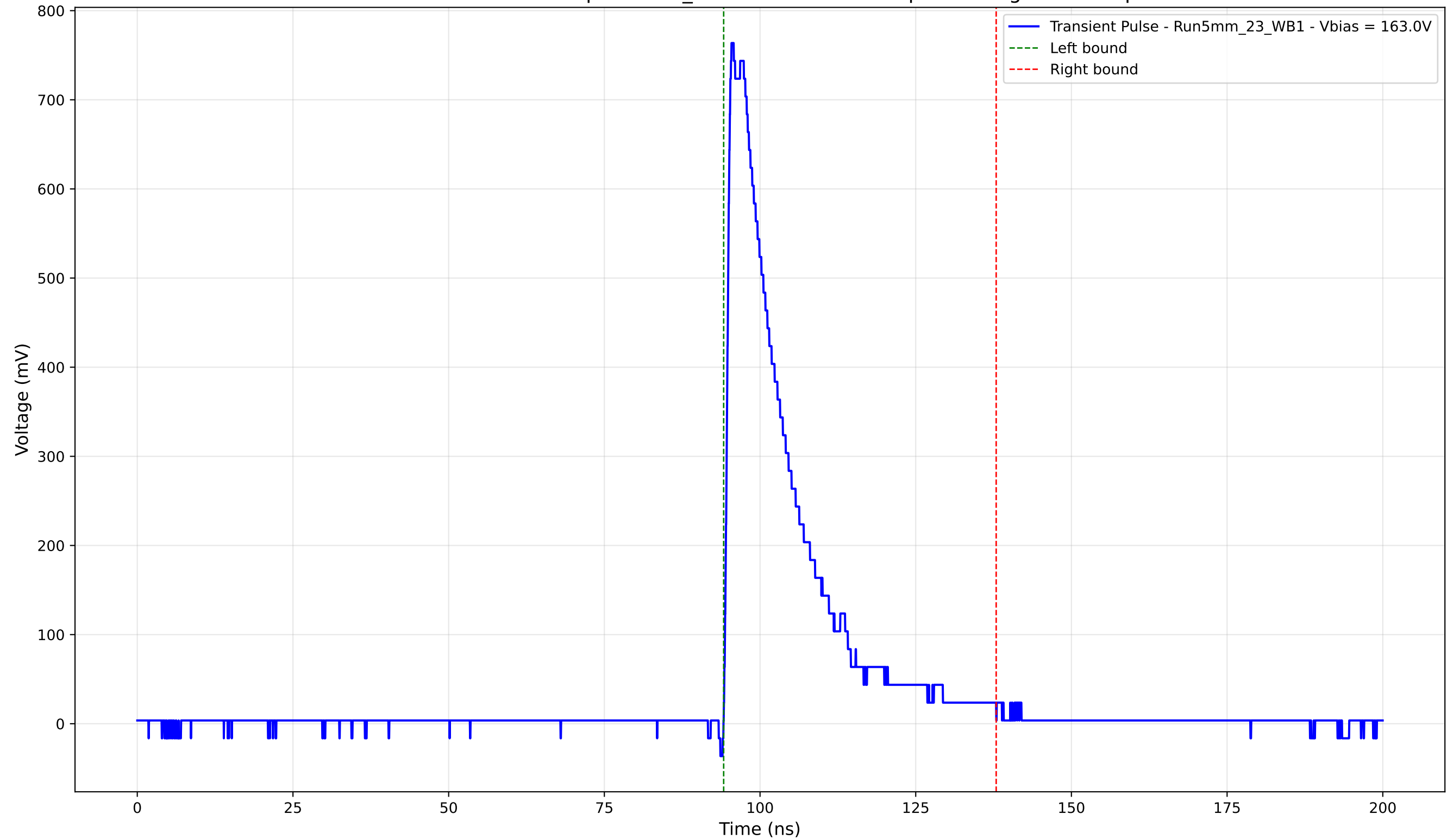
Transient Pulse - Sample: 5mm_23 - Position: 3315.0 \mu\text{m} - Charge: 161.14 pC
