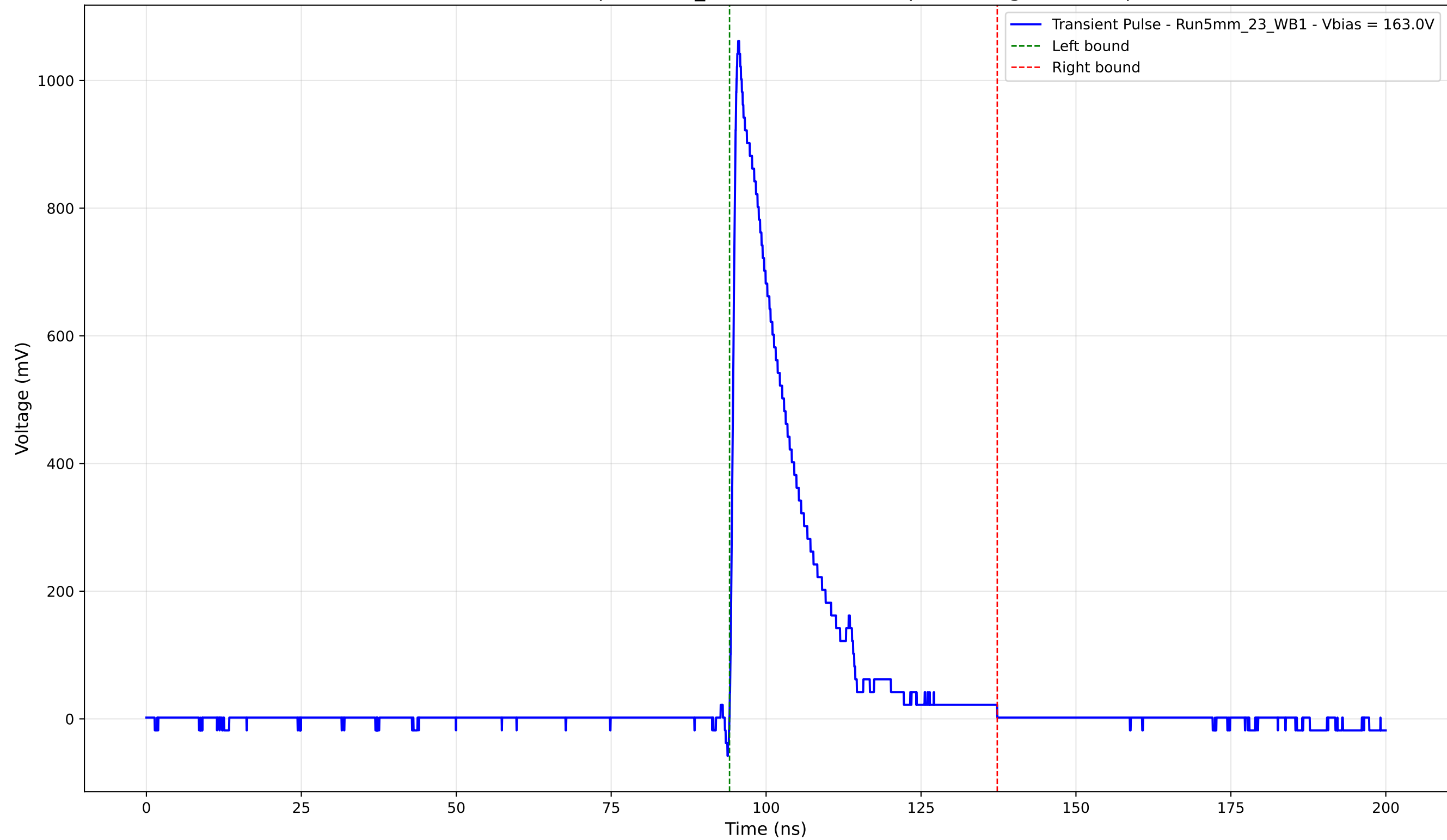
Transient Pulse - Sample: 5mm_23 - Position: 445.0 \mu\text{m} - Charge: 200.49 pC
