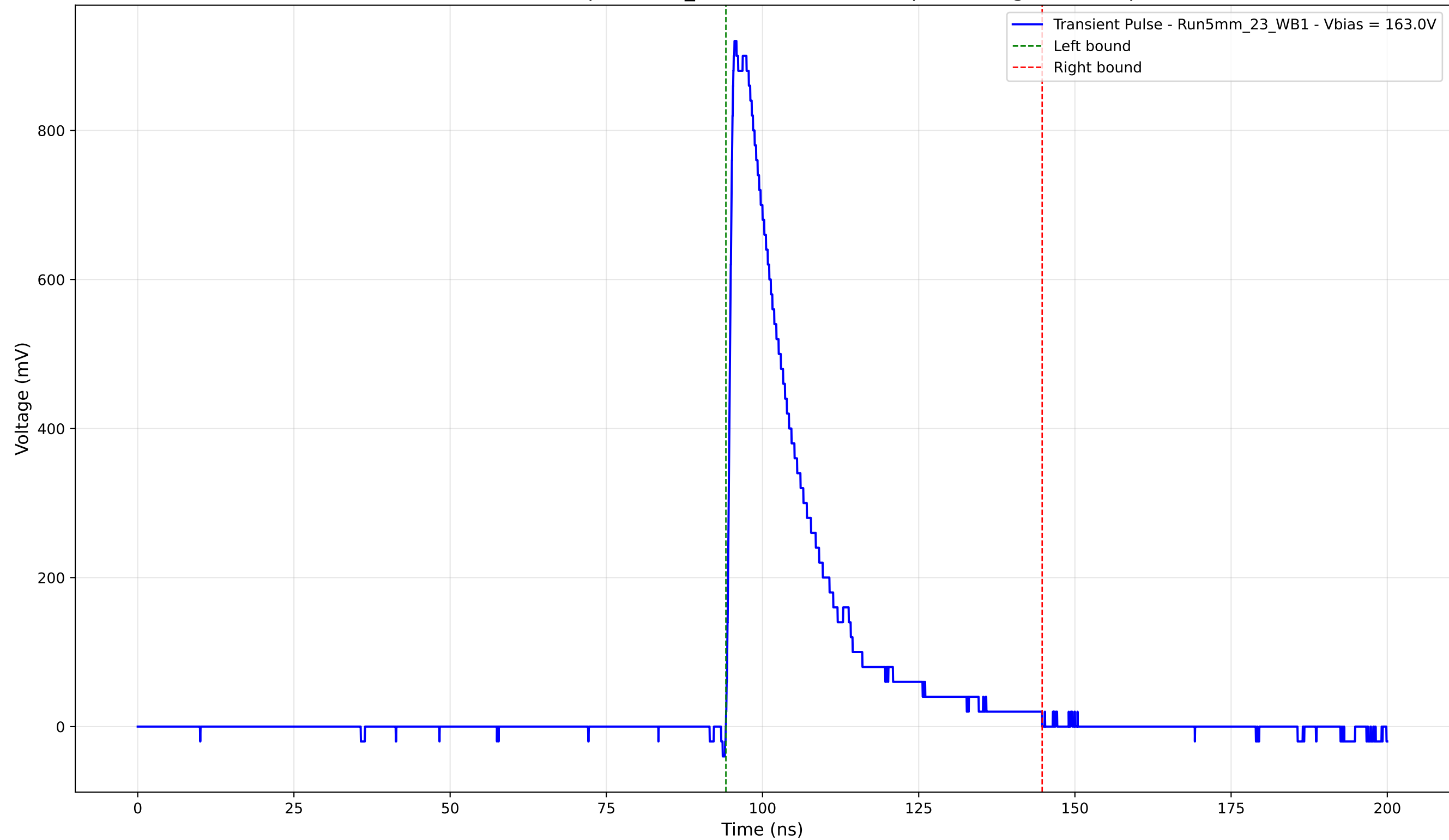
Transient Pulse - Sample: 5mm_23 - Position: 3385.0 \mu\text{m} - Charge: 210.86 pC
