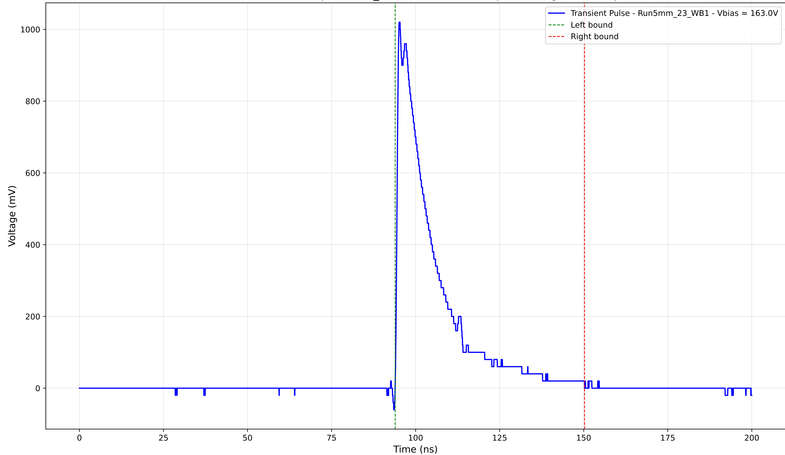
Transient Pulse - Sample: 5mm_23 - Position: 2500.0 \mu\text{m} - Charge: 234.15 pC
