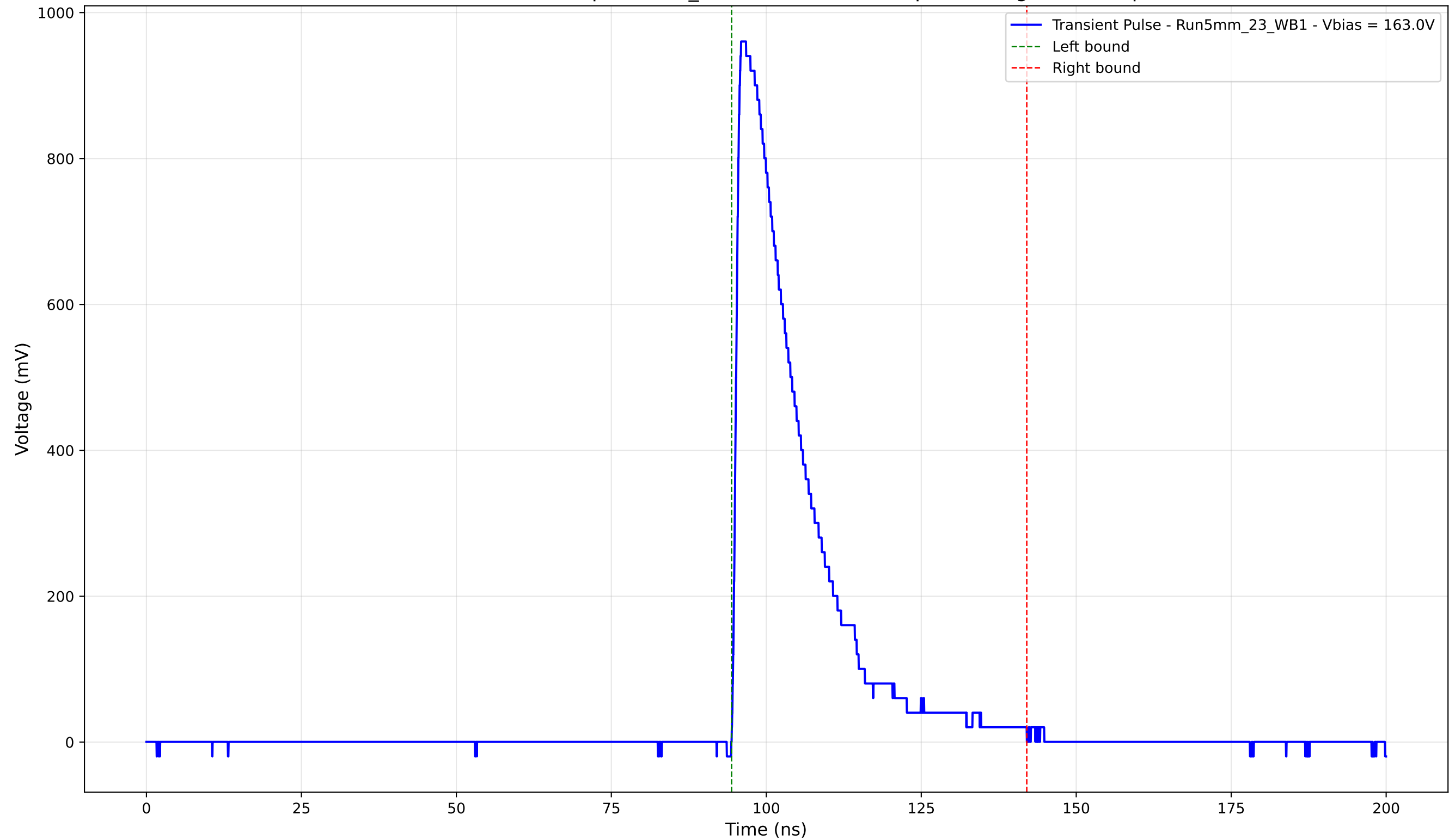
Transient Pulse - Sample: 5mm_23 - Position: 1365.0 \mu\text{m} - Charge: 223.51 pC
