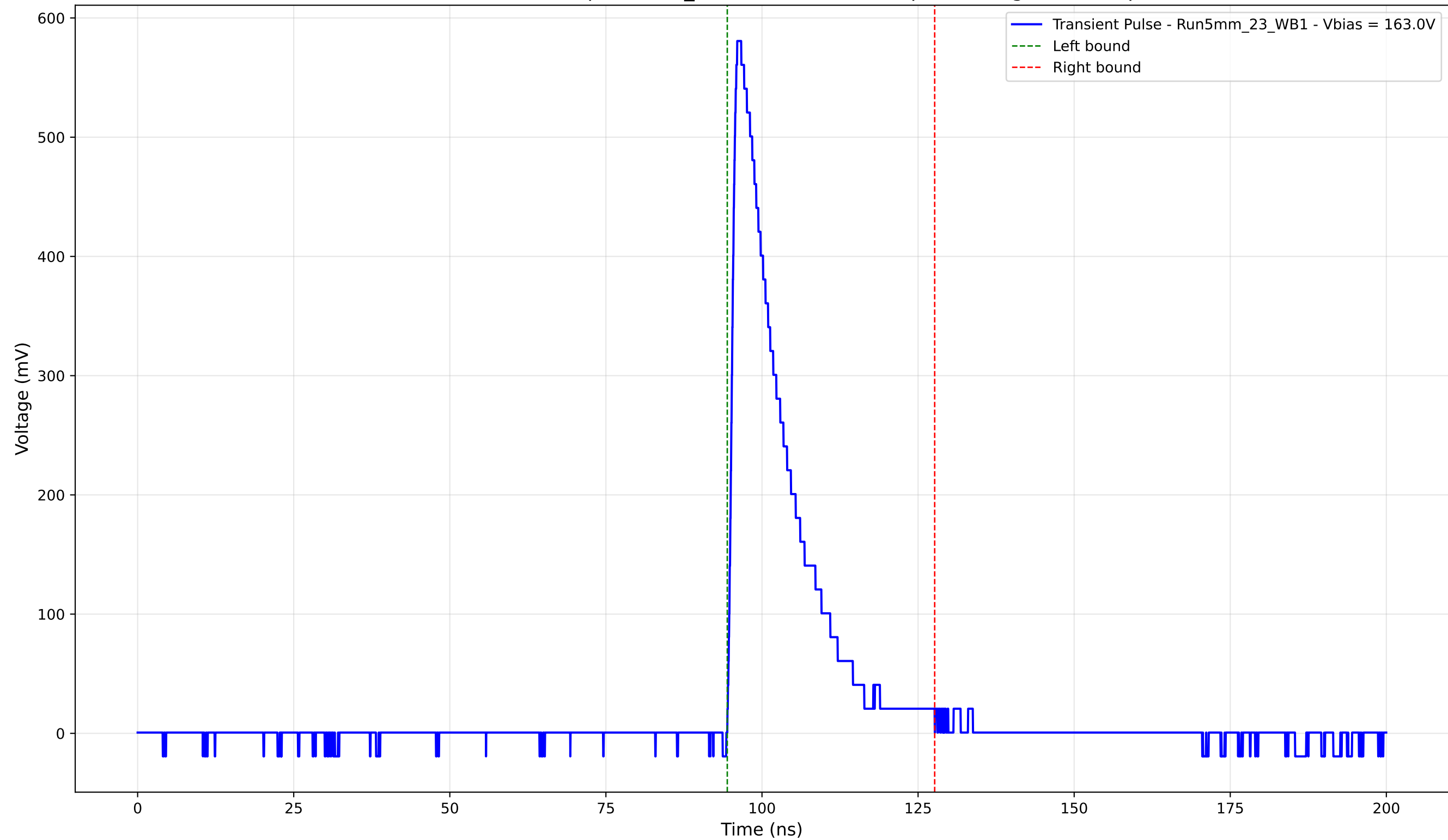
Transient Pulse - Sample: 5mm_23 - Position: 4210.0 \mu\text{m} - Charge: 106.71 pC
