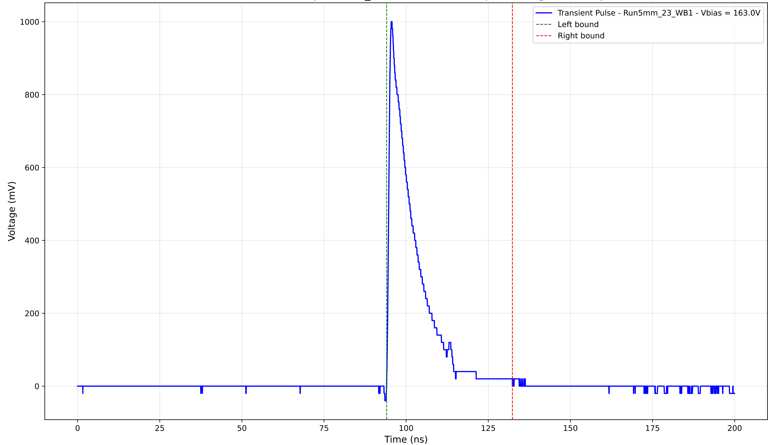
Transient Pulse - Sample: 5mm_23 - Position: 4965.0 \mu\text{m} - Charge: 167.08 pC
