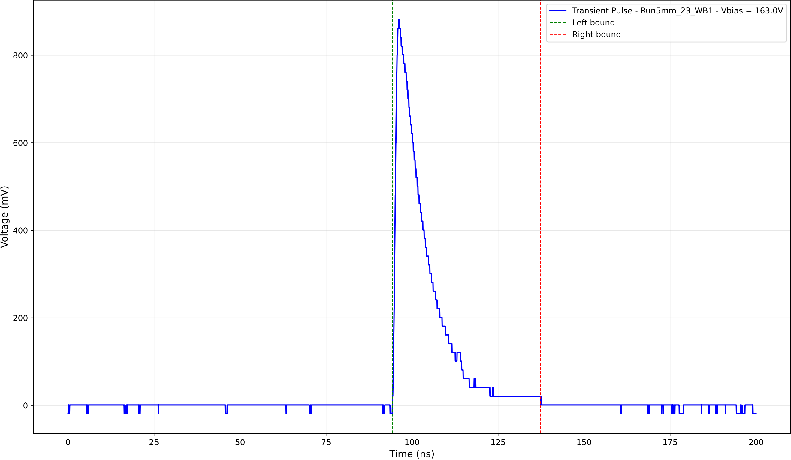
Transient Pulse - Sample: 5mm_23 - Position: 4355.0 \mu\text{m} - Charge: 170.15 pC
