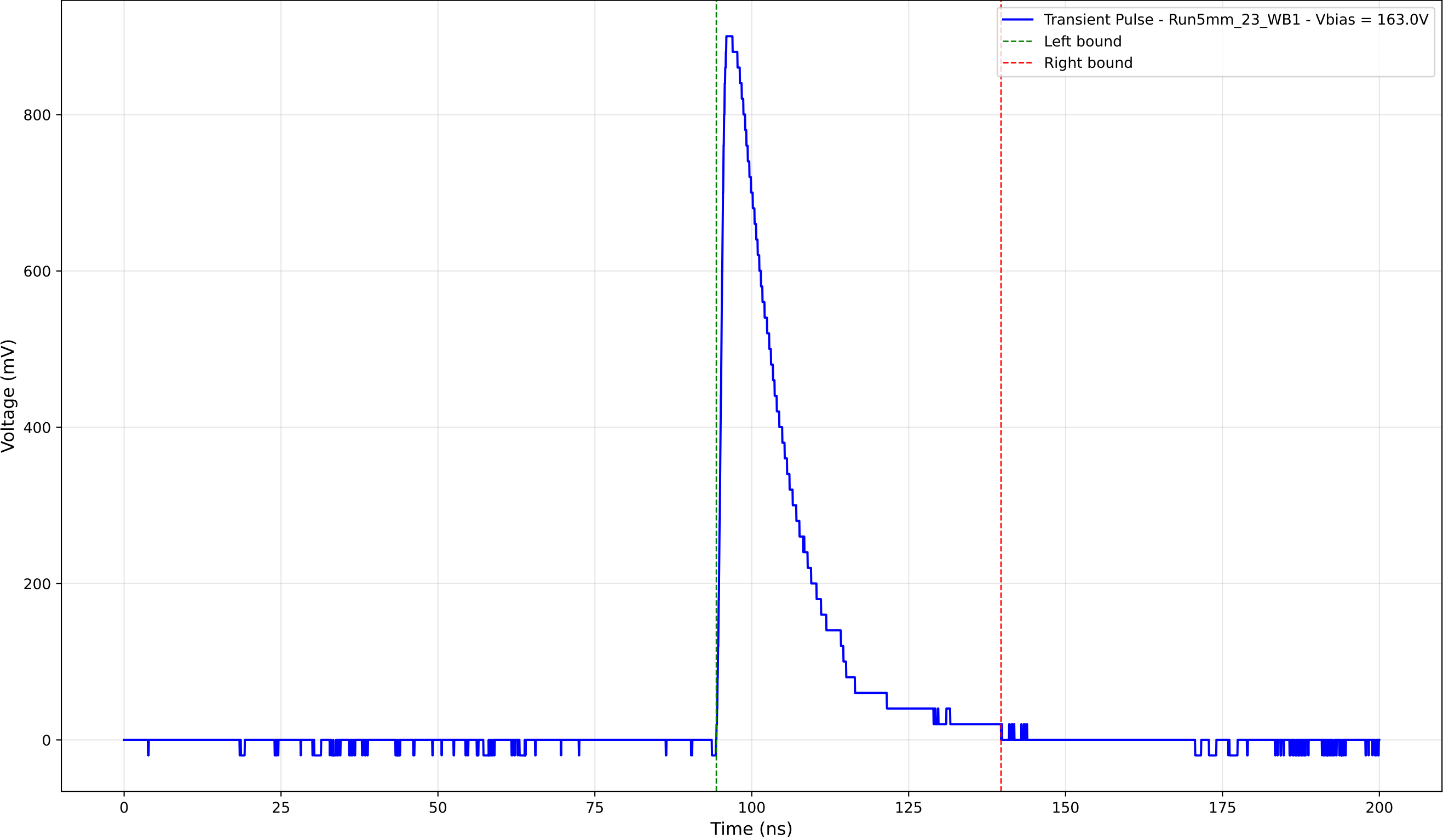
Transient Pulse - Sample: 5mm_23 - Position: 3965.0 \mu\text{m} - Charge: 197.37 pC
