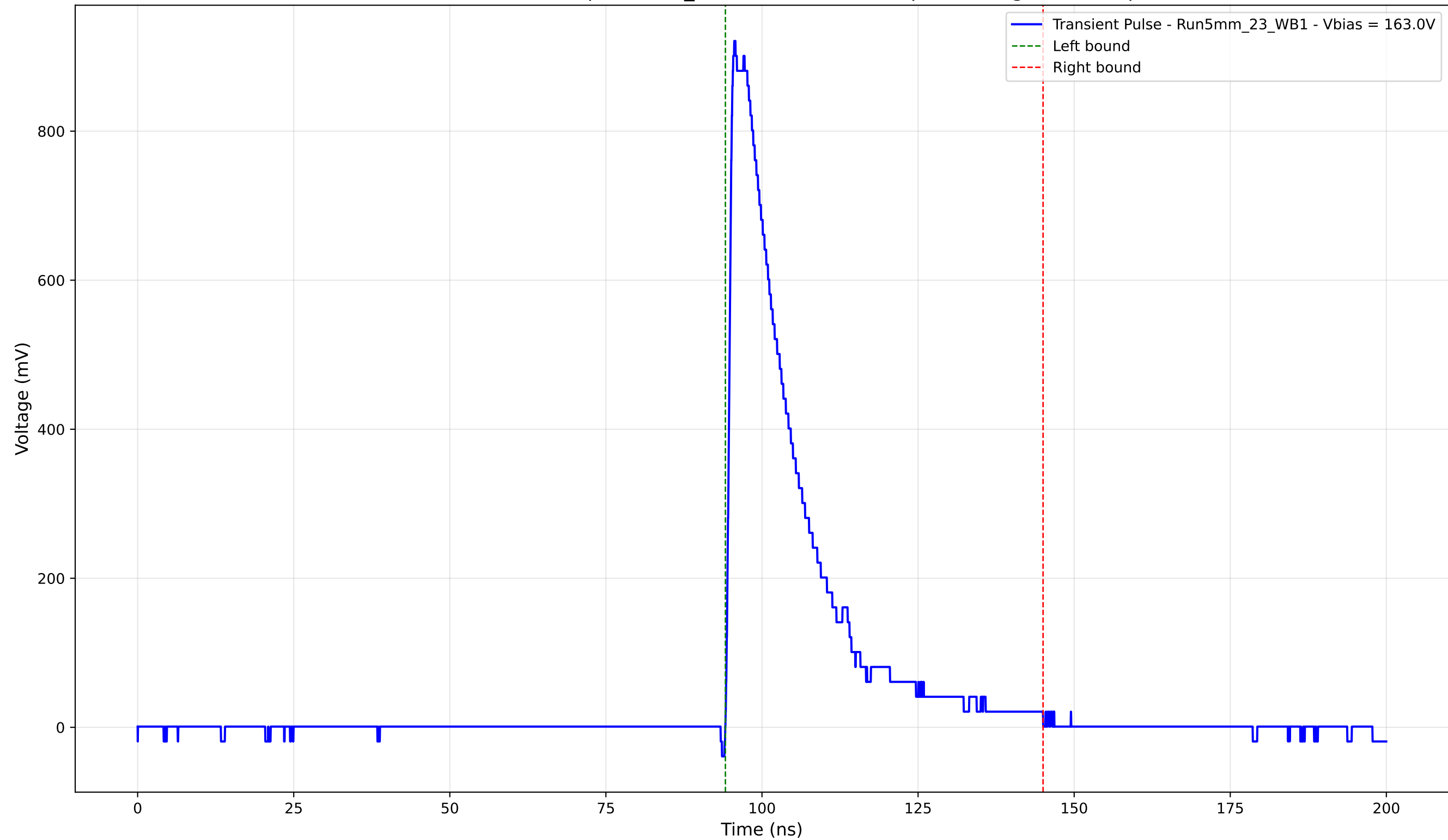
Transient Pulse - Sample: 5mm_23 - Position: 3365.0 \mu\text{m} - Charge: 208.46 pC
