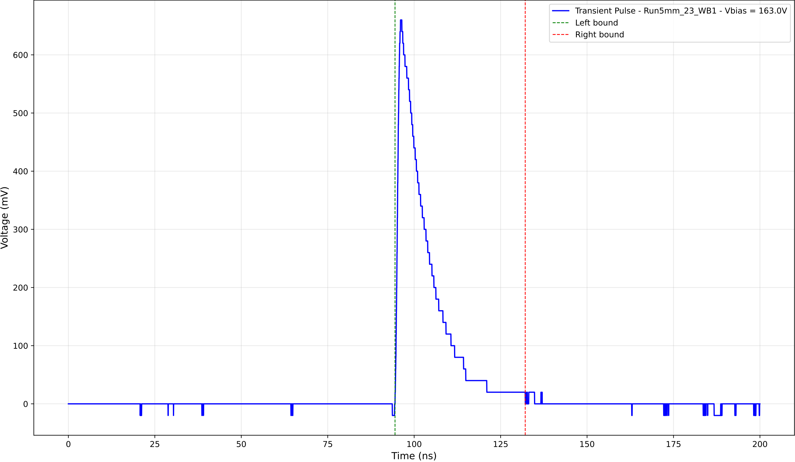
Transient Pulse - Sample: 5mm_23 - Position: 1175.0 \mu\text{m} - Charge: 122.92 pC
