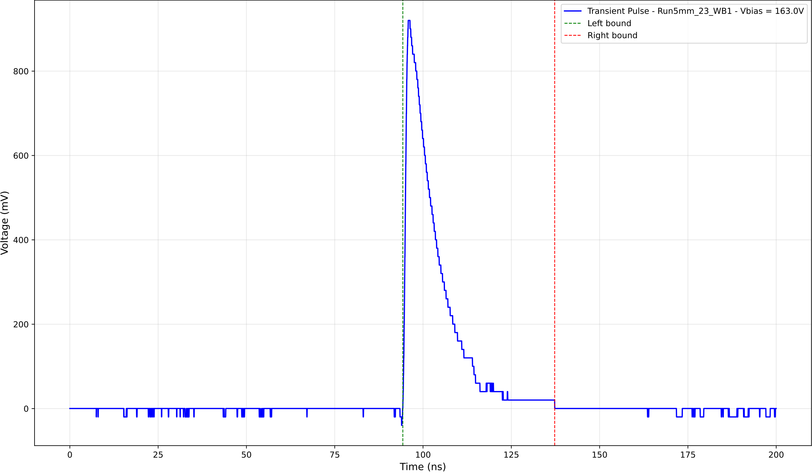
Transient Pulse - Sample: 5mm_23 - Position: 4515.0 \mu\text{m} - Charge: 178.63 pC
