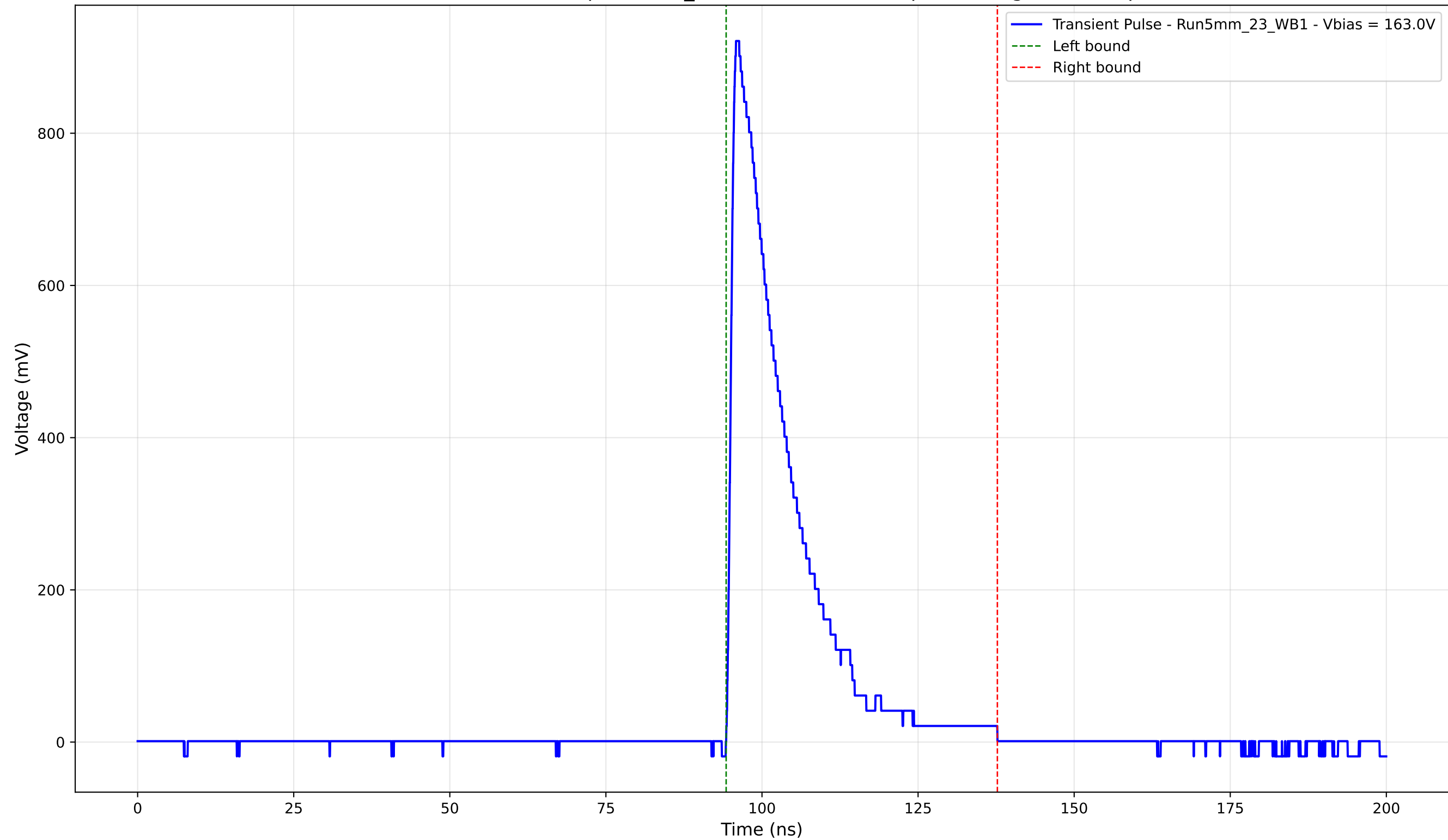
Transient Pulse - Sample: 5mm_23 - Position: 4505.0 \mu\text{m} - Charge: 180.84 pC
