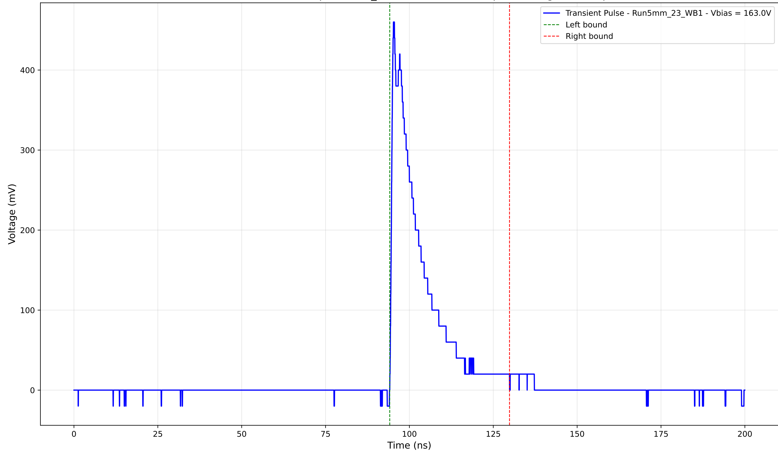
Transient Pulse - Sample: 5mm_23 - Position: 2270.0 \mu\text{m} - Charge: 82.82 pC
