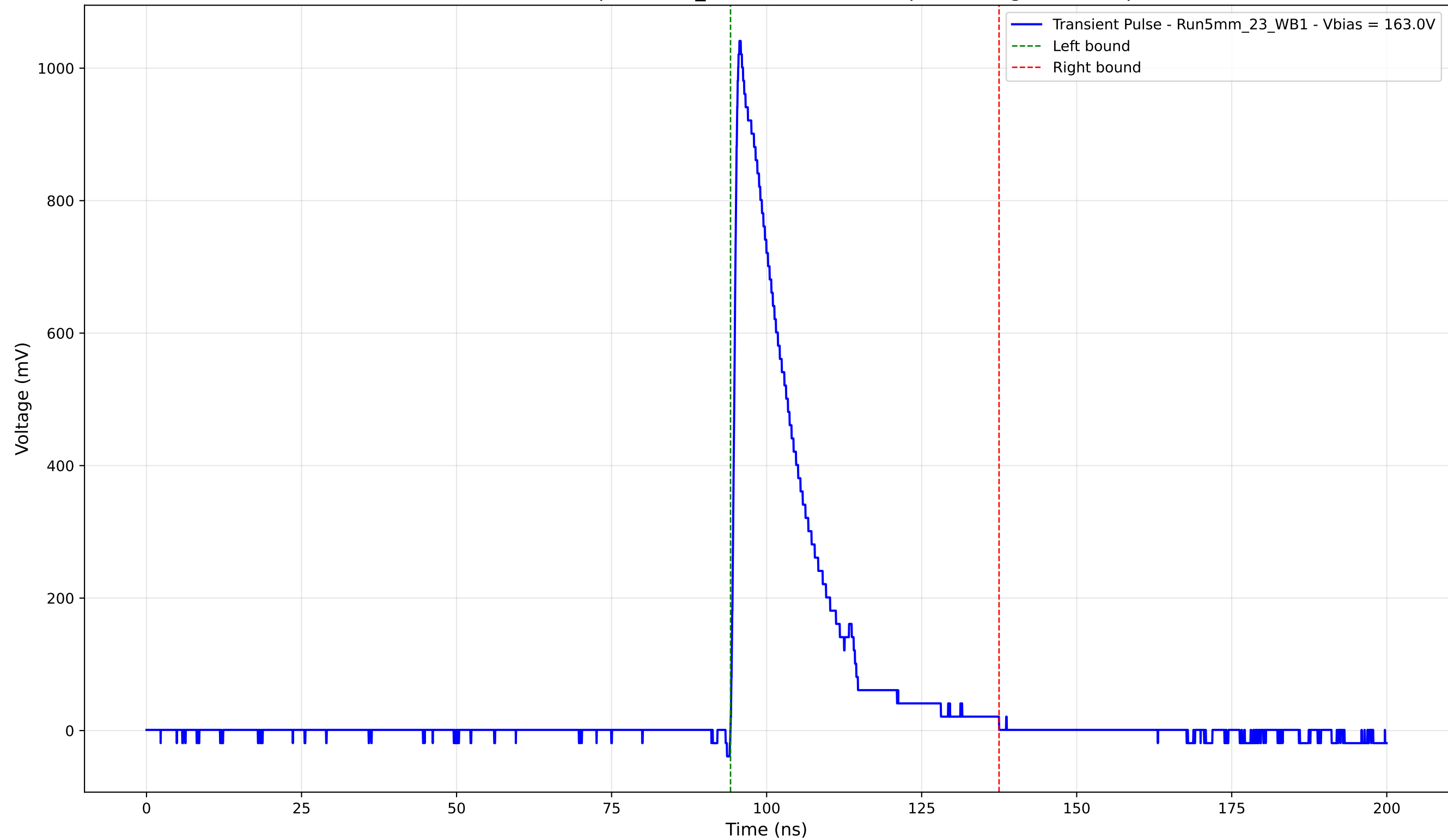
Transient Pulse - Sample: 5mm_23 - Position: 620.0 \mu\text{m} - Charge: 210.01 pC
