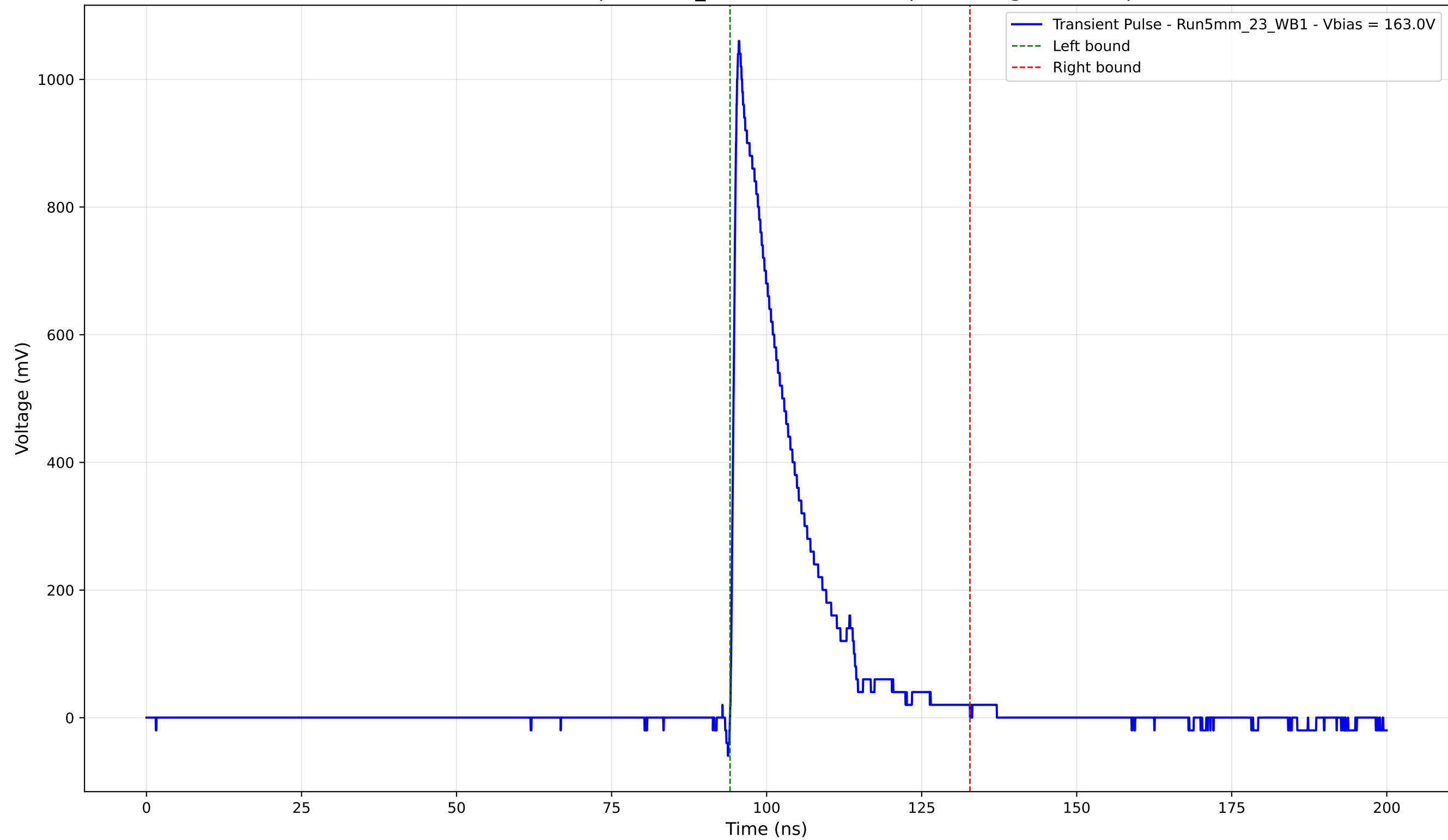
Transient Pulse - Sample: 5mm_23 - Position: 455.0 \mu\text{m} - Charge: 197.24 pC
