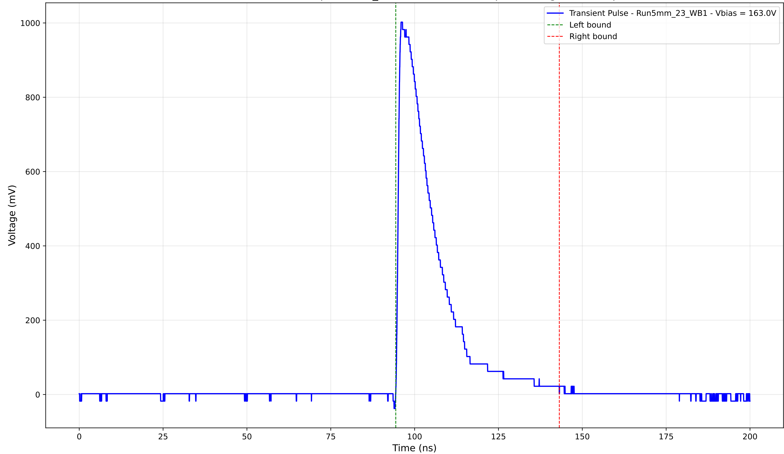
Transient Pulse - Sample: 5mm_23 - Position: 1465.0 \mu\text{m} - Charge: 244.92 pC
