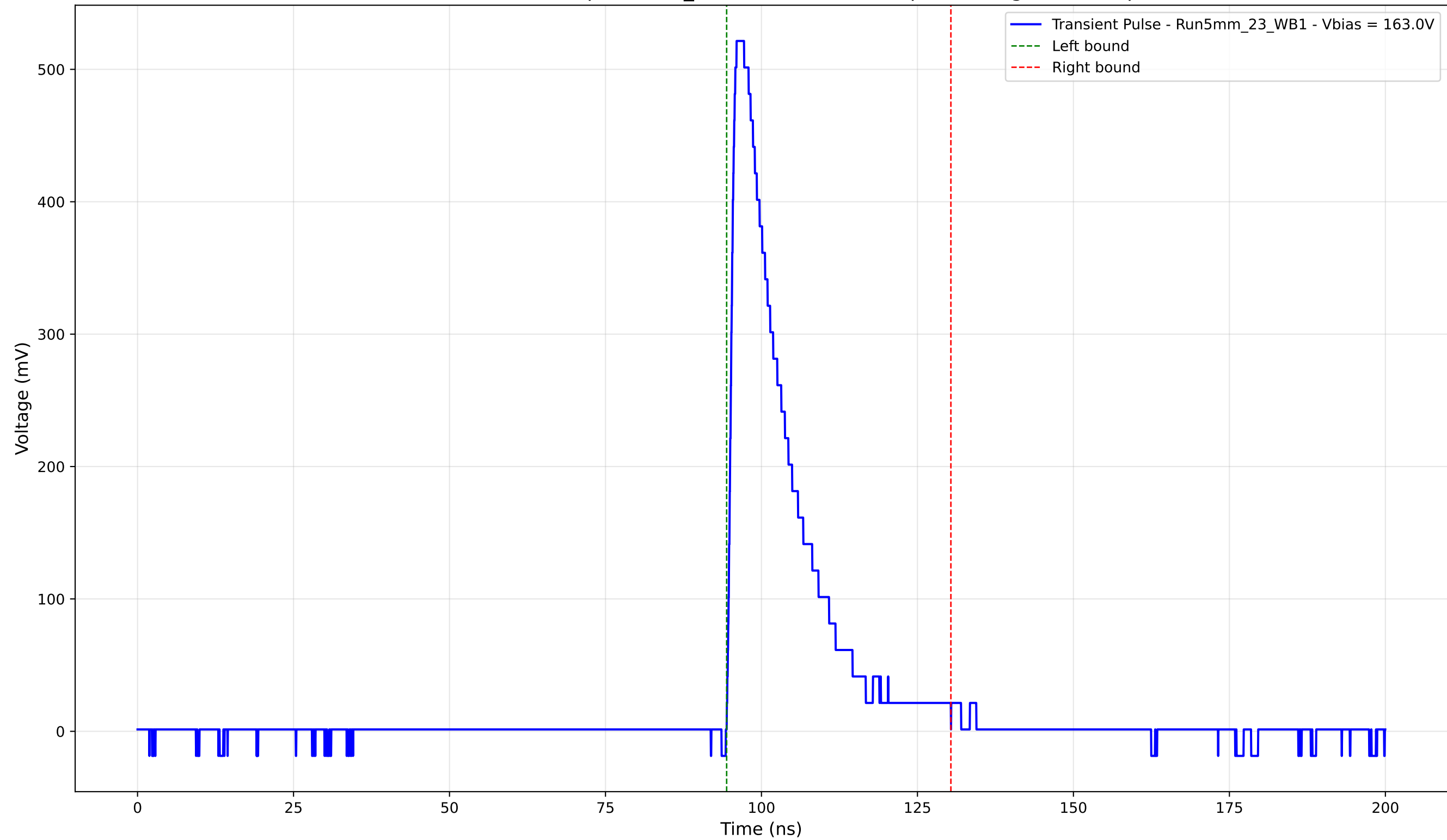
Transient Pulse - Sample: 5mm_23 - Position: 3800.0 \mu\text{m} - Charge: 103.25 pC
