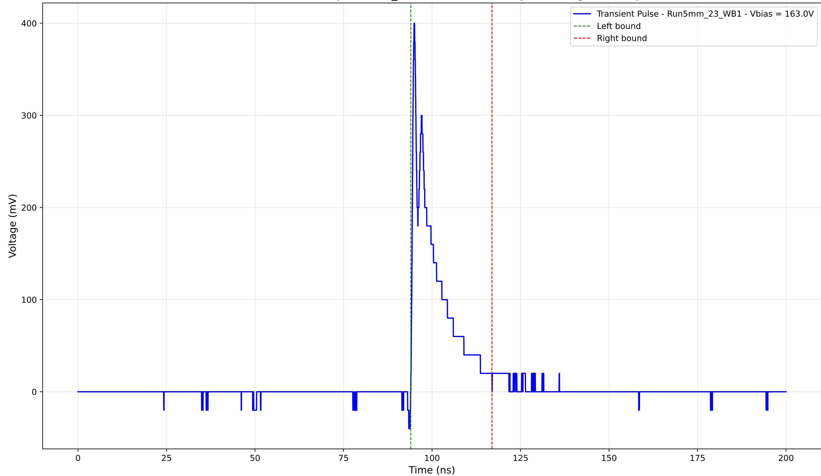
Transient Pulse - Sample: 5mm_23 - Position: 2760.0 \mu\text{m} - Charge: 49.12 pC
