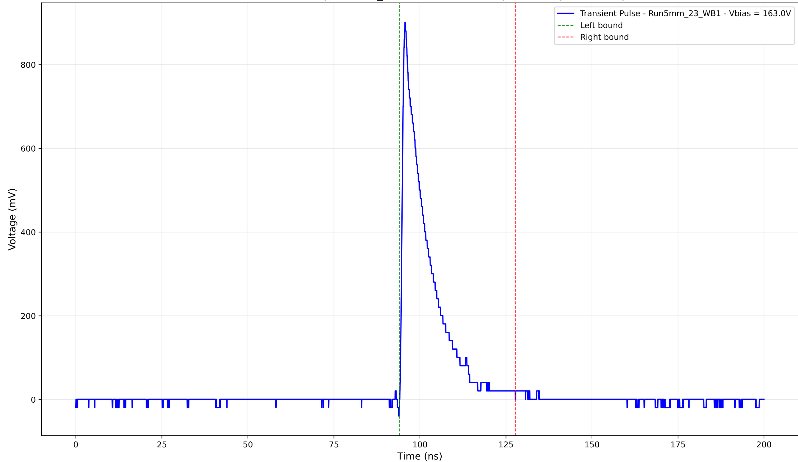
Transient Pulse - Sample: 5mm_23 - Position: 4835.0 \mu\text{m} - Charge: 142.23 pC
