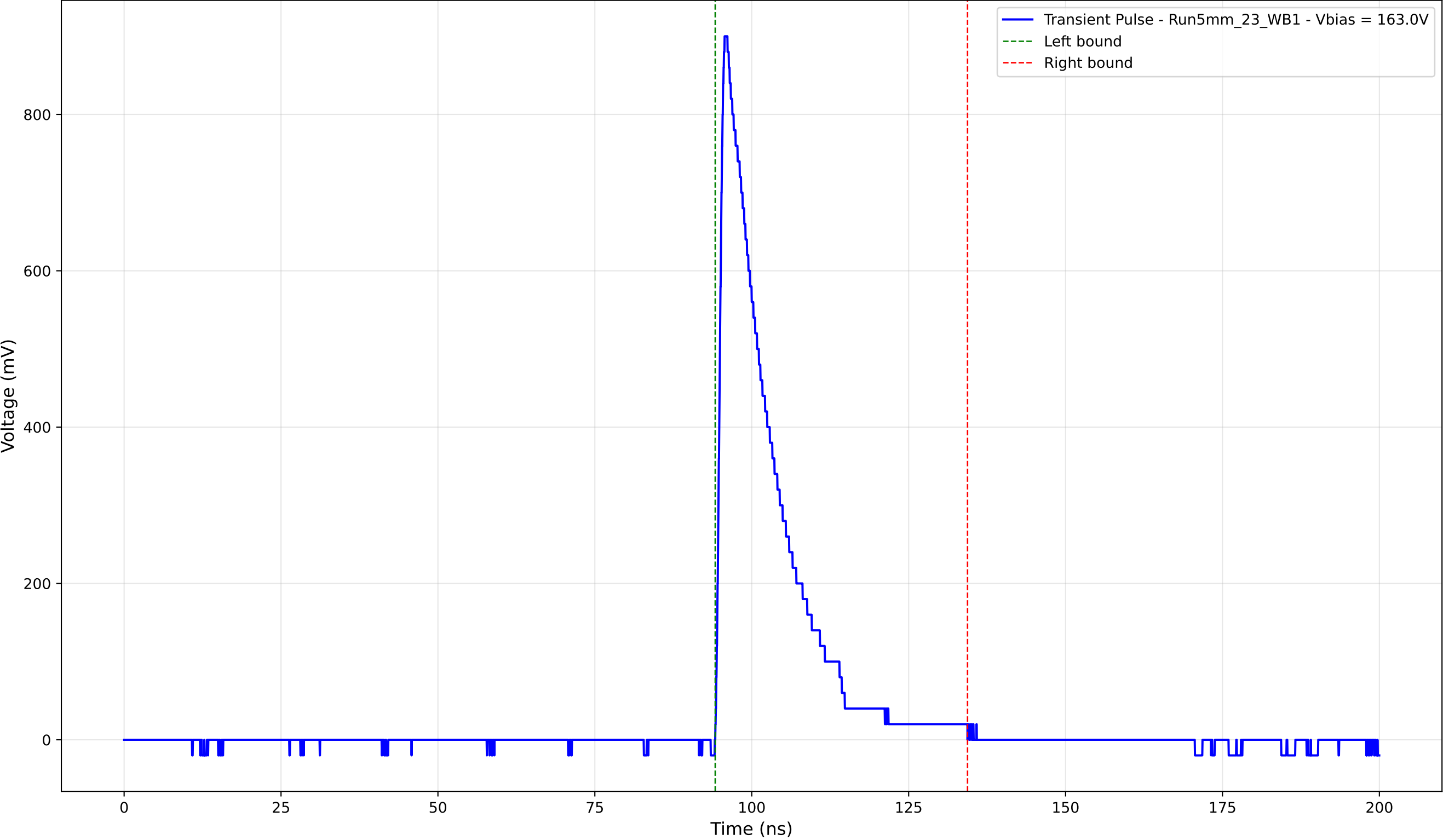
Transient Pulse - Sample: 5mm_23 - Position: 4680.0 \mu\text{m} - Charge: 160.98 pC
