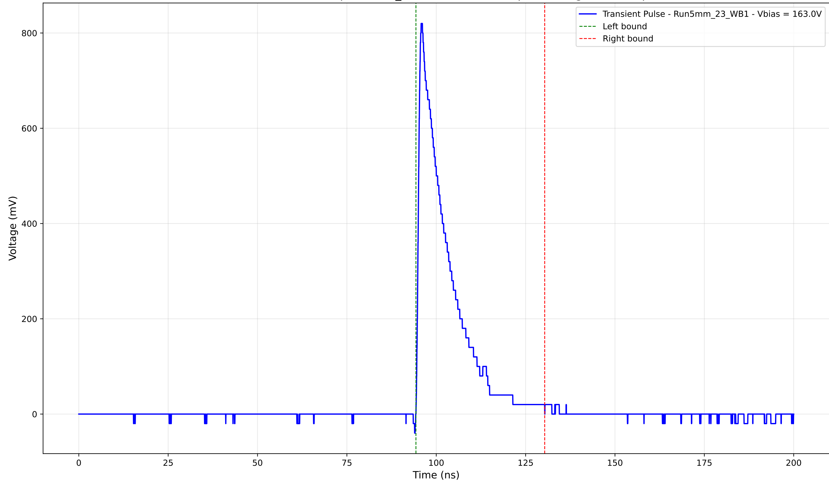
Transient Pulse - Sample: 5mm_23 - Position: 775.0 \mu\text{m} - Charge: 143.86 pC
