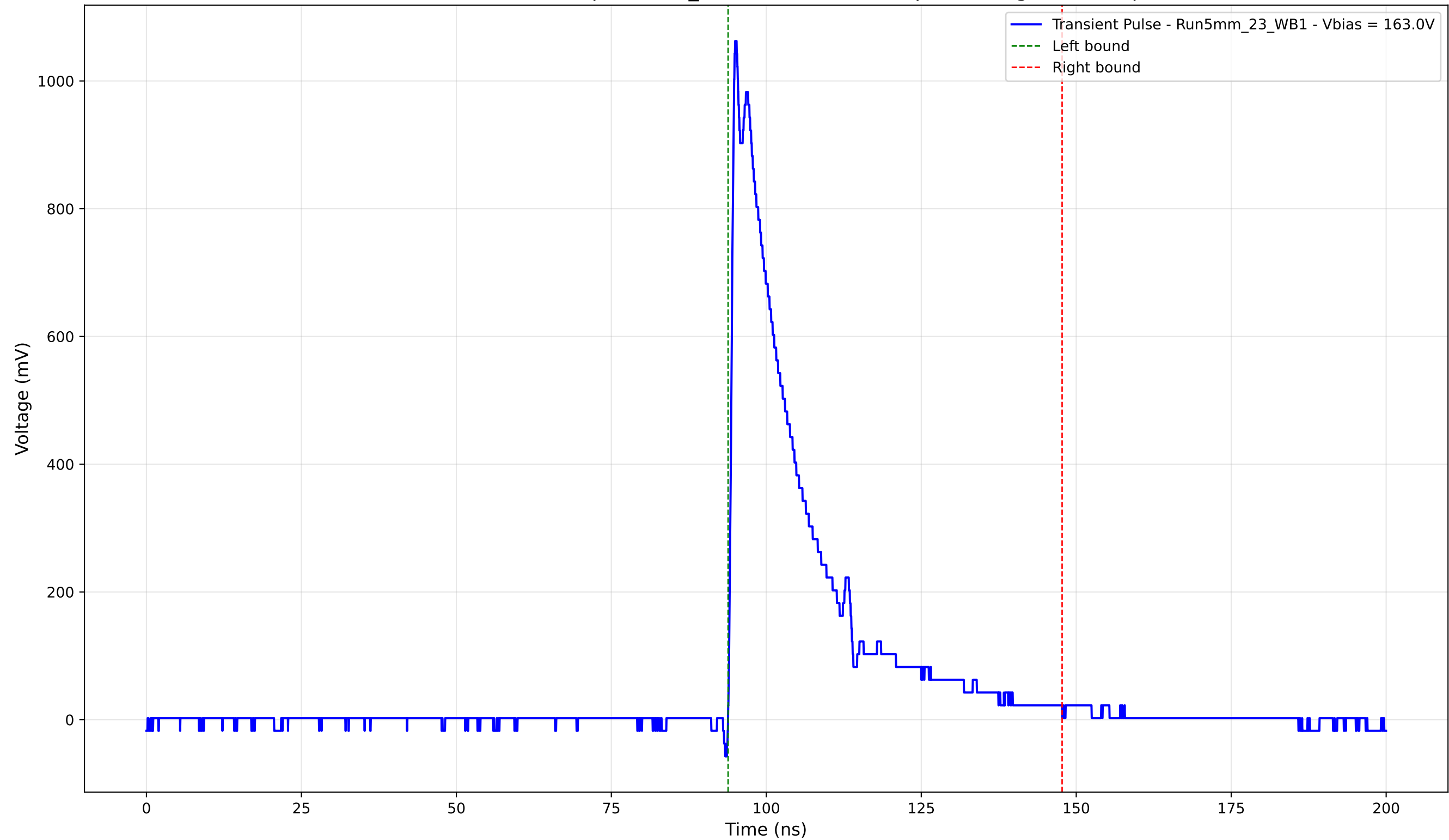
Transient Pulse - Sample: 5mm_23 - Position: 2645.0 \mu\text{m} - Charge: 238.75 pC
