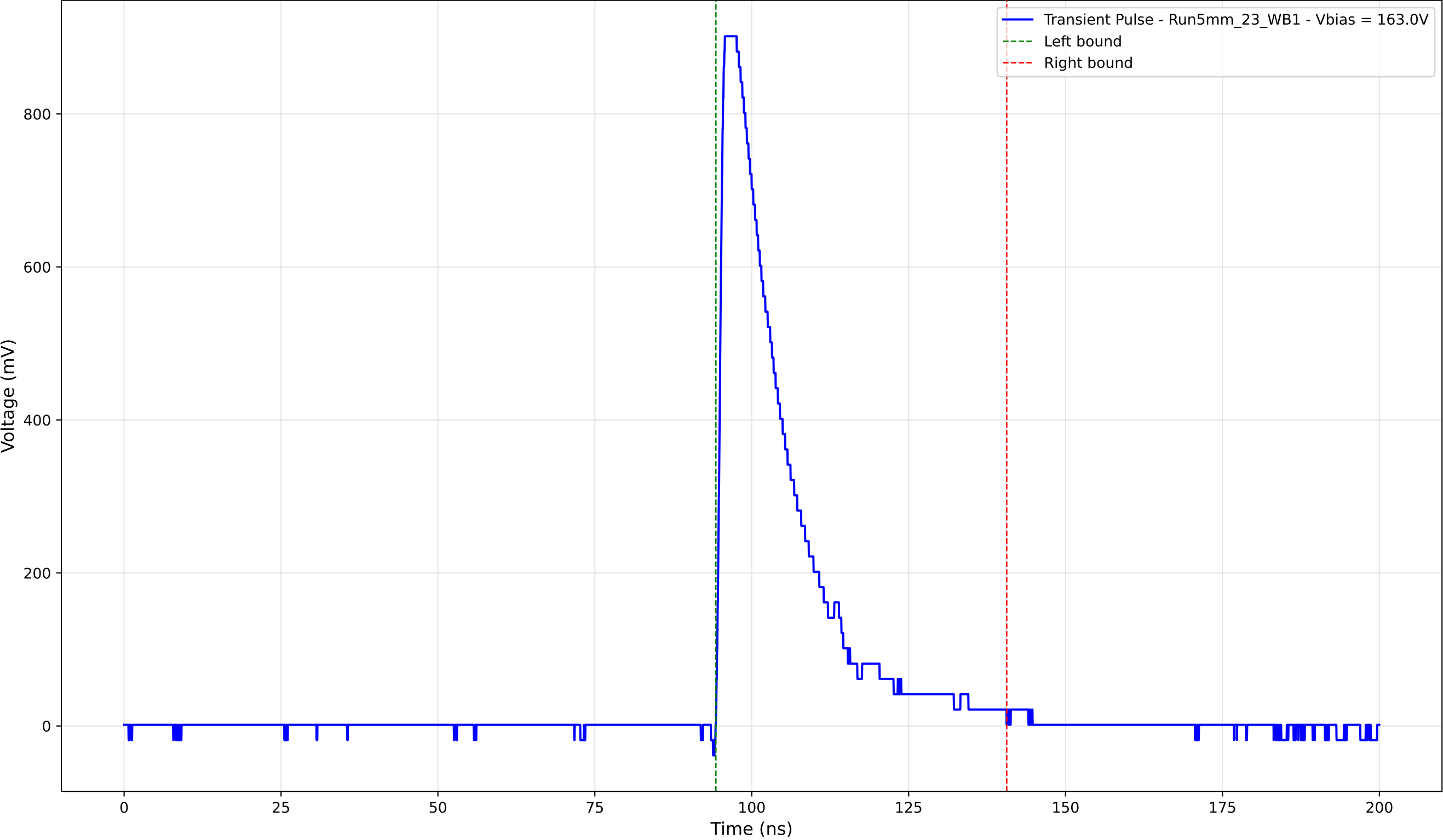
Transient Pulse - Sample: 5mm_23 - Position: 3615.0 \mu\text{m} - Charge: 208.13 pC
