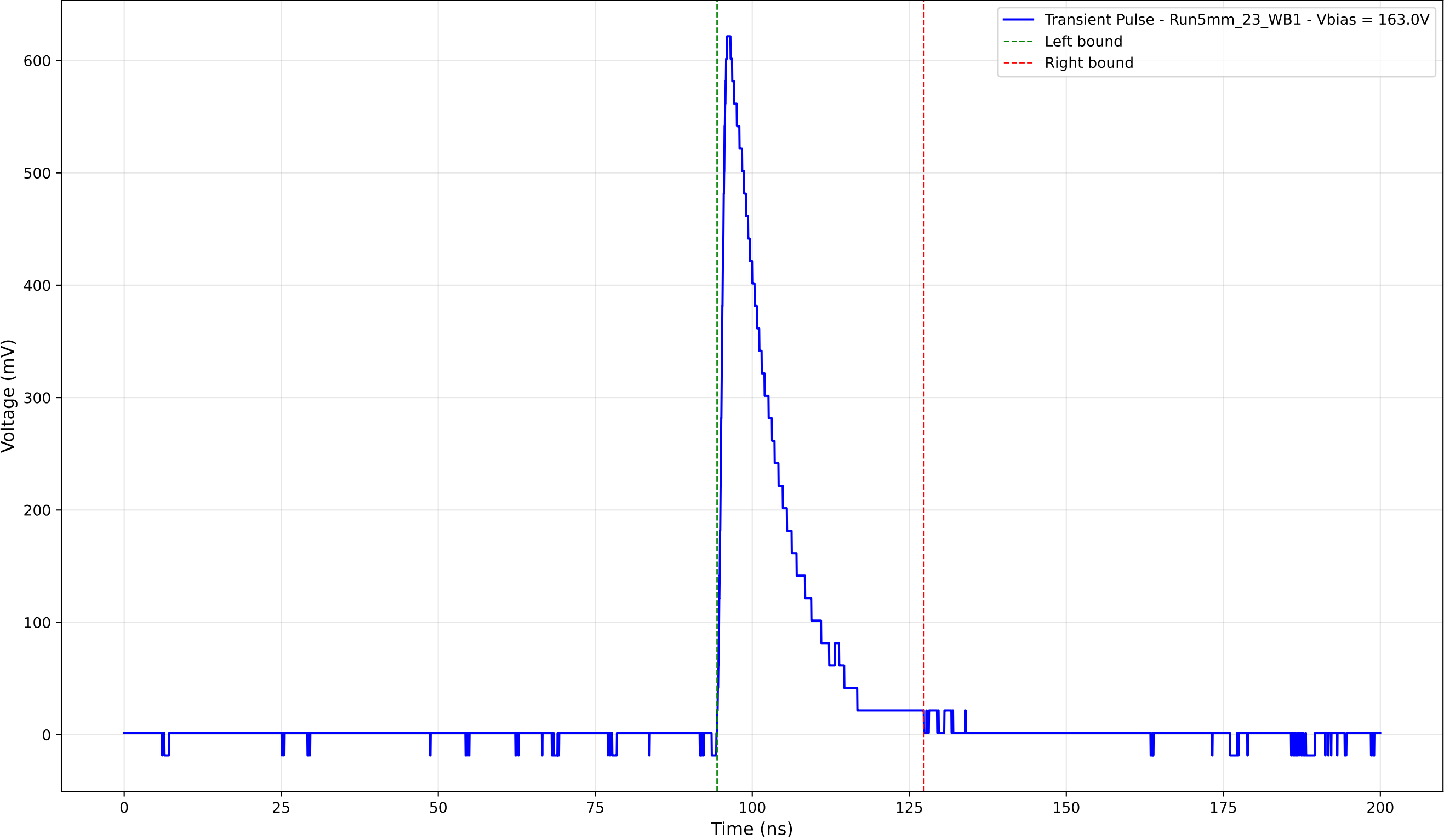
Transient Pulse - Sample: 5mm_23 - Position: 4315.0 \mu\text{m} - Charge: 110.87 pC
