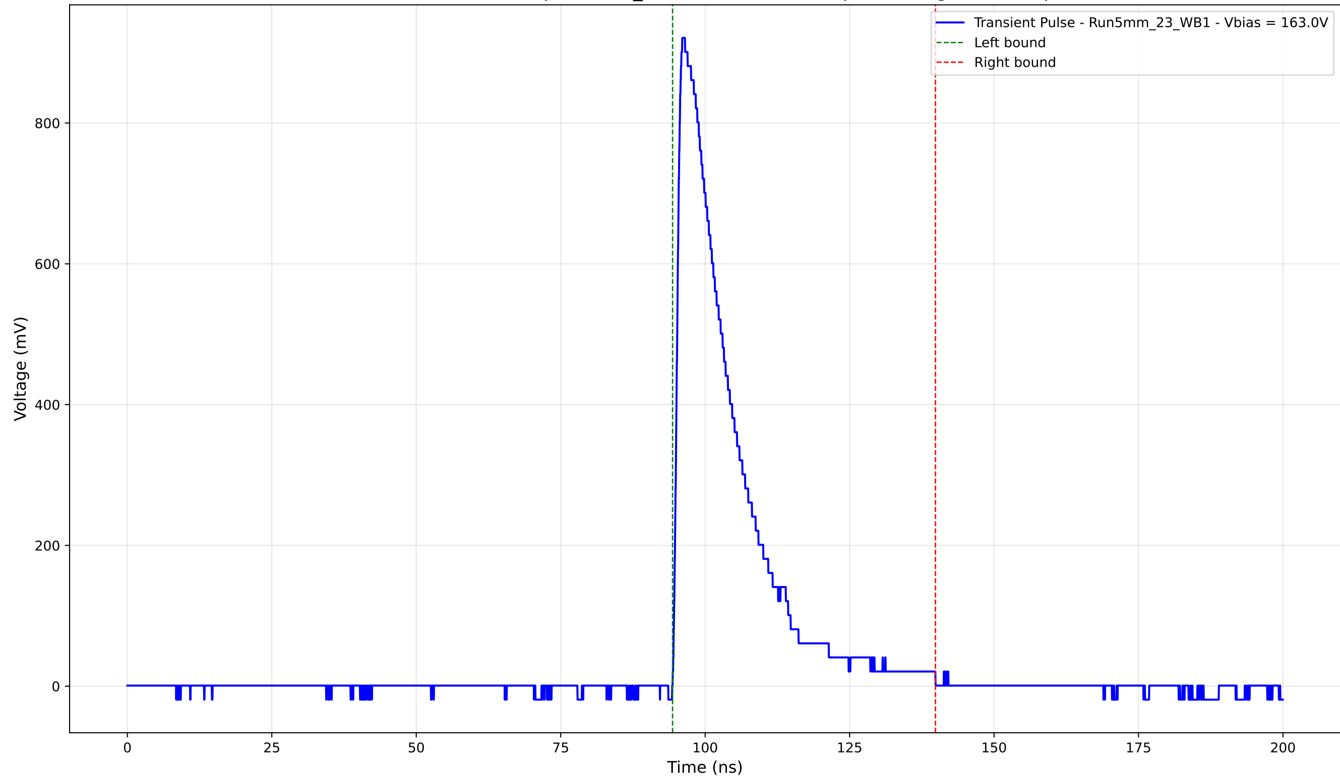
Transient Pulse - Sample: 5mm_23 - Position: 4115.0 \mu\text{m} - Charge: 195.89 pC
