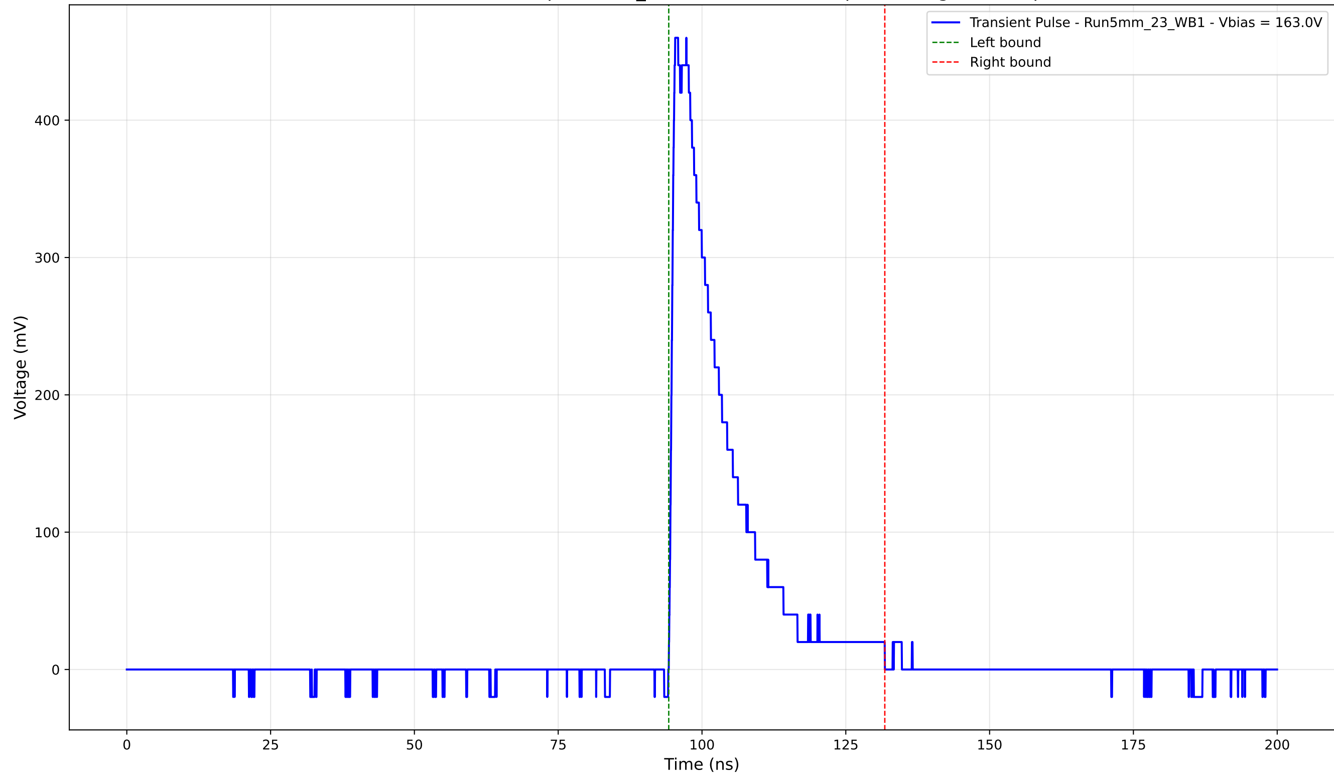
Transient Pulse - Sample: 5mm_23 - Position: 3285.0 \mu\text{m} - Charge: 90.39 pC
