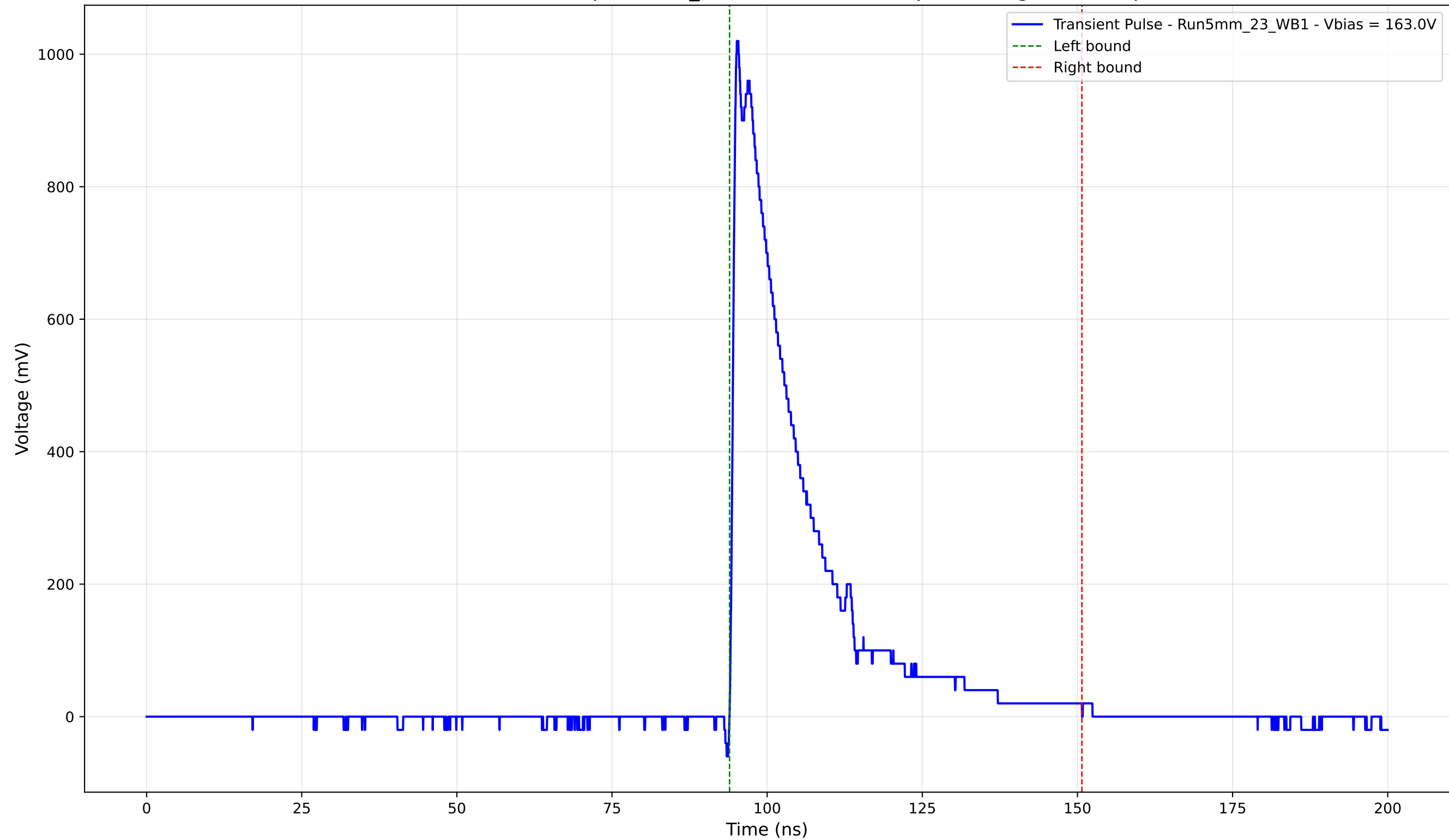
Transient Pulse - Sample: 5mm_23 - Position: 3005.0 \mu\text{m} - Charge: 231.74 pC
