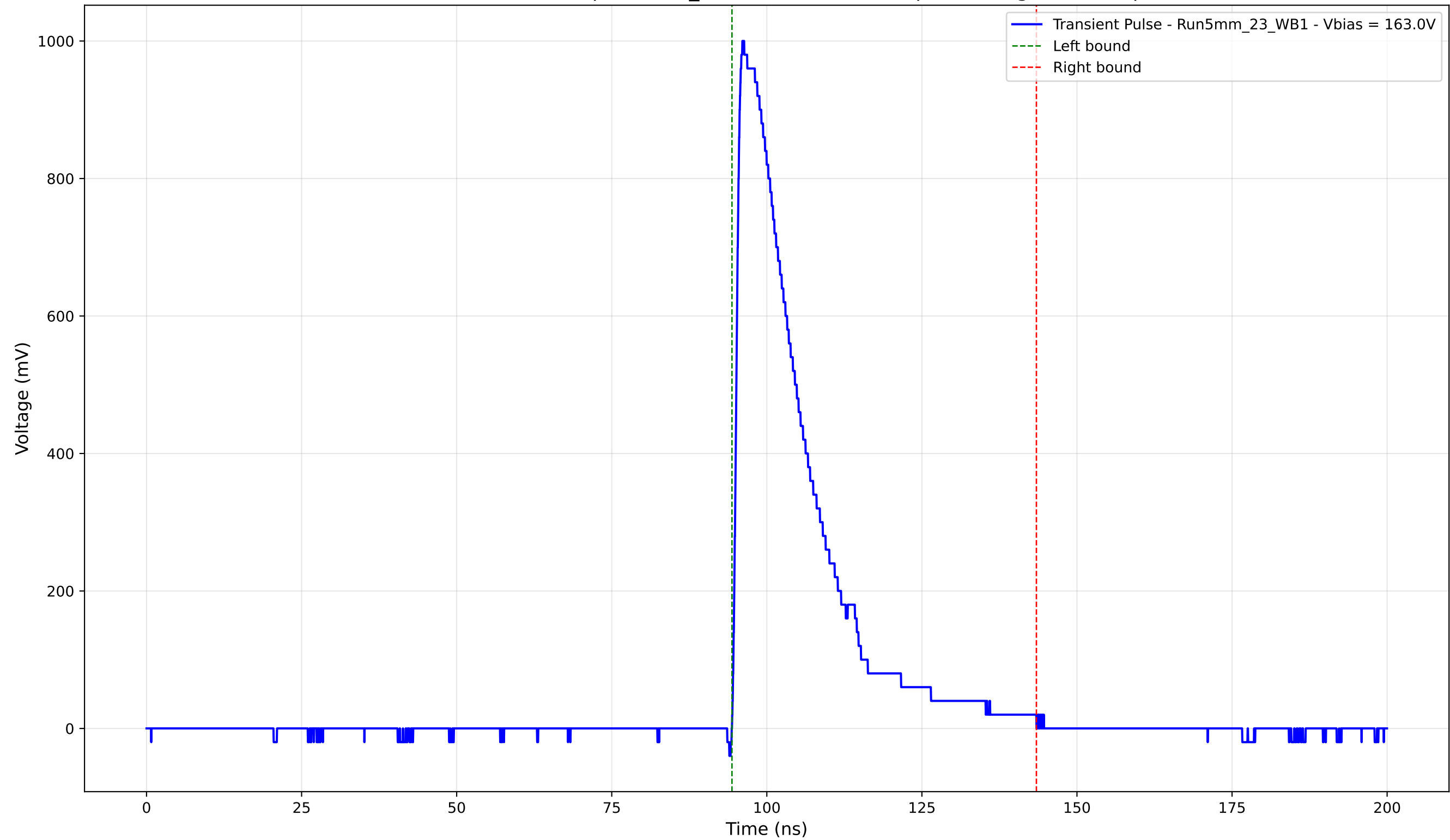
Transient Pulse - Sample: 5mm_23 - Position: 1445.0 \mu\text{m} - Charge: 239.03 pC
