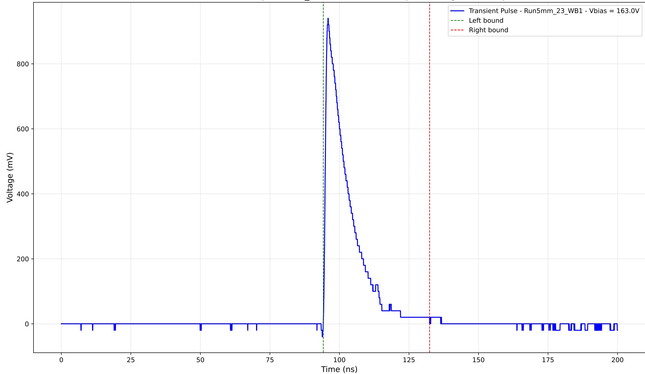
Transient Pulse - Sample: 5mm_23 - Position: 4650.0 \mu\text{m} - Charge: 170.60 pC
