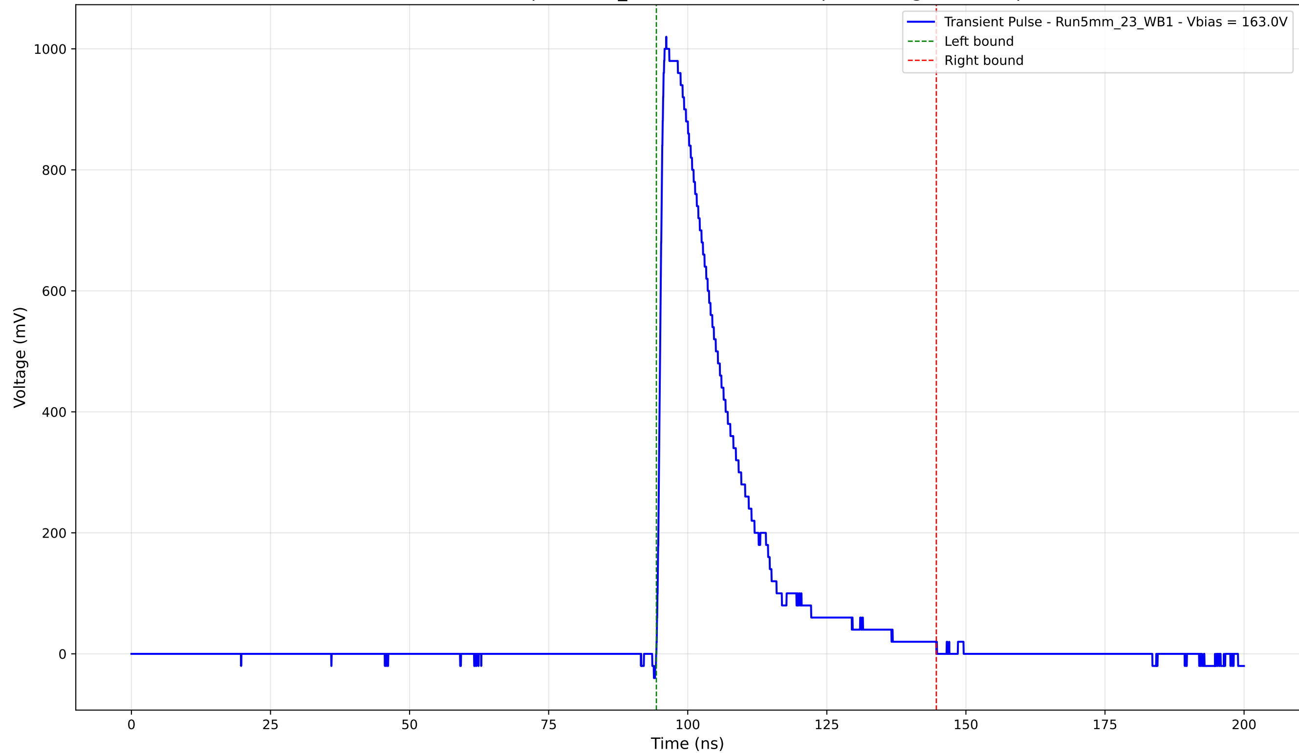
Transient Pulse - Sample: 5mm_23 - Position: 1540.0 \mu\text{m} - Charge: 255.18 pC
