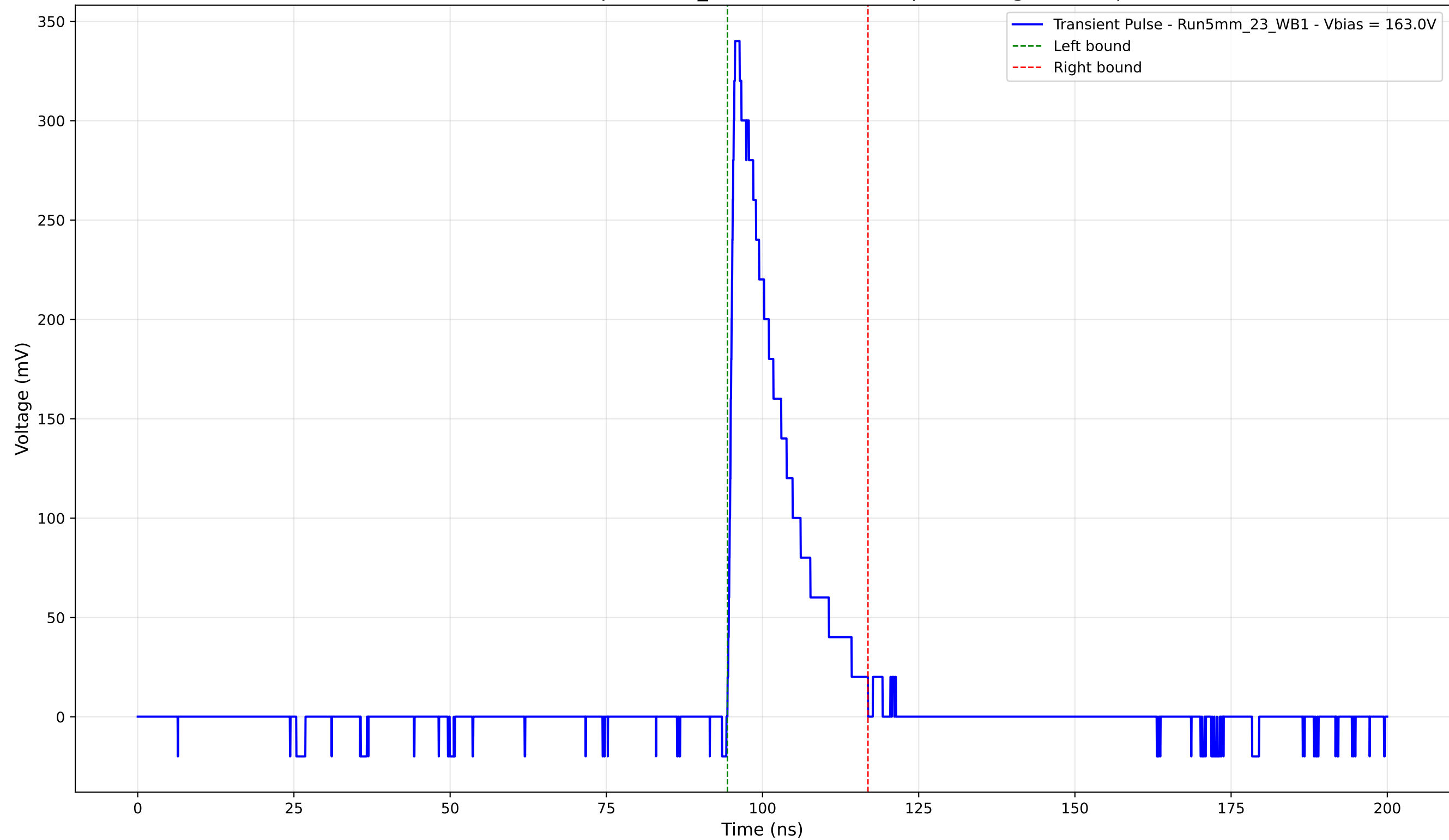
Transient Pulse - Sample: 5mm_23 - Position: 740.0 \mu\text{m} - Charge: 57.27 pC
