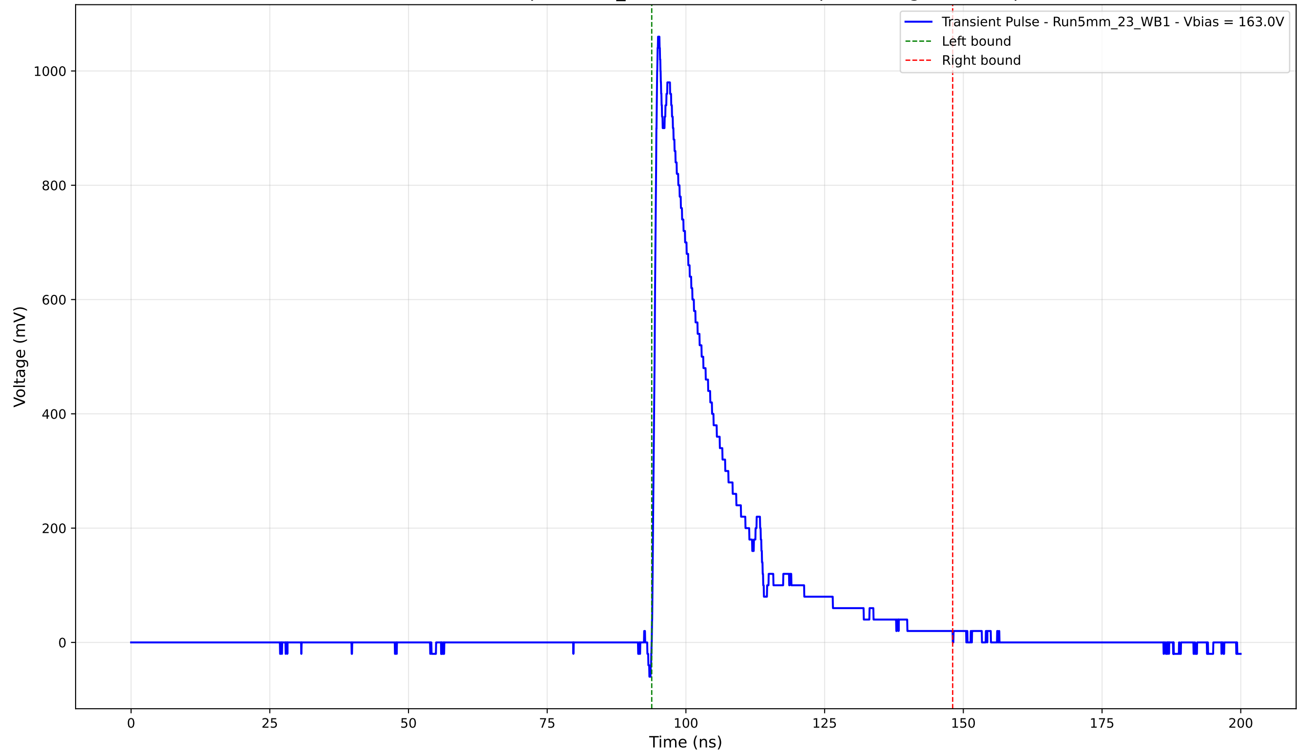
Transient Pulse - Sample: 5mm_23 - Position: 2860.0 \mu\text{m} - Charge: 240.10 pC
