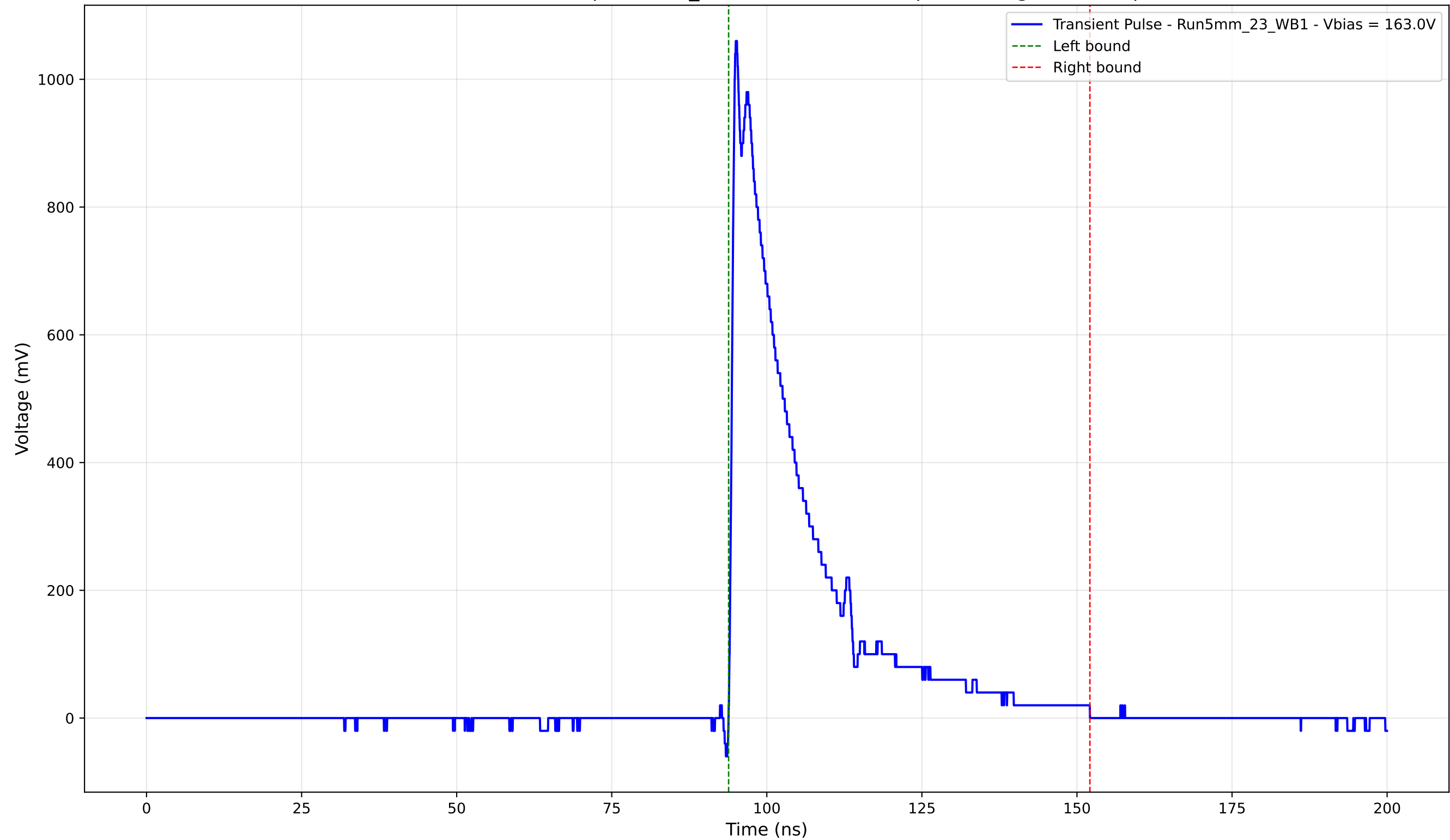
Transient Pulse - Sample: 5mm_23 - Position: 2650.0 \mu\text{m} - Charge: 236.46 pC
