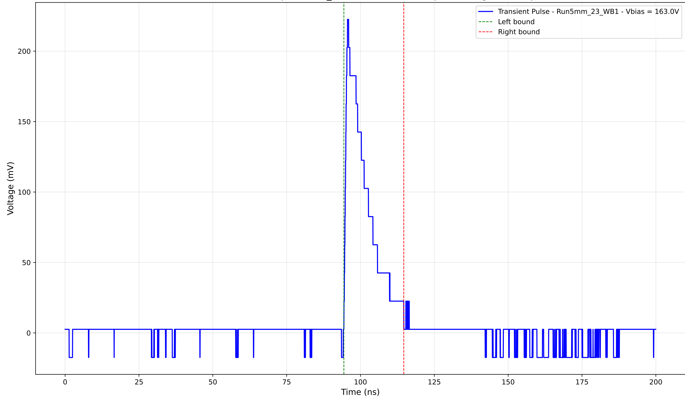
Transient Pulse - Sample: 5mm_23 - Position: 4760.0 \mu\text{m} - Charge: 34.72 pC
