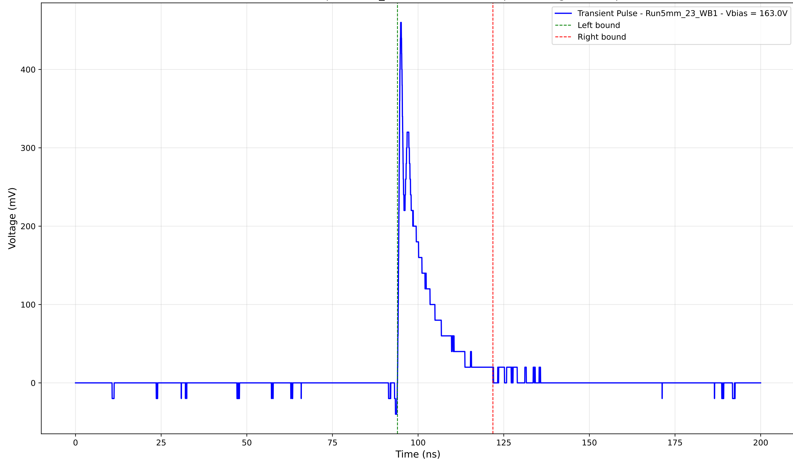
Transient Pulse - Sample: 5mm_23 - Position: 2765.0 \mu\text{m} - Charge: 56.77 pC
