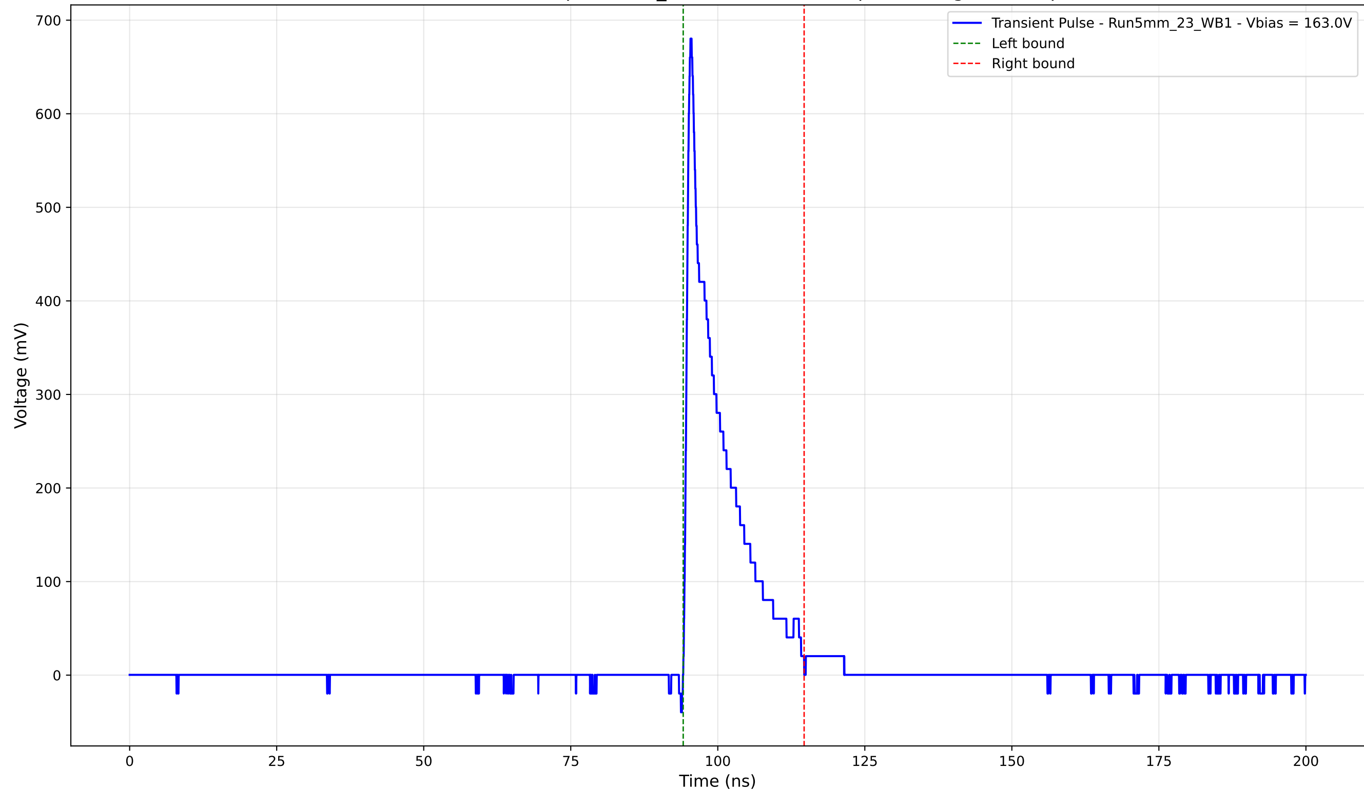
Transient Pulse - Sample: 5mm_23 - Position: 310.0 \mu\text{m} - Charge: 82.91 pC
