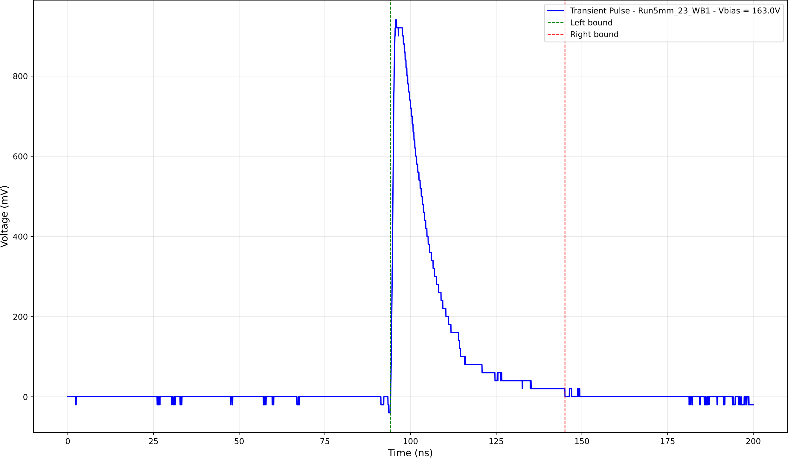
Transient Pulse - Sample: 5mm_23 - Position: 3465.0 \mu\text{m} - Charge: 219.16 pC
