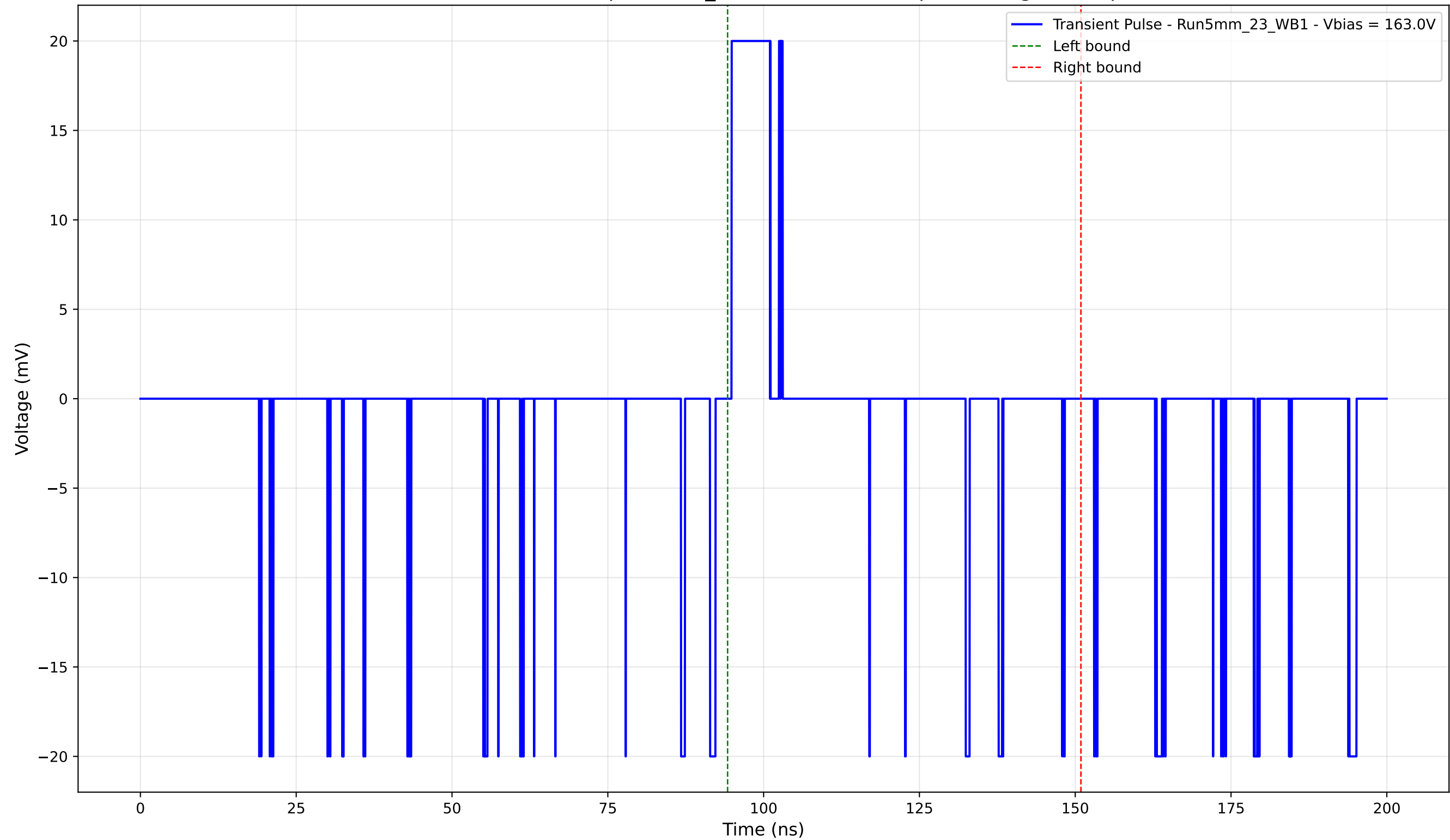
Transient Pulse - Sample: 5mm_23 - Position: 230.0 \mu\text{m} - Charge: 2.01 pC
