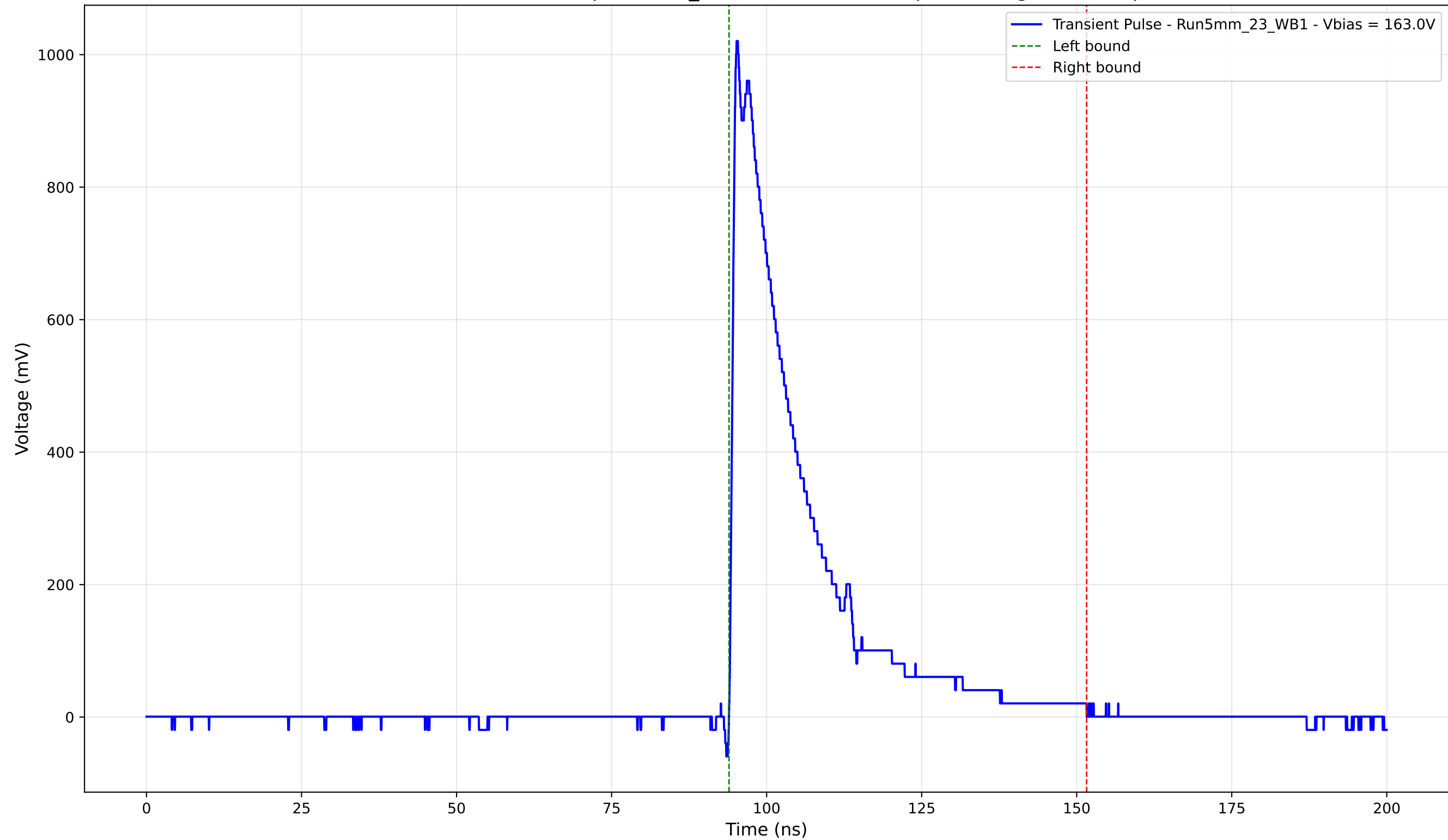
Transient Pulse - Sample: 5mm_23 - Position: 2465.0 \mu\text{m} - Charge: 233.06 pC
