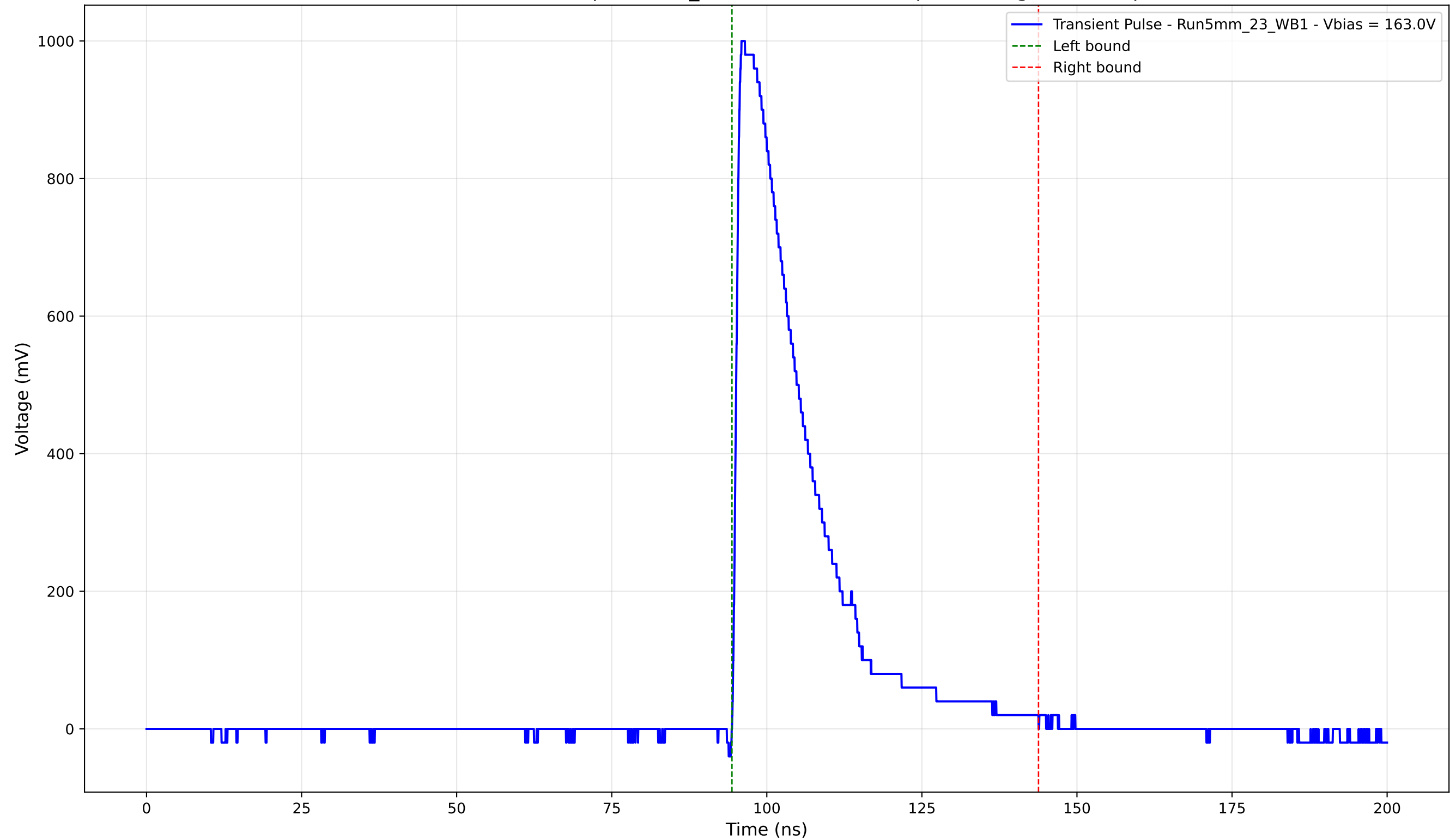
Transient Pulse - Sample: 5mm_23 - Position: 1480.0 \mu\text{m} - Charge: 246.82 pC
