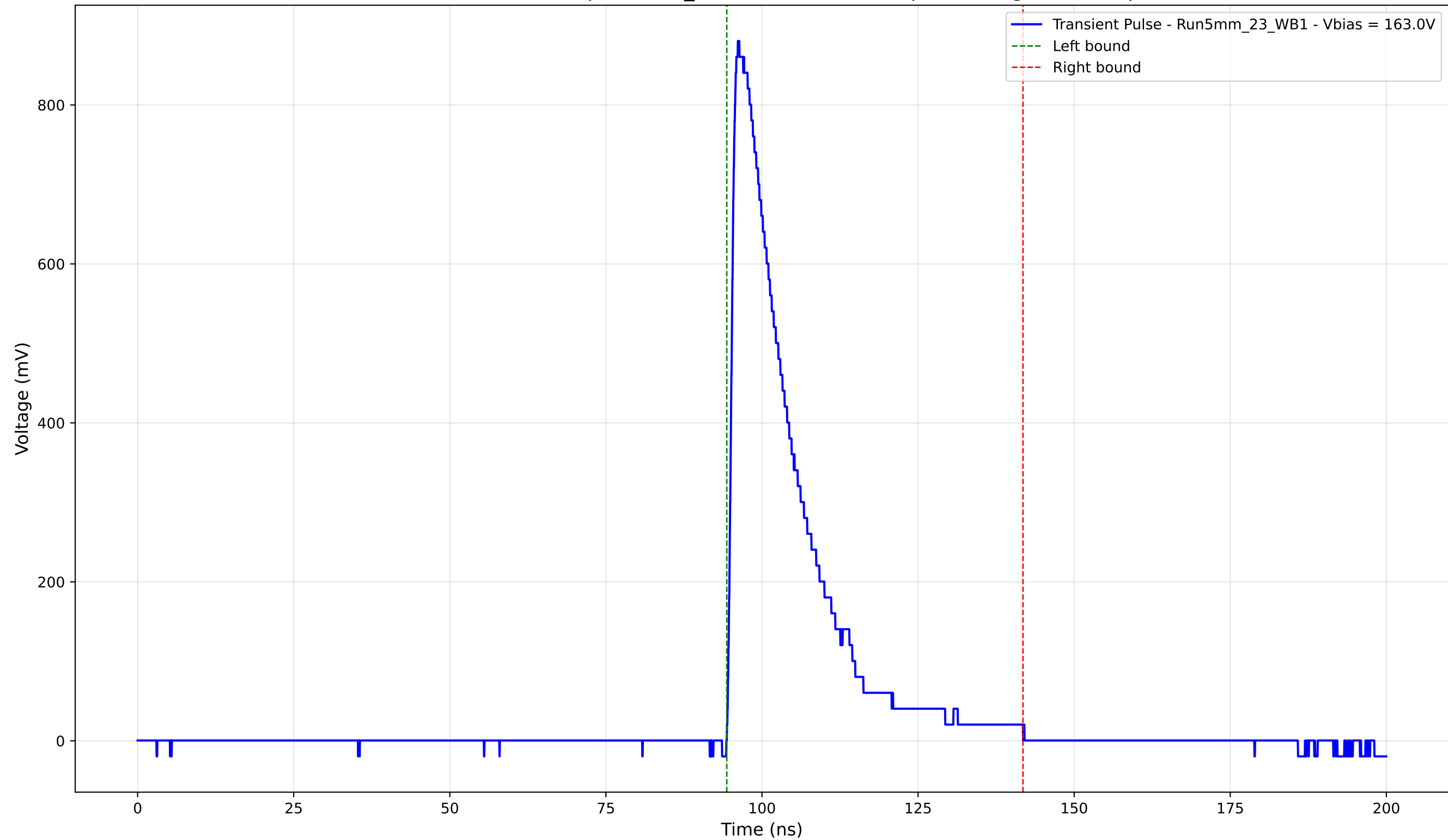
Transient Pulse - Sample: 5mm_23 - Position: 1655.0 \mu\text{m} - Charge: 190.08 pC
