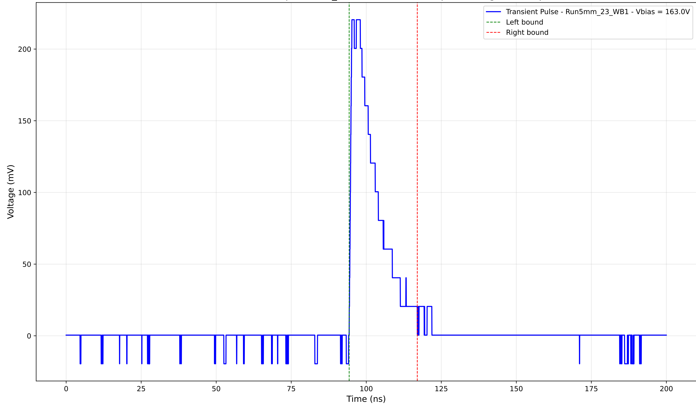
Transient Pulse - Sample: 5mm_23 - Position: 3260.0 \mu\text{m} - Charge: 42.22 pC
