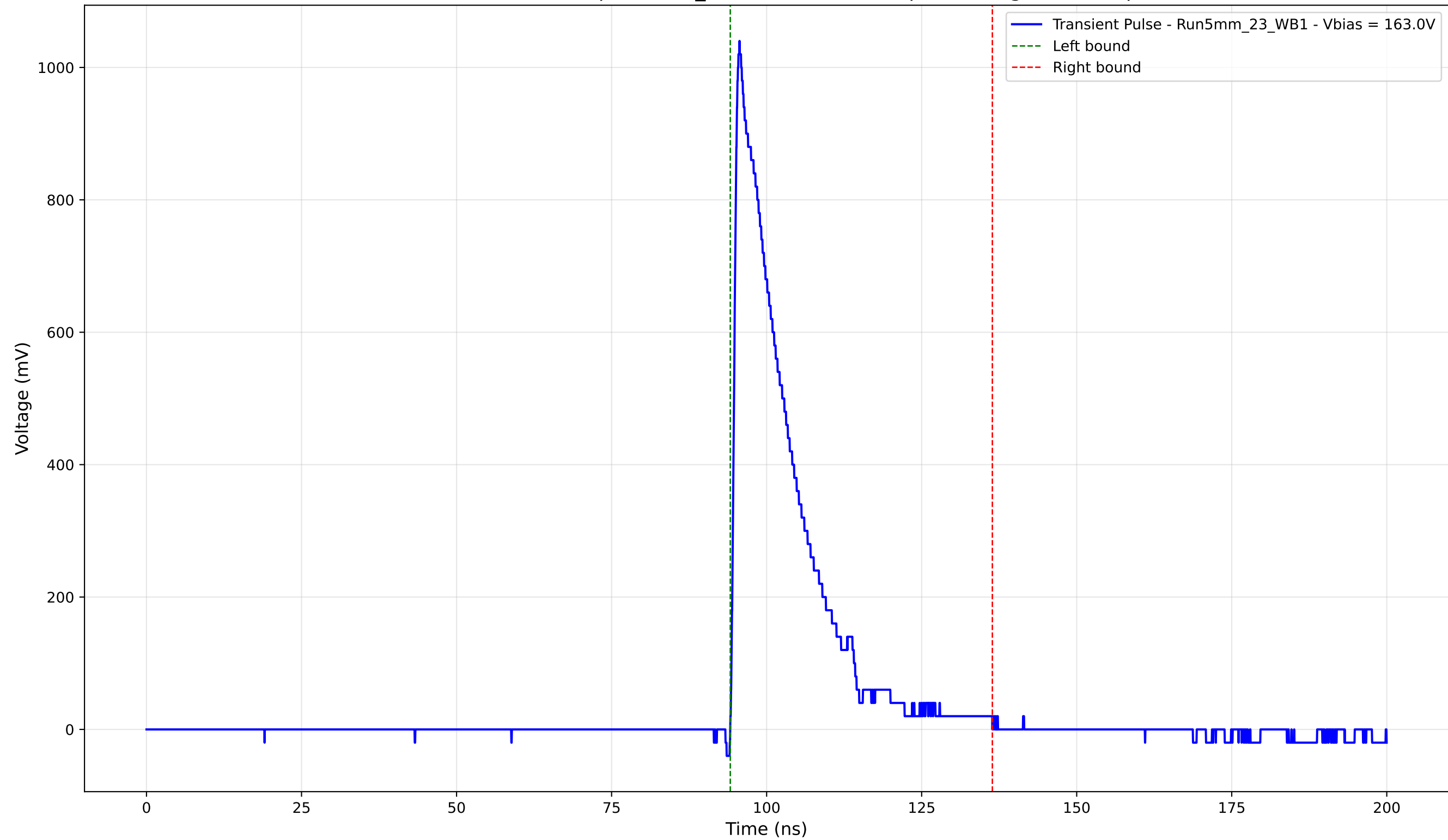
Transient Pulse - Sample: 5mm_23 - Position: 535.0 \mu\text{m} - Charge: 195.53 pC
