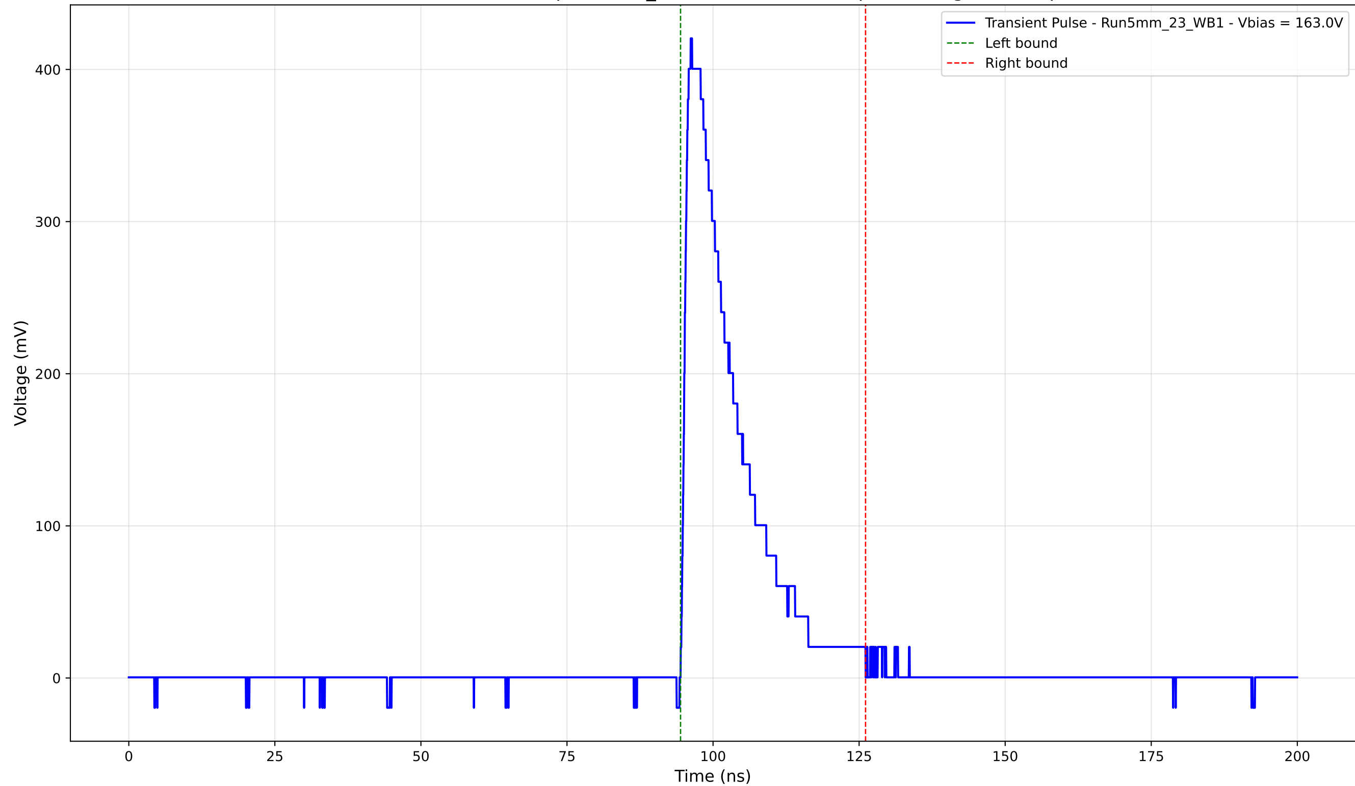
Transient Pulse - Sample: 5mm_23 - Position: 1695.0 \mu\text{m} - Charge: 80.85 pC
