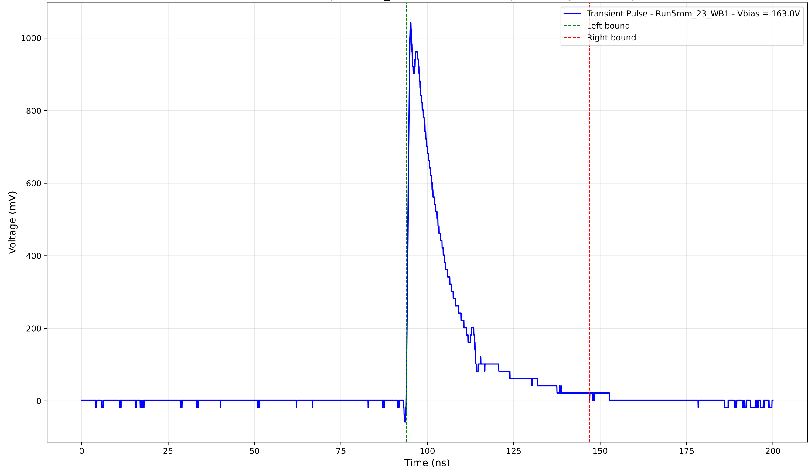
Transient Pulse - Sample: 5mm_23 - Position: 2960.0 \mu\text{m} - Charge: 234.12 pC
