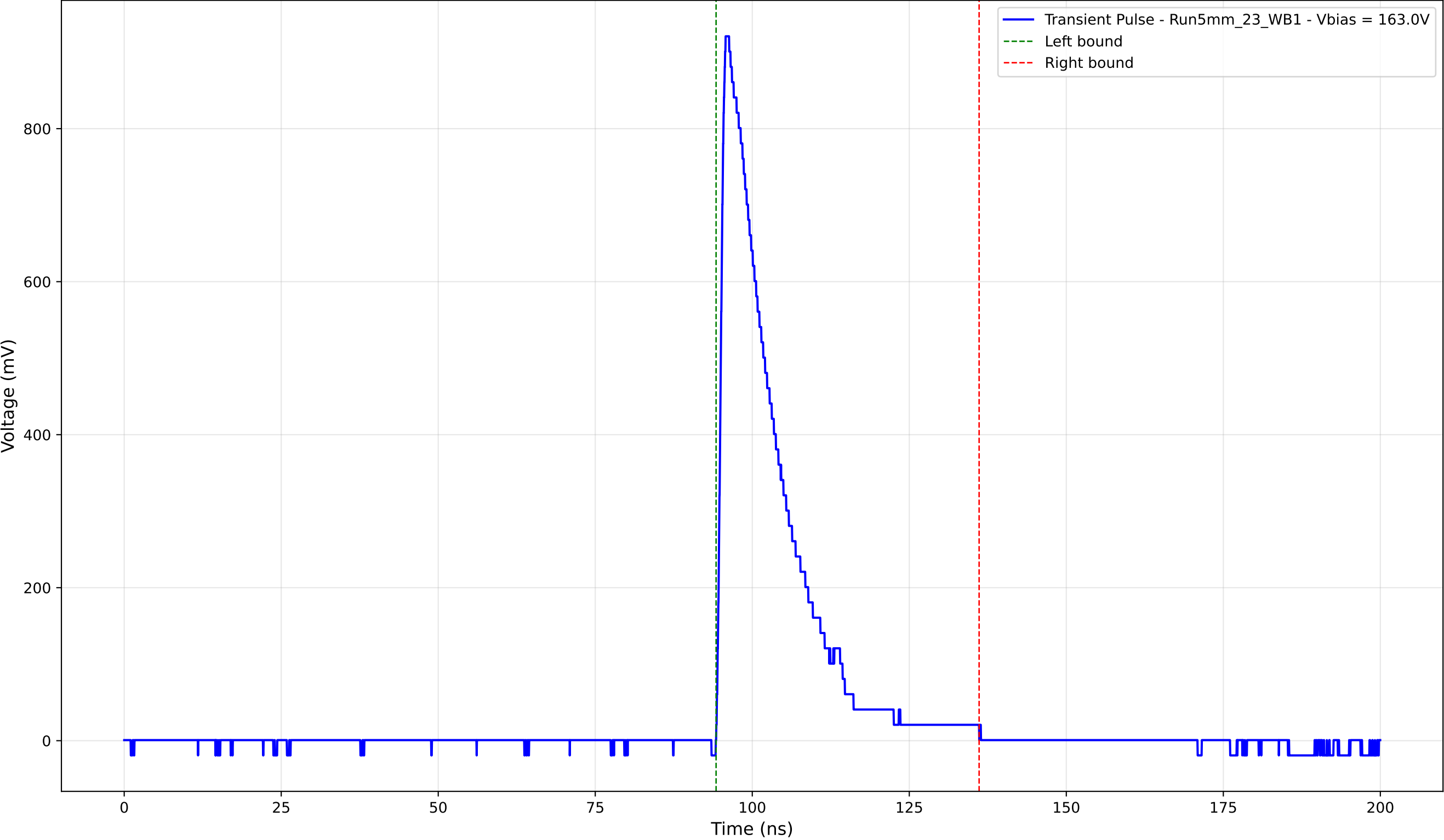
Transient Pulse - Sample: 5mm_23 - Position: 4560.0 \mu\text{m} - Charge: 177.25 pC
