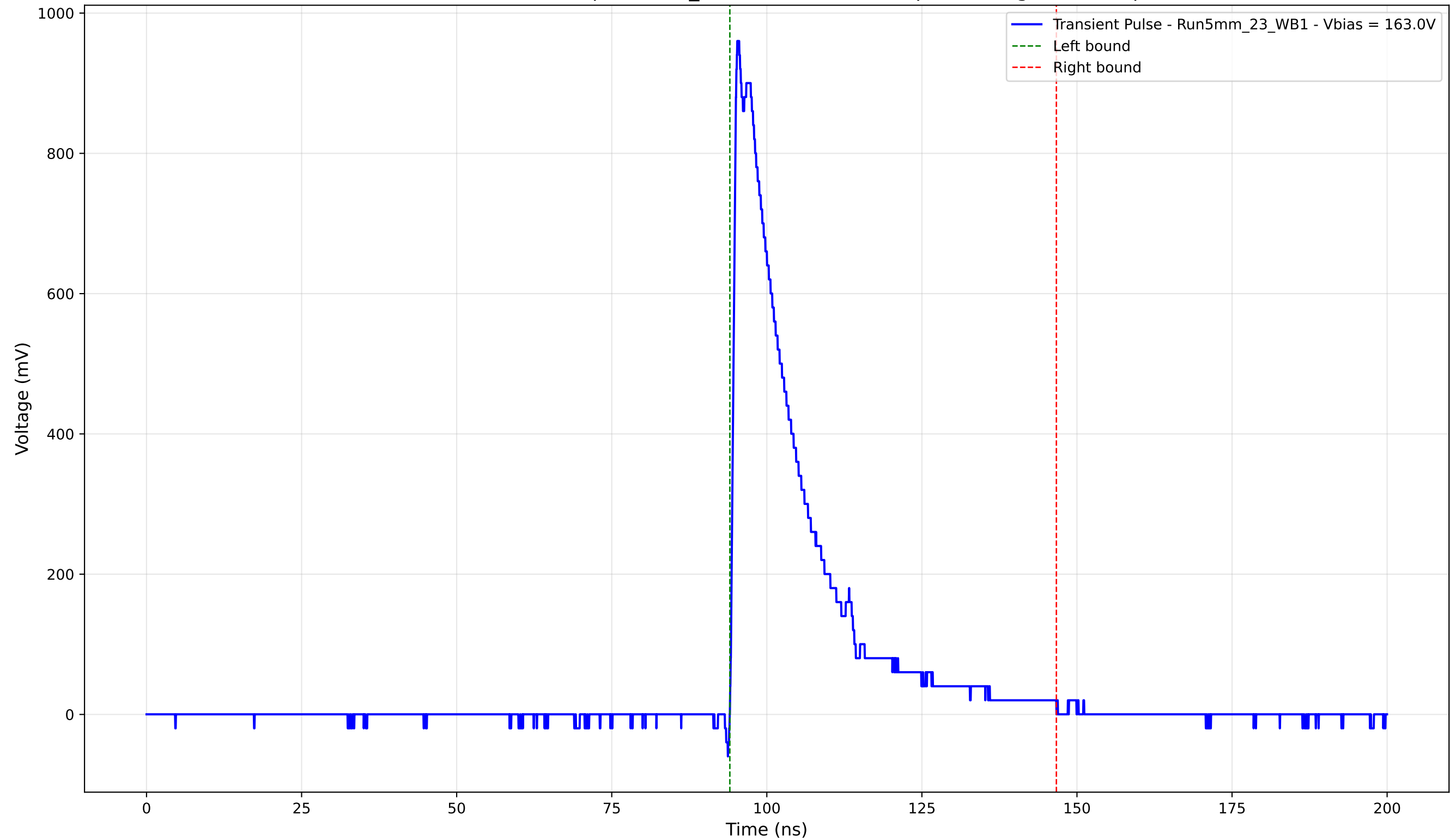
Transient Pulse - Sample: 5mm_23 - Position: 3155.0 \mu\text{m} - Charge: 209.19 pC
