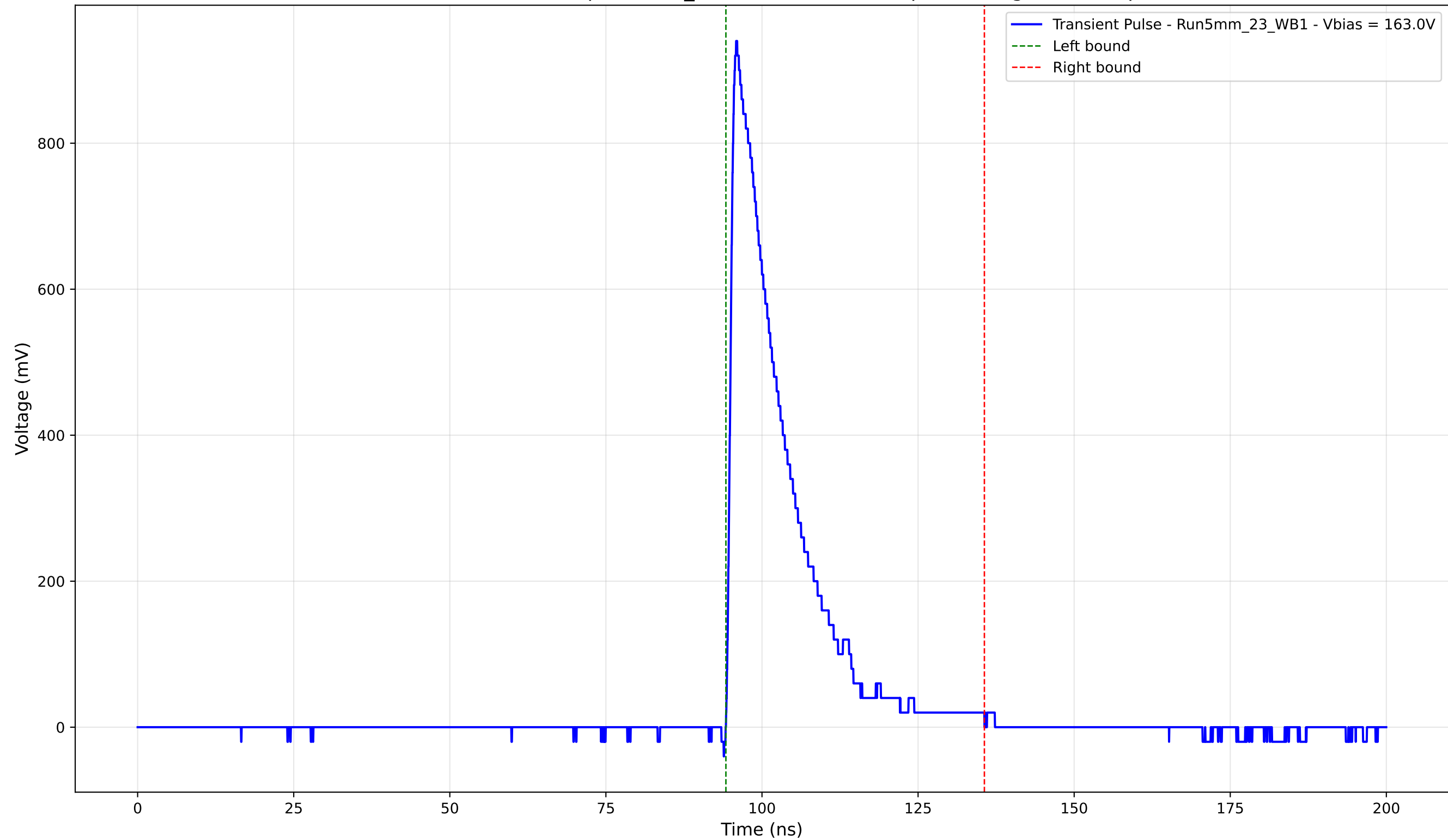
Transient Pulse - Sample: 5mm_23 - Position: 4605.0 \mu\text{m} - Charge: 176.10 pC
