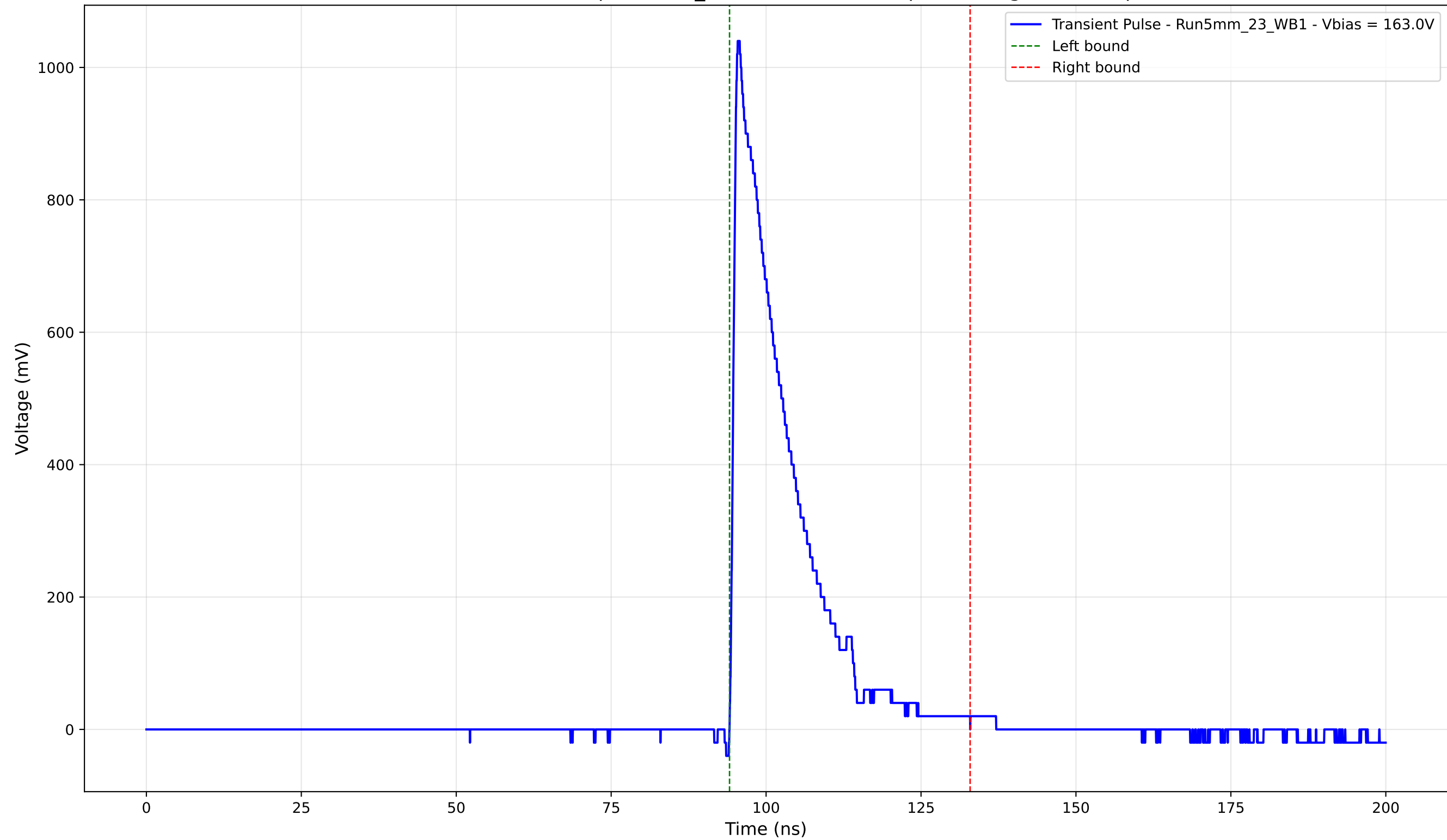
Transient Pulse - Sample: 5mm_23 - Position: 475.0 \mu\text{m} - Charge: 194.24 pC
