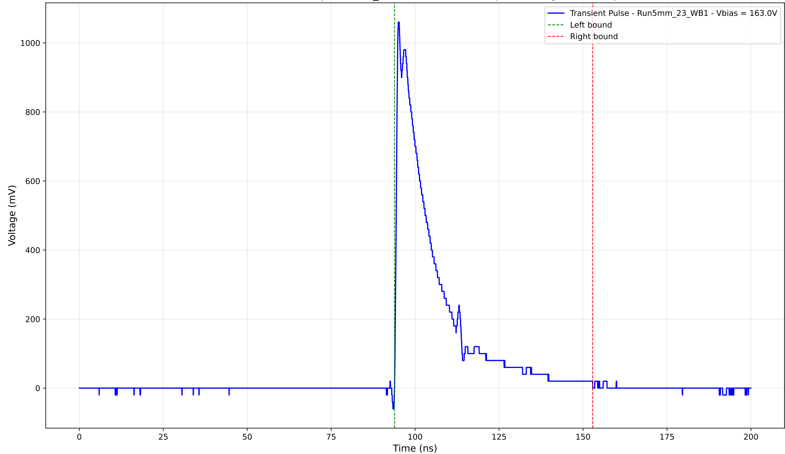
Transient Pulse - Sample: 5mm_23 - Position: 2620.0 \mu\text{m} - Charge: 244.51 pC
