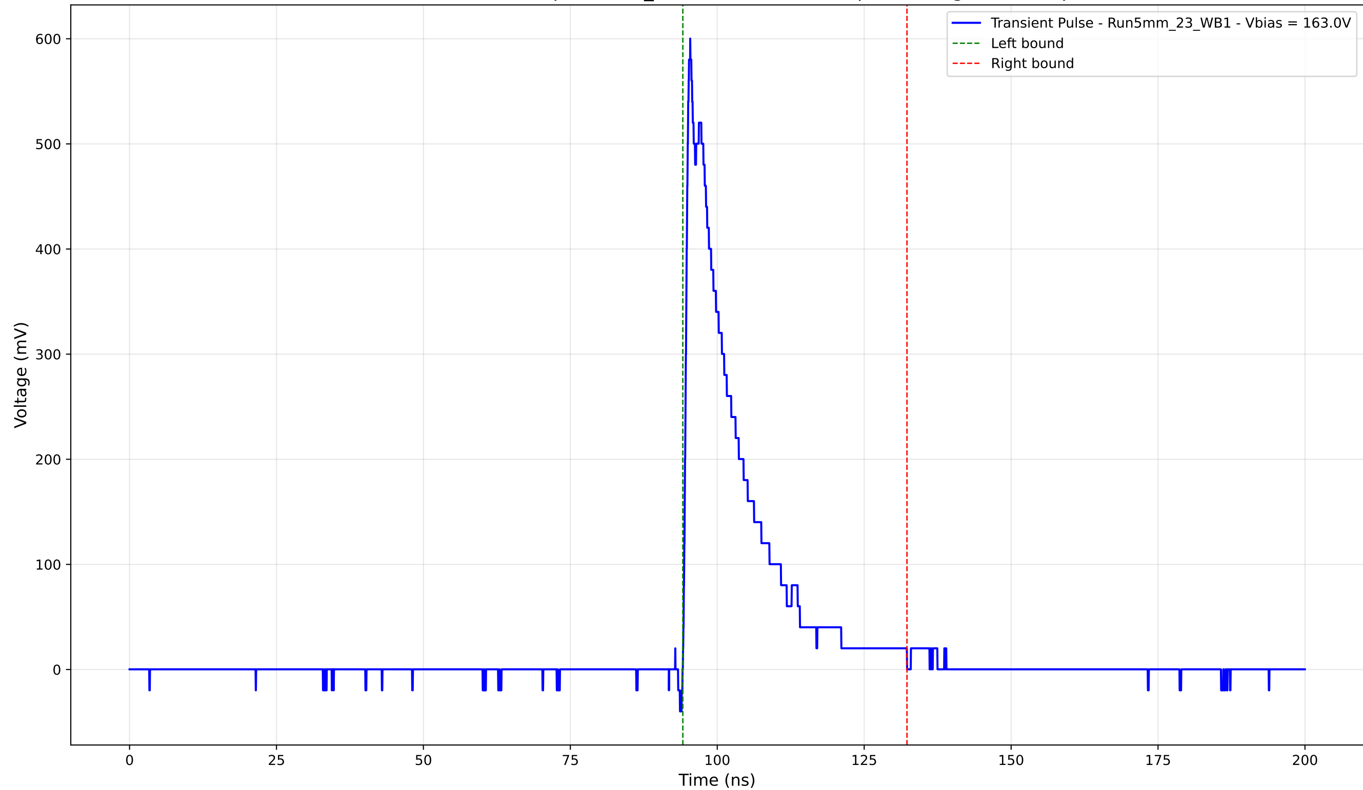
Transient Pulse - Sample: 5mm_23 - Position: 3205.0 \mu\text{m} - Charge: 105.27 pC
