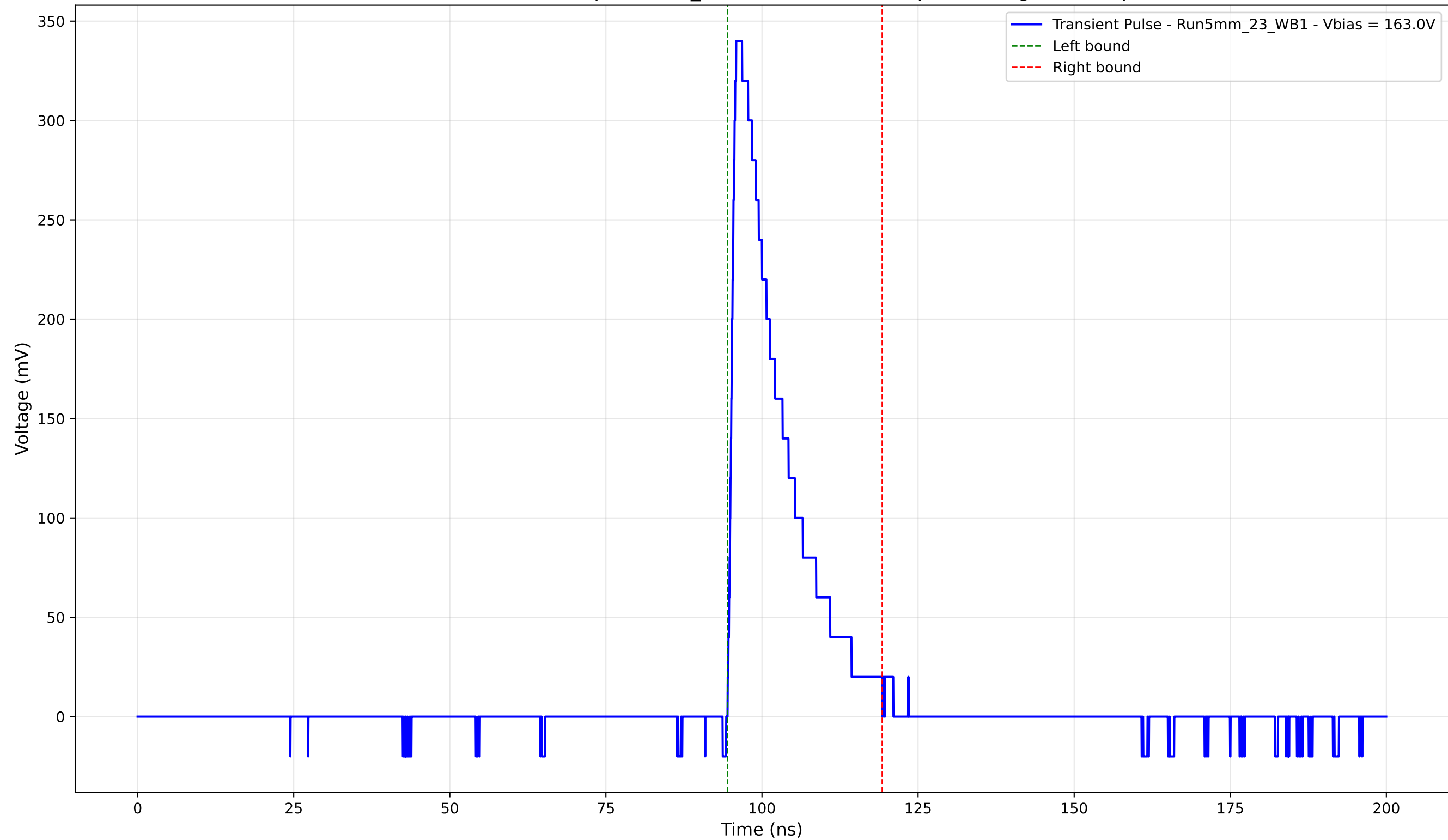
Transient Pulse - Sample: 5mm_23 - Position: 4290.0 \mu\text{m} - Charge: 60.24 pC
