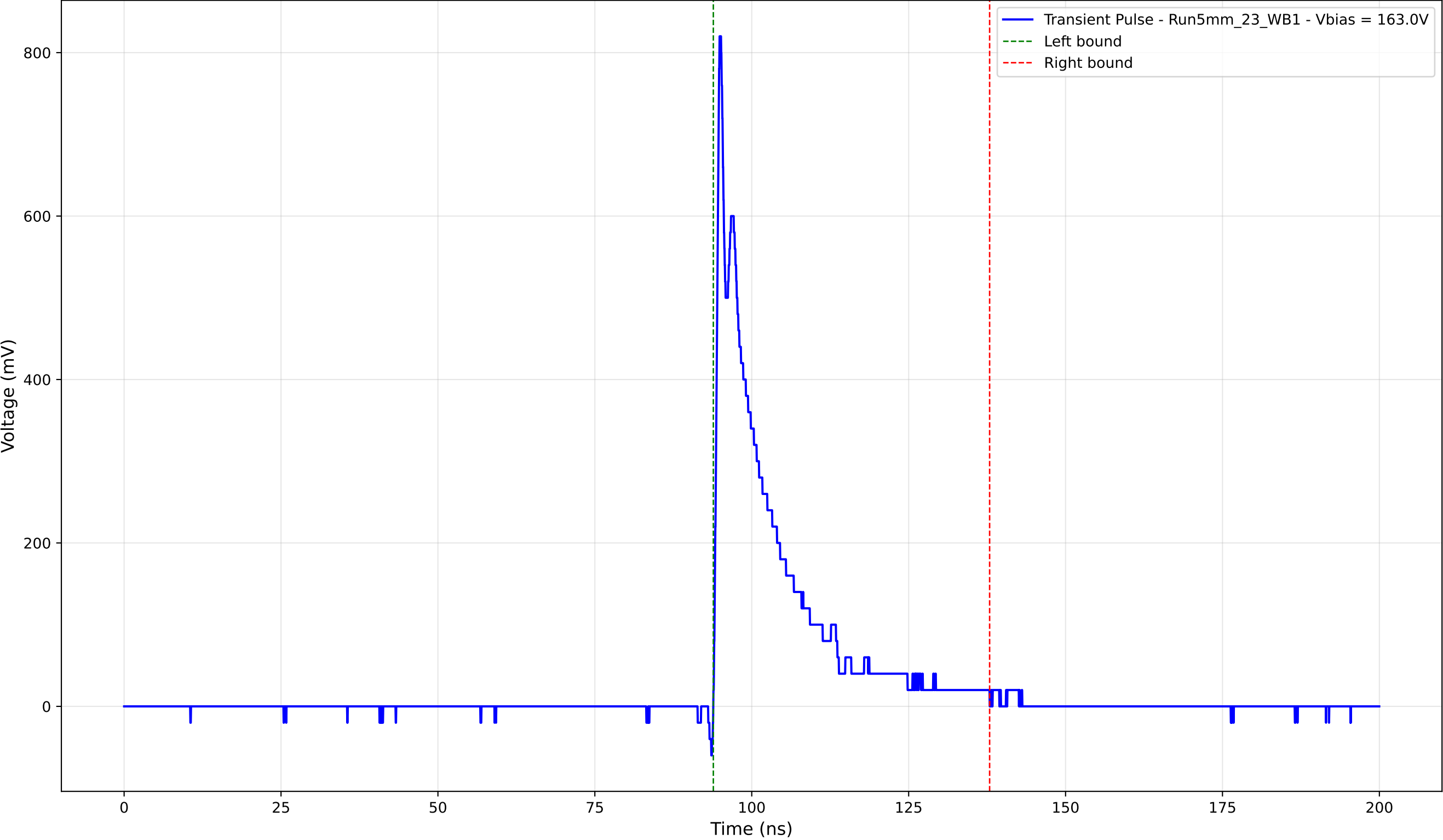
Transient Pulse - Sample: 5mm_23 - Position: 2705.0 \mu\text{m} - Charge: 121.33 pC
