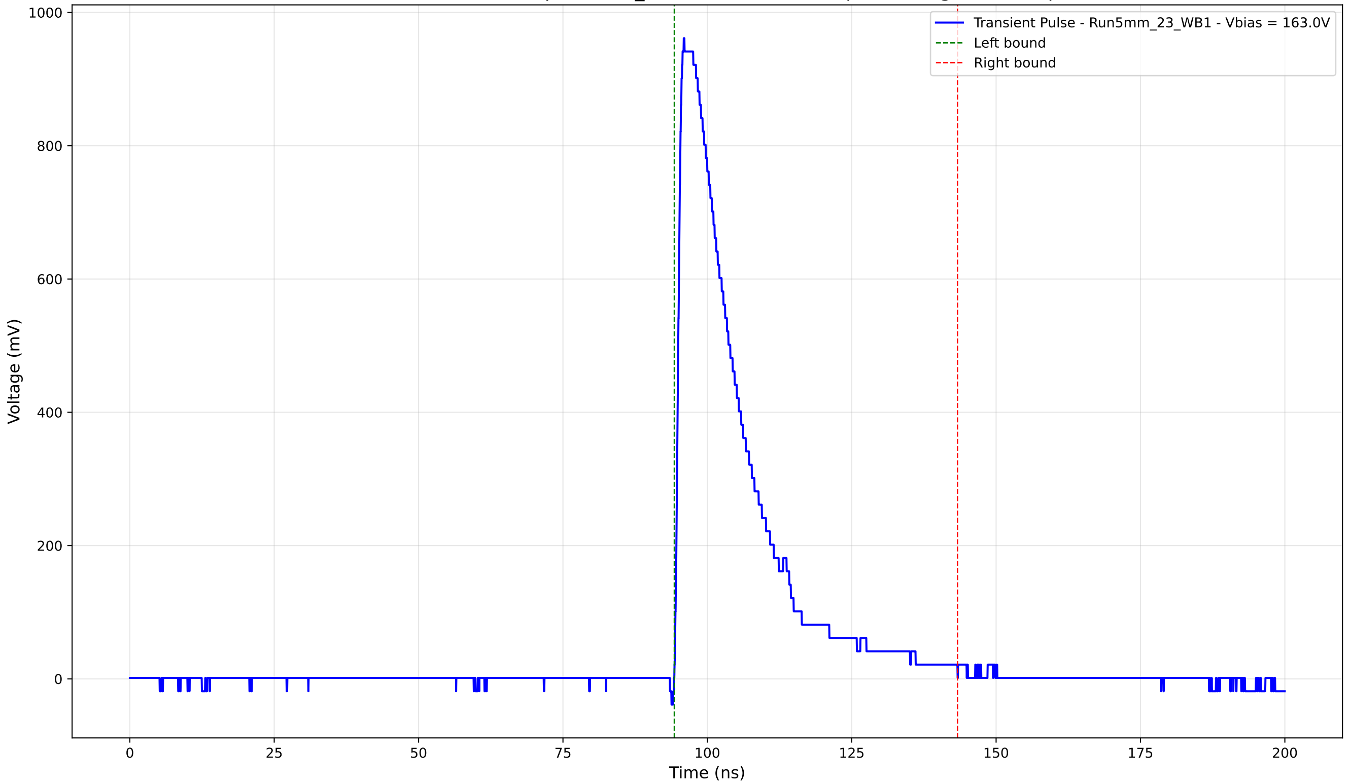
Transient Pulse - Sample: 5mm_23 - Position: 1845.0 \mu\text{m} - Charge: 228.56 pC
