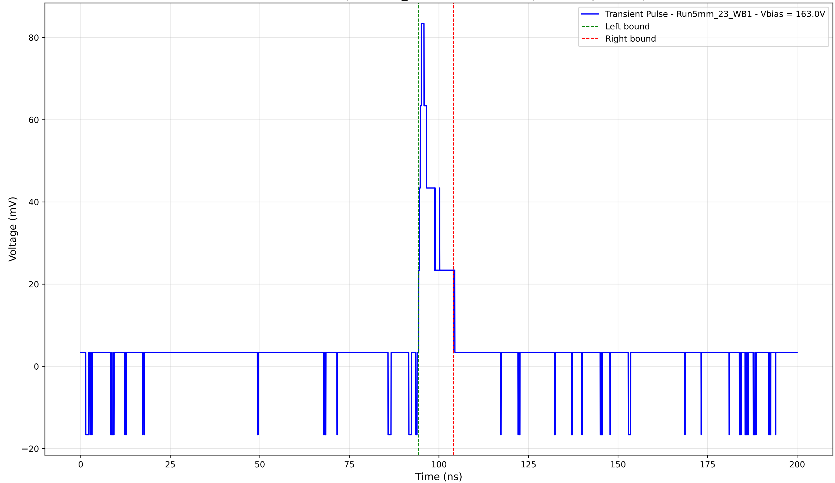
Transient Pulse - Sample: 5mm_23 - Position: 5215.0 \mu\text{m} - Charge: 7.30 pC
