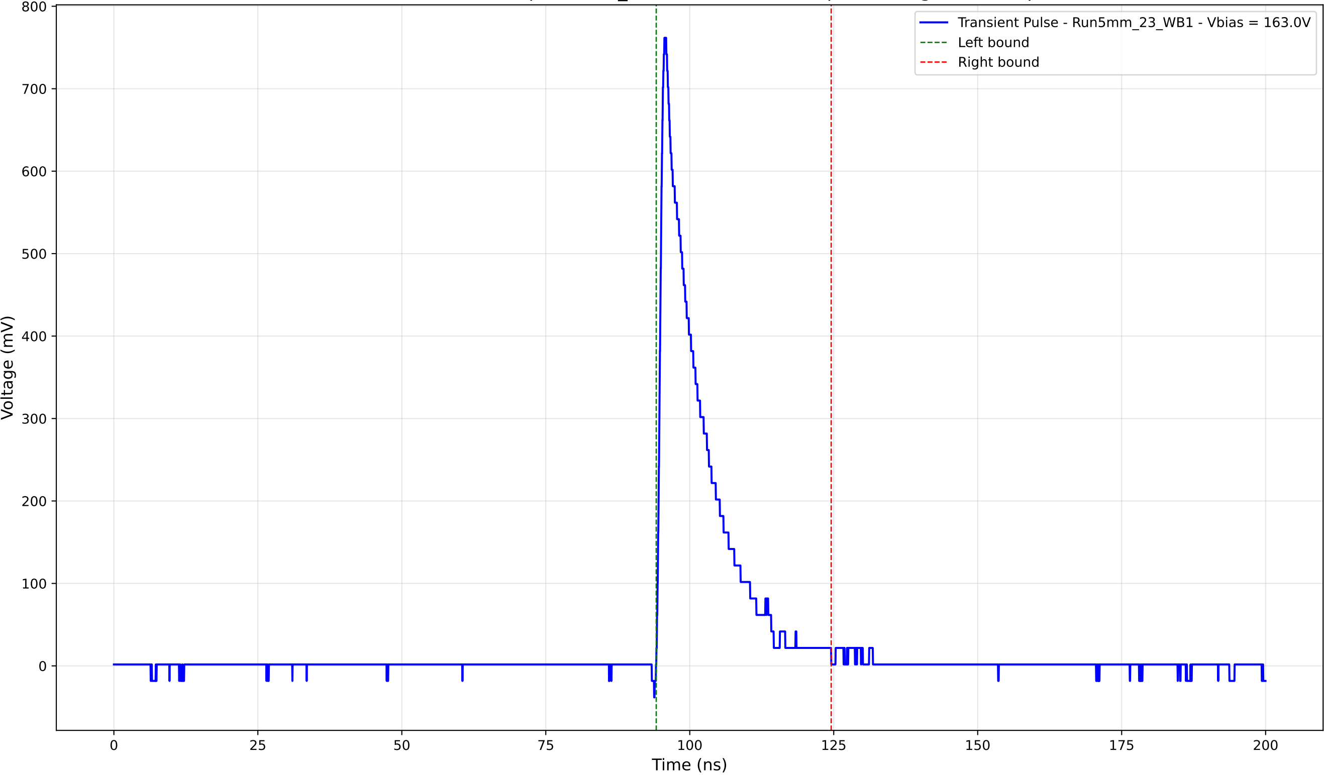
Transient Pulse - Sample: 5mm_23 - Position: 4820.0 \mu\text{m} - Charge: 114.92 pC
