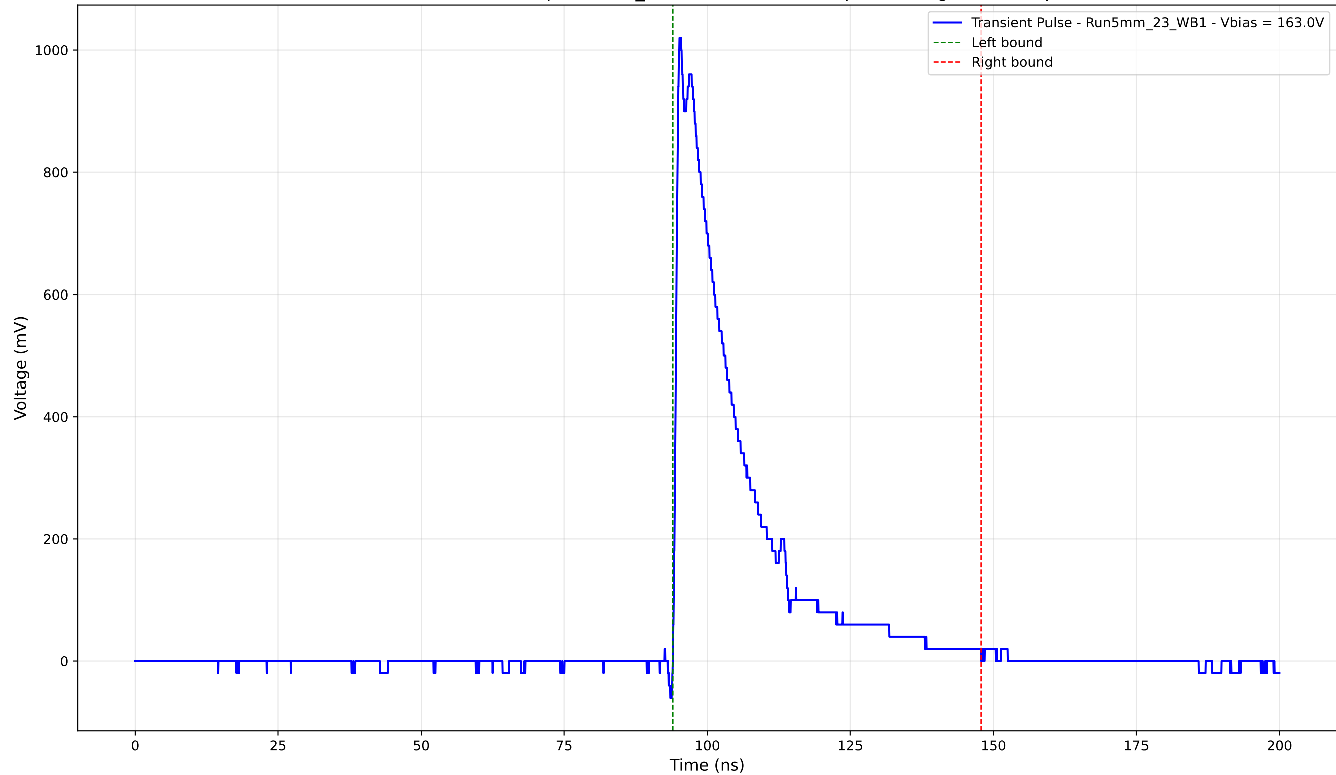
Transient Pulse - Sample: 5mm_23 - Position: 2995.0 \mu\text{m} - Charge: 231.28 pC
