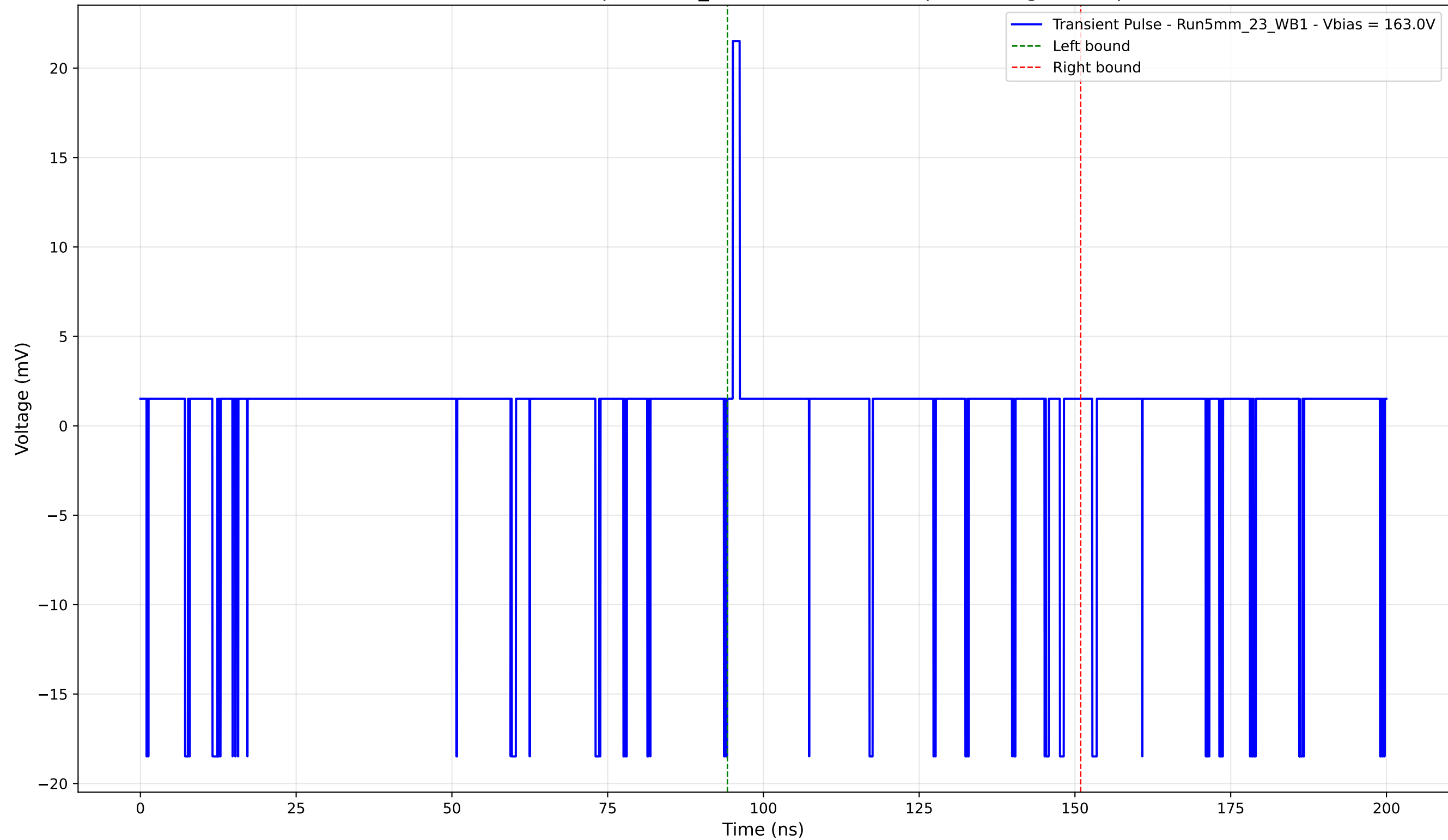
Transient Pulse - Sample: 5mm_23 - Position: 5280.0 \mu\text{m} - Charge: 1.12 pC
