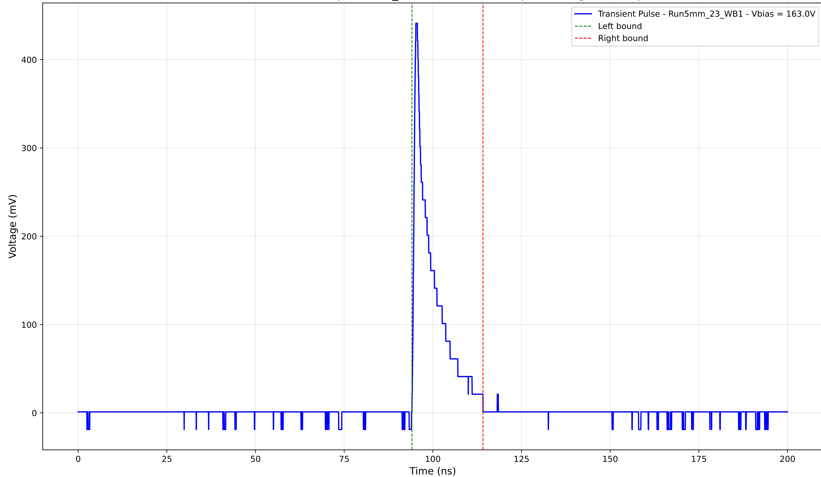
Transient Pulse - Sample: 5mm_23 - Position: 5175.0 \mu\text{m} - Charge: 48.18 pC
