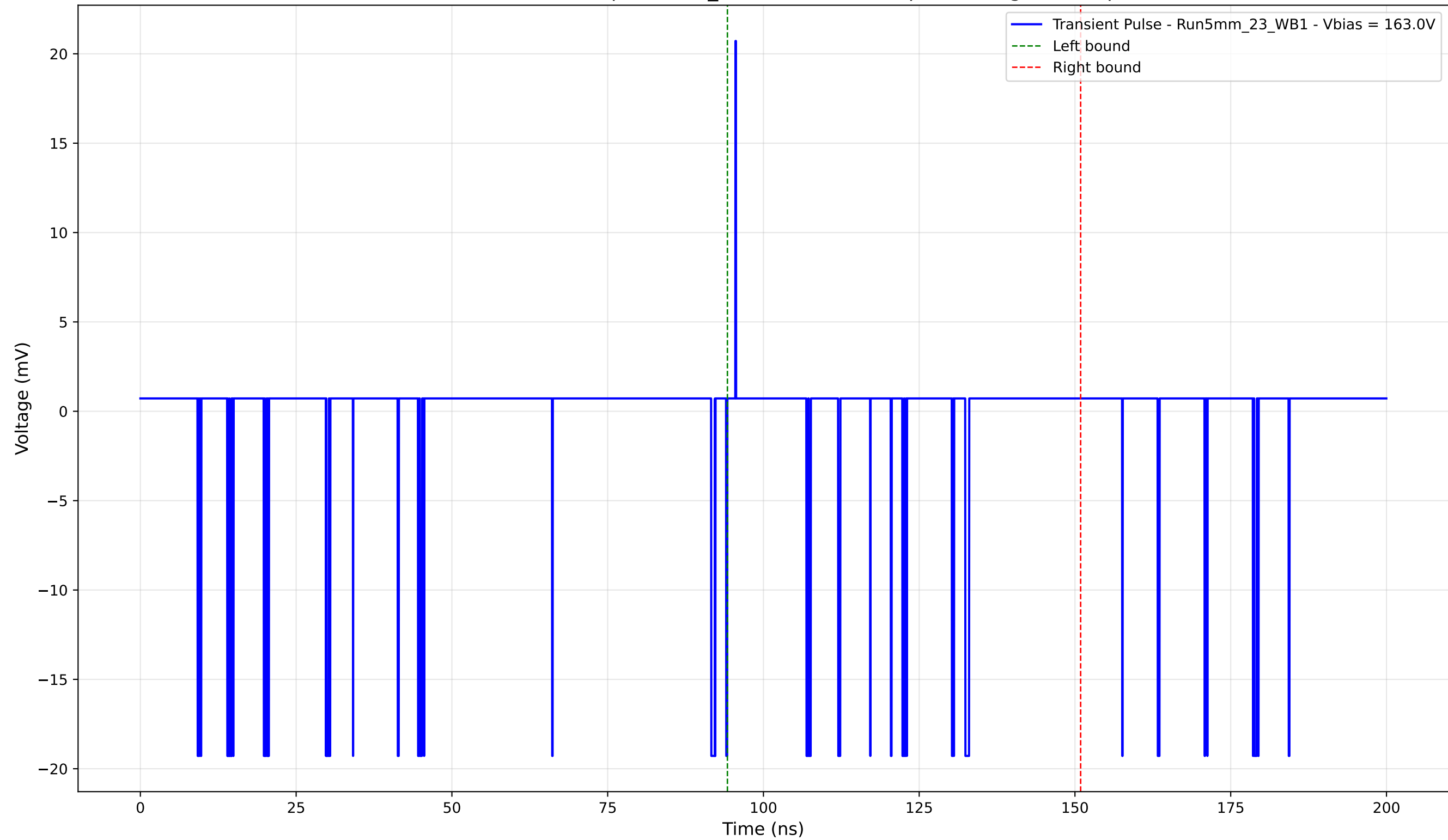
Transient Pulse - Sample: 5mm_23 - Position: 55.0 \mu\text{m} - Charge: -0.14 pC
