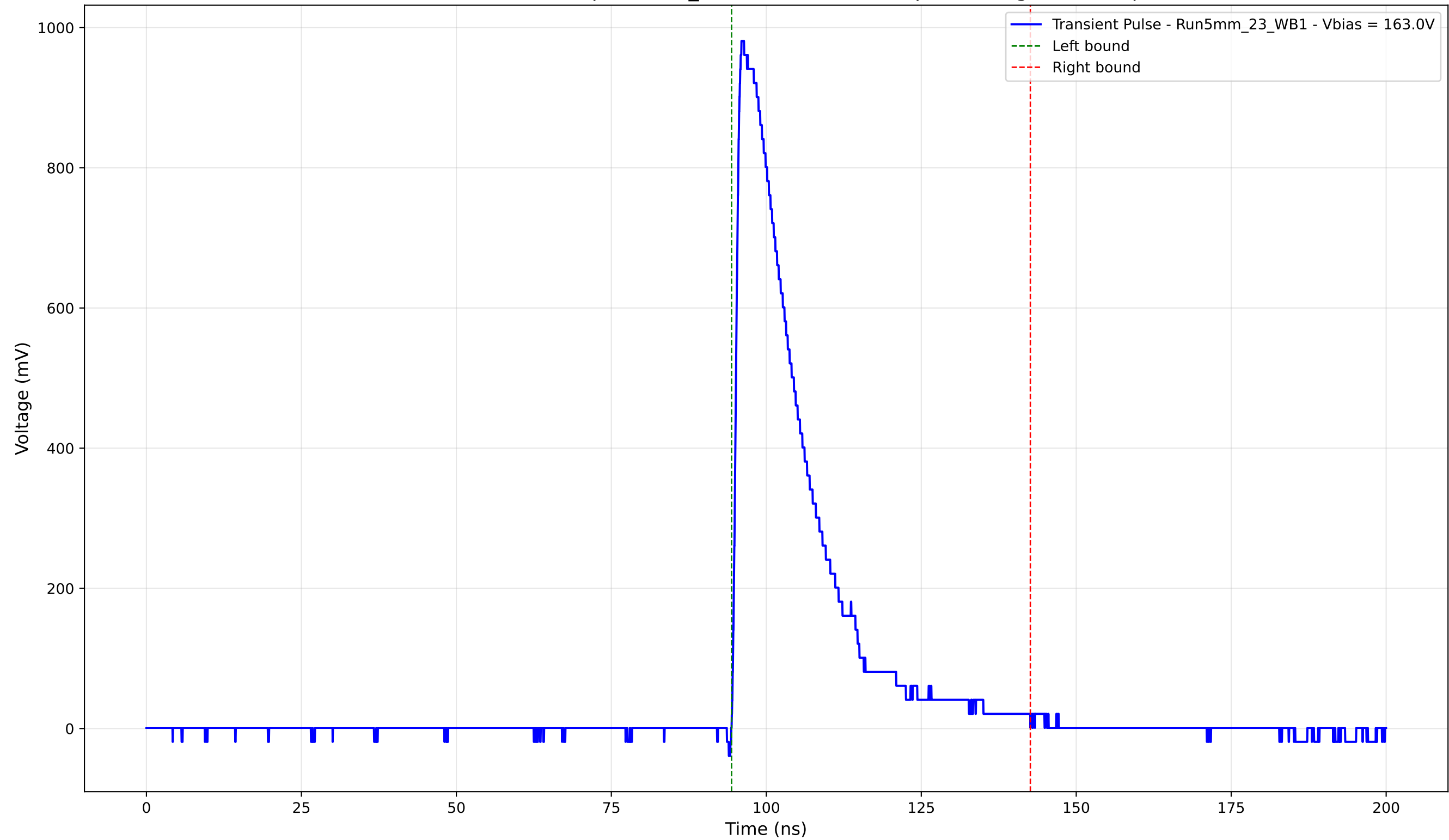
Transient Pulse - Sample: 5mm_23 - Position: 1390.0 \mu\text{m} - Charge: 229.41 pC
