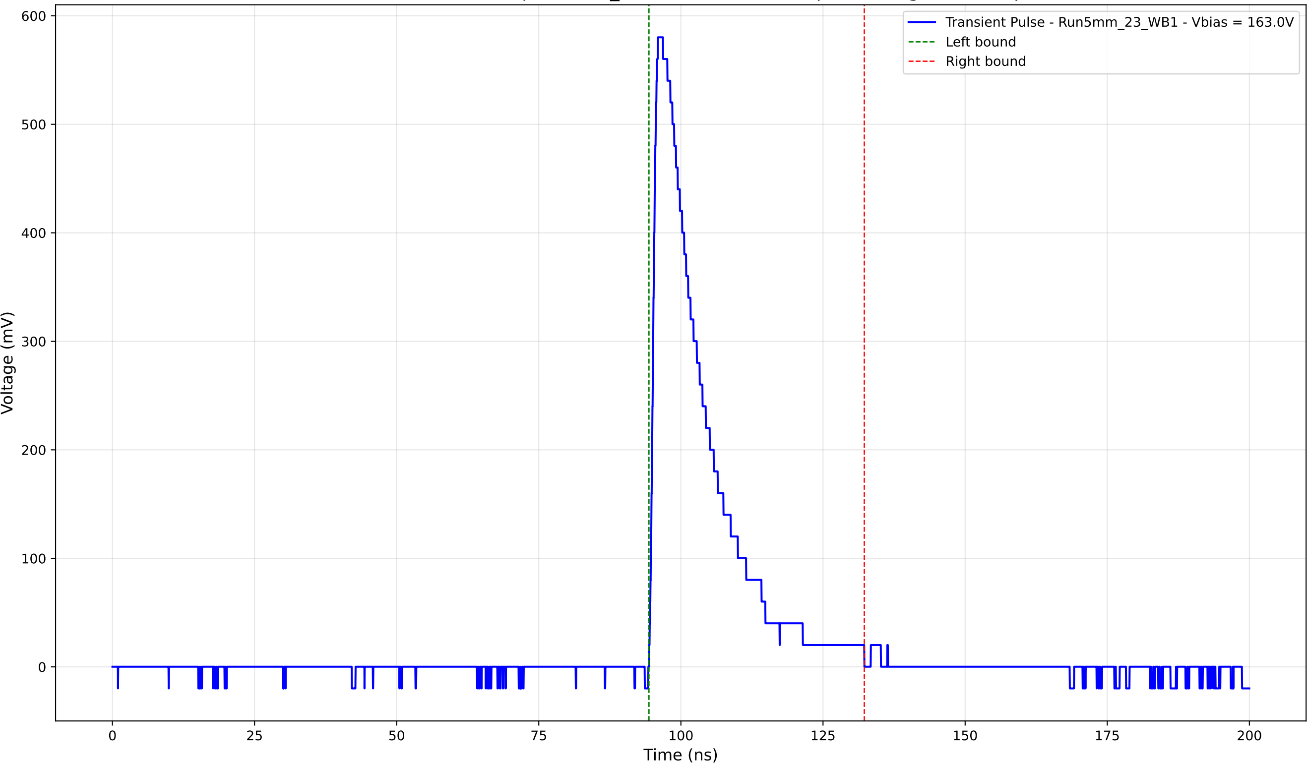
Transient Pulse - Sample: 5mm_23 - Position: 3805.0 \mu\text{m} - Charge: 115.56 pC
