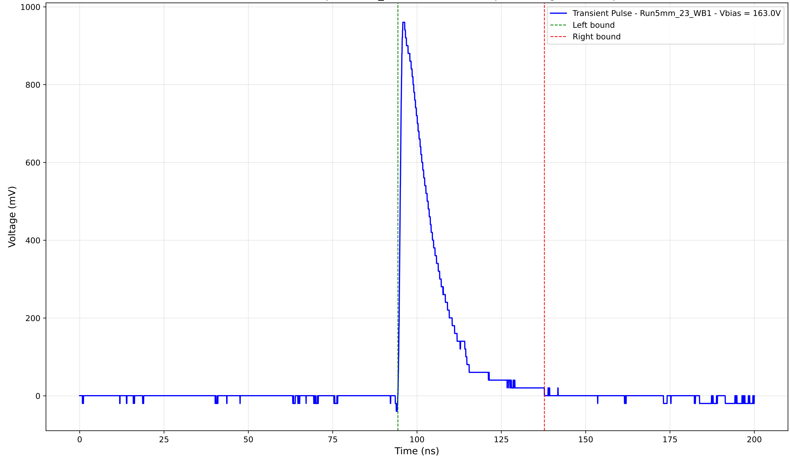
Transient Pulse - Sample: 5mm_23 - Position: 945.0 \mu\text{m} - Charge: 201.54 pC
