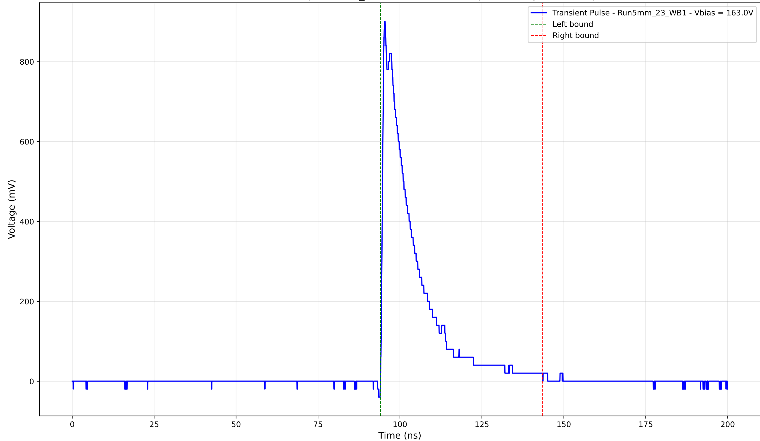
Transient Pulse - Sample: 5mm_23 - Position: 2310.0 \mu\text{m} - Charge: 182.70 pC
