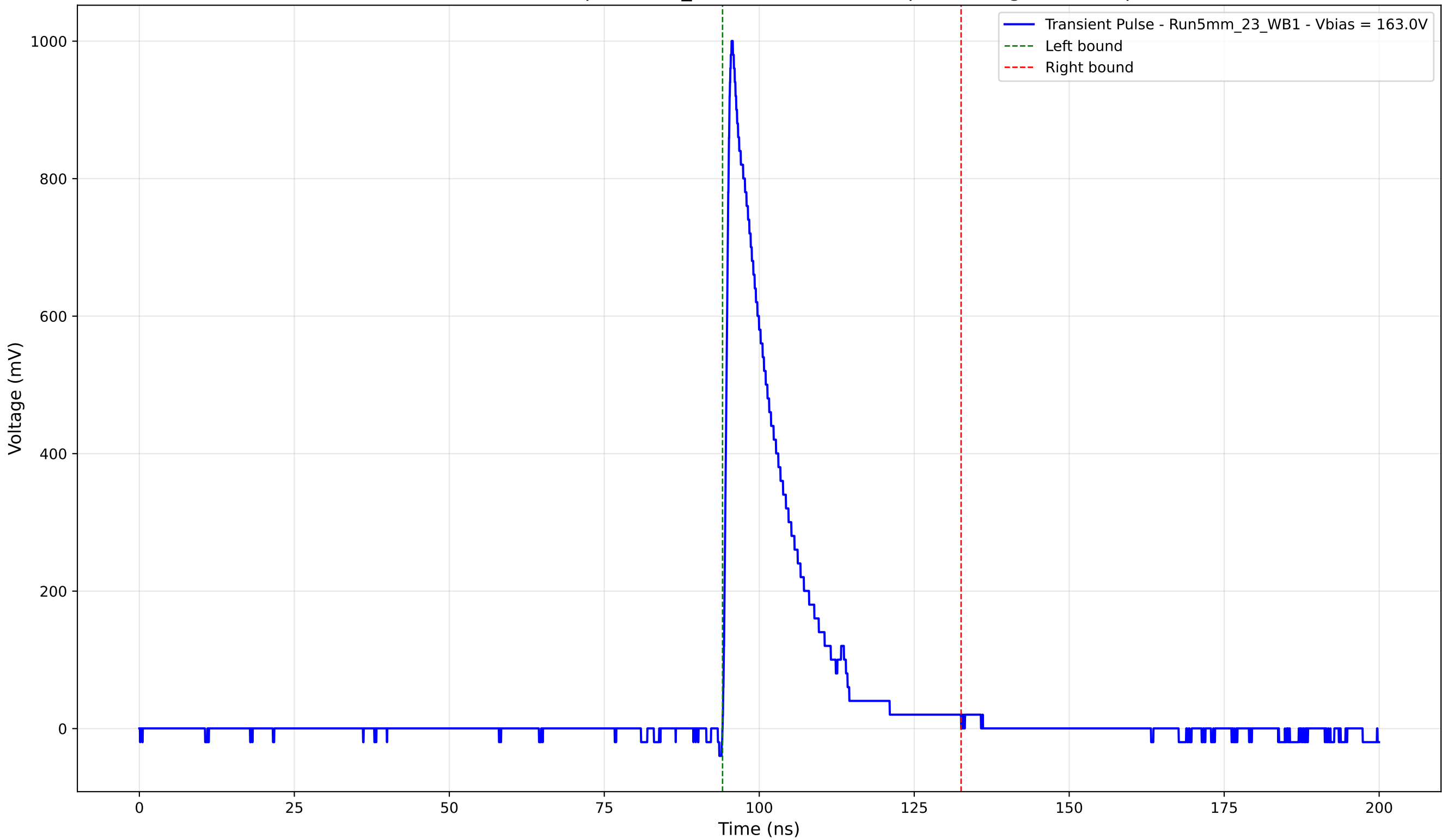
Transient Pulse - Sample: 5mm_23 - Position: 4920.0 \mu\text{m} - Charge: 169.08 pC
