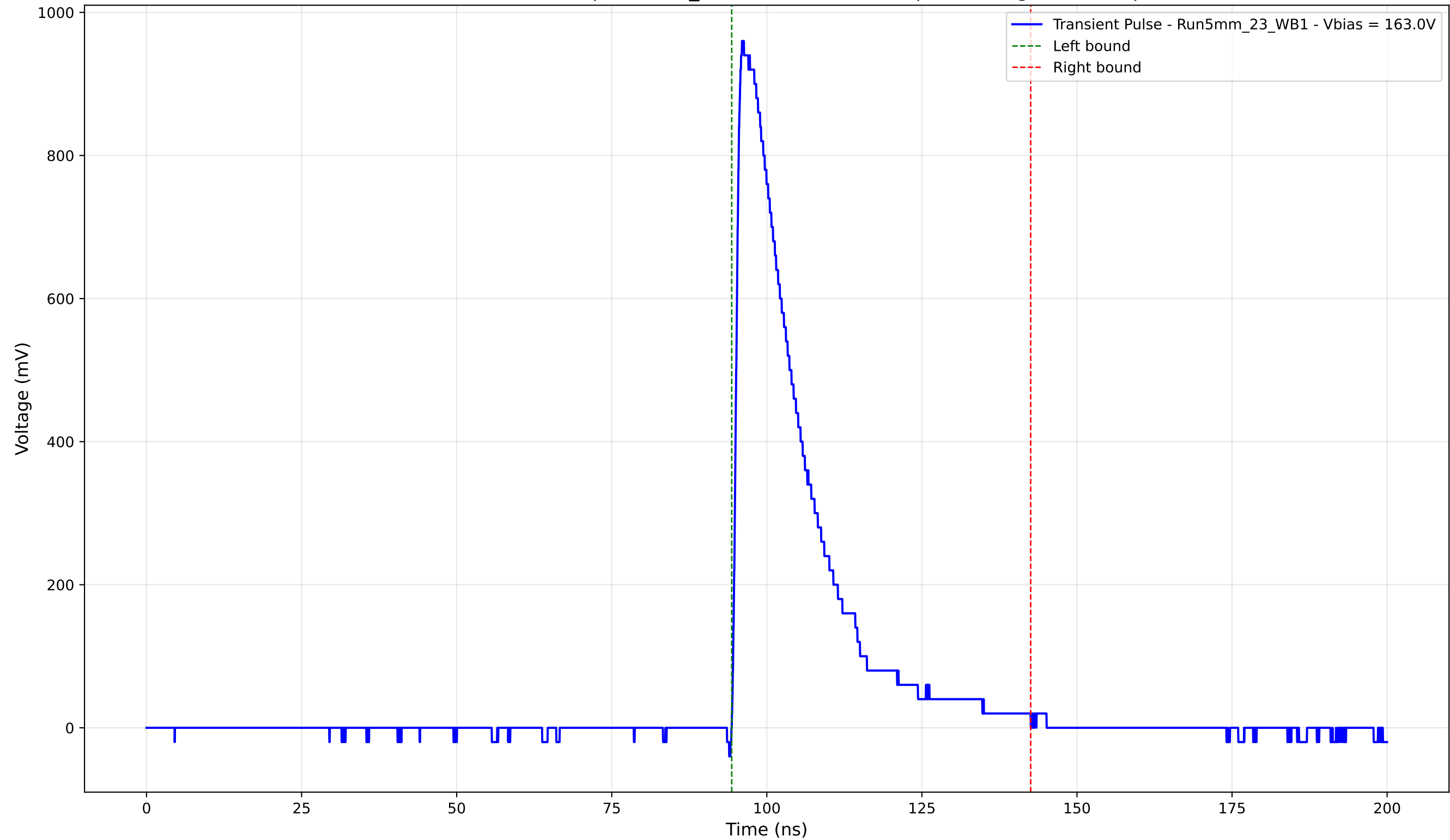
Transient Pulse - Sample: 5mm_23 - Position: 1640.0 \mu\text{m} - Charge: 222.74 pC
