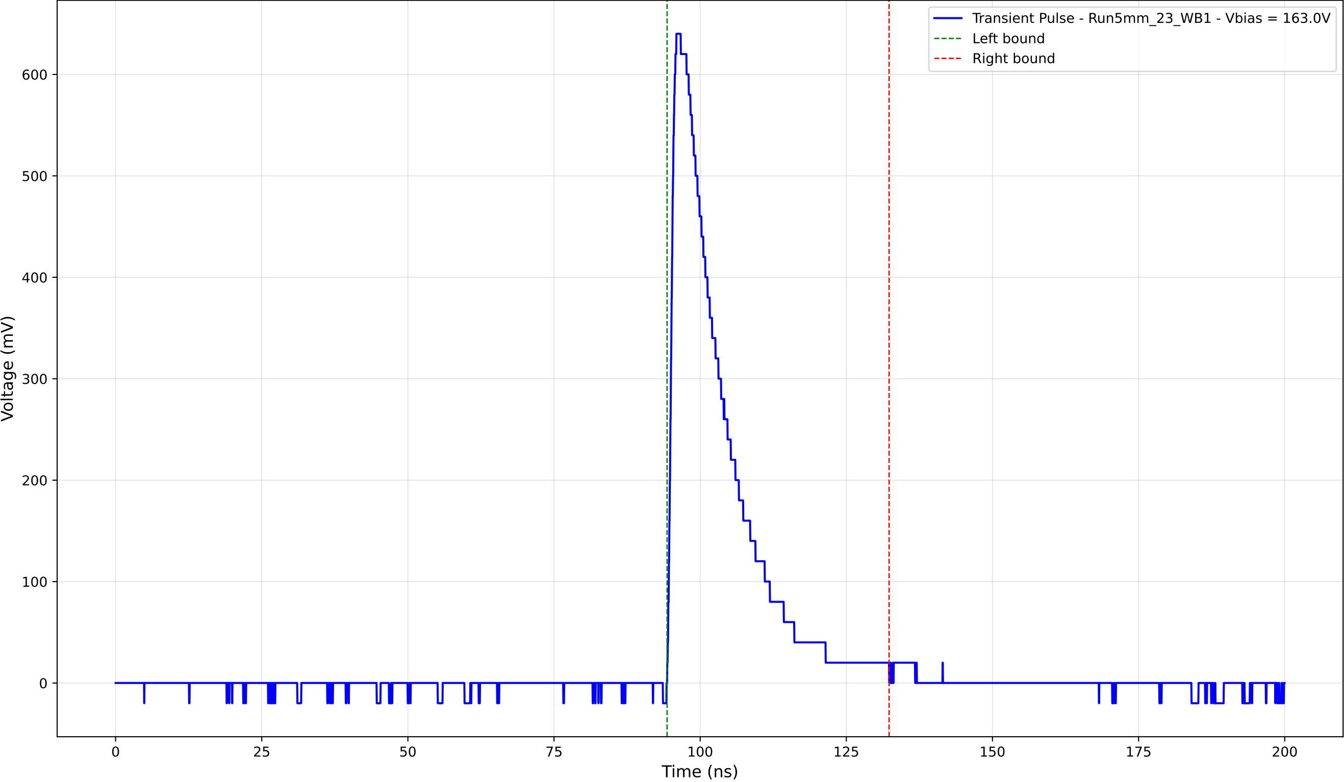
Transient Pulse - Sample: 5mm_23 - Position: 3700.0 \mu\text{m} - Charge: 128.09 pC
