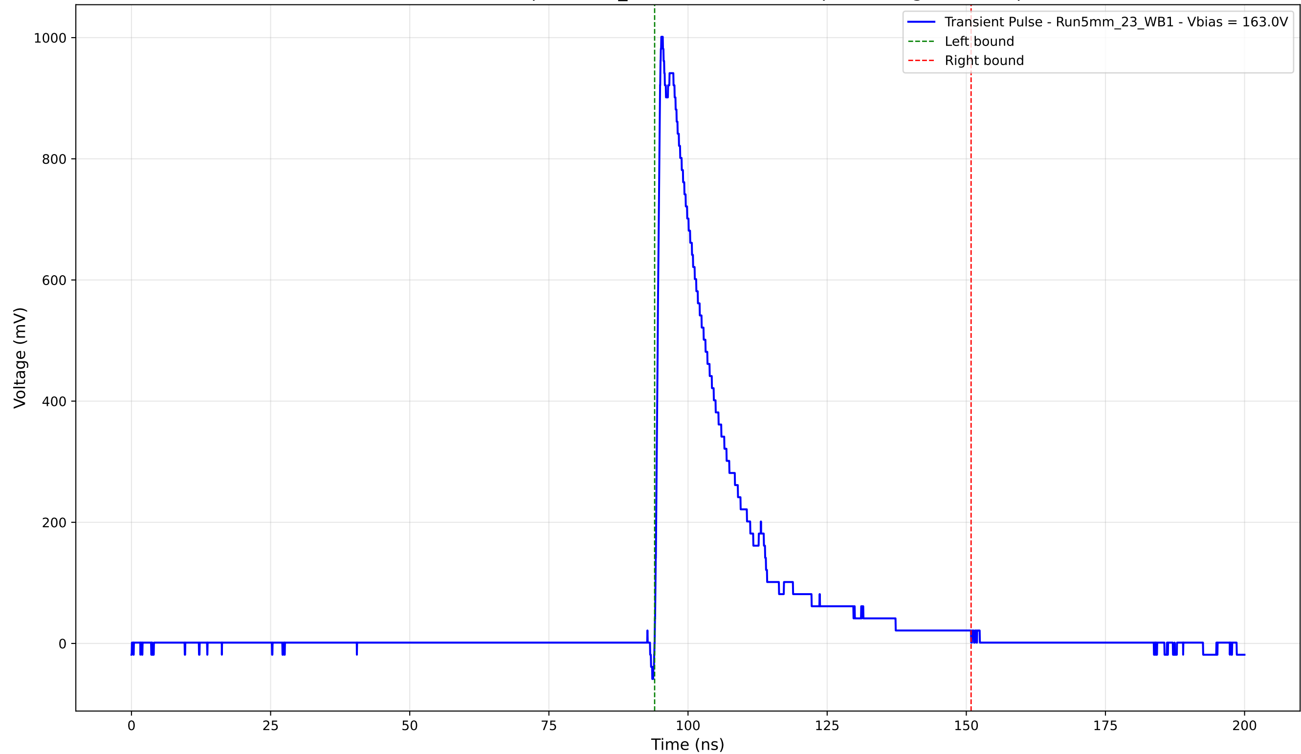
Transient Pulse - Sample: 5mm_23 - Position: 2395.0 \mu\text{m} - Charge: 230.51 pC
