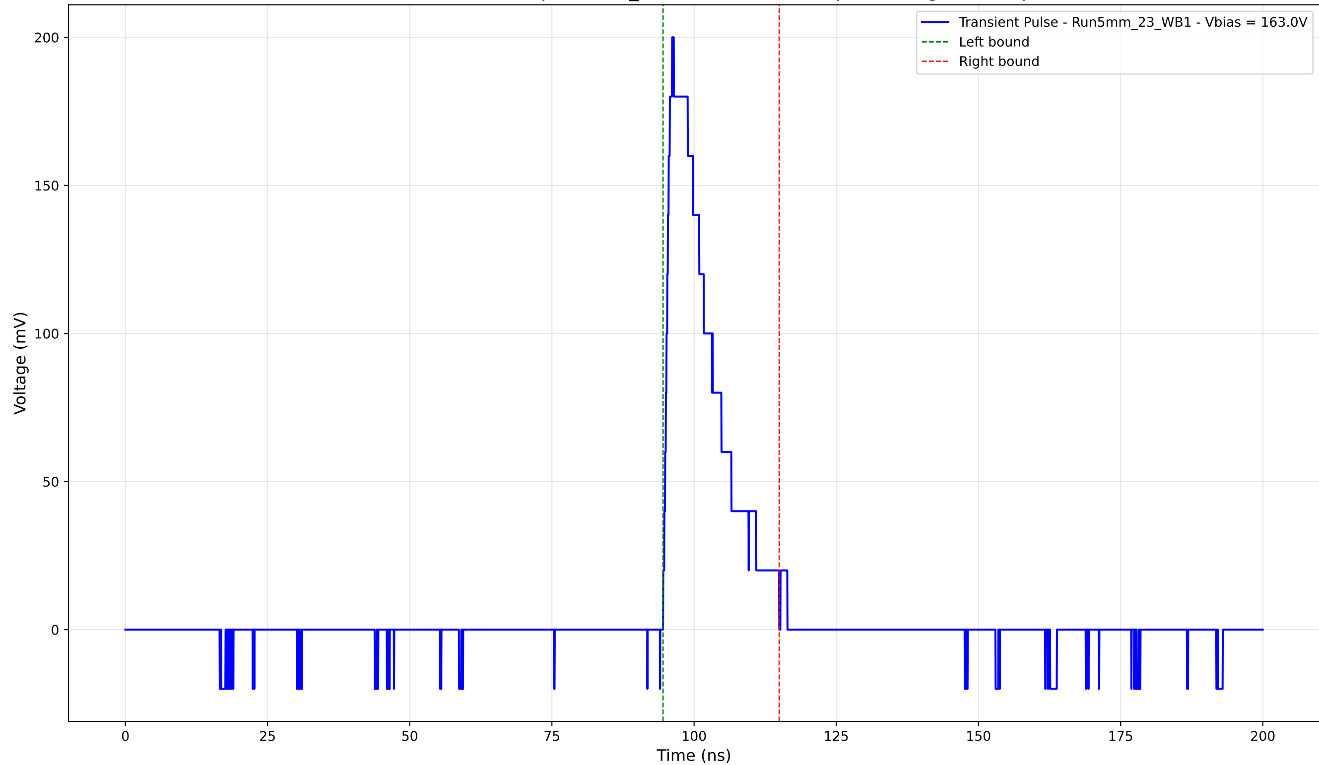
Transient Pulse - Sample: 5mm_23 - Position: 4270.0 \mu\text{m} - Charge: 34.30 pC
