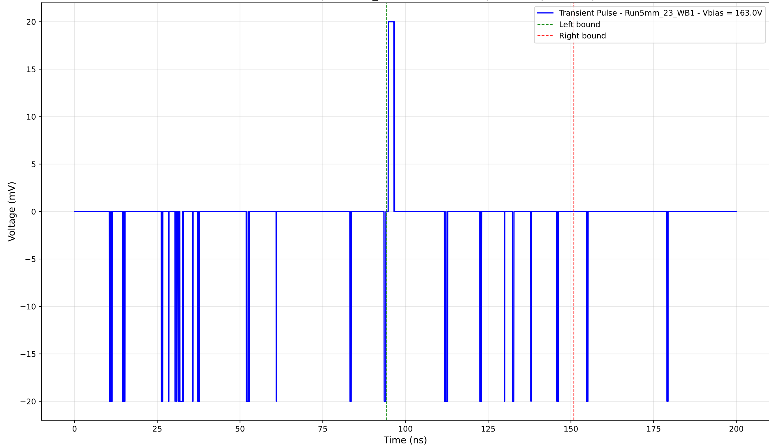
Transient Pulse - Sample: 5mm_23 - Position: 110.0 \mu\text{m} - Charge: -0.07 pC
