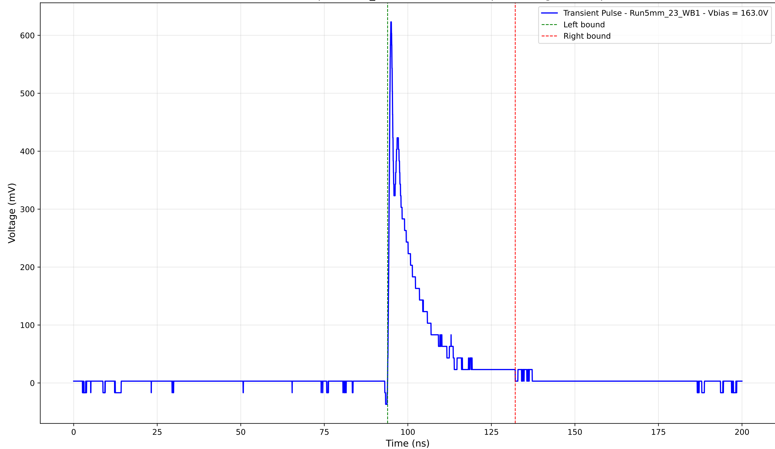
Transient Pulse - Sample: 5mm_23 - Position: 2775.0 \mu\text{m} - Charge: 82.51 pC
