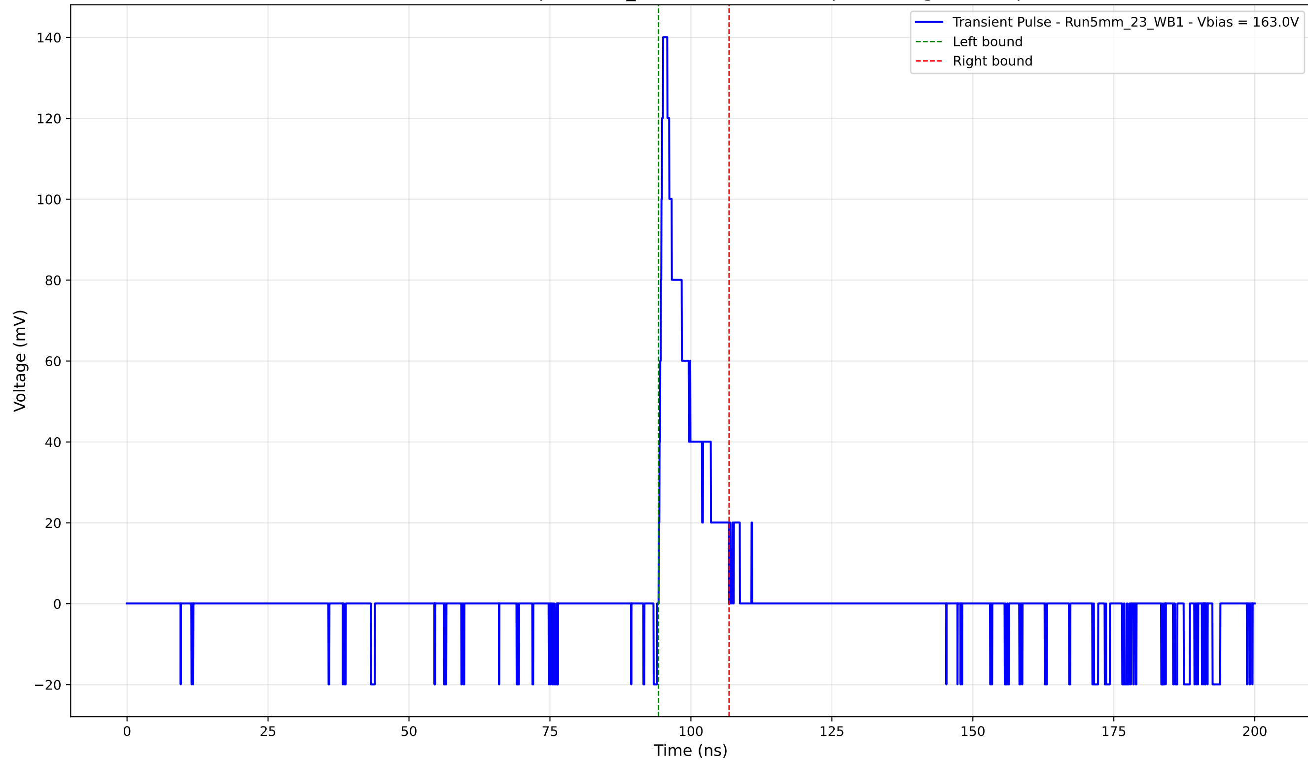
Transient Pulse - Sample: 5mm_23 - Position: 5200.0 \mu\text{m} - Charge: 13.69 pC
