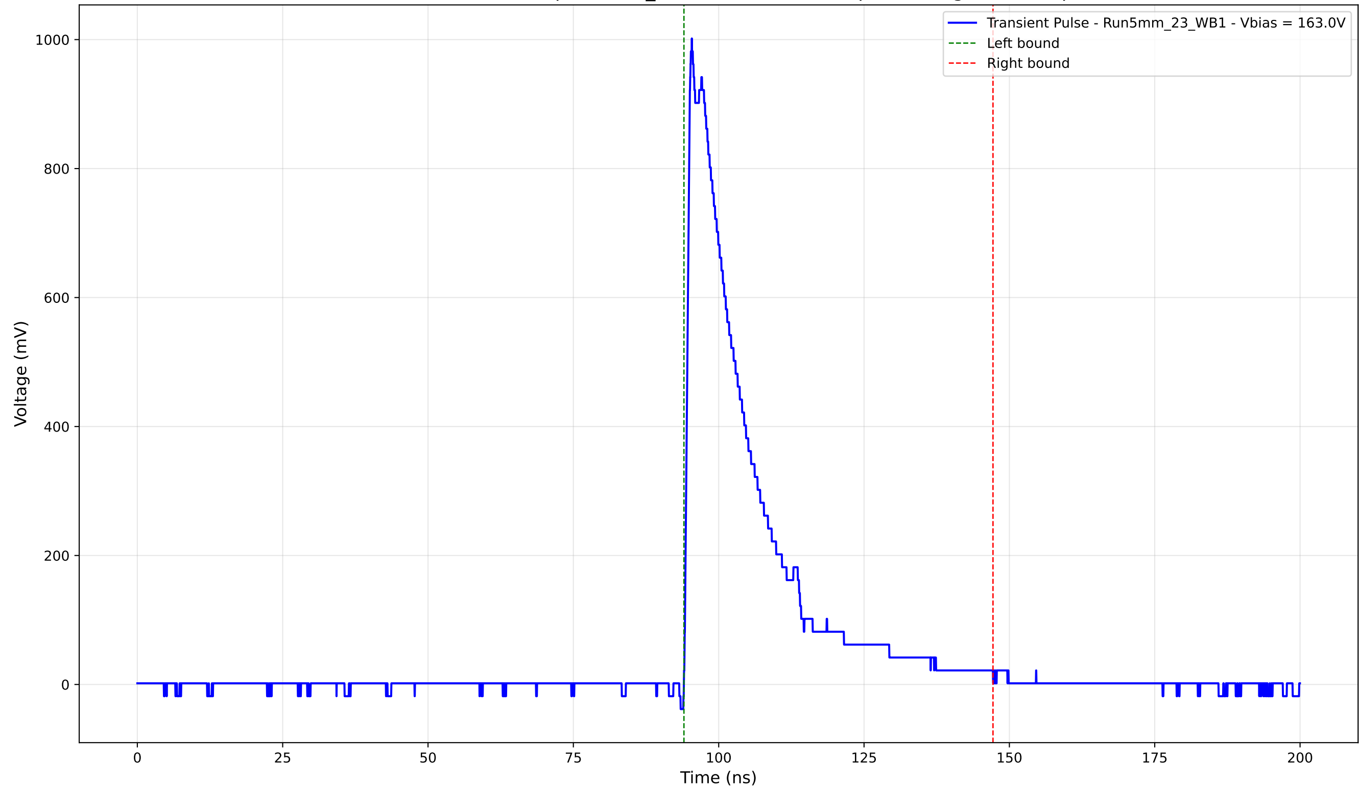
Transient Pulse - Sample: 5mm_23 - Position: 3130.0 \mu\text{m} - Charge: 222.53 pC
