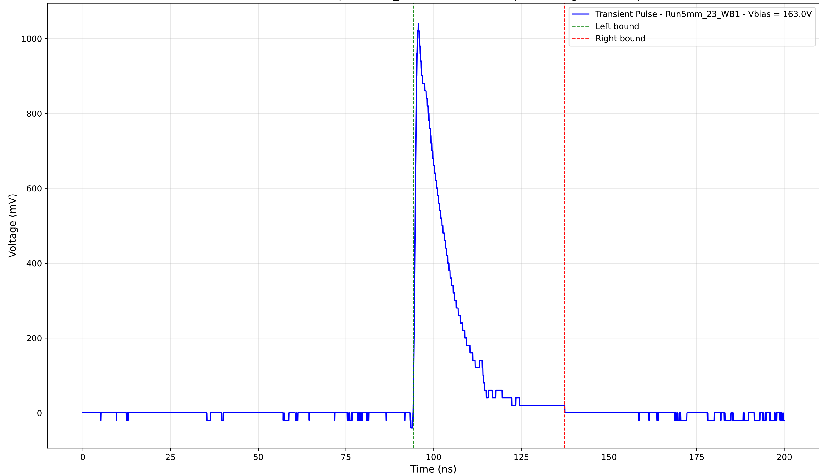
Transient Pulse - Sample: 5mm_23 - Position: 525.0 \mu\text{m} - Charge: 194.19 pC
