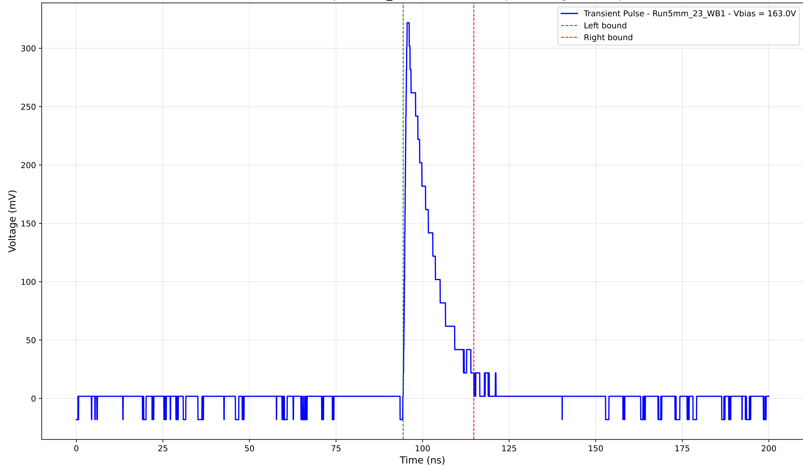
Transient Pulse - Sample: 5mm_23 - Position: 705.0 \mu\text{m} - Charge: 50.17 pC
