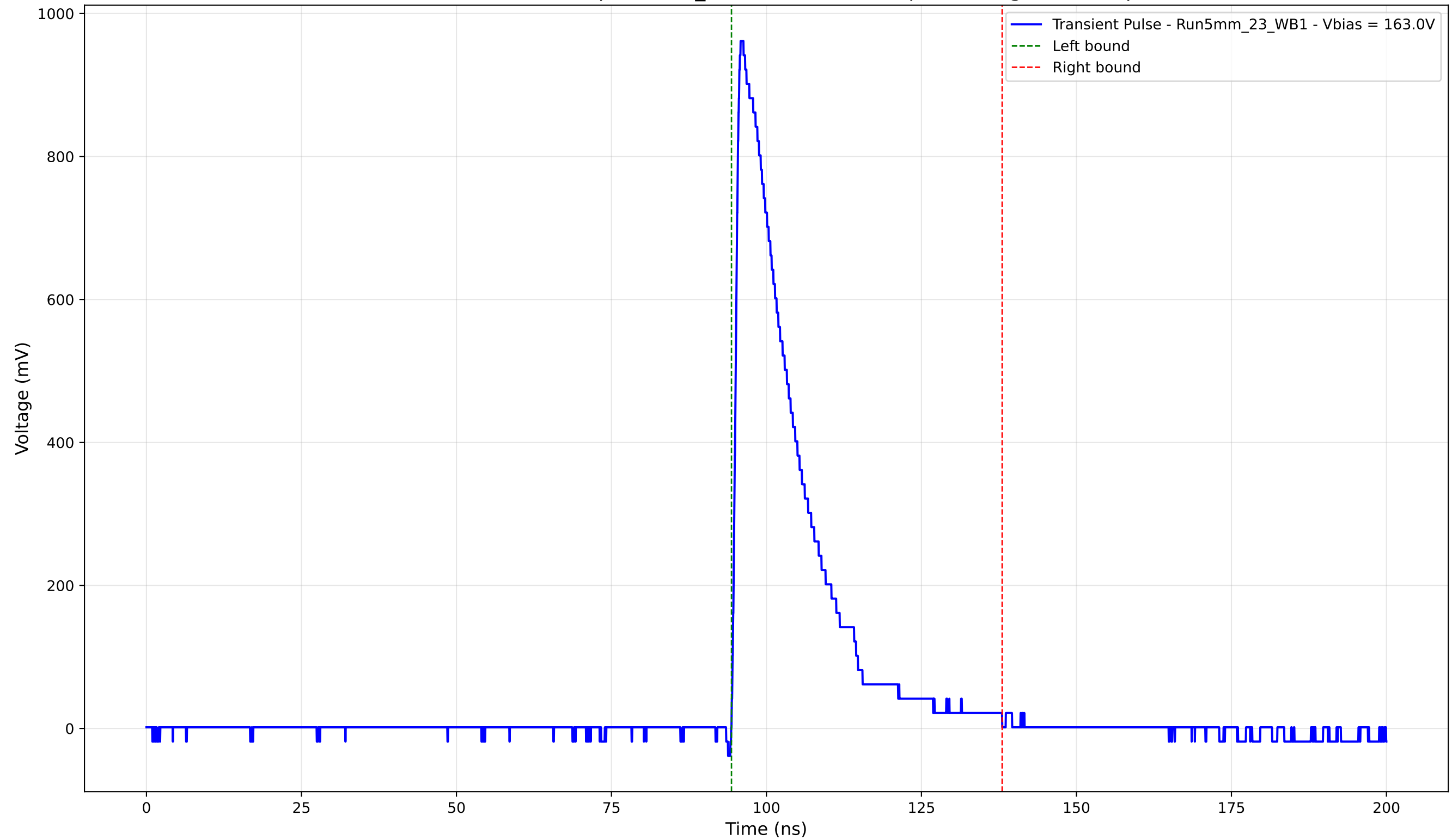
Transient Pulse - Sample: 5mm_23 - Position: 965.0 \mu\text{m} - Charge: 201.97 pC
