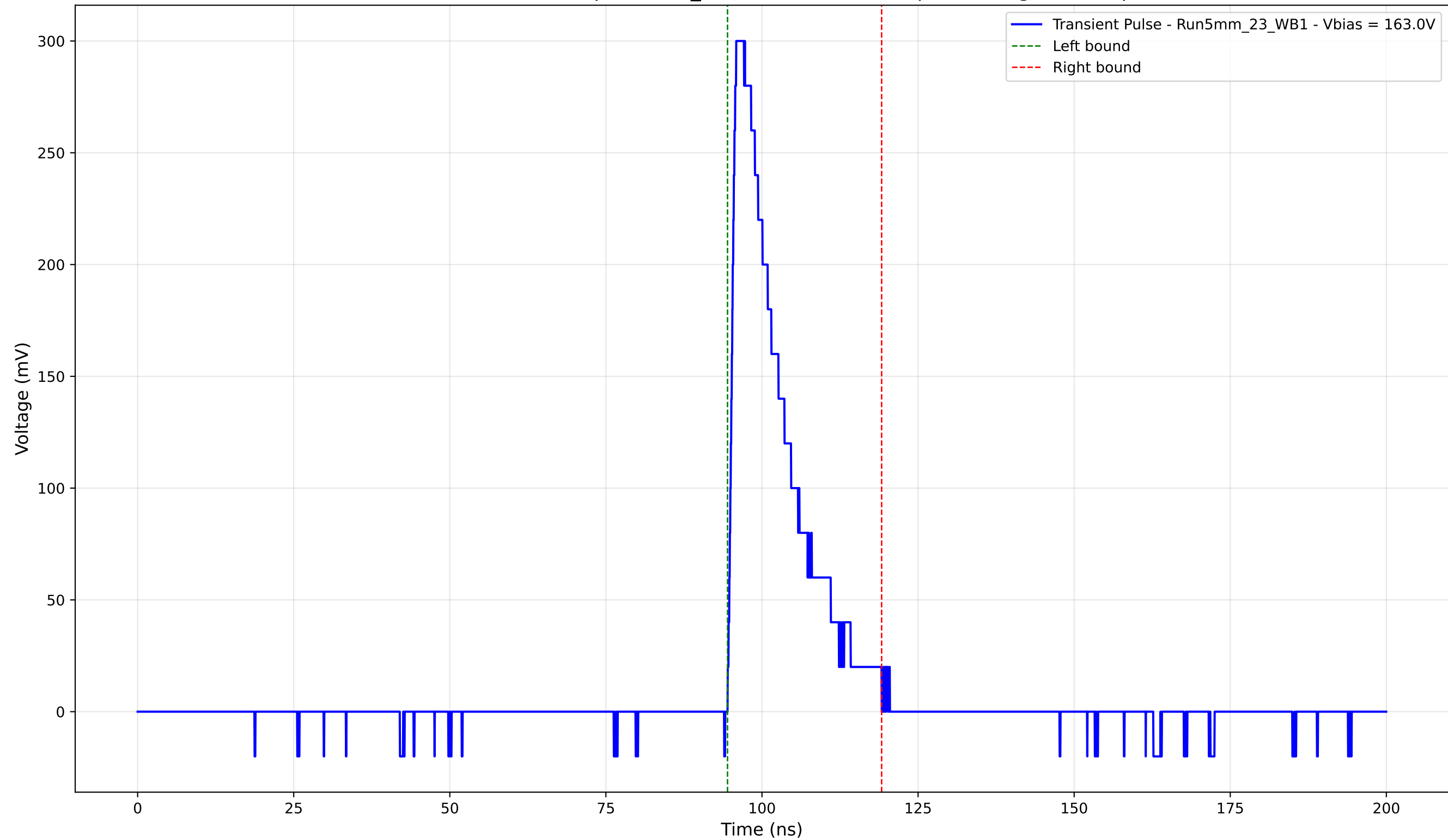
Transient Pulse - Sample: 5mm_23 - Position: 4235.0 \mu\text{m} - Charge: 54.81 pC
