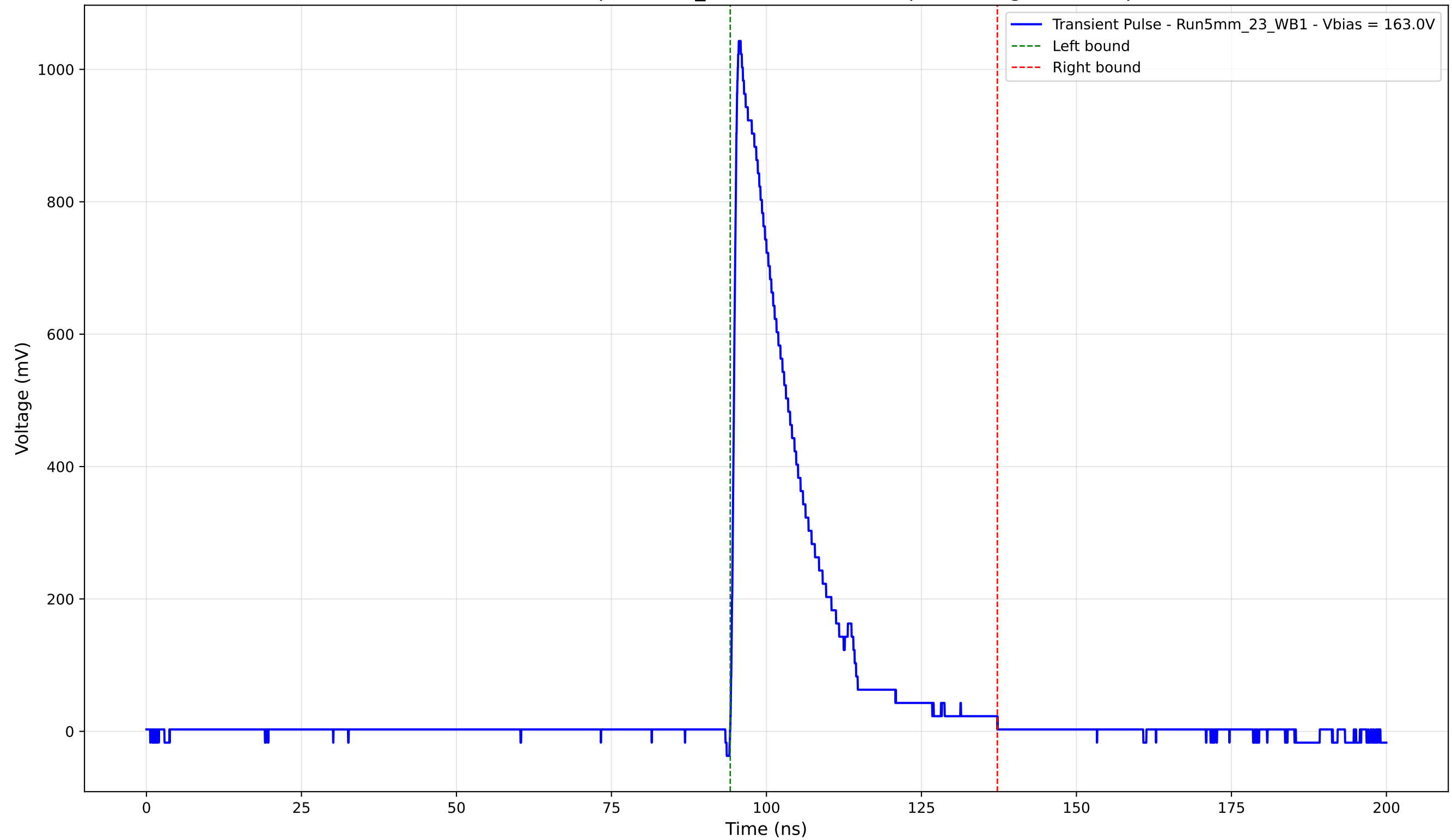
Transient Pulse - Sample: 5mm_23 - Position: 595.0 \mu\text{m} - Charge: 212.79 pC
