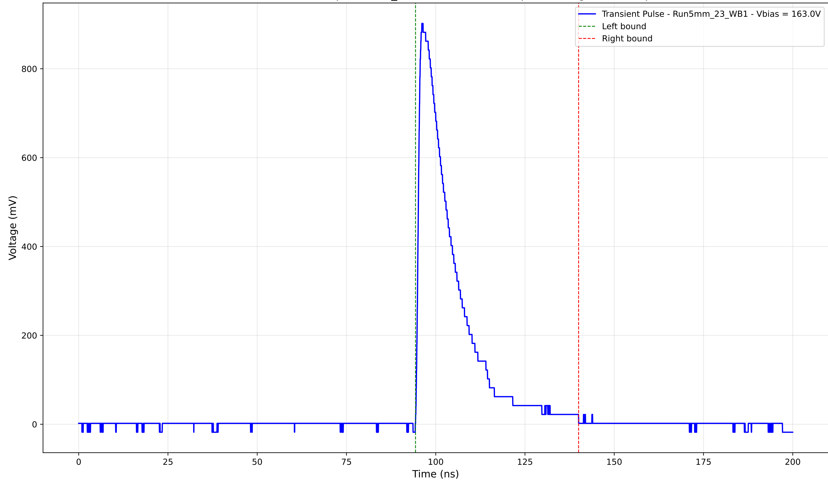
Transient Pulse - Sample: 5mm_23 - Position: 3875.0 \mu\text{m} - Charge: 196.79 pC
