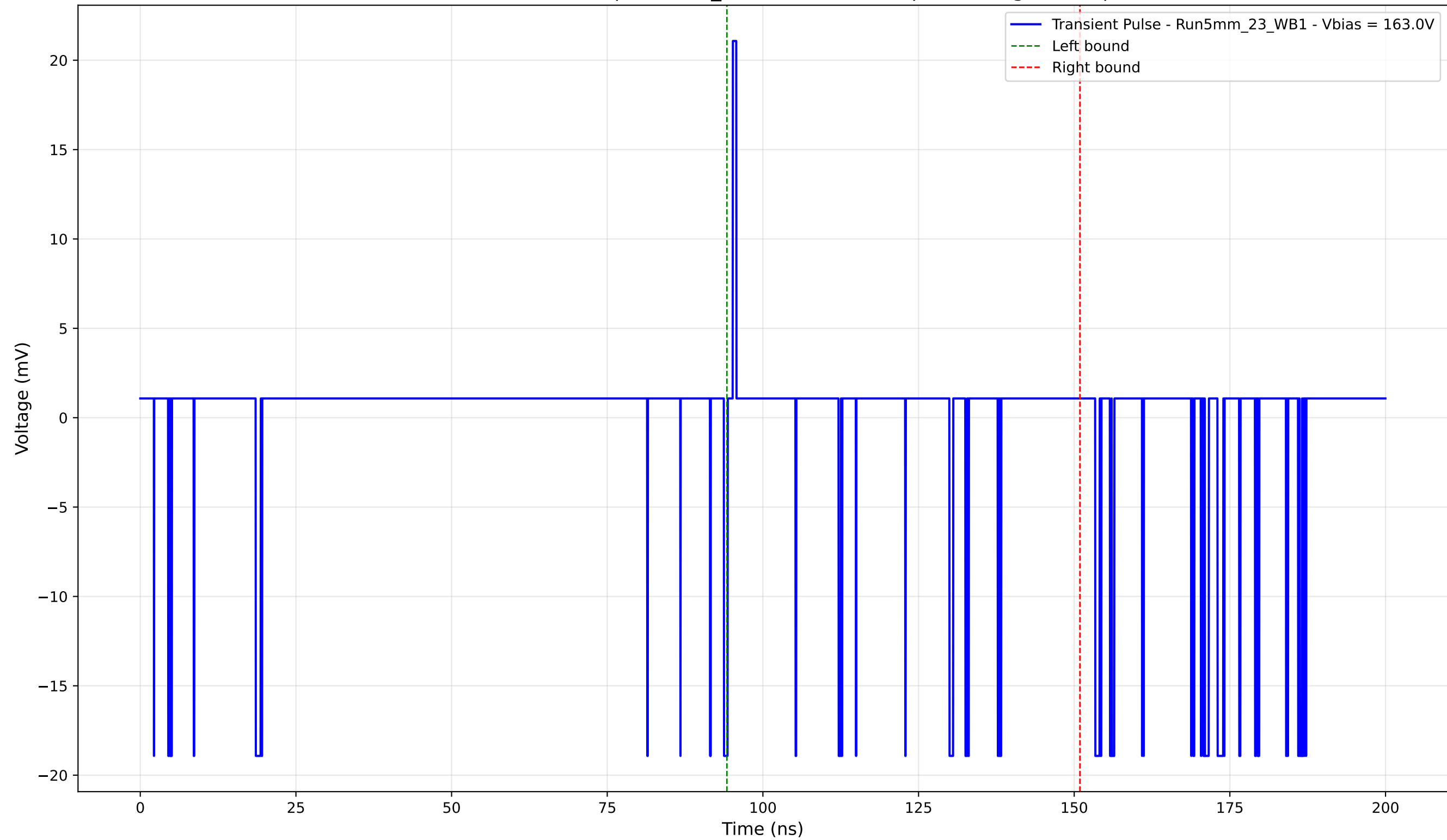
Transient Pulse - Sample: 5mm_23 - Position: 80.0 \mu\text{m} - Charge: 0.55 pC
