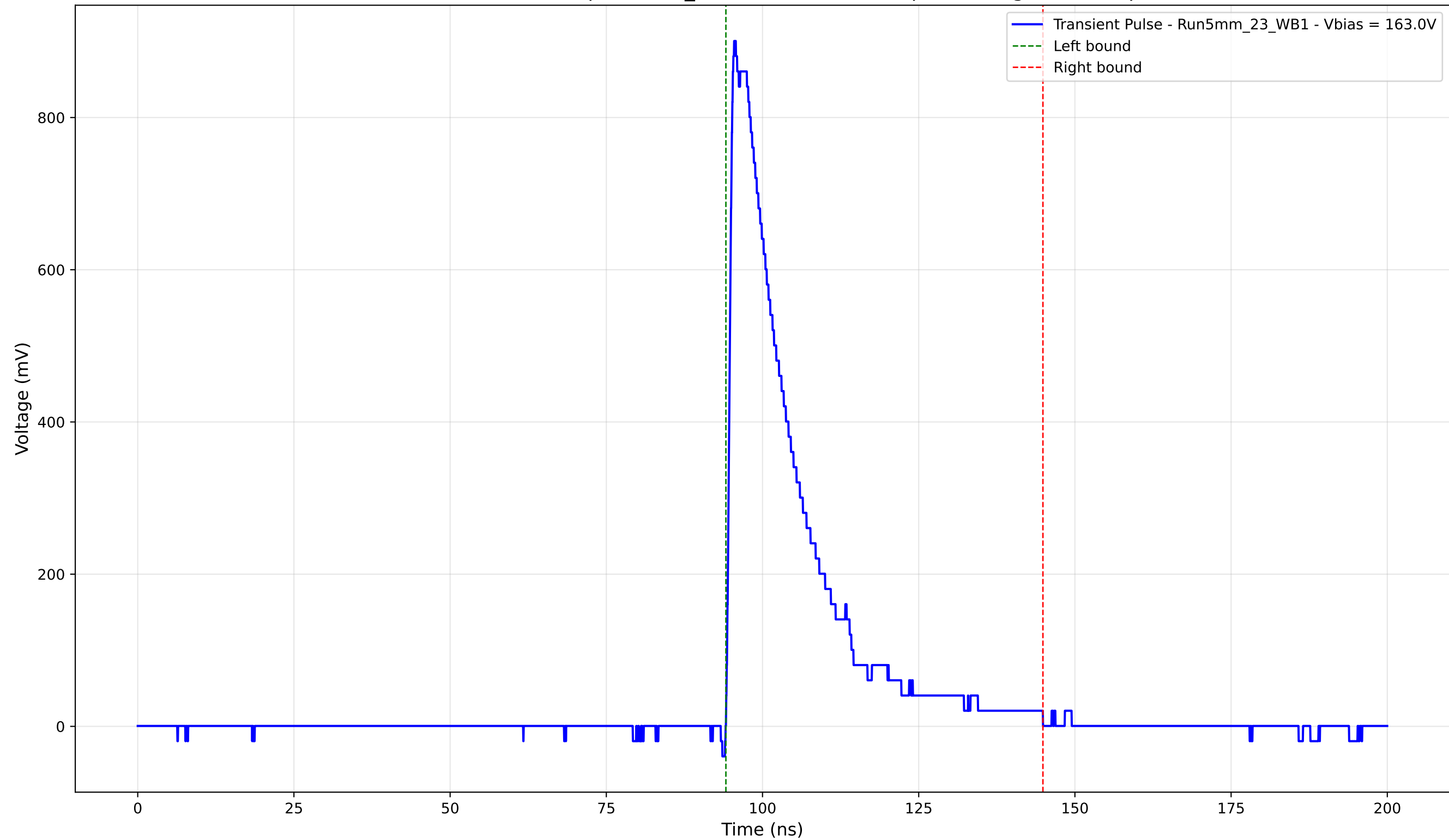
Transient Pulse - Sample: 5mm_23 - Position: 2165.0 \mu\text{m} - Charge: 198.42 pC
