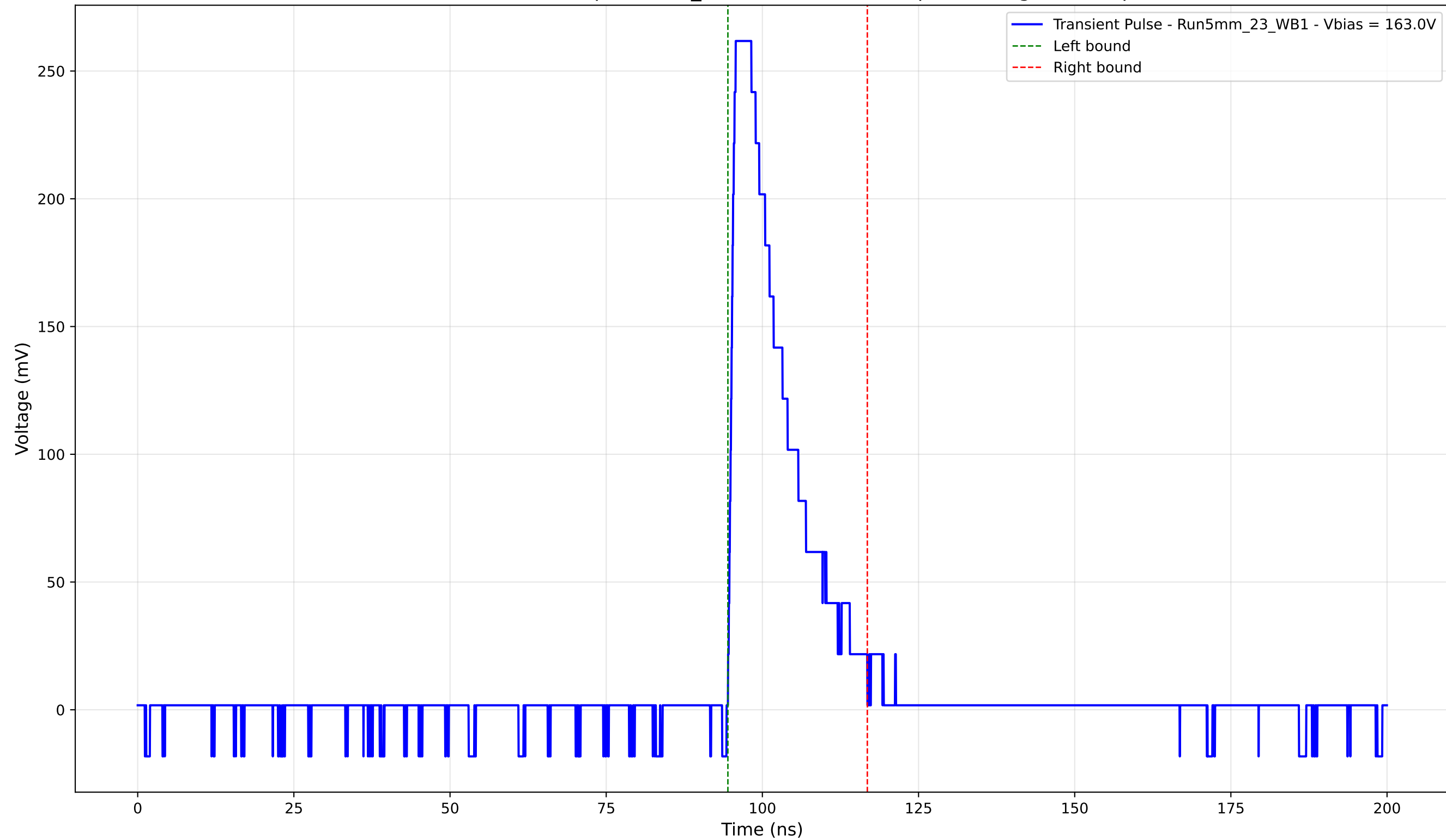
Transient Pulse - Sample: 5mm_23 - Position: 3735.0 \mu\text{m} - Charge: 50.58 pC
