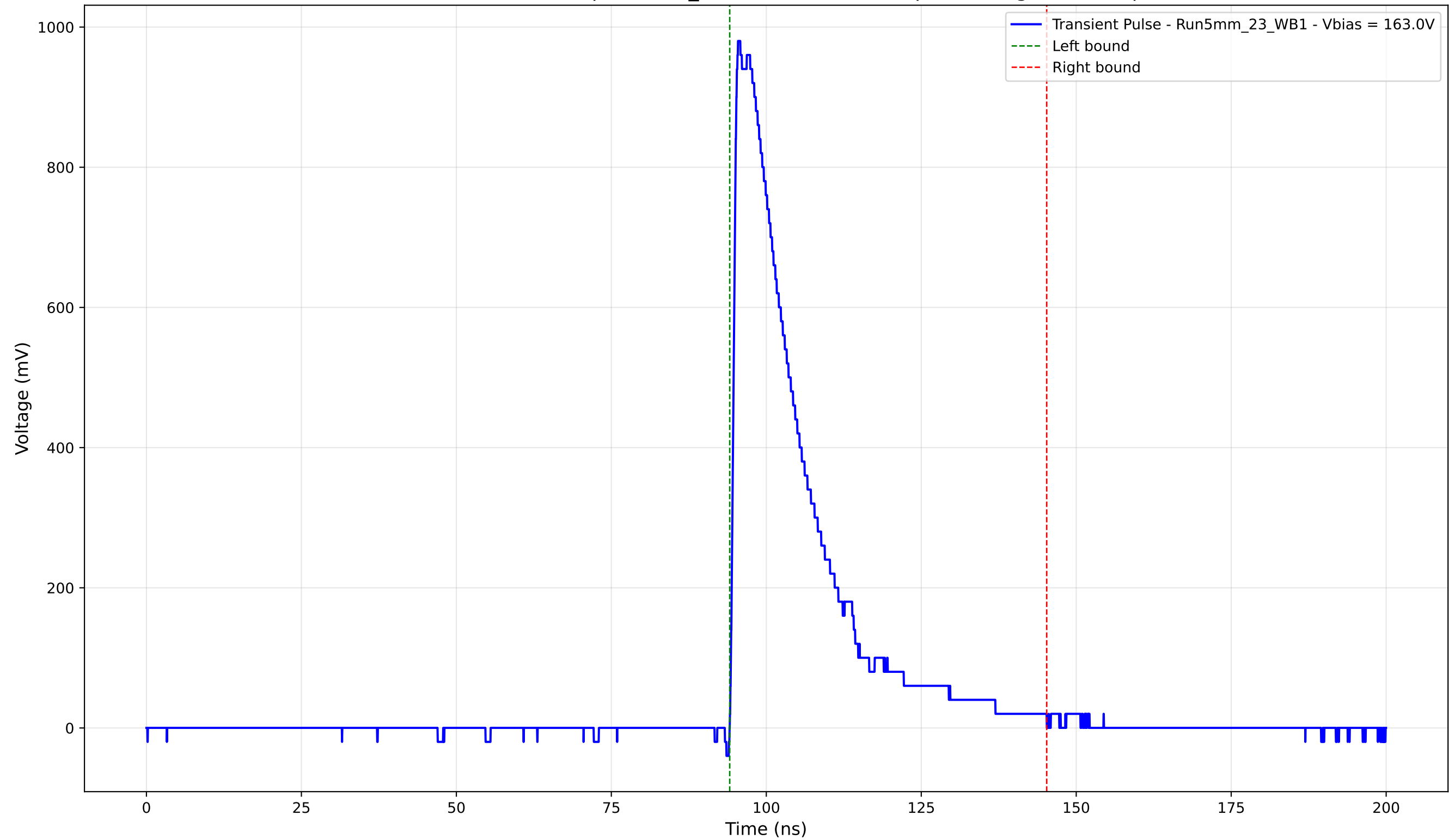
Transient Pulse - Sample: 5mm_23 - Position: 2135.0 \mu\text{m} - Charge: 235.73 pC
