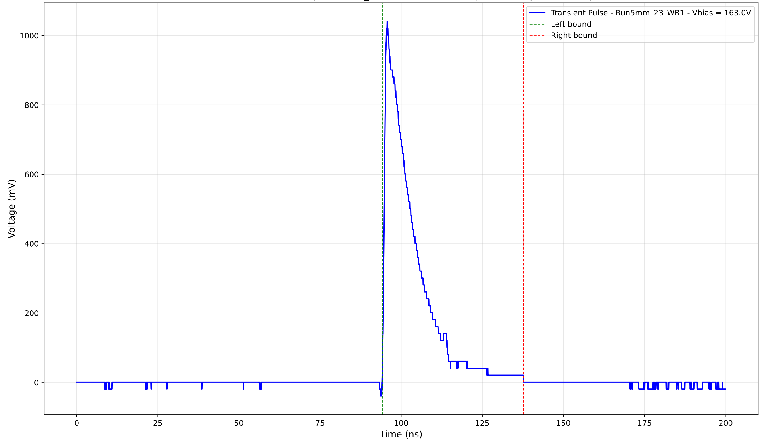
Transient Pulse - Sample: 5mm_23 - Position: 550.0 \mu\text{m} - Charge: 200.54 pC
