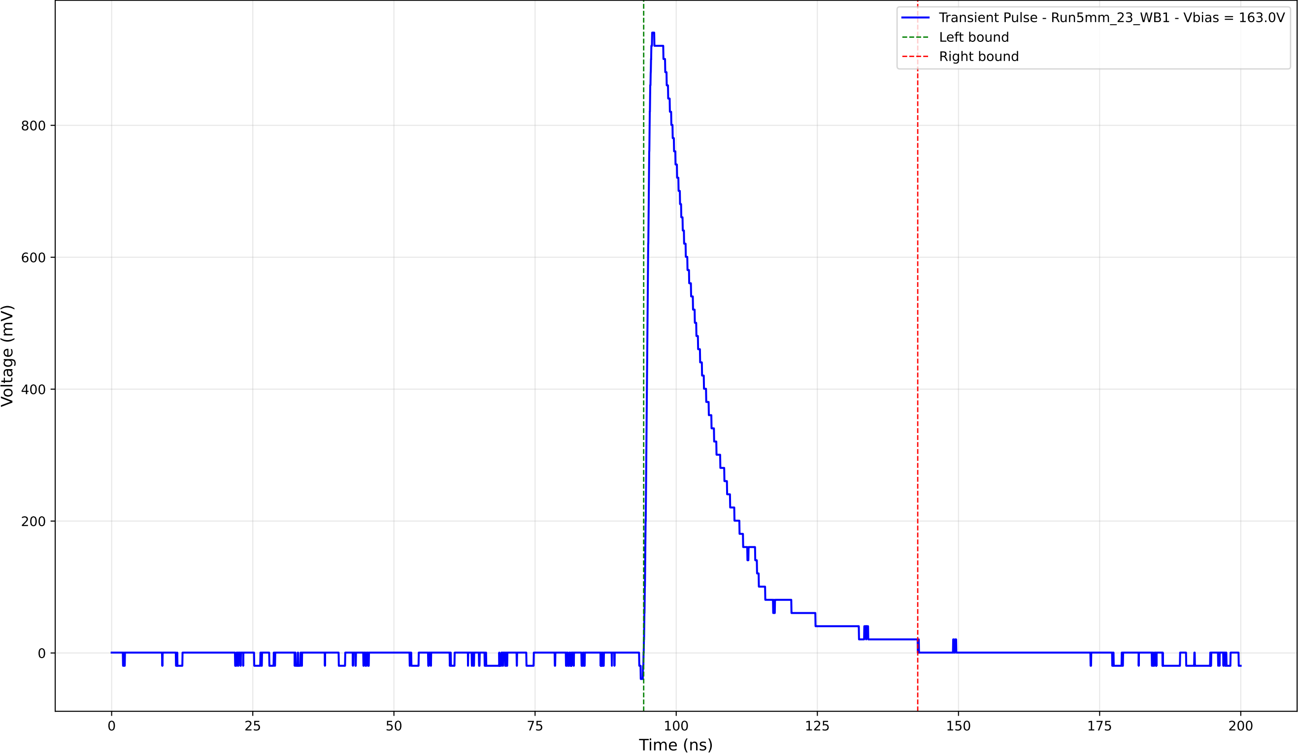
Transient Pulse - Sample: 5mm_23 - Position: 3555.0 \mu\text{m} - Charge: 218.01 pC
