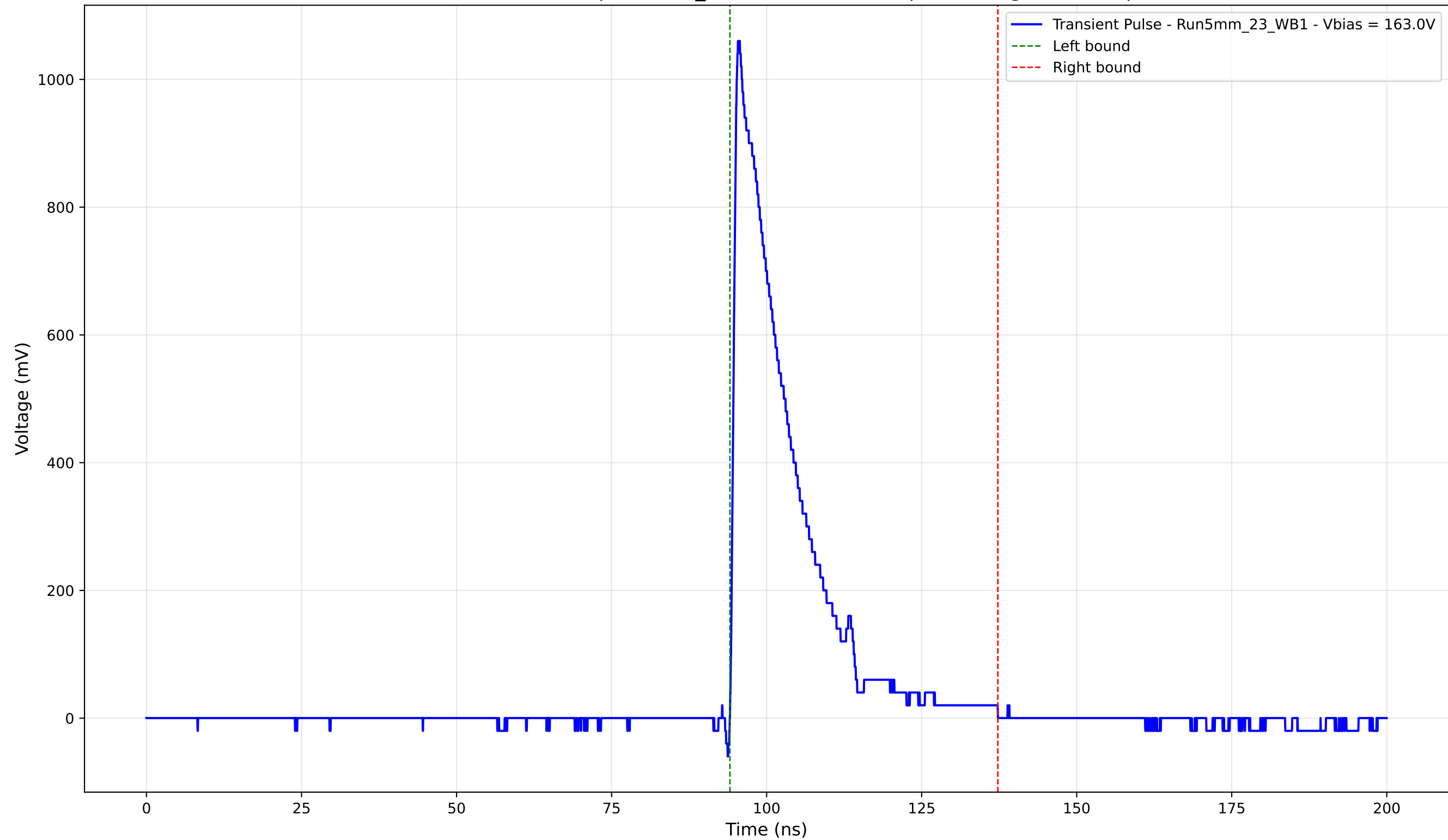
Transient Pulse - Sample: 5mm_23 - Position: 420.0 \mu\text{m} - Charge: 203.35 pC
