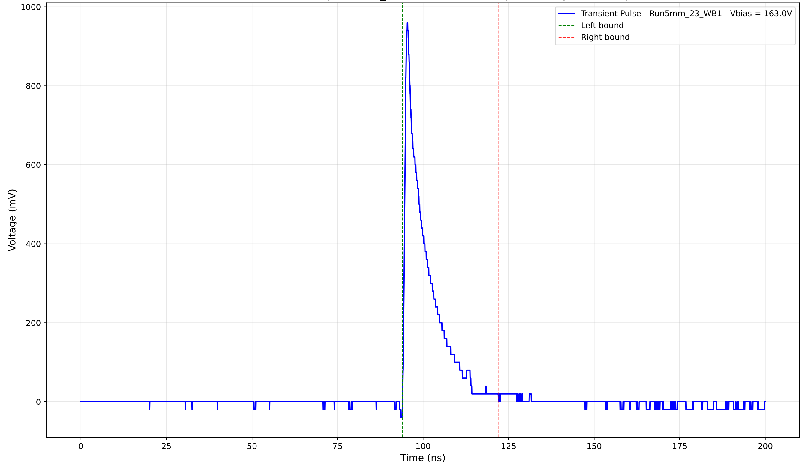
Transient Pulse - Sample: 5mm_23 - Position: 5140.0 \mu\text{m} - Charge: 126.64 pC
