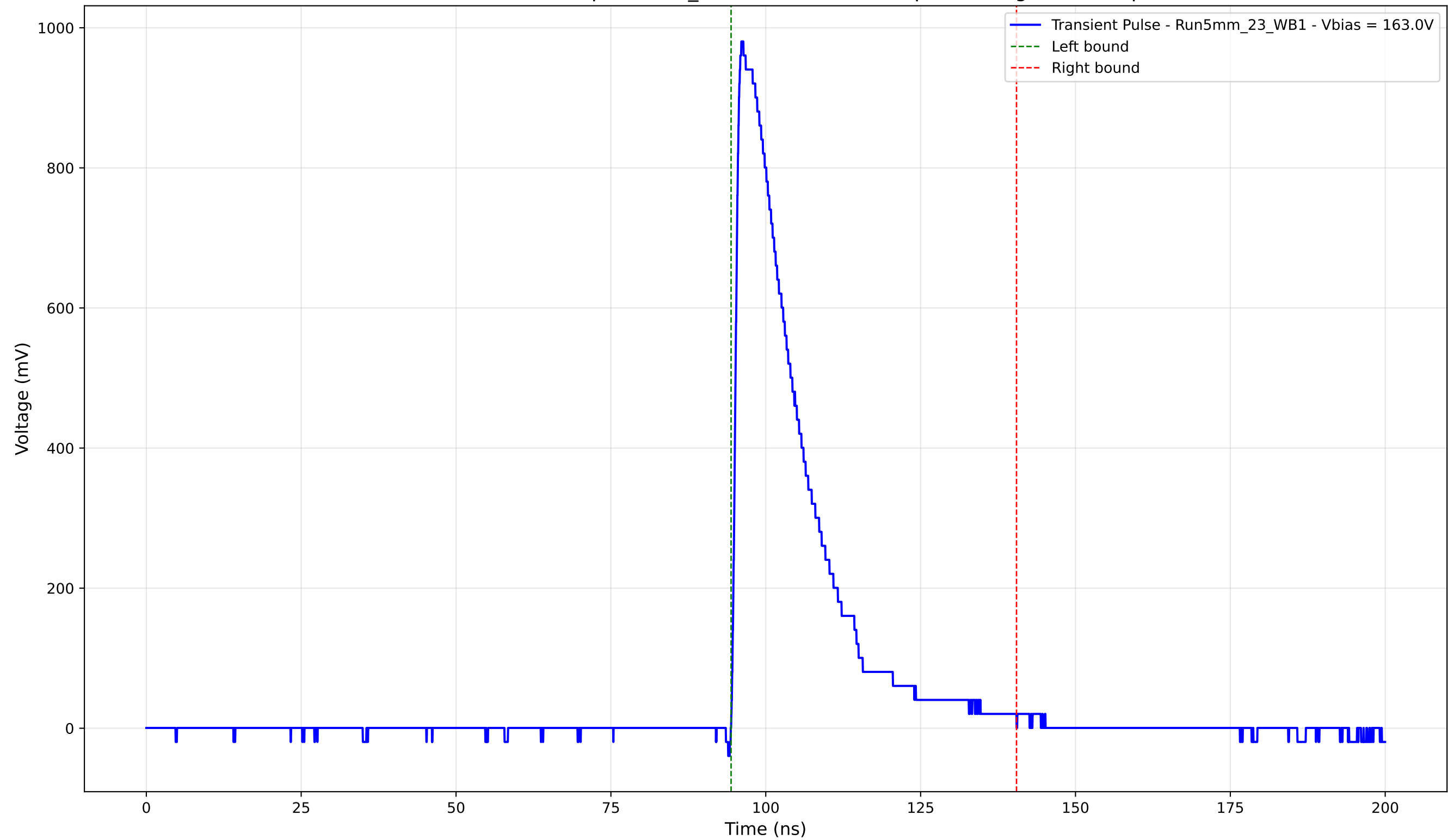
Transient Pulse - Sample: 5mm_23 - Position: 1380.0 \mu\text{m} - Charge: 226.09 pC
