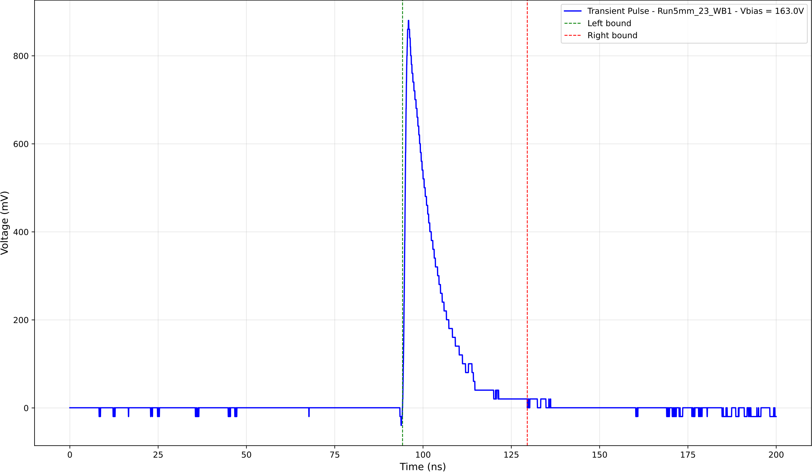
Transient Pulse - Sample: 5mm_23 - Position: 4690.0 \mu\text{m} - Charge: 149.69 pC
