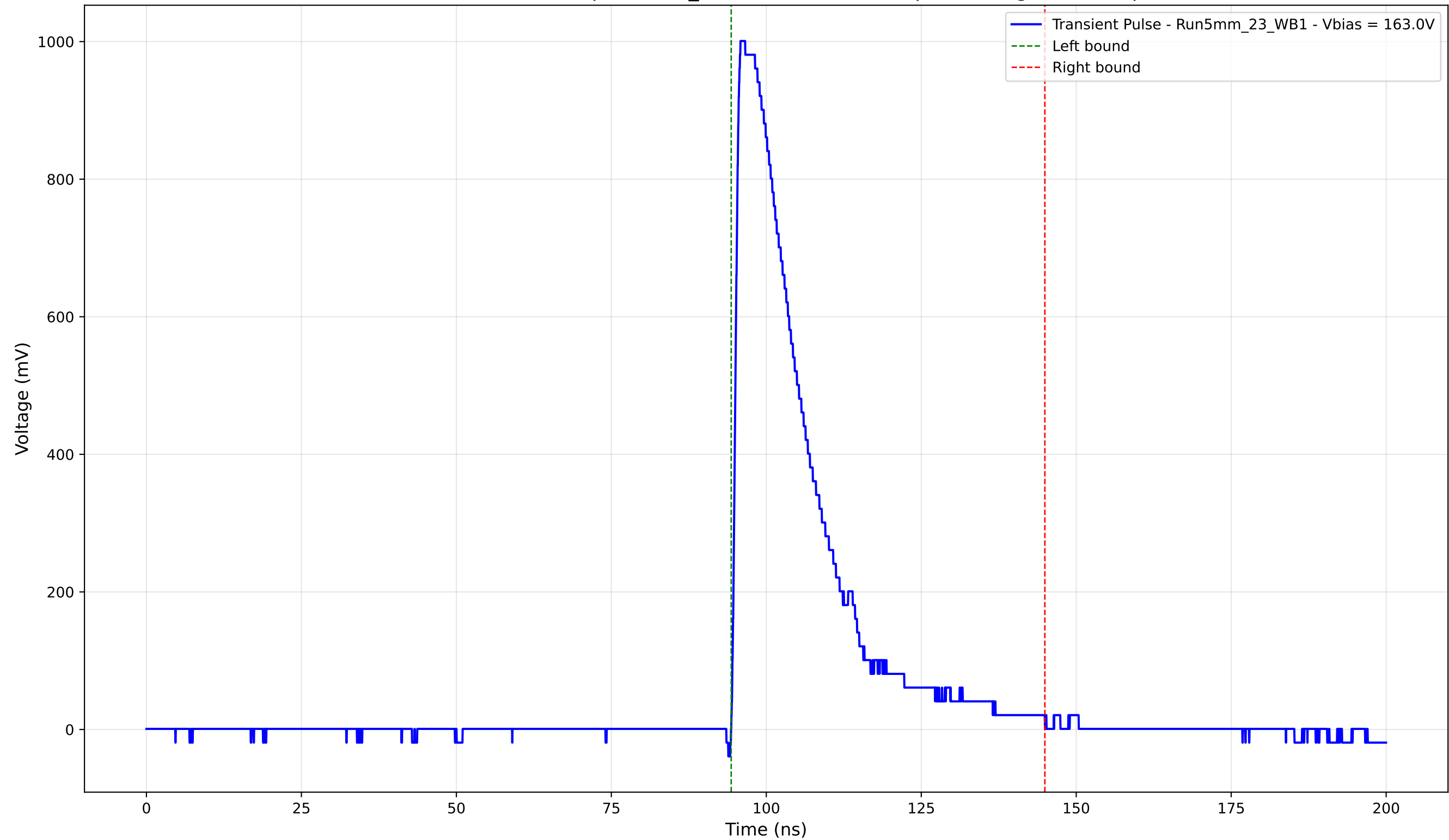
Transient Pulse - Sample: 5mm_23 - Position: 1585.0 \mu\text{m} - Charge: 253.28 pC
