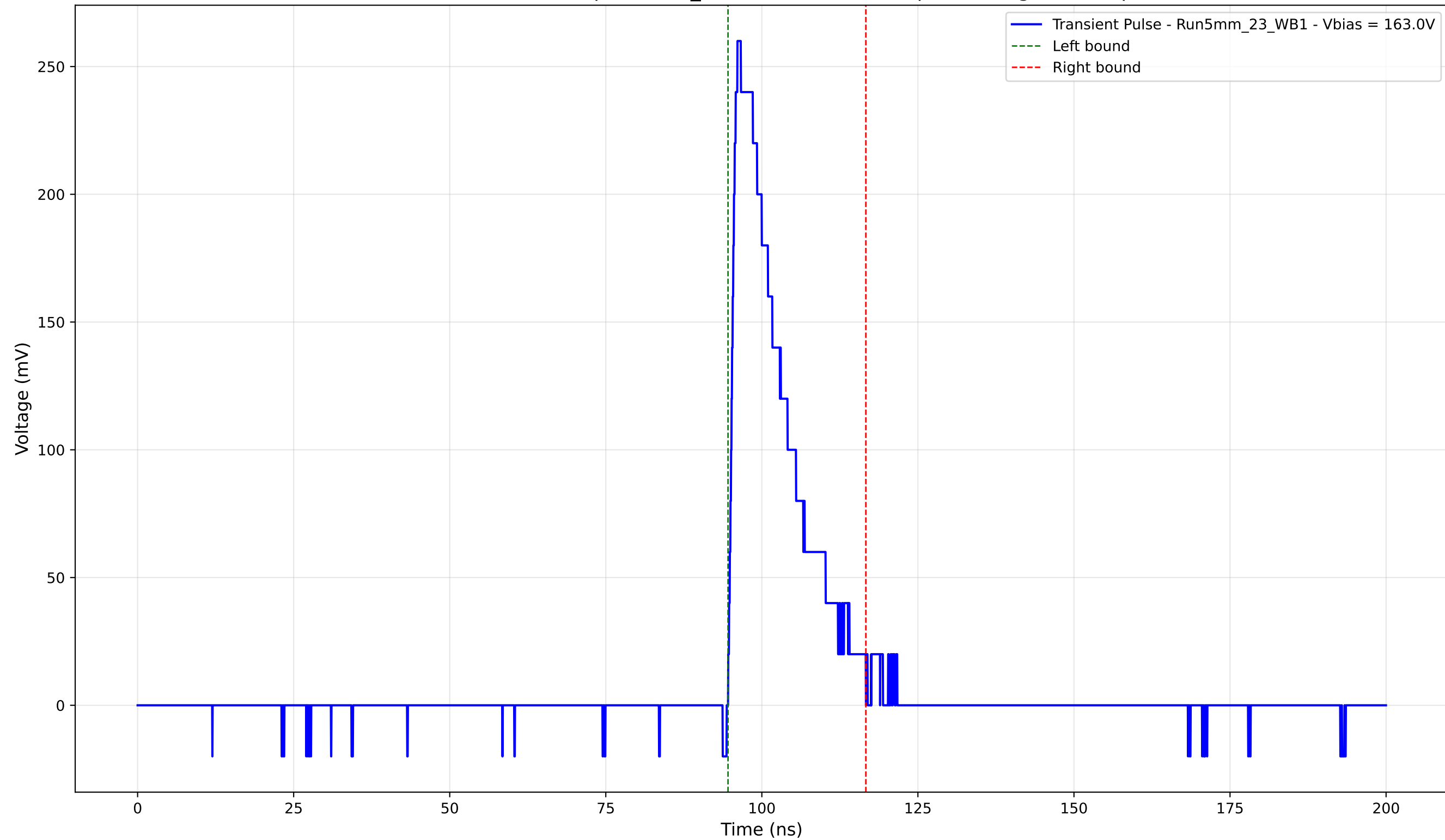
Transient Pulse - Sample: 5mm_23 - Position: 1240.0 \mu\text{m} - Charge: 47.33 pC
