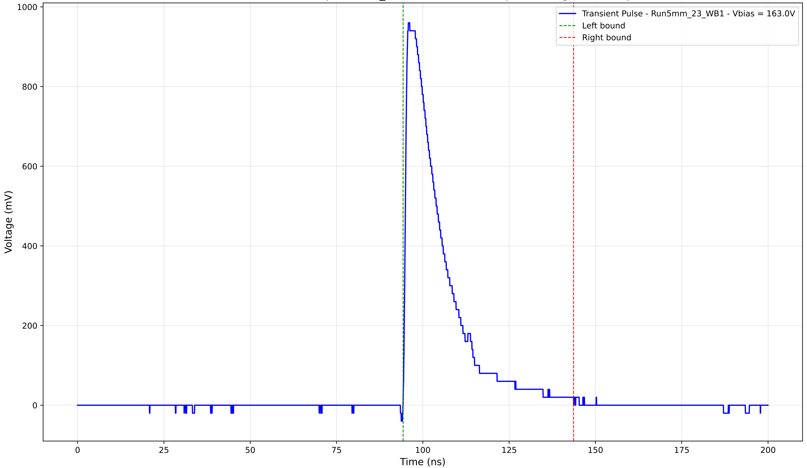
Transient Pulse - Sample: 5mm_23 - Position: 1870.0 \mu\text{m} - Charge: 229.77 pC
