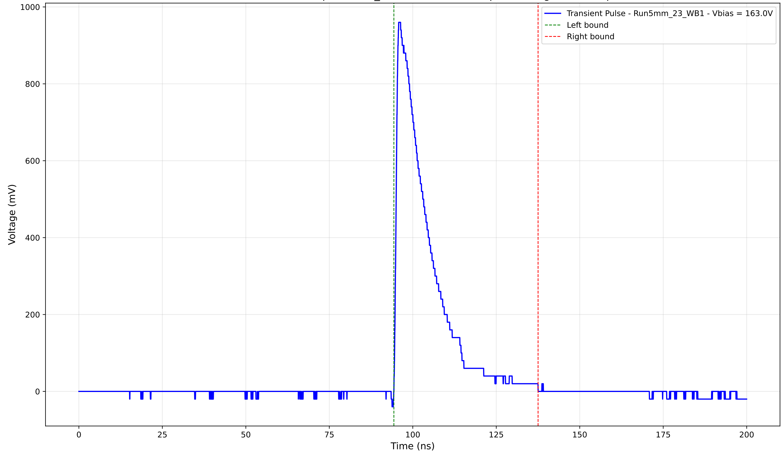
Transient Pulse - Sample: 5mm_23 - Position: 930.0 \mu\text{m} - Charge: 200.68 pC
