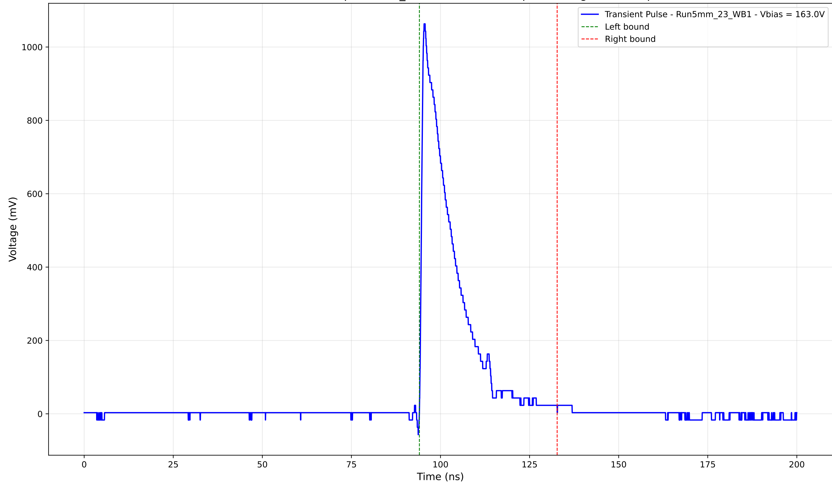
Transient Pulse - Sample: 5mm_23 - Position: 415.0 \mu\text{m} - Charge: 202.49 pC
