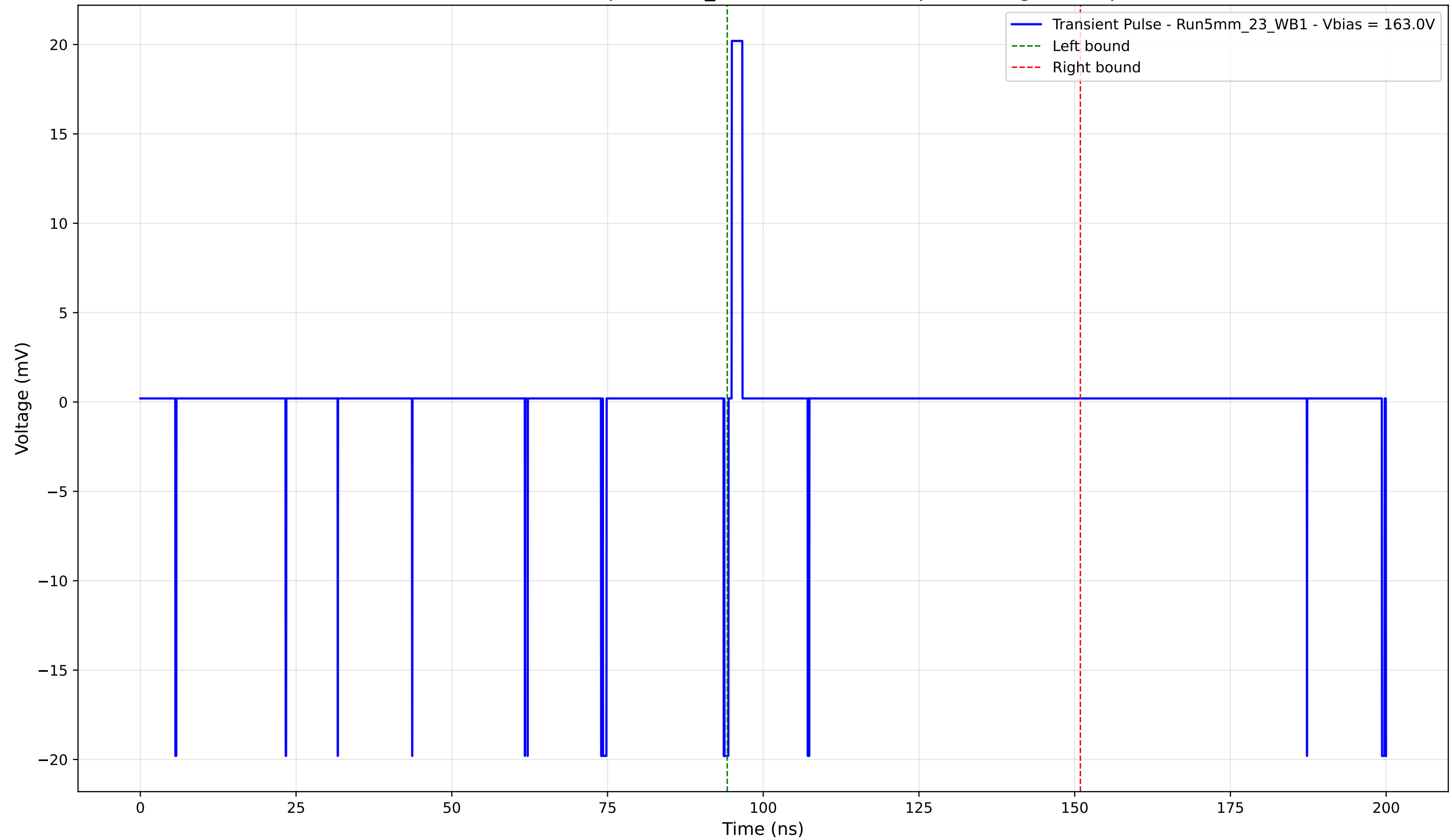
Transient Pulse - Sample: 5mm_23 - Position: 105.0 \mu\text{m} - Charge: 0.79 pC
