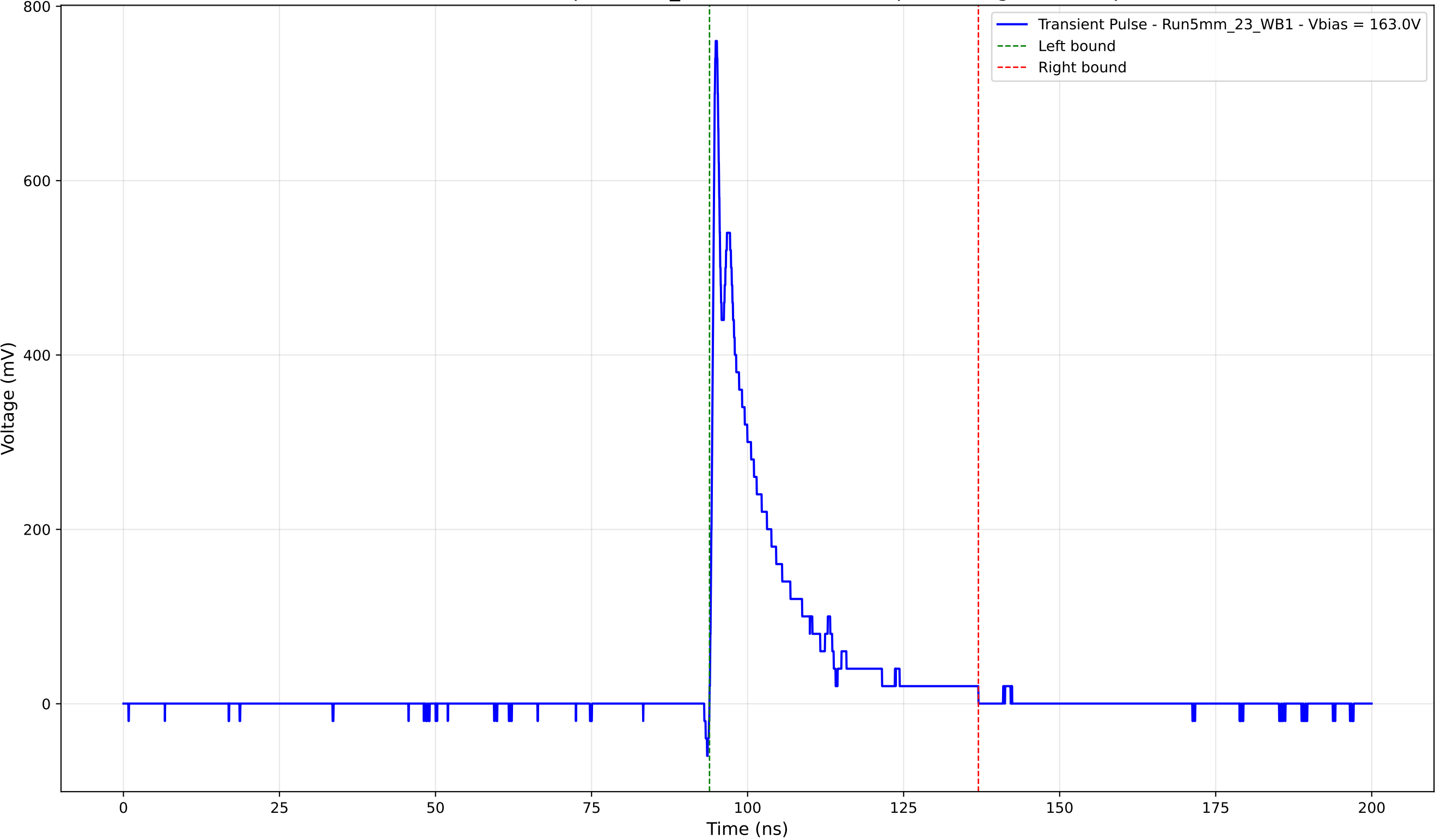
Transient Pulse - Sample: 5mm_23 - Position: 2785.0 \mu\text{m} - Charge: 108.60 pC
