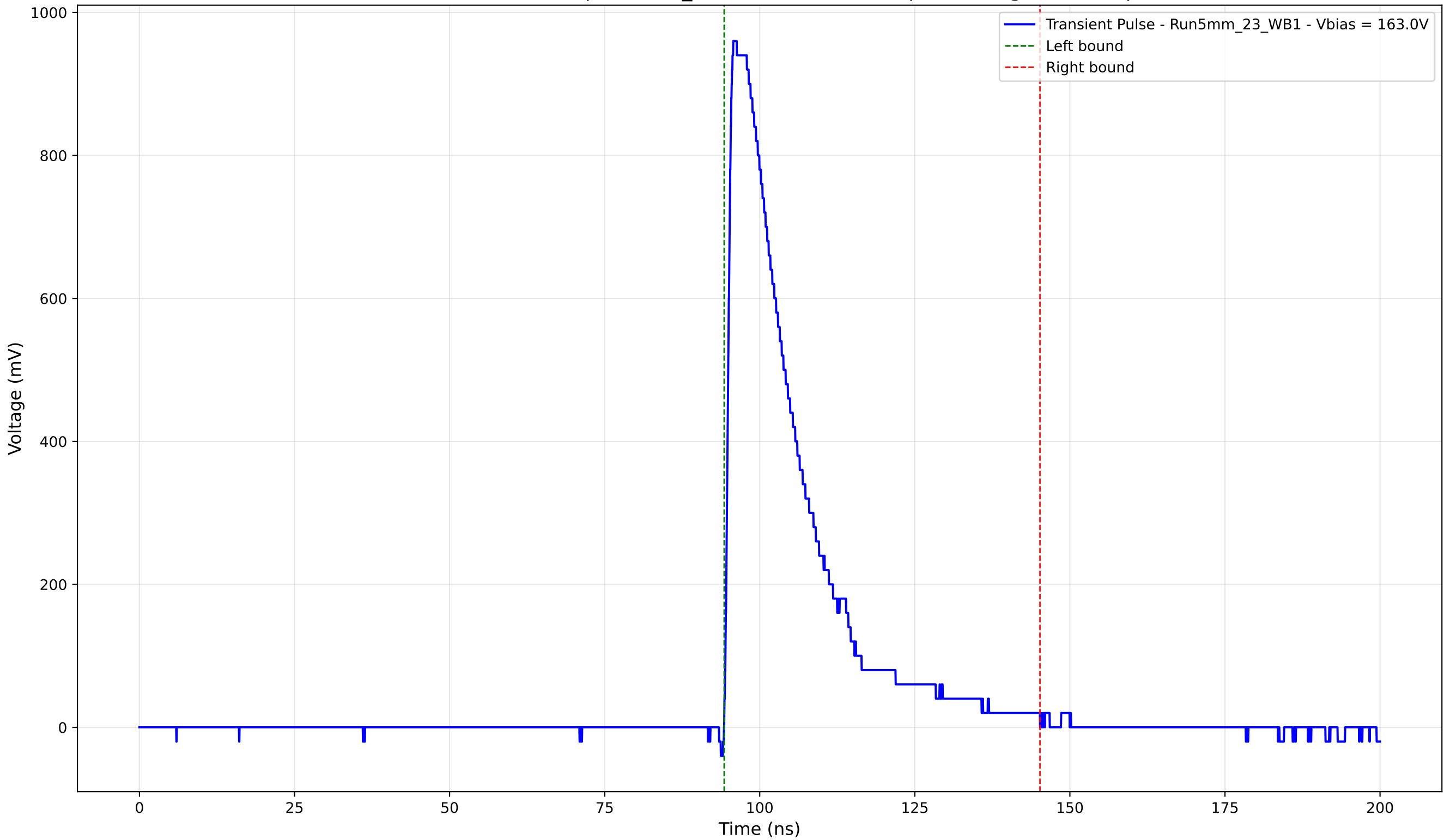
Transient Pulse - Sample: 5mm_23 - Position: 1890.0 \mu\text{m} - Charge: 234.00 pC
