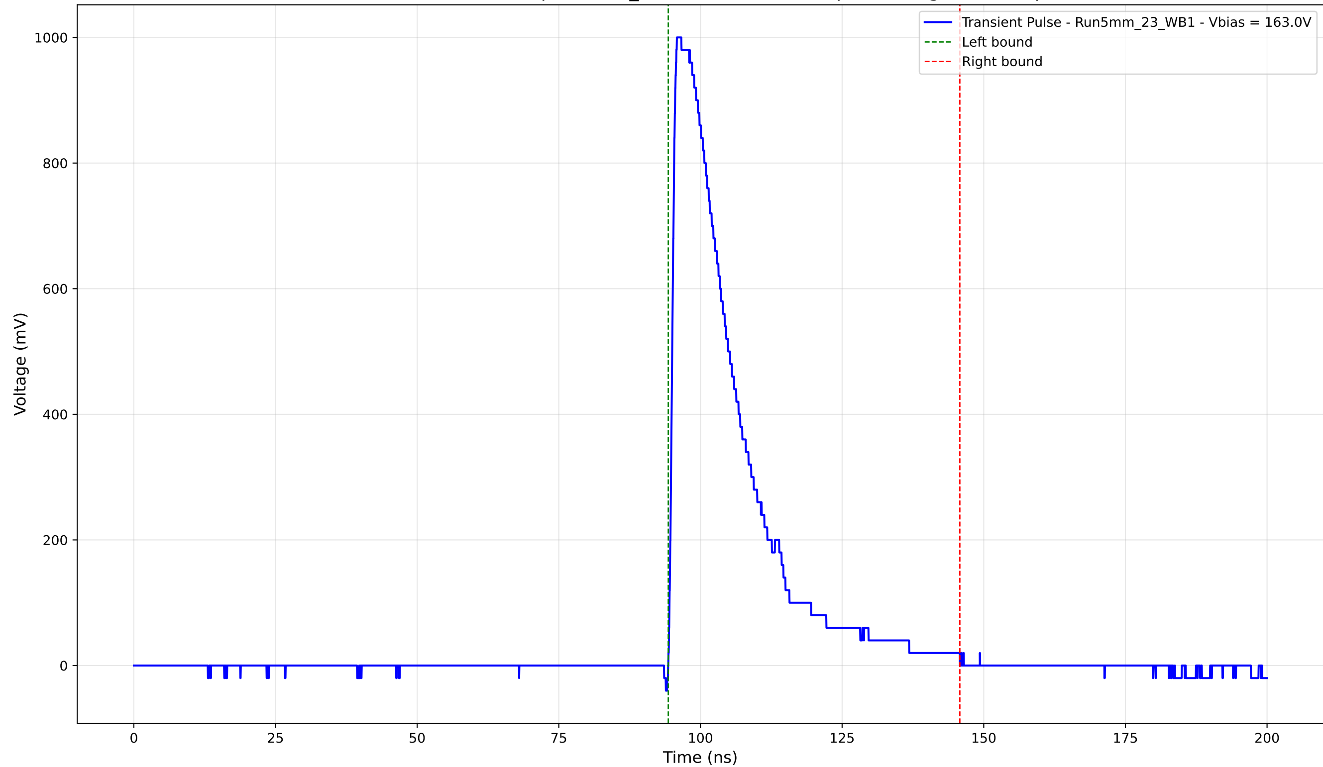
Transient Pulse - Sample: 5mm_23 - Position: 1595.0 \mu\text{m} - Charge: 252.98 pC
