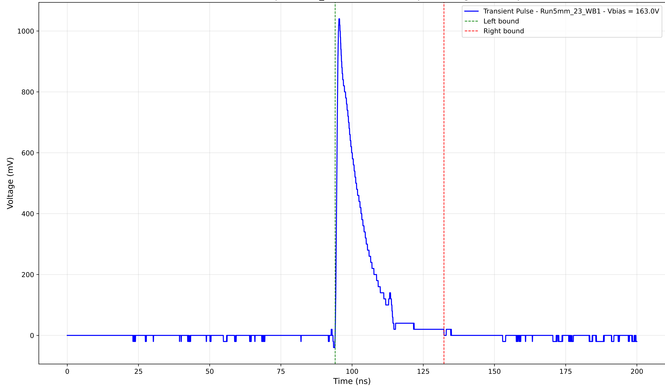
Transient Pulse - Sample: 5mm_23 - Position: 355.0 \mu\text{m} - Charge: 175.15 pC
