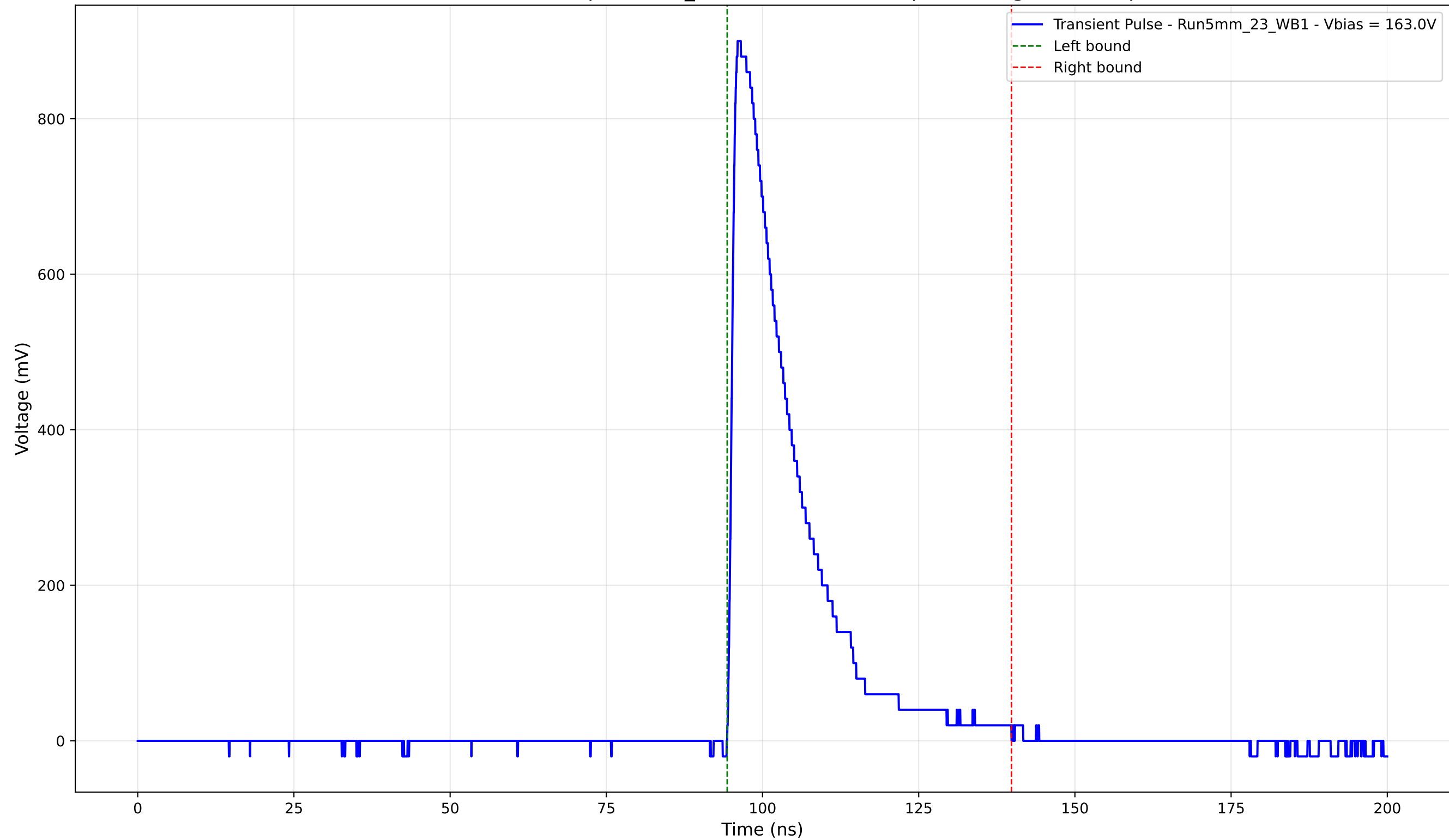
Transient Pulse - Sample: 5mm_23 - Position: 3890.0 \mu\text{m} - Charge: 196.32 pC
