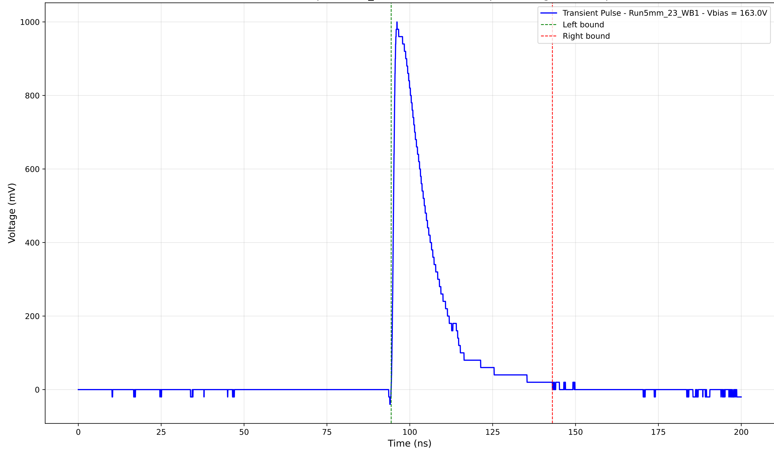
Transient Pulse - Sample: 5mm_23 - Position: 1430.0 \mu\text{m} - Charge: 236.30 pC
