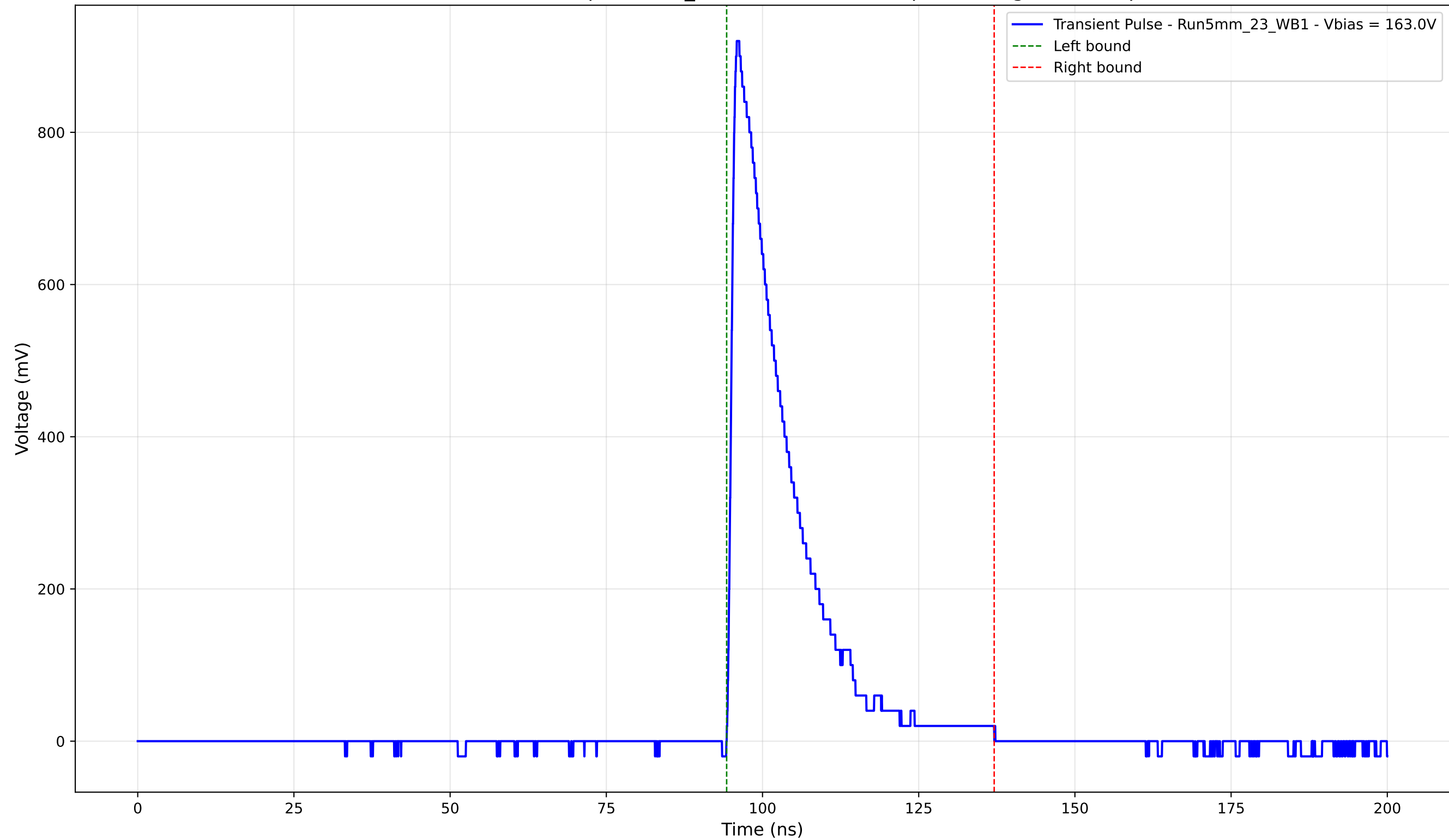
Transient Pulse - Sample: 5mm_23 - Position: 4500.0 \mu\text{m} - Charge: 178.00 pC
