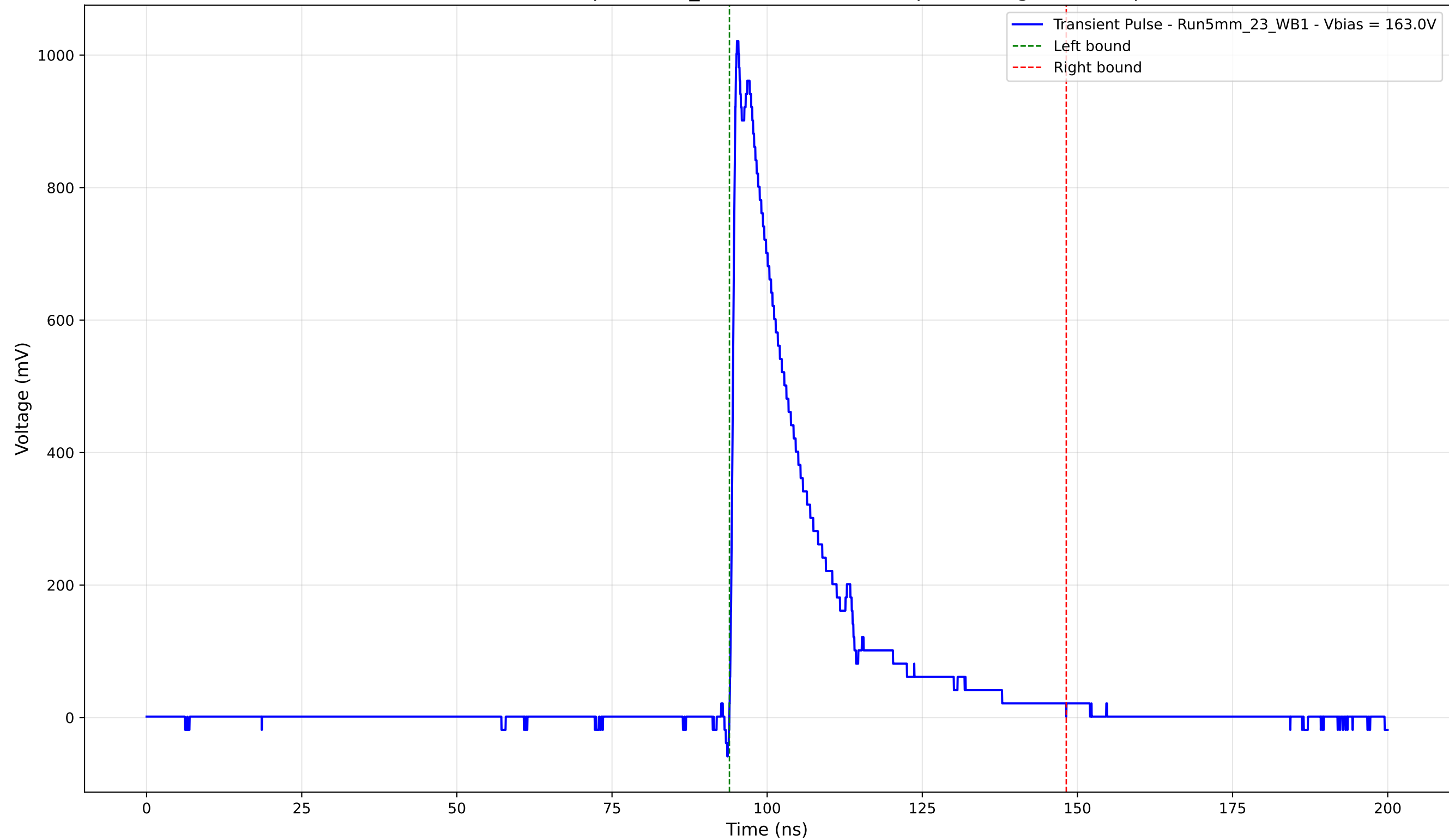
Transient Pulse - Sample: 5mm_23 - Position: 2480.0 \mu\text{m} - Charge: 232.20 pC
