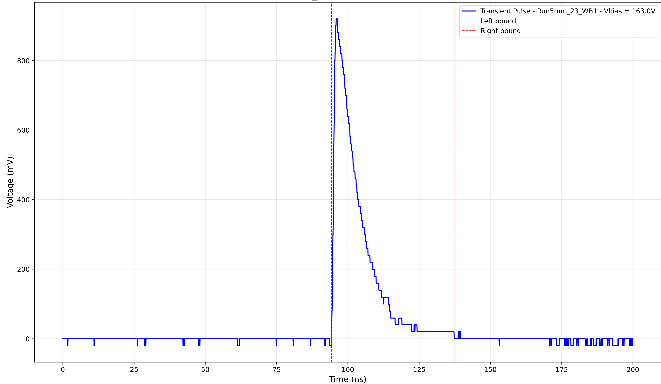
Transient Pulse - Sample: 5mm_23 - Position: 4465.0 \mu\text{m} - Charge: 178.97 pC
