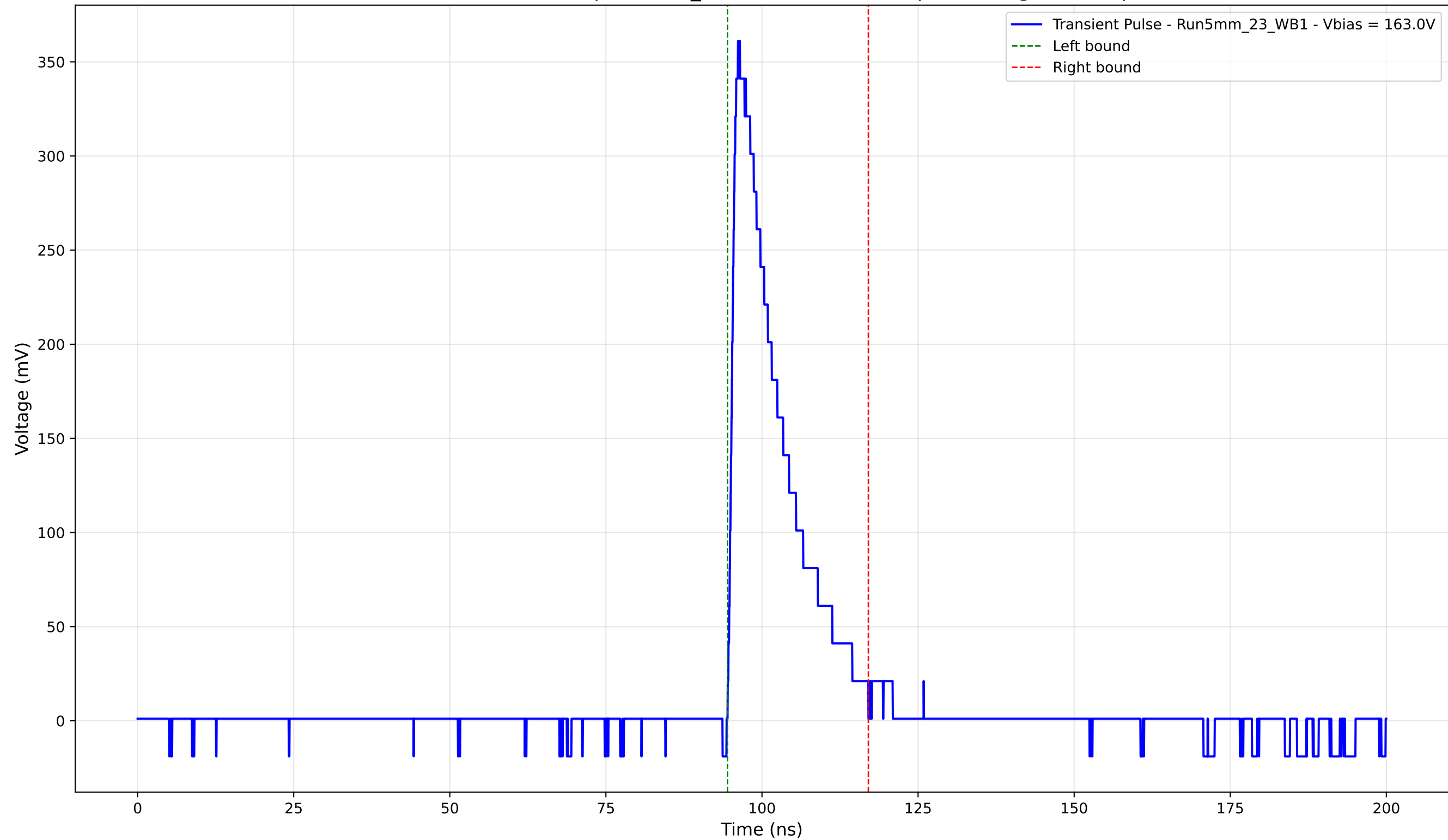
Transient Pulse - Sample: 5mm_23 - Position: 4230.0 \mu\text{m} - Charge: 61.39 pC
