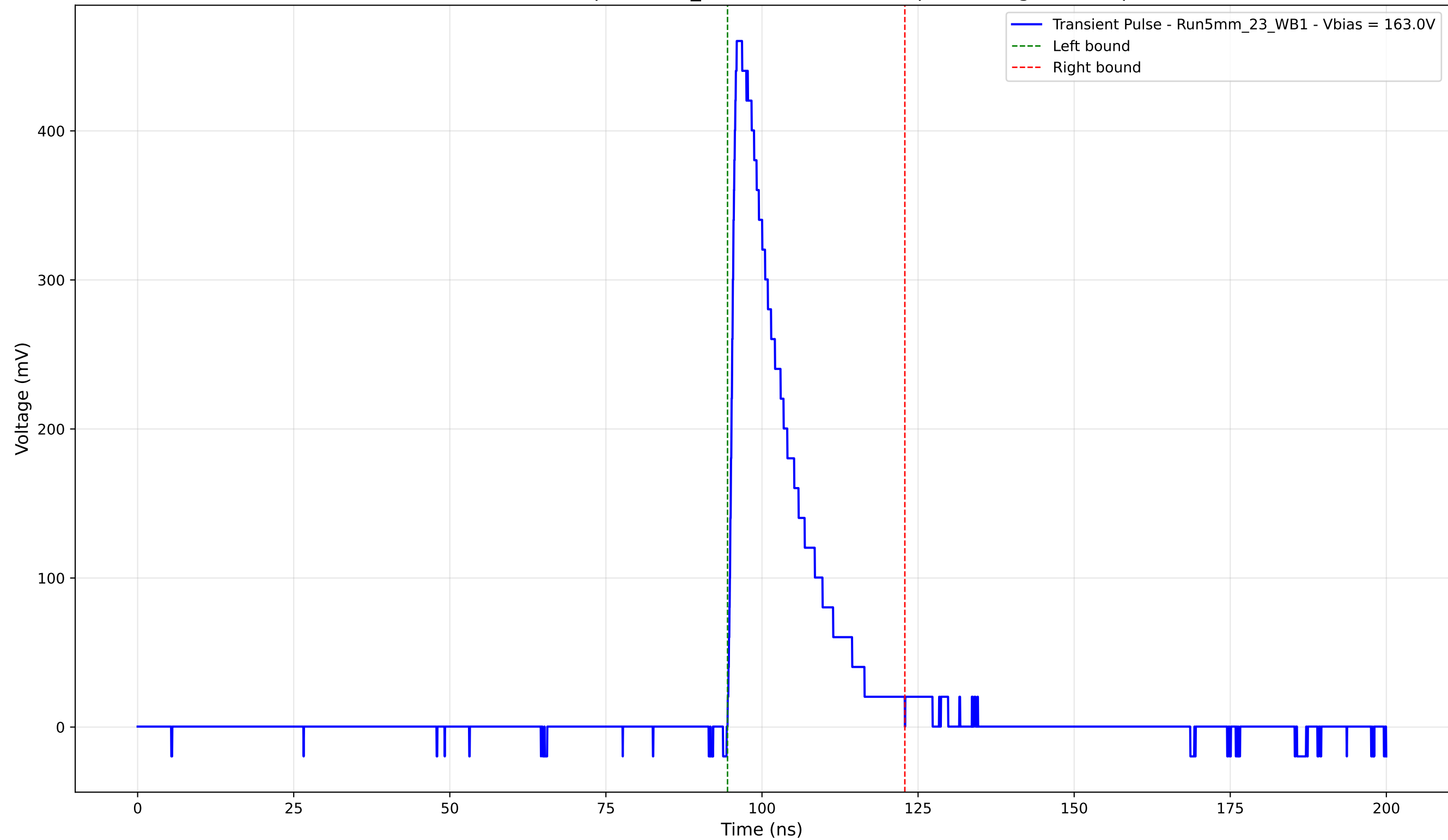
Transient Pulse - Sample: 5mm_23 - Position: 1260.0 \mu\text{m} - Charge: 87.07 pC
