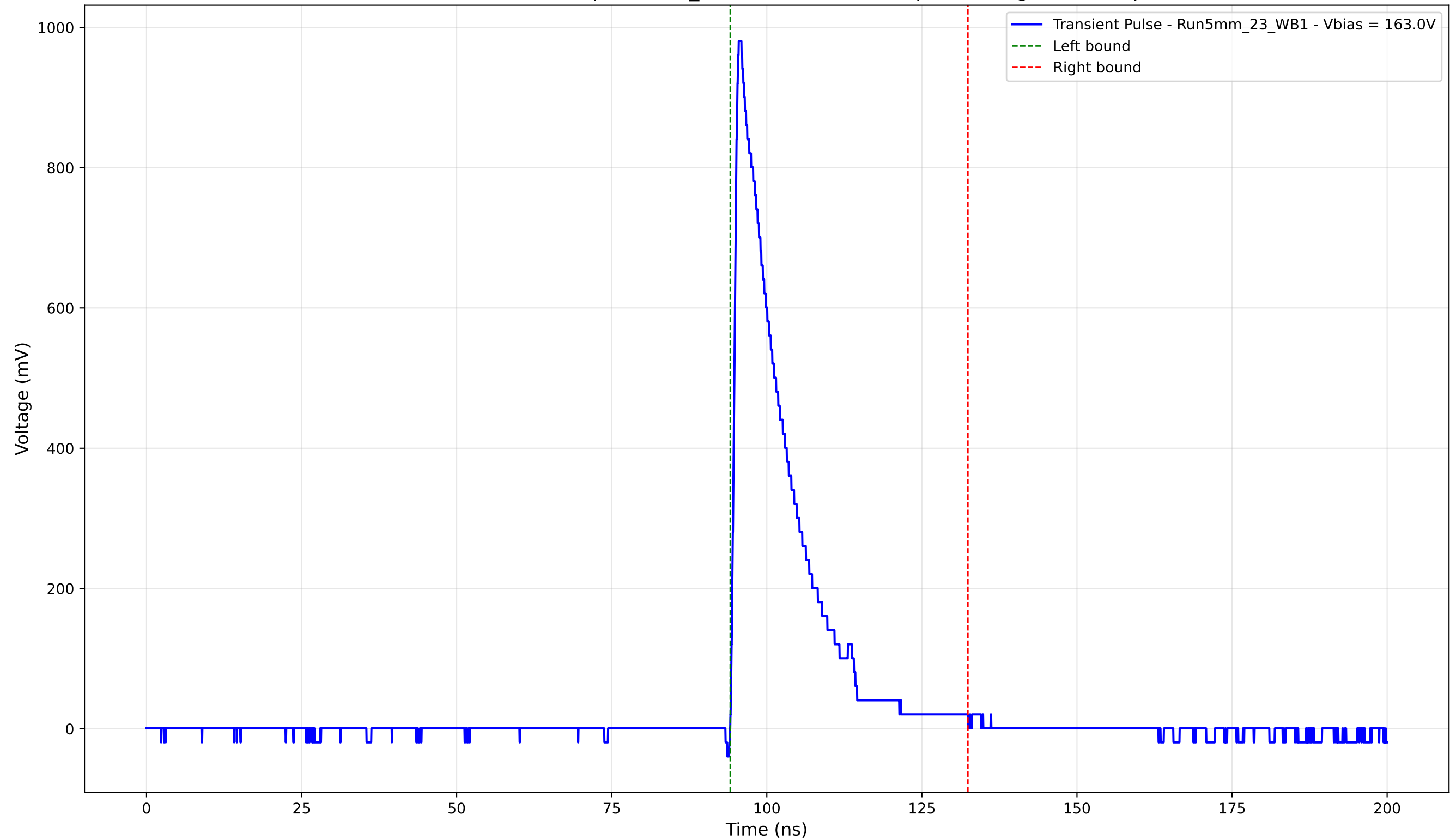
Transient Pulse - Sample: 5mm_23 - Position: 4880.0 \mu\text{m} - Charge: 171.11 pC
