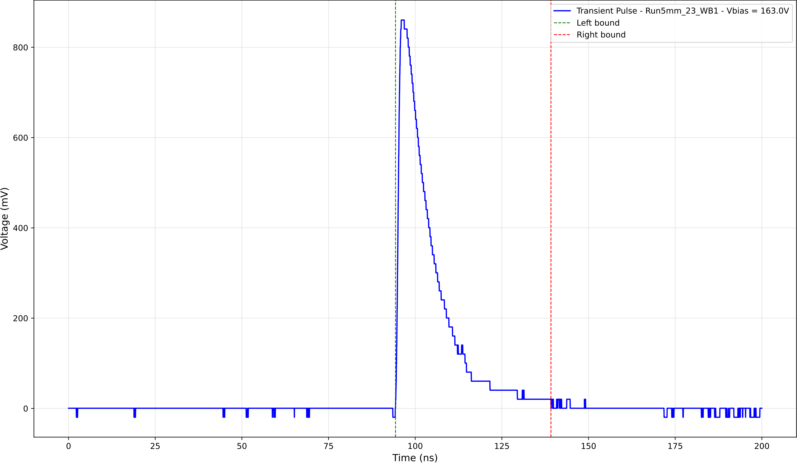
Transient Pulse - Sample: 5mm_23 - Position: 3850.0 \mu\text{m} - Charge: 186.27 pC
