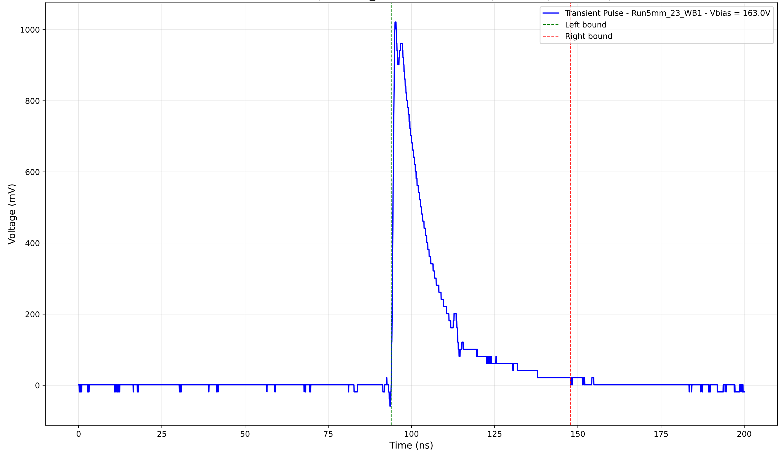
Transient Pulse - Sample: 5mm_23 - Position: 2980.0 \mu\text{m} - Charge: 233.22 pC
