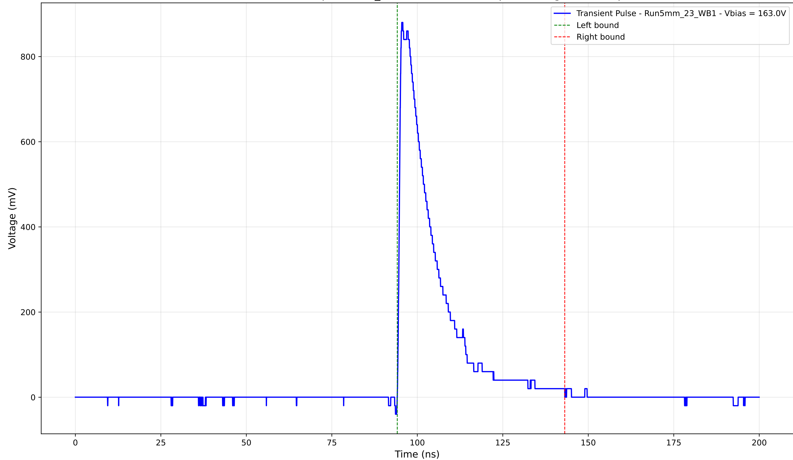
Transient Pulse - Sample: 5mm_23 - Position: 3340.0 \mu\text{m} - Charge: 193.88 pC
