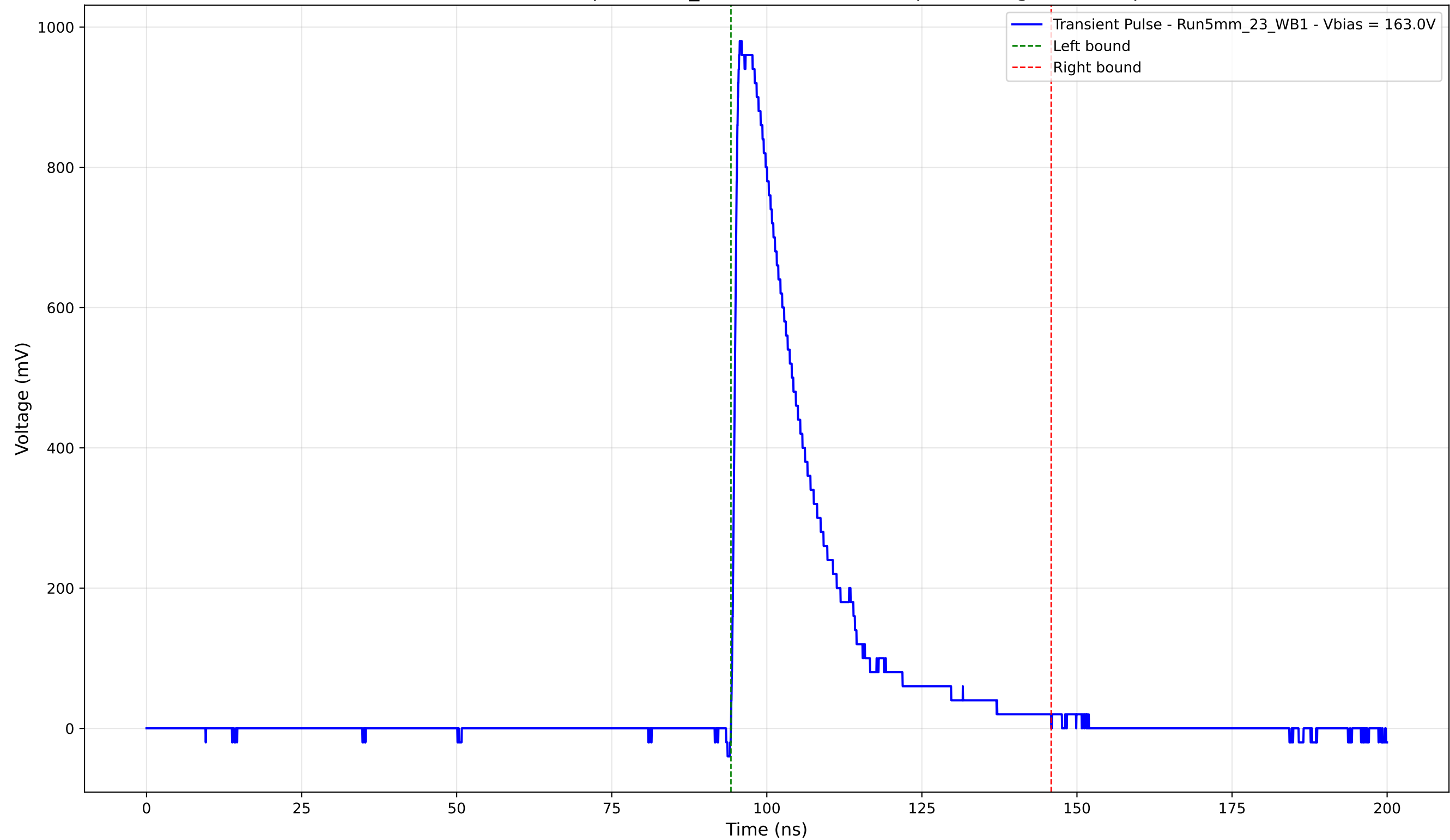
Transient Pulse - Sample: 5mm_23 - Position: 1985.0 \mu\text{m} - Charge: 240.16 pC
