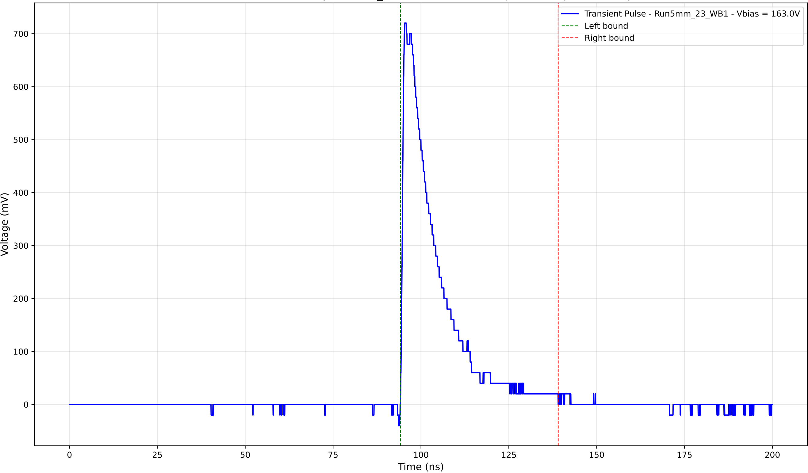
Transient Pulse - Sample: 5mm_23 - Position: 2185.0 \mu\text{m} - Charge: 149.62 pC
