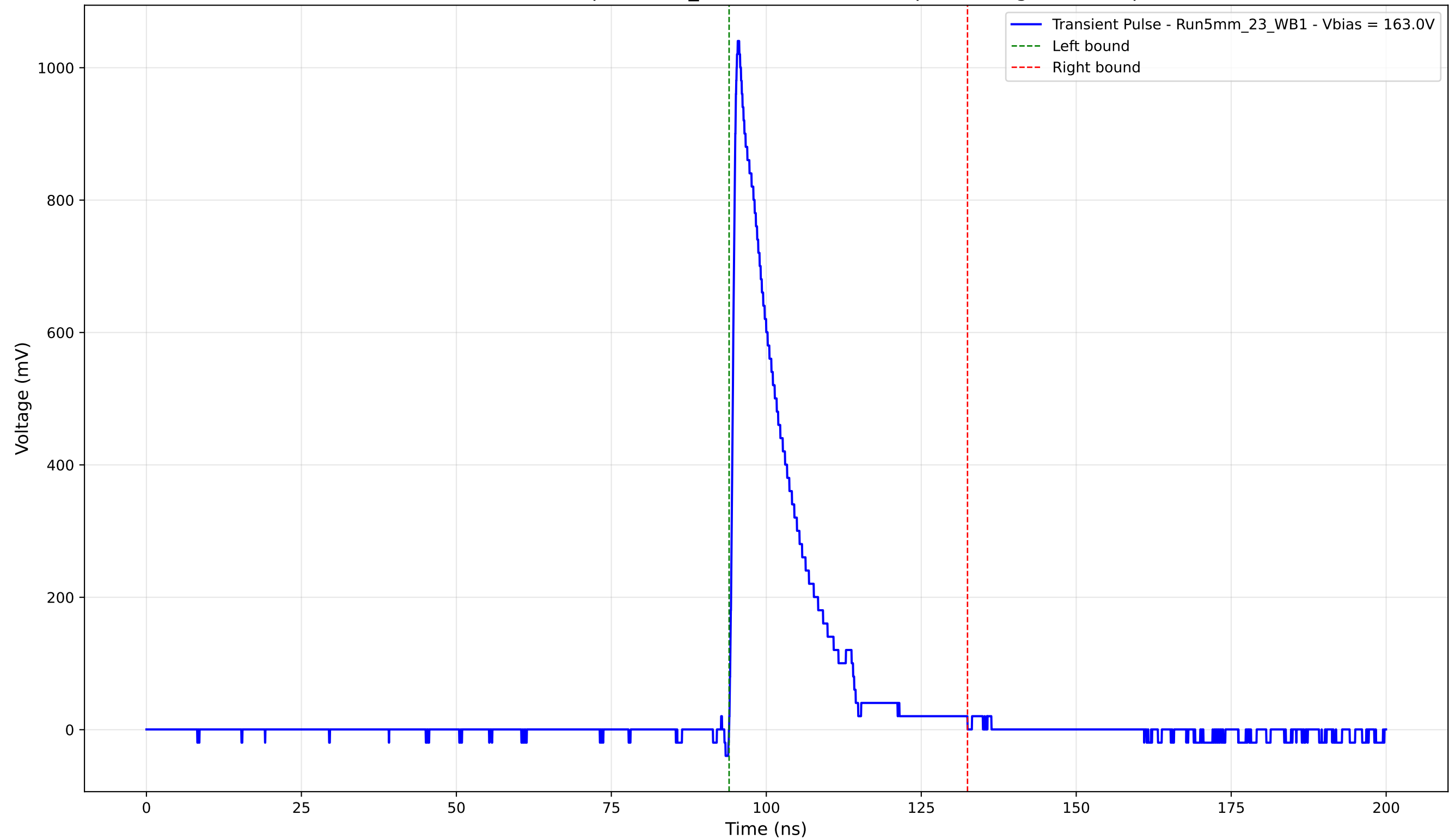
Transient Pulse - Sample: 5mm_23 - Position: 5035.0 \mu\text{m} - Charge: 177.48 pC
