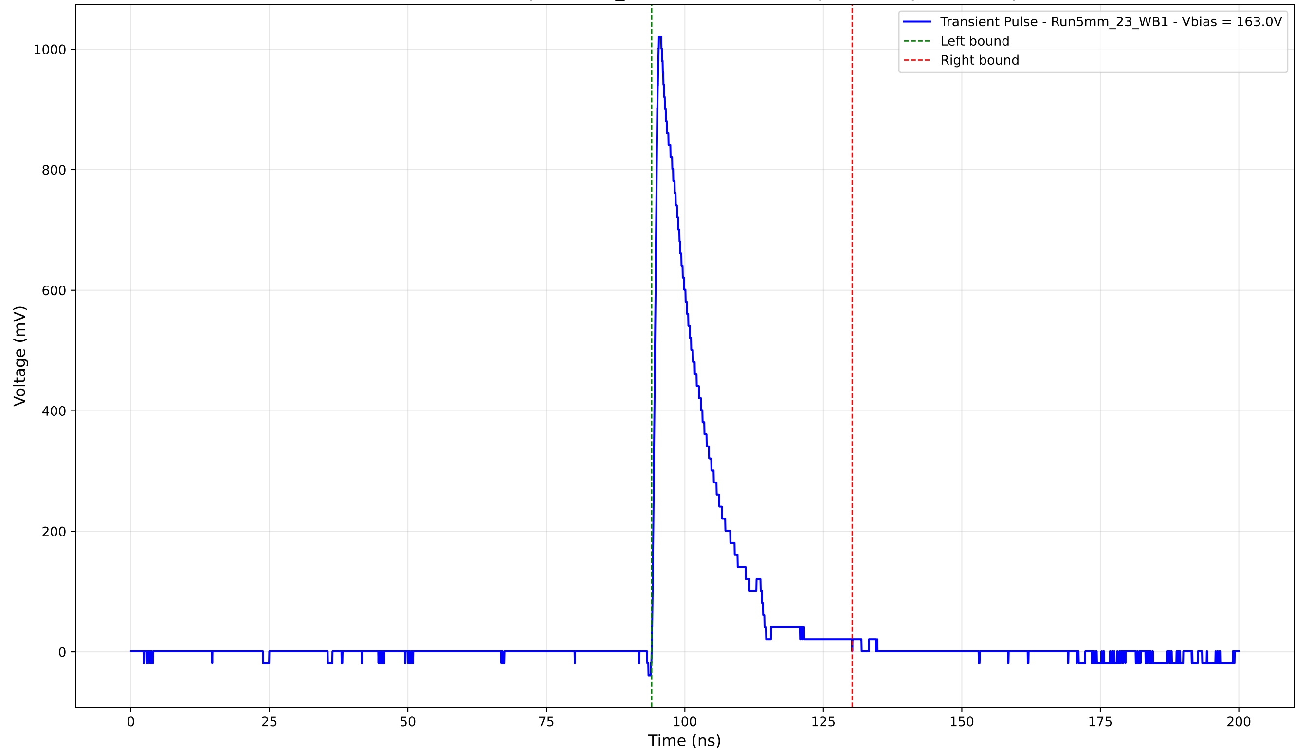
Transient Pulse - Sample: 5mm_23 - Position: 5025.0 \mu\text{m} - Charge: 173.43 pC
