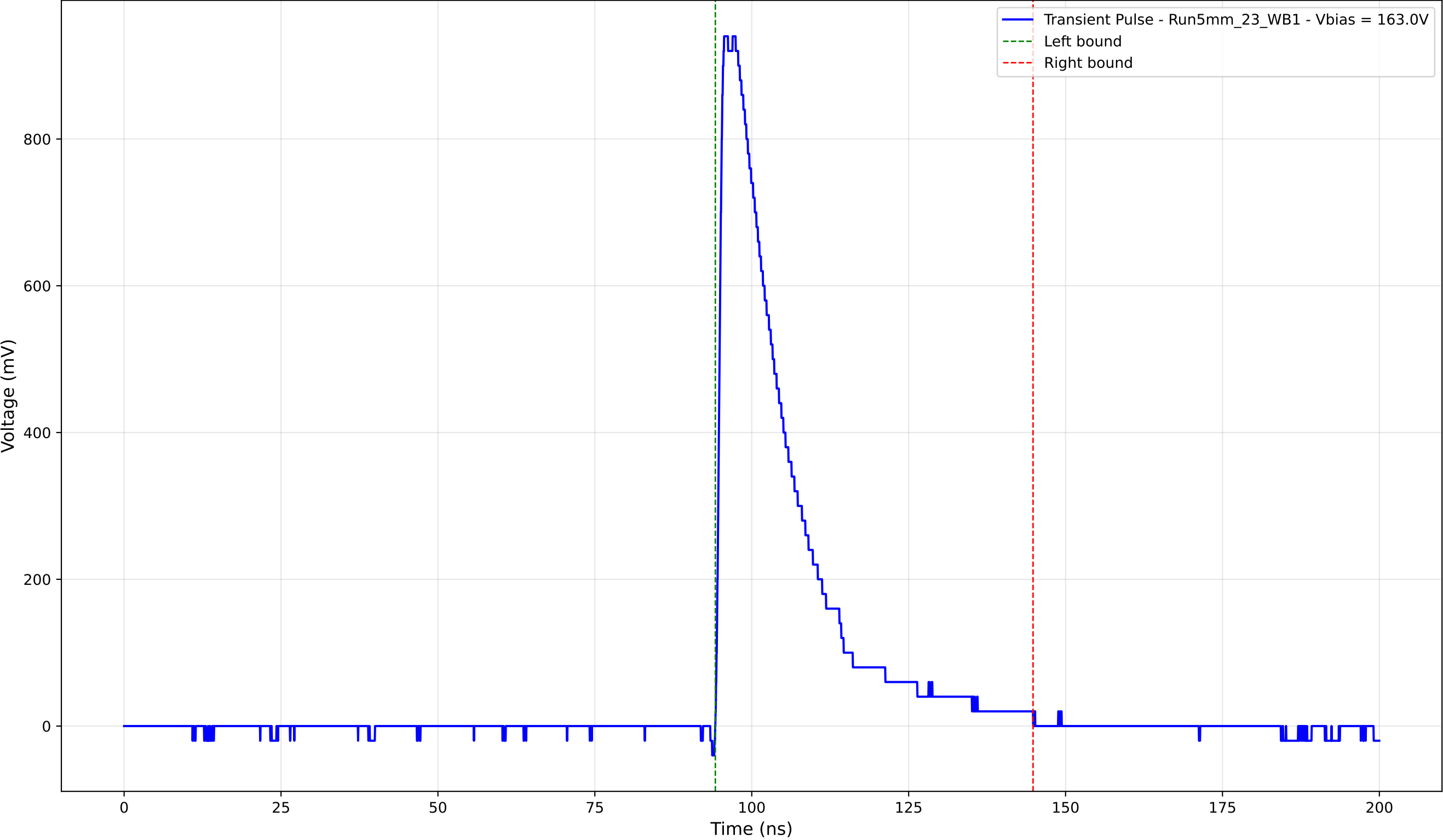
Transient Pulse - Sample: 5mm_23 - Position: 3500.0 \mu\text{m} - Charge: 223.28 pC
