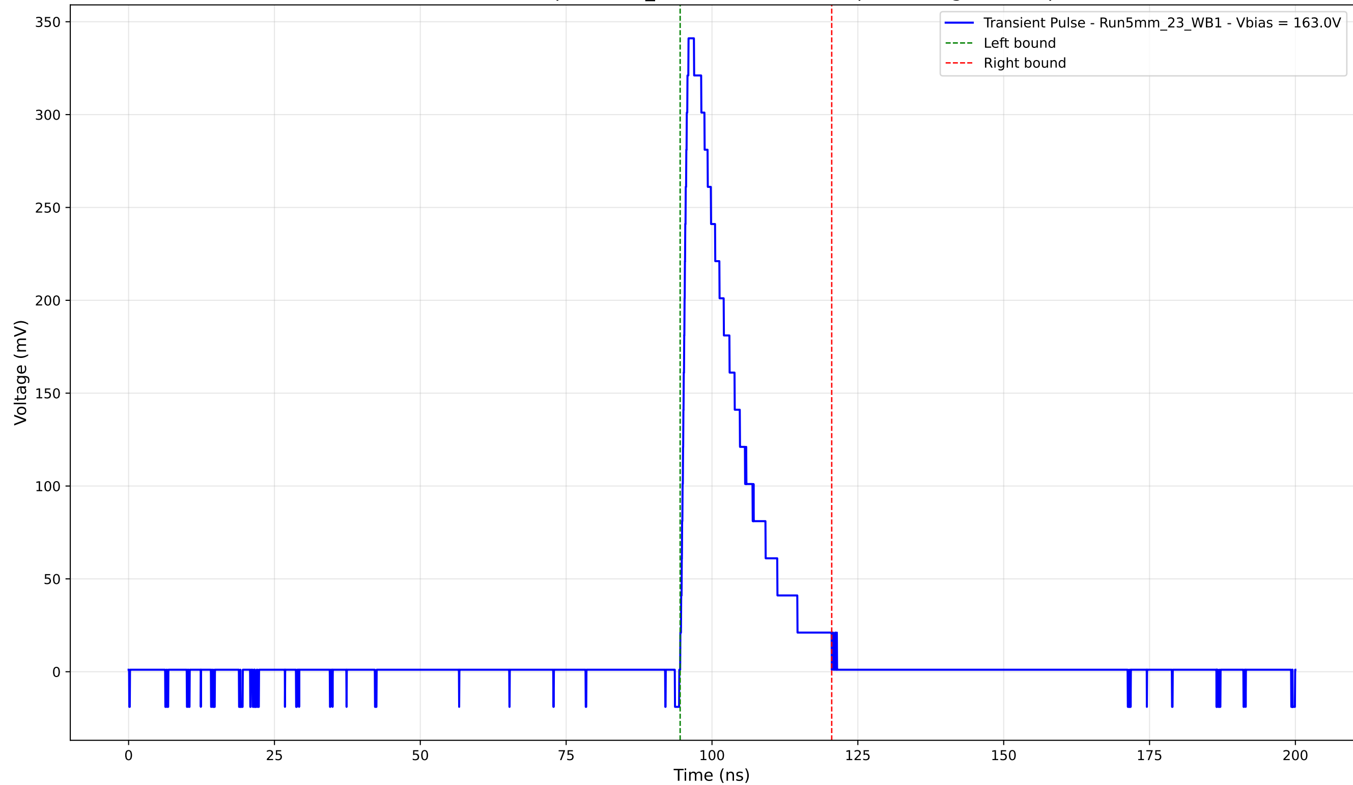
Transient Pulse - Sample: 5mm_23 - Position: 1250.0 \mu\text{m} - Charge: 63.69 pC
