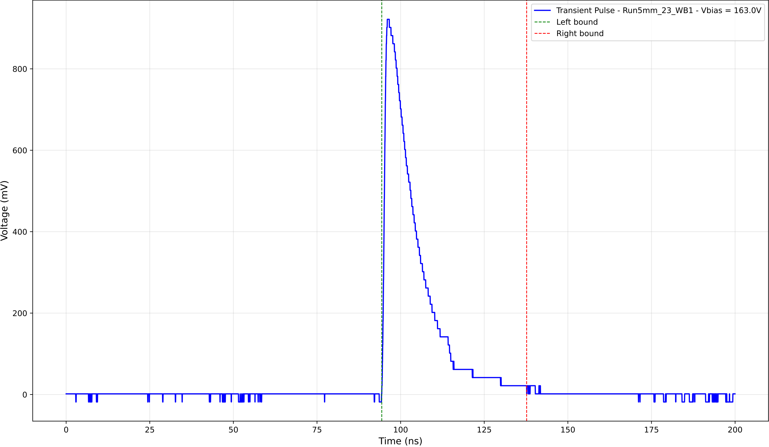
Transient Pulse - Sample: 5mm_23 - Position: 4110.0 \mu\text{m} - Charge: 197.72 pC
