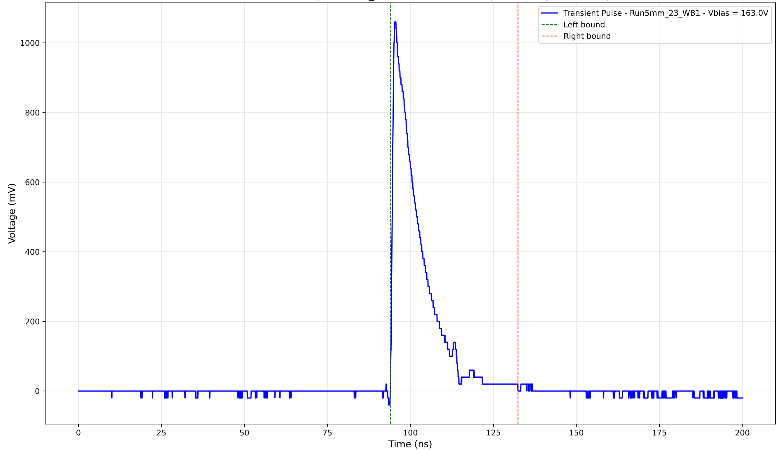
Transient Pulse - Sample: 5mm_23 - Position: 5085.0 \mu\text{m} - Charge: 187.28 pC
