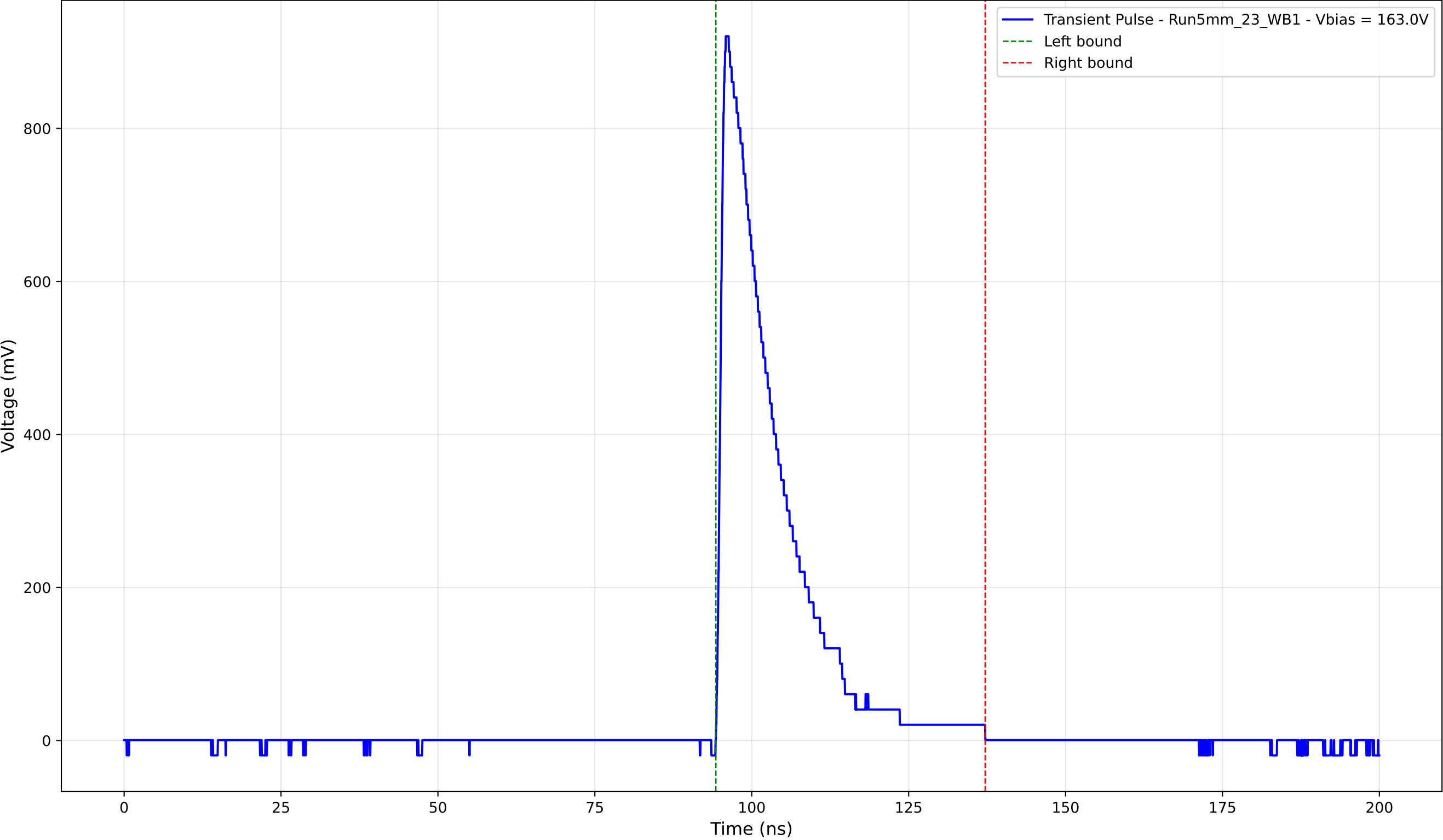
Transient Pulse - Sample: 5mm_23 - Position: 4490.0 \mu\text{m} - Charge: 178.92 pC
