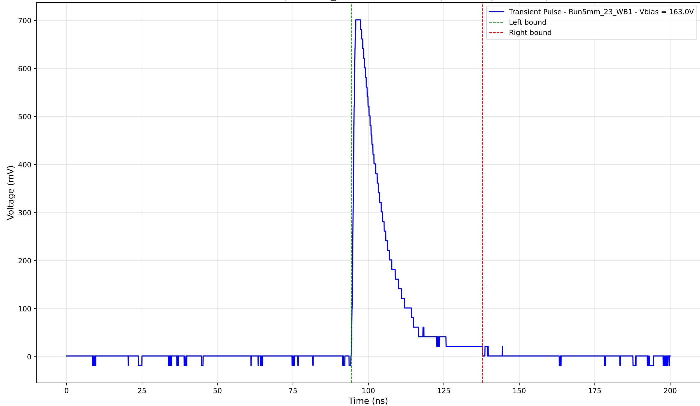
Transient Pulse - Sample: 5mm_23 - Position: 1785.0 \mu\text{m} - Charge: 150.00 pC
