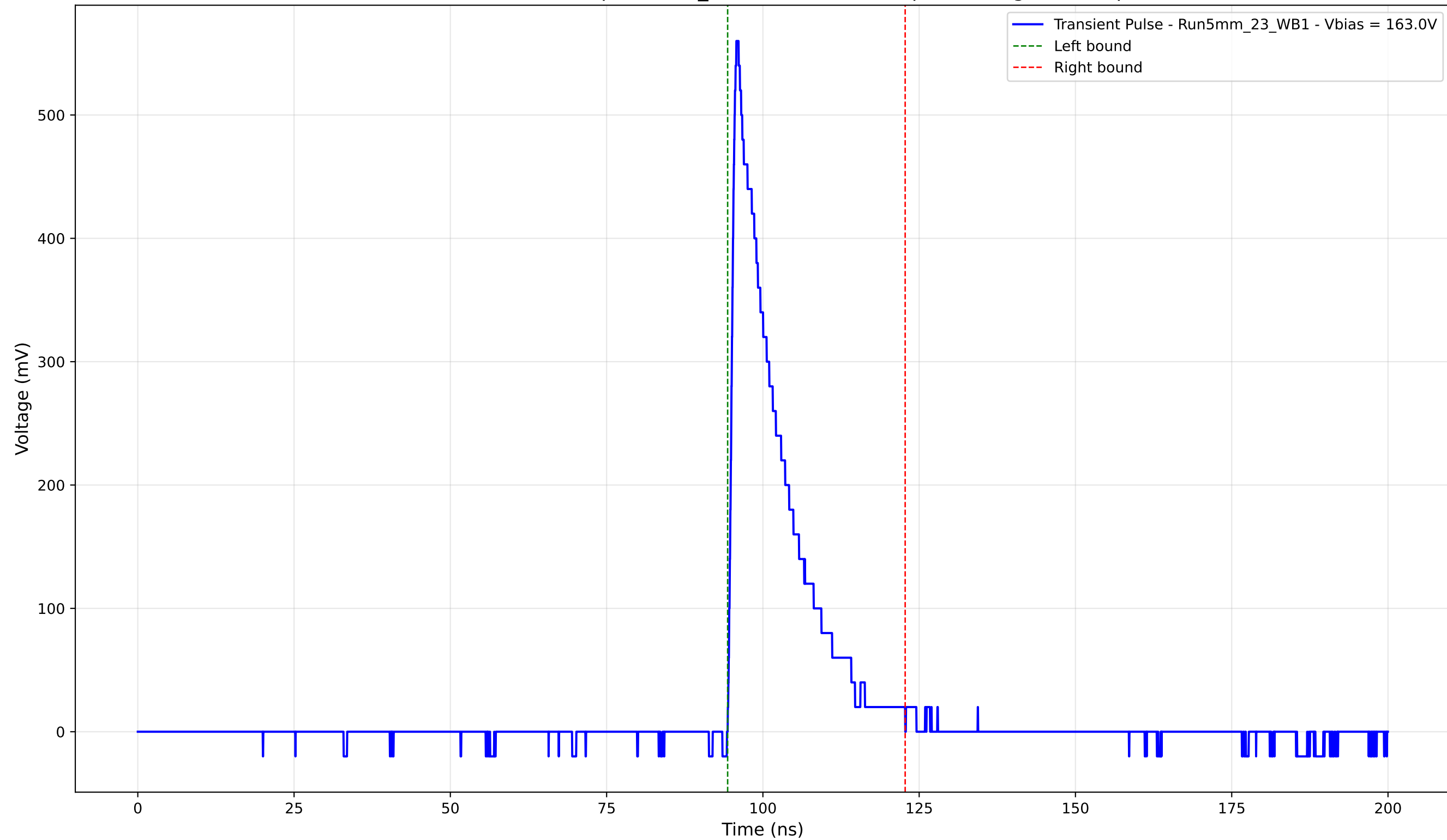
Transient Pulse - Sample: 5mm_23 - Position: 755.0 \mu\text{m} - Charge: 91.40 pC
