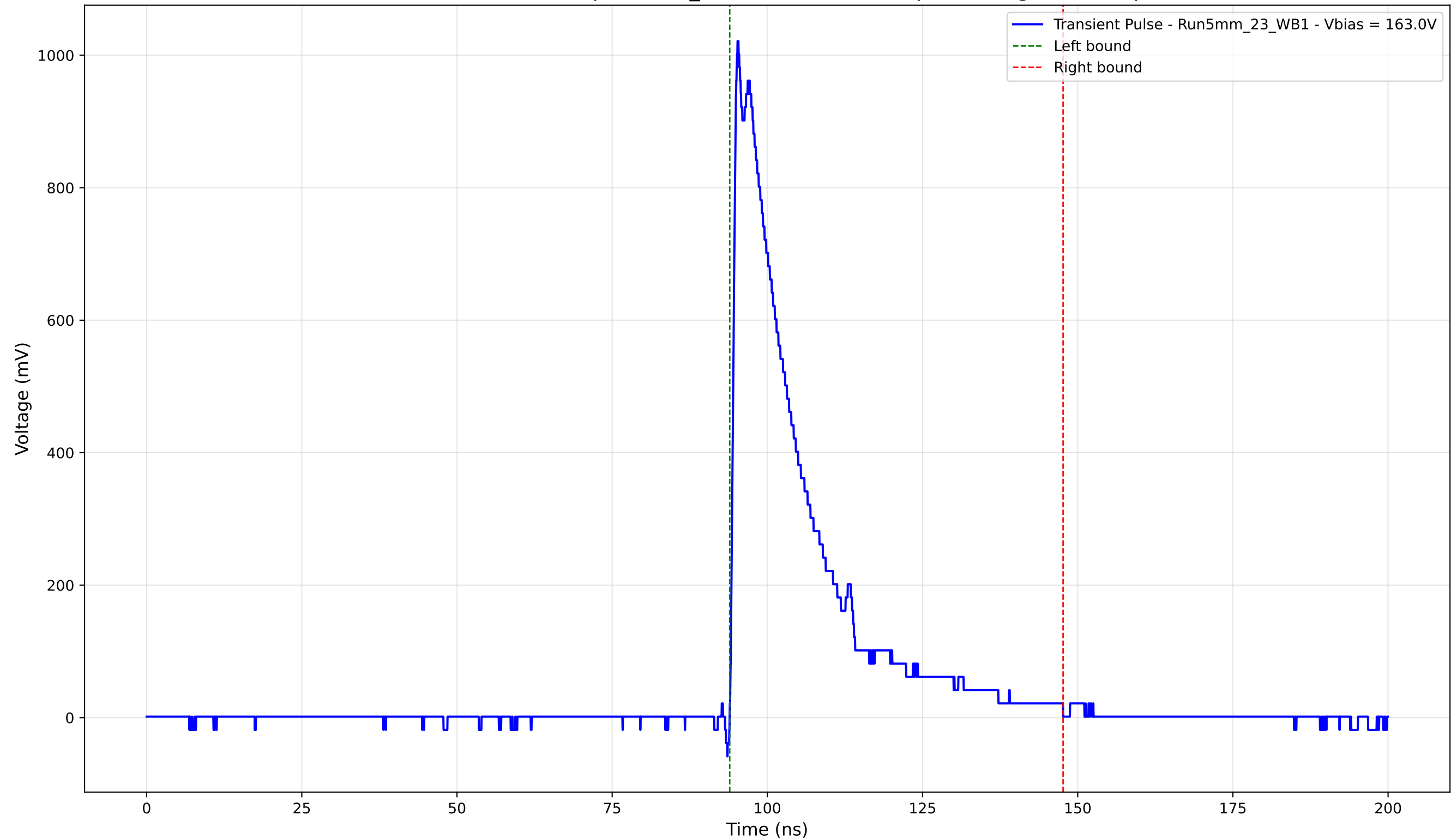
Transient Pulse - Sample: 5mm_23 - Position: 2445.0 \mu\text{m} - Charge: 231.89 pC
