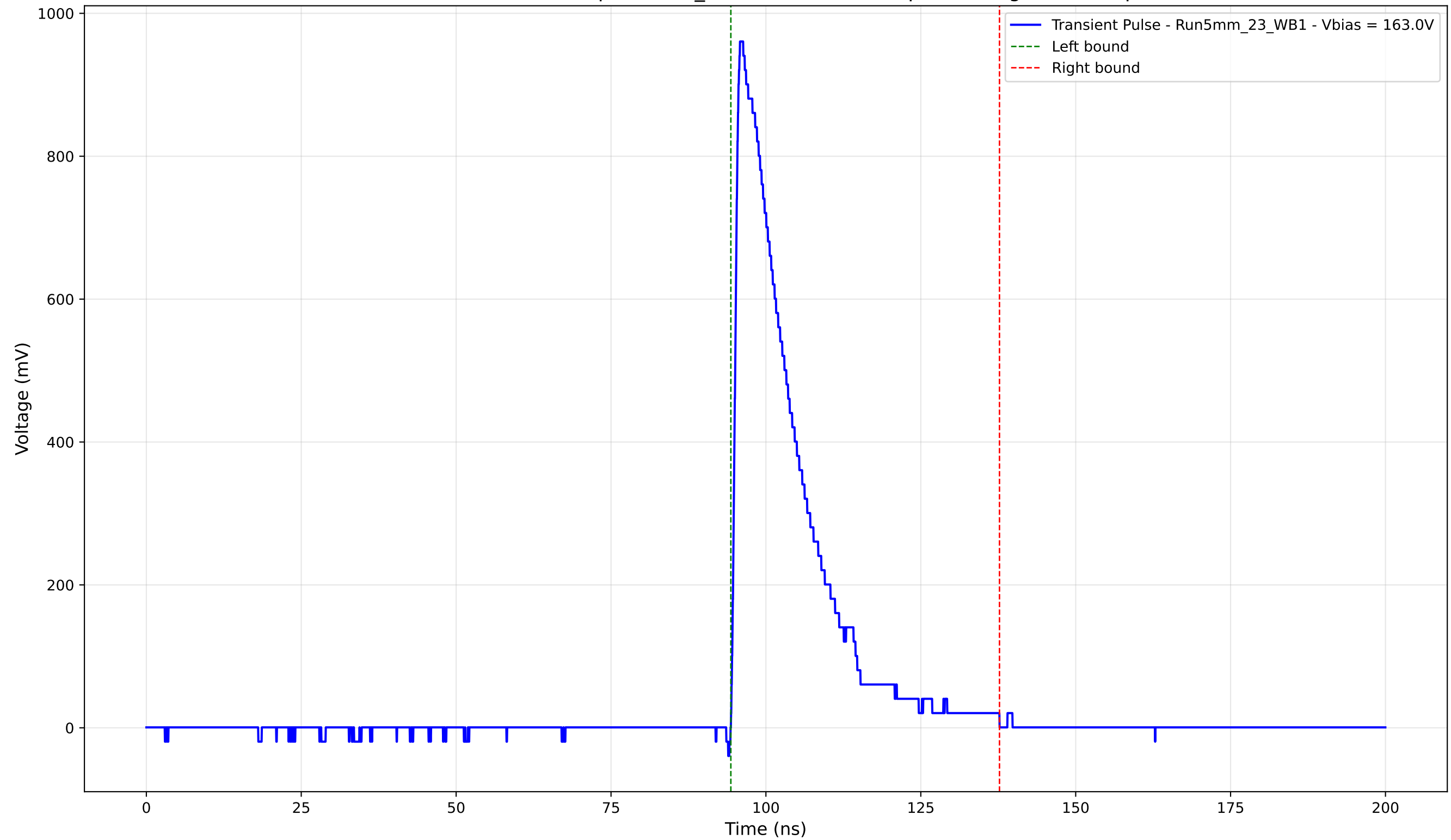
Transient Pulse - Sample: 5mm_23 - Position: 950.0 \mu\text{m} - Charge: 200.44 pC
