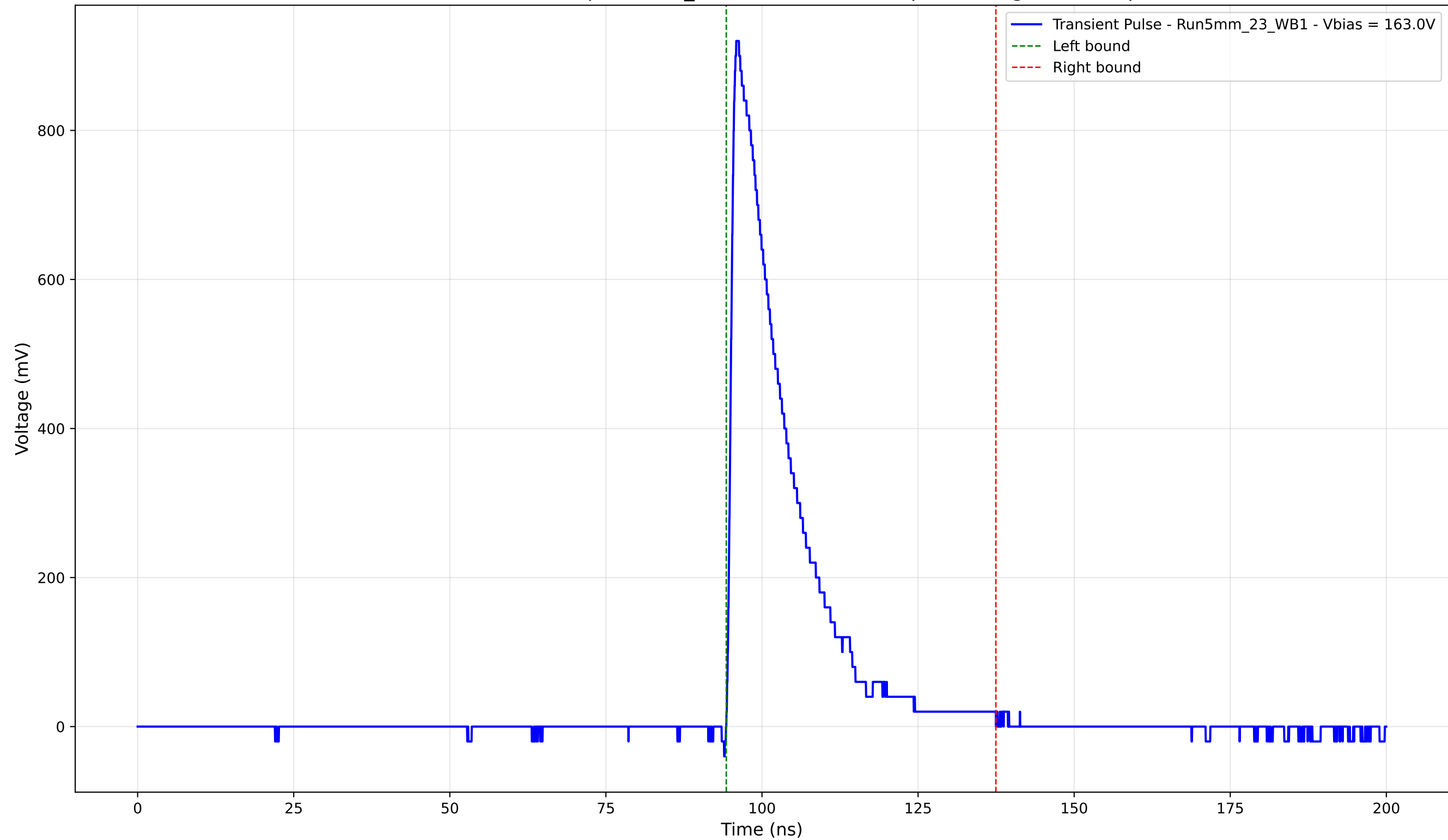
Transient Pulse - Sample: 5mm_23 - Position: 4495.0 \mu\text{m} - Charge: 180.11 pC
