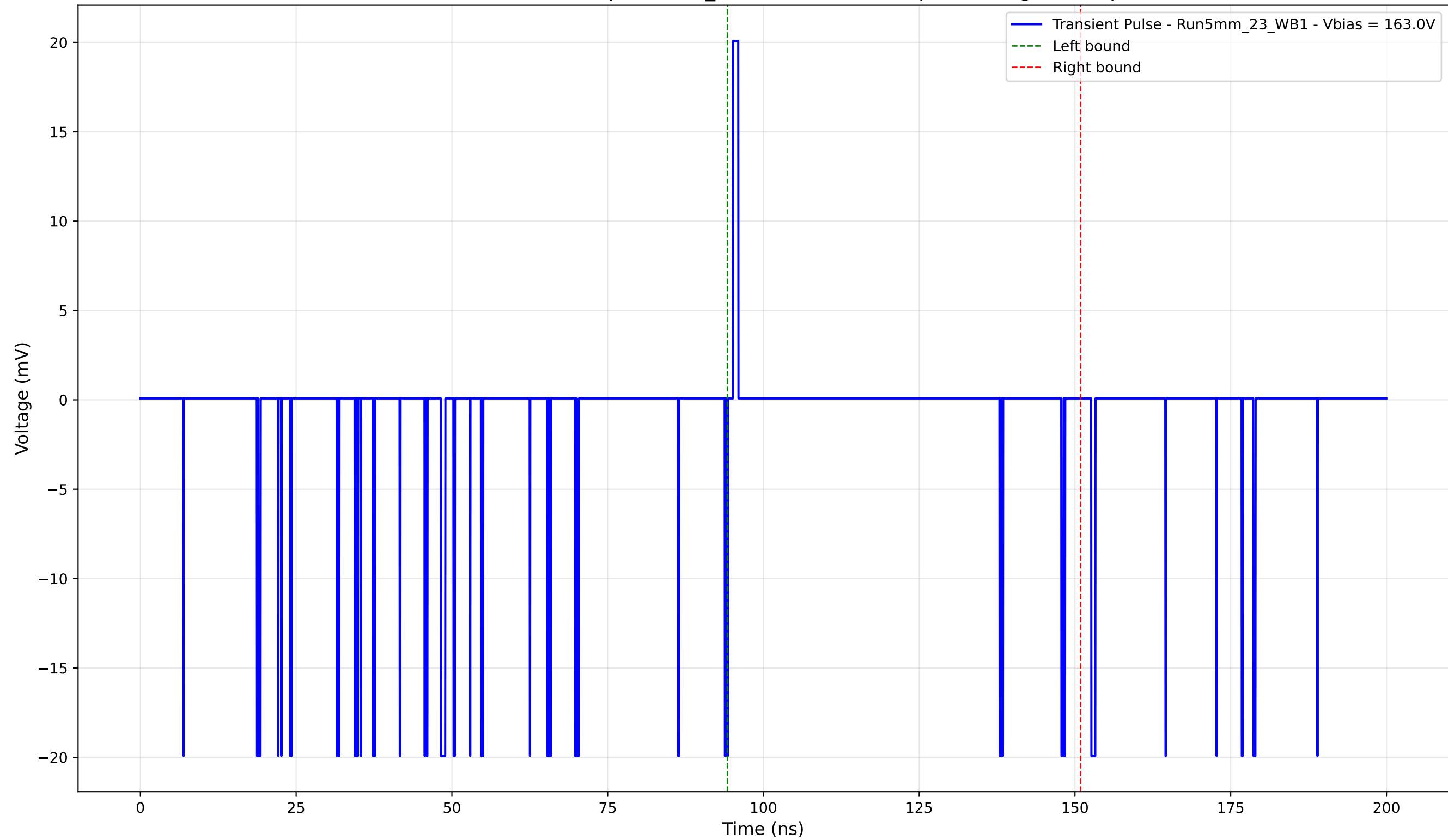
Transient Pulse - Sample: 5mm_23 - Position: 150.0 \mu\text{m} - Charge: 0.08 pC
