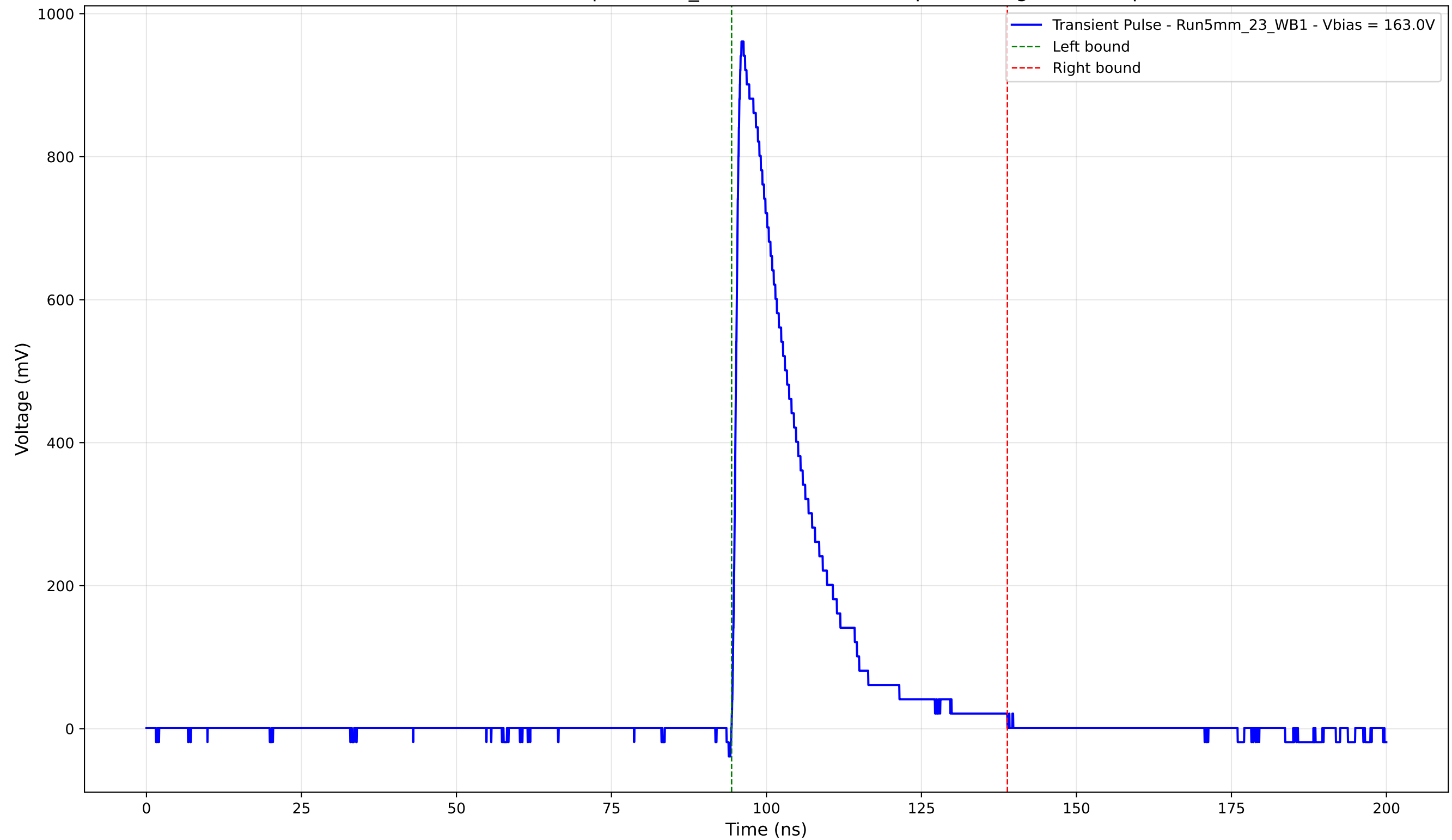
Transient Pulse - Sample: 5mm_23 - Position: 1085.0 \mu\text{m} - Charge: 203.37 pC
