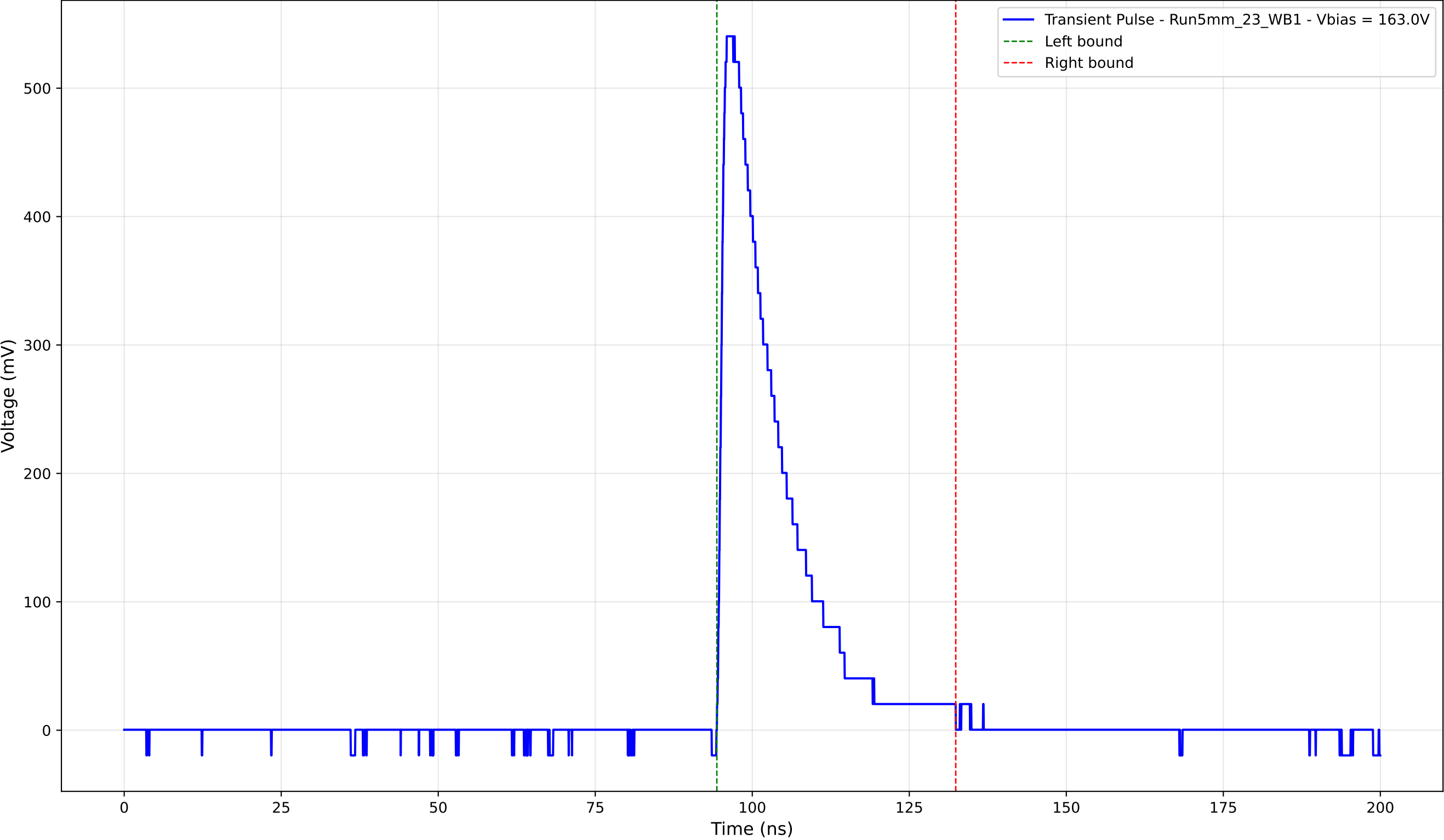
Transient Pulse - Sample: 5mm_23 - Position: 1770.0 \mu\text{m} - Charge: 109.84 pC
