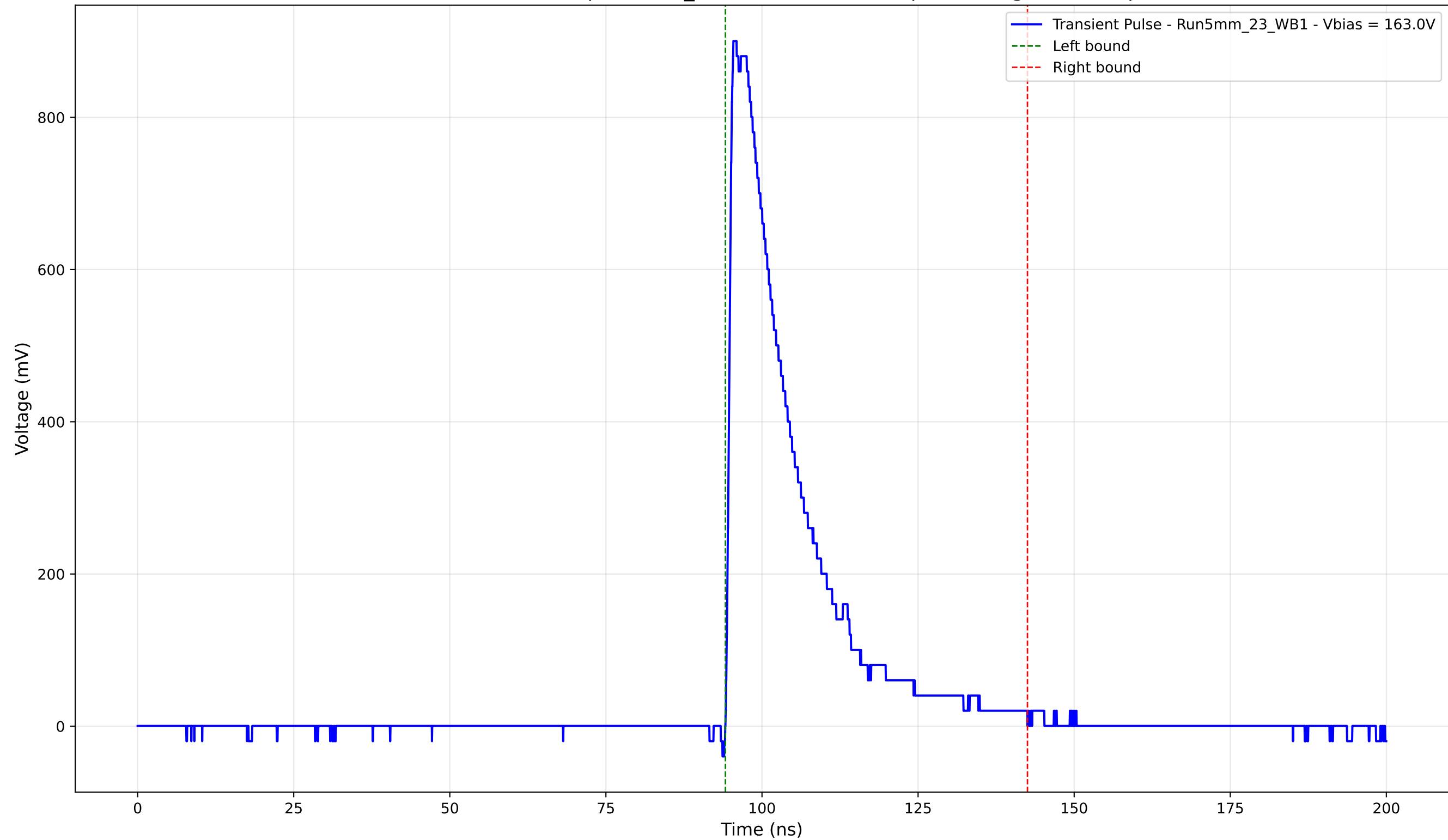
Transient Pulse - Sample: 5mm_23 - Position: 3360.0 \mu\text{m} - Charge: 204.52 pC
