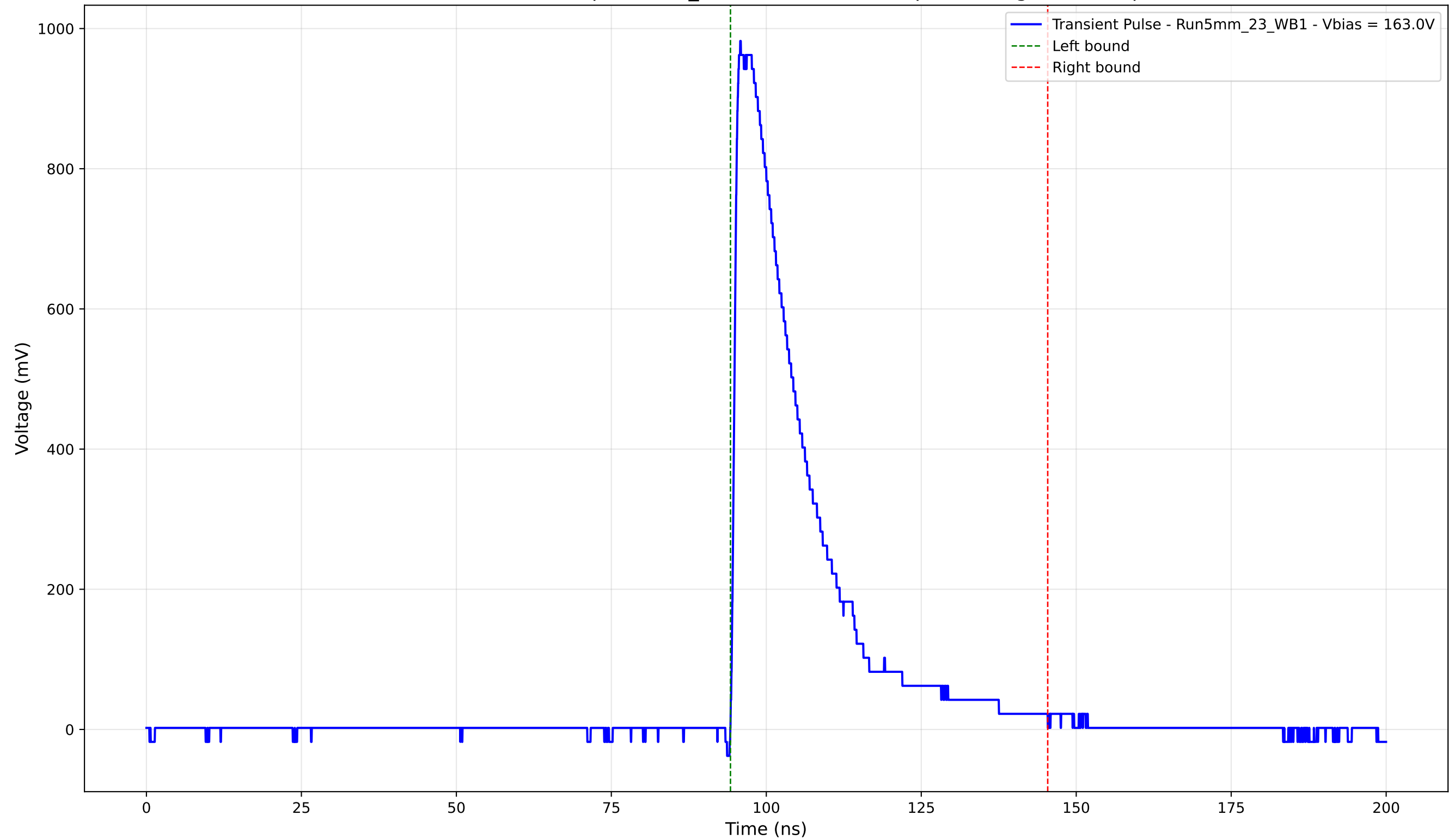
Transient Pulse - Sample: 5mm_23 - Position: 1955.0 \mu\text{m} - Charge: 240.64 pC
