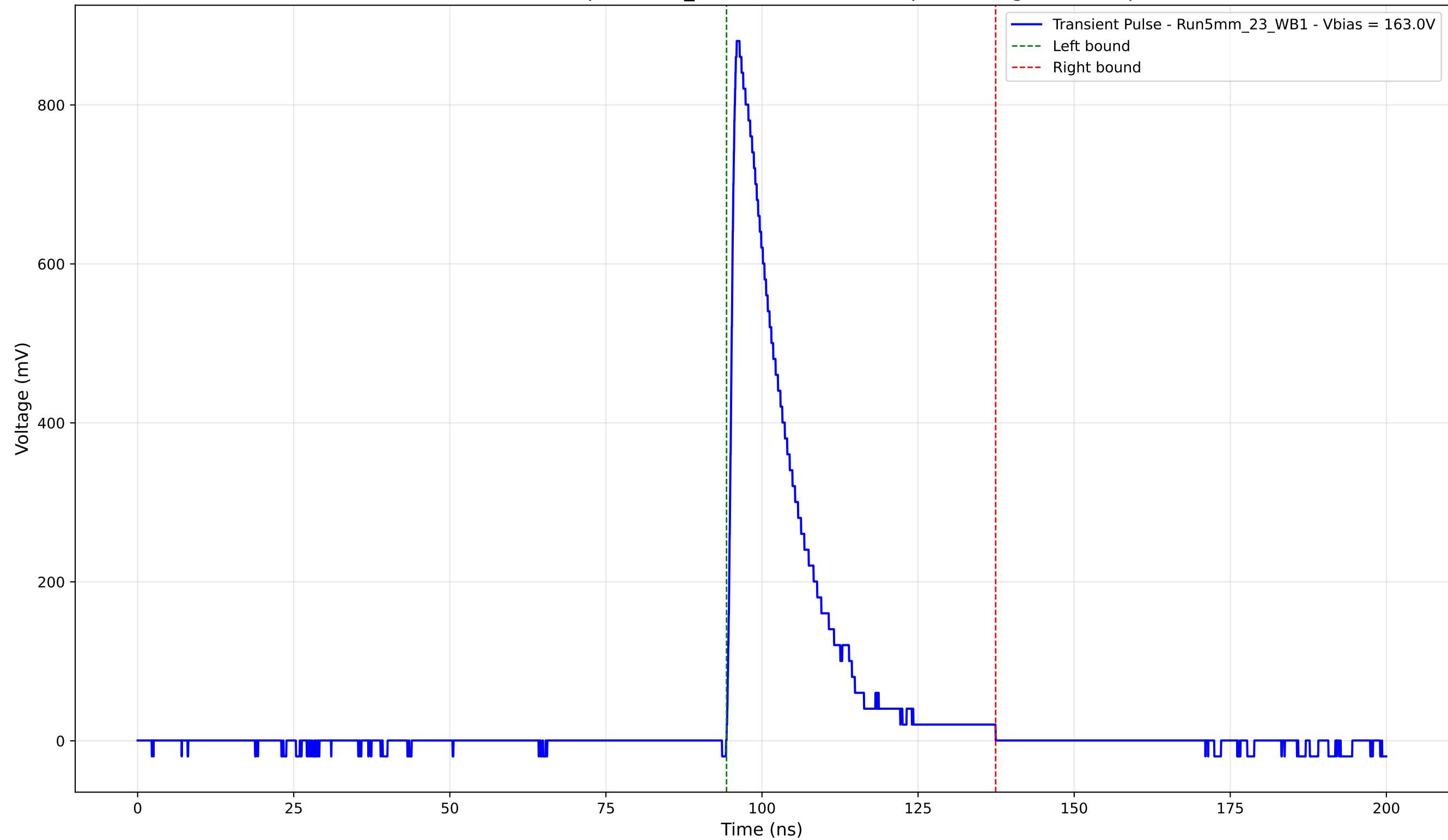
Transient Pulse - Sample: 5mm_23 - Position: 4360.0 \mu\text{m} - Charge: 172.03 pC
