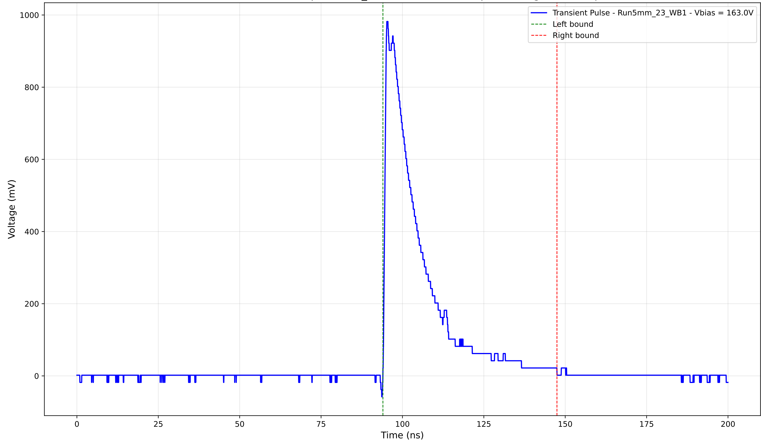
Transient Pulse - Sample: 5mm_23 - Position: 3120.0 \mu\text{m} - Charge: 223.64 pC
