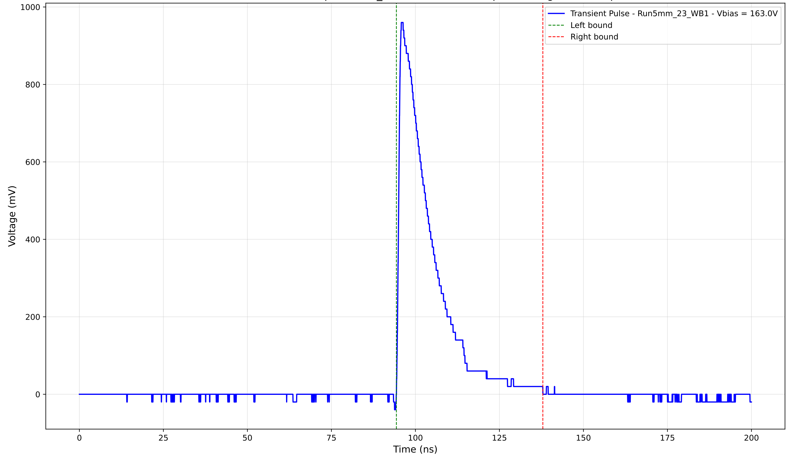
Transient Pulse - Sample: 5mm_23 - Position: 935.0 \mu\text{m} - Charge: 200.94 pC
