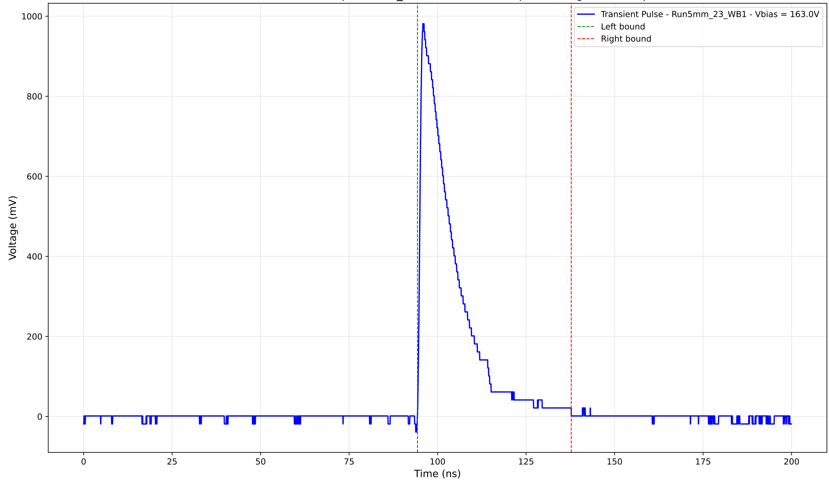
Transient Pulse - Sample: 5mm_23 - Position: 900.0 \mu\text{m} - Charge: 203.13 pC
