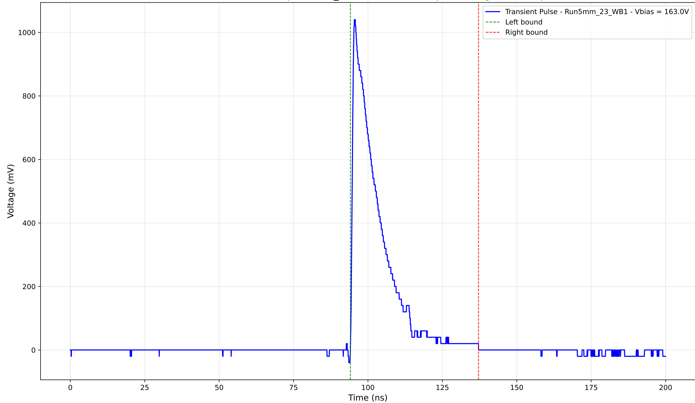
Transient Pulse - Sample: 5mm_23 - Position: 470.0 \mu\text{m} - Charge: 196.60 pC
