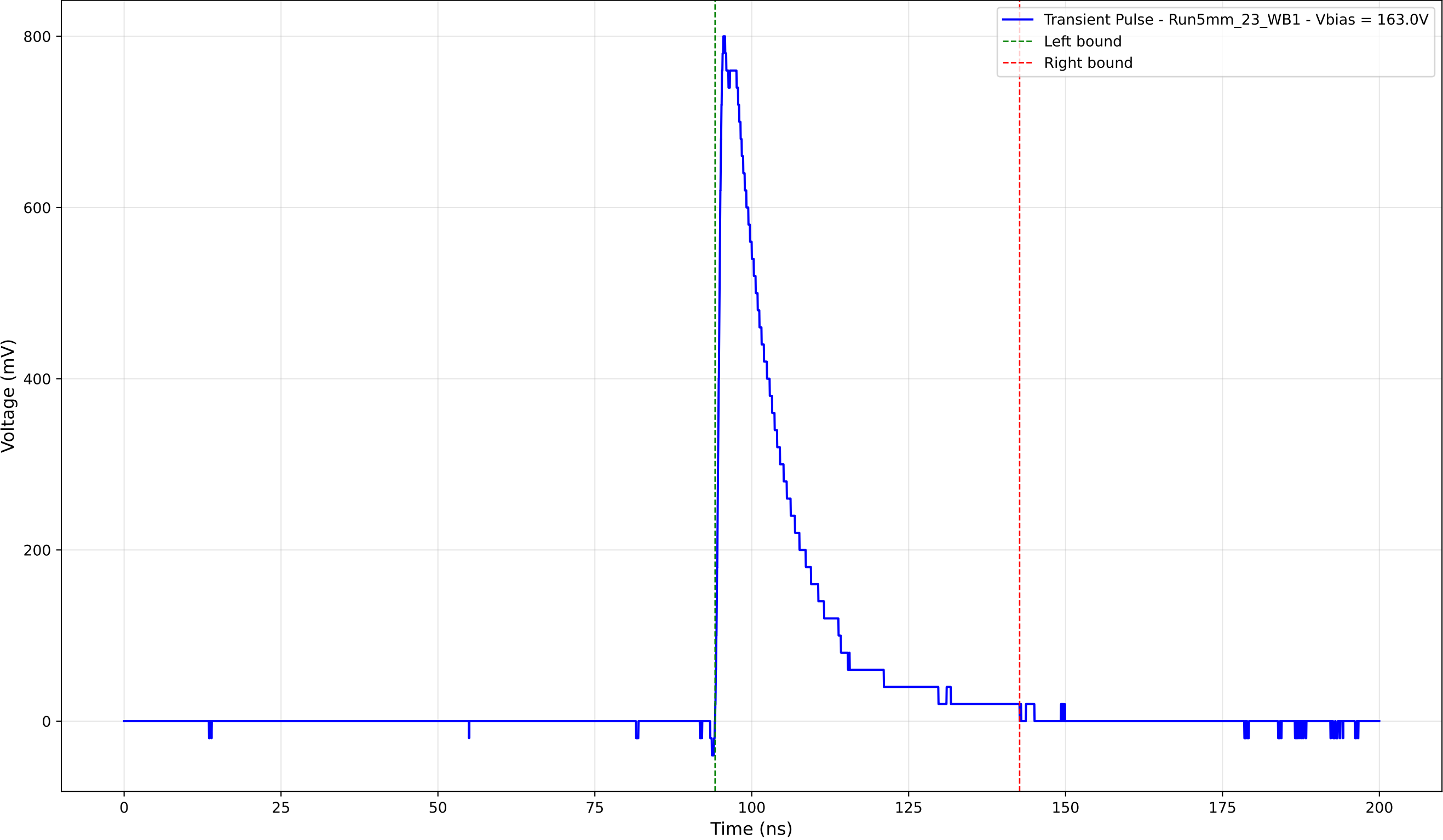
Transient Pulse - Sample: 5mm_23 - Position: 3320.0 \mu\text{m} - Charge: 169.19 pC
