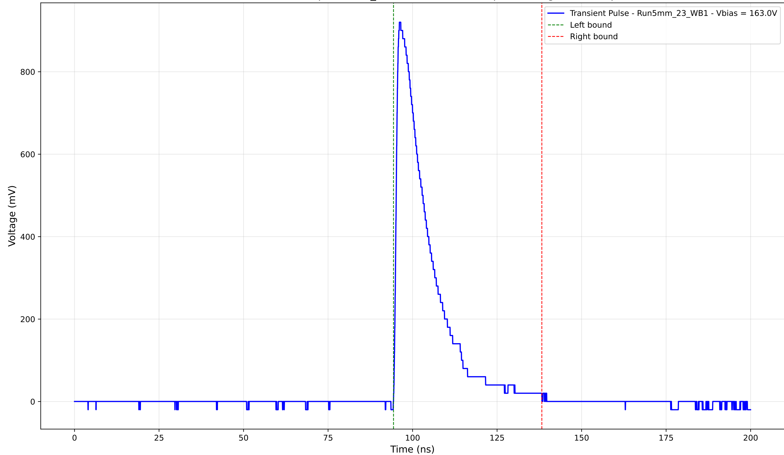
Transient Pulse - Sample: 5mm_23 - Position: 4005.0 \mu\text{m} - Charge: 196.84 pC
