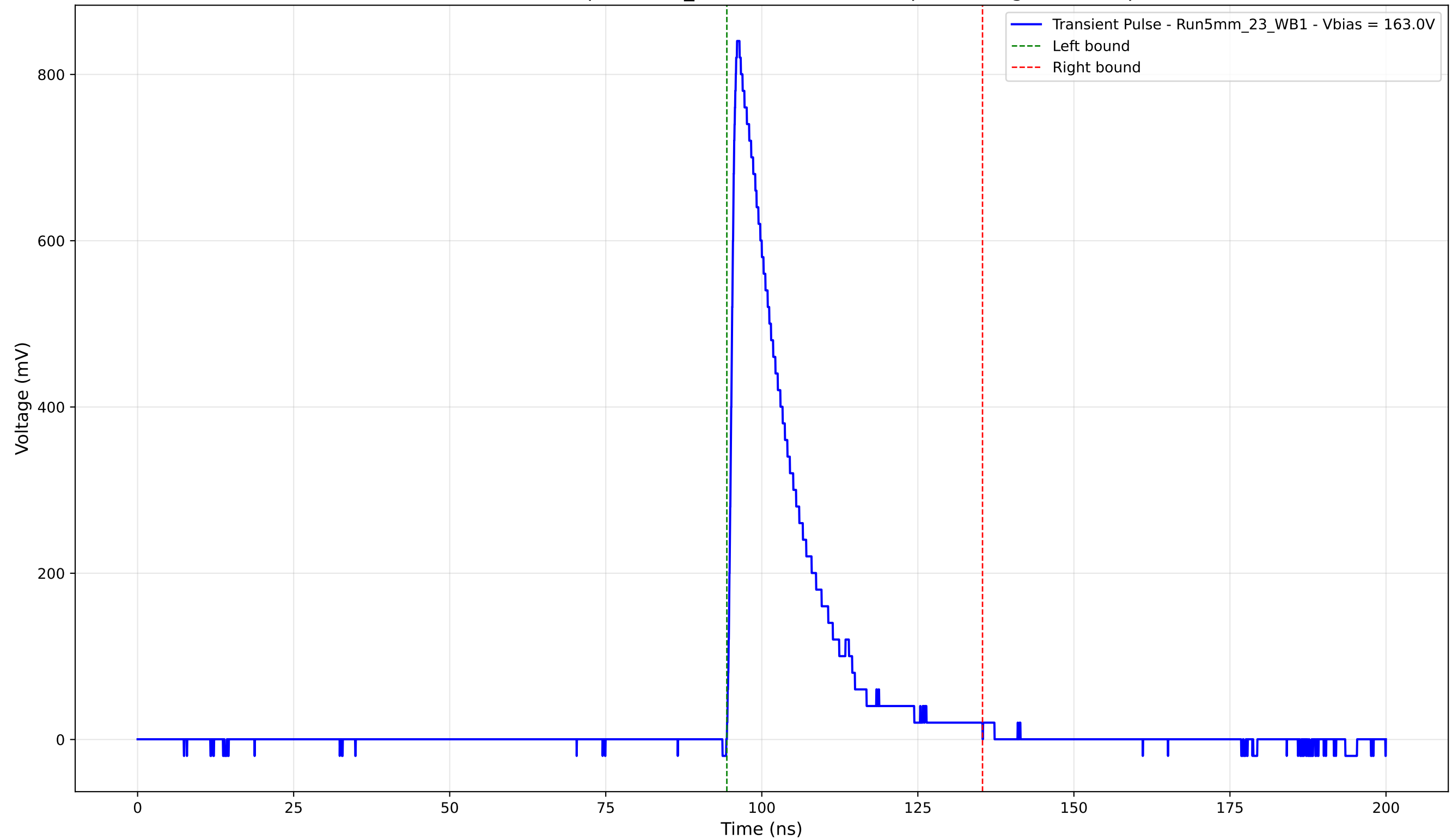
Transient Pulse - Sample: 5mm_23 - Position: 1155.0 \mu\text{m} - Charge: 163.53 pC
