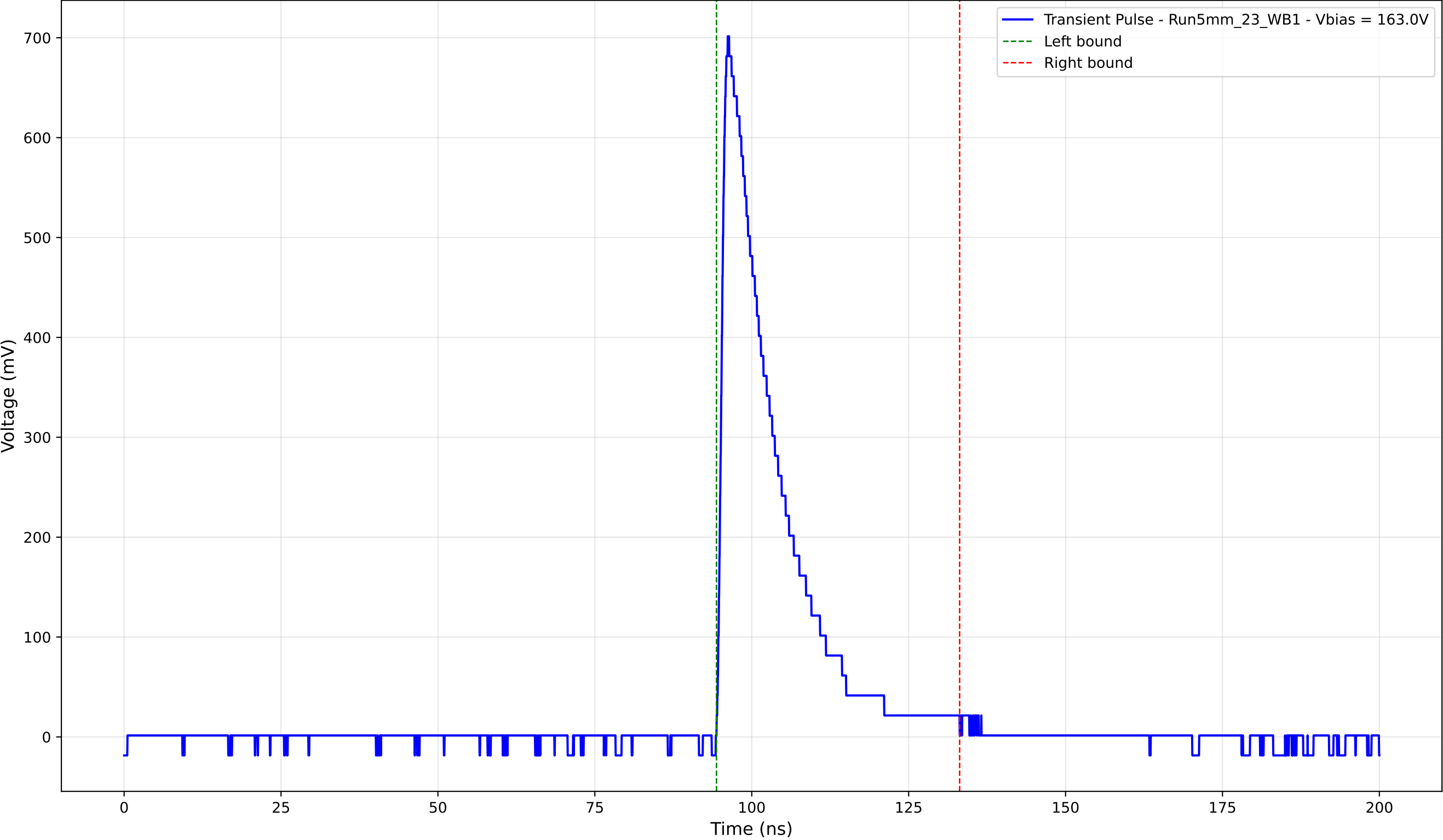
Transient Pulse - Sample: 5mm_23 - Position: 4200.0 \mu\text{m} - Charge: 131.38 pC
