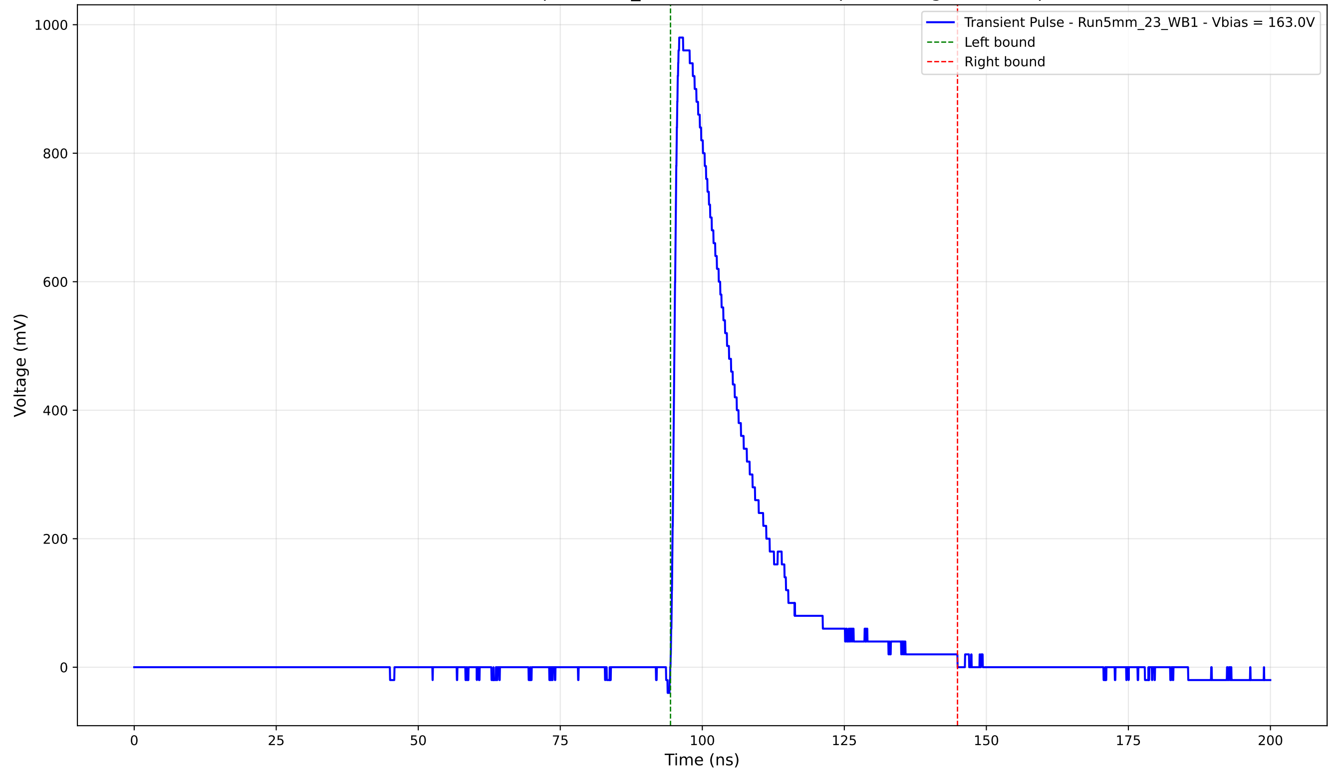
Transient Pulse - Sample: 5mm_23 - Position: 1425.0 \mu\text{m} - Charge: 235.92 pC
