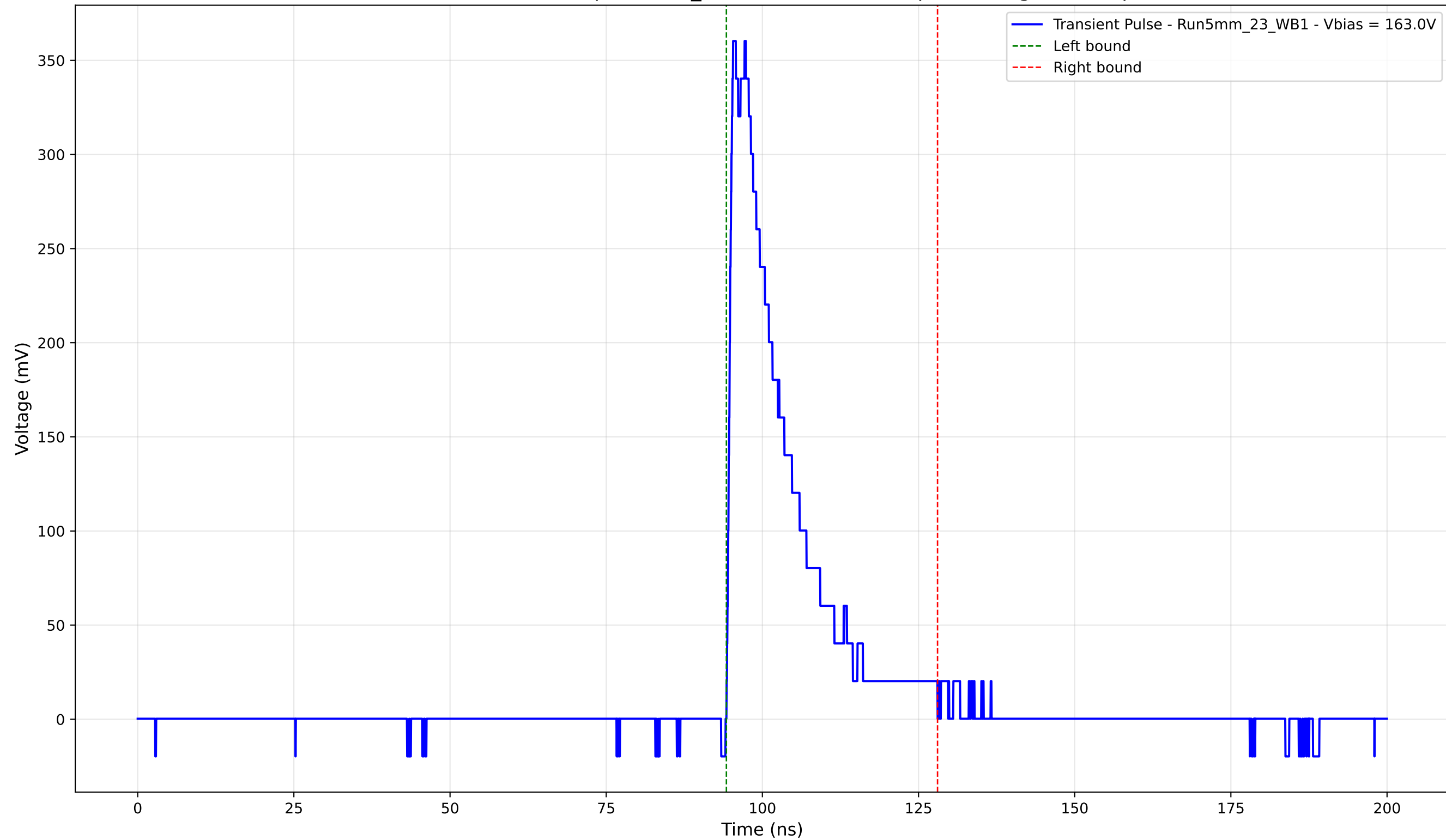
Transient Pulse - Sample: 5mm_23 - Position: 2215.0 \mu\text{m} - Charge: 70.05 pC
