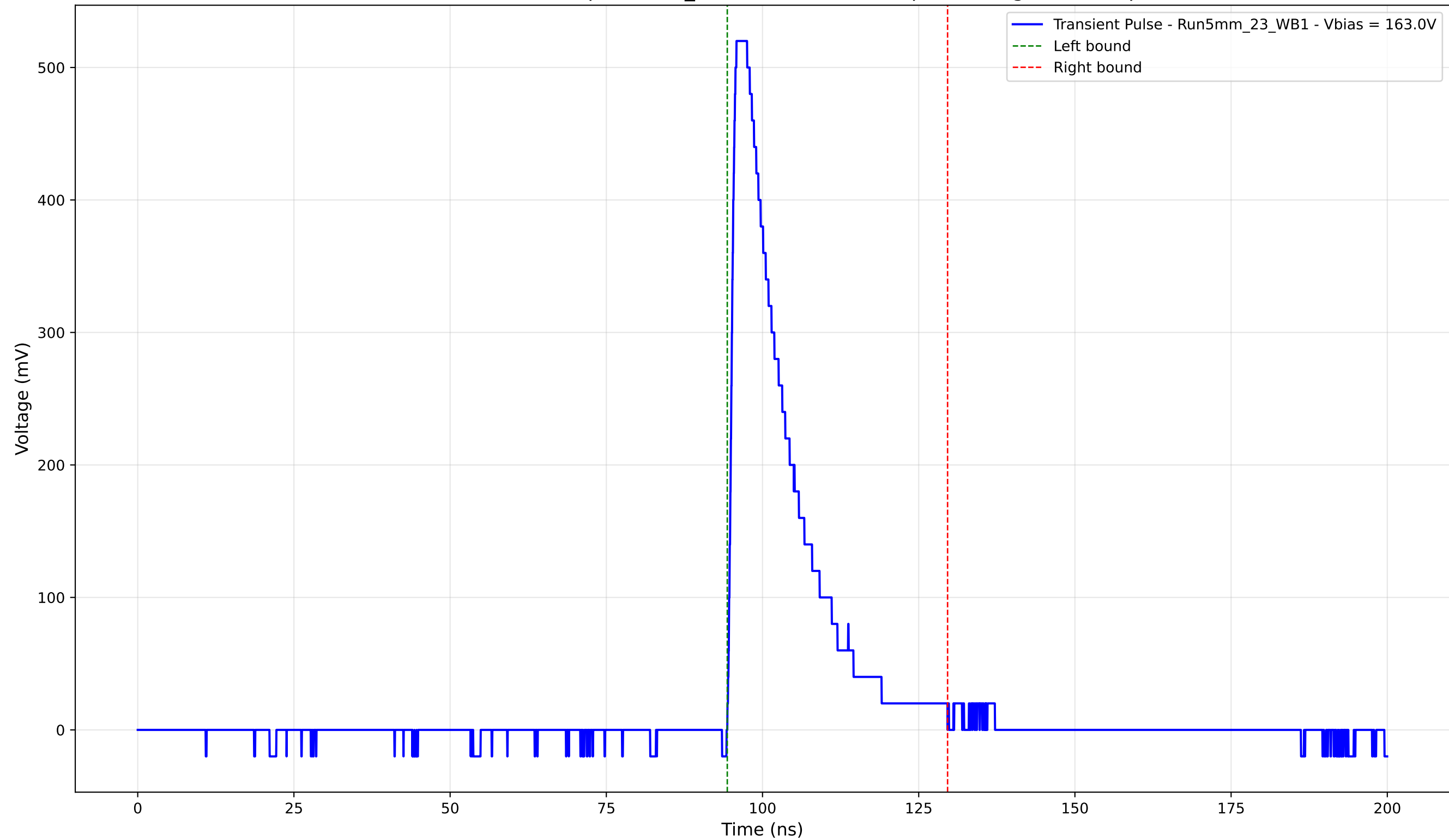
Transient Pulse - Sample: 5mm_23 - Position: 3710.0 \mu\text{m} - Charge: 103.54 pC
