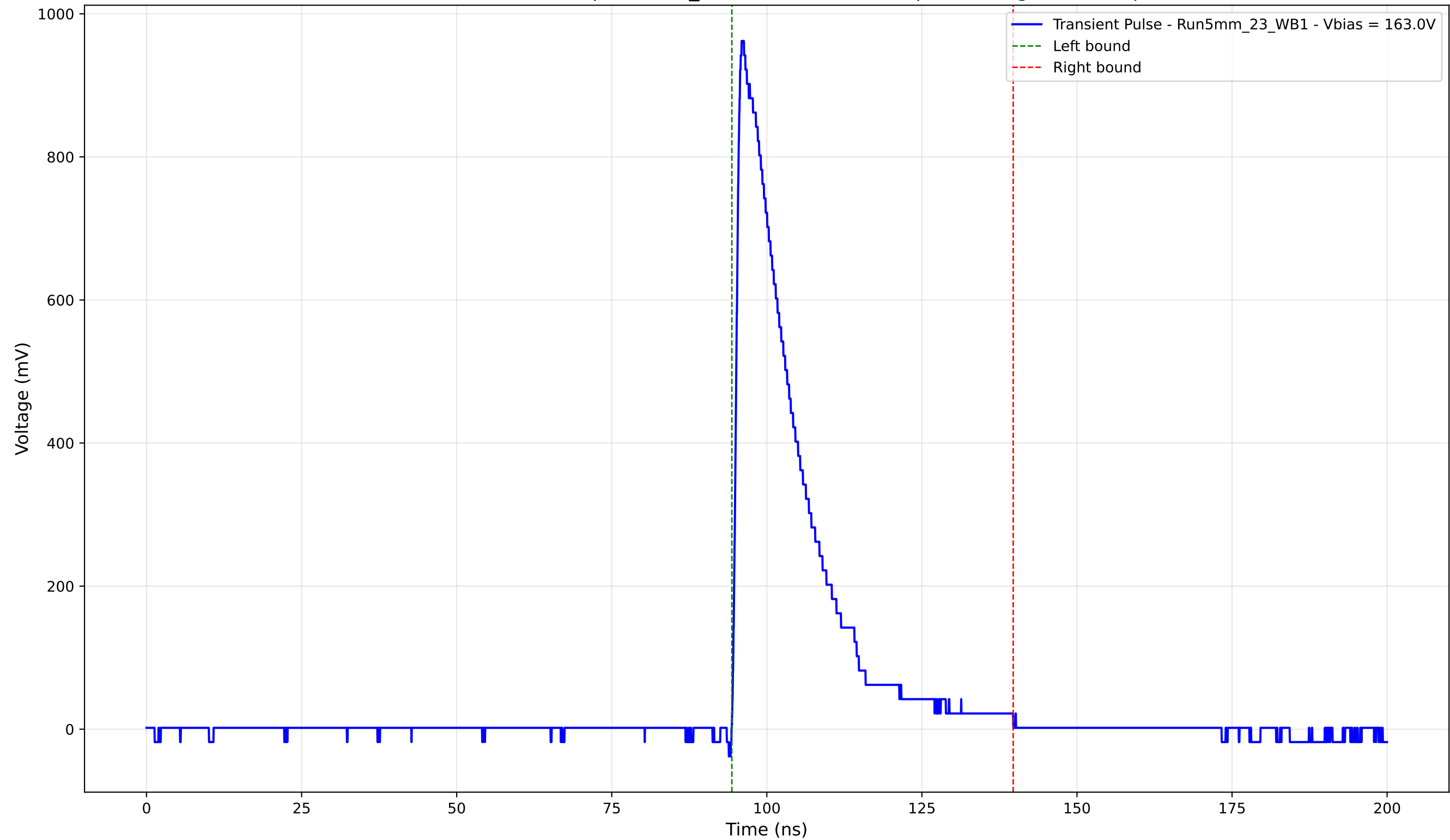
Transient Pulse - Sample: 5mm_23 - Position: 1015.0 \mu\text{m} - Charge: 203.31 pC
