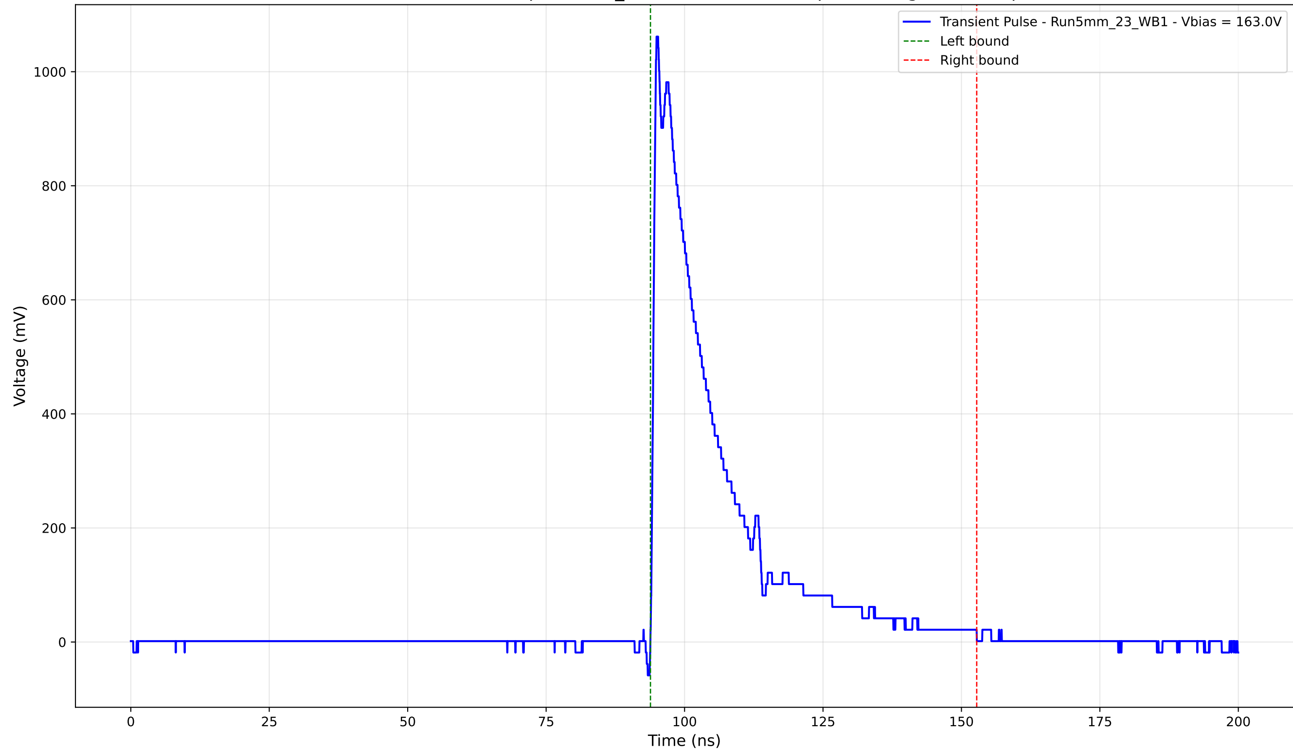
Transient Pulse - Sample: 5mm_23 - Position: 2640.0 \mu\text{m} - Charge: 243.26 pC
