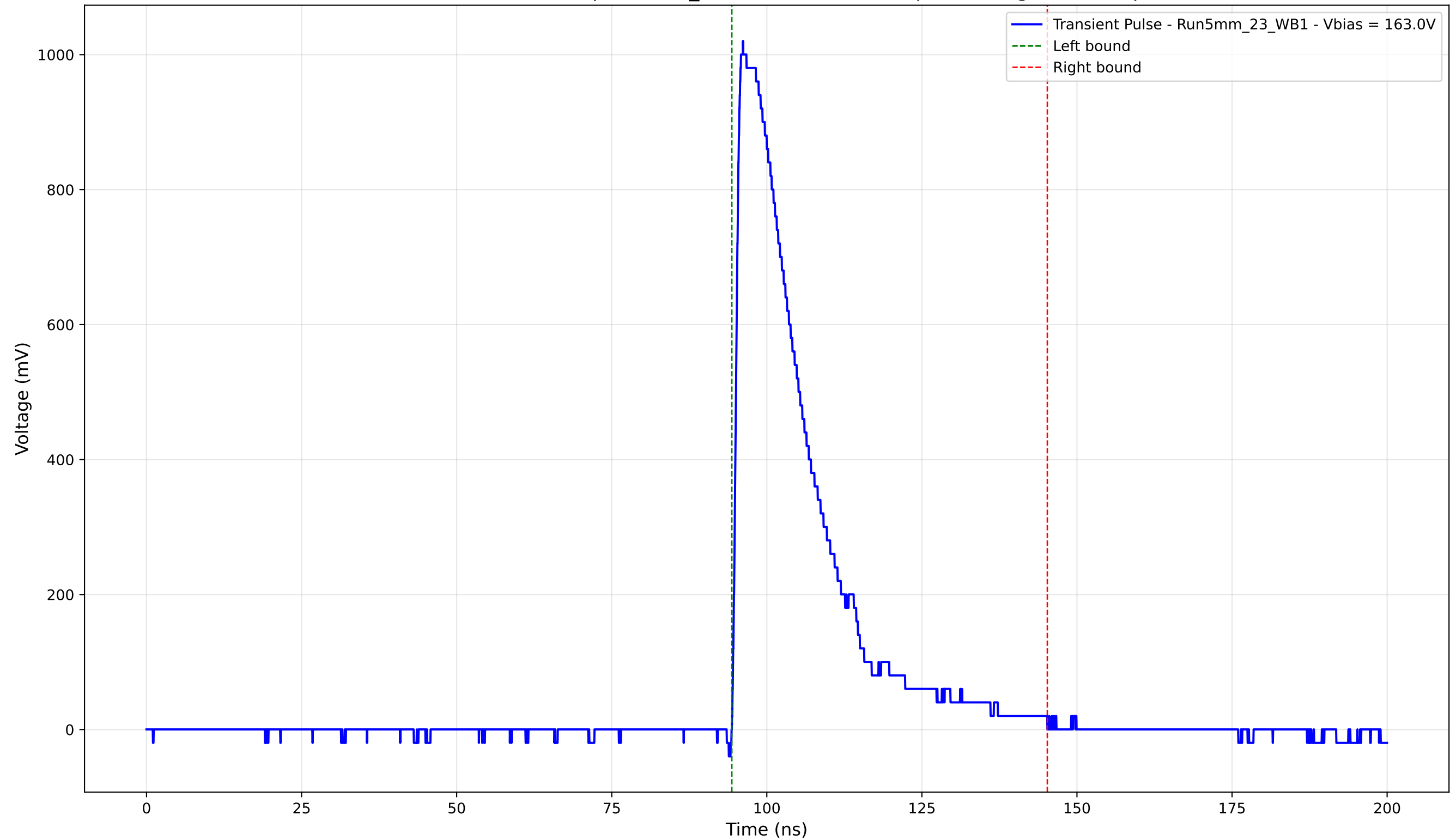
Transient Pulse - Sample: 5mm_23 - Position: 1555.0 \mu\text{m} - Charge: 254.44 pC
