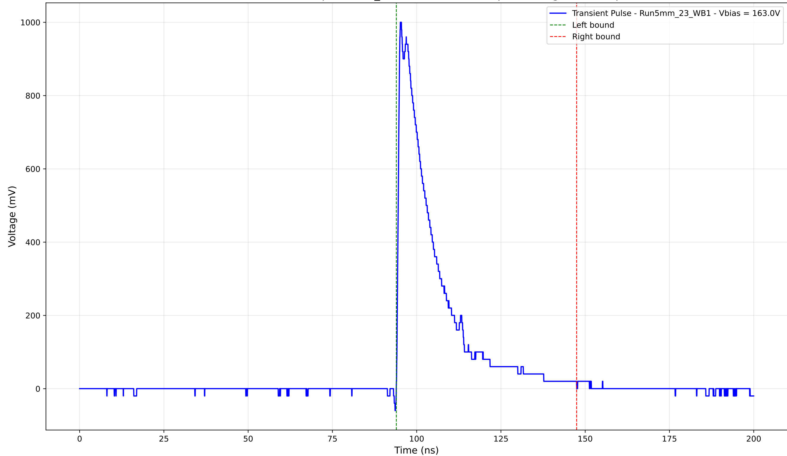
Transient Pulse - Sample: 5mm_23 - Position: 2425.0 \mu\text{m} - Charge: 228.27 pC
