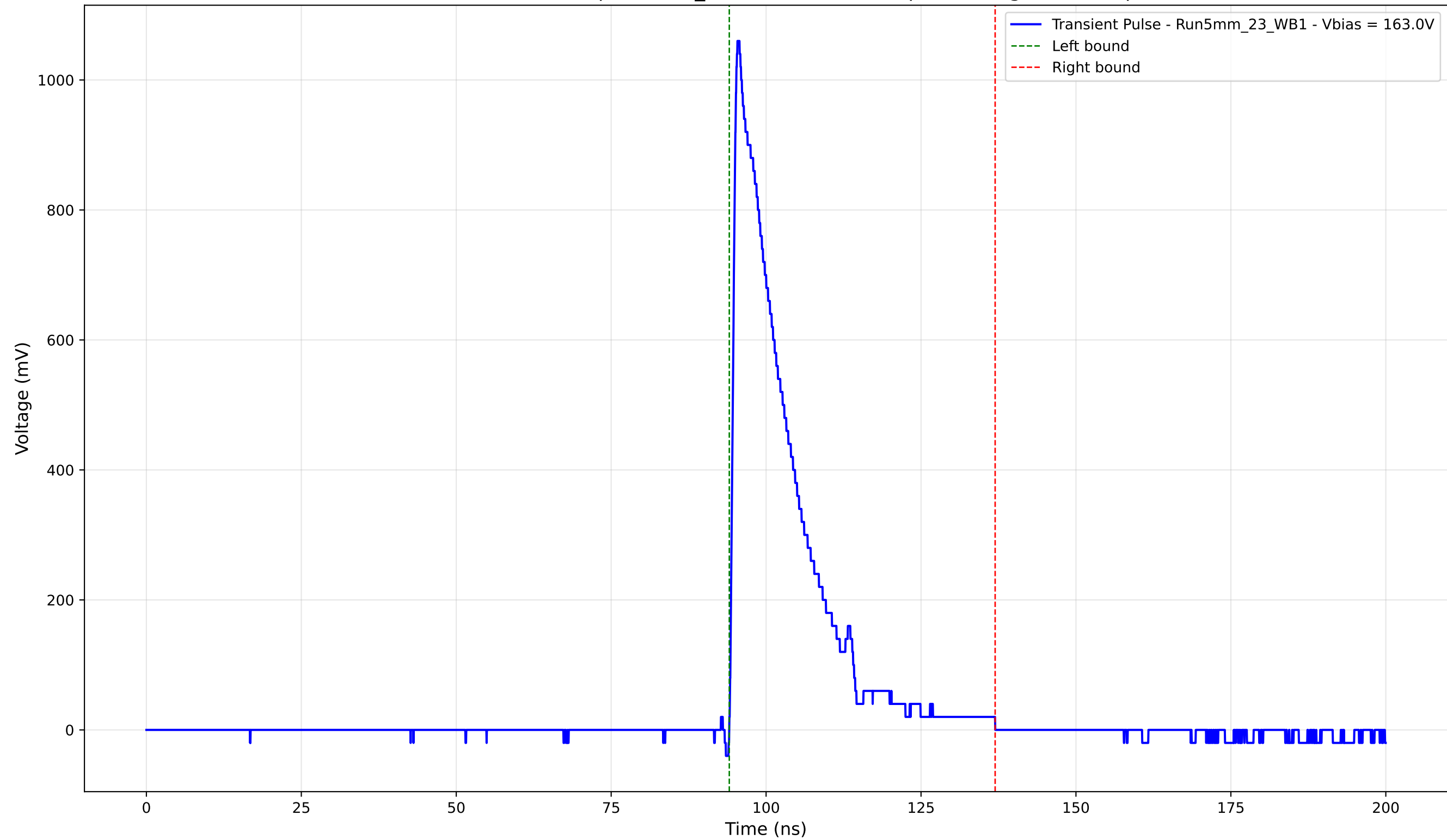
Transient Pulse - Sample: 5mm_23 - Position: 410.0 \mu\text{m} - Charge: 201.81 pC
