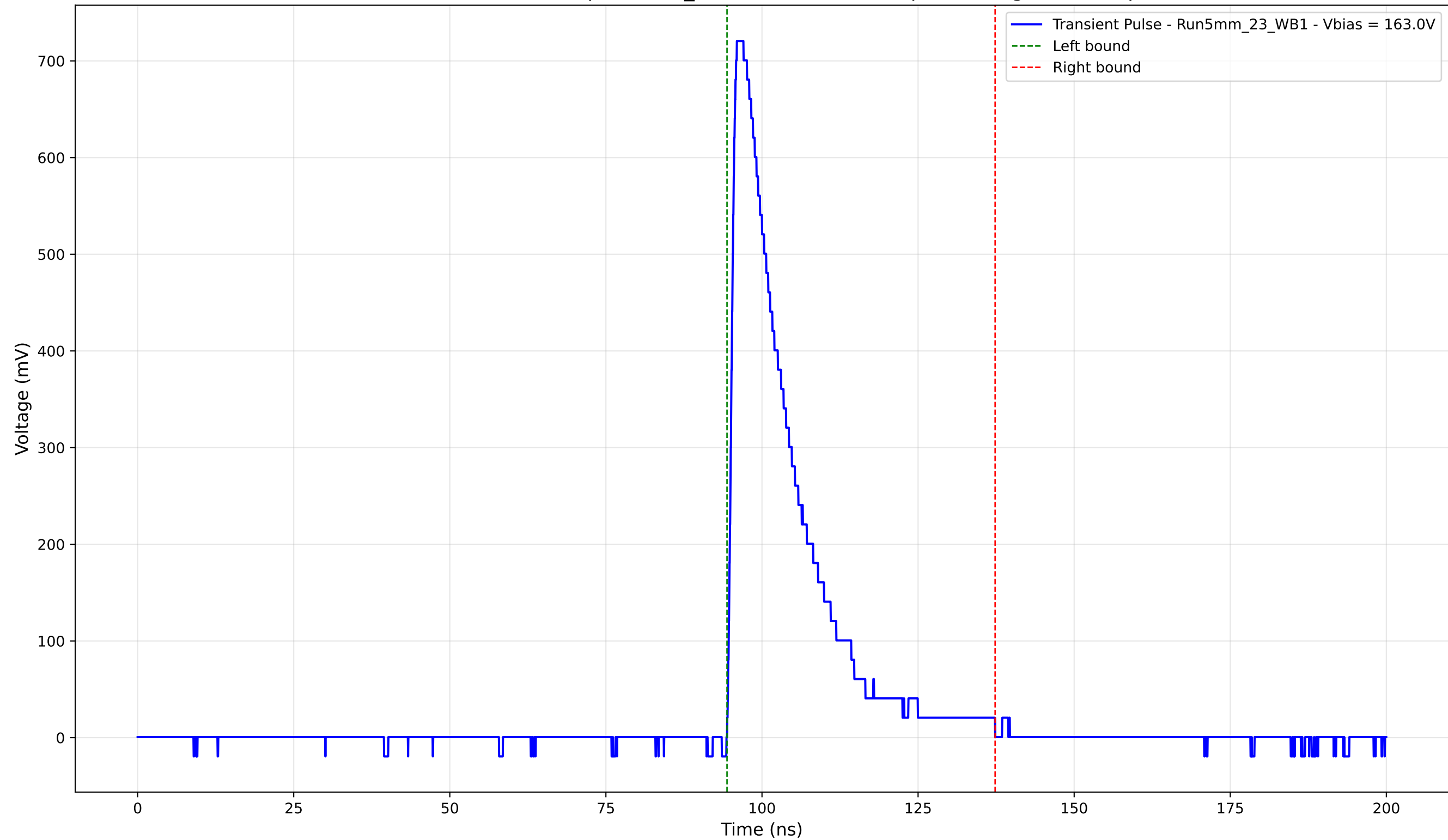
Transient Pulse - Sample: 5mm_23 - Position: 1670.0 \mu\text{m} - Charge: 149.61 pC
