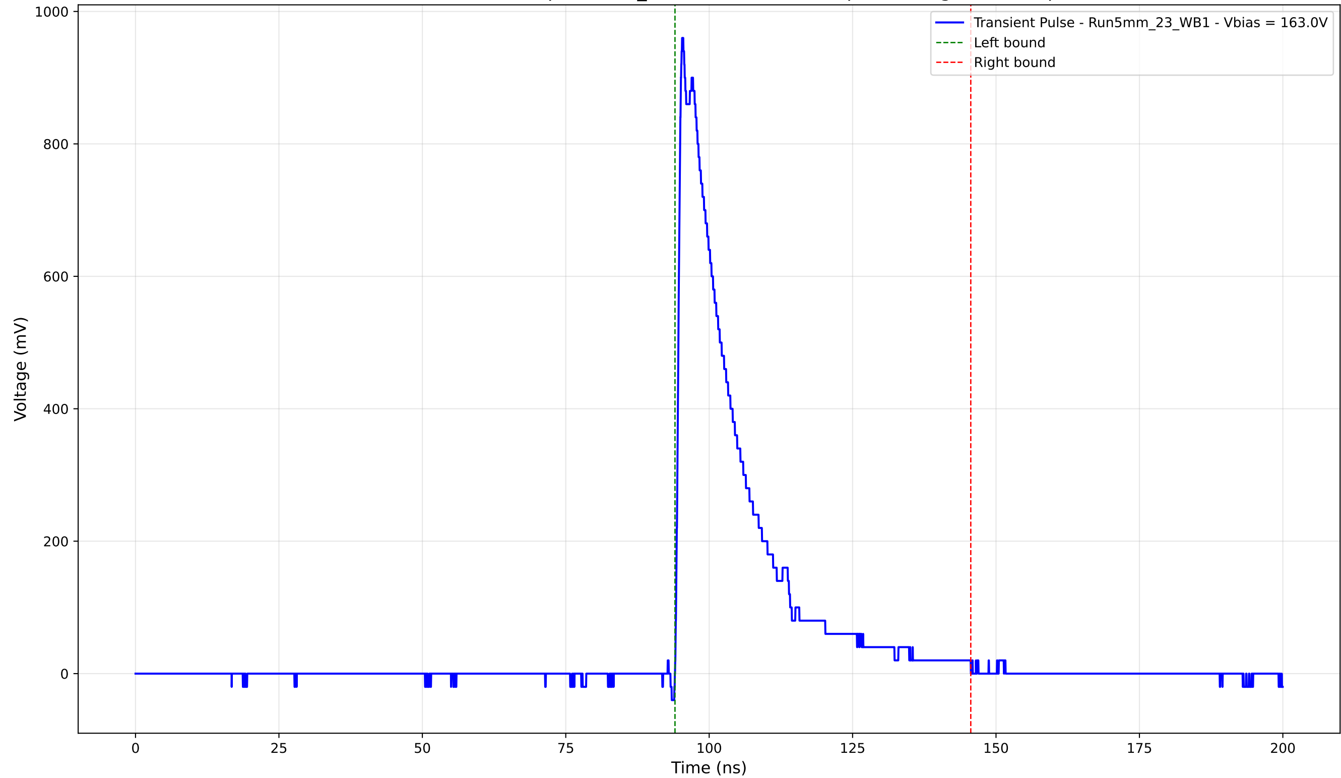
Transient Pulse - Sample: 5mm_23 - Position: 3160.0 \mu\text{m} - Charge: 204.70 pC
