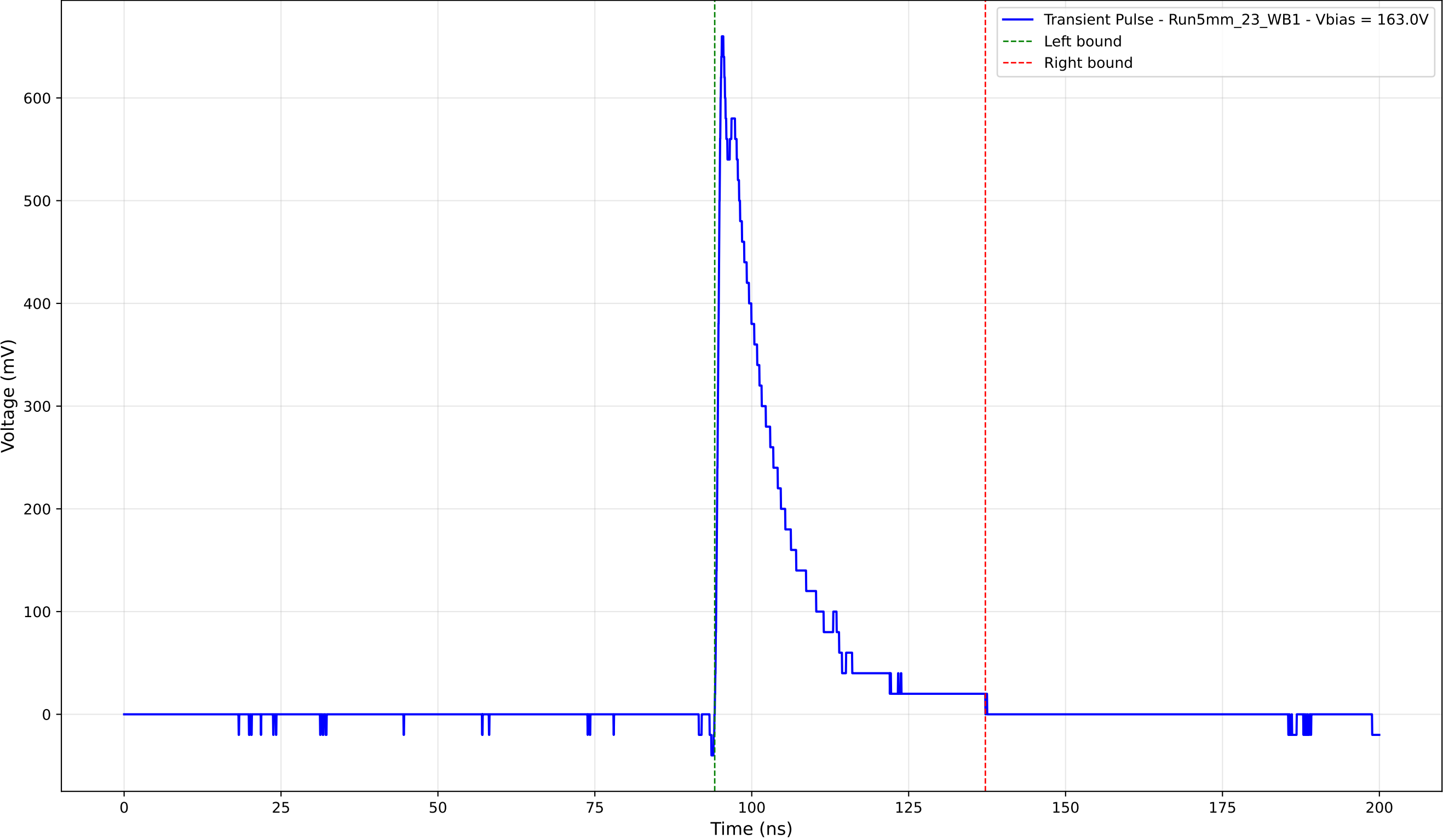
Transient Pulse - Sample: 5mm_23 - Position: 2285.0 \mu\text{m} - Charge: 120.96 pC
