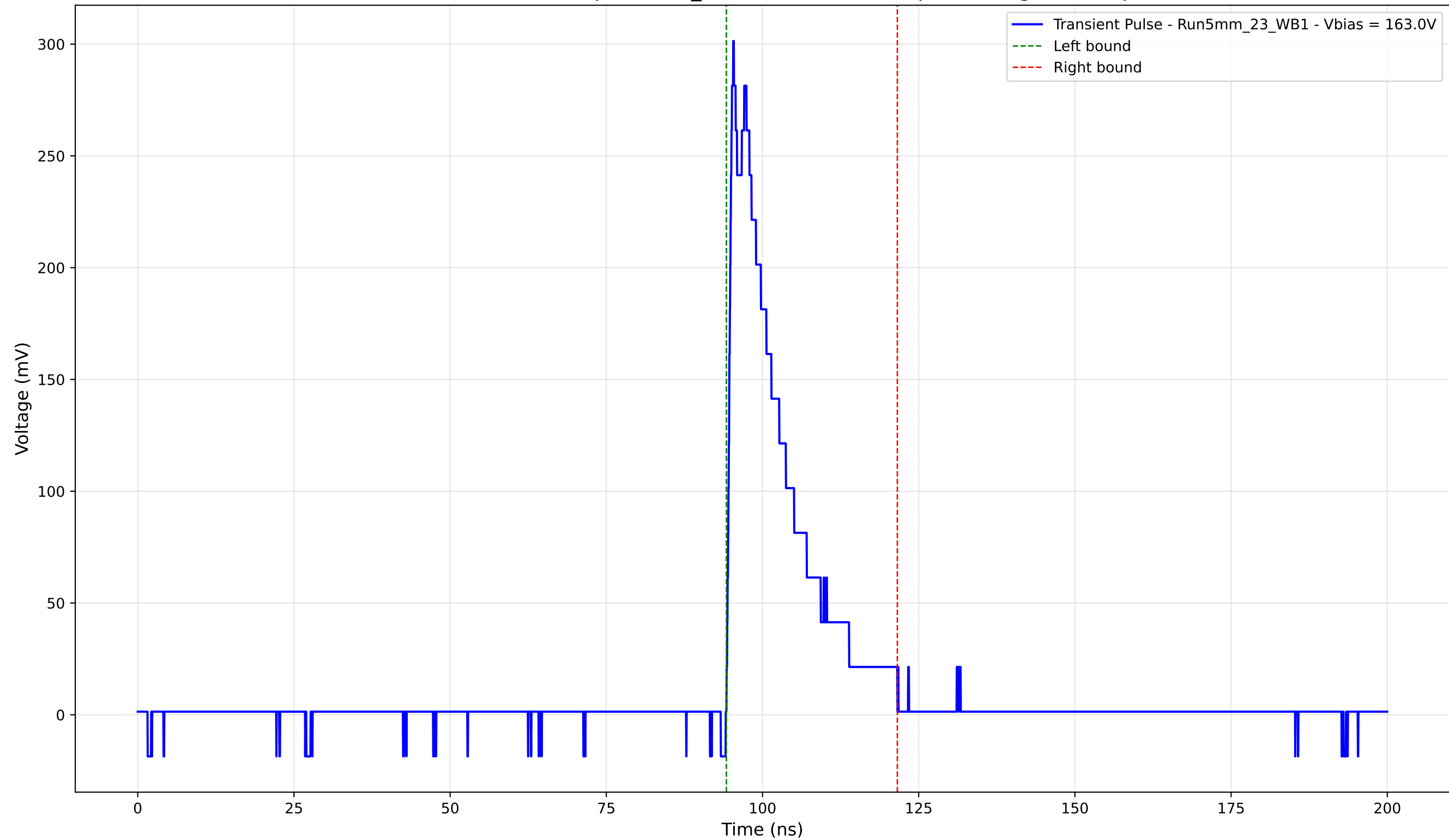
Transient Pulse - Sample: 5mm_23 - Position: 2255.0 \mu\text{m} - Charge: 52.92 pC
