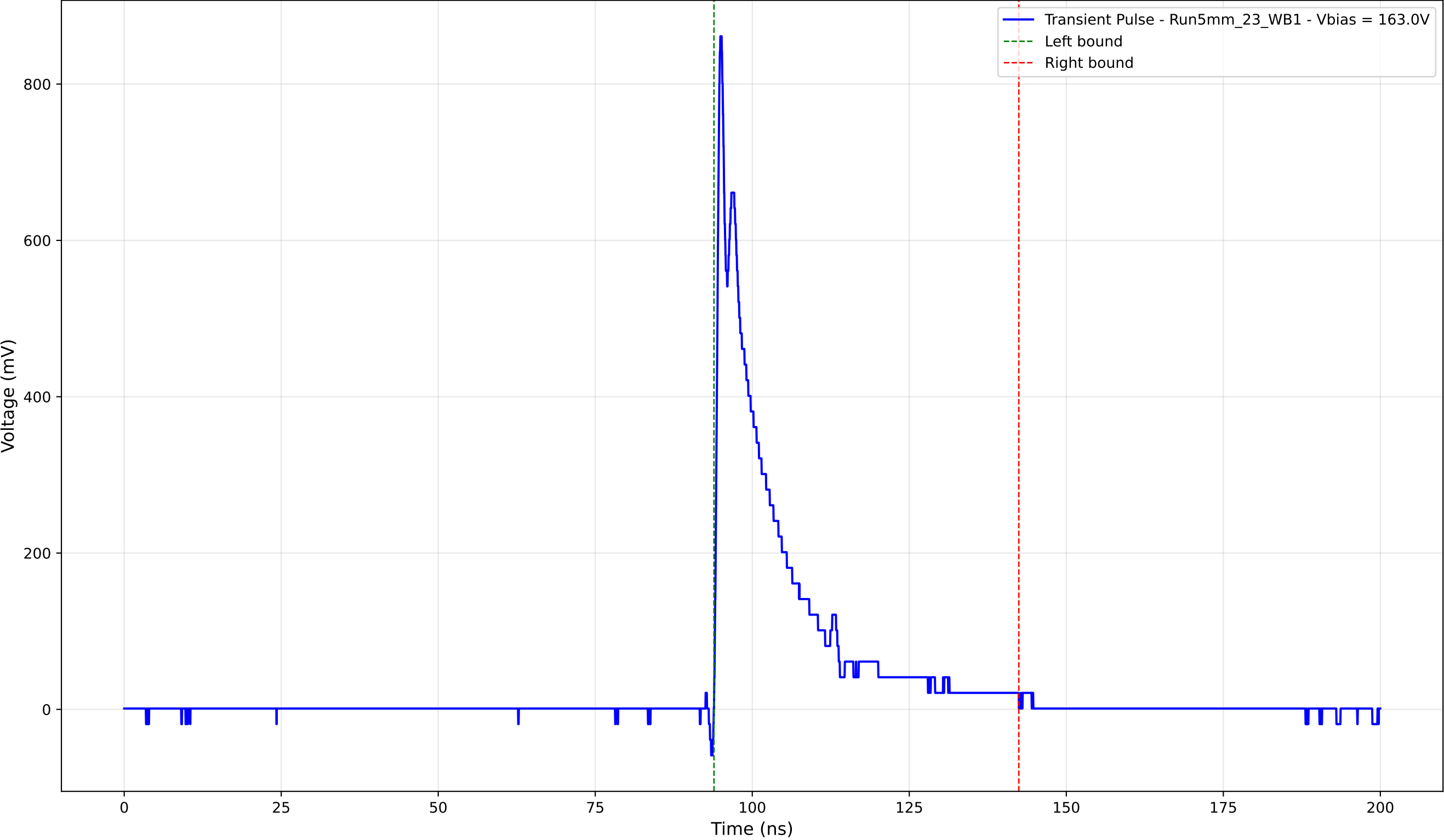
Transient Pulse - Sample: 5mm_23 - Position: 2700.0 \mu\text{m} - Charge: 137.45 pC
