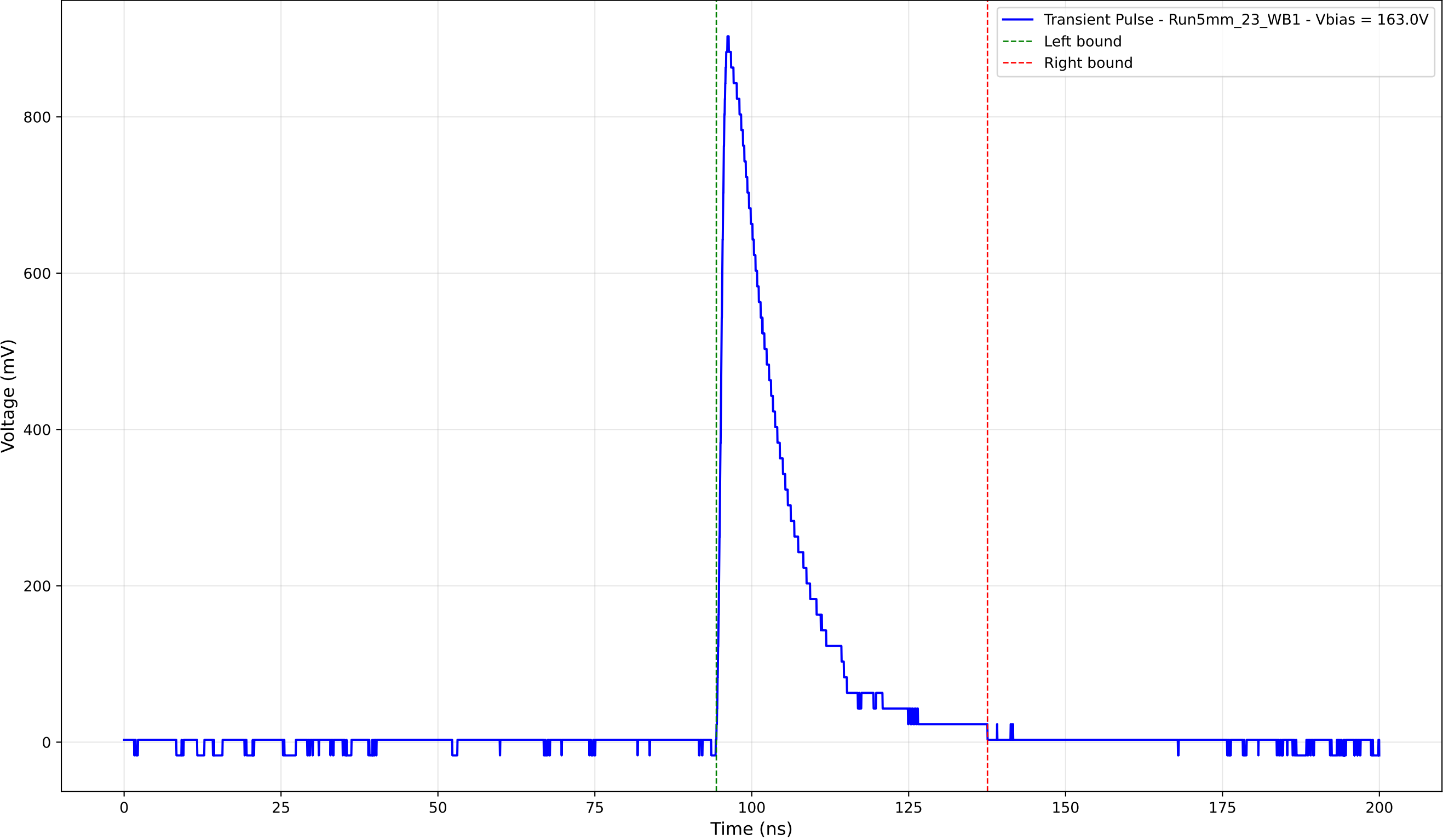
Transient Pulse - Sample: 5mm_23 - Position: 4165.0 \mu\text{m} - Charge: 183.90 pC
