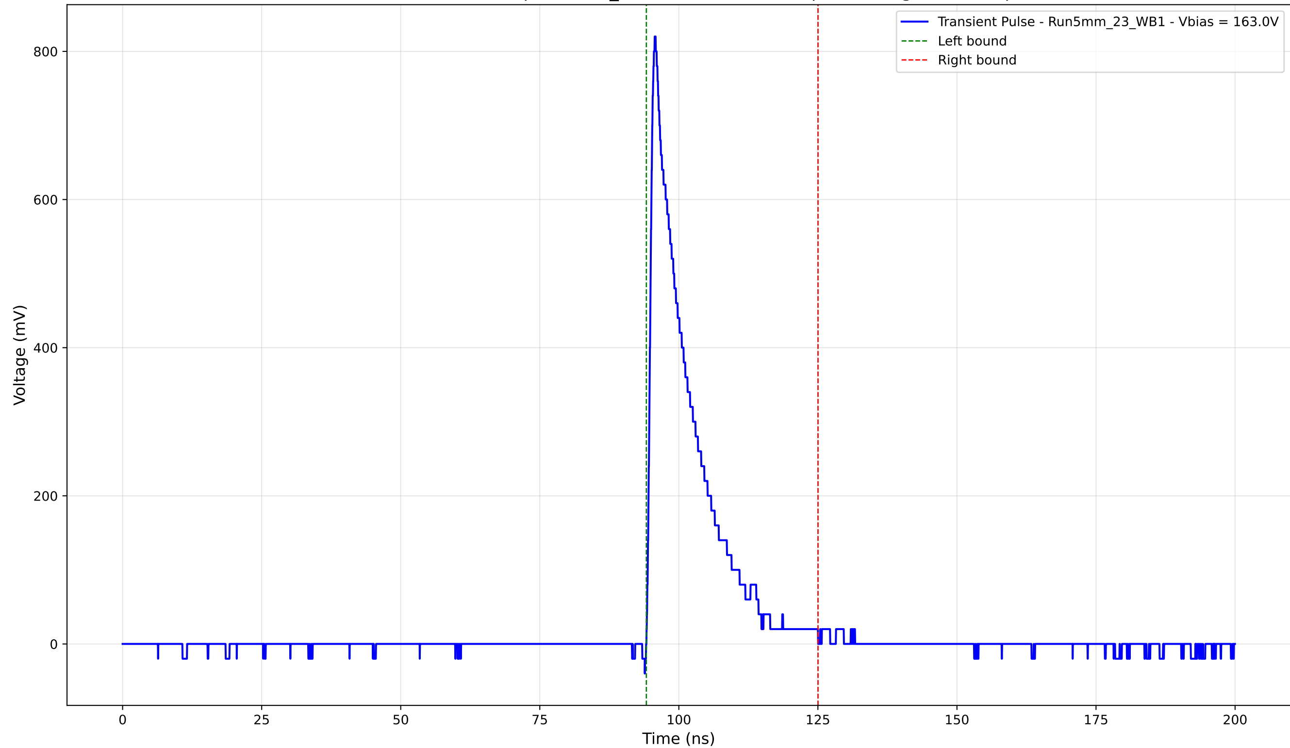
Transient Pulse - Sample: 5mm_23 - Position: 4825.0 \mu\text{m} - Charge: 124.23 pC
