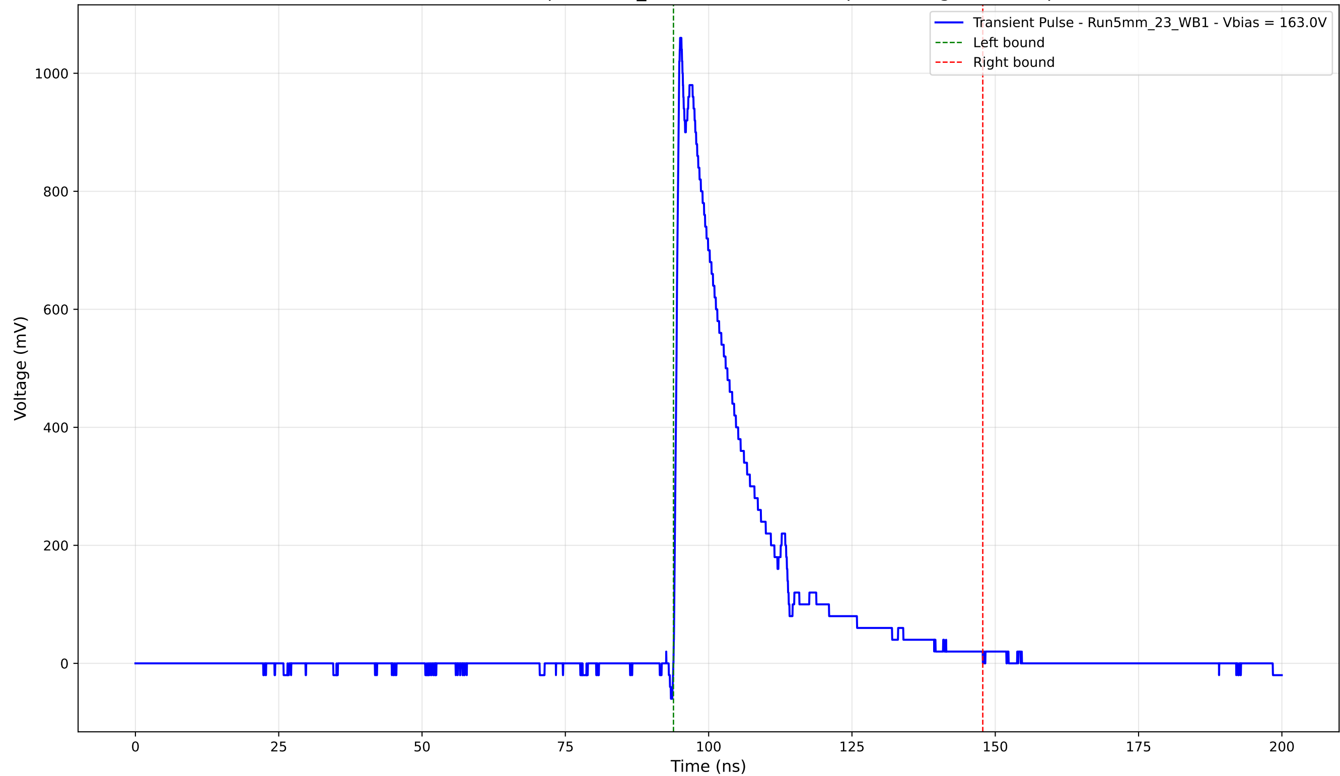
Transient Pulse - Sample: 5mm_23 - Position: 2605.0 \mu\text{m} - Charge: 240.95 pC
