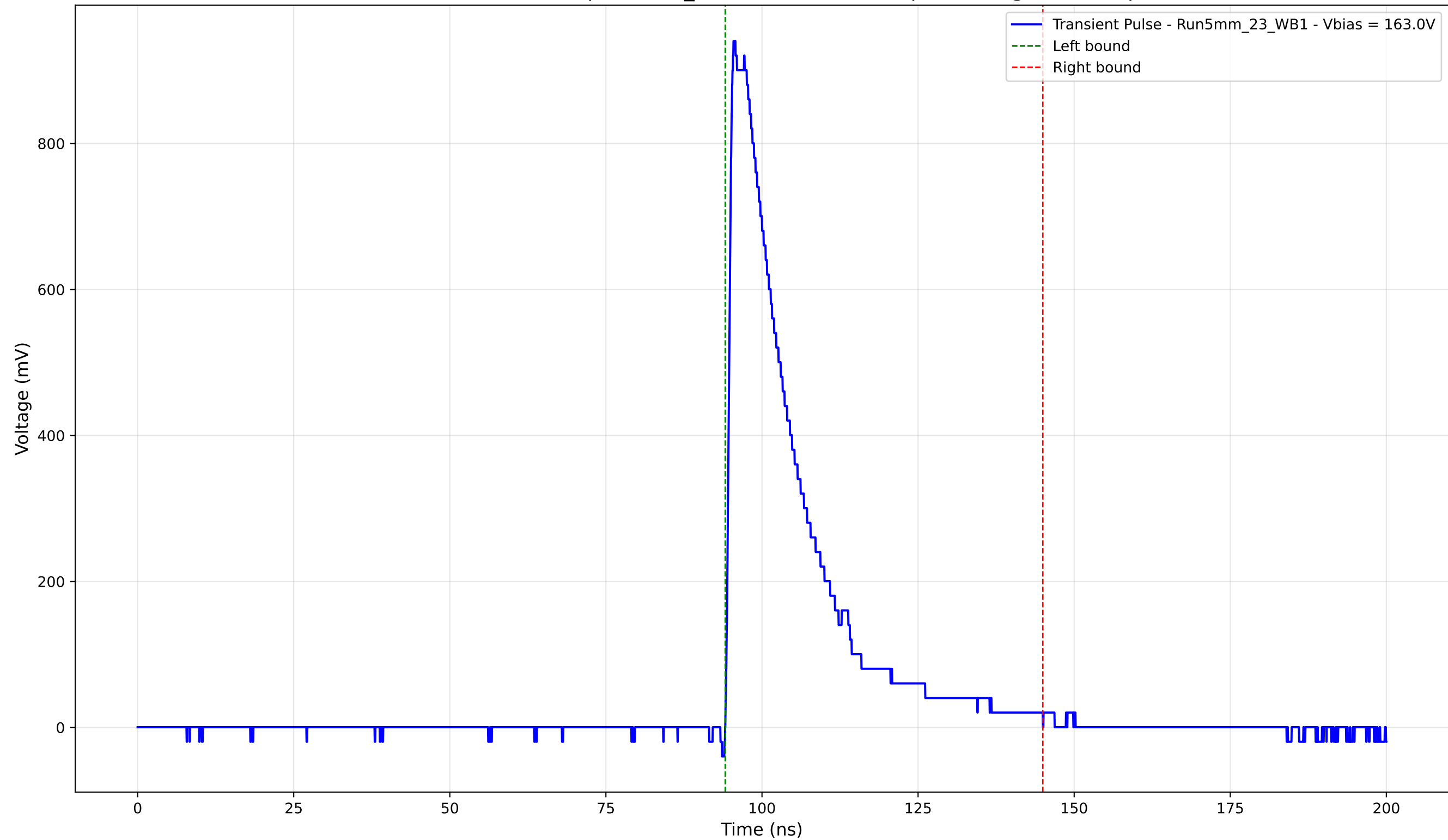
Transient Pulse - Sample: 5mm_23 - Position: 2155.0 \mu\text{m} - Charge: 215.13 pC
