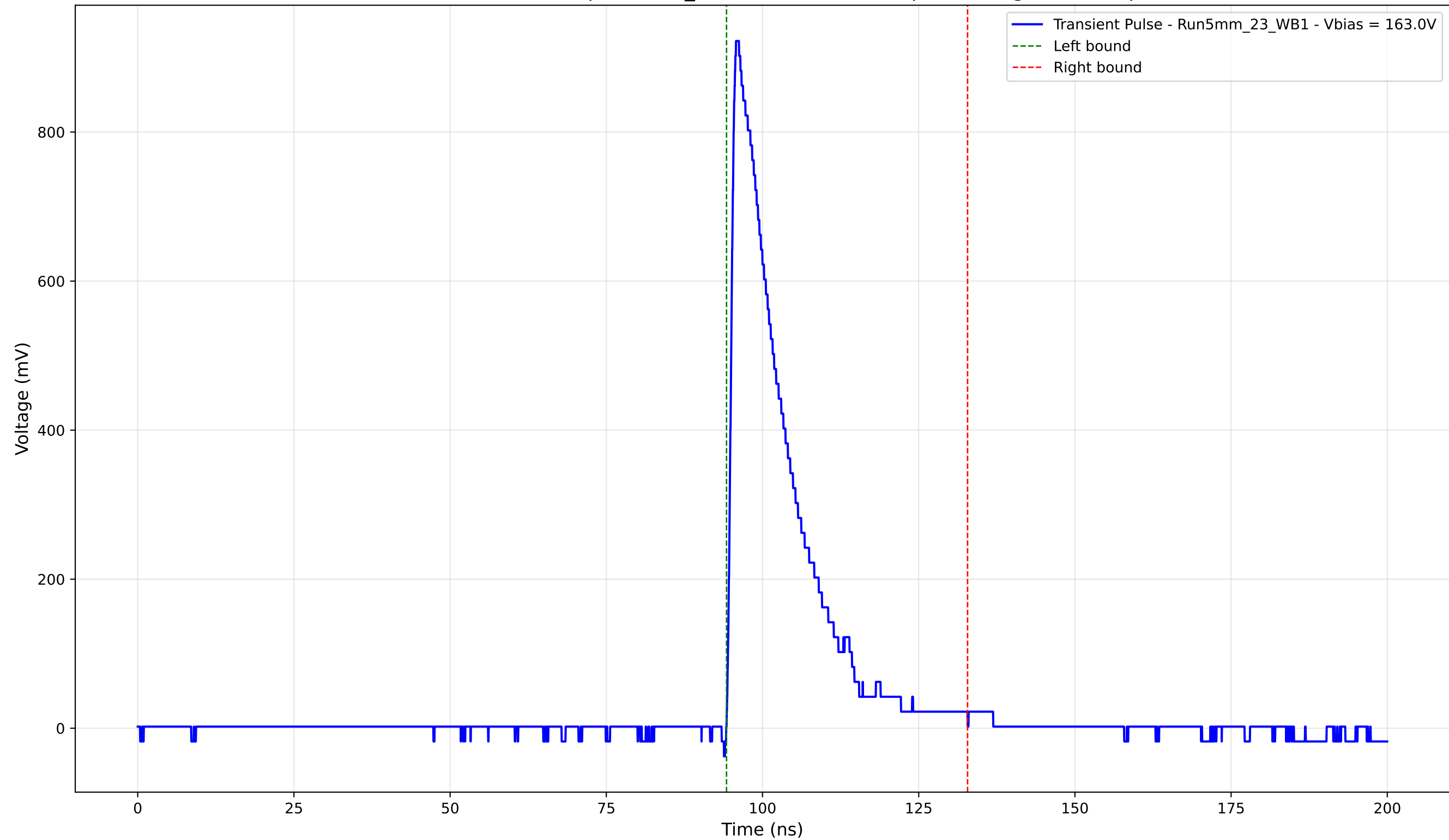
Transient Pulse - Sample: 5mm_23 - Position: 4590.0 \mu\text{m} - Charge: 175.09 pC
