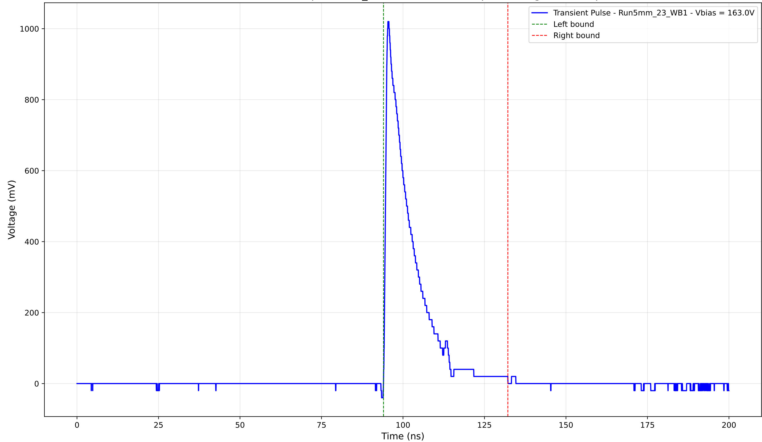
Transient Pulse - Sample: 5mm_23 - Position: 5015.0 \mu\text{m} - Charge: 171.56 pC
