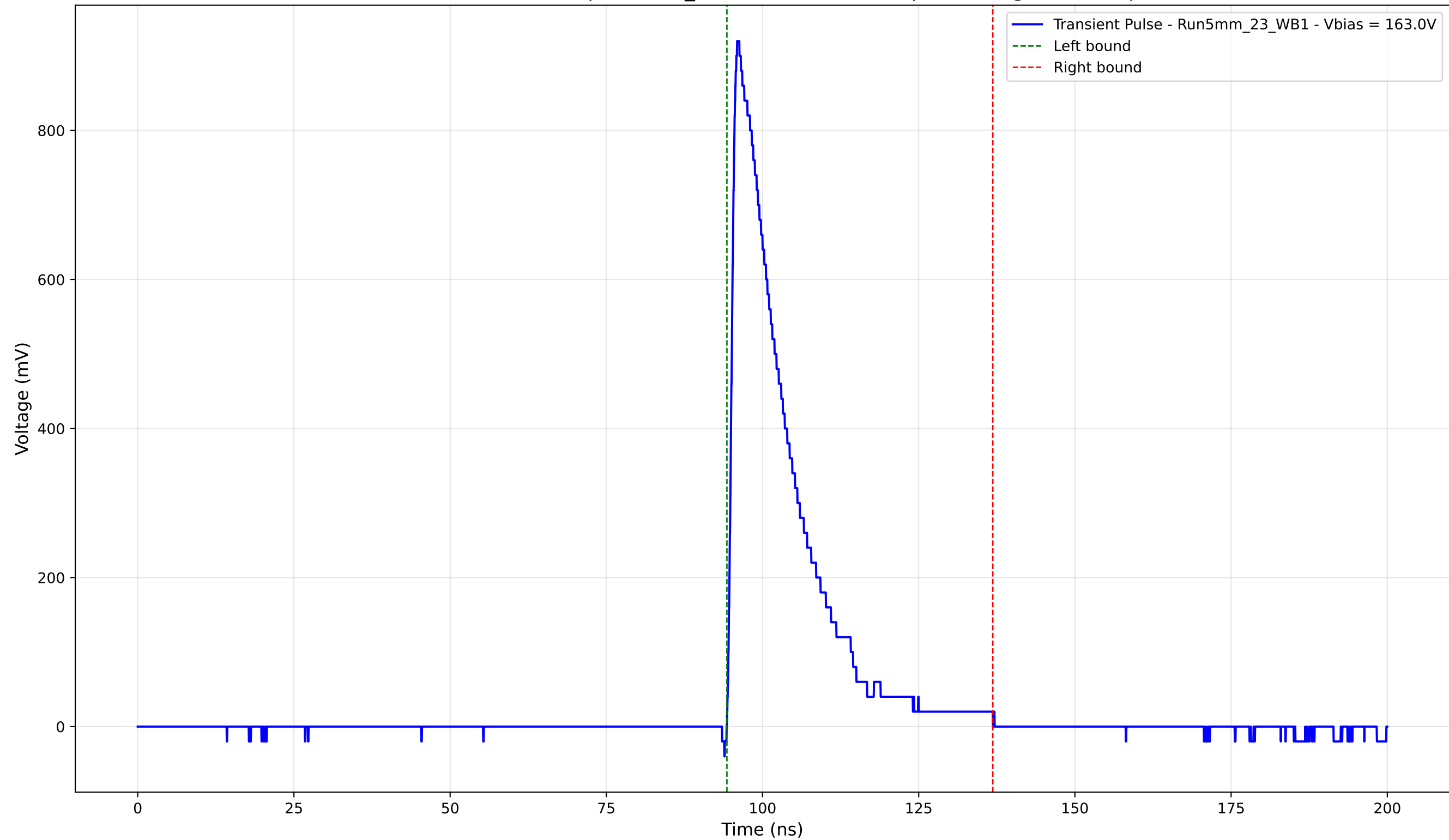
Transient Pulse - Sample: 5mm_23 - Position: 4440.0 \mu\text{m} - Charge: 179.94 pC
