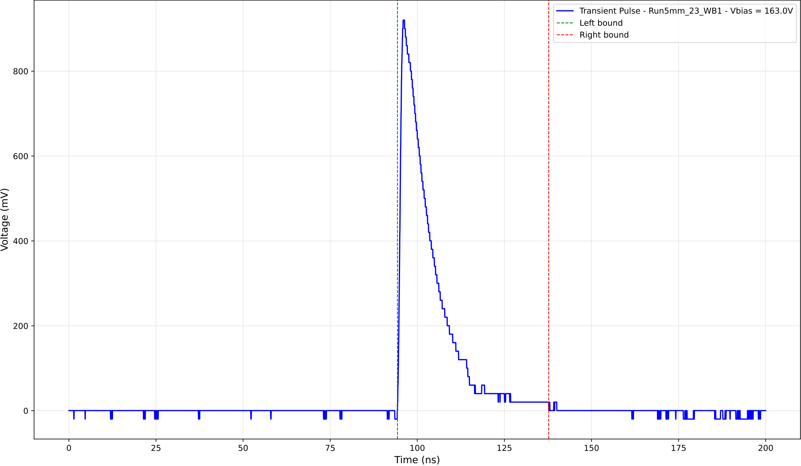
Transient Pulse - Sample: 5mm_23 - Position: 4435.0 \mu\text{m} - Charge: 181.51 pC
