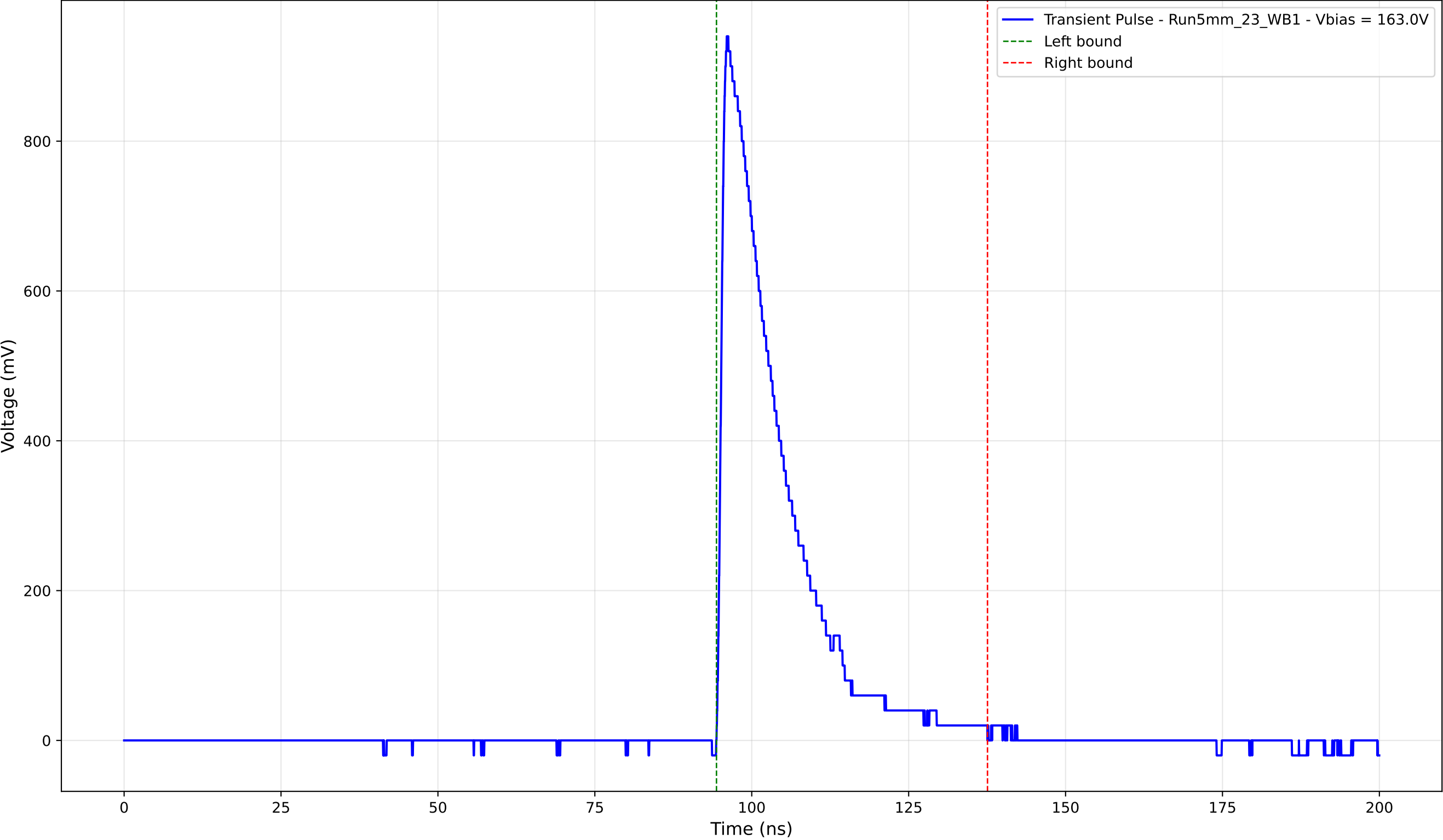
Transient Pulse - Sample: 5mm_23 - Position: 1130.0 \mu\text{m} - Charge: 194.10 pC
