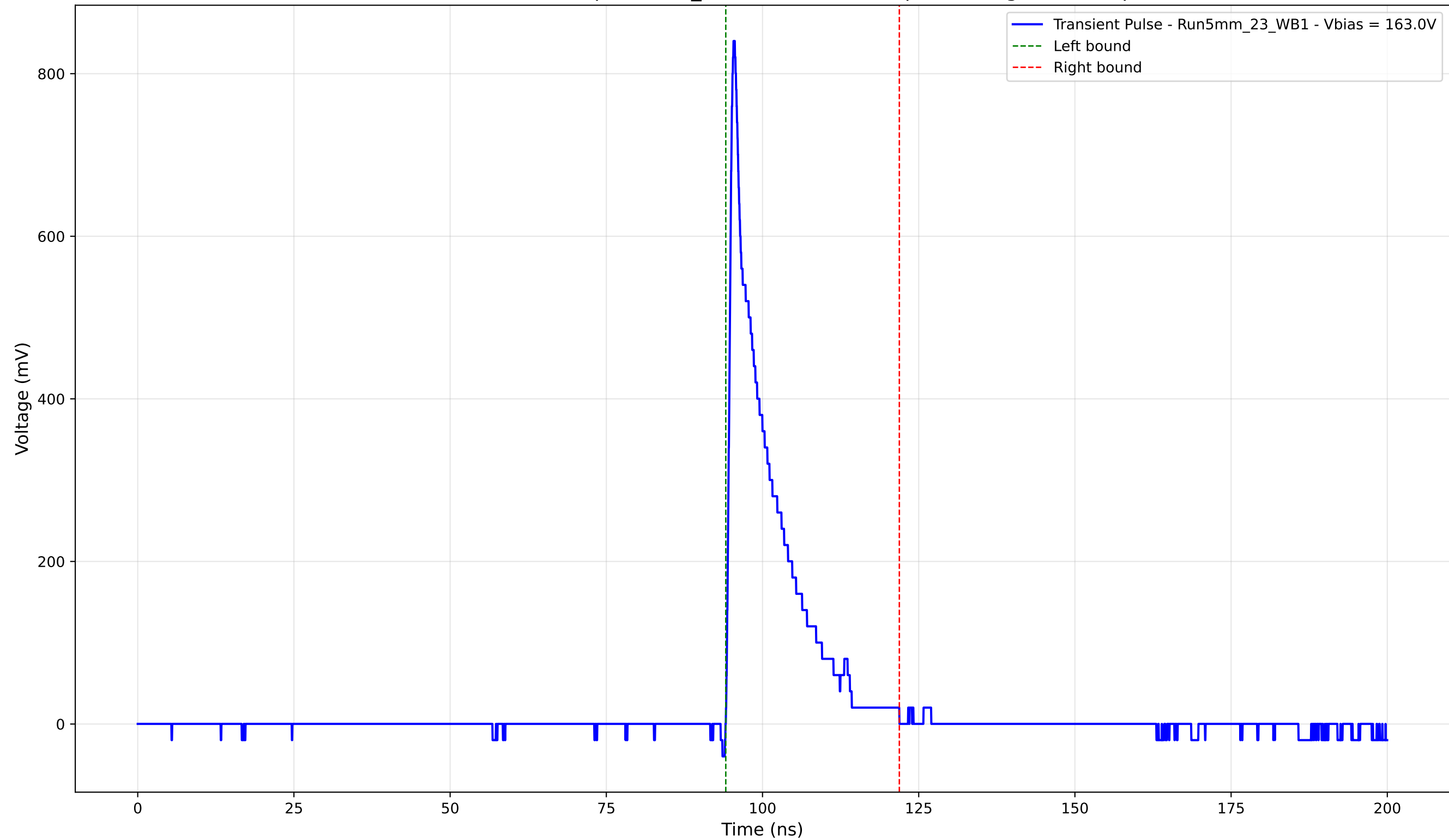
Transient Pulse - Sample: 5mm_23 - Position: 320.0 \mu\text{m} - Charge: 108.99 pC
