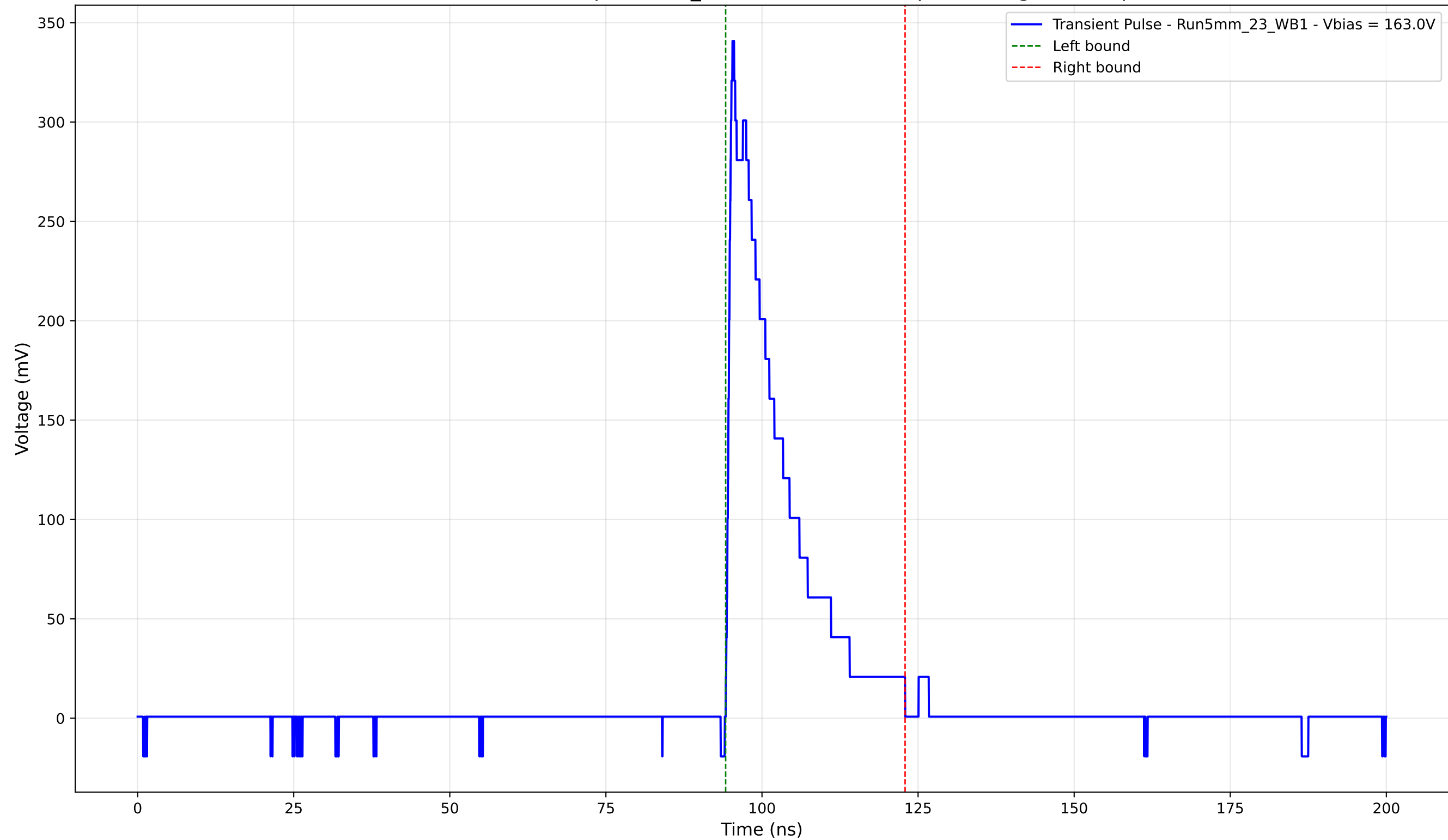
Transient Pulse - Sample: 5mm_23 - Position: 3225.0 \mu\text{m} - Charge: 58.67 pC
