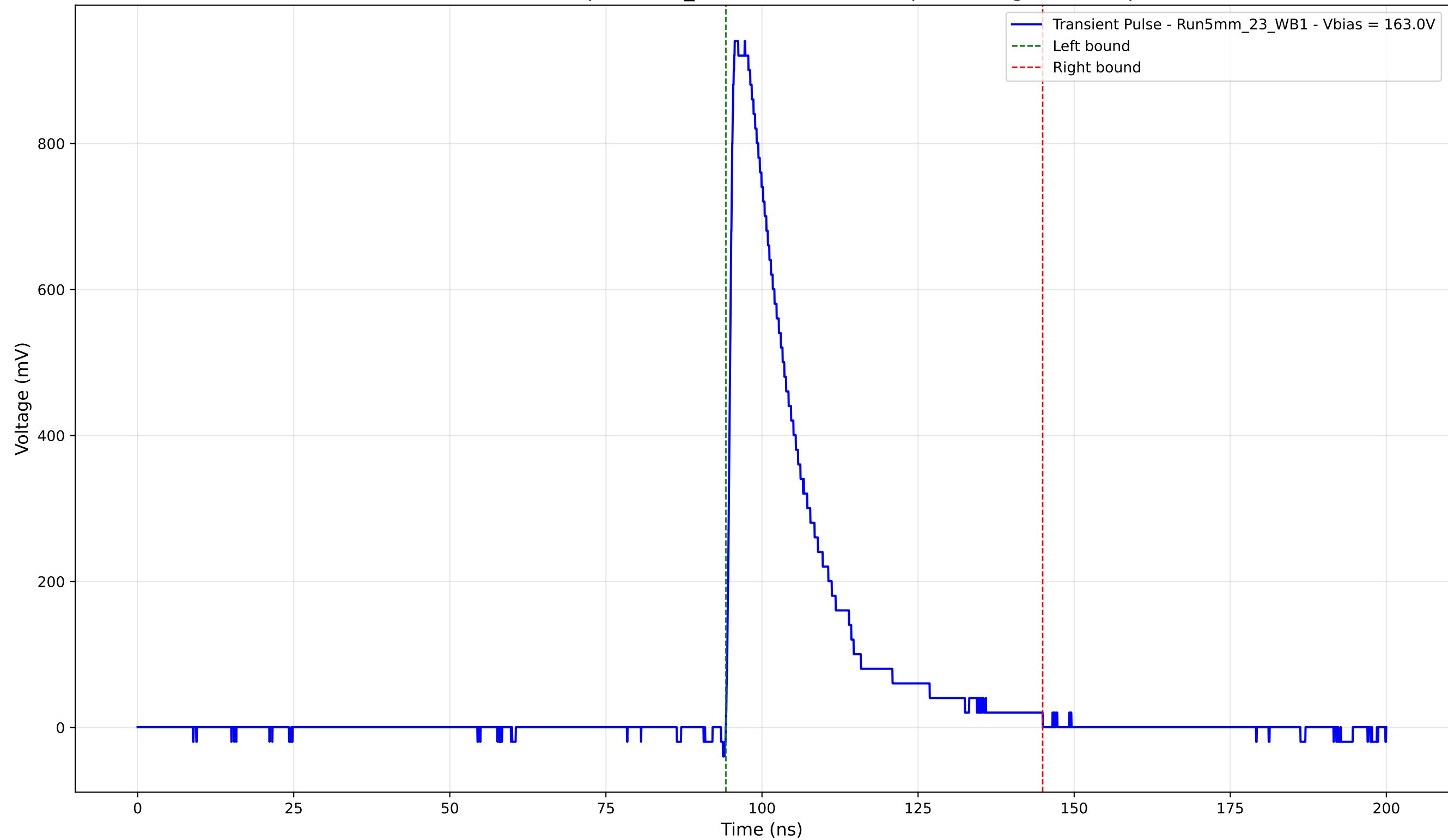
Transient Pulse - Sample: 5mm_23 - Position: 3520.0 \mu\text{m} - Charge: 221.84 pC
