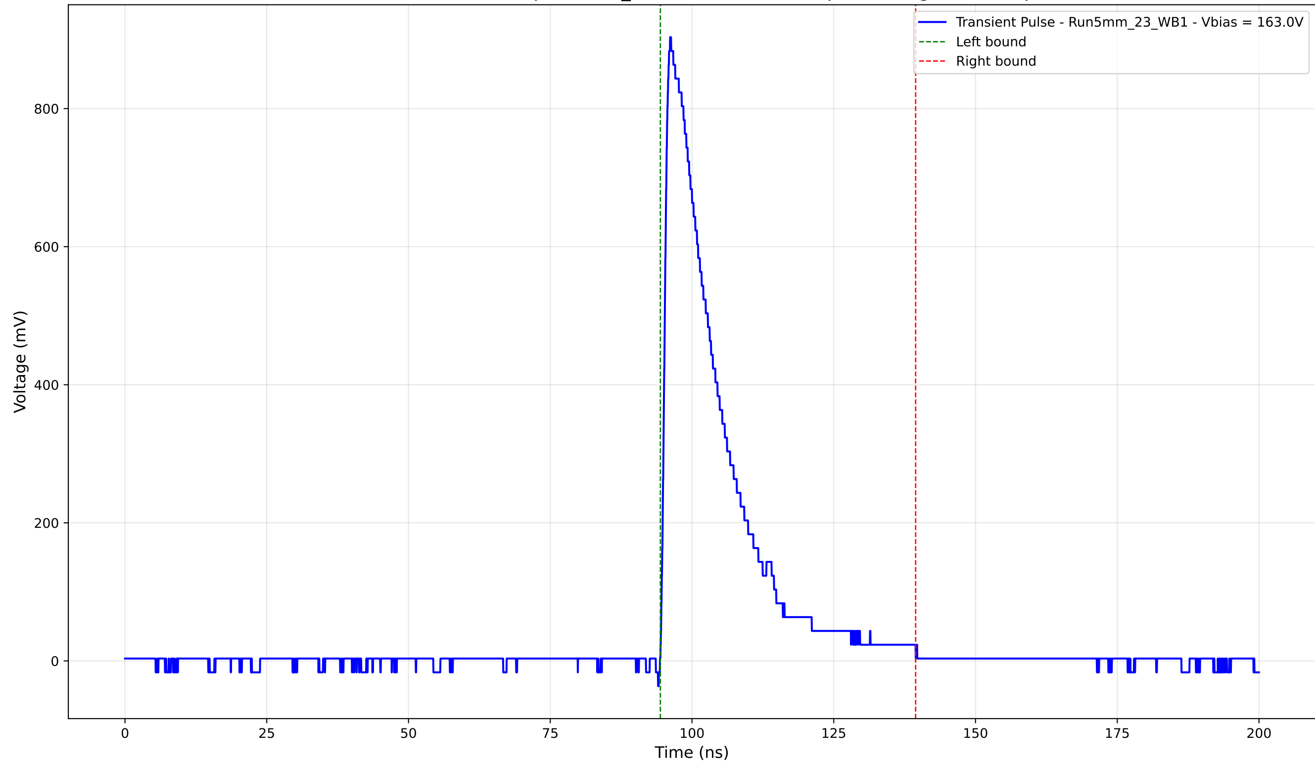
Transient Pulse - Sample: 5mm_23 - Position: 1305.0 \mu\text{m} - Charge: 192.14 pC
