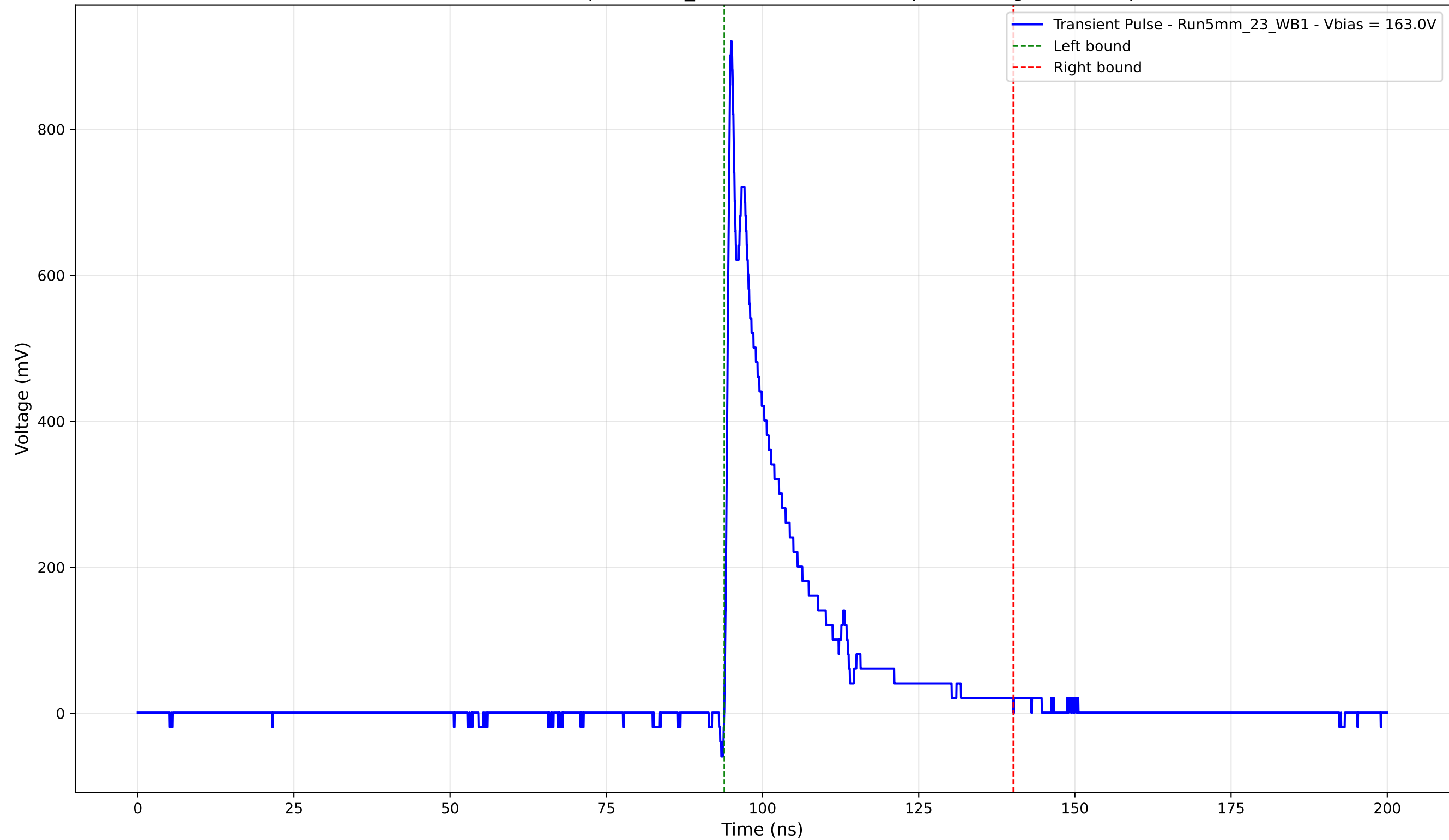
Transient Pulse - Sample: 5mm_23 - Position: 2695.0 \mu\text{m} - Charge: 150.37 pC
