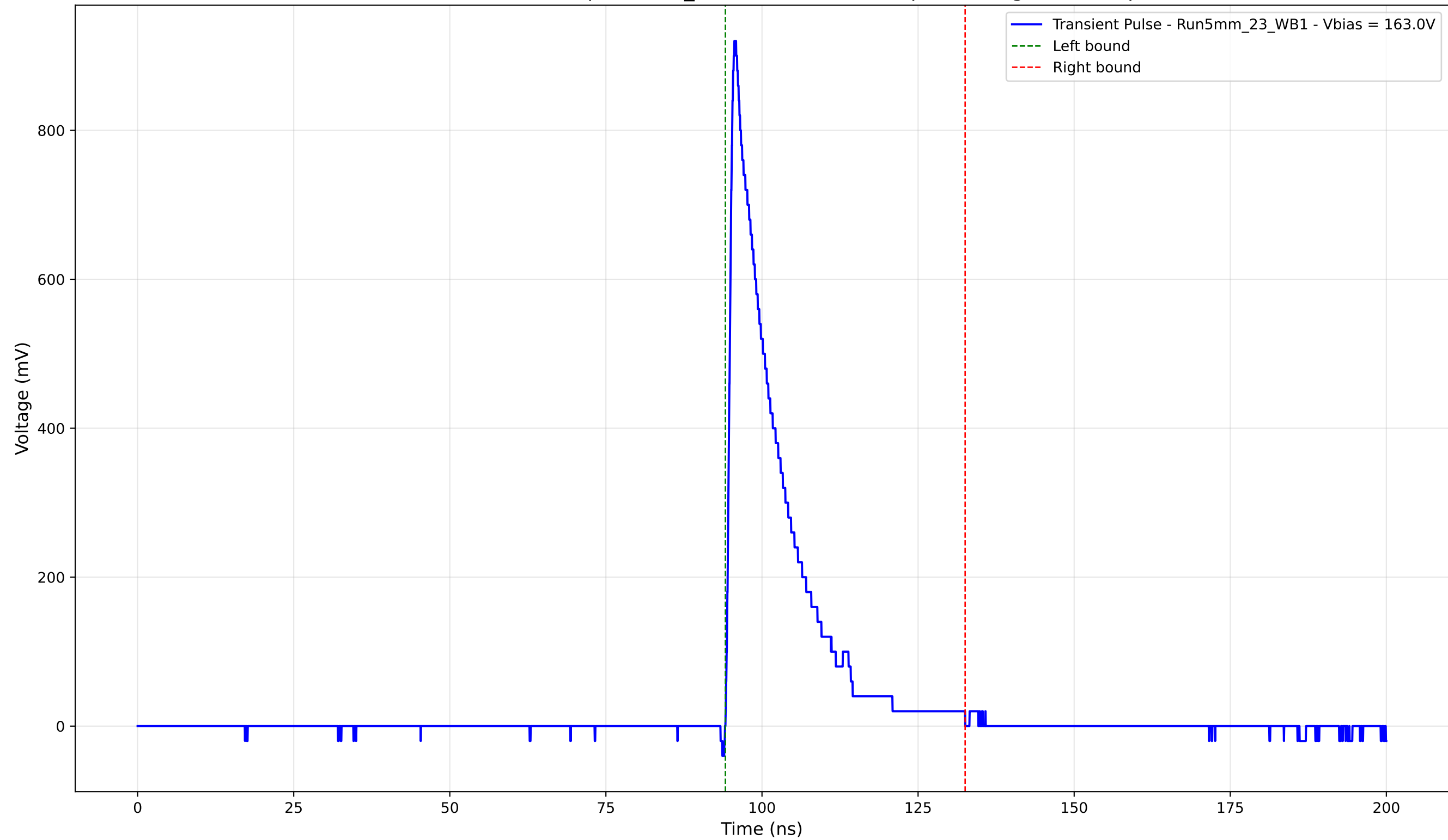
Transient Pulse - Sample: 5mm_23 - Position: 4840.0 \mu\text{m} - Charge: 150.86 pC
