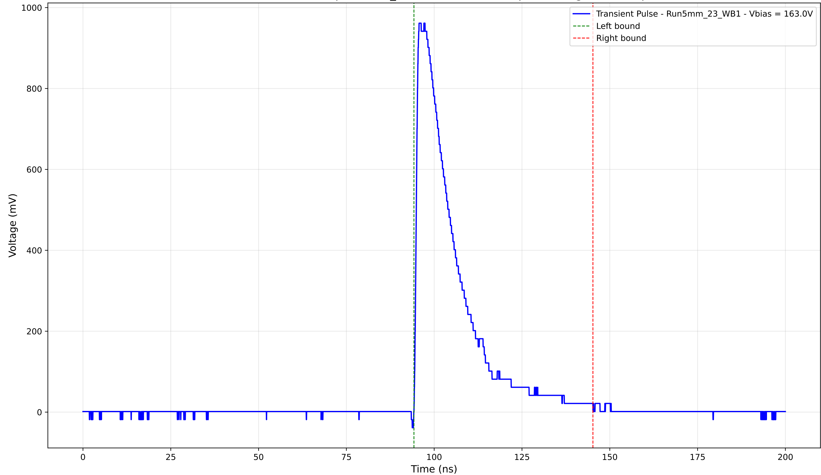
Transient Pulse - Sample: 5mm_23 - Position: 1905.0 \mu\text{m} - Charge: 235.83 pC
