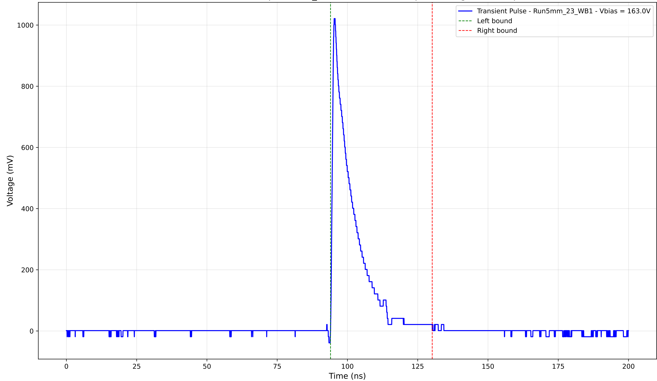
Transient Pulse - Sample: 5mm_23 - Position: 5125.0 \mu\text{m} - Charge: 157.99 pC
