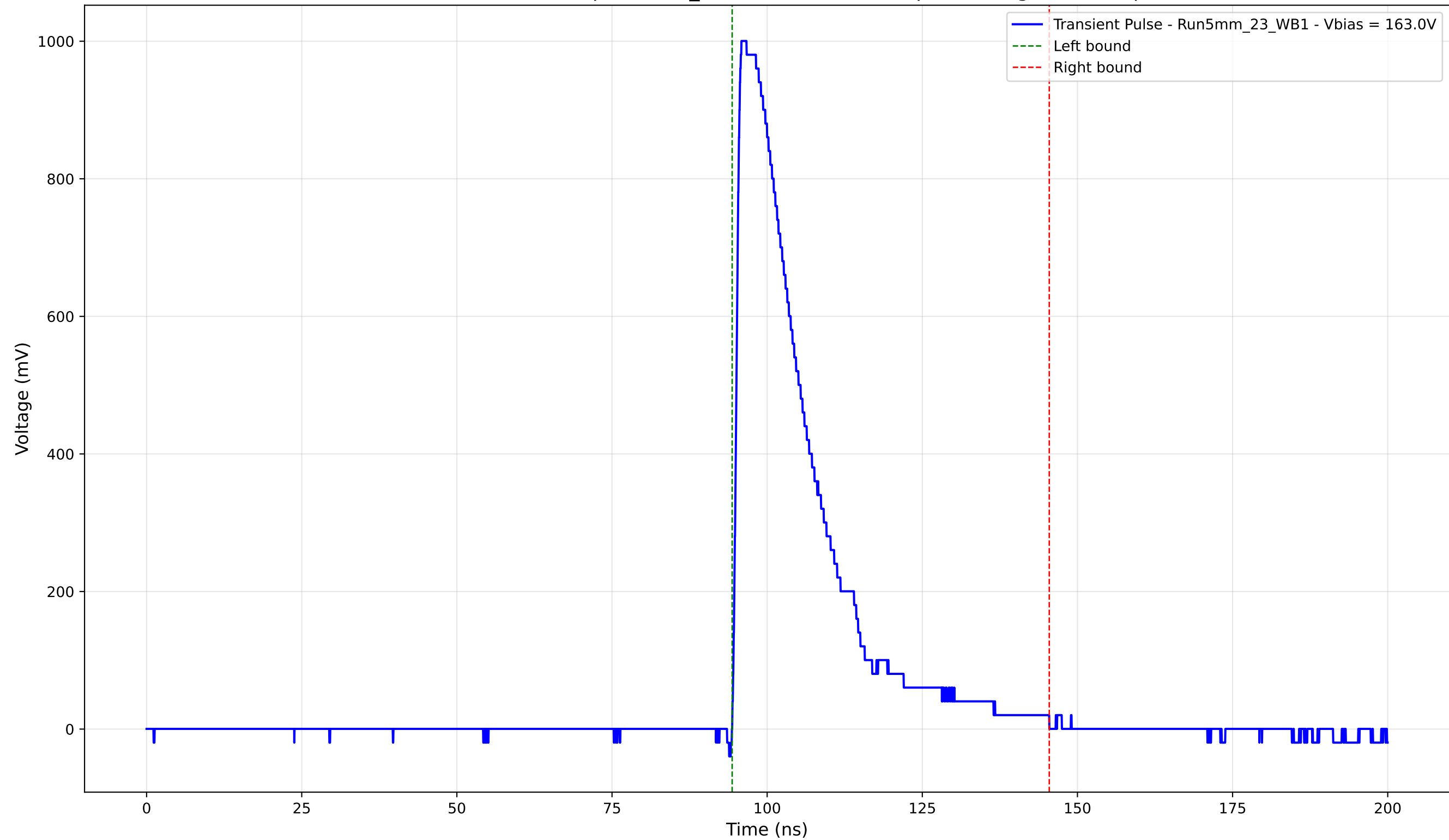
Transient Pulse - Sample: 5mm_23 - Position: 1550.0 \mu\text{m} - Charge: 254.25 pC
