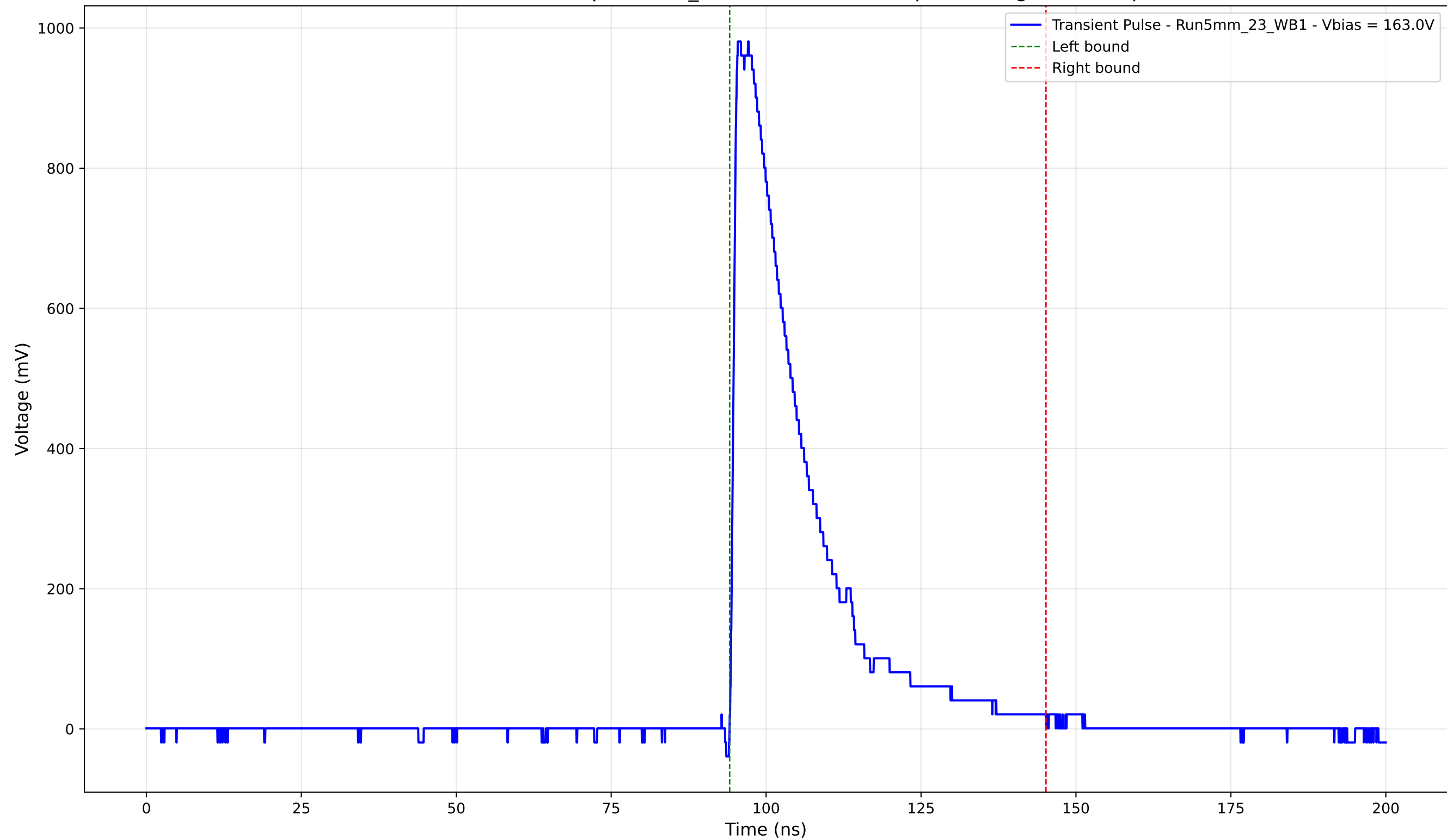
Transient Pulse - Sample: 5mm_23 - Position: 2105.0 \mu\text{m} - Charge: 243.14 pC
