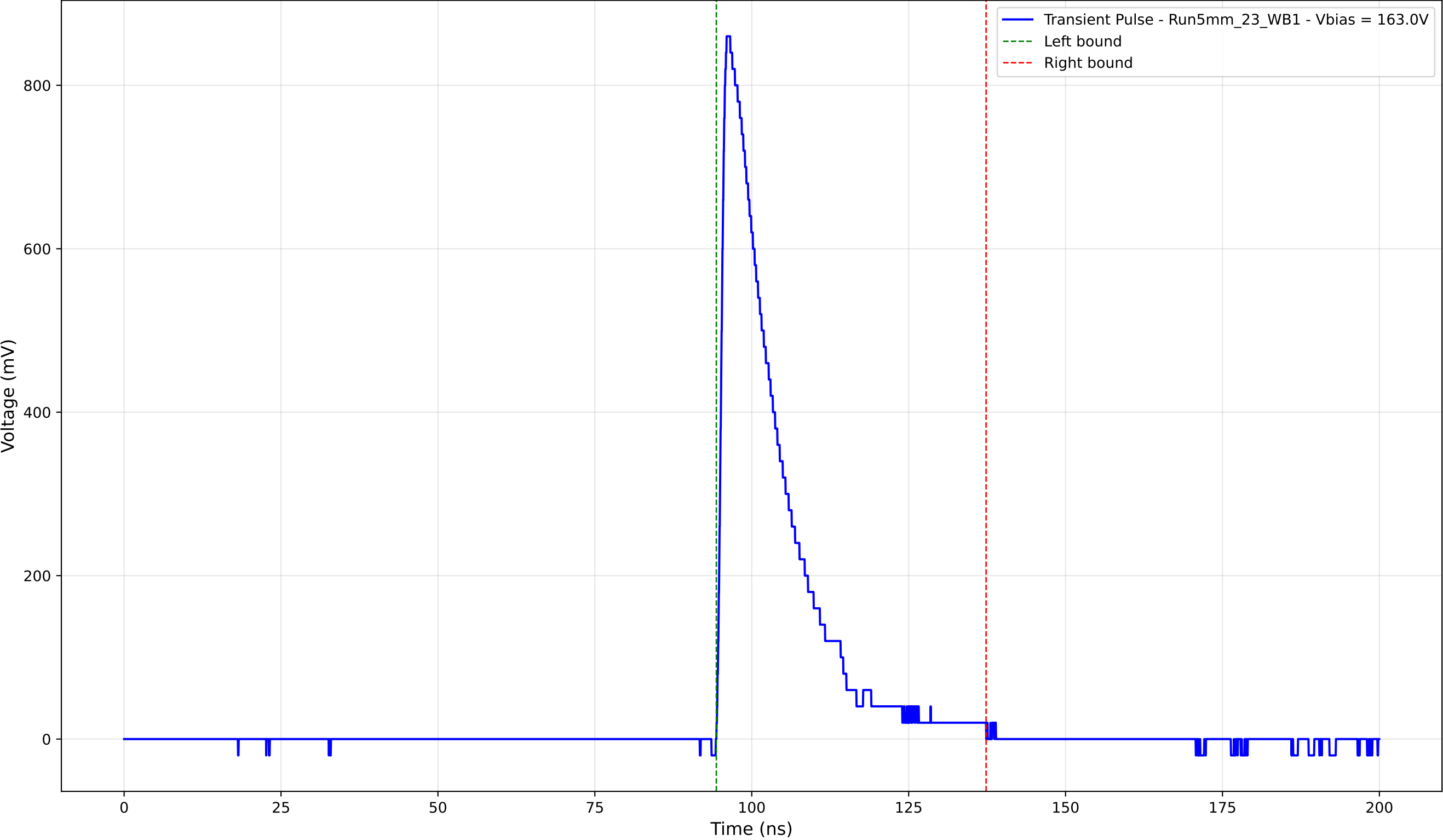
Transient Pulse - Sample: 5mm_23 - Position: 4175.0 \mu\text{m} - Charge: 172.79 pC
