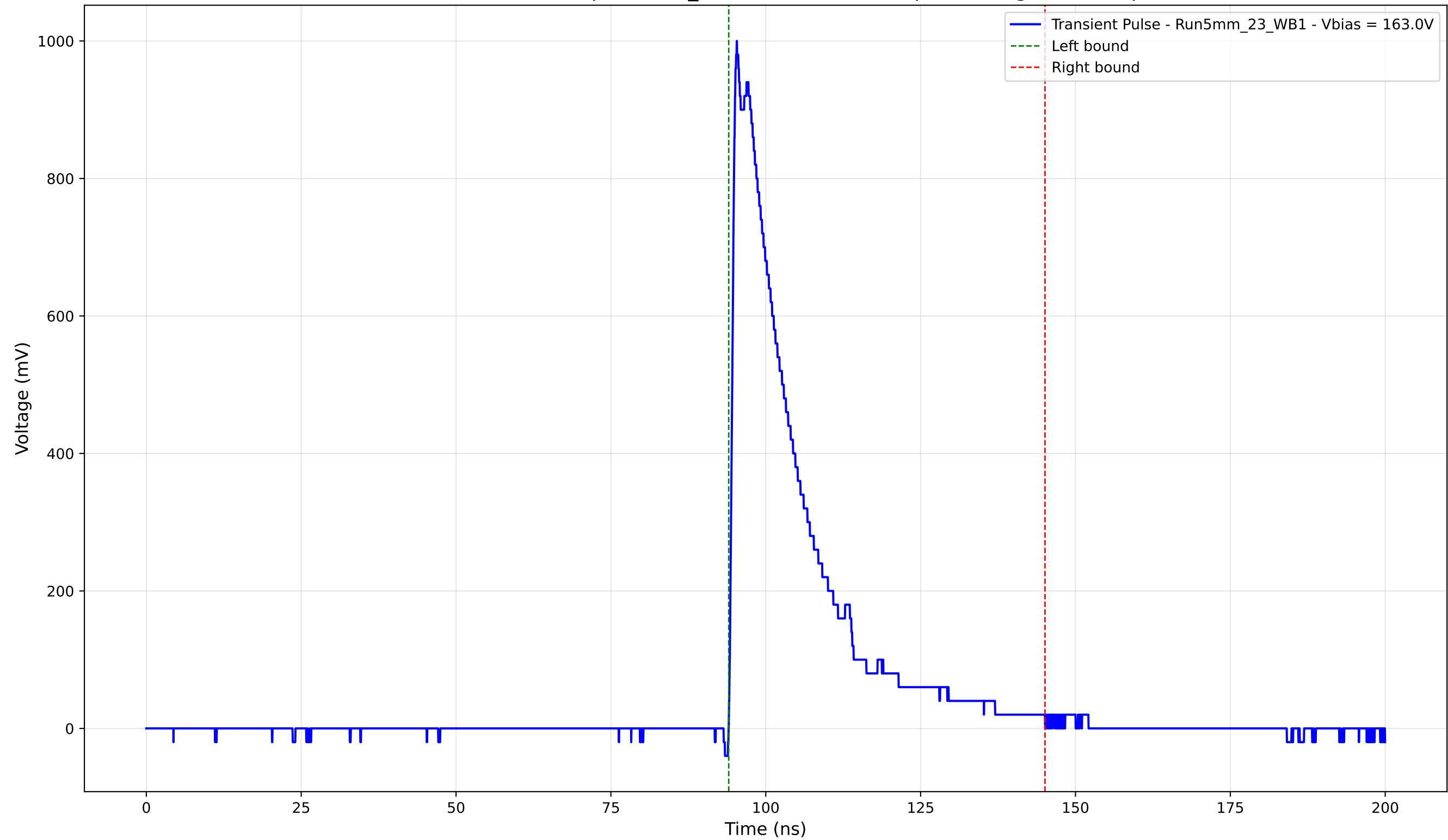
Transient Pulse - Sample: 5mm_23 - Position: 3125.0 \mu\text{m} - Charge: 220.73 pC
