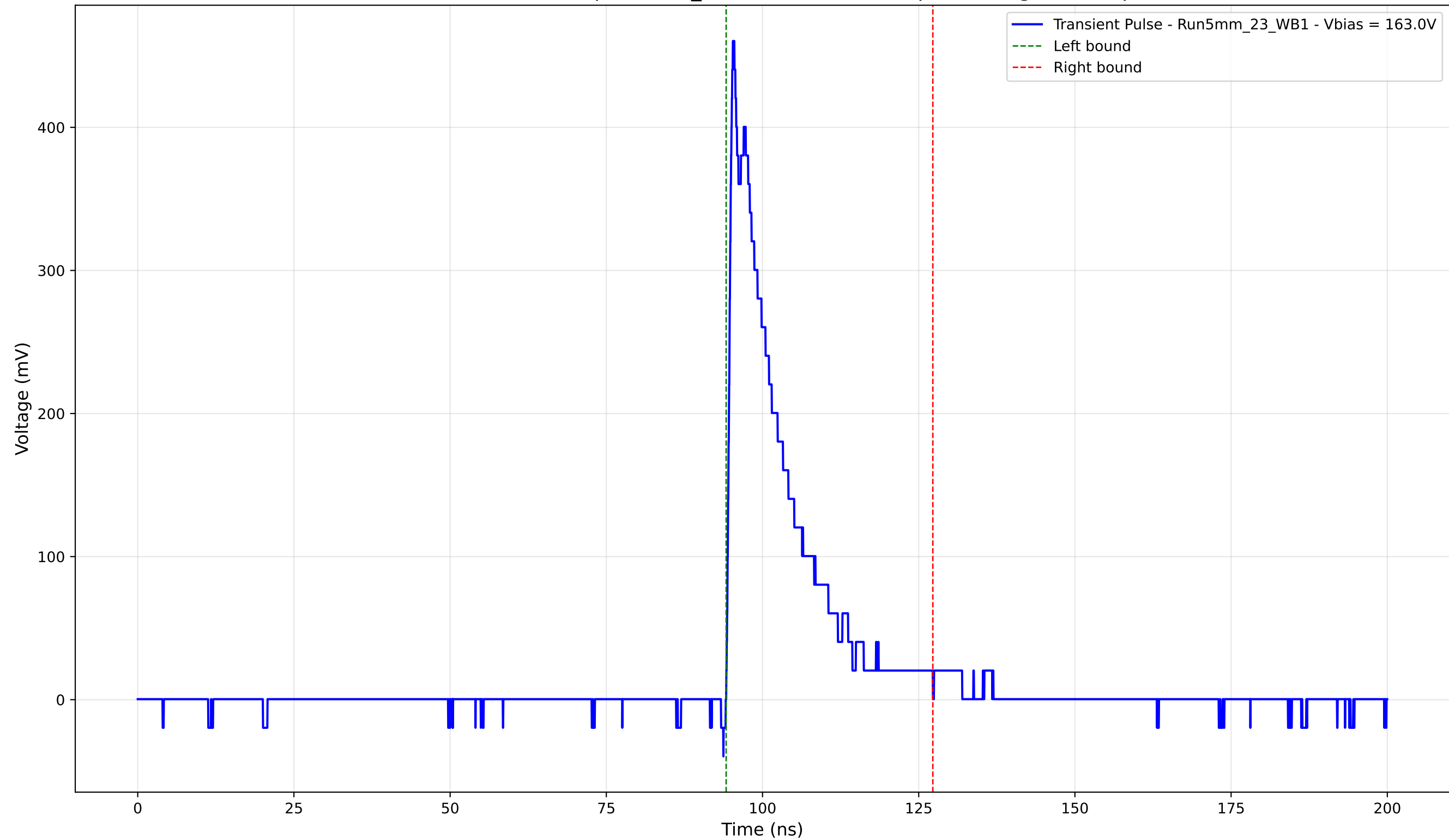
Transient Pulse - Sample: 5mm_23 - Position: 3215.0 \mu\text{m} - Charge: 78.55 pC
