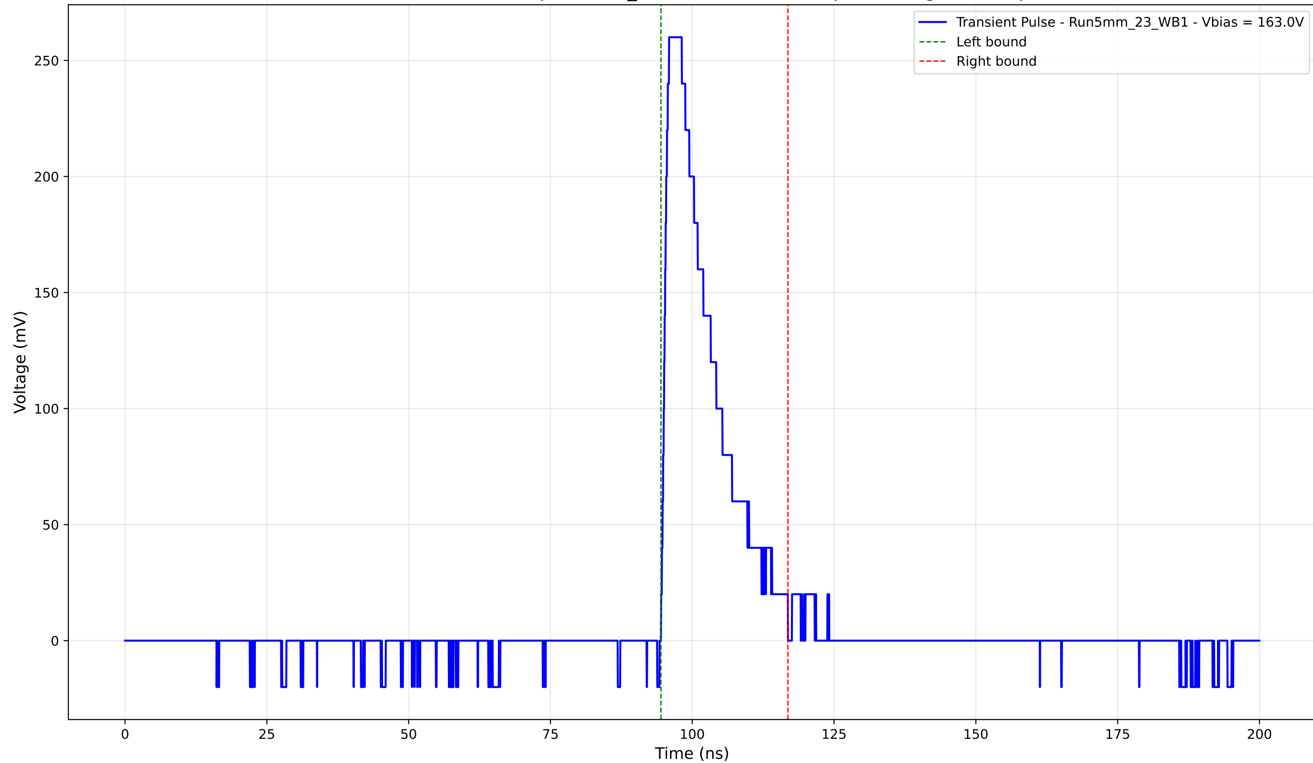
Transient Pulse - Sample: 5mm_23 - Position: 3775.0 \mu\text{m} - Charge: 49.19 pC
