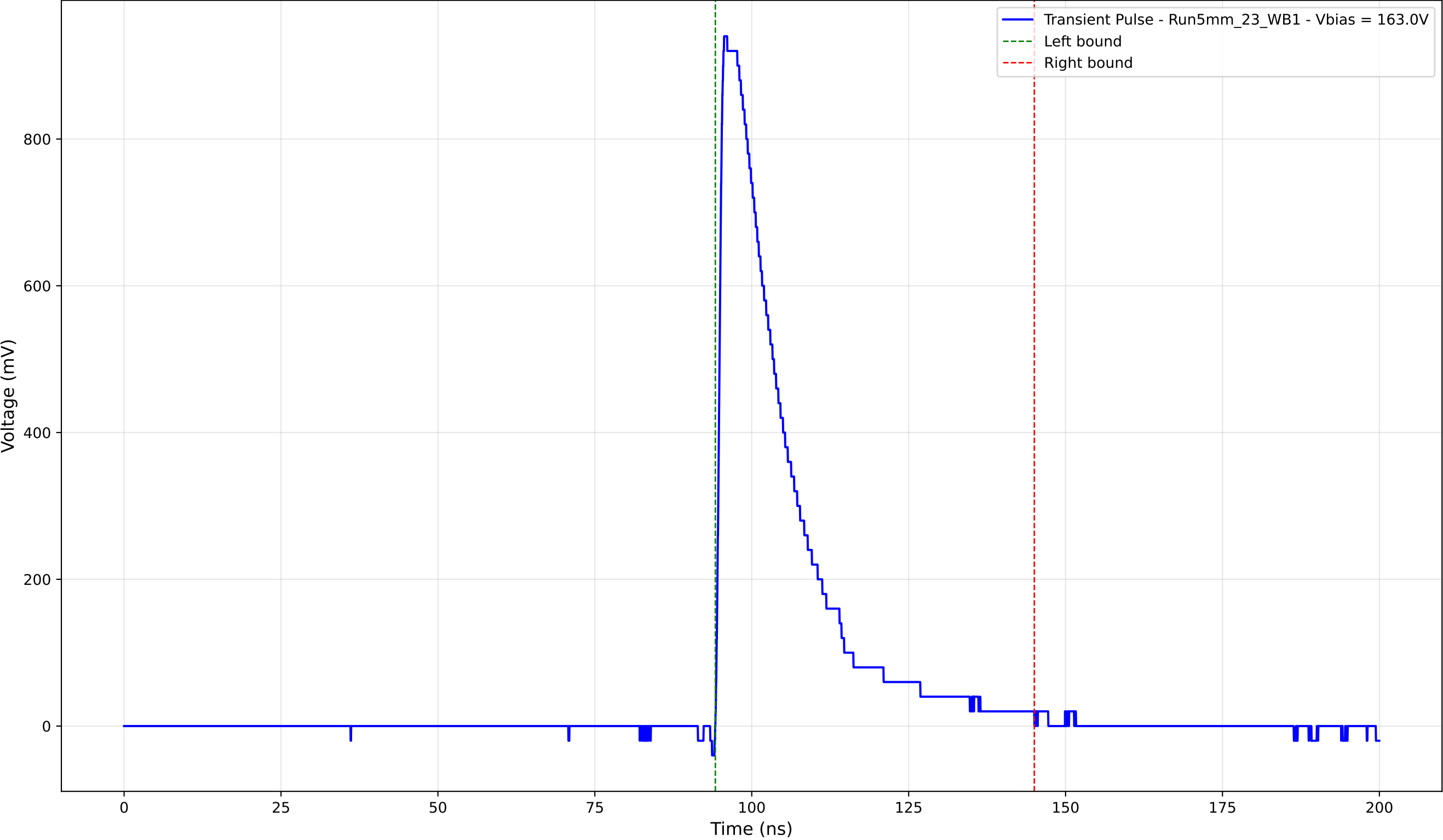
Transient Pulse - Sample: 5mm_23 - Position: 3480.0 \mu\text{m} - Charge: 222.23 pC
