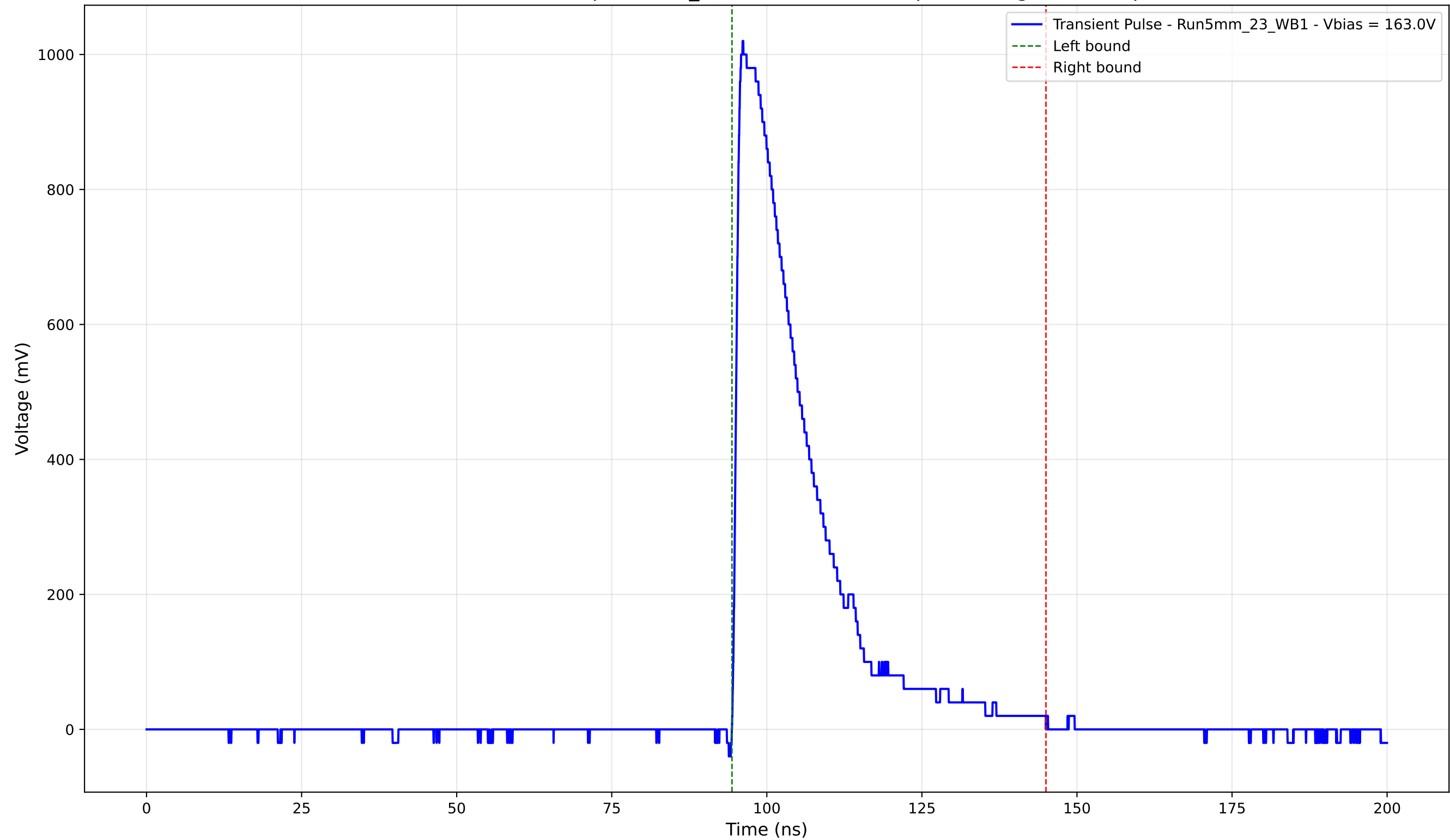
Transient Pulse - Sample: 5mm_23 - Position: 1510.0 \mu\text{m} - Charge: 252.02 pC
