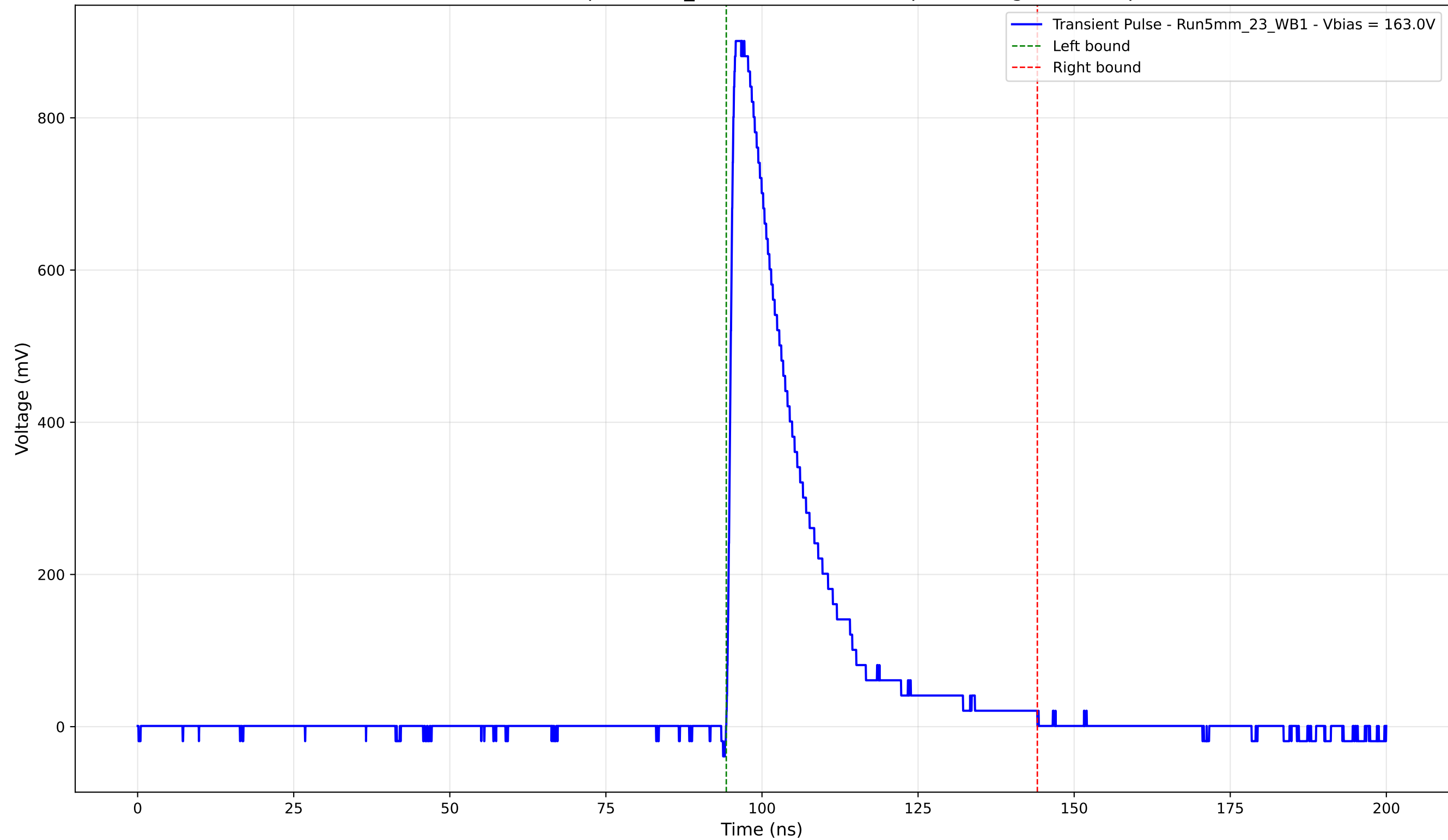
Transient Pulse - Sample: 5mm_23 - Position: 3635.0 \mu\text{m} - Charge: 204.74 pC
