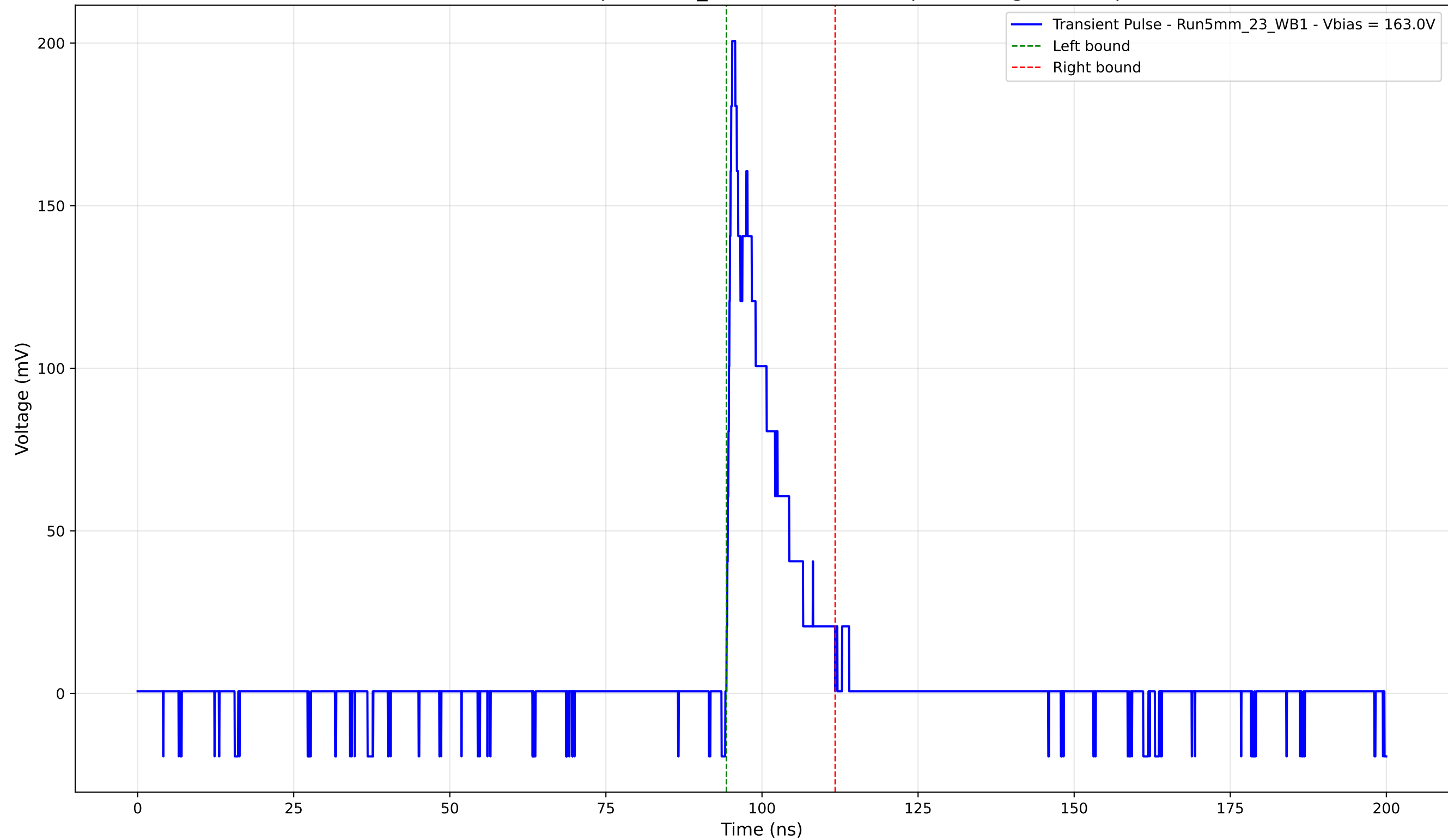
Transient Pulse - Sample: 5mm_23 - Position: 280.0 \mu\text{m} - Charge: 25.57 pC
