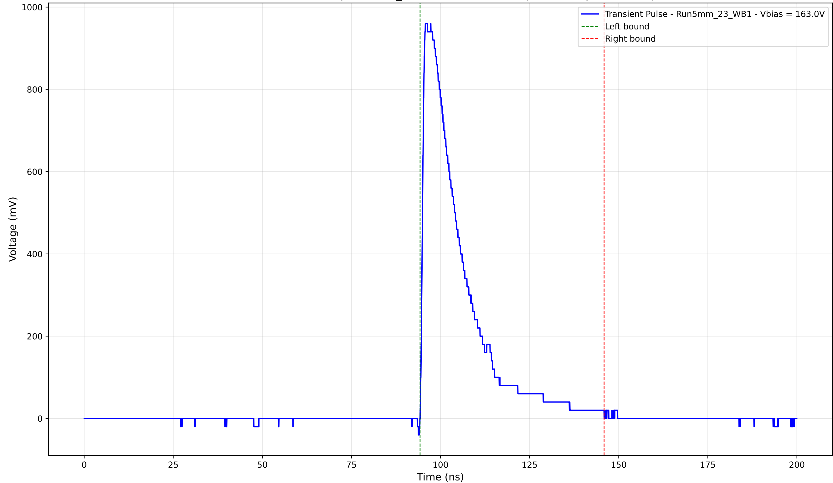
Transient Pulse - Sample: 5mm_23 - Position: 1875.0 \mu\text{m} - Charge: 233.55 pC
