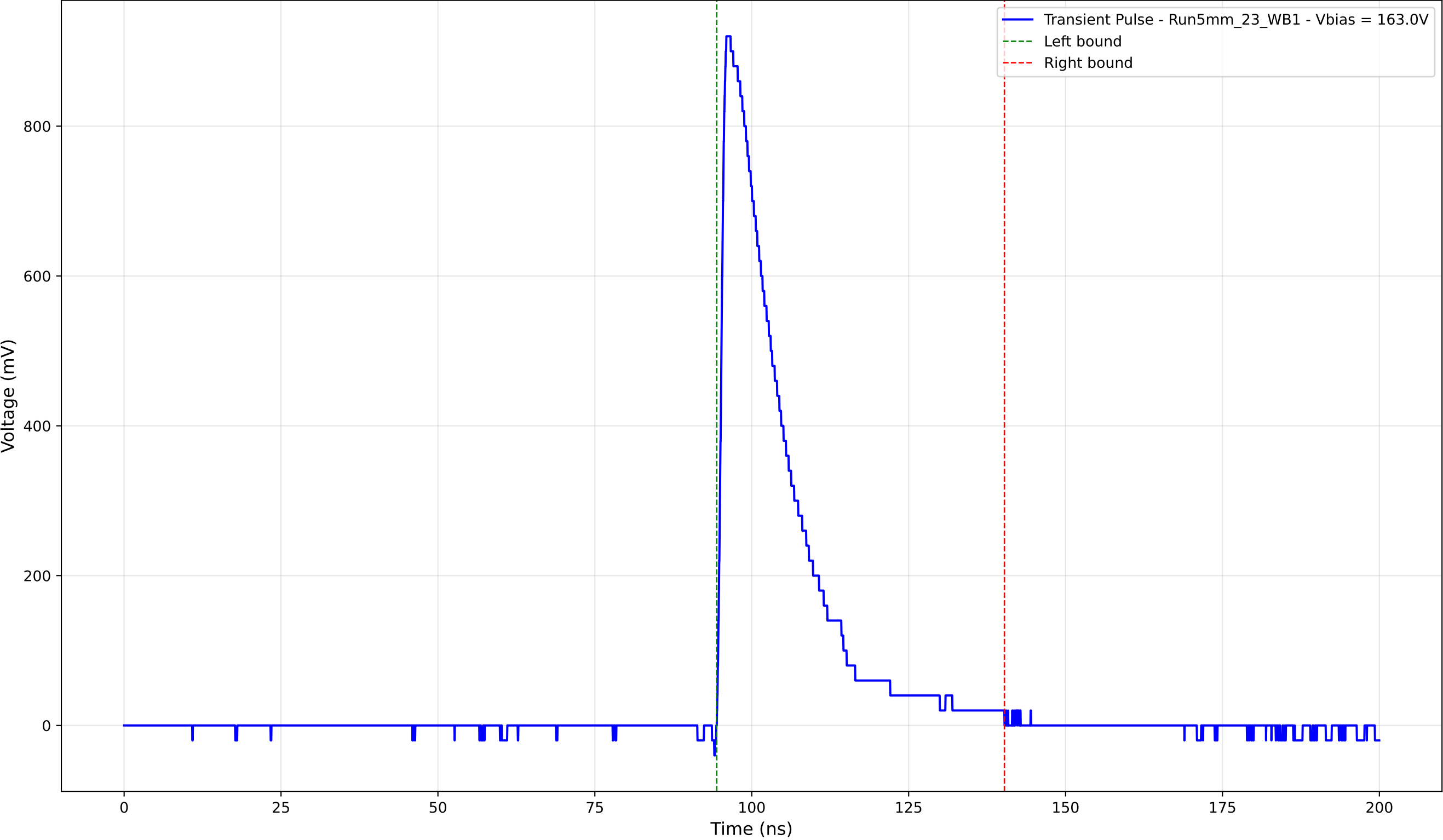
Transient Pulse - Sample: 5mm_23 - Position: 1315.0 \mu\text{m} - Charge: 202.00 pC
