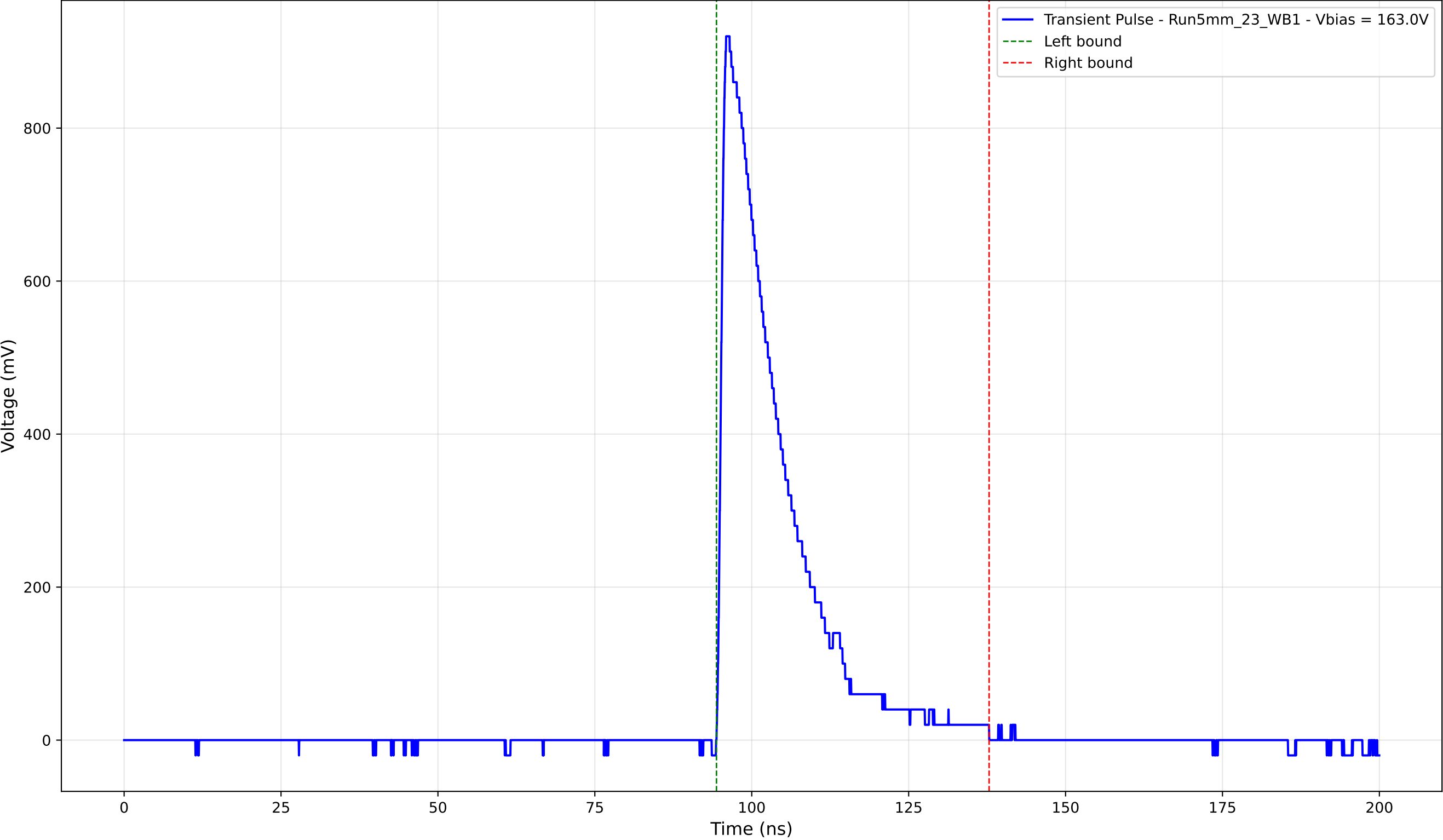
Transient Pulse - Sample: 5mm_23 - Position: 1135.0 \mu\text{m} - Charge: 191.81 pC
