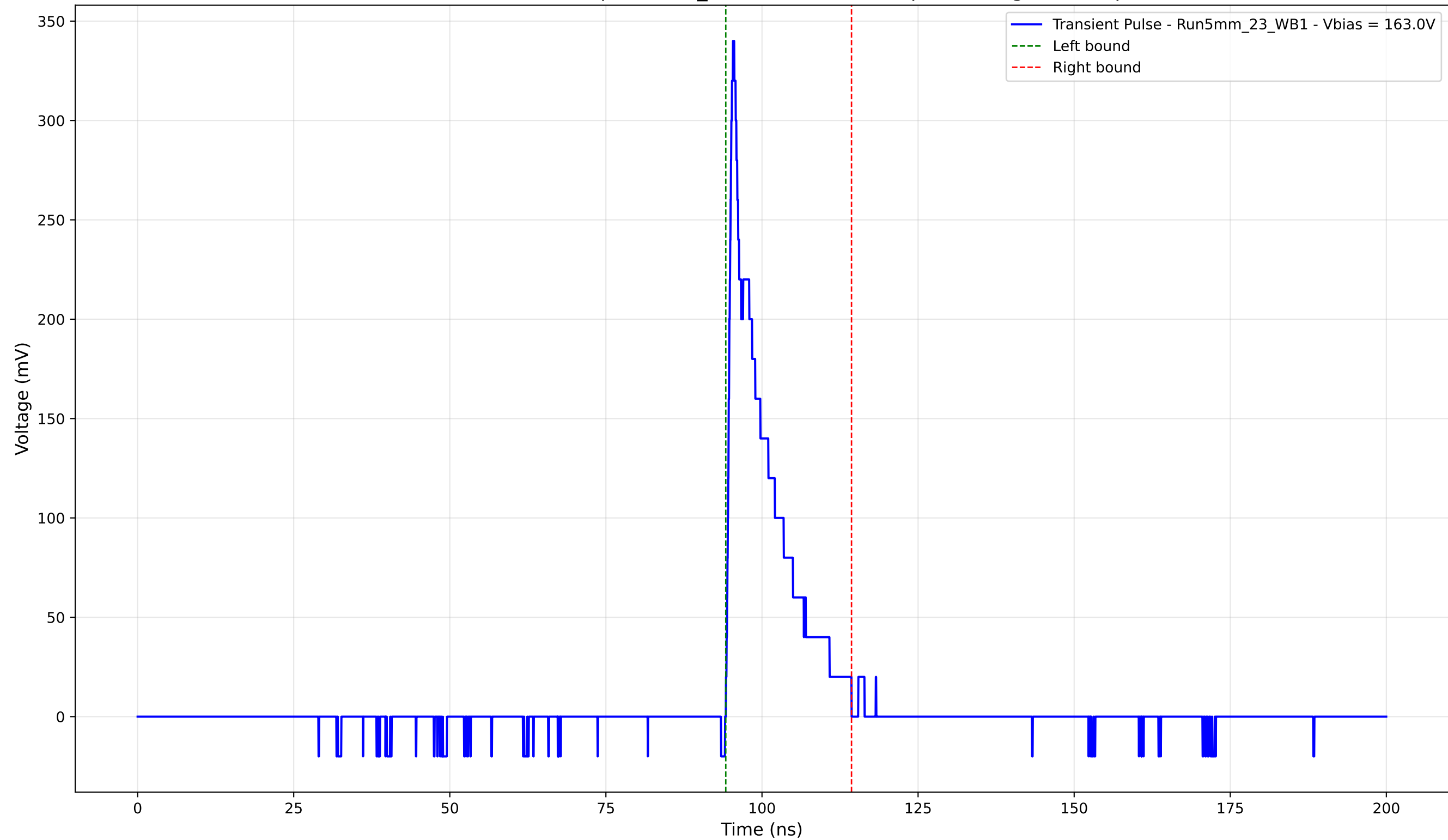
Transient Pulse - Sample: 5mm_23 - Position: 290.0 \mu\text{m} - Charge: 41.41 pC
