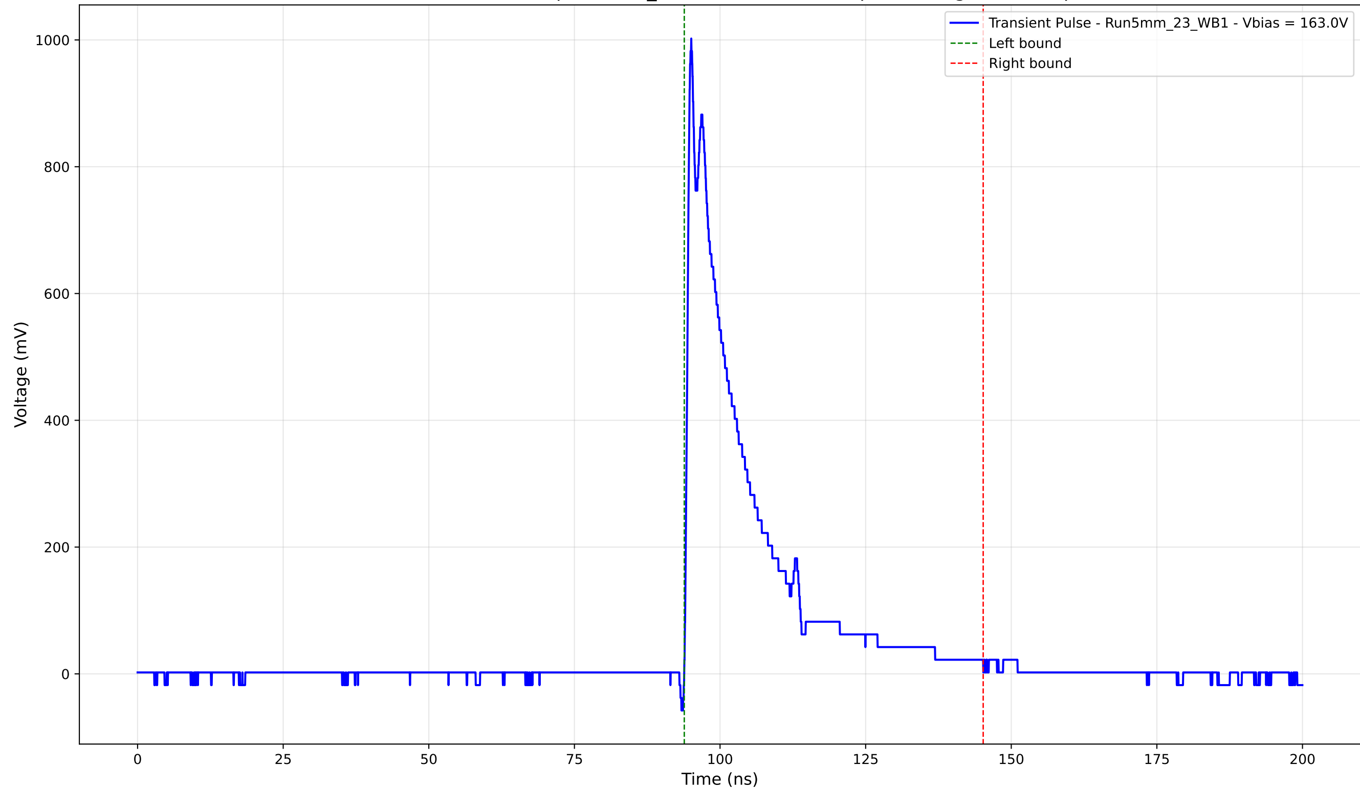
Transient Pulse - Sample: 5mm_23 - Position: 2815.0 \mu\text{m} - Charge: 193.41 pC
