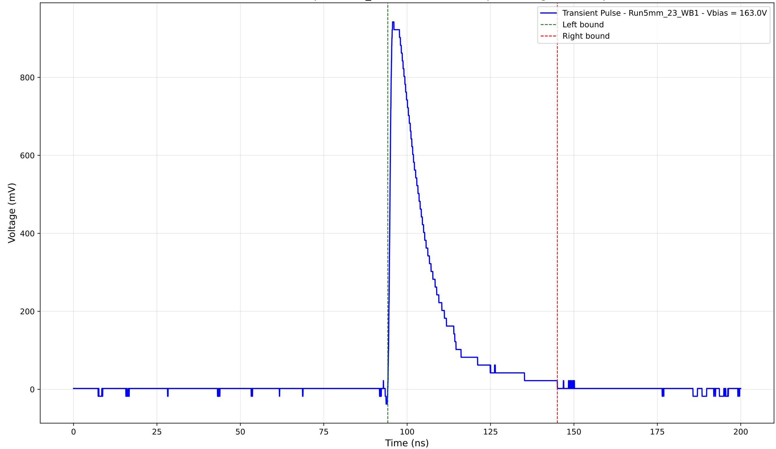
Transient Pulse - Sample: 5mm_23 - Position: 3485.0 \mu\text{m} - Charge: 222.70 pC
