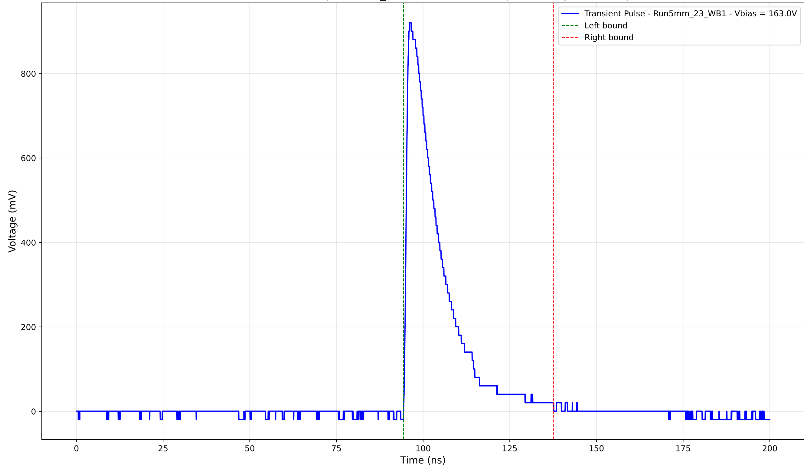
Transient Pulse - Sample: 5mm_23 - Position: 4055.0 \mu\text{m} - Charge: 197.21 pC
