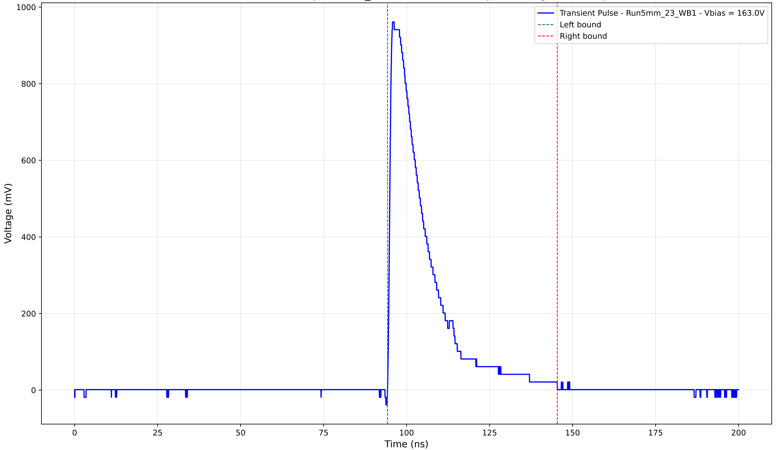
Transient Pulse - Sample: 5mm_23 - Position: 1885.0 \mu\text{m} - Charge: 233.91 pC
