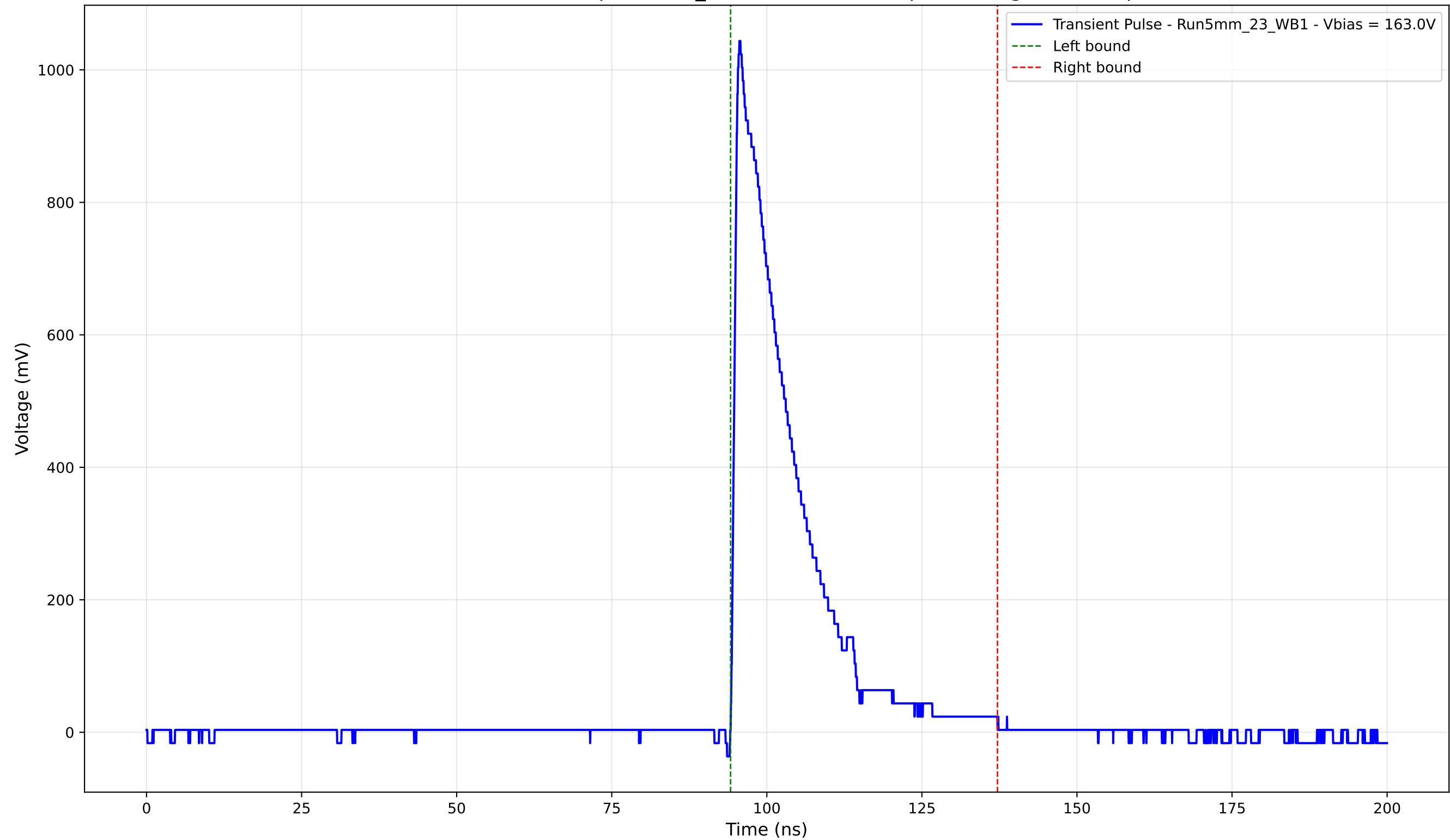
Transient Pulse - Sample: 5mm_23 - Position: 565.0 \mu\text{m} - Charge: 205.16 pC
