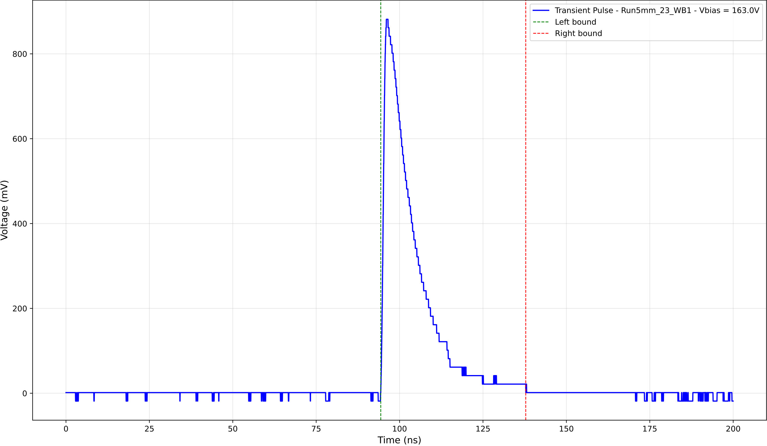
Transient Pulse - Sample: 5mm_23 - Position: 4170.0 \mu\text{m} - Charge: 178.94 pC
