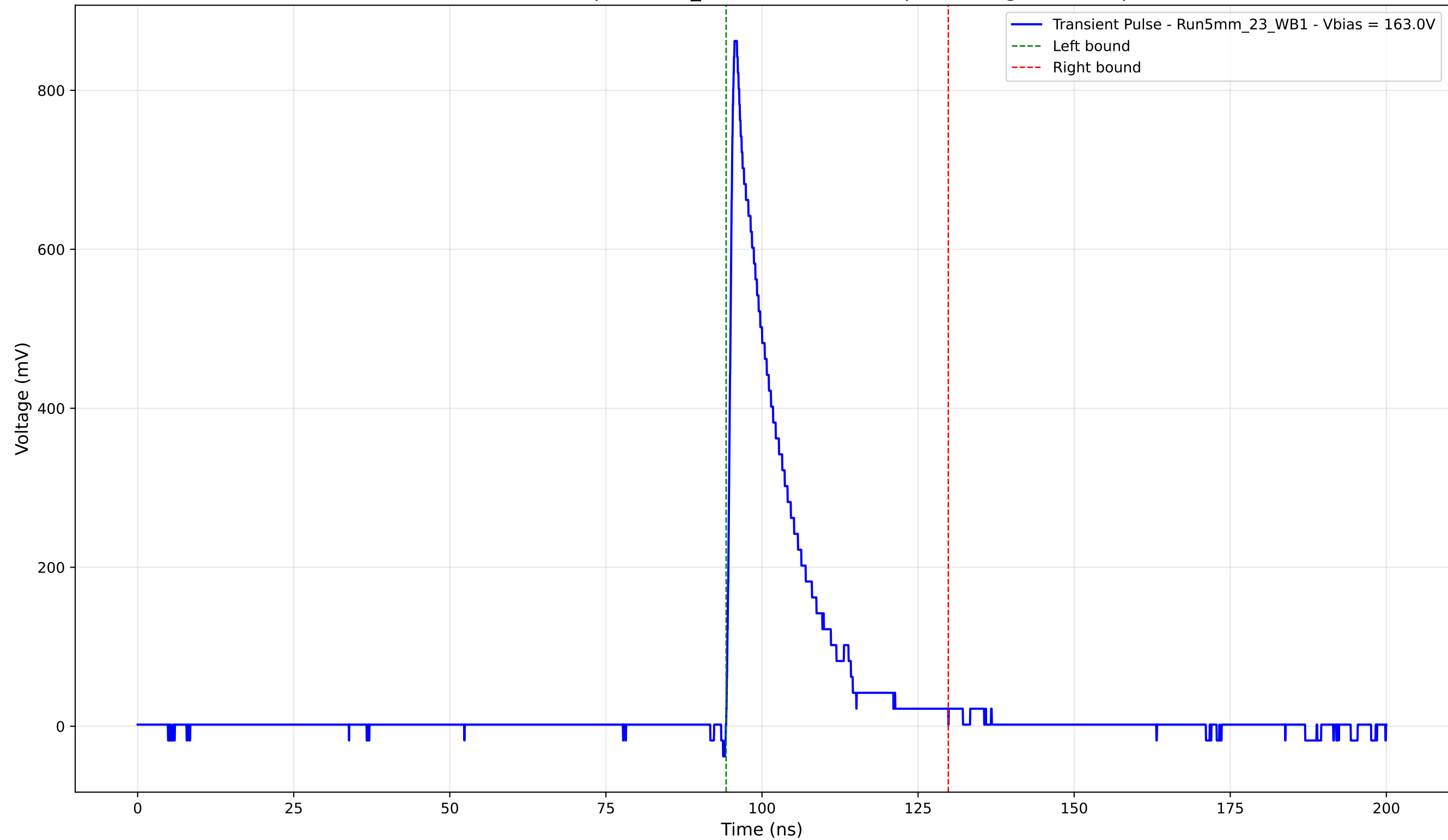
Transient Pulse - Sample: 5mm_23 - Position: 665.0 \mu\text{m} - Charge: 143.91 pC
