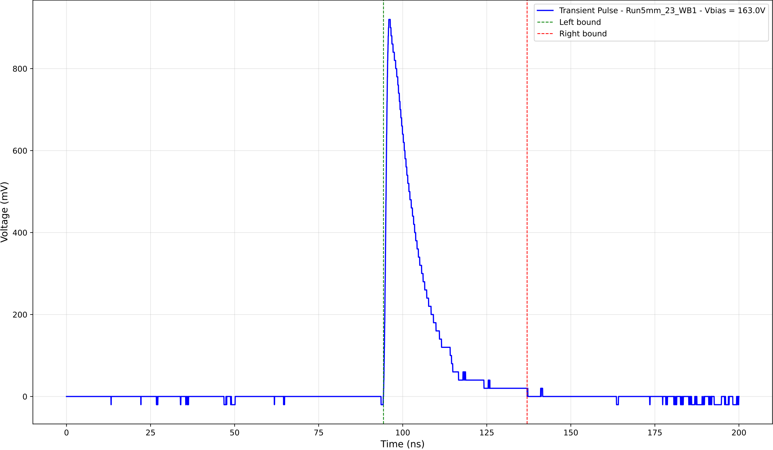
Transient Pulse - Sample: 5mm_23 - Position: 4480.0 \mu\text{m} - Charge: 179.14 pC
