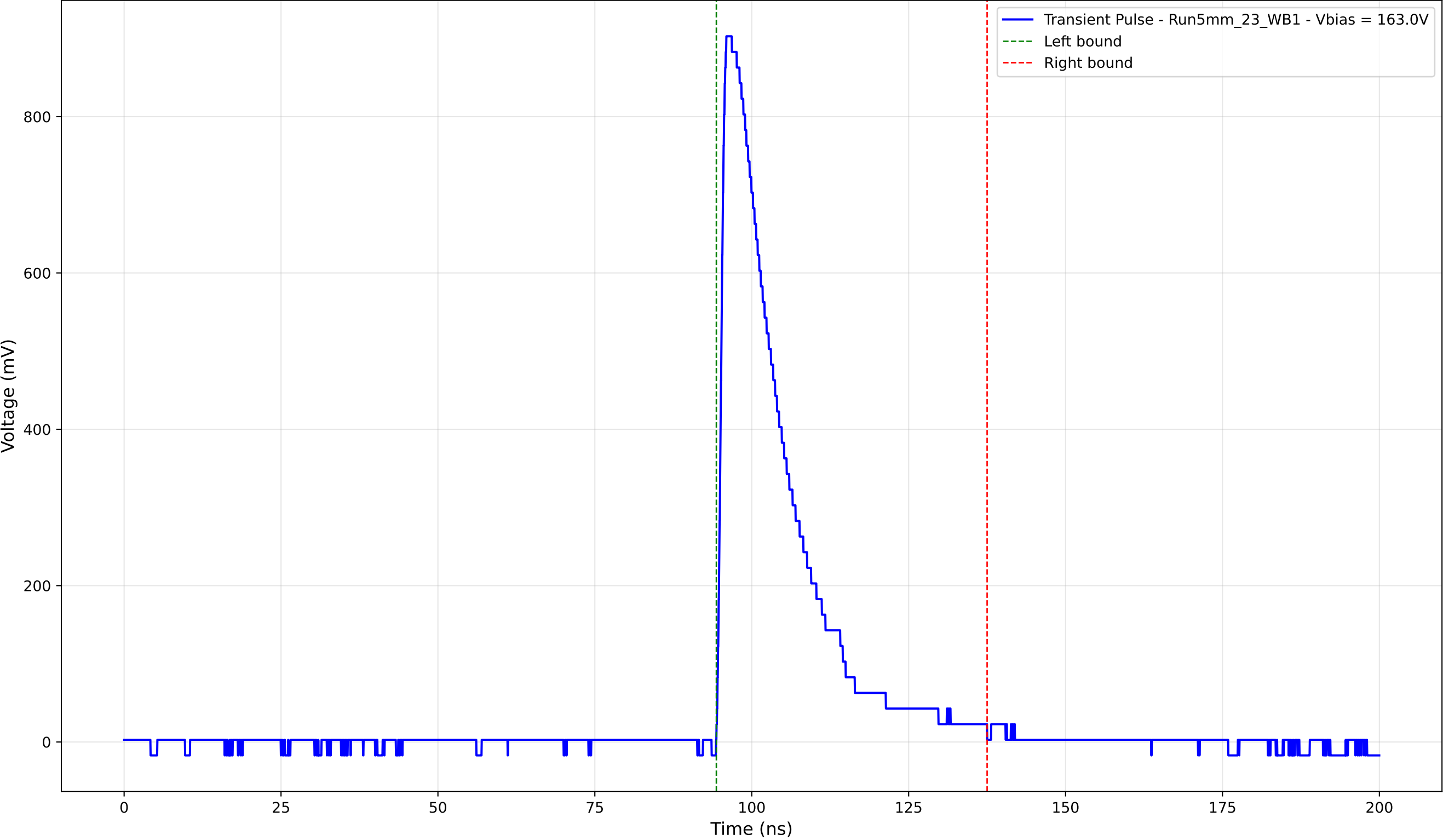
Transient Pulse - Sample: 5mm_23 - Position: 3975.0 \mu\text{m} - Charge: 198.31 pC
