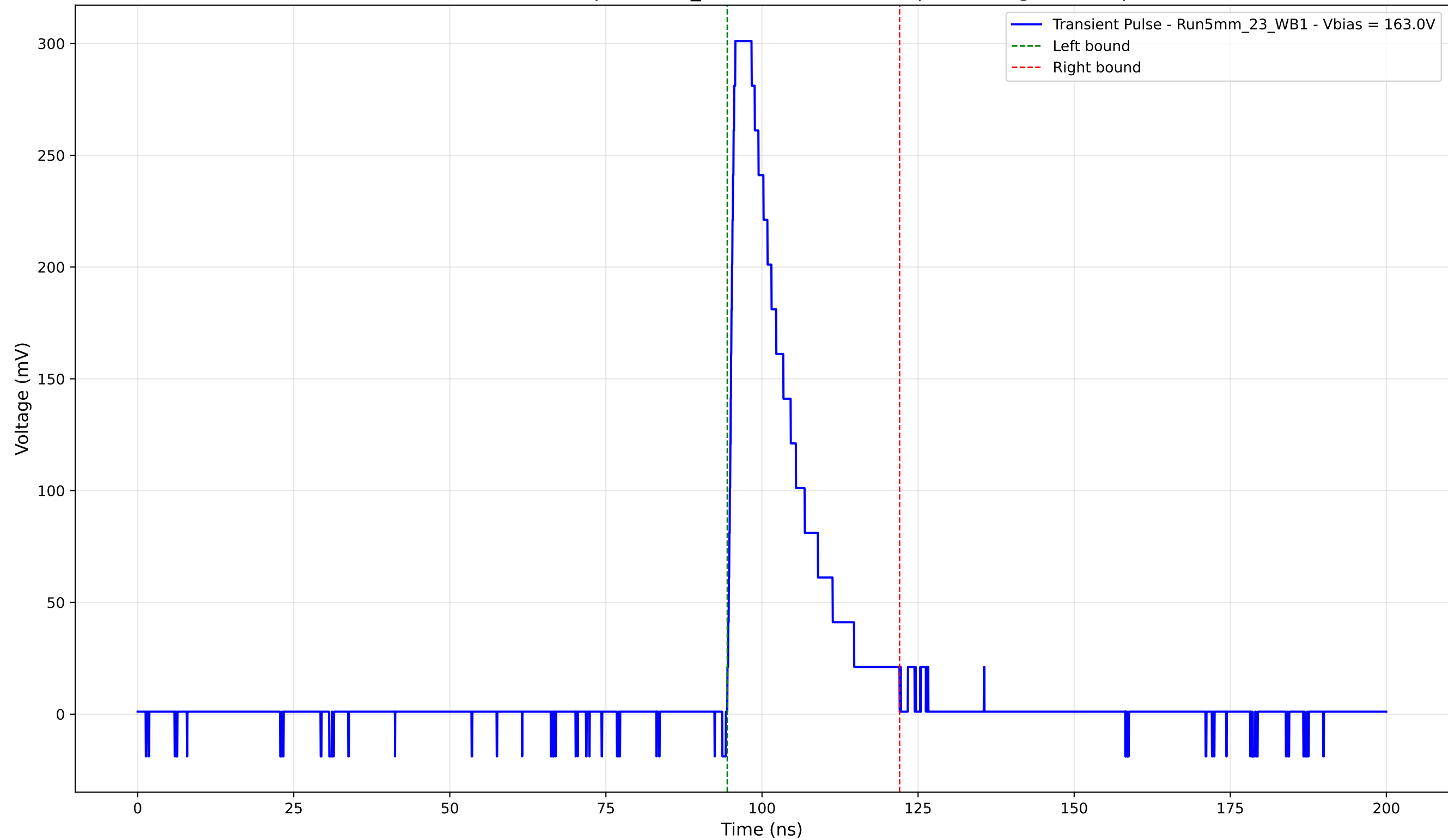
Transient Pulse - Sample: 5mm_23 - Position: 1750.0 \mu\text{m} - Charge: 61.85 pC
