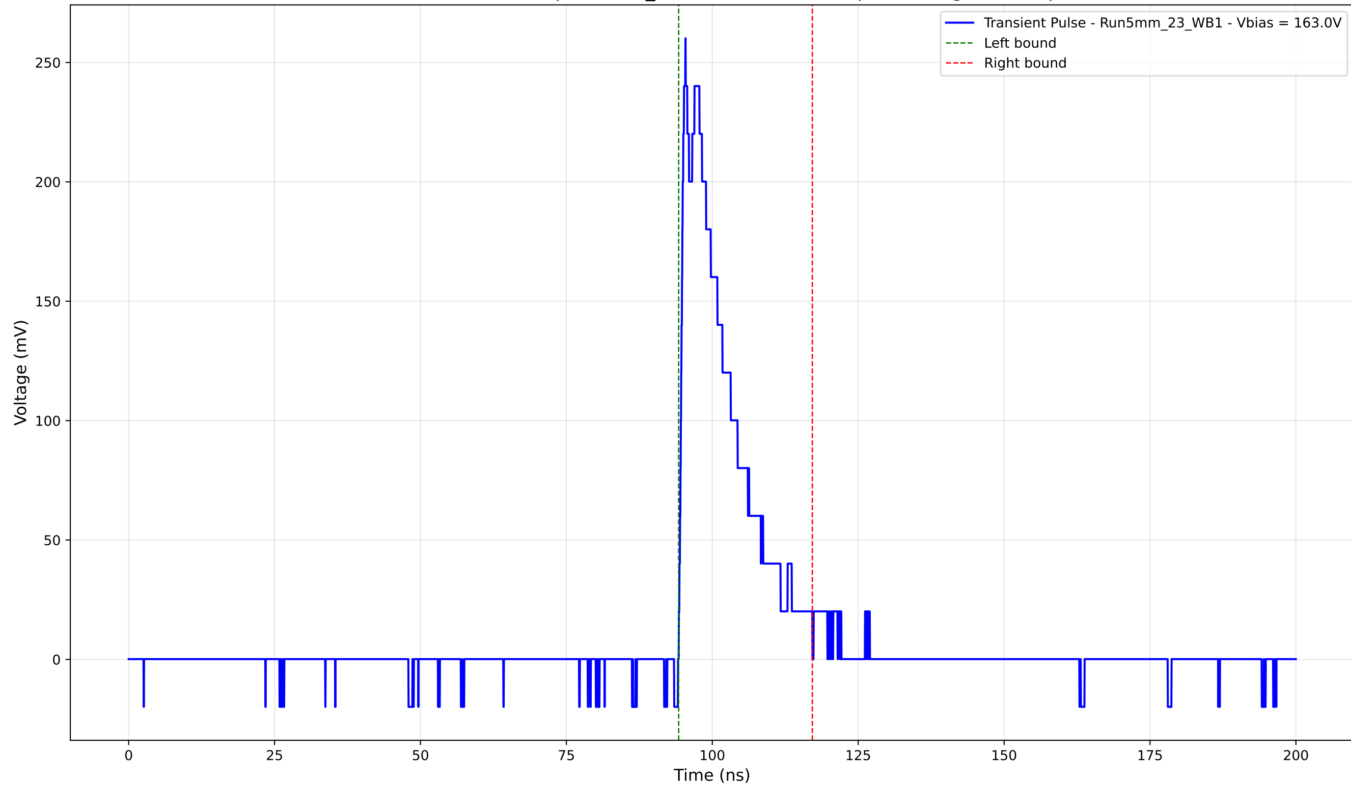
Transient Pulse - Sample: 5mm_23 - Position: 2250.0 \mu\text{m} - Charge: 44.55 pC
