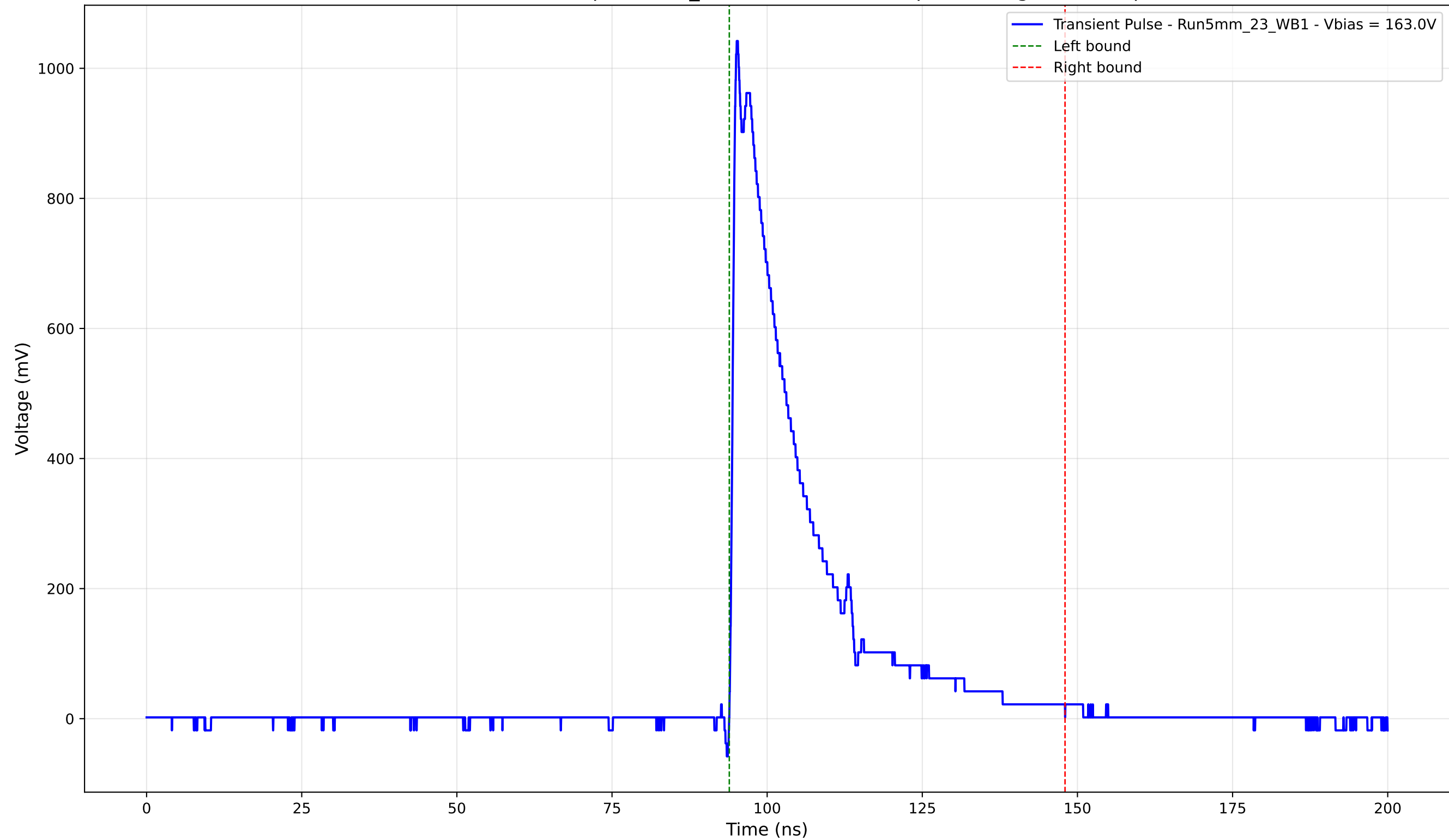
Transient Pulse - Sample: 5mm_23 - Position: 2950.0 \mu\text{m} - Charge: 235.91 pC
