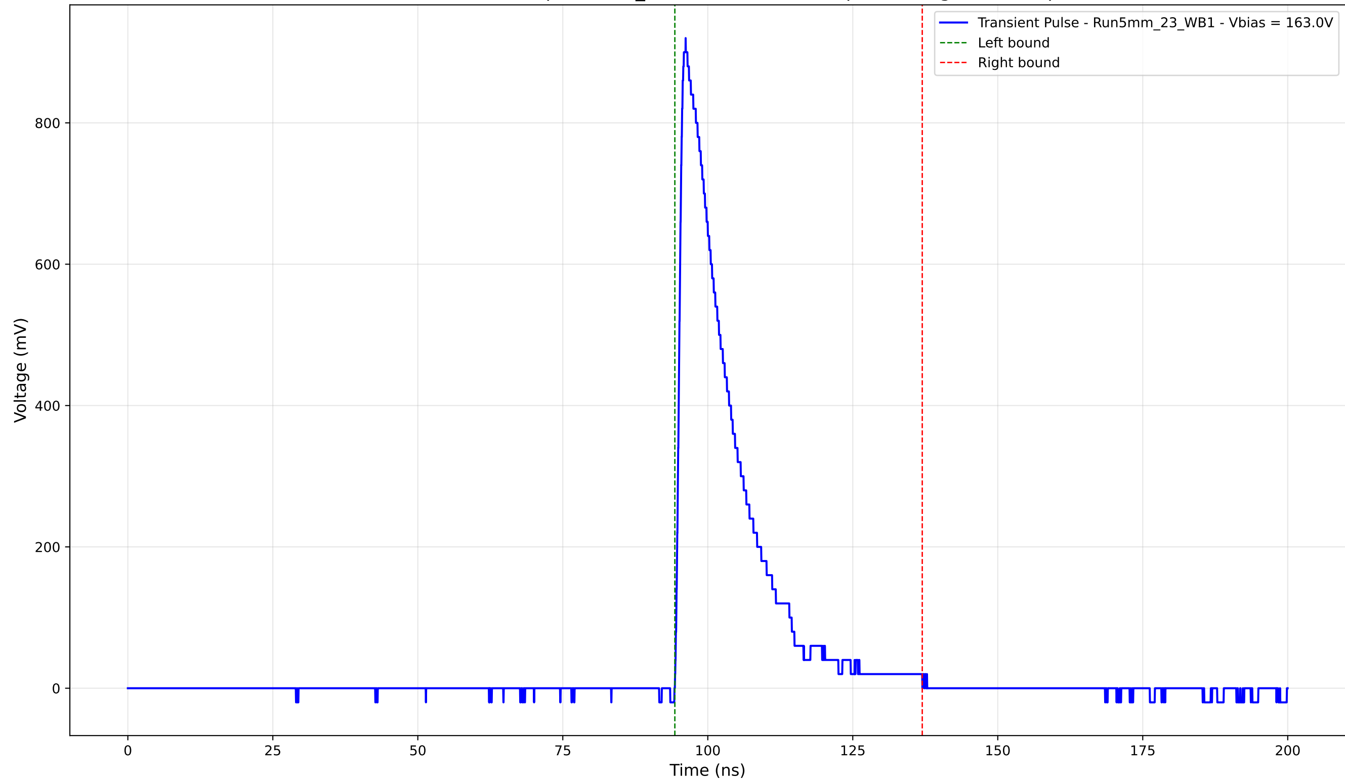
Transient Pulse - Sample: 5mm_23 - Position: 4400.0 \mu\text{m} - Charge: 179.77 pC
