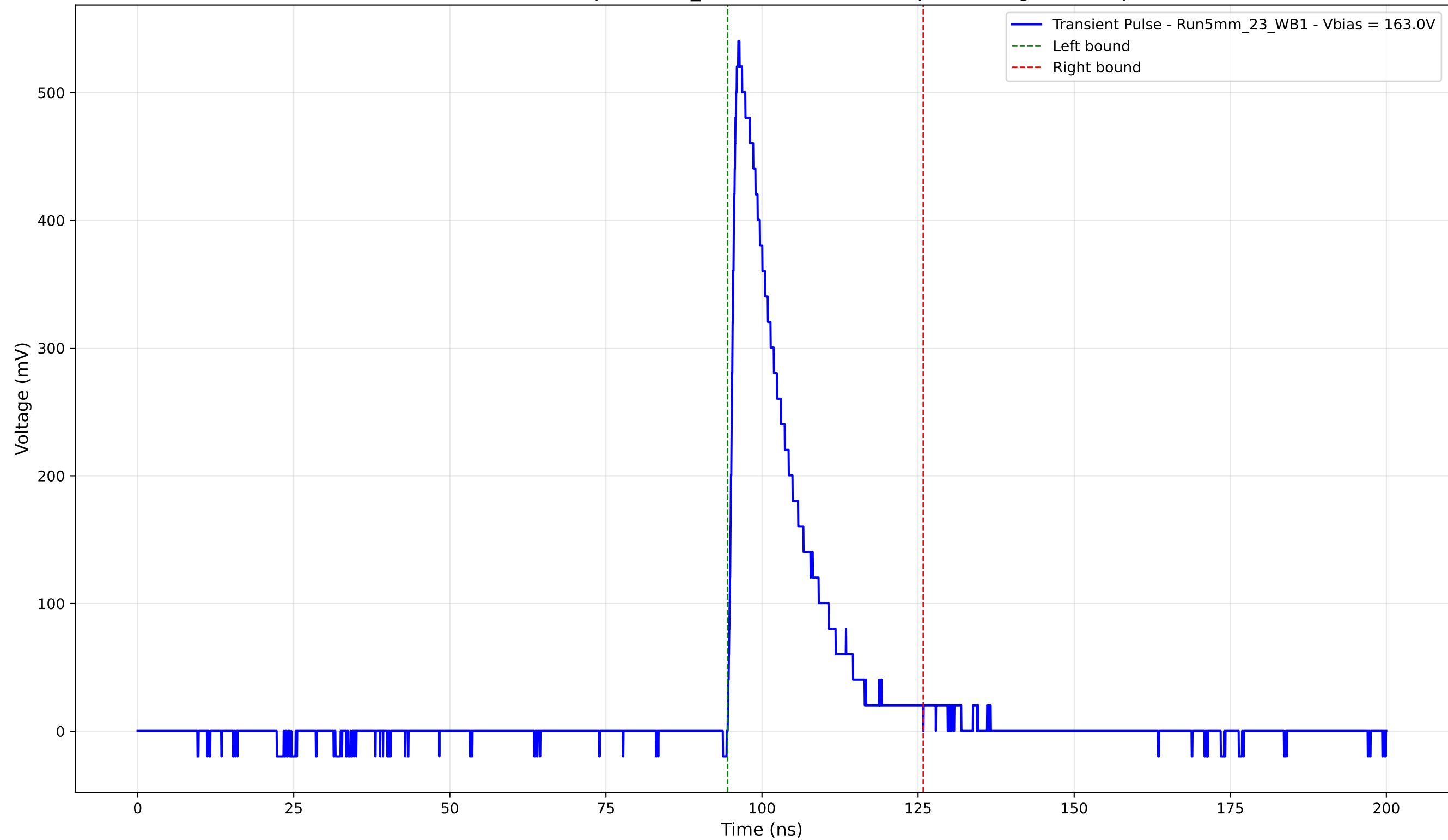
Transient Pulse - Sample: 5mm_23 - Position: 1265.0 \mu\text{m} - Charge: 98.53 pC
