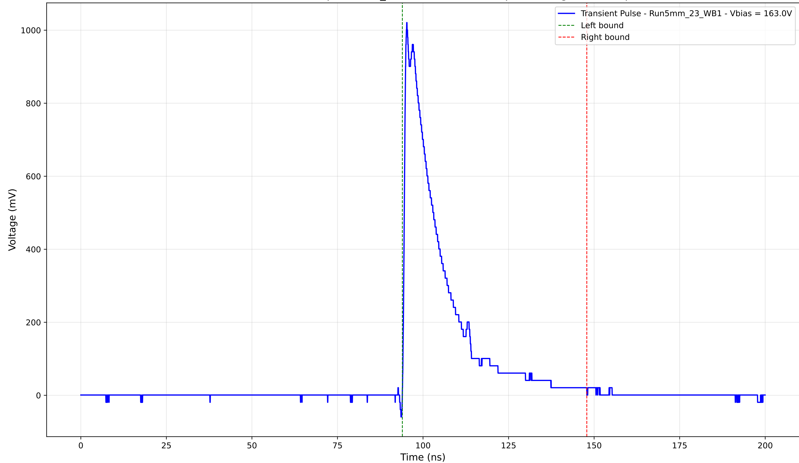
Transient Pulse - Sample: 5mm_23 - Position: 2435.0 \mu\text{m} - Charge: 229.76 pC
