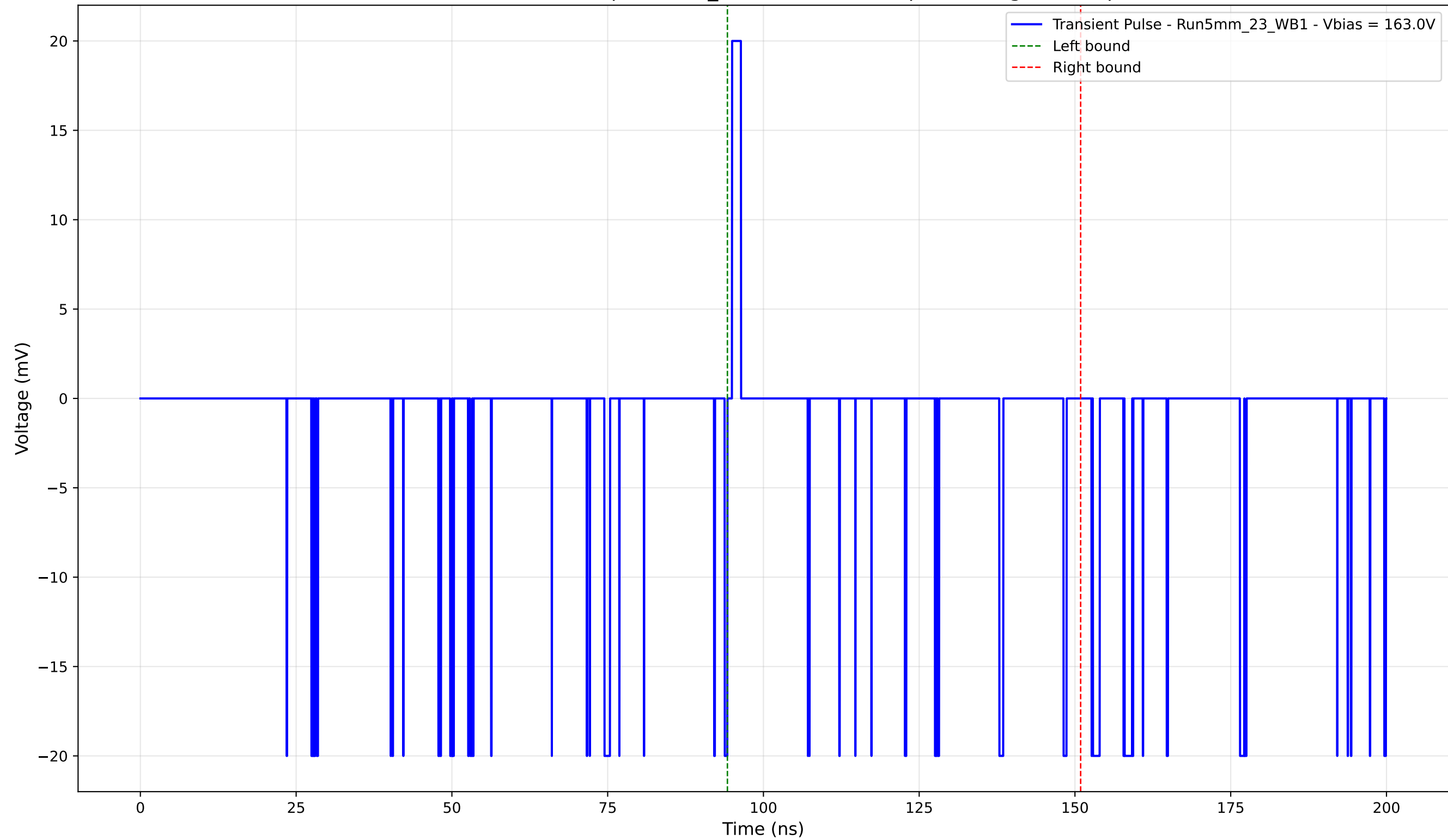
Transient Pulse - Sample: 5mm_23 - Position: 95.0 \mu\text{m} - Charge: -0.23 pC
