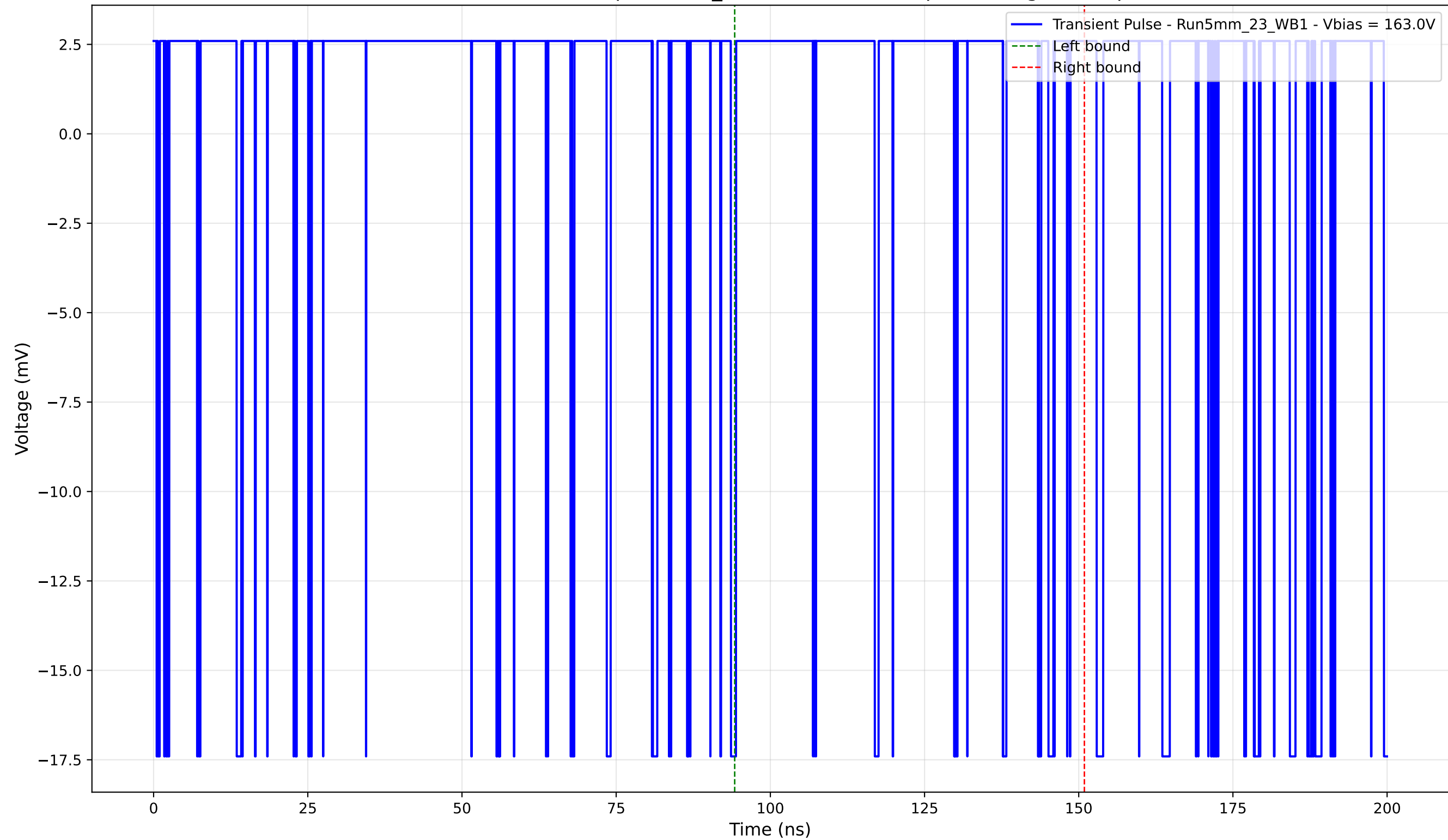
Transient Pulse - Sample: 5mm_23 - Position: 180.0 \mu\text{m} - Charge: 1.46 pC
