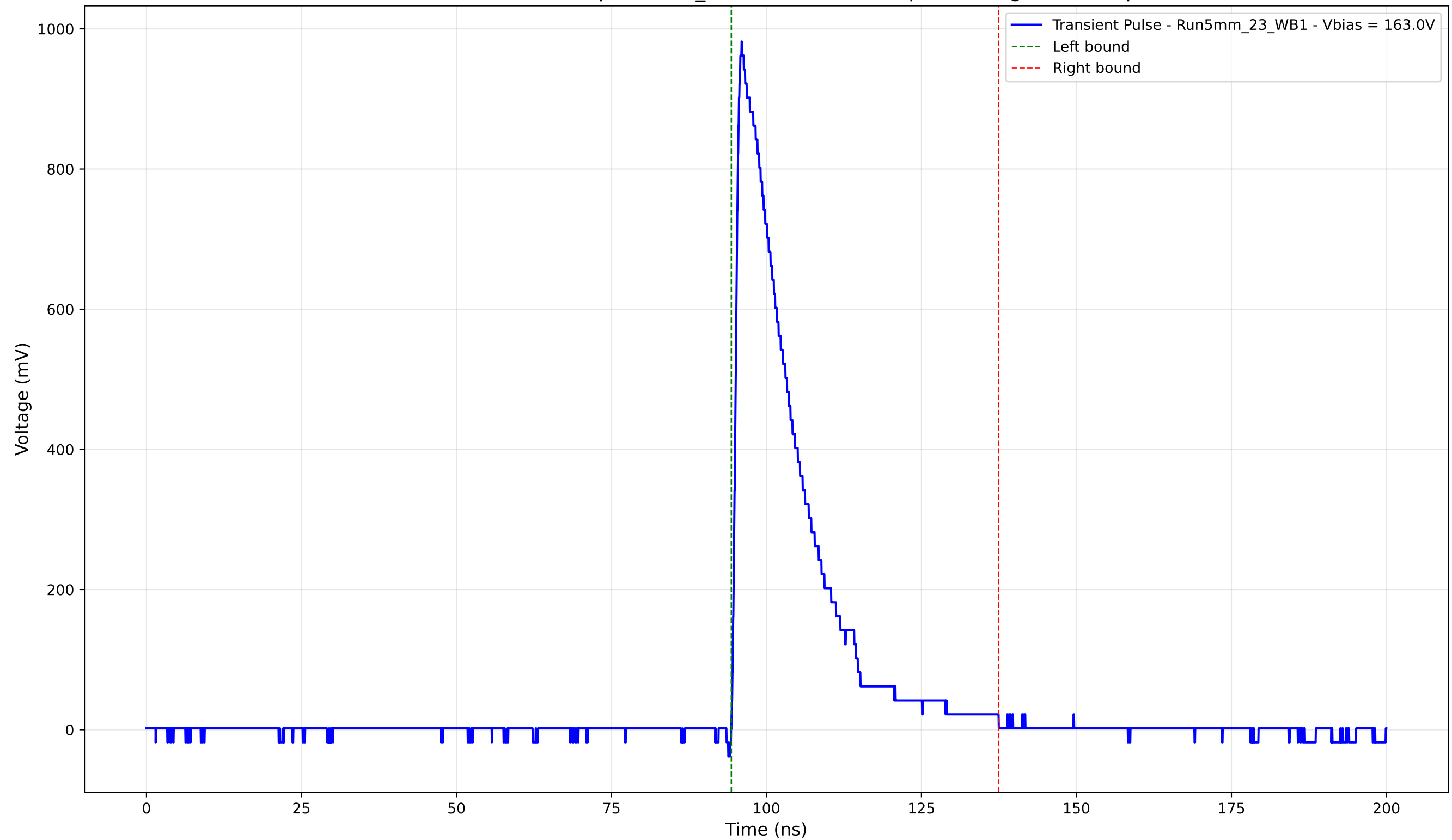
Transient Pulse - Sample: 5mm_23 - Position: 960.0 \mu\text{m} - Charge: 202.72 pC
