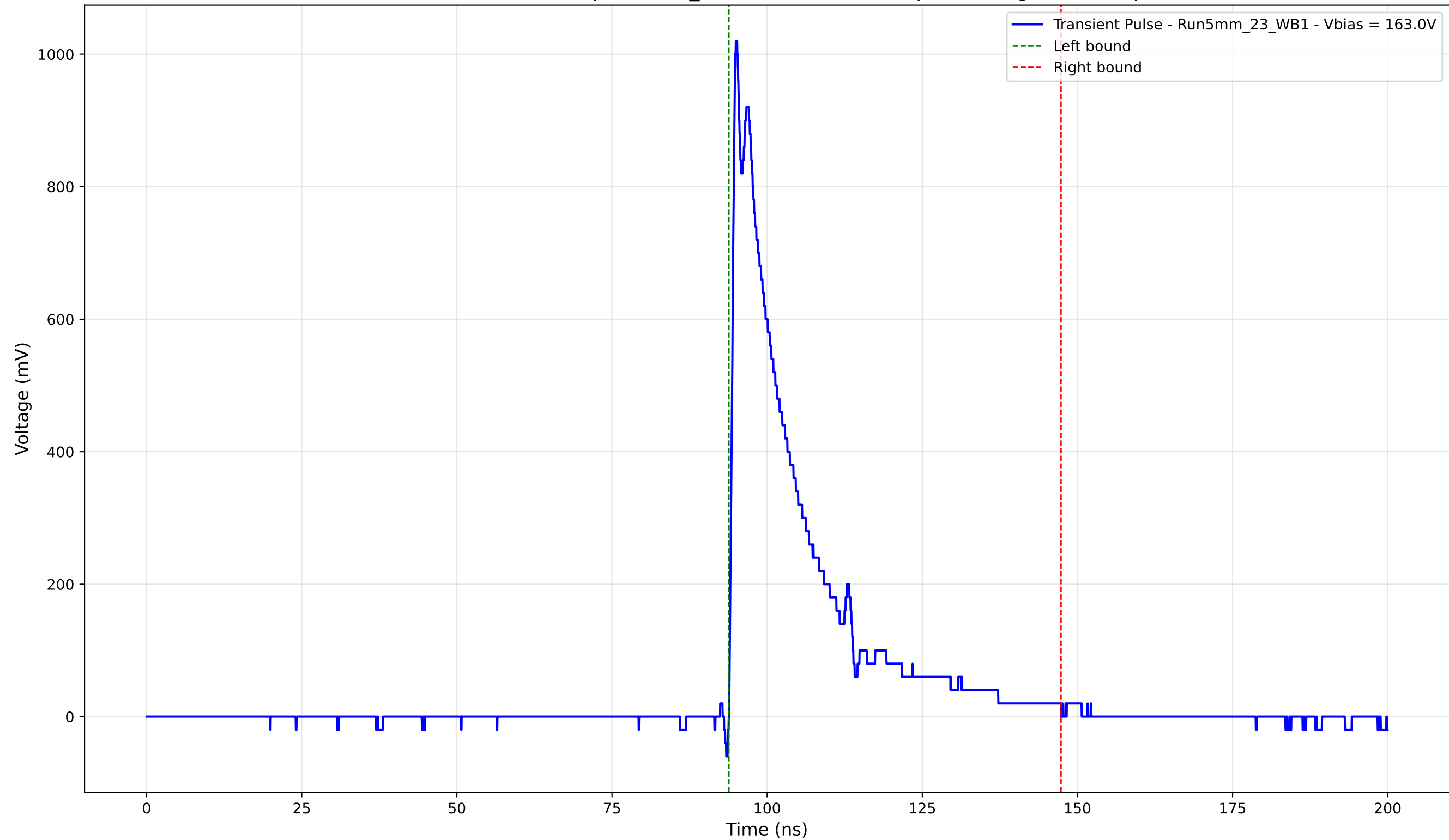
Transient Pulse - Sample: 5mm_23 - Position: 2670.0 \mu\text{m} - Charge: 209.24 pC
