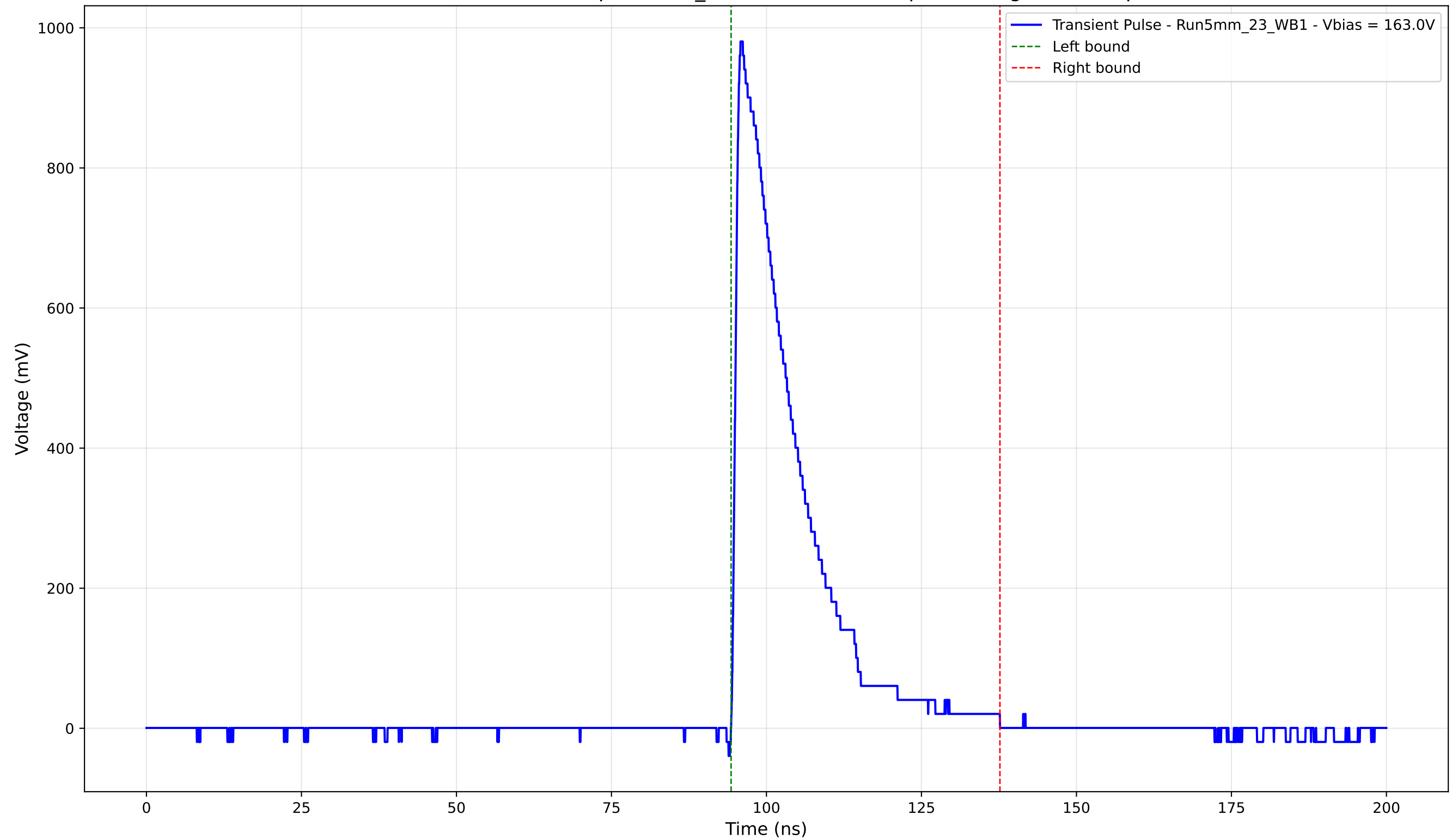
Transient Pulse - Sample: 5mm_23 - Position: 895.0 \mu\text{m} - Charge: 202.92 pC
