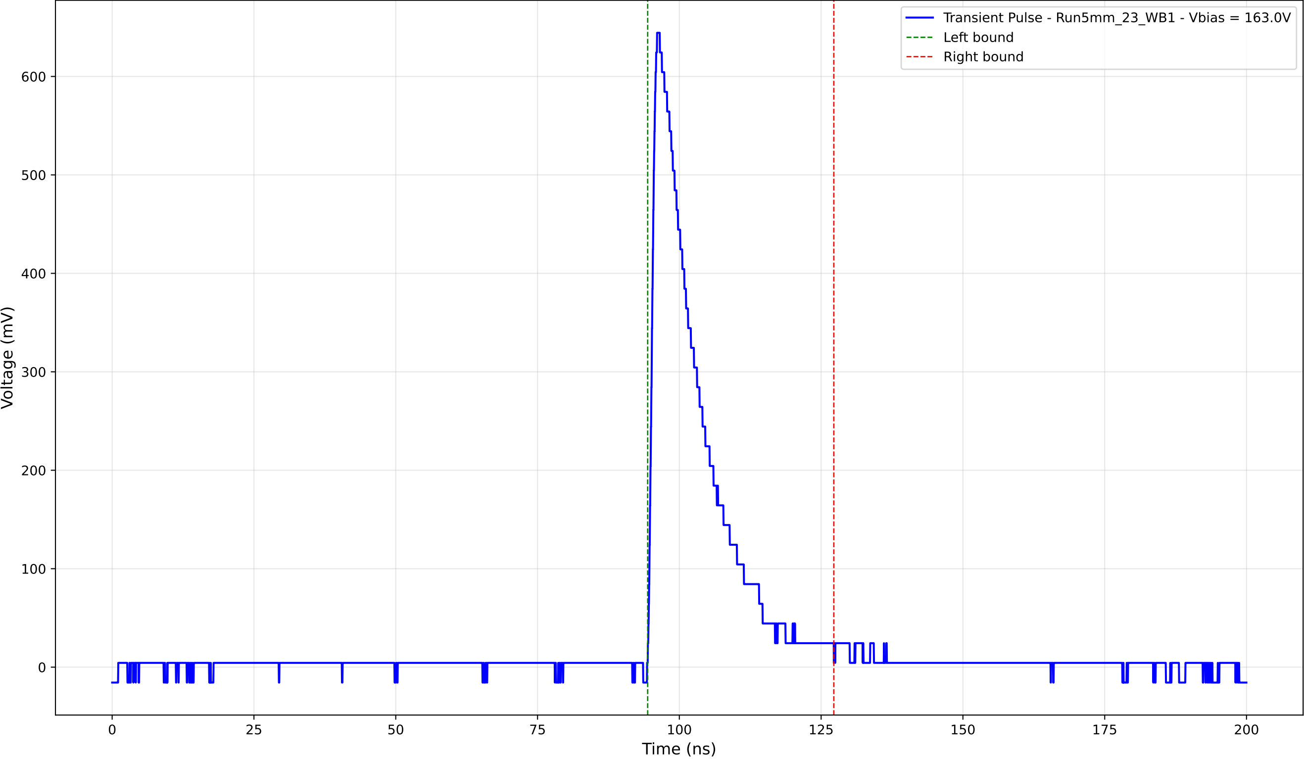
Transient Pulse - Sample: 5mm_23 - Position: 4205.0 \mu\text{m} - Charge: 119.69 pC
