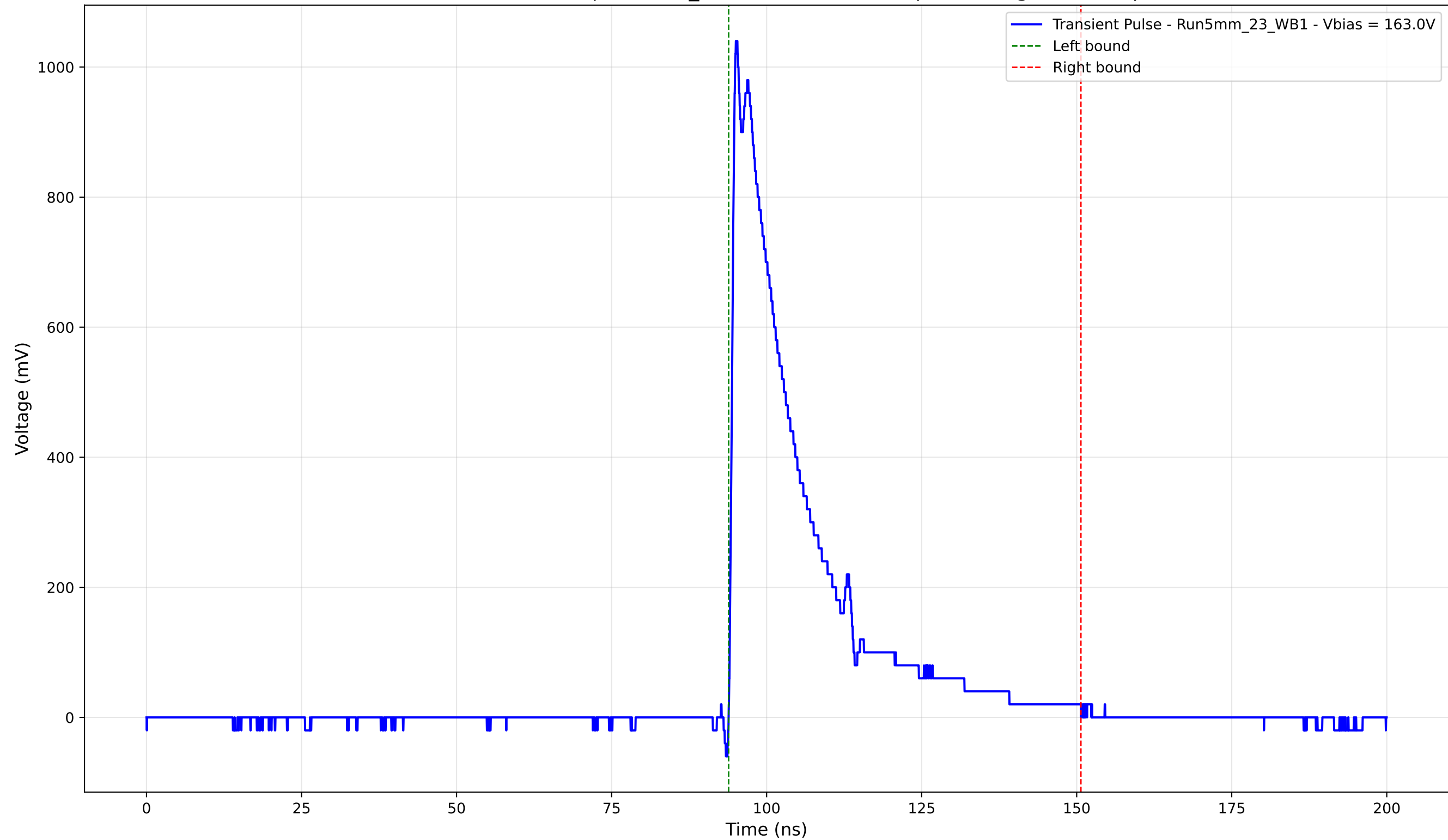
Transient Pulse - Sample: 5mm_23 - Position: 2925.0 \mu\text{m} - Charge: 236.79 pC
