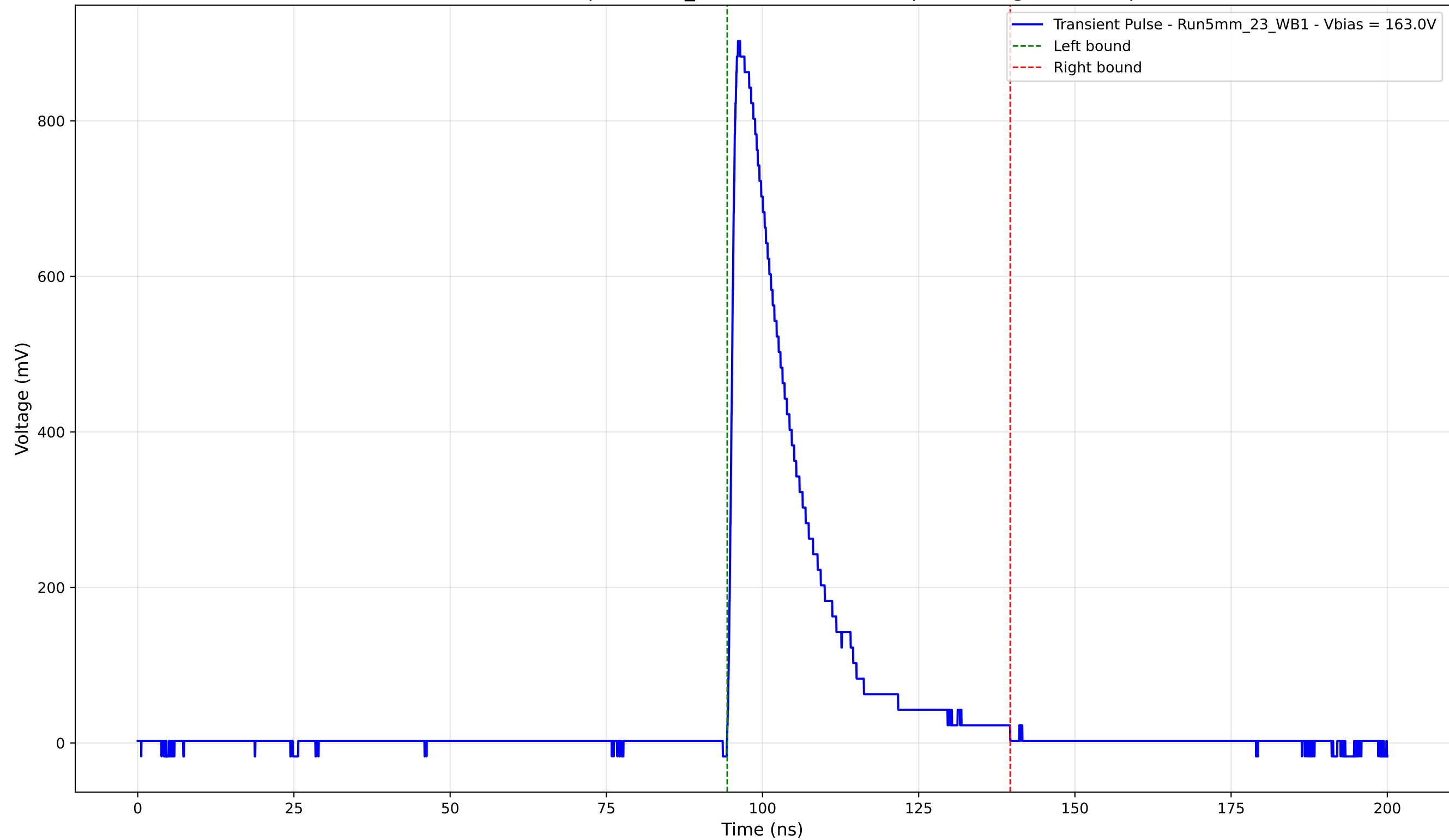
Transient Pulse - Sample: 5mm_23 - Position: 3880.0 \mu\text{m} - Charge: 197.39 pC
