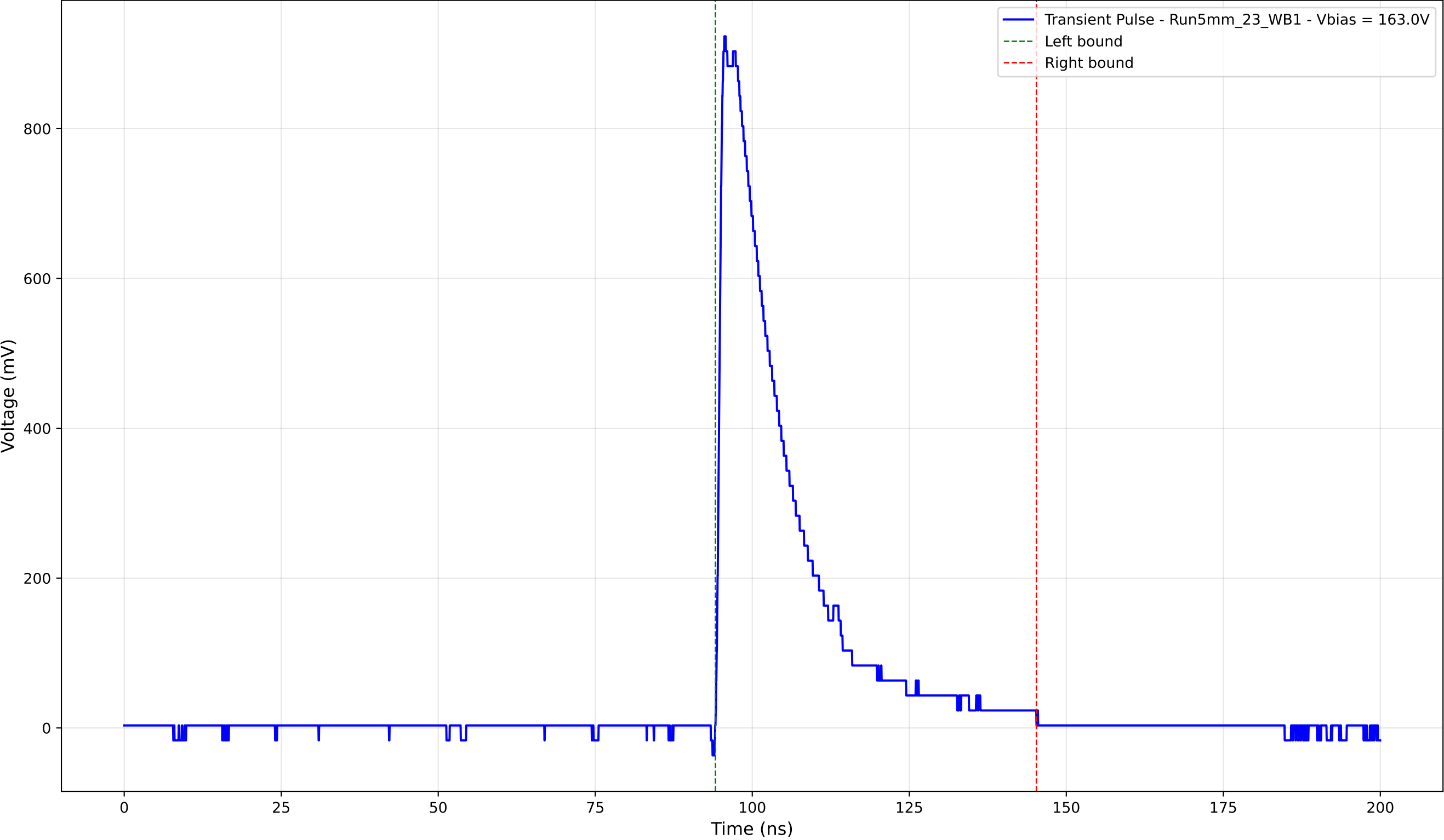
Transient Pulse - Sample: 5mm_23 - Position: 3375.0 \mu\text{m} - Charge: 211.85 pC
