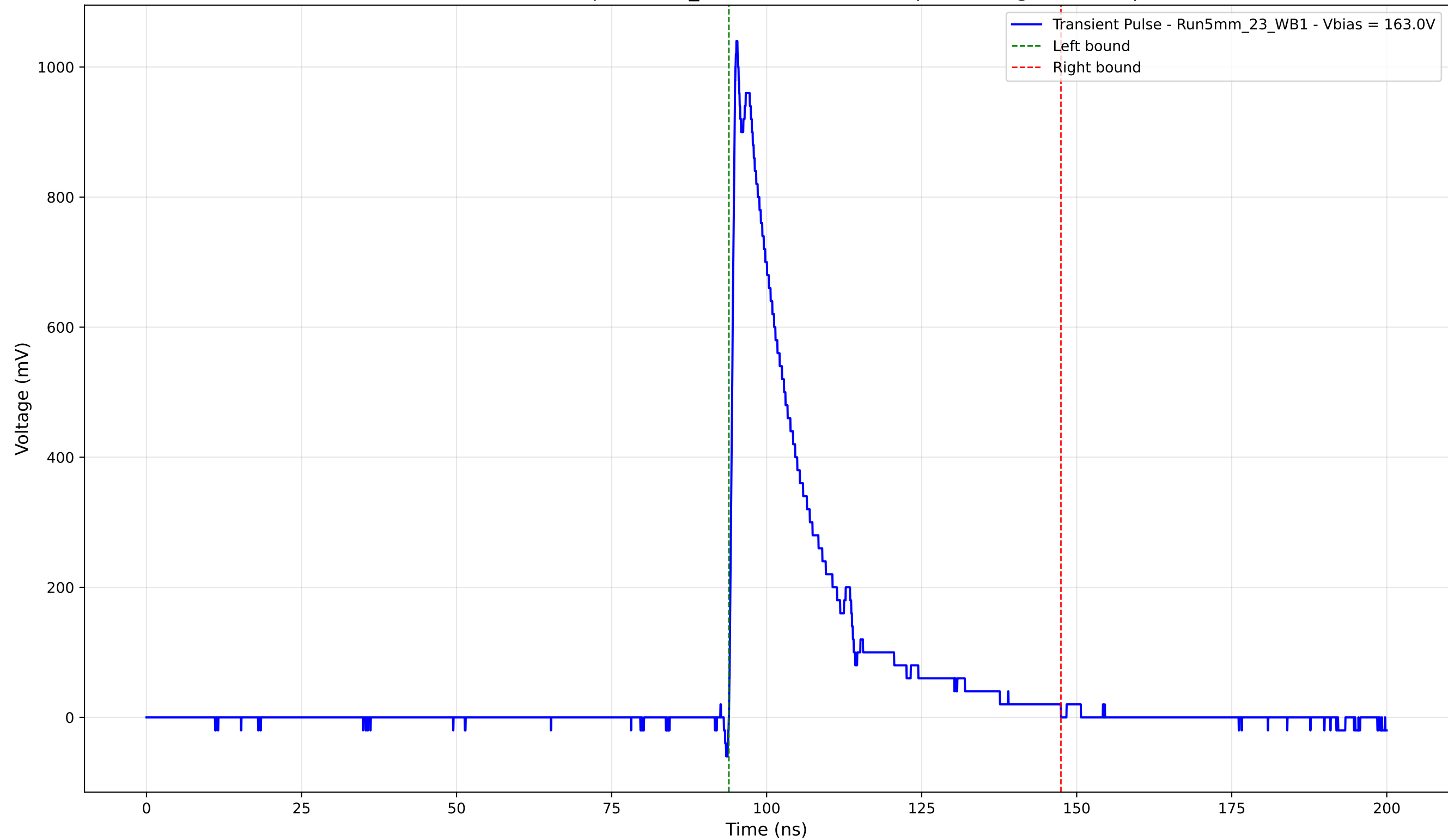
Transient Pulse - Sample: 5mm_23 - Position: 2955.0 \mu\text{m} - Charge: 232.84 pC
