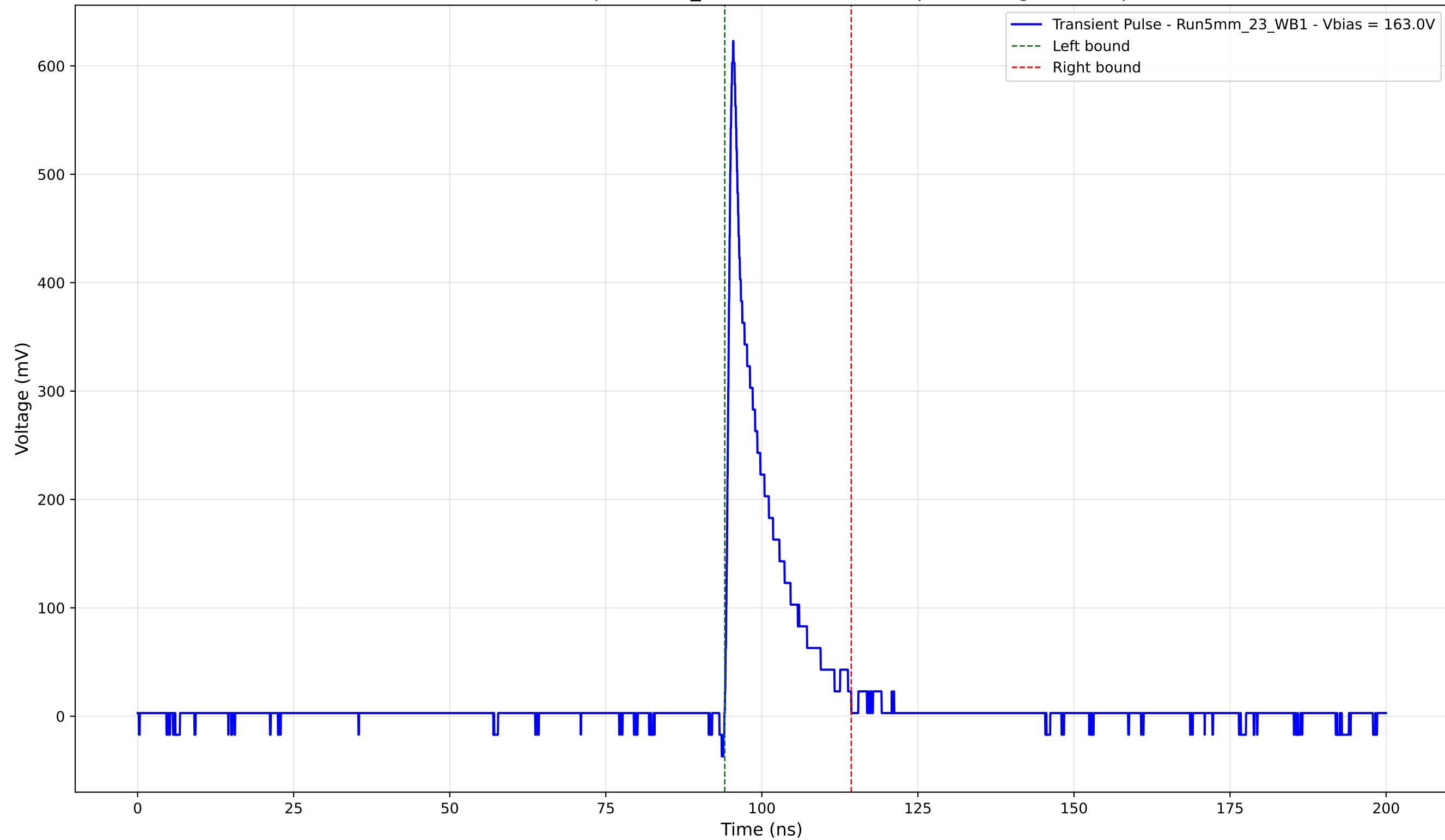
Transient Pulse - Sample: 5mm_23 - Position: 5165.0 \mu\text{m} - Charge: 68.56 pC
