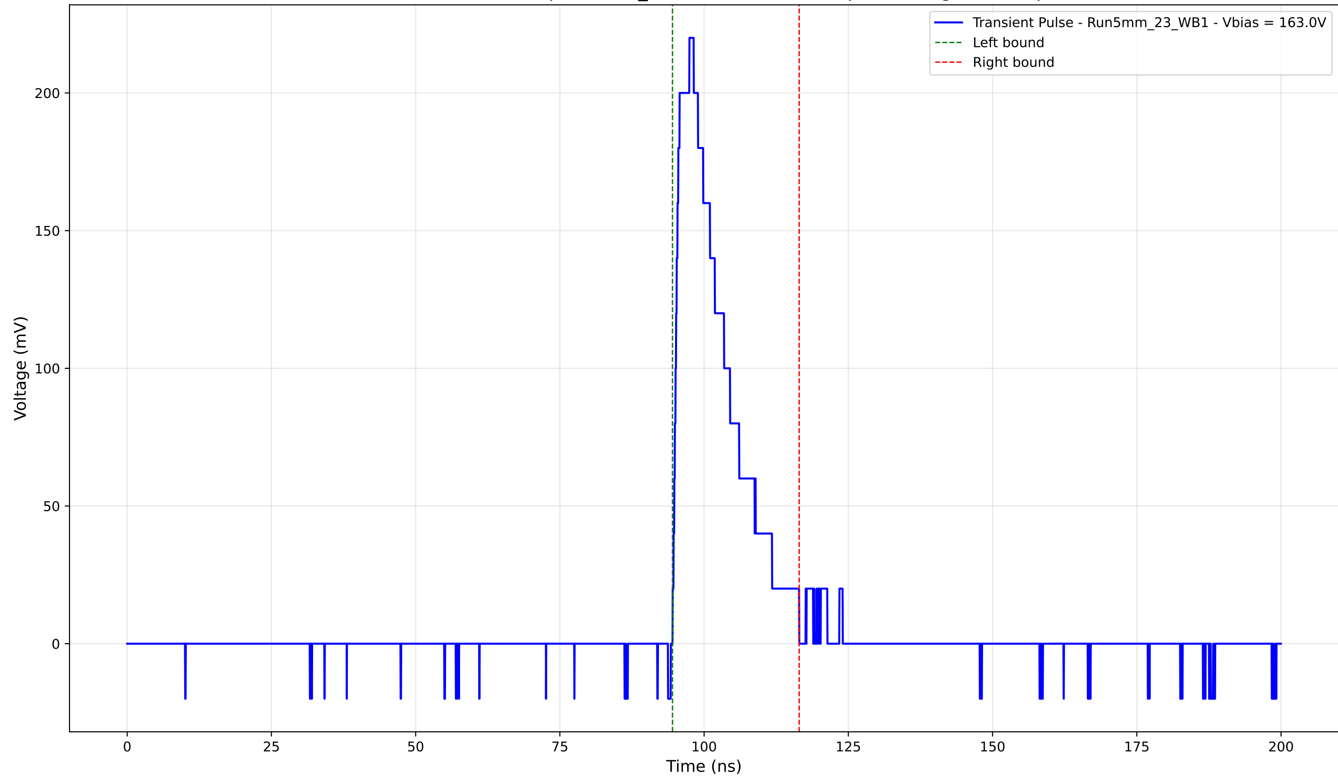
Transient Pulse - Sample: 5mm_23 - Position: 1725.0 \mu\text{m} - Charge: 41.02 pC
