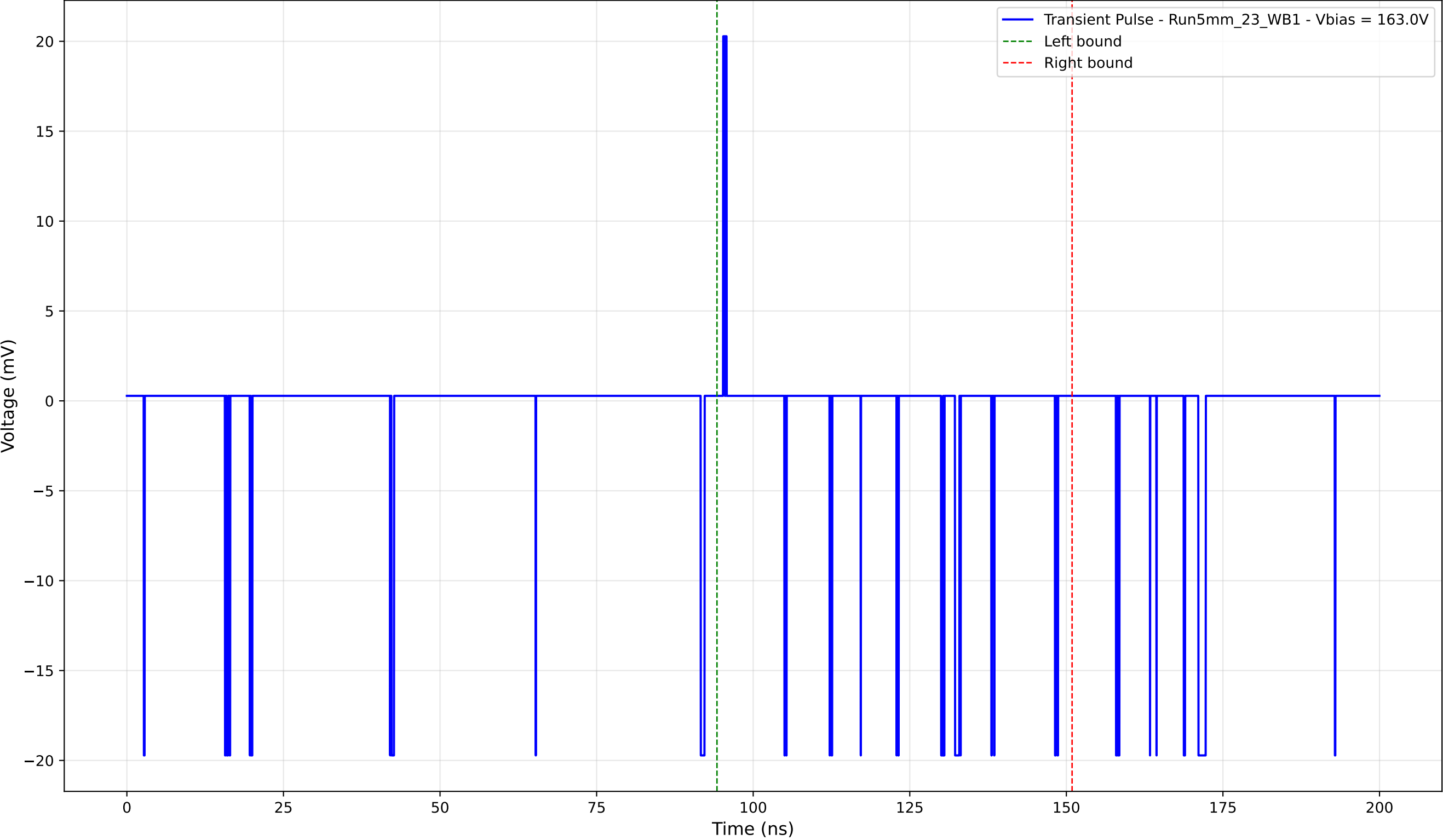
Transient Pulse - Sample: 5mm_23 - Position: 175.0 \mu\text{m} - Charge: -0.35 pC
