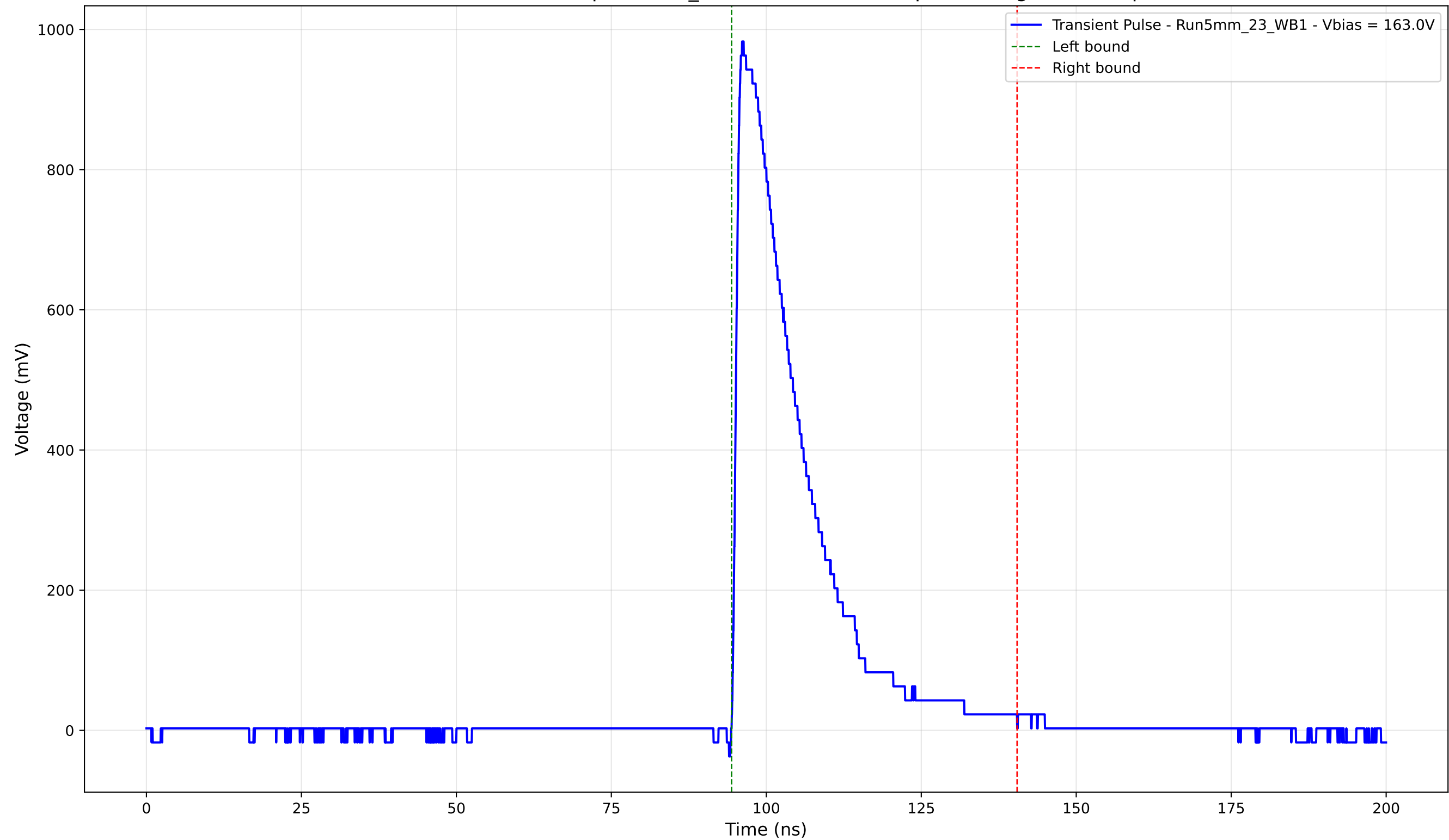
Transient Pulse - Sample: 5mm_23 - Position: 1375.0 \mu\text{m} - Charge: 226.26 pC
