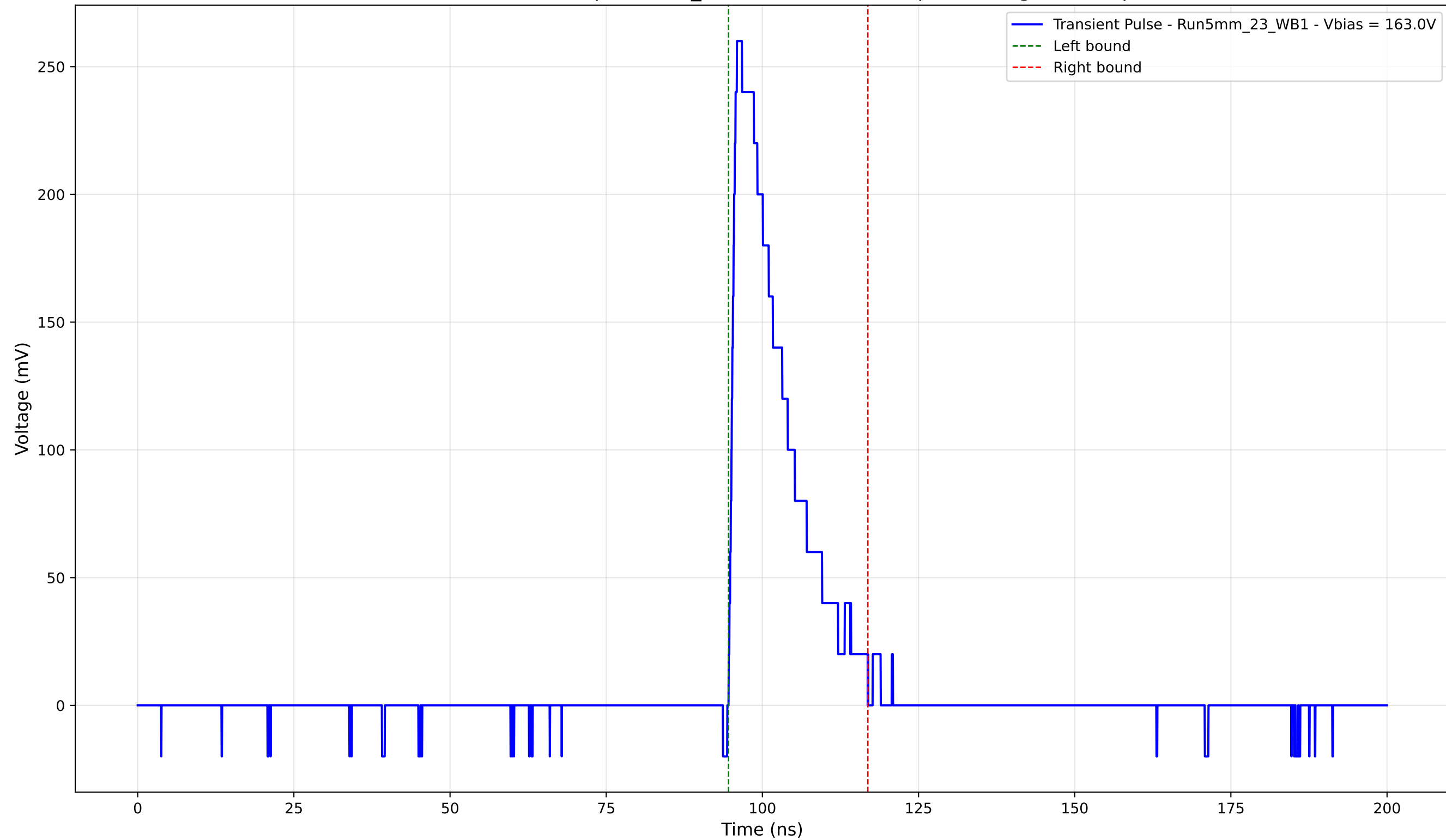
Transient Pulse - Sample: 5mm_23 - Position: 1210.0 \mu\text{m} - Charge: 47.51 pC
