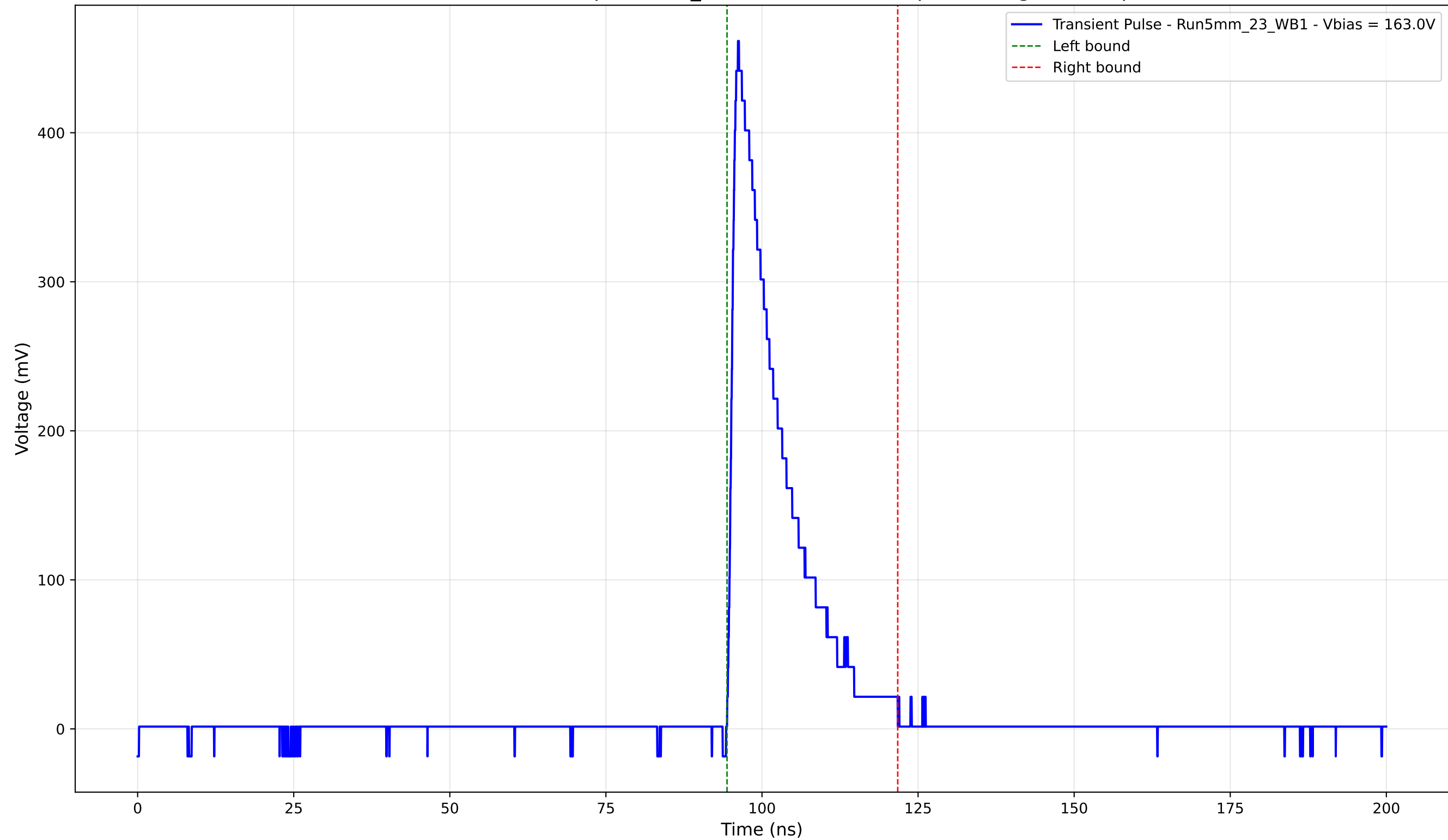
Transient Pulse - Sample: 5mm_23 - Position: 4300.0 \mu\text{m} - Charge: 78.78 pC
