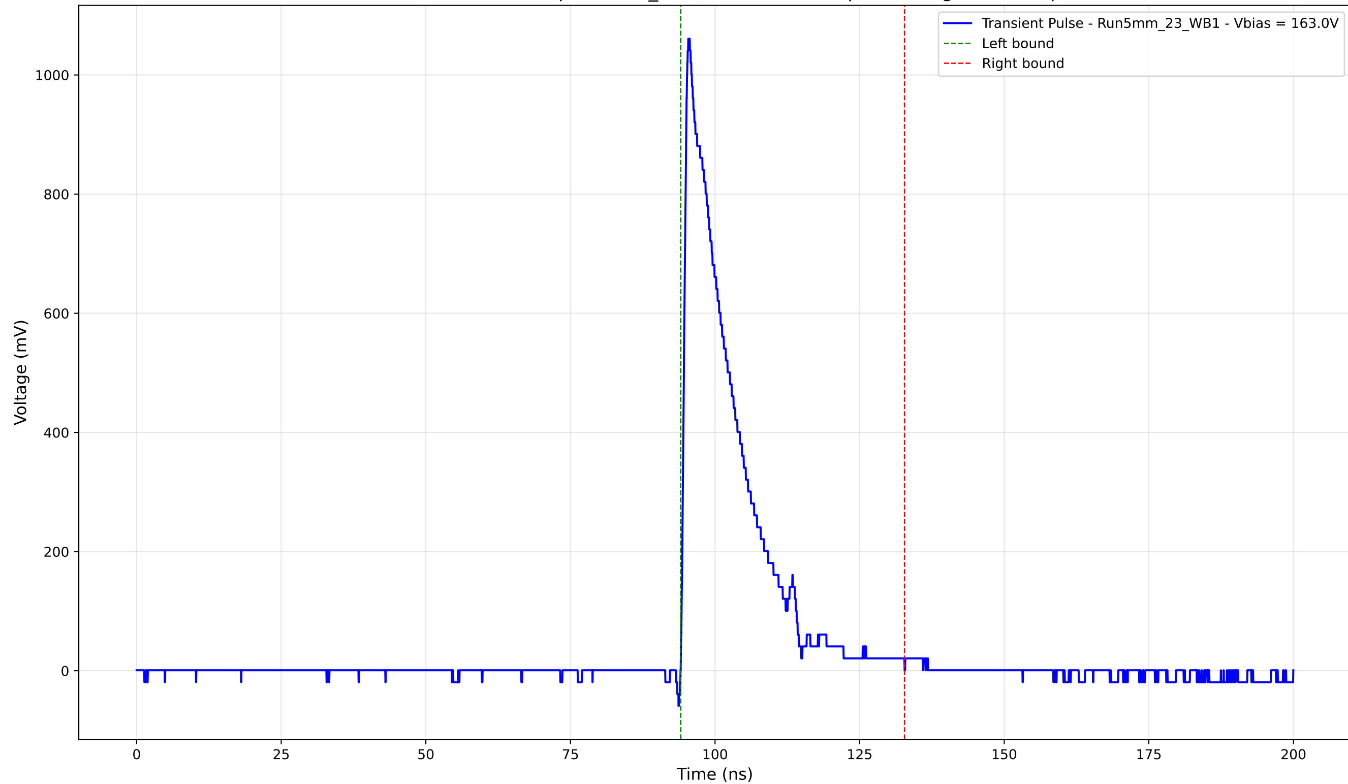
Transient Pulse - Sample: 5mm_23 - Position: 375.0 \mu\text{m} - Charge: 191.91 pC
