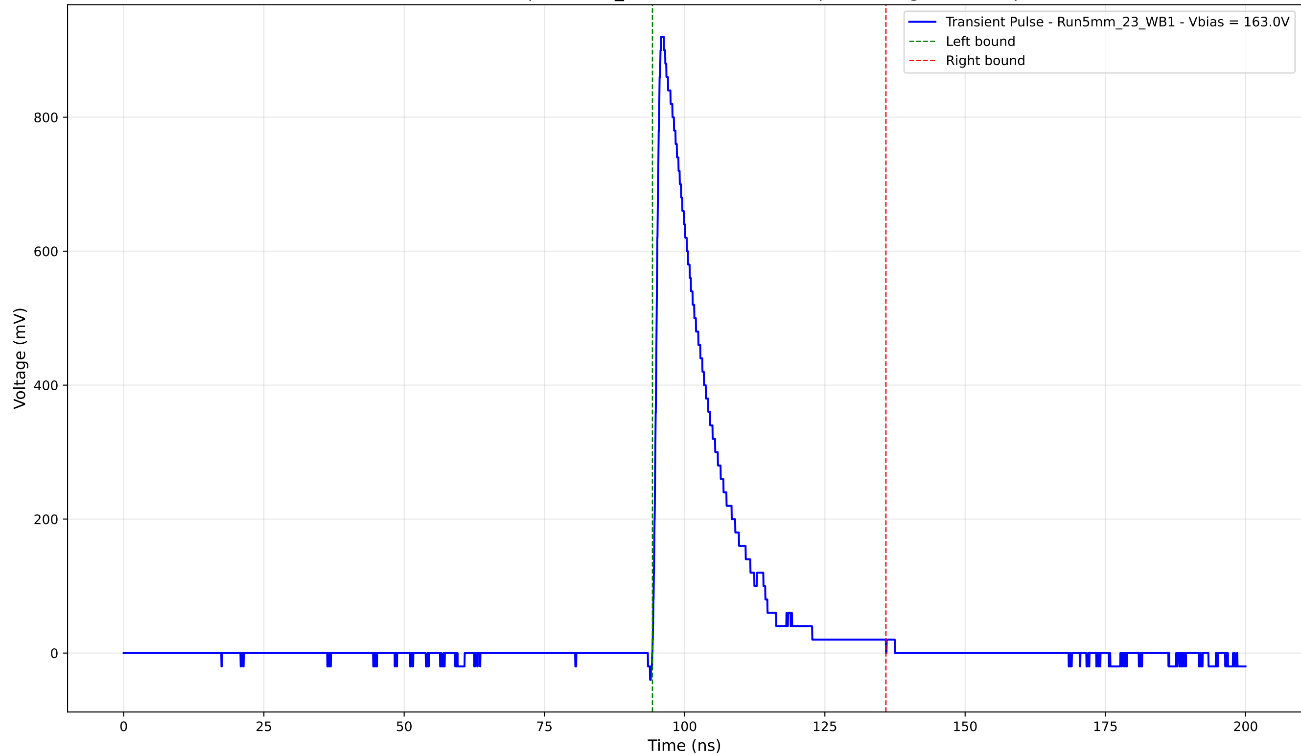
Transient Pulse - Sample: 5mm_23 - Position: 4555.0 \mu\text{m} - Charge: 176.91 pC
