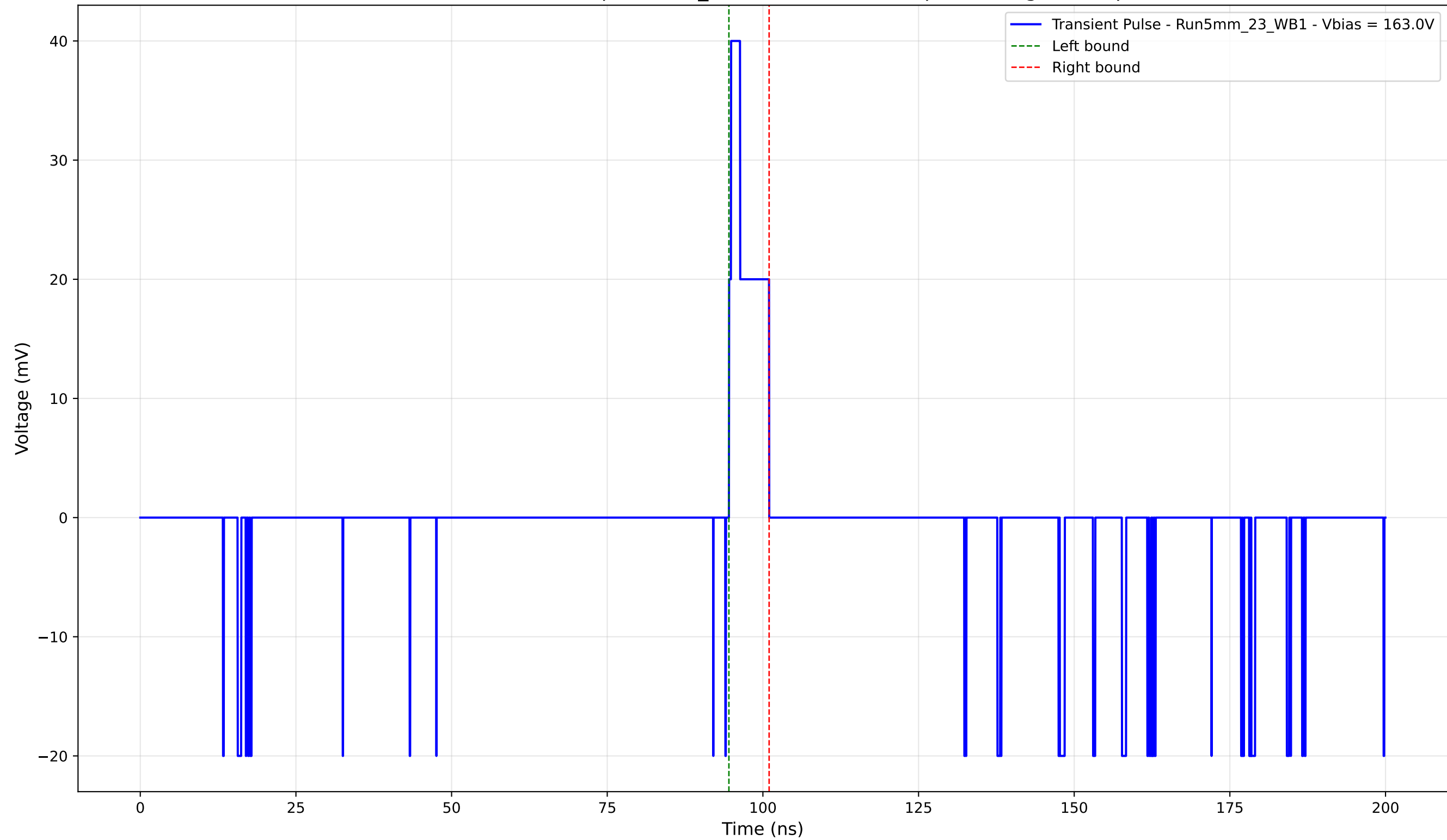
Transient Pulse - Sample: 5mm_23 - Position: 5235.0 \mu\text{m} - Charge: 3.16 pC
