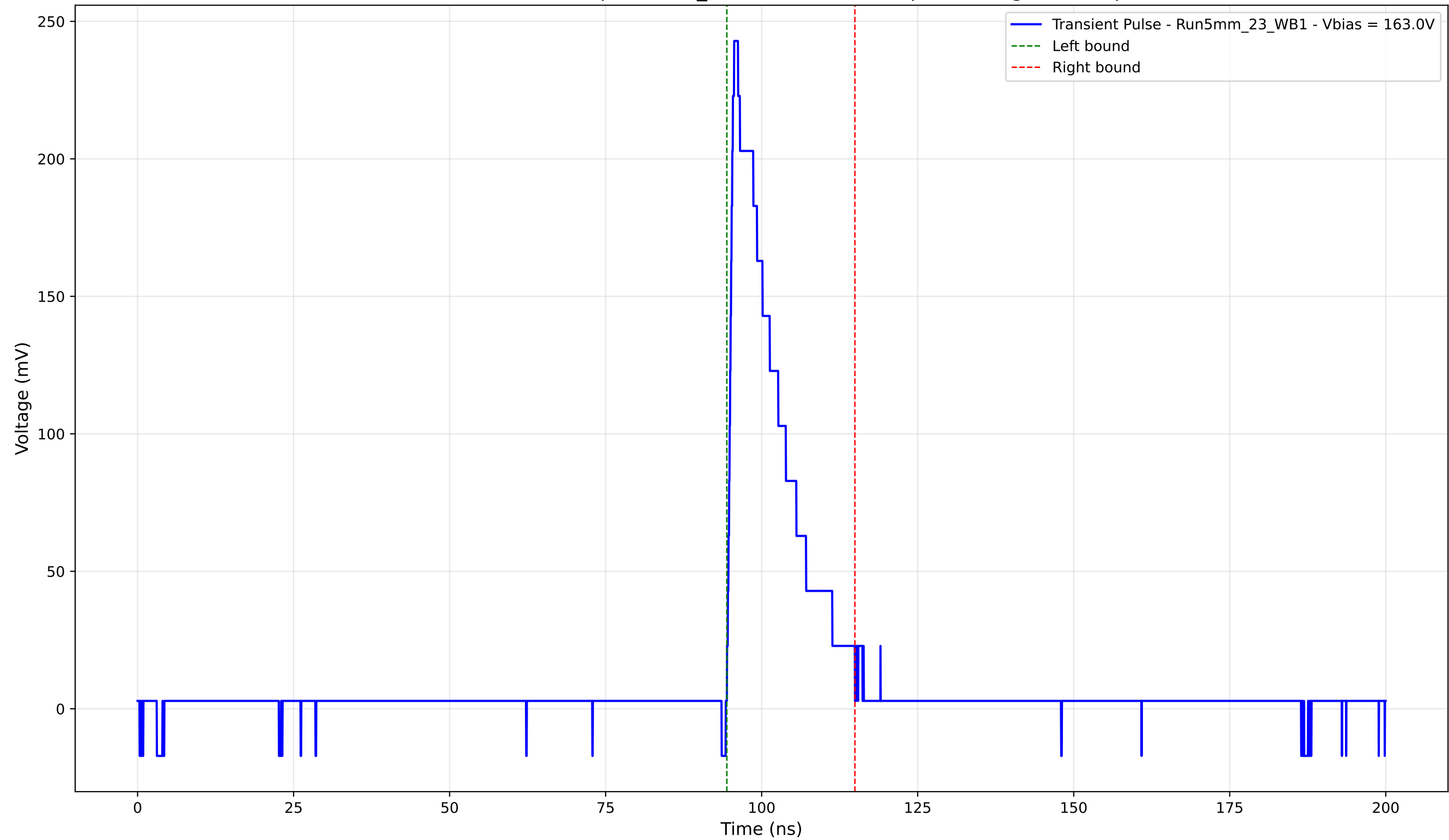
Transient Pulse - Sample: 5mm_23 - Position: 715.0 \mu\text{m} - Charge: 40.28 pC
