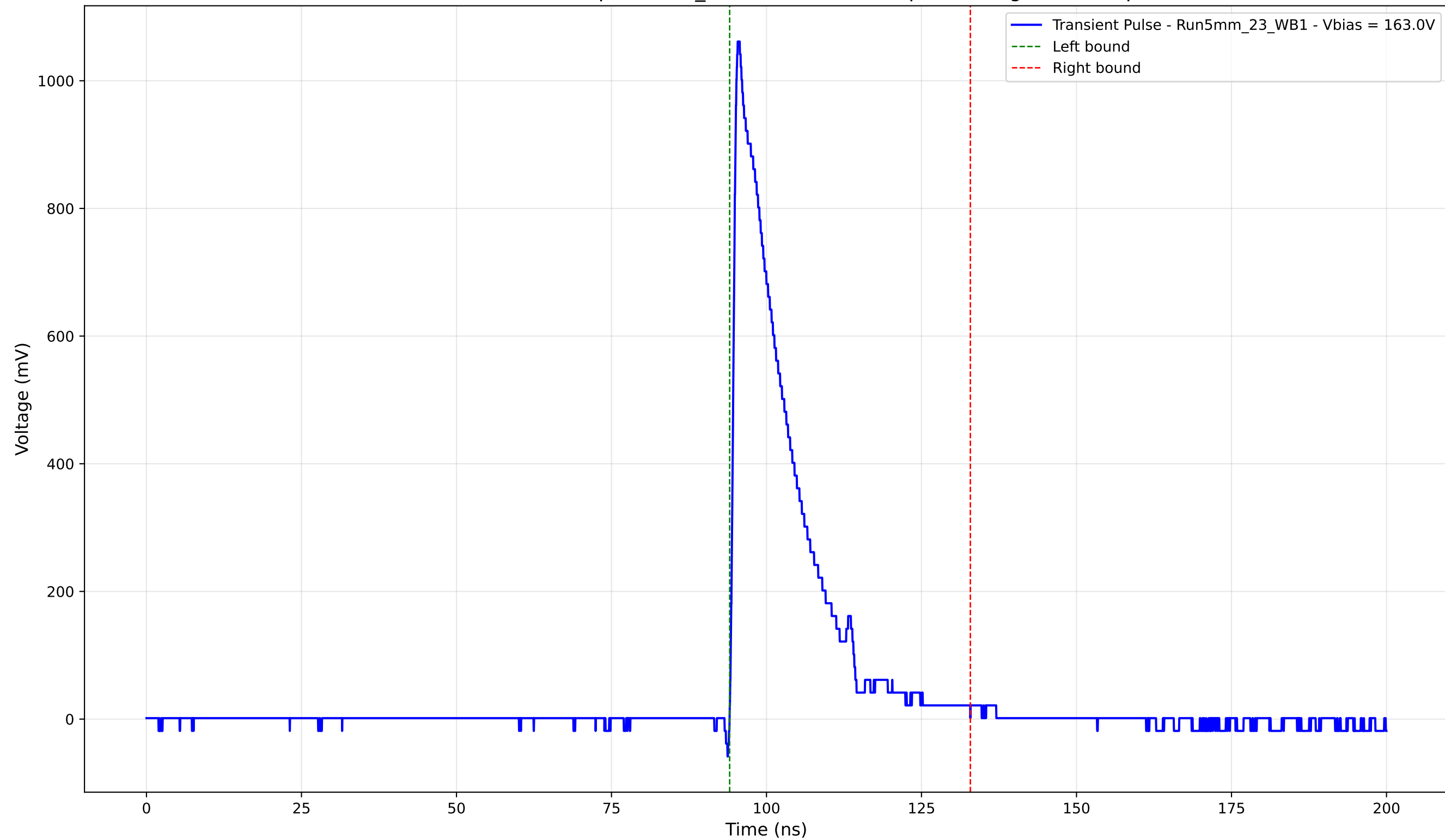
Transient Pulse - Sample: 5mm_23 - Position: 400.0 \mu\text{m} - Charge: 199.49 pC
