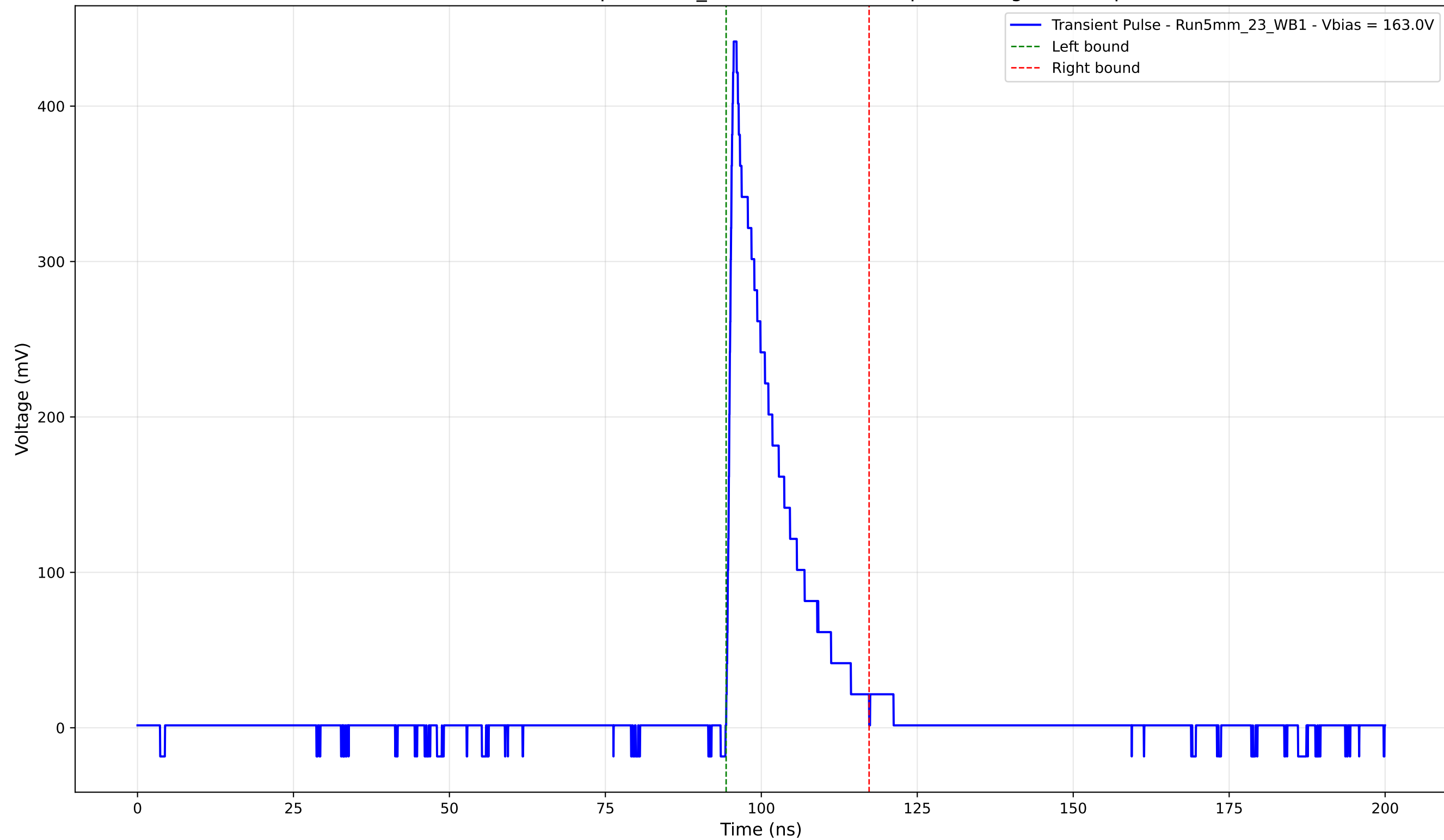
Transient Pulse - Sample: 5mm_23 - Position: 695.0 \mu\text{m} - Charge: 67.36 pC
