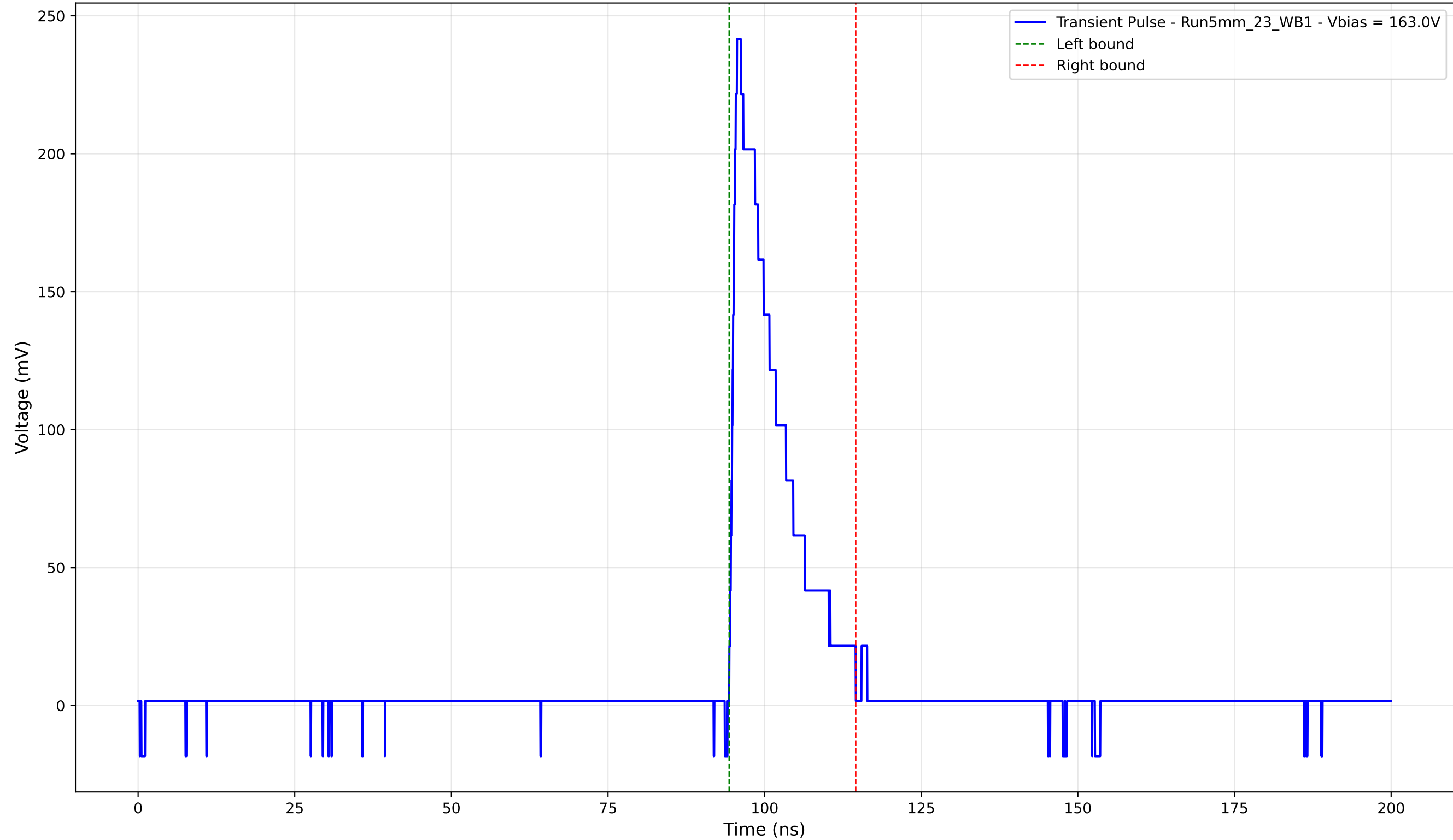
Transient Pulse - Sample: 5mm_23 - Position: 4755.0 \mu\text{m} - Charge: 37.77 pC
