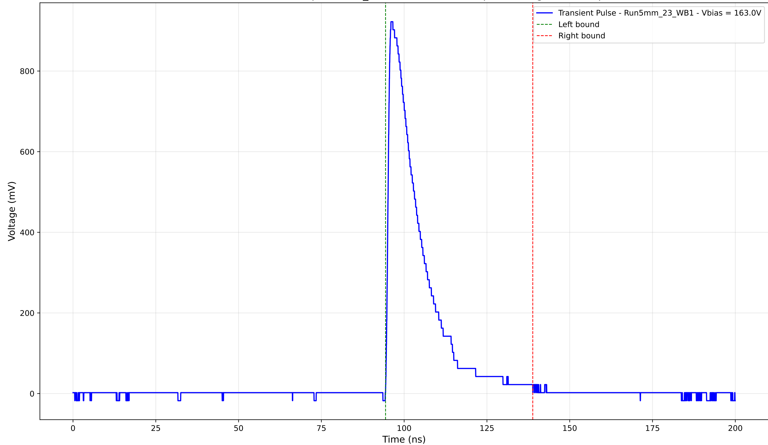
Transient Pulse - Sample: 5mm_23 - Position: 4065.0 \mu\text{m} - Charge: 200.23 pC
