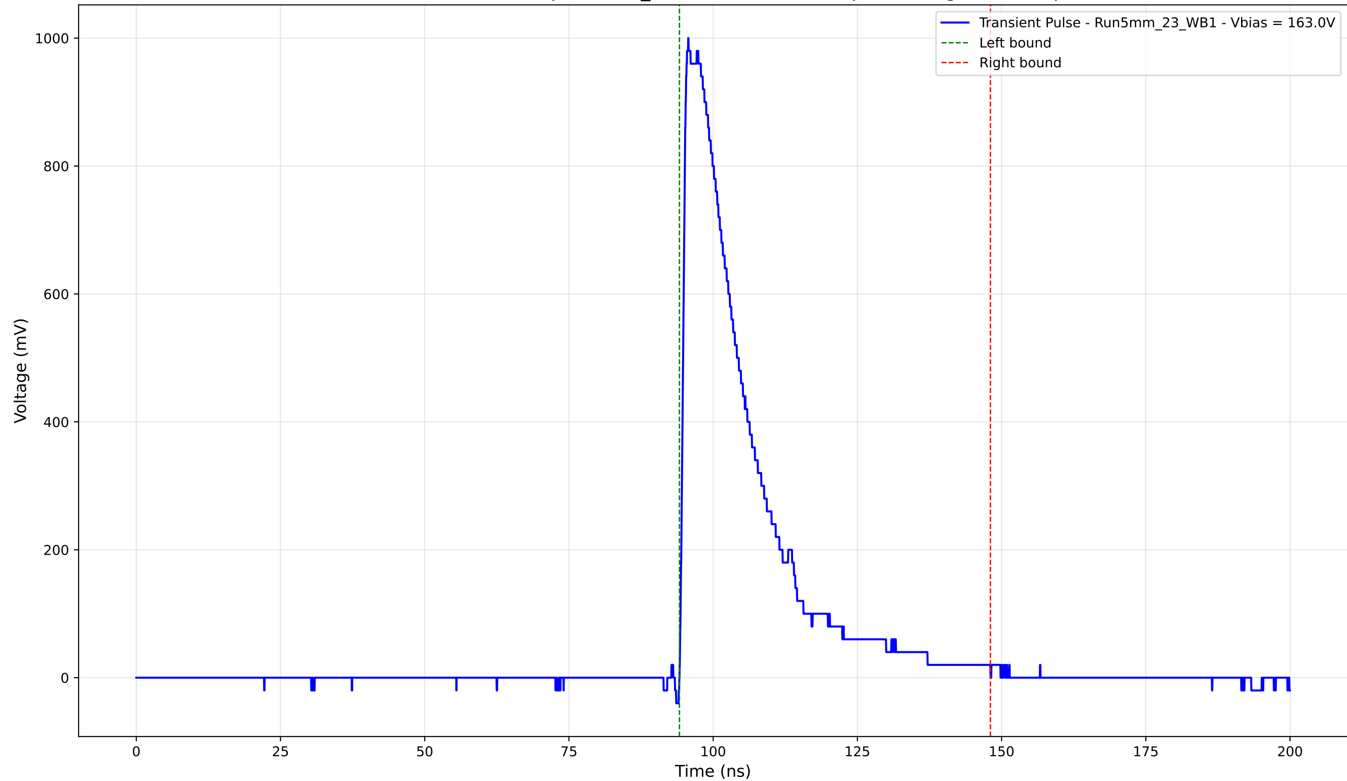
Transient Pulse - Sample: 5mm_23 - Position: 2065.0 \mu\text{m} - Charge: 246.52 pC
