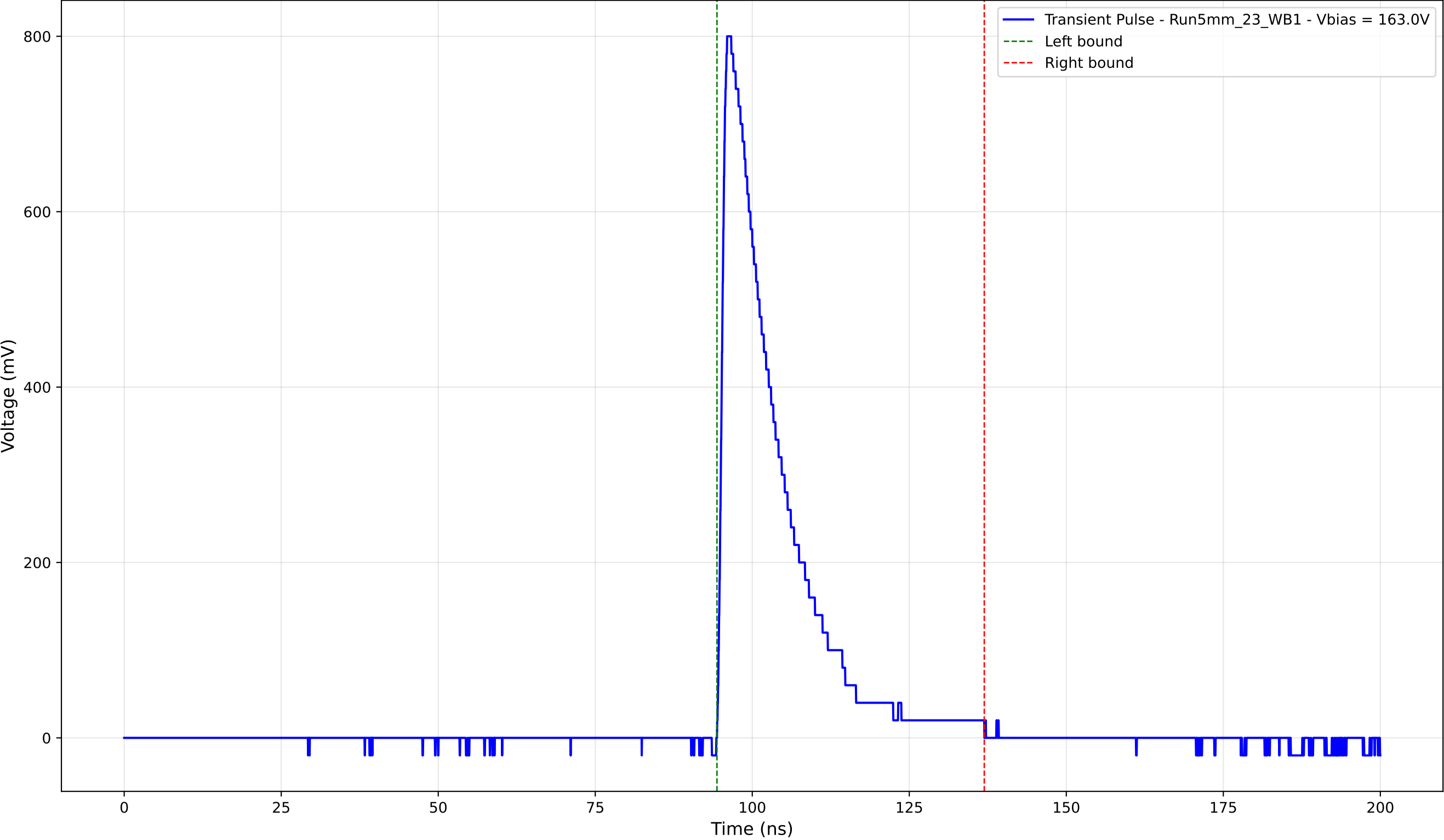
Transient Pulse - Sample: 5mm_23 - Position: 4185.0 \mu\text{m} - Charge: 156.95 pC
