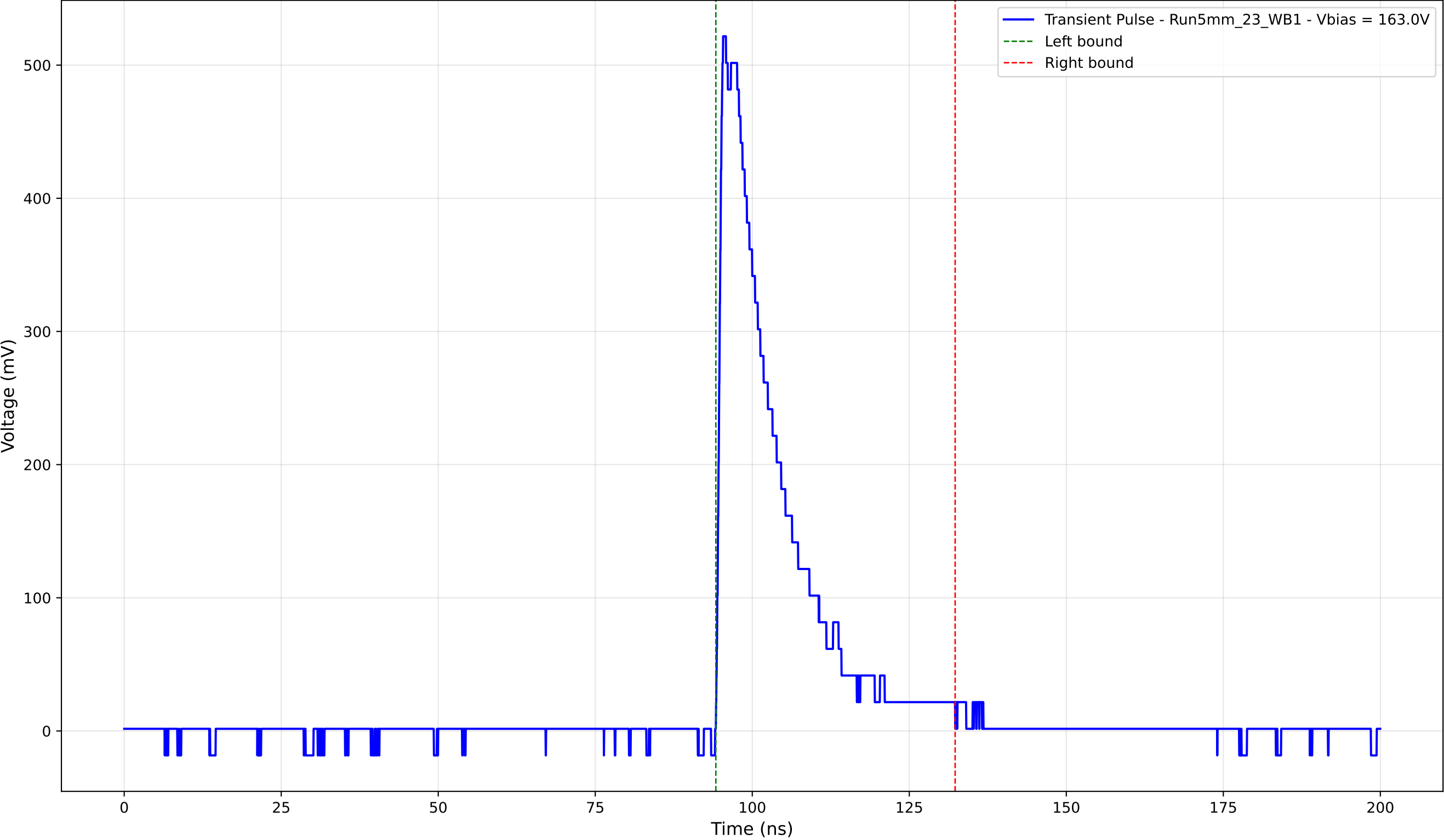
Transient Pulse - Sample: 5mm_23 - Position: 3290.0 \mu\text{m} - Charge: 104.18 pC
