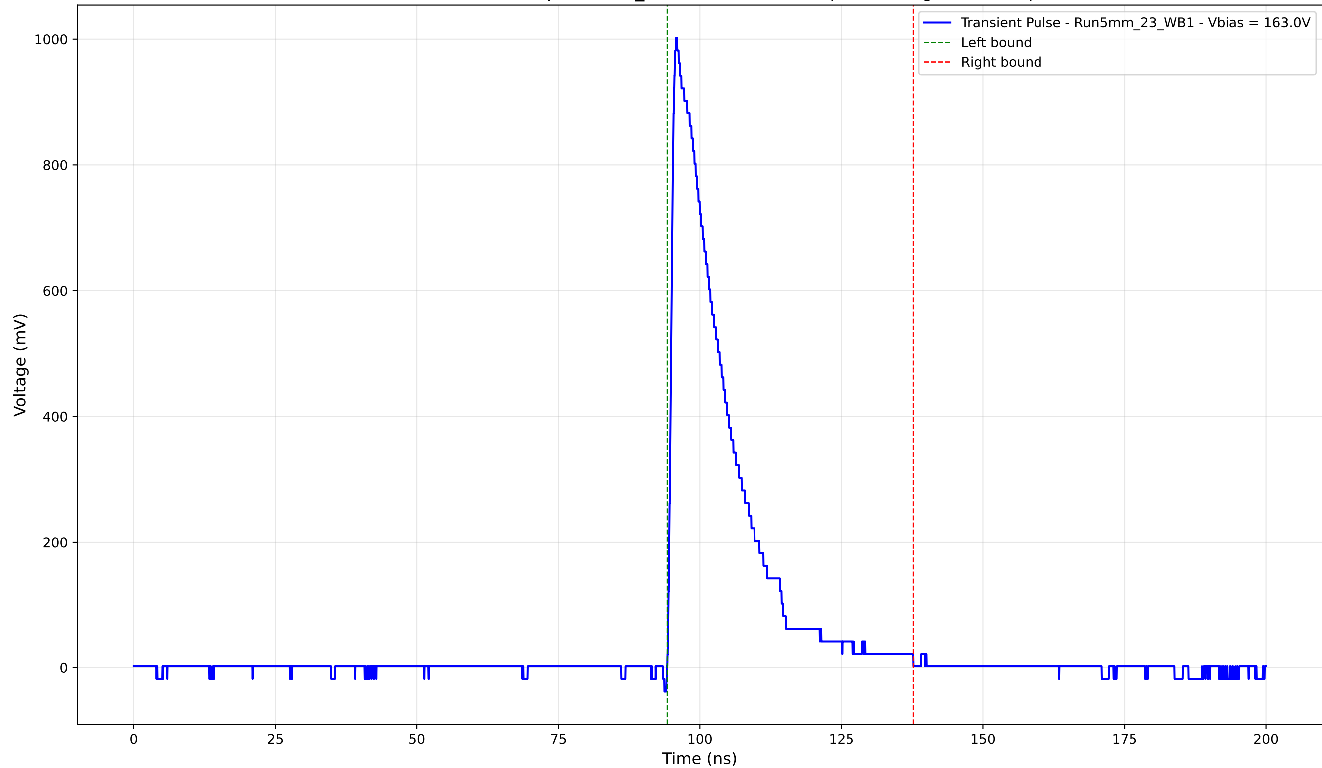
Transient Pulse - Sample: 5mm_23 - Position: 845.0 \mu\text{m} - Charge: 207.83 pC
