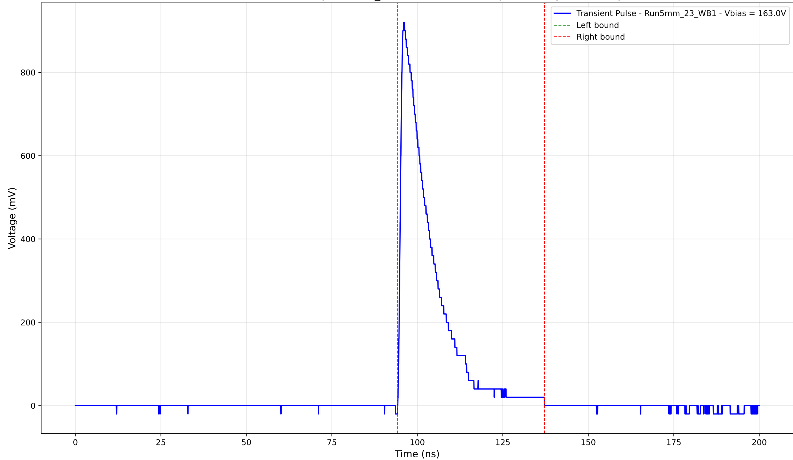
Transient Pulse - Sample: 5mm_23 - Position: 4475.0 \mu\text{m} - Charge: 179.26 pC
