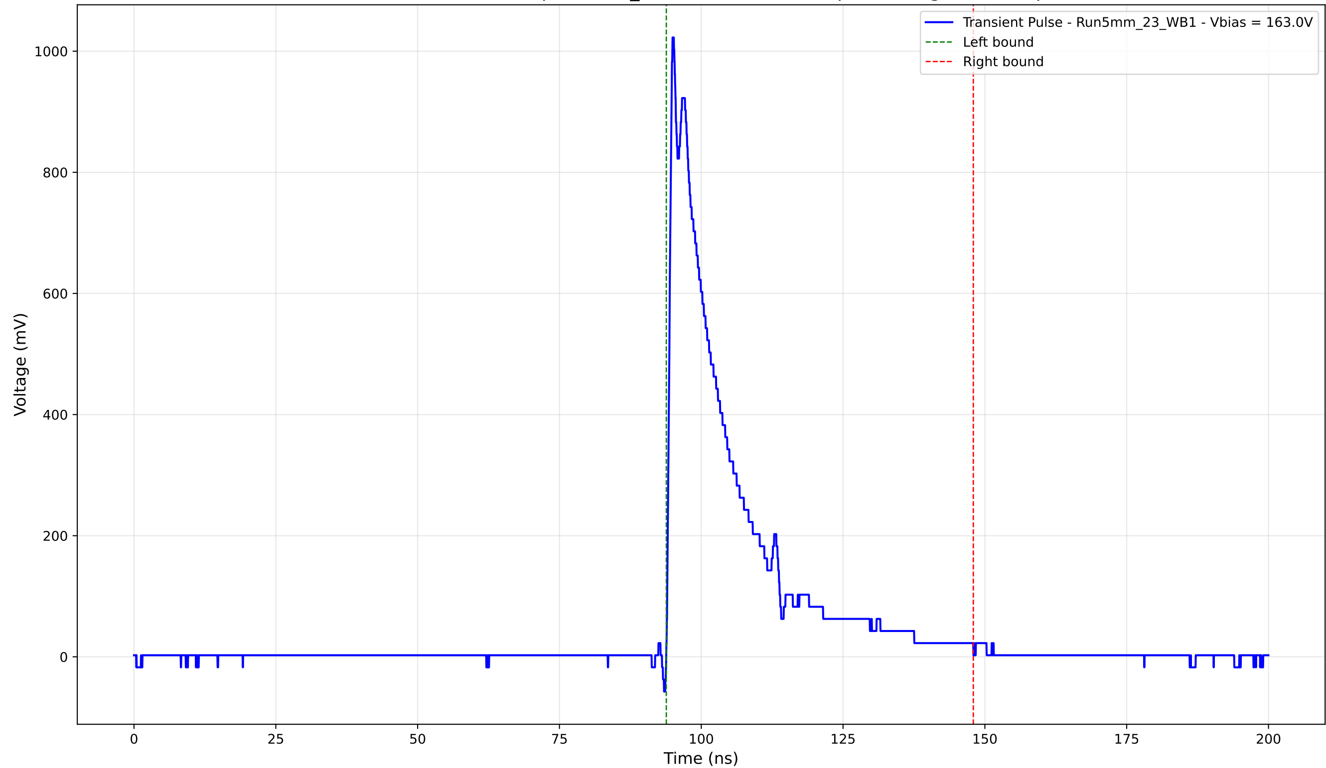
Transient Pulse - Sample: 5mm_23 - Position: 2825.0 \mu\text{m} - Charge: 213.28 pC
