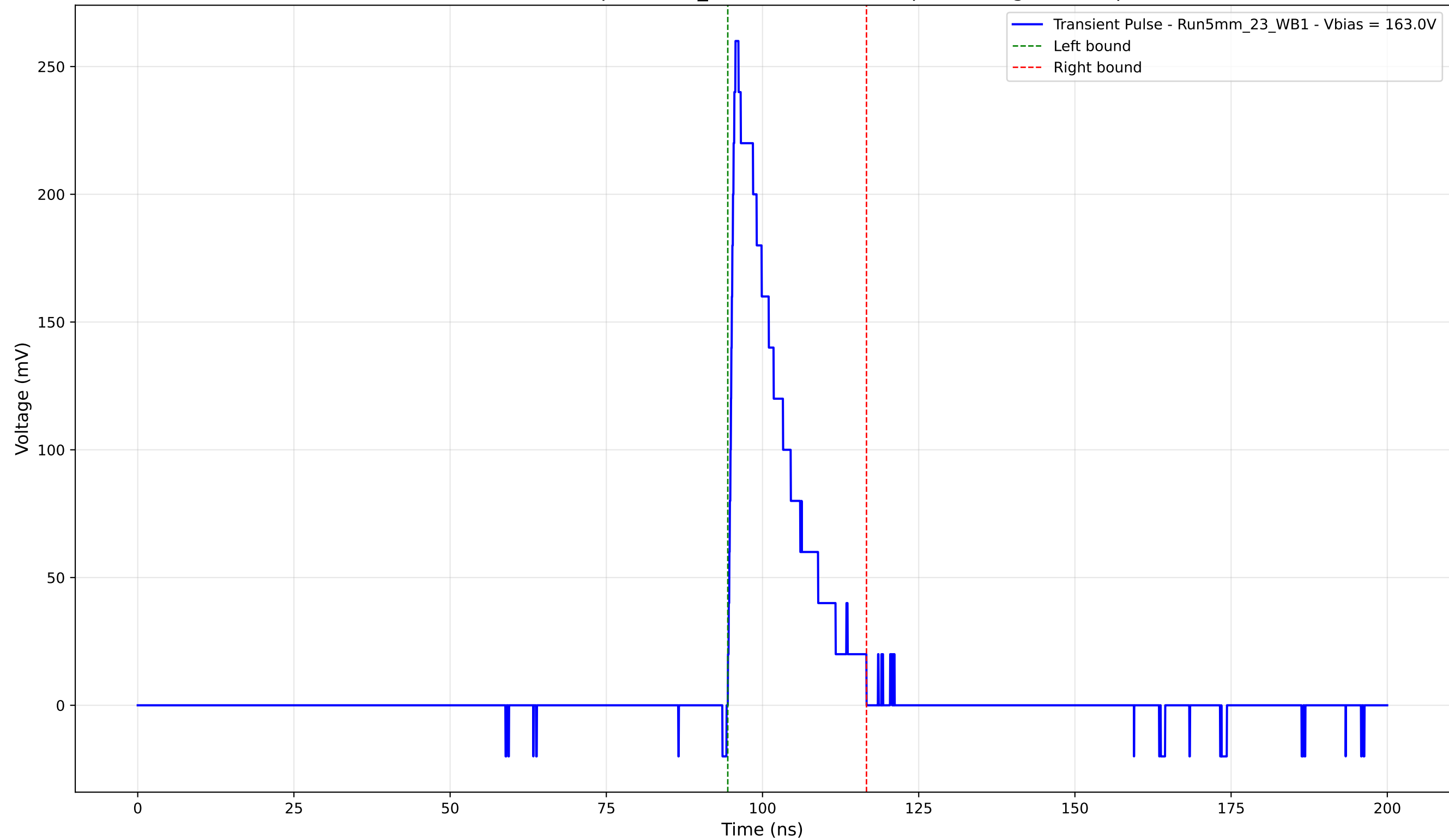
Transient Pulse - Sample: 5mm_23 - Position: 730.0 \mu\text{m} - Charge: 43.56 pC
