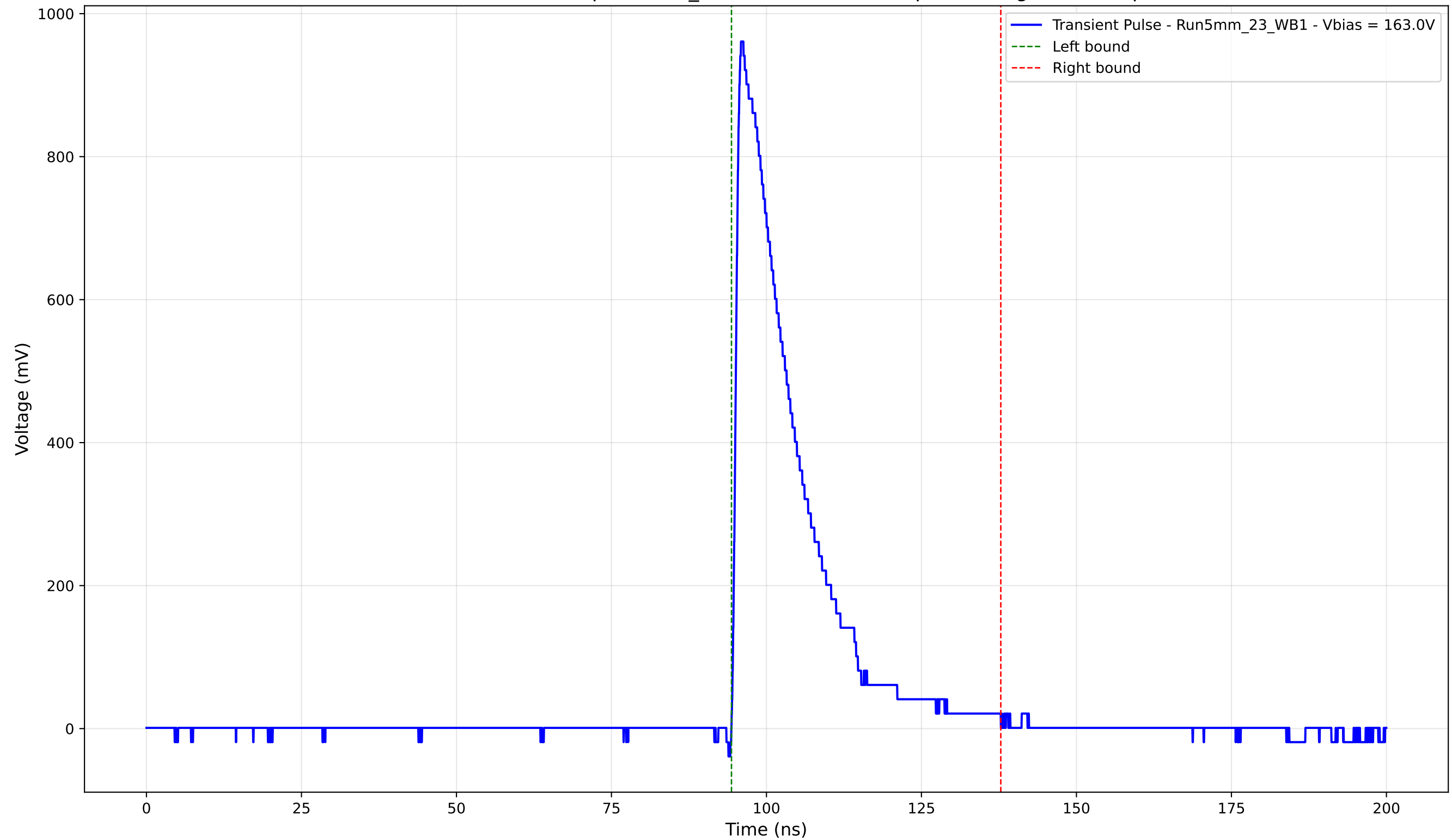
Transient Pulse - Sample: 5mm_23 - Position: 1005.0 \mu\text{m} - Charge: 200.87 pC
