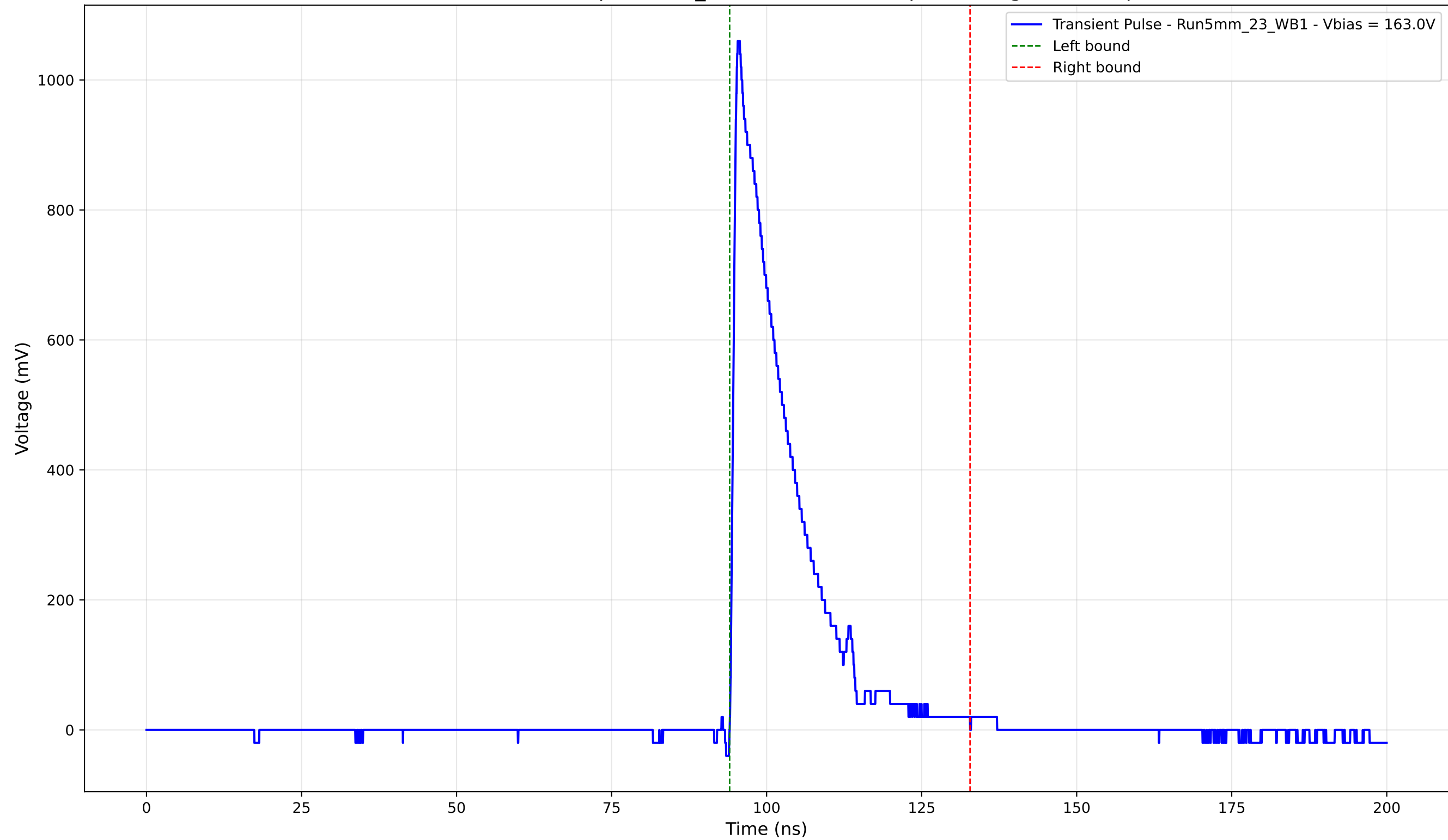
Transient Pulse - Sample: 5mm_23 - Position: 390.0 \mu\text{m} - Charge: 197.59 pC
