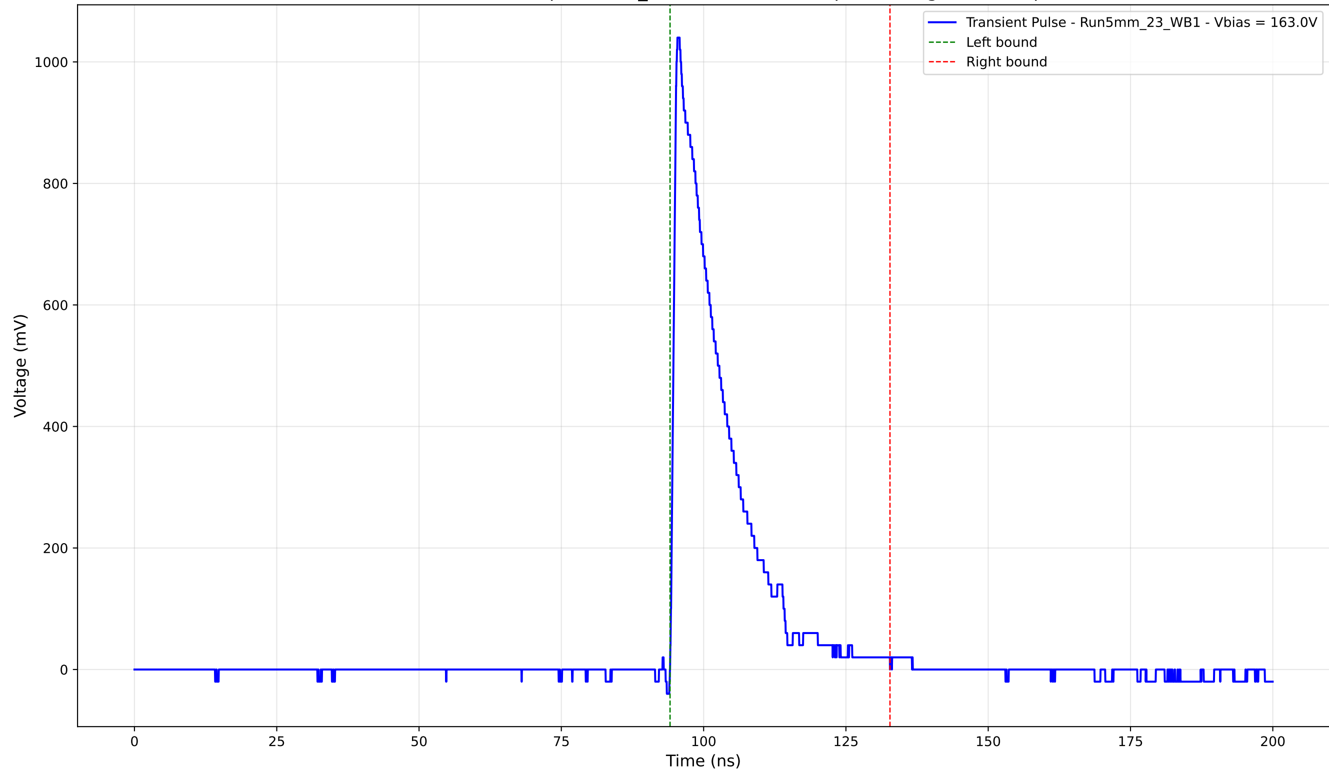
Transient Pulse - Sample: 5mm_23 - Position: 465.0 \mu\text{m} - Charge: 196.04 pC
