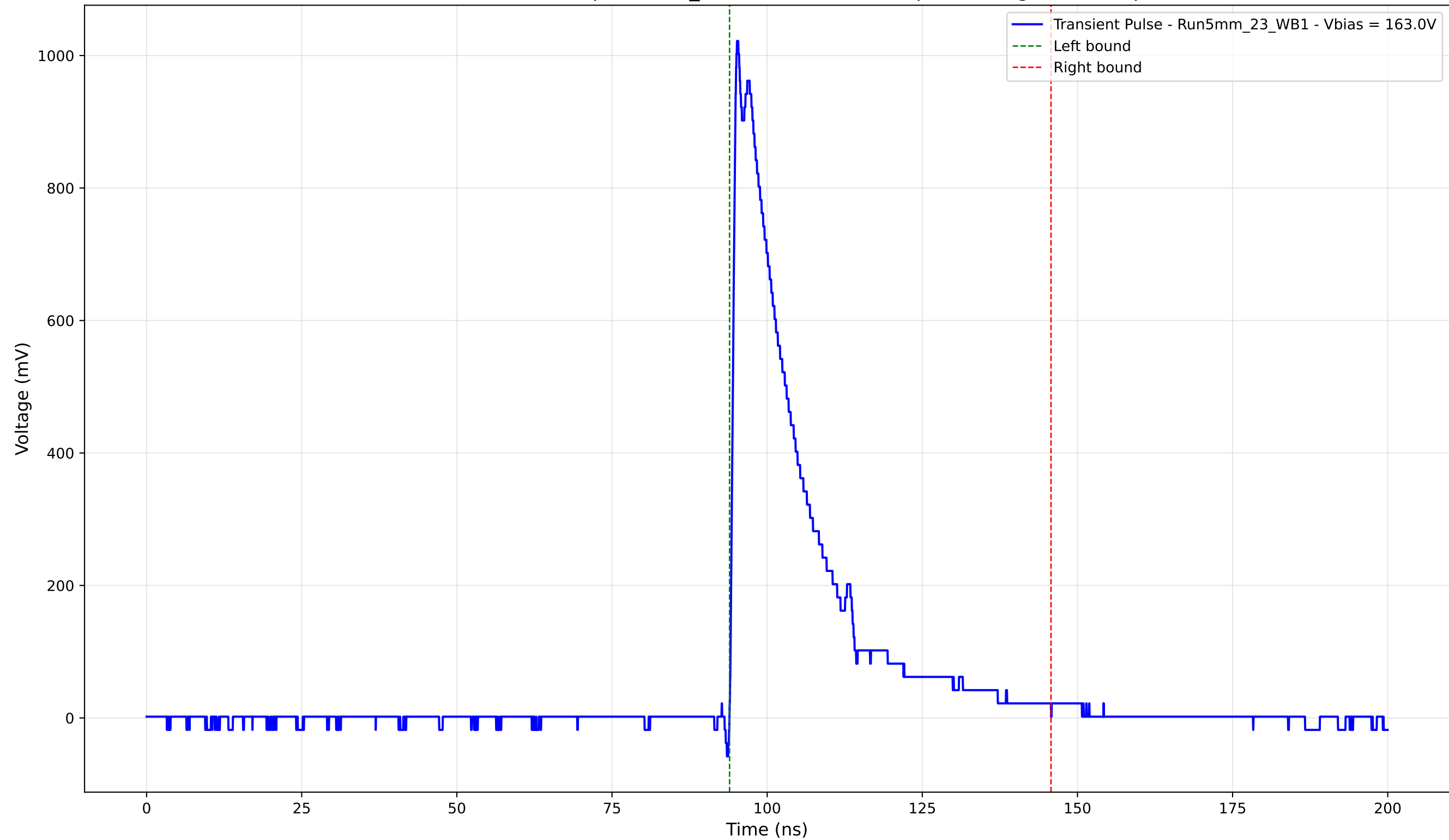
Transient Pulse - Sample: 5mm_23 - Position: 3010.0 \mu\text{m} - Charge: 231.07 pC
