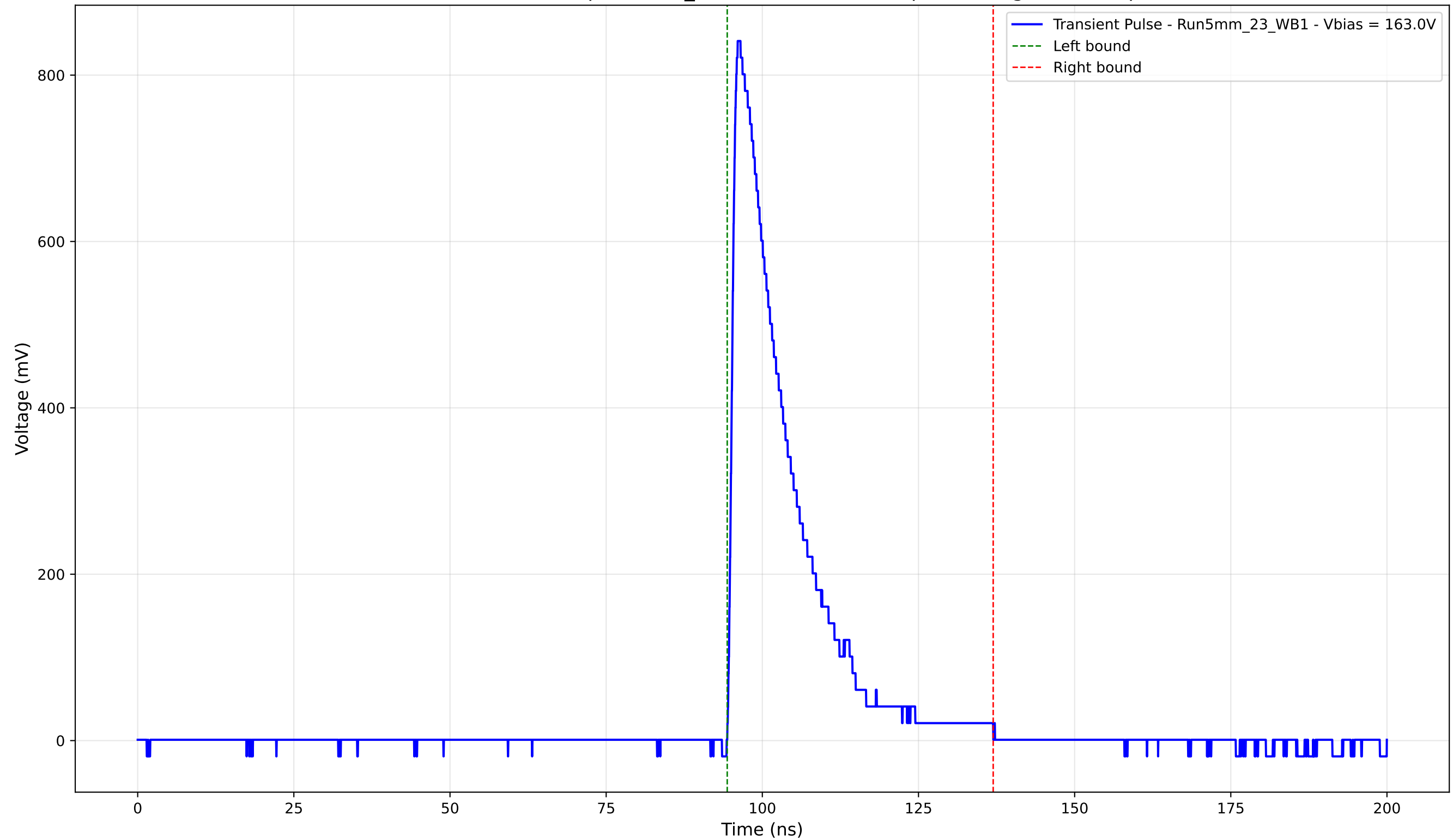
Transient Pulse - Sample: 5mm_23 - Position: 4180.0 \mu\text{m} - Charge: 165.72 pC
