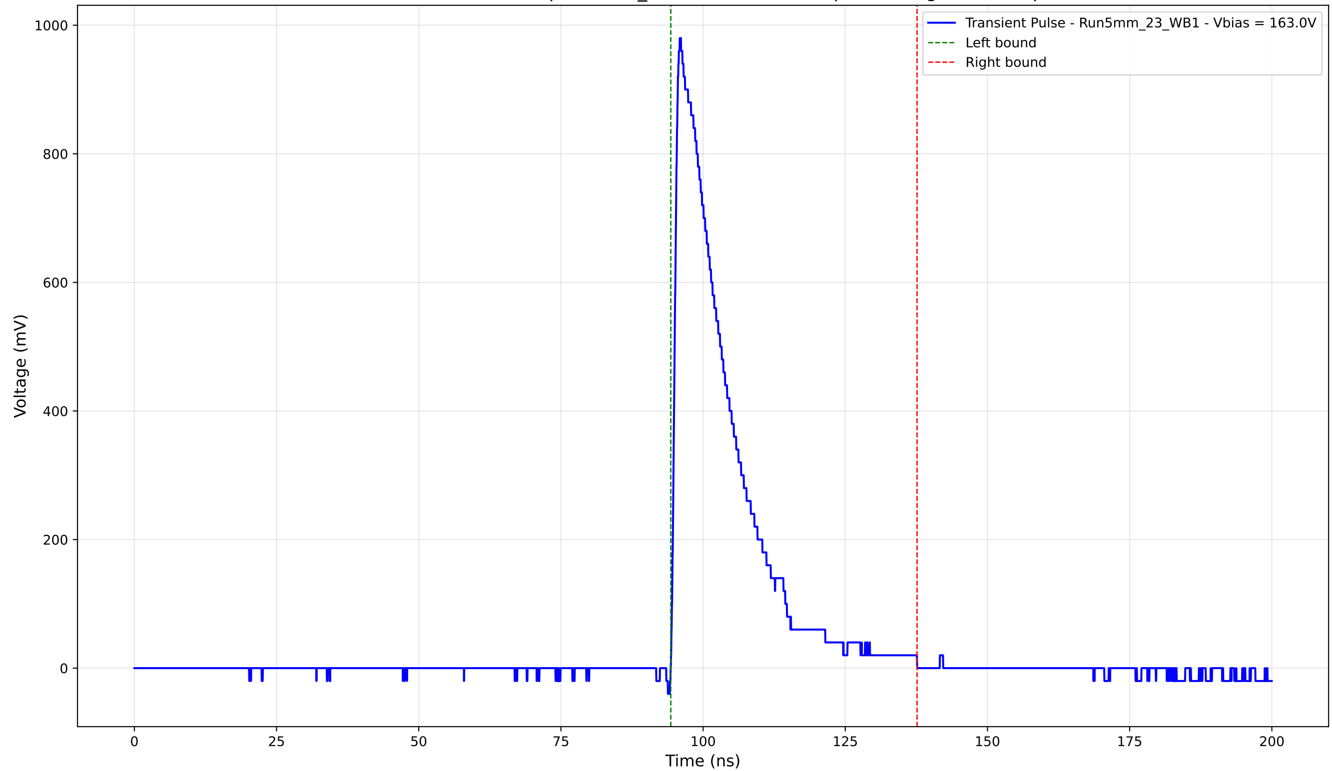
Transient Pulse - Sample: 5mm_23 - Position: 905.0 \mu\text{m} - Charge: 201.52 pC
