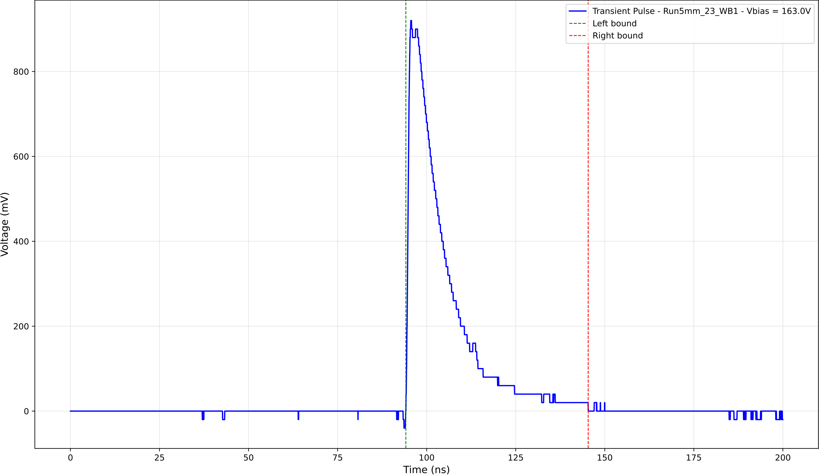
Transient Pulse - Sample: 5mm_23 - Position: 3380.0 \mu\text{m} - Charge: 208.86 pC
