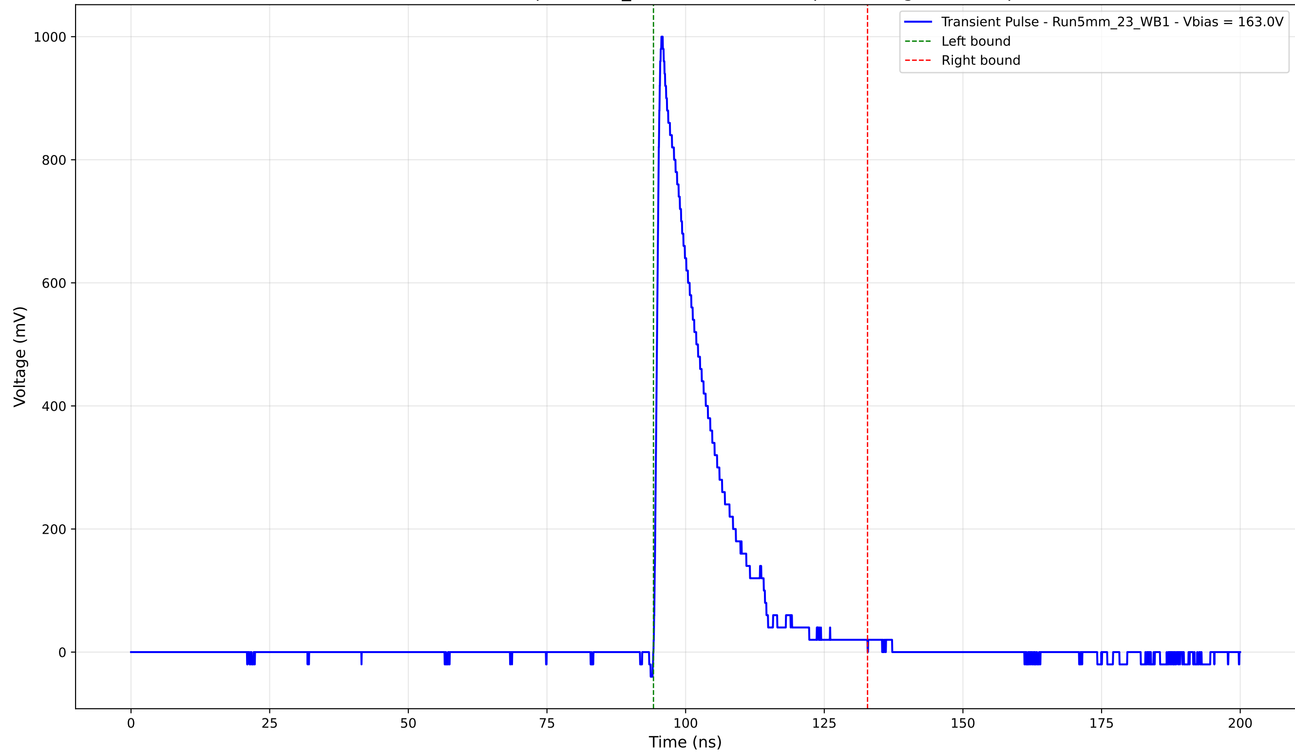
Transient Pulse - Sample: 5mm_23 - Position: 645.0 \mu\text{m} - Charge: 182.29 pC
