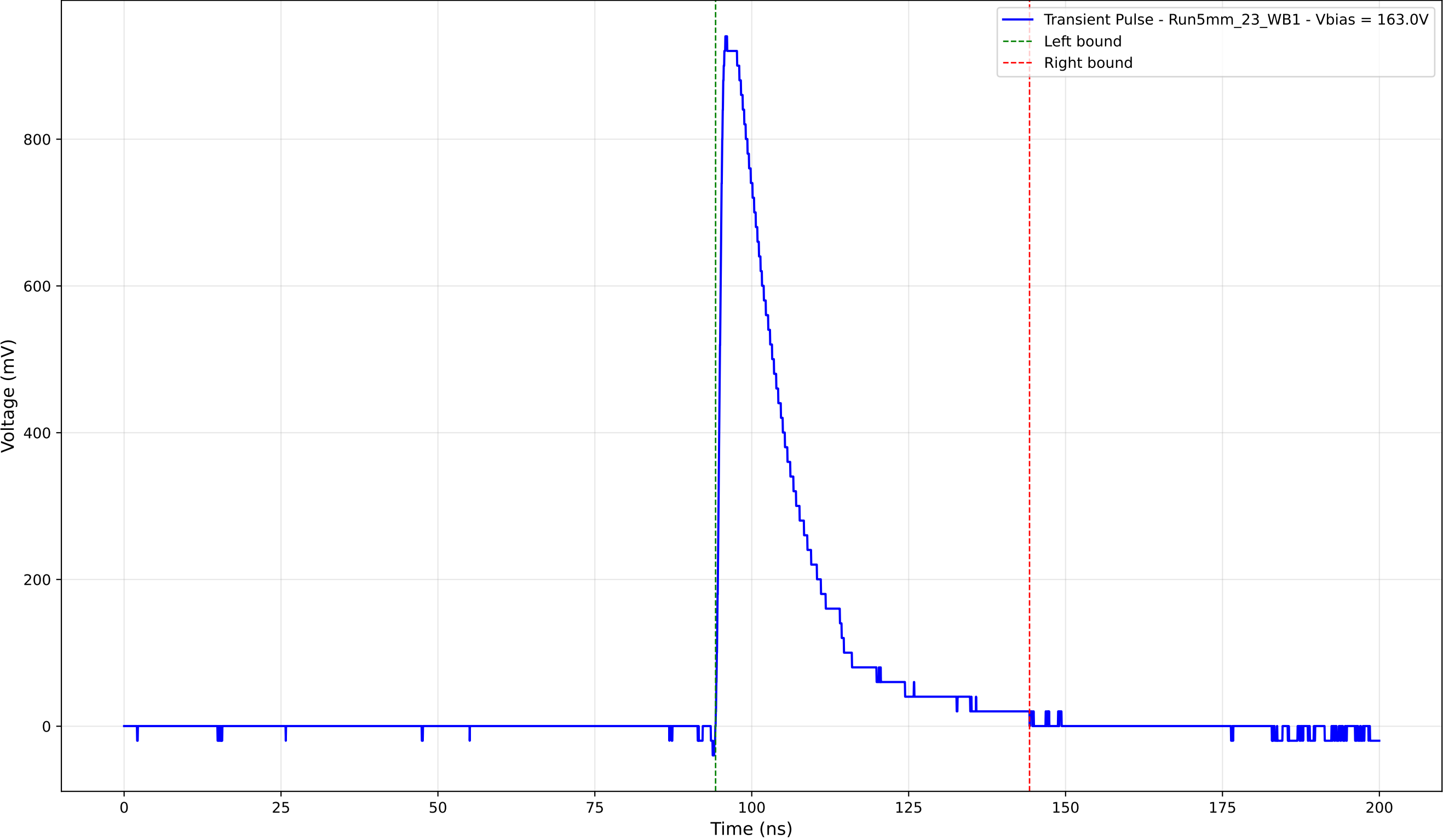
Transient Pulse - Sample: 5mm_23 - Position: 3565.0 \mu\text{m} - Charge: 218.20 pC
