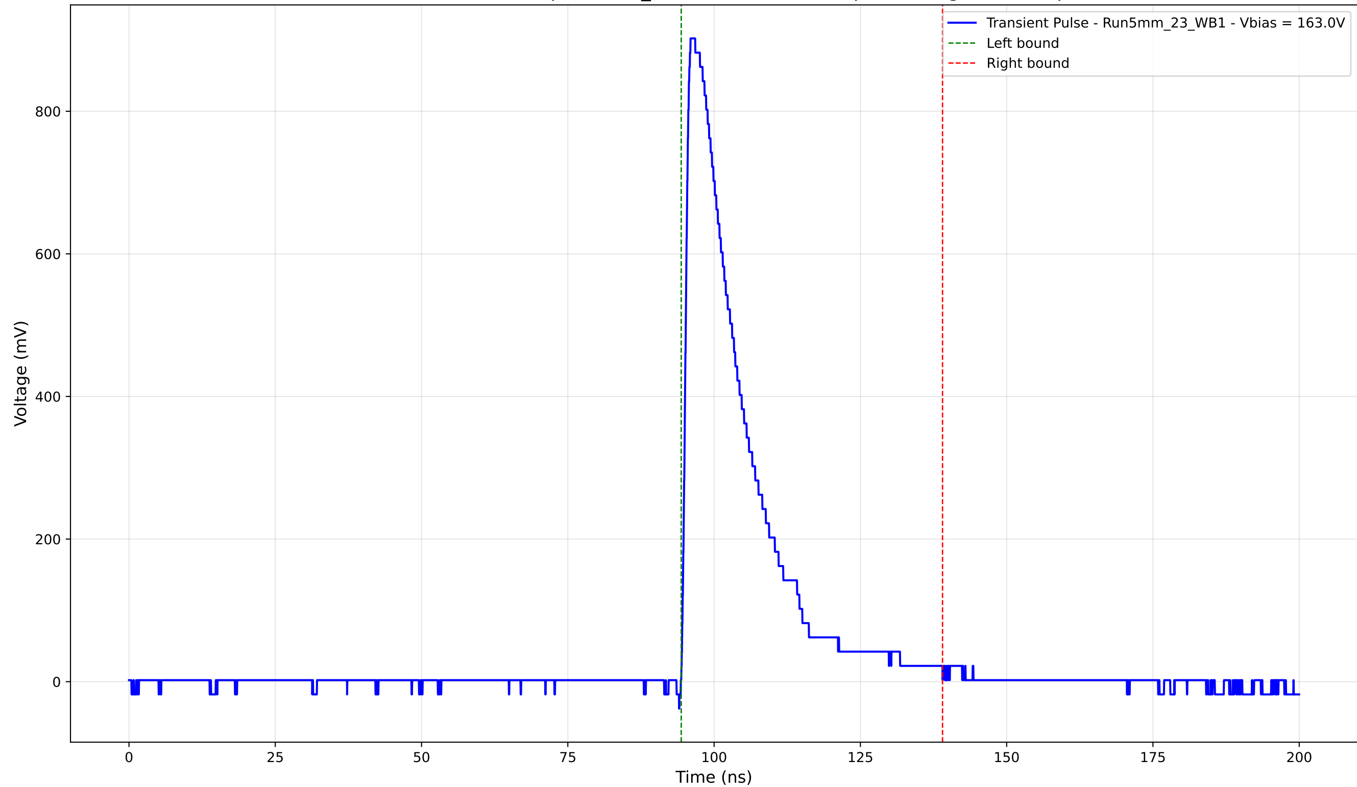
Transient Pulse - Sample: 5mm_23 - Position: 3955.0 \mu\text{m} - Charge: 198.75 pC
