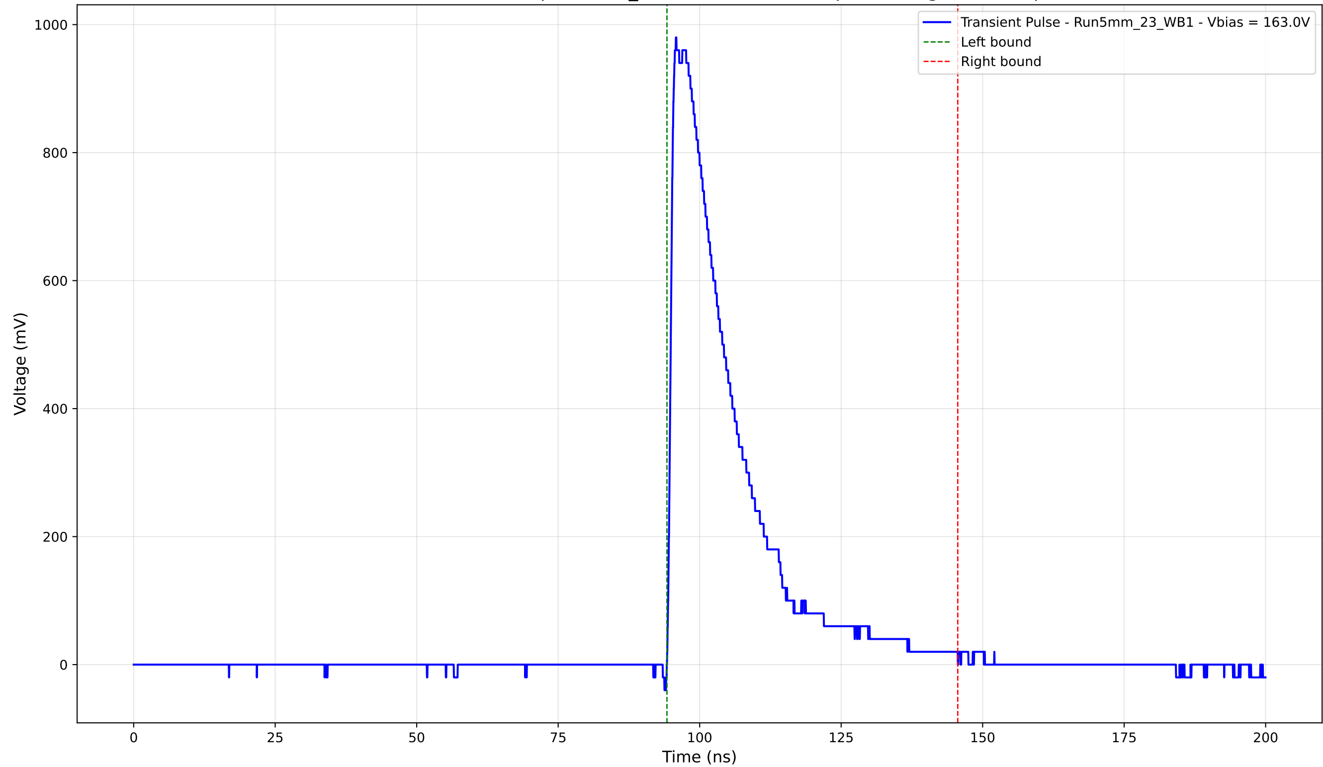
Transient Pulse - Sample: 5mm_23 - Position: 1945.0 \mu\text{m} - Charge: 238.11 pC
