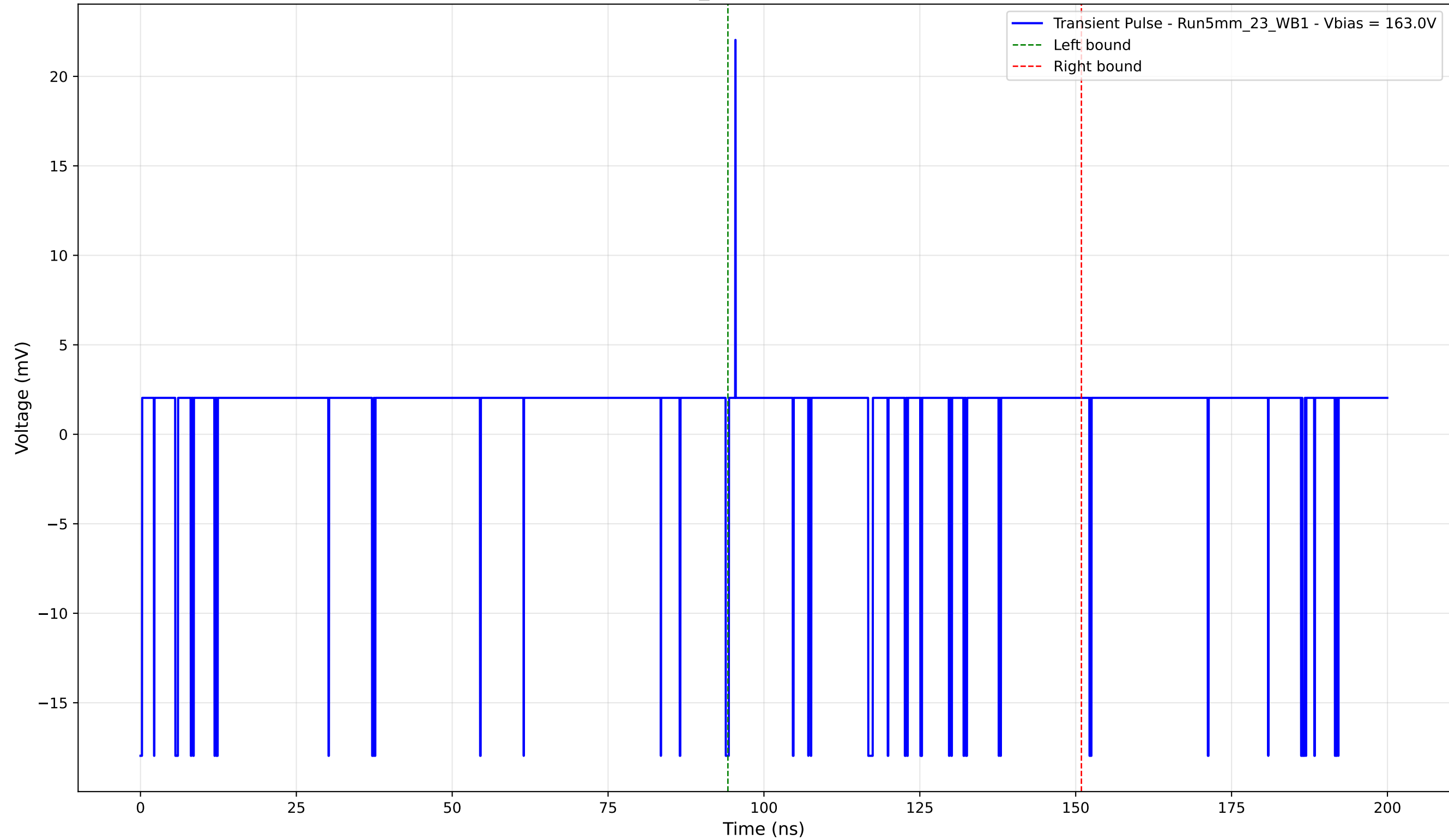
Transient Pulse - Sample: 5mm_23 - Position: 5295.0 \mu\text{m} - Charge: 1.28 pC
