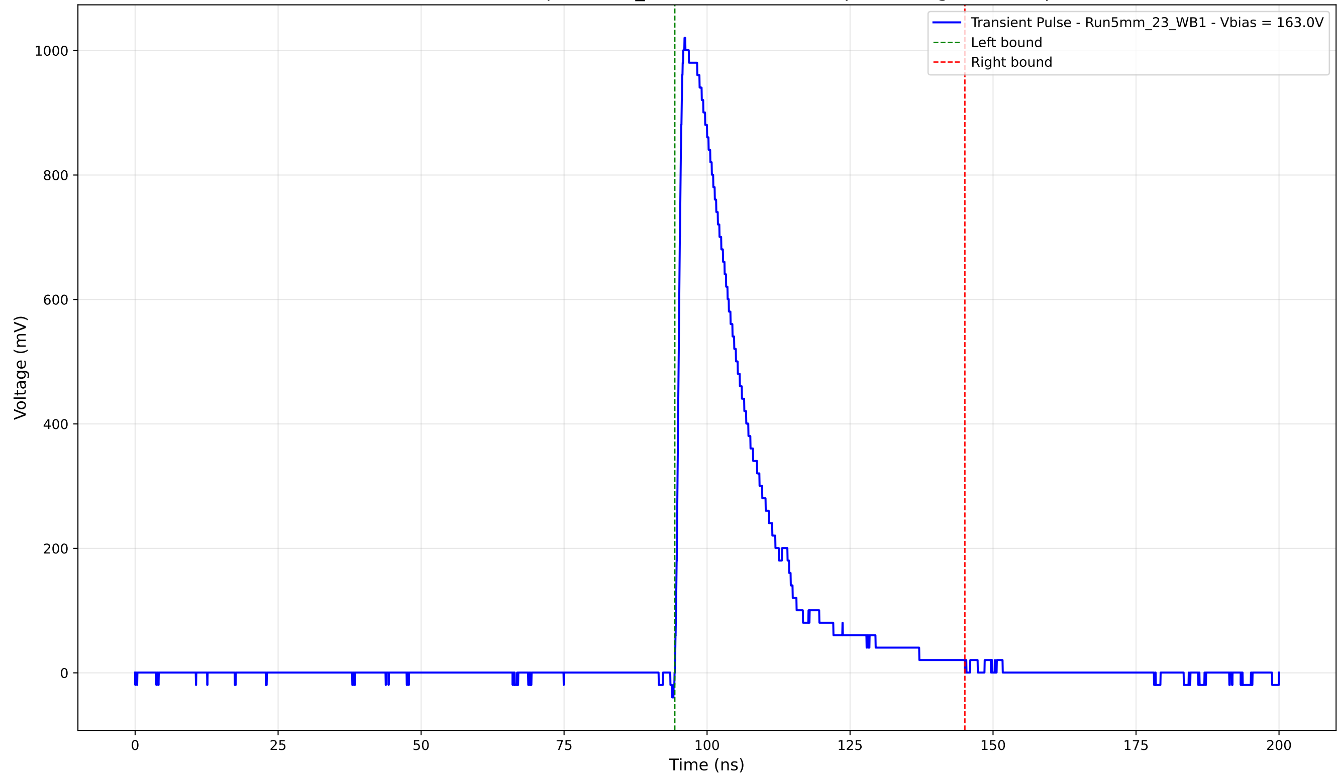
Transient Pulse - Sample: 5mm_23 - Position: 1535.0 \mu\text{m} - Charge: 255.13 pC
