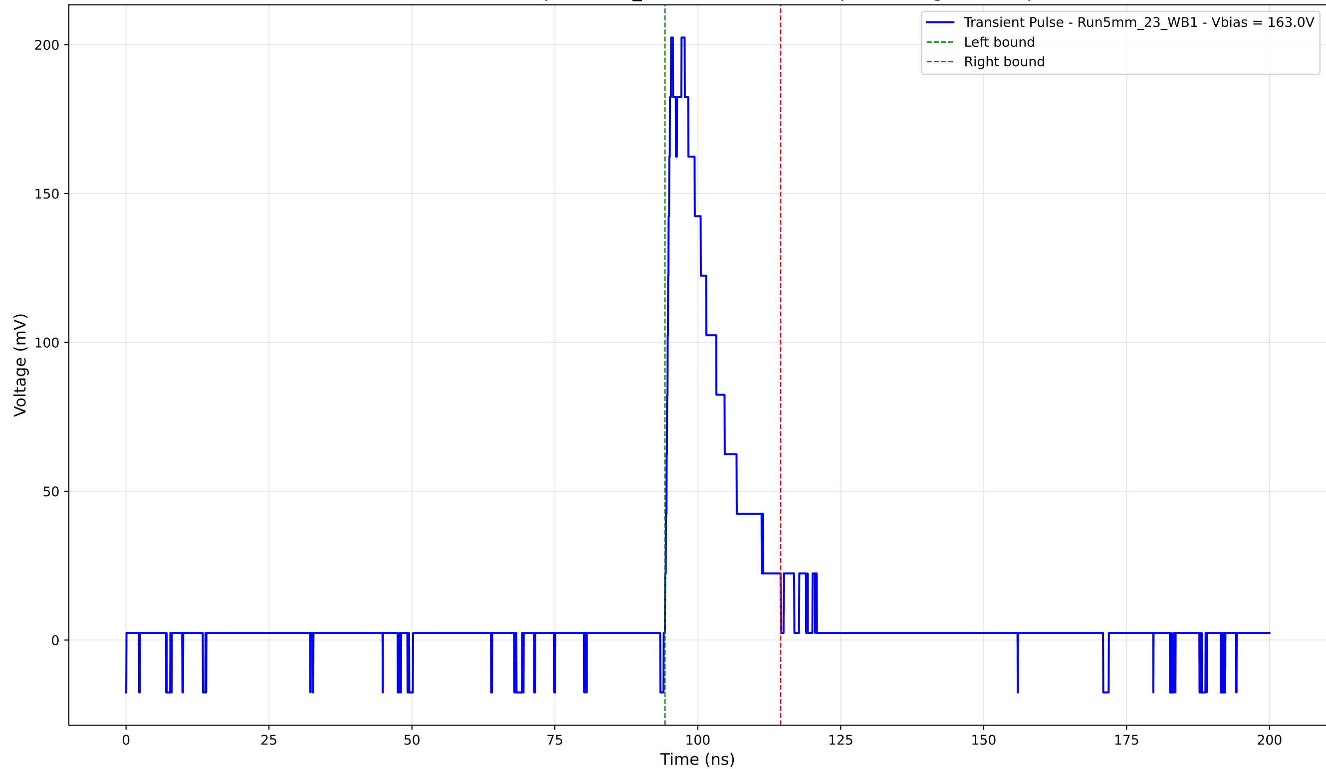
Transient Pulse - Sample: 5mm_23 - Position: 3250.0 \mu\text{m} - Charge: 36.43 pC
