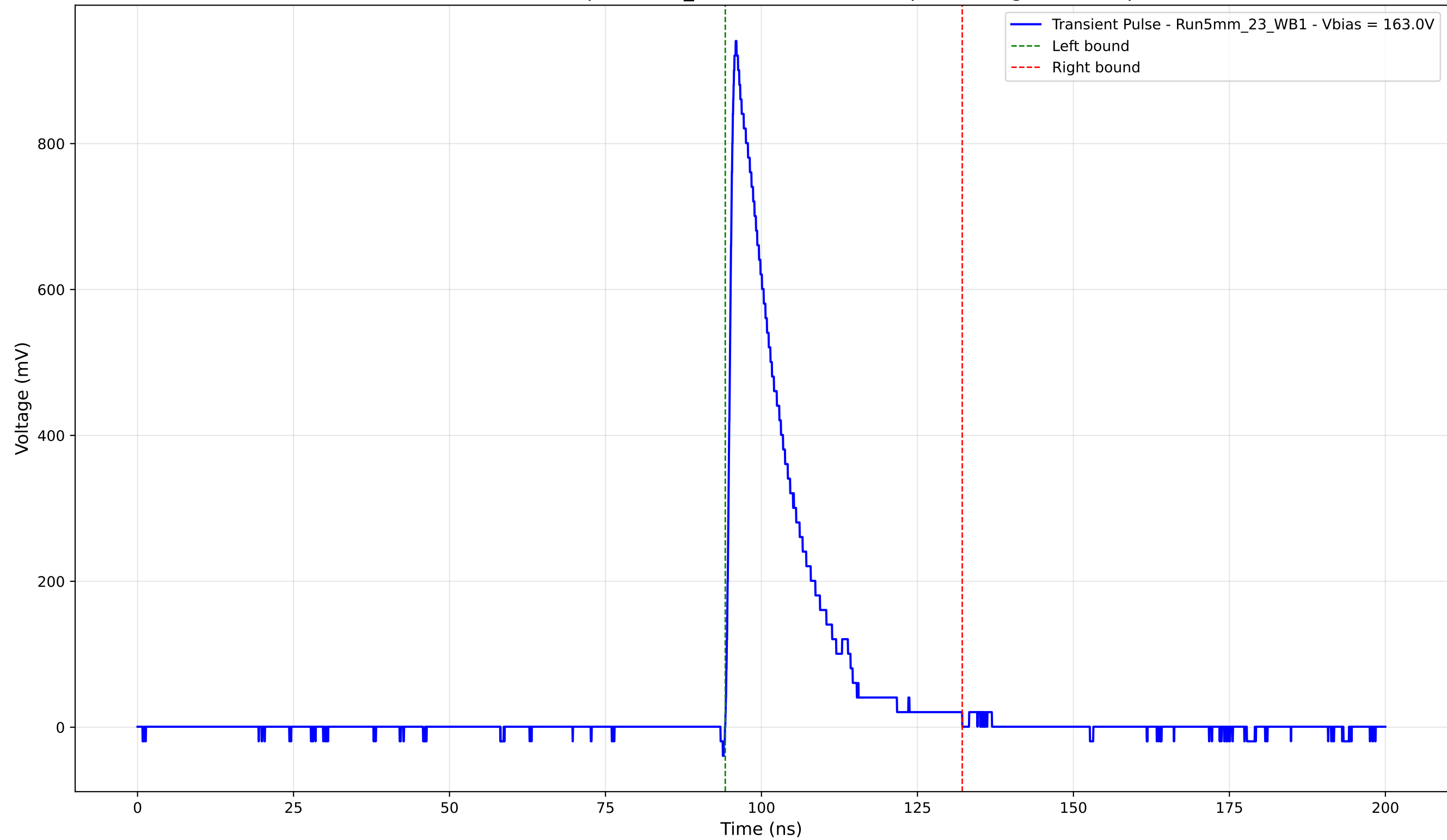
Transient Pulse - Sample: 5mm_23 - Position: 4640.0 \mu\text{m} - Charge: 171.29 pC
