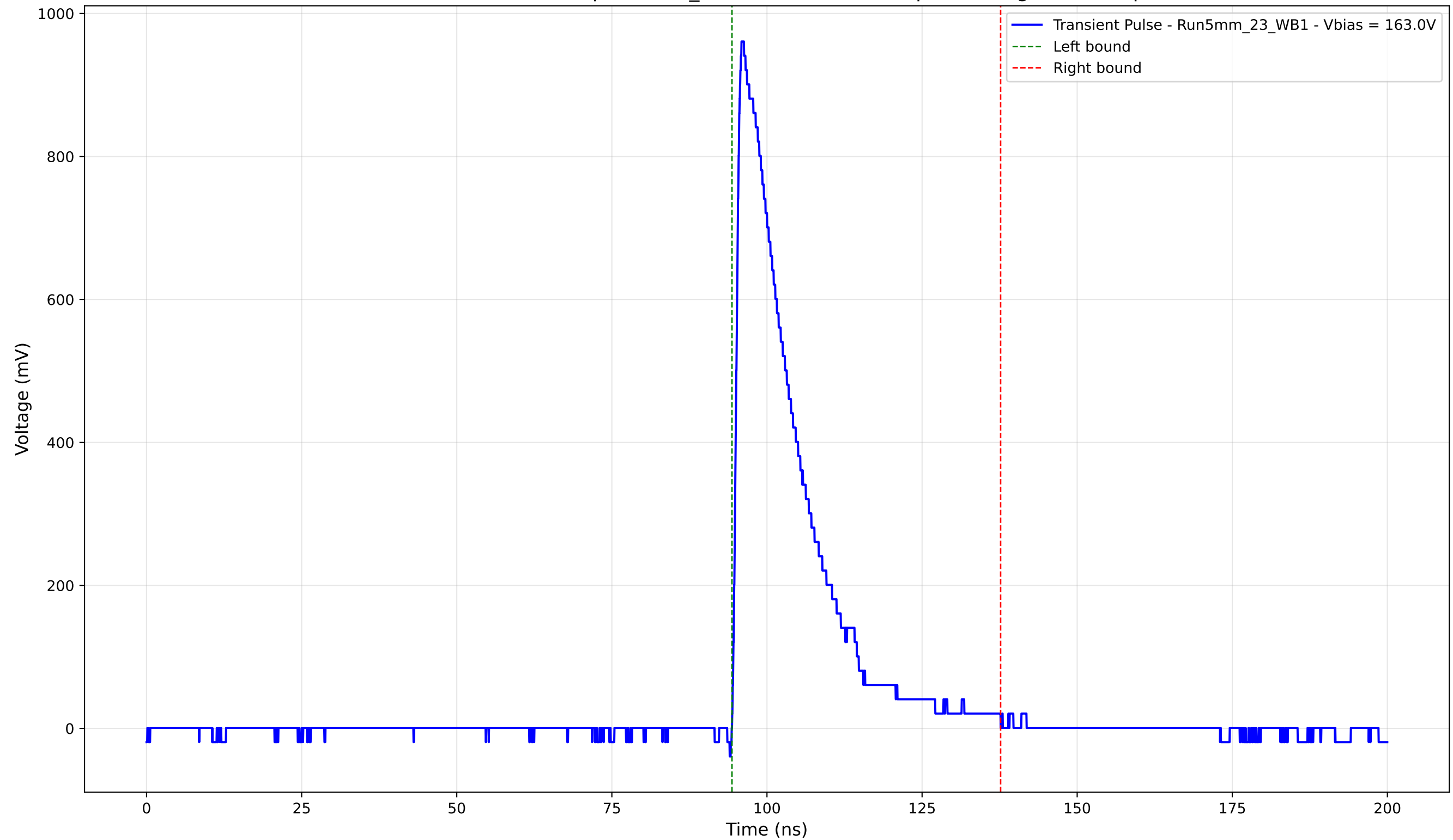
Transient Pulse - Sample: 5mm_23 - Position: 1000.0 \mu\text{m} - Charge: 200.31 pC
