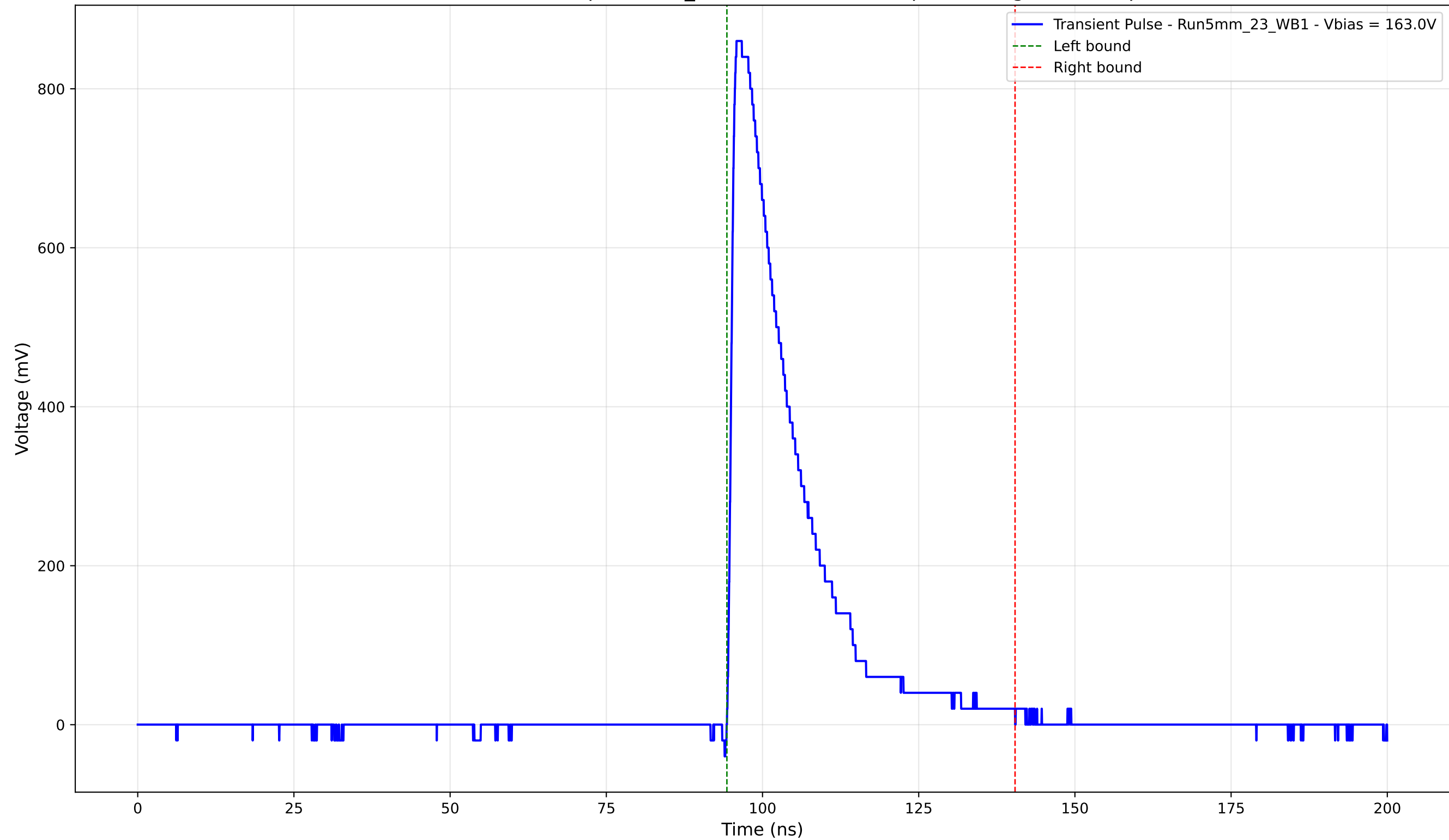
Transient Pulse - Sample: 5mm_23 - Position: 1805.0 \mu\text{m} - Charge: 192.02 pC
