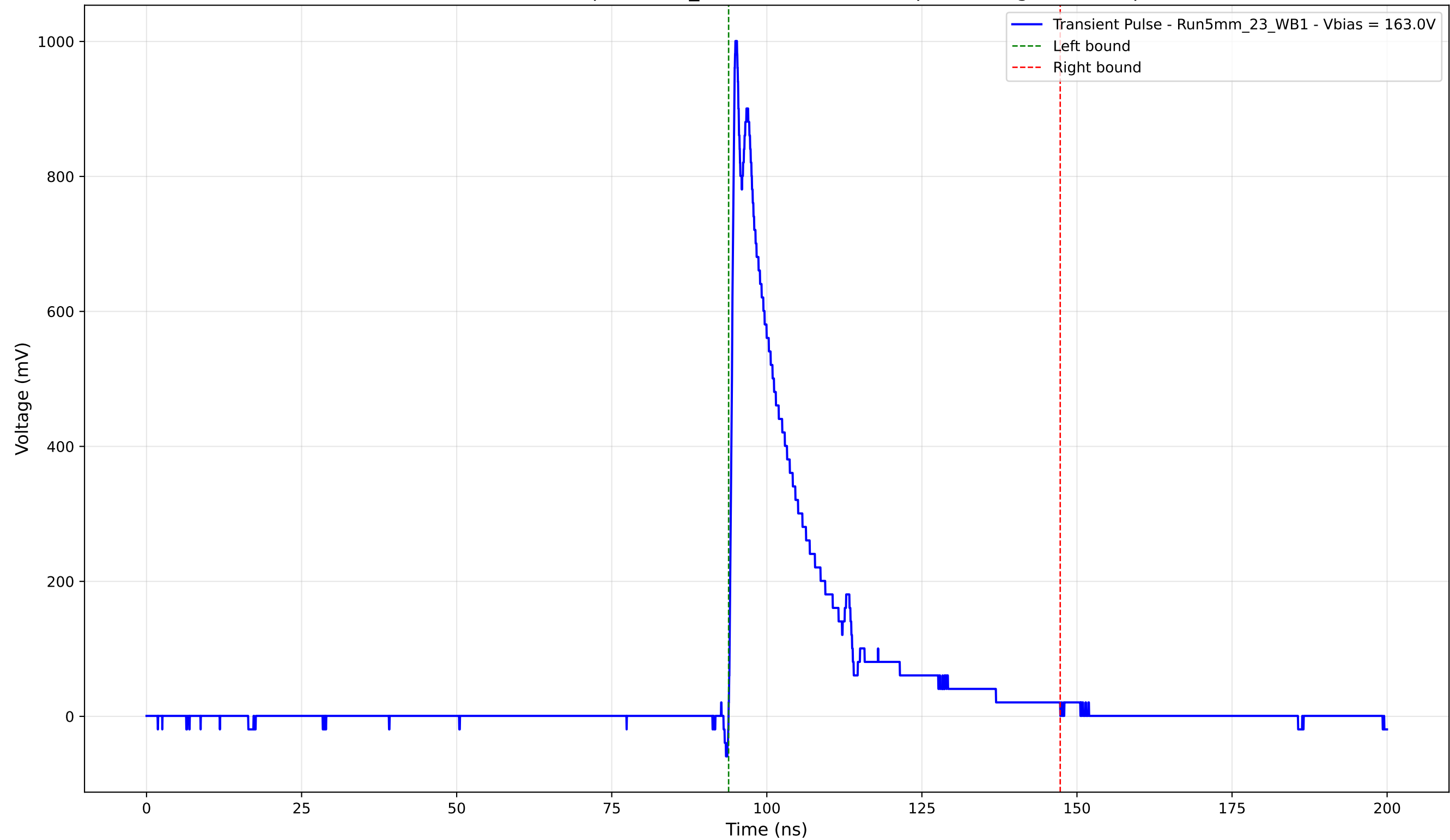
Transient Pulse - Sample: 5mm_23 - Position: 2675.0 \mu\text{m} - Charge: 200.41 pC
