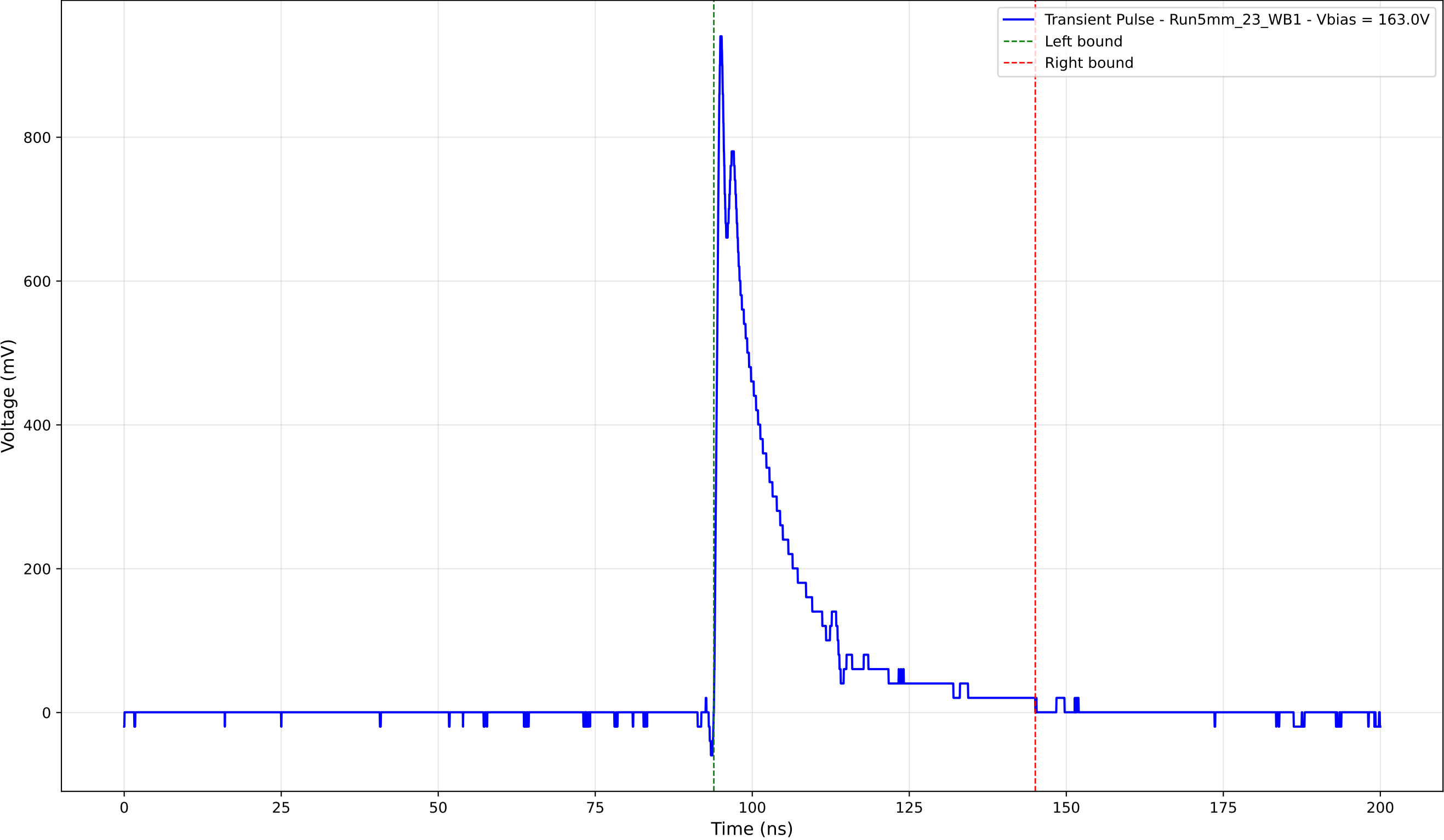
Transient Pulse - Sample: 5mm_23 - Position: 2690.0 \mu\text{m} - Charge: 164.14 pC
