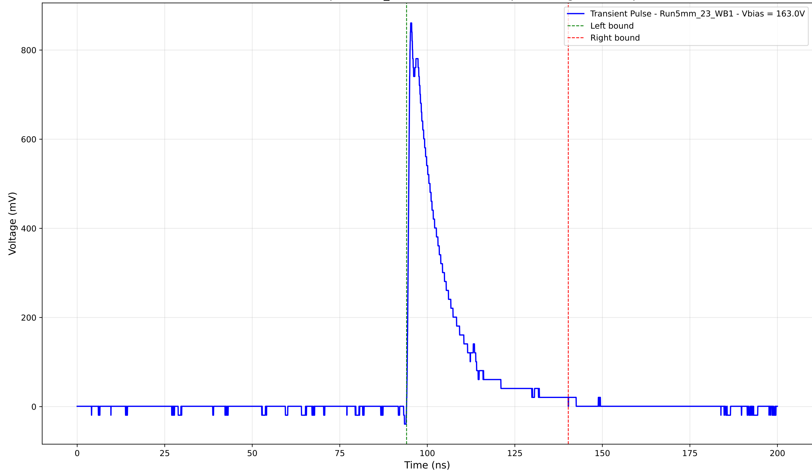
Transient Pulse - Sample: 5mm_23 - Position: 3180.0 \mu\text{m} - Charge: 170.47 pC
