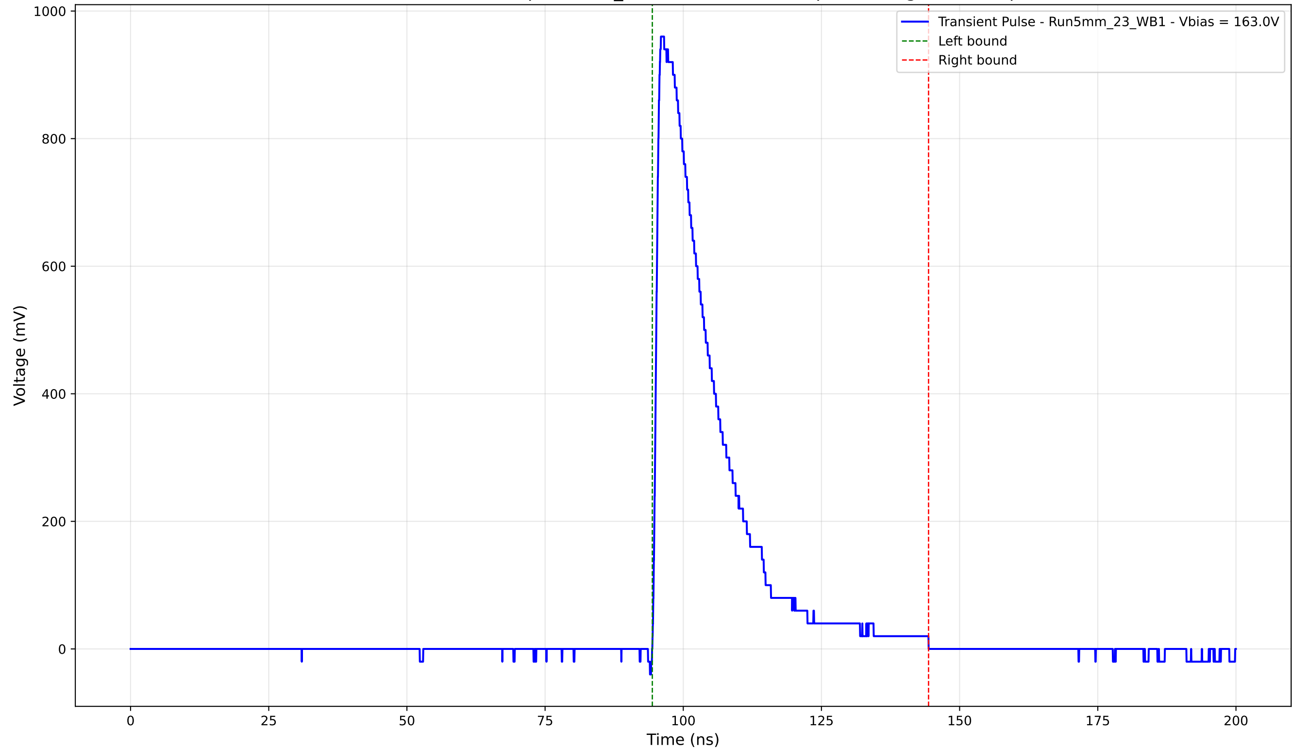
Transient Pulse - Sample: 5mm_23 - Position: 1355.0 \mu\text{m} - Charge: 222.48 pC
