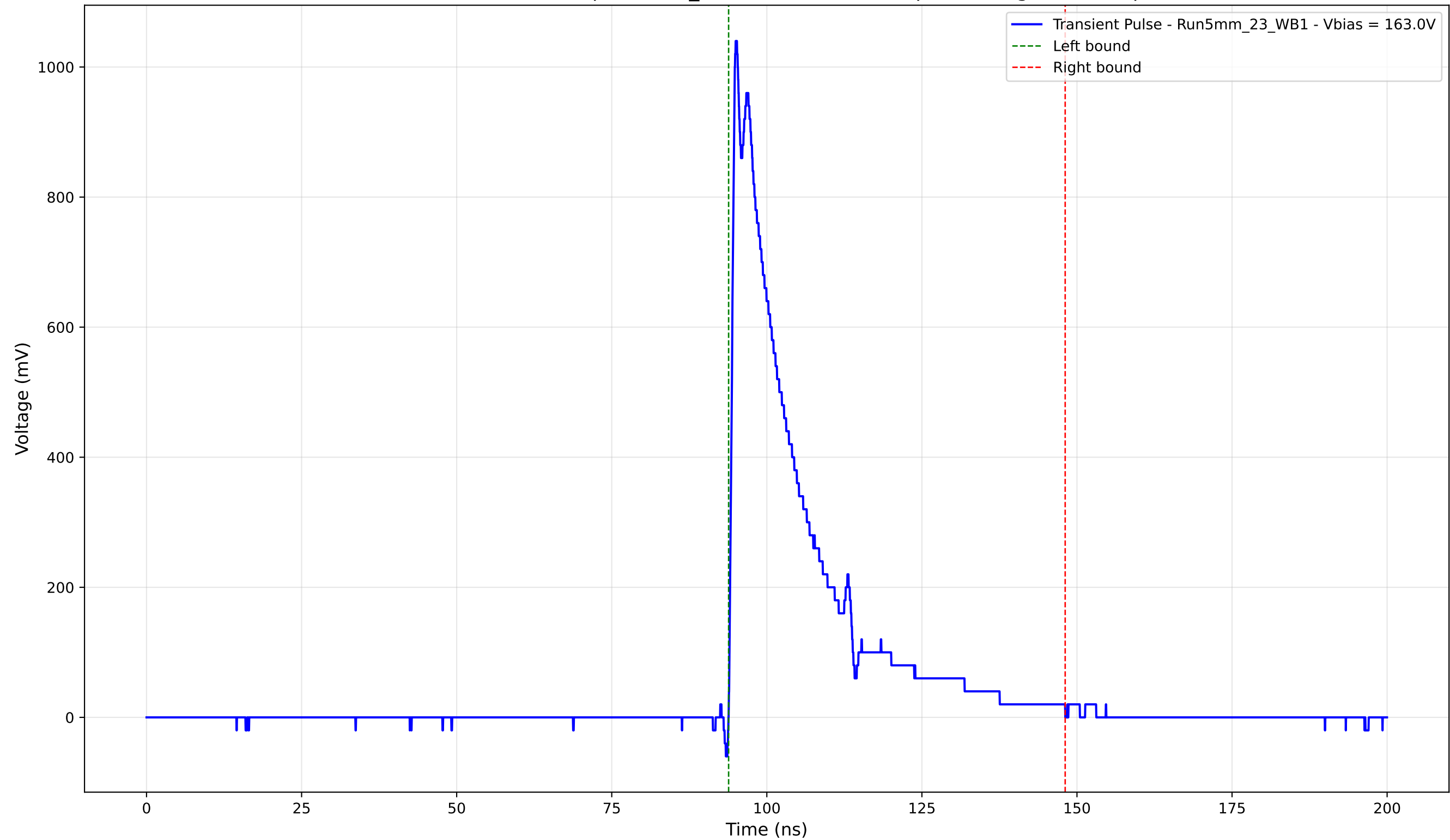
Transient Pulse - Sample: 5mm_23 - Position: 2660.0 \mu\text{m} - Charge: 224.11 pC
