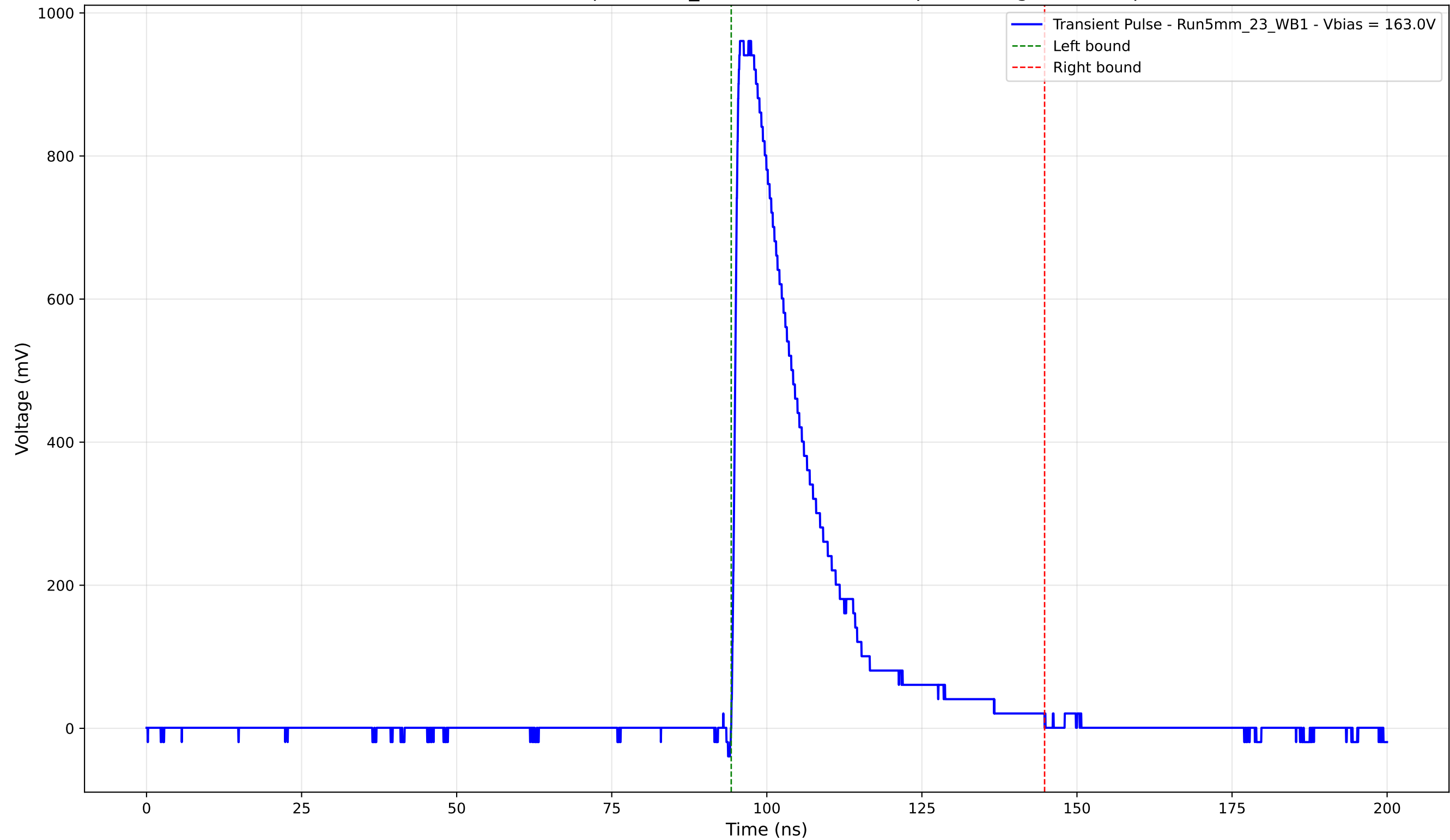
Transient Pulse - Sample: 5mm_23 - Position: 1920.0 \mu\text{m} - Charge: 235.42 pC
