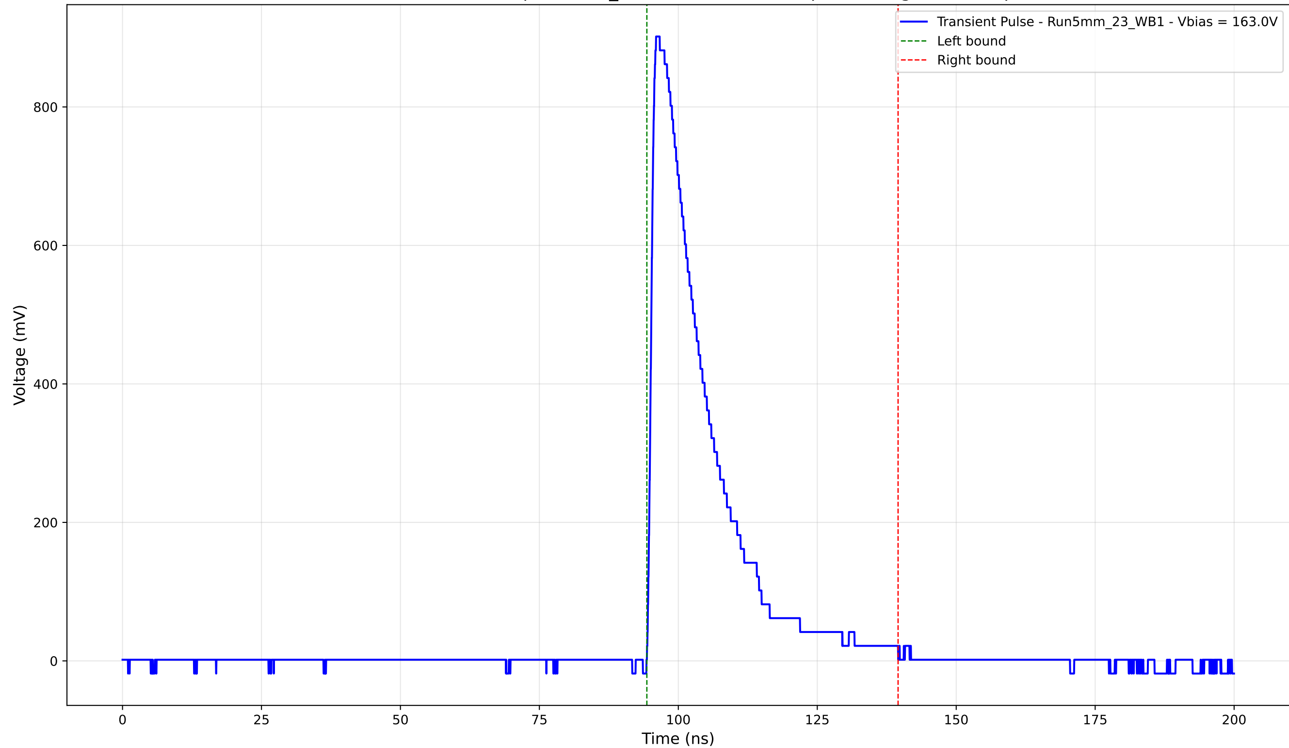
Transient Pulse - Sample: 5mm_23 - Position: 3900.0 \mu\text{m} - Charge: 198.18 pC
