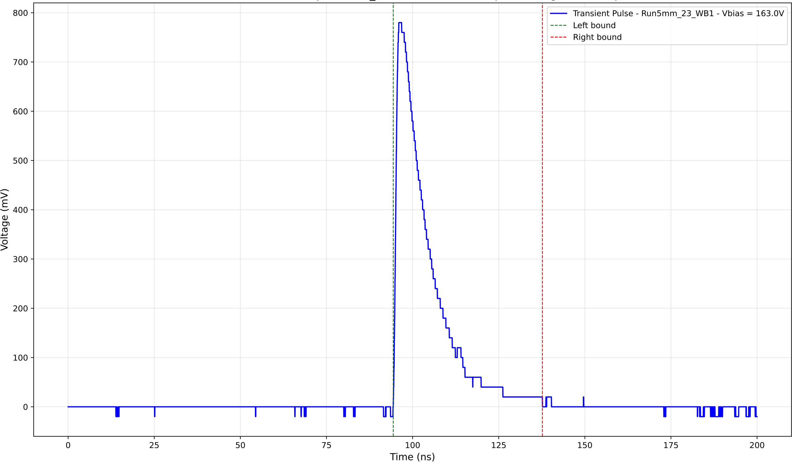
Transient Pulse - Sample: 5mm_23 - Position: 1665.0 \mu\text{m} - Charge: 163.98 pC
