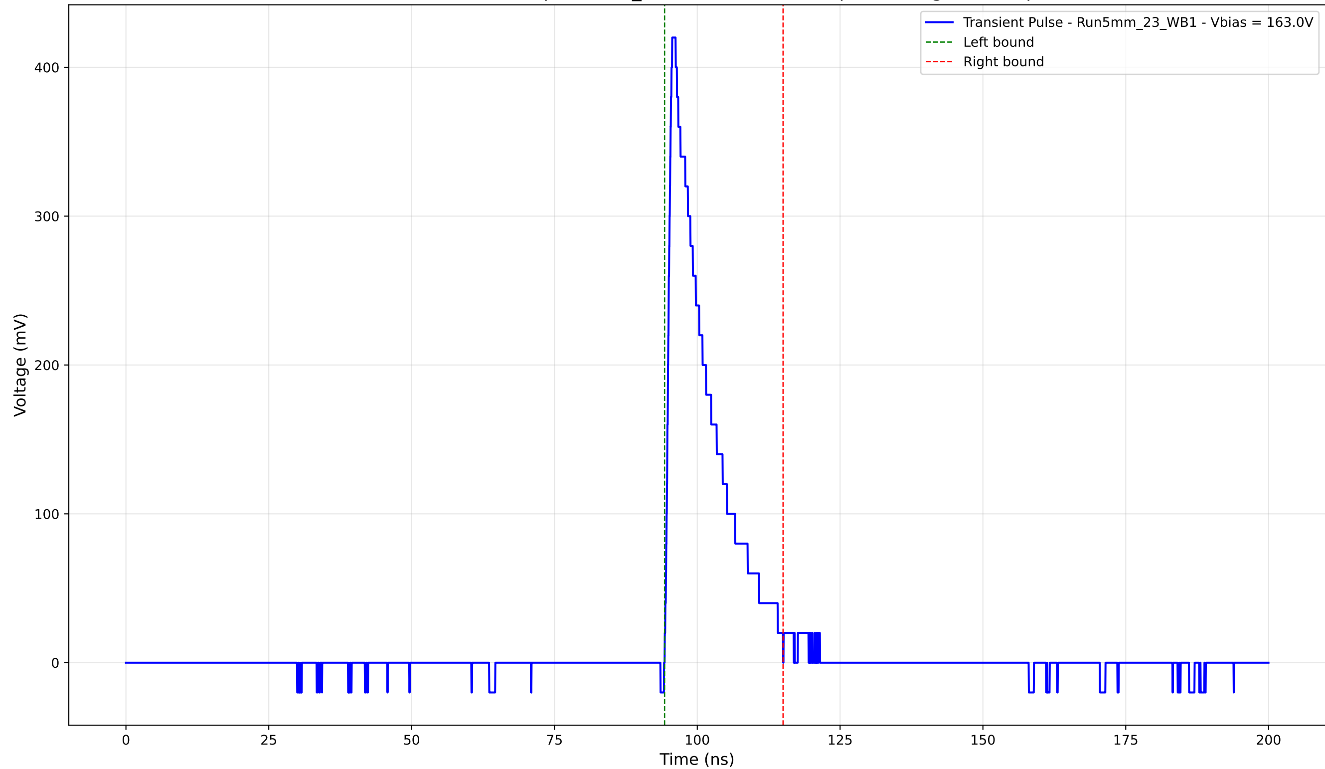
Transient Pulse - Sample: 5mm_23 - Position: 4735.0 \mu\text{m} - Charge: 64.16 pC
