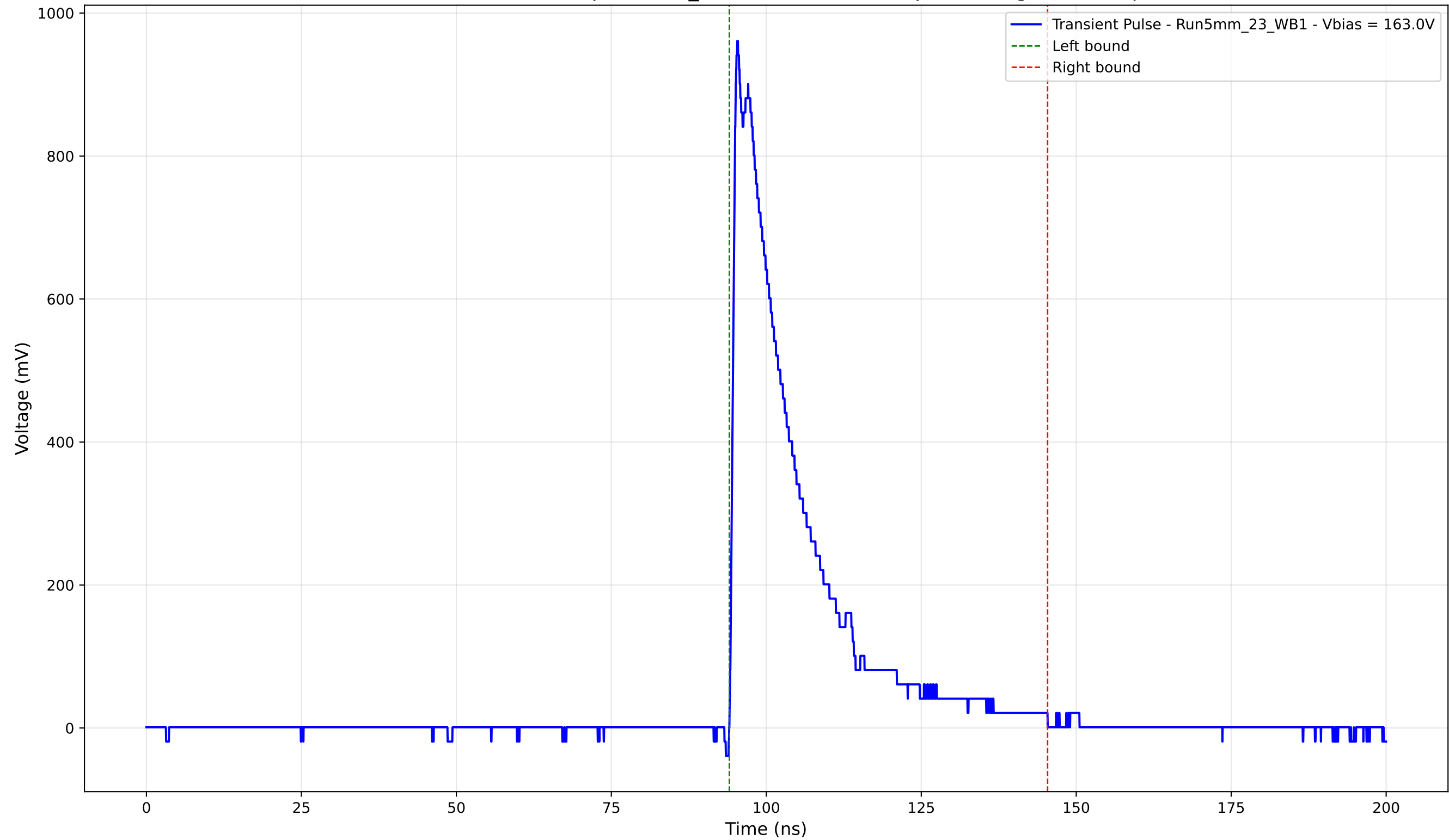
Transient Pulse - Sample: 5mm_23 - Position: 2325.0 \mu\text{m} - Charge: 206.48 pC
