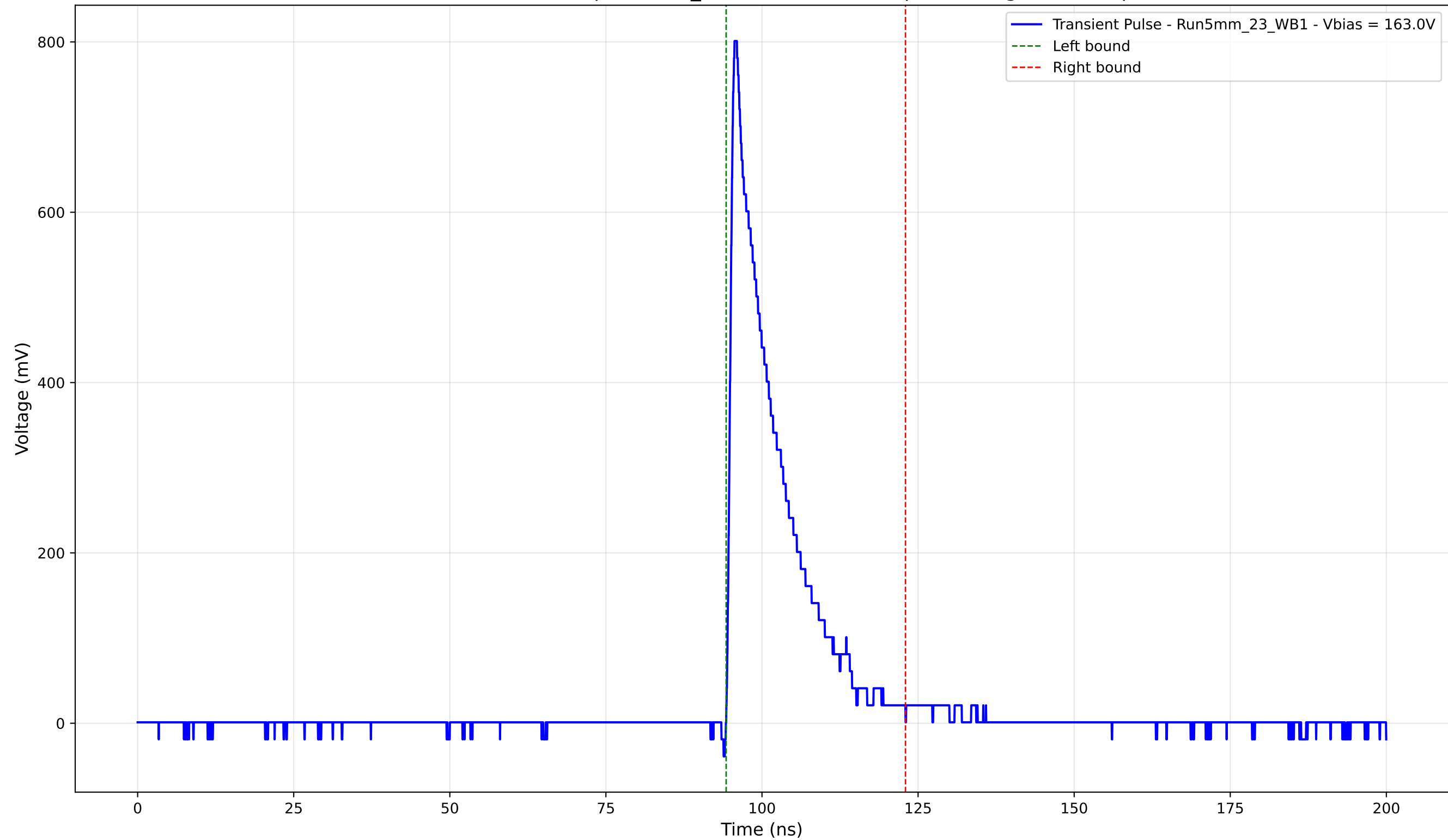
Transient Pulse - Sample: 5mm_23 - Position: 670.0 \mu\text{m} - Charge: 126.61 pC
