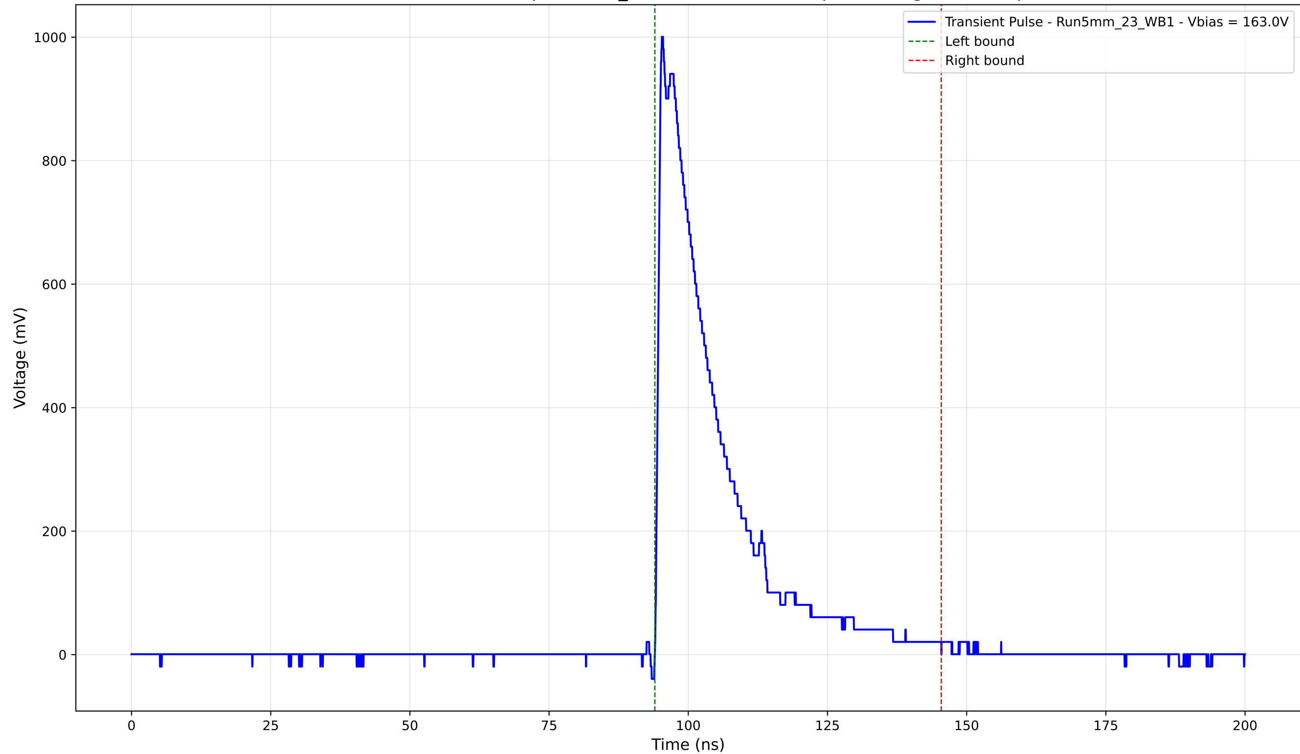
Transient Pulse - Sample: 5mm_23 - Position: 2365.0 \mu\text{m} - Charge: 226.11 pC
