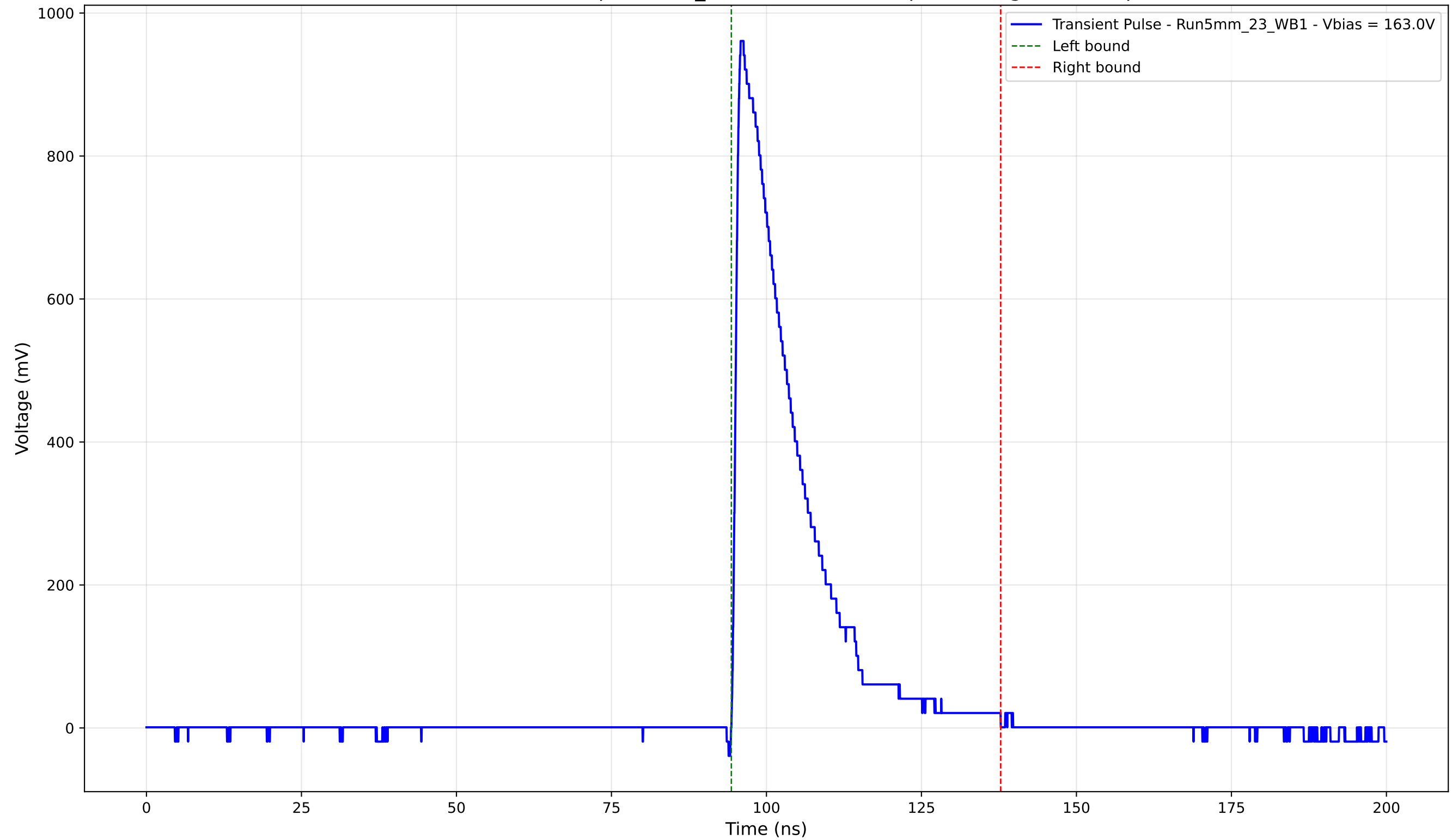
Transient Pulse - Sample: 5mm_23 - Position: 970.0 \mu\text{m} - Charge: 201.27 pC
