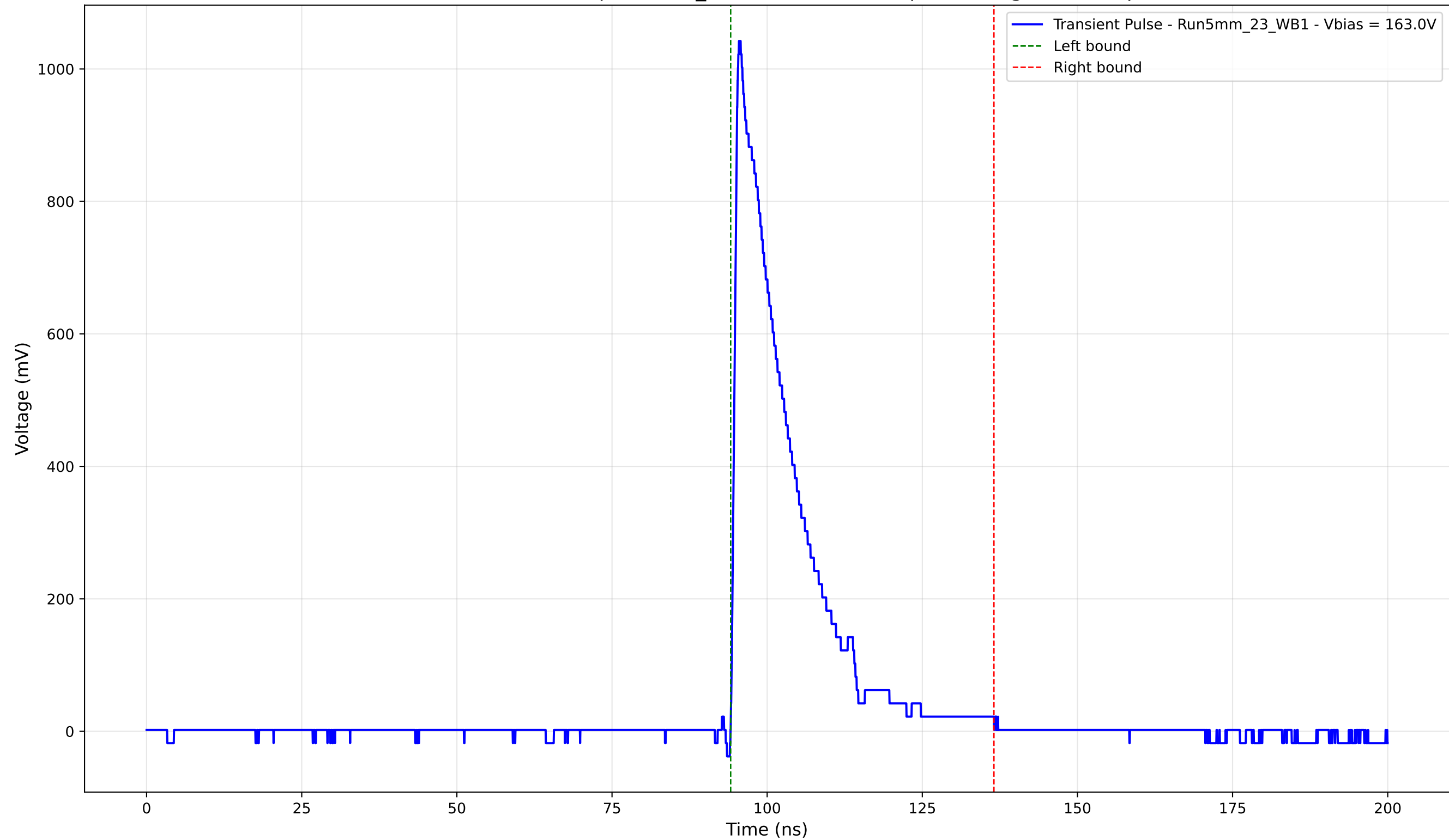
Transient Pulse - Sample: 5mm_23 - Position: 480.0 \mu\text{m} - Charge: 197.17 pC
