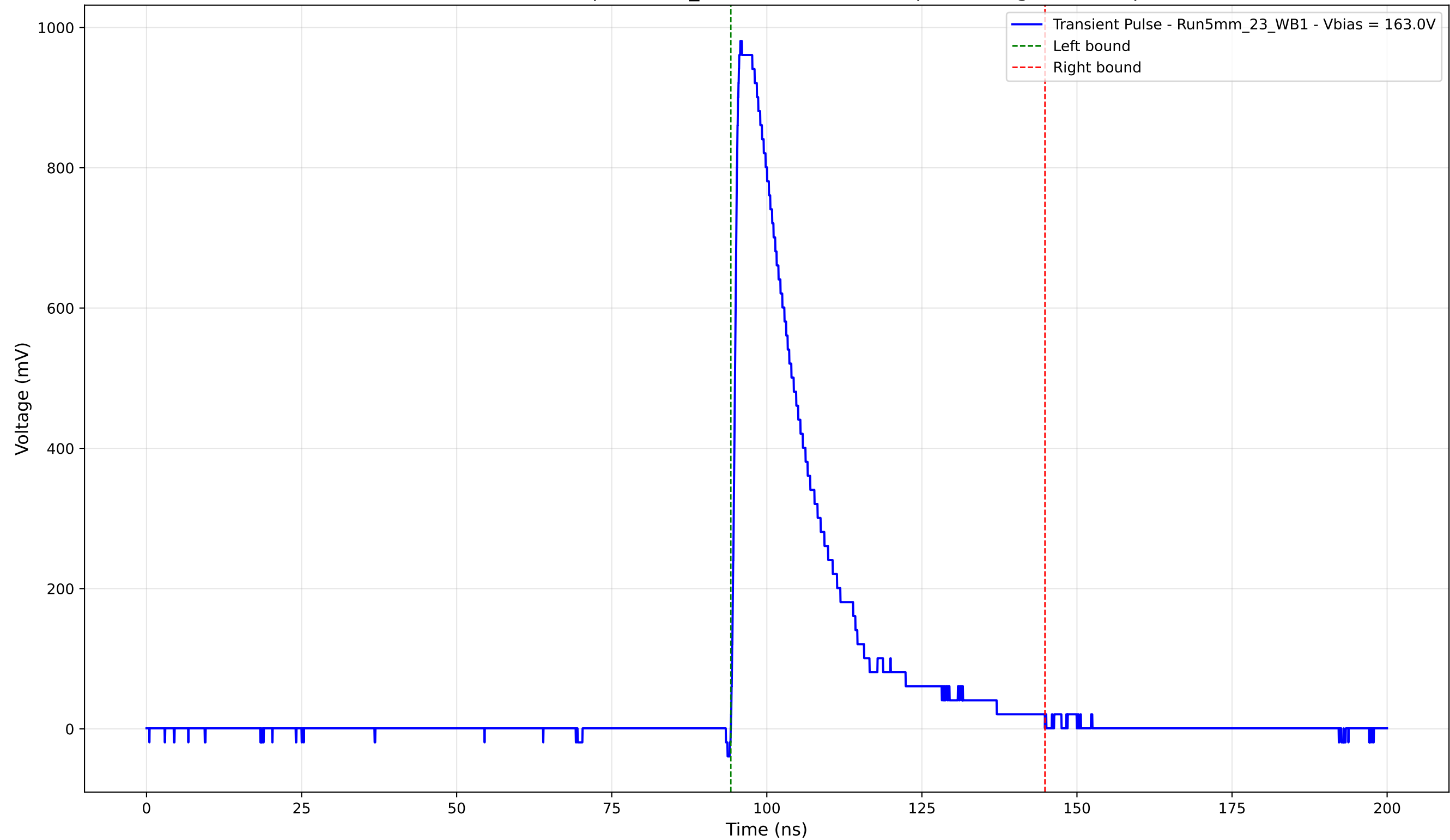
Transient Pulse - Sample: 5mm_23 - Position: 1970.0 \mu\text{m} - Charge: 240.42 pC
