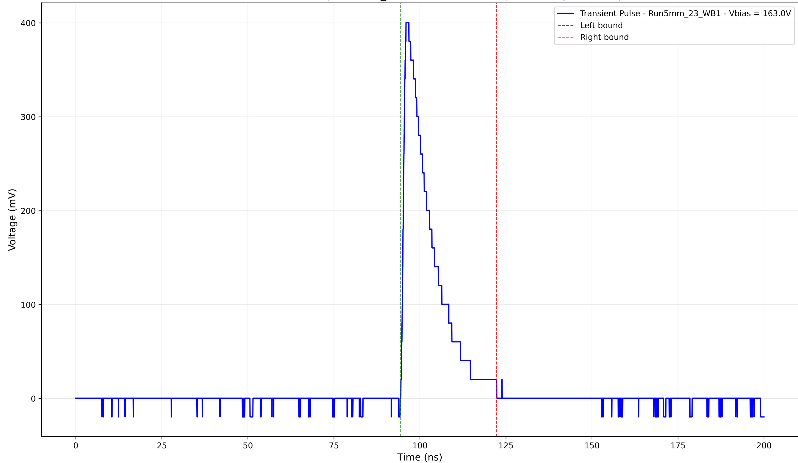
Transient Pulse - Sample: 5mm_23 - Position: 4225.0 \mu\text{m} - Charge: 71.68 pC
