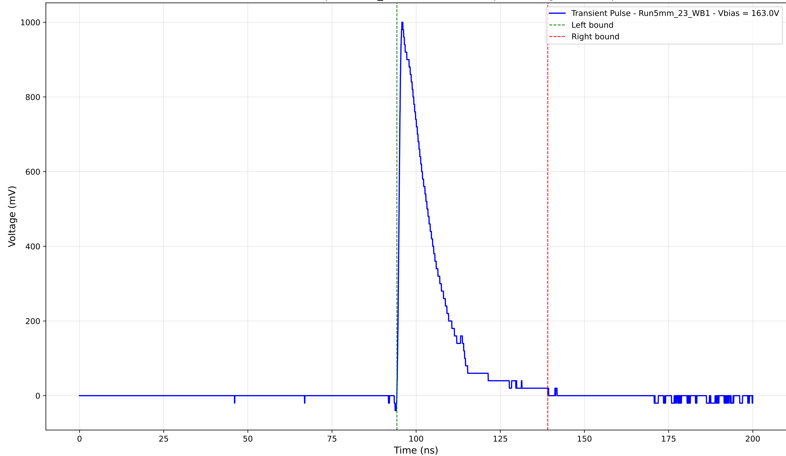
Transient Pulse - Sample: 5mm_23 - Position: 840.0 \mu\text{m} - Charge: 208.83 pC
