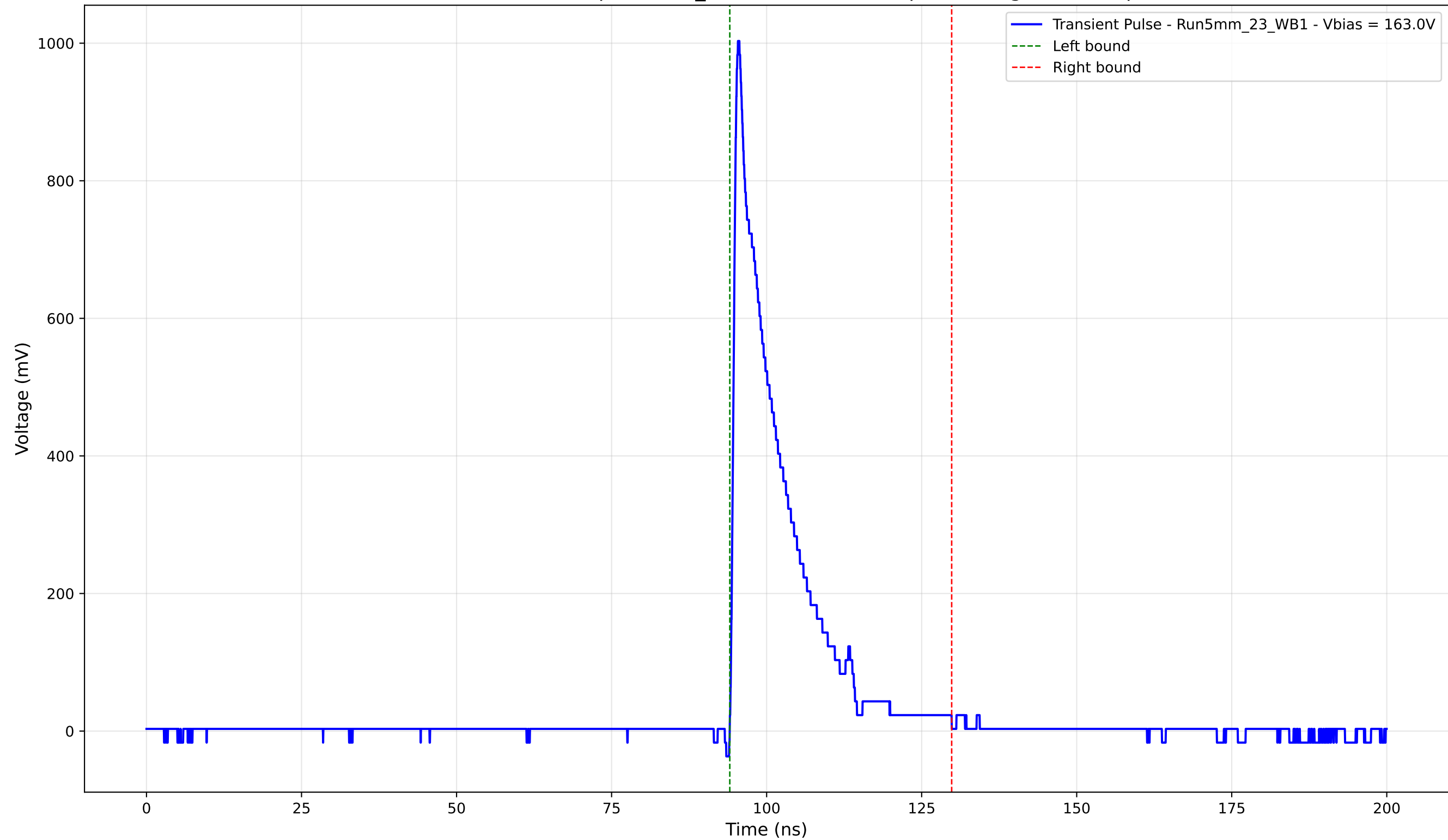
Transient Pulse - Sample: 5mm_23 - Position: 340.0 \mu\text{m} - Charge: 156.06 pC
