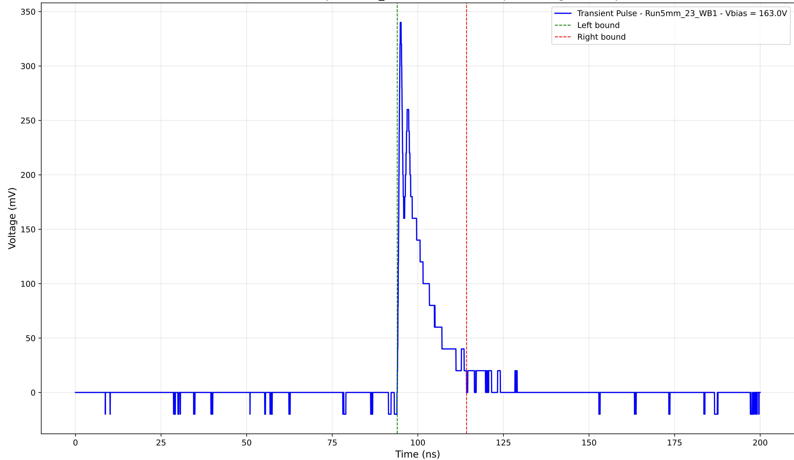
Transient Pulse - Sample: 5mm_23 - Position: 2745.0 \mu\text{m} - Charge: 41.35 pC
