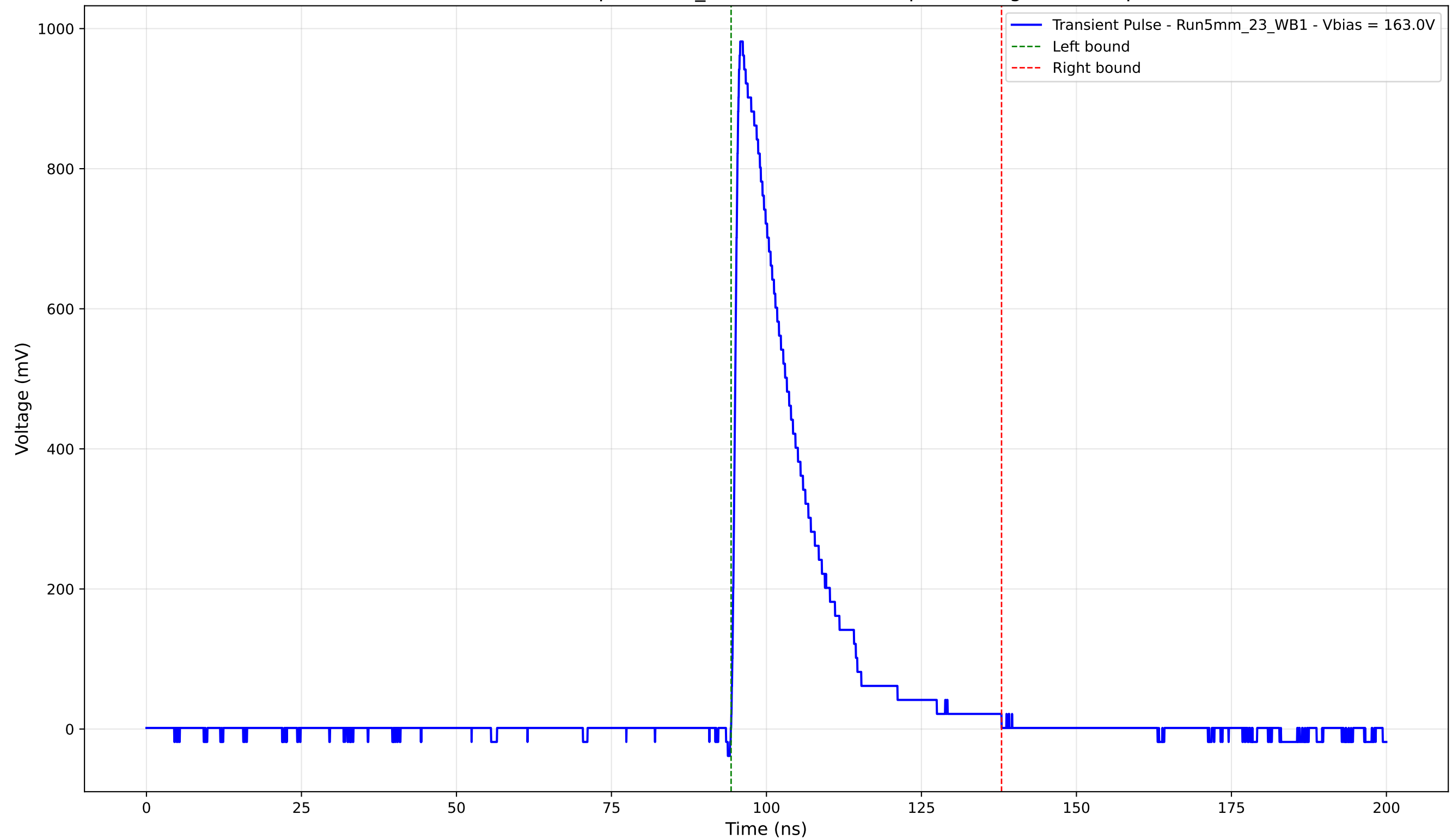
Transient Pulse - Sample: 5mm_23 - Position: 880.0 \mu\text{m} - Charge: 204.39 pC
