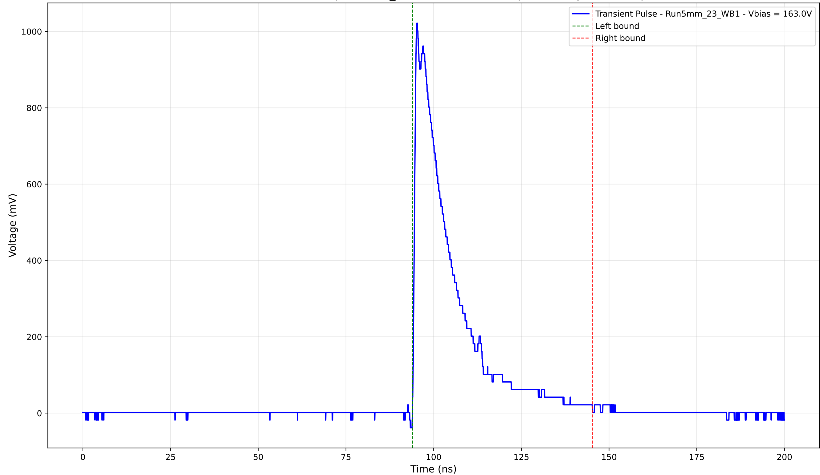
Transient Pulse - Sample: 5mm_23 - Position: 3045.0 \mu\text{m} - Charge: 230.36 pC
