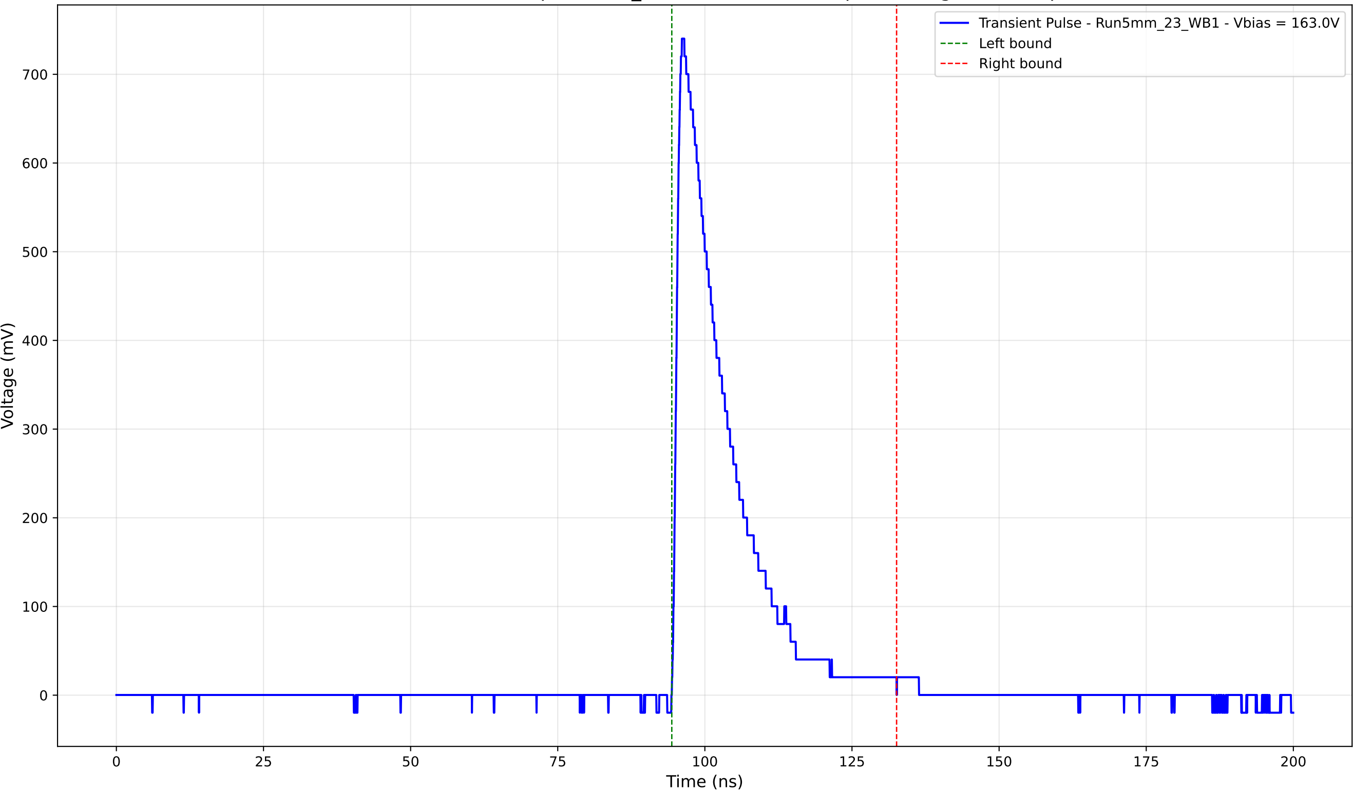
Transient Pulse - Sample: 5mm_23 - Position: 4195.0 \mu\text{m} - Charge: 139.27 pC
