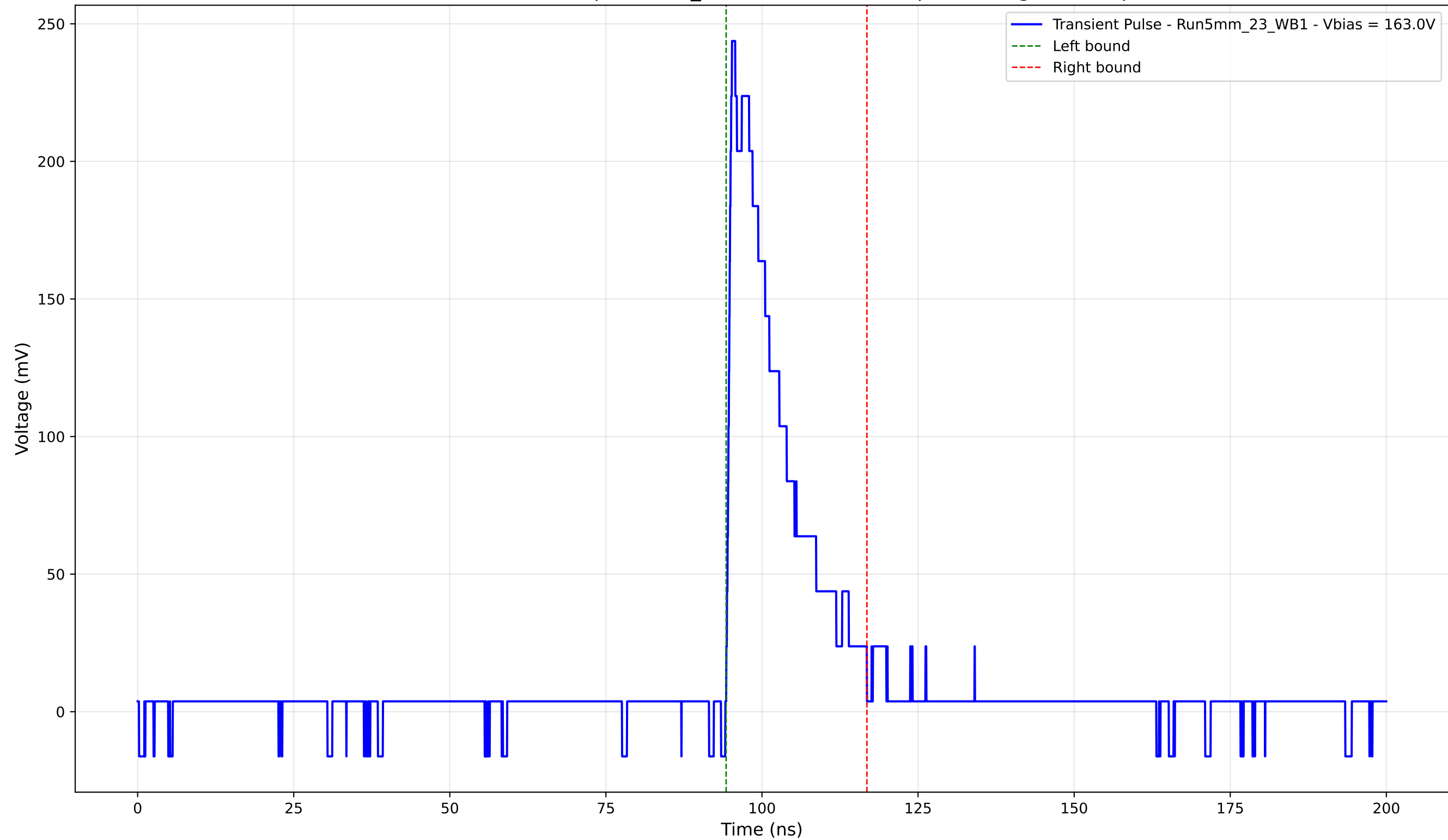
Transient Pulse - Sample: 5mm_23 - Position: 3235.0 \mu\text{m} - Charge: 44.17 pC
