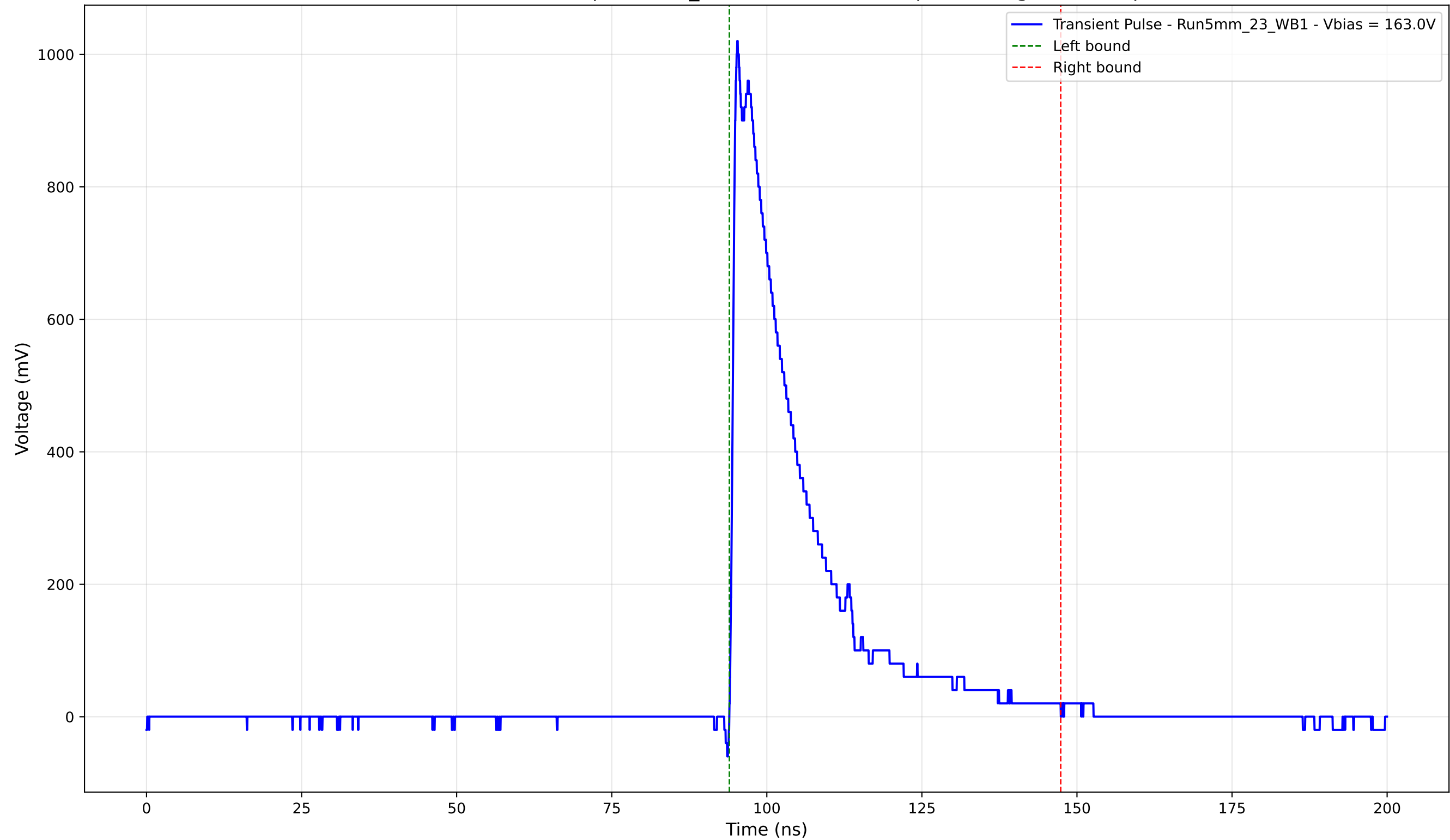
Transient Pulse - Sample: 5mm_23 - Position: 3050.0 \mu\text{m} - Charge: 229.61 pC
