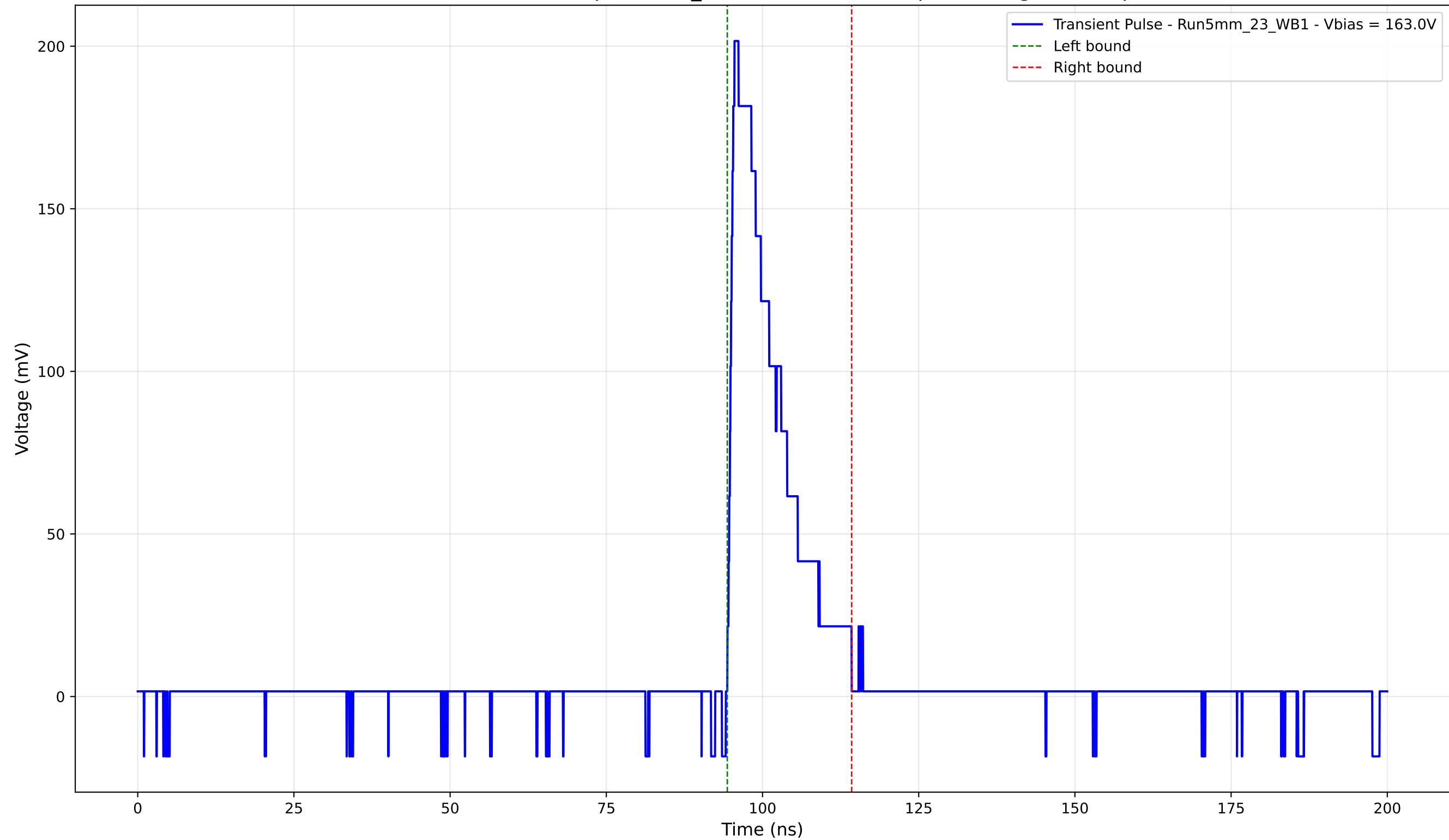
Transient Pulse - Sample: 5mm_23 - Position: 4765.0 \mu\text{m} - Charge: 32.85 pC
