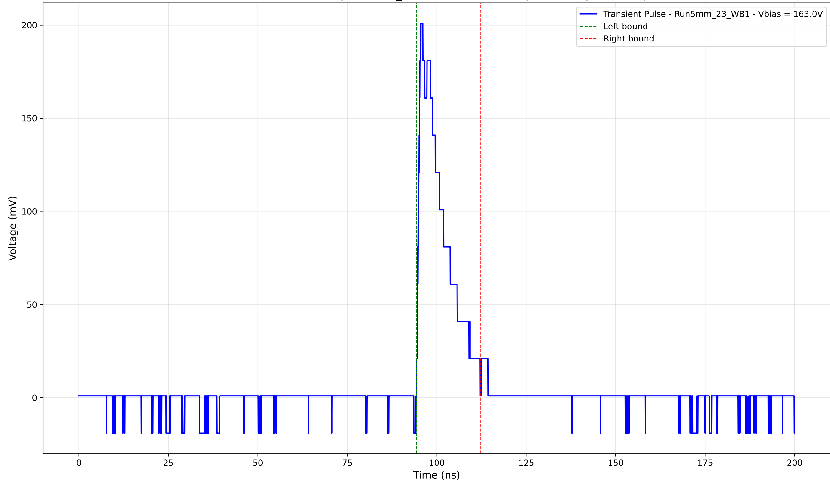
Transient Pulse - Sample: 5mm_23 - Position: 4770.0 \mu\text{m} - Charge: 30.80 pC
