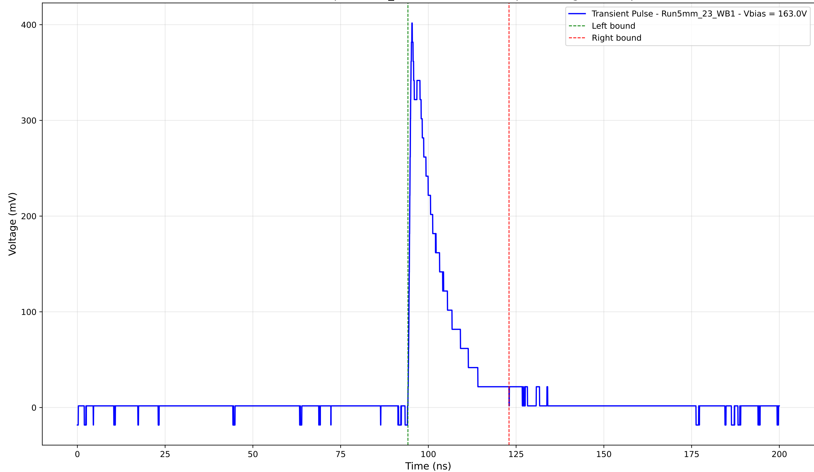
Transient Pulse - Sample: 5mm_23 - Position: 3220.0 \mu\text{m} - Charge: 66.96 pC
