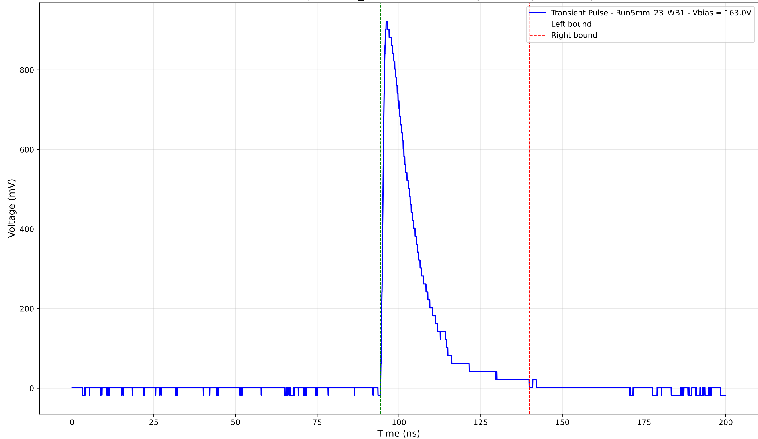
Transient Pulse - Sample: 5mm_23 - Position: 4000.0 \mu\text{m} - Charge: 200.01 pC
