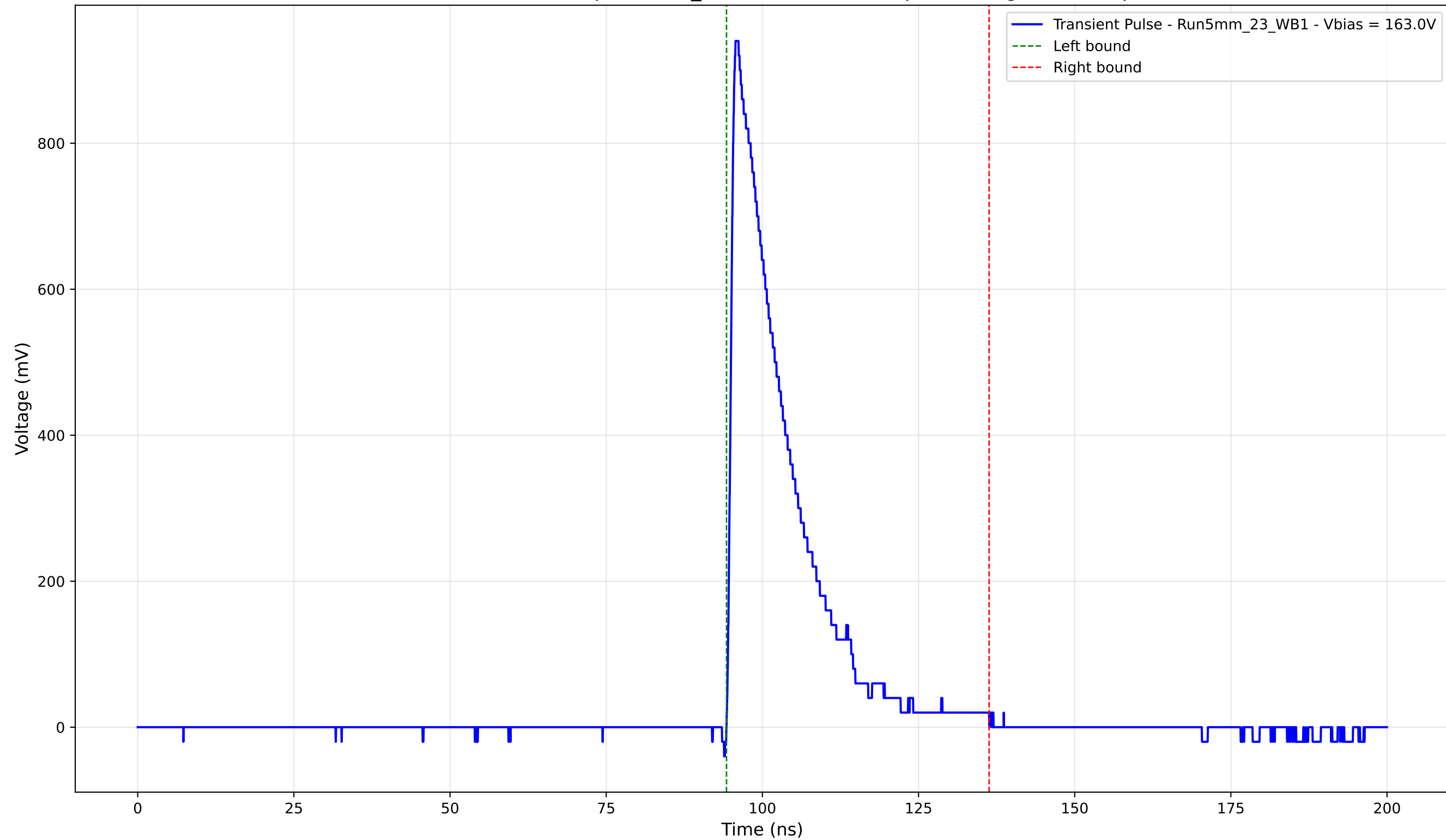
Transient Pulse - Sample: 5mm_23 - Position: 795.0 \mu\text{m} - Charge: 181.95 pC
