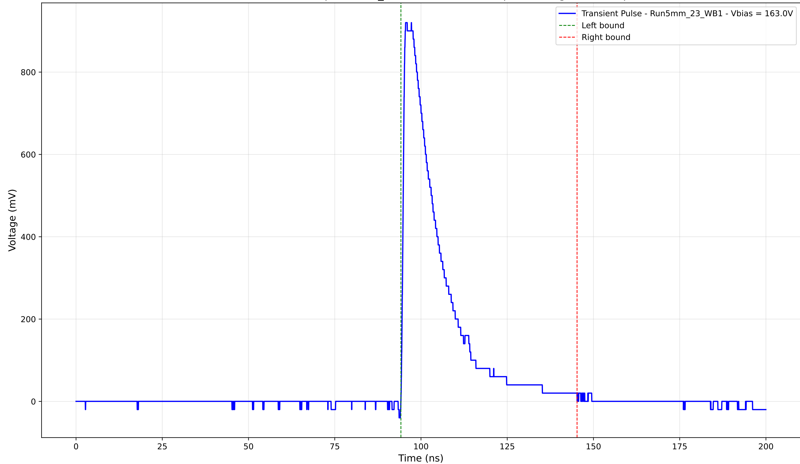
Transient Pulse - Sample: 5mm_23 - Position: 3430.0 \mu\text{m} - Charge: 214.21 pC
