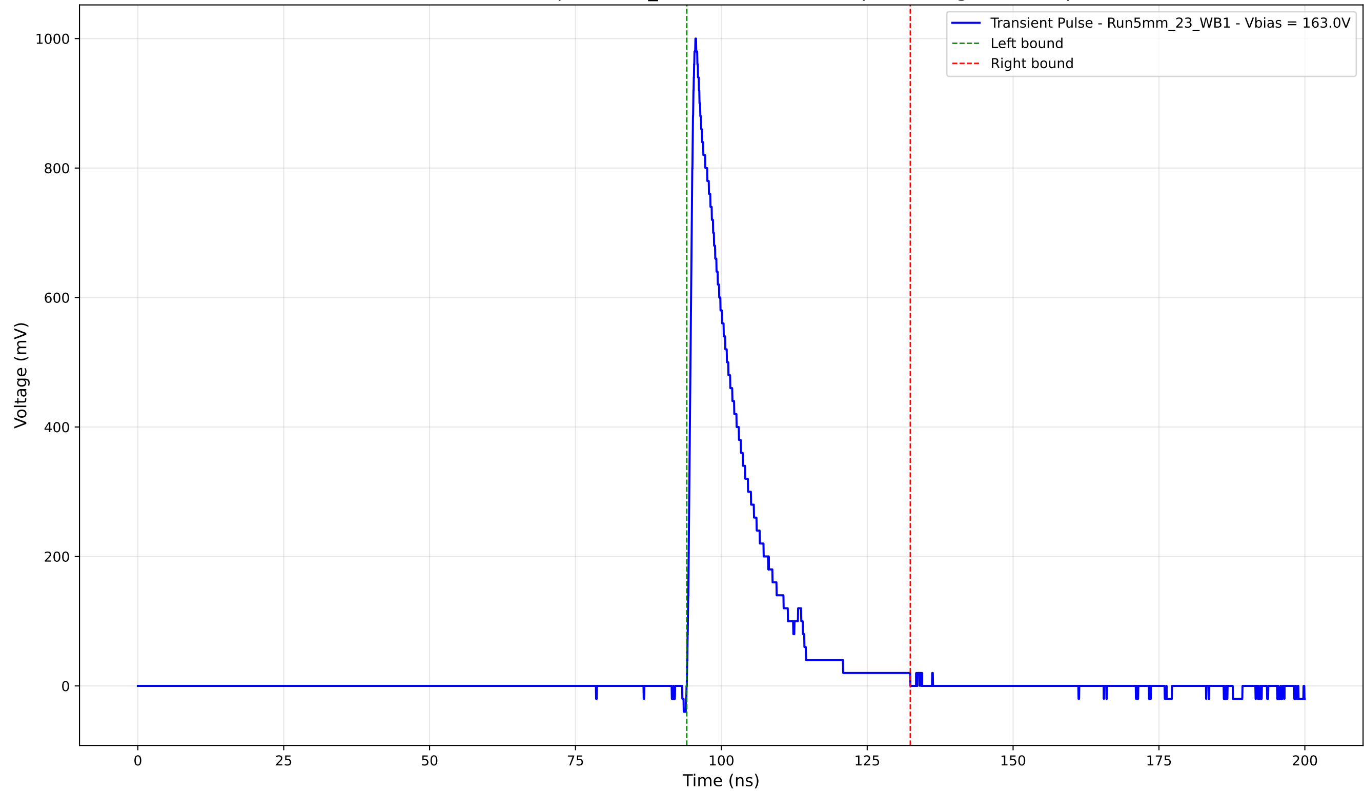
Transient Pulse - Sample: 5mm_23 - Position: 4935.0 \mu\text{m} - Charge: 167.44 pC
