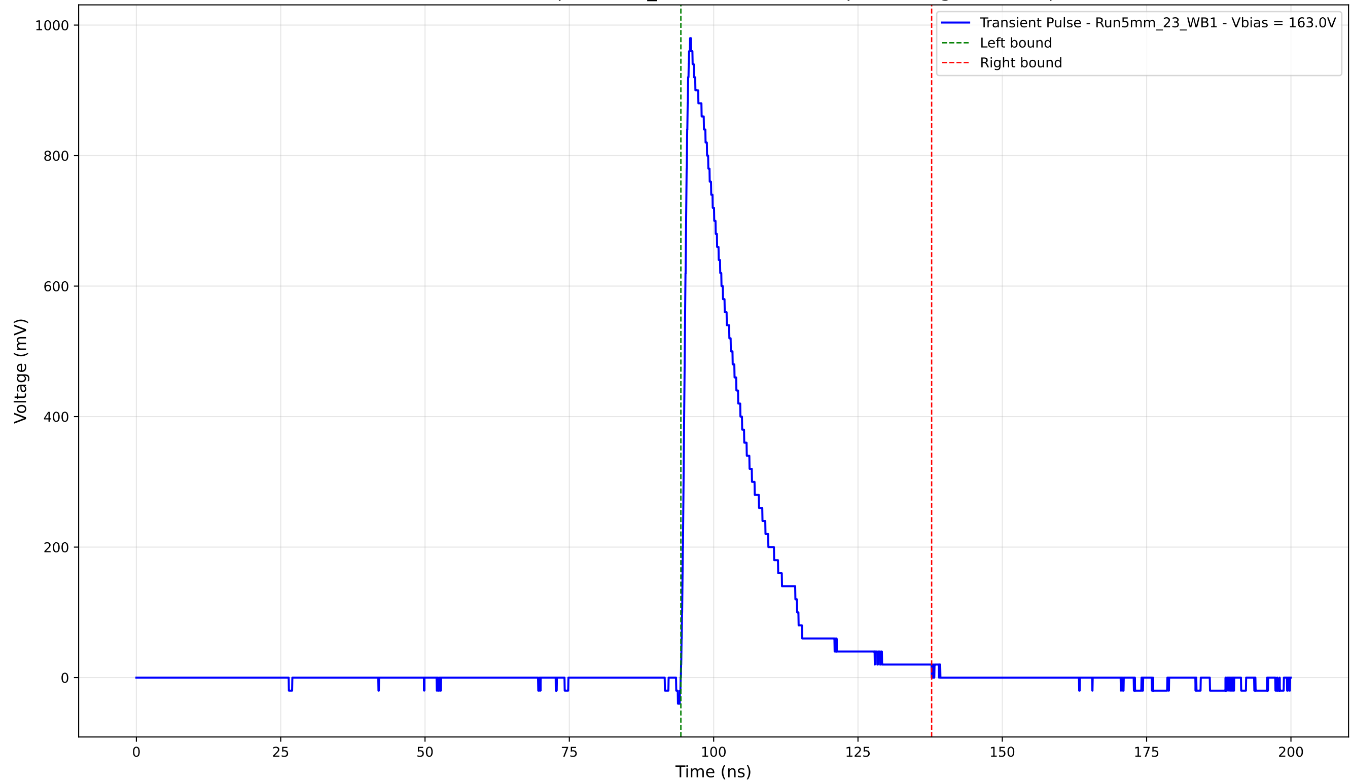
Transient Pulse - Sample: 5mm_23 - Position: 915.0 \mu\text{m} - Charge: 201.70 pC
