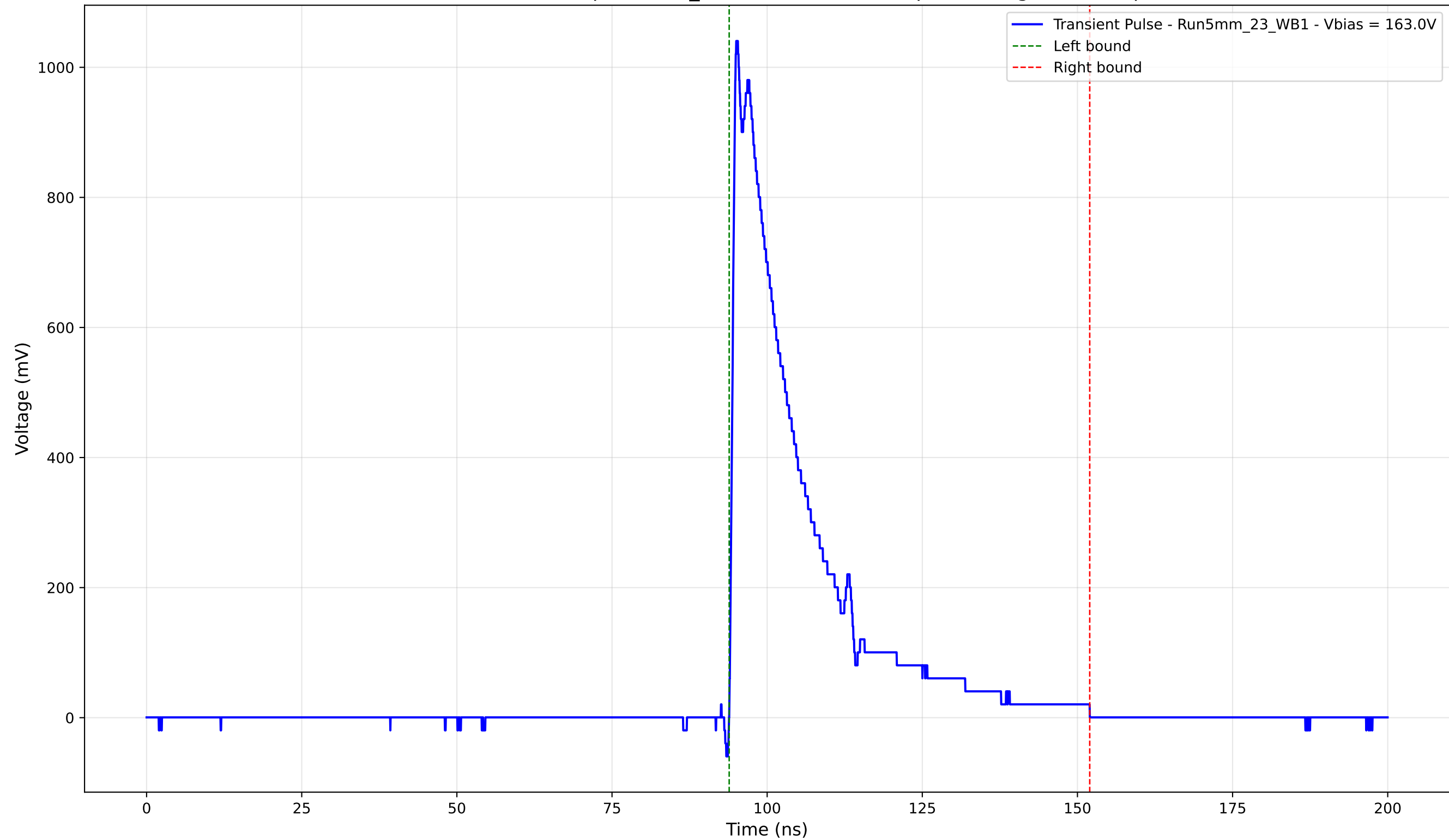
Transient Pulse - Sample: 5mm_23 - Position: 2920.0 \mu\text{m} - Charge: 238.92 pC
