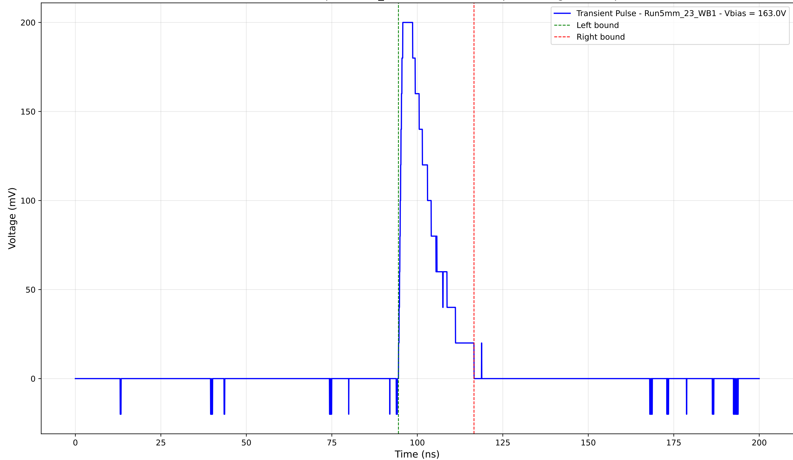
Transient Pulse - Sample: 5mm_23 - Position: 3745.0 \mu\text{m} - Charge: 39.28 pC
