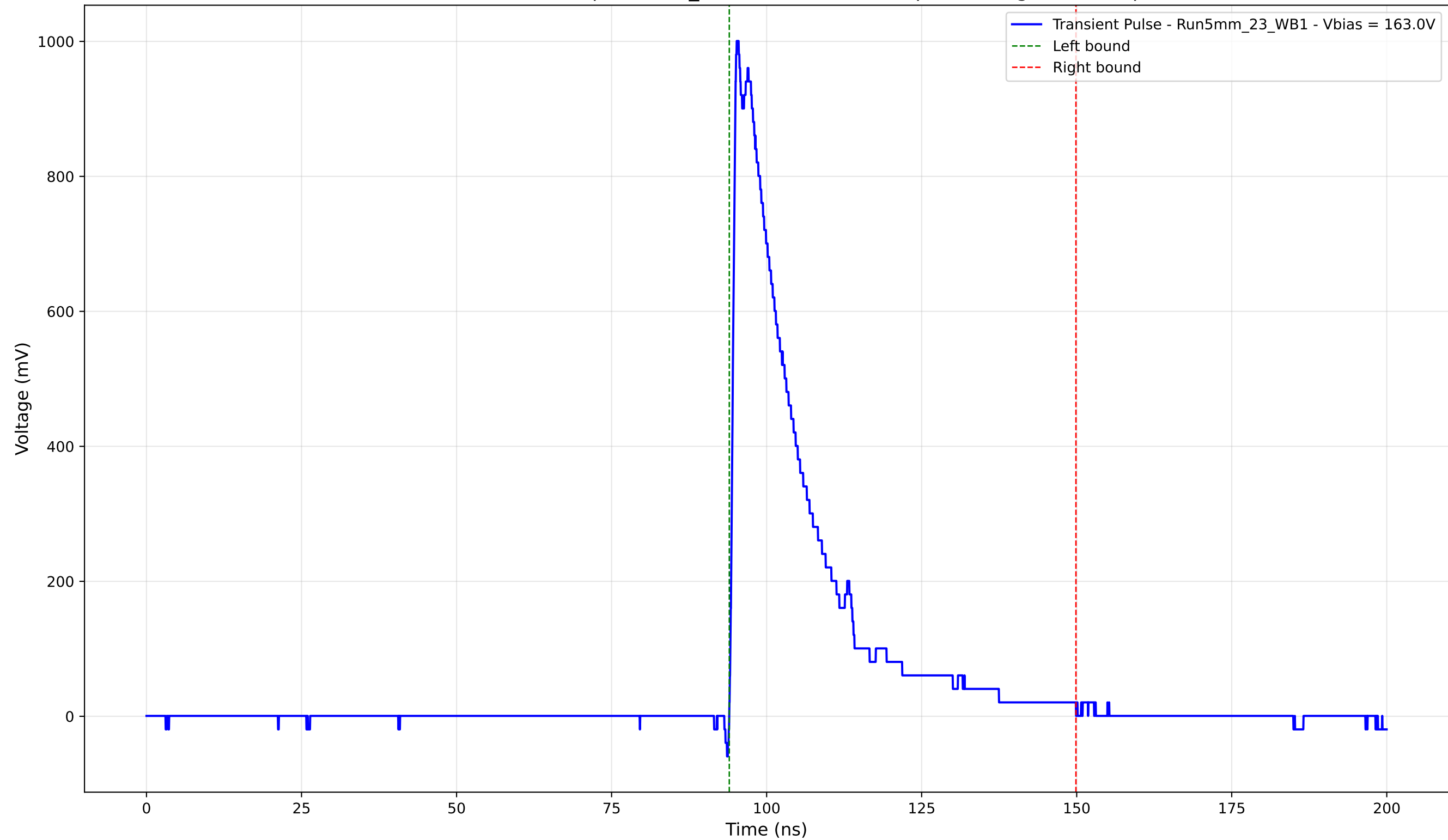
Transient Pulse - Sample: 5mm_23 - Position: 2400.0 \mu\text{m} - Charge: 230.40 pC
