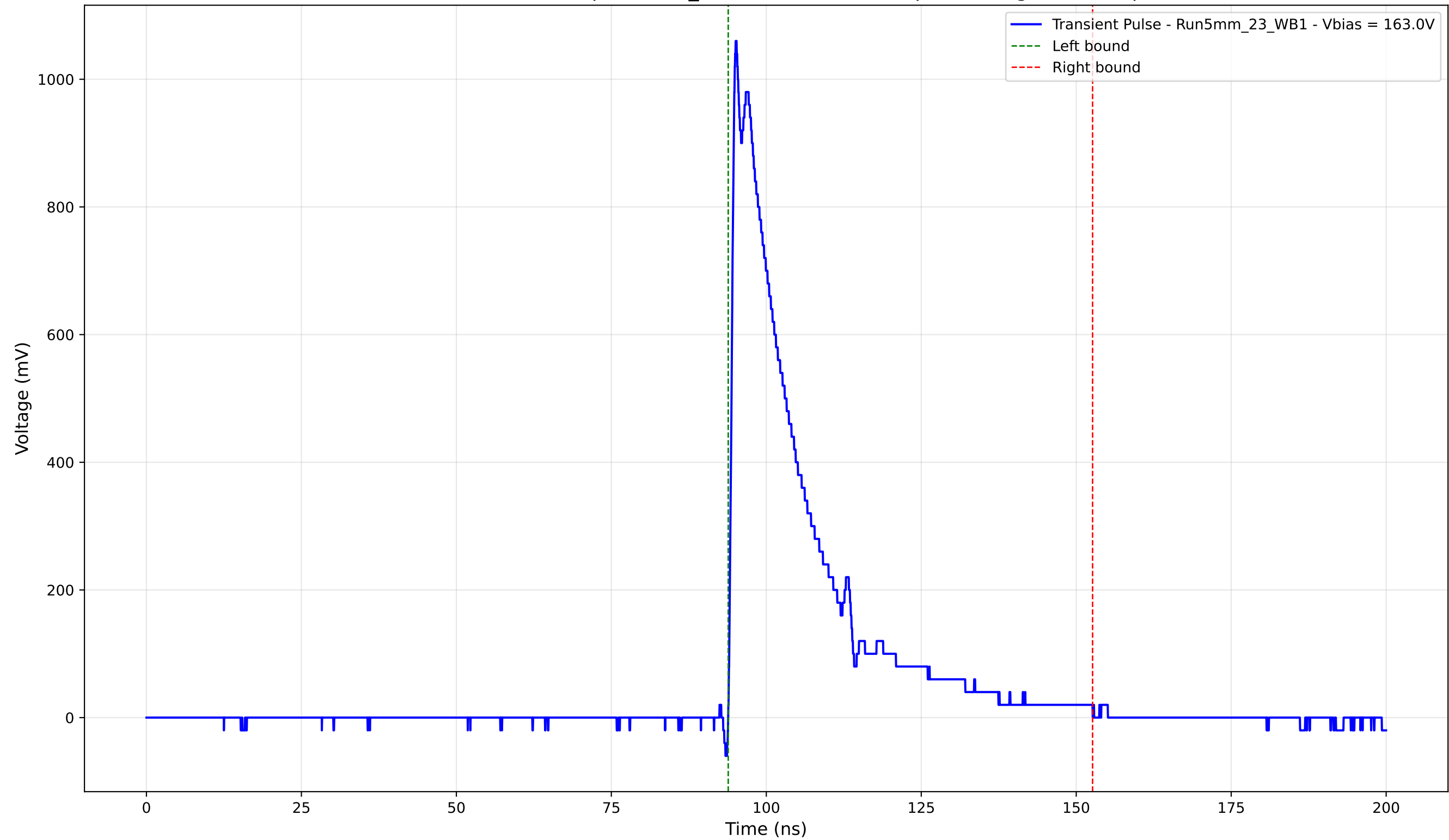
Transient Pulse - Sample: 5mm_23 - Position: 2585.0 \mu\text{m} - Charge: 241.38 pC
