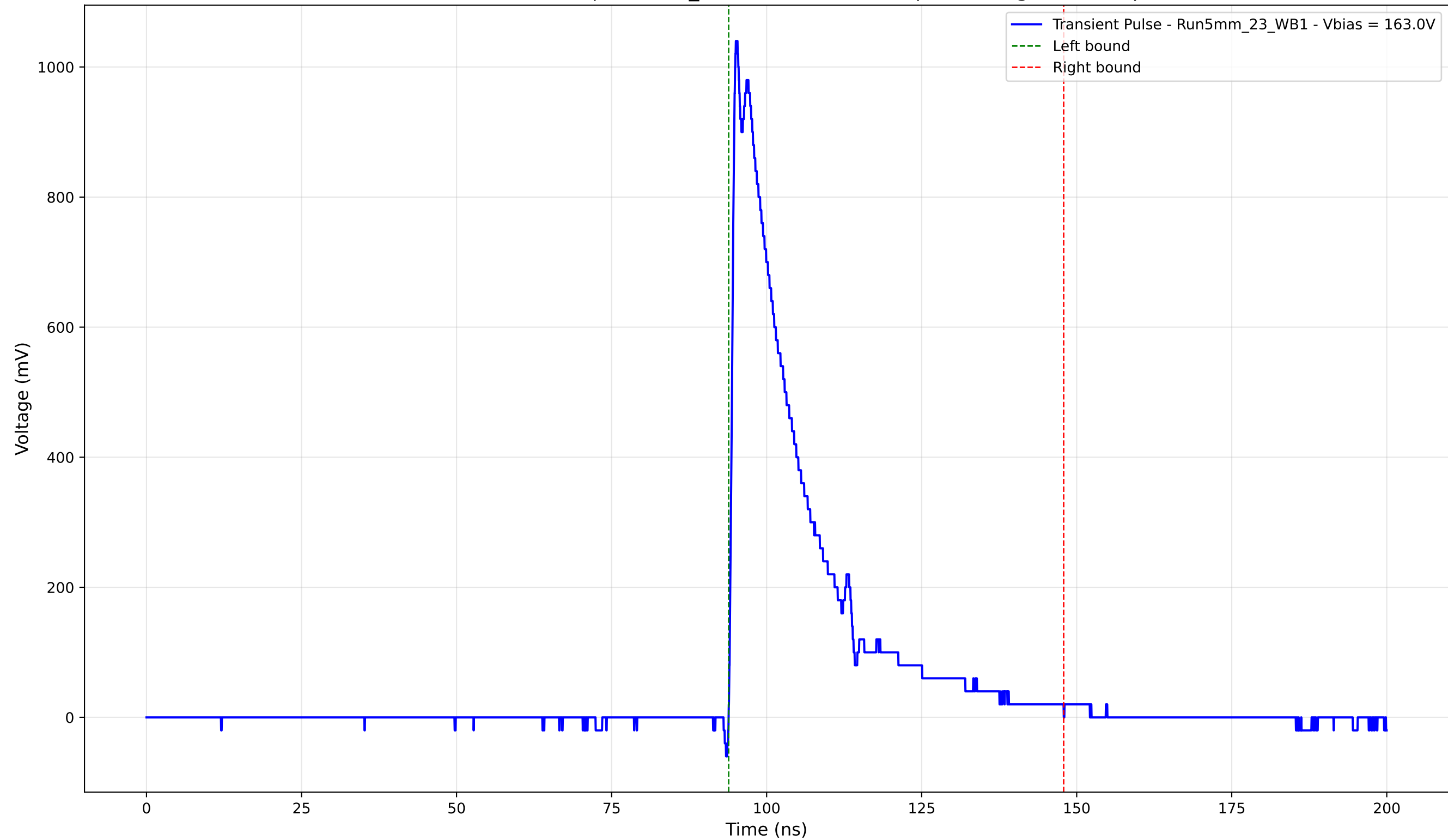
Transient Pulse - Sample: 5mm_23 - Position: 2560.0 \mu\text{m} - Charge: 238.30 pC
