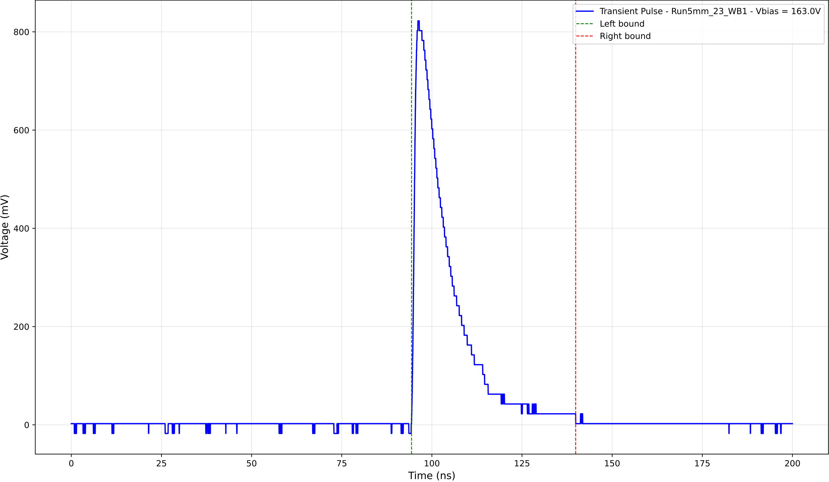
Transient Pulse - Sample: 5mm_23 - Position: 3835.0 \mu\text{m} - Charge: 173.69 pC
