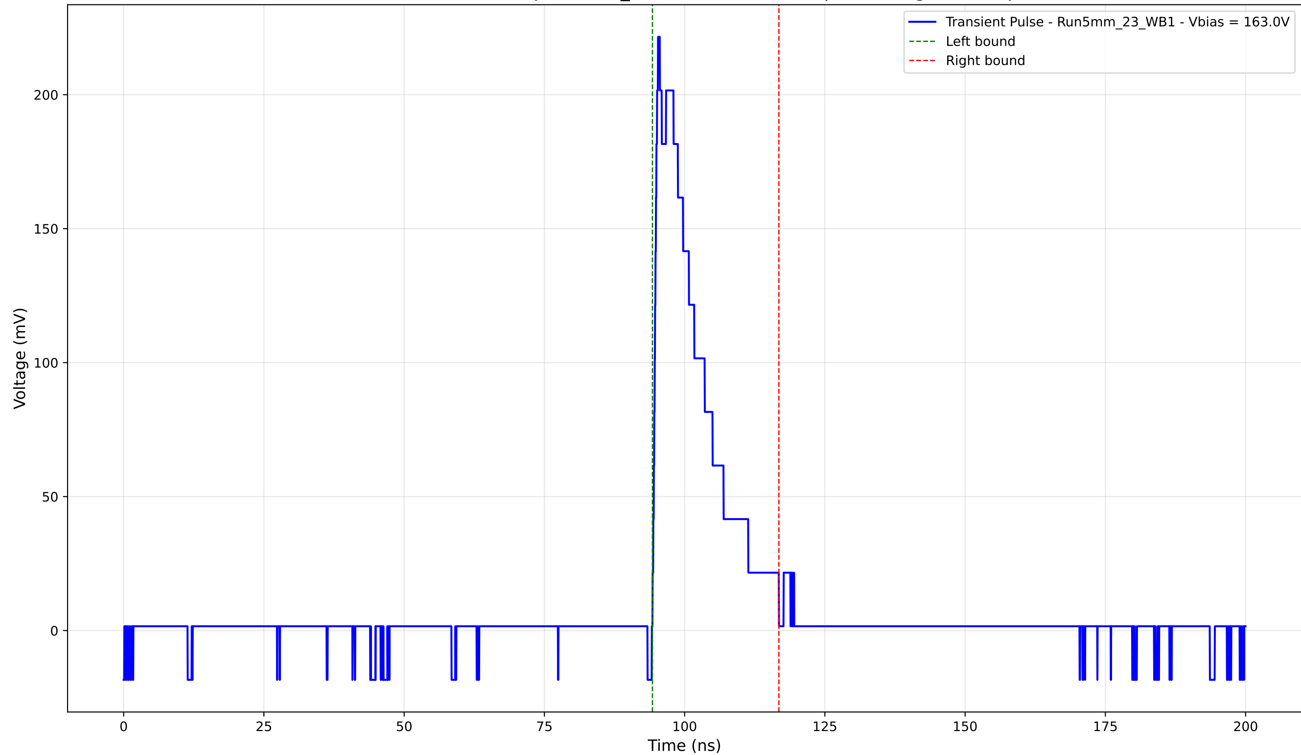
Transient Pulse - Sample: 5mm_23 - Position: 3240.0 \mu\text{m} - Charge: 38.87 pC
