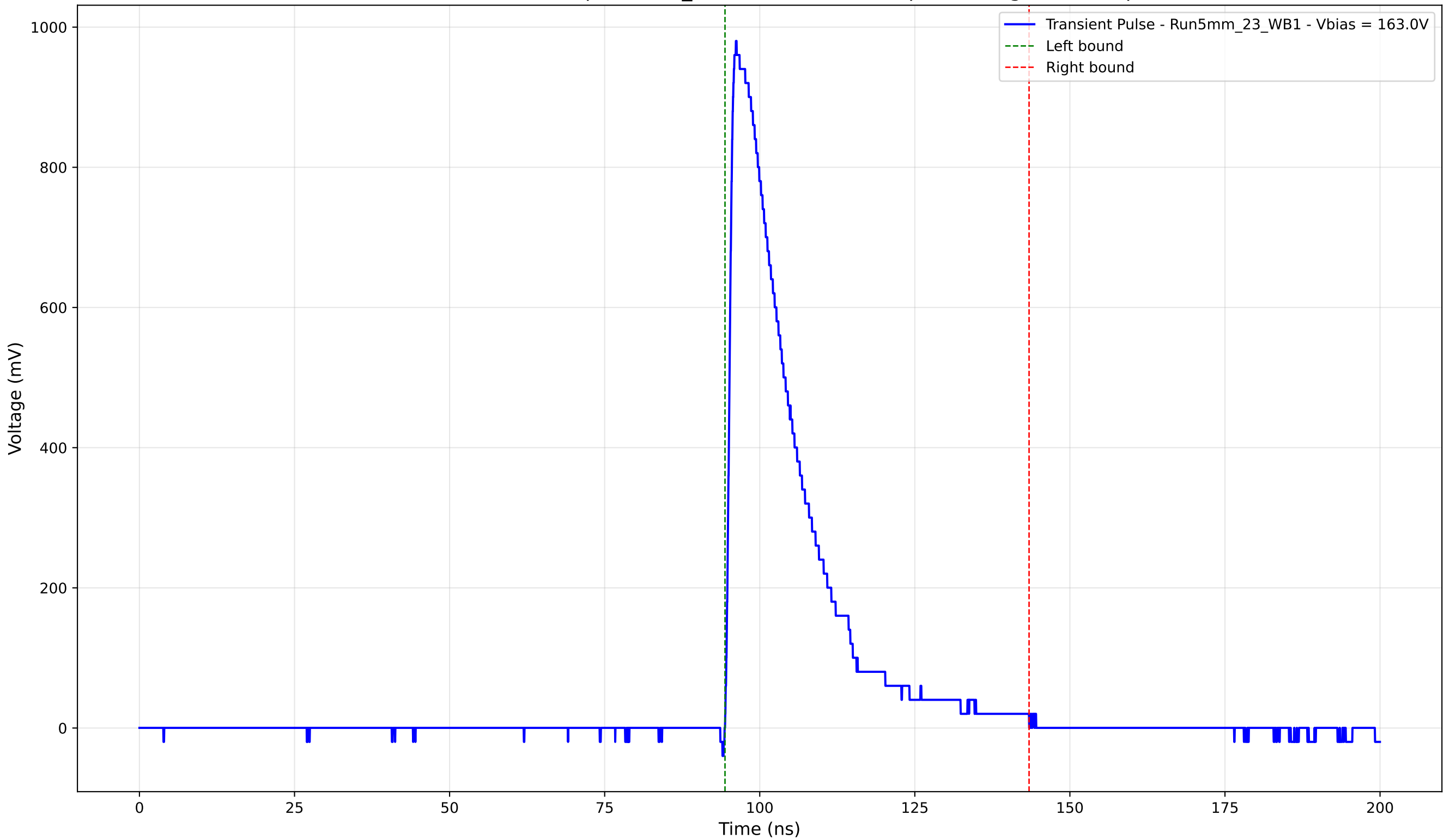
Transient Pulse - Sample: 5mm_23 - Position: 1370.0 \mu\text{m} - Charge: 225.27 pC
