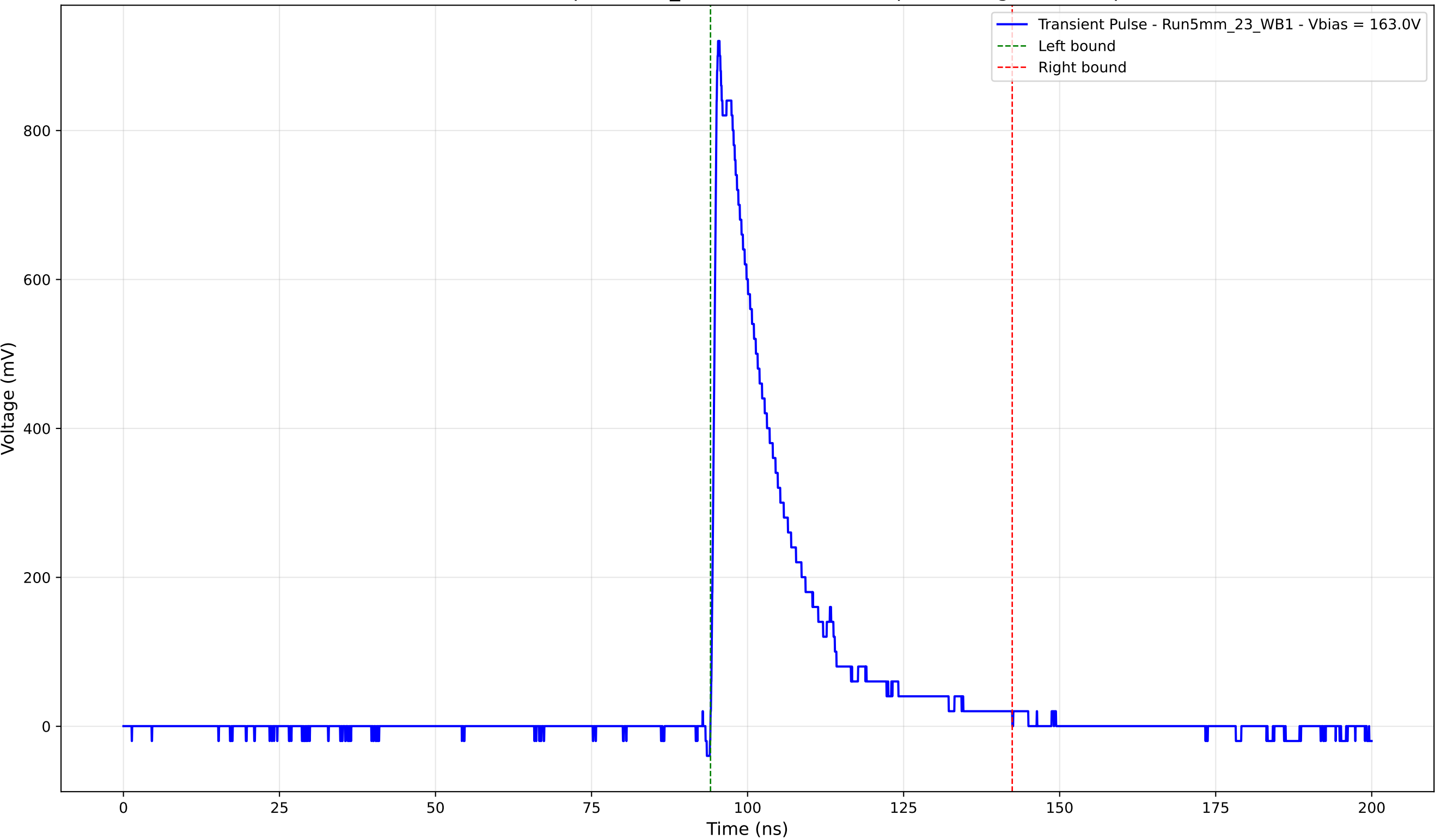
Transient Pulse - Sample: 5mm_23 - Position: 3170.0 \mu\text{m} - Charge: 189.69 pC
