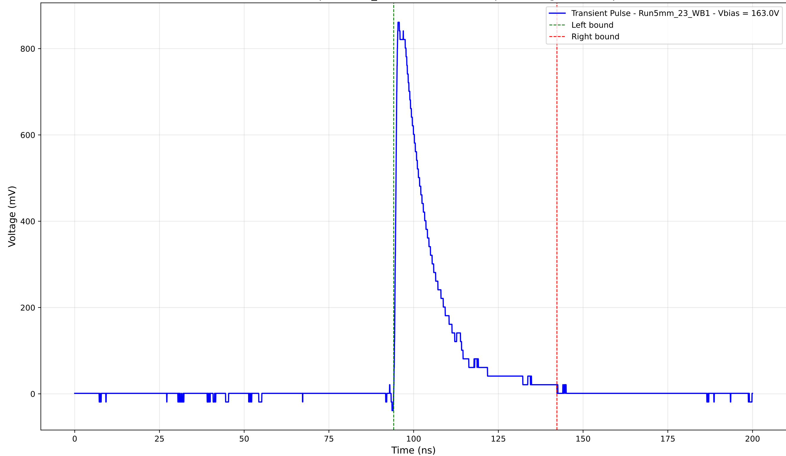
Transient Pulse - Sample: 5mm_23 - Position: 2170.0 \mu\text{m} - Charge: 187.69 pC
