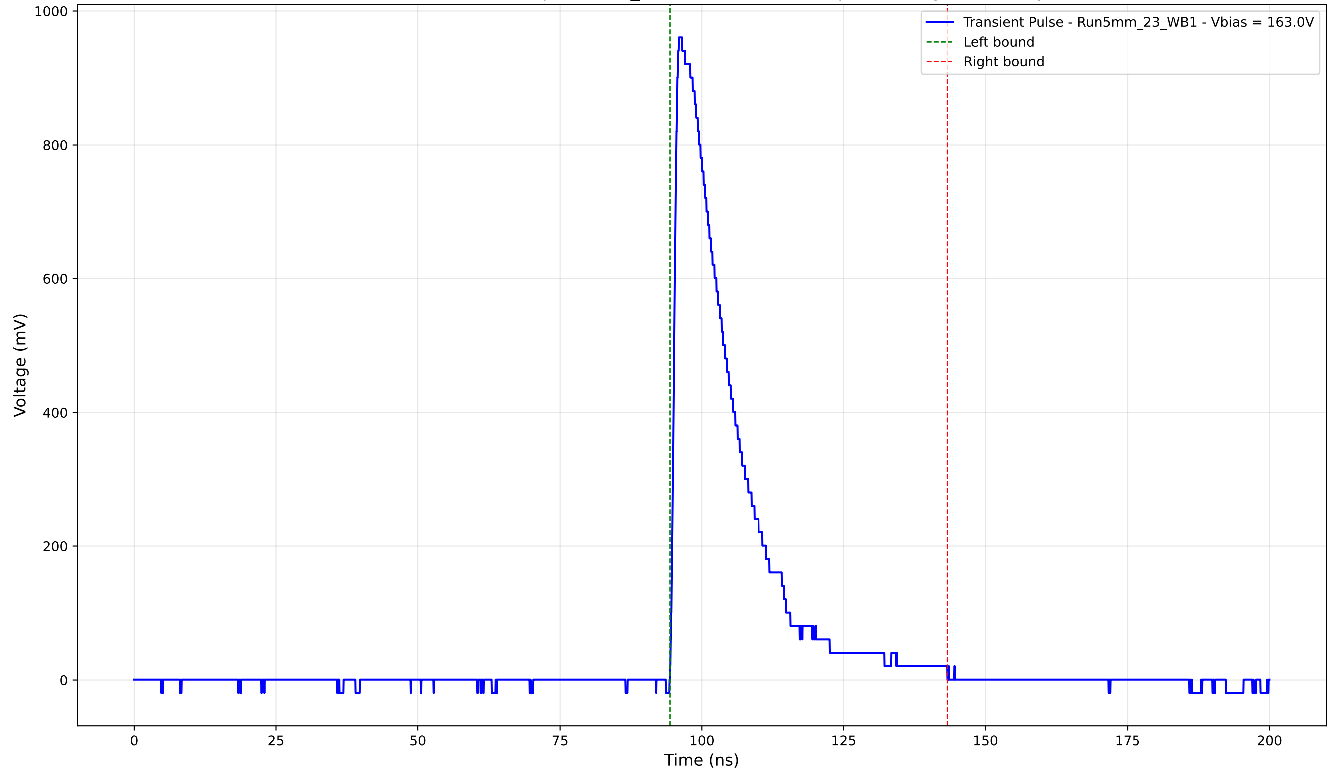
Transient Pulse - Sample: 5mm_23 - Position: 1345.0 \mu\text{m} - Charge: 220.80 pC
