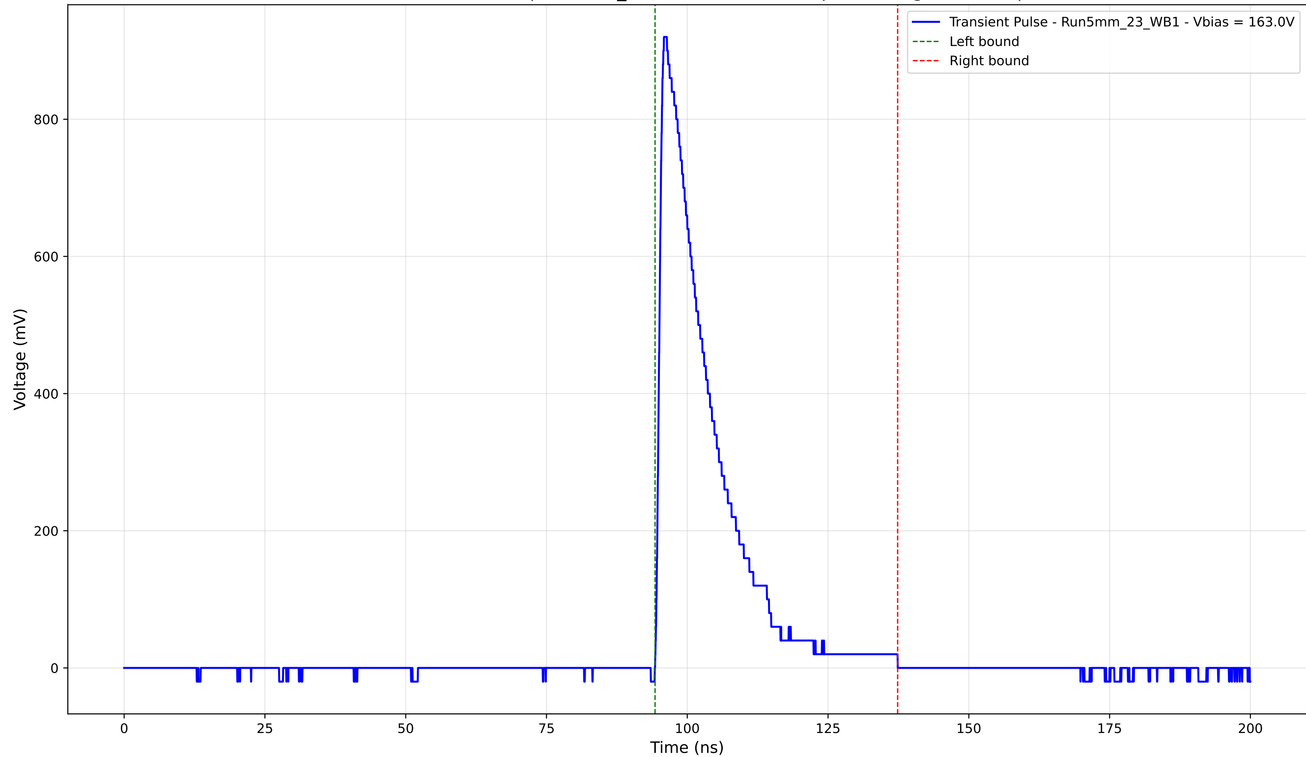
Transient Pulse - Sample: 5mm_23 - Position: 4470.0 \mu\text{m} - Charge: 180.06 pC
