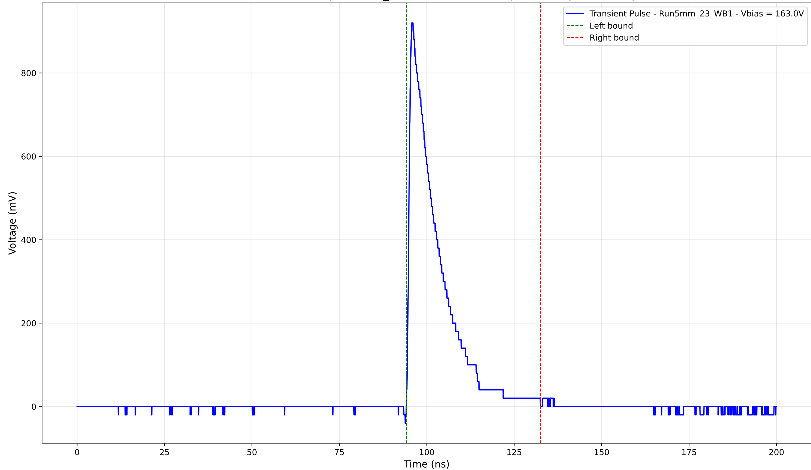
Transient Pulse - Sample: 5mm_23 - Position: 4675.0 \mu\text{m} - Charge: 164.54 pC
