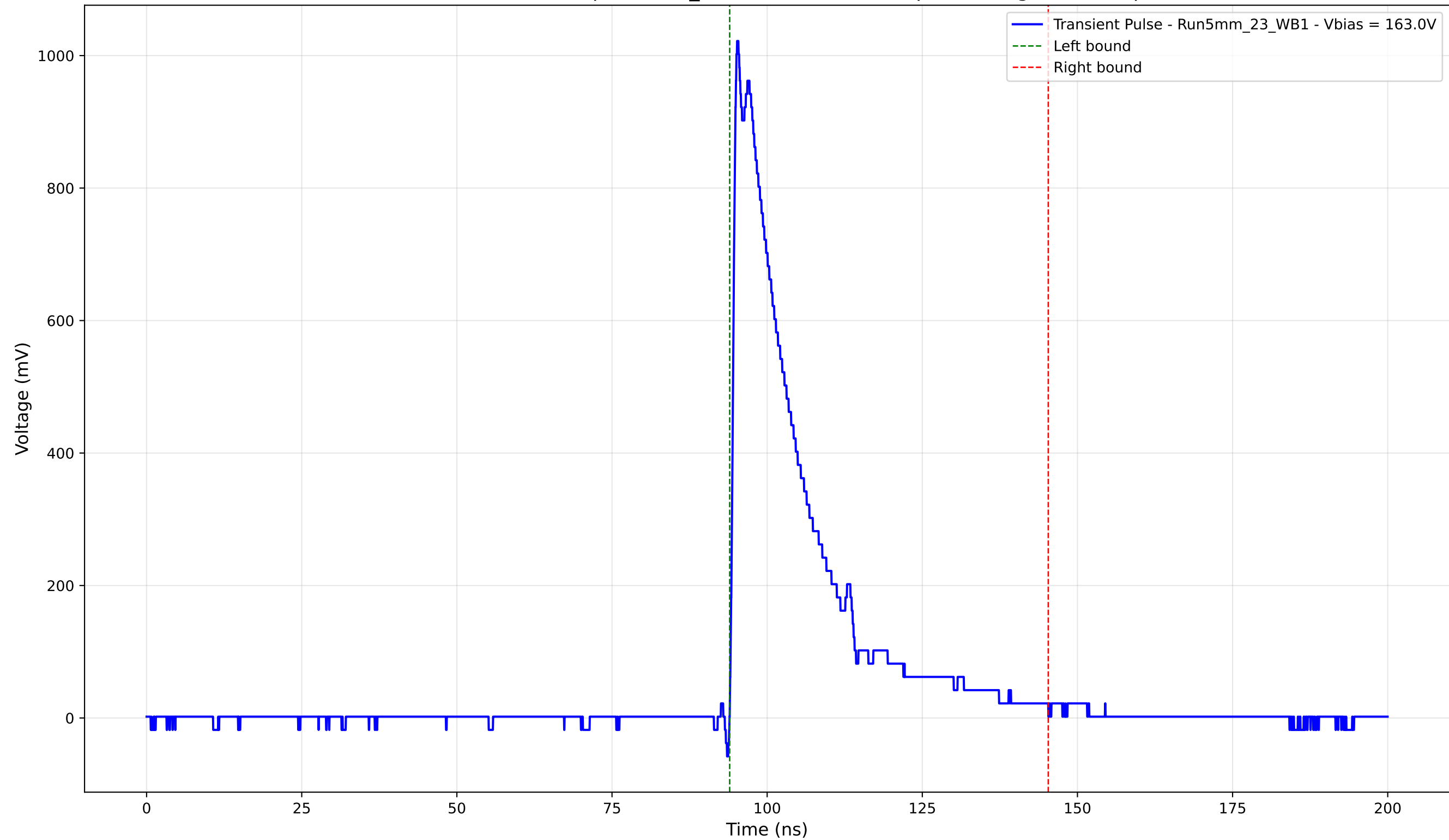
Transient Pulse - Sample: 5mm_23 - Position: 3025.0 \mu\text{m} - Charge: 230.33 pC
