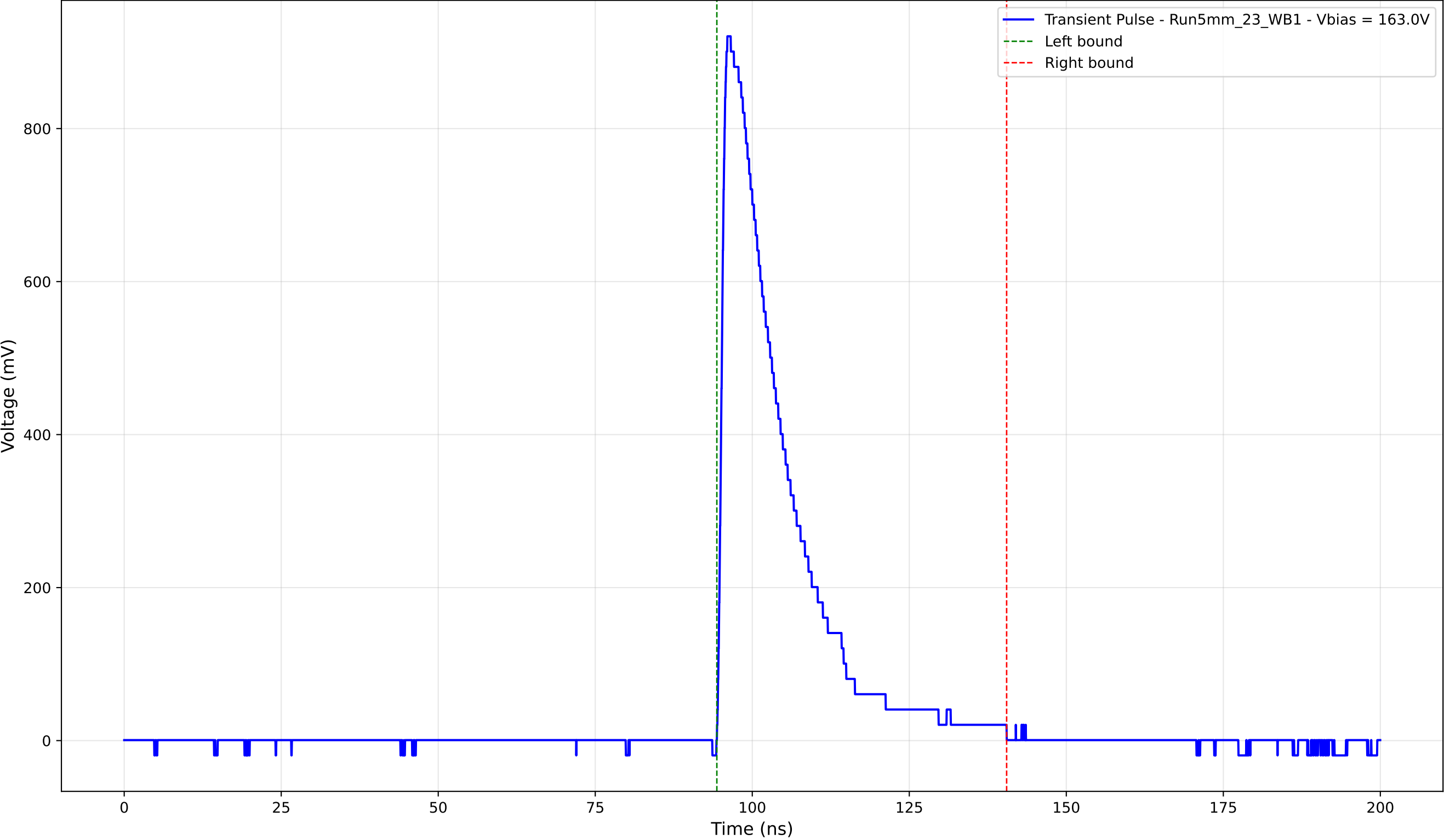
Transient Pulse - Sample: 5mm_23 - Position: 4025.0 \mu\text{m} - Charge: 199.75 pC
