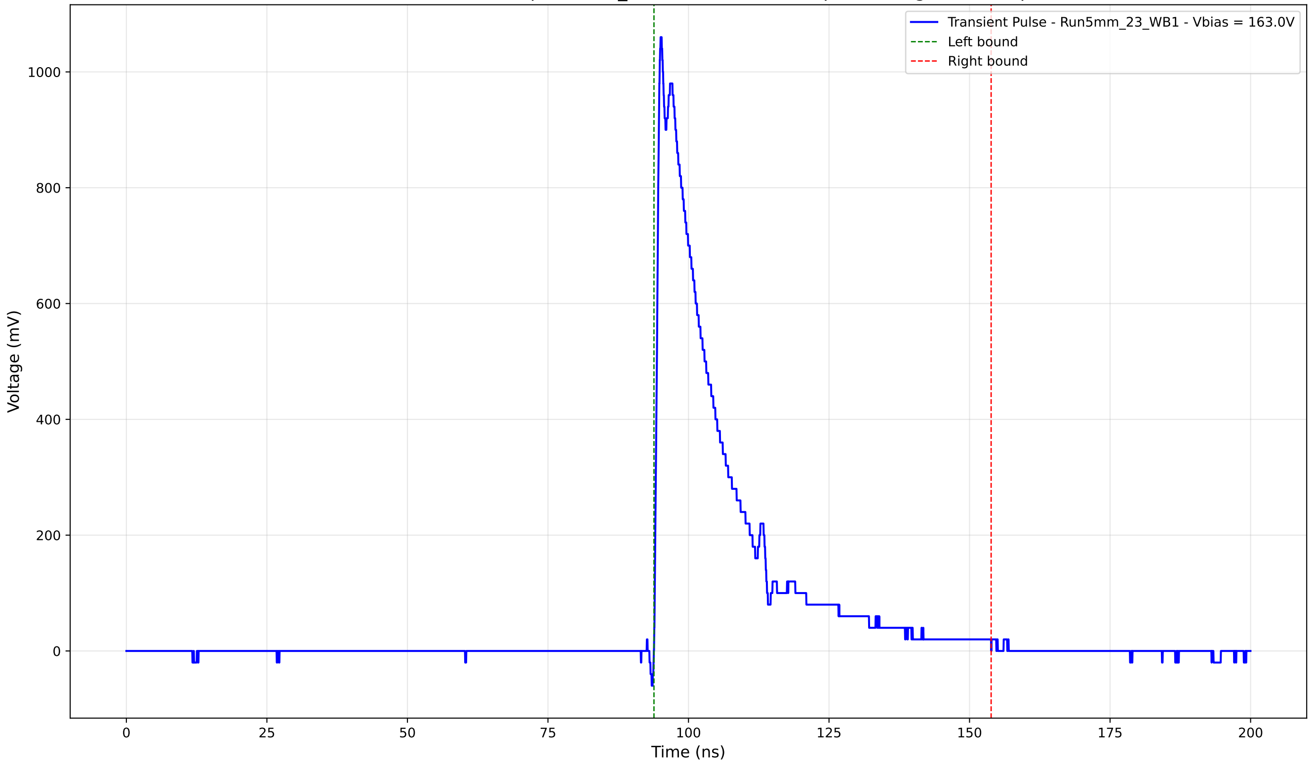
Transient Pulse - Sample: 5mm_23 - Position: 2890.0 \mu\text{m} - Charge: 242.98 pC
