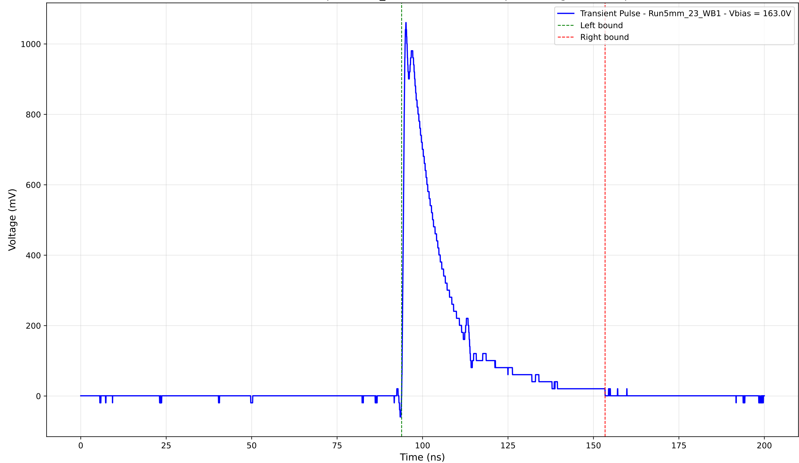
Transient Pulse - Sample: 5mm_23 - Position: 2575.0 \mu\text{m} - Charge: 242.81 pC
