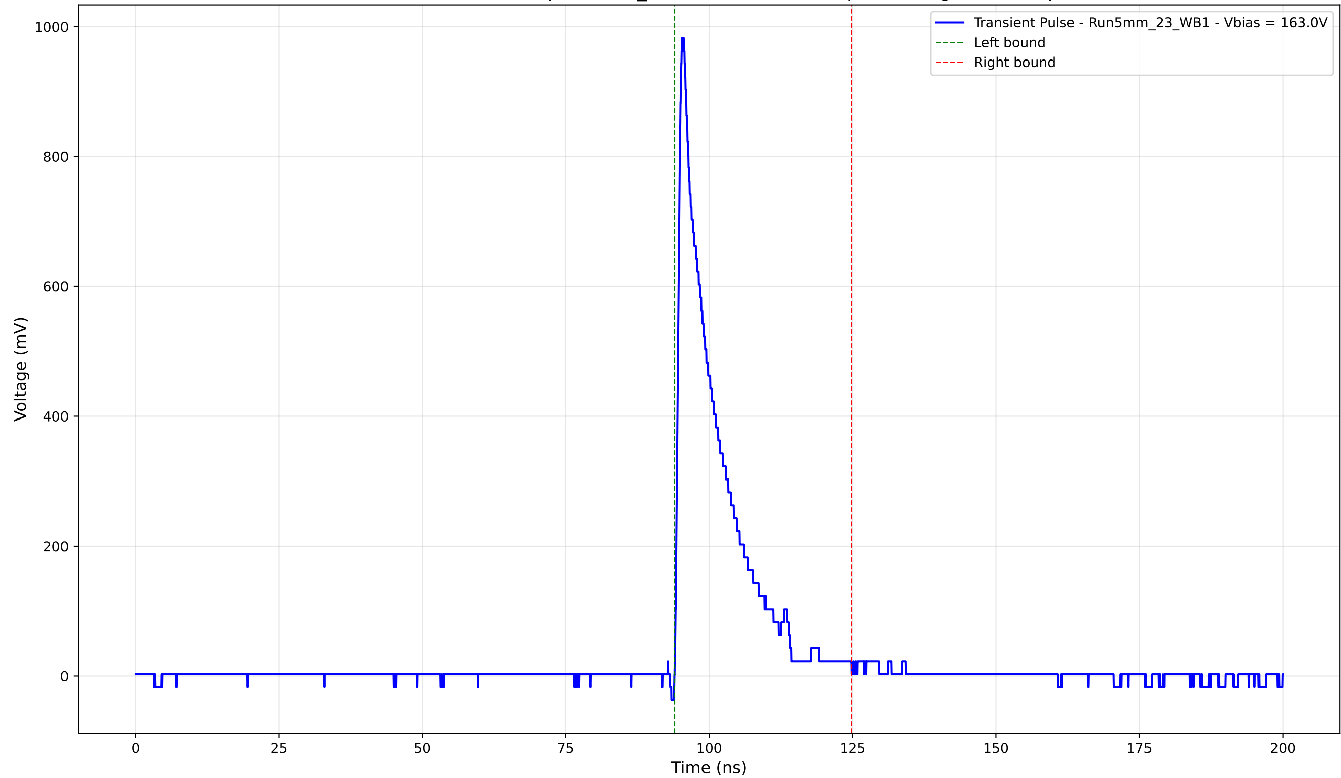
Transient Pulse - Sample: 5mm_23 - Position: 5135.0 \mu\text{m} - Charge: 139.53 pC
