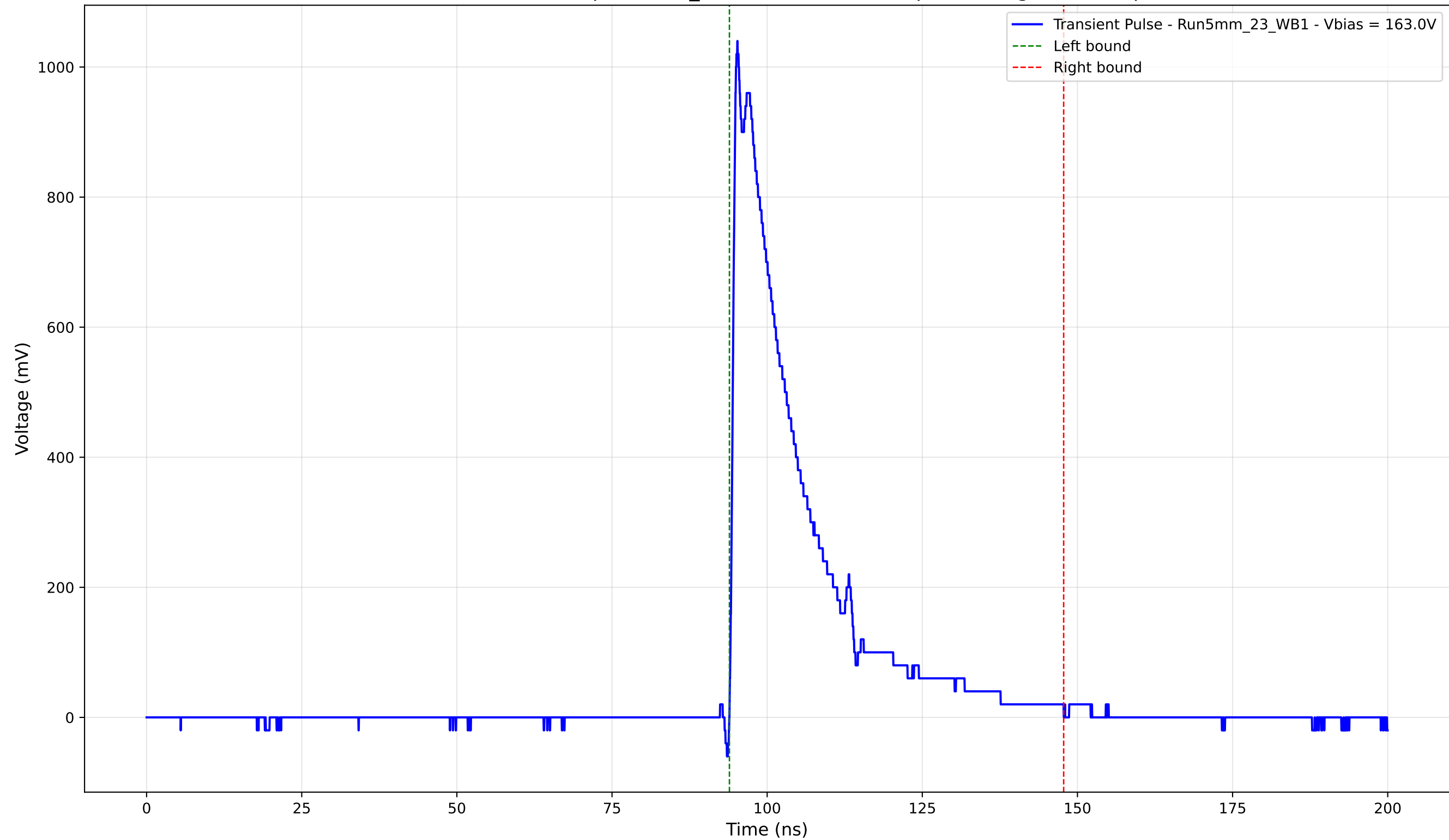
Transient Pulse - Sample: 5mm_23 - Position: 2965.0 \mu\text{m} - Charge: 232.39 pC
