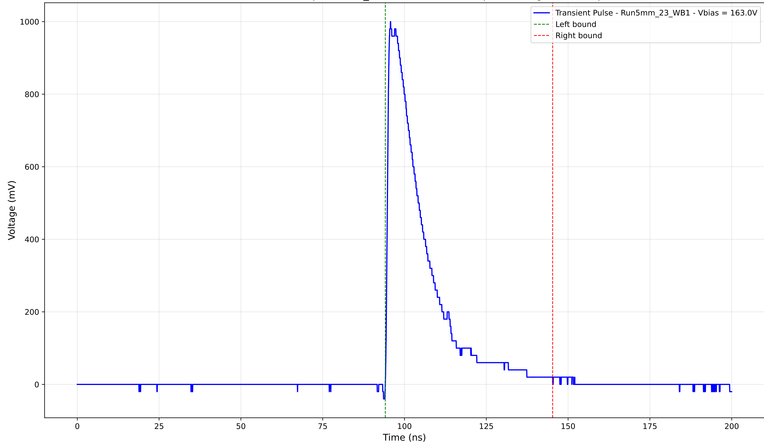
Transient Pulse - Sample: 5mm_23 - Position: 2060.0 \mu\text{m} - Charge: 245.89 pC
