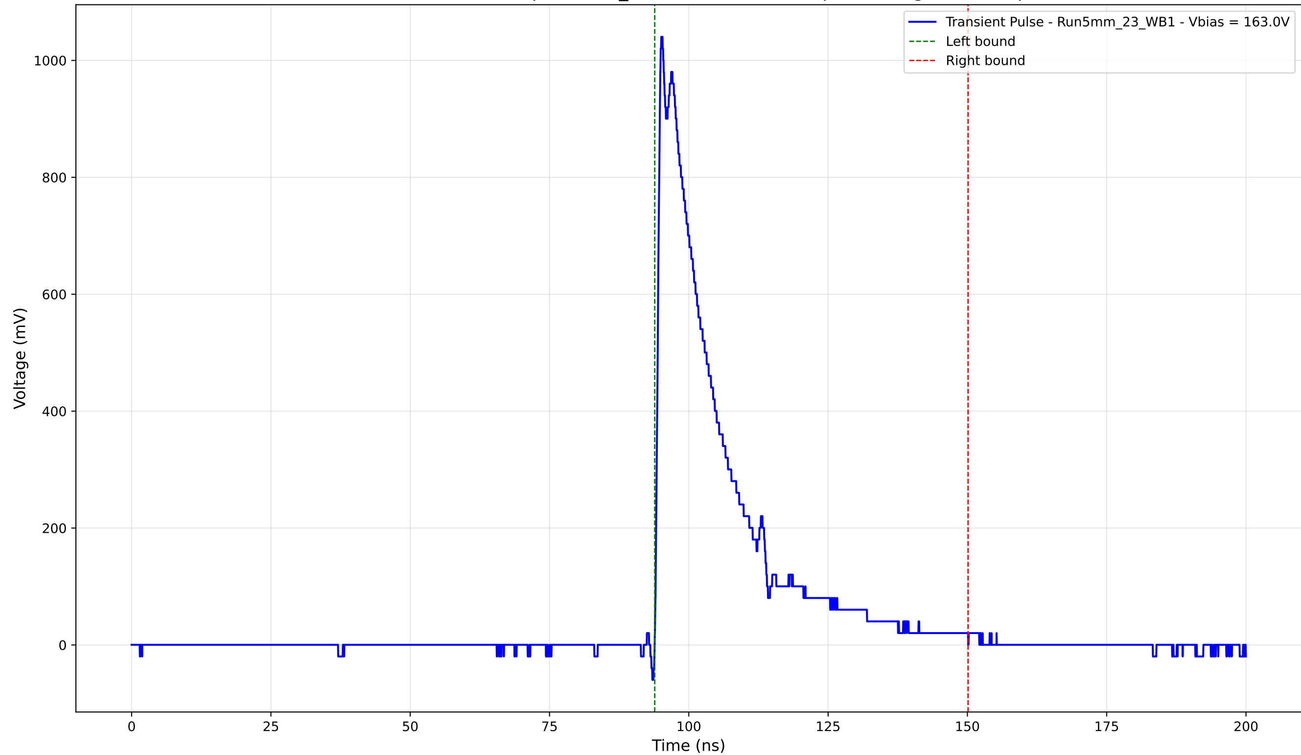
Transient Pulse - Sample: 5mm_23 - Position: 2550.0 \mu\text{m} - Charge: 238.25 pC
