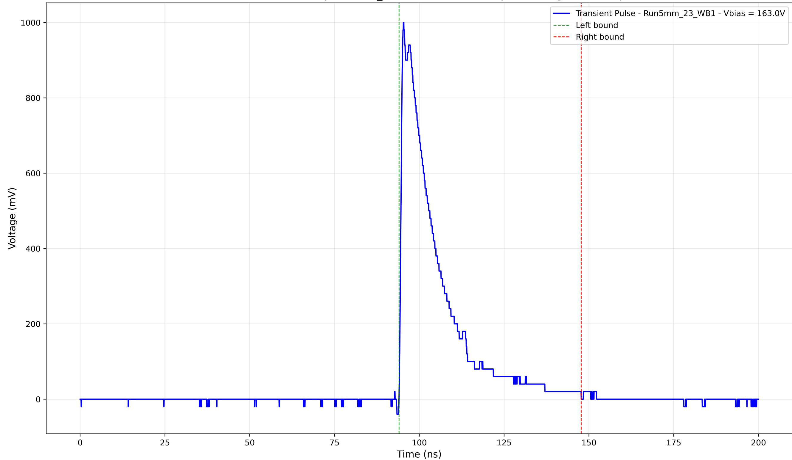
Transient Pulse - Sample: 5mm_23 - Position: 2355.0 \mu\text{m} - Charge: 225.05 pC
