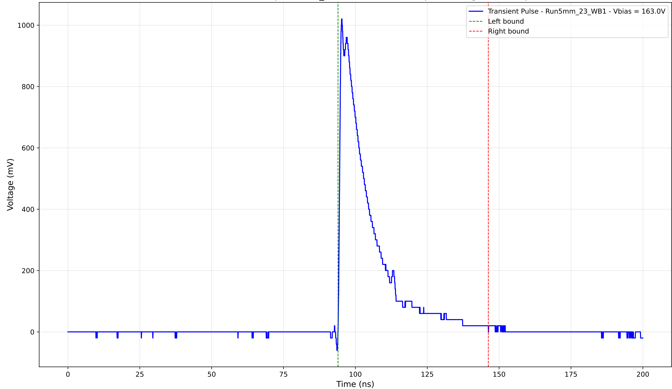
Transient Pulse - Sample: 5mm_23 - Position: 3035.0 \mu\text{m} - Charge: 229.17 pC
