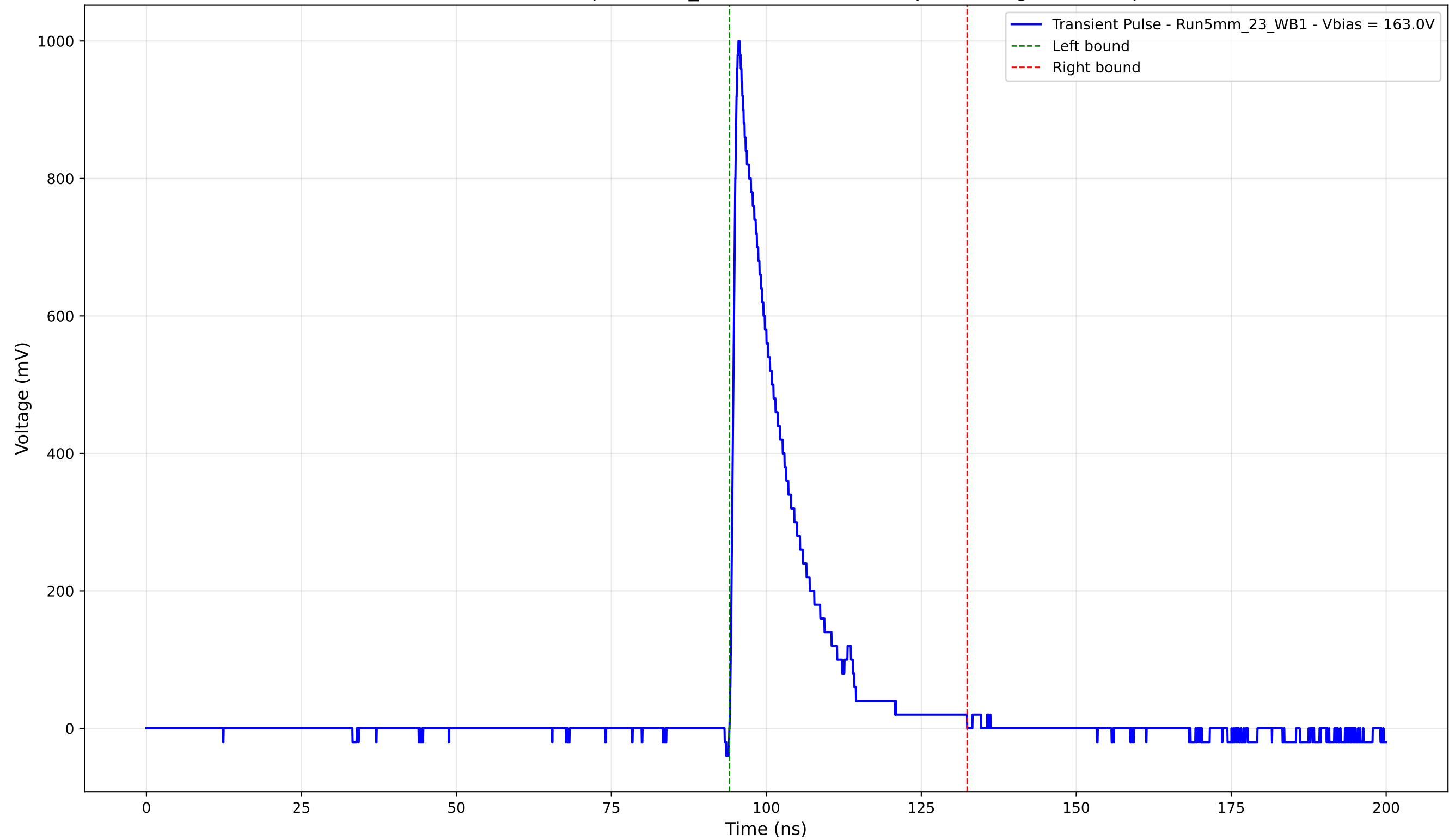
Transient Pulse - Sample: 5mm_23 - Position: 4955.0 \mu\text{m} - Charge: 166.45 pC
