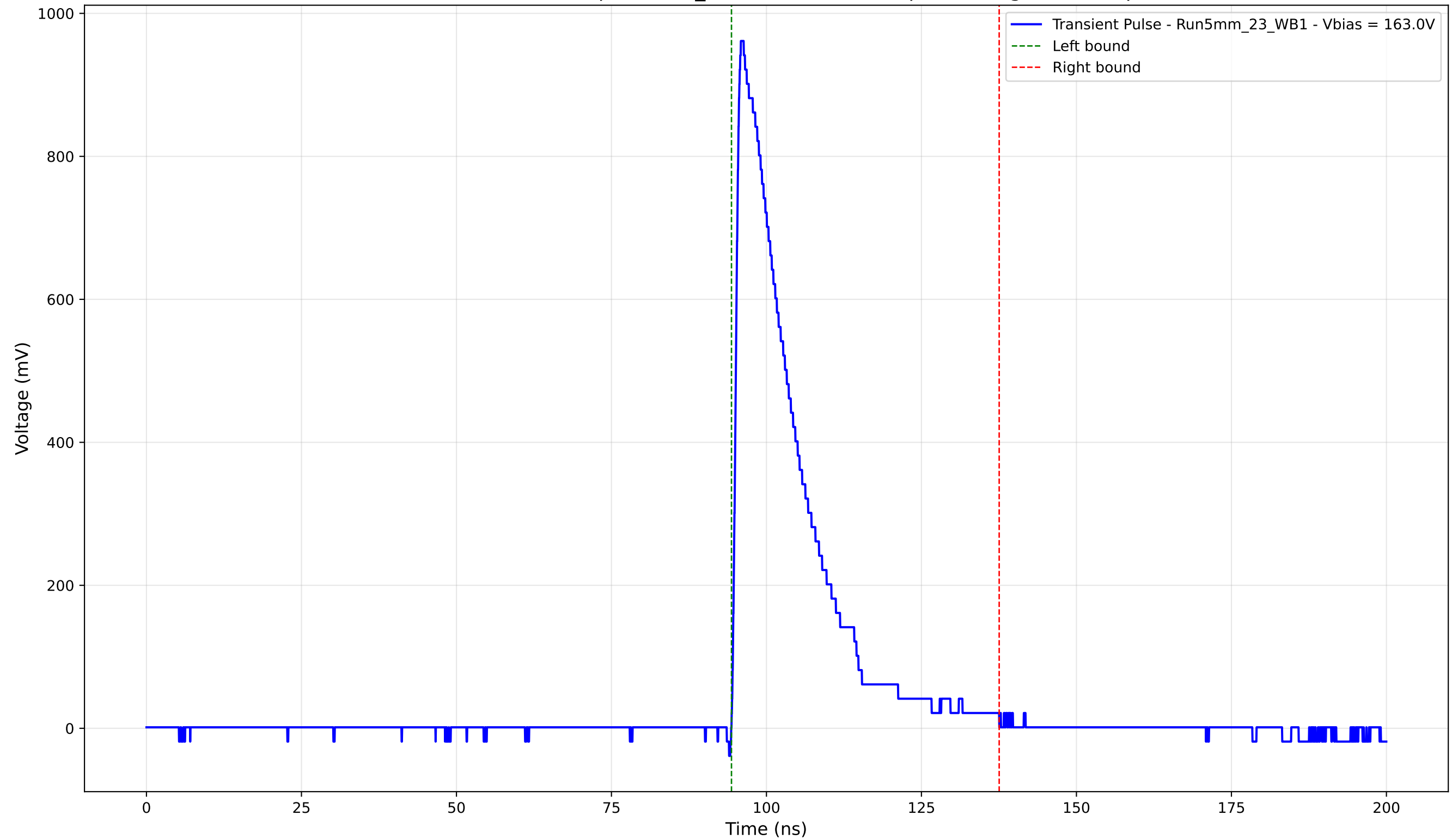
Transient Pulse - Sample: 5mm_23 - Position: 995.0 \mu\text{m} - Charge: 202.01 pC
