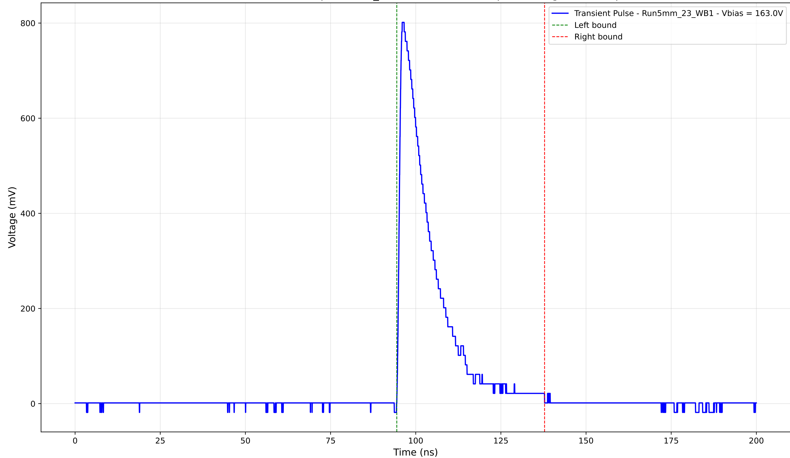
Transient Pulse - Sample: 5mm_23 - Position: 1290.0 \mu\text{m} - Charge: 165.09 pC
