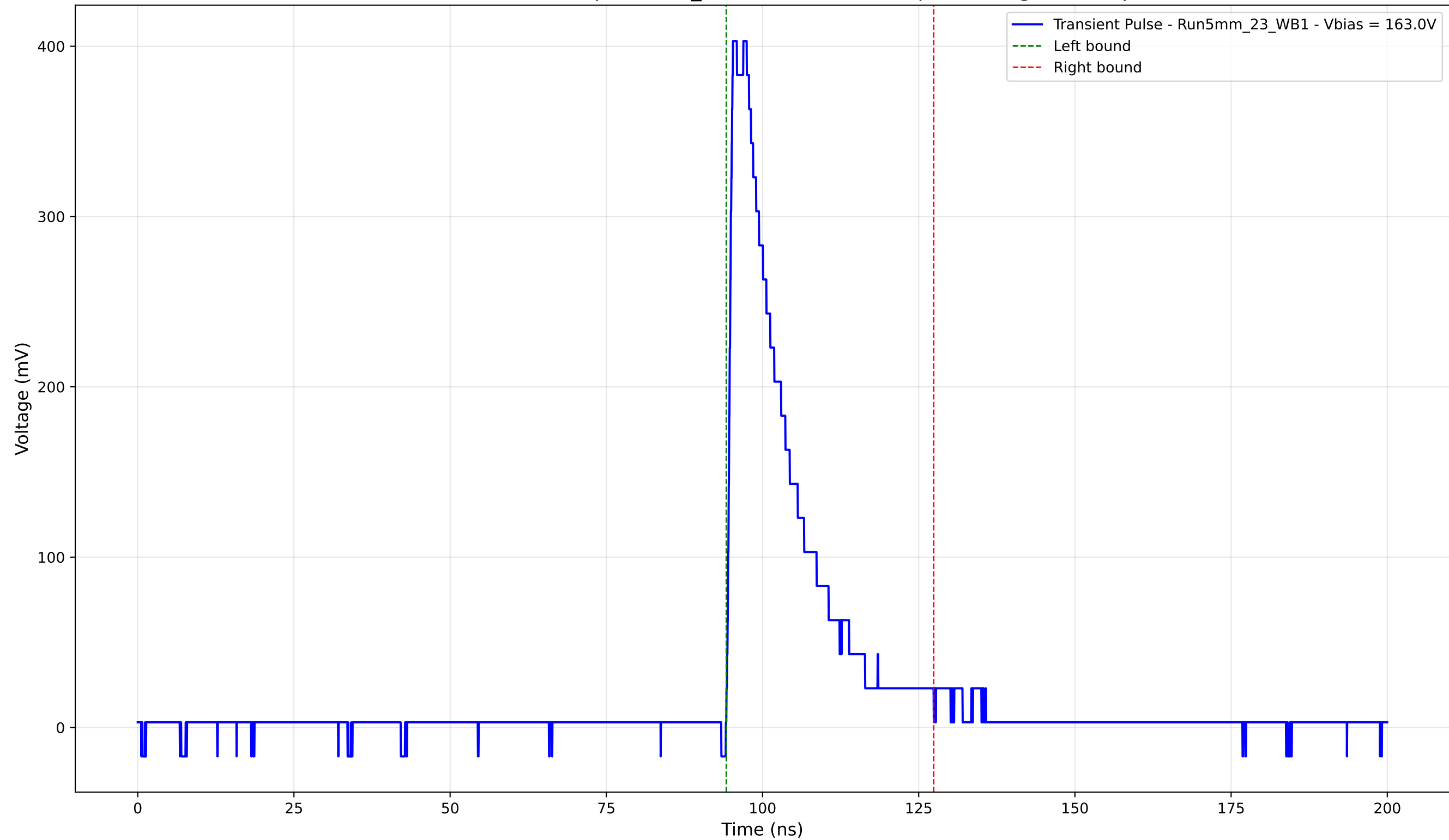
Transient Pulse - Sample: 5mm_23 - Position: 2210.0 \mu\text{m} - Charge: 81.35 pC
