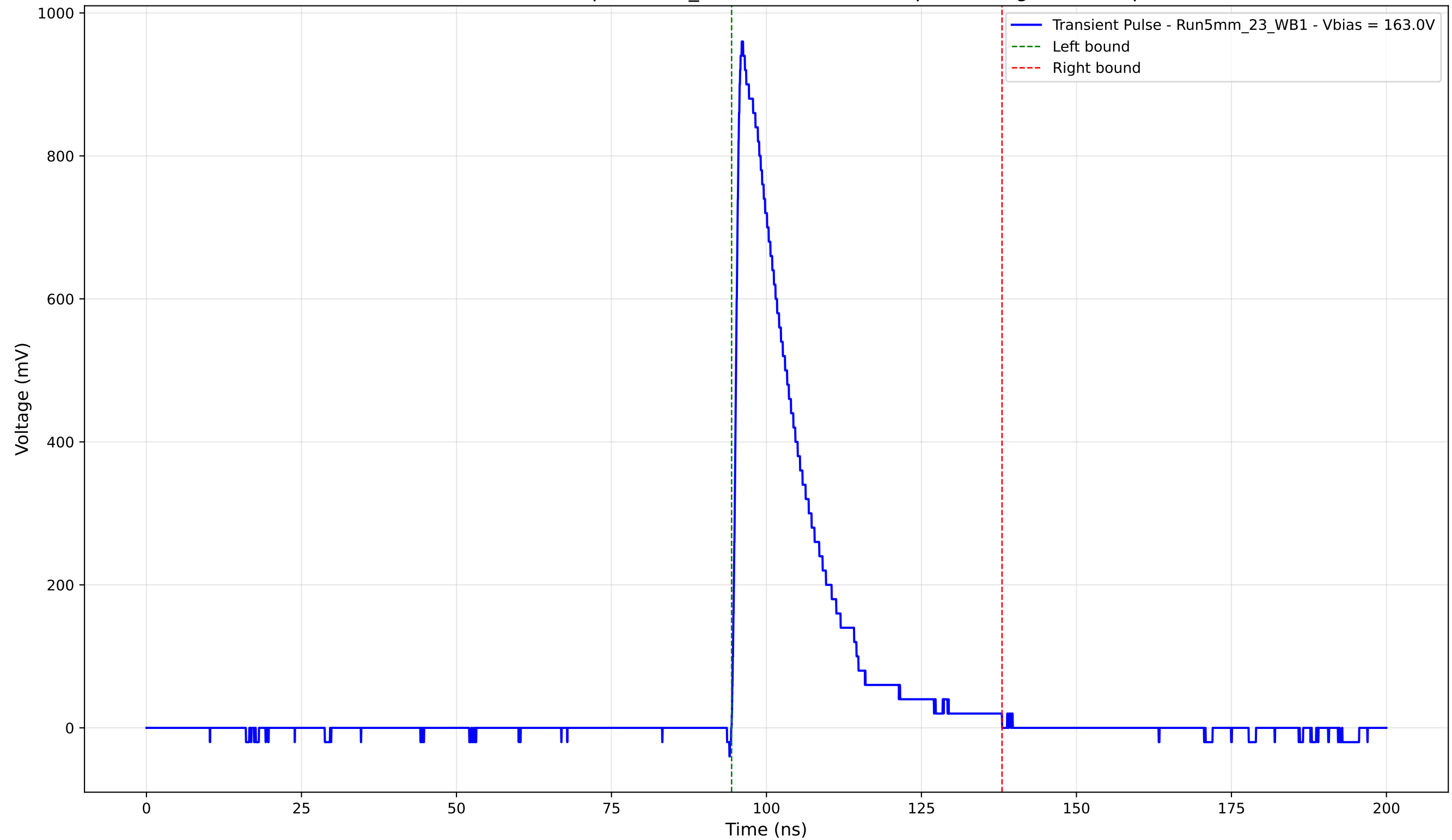
Transient Pulse - Sample: 5mm_23 - Position: 1060.0 \mu\text{m} - Charge: 200.74 pC
