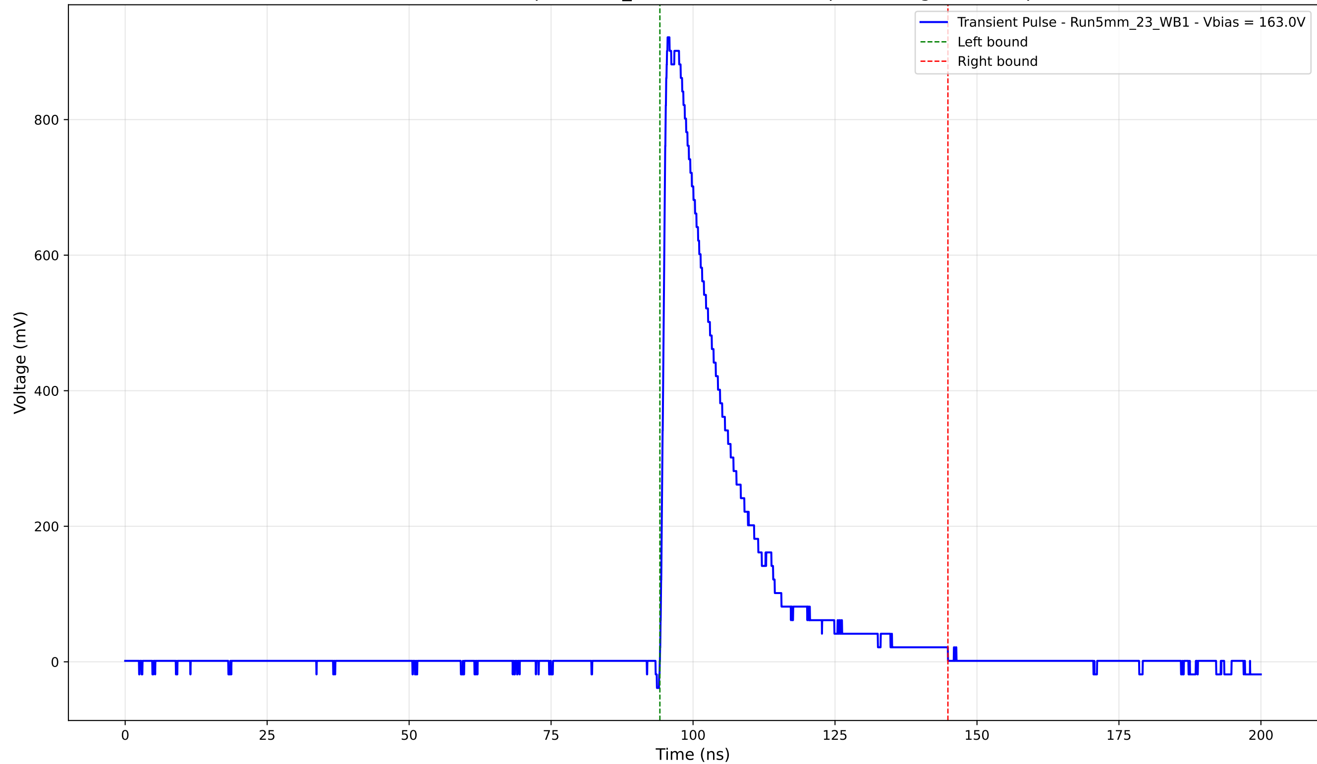
Transient Pulse - Sample: 5mm_23 - Position: 3390.0 \mu\text{m} - Charge: 212.19 pC
