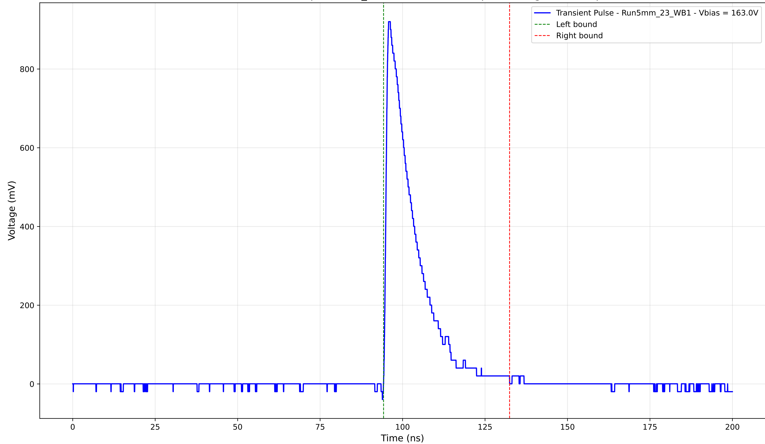
Transient Pulse - Sample: 5mm_23 - Position: 4570.0 \mu\text{m} - Charge: 174.48 pC
