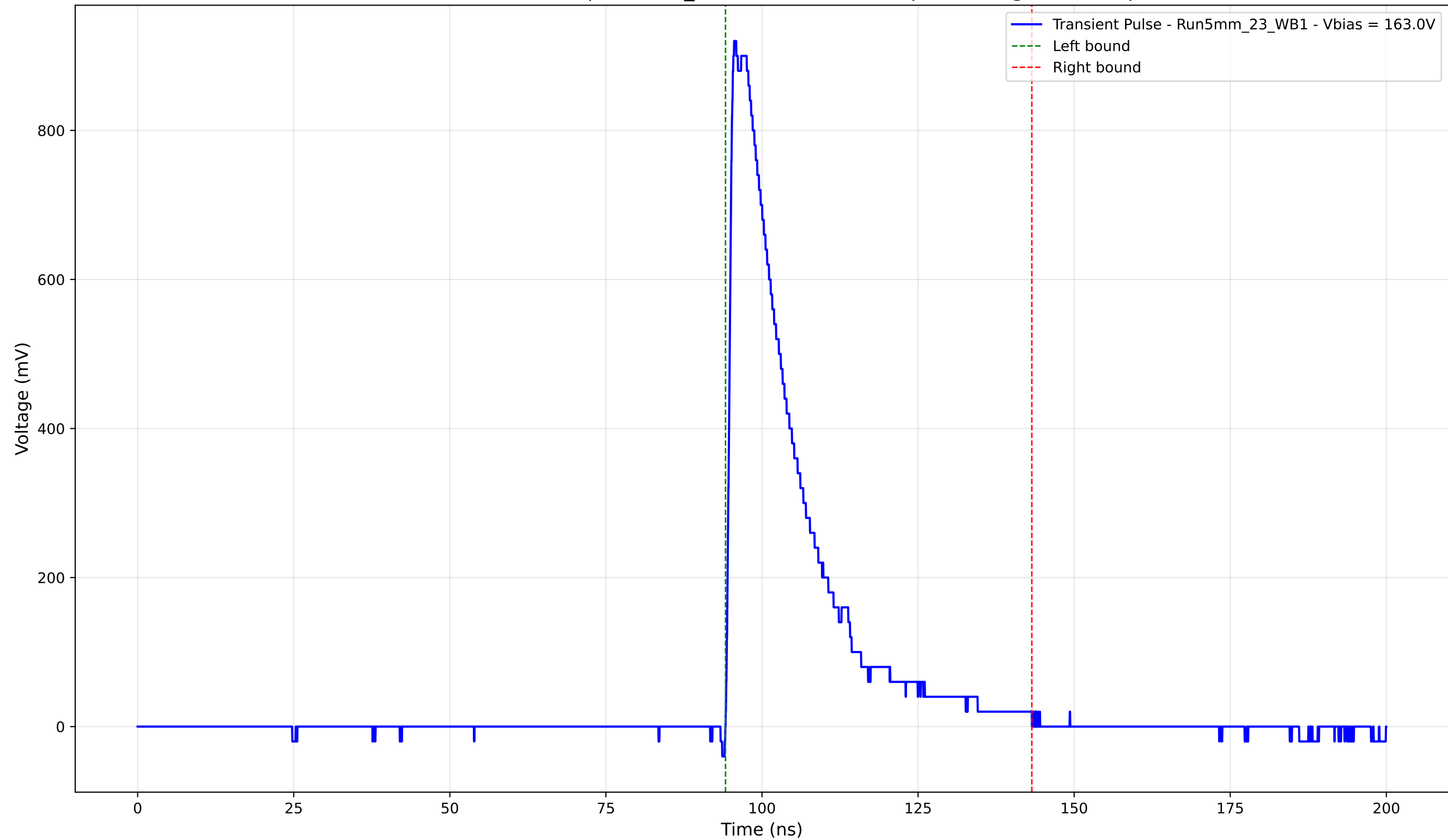
Transient Pulse - Sample: 5mm_23 - Position: 3400.0 \mu\text{m} - Charge: 210.34 pC
