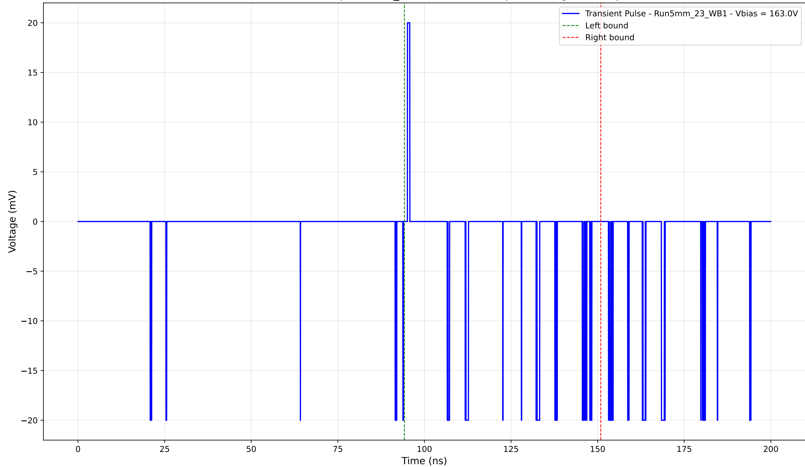
Transient Pulse - Sample: 5mm_23 - Position: 75.0 \mu\text{m} - Charge: -1.20 pC
