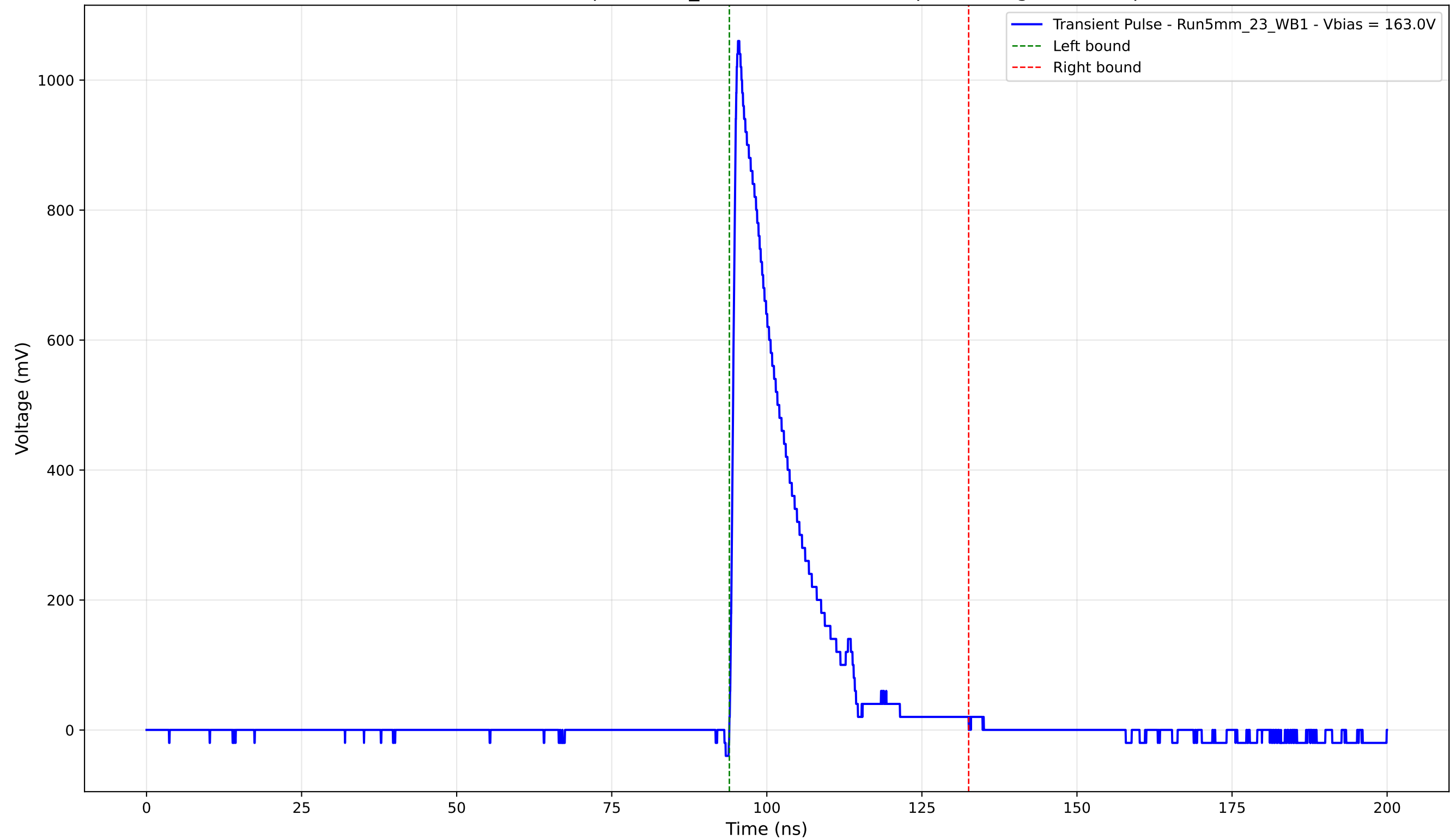
Transient Pulse - Sample: 5mm_23 - Position: 5065.0 \mu\text{m} - Charge: 185.07 pC
