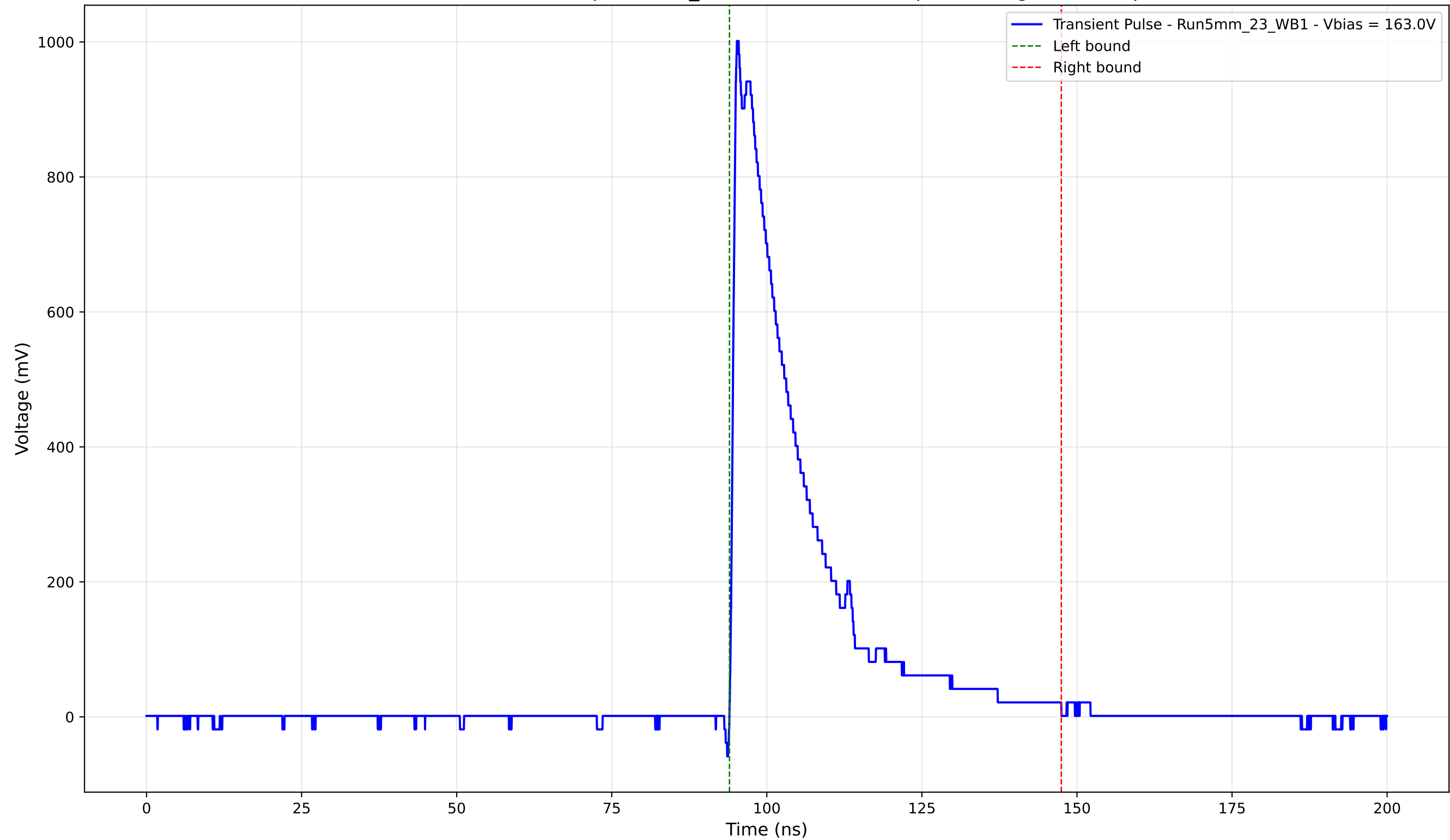
Transient Pulse - Sample: 5mm_23 - Position: 2405.0 \mu\text{m} - Charge: 228.48 pC
