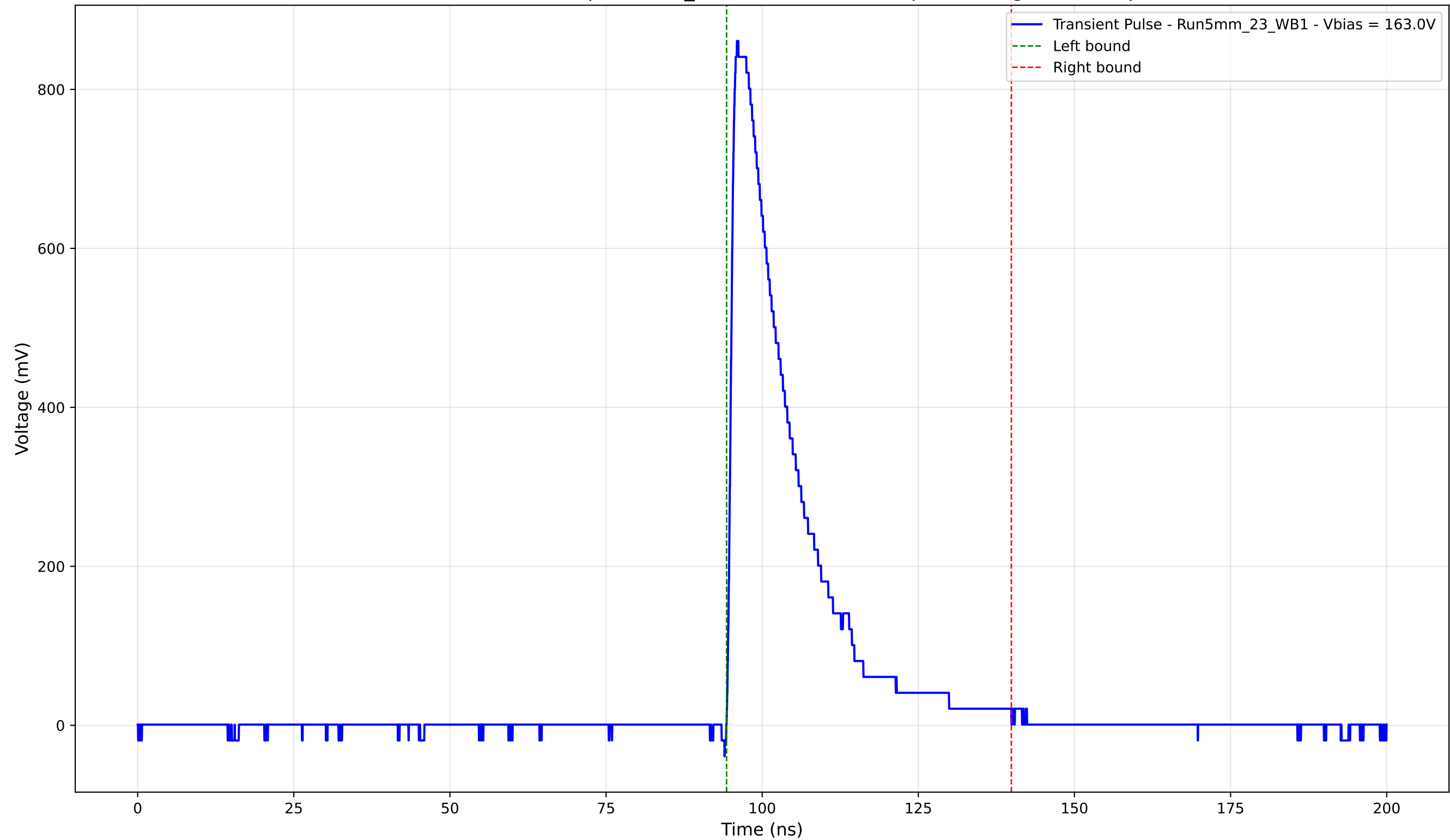
Transient Pulse - Sample: 5mm_23 - Position: 3670.0 \mu\text{m} - Charge: 185.91 pC
