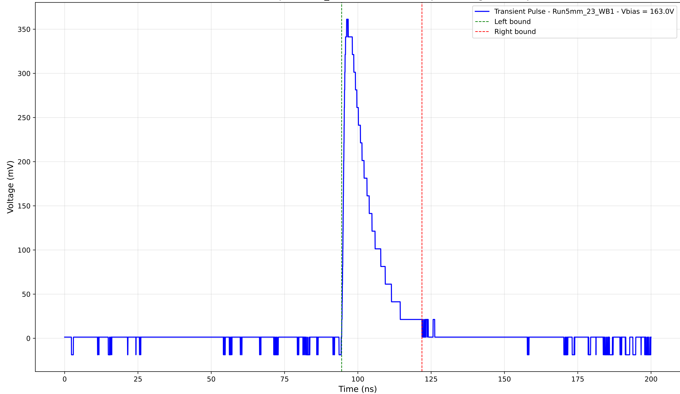
Transient Pulse - Sample: 5mm_23 - Position: 3785.0 \mu\text{m} - Charge: 67.23 pC
