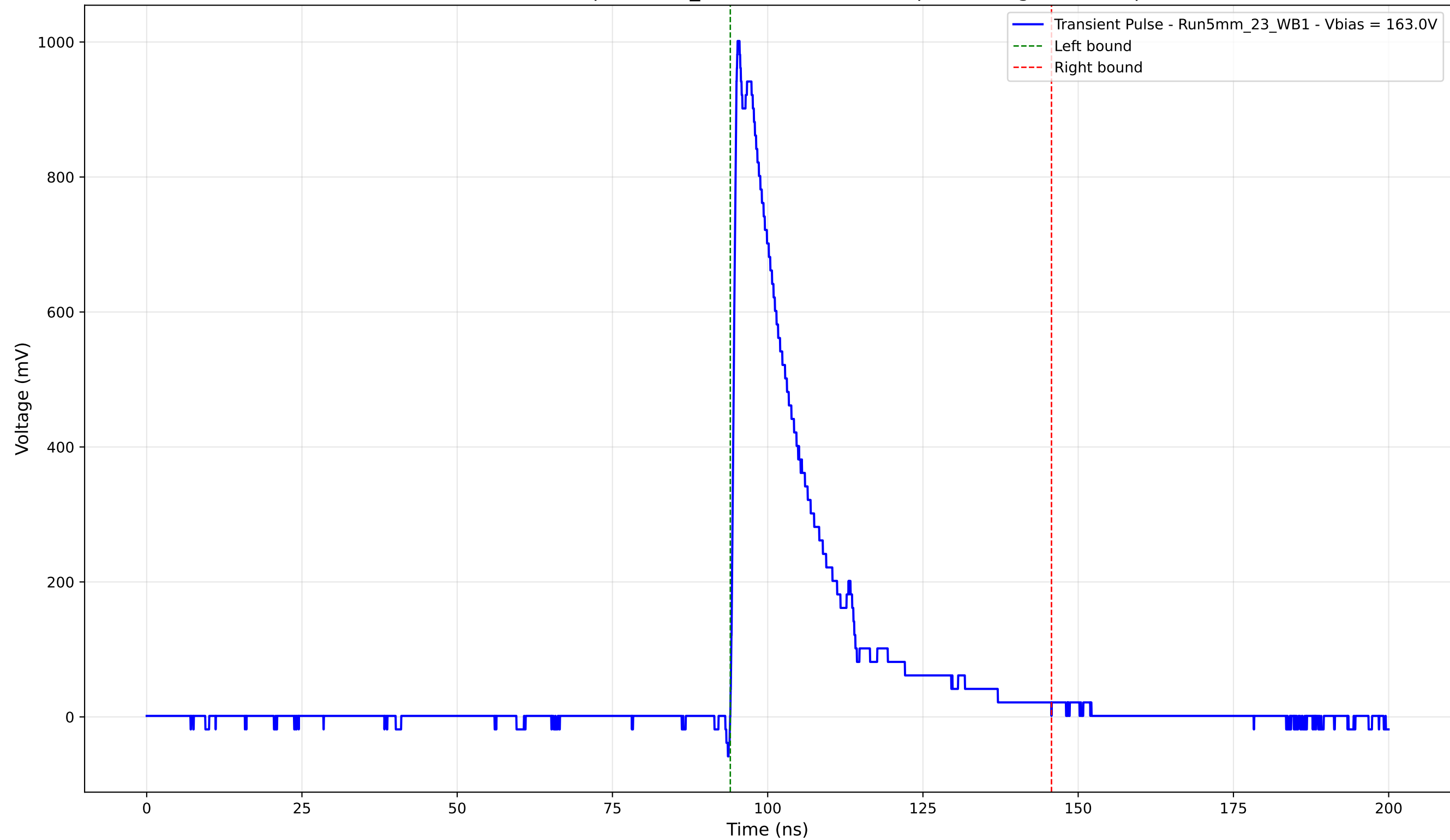
Transient Pulse - Sample: 5mm_23 - Position: 3065.0 \mu\text{m} - Charge: 228.32 pC
