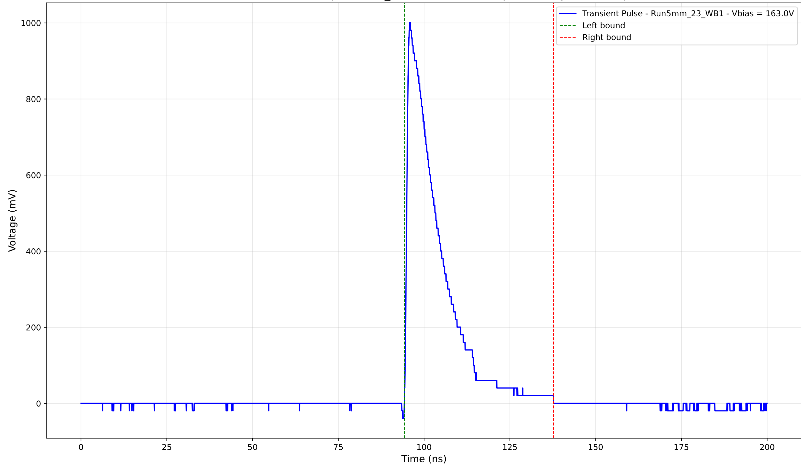
Transient Pulse - Sample: 5mm_23 - Position: 835.0 \mu\text{m} - Charge: 206.70 pC
