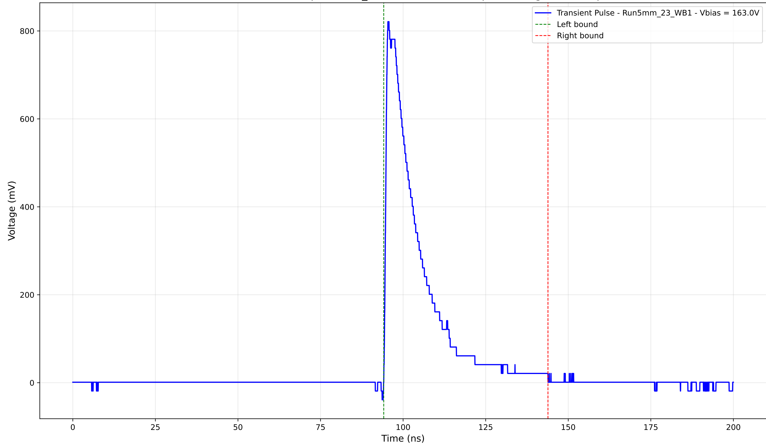
Transient Pulse - Sample: 5mm_23 - Position: 2175.0 \mu\text{m} - Charge: 176.64 pC
