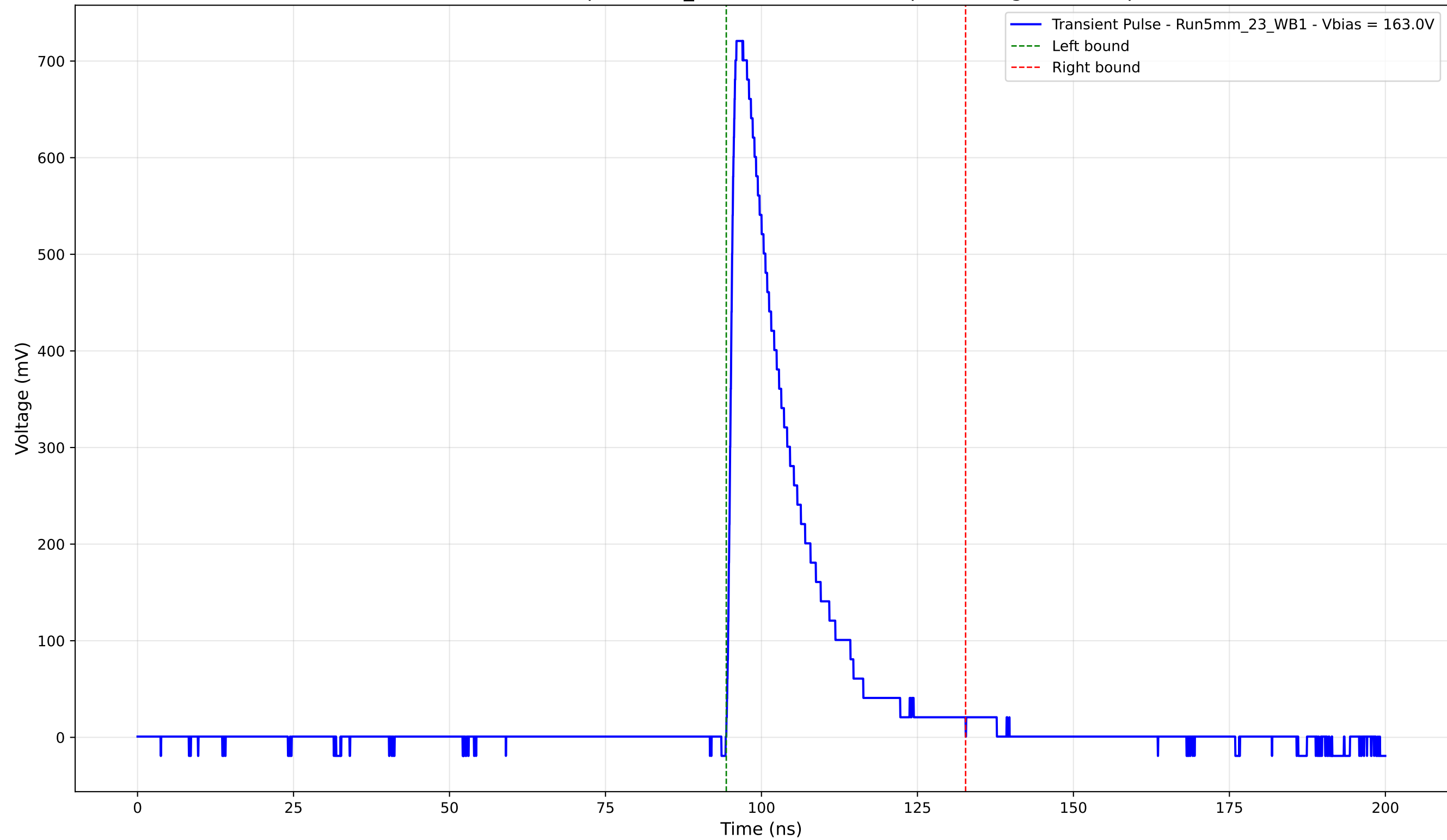
Transient Pulse - Sample: 5mm_23 - Position: 3820.0 \mu\text{m} - Charge: 146.21 pC
