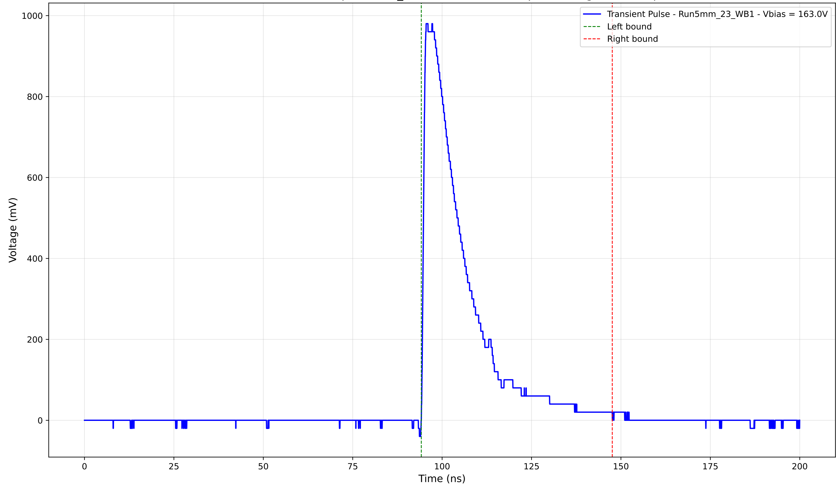
Transient Pulse - Sample: 5mm_23 - Position: 2030.0 \mu\text{m} - Charge: 245.22 pC
