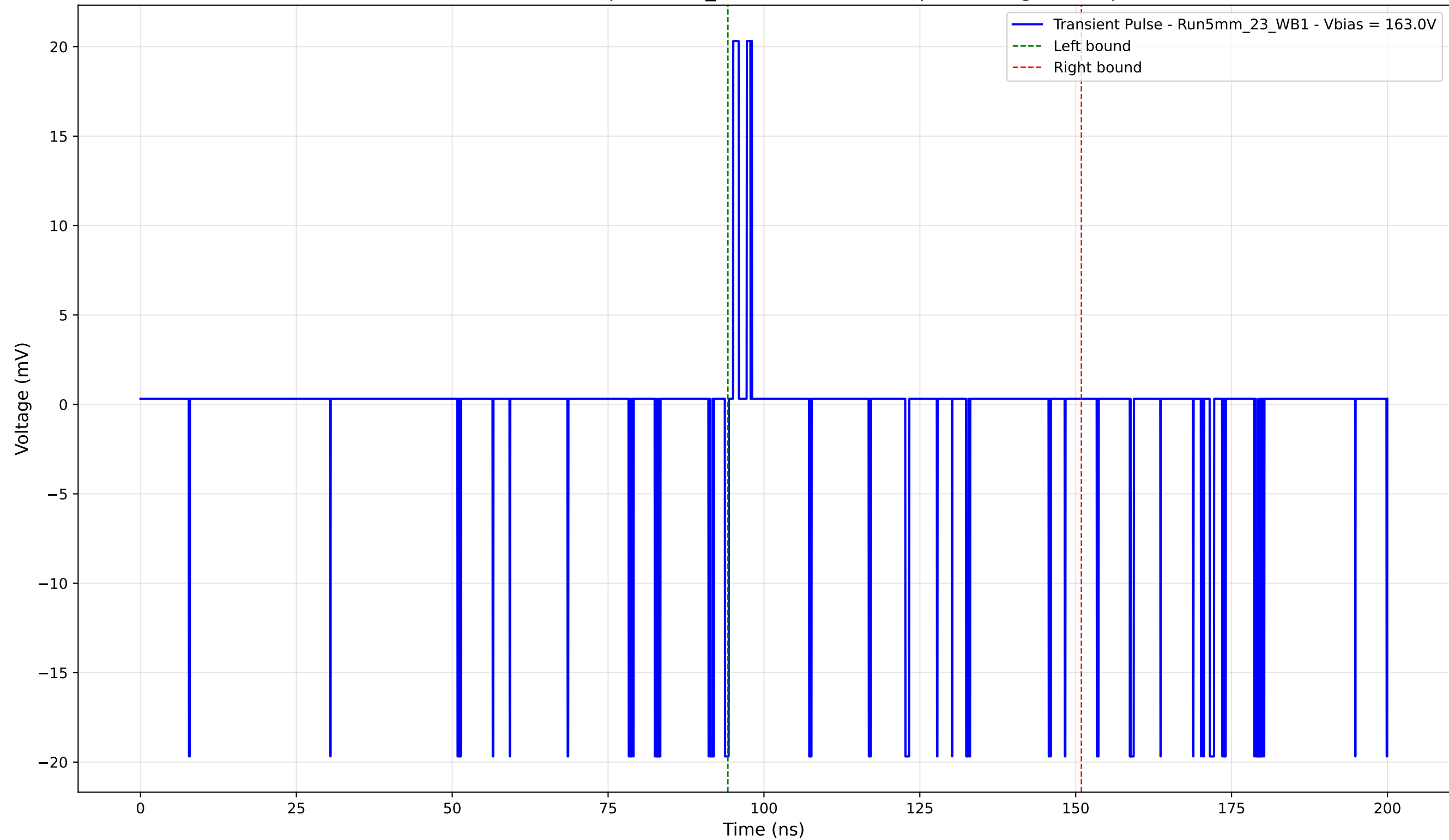
Transient Pulse - Sample: 5mm_23 - Position: 215.0 \mu\text{m} - Charge: 0.09 pC
