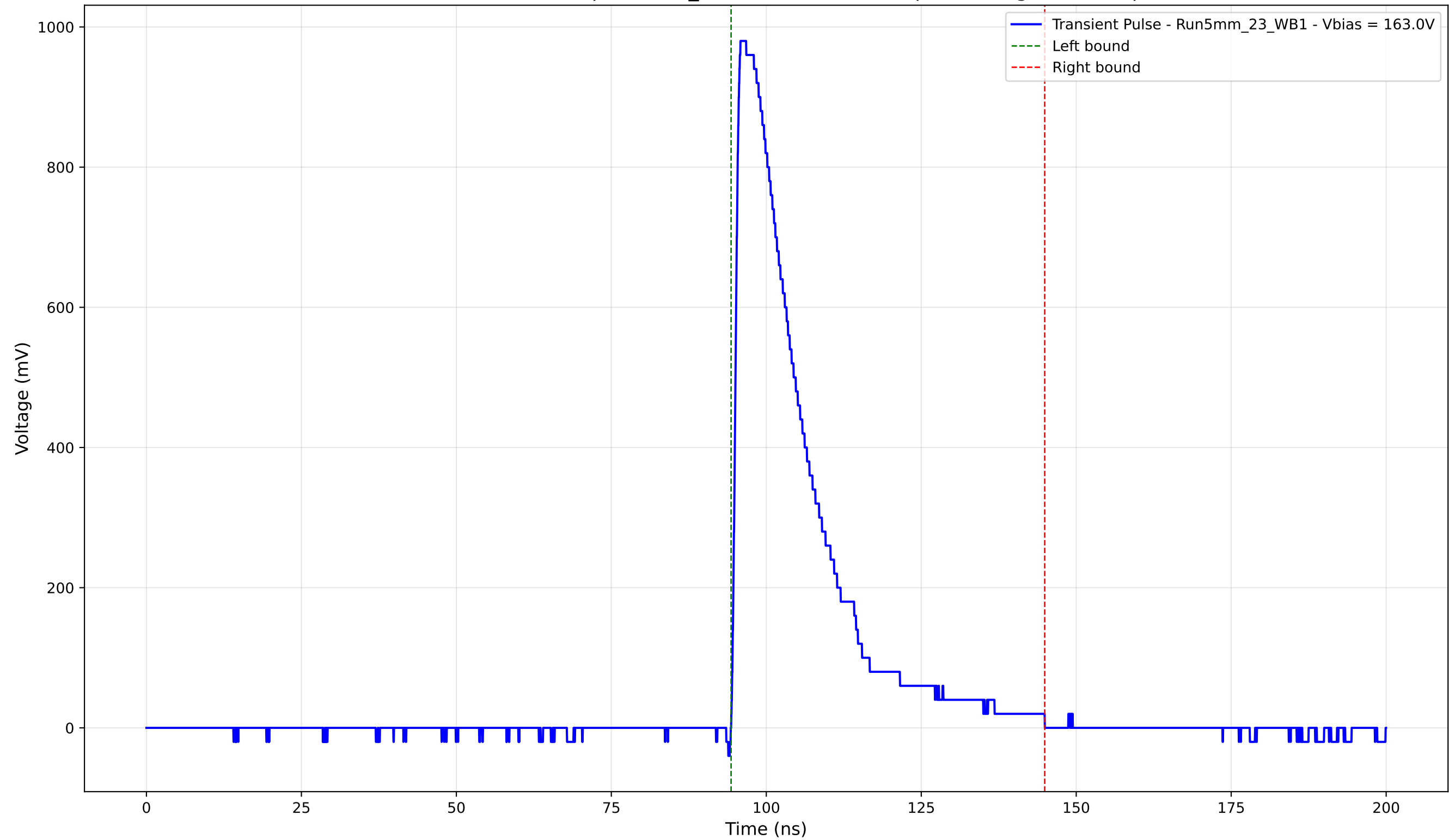
Transient Pulse - Sample: 5mm_23 - Position: 1625.0 \mu\text{m} - Charge: 241.10 pC
