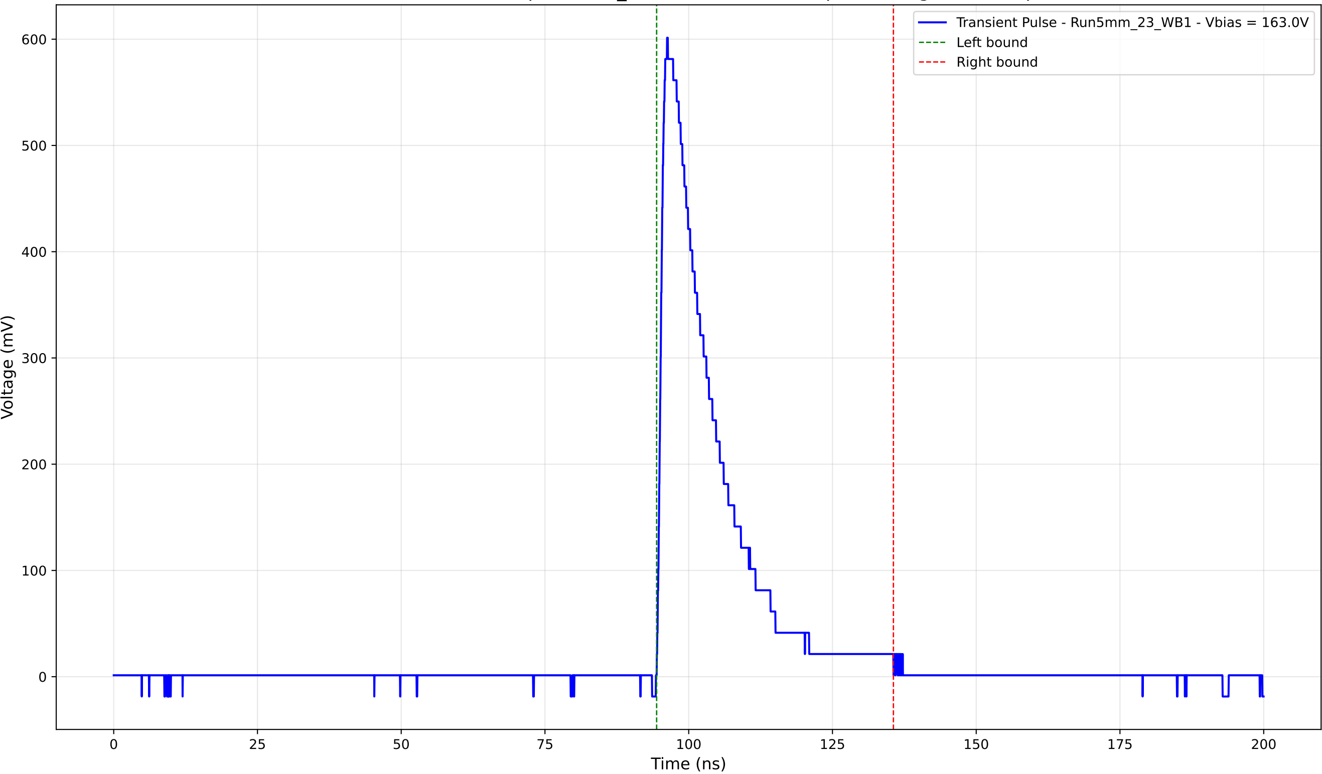
Transient Pulse - Sample: 5mm_23 - Position: 1680.0 \mu\text{m} - Charge: 120.25 pC
