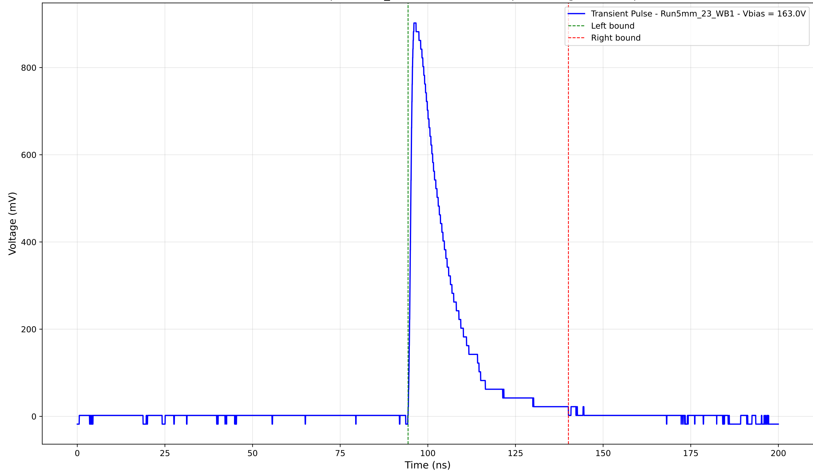
Transient Pulse - Sample: 5mm_23 - Position: 3905.0 \mu\text{m} - Charge: 197.77 pC
