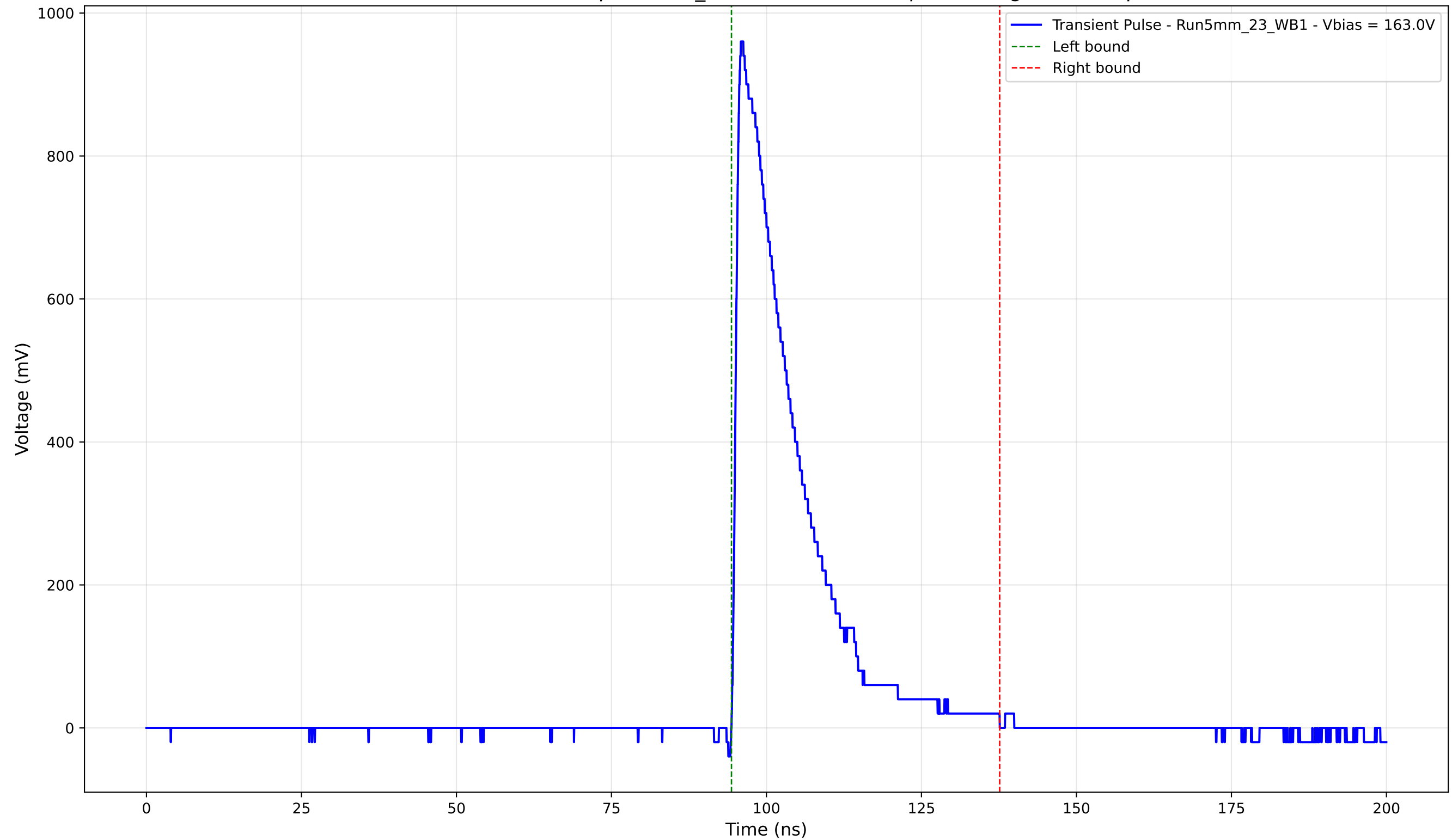
Transient Pulse - Sample: 5mm_23 - Position: 985.0 \mu\text{m} - Charge: 199.88 pC
