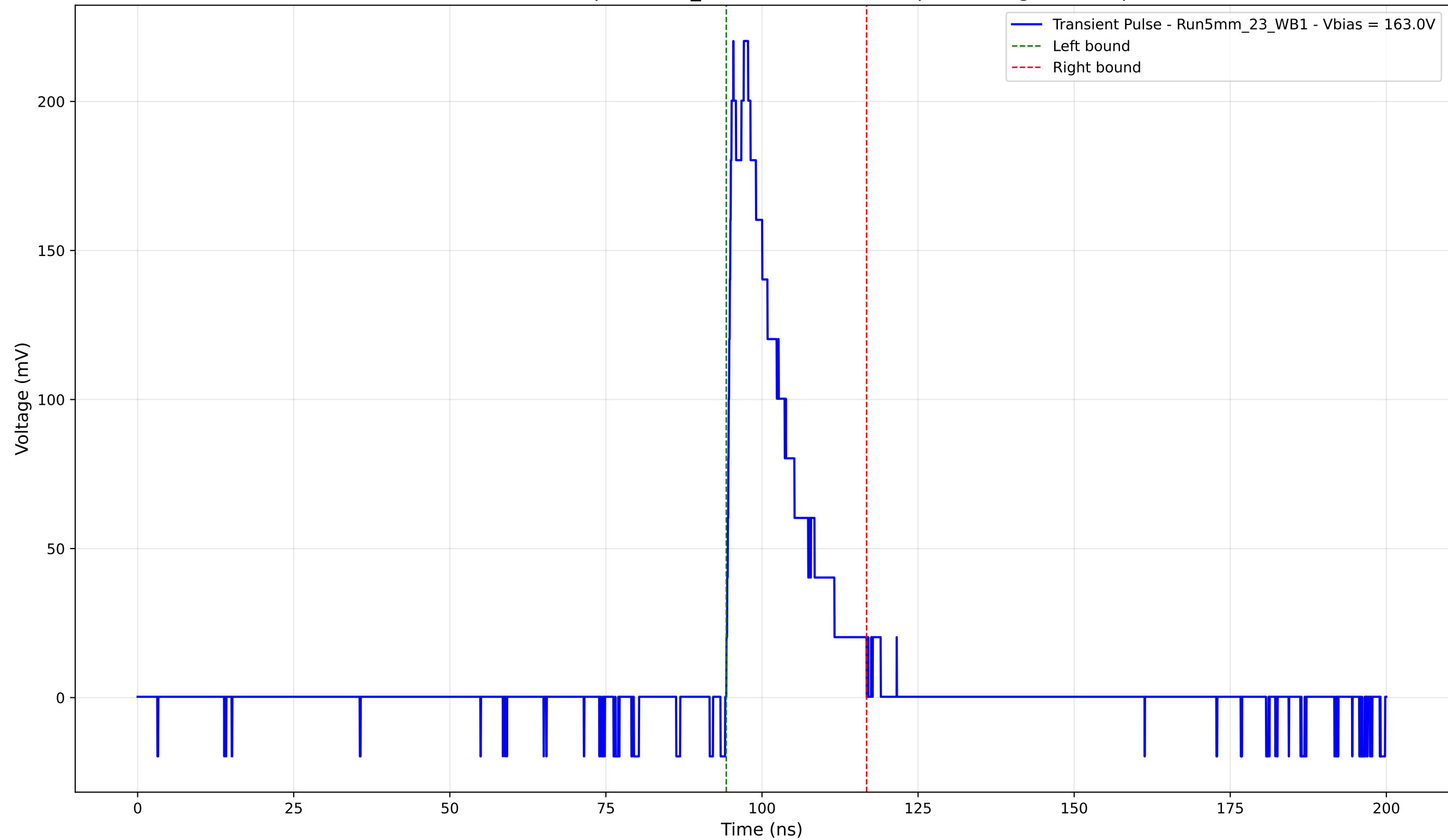
Transient Pulse - Sample: 5mm_23 - Position: 2240.0 \mu\text{m} - Charge: 39.61 pC
