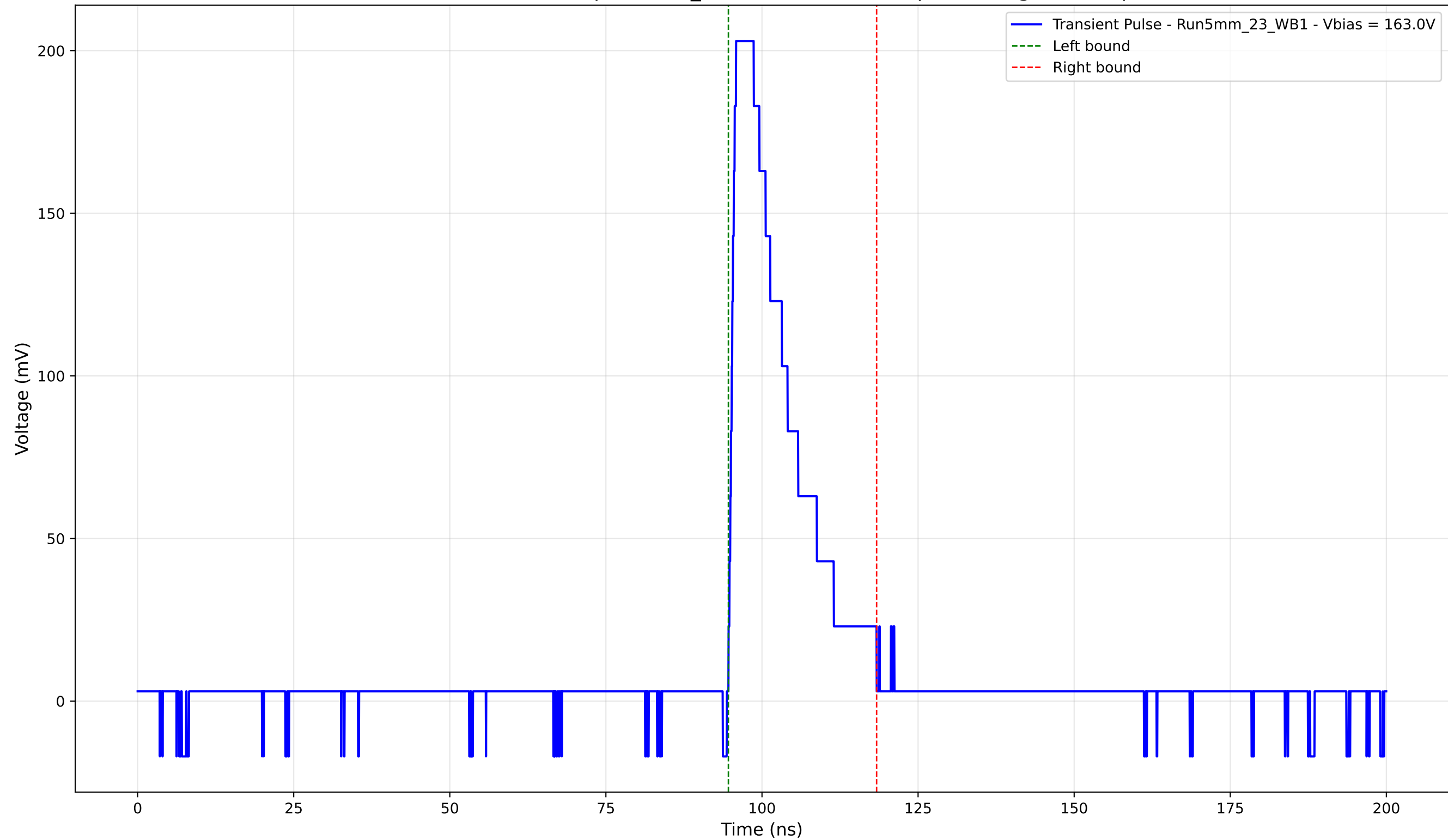
Transient Pulse - Sample: 5mm_23 - Position: 1220.0 \mu\text{m} - Charge: 41.37 pC
