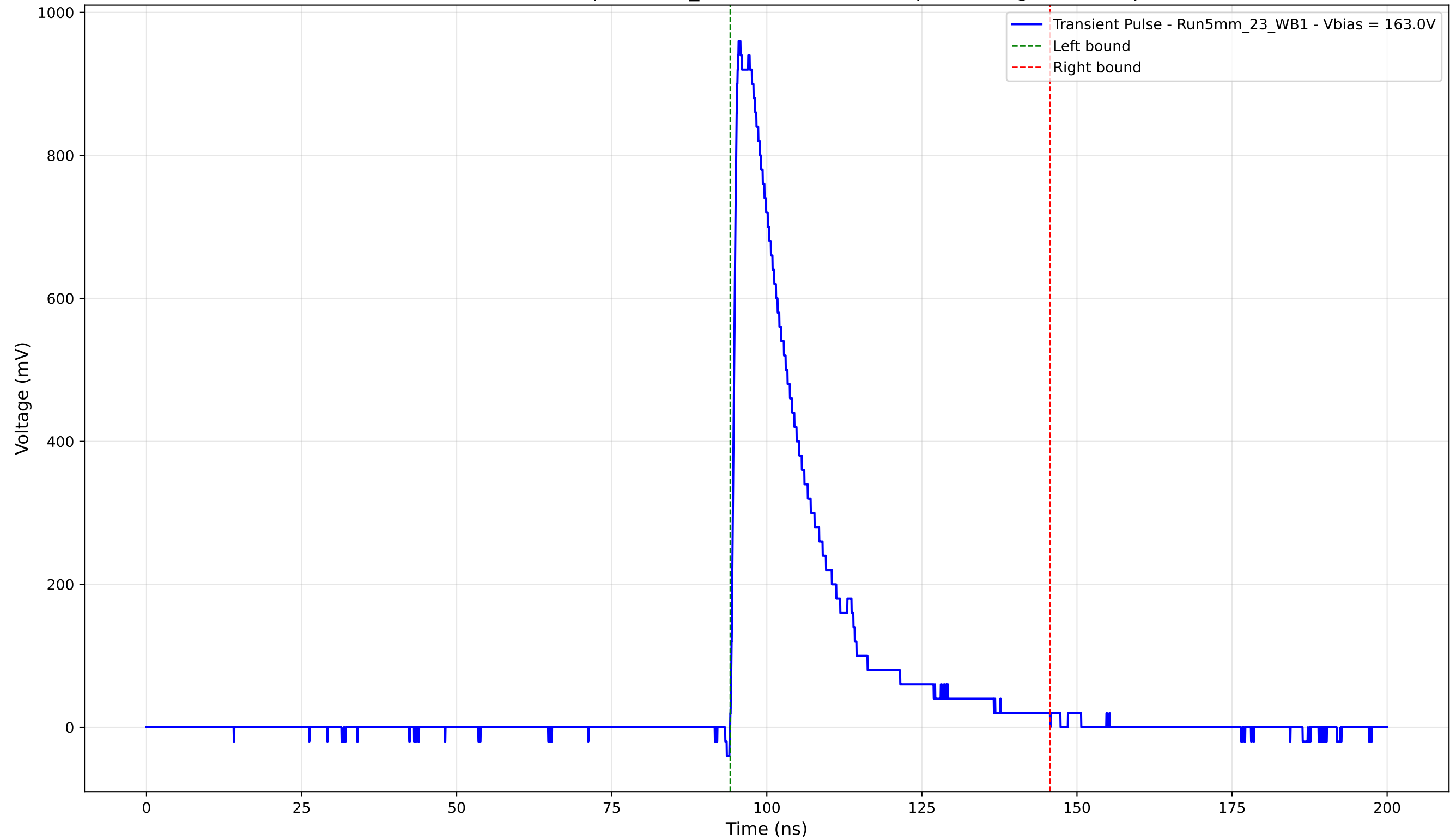
Transient Pulse - Sample: 5mm_23 - Position: 2150.0 \mu\text{m} - Charge: 223.66 pC
