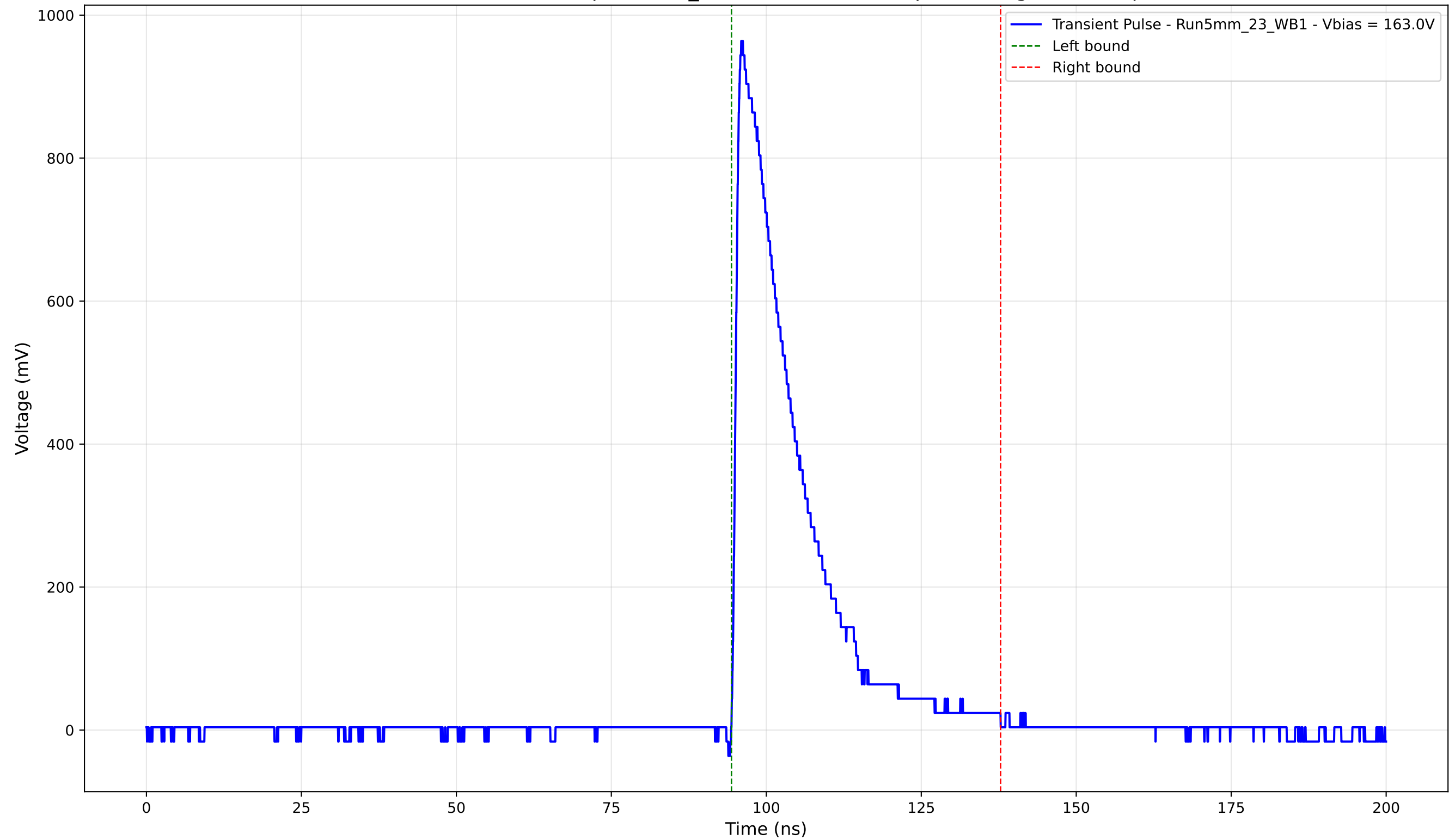
Transient Pulse - Sample: 5mm_23 - Position: 1025.0 \mu\text{m} - Charge: 203.41 pC
