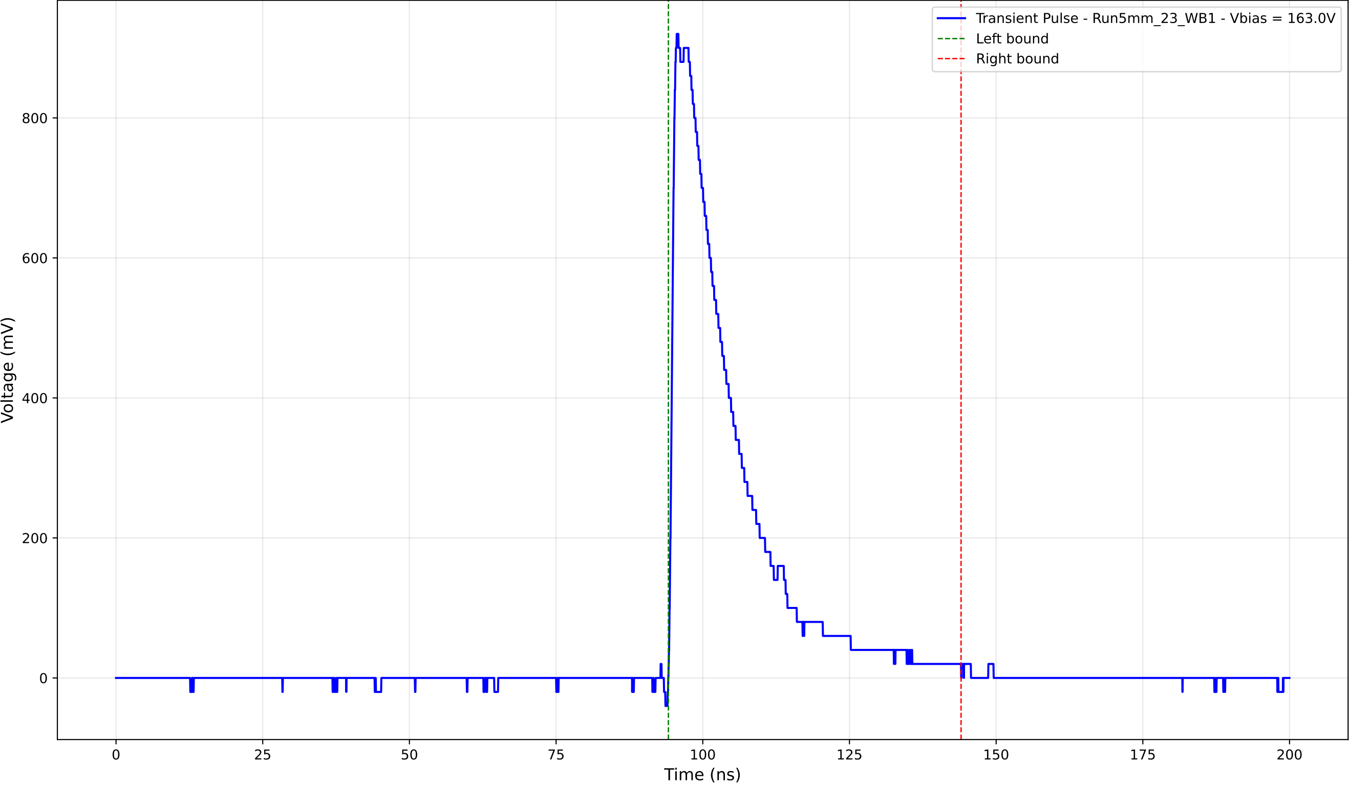
Transient Pulse - Sample: 5mm_23 - Position: 3395.0 \mu\text{m} - Charge: 211.05 pC
