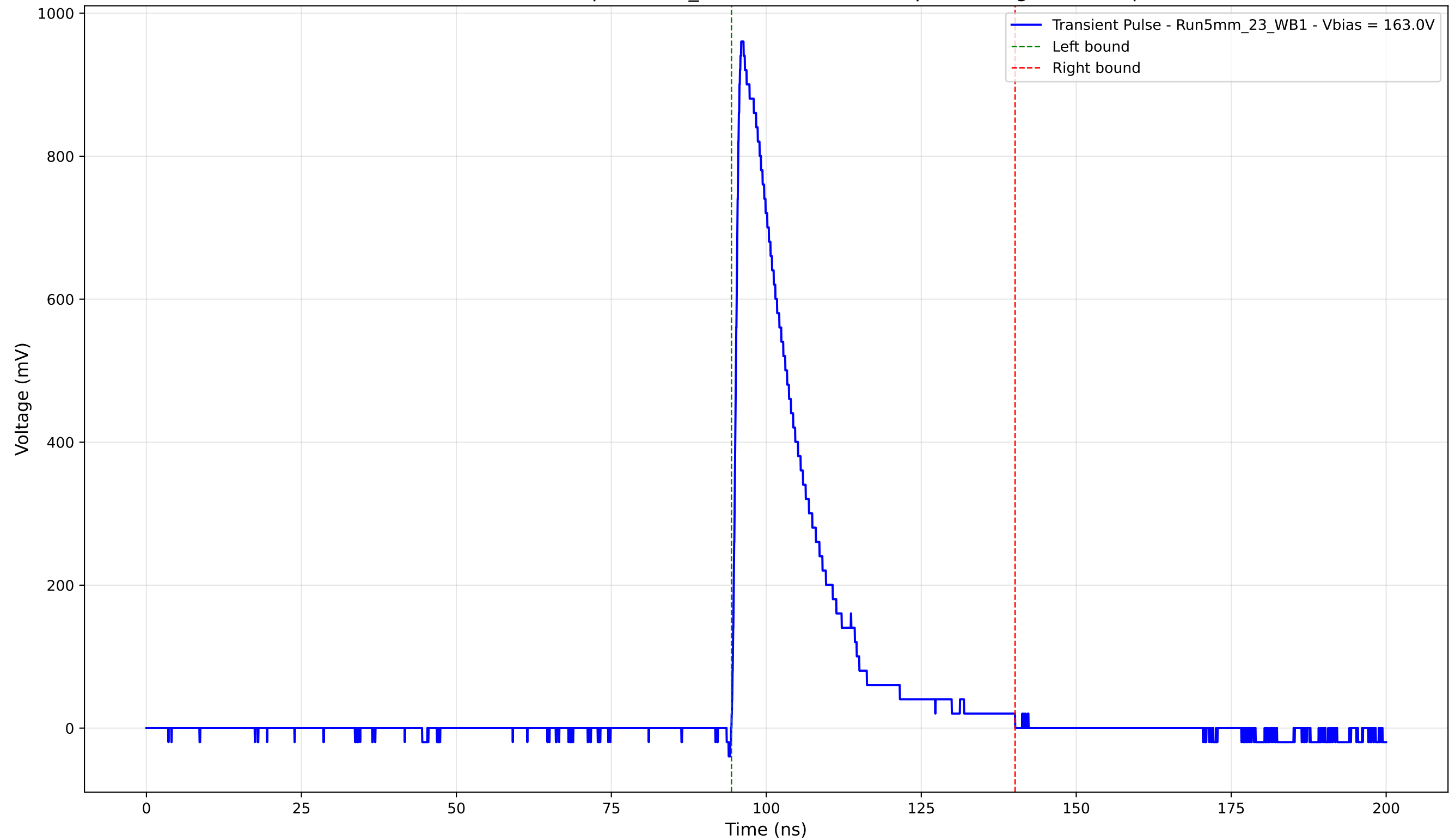
Transient Pulse - Sample: 5mm_23 - Position: 1070.0 \mu\text{m} - Charge: 204.35 pC
