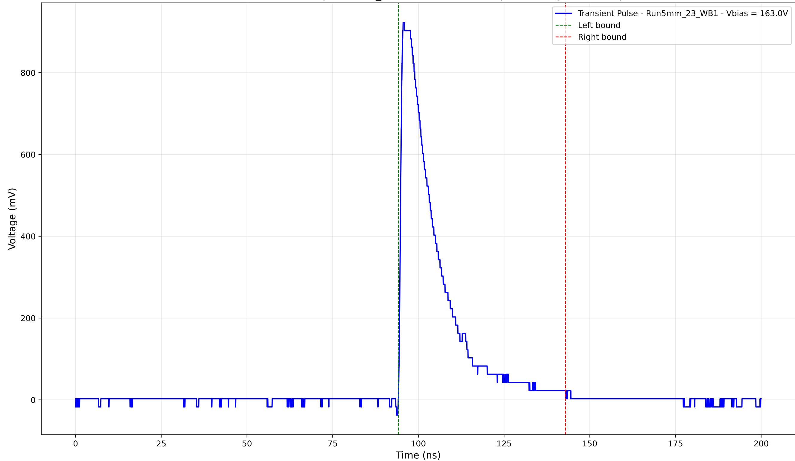
Transient Pulse - Sample: 5mm_23 - Position: 3425.0 \mu\text{m} - Charge: 214.58 pC
