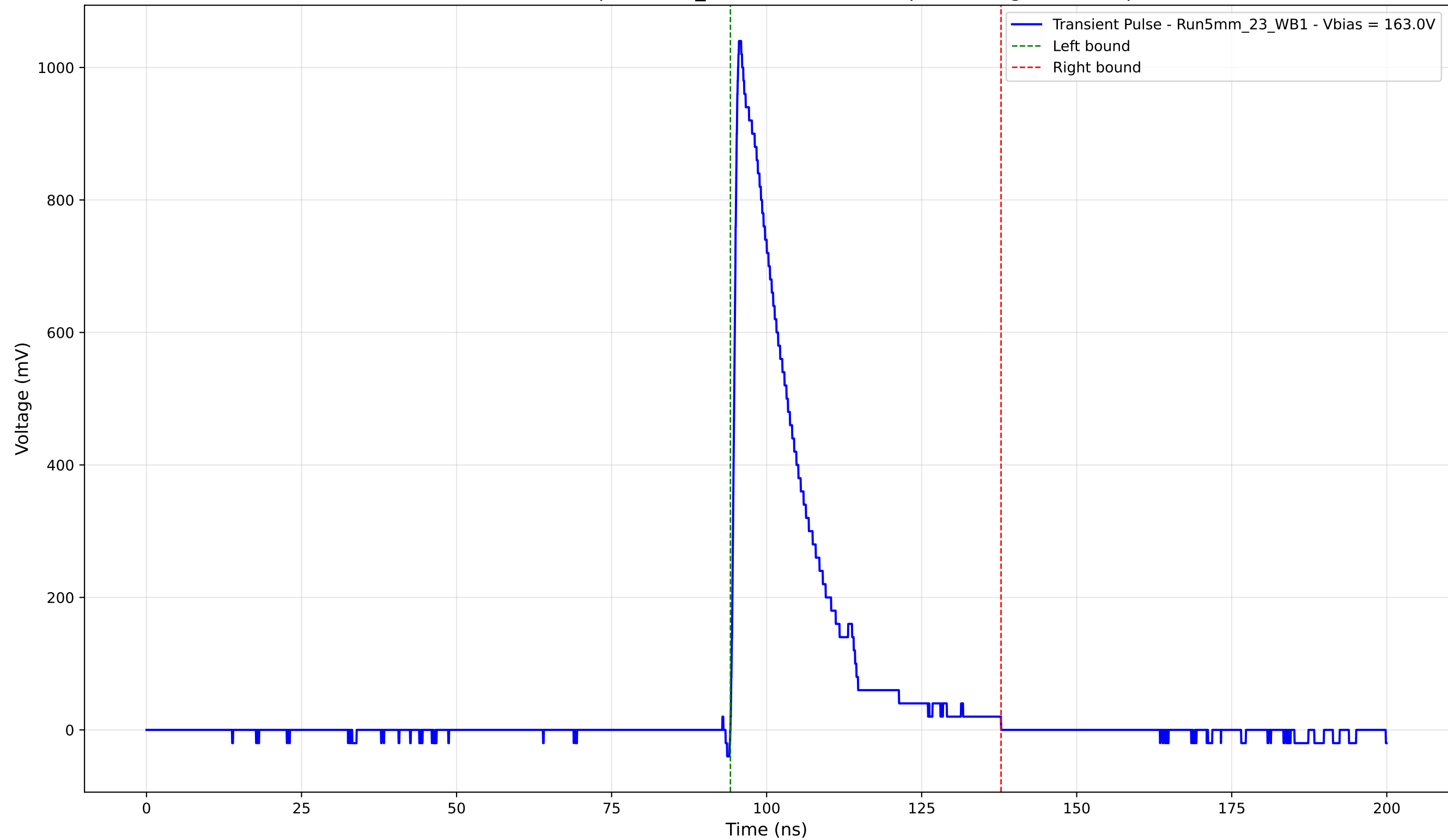
Transient Pulse - Sample: 5mm_23 - Position: 615.0 \mu\text{m} - Charge: 211.07 pC
