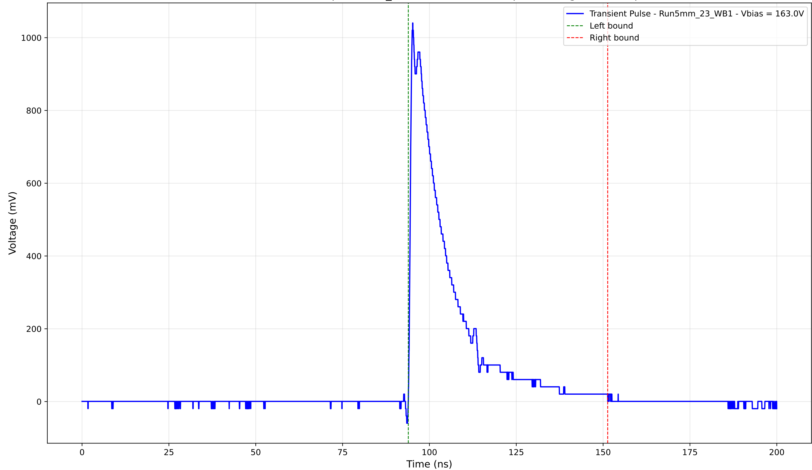
Transient Pulse - Sample: 5mm_23 - Position: 2975.0 \mu\text{m} - Charge: 234.07 pC
