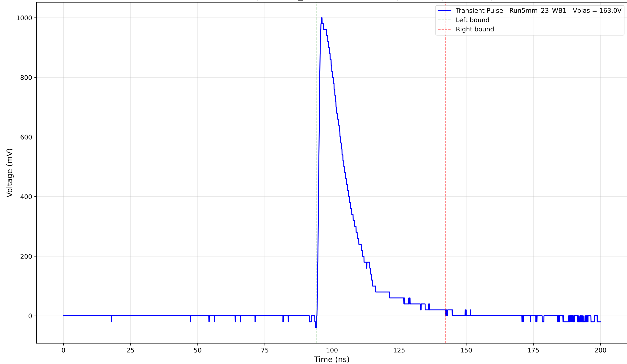
Transient Pulse - Sample: 5mm_23 - Position: 1435.0 \mu\text{m} - Charge: 237.27 pC
