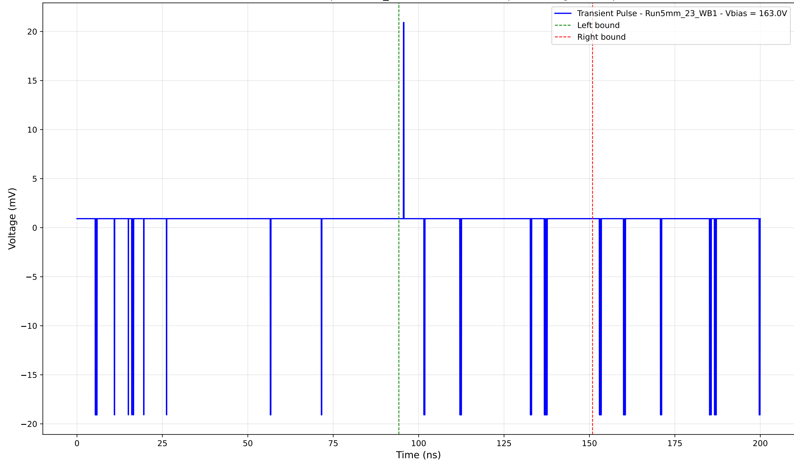
Transient Pulse - Sample: 5mm_23 - Position: 5300.0 \mu\text{m} - Charge: 0.66 pC
