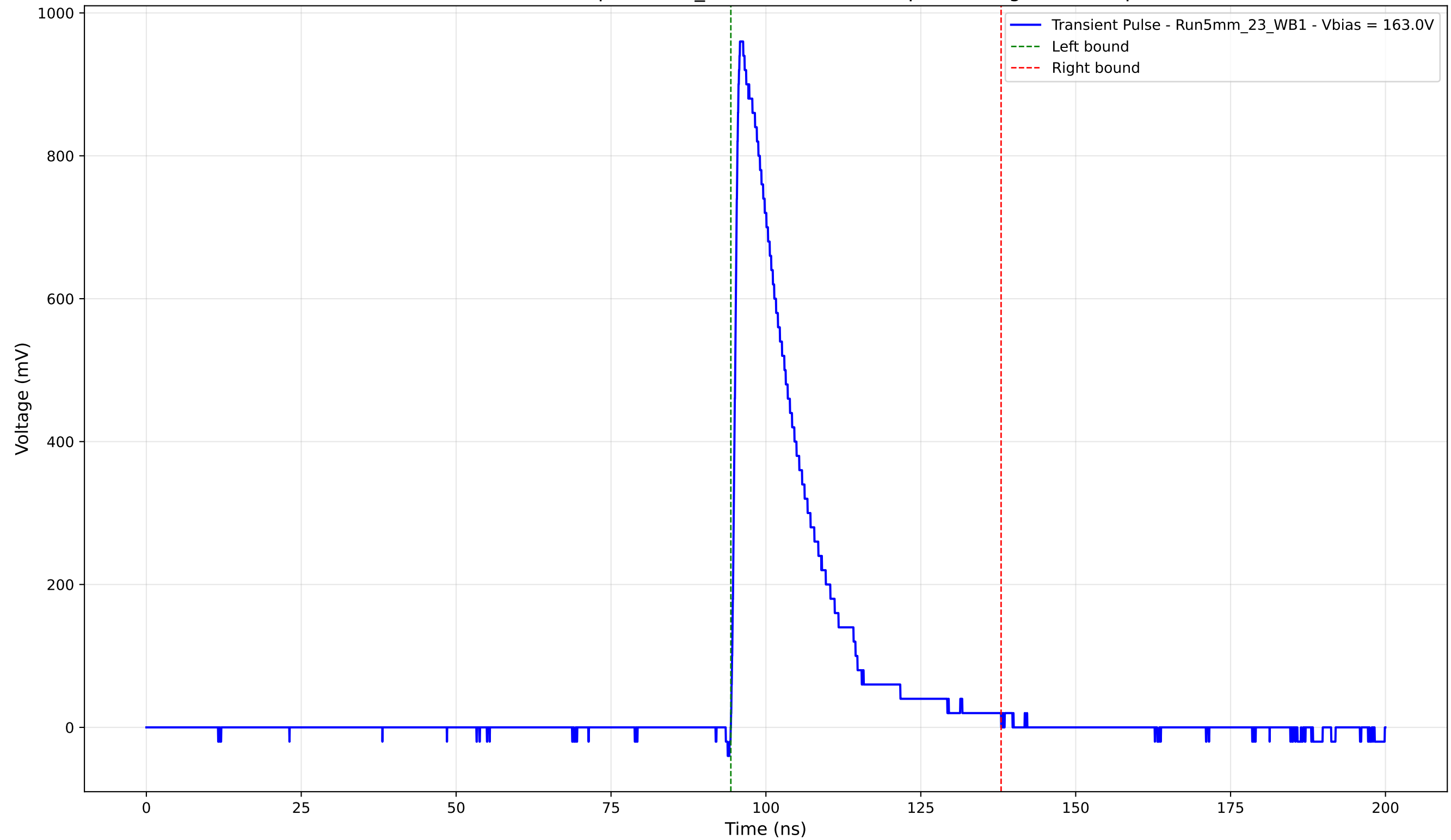
Transient Pulse - Sample: 5mm_23 - Position: 955.0 \mu\text{m} - Charge: 201.80 pC
