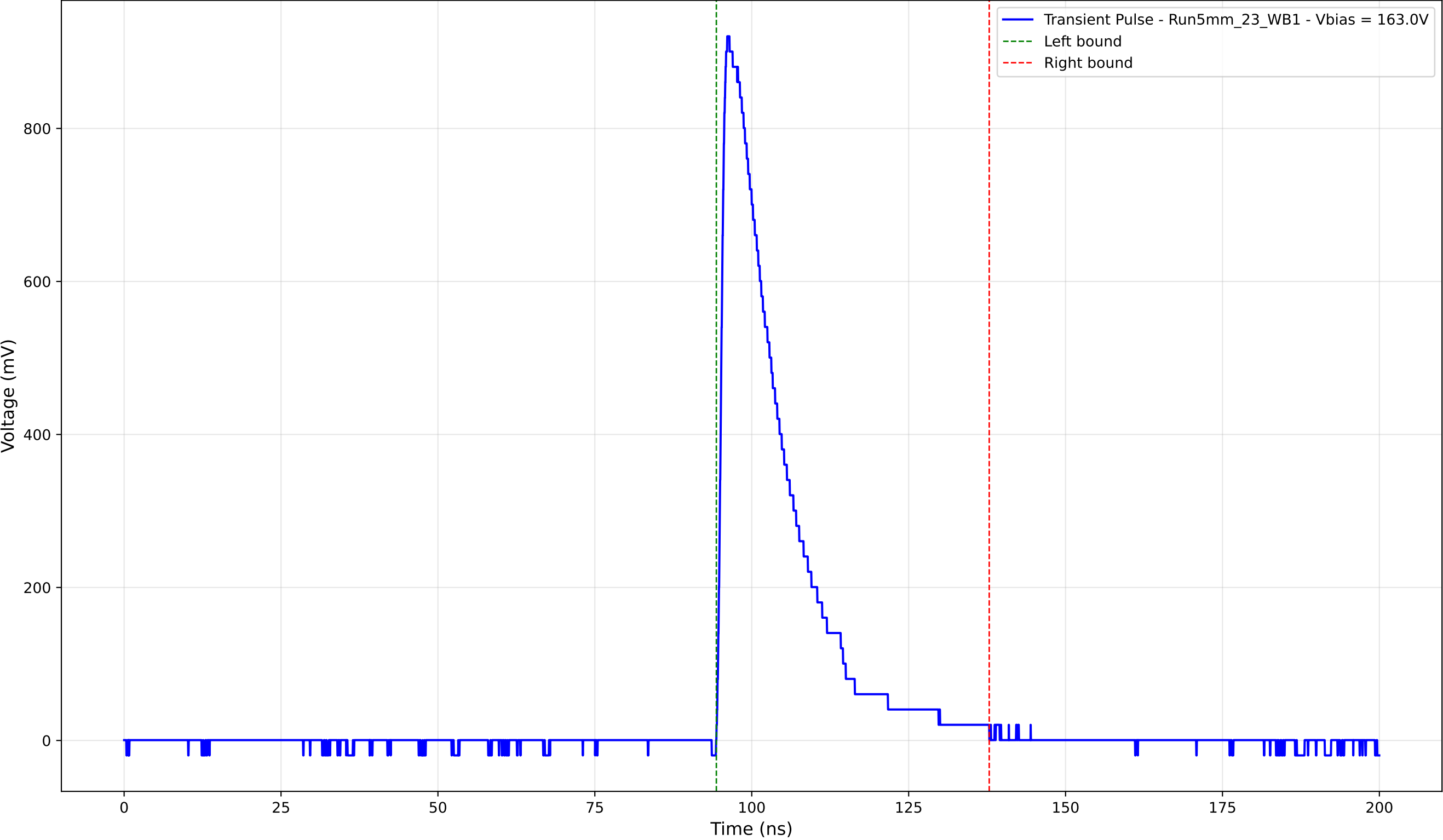
Transient Pulse - Sample: 5mm_23 - Position: 3995.0 \mu\text{m} - Charge: 197.65 pC
