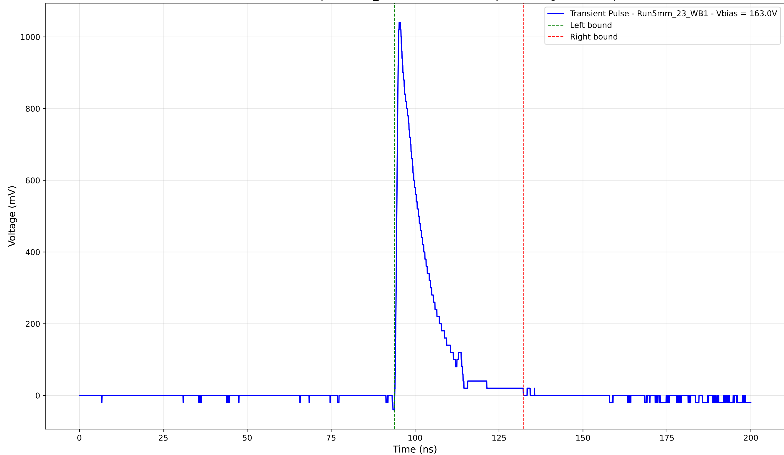
Transient Pulse - Sample: 5mm_23 - Position: 5115.0 \mu\text{m} - Charge: 171.58 pC
