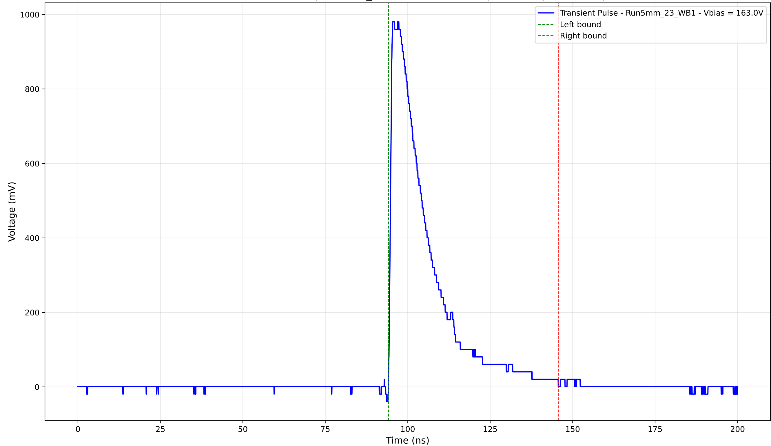
Transient Pulse - Sample: 5mm_23 - Position: 2095.0 \mu\text{m} - Charge: 245.77 pC
