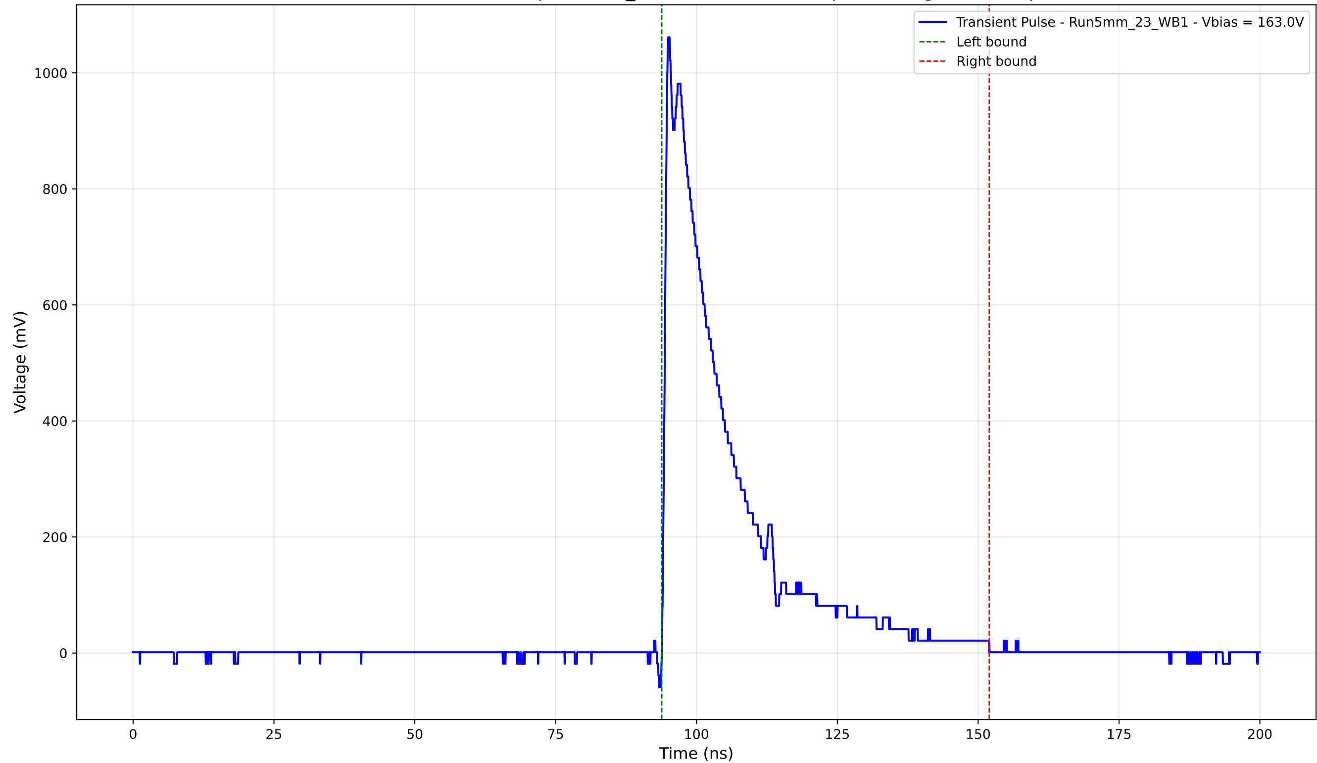
Transient Pulse - Sample: 5mm_23 - Position: 2865.0 \mu\text{m} - Charge: 243.19 pC
