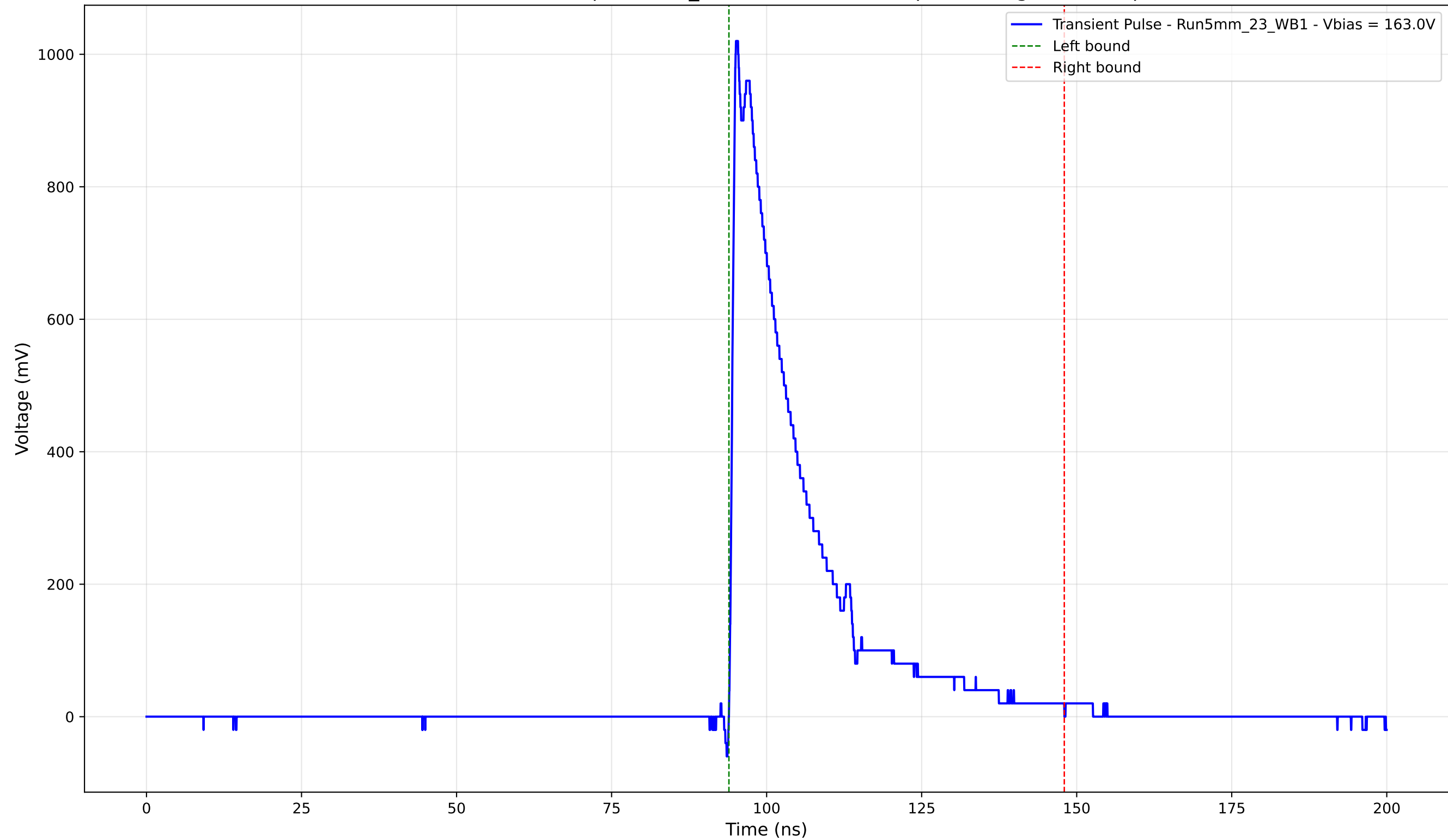
Transient Pulse - Sample: 5mm_23 - Position: 2515.0 \mu\text{m} - Charge: 232.94 pC
