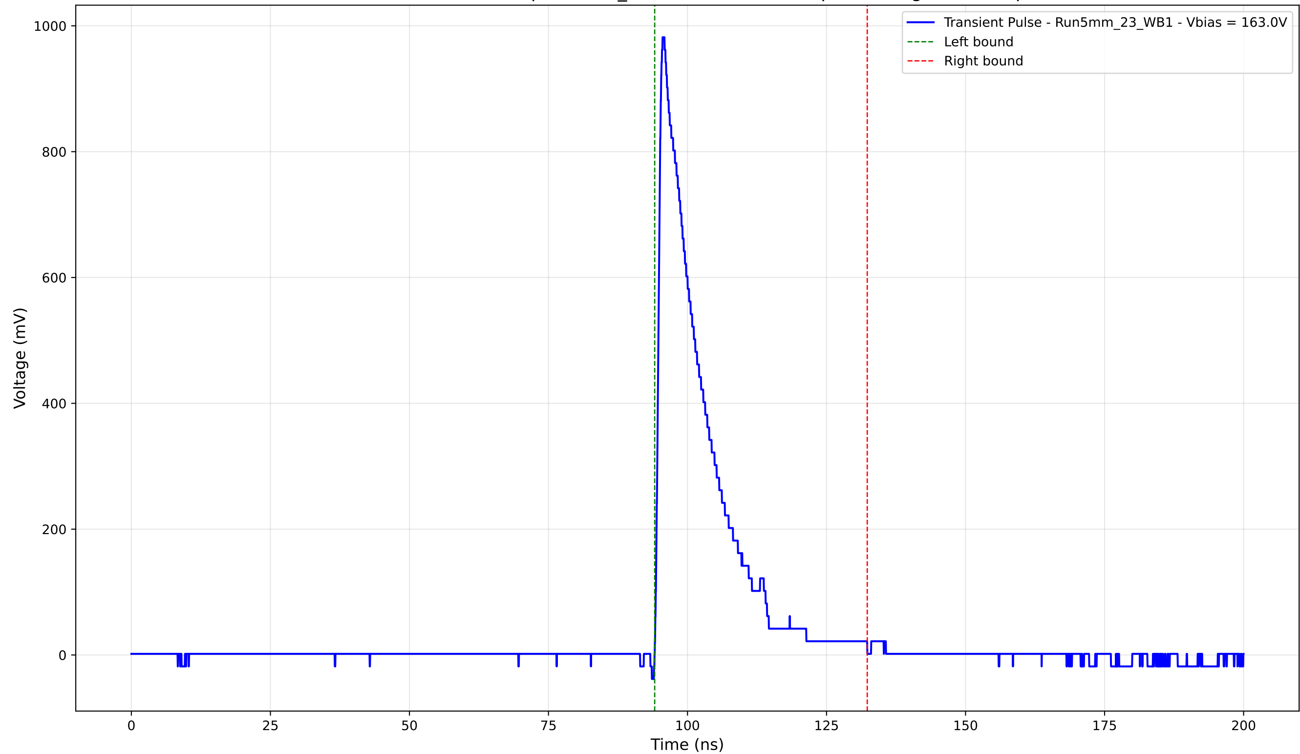
Transient Pulse - Sample: 5mm_23 - Position: 4870.0 \mu\text{m} - Charge: 171.22 pC
