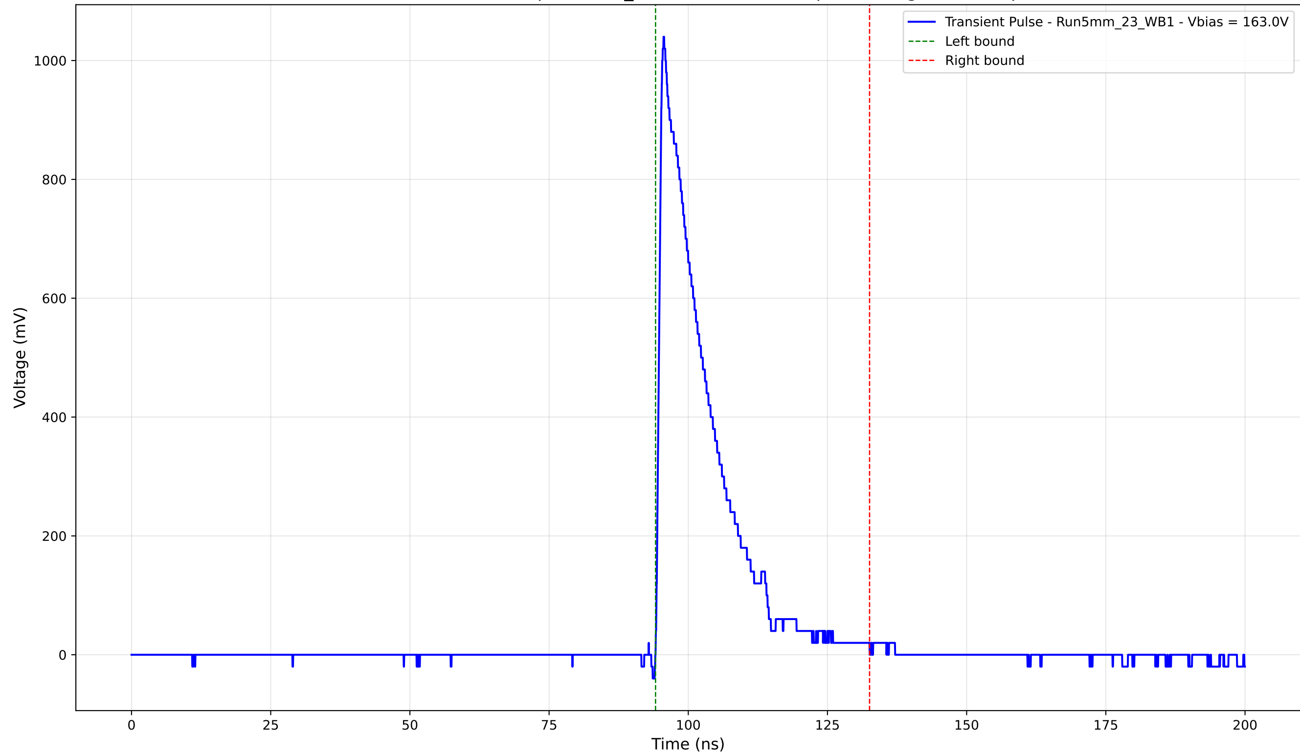
Transient Pulse - Sample: 5mm_23 - Position: 510.0 \mu\text{m} - Charge: 192.73 pC
