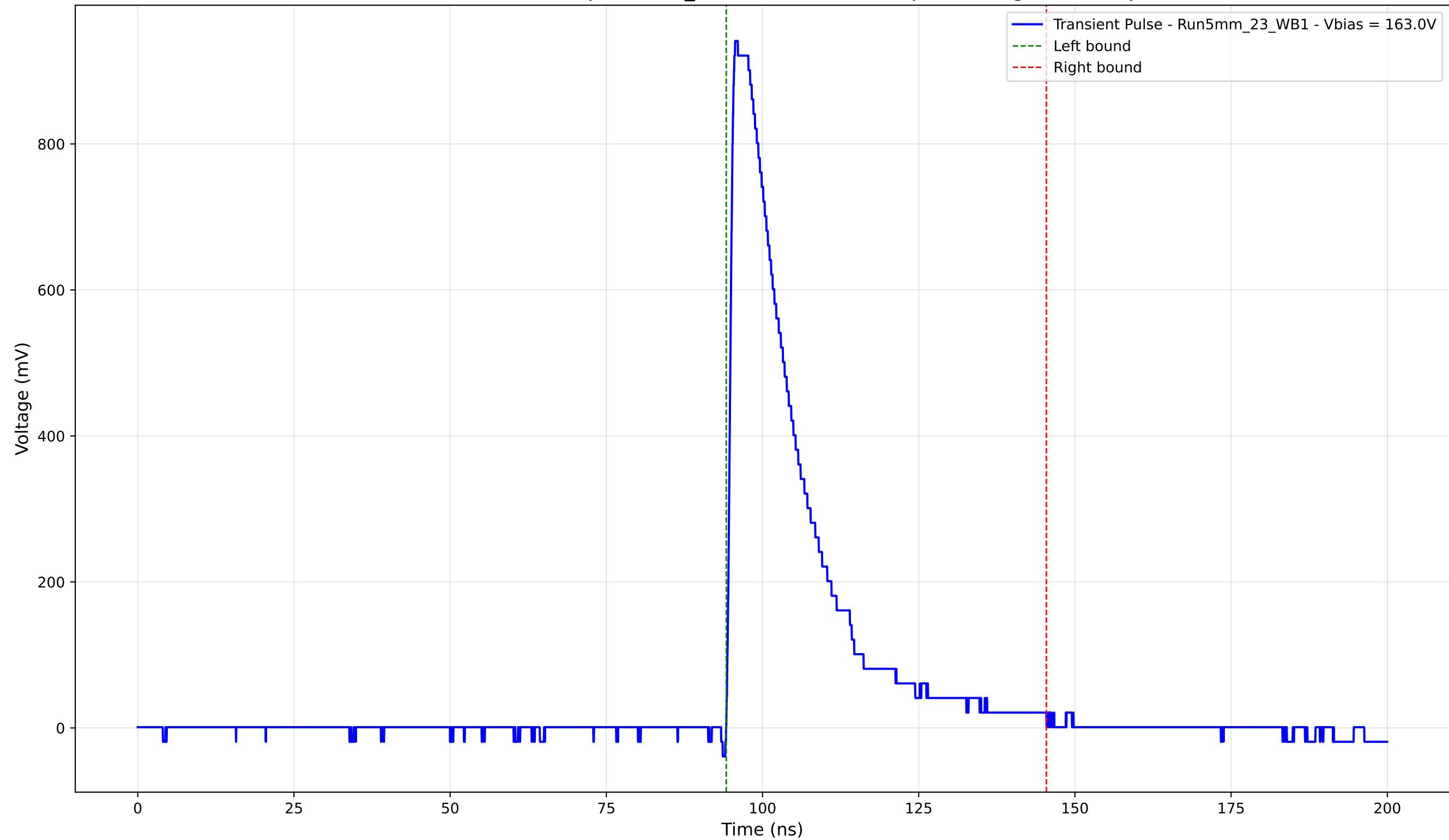
Transient Pulse - Sample: 5mm_23 - Position: 3475.0 \mu\text{m} - Charge: 222.17 pC
