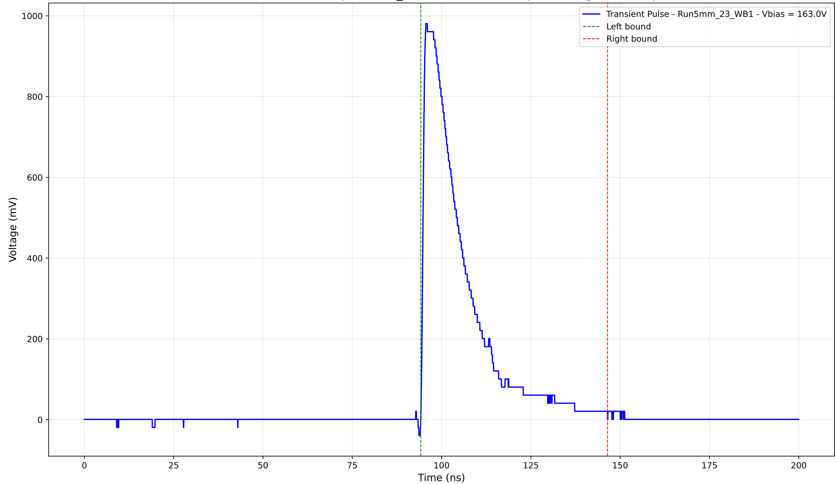
Transient Pulse - Sample: 5mm_23 - Position: 2005.0 \mu\text{m} - Charge: 244.53 pC
