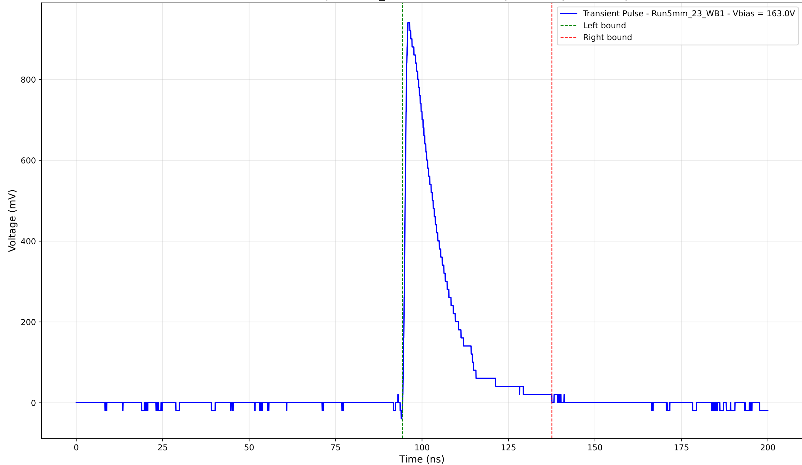
Transient Pulse - Sample: 5mm_23 - Position: 1120.0 \mu\text{m} - Charge: 199.55 pC
