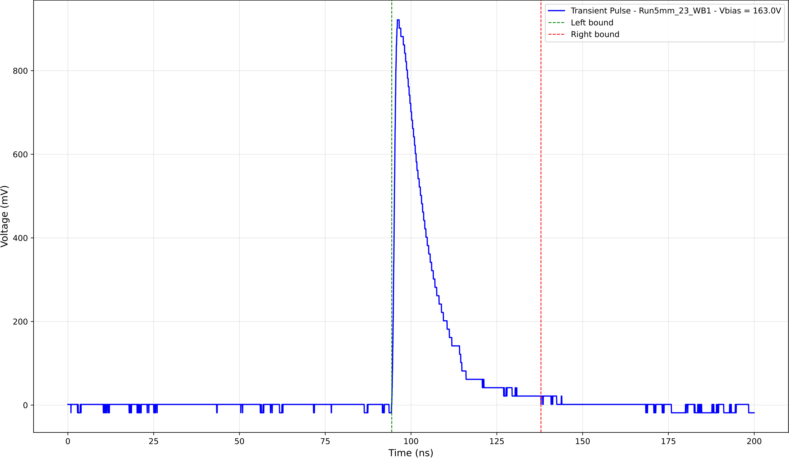
Transient Pulse - Sample: 5mm_23 - Position: 4095.0 \mu\text{m} - Charge: 197.14 pC
