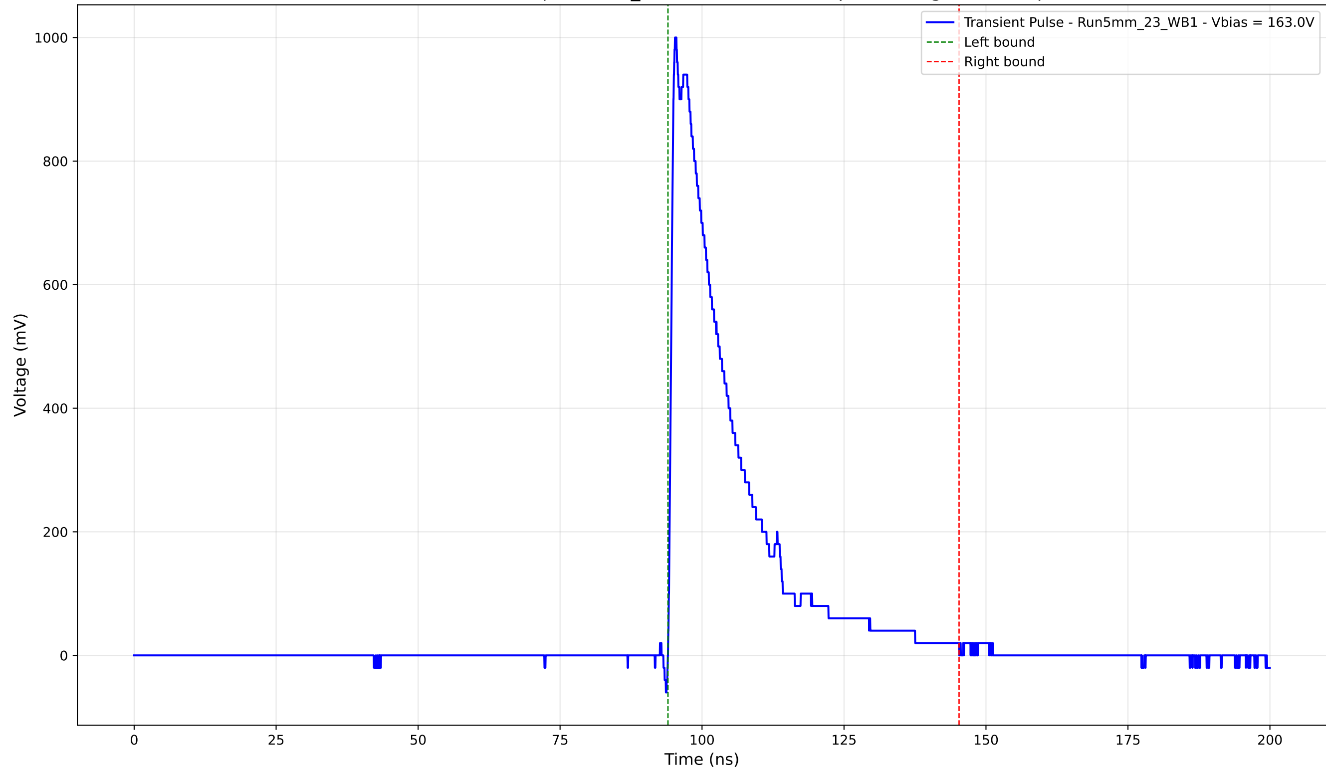
Transient Pulse - Sample: 5mm_23 - Position: 2380.0 \mu\text{m} - Charge: 226.52 pC
