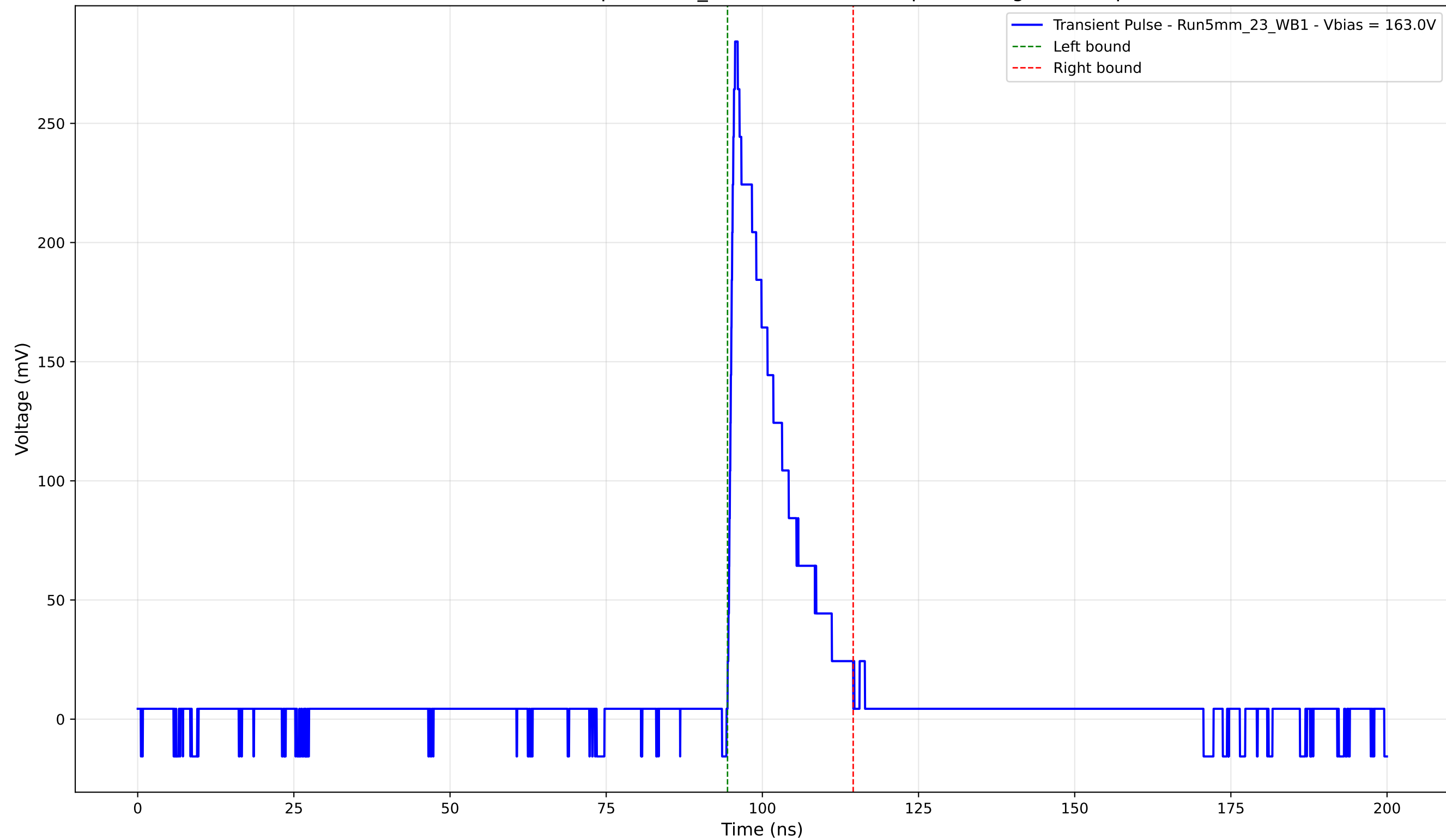
Transient Pulse - Sample: 5mm_23 - Position: 710.0 \mu\text{m} - Charge: 44.19 pC
