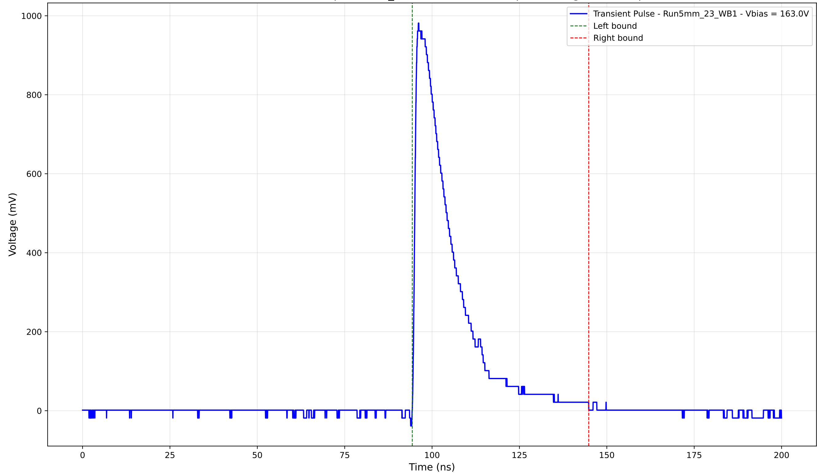
Transient Pulse - Sample: 5mm_23 - Position: 1635.0 \mu\text{m} - Charge: 232.21 pC
