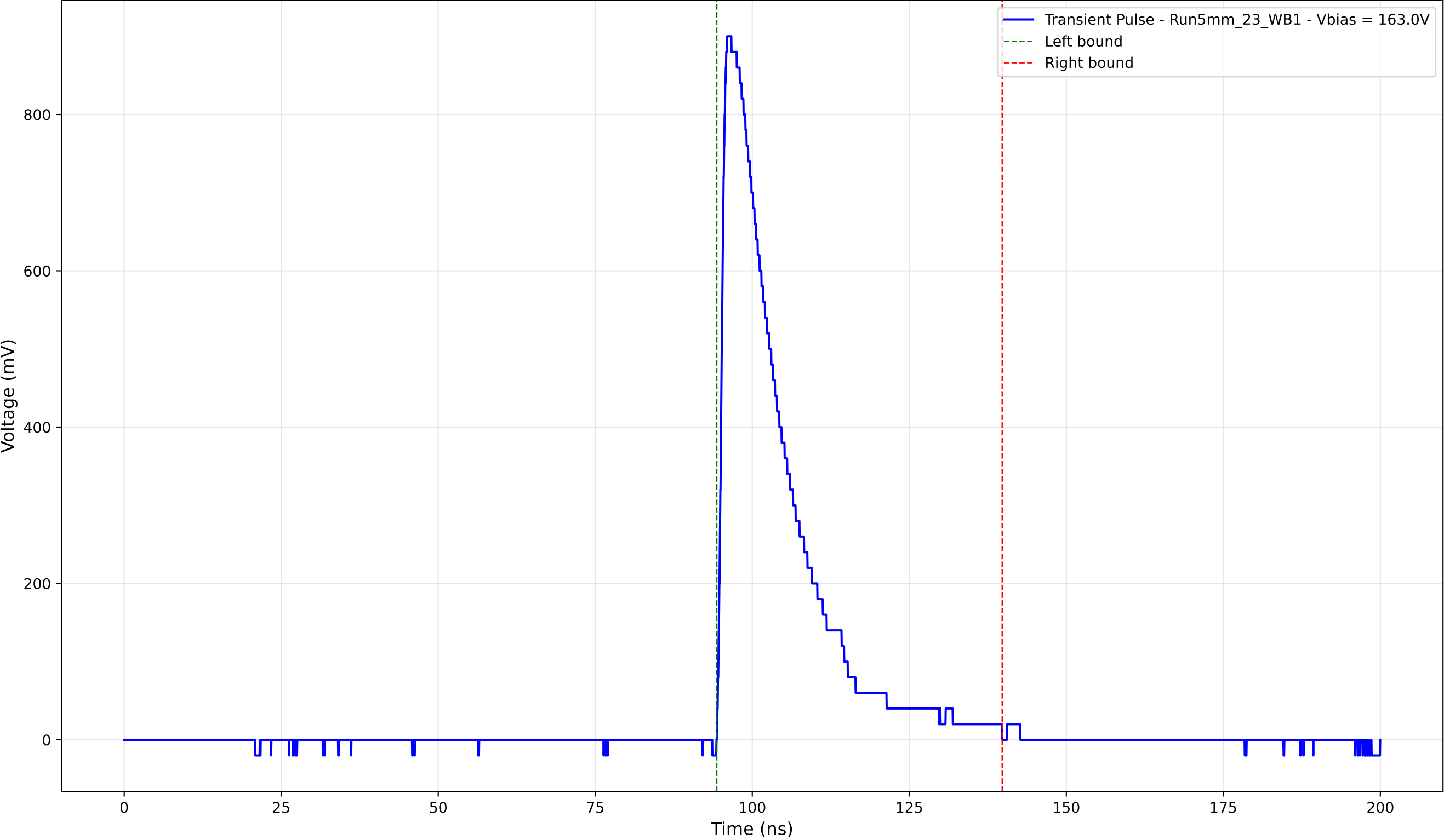
Transient Pulse - Sample: 5mm_23 - Position: 3910.0 \mu\text{m} - Charge: 196.93 pC
