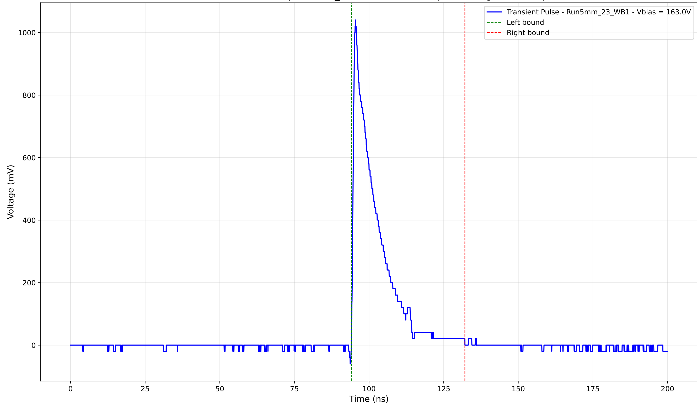
Transient Pulse - Sample: 5mm_23 - Position: 350.0 \mu\text{m} - Charge: 168.88 pC
