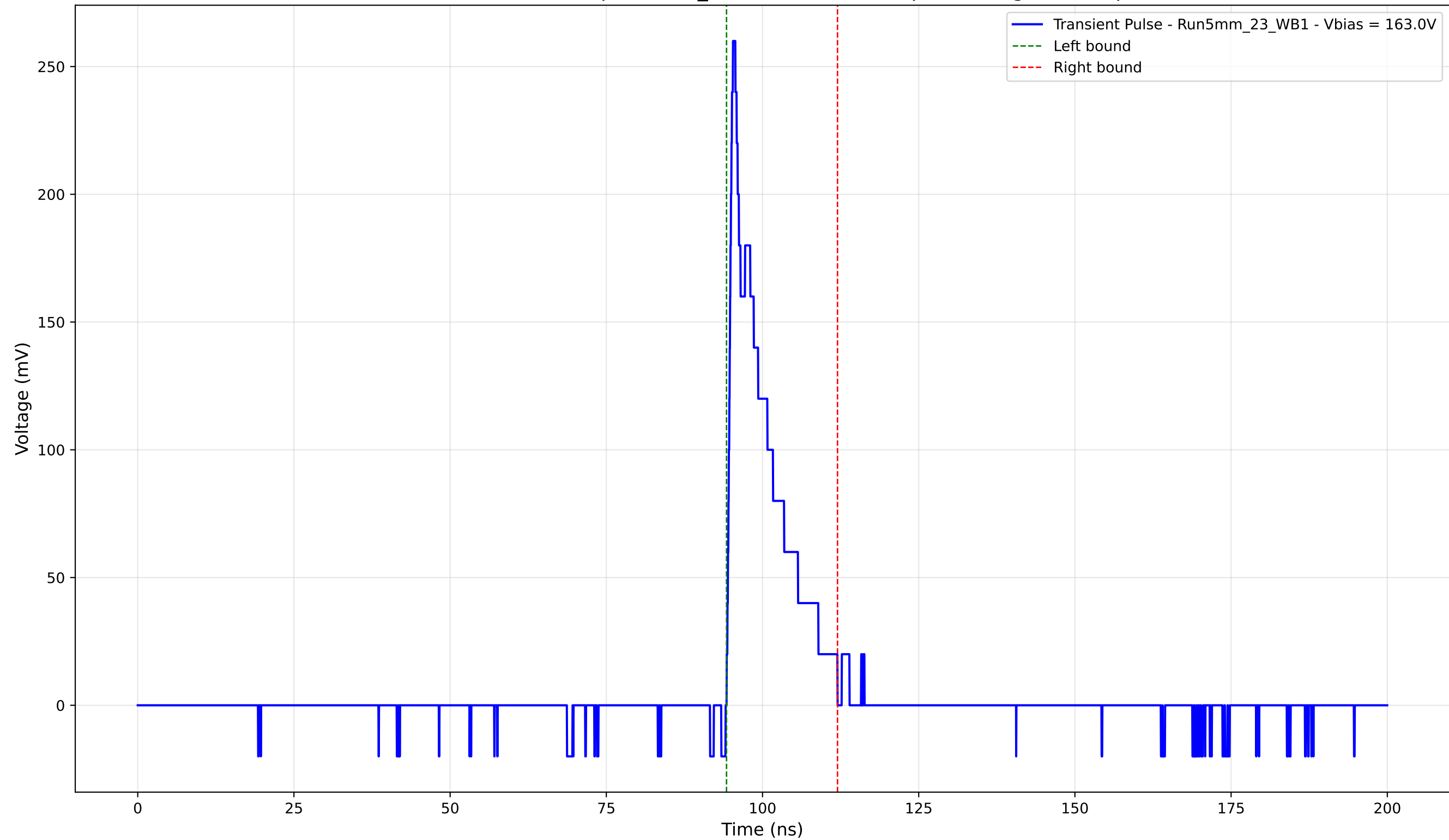
Transient Pulse - Sample: 5mm_23 - Position: 285.0 \mu\text{m} - Charge: 31.95 pC
