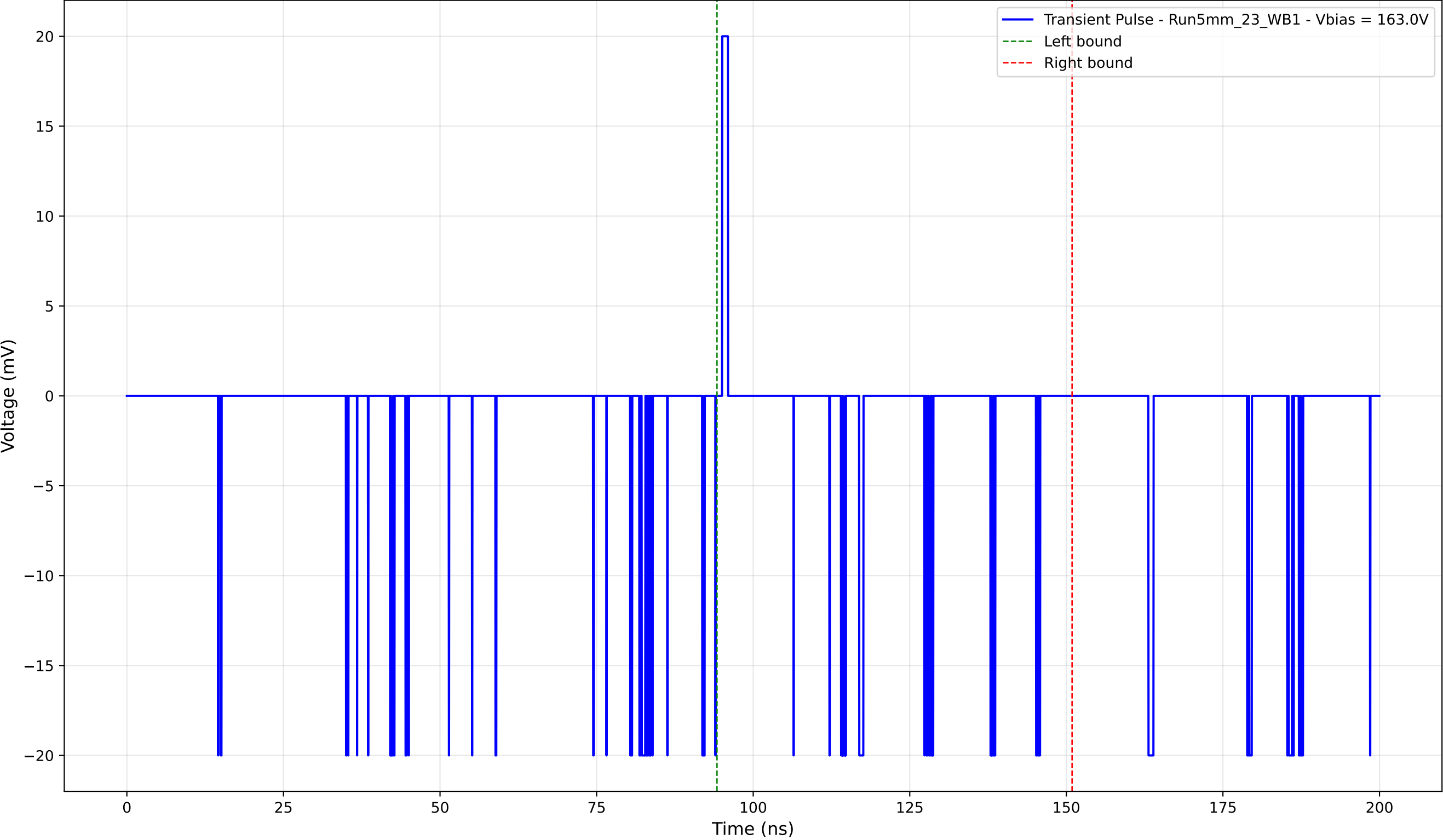
Transient Pulse - Sample: 5mm_23 - Position: 155.0 \mu\text{m} - Charge: -0.95 pC
