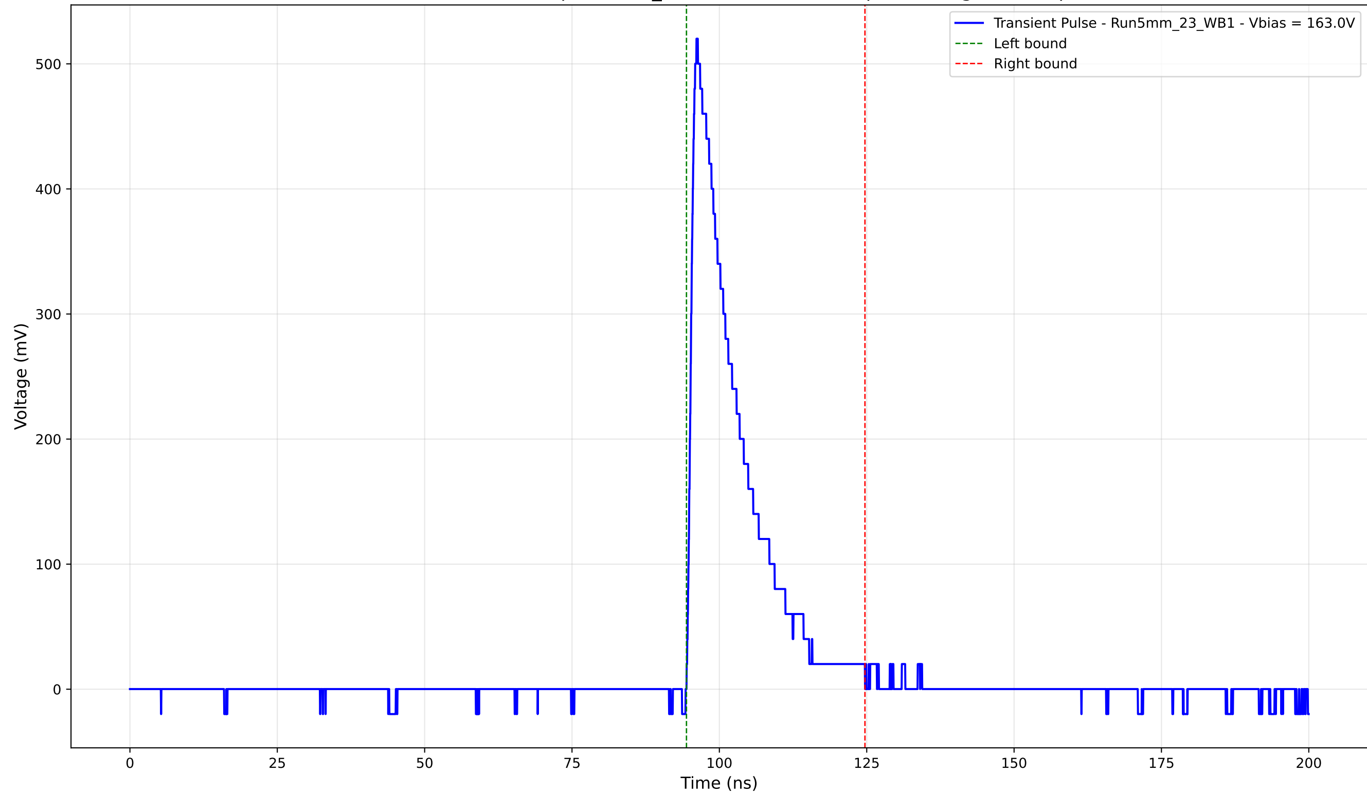
Transient Pulse - Sample: 5mm_23 - Position: 4305.0 \mu\text{m} - Charge: 89.99 pC
