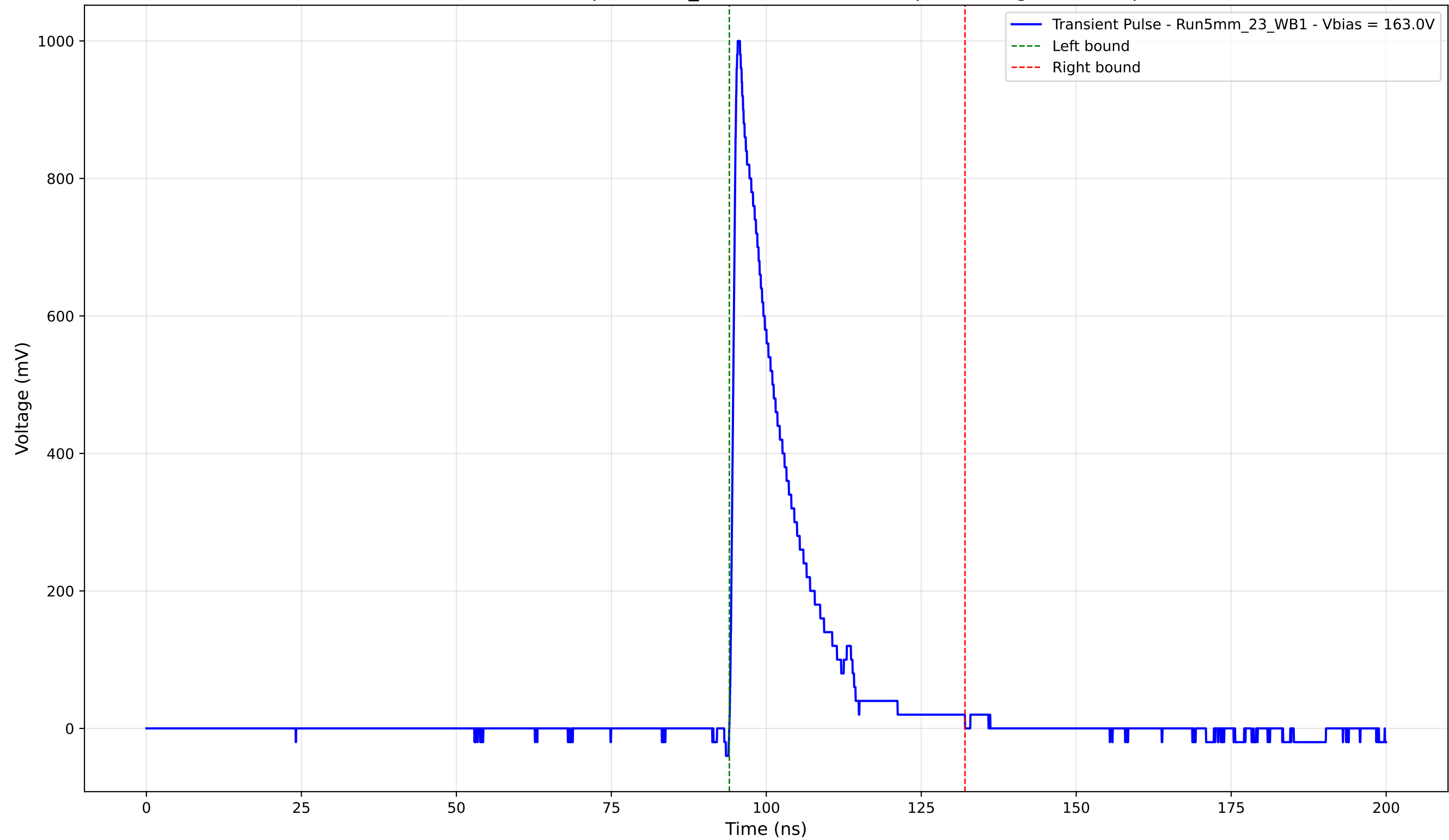
Transient Pulse - Sample: 5mm_23 - Position: 4990.0 \mu\text{m} - Charge: 167.58 pC
