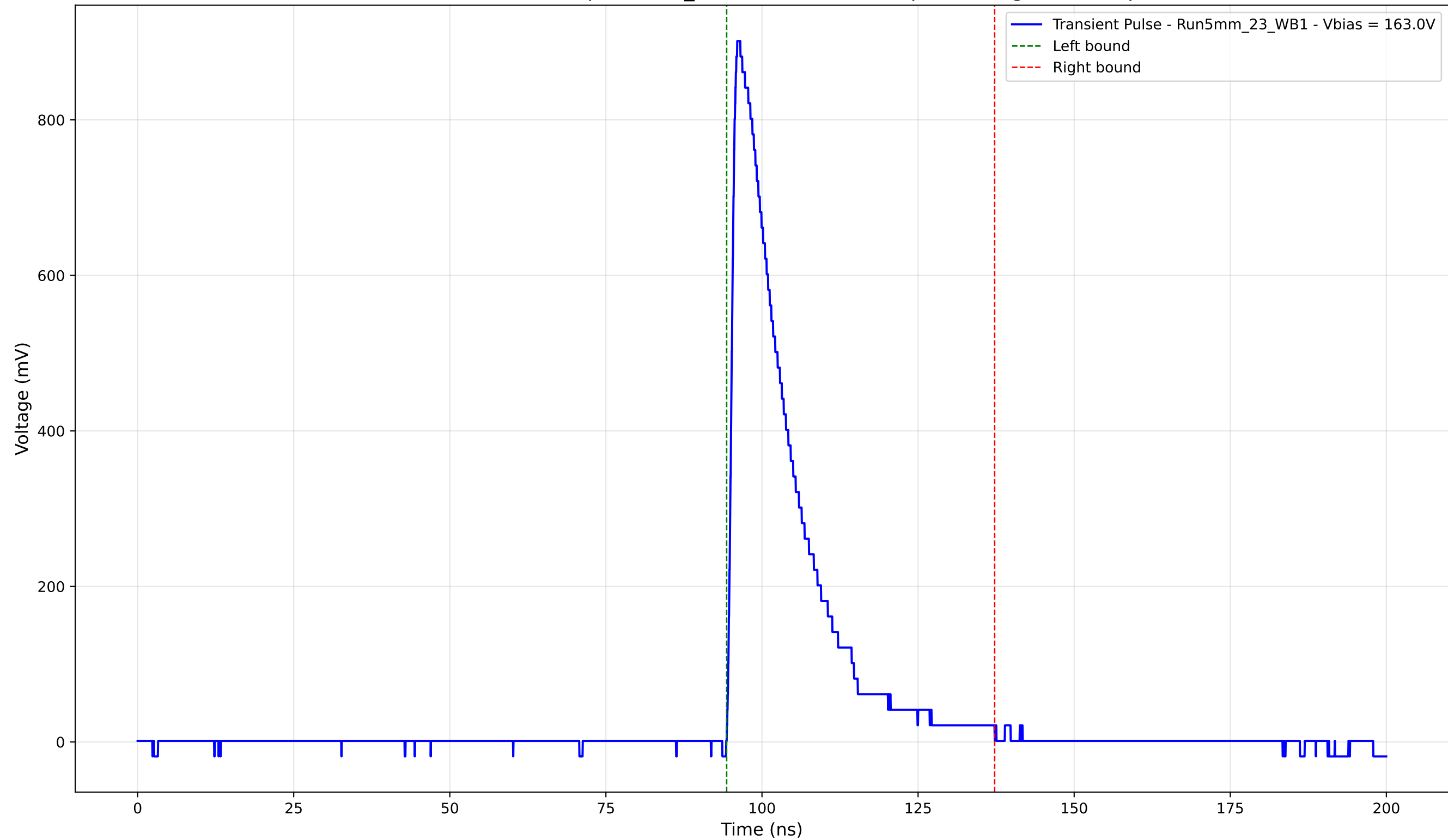
Transient Pulse - Sample: 5mm_23 - Position: 4160.0 \mu\text{m} - Charge: 185.43 pC
