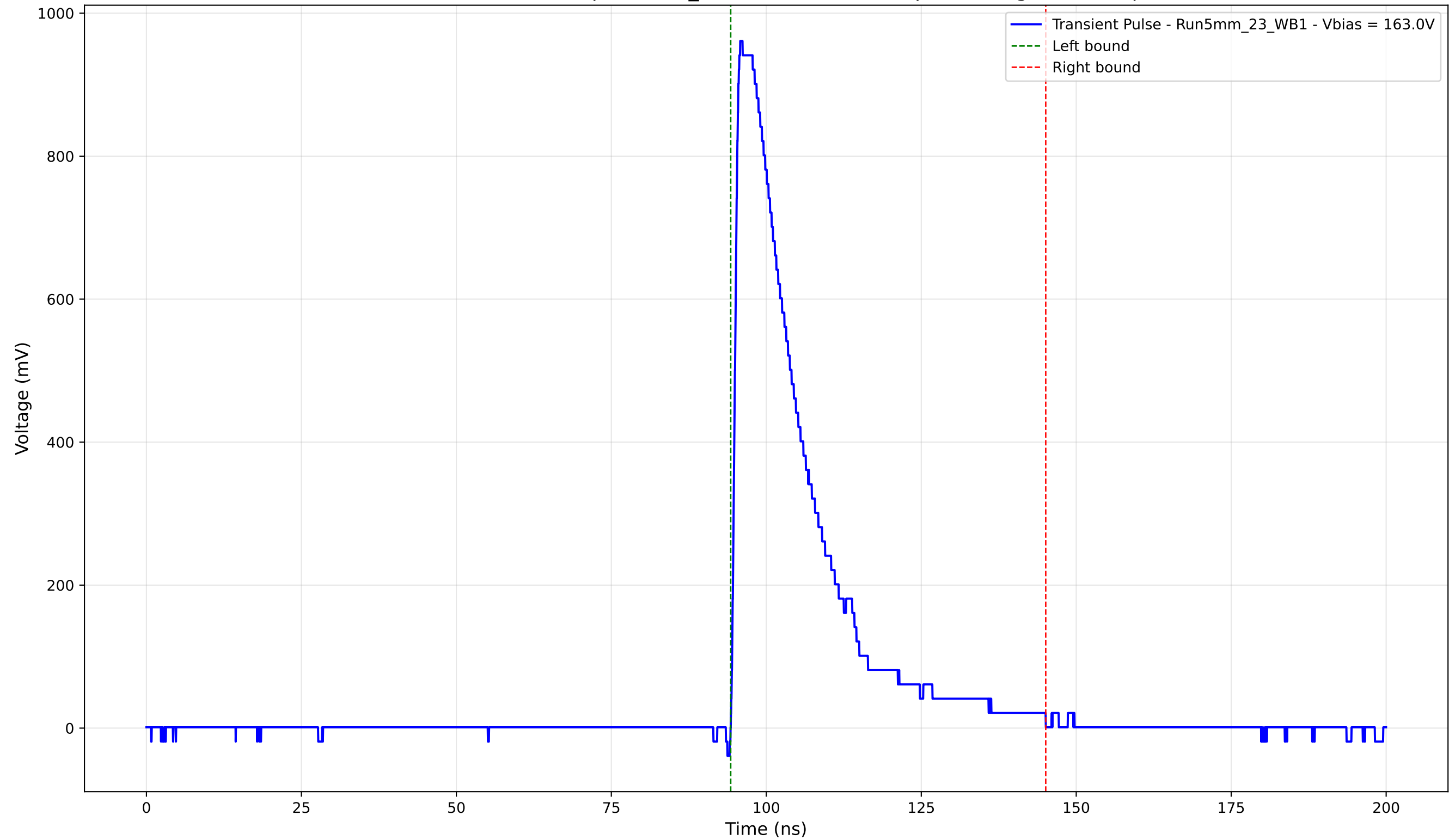
Transient Pulse - Sample: 5mm_23 - Position: 1860.0 \mu\text{m} - Charge: 231.62 pC
