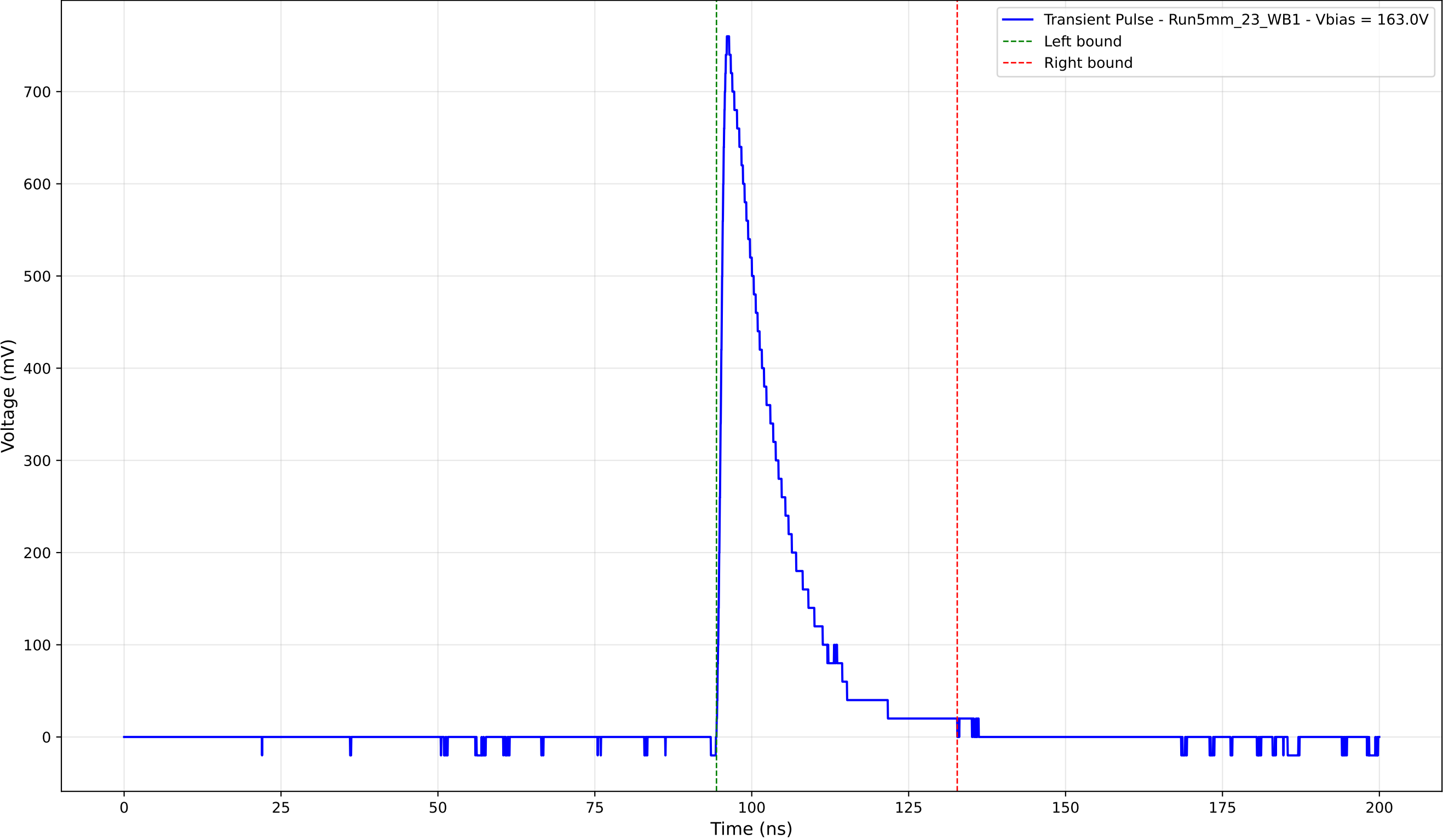
Transient Pulse - Sample: 5mm_23 - Position: 4330.0 \mu\text{m} - Charge: 139.92 pC
