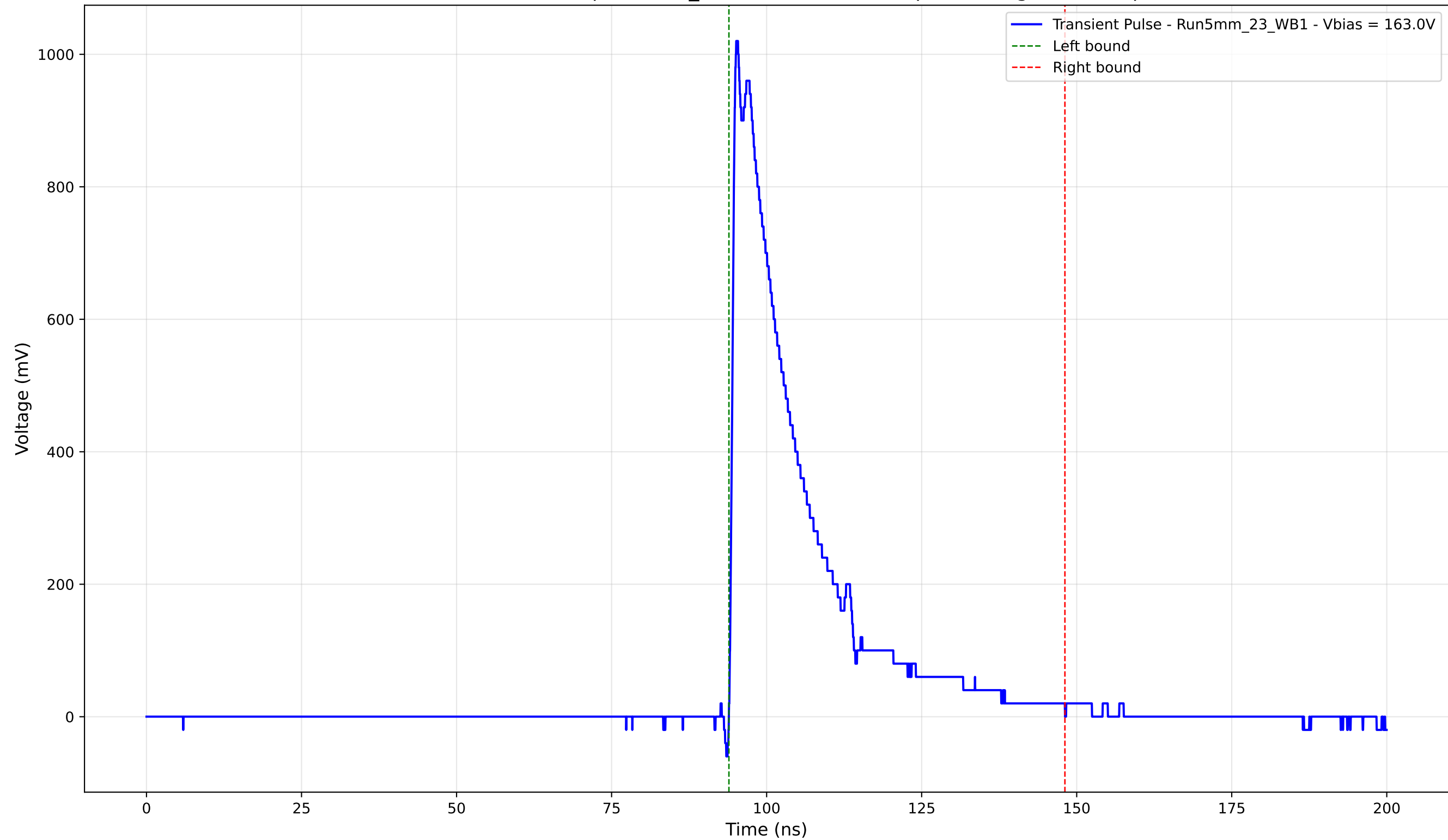
Transient Pulse - Sample: 5mm_23 - Position: 2495.0 \mu\text{m} - Charge: 232.40 pC
