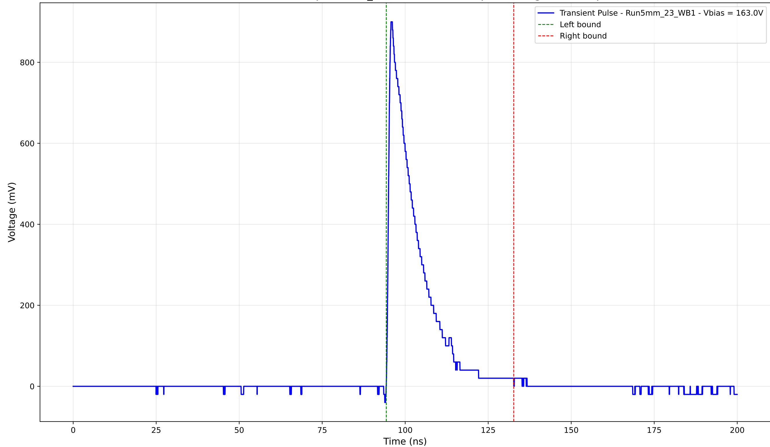
Transient Pulse - Sample: 5mm_23 - Position: 785.0 \mu\text{m} - Charge: 164.94 pC
