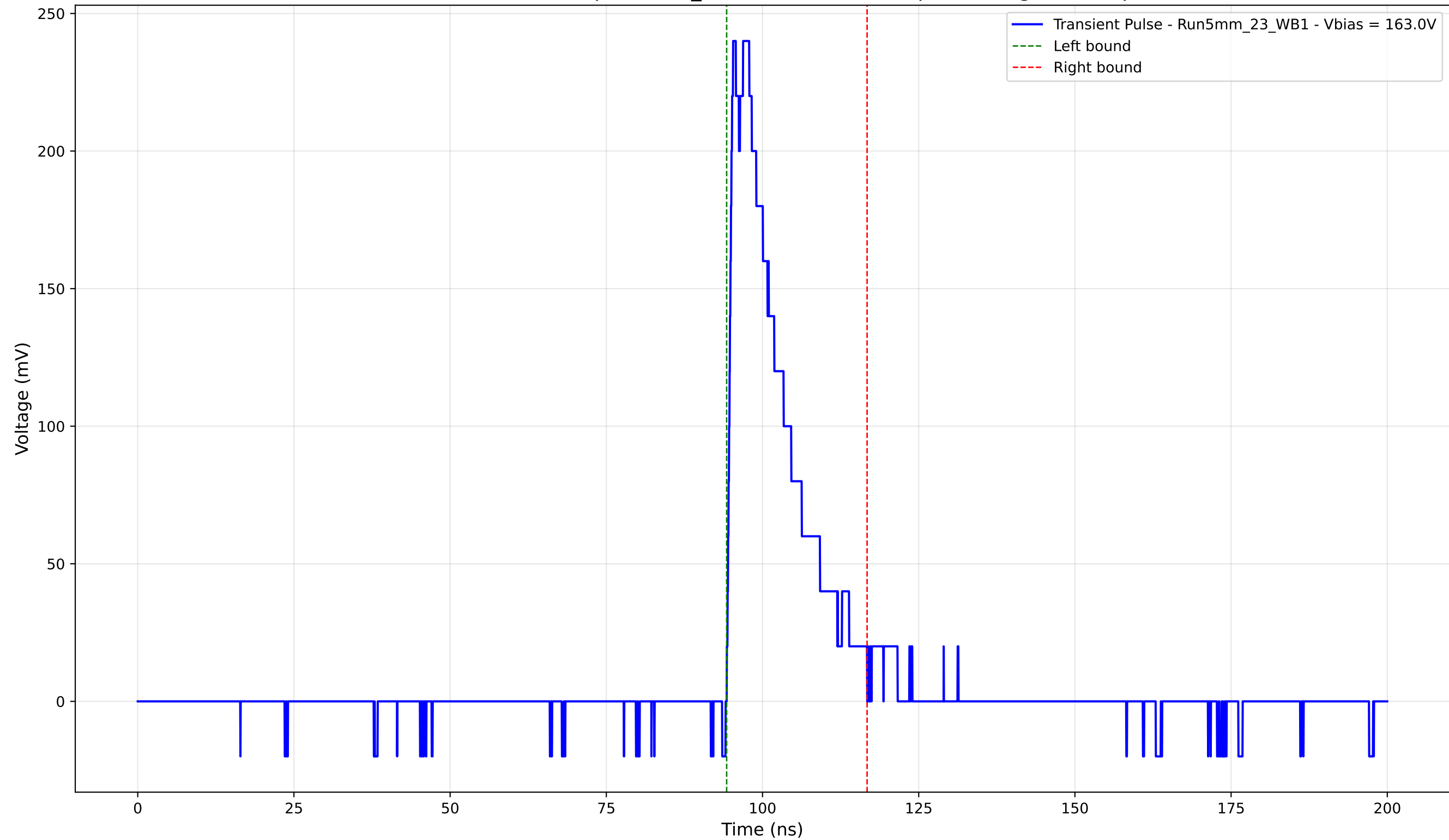
Transient Pulse - Sample: 5mm_23 - Position: 2230.0 \mu\text{m} - Charge: 45.18 pC
