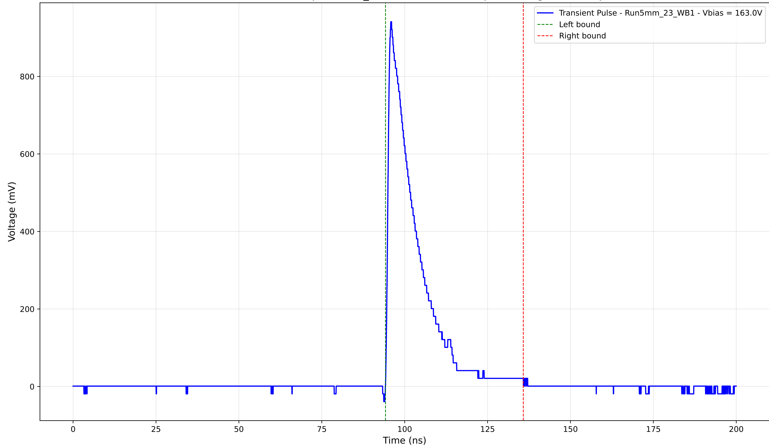
Transient Pulse - Sample: 5mm_23 - Position: 4630.0 \mu\text{m} - Charge: 174.23 pC
