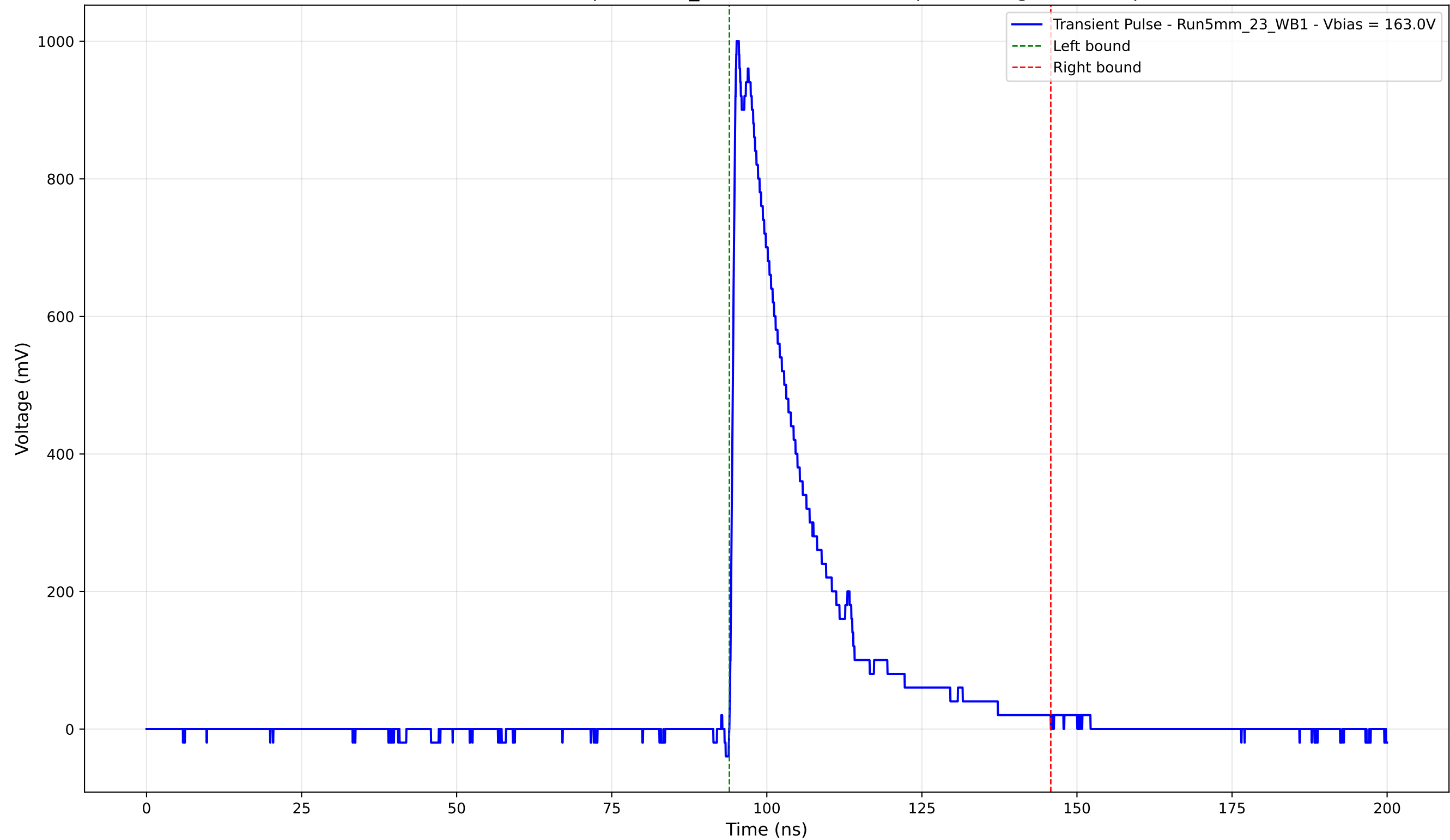
Transient Pulse - Sample: 5mm_23 - Position: 3060.0 \mu\text{m} - Charge: 227.95 pC
