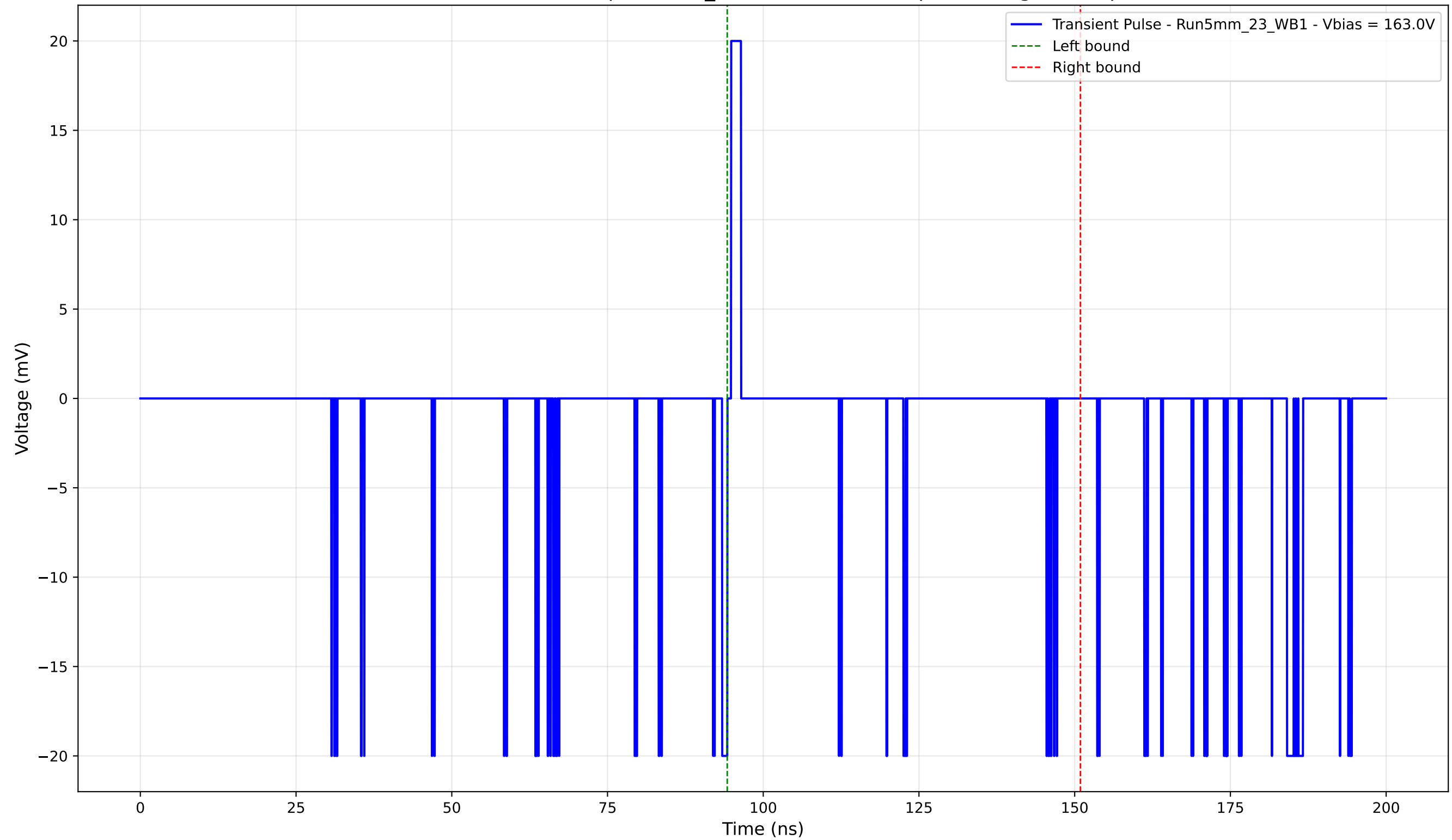
Transient Pulse - Sample: 5mm_23 - Position: 120.0 \mu\text{m} - Charge: 0.06 pC
