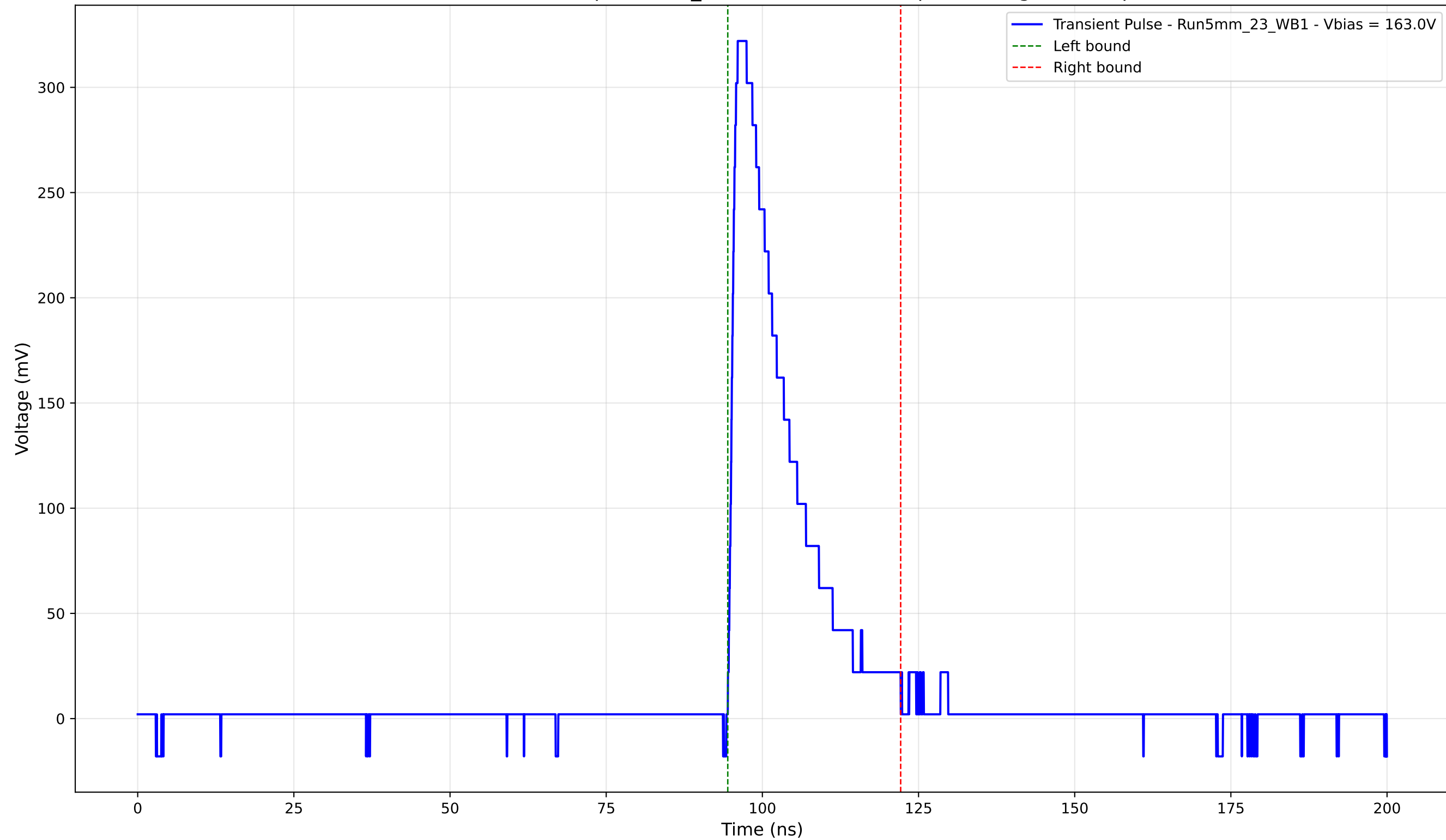
Transient Pulse - Sample: 5mm_23 - Position: 1705.0 \mu\text{m} - Charge: 62.84 pC
