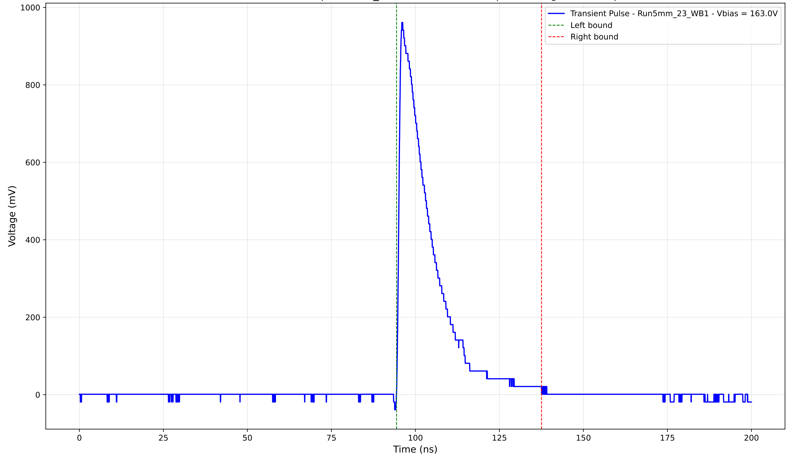
Transient Pulse - Sample: 5mm_23 - Position: 1035.0 \mu\text{m} - Charge: 201.44 pC
