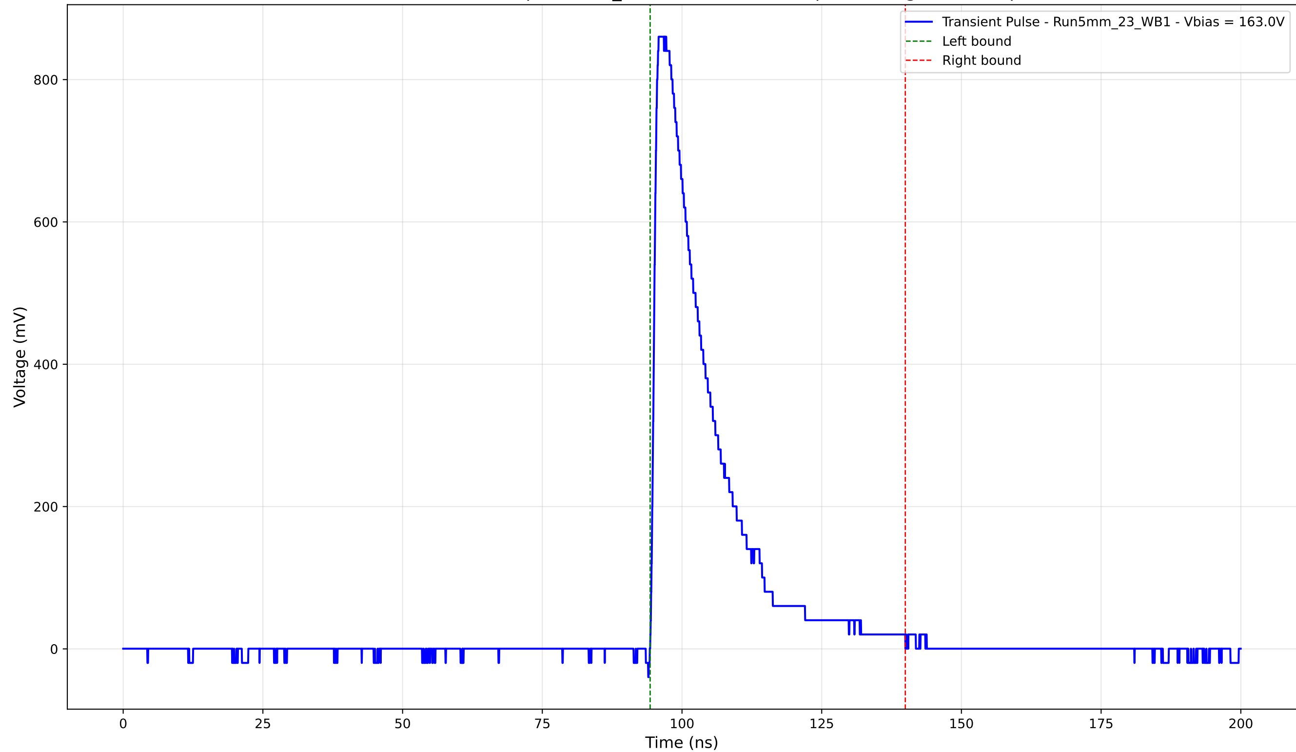
Transient Pulse - Sample: 5mm_23 - Position: 3665.0 \mu\text{m} - Charge: 189.71 pC
