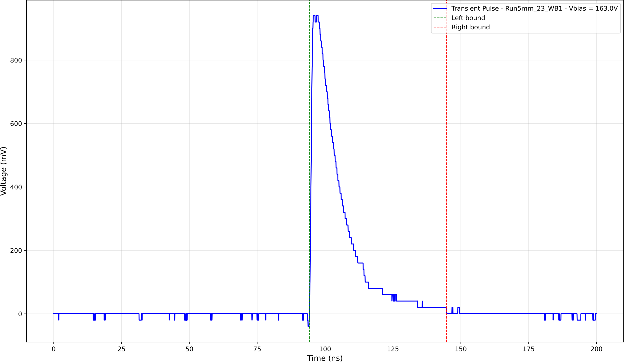
Transient Pulse - Sample: 5mm_23 - Position: 3535.0 \mu\text{m} - Charge: 222.63 pC
