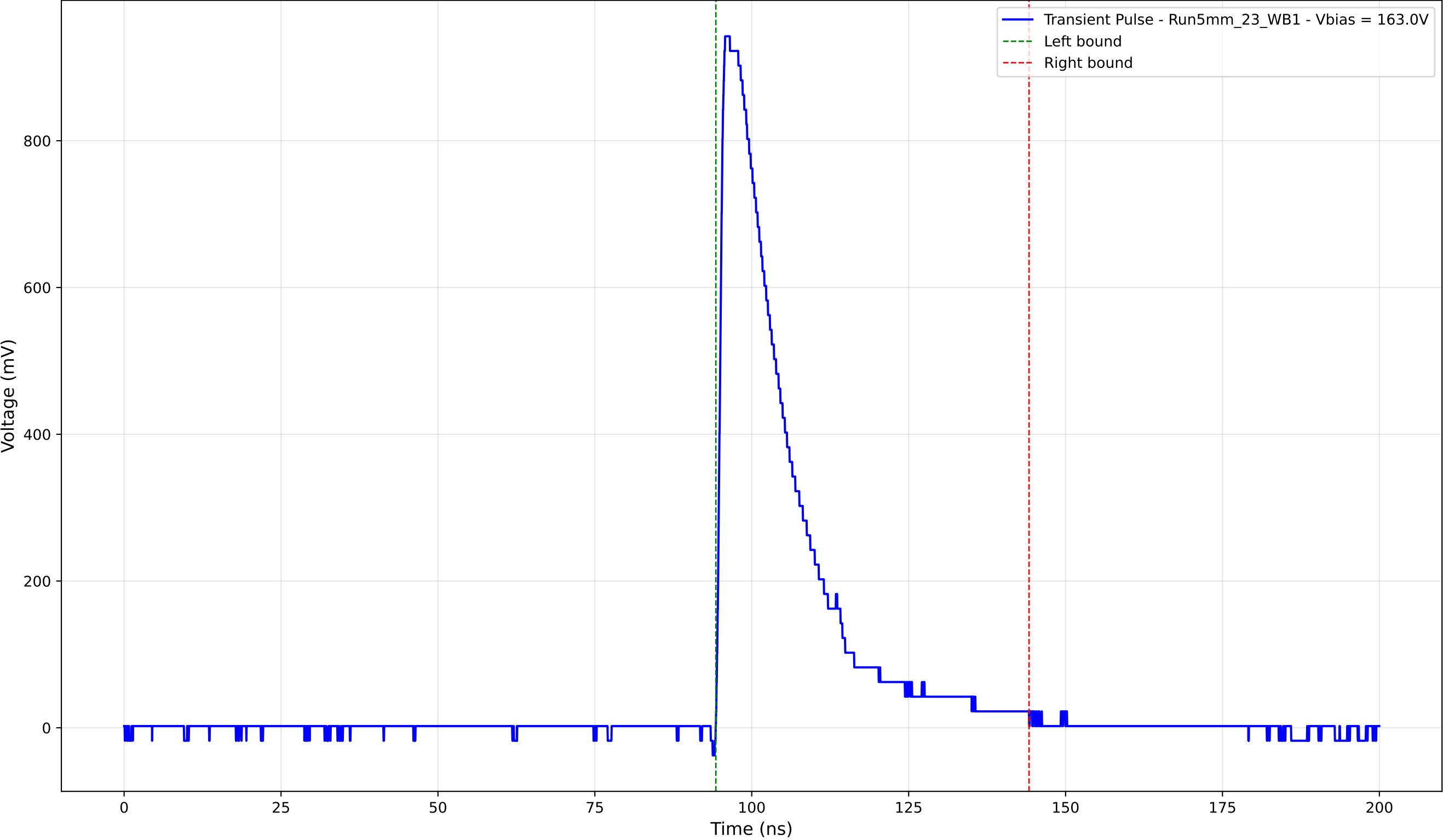
Transient Pulse - Sample: 5mm_23 - Position: 1835.0 \mu\text{m} - Charge: 225.85 pC
