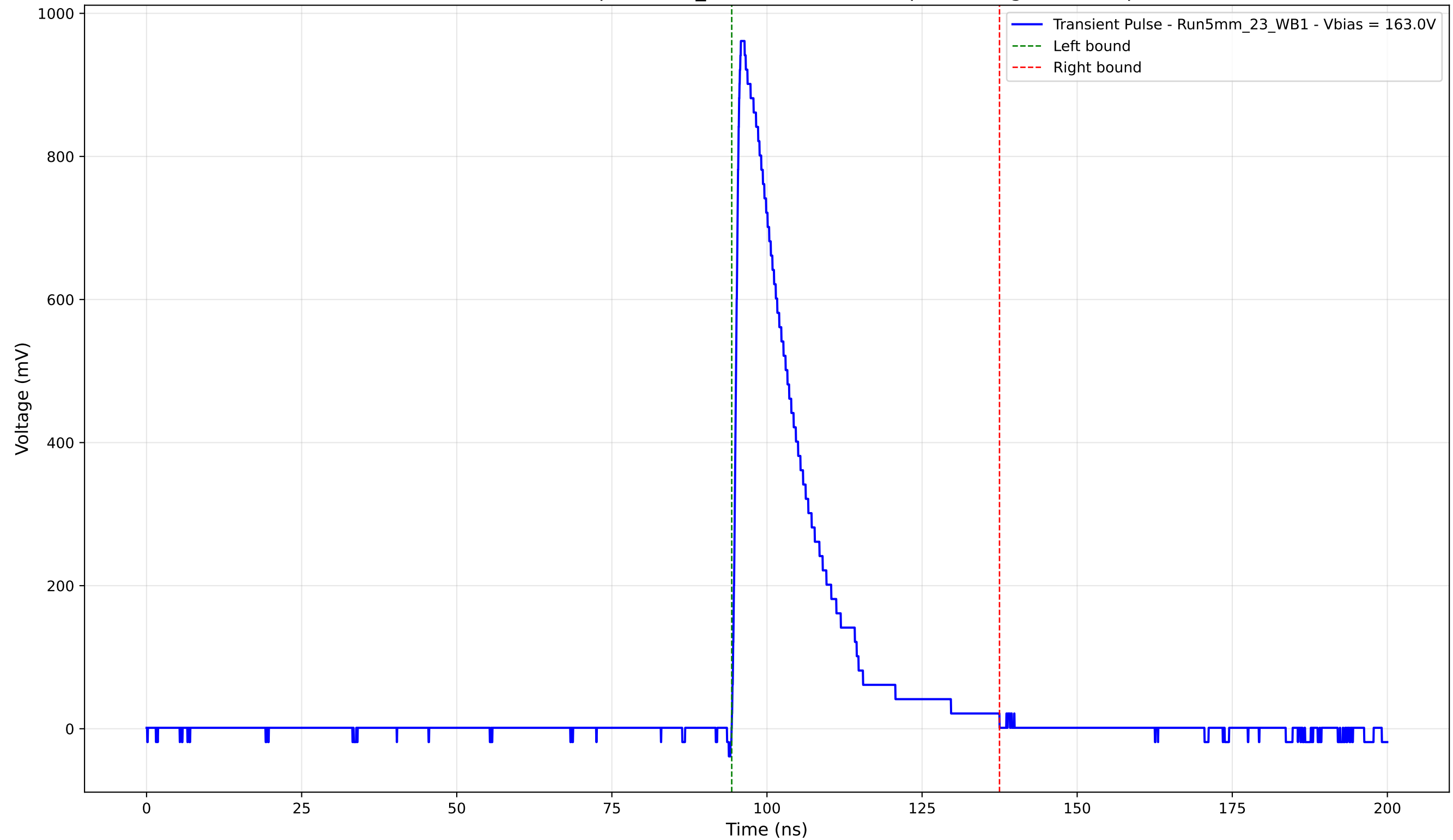
Transient Pulse - Sample: 5mm_23 - Position: 940.0 \mu\text{m} - Charge: 203.04 pC
