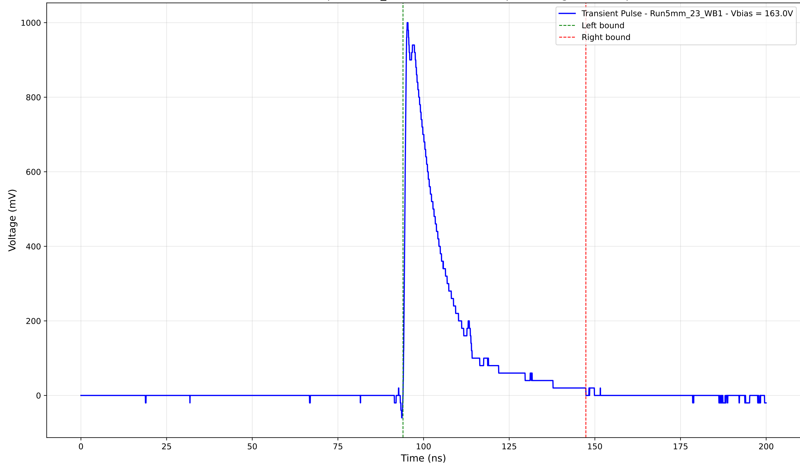
Transient Pulse - Sample: 5mm_23 - Position: 3090.0 \mu\text{m} - Charge: 226.00 pC
