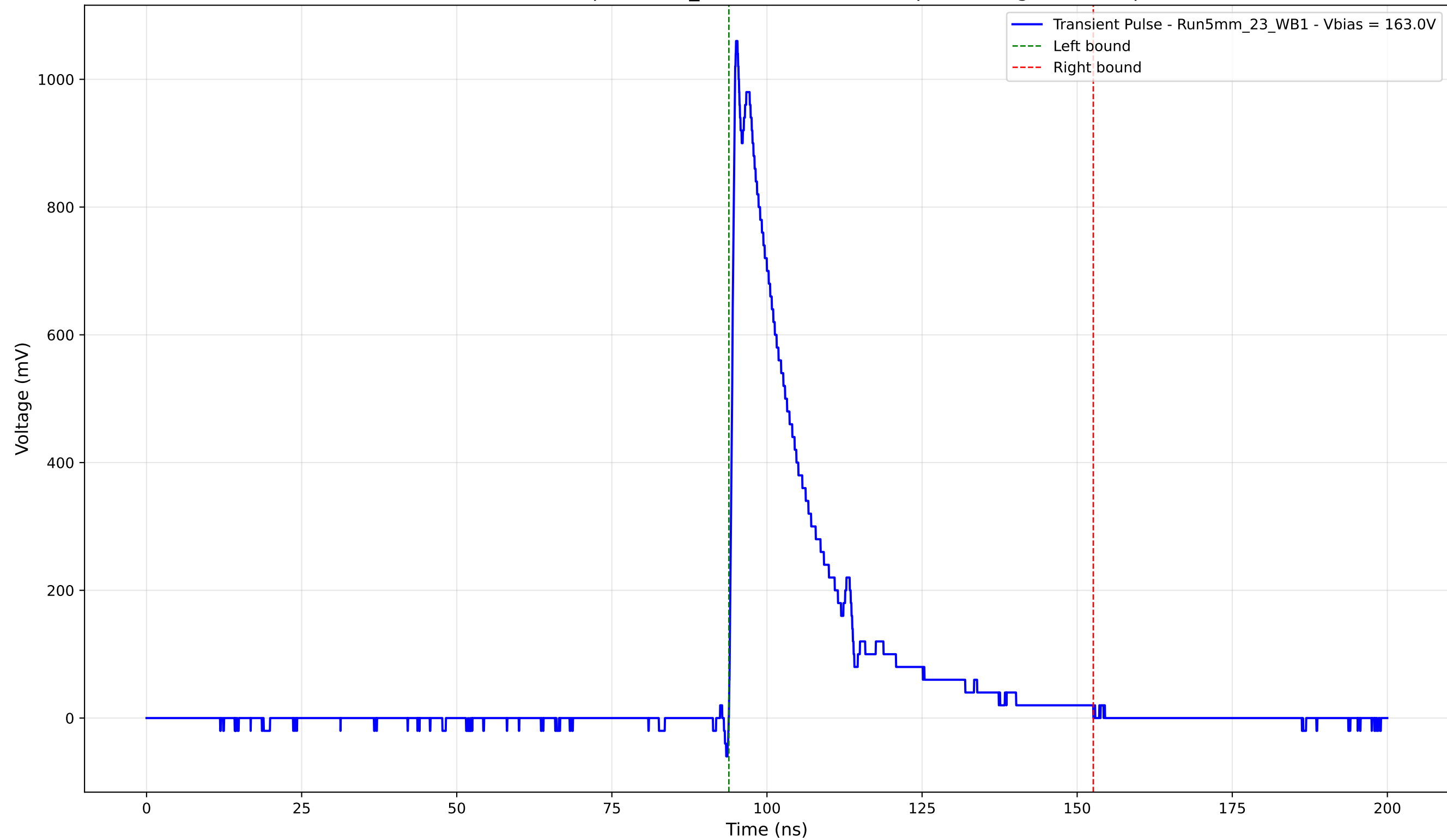
Transient Pulse - Sample: 5mm_23 - Position: 2885.0 \mu\text{m} - Charge: 242.10 pC
