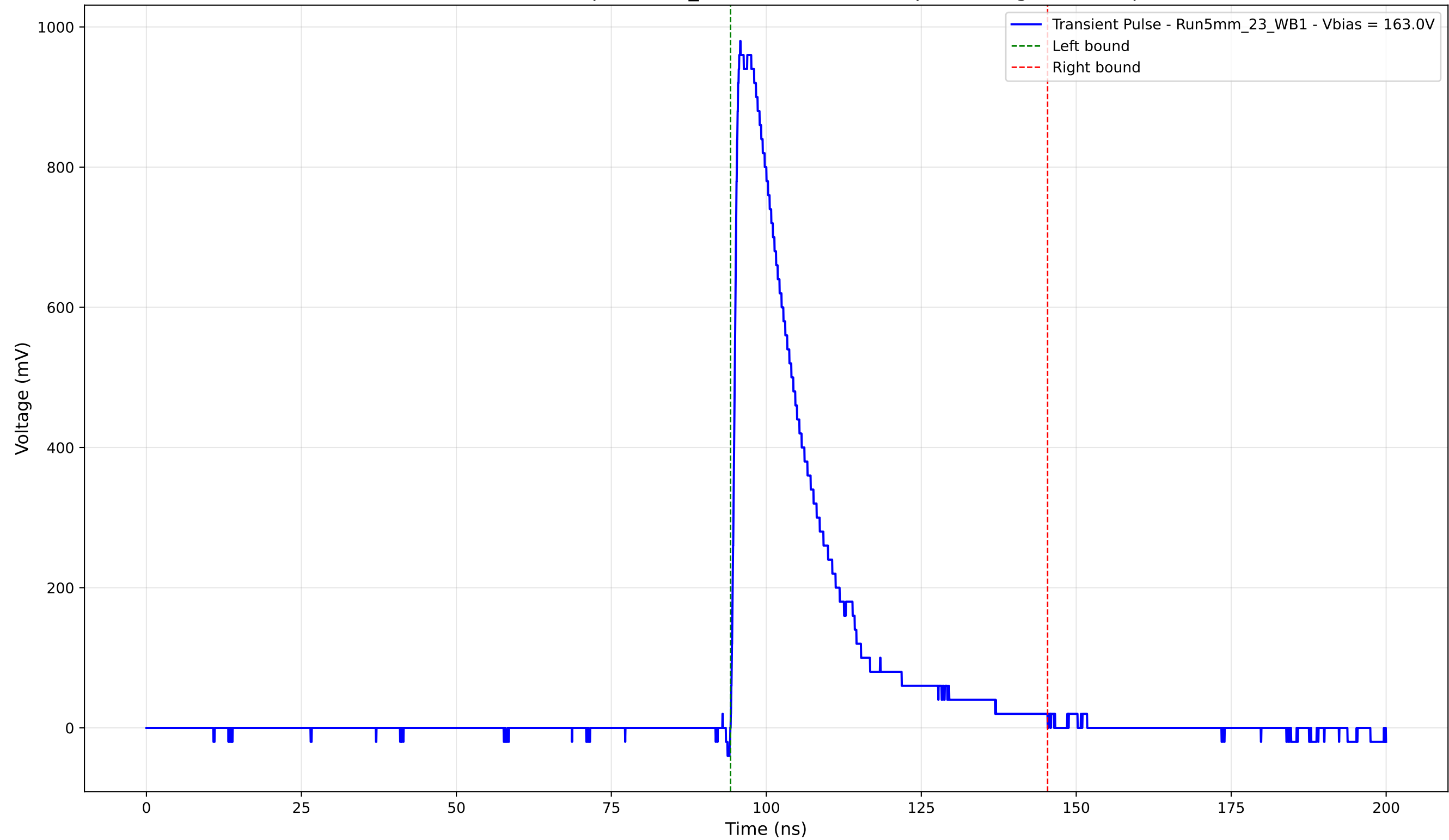
Transient Pulse - Sample: 5mm_23 - Position: 1935.0 \mu\text{m} - Charge: 237.29 pC
