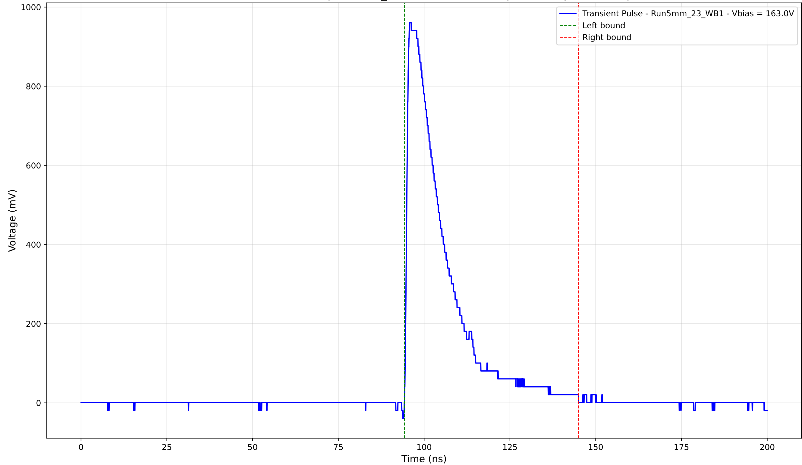
Transient Pulse - Sample: 5mm_23 - Position: 1865.0 \mu\text{m} - Charge: 232.71 pC
