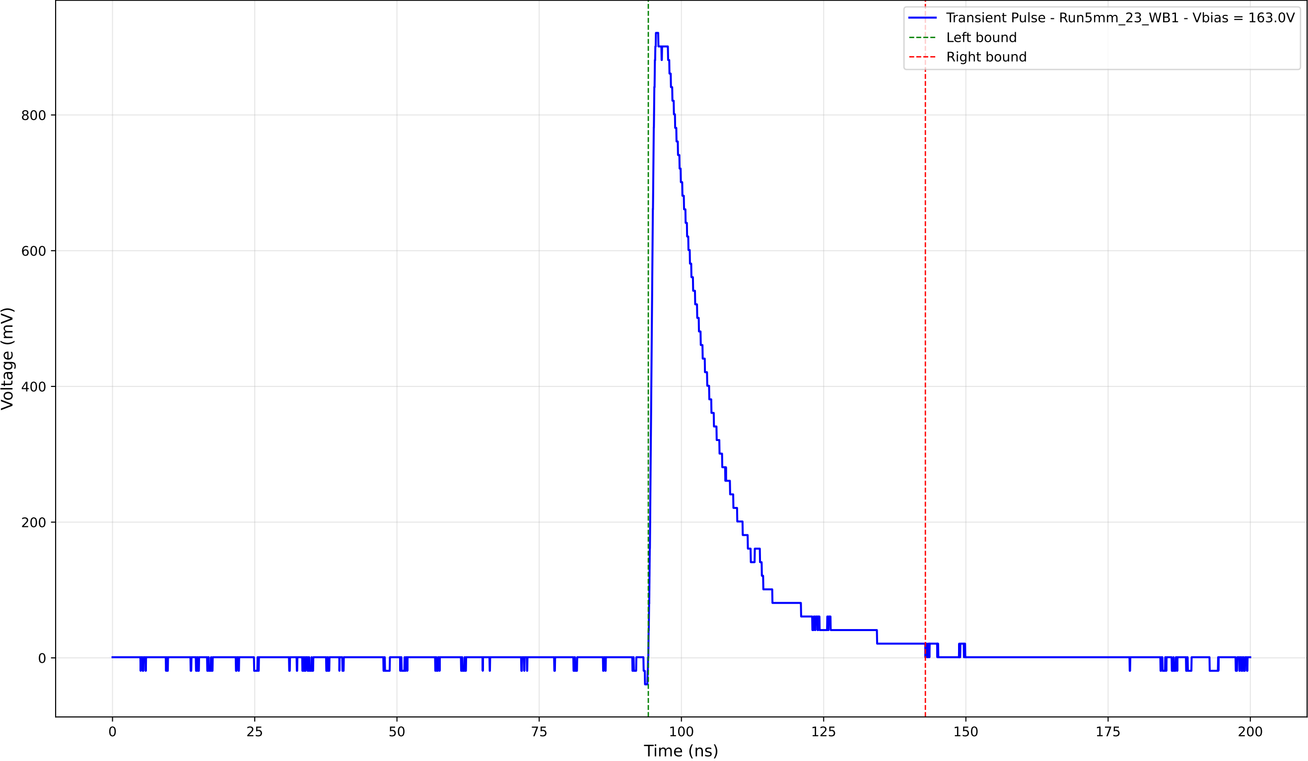
Transient Pulse - Sample: 5mm_23 - Position: 3410.0 \mu\text{m} - Charge: 212.61 pC
