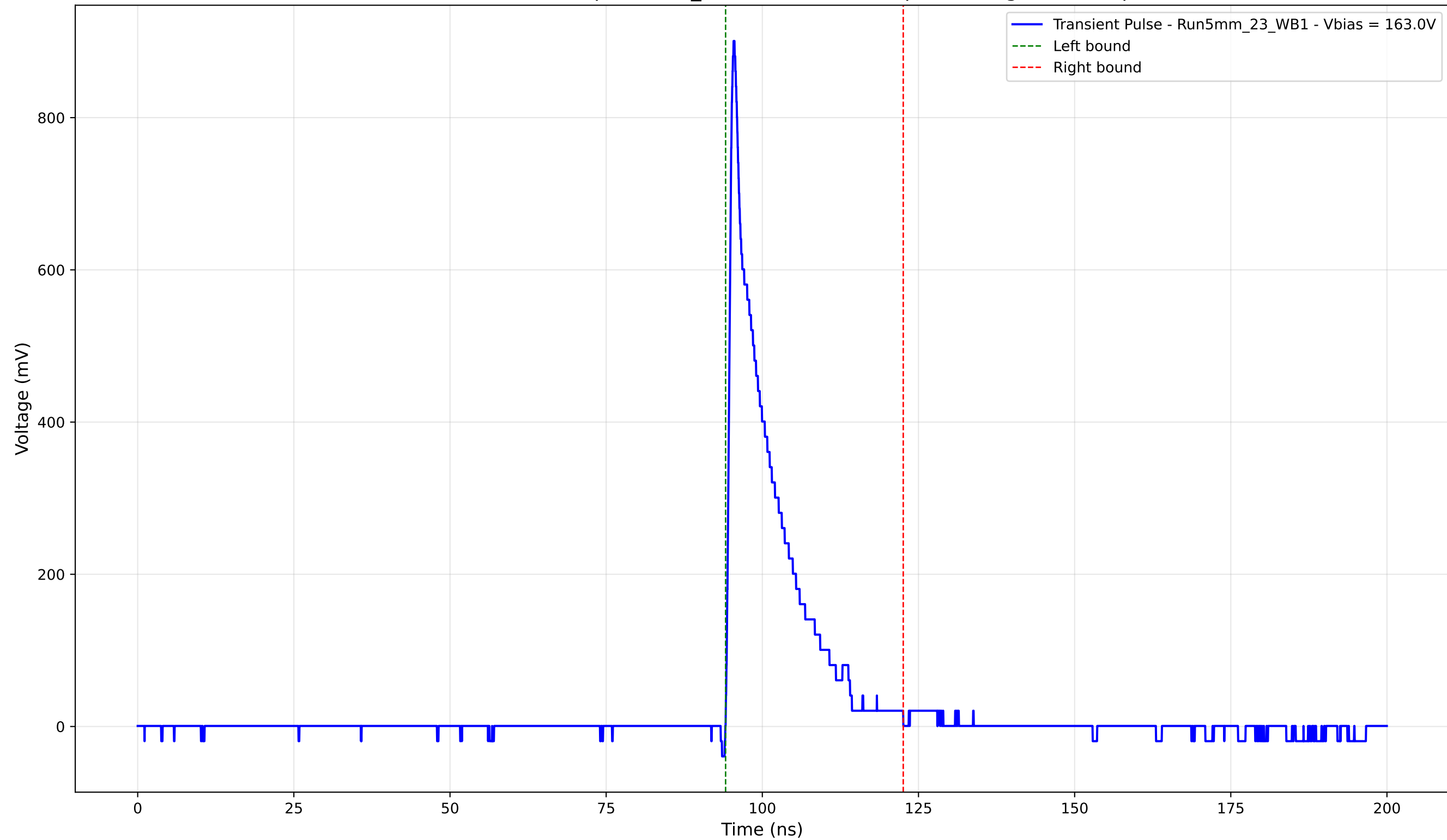
Transient Pulse - Sample: 5mm_23 - Position: 325.0 \mu\text{m} - Charge: 120.72 pC
