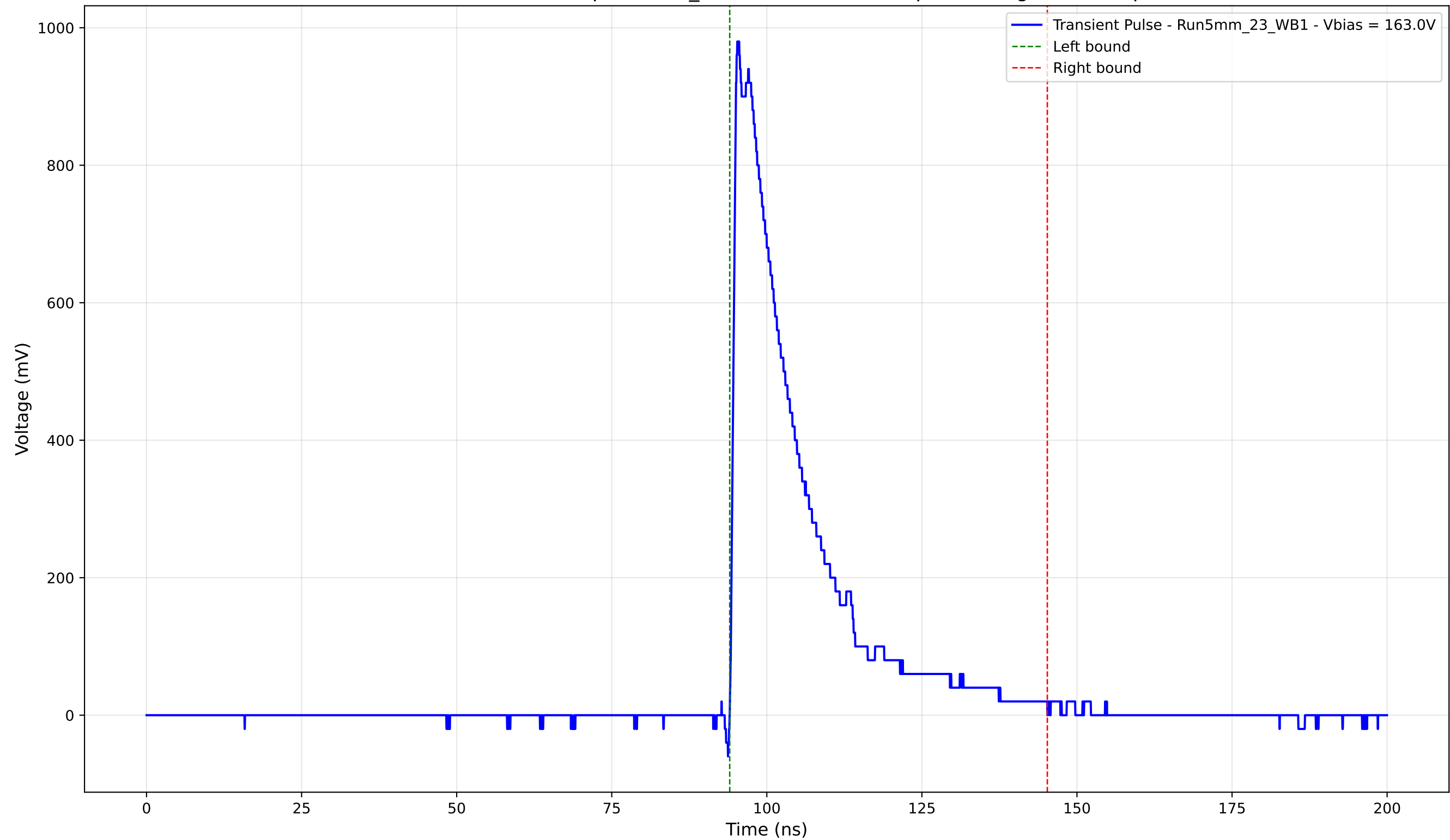
Transient Pulse - Sample: 5mm_23 - Position: 2345.0 \mu\text{m} - Charge: 222.54 pC
