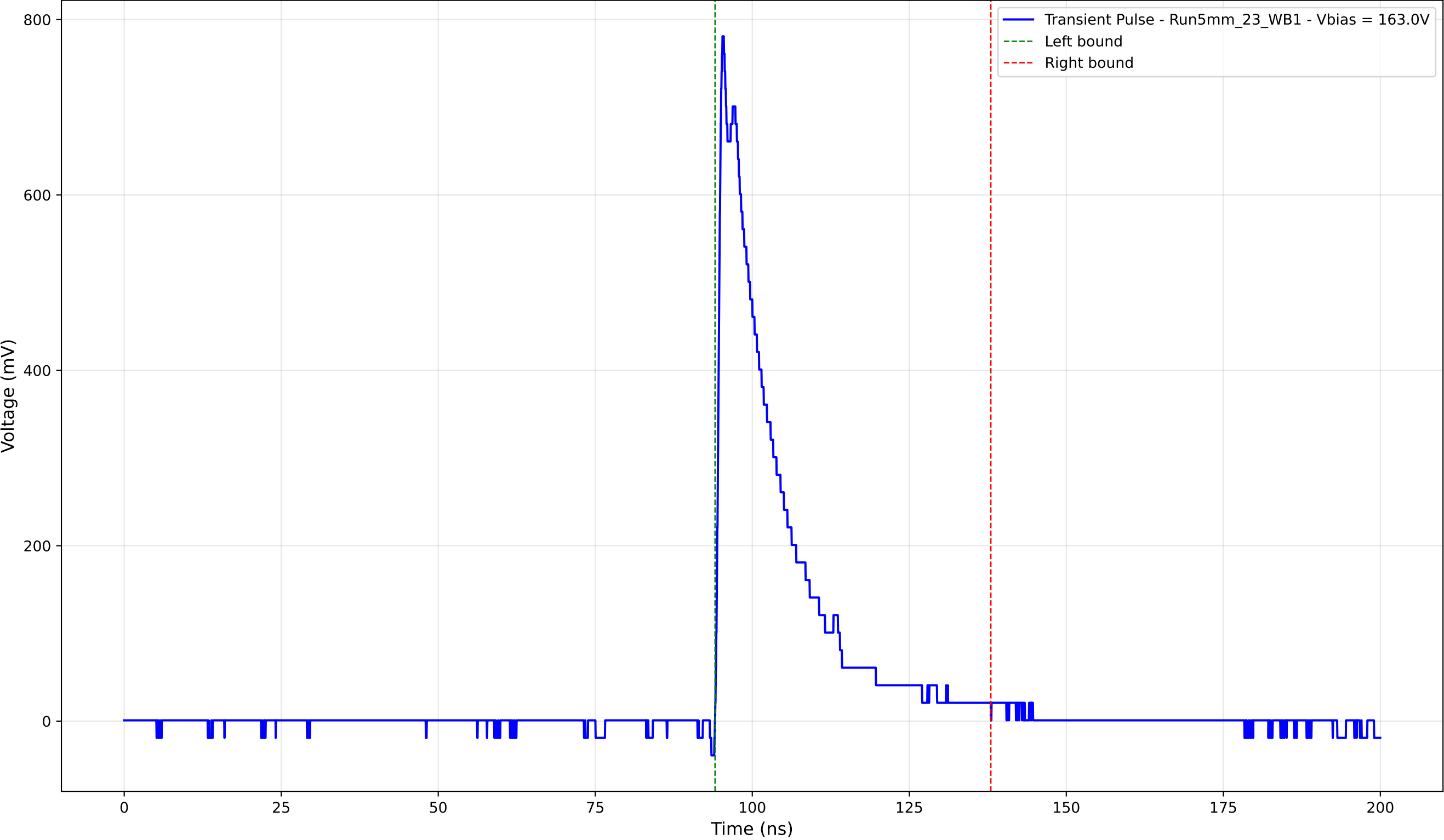
Transient Pulse - Sample: 5mm_23 - Position: 2295.0 \mu\text{m} - Charge: 150.04 pC
