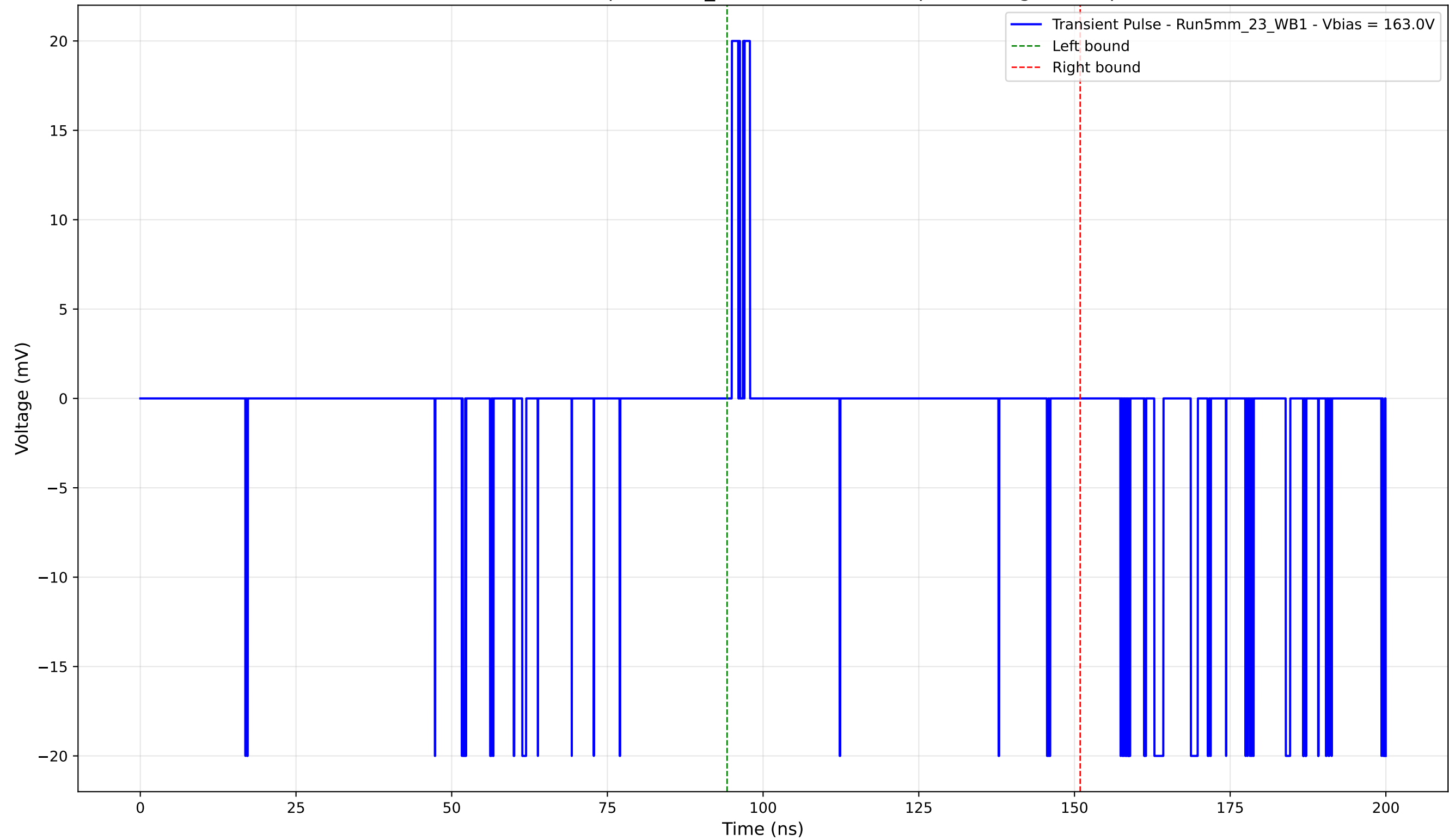
Transient Pulse - Sample: 5mm_23 - Position: 220.0 \mu\text{m} - Charge: 0.63 pC
