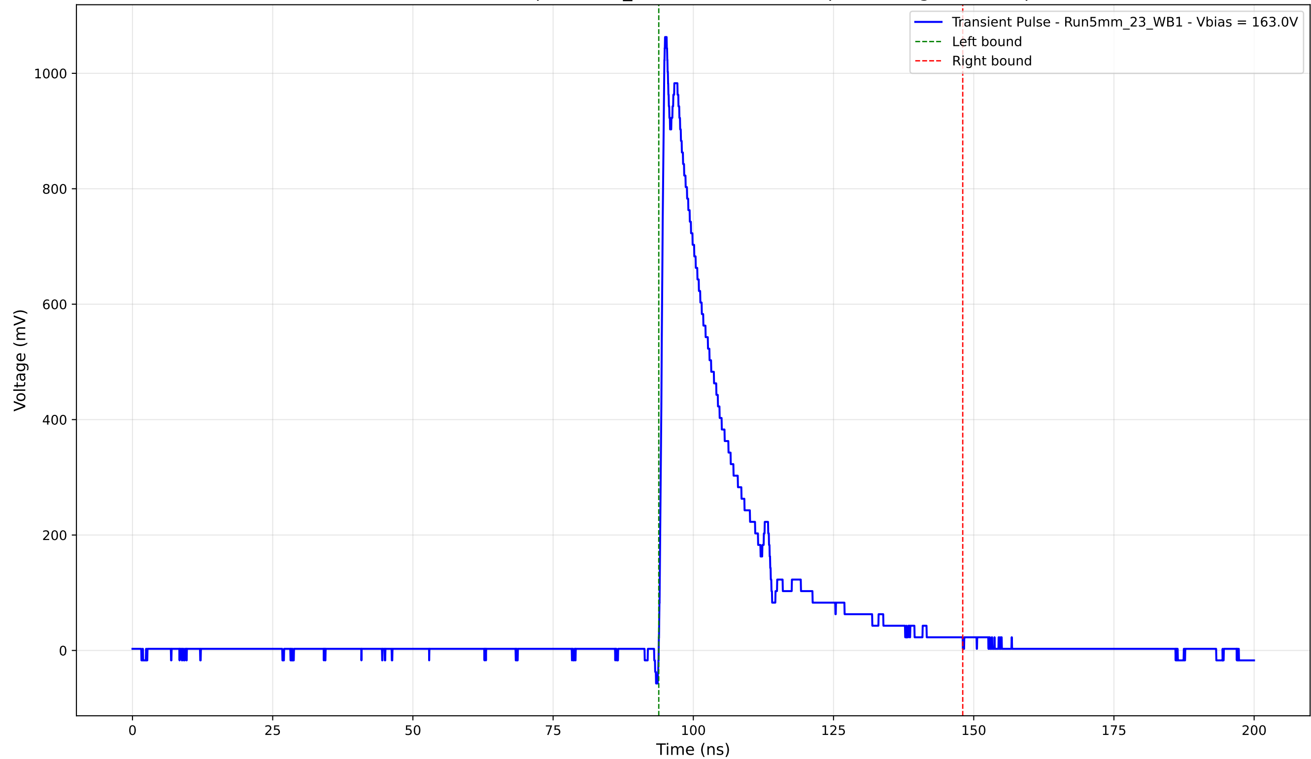
Transient Pulse - Sample: 5mm_23 - Position: 2630.0 \mu\text{m} - Charge: 244.61 pC
