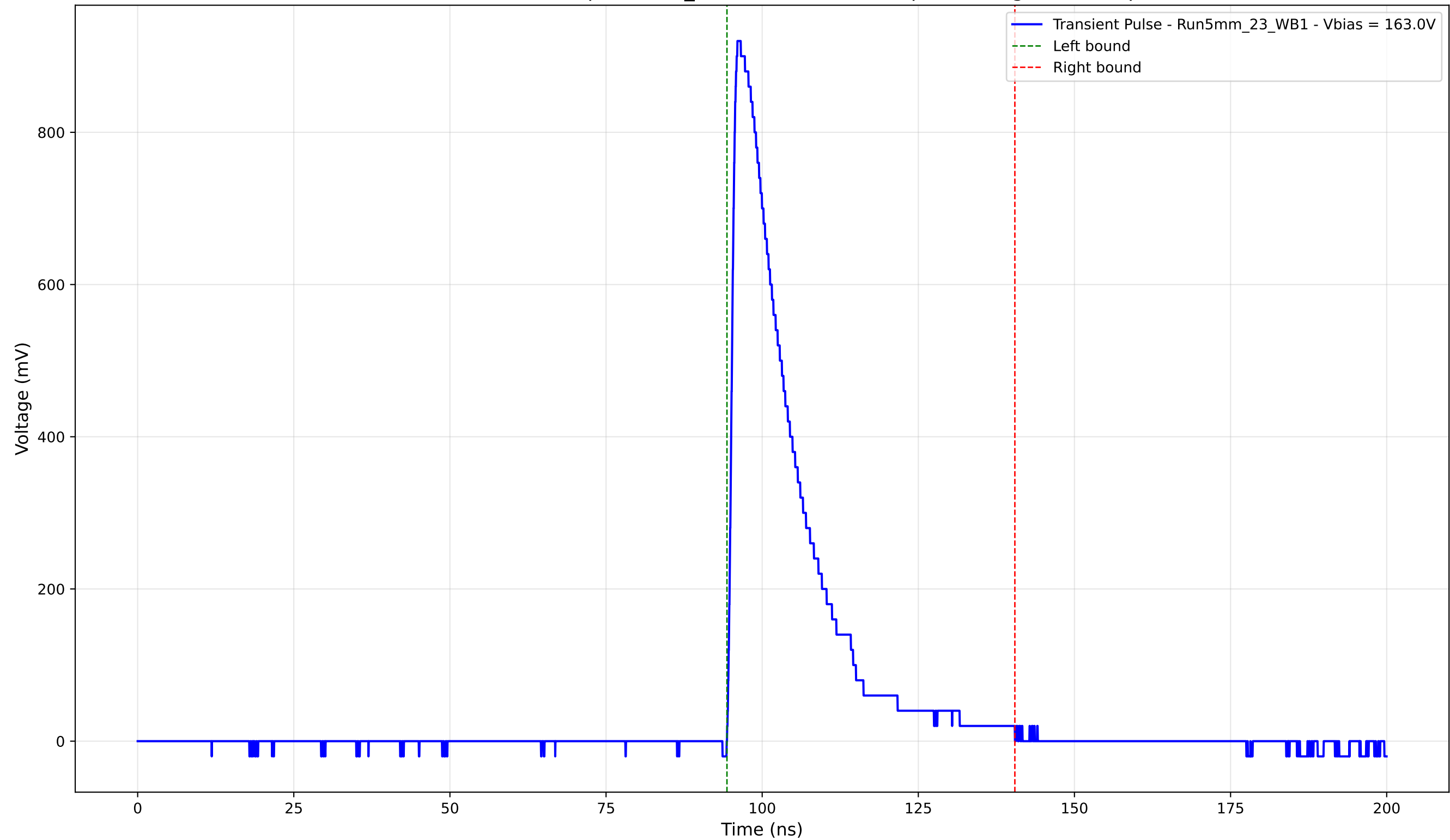
Transient Pulse - Sample: 5mm_23 - Position: 4020.0 \mu\text{m} - Charge: 199.32 pC
