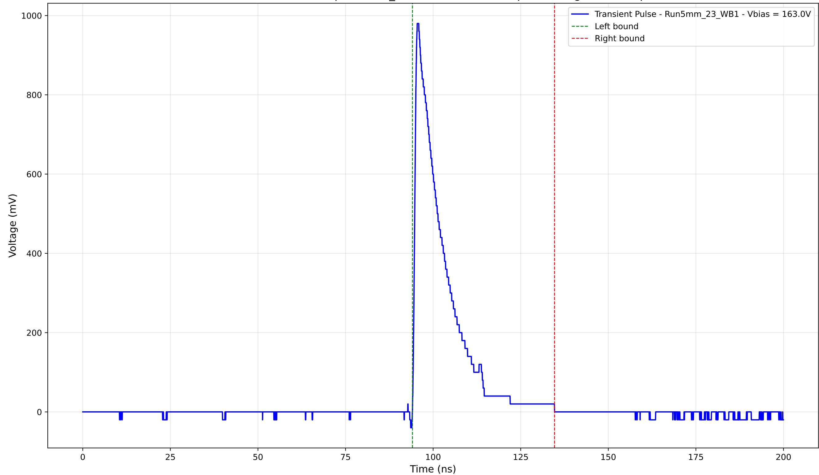
Transient Pulse - Sample: 5mm_23 - Position: 4885.0 \mu\text{m} - Charge: 172.06 pC
