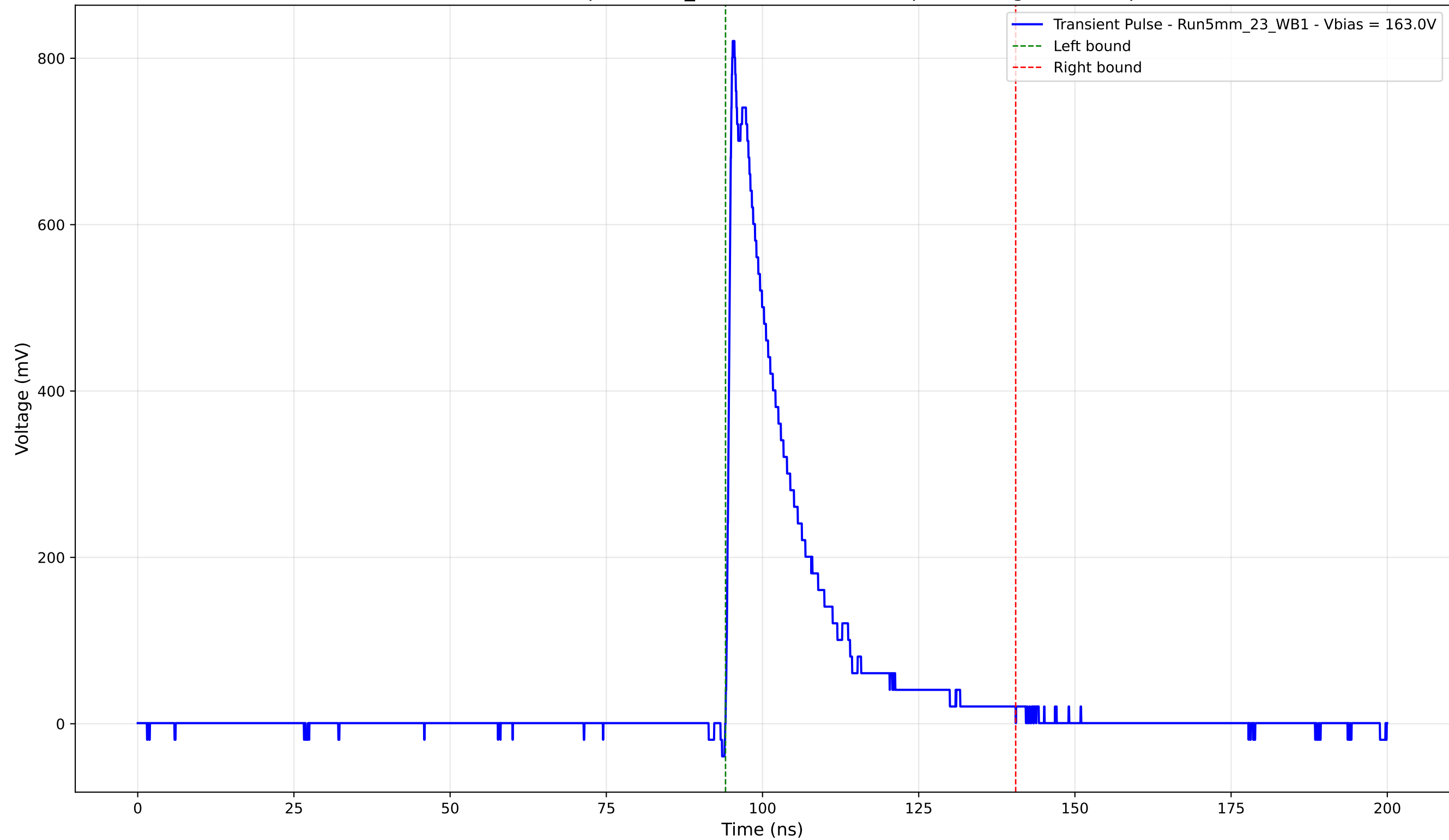
Transient Pulse - Sample: 5mm_23 - Position: 2300.0 \mu\text{m} - Charge: 161.91 pC
