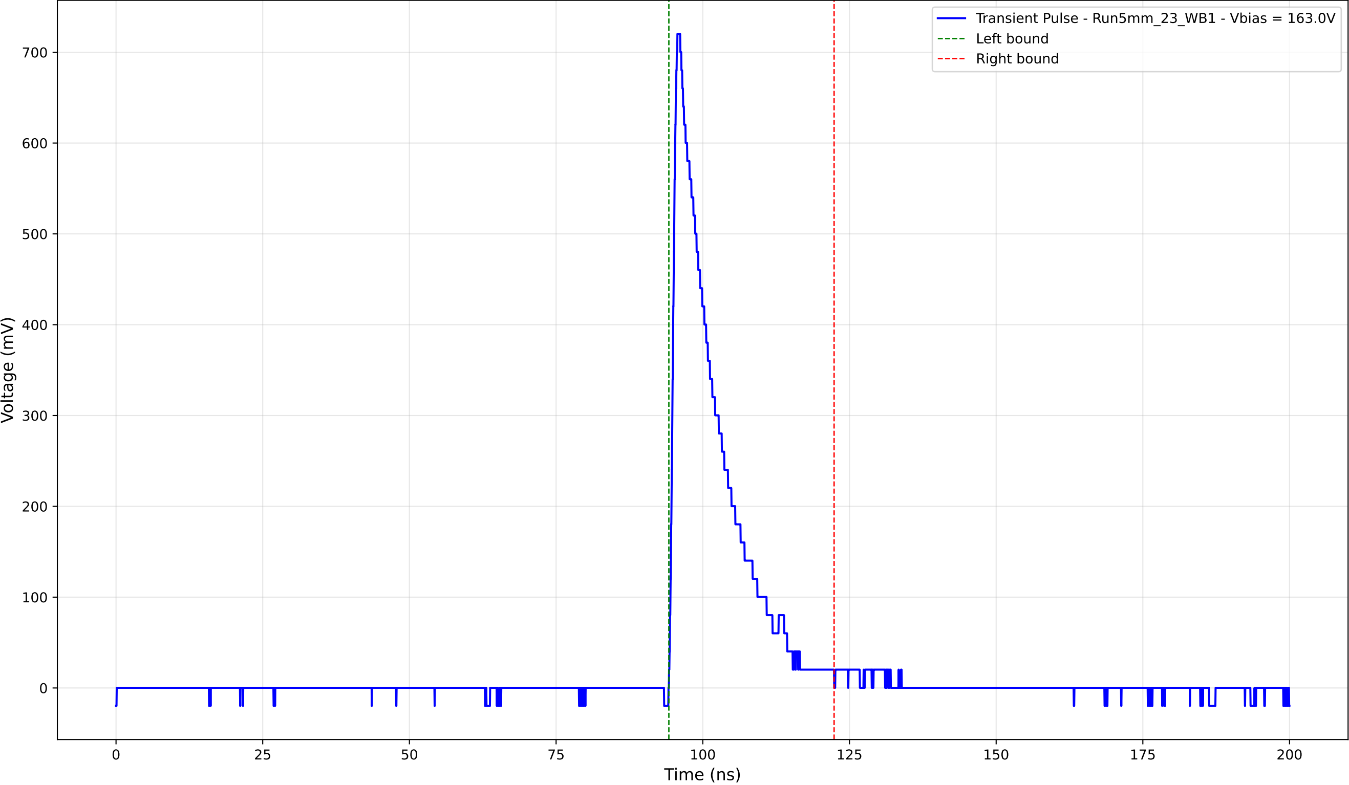
Transient Pulse - Sample: 5mm_23 - Position: 4710.0 \mu\text{m} - Charge: 115.74 pC
