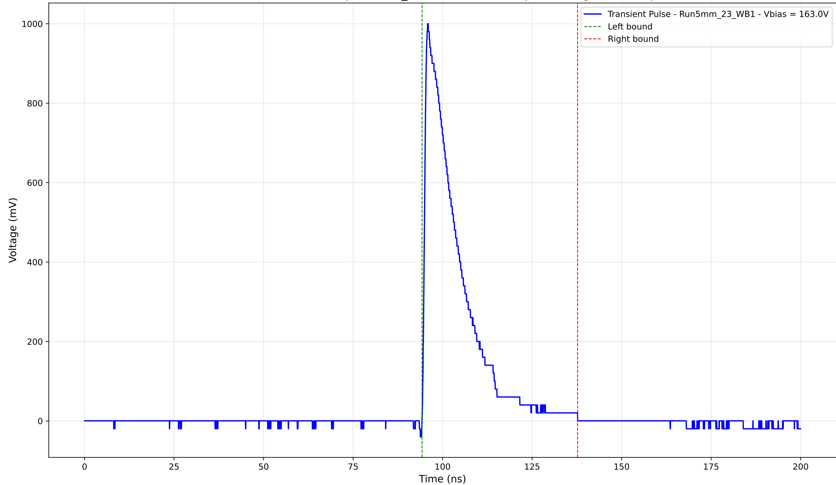
Transient Pulse - Sample: 5mm_23 - Position: 820.0 \mu\text{m} - Charge: 204.34 pC
