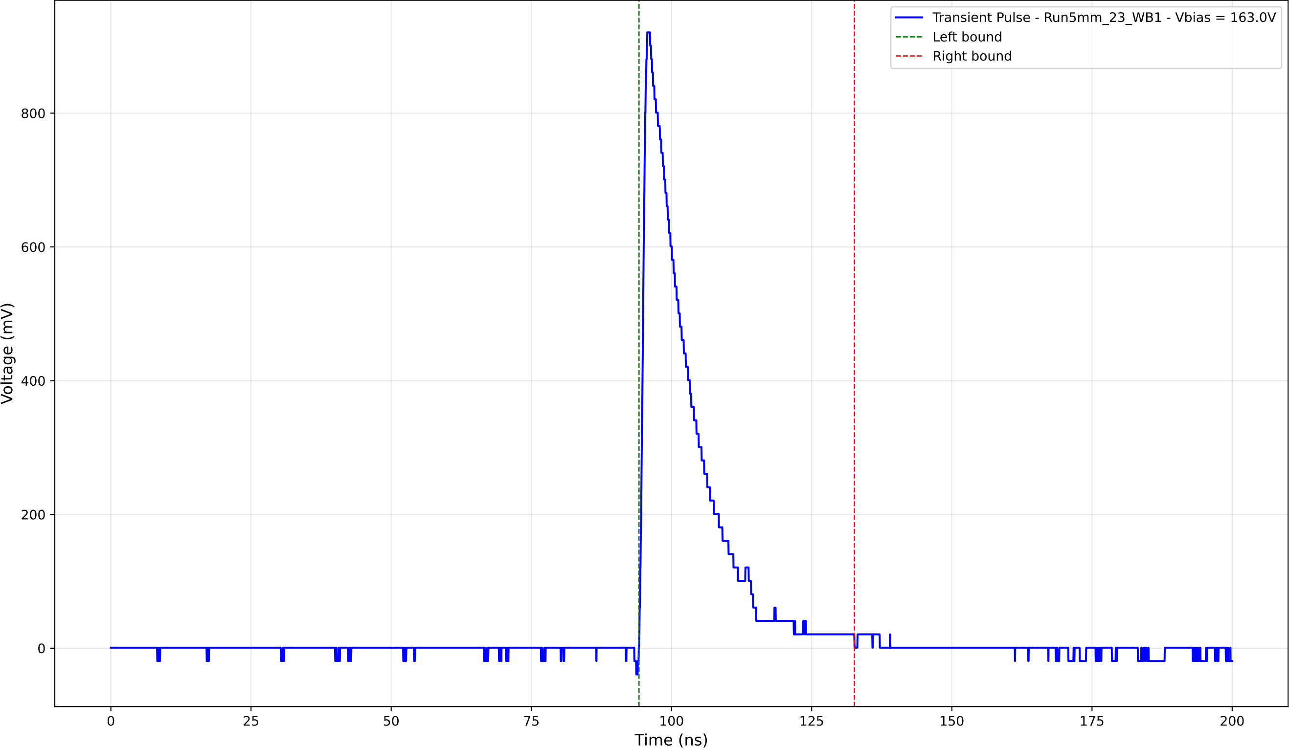
Transient Pulse - Sample: 5mm_23 - Position: 4670.0 \mu\text{m} - Charge: 167.80 pC
