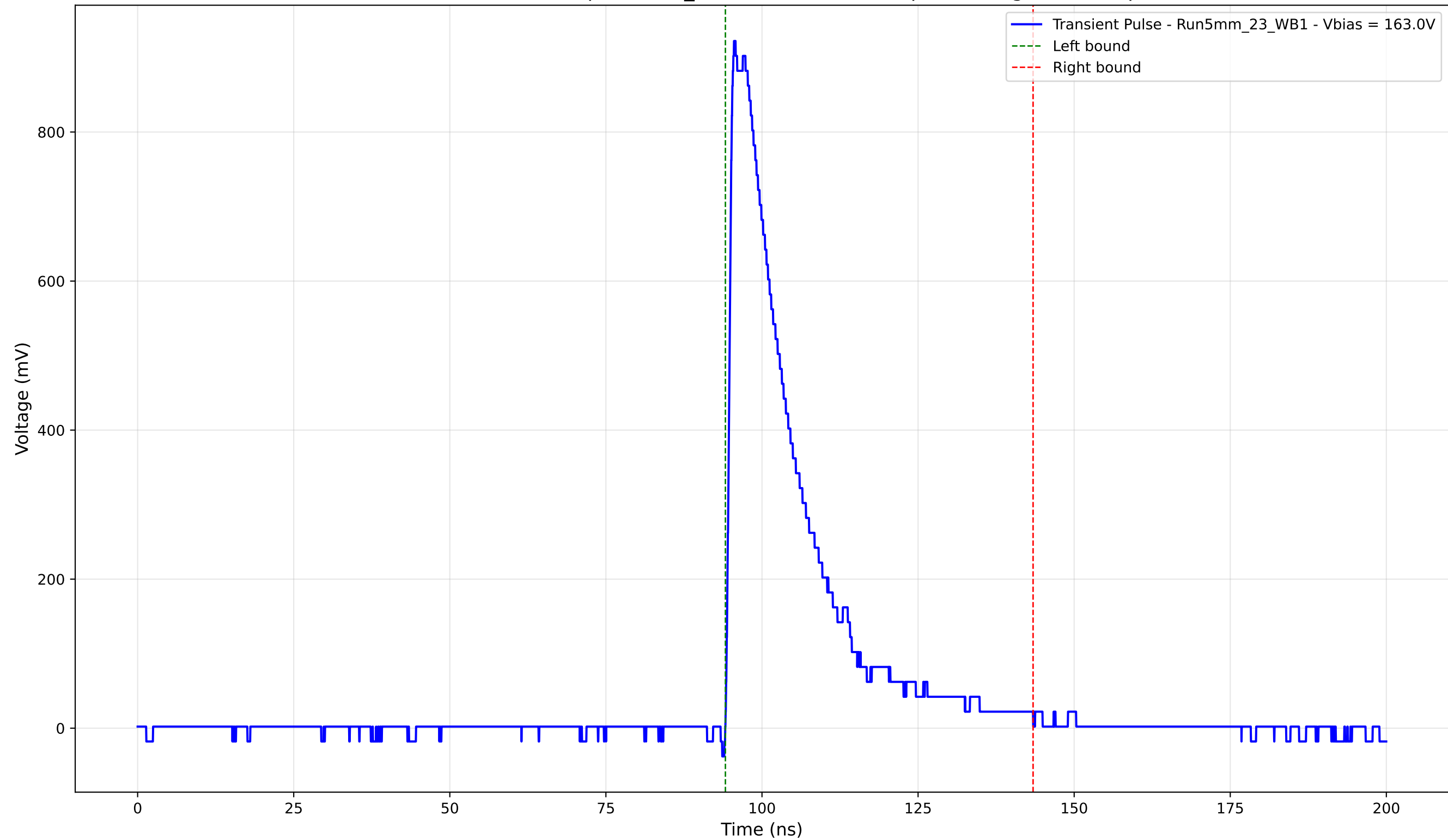
Transient Pulse - Sample: 5mm_23 - Position: 3370.0 \mu\text{m} - Charge: 209.98 pC
