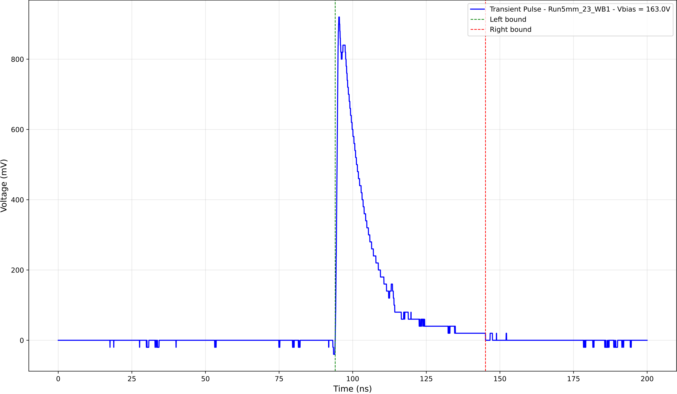
Transient Pulse - Sample: 5mm_23 - Position: 2315.0 \mu\text{m} - Charge: 191.31 pC
