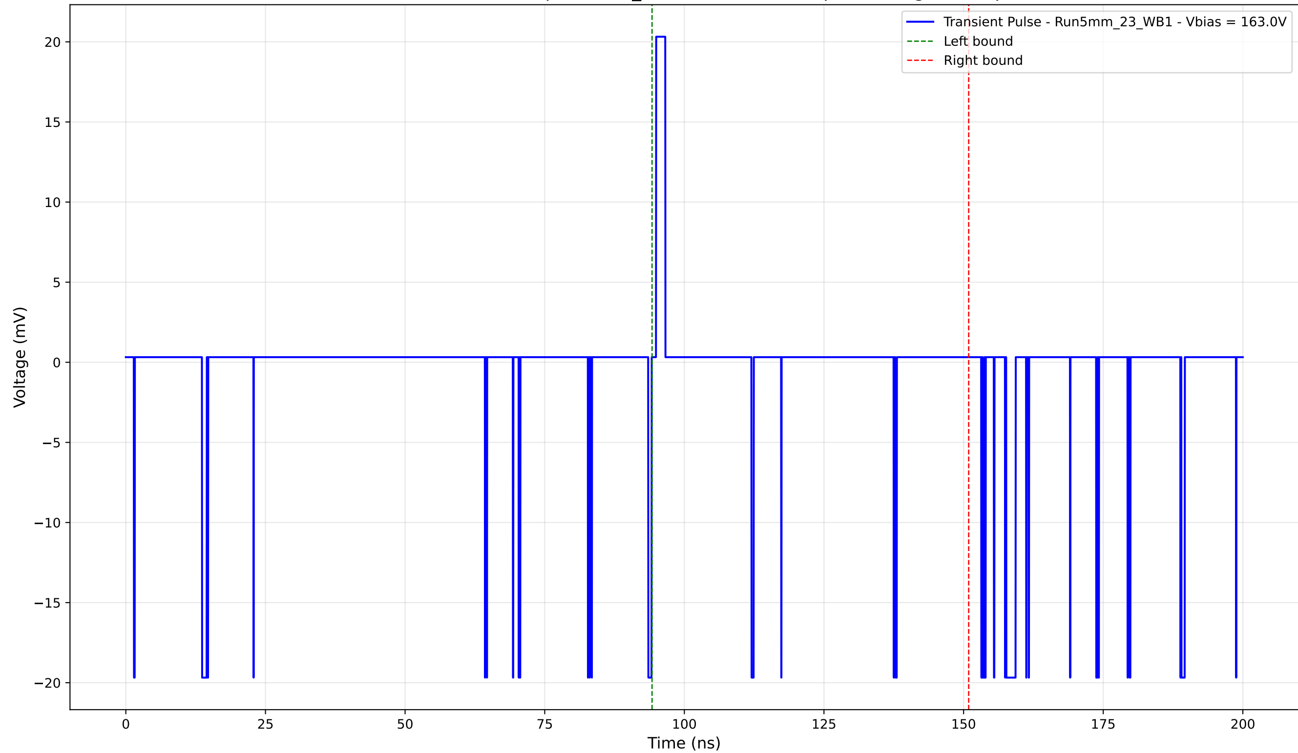
Transient Pulse - Sample: 5mm_23 - Position: 145.0 \mu\text{m} - Charge: 0.71 pC
