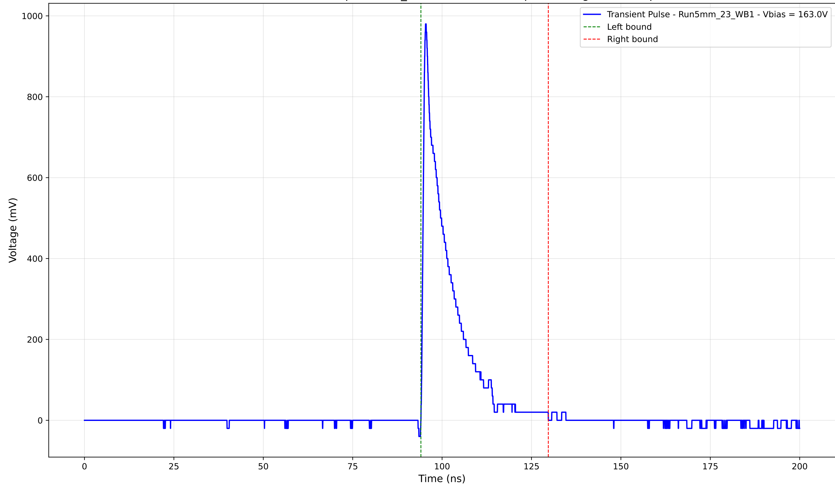
Transient Pulse - Sample: 5mm_23 - Position: 335.0 \mu\text{m} - Charge: 145.06 pC
