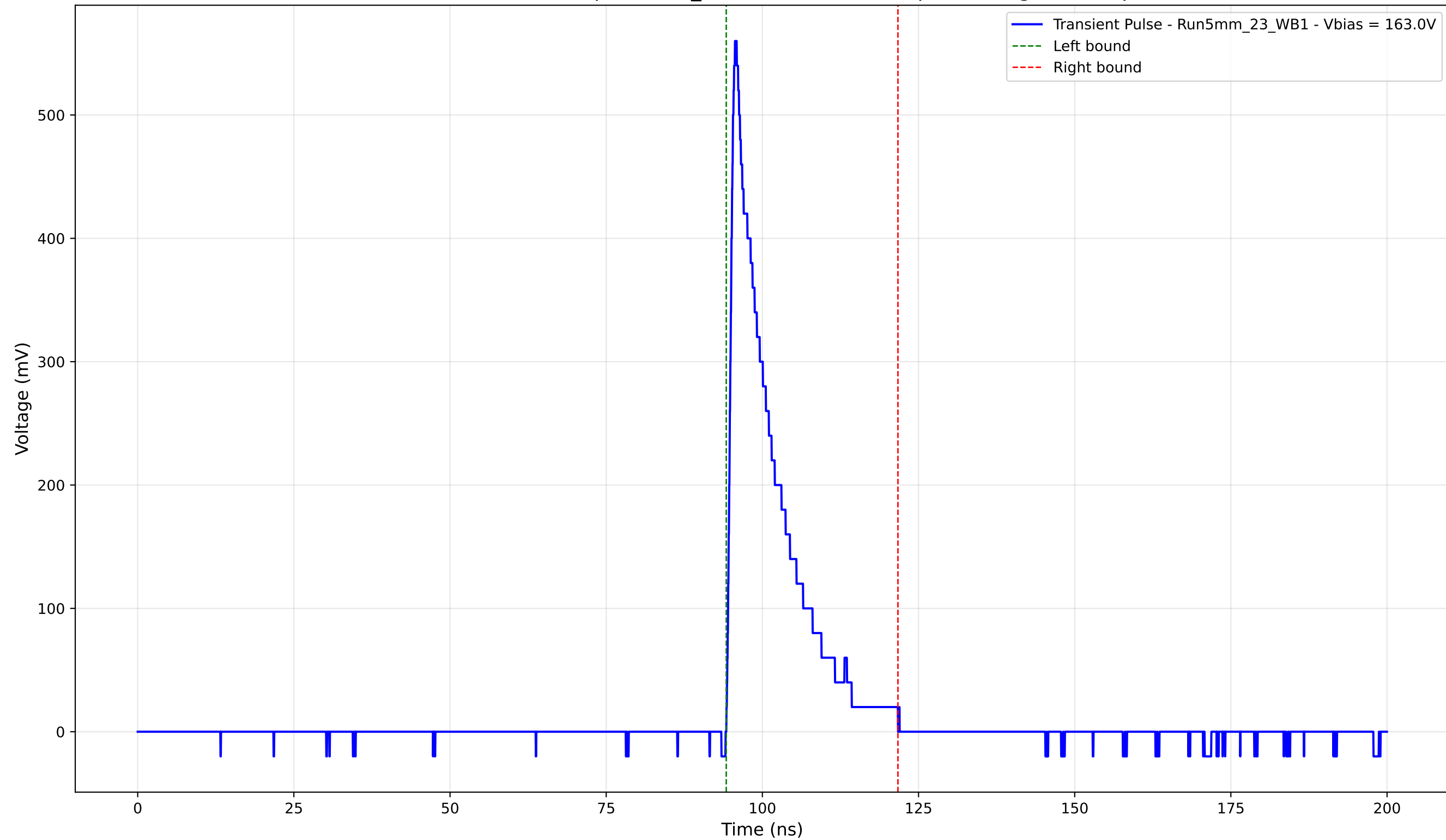
Transient Pulse - Sample: 5mm_23 - Position: 4805.0 \mu\text{m} - Charge: 81.61 pC
