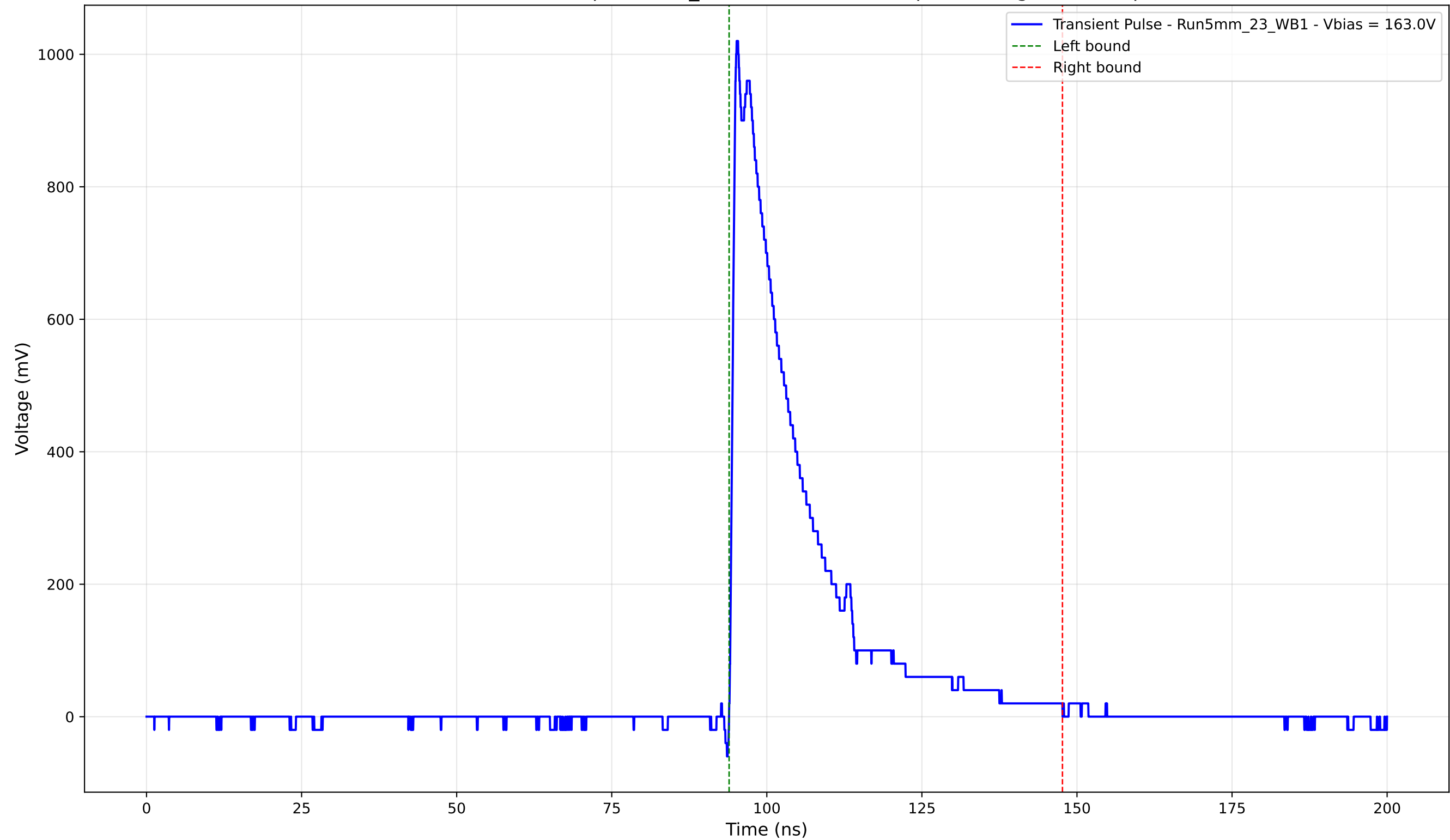
Transient Pulse - Sample: 5mm_23 - Position: 3000.0 \mu\text{m} - Charge: 229.87 pC
