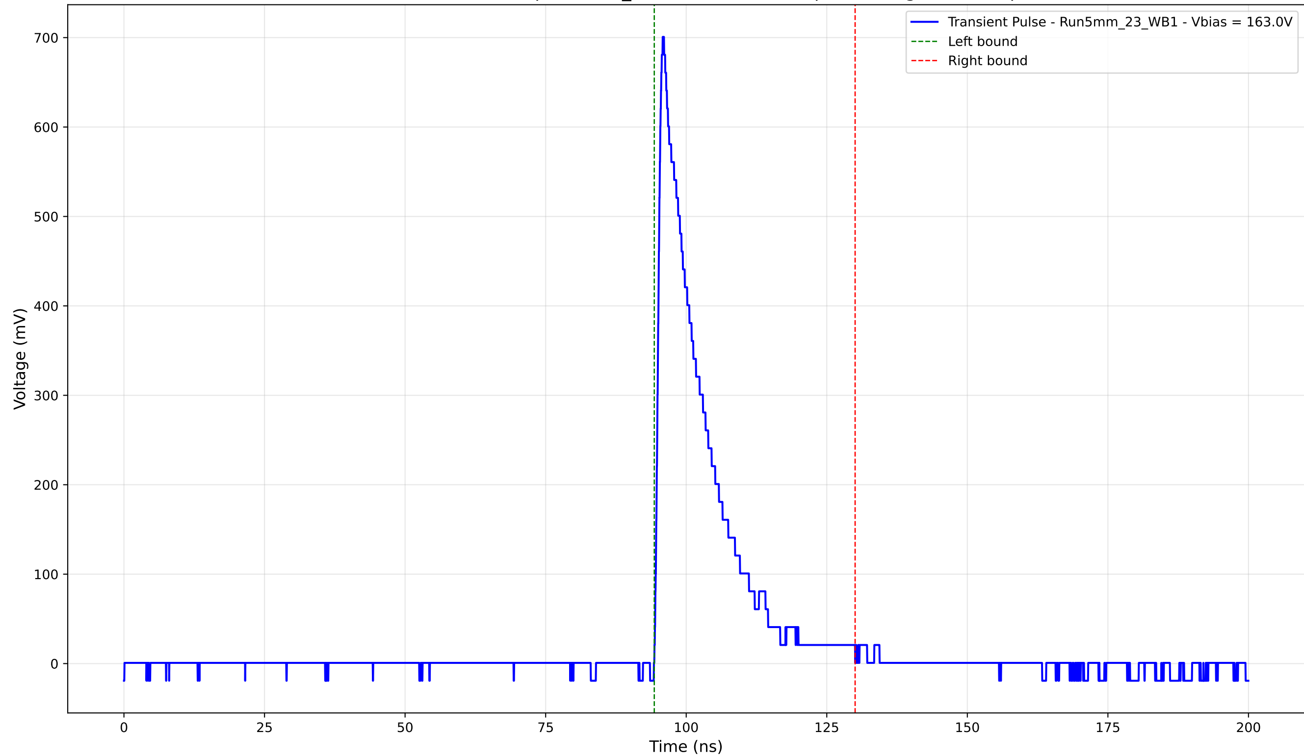
Transient Pulse - Sample: 5mm_23 - Position: 765.0 \mu\text{m} - Charge: 118.92 pC
