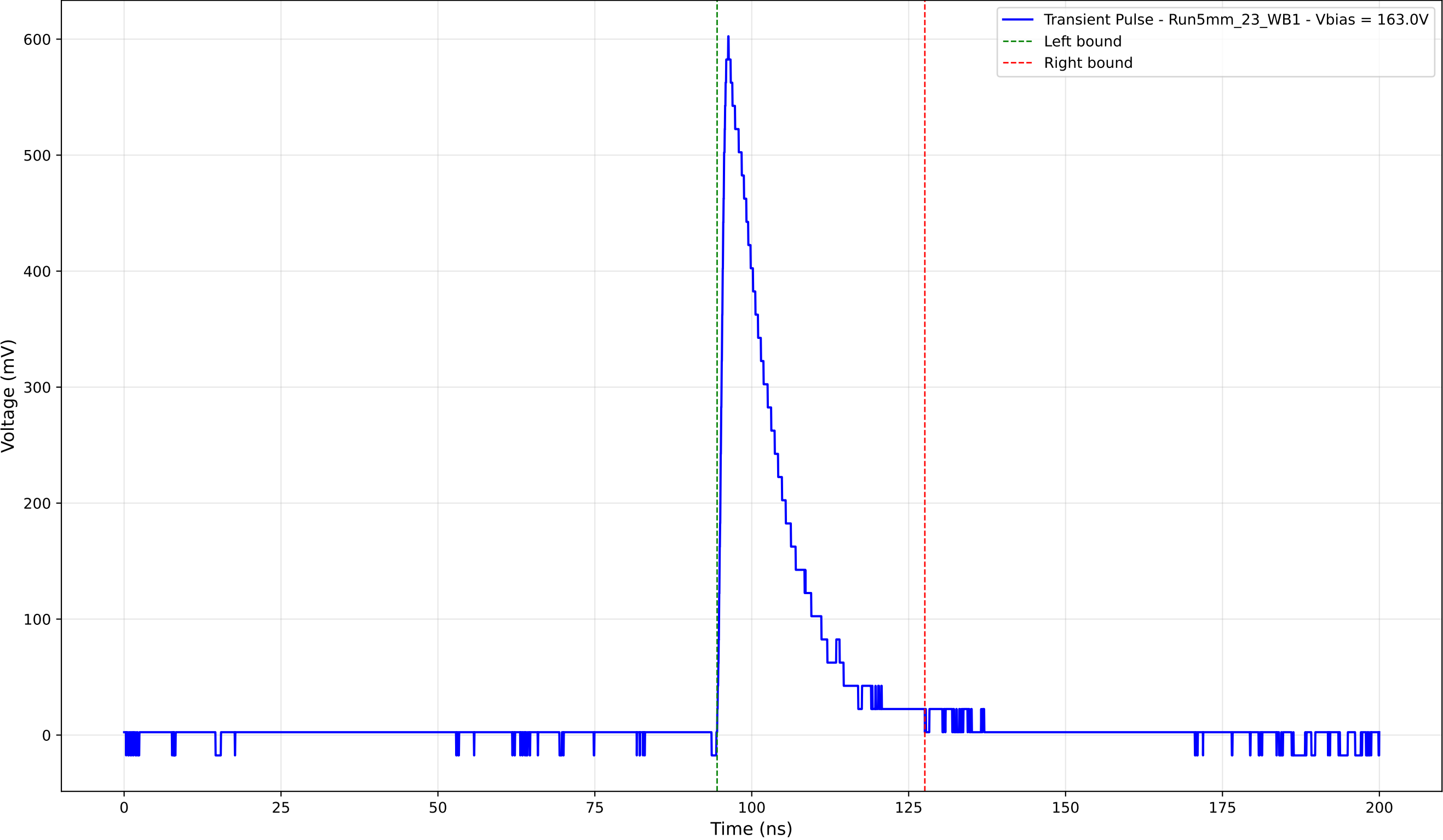
Transient Pulse - Sample: 5mm_23 - Position: 1180.0 \mu\text{m} - Charge: 109.13 pC
