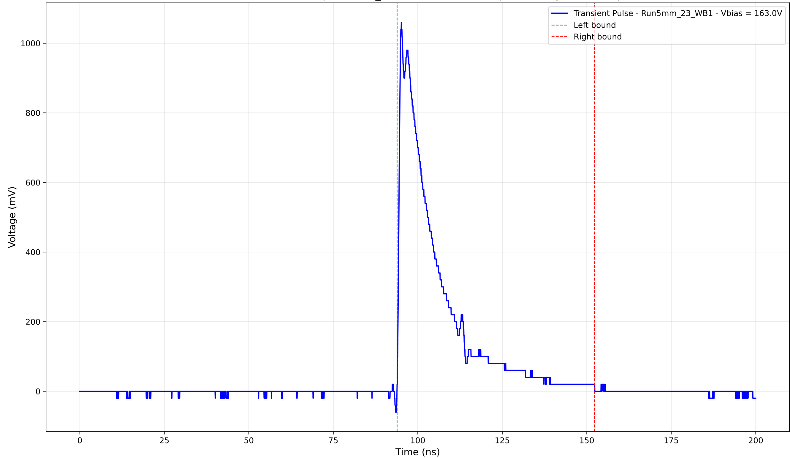
Transient Pulse - Sample: 5mm_23 - Position: 2910.0 \mu\text{m} - Charge: 239.72 pC
