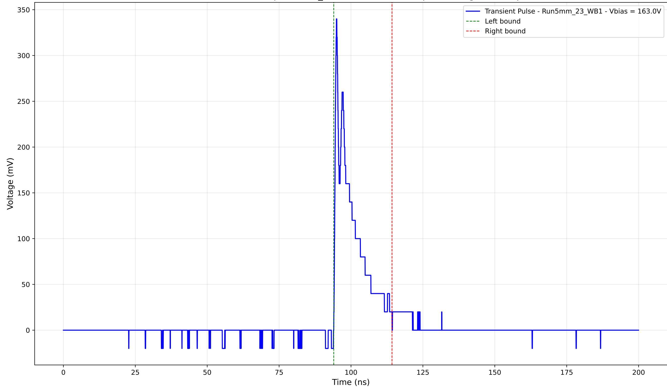
Transient Pulse - Sample: 5mm_23 - Position: 2750.0 \mu\text{m} - Charge: 40.86 pC
