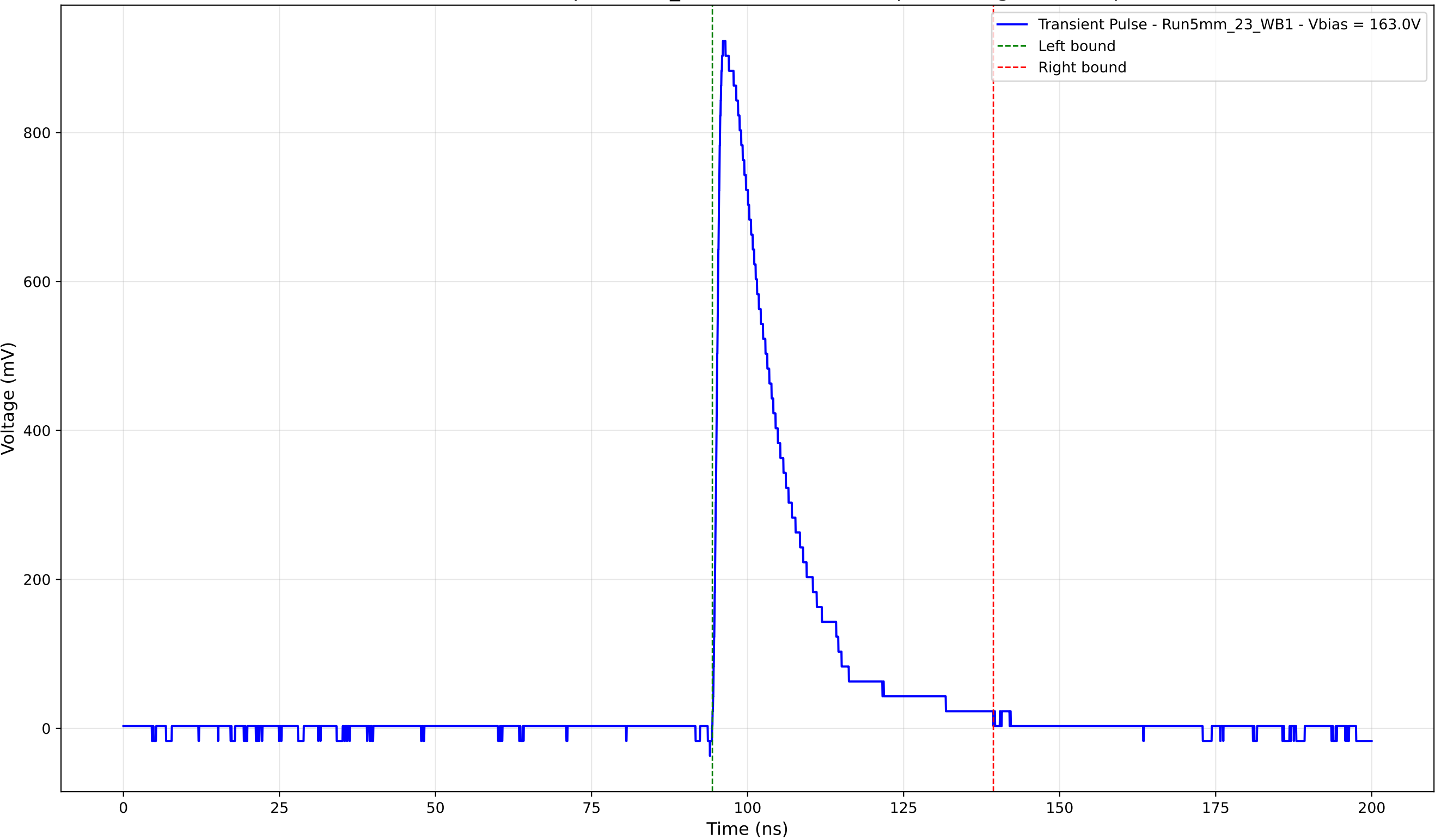
Transient Pulse - Sample: 5mm_23 - Position: 3980.0 \mu\text{m} - Charge: 202.04 pC
