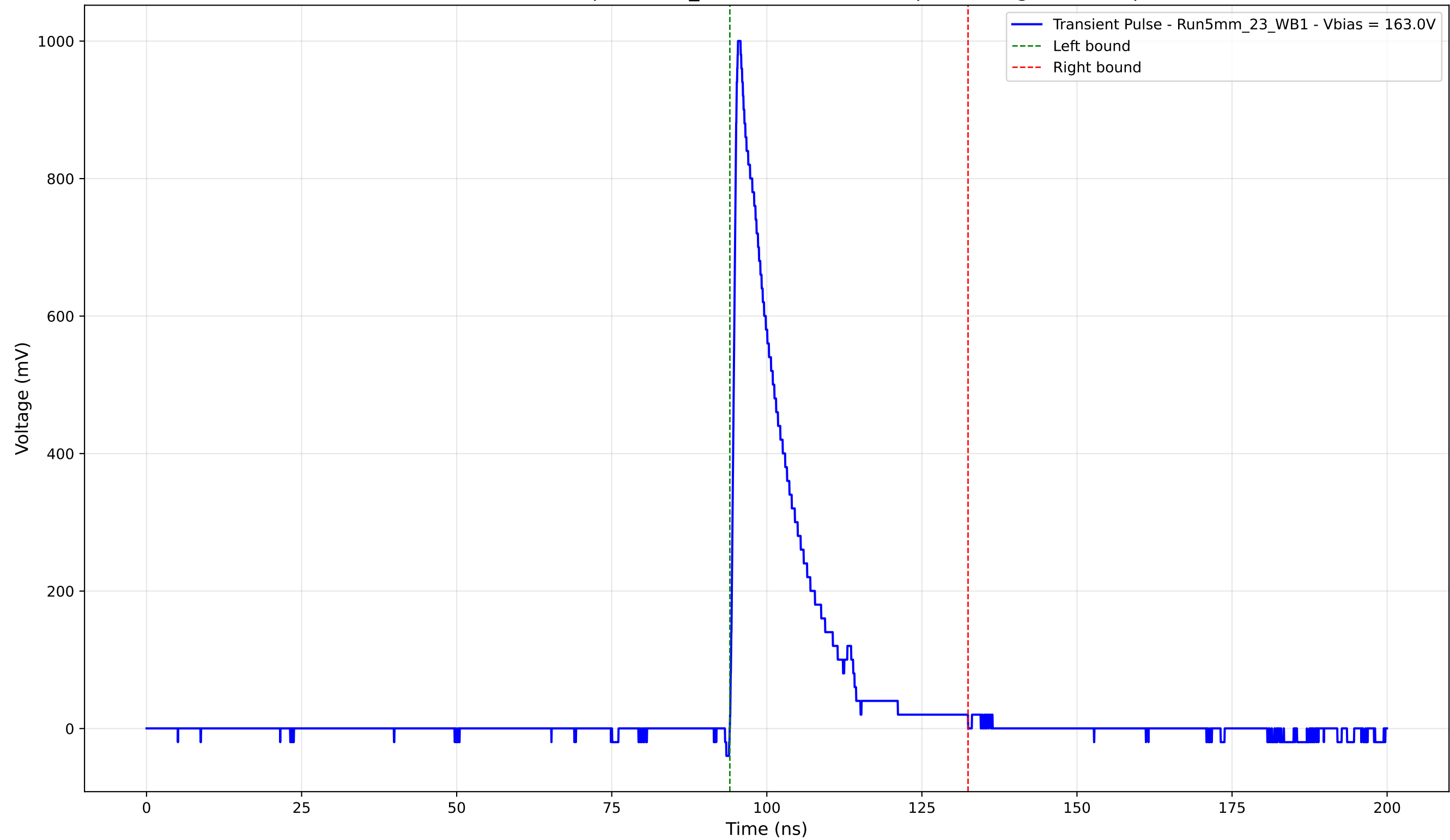
Transient Pulse - Sample: 5mm_23 - Position: 4995.0 \mu\text{m} - Charge: 168.45 pC
