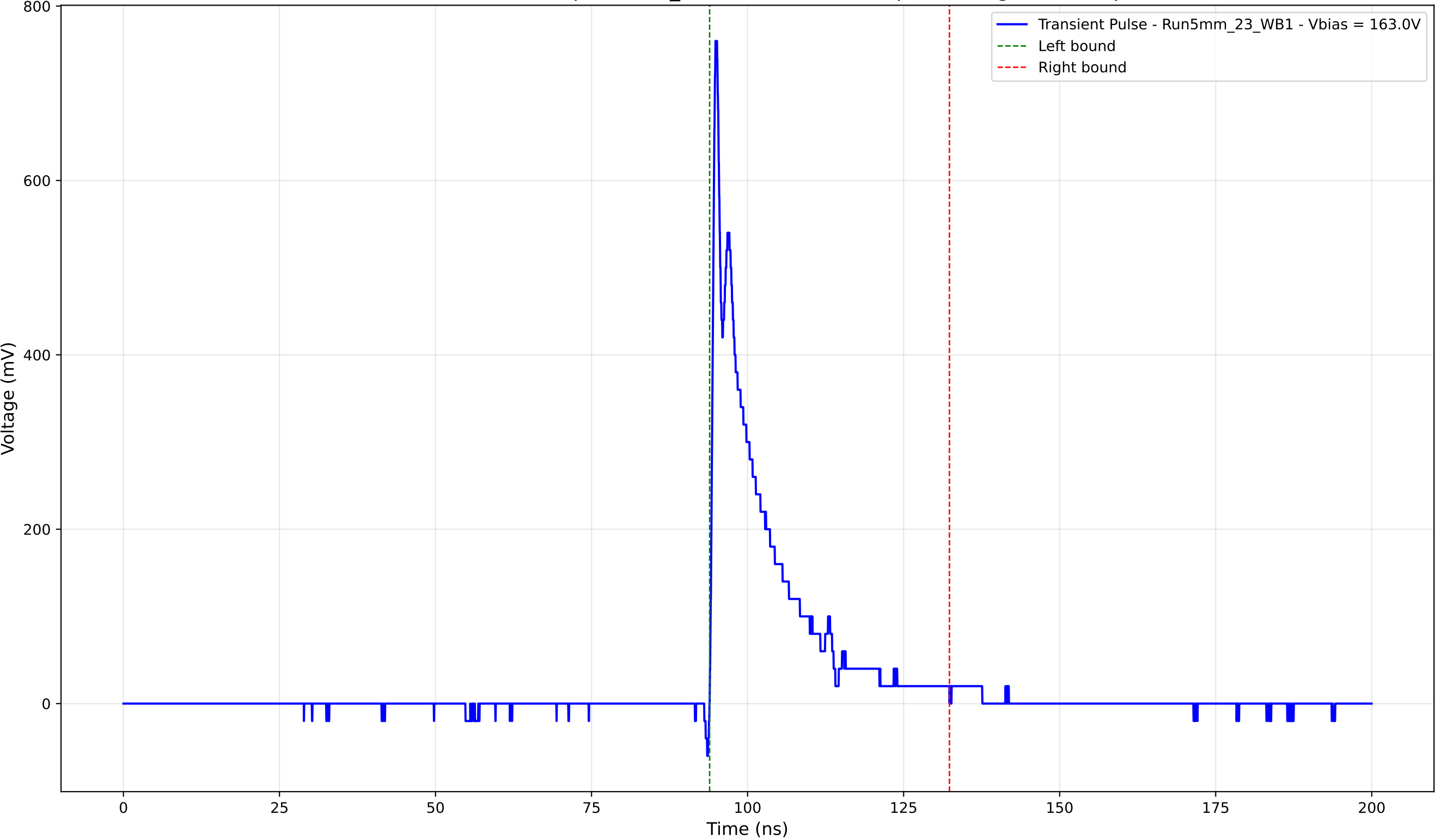
Transient Pulse - Sample: 5mm_23 - Position: 2710.0 \mu\text{m} - Charge: 104.50 pC
