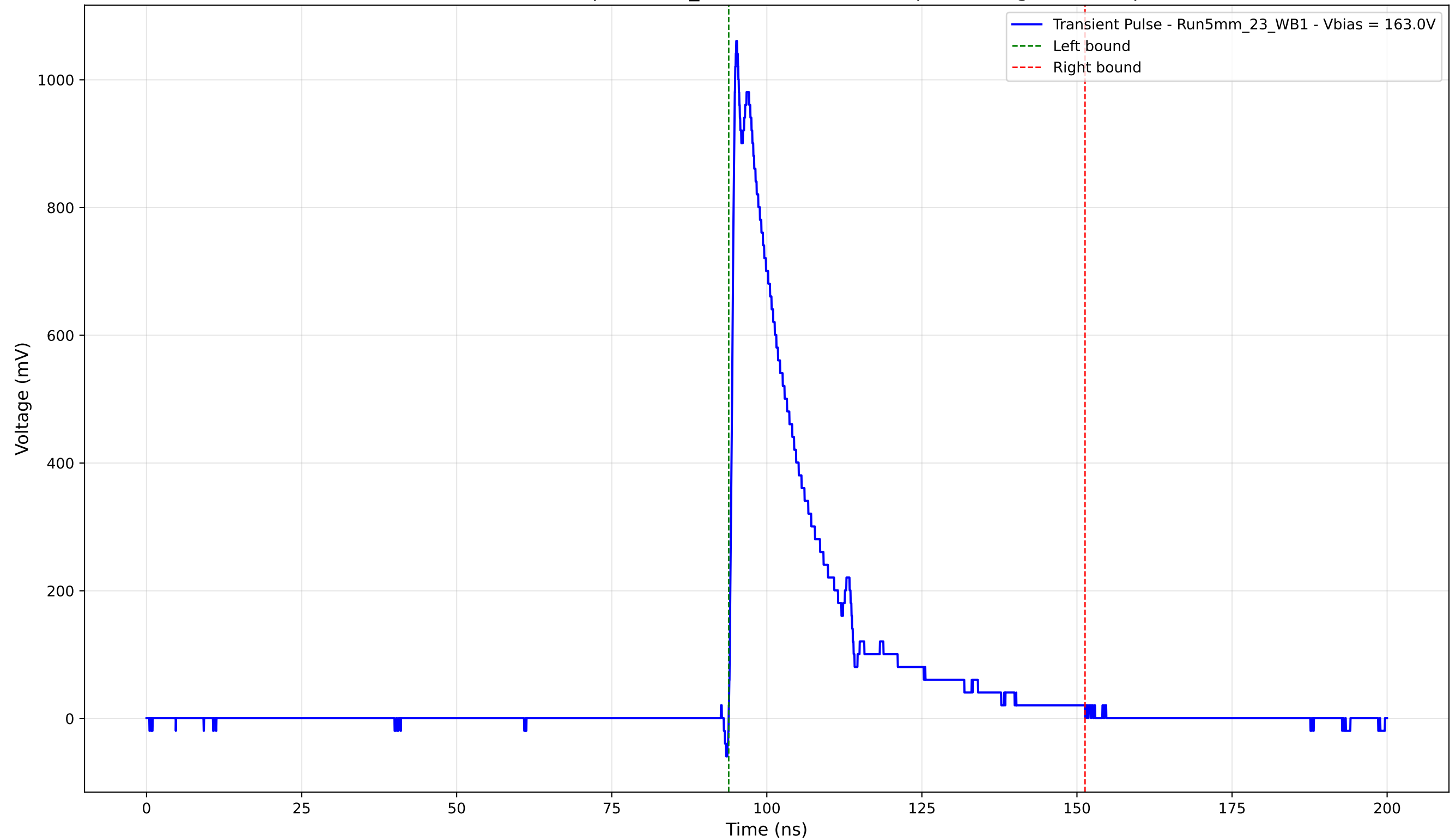
Transient Pulse - Sample: 5mm_23 - Position: 2905.0 \mu\text{m} - Charge: 241.43 pC
