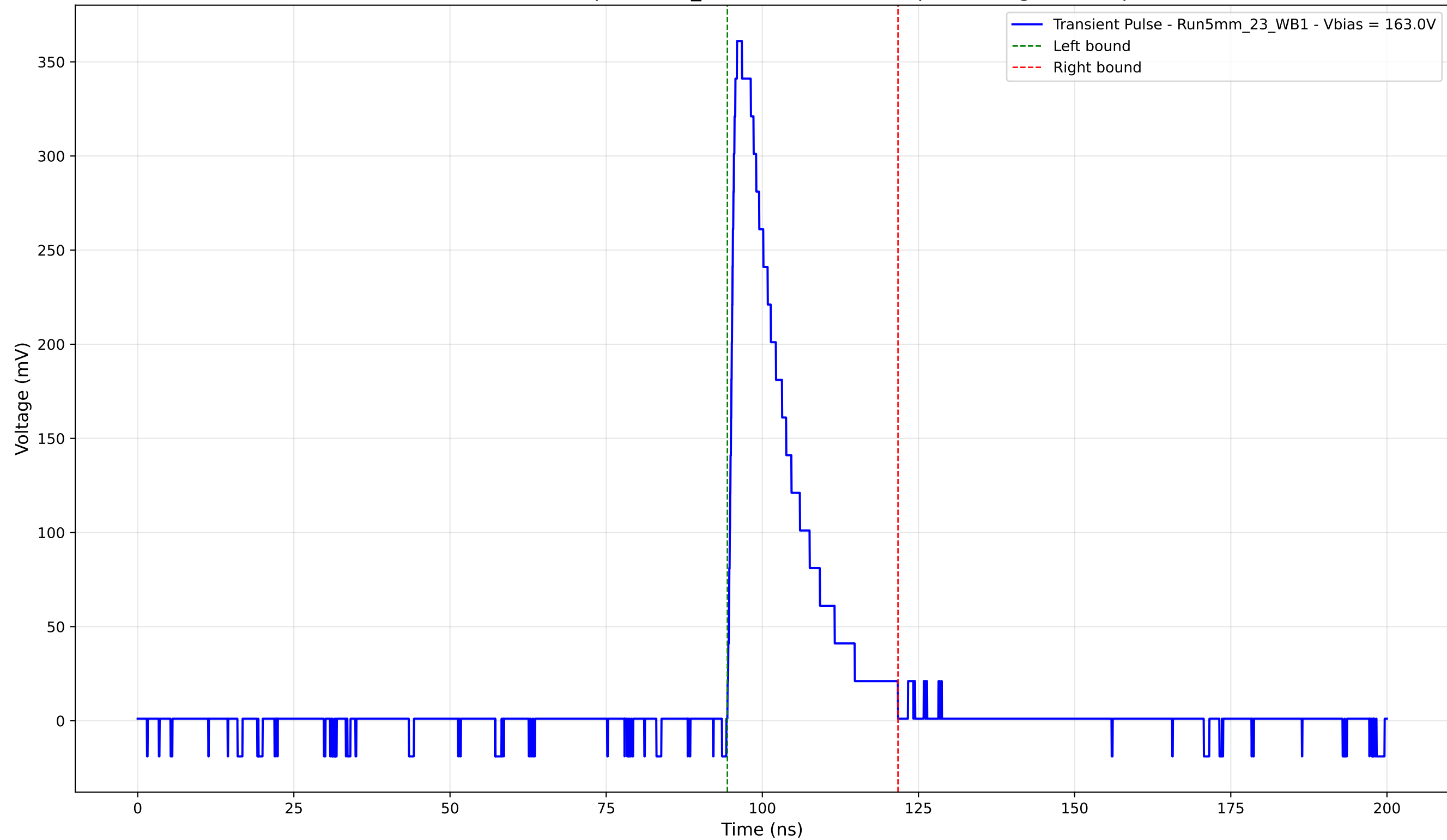
Transient Pulse - Sample: 5mm_23 - Position: 3725.0 \mu\text{m} - Charge: 67.62 pC
