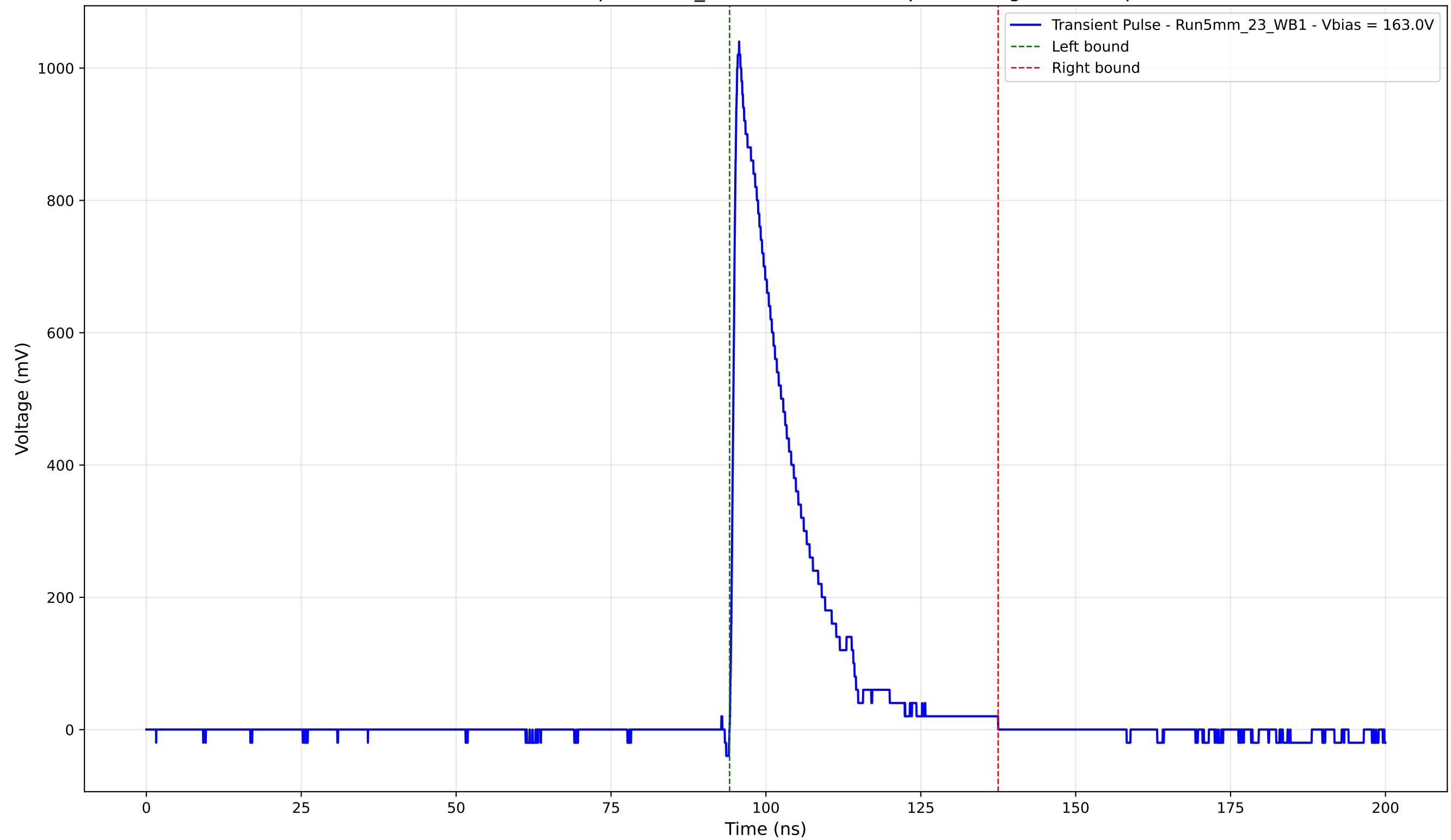
Transient Pulse - Sample: 5mm_23 - Position: 540.0 \mu\text{m} - Charge: 196.21 pC
