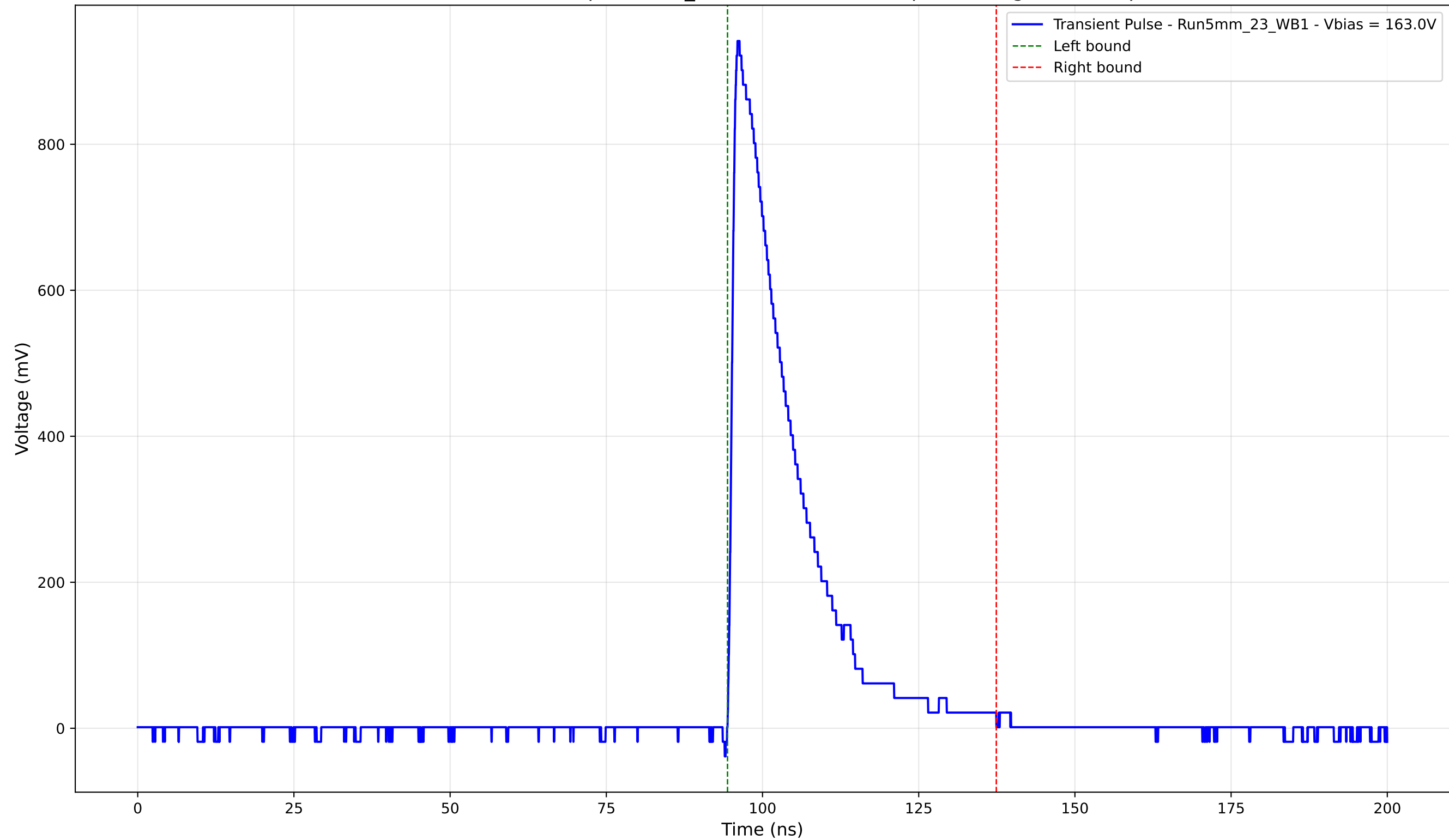
Transient Pulse - Sample: 5mm_23 - Position: 1125.0 \mu\text{m} - Charge: 196.94 pC
