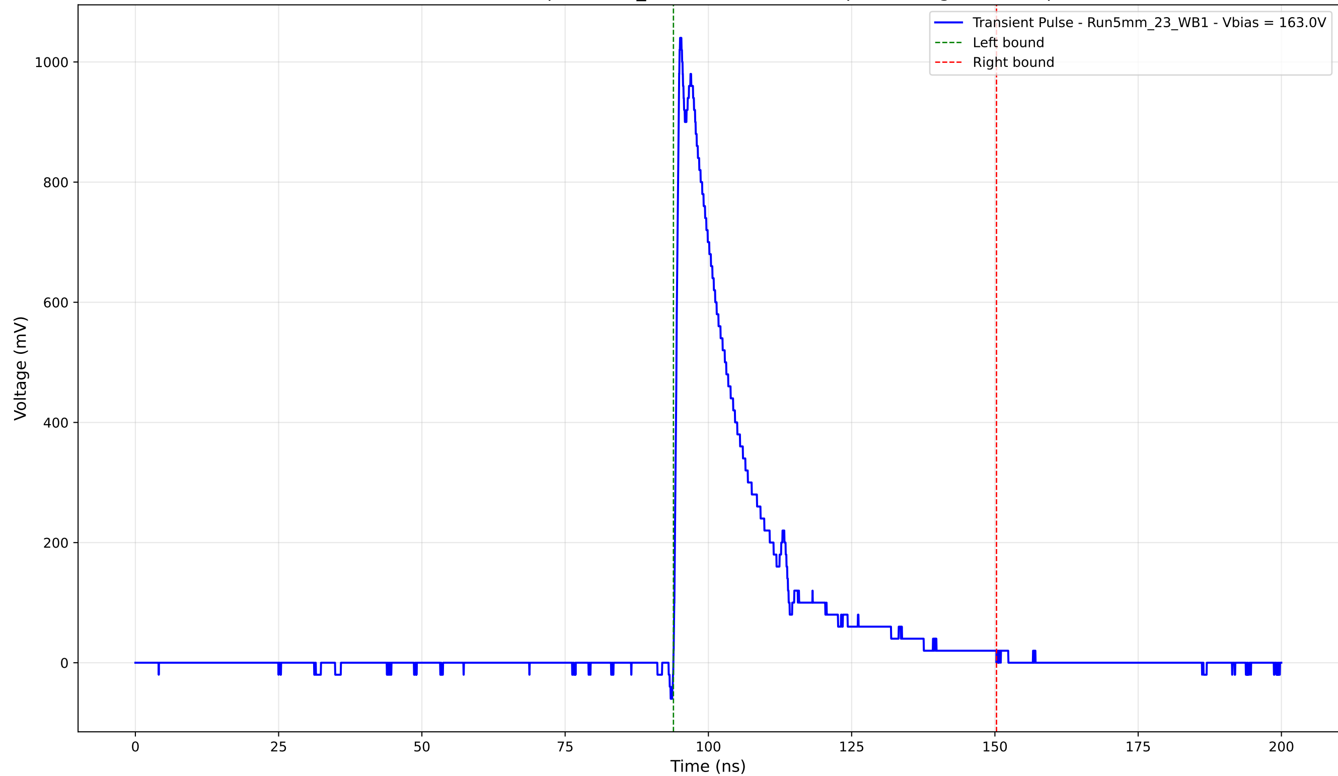
Transient Pulse - Sample: 5mm_23 - Position: 2940.0 \mu\text{m} - Charge: 236.23 pC
