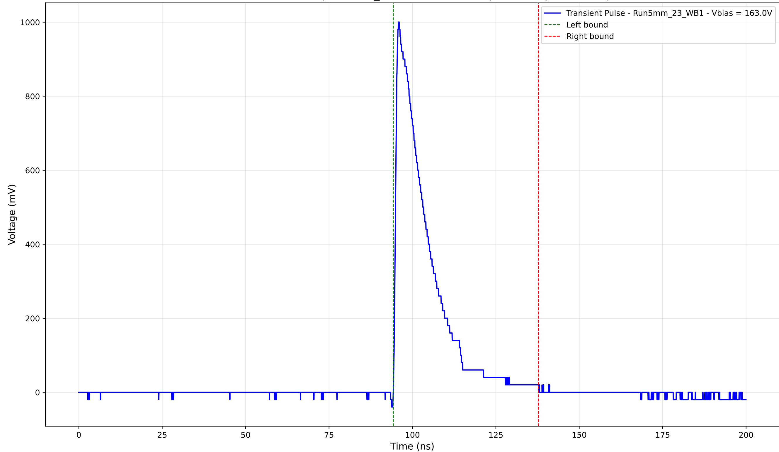
Transient Pulse - Sample: 5mm_23 - Position: 830.0 \mu\text{m} - Charge: 206.28 pC
