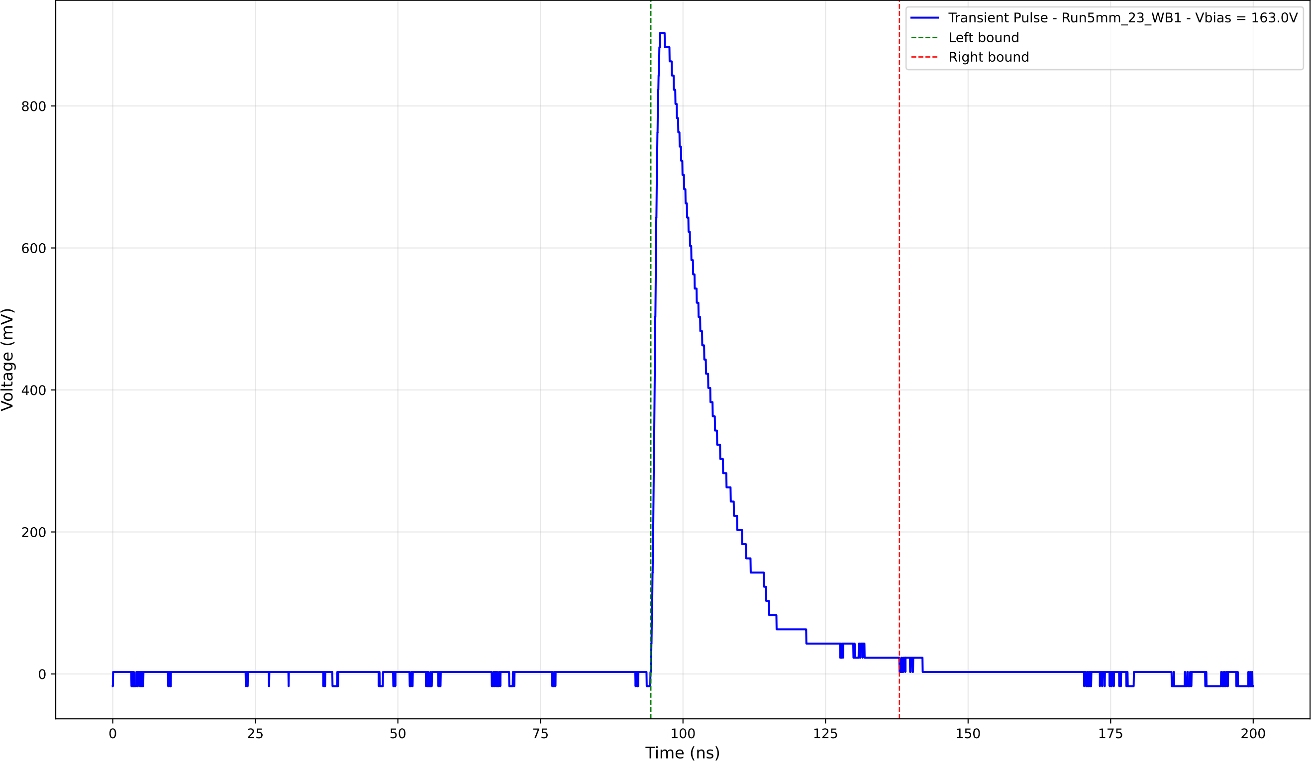
Transient Pulse - Sample: 5mm_23 - Position: 3930.0 \mu\text{m} - Charge: 199.40 pC
