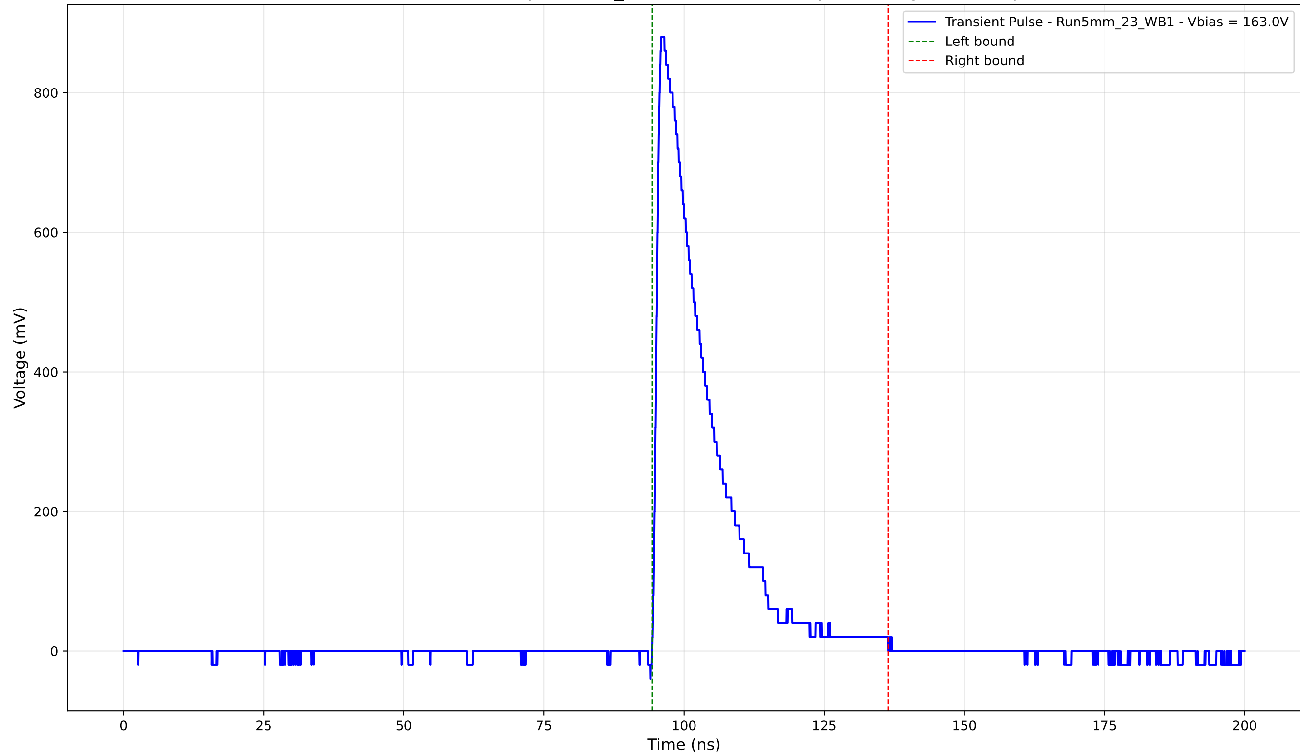
Transient Pulse - Sample: 5mm_23 - Position: 4365.0 \mu\text{m} - Charge: 174.14 pC
