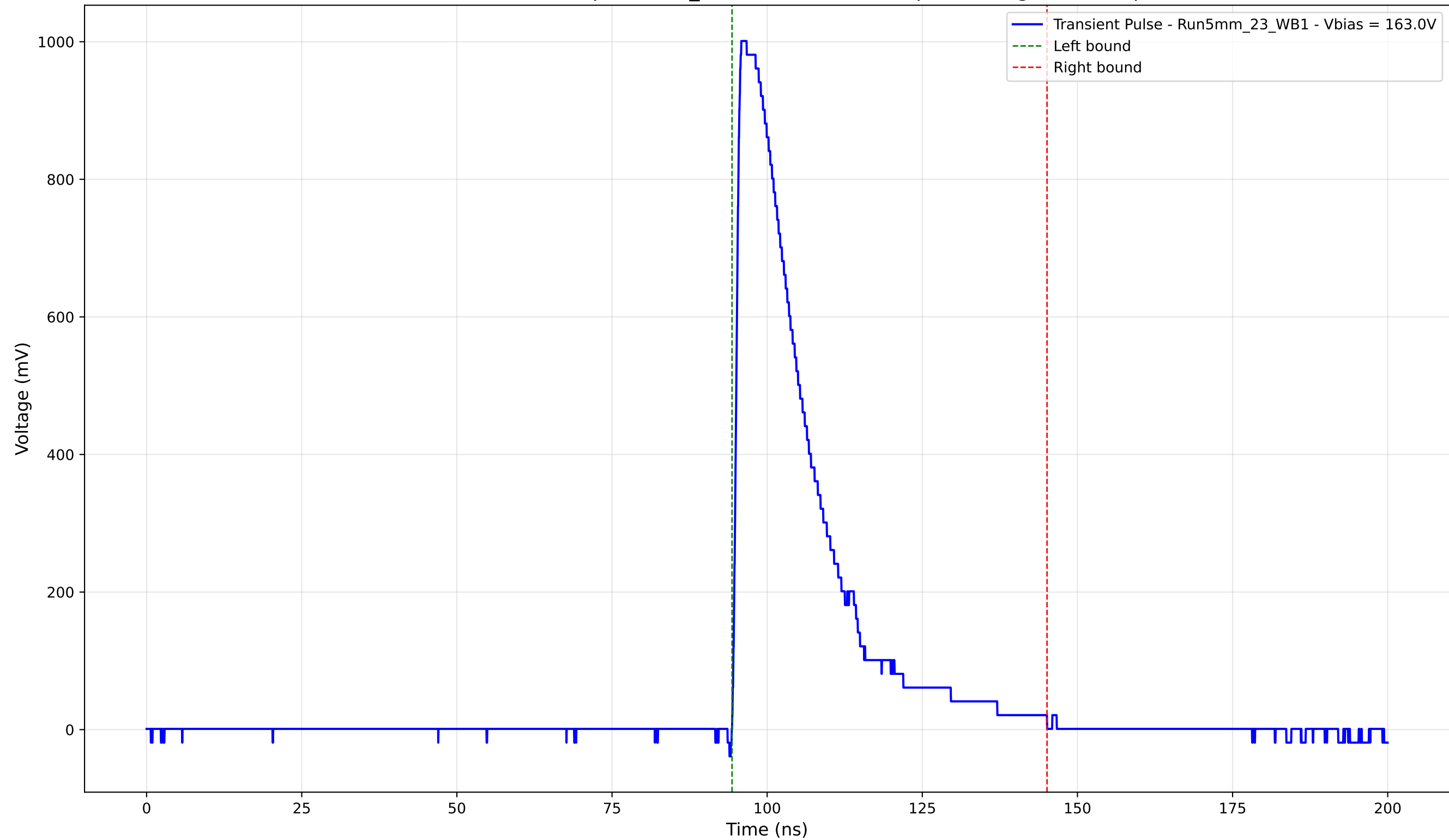
Transient Pulse - Sample: 5mm_23 - Position: 1580.0 \mu\text{m} - Charge: 255.85 pC
