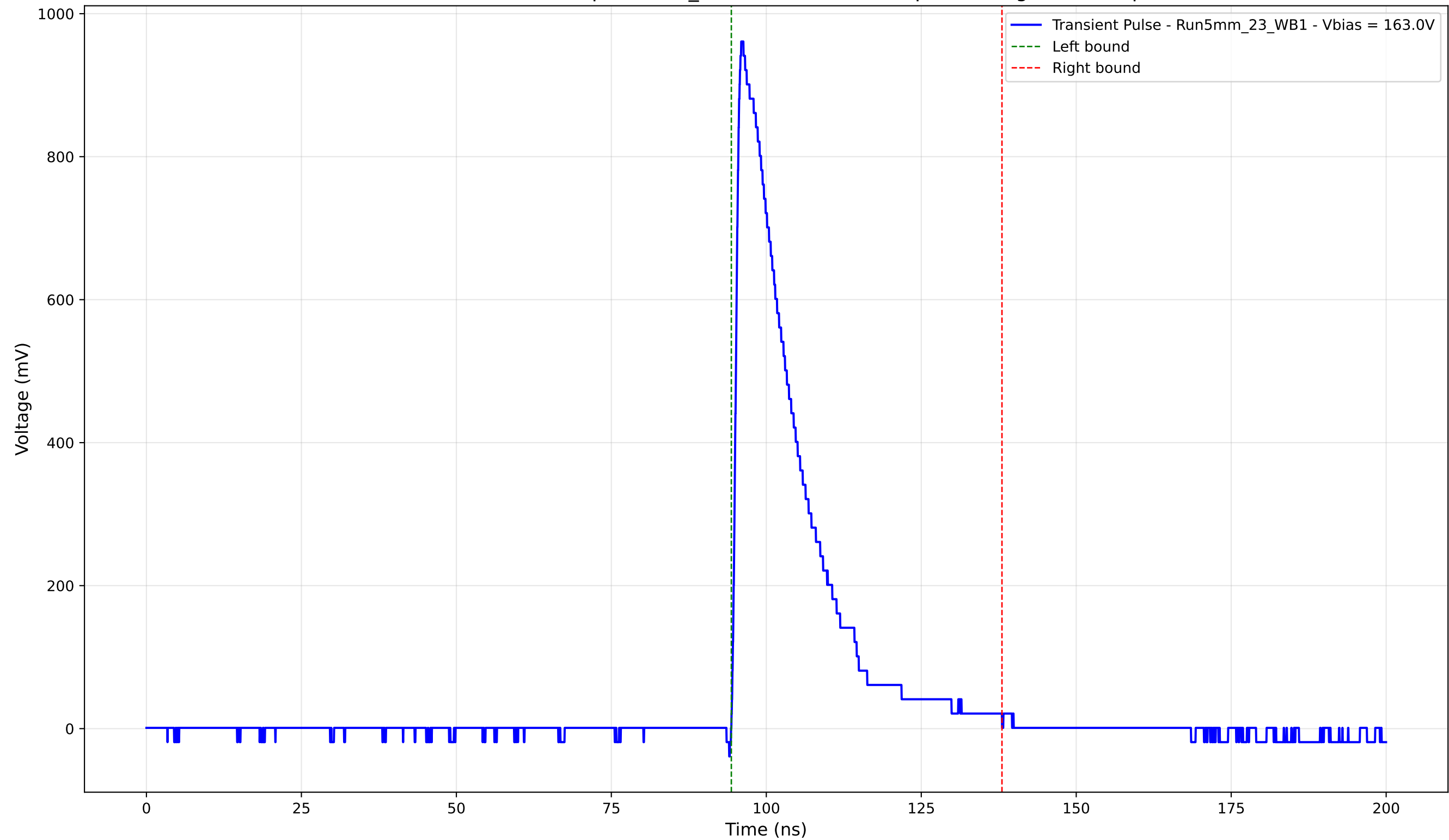
Transient Pulse - Sample: 5mm_23 - Position: 1065.0 \mu\text{m} - Charge: 204.16 pC
