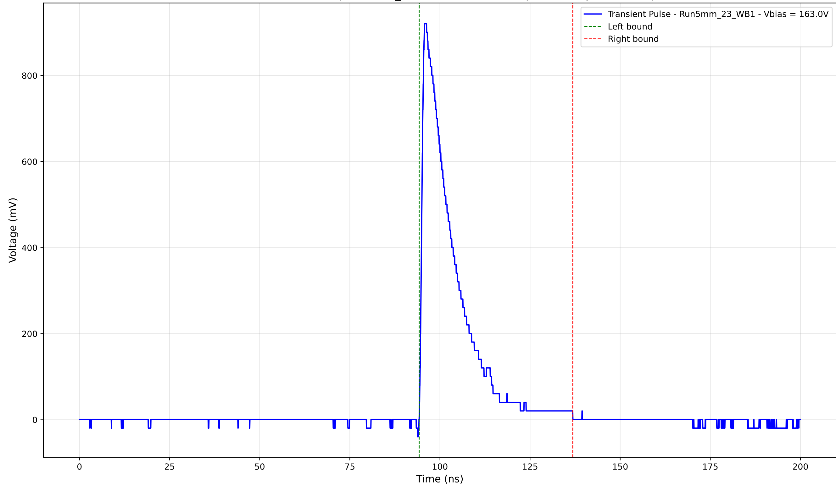
Transient Pulse - Sample: 5mm_23 - Position: 4580.0 \mu\text{m} - Charge: 176.36 pC
