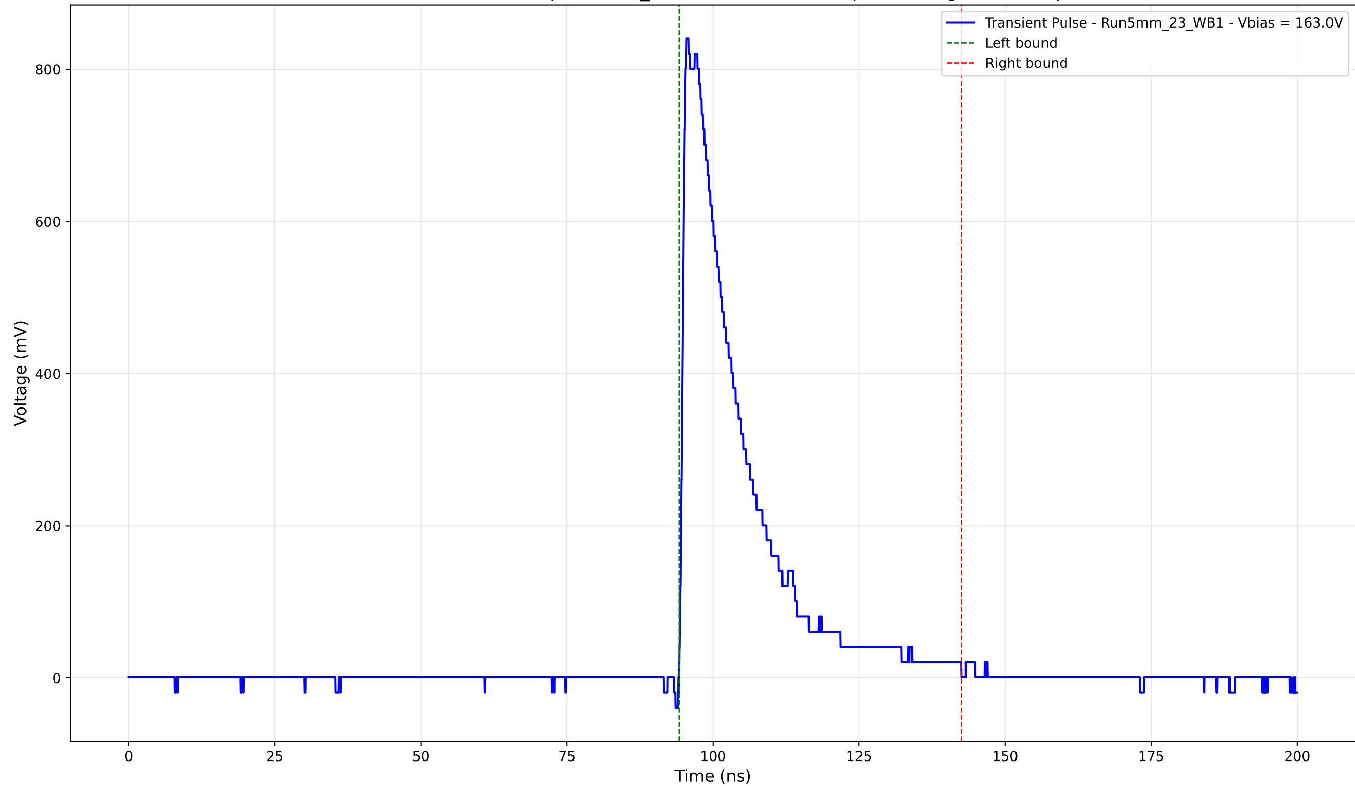
Transient Pulse - Sample: 5mm_23 - Position: 3330.0 \mu\text{m} - Charge: 183.09 pC
