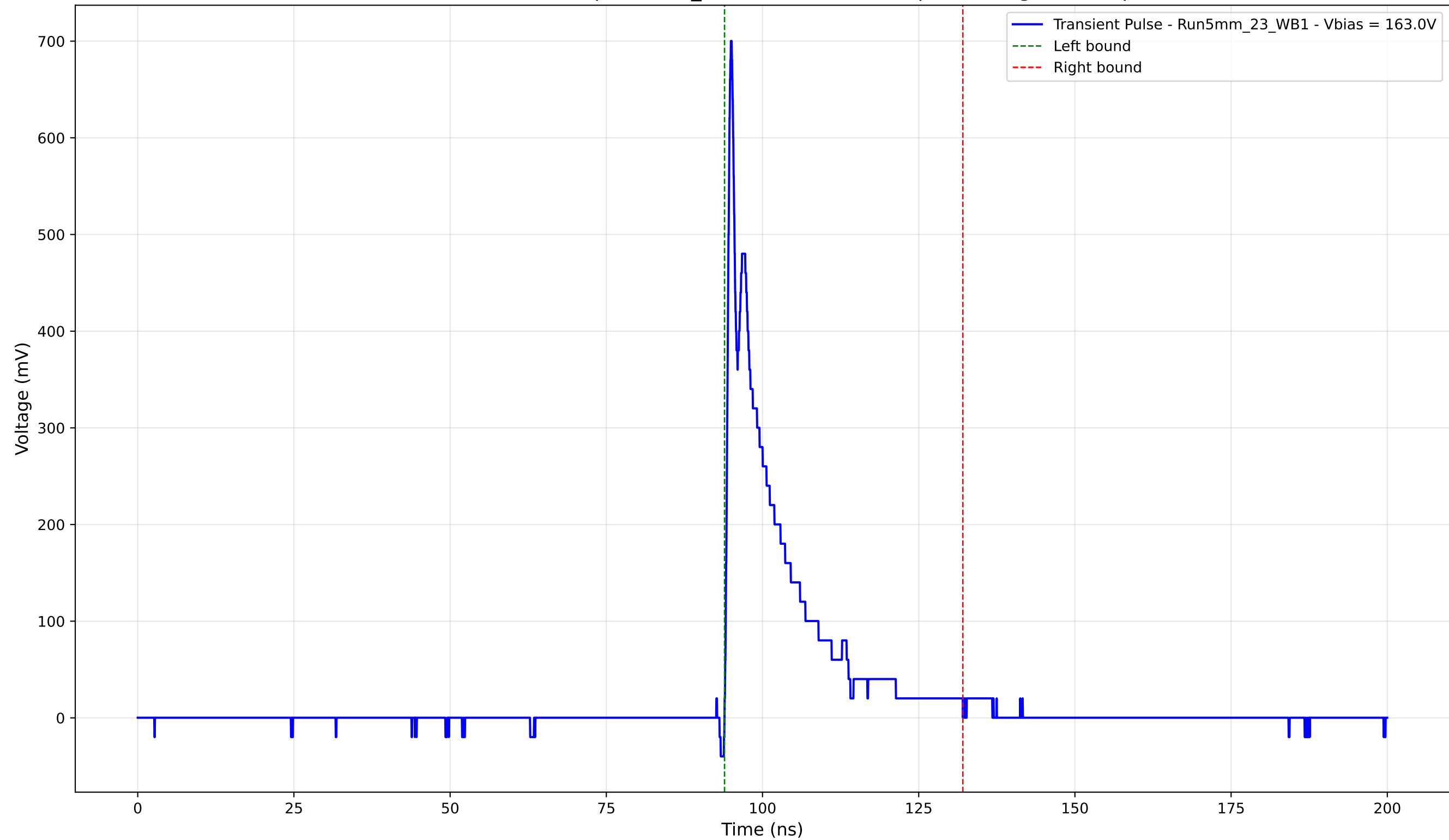
Transient Pulse - Sample: 5mm_23 - Position: 2780.0 \mu\text{m} - Charge: 94.31 pC
