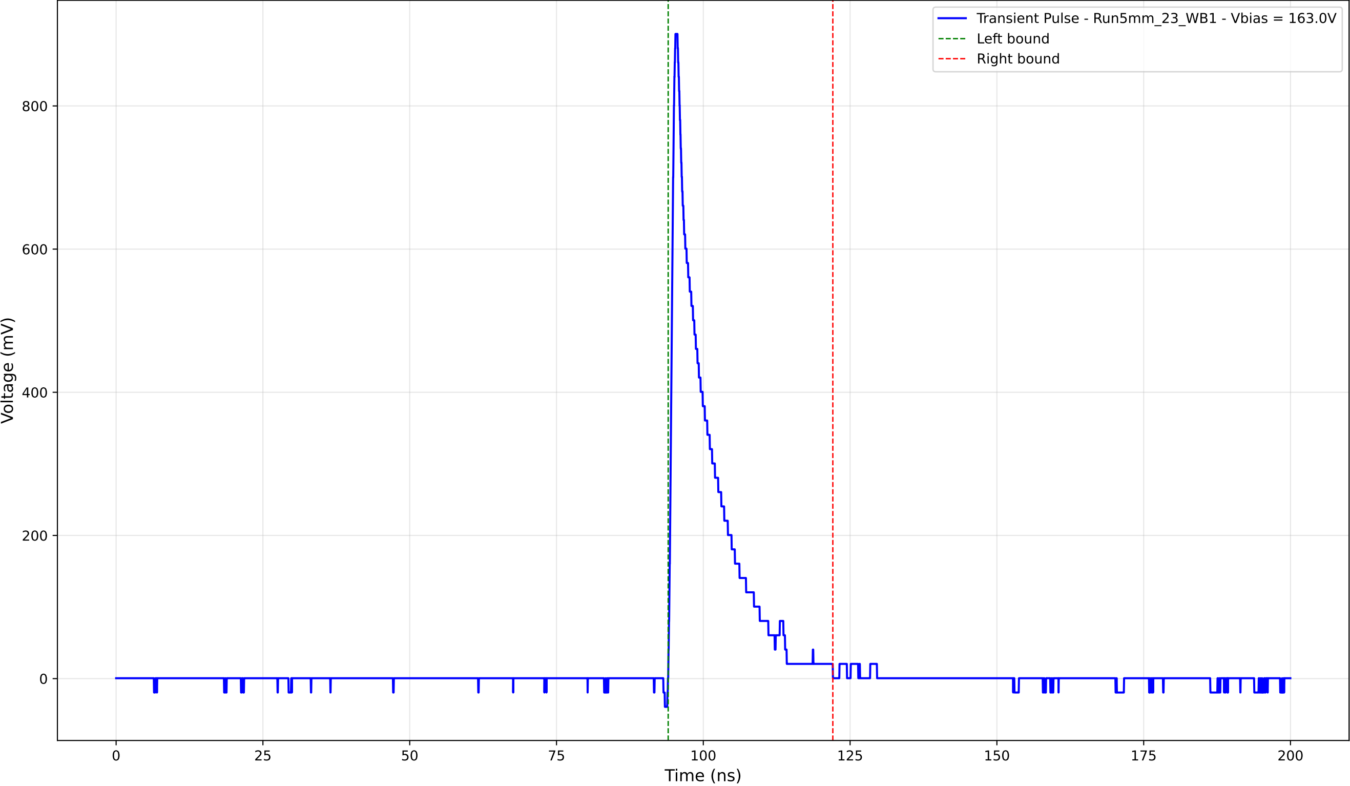
Transient Pulse - Sample: 5mm_23 - Position: 5145.0 \mu\text{m} - Charge: 116.61 pC
