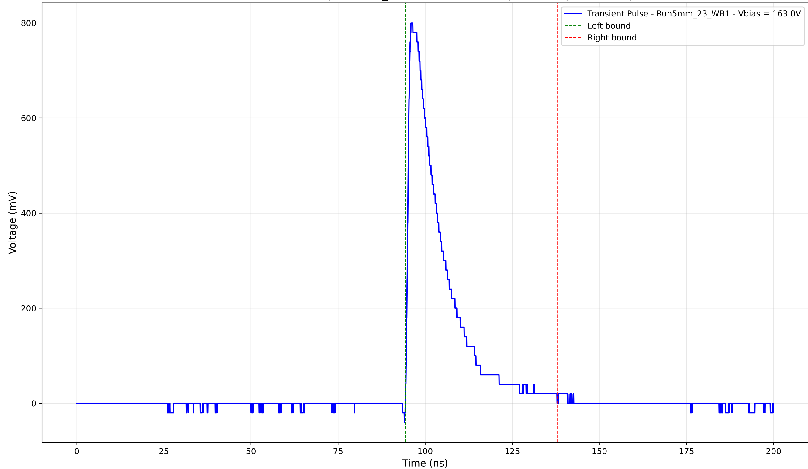
Transient Pulse - Sample: 5mm_23 - Position: 1795.0 \mu\text{m} - Charge: 172.23 pC
