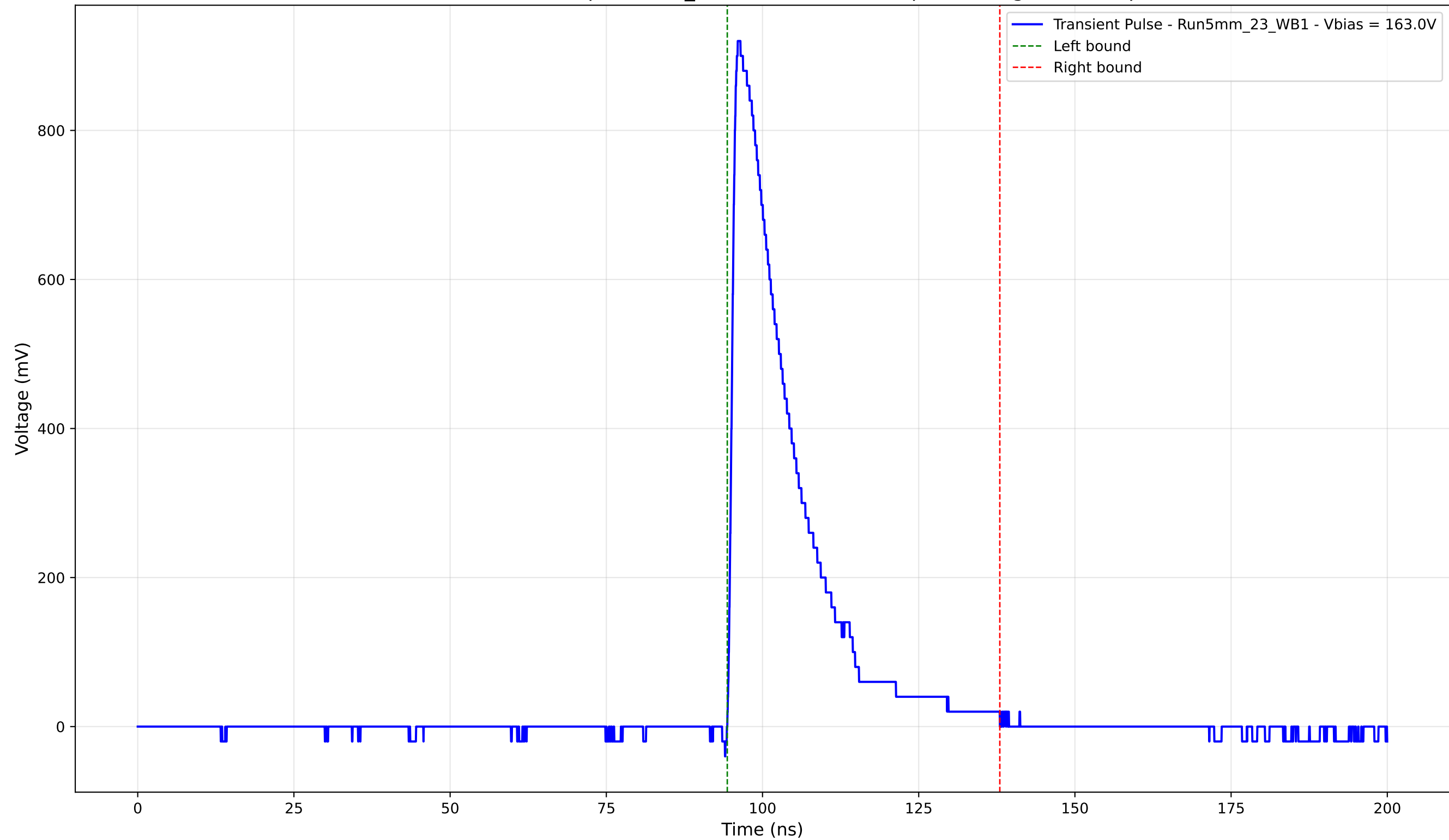
Transient Pulse - Sample: 5mm_23 - Position: 4135.0 \mu\text{m} - Charge: 193.91 pC
