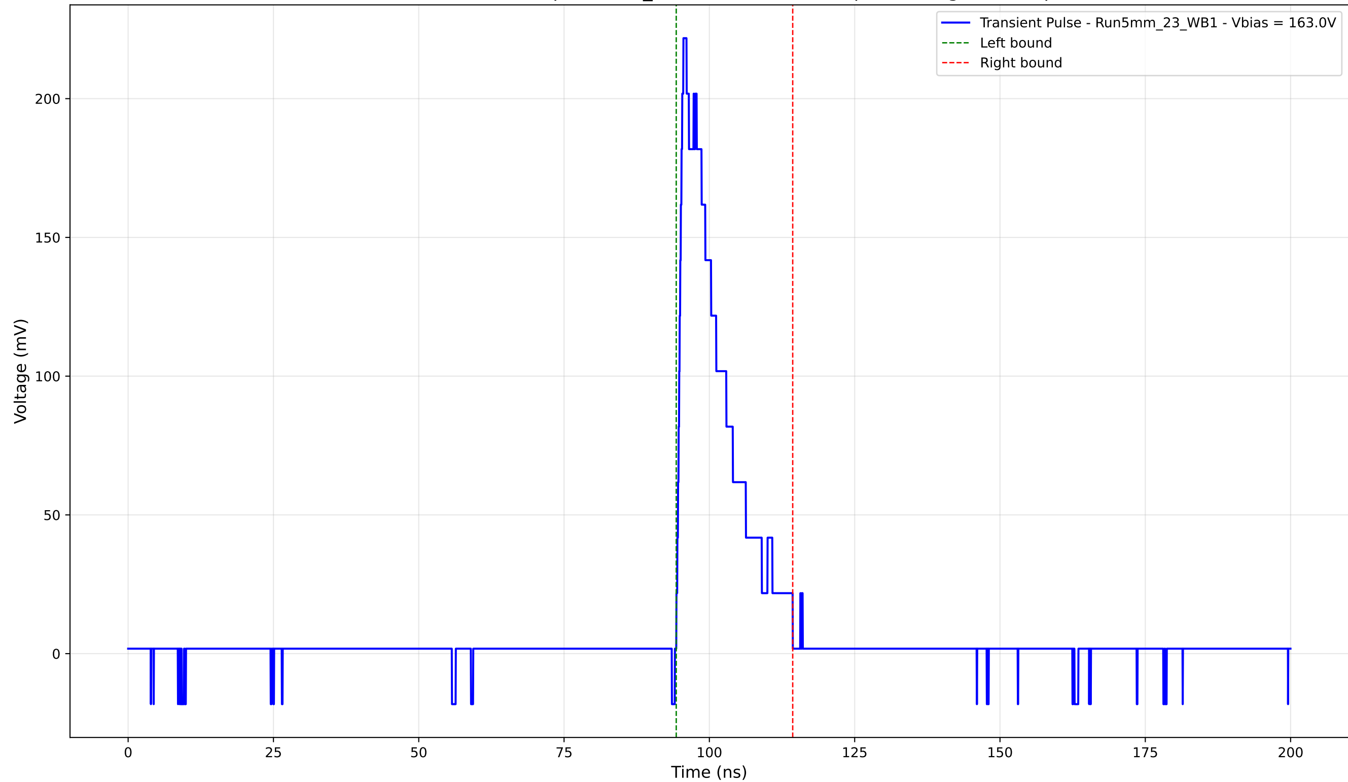
Transient Pulse - Sample: 5mm_23 - Position: 4775.0 \mu\text{m} - Charge: 35.08 pC
