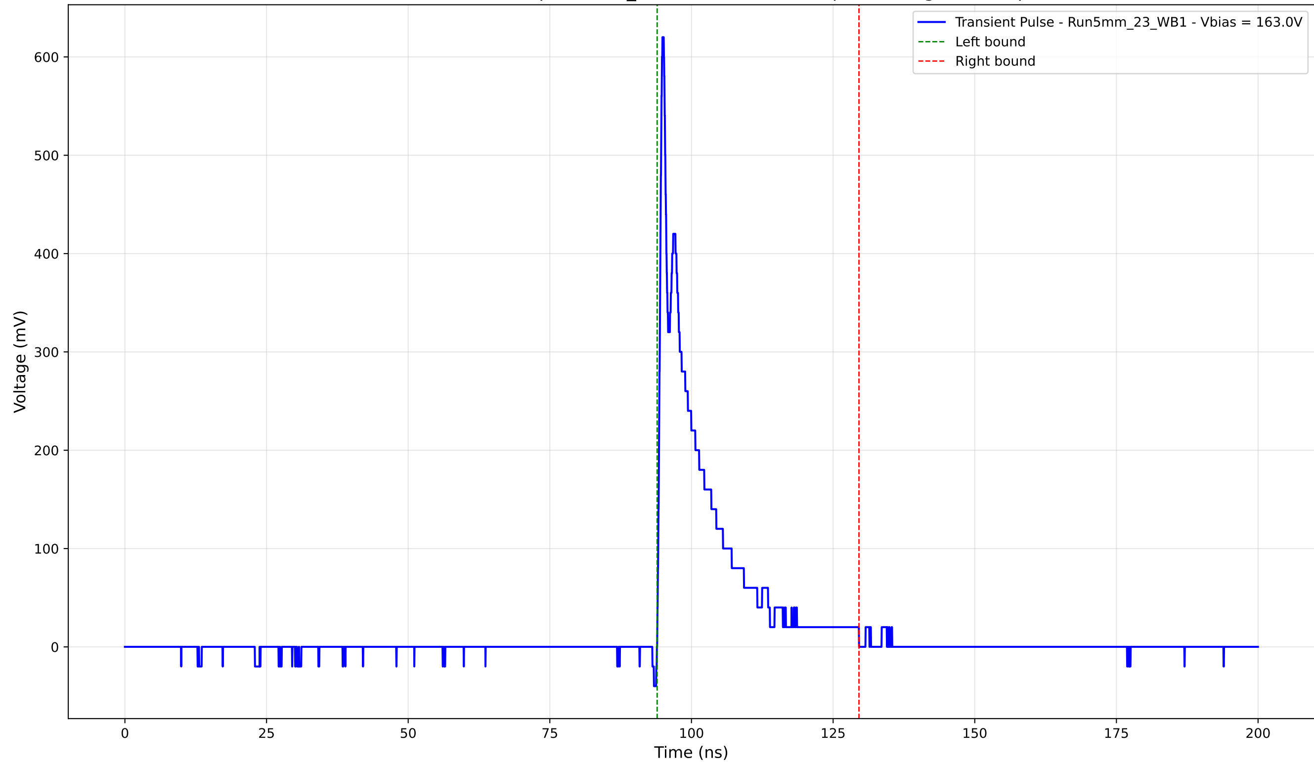
Transient Pulse - Sample: 5mm_23 - Position: 2720.0 \mu\text{m} - Charge: 78.78 pC
