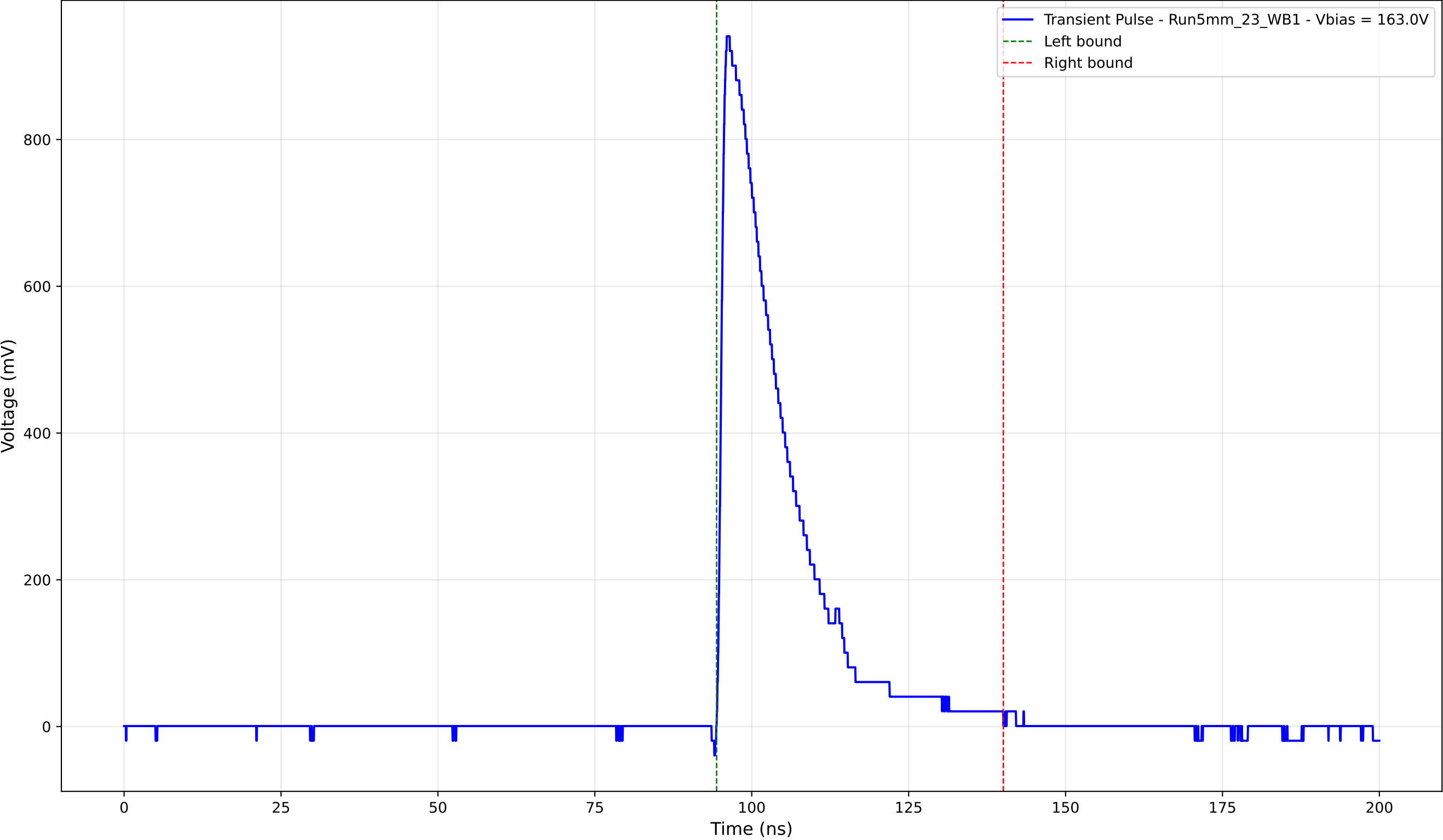
Transient Pulse - Sample: 5mm_23 - Position: 1320.0 \mu\text{m} - Charge: 206.59 pC
