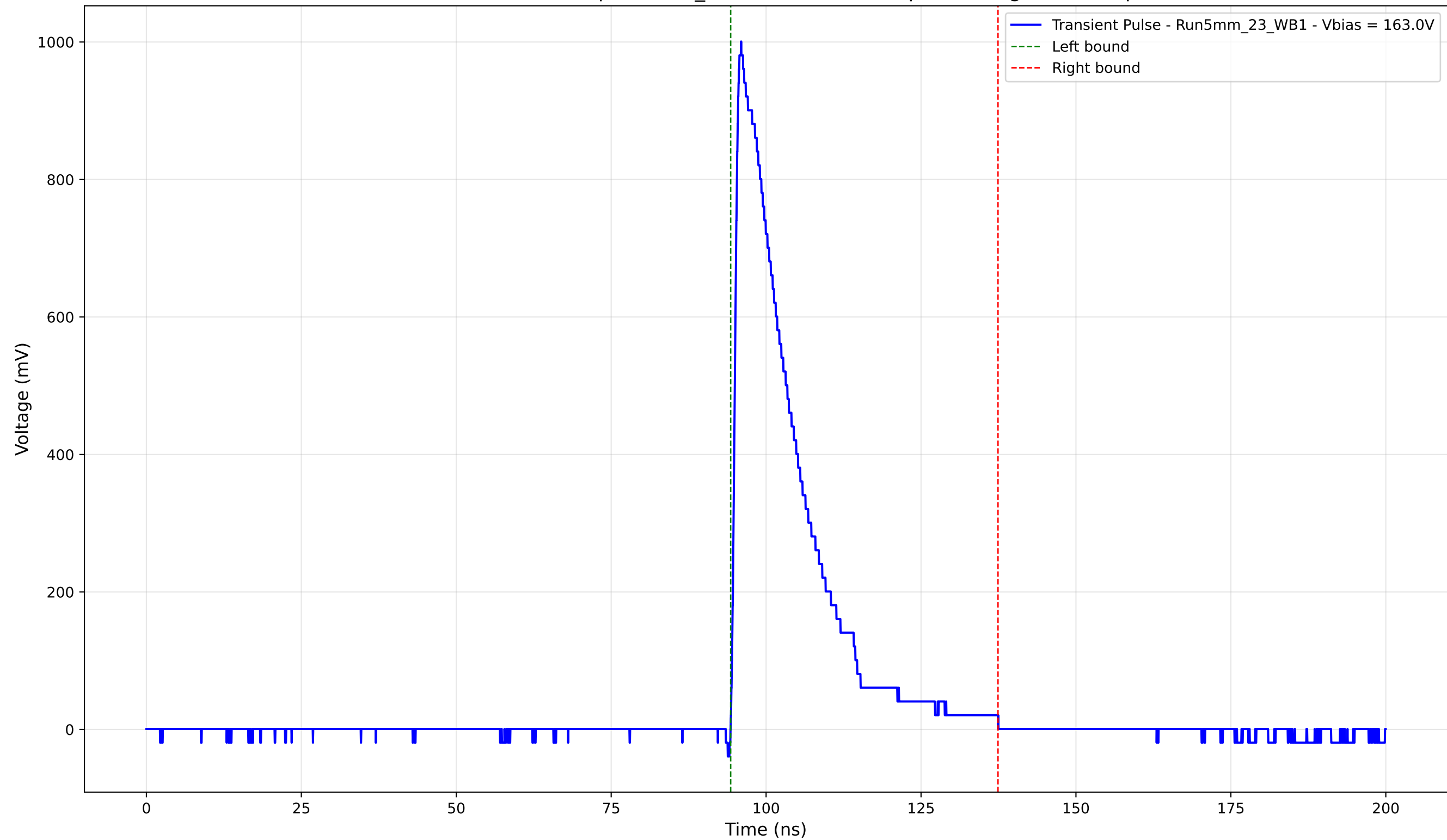
Transient Pulse - Sample: 5mm_23 - Position: 860.0 \mu\text{m} - Charge: 206.12 pC
