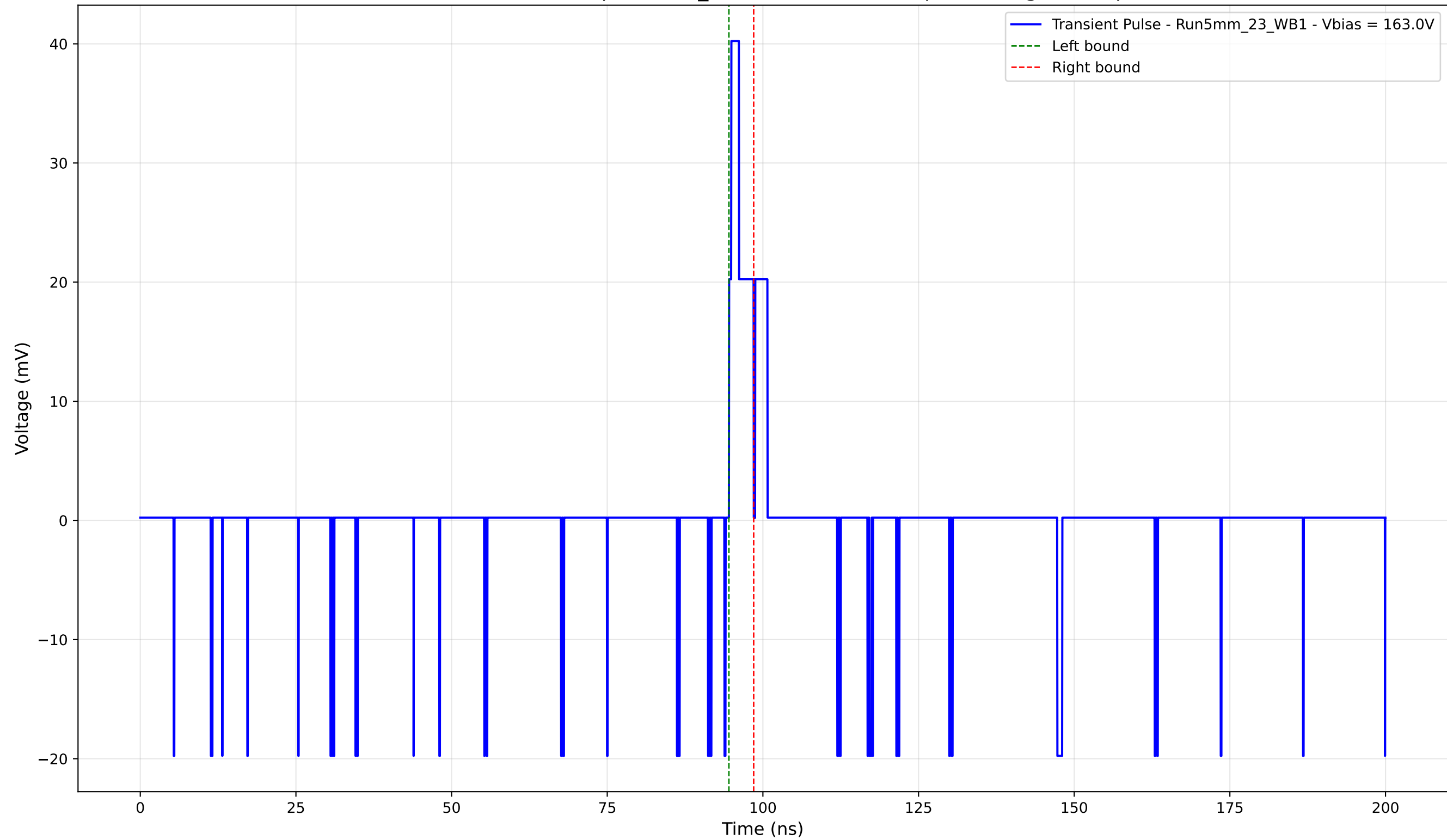
Transient Pulse - Sample: 5mm_23 - Position: 5240.0 \mu\text{m} - Charge: 2.10 pC
