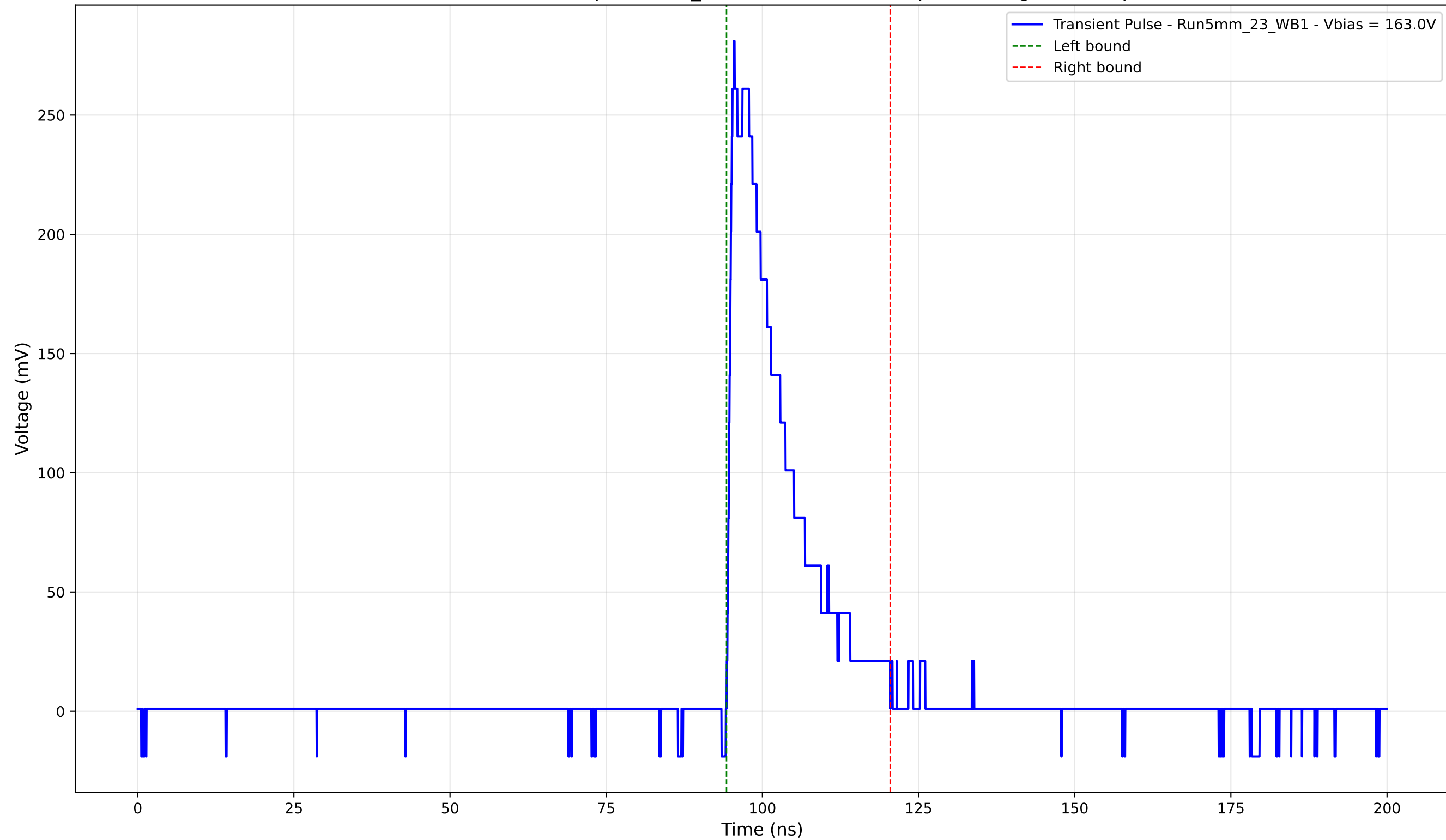
Transient Pulse - Sample: 5mm_23 - Position: 3265.0 \mu\text{m} - Charge: 51.40 pC
