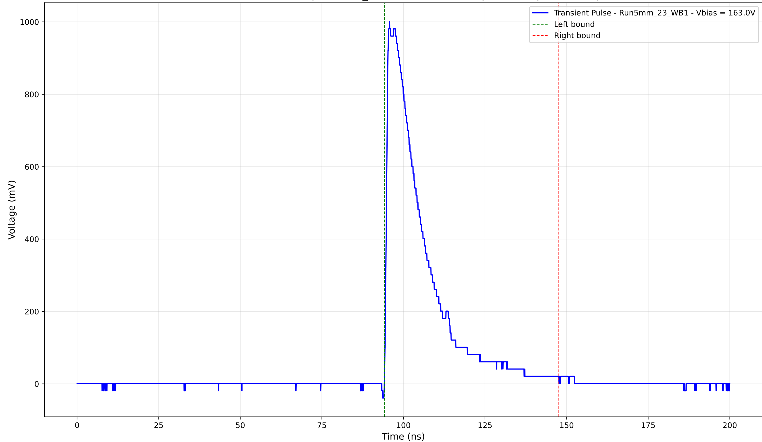
Transient Pulse - Sample: 5mm_23 - Position: 2050.0 \mu\text{m} - Charge: 248.62 pC
