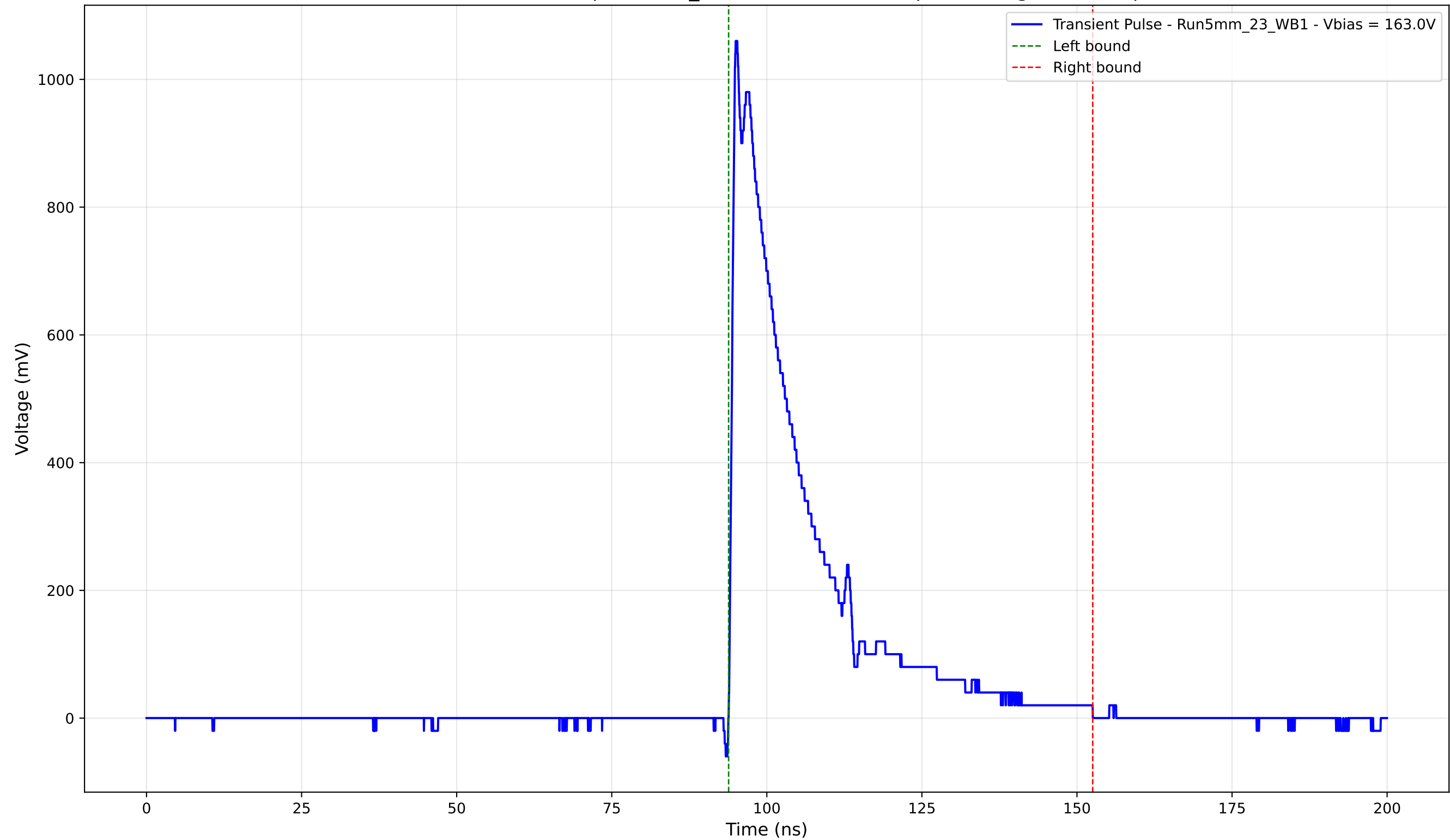
Transient Pulse - Sample: 5mm_23 - Position: 2625.0 \mu\text{m} - Charge: 244.27 pC
