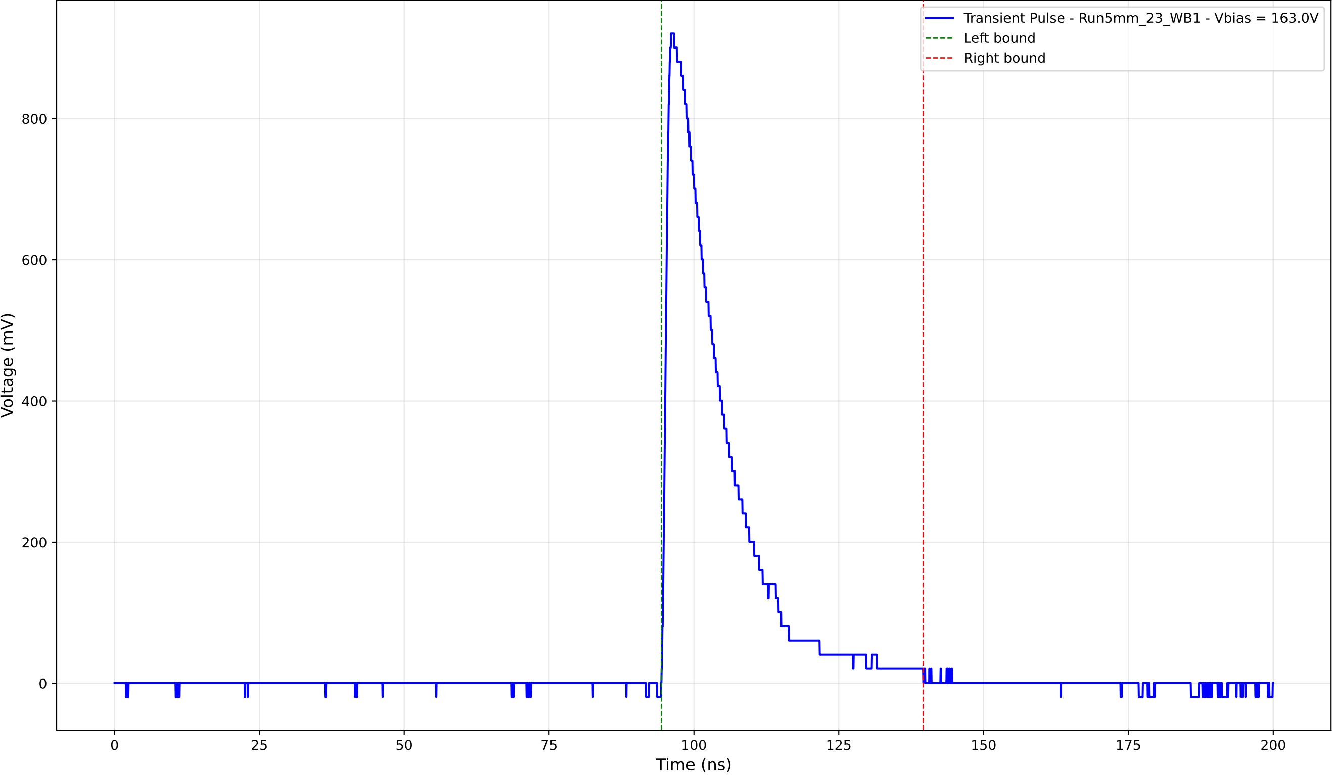
Transient Pulse - Sample: 5mm_23 - Position: 4030.0 \mu\text{m} - Charge: 199.37 pC
