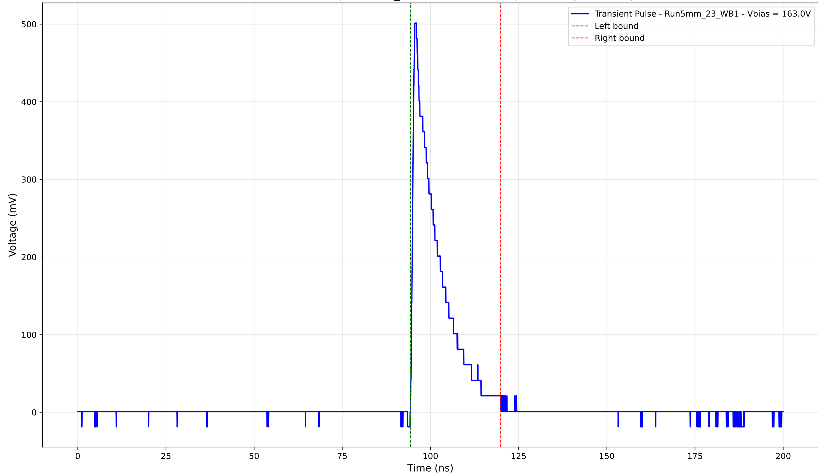
Transient Pulse - Sample: 5mm_23 - Position: 690.0 \mu\text{m} - Charge: 76.17 pC
