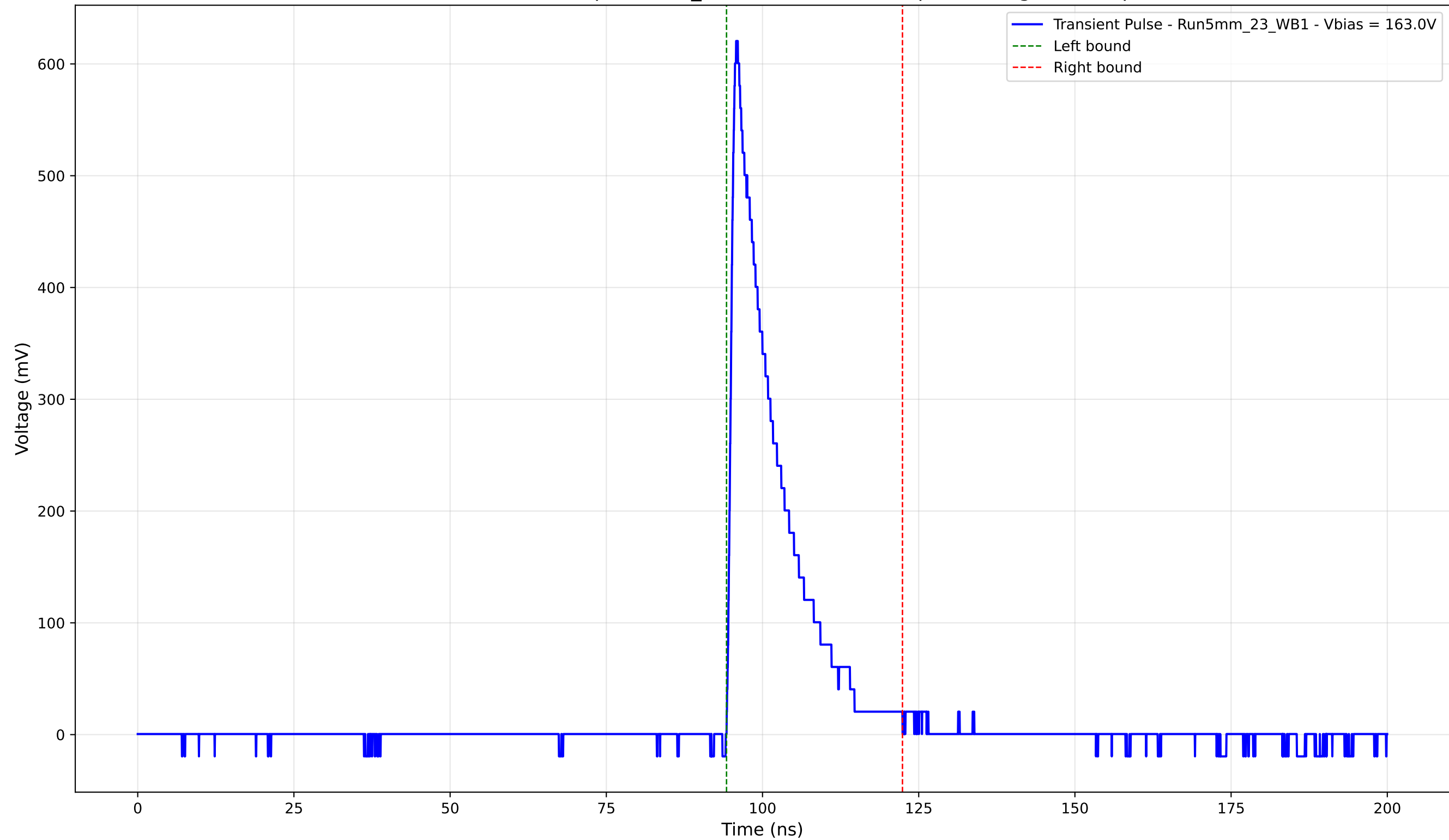
Transient Pulse - Sample: 5mm_23 - Position: 4720.0 \mu\text{m} - Charge: 96.44 pC
