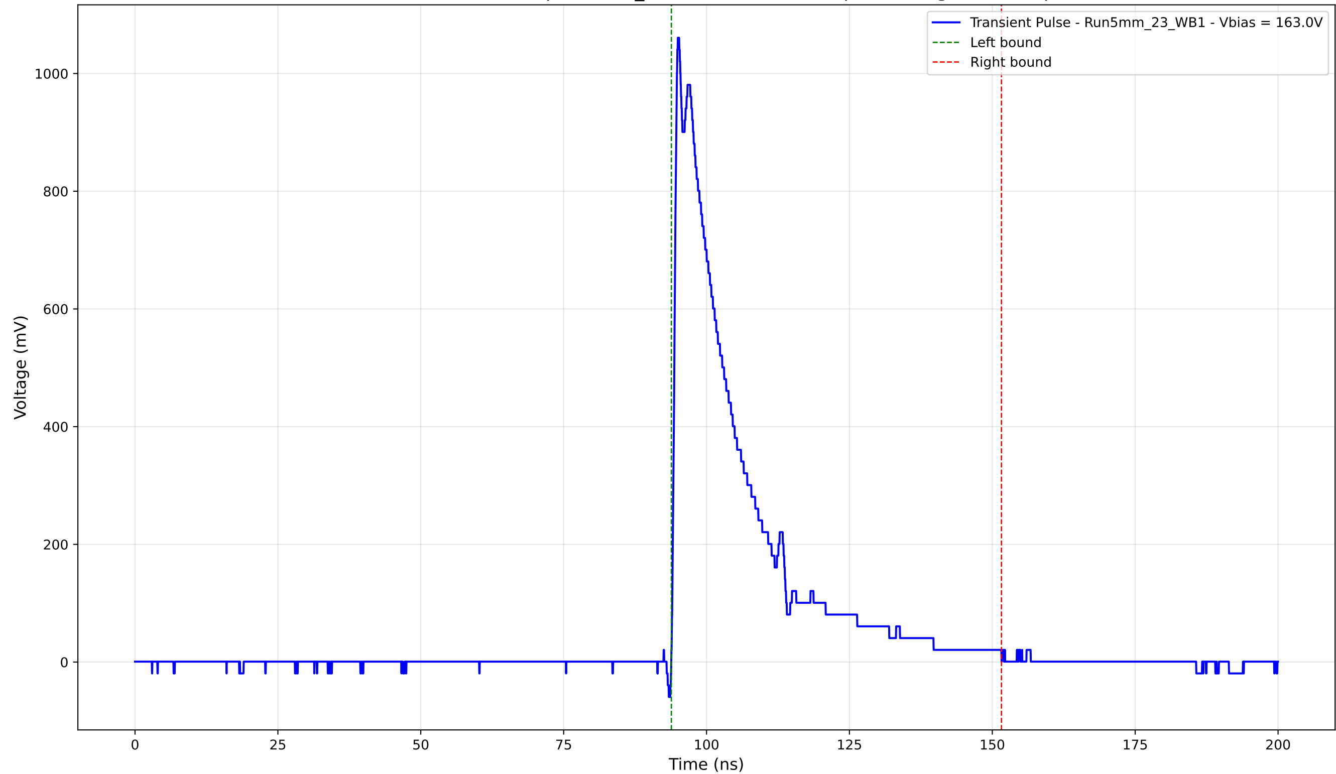
Transient Pulse - Sample: 5mm_23 - Position: 2855.0 \mu\text{m} - Charge: 240.58 pC
