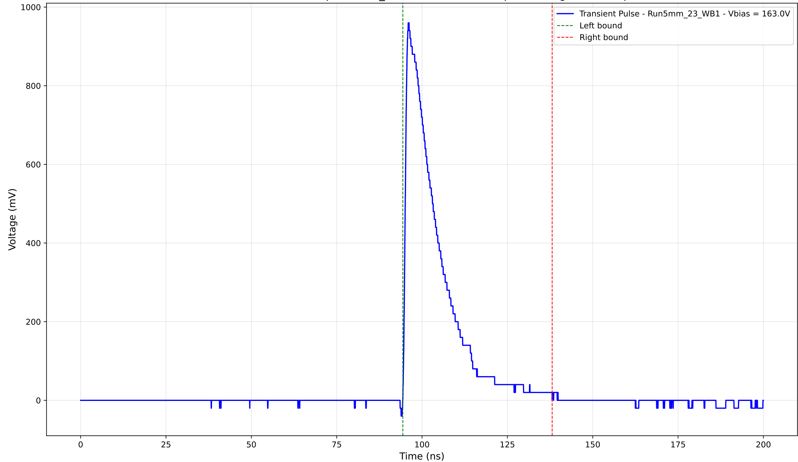
Transient Pulse - Sample: 5mm_23 - Position: 1045.0 \mu\text{m} - Charge: 201.49 pC
