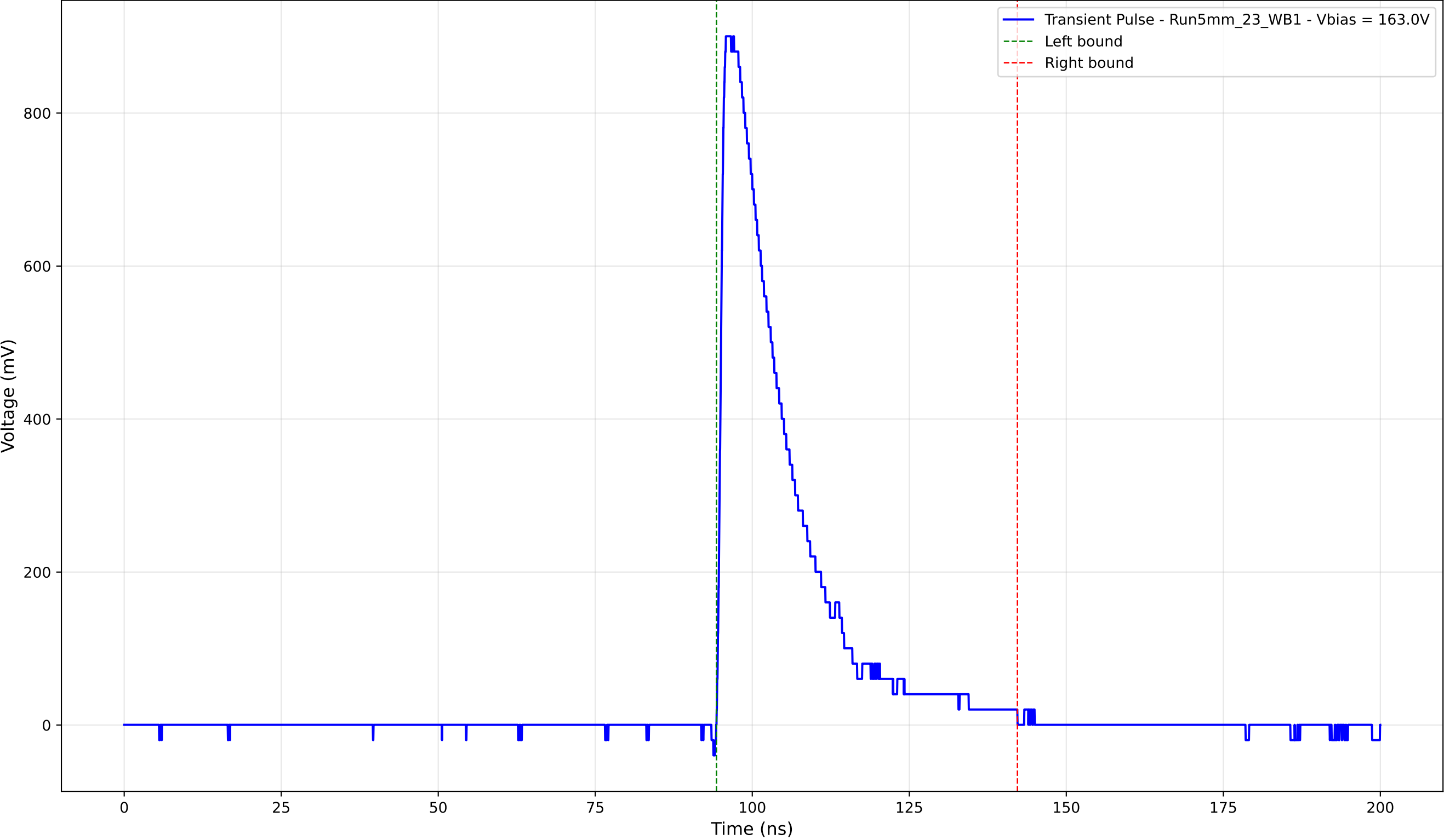
Transient Pulse - Sample: 5mm_23 - Position: 1815.0 \mu\text{m} - Charge: 207.98 pC
