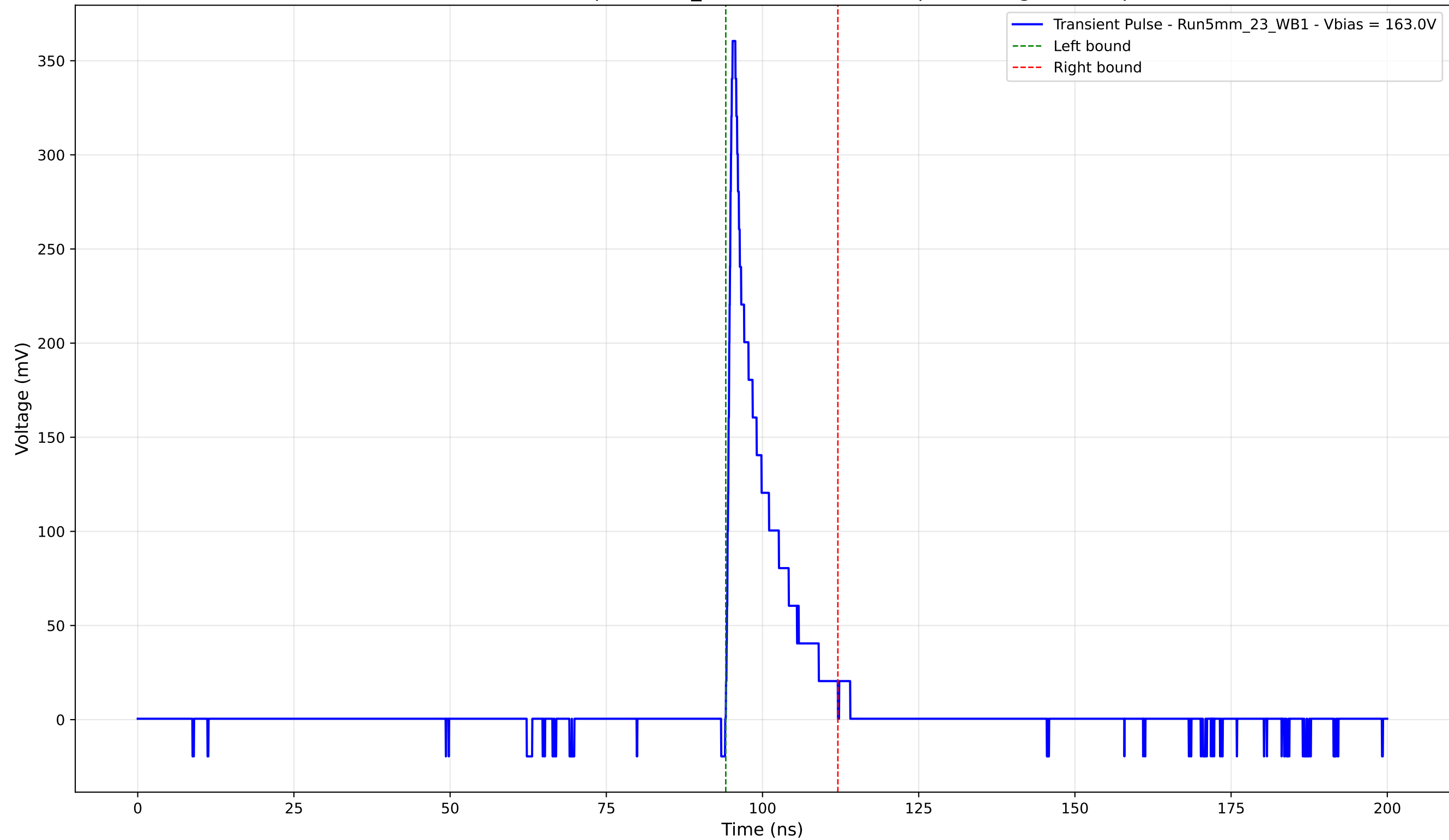
Transient Pulse - Sample: 5mm_23 - Position: 5180.0 \mu\text{m} - Charge: 38.37 pC
