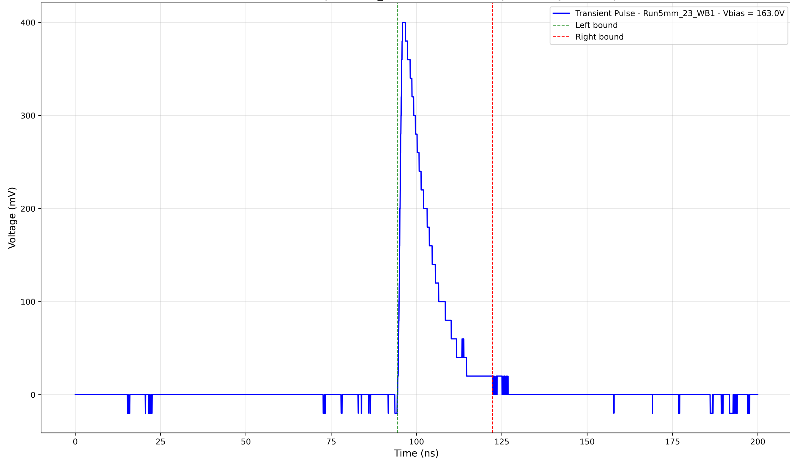
Transient Pulse - Sample: 5mm_23 - Position: 1195.0 \mu\text{m} - Charge: 72.58 pC
