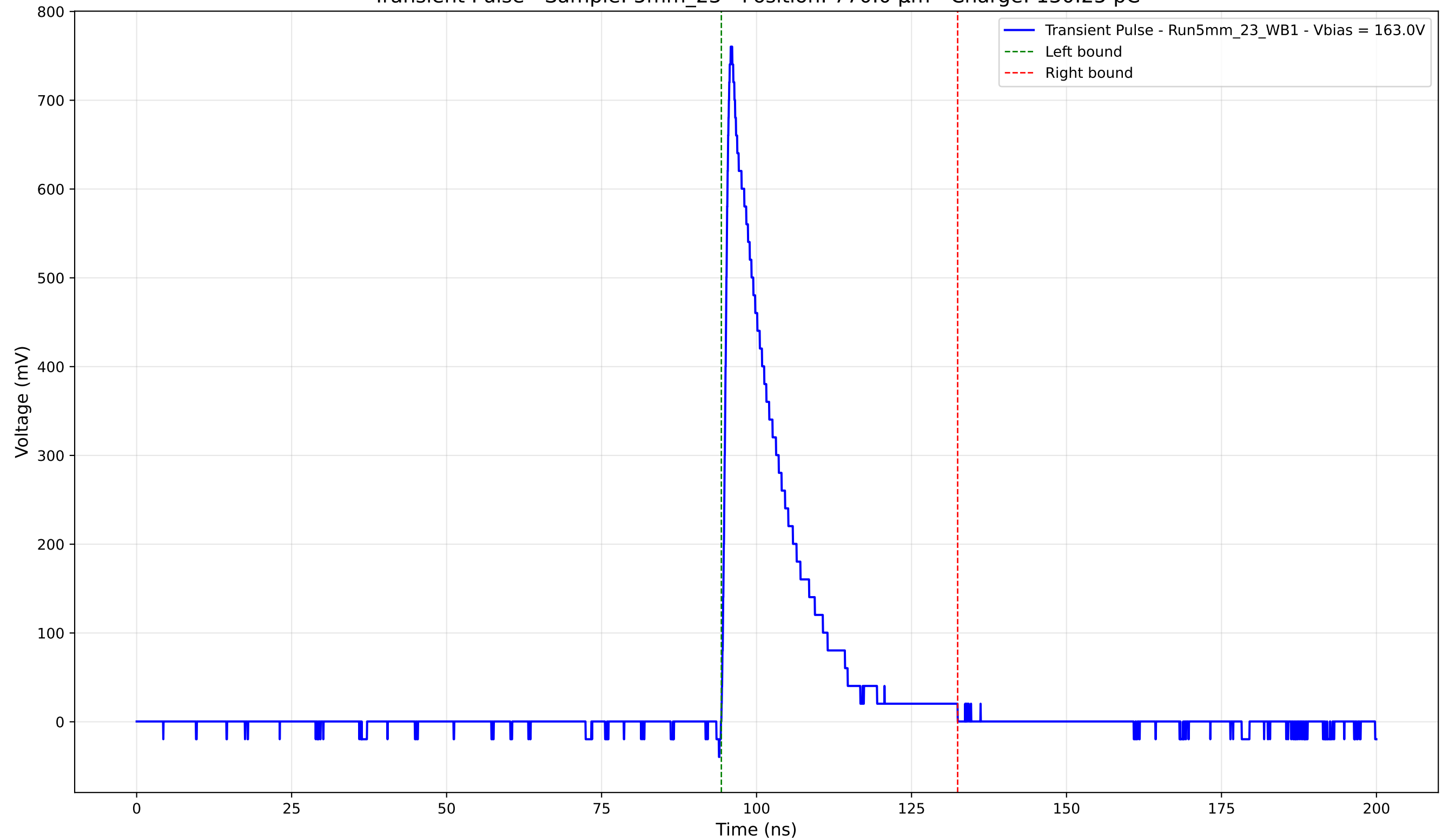
Transient Pulse - Sample: 5mm_23 - Position: 770.0 \mu\text{m} - Charge: 130.25 pC
