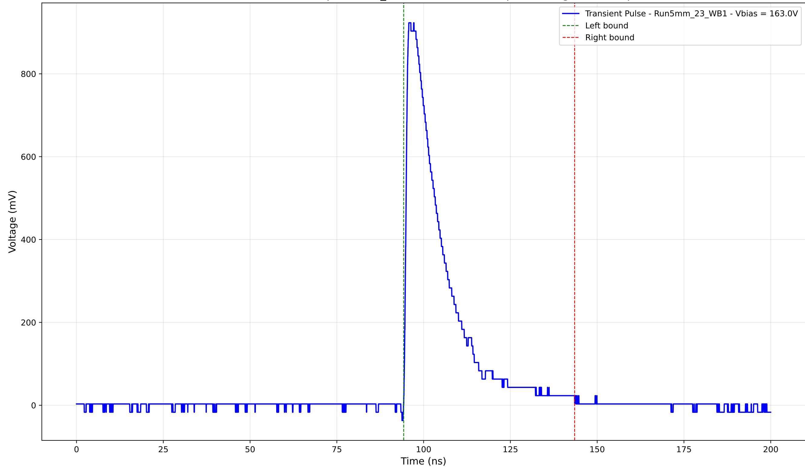
Transient Pulse - Sample: 5mm_23 - Position: 3585.0 \mu\text{m} - Charge: 214.92 pC
