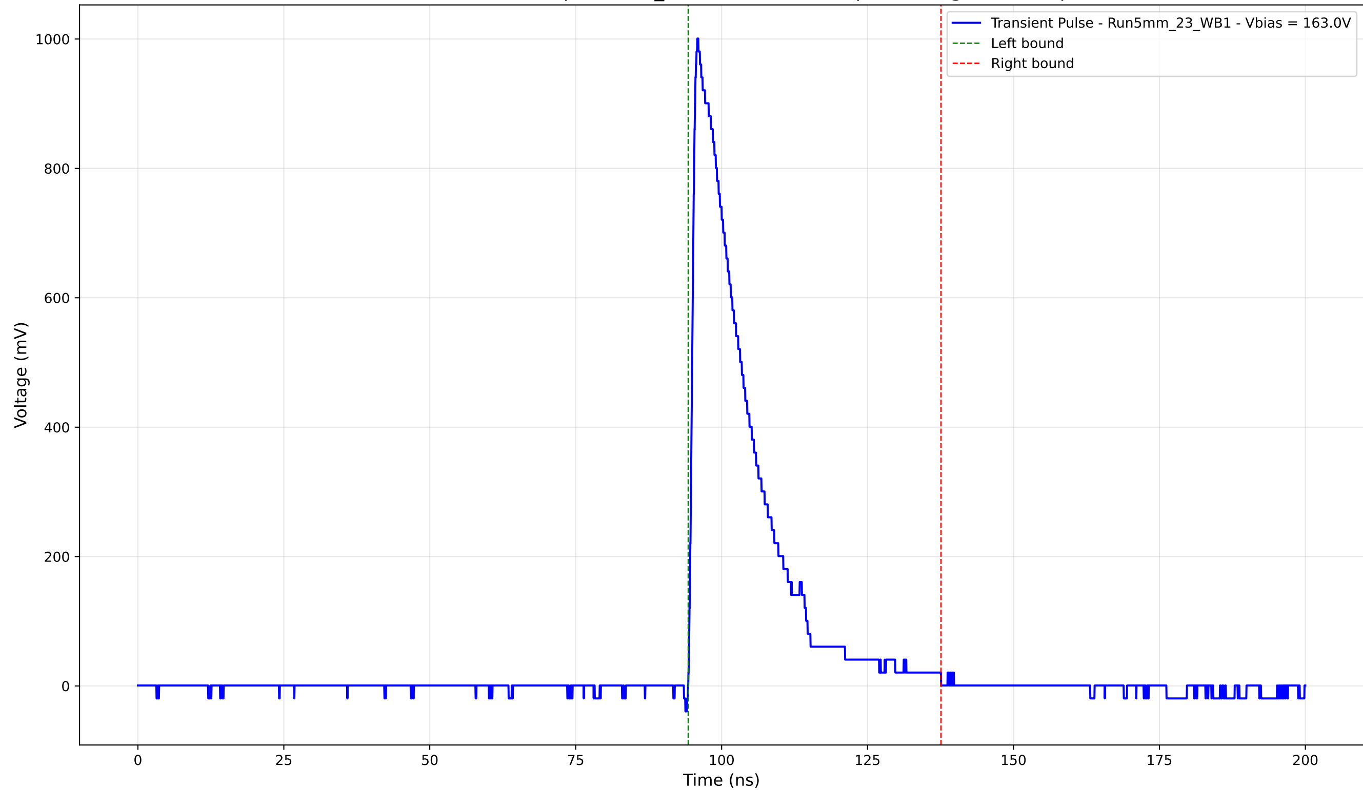
Transient Pulse - Sample: 5mm_23 - Position: 850.0 \mu\text{m} - Charge: 207.06 pC
