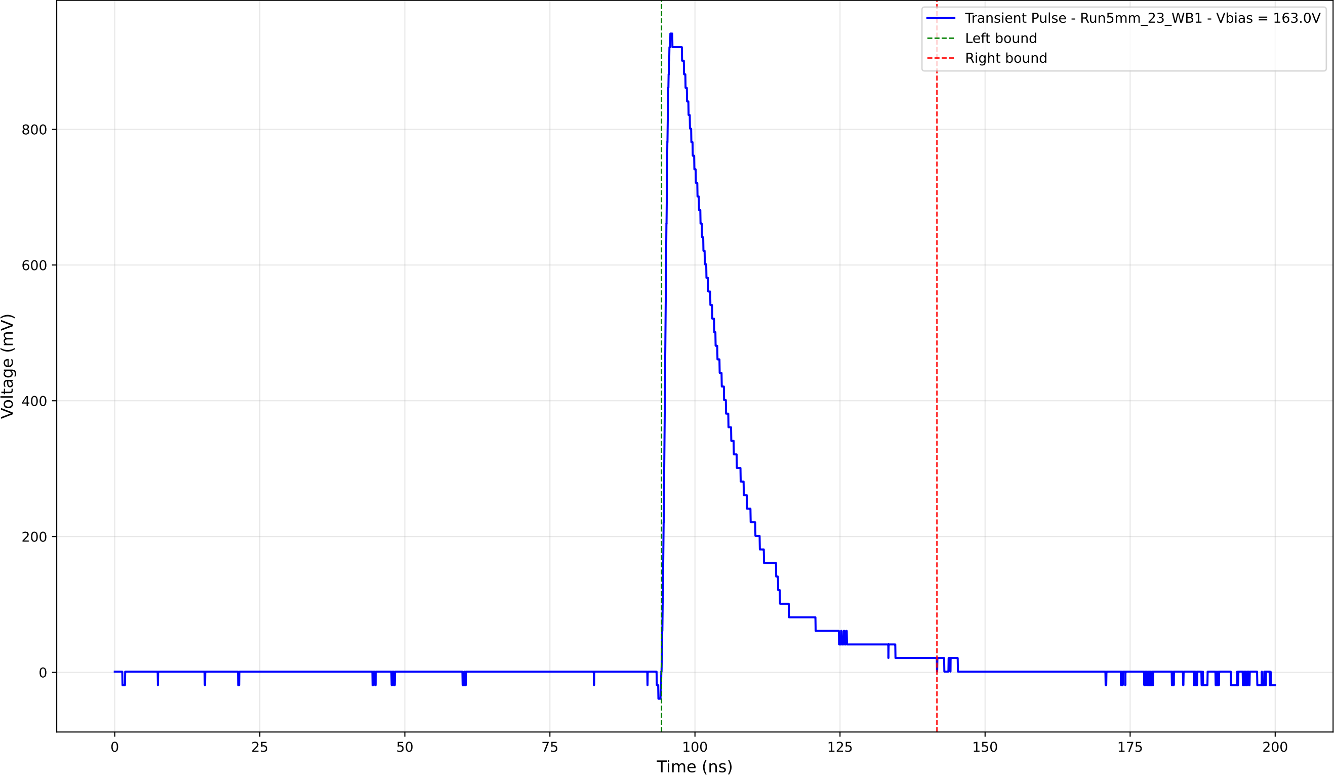
Transient Pulse - Sample: 5mm_23 - Position: 3545.0 \mu\text{m} - Charge: 219.64 pC
