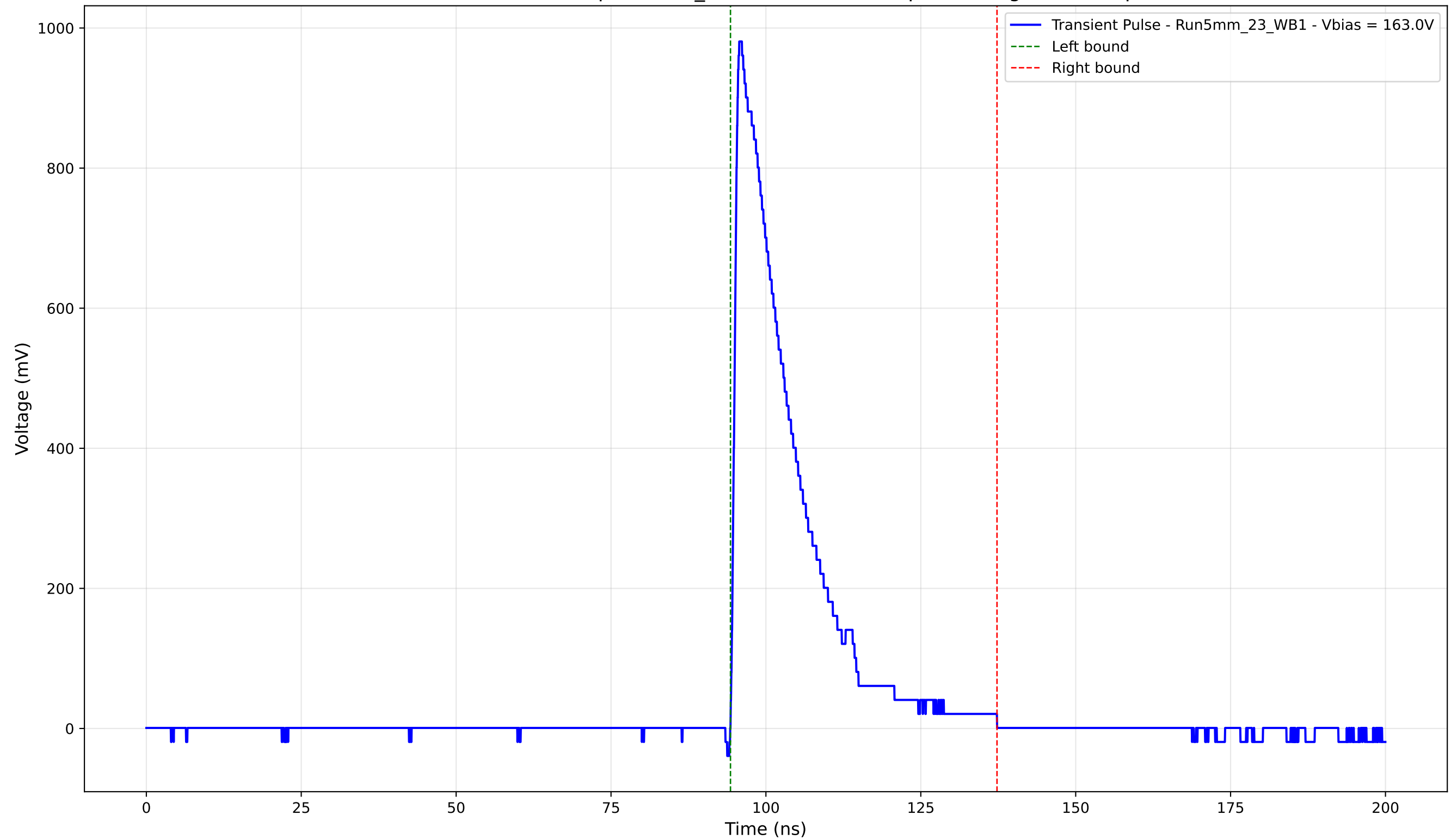
Transient Pulse - Sample: 5mm_23 - Position: 810.0 \mu\text{m} - Charge: 199.19 pC
