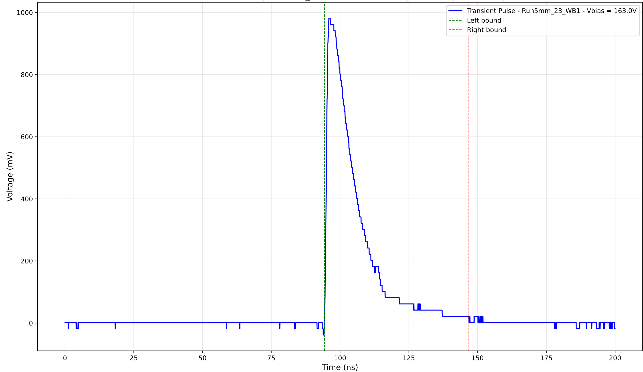
Transient Pulse - Sample: 5mm_23 - Position: 1630.0 \mu\text{m} - Charge: 239.13 pC
