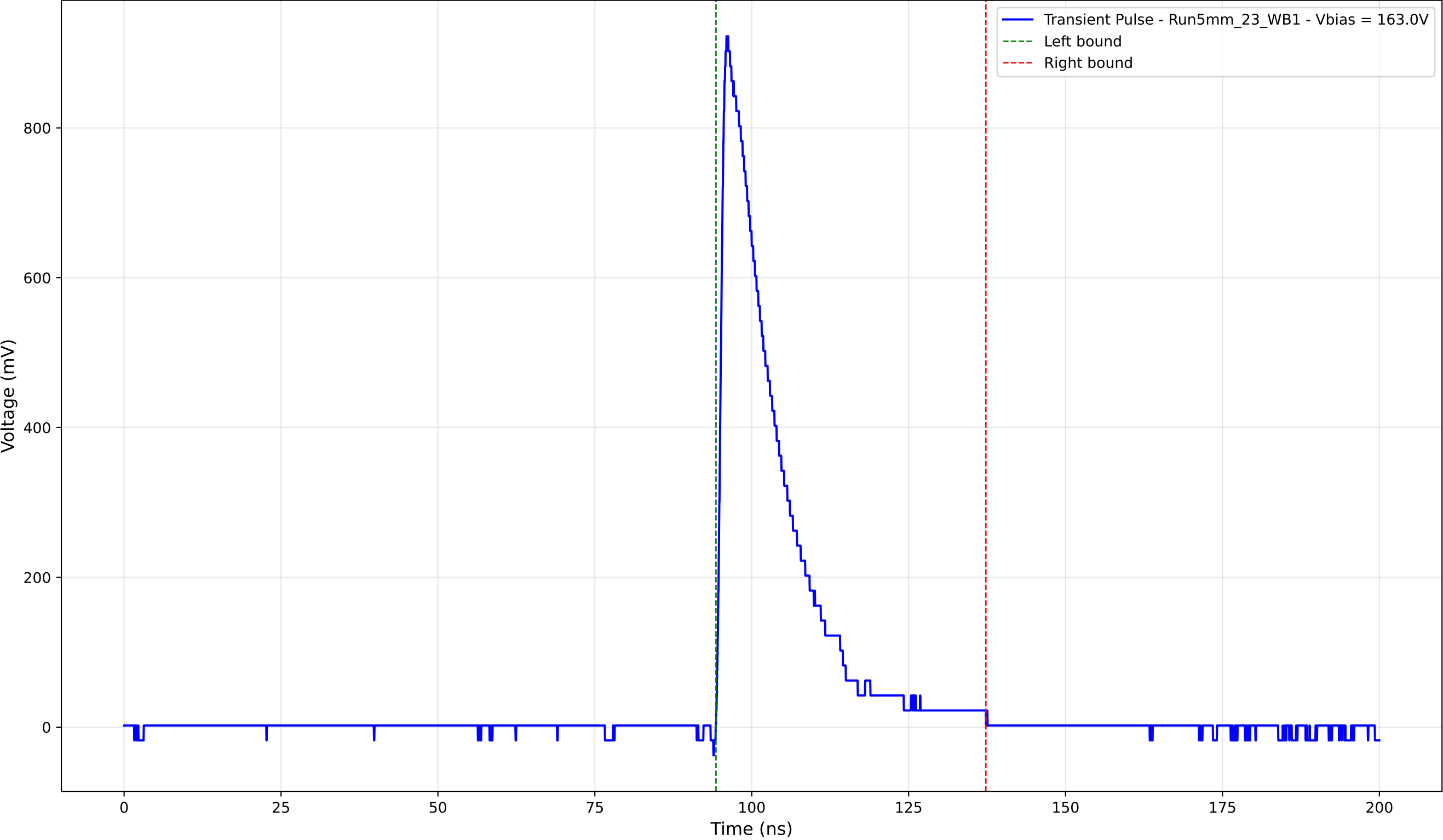
Transient Pulse - Sample: 5mm_23 - Position: 4430.0 \mu\text{m} - Charge: 181.61 pC
