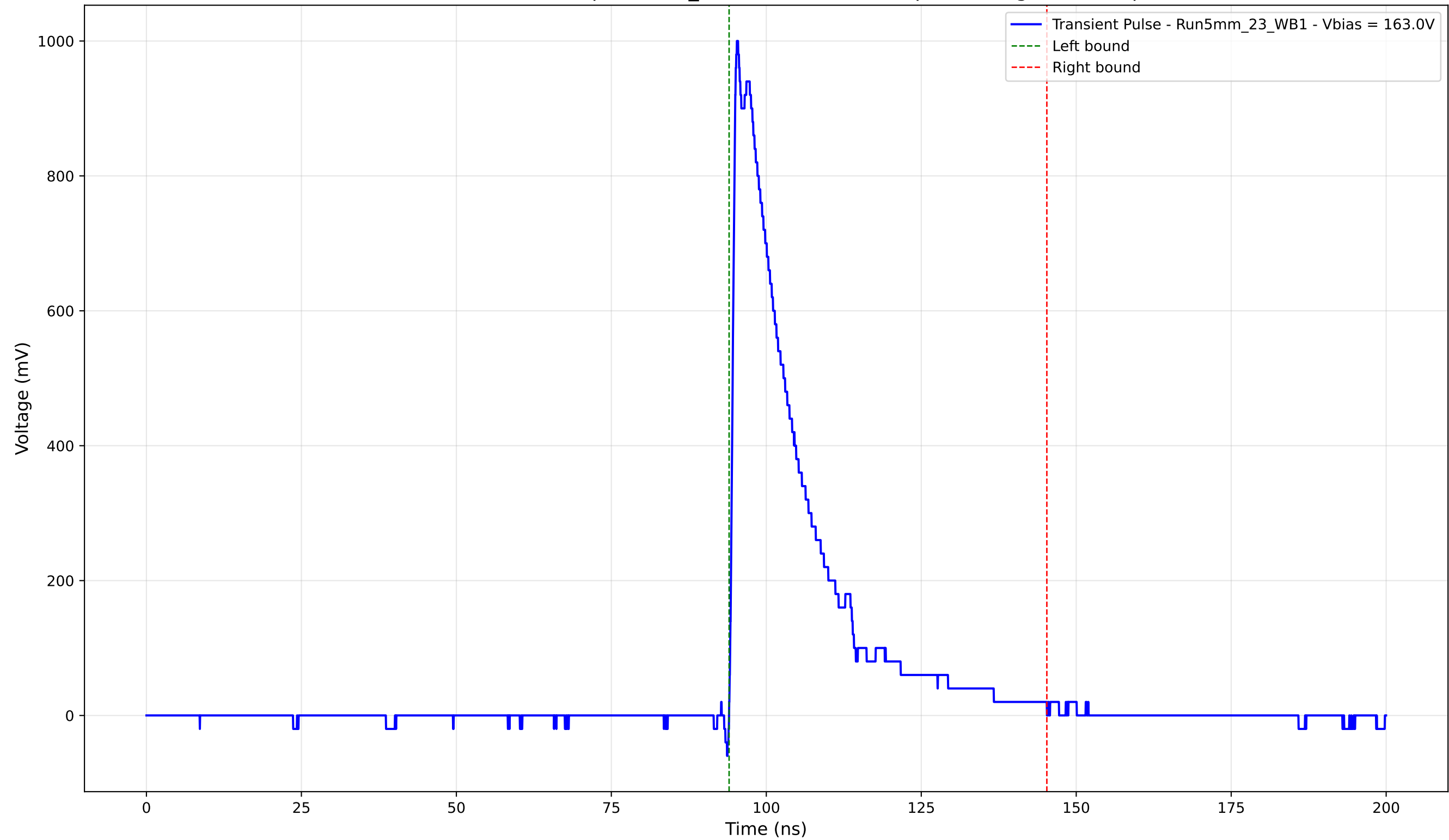
Transient Pulse - Sample: 5mm_23 - Position: 3105.0 \mu\text{m} - Charge: 223.29 pC
