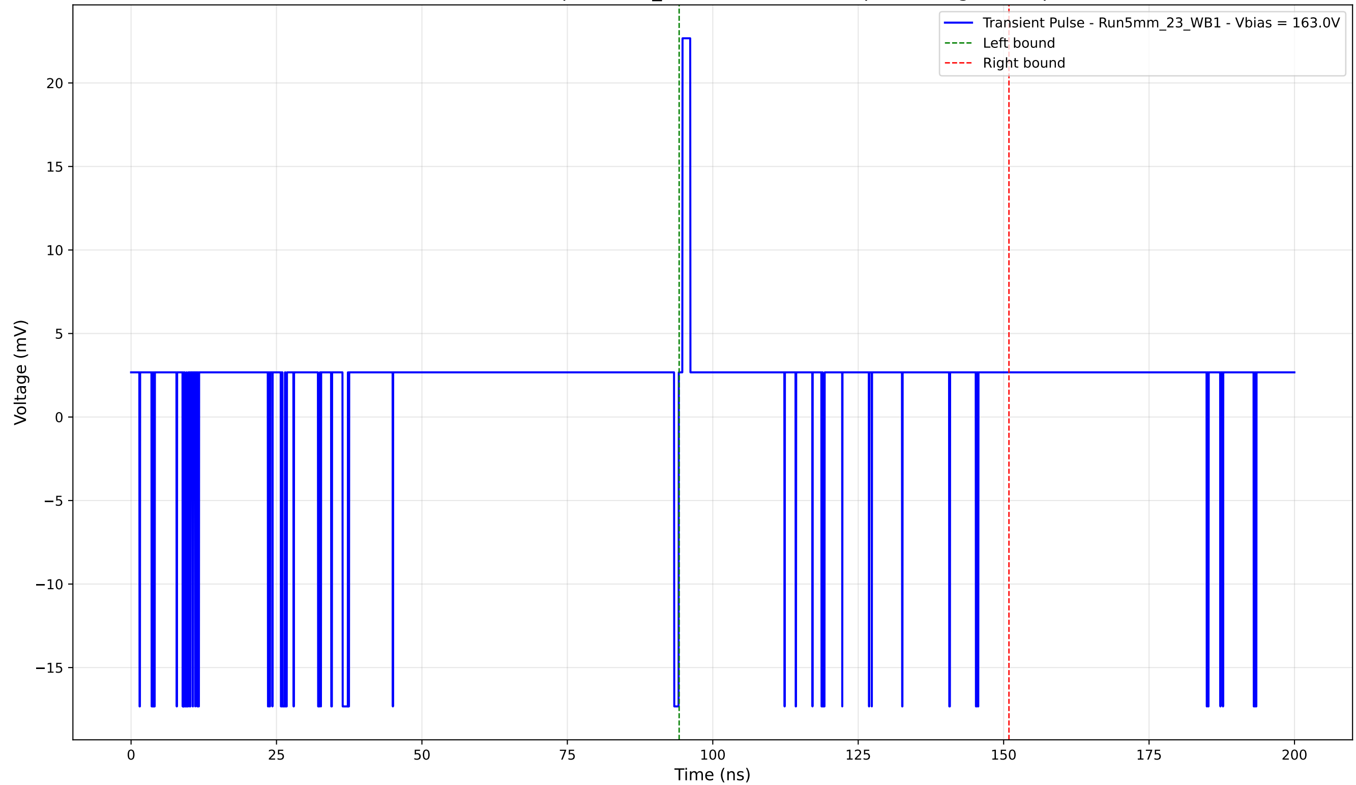
Transient Pulse - Sample: 5mm_23 - Position: 5275.0 \mu\text{m} - Charge: 3.09 pC
