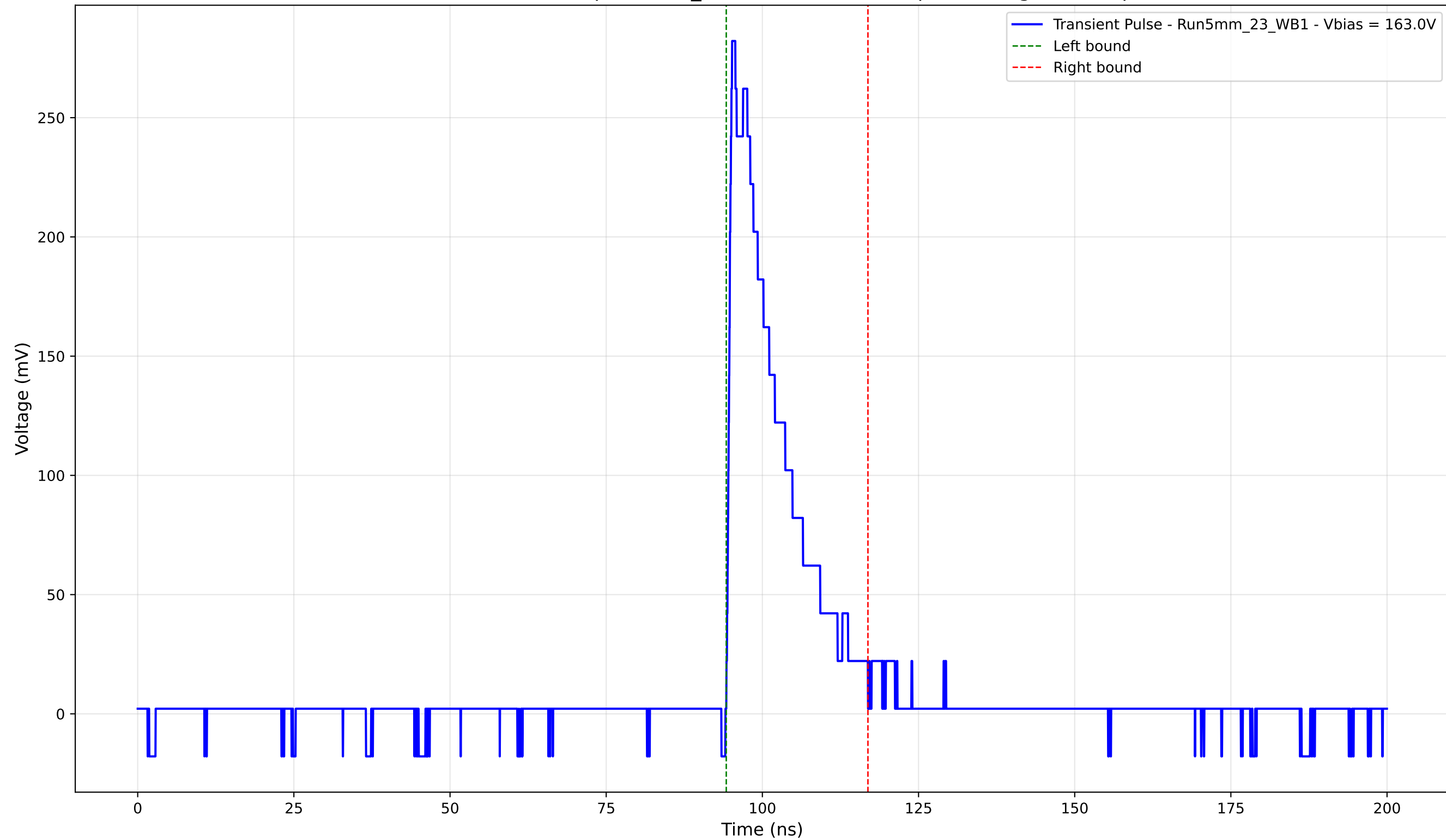
Transient Pulse - Sample: 5mm_23 - Position: 3230.0 \mu\text{m} - Charge: 48.94 pC
