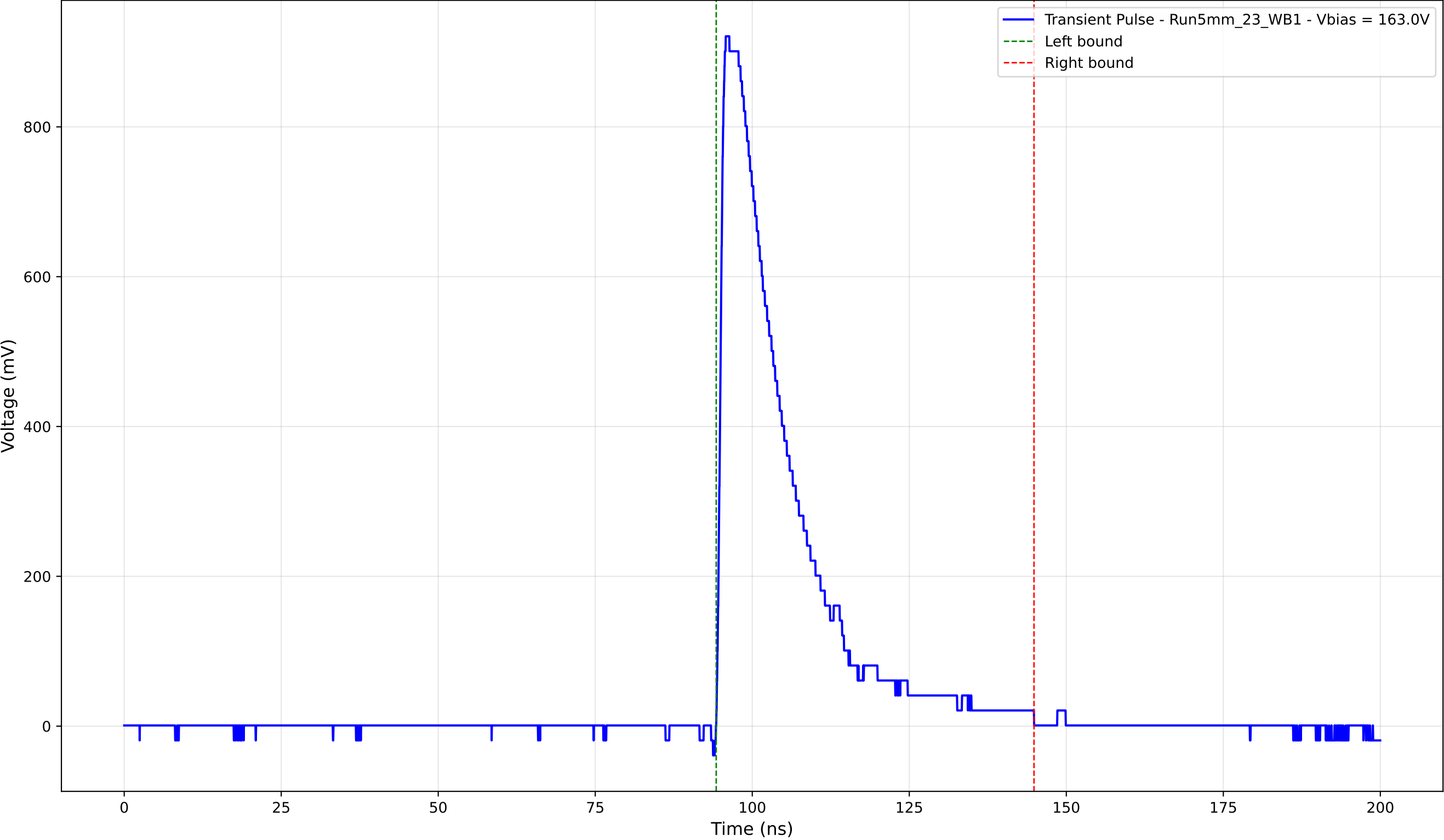
Transient Pulse - Sample: 5mm_23 - Position: 3595.0 \mu\text{m} - Charge: 213.52 pC
