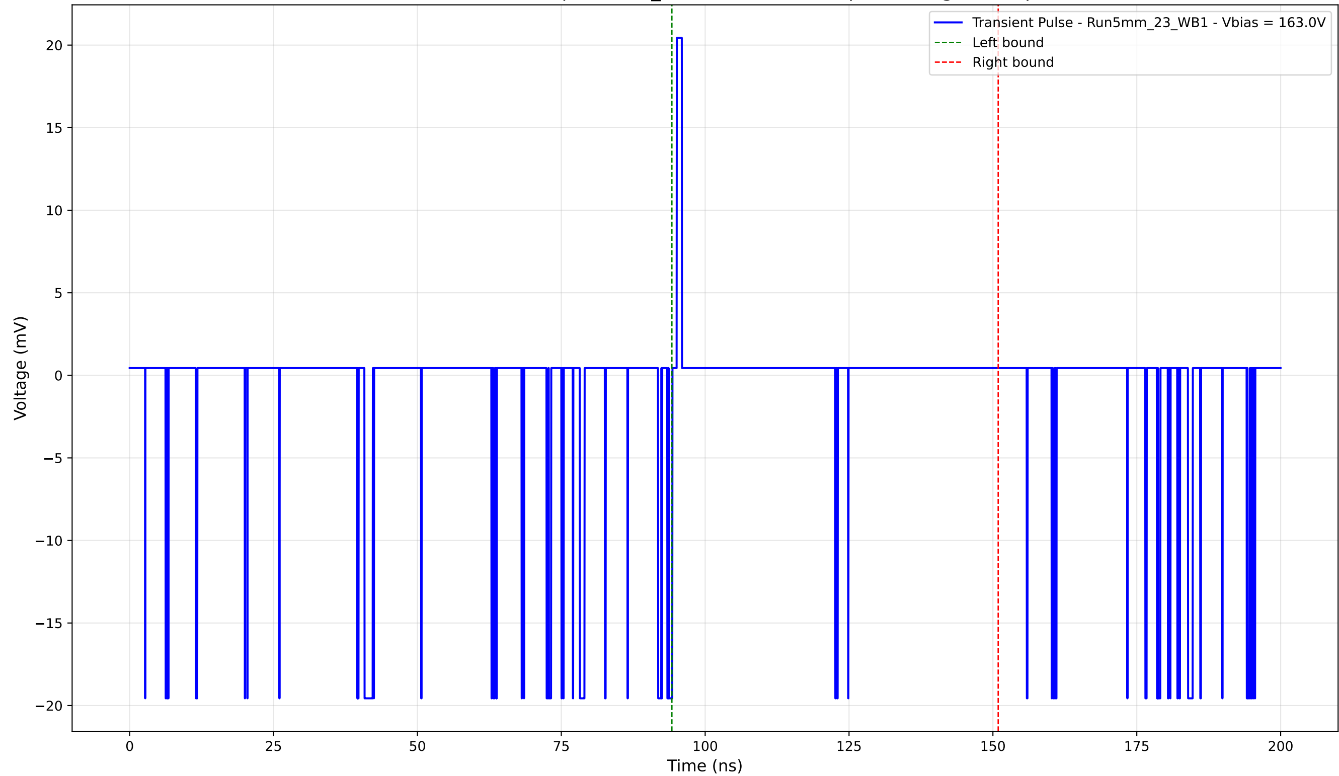
Transient Pulse - Sample: 5mm_23 - Position: 210.0 \mu\text{m} - Charge: 0.70 pC
