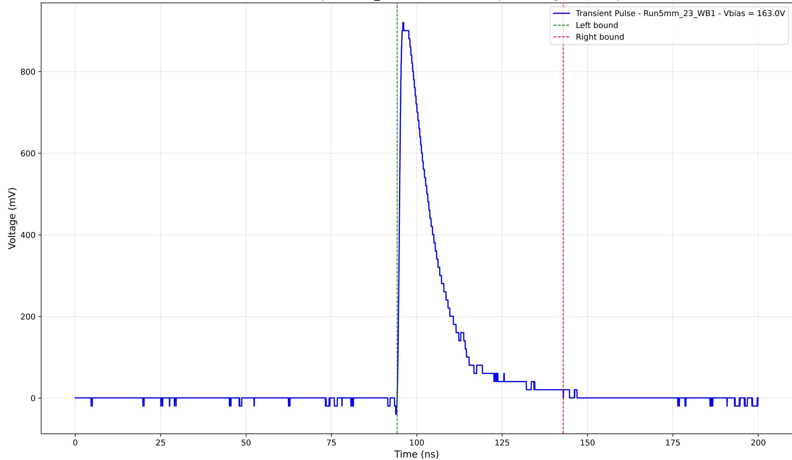
Transient Pulse - Sample: 5mm_23 - Position: 3610.0 \mu\text{m} - Charge: 208.65 pC
