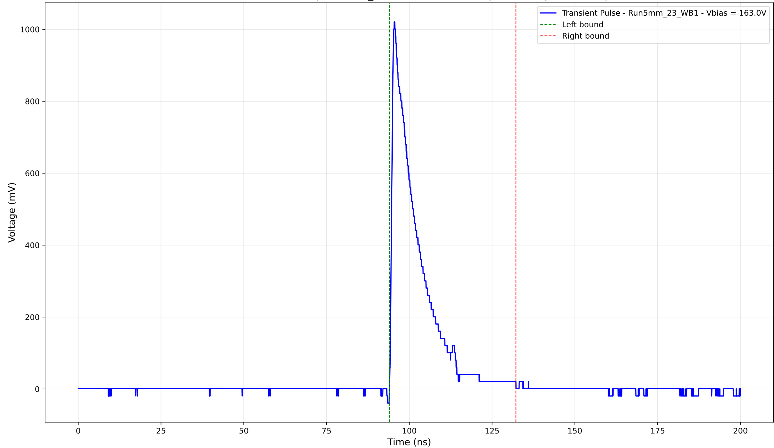
Transient Pulse - Sample: 5mm_23 - Position: 5005.0 \mu\text{m} - Charge: 170.45 pC
