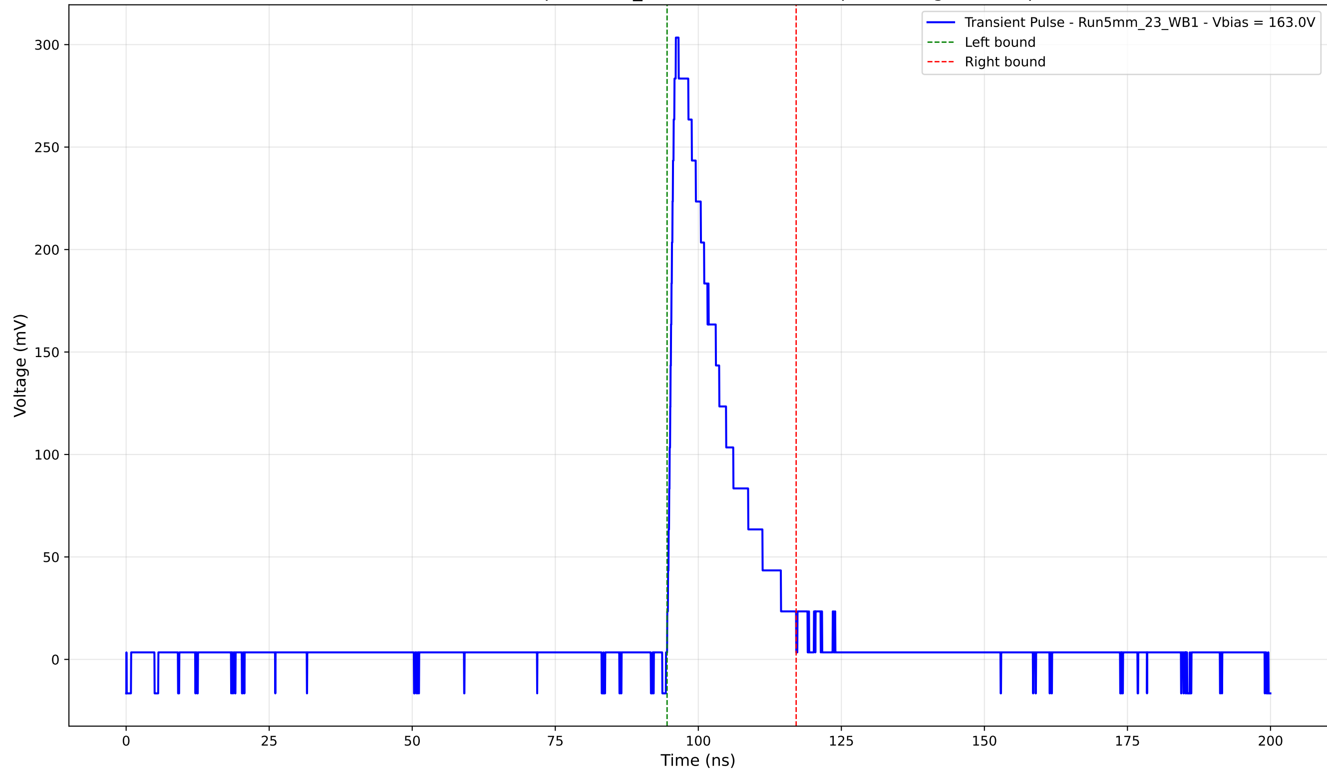
Transient Pulse - Sample: 5mm_23 - Position: 1245.0 \mu\text{m} - Charge: 56.31 pC
