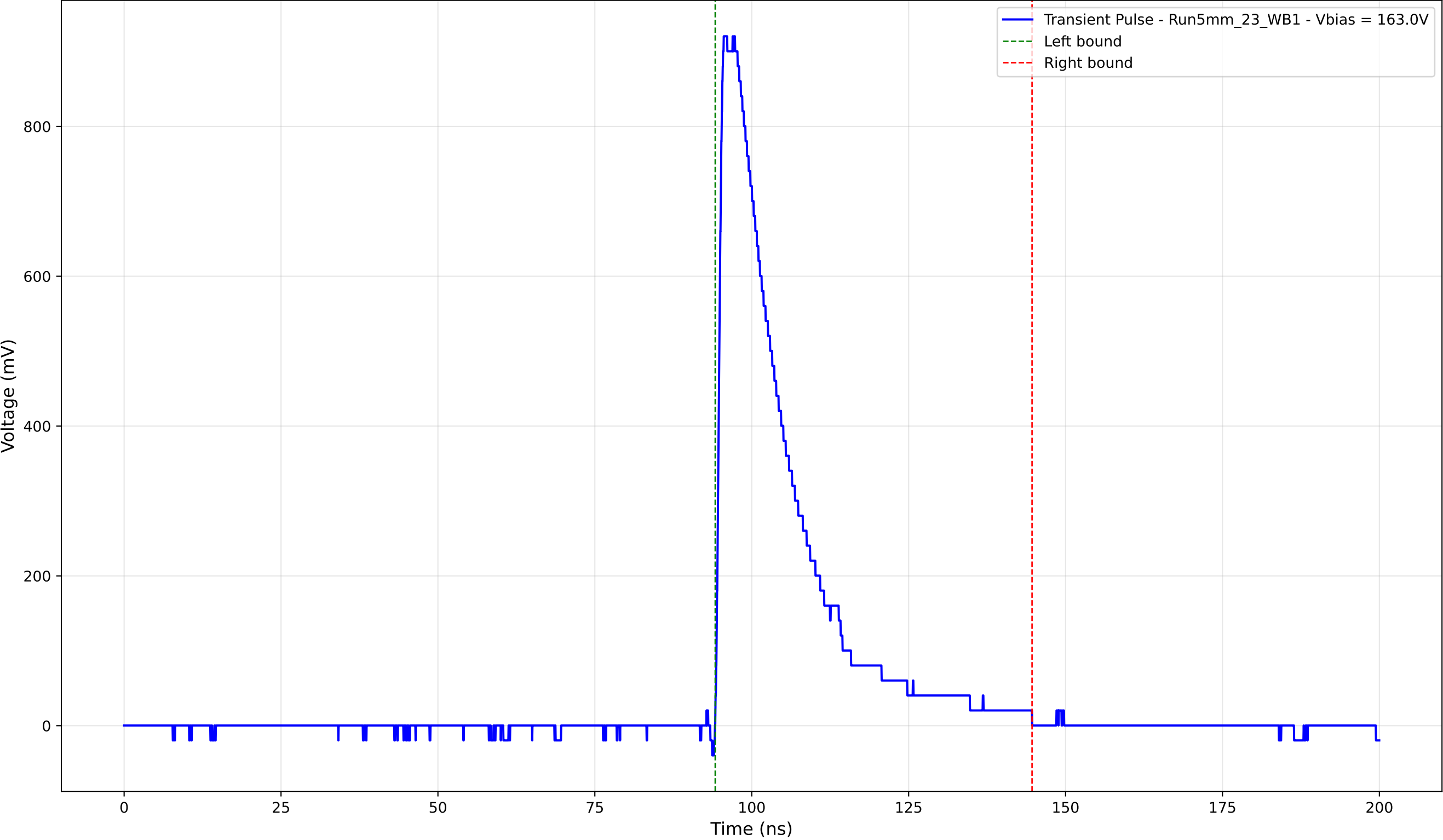
Transient Pulse - Sample: 5mm_23 - Position: 3440.0 \mu\text{m} - Charge: 215.42 pC
