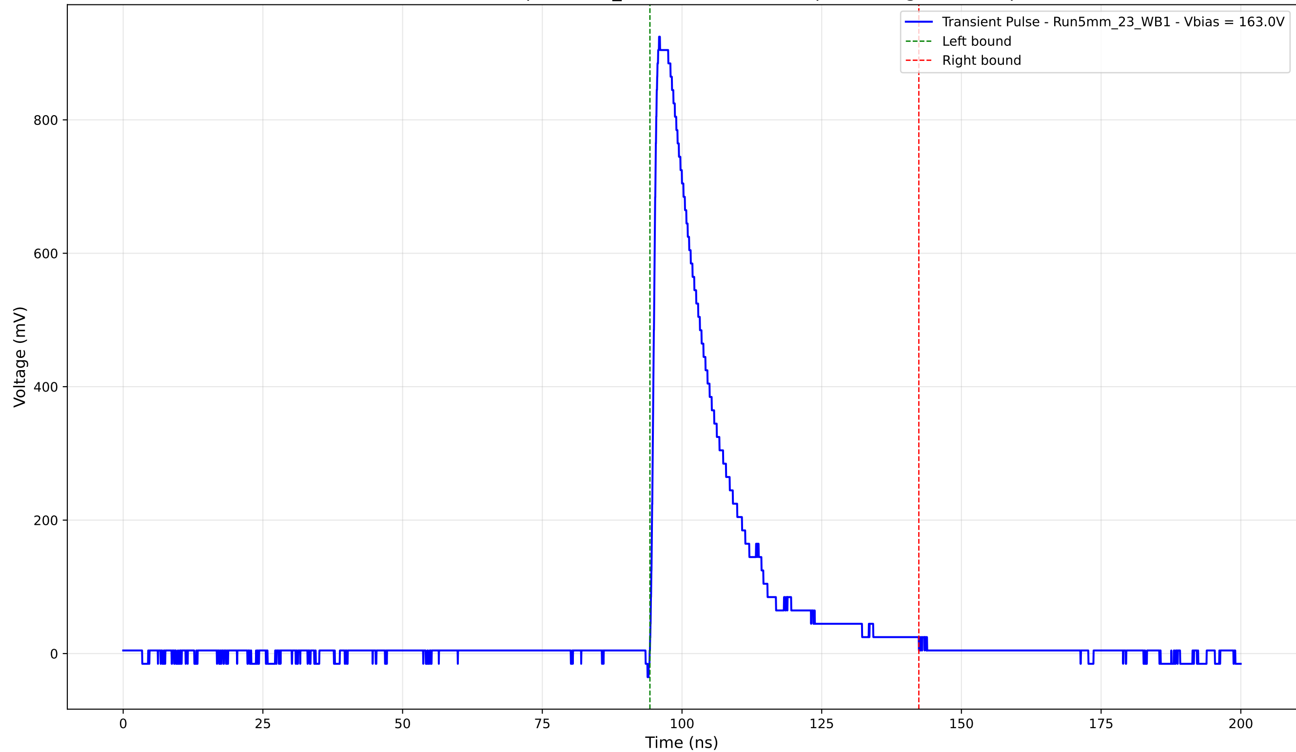
Transient Pulse - Sample: 5mm_23 - Position: 3620.0 \mu\text{m} - Charge: 211.14 pC
