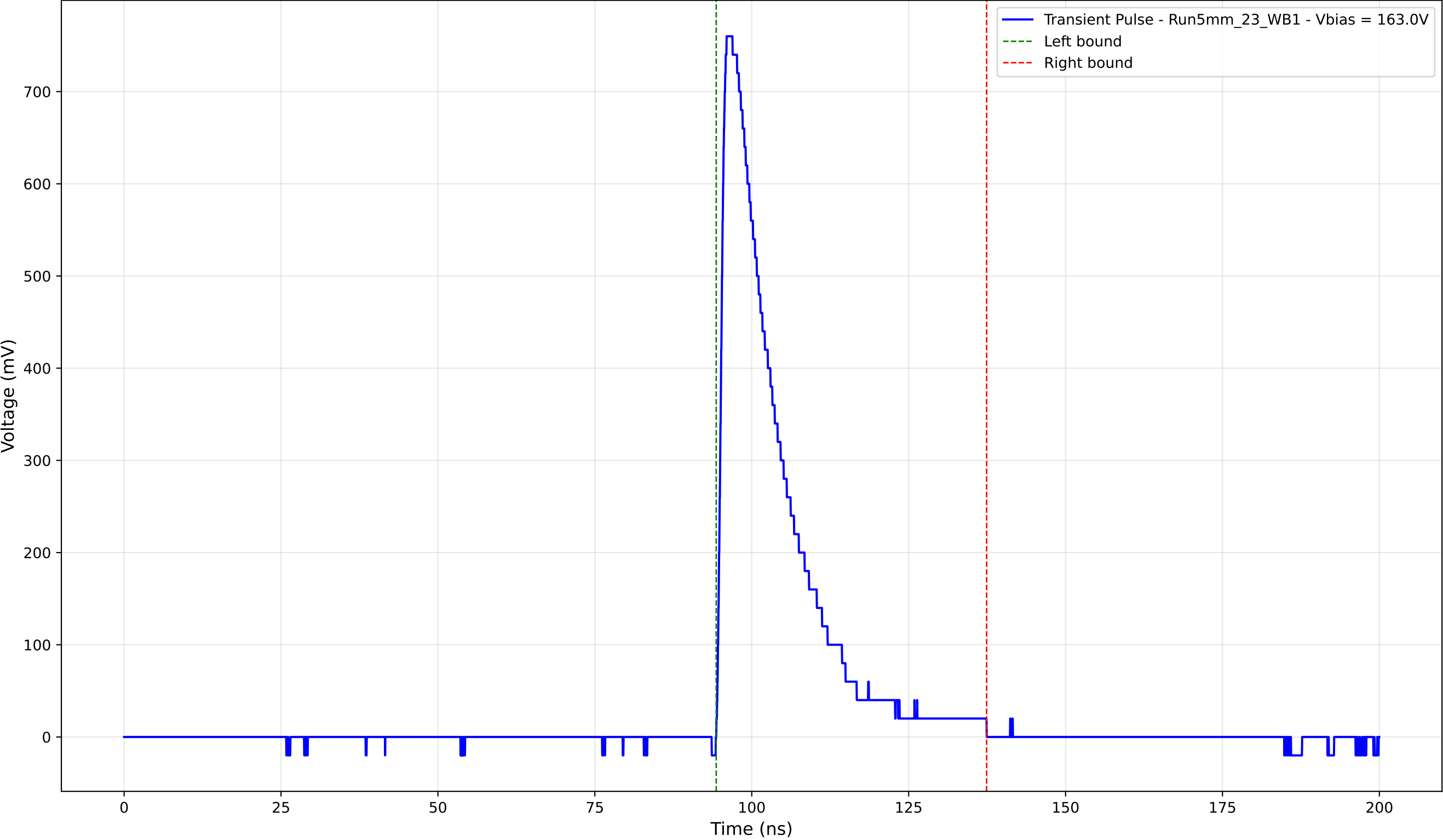
Transient Pulse - Sample: 5mm_23 - Position: 3825.0 \mu\text{m} - Charge: 156.00 pC
