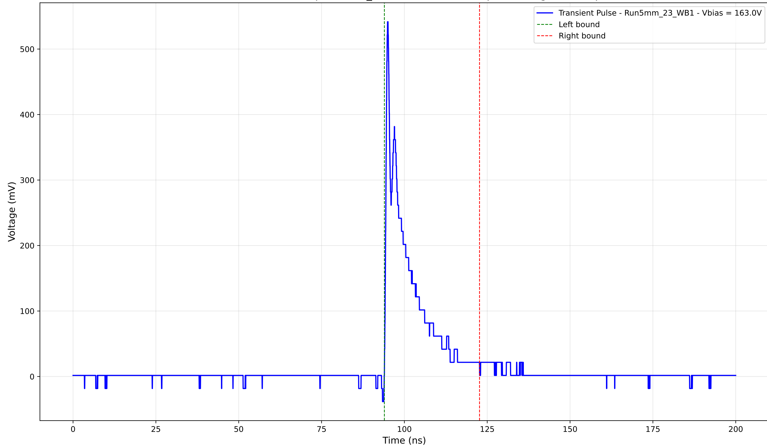
Transient Pulse - Sample: 5mm_23 - Position: 2770.0 \mu\text{m} - Charge: 67.49 pC
