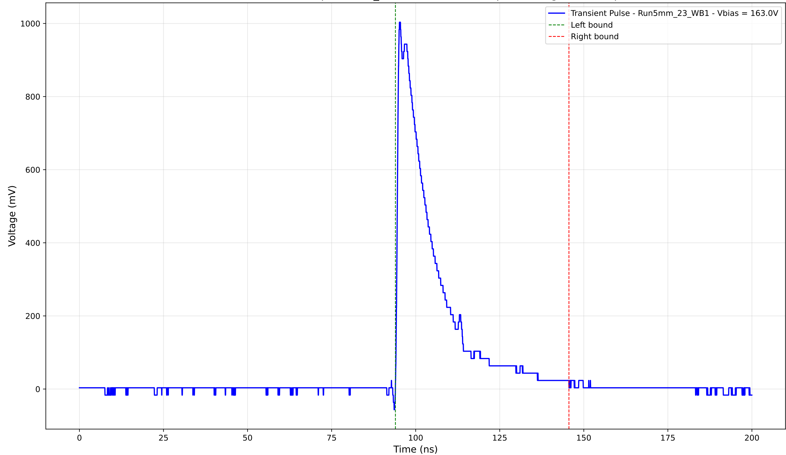
Transient Pulse - Sample: 5mm_23 - Position: 3070.0 \mu\text{m} - Charge: 229.51 pC
