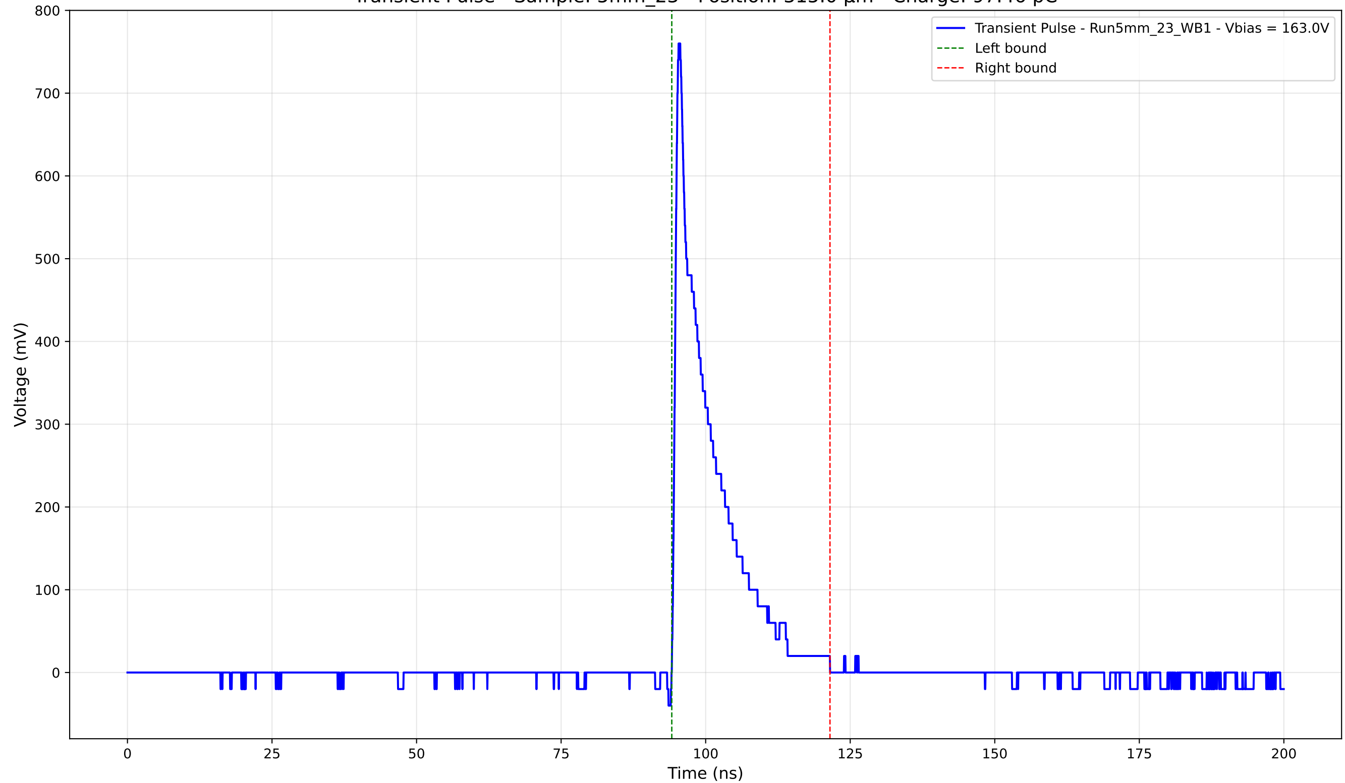
Transient Pulse - Sample: 5mm_23 - Position: 315.0 \mu\text{m} - Charge: 97.46 pC
