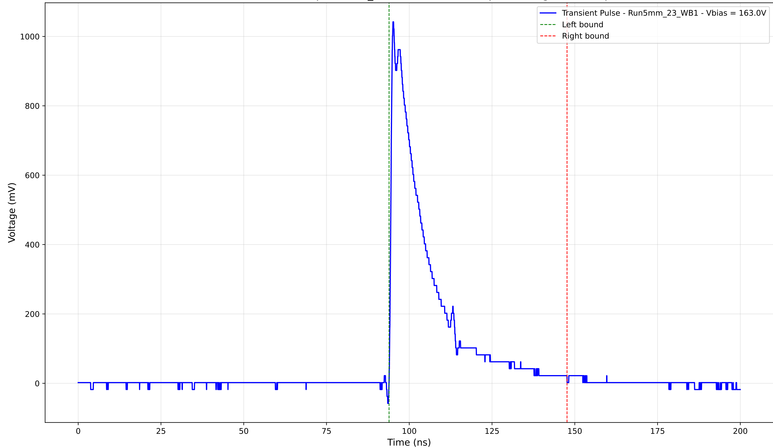
Transient Pulse - Sample: 5mm_23 - Position: 2945.0 \mu\text{m} - Charge: 235.46 pC
