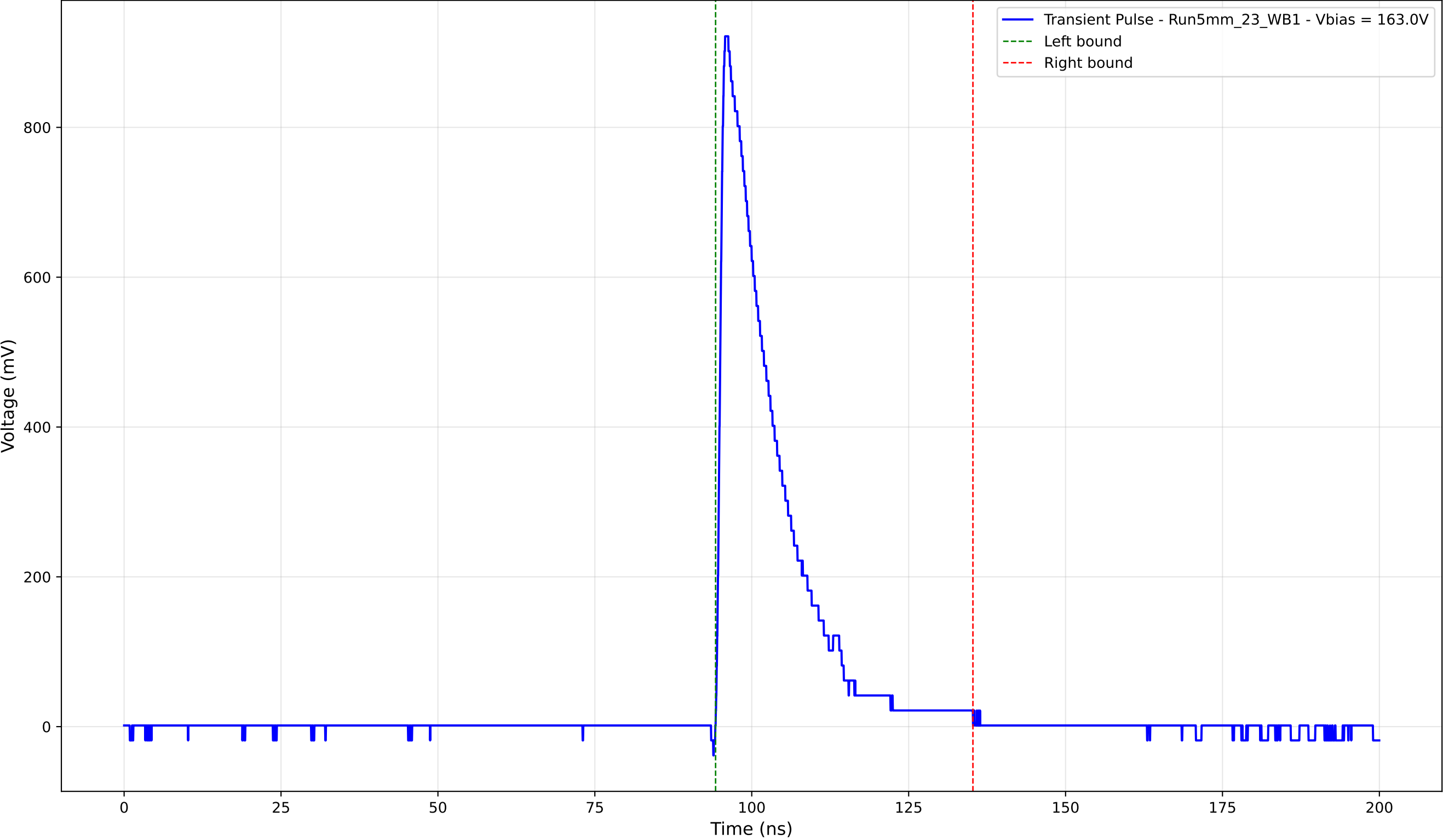
Transient Pulse - Sample: 5mm_23 - Position: 4585.0 \mu\text{m} - Charge: 175.80 pC
