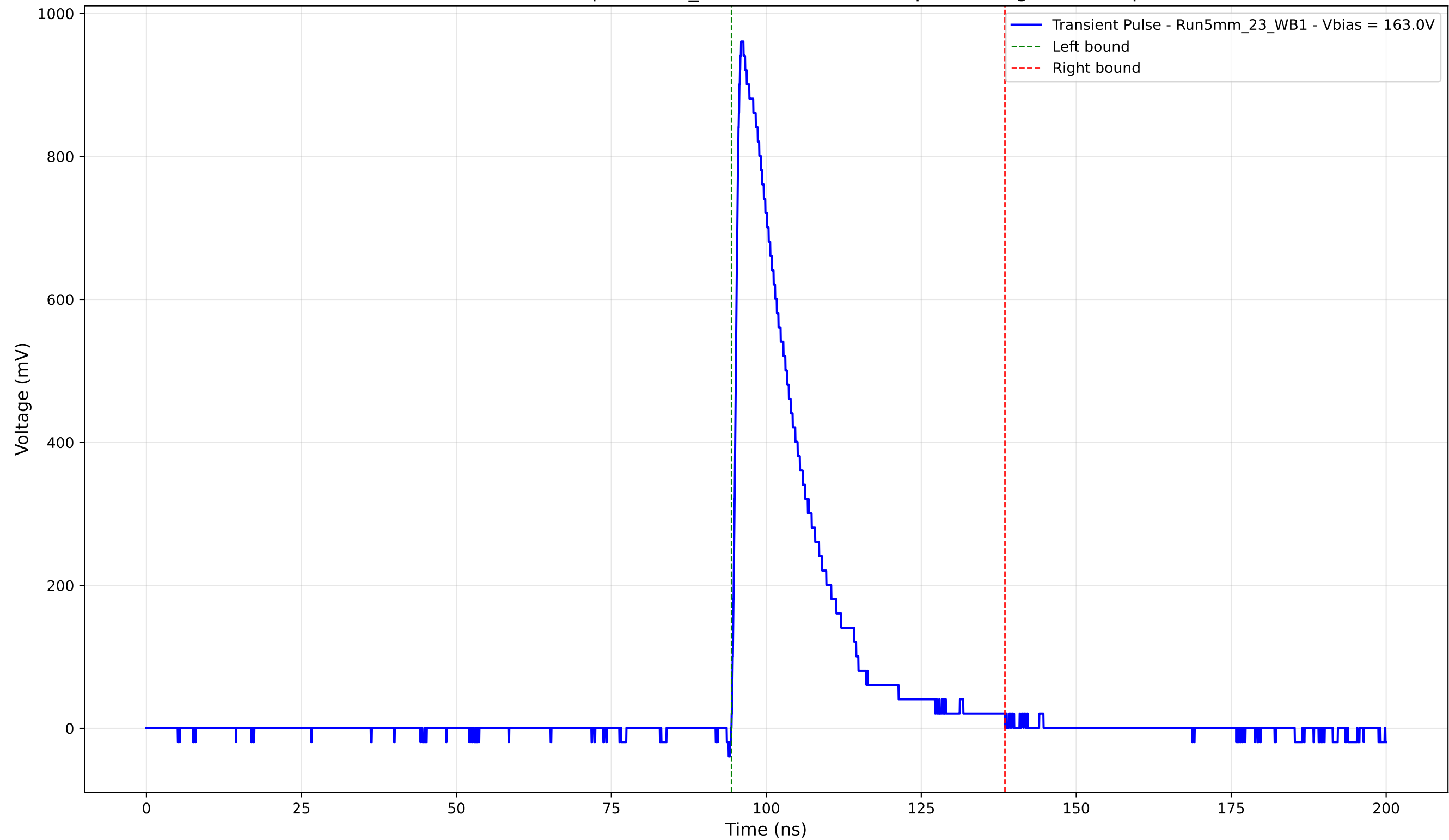
Transient Pulse - Sample: 5mm_23 - Position: 1055.0 \mu\text{m} - Charge: 202.46 pC
