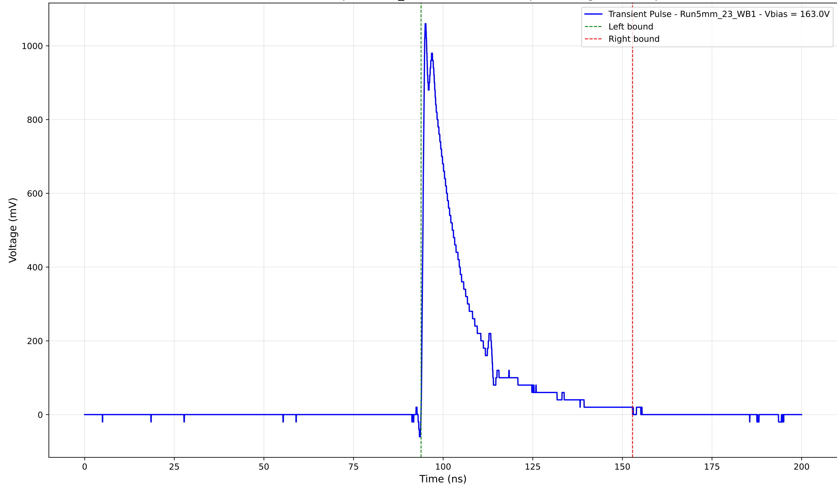
Transient Pulse - Sample: 5mm_23 - Position: 2845.0 \mu\text{m} - Charge: 235.65 pC
