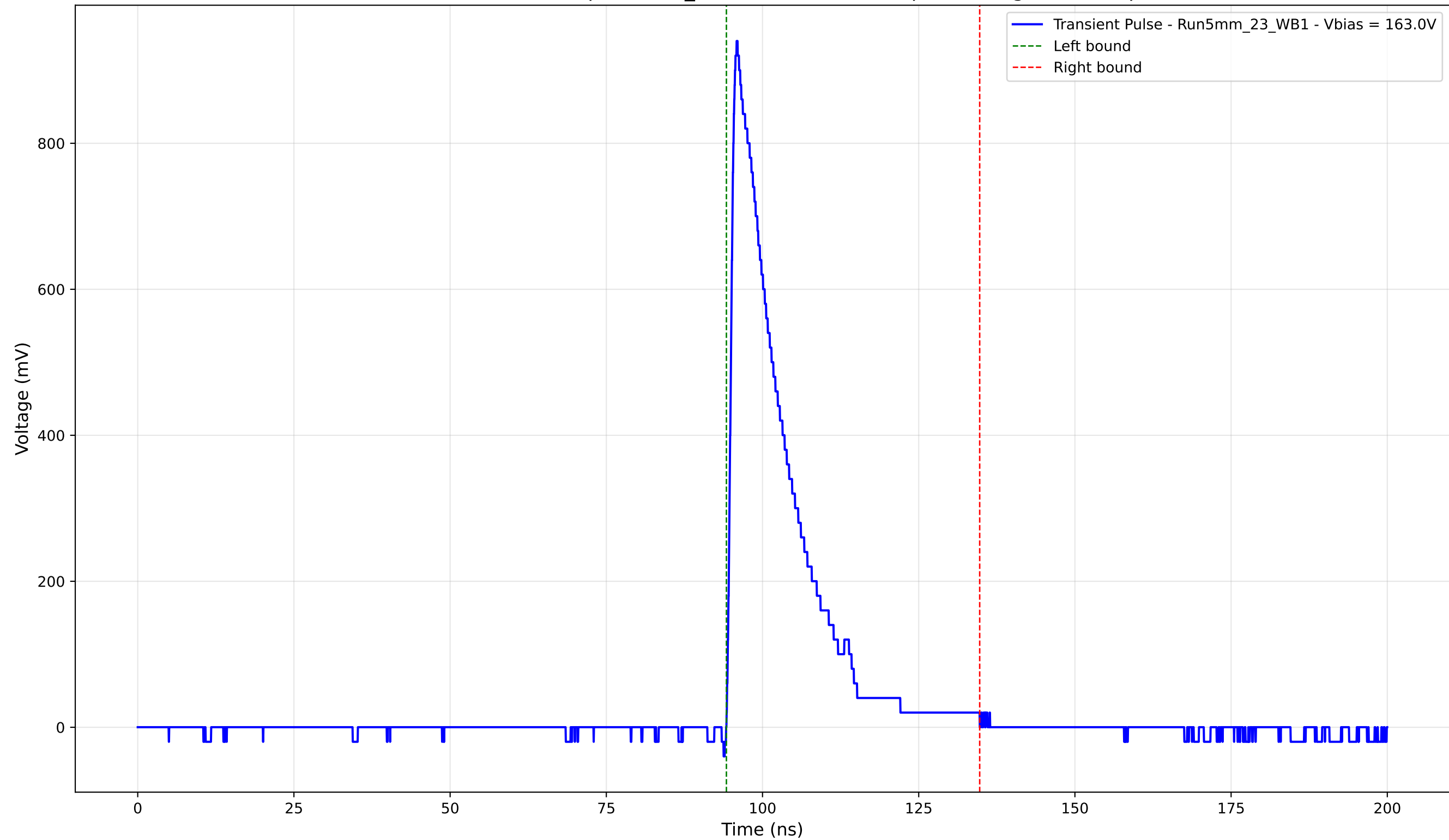
Transient Pulse - Sample: 5mm_23 - Position: 4635.0 \mu\text{m} - Charge: 172.32 pC
