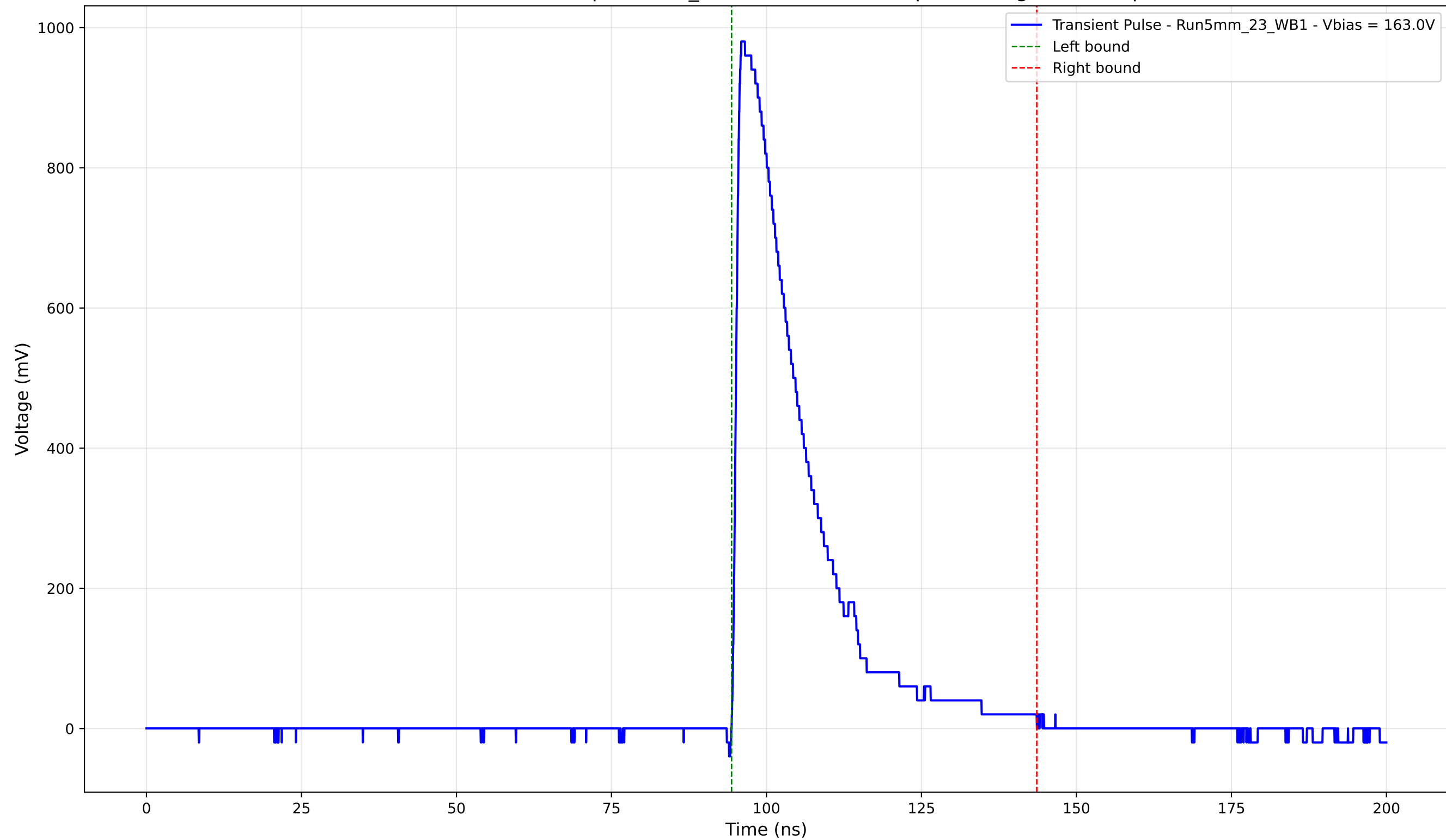
Transient Pulse - Sample: 5mm_23 - Position: 1420.0 \mu\text{m} - Charge: 234.22 pC
