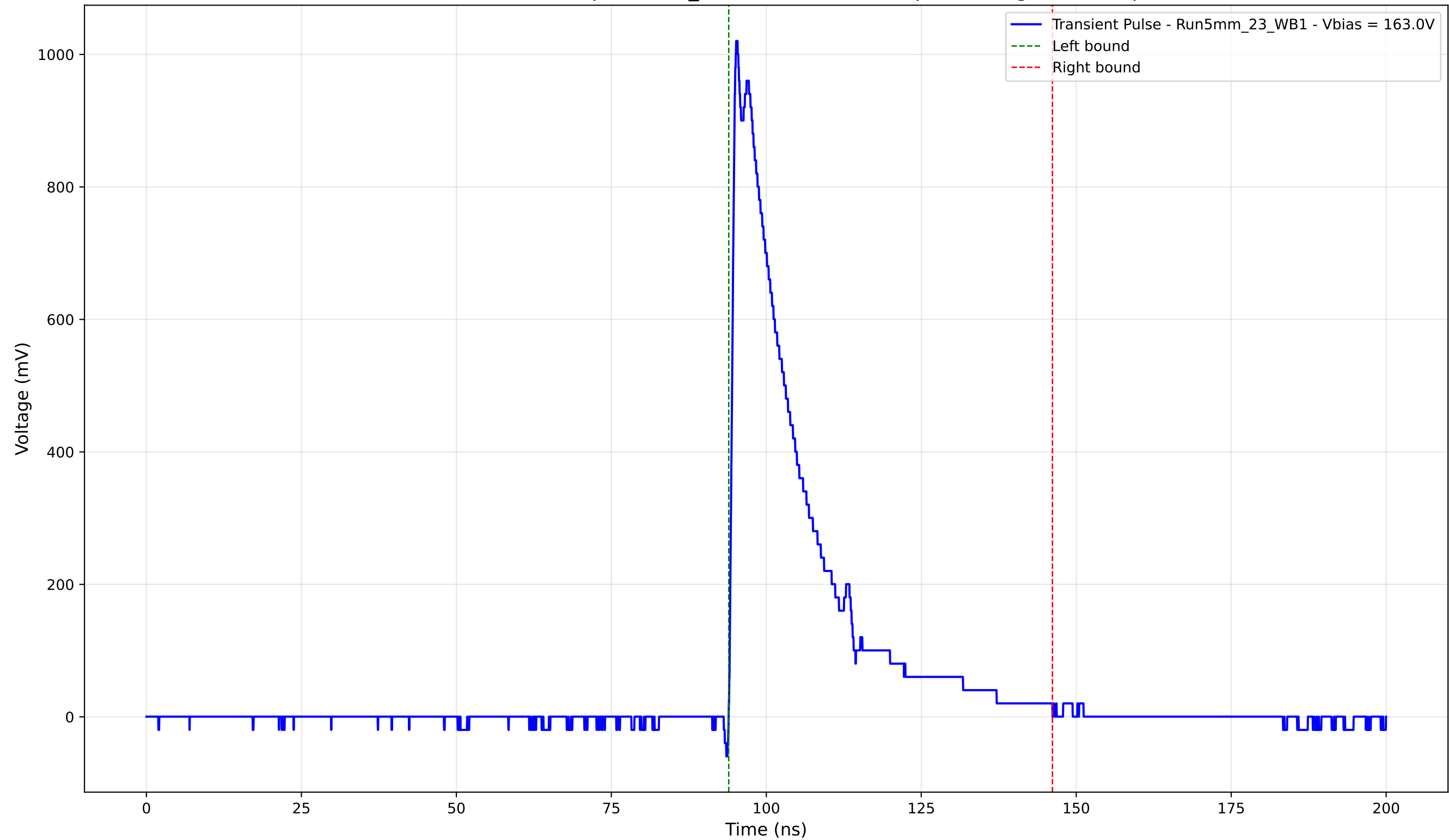
Transient Pulse - Sample: 5mm_23 - Position: 3015.0 \mu\text{m} - Charge: 230.29 pC
