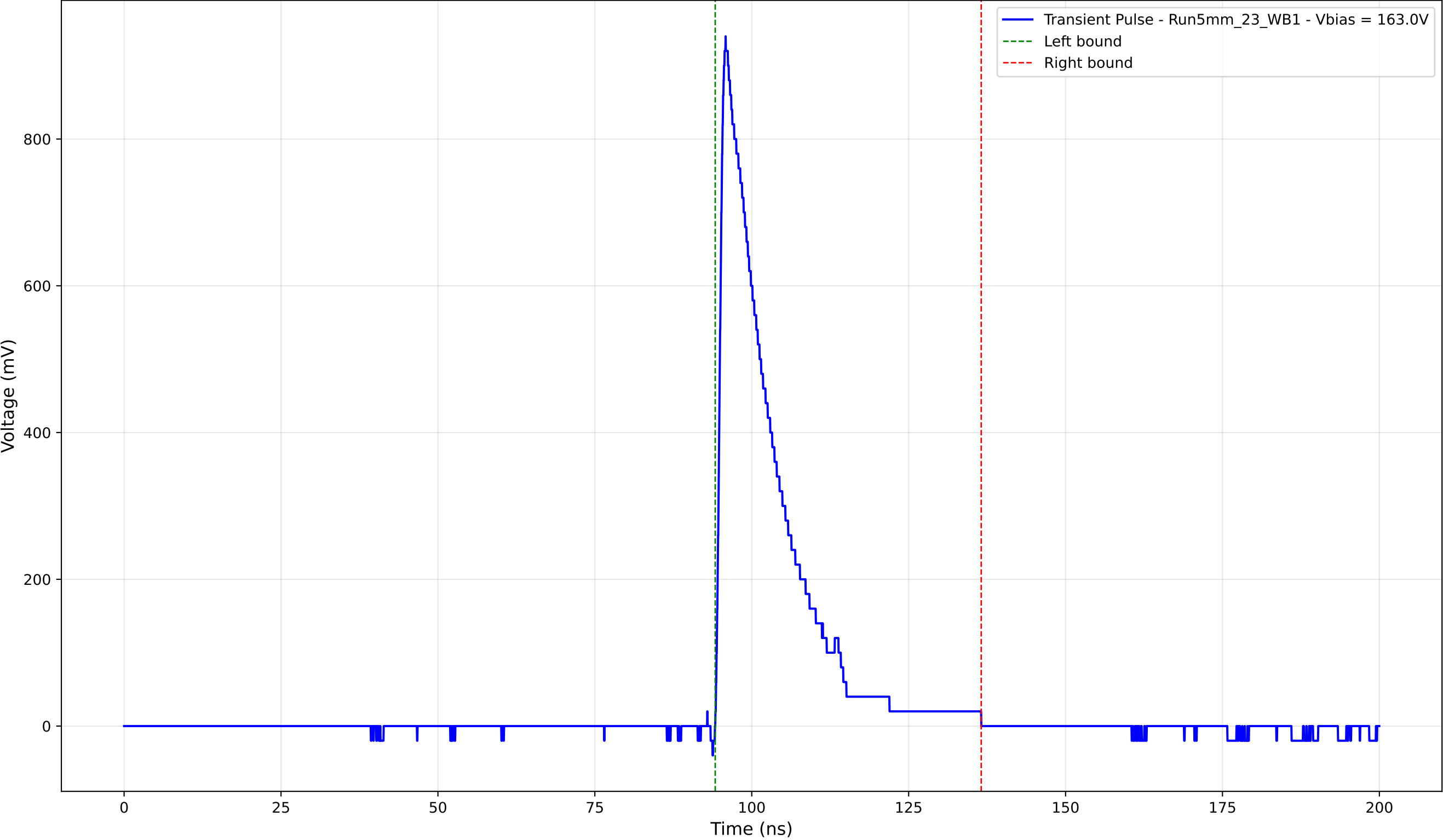
Transient Pulse - Sample: 5mm_23 - Position: 4665.0 \mu\text{m} - Charge: 169.27 pC
