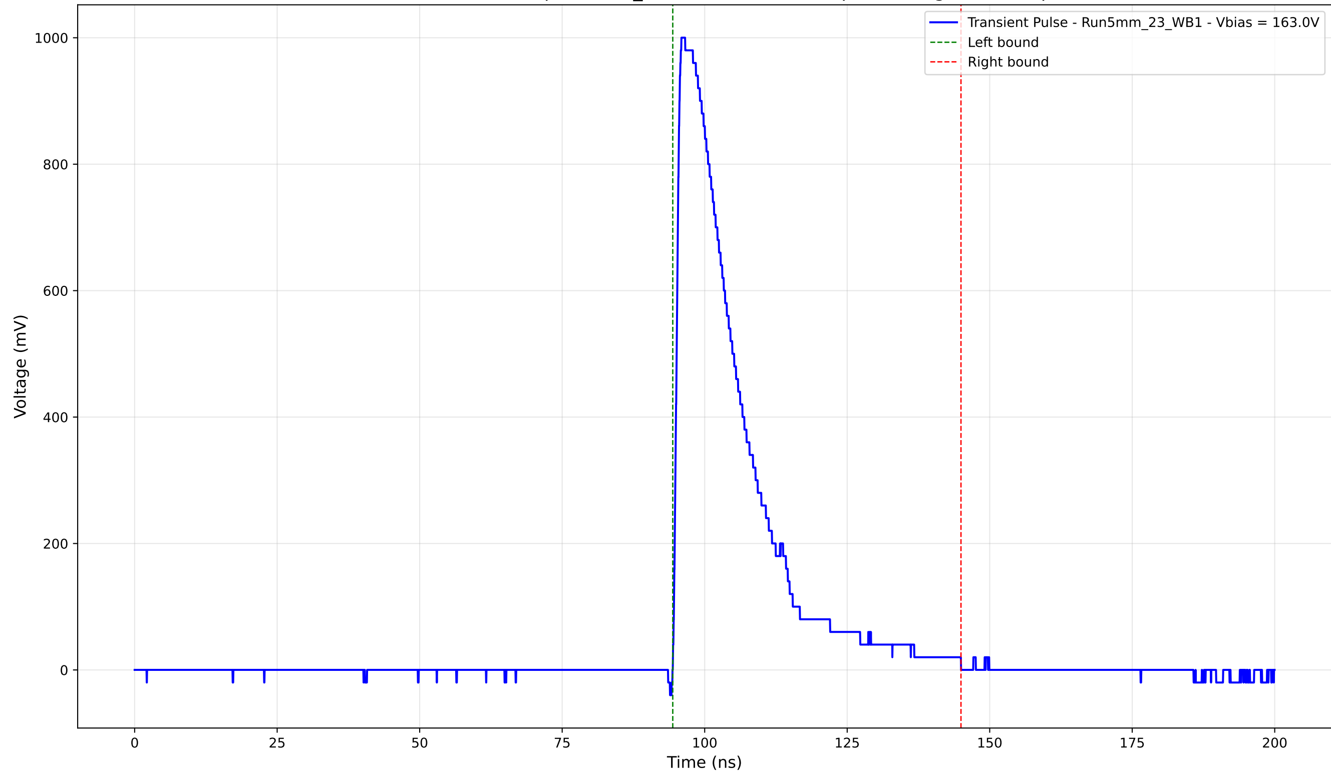
Transient Pulse - Sample: 5mm_23 - Position: 1485.0 \mu\text{m} - Charge: 248.26 pC
