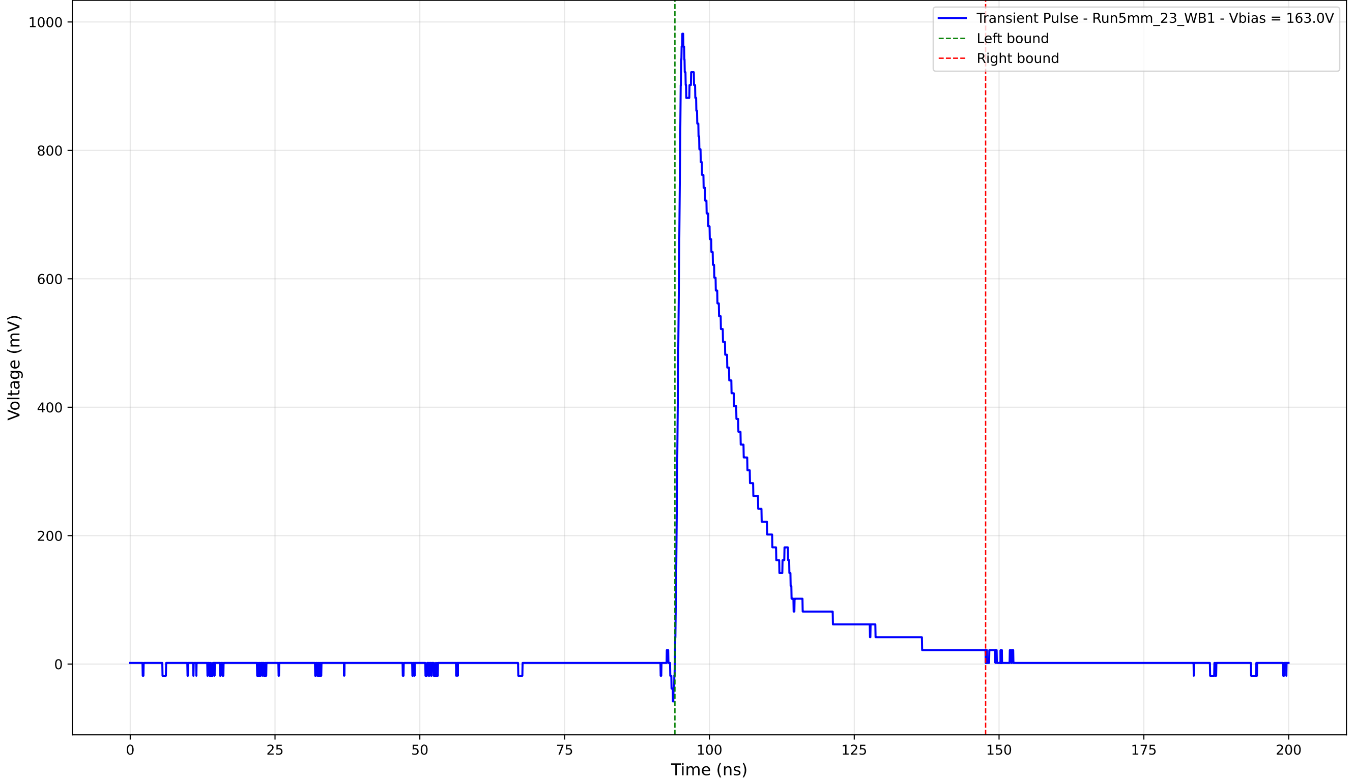
Transient Pulse - Sample: 5mm_23 - Position: 2335.0 \mu\text{m} - Charge: 218.49 pC
