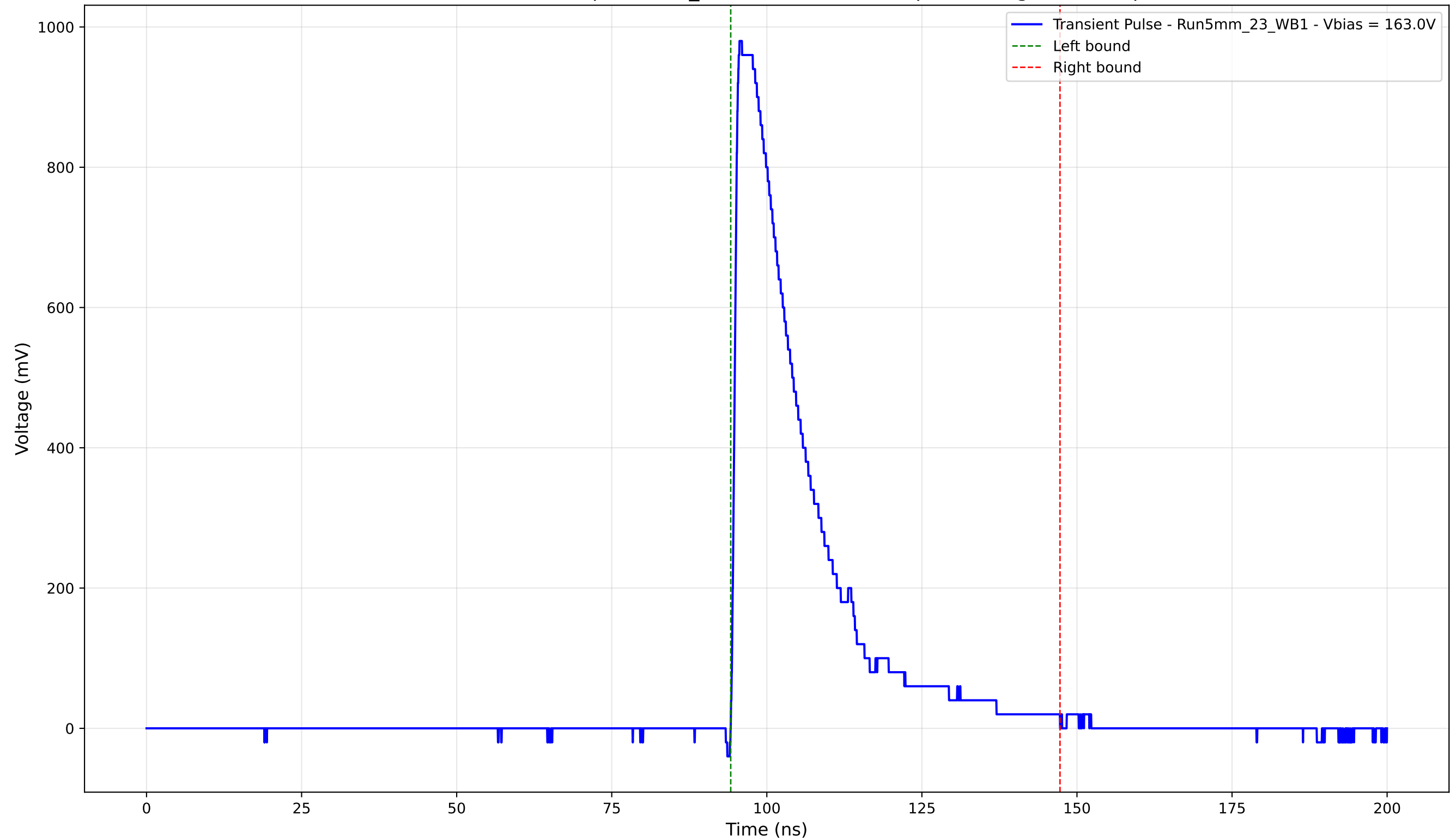
Transient Pulse - Sample: 5mm_23 - Position: 2010.0 \mu\text{m} - Charge: 242.76 pC
