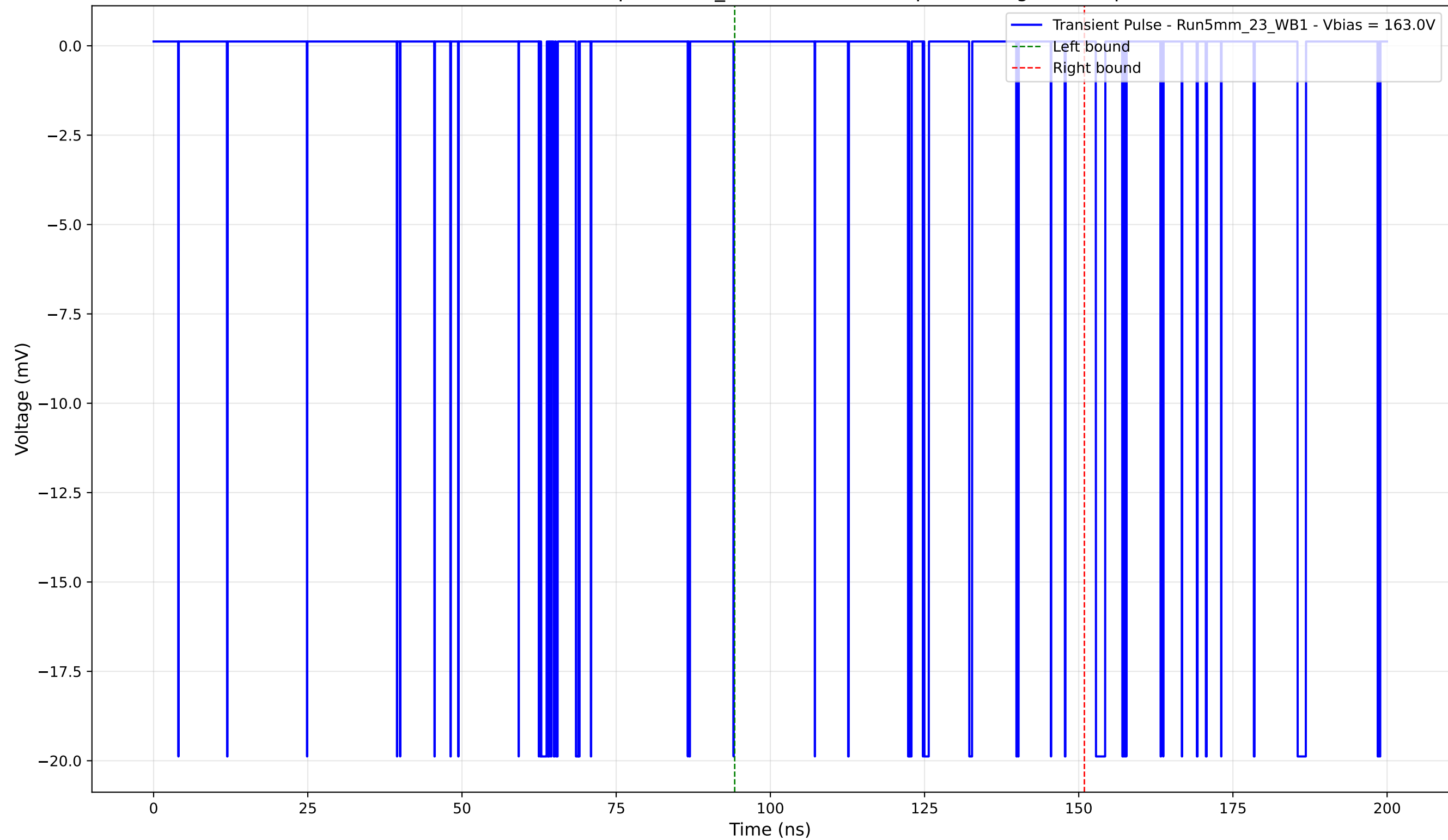
Transient Pulse - Sample: 5mm_23- Position: 50.0 \mu\text{m} - Charge: -0.83 pC
