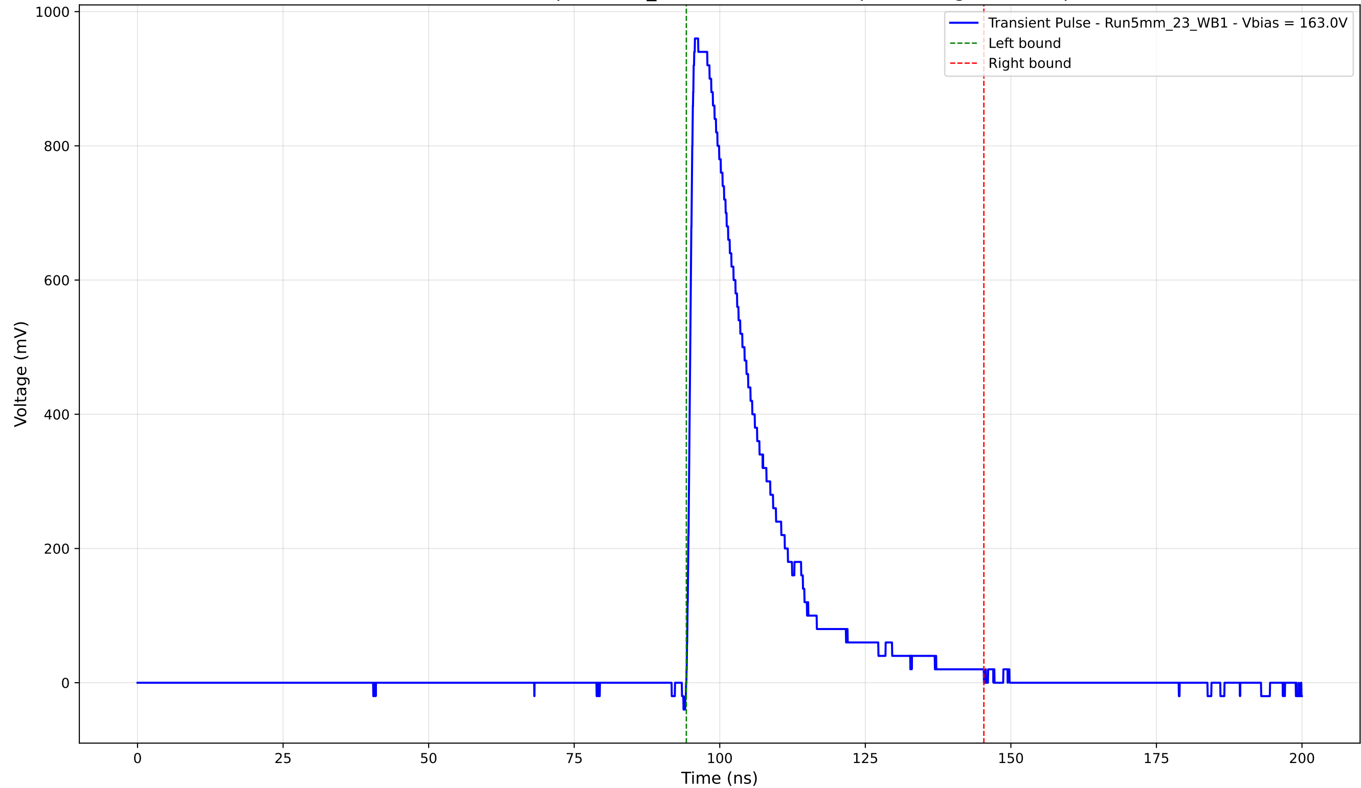
Transient Pulse - Sample: 5mm_23 - Position: 1880.0 \mu\text{m} - Charge: 234.14 pC
