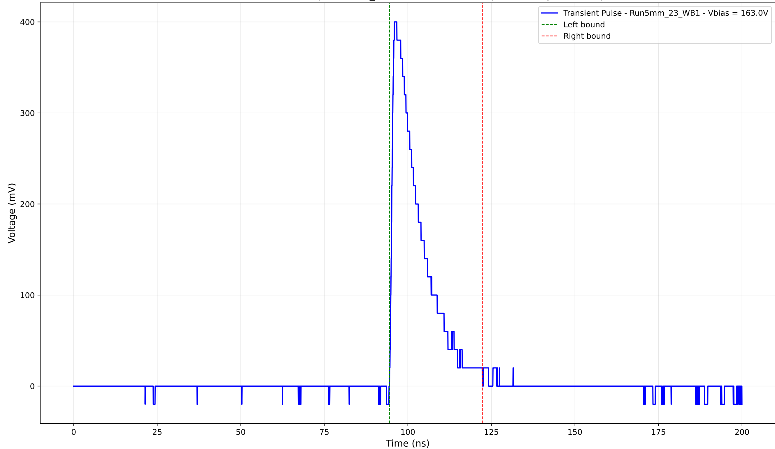
Transient Pulse - Sample: 5mm_23 - Position: 1255.0 \mu\text{m} - Charge: 75.07 pC
