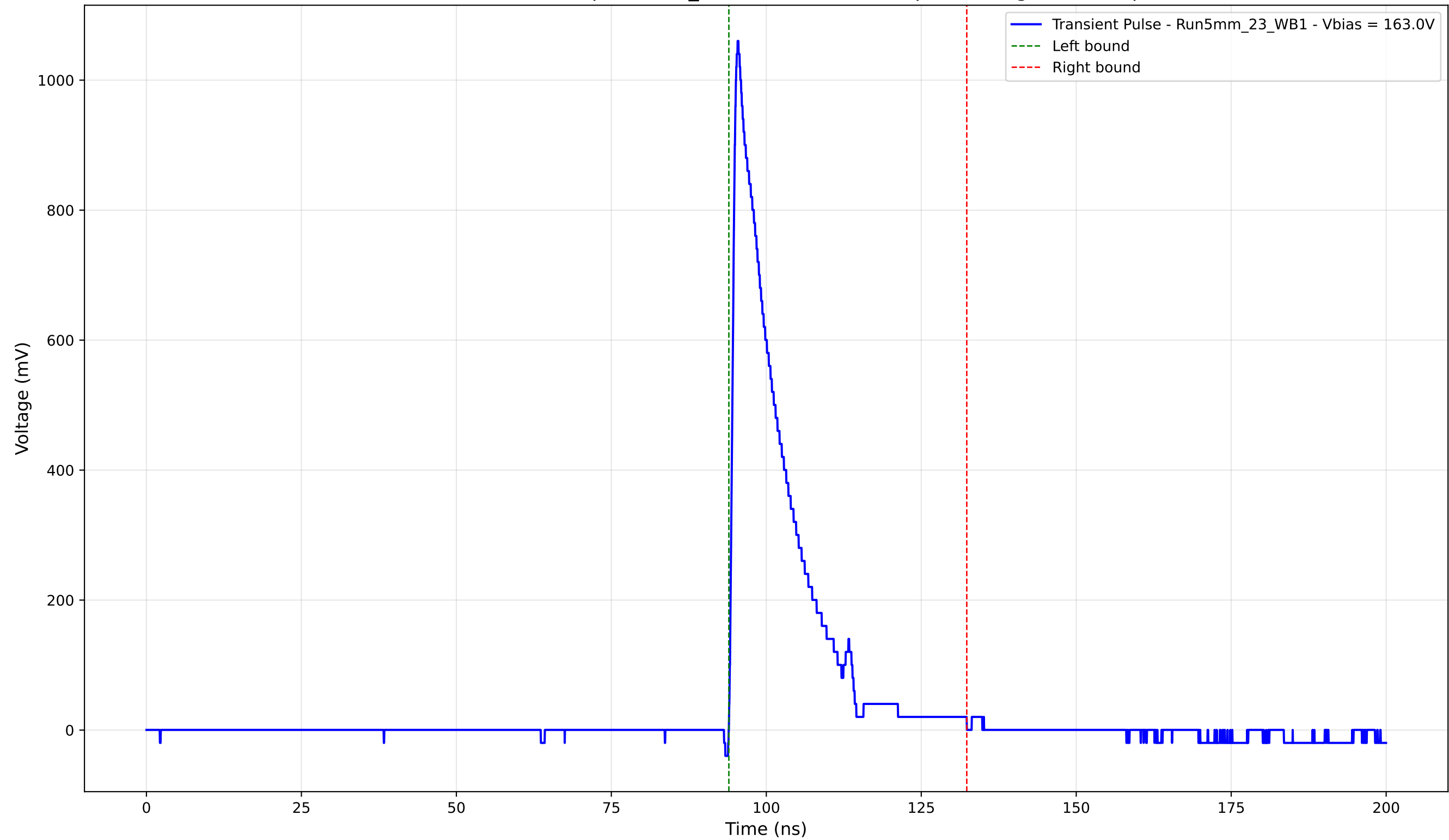
Transient Pulse - Sample: 5mm_23 - Position: 5110.0 \mu\text{m} - Charge: 176.21 pC
