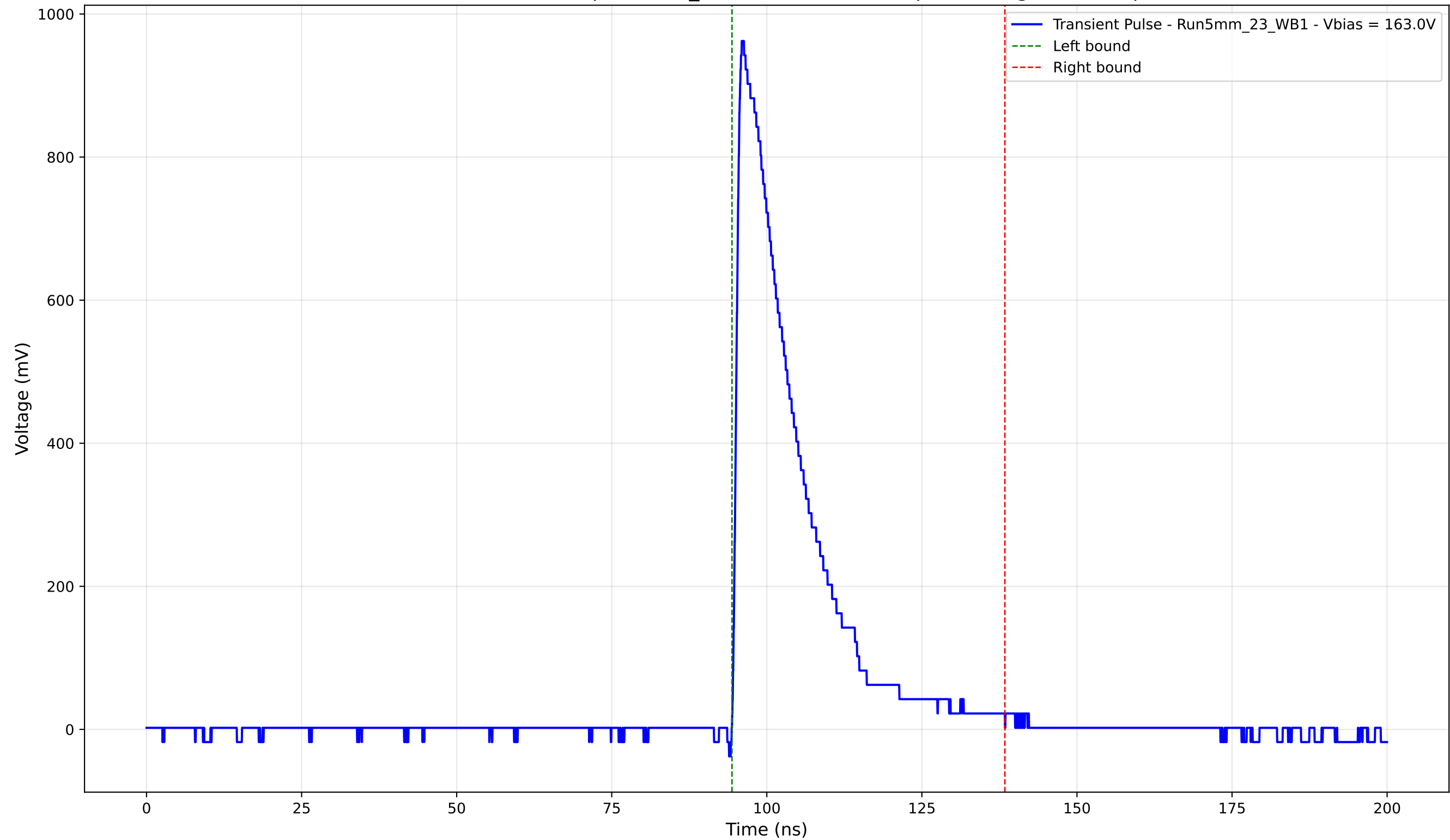
Transient Pulse - Sample: 5mm_23 - Position: 1090.0 \mu\text{m} - Charge: 204.67 pC
