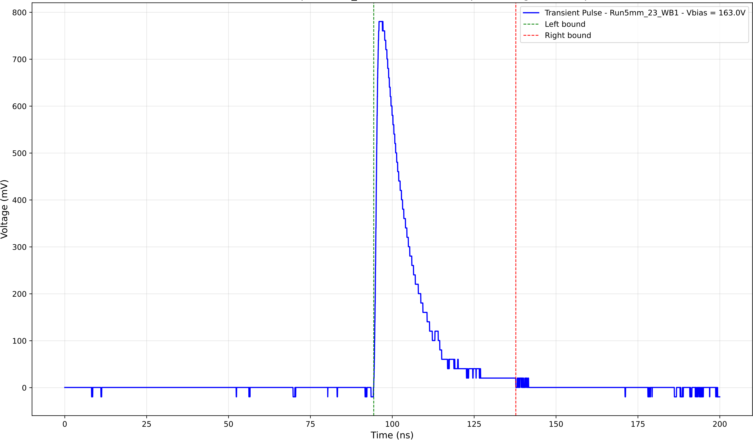
Transient Pulse - Sample: 5mm_23 - Position: 3830.0 \mu\text{m} - Charge: 163.62 pC
