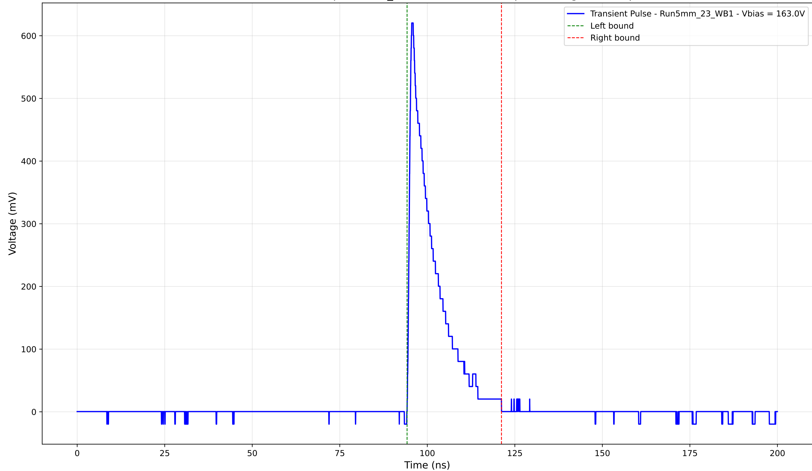
Transient Pulse - Sample: 5mm_23 - Position: 4810.0 \mu\text{m} - Charge: 90.99 pC
