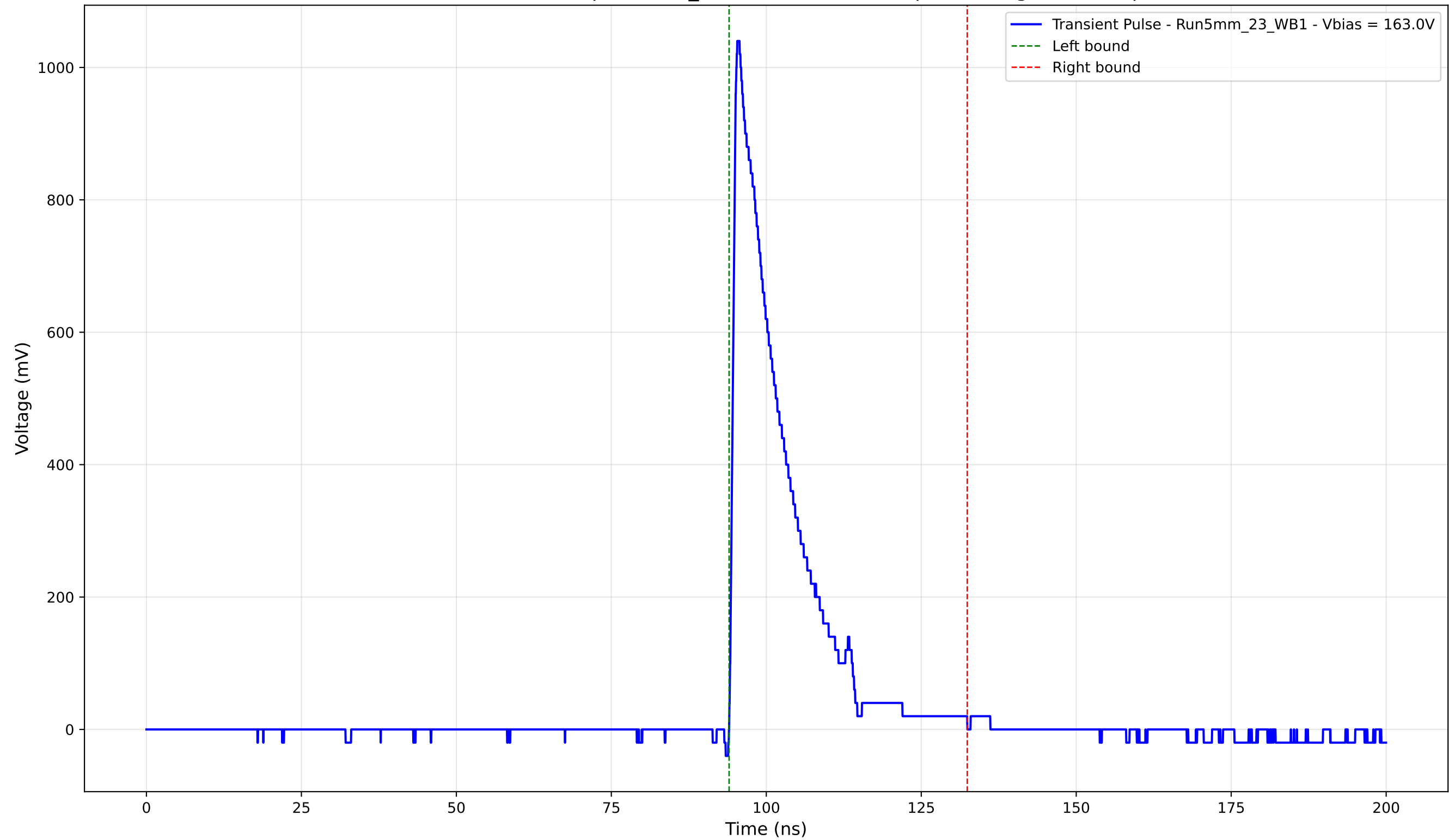
Transient Pulse - Sample: 5mm_23 - Position: 5050.0 \mu\text{m} - Charge: 180.82 pC
