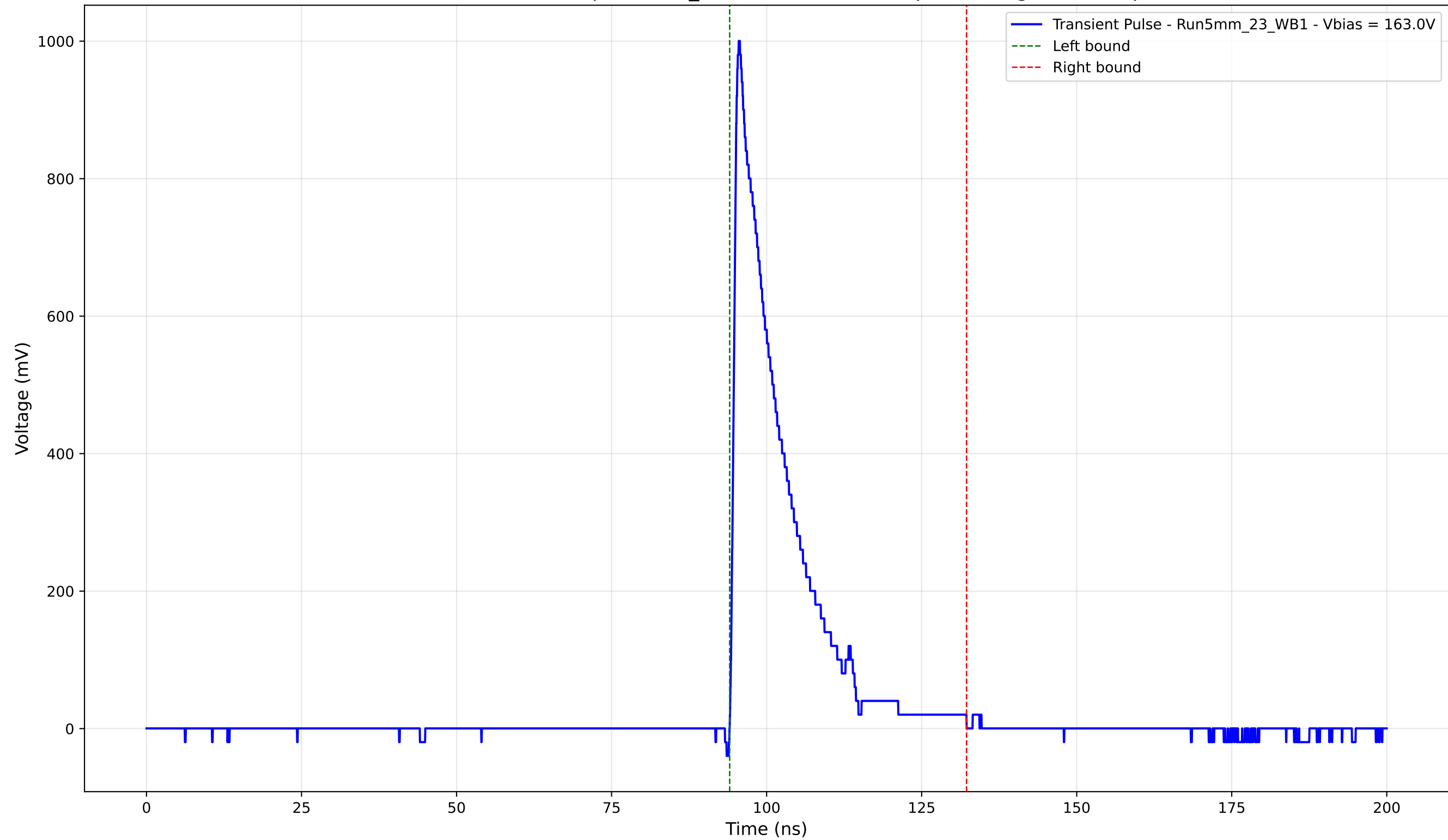
Transient Pulse - Sample: 5mm_23 - Position: 4960.0 \mu\text{m} - Charge: 165.82 pC
