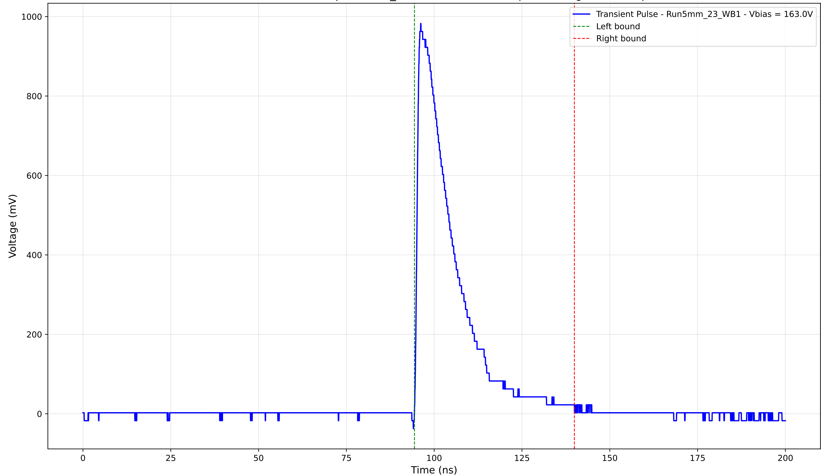
Transient Pulse - Sample: 5mm_23 - Position: 1360.0 \mu\text{m} - Charge: 223.60 pC
