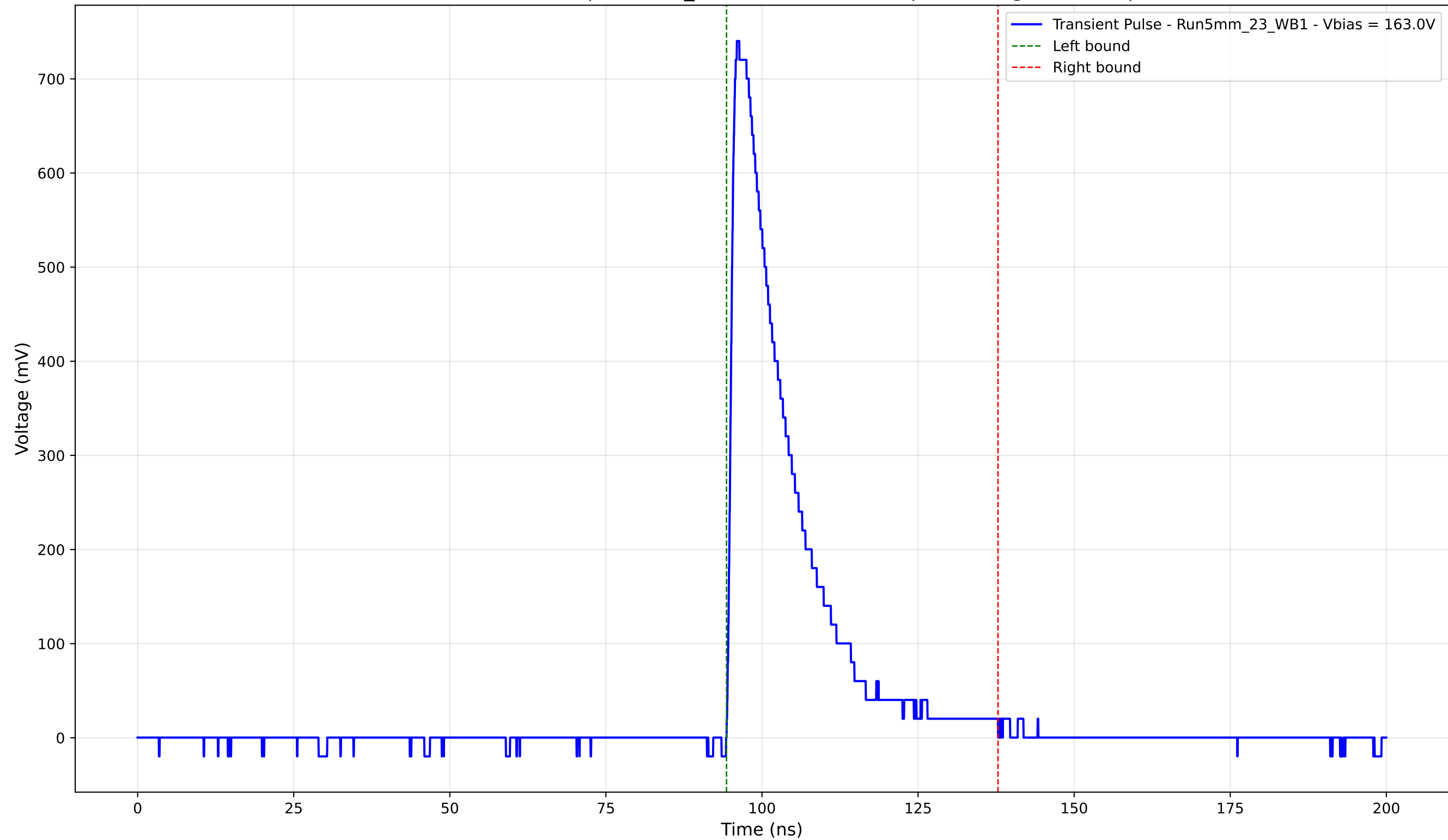
Transient Pulse - Sample: 5mm_23 - Position: 3690.0 \mu\text{m} - Charge: 151.92 pC
