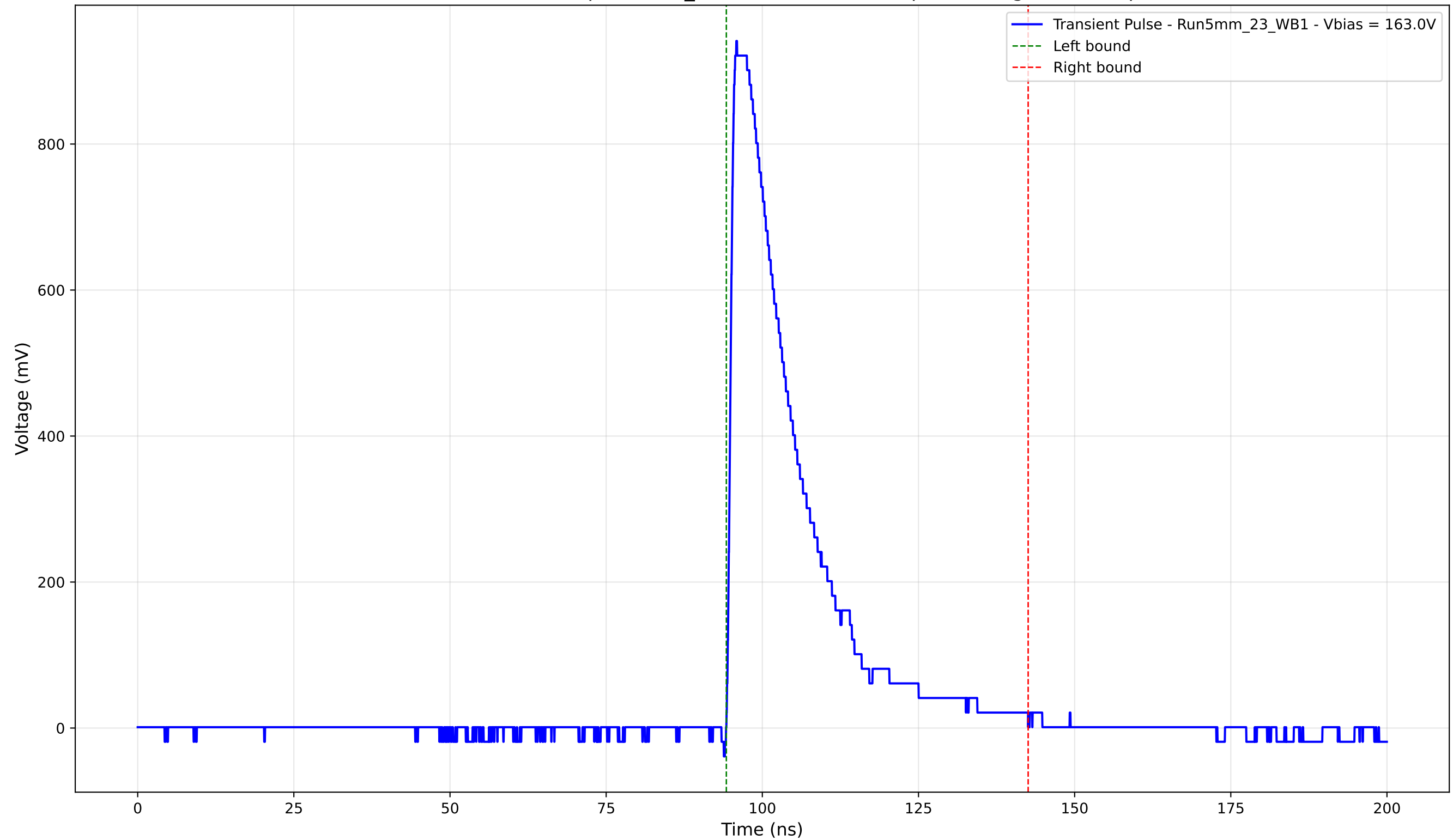
Transient Pulse - Sample: 5mm_23 - Position: 3570.0 \mu\text{m} - Charge: 217.29 pC
