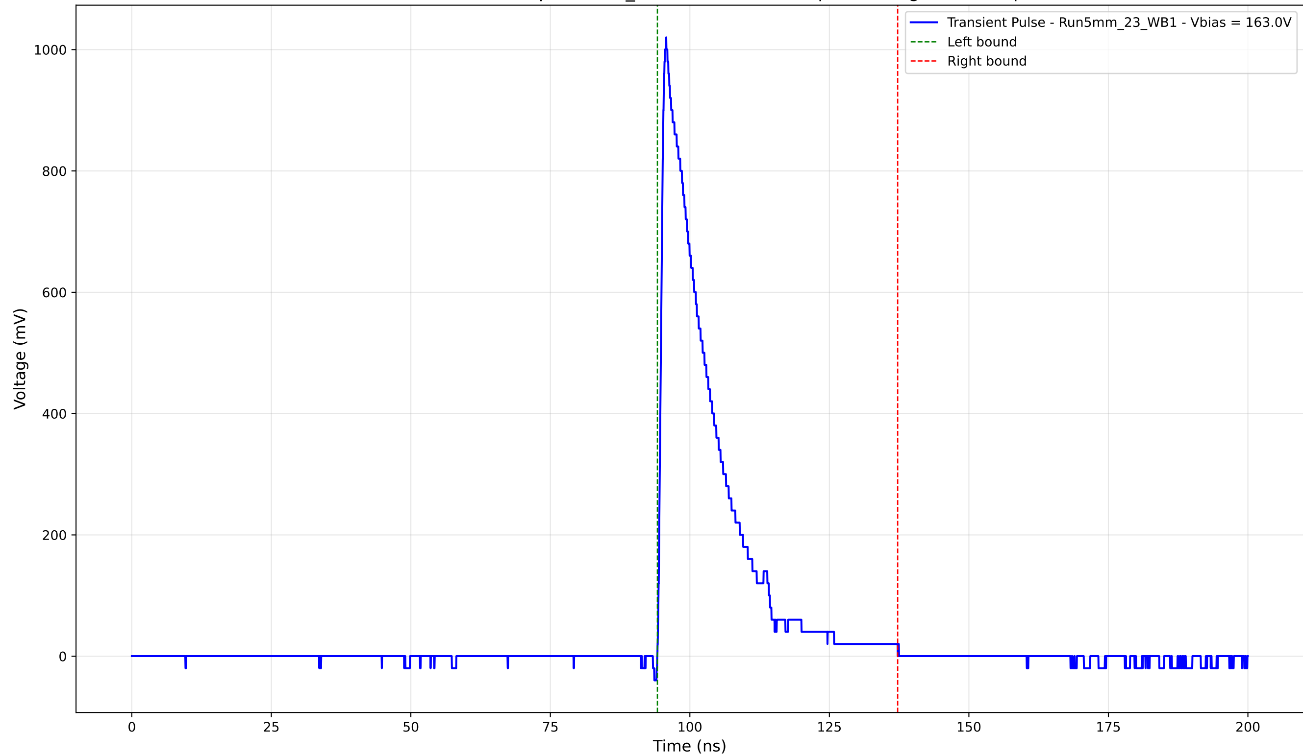
Transient Pulse - Sample: 5mm_23 - Position: 640.0 \mu\text{m} - Charge: 192.95 pC
