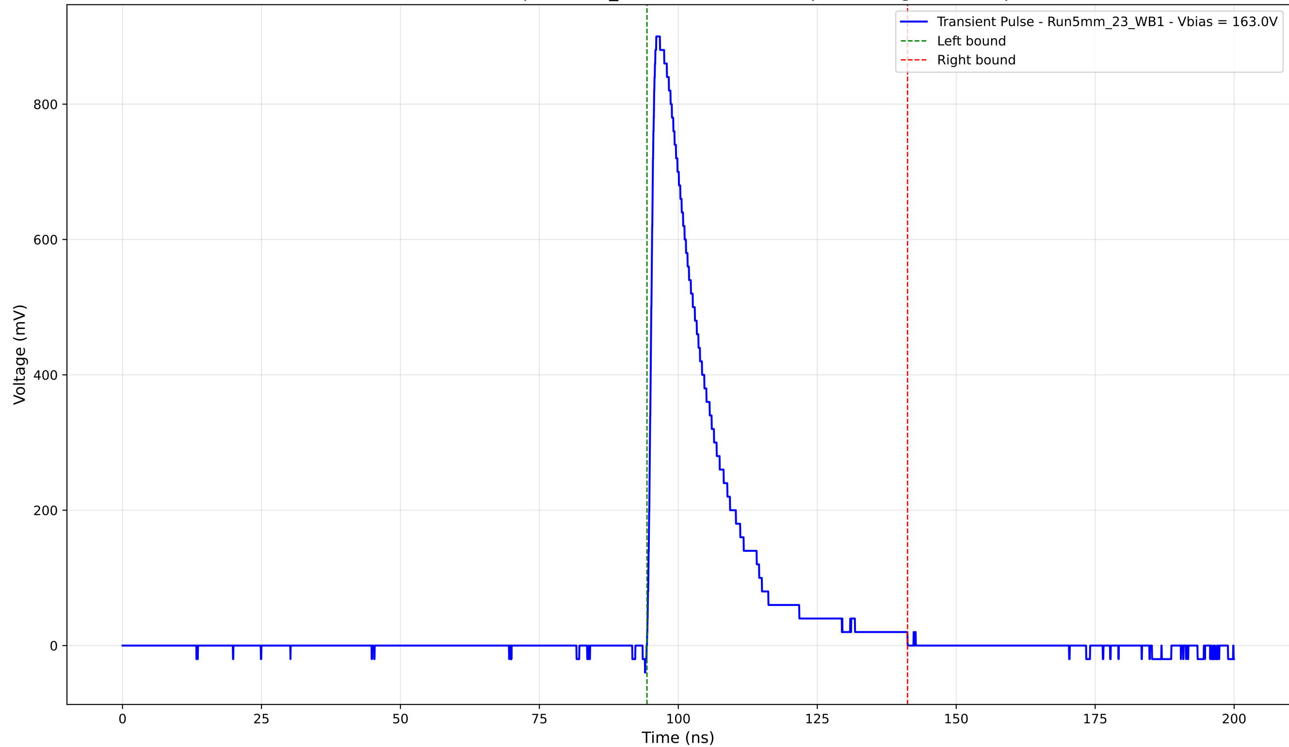
Transient Pulse - Sample: 5mm_23 - Position: 3915.0 \mu\text{m} - Charge: 196.52 pC
