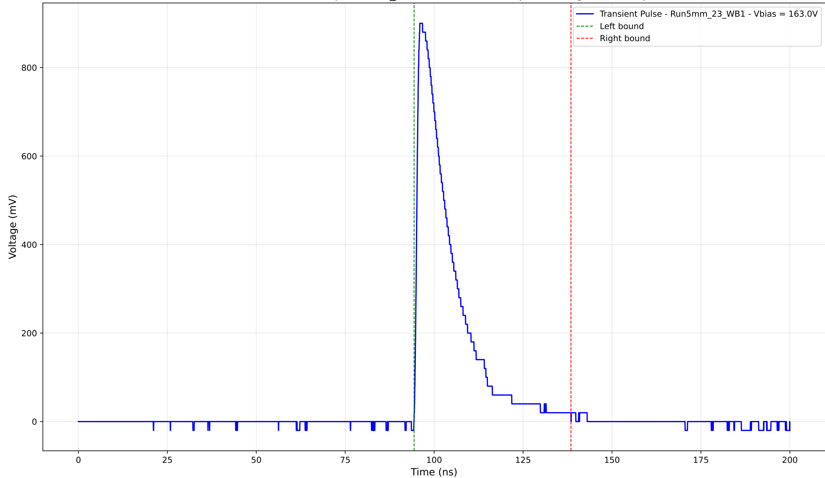
Transient Pulse - Sample: 5mm_23 - Position: 3945.0 \mu\text{m} - Charge: 196.08 pC
