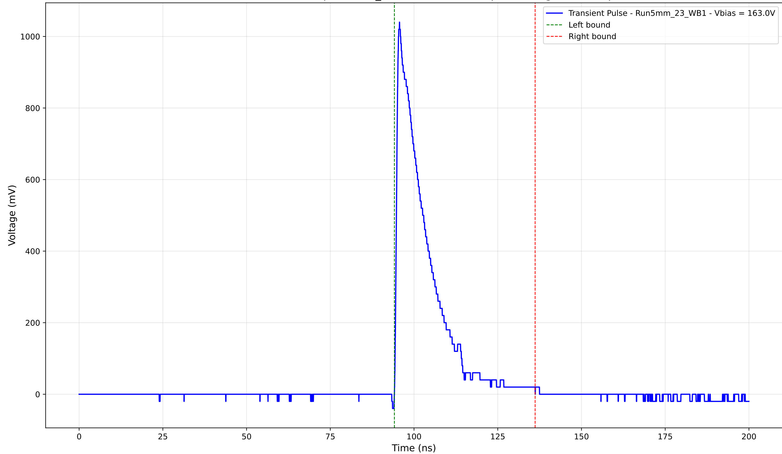
Transient Pulse - Sample: 5mm_23 - Position: 545.0 \mu\text{m} - Charge: 197.38 pC
