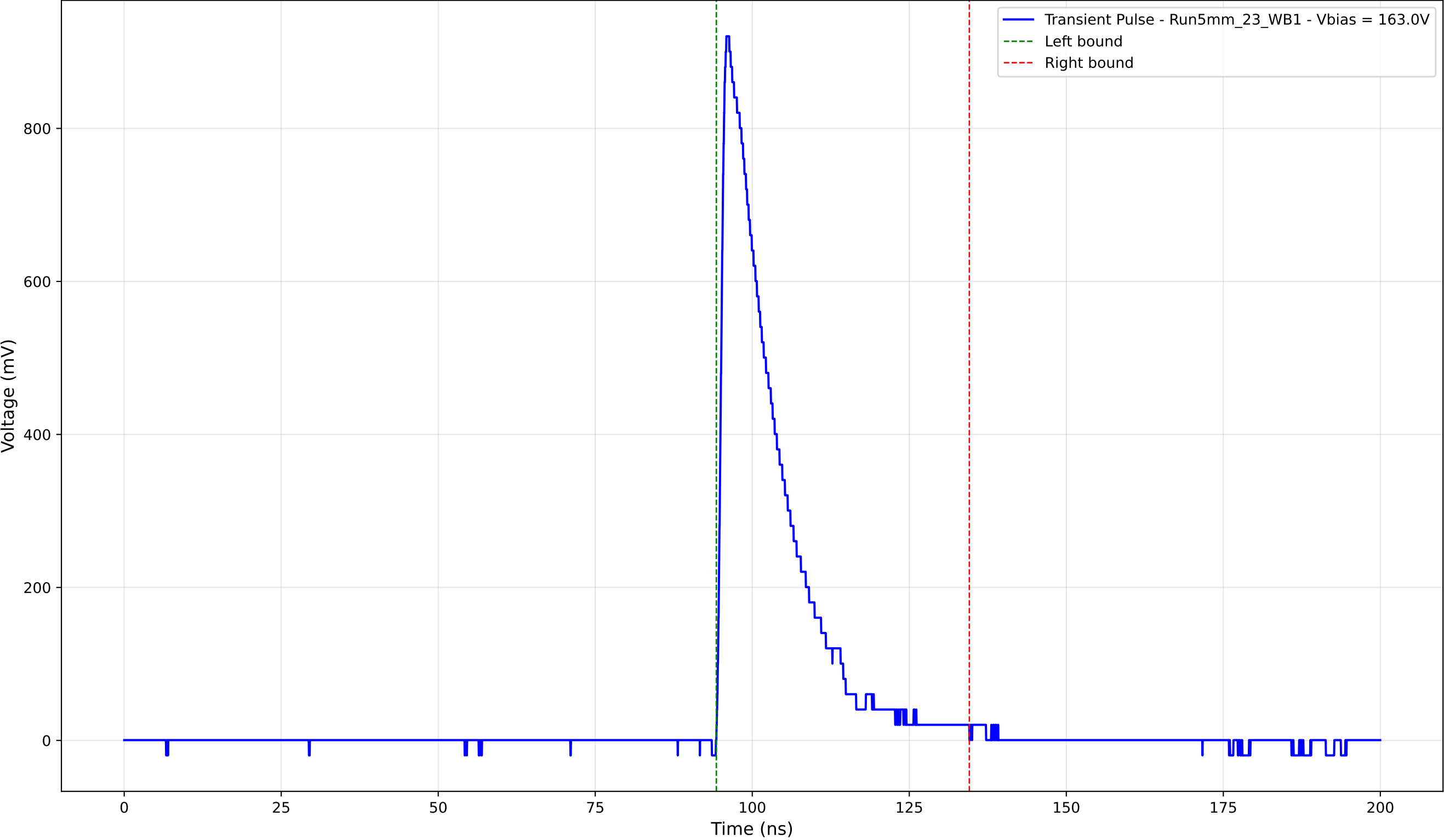
Transient Pulse - Sample: 5mm_23 - Position: 4485.0 \mu\text{m} - Charge: 178.94 pC
