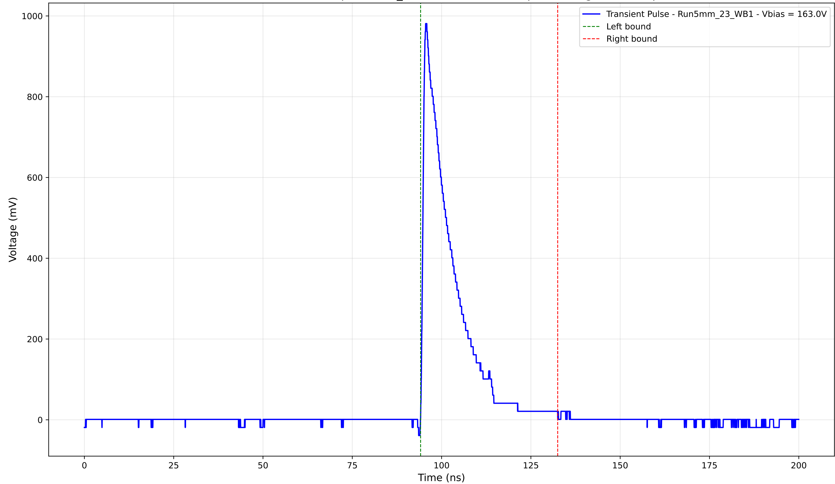
Transient Pulse - Sample: 5mm_23 - Position: 4865.0 \mu\text{m} - Charge: 169.43 pC
