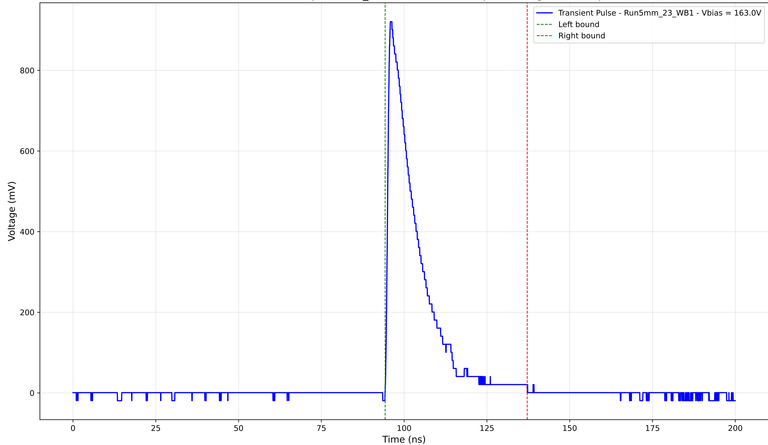
Transient Pulse - Sample: 5mm_23 - Position: 4510.0 \mu\text{m} - Charge: 179.46 pC
