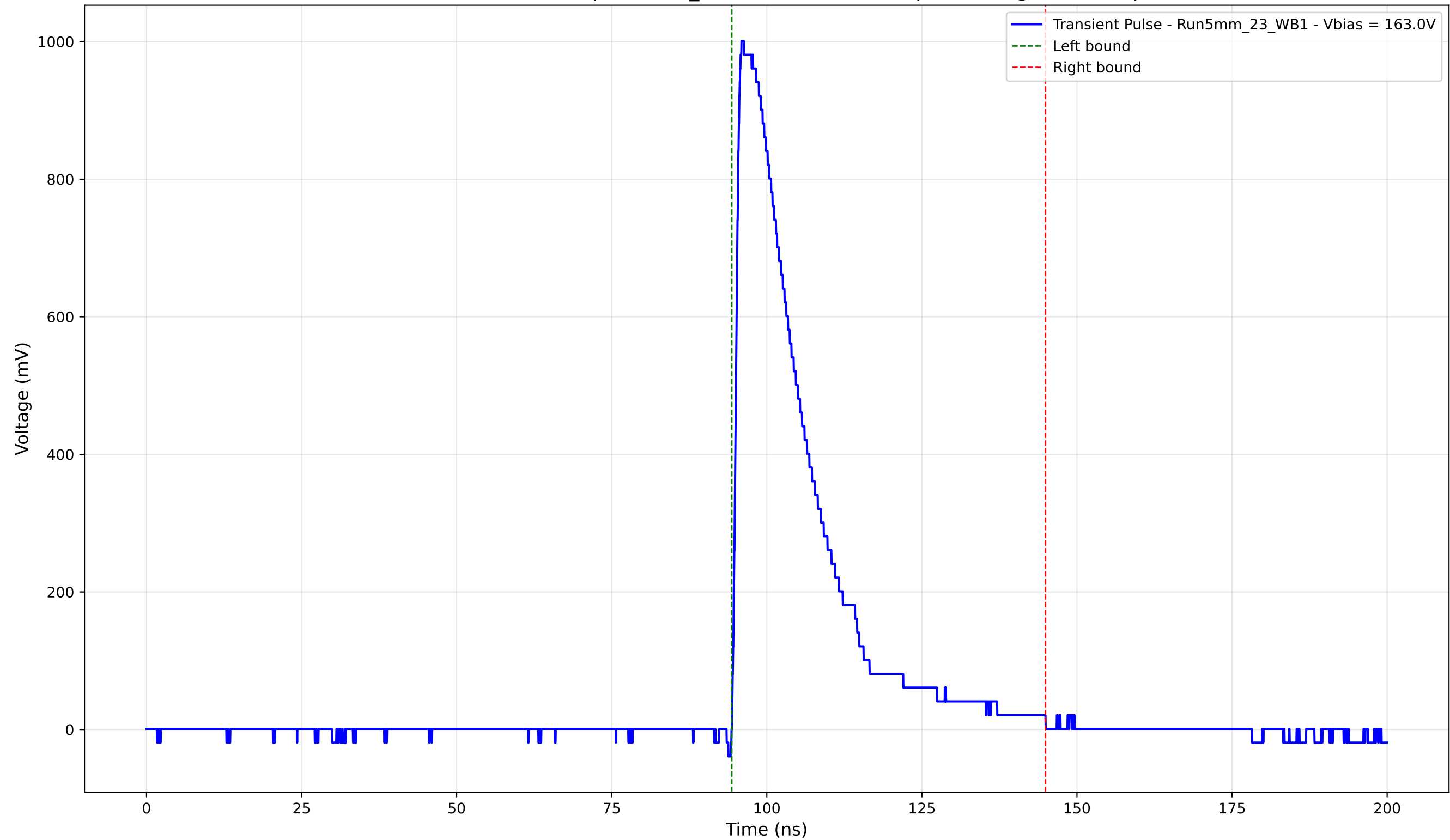
Transient Pulse - Sample: 5mm_23 - Position: 1615.0 \mu\text{m} - Charge: 246.79 pC
