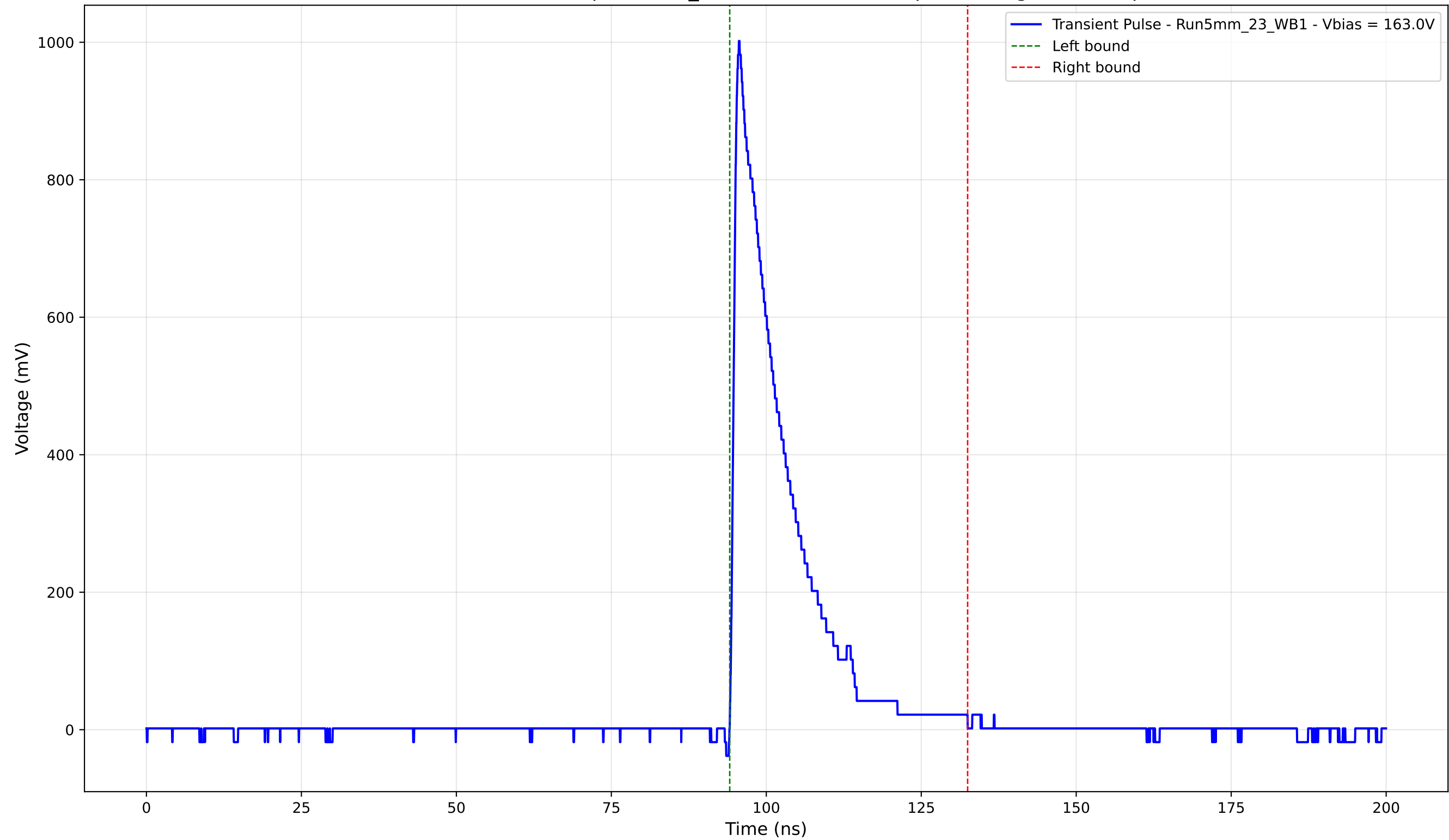
Transient Pulse - Sample: 5mm_23 - Position: 4905.0 \mu\text{m} - Charge: 171.59 pC
