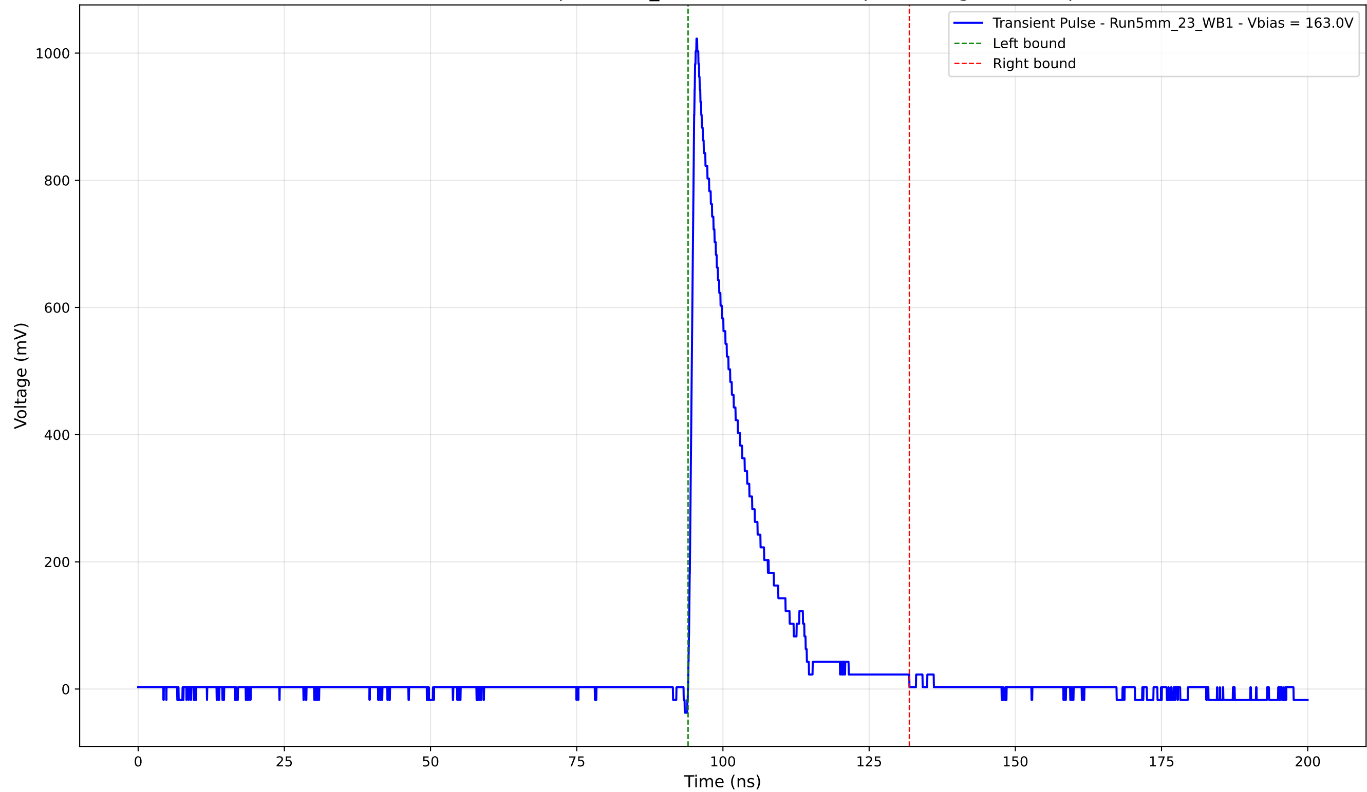
Transient Pulse - Sample: 5mm_23 - Position: 5000.0 \mu\text{m} - Charge: 170.12 pC
