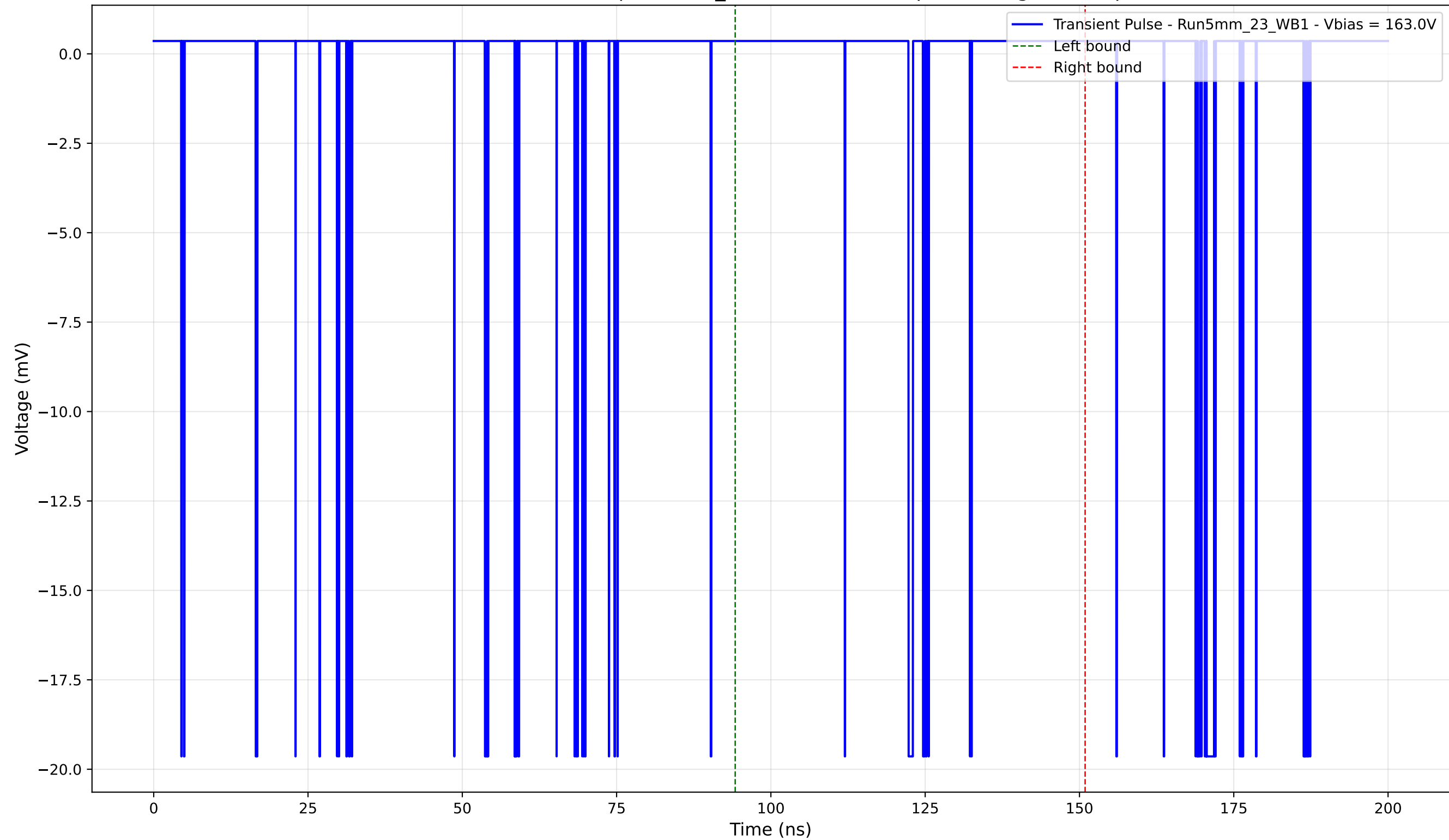
Transient Pulse - Sample: 5mm_23- Position: 25.0 \mu\text{m} - Charge: -0.17 pC
