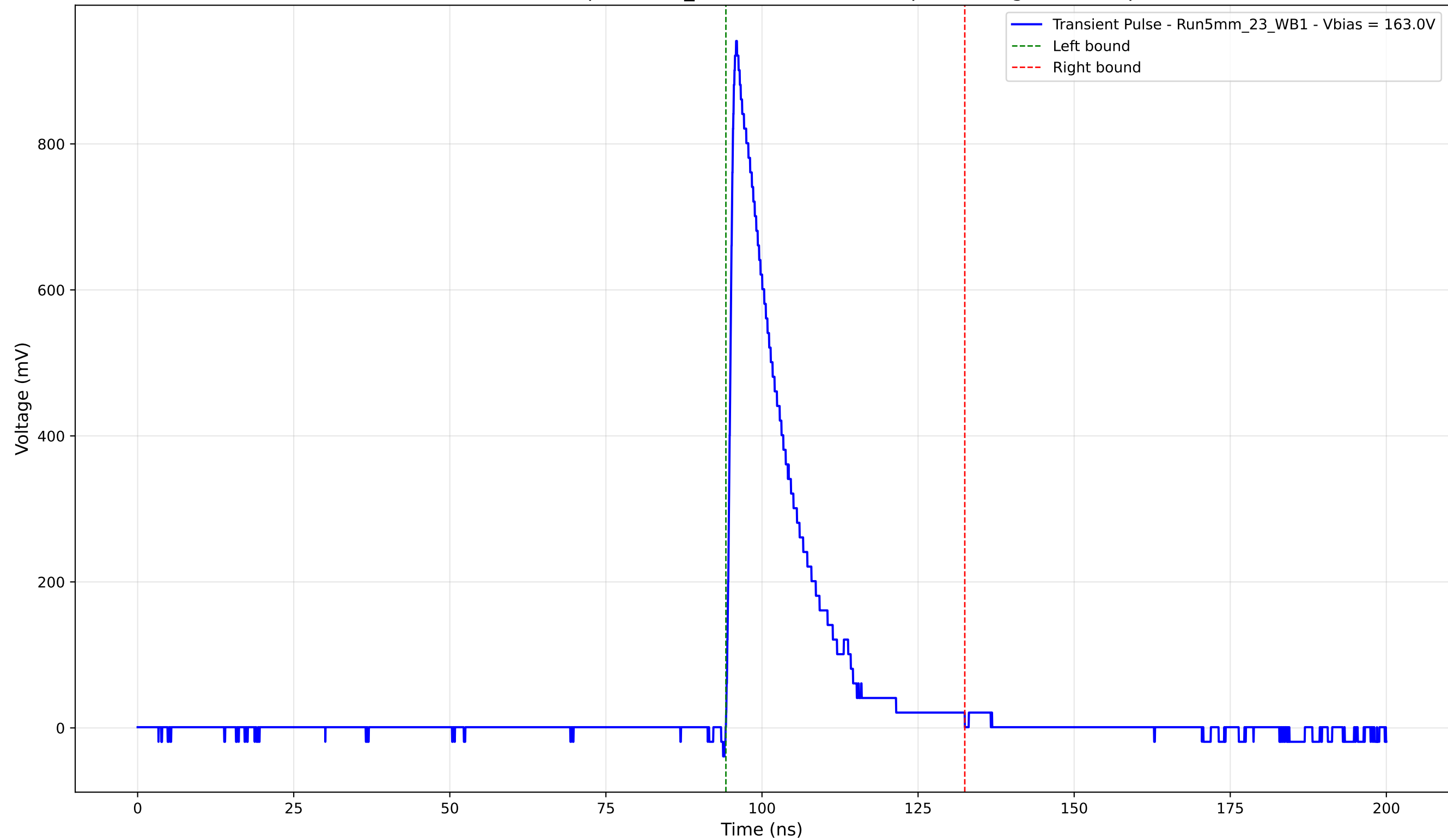
Transient Pulse - Sample: 5mm_23 - Position: 4645.0 \mu\text{m} - Charge: 171.11 pC
