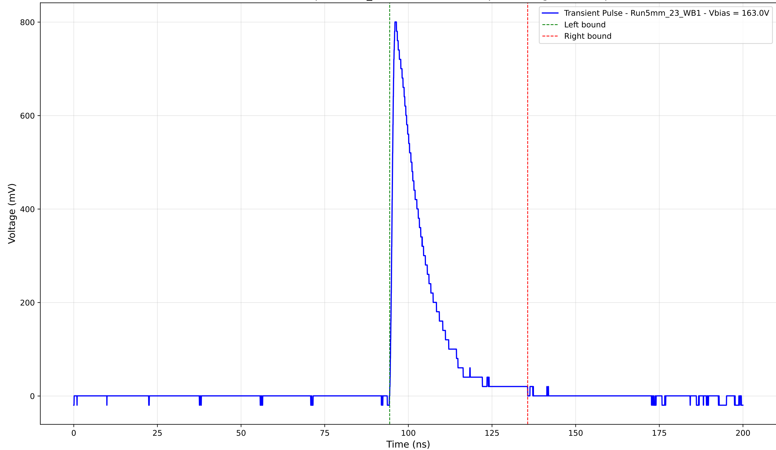
Transient Pulse - Sample: 5mm_23 - Position: 1160.0 \mu\text{m} - Charge: 154.60 pC
