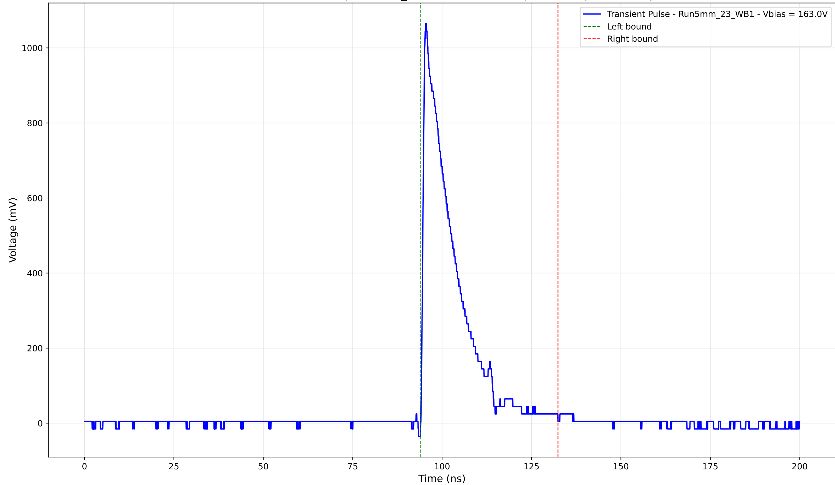
Transient Pulse - Sample: 5mm_23 - Position: 380.0 \mu\text{m} - Charge: 197.40 pC
