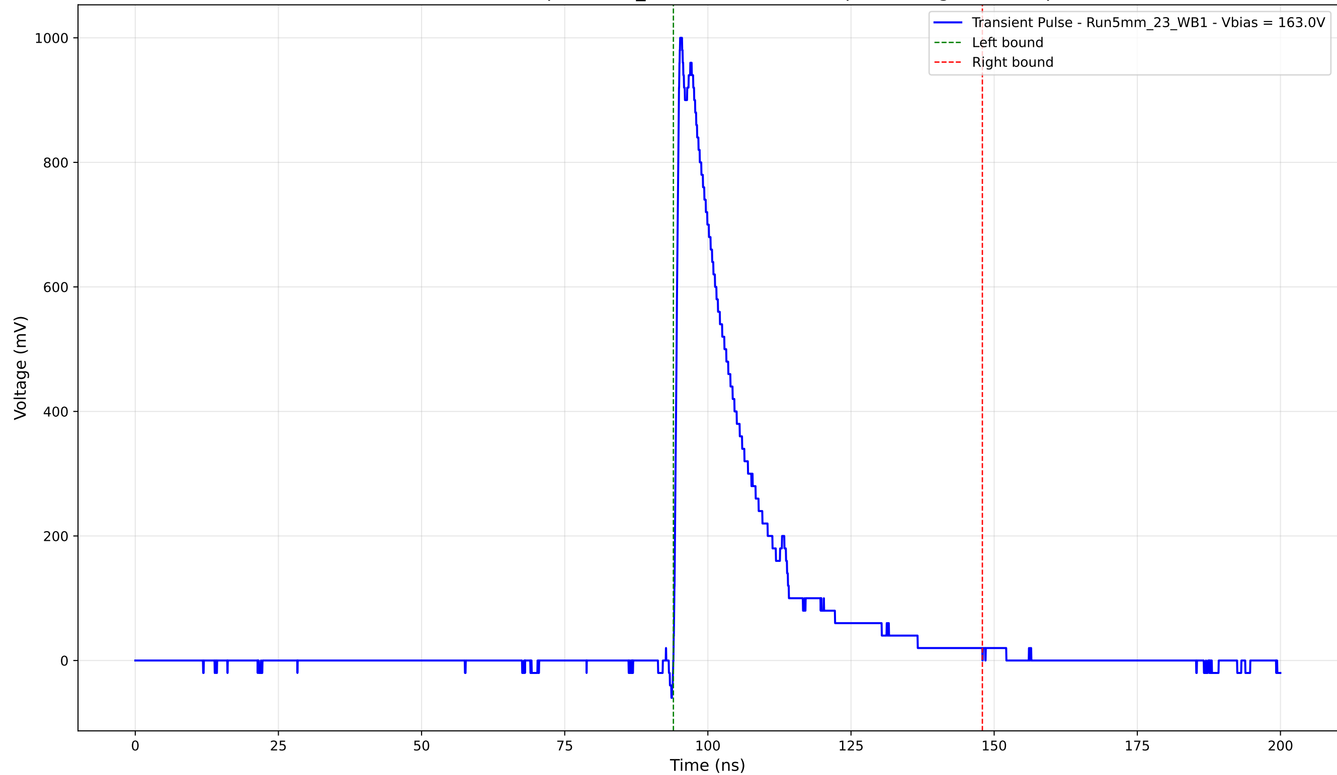
Transient Pulse - Sample: 5mm_23 - Position: 2410.0 \mu\text{m} - Charge: 229.41 pC
