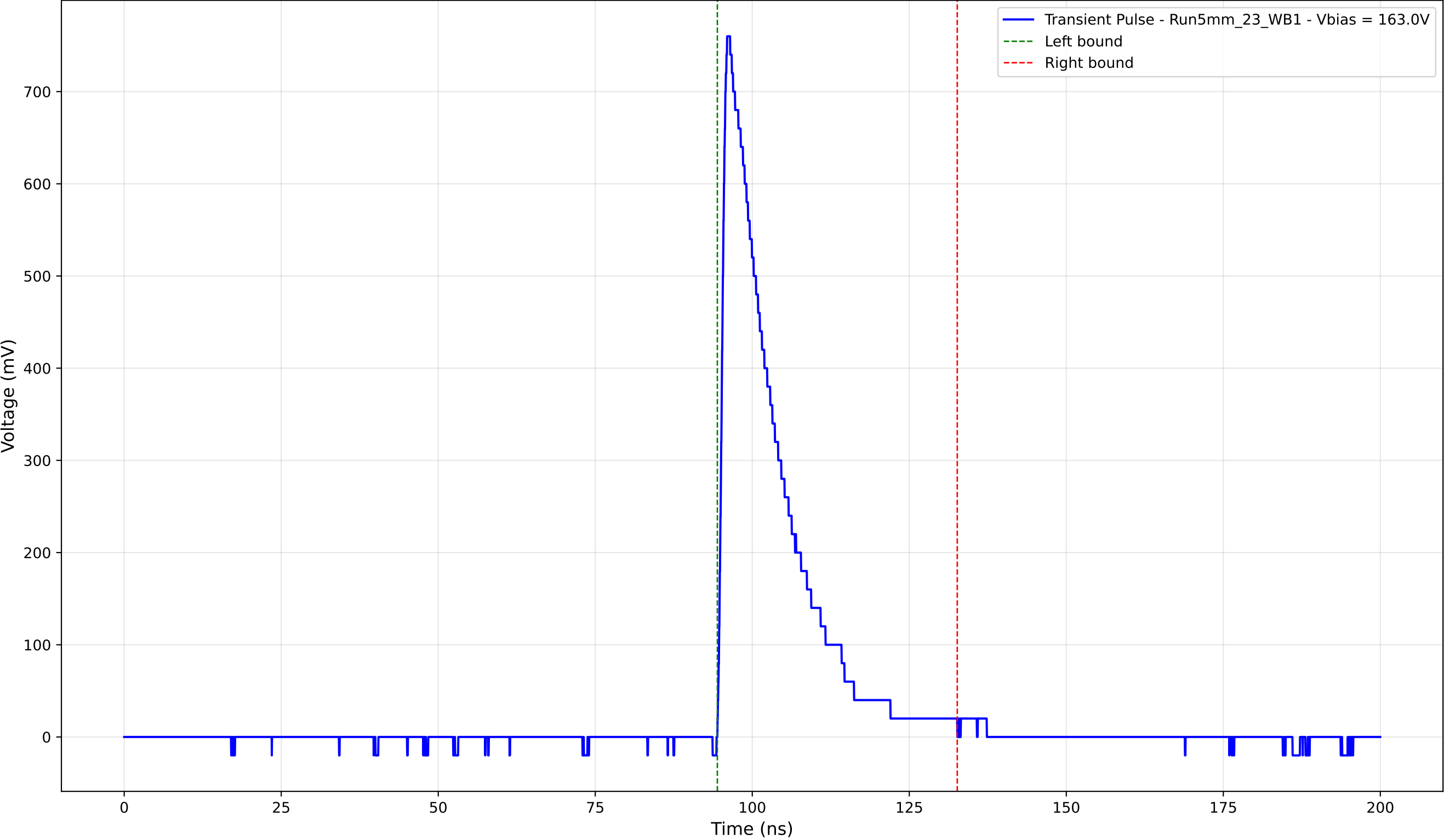
Transient Pulse - Sample: 5mm_23 - Position: 1165.0 \mu\text{m} - Charge: 144.52 pC
