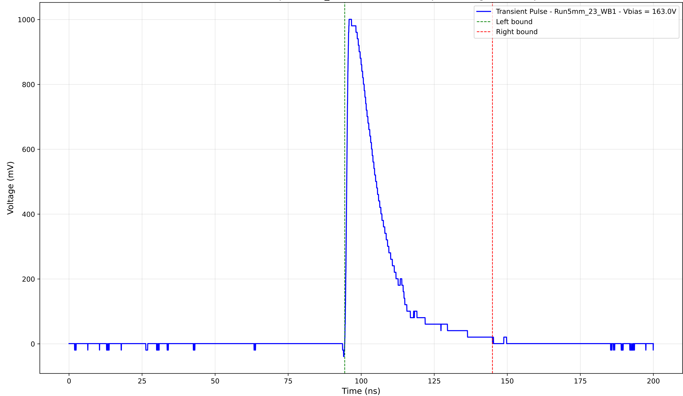
Transient Pulse - Sample: 5mm_23 - Position: 1505.0 \mu\text{m} - Charge: 252.73 pC
