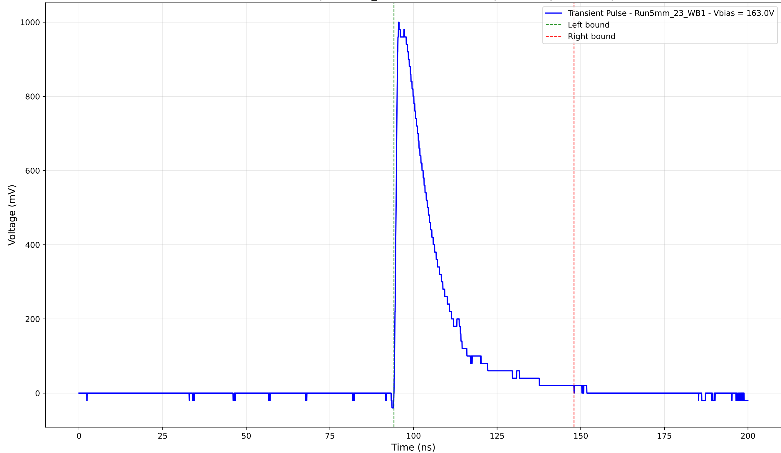
Transient Pulse - Sample: 5mm_23 - Position: 2070.0 \mu\text{m} - Charge: 246.34 pC
