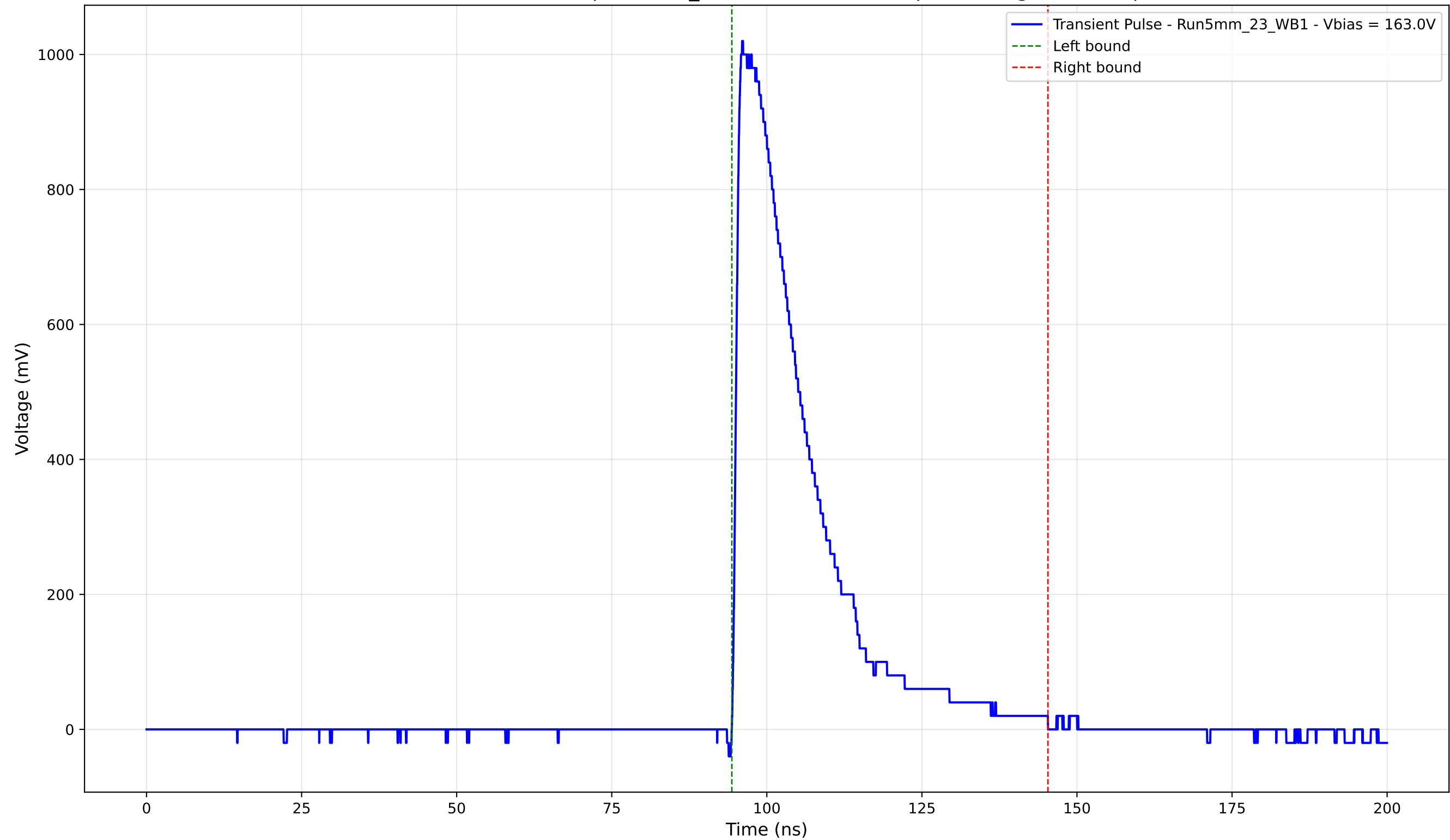
Transient Pulse - Sample: 5mm_23 - Position: 1530.0 \mu\text{m} - Charge: 255.36 pC
