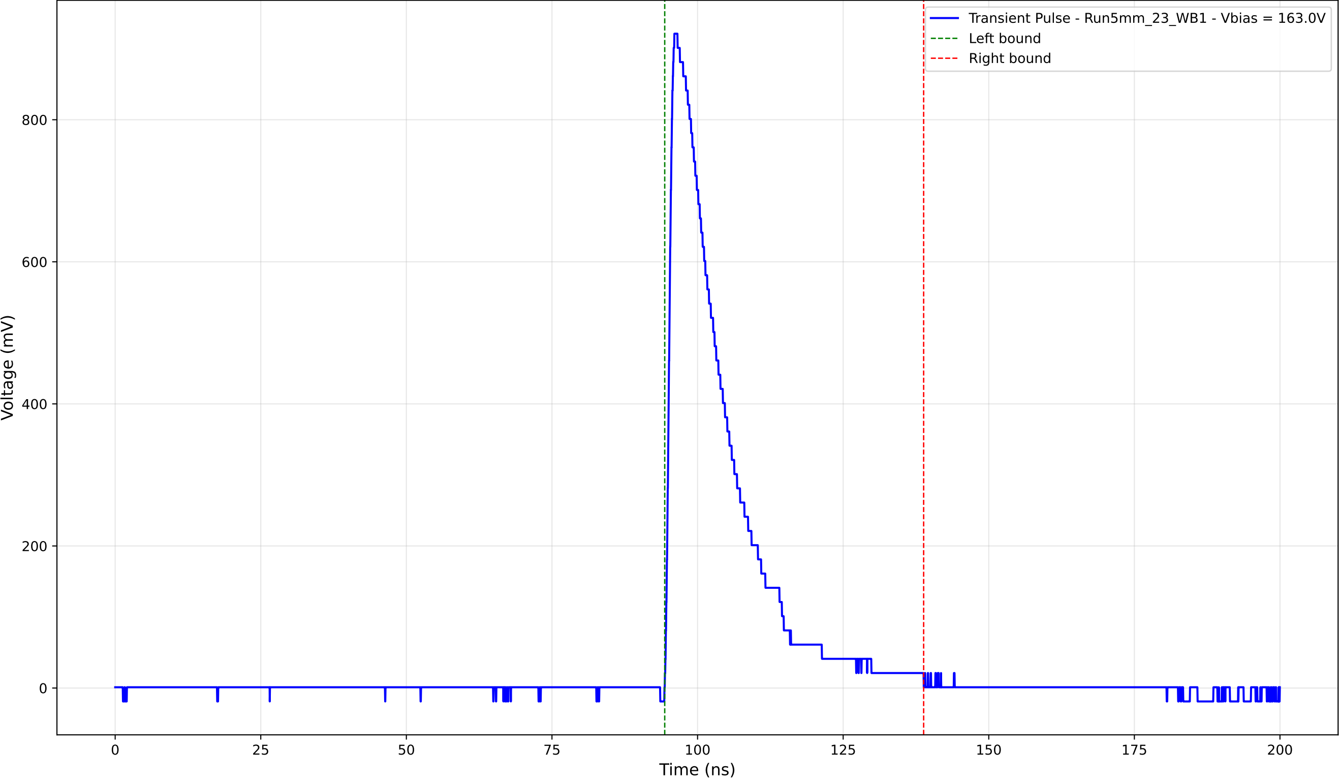
Transient Pulse - Sample: 5mm_23 - Position: 4125.0 \mu\text{m} - Charge: 195.79 pC
