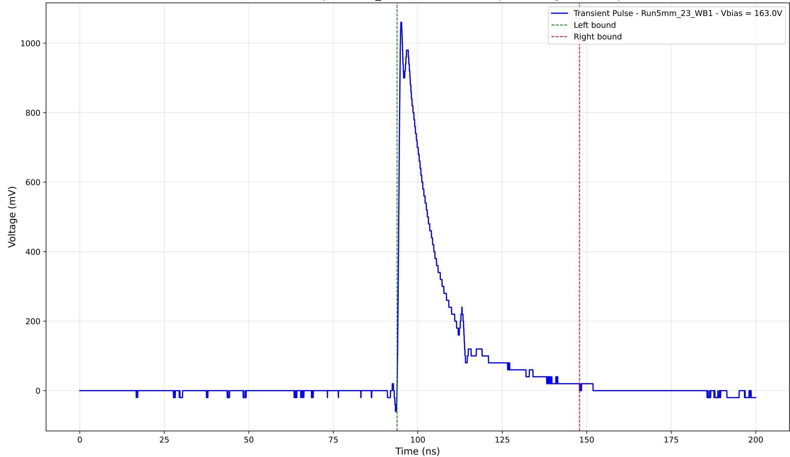
Transient Pulse - Sample: 5mm_23 - Position: 2875.0 \mu\text{m} - Charge: 240.33 pC
