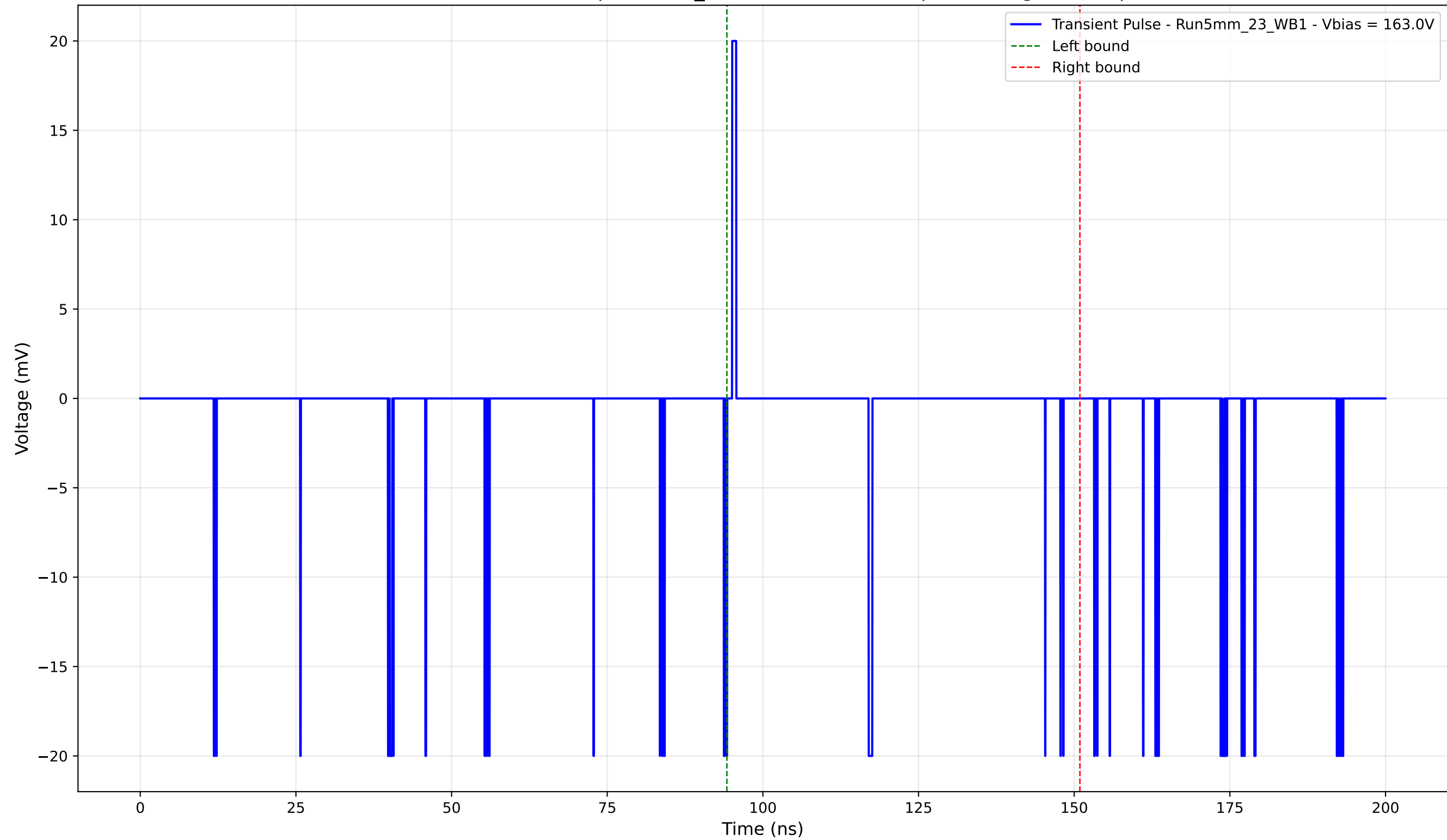
Transient Pulse - Sample: 5mm_23 - Position: 5290.0 \mu\text{m} - Charge: -0.05 pC
