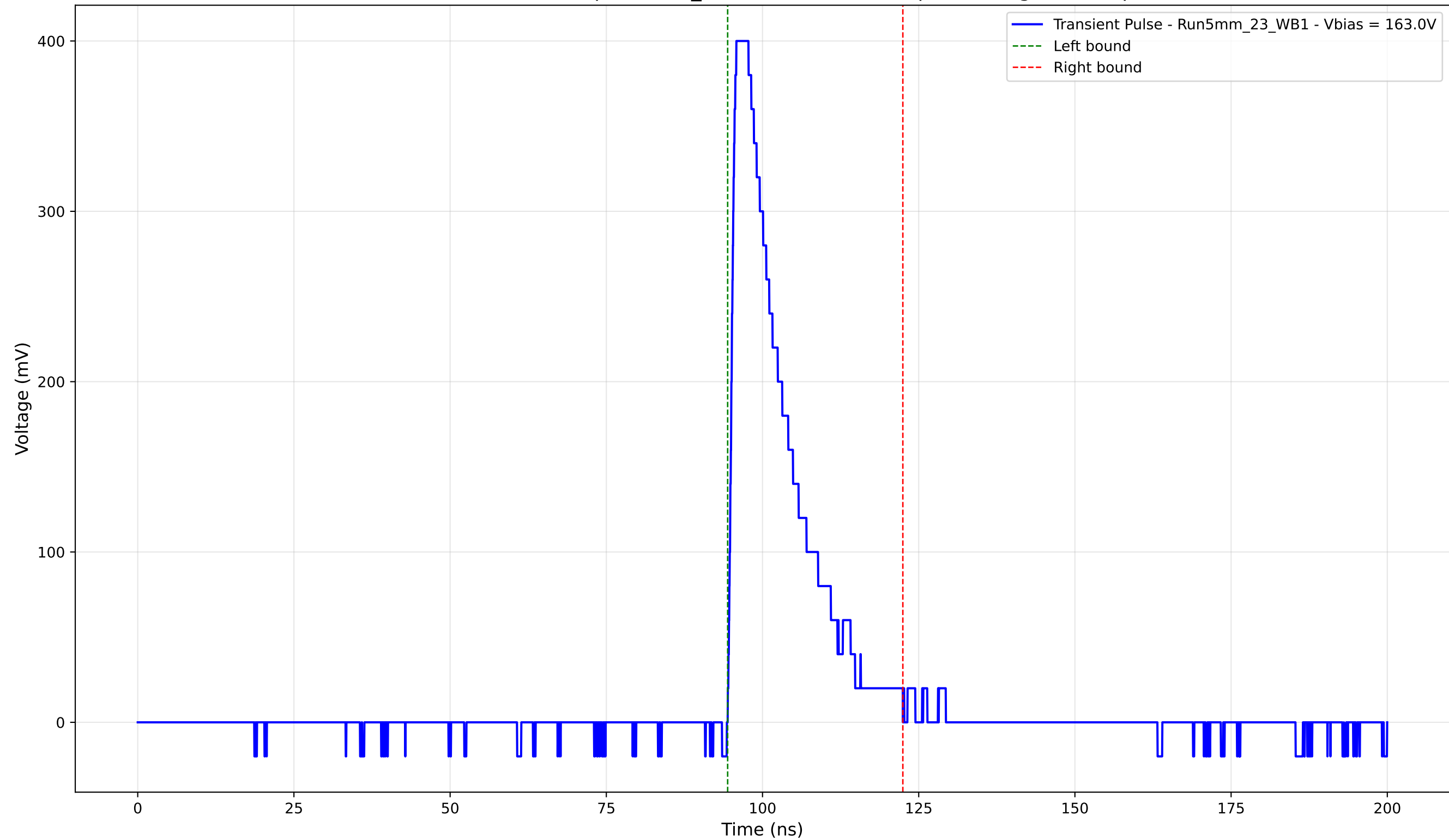
Transient Pulse - Sample: 5mm_23 - Position: 3720.0 \mu\text{m} - Charge: 77.28 pC
