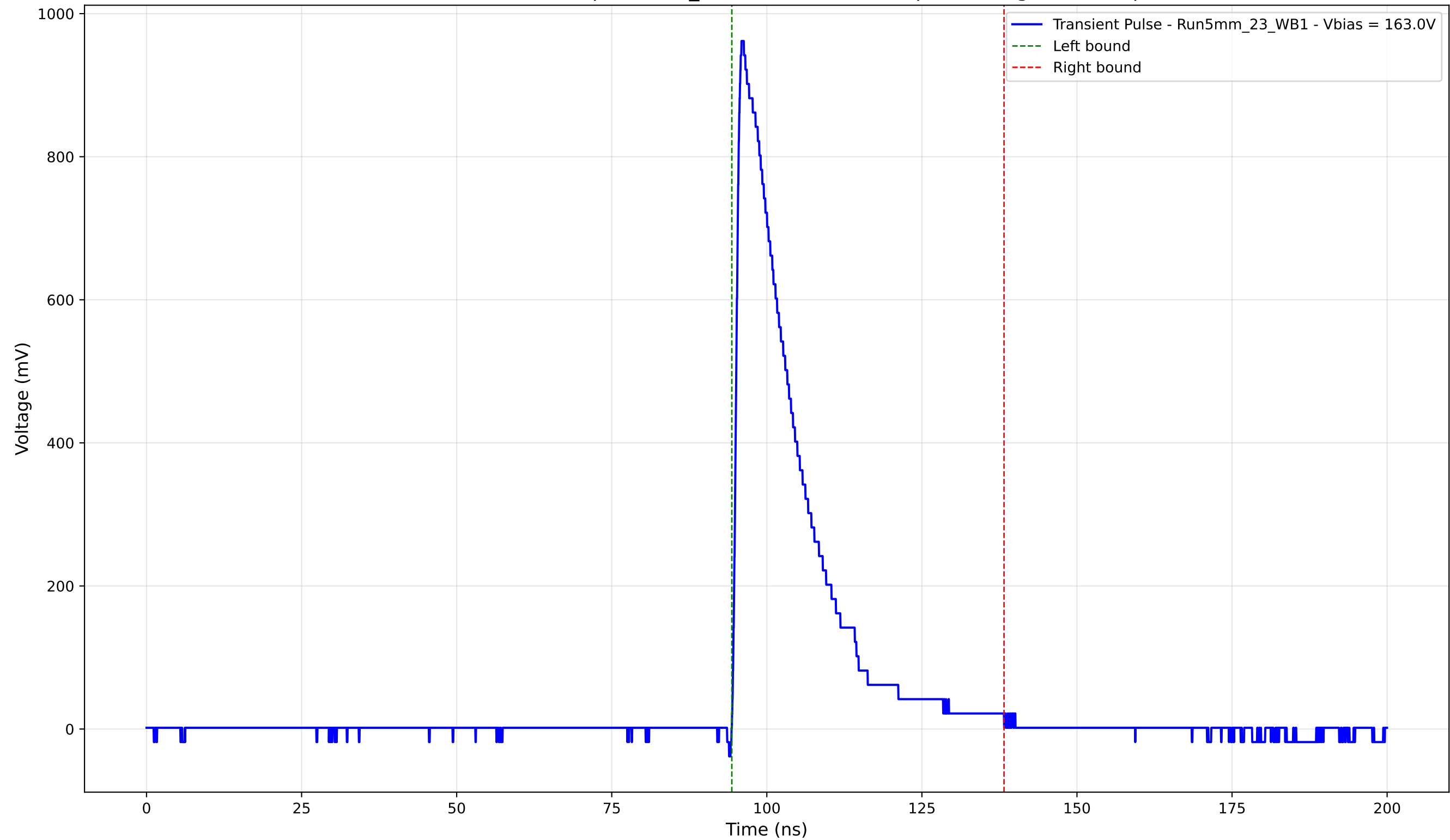
Transient Pulse - Sample: 5mm_23 - Position: 1020.0 \mu\text{m} - Charge: 201.89 pC
