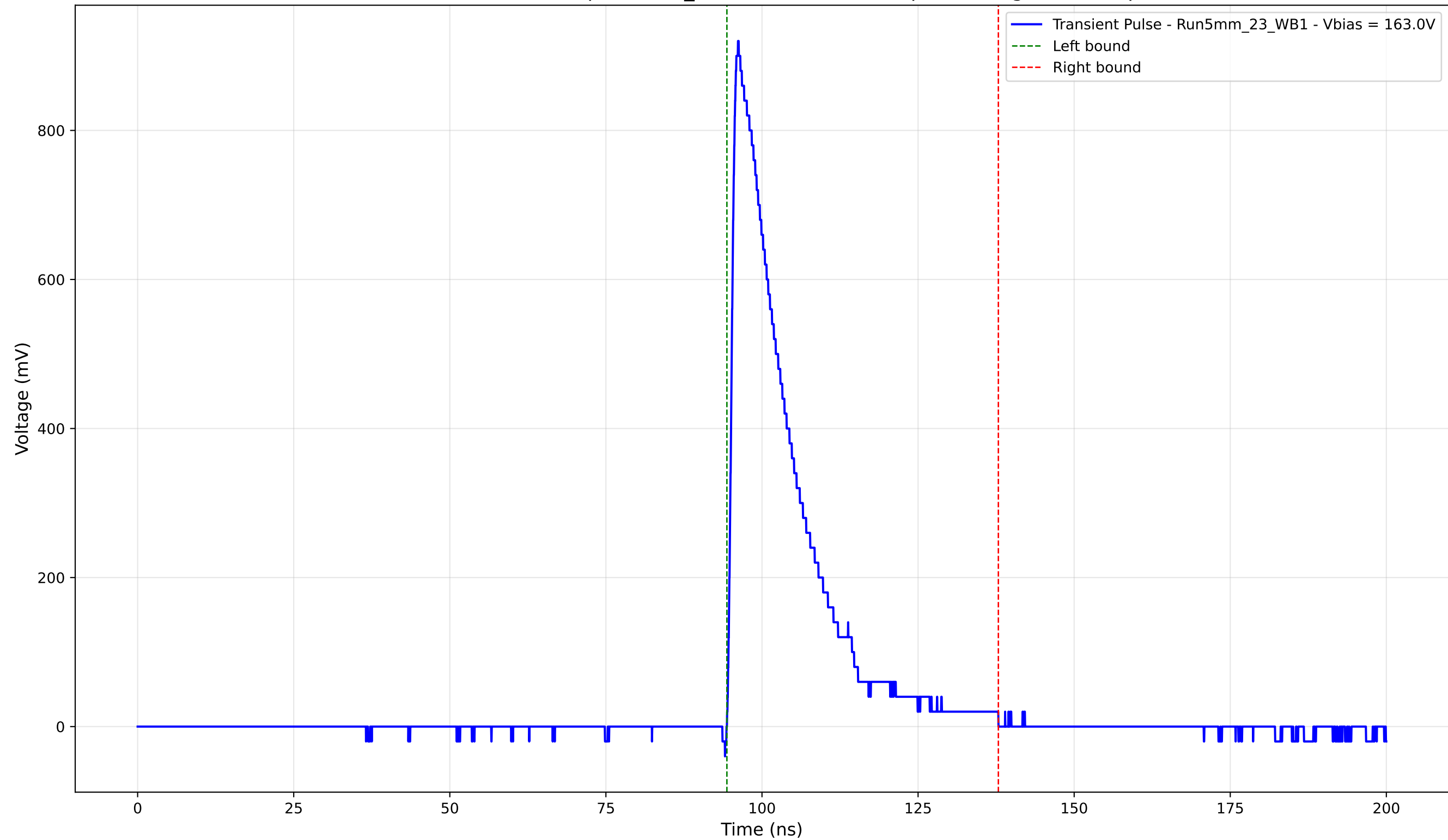
Transient Pulse - Sample: 5mm_23 - Position: 1140.0 \mu\text{m} - Charge: 185.84 pC
