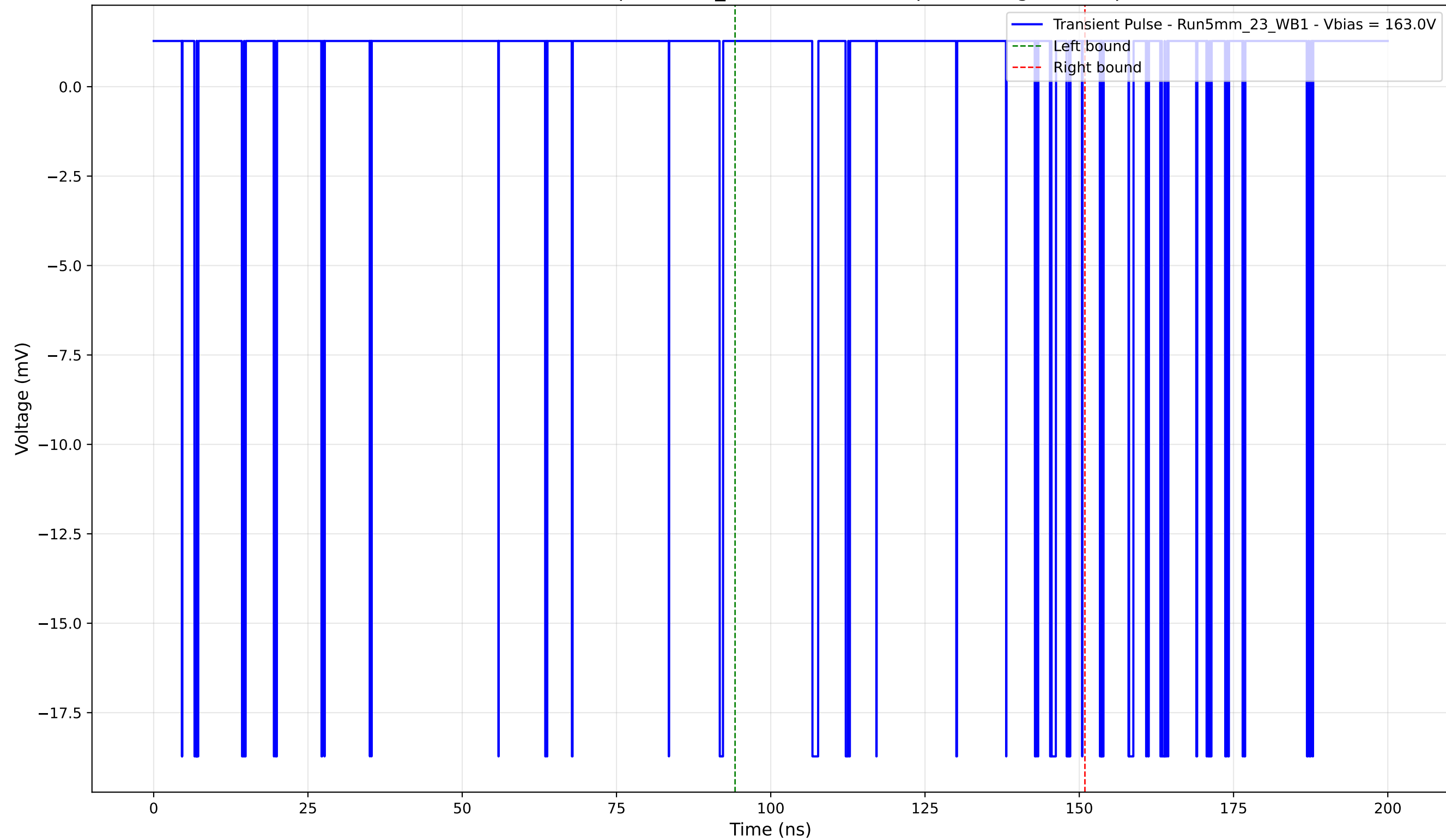
Transient Pulse - Sample: 5mm_23- Position: 30.0 \mu\text{m} - Charge: -0.01 pC
