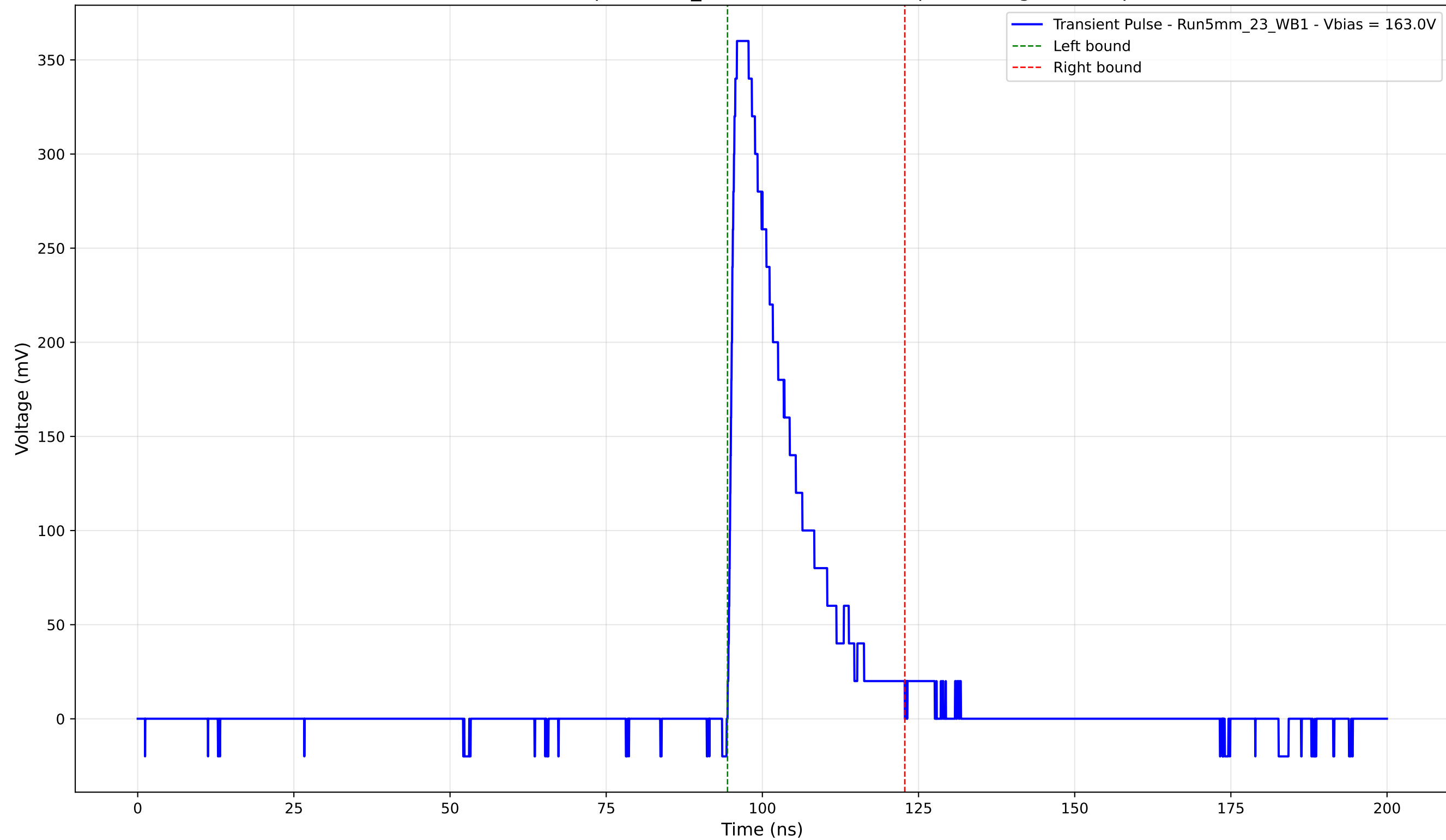
Transient Pulse - Sample: 5mm_23 - Position: 1755.0 \mu\text{m} - Charge: 71.29 pC
