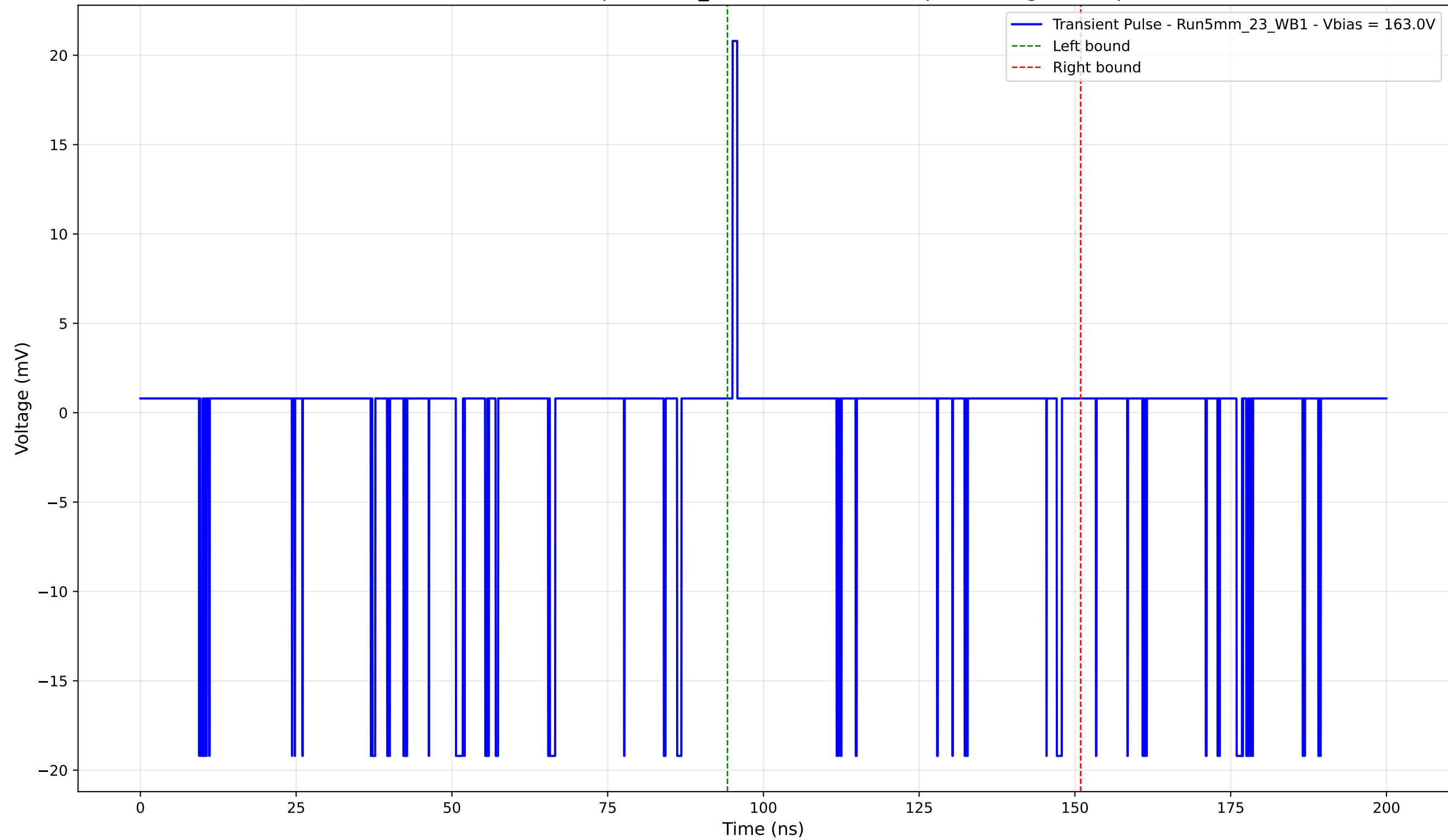
Transient Pulse - Sample: 5mm_23 - Position: 5285.0 \mu\text{m} - Charge: 0.44 pC
