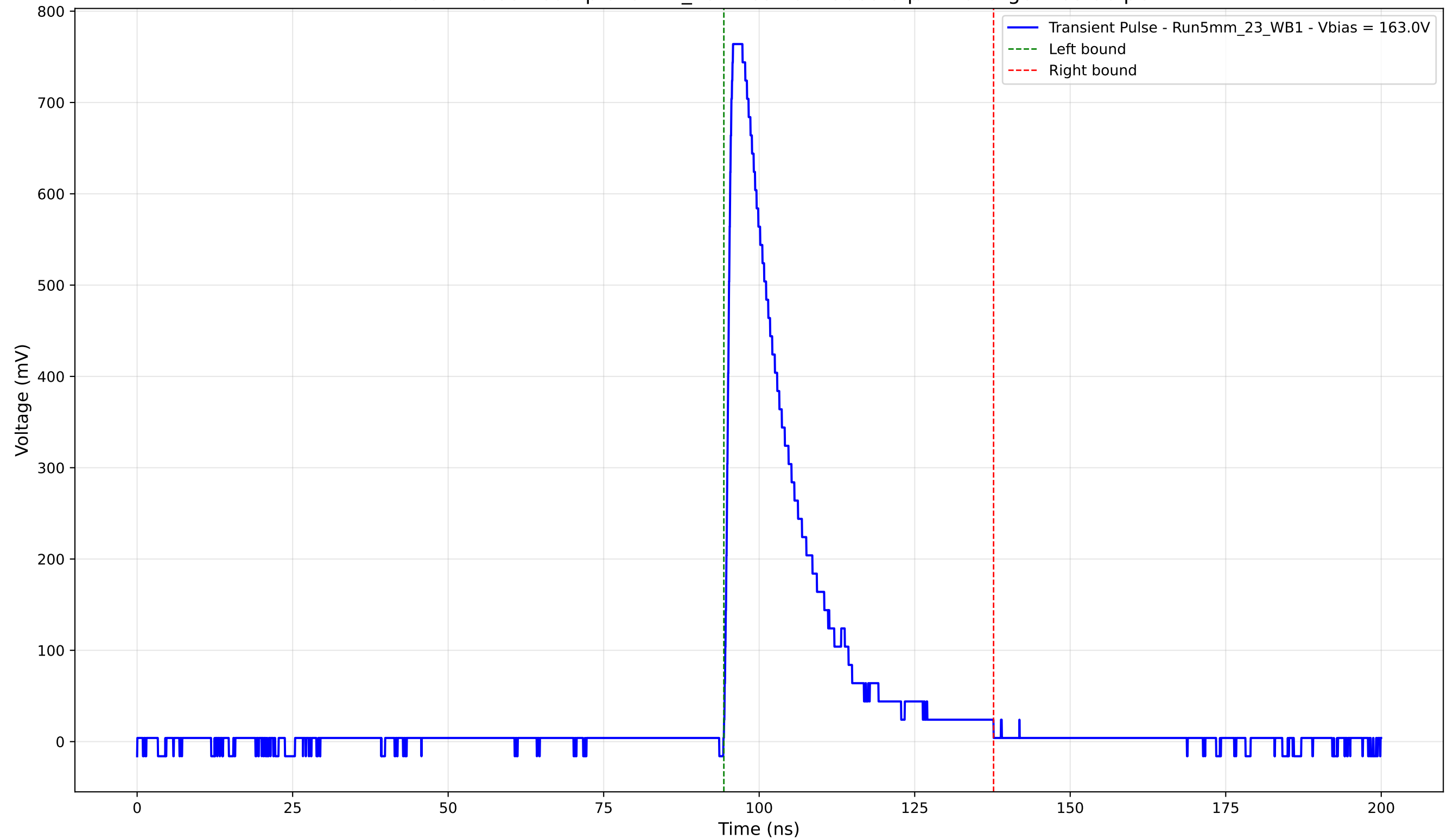
Transient Pulse - Sample: 5mm_23 - Position: 3685.0 \mu\text{m} - Charge: 163.56 pC
