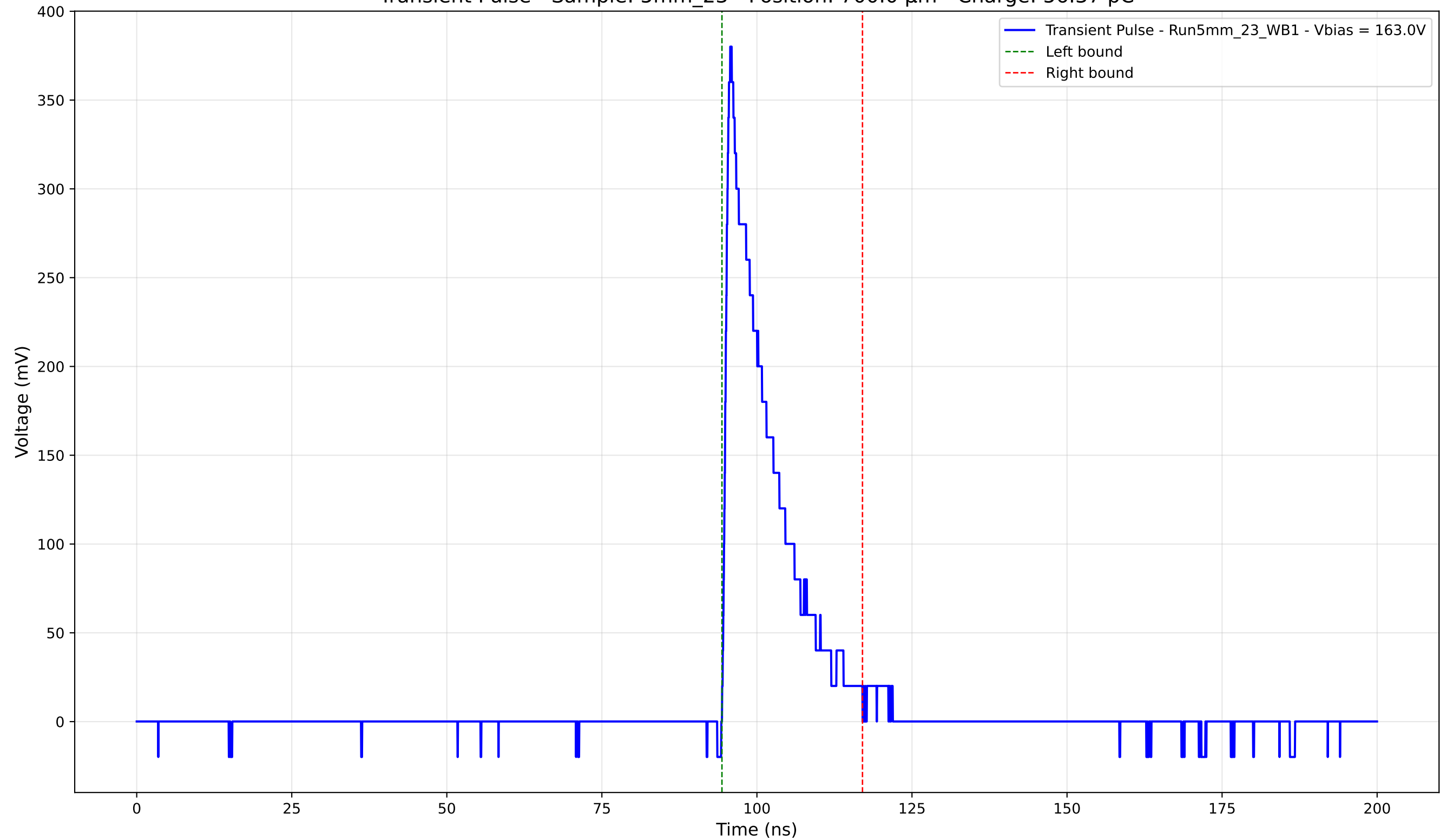
Transient Pulse - Sample: 5mm_23 - Position: 700.0 \mu\text{m} - Charge: 56.37 pC
