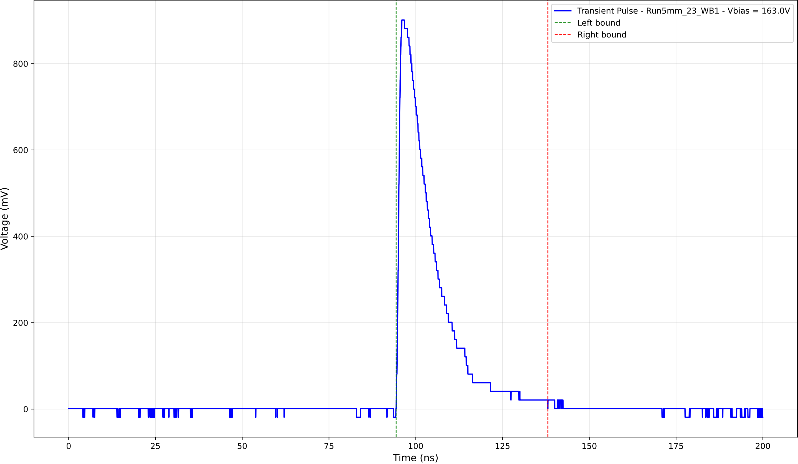
Transient Pulse - Sample: 5mm_23 - Position: 3925.0 \mu\text{m} - Charge: 196.78 pC
