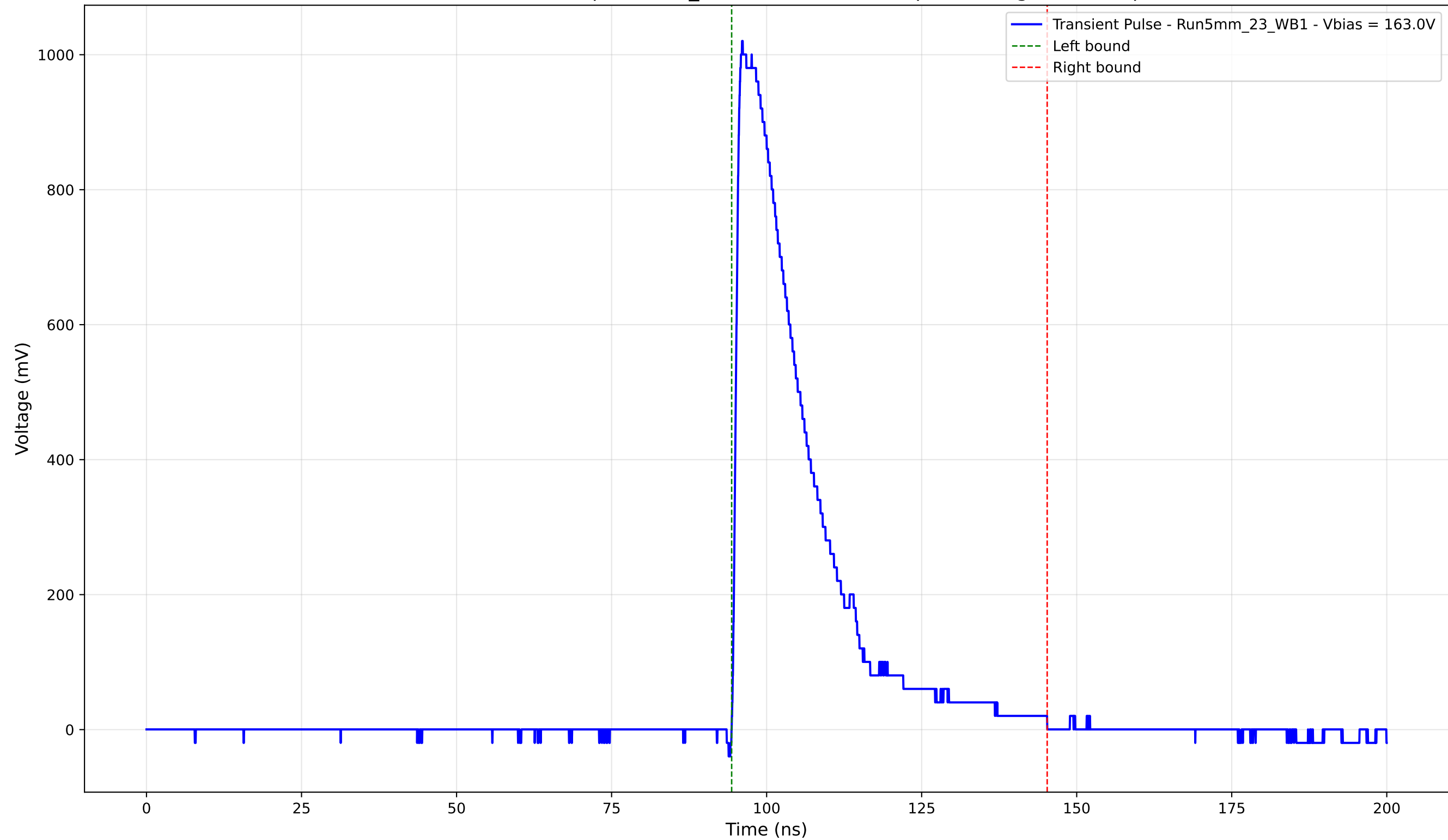
Transient Pulse - Sample: 5mm_23 - Position: 1525.0 \mu\text{m} - Charge: 253.64 pC
