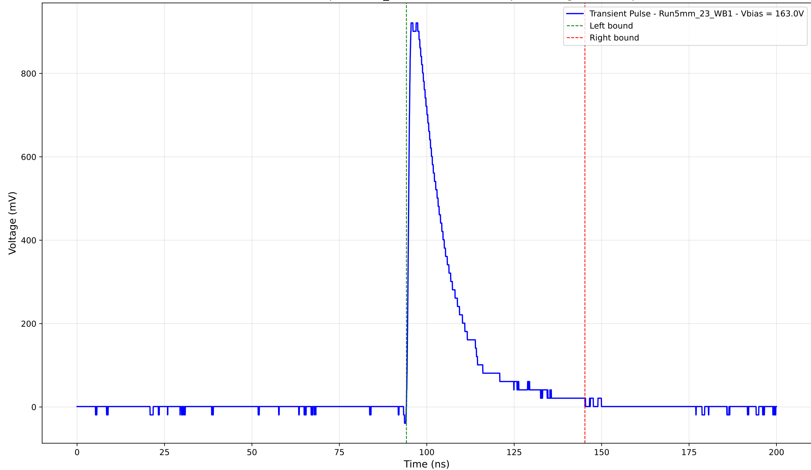
Transient Pulse - Sample: 5mm_23 - Position: 3435.0 \mu\text{m} - Charge: 217.05 pC
