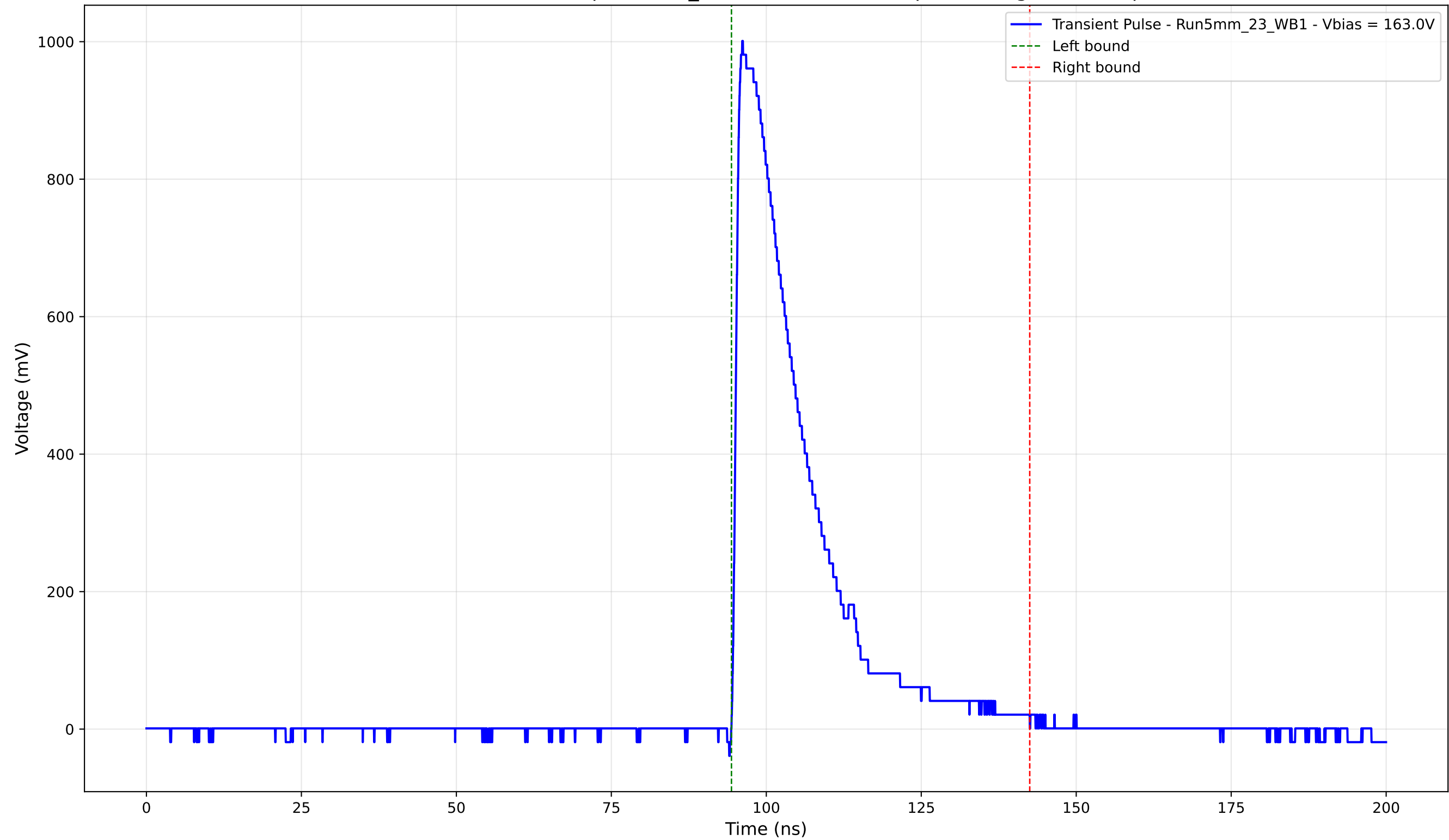
Transient Pulse - Sample: 5mm_23 - Position: 1440.0 \mu\text{m} - Charge: 238.24 pC
