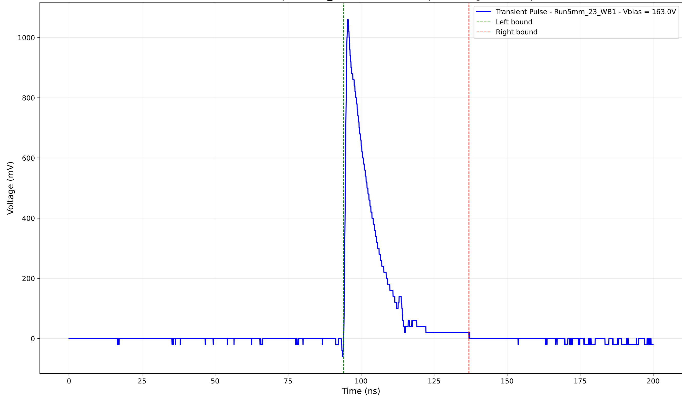
Transient Pulse - Sample: 5mm_23 - Position: 370.0 \mu\text{m} - Charge: 190.30 pC
