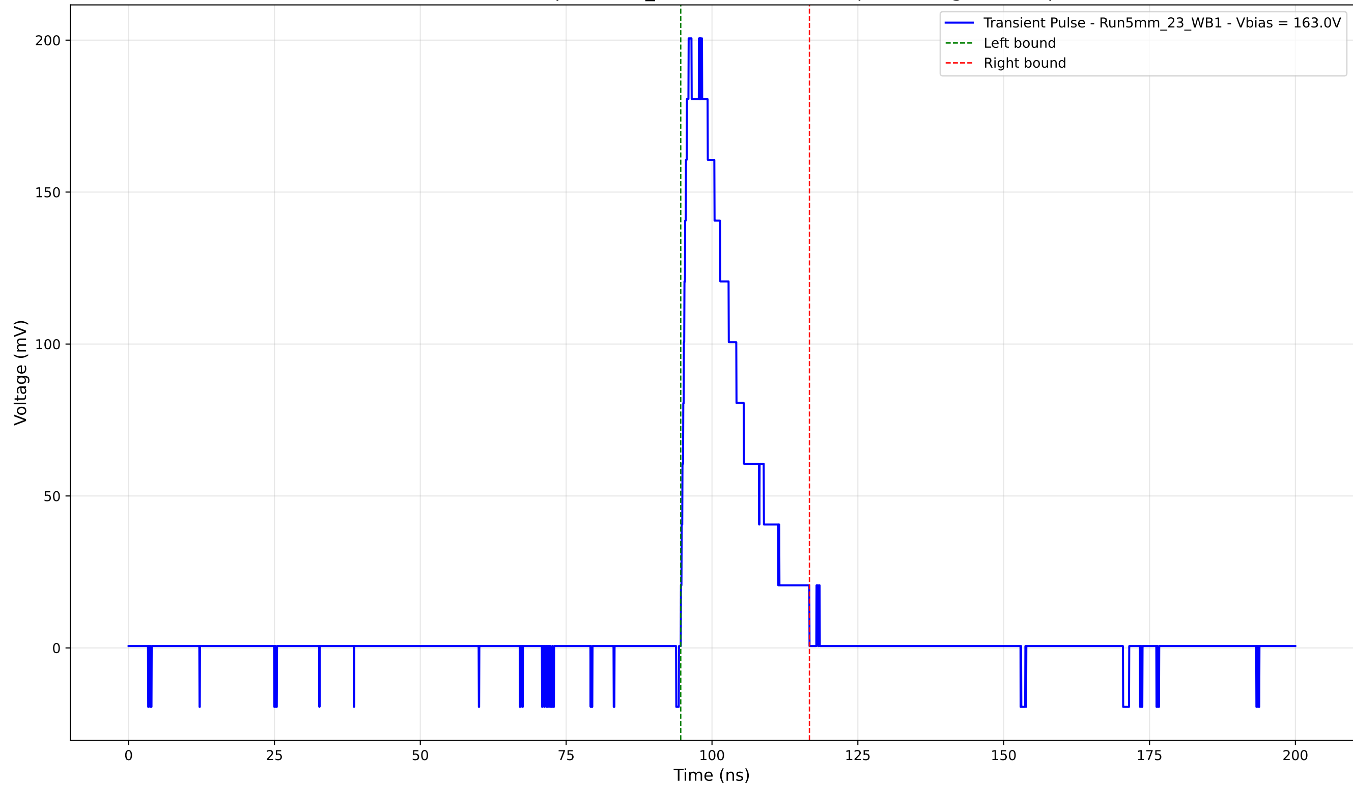
Transient Pulse - Sample: 5mm_23 - Position: 1225.0 \mu\text{m} - Charge: 38.22 pC
