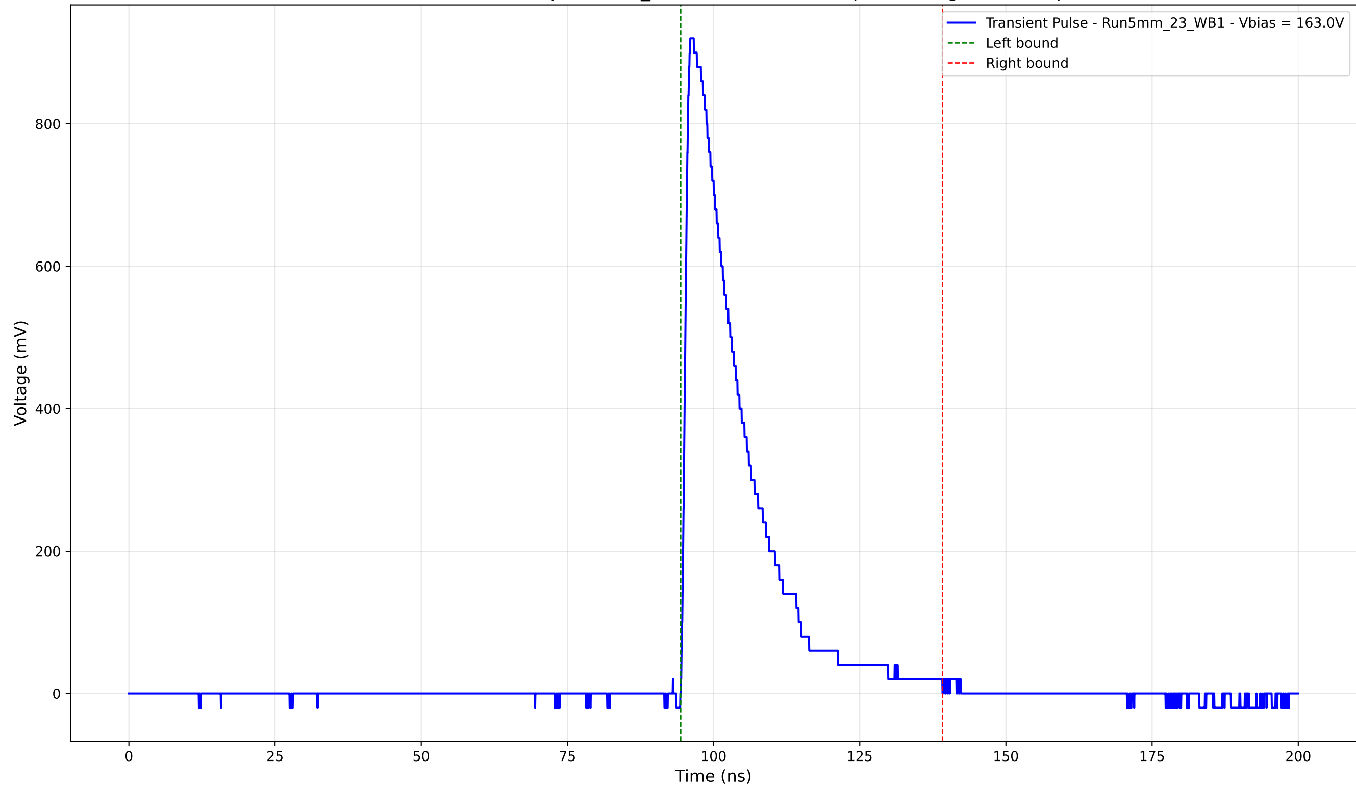
Transient Pulse - Sample: 5mm_23 - Position: 4060.0 \mu\text{m} - Charge: 198.24 pC
