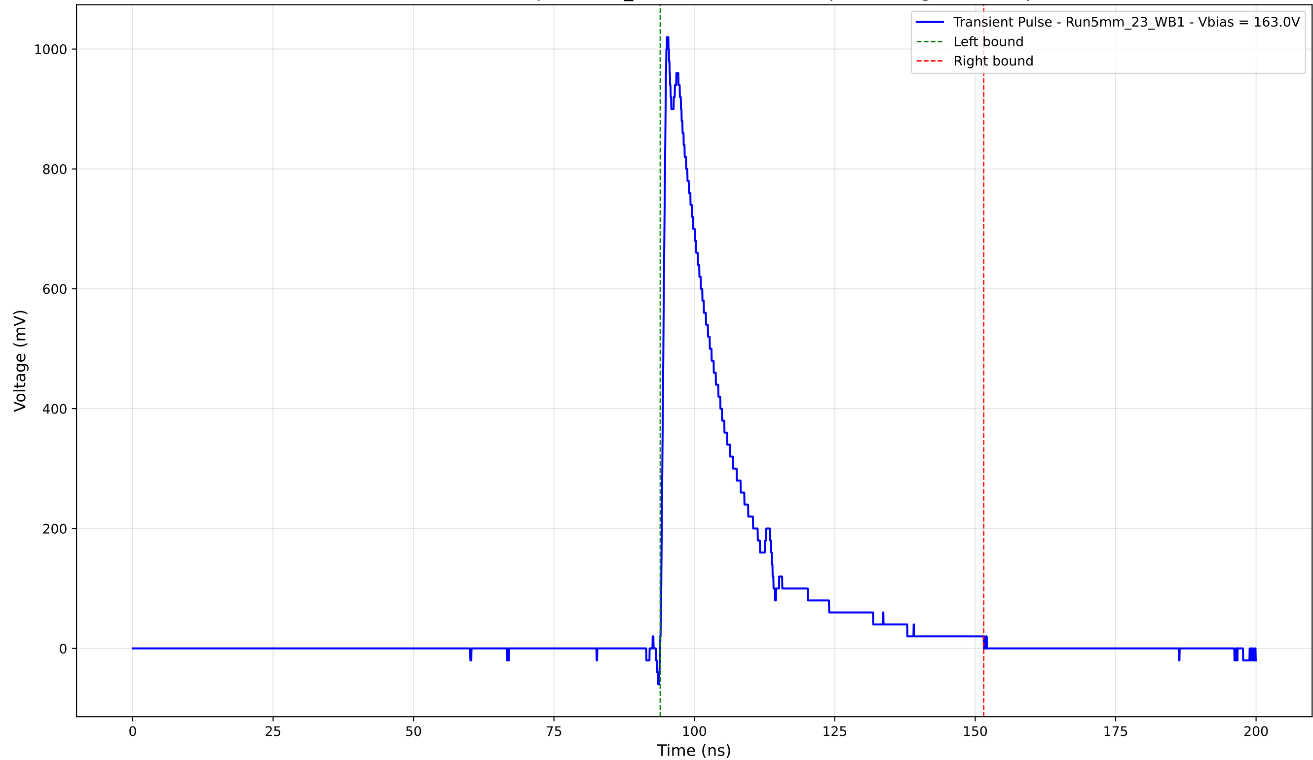
Transient Pulse - Sample: 5mm_23 - Position: 2485.0 \mu\text{m} - Charge: 233.22 pC
