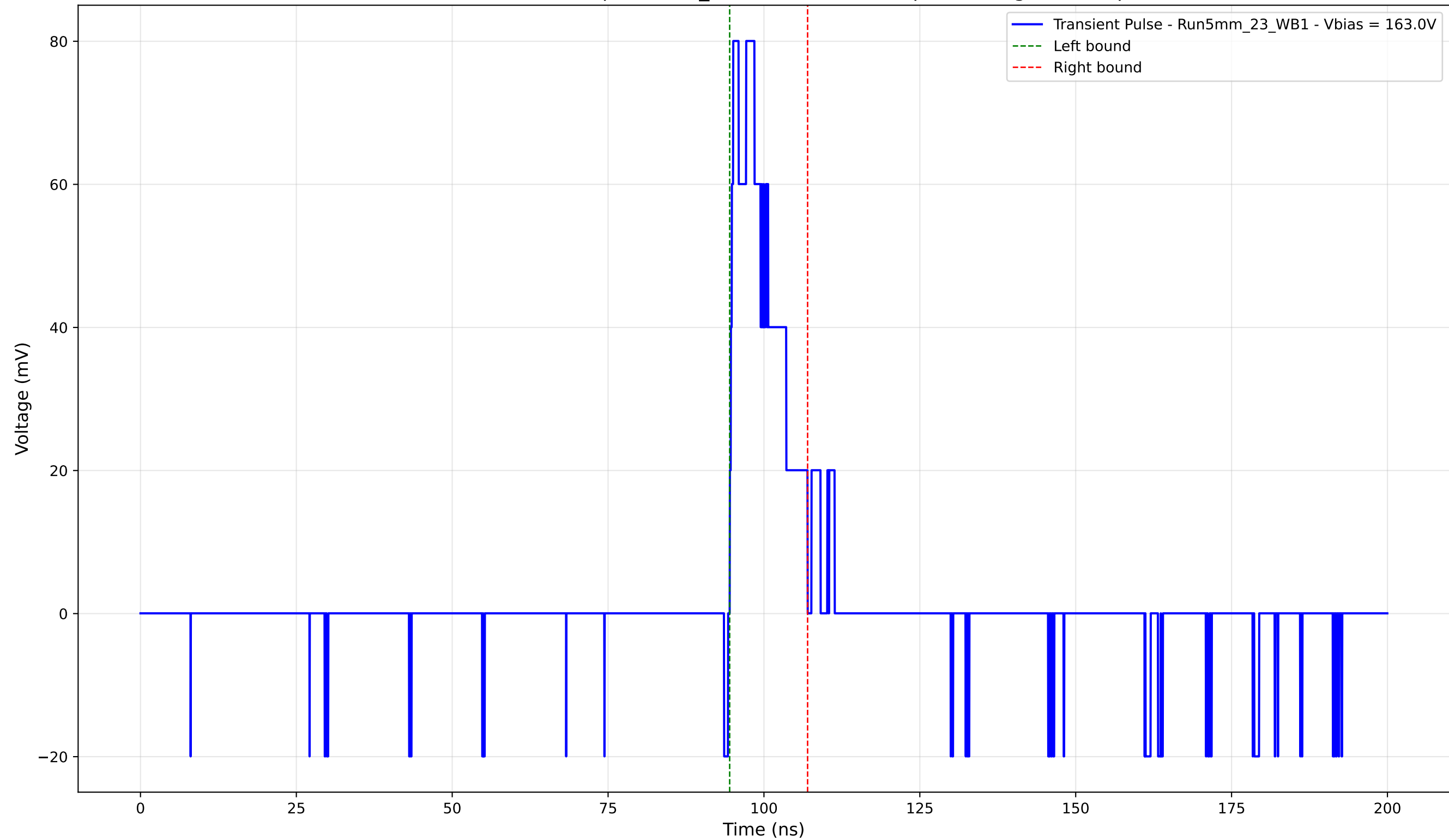
Transient Pulse - Sample: 5mm_23 - Position: 265.0 \mu\text{m} - Charge: 11.43 pC
