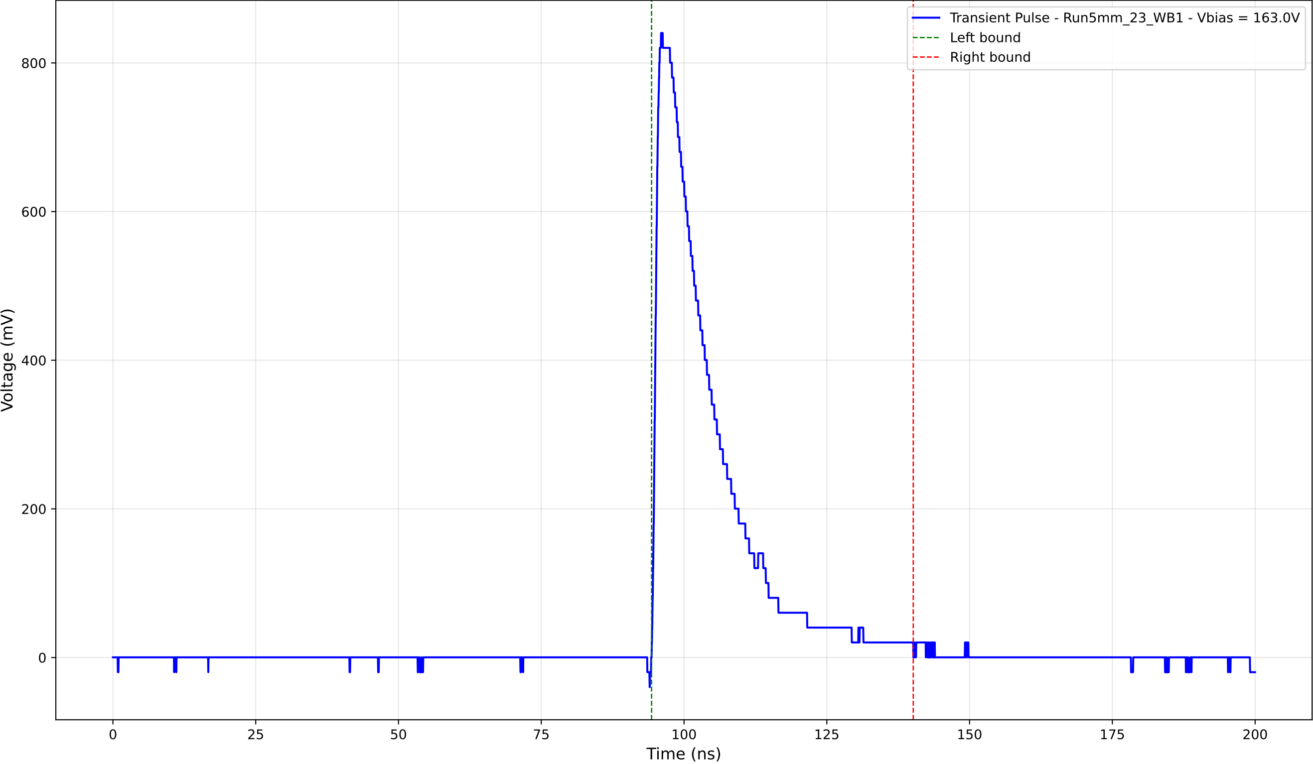
Transient Pulse - Sample: 5mm_23 - Position: 1800.0 \mu\text{m} - Charge: 183.46 pC
