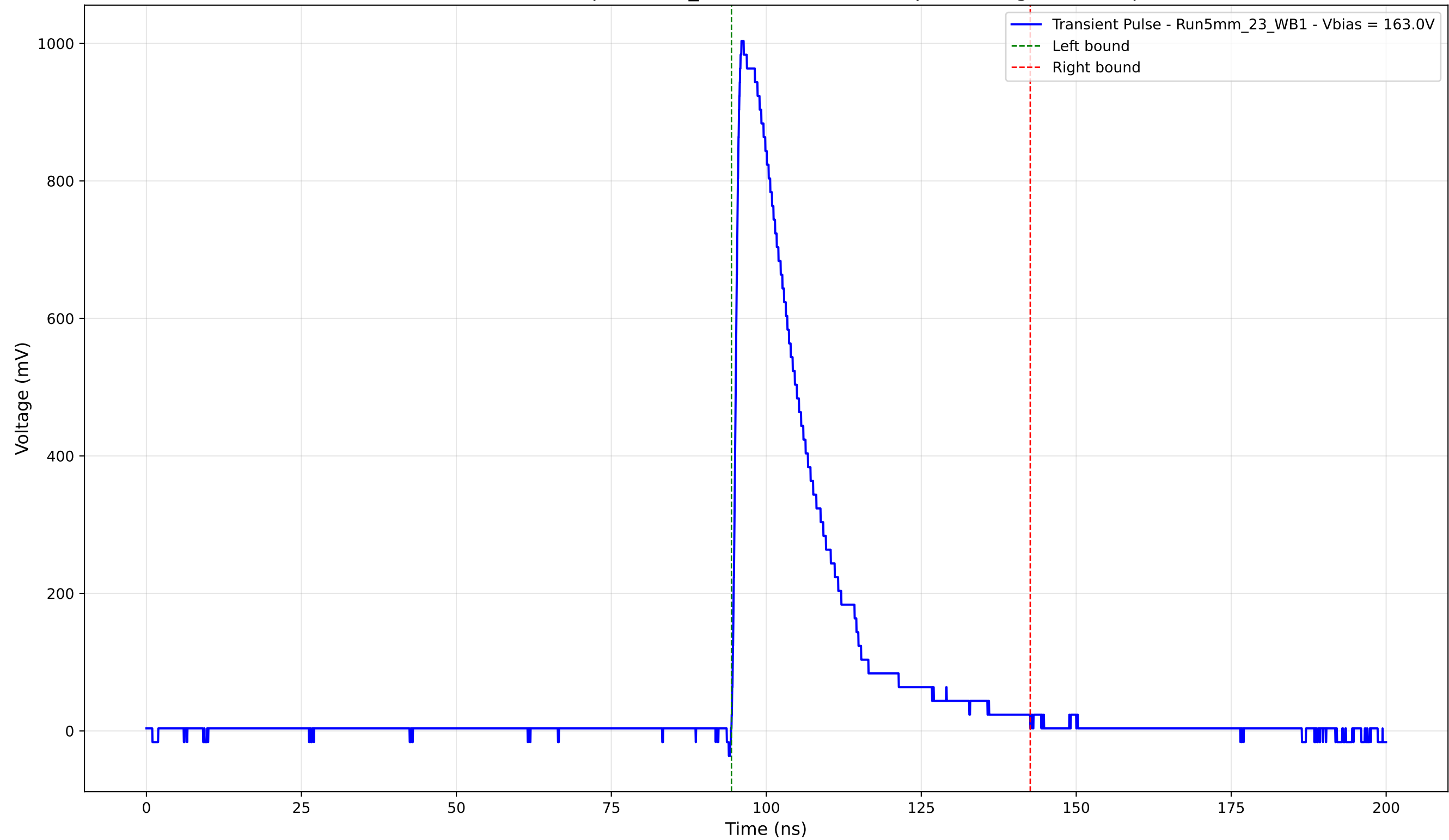
Transient Pulse - Sample: 5mm_23 - Position: 1460.0 \mu\text{m} - Charge: 244.94 pC
