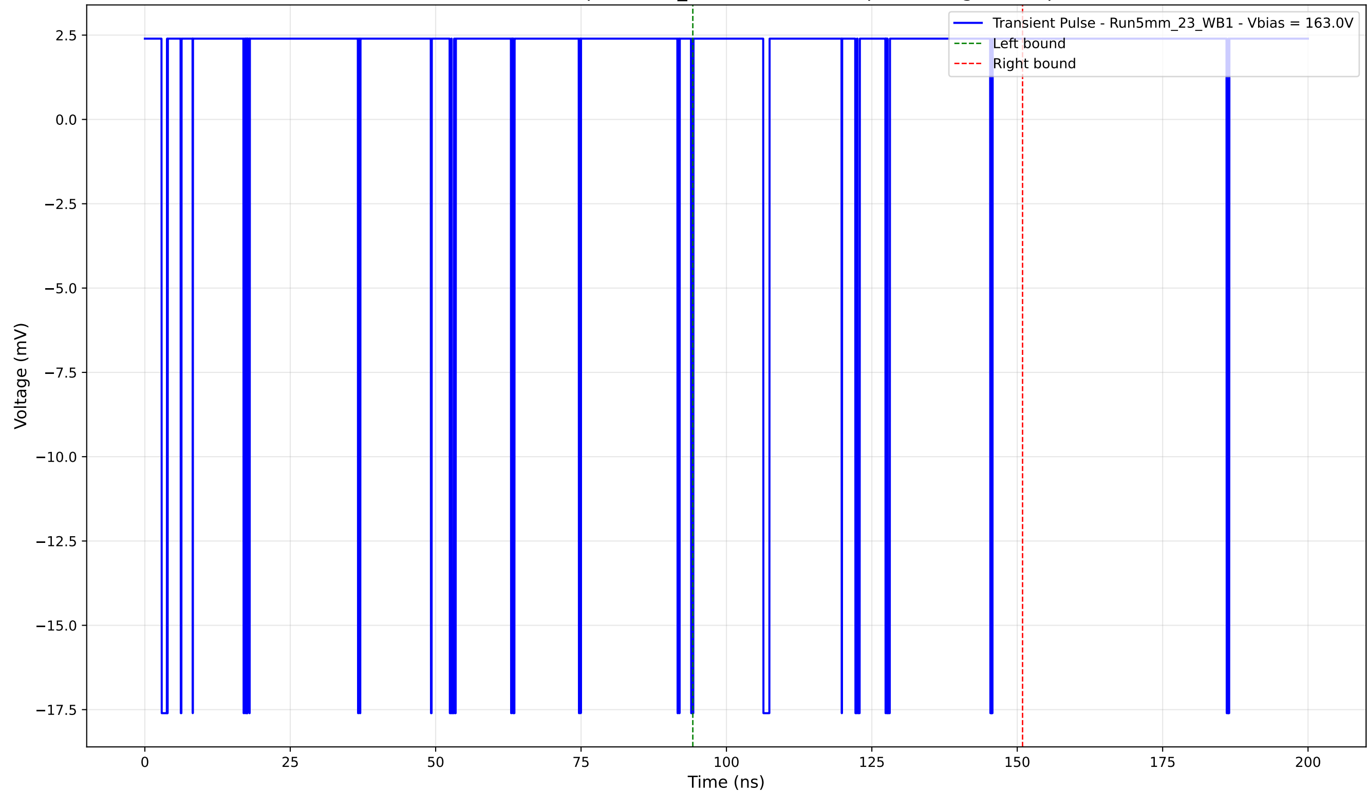
Transient Pulse - Sample: 5mm_23 - Position: 60.0 \mu\text{m} - Charge: 1.61 pC
