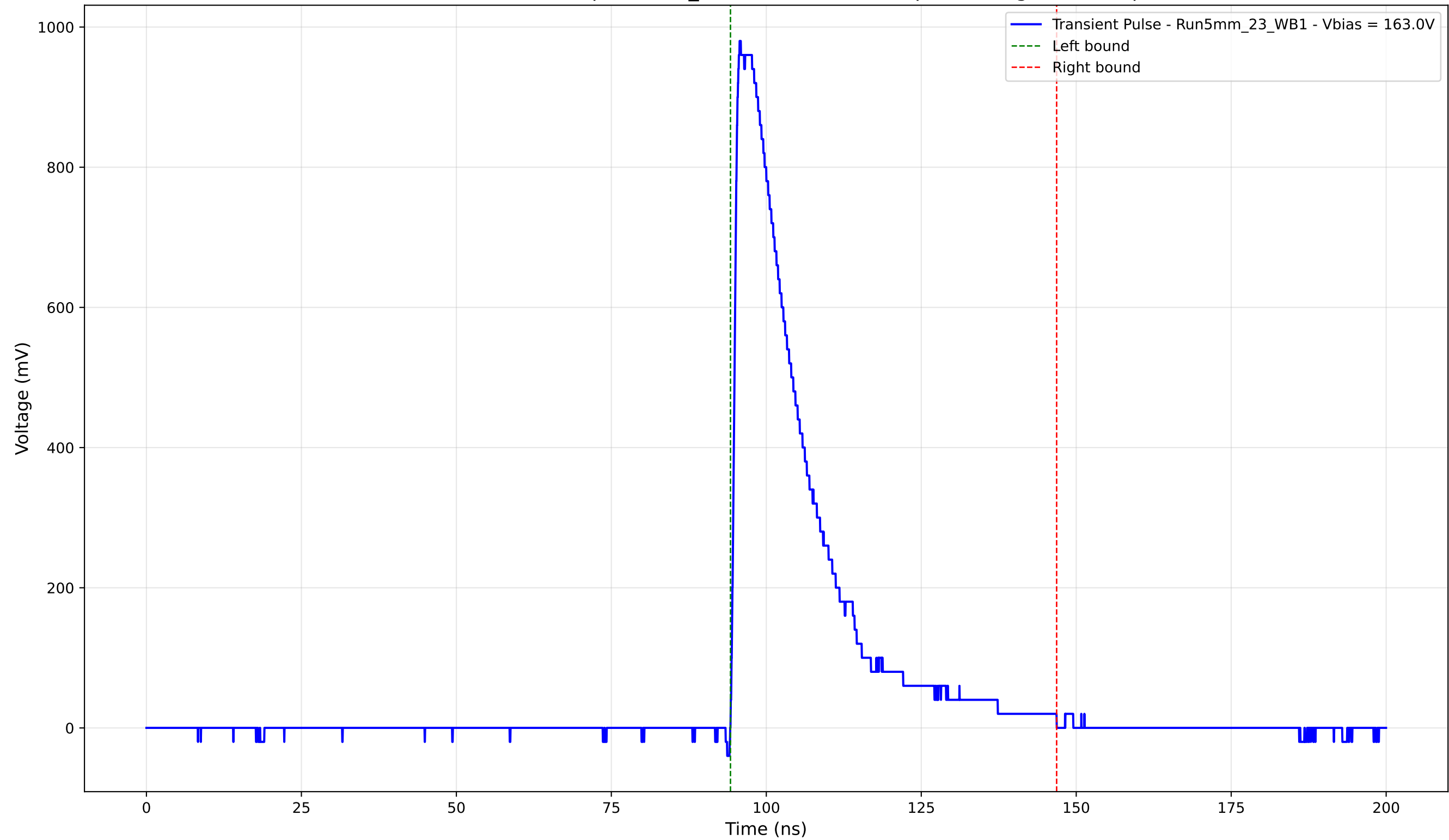
Transient Pulse - Sample: 5mm_23 - Position: 1960.0 \mu\text{m} - Charge: 239.74 pC
