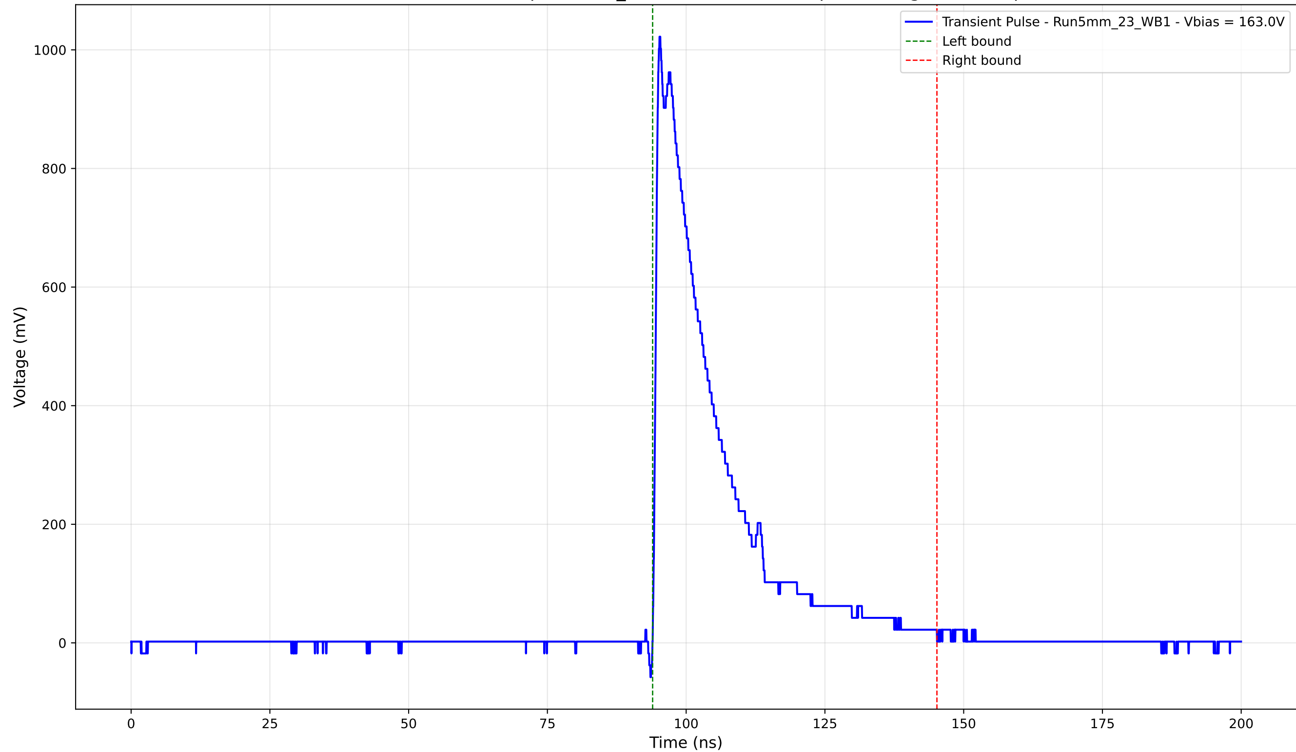
Transient Pulse - Sample: 5mm_23 - Position: 2450.0 \mu\text{m} - Charge: 231.26 pC
