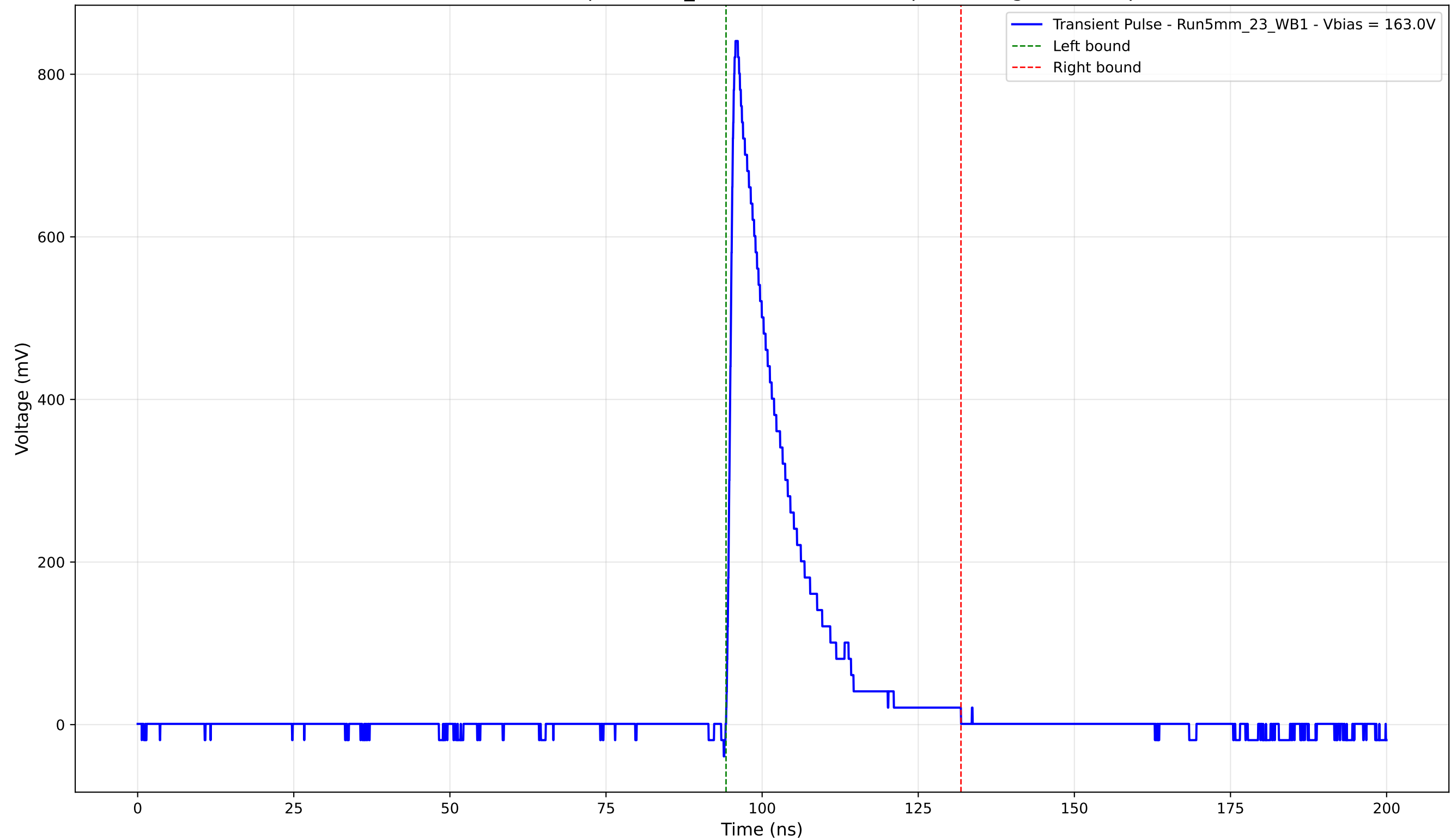
Transient Pulse - Sample: 5mm_23 - Position: 4695.0 \mu\text{m} - Charge: 144.55 pC
