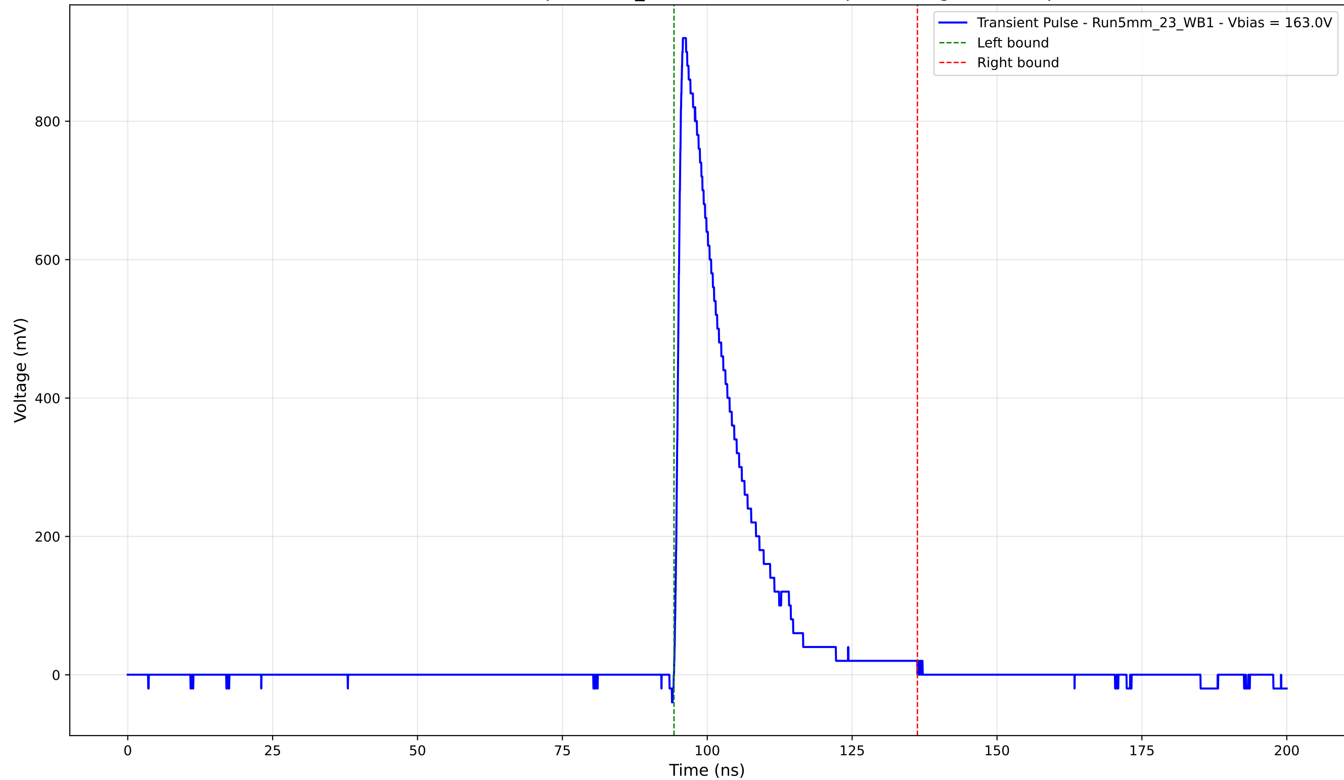
Transient Pulse - Sample: 5mm_23 - Position: 4540.0 \mu\text{m} - Charge: 177.50 pC
