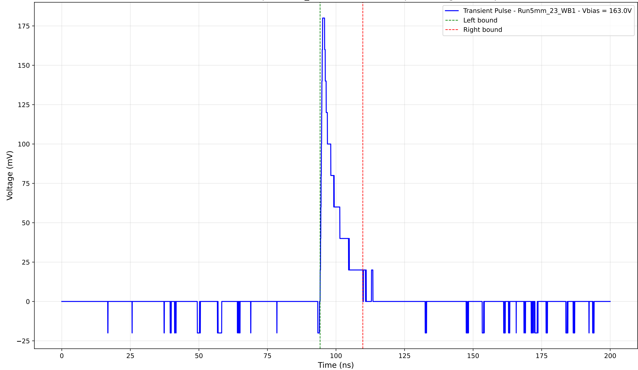
Transient Pulse - Sample: 5mm_23 -Position: 5195.0 \mu\text{m} - Charge: 18.65 pC
