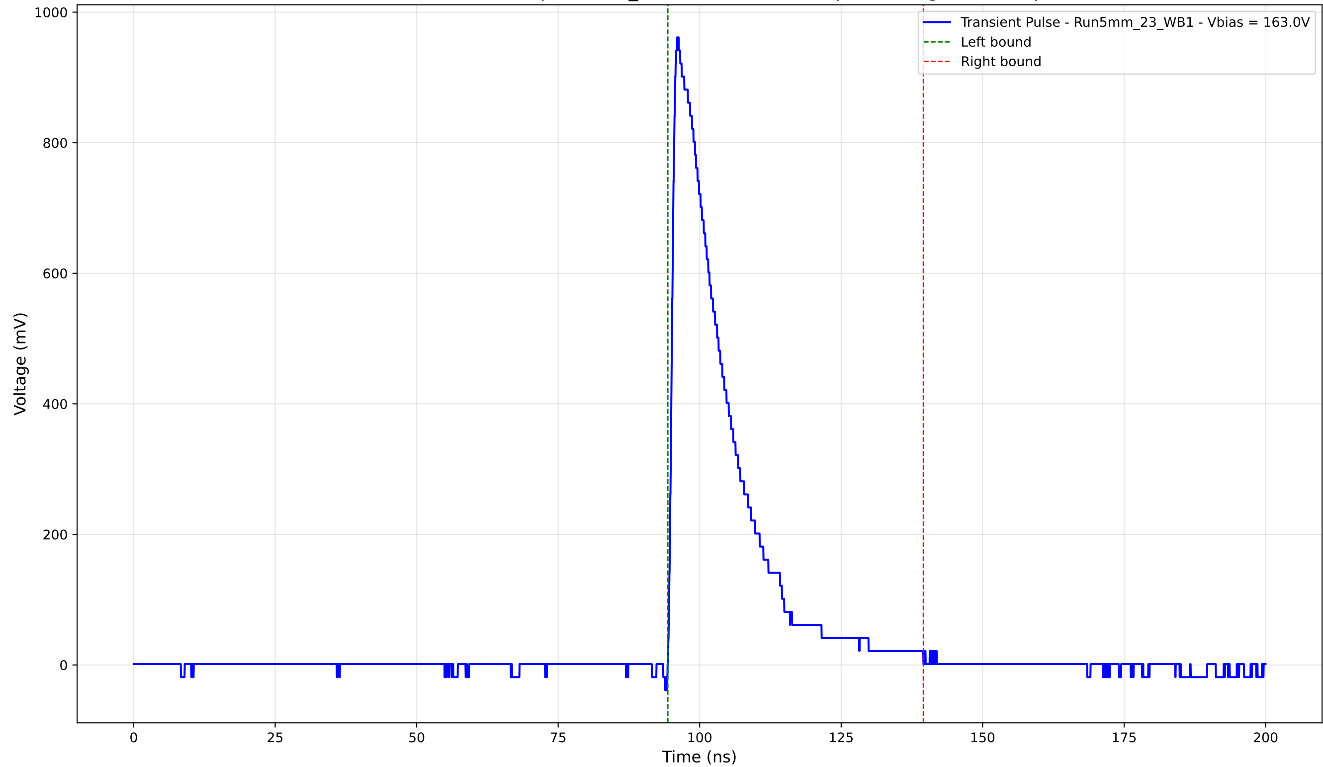
Transient Pulse - Sample: 5mm_23 - Position: 1080.0 \mu\text{m} - Charge: 204.28 pC
