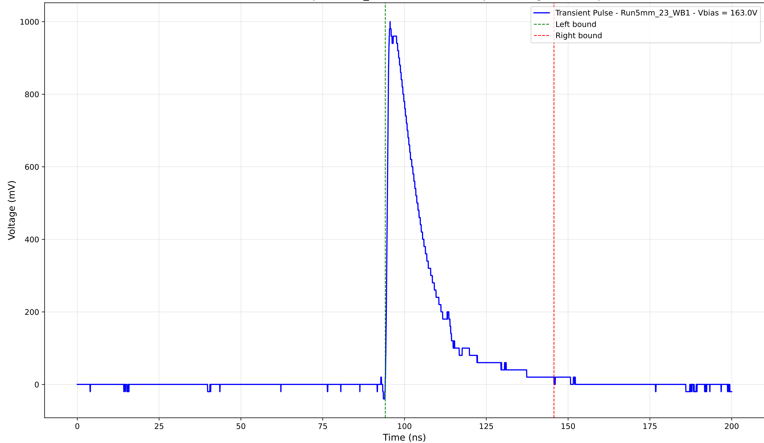
Transient Pulse - Sample: 5mm_23 - Position: 2125.0 \mu\text{m} - Charge: 239.53 pC
