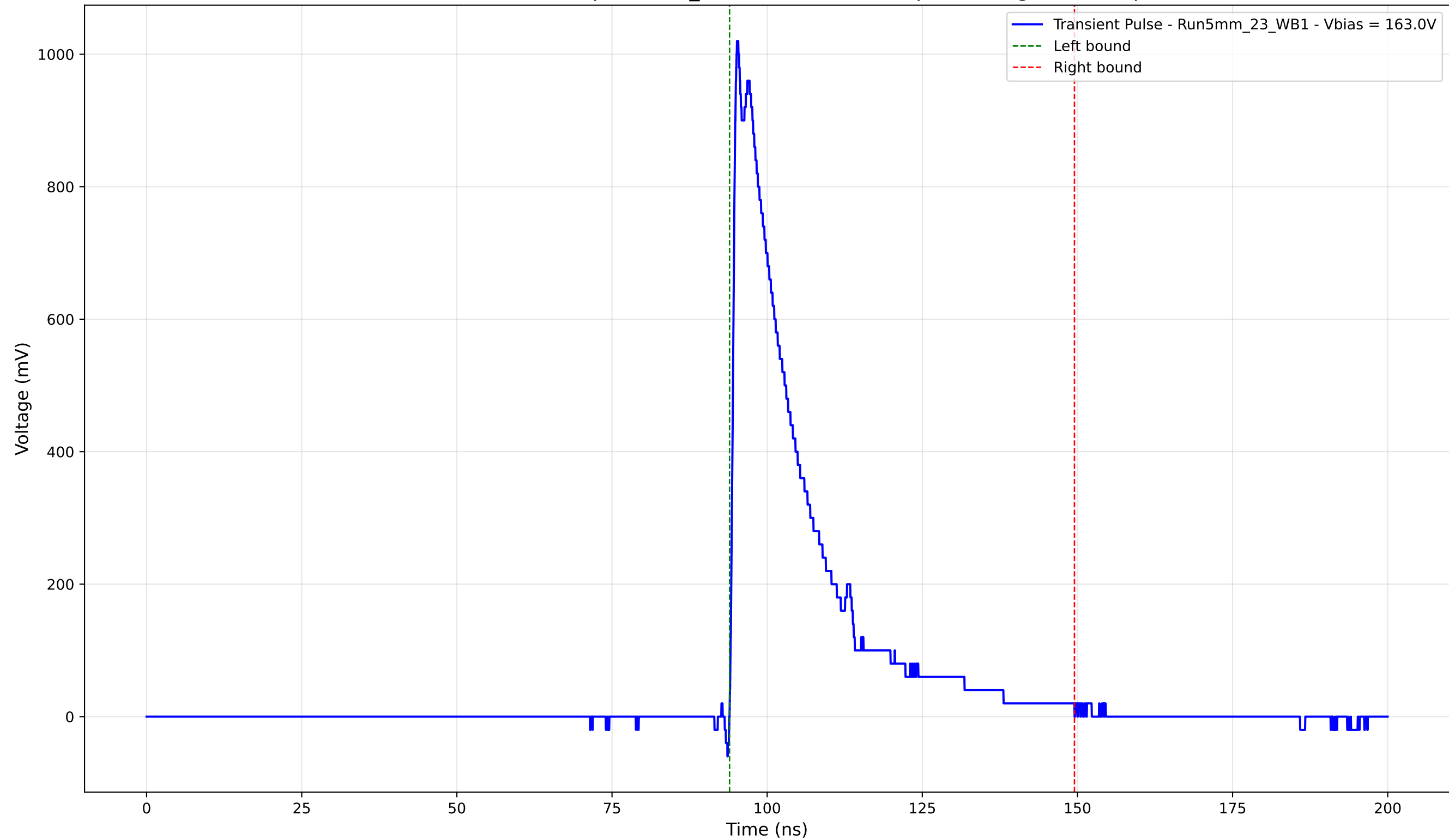
Transient Pulse - Sample: 5mm_23 - Position: 2475.0 \mu\text{m} - Charge: 231.62 pC
