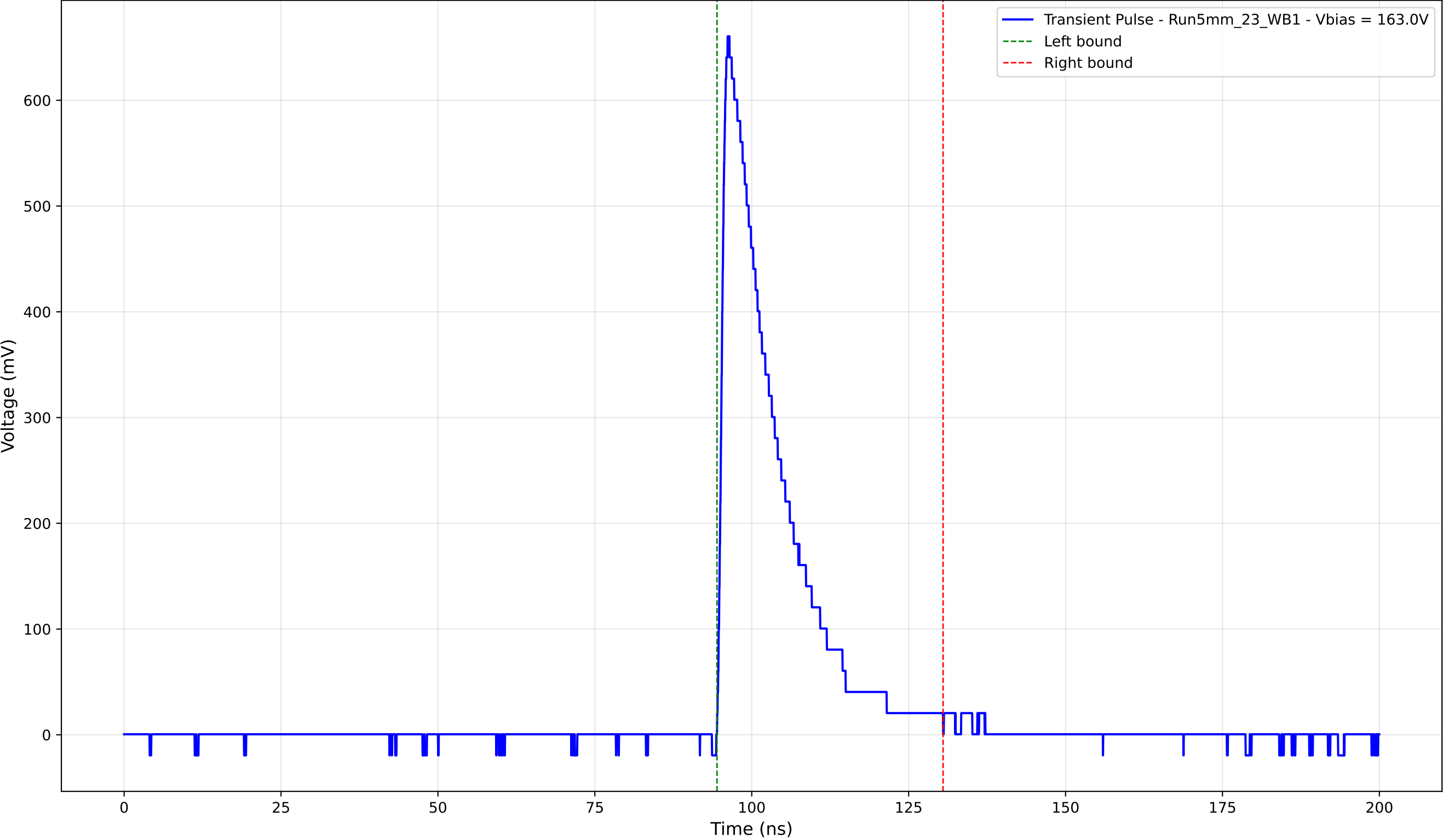
Transient Pulse - Sample: 5mm_23 - Position: 1275.0 \mu\text{m} - Charge: 125.69 pC
