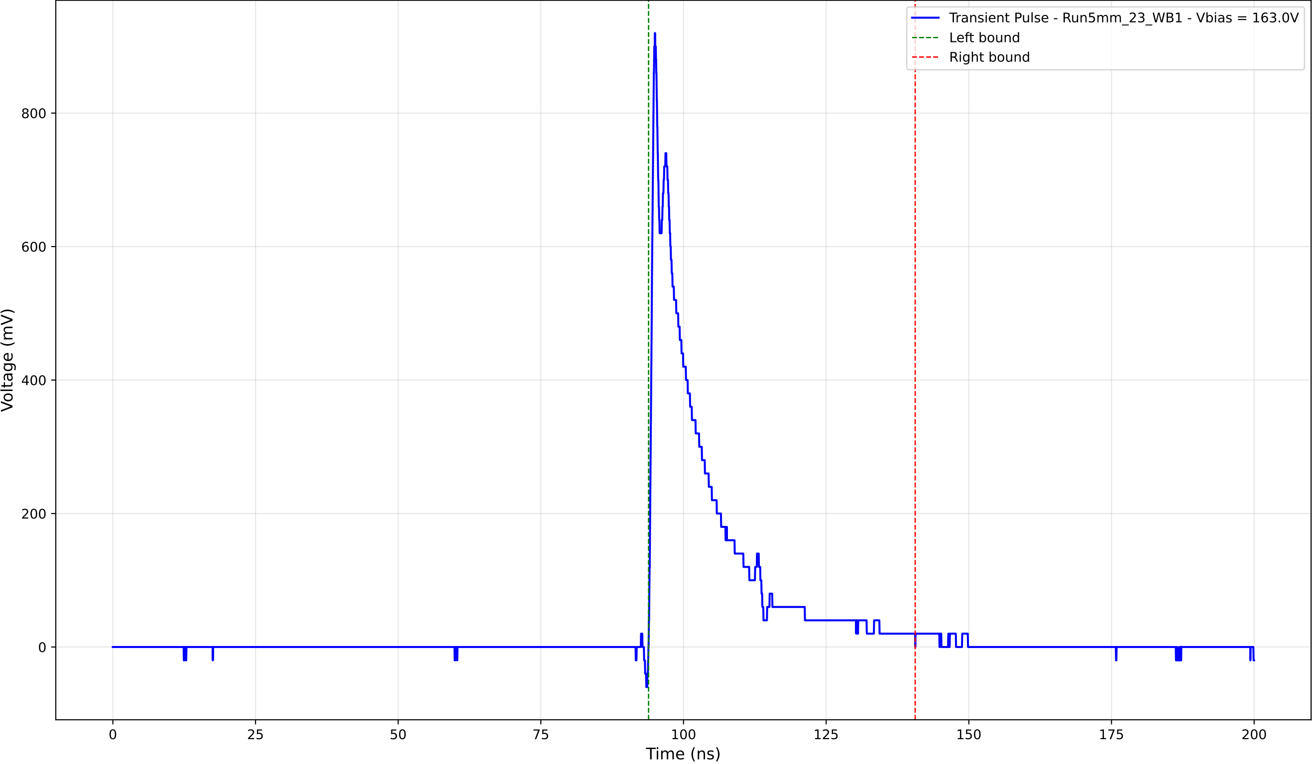
Transient Pulse - Sample: 5mm_23 - Position: 2800.0 \mu\text{m} - Charge: 151.80 pC
