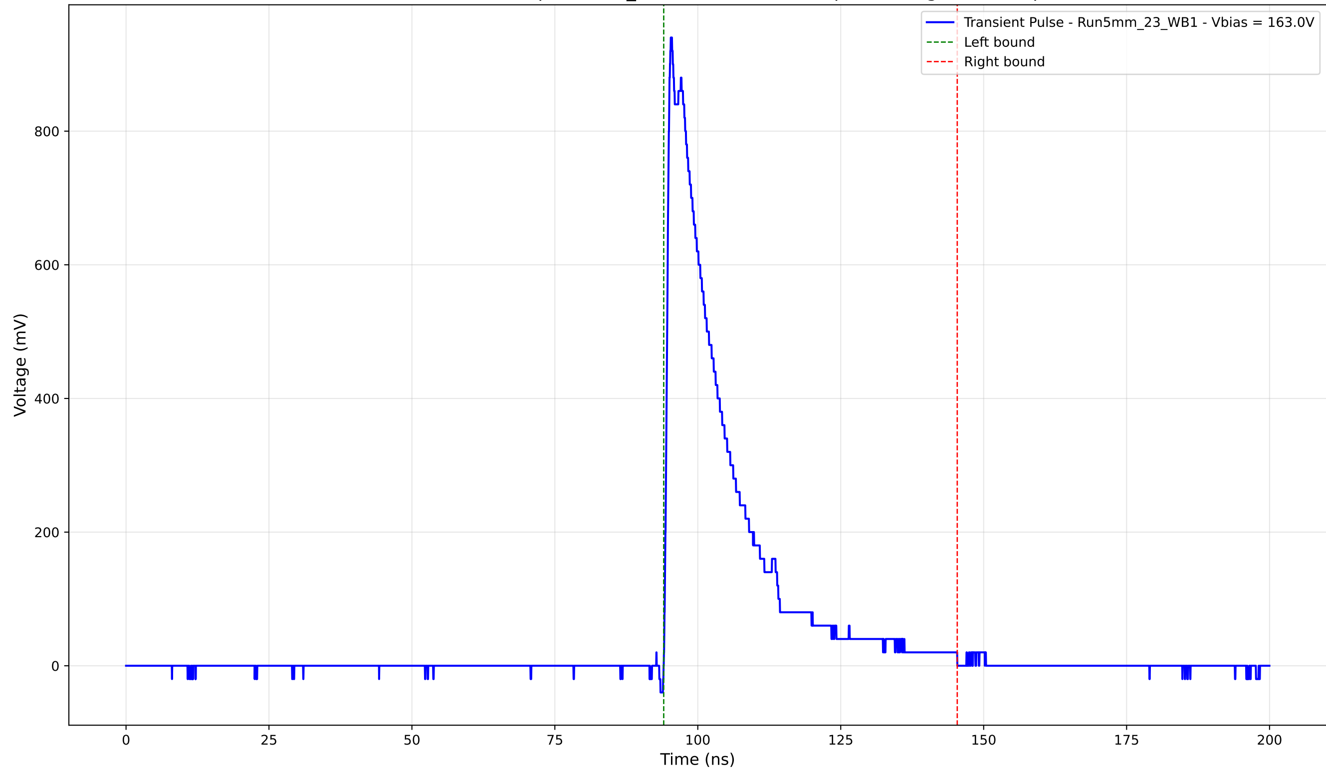
Transient Pulse - Sample: 5mm_23 - Position: 2320.0 \mu\text{m} - Charge: 198.81 pC
