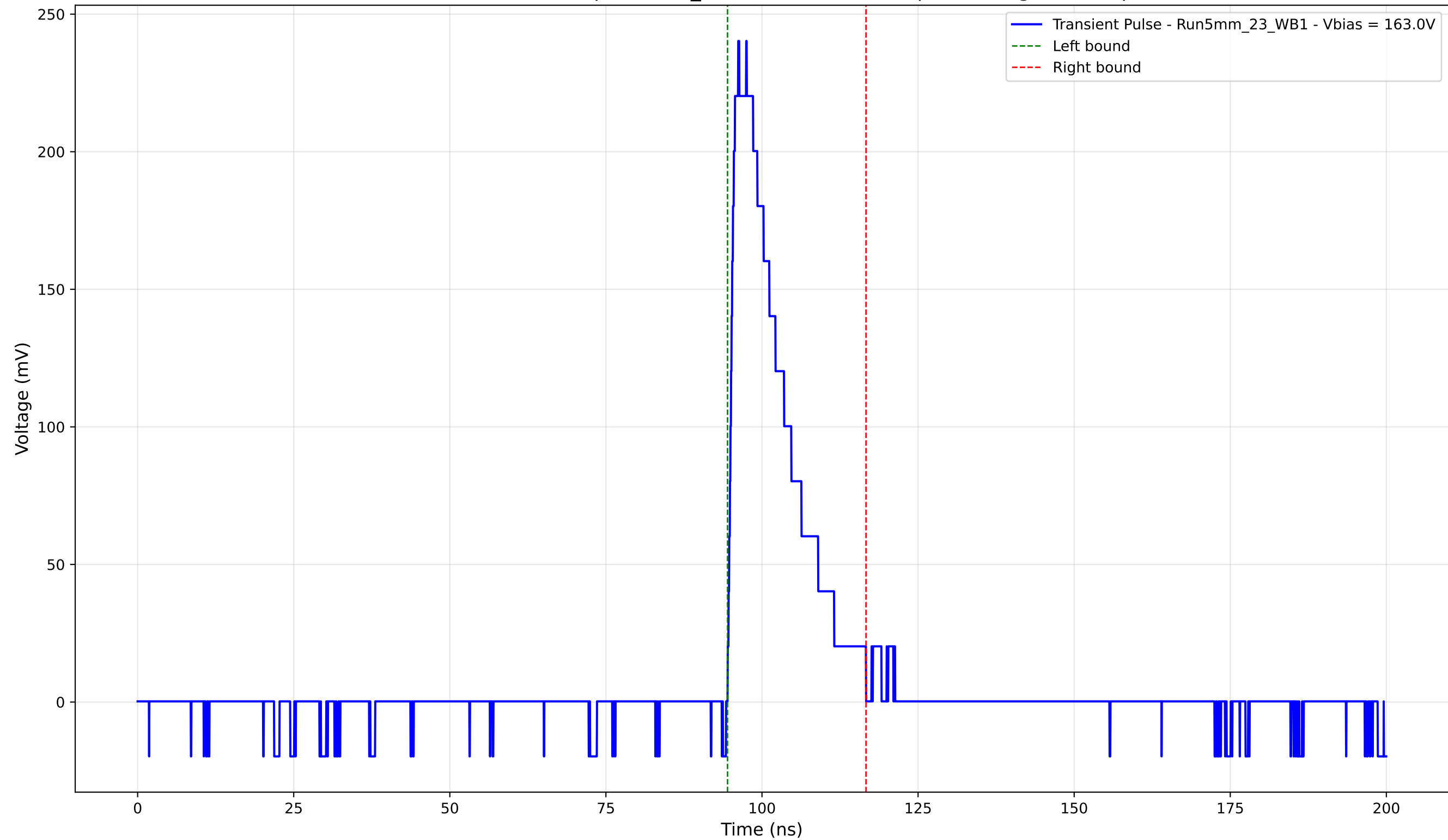
Transient Pulse - Sample: 5mm_23 - Position: 3740.0 \mu\text{m} - Charge: 43.29 pC
