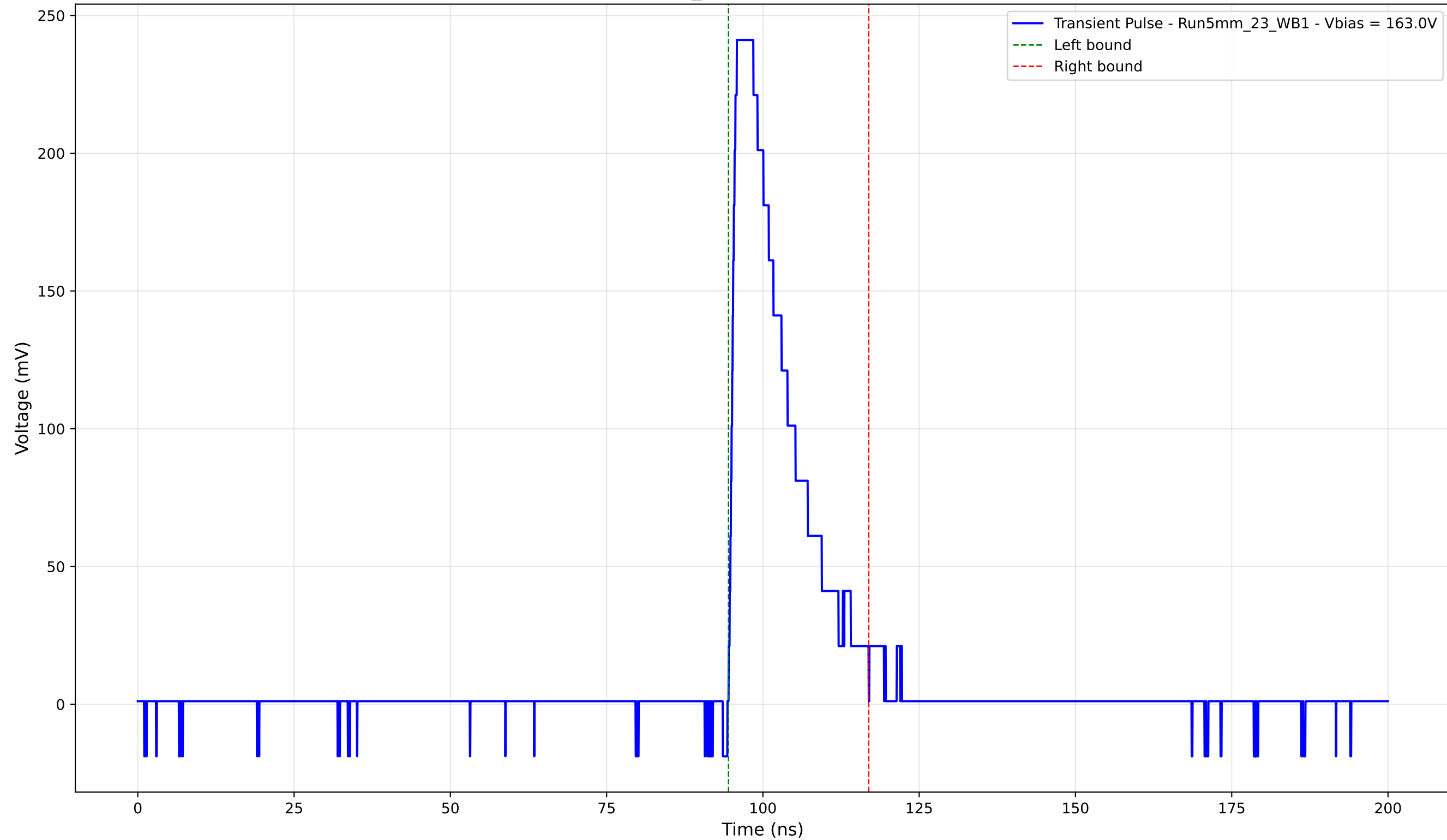
Transient Pulse - Sample: 5mm_23 - Position: 1715.0 \mu\text{m} - Charge: 47.58 pC
