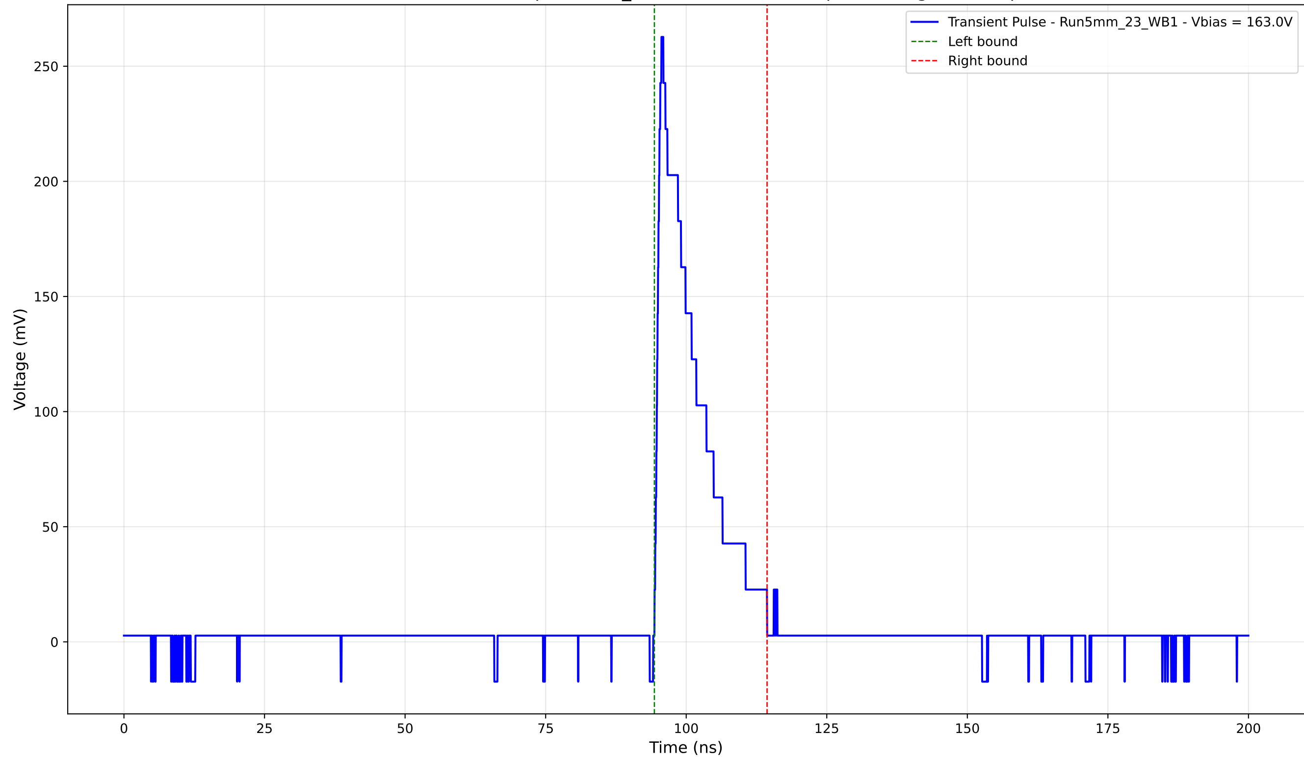
Transient Pulse - Sample: 5mm_23 - Position: 4780.0 \mu\text{m} - Charge: 39.11 pC
