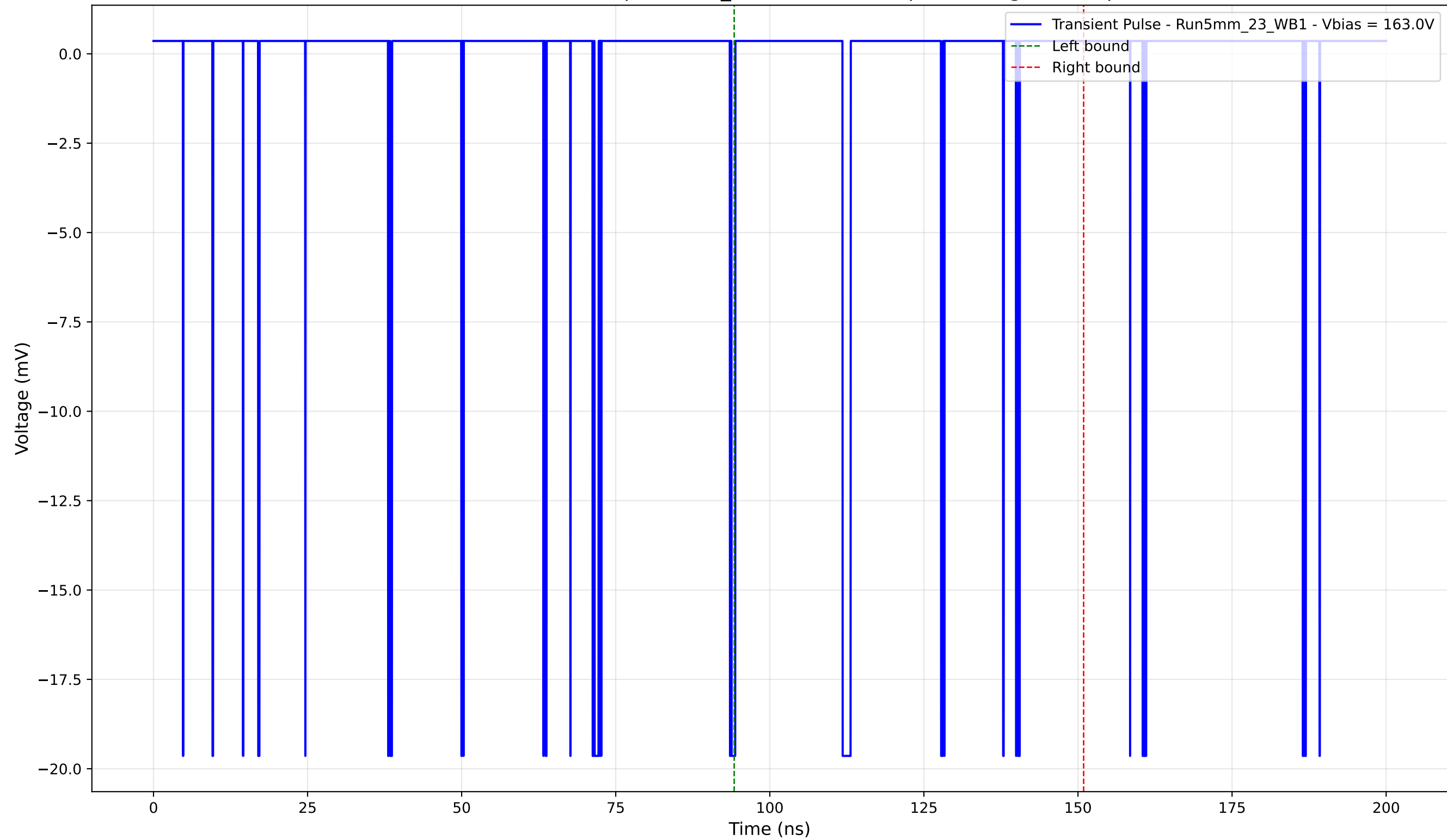
Transient Pulse - Sample: 5mm_23 - Position: 5.0 \mu\text{m} - Charge: -0.52 pC
