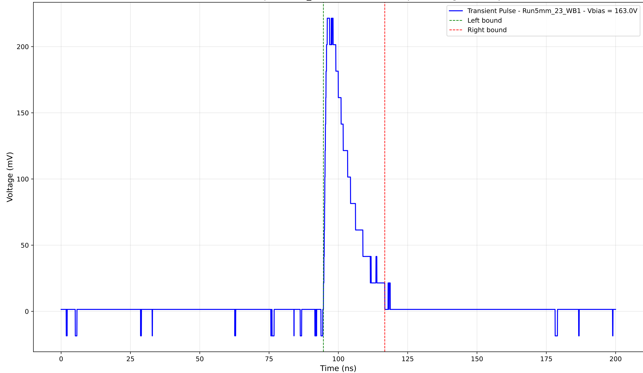
Transient Pulse - Sample: 5mm_23 - Position: 1235.0 \mu\text{m} - Charge: 41.85 pC
