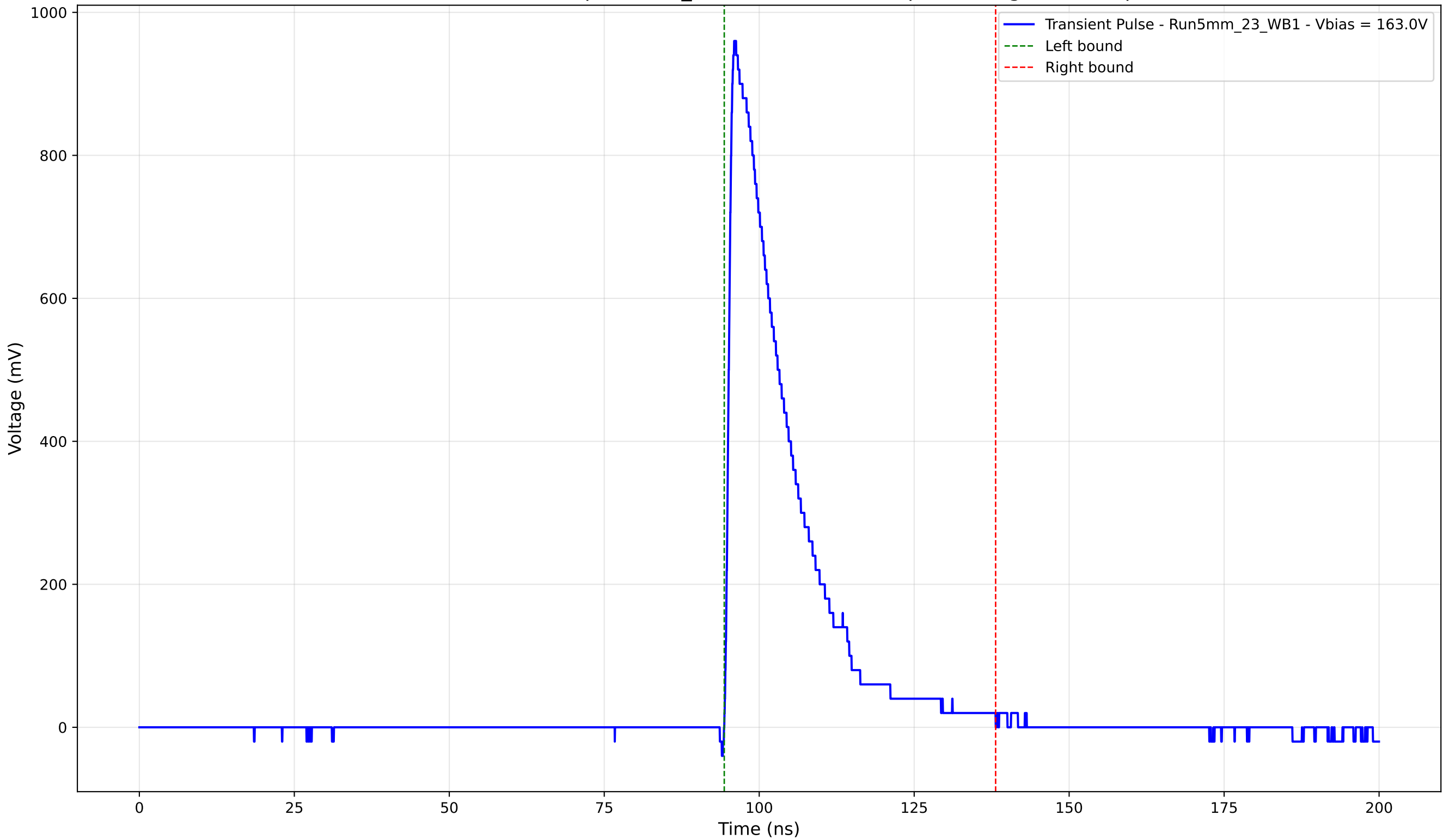
Transient Pulse - Sample: 5mm_23 - Position: 1050.0 \mu\text{m} - Charge: 202.33 pC
