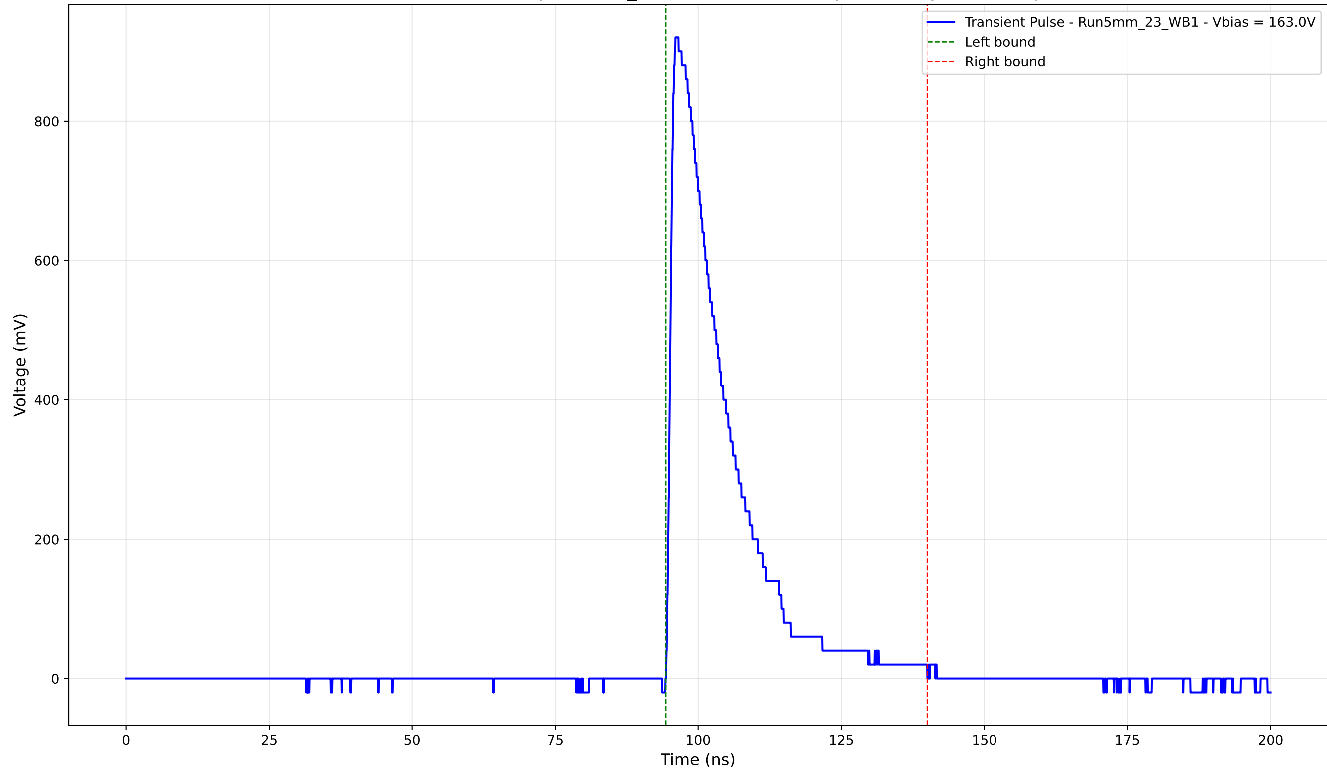
Transient Pulse - Sample: 5mm_23 - Position: 4045.0 \mu\text{m} - Charge: 198.48 pC
