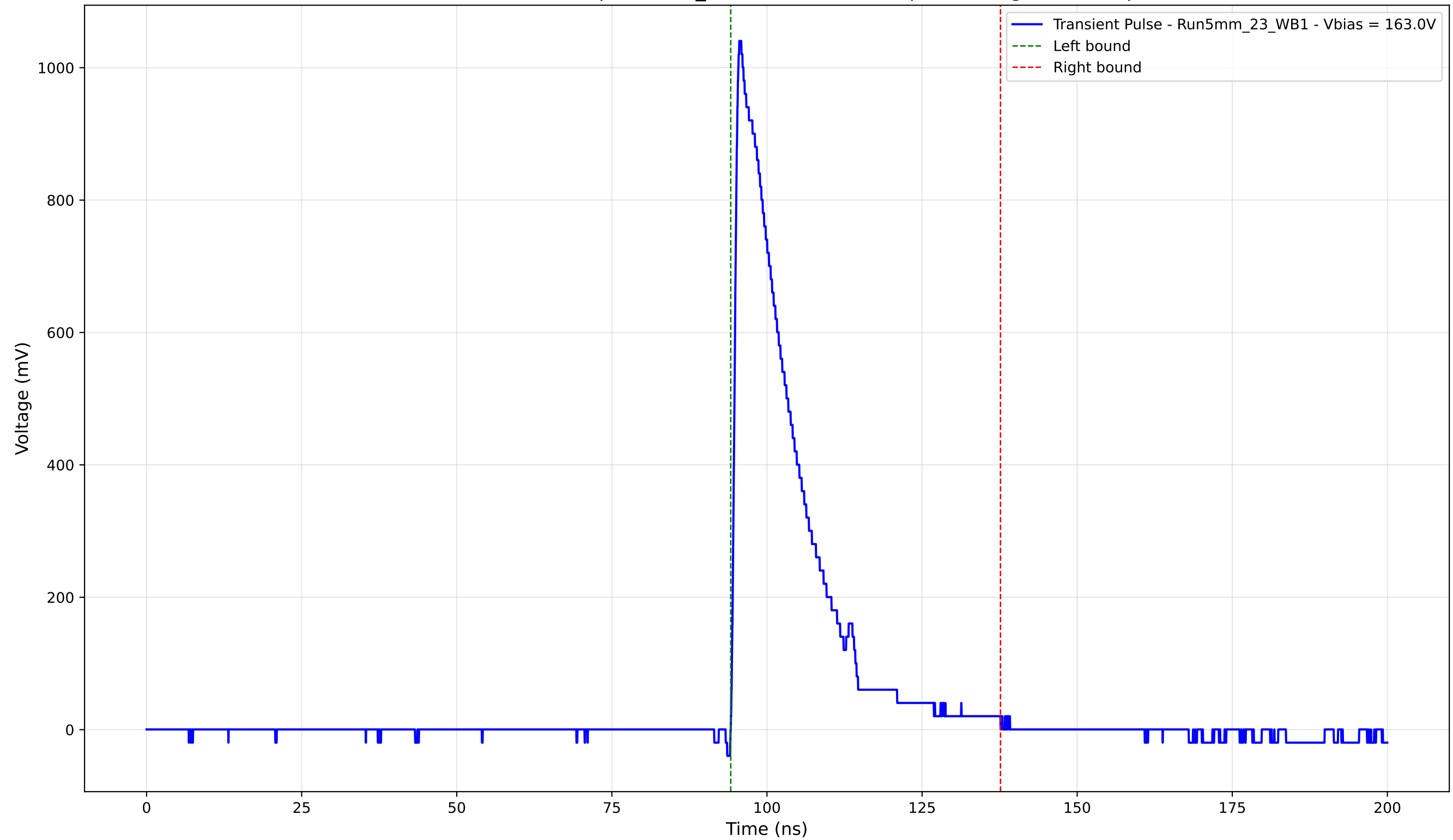
Transient Pulse - Sample: 5mm_23 - Position: 605.0 \mu\text{m} - Charge: 210.94 pC
