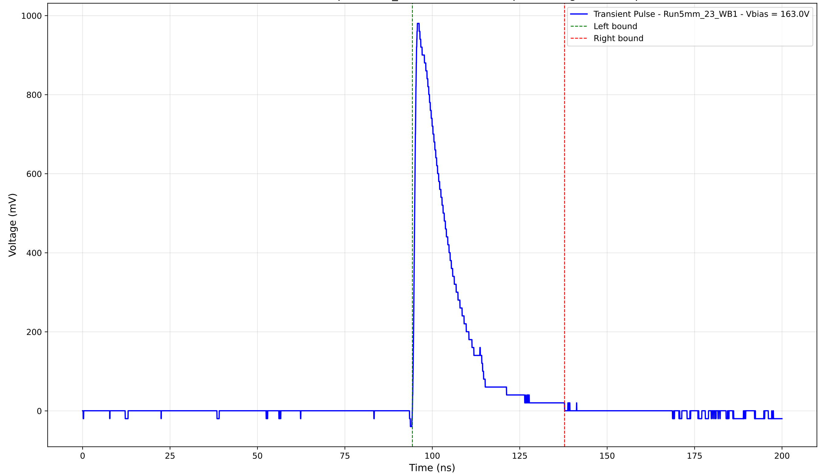
Transient Pulse - Sample: 5mm_23 - Position: 865.0 \mu\text{m} - Charge: 204.66 pC
