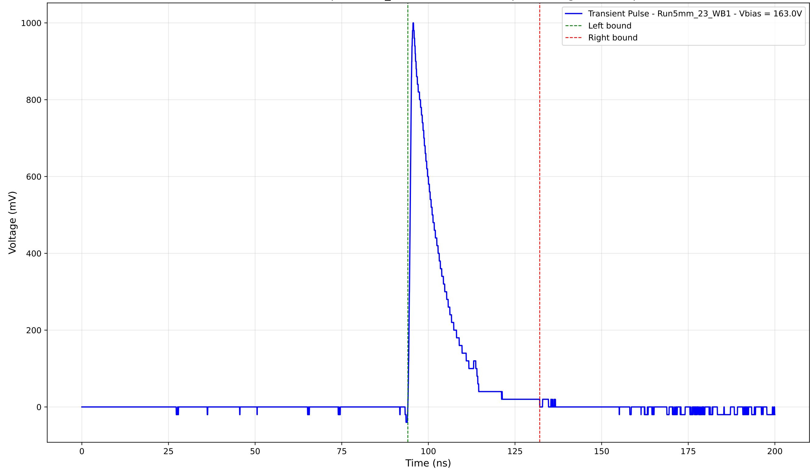
Transient Pulse - Sample: 5mm_23 - Position: 4910.0 \mu\text{m} - Charge: 169.85 pC
