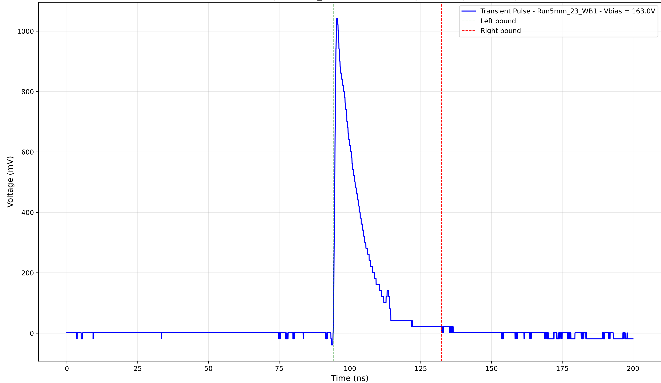
Transient Pulse - Sample: 5mm_23 - Position: 360.0 \mu\text{m} - Charge: 180.71 pC
