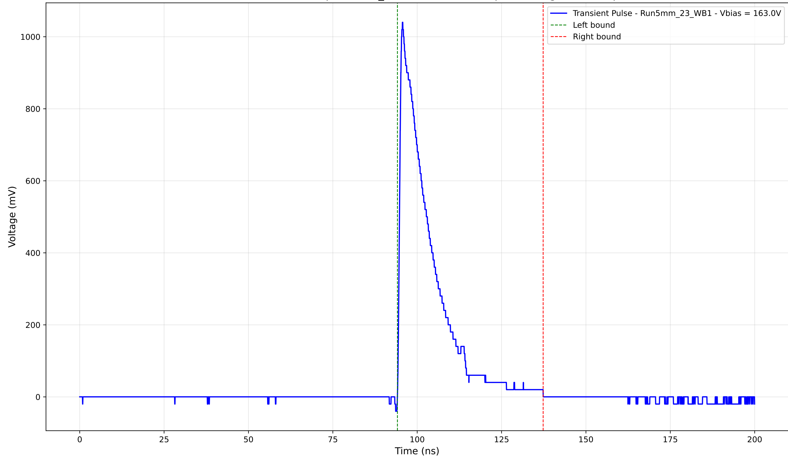
Transient Pulse - Sample: 5mm_23 - Position: 555.0 \mu\text{m} - Charge: 200.88 pC
