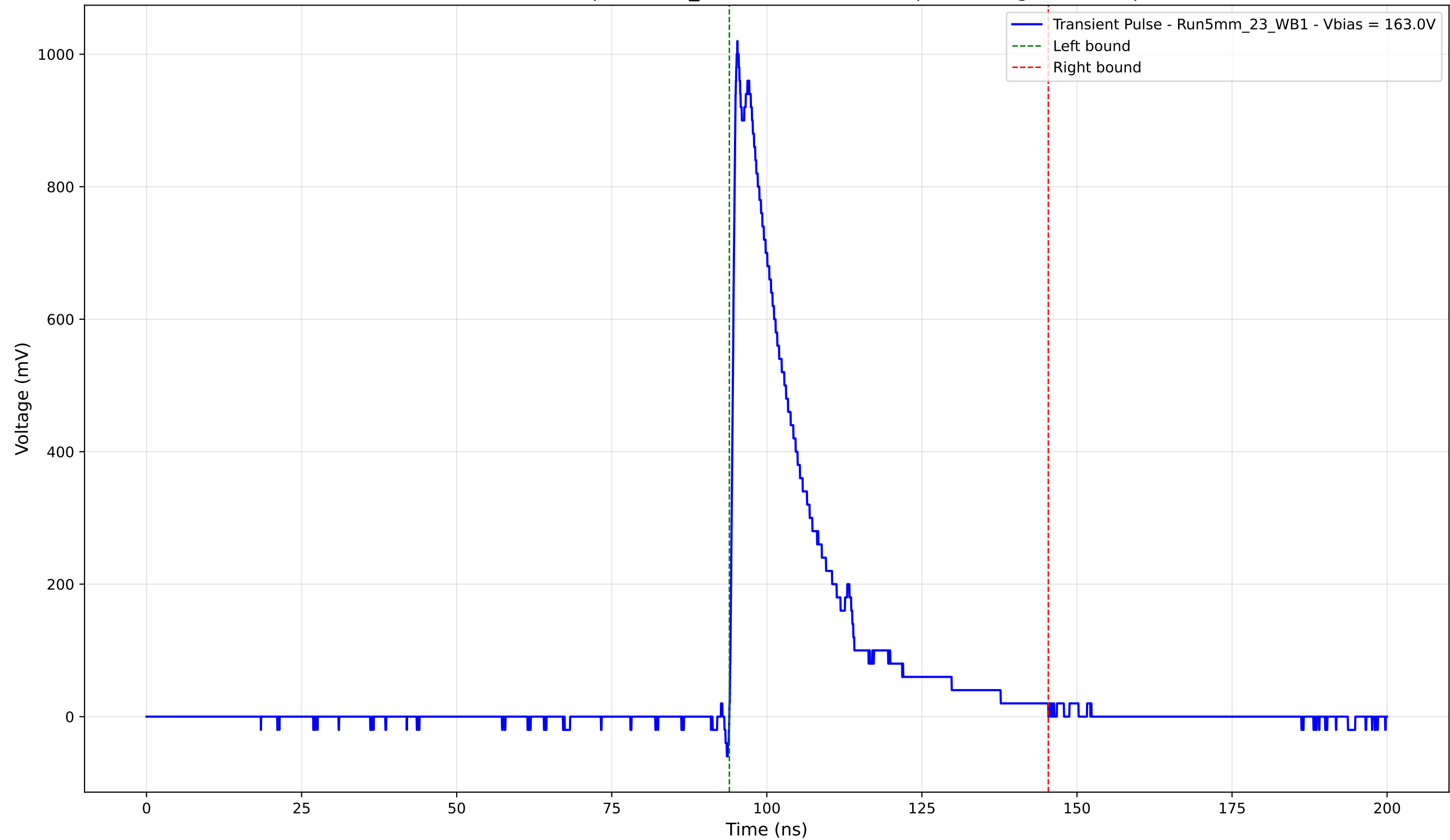
Transient Pulse - Sample: 5mm_23 - Position: 2430.0 \mu\text{m} - Charge: 227.23 pC
