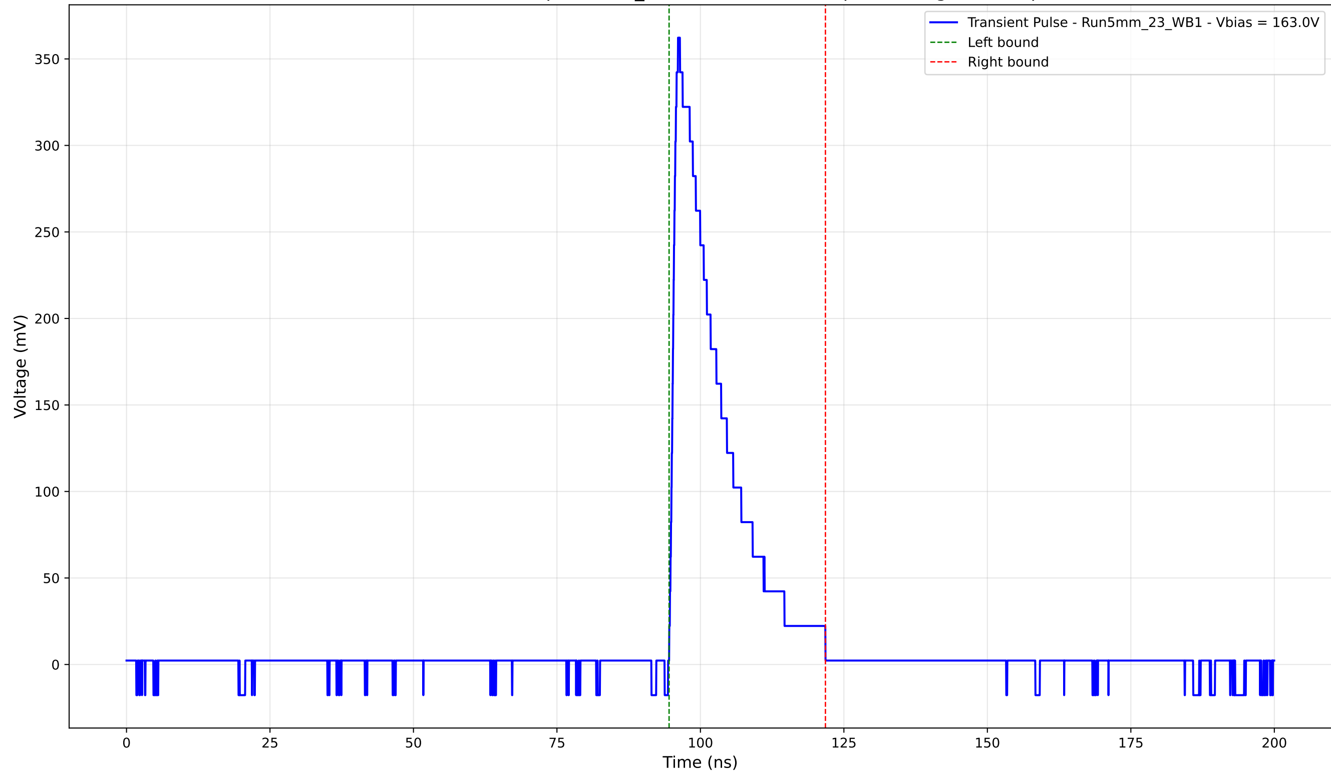
Transient Pulse - Sample: 5mm_23 - Position: 1200.0 \mu\text{m} - Charge: 64.76 pC
