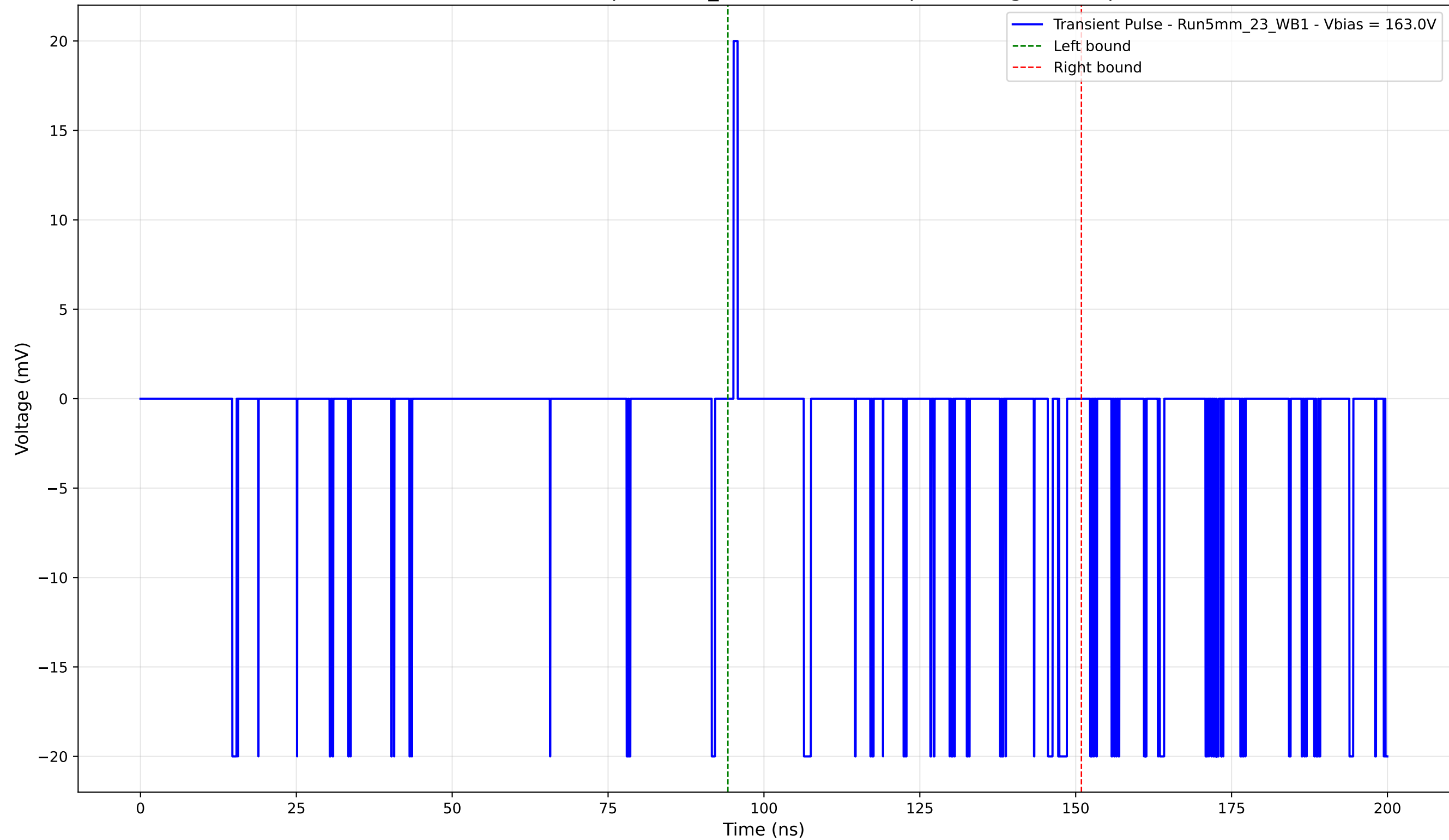
Transient Pulse - Sample: 5mm_23 - Position: 70.0 \mu\text{m} - Charge: -2.02 pC
