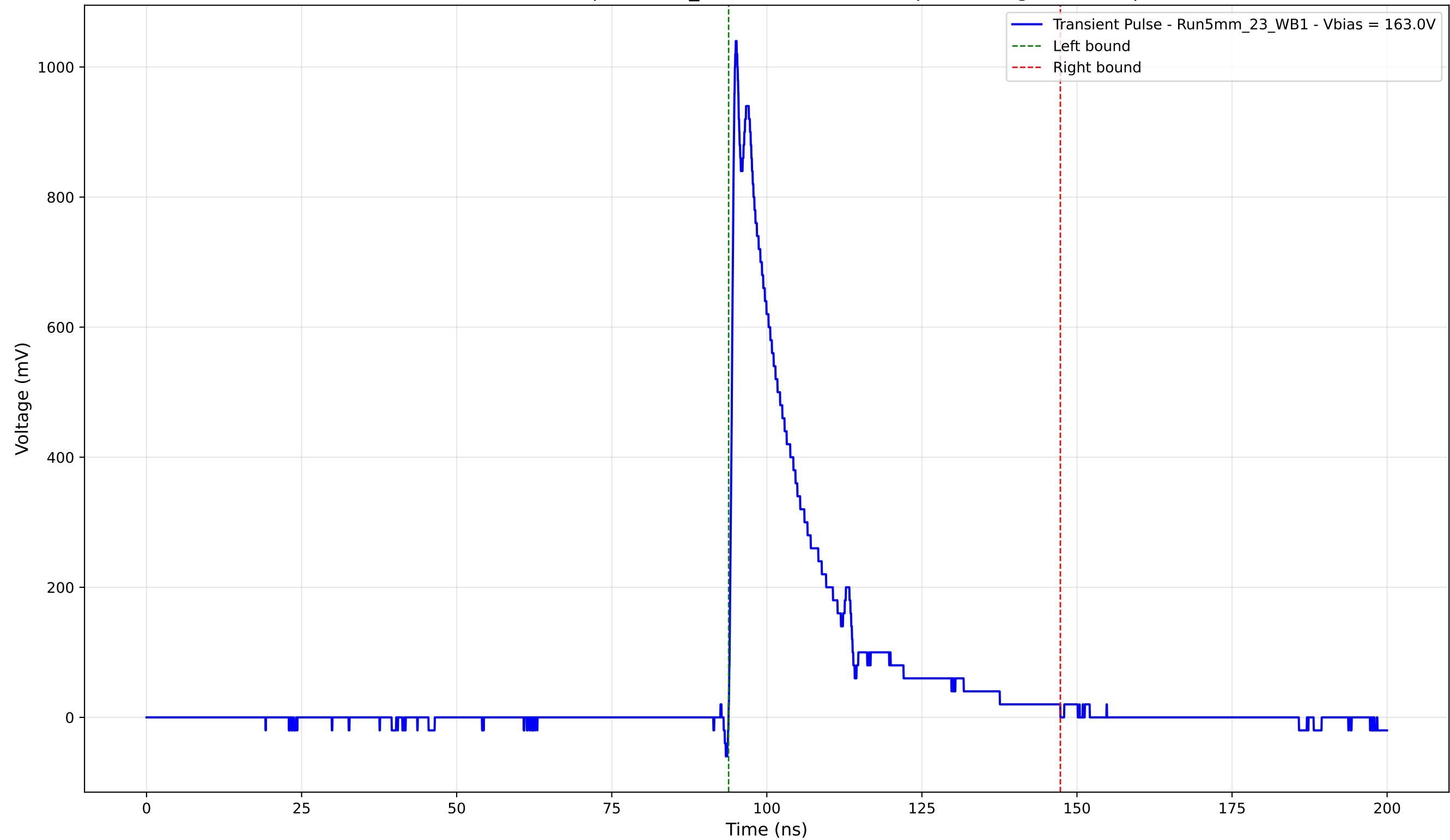
Transient Pulse - Sample: 5mm_23 - Position: 2830.0 \mu\text{m} - Charge: 217.74 pC
