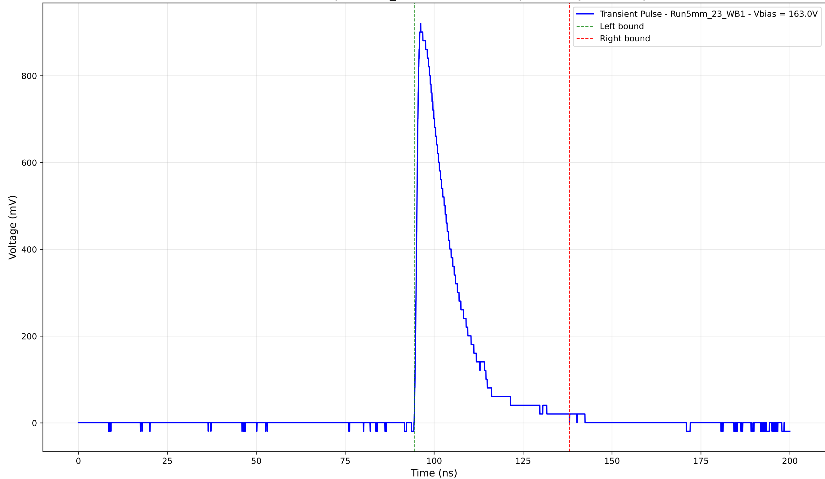
Transient Pulse - Sample: 5mm_23 - Position: 3970.0 \mu\text{m} - Charge: 197.19 pC
