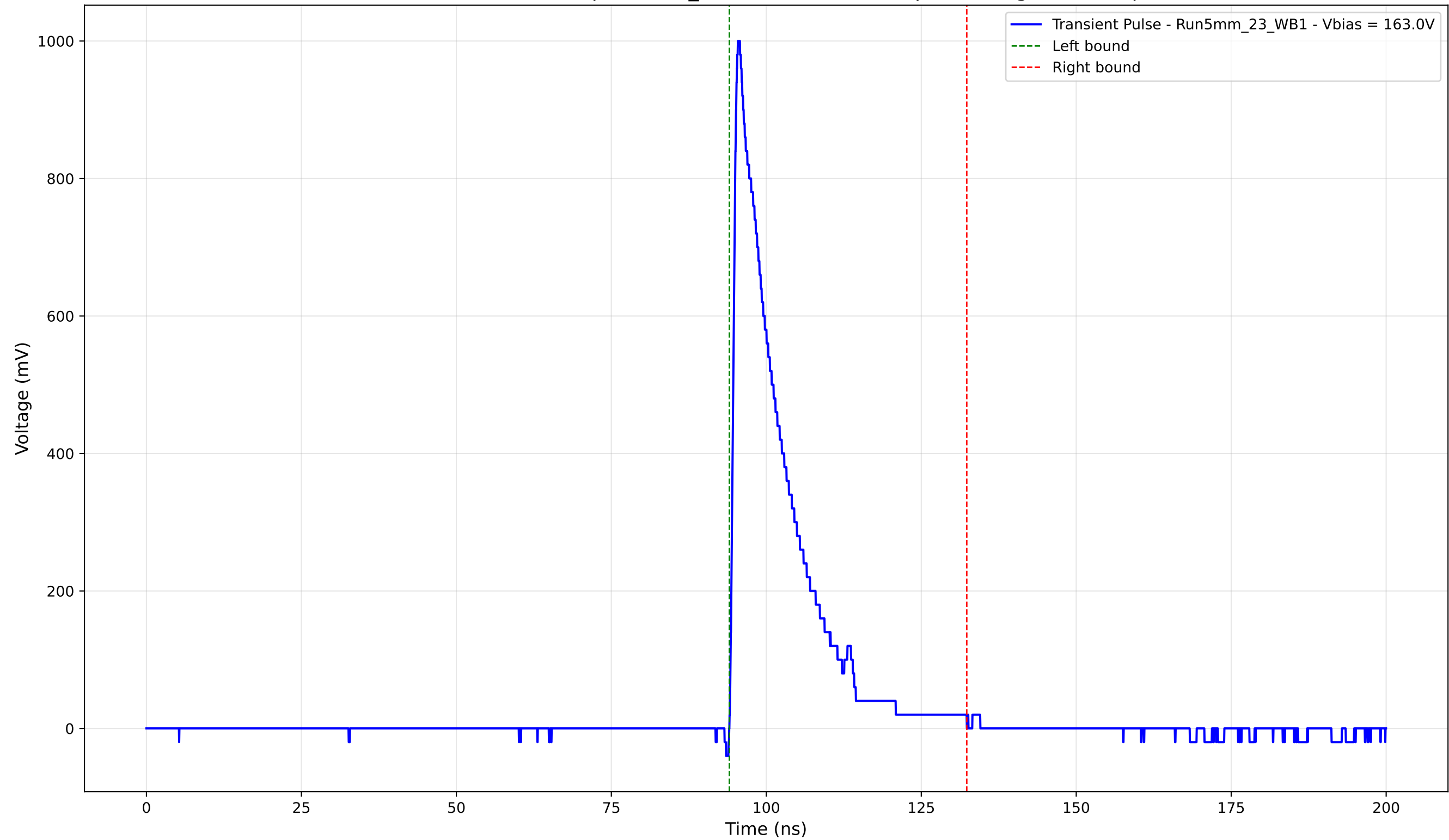
Transient Pulse - Sample: 5mm_23 - Position: 4985.0 \mu\text{m} - Charge: 167.36 pC
