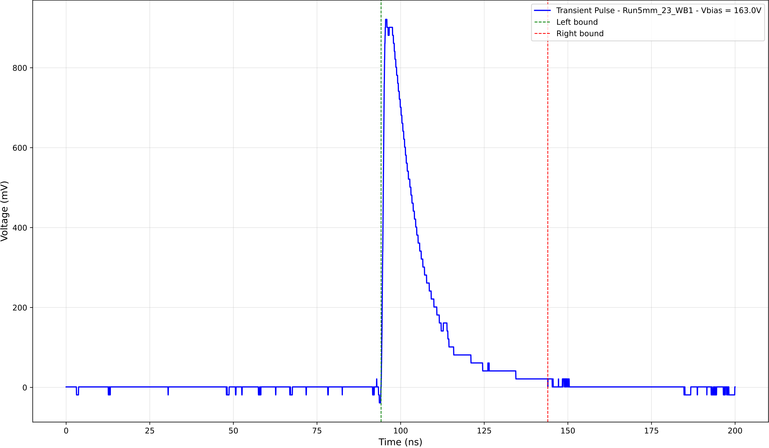
Transient Pulse - Sample: 5mm_23 - Position: 3405.0 \mu\text{m} - Charge: 213.11 pC
