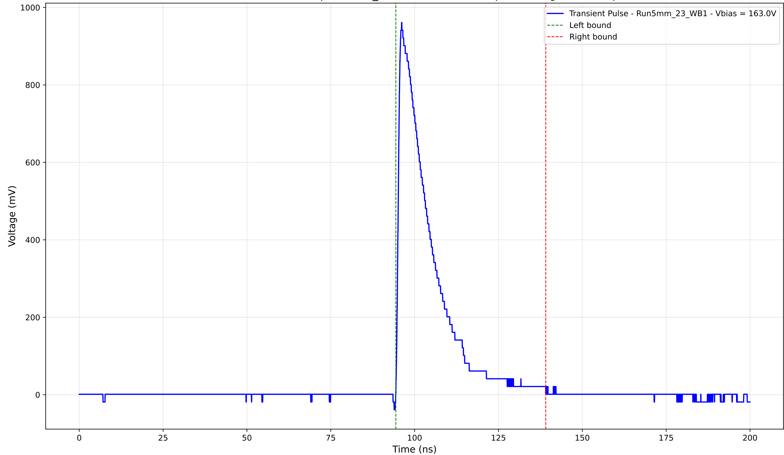
Transient Pulse - Sample: 5mm_23 - Position: 1115.0 \mu\text{m} - Charge: 201.27 pC
