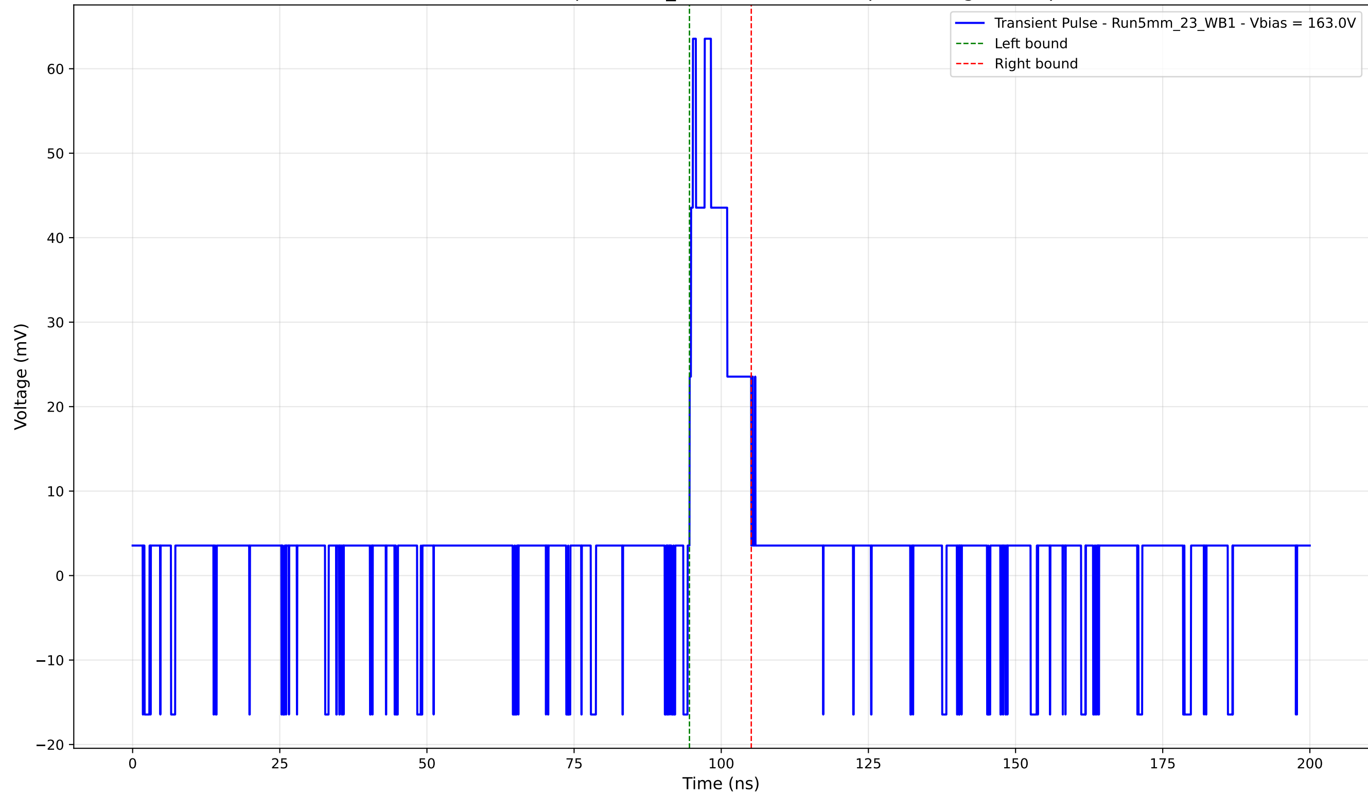
Transient Pulse - Sample: 5mm_23 - Position: 255.0 \mu\text{m} - Charge: 8.04 pC
