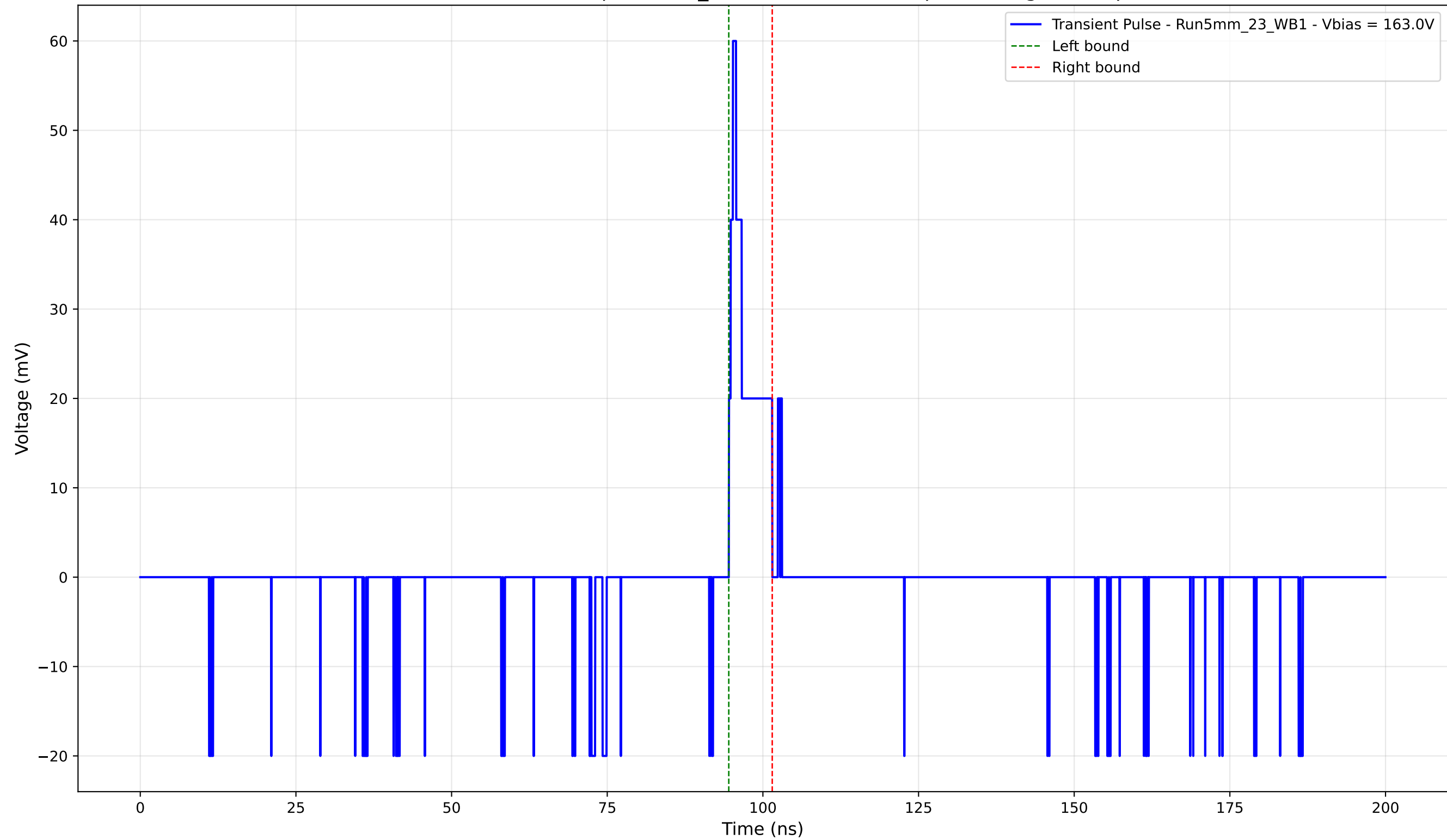
Transient Pulse - Sample: 5mm_23 - Position: 5230.0 \mu\text{m} - Charge: 3.70 pC
