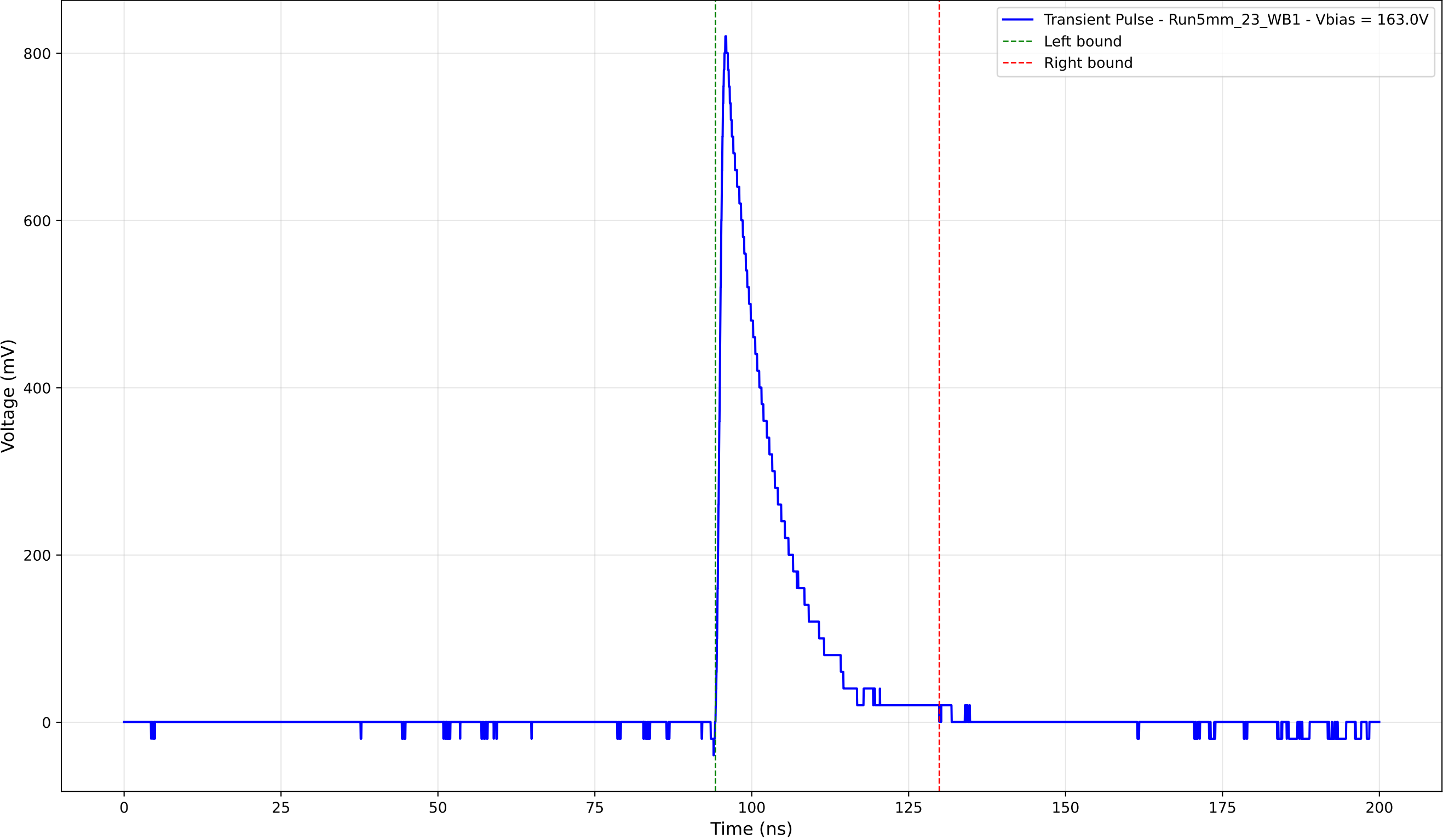
Transient Pulse - Sample: 5mm_23 - Position: 4700.0 \mu\text{m} - Charge: 135.82 pC
