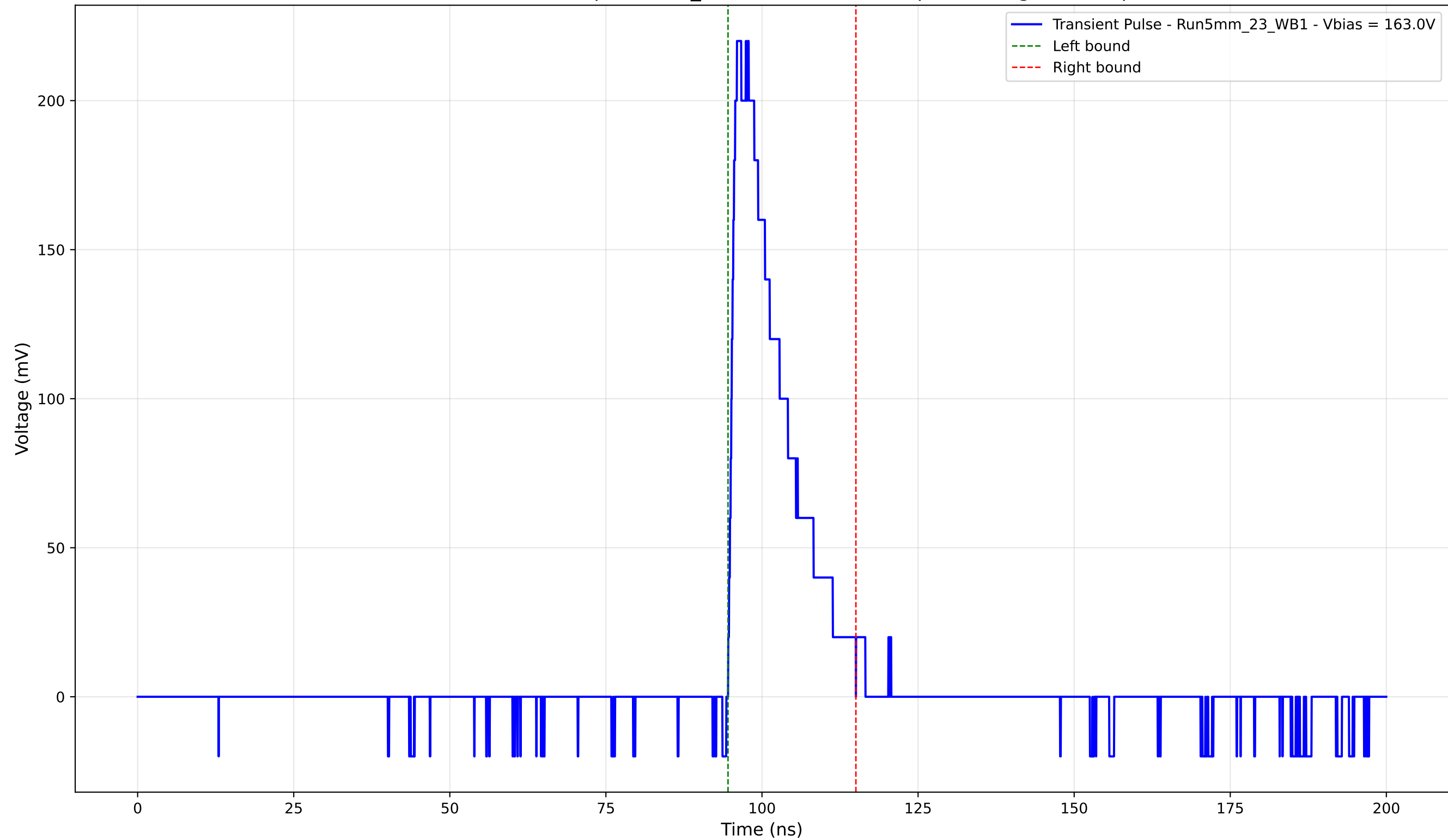
Transient Pulse - Sample: 5mm_23 - Position: 4275.0 \mu\text{m} - Charge: 38.68 pC
