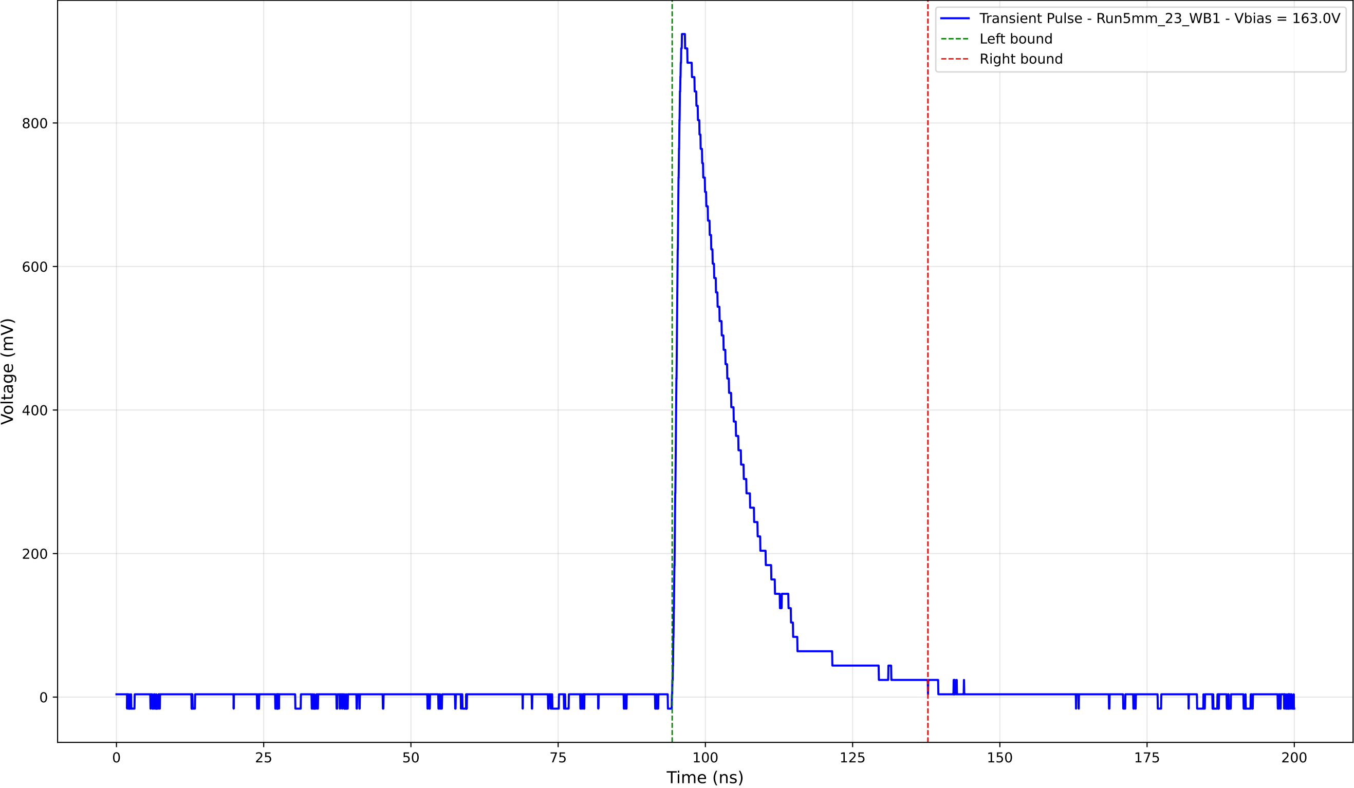
Transient Pulse - Sample: 5mm_23 - Position: 4100.0 \mu\text{m} - Charge: 199.54 pC
