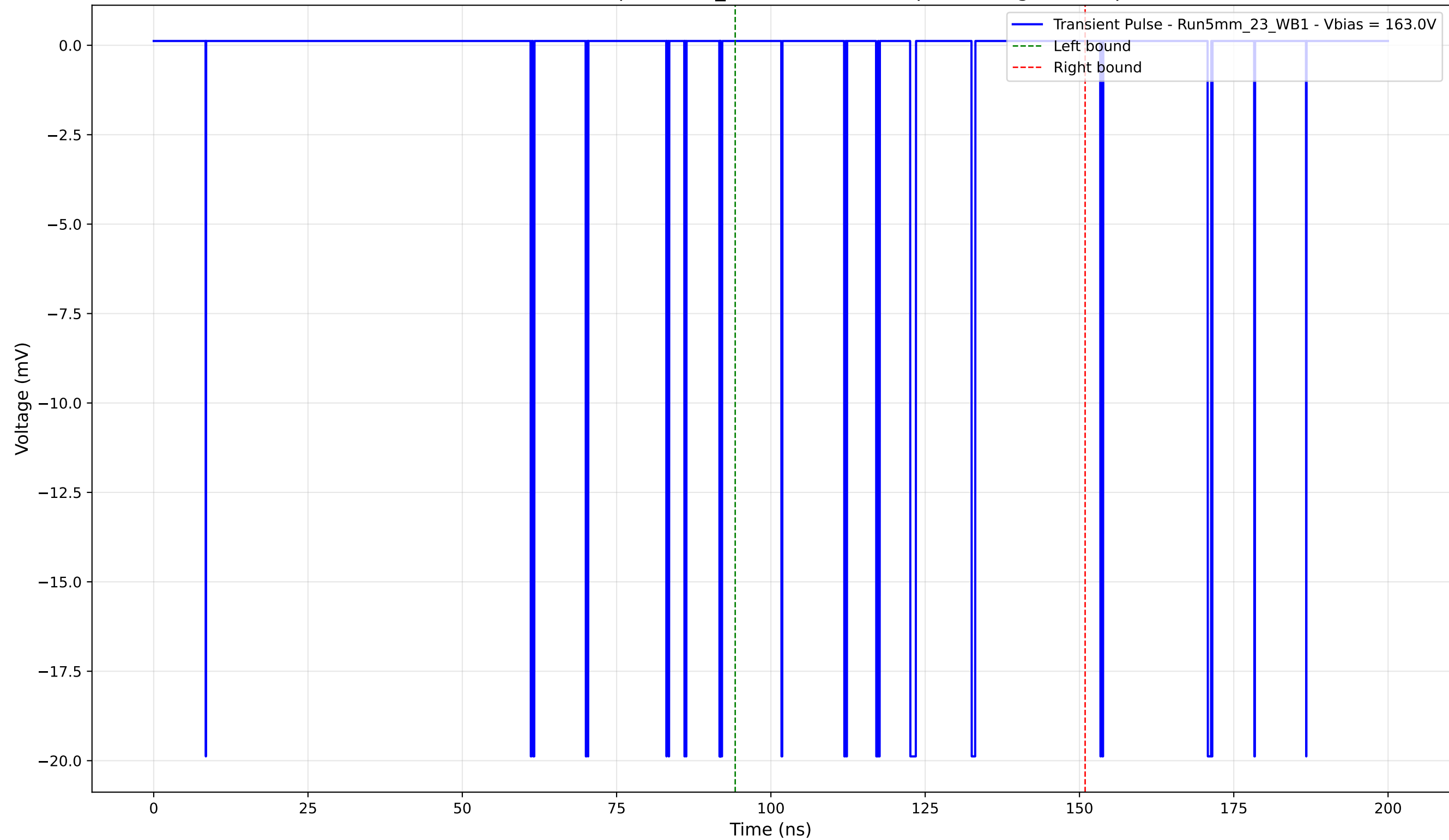
Transient Pulse - Sample: 5mm_23- Position: 10.0 \mu\text{m} - Charge: -0.84 pC
