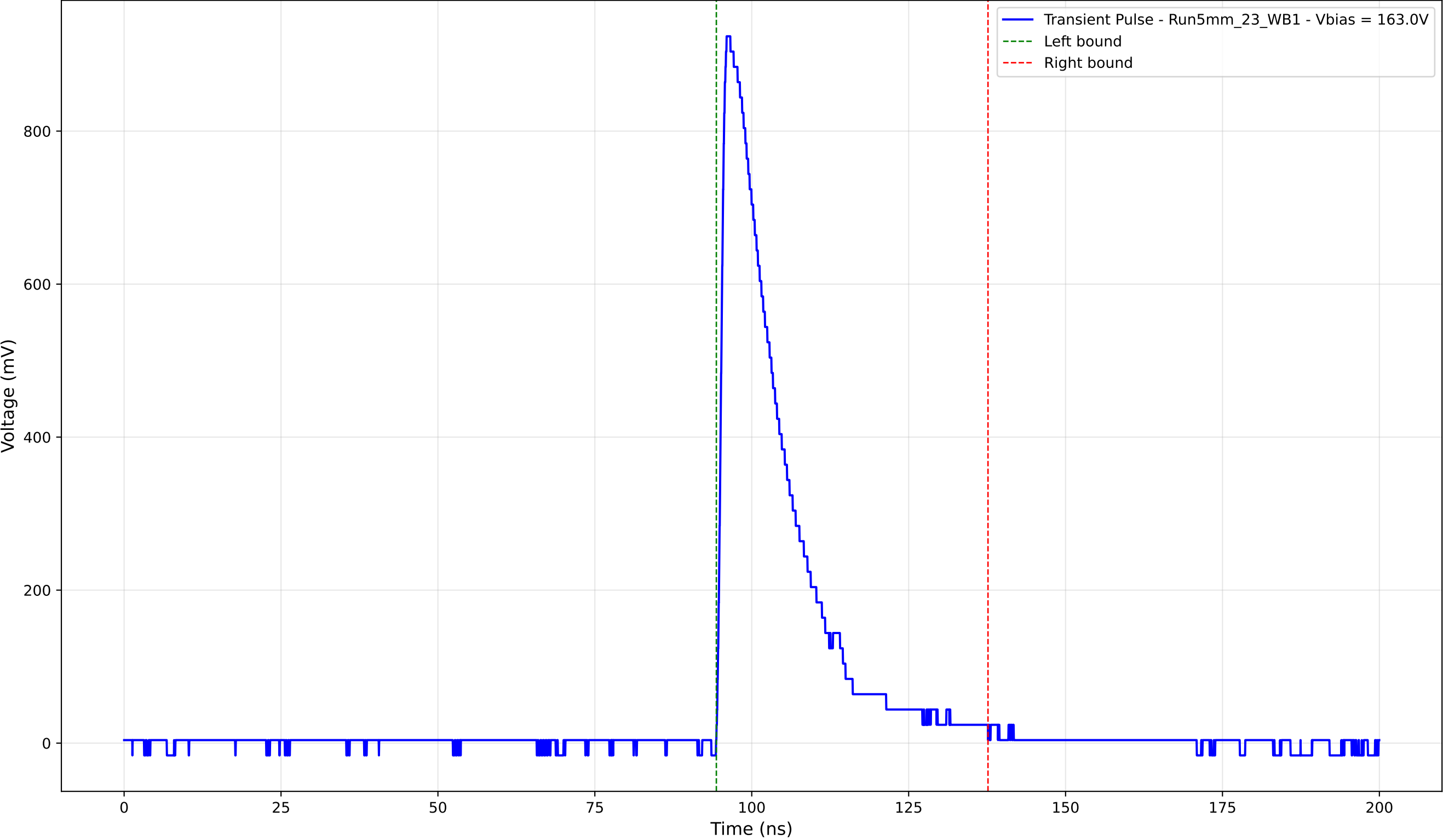
Transient Pulse - Sample: 5mm_23 - Position: 4085.0 \mu\text{m} - Charge: 199.87 pC
