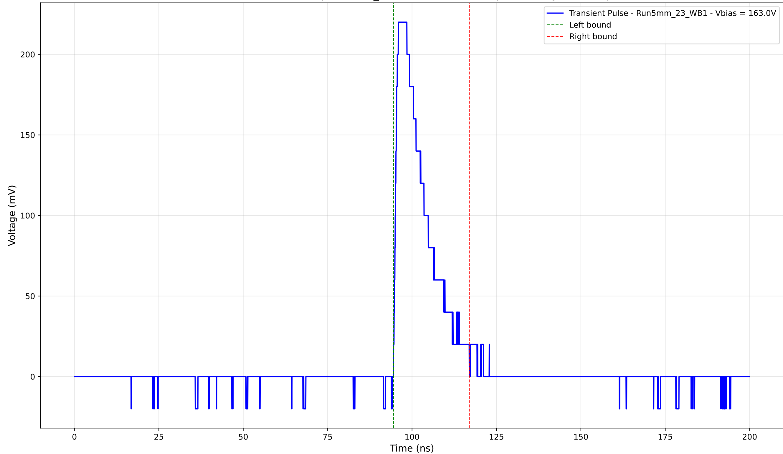
Transient Pulse - Sample: 5mm_23 - Position: 1720.0 \mu\text{m} - Charge: 43.71 pC
