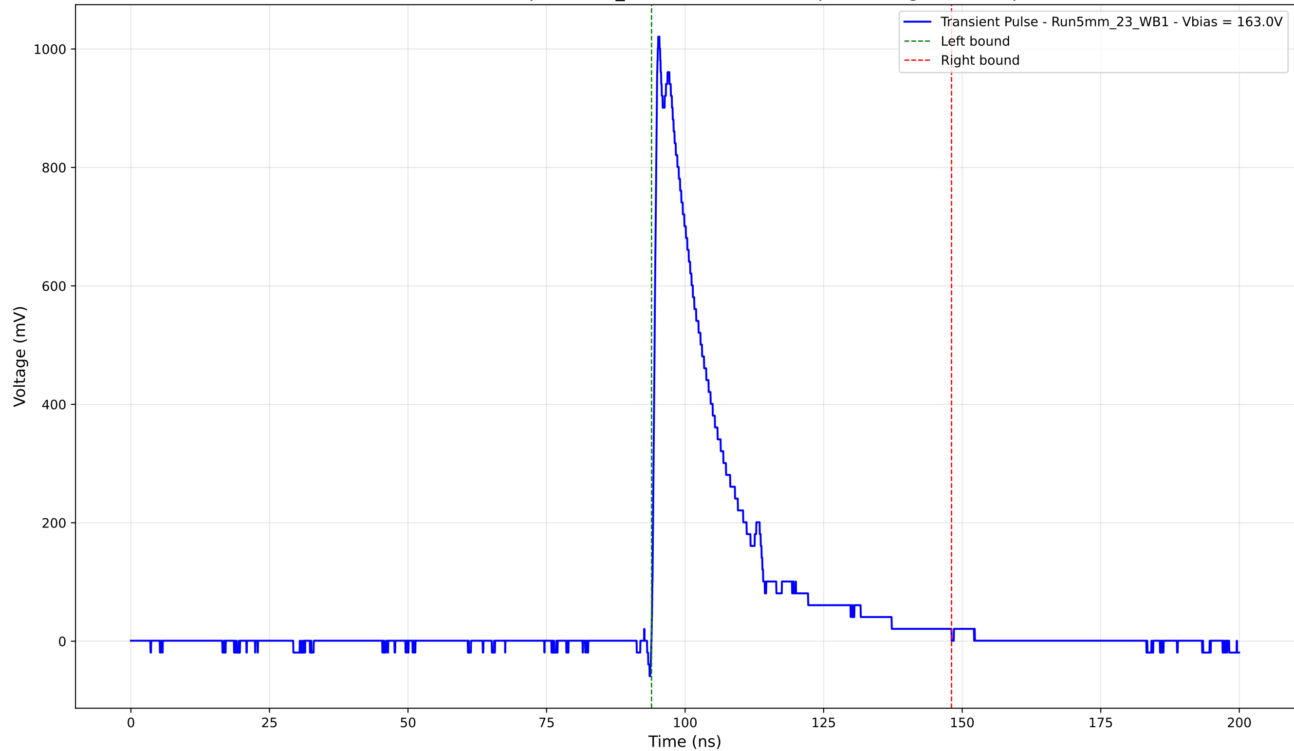
Transient Pulse - Sample: 5mm_23 - Position: 3020.0 \mu\text{m} - Charge: 230.45 pC
