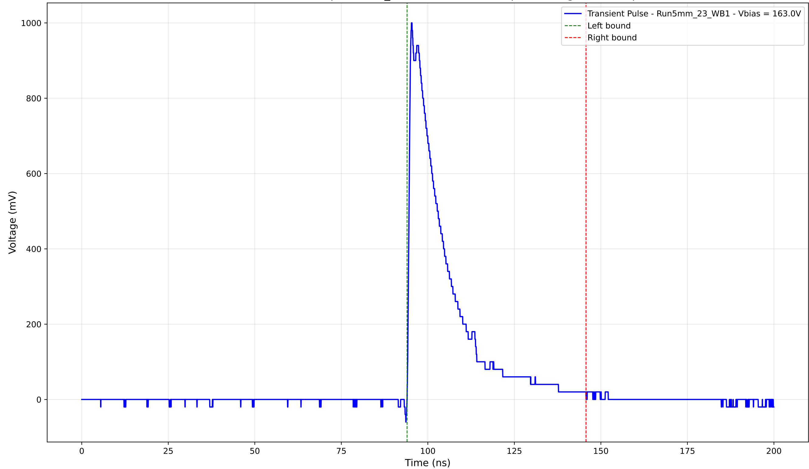
Transient Pulse - Sample: 5mm_23 - Position: 3100.0 \mu\text{m} - Charge: 223.82 pC
