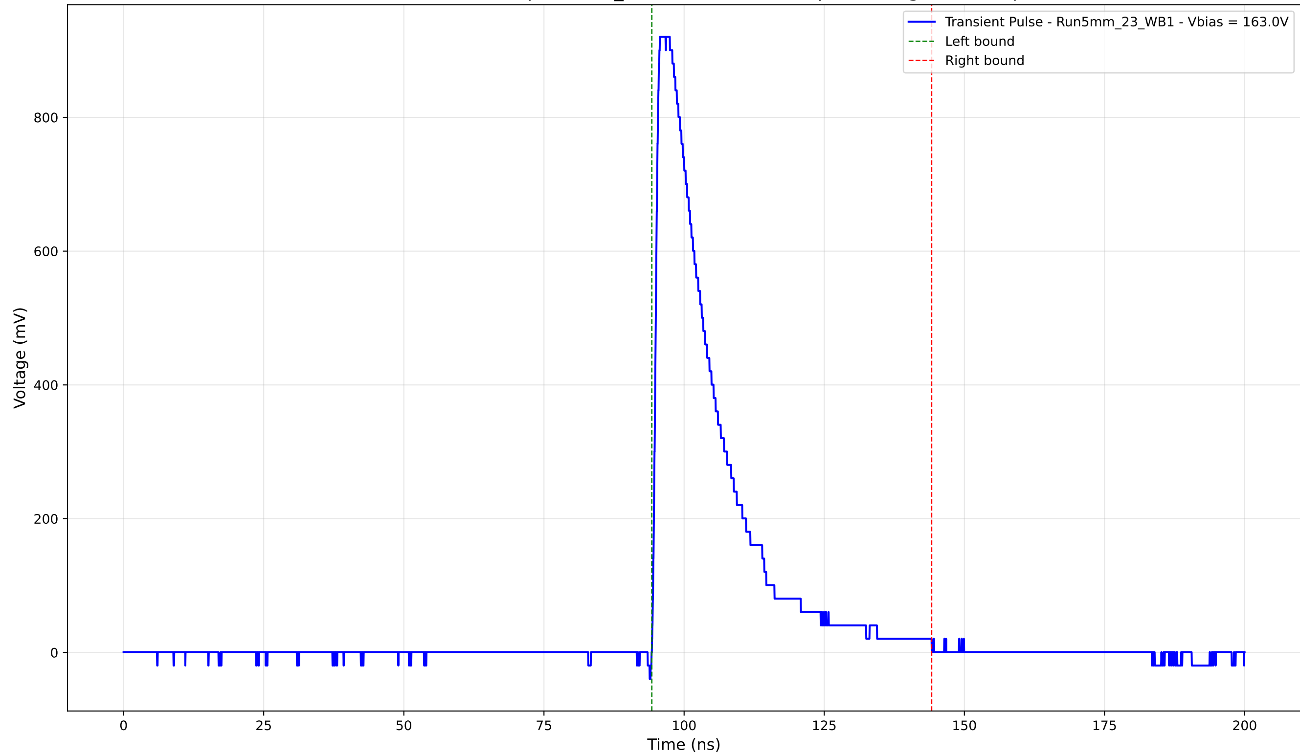
Transient Pulse - Sample: 5mm_23 - Position: 3575.0 \mu\text{m} - Charge: 216.92 pC
