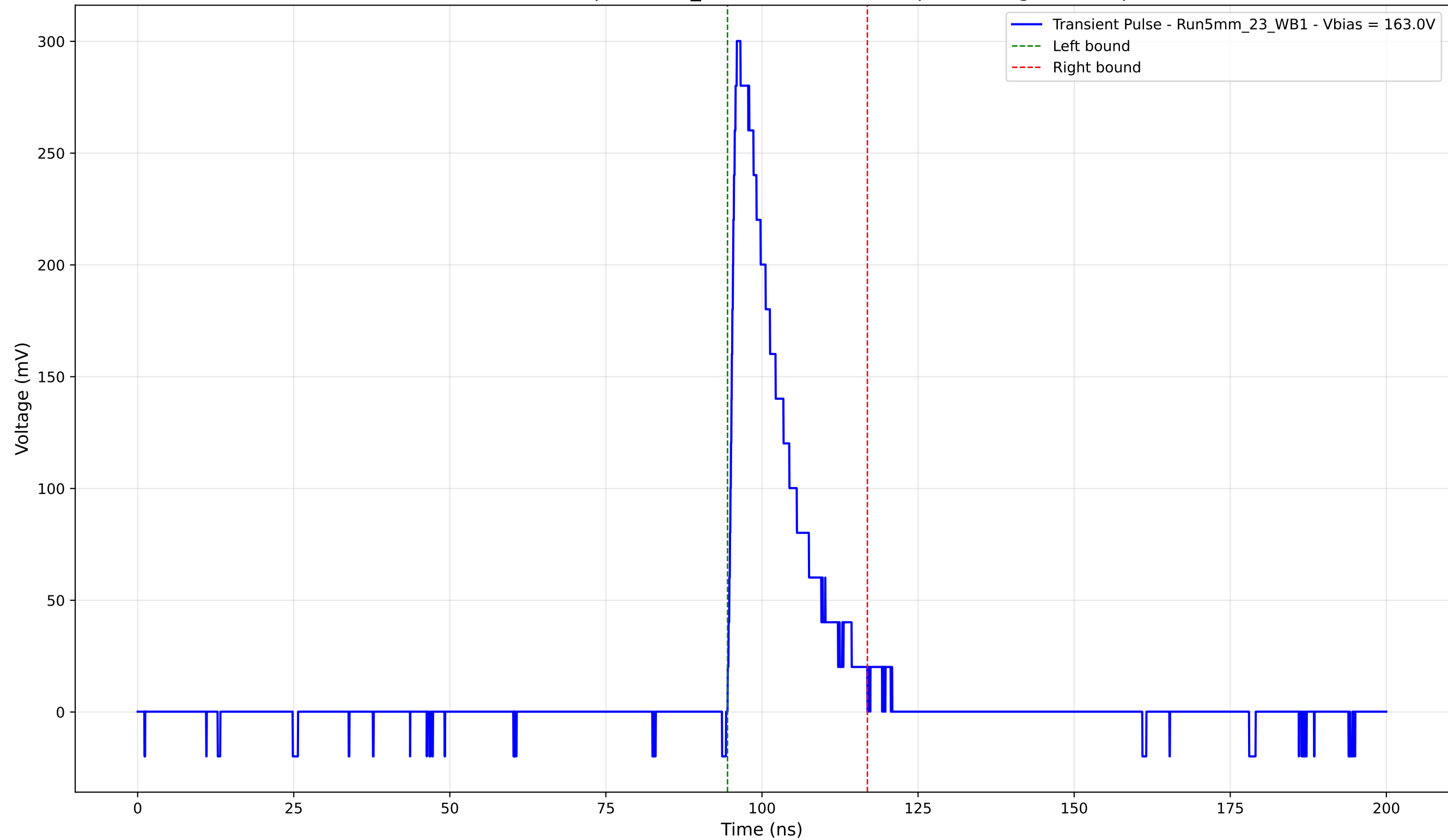
Transient Pulse - Sample: 5mm_23 - Position: 4285.0 \mu\text{m} - Charge: 51.84 pC
