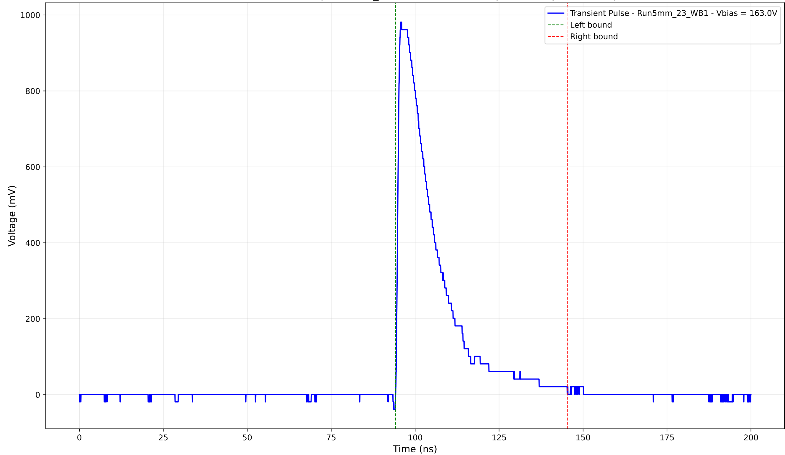
Transient Pulse - Sample: 5mm_23 - Position: 1975.0 \mu\text{m} - Charge: 241.85 pC
