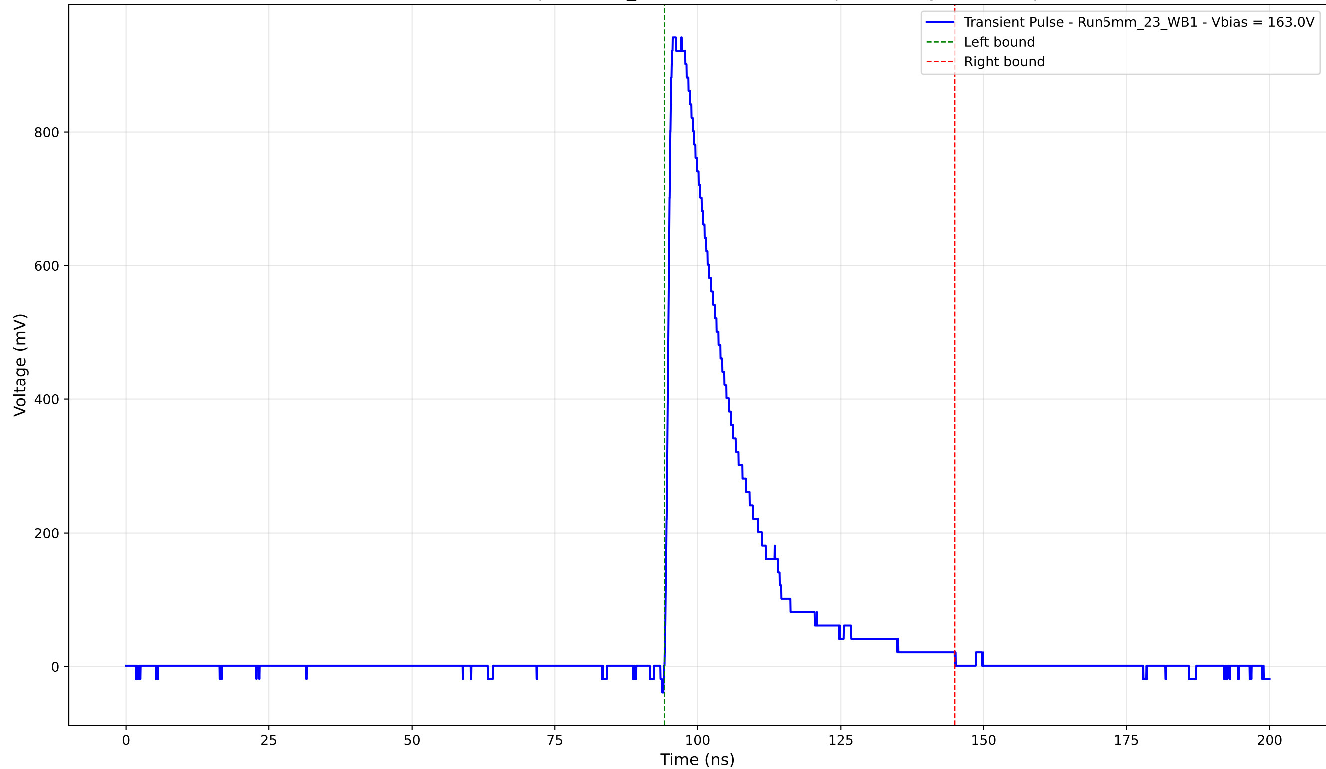
Transient Pulse - Sample: 5mm_23 - Position: 3515.0 \mu\text{m} - Charge: 223.13 pC
