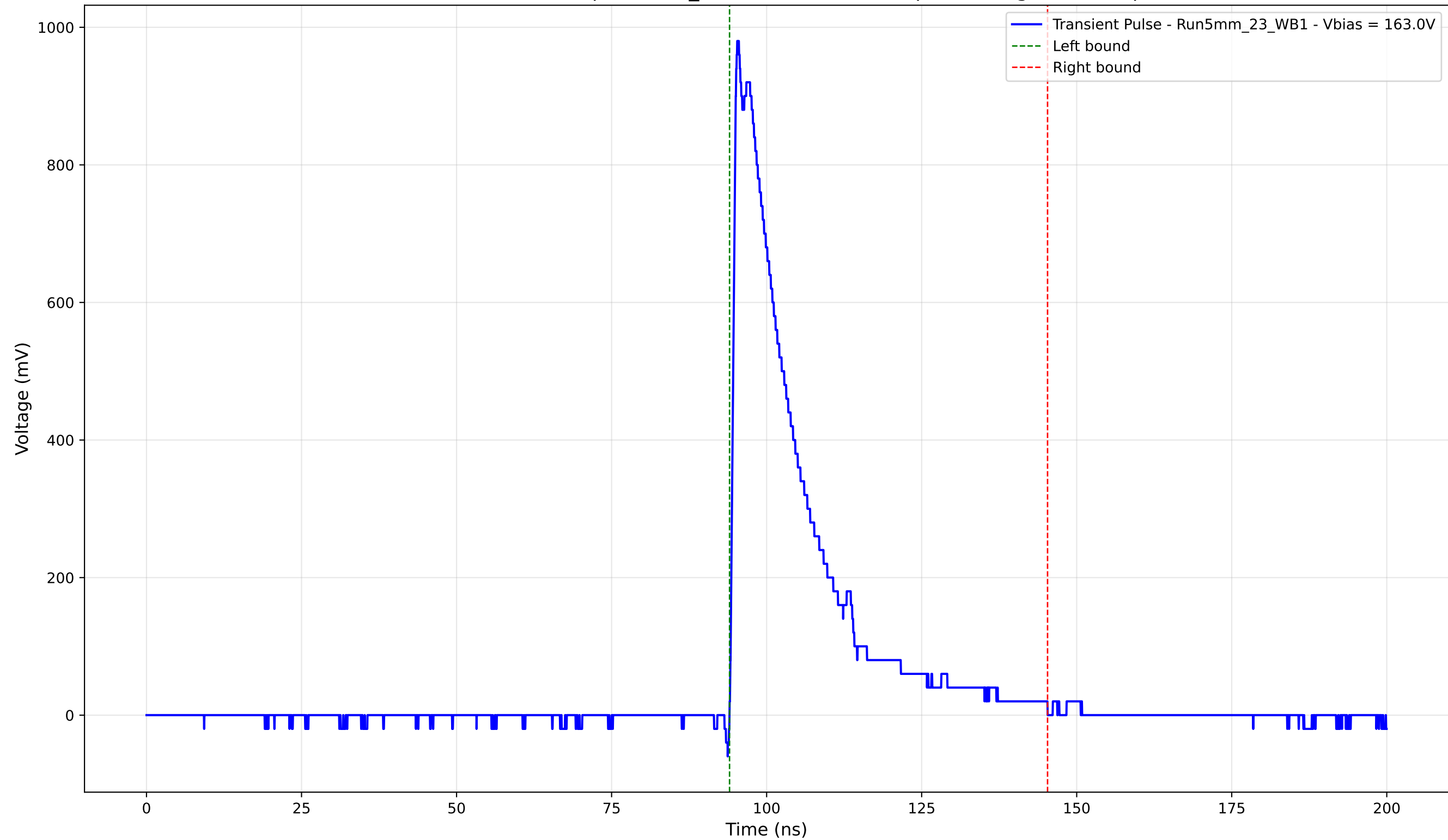
Transient Pulse - Sample: 5mm_23 - Position: 3135.0 \mu\text{m} - Charge: 217.24 pC
