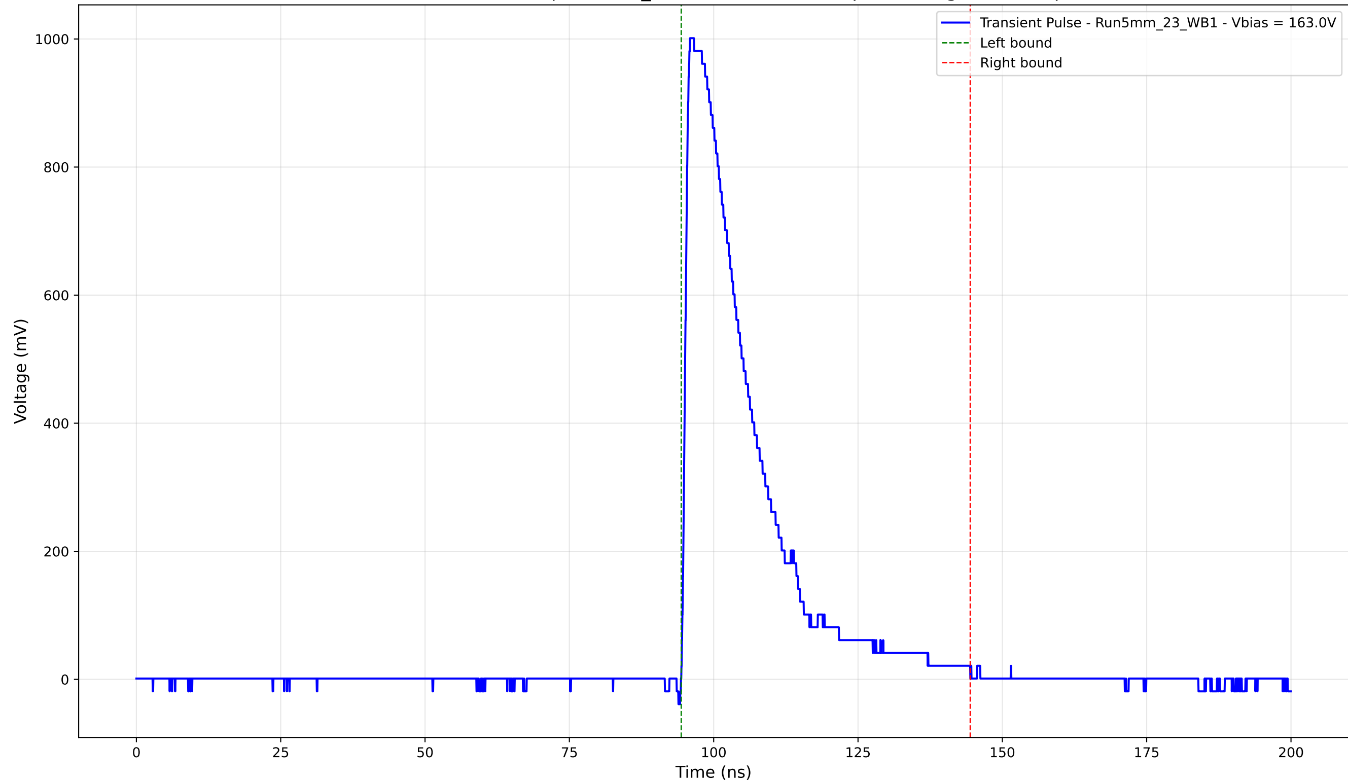
Transient Pulse - Sample: 5mm_23 - Position: 1490.0 \mu\text{m} - Charge: 250.78 pC
