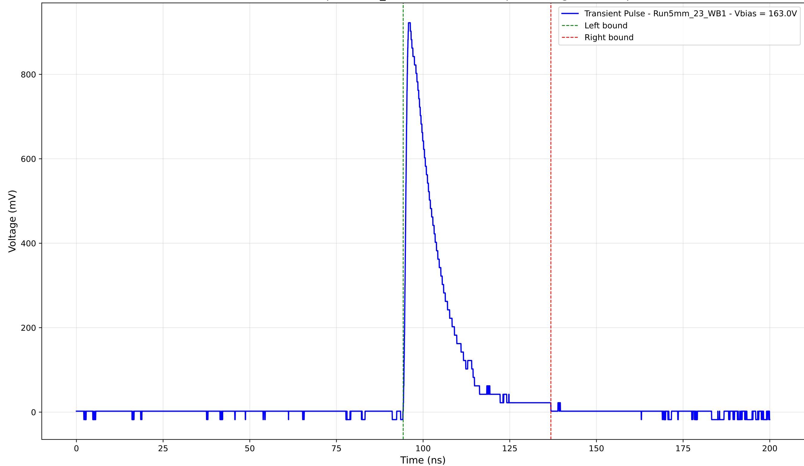
Transient Pulse - Sample: 5mm_23 - Position: 4520.0 \mu\text{m} - Charge: 179.98 pC
