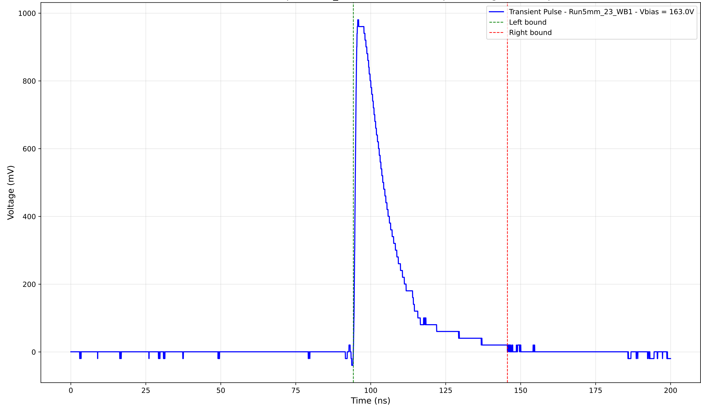
Transient Pulse - Sample: 5mm_23 - Position: 1980.0 \mu\text{m} - Charge: 240.55 pC
