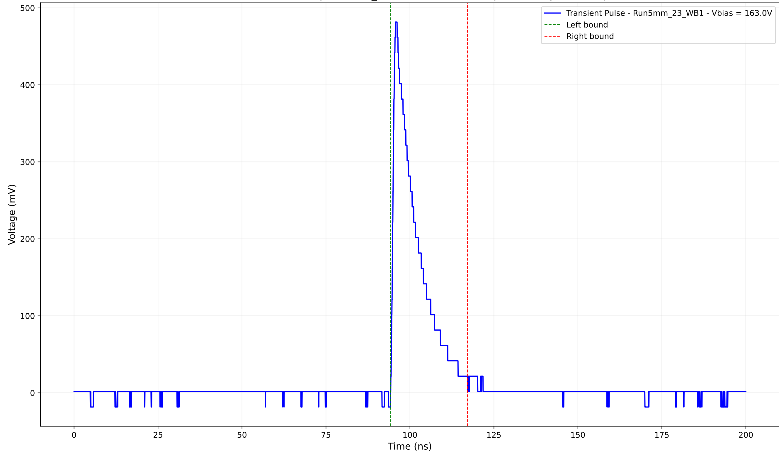
Transient Pulse - Sample: 5mm_23 - Position: 4730.0 \mu\text{m} - Charge: 73.65 pC
