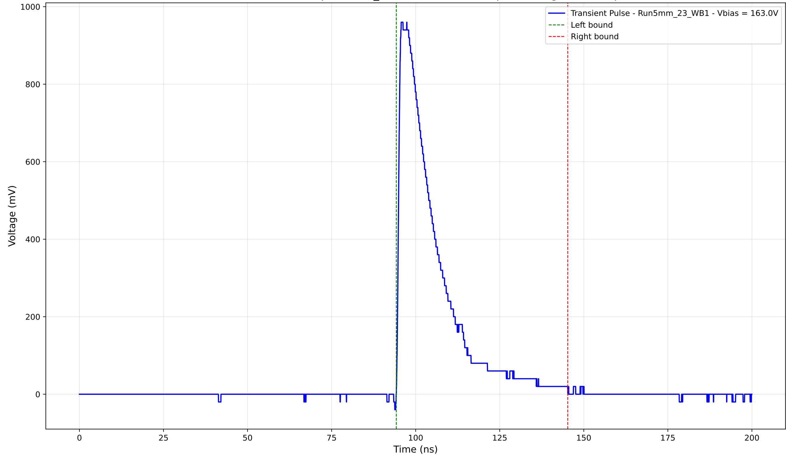
Transient Pulse - Sample: 5mm_23 - Position: 1910.0 \mu\text{m} - Charge: 233.58 pC
