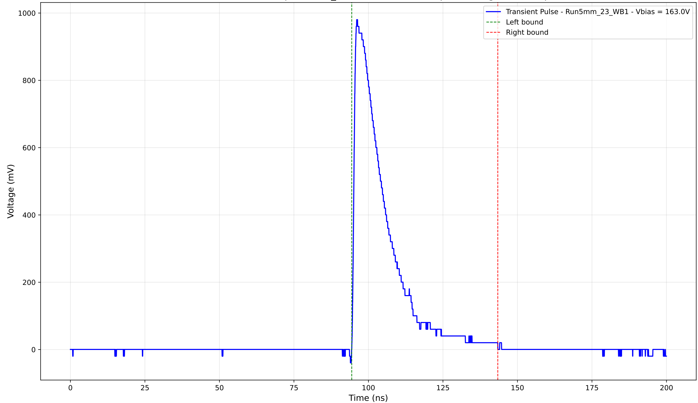
Transient Pulse - Sample: 5mm_23 - Position: 1385.0 \mu\text{m} - Charge: 226.82 pC
