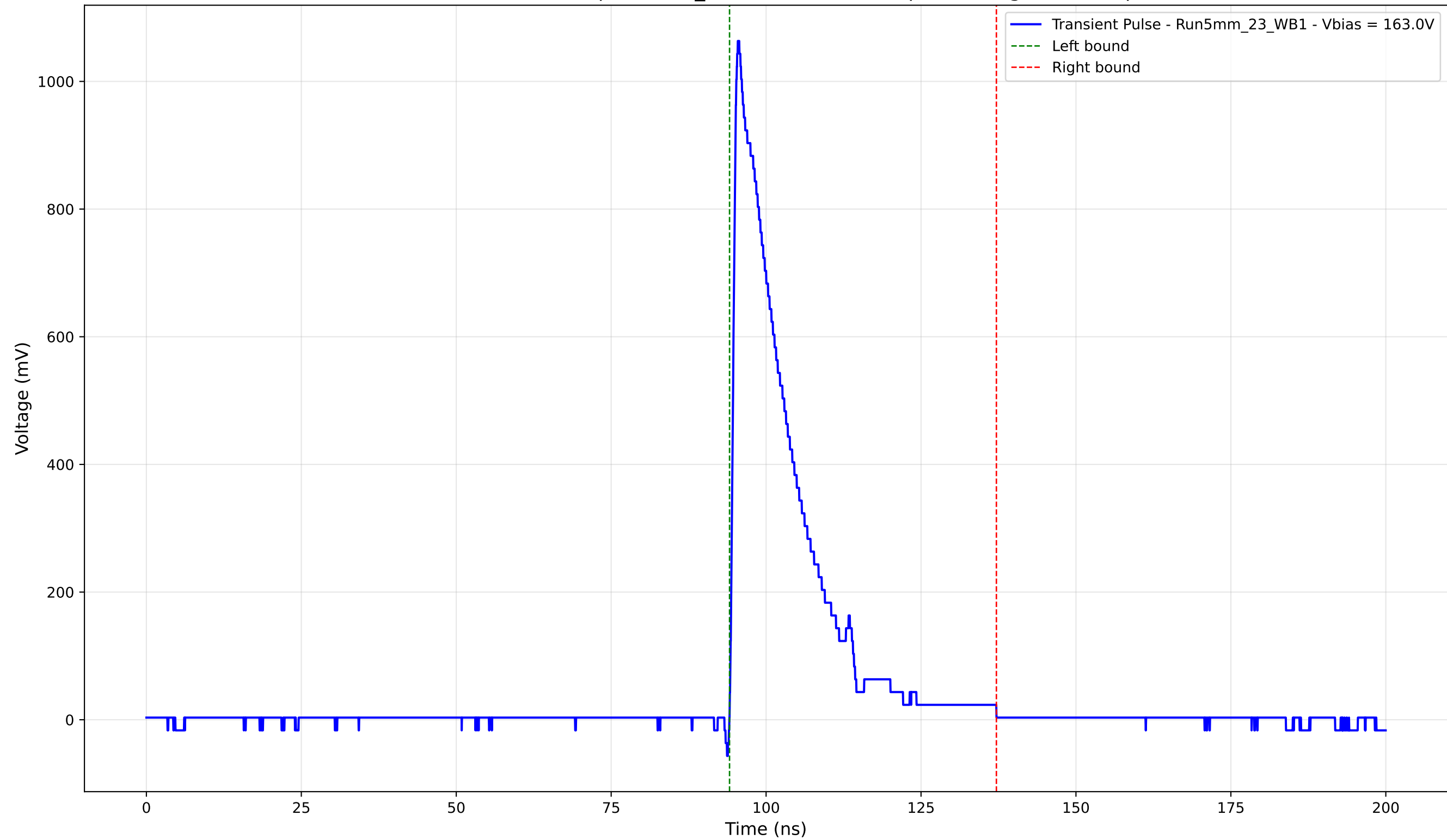
Transient Pulse - Sample: 5mm_23 - Position: 435.0 \mu\text{m} - Charge: 202.85 pC
