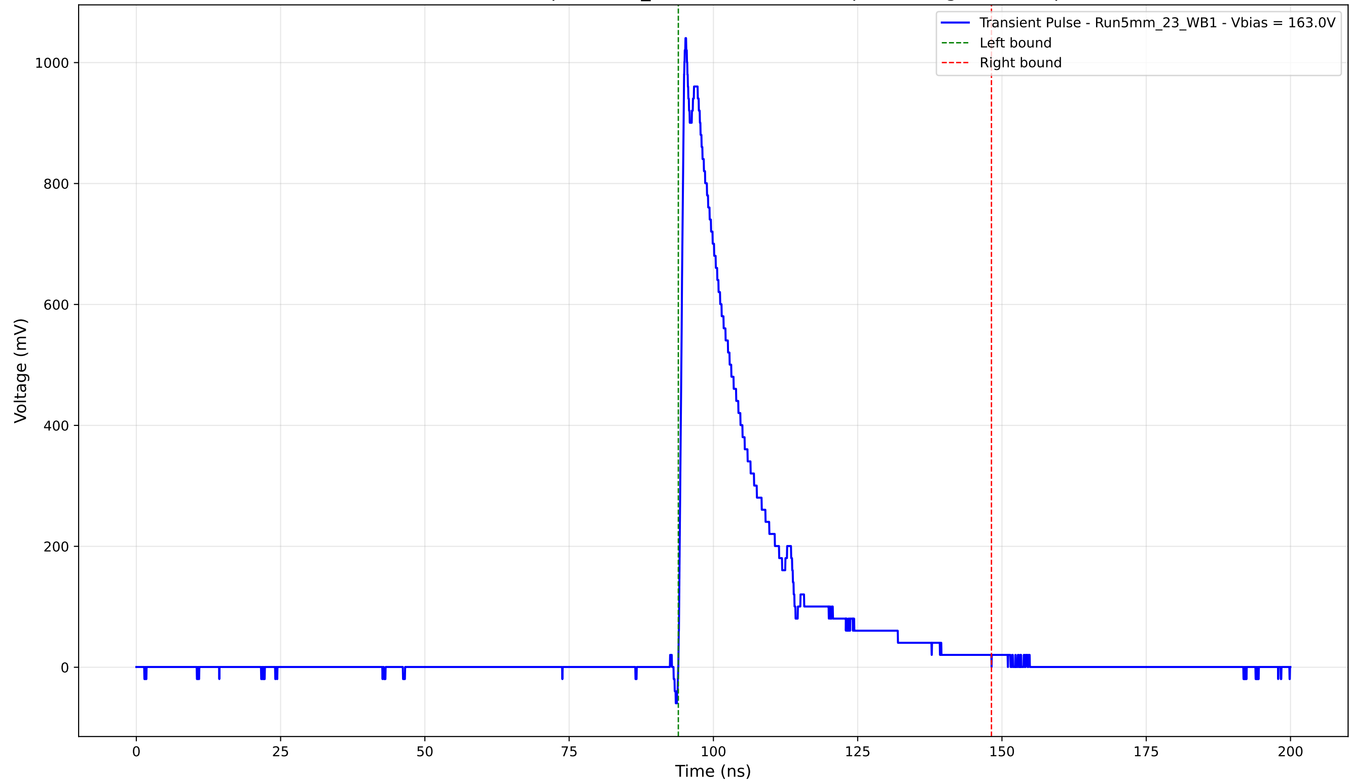
Transient Pulse - Sample: 5mm_23 - Position: 2520.0 \mu\text{m} - Charge: 234.87 pC
