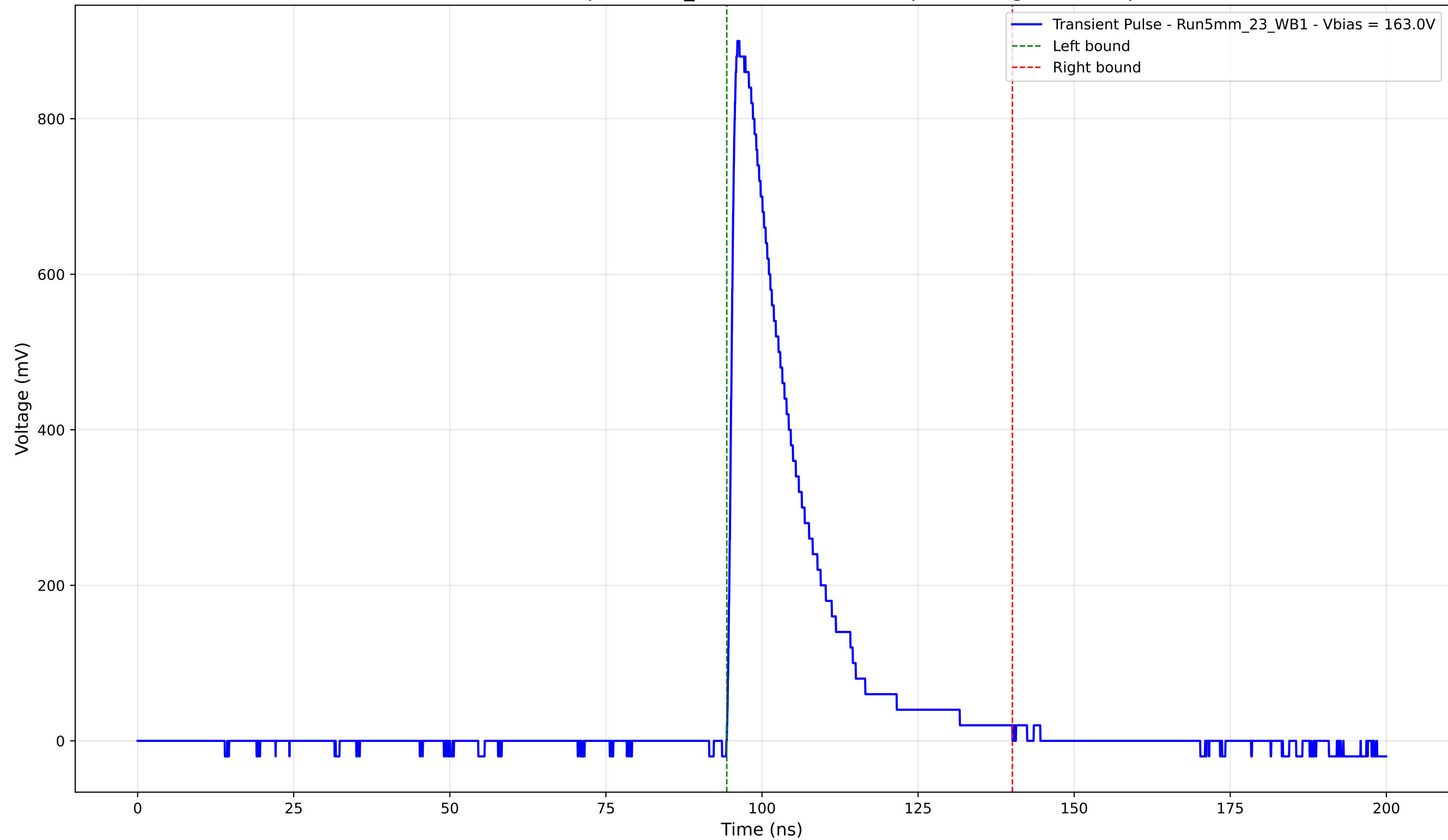
Transient Pulse - Sample: 5mm_23 - Position: 3885.0 \mu\text{m} - Charge: 196.16 pC
