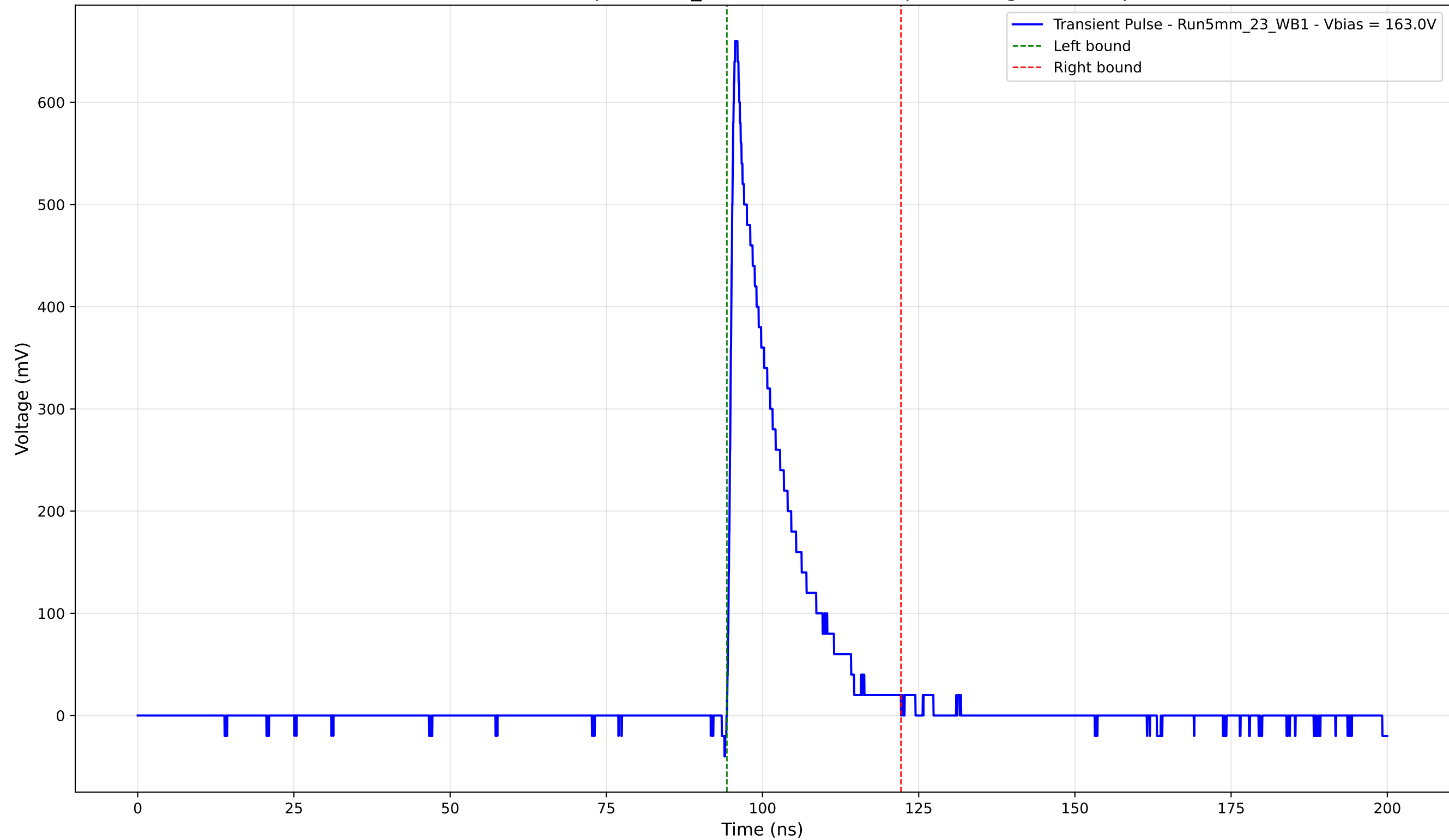
Transient Pulse - Sample: 5mm_23 - Position: 680.0 \mu\text{m} - Charge: 100.37 pC
