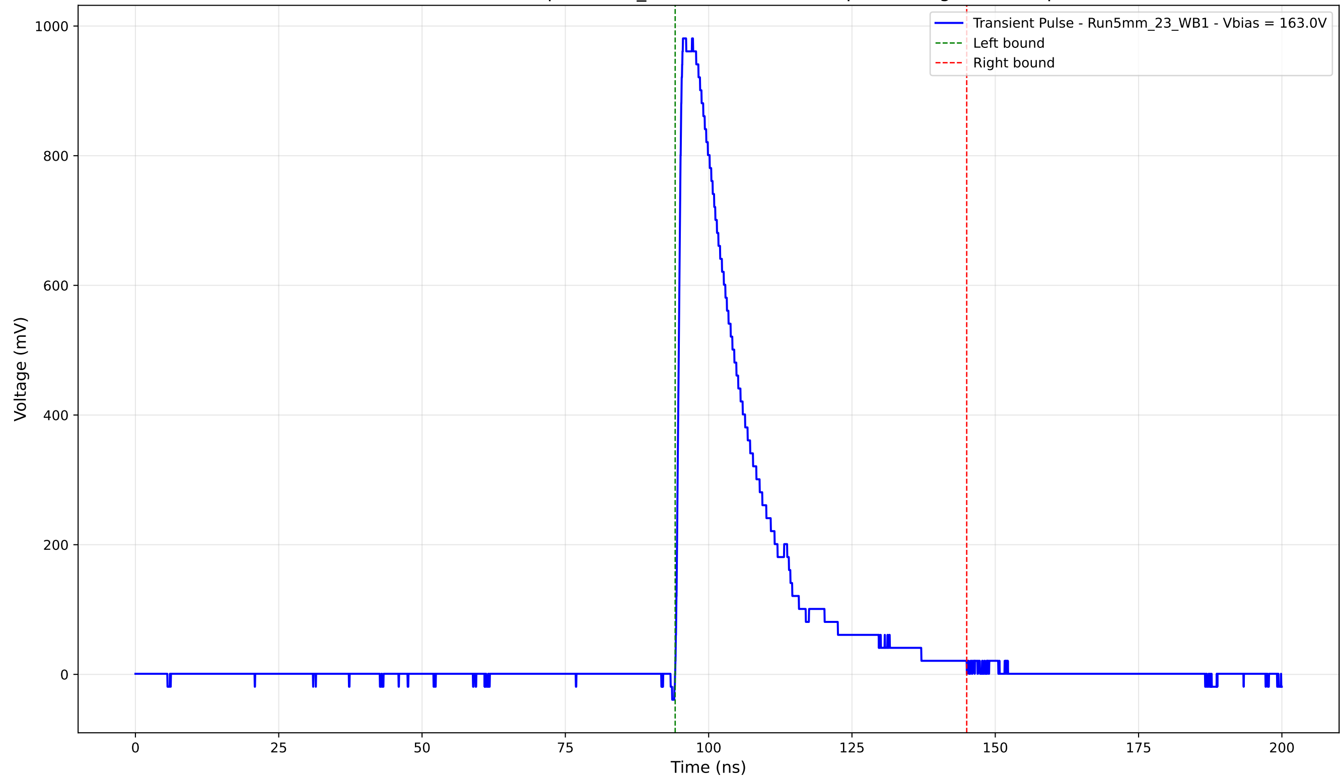
Transient Pulse - Sample: 5mm_23 - Position: 2035.0 \mu\text{m} - Charge: 245.68 pC
