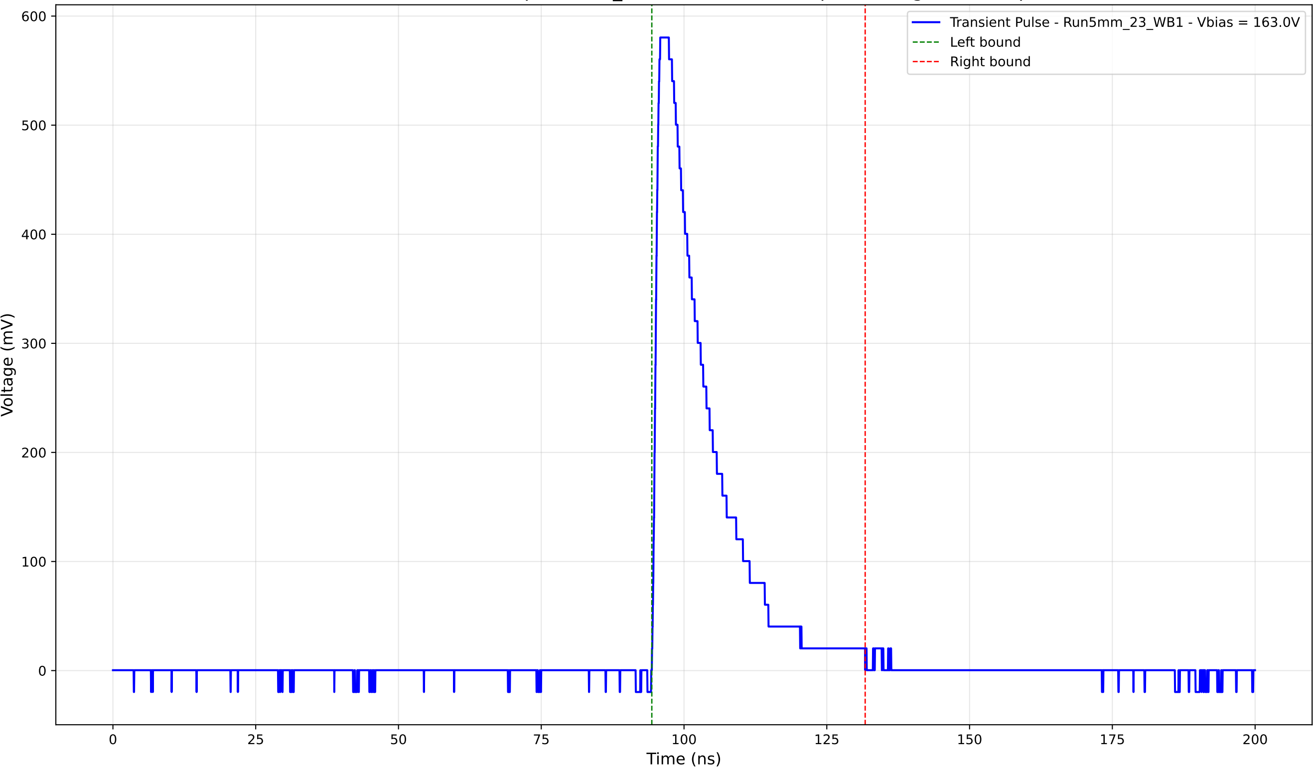
Transient Pulse - Sample: 5mm_23 - Position: 3705.0 \mu\text{m} - Charge: 117.10 pC
