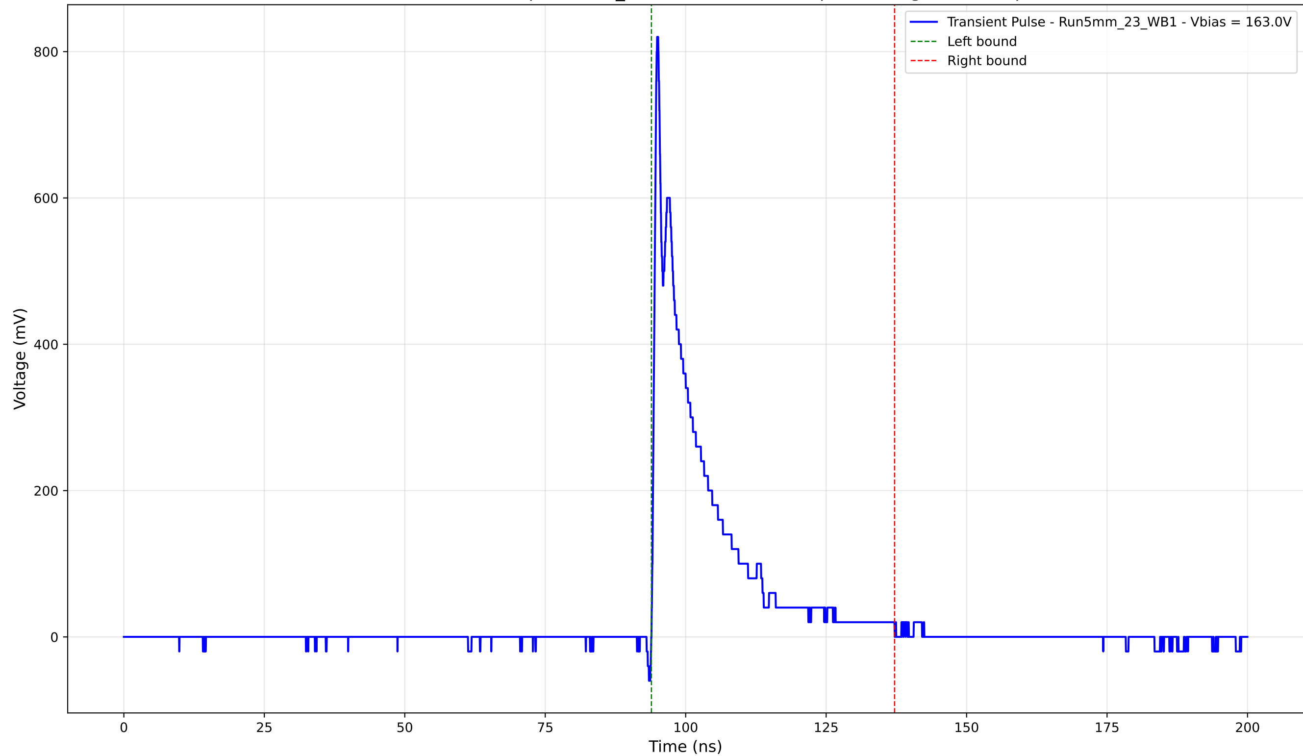
Transient Pulse - Sample: 5mm_23 - Position: 2790.0 \mu\text{m} - Charge: 121.46 pC
