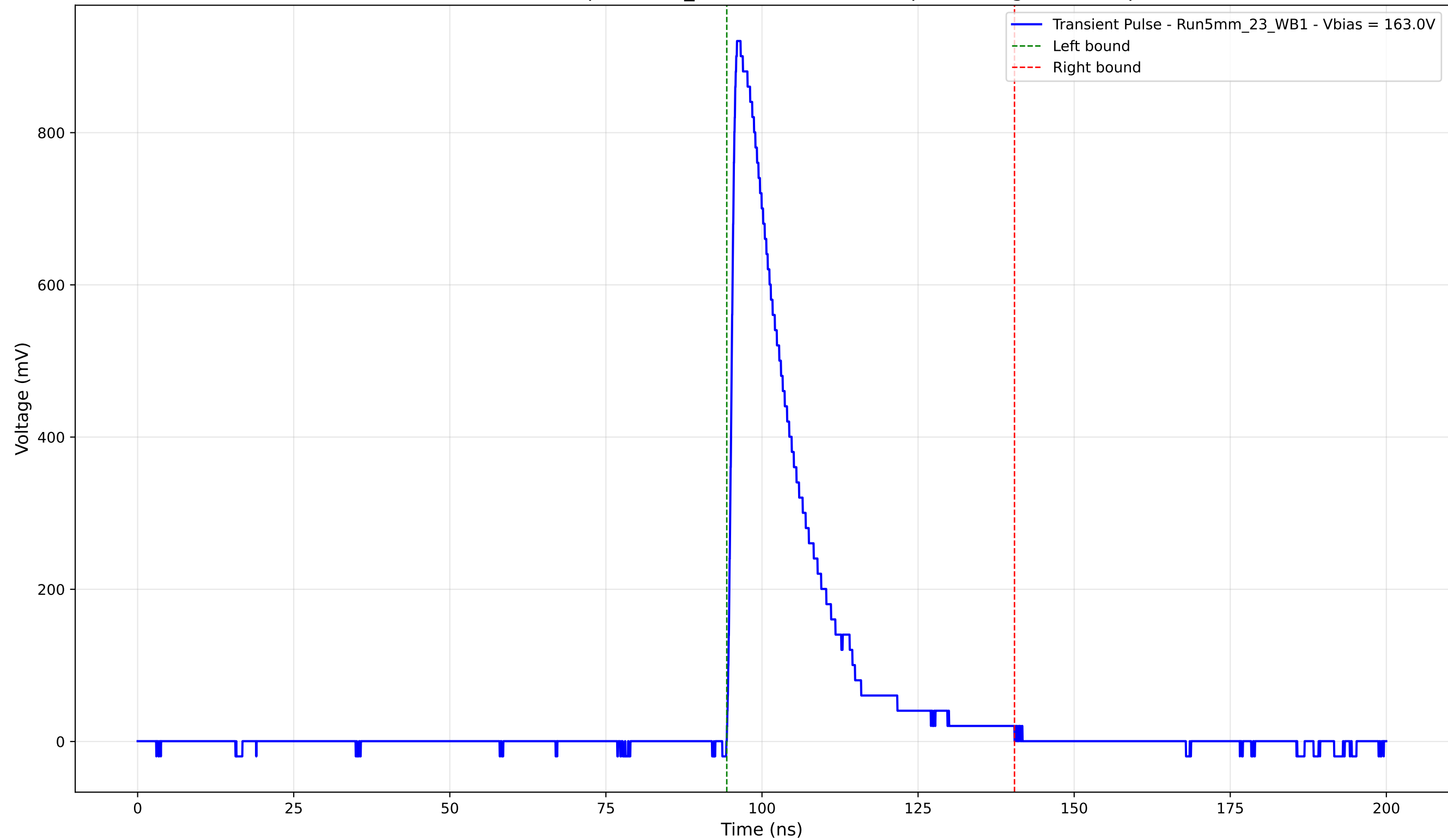
Transient Pulse - Sample: 5mm_23 - Position: 4105.0 \mu\text{m} - Charge: 197.49 pC
