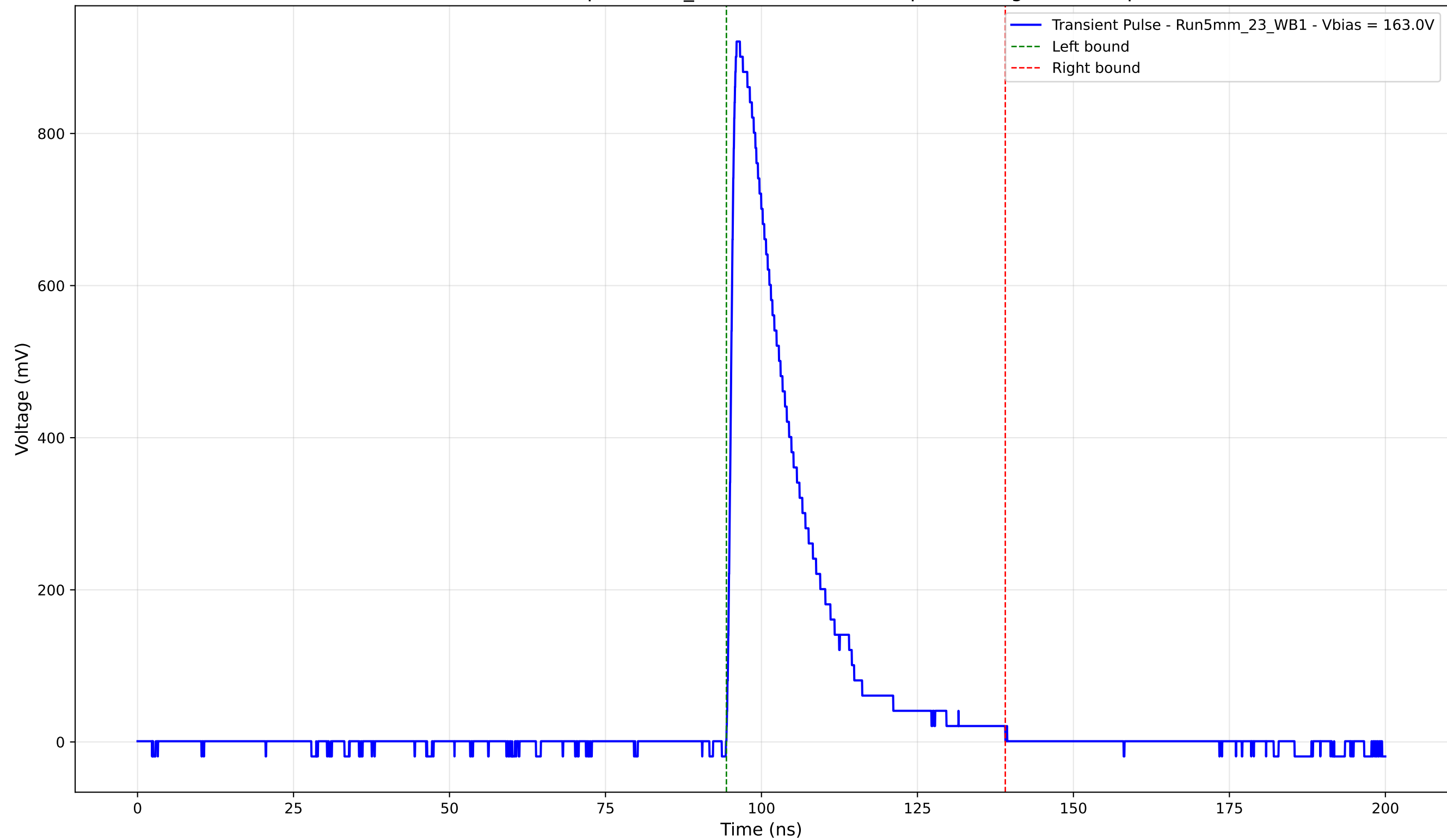
Transient Pulse - Sample: 5mm_23 - Position: 4080.0 \mu\text{m} - Charge: 197.53 pC
