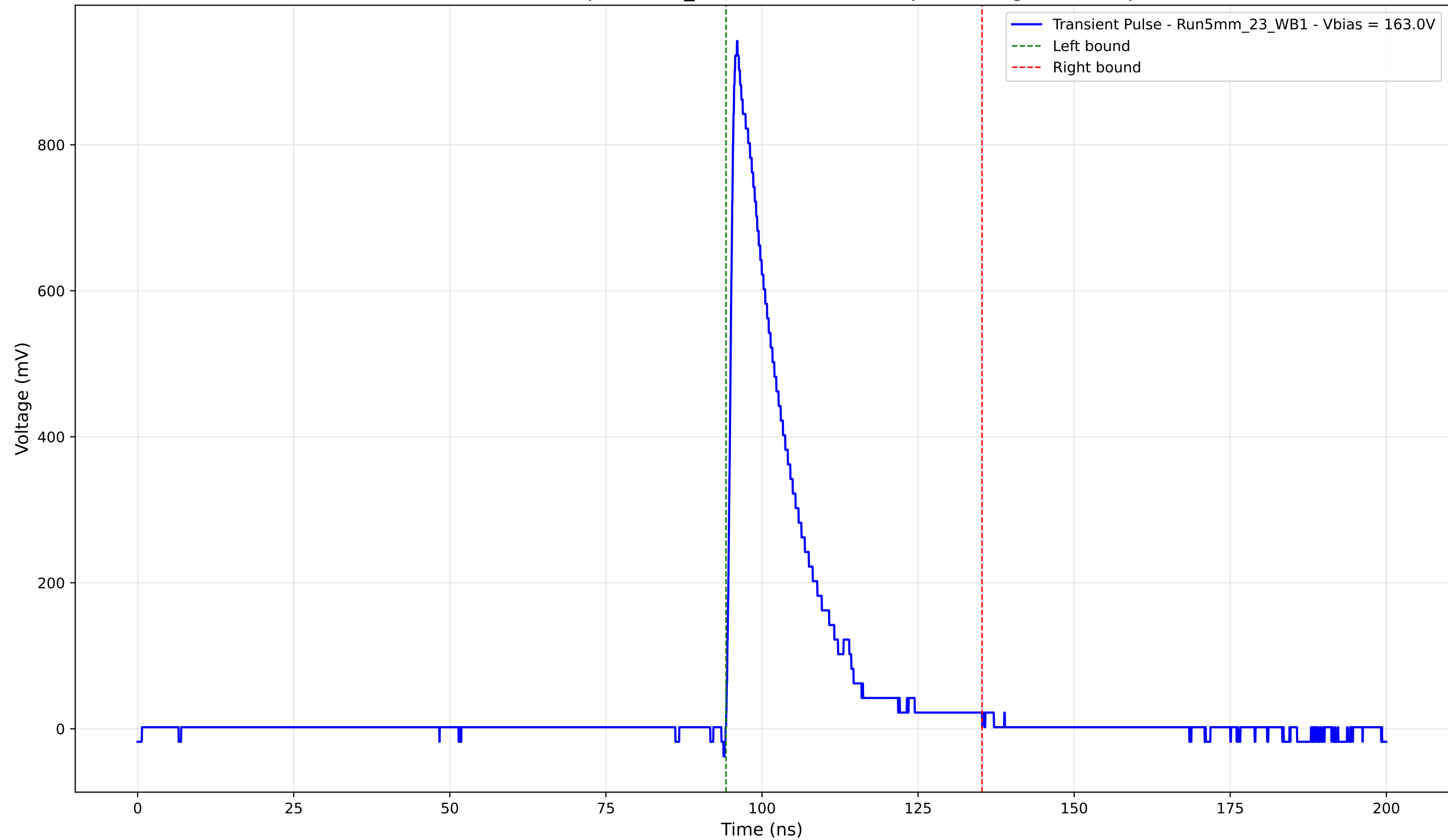
Transient Pulse - Sample: 5mm_23 - Position: 4595.0 \mu\text{m} - Charge: 177.42 pC
