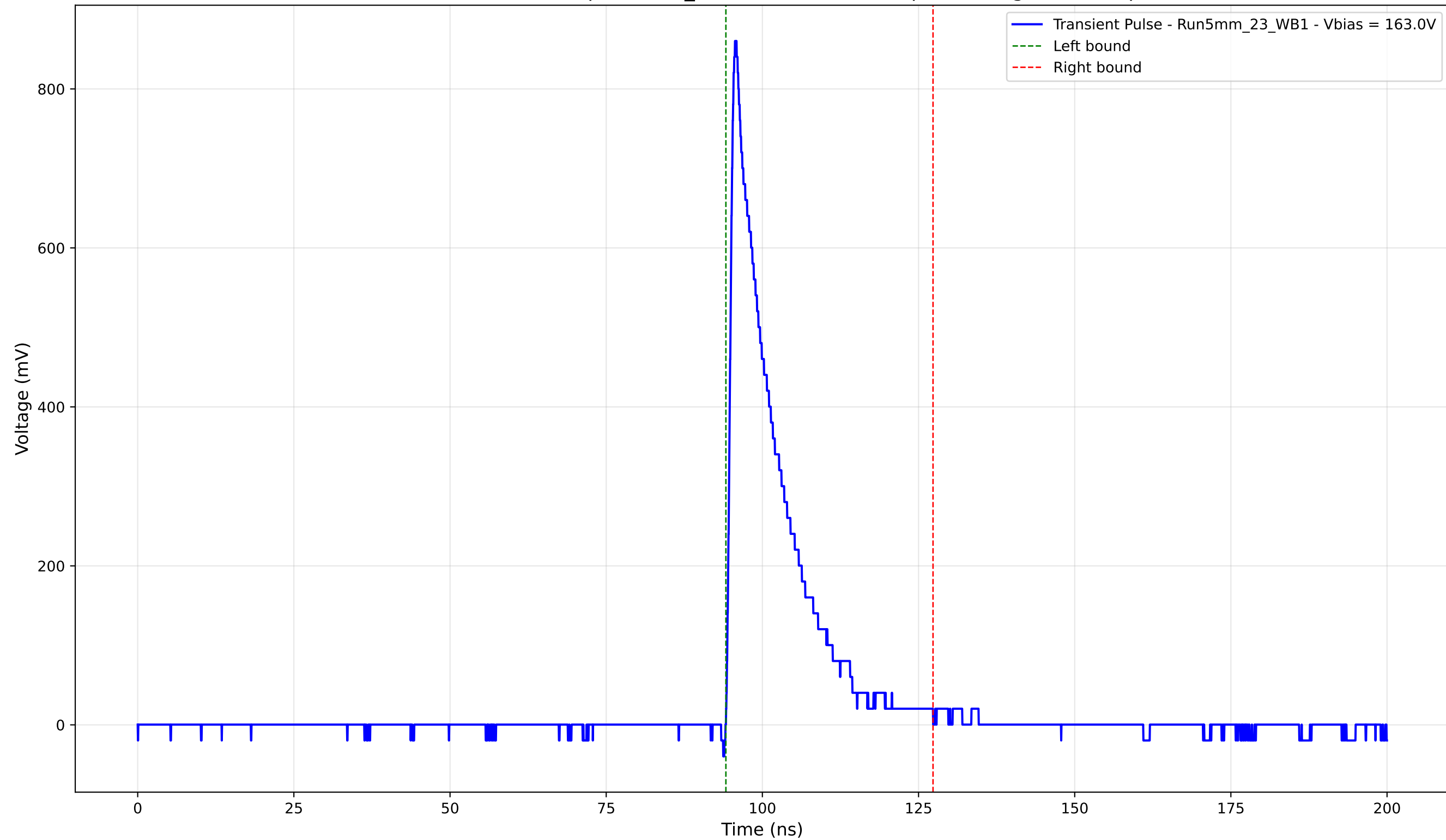
Transient Pulse - Sample: 5mm_23 - Position: 4830.0 \mu\text{m} - Charge: 134.81 pC
