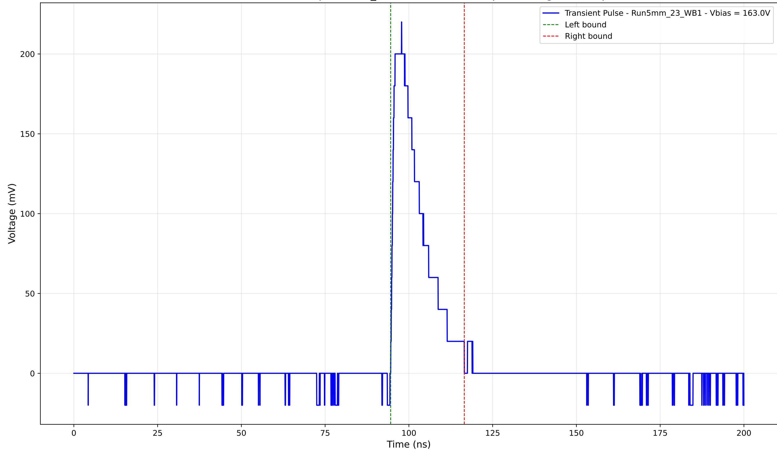
Transient Pulse - Sample: 5mm_23 - Position: 1730.0 \mu\text{m} - Charge: 39.88 pC
