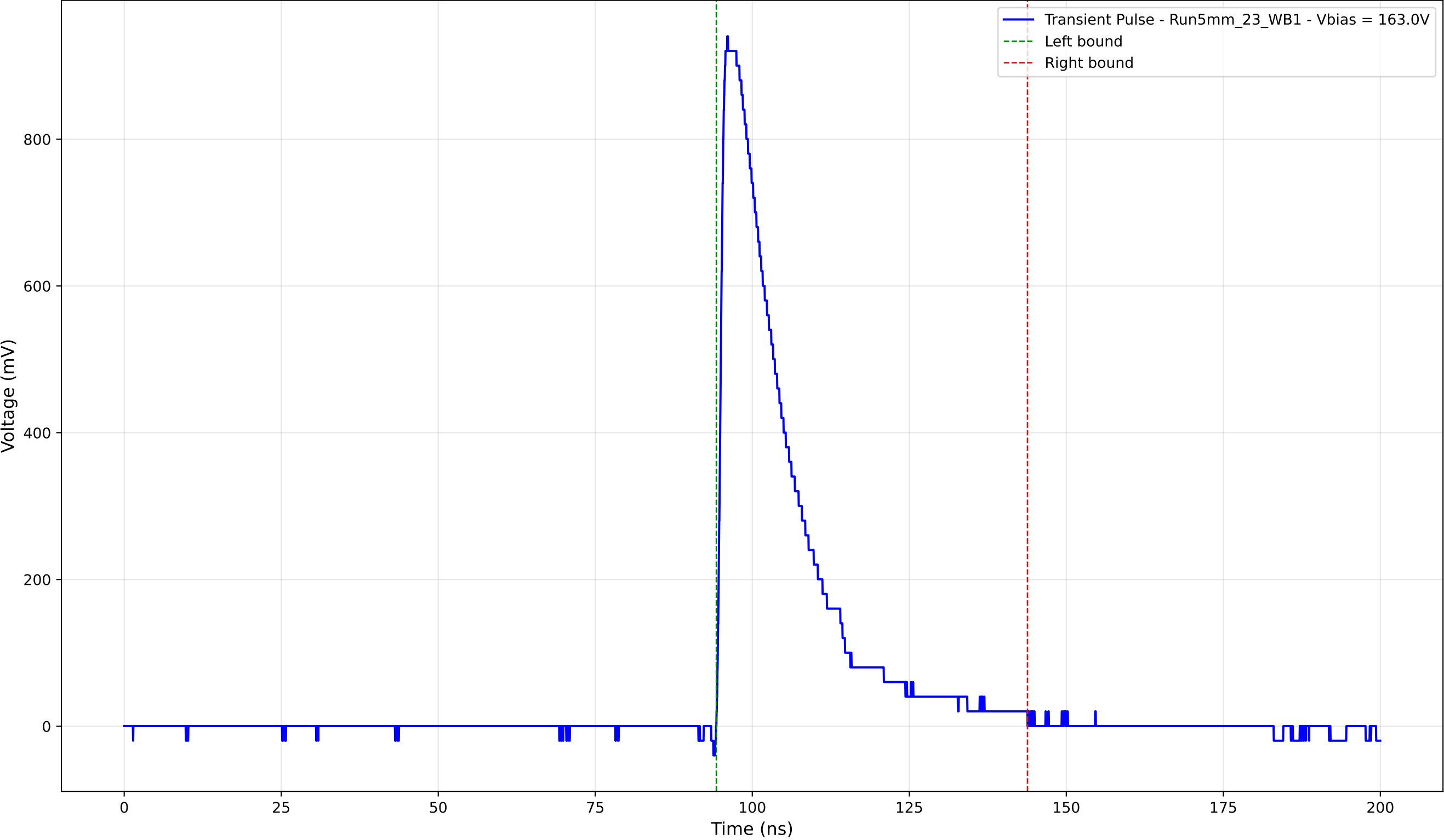
Transient Pulse - Sample: 5mm_23 - Position: 1825.0 \mu\text{m} - Charge: 218.03 pC
