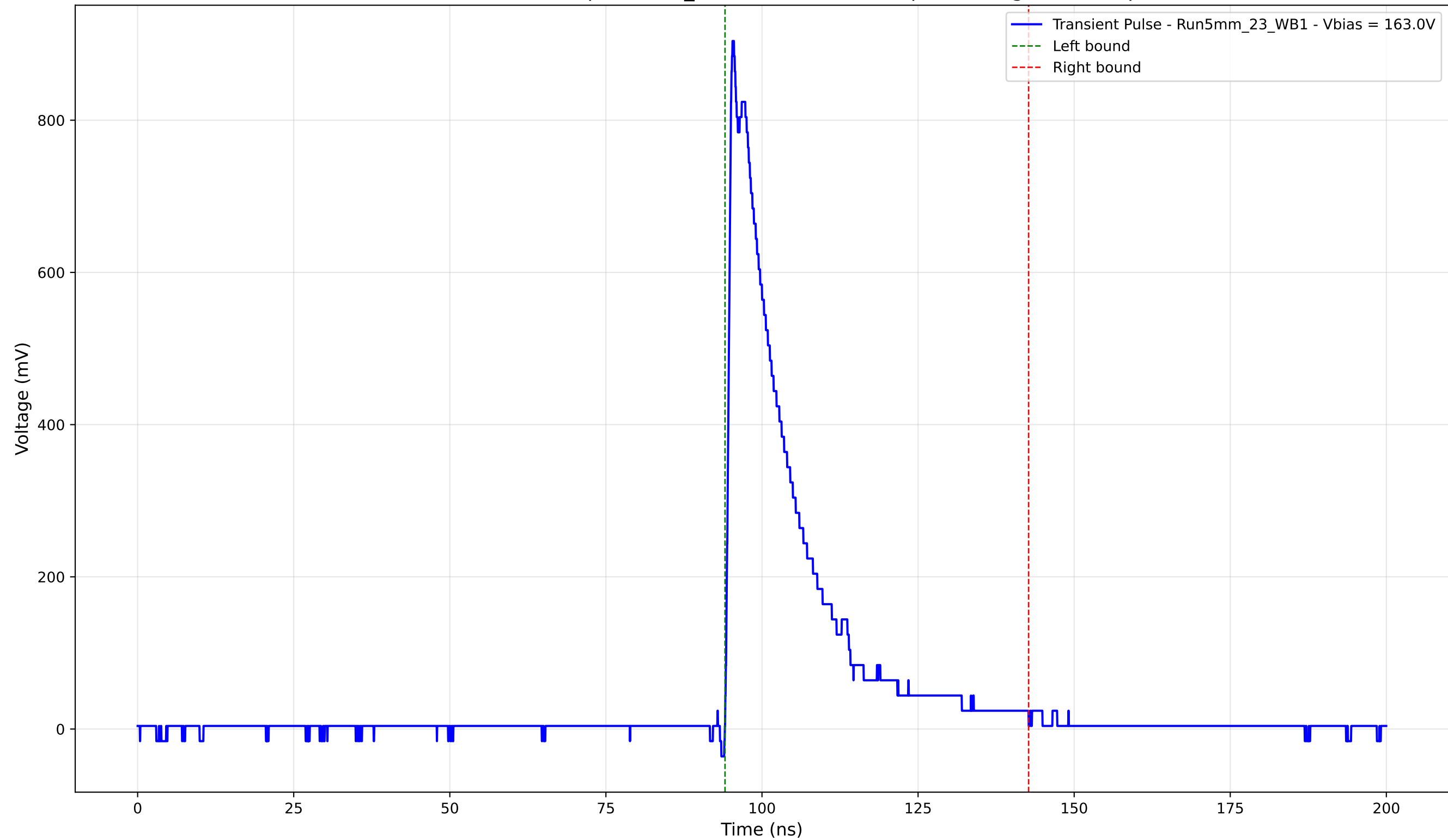
Transient Pulse - Sample: 5mm_23 - Position: 3175.0 \mu\text{m} - Charge: 185.16 pC
