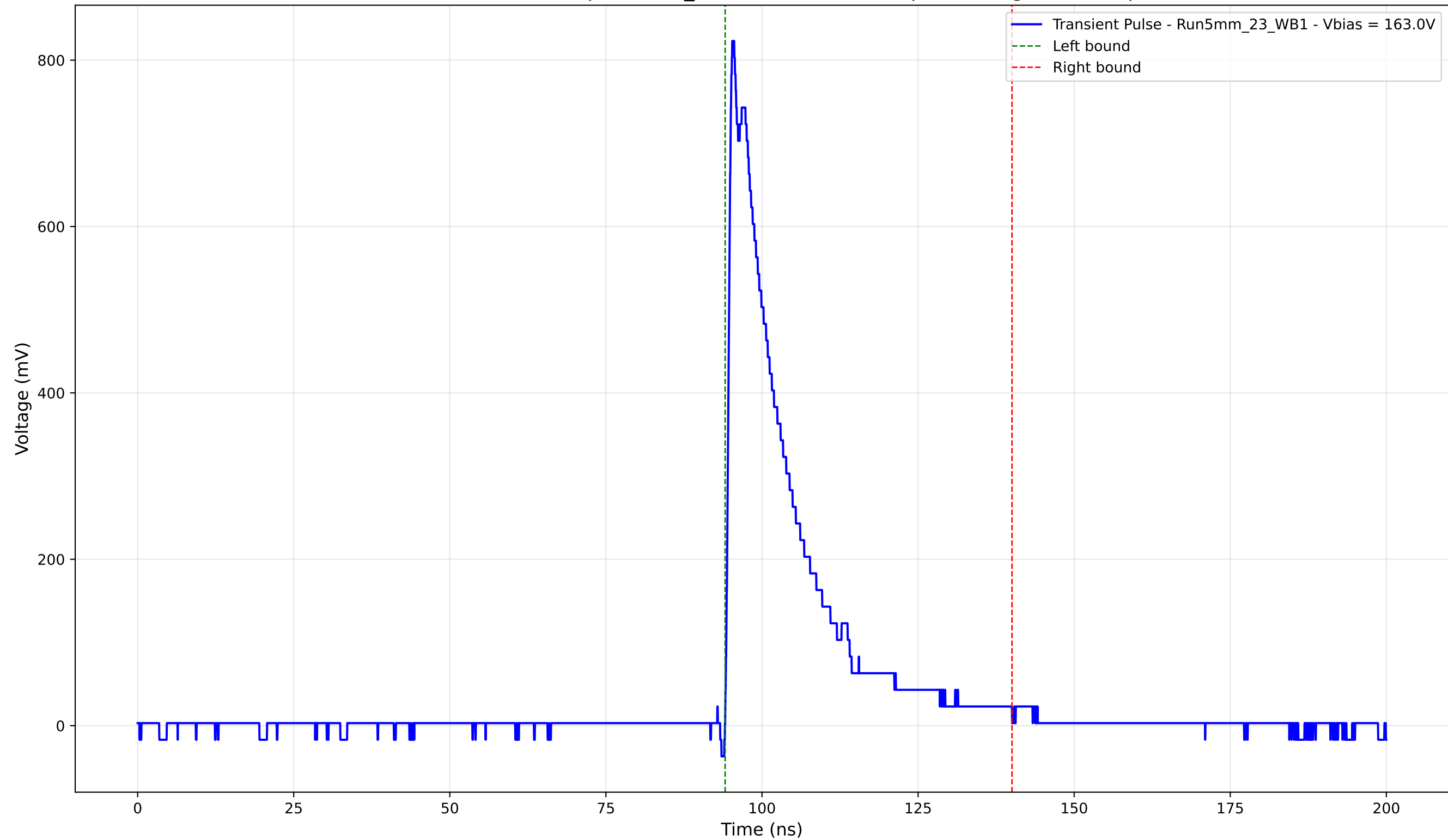
Transient Pulse - Sample: 5mm_23 - Position: 3185.0 \mu\text{m} - Charge: 162.35 pC
