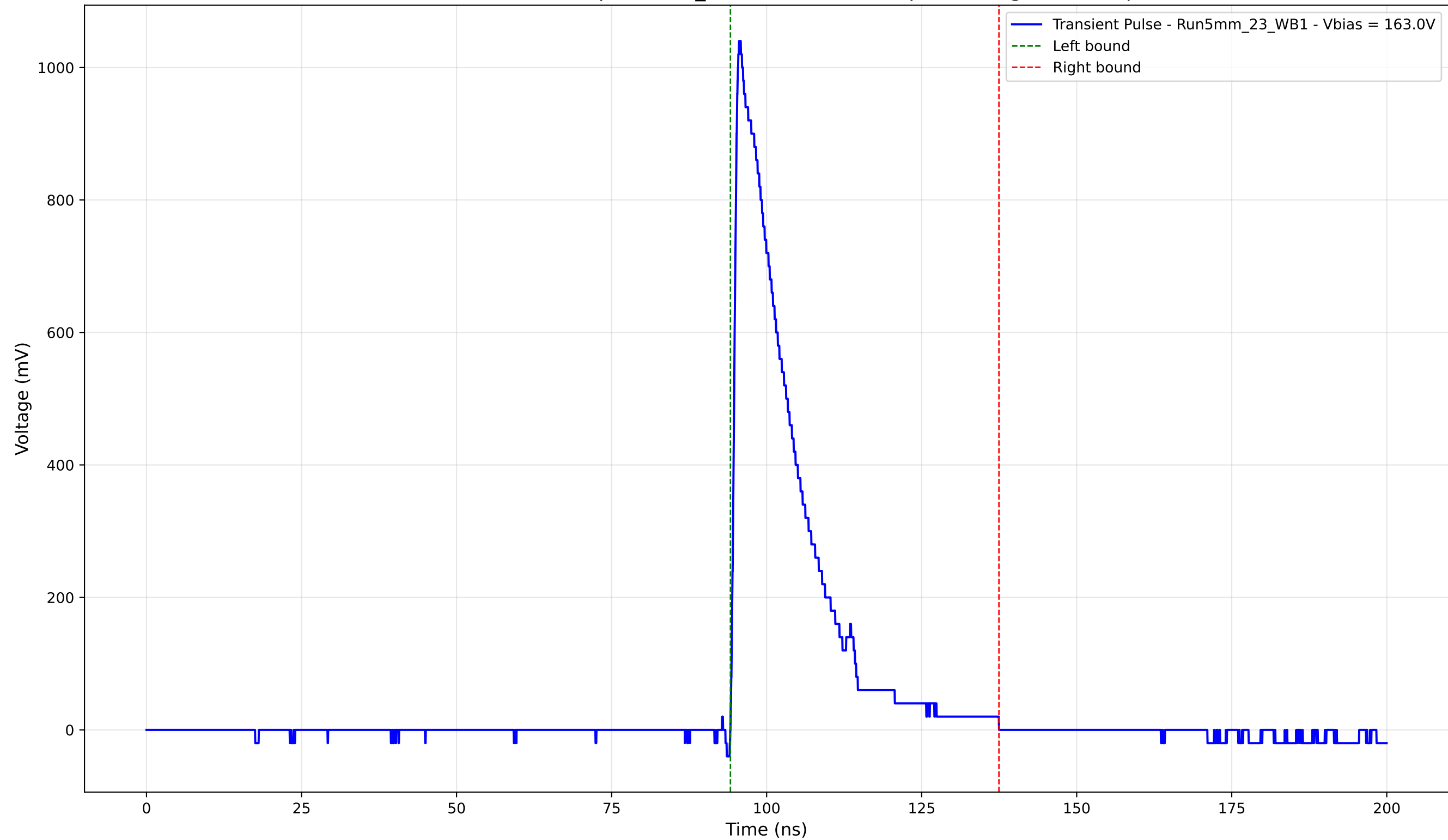
Transient Pulse - Sample: 5mm_23 - Position: 590.0 \mu\text{m} - Charge: 208.62 pC
