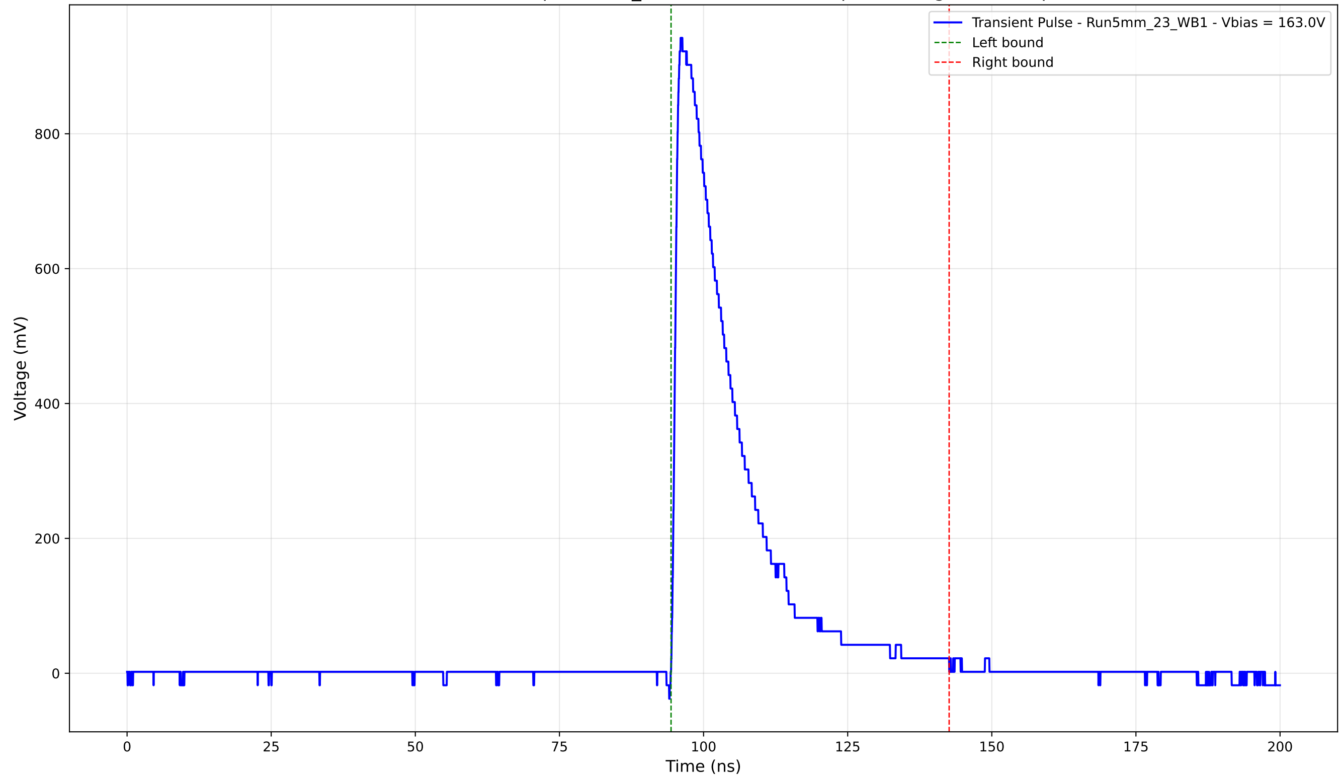
Transient Pulse - Sample: 5mm_23 - Position: 1645.0 \mu\text{m} - Charge: 215.64 pC
