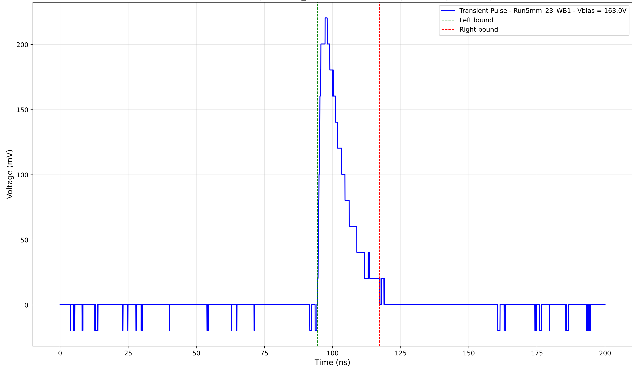
Transient Pulse - Sample: 5mm_23 - Position: 1735.0 \mu\text{m} - Charge: 41.91 pC
