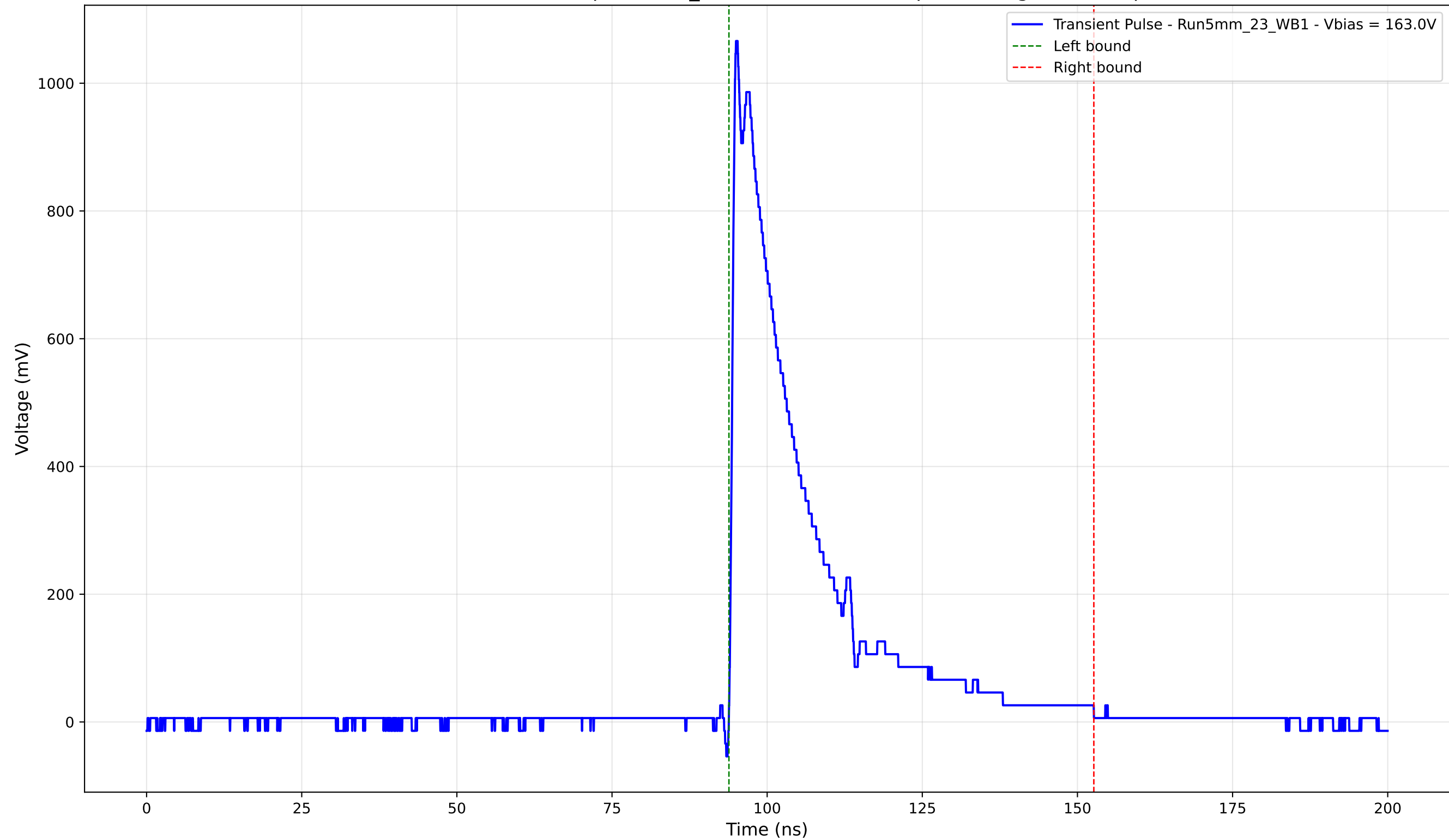
Transient Pulse - Sample: 5mm_23 - Position: 2635.0 \mu\text{m} - Charge: 248.66 pC
