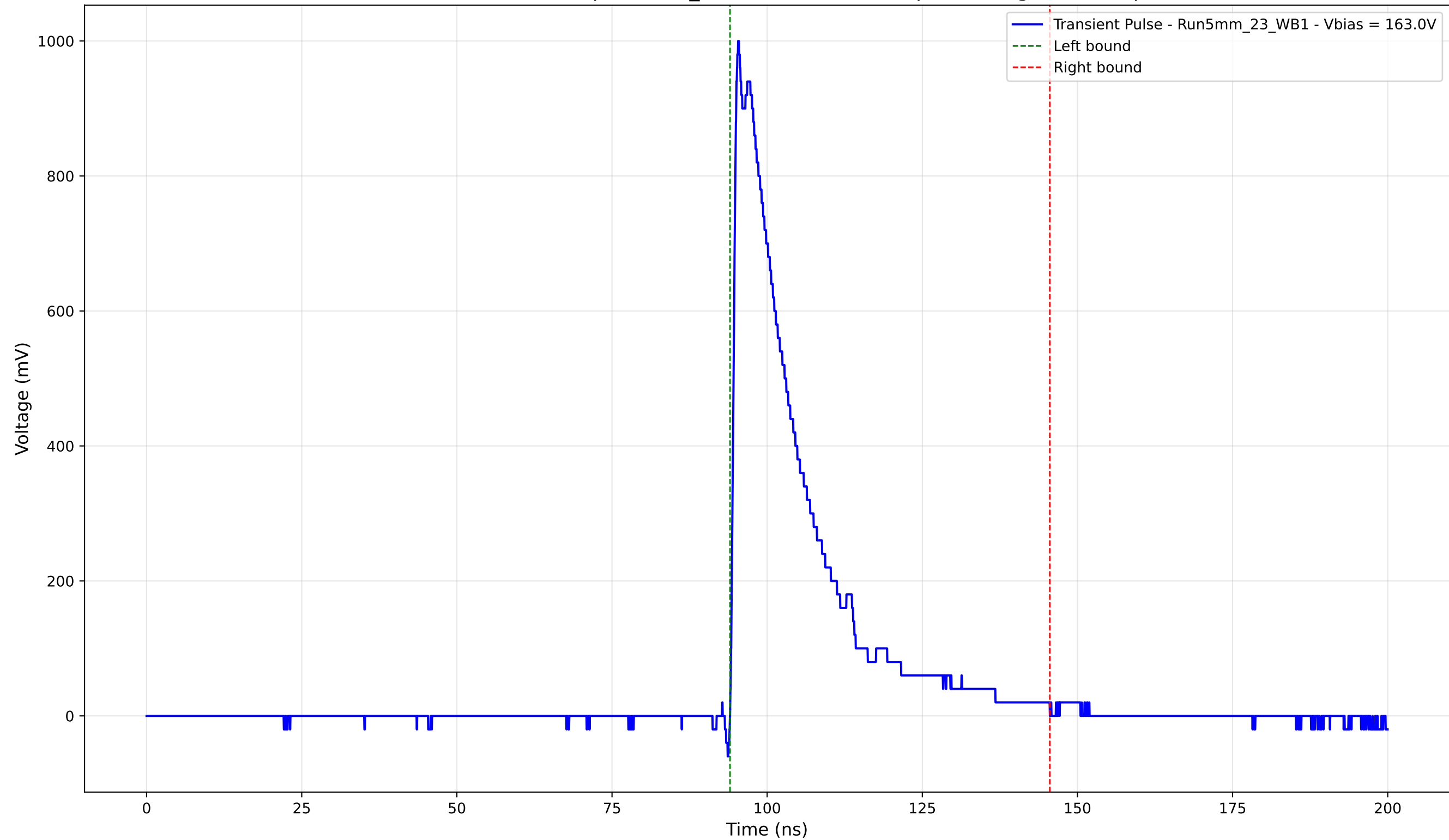
Transient Pulse - Sample: 5mm_23 - Position: 2360.0 \mu\text{m} - Charge: 224.22 pC
