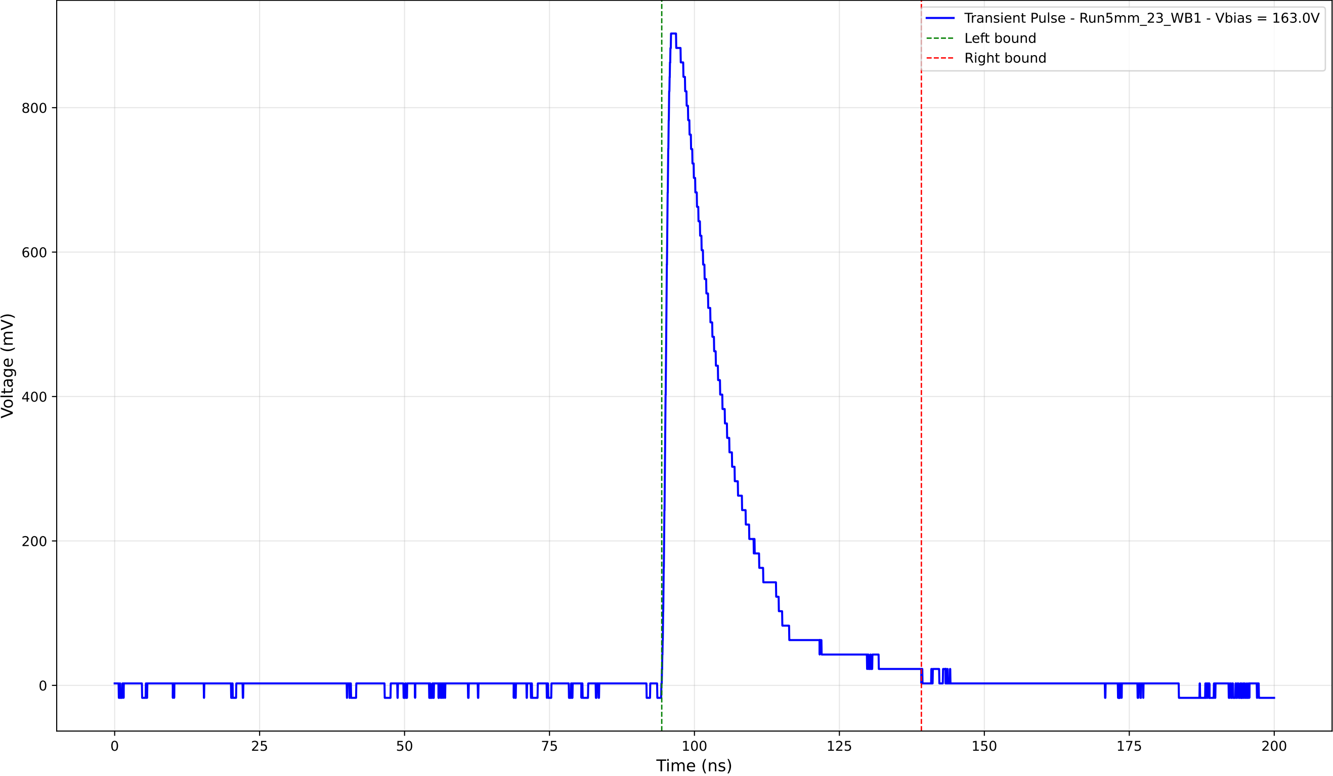
Transient Pulse - Sample: 5mm_23 - Position: 3940.0 \mu\text{m} - Charge: 199.89 pC
