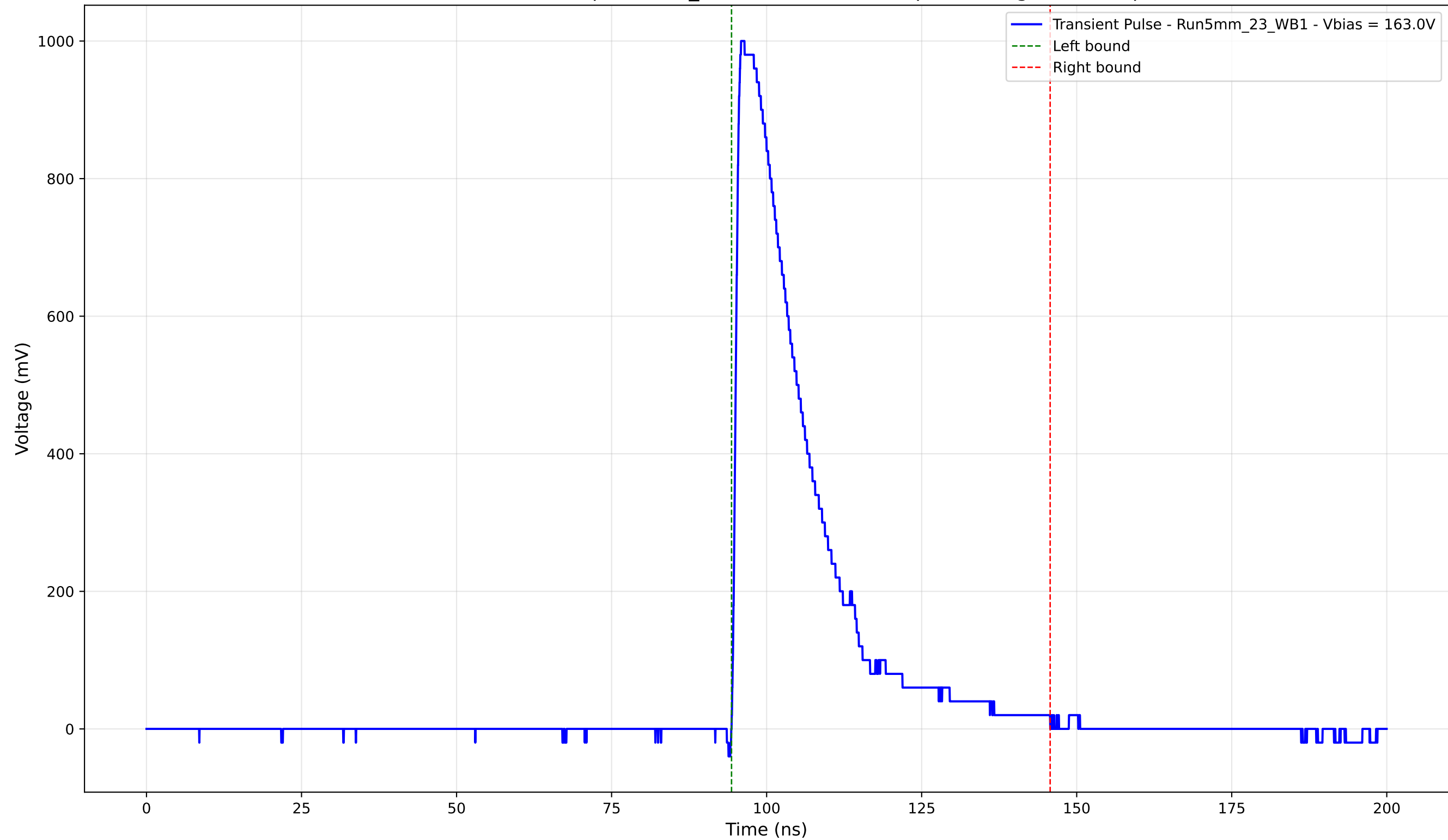
Transient Pulse - Sample: 5mm_23 - Position: 1610.0 \mu\text{m} - Charge: 249.65 pC
