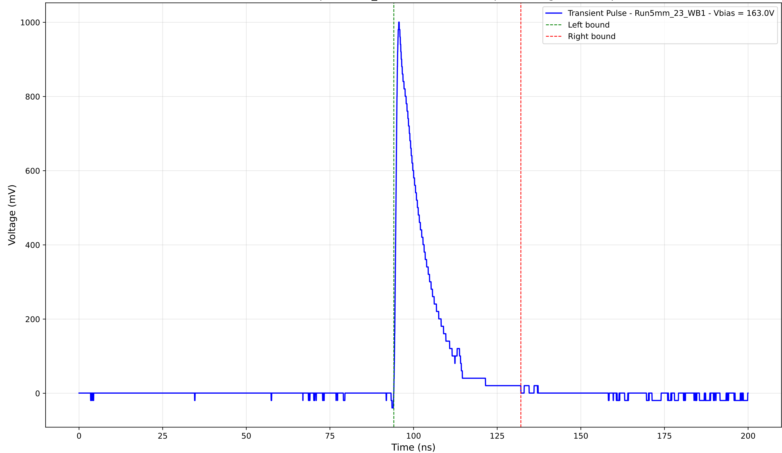
Transient Pulse - Sample: 5mm_23 - Position: 4900.0 \mu\text{m} - Charge: 170.76 pC
