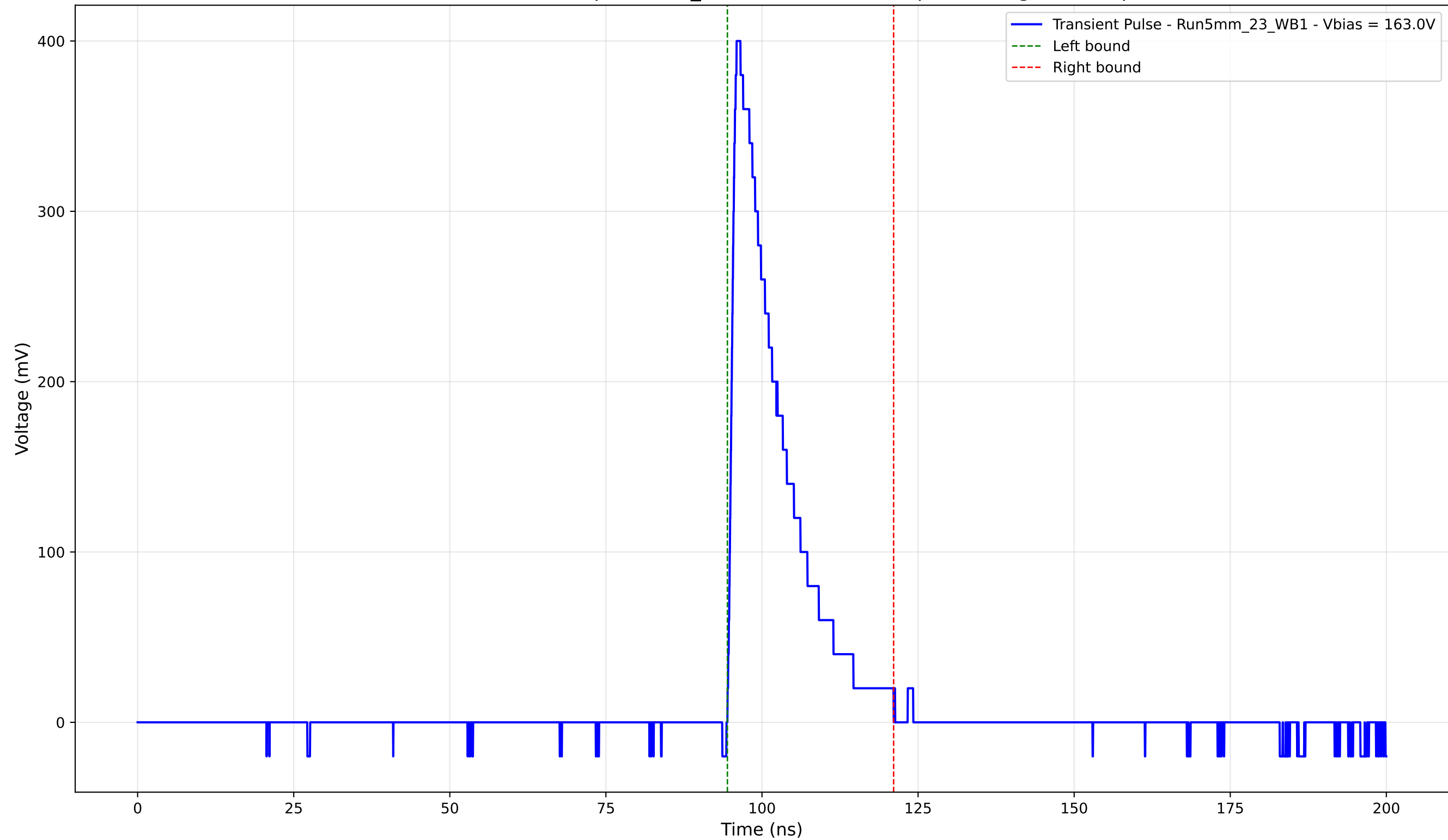
Transient Pulse - Sample: 5mm_23 - Position: 4295.0 \mu\text{m} - Charge: 69.05 pC
