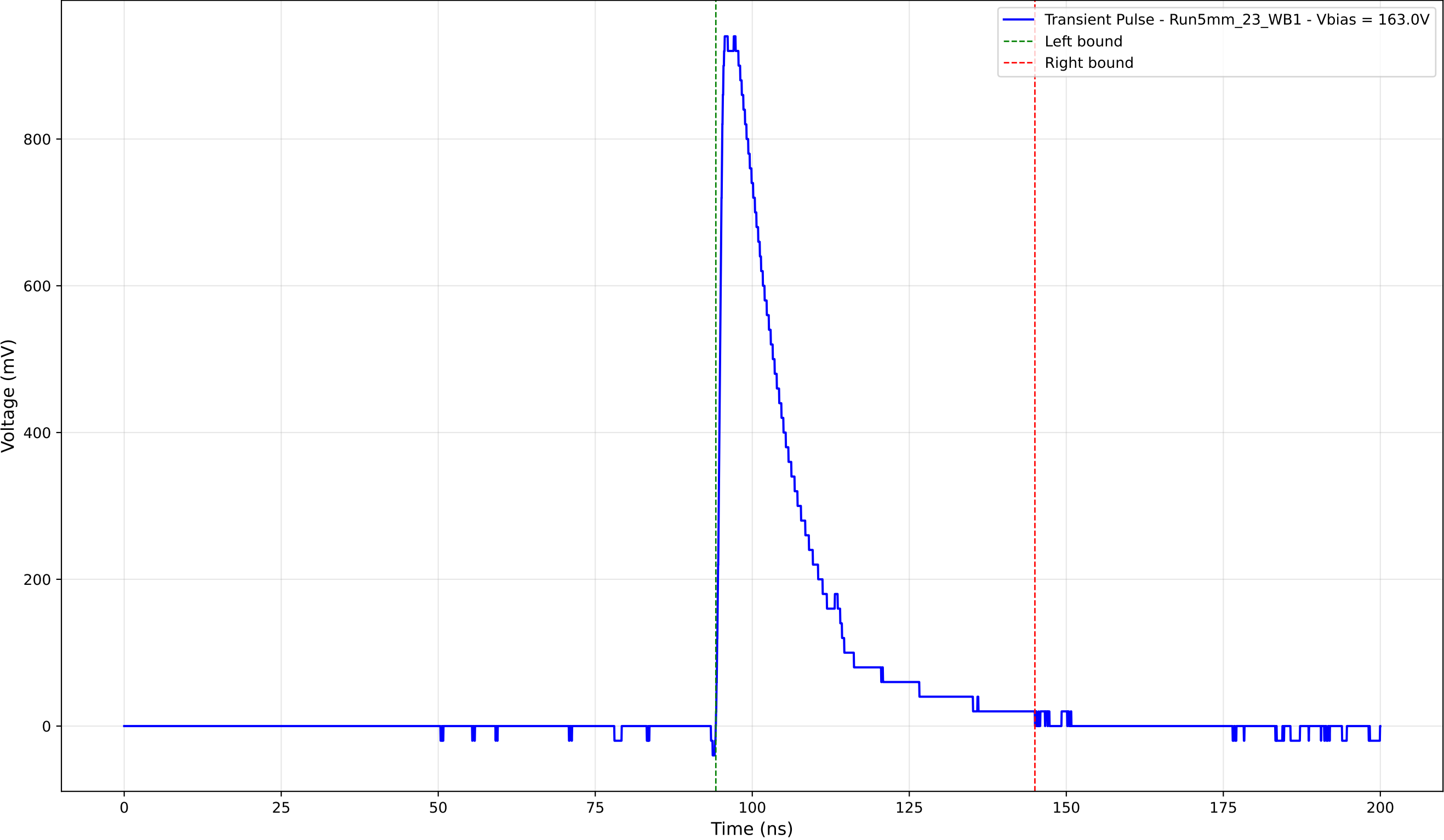
Transient Pulse - Sample: 5mm_23 - Position: 3490.0 \mu\text{m} - Charge: 222.21 pC
