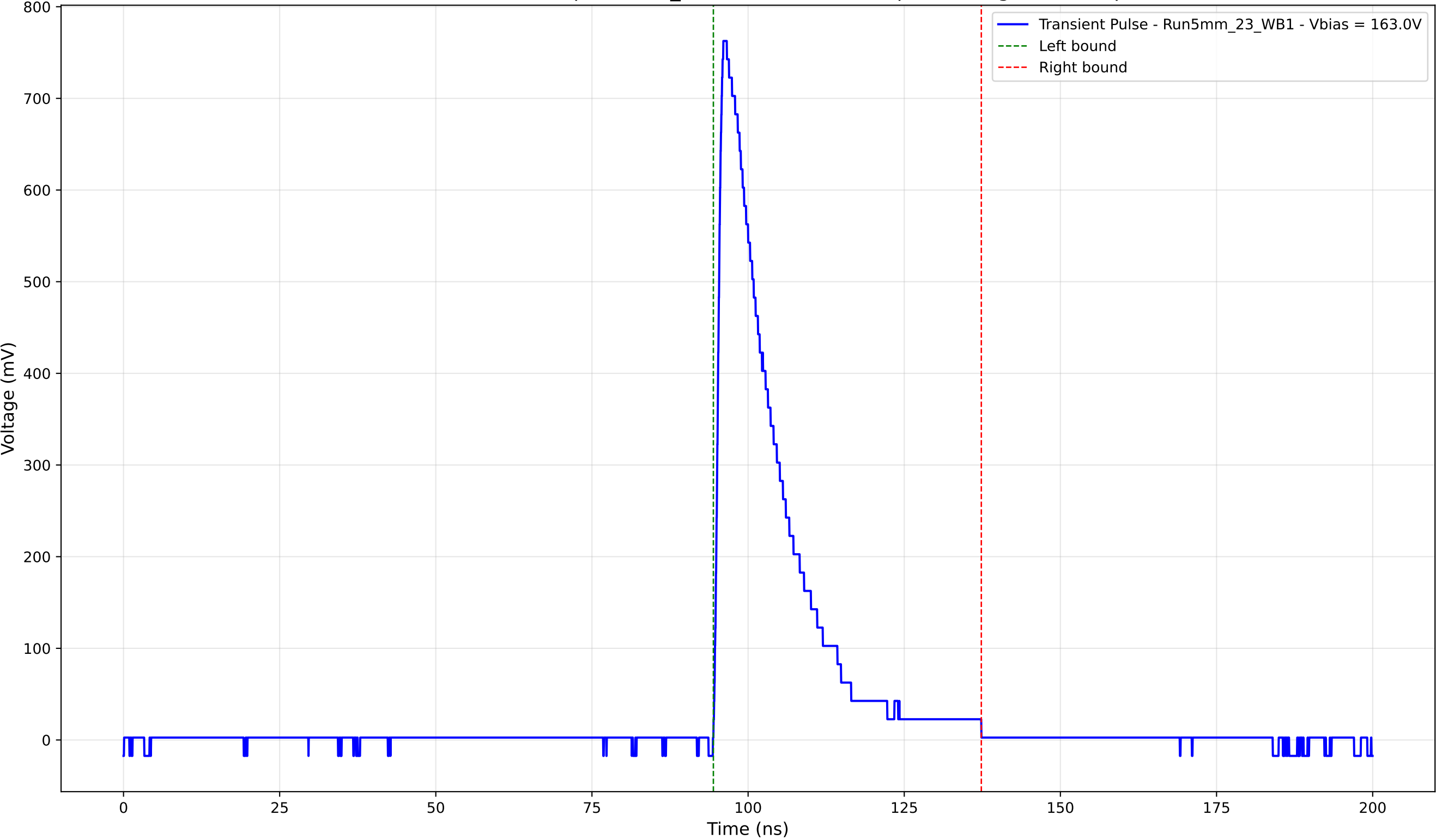
Transient Pulse - Sample: 5mm_23 - Position: 1285.0 \mu\text{m} - Charge: 153.96 pC
