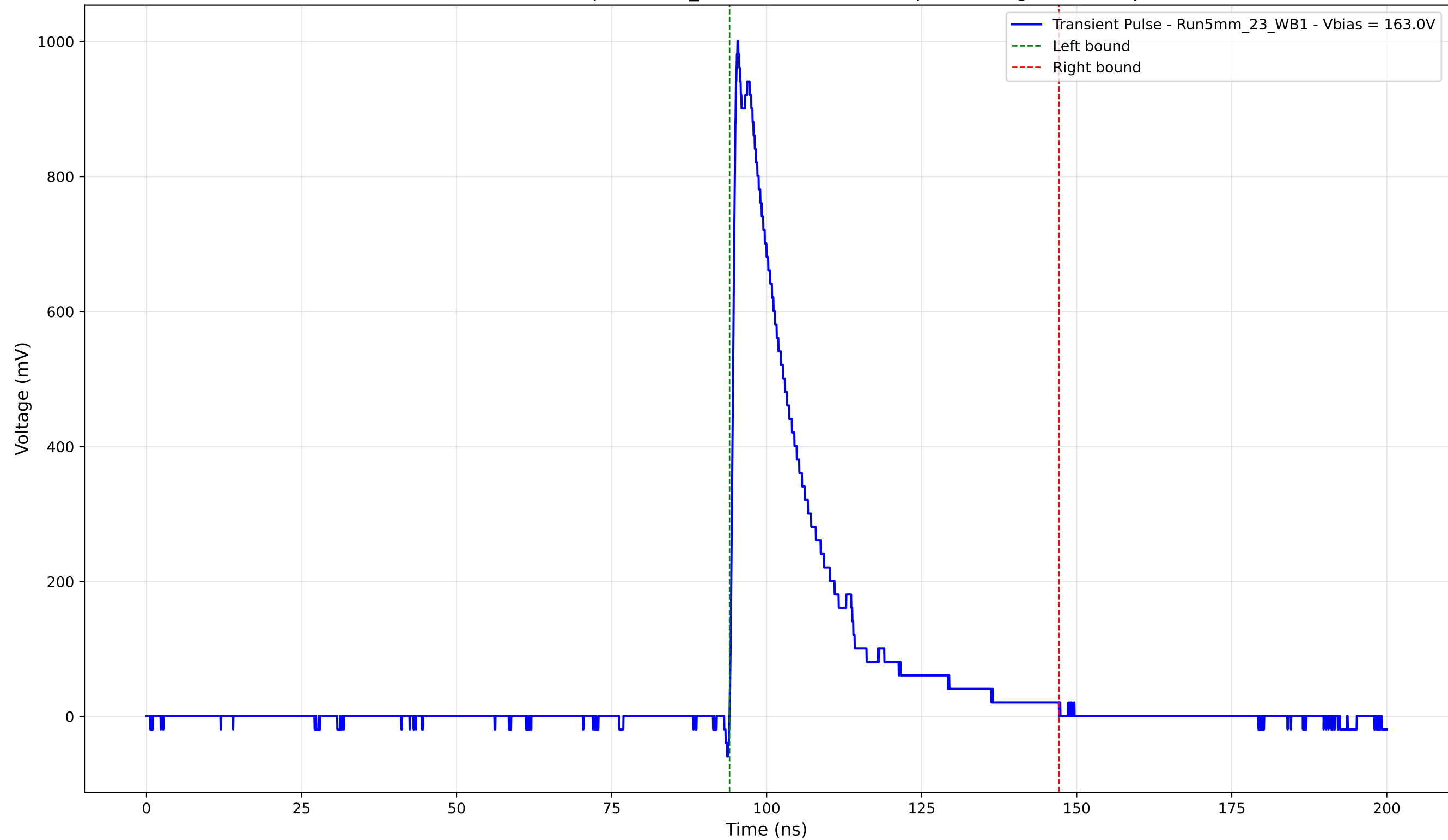
Transient Pulse - Sample: 5mm_23 - Position: 3115.0 \mu\text{m} - Charge: 223.37 pC
