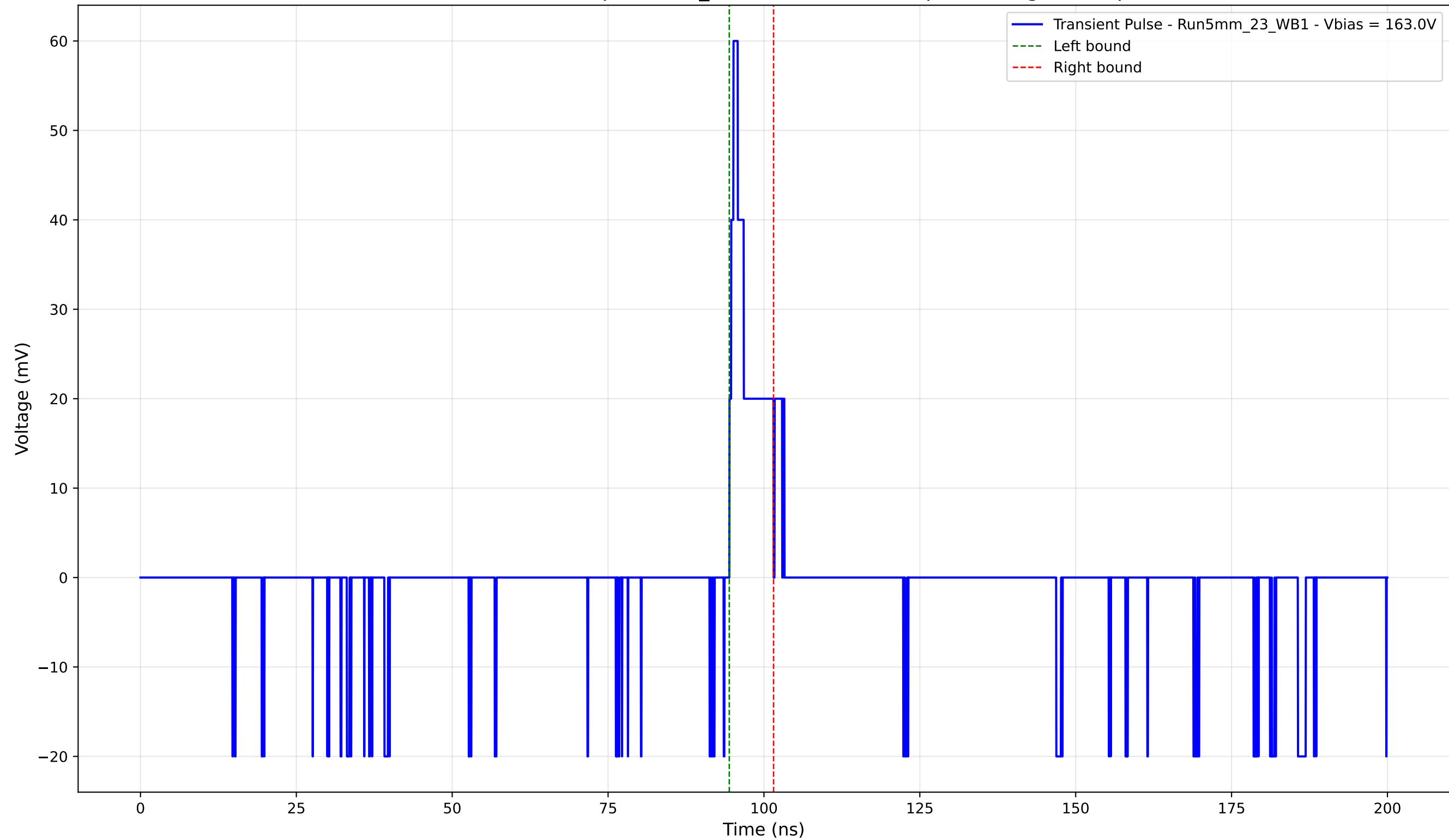
Transient Pulse - Sample: 5mm_23 - Position: 5225.0 \mu\text{m} - Charge: 3.92 pC
