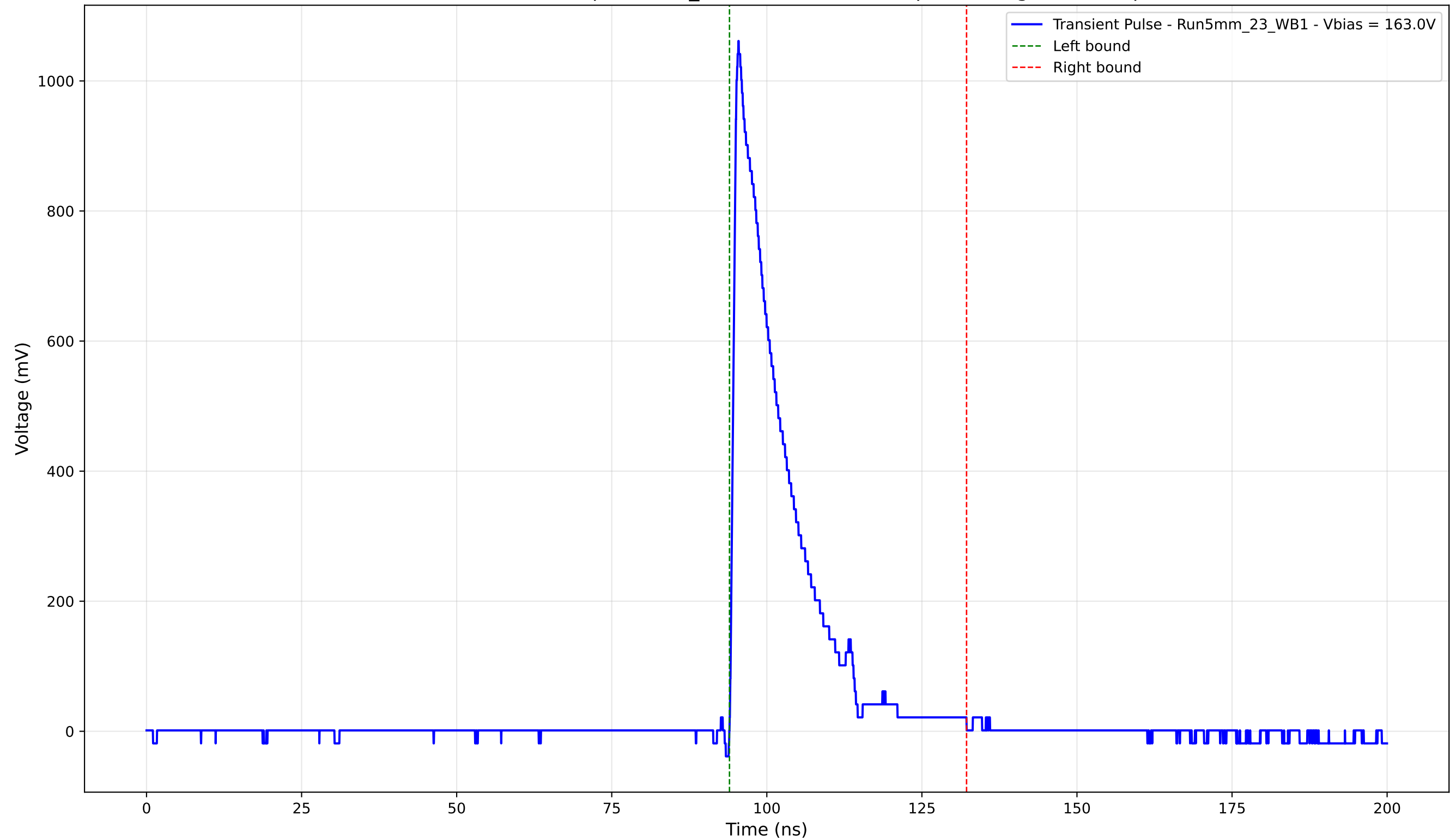
Transient Pulse - Sample: 5mm_23 - Position: 5055.0 \mu\text{m} - Charge: 182.63 pC
