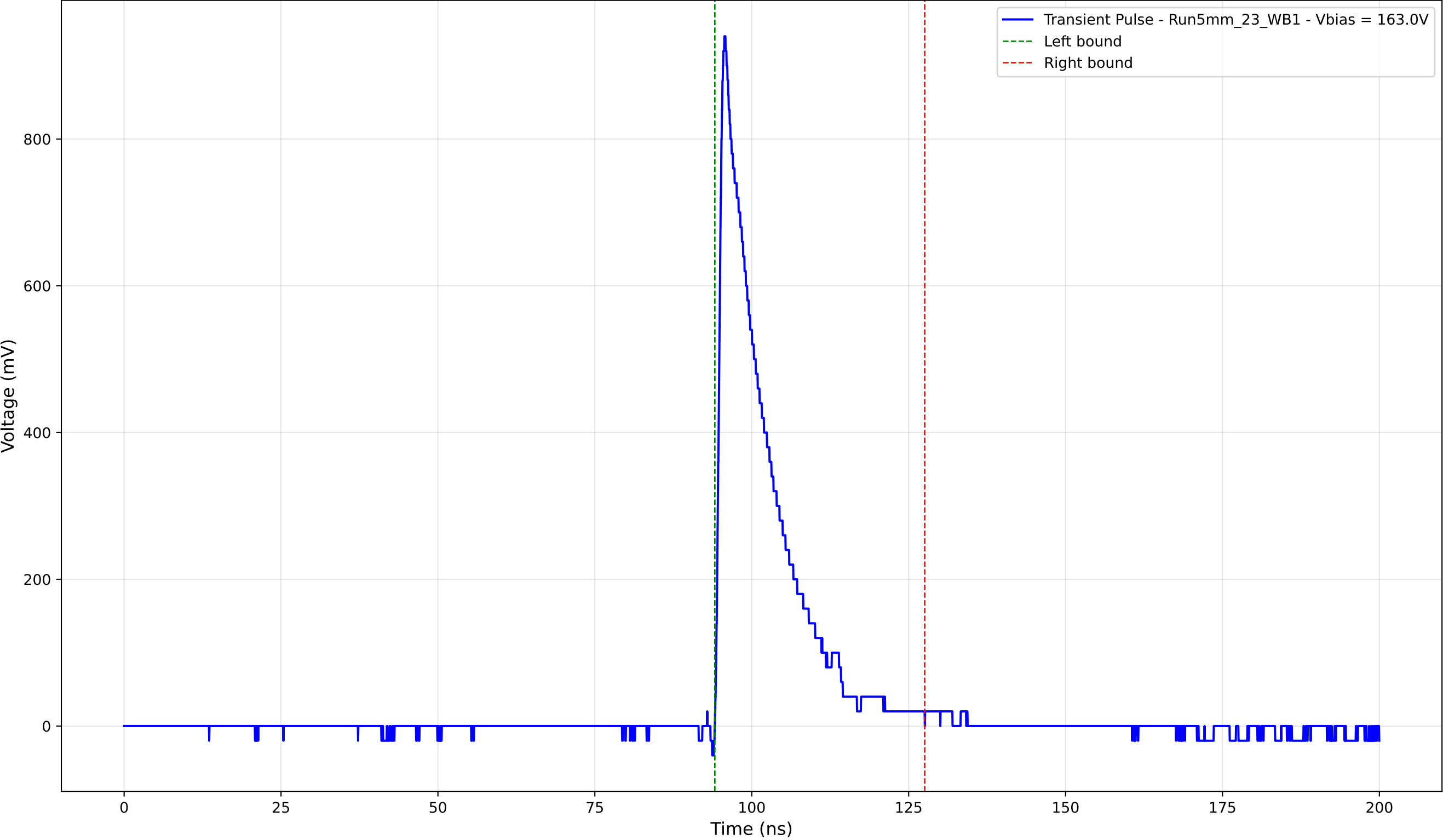
Transient Pulse - Sample: 5mm_23 - Position: 4845.0 \mu\text{m} - Charge: 152.49 pC
