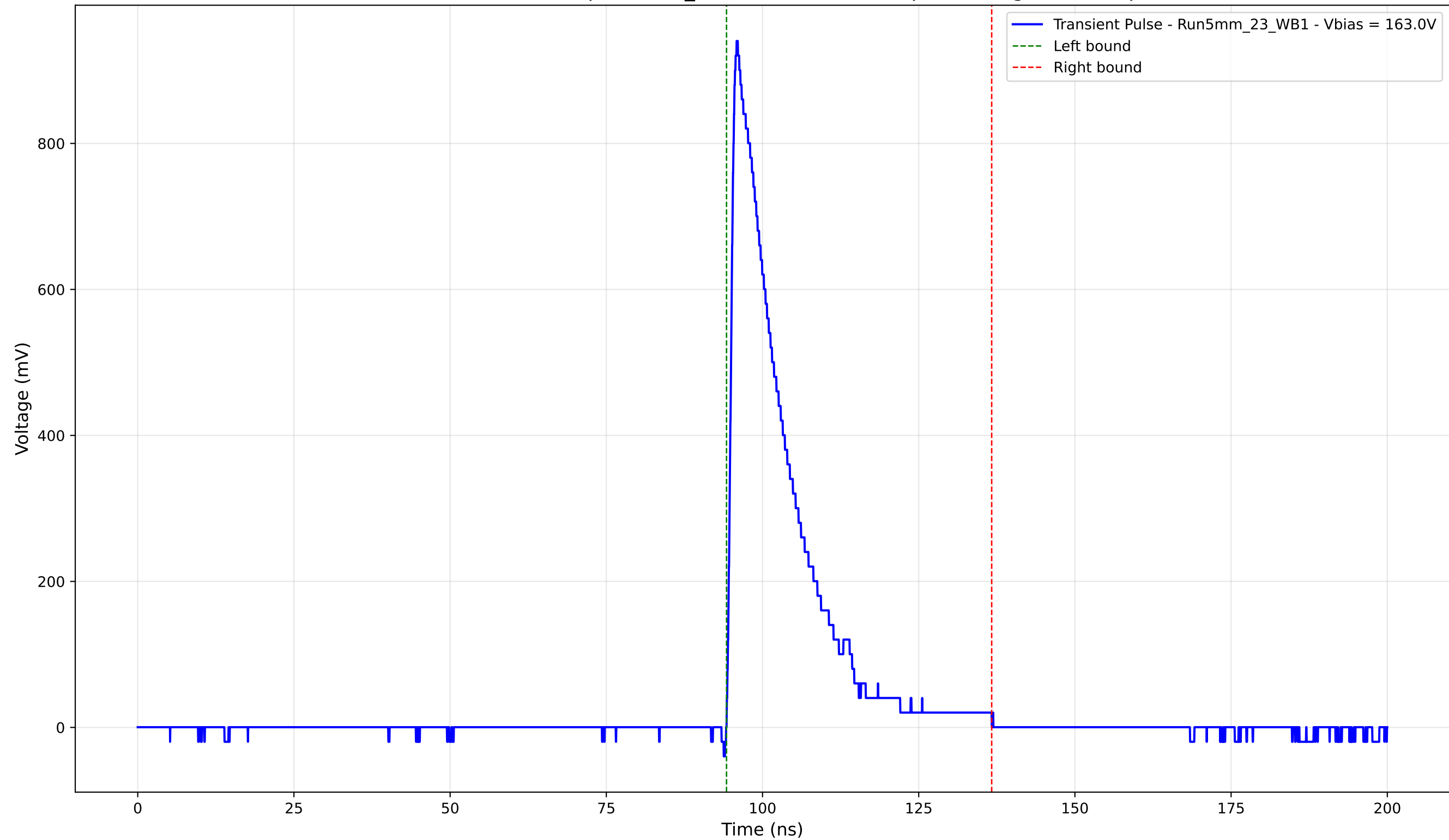
Transient Pulse - Sample: 5mm_23 - Position: 4615.0 \mu\text{m} - Charge: 175.27 pC
