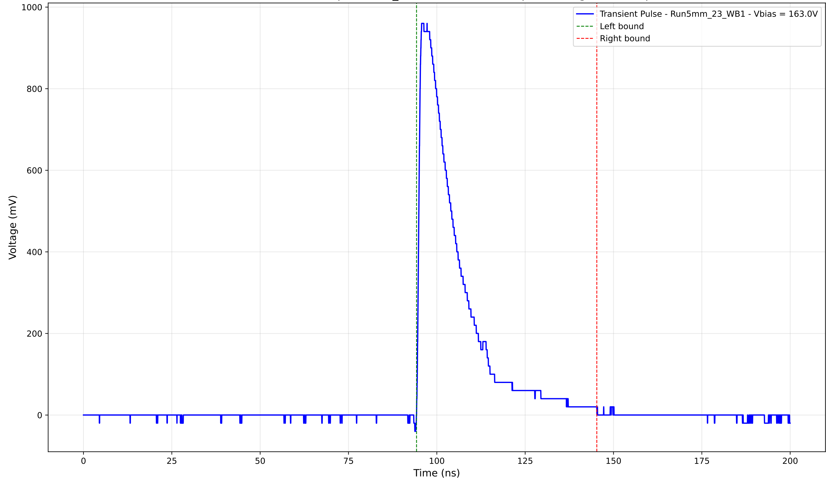
Transient Pulse - Sample: 5mm_23 - Position: 1900.0 \mu\text{m} - Charge: 234.65 pC
