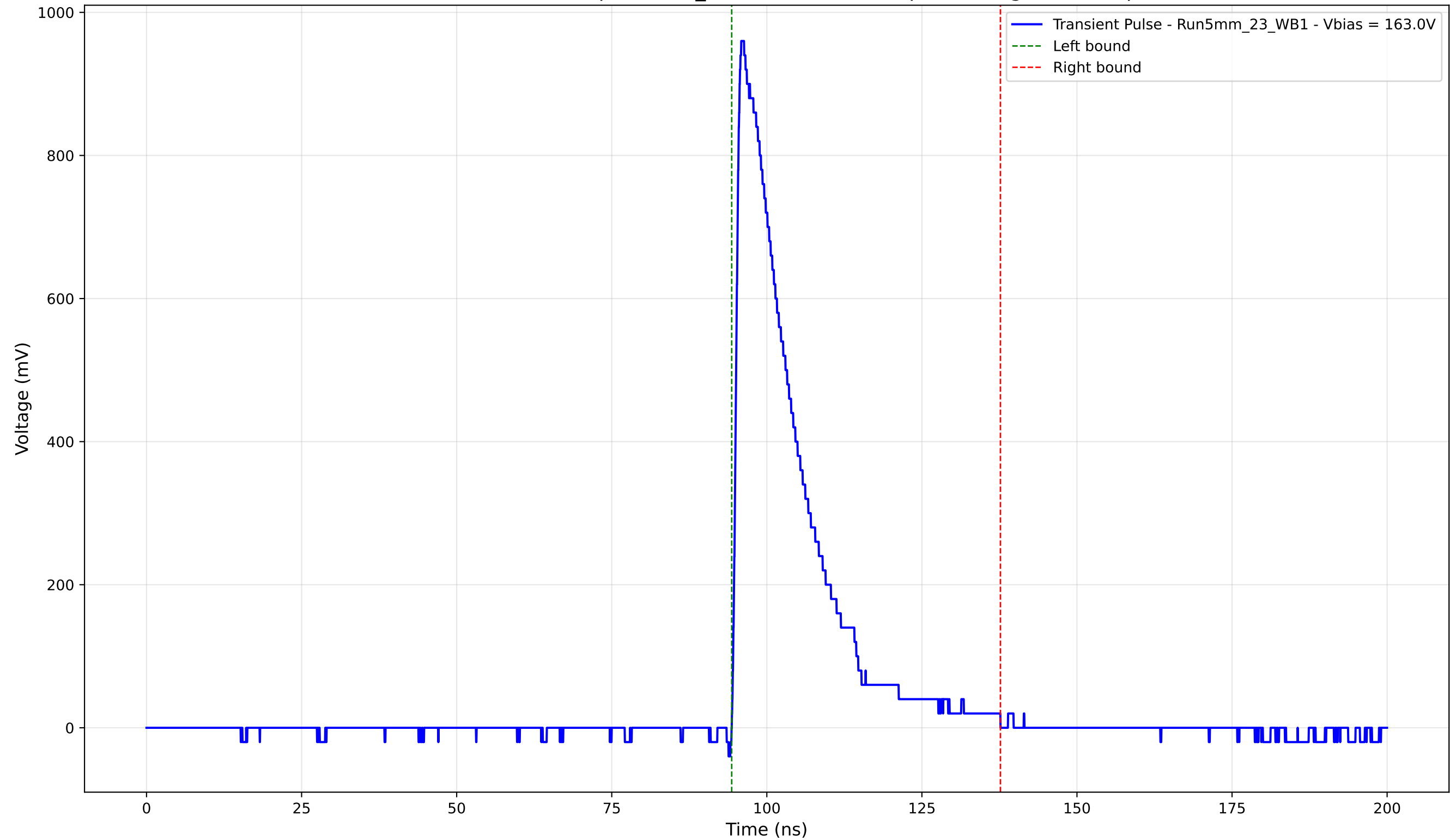
Transient Pulse - Sample: 5mm_23 - Position: 980.0 \mu\text{m} - Charge: 200.99 pC
