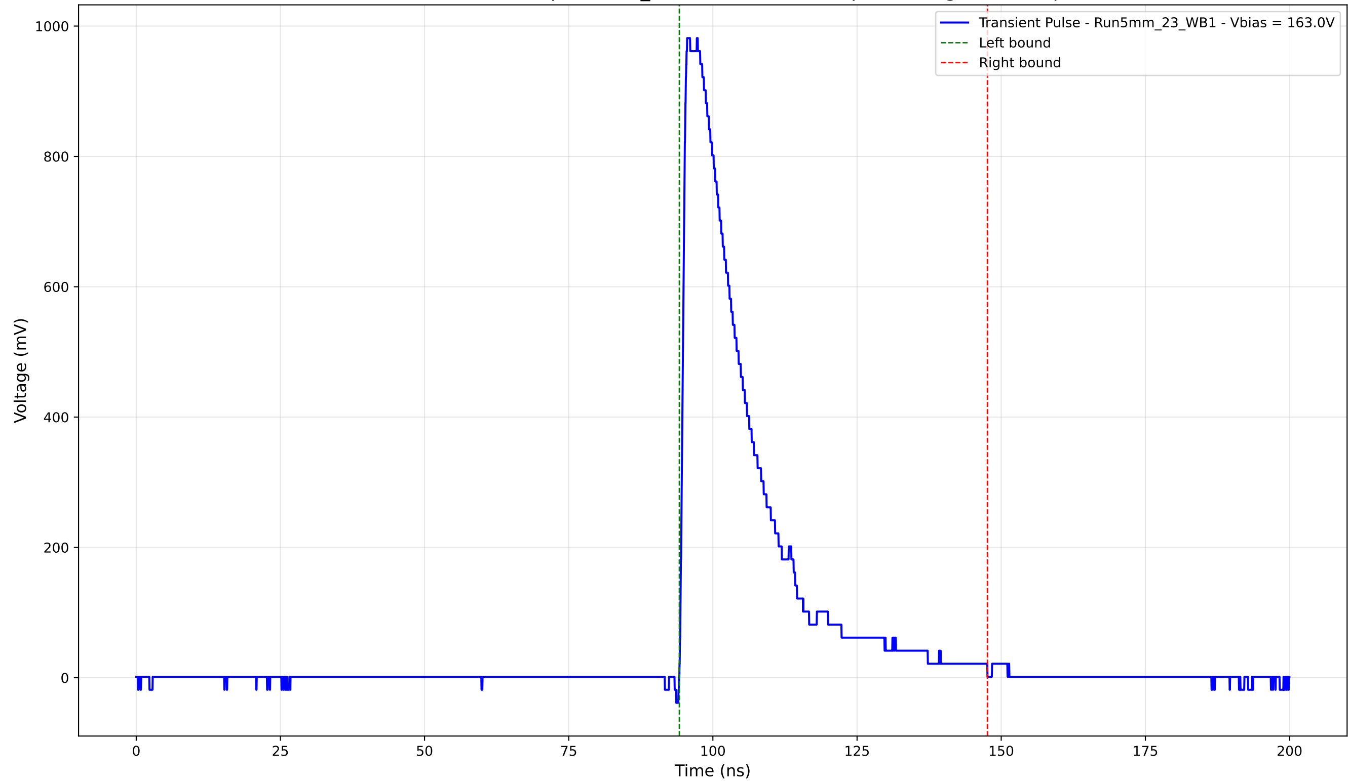
Transient Pulse - Sample: 5mm_23 - Position: 2025.0 \mu\text{m} - Charge: 246.26 pC
