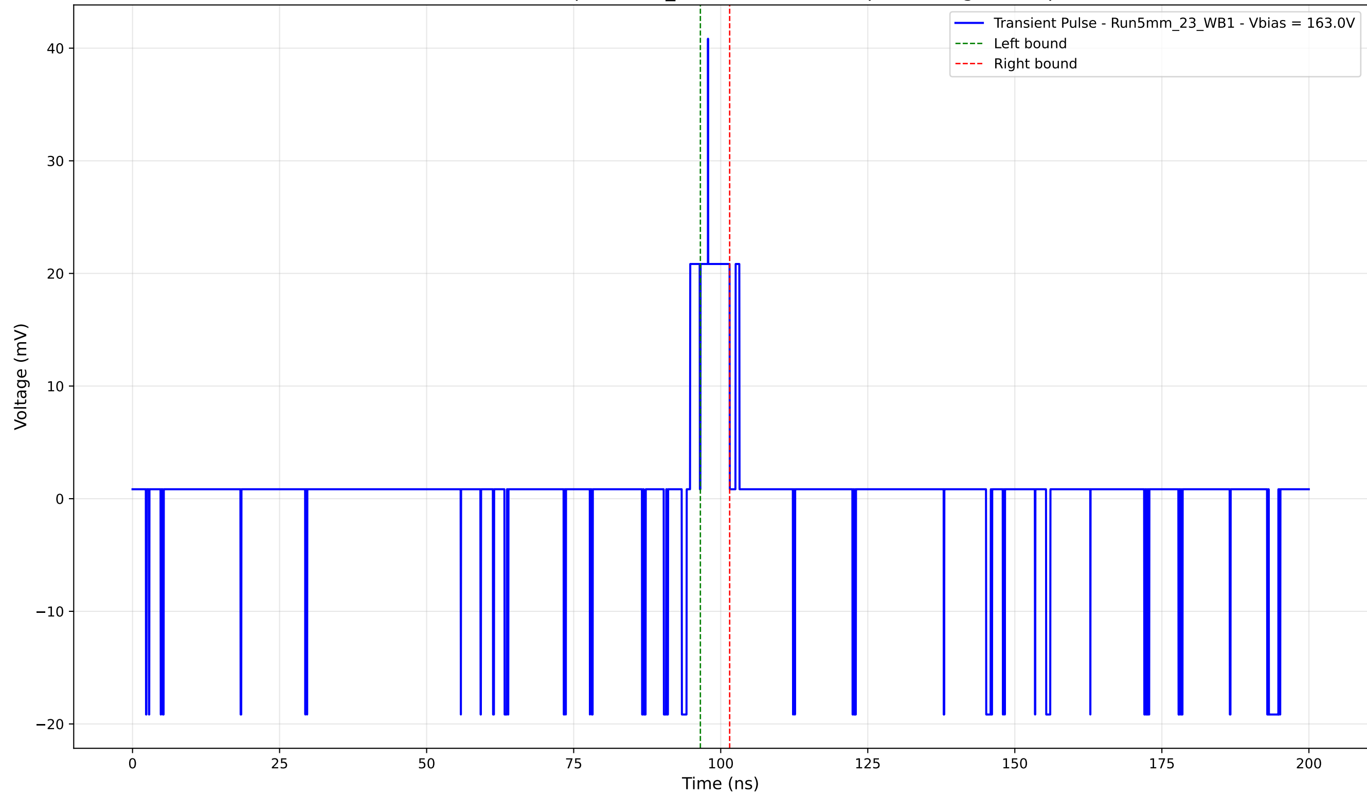
Transient Pulse - Sample: 5mm_23 - Position: 235.0 \mu\text{m} - Charge: 2.08 pC
