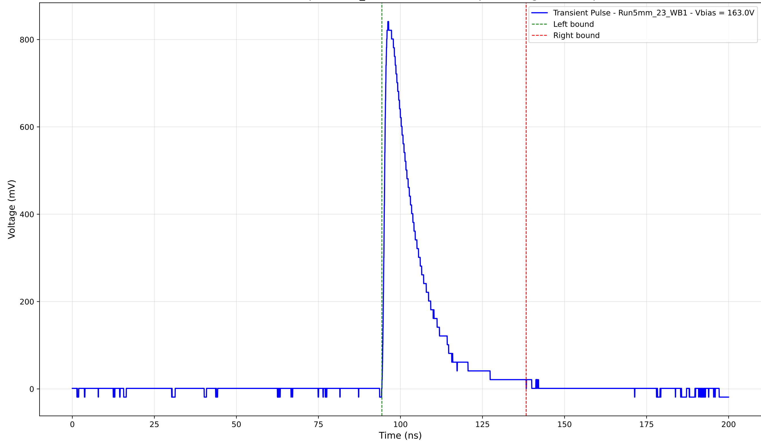
Transient Pulse - Sample: 5mm_23 - Position: 3840.0 \mu\text{m} - Charge: 177.06 pC
