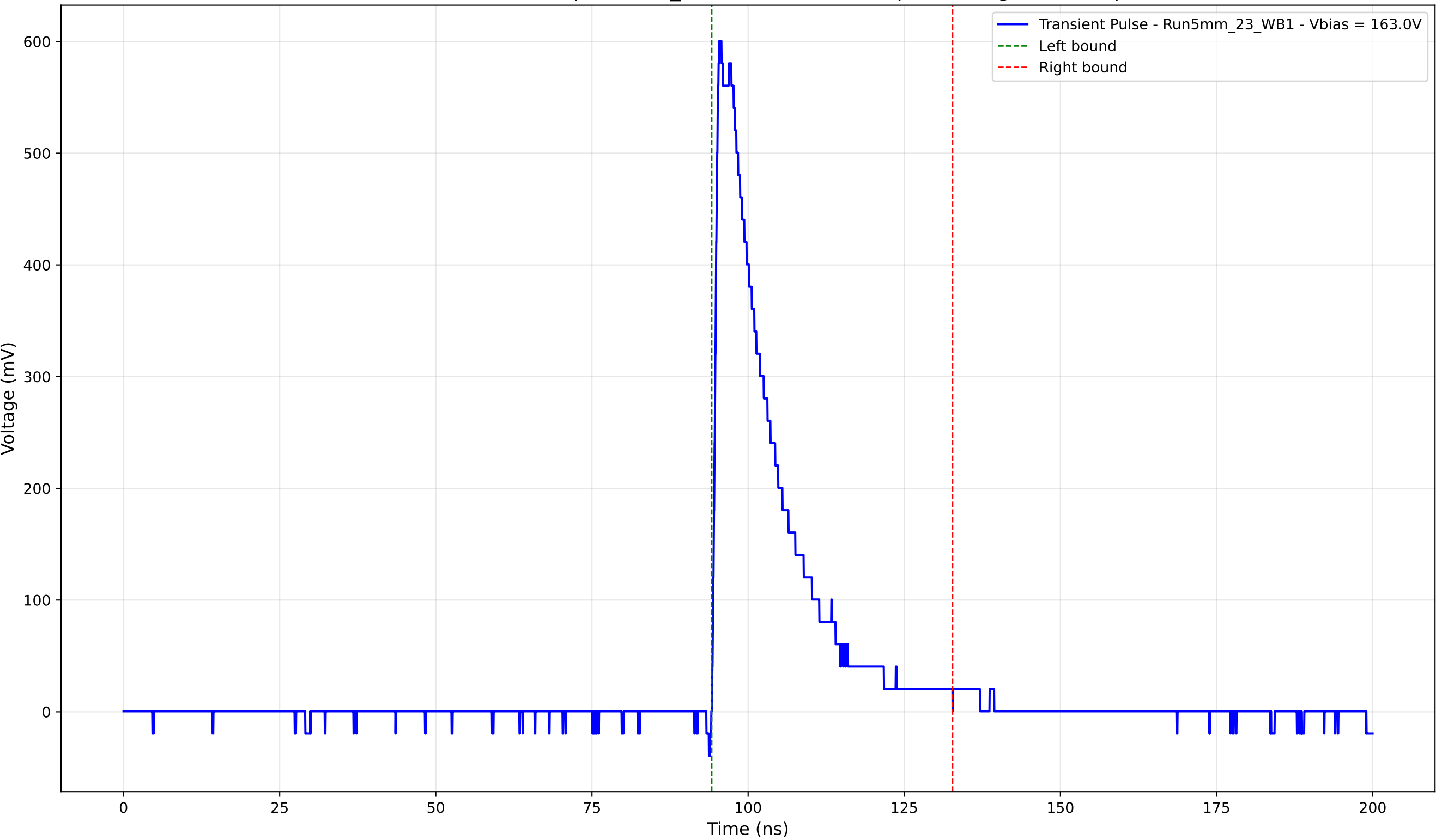
Transient Pulse - Sample: 5mm_23 - Position: 2195.0 \mu\text{m} - Charge: 118.88 pC
