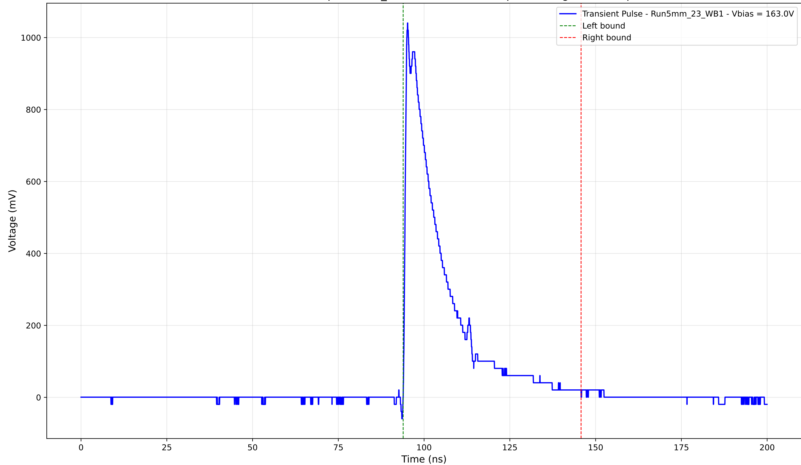
Transient Pulse - Sample: 5mm_23 - Position: 2525.0 \mu\text{m} - Charge: 233.00 pC
