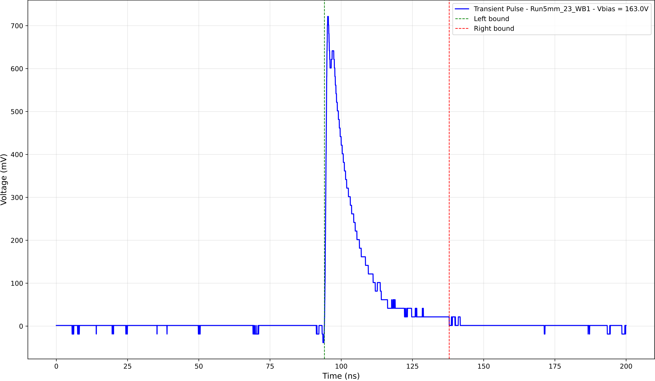
Transient Pulse - Sample: 5mm_23 - Position: 2290.0 \mu\text{m} - Charge: 135.74 pC
