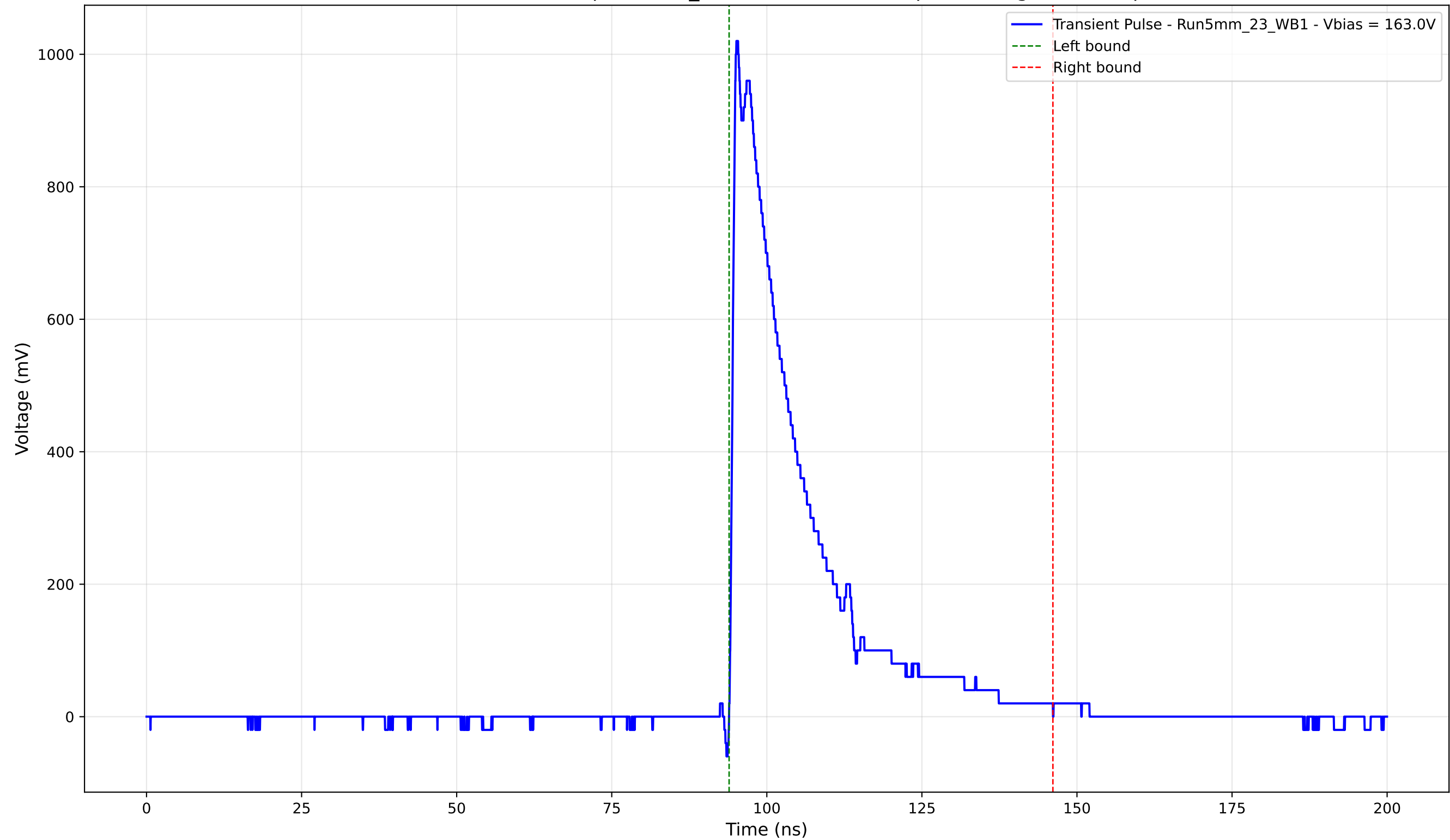
Transient Pulse - Sample: 5mm_23 - Position: 2985.0 \mu\text{m} - Charge: 231.79 pC
