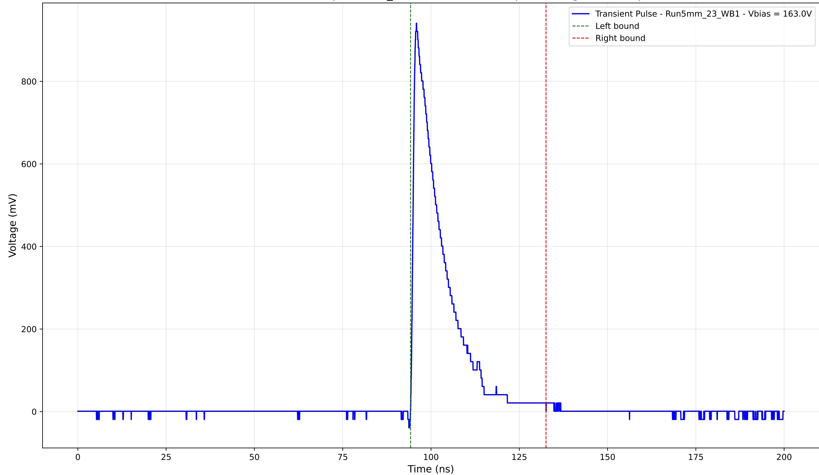
Transient Pulse - Sample: 5mm_23 - Position: 4655.0 \mu\text{m} - Charge: 169.29 pC
