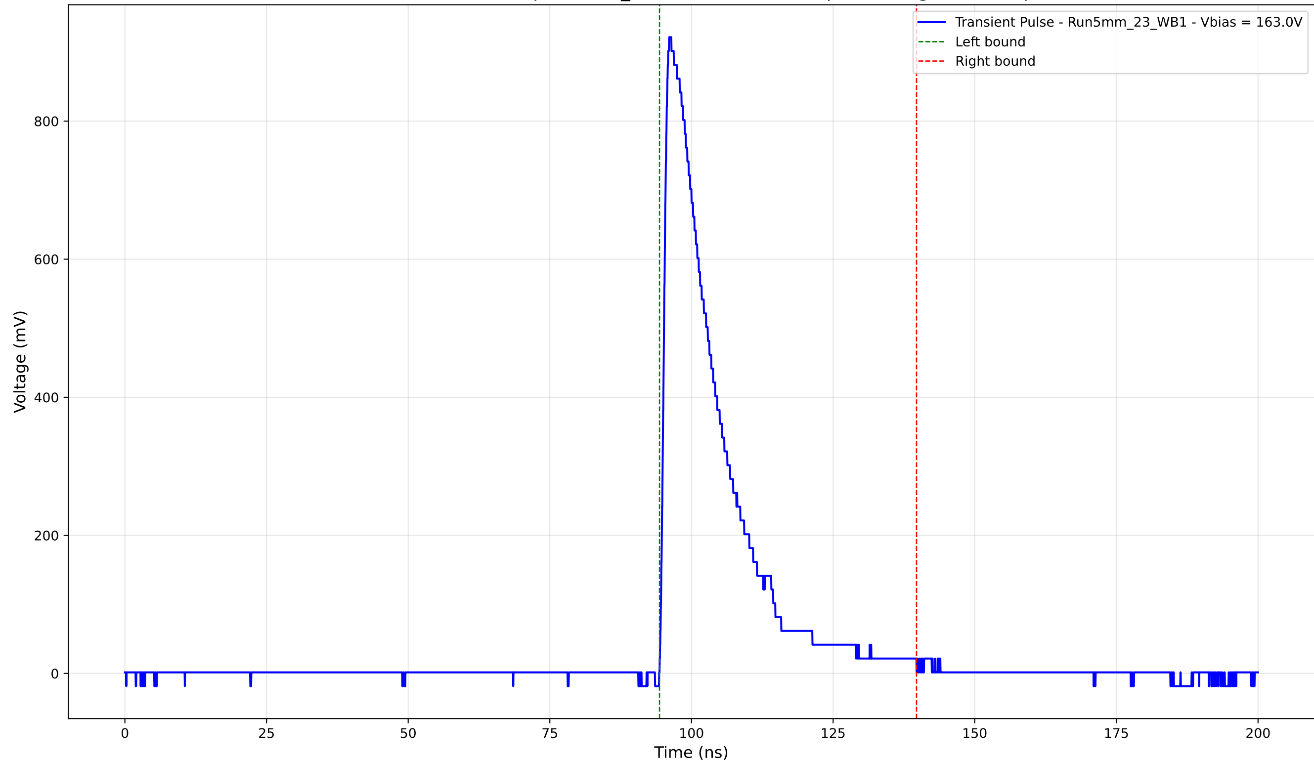
Transient Pulse - Sample: 5mm_23 - Position: 4140.0 \mu\text{m} - Charge: 195.22 pC
