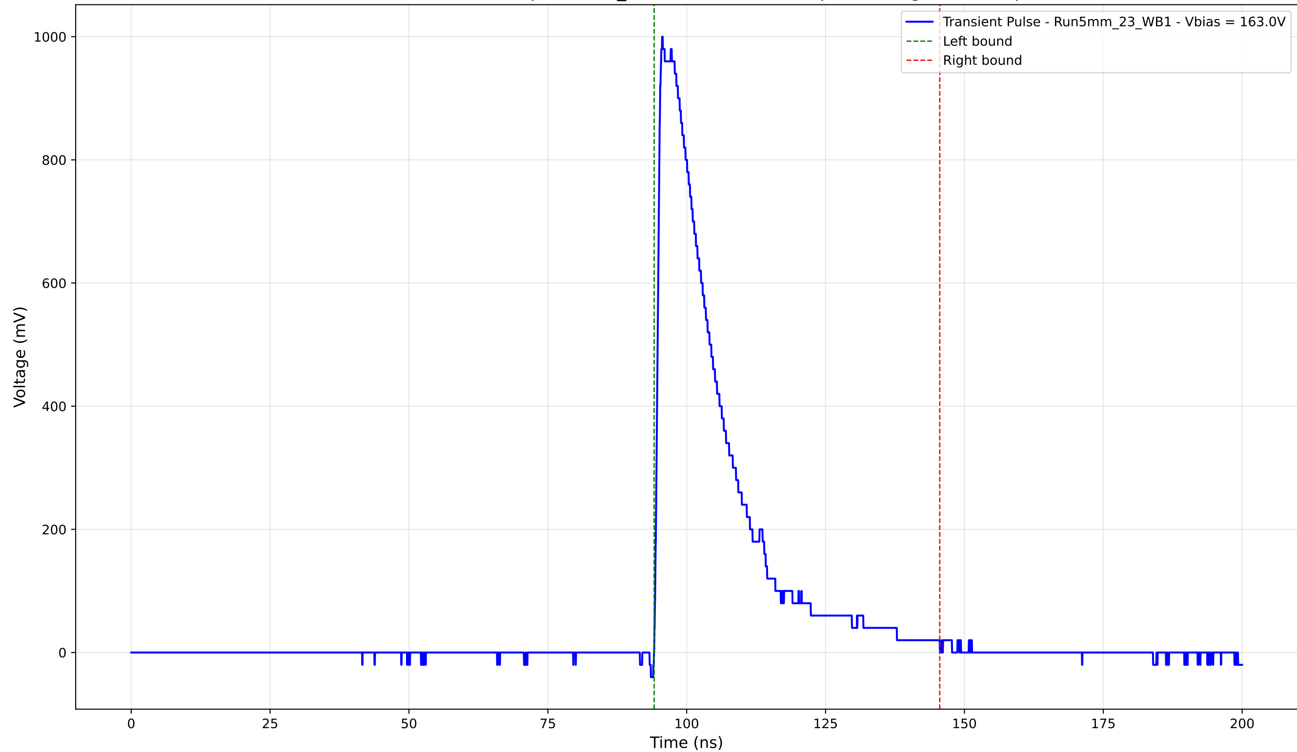
Transient Pulse - Sample: 5mm_23 - Position: 2085.0 \mu\text{m} - Charge: 244.96 pC
