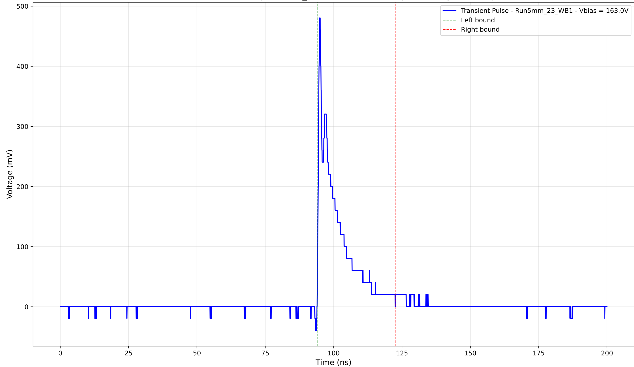
Transient Pulse - Sample: 5mm_23 - Position: 2730.0 \mu\text{m} - Charge: 58.93 pC
