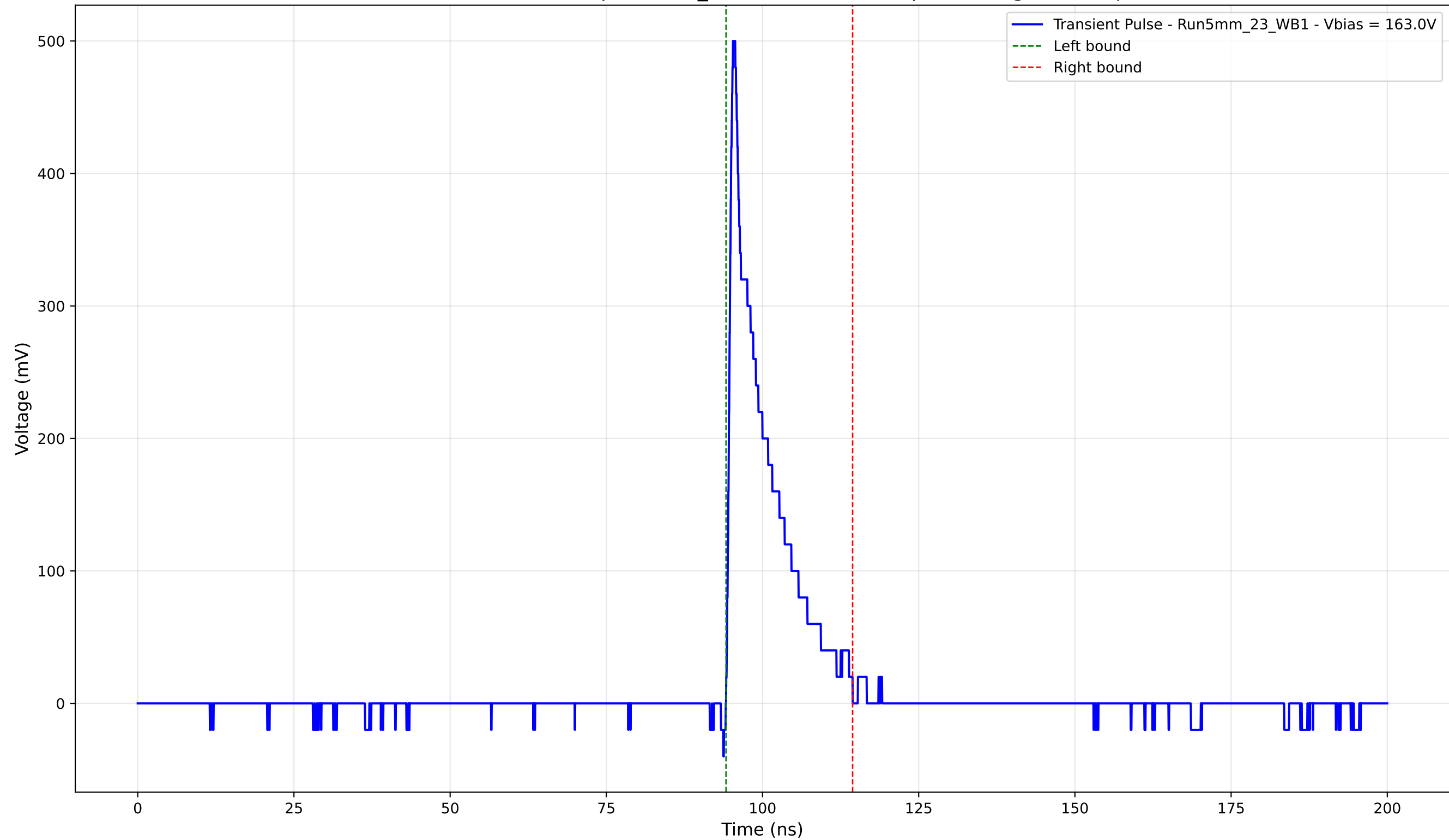
Transient Pulse - Sample: 5mm_23 - Position: 300.0 \mu\text{m} - Charge: 60.90 pC
