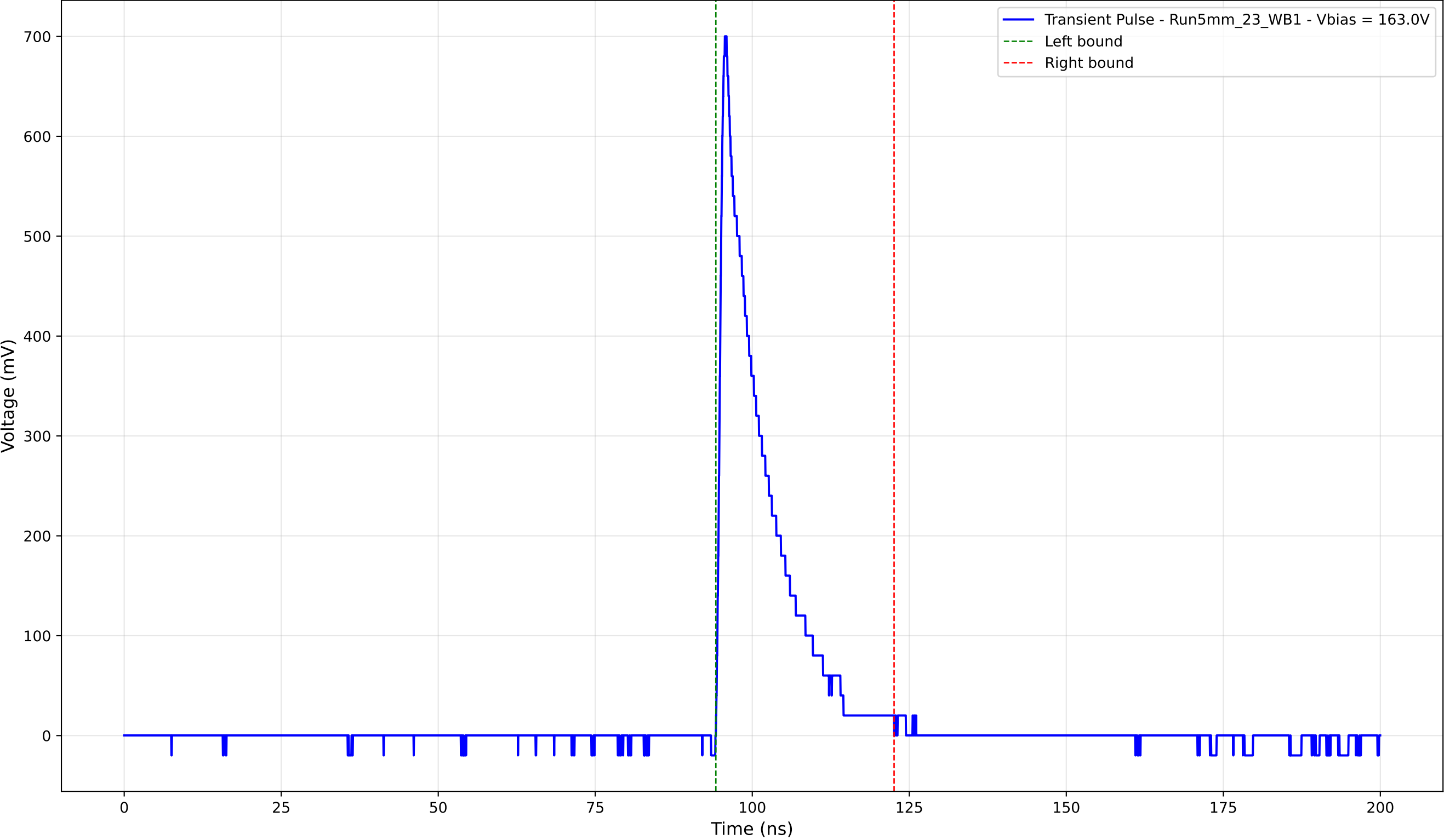
Transient Pulse - Sample: 5mm_23 - Position: 4815.0 \mu\text{m} - Charge: 102.60 pC
