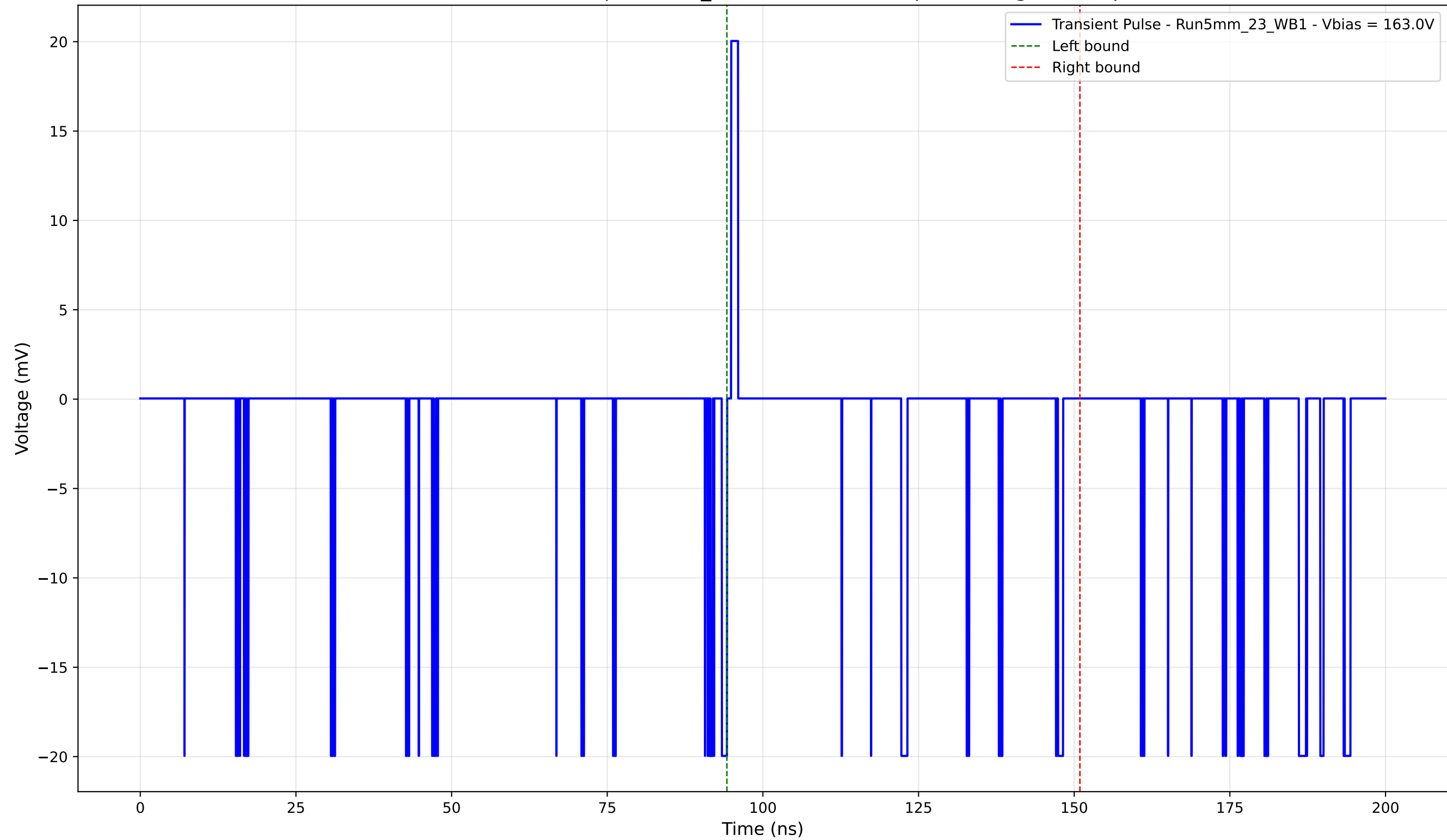
Transient Pulse - Sample: 5mm_23 - Position: 160.0 \mu\text{m} - Charge: -0.63 pC
