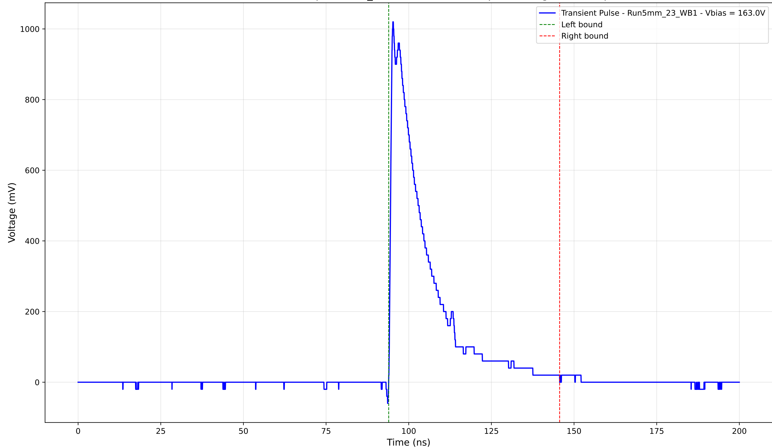
Transient Pulse - Sample: 5mm_23 - Position: 3030.0 \mu\text{m} - Charge: 229.15 pC
