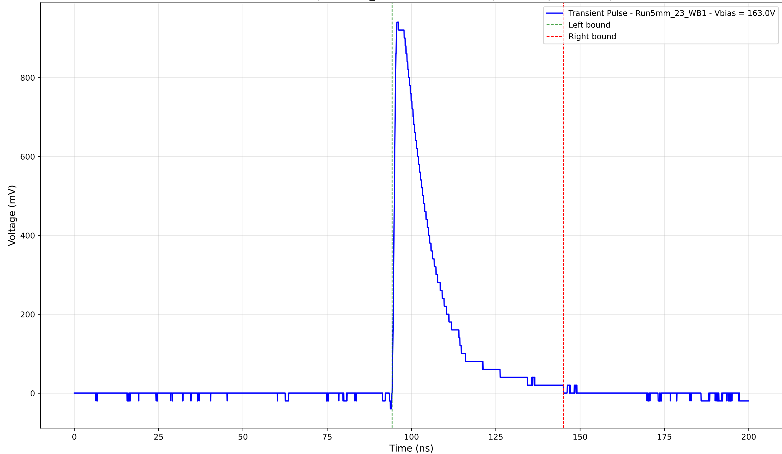
Transient Pulse - Sample: 5mm_23 - Position: 3540.0 \mu\text{m} - Charge: 221.94 pC
