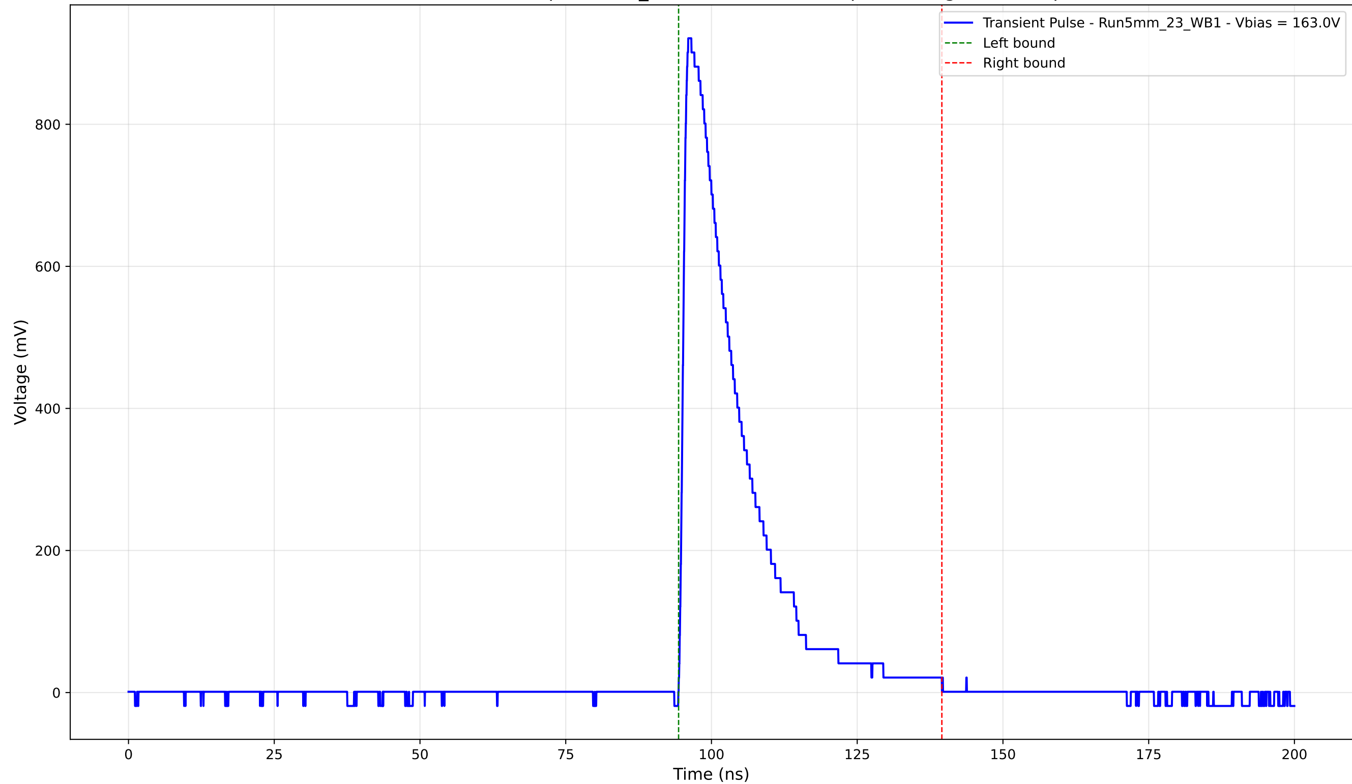
Transient Pulse - Sample: 5mm_23 - Position: 4070.0 \mu\text{m} - Charge: 198.51 pC
