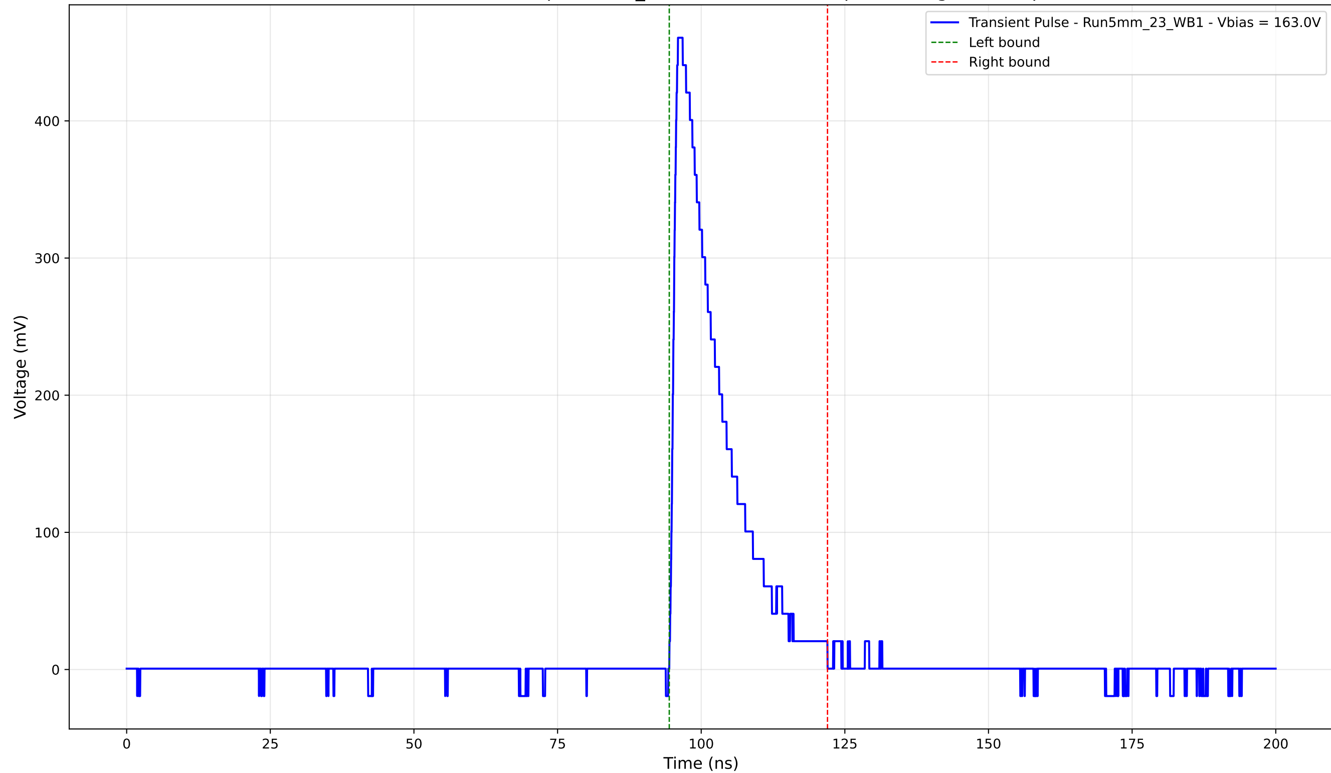
Transient Pulse - Sample: 5mm_23 - Position: 4220.0 \mu\text{m} - Charge: 83.04 pC
