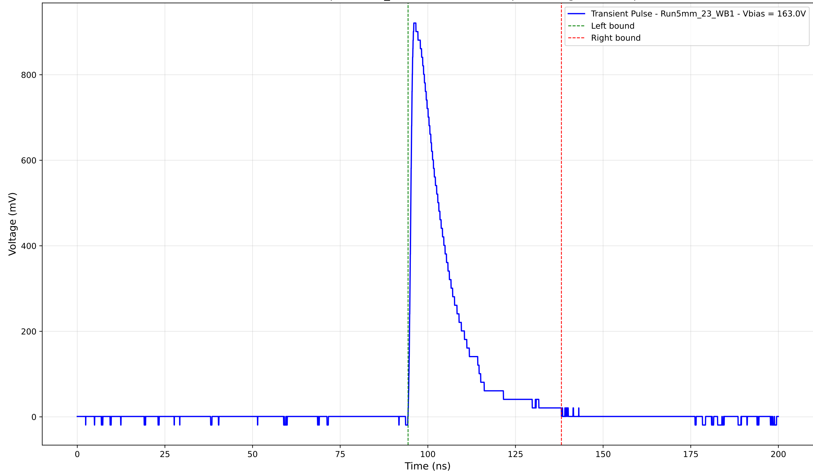
Transient Pulse - Sample: 5mm_23 - Position: 4050.0 \mu\text{m} - Charge: 199.73 pC
