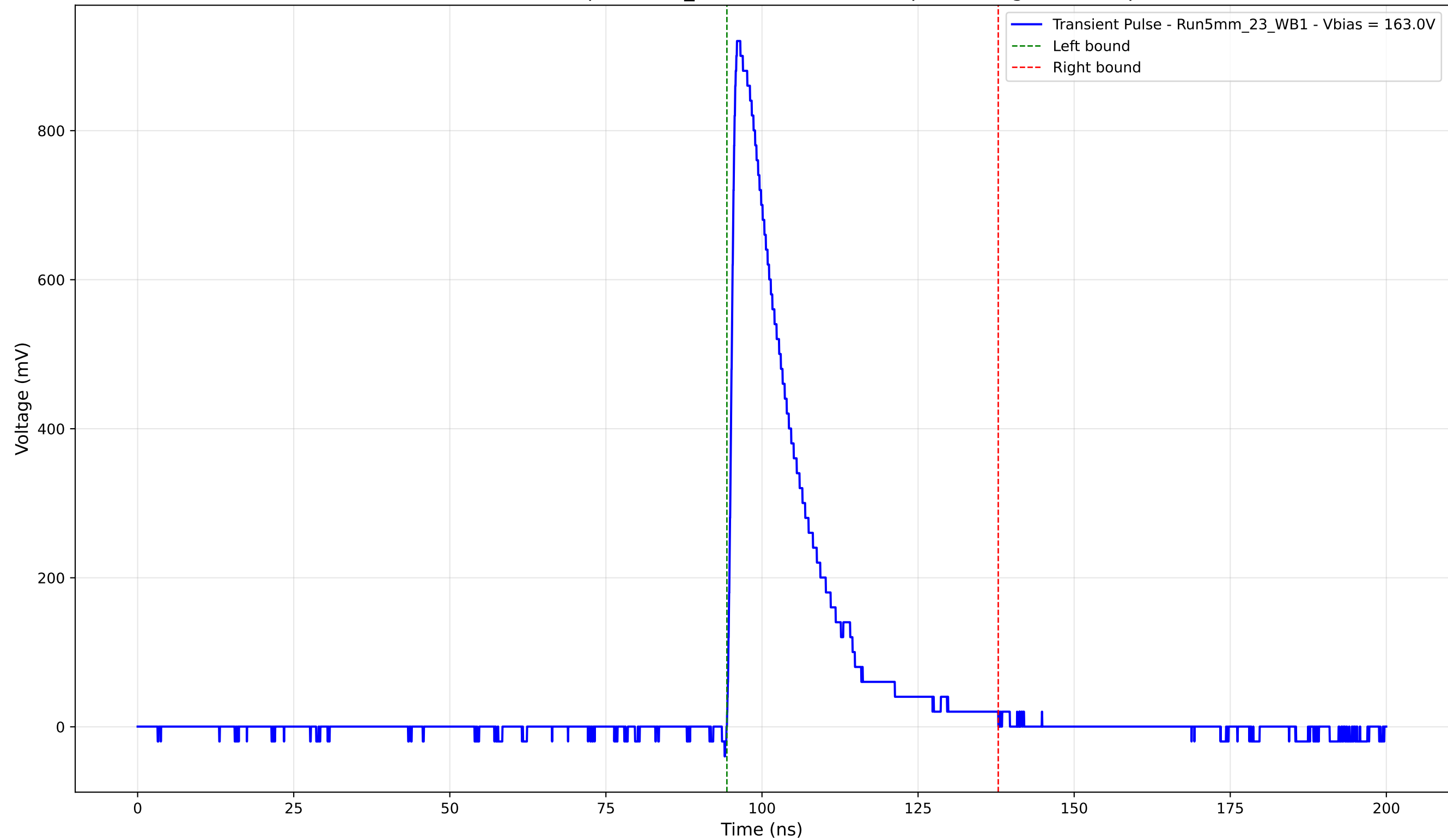
Transient Pulse - Sample: 5mm_23 - Position: 4120.0 \mu\text{m} - Charge: 195.03 pC
