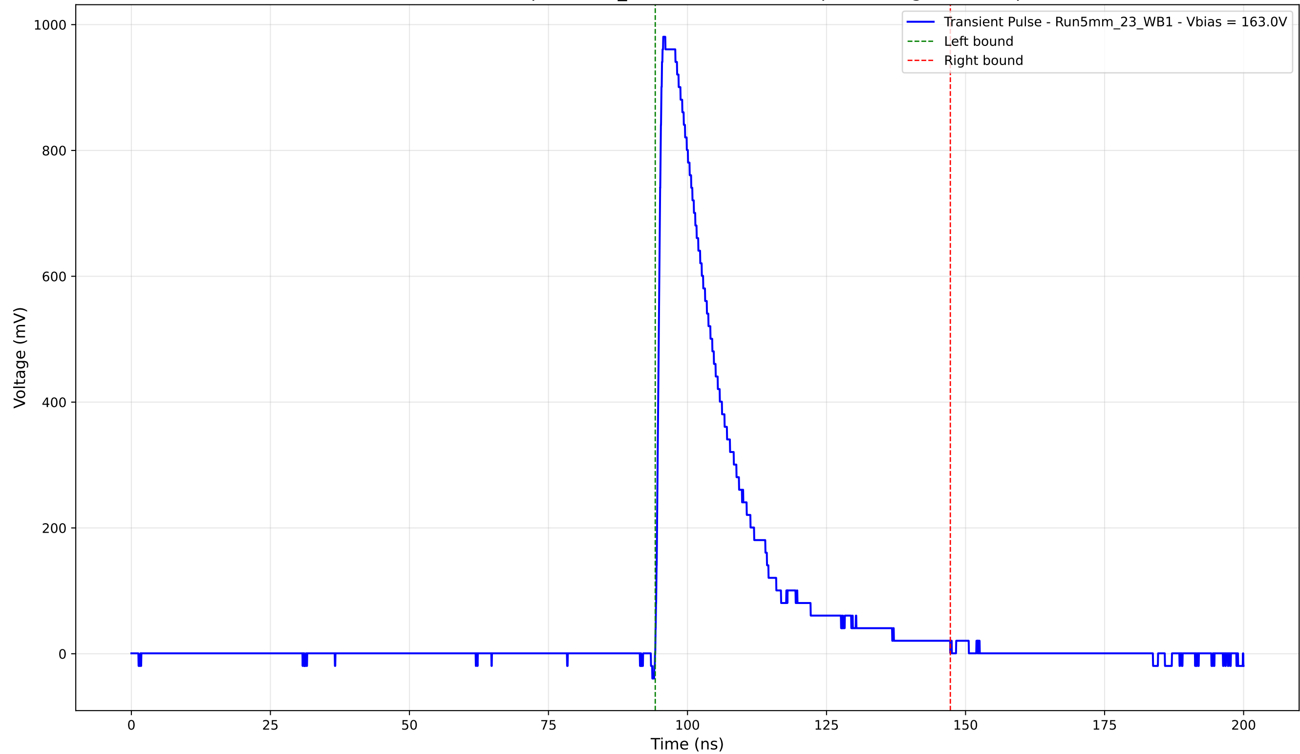
Transient Pulse - Sample: 5mm_23 - Position: 1990.0 \mu\text{m} - Charge: 242.95 pC
