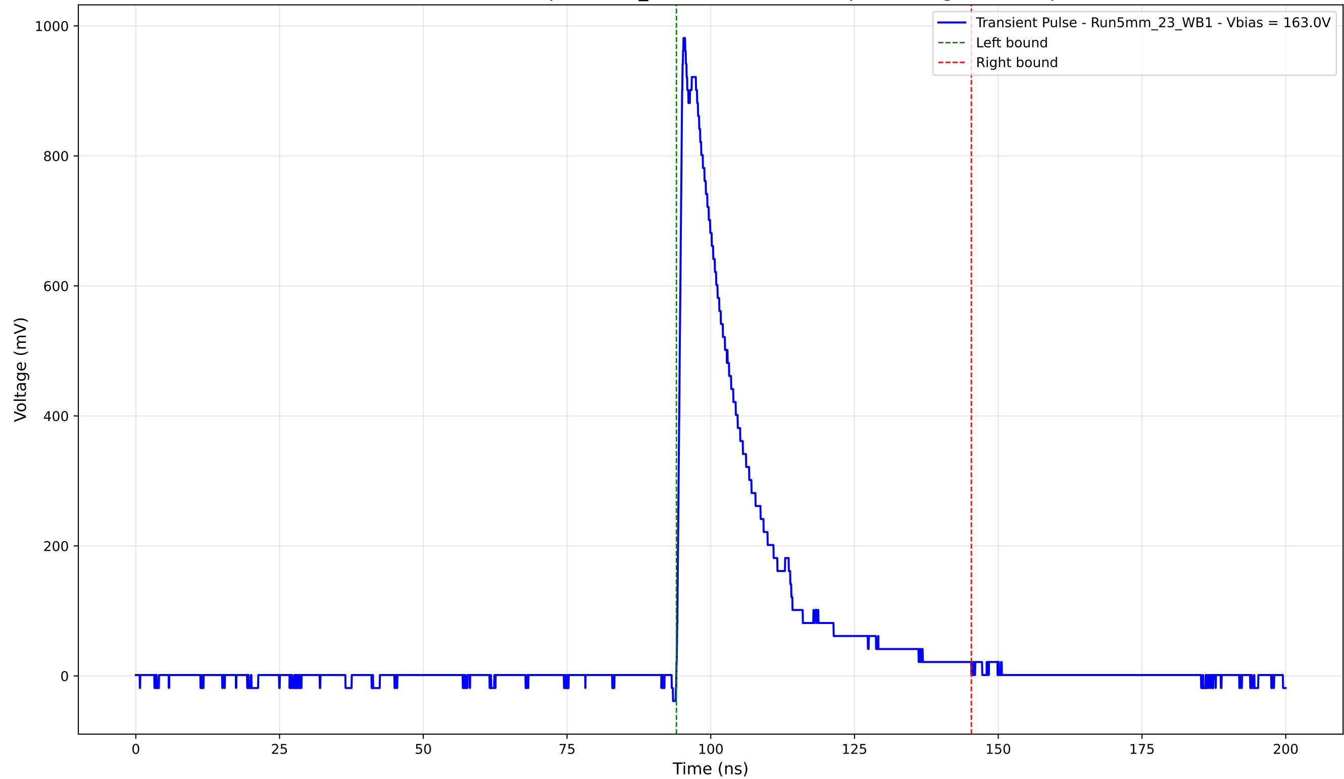
Transient Pulse - Sample: 5mm_23 - Position: 2340.0 \mu\text{m} - Charge: 220.02 pC
