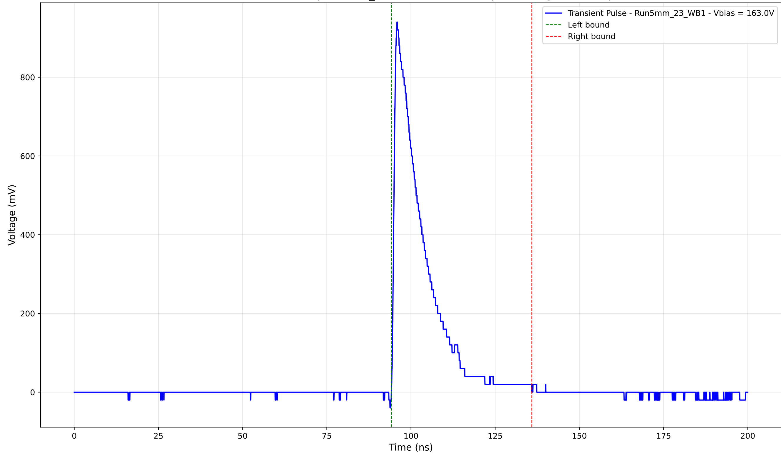
Transient Pulse - Sample: 5mm_23 - Position: 4620.0 \mu\text{m} - Charge: 174.28 pC
