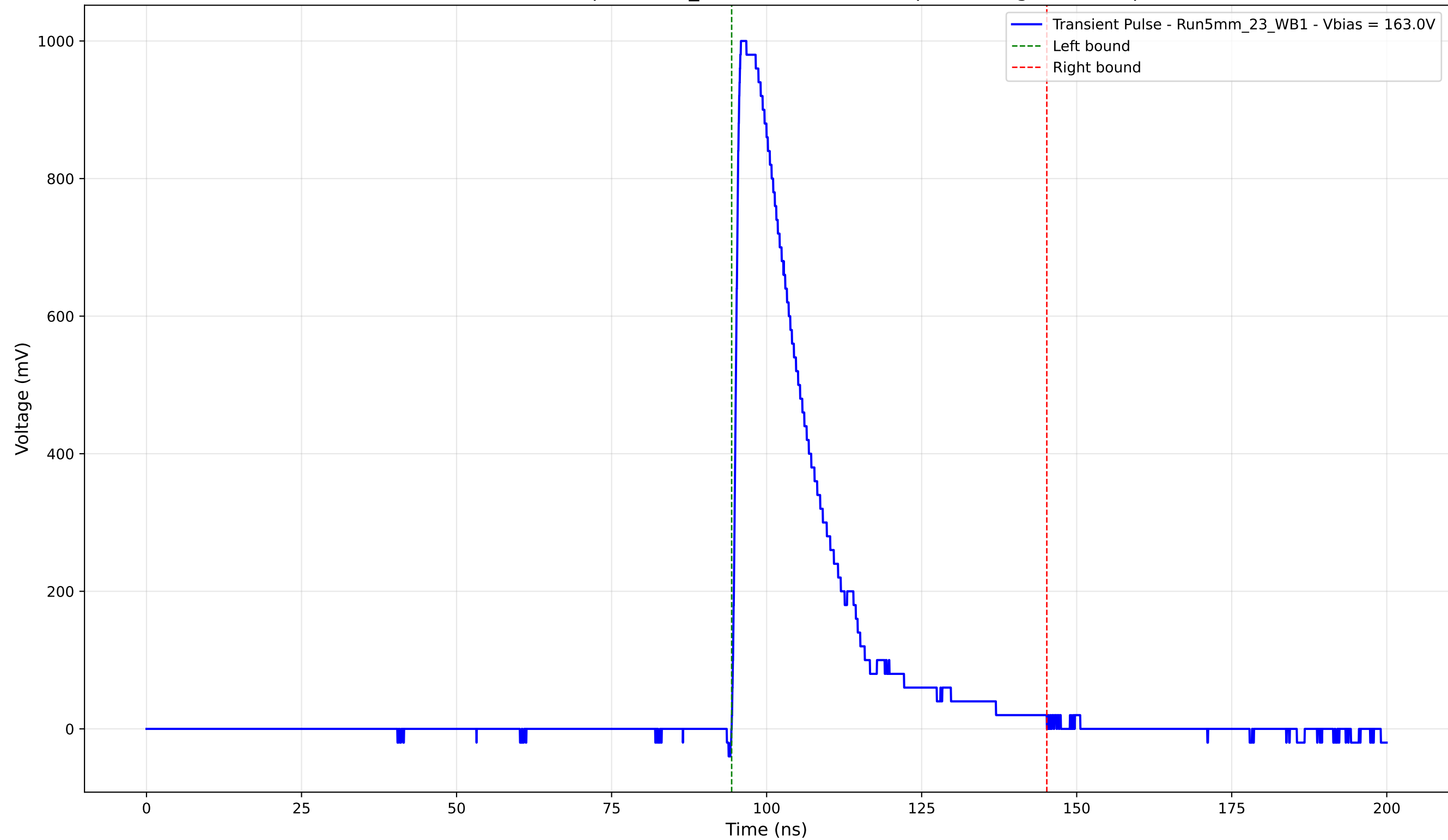
Transient Pulse - Sample: 5mm_23 - Position: 1545.0 \mu\text{m} - Charge: 254.30 pC
