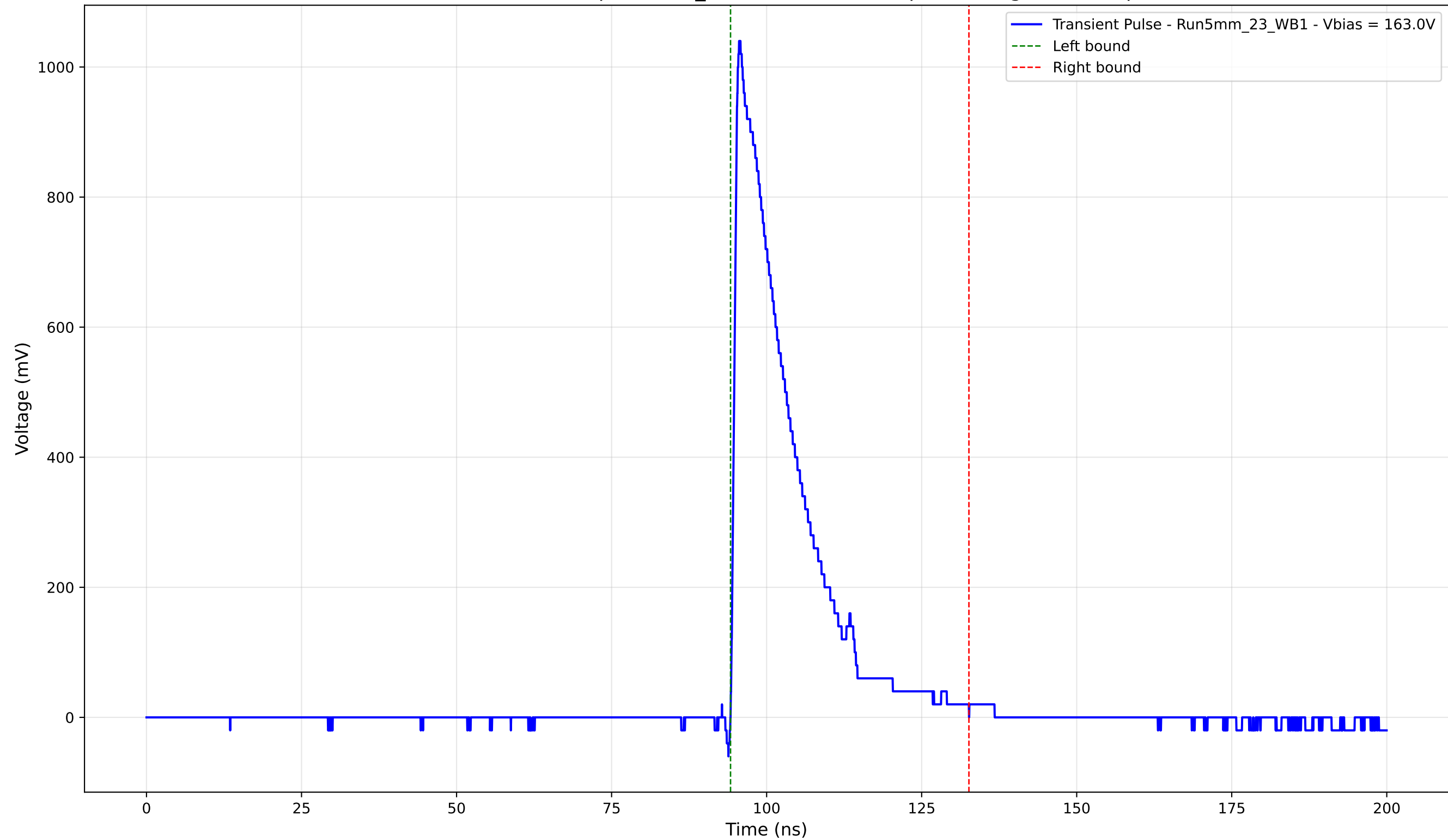
Transient Pulse - Sample: 5mm_23 - Position: 580.0 \mu\text{m} - Charge: 204.46 pC
