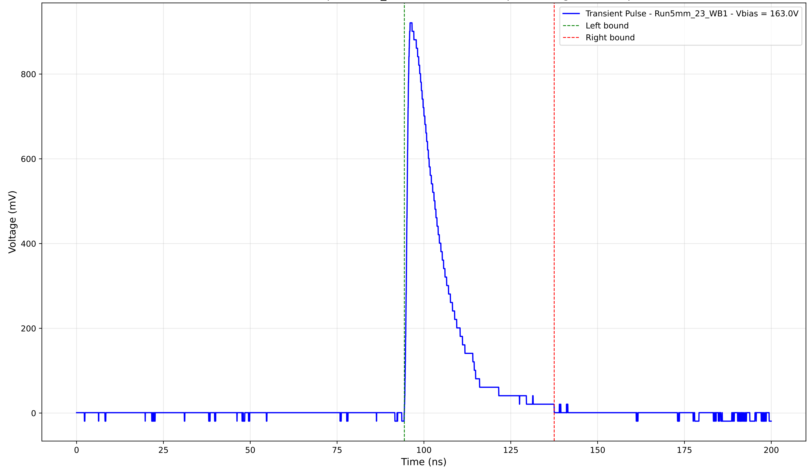
Transient Pulse - Sample: 5mm_23 - Position: 4035.0 \mu\text{m} - Charge: 198.05 pC
