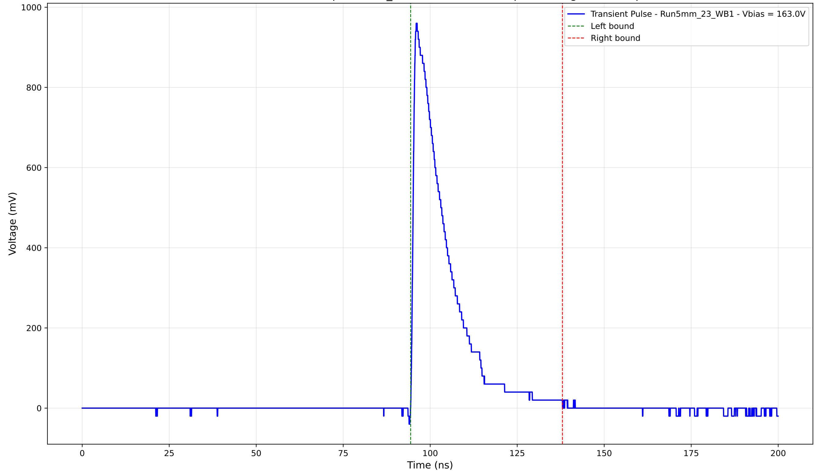
Transient Pulse - Sample: 5mm_23 - Position: 1040.0 \mu\text{m} - Charge: 200.77 pC
