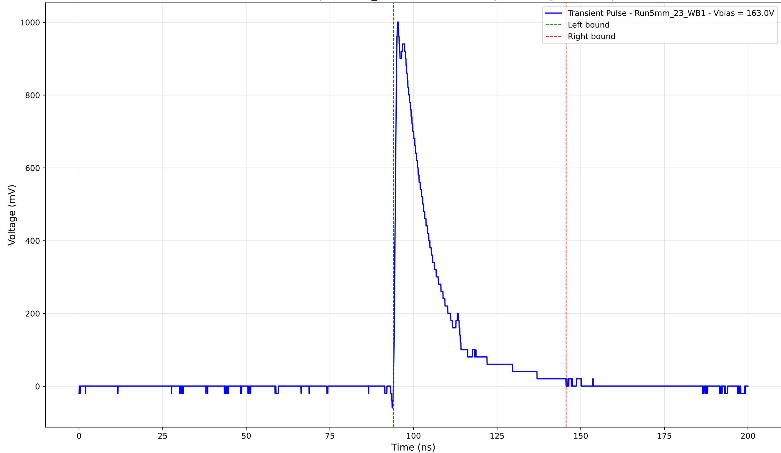
Transient Pulse - Sample: 5mm_23 - Position: 3095.0 \mu\text{m} - Charge: 225.04 pC
