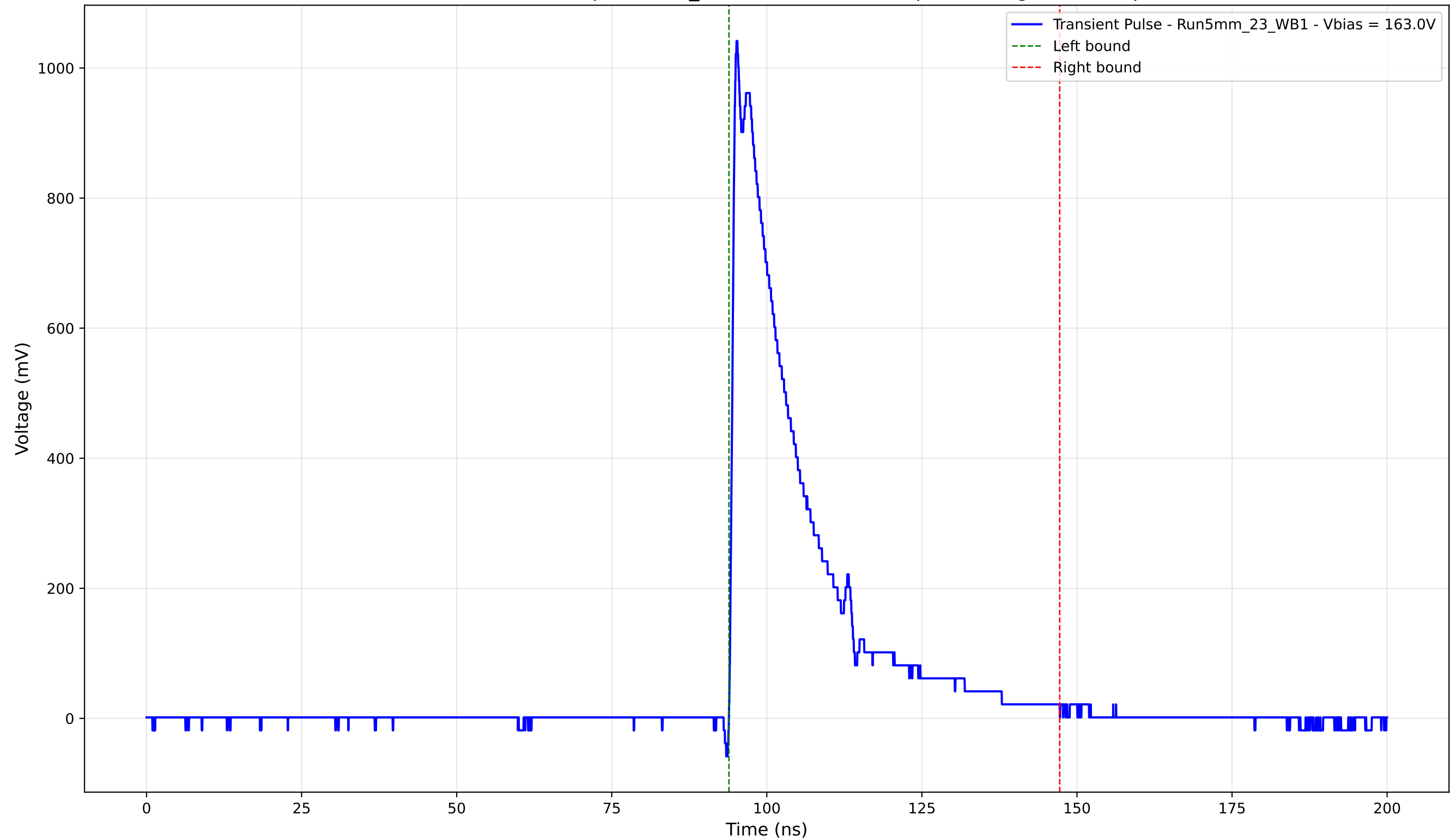
Transient Pulse - Sample: 5mm_23 - Position: 2535.0 \mu\text{m} - Charge: 235.42 pC
