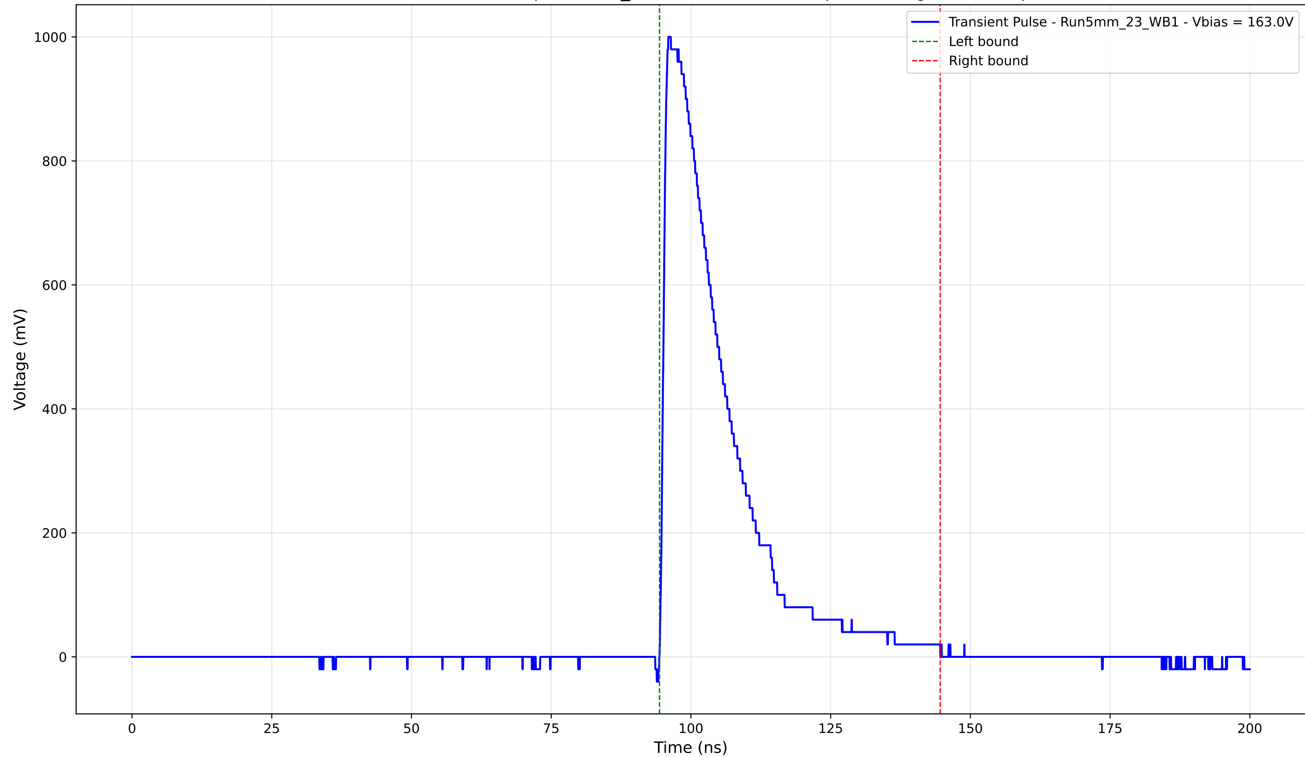
Transient Pulse - Sample: 5mm_23 - Position: 1470.0 \mu\text{m} - Charge: 245.34 pC
