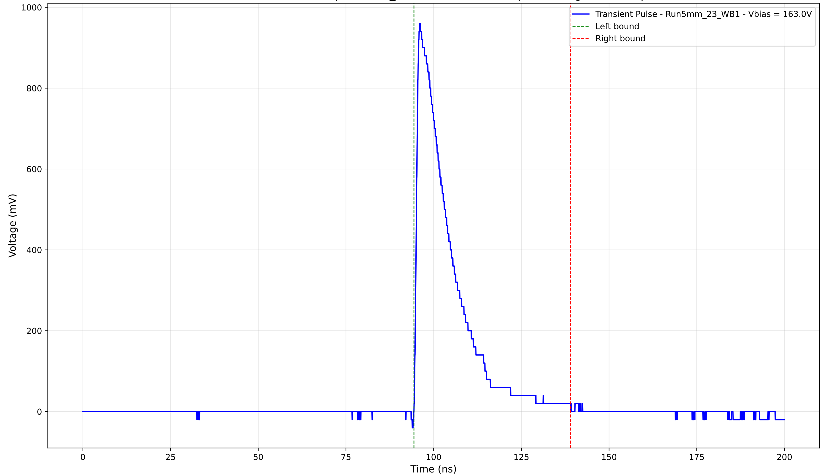
Transient Pulse - Sample: 5mm_23 - Position: 1075.0 \mu\text{m} - Charge: 203.34 pC
