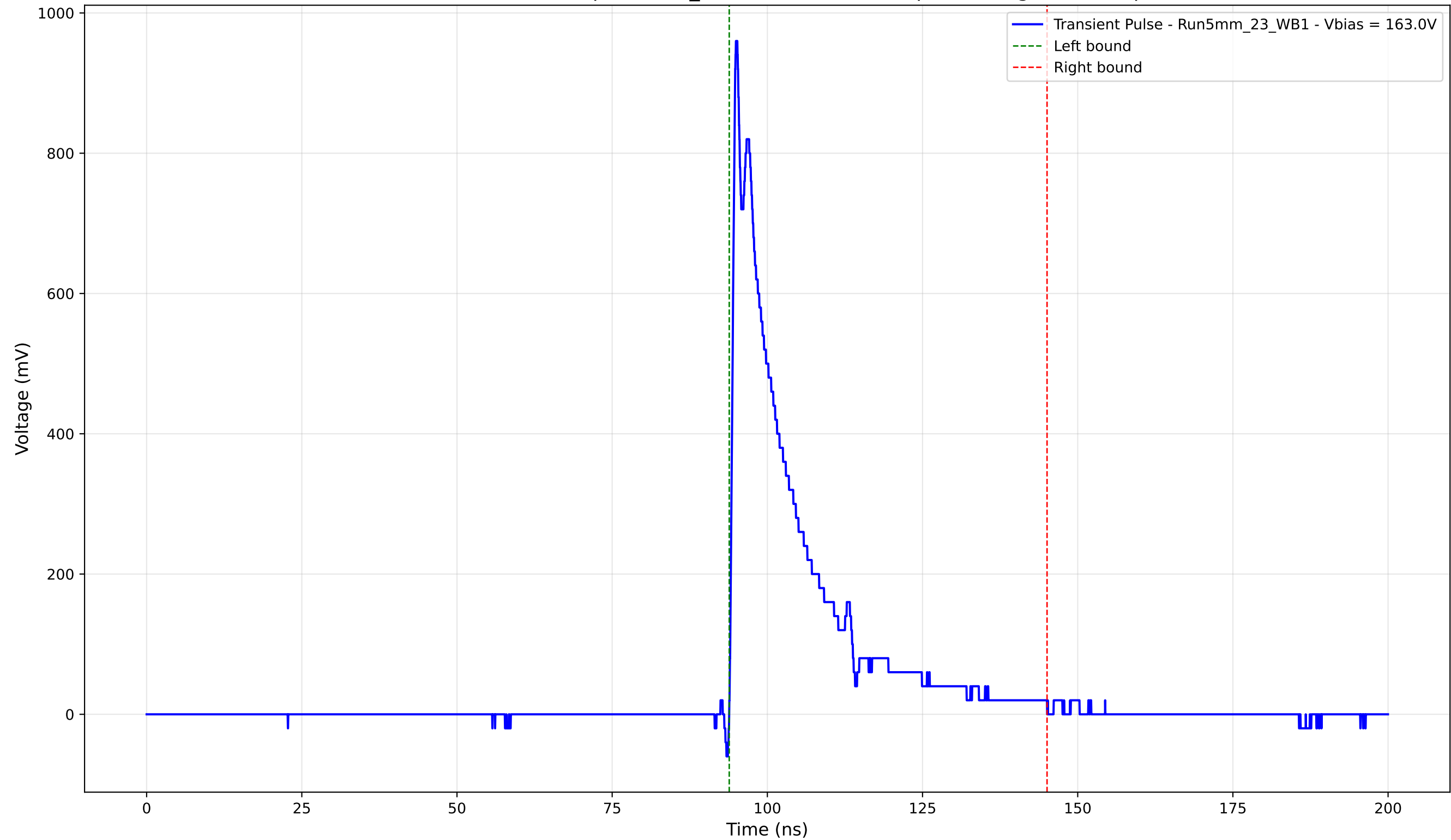
Transient Pulse - Sample: 5mm_23 - Position: 2685.0 \mu\text{m} - Charge: 177.06 pC
