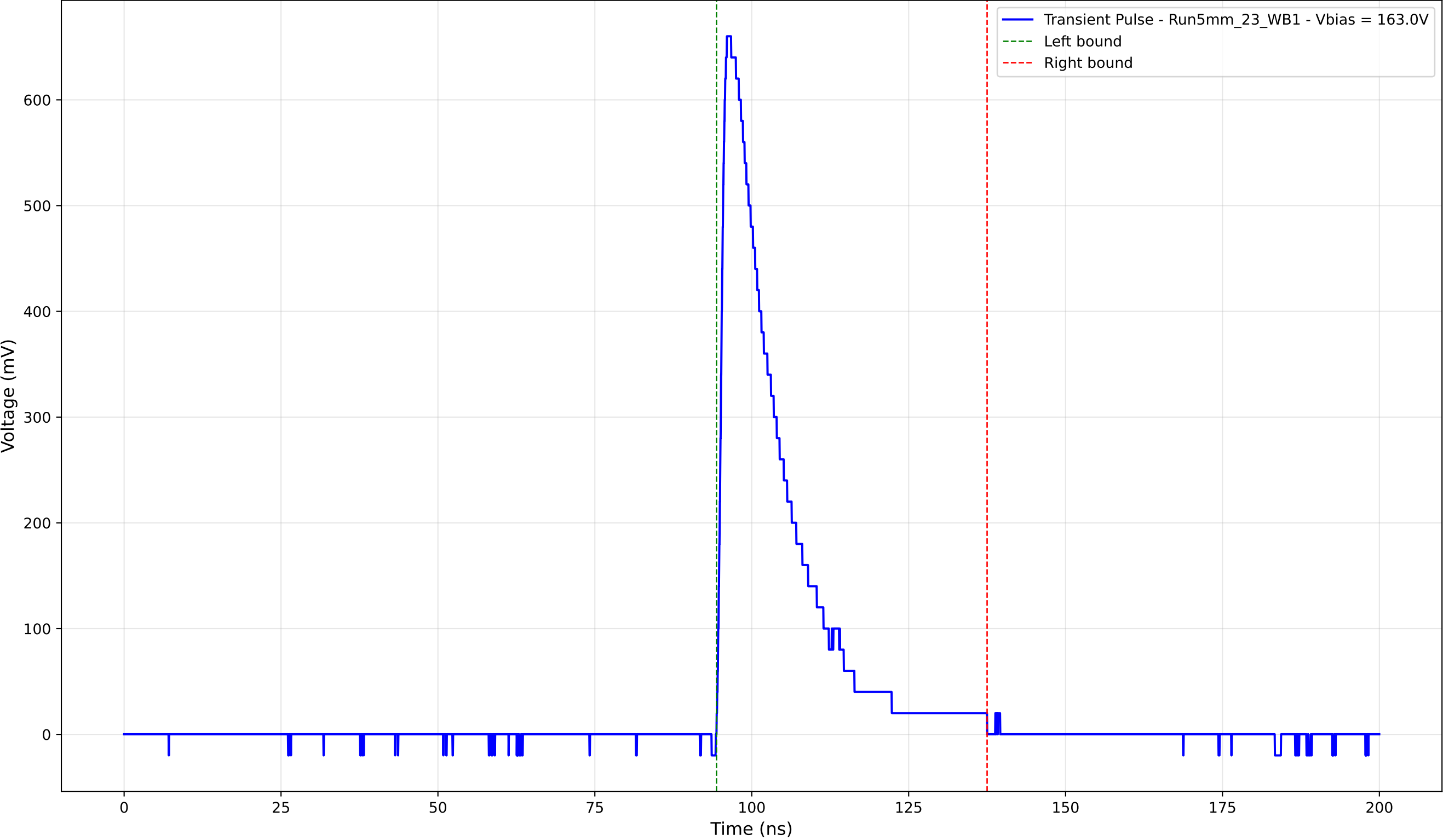
Transient Pulse - Sample: 5mm_23 - Position: 1675.0 \mu\text{m} - Charge: 135.14 pC
