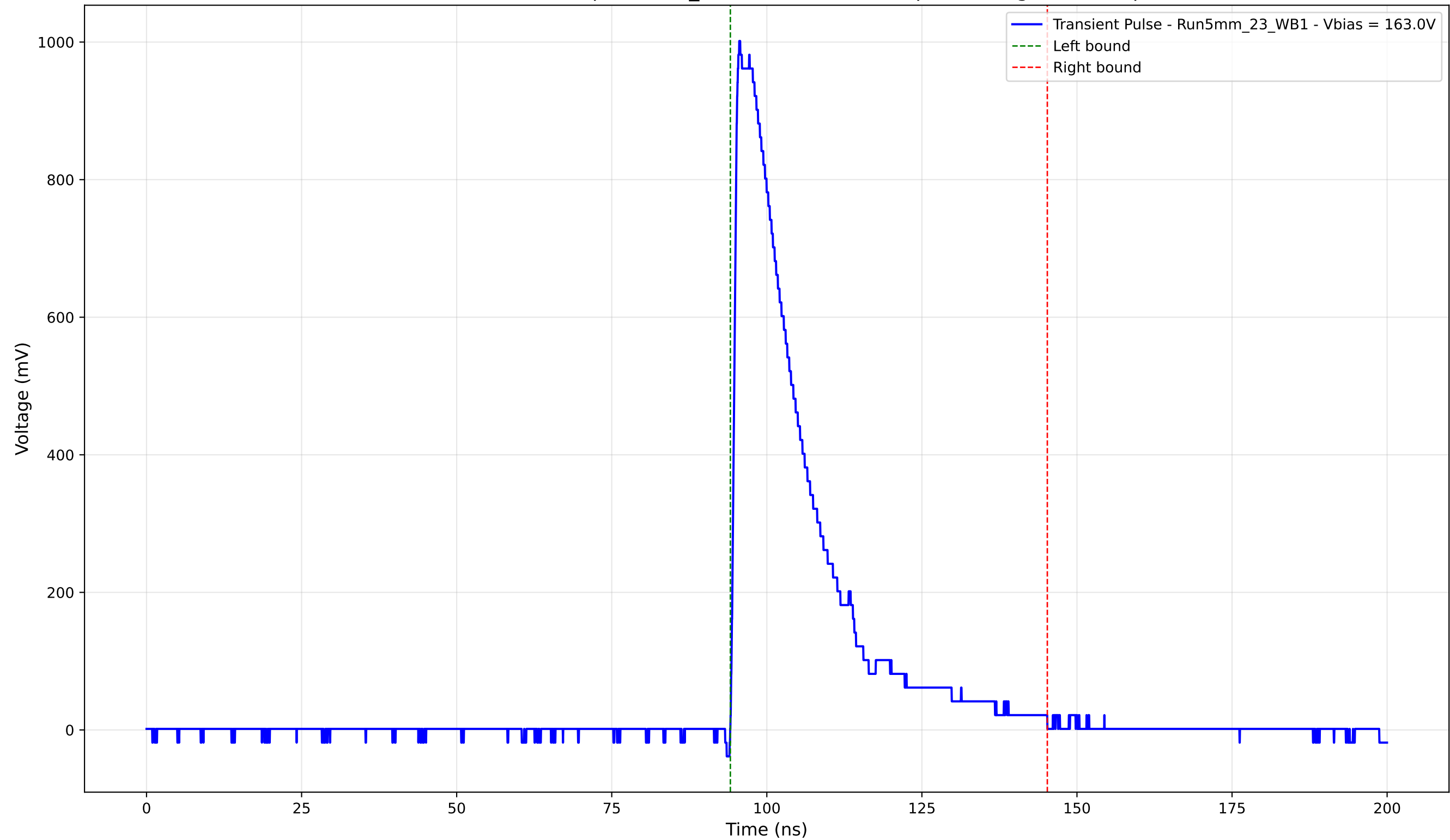
Transient Pulse - Sample: 5mm_23 - Position: 2110.0 \mu\text{m} - Charge: 243.78 pC
