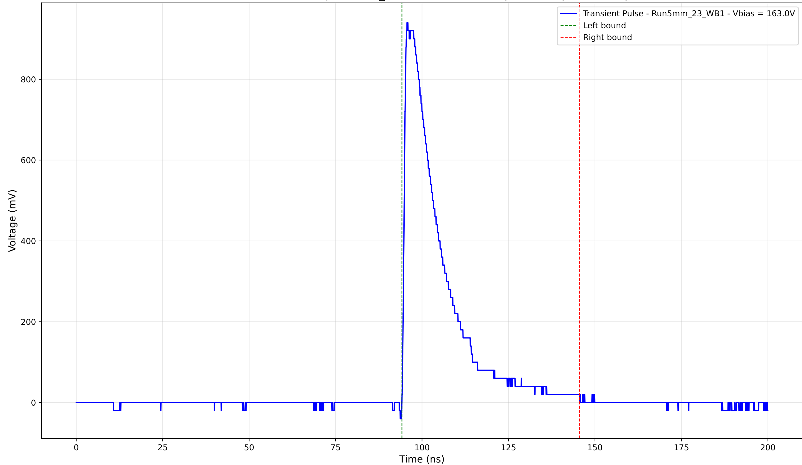
Transient Pulse - Sample: 5mm_23 - Position: 3460.0 \mu\text{m} - Charge: 219.82 pC
