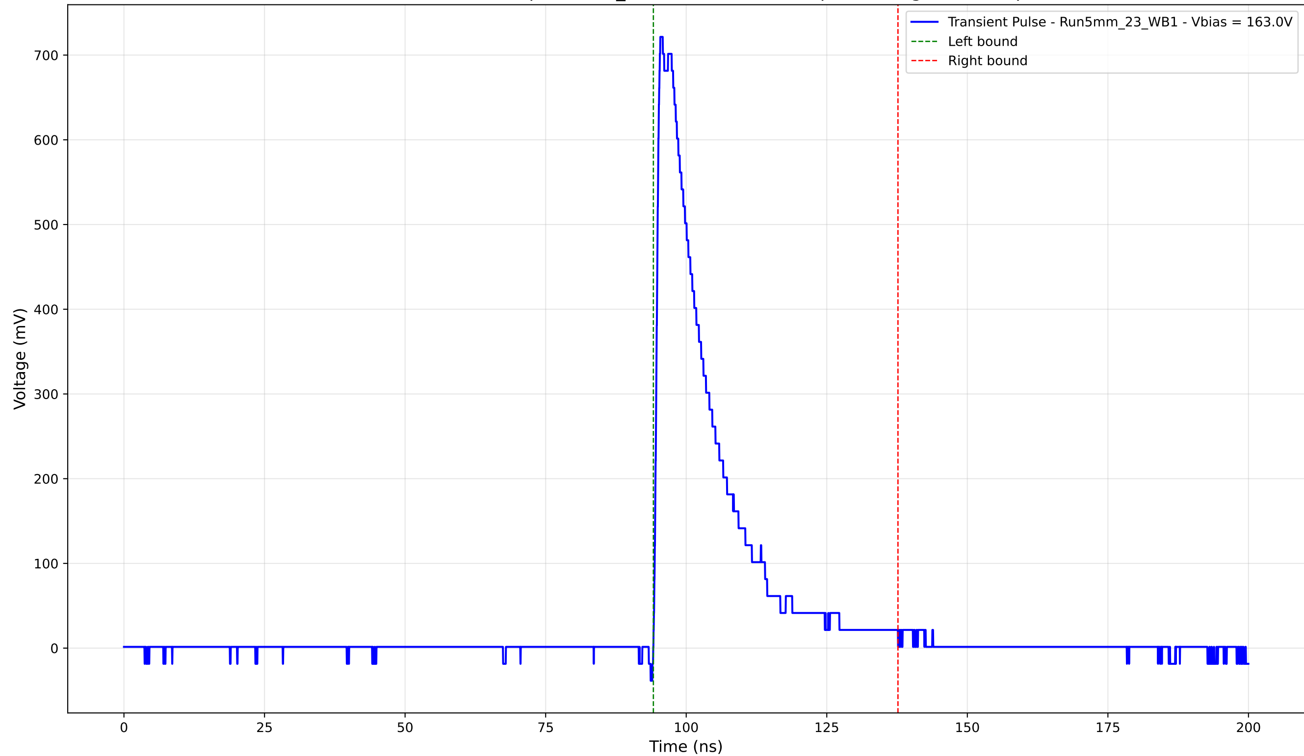
Transient Pulse - Sample: 5mm_23 - Position: 3310.0 \mu\text{m} - Charge: 149.38 pC
