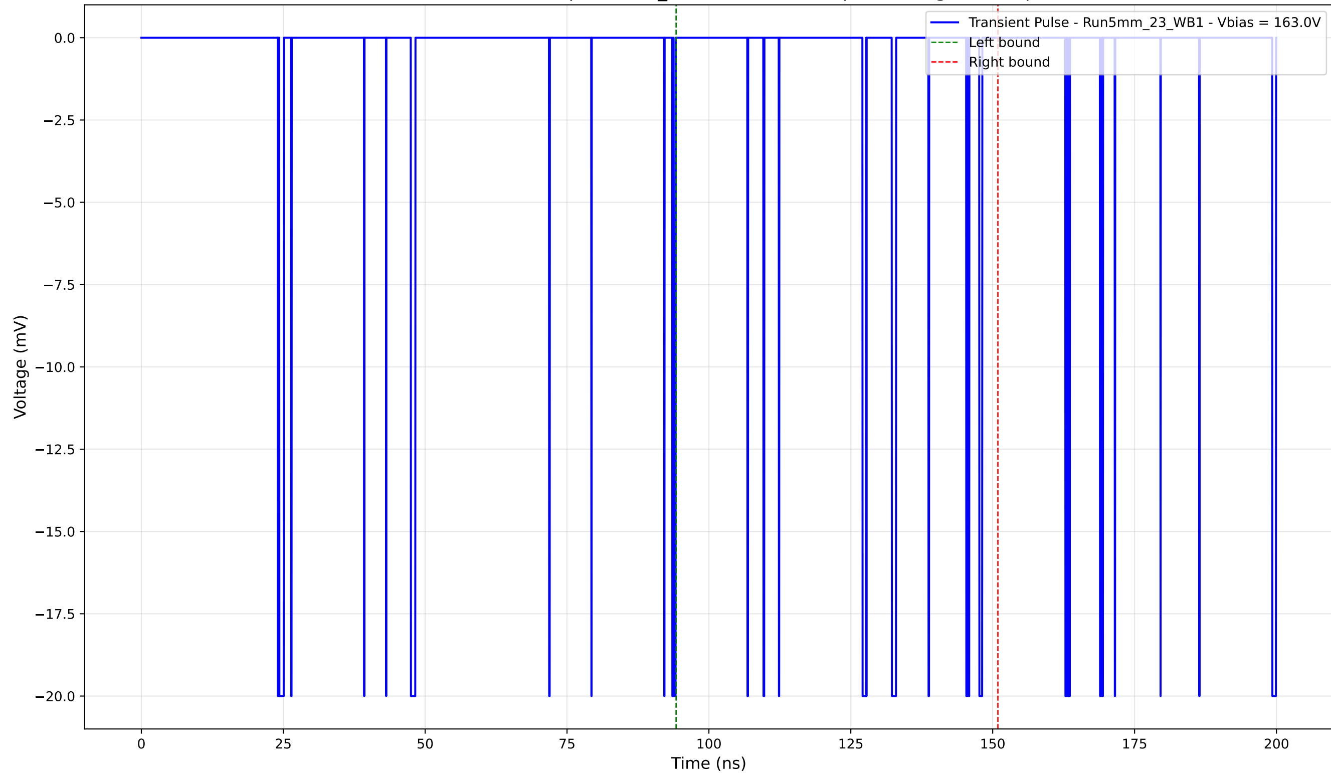
Transient Pulse - Sample: 5mm_23- Position: 40.0 \mu\text{m} - Charge: -1.10 pC
