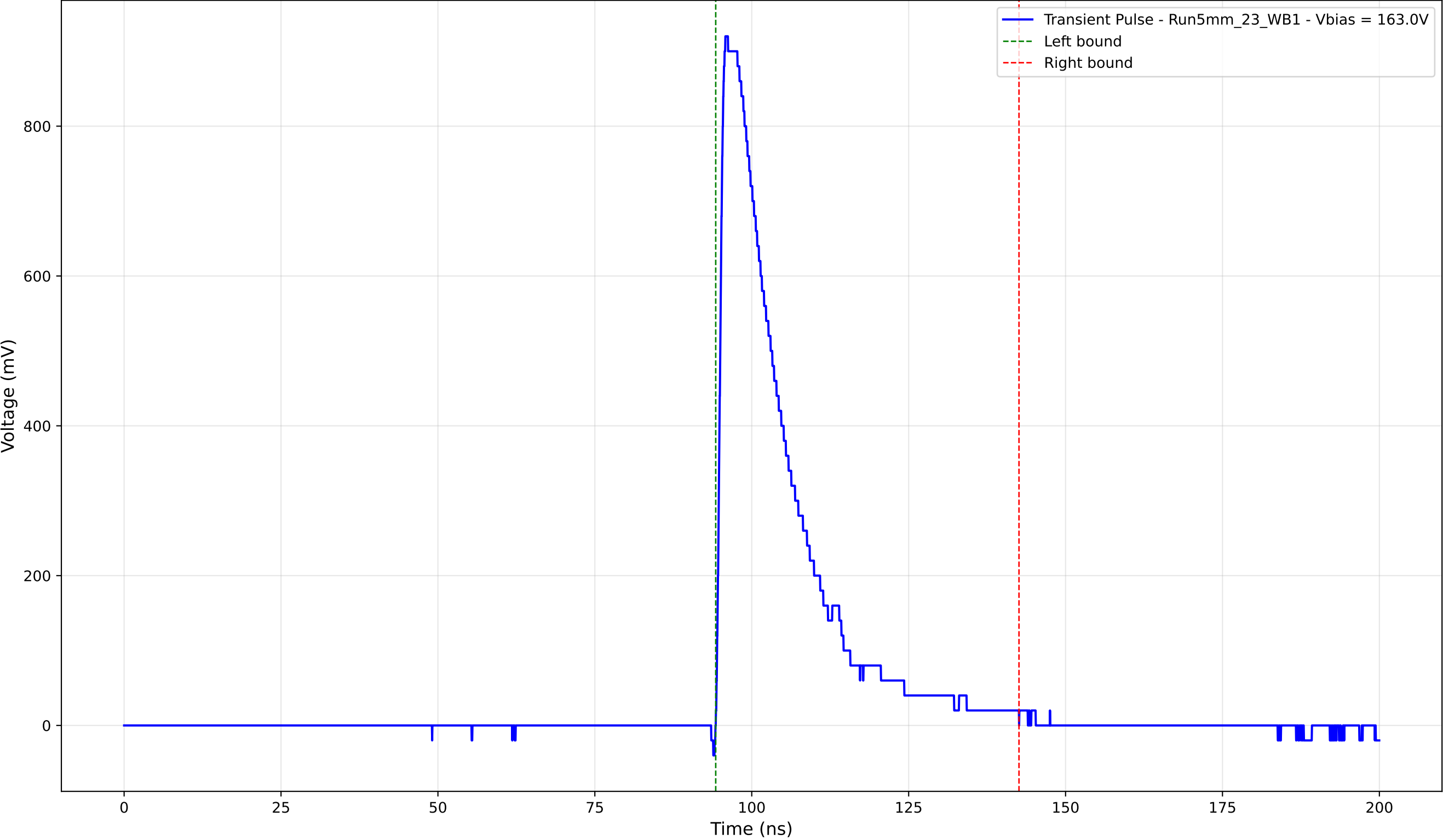
Transient Pulse - Sample: 5mm_23 - Position: 3600.0 \mu\text{m} - Charge: 211.02 pC
