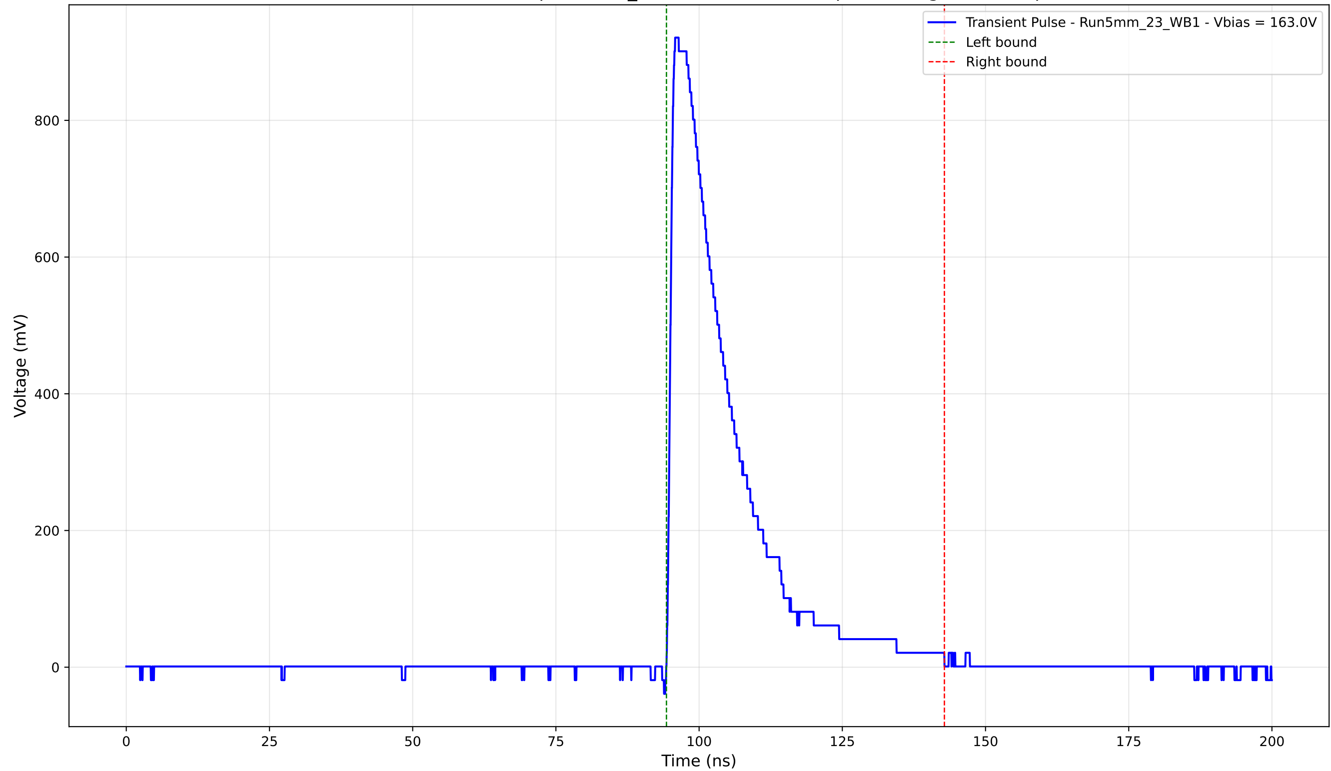
Transient Pulse - Sample: 5mm_23 - Position: 1820.0 \mu\text{m} - Charge: 214.97 pC
