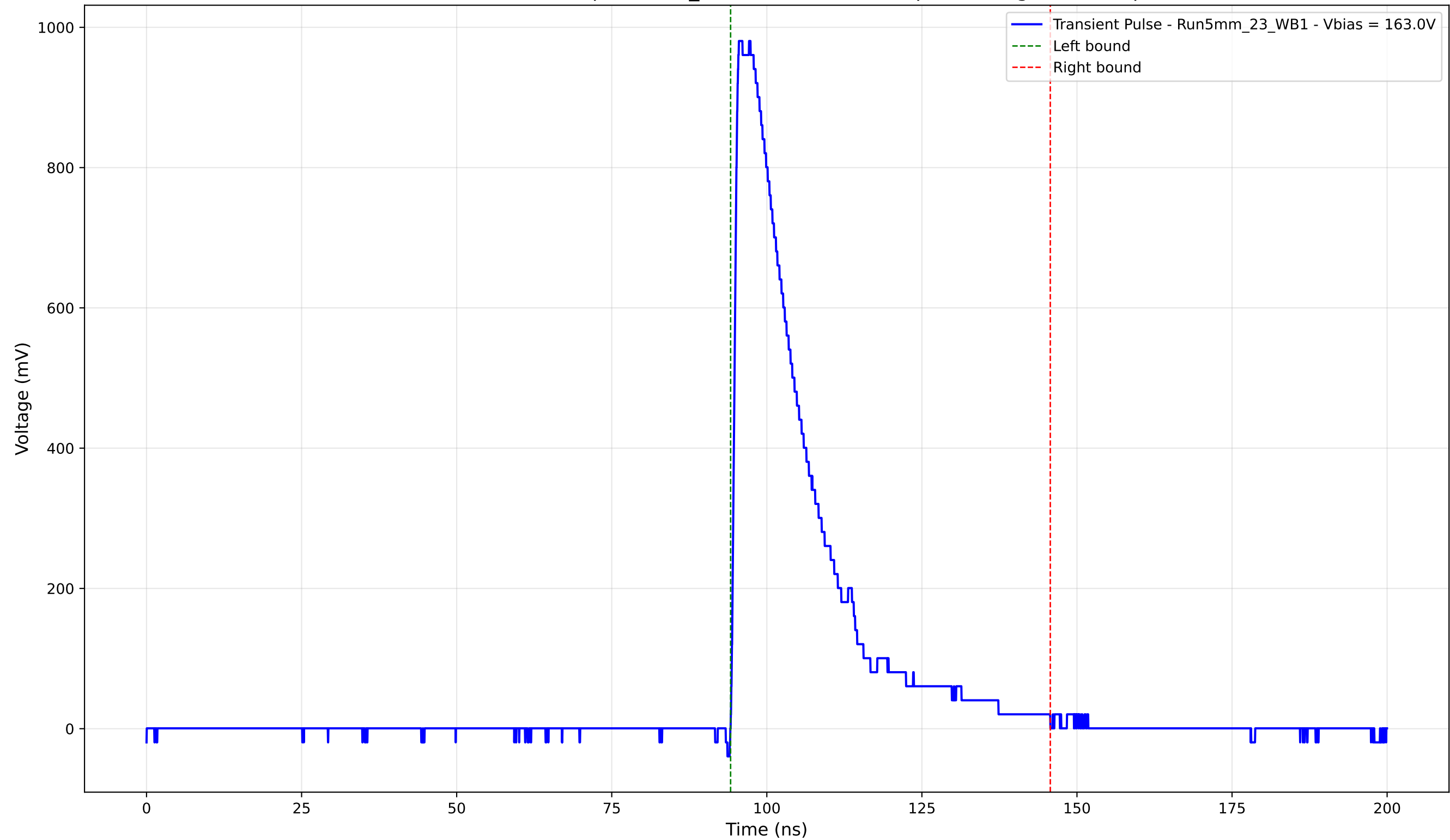
Transient Pulse - Sample: 5mm_23 - Position: 2040.0 \mu\text{m} - Charge: 245.61 pC
