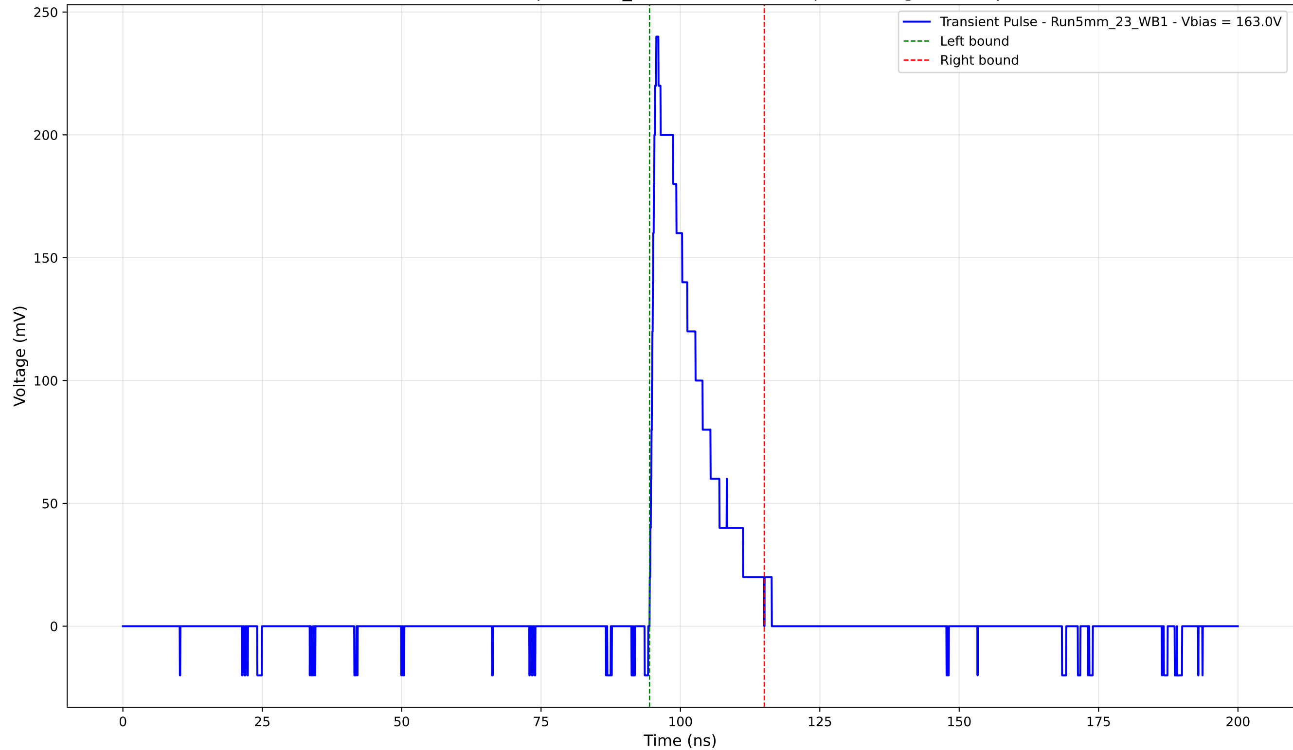
Transient Pulse - Sample: 5mm_23 - Position: 725.0 \mu\text{m} - Charge: 38.90 pC
