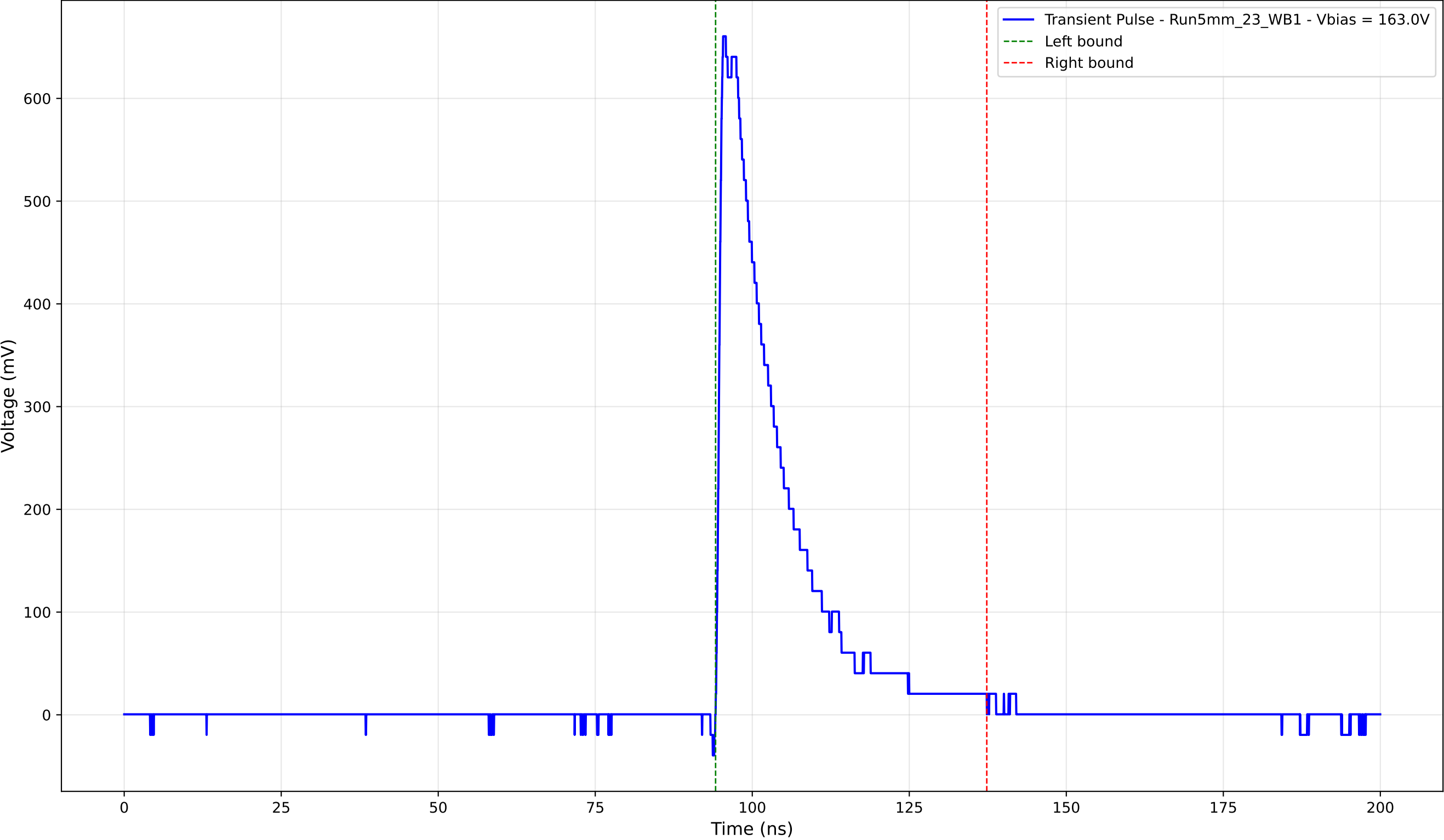
Transient Pulse - Sample: 5mm_23 - Position: 2190.0 \mu\text{m} - Charge: 136.03 pC
