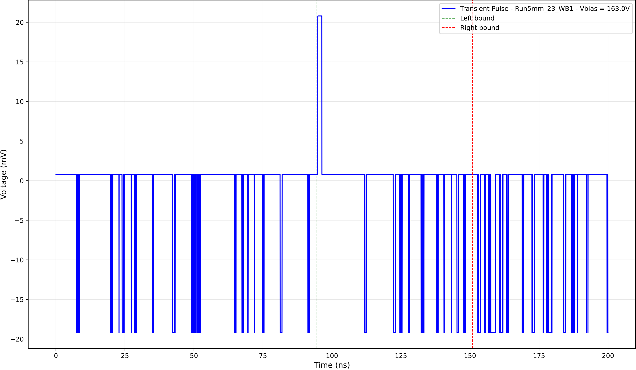
Transient Pulse - Sample: 5mm_23 - Position: 135.0 \mu\text{m} - Charge: -0.47 pC
