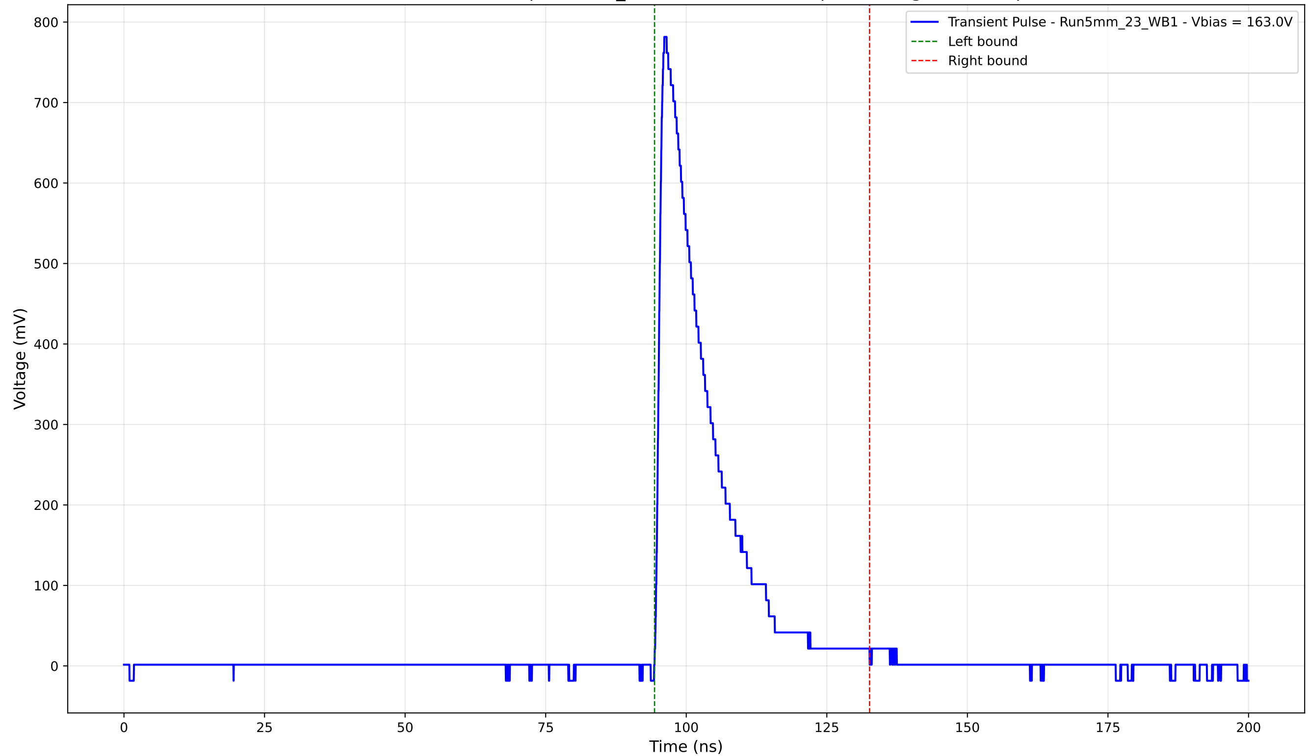
Transient Pulse - Sample: 5mm_23 - Position: 4190.0 \mu\text{m} - Charge: 149.25 pC
