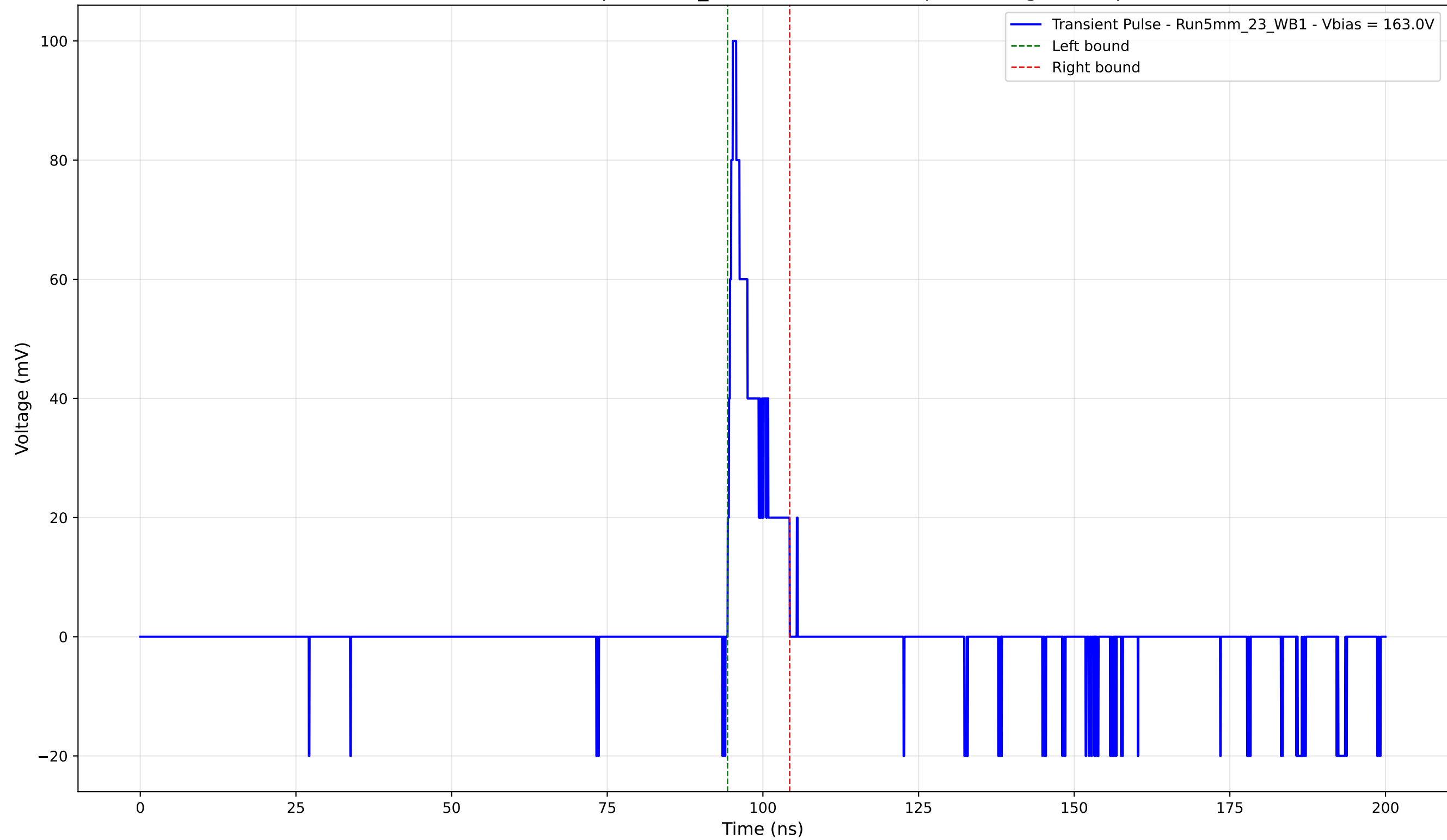
Transient Pulse - Sample: 5mm_23 - Position: 5210.0 \mu\text{m} - Charge: 8.09 pC
