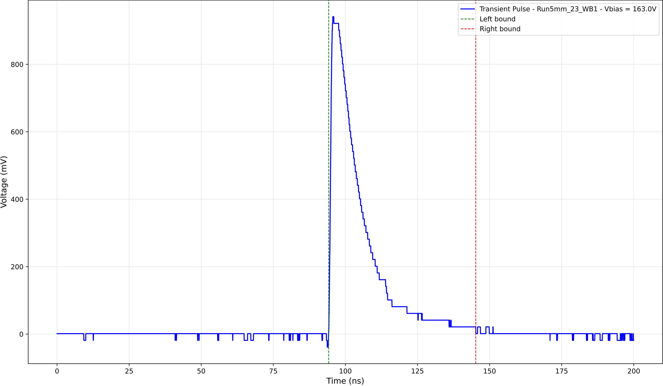
Transient Pulse - Sample: 5mm_23 - Position: 3470.0 \mu\text{m} - Charge: 221.75 pC
