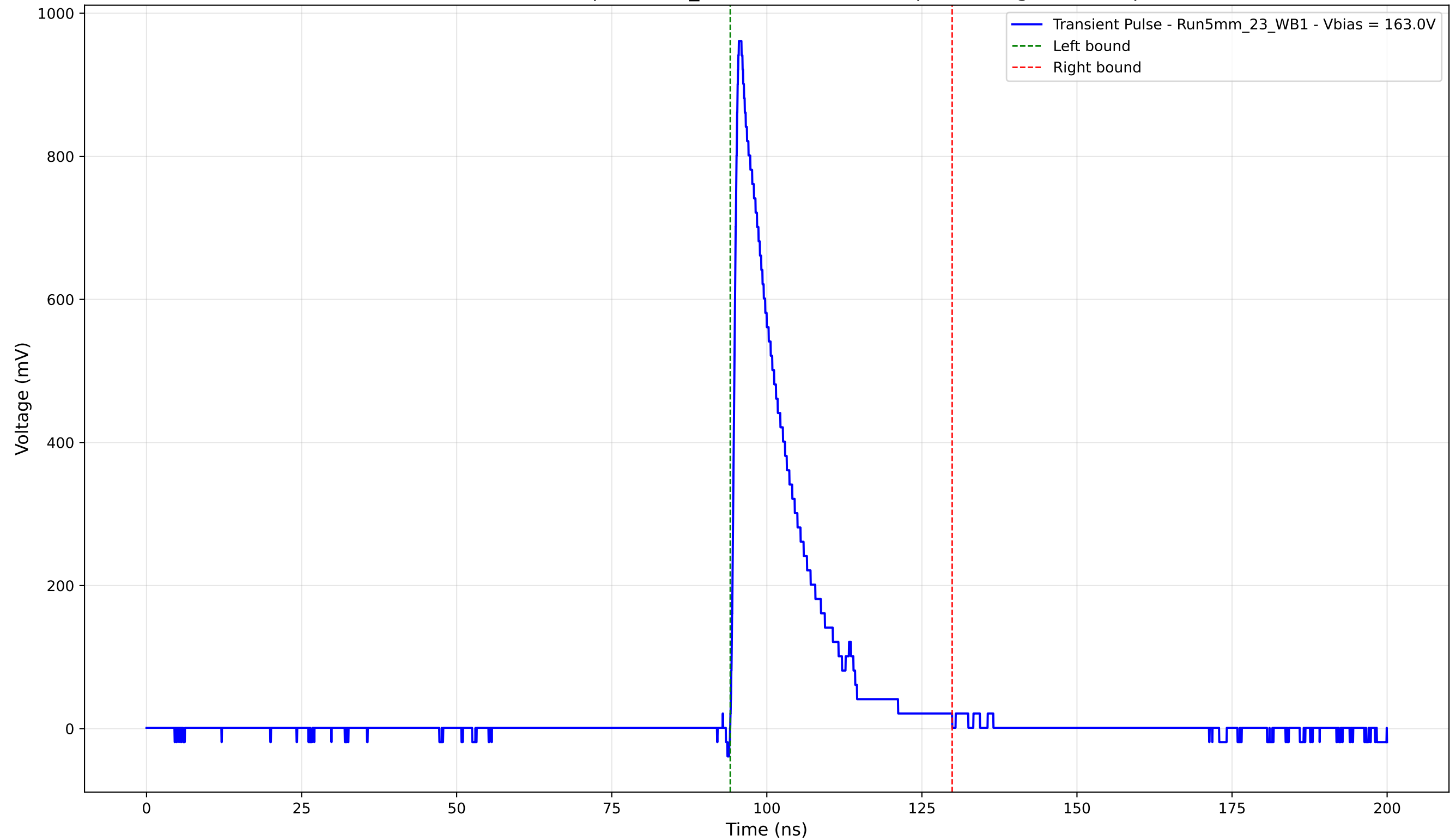
Transient Pulse - Sample: 5mm_23 - Position: 4855.0 \mu\text{m} - Charge: 163.92 pC
