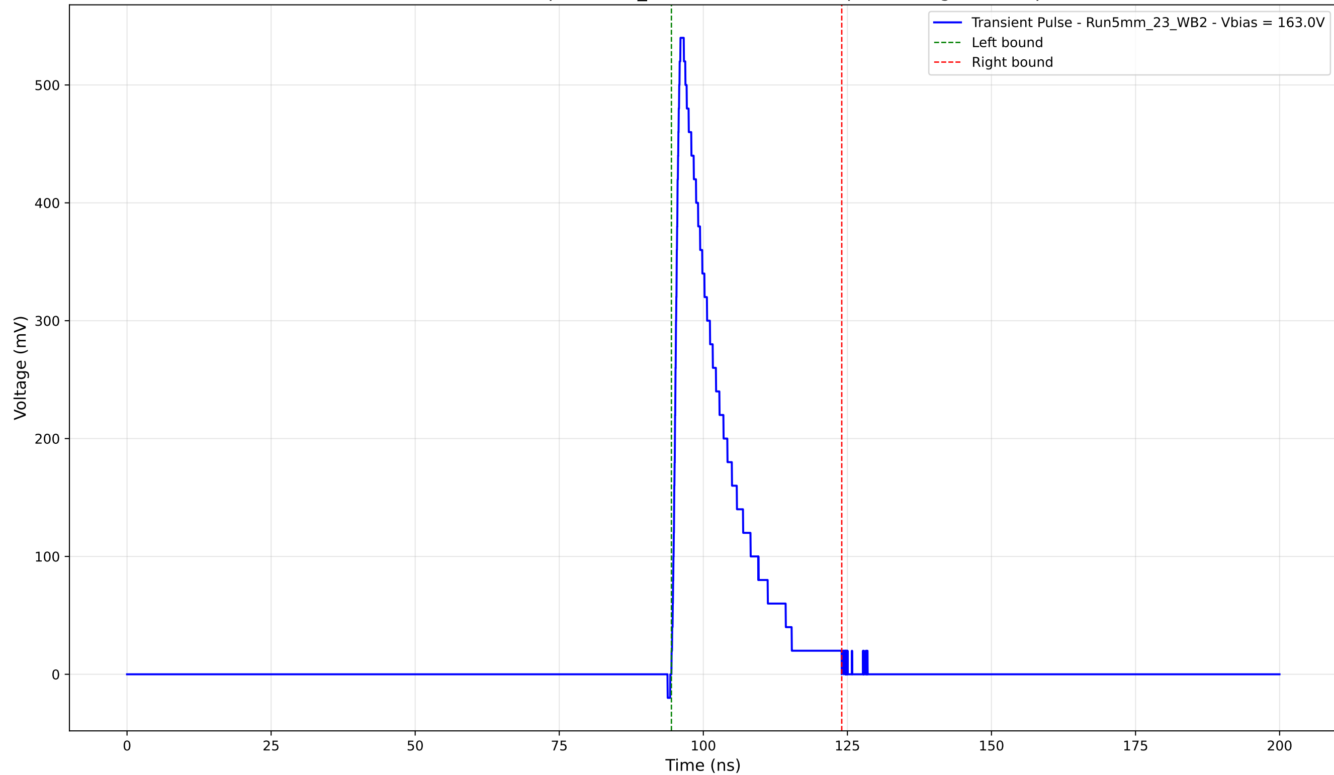
Transient Pulse - Sample: 5mm_23 - Position: 4085.0 \mu\text{m} - Charge: 90.74 pC
