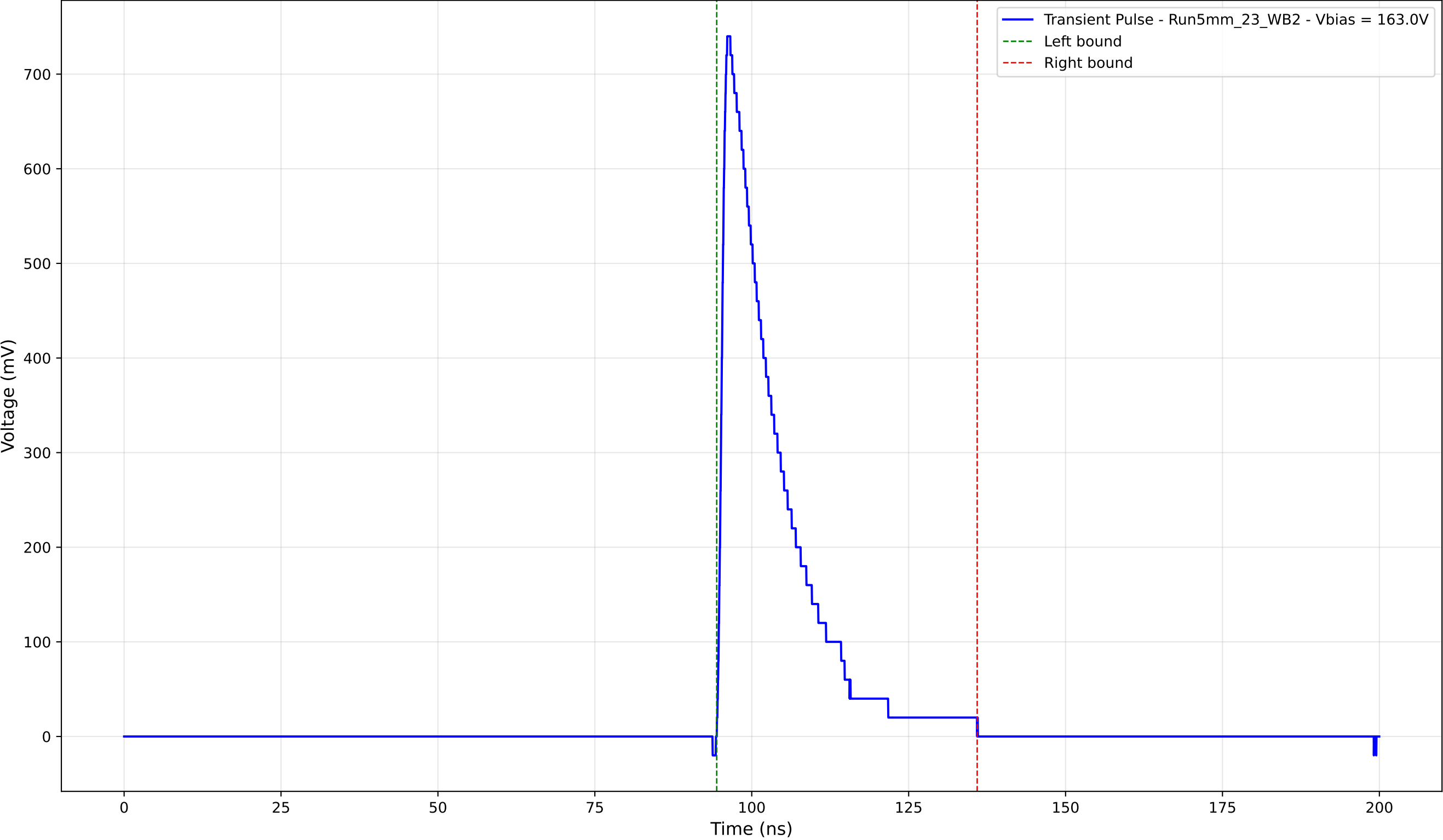
Transient Pulse - Sample: 5mm_23 - Position: 1060.0 \mu\text{m} - Charge: 143.68 pC
