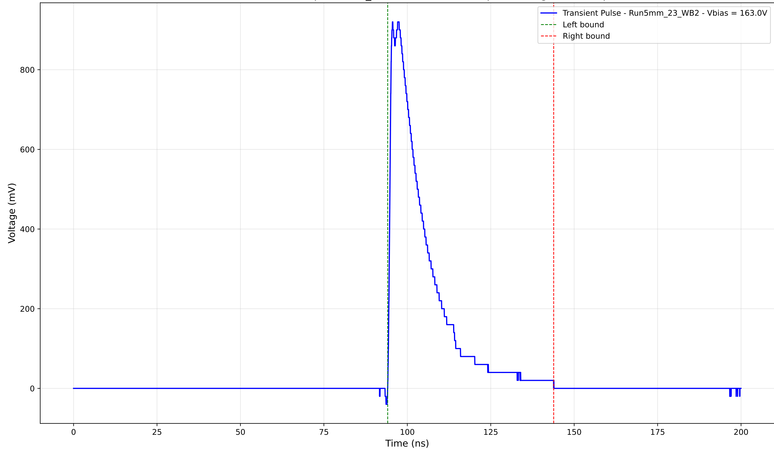
Transient Pulse - Sample: 5mm_23 - Position: 3225.0 \mu\text{m} - Charge: 216.50 pC
