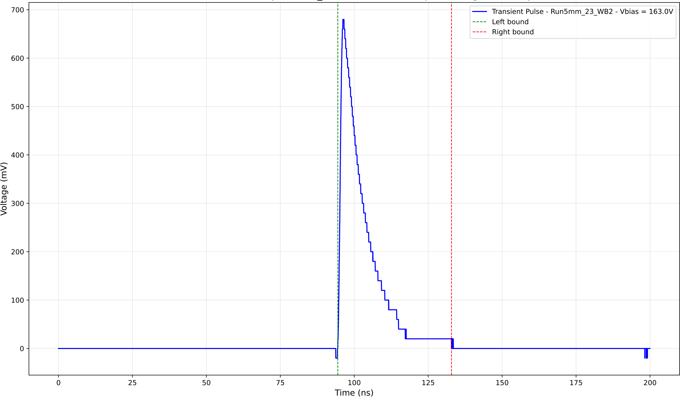
Transient Pulse - Sample: 5mm_23 - Position: 3975.0 \mu\text{m} - Charge: 121.65 pC
