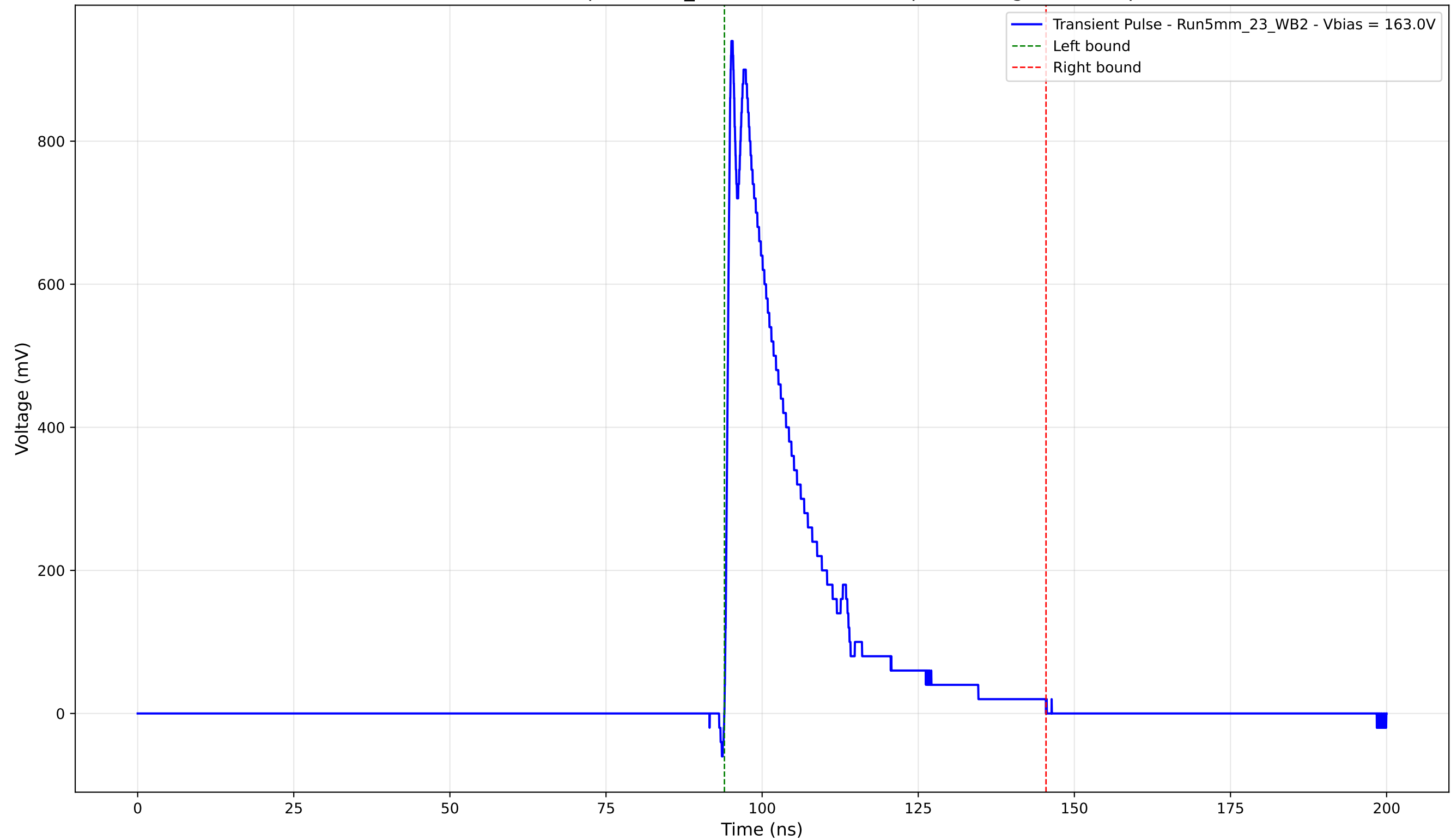
Transient Pulse - Sample: 5mm_23 - Position: 2165.0 \mu\text{m} - Charge: 205.58 pC
