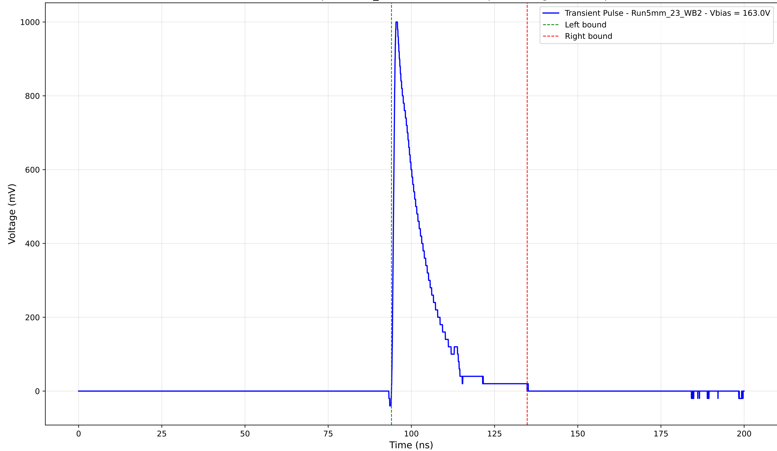
Transient Pulse - Sample: 5mm_23 - Position: 205.0 \mu\text{m} - Charge: 176.42 pC
