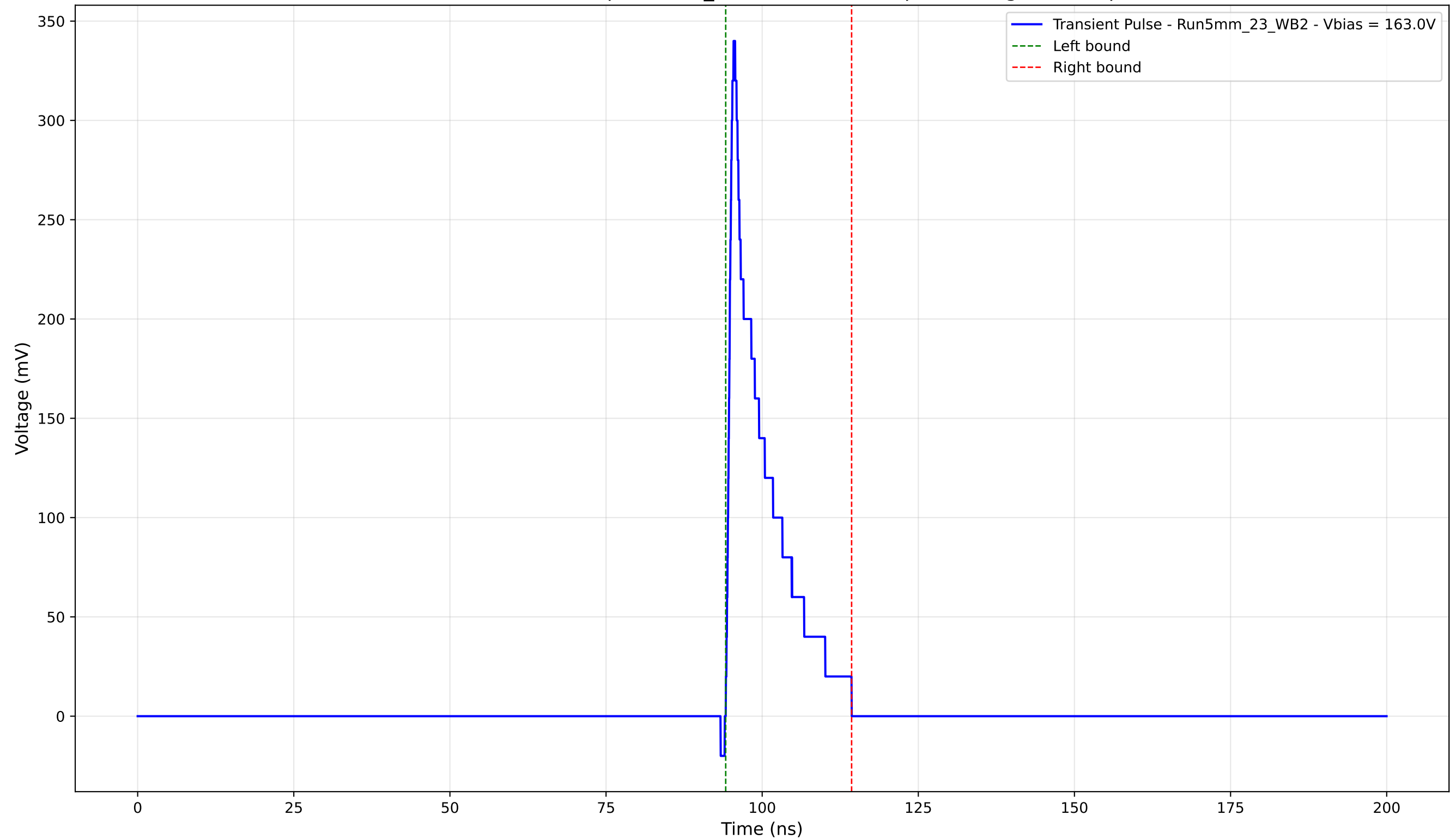
Transient Pulse - Sample: 5mm_23 - Position: 60.0 \mu\text{m} - Charge: 40.39 pC
