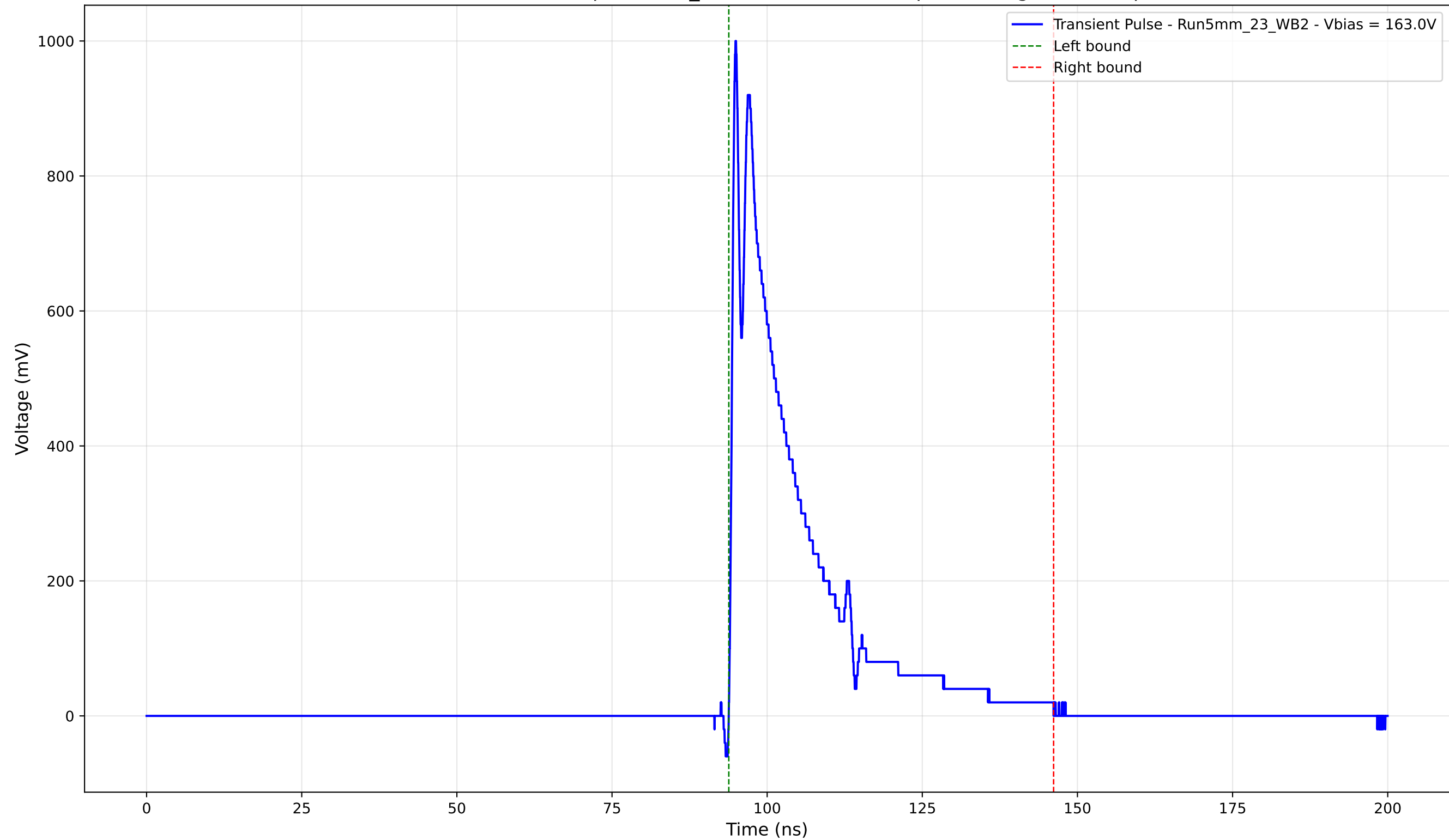
Transient Pulse - Sample: 5mm_23 - Position: 2630.0 \mu\text{m} - Charge: 199.61 pC
