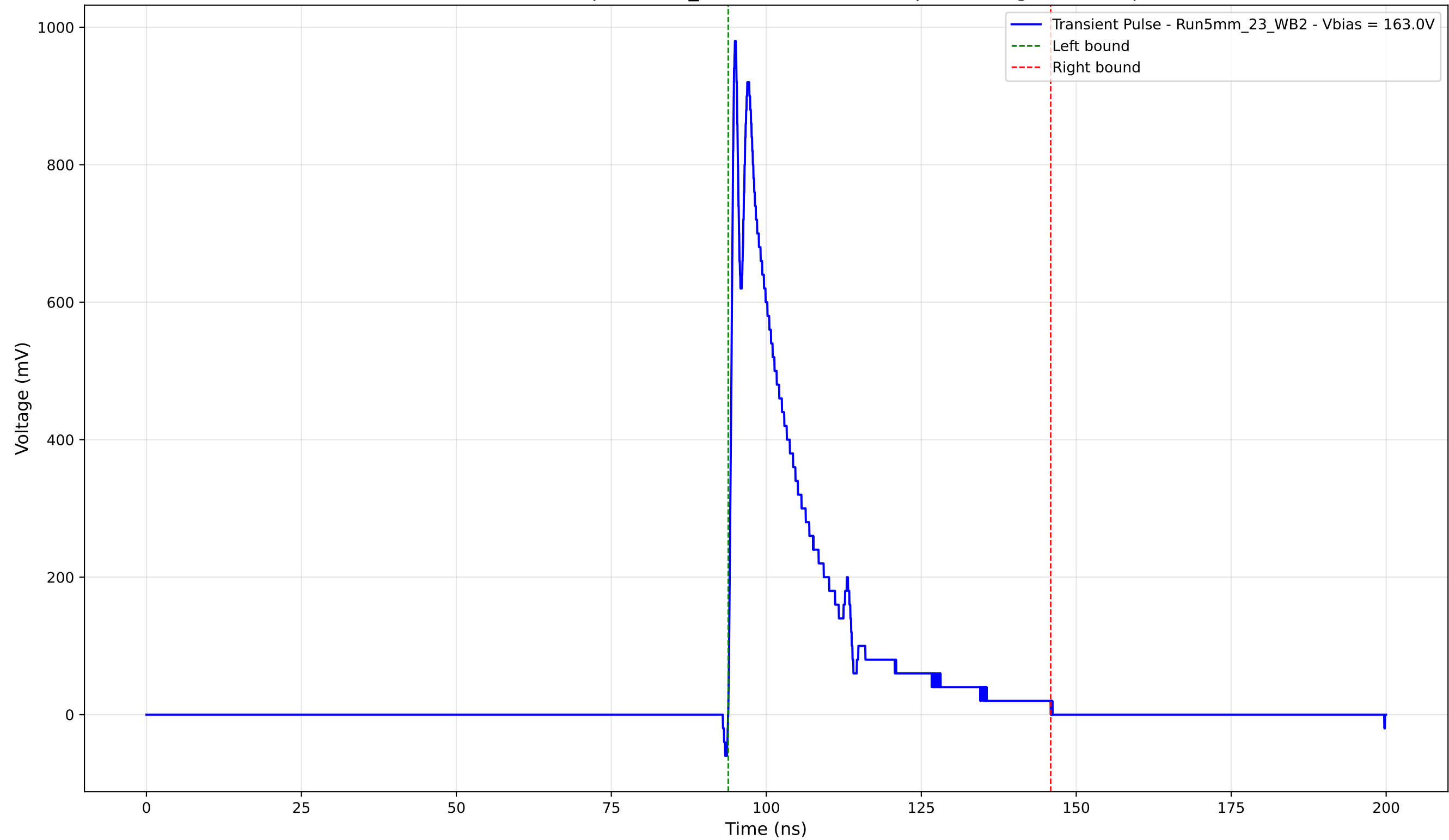
Transient Pulse - Sample: 5mm_23 - Position: 2695.0 \mu\text{m} - Charge: 201.64 pC
