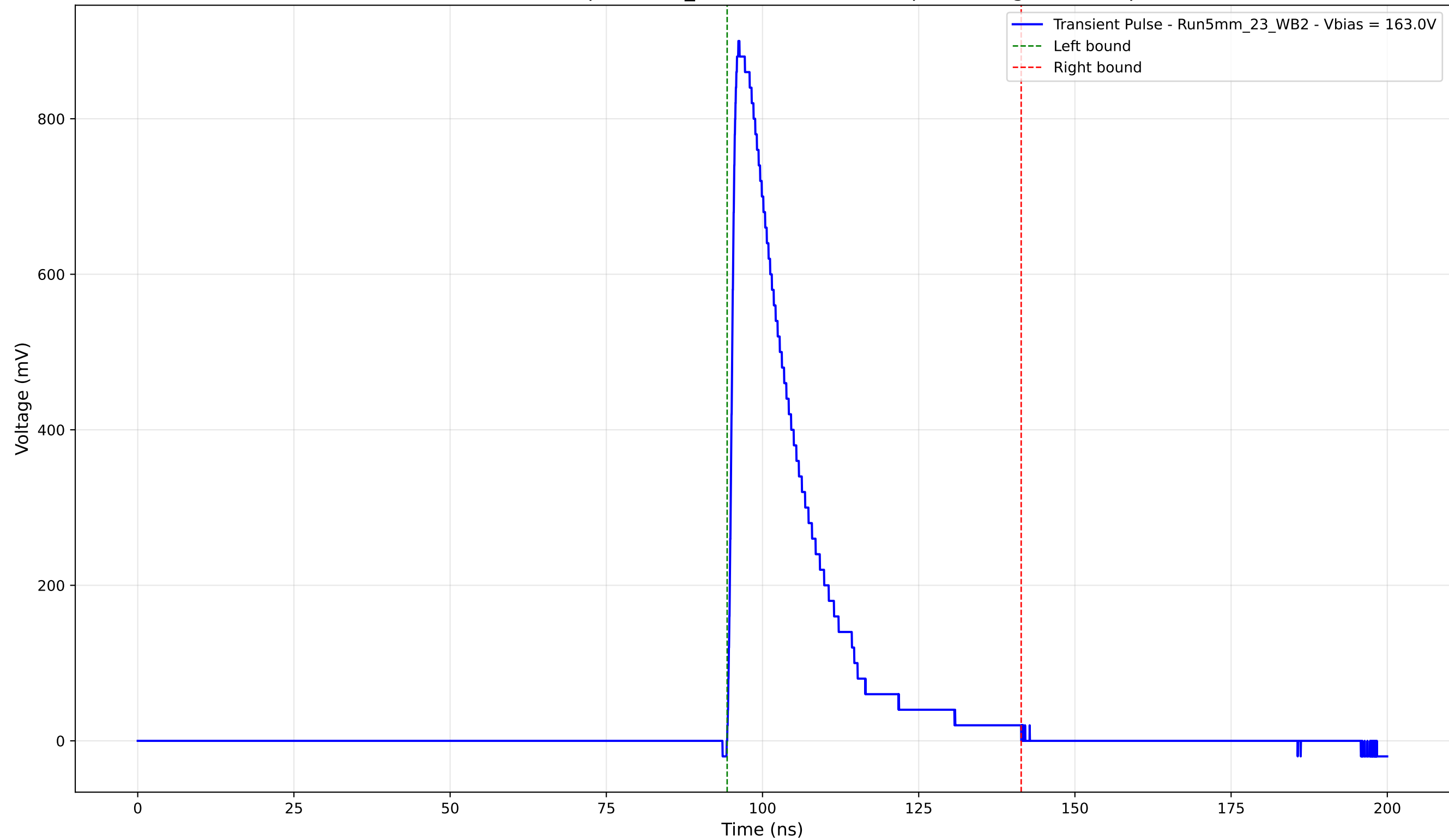
Transient Pulse - Sample: 5mm_23 - Position: 1350.0 \mu\text{m} - Charge: 199.62 pC
