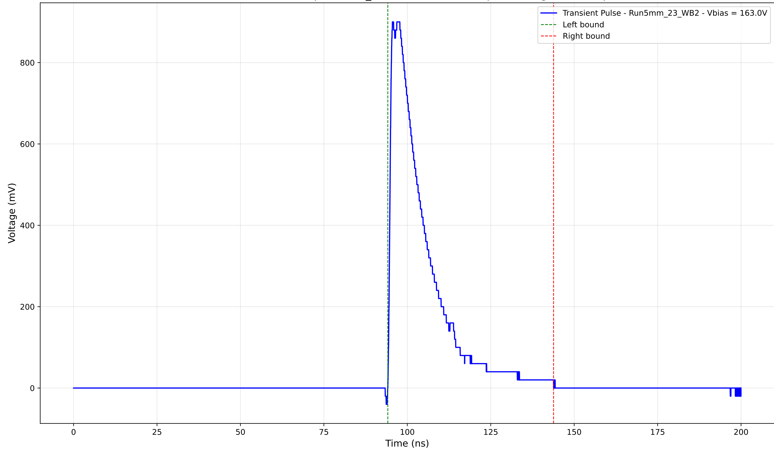
Transient Pulse - Sample: 5mm_23 - Position: 3275.0 \mu\text{m} - Charge: 212.35 pC
