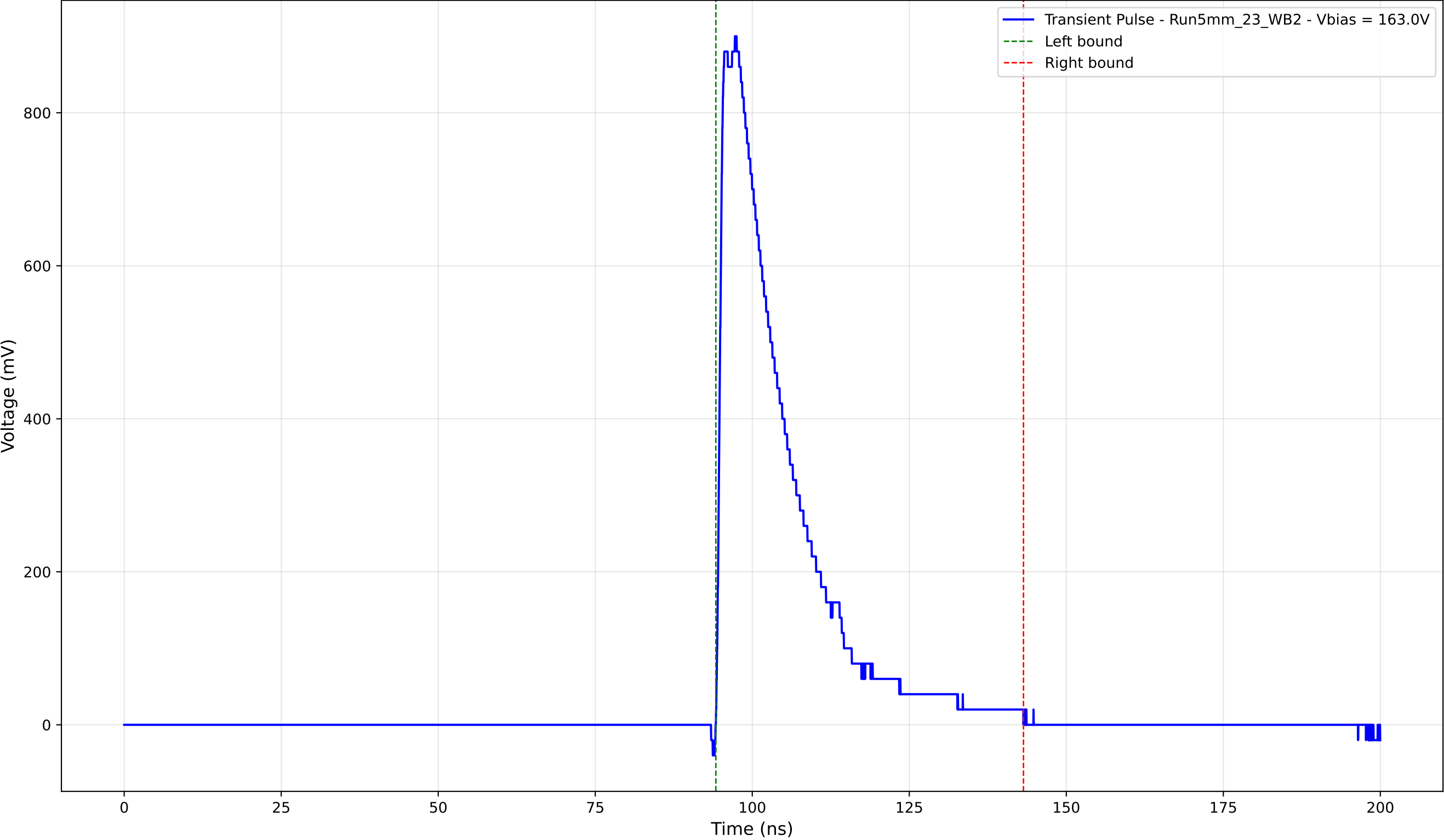
Transient Pulse - Sample: 5mm_23 - Position: 1715.0 \mu\text{m} - Charge: 210.20 pC
