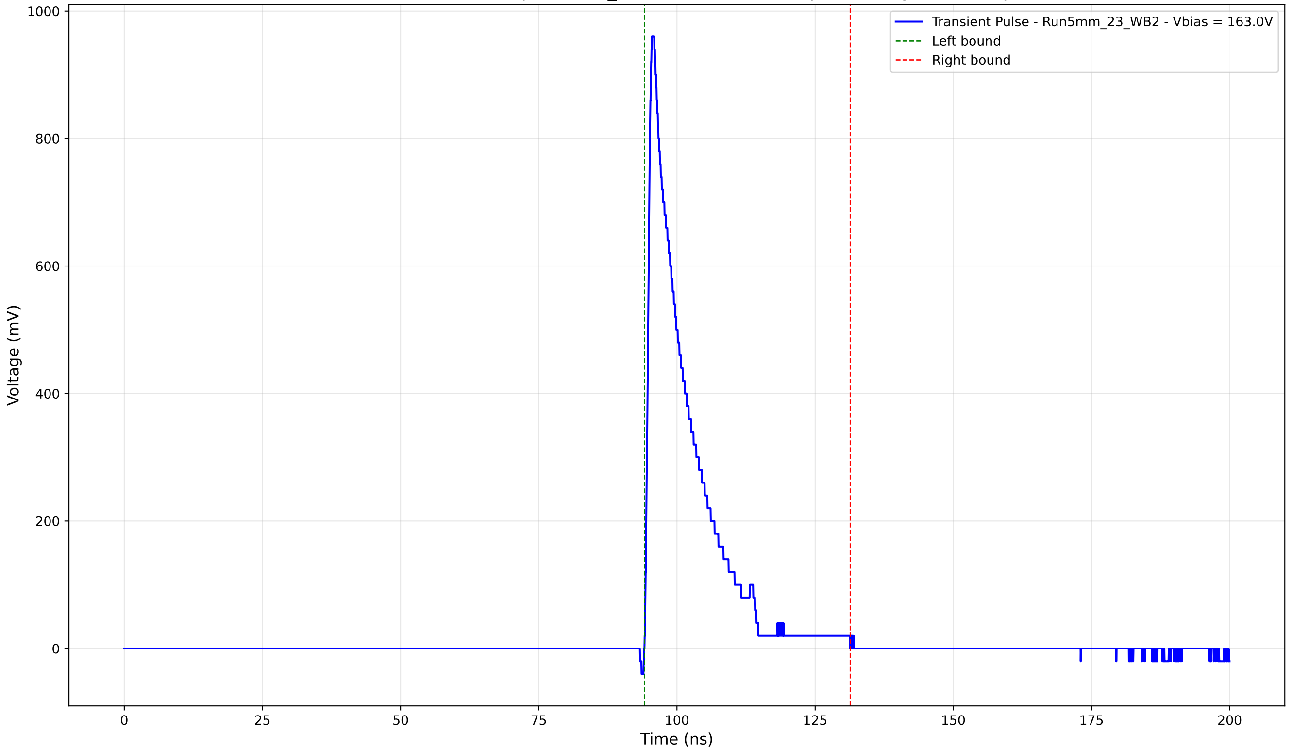
Transient Pulse - Sample: 5mm_23 - Position: 4780.0 \mu\text{m} - Charge: 146.86 pC
