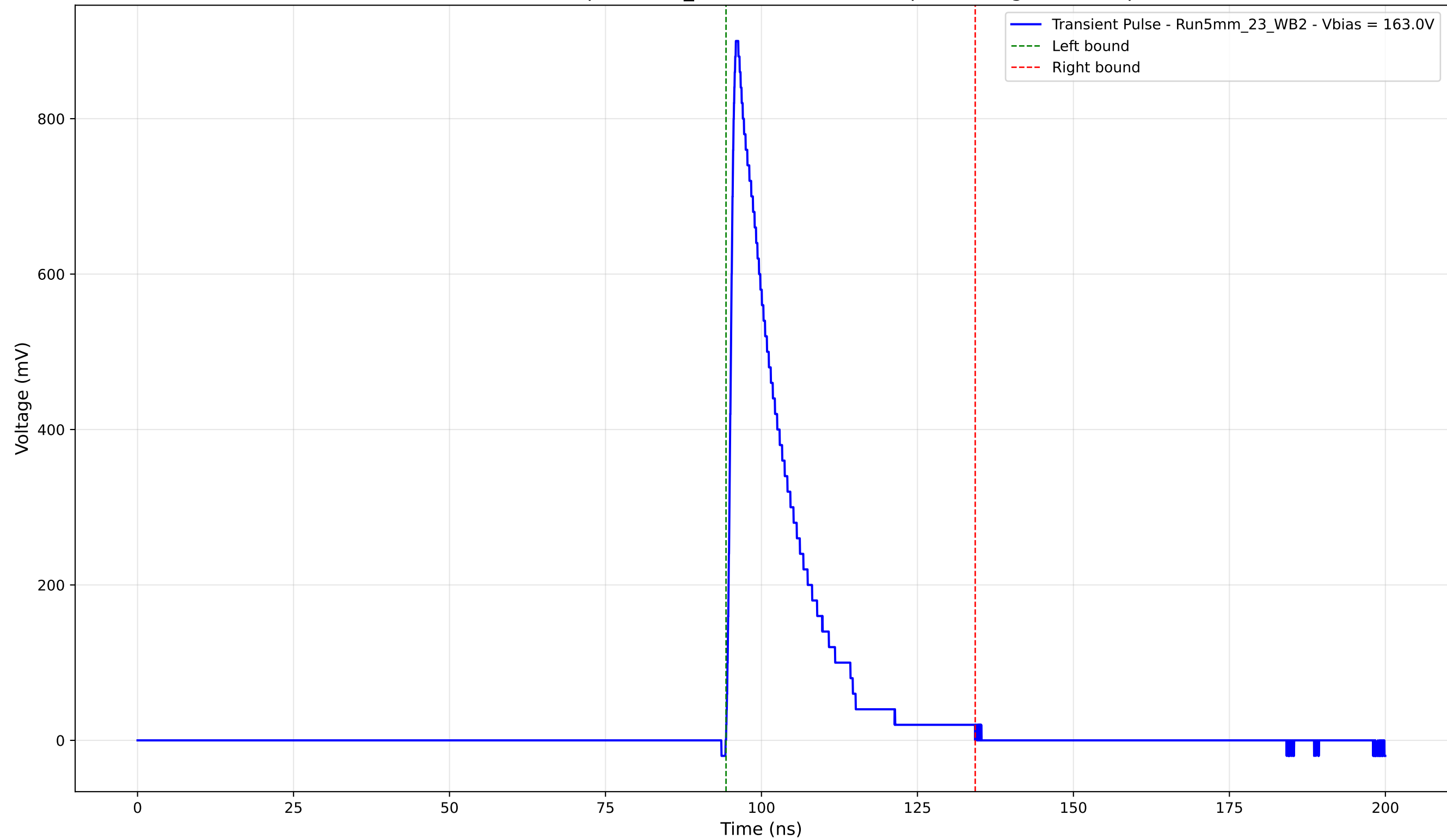
Transient Pulse - Sample: 5mm_23 - Position: 4360.0 \mu\text{m} - Charge: 159.82 pC
