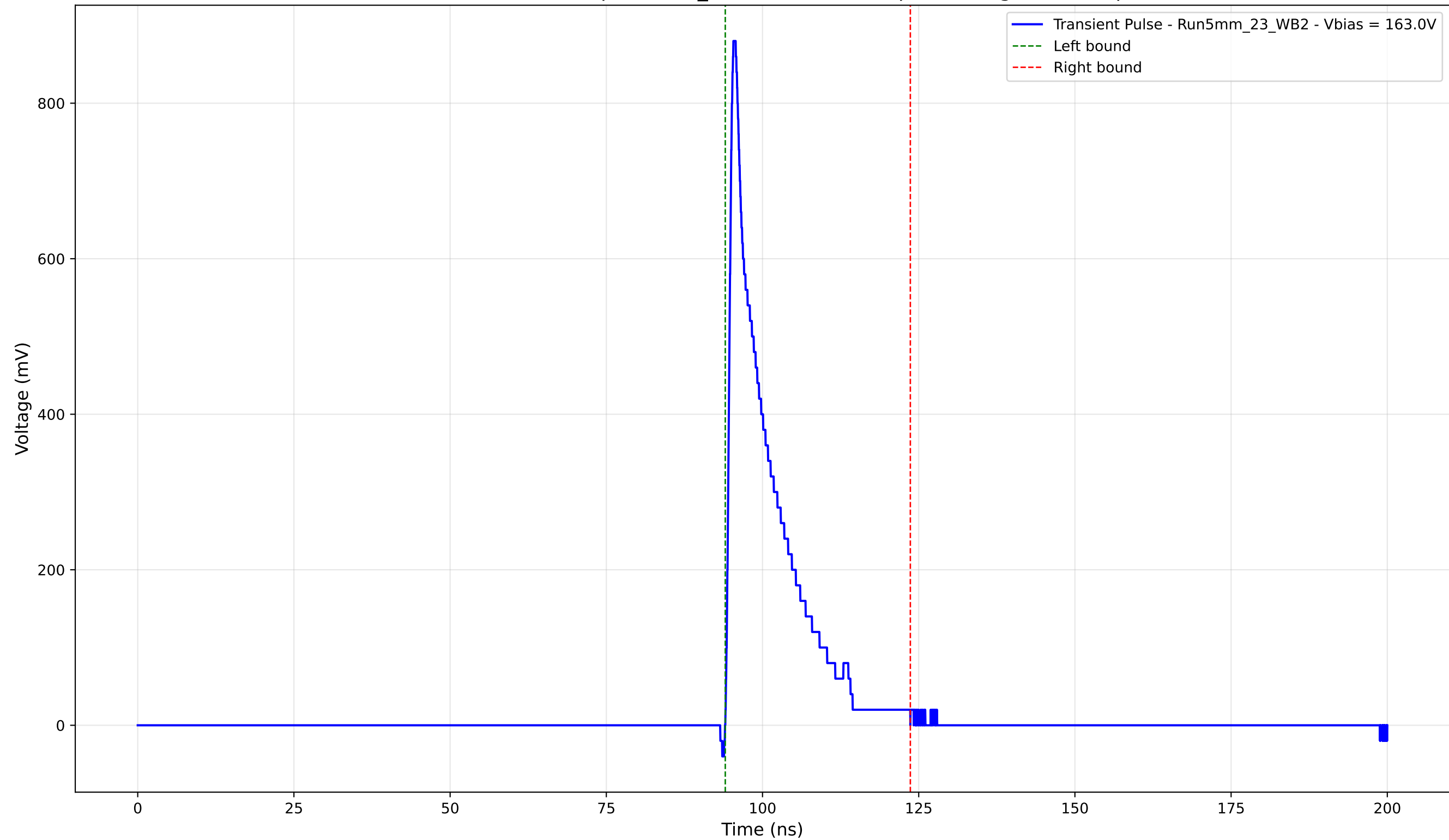
Transient Pulse - Sample: 5mm_23 - Position: 95.0 \mu\text{m} - Charge: 119.42 pC
