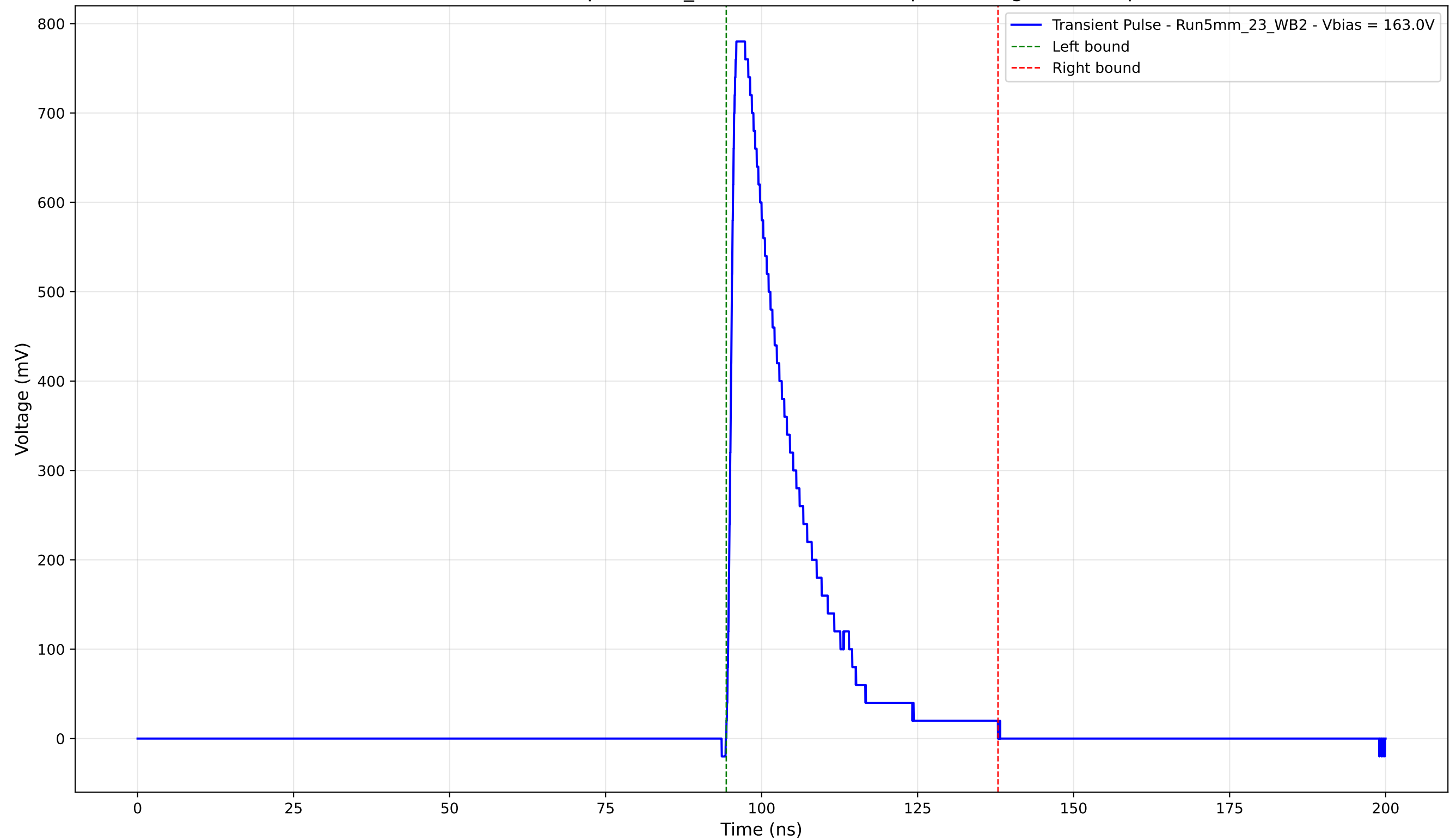
Transient Pulse - Sample: 5mm_23 - Position: 3620.0 \mu\text{m} - Charge: 163.54 pC
