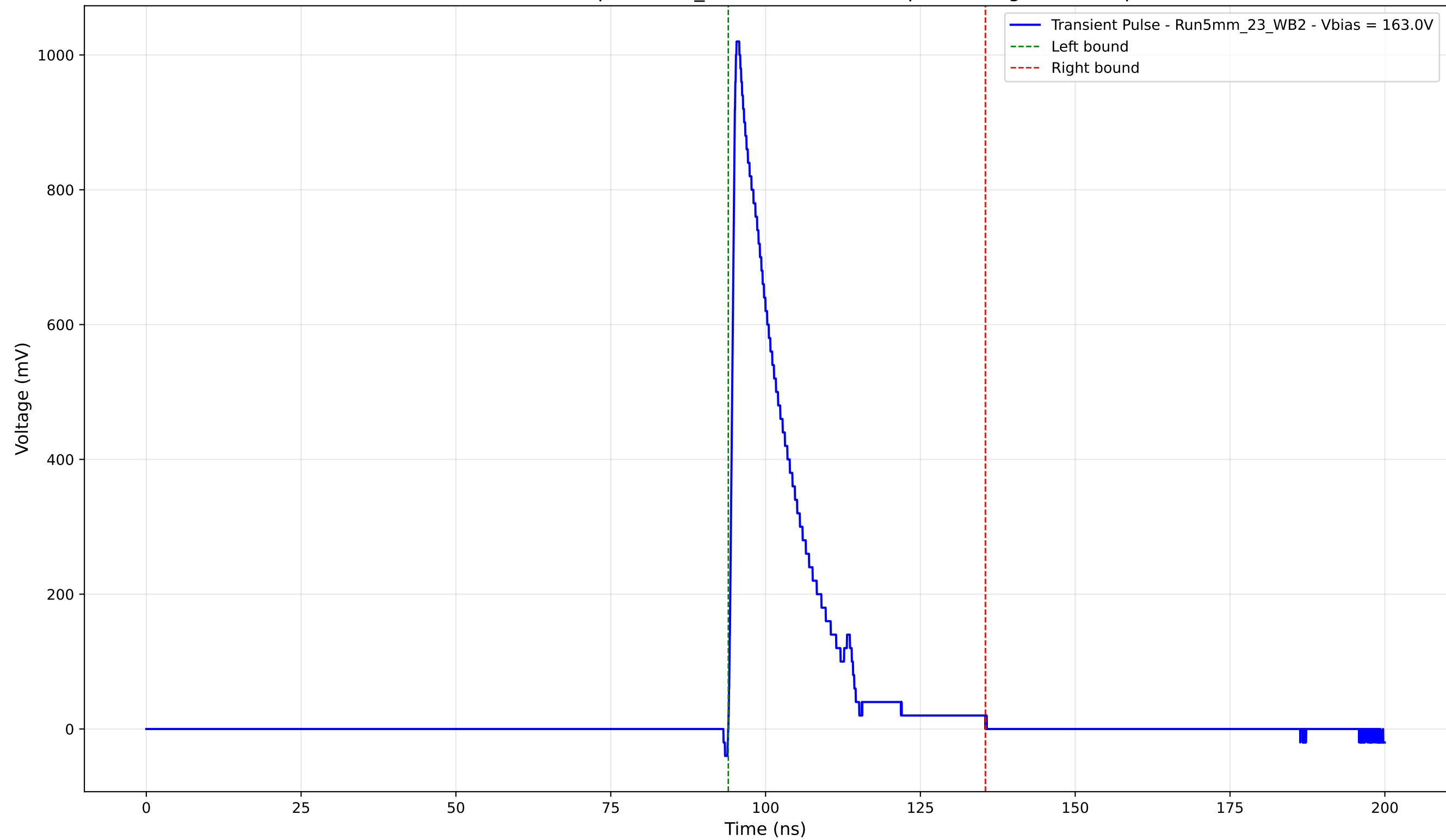
Transient Pulse - Sample: 5mm_23 - Position: 160.0 \mu\text{m} - Charge: 184.66 pC
