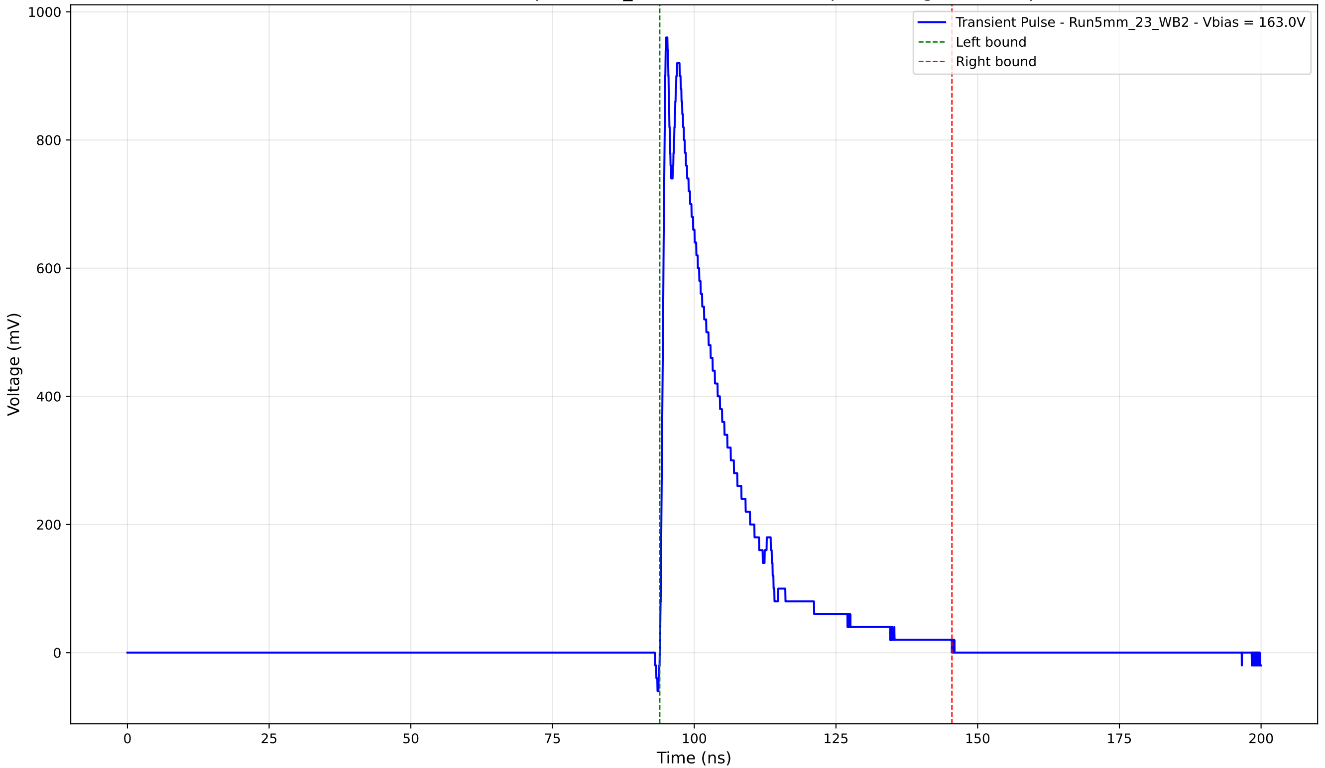
Transient Pulse - Sample: 5mm_23 - Position: 2840.0 \mu\text{m} - Charge: 211.58 pC
