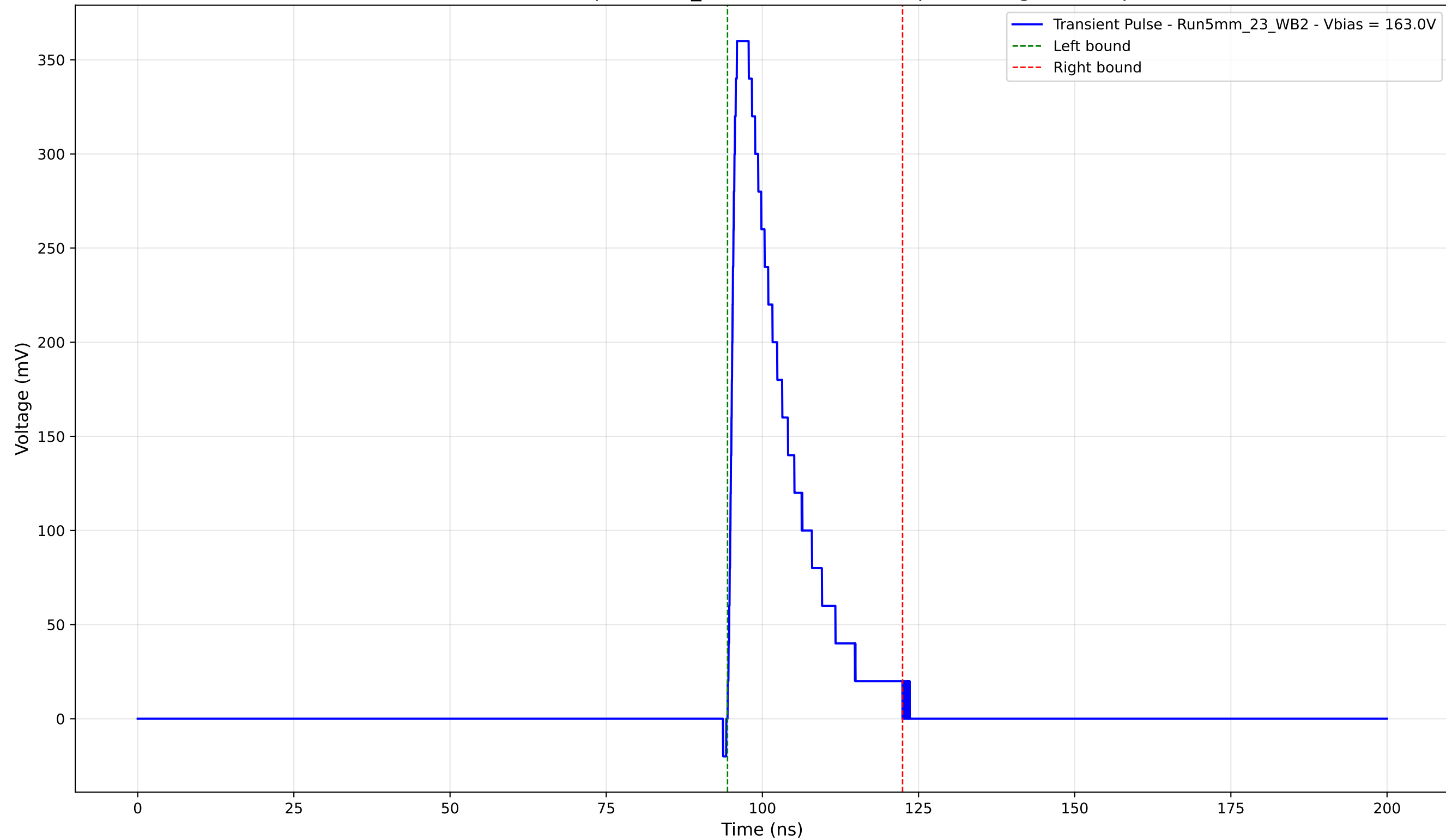
Transient Pulse - Sample: 5mm_23 - Position: 3560.0 \mu\text{m} - Charge: 68.88 pC
