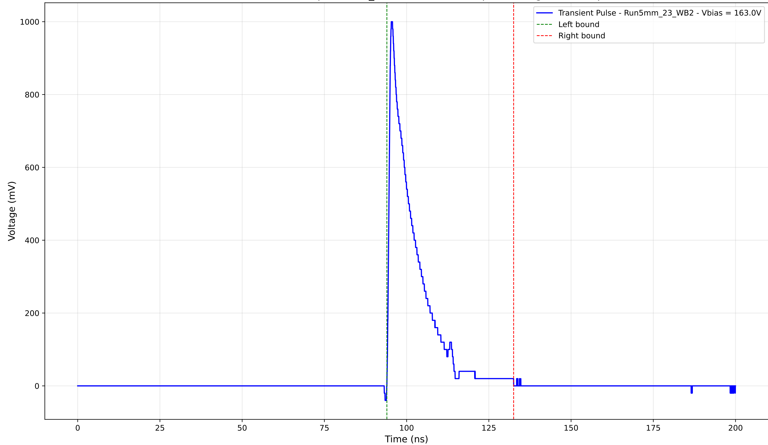
Transient Pulse - Sample: 5mm_23 - Position: 120.0 \mu\text{m} - Charge: 164.01 pC
