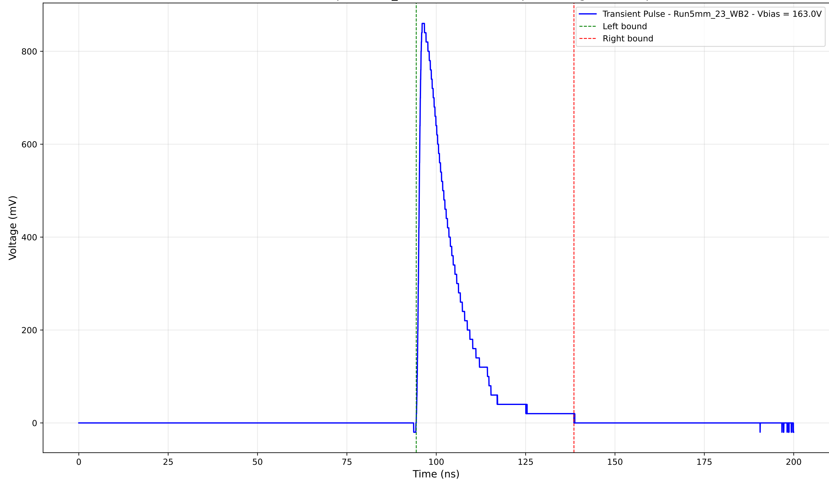
Transient Pulse - Sample: 5mm_23 - Position: 3820.0 \mu\text{m} - Charge: 176.00 pC
