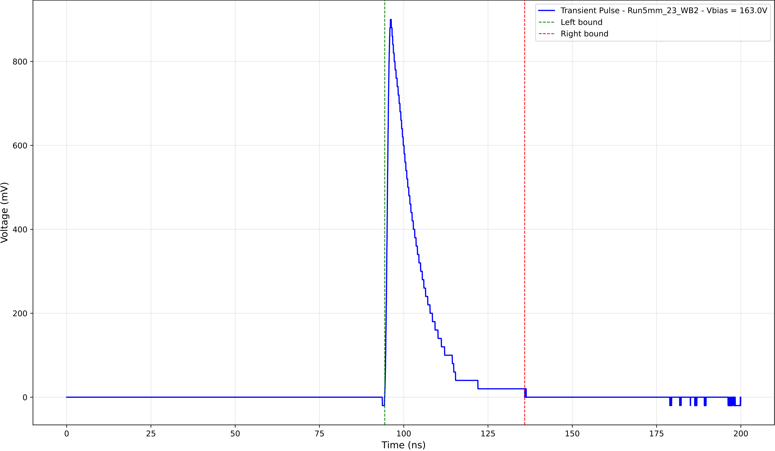
Transient Pulse - Sample: 5mm_23 - Position: 4235.0 \mu\text{m} - Charge: 164.02 pC
