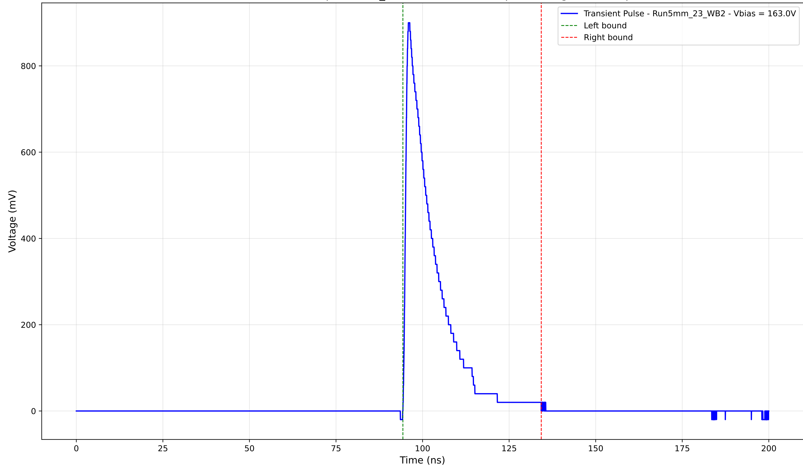
Transient Pulse - Sample: 5mm_23 - Position: 4355.0 \mu\text{m} - Charge: 160.17 pC
