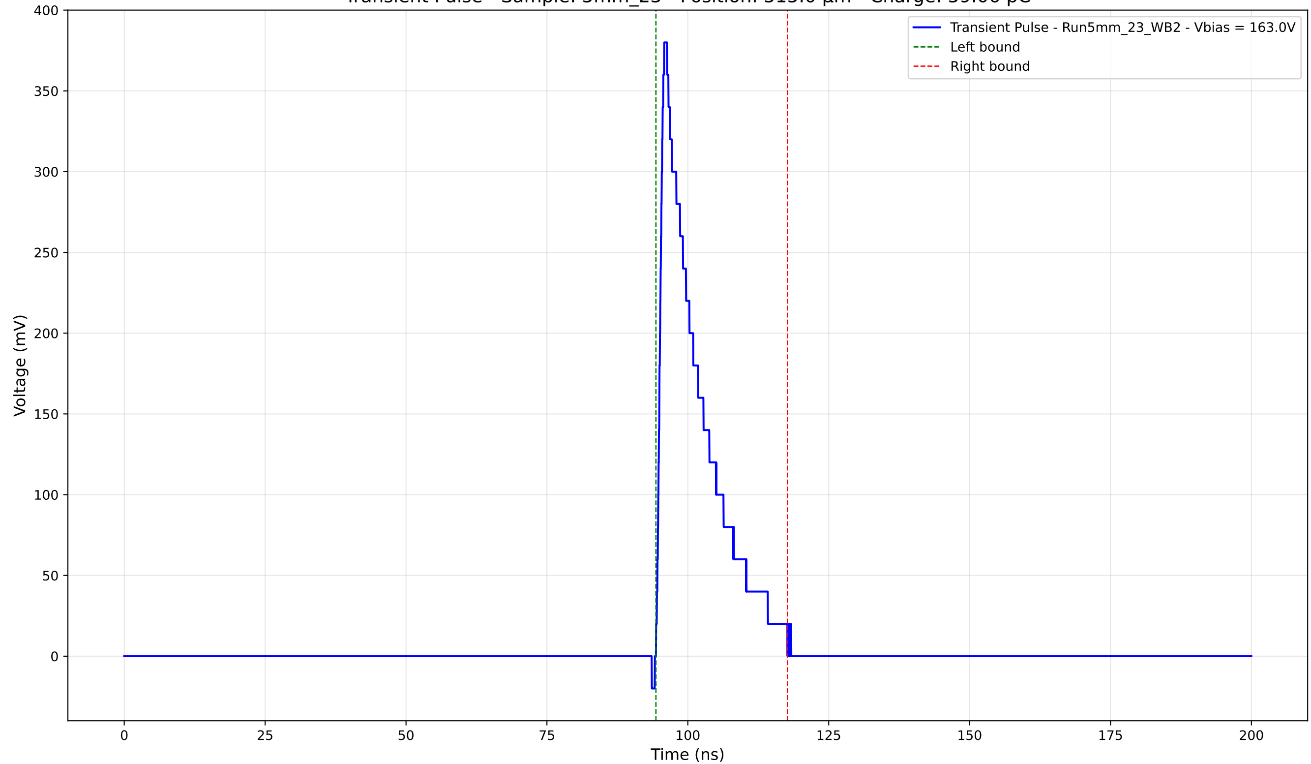
Transient Pulse - Sample: 5mm_23 - Position: 515.0 \mu\text{m} - Charge: 59.06 pC
