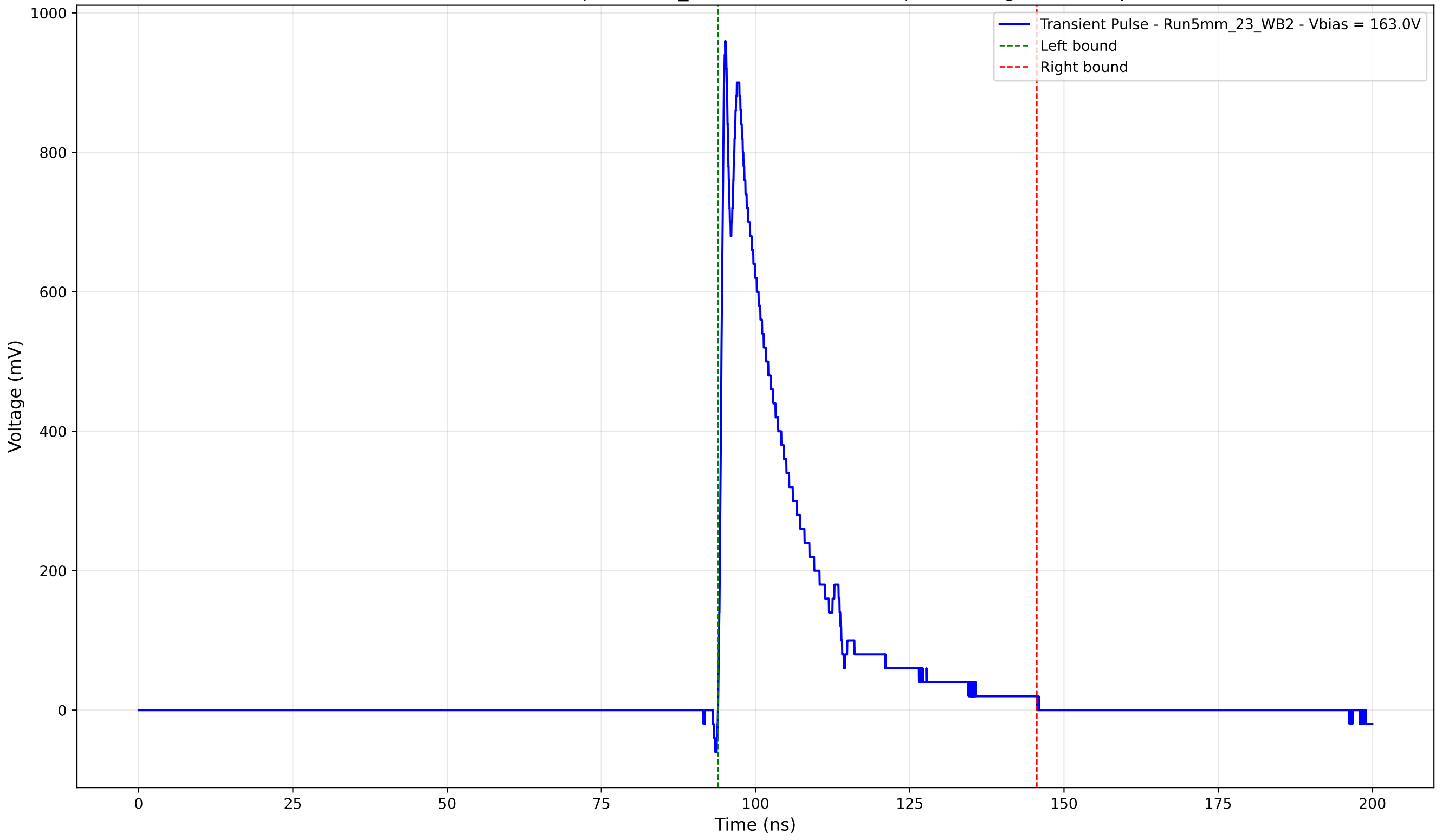
Transient Pulse - Sample: 5mm_23 - Position: 2235.0 \mu\text{m} - Charge: 204.72 pC
