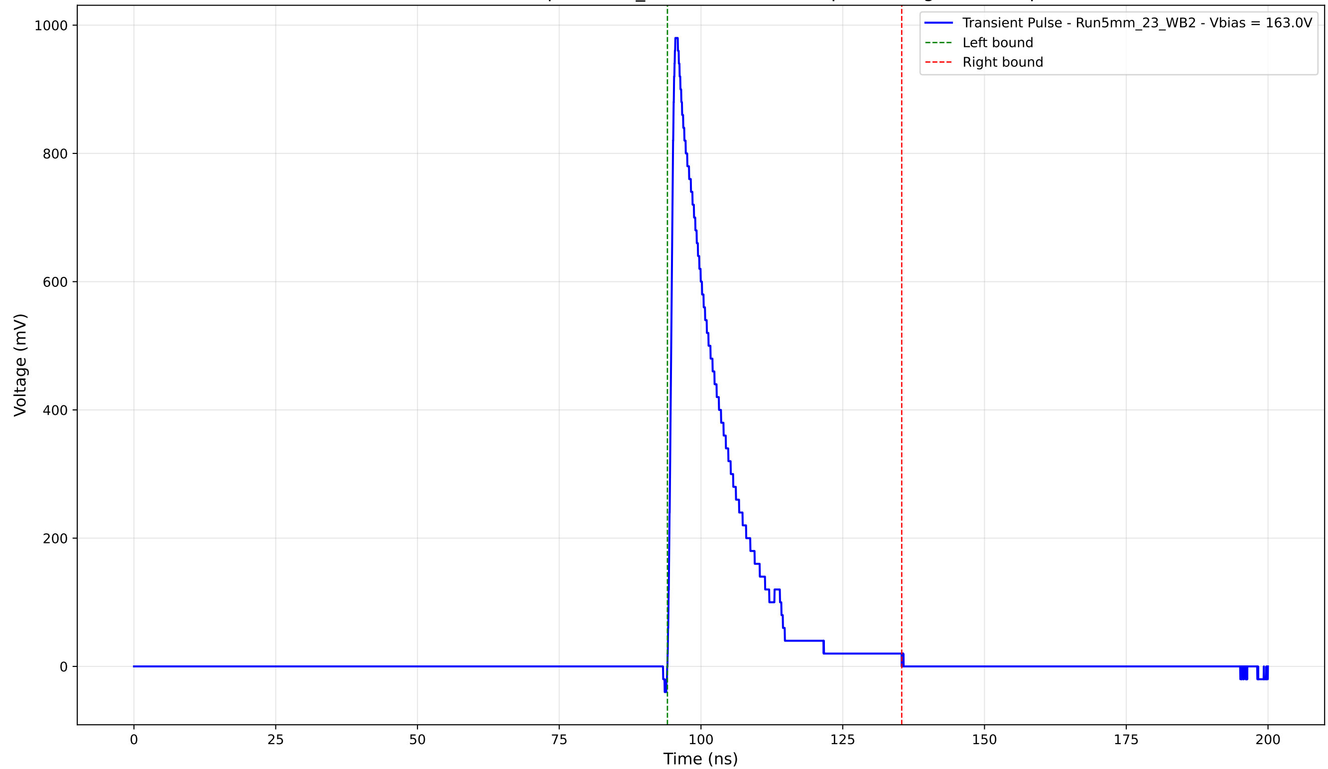
Transient Pulse - Sample: 5mm_23 - Position: 290.0 \mu\text{m} - Charge: 175.86 pC
