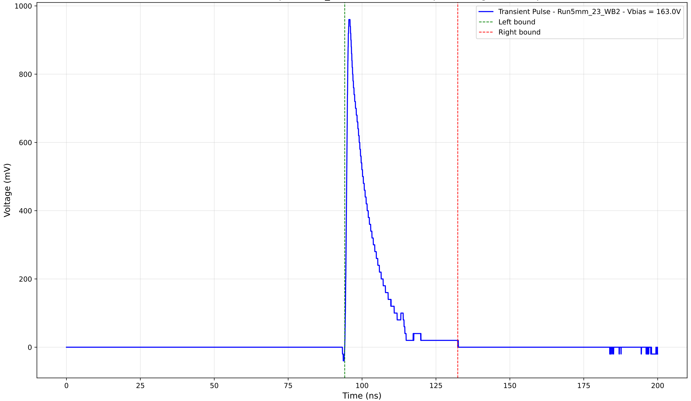
Transient Pulse - Sample: 5mm_23 - Position: 4725.0 \mu\text{m} - Charge: 152.19 pC
