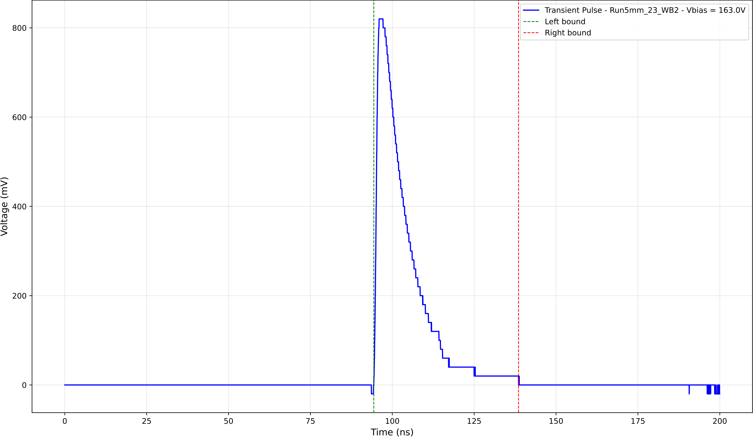
Transient Pulse - Sample: 5mm_23 - Position: 3665.0 \mu\text{m} - Charge: 172.95 pC
