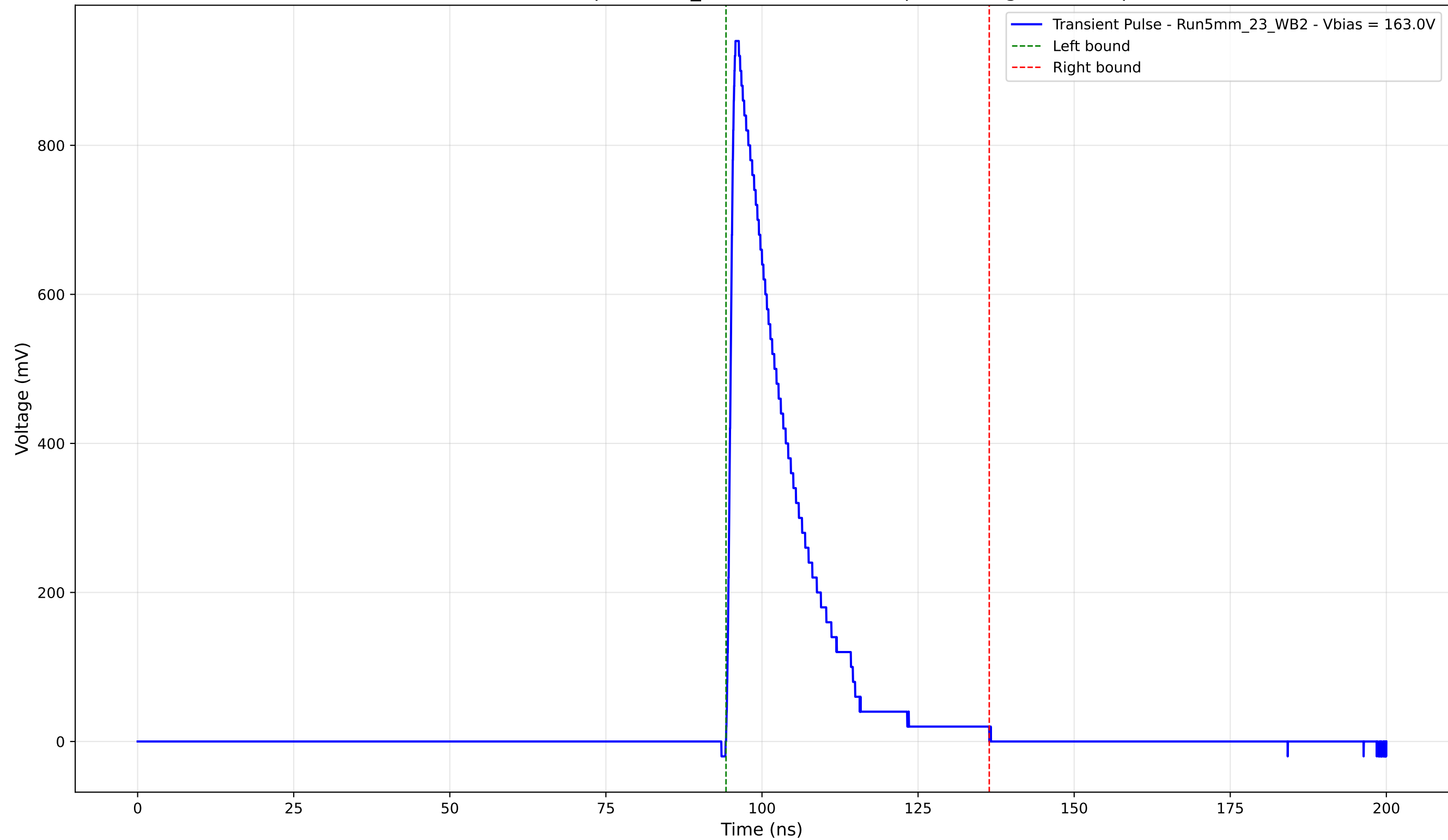
Transient Pulse - Sample: 5mm_23 - Position: 585.0 \mu\text{m} - Charge: 182.35 pC
