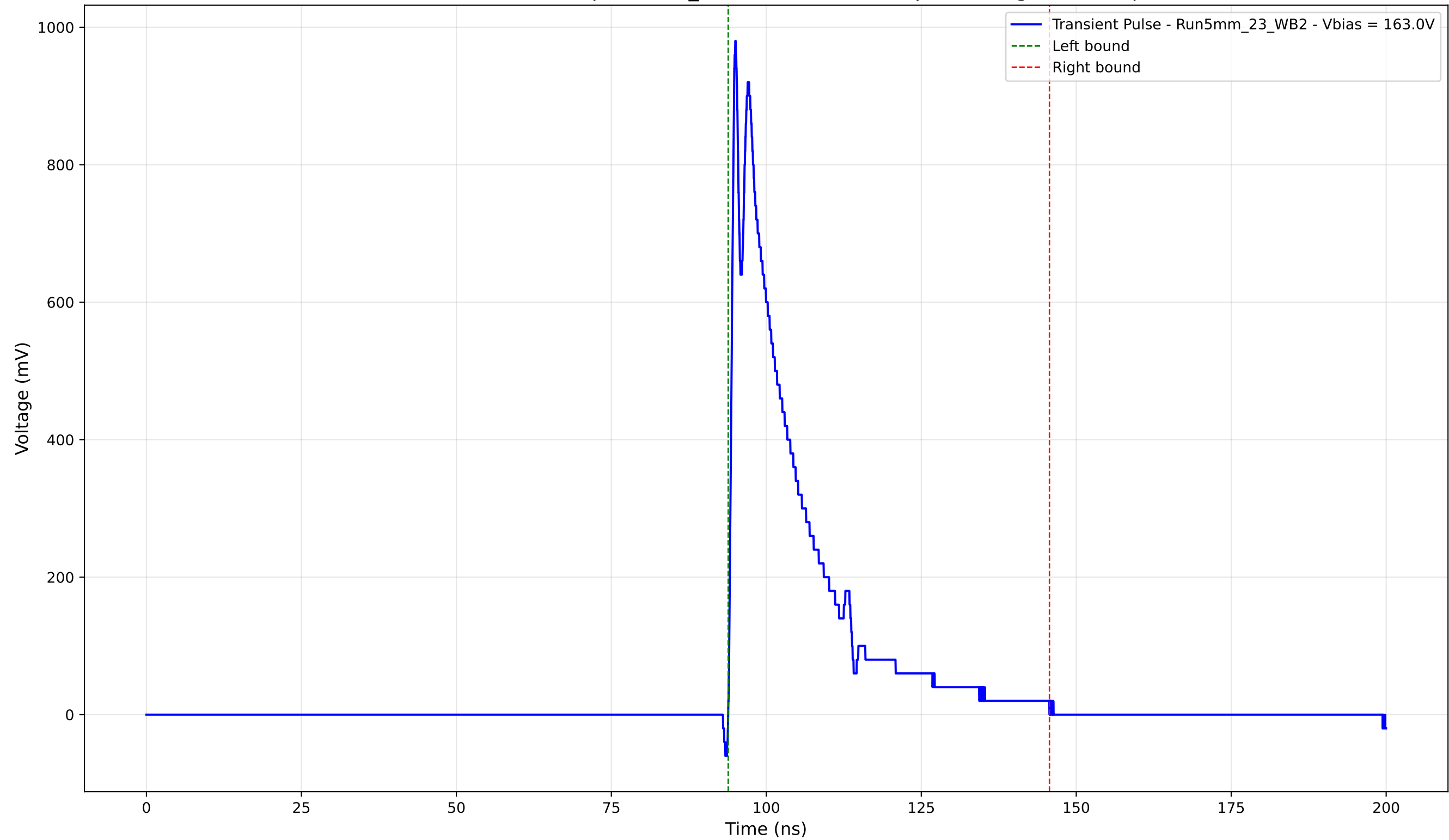
Transient Pulse - Sample: 5mm_23 - Position: 2720.0 \mu\text{m} - Charge: 201.77 pC
