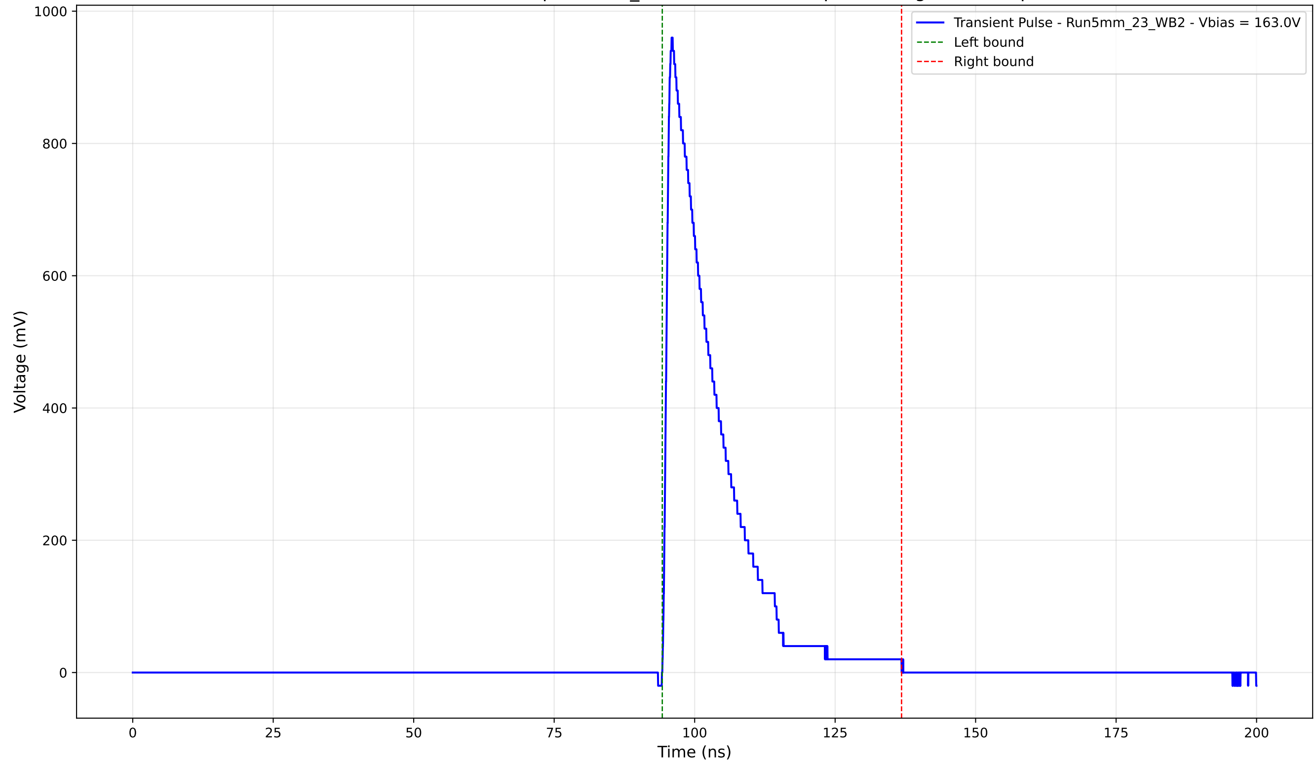
Transient Pulse - Sample: 5mm_23 - Position: 590.0 \mu\text{m} - Charge: 184.36 pC
