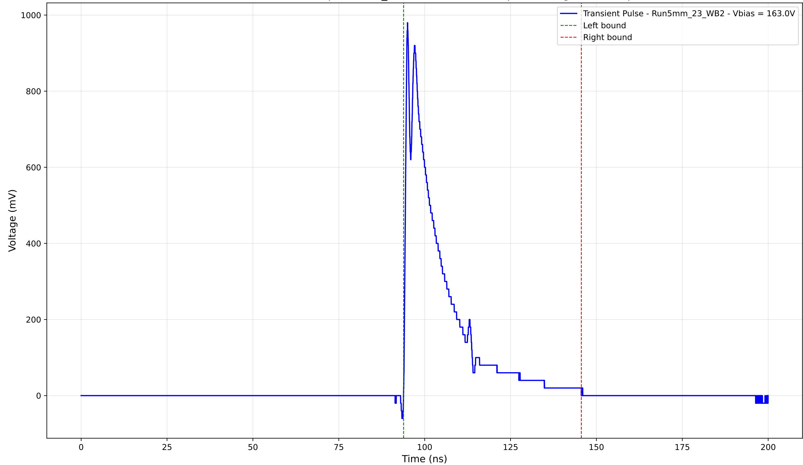
Transient Pulse - Sample: 5mm_23 - Position: 2325.0 \mu\text{m} - Charge: 202.20 pC
