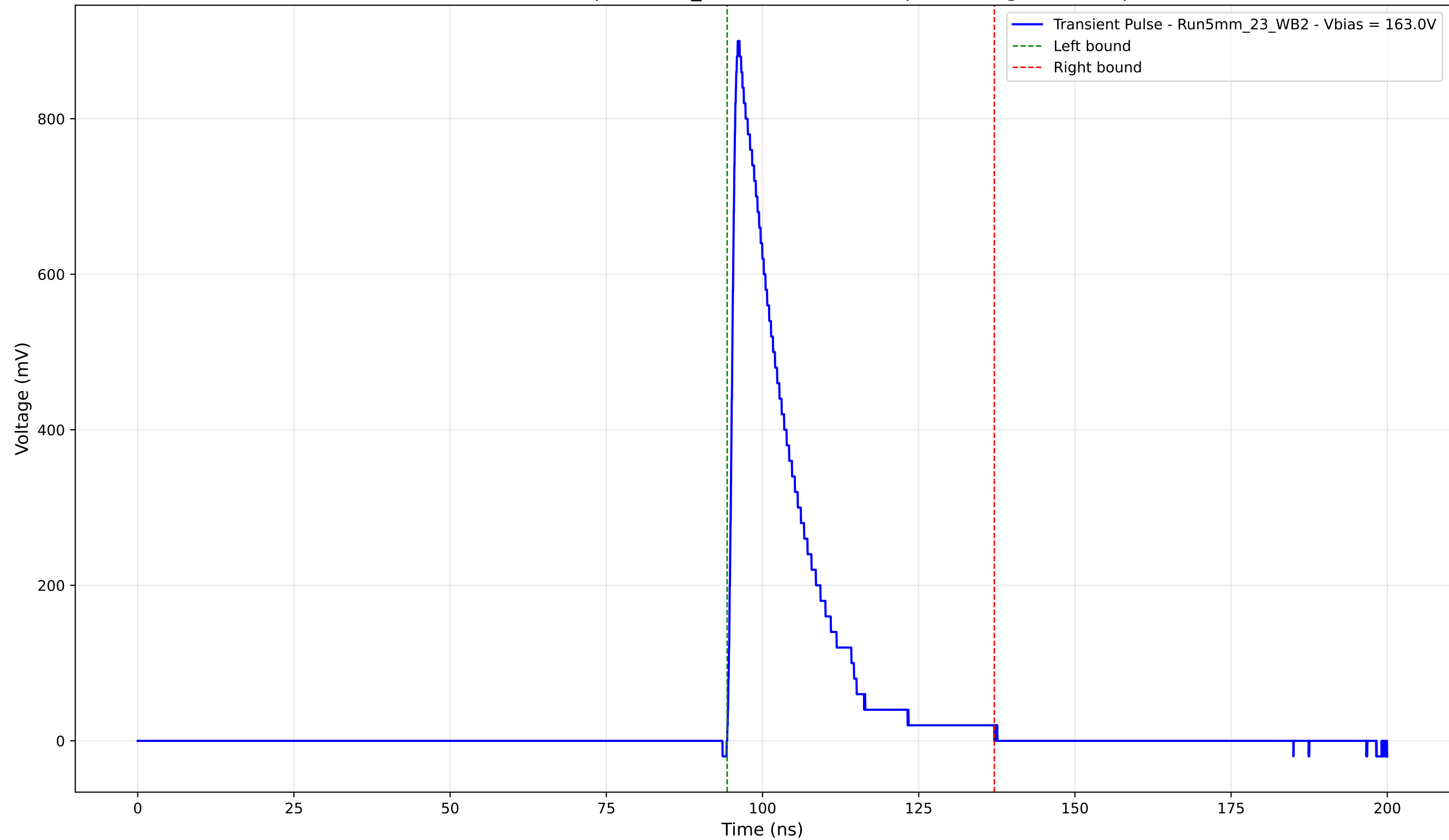
Transient Pulse - Sample: 5mm_23 - Position: 780.0 \mu\text{m} - Charge: 174.10 pC
