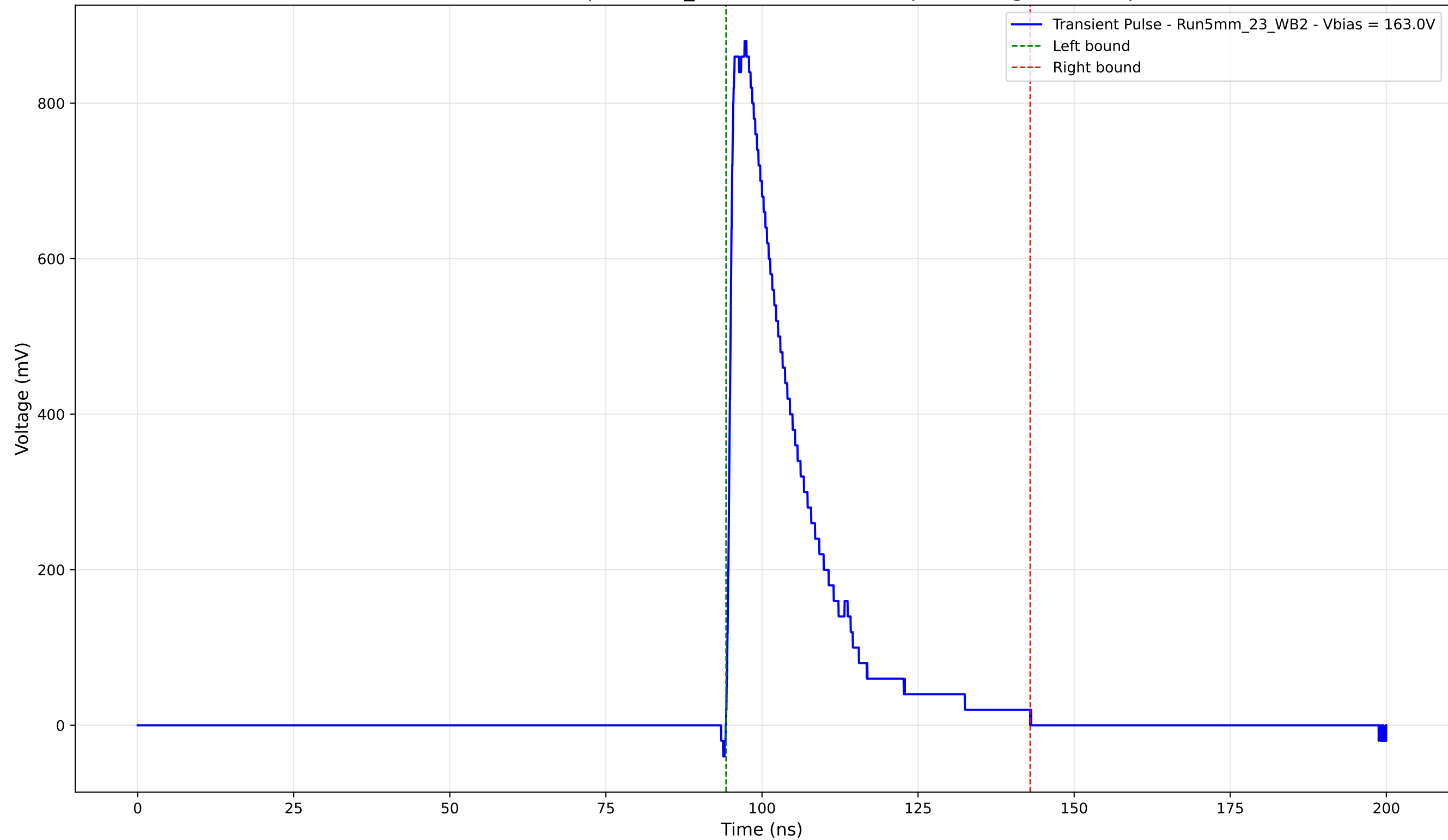
Transient Pulse - Sample: 5mm_23 - Position: 1650.0 \mu\text{m} - Charge: 202.60 pC
