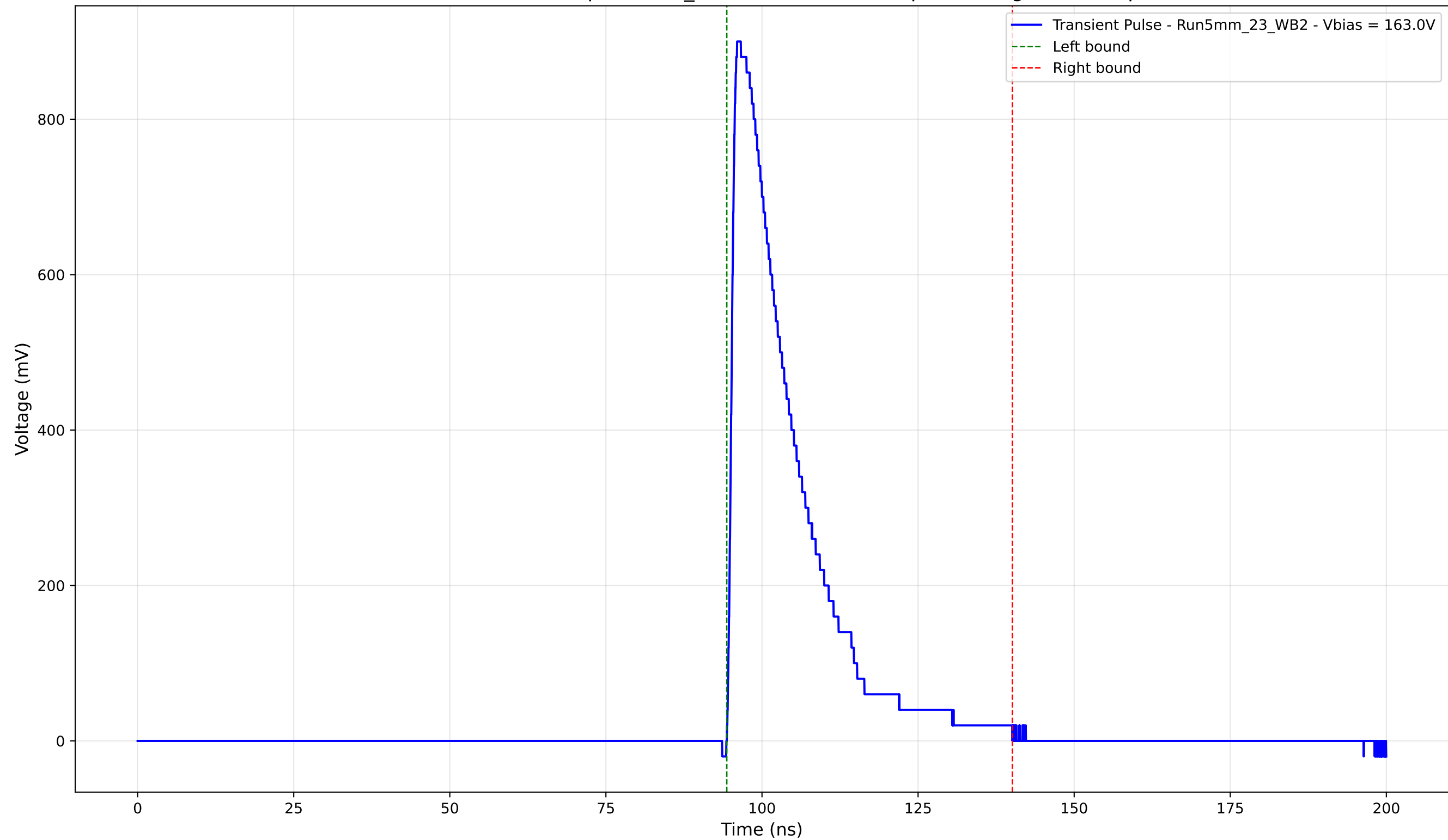
Transient Pulse - Sample: 5mm_23 - Position: 1295.0 \mu\text{m} - Charge: 200.62 pC
