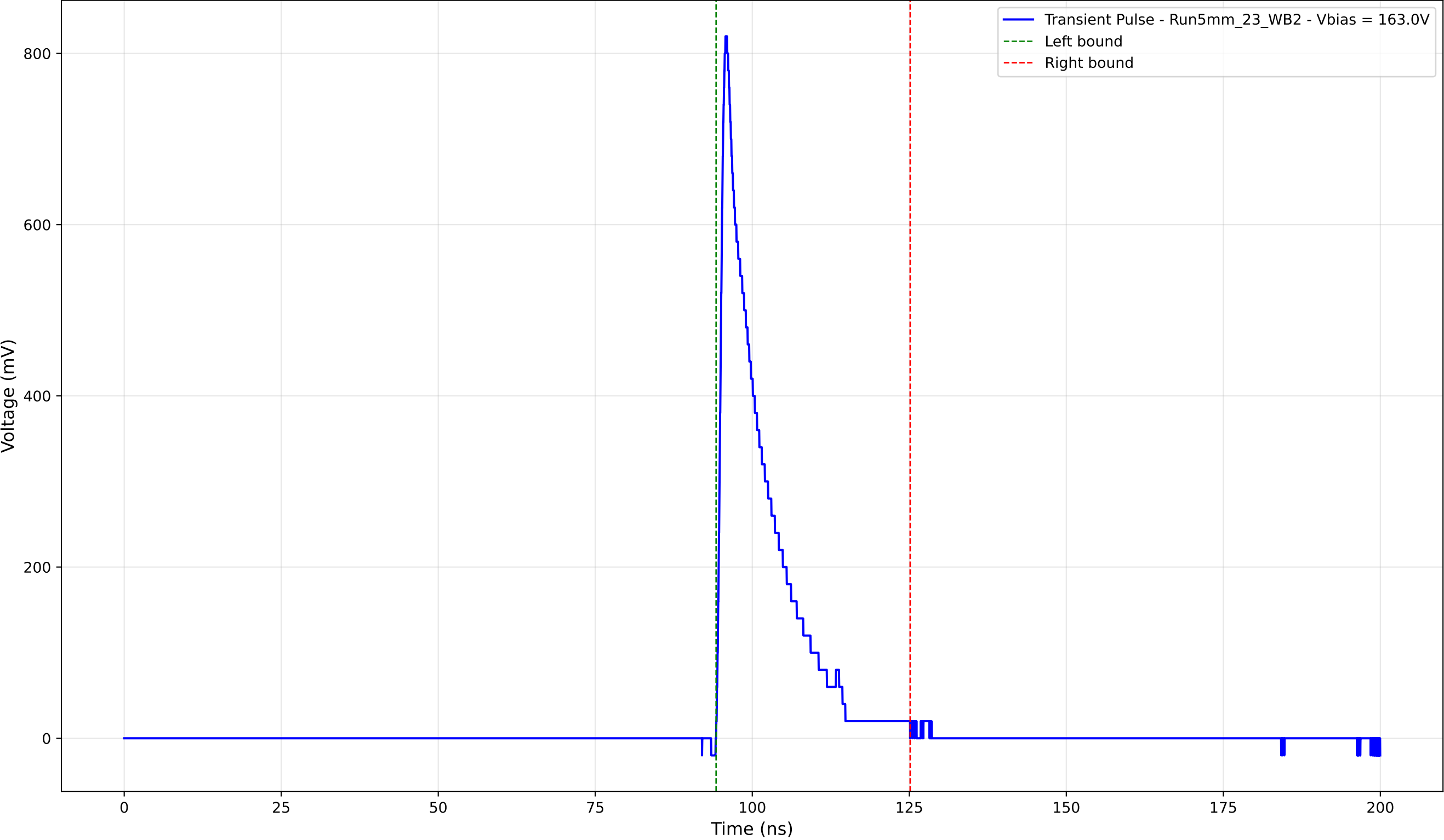
Transient Pulse - Sample: 5mm_23 - Position: 4600.0 \mu\text{m} - Charge: 118.10 pC
