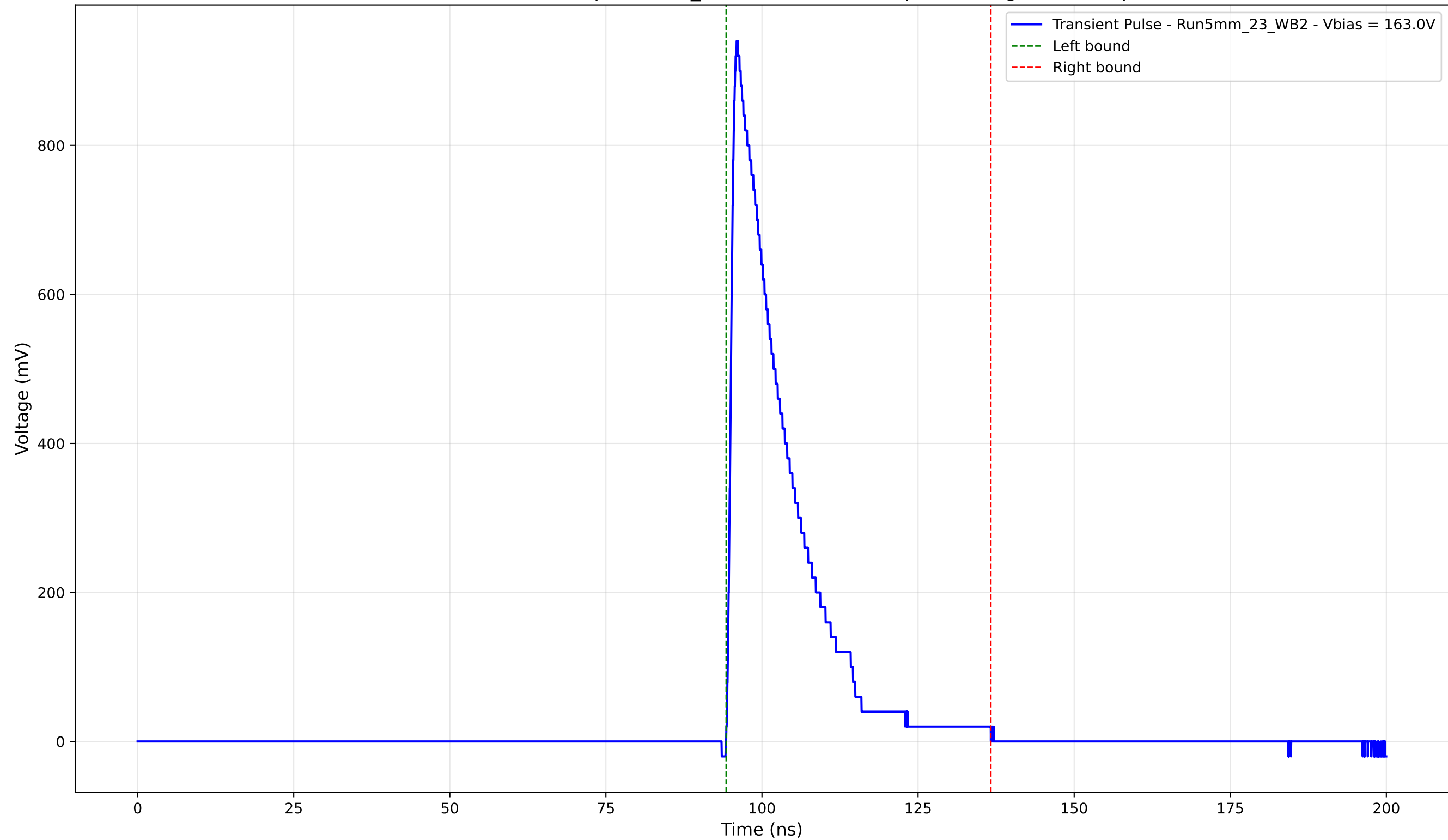
Transient Pulse - Sample: 5mm_23 - Position: 635.0 \mu\text{m} - Charge: 179.36 pC
