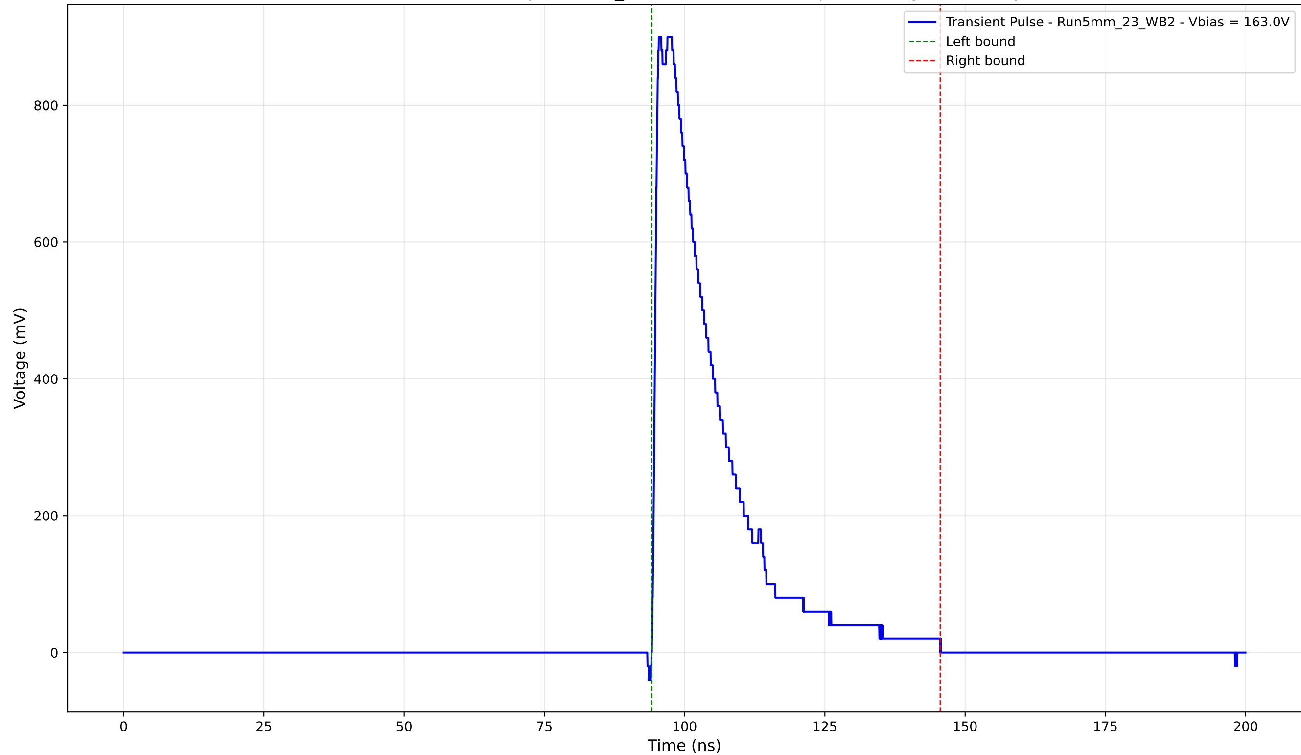
Transient Pulse - Sample: 5mm_23 - Position: 1820.0 \mu\text{m} - Charge: 220.29 pC
