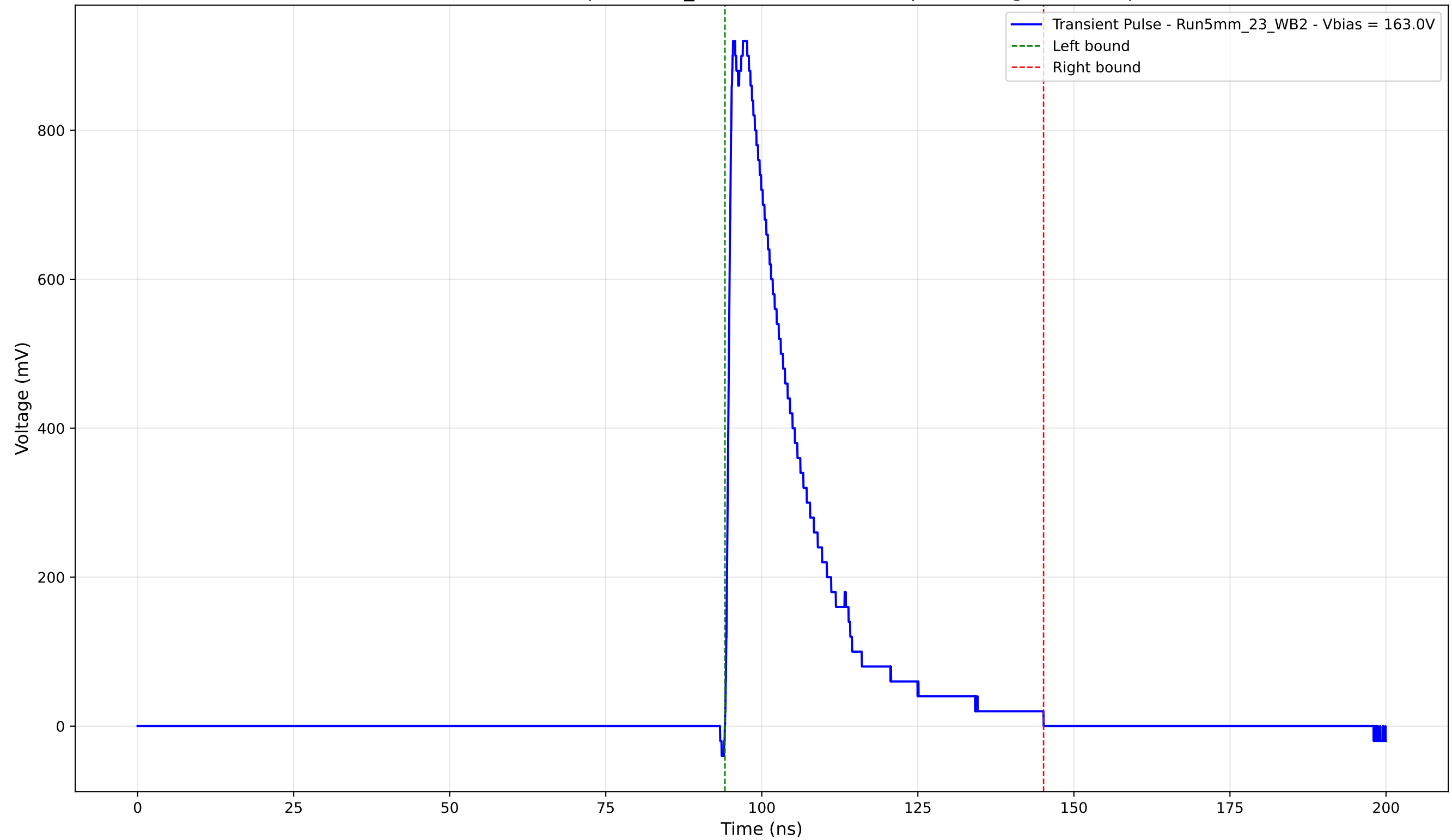
Transient Pulse - Sample: 5mm_23 - Position: 3190.0 \mu\text{m} - Charge: 219.73 pC
