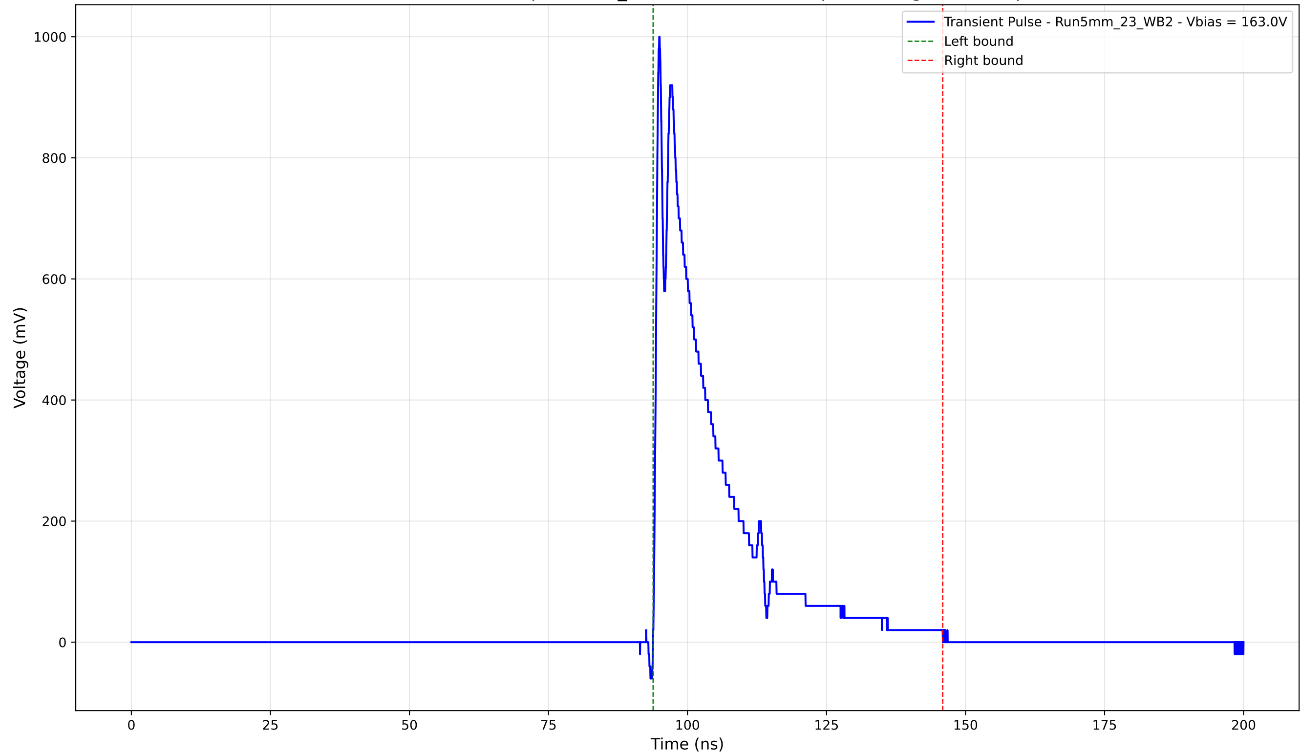
Transient Pulse - Sample: 5mm_23 - Position: 2645.0 \mu\text{m} - Charge: 201.25 pC
