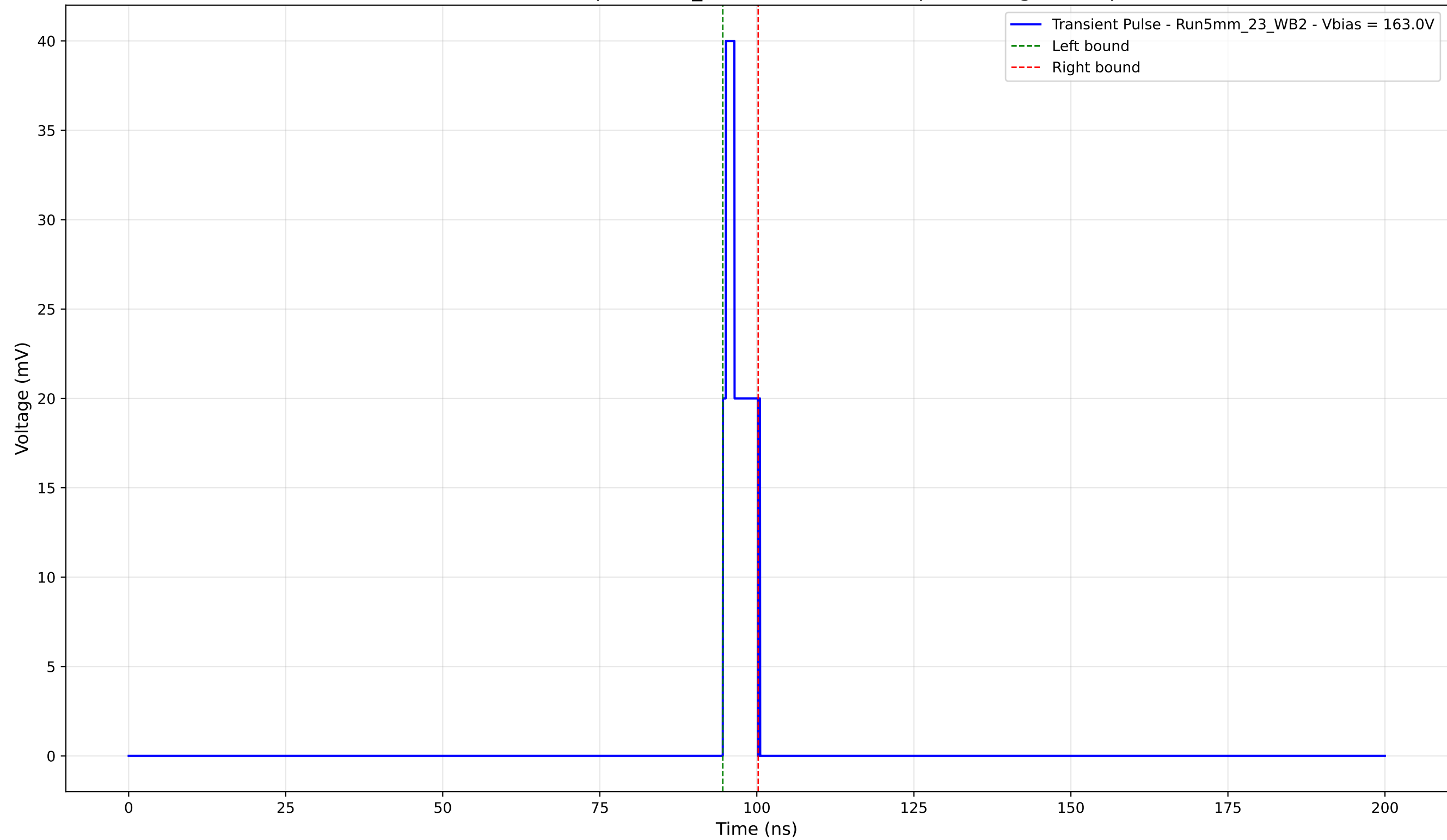
Transient Pulse - Sample: 5mm_23 - Position: 5005.0 \mu\text{m} - Charge: 2.80 pC
