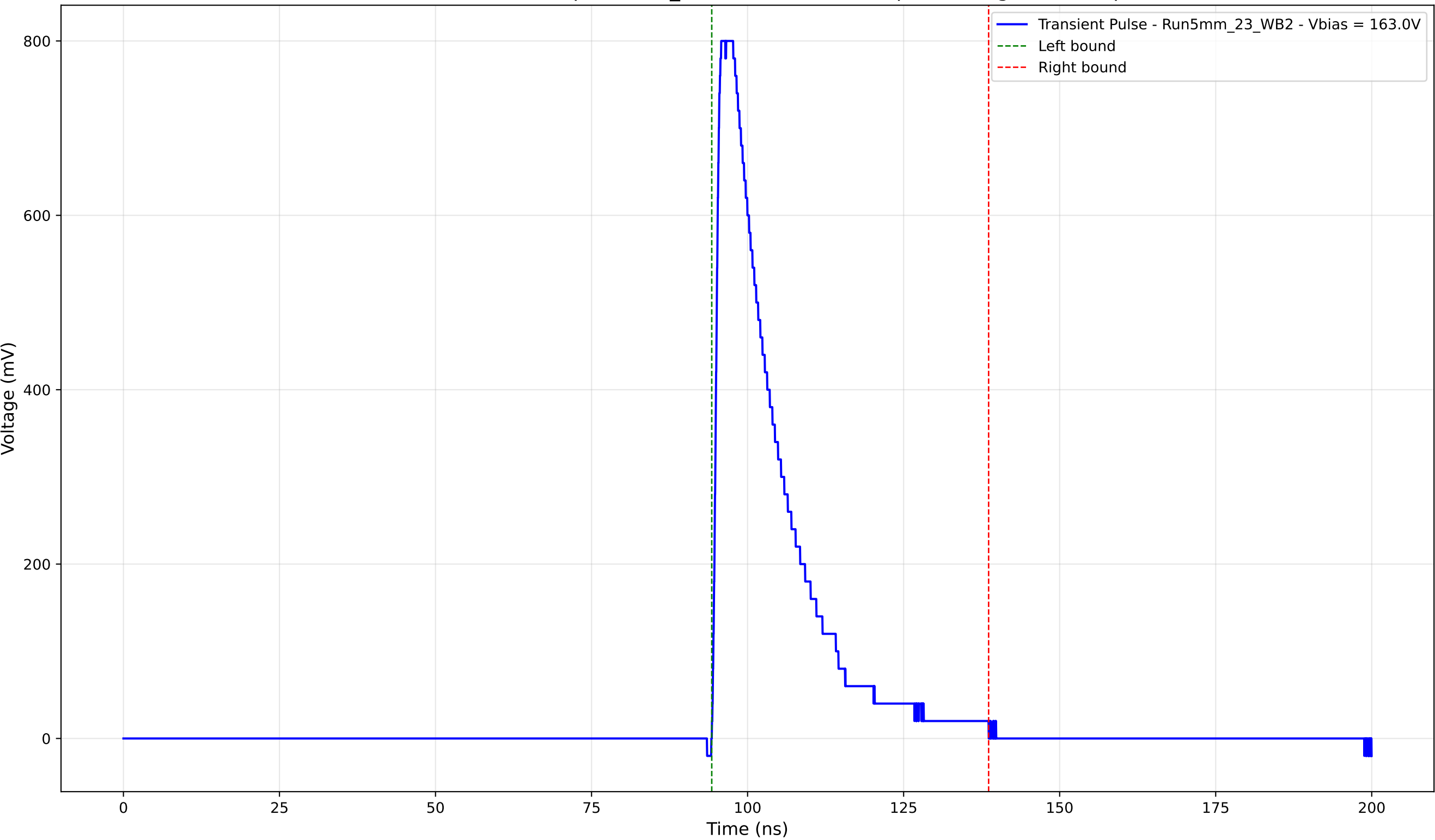
Transient Pulse - Sample: 5mm_23 - Position: 3430.0 \mu\text{m} - Charge: 174.70 pC
