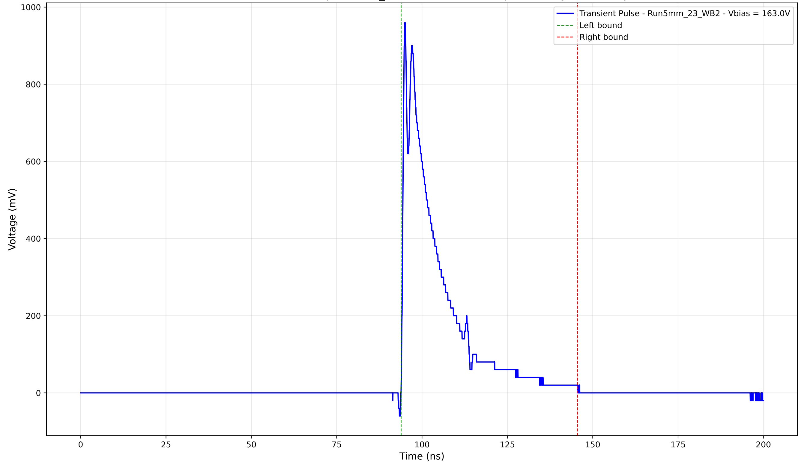
Transient Pulse - Sample: 5mm_23 - Position: 2335.0 \mu\text{m} - Charge: 199.70 pC
