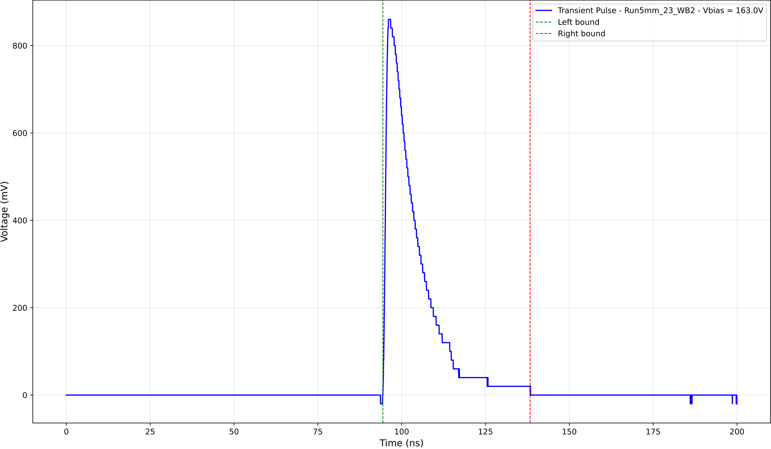
Transient Pulse - Sample: 5mm_23 - Position: 3785.0 \mu\text{m} - Charge: 177.13 pC
