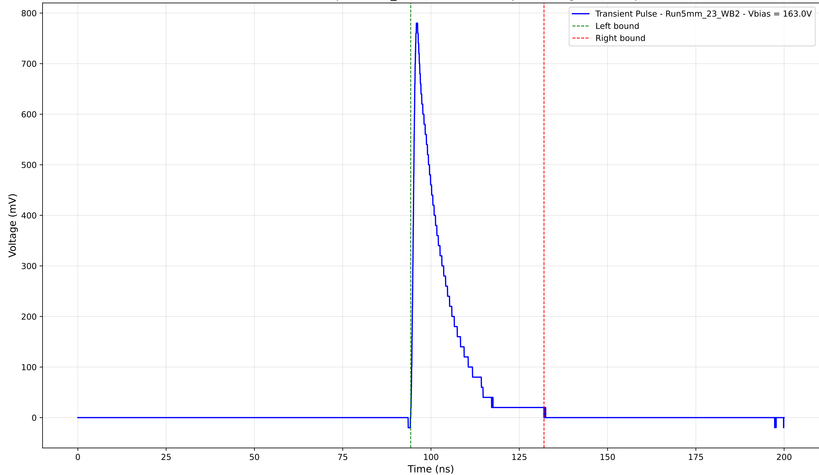
Transient Pulse - Sample: 5mm_23 - Position: 545.0 \mu\text{m} - Charge: 130.86 pC
