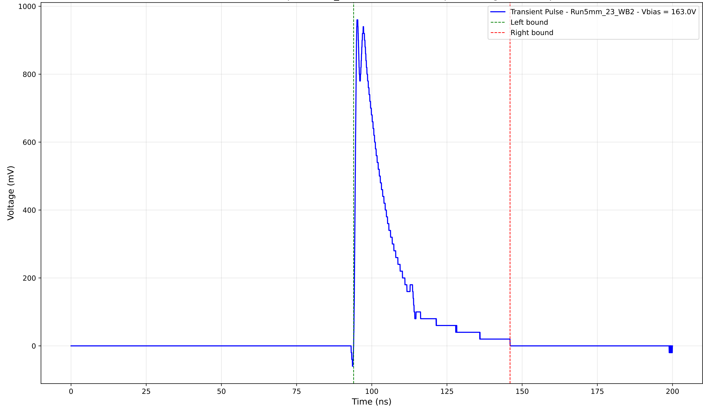
Transient Pulse - Sample: 5mm_23 - Position: 2890.0 \mu\text{m} - Charge: 218.52 pC
