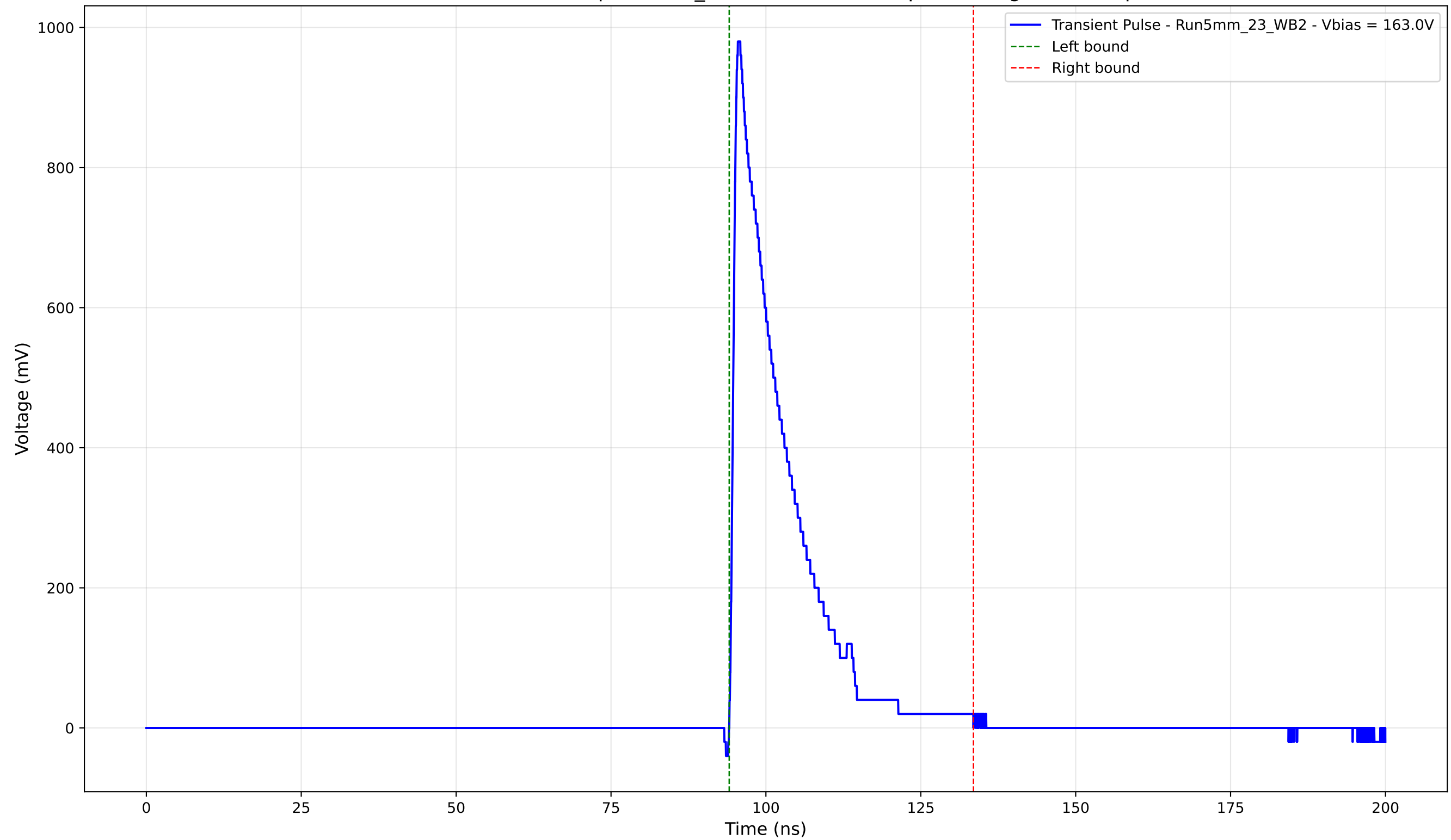
Transient Pulse - Sample: 5mm_23 - Position: 270.0 \mu\text{m} - Charge: 172.55 pC
