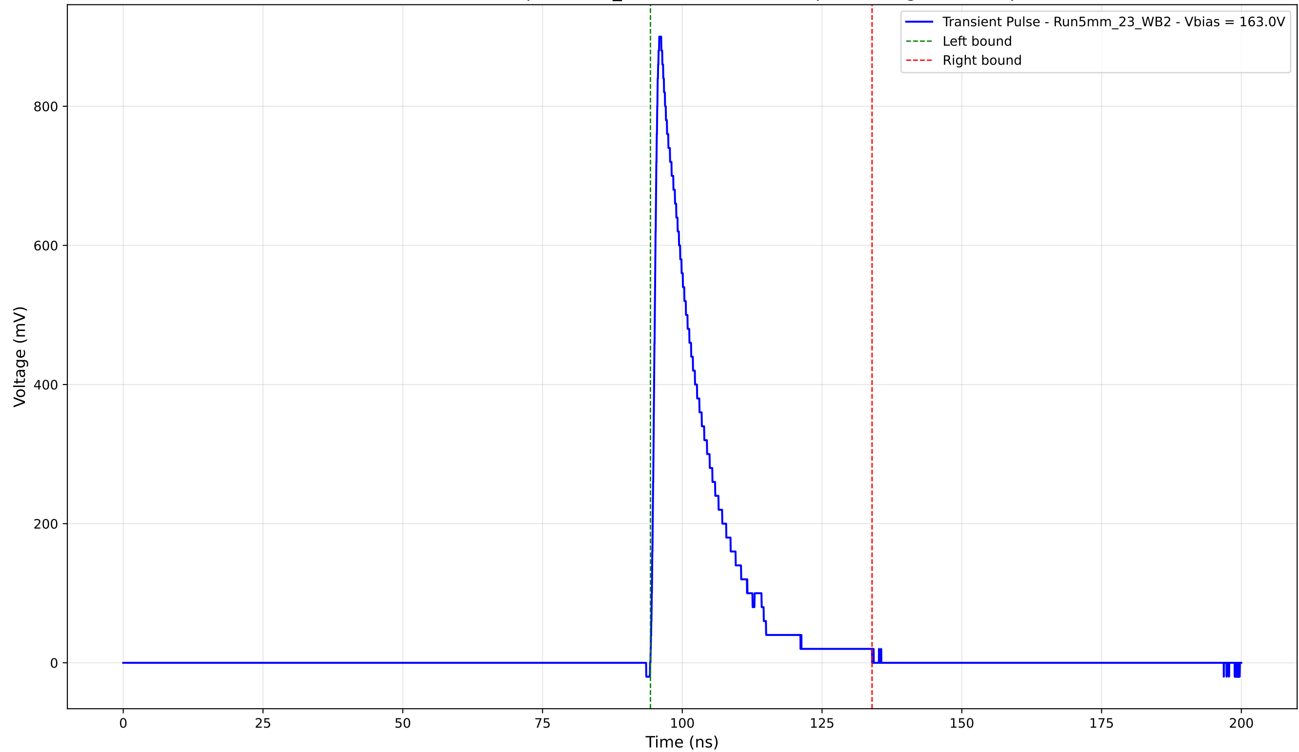
Transient Pulse - Sample: 5mm_23 - Position: 4405.0 \mu\text{m} - Charge: 156.34 pC
