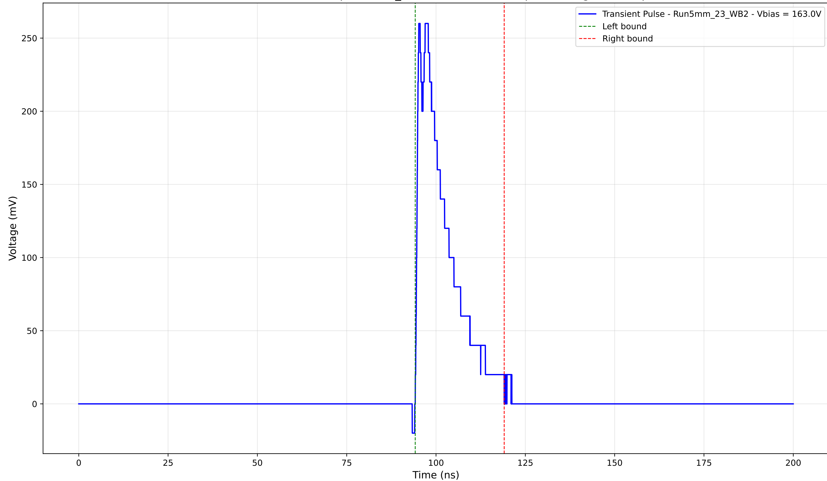
Transient Pulse - Sample: 5mm_23 - Position: 3040.0 \mu\text{m} - Charge: 49.17 pC
