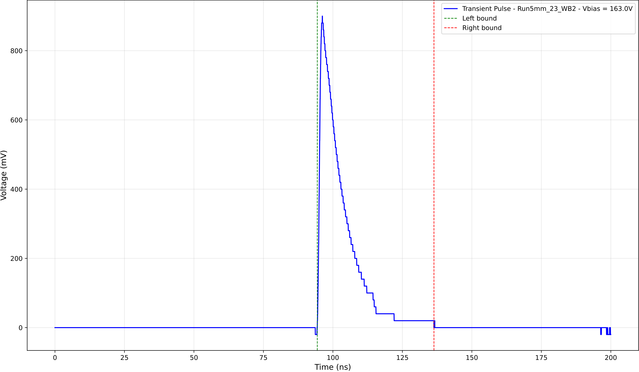
Transient Pulse - Sample: 5mm_23 - Position: 4210.0 \mu\text{m} - Charge: 164.30 pC
