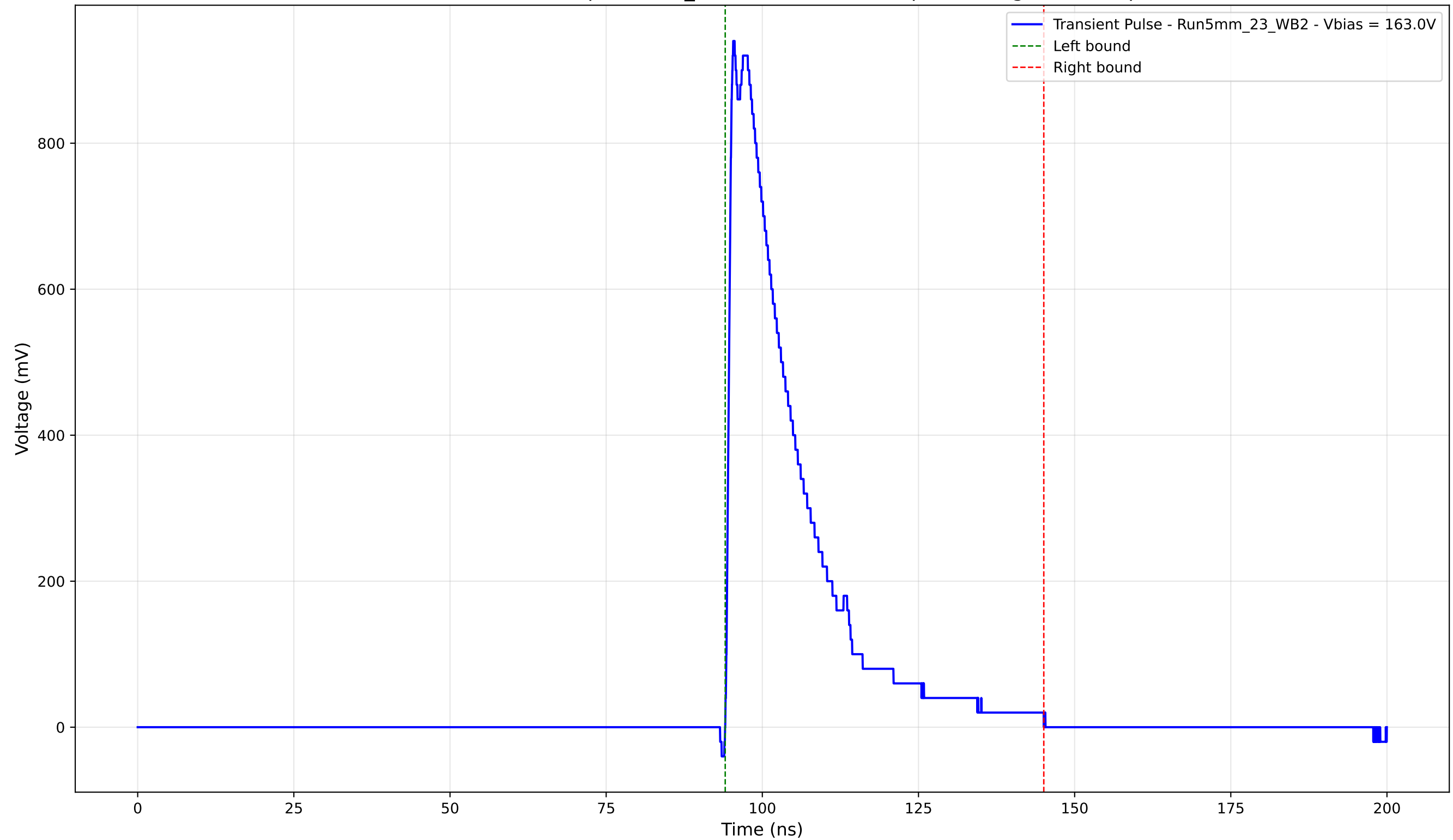
Transient Pulse - Sample: 5mm_23 - Position: 3120.0 \mu\text{m} - Charge: 221.02 pC
