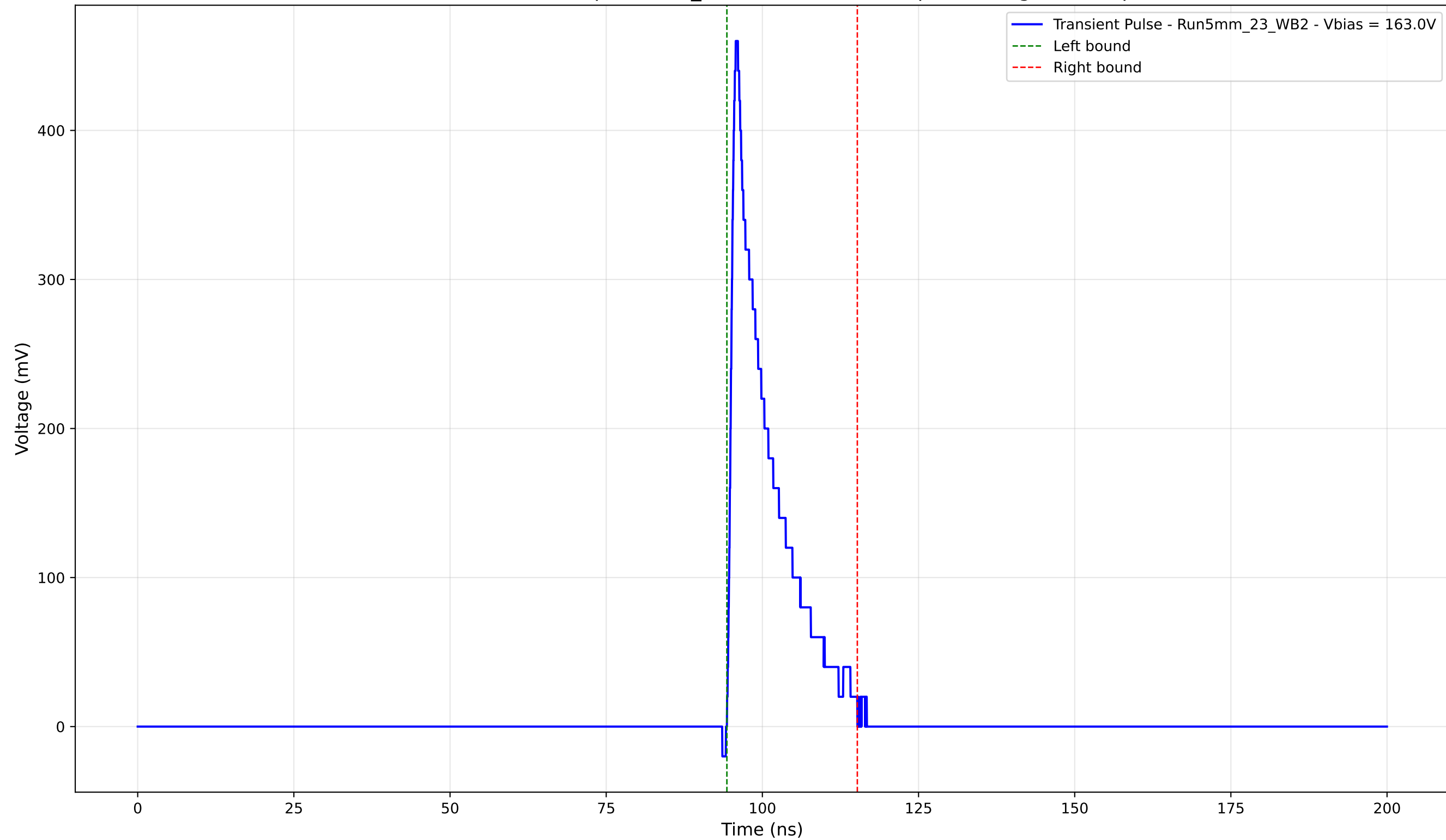
Transient Pulse - Sample: 5mm_23 - Position: 4570.0 \mu\text{m} - Charge: 60.98 pC
