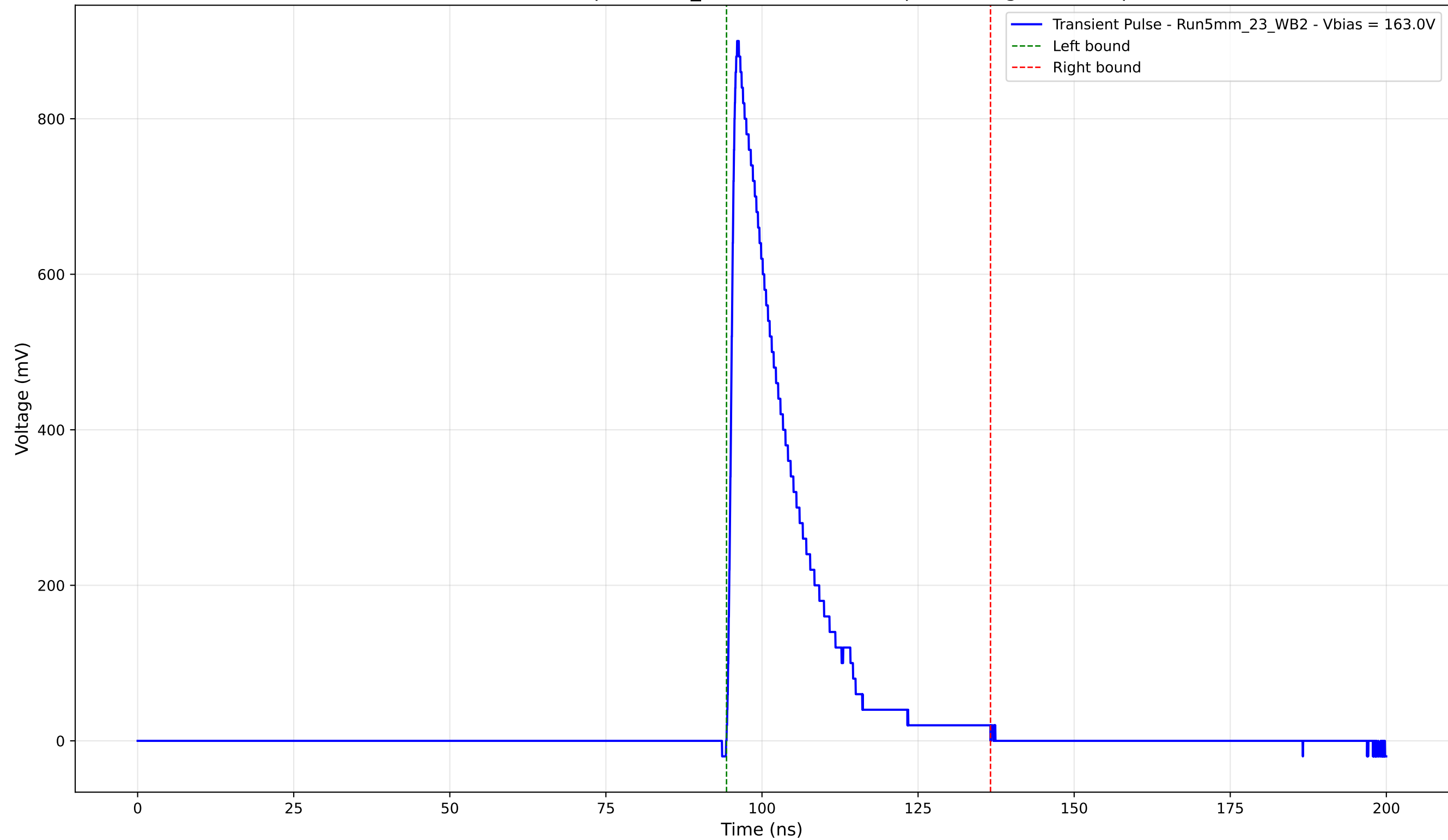
Transient Pulse - Sample: 5mm_23 - Position: 740.0 \mu\text{m} - Charge: 172.38 pC
