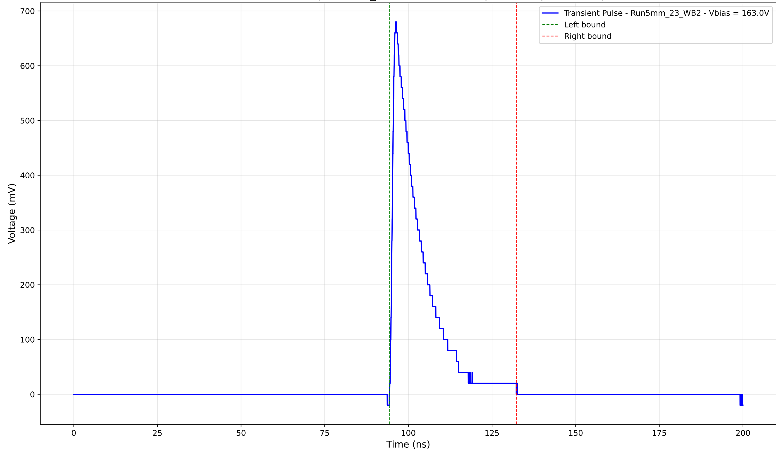
Transient Pulse - Sample: 5mm_23 - Position: 935.0 \mu\text{m} - Charge: 122.27 pC
