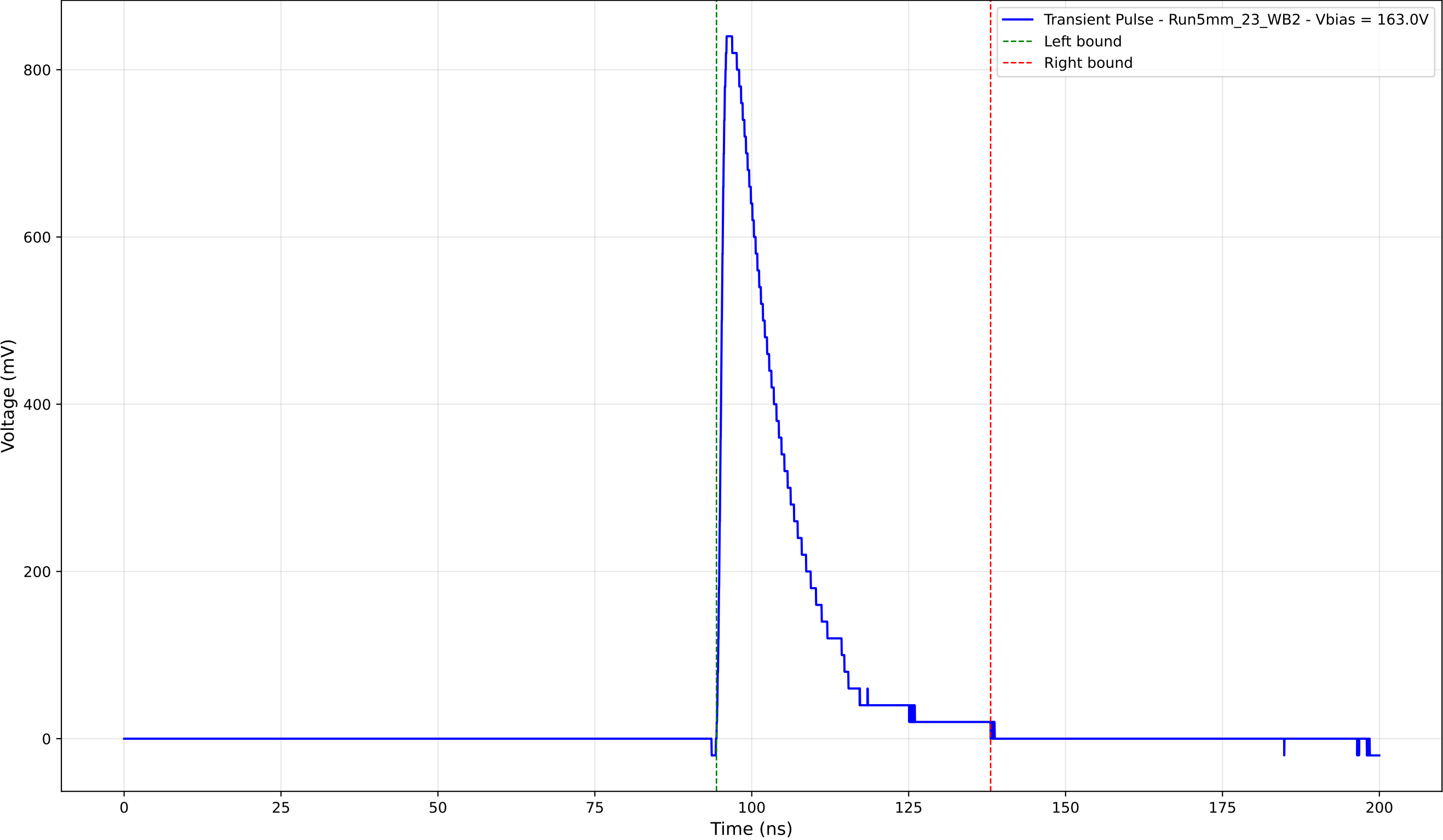
Transient Pulse - Sample: 5mm_23 - Position: 3715.0 \mu\text{m} - Charge: 175.62 pC
