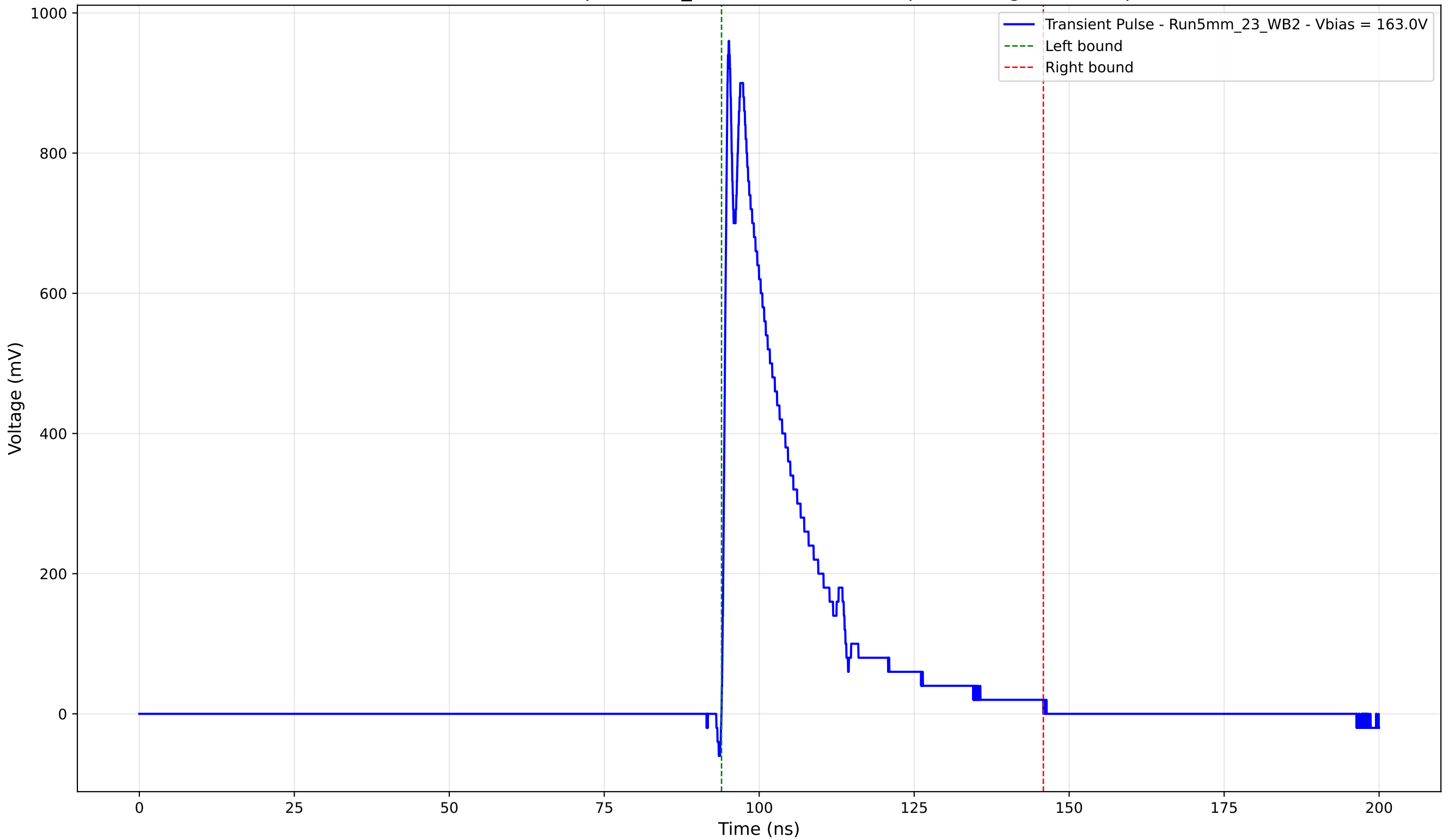
Transient Pulse - Sample: 5mm_23 - Position: 2230.0 \mu\text{m} - Charge: 205.10 pC
