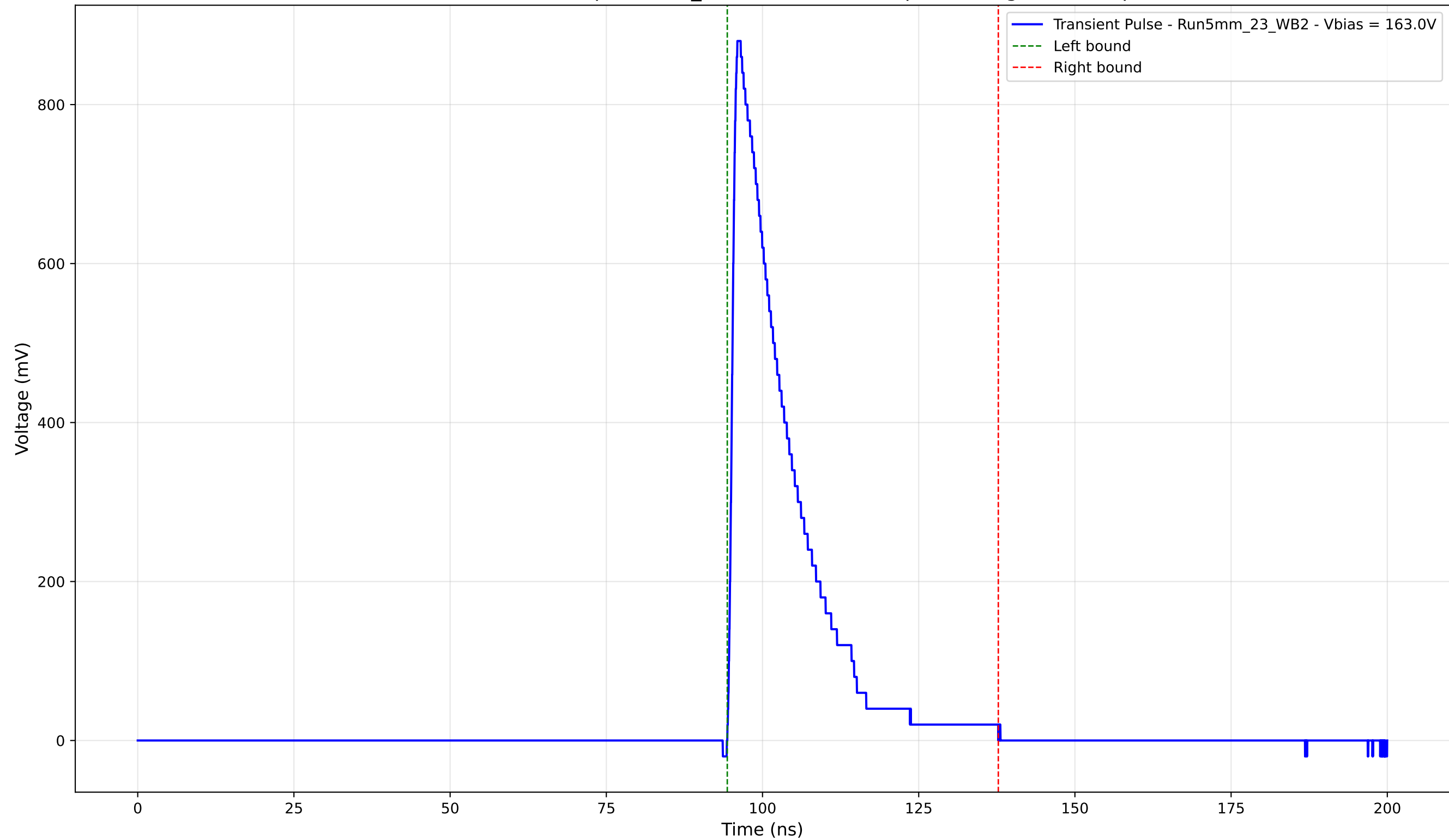
Transient Pulse - Sample: 5mm_23 - Position: 855.0 \mu\text{m} - Charge: 173.86 pC
