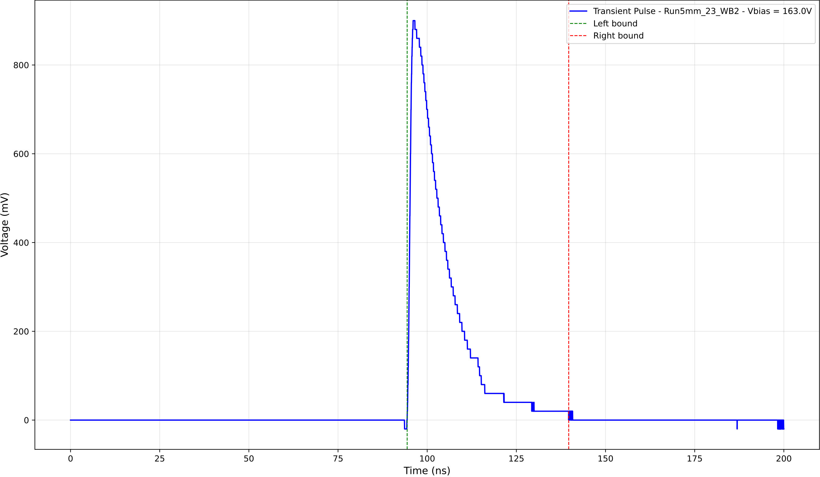
Transient Pulse - Sample: 5mm_23 - Position: 1205.0 \mu\text{m} - Charge: 196.60 pC
