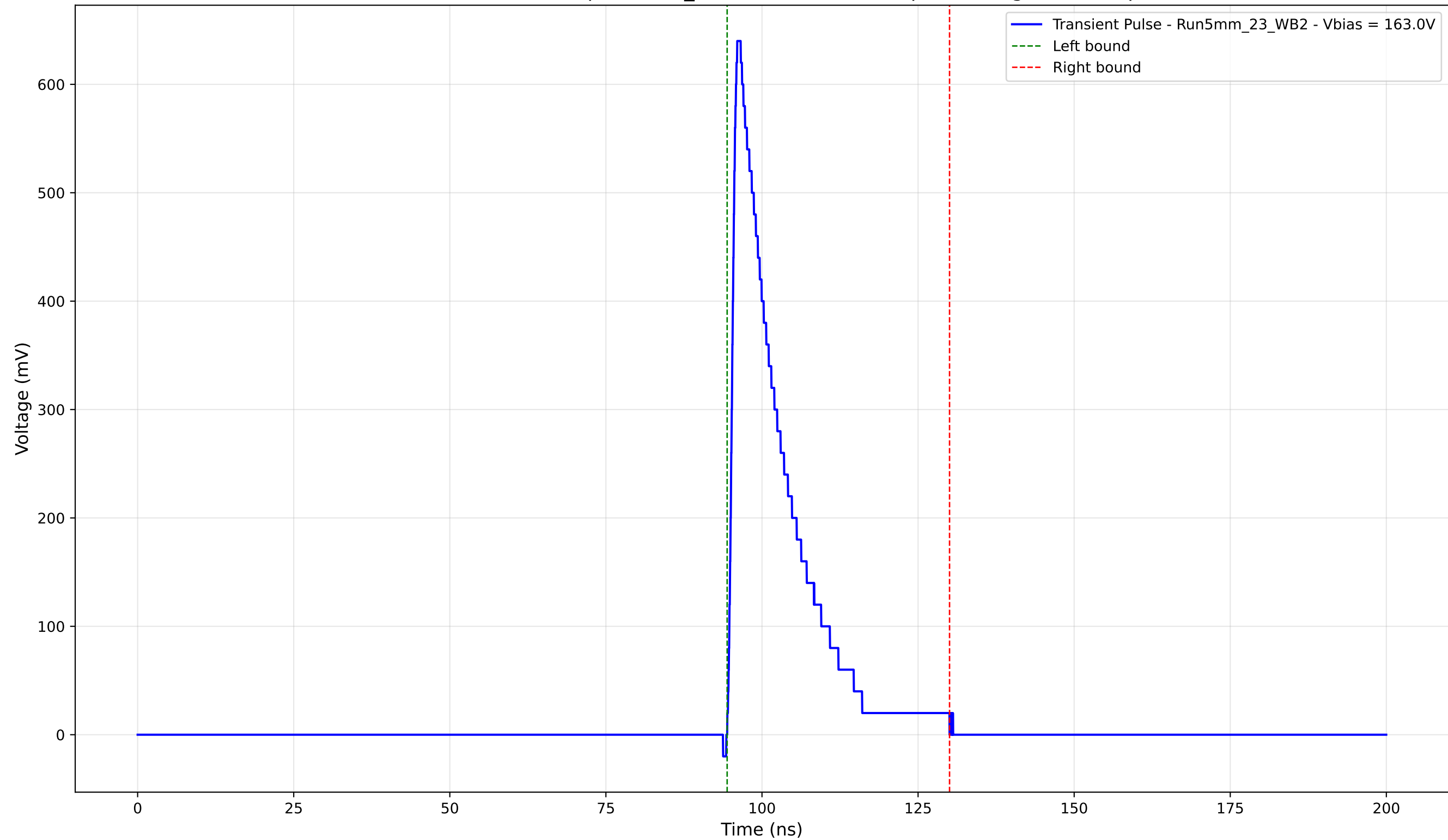
Transient Pulse - Sample: 5mm_23 - Position: 4095.0 \mu\text{m} - Charge: 110.16 pC
