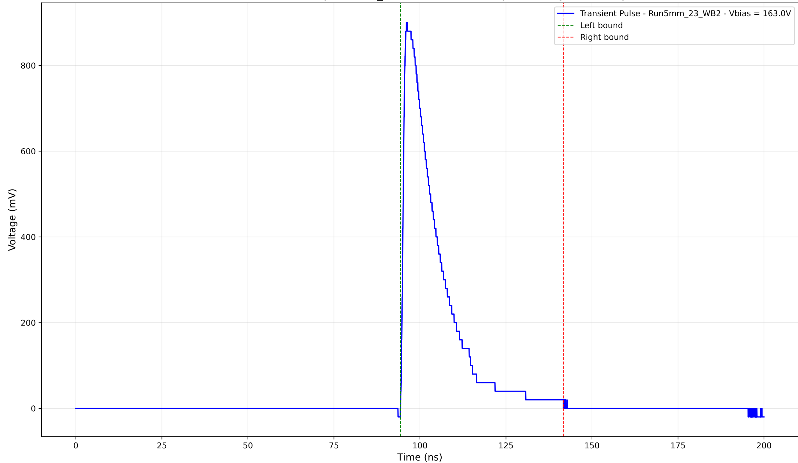
Transient Pulse - Sample: 5mm_23 - Position: 1345.0 \mu\text{m} - Charge: 200.54 pC
