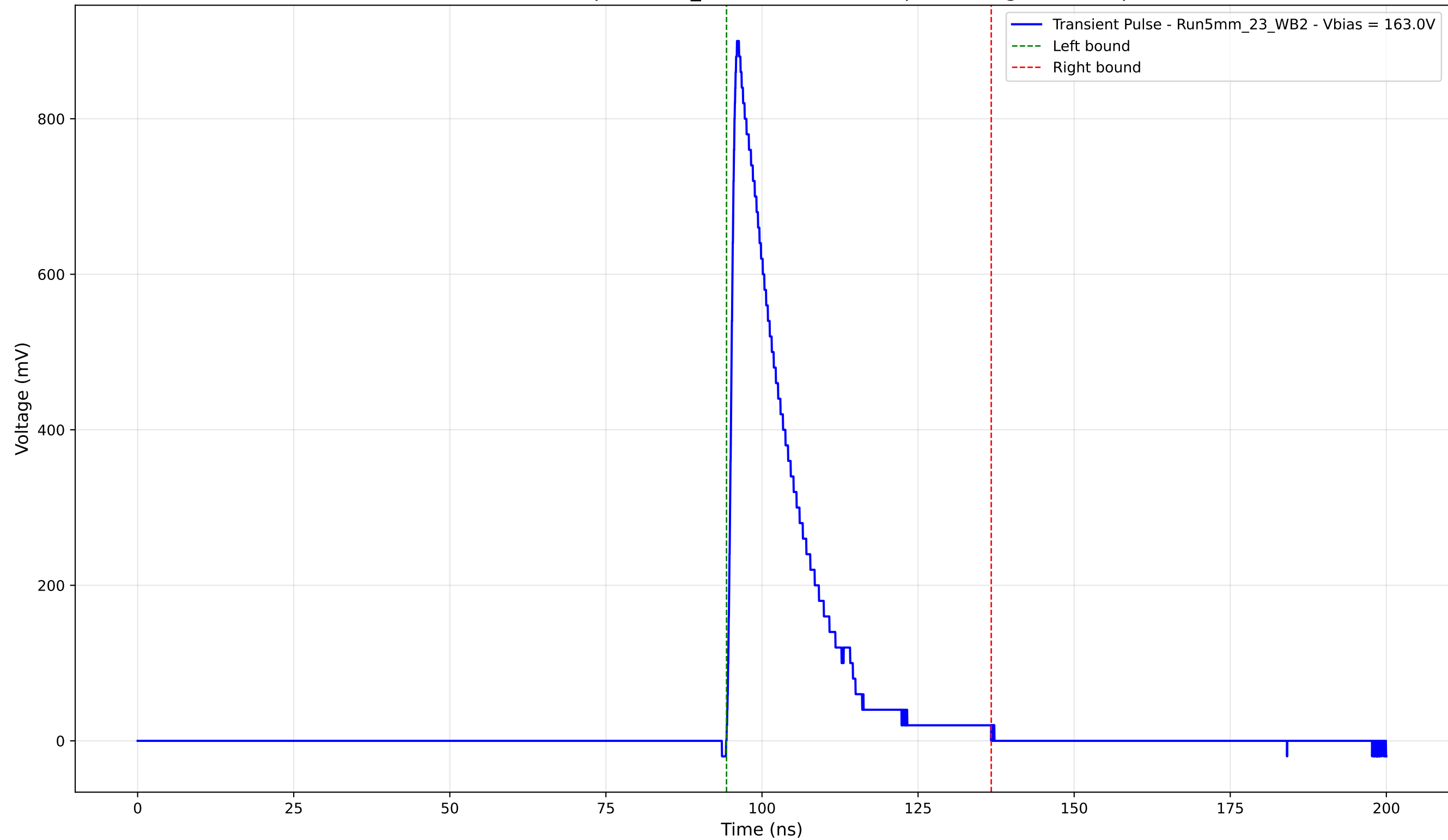
Transient Pulse - Sample: 5mm_23 - Position: 735.0 \mu\text{m} - Charge: 172.22 pC
