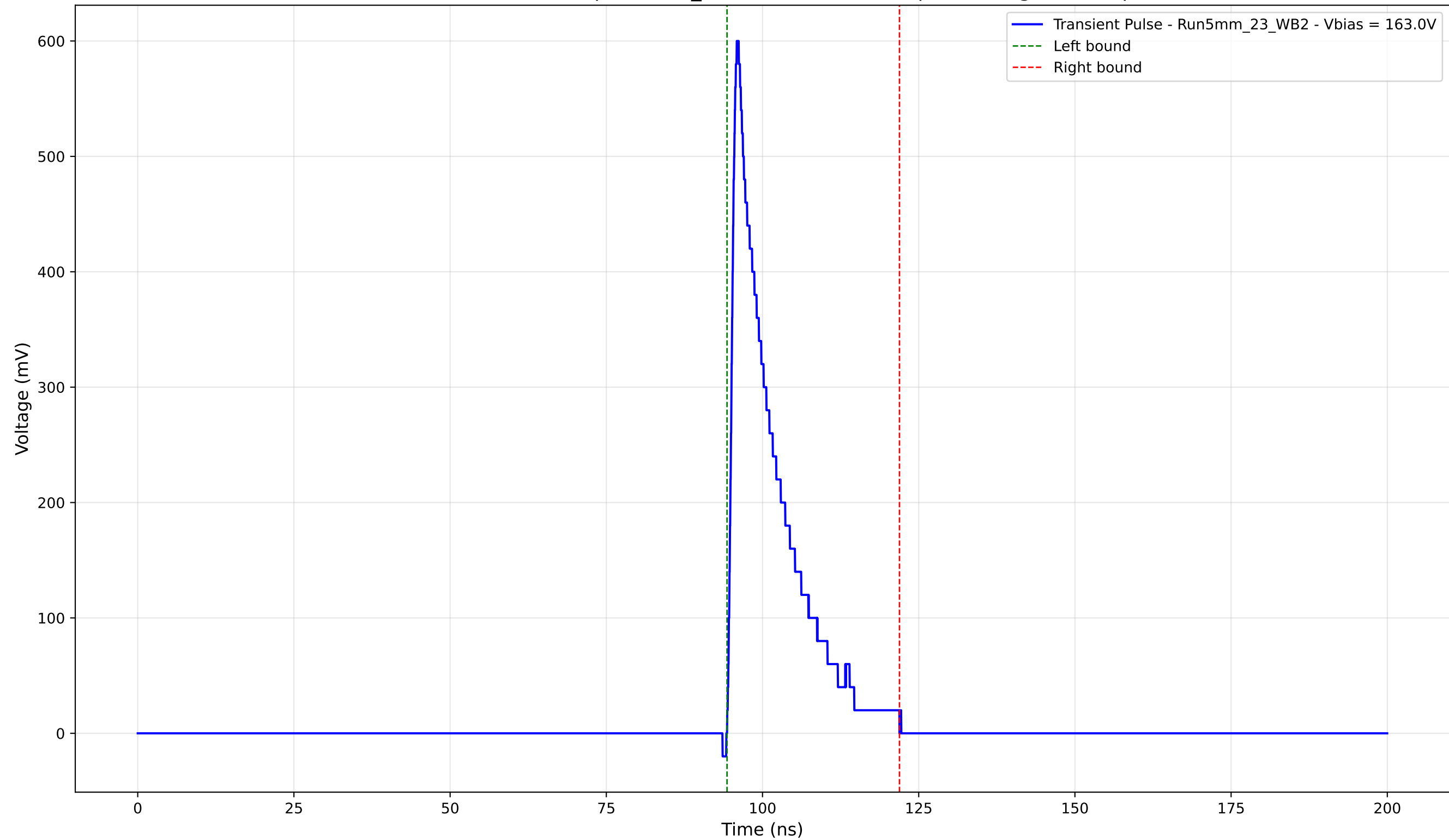
Transient Pulse - Sample: 5mm_23 - Position: 4490.0 \mu\text{m} - Charge: 87.95 pC
