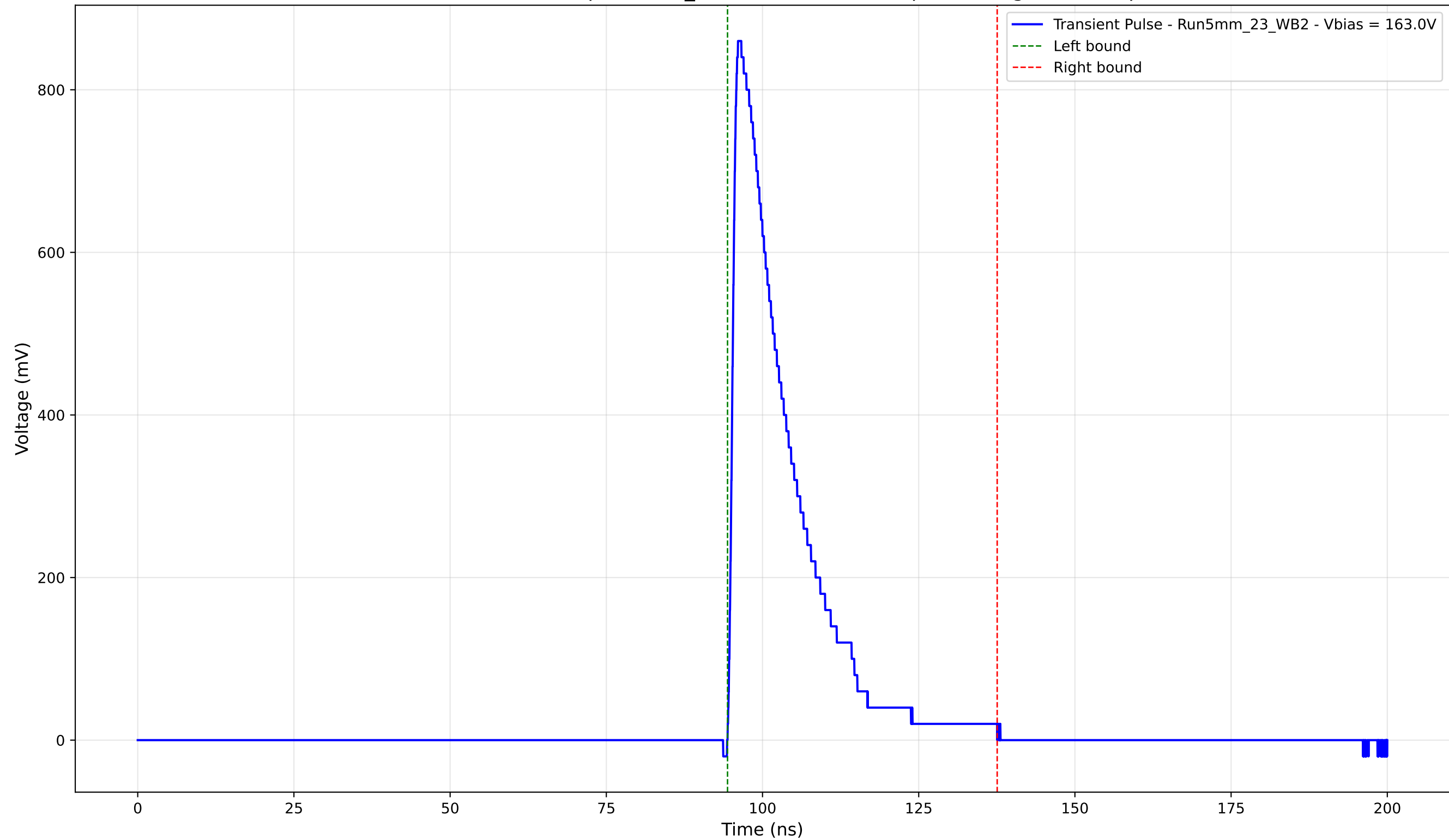
Transient Pulse - Sample: 5mm_23 - Position: 3870.0 \mu\text{m} - Charge: 172.38 pC
