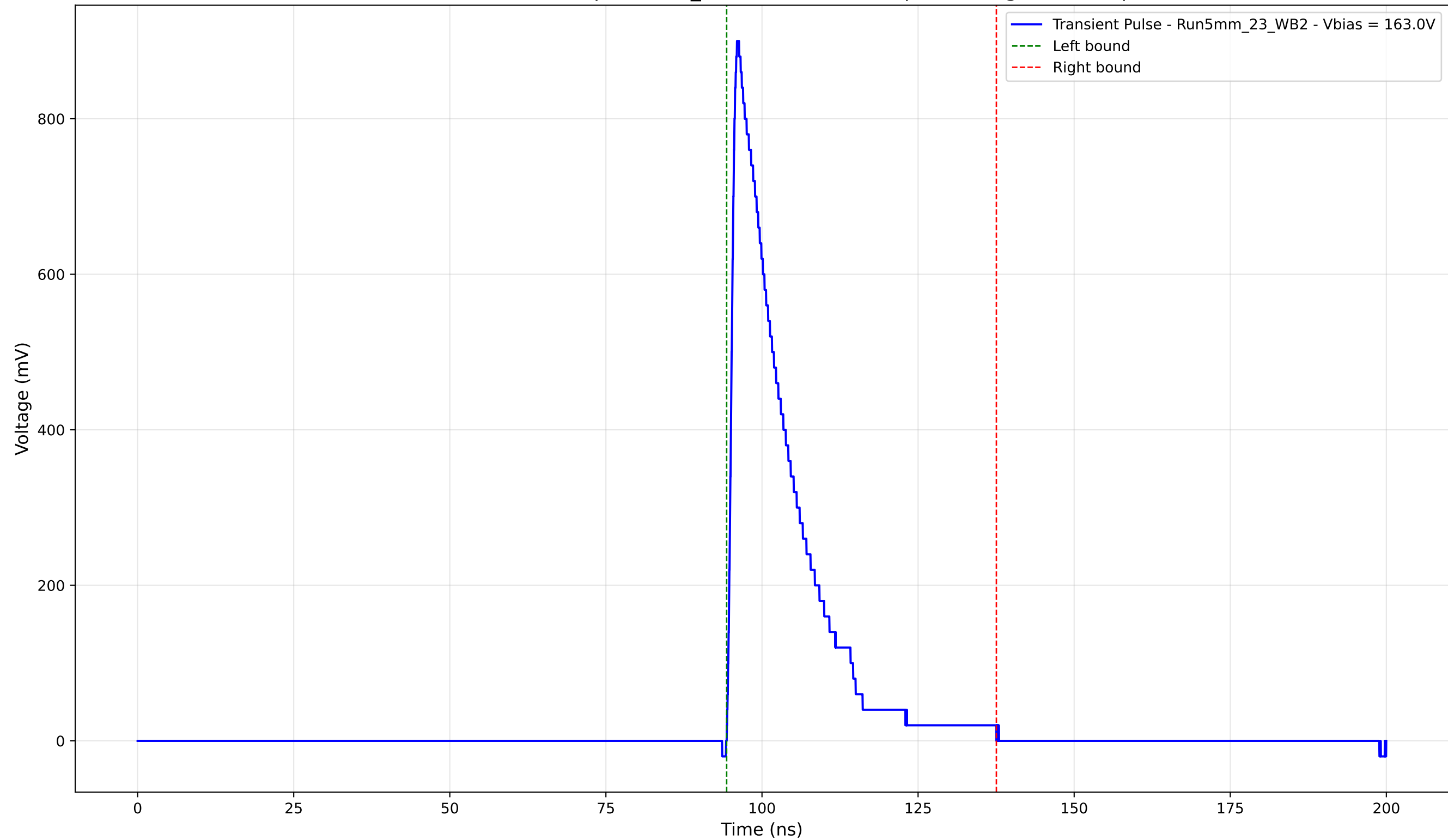
Transient Pulse - Sample: 5mm_23 - Position: 750.0 \mu\text{m} - Charge: 173.22 pC
