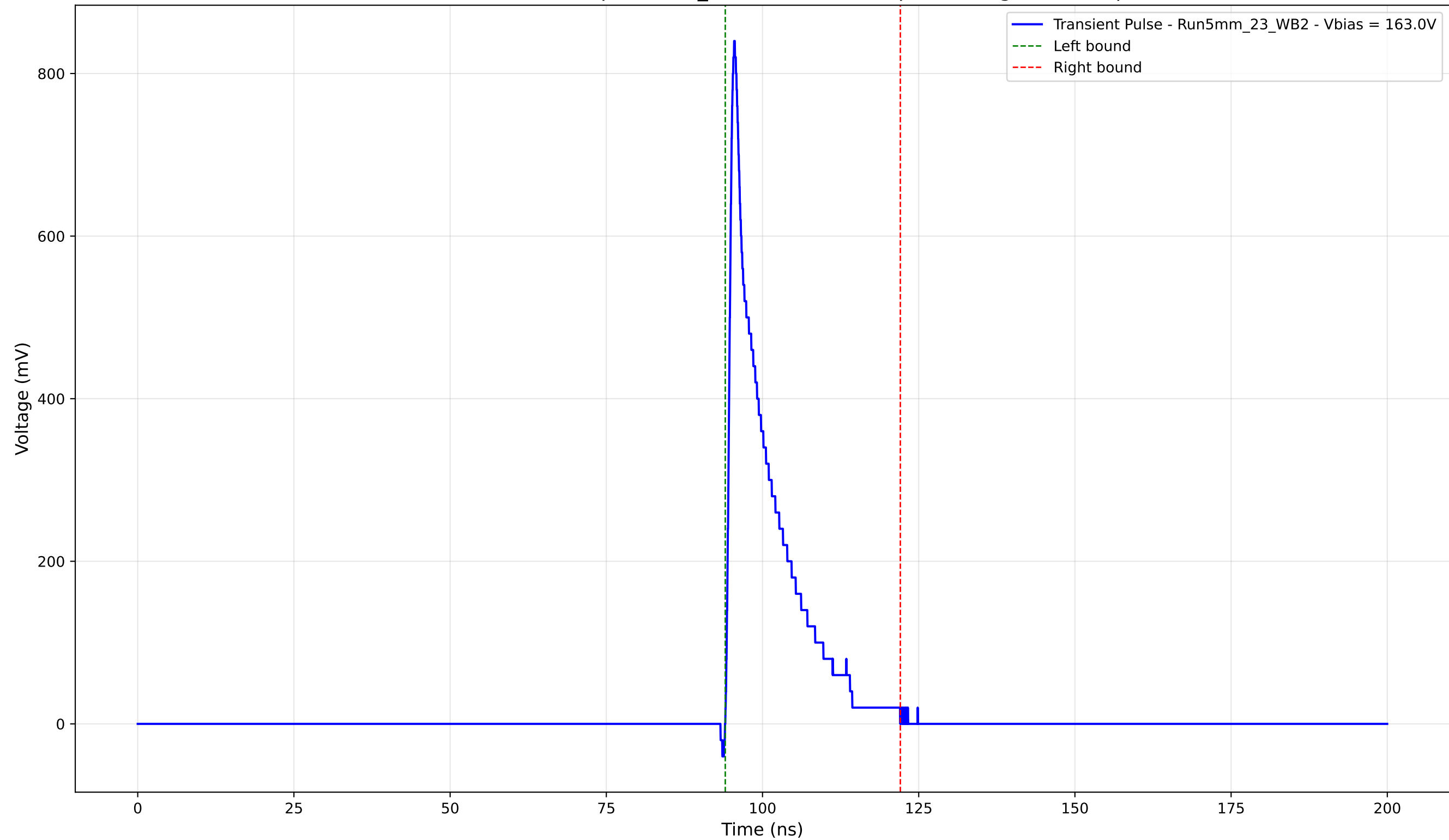
Transient Pulse - Sample: 5mm_23 - Position: 90.0 \mu\text{m} - Charge: 108.28 pC
