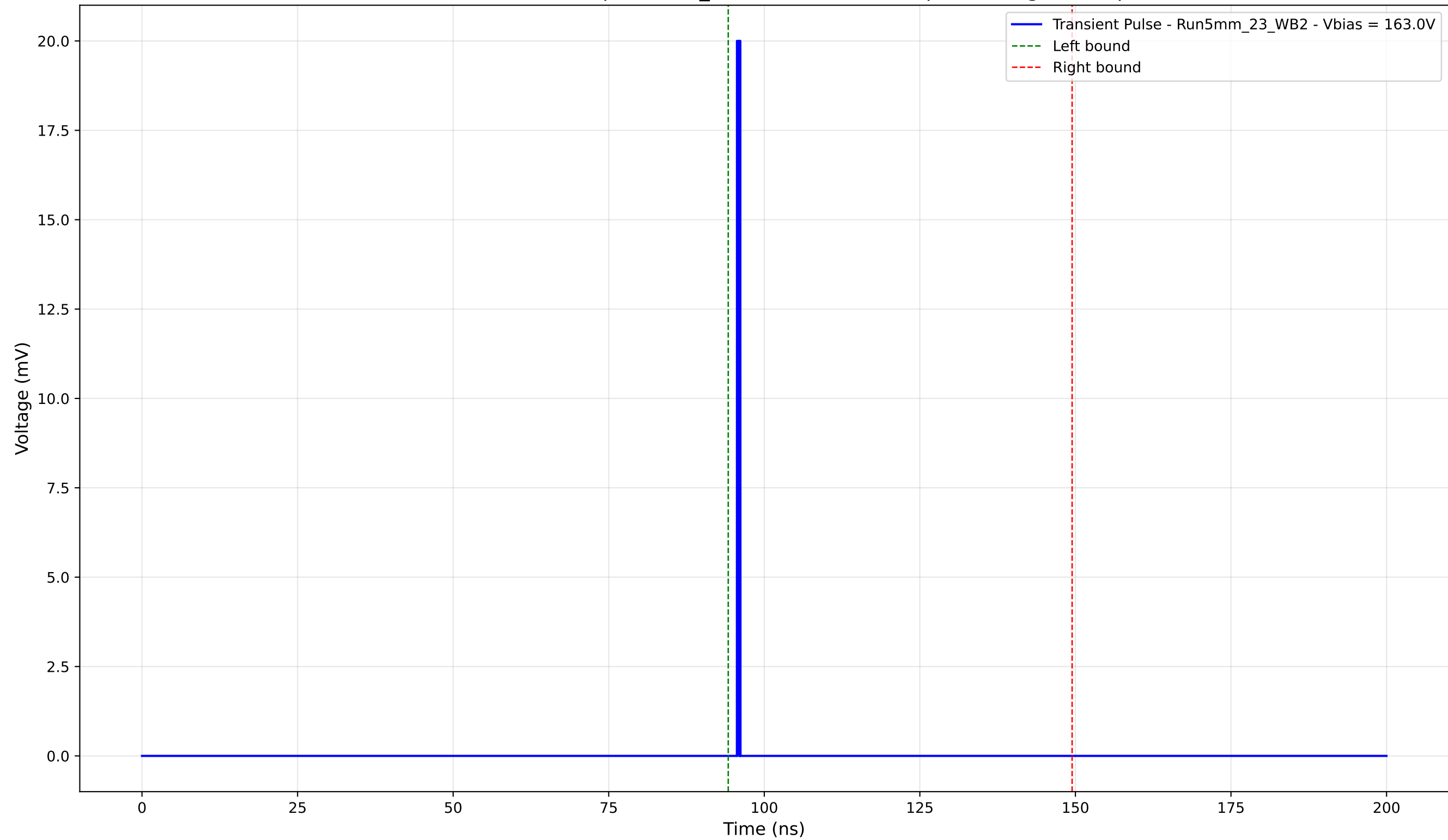
Transient Pulse - Sample: 5mm_23 - Position: 5055.0 \mu\text{m} - Charge: 0.18 pC
