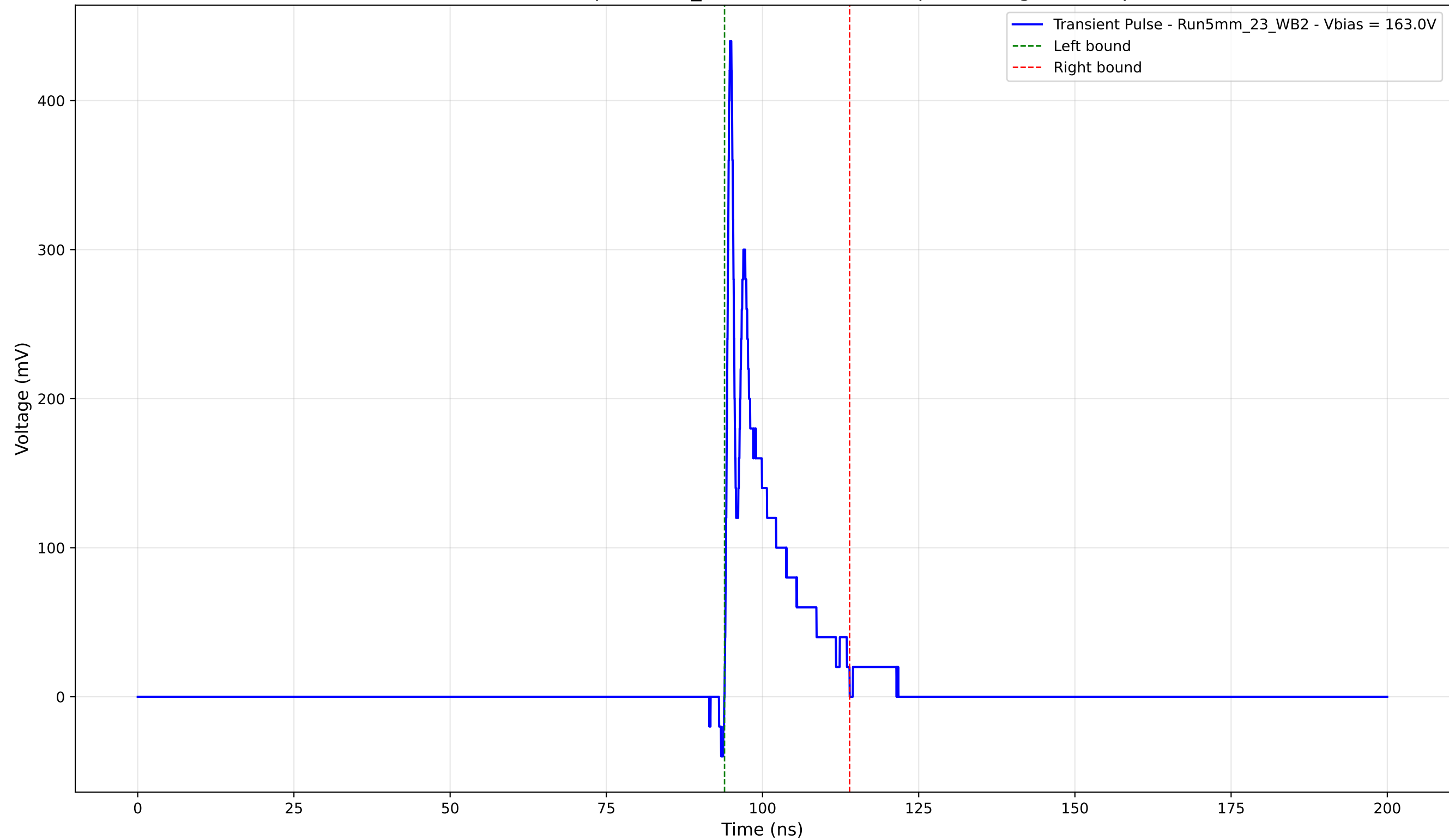
Transient Pulse - Sample: 5mm_23 - Position: 2500.0 \mu\text{m} - Charge: 45.53 pC
