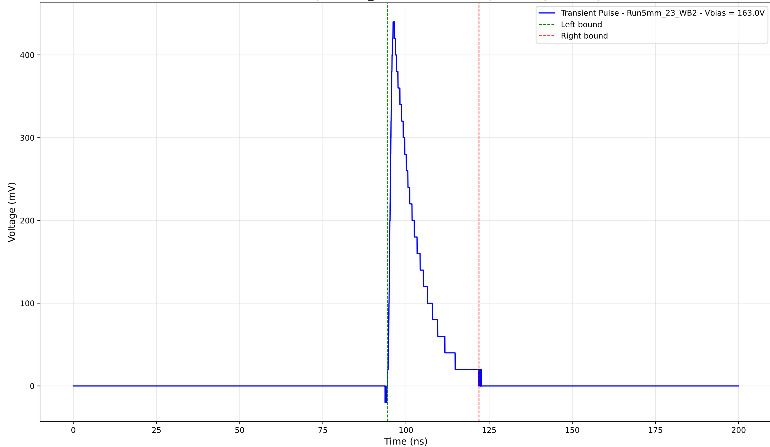
Transient Pulse - Sample: 5mm_23 - Position: 4075.0 \mu\text{m} - Charge: 71.74 pC
