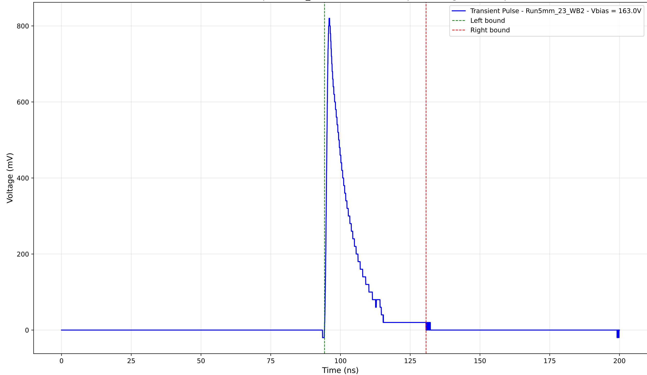
Transient Pulse - Sample: 5mm_23 - Position: 4465.0 \mu\text{m} - Charge: 129.03 pC
