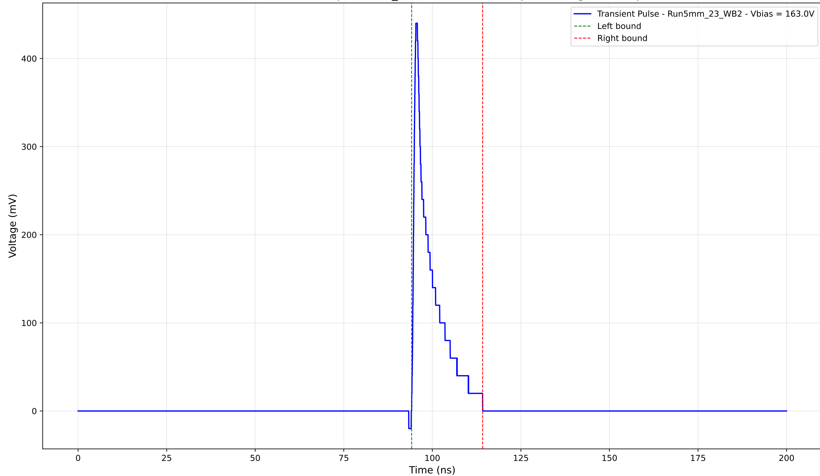
Transient Pulse - Sample: 5mm_23 - Position: 4940.0 \mu\text{m} - Charge: 46.41 pC
