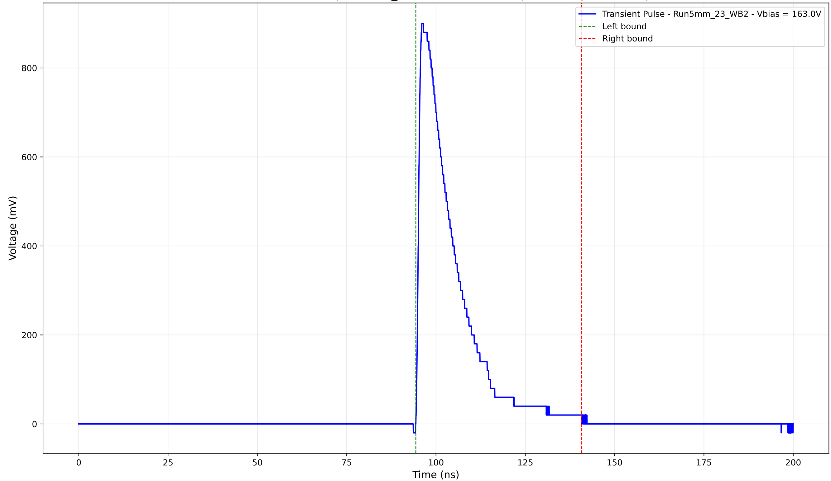
Transient Pulse - Sample: 5mm_23 - Position: 1330.0 \mu\text{m} - Charge: 200.96 pC
