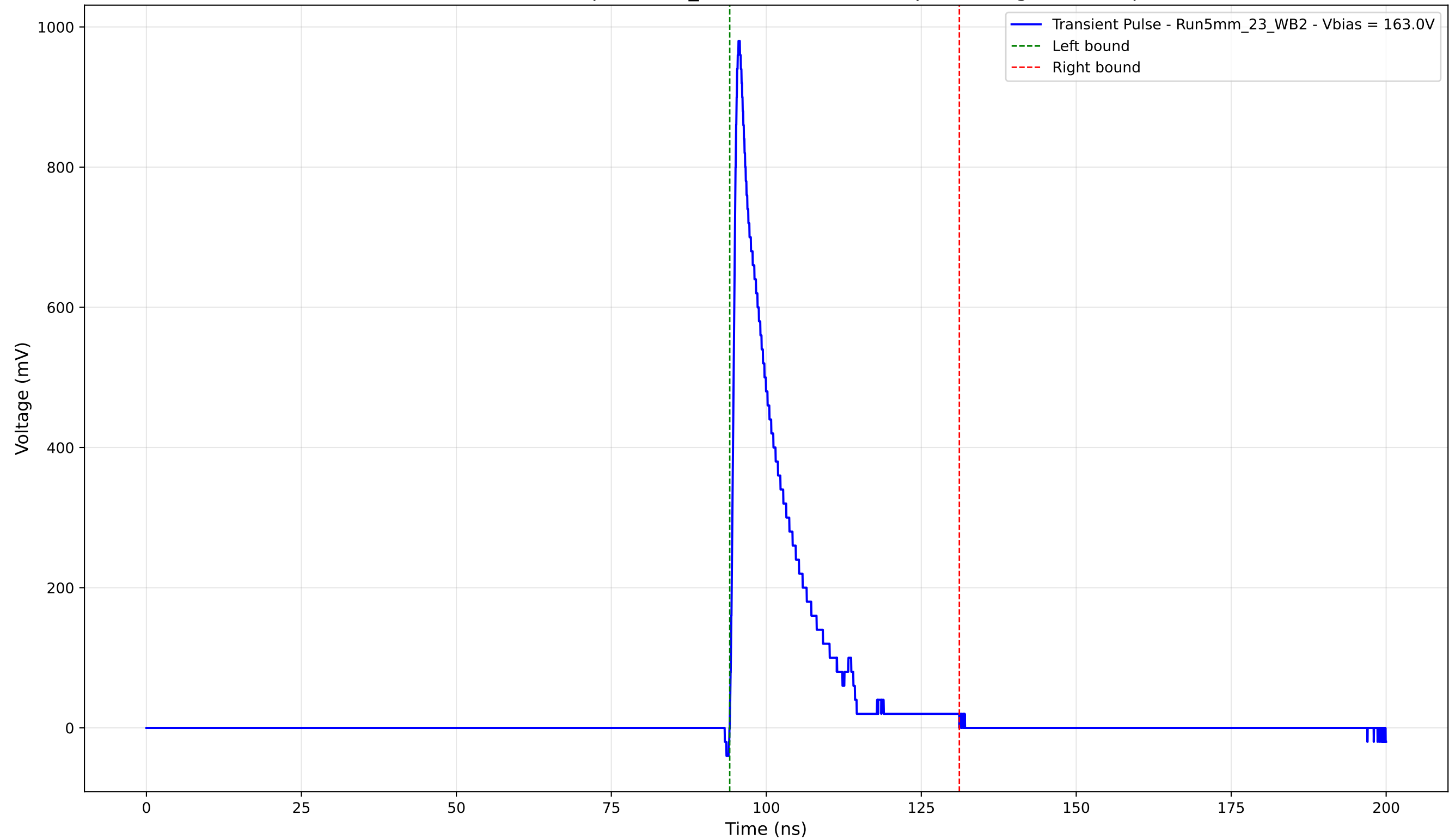
Transient Pulse - Sample: 5mm_23 - Position: 4830.0 \mu\text{m} - Charge: 144.26 pC
