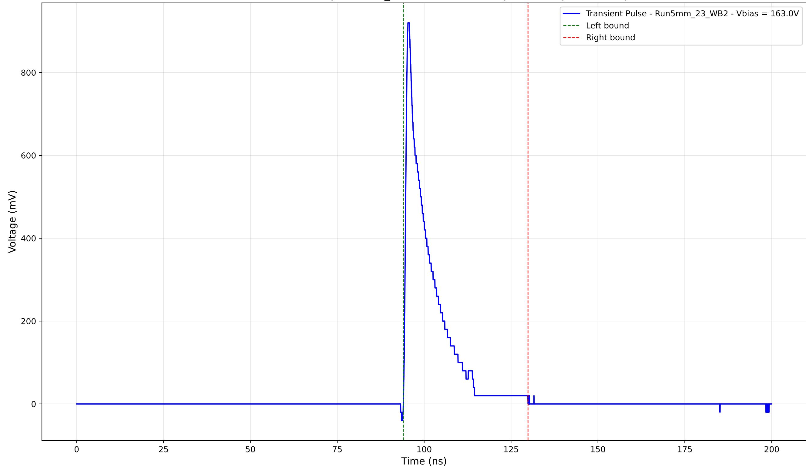
Transient Pulse - Sample: 5mm_23 - Position: 100.0 \mu\text{m} - Charge: 131.70 pC
