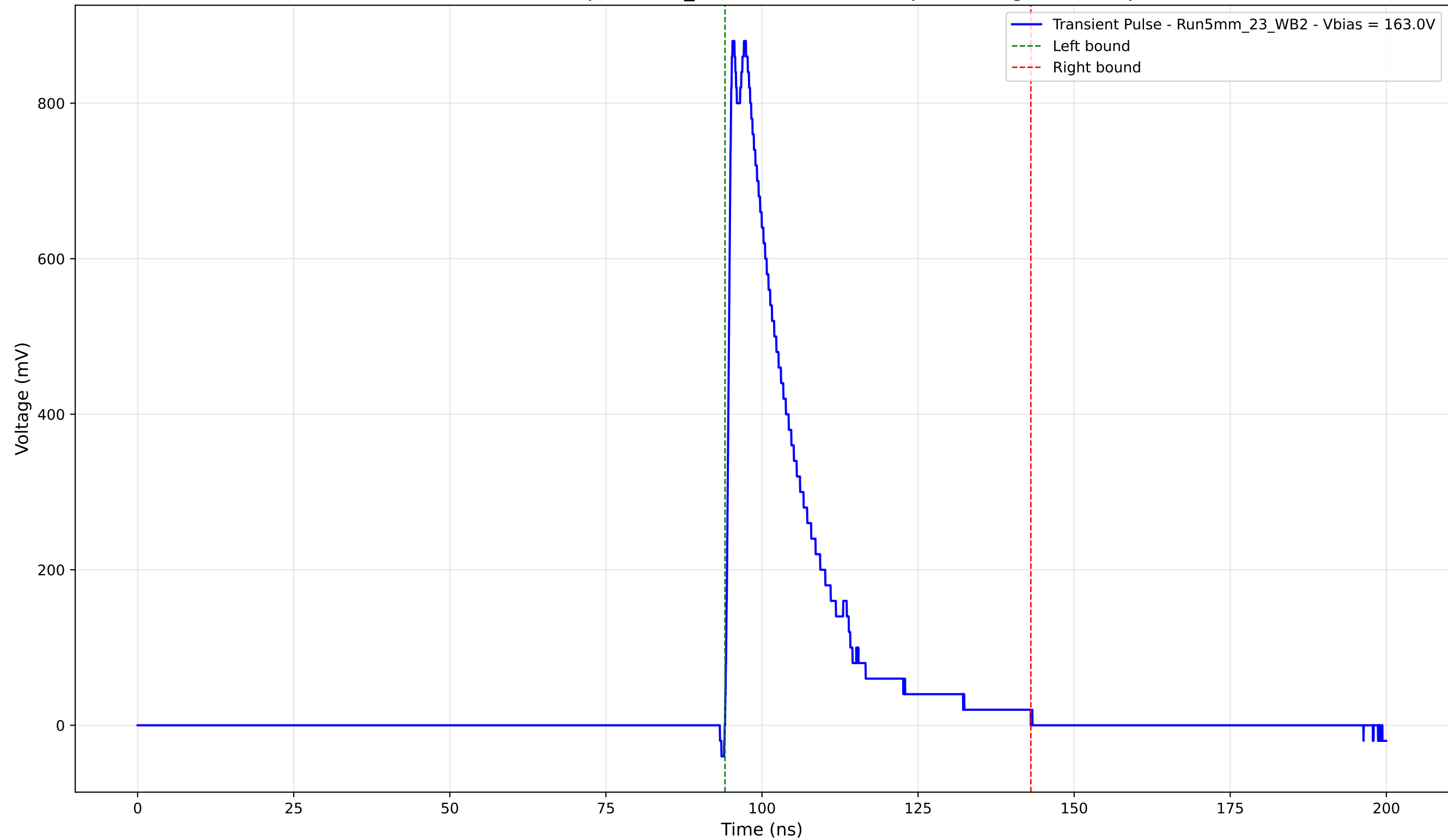
Transient Pulse - Sample: 5mm_23 - Position: 3100.0 \mu\text{m} - Charge: 197.69 pC
