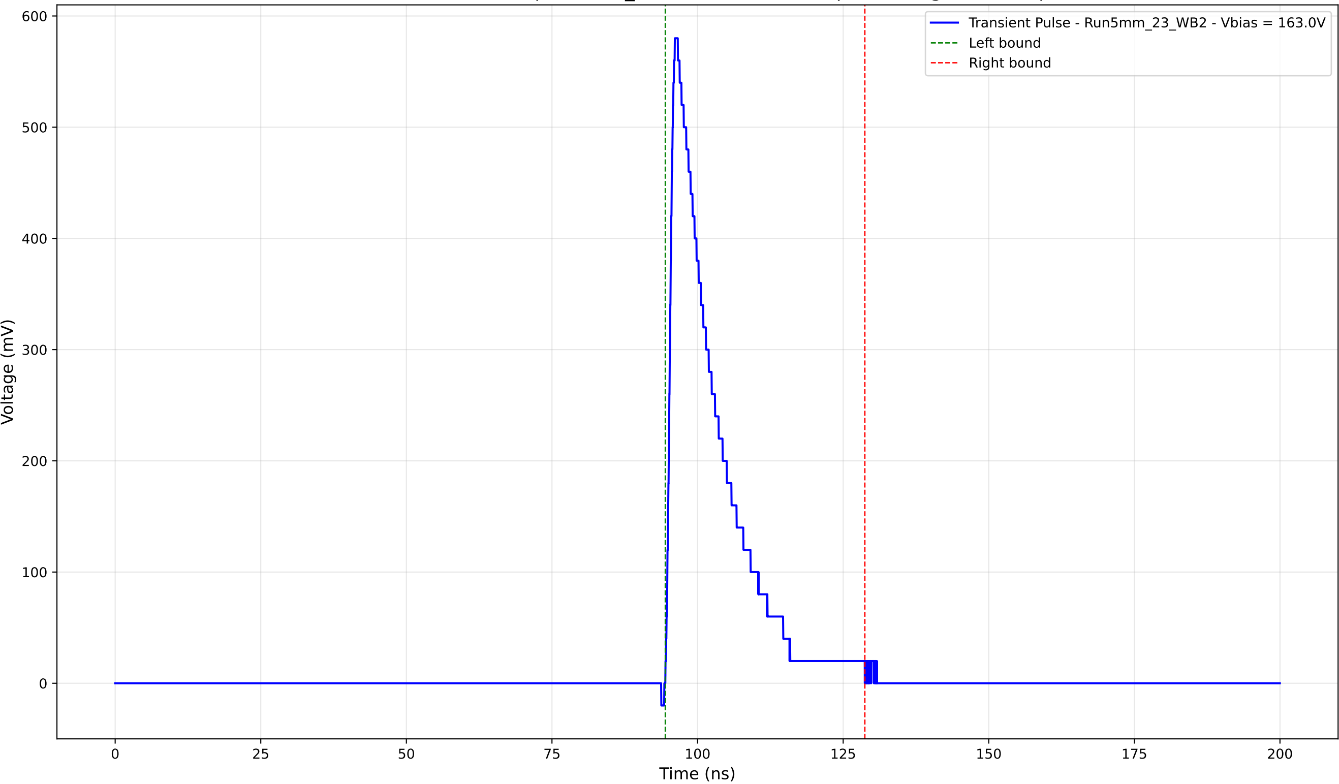
Transient Pulse - Sample: 5mm_23 - Position: 3985.0 \mu\text{m} - Charge: 101.87 pC
