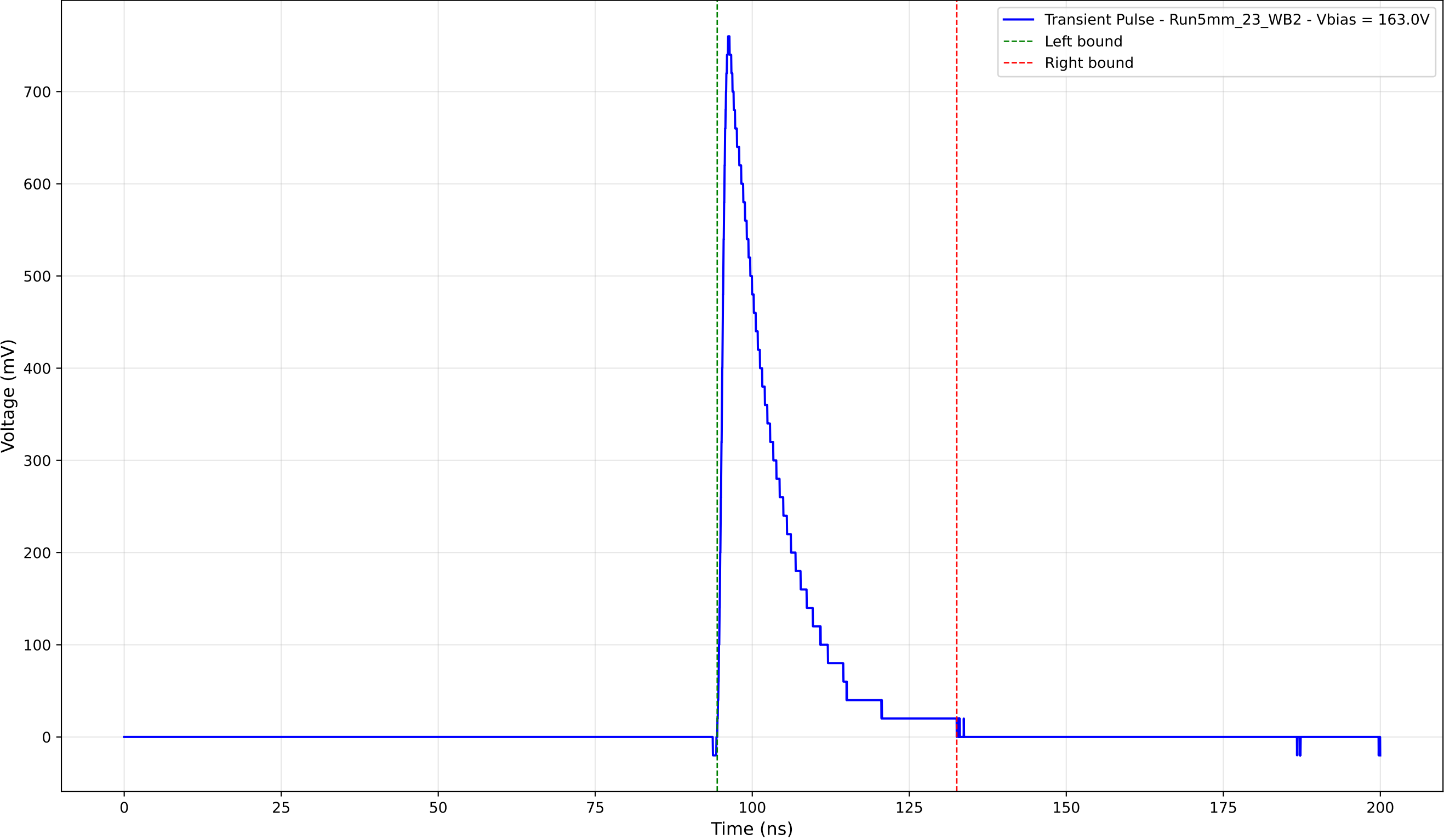
Transient Pulse - Sample: 5mm_23 - Position: 4110.0 \mu\text{m} - Charge: 133.37 pC
