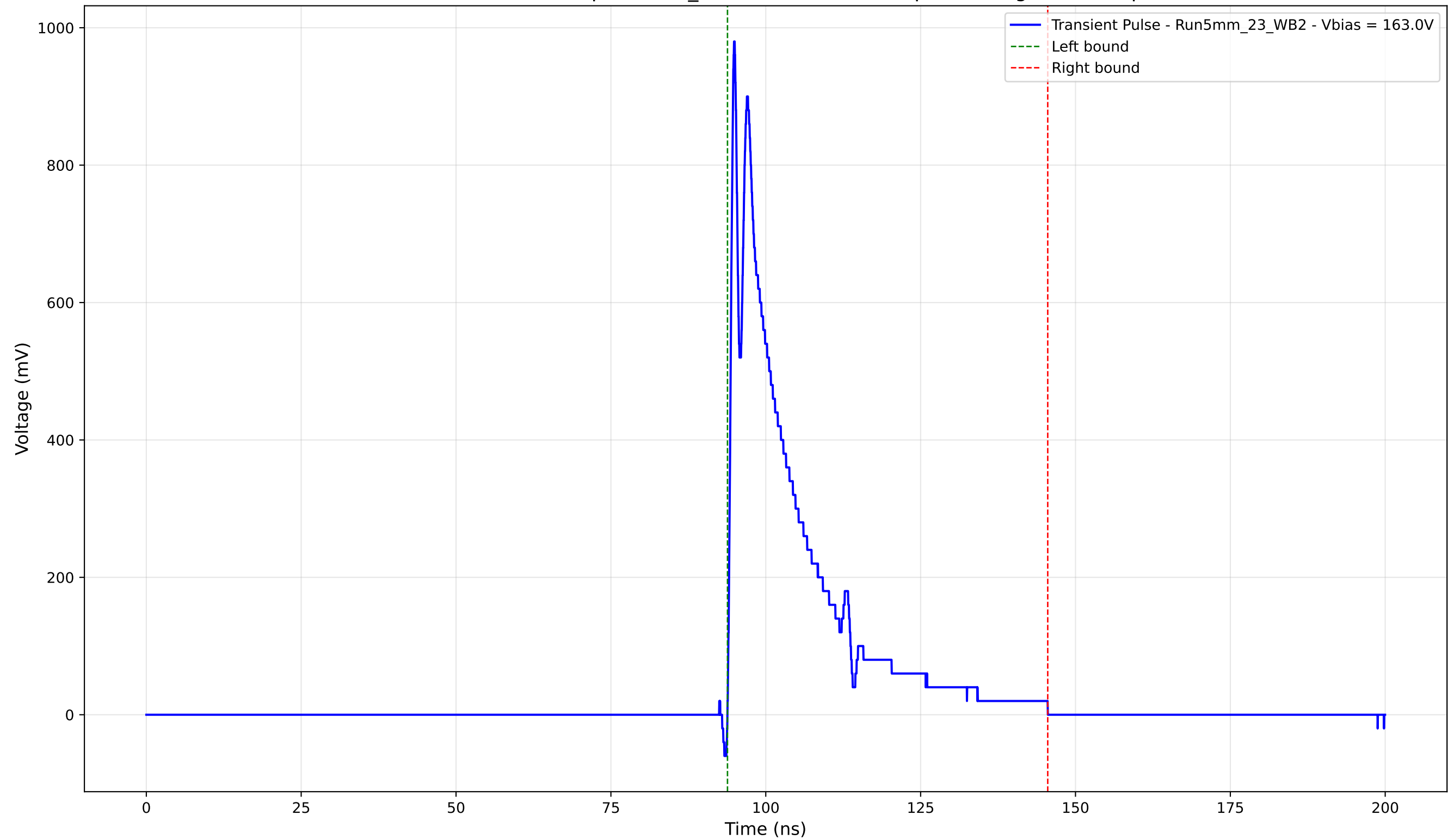
Transient Pulse - Sample: 5mm_23 - Position: 2605.0 \mu\text{m} - Charge: 186.57 pC
