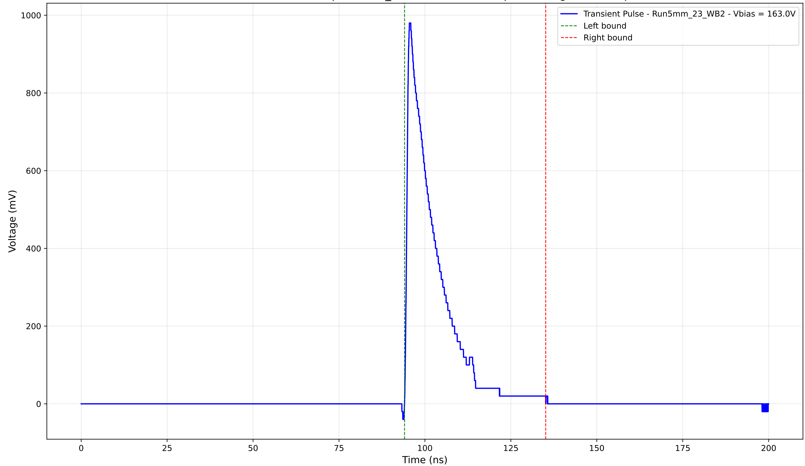
Transient Pulse - Sample: 5mm_23 - Position: 285.0 \mu\text{m} - Charge: 174.82 pC
