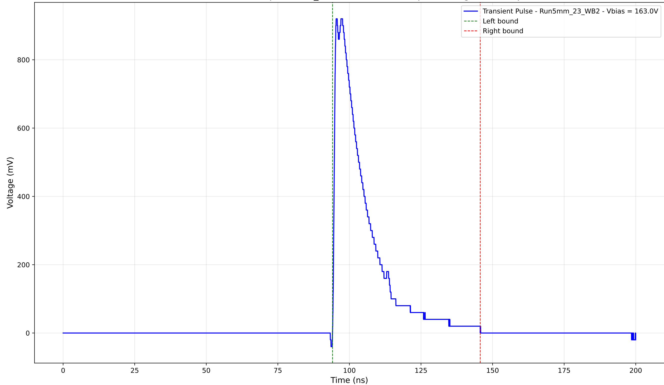
Transient Pulse - Sample: 5mm_23 - Position: 1860.0 \mu\text{m} - Charge: 222.82 pC
