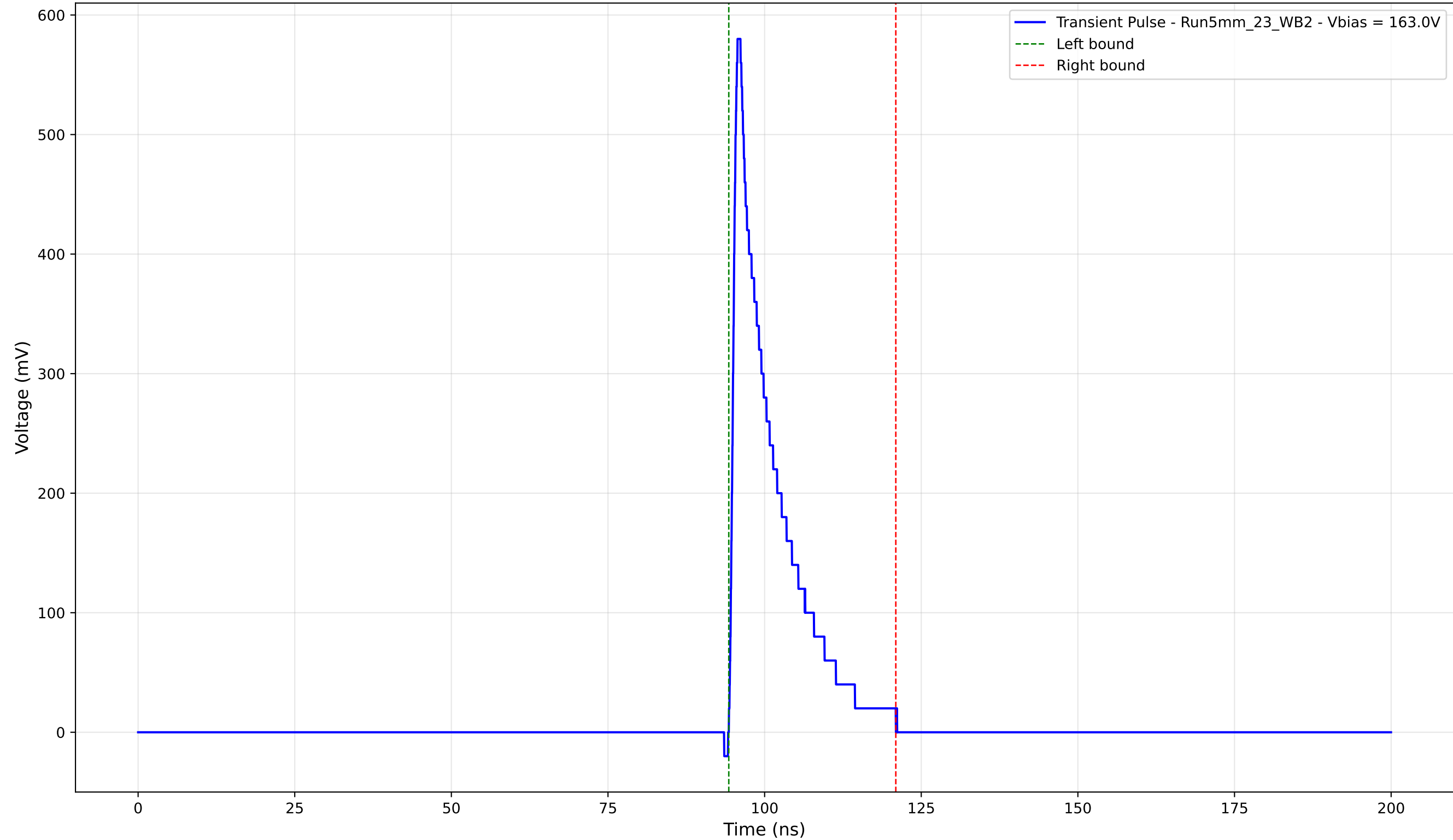
Transient Pulse - Sample: 5mm_23 - Position: 4580.0 \mu\text{m} - Charge: 80.38 pC
