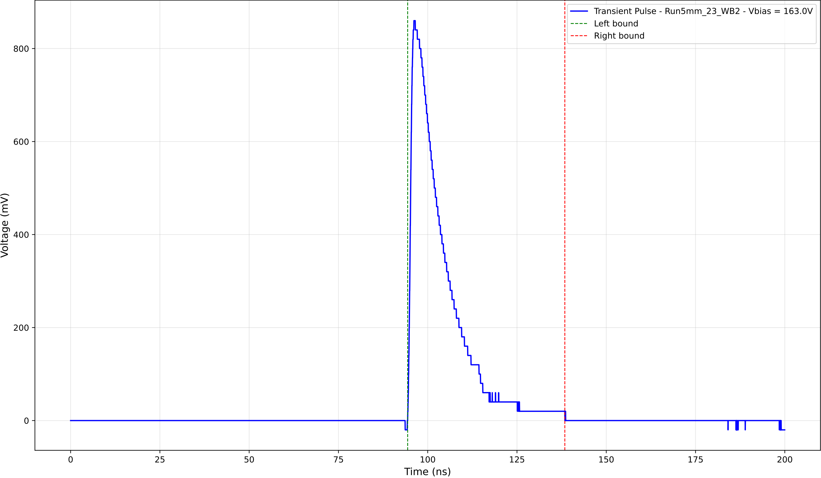
Transient Pulse - Sample: 5mm_23 - Position: 3735.0 \mu\text{m} - Charge: 177.05 pC
