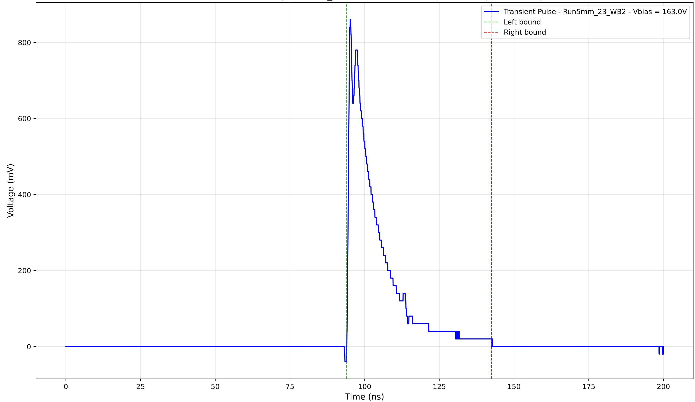
Transient Pulse - Sample: 5mm_23 - Position: 2085.0 \mu\text{m} - Charge: 170.69 pC
