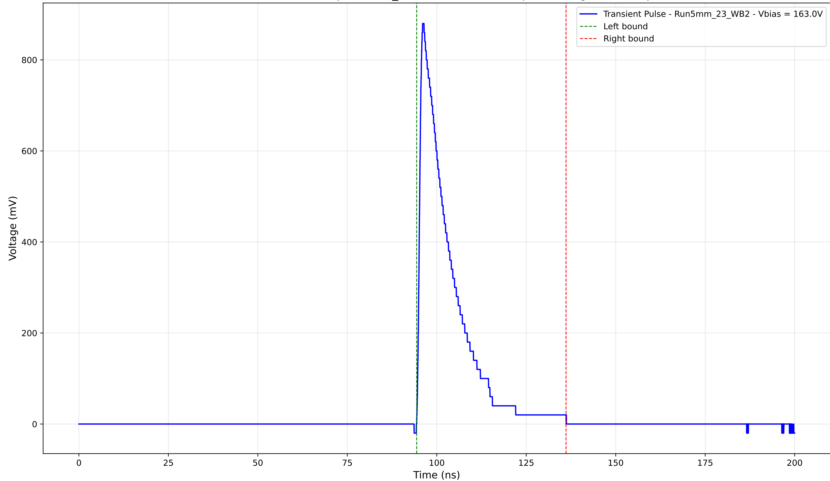
Transient Pulse - Sample: 5mm_23 - Position: 4175.0 \mu\text{m} - Charge: 163.02 pC
