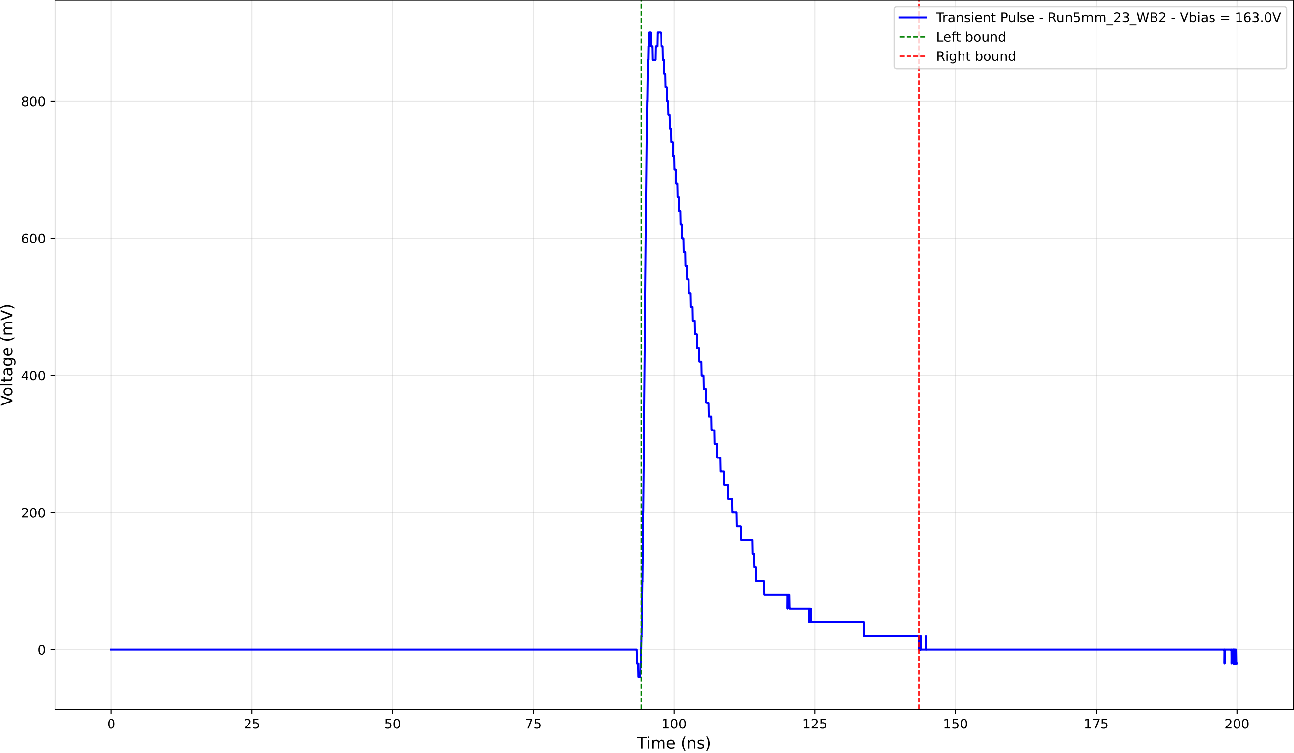
Transient Pulse - Sample: 5mm_23 - Position: 1745.0 \mu\text{m} - Charge: 214.02 pC
