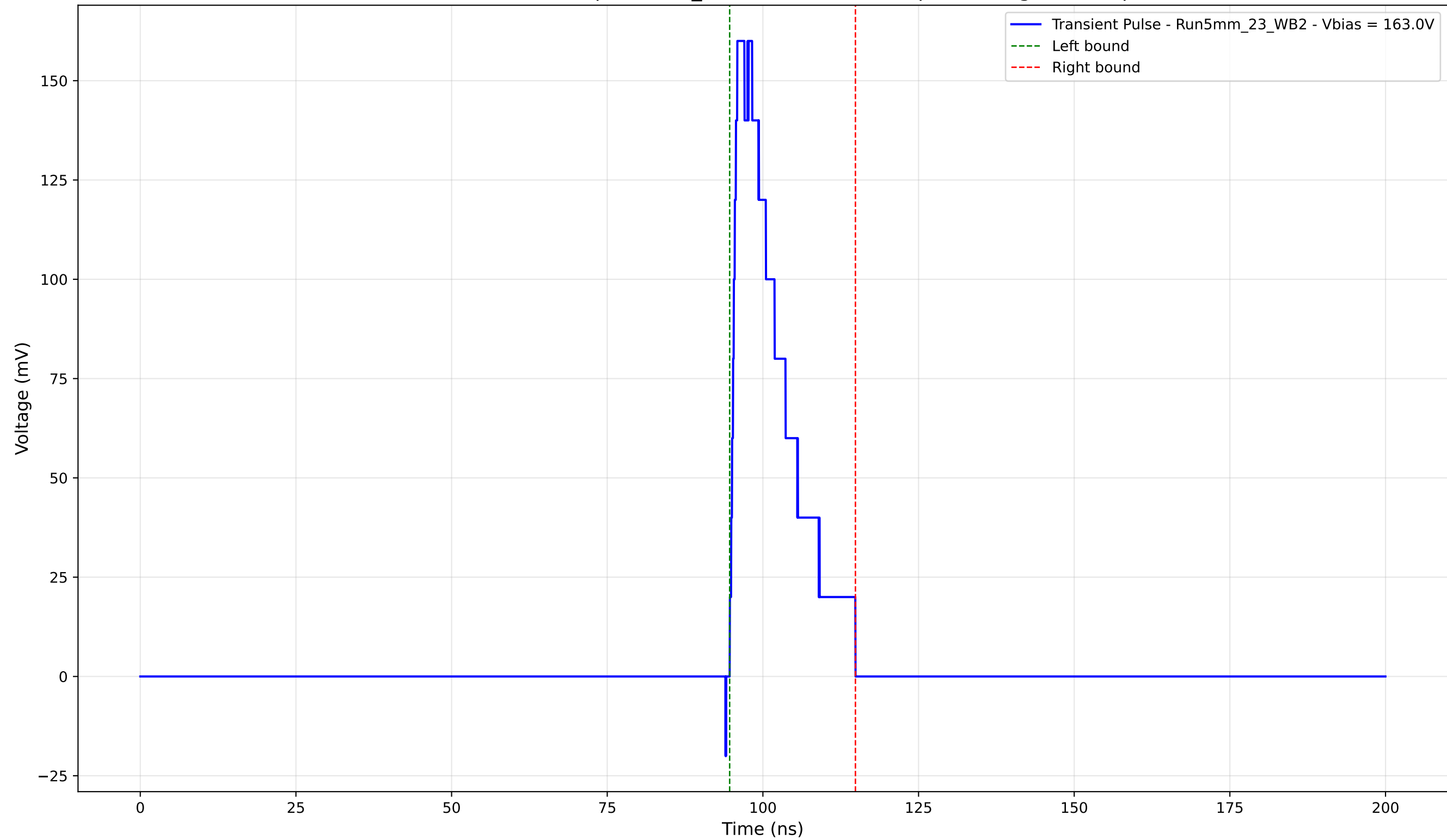
Transient Pulse - Sample: 5mm_23 -Position: 4035.0 \mu\text{m} - Charge: 28.12 pC
