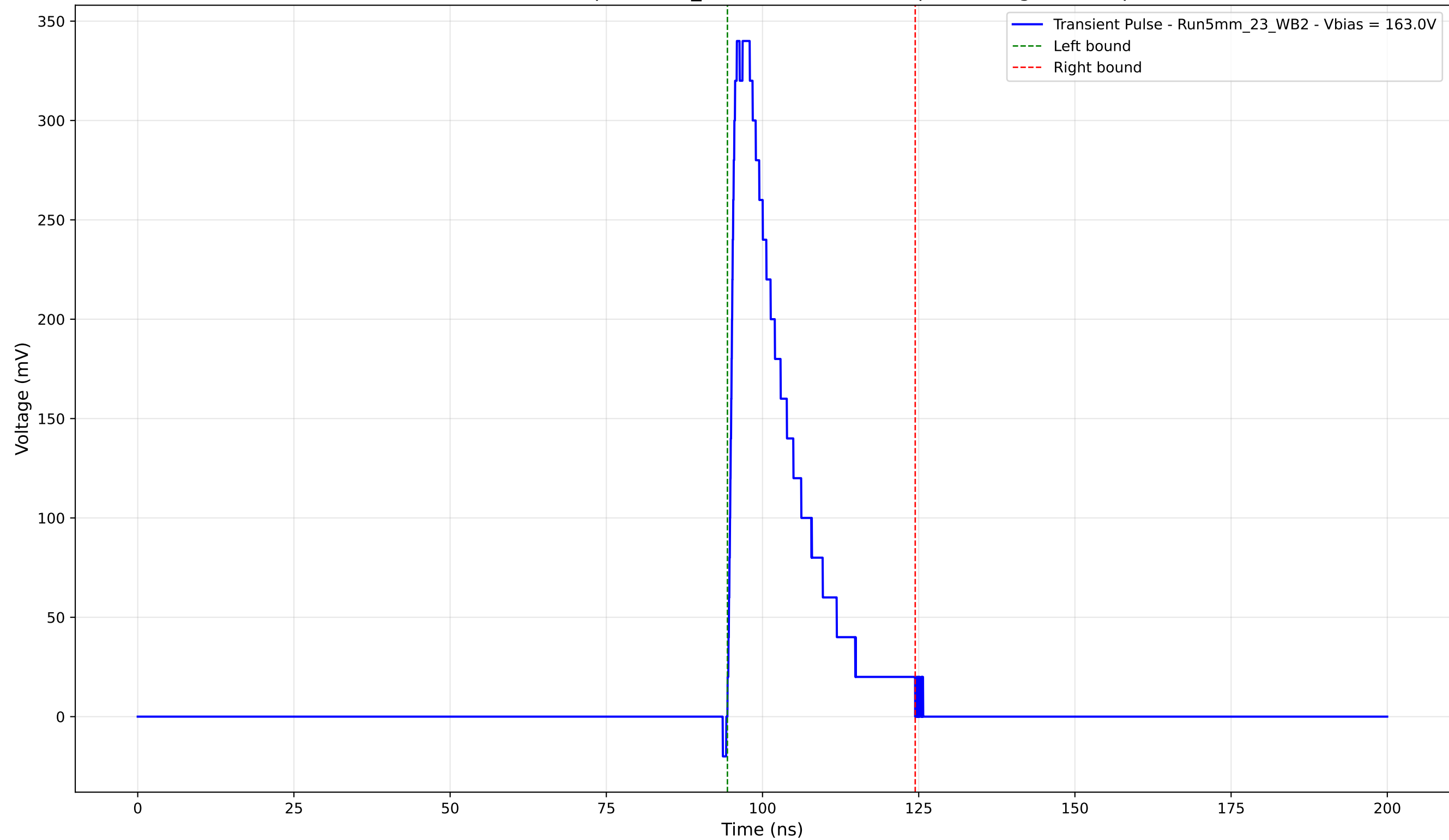
Transient Pulse - Sample: 5mm_23 - Position: 1530.0 \mu\text{m} - Charge: 67.58 pC
