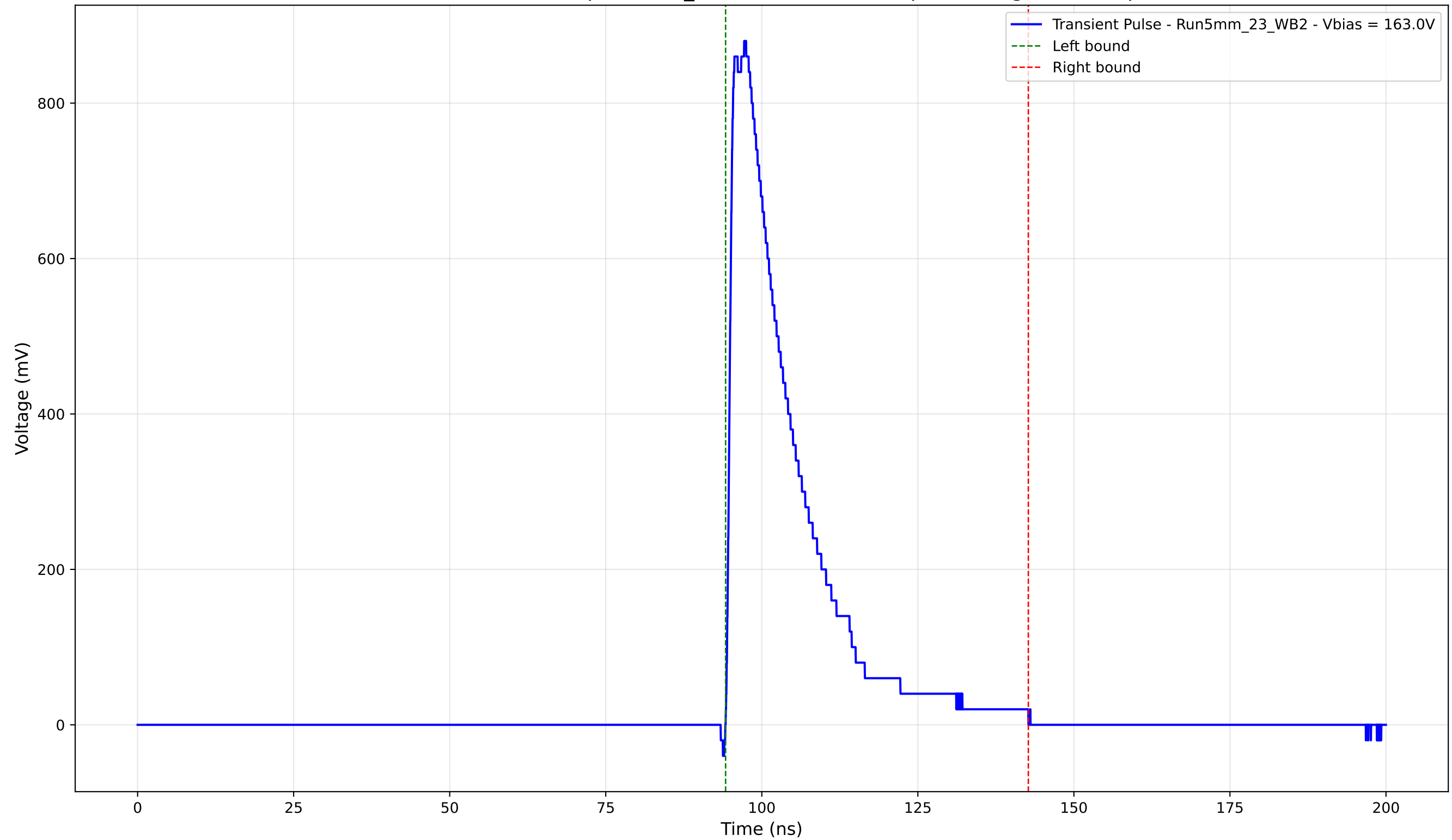
Transient Pulse - Sample: 5mm_23 - Position: 3340.0 \mu\text{m} - Charge: 198.56 pC
