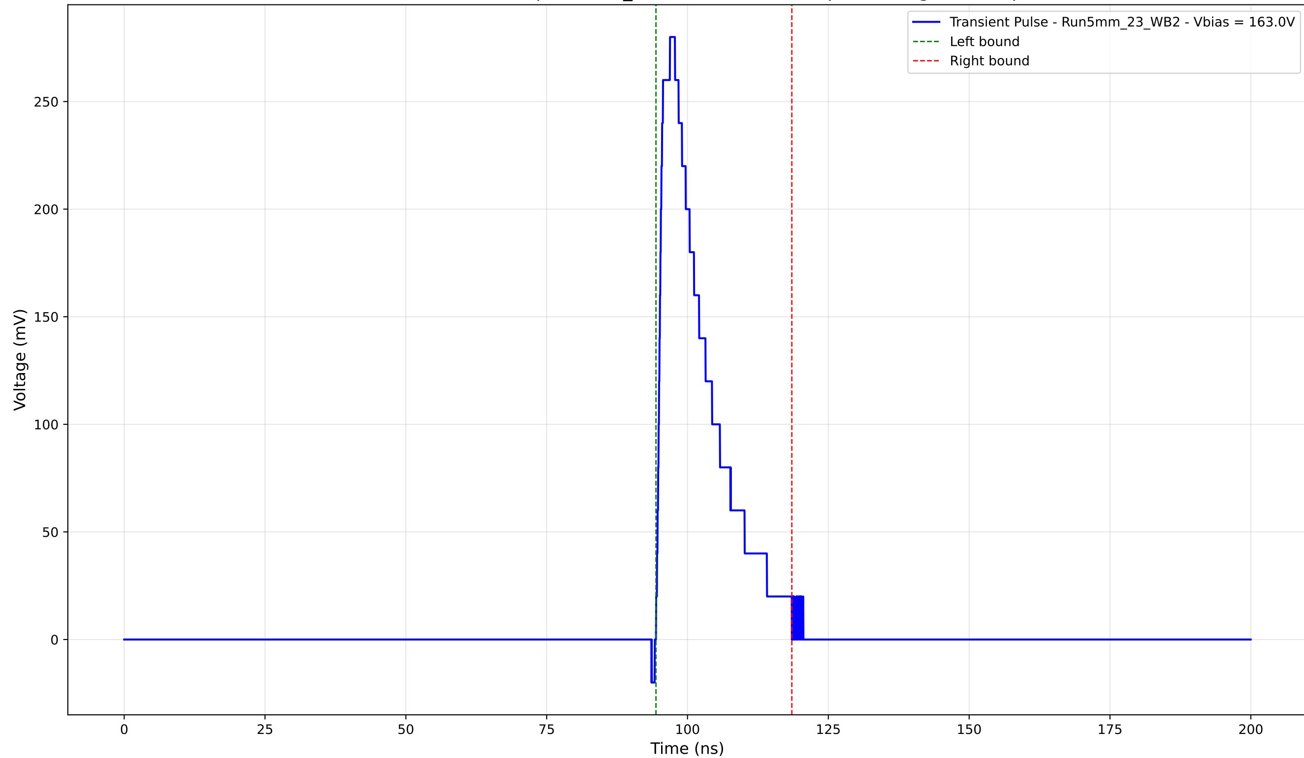
Transient Pulse - Sample: 5mm_23 - Position: 3500.0 \mu\text{m} - Charge: 52.02 pC
