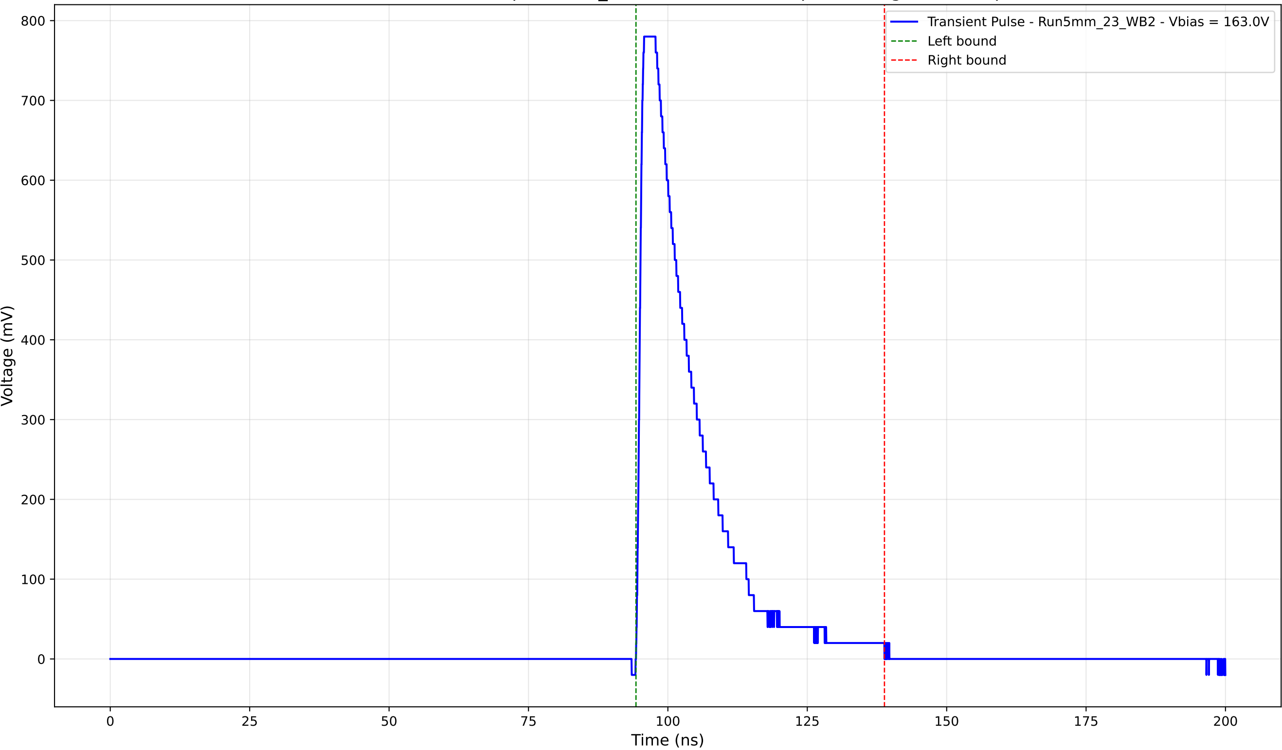
Transient Pulse - Sample: 5mm_23 - Position: 3435.0 \mu\text{m} - Charge: 170.76 pC
