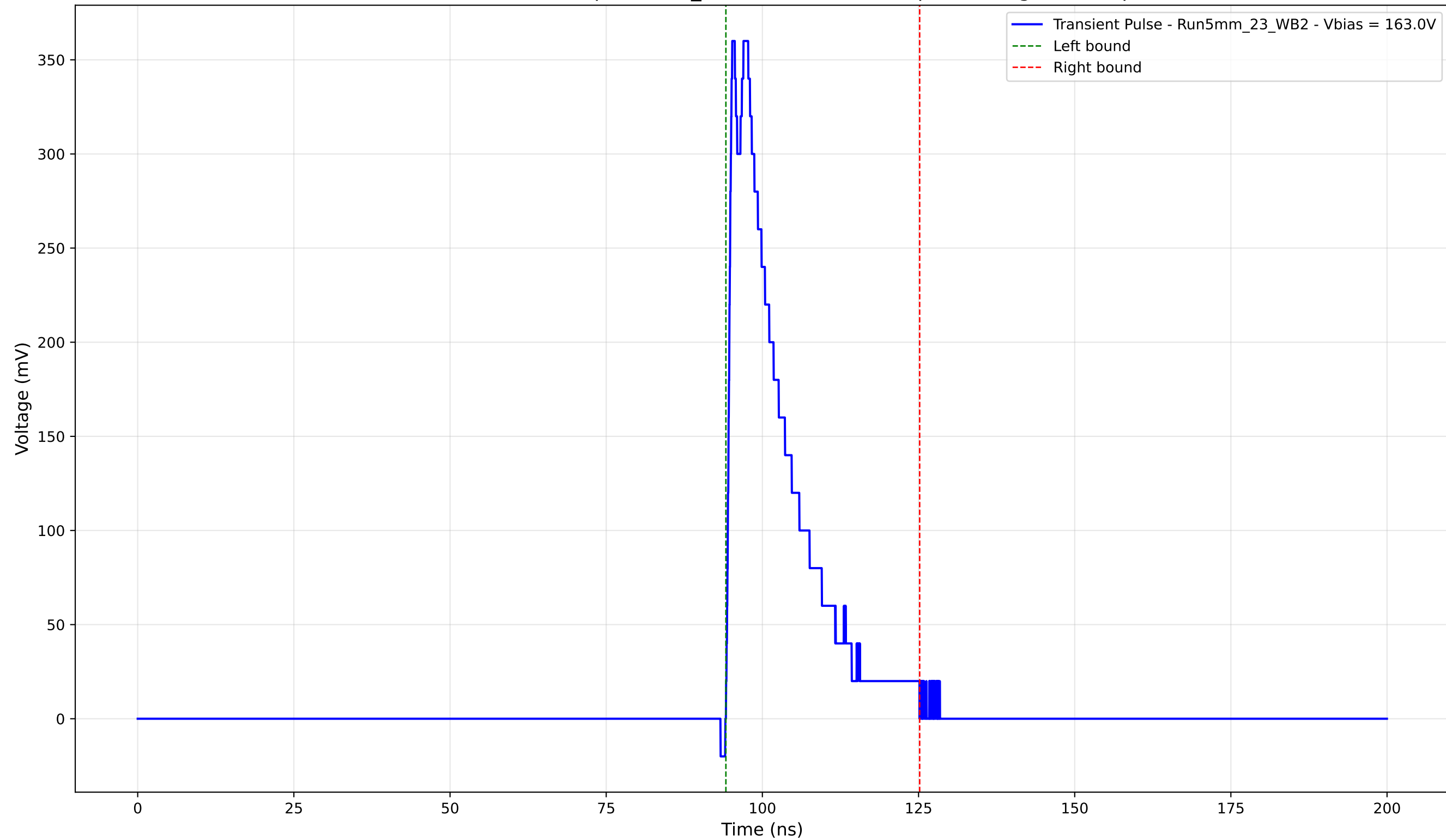
Transient Pulse - Sample: 5mm_23 - Position: 3050.0 \mu\text{m} - Charge: 69.62 pC
