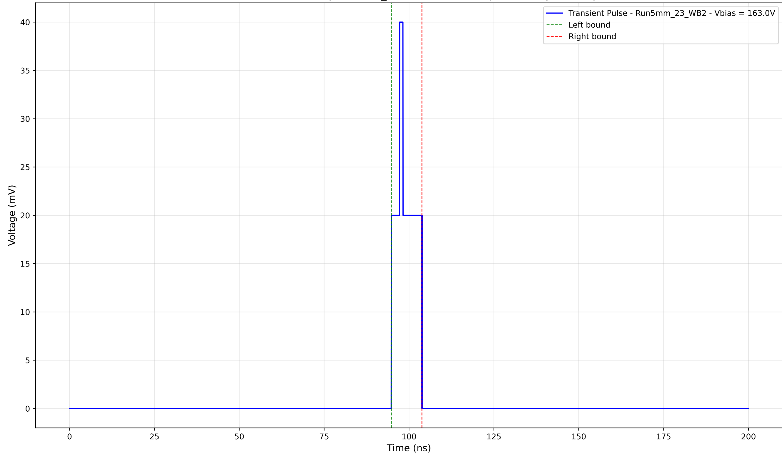
Transient Pulse - Sample: 5mm_23 - Position: 10.0 \mu\text{m} - Charge: 4.01 pC
