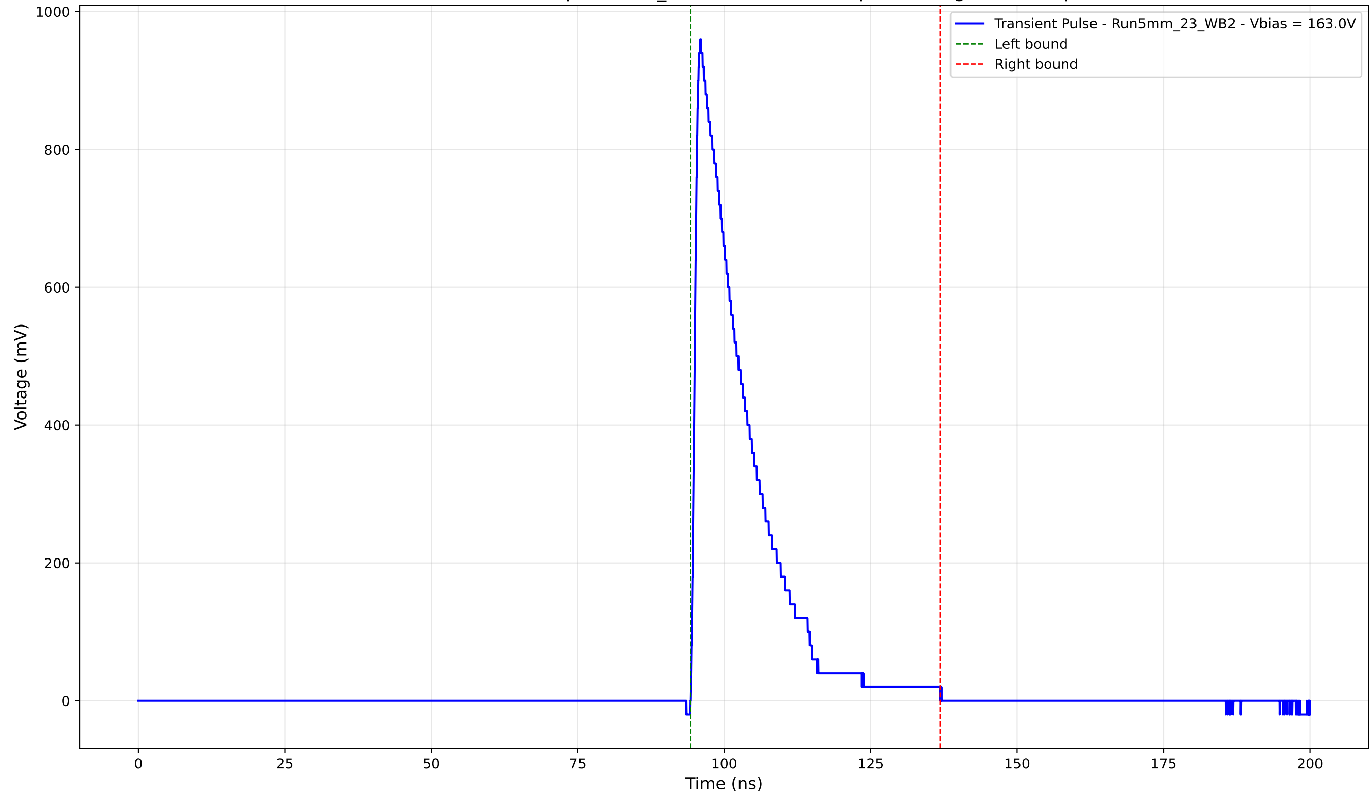
Transient Pulse - Sample: 5mm_23 - Position: 605.0 \mu\text{m} - Charge: 184.75 pC
