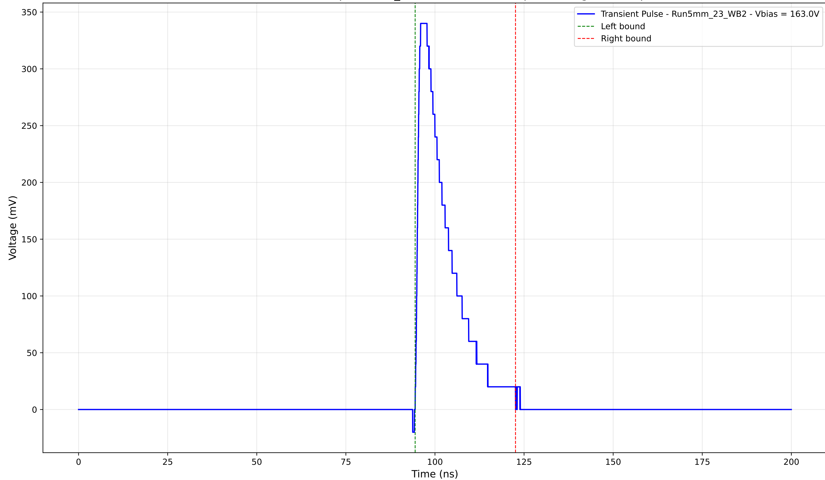
Transient Pulse - Sample: 5mm_23 - Position: 1470.0 \mu\text{m} - Charge: 65.86 pC
