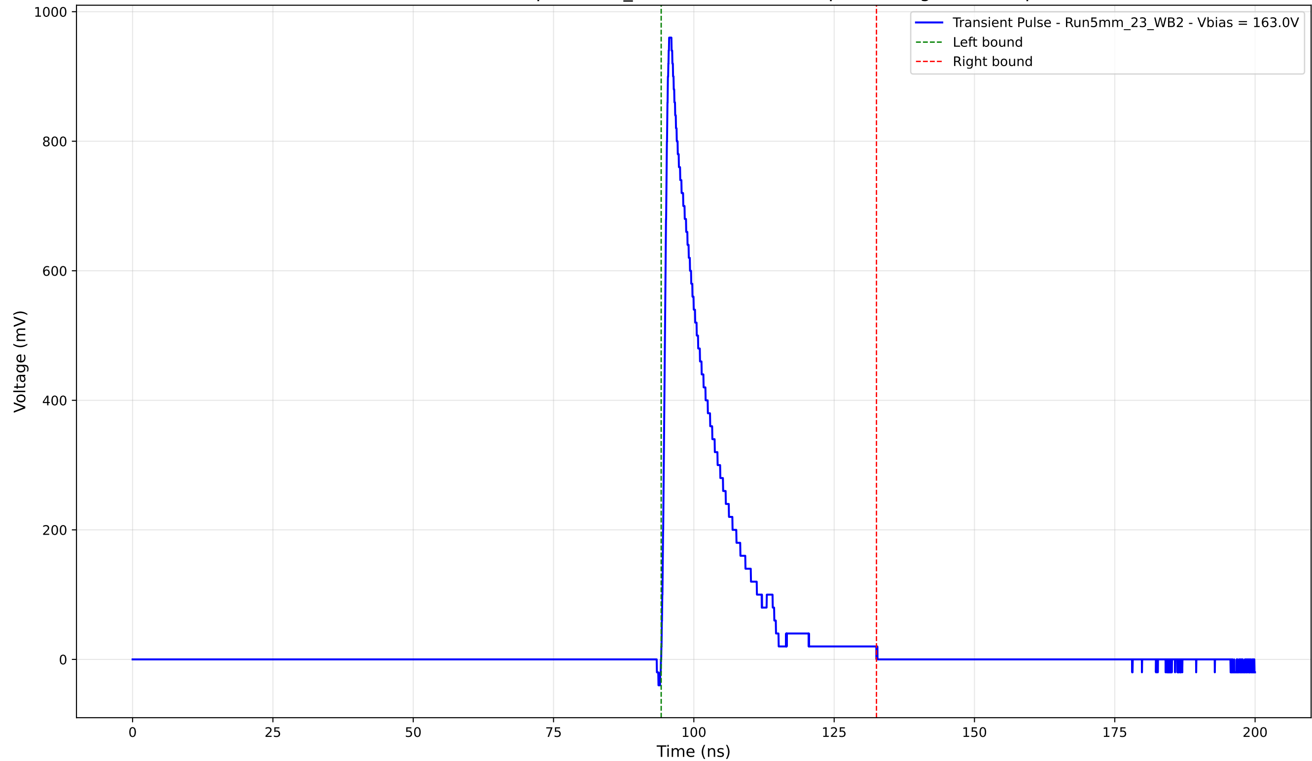
Transient Pulse - Sample: 5mm_23 - Position: 4660.0 \mu\text{m} - Charge: 157.31 pC
