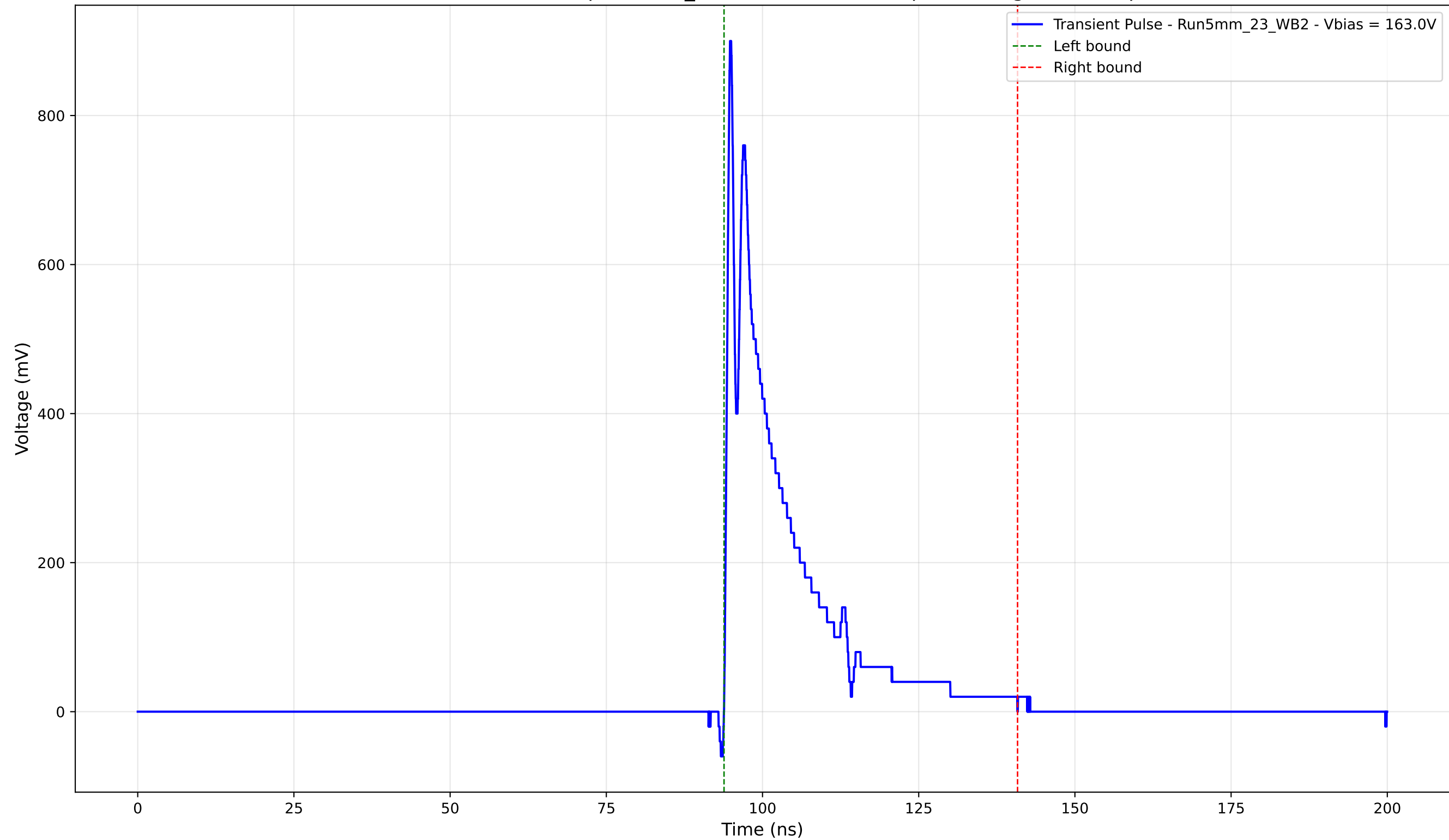
Transient Pulse - Sample: 5mm_23 - Position: 2580.0 \mu\text{m} - Charge: 147.81 pC
