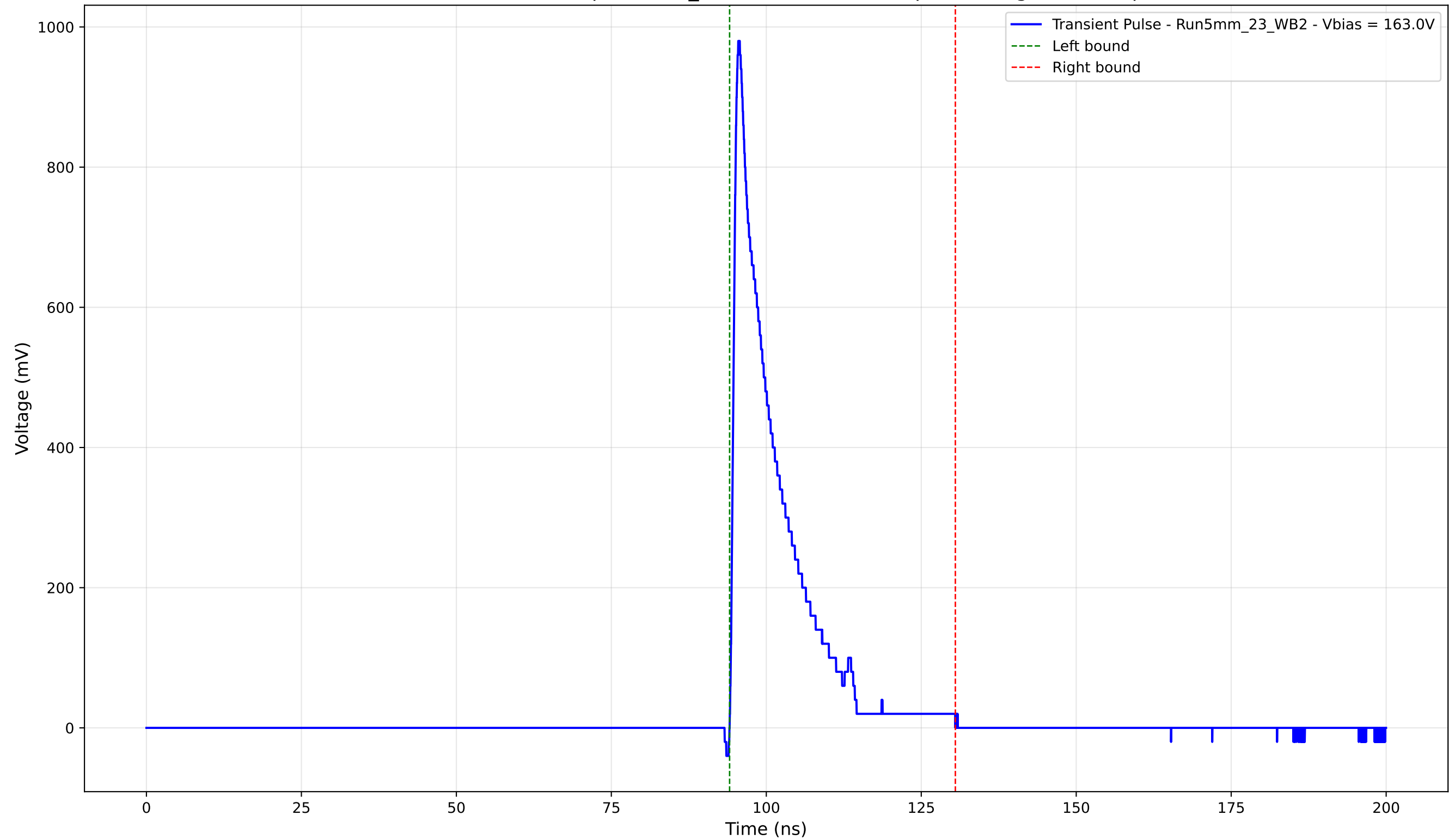
Transient Pulse - Sample: 5mm_23 - Position: 4845.0 \mu\text{m} - Charge: 142.14 pC
