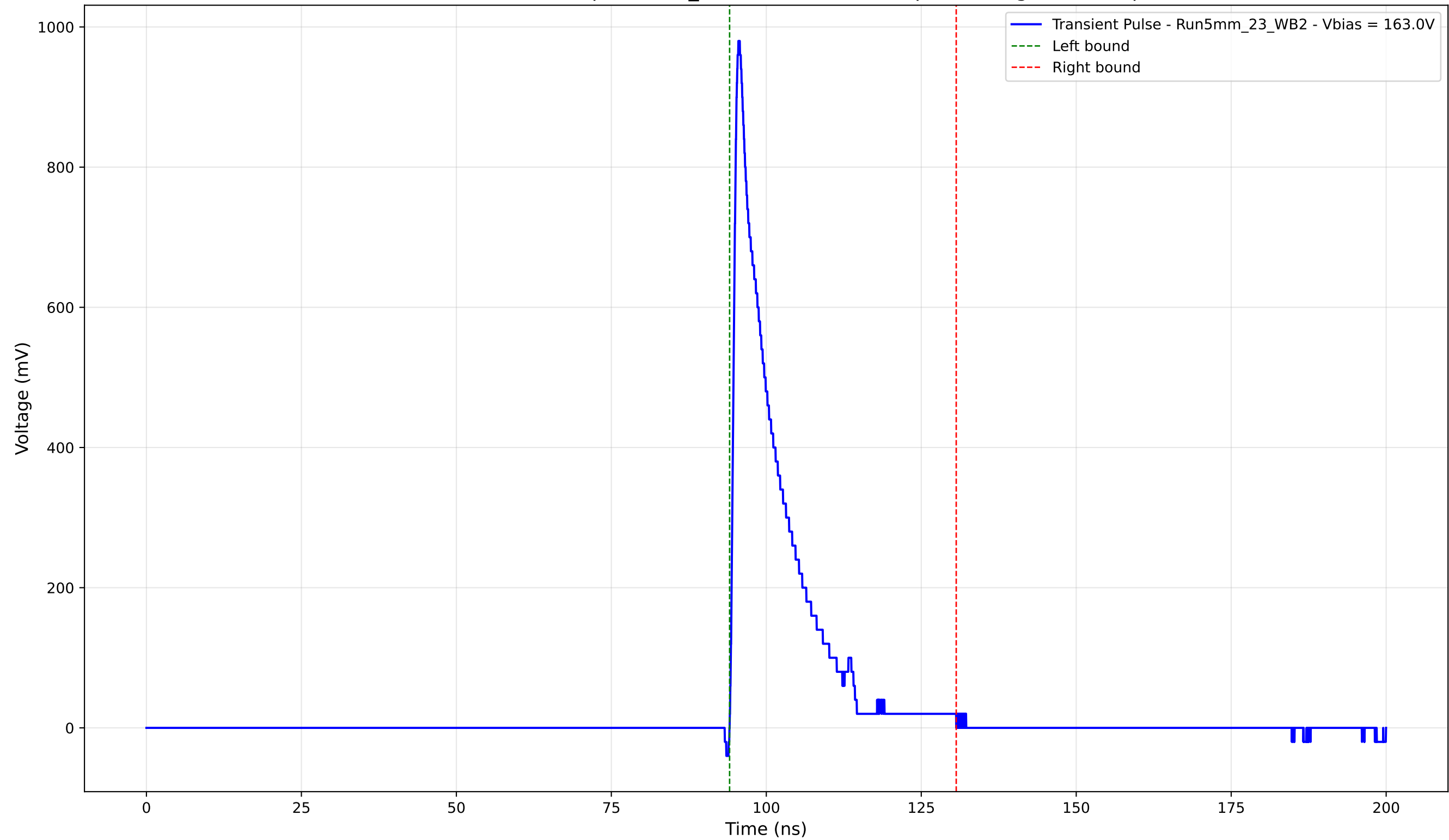
Transient Pulse - Sample: 5mm_23 - Position: 4835.0 \mu\text{m} - Charge: 143.77 pC
