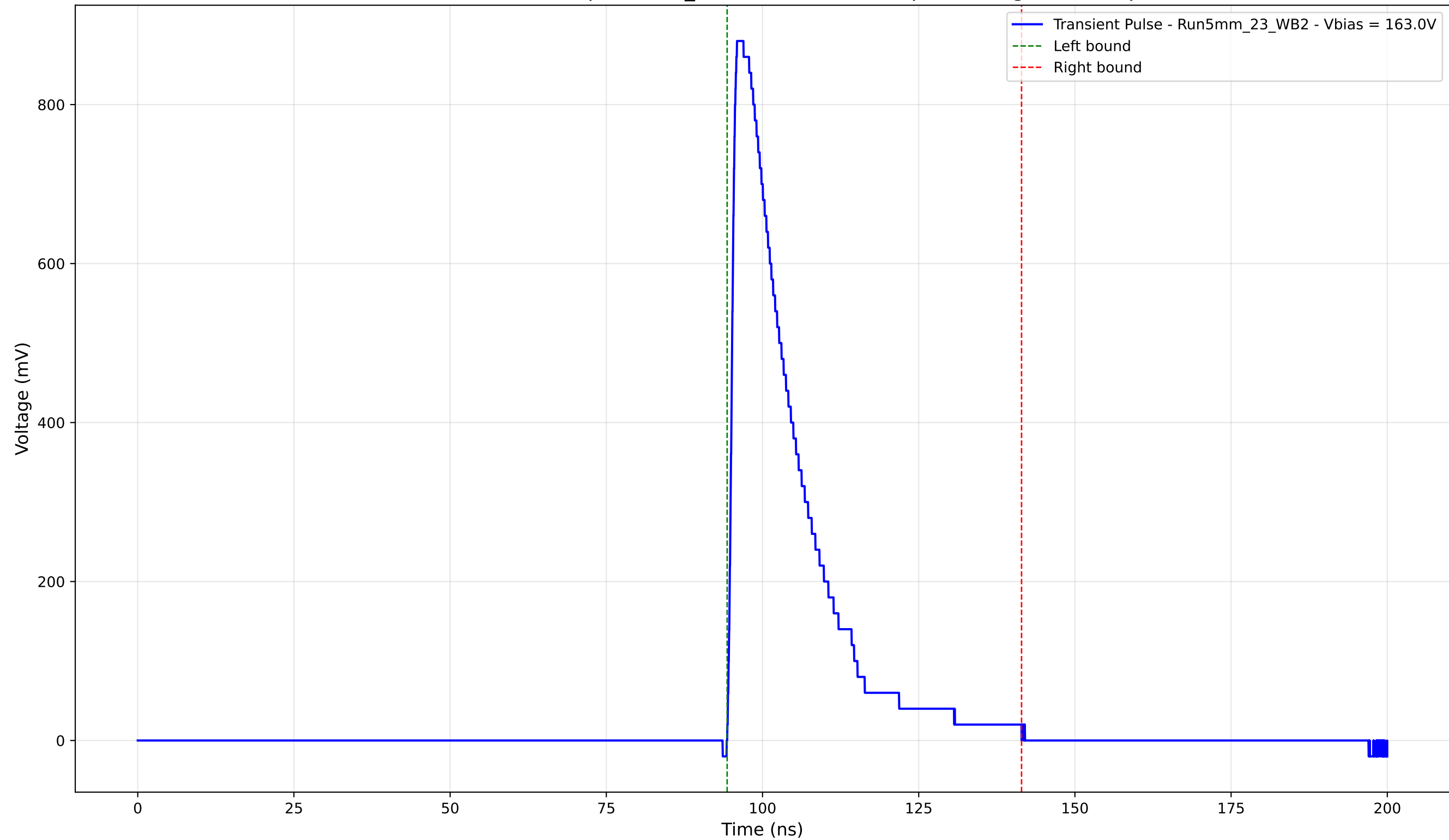
Transient Pulse - Sample: 5mm_23 - Position: 1370.0 \mu\text{m} - Charge: 198.61 pC
