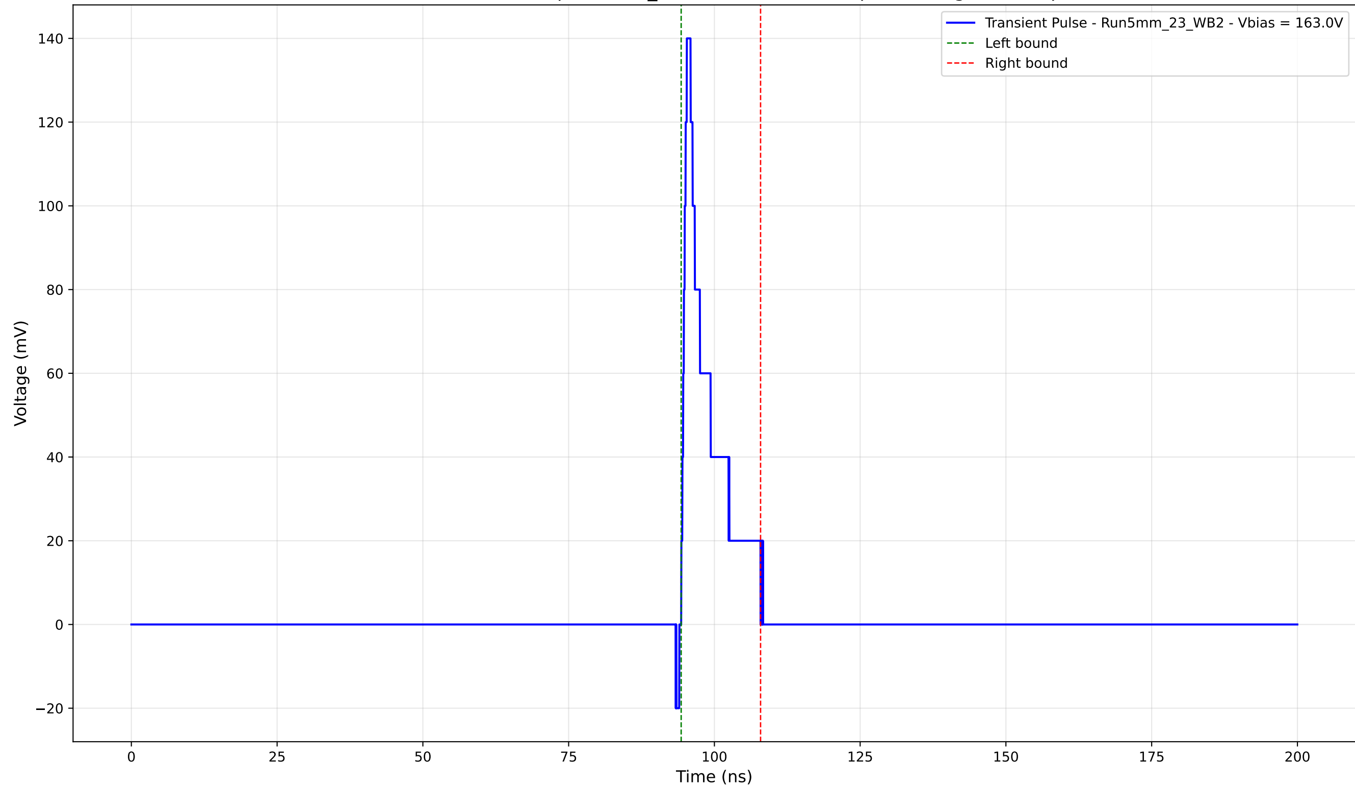
Transient Pulse - Sample: 5mm_23 - Position: 4970.0 \mu\text{m} - Charge: 13.07 pC
