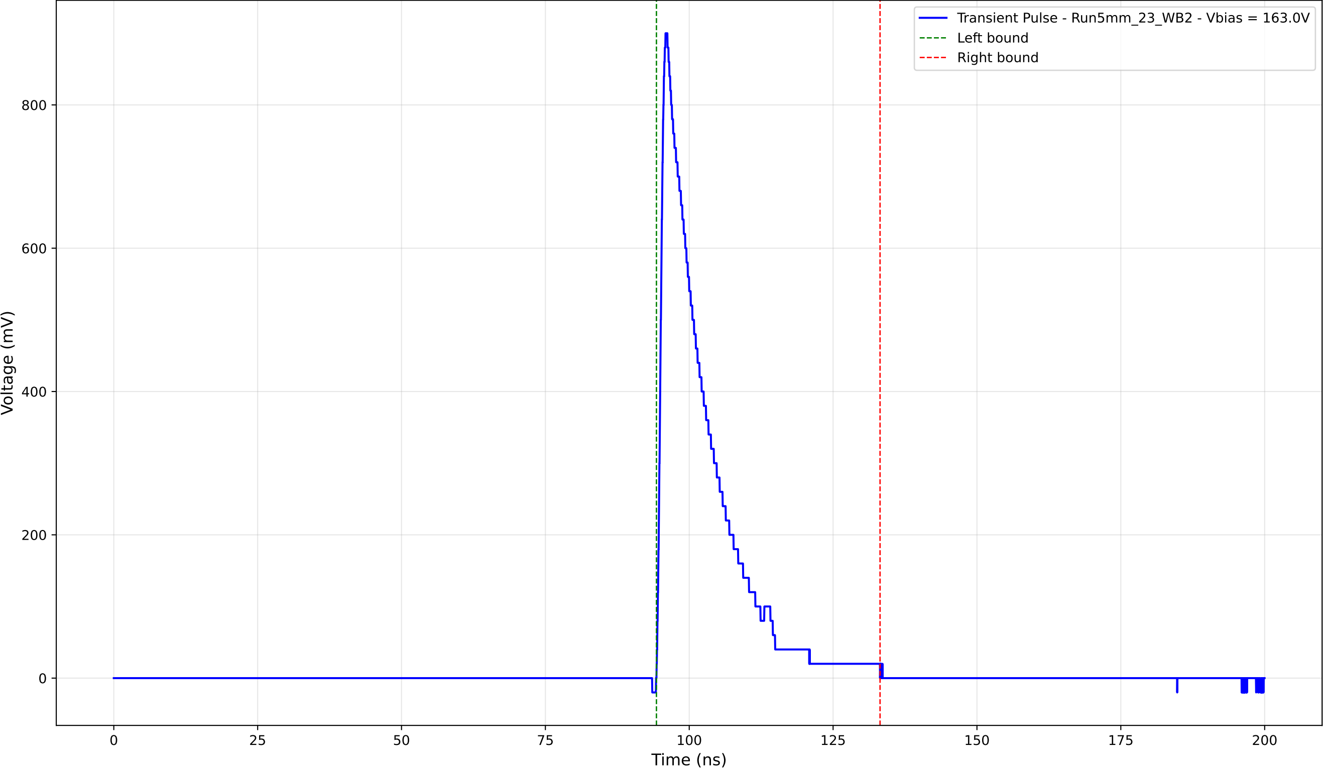
Transient Pulse - Sample: 5mm_23 - Position: 4420.0 \mu\text{m} - Charge: 154.10 pC
