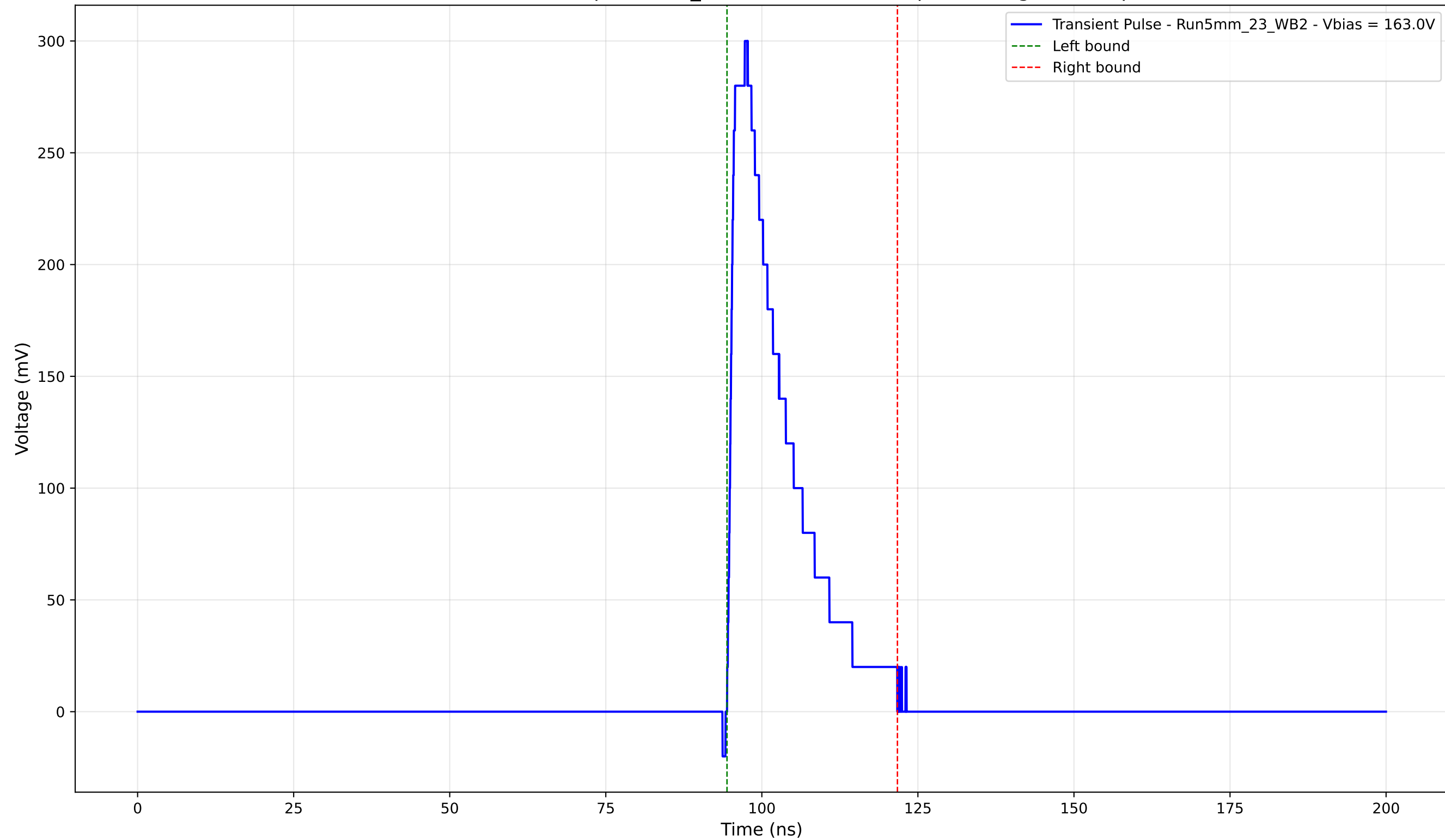
Transient Pulse - Sample: 5mm_23 - Position: 1525.0 \mu\text{m} - Charge: 57.36 pC
