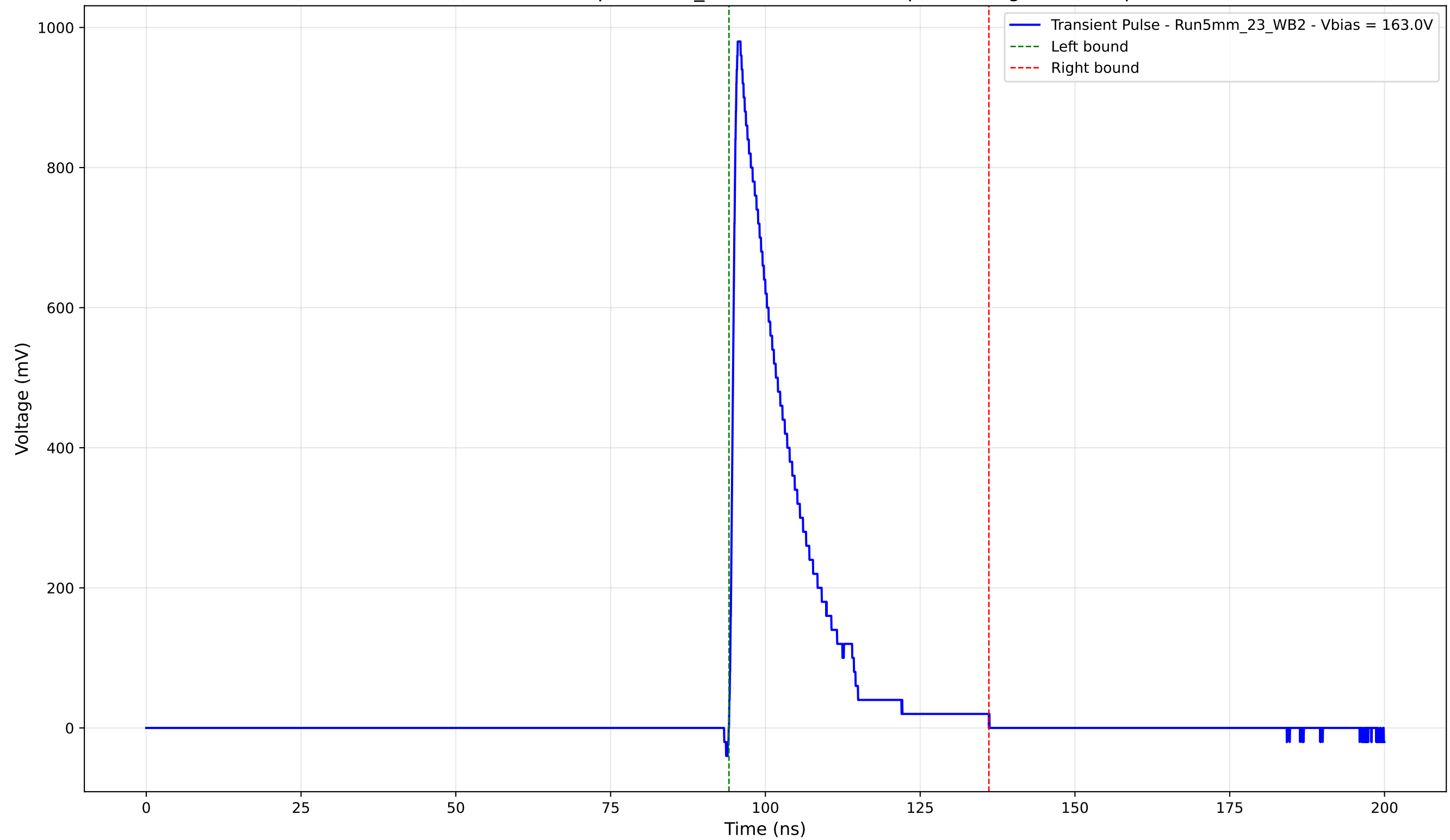
Transient Pulse - Sample: 5mm_23 - Position: 355.0 \mu\text{m} - Charge: 181.34 pC
