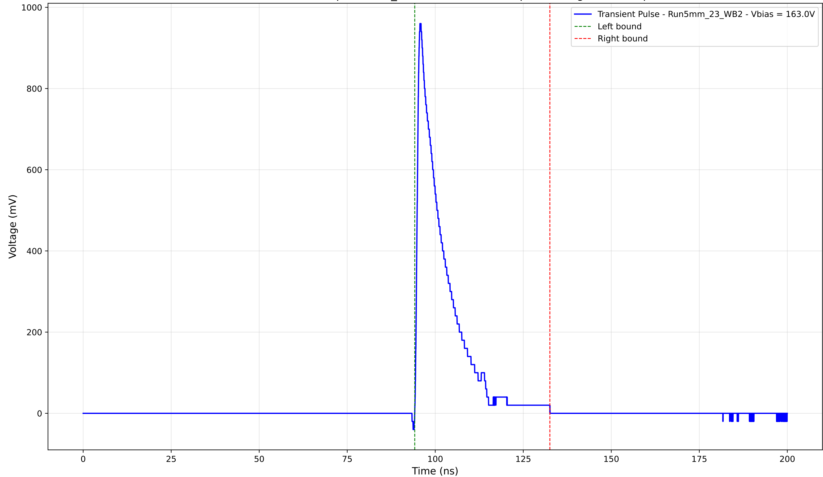
Transient Pulse - Sample: 5mm_23 - Position: 4645.0 \mu\text{m} - Charge: 156.44 pC
