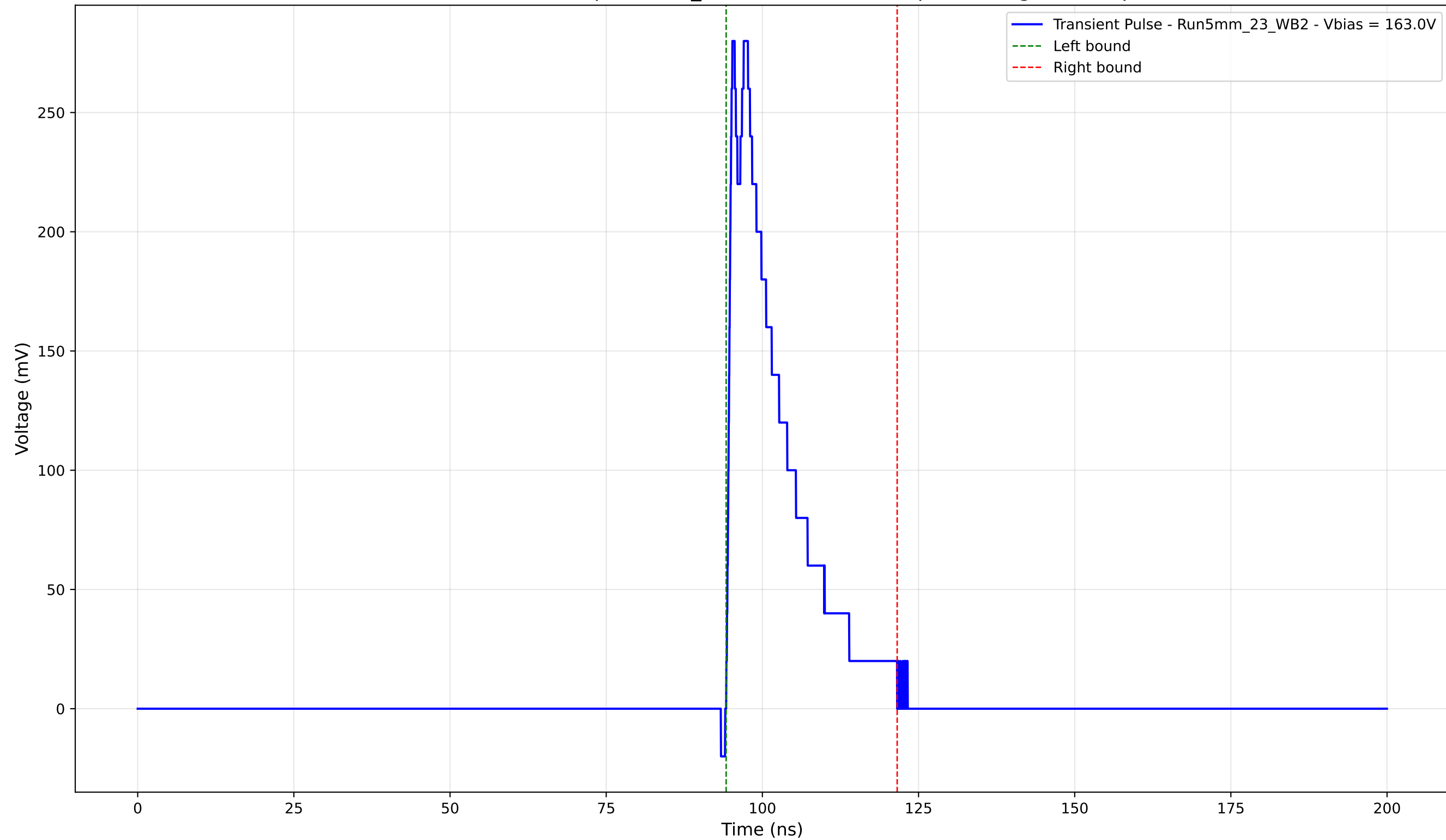
Transient Pulse - Sample: 5mm_23 - Position: 1990.0 \mu\text{m} - Charge: 52.48 pC
