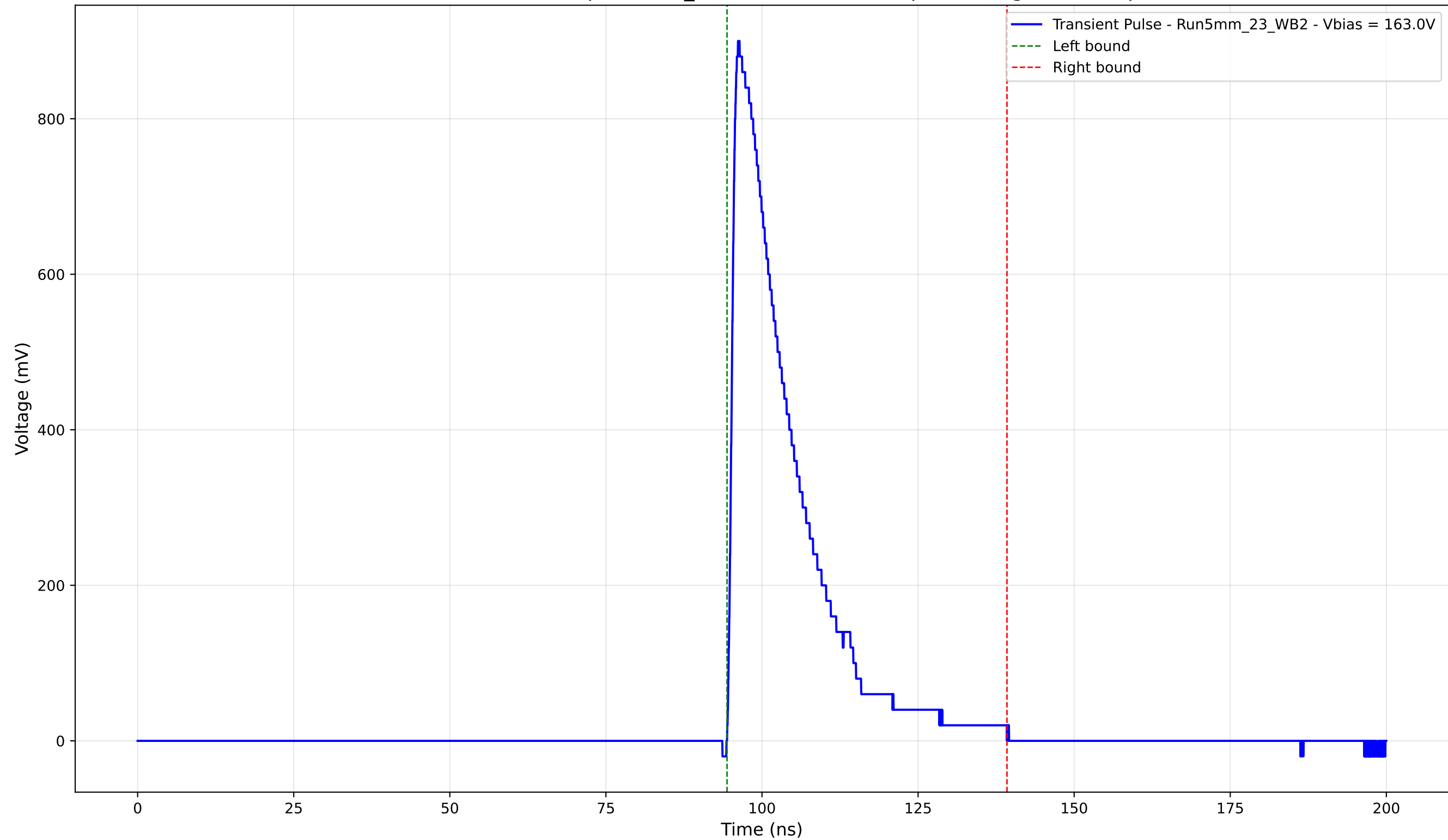
Transient Pulse - Sample: 5mm_23 - Position: 1155.0 \mu\text{m} - Charge: 191.78 pC
