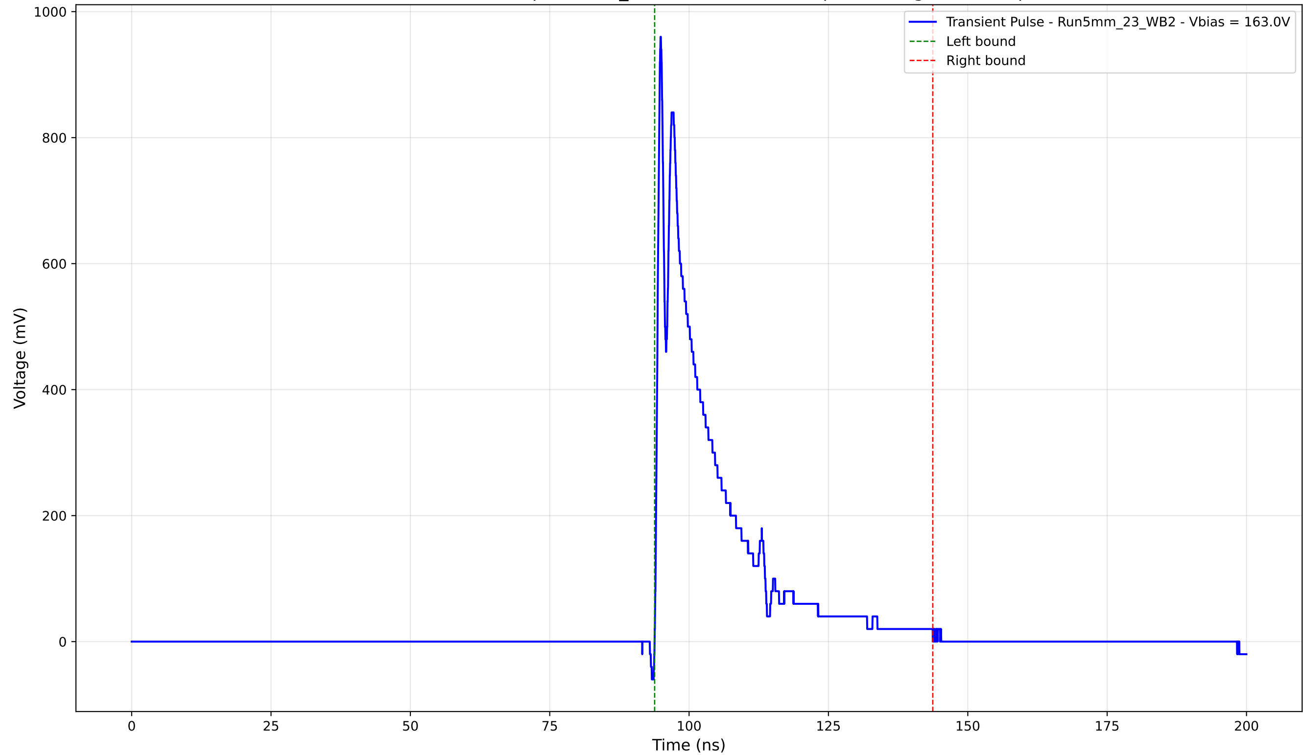
Transient Pulse - Sample: 5mm_23 - Position: 2440.0 \mu\text{m} - Charge: 171.24 pC
