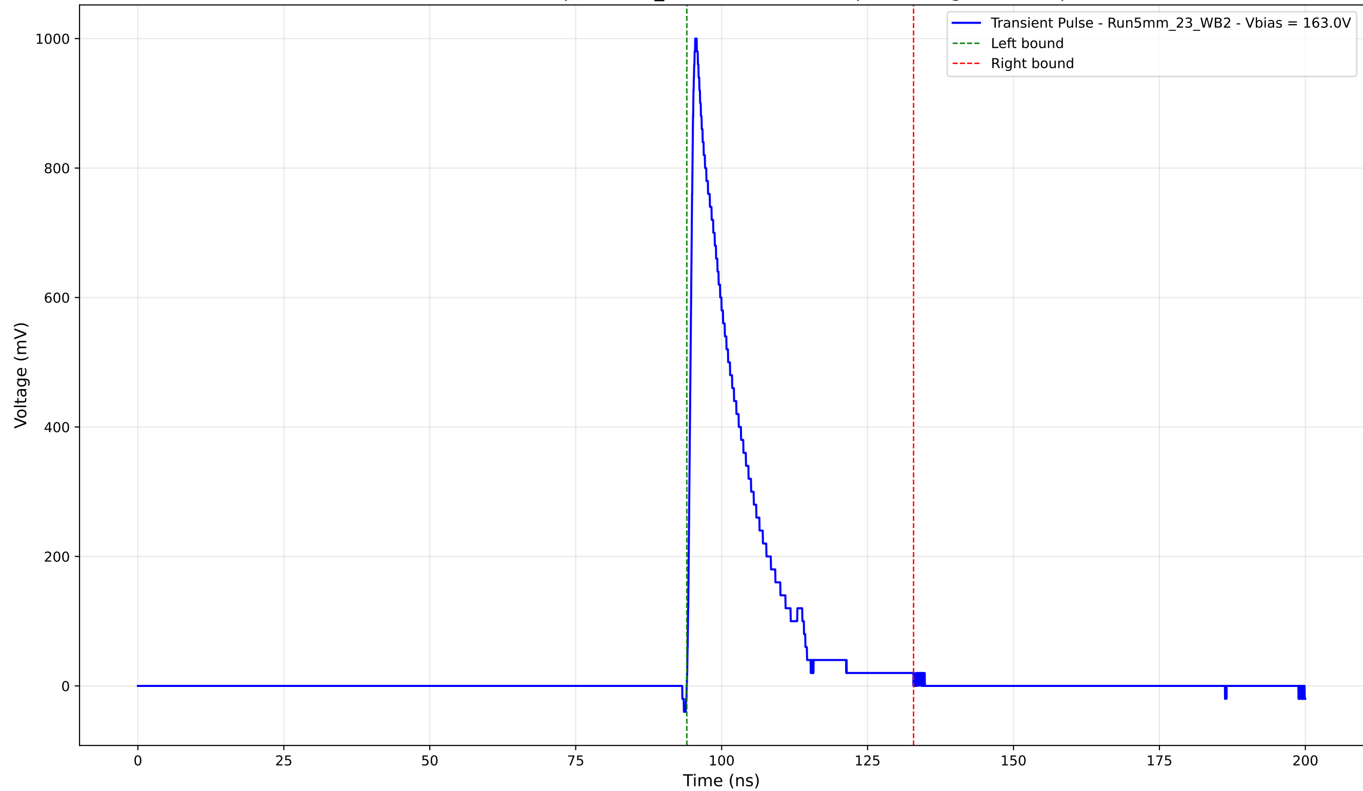
Transient Pulse - Sample: 5mm_23 - Position: 225.0 \mu\text{m} - Charge: 172.19 pC
