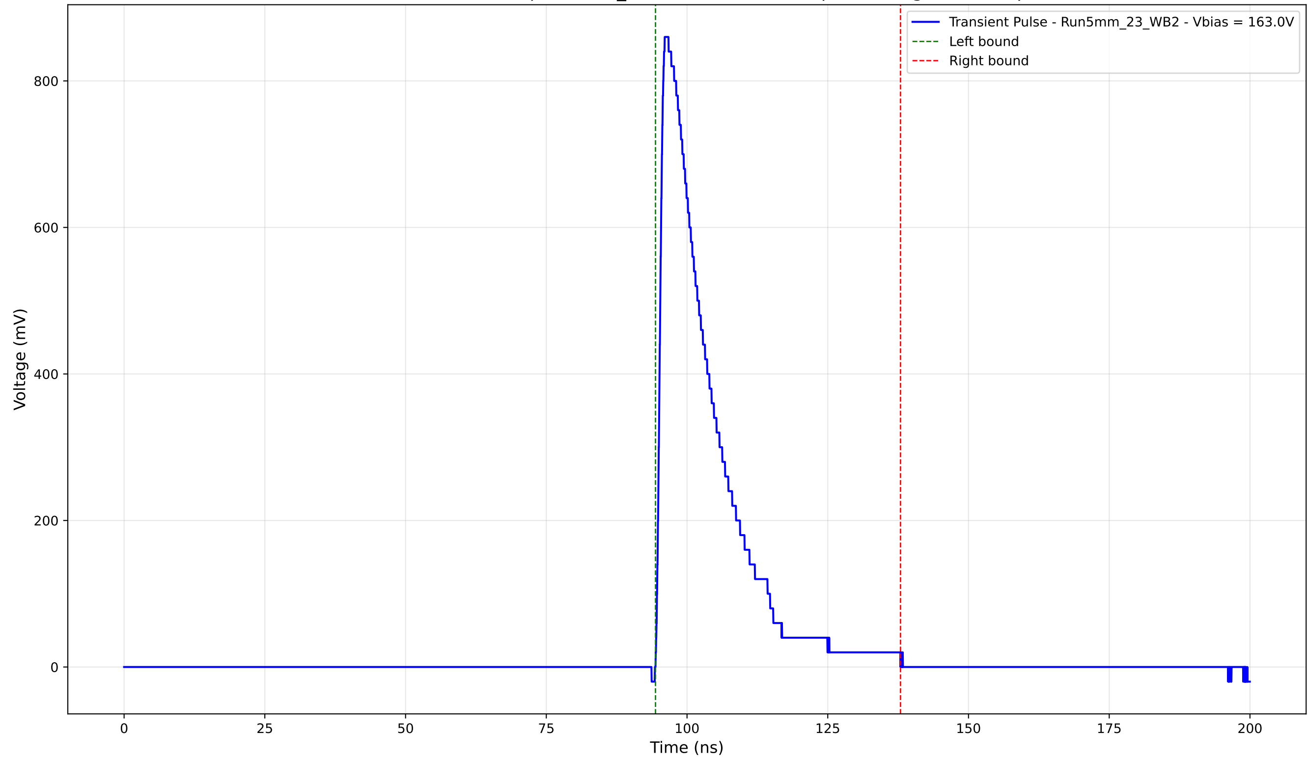
Transient Pulse - Sample: 5mm_23 - Position: 3815.0 \mu\text{m} - Charge: 176.11 pC
