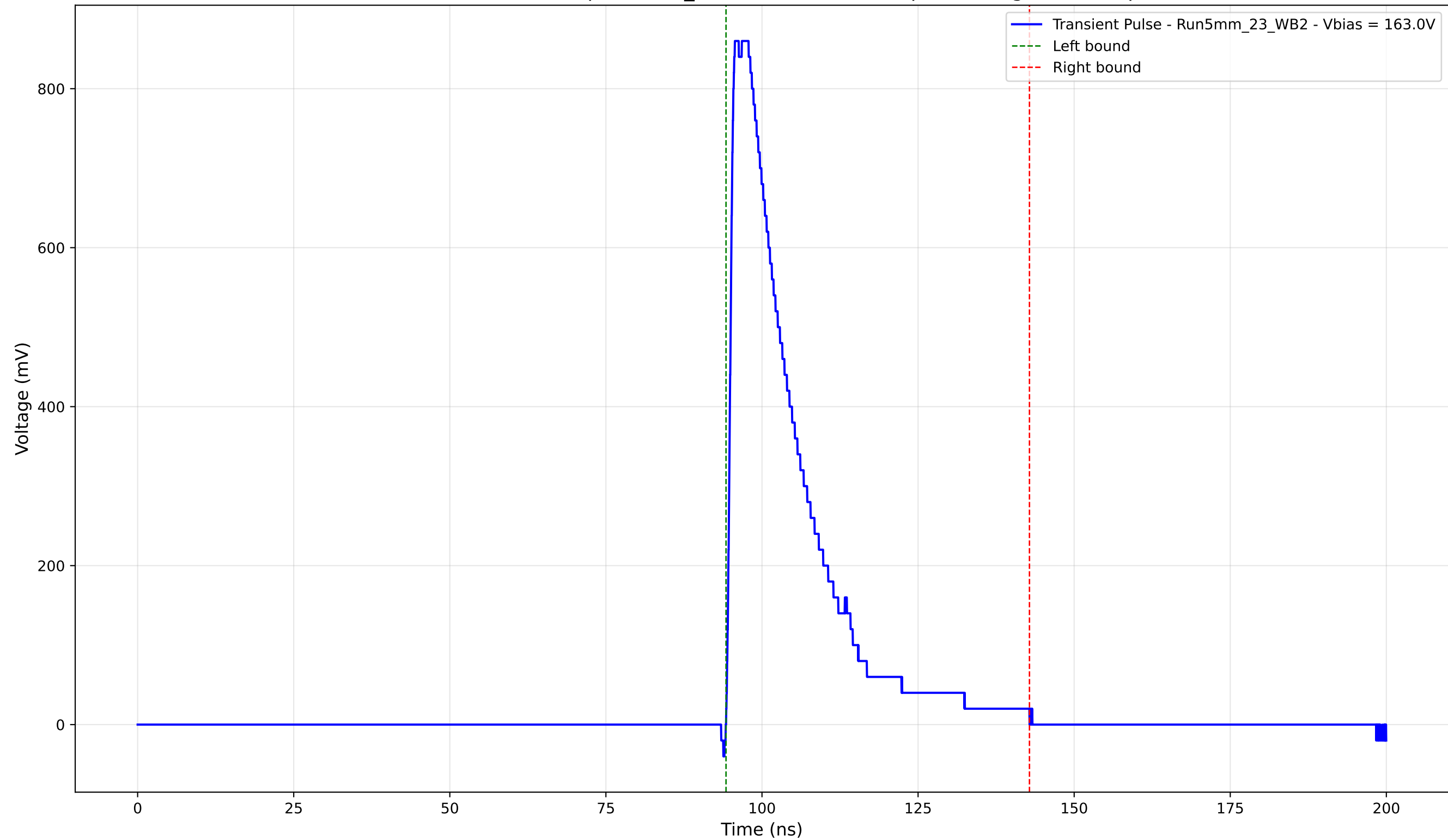
Transient Pulse - Sample: 5mm_23 - Position: 1635.0 \mu\text{m} - Charge: 200.89 pC
