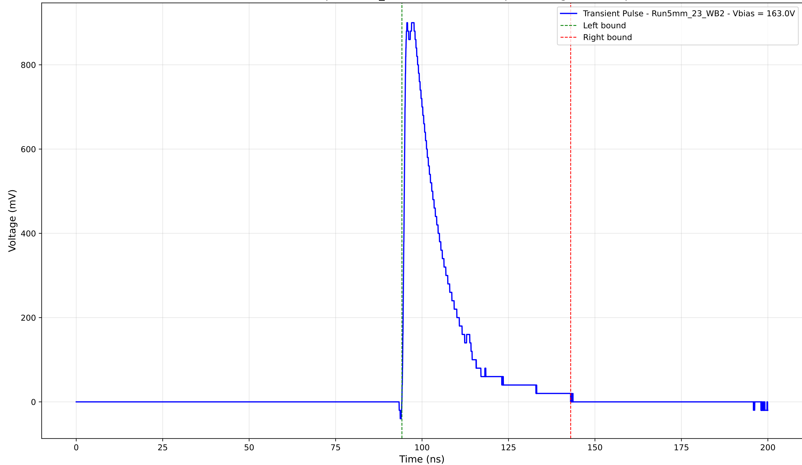
Transient Pulse - Sample: 5mm_23 - Position: 3290.0 \mu\text{m} - Charge: 209.07 pC
