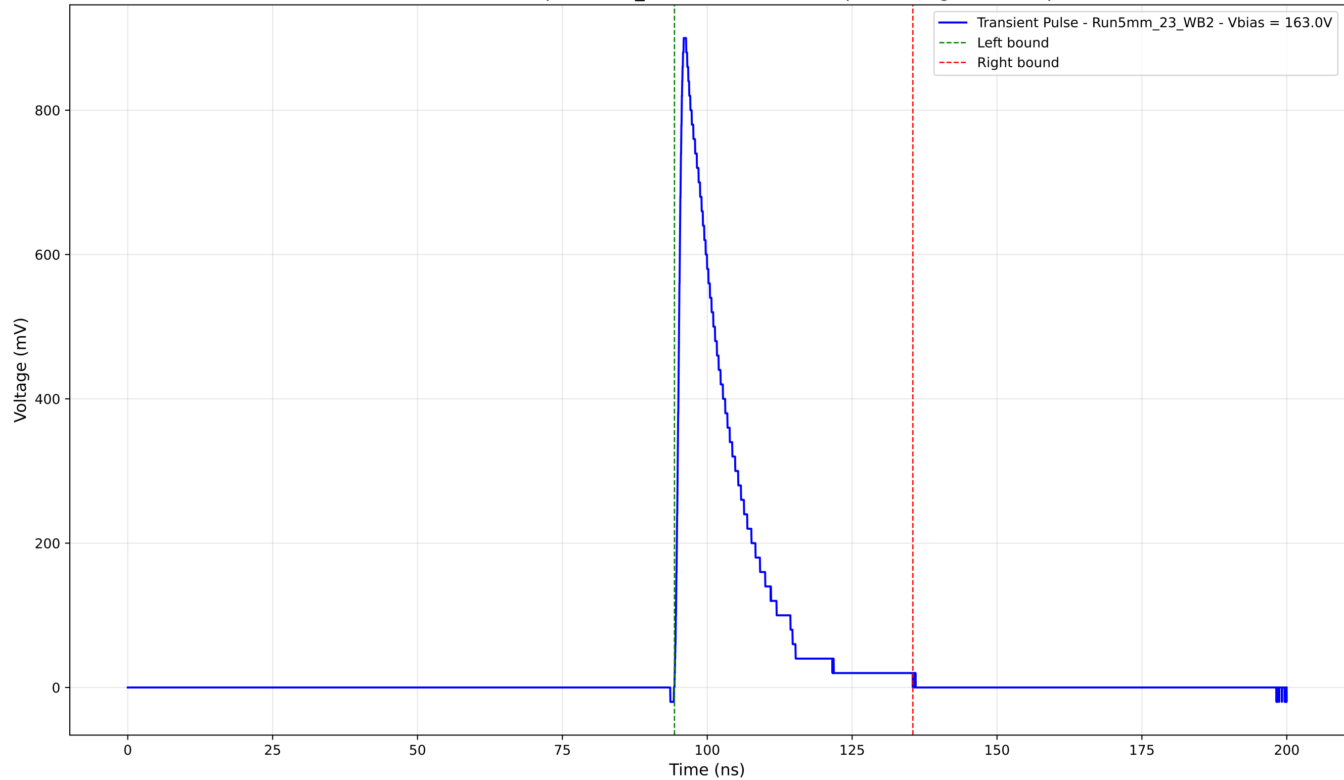
Transient Pulse - Sample: 5mm_23 - Position: 4315.0 \mu\text{m} - Charge: 162.39 pC
