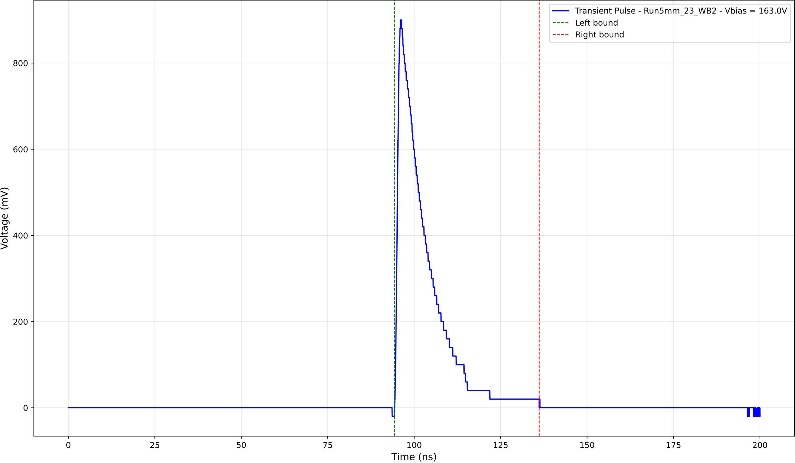
Transient Pulse - Sample: 5mm_23 - Position: 4245.0 \mu\text{m} - Charge: 164.14 pC
