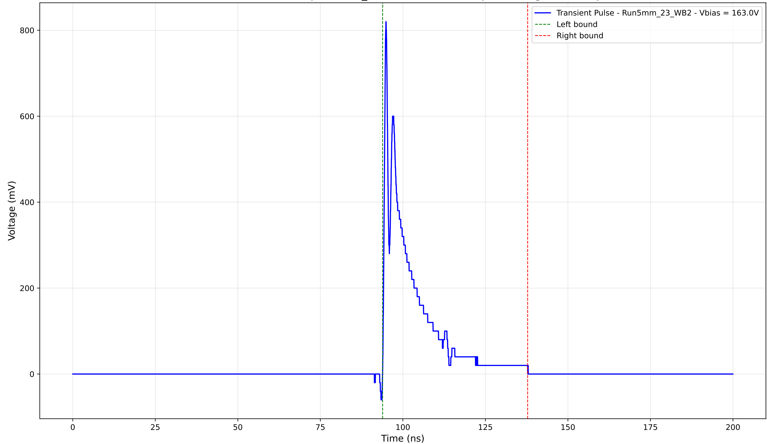
Transient Pulse - Sample: 5mm_23 - Position: 2470.0 \mu\text{m} - Charge: 111.81 pC
