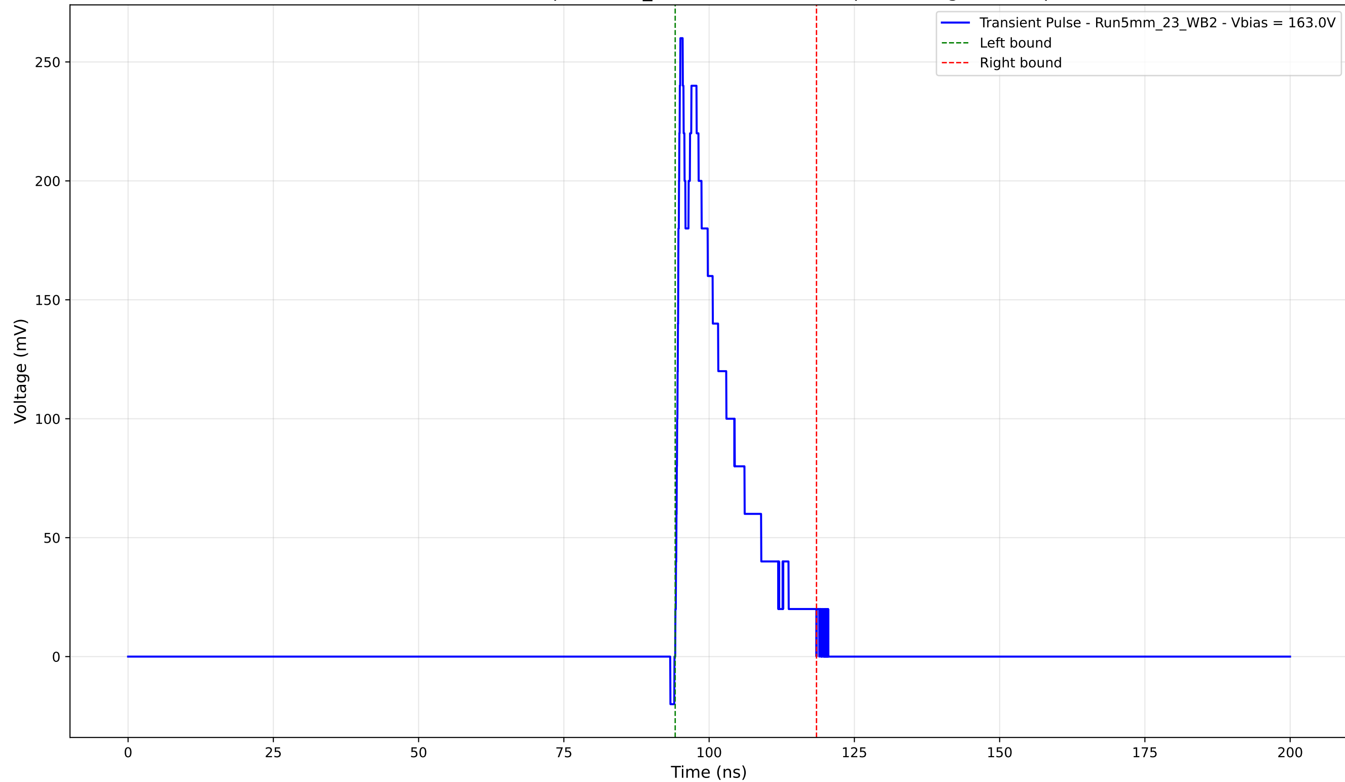
Transient Pulse - Sample: 5mm_23 - Position: 3010.0 \mu\text{m} - Charge: 45.28 pC
