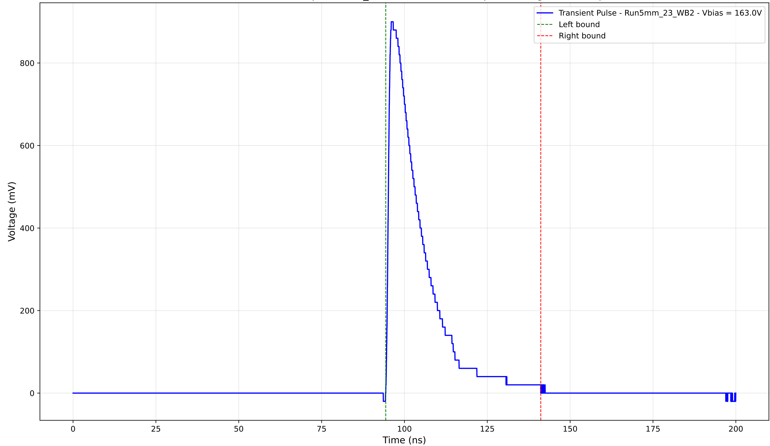
Transient Pulse - Sample: 5mm_23 - Position: 1300.0 \mu\text{m} - Charge: 201.05 pC
