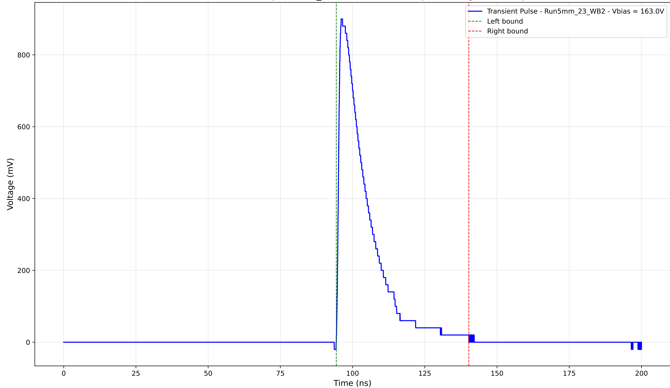
Transient Pulse - Sample: 5mm_23 - Position: 1320.0 \mu\text{m} - Charge: 200.36 pC
