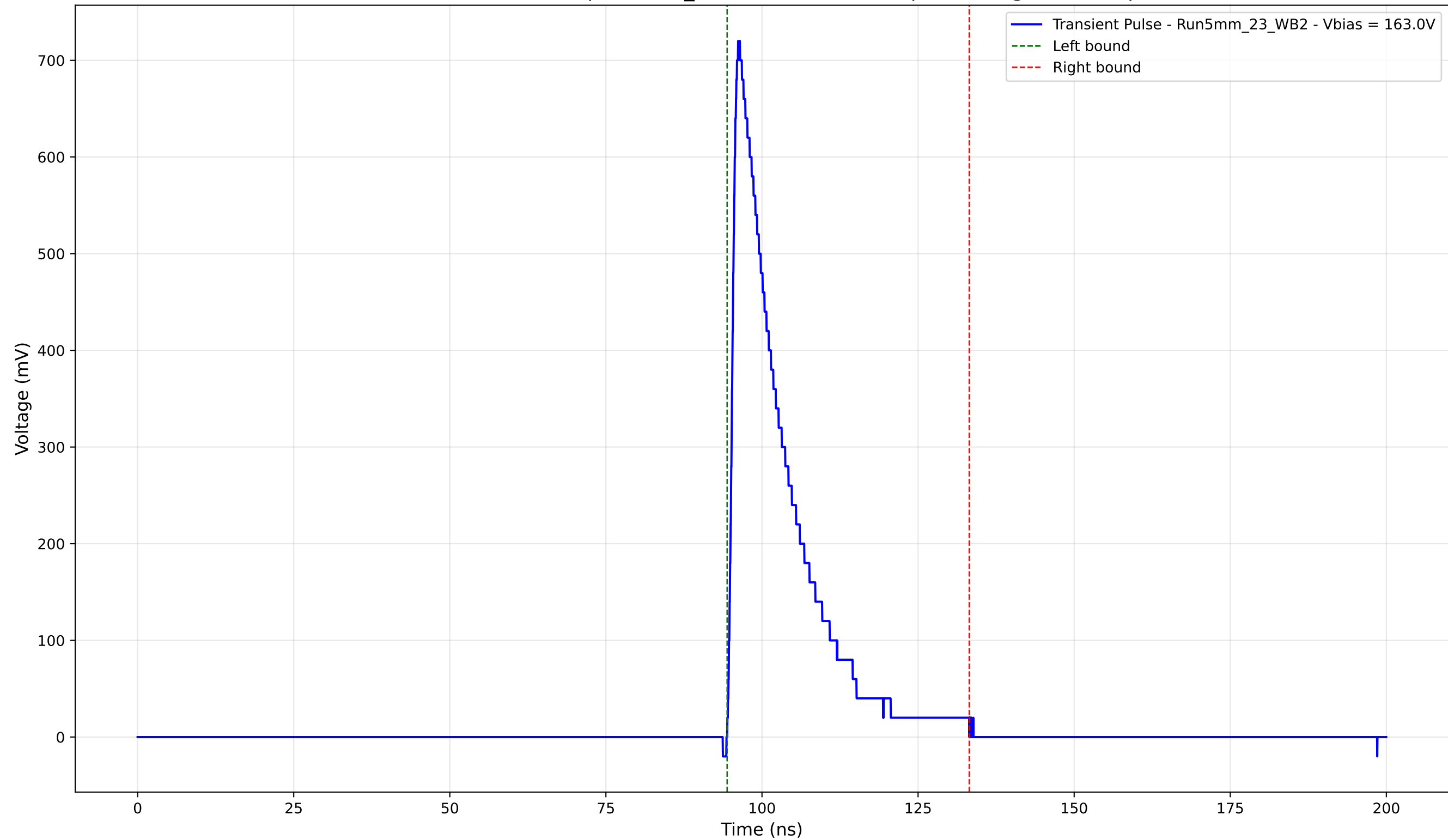
Transient Pulse - Sample: 5mm_23 - Position: 3970.0 \mu\text{m} - Charge: 130.38 pC
