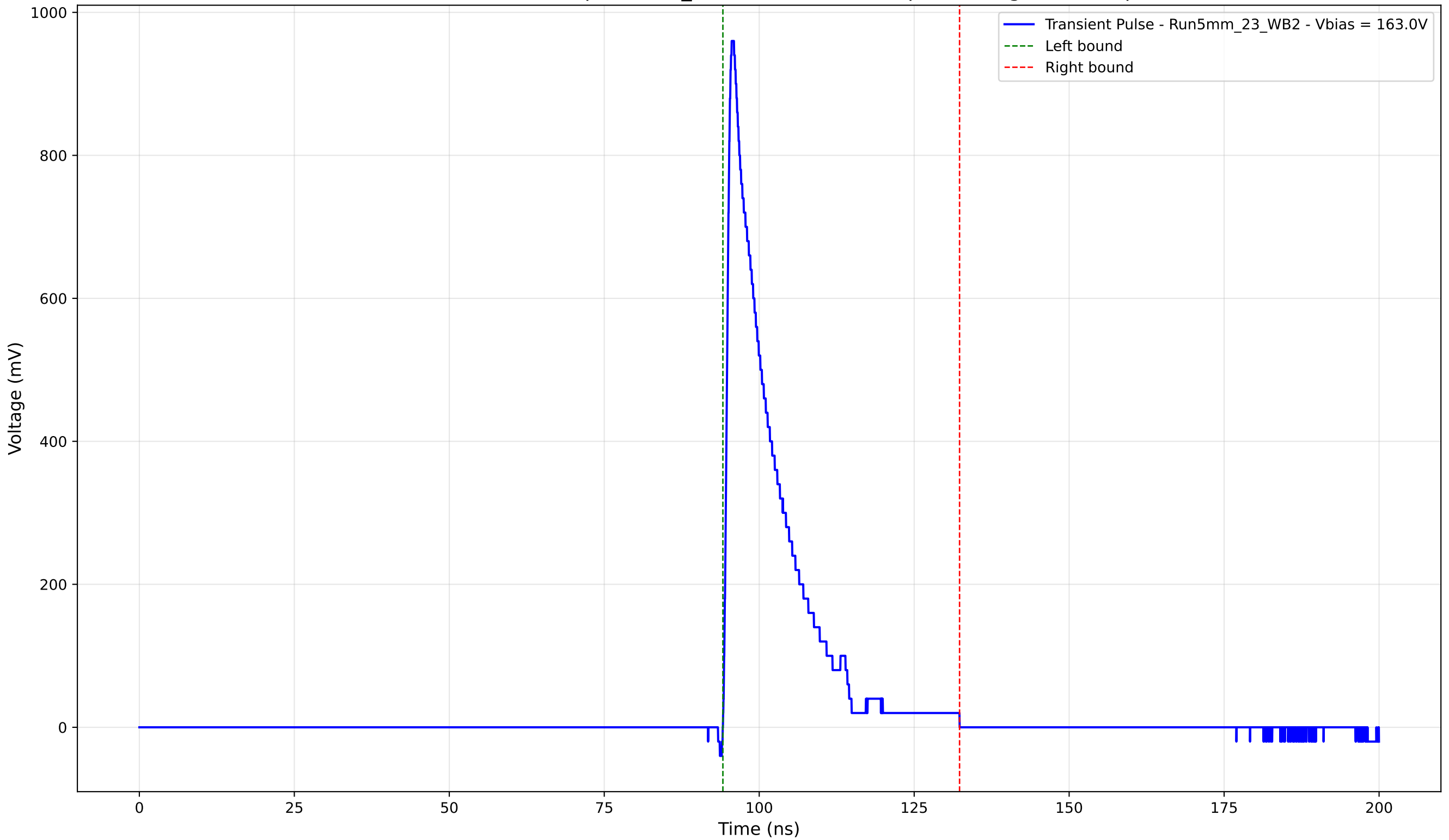
Transient Pulse - Sample: 5mm_23 - Position: 4720.0 \mu\text{m} - Charge: 151.98 pC
