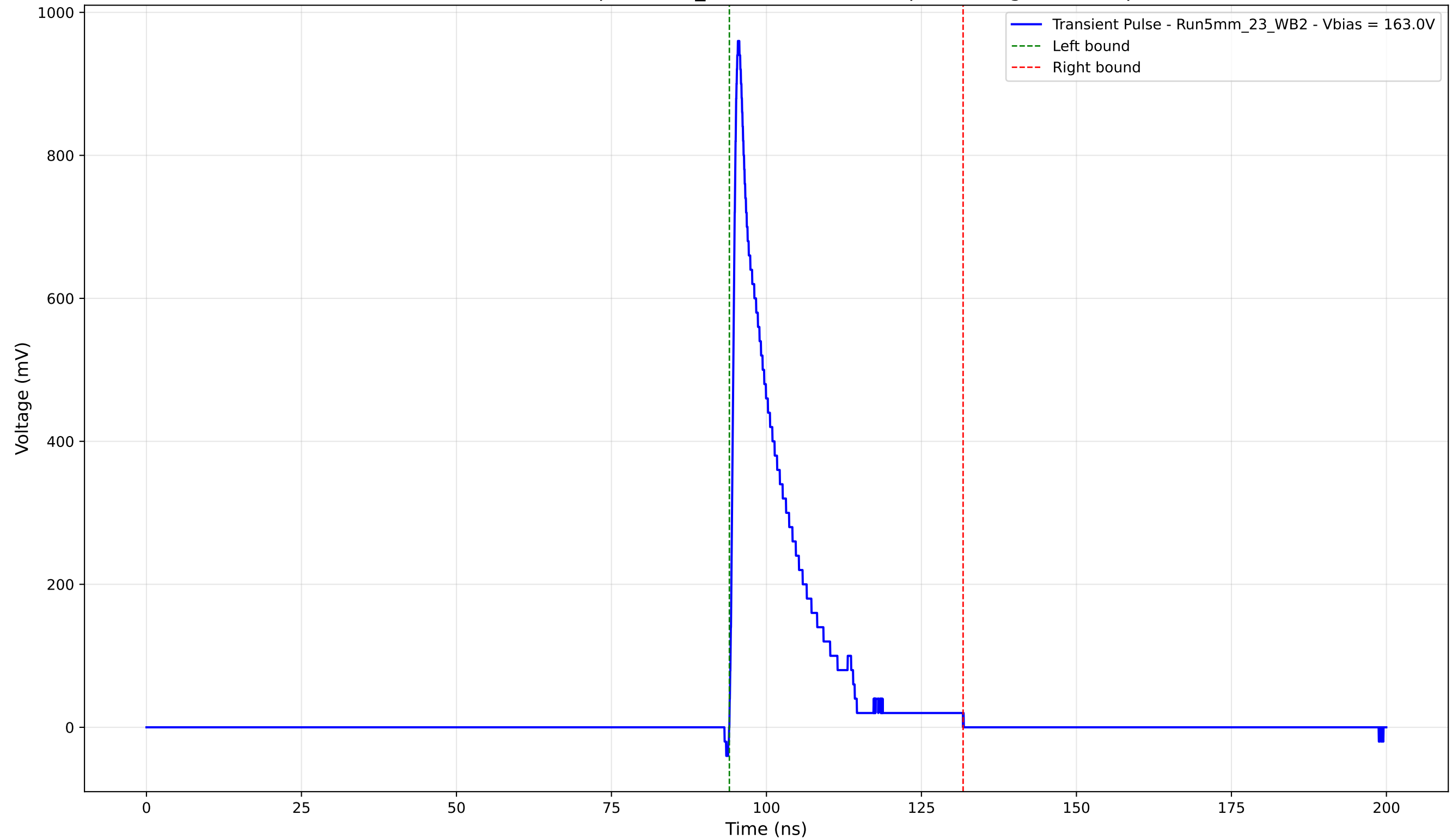
Transient Pulse - Sample: 5mm_23 - Position: 105.0 \mu\text{m} - Charge: 141.63 pC
