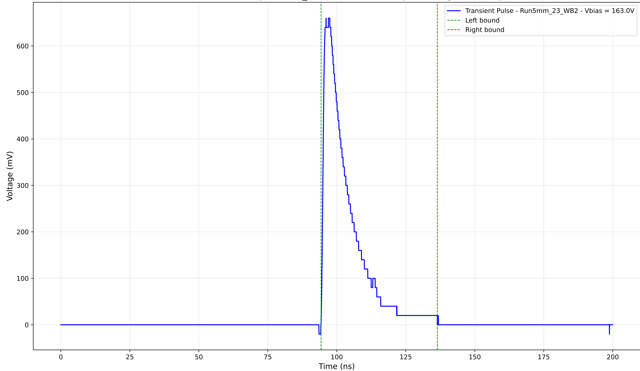
Transient Pulse - Sample: 5mm_23 - Position: 3460.0 \mu\text{m} - Charge: 134.97 pC
