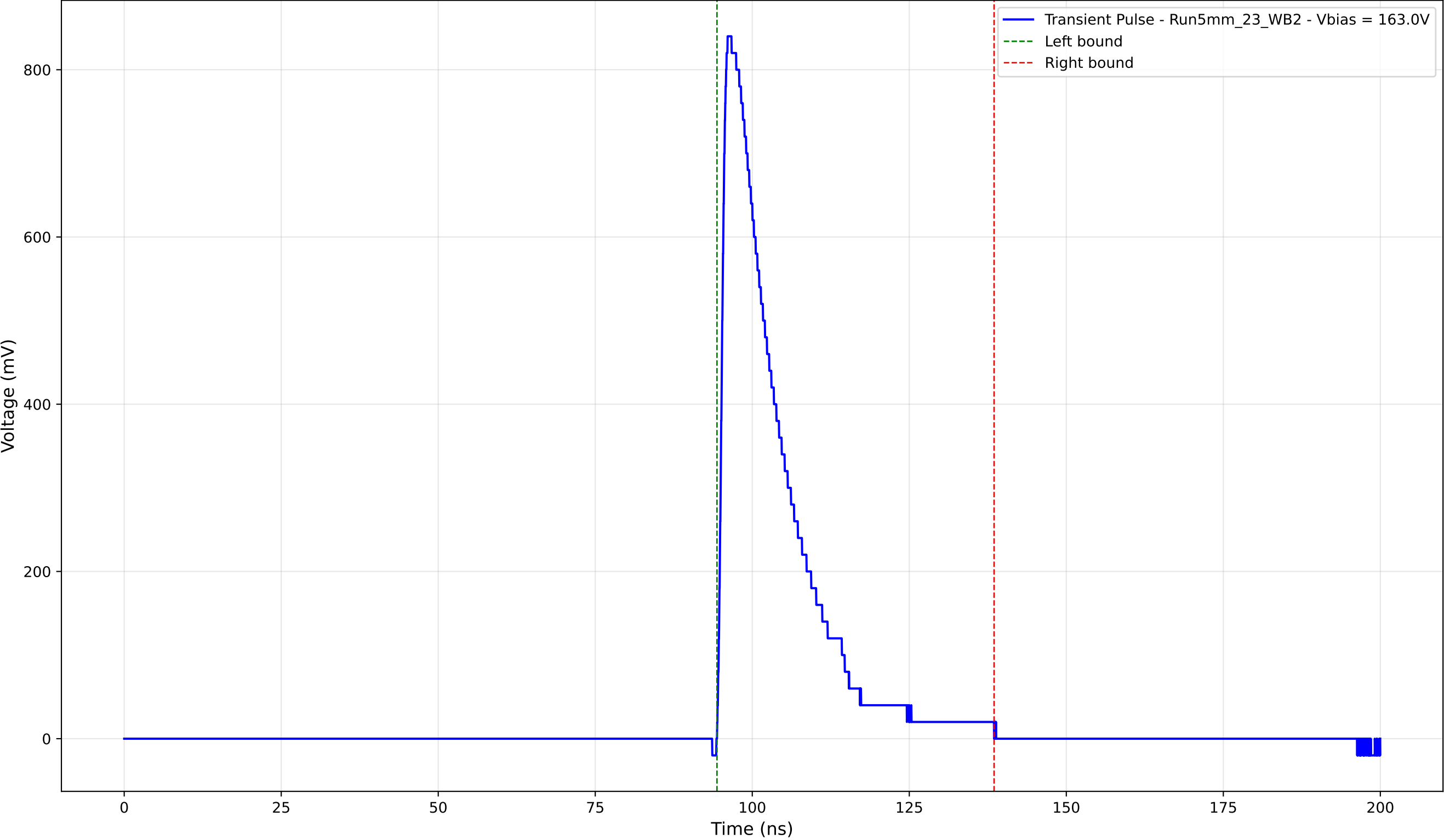
Transient Pulse - Sample: 5mm_23 - Position: 3695.0 \mu\text{m} - Charge: 174.47 pC
