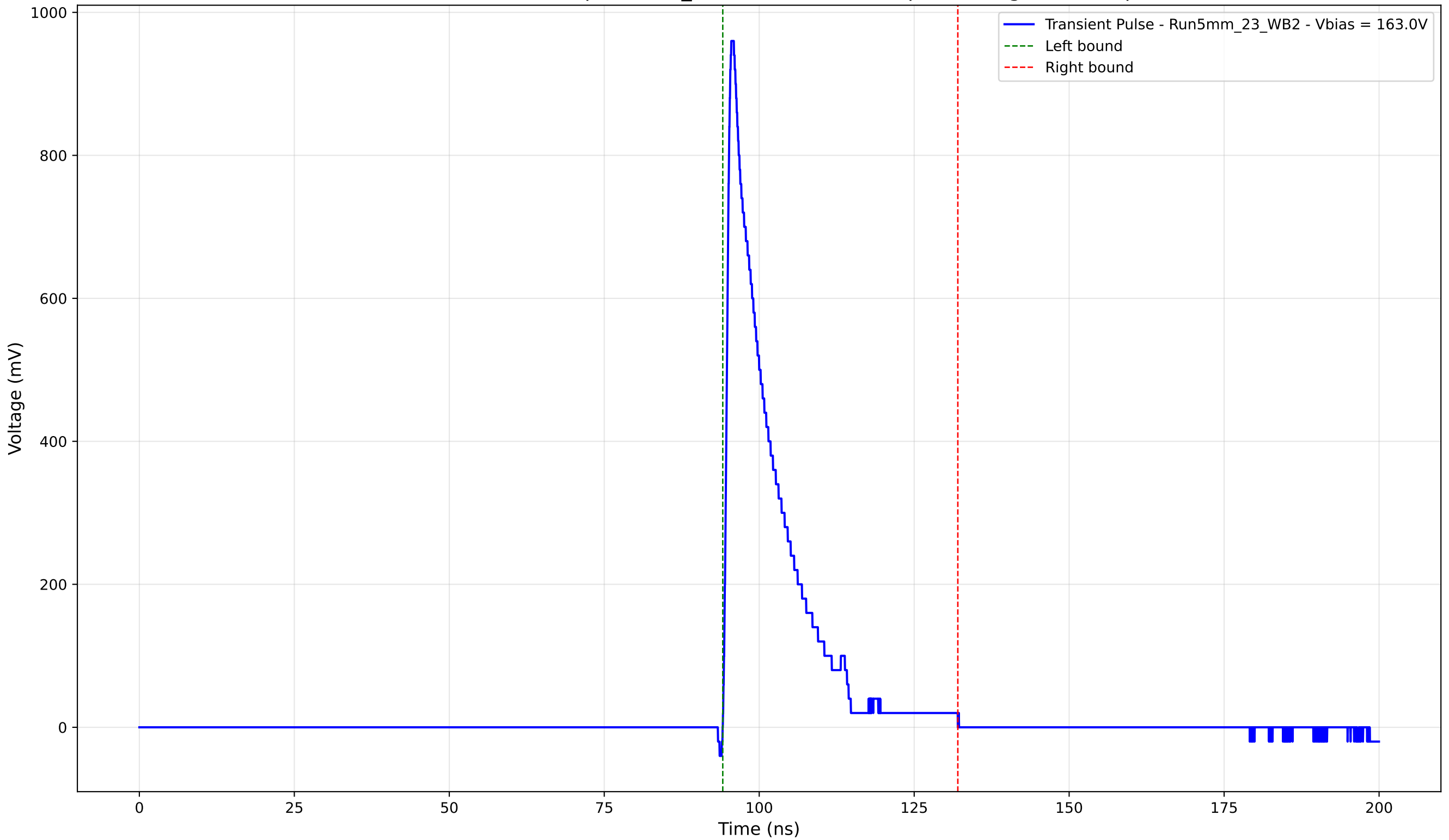
Transient Pulse - Sample: 5mm_23 - Position: 4760.0 \mu\text{m} - Charge: 148.63 pC
