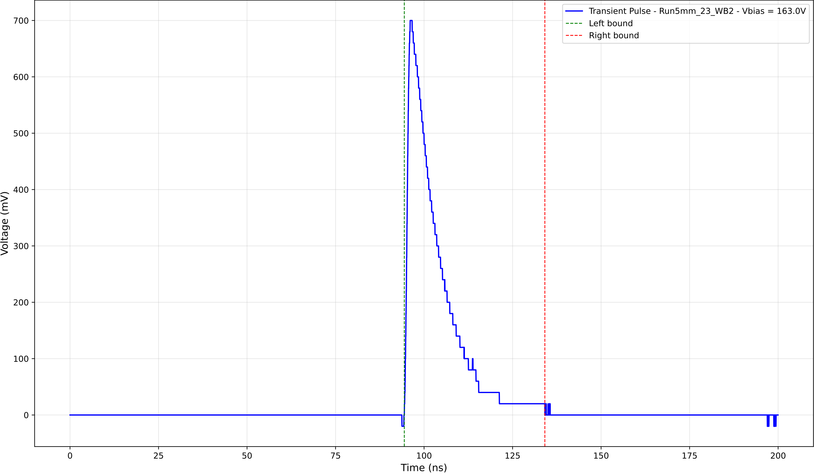
Transient Pulse - Sample: 5mm_23 - Position: 1055.0 \mu\text{m} - Charge: 134.33 pC
