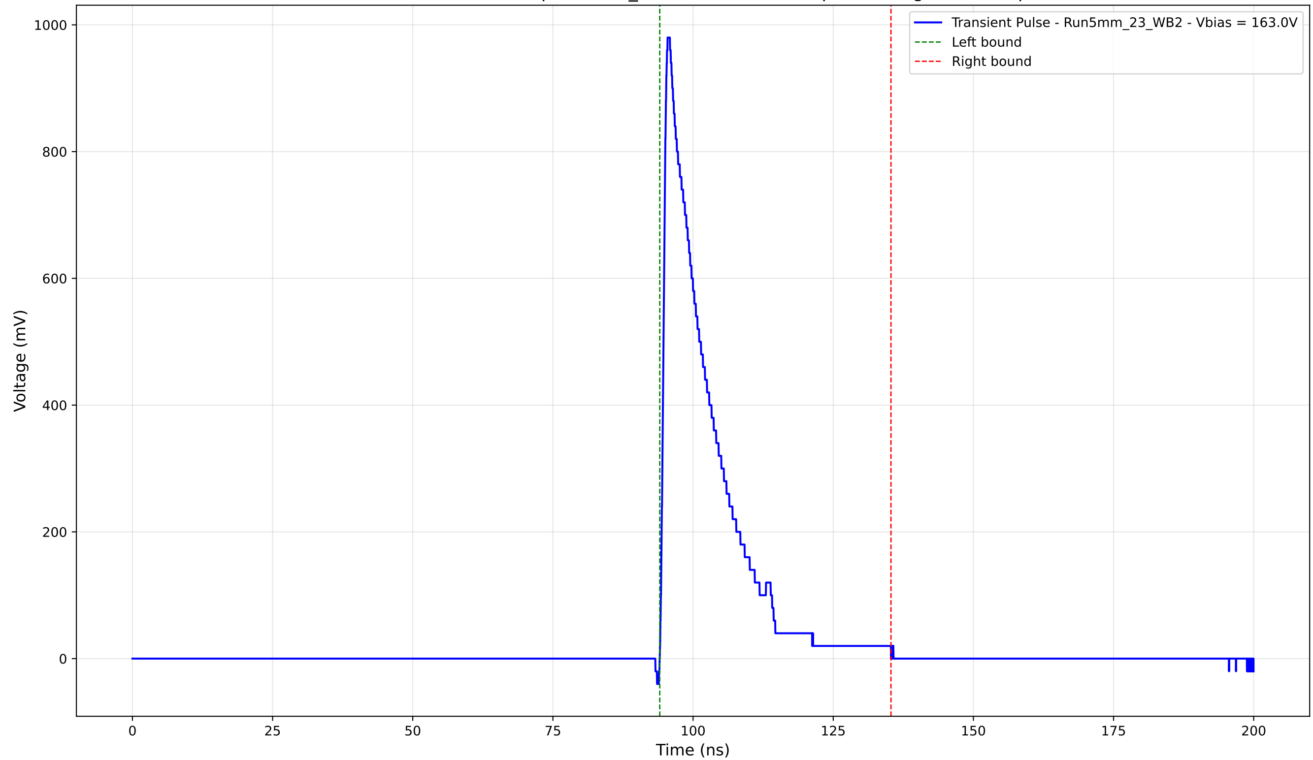
Transient Pulse - Sample: 5mm_23 - Position: 255.0 \mu\text{m} - Charge: 172.14 pC
