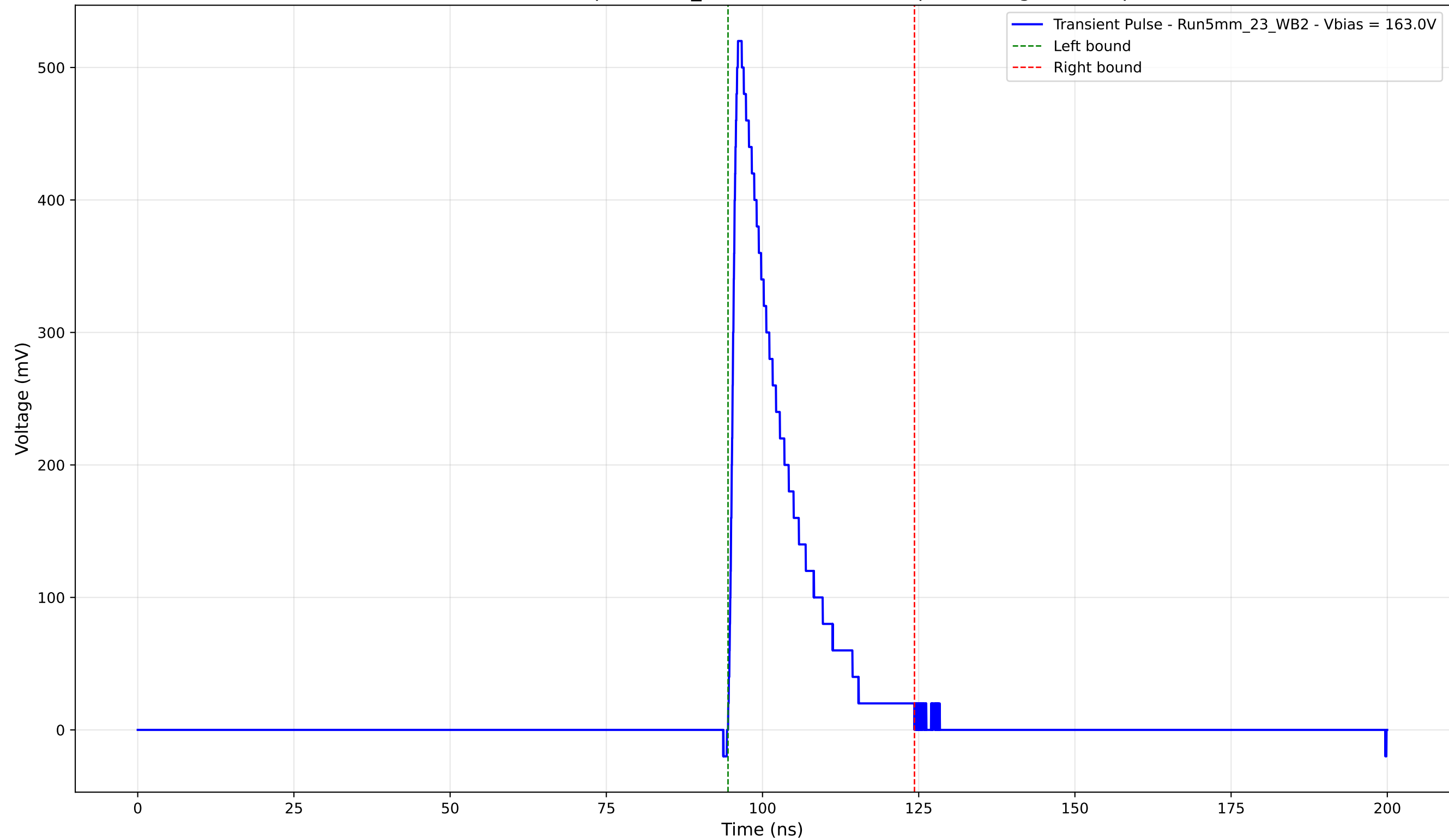
Transient Pulse - Sample: 5mm_23 - Position: 3990.0 \mu\text{m} - Charge: 89.89 pC
