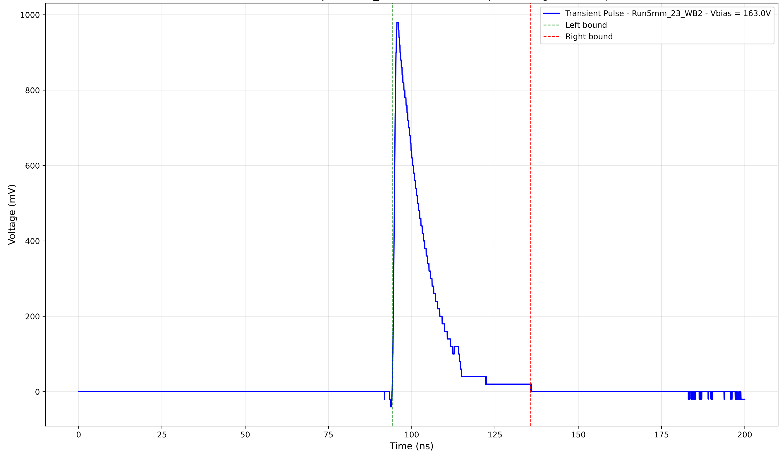
Transient Pulse - Sample: 5mm_23 - Position: 370.0 \mu\text{m} - Charge: 181.08 pC
