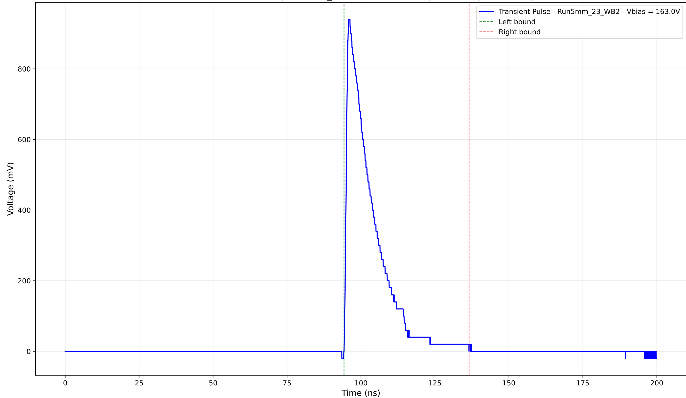
Transient Pulse - Sample: 5mm_23 - Position: 620.0 \mu\text{m} - Charge: 182.54 pC
