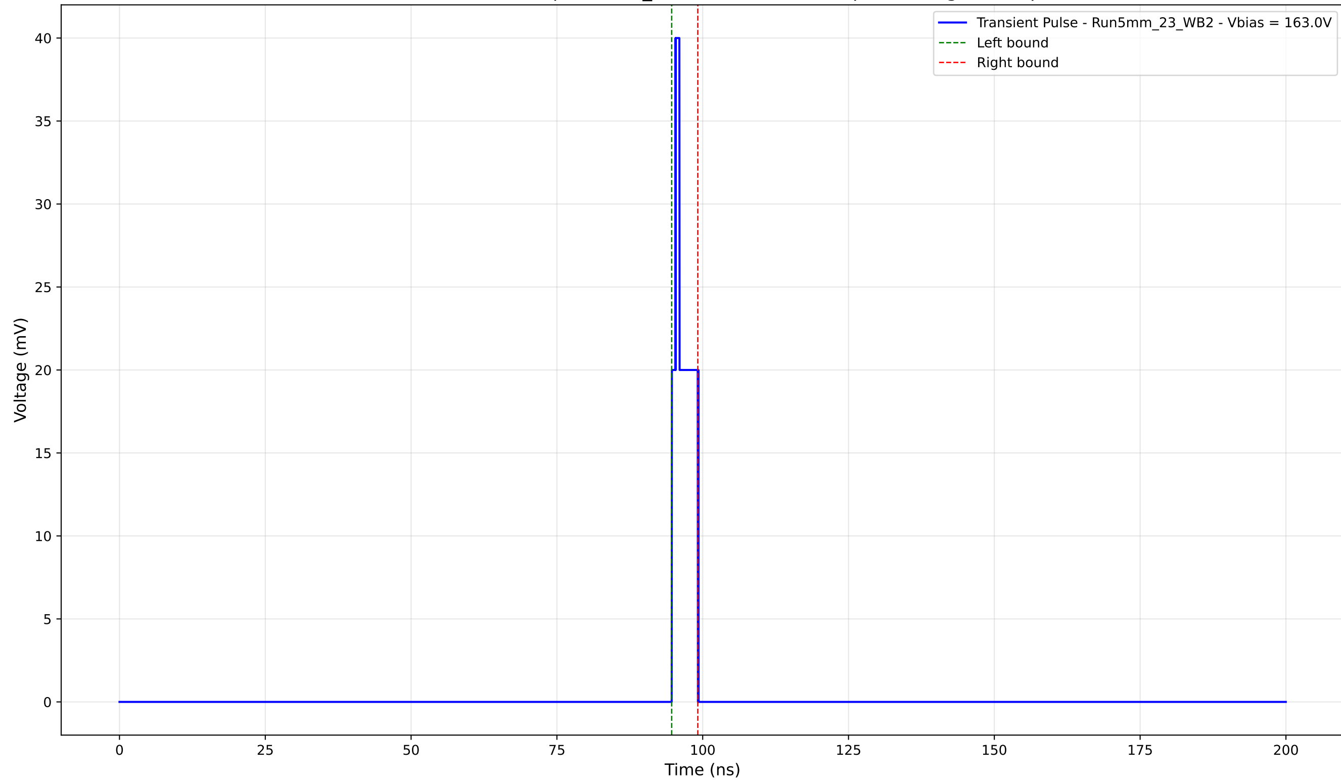
Transient Pulse - Sample: 5mm_23 - Position: 5015.0 \mu\text{m} - Charge: 2.05 pC
