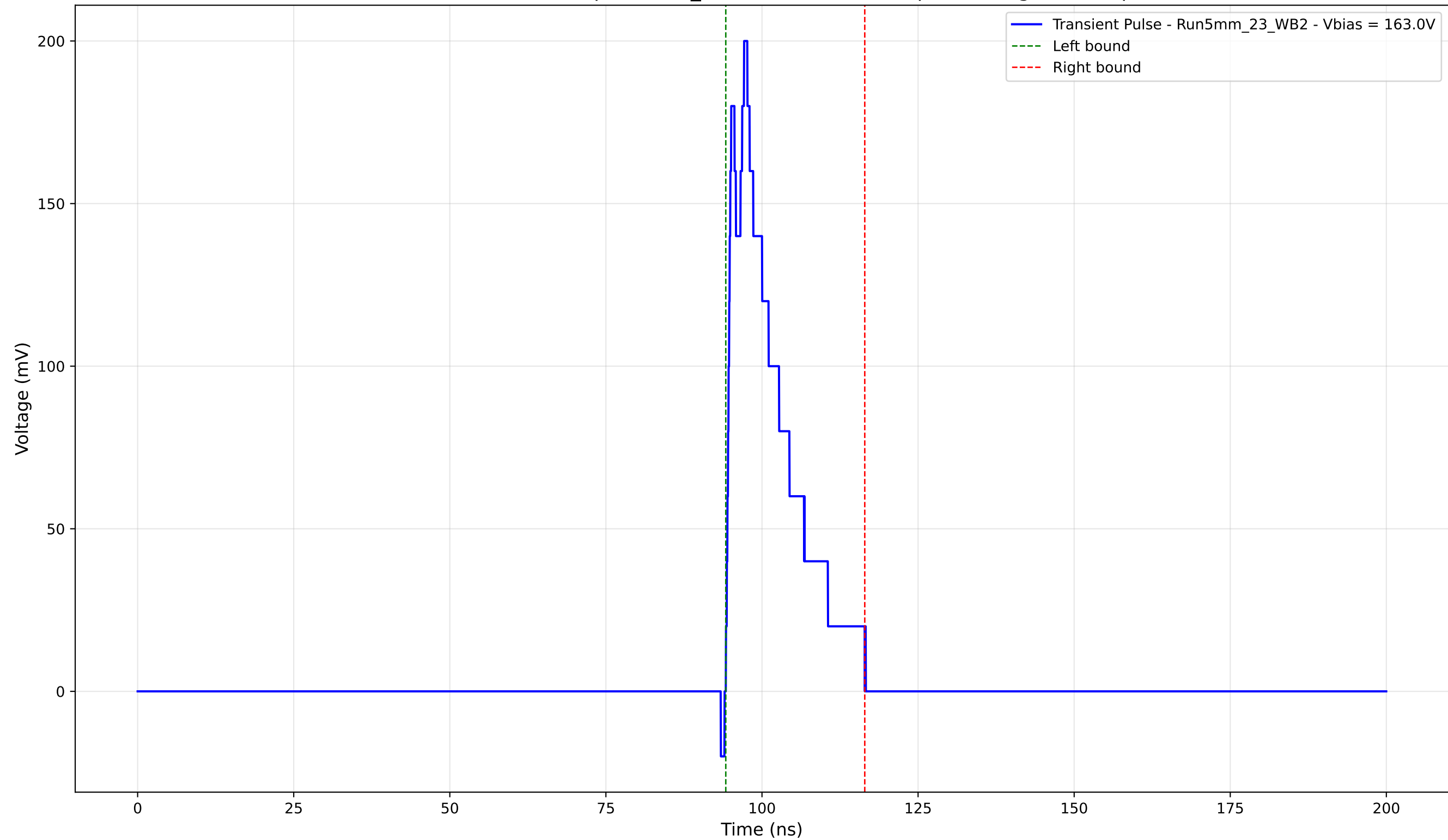
Transient Pulse - Sample: 5mm_23 - Position: 2010.0 \mu\text{m} - Charge: 34.17 pC
