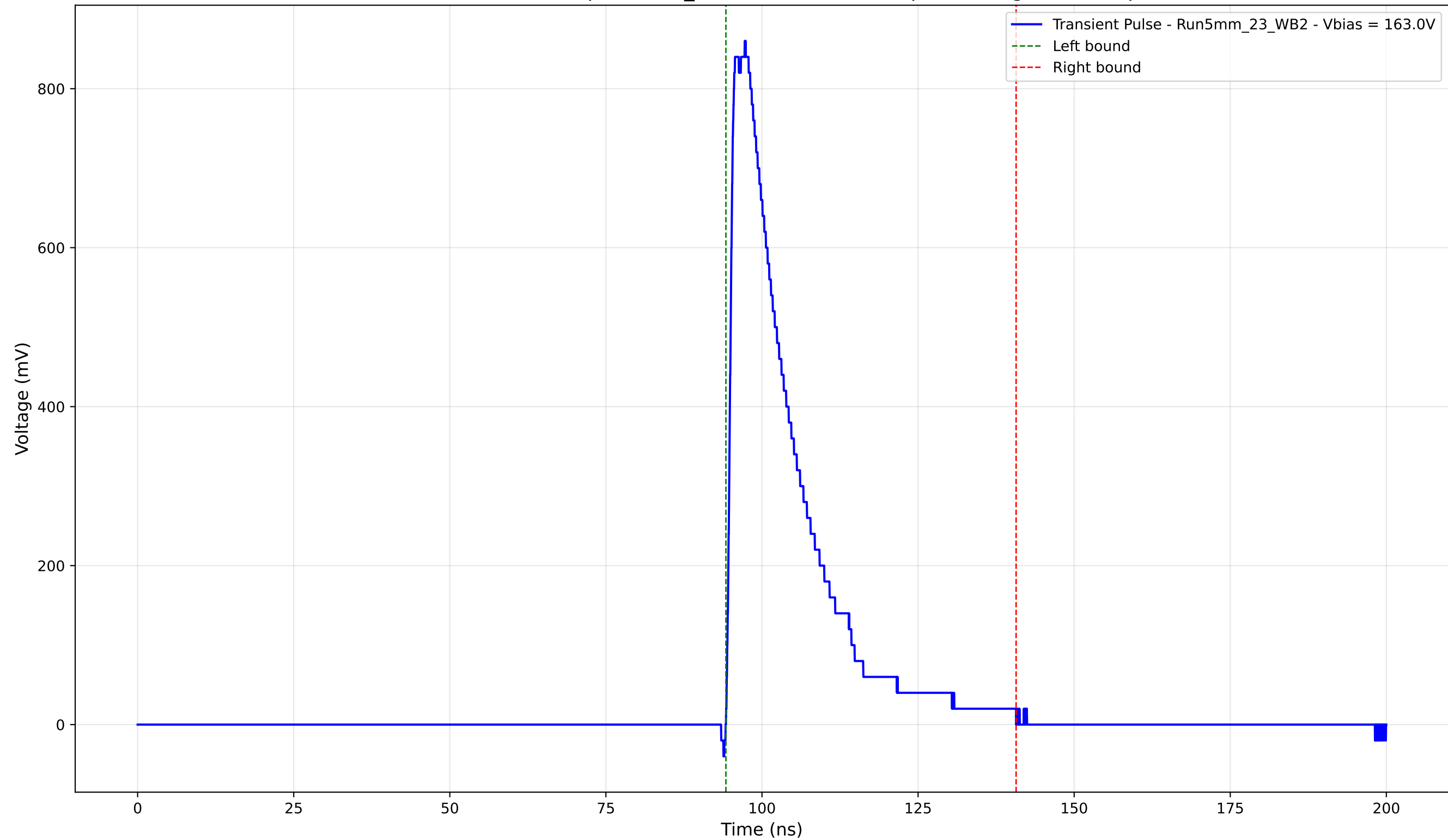
Transient Pulse - Sample: 5mm_23 - Position: 3375.0 \mu\text{m} - Charge: 190.84 pC
