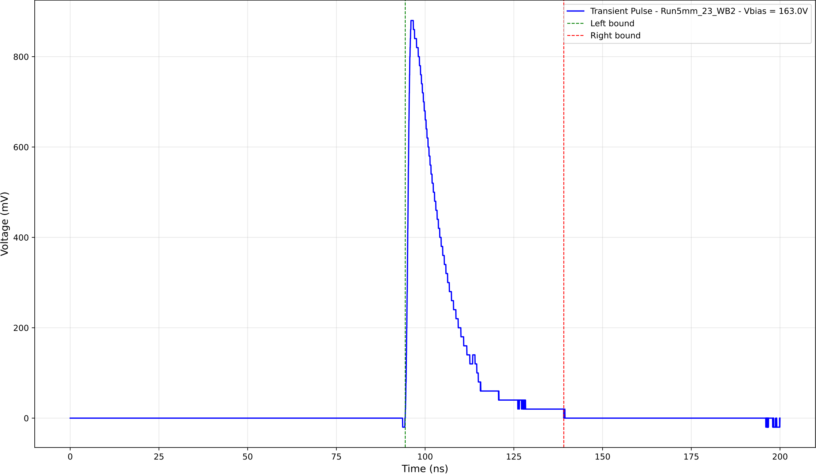
Transient Pulse - Sample: 5mm_23 - Position: 1120.0 \mu\text{m} - Charge: 187.70 pC
