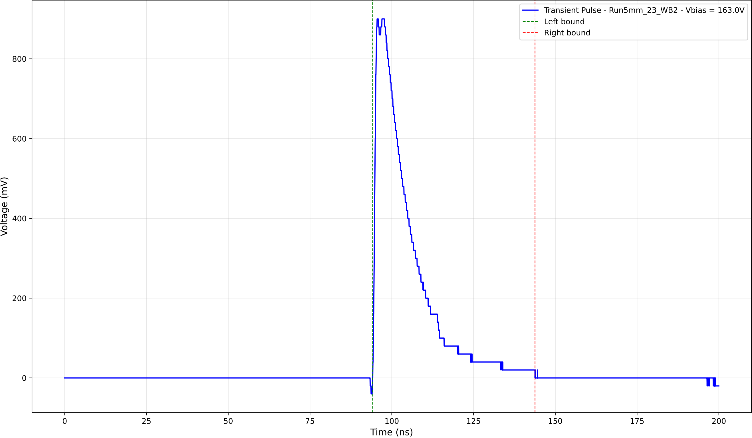
Transient Pulse - Sample: 5mm_23 - Position: 1755.0 \mu\text{m} - Charge: 214.96 pC
