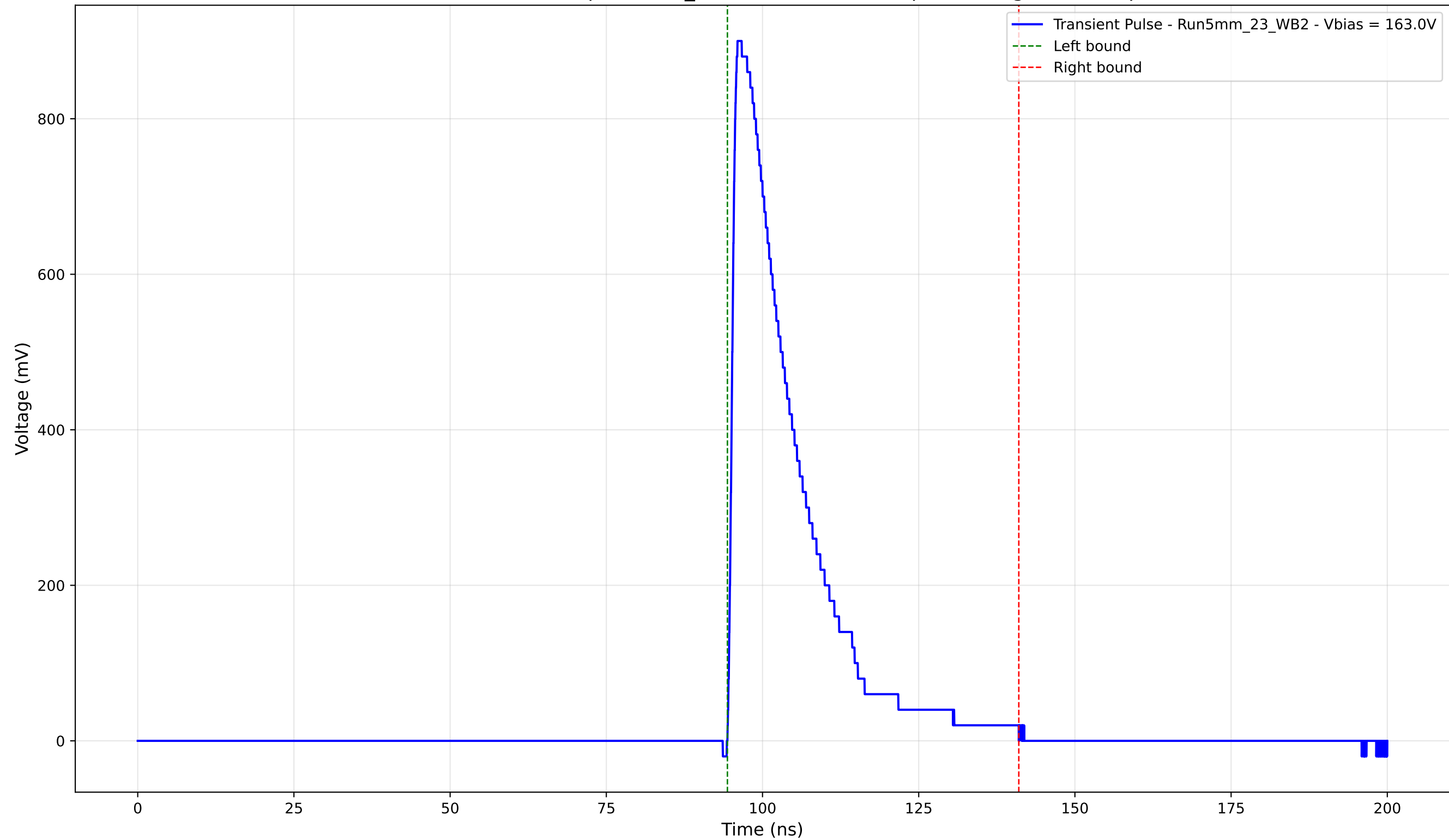
Transient Pulse - Sample: 5mm_23 - Position: 1280.0 \mu\text{m} - Charge: 201.01 pC
