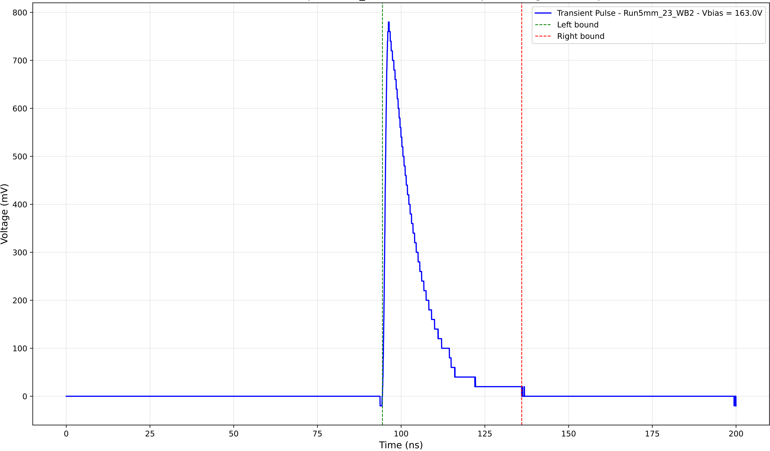
Transient Pulse - Sample: 5mm_23 - Position: 1065.0 \mu\text{m} - Charge: 150.59 pC
