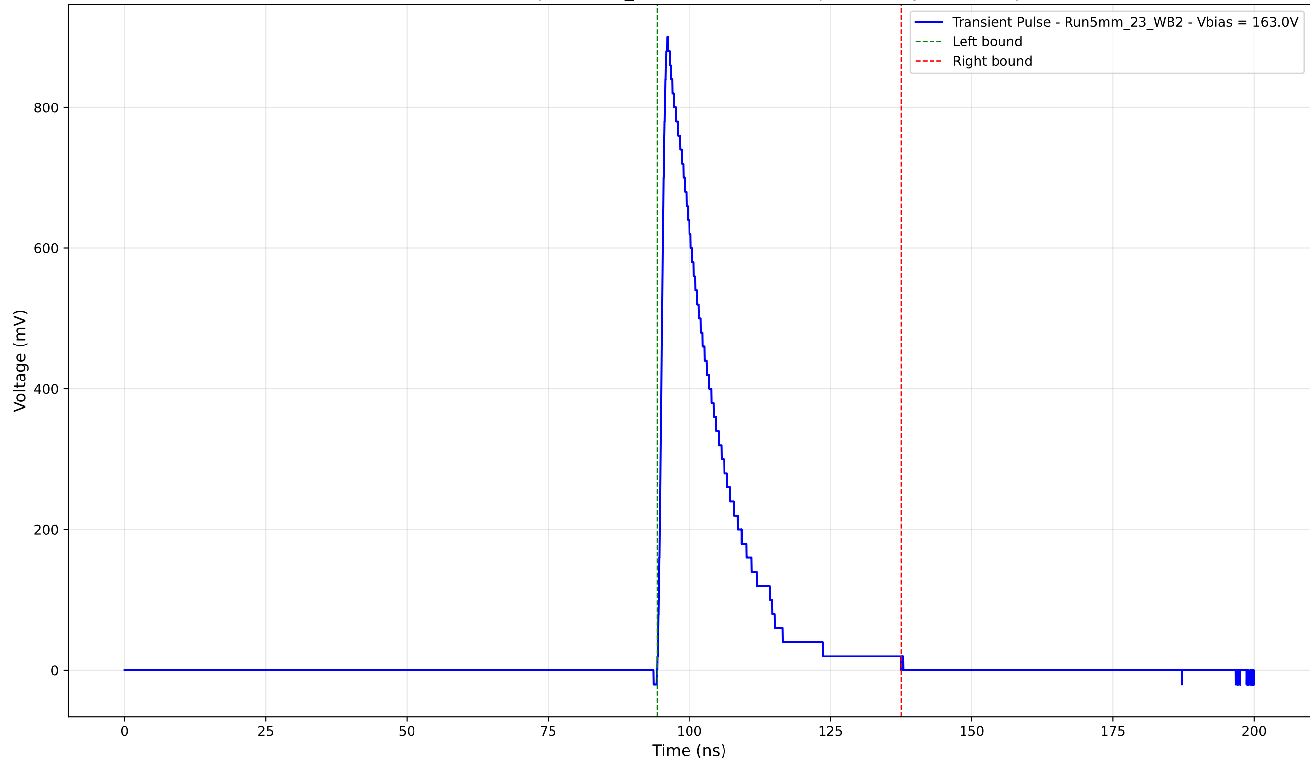
Transient Pulse - Sample: 5mm_23 - Position: 825.0 \mu\text{m} - Charge: 174.34 pC
