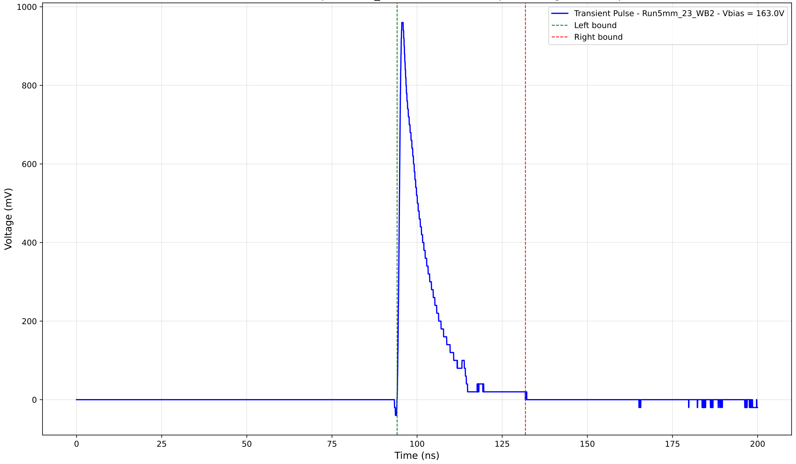
Transient Pulse - Sample: 5mm_23 - Position: 4740.0 \mu\text{m} - Charge: 150.18 pC
