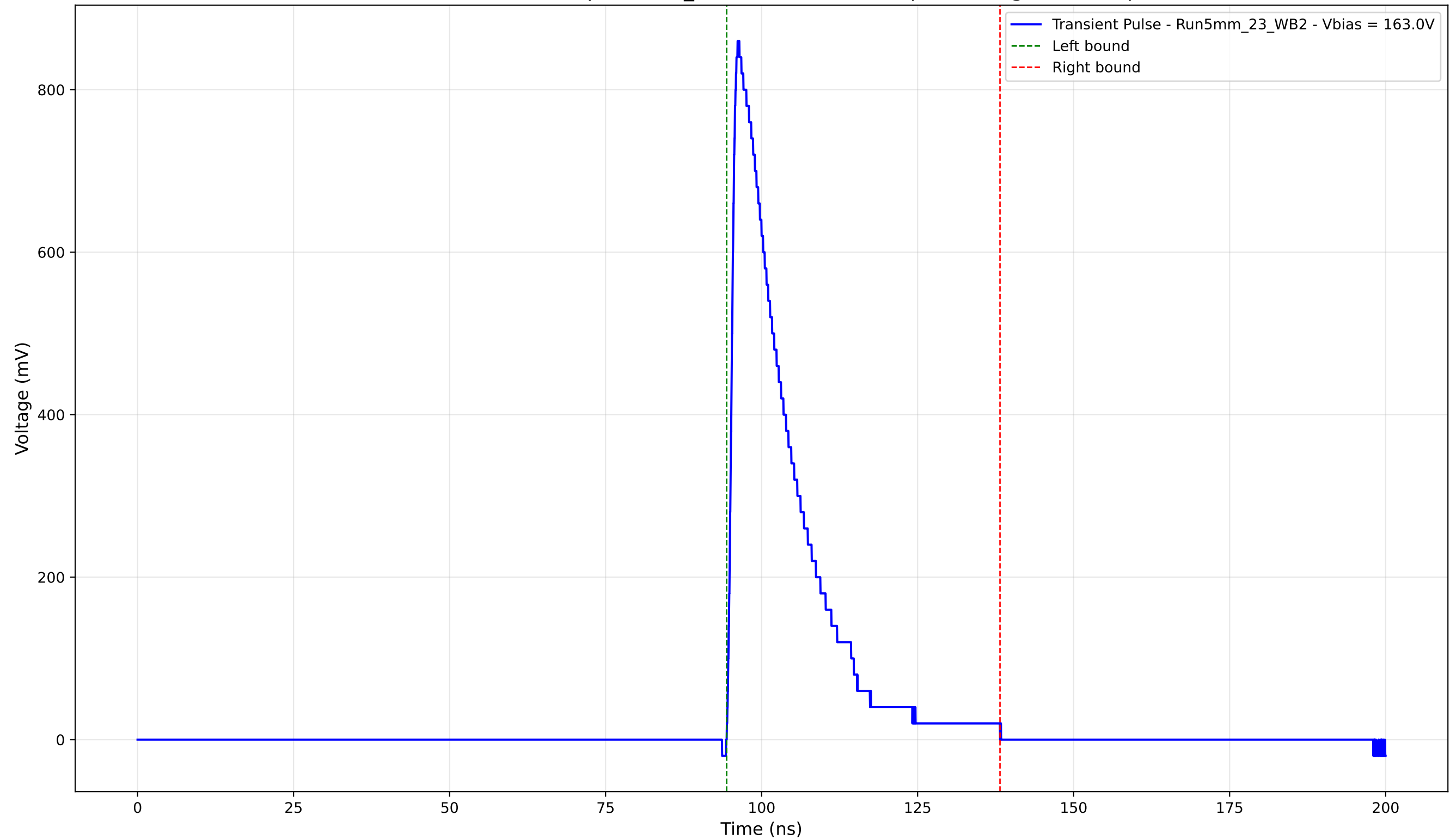
Transient Pulse - Sample: 5mm_23 - Position: 1085.0 \mu\text{m} - Charge: 173.78 pC
