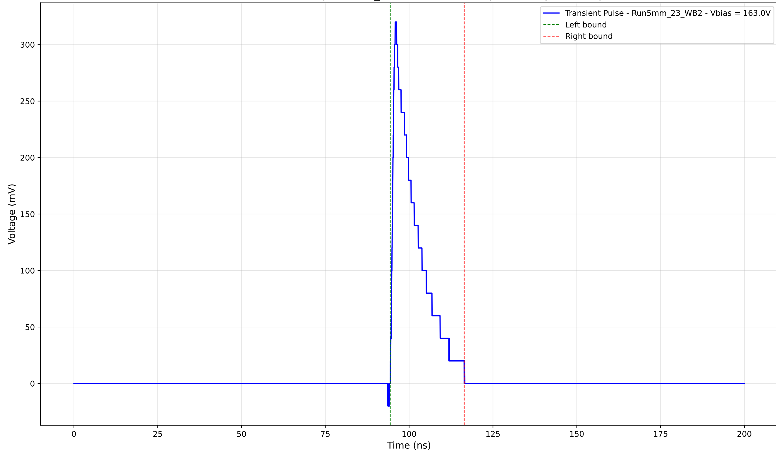
Transient Pulse - Sample: 5mm_23 - Position: 510.0 \mu\text{m} - Charge: 48.83 pC
