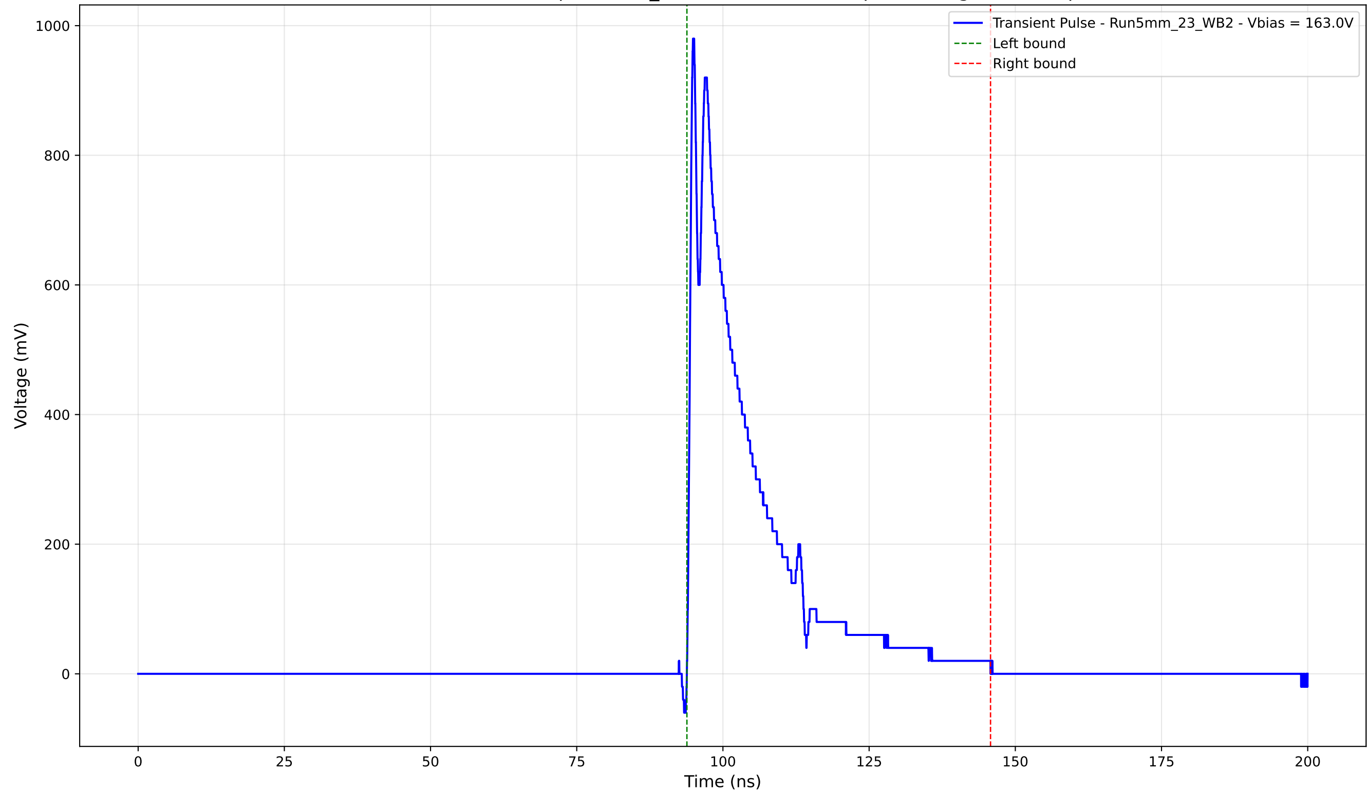
Transient Pulse - Sample: 5mm_23 - Position: 2665.0 \mu\text{m} - Charge: 201.50 pC
