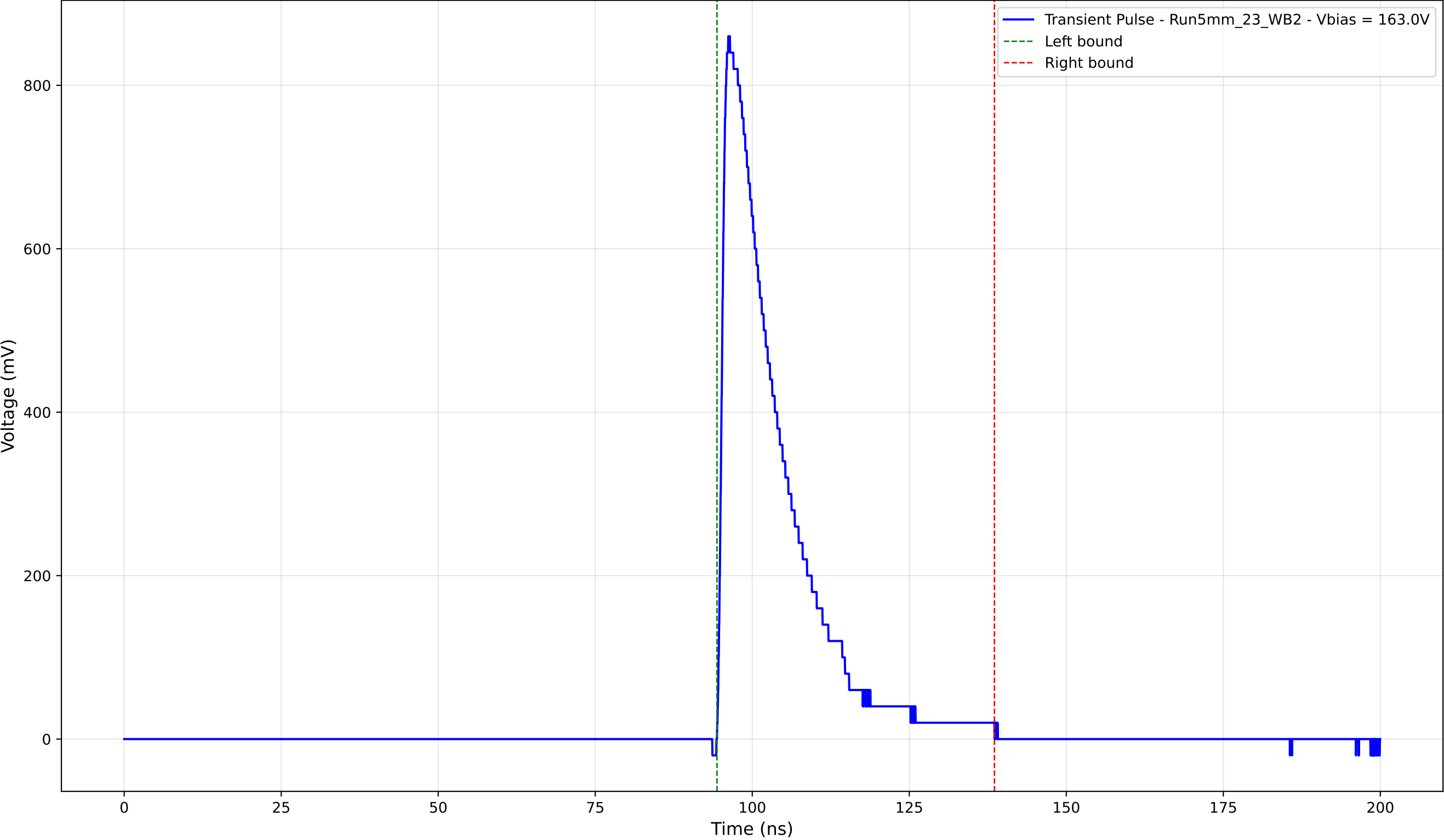
Transient Pulse - Sample: 5mm_23 - Position: 3730.0 \mu\text{m} - Charge: 177.16 pC
