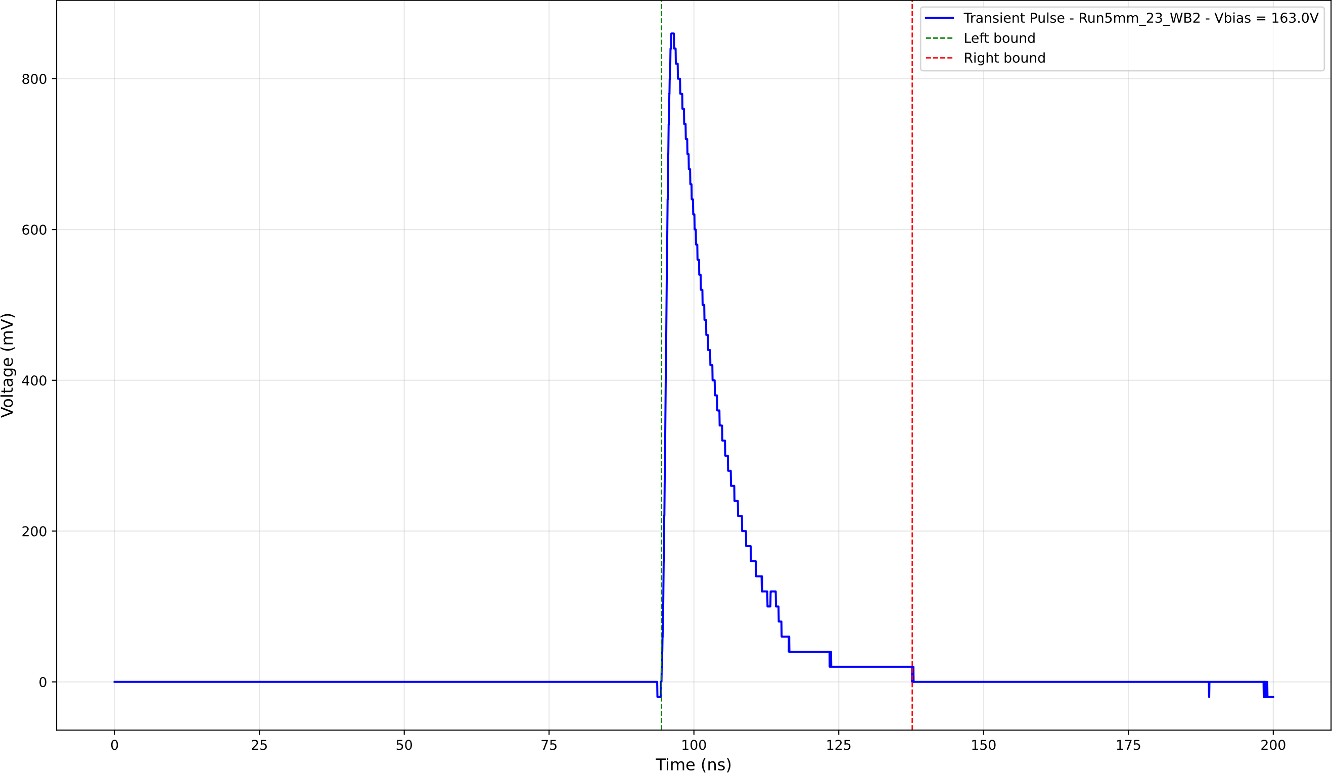
Transient Pulse - Sample: 5mm_23 - Position: 3910.0 \mu\text{m} - Charge: 169.29 pC
