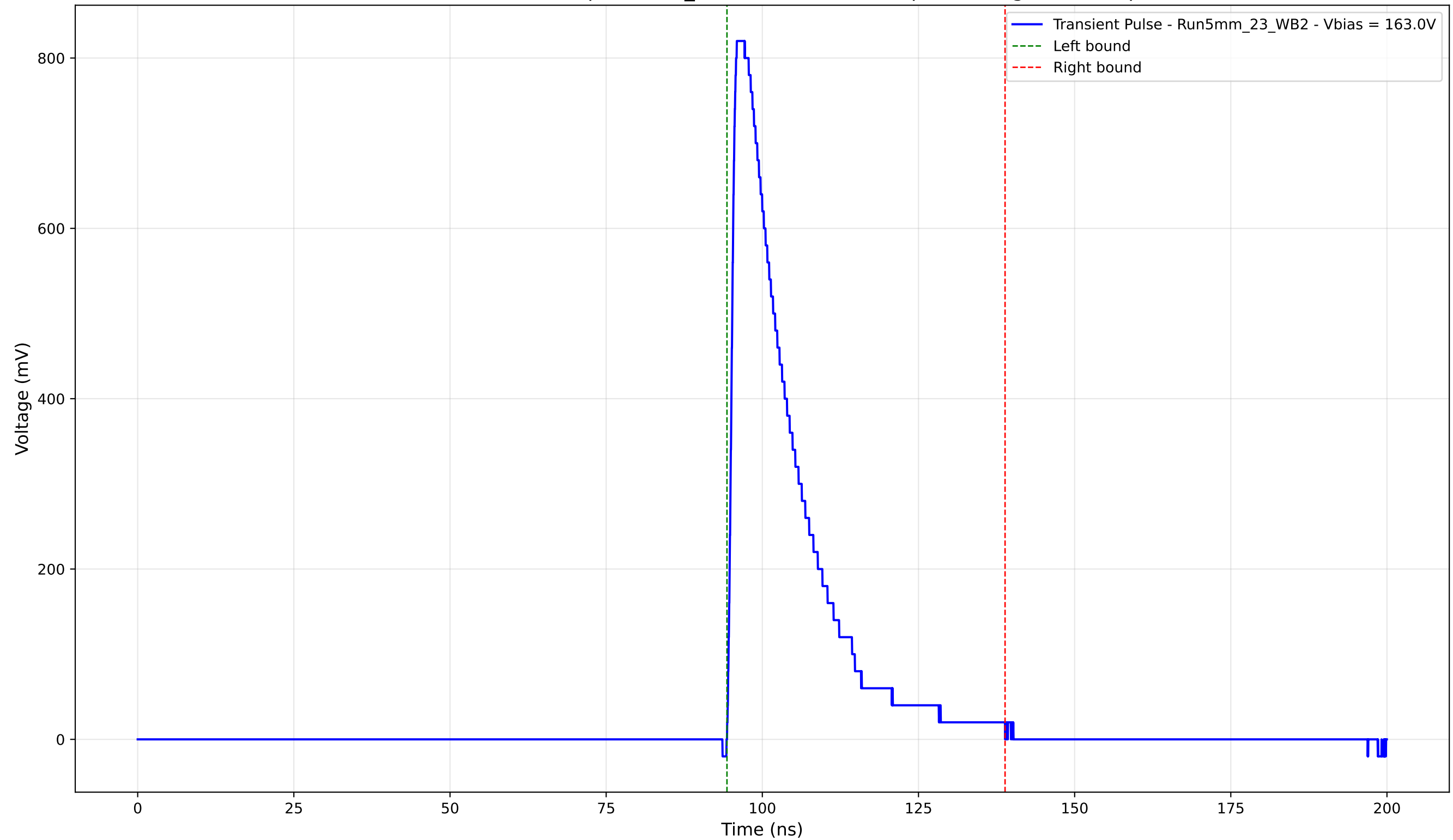
Transient Pulse - Sample: 5mm_23 - Position: 1415.0 \mu\text{m} - Charge: 179.14 pC
