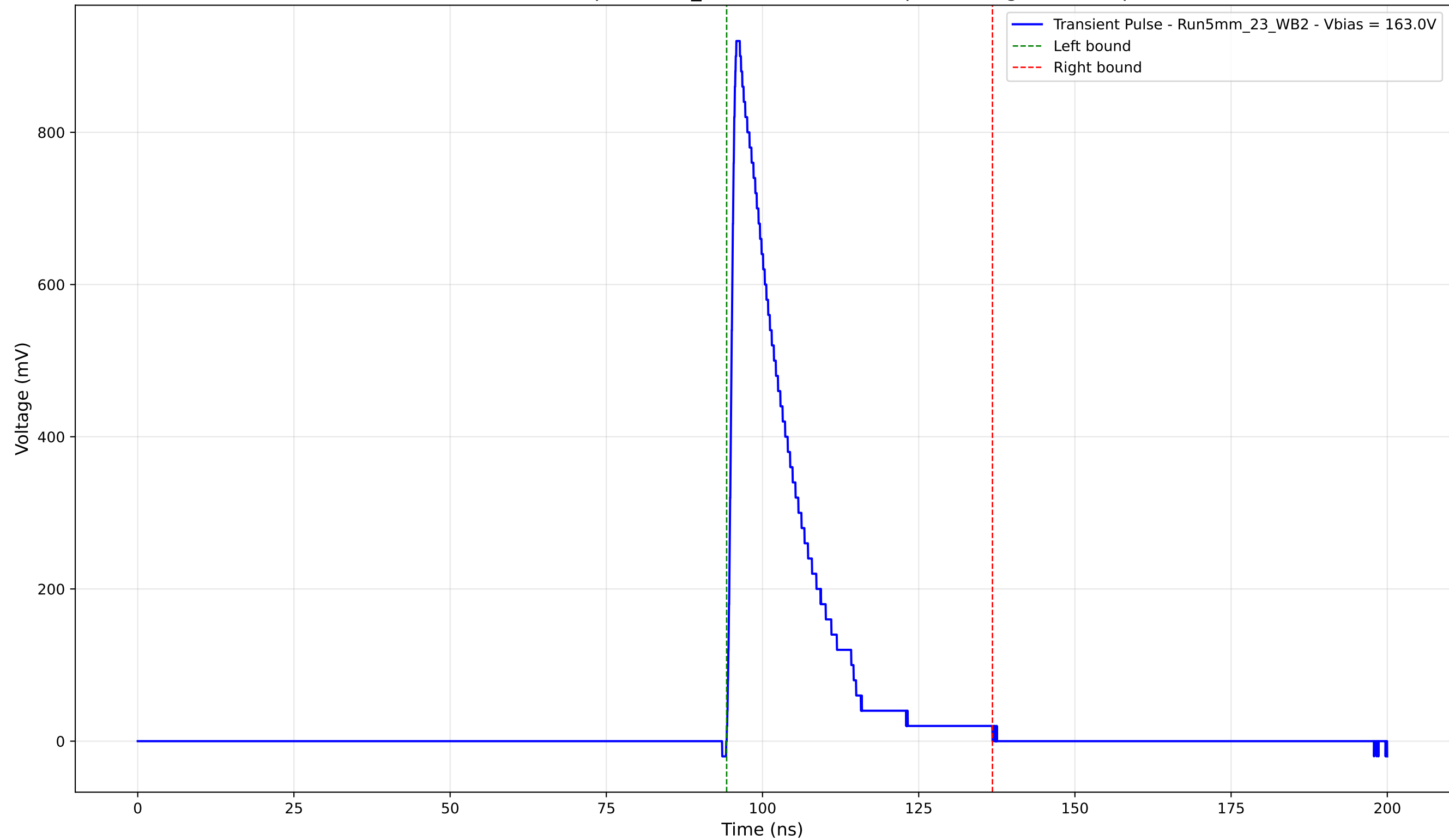
Transient Pulse - Sample: 5mm_23 - Position: 640.0 \mu\text{m} - Charge: 178.43 pC
