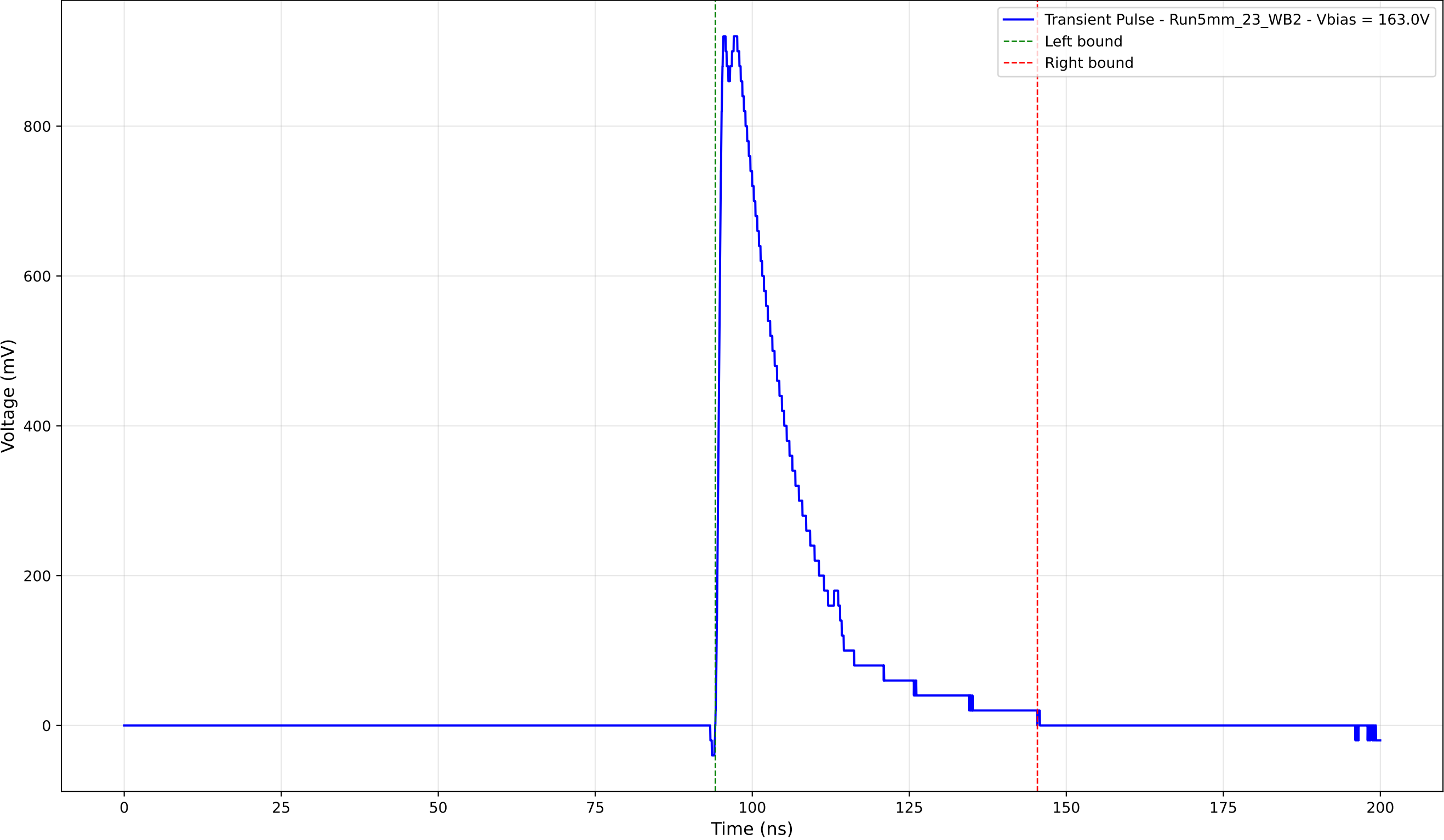
Transient Pulse - Sample: 5mm_23 - Position: 1840.0 \mu\text{m} - Charge: 222.46 pC
