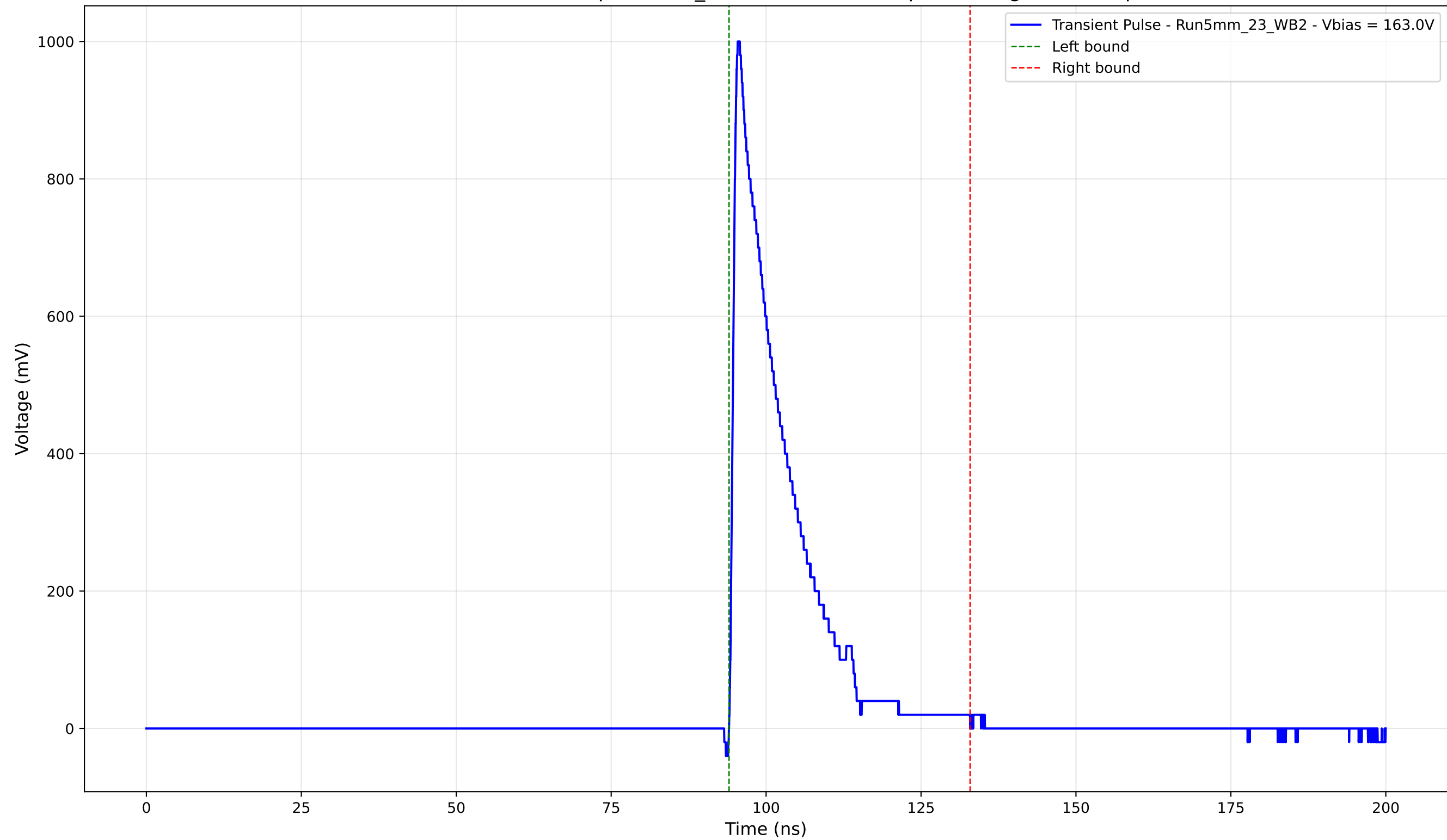
Transient Pulse - Sample: 5mm_23 - Position: 210.0 \mu\text{m} - Charge: 174.39 pC
