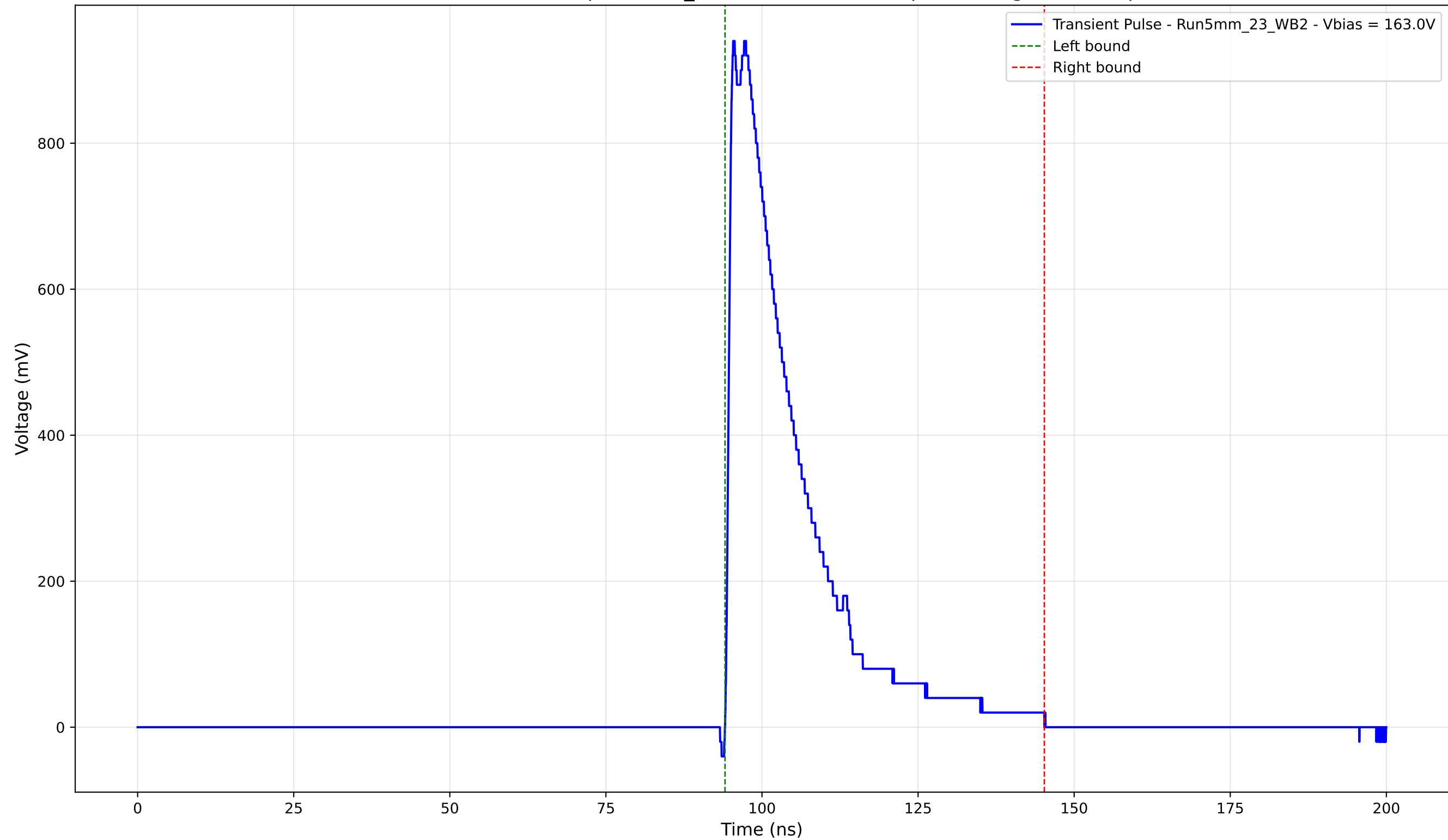
Transient Pulse - Sample: 5mm_23 - Position: 3160.0 \mu\text{m} - Charge: 224.55 pC
