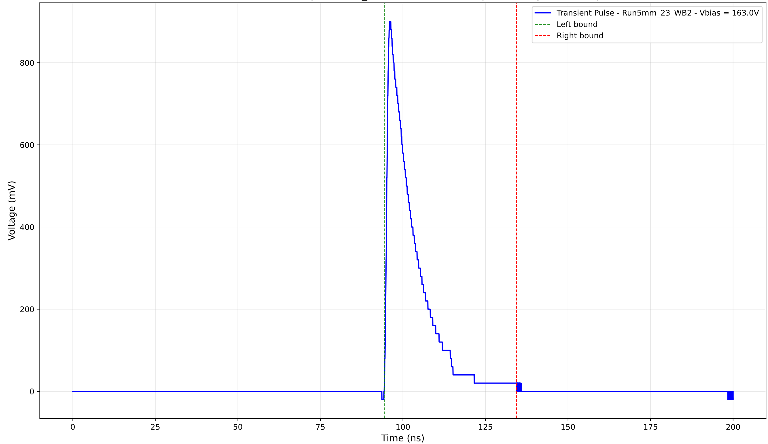
Transient Pulse - Sample: 5mm_23 - Position: 4330.0 \mu\text{m} - Charge: 161.38 pC
