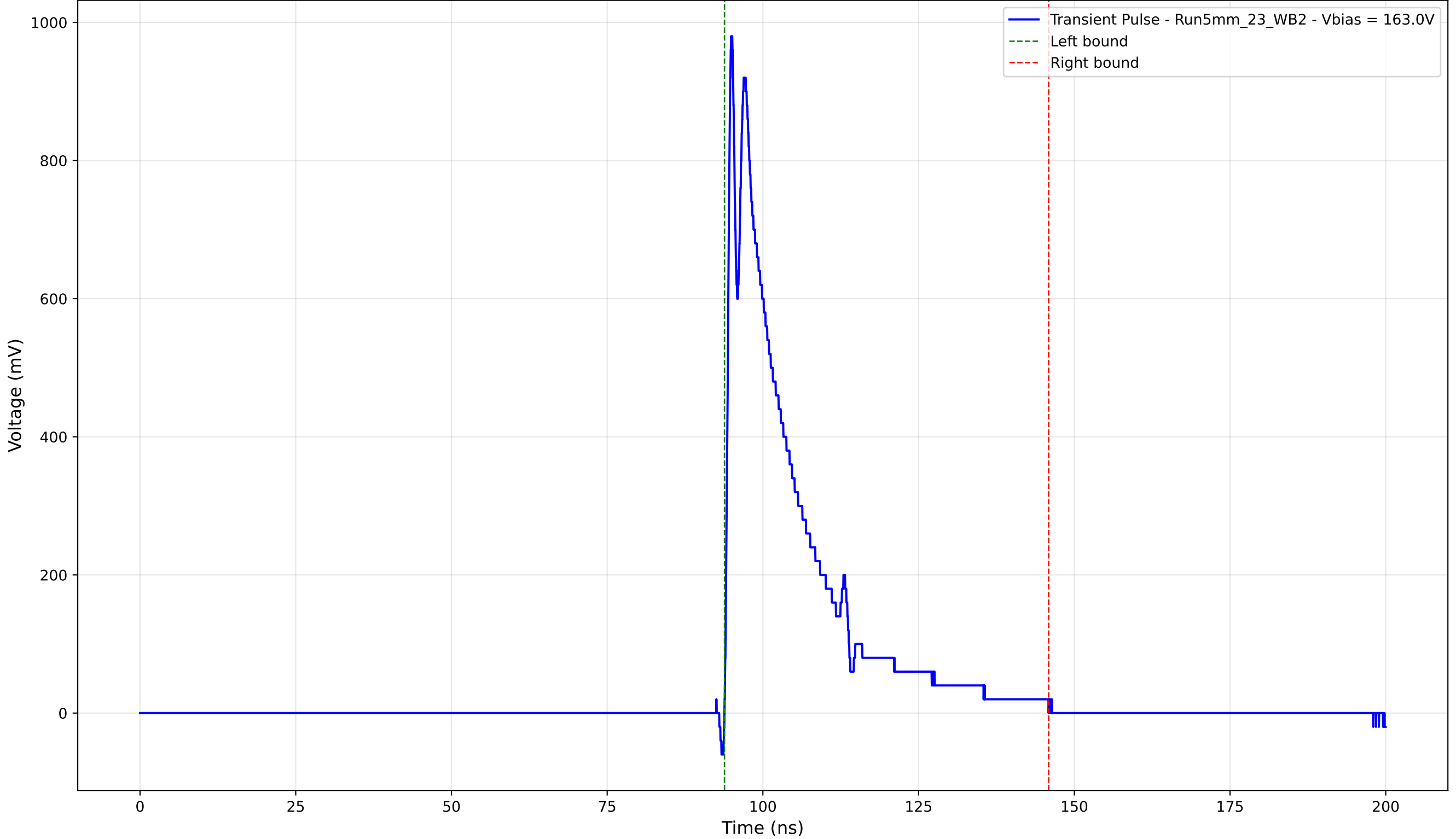
Transient Pulse - Sample: 5mm_23 - Position: 2680.0 \mu\text{m} - Charge: 201.49 pC
