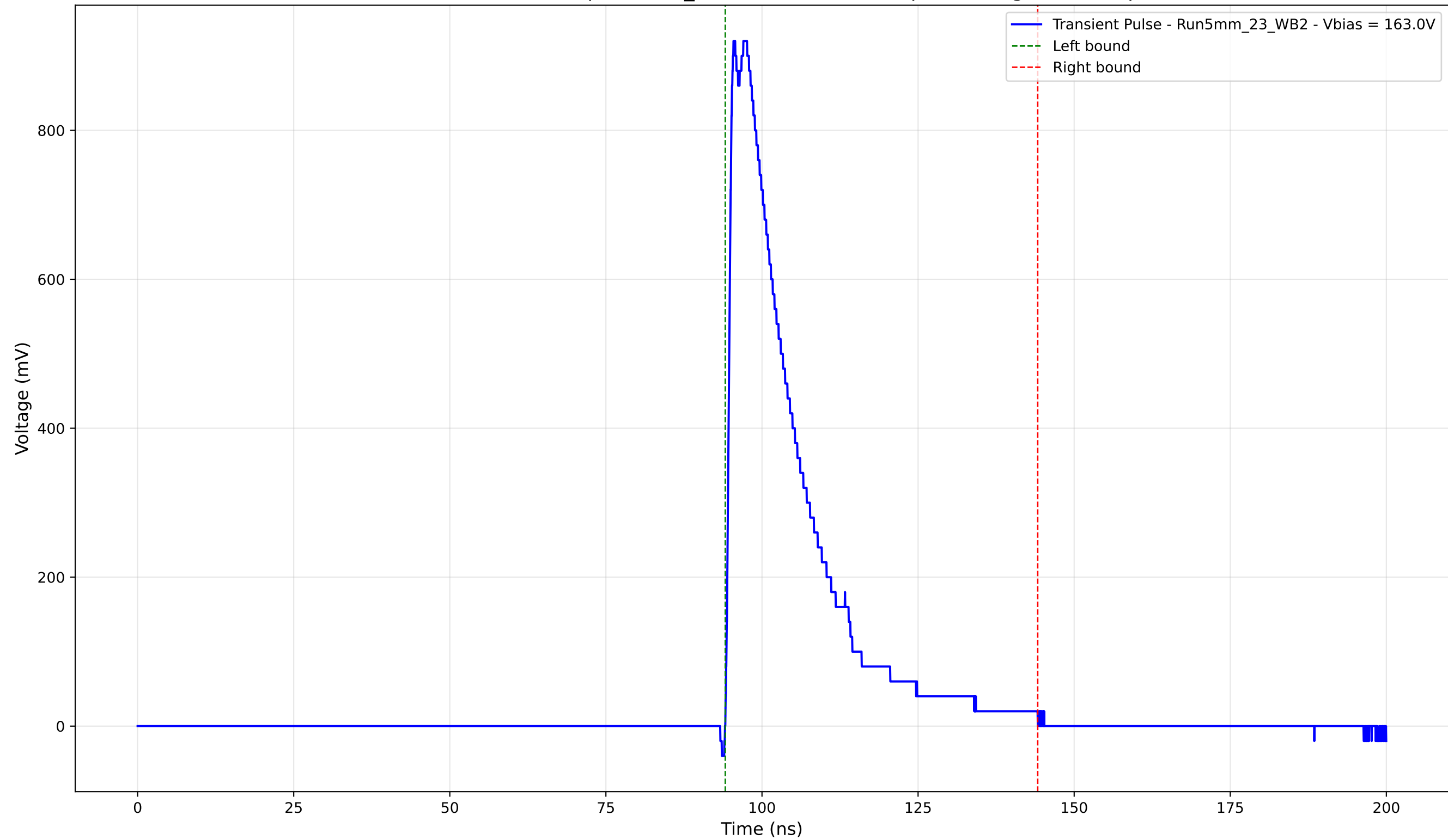
Transient Pulse - Sample: 5mm_23 - Position: 3200.0 \mu\text{m} - Charge: 218.04 pC
