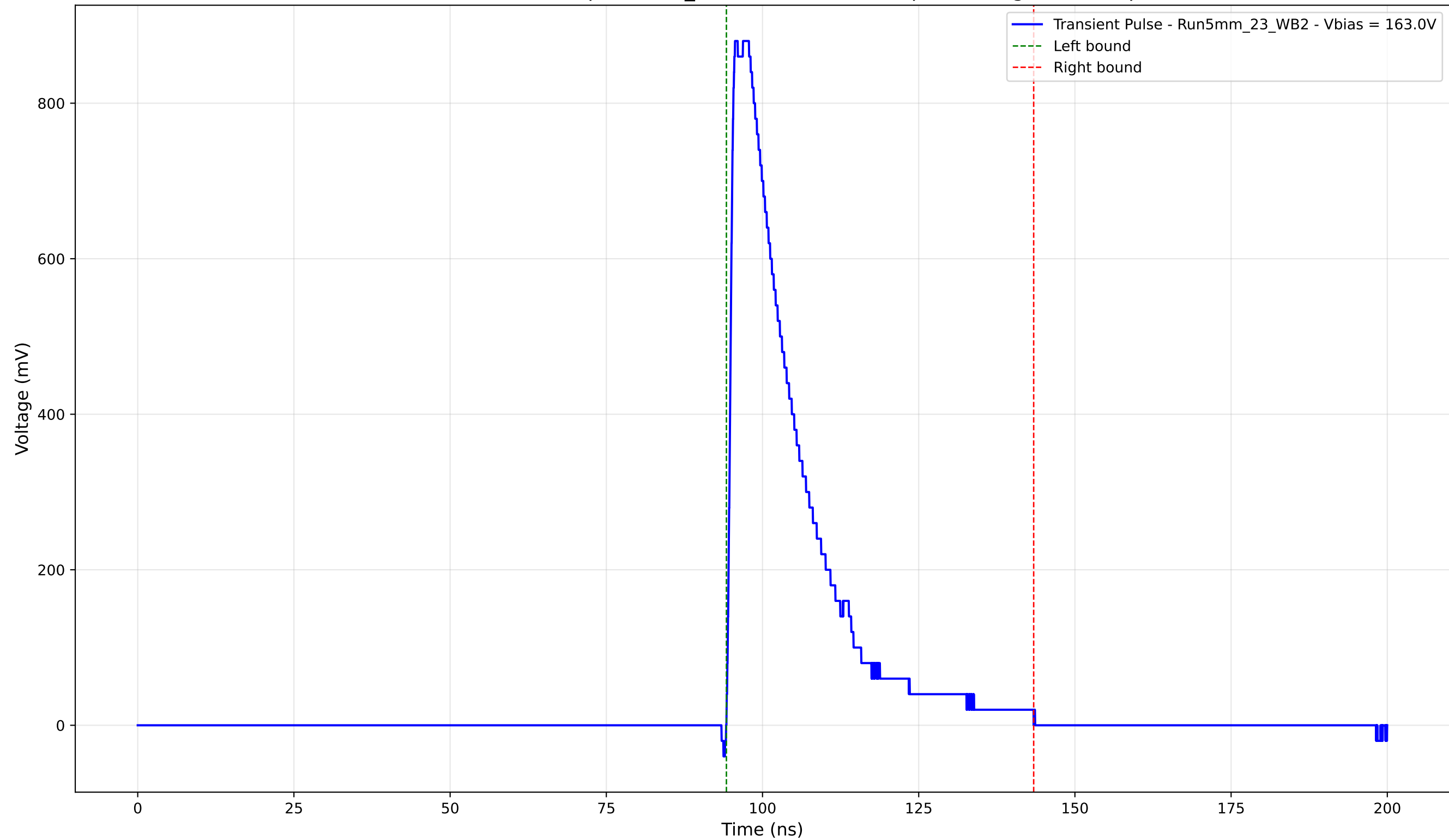
Transient Pulse - Sample: 5mm_23 - Position: 1695.0 \mu\text{m} - Charge: 208.38 pC
