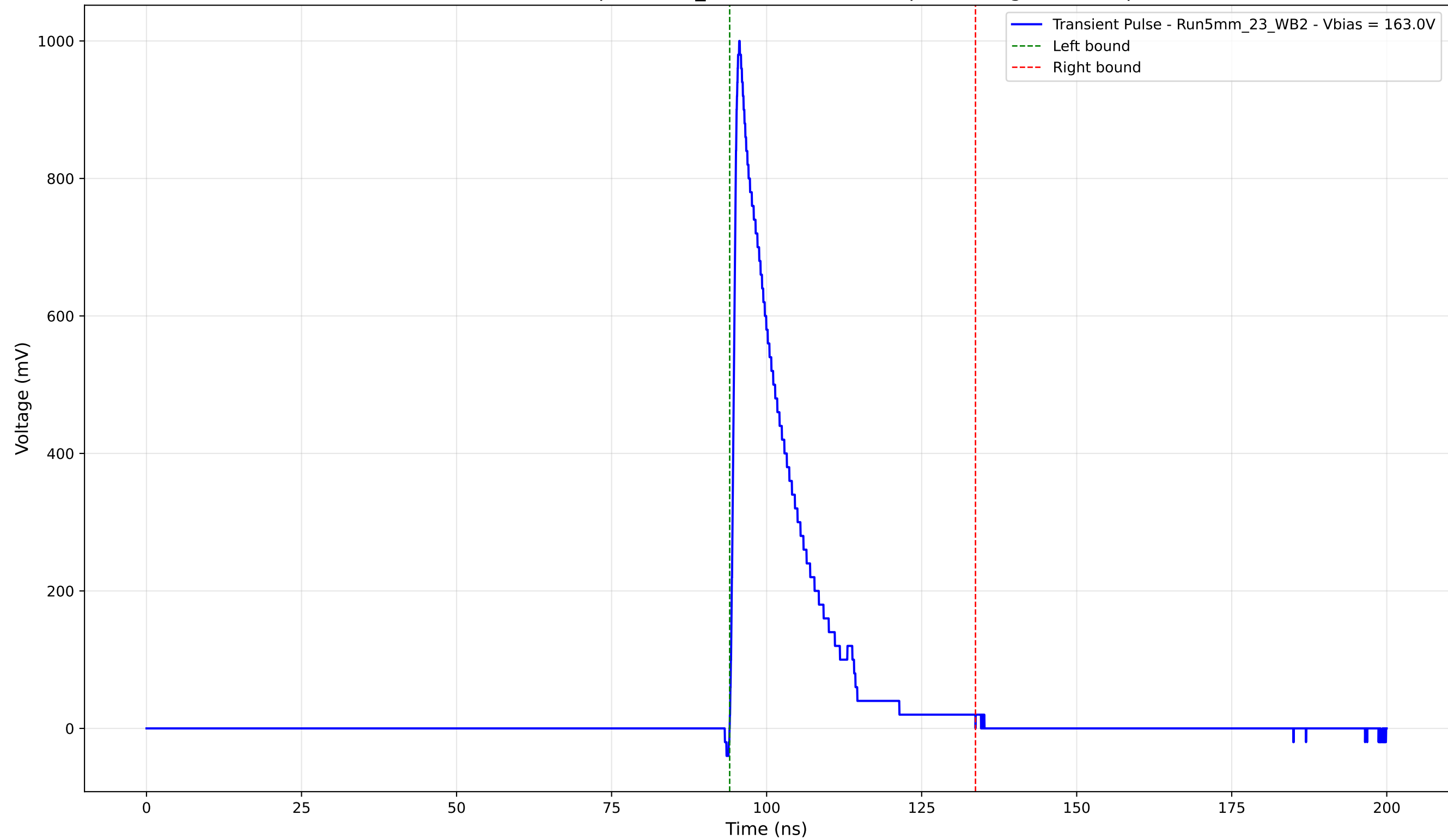
Transient Pulse - Sample: 5mm_23 - Position: 235.0 \mu\text{m} - Charge: 171.58 pC
