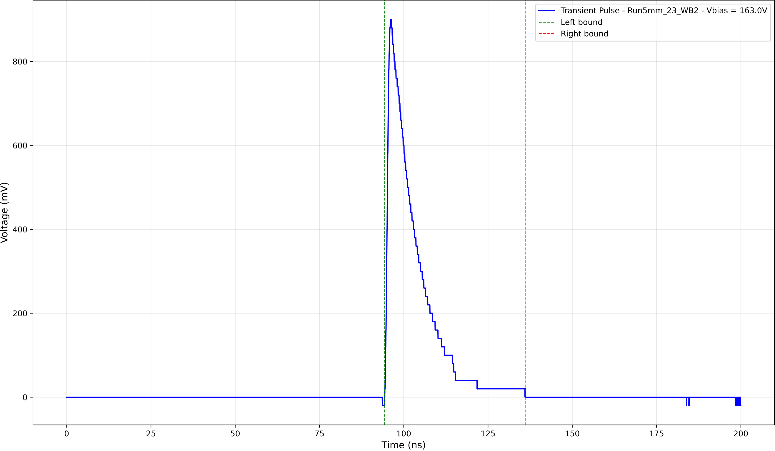
Transient Pulse - Sample: 5mm_23 - Position: 4255.0 \mu\text{m} - Charge: 164.07 pC
