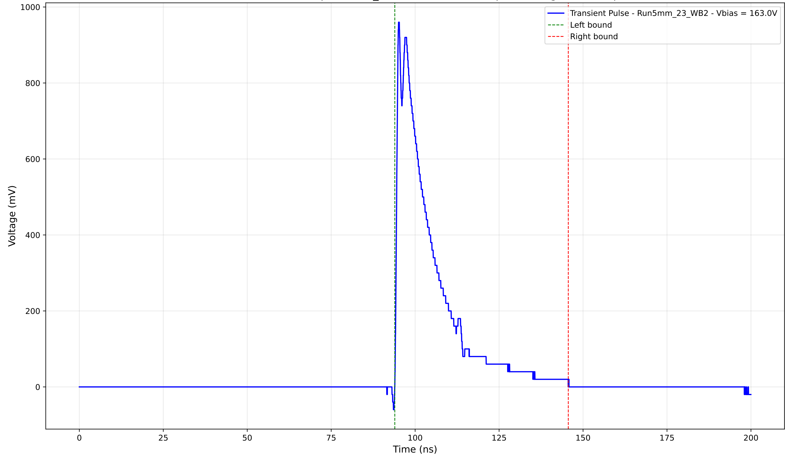
Transient Pulse - Sample: 5mm_23 - Position: 2850.0 \mu\text{m} - Charge: 213.44 pC
