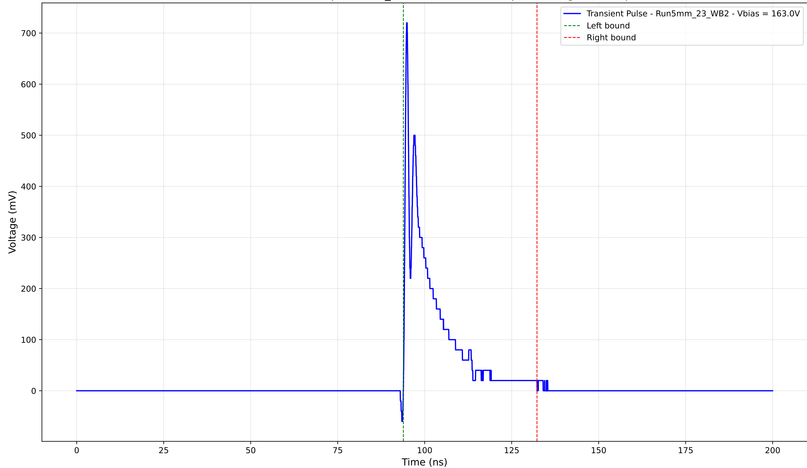
Transient Pulse - Sample: 5mm_23 - Position: 2555.0 \mu\text{m} - Charge: 89.50 pC
