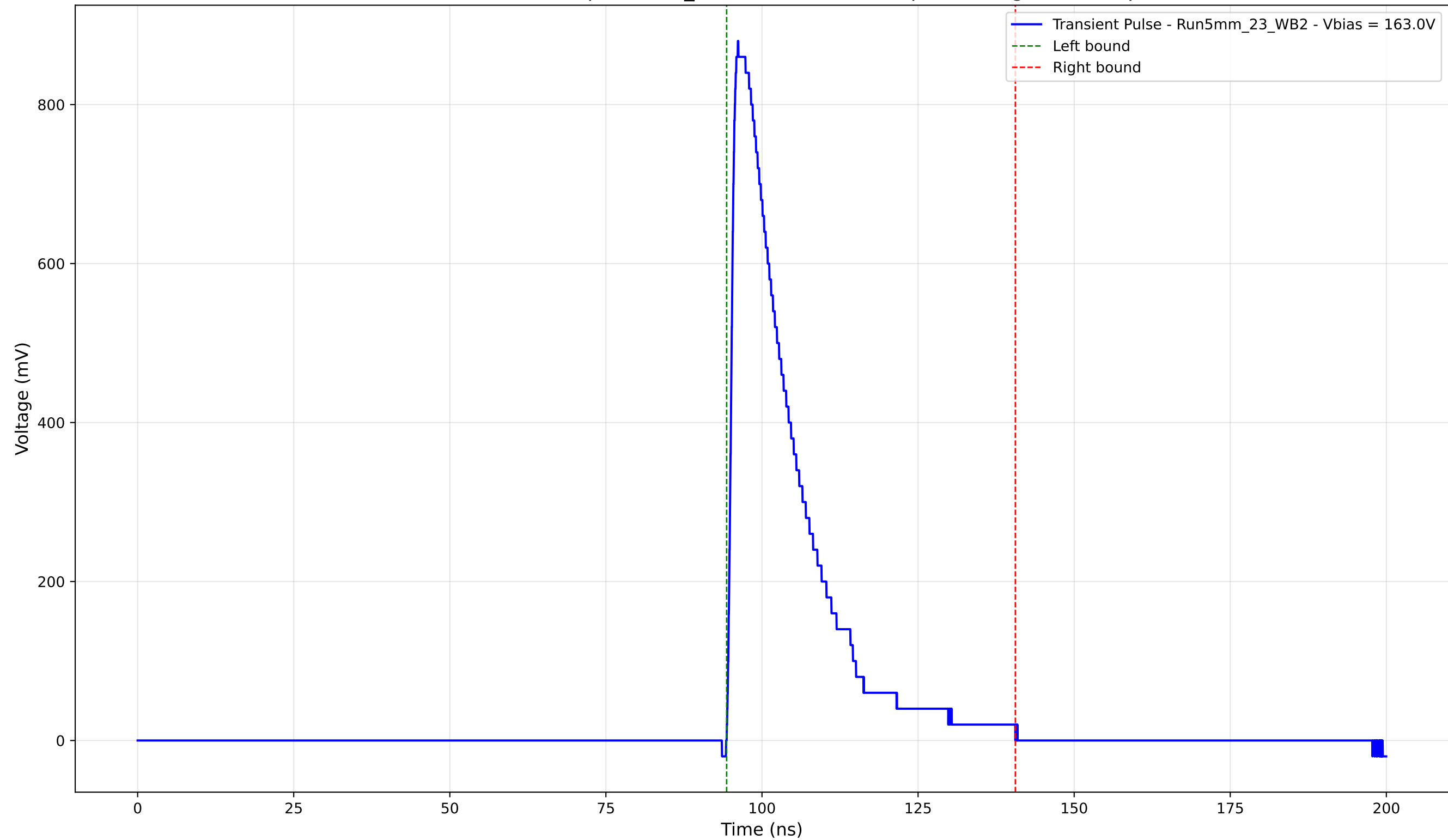
Transient Pulse - Sample: 5mm_23 - Position: 1395.0 \mu\text{m} - Charge: 193.37 pC
