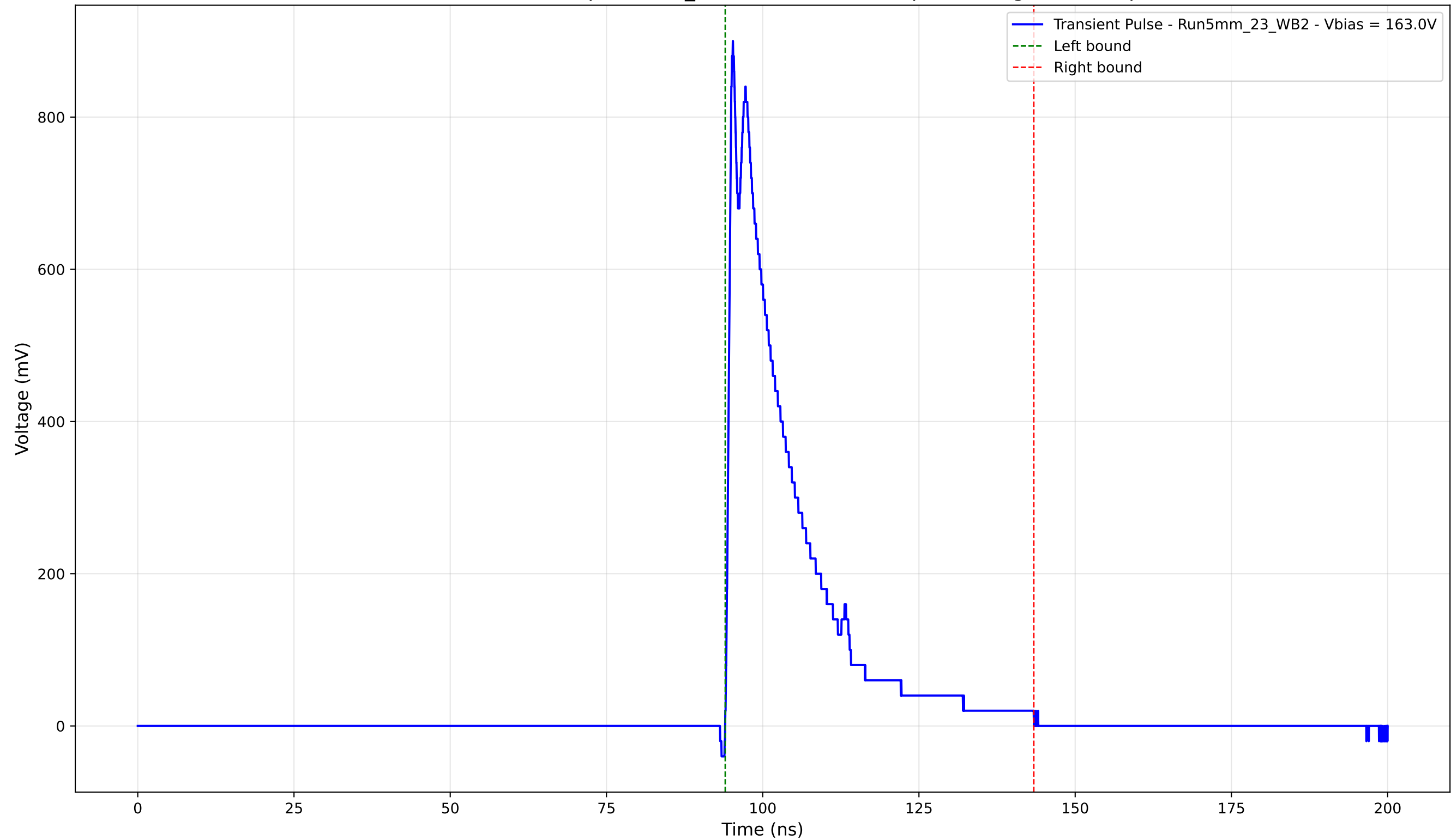
Transient Pulse - Sample: 5mm_23 - Position: 2095.0 \mu\text{m} - Charge: 182.65 pC
