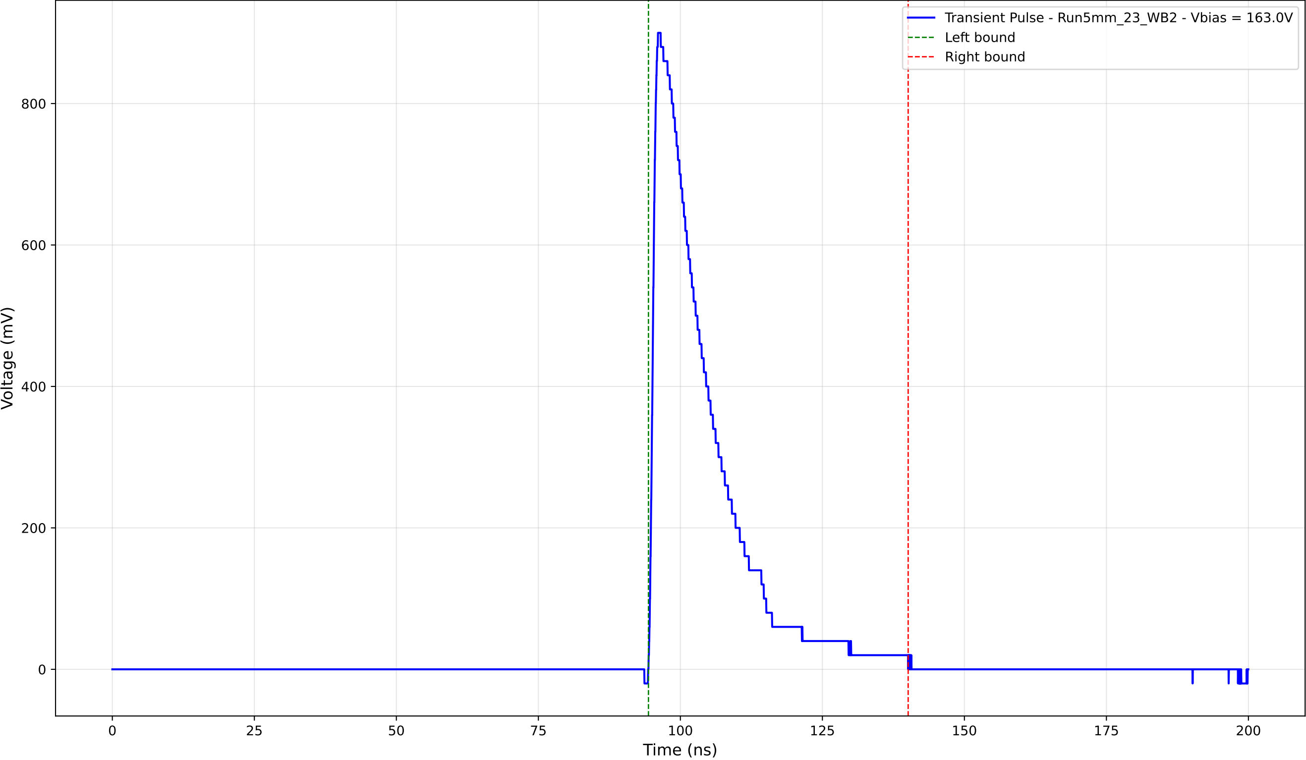
Transient Pulse - Sample: 5mm_23 - Position: 1195.0 \mu\text{m} - Charge: 196.15 pC
