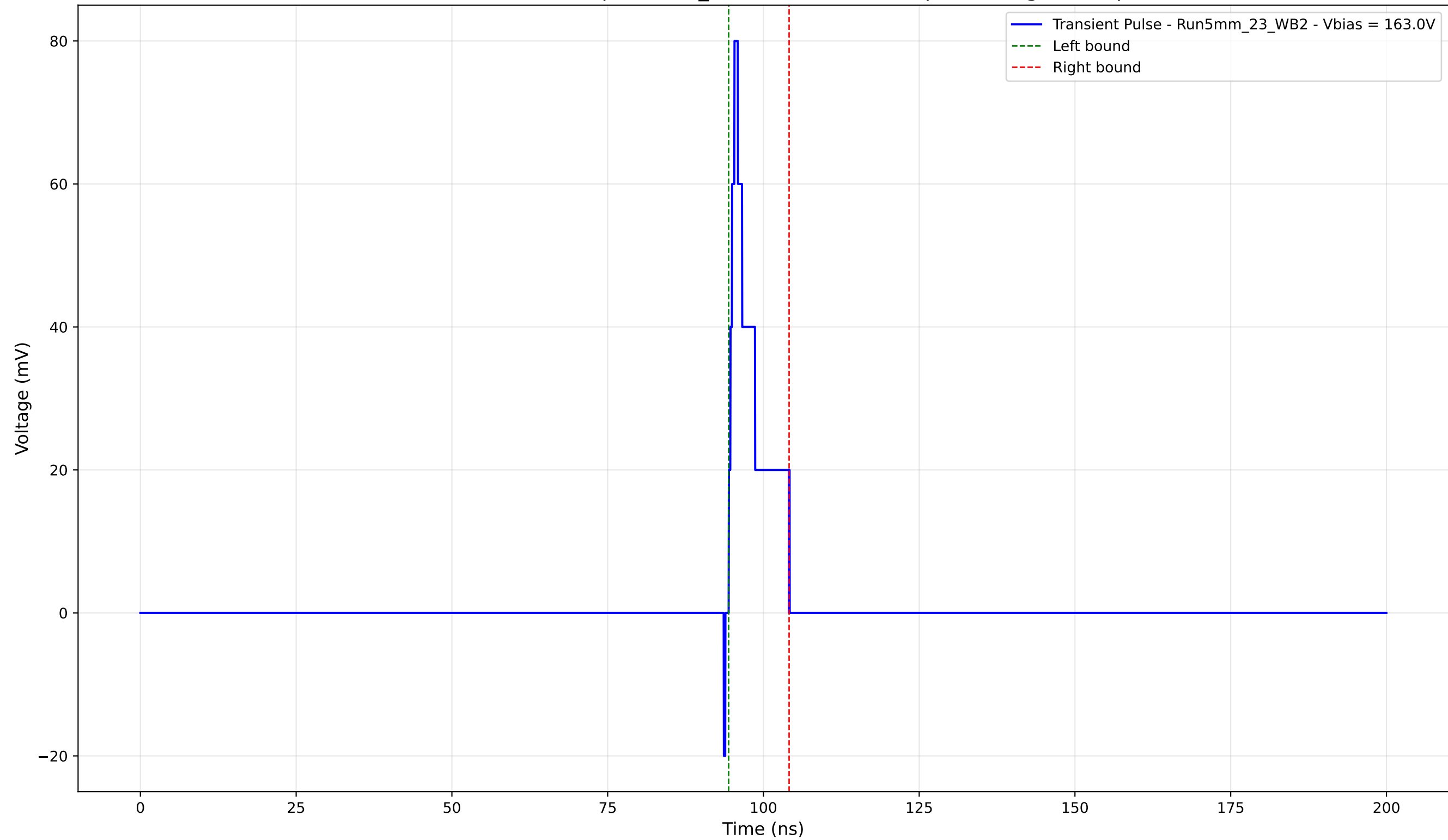
Transient Pulse - Sample: 5mm_23 - Position: 4985.0 \mu\text{m} - Charge: 6.33 pC
