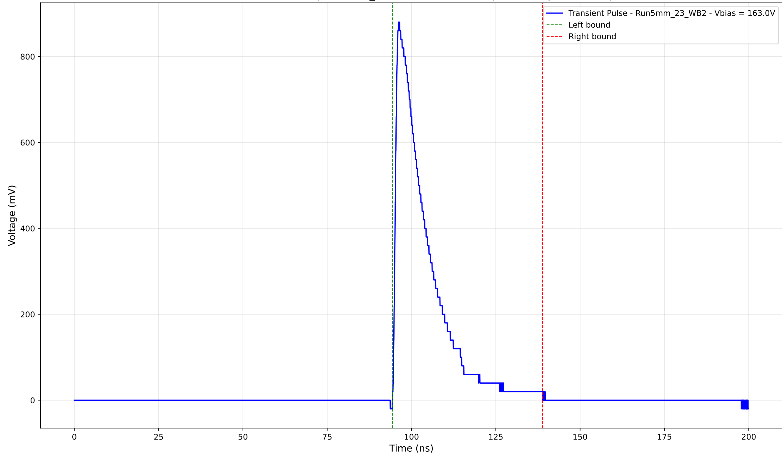
Transient Pulse - Sample: 5mm_23 - Position: 1100.0 \mu\text{m} - Charge: 182.89 pC
