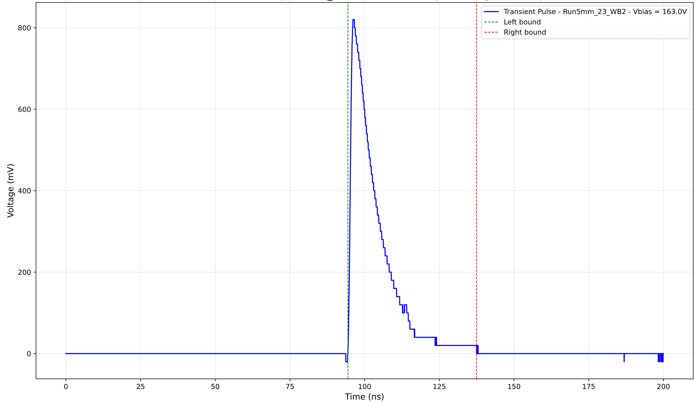
Transient Pulse - Sample: 5mm_23 - Position: 1075.0 \mu\text{m} - Charge: 164.14 pC
