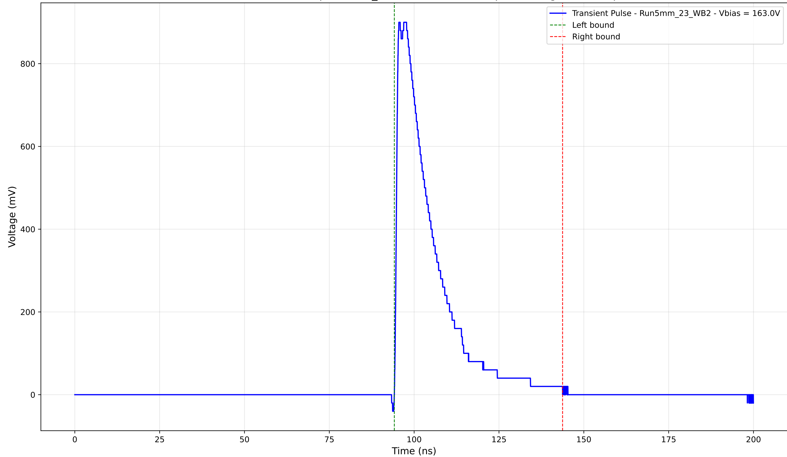
Transient Pulse - Sample: 5mm_23 - Position: 1765.0 \mu\text{m} - Charge: 216.16 pC
