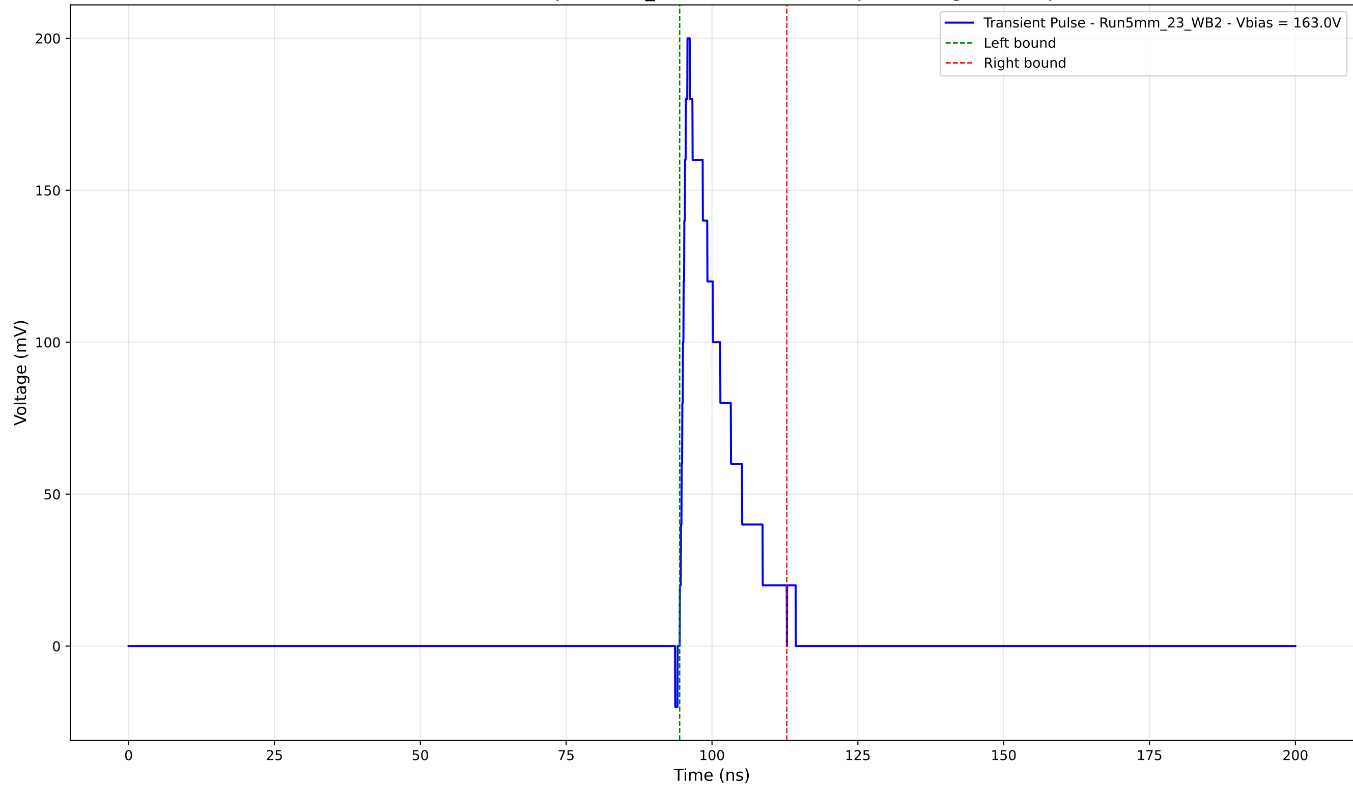
Transient Pulse - Sample: 5mm_23 - Position: 4535.0 \mu\text{m} - Charge: 28.45 pC
