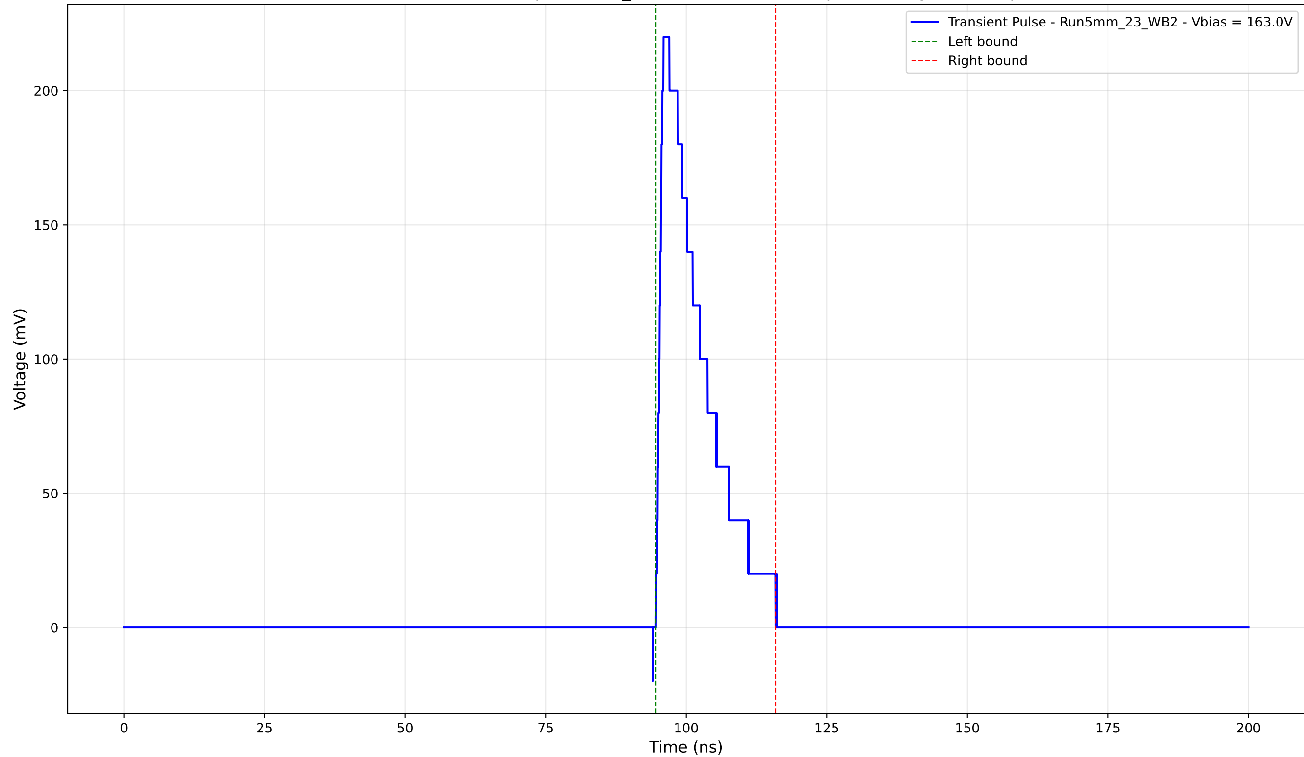
Transient Pulse - Sample: 5mm_23 - Position: 4020.0 \mu\text{m} - Charge: 37.74 pC
