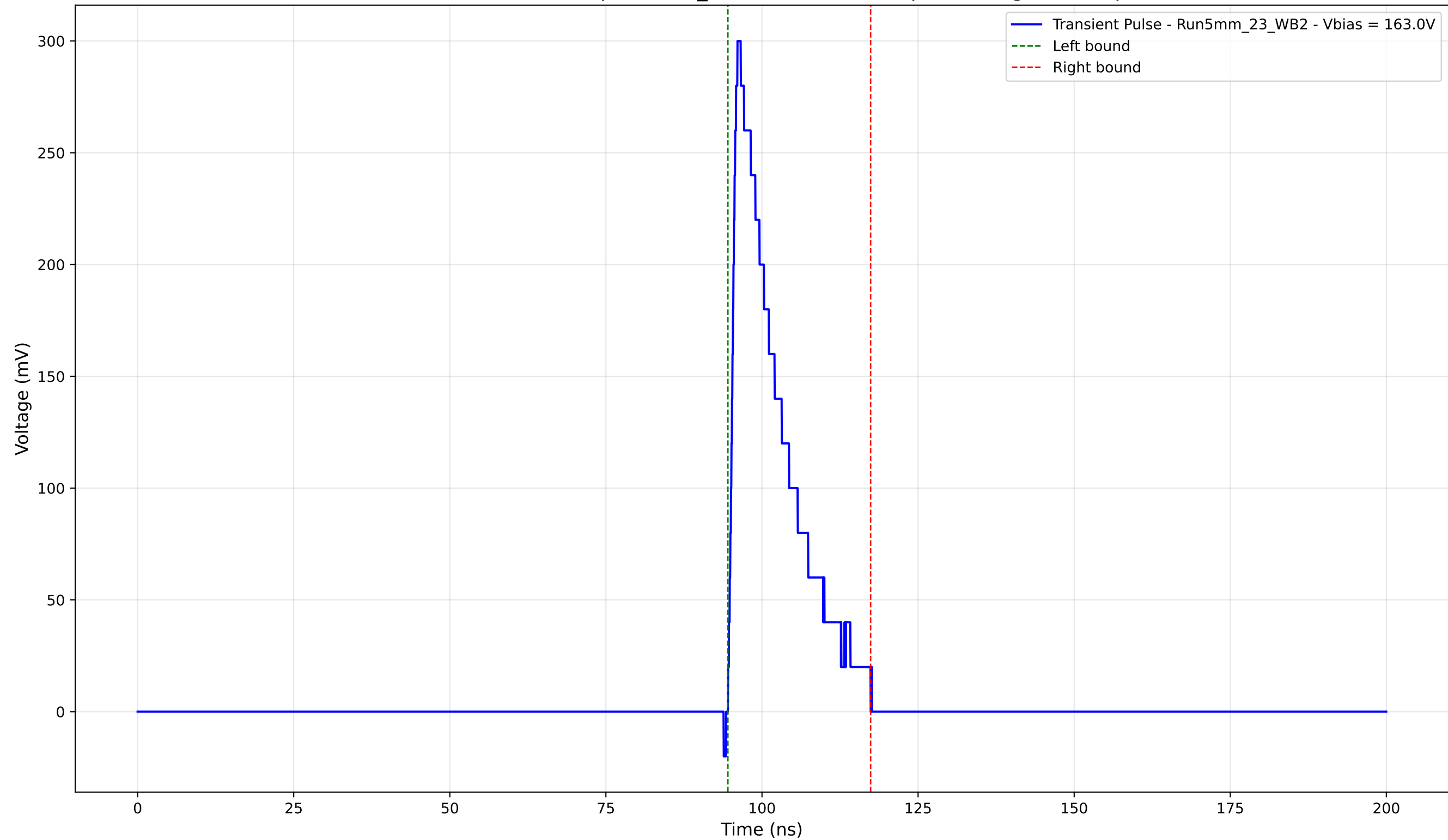
Transient Pulse - Sample: 5mm_23 - Position: 970.0 \mu\text{m} - Charge: 50.51 pC
