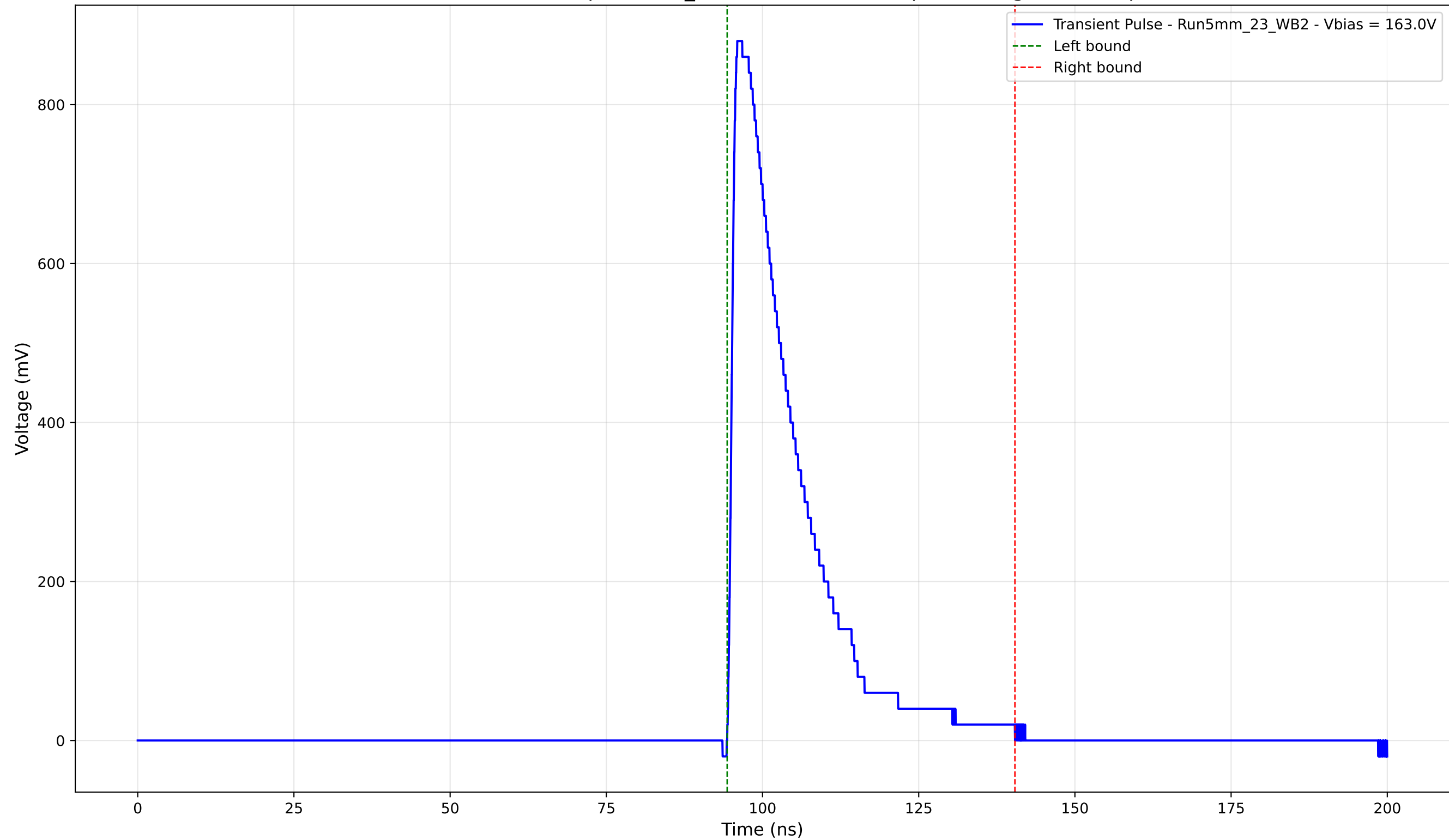
Transient Pulse - Sample: 5mm_23 - Position: 1375.0 \mu\text{m} - Charge: 197.22 pC
