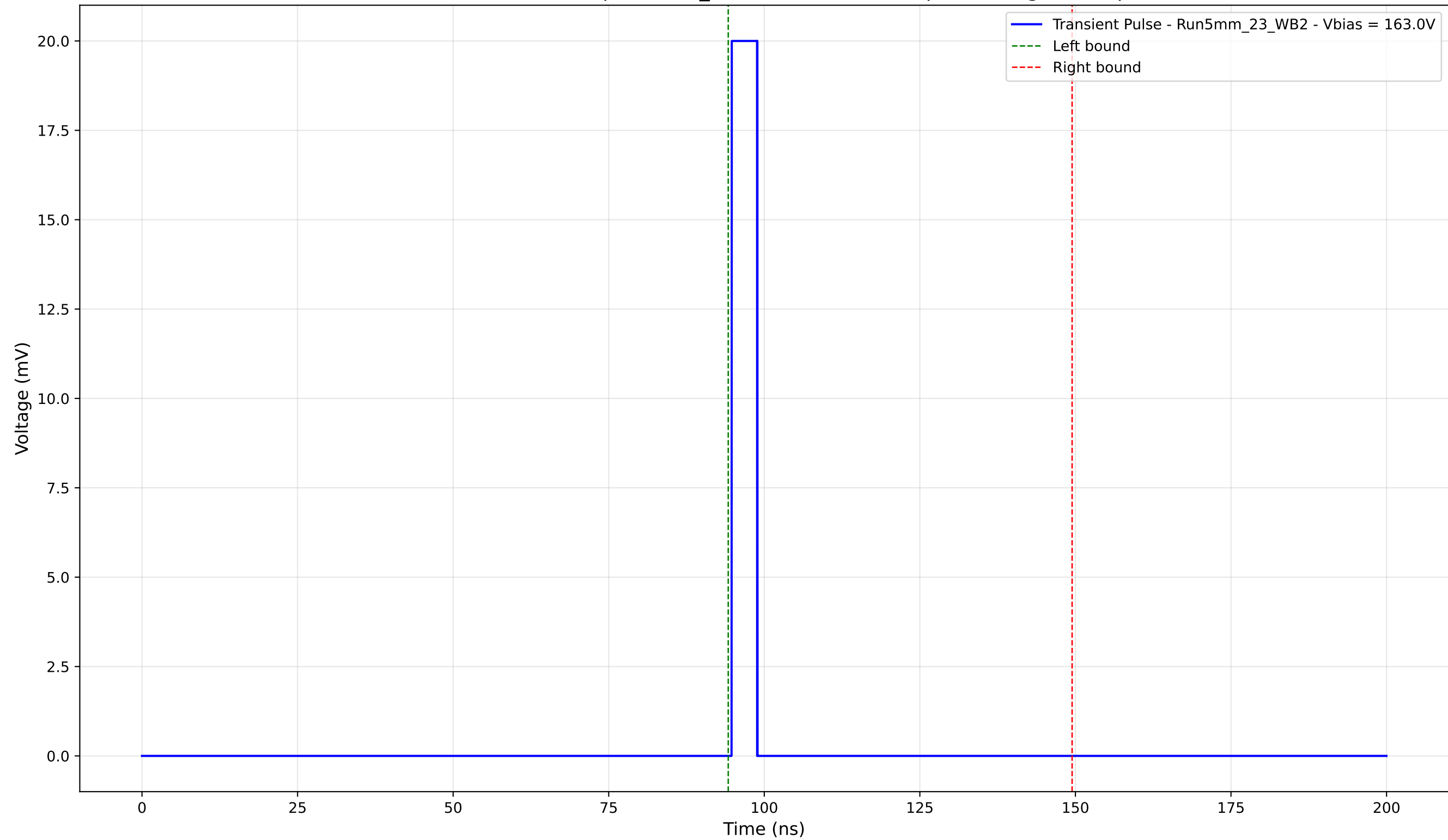
Transient Pulse - Sample: 5mm_23 - Position: 5020.0 \mu\text{m} - Charge: 1.65 pC
