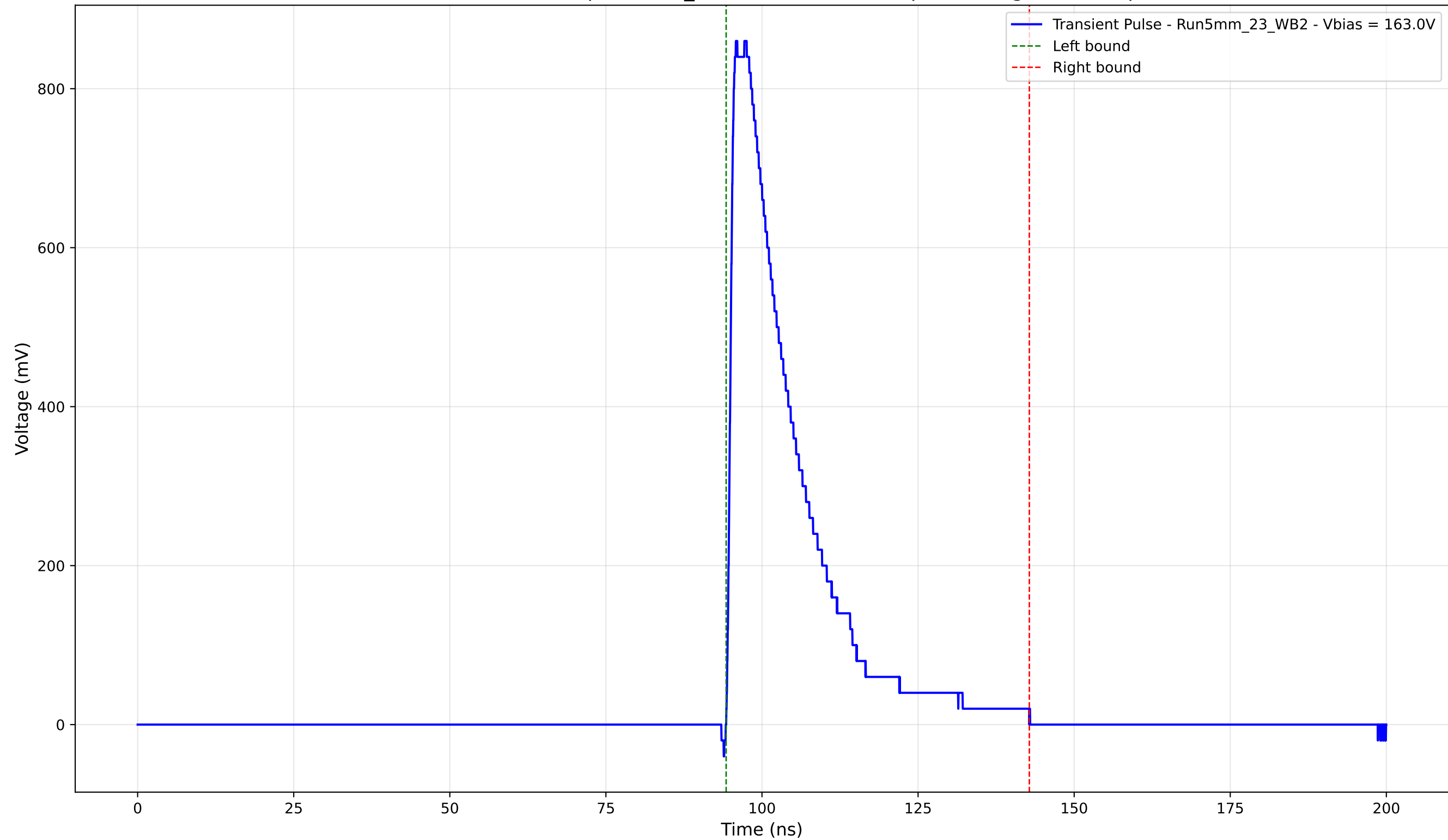
Transient Pulse - Sample: 5mm_23 - Position: 1610.0 \mu\text{m} - Charge: 196.54 pC
