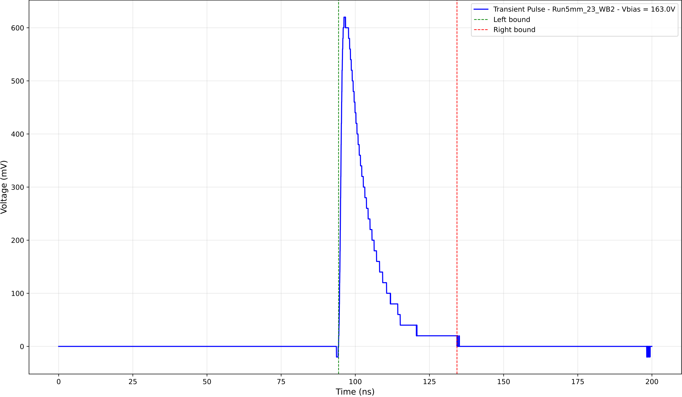
Transient Pulse - Sample: 5mm_23 - Position: 3585.0 \mu\text{m} - Charge: 122.81 pC
