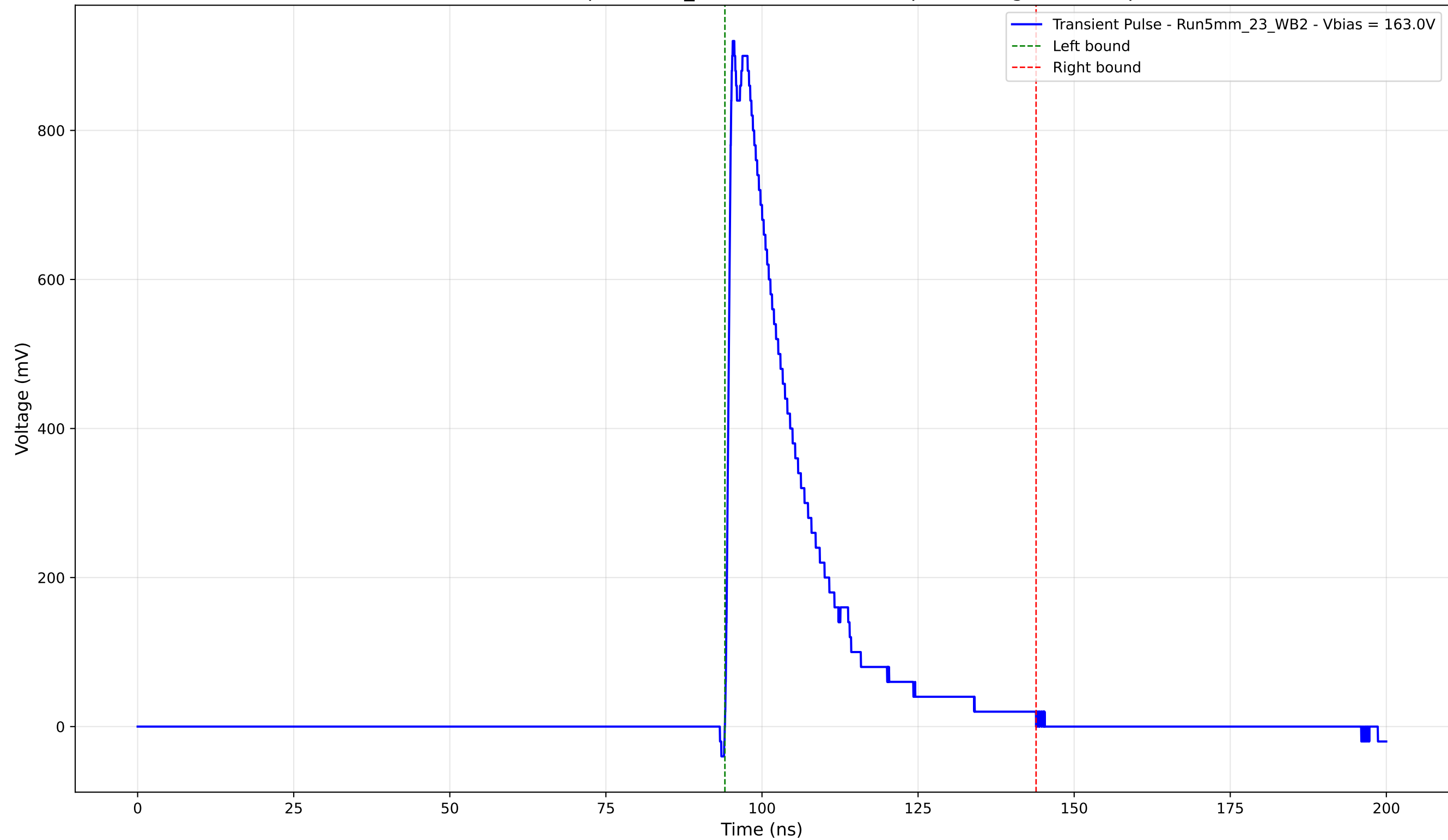
Transient Pulse - Sample: 5mm_23 - Position: 3110.0 \mu\text{m} - Charge: 212.50 pC
