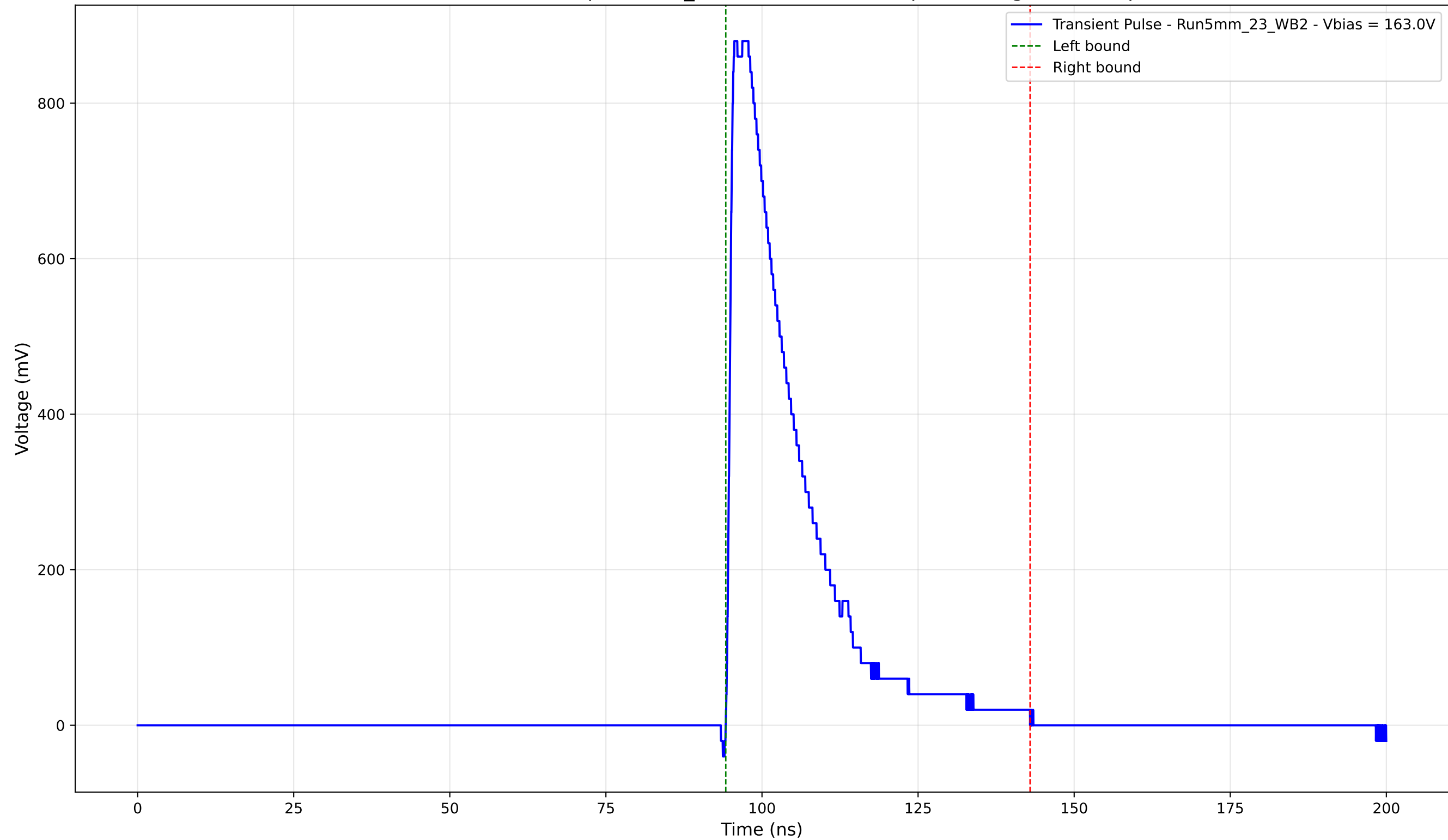
Transient Pulse - Sample: 5mm_23 - Position: 1700.0 \mu\text{m} - Charge: 208.31 pC
