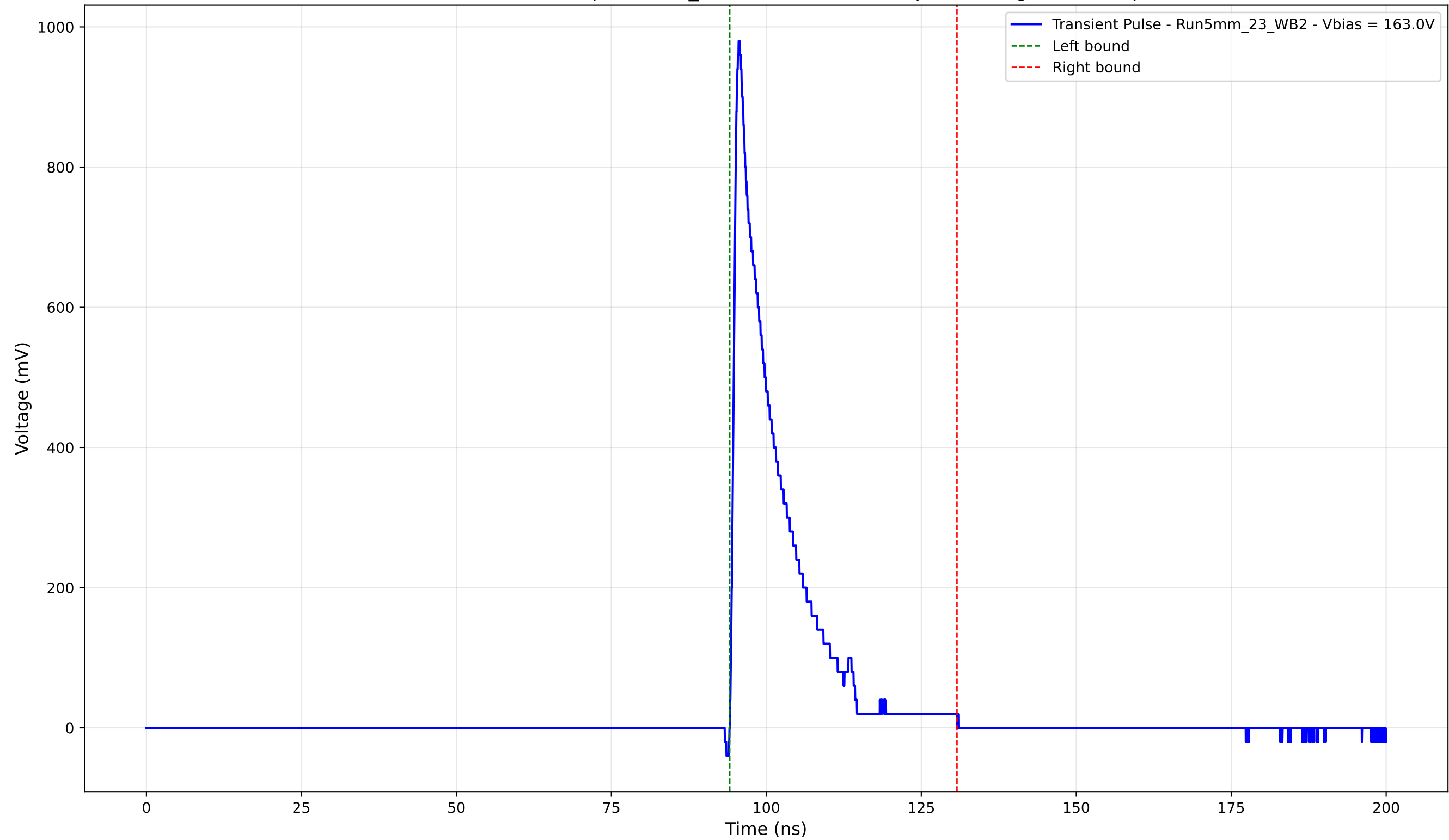
Transient Pulse - Sample: 5mm_23 - Position: 4820.0 \mu\text{m} - Charge: 144.61 pC
