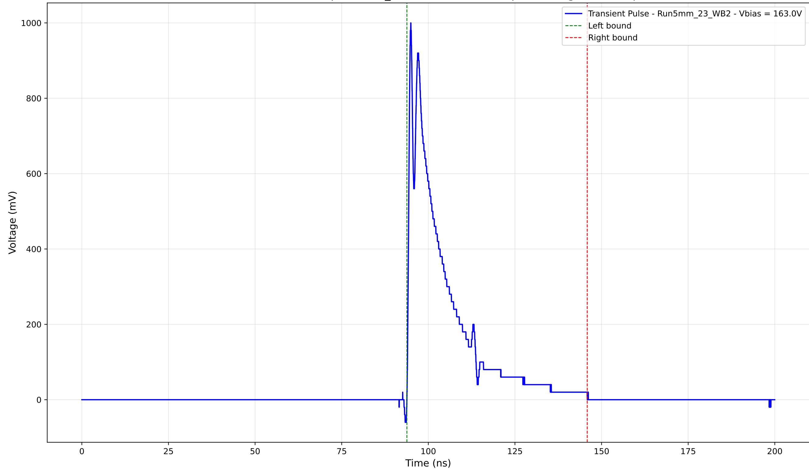
Transient Pulse - Sample: 5mm_23 - Position: 2405.0 \mu\text{m} - Charge: 197.35 pC
