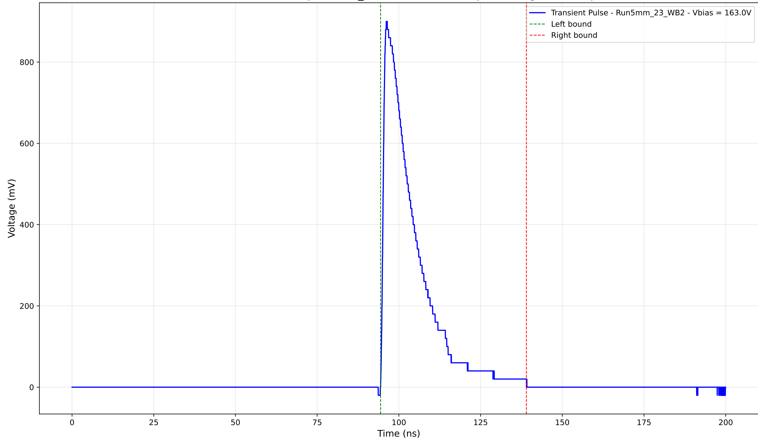
Transient Pulse - Sample: 5mm_23 - Position: 1160.0 \mu\text{m} - Charge: 192.74 pC
