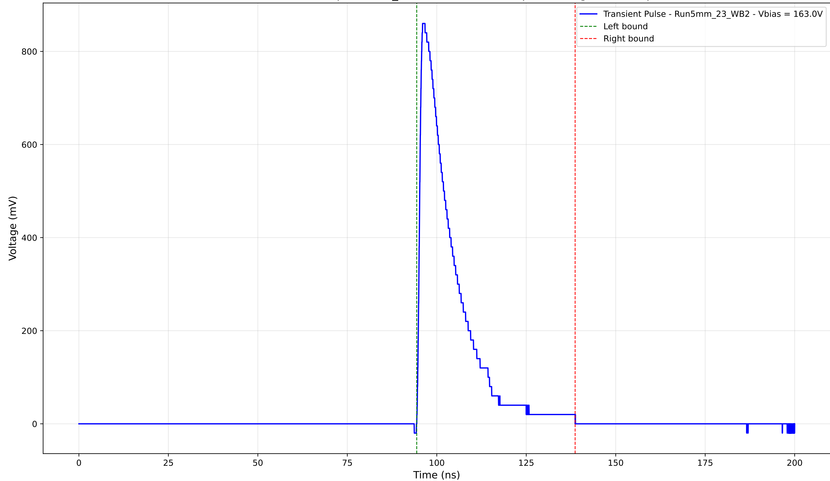
Transient Pulse - Sample: 5mm_23 - Position: 3790.0 \mu\text{m} - Charge: 177.14 pC
