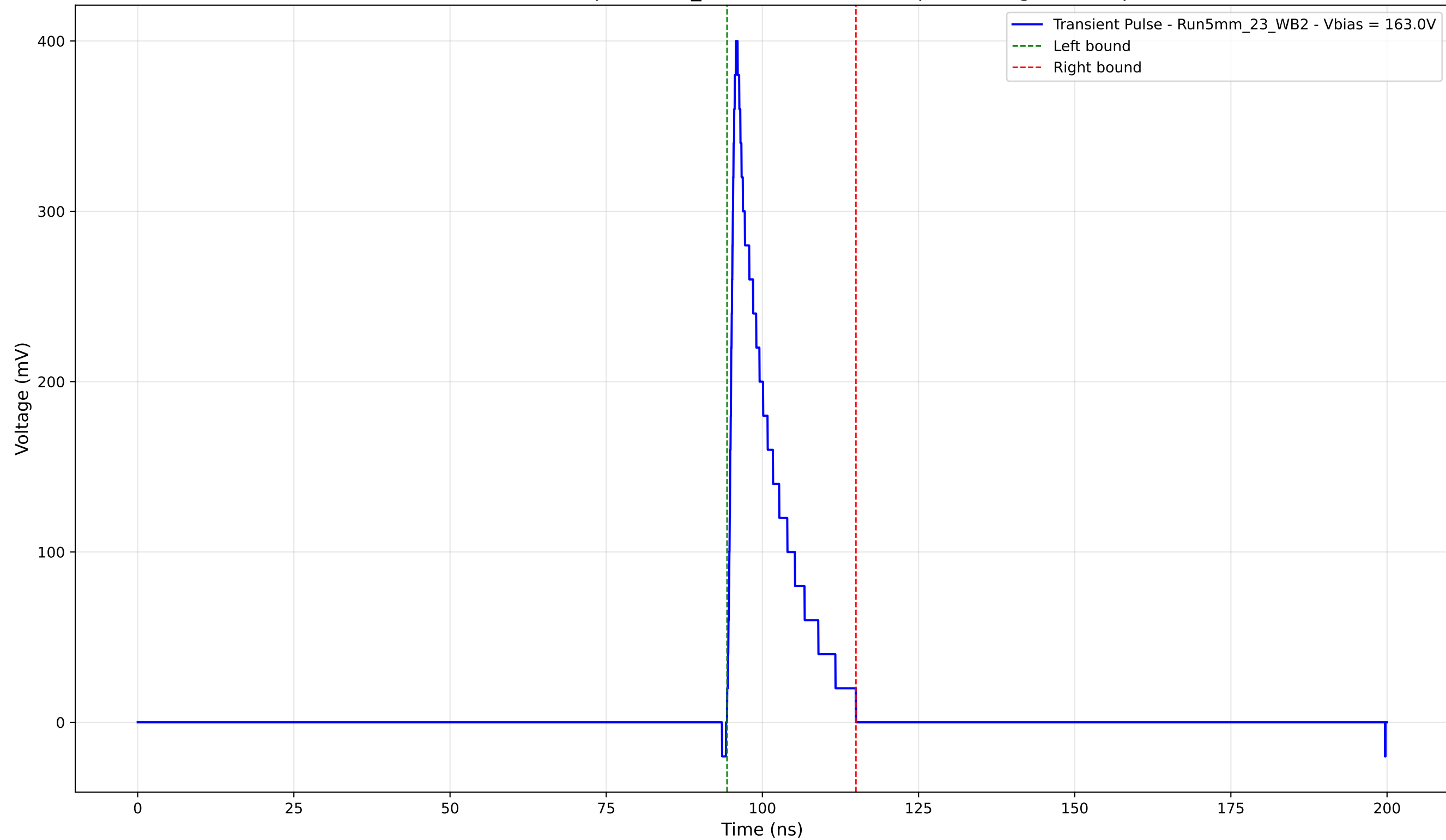
Transient Pulse - Sample: 5mm_23 - Position: 4565.0 \mu\text{m} - Charge: 52.49 pC
