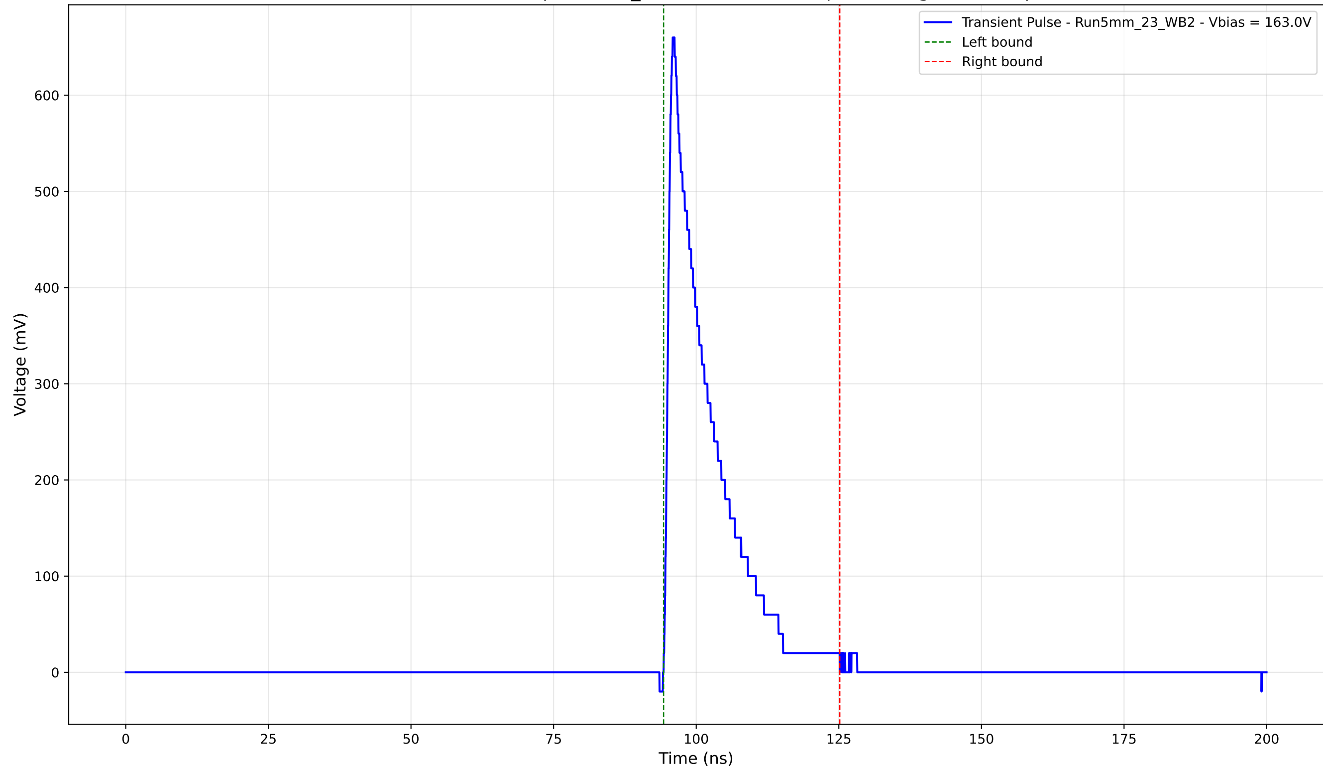
Transient Pulse - Sample: 5mm_23 - Position: 535.0 \mu\text{m} - Charge: 105.10 pC
