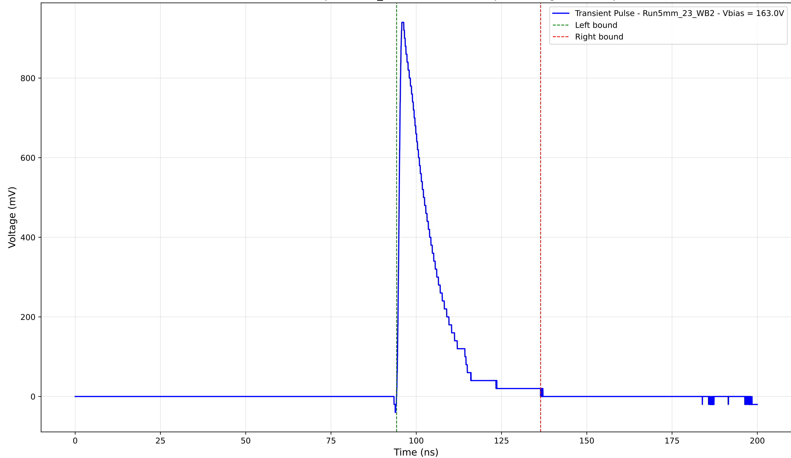
Transient Pulse - Sample: 5mm_23 - Position: 610.0 \mu\text{m} - Charge: 184.25 pC
