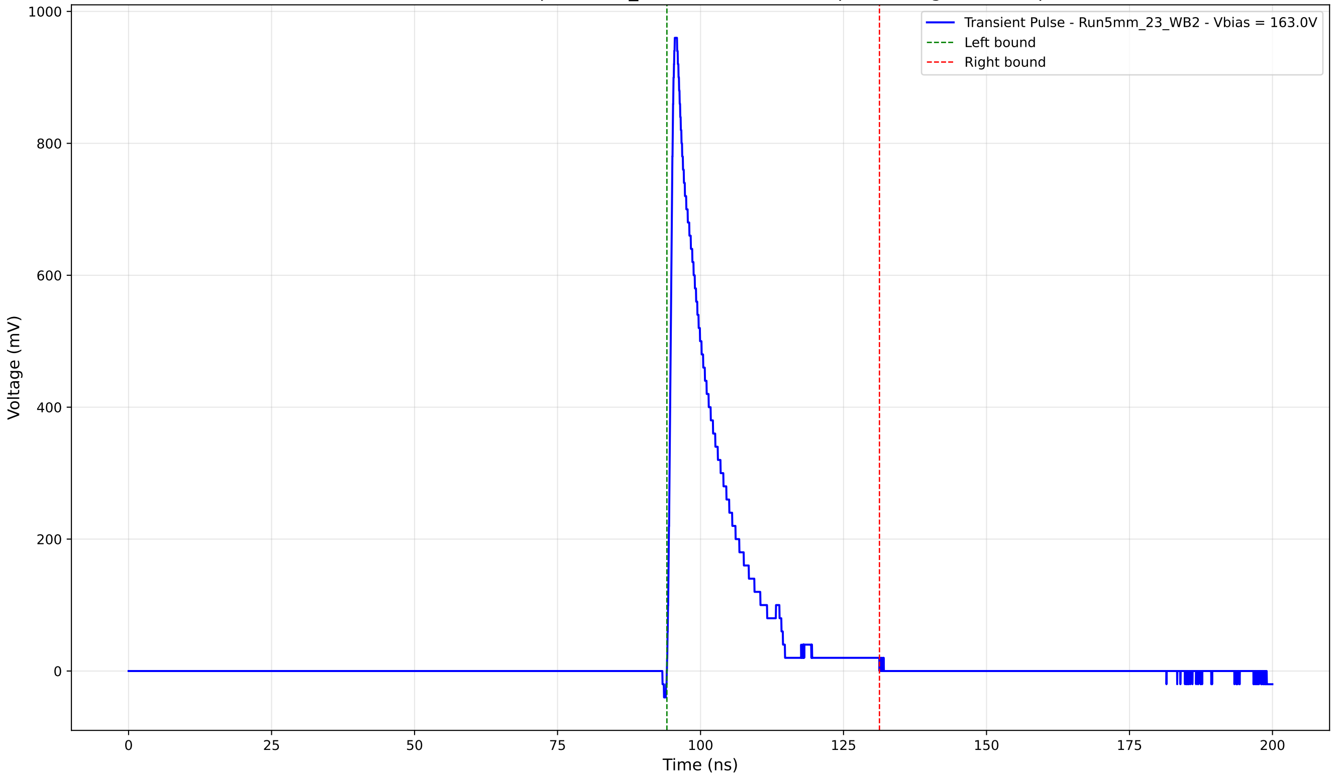
Transient Pulse - Sample: 5mm_23 - Position: 4770.0 \mu\text{m} - Charge: 147.31 pC
