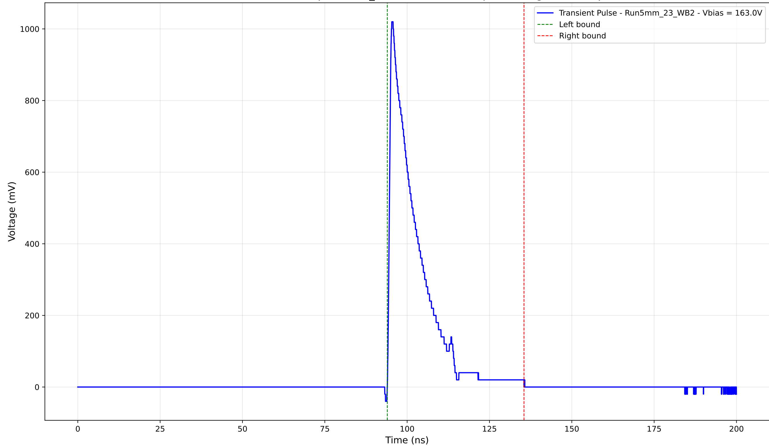
Transient Pulse - Sample: 5mm_23 - Position: 140.0 \mu\text{m} - Charge: 180.65 pC
