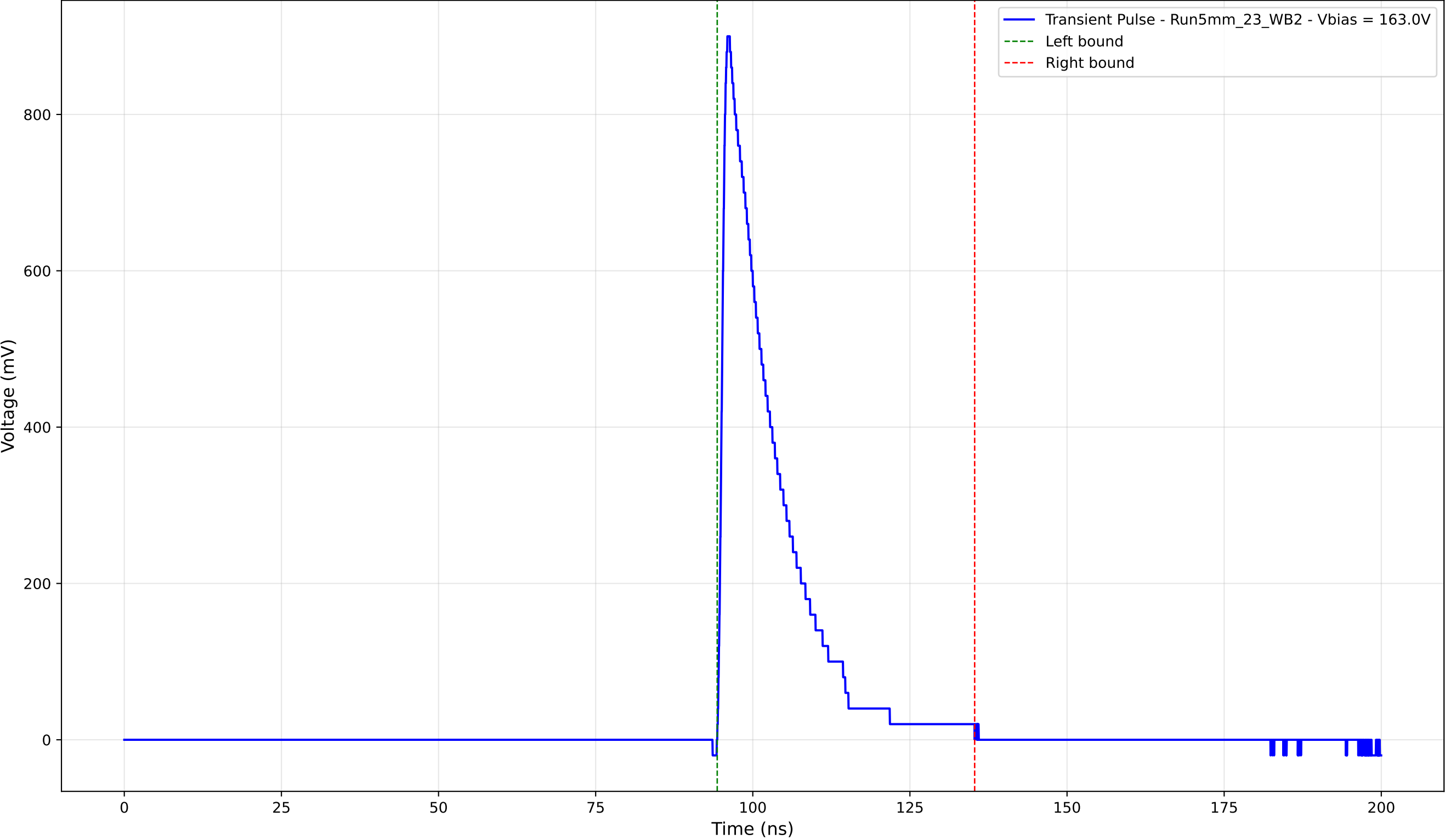
Transient Pulse - Sample: 5mm_23 - Position: 4295.0 \mu\text{m} - Charge: 162.75 pC
