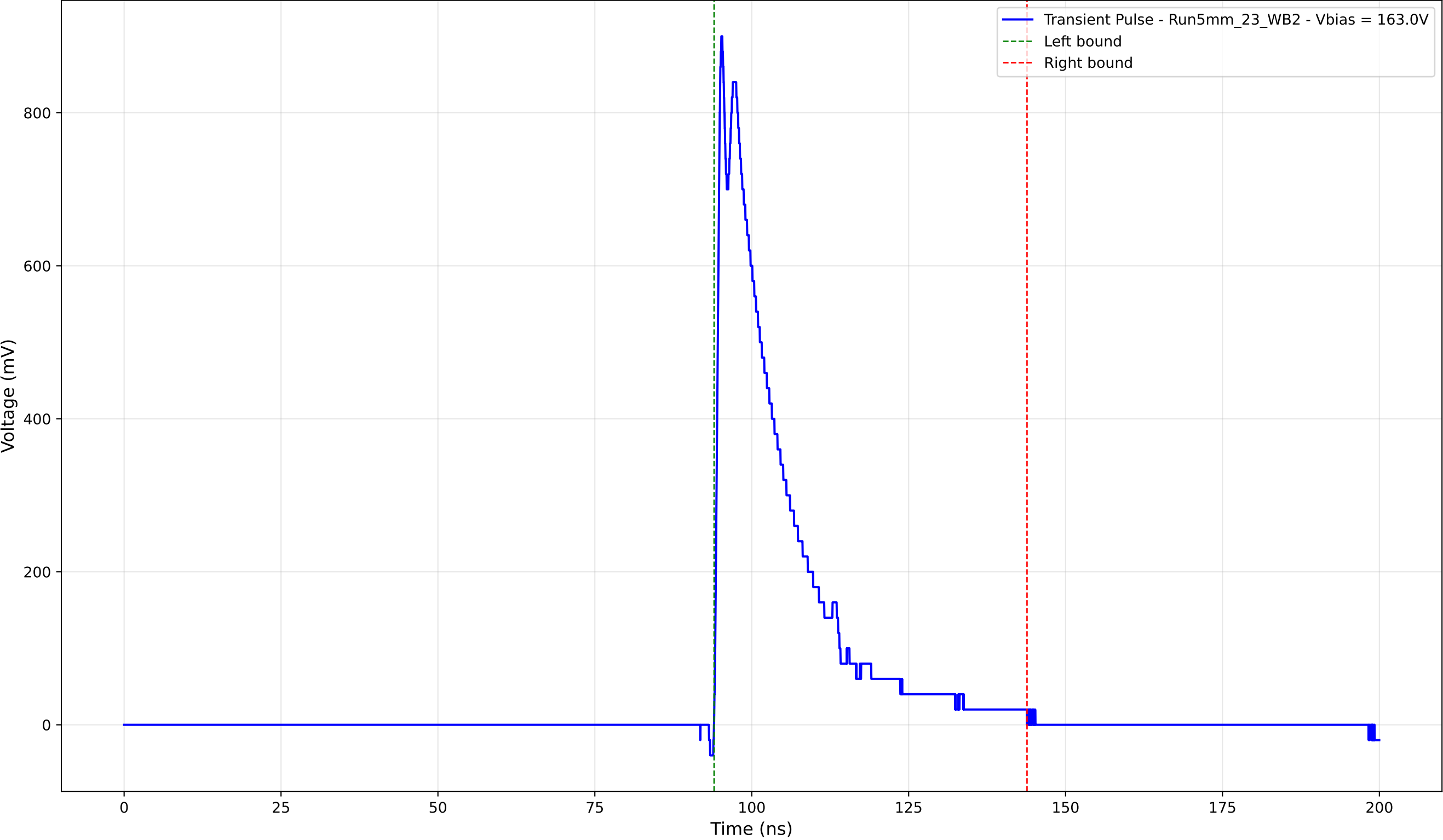
Transient Pulse - Sample: 5mm_23 - Position: 2105.0 \mu\text{m} - Charge: 190.94 pC
