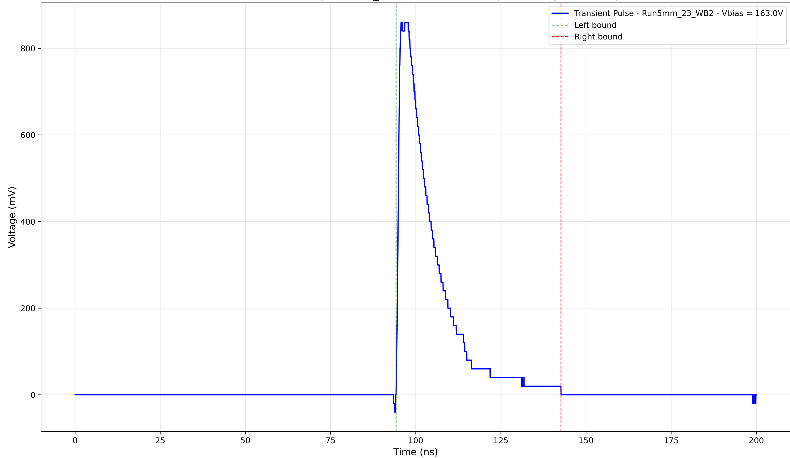
Transient Pulse - Sample: 5mm_23 - Position: 3350.0 \mu\text{m} - Charge: 196.35 pC
