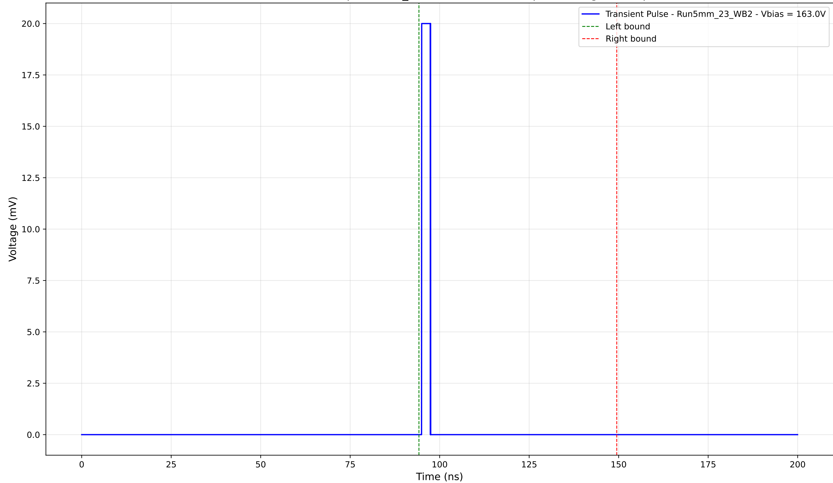
Transient Pulse - Sample: 5mm_23 - Position: 5035.0 \mu\text{m} - Charge: 0.98 pC
