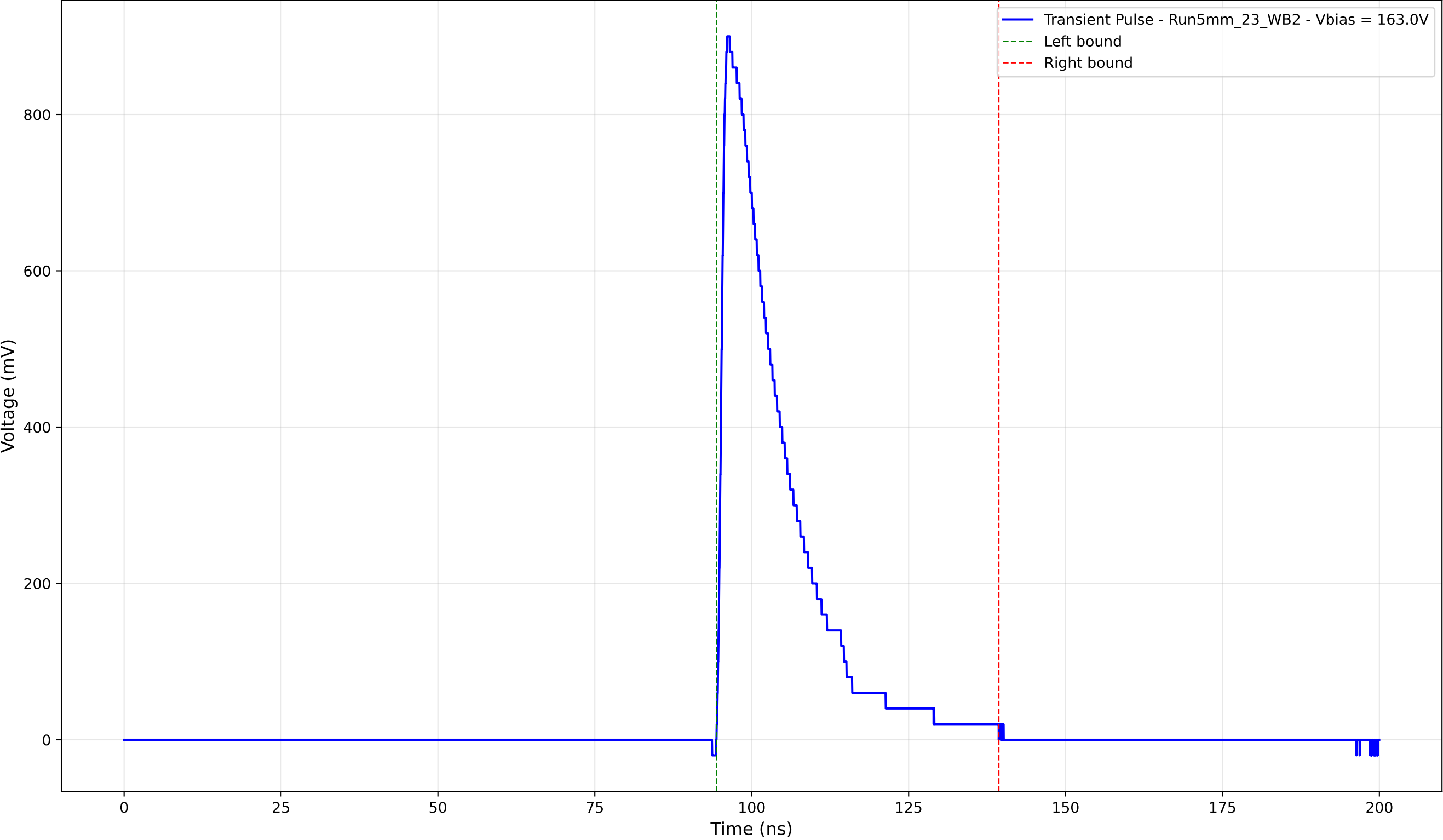
Transient Pulse - Sample: 5mm_23 - Position: 1175.0 \mu\text{m} - Charge: 194.20 pC
