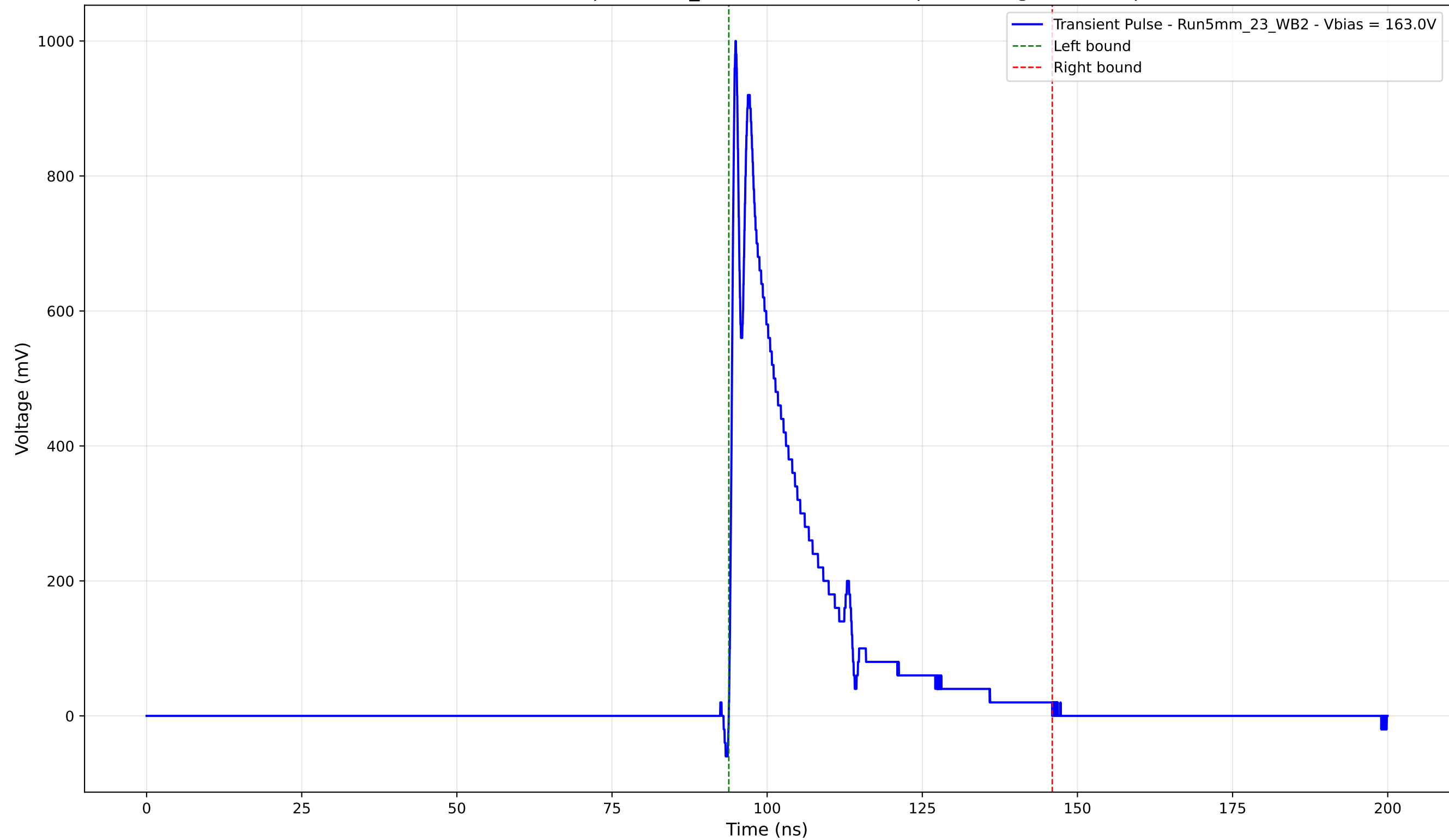
Transient Pulse - Sample: 5mm_23 - Position: 2625.0 \mu\text{m} - Charge: 198.13 pC
