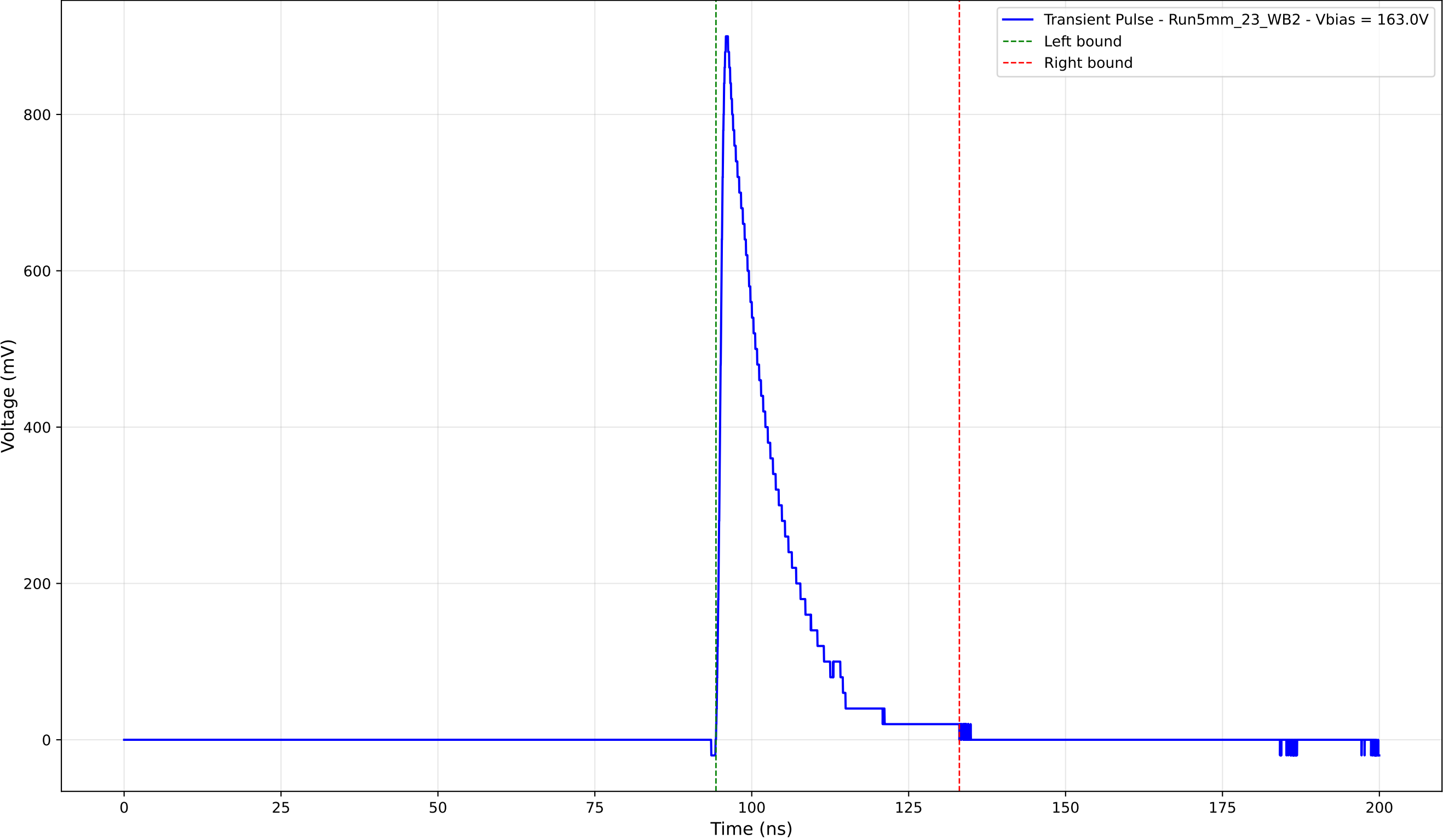
Transient Pulse - Sample: 5mm_23 - Position: 4415.0 \mu\text{m} - Charge: 154.71 pC
