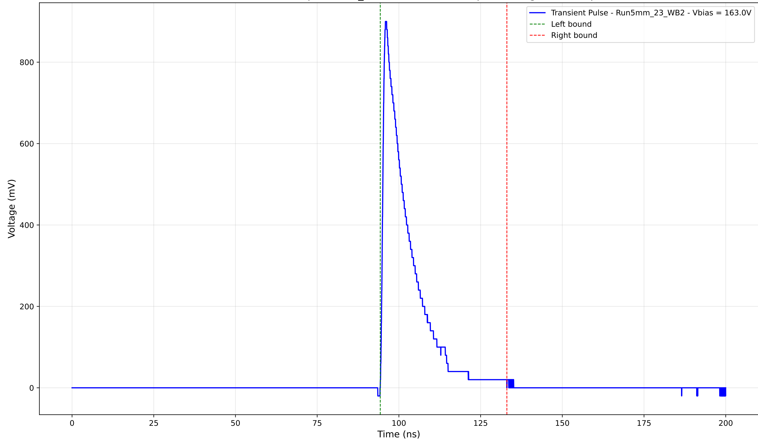
Transient Pulse - Sample: 5mm_23 - Position: 4395.0 \mu\text{m} - Charge: 157.04 pC
