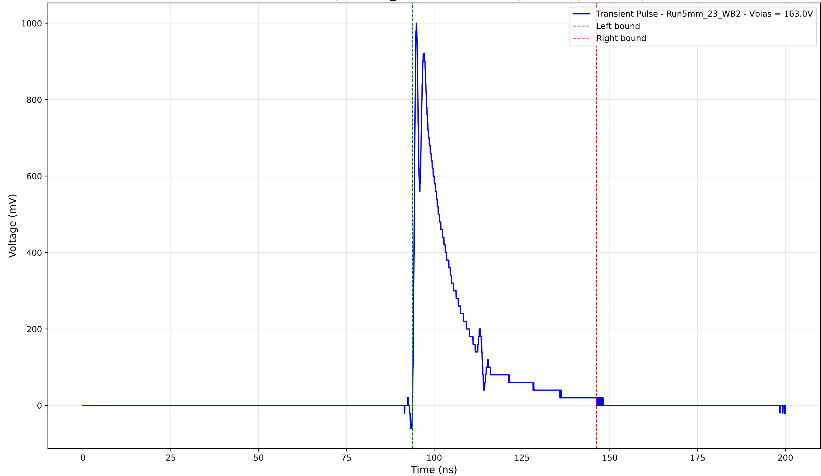
Transient Pulse - Sample: 5mm_23 - Position: 2635.0 \mu\text{m} - Charge: 200.88 pC
