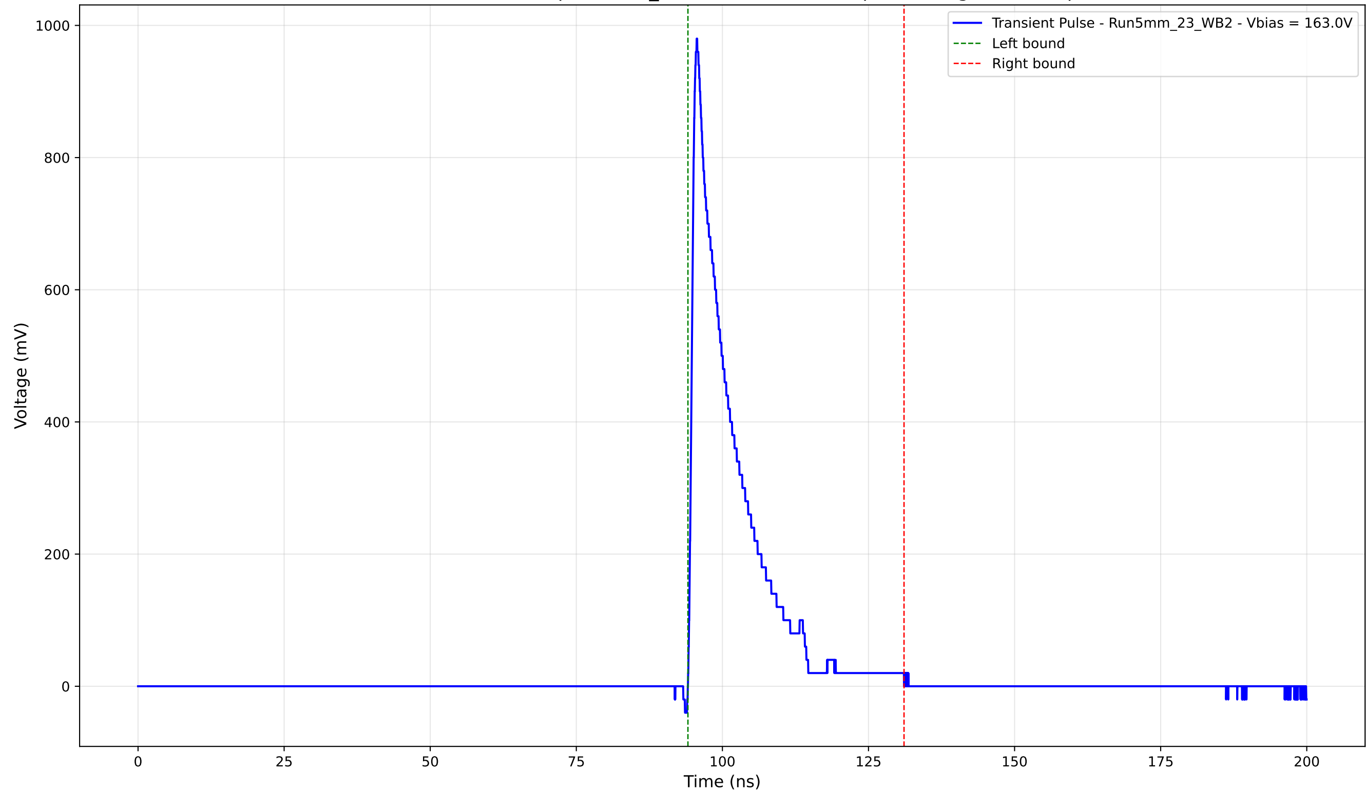
Transient Pulse - Sample: 5mm_23 - Position: 4795.0 \mu\text{m} - Charge: 146.30 pC
