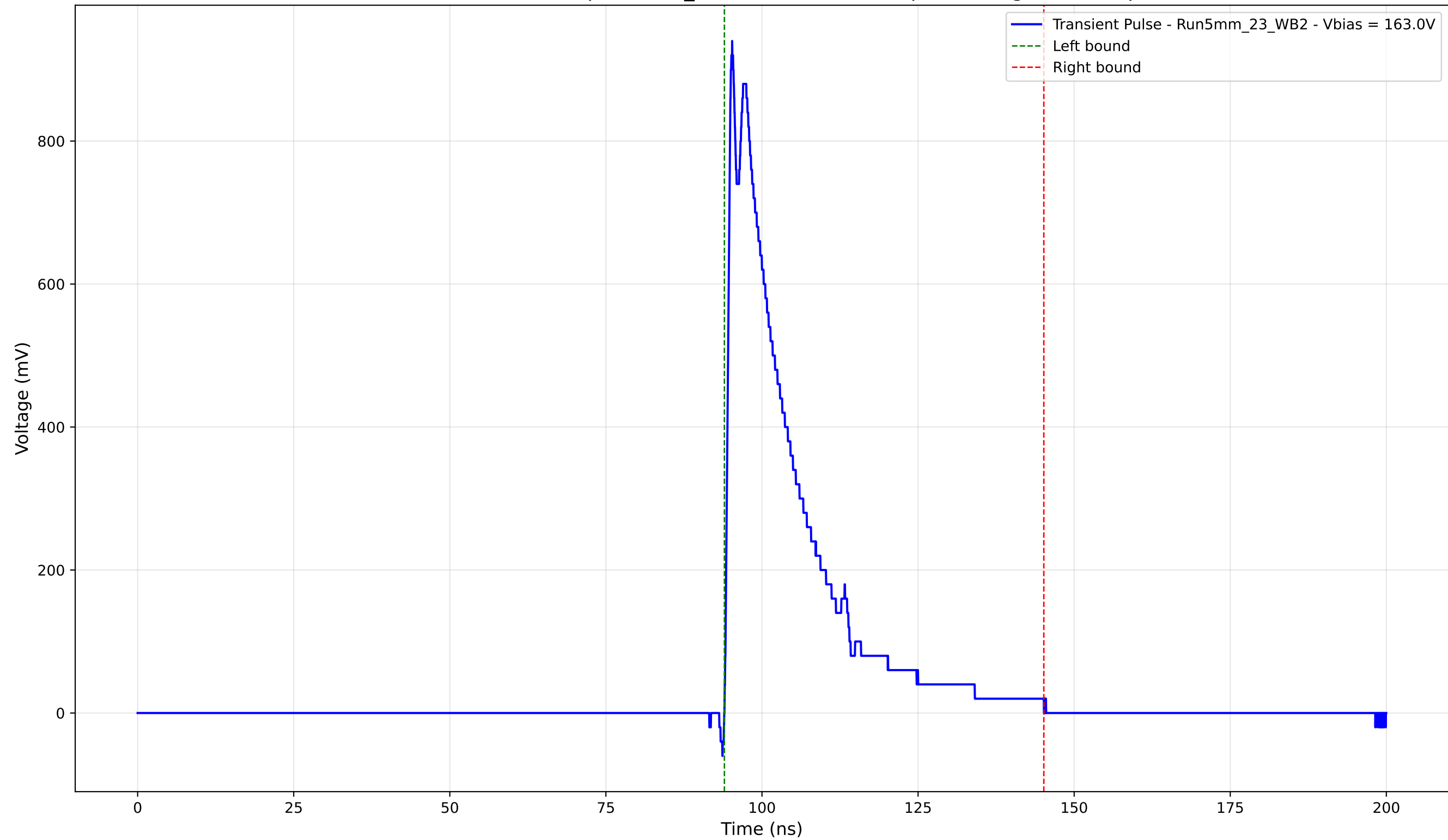
Transient Pulse - Sample: 5mm_23 - Position: 2120.0 \mu\text{m} - Charge: 201.46 pC
