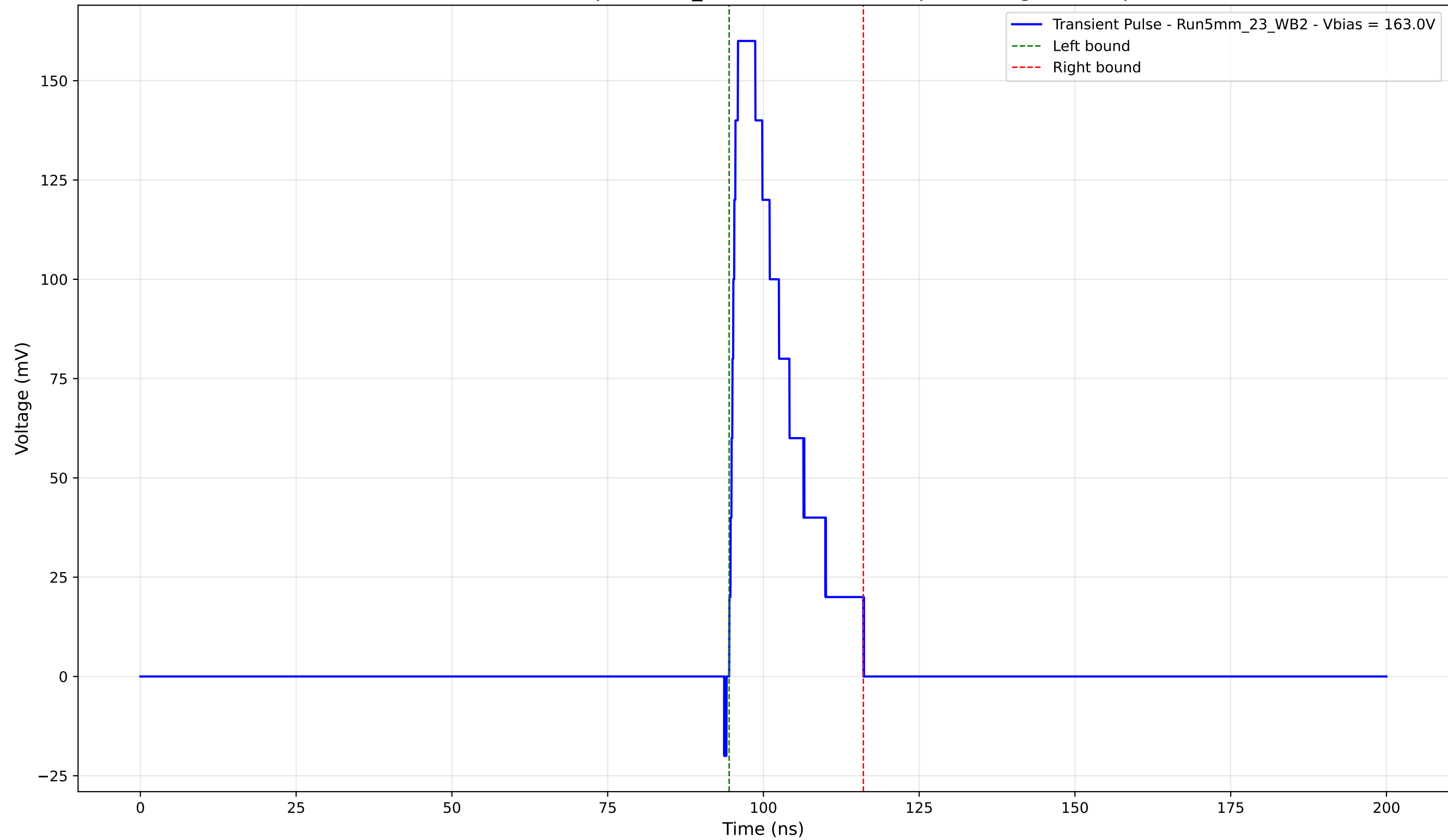
Transient Pulse - Sample: 5mm_23 -Position: 3520.0 \mu\text{m} - Charge: 31.06 pC
