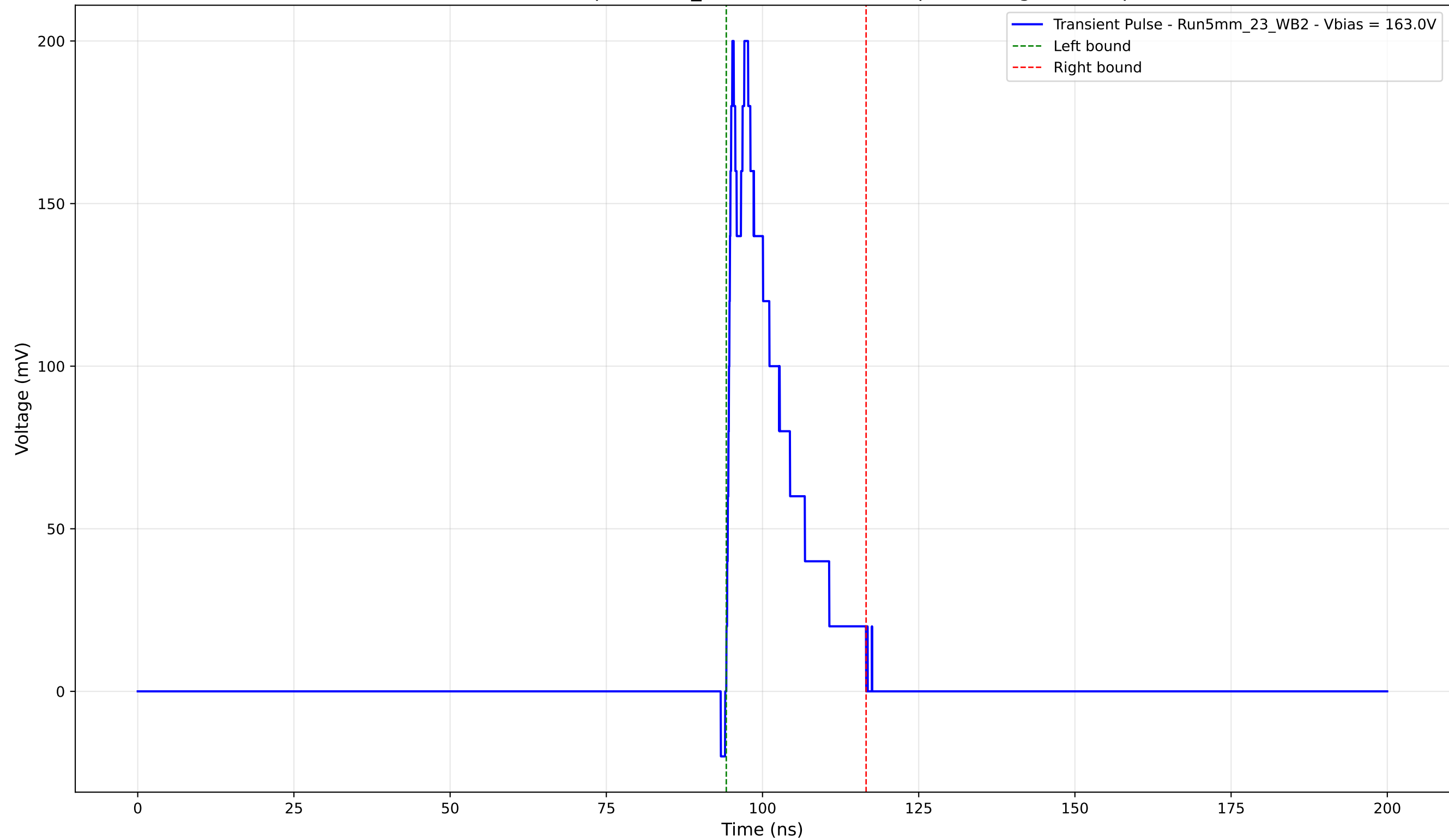
Transient Pulse - Sample: 5mm_23 - Position: 2015.0 \mu\text{m} - Charge: 34.62 pC
