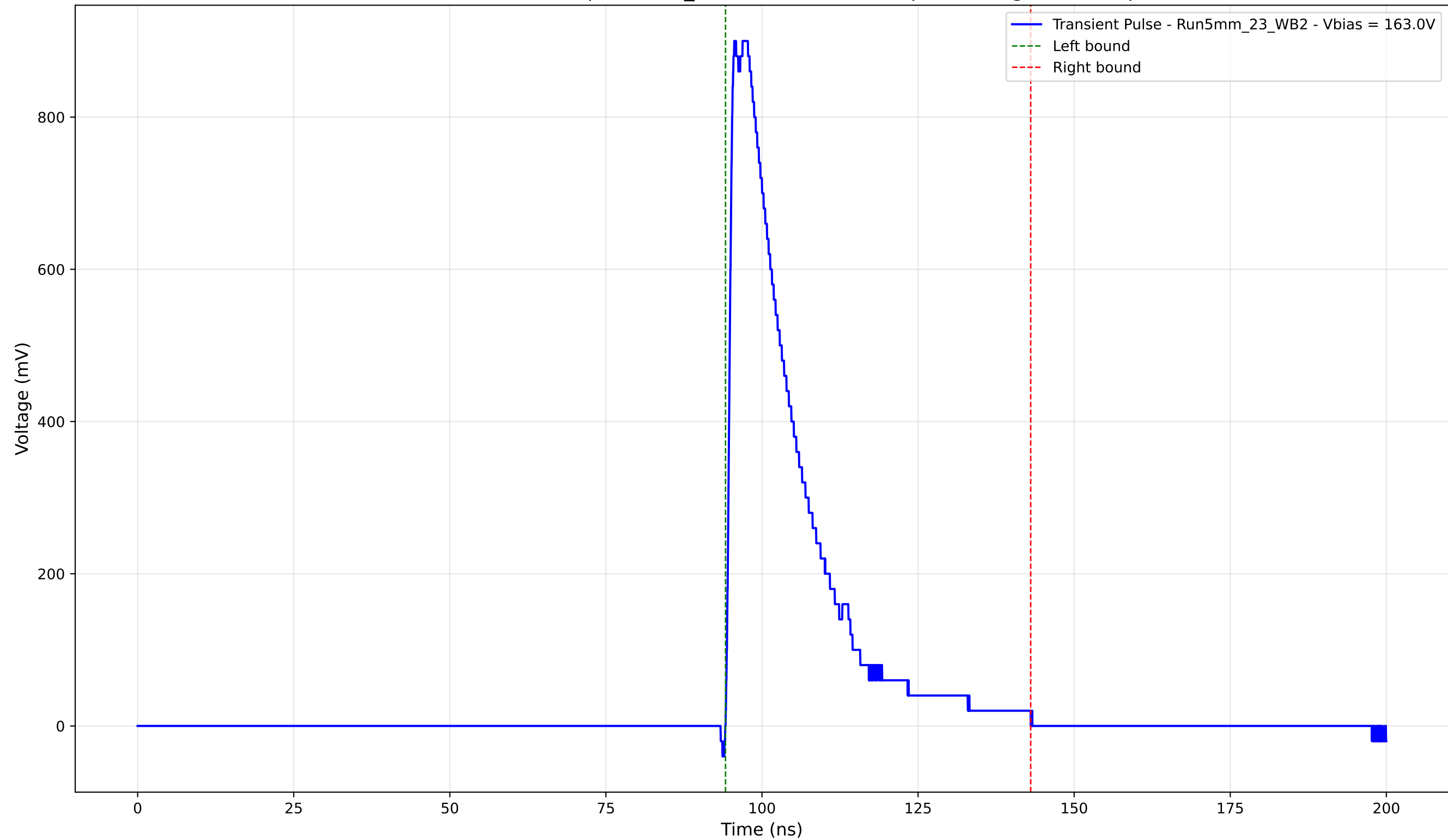
Transient Pulse - Sample: 5mm_23 - Position: 3280.0 \mu\text{m} - Charge: 211.04 pC
