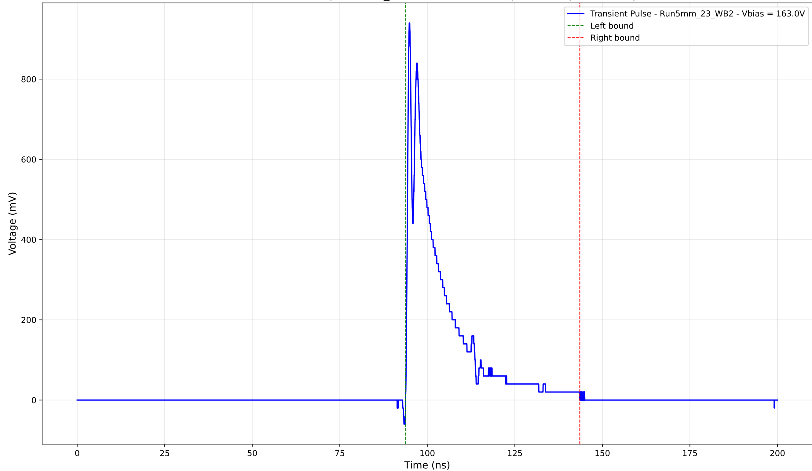
Transient Pulse - Sample: 5mm_23 - Position: 2590.0 \mu\text{m} - Charge: 166.27 pC
