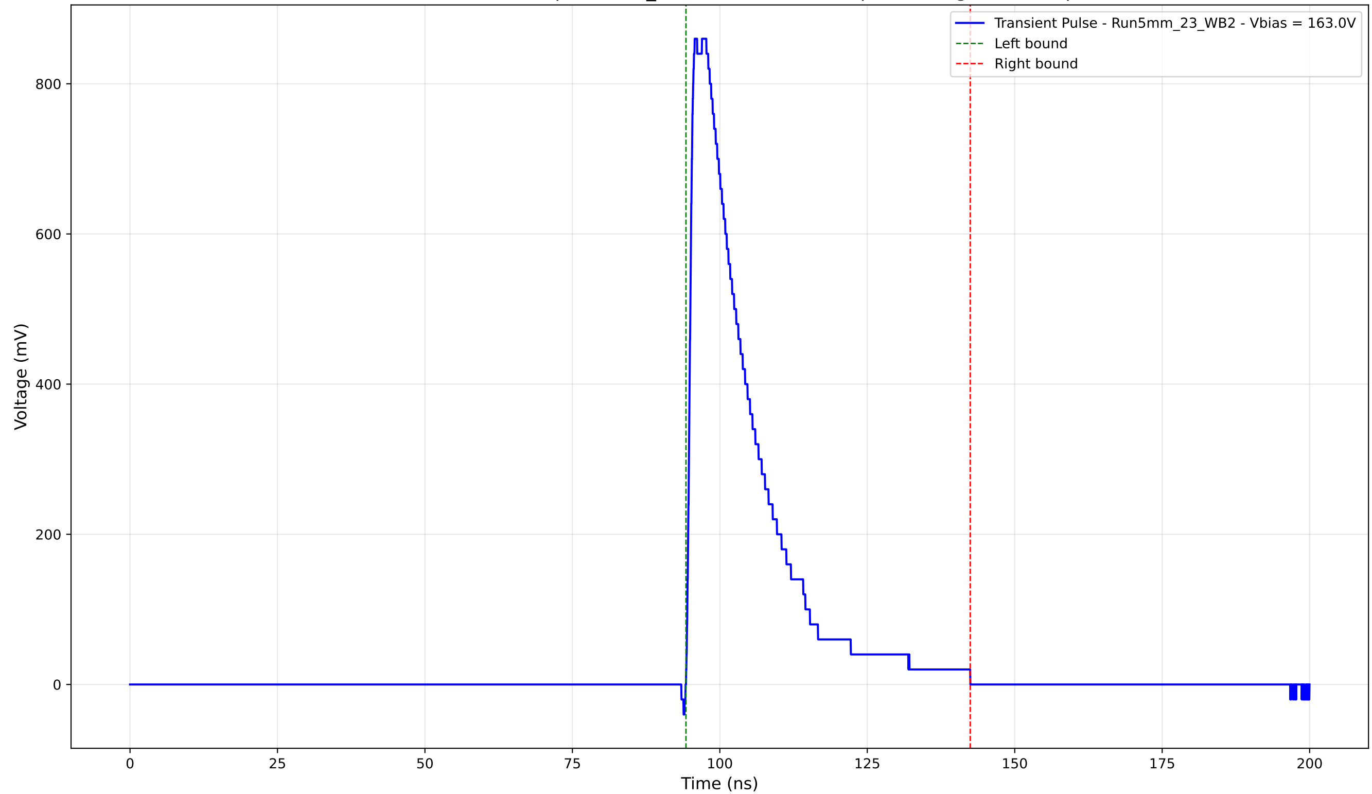
Transient Pulse - Sample: 5mm_23 - Position: 1620.0 \mu\text{m} - Charge: 198.05 pC
