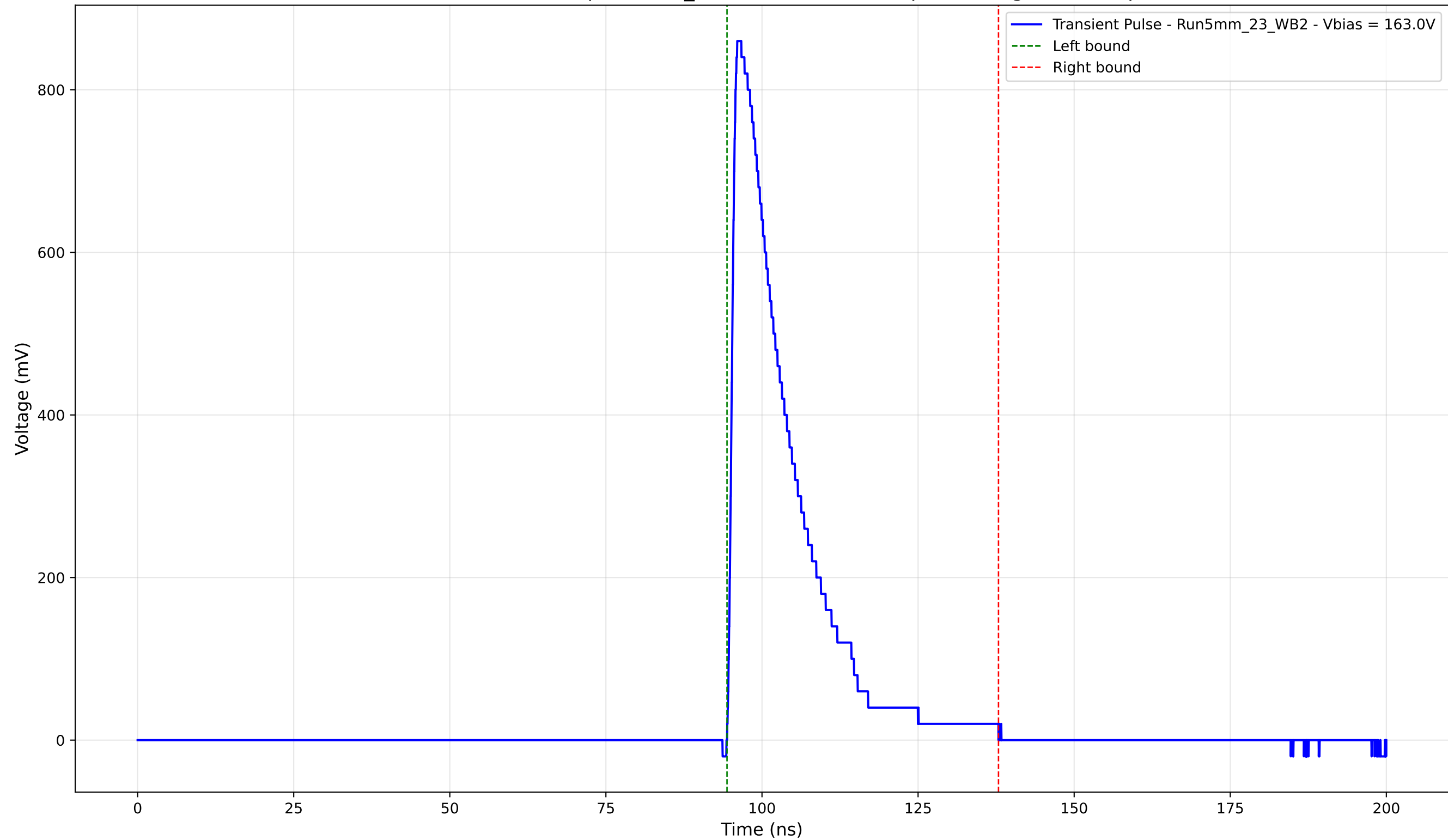
Transient Pulse - Sample: 5mm_23 - Position: 3805.0 \mu\text{m} - Charge: 176.26 pC
