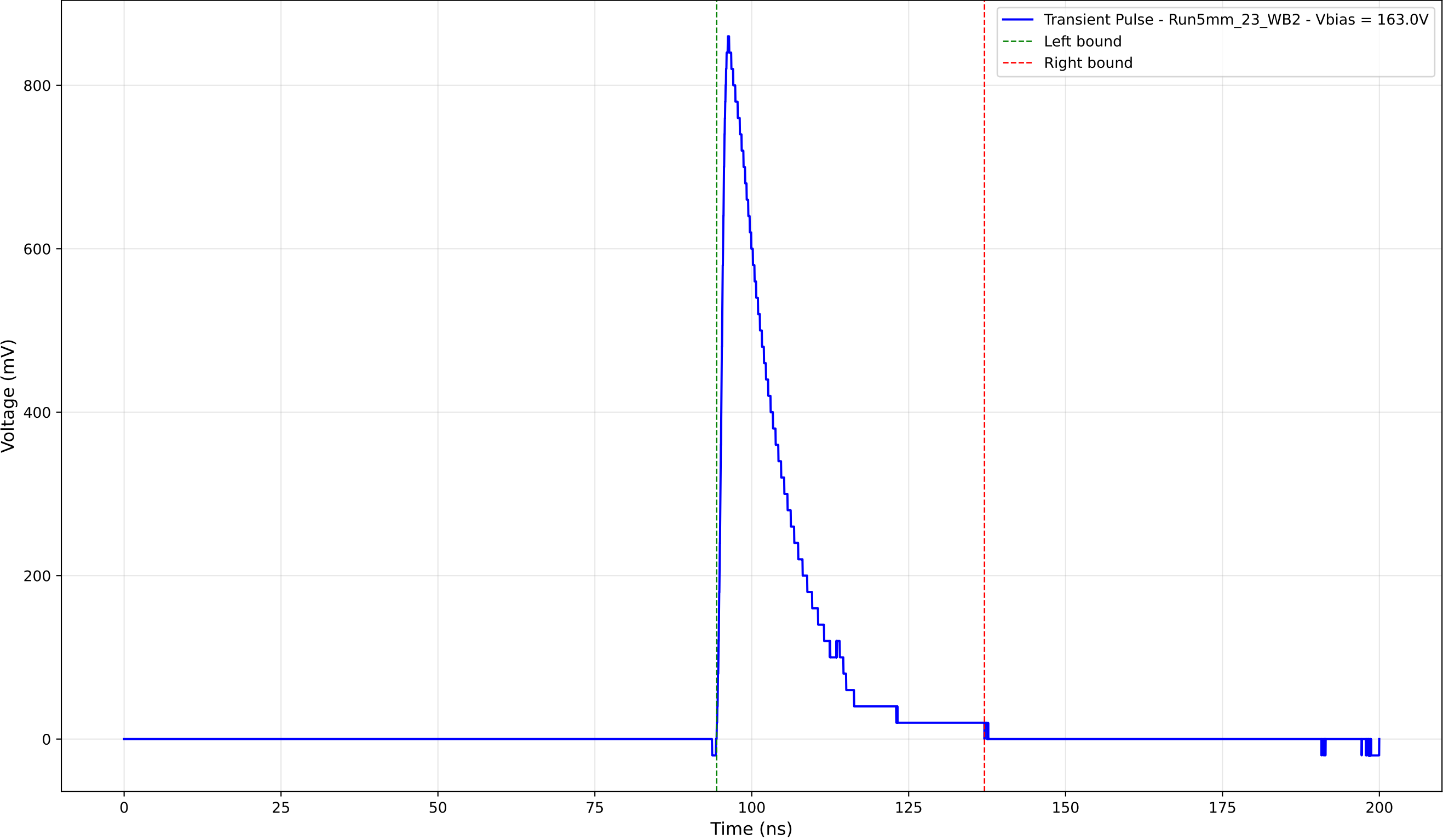
Transient Pulse - Sample: 5mm_23 - Position: 3930.0 \mu\text{m} - Charge: 165.53 pC
