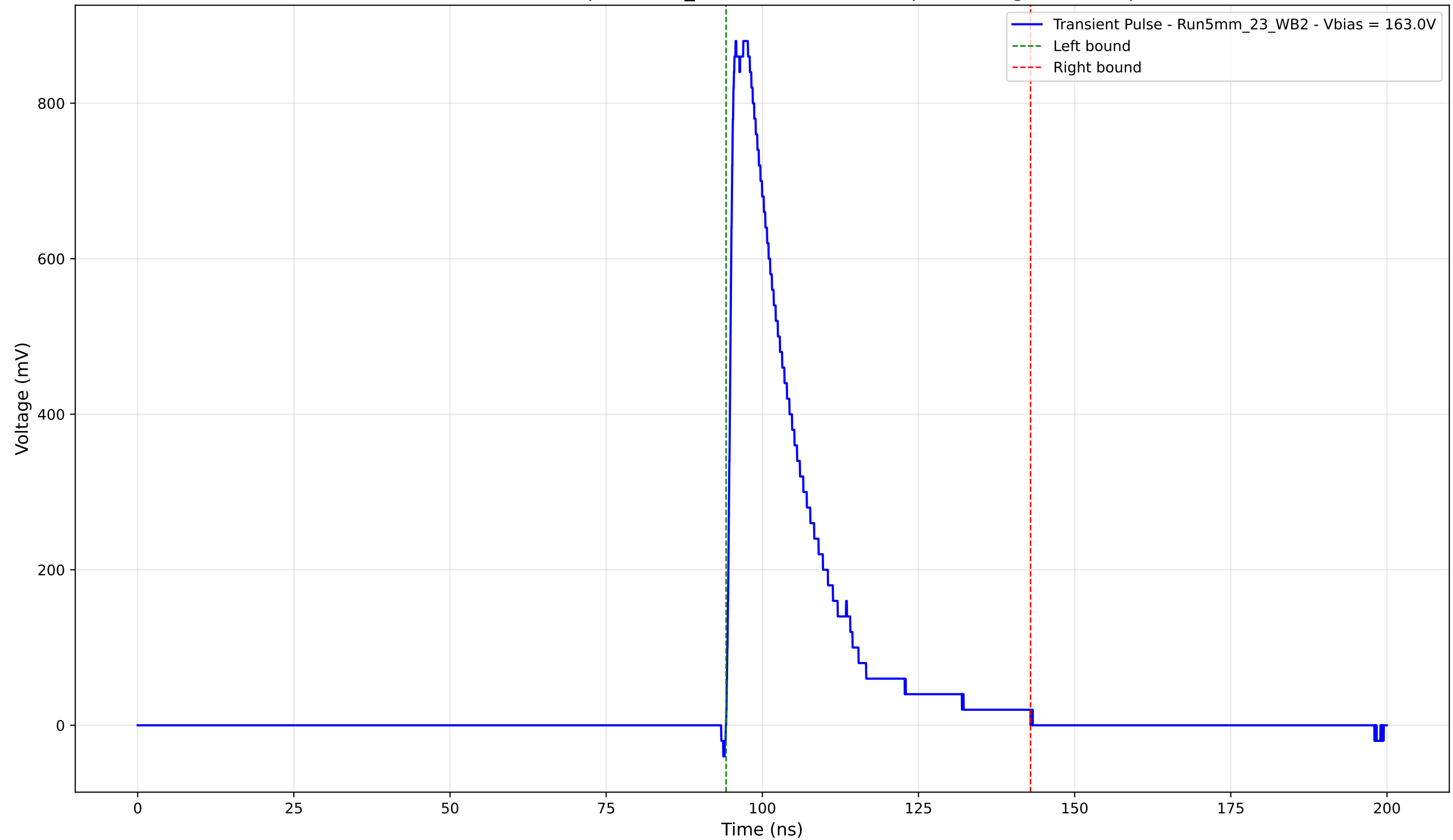
Transient Pulse - Sample: 5mm_23 - Position: 3325.0 \mu\text{m} - Charge: 202.04 pC
