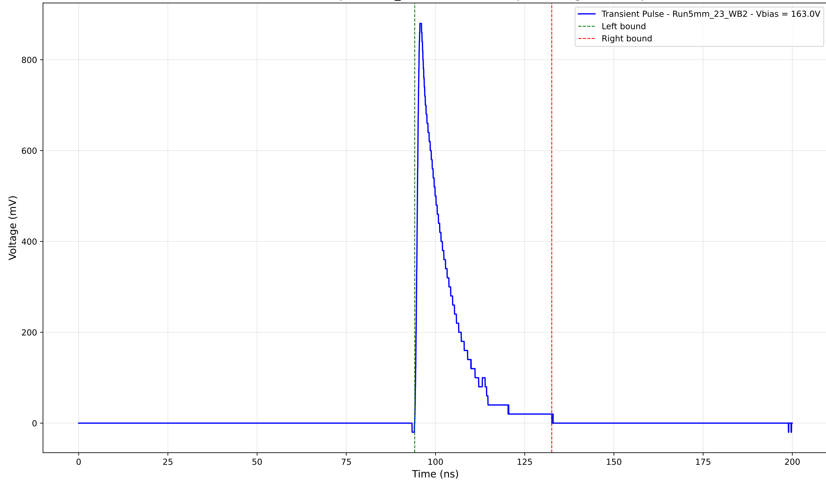
Transient Pulse - Sample: 5mm_23 - Position: 420.0 \mu\text{m} - Charge: 146.42 pC
