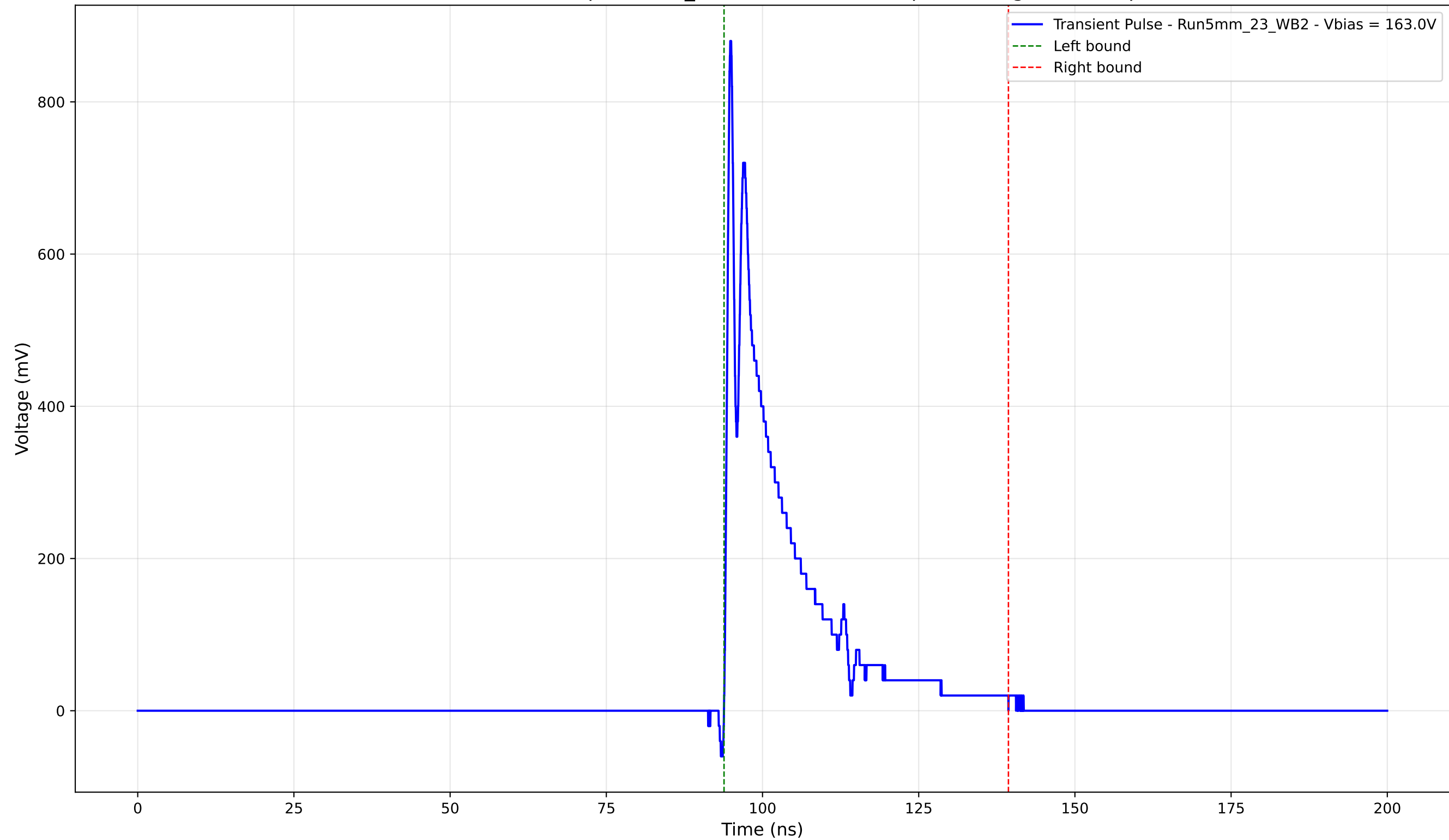
Transient Pulse - Sample: 5mm_23 - Position: 2575.0 \mu\text{m} - Charge: 137.59 pC
