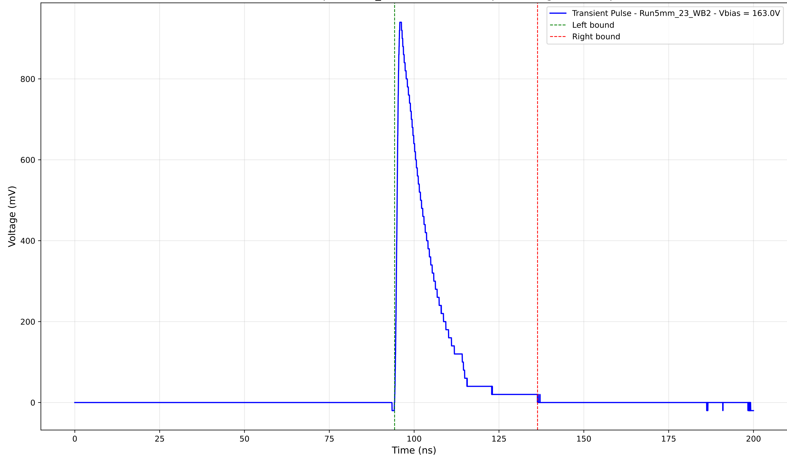
Transient Pulse - Sample: 5mm_23 - Position: 580.0 \mu\text{m} - Charge: 180.13 pC
