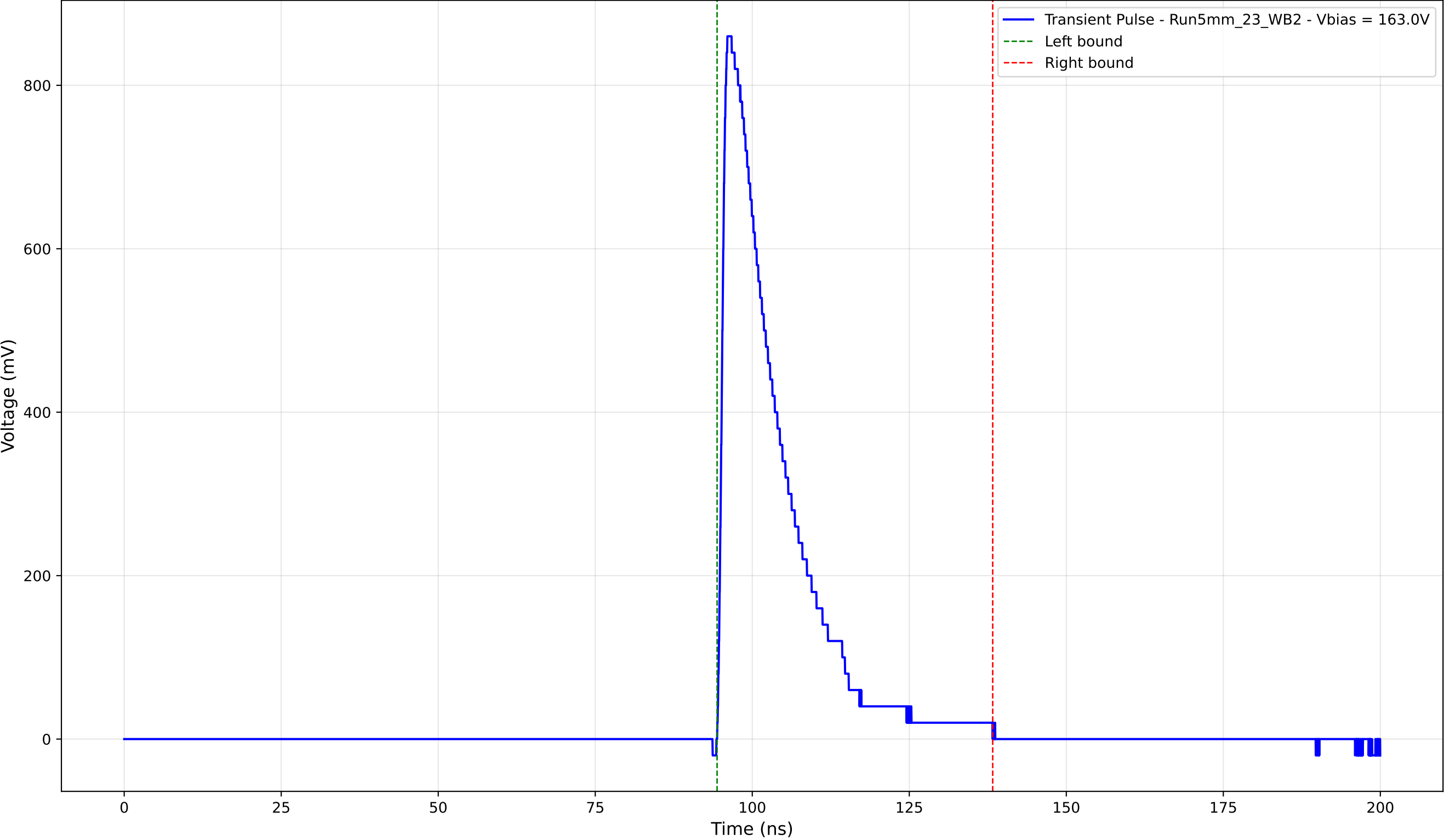
Transient Pulse - Sample: 5mm_23 - Position: 3795.0 \mu\text{m} - Charge: 176.56 pC
