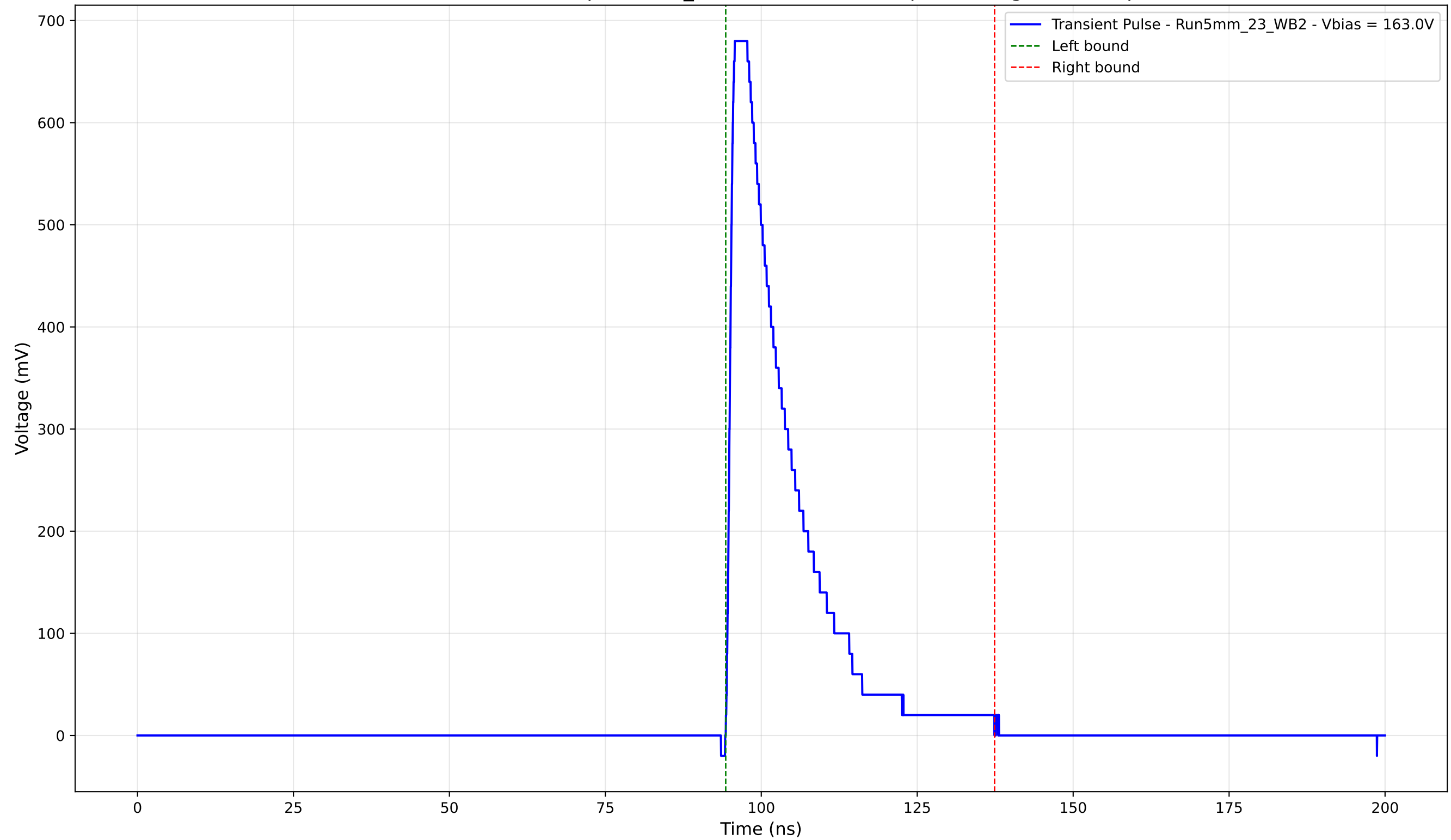
Transient Pulse - Sample: 5mm_23 - Position: 3455.0 \mu\text{m} - Charge: 143.25 pC
