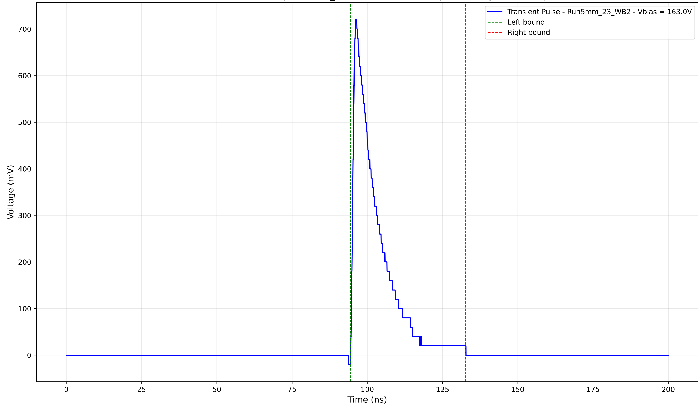
Transient Pulse - Sample: 5mm_23 - Position: 4105.0 \mu\text{m} - Charge: 126.40 pC
