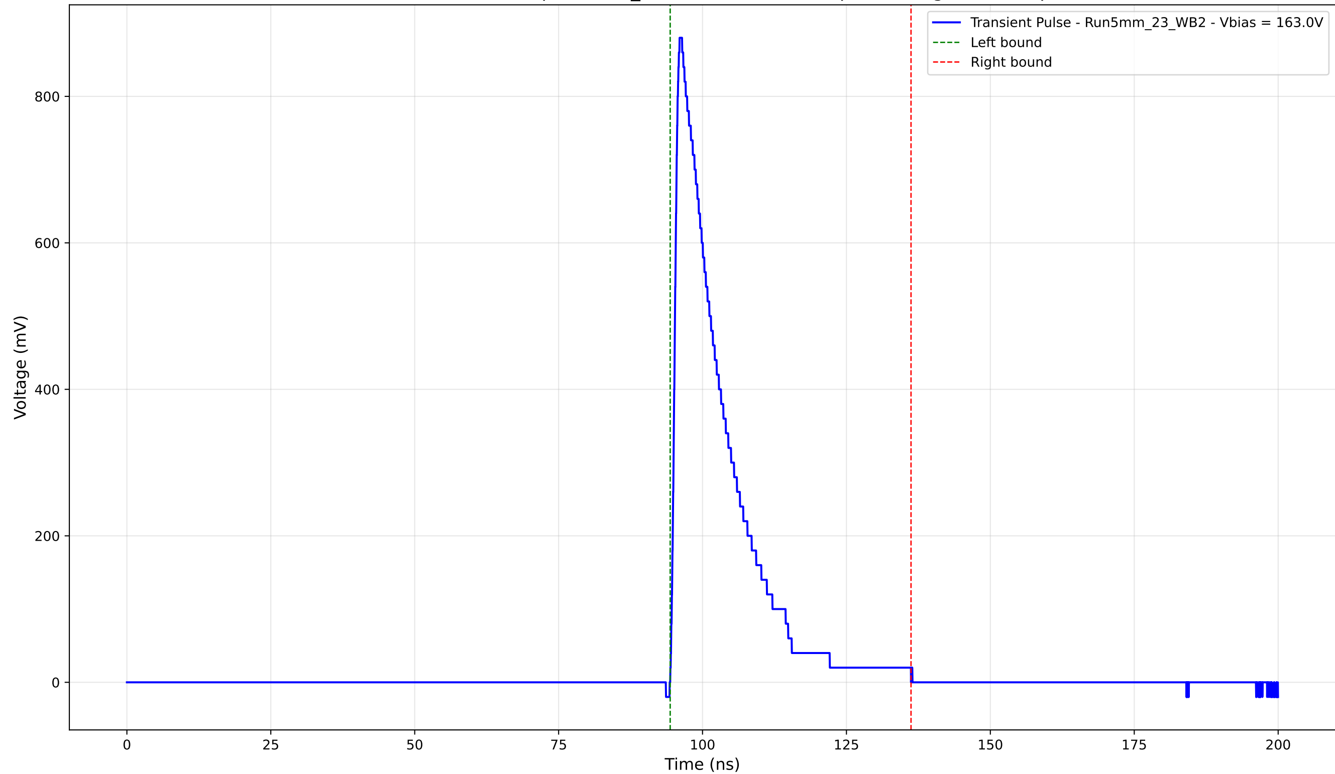
Transient Pulse - Sample: 5mm_23 - Position: 4185.0 \mu\text{m} - Charge: 163.22 pC
