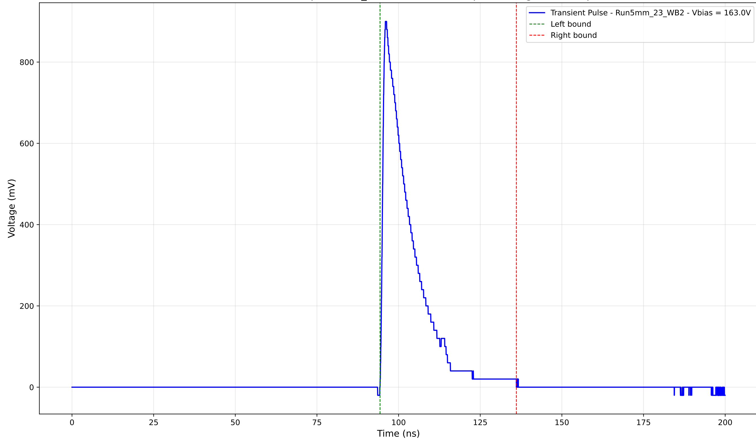
Transient Pulse - Sample: 5mm_23 - Position: 715.0 \mu\text{m} - Charge: 171.46 pC
