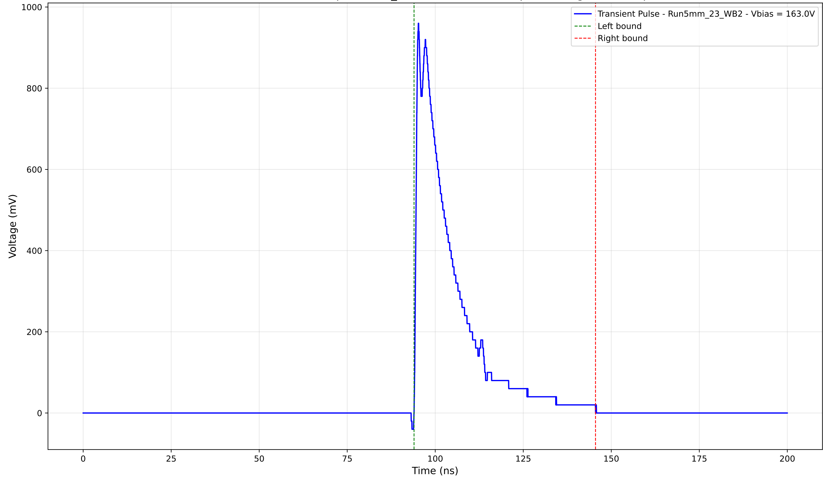
Transient Pulse - Sample: 5mm_23 - Position: 2930.0 \mu\text{m} - Charge: 210.54 pC
