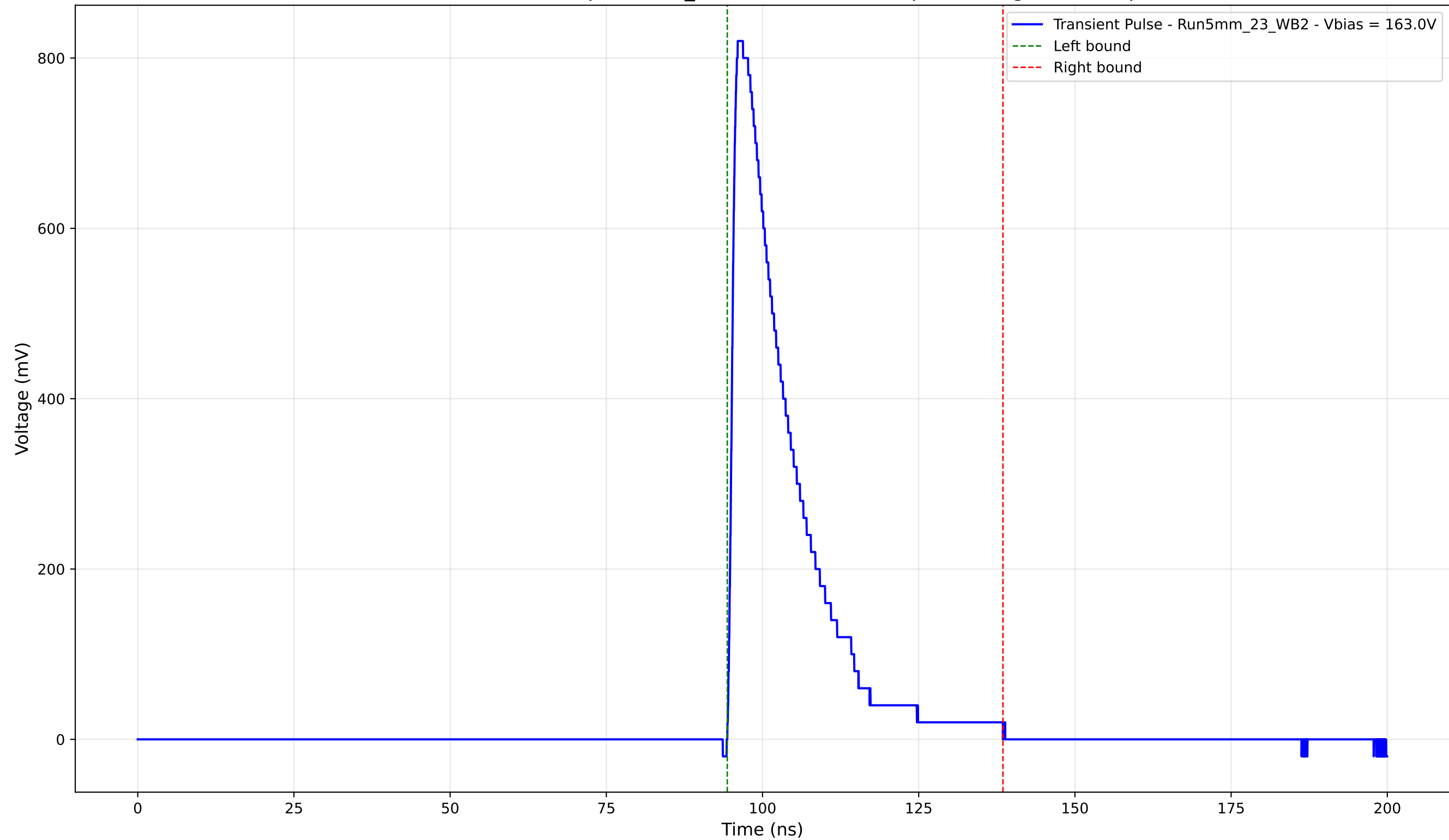
Transient Pulse - Sample: 5mm_23 - Position: 3650.0 \mu\text{m} - Charge: 171.62 pC
