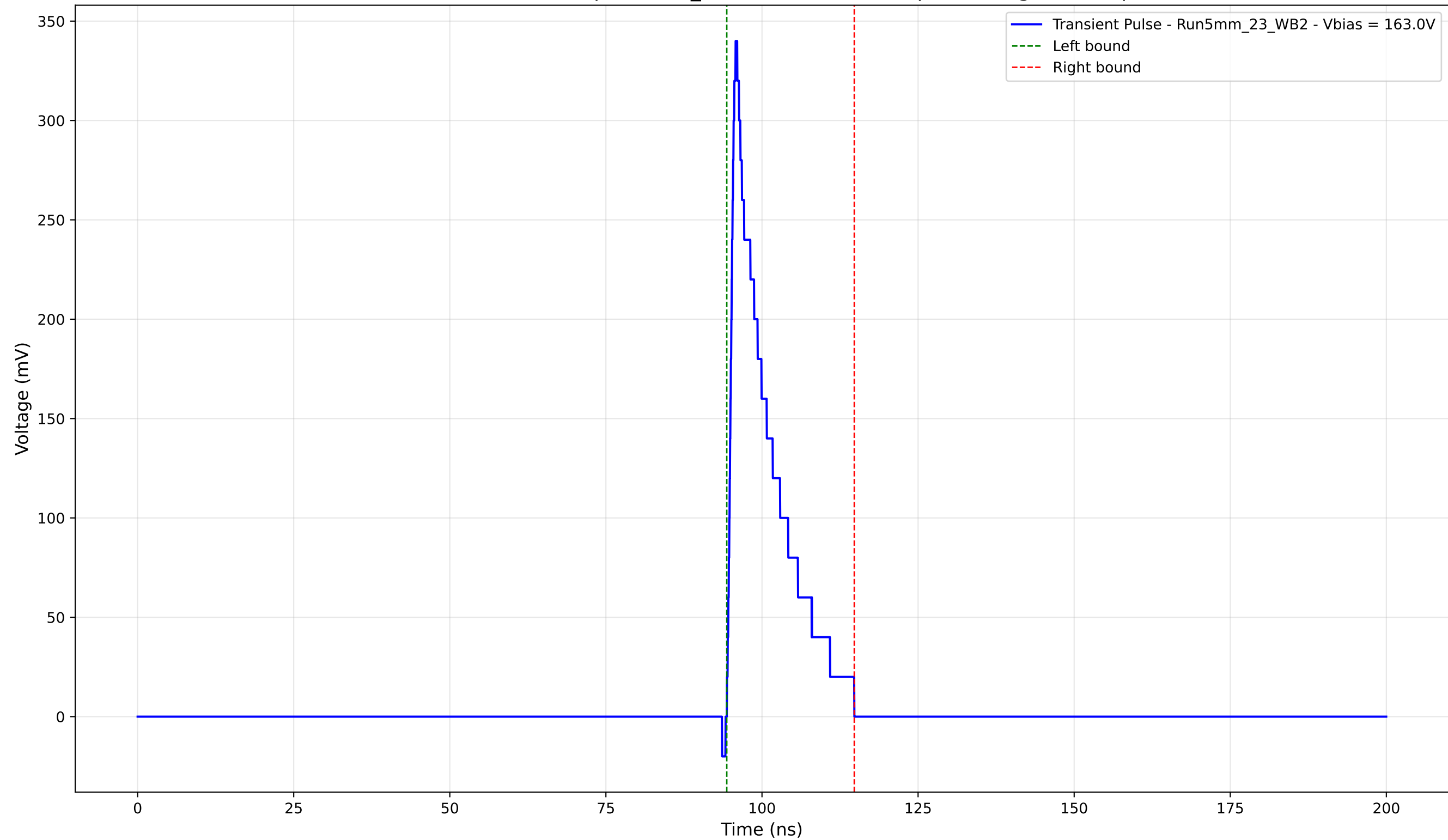
Transient Pulse - Sample: 5mm_23 - Position: 4560.0 \mu\text{m} - Charge: 45.02 pC
