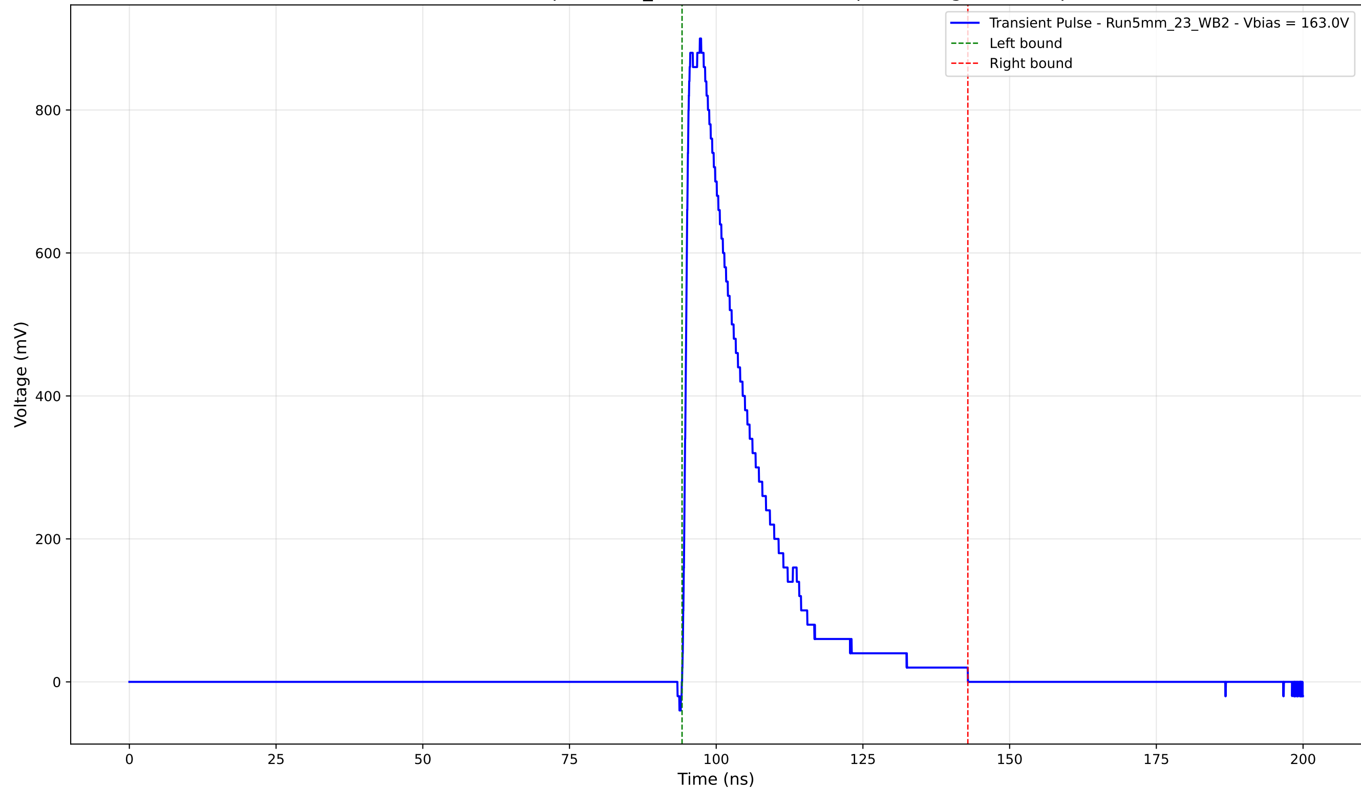
Transient Pulse - Sample: 5mm_23 - Position: 3310.0 \mu\text{m} - Charge: 205.42 pC
