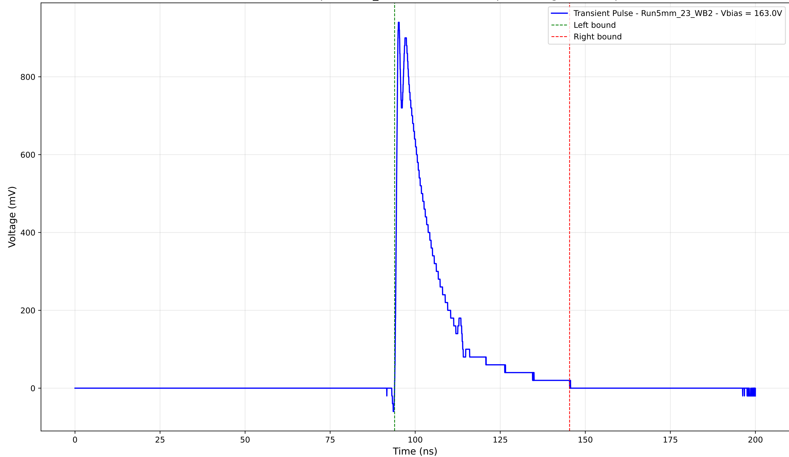
Transient Pulse - Sample: 5mm_23 - Position: 2180.0 \mu\text{m} - Charge: 205.78 pC
