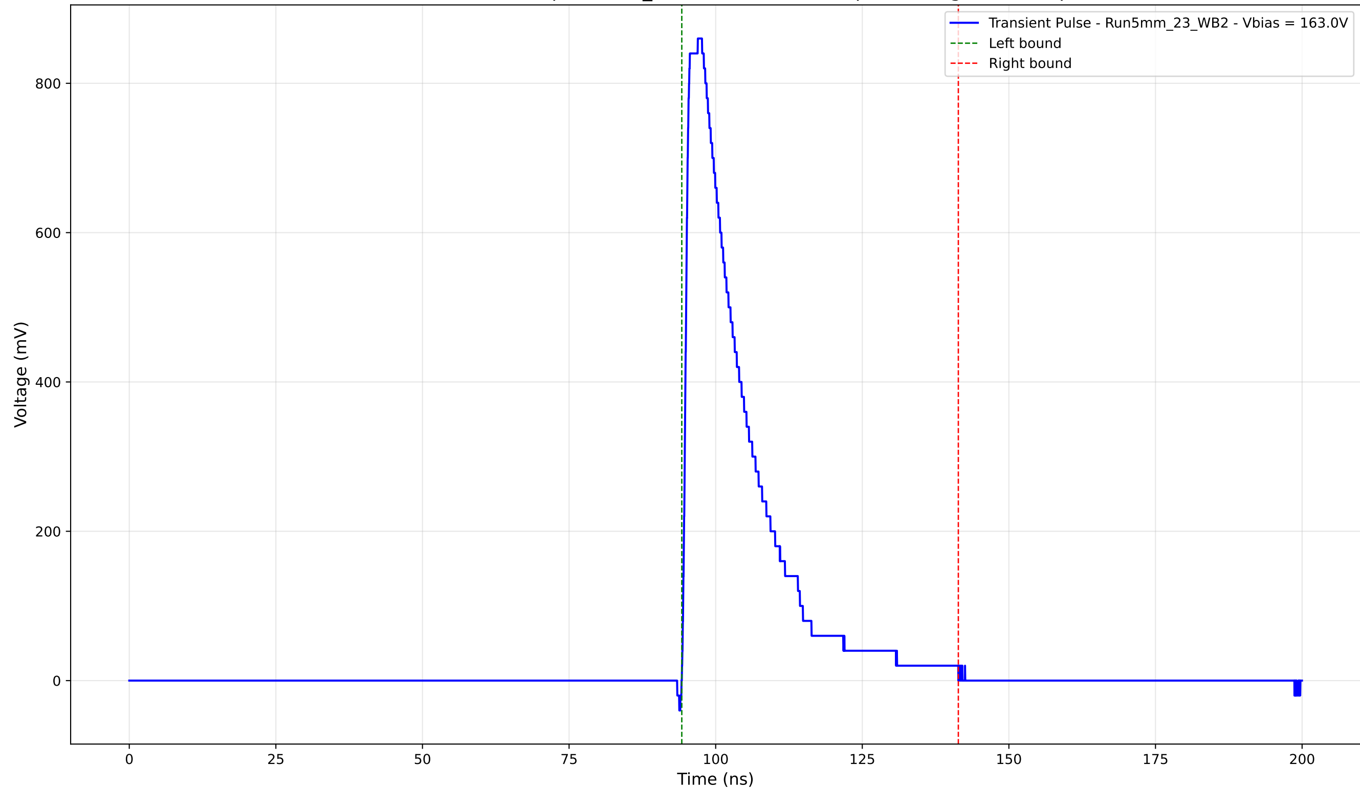
Transient Pulse - Sample: 5mm_23 - Position: 3360.0 \mu\text{m} - Charge: 193.81 pC
