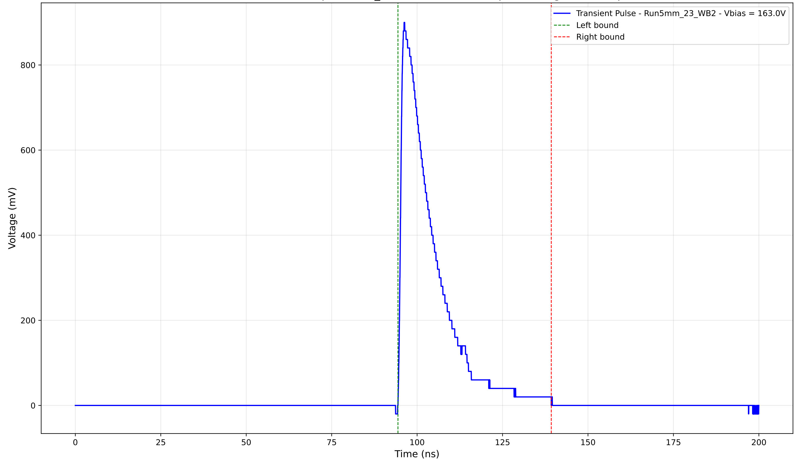
Transient Pulse - Sample: 5mm_23 - Position: 1140.0 \mu\text{m} - Charge: 190.89 pC
