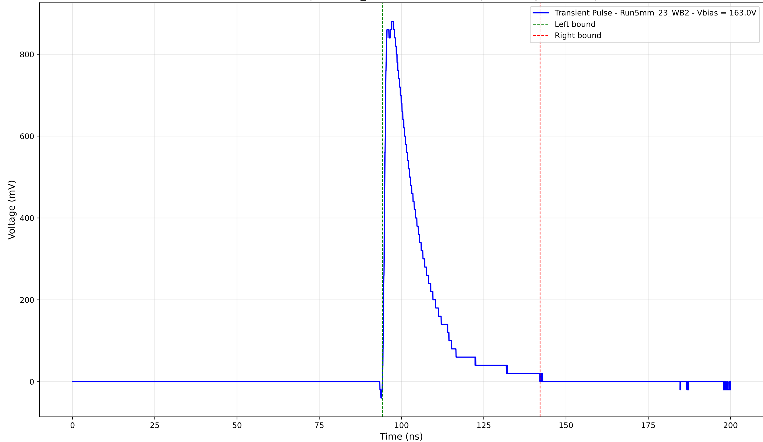
Transient Pulse - Sample: 5mm_23 - Position: 3335.0 \mu\text{m} - Charge: 199.68 pC
