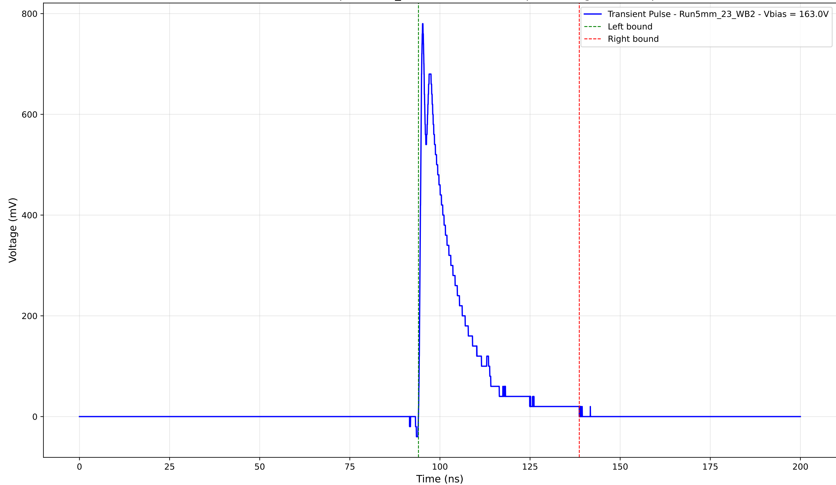
Transient Pulse - Sample: 5mm_23 - Position: 2070.0 \mu\text{m} - Charge: 142.23 pC
