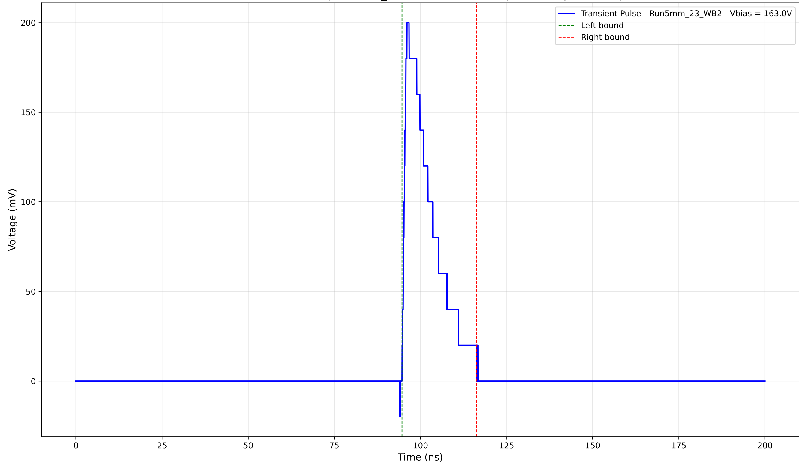
Transient Pulse - Sample: 5mm_23 - Position: 1005.0 \mu\text{m} - Charge: 35.80 pC
