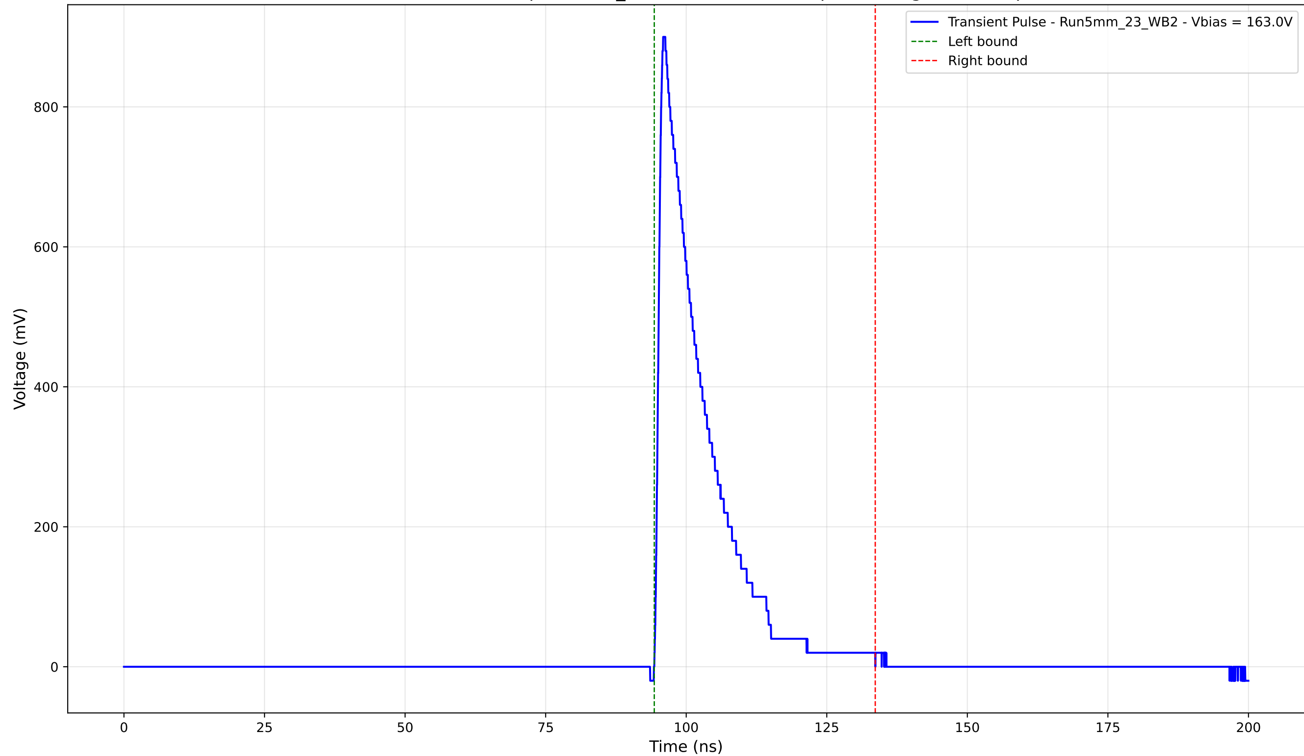
Transient Pulse - Sample: 5mm_23 - Position: 4365.0 \mu\text{m} - Charge: 159.17 pC
