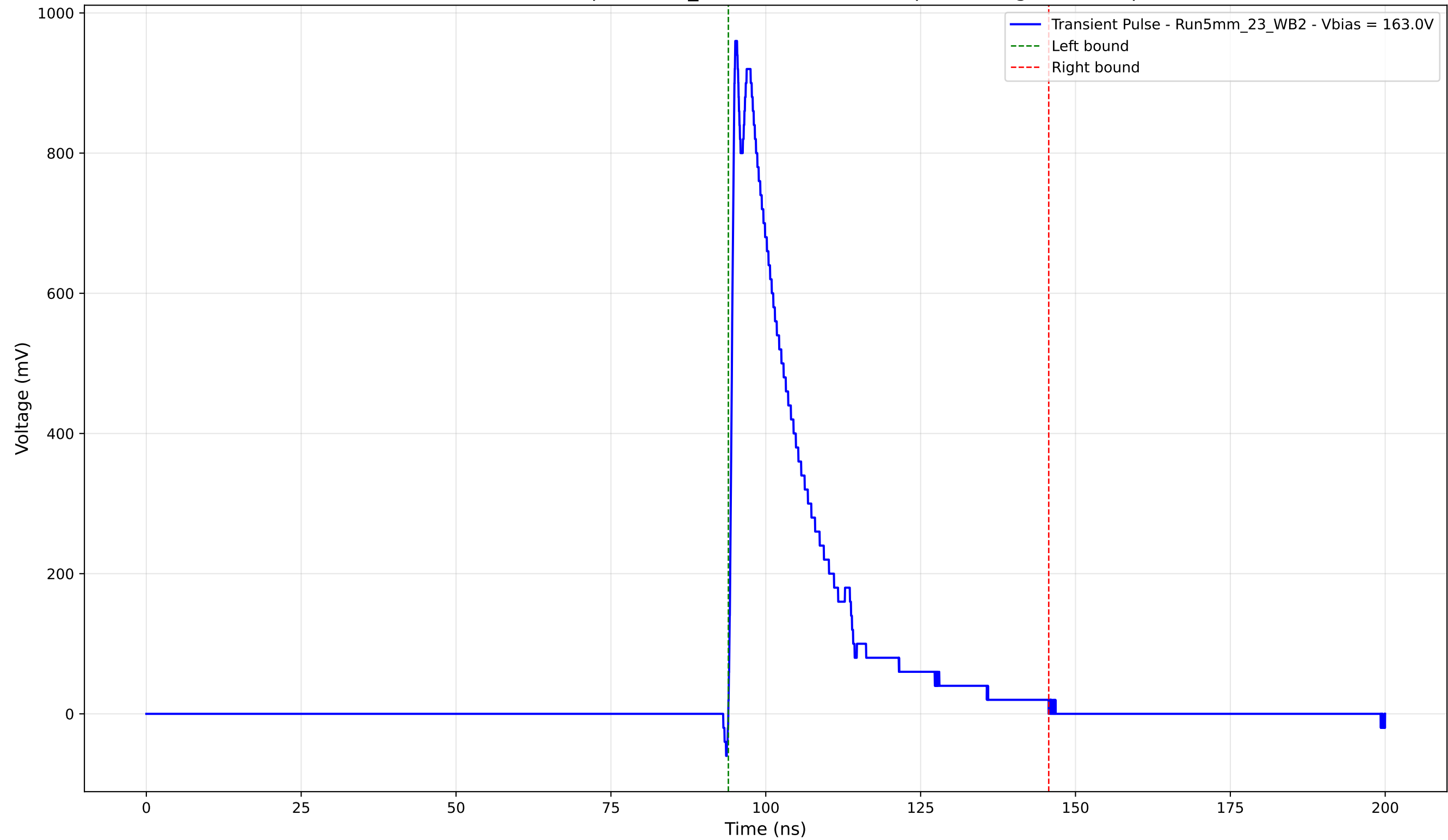
Transient Pulse - Sample: 5mm_23 - Position: 2915.0 \mu\text{m} - Charge: 218.26 pC
