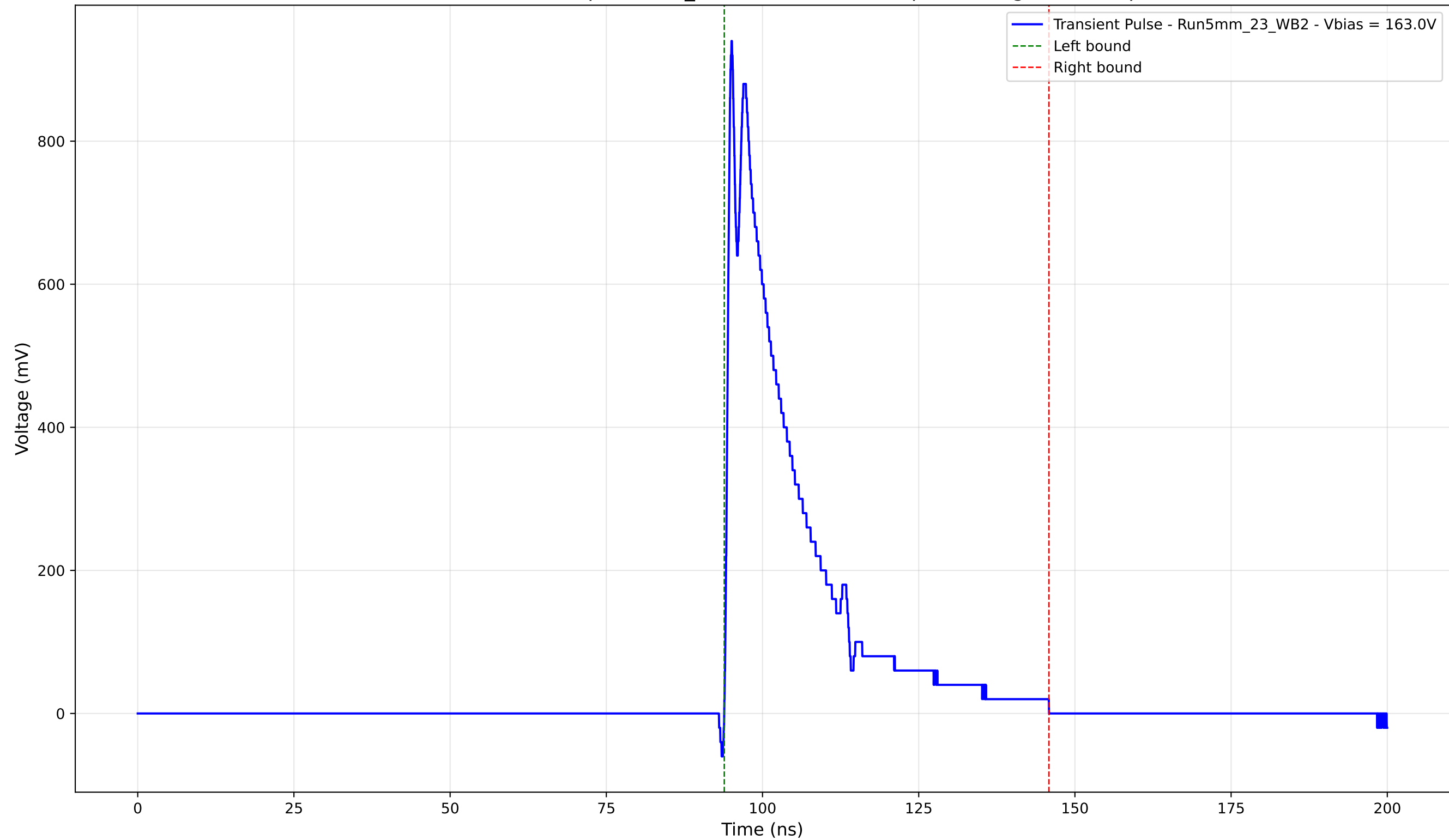
Transient Pulse - Sample: 5mm_23 - Position: 2280.0 \mu\text{m} - Charge: 200.58 pC
