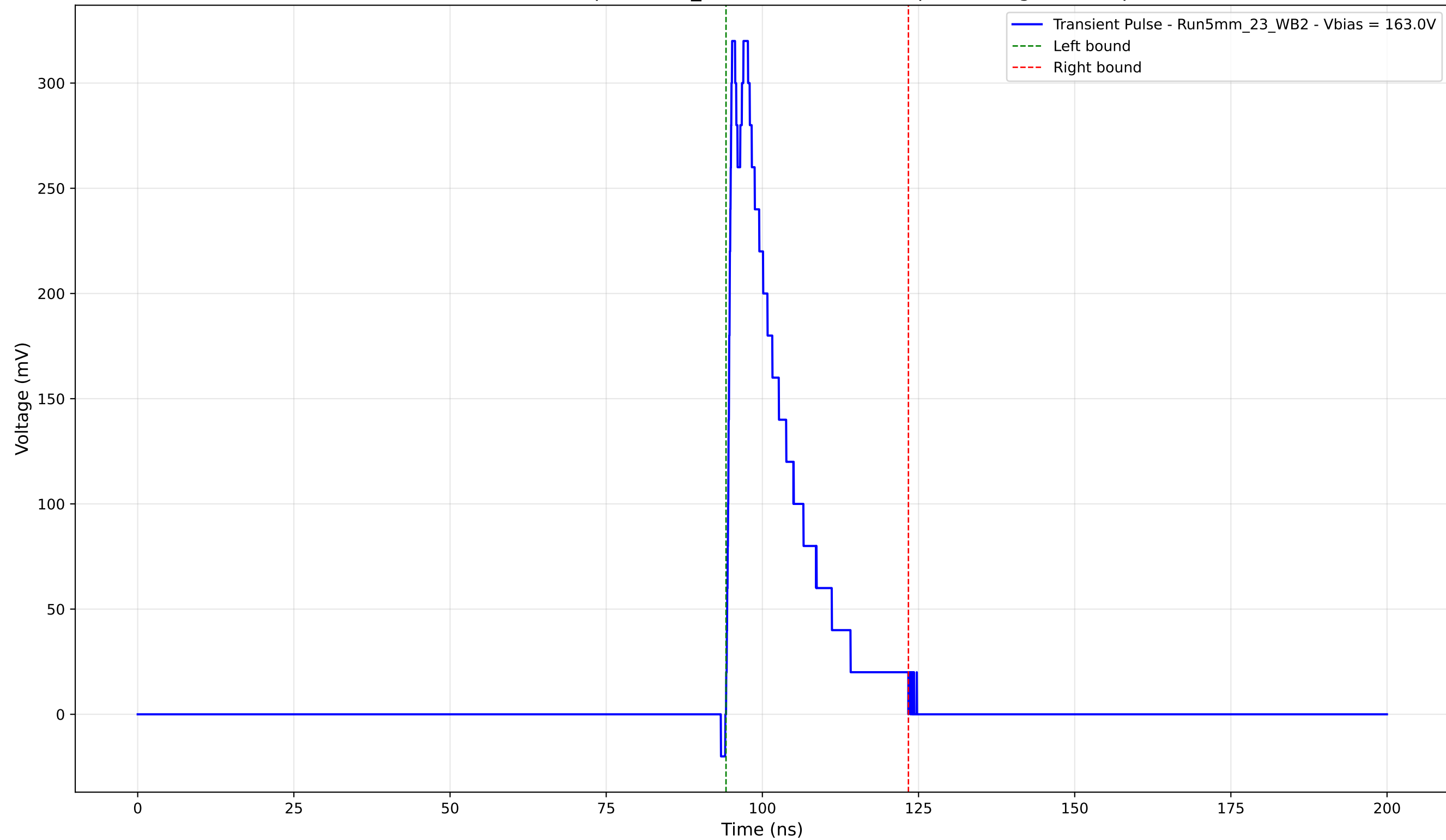
Transient Pulse - Sample: 5mm_23 - Position: 1985.0 \mu\text{m} - Charge: 61.05 pC
