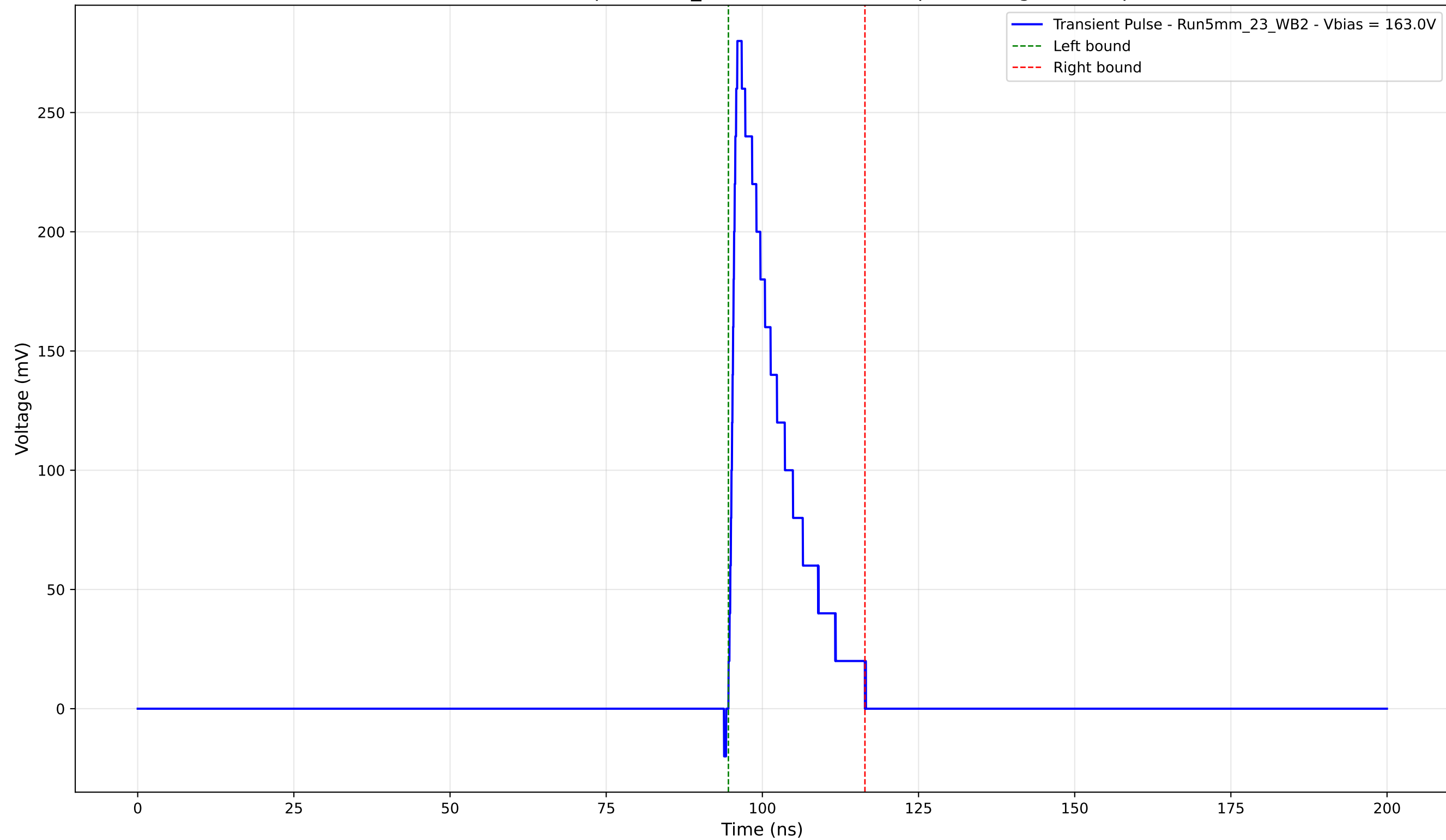
Transient Pulse - Sample: 5mm_23 - Position: 4060.0 \mu\text{m} - Charge: 45.38 pC
