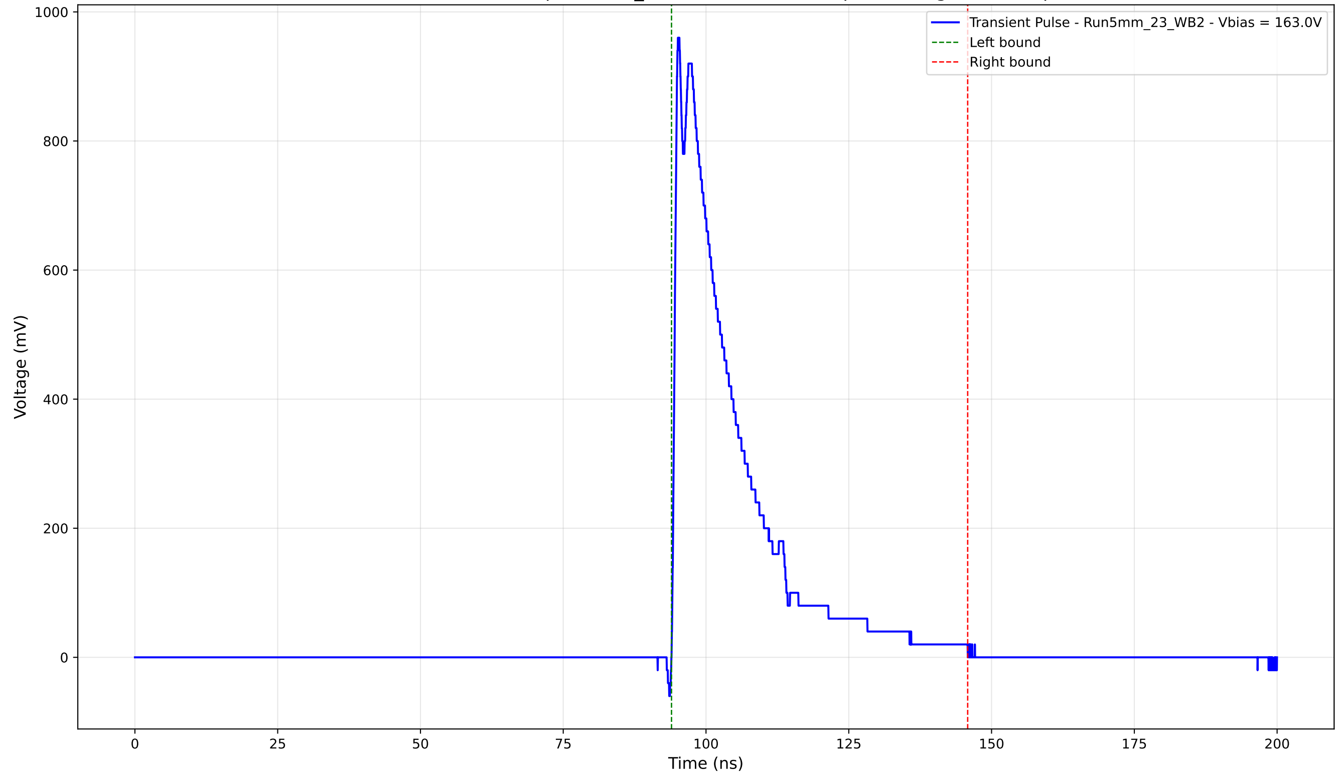
Transient Pulse - Sample: 5mm_23 - Position: 2885.0 \mu\text{m} - Charge: 217.80 pC
