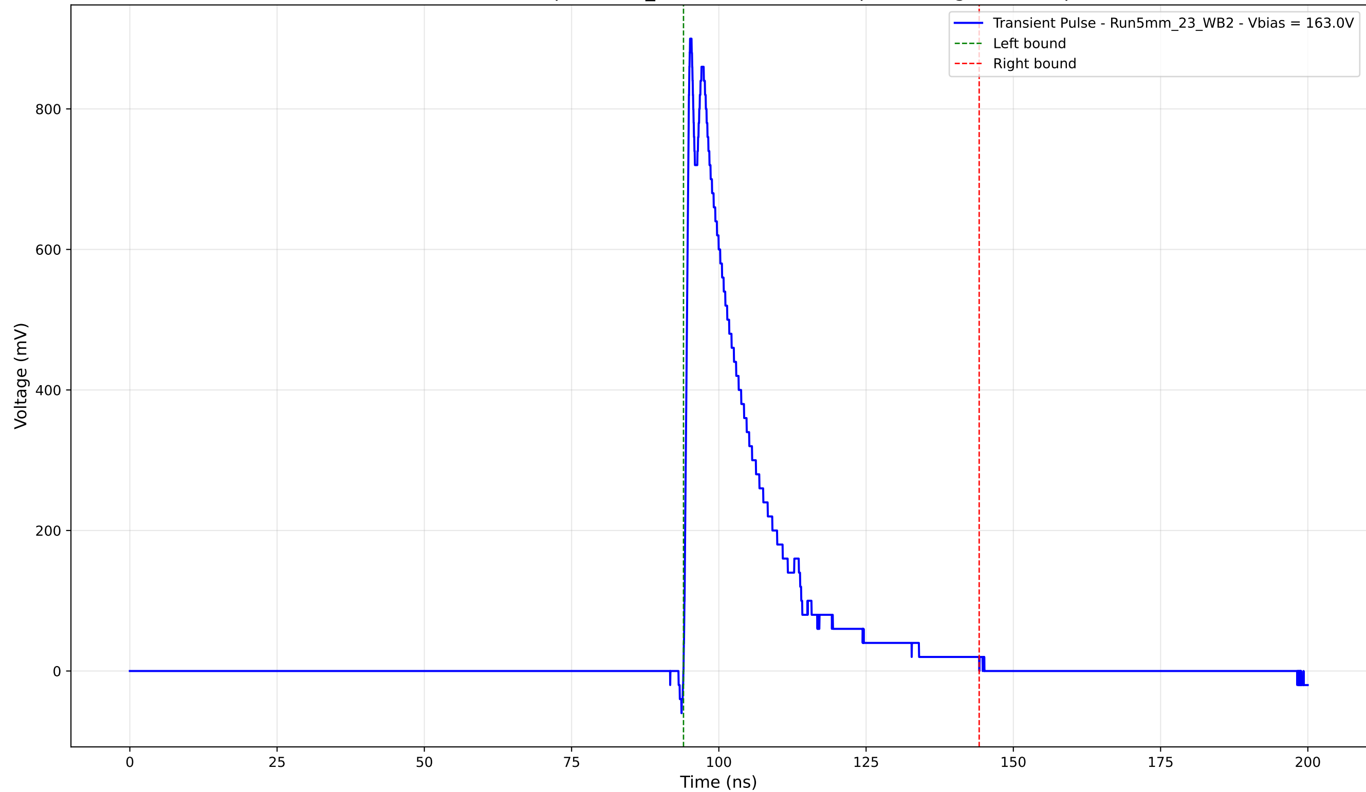
Transient Pulse - Sample: 5mm_23 - Position: 2110.0 \mu\text{m} - Charge: 194.67 pC
