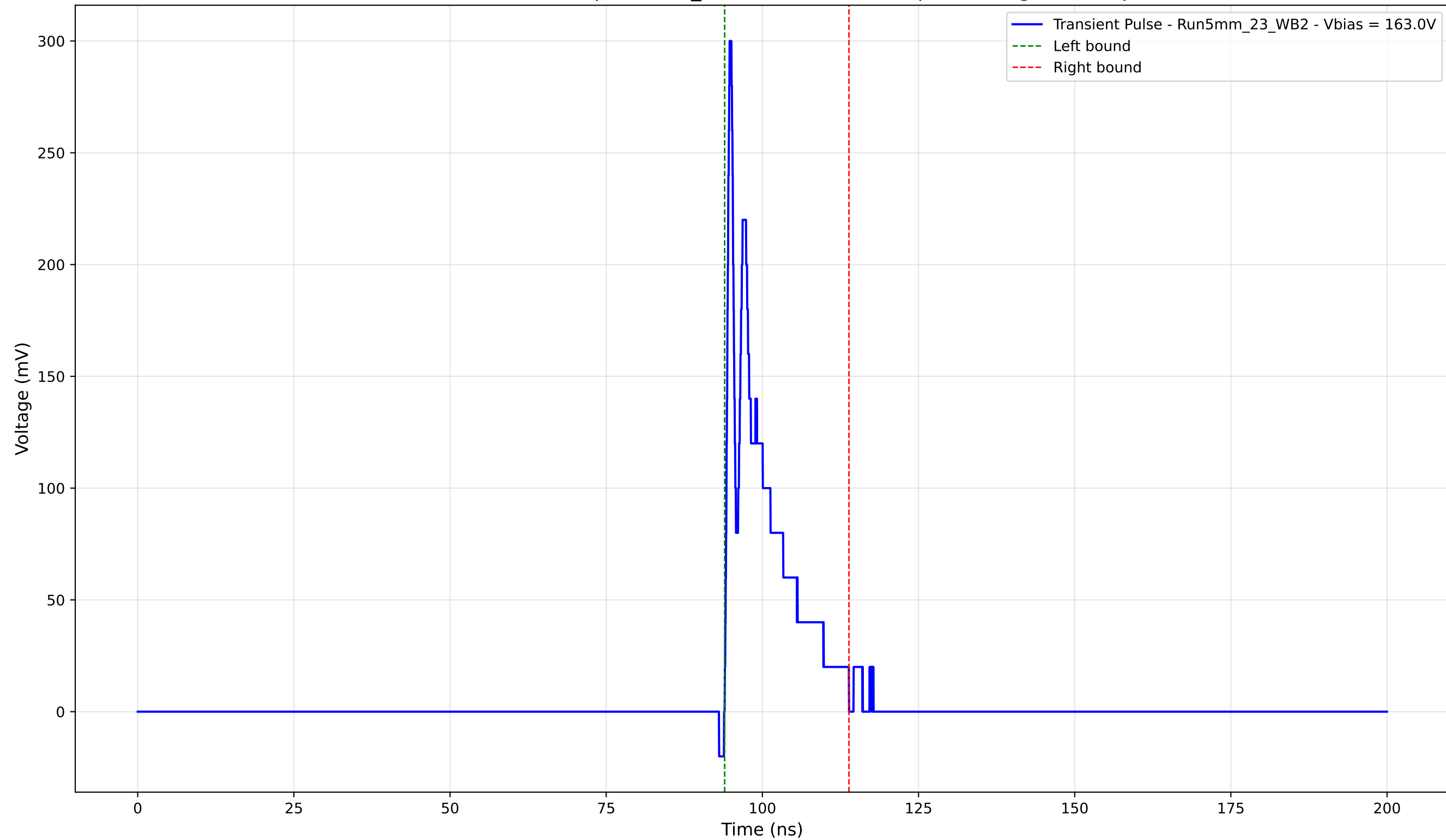
Transient Pulse - Sample: 5mm_23 - Position: 2520.0 \mu\text{m} - Charge: 32.48 pC
