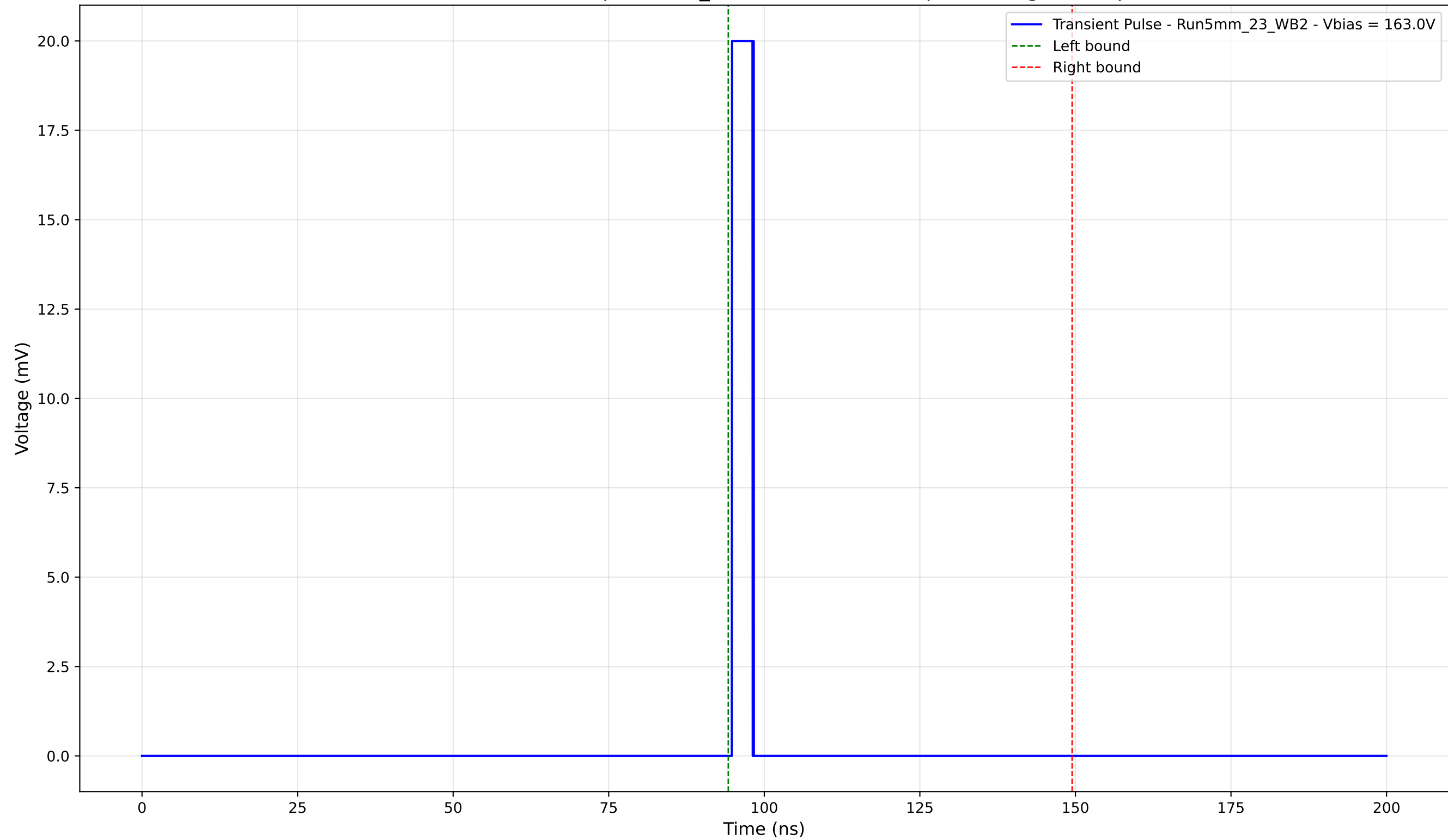
Transient Pulse - Sample: 5mm_23 - Position: 5025.0 \mu\text{m} - Charge: 1.34 pC
