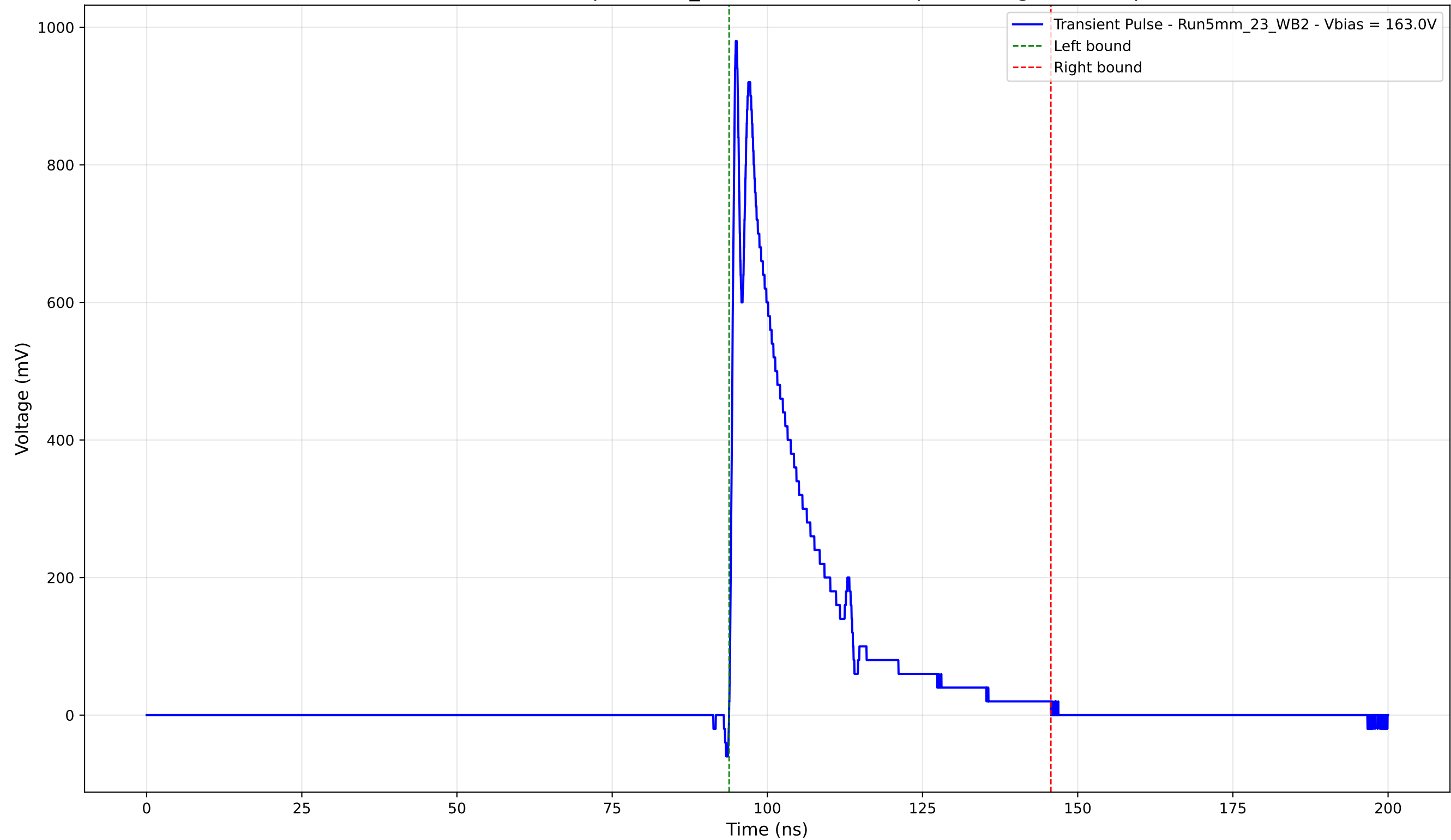
Transient Pulse - Sample: 5mm_23 - Position: 2360.0 \mu\text{m} - Charge: 201.30 pC
