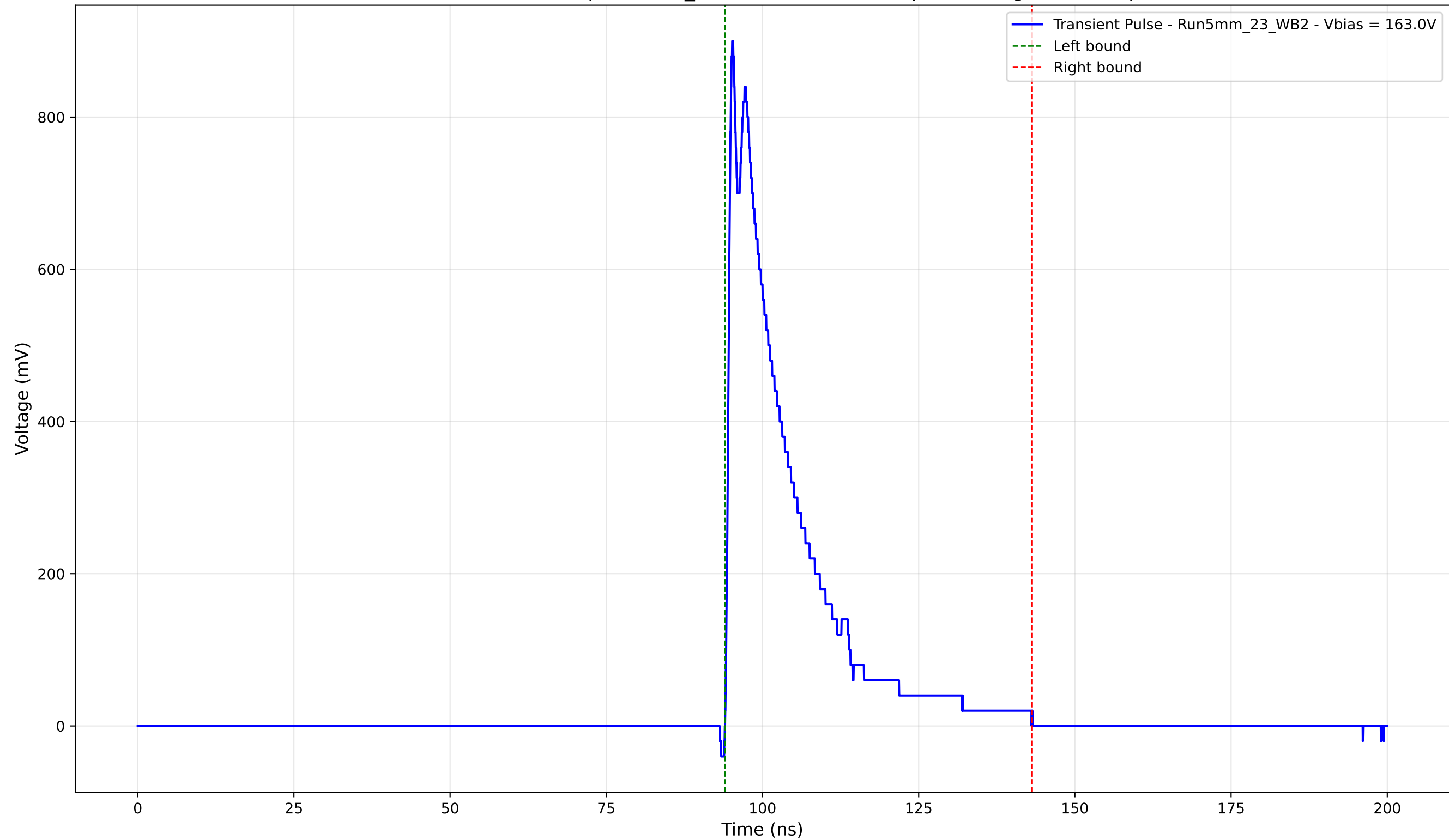
Transient Pulse - Sample: 5mm_23 - Position: 2950.0 \mu\text{m} - Charge: 181.87 pC
