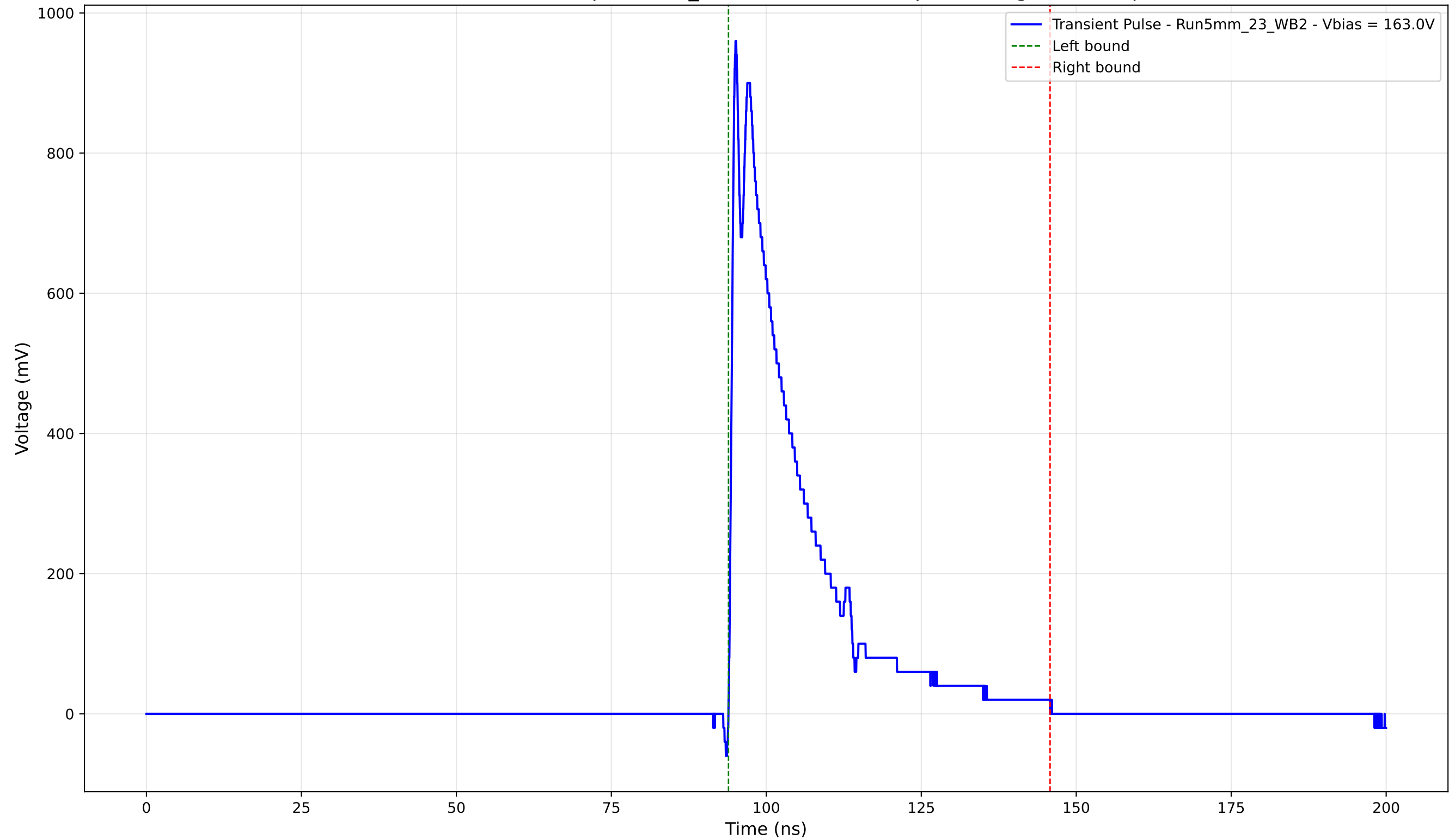
Transient Pulse - Sample: 5mm_23 - Position: 2255.0 \mu\text{m} - Charge: 205.06 pC
