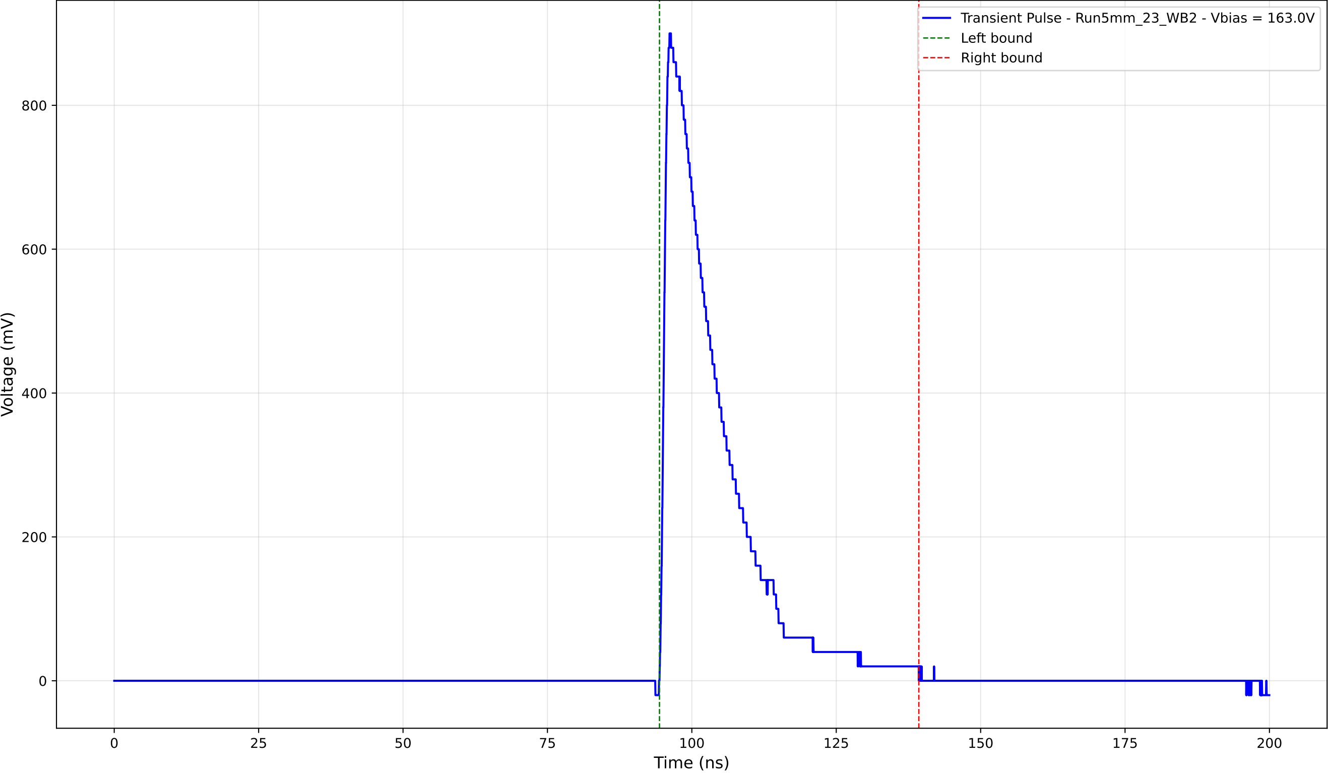
Transient Pulse - Sample: 5mm_23 - Position: 1150.0 \mu\text{m} - Charge: 191.69 pC
