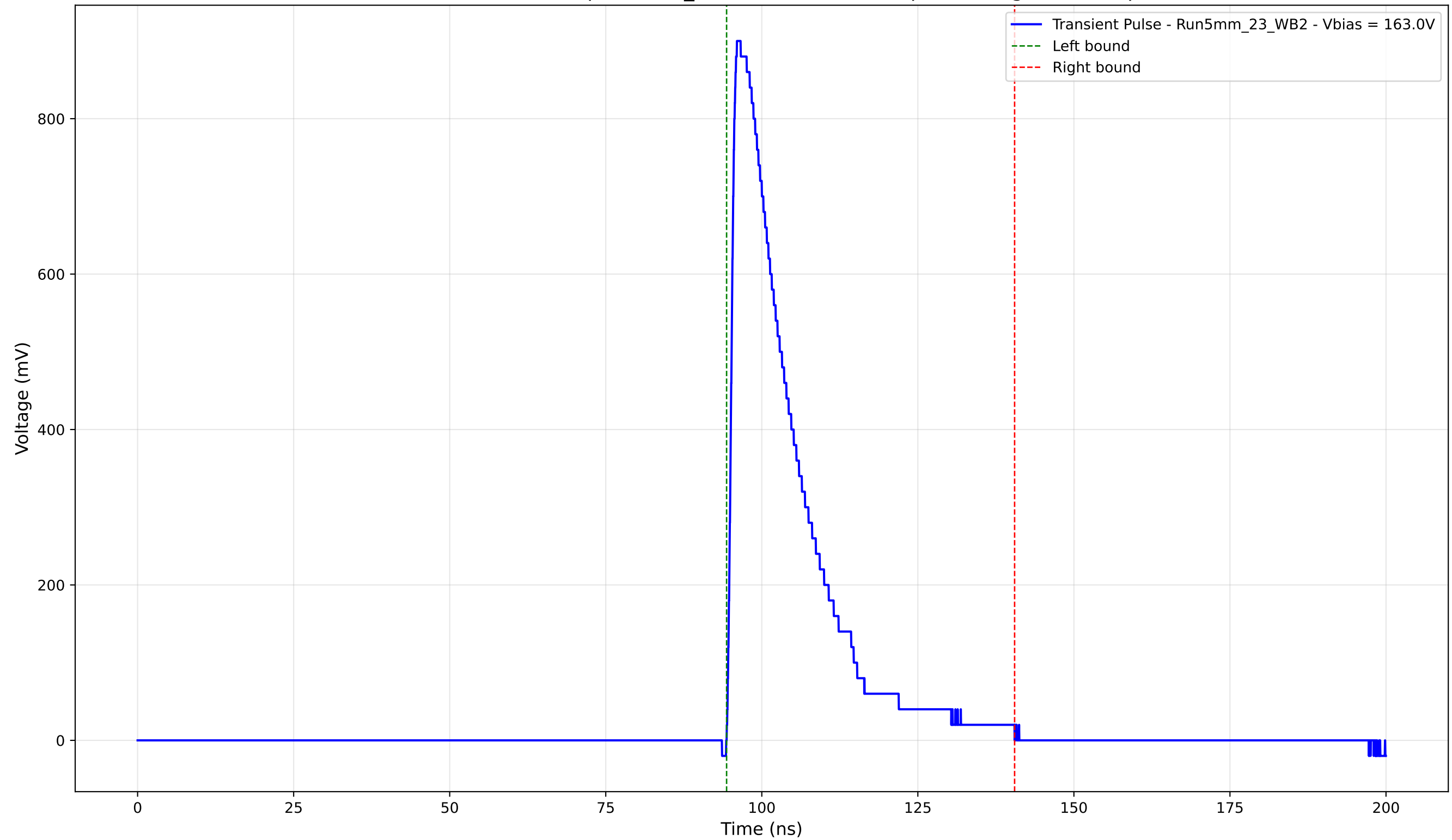
Transient Pulse - Sample: 5mm_23 - Position: 1310.0 \mu\text{m} - Charge: 201.07 pC
