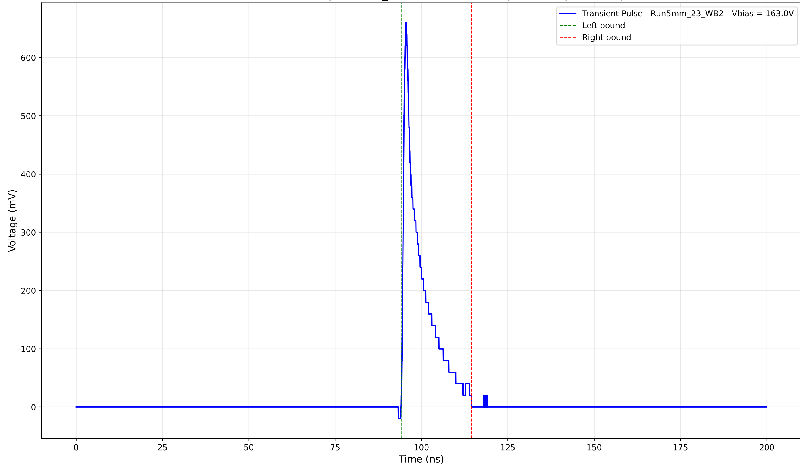
Transient Pulse - Sample: 5mm_23 - Position: 4925.0 \mu\text{m} - Charge: 71.12 pC
