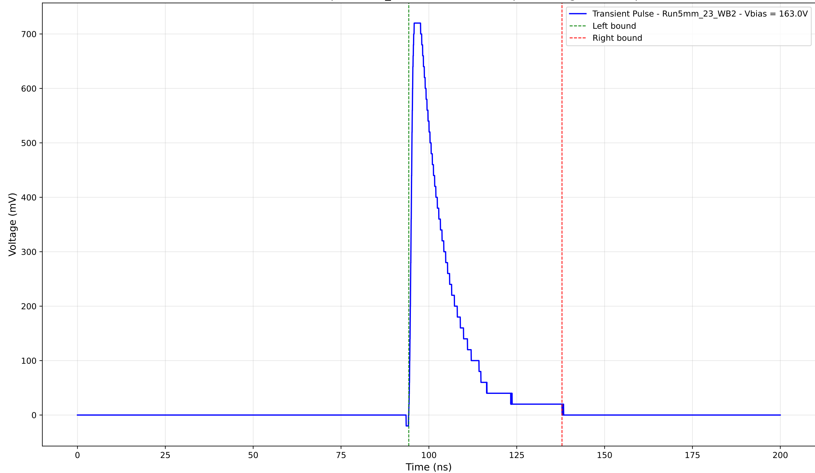
Transient Pulse - Sample: 5mm_23 - Position: 3450.0 \mu\text{m} - Charge: 151.39 pC
