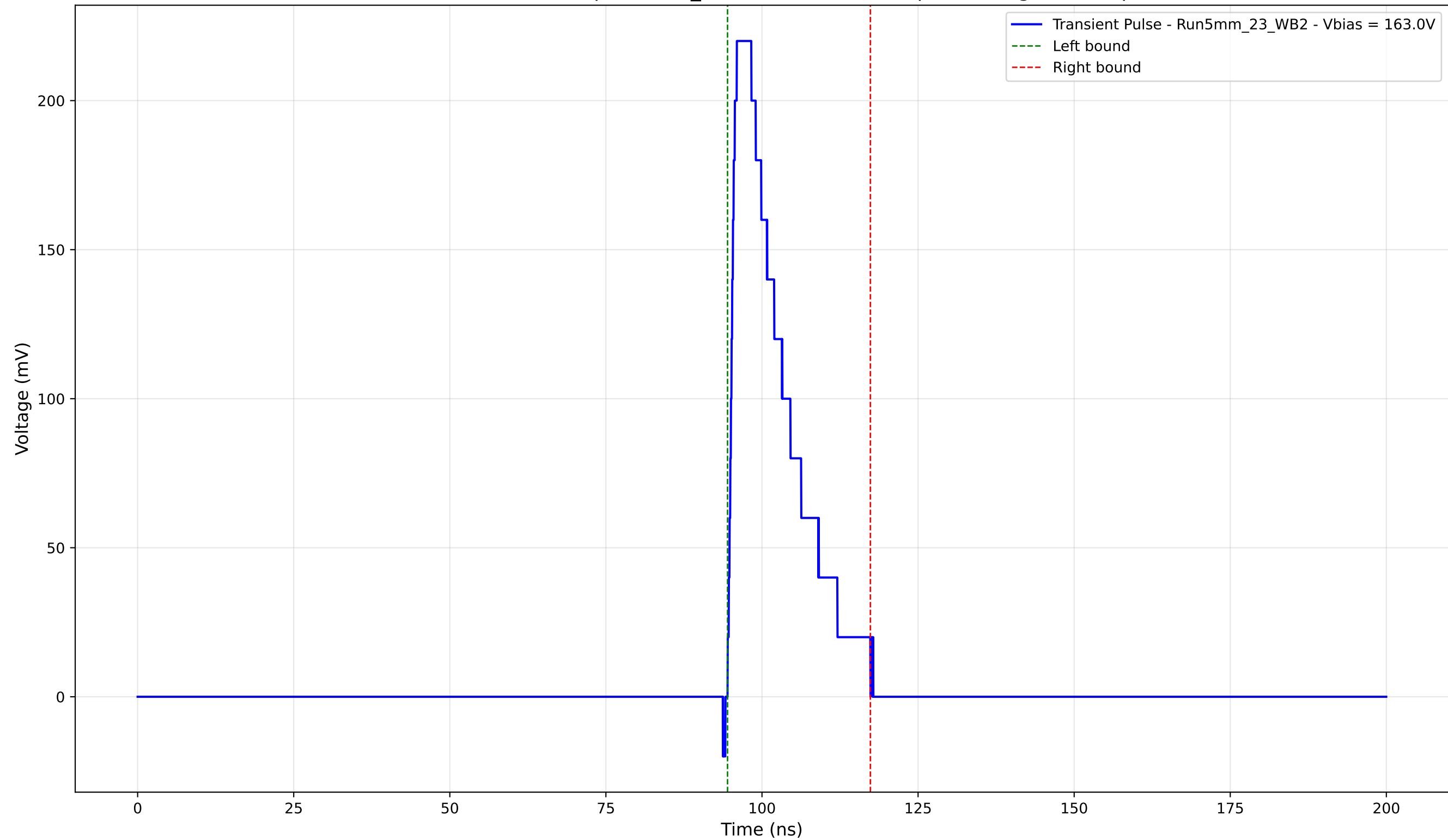
Transient Pulse - Sample: 5mm_23 - Position: 1485.0 \mu\text{m} - Charge: 42.36 pC
