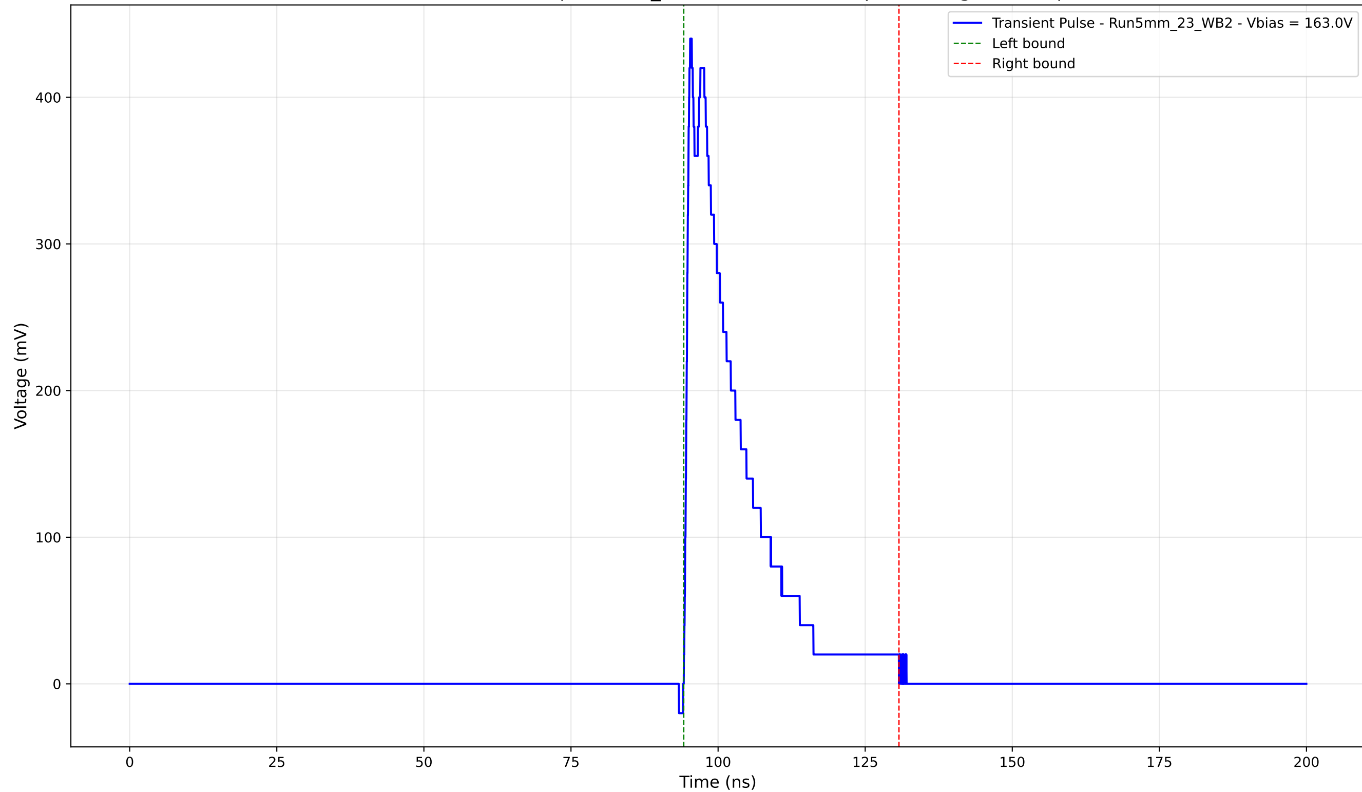
Transient Pulse - Sample: 5mm_23 - Position: 1975.0 \mu\text{m} - Charge: 83.86 pC
