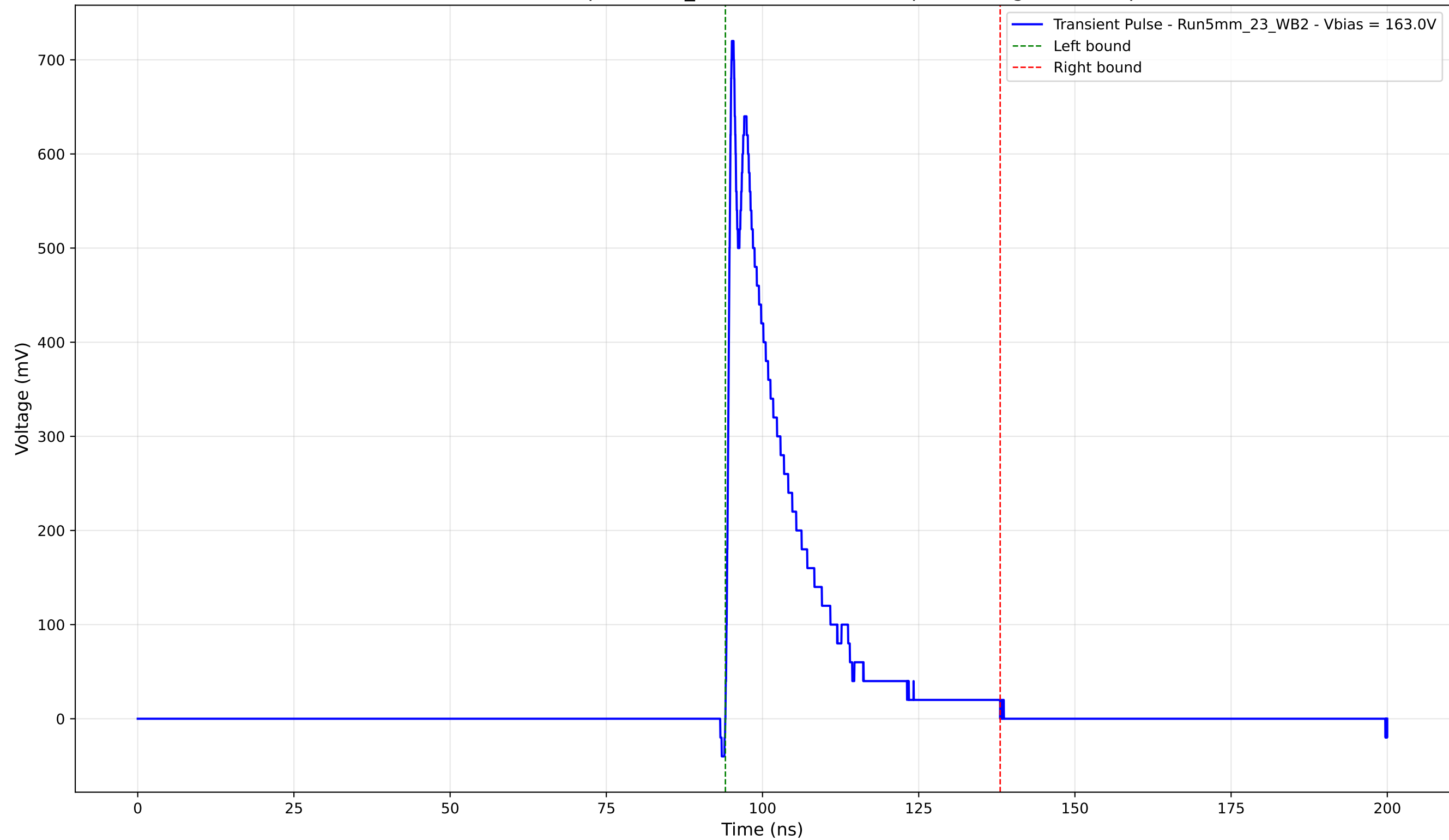
Transient Pulse - Sample: 5mm_23 - Position: 2065.0 \mu\text{m} - Charge: 130.94 pC
