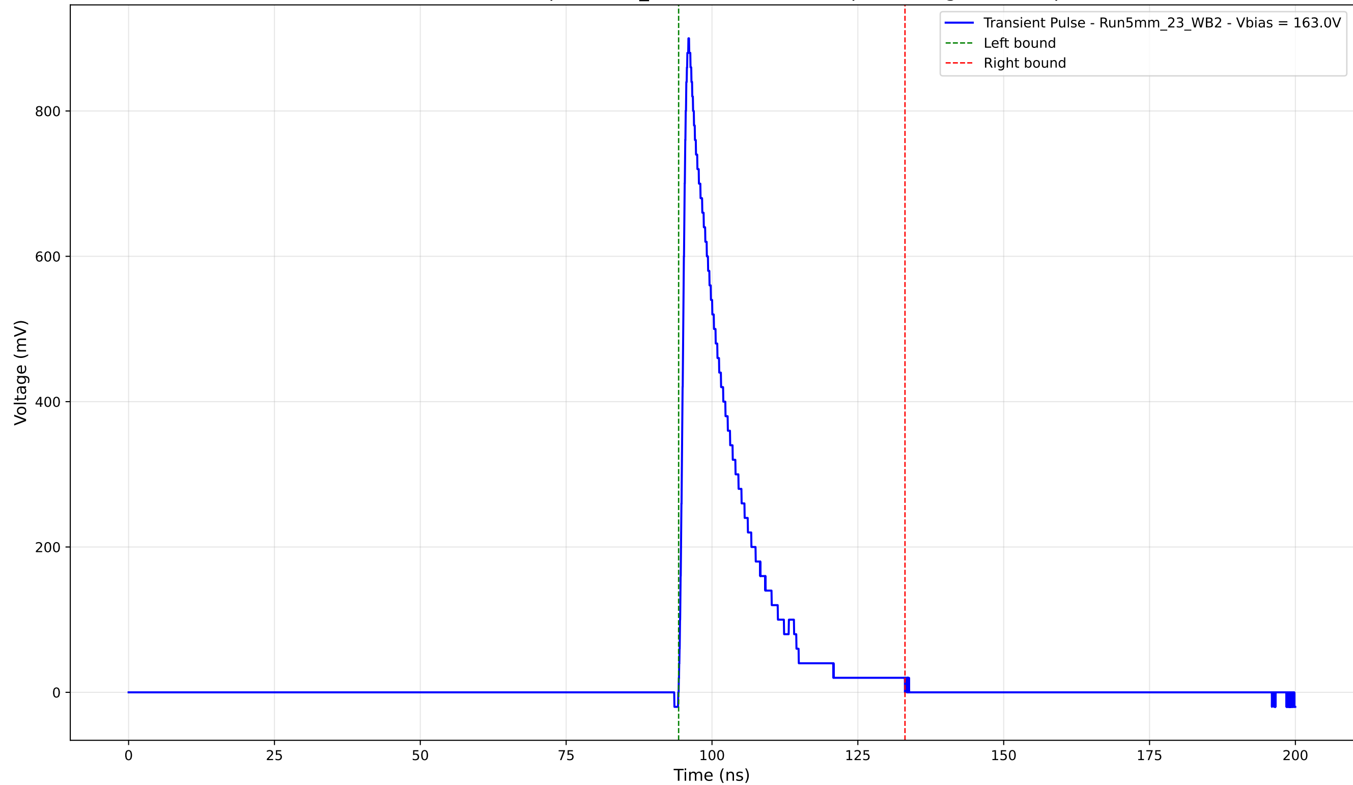
Transient Pulse - Sample: 5mm_23 - Position: 4440.0 \mu\text{m} - Charge: 150.82 pC
