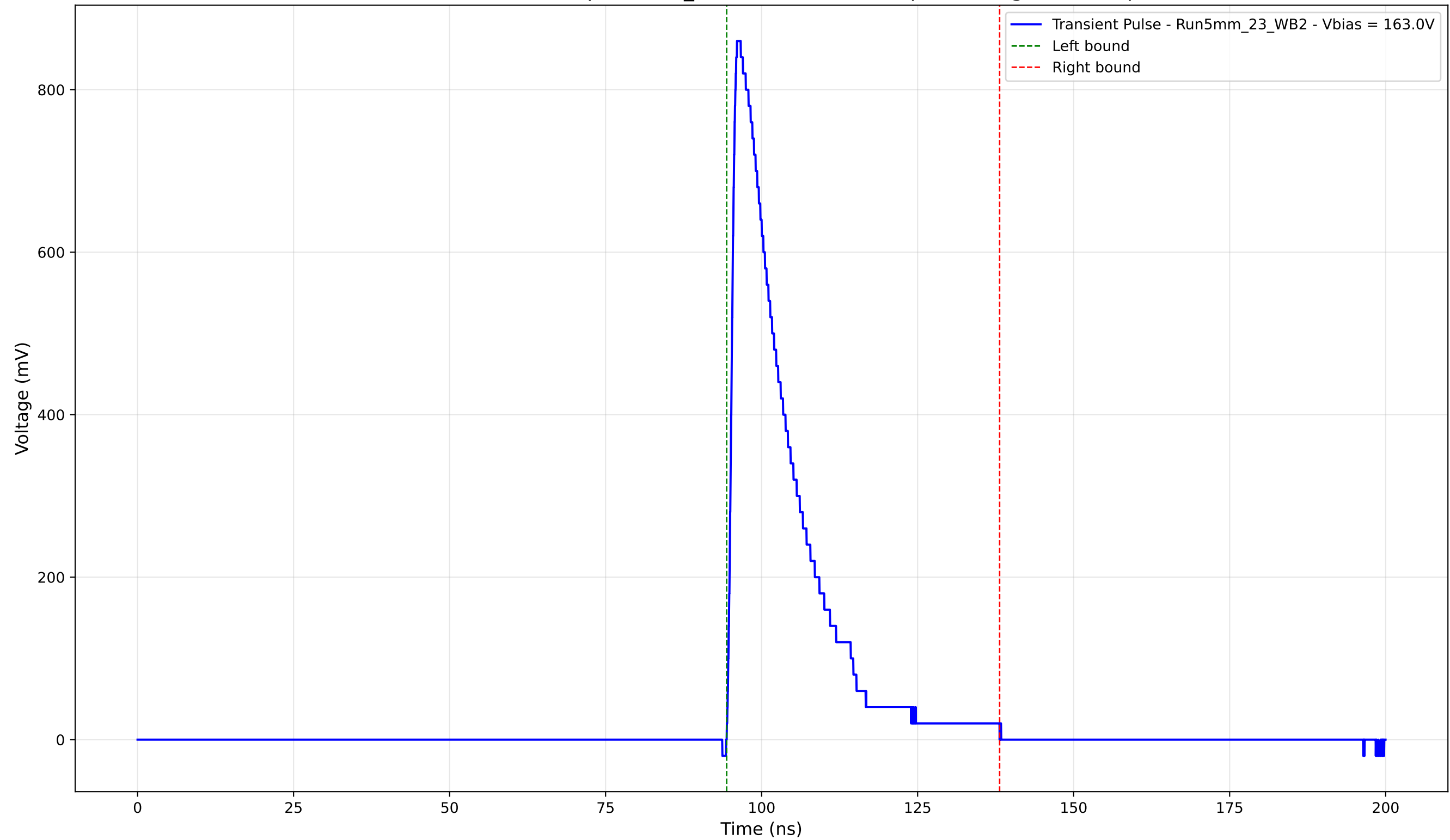
Transient Pulse - Sample: 5mm_23 - Position: 3860.0 \mu\text{m} - Charge: 173.47 pC
