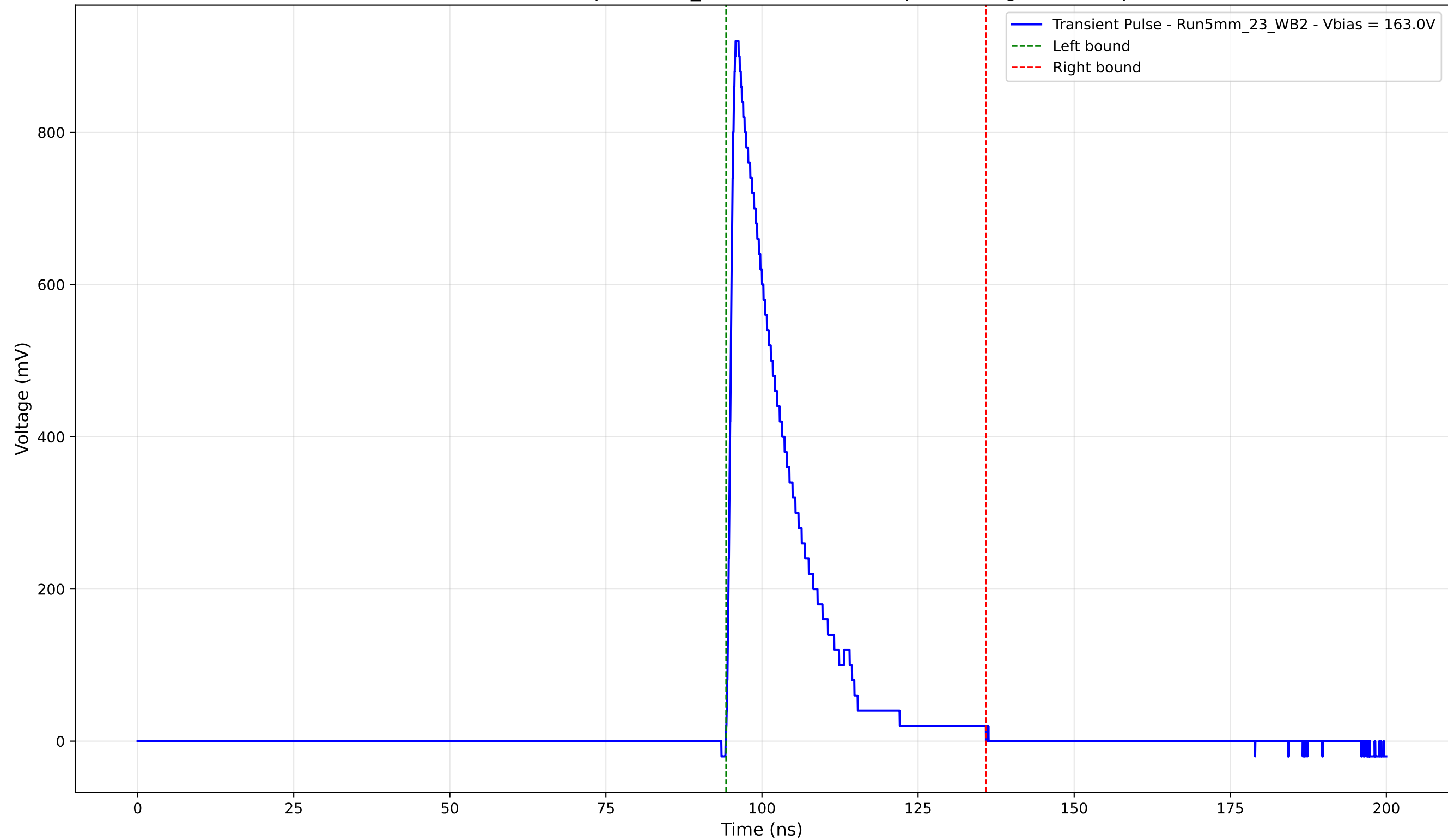
Transient Pulse - Sample: 5mm_23 - Position: 570.0 \mu\text{m} - Charge: 171.81 pC
