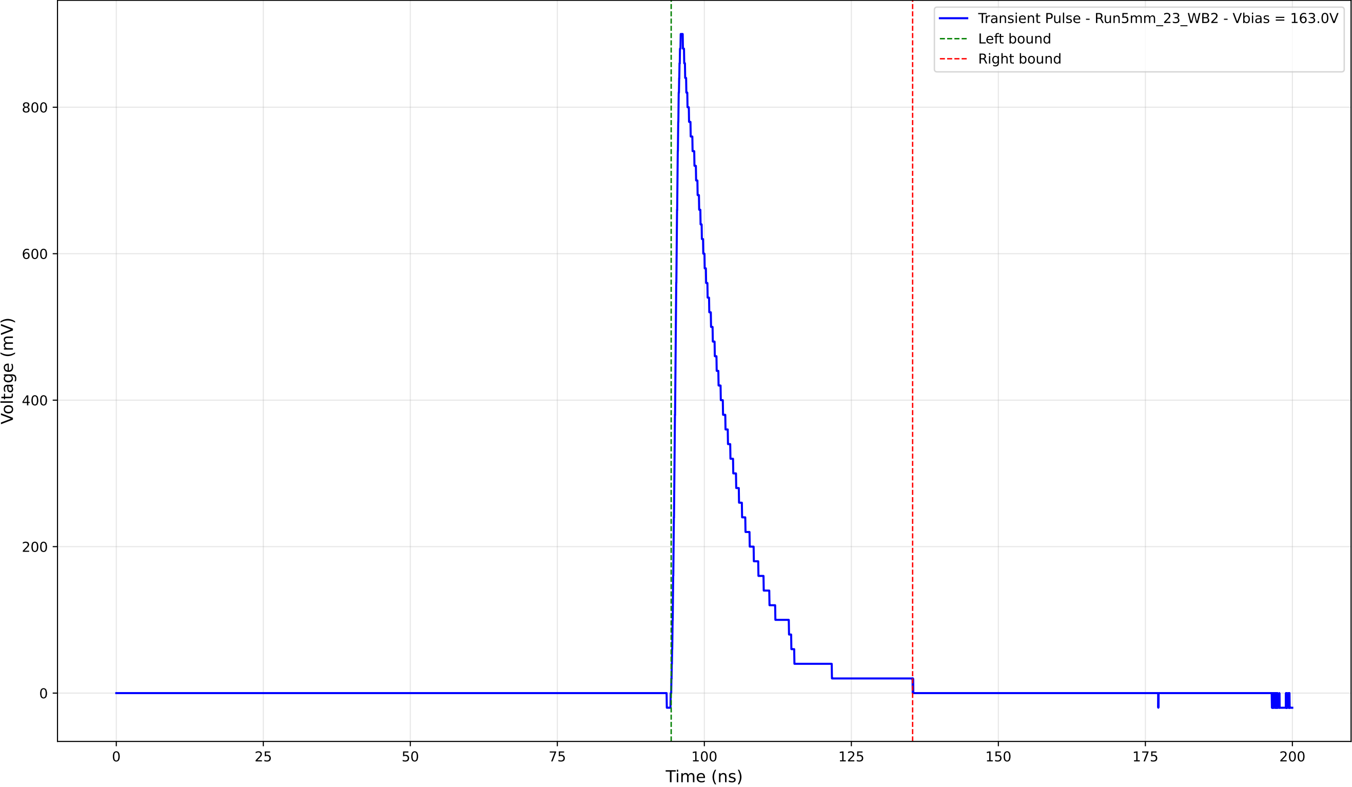
Transient Pulse - Sample: 5mm_23 - Position: 4275.0 \mu\text{m} - Charge: 163.18 pC
