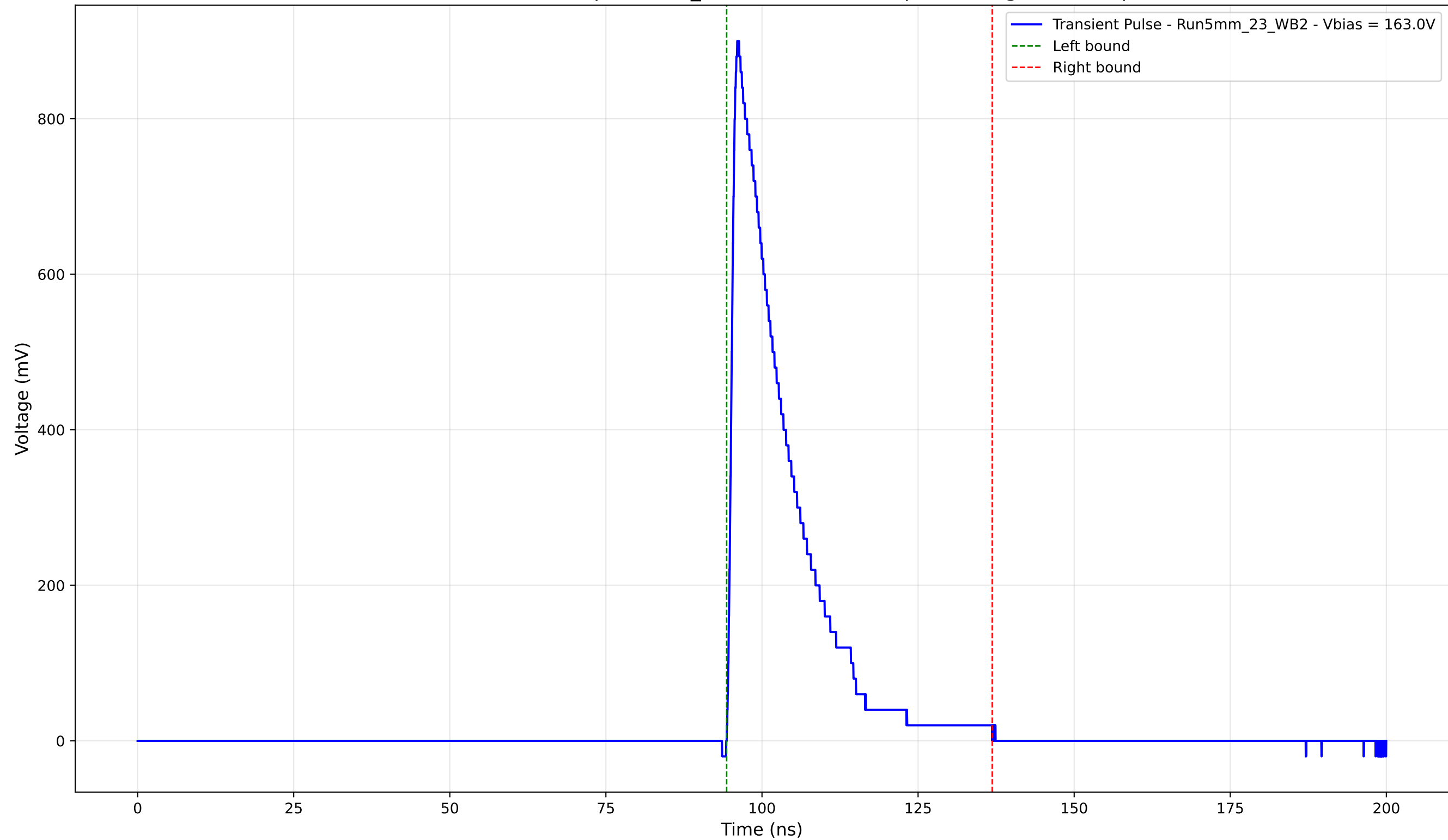
Transient Pulse - Sample: 5mm_23 - Position: 785.0 \mu\text{m} - Charge: 173.92 pC
