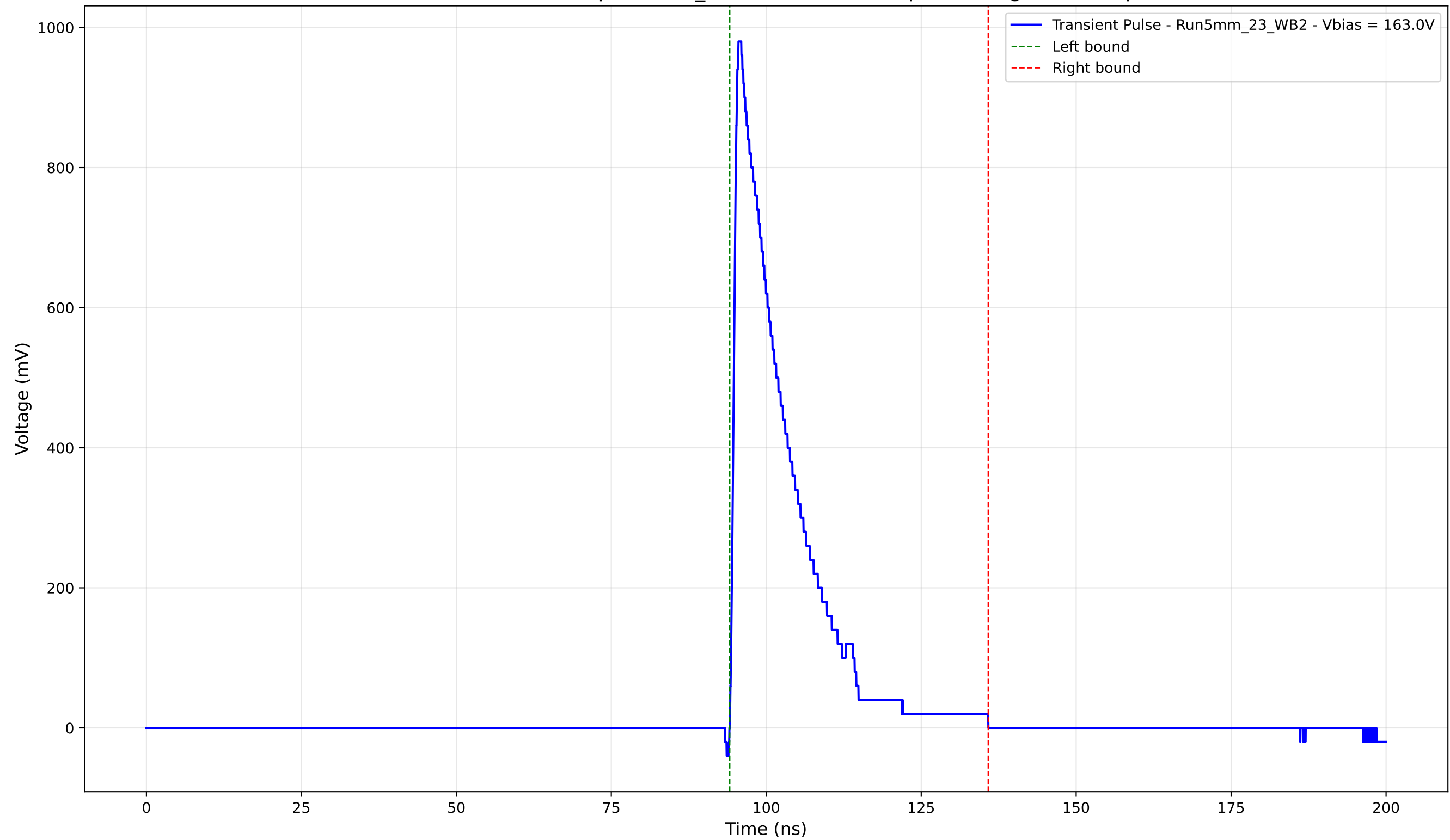
Transient Pulse - Sample: 5mm_23 - Position: 335.0 \mu\text{m} - Charge: 180.11 pC
