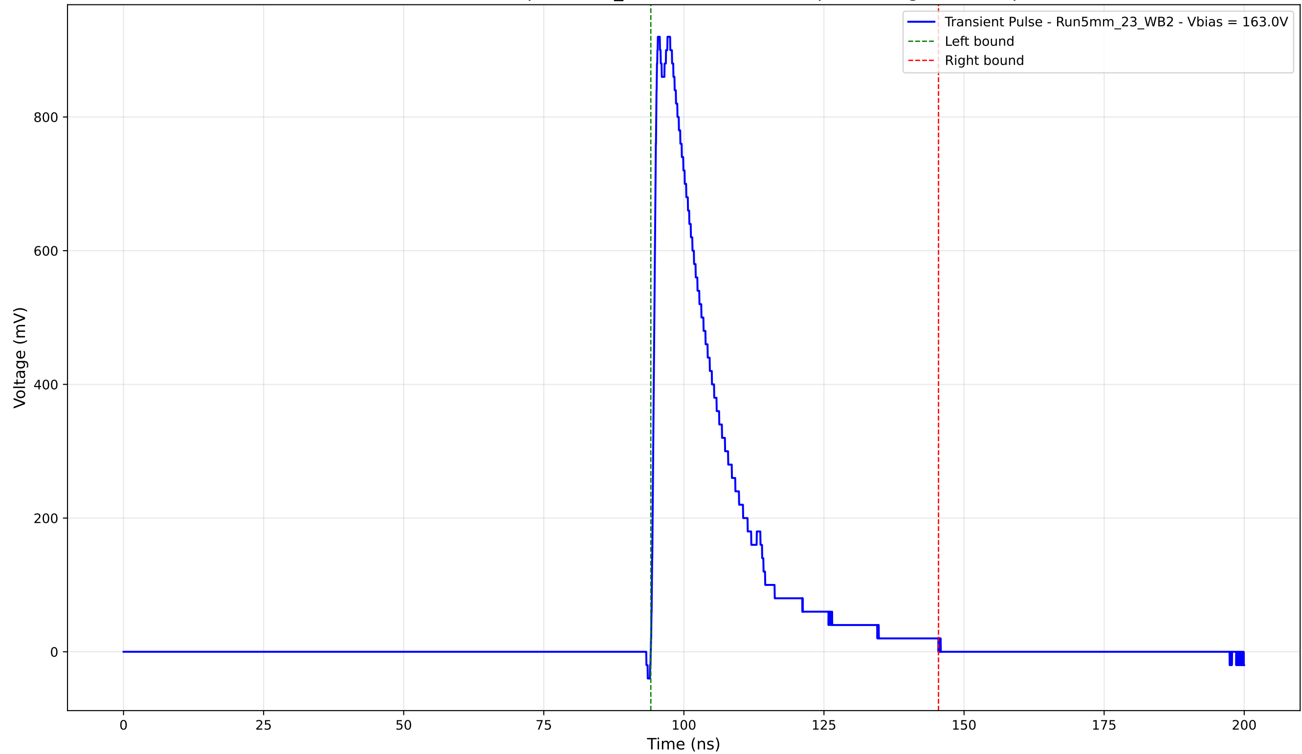
Transient Pulse - Sample: 5mm_23 - Position: 1870.0 \mu\text{m} - Charge: 221.82 pC
