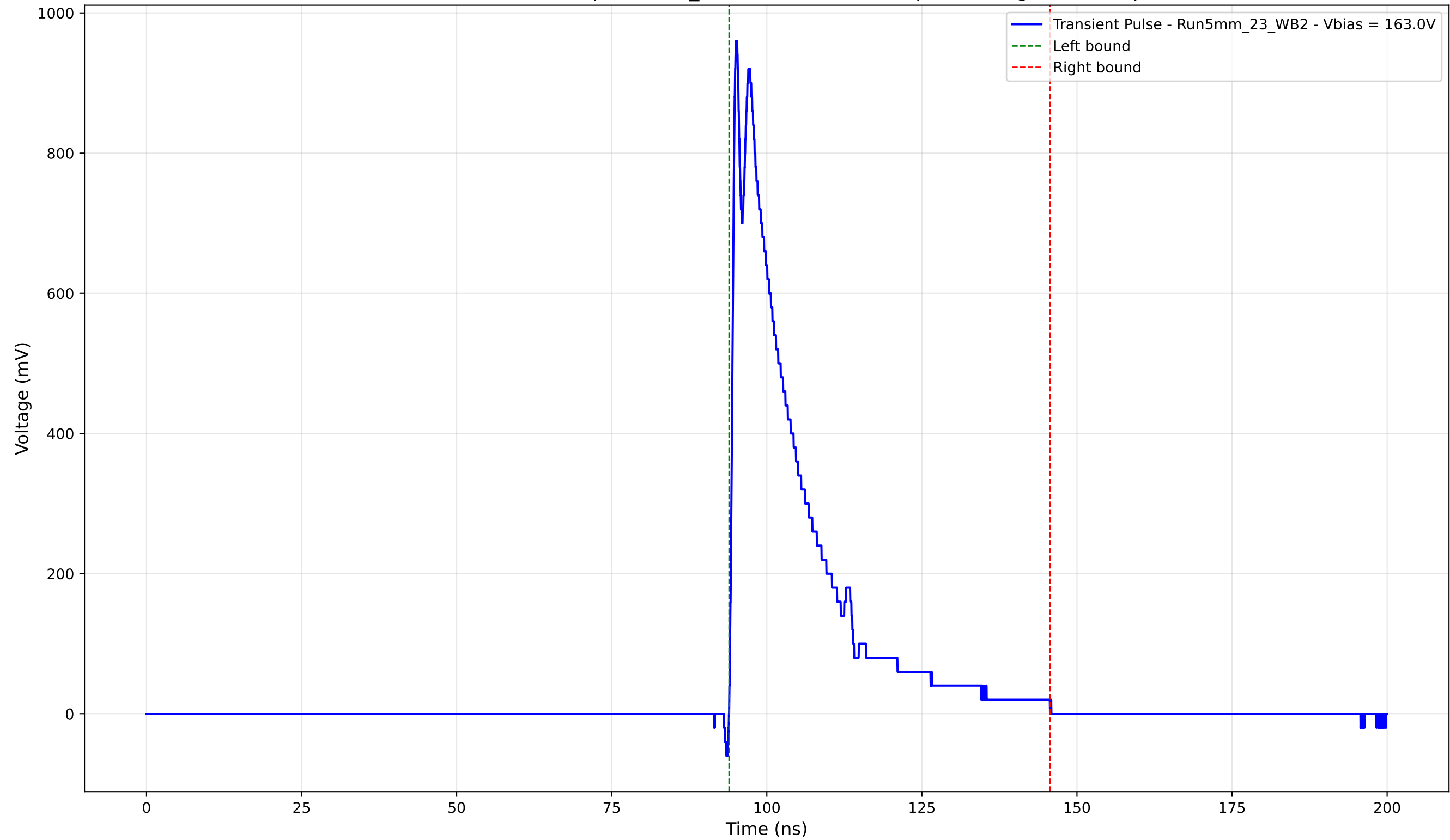
Transient Pulse - Sample: 5mm_23 - Position: 2805.0 \mu\text{m} - Charge: 207.42 pC
