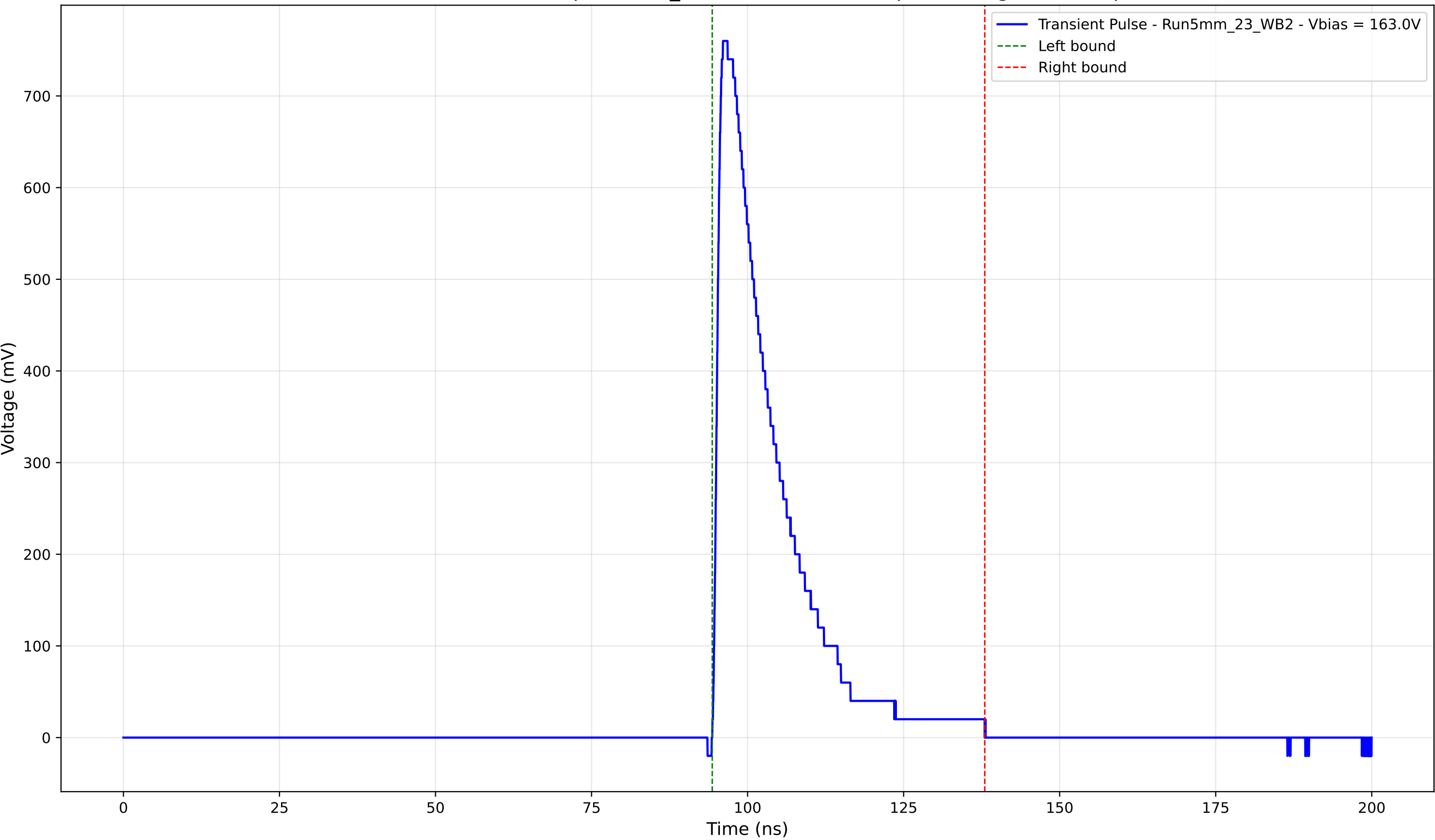
Transient Pulse - Sample: 5mm_23 - Position: 3610.0 \mu\text{m} - Charge: 156.05 pC
