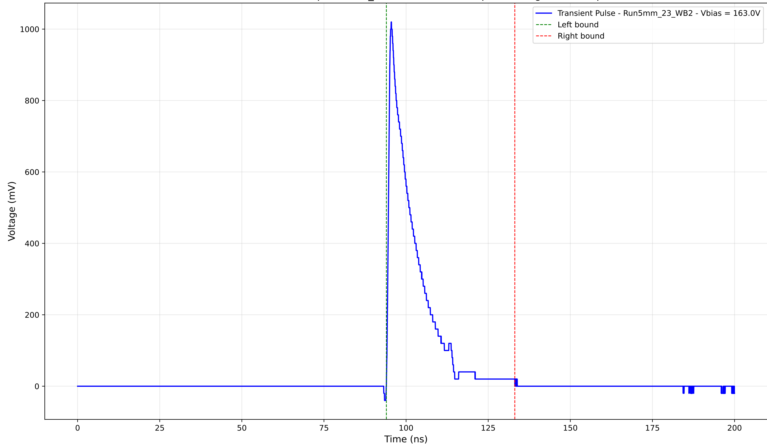
Transient Pulse - Sample: 5mm_23 - Position: 125.0 \mu\text{m} - Charge: 169.16 pC
