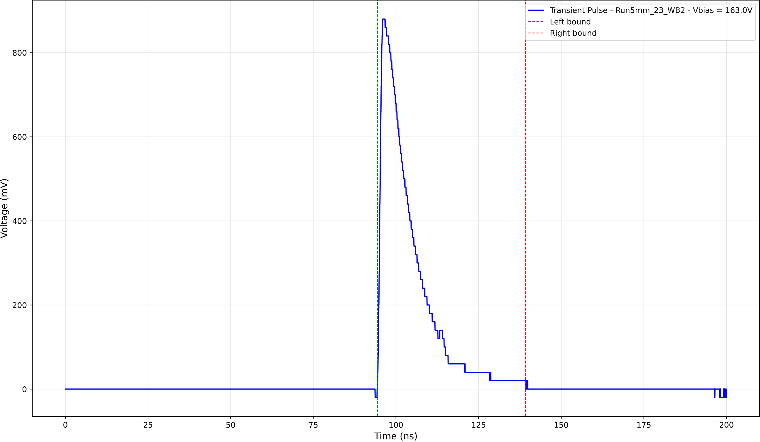
Transient Pulse - Sample: 5mm_23 - Position: 1130.0 \mu\text{m} - Charge: 189.30 pC
