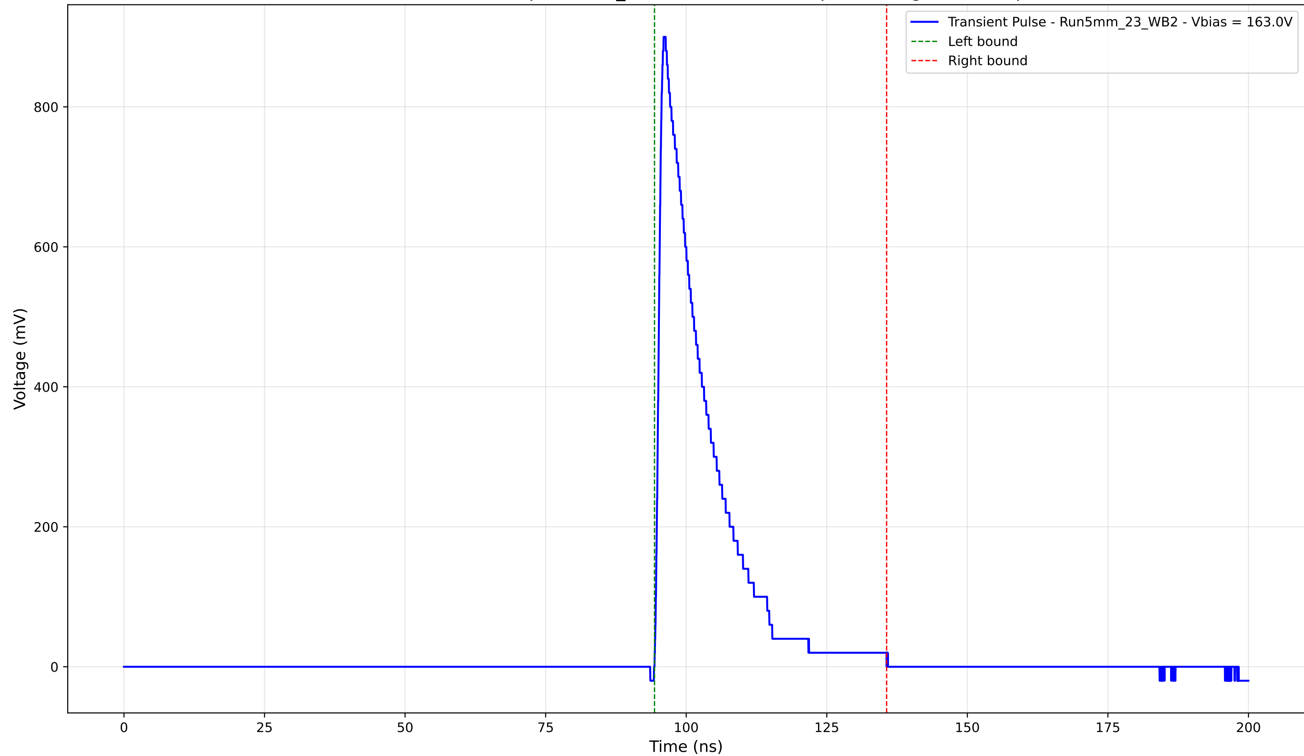
Transient Pulse - Sample: 5mm_23 - Position: 4280.0 \mu\text{m} - Charge: 163.30 pC
