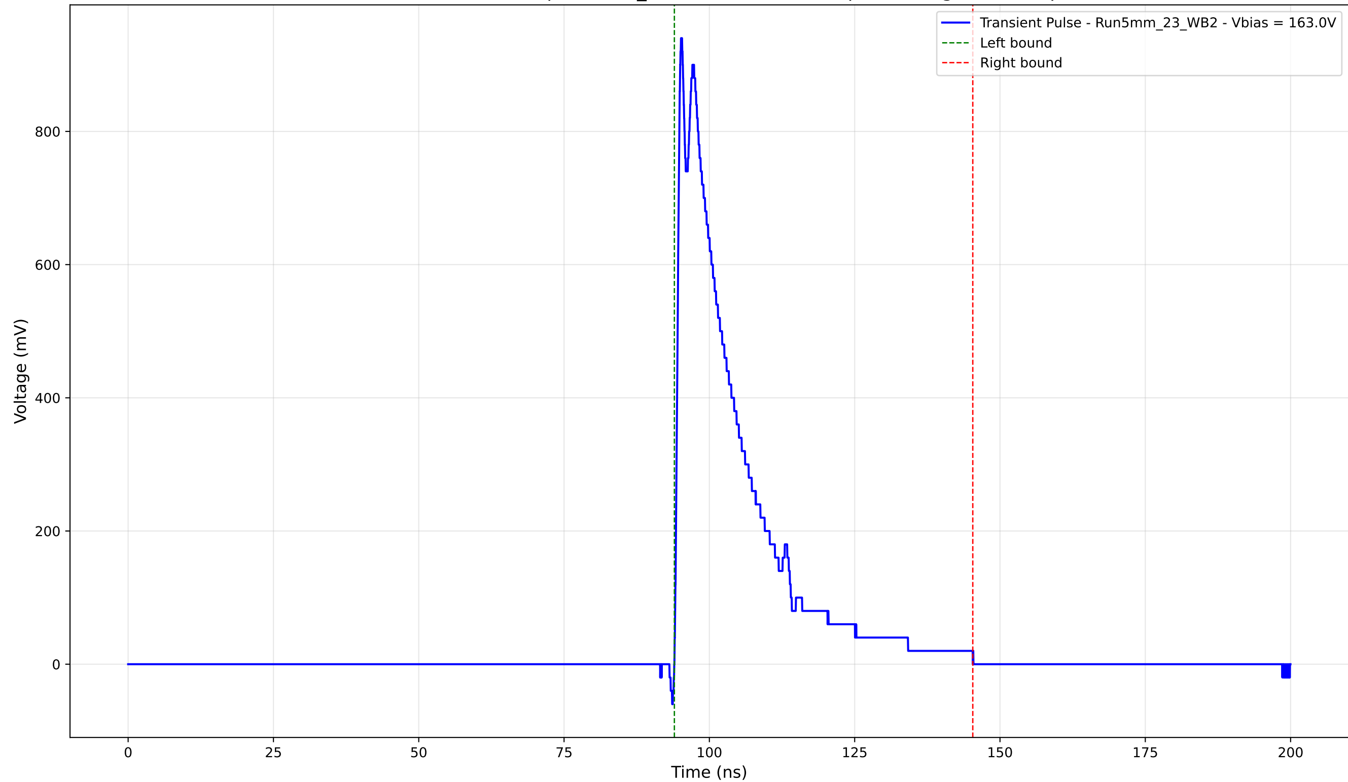
Transient Pulse - Sample: 5mm_23 - Position: 2140.0 \mu\text{m} - Charge: 204.27 pC
