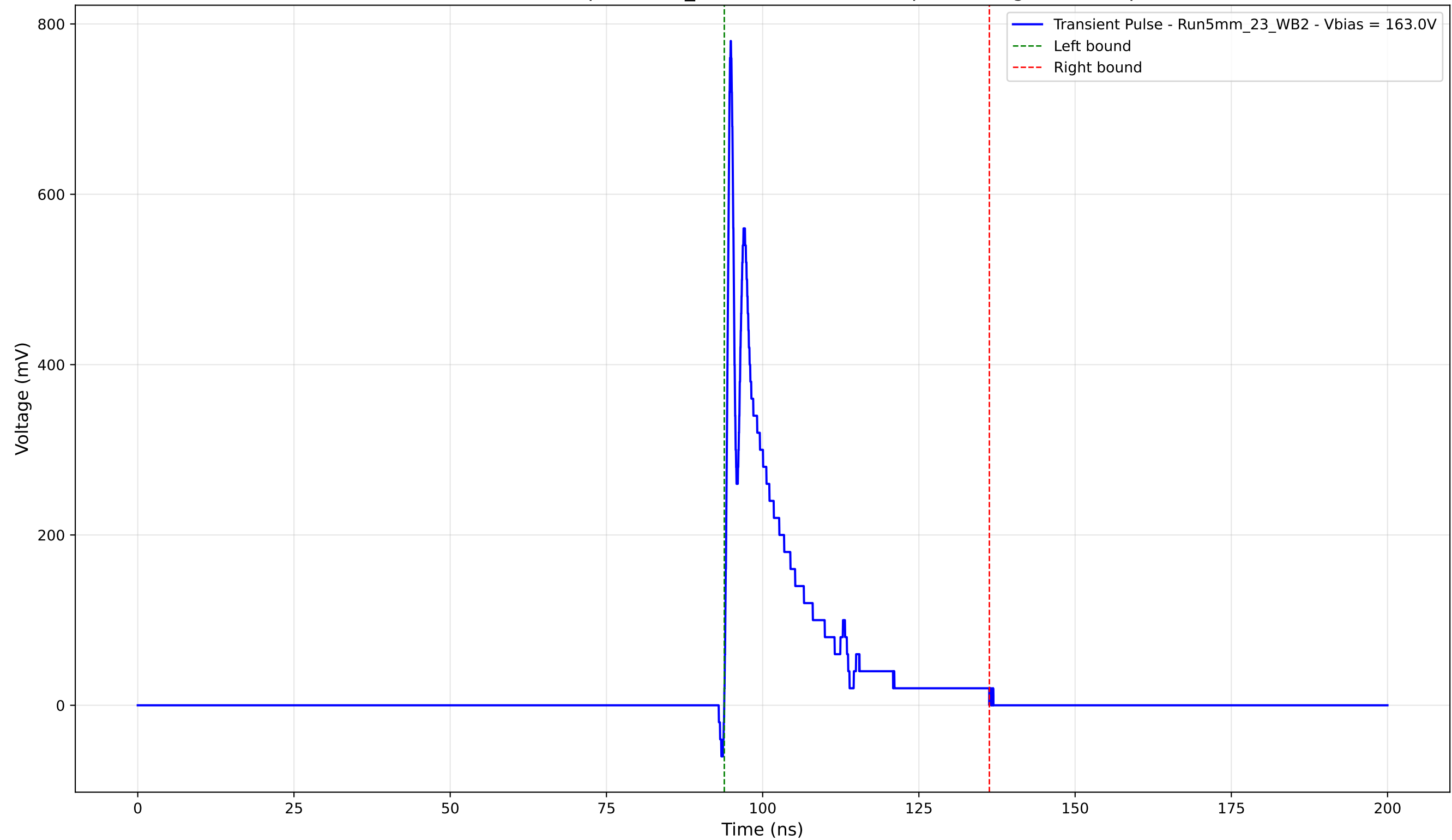
Transient Pulse - Sample: 5mm_23 - Position: 2560.0 \mu\text{m} - Charge: 101.80 pC
