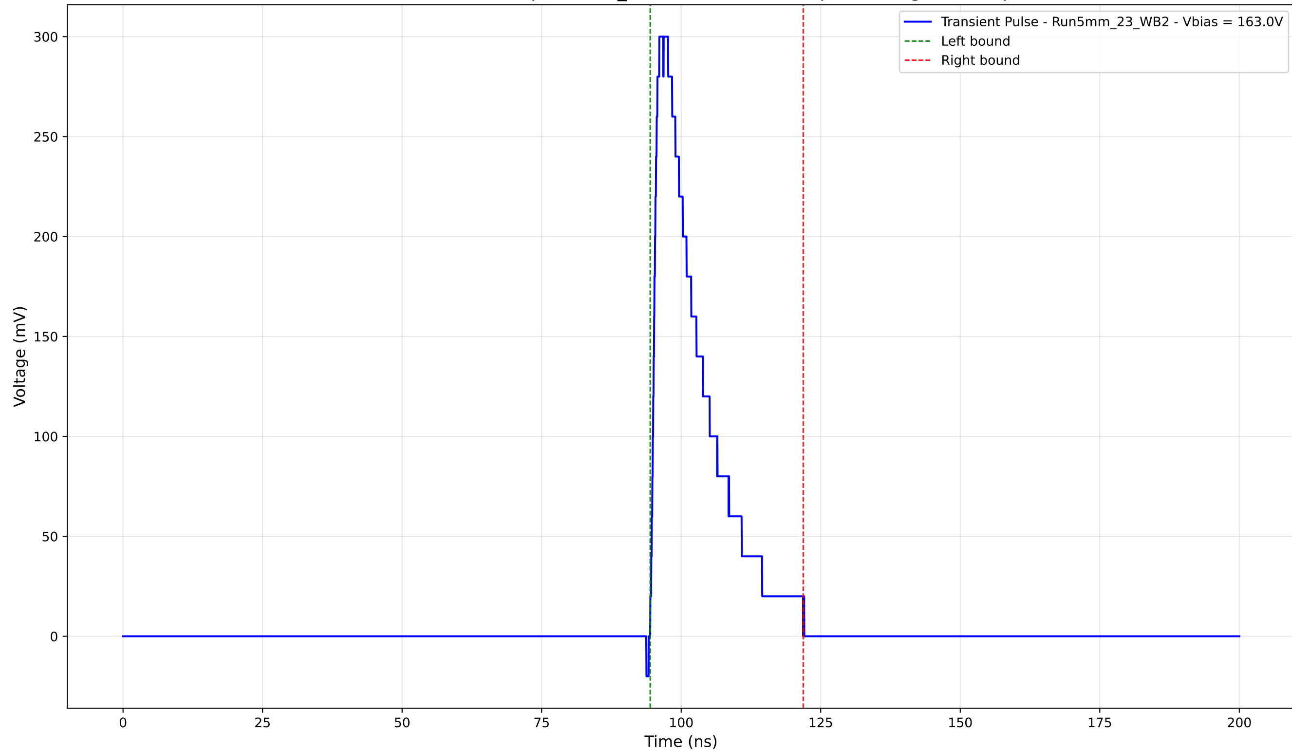
Transient Pulse - Sample: 5mm_23 - Position: 1475.0 \mu\text{m} - Charge: 57.64 pC
