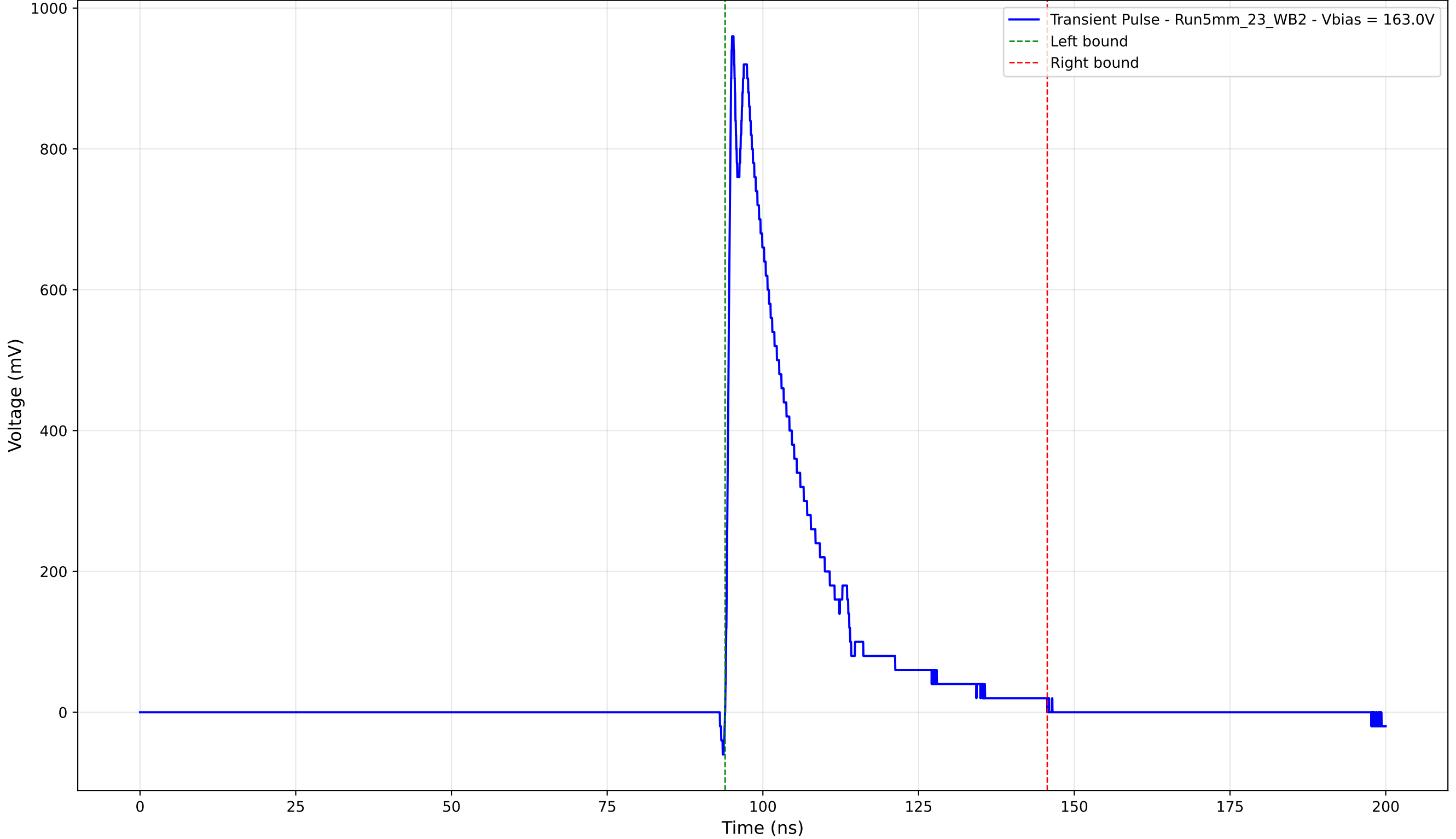
Transient Pulse - Sample: 5mm_23 - Position: 2855.0 \mu\text{m} - Charge: 214.09 pC
