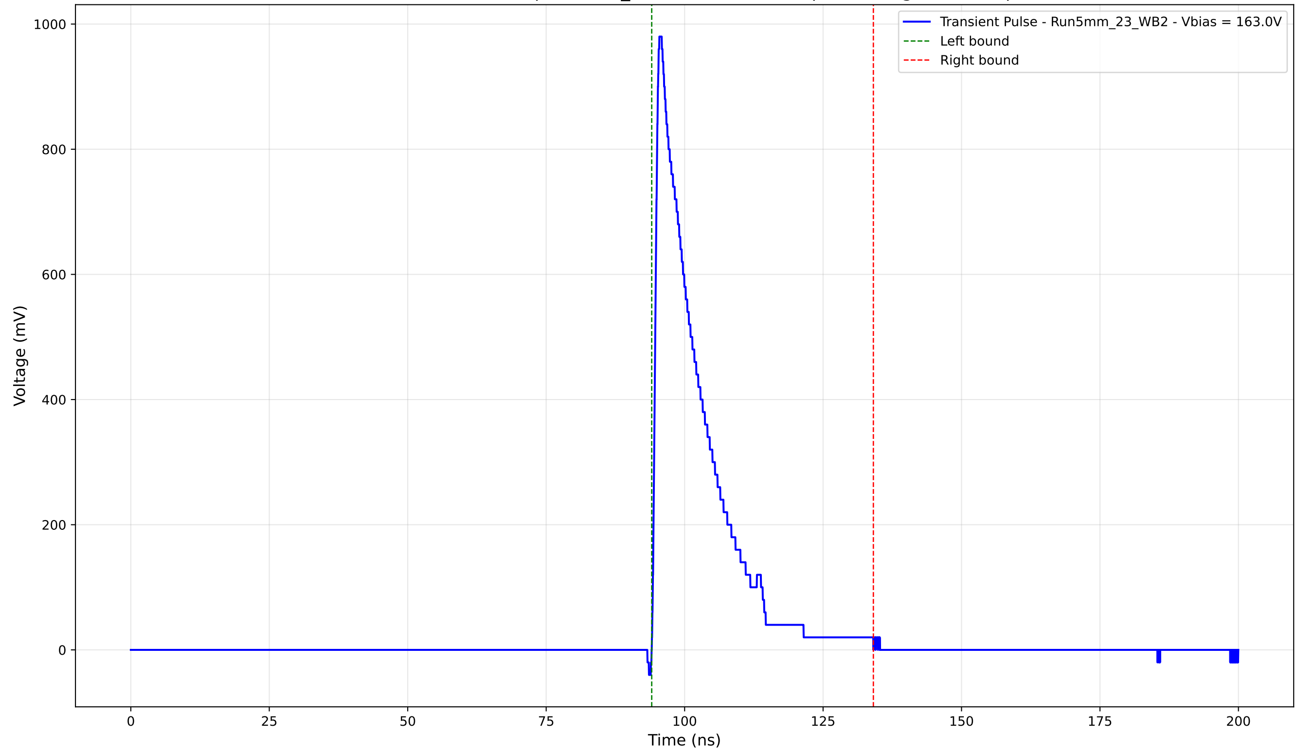
Transient Pulse - Sample: 5mm_23 - Position: 245.0 \mu\text{m} - Charge: 171.67 pC
