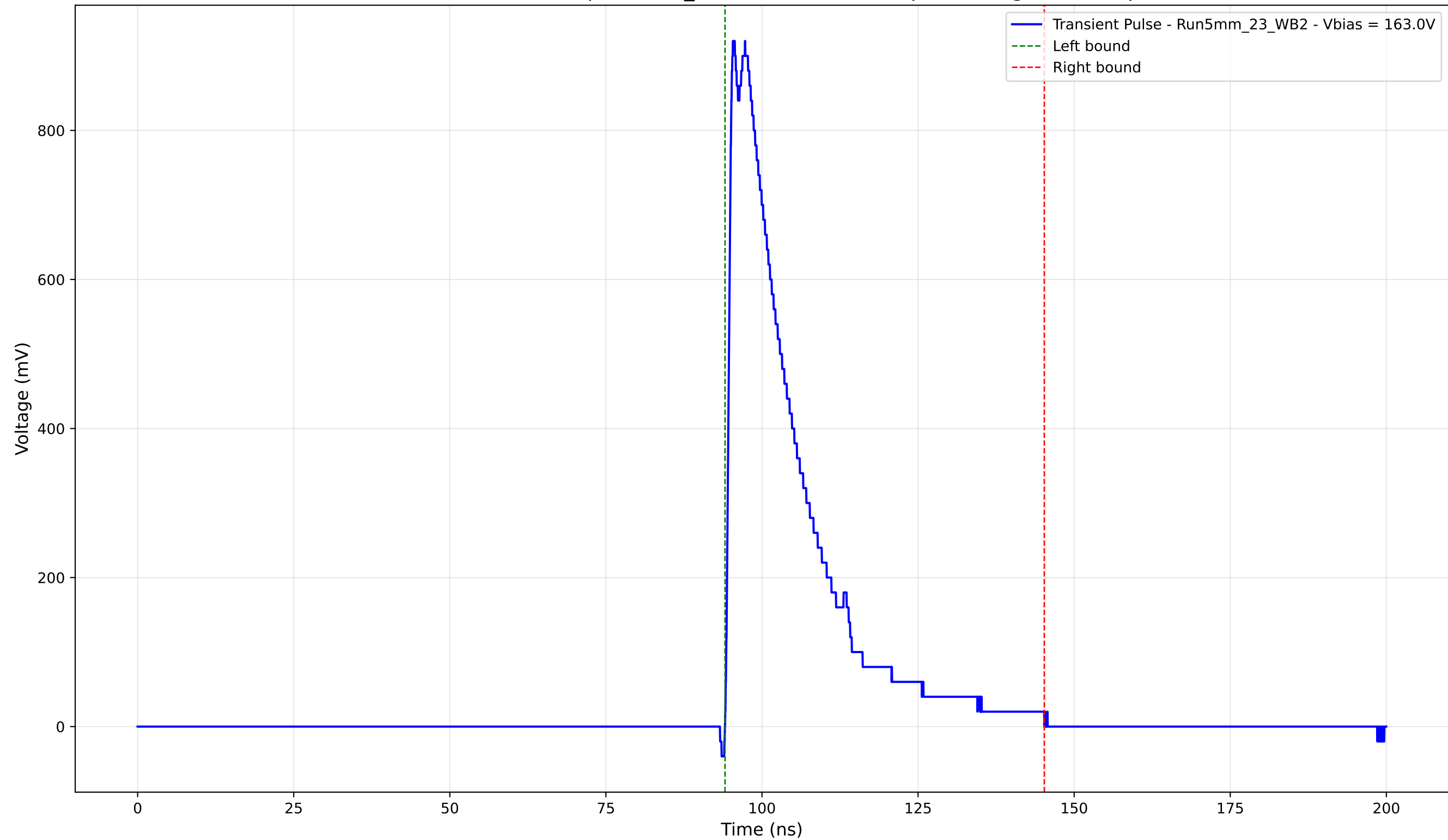
Transient Pulse - Sample: 5mm_23 - Position: 1900.0 \mu\text{m} - Charge: 218.01 pC
