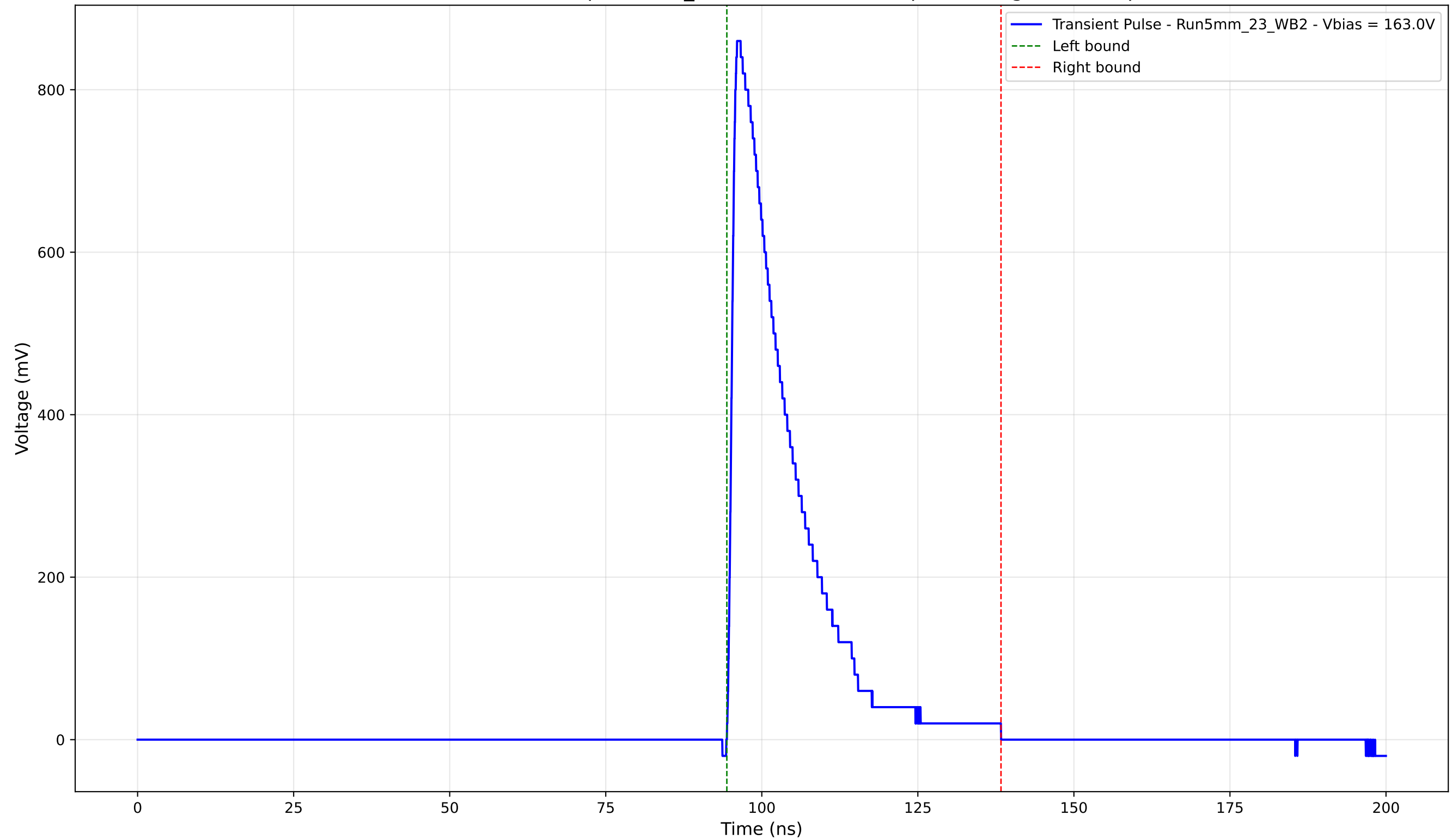
Transient Pulse - Sample: 5mm_23 - Position: 1090.0 \mu\text{m} - Charge: 177.21 pC
