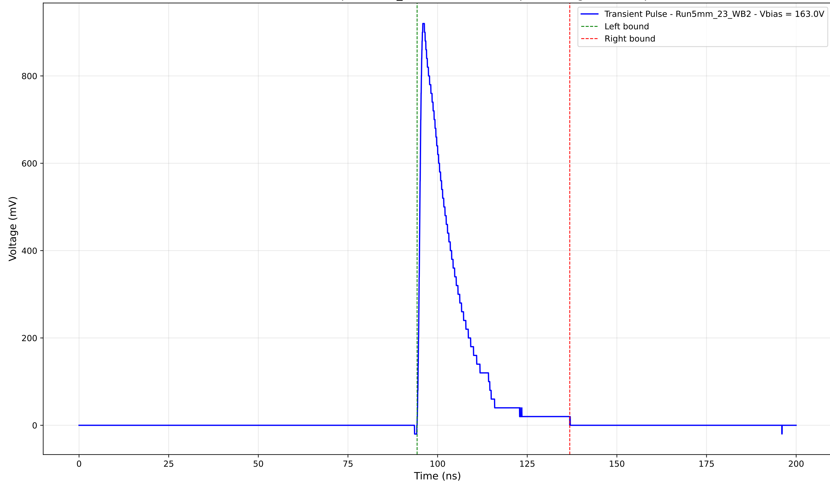
Transient Pulse - Sample: 5mm_23 - Position: 650.0 \mu\text{m} - Charge: 176.82 pC
