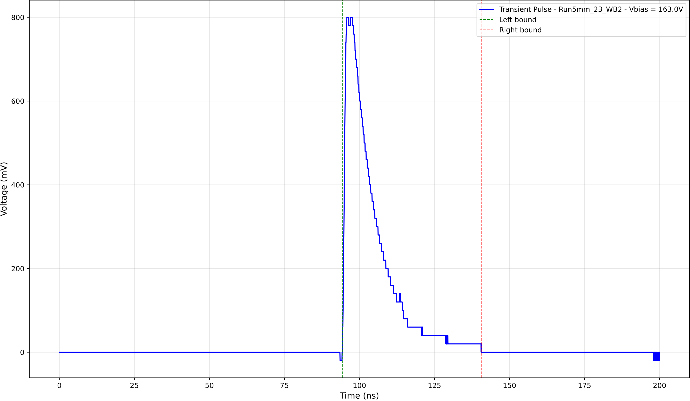
Transient Pulse - Sample: 5mm_23 - Position: 1585.0 \mu\text{m} - Charge: 178.71 pC
