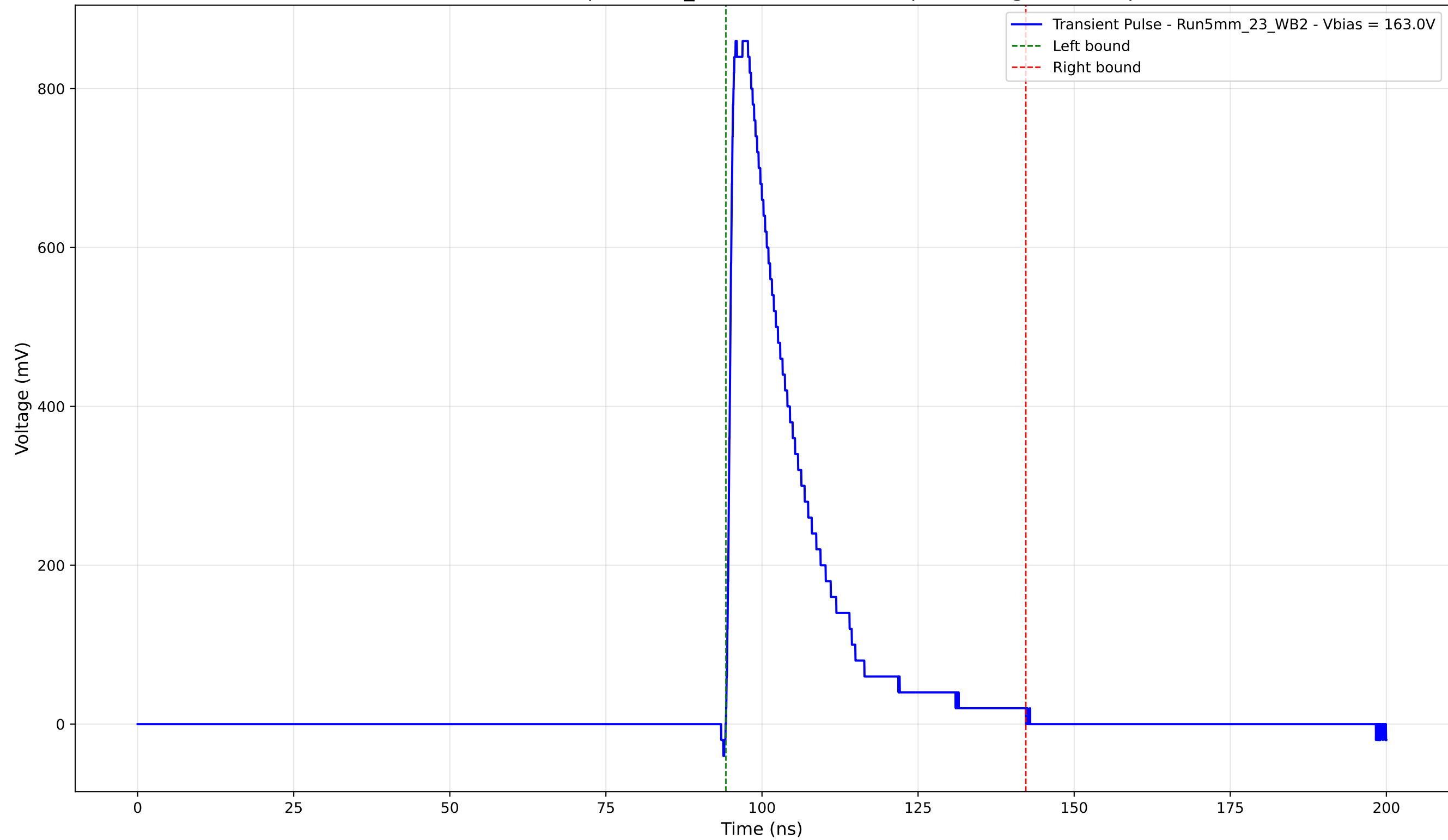
Transient Pulse - Sample: 5mm_23 - Position: 3355.0 \mu\text{m} - Charge: 195.52 pC
