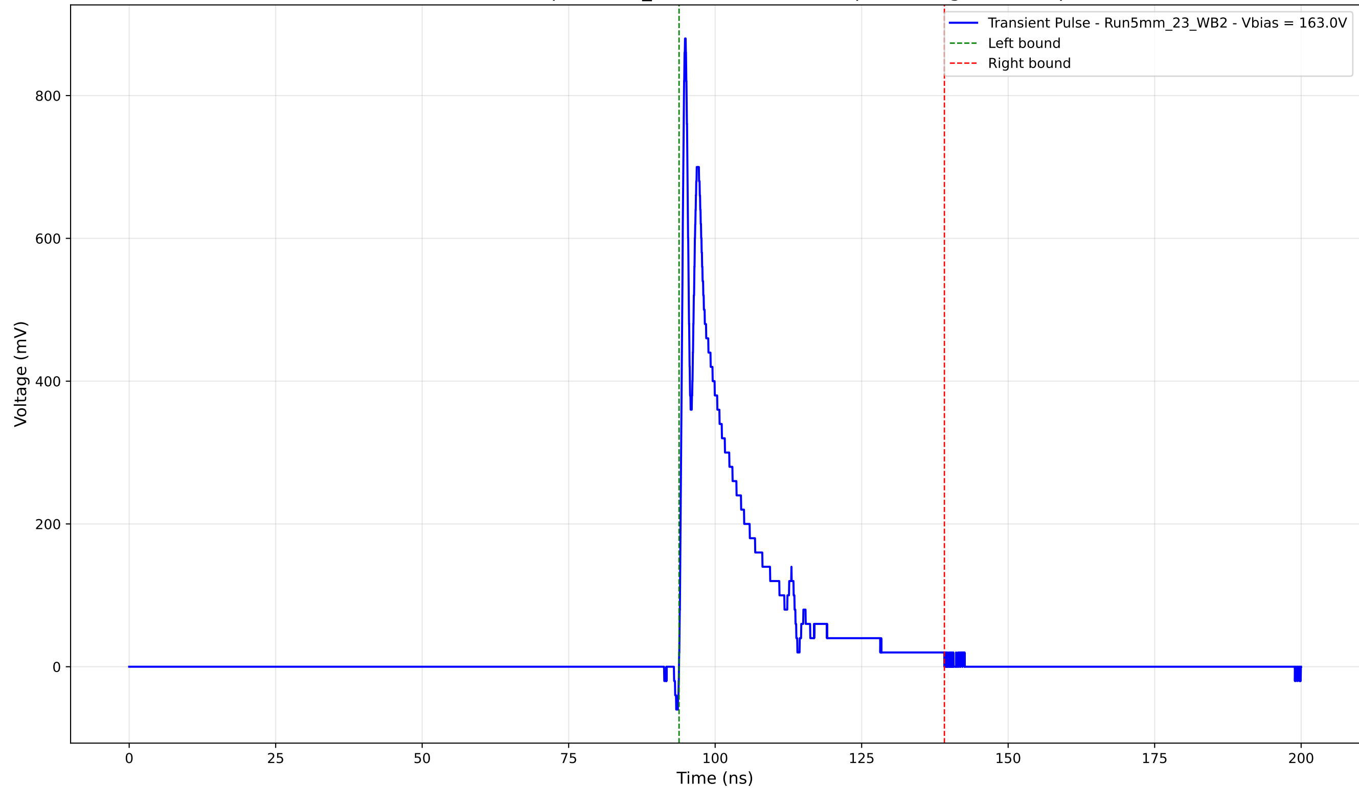
Transient Pulse - Sample: 5mm_23 - Position: 2460.0 \mu\text{m} - Charge: 134.56 pC
