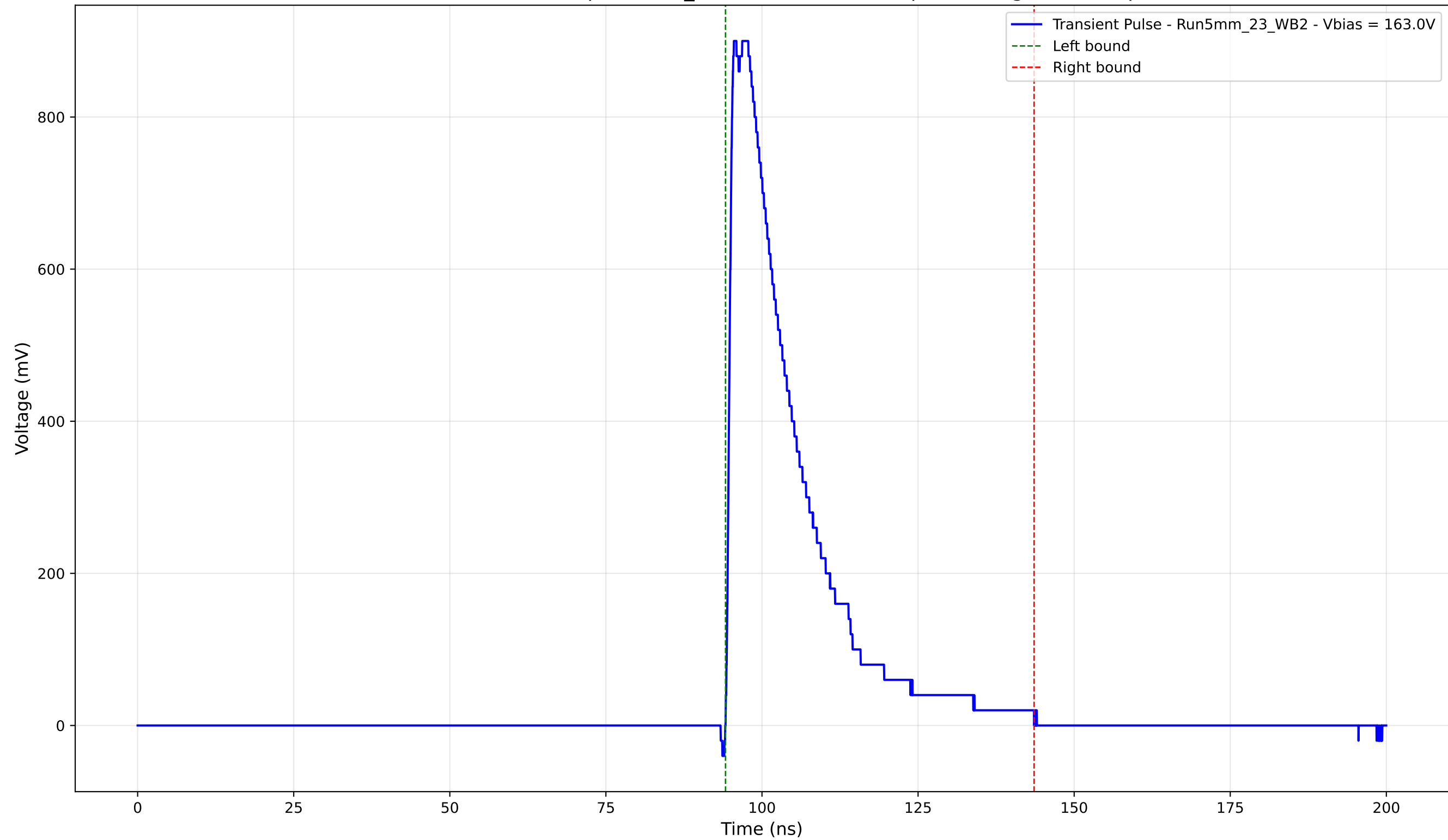
Transient Pulse - Sample: 5mm_23 - Position: 3265.0 \mu\text{m} - Charge: 213.82 pC
