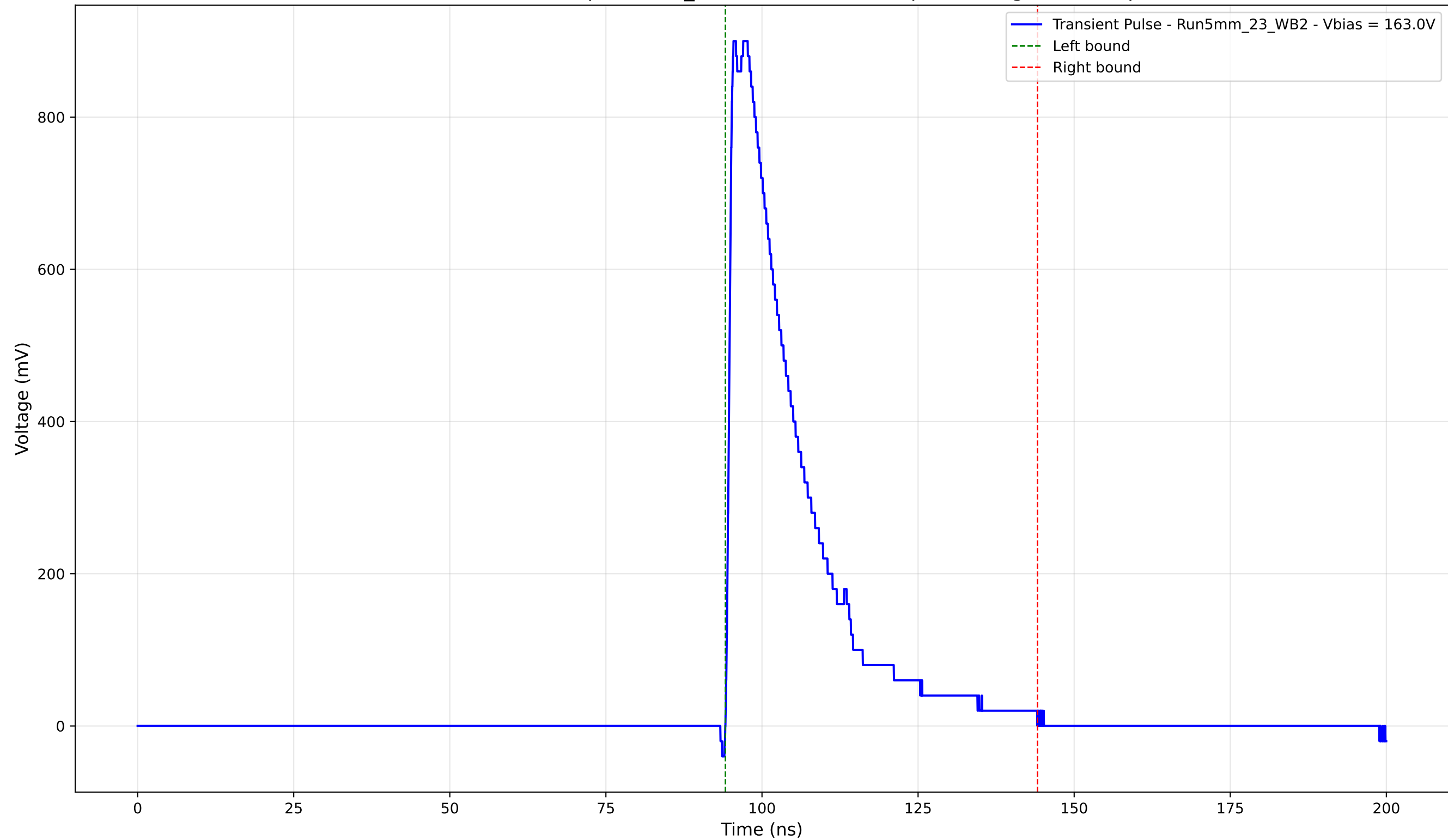
Transient Pulse - Sample: 5mm_23 - Position: 1805.0 \mu\text{m} - Charge: 218.62 pC
