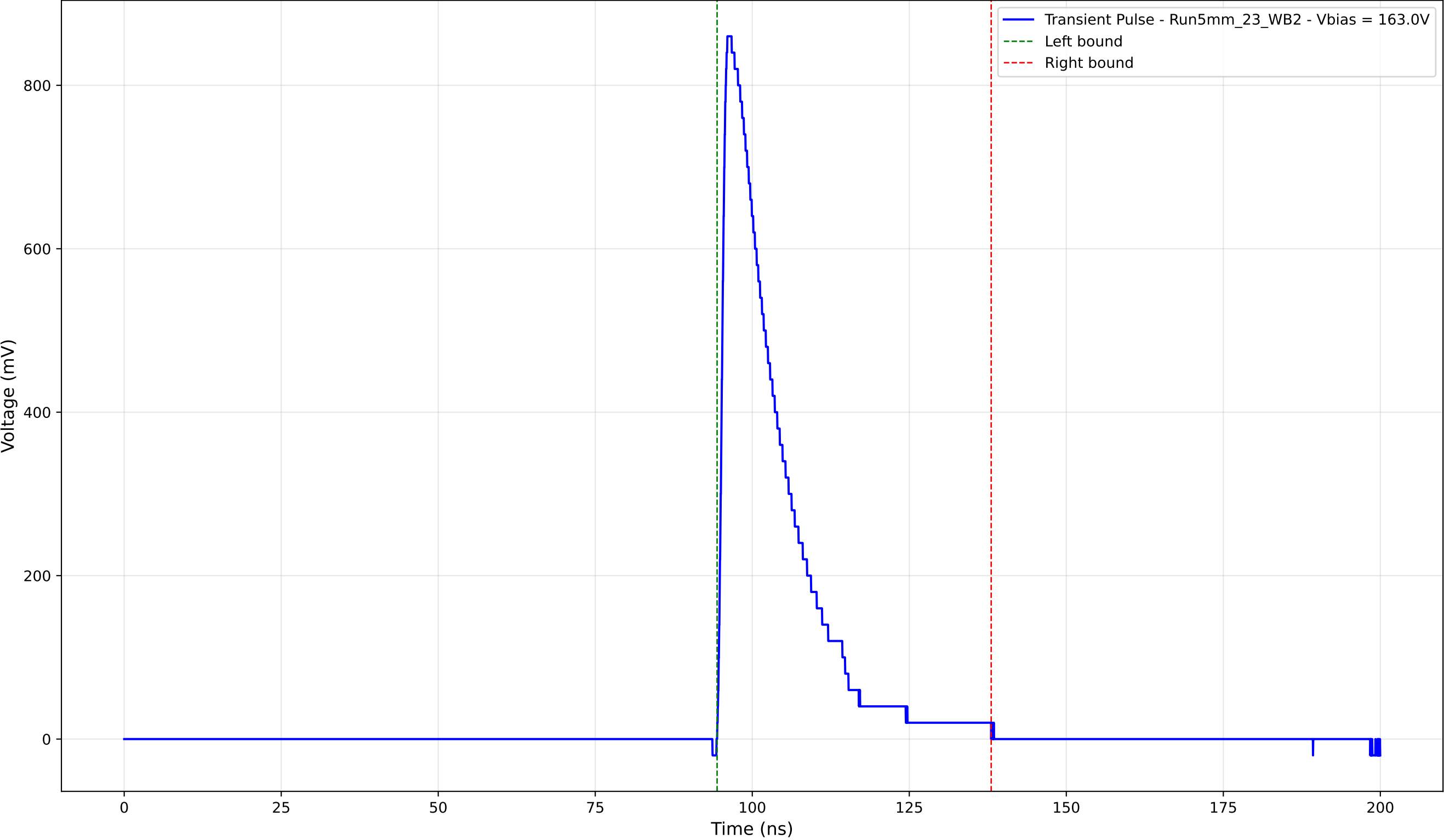
Transient Pulse - Sample: 5mm_23 - Position: 3800.0 \mu\text{m} - Charge: 176.28 pC
