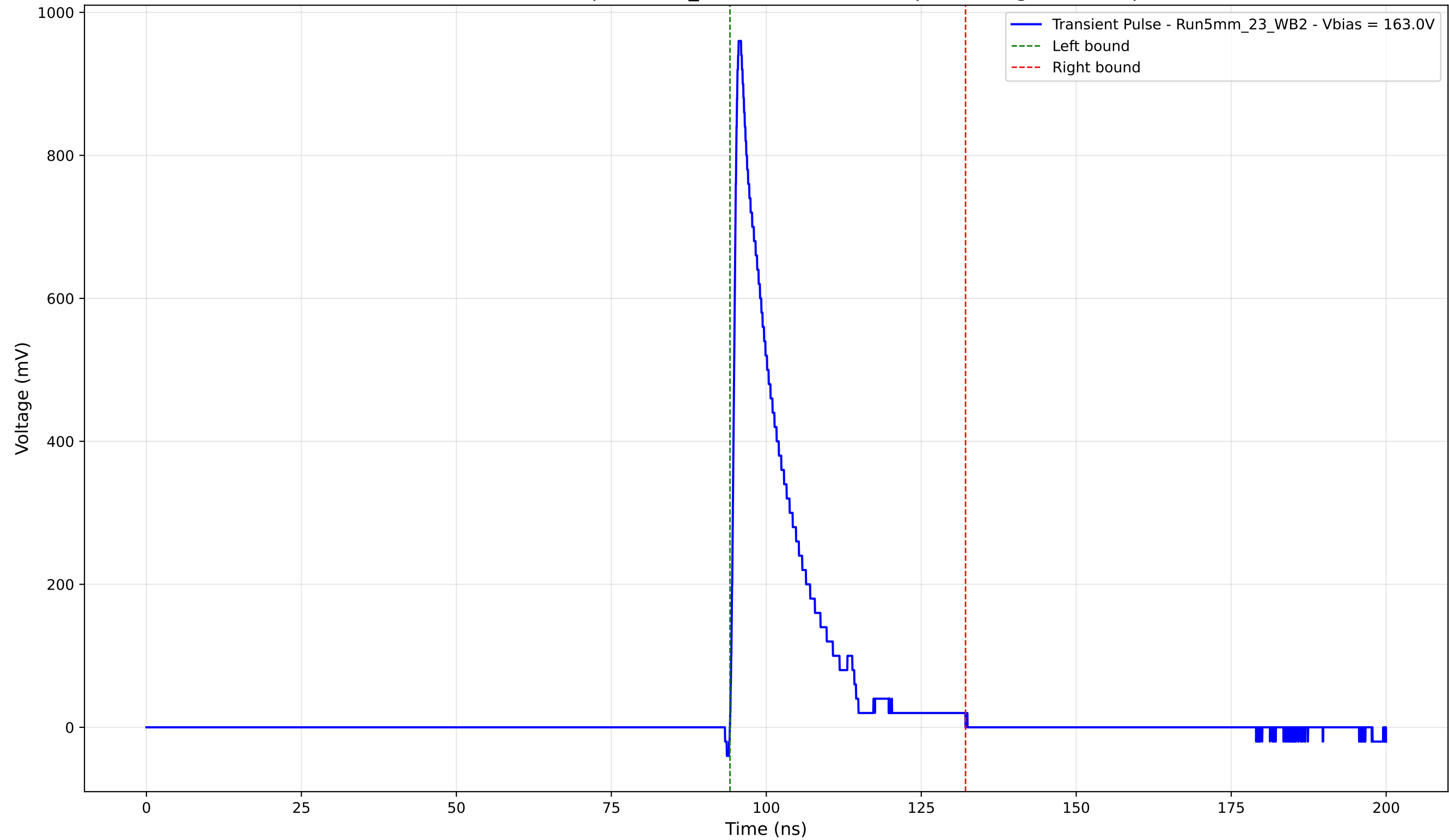
Transient Pulse - Sample: 5mm_23 - Position: 4730.0 \mu\text{m} - Charge: 151.36 pC
