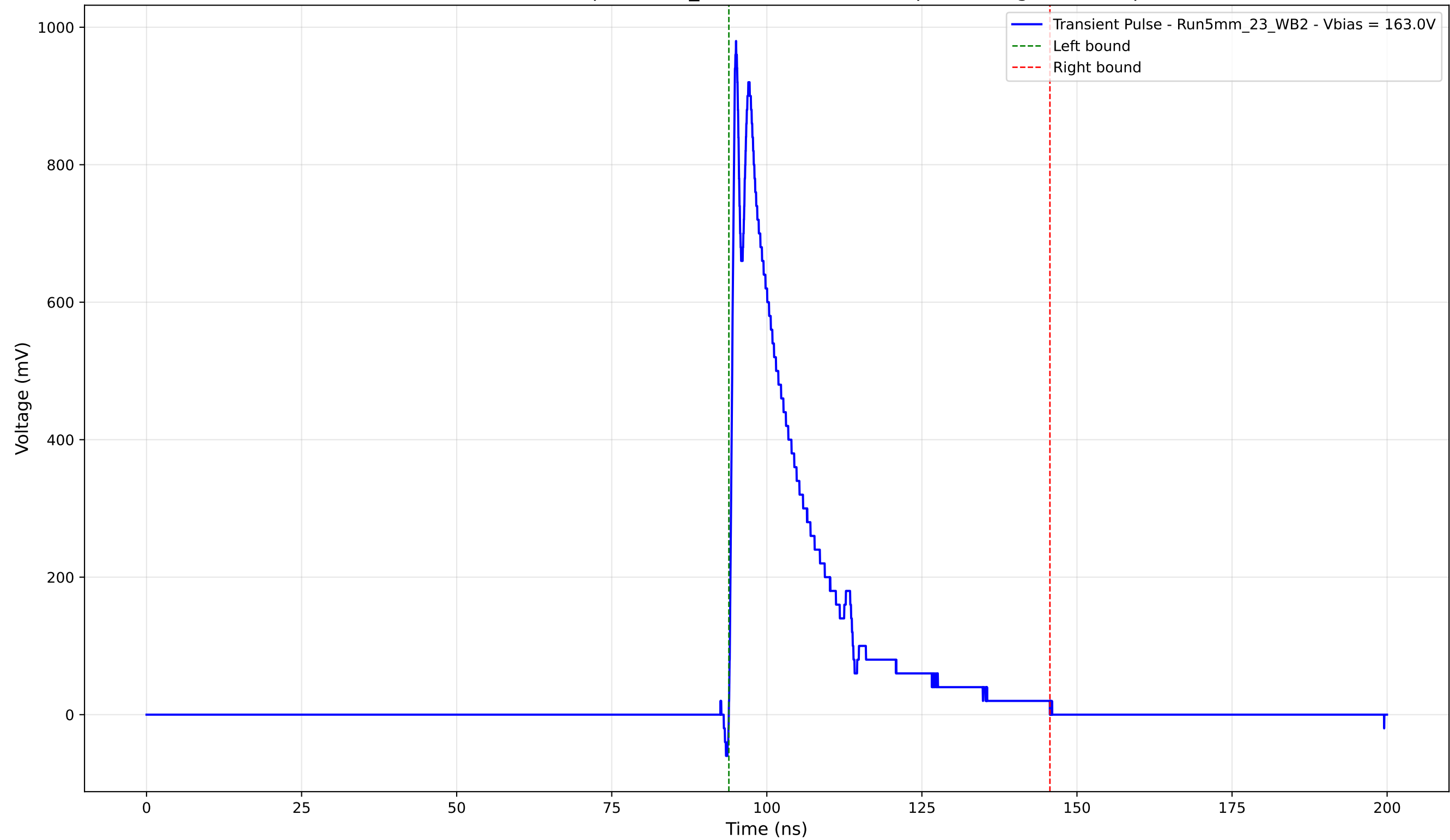
Transient Pulse - Sample: 5mm_23 - Position: 2745.0 \mu\text{m} - Charge: 203.21 pC
