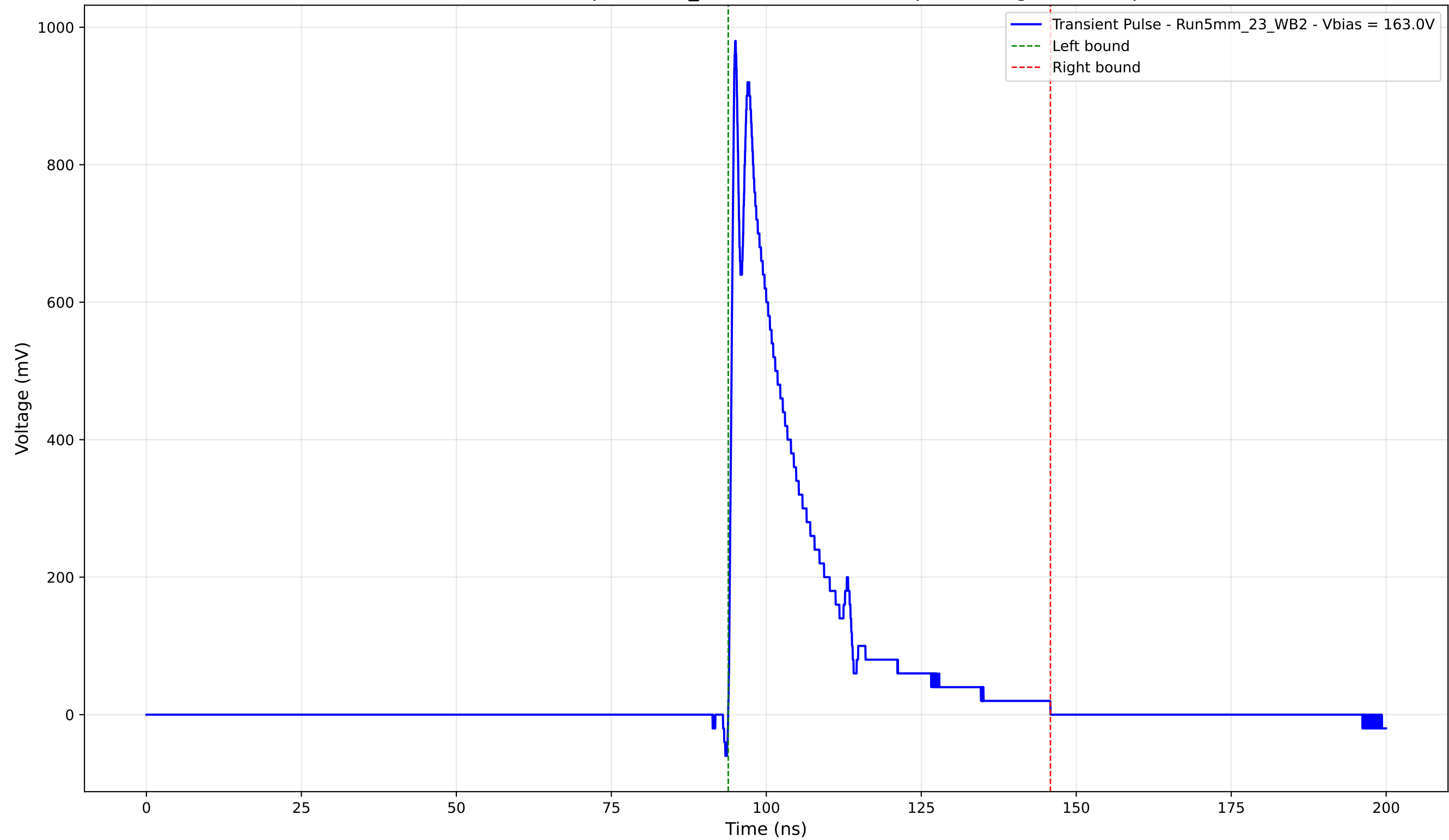
Transient Pulse - Sample: 5mm_23 - Position: 2320.0 \mu\text{m} - Charge: 203.01 pC
