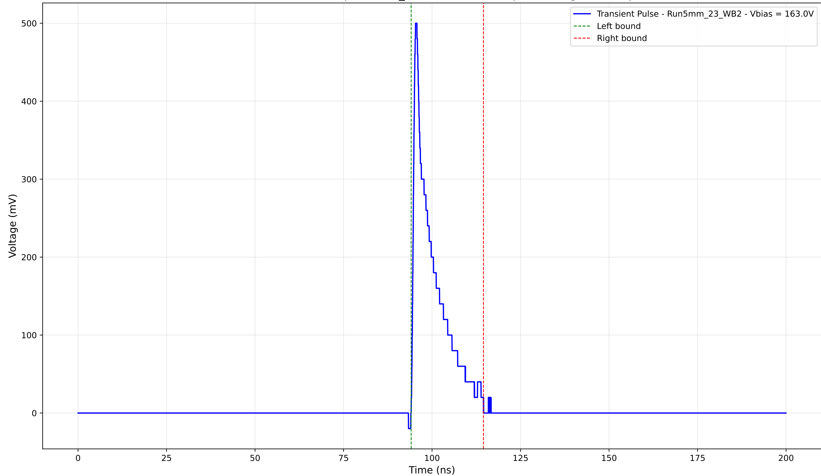
Transient Pulse - Sample: 5mm_23 - Position: 70.0 \mu\text{m} - Charge: 59.93 pC
