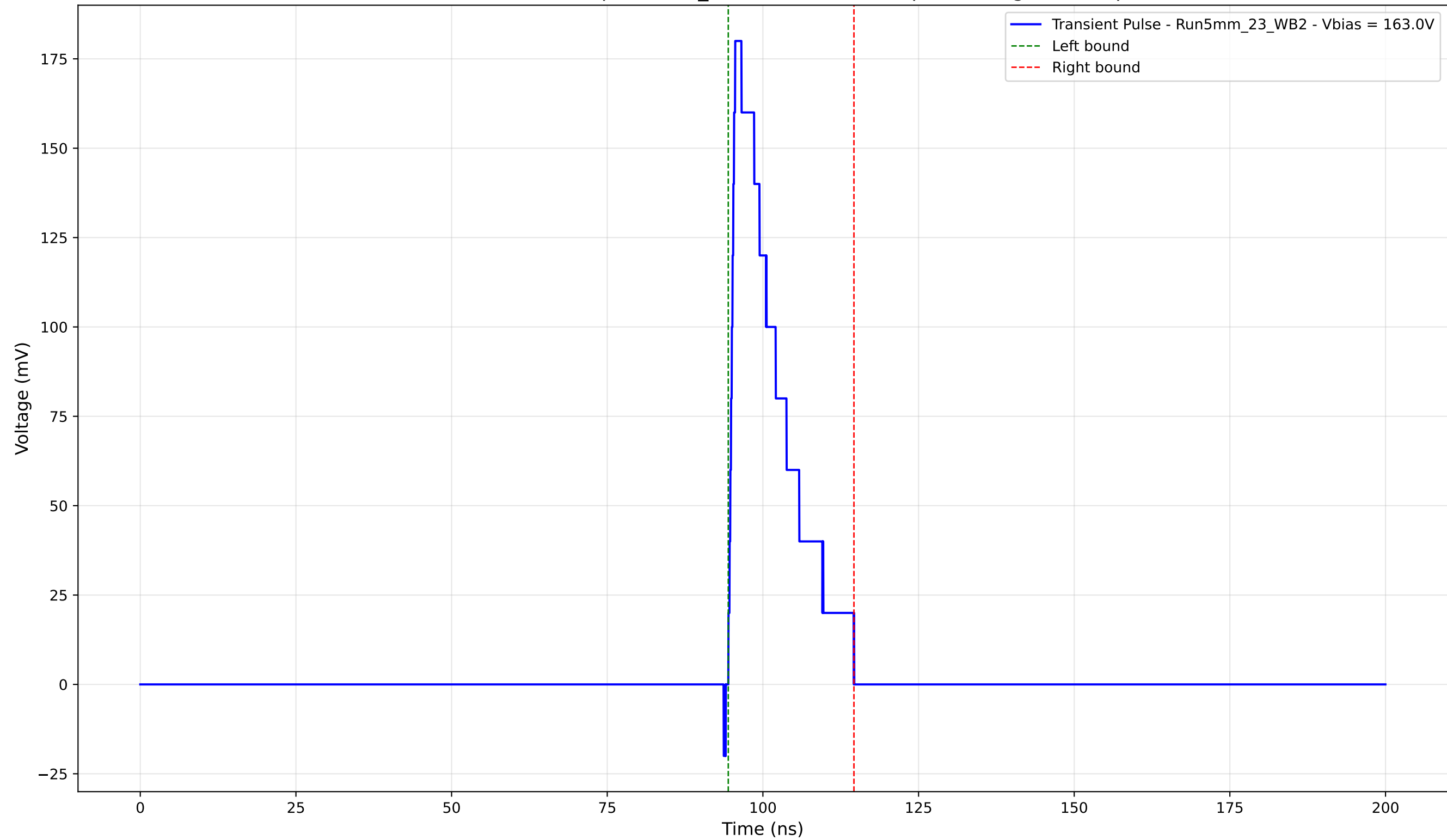
Transient Pulse - Sample: 5mm_23 - Position: 490.0 \mu\text{m} - Charge: 30.46 pC
