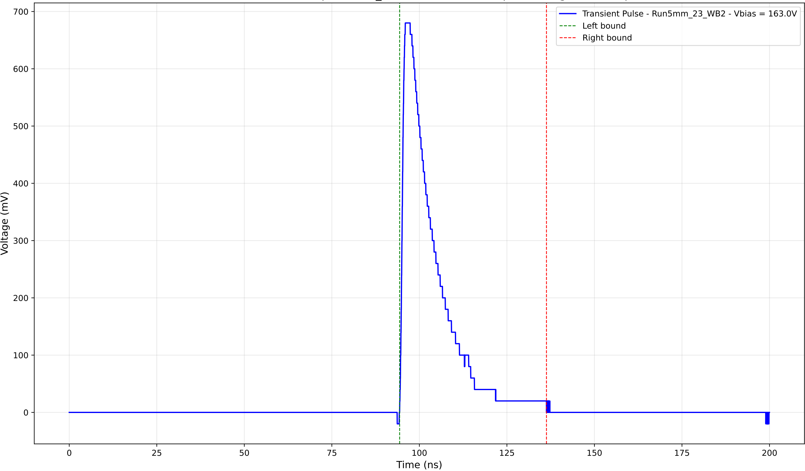
Transient Pulse - Sample: 5mm_23 - Position: 3595.0 \mu\text{m} - Charge: 139.00 pC
