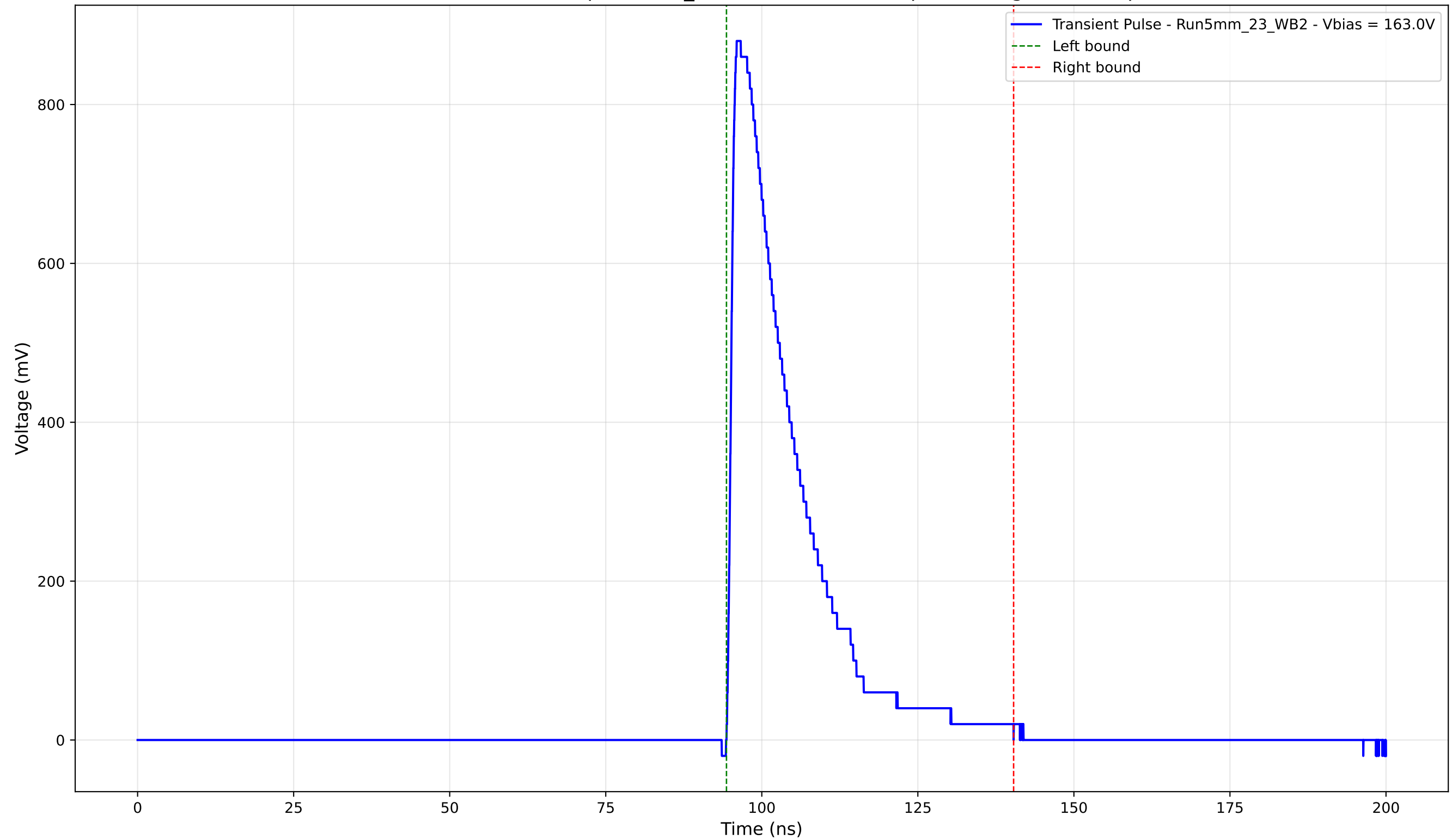
Transient Pulse - Sample: 5mm_23 - Position: 1385.0 \mu\text{m} - Charge: 195.91 pC
