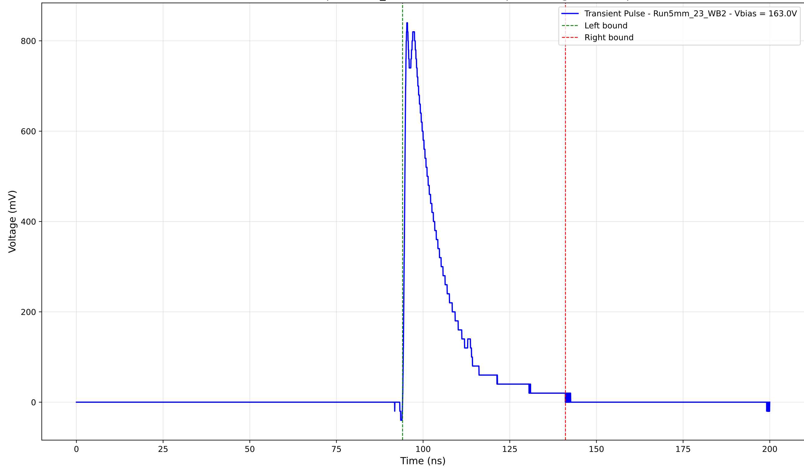
Transient Pulse - Sample: 5mm_23 - Position: 3090.0 \mu\text{m} - Charge: 180.22 pC
