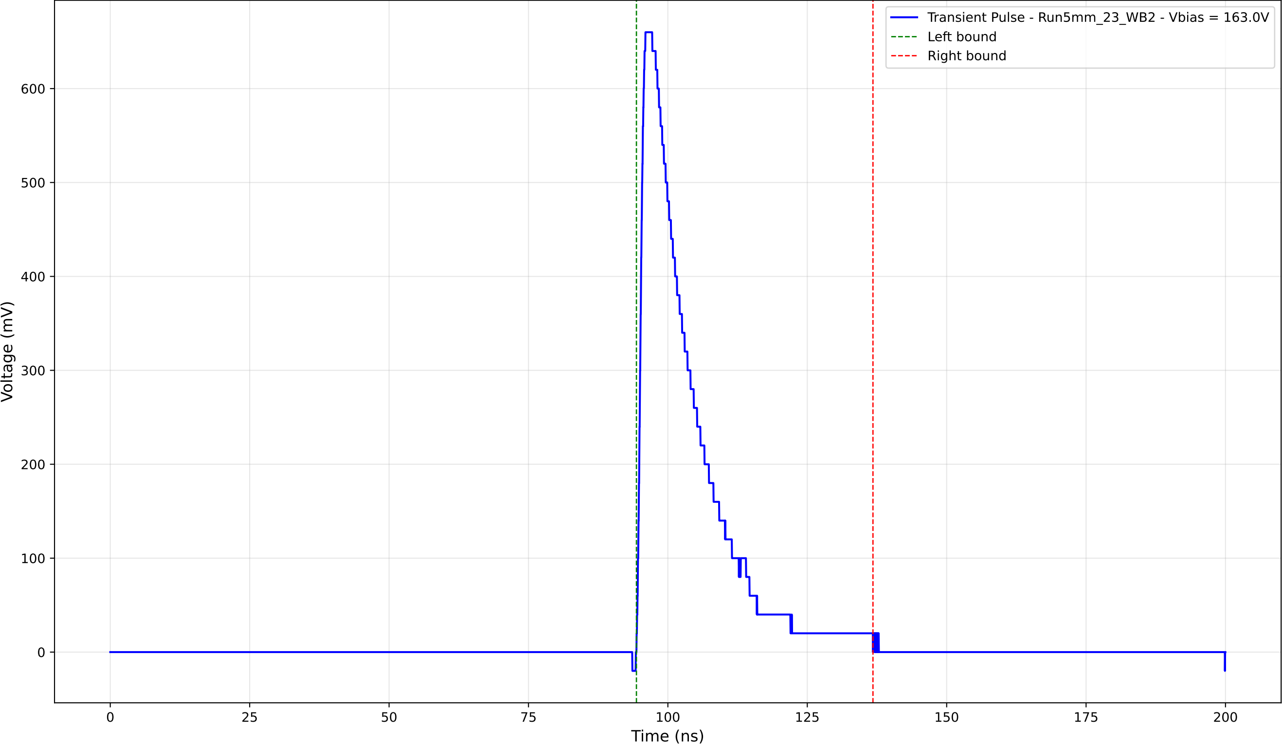
Transient Pulse - Sample: 5mm_23 - Position: 1440.0 \mu\text{m} - Charge: 136.49 pC
