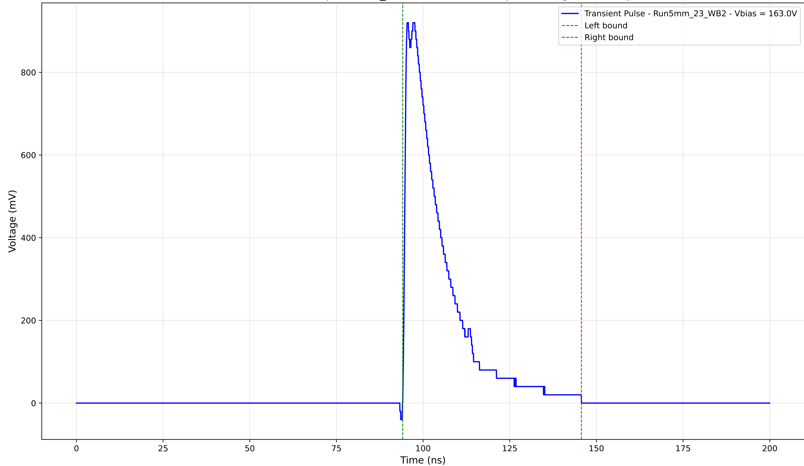
Transient Pulse - Sample: 5mm_23 - Position: 1855.0 \mu\text{m} - Charge: 223.12 pC
