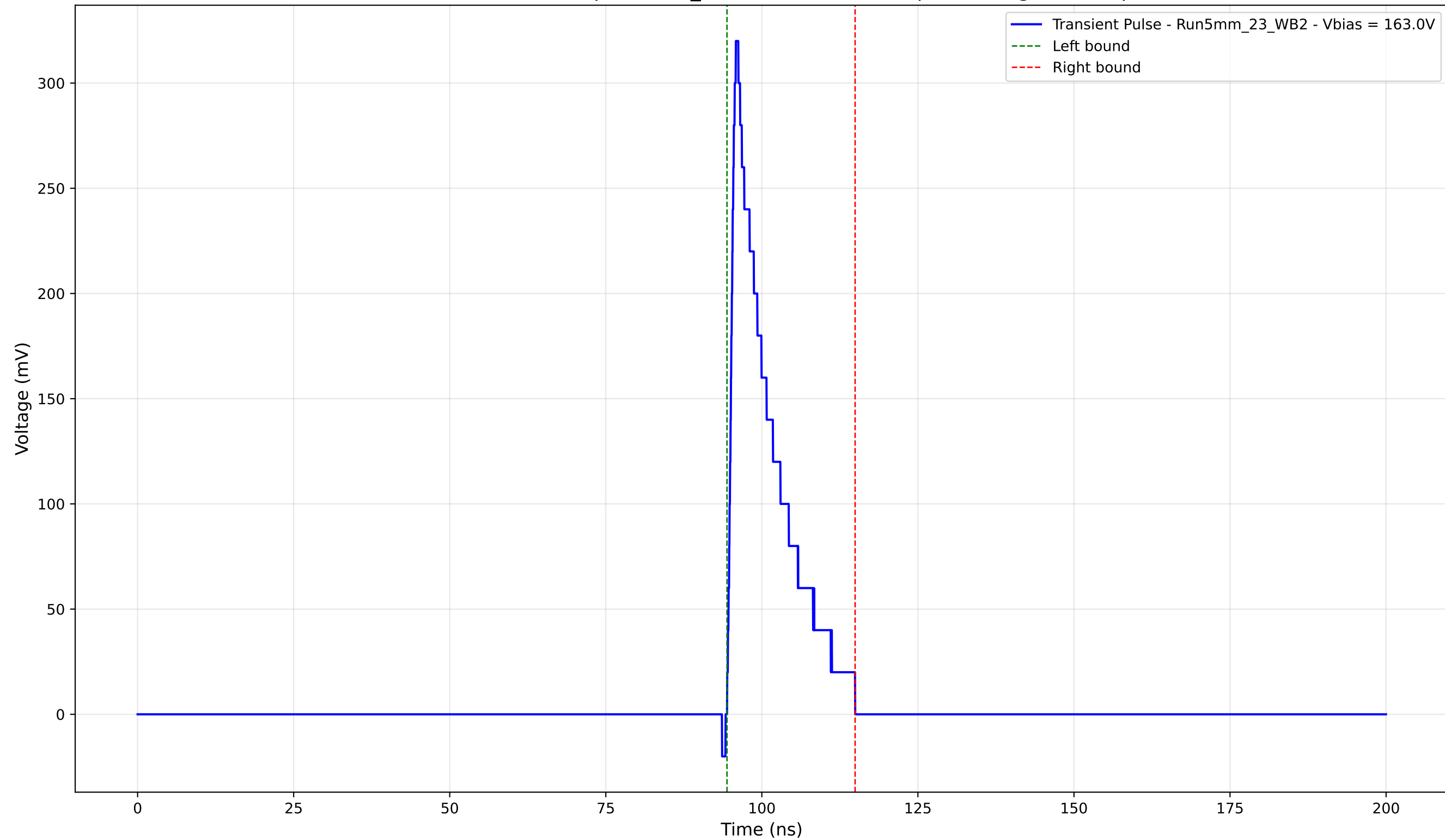
Transient Pulse - Sample: 5mm_23 - Position: 4515.0 \mu\text{m} - Charge: 44.49 pC
