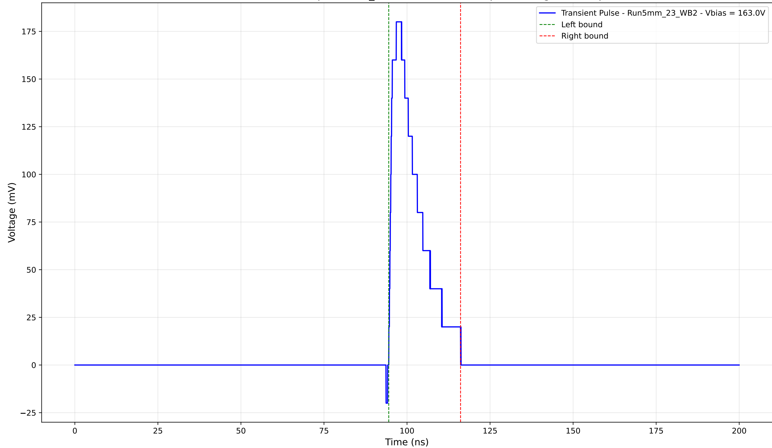
Transient Pulse - Sample: 5mm_23 -Position: 3515.0 \mu\text{m} - Charge: 33.63 pC
