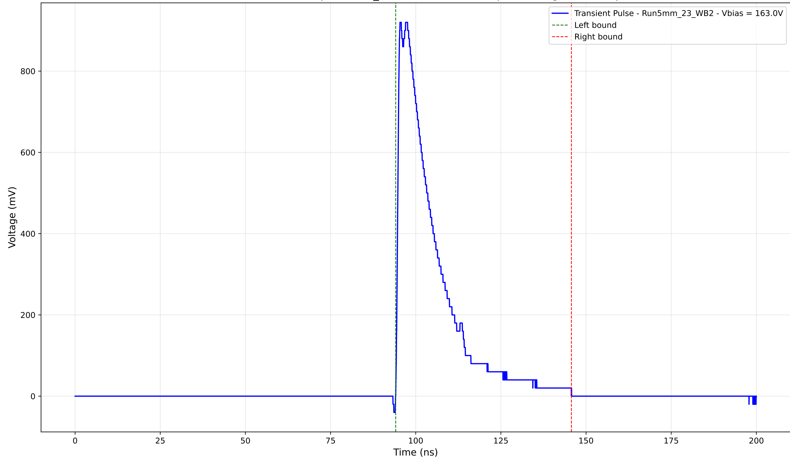
Transient Pulse - Sample: 5mm_23 - Position: 1850.0 \mu\text{m} - Charge: 223.25 pC
