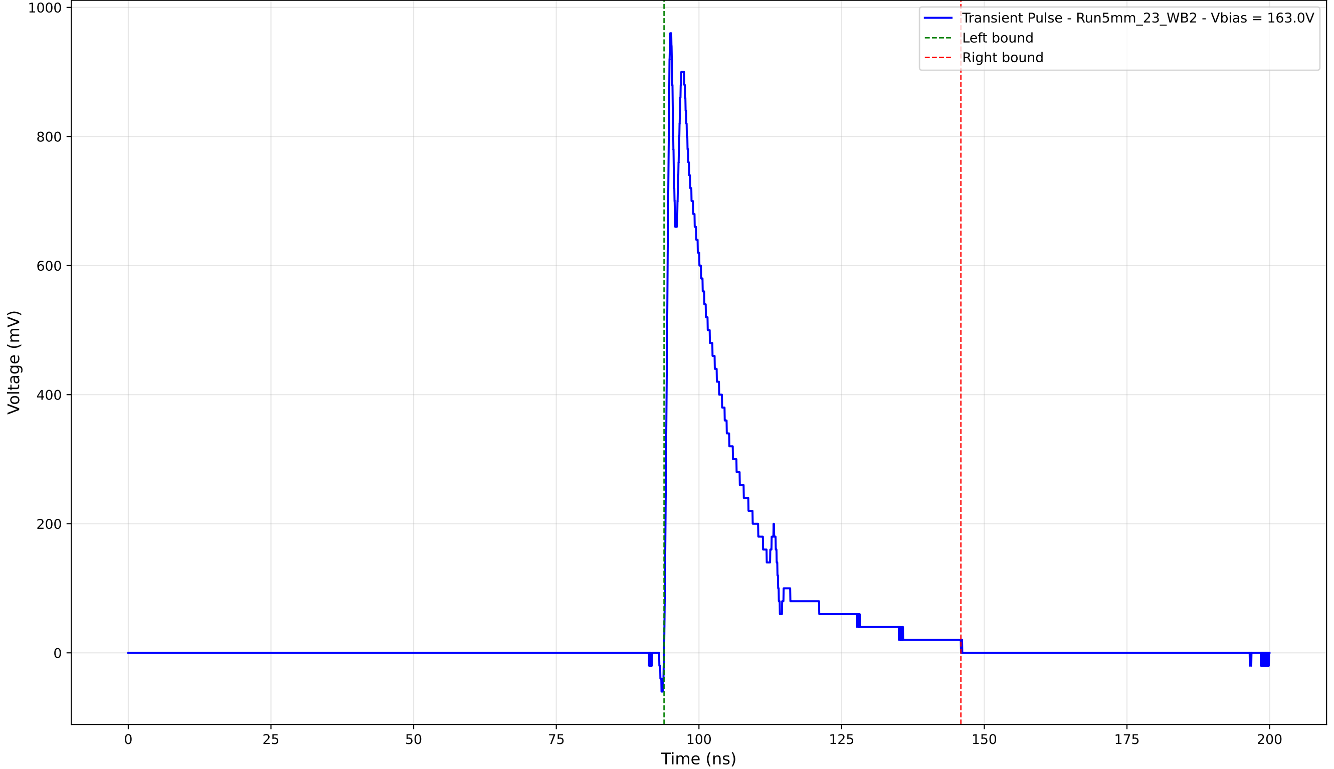
Transient Pulse - Sample: 5mm_23 - Position: 2290.0 \mu\text{m} - Charge: 204.18 pC
