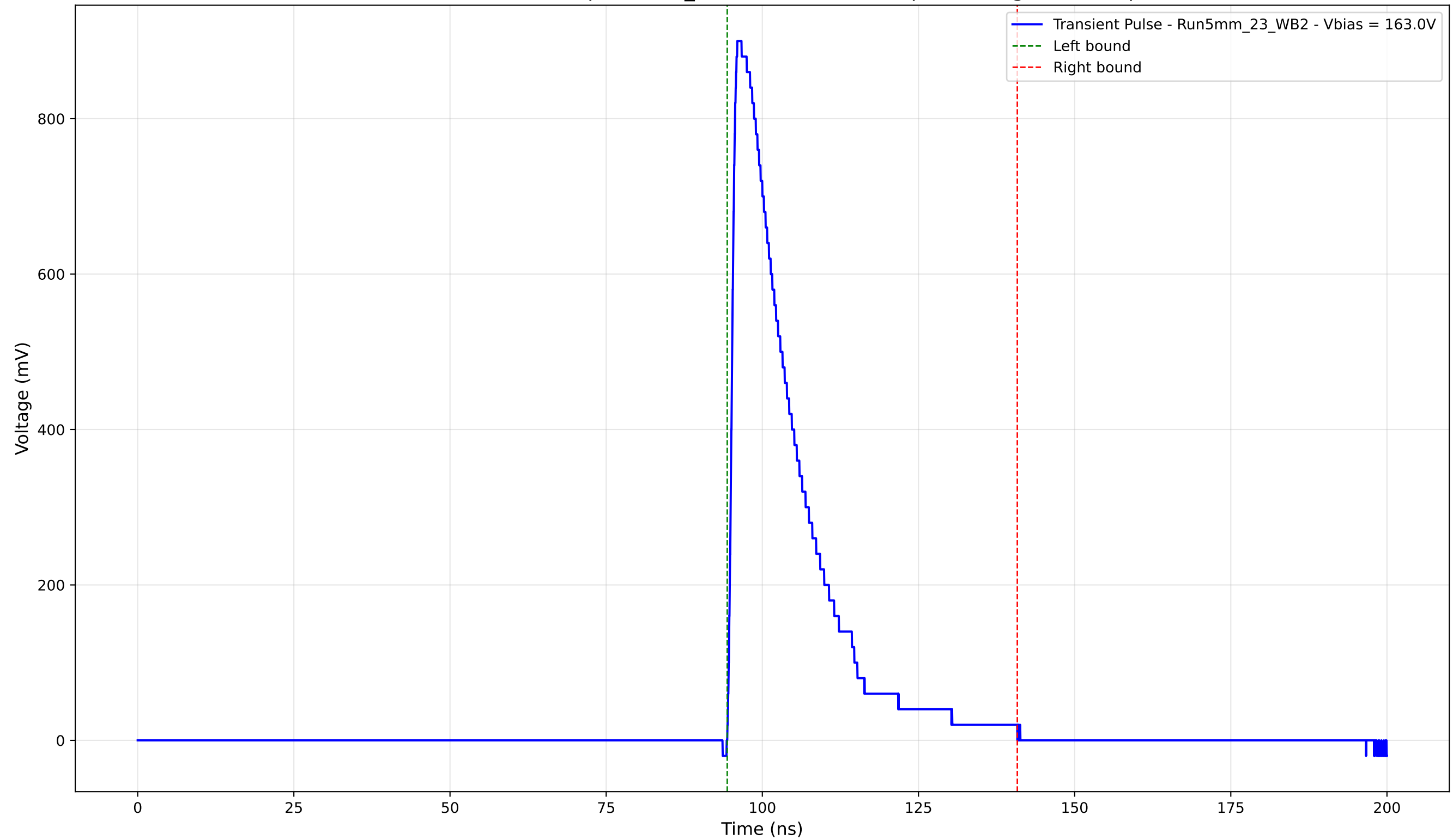
Transient Pulse - Sample: 5mm_23 - Position: 1270.0 \mu\text{m} - Charge: 200.69 pC
