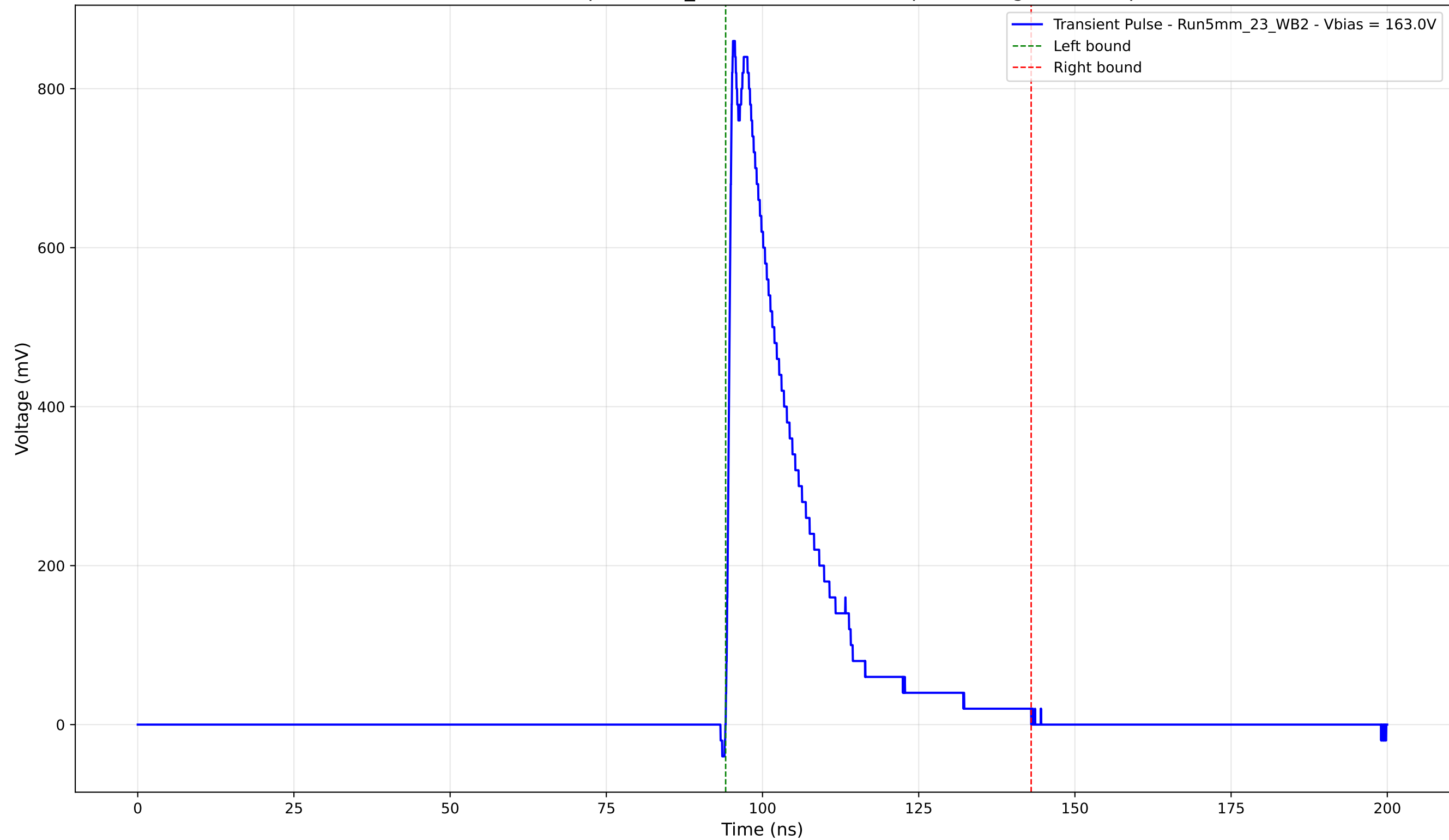
Transient Pulse - Sample: 5mm_23 - Position: 1930.0 \mu\text{m} - Charge: 190.36 pC
