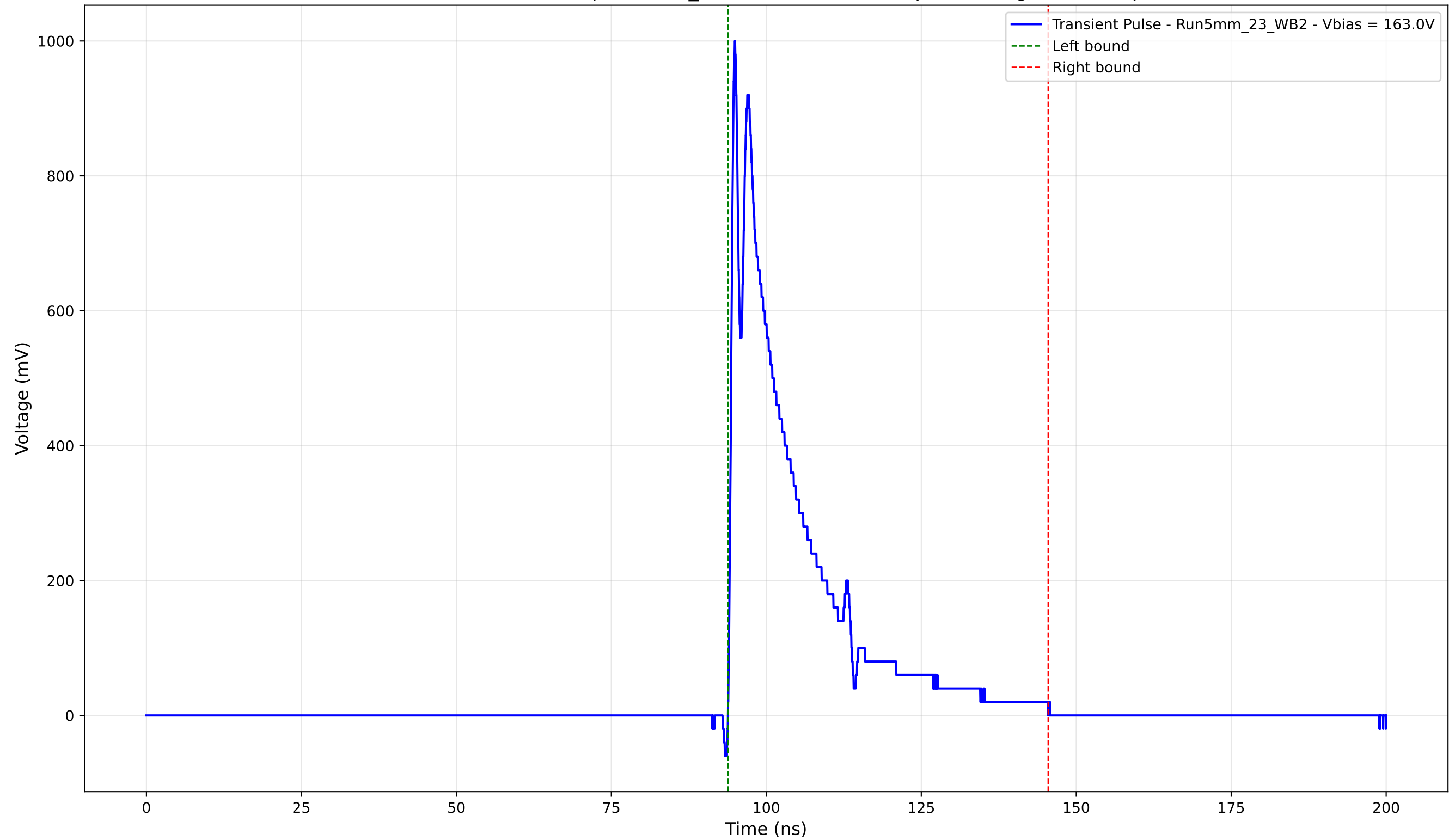
Transient Pulse - Sample: 5mm_23 - Position: 2410.0 \mu\text{m} - Charge: 195.90 pC
