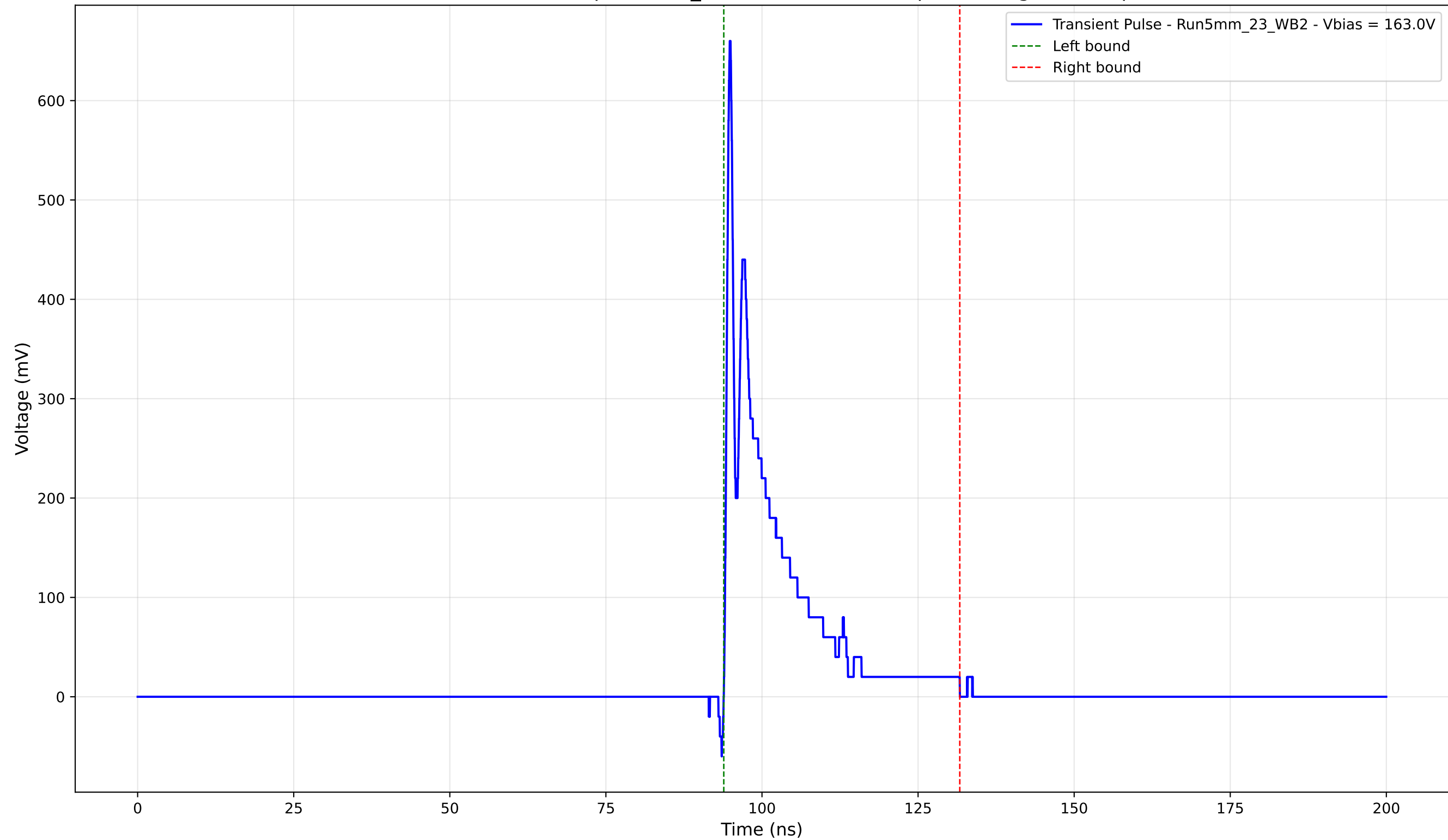
Transient Pulse - Sample: 5mm_23 - Position: 2550.0 \mu\text{m} - Charge: 78.36 pC
