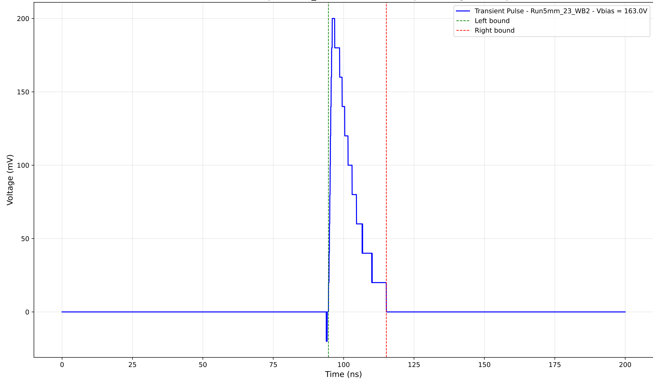
Transient Pulse - Sample: 5mm_23 - Position: 4050.0 \mu\text{m} - Charge: 33.45 pC
