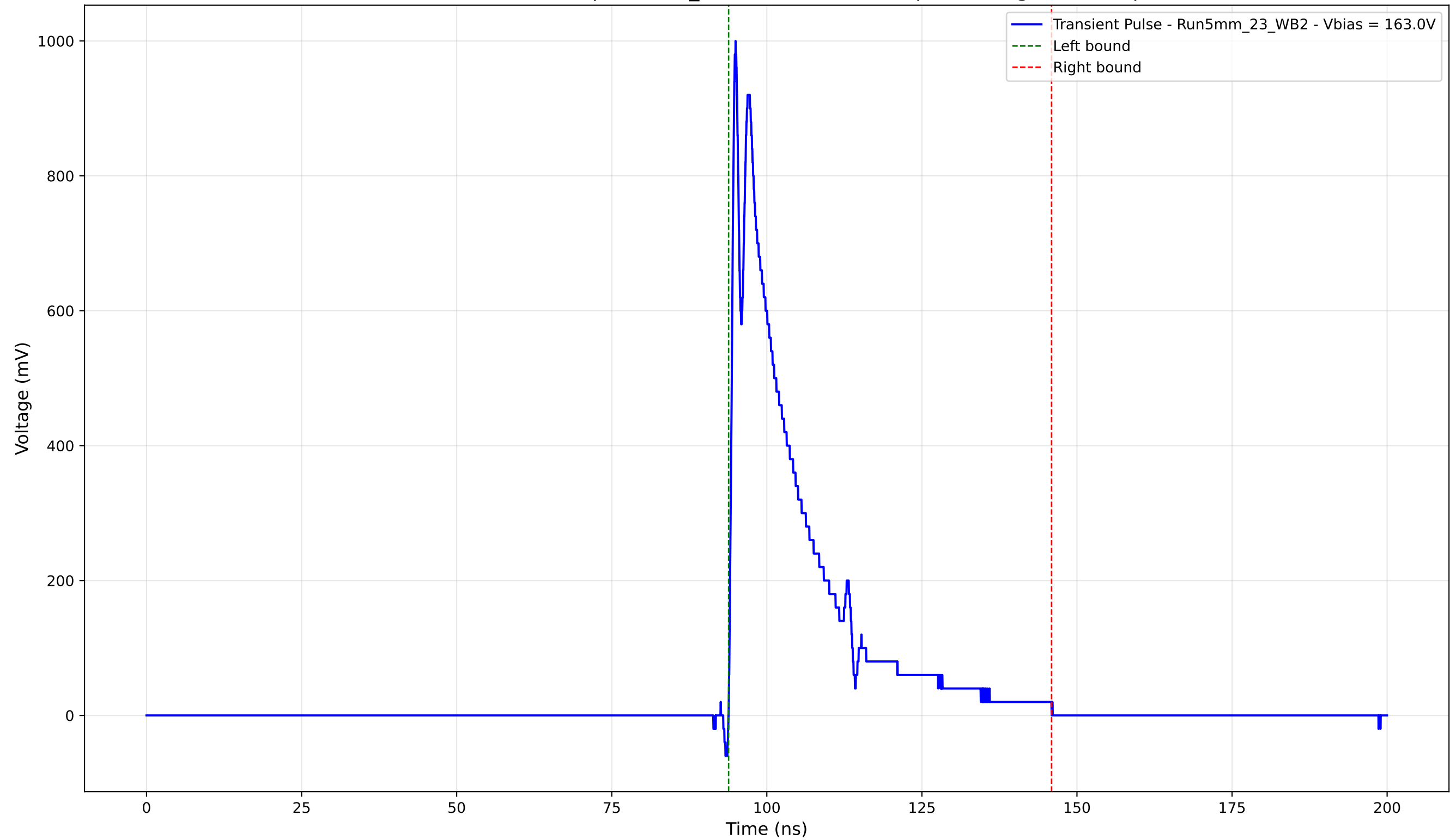
Transient Pulse - Sample: 5mm_23 - Position: 2655.0 \mu\text{m} - Charge: 200.89 pC
