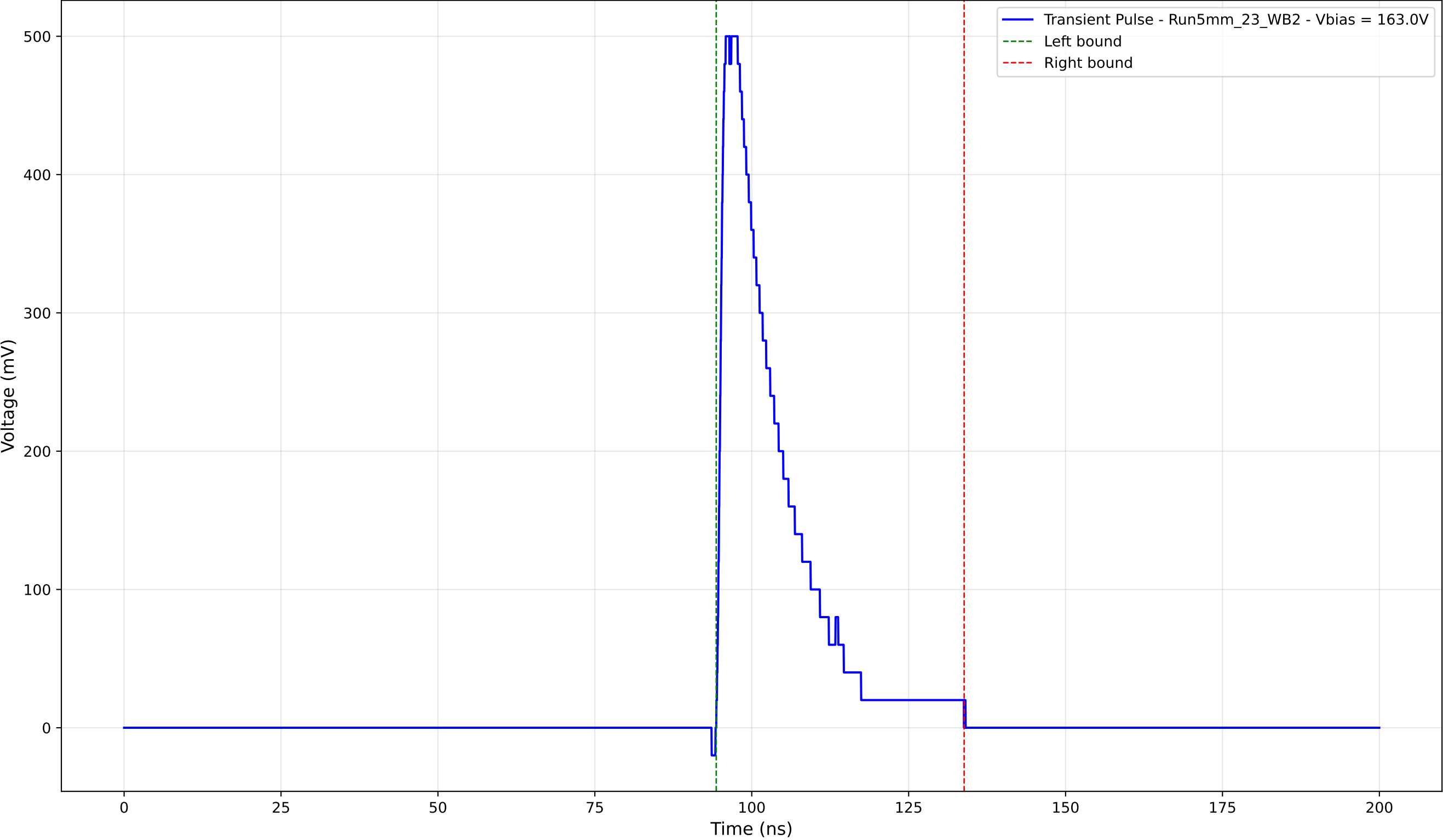
Transient Pulse - Sample: 5mm_23 - Position: 1545.0 \mu\text{m} - Charge: 102.98 pC
