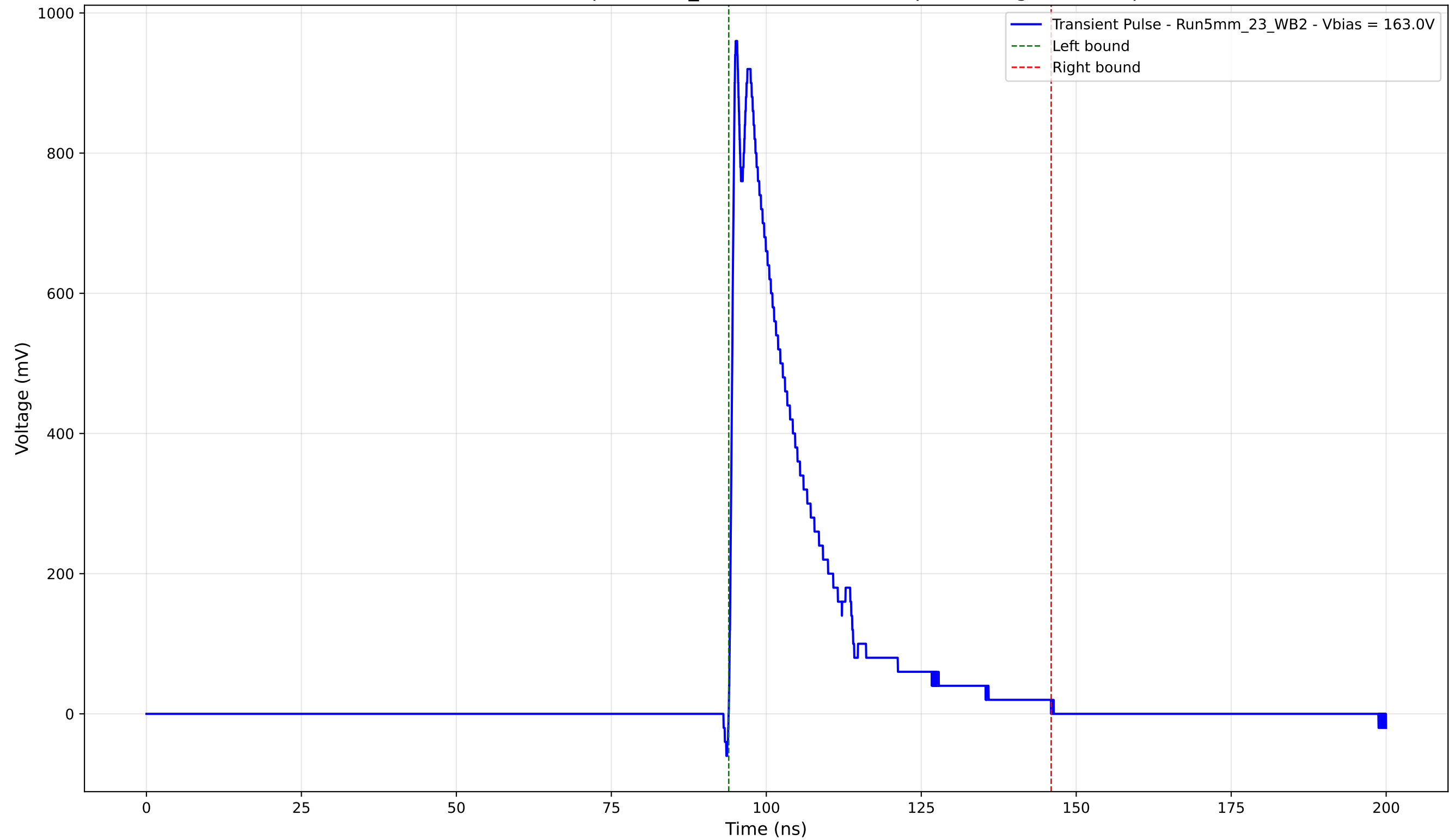
Transient Pulse - Sample: 5mm_23 - Position: 2860.0 \mu\text{m} - Charge: 214.56 pC
