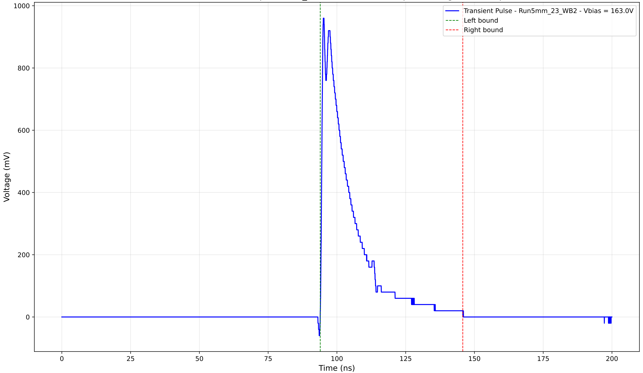
Transient Pulse - Sample: 5mm_23 - Position: 2865.0 \mu\text{m} - Charge: 214.88 pC
