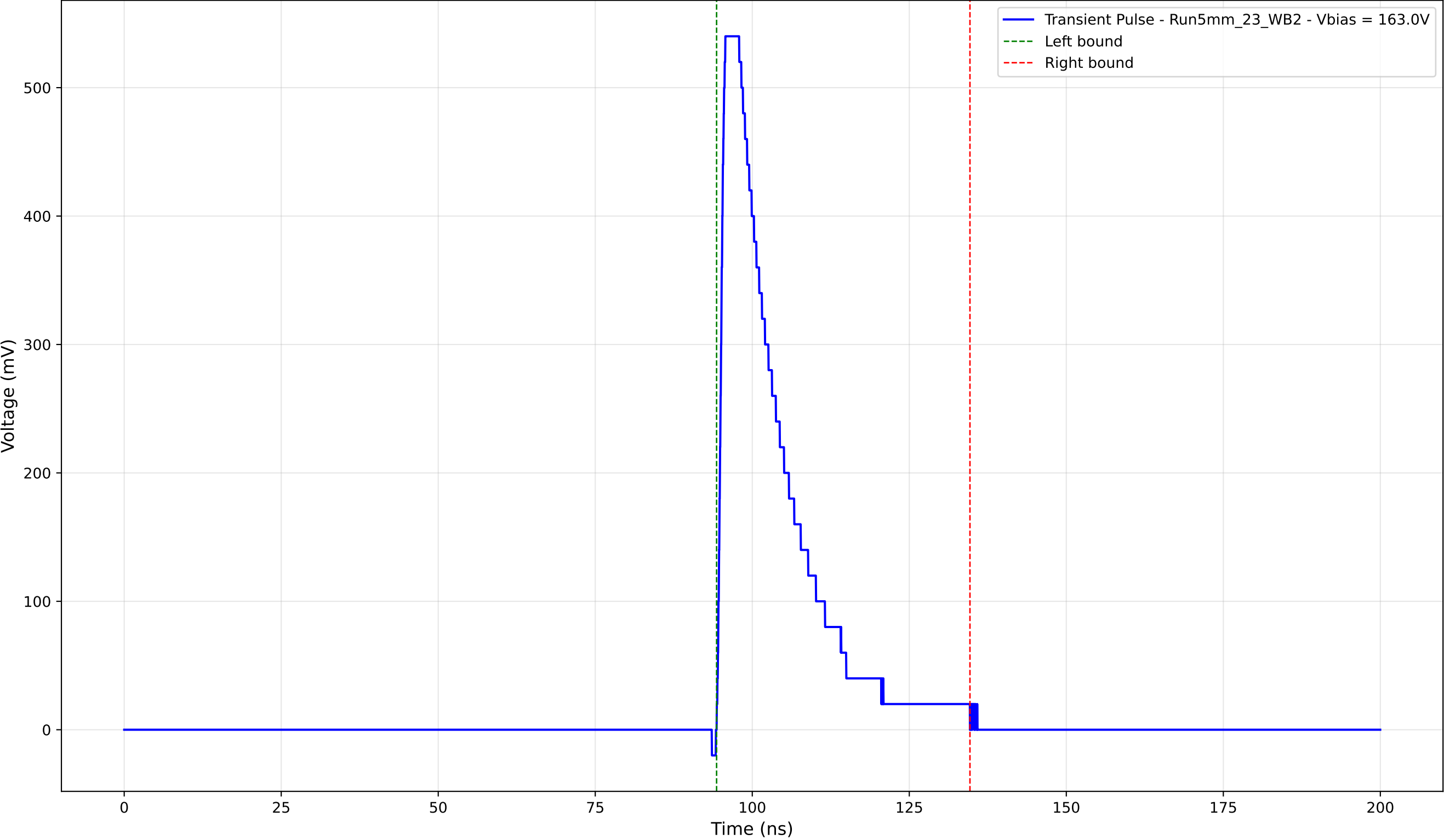
Transient Pulse - Sample: 5mm_23 - Position: 1550.0 \mu\text{m} - Charge: 114.74 pC
