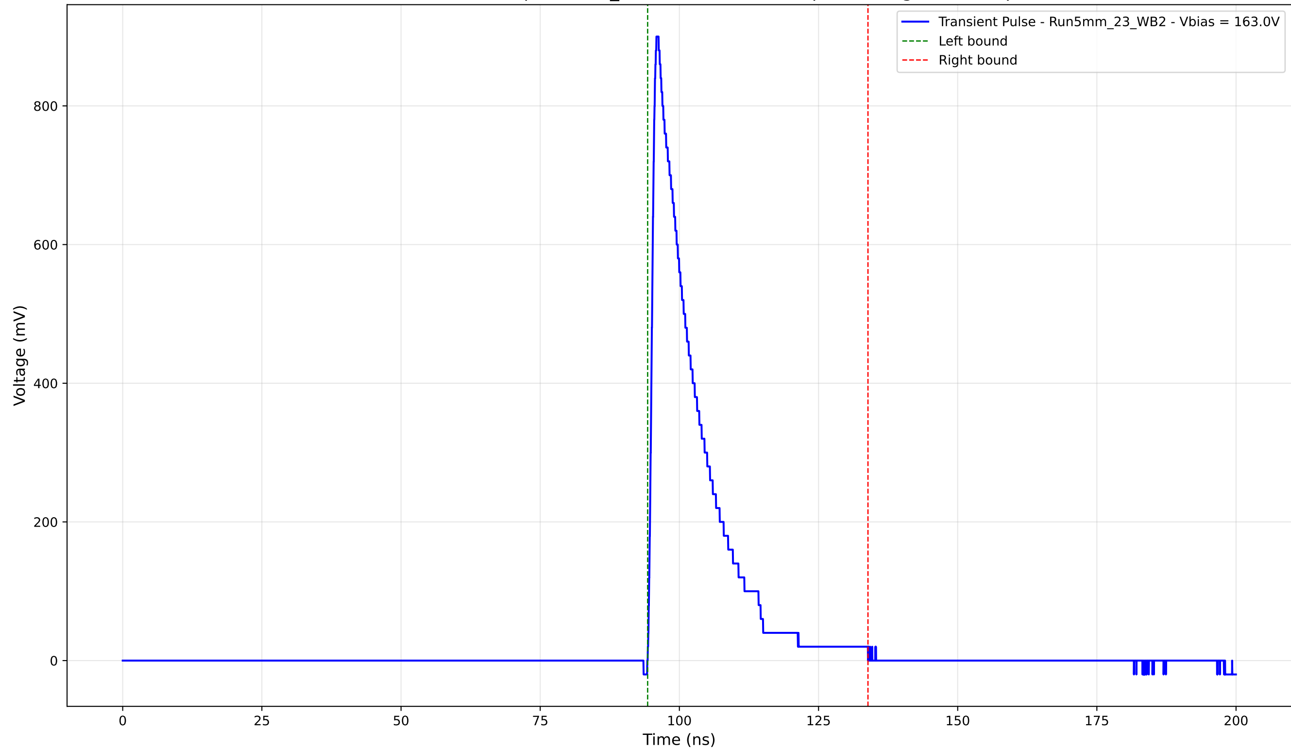
Transient Pulse - Sample: 5mm_23 - Position: 4385.0 \mu\text{m} - Charge: 157.86 pC
