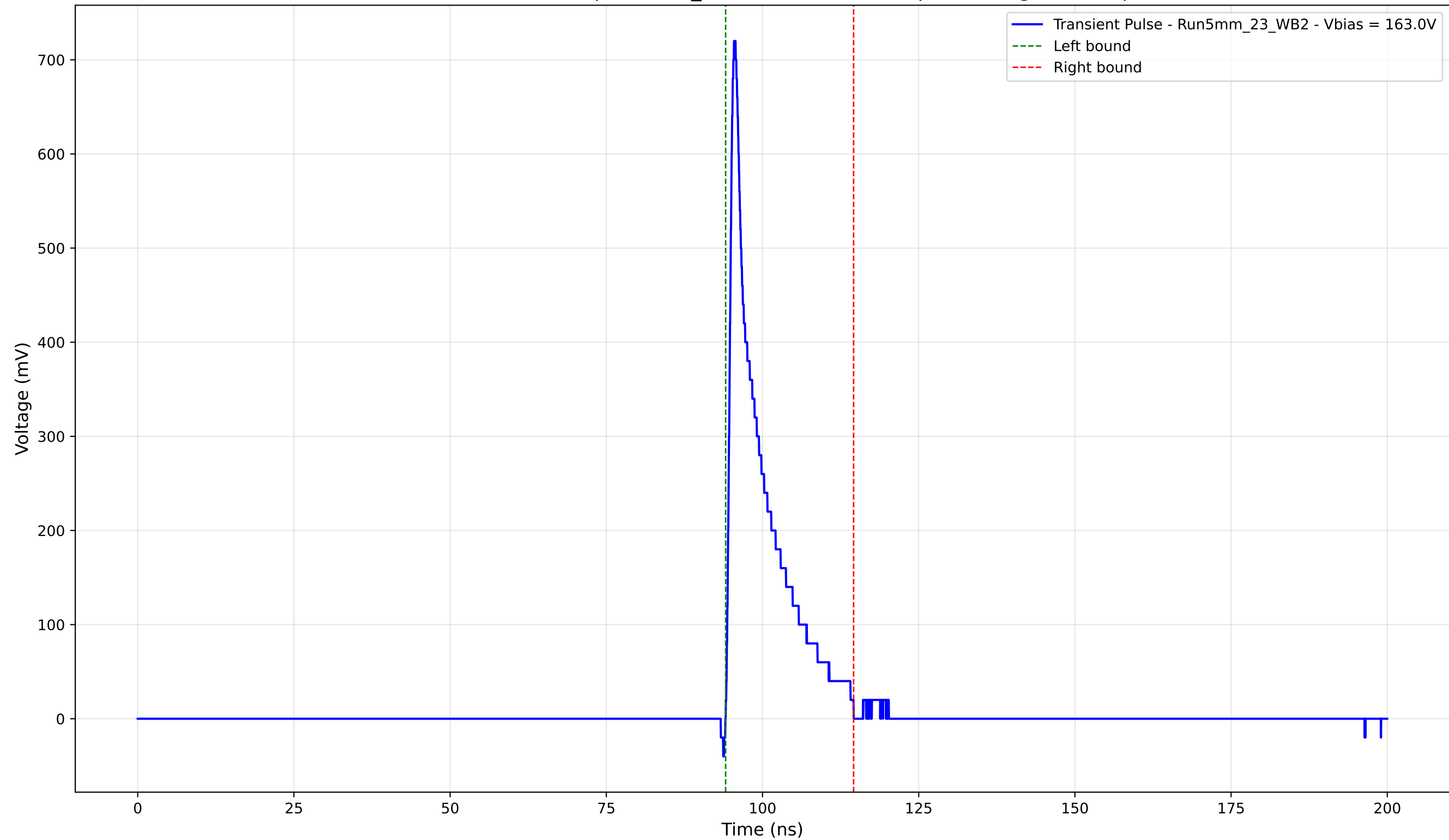
Transient Pulse - Sample: 5mm_23 - Position: 4920.0 \mu\text{m} - Charge: 79.63 pC
