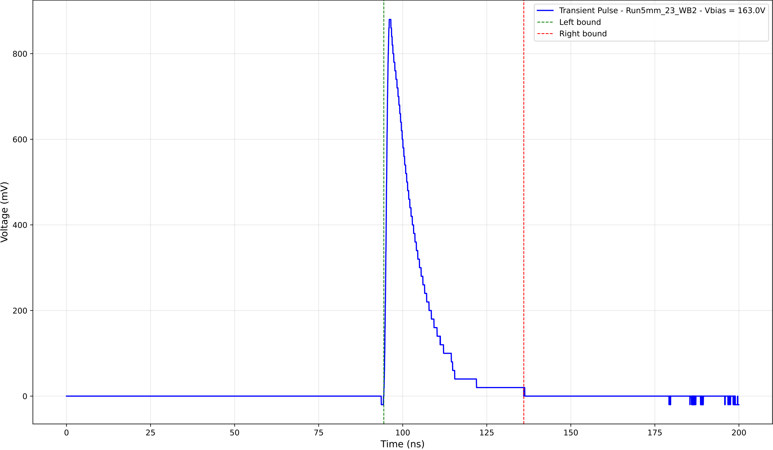
Transient Pulse - Sample: 5mm_23 - Position: 4190.0 \mu\text{m} - Charge: 163.25 pC
