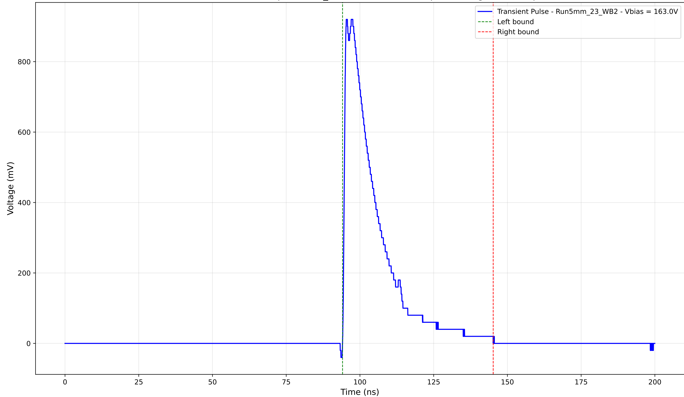
Transient Pulse - Sample: 5mm_23 - Position: 1865.0 \mu\text{m} - Charge: 222.48 pC
