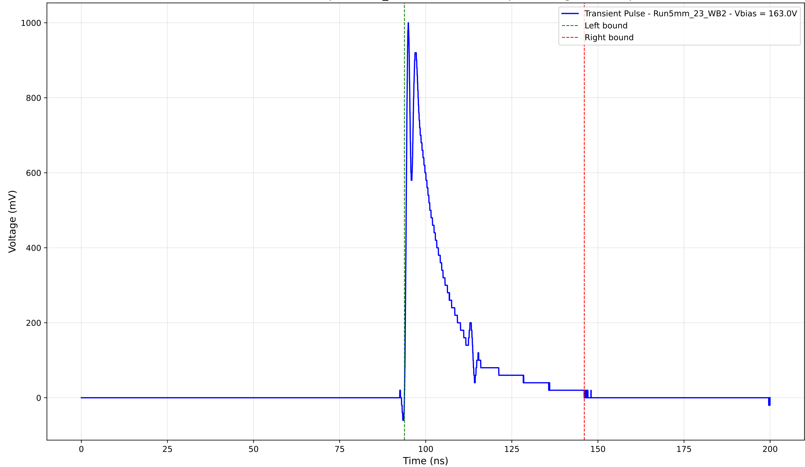
Transient Pulse - Sample: 5mm_23 - Position: 2640.0 \mu\text{m} - Charge: 201.50 pC
