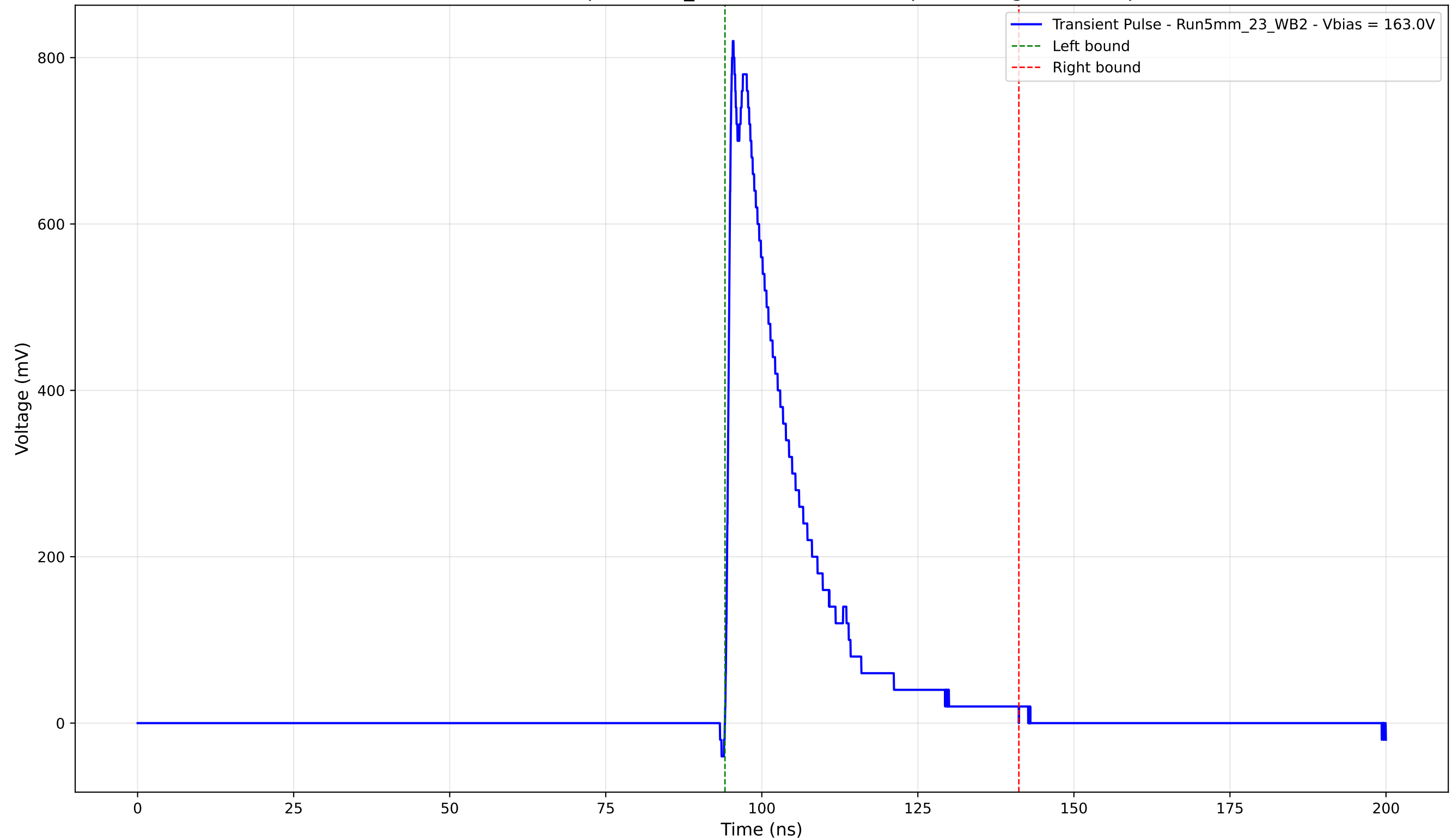
Transient Pulse - Sample: 5mm_23 - Position: 1940.0 \mu\text{m} - Charge: 172.67 pC
