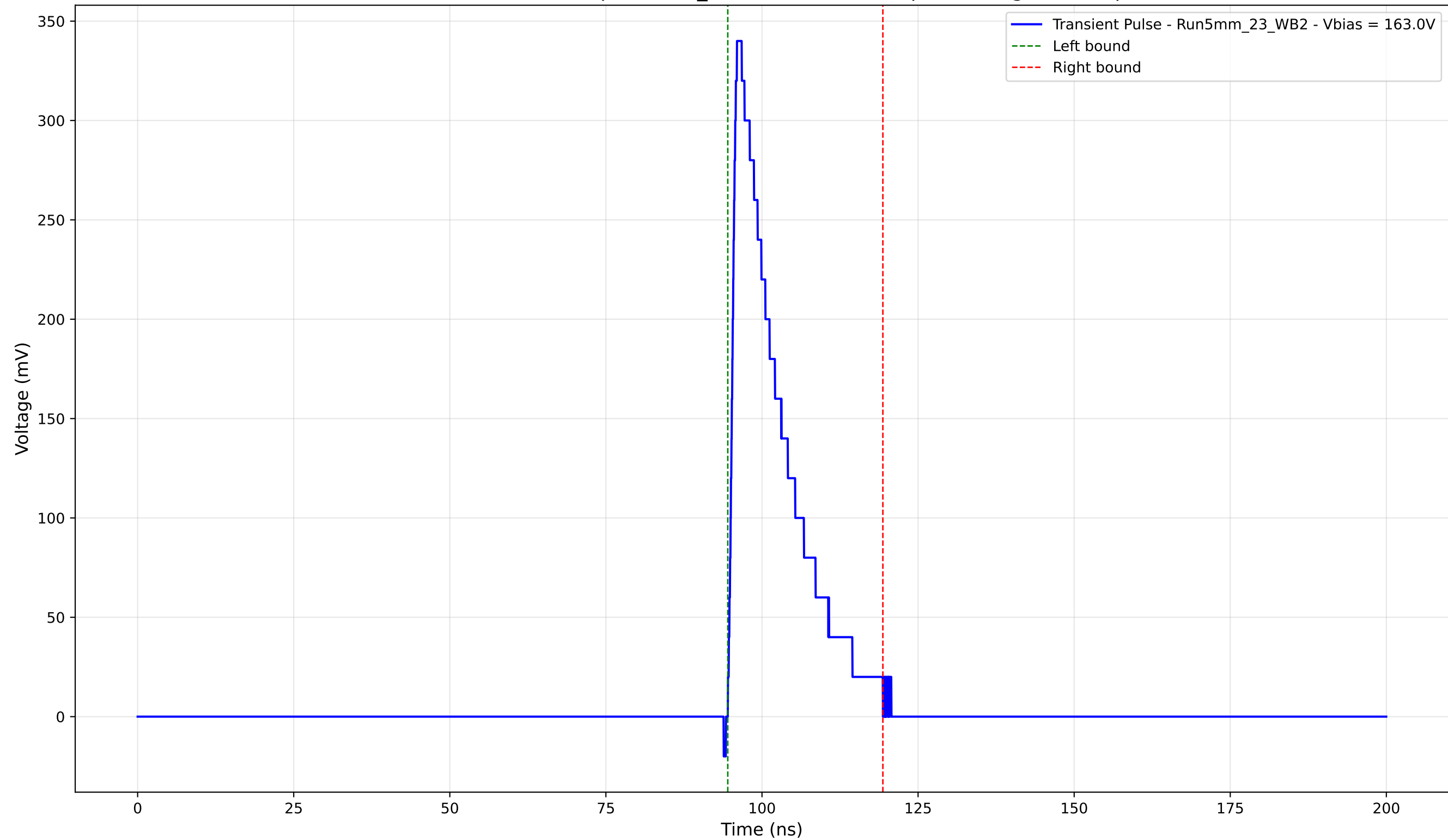
Transient Pulse - Sample: 5mm_23 - Position: 965.0 \mu\text{m} - Charge: 58.83 pC
