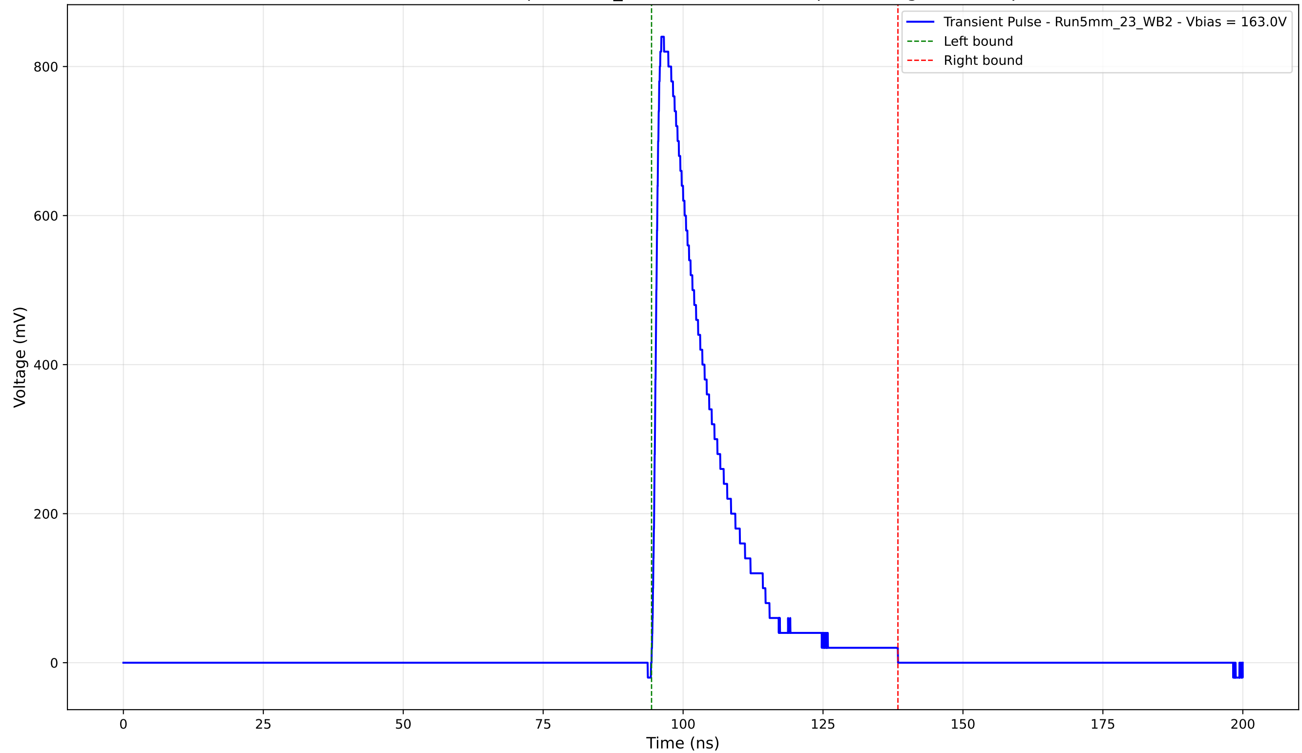
Transient Pulse - Sample: 5mm_23 - Position: 3680.0 \mu\text{m} - Charge: 174.19 pC
