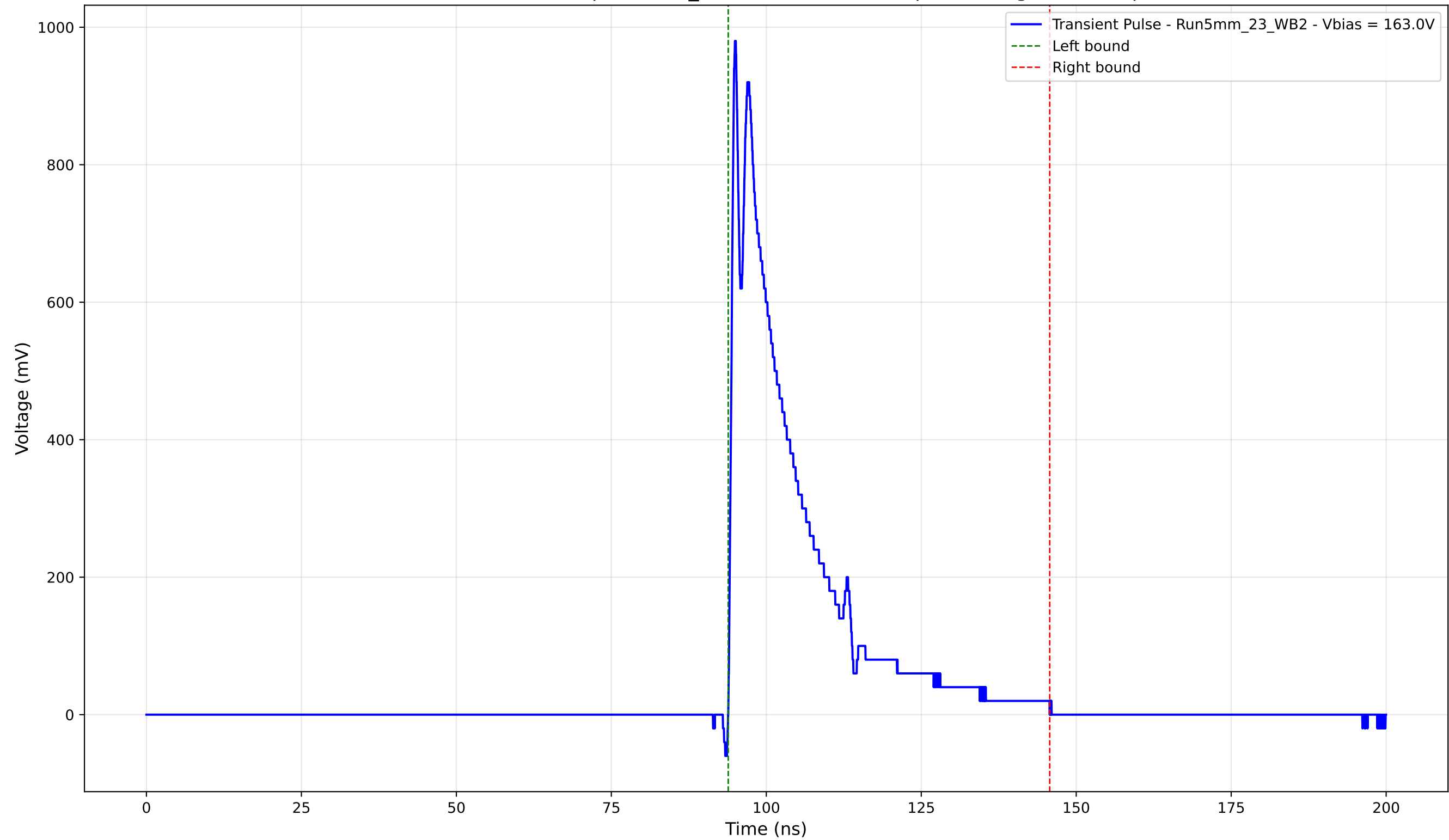
Transient Pulse - Sample: 5mm_23 - Position: 2345.0 \mu\text{m} - Charge: 202.13 pC
