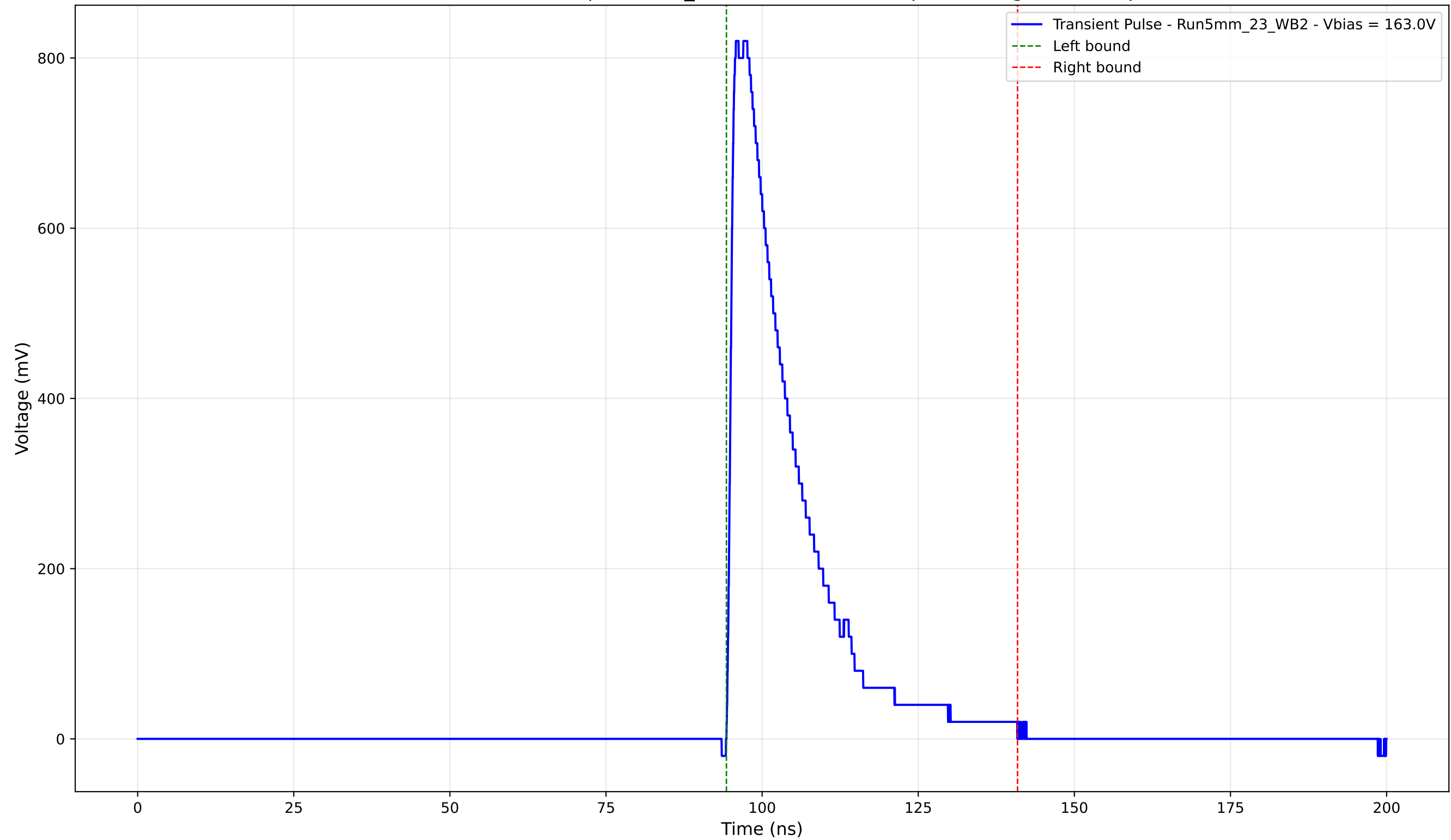
Transient Pulse - Sample: 5mm_23 - Position: 1590.0 \mu\text{m} - Charge: 184.04 pC
