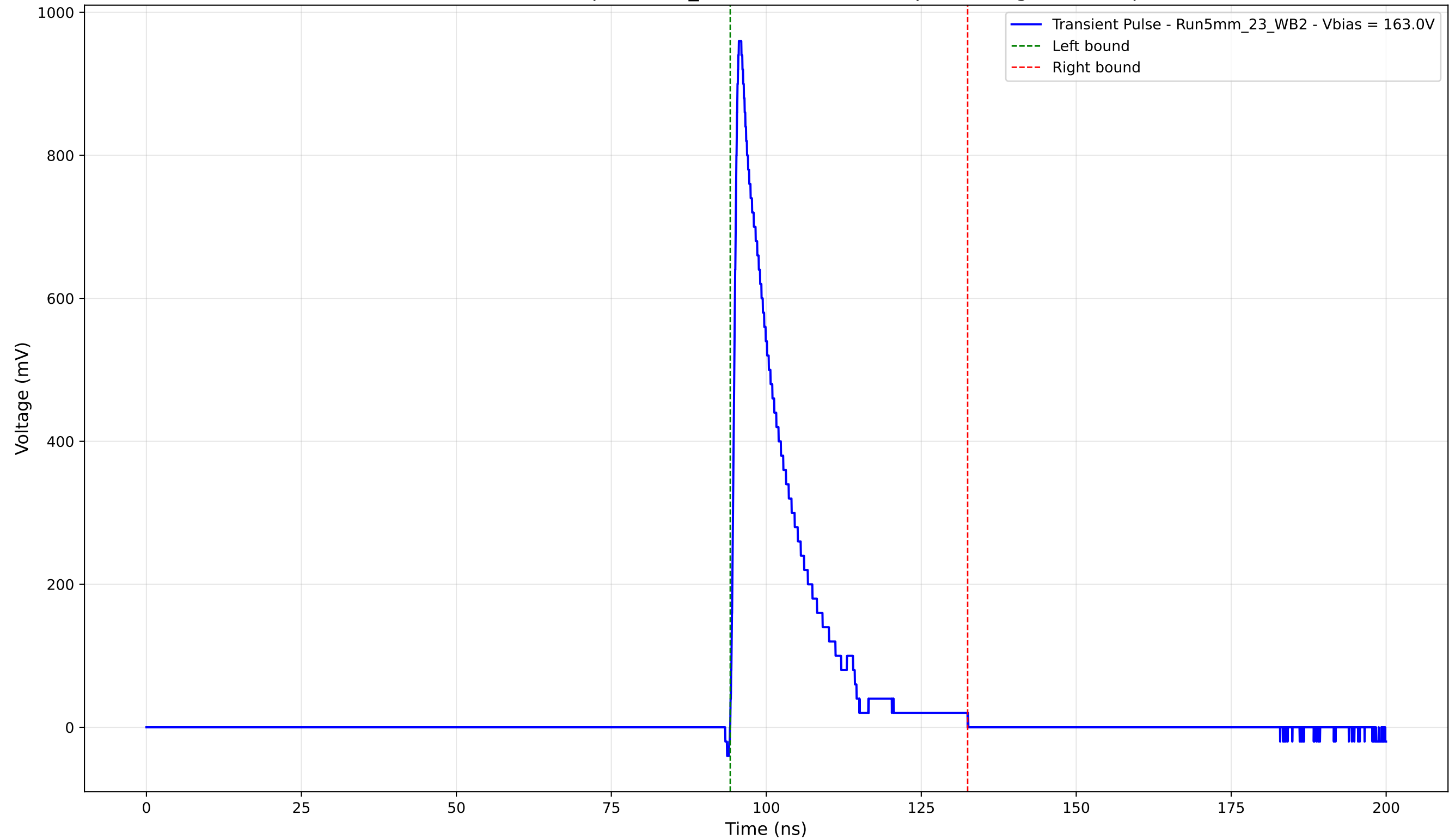
Transient Pulse - Sample: 5mm_23 - Position: 4680.0 \mu\text{m} - Charge: 155.98 pC
