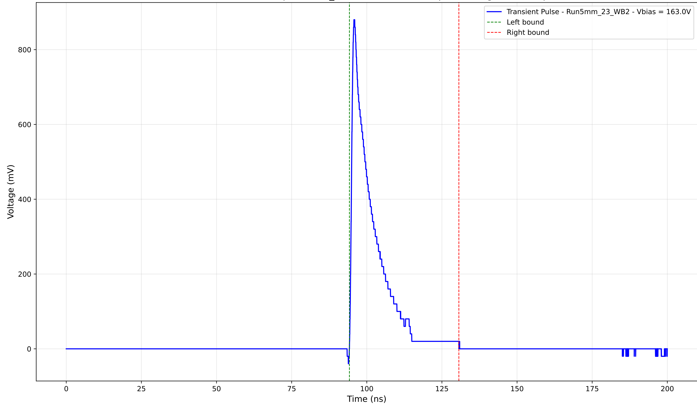
Transient Pulse - Sample: 5mm_23 - Position: 4610.0 \mu\text{m} - Charge: 132.66 pC
