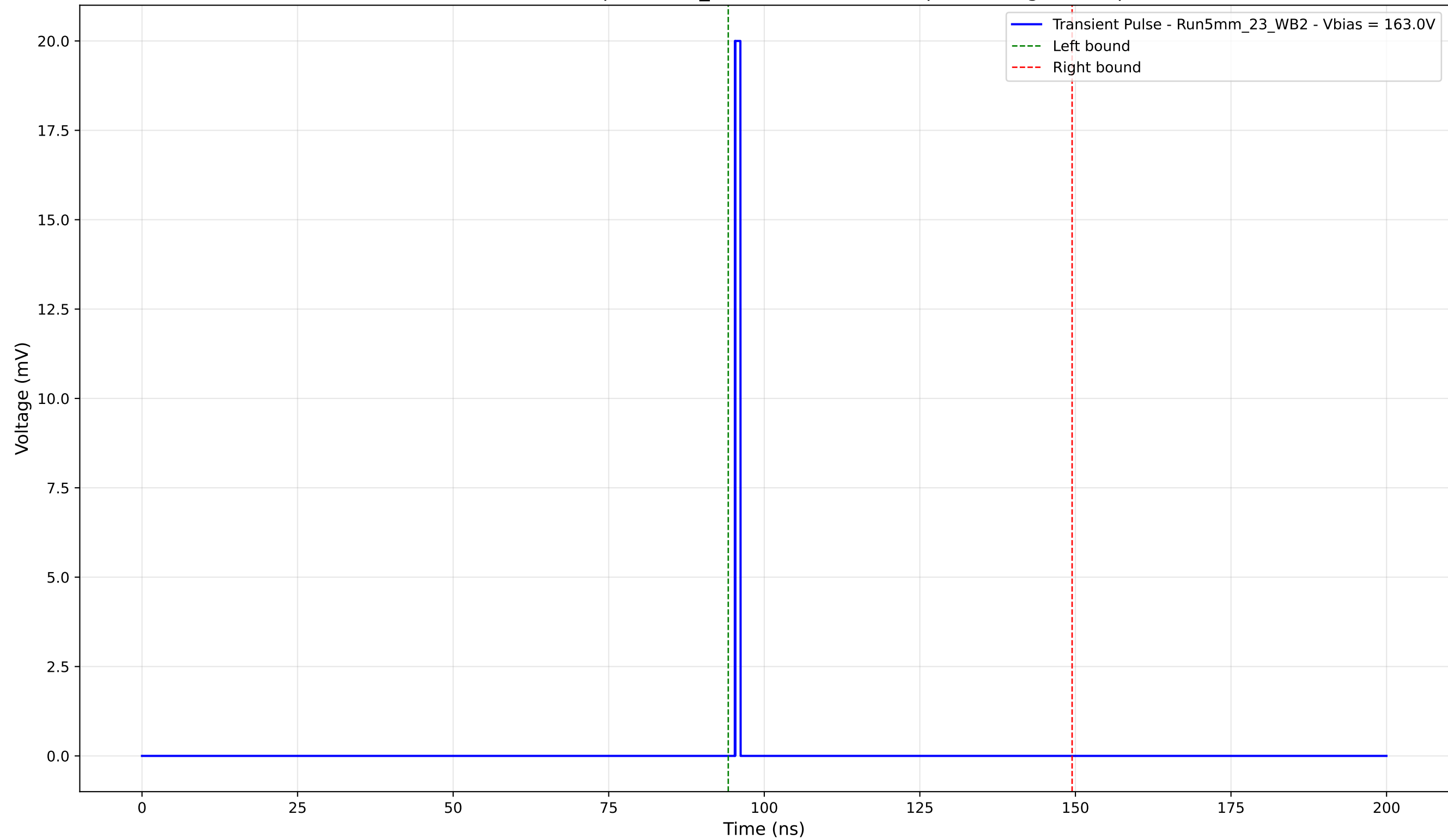
Transient Pulse - Sample: 5mm_23 - Position: 5050.0 \mu\text{m} - Charge: 0.34 pC
