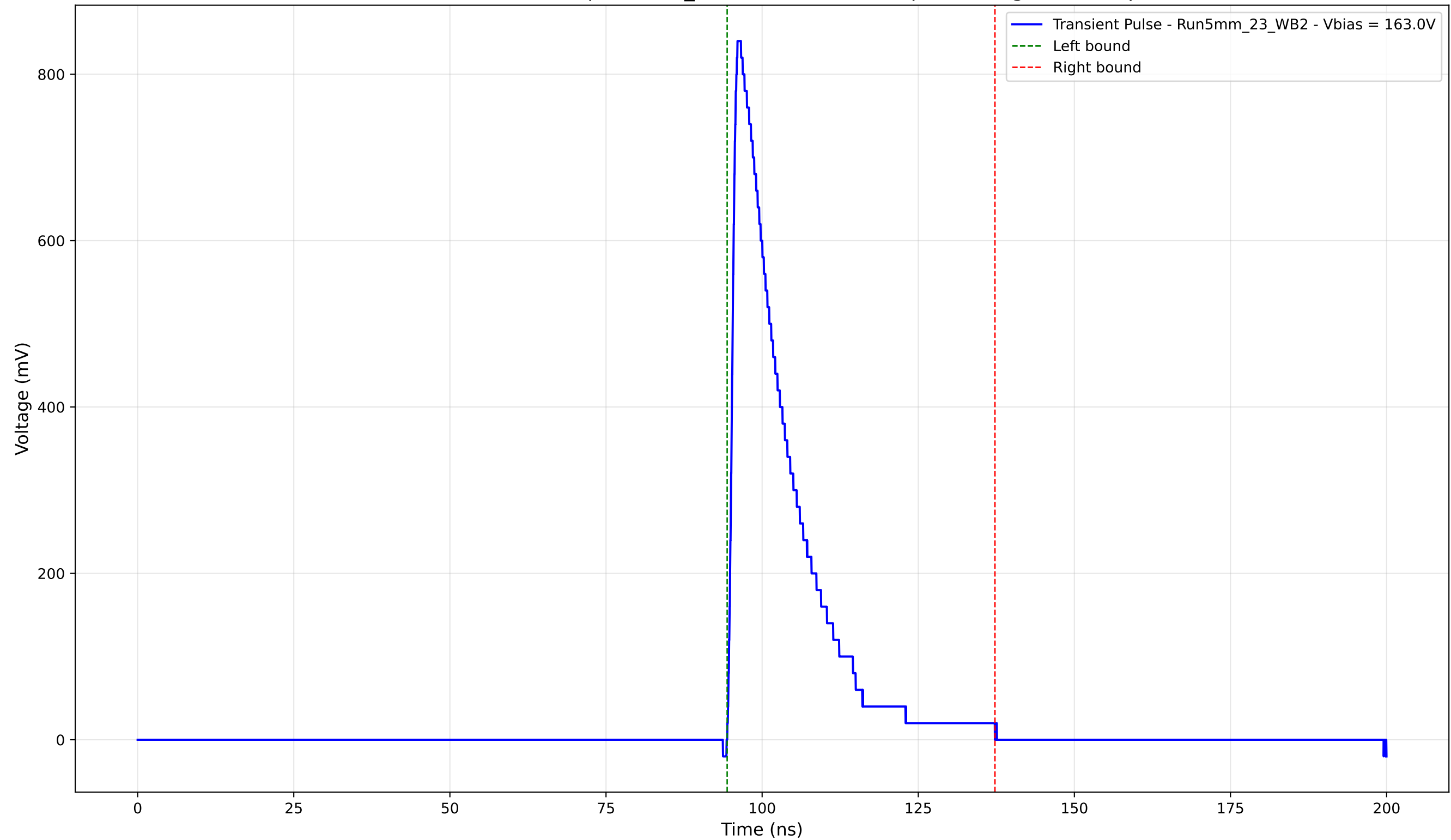
Transient Pulse - Sample: 5mm_23 - Position: 3940.0 \mu\text{m} - Charge: 162.44 pC
