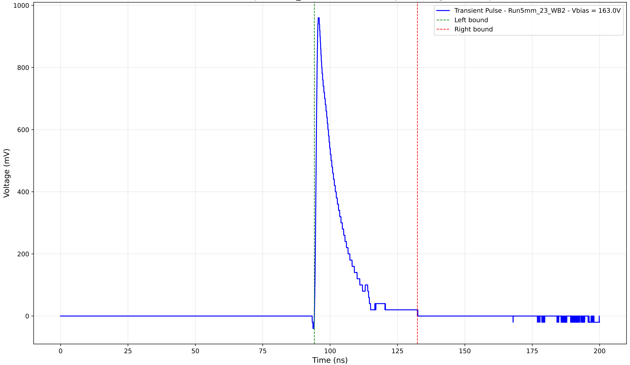
Transient Pulse - Sample: 5mm_23 - Position: 4690.0 \mu\text{m} - Charge: 155.14 pC
