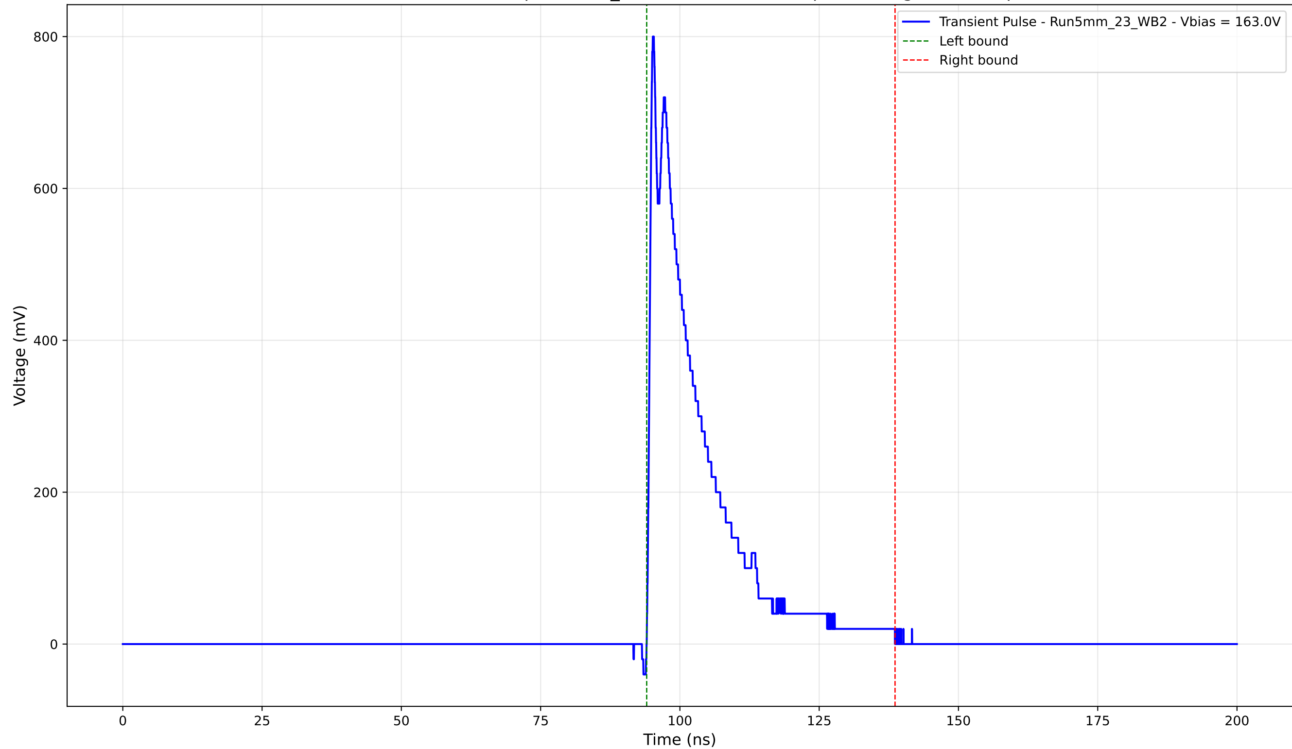
Transient Pulse - Sample: 5mm_23 - Position: 2965.0 \mu\text{m} - Charge: 148.35 pC
