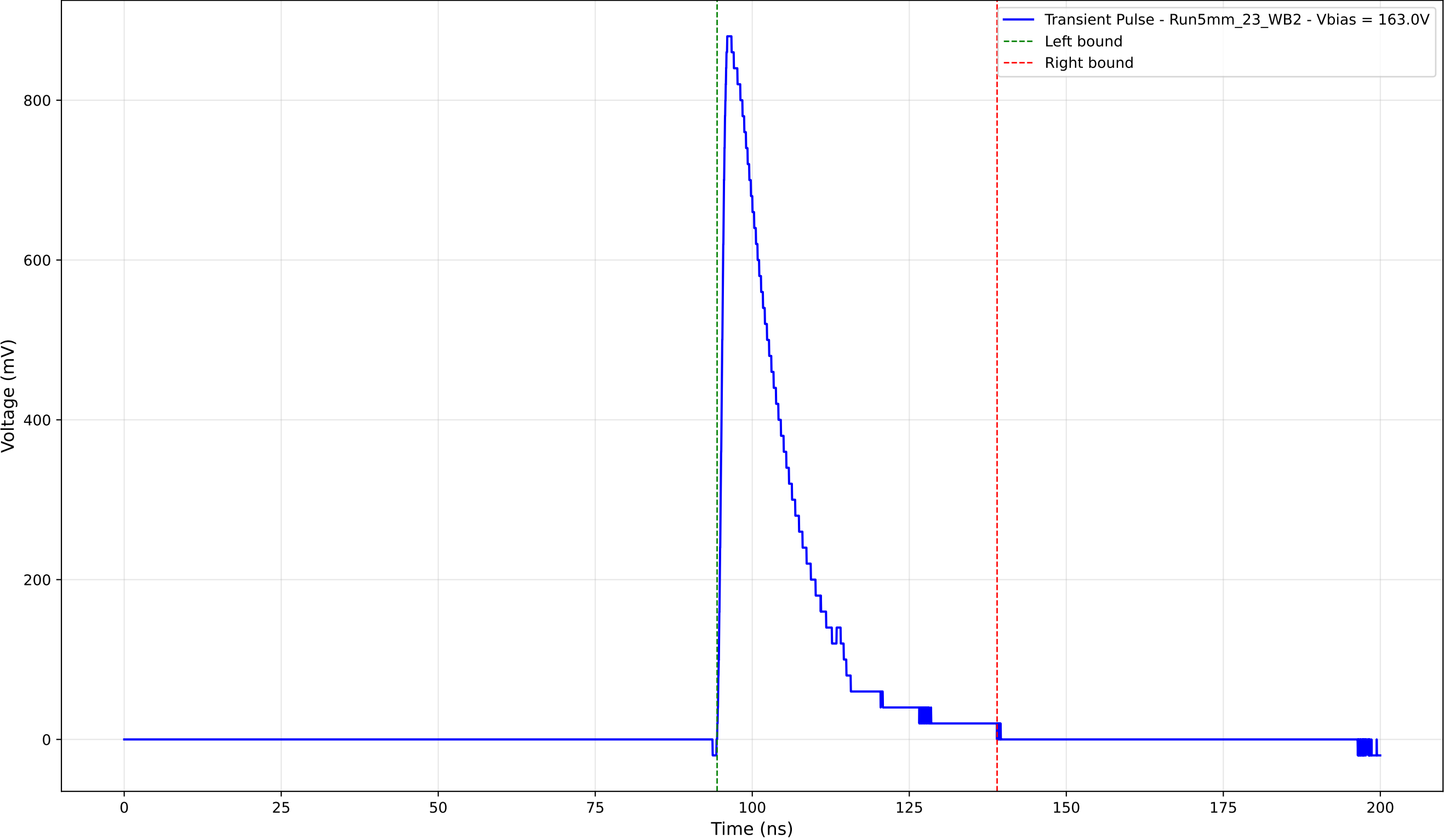
Transient Pulse - Sample: 5mm_23 - Position: 1125.0 \mu\text{m} - Charge: 188.03 pC
