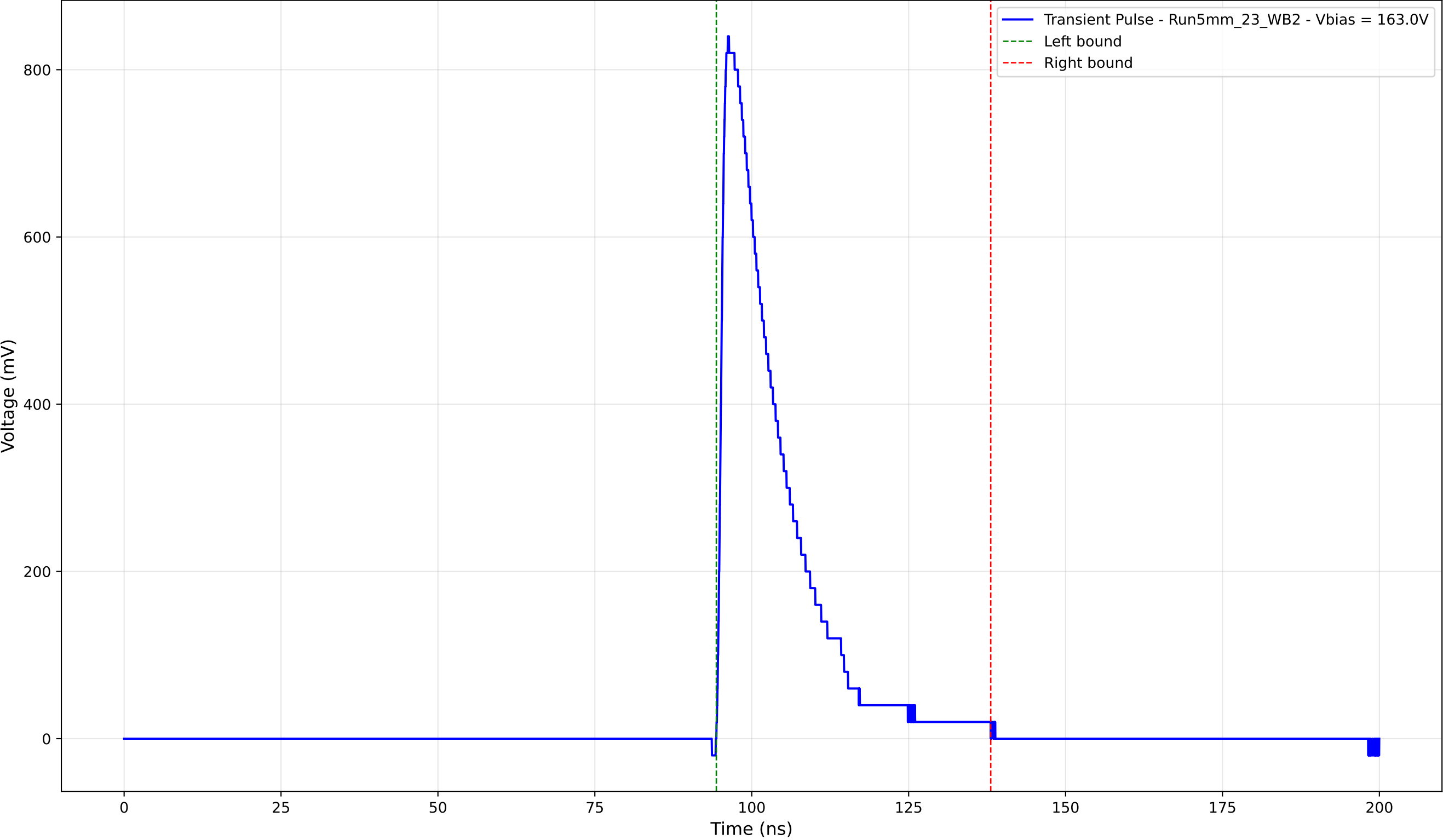
Transient Pulse - Sample: 5mm_23 - Position: 3670.0 \mu\text{m} - Charge: 173.26 pC
