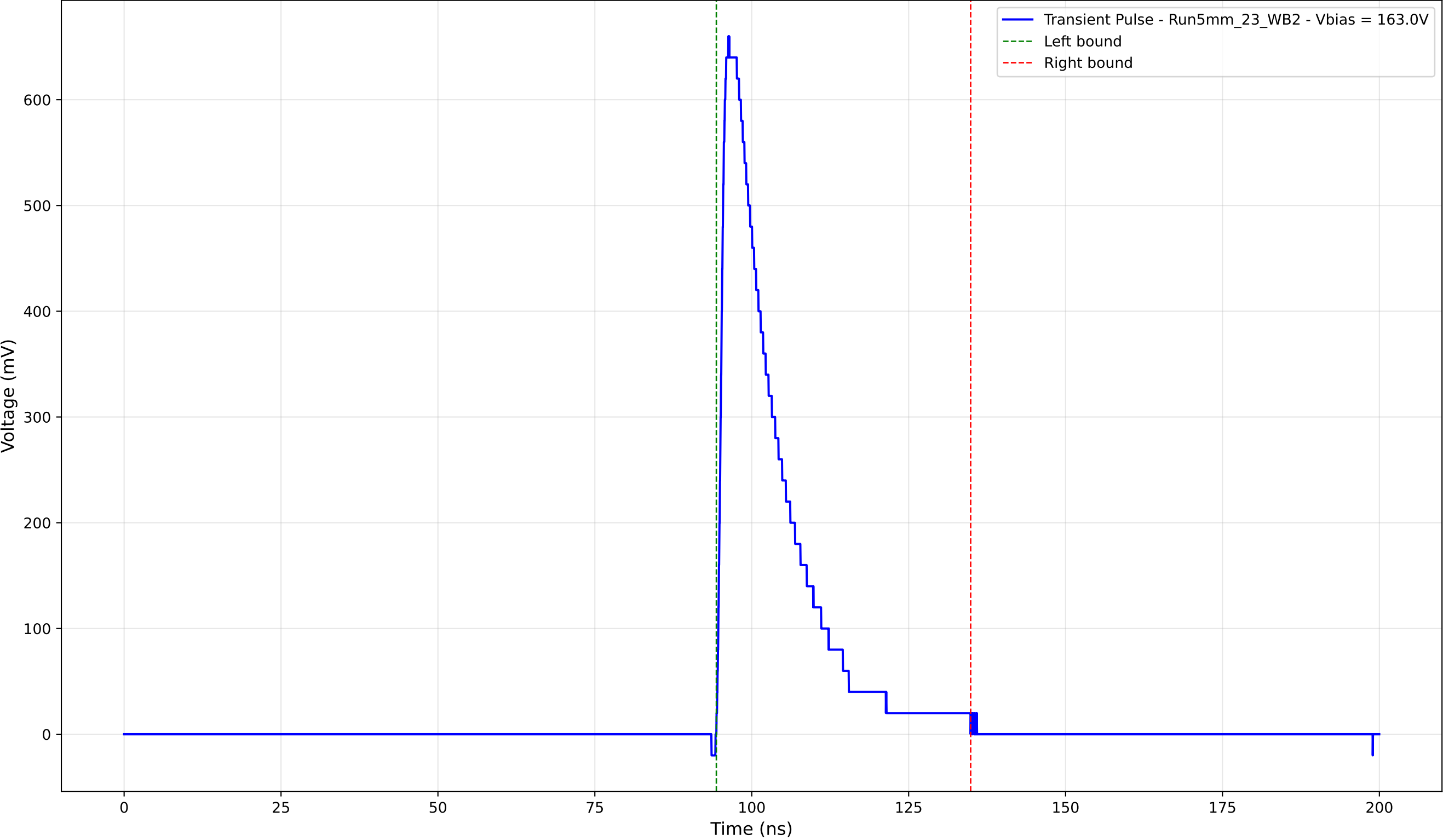
Transient Pulse - Sample: 5mm_23 - Position: 3590.0 \mu\text{m} - Charge: 130.81 pC
