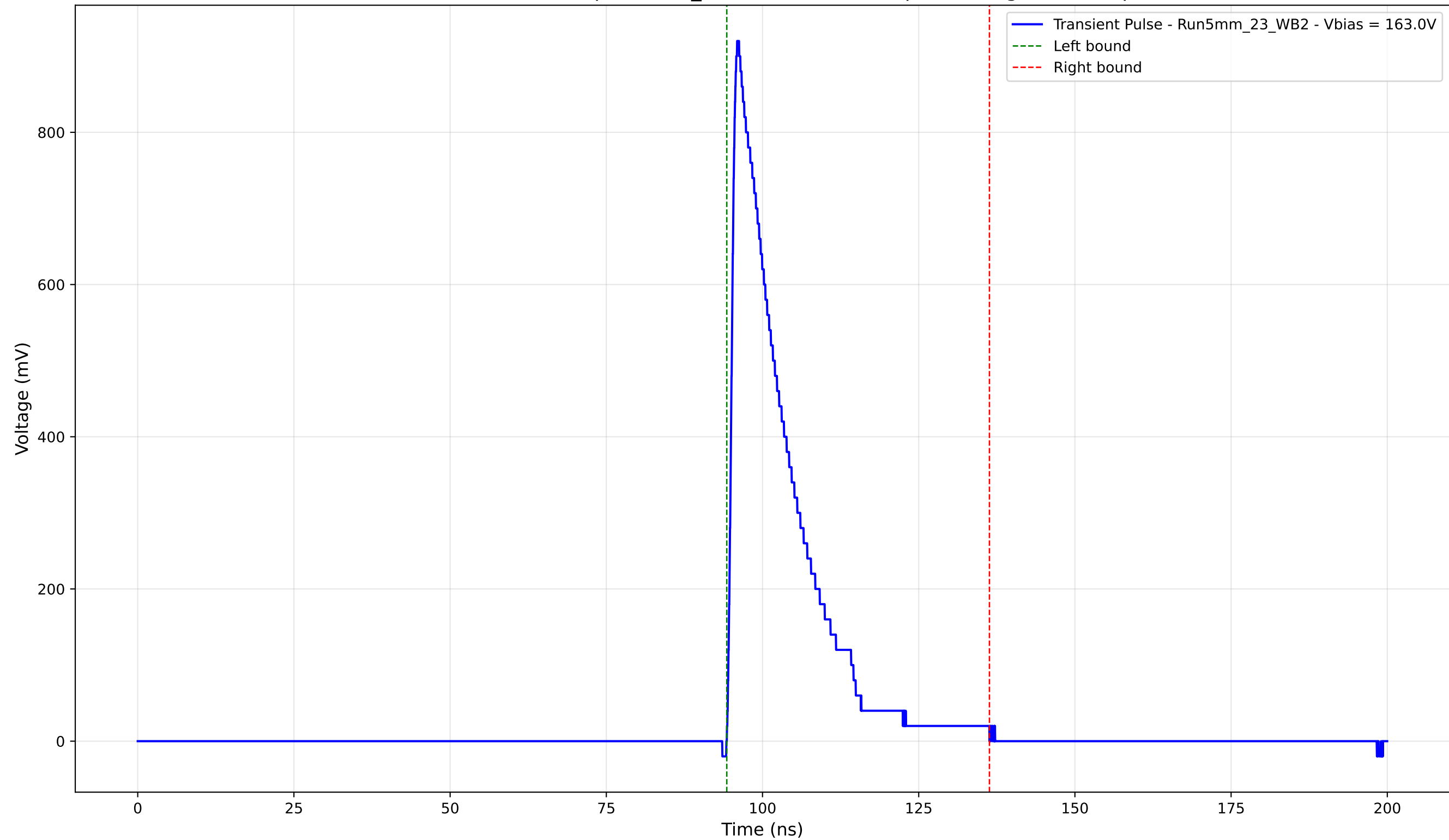
Transient Pulse - Sample: 5mm_23 - Position: 660.0 \mu\text{m} - Charge: 174.84 pC
