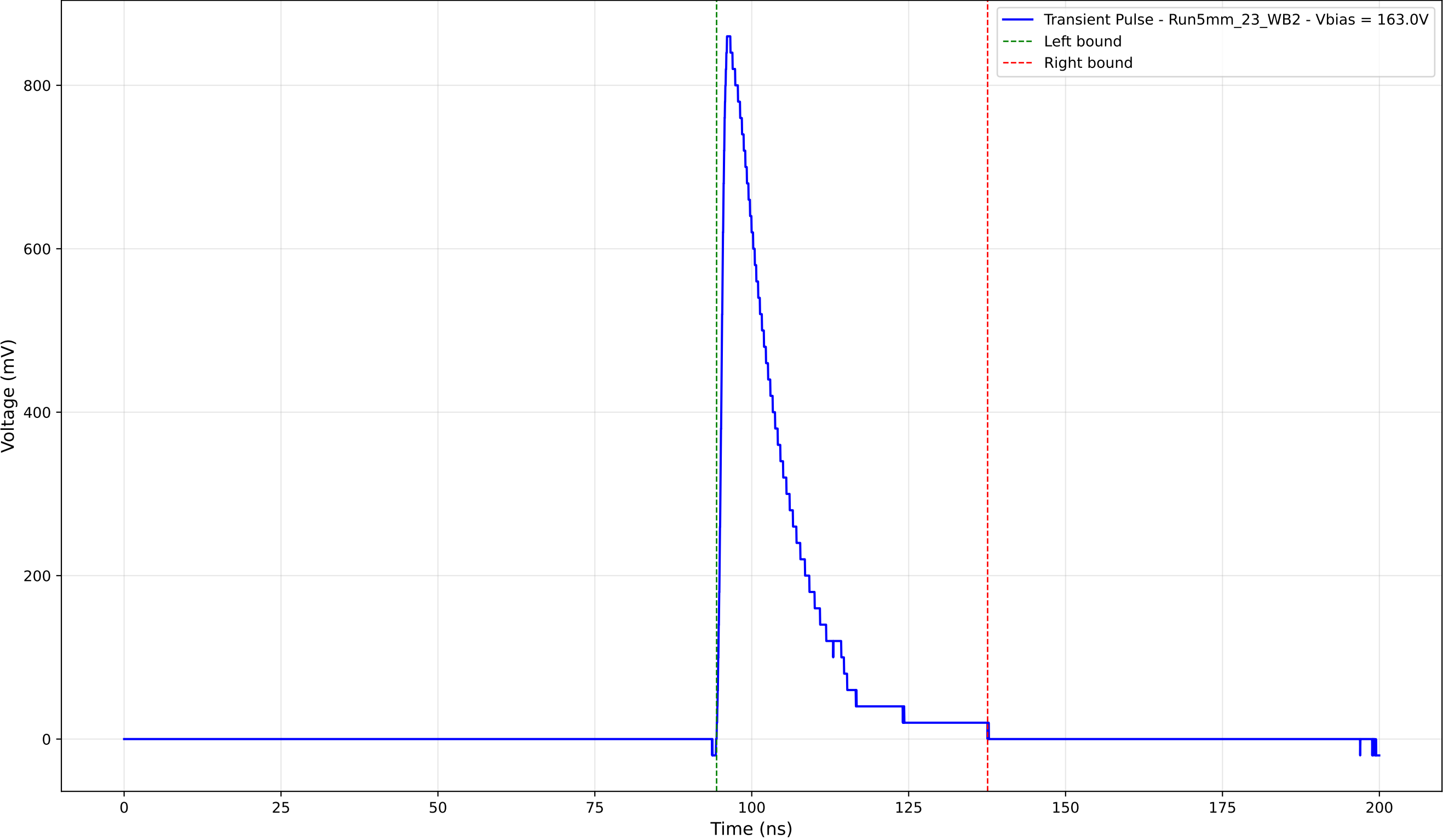
Transient Pulse - Sample: 5mm_23 - Position: 3880.0 \mu\text{m} - Charge: 171.94 pC
