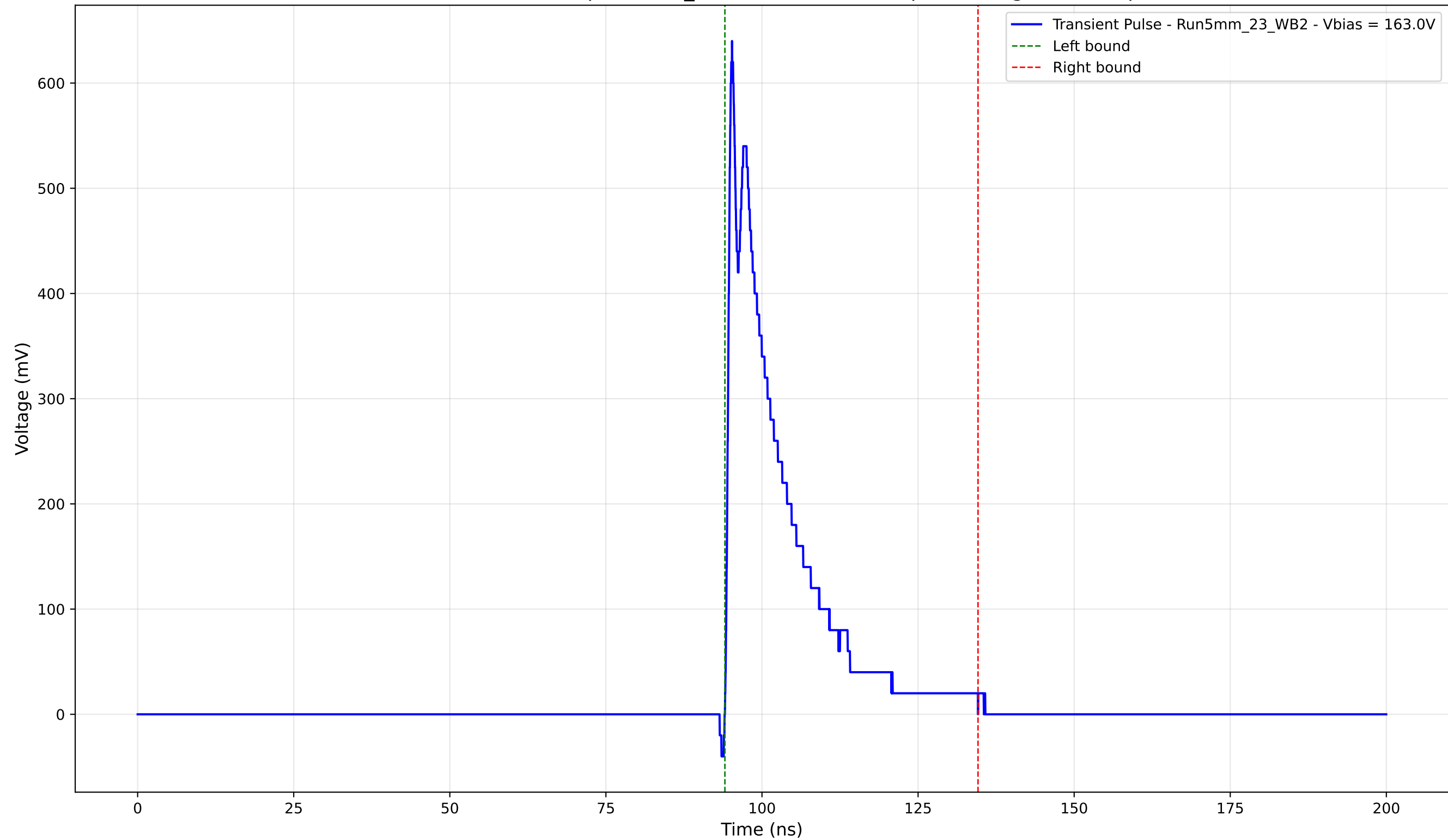
Transient Pulse - Sample: 5mm_23 - Position: 2980.0 \mu\text{m} - Charge: 109.11 pC
