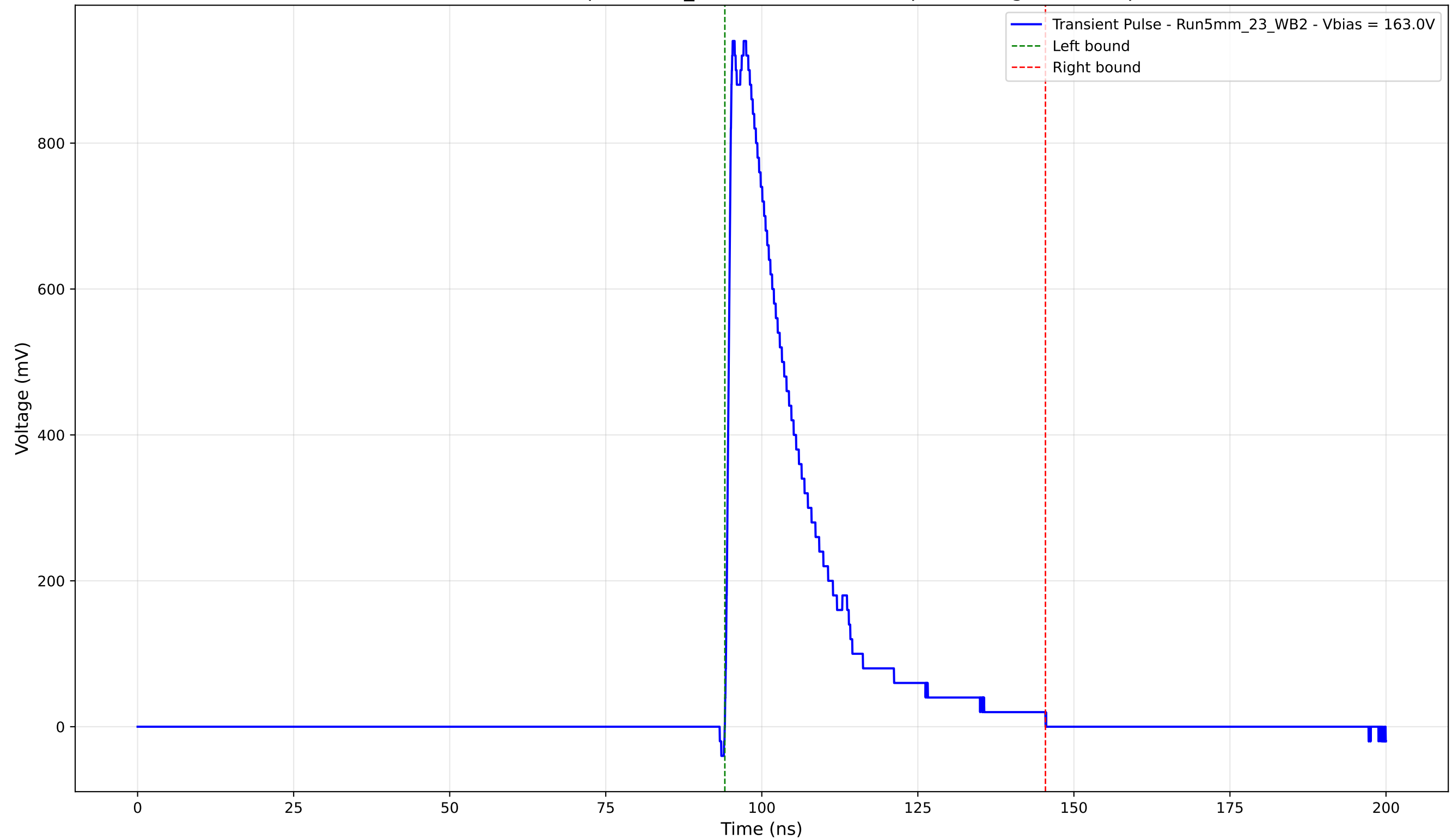
Transient Pulse - Sample: 5mm_23 - Position: 3150.0 \mu\text{m} - Charge: 225.79 pC
