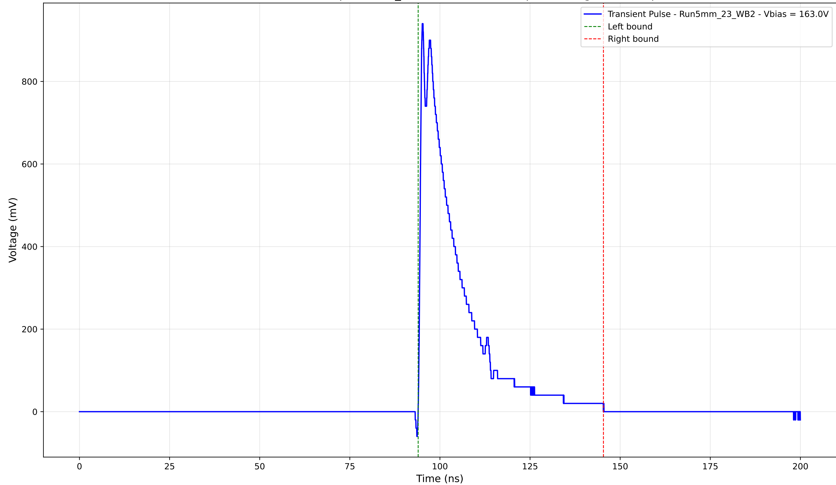
Transient Pulse - Sample: 5mm_23 - Position: 2150.0 \mu\text{m} - Charge: 205.17 pC
