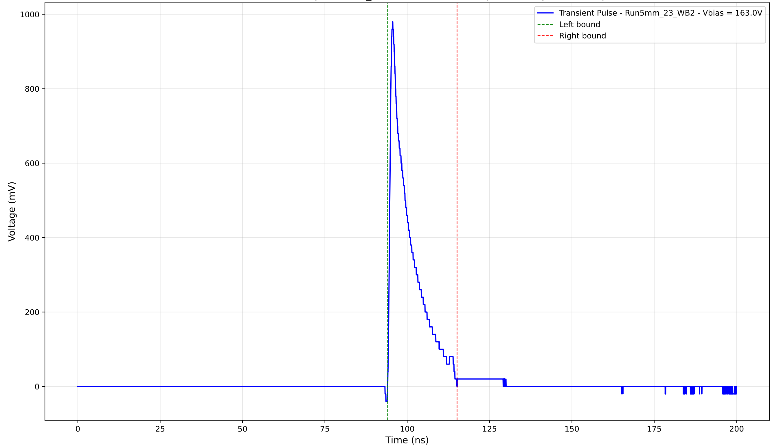
Transient Pulse - Sample: 5mm_23 - Position: 4870.0 \mu\text{m} - Charge: 130.95 pC
