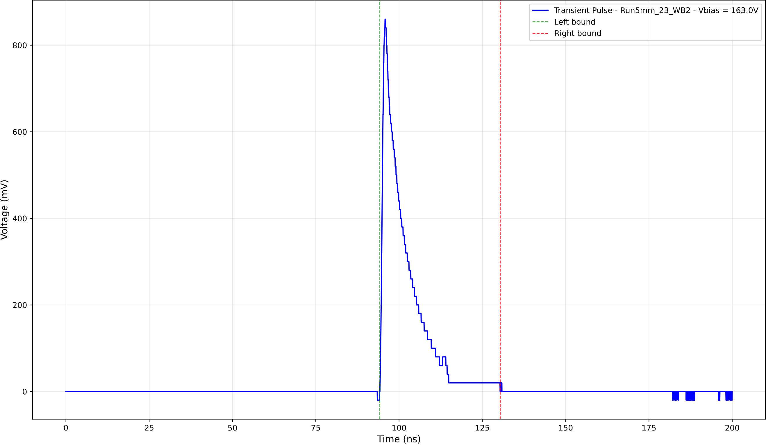
Transient Pulse - Sample: 5mm_23 - Position: 4605.0 \mu\text{m} - Charge: 126.94 pC
