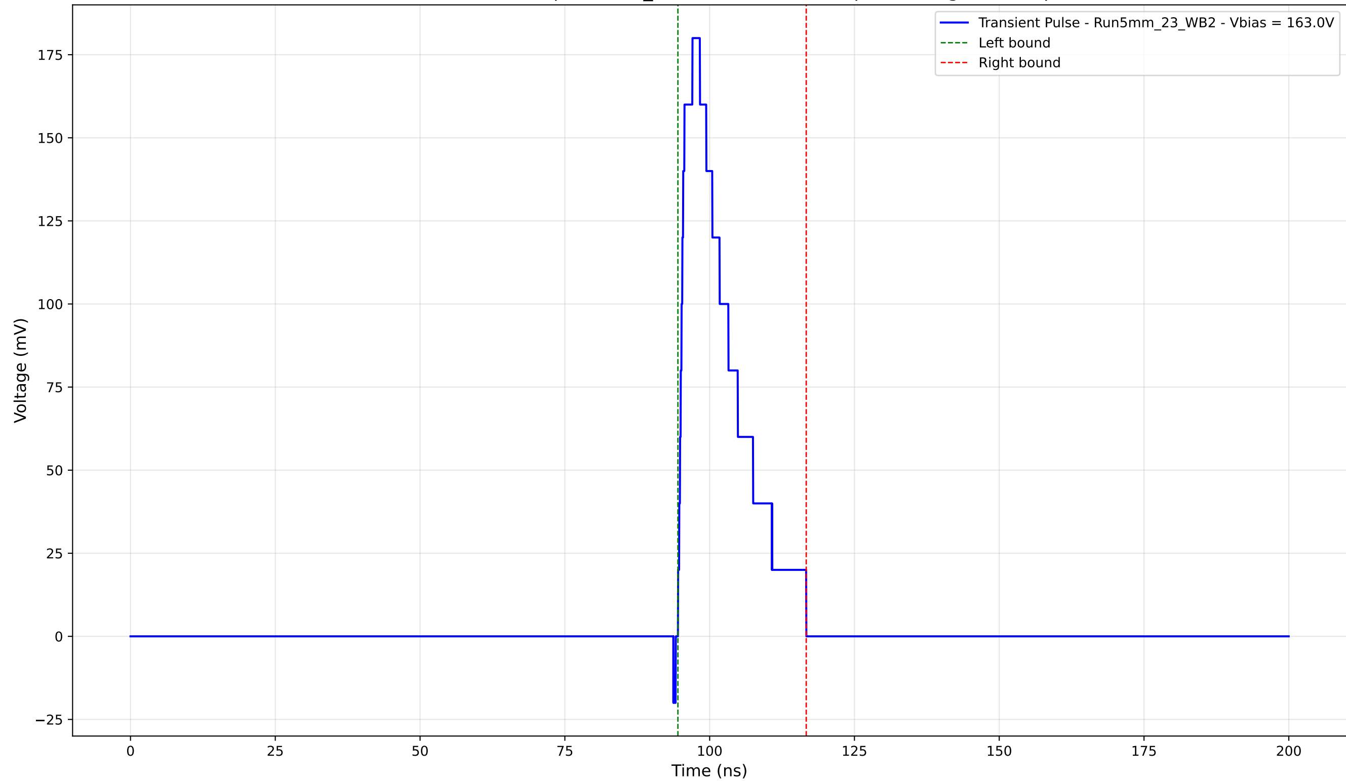
Transient Pulse - Sample: 5mm_23 -Position: 1495.0 \mu\text{m} - Charge: 34.13 pC
