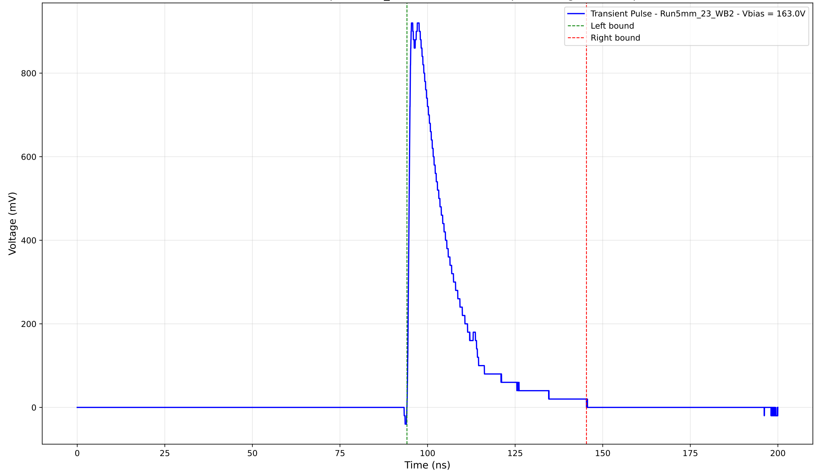
Transient Pulse - Sample: 5mm_23 - Position: 1835.0 \mu\text{m} - Charge: 222.40 pC
