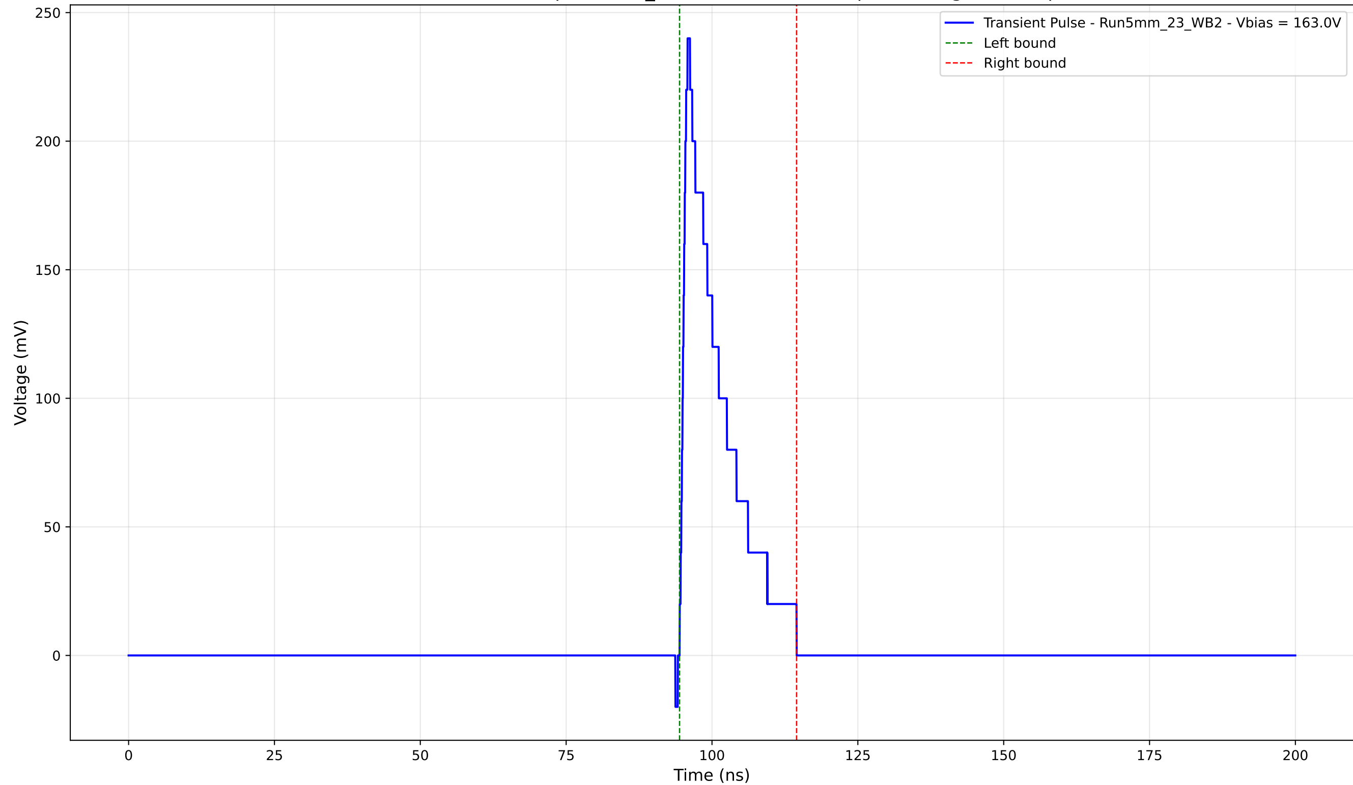
Transient Pulse - Sample: 5mm_23 - Position: 4525.0 \mu\text{m} - Charge: 33.91 pC
