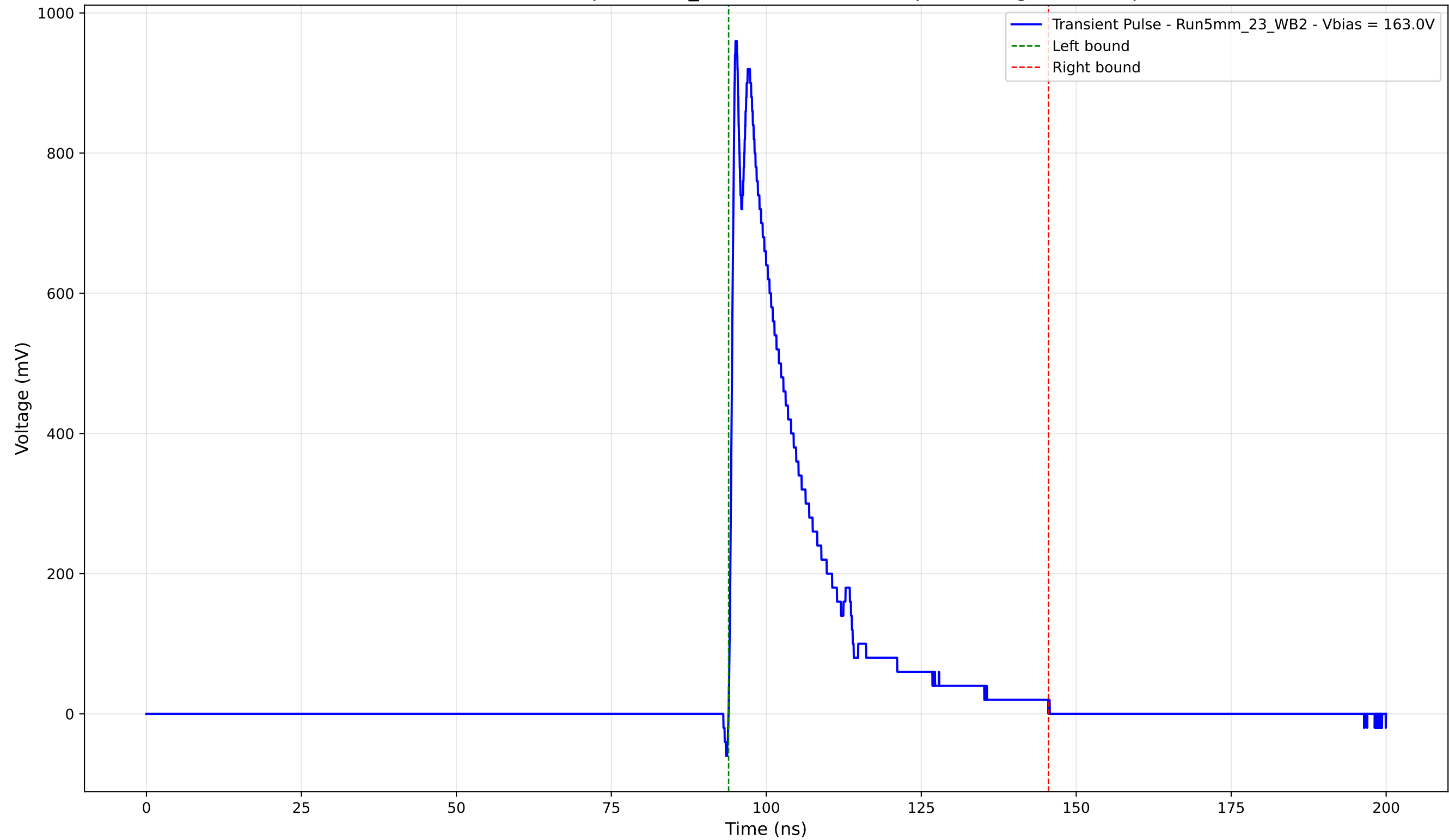
Transient Pulse - Sample: 5mm_23 - Position: 2825.0 \mu\text{m} - Charge: 210.12 pC
