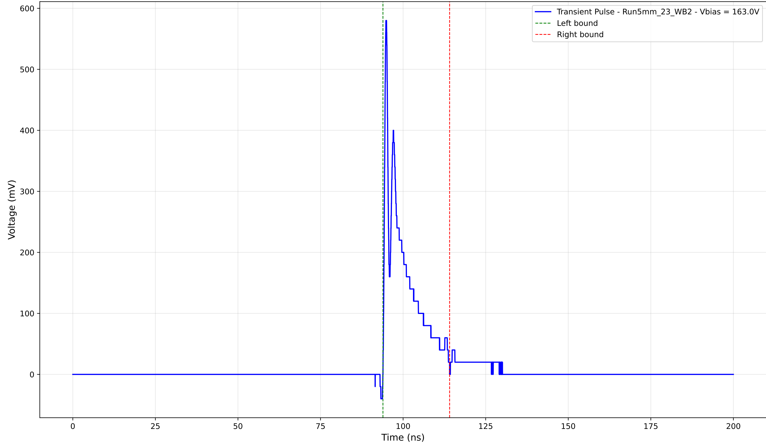
Transient Pulse - Sample: 5mm_23 - Position: 2545.0 \mu\text{m} - Charge: 61.50 pC
