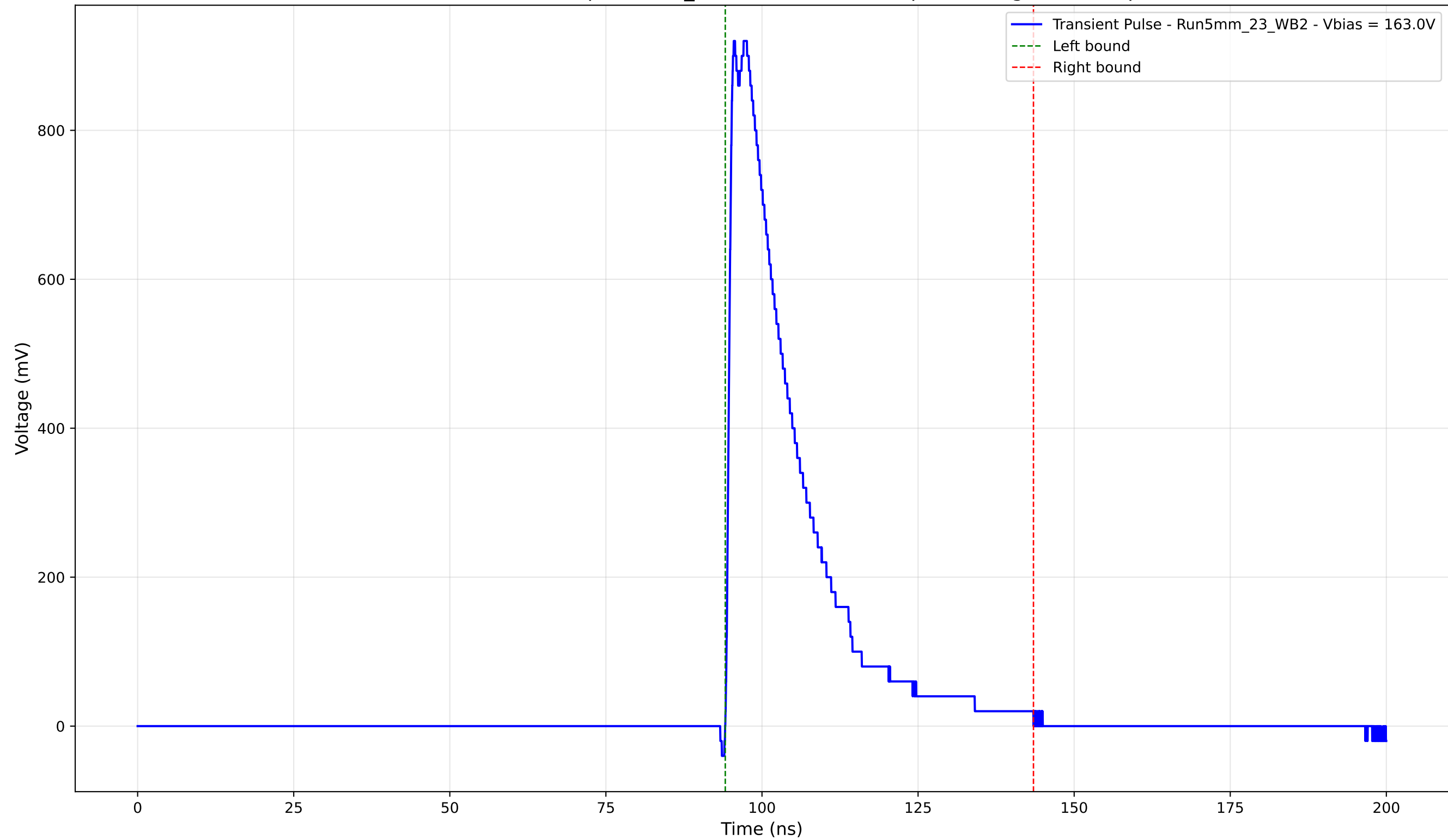
Transient Pulse - Sample: 5mm_23 - Position: 3210.0 \mu\text{m} - Charge: 217.02 pC
