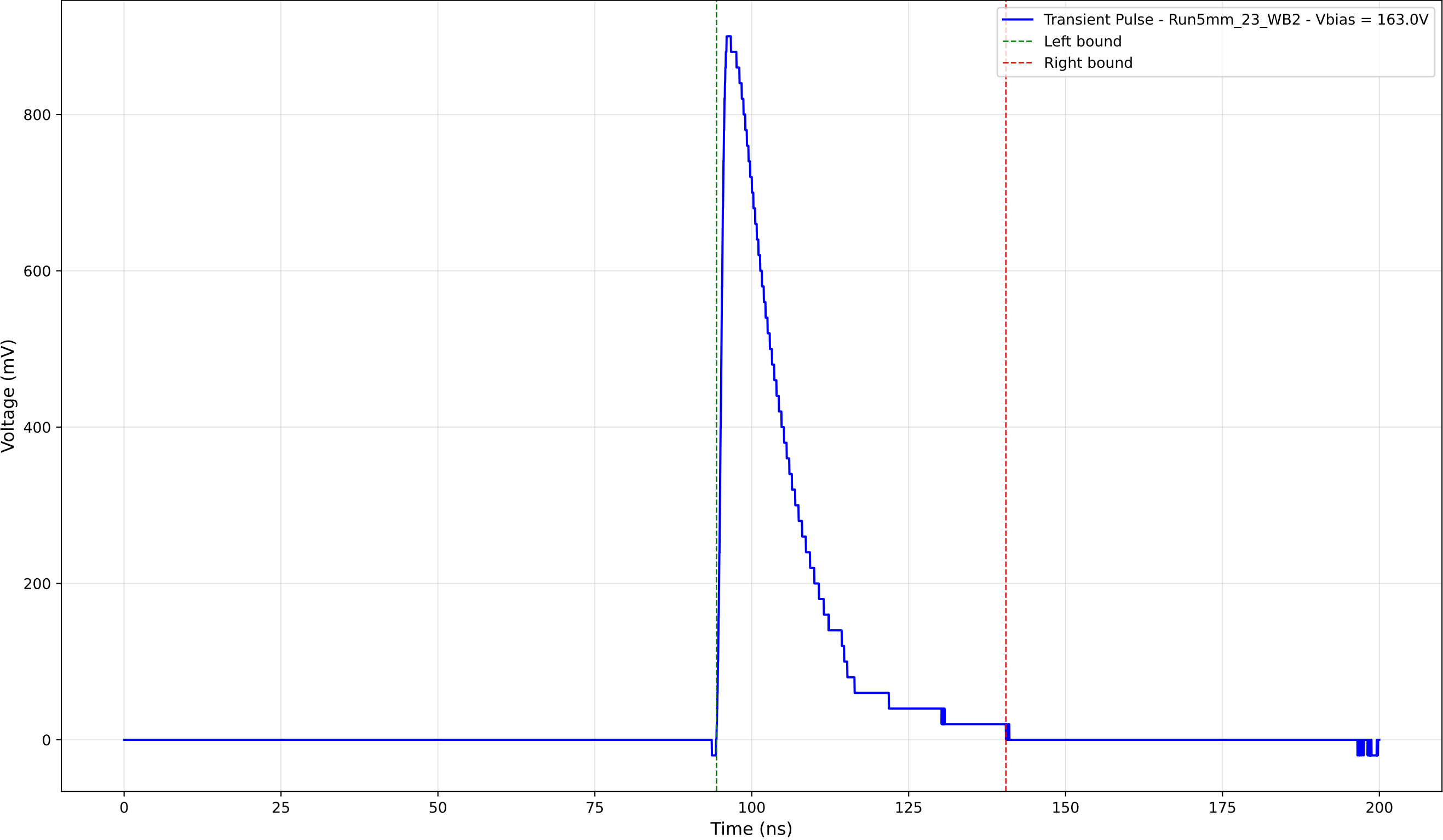
Transient Pulse - Sample: 5mm_23 - Position: 1275.0 \mu\text{m} - Charge: 200.83 pC
