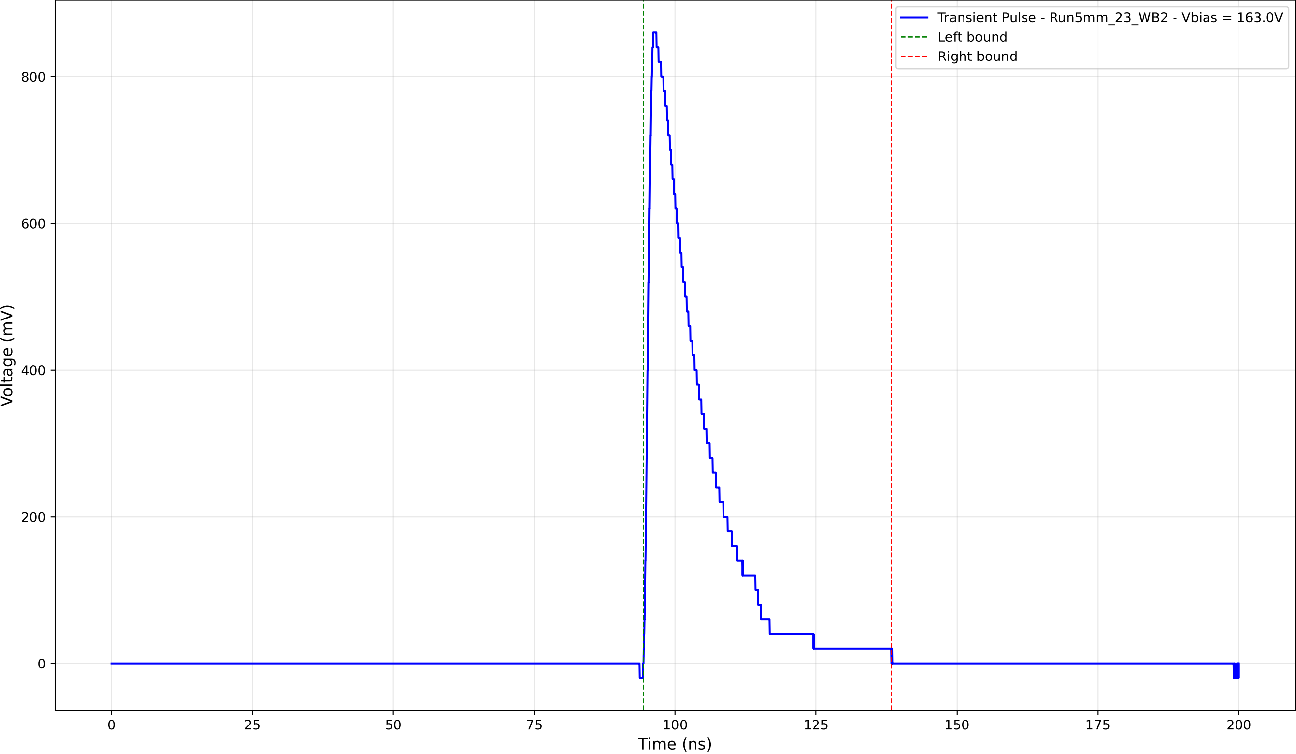
Transient Pulse - Sample: 5mm_23 - Position: 3855.0 \mu\text{m} - Charge: 173.94 pC
