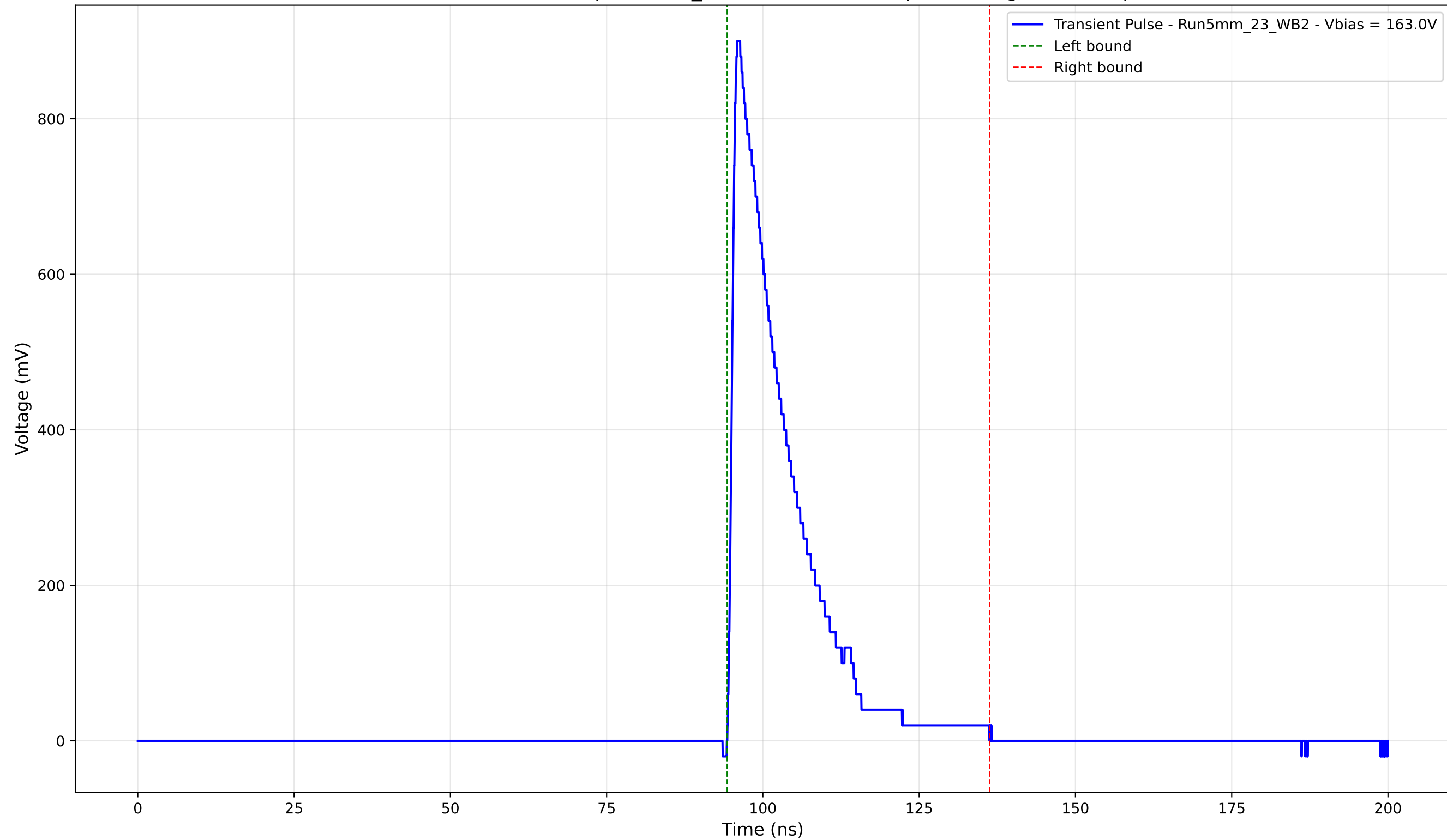
Transient Pulse - Sample: 5mm_23 - Position: 680.0 \mu\text{m} - Charge: 171.98 pC
