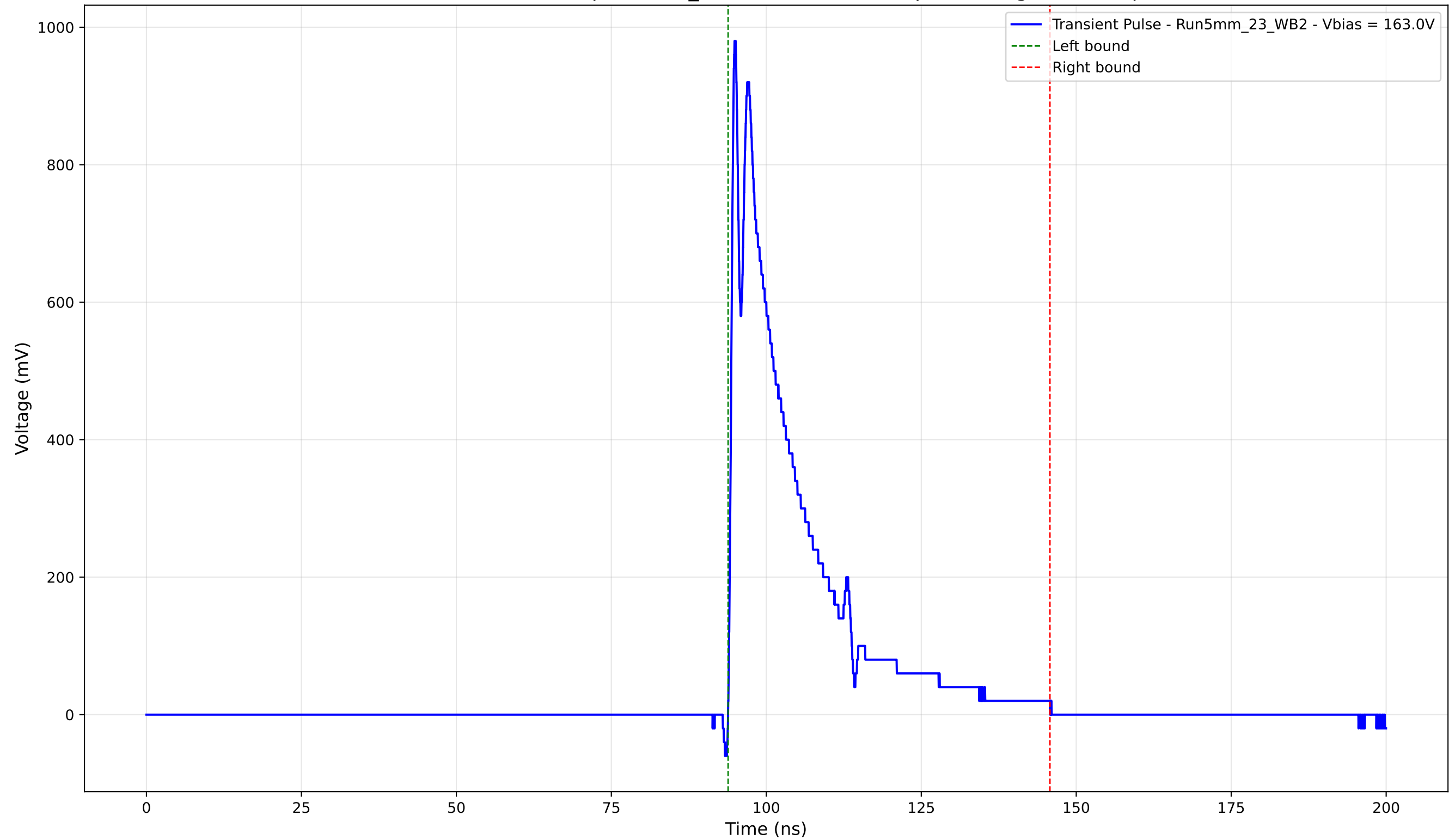
Transient Pulse - Sample: 5mm_23 - Position: 2380.0 \mu\text{m} - Charge: 199.89 pC
