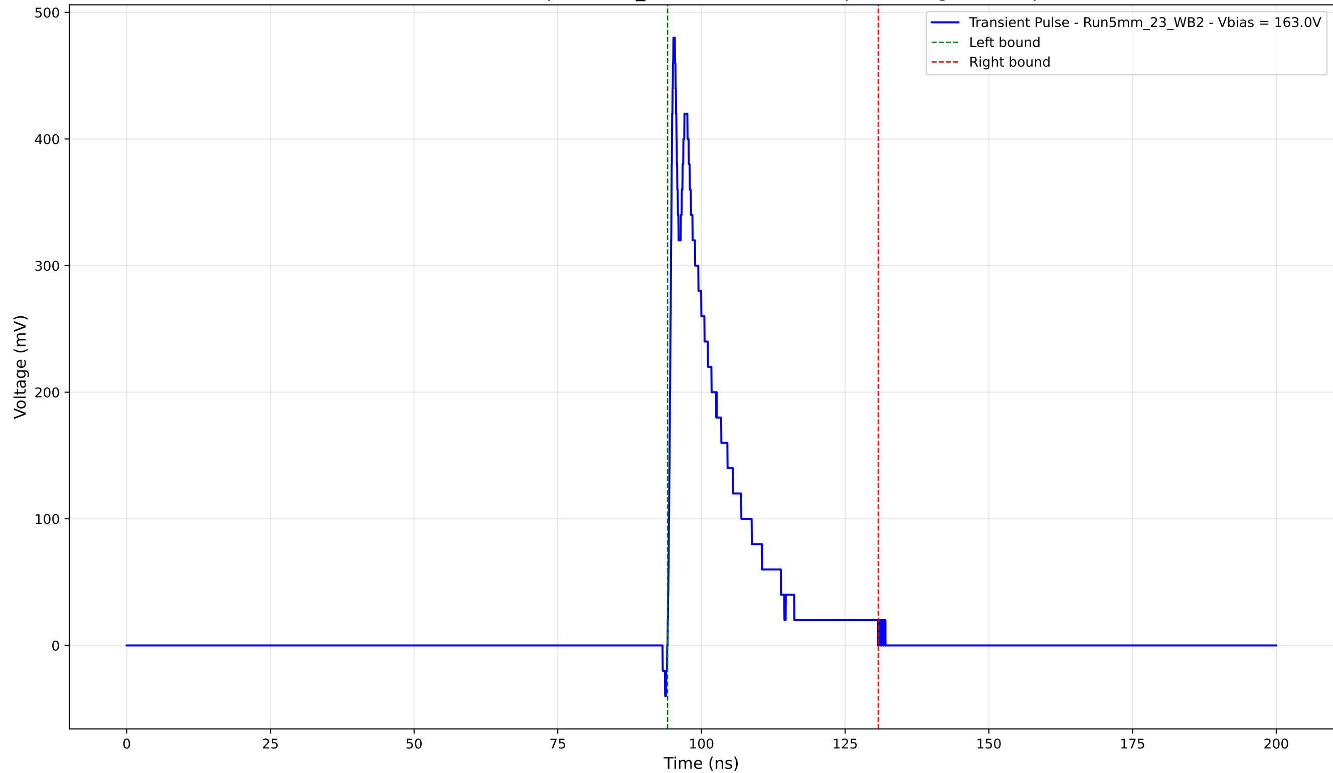
Transient Pulse - Sample: 5mm_23 - Position: 2045.0 \mu\text{m} - Charge: 82.31 pC
