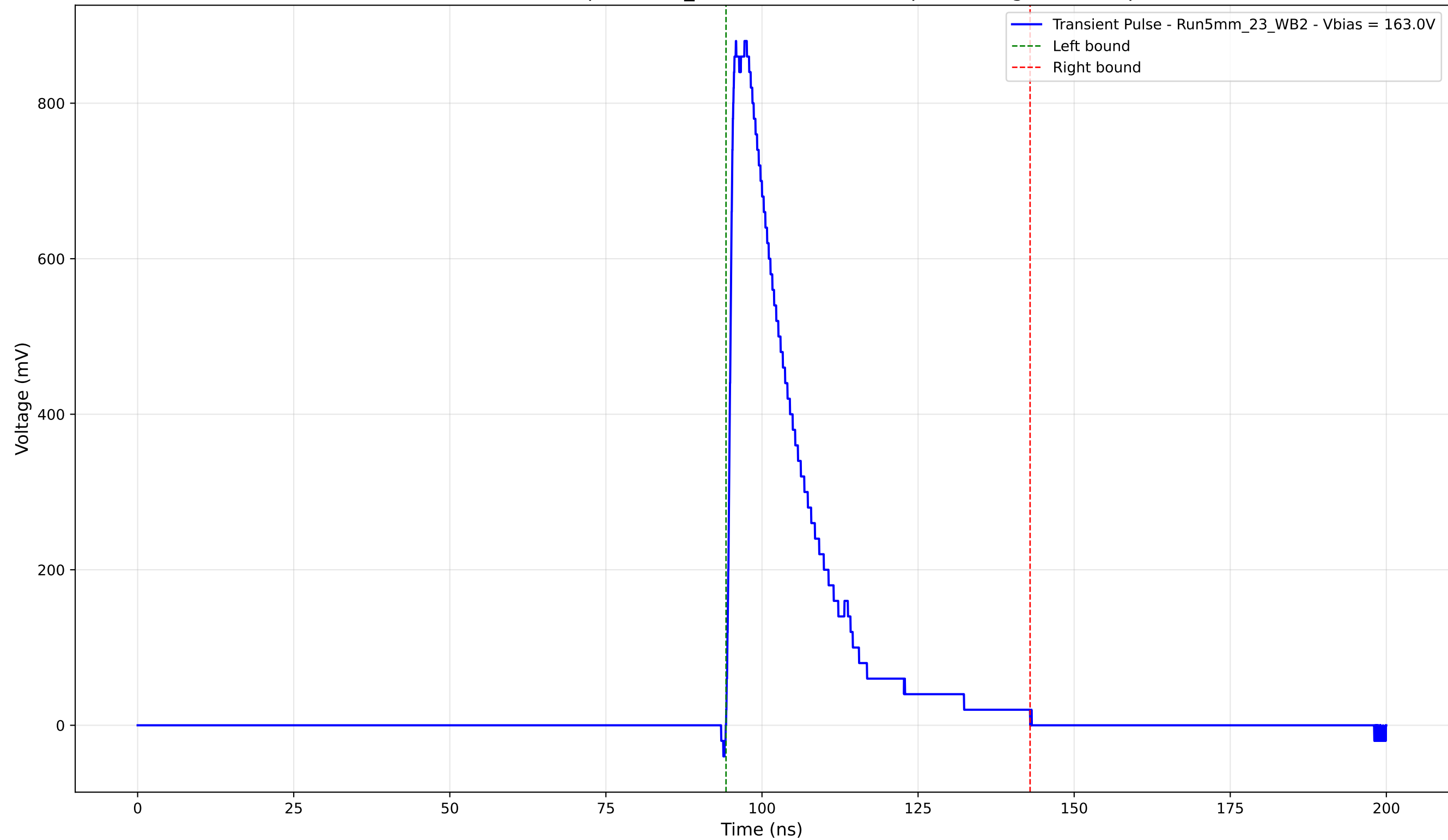
Transient Pulse - Sample: 5mm_23 - Position: 1655.0 \mu\text{m} - Charge: 203.03 pC
