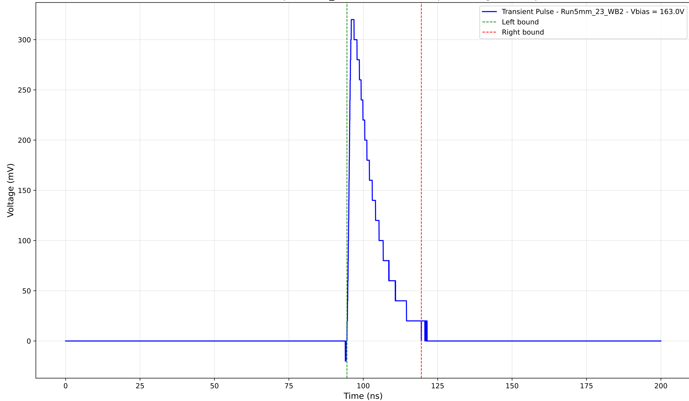
Transient Pulse - Sample: 5mm_23 - Position: 1020.0 \mu\text{m} - Charge: 58.06 pC
