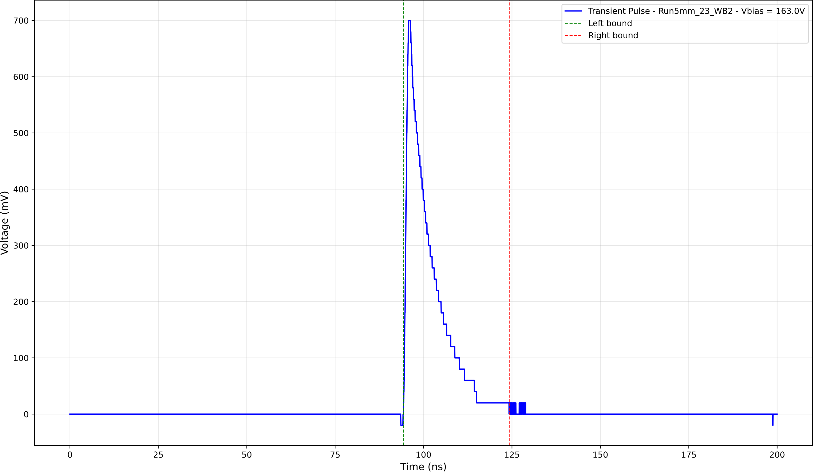
Transient Pulse - Sample: 5mm_23 - Position: 4480.0 \mu\text{m} - Charge: 106.10 pC
