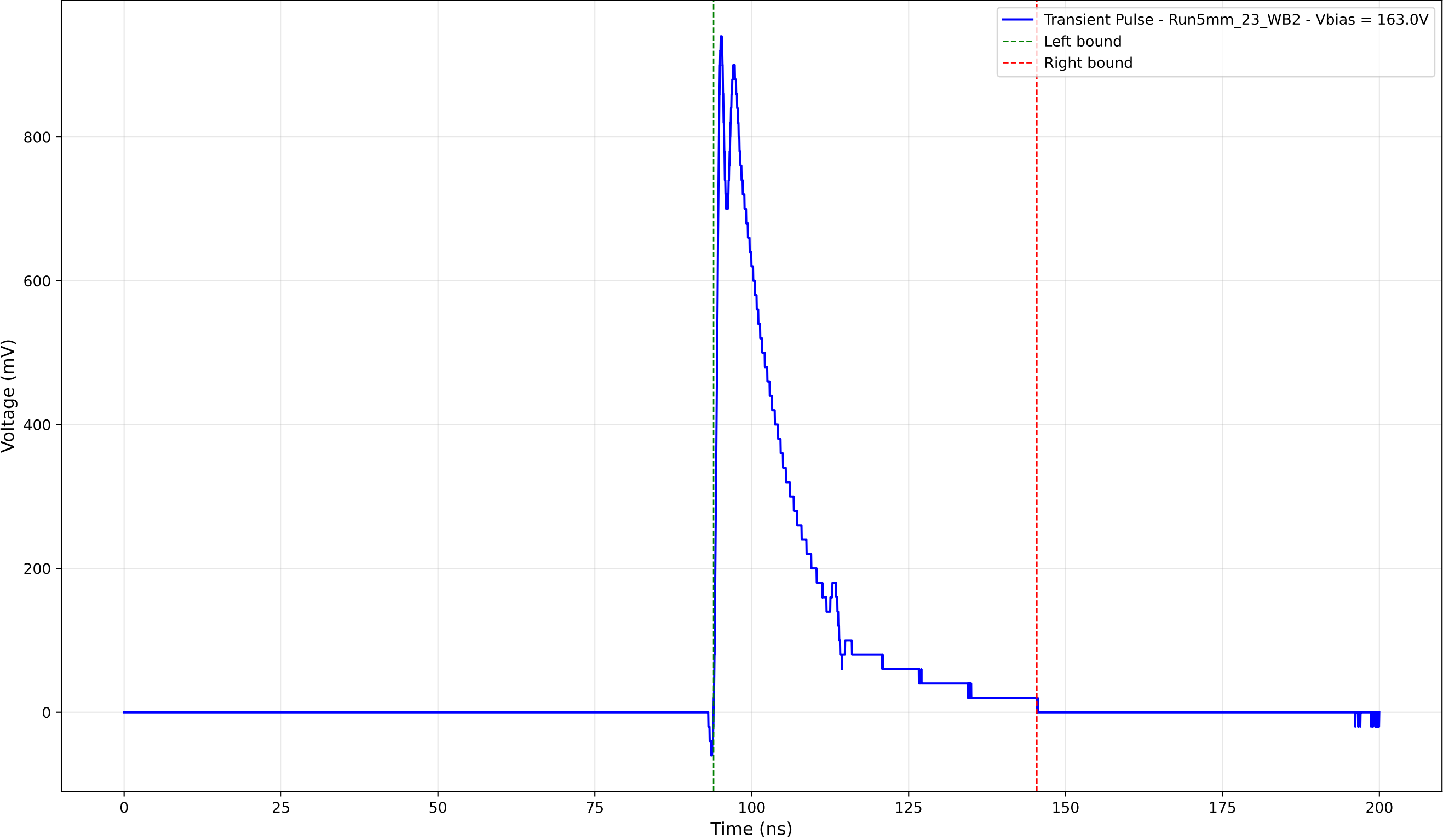
Transient Pulse - Sample: 5mm_23 - Position: 2210.0 \mu\text{m} - Charge: 203.99 pC
