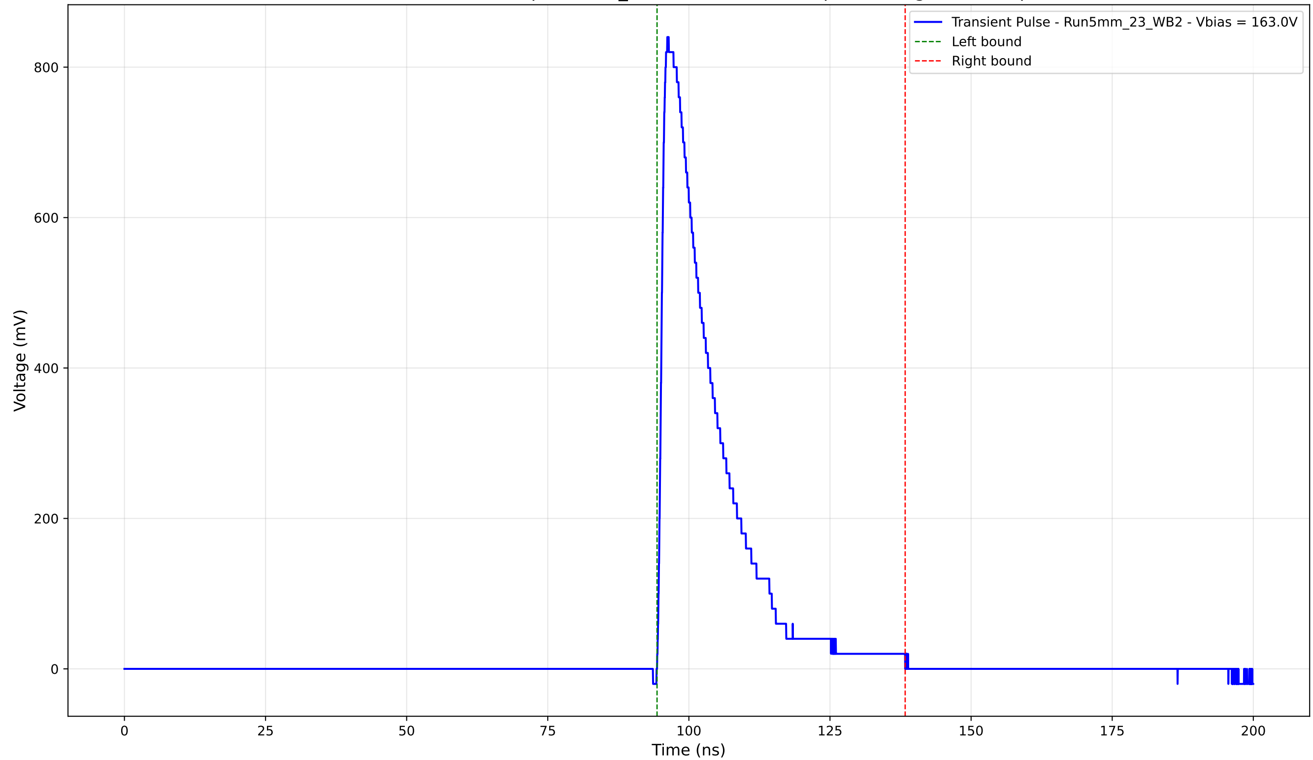
Transient Pulse - Sample: 5mm_23 - Position: 3675.0 \mu\text{m} - Charge: 173.65 pC
