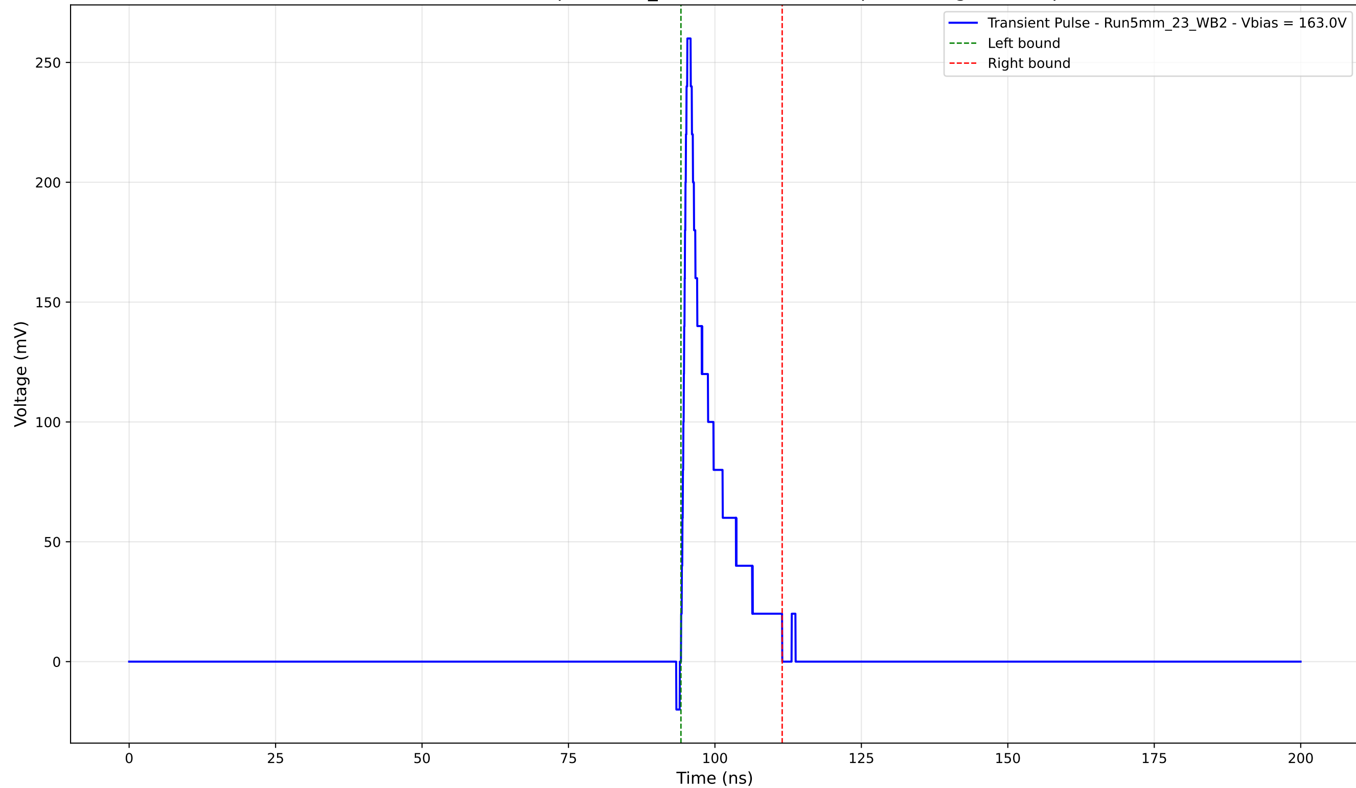
Transient Pulse - Sample: 5mm_23 - Position: 4955.0 \mu\text{m} - Charge: 26.30 pC
