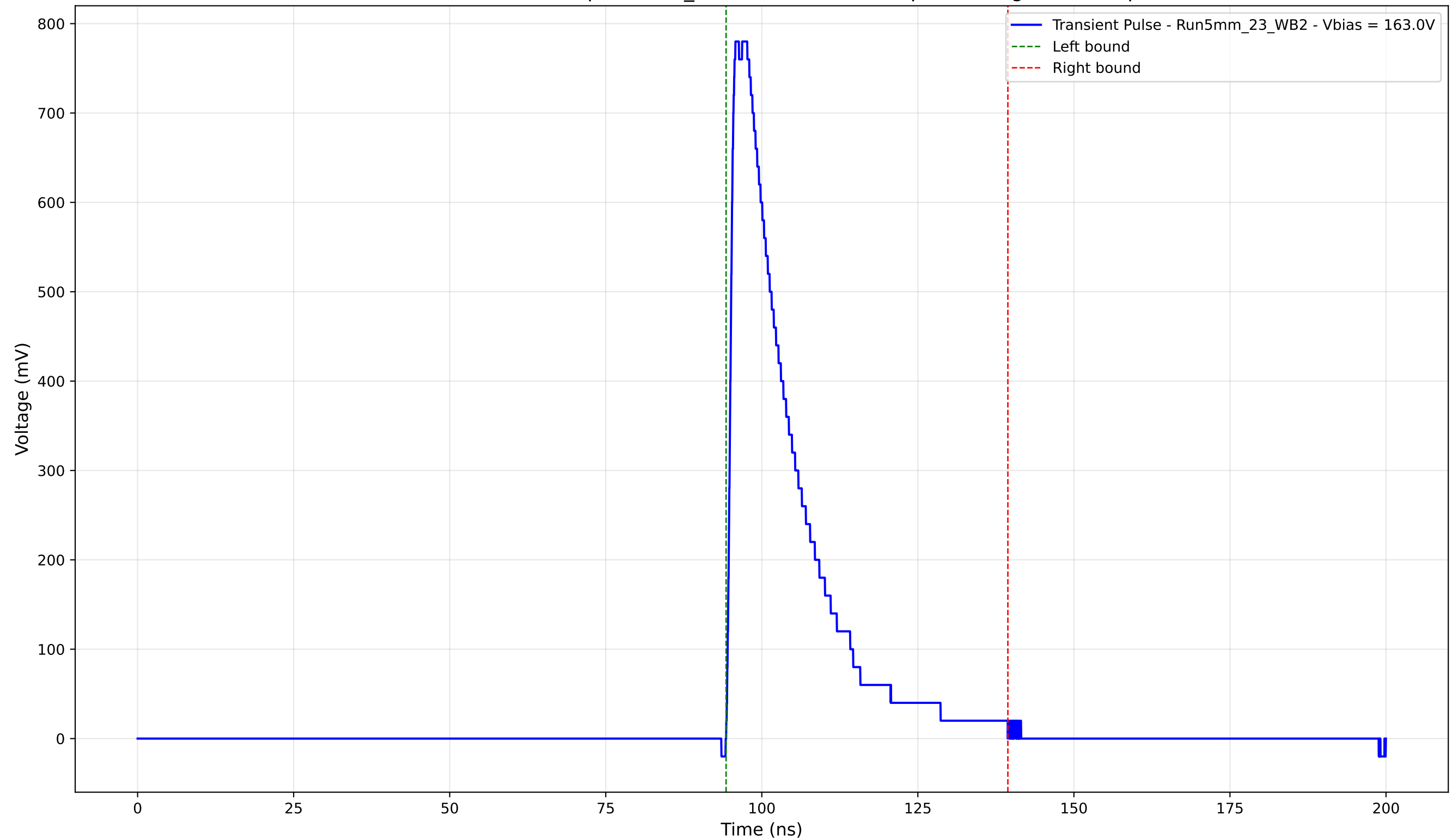
Transient Pulse - Sample: 5mm_23 - Position: 1580.0 \mu\text{m} - Charge: 172.86 pC
