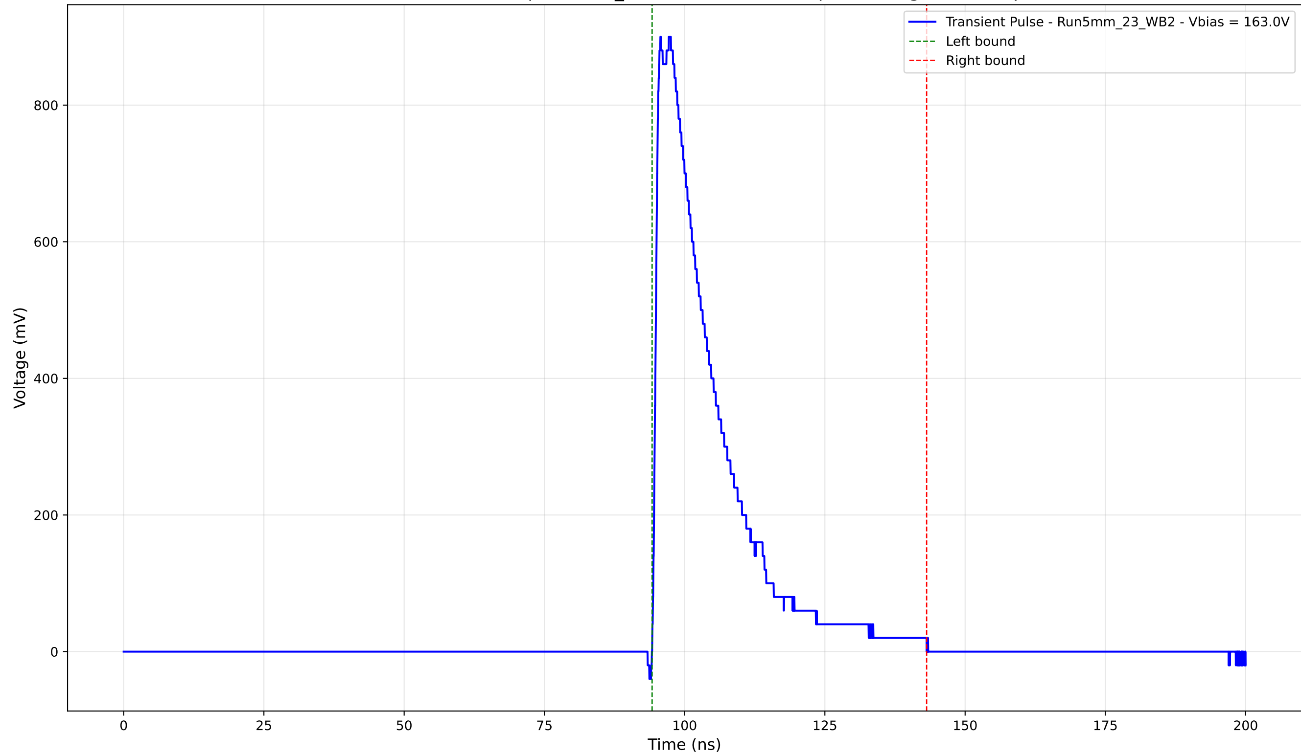
Transient Pulse - Sample: 5mm_23 - Position: 1725.0 \mu\text{m} - Charge: 210.88 pC
