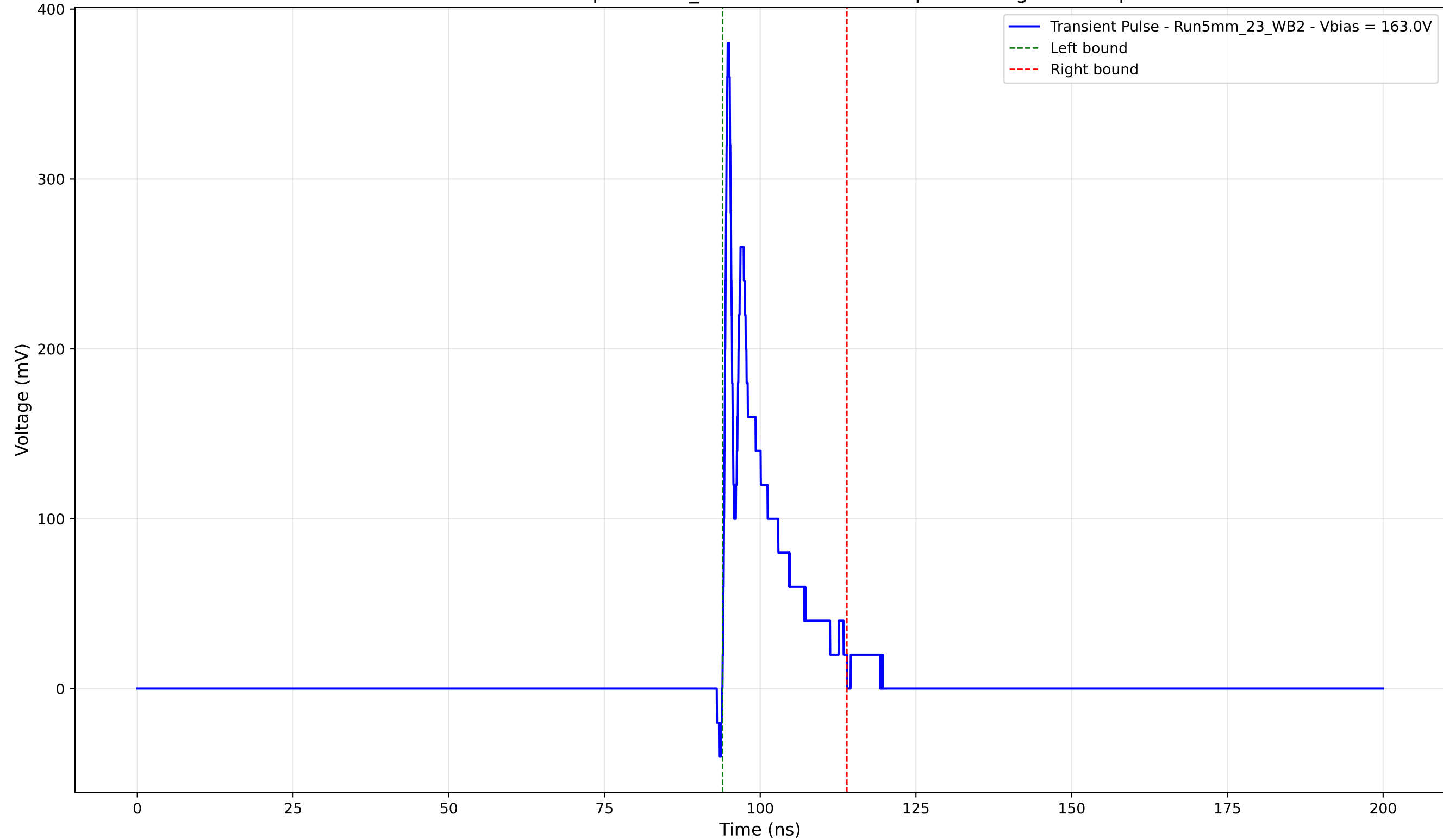
Transient Pulse - Sample: 5mm_23 - Position: 2505.0 \mu\text{m} - Charge: 40.15 pC
