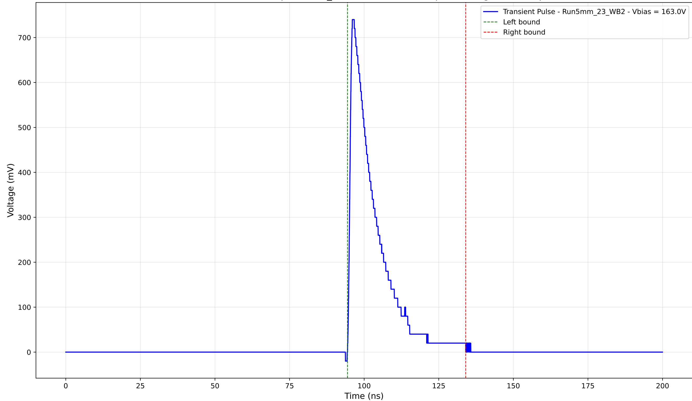
Transient Pulse - Sample: 5mm_23 - Position: 3965.0 \mu\text{m} - Charge: 137.78 pC
