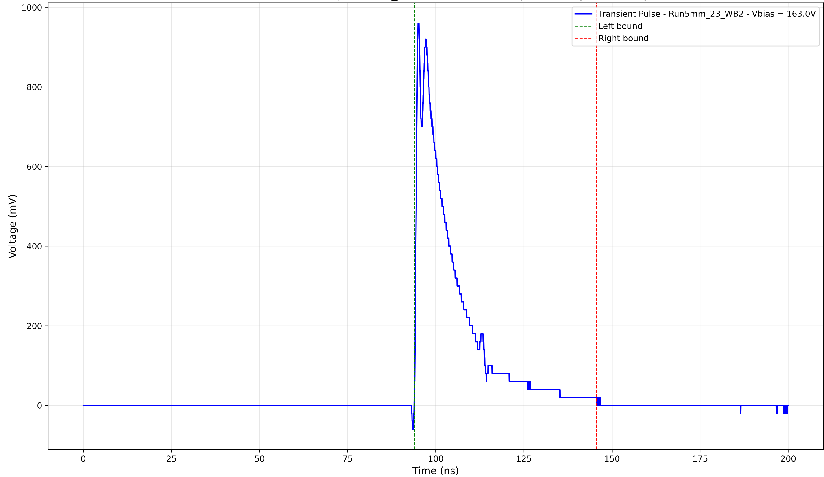
Transient Pulse - Sample: 5mm_23 - Position: 2790.0 \mu\text{m} - Charge: 206.21 pC
