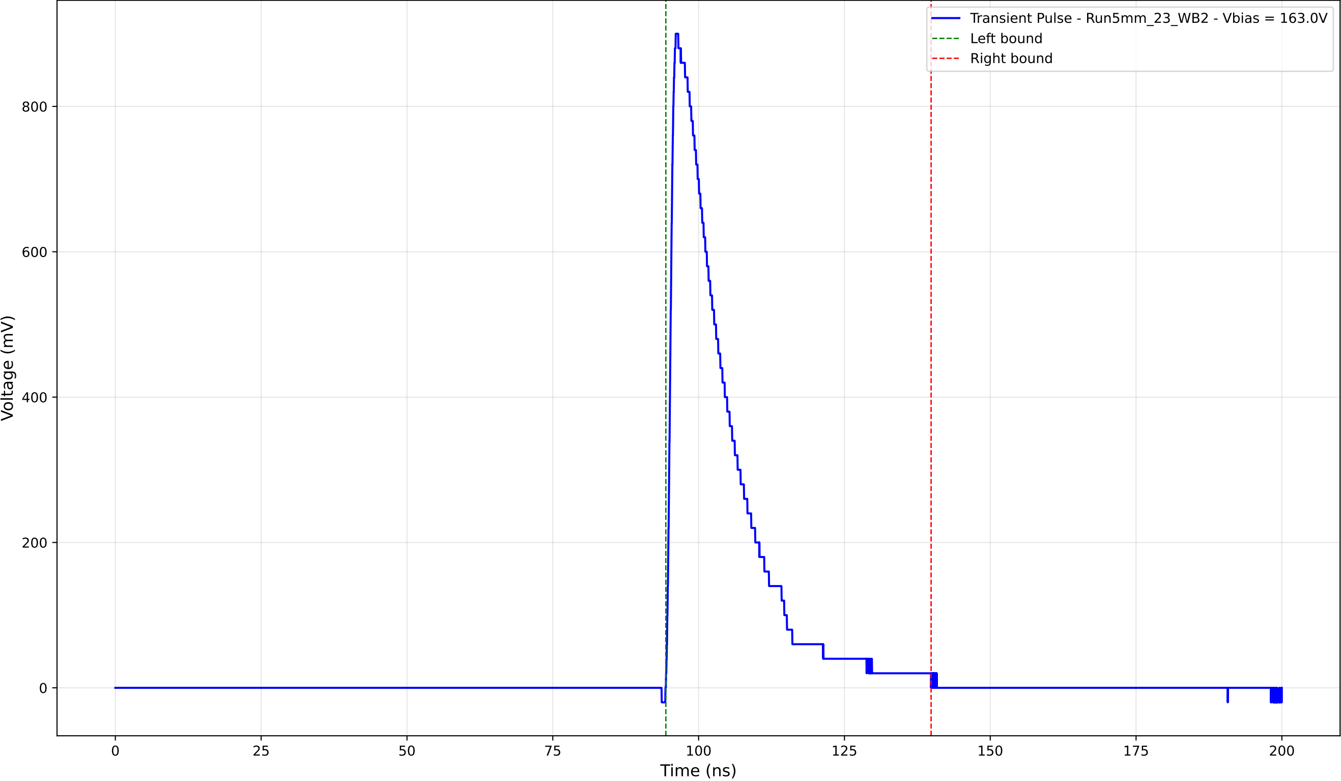
Transient Pulse - Sample: 5mm_23 - Position: 1190.0 \mu\text{m} - Charge: 195.45 pC
