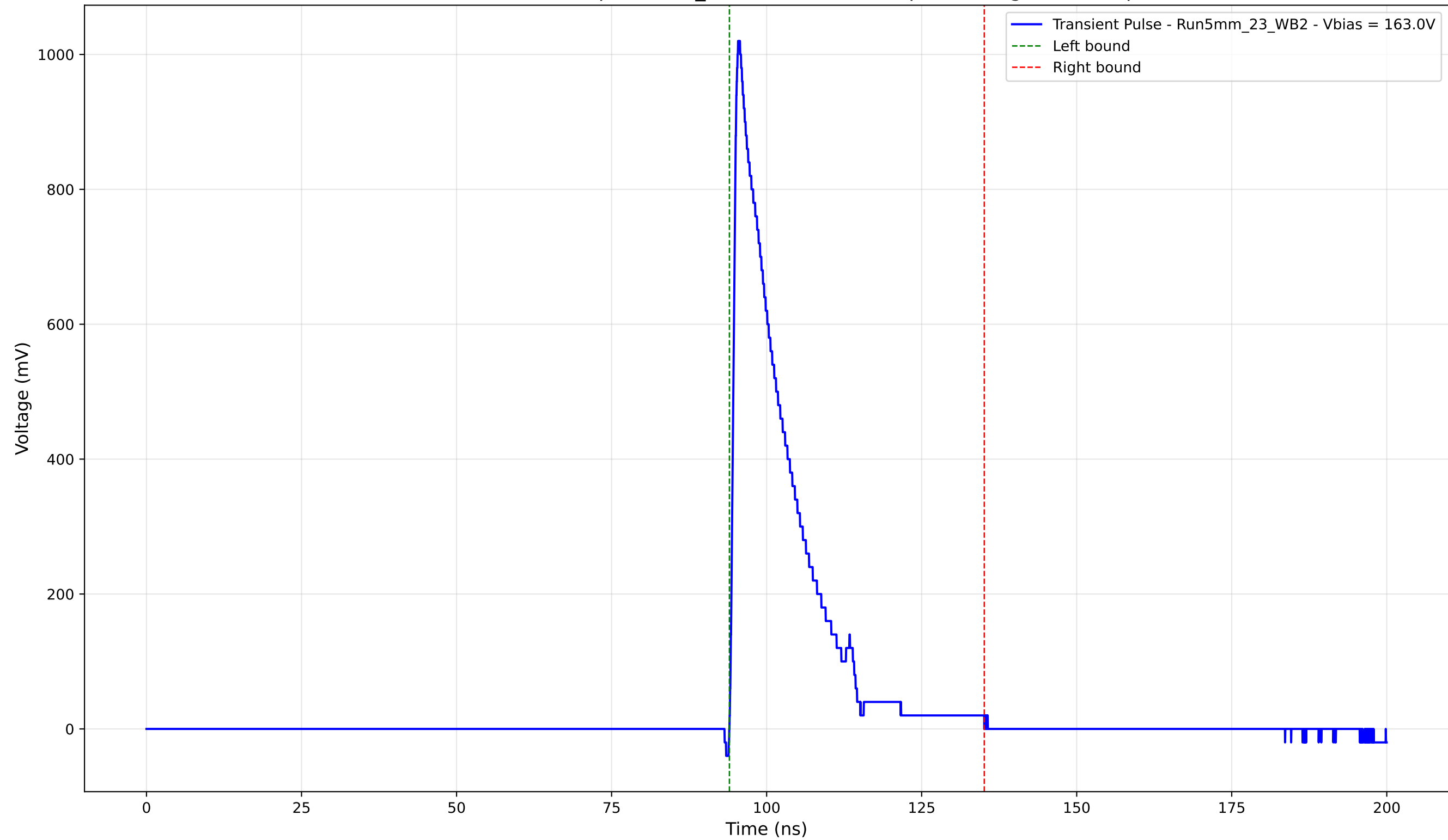
Transient Pulse - Sample: 5mm_23 - Position: 185.0 \mu\text{m} - Charge: 180.84 pC
