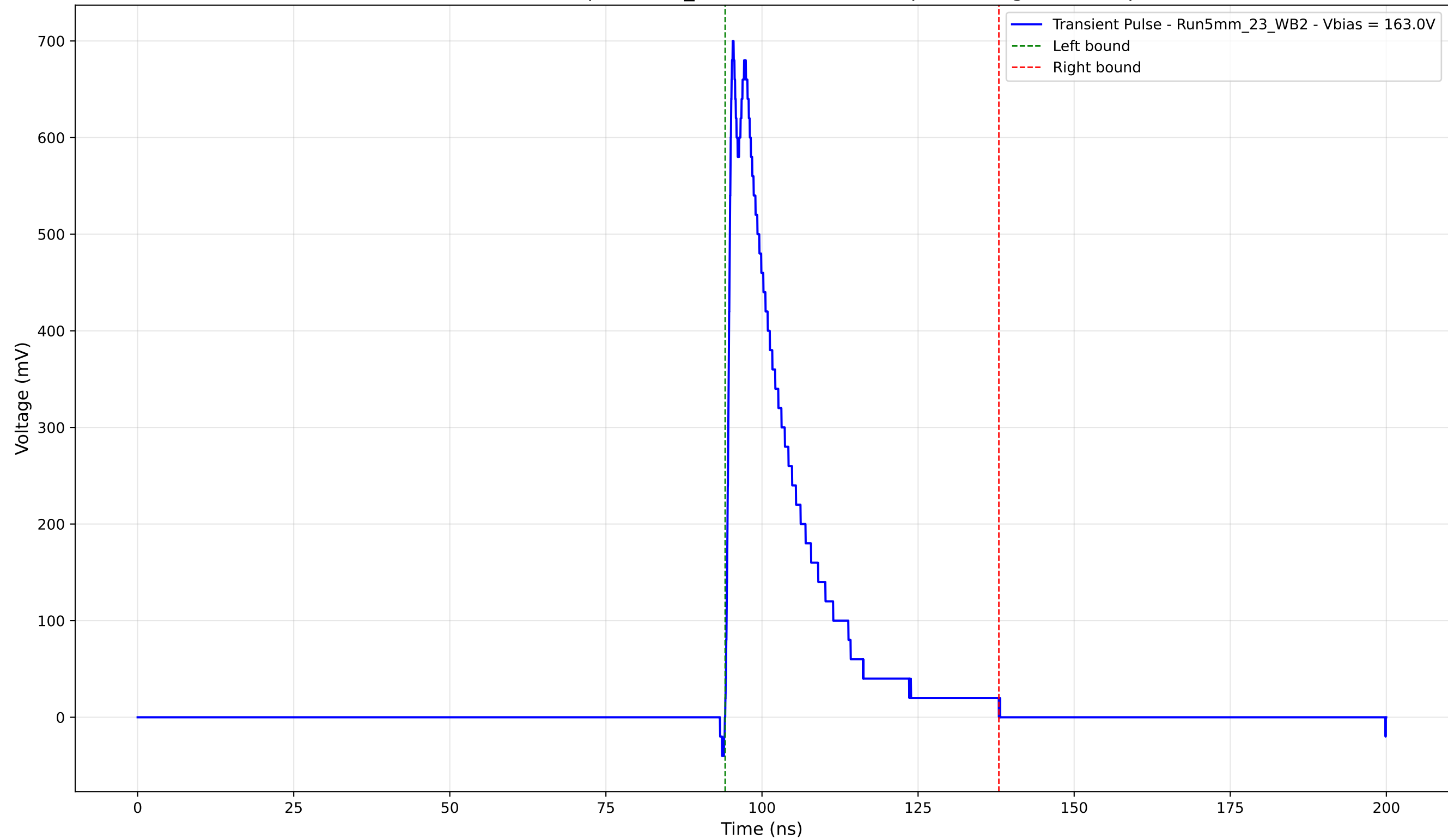
Transient Pulse - Sample: 5mm_23 - Position: 3075.0 \mu\text{m} - Charge: 139.74 pC
