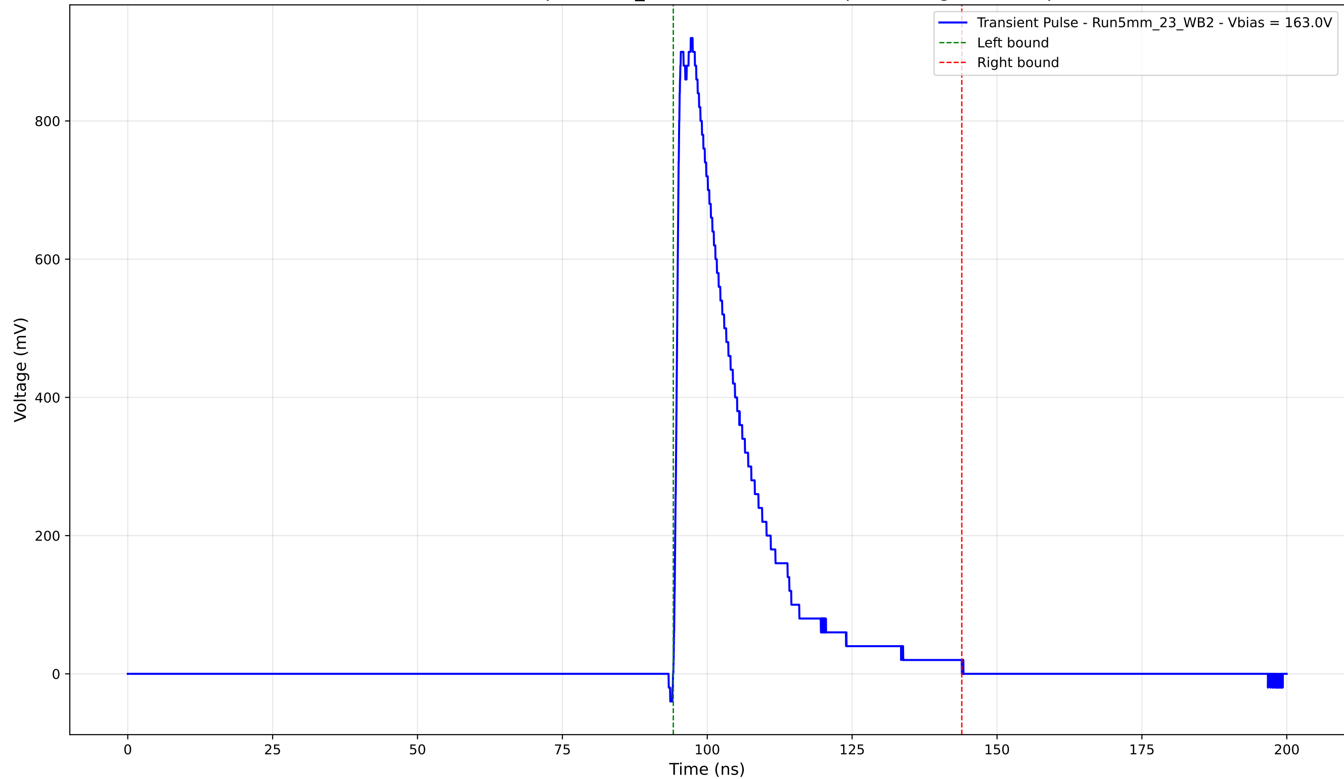
Transient Pulse - Sample: 5mm_23 - Position: 3240.0 \mu\text{m} - Charge: 215.10 pC
