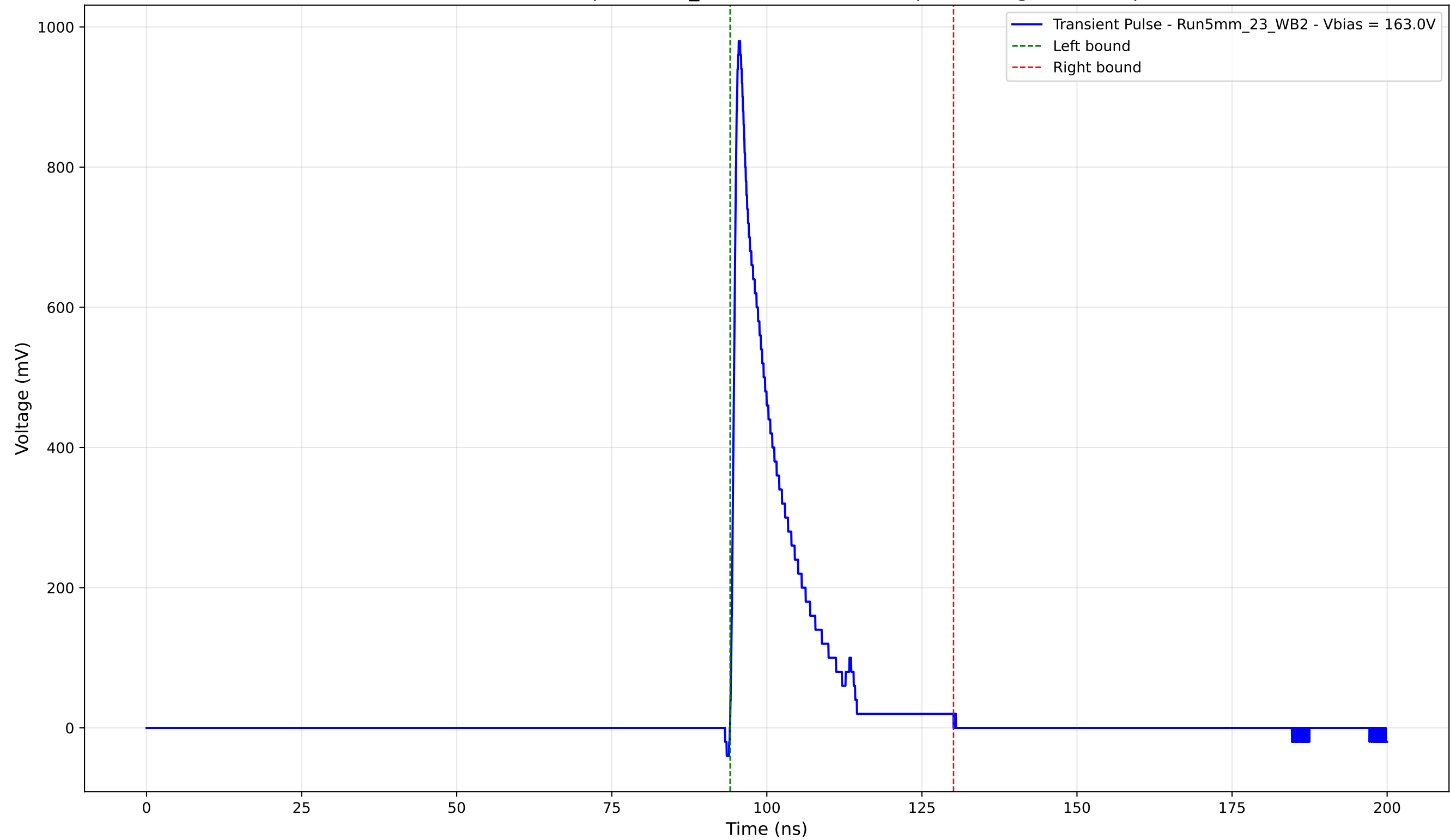
Transient Pulse - Sample: 5mm_23 - Position: 4860.0 \mu\text{m} - Charge: 140.04 pC
