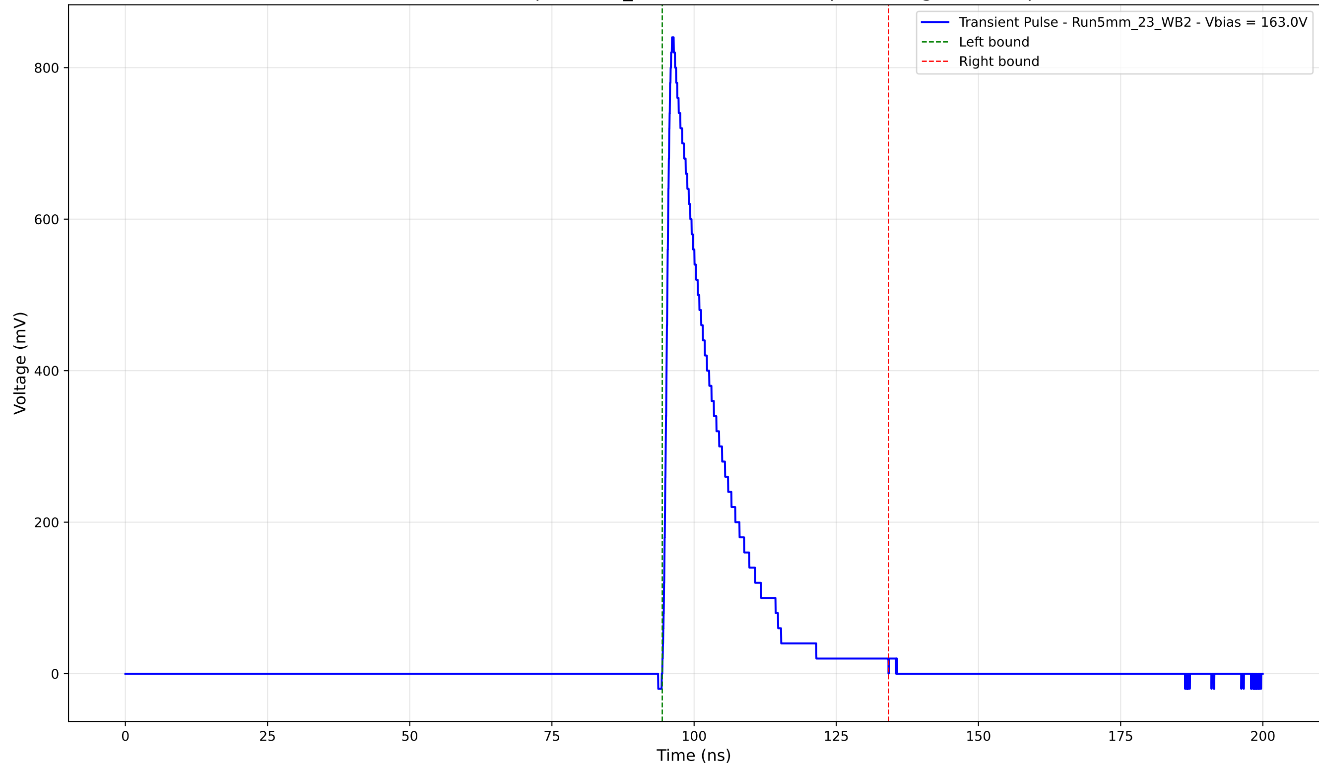
Transient Pulse - Sample: 5mm_23 - Position: 4130.0 \mu\text{m} - Charge: 152.11 pC
