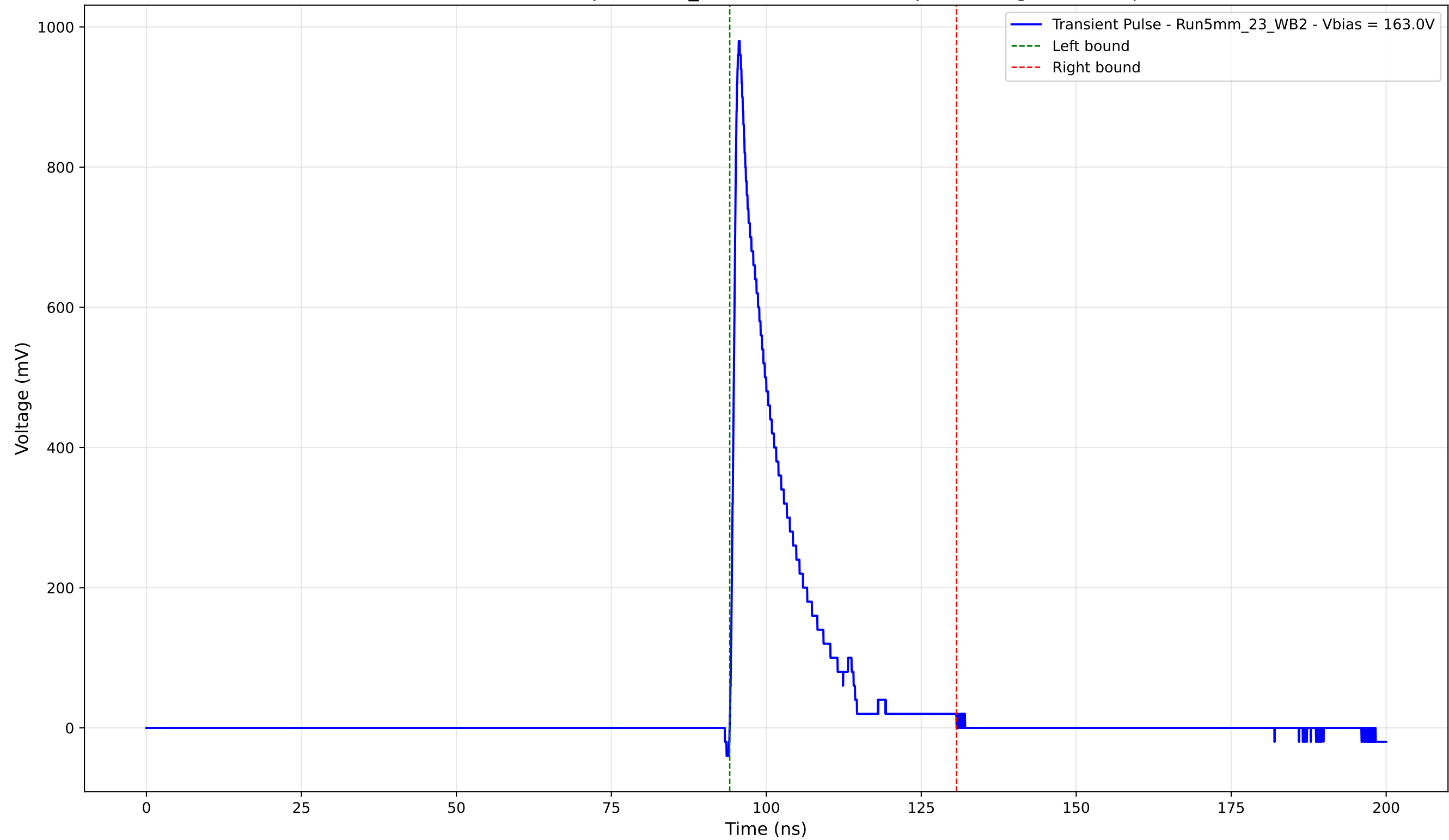
Transient Pulse - Sample: 5mm_23 - Position: 4810.0 \mu\text{m} - Charge: 145.21 pC
