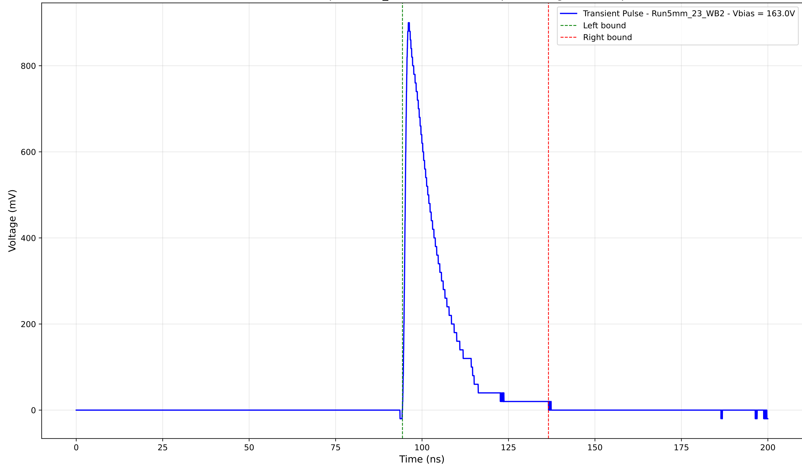
Transient Pulse - Sample: 5mm_23 - Position: 775.0 \mu\text{m} - Charge: 173.46 pC
