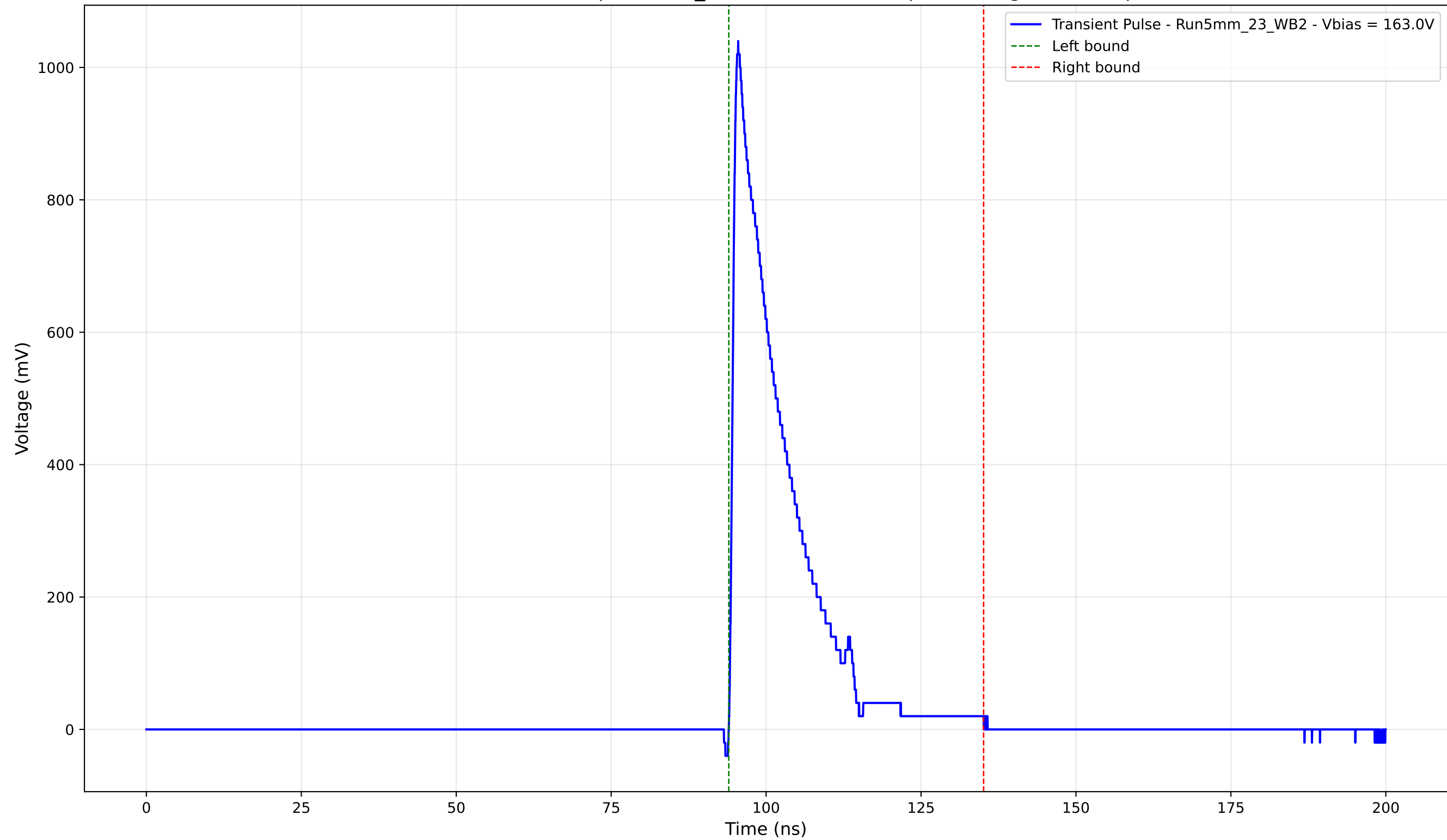
Transient Pulse - Sample: 5mm_23 - Position: 145.0 \mu\text{m} - Charge: 182.19 pC
