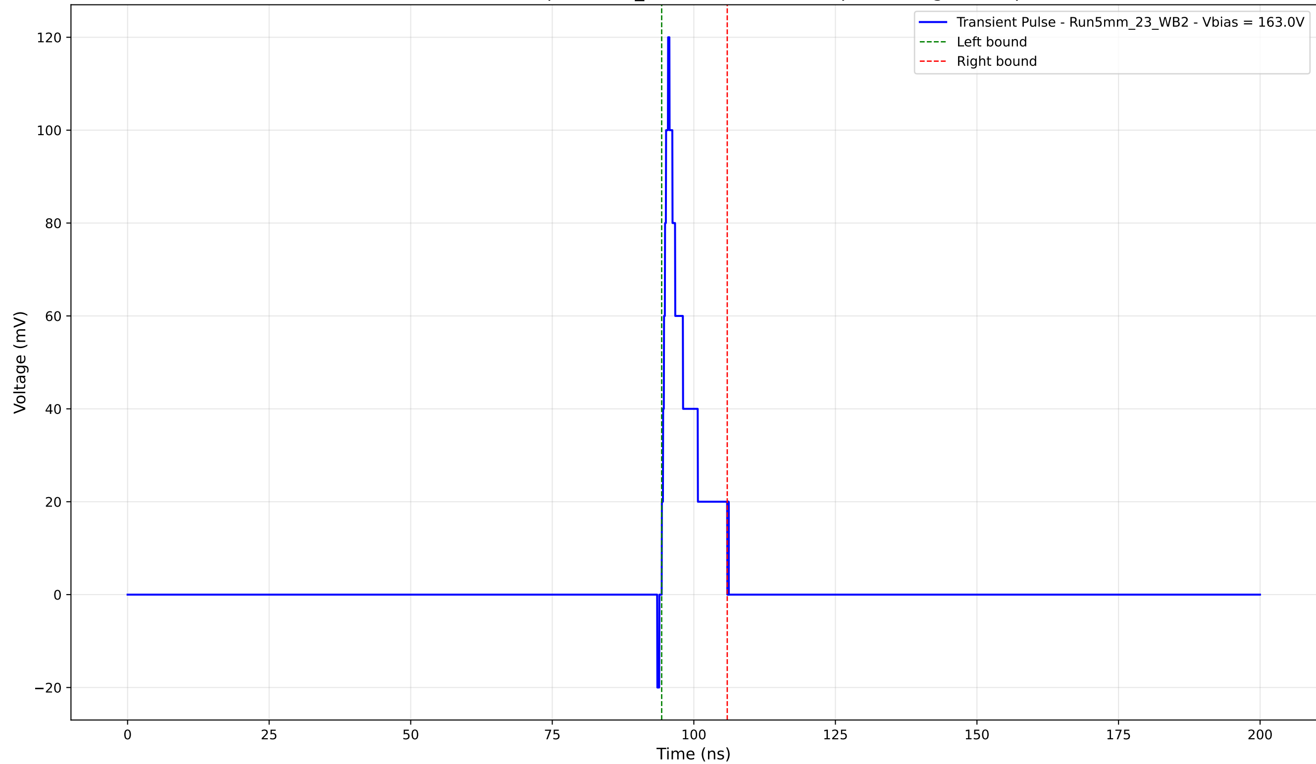
Transient Pulse - Sample: 5mm_23 - Position: 4975.0 \mu\text{m} - Charge: 9.70 pC
