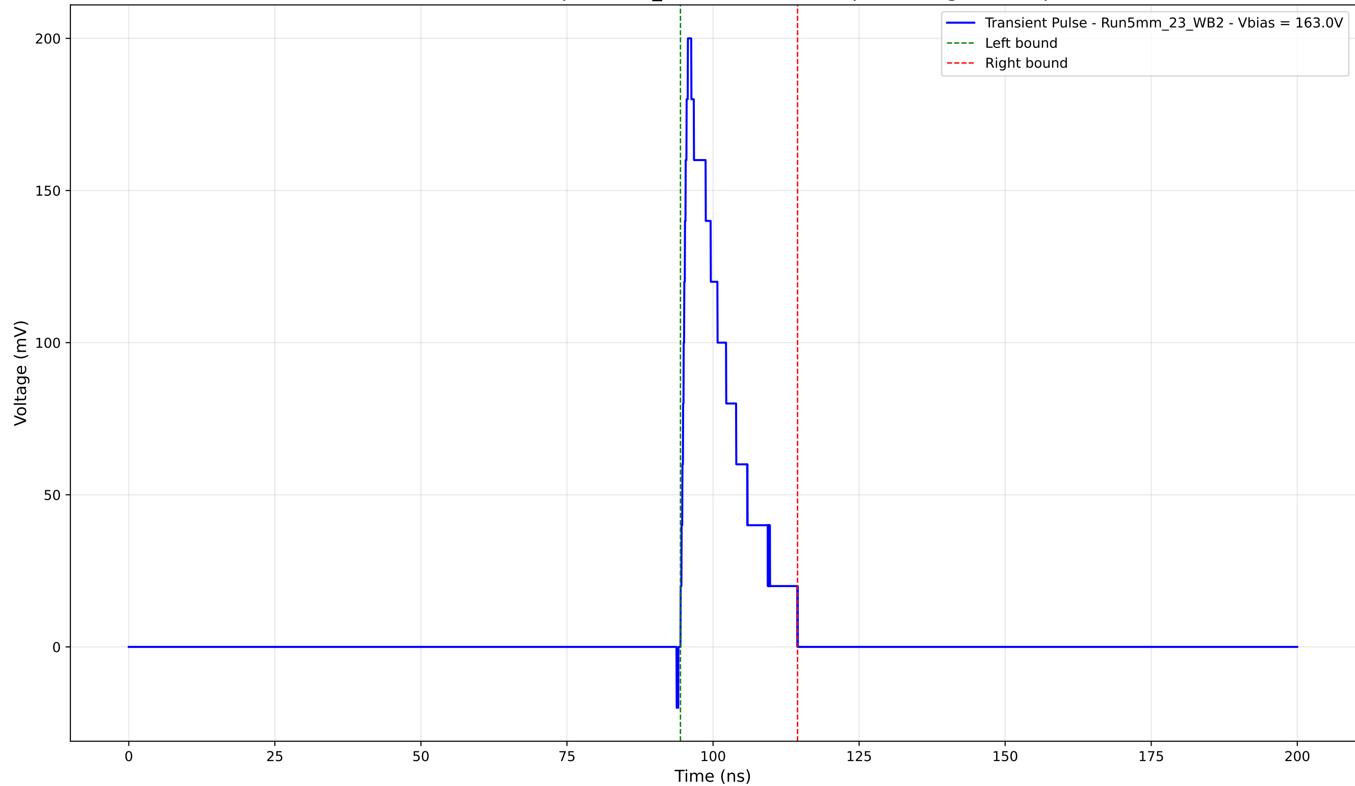
Transient Pulse - Sample: 5mm_23 - Position: 485.0 \mu\text{m} - Charge: 31.14 pC
