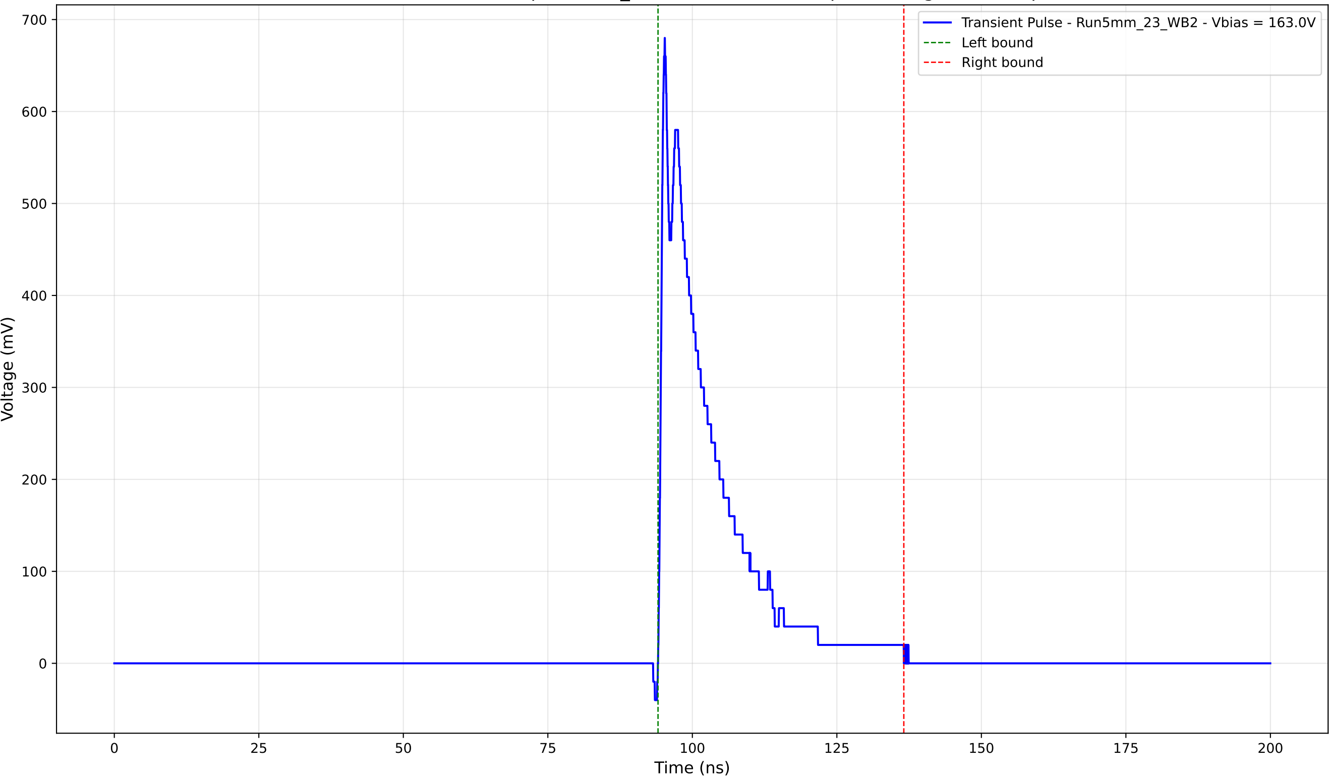
Transient Pulse - Sample: 5mm_23 - Position: 2060.0 \mu\text{m} - Charge: 118.72 pC
