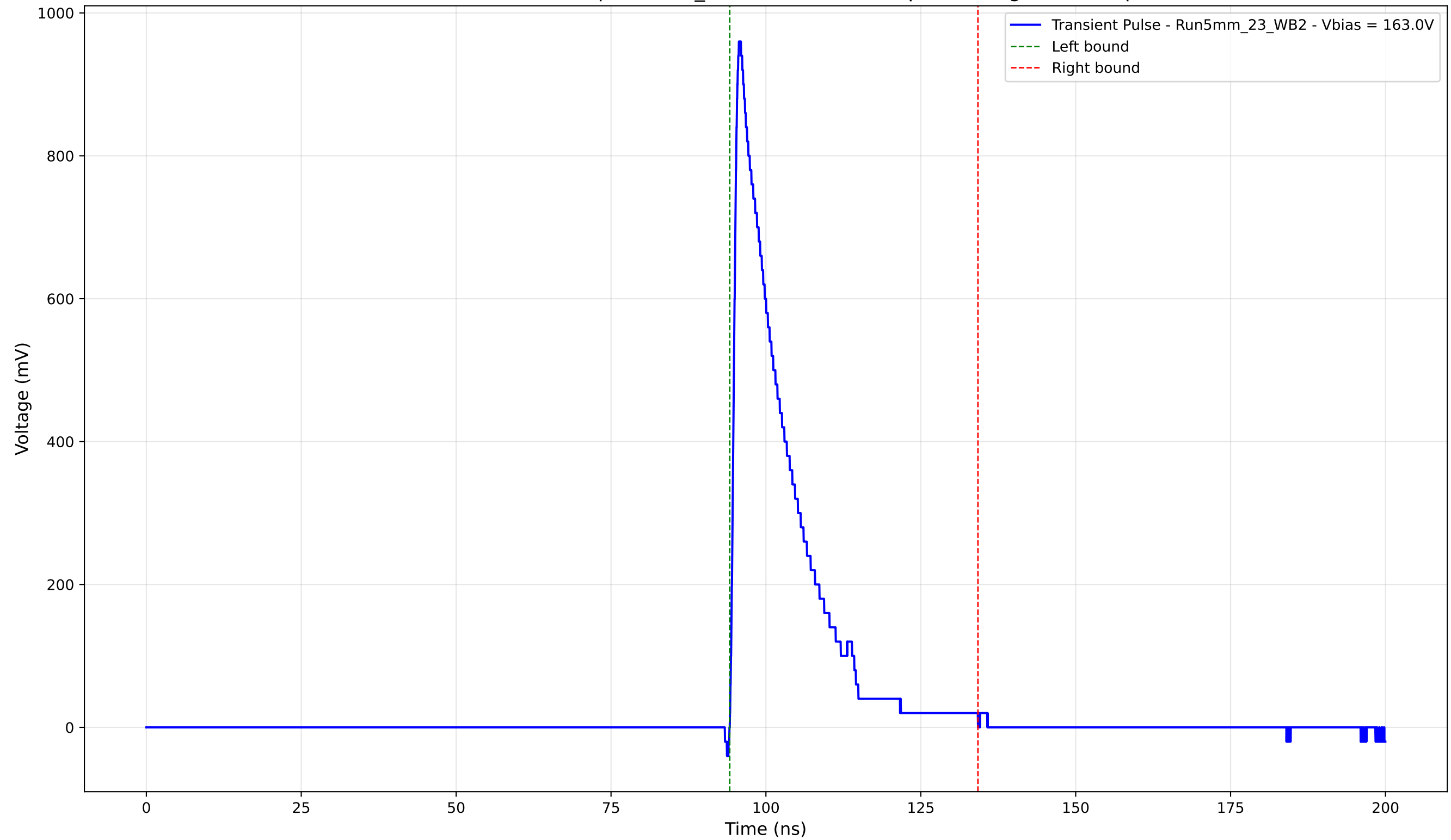
Transient Pulse - Sample: 5mm_23 - Position: 400.0 \mu\text{m} - Charge: 171.04 pC
