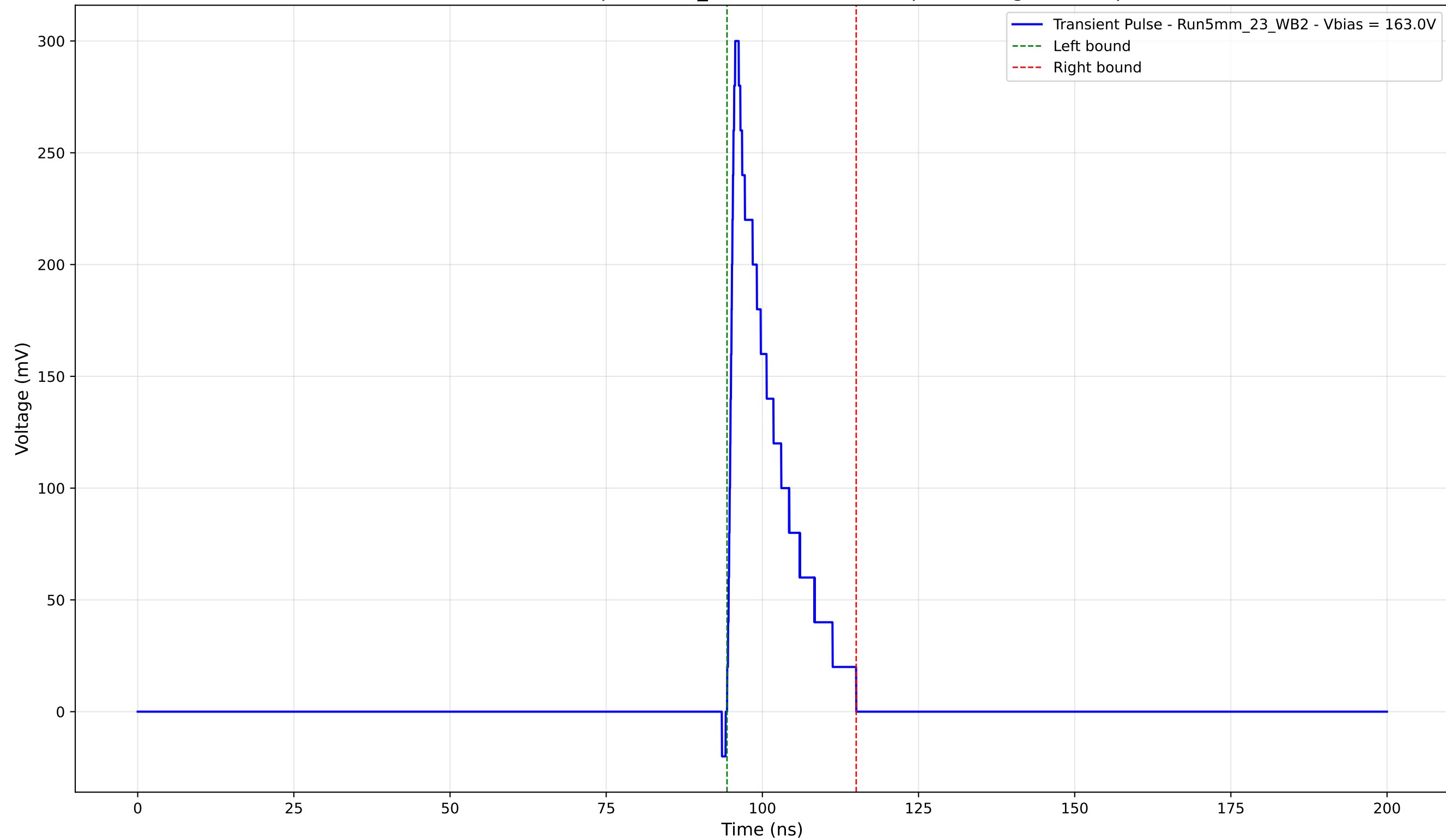
Transient Pulse - Sample: 5mm_23 - Position: 470.0 \mu\text{m} - Charge: 43.84 pC
