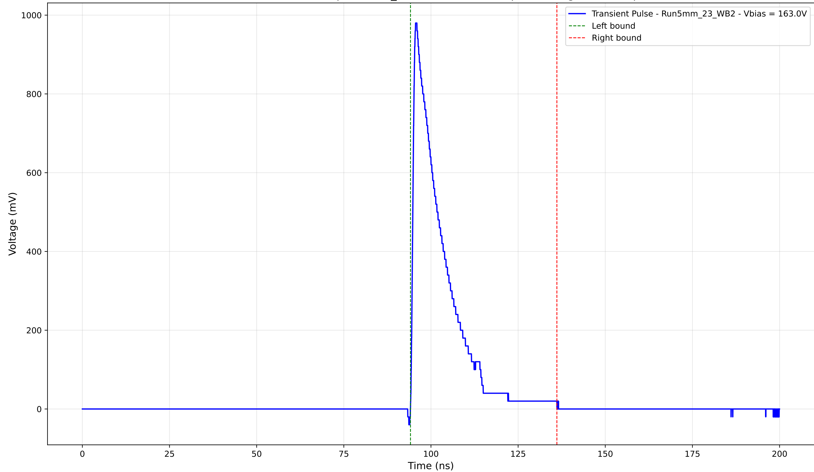
Transient Pulse - Sample: 5mm_23 - Position: 375.0 \mu\text{m} - Charge: 180.92 pC
