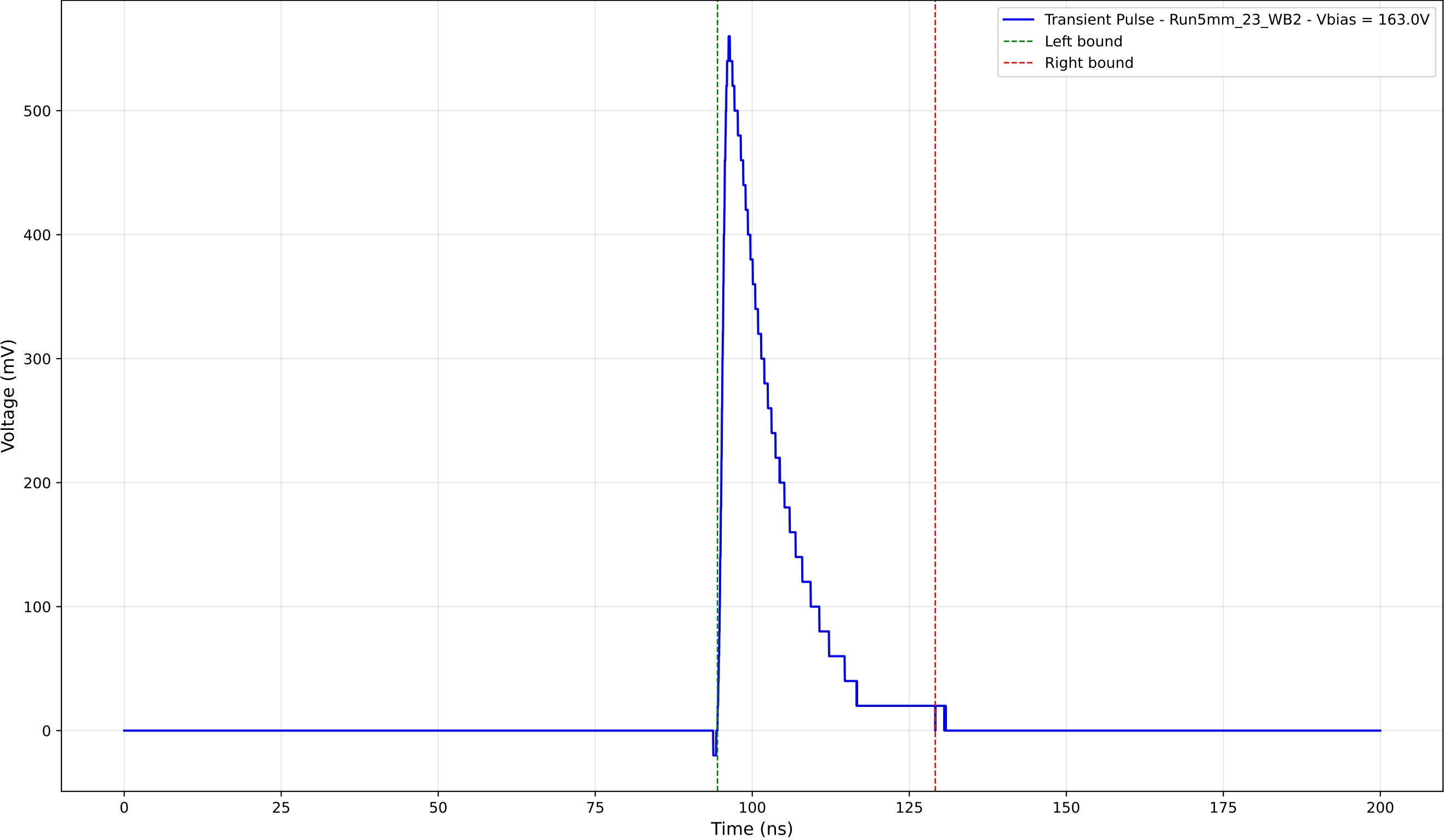
Transient Pulse - Sample: 5mm_23 - Position: 1040.0 \mu\text{m} - Charge: 101.06 pC
