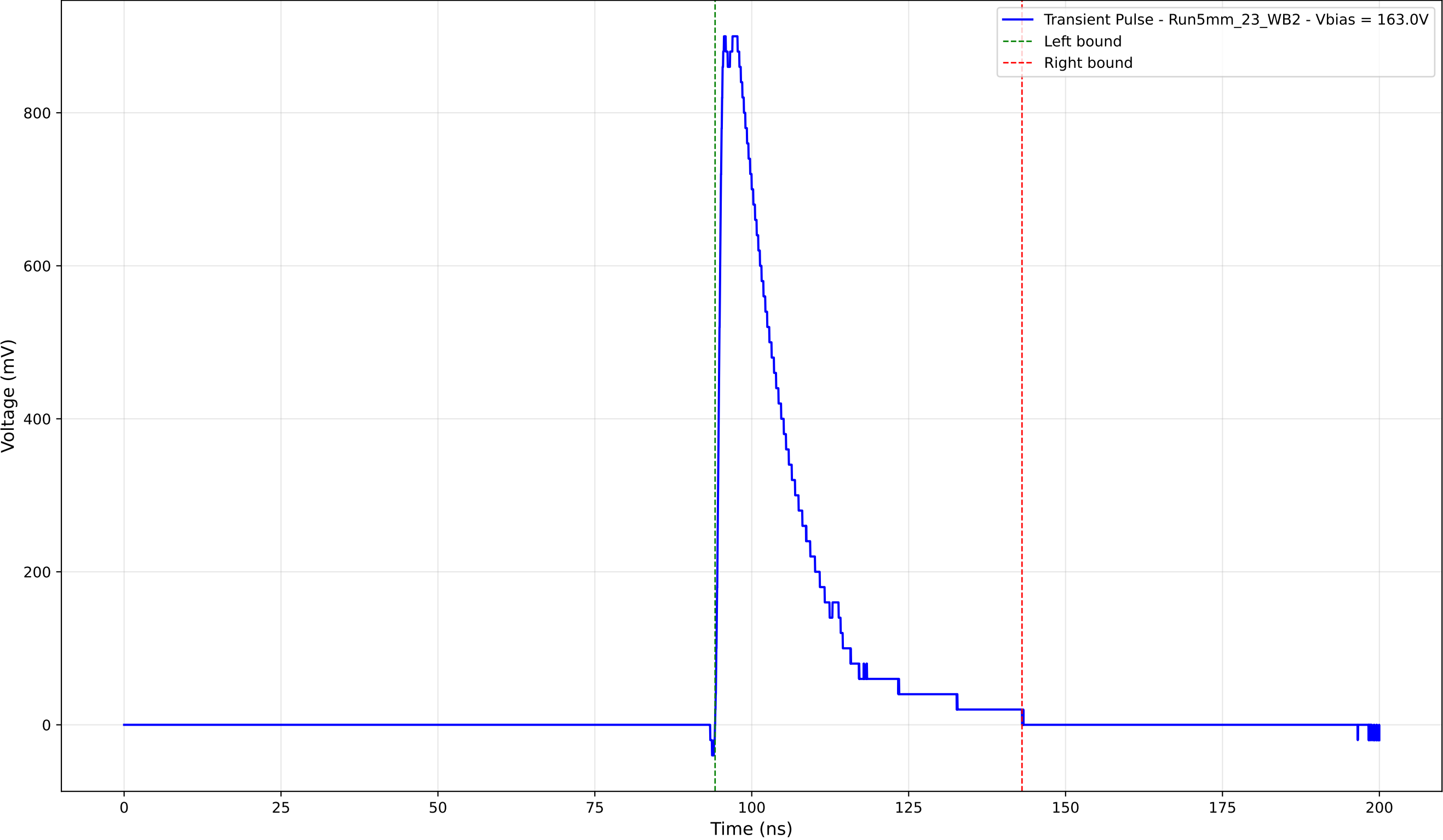
Transient Pulse - Sample: 5mm_23 - Position: 3285.0 \mu\text{m} - Charge: 209.94 pC
