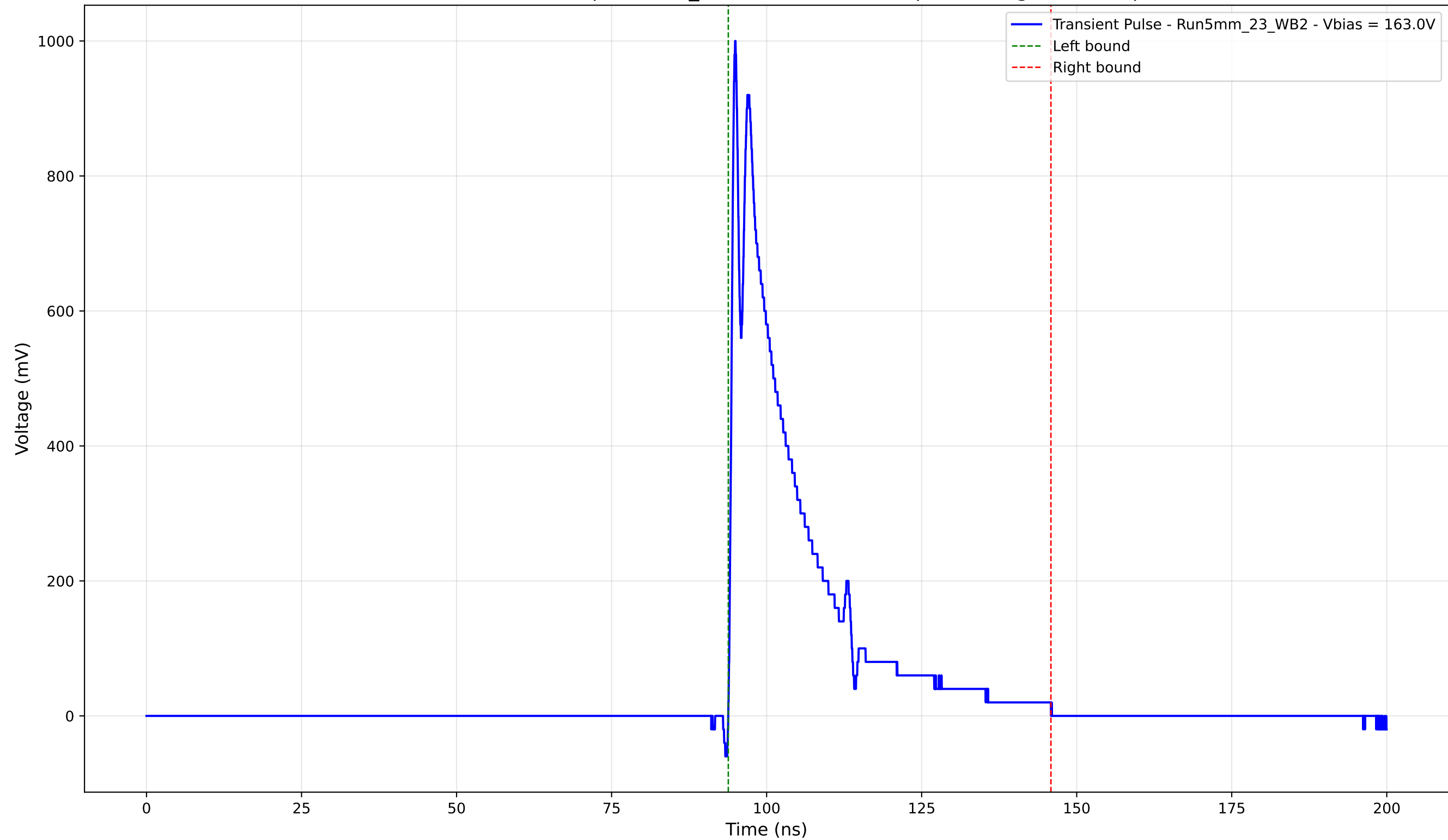
Transient Pulse - Sample: 5mm_23 - Position: 2400.0 \mu\text{m} - Charge: 198.46 pC
