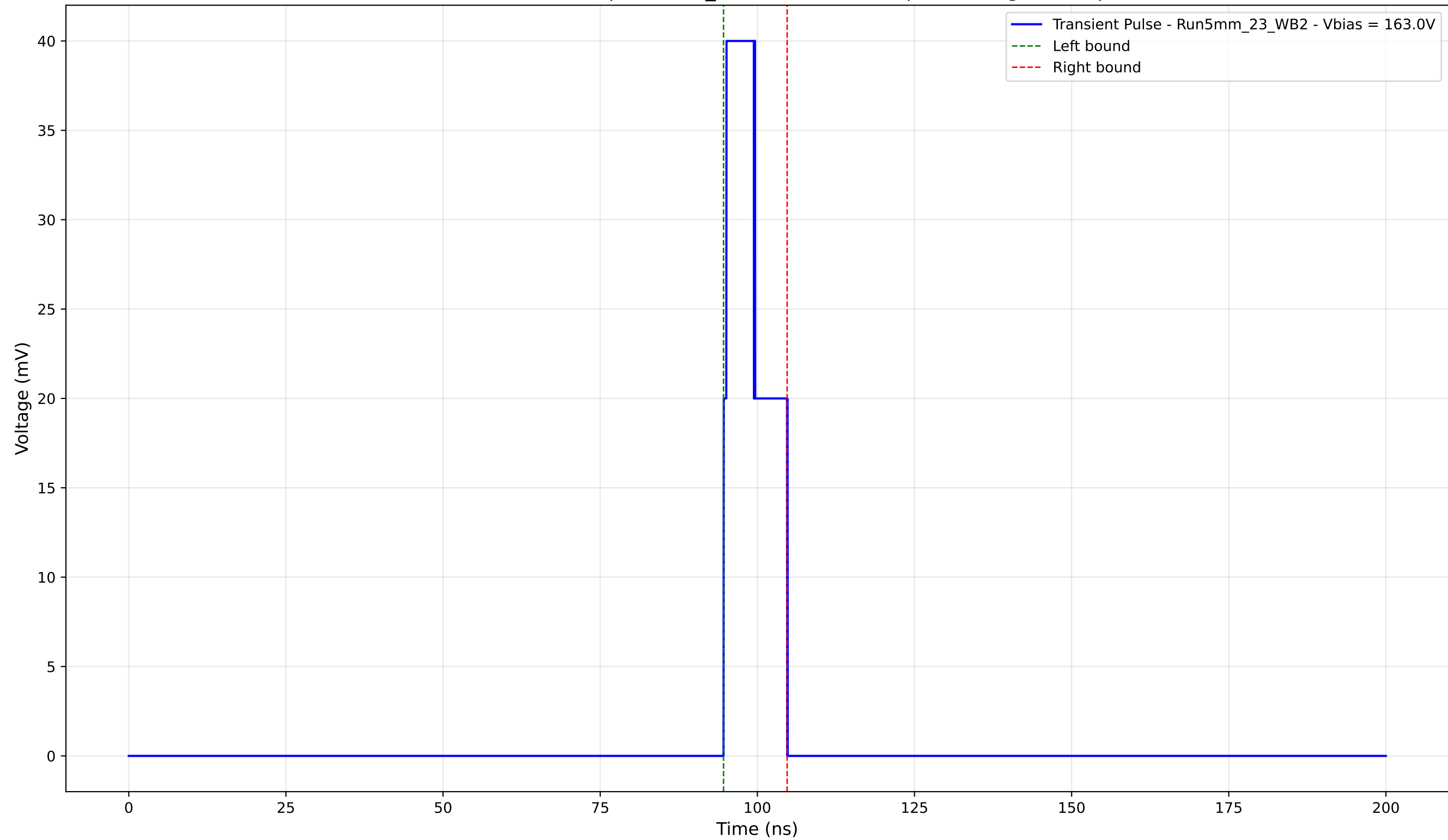
Transient Pulse - Sample: 5mm_23 - Position: 20.0 \mu\text{m} - Charge: 5.82 pC
