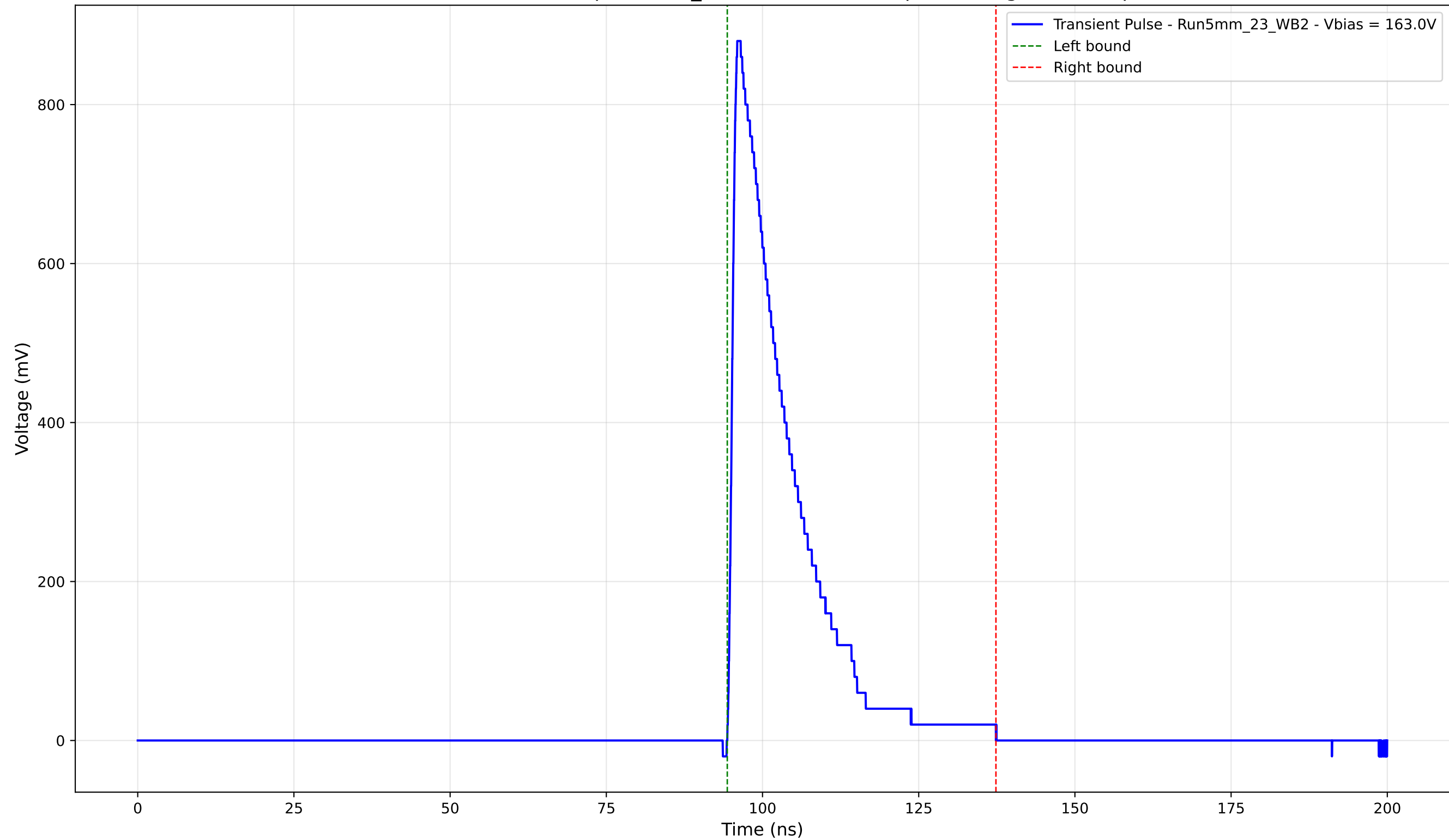
Transient Pulse - Sample: 5mm_23 - Position: 840.0 \mu\text{m} - Charge: 173.96 pC
