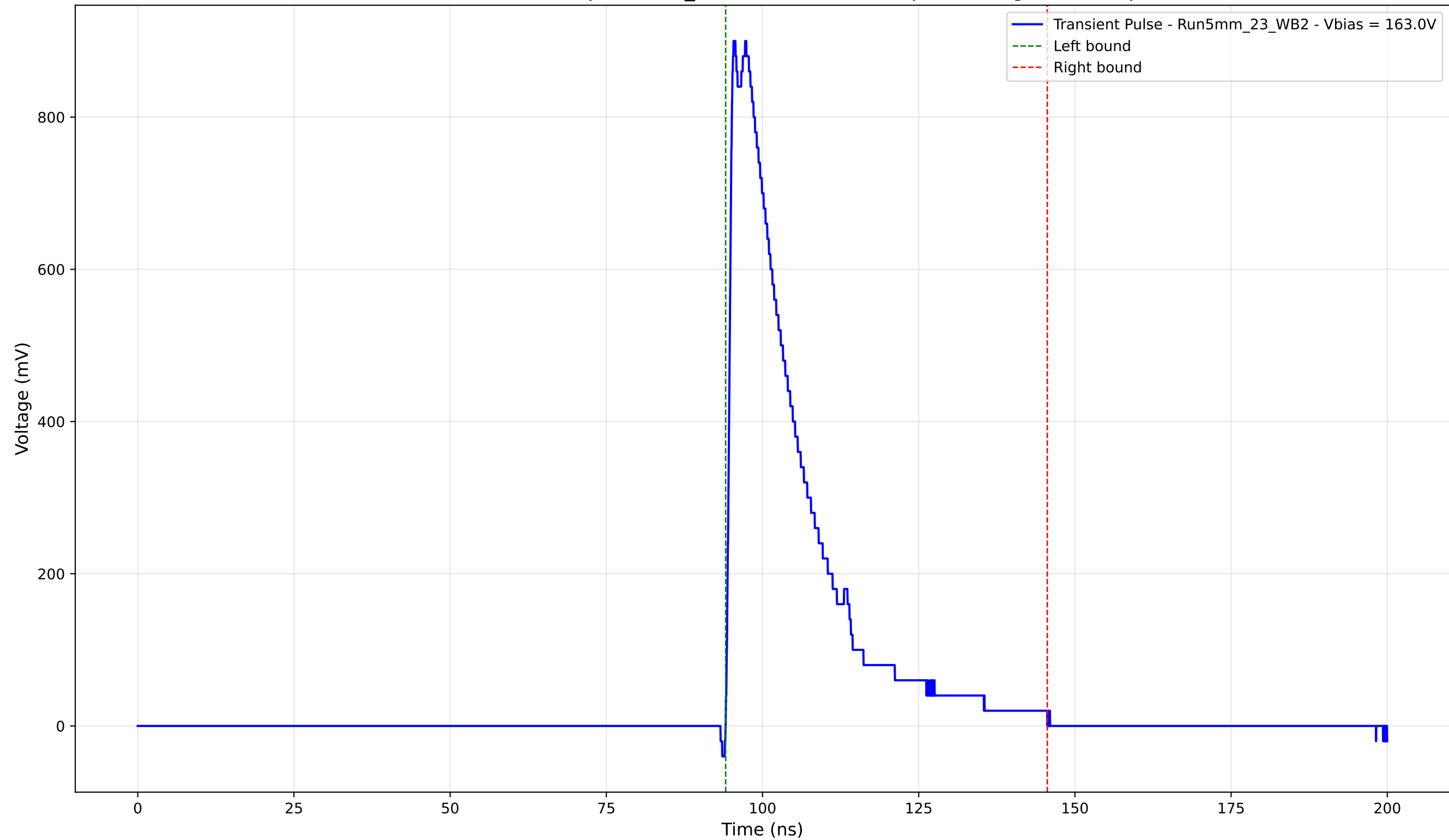
Transient Pulse - Sample: 5mm_23 - Position: 1880.0 \mu\text{m} - Charge: 217.76 pC
