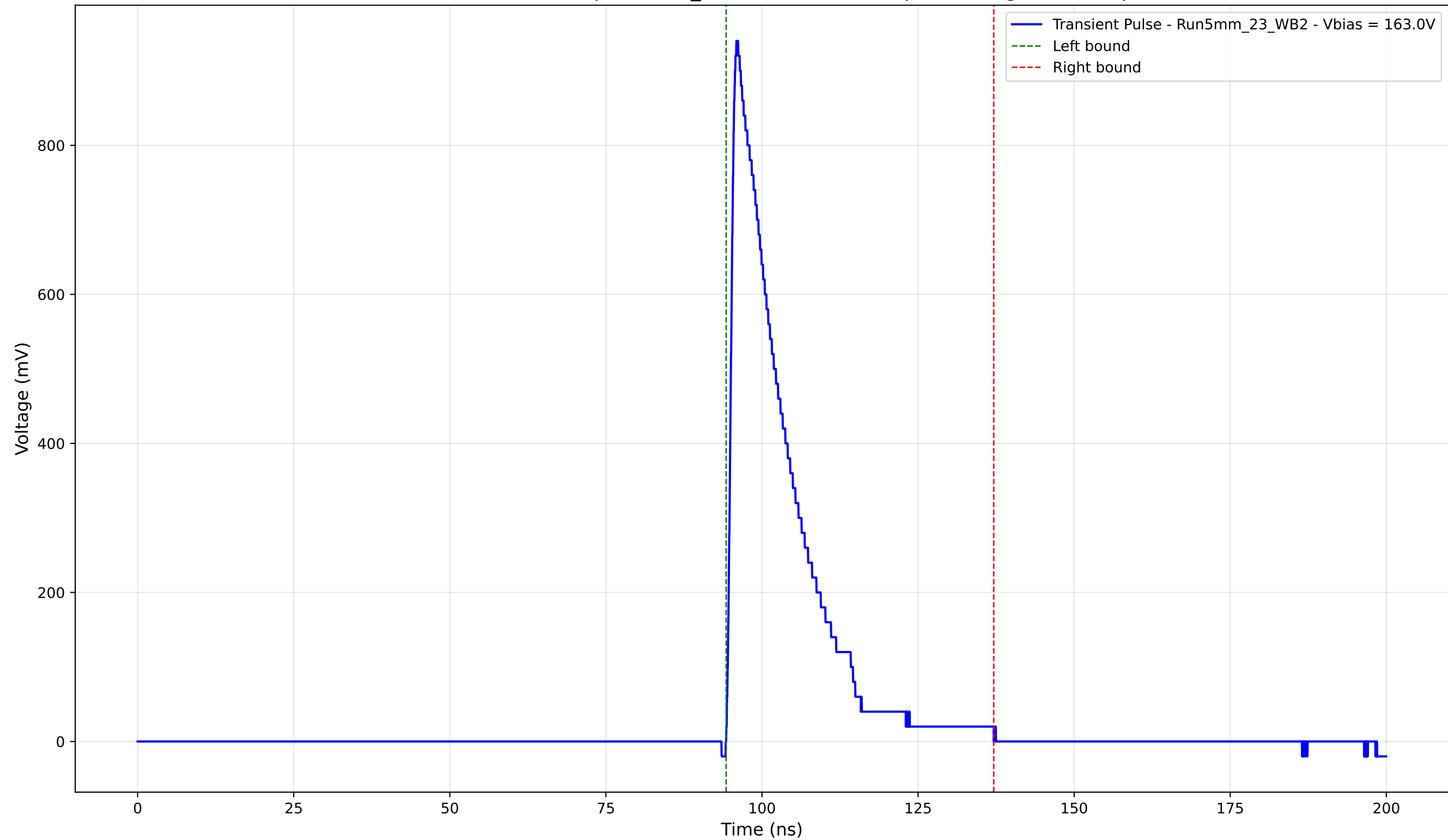
Transient Pulse - Sample: 5mm_23 - Position: 630.0 \mu\text{m} - Charge: 180.49 pC
