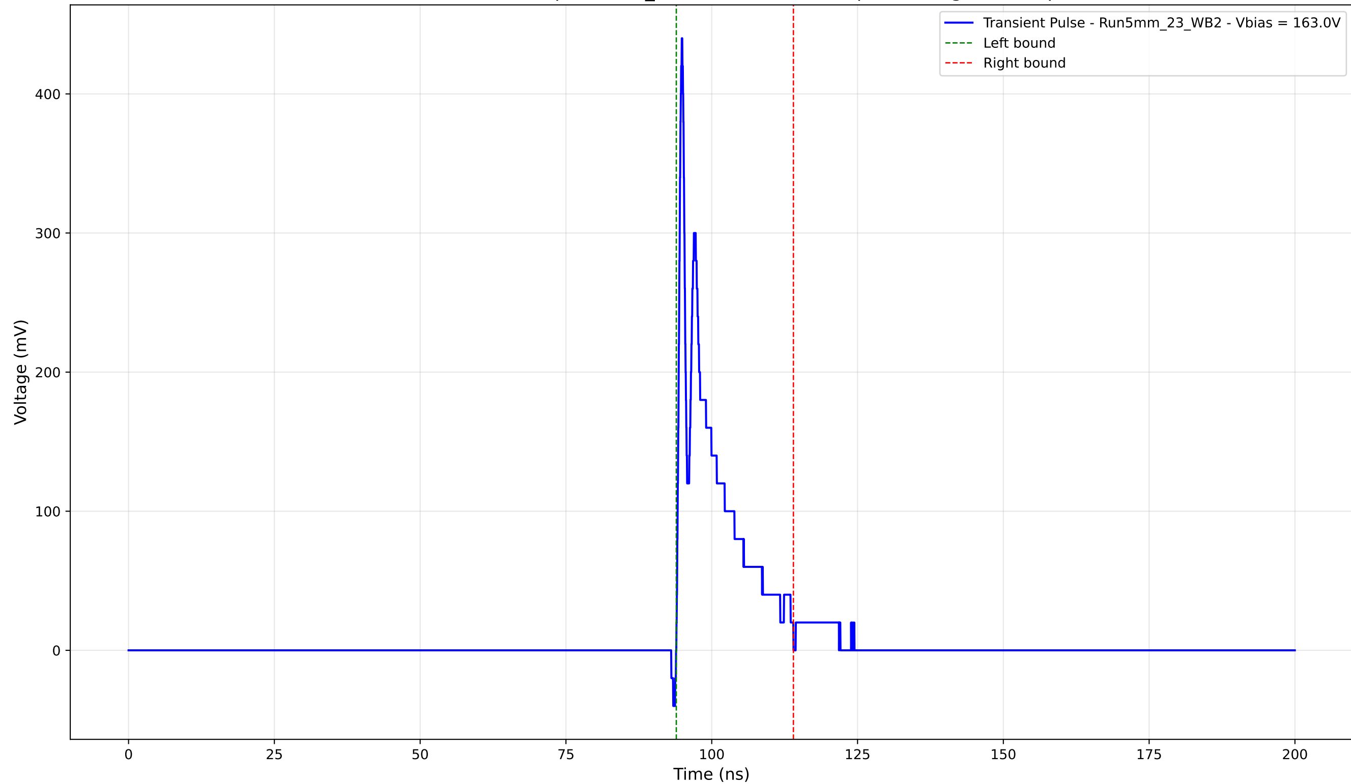
Transient Pulse - Sample: 5mm_23 - Position: 2535.0 \mu\text{m} - Charge: 45.51 pC
