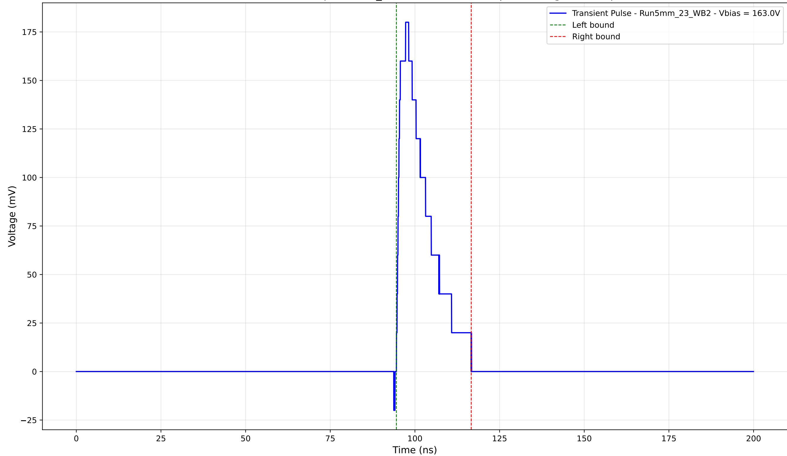
Transient Pulse - Sample: 5mm_23 -Position: 1505.0 \mu\text{m} - Charge: 33.58 pC
