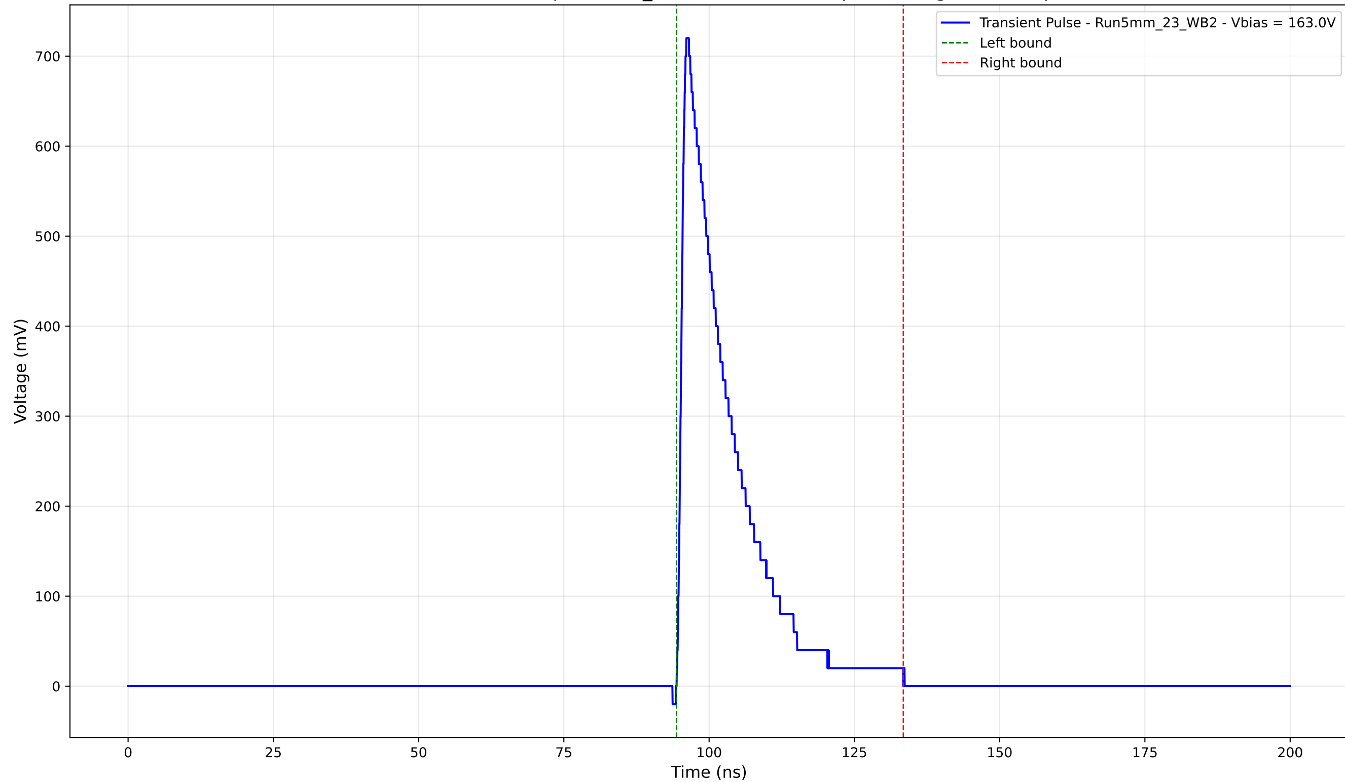
Transient Pulse - Sample: 5mm_23 - Position: 930.0 \mu\text{m} - Charge: 131.74 pC
