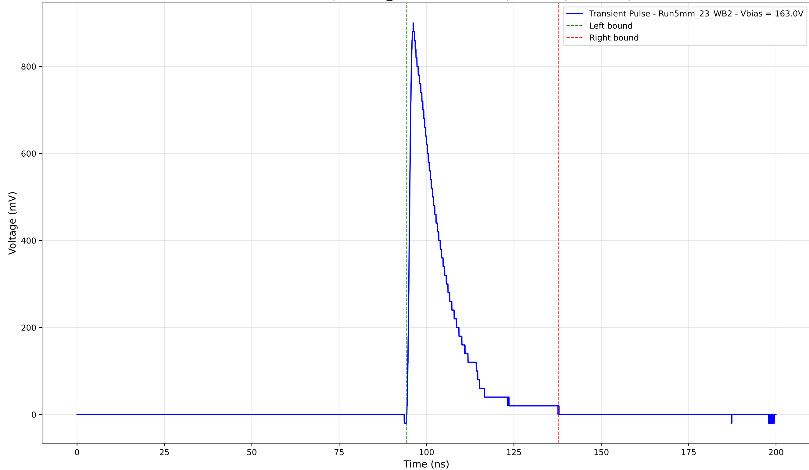
Transient Pulse - Sample: 5mm_23 - Position: 830.0 \mu\text{m} - Charge: 174.16 pC
