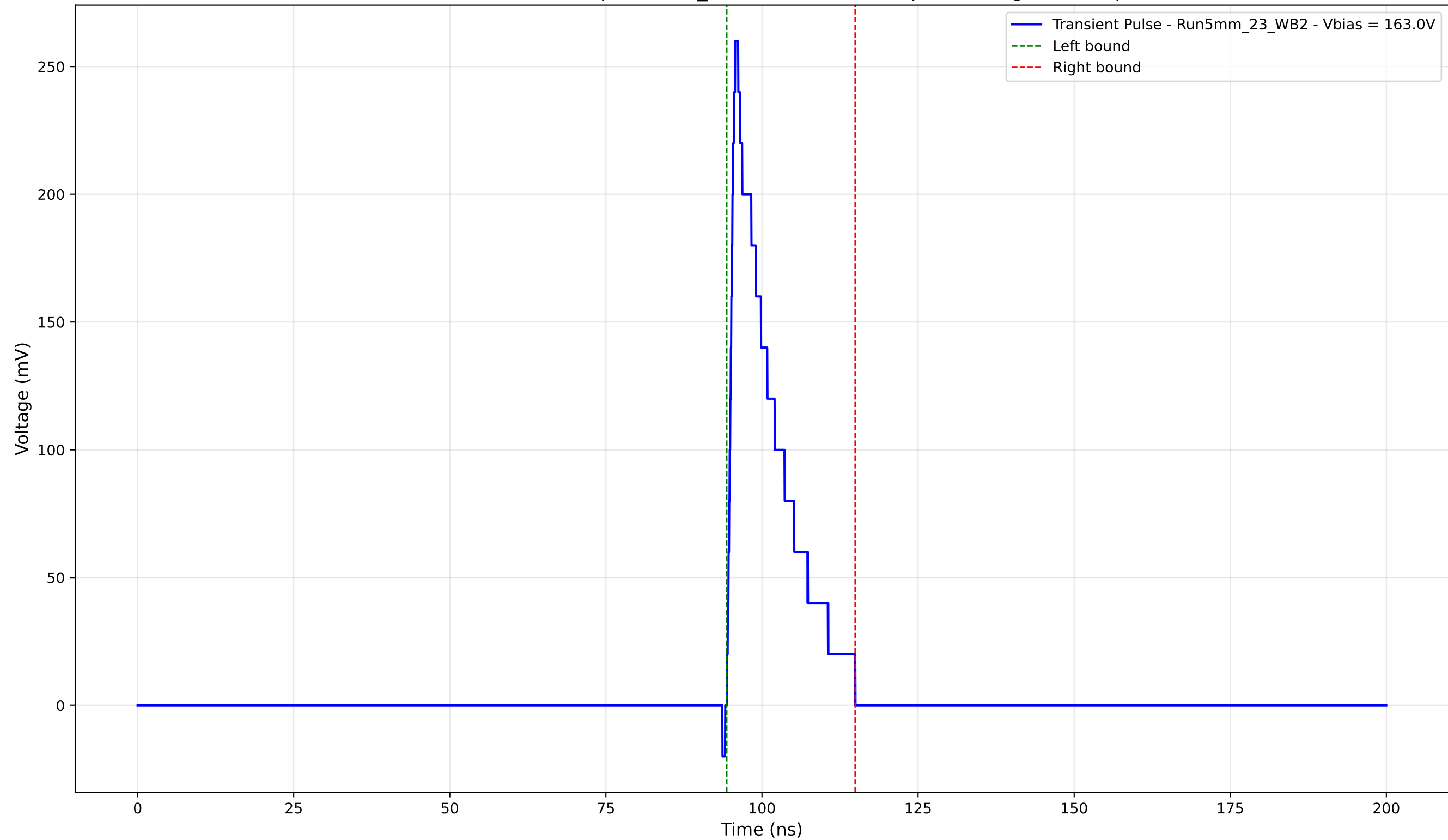
Transient Pulse - Sample: 5mm_23 - Position: 475.0 \mu\text{m} - Charge: 38.46 pC
