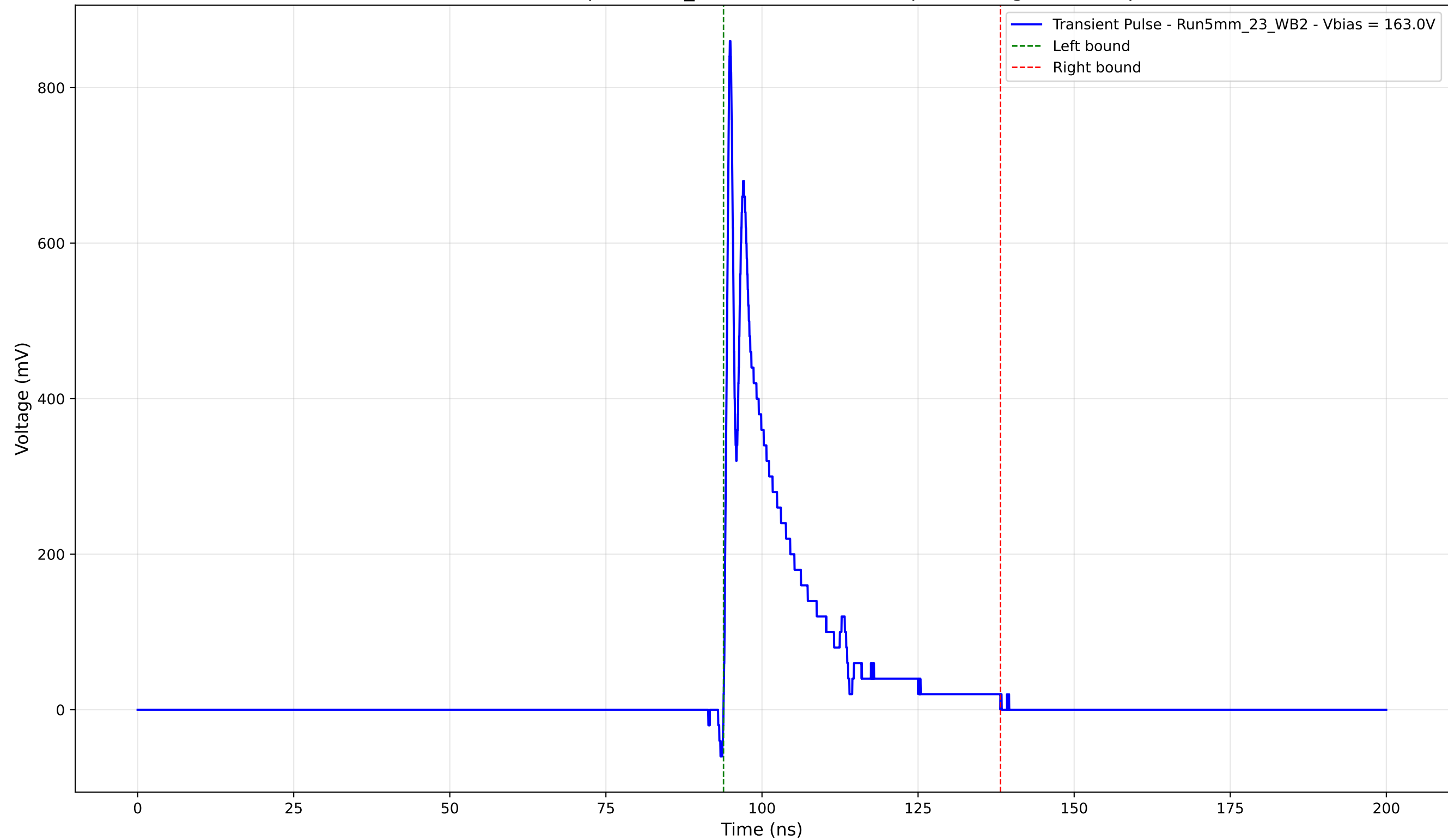
Transient Pulse - Sample: 5mm_23 - Position: 2570.0 \mu\text{m} - Charge: 125.07 pC
