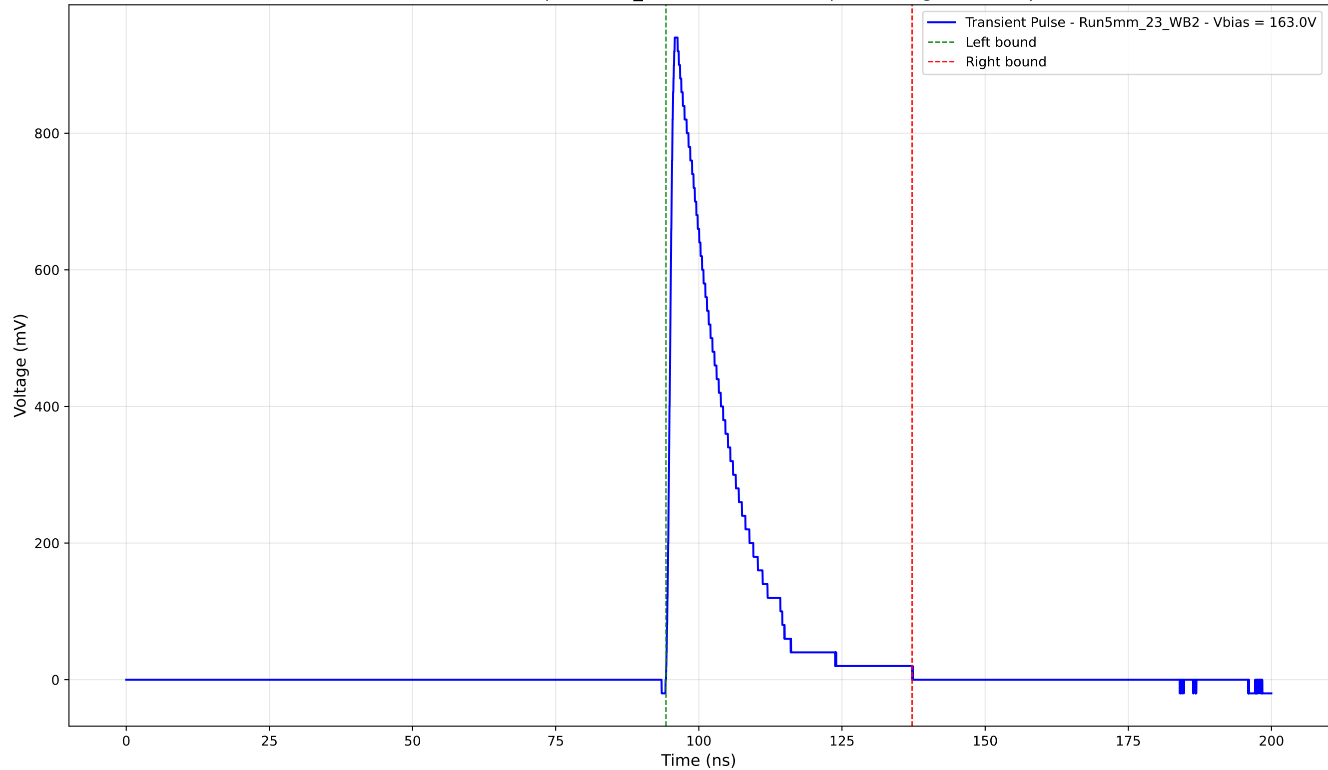
Transient Pulse - Sample: 5mm_23 - Position: 615.0 \mu\text{m} - Charge: 183.52 pC
