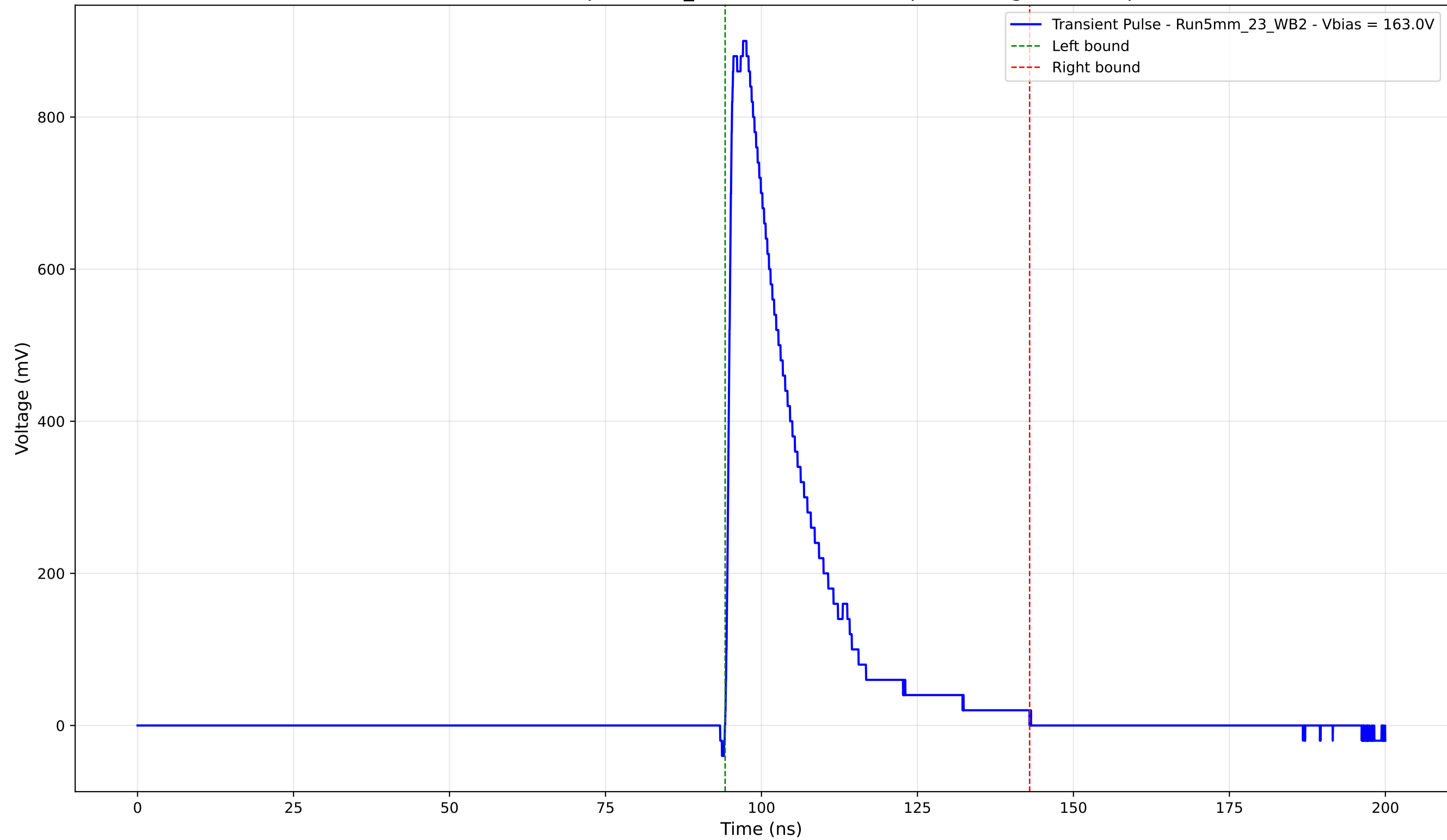
Transient Pulse - Sample: 5mm_23 - Position: 3300.0 \mu\text{m} - Charge: 206.92 pC
