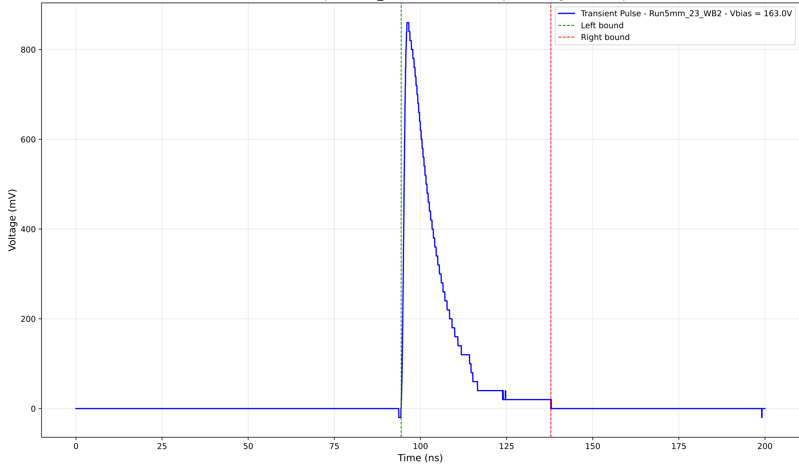
Transient Pulse - Sample: 5mm_23 - Position: 3885.0 \mu\text{m} - Charge: 171.74 pC
