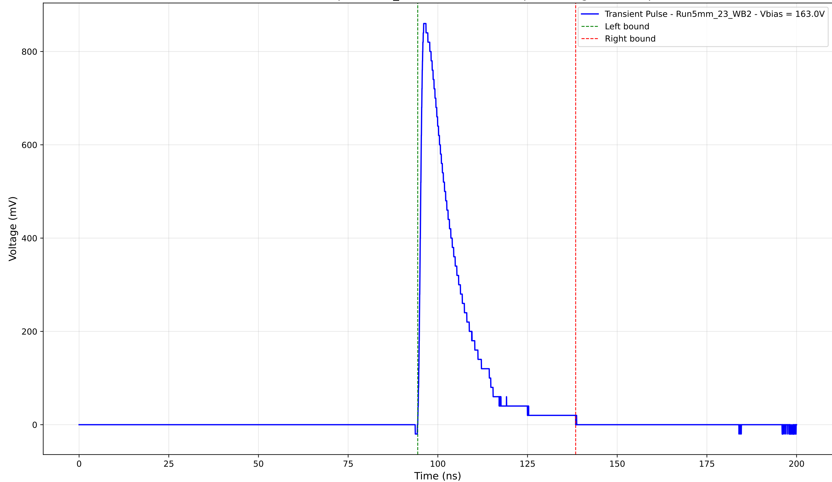
Transient Pulse - Sample: 5mm_23 - Position: 3775.0 \mu\text{m} - Charge: 177.35 pC
