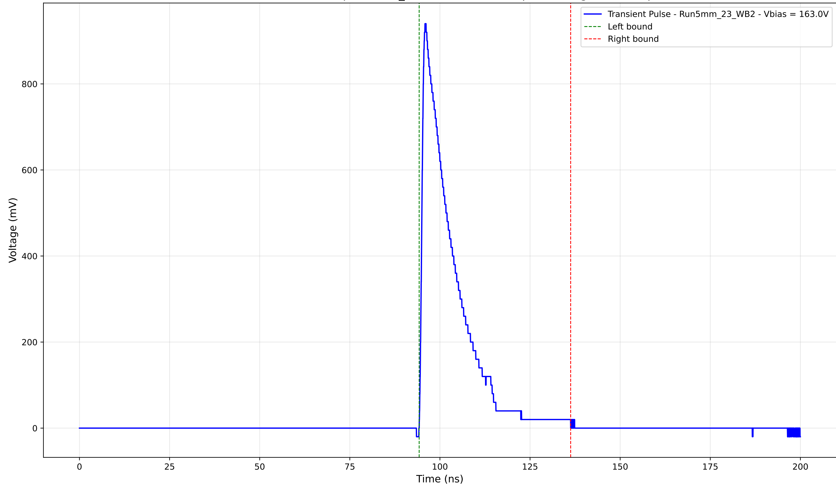
Transient Pulse - Sample: 5mm_23 - Position: 575.0 \mu\text{m} - Charge: 176.61 pC
