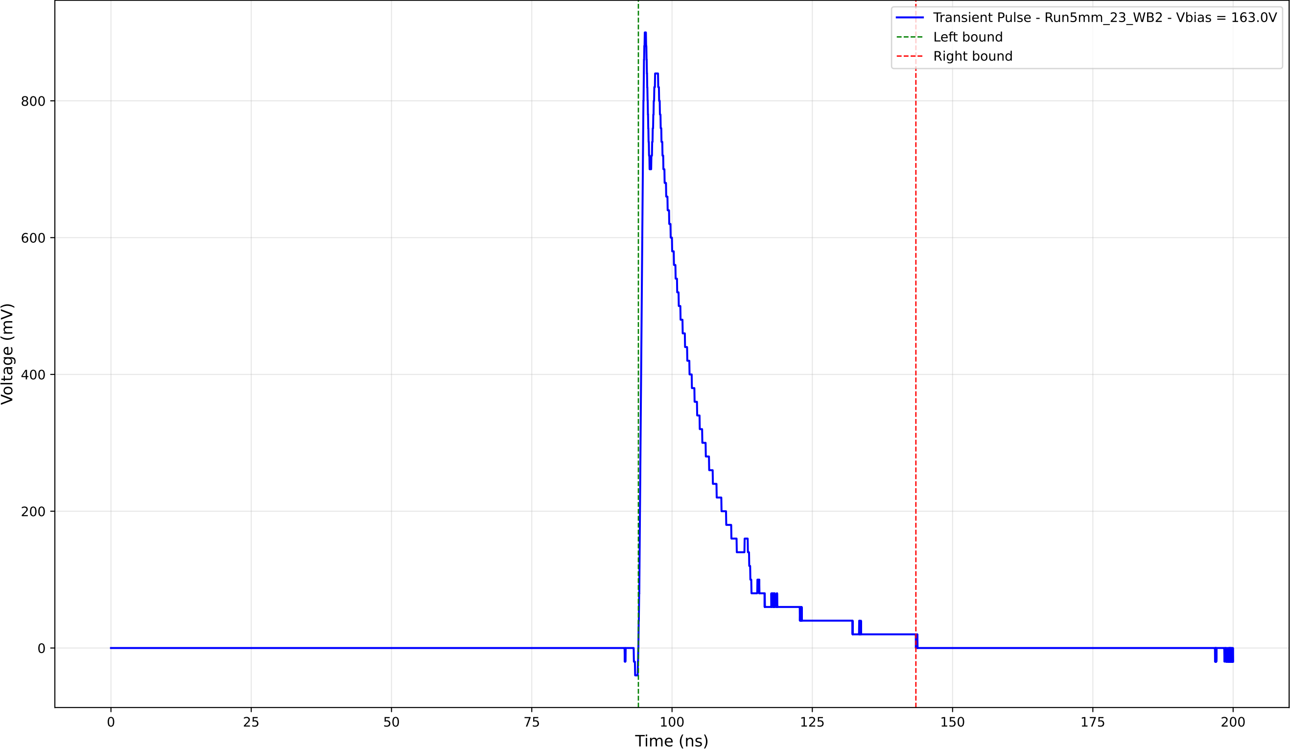
Transient Pulse - Sample: 5mm_23 - Position: 2100.0 \mu\text{m} - Charge: 188.28 pC
