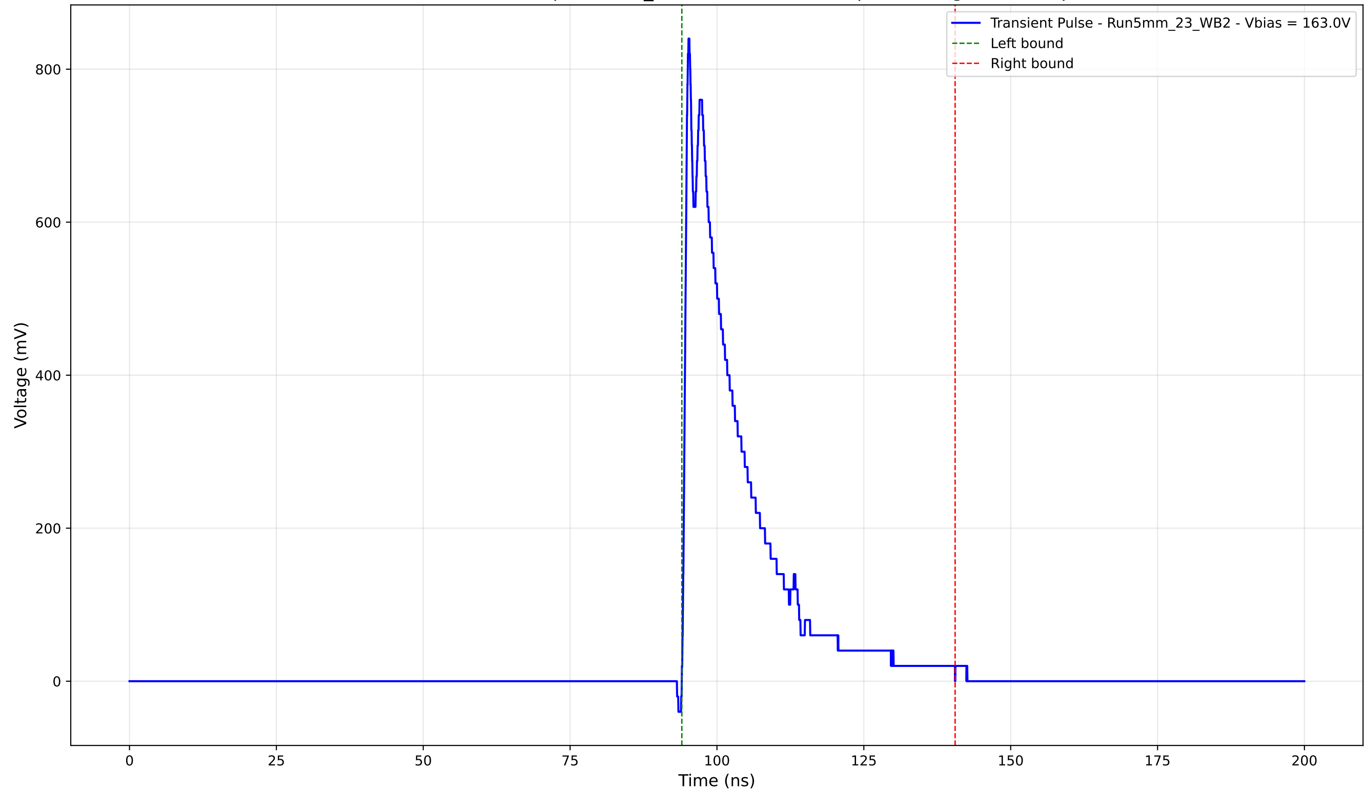
Transient Pulse - Sample: 5mm_23 - Position: 2080.0 \mu\text{m} - Charge: 162.98 pC
