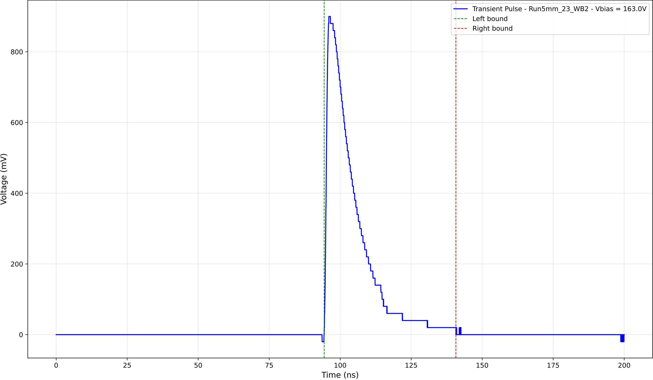
Transient Pulse - Sample: 5mm_23 - Position: 1315.0 \mu\text{m} - Charge: 200.94 pC
