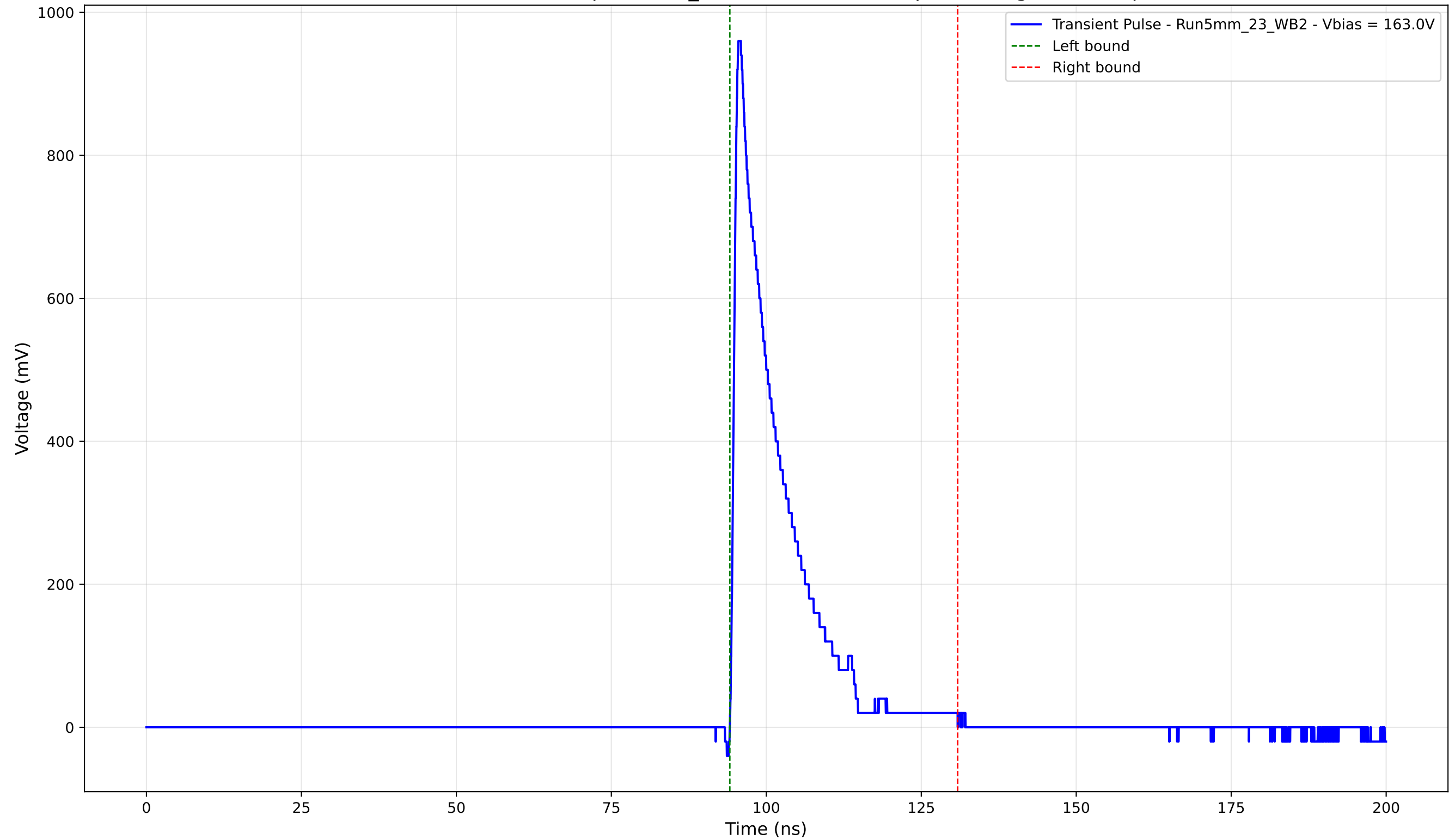
Transient Pulse - Sample: 5mm_23 - Position: 4755.0 \mu\text{m} - Charge: 148.32 pC
