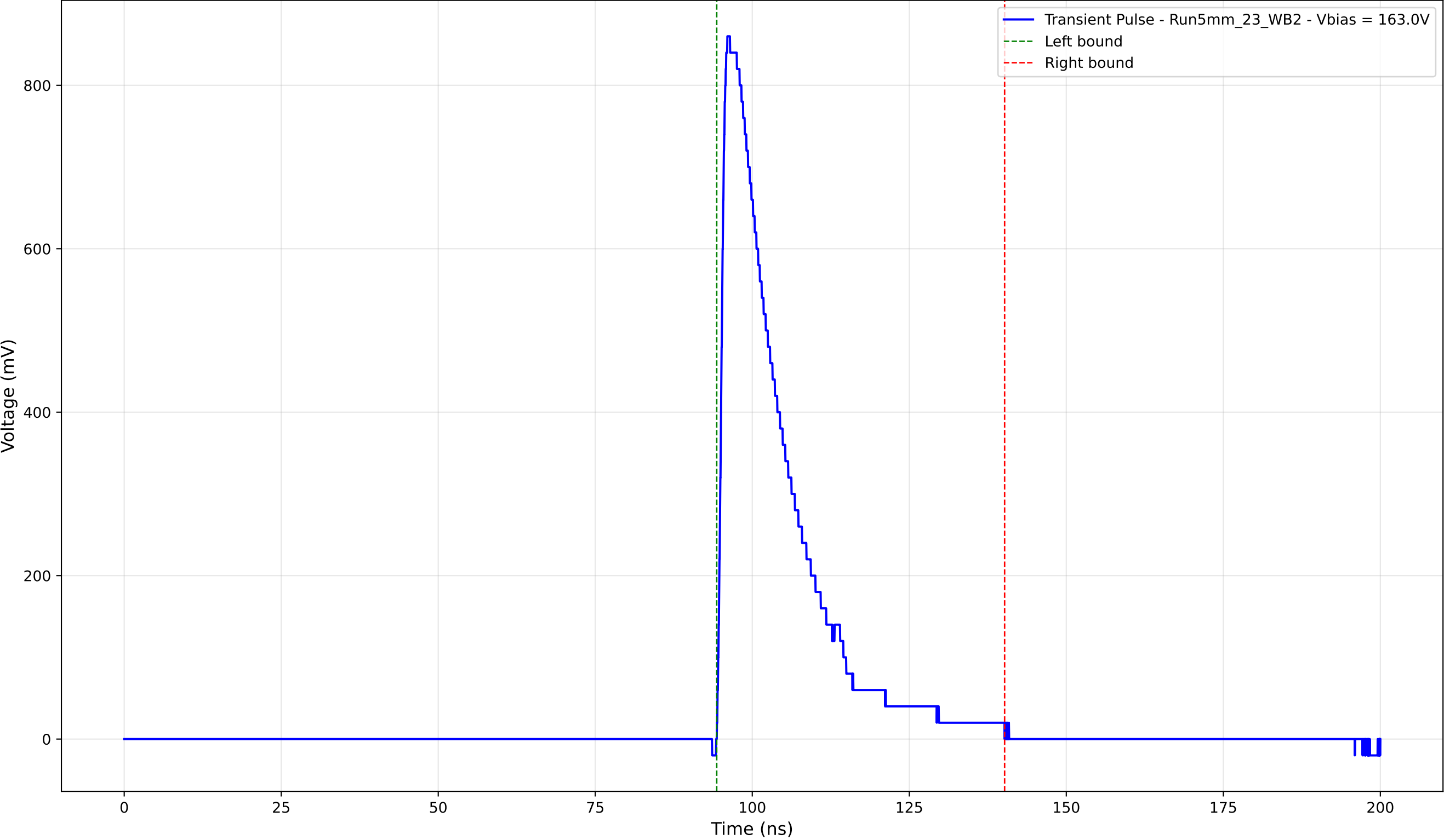
Transient Pulse - Sample: 5mm_23 - Position: 1405.0 \mu\text{m} - Charge: 188.26 pC
