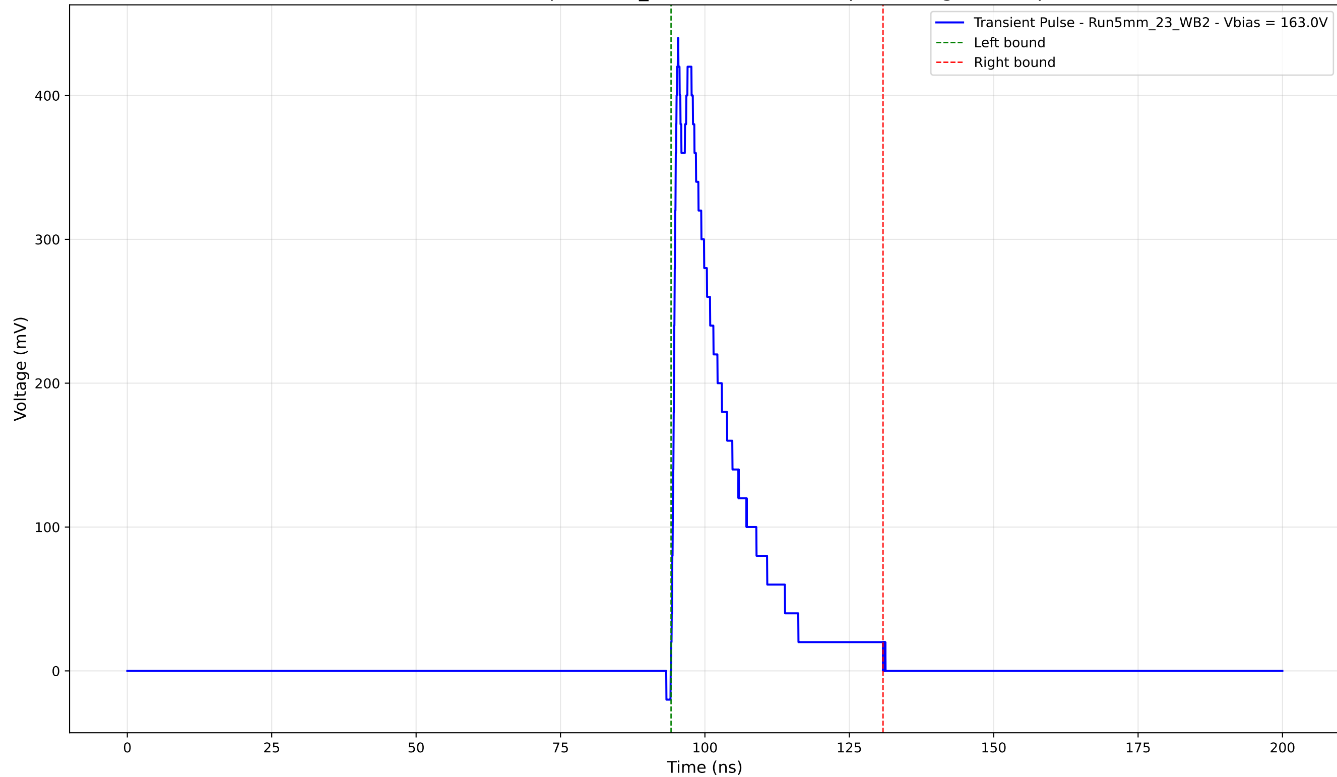
Transient Pulse - Sample: 5mm_23 - Position: 3055.0 \mu\text{m} - Charge: 83.85 pC
