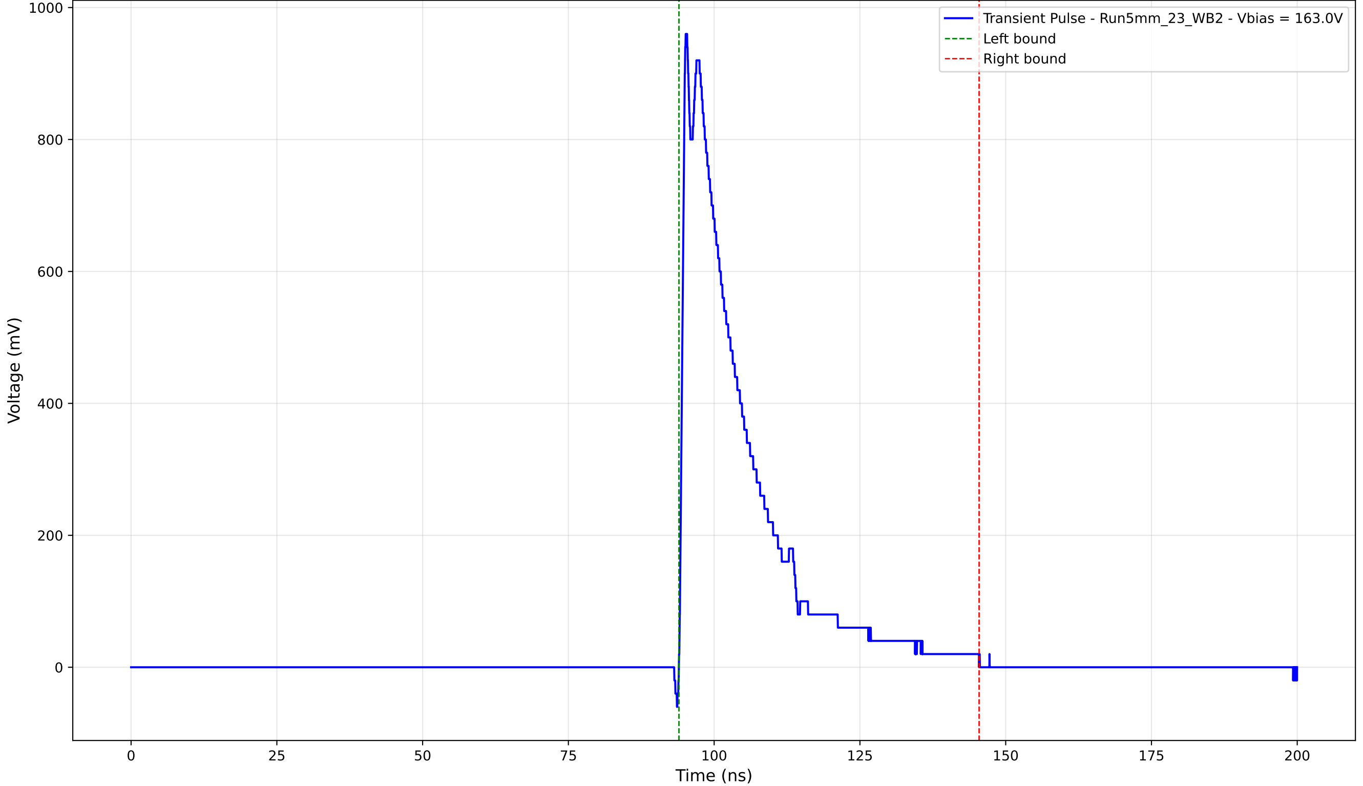
Transient Pulse - Sample: 5mm_23 - Position: 2920.0 \mu\text{m} - Charge: 216.08 pC
