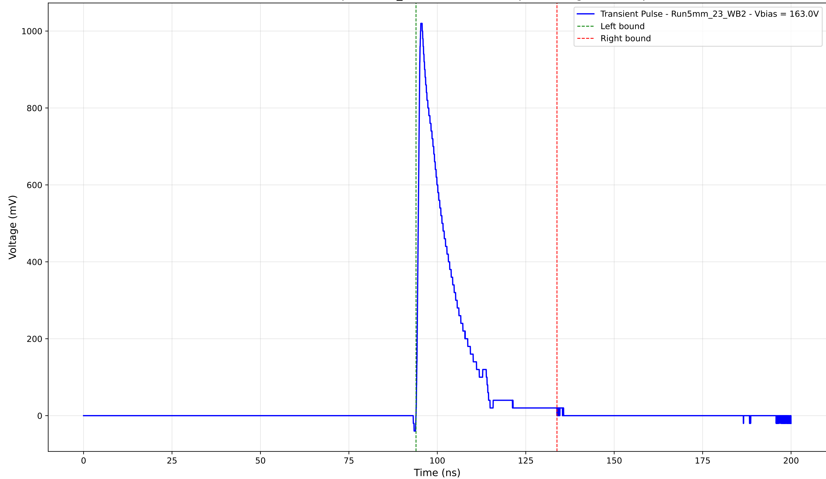
Transient Pulse - Sample: 5mm_23 - Position: 135.0 \mu\text{m} - Charge: 177.18 pC
