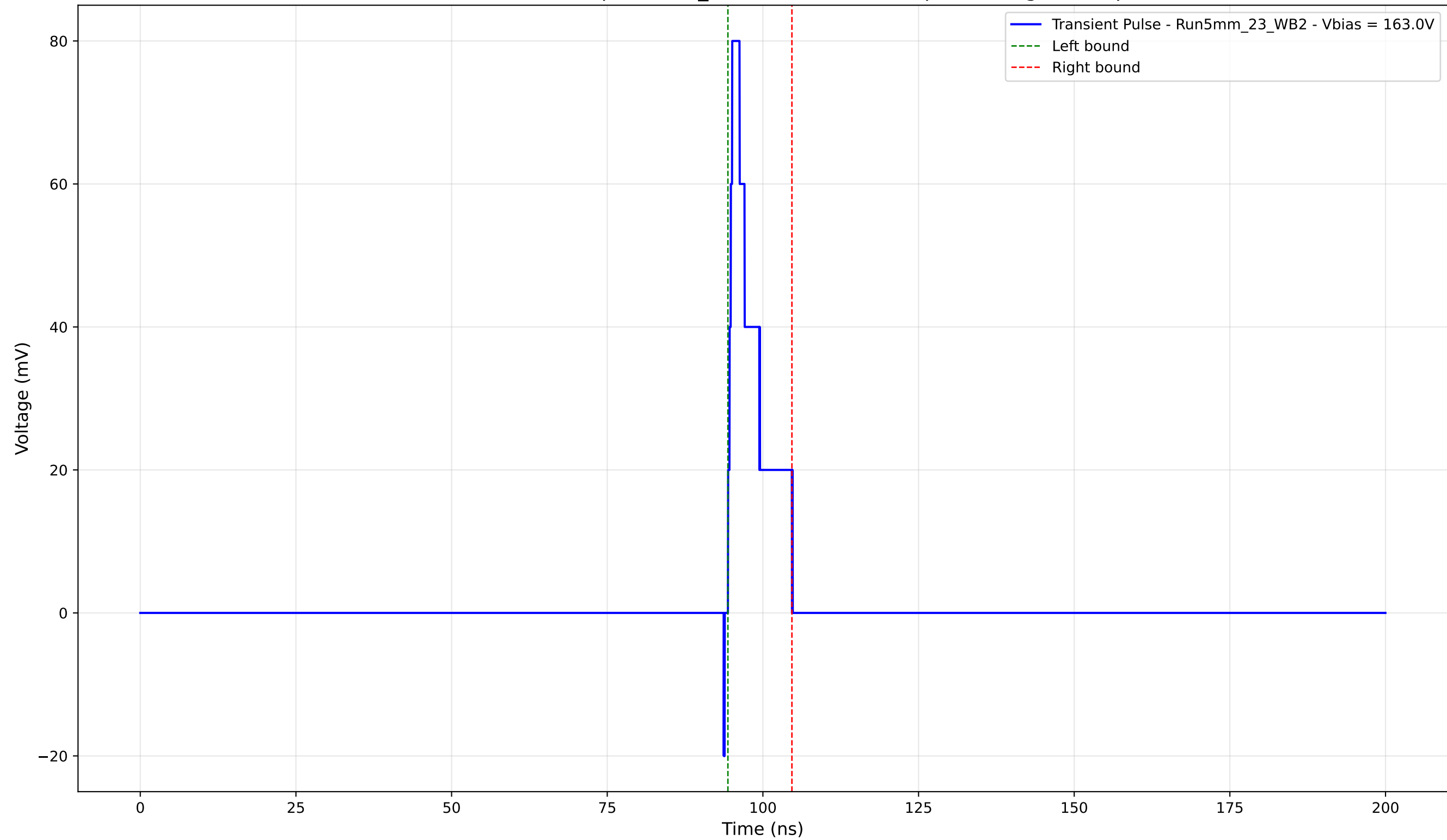
Transient Pulse - Sample: 5mm_23 - Position: 4980.0 \mu\text{m} - Charge: 7.42 pC
