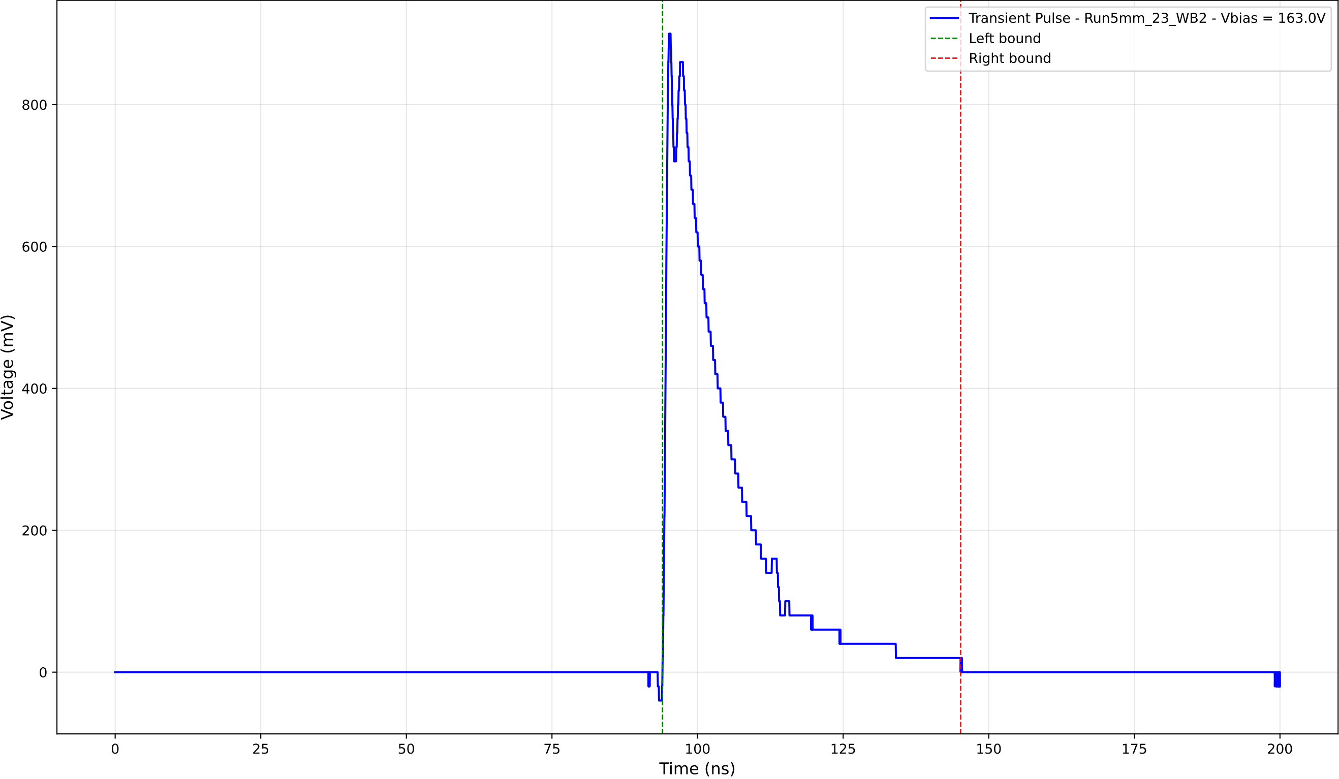
Transient Pulse - Sample: 5mm_23 - Position: 2115.0 \mu\text{m} - Charge: 196.93 pC
