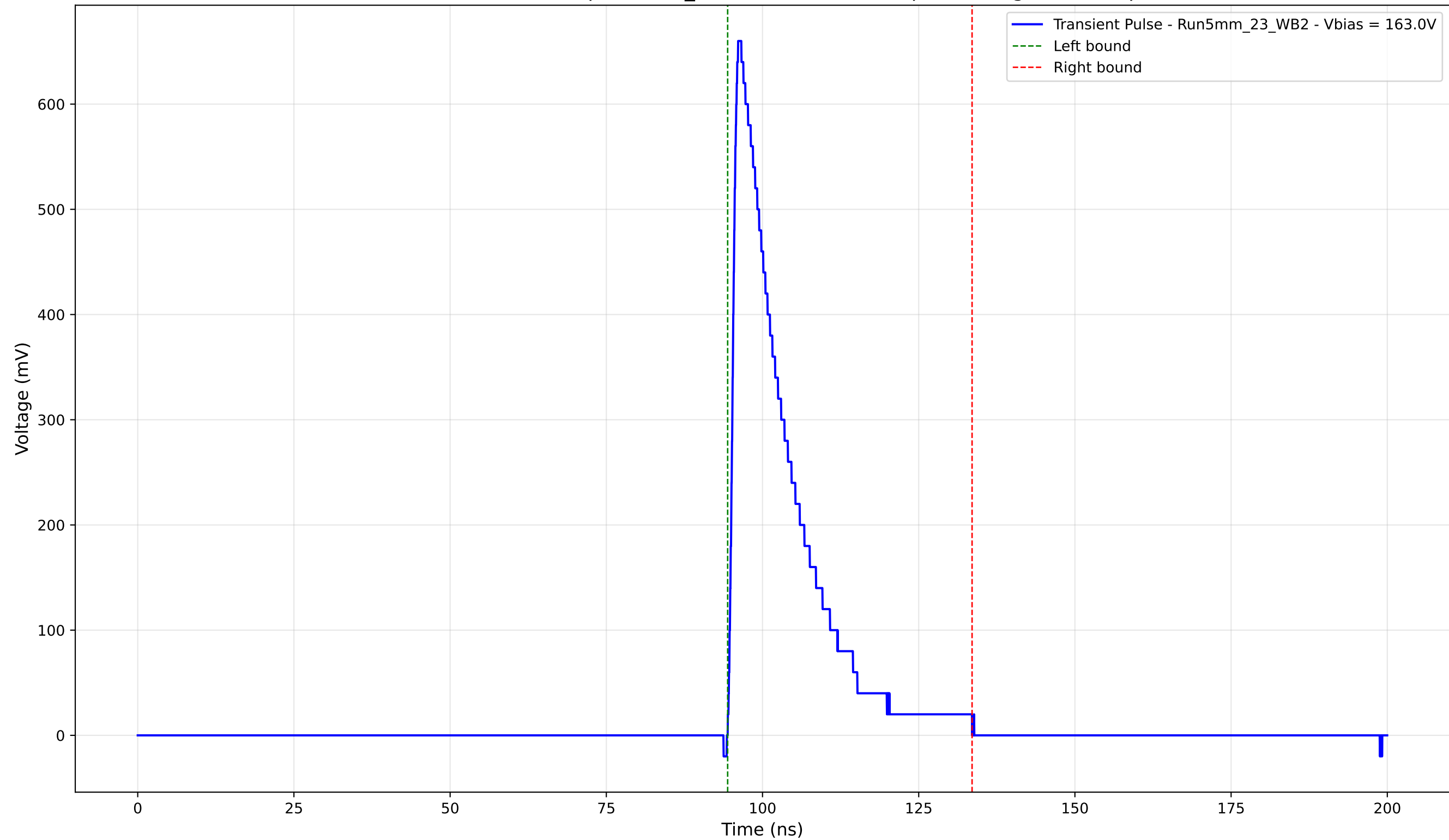
Transient Pulse - Sample: 5mm_23 - Position: 1050.0 \mu\text{m} - Charge: 125.38 pC
