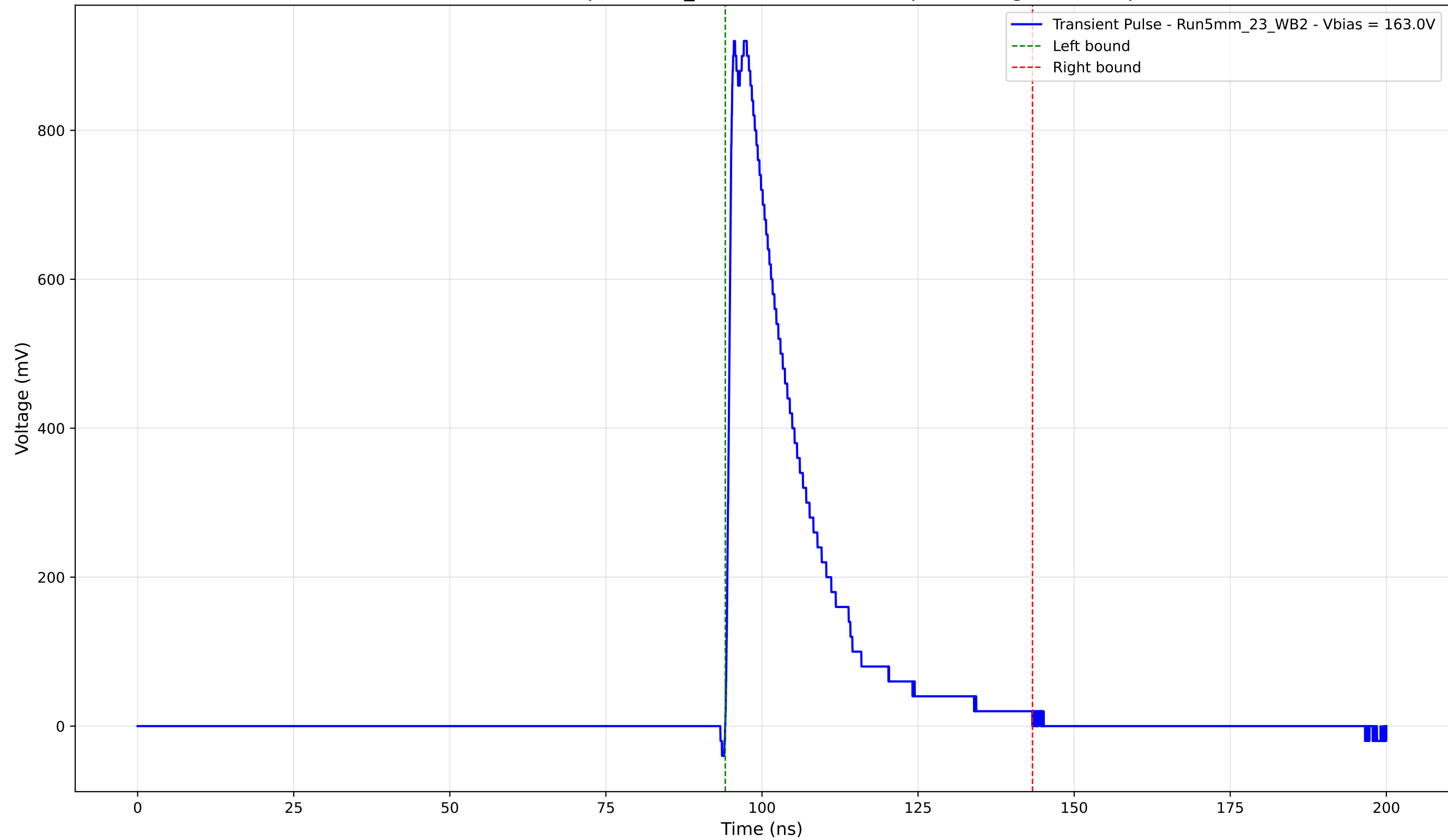
Transient Pulse - Sample: 5mm_23 - Position: 3215.0 \mu\text{m} - Charge: 216.59 pC
