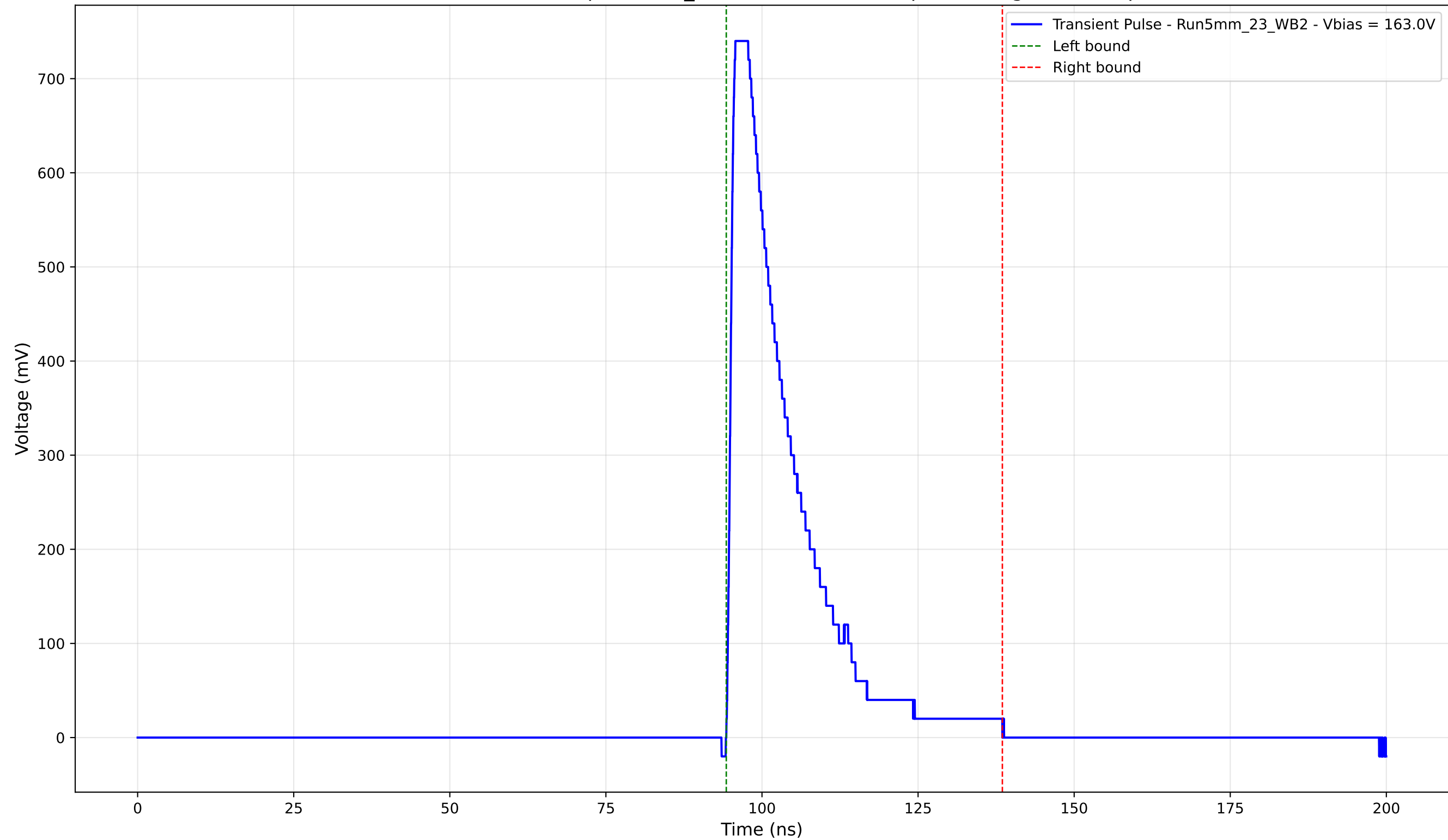
Transient Pulse - Sample: 5mm_23 - Position: 3445.0 \mu\text{m} - Charge: 158.42 pC
