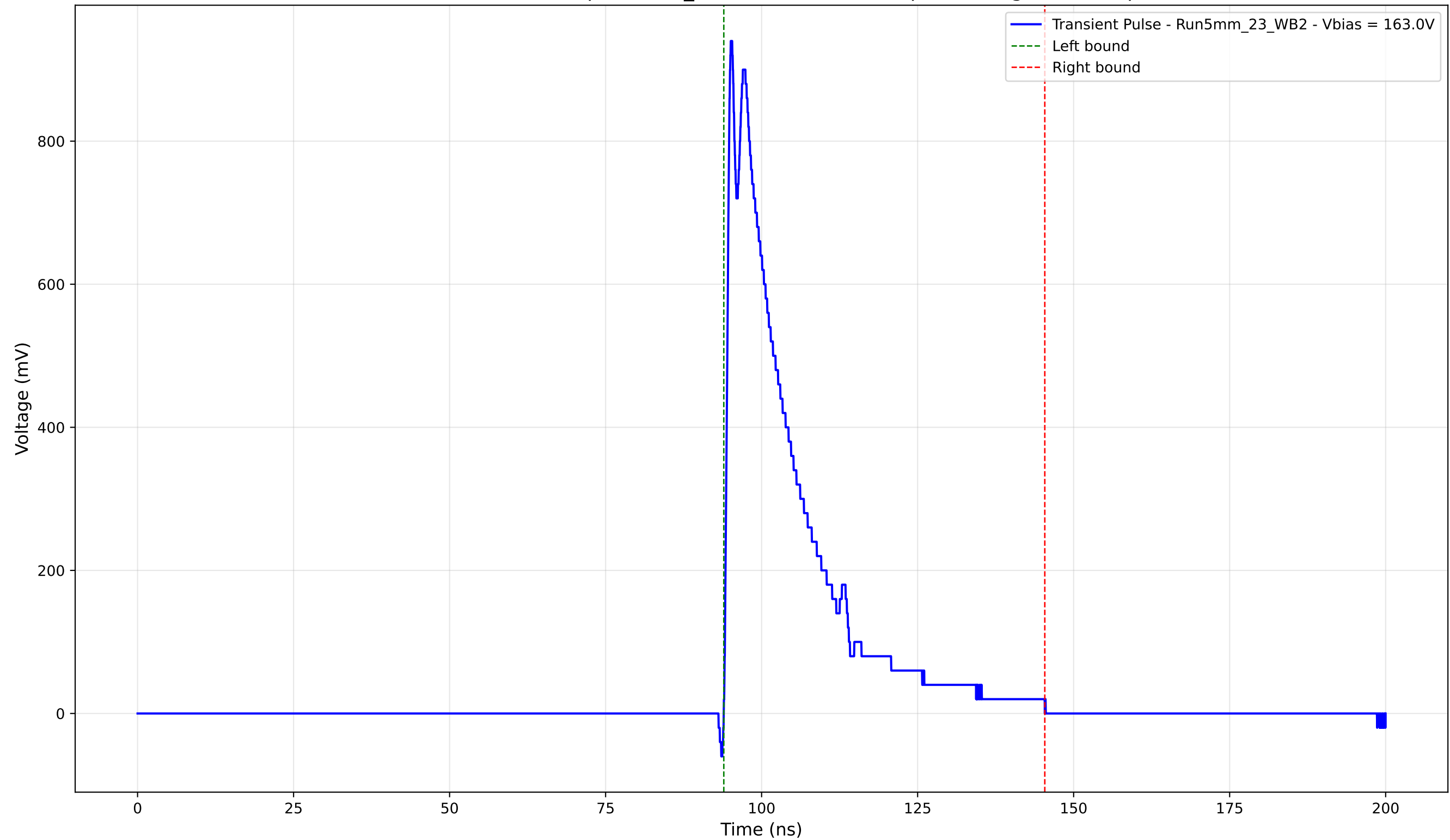
Transient Pulse - Sample: 5mm_23 - Position: 2175.0 \mu\text{m} - Charge: 205.70 pC
