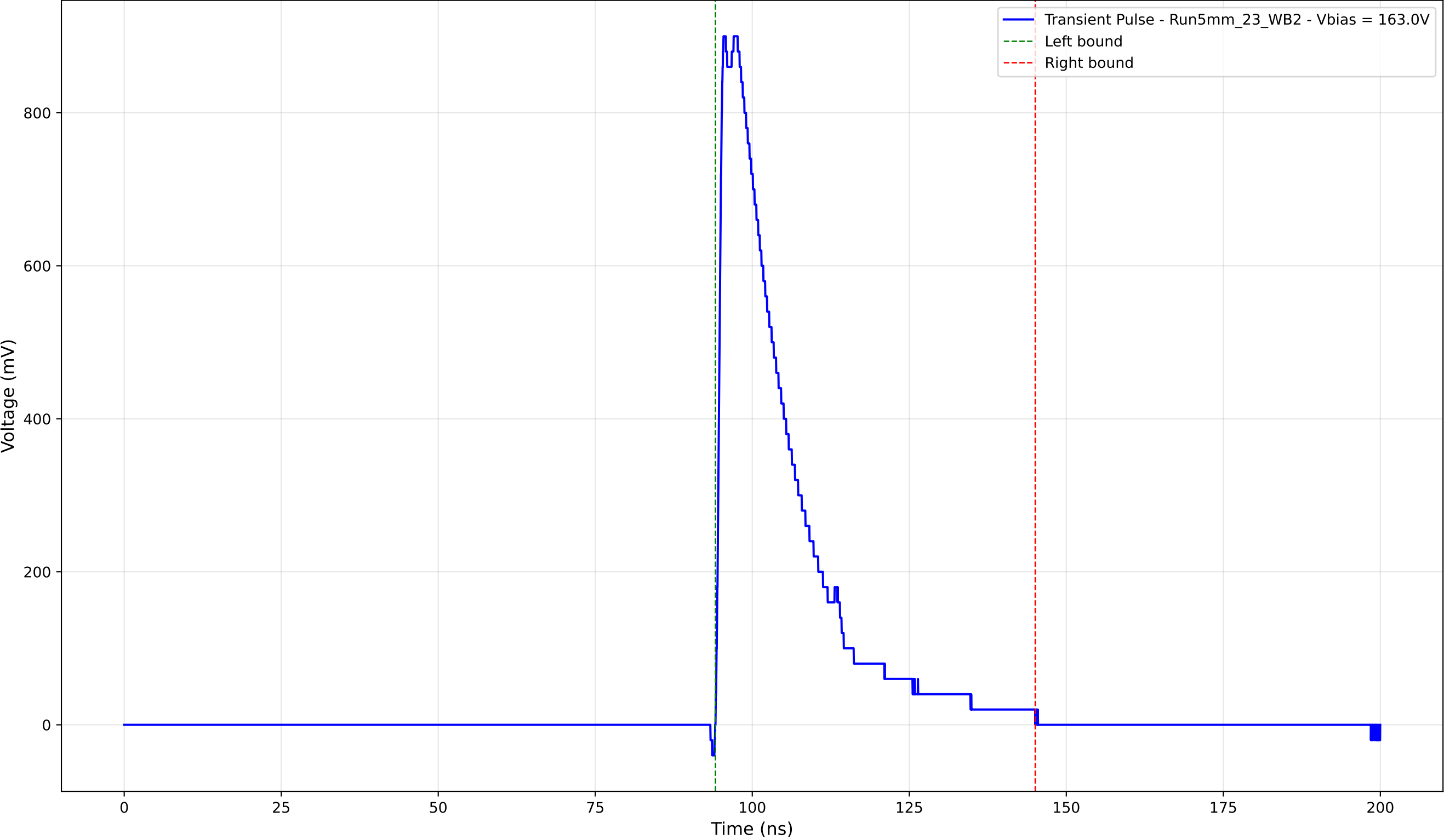
Transient Pulse - Sample: 5mm_23 - Position: 1815.0 \mu\text{m} - Charge: 218.91 pC
