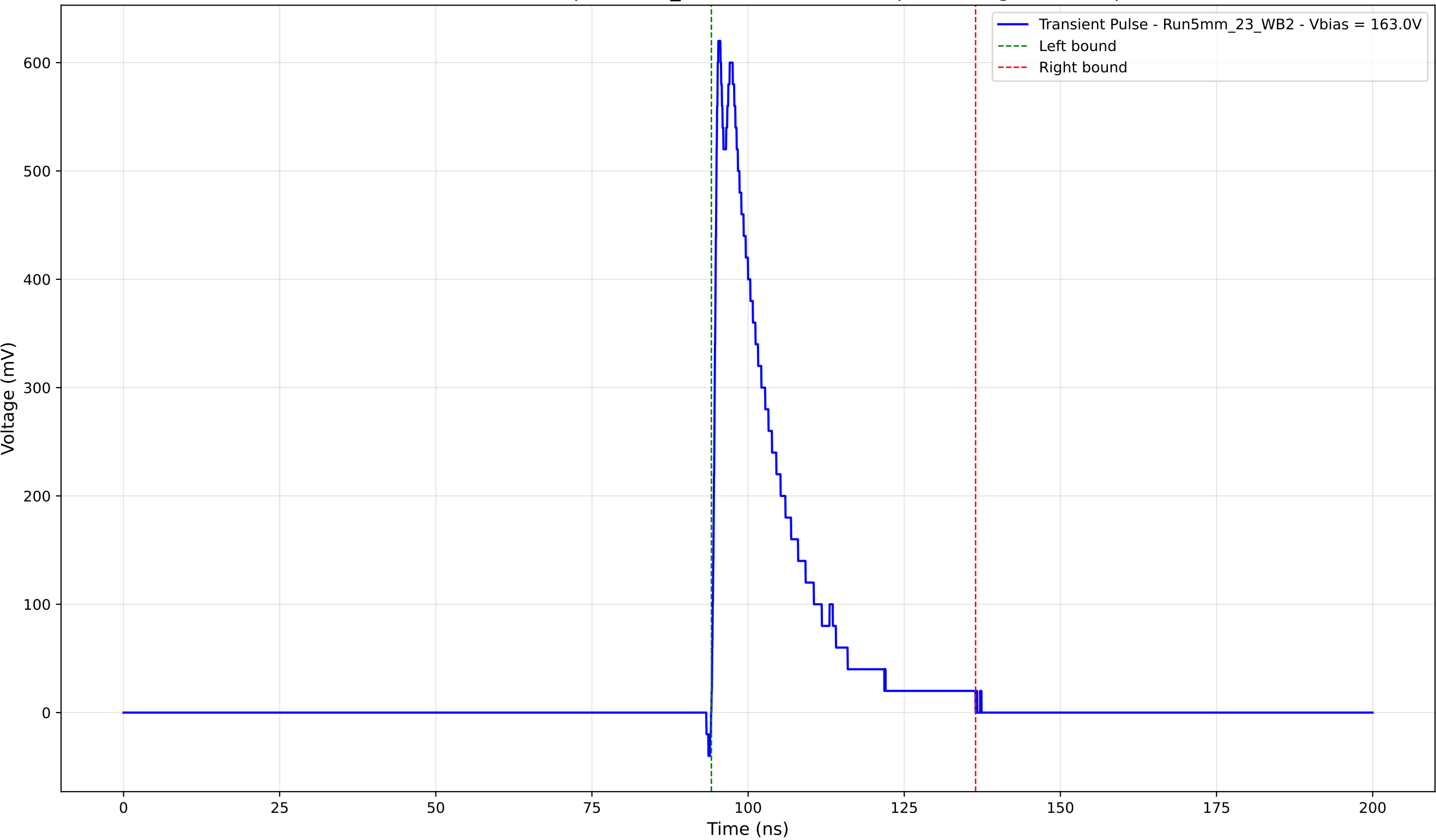
Transient Pulse - Sample: 5mm_23 - Position: 1960.0 \mu\text{m} - Charge: 124.02 pC
