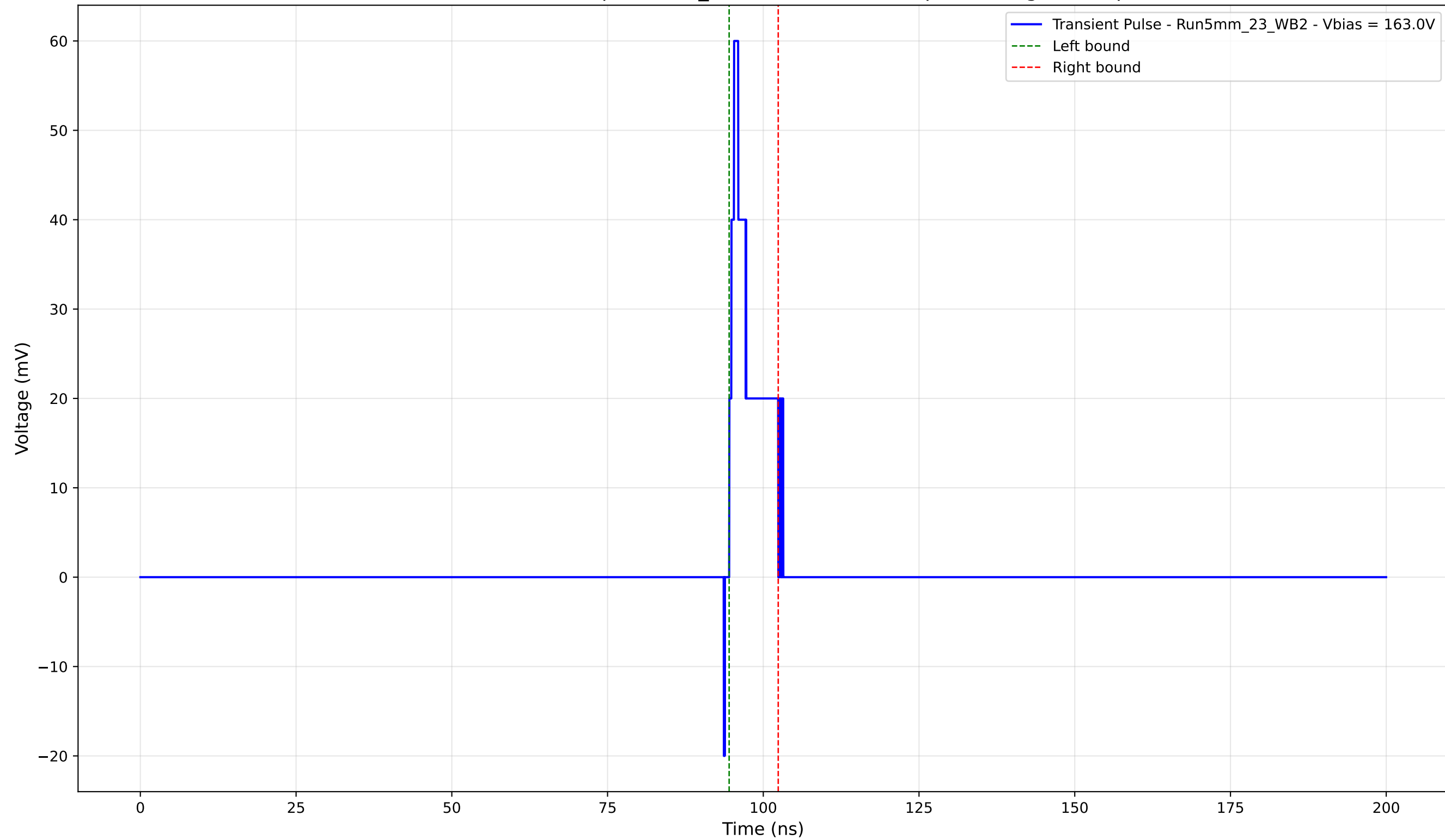
Transient Pulse - Sample: 5mm_23 - Position: 4995.0 \mu\text{m} - Charge: 4.36 pC
