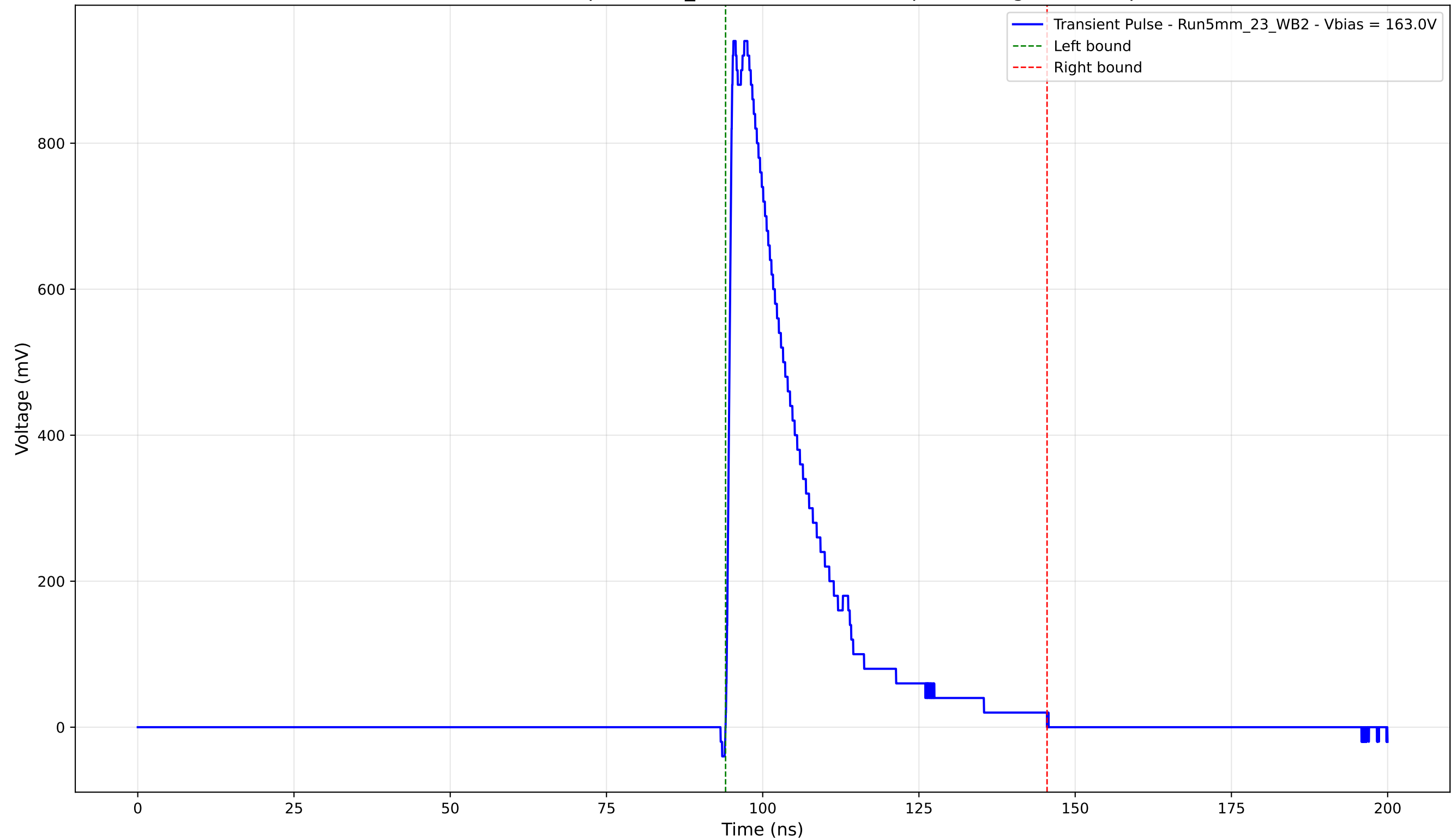
Transient Pulse - Sample: 5mm_23 - Position: 3140.0 \mu\text{m} - Charge: 226.61 pC
