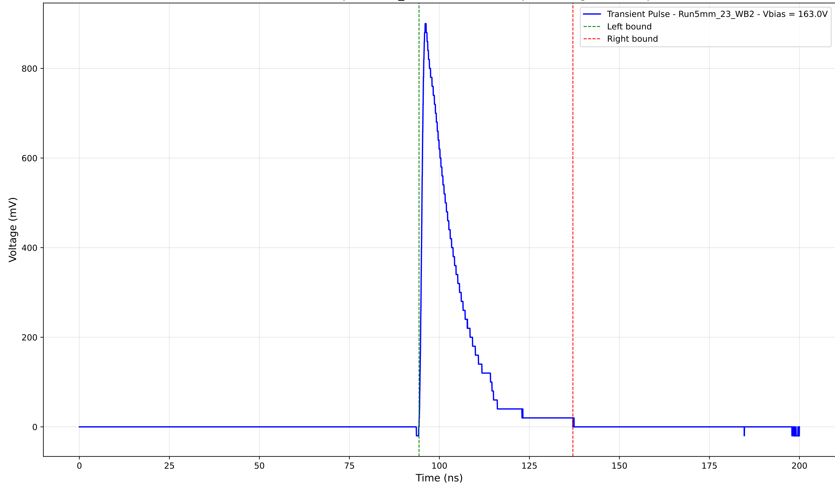
Transient Pulse - Sample: 5mm_23 - Position: 760.0 \mu\text{m} - Charge: 172.96 pC
