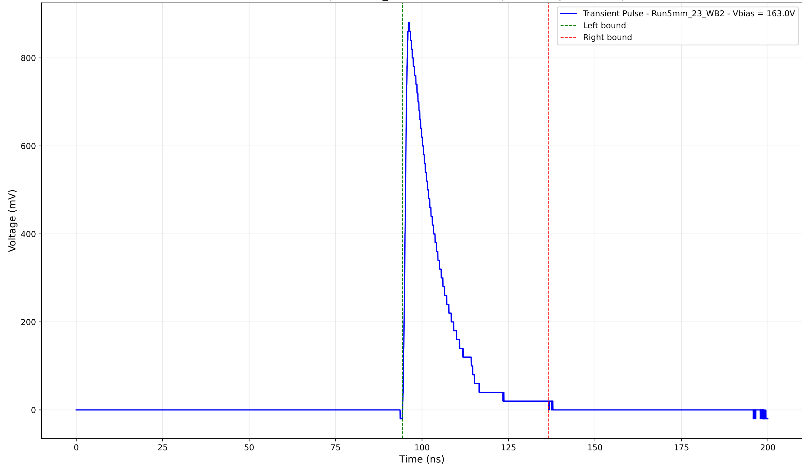
Transient Pulse - Sample: 5mm_23 - Position: 880.0 \mu\text{m} - Charge: 171.34 pC
