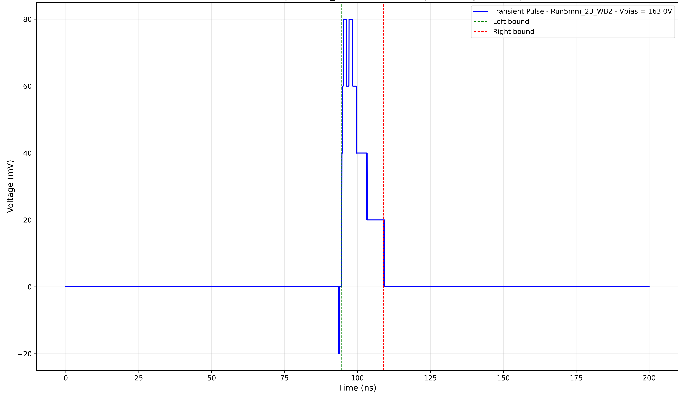
Transient Pulse - Sample: 5mm_23 - Position: 35.0 \mu\text{m} - Charge: 12.05 pC
