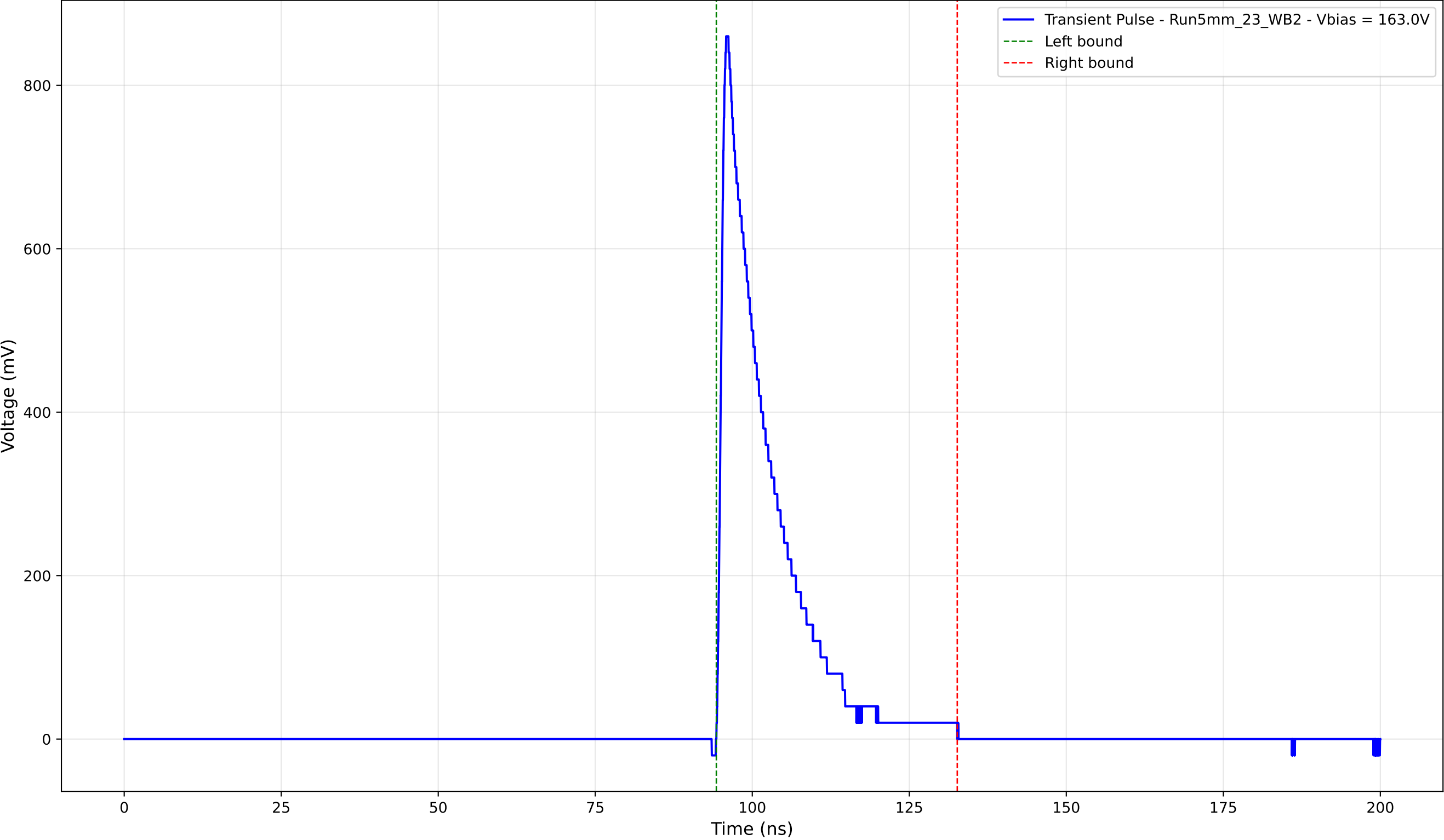
Transient Pulse - Sample: 5mm_23 - Position: 4455.0 \mu\text{m} - Charge: 141.66 pC
