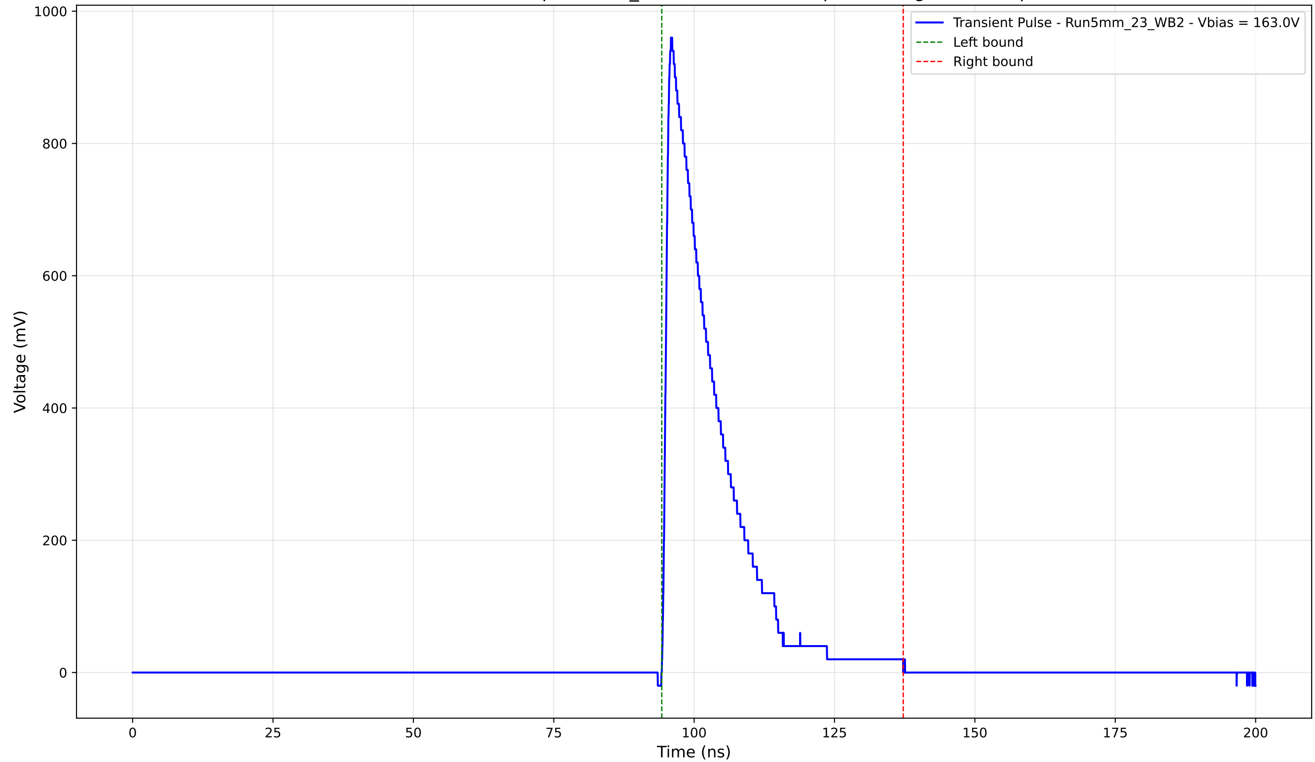
Transient Pulse - Sample: 5mm_23 - Position: 595.0 \mu\text{m} - Charge: 185.46 pC
