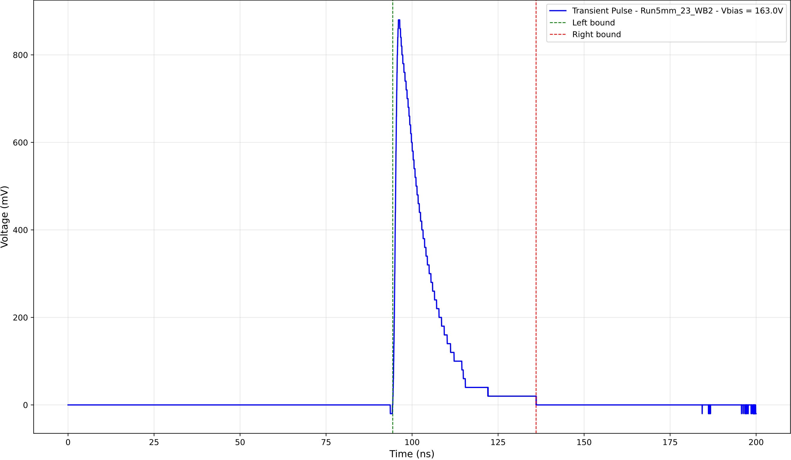
Transient Pulse - Sample: 5mm_23 - Position: 4170.0 \mu\text{m} - Charge: 162.78 pC
