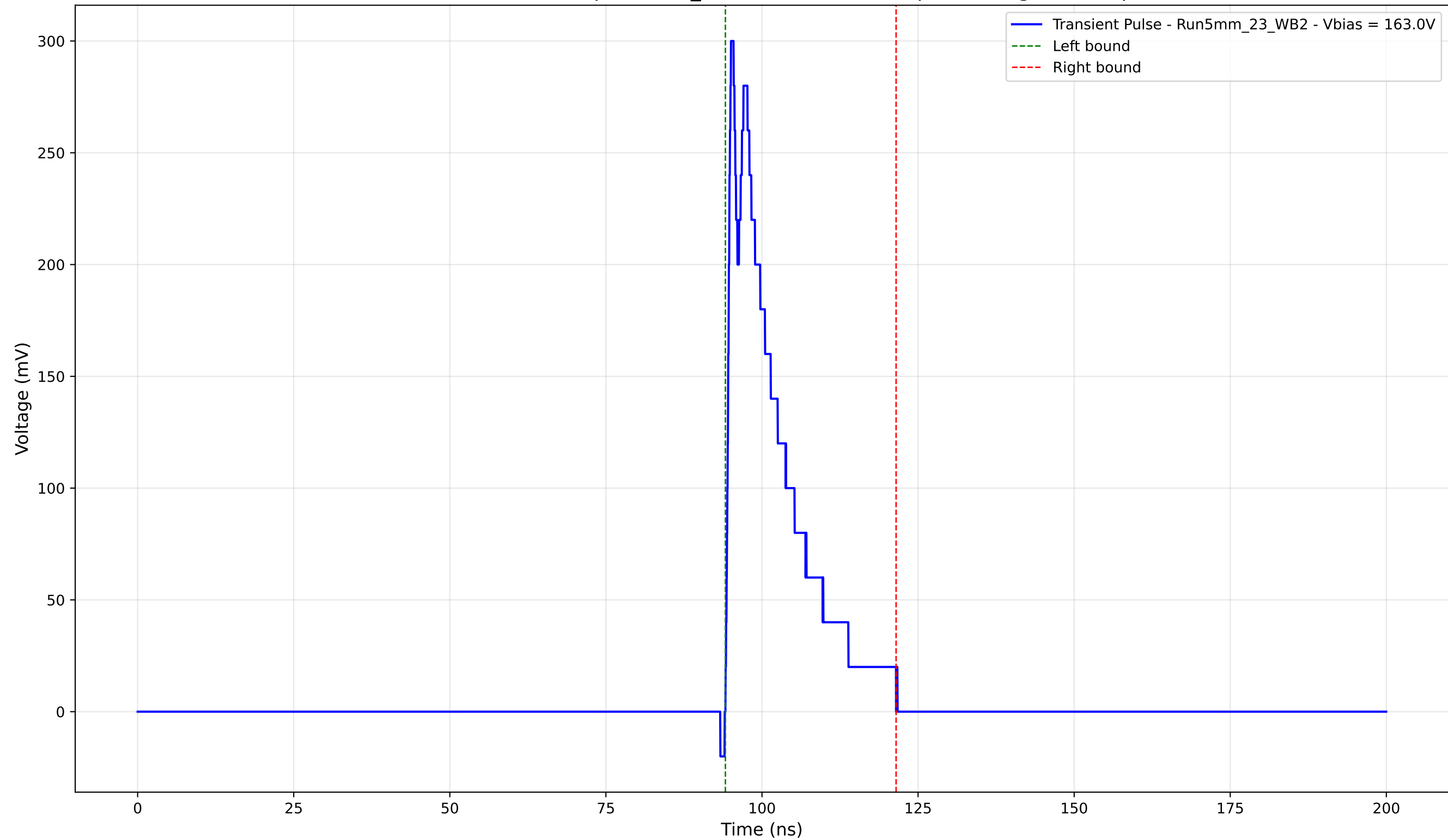
Transient Pulse - Sample: 5mm_23 - Position: 3005.0 \mu\text{m} - Charge: 52.48 pC
