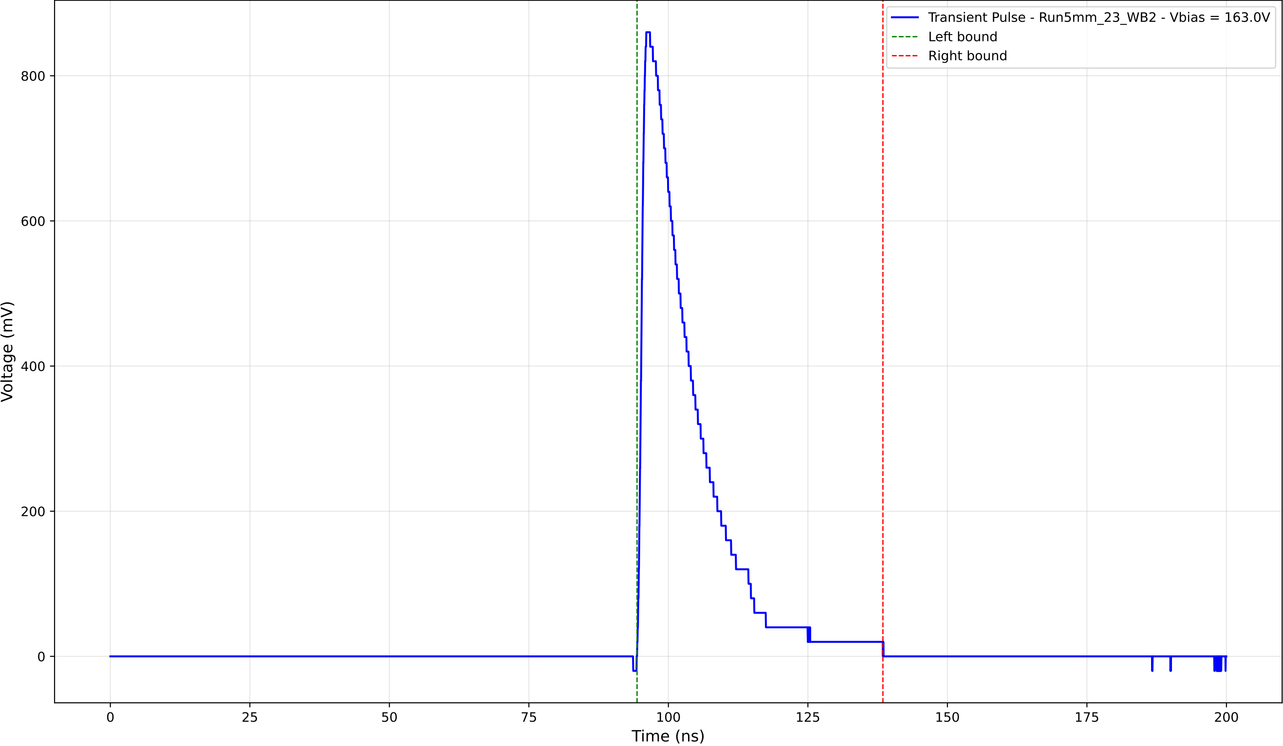
Transient Pulse - Sample: 5mm_23 - Position: 3780.0 \mu\text{m} - Charge: 177.42 pC
