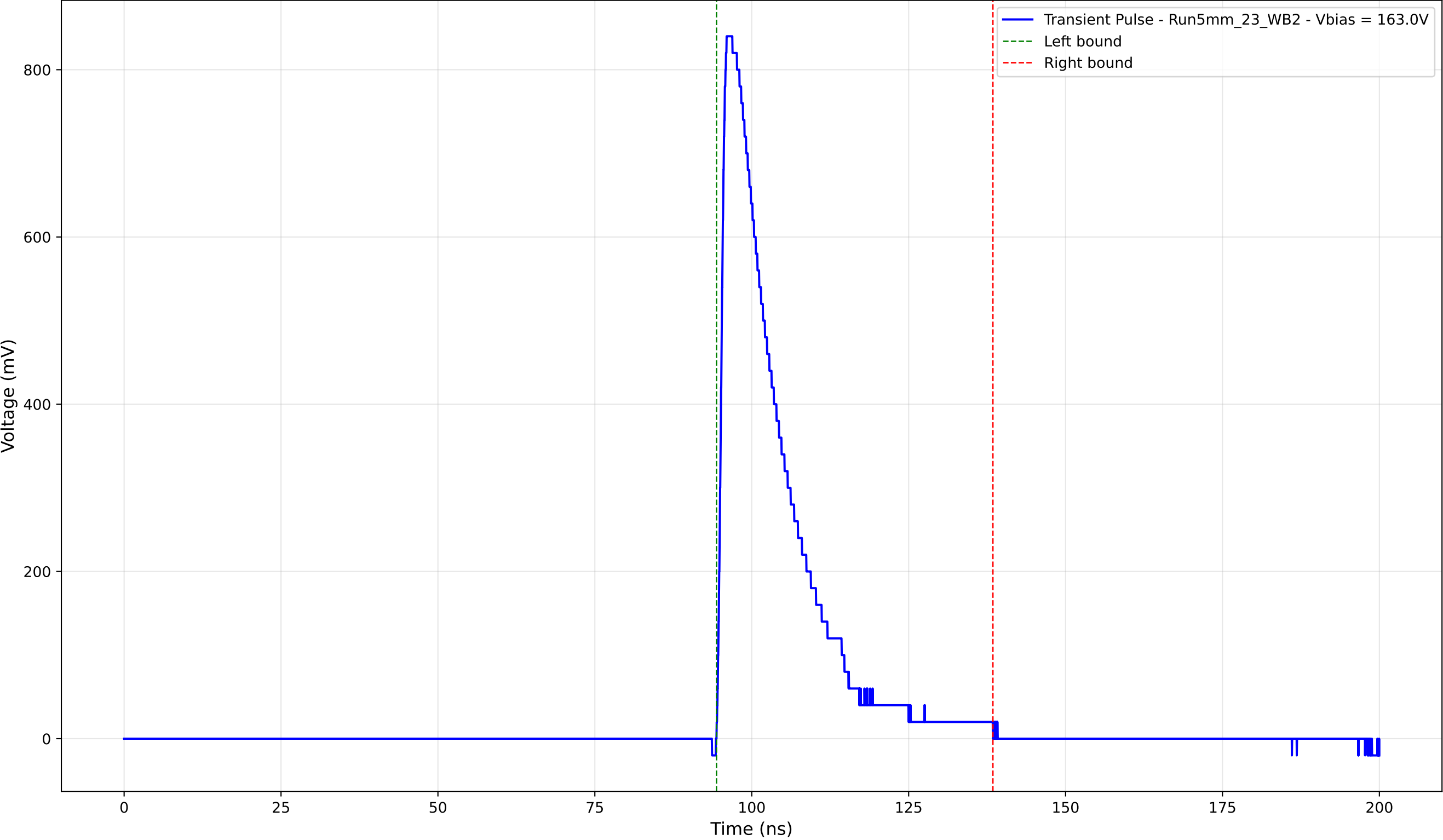
Transient Pulse - Sample: 5mm_23 - Position: 3720.0 \mu\text{m} - Charge: 175.91 pC
