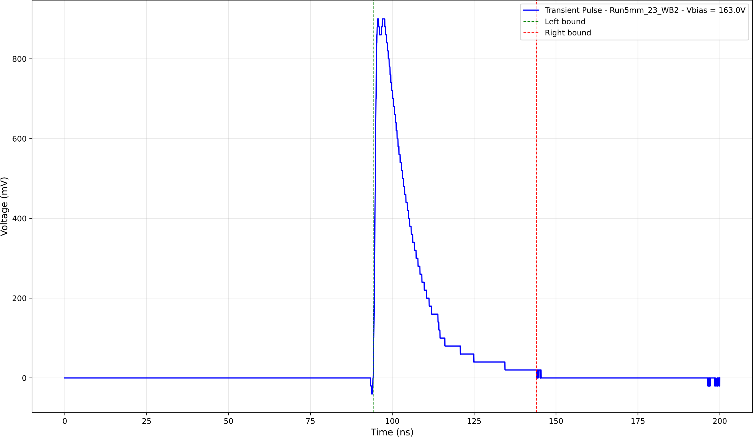
Transient Pulse - Sample: 5mm_23 - Position: 1790.0 \mu\text{m} - Charge: 217.16 pC
