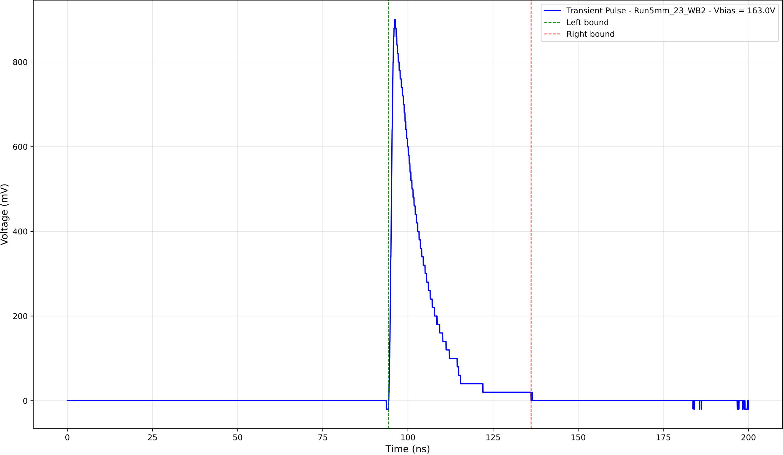
Transient Pulse - Sample: 5mm_23 - Position: 4225.0 \mu\text{m} - Charge: 164.34 pC
