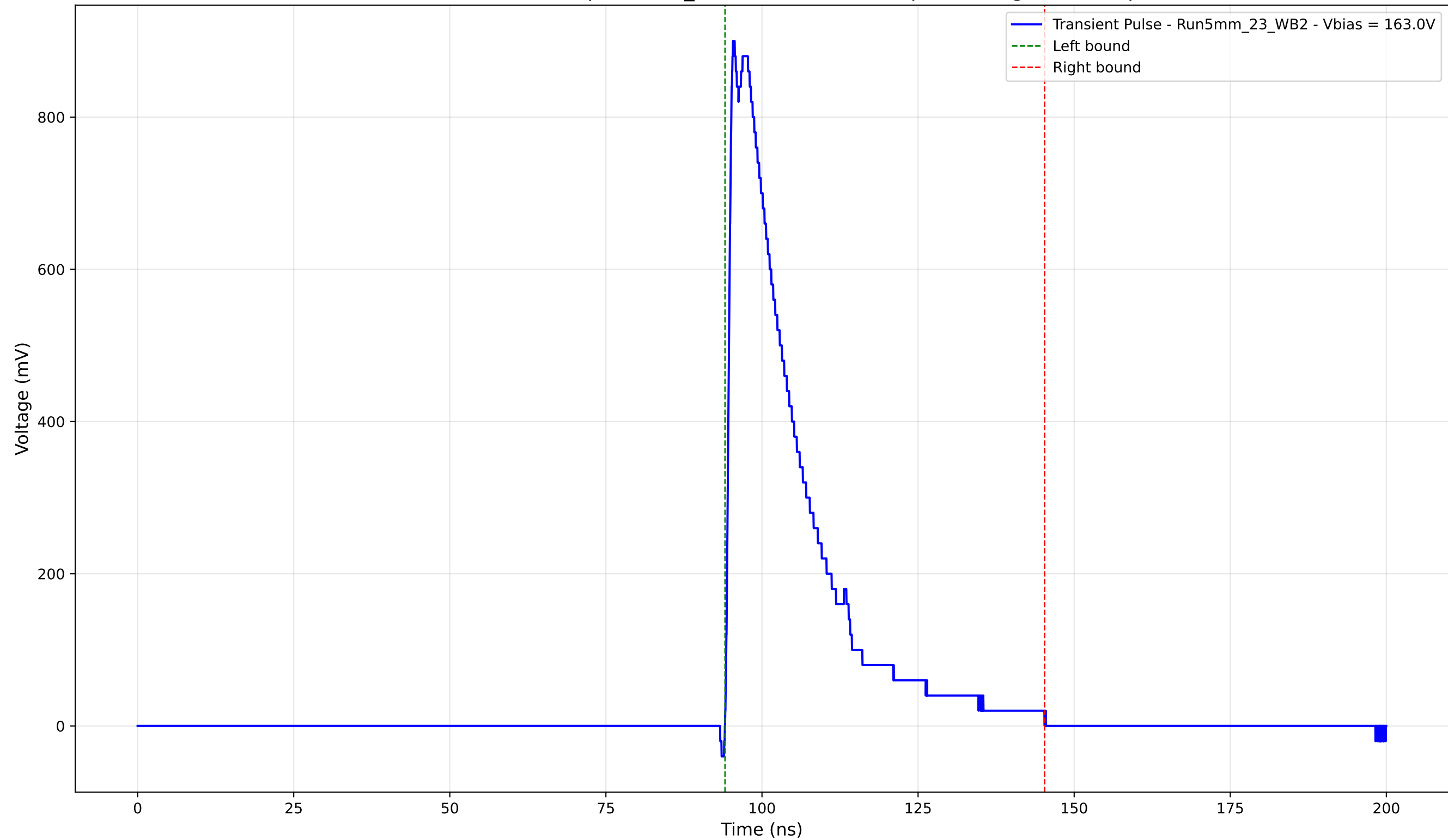
Transient Pulse - Sample: 5mm_23 - Position: 1890.0 \mu\text{m} - Charge: 216.24 pC
