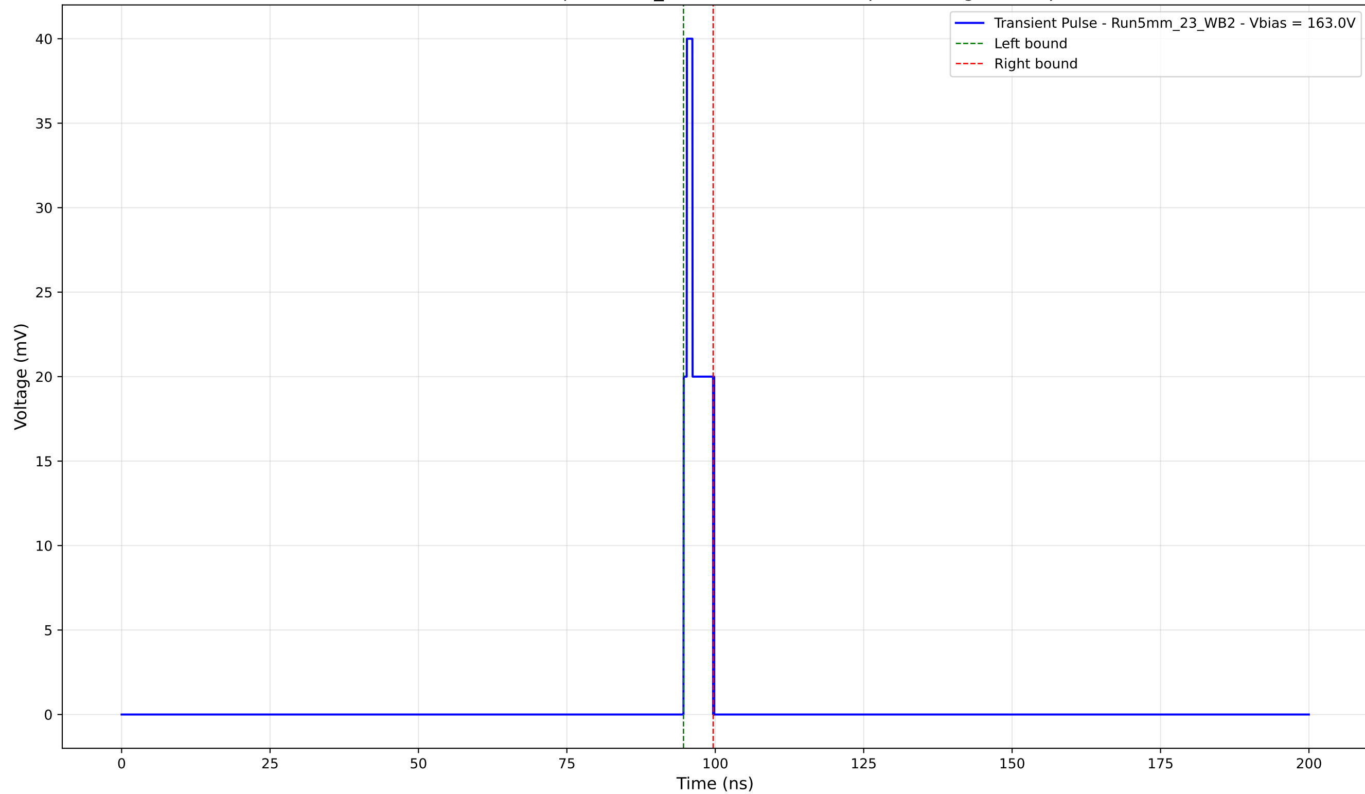
Transient Pulse - Sample: 5mm_23 - Position: 5010.0 \mu\text{m} - Charge: 2.38 pC
