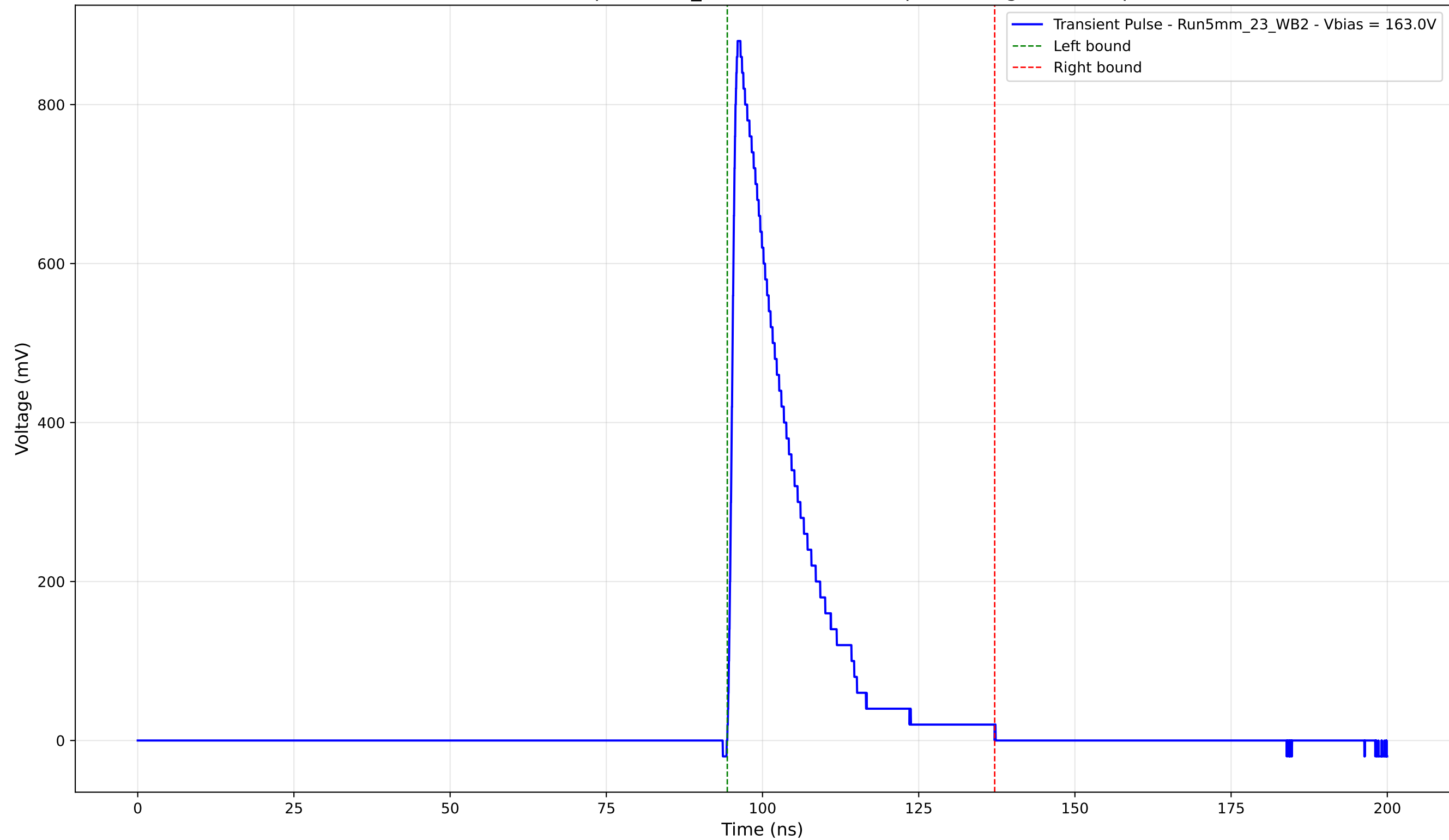
Transient Pulse - Sample: 5mm_23 - Position: 870.0 \mu\text{m} - Charge: 172.71 pC
