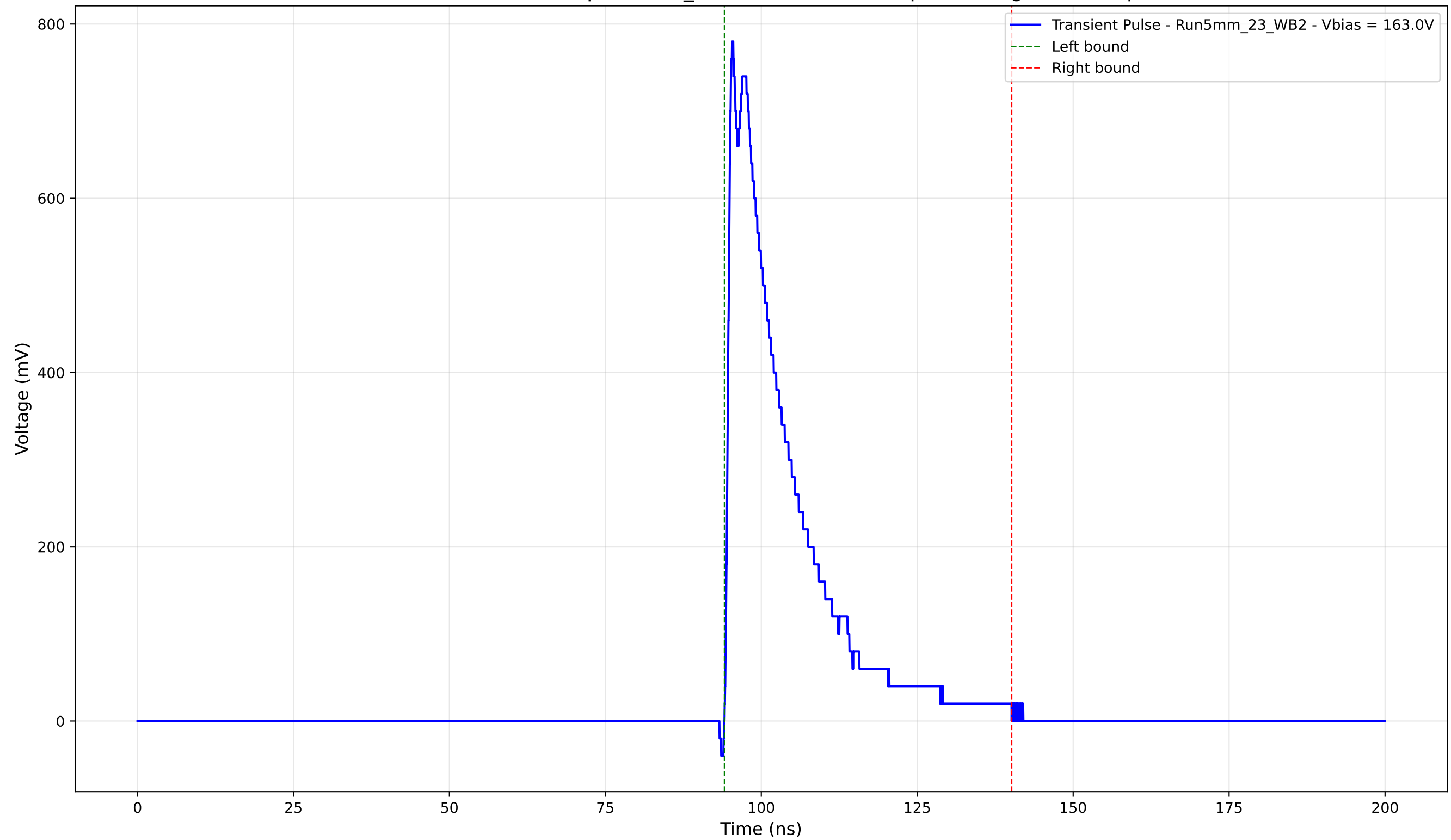
Transient Pulse - Sample: 5mm_23 - Position: 1945.0 \mu\text{m} - Charge: 162.59 pC
