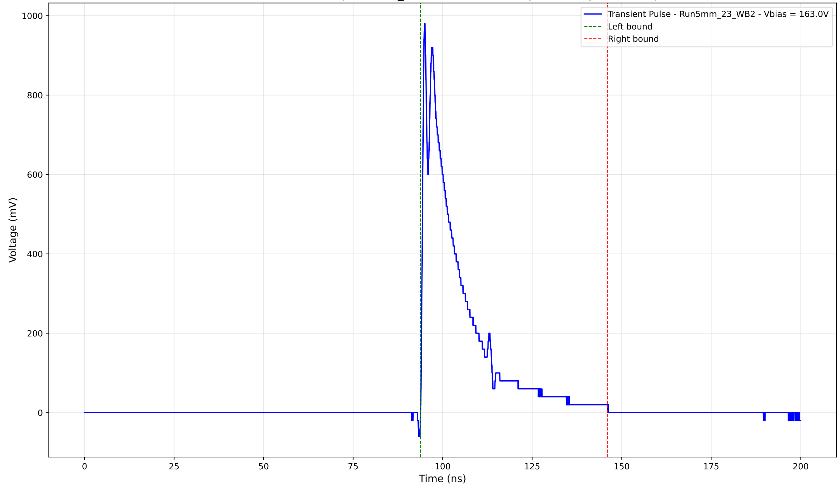
Transient Pulse - Sample: 5mm_23 - Position: 2355.0 \mu\text{m} - Charge: 201.41 pC
