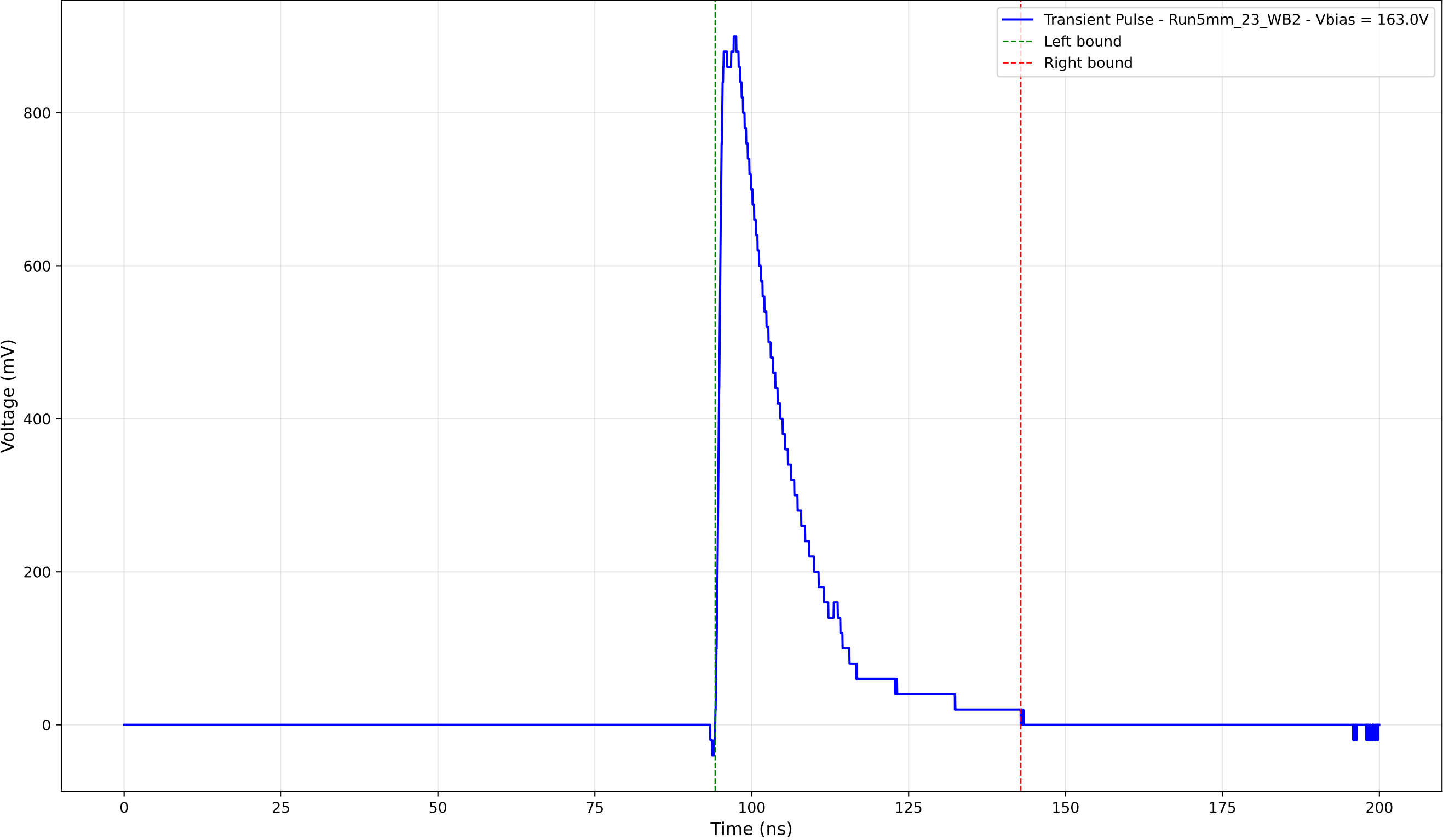
Transient Pulse - Sample: 5mm_23 - Position: 3305.0 \mu\text{m} - Charge: 206.12 pC
