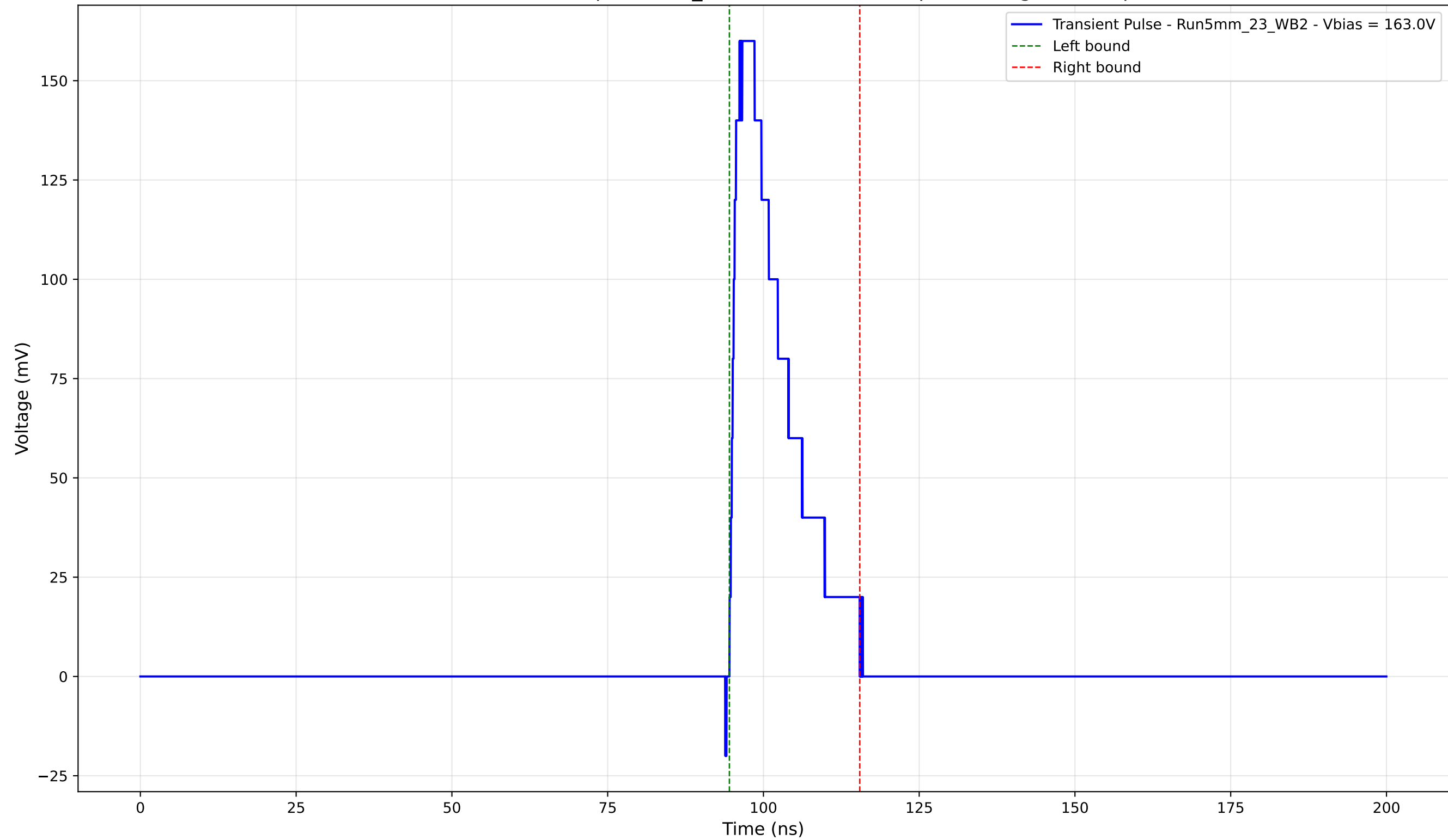
Transient Pulse - Sample: 5mm_23 -Position: 3530.0 \mu\text{m} - Charge: 30.03 pC
