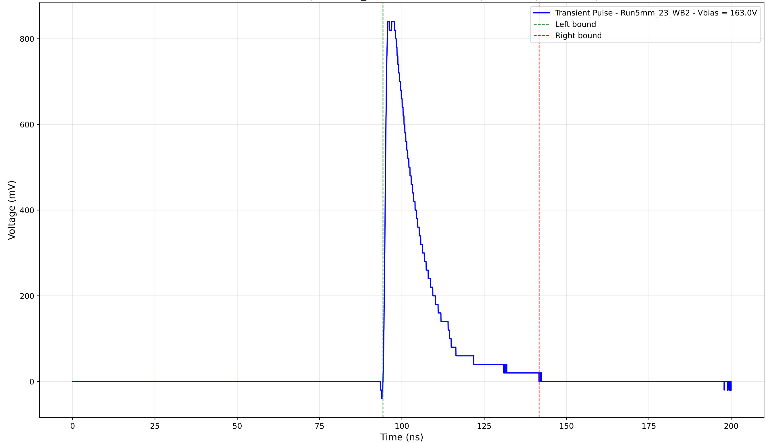
Transient Pulse - Sample: 5mm_23 - Position: 1600.0 \mu\text{m} - Charge: 191.64 pC
