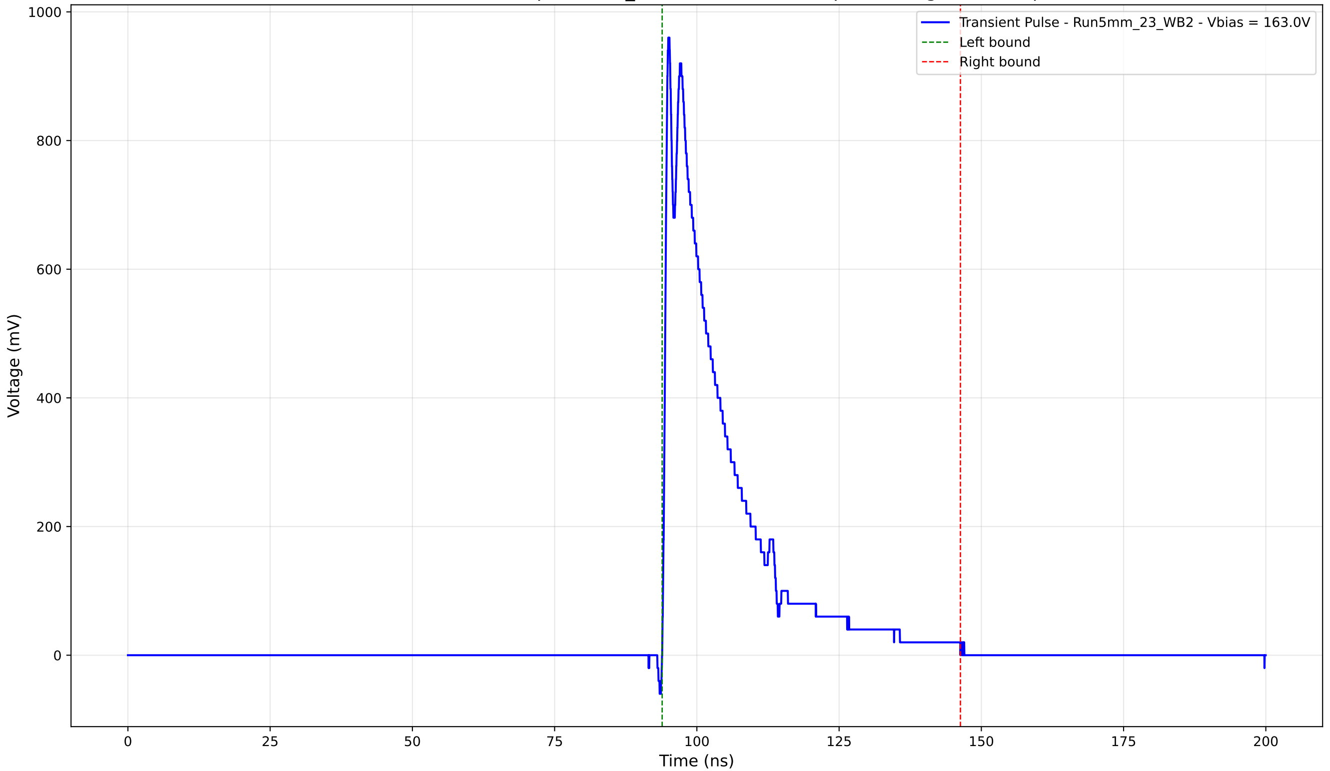
Transient Pulse - Sample: 5mm_23 - Position: 2770.0 \mu\text{m} - Charge: 205.43 pC
