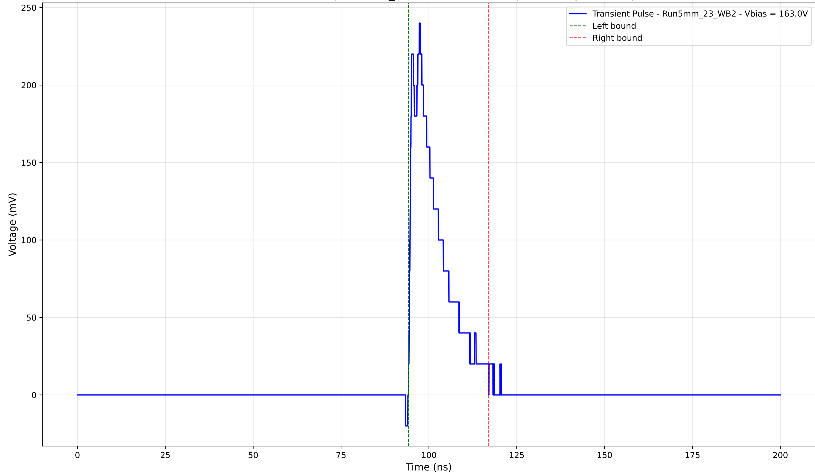
Transient Pulse - Sample: 5mm_23 - Position: 3035.0 \mu\text{m} - Charge: 41.88 pC
