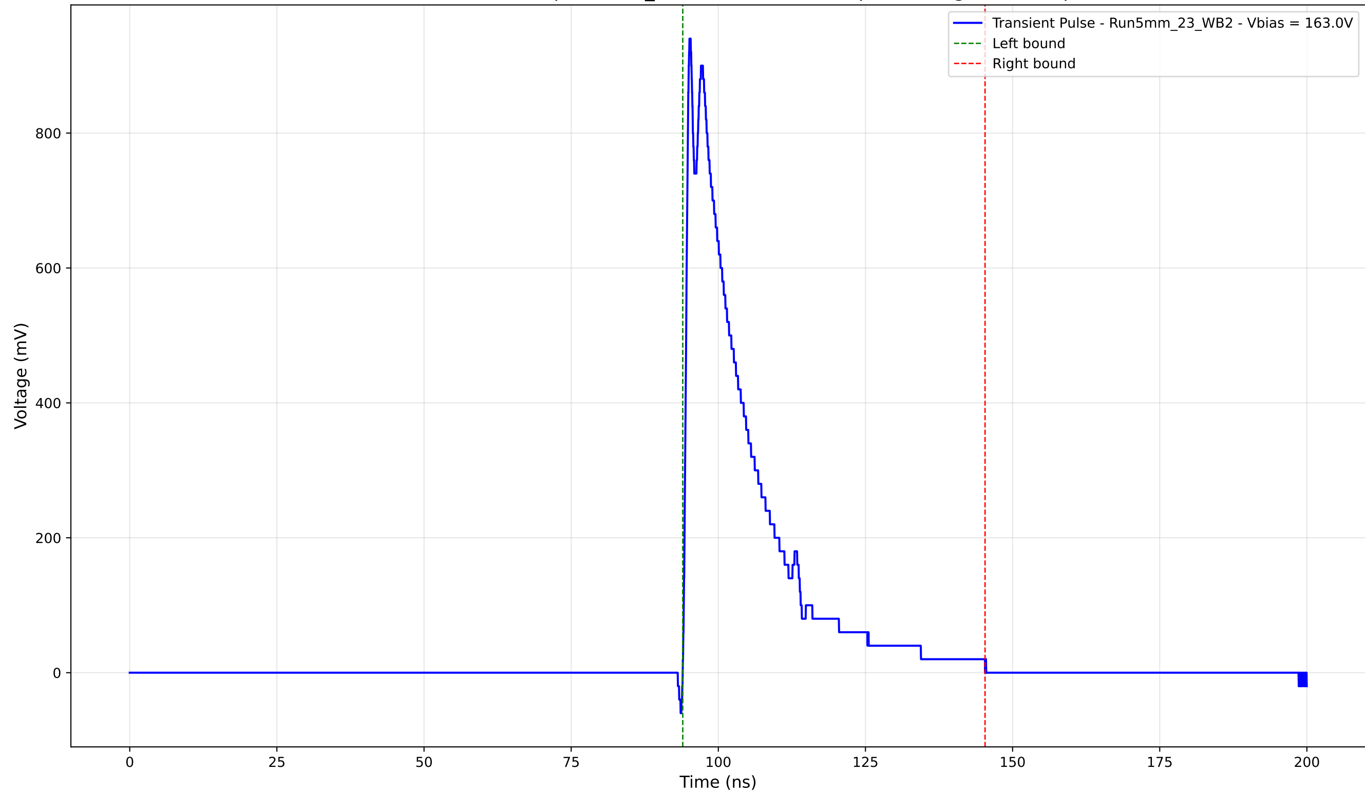
Transient Pulse - Sample: 5mm_23 - Position: 2145.0 \mu\text{m} - Charge: 204.92 pC
