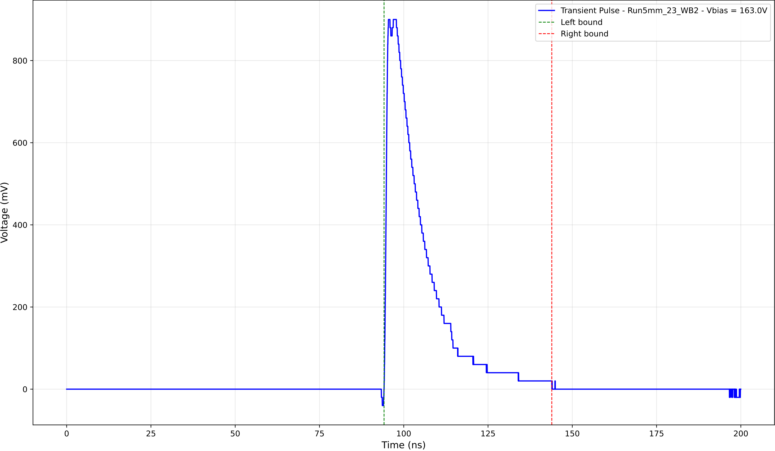
Transient Pulse - Sample: 5mm_23 - Position: 1775.0 \mu\text{m} - Charge: 217.05 pC
