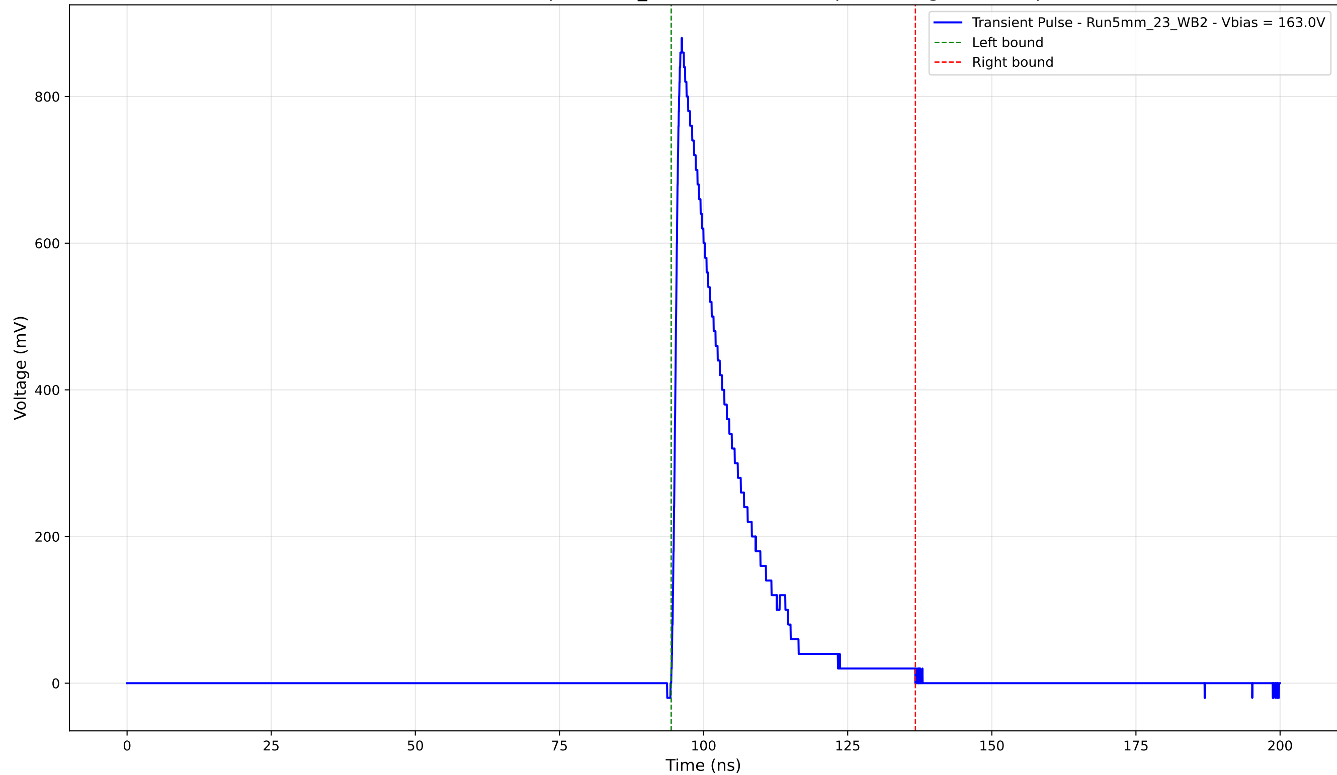
Transient Pulse - Sample: 5mm_23 - Position: 895.0 \mu\text{m} - Charge: 168.69 pC
