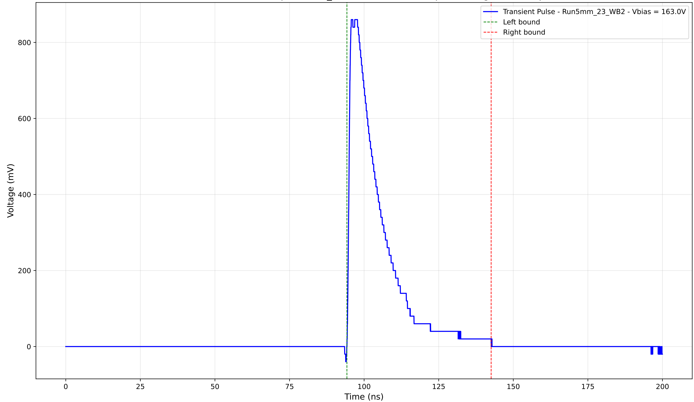
Transient Pulse - Sample: 5mm_23 - Position: 1625.0 \mu\text{m} - Charge: 199.39 pC
