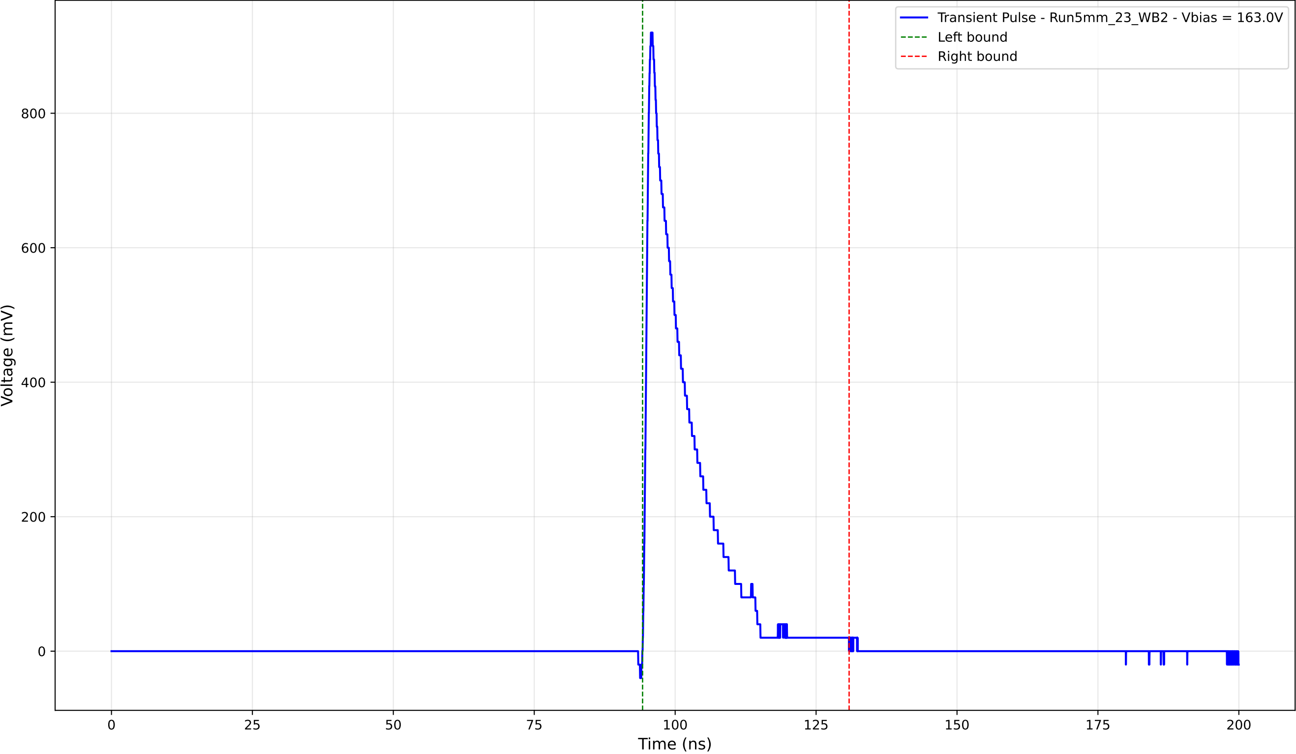
Transient Pulse - Sample: 5mm_23 - Position: 4620.0 \mu\text{m} - Charge: 142.73 pC
