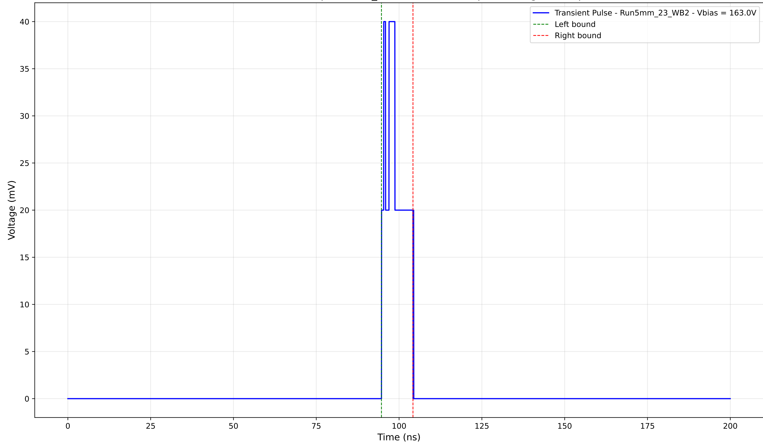
Transient Pulse - Sample: 5mm_23 - Position: 15.0 \mu\text{m} - Charge: 4.74 pC
