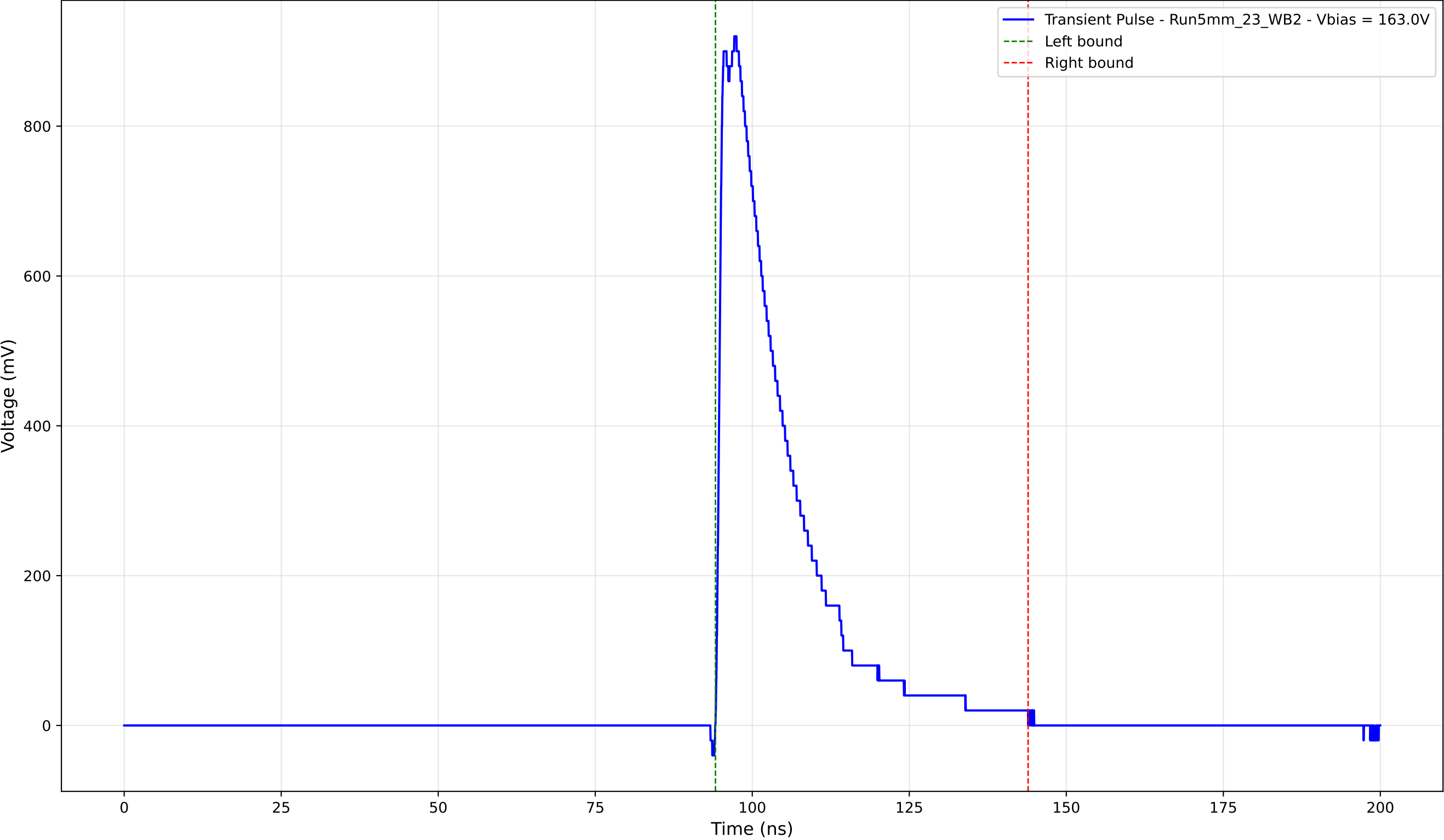
Transient Pulse - Sample: 5mm_23 - Position: 3245.0 \mu\text{m} - Charge: 215.68 pC
