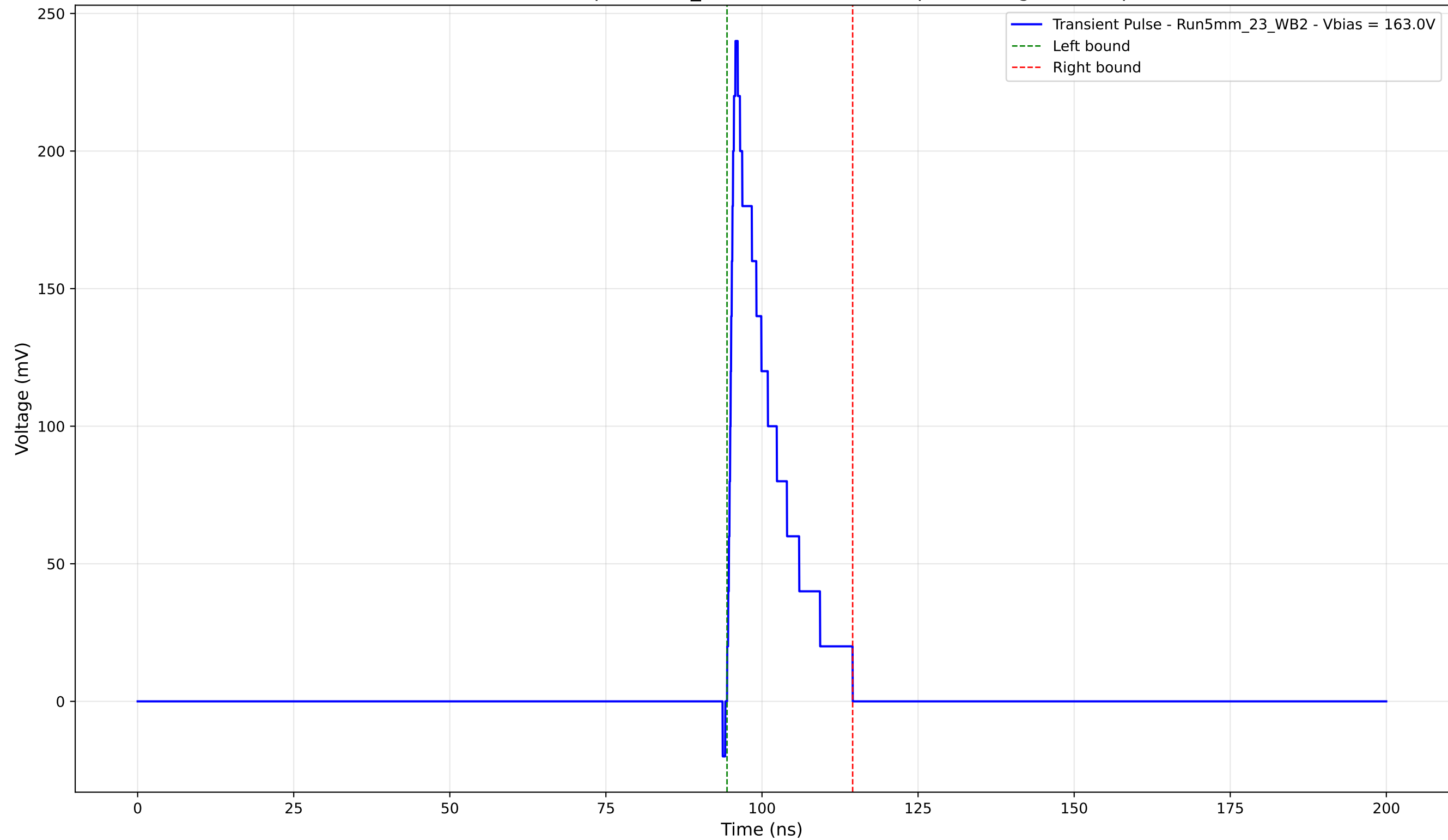
Transient Pulse - Sample: 5mm_23 - Position: 4550.0 \mu\text{m} - Charge: 33.38 pC
