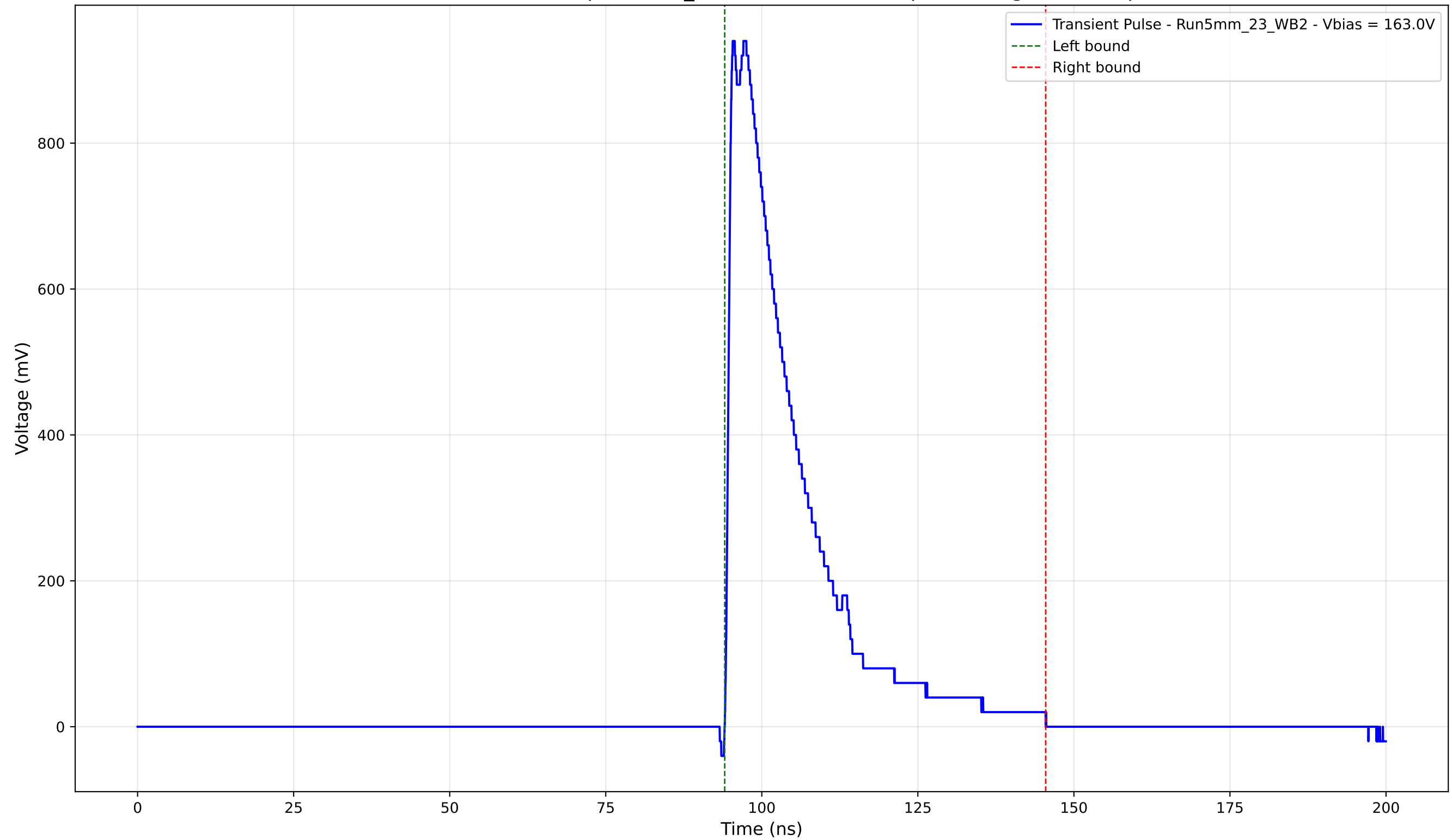
Transient Pulse - Sample: 5mm_23 - Position: 3145.0 \mu\text{m} - Charge: 226.29 pC
