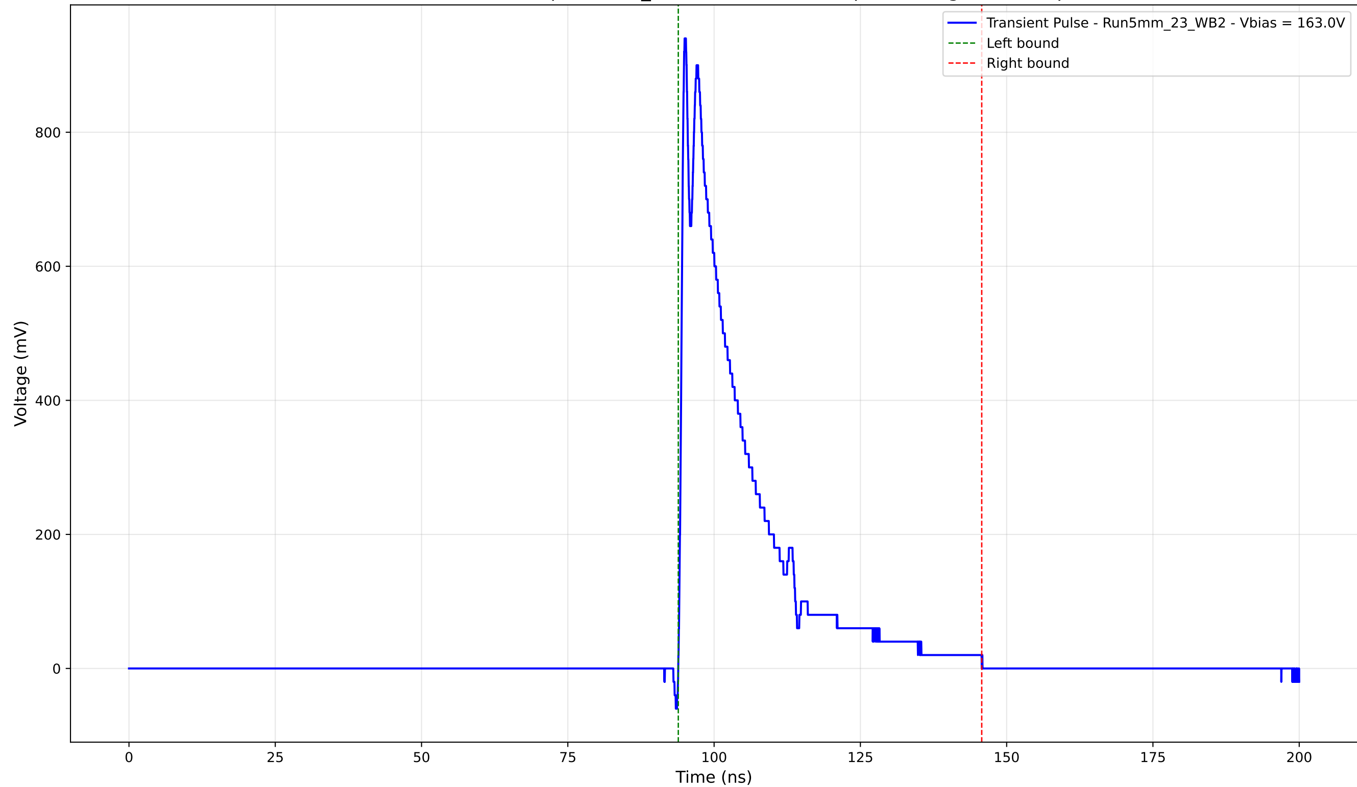
Transient Pulse - Sample: 5mm_23 - Position: 2275.0 \mu\text{m} - Charge: 202.86 pC
