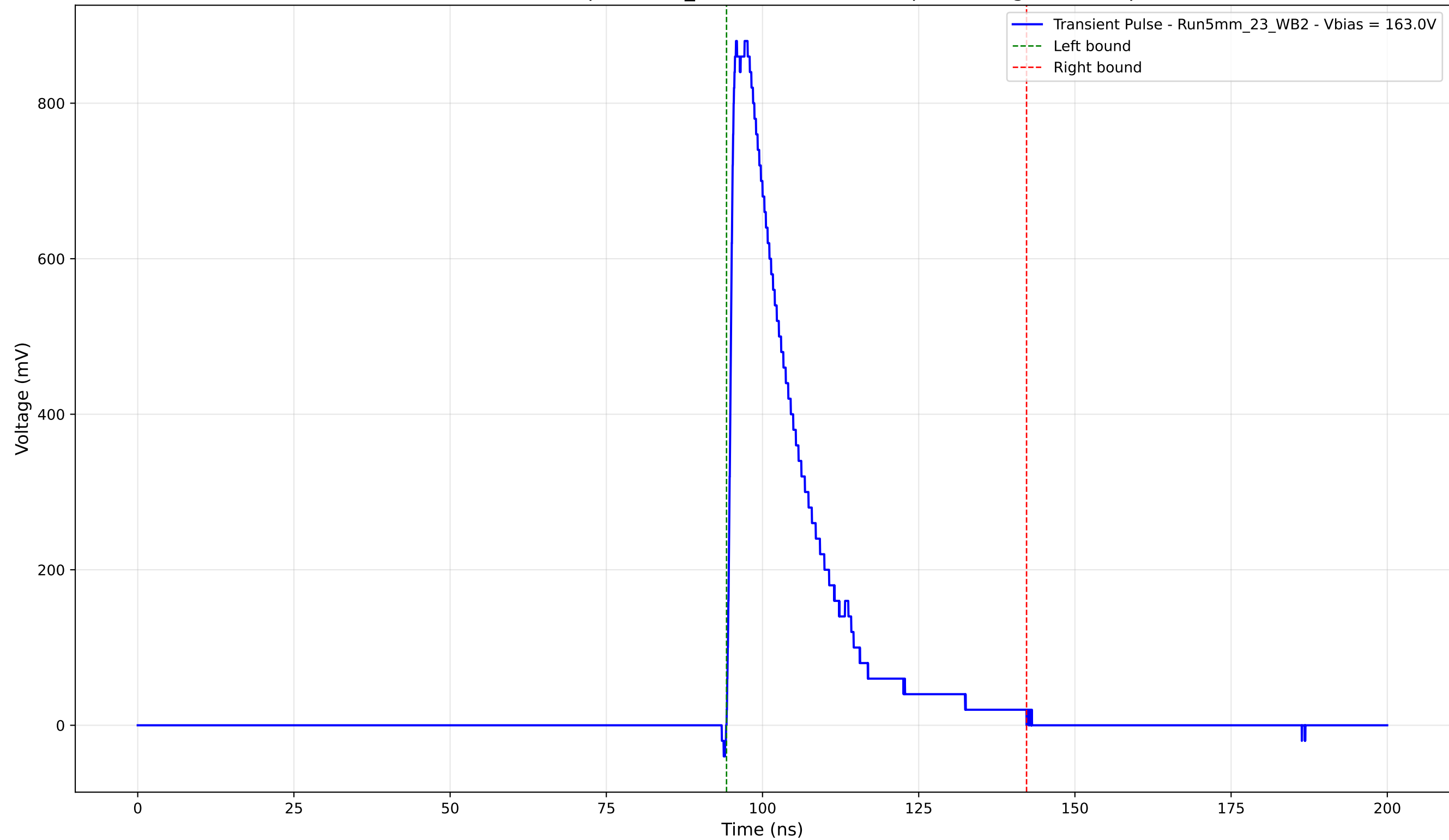
Transient Pulse - Sample: 5mm_23 - Position: 1660.0 \mu\text{m} - Charge: 203.22 pC
