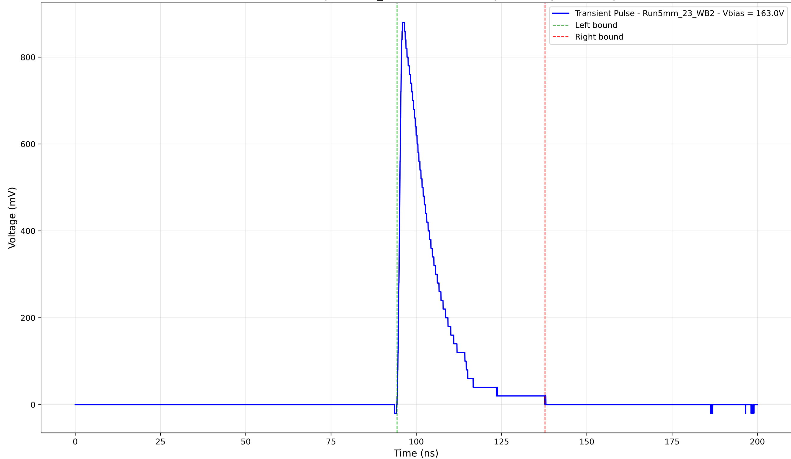
Transient Pulse - Sample: 5mm_23 - Position: 835.0 \mu\text{m} - Charge: 174.23 pC
