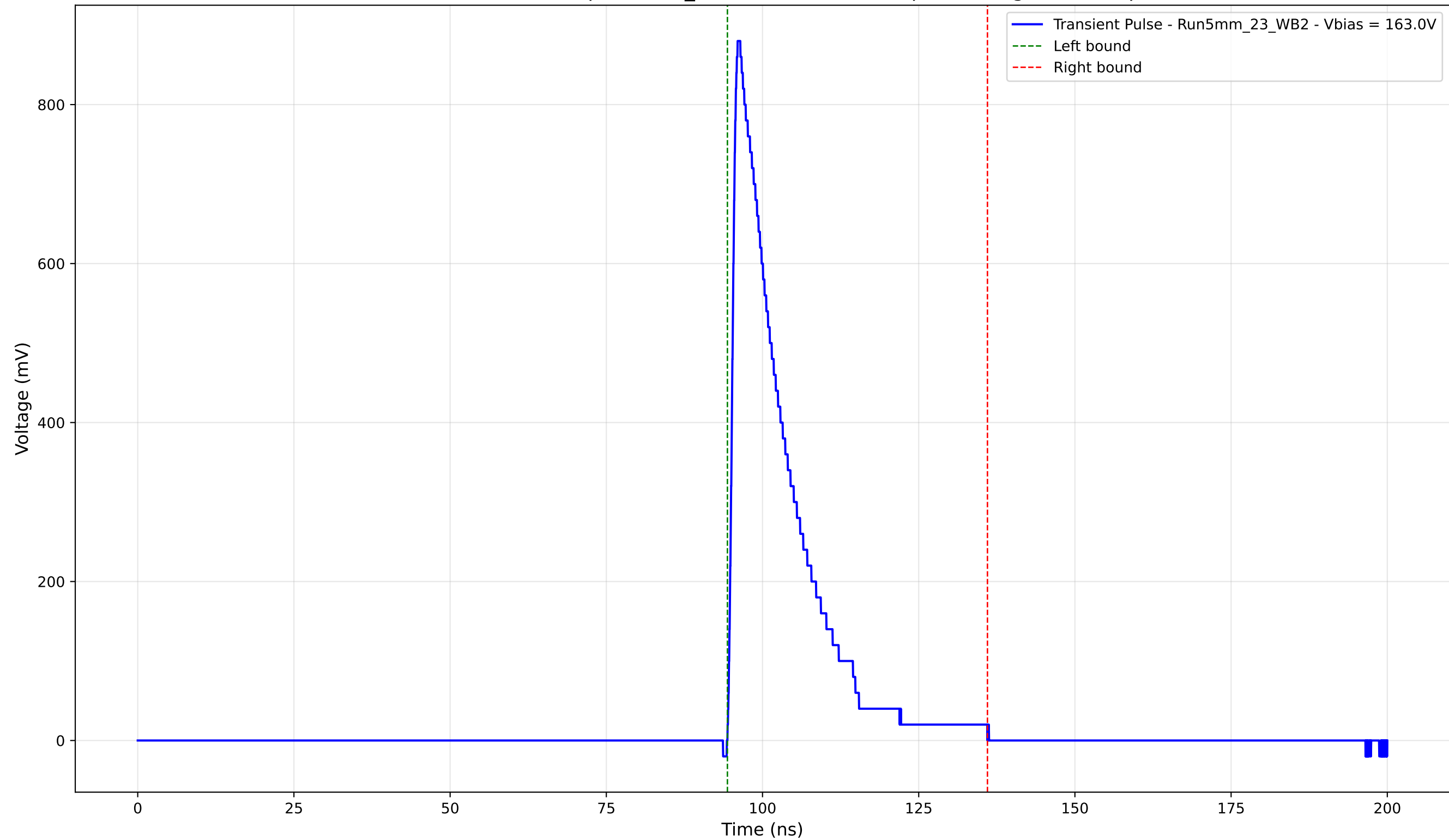
Transient Pulse - Sample: 5mm_23 - Position: 4180.0 \mu\text{m} - Charge: 163.28 pC
