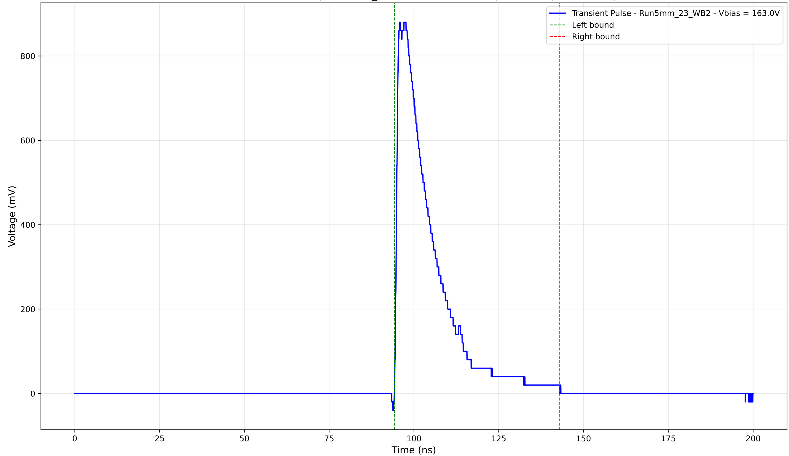
Transient Pulse - Sample: 5mm_23 - Position: 1665.0 \mu\text{m} - Charge: 204.46 pC
