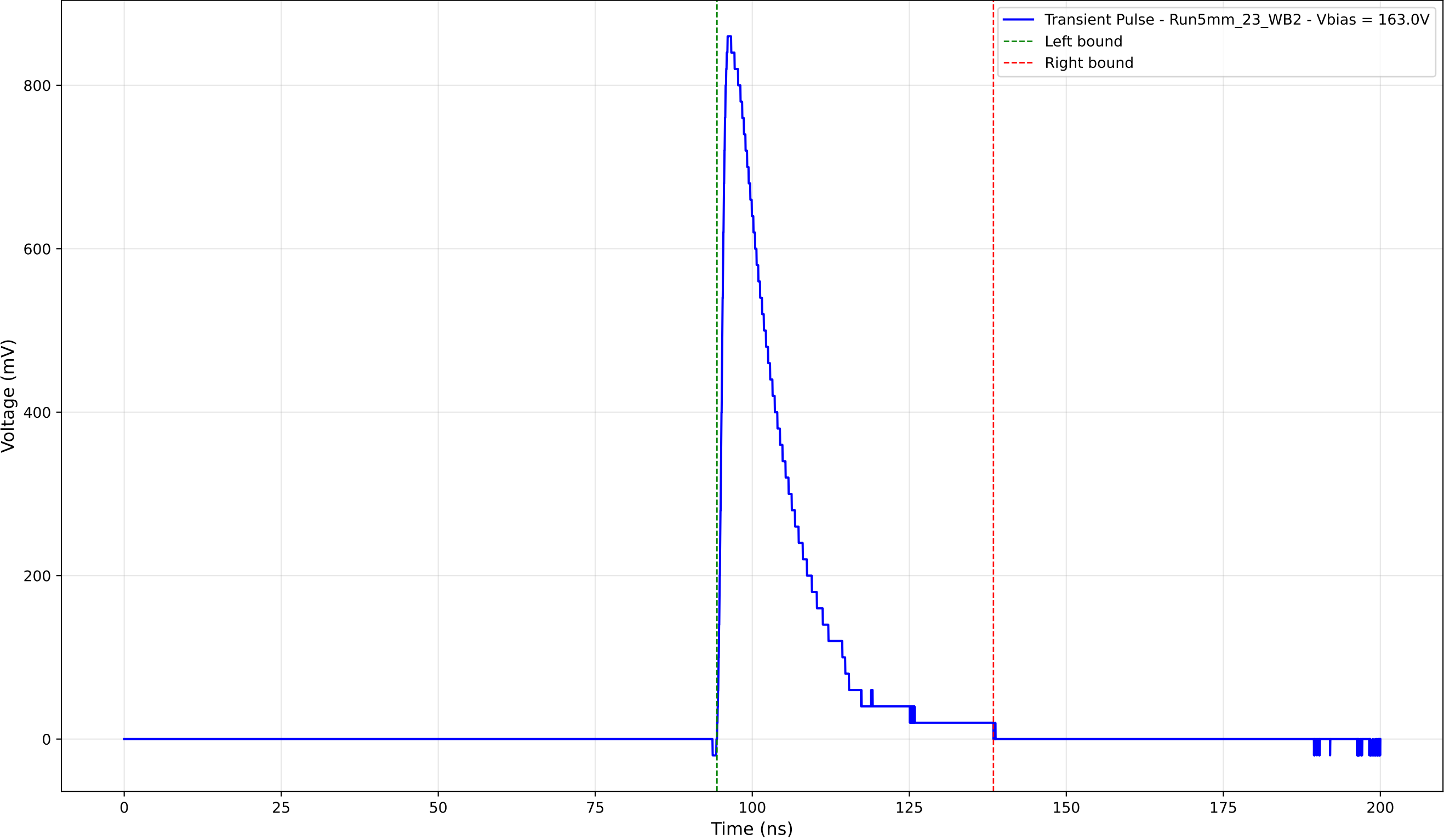
Transient Pulse - Sample: 5mm_23 - Position: 3755.0 \mu\text{m} - Charge: 177.30 pC
