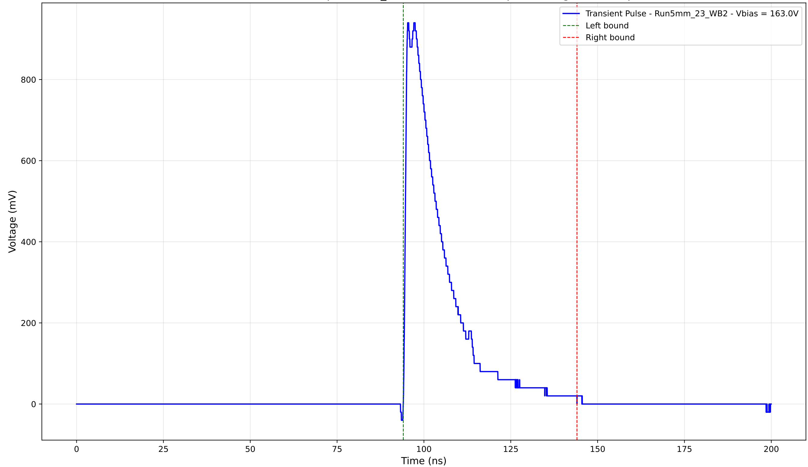
Transient Pulse - Sample: 5mm_23 - Position: 3130.0 \mu\text{m} - Charge: 225.04 pC
