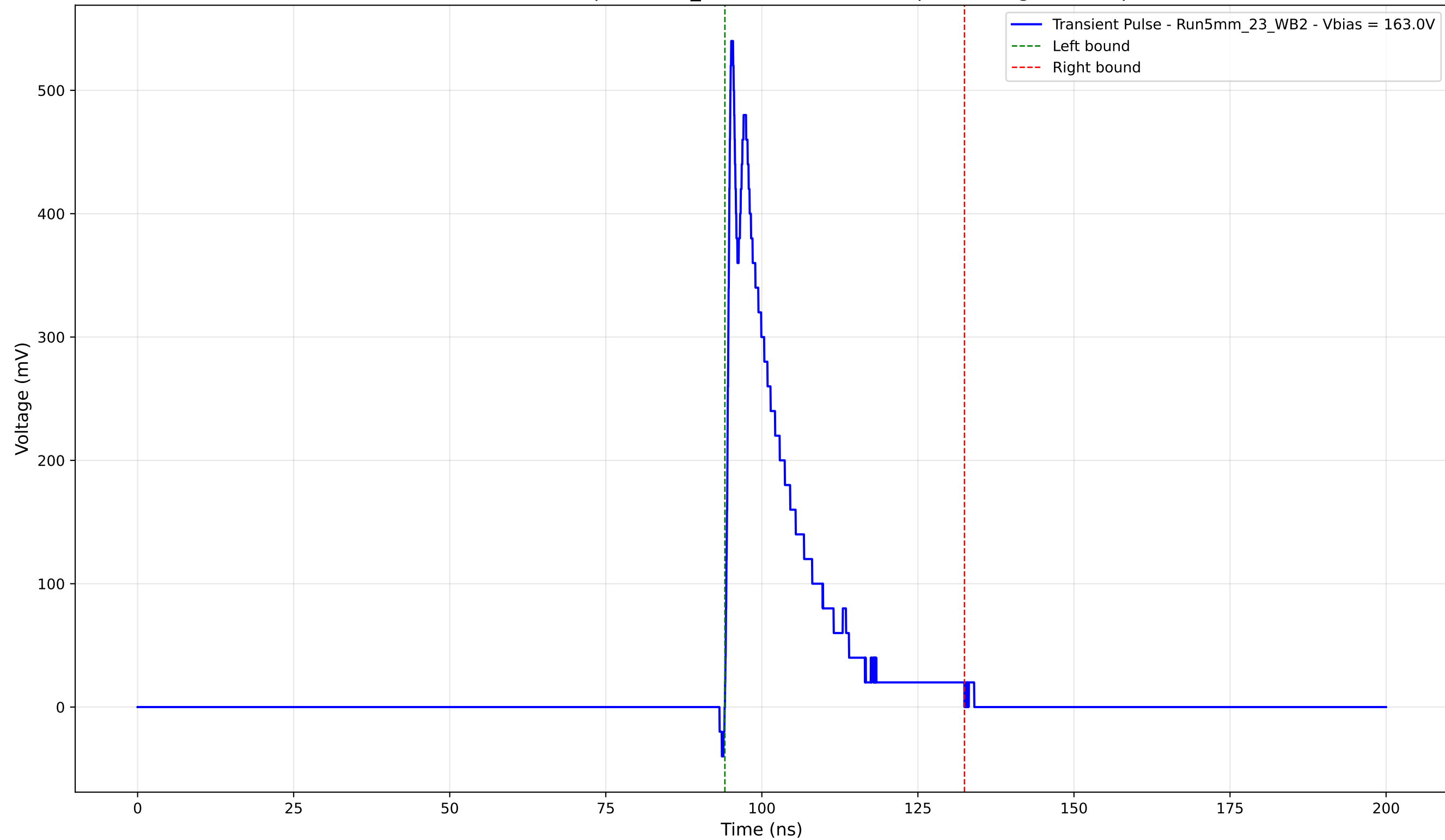
Transient Pulse - Sample: 5mm_23 - Position: 2050.0 \mu\text{m} - Charge: 93.98 pC
