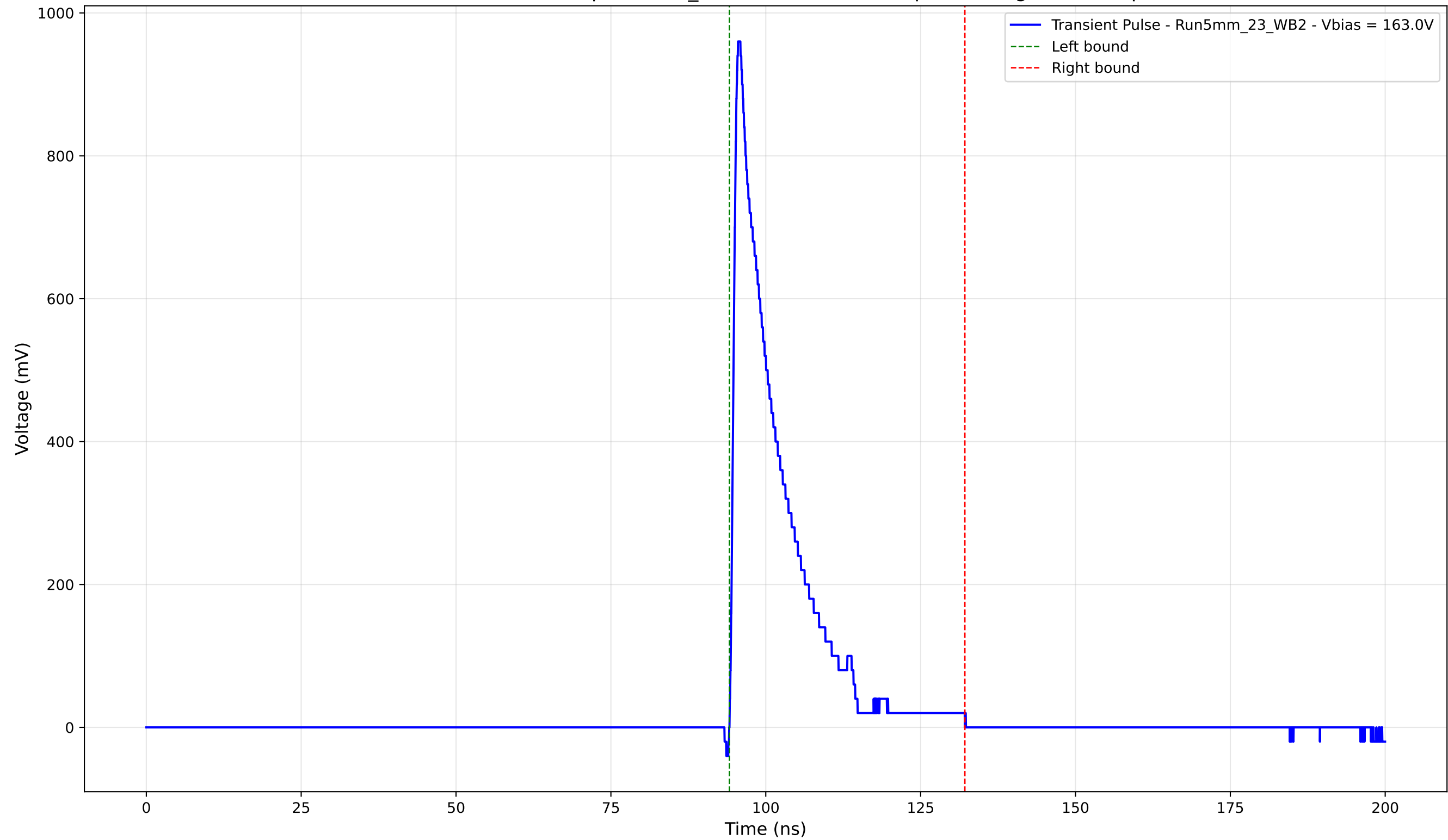
Transient Pulse - Sample: 5mm_23 - Position: 4745.0 \mu\text{m} - Charge: 149.70 pC
