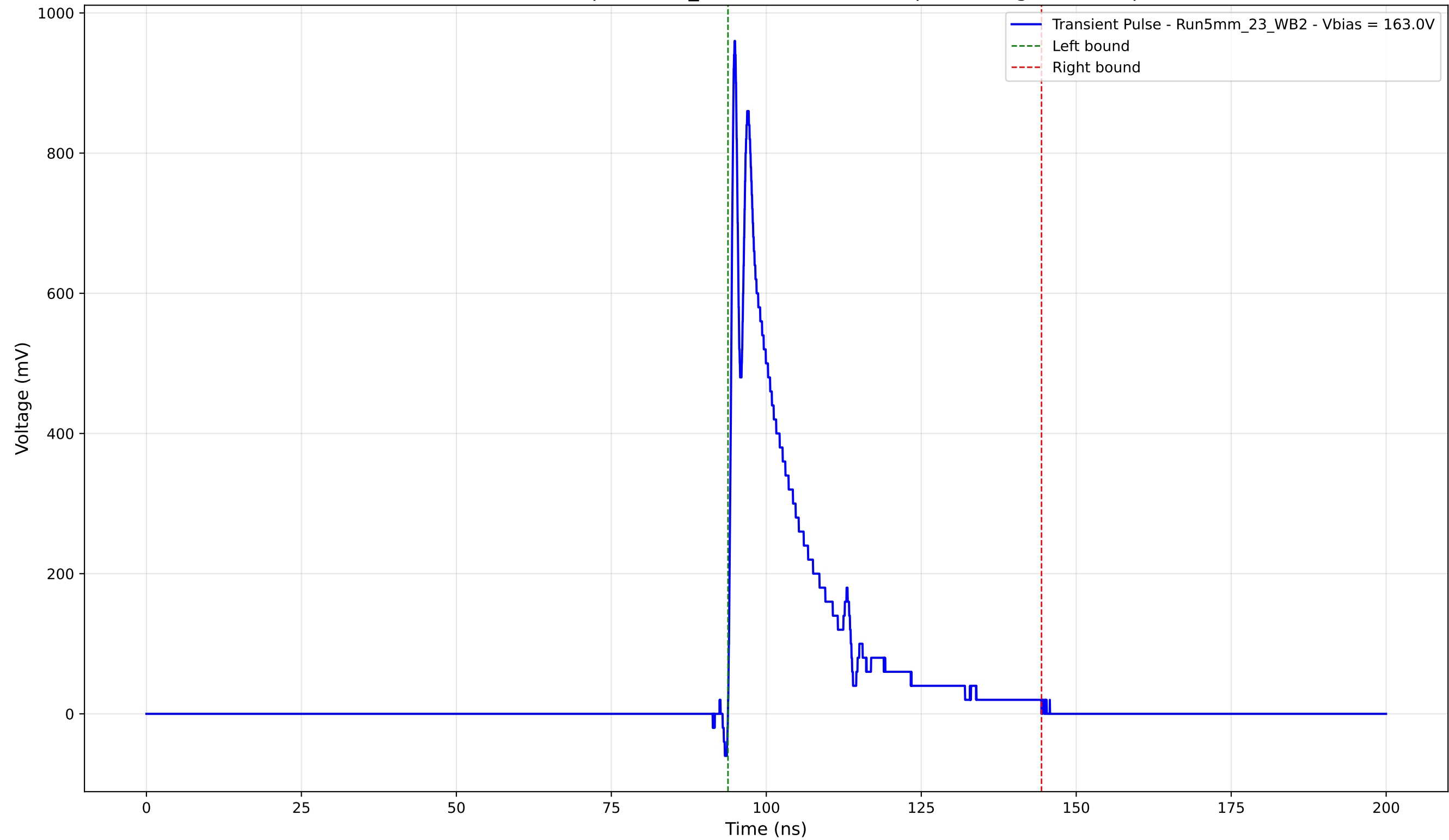
Transient Pulse - Sample: 5mm_23 - Position: 2595.0 \mu\text{m} - Charge: 173.90 pC
