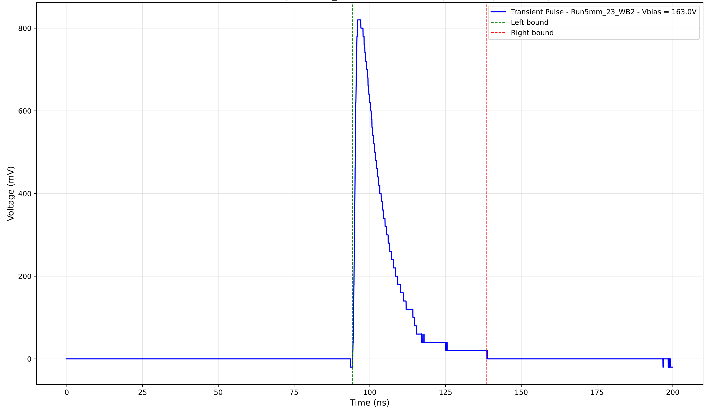
Transient Pulse - Sample: 5mm_23 - Position: 3660.0 \mu\text{m} - Charge: 172.92 pC
