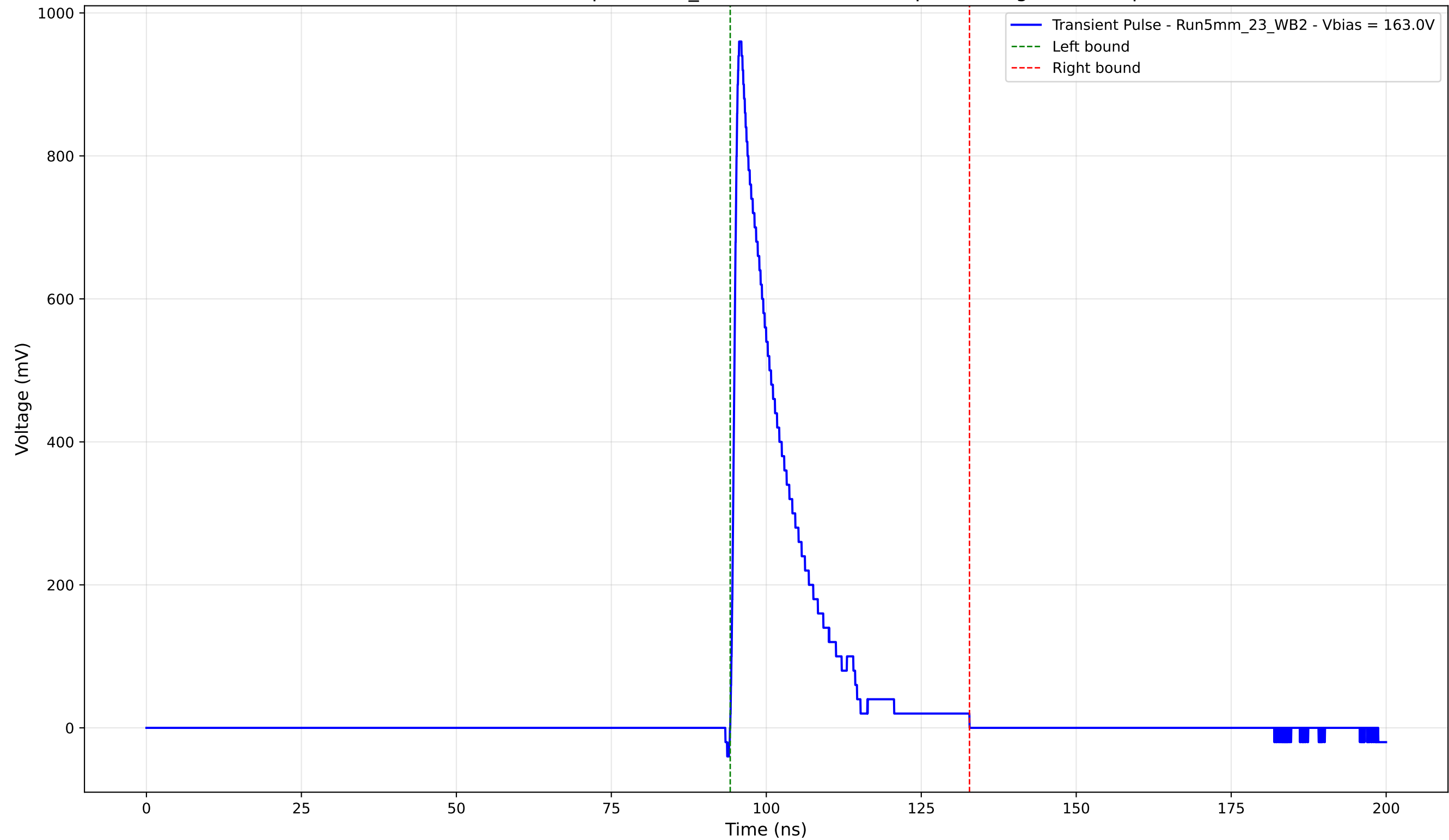
Transient Pulse - Sample: 5mm_23 - Position: 4655.0 \mu\text{m} - Charge: 157.68 pC
