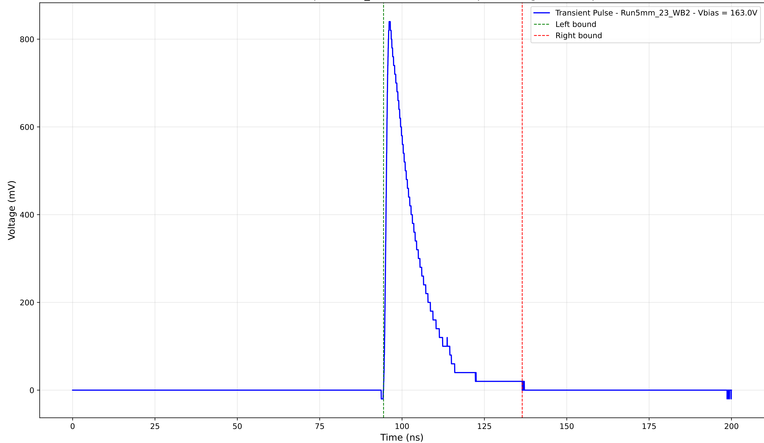
Transient Pulse - Sample: 5mm_23 - Position: 910.0 \mu\text{m} - Charge: 159.58 pC
