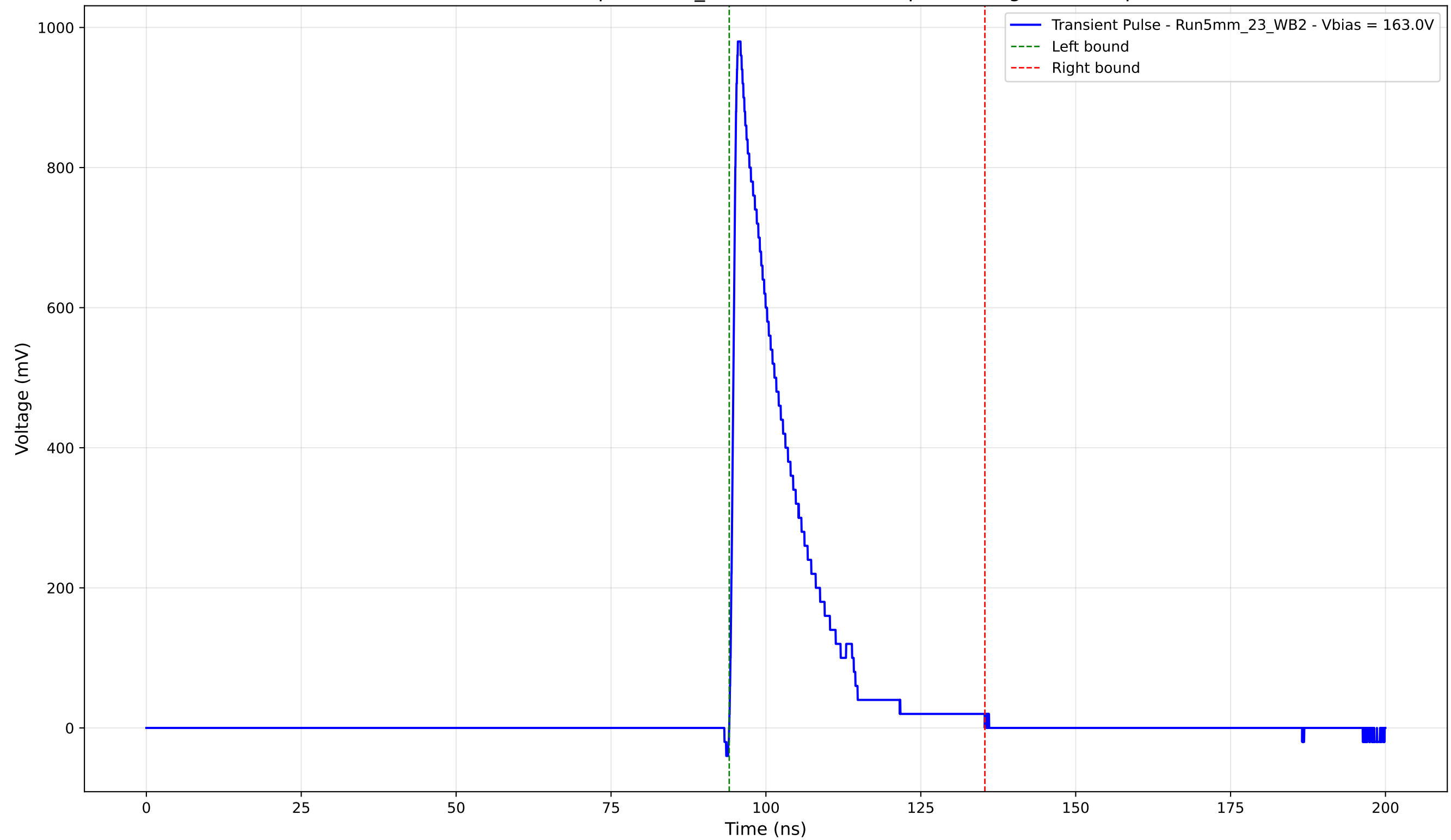
Transient Pulse - Sample: 5mm_23 - Position: 295.0 \mu\text{m} - Charge: 176.02 pC
