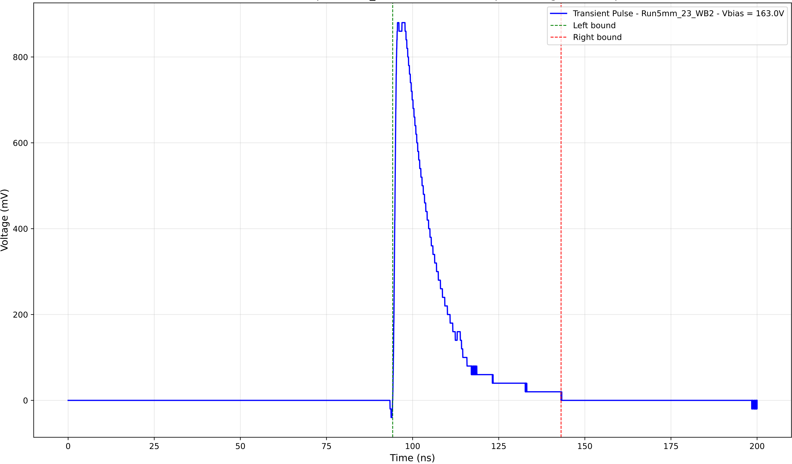
Transient Pulse - Sample: 5mm_23 - Position: 1690.0 \mu\text{m} - Charge: 207.02 pC
