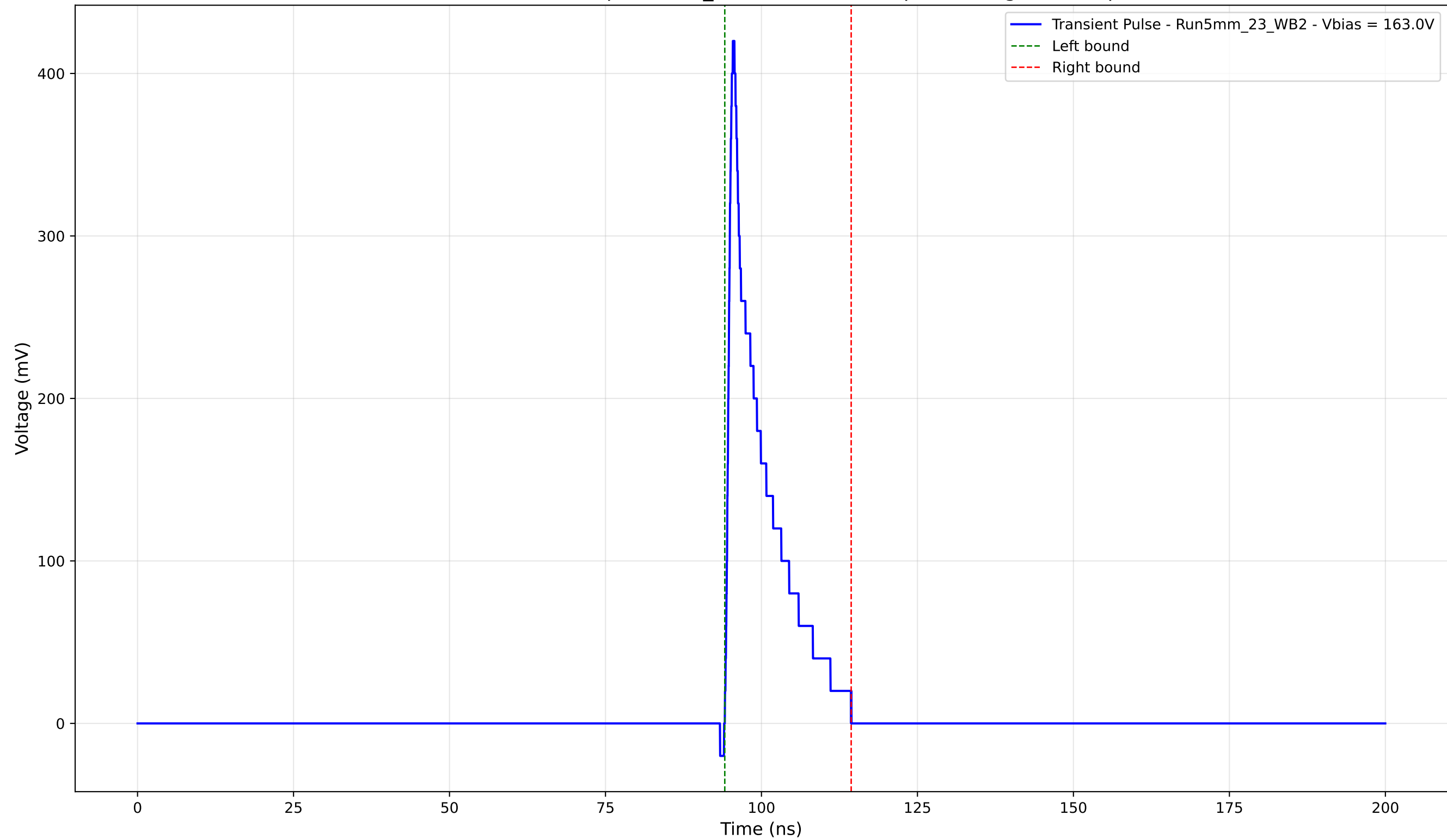
Transient Pulse - Sample: 5mm_23 - Position: 65.0 \mu\text{m} - Charge: 49.39 pC
