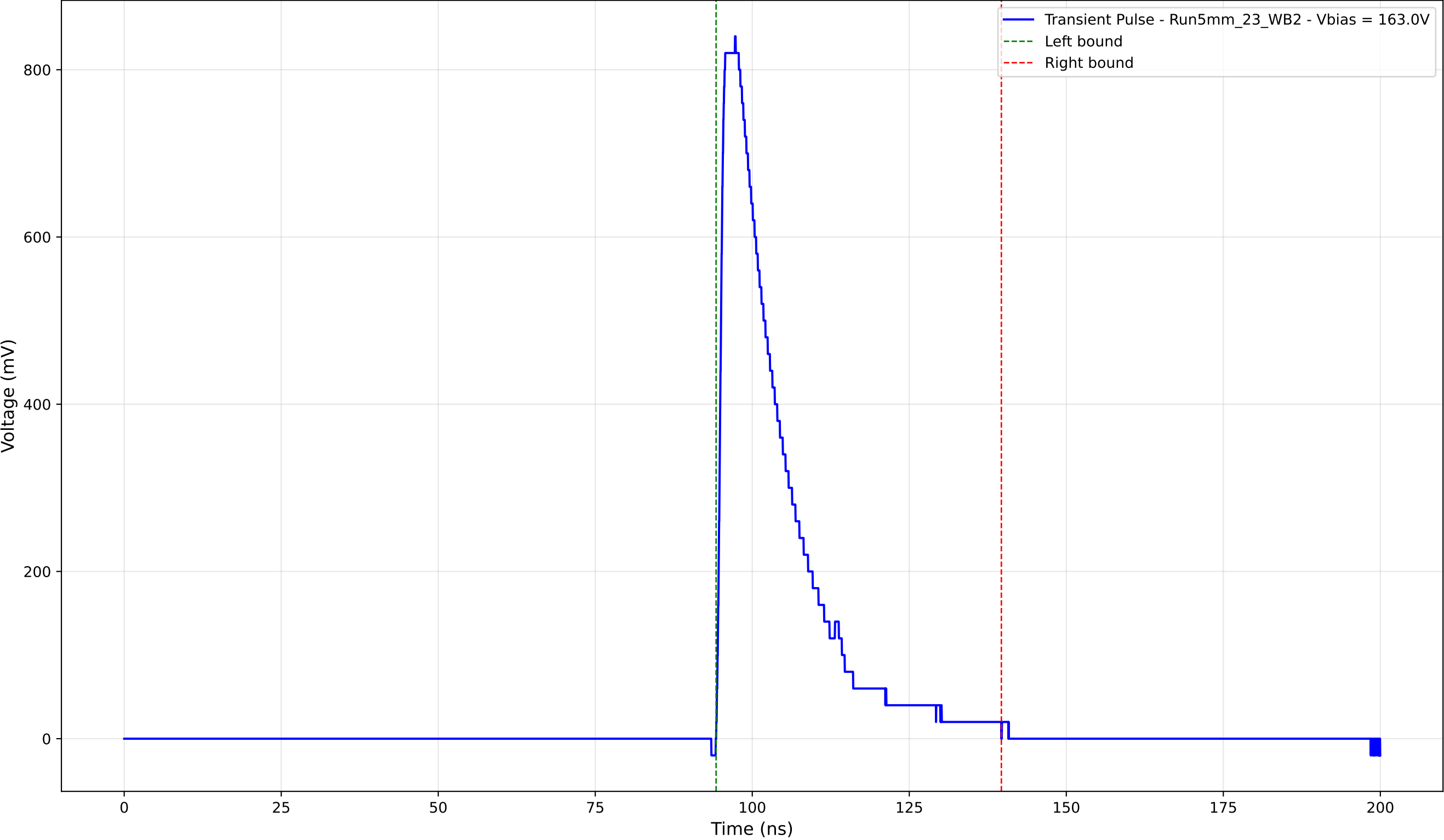
Transient Pulse - Sample: 5mm_23 - Position: 3405.0 \mu\text{m} - Charge: 184.16 pC
