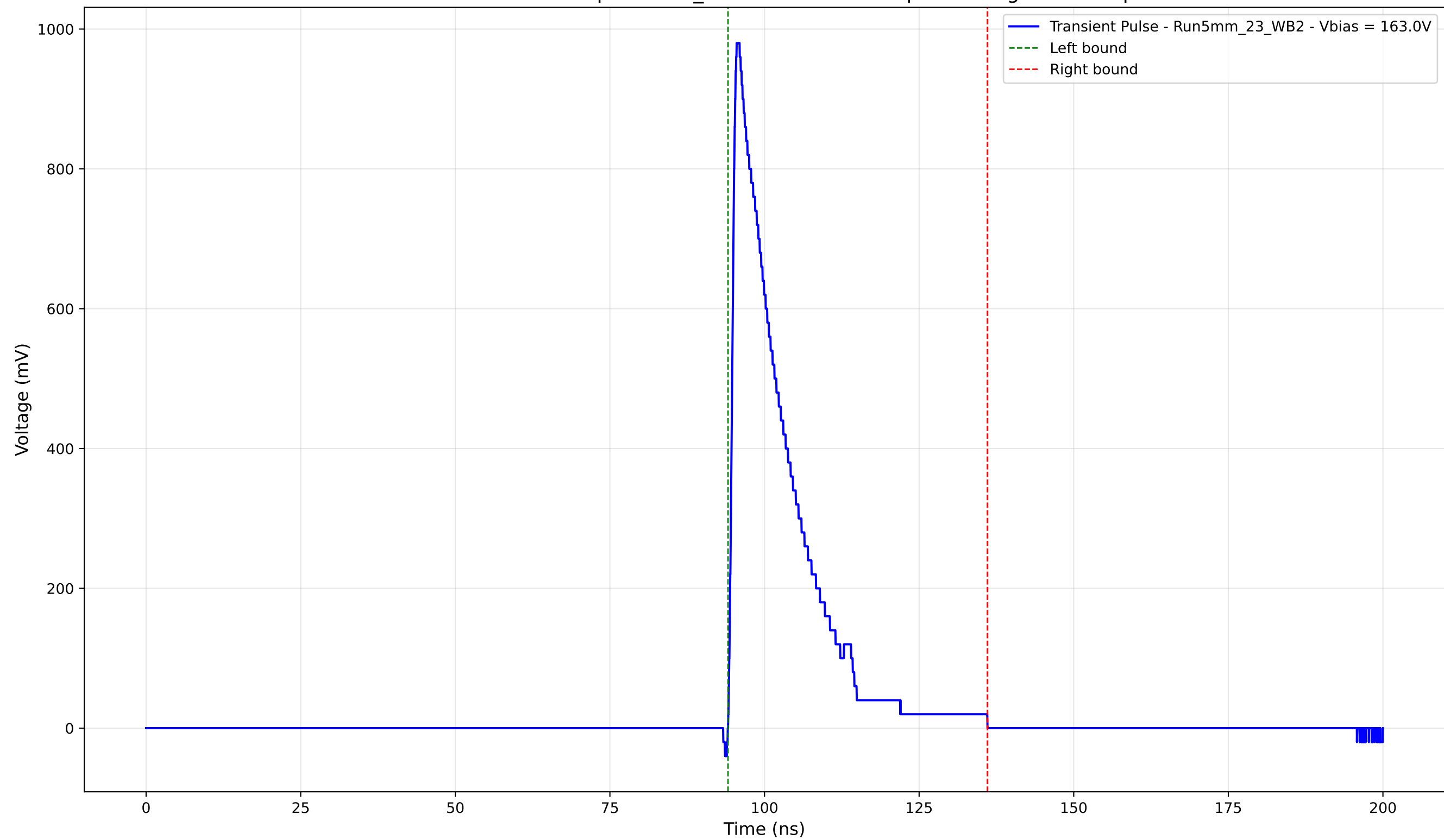
Transient Pulse - Sample: 5mm_23 - Position: 330.0 \mu\text{m} - Charge: 179.97 pC
