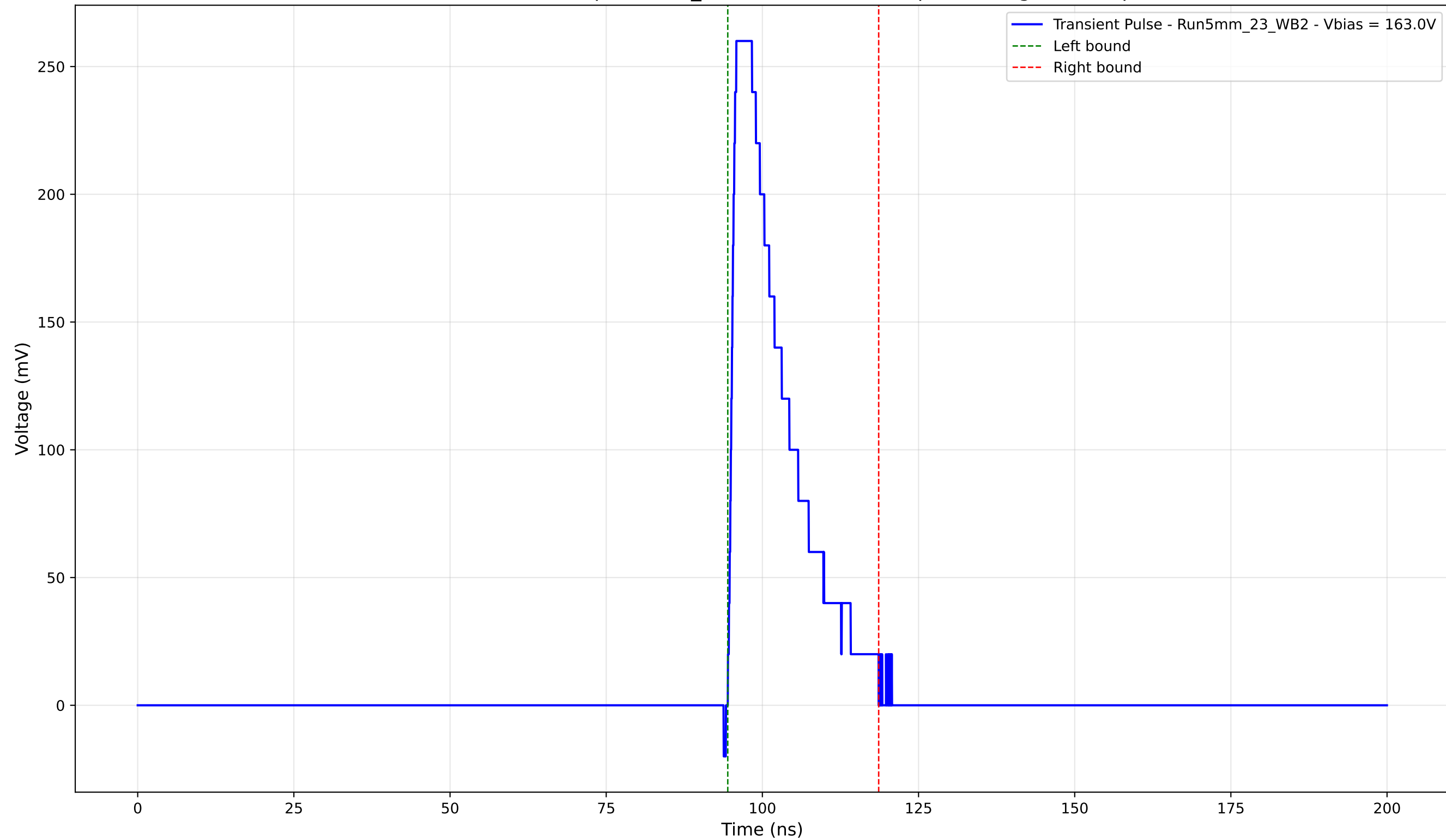
Transient Pulse - Sample: 5mm_23 - Position: 3550.0 \mu\text{m} - Charge: 50.72 pC
