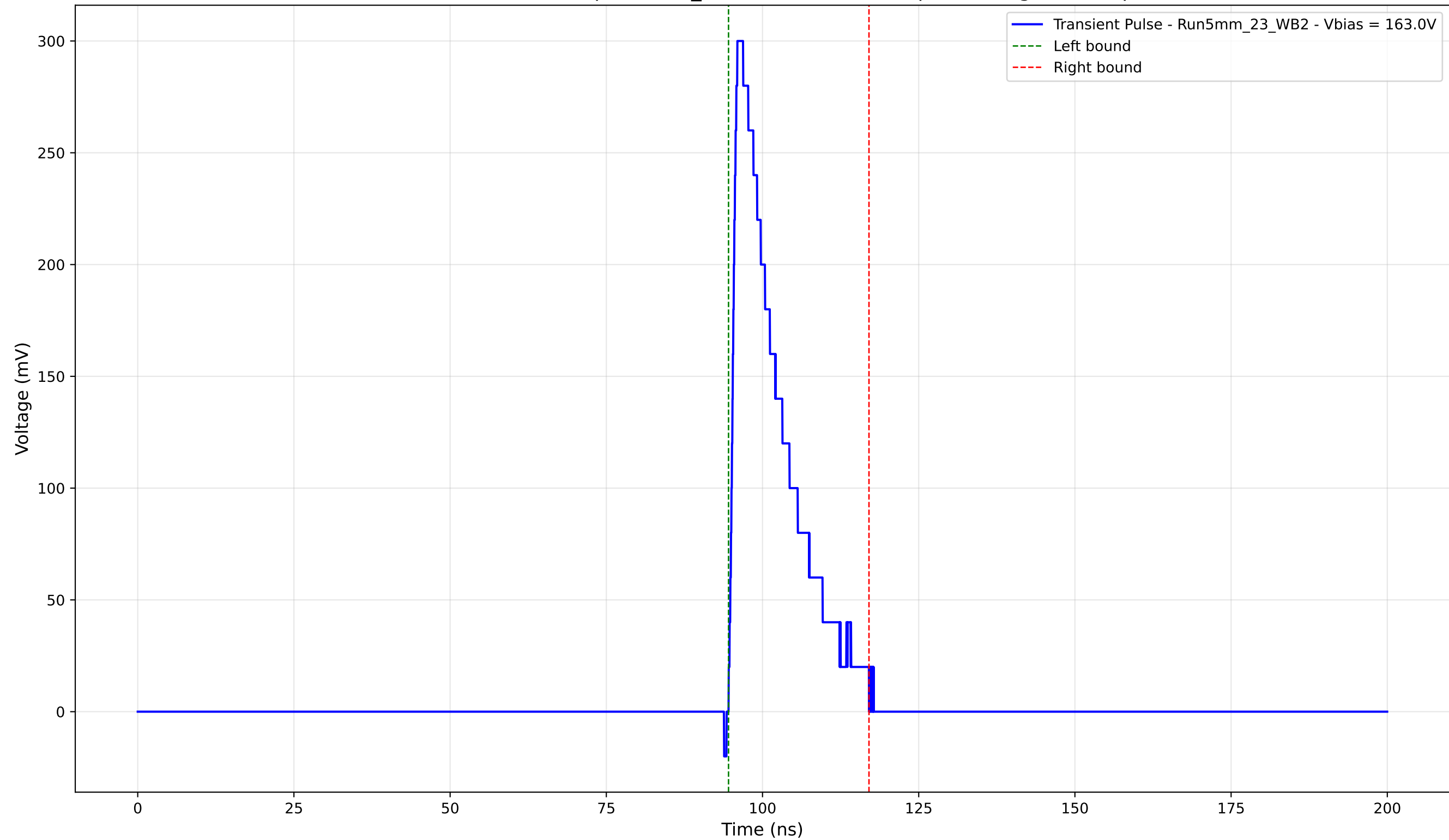
Transient Pulse - Sample: 5mm_23 - Position: 4010.0 \mu\text{m} - Charge: 50.88 pC
