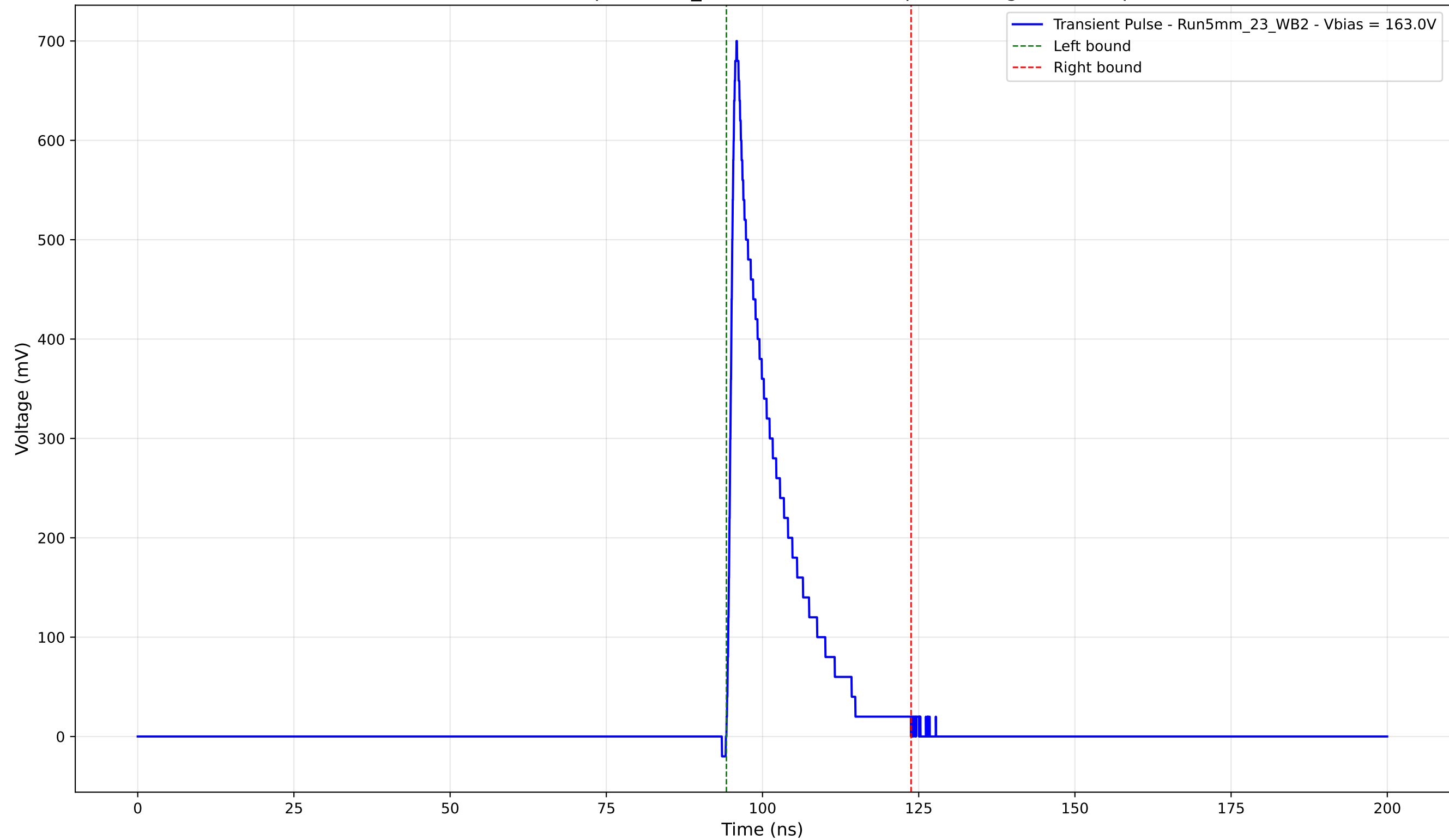
Transient Pulse - Sample: 5mm_23 - Position: 440.0 \mu\text{m} - Charge: 103.28 pC
