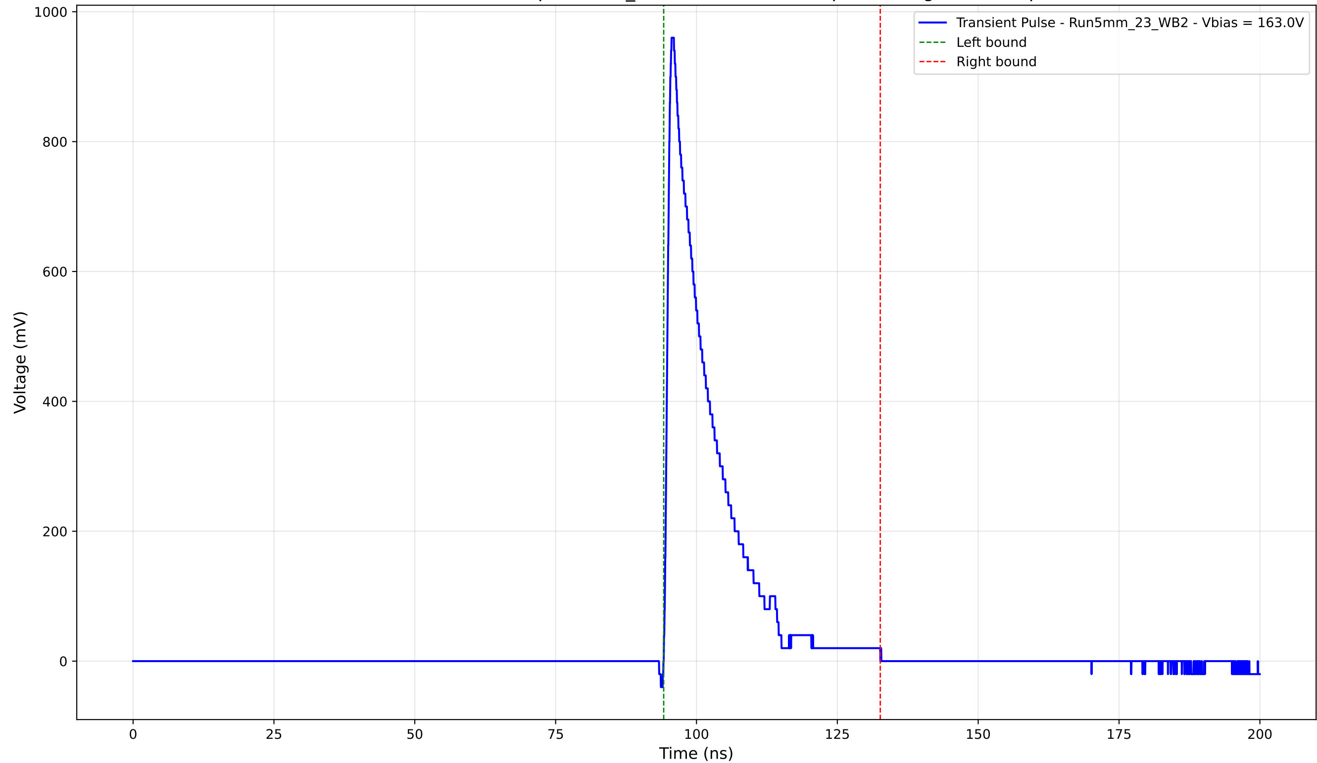
Transient Pulse - Sample: 5mm_23 - Position: 4675.0 \mu\text{m} - Charge: 156.66 pC
