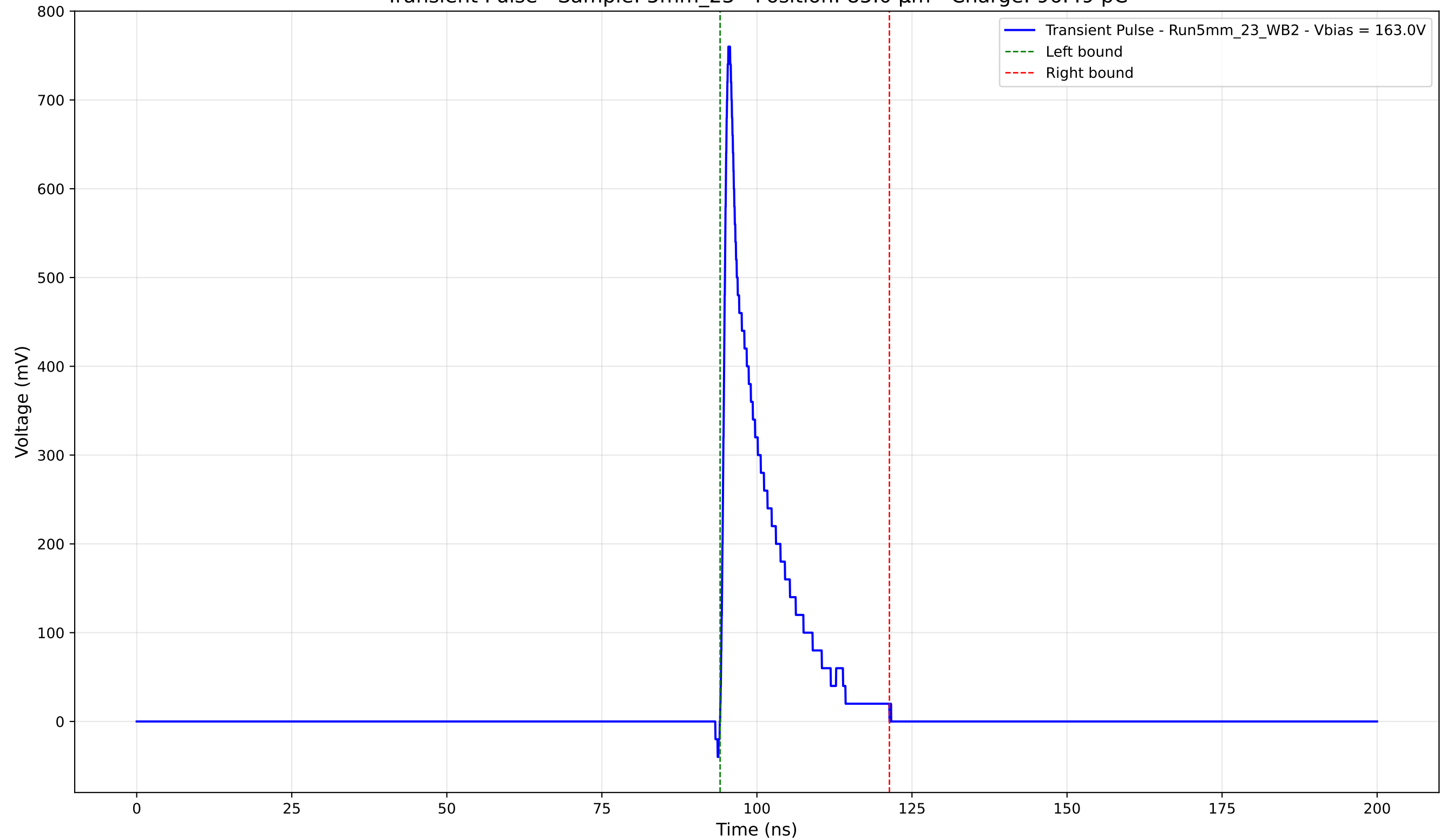
Transient Pulse - Sample: 5mm_23 - Position: 85.0 \mu\text{m} - Charge: 96.49 pC
