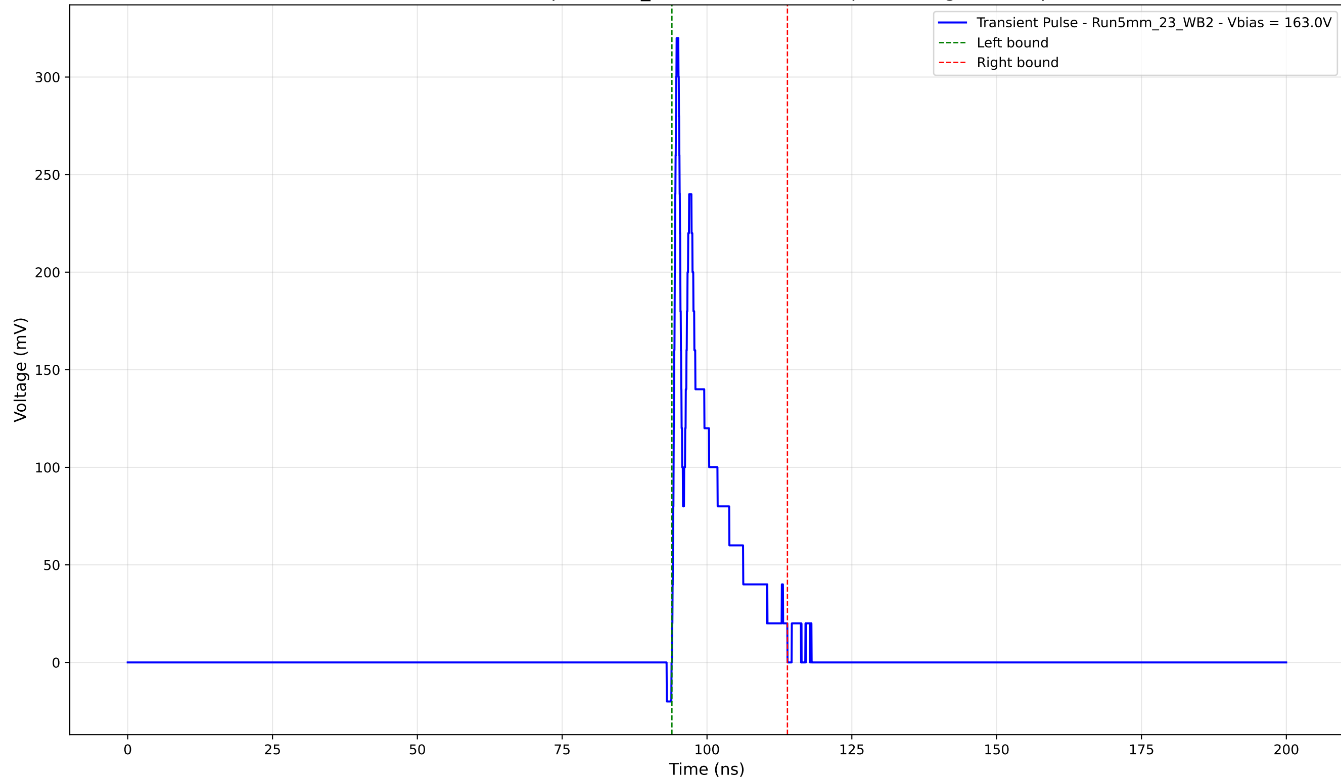
Transient Pulse - Sample: 5mm_23 - Position: 2525.0 \mu\text{m} - Charge: 35.14 pC
