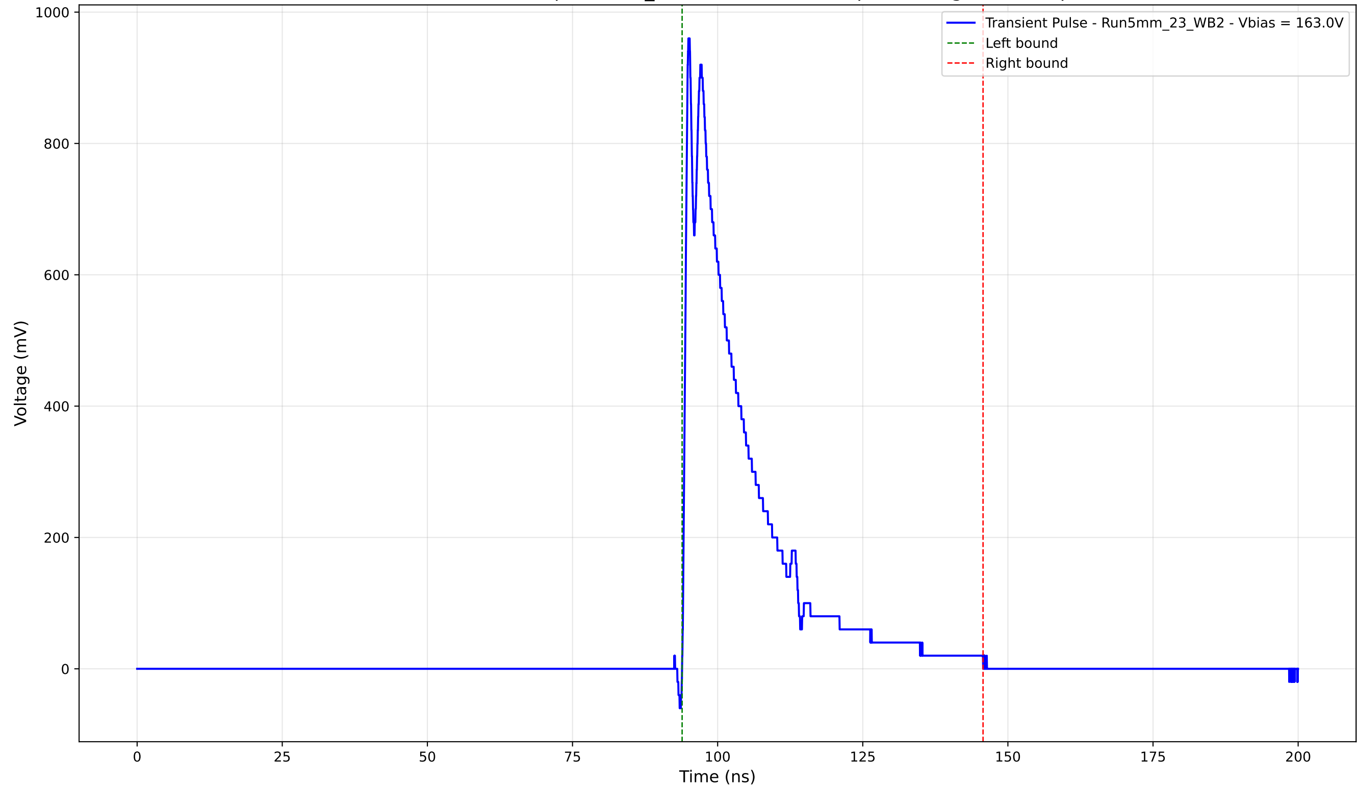
Transient Pulse - Sample: 5mm_23 - Position: 2760.0 \mu\text{m} - Charge: 204.08 pC
