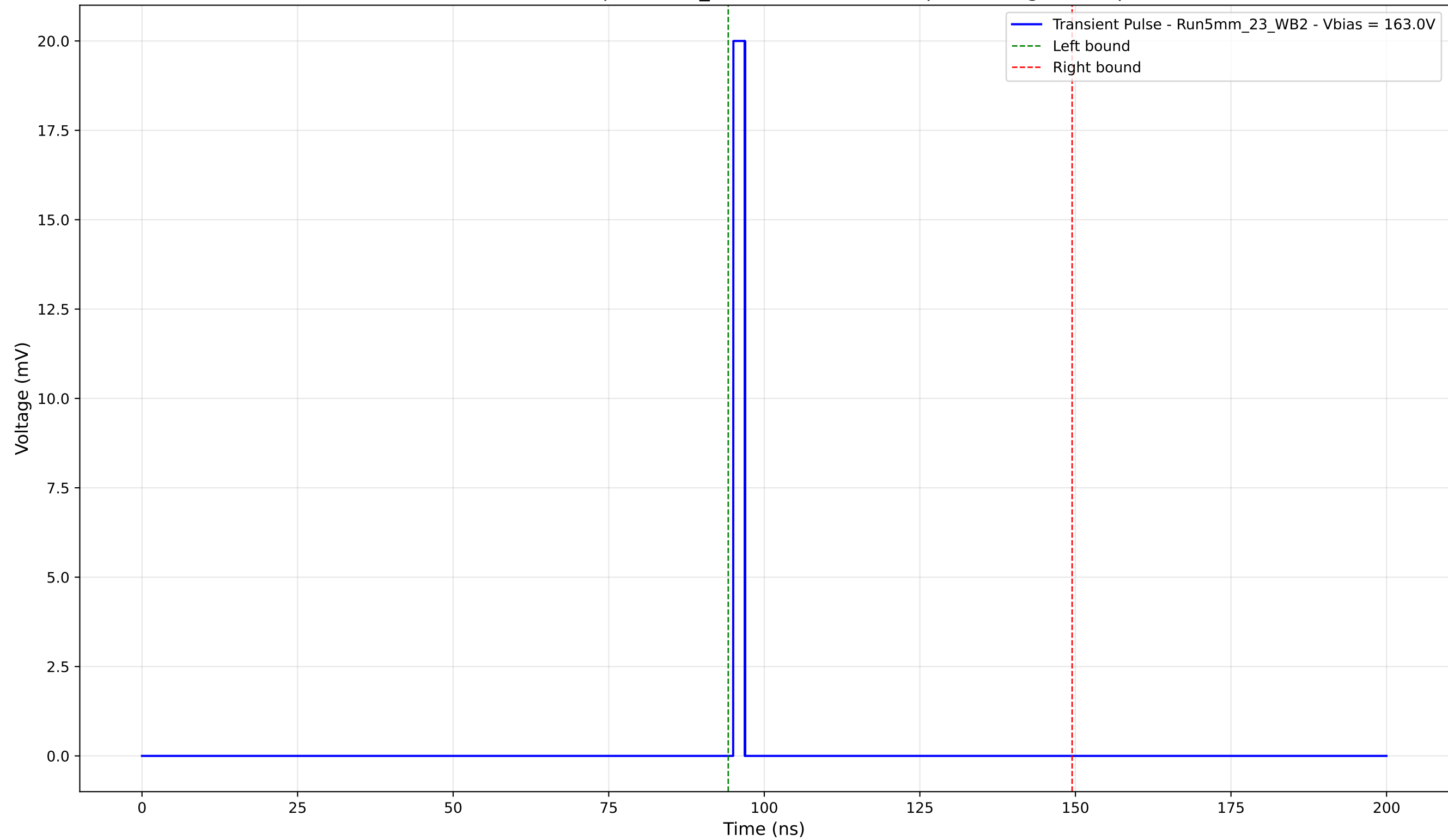
Transient Pulse - Sample: 5mm_23 - Position: 5040.0 \mu\text{m} - Charge: 0.74 pC
