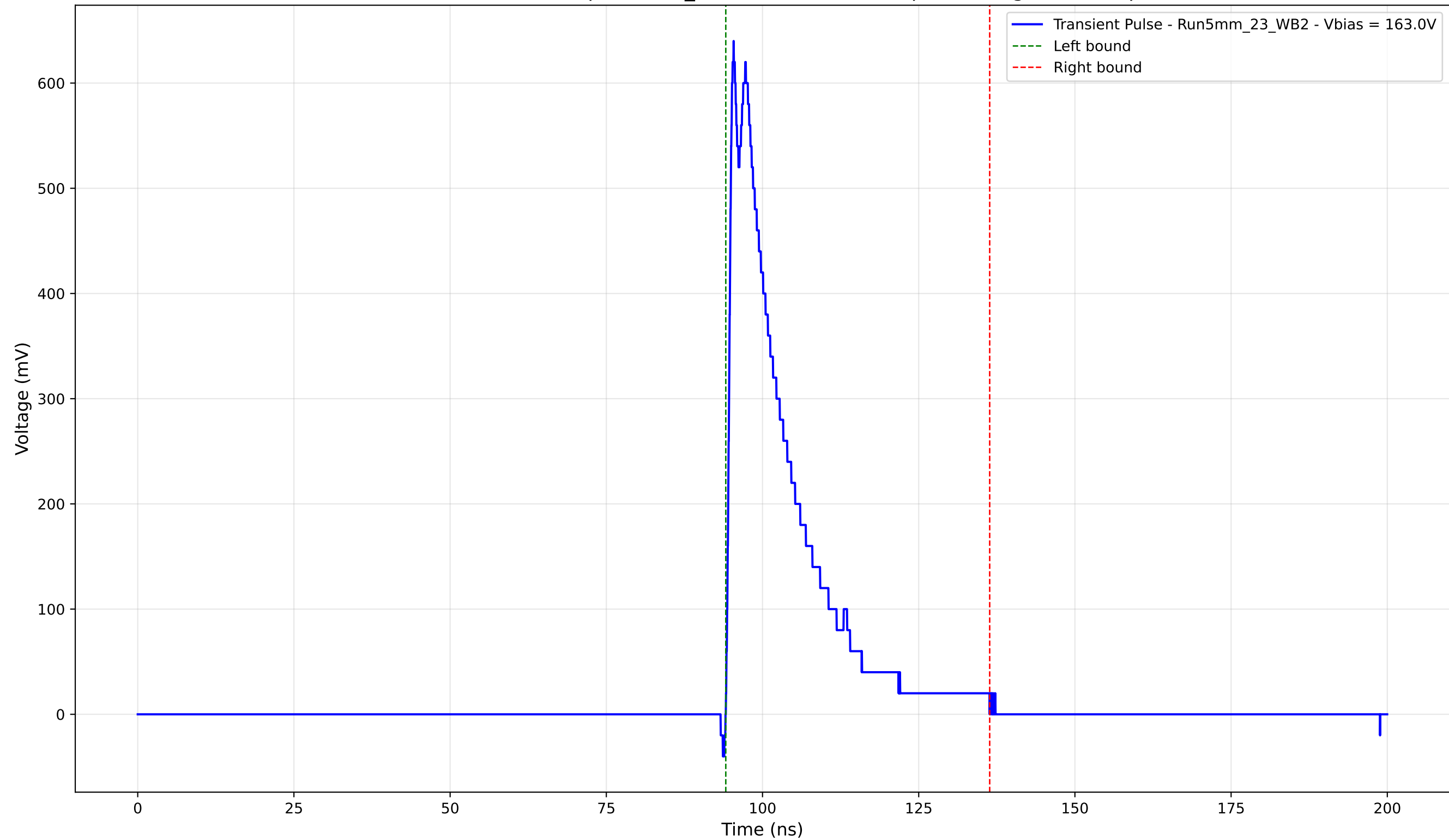
Transient Pulse - Sample: 5mm_23 - Position: 3070.0 \mu\text{m} - Charge: 125.30 pC
