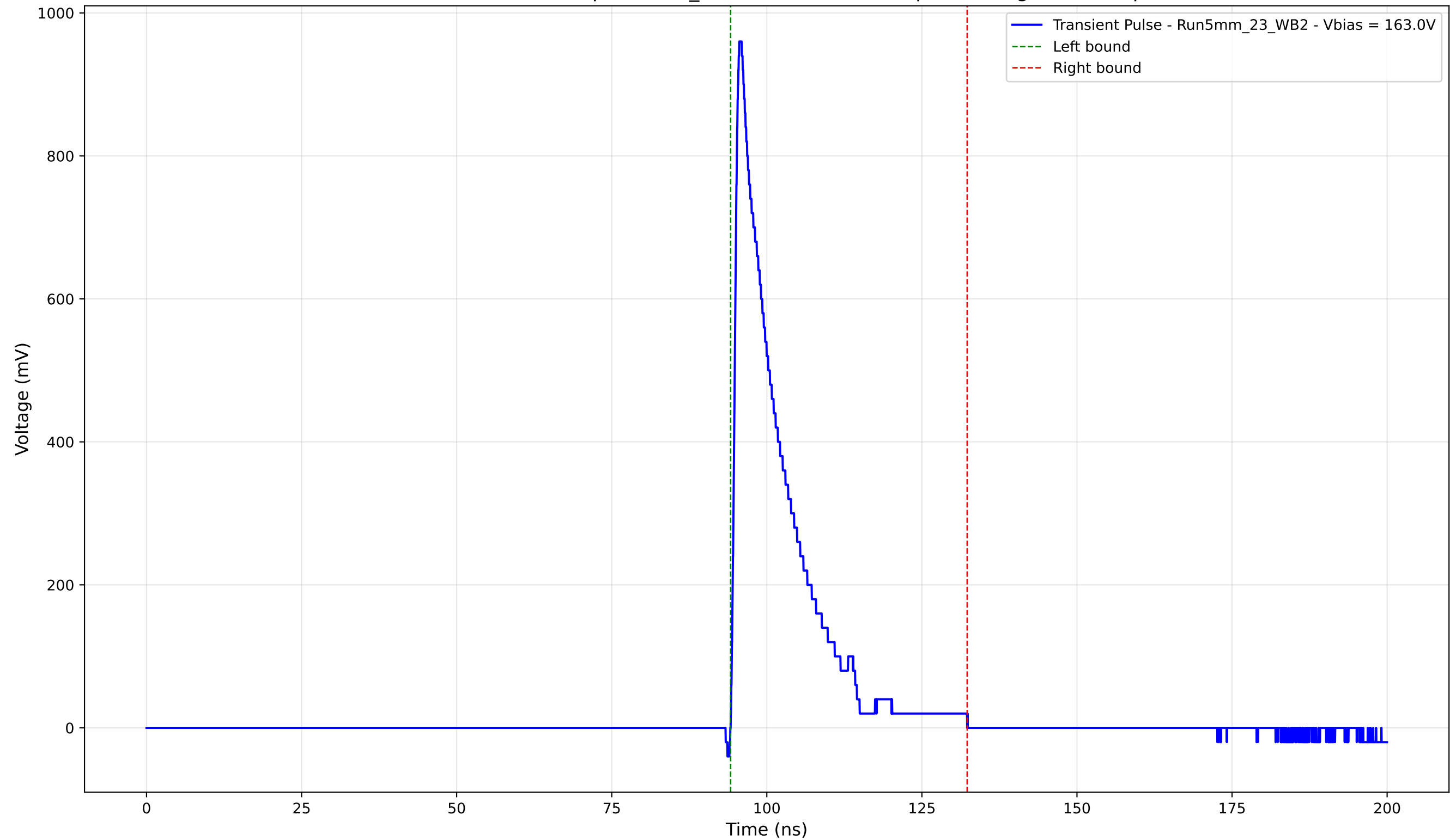
Transient Pulse - Sample: 5mm_23 - Position: 4710.0 \mu\text{m} - Charge: 152.86 pC
