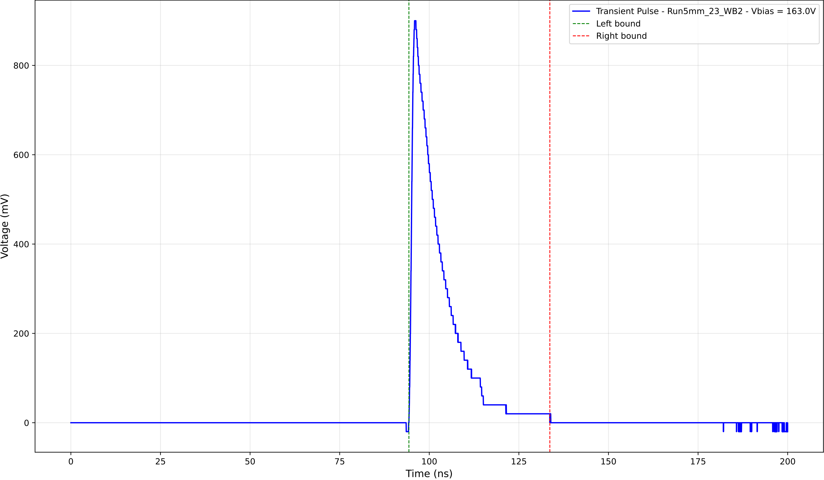
Transient Pulse - Sample: 5mm_23 - Position: 4370.0 \mu\text{m} - Charge: 158.67 pC
