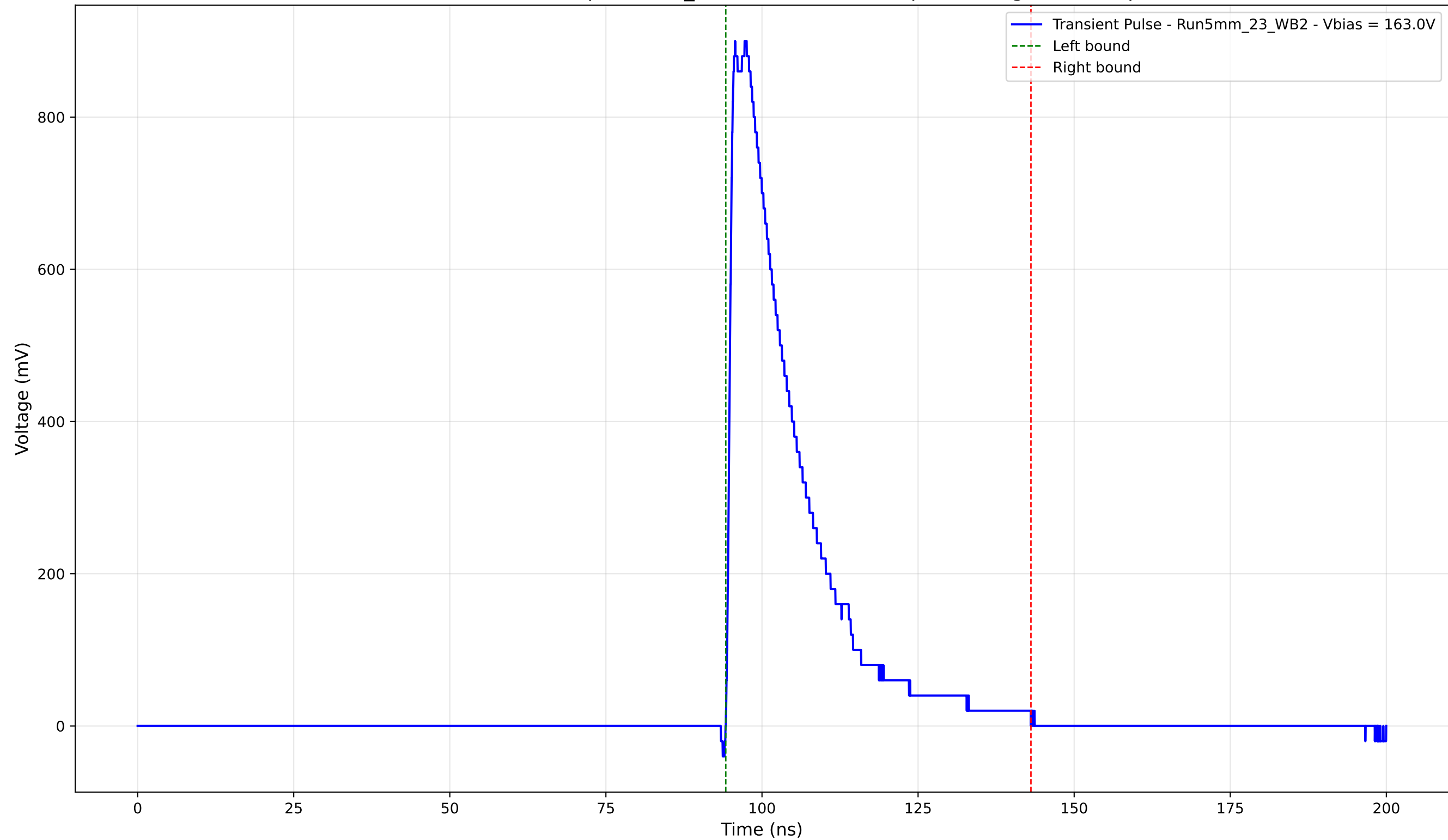
Transient Pulse - Sample: 5mm_23 - Position: 1720.0 \mu\text{m} - Charge: 210.58 pC
