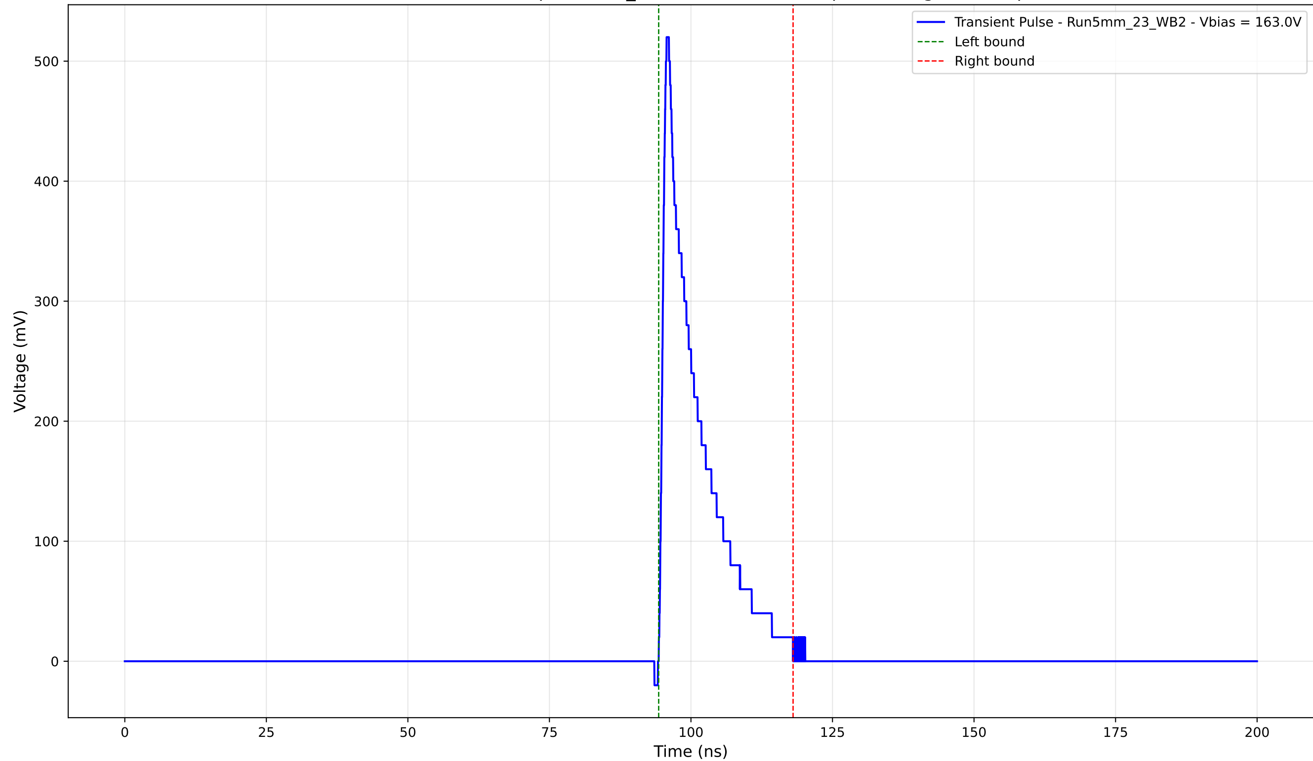
Transient Pulse - Sample: 5mm_23 - Position: 4575.0 \mu\text{m} - Charge: 70.59 pC
