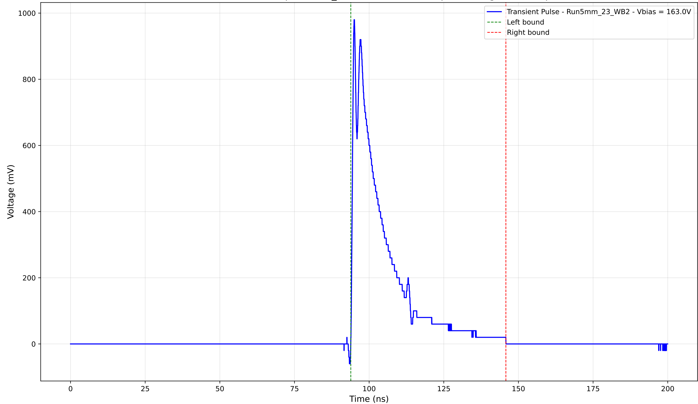
Transient Pulse - Sample: 5mm_23 - Position: 2710.0 \mu\text{m} - Charge: 202.17 pC
