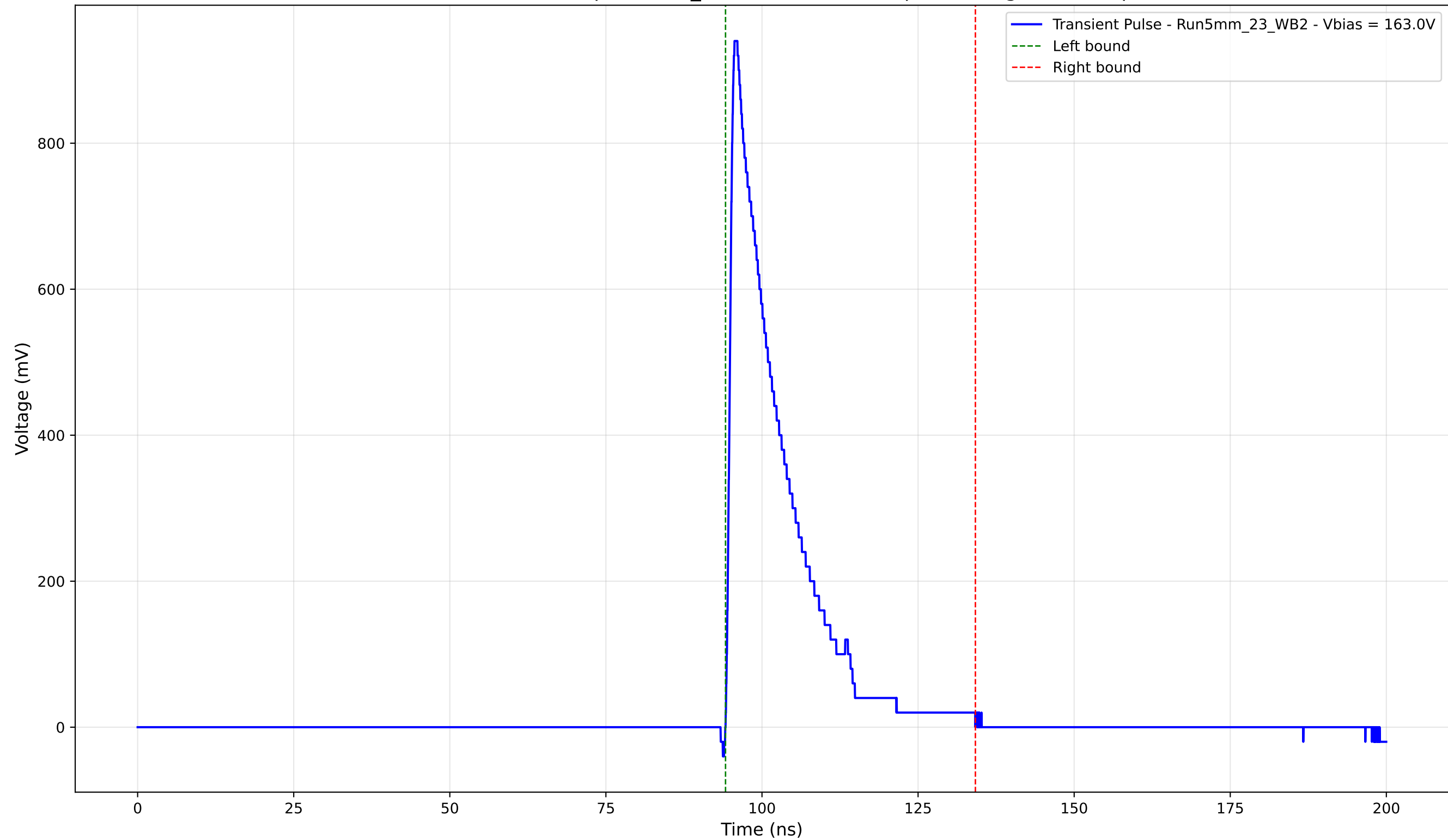
Transient Pulse - Sample: 5mm_23 - Position: 405.0 \mu\text{m} - Charge: 166.44 pC
