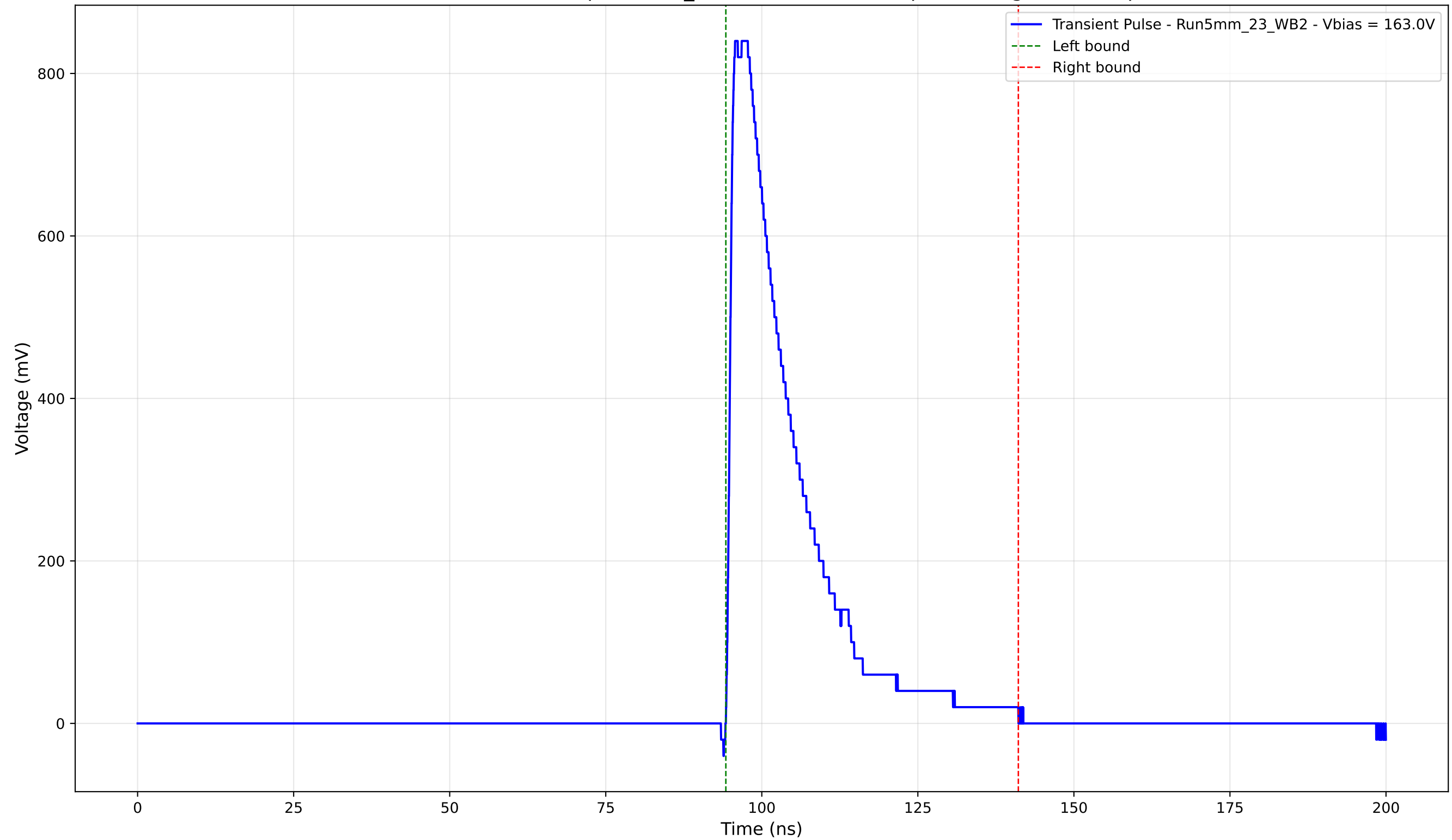
Transient Pulse - Sample: 5mm_23 - Position: 3380.0 \mu\text{m} - Charge: 189.87 pC
