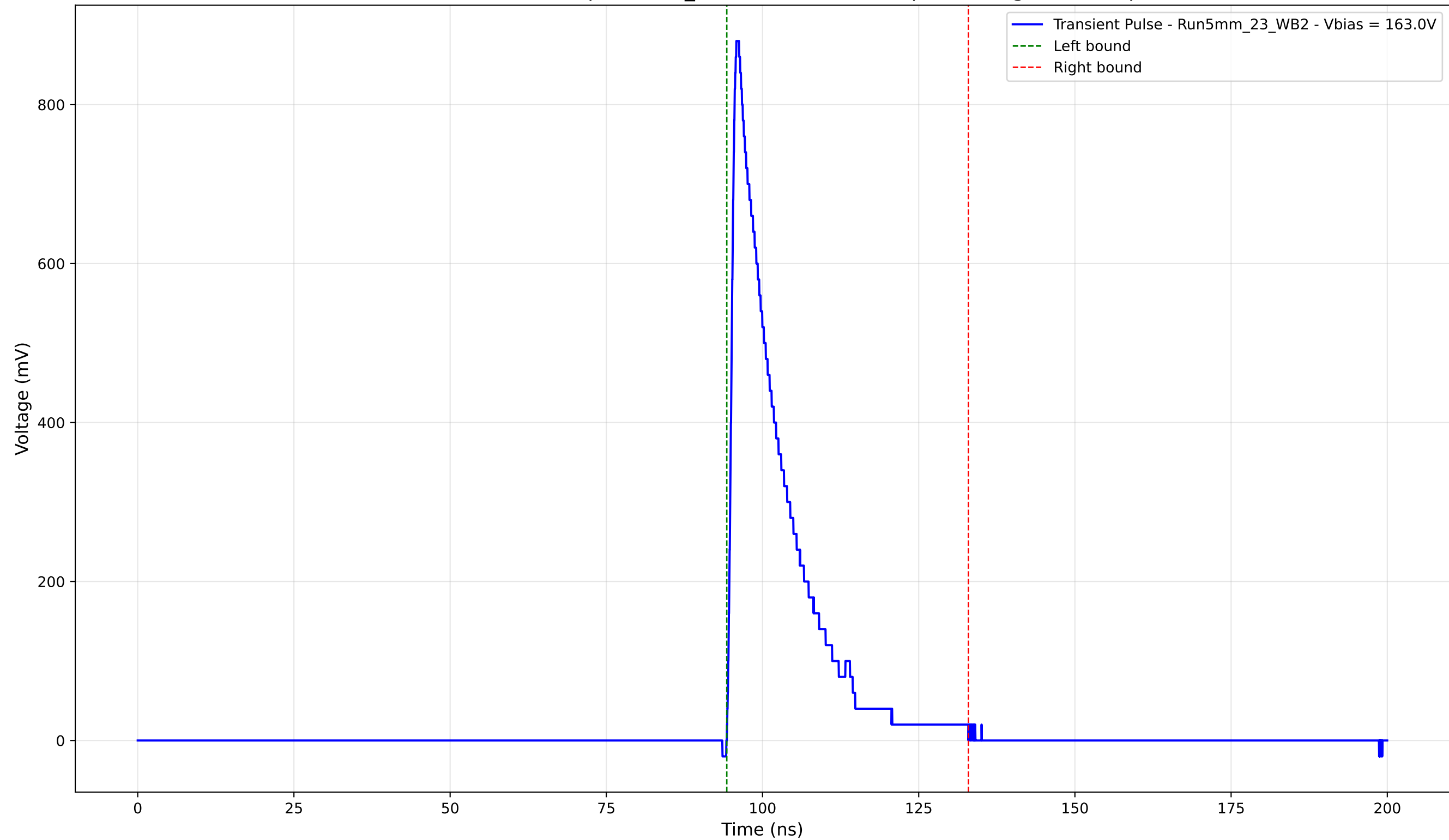
Transient Pulse - Sample: 5mm_23 - Position: 4445.0 \mu\text{m} - Charge: 148.95 pC
