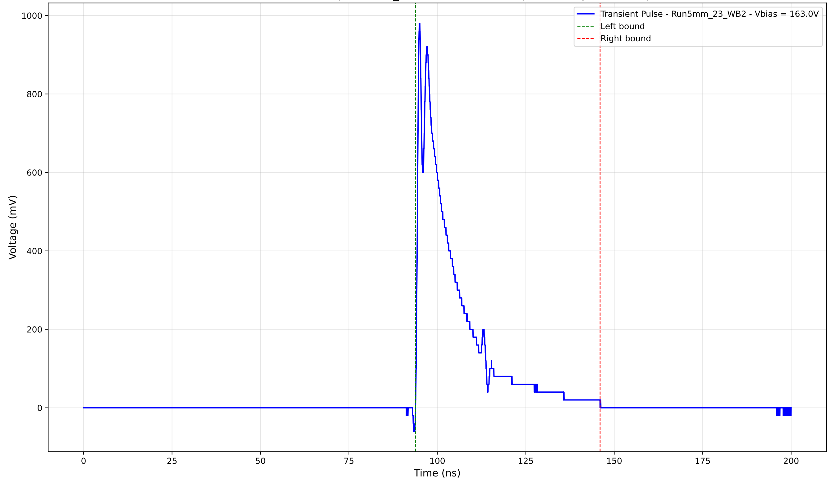
Transient Pulse - Sample: 5mm_23 - Position: 2370.0 \mu\text{m} - Charge: 200.73 pC
