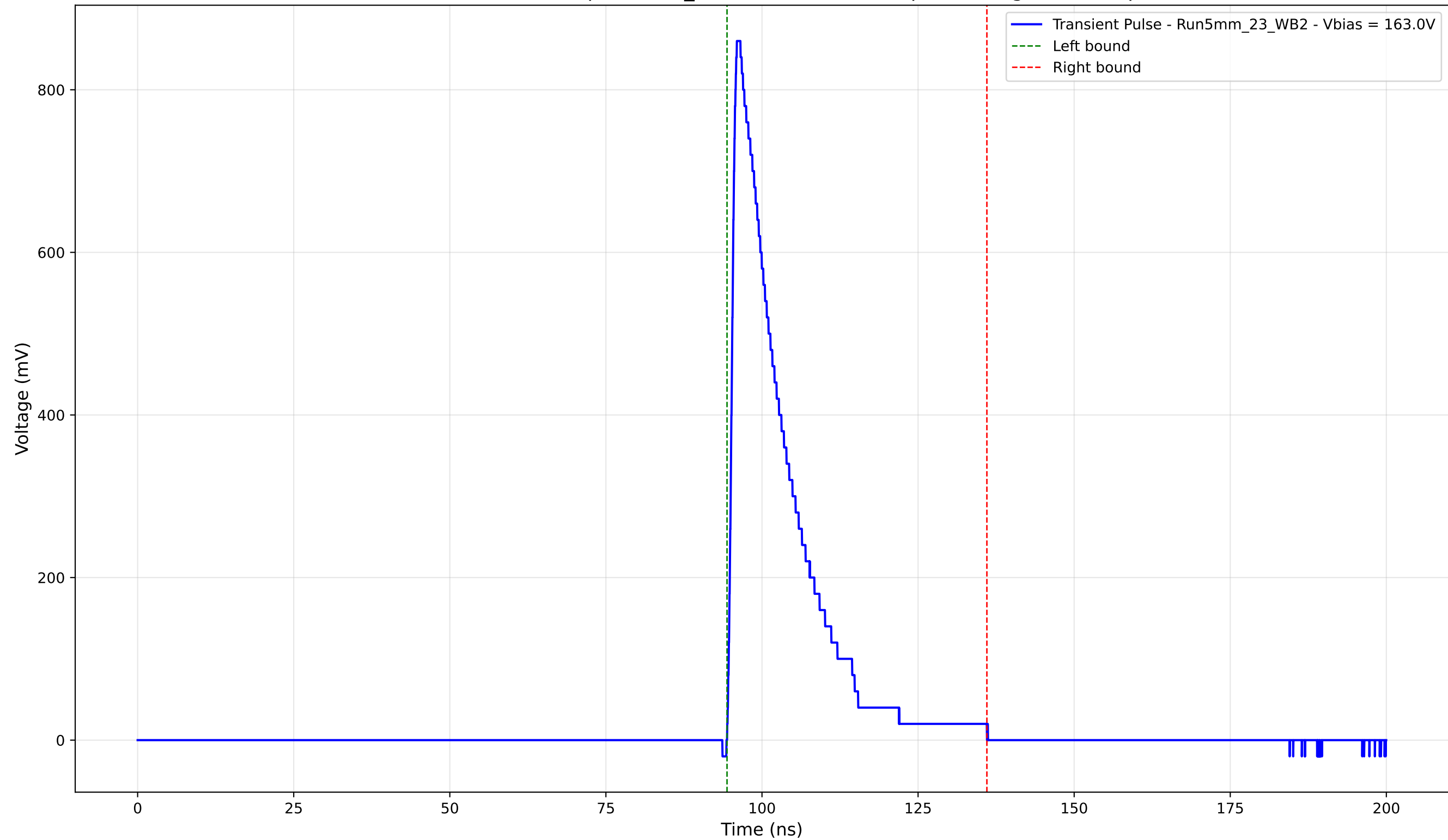
Transient Pulse - Sample: 5mm_23 - Position: 4155.0 \mu\text{m} - Charge: 160.62 pC
