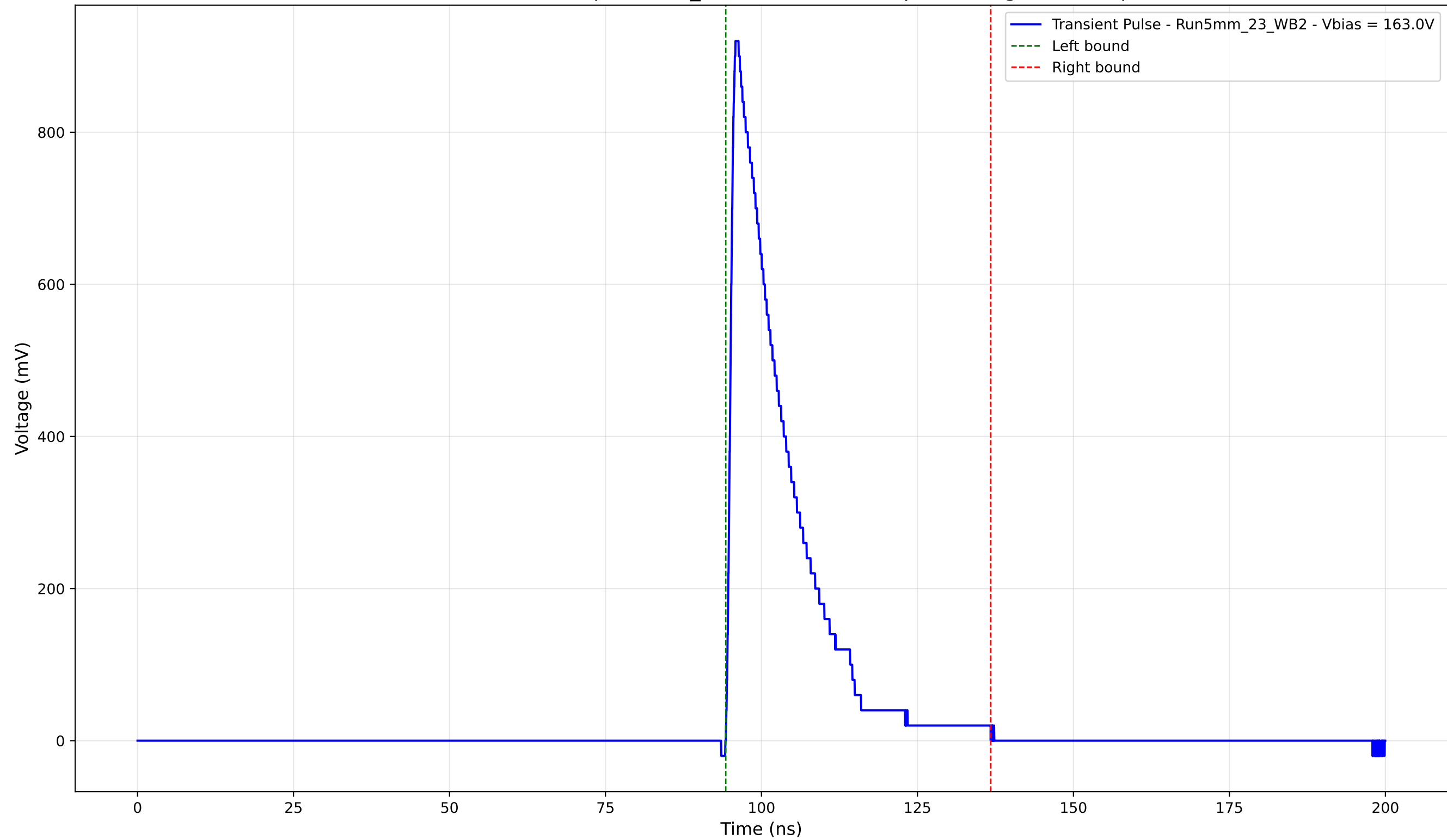
Transient Pulse - Sample: 5mm_23 - Position: 645.0 \mu\text{m} - Charge: 177.43 pC
