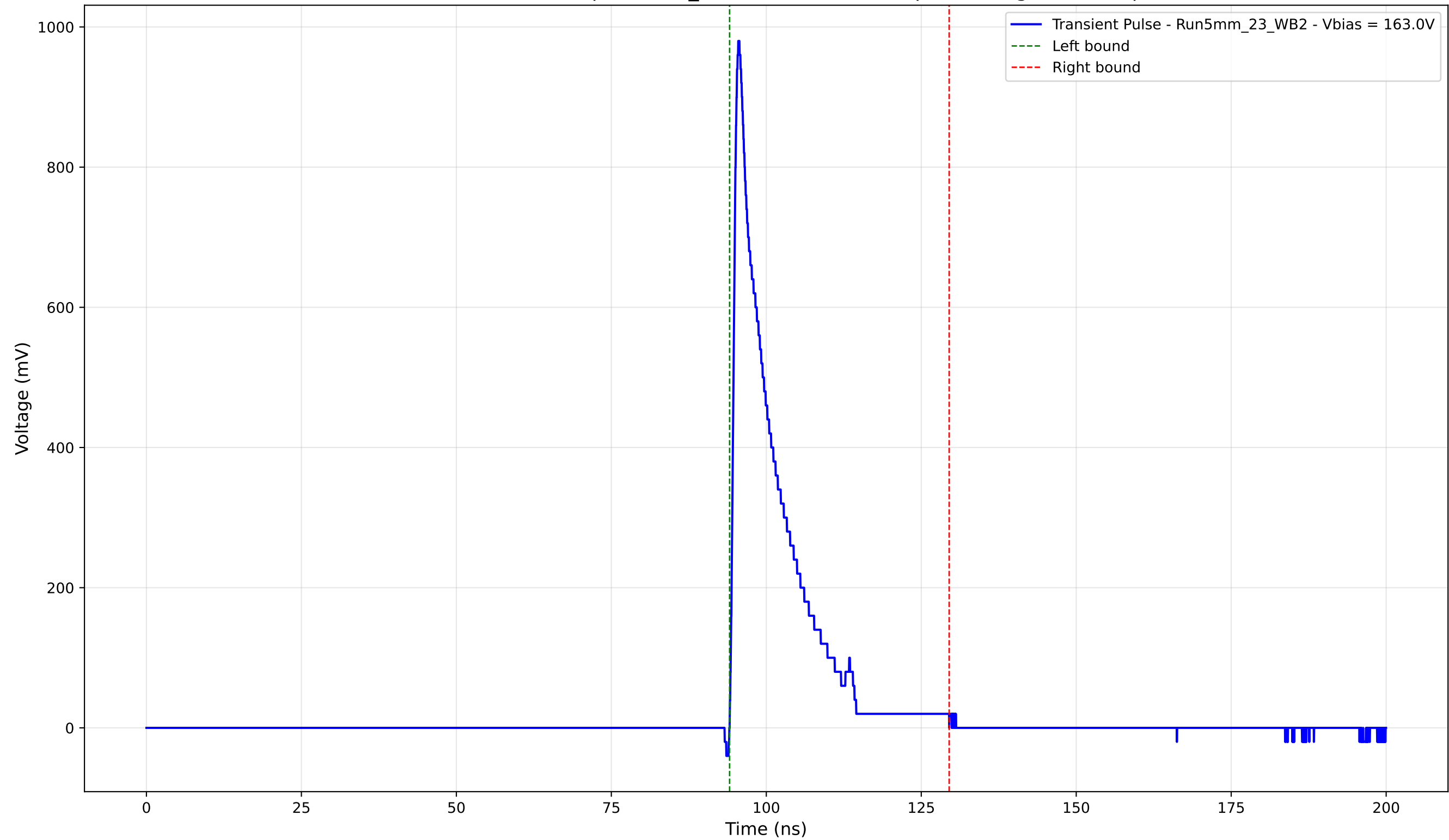
Transient Pulse - Sample: 5mm_23 - Position: 4865.0 \mu\text{m} - Charge: 138.27 pC
