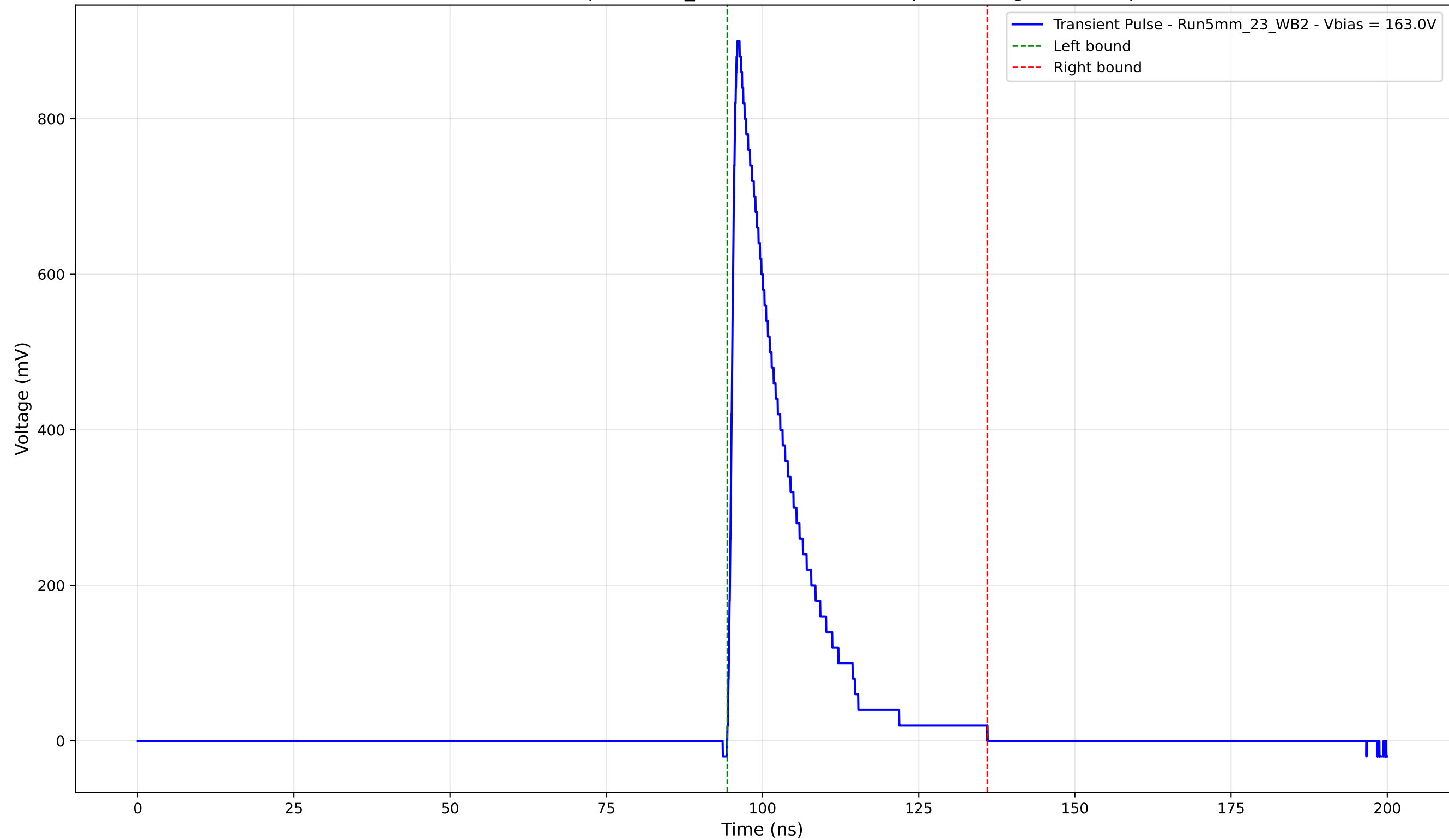
Transient Pulse - Sample: 5mm_23 - Position: 4260.0 \mu\text{m} - Charge: 163.99 pC
