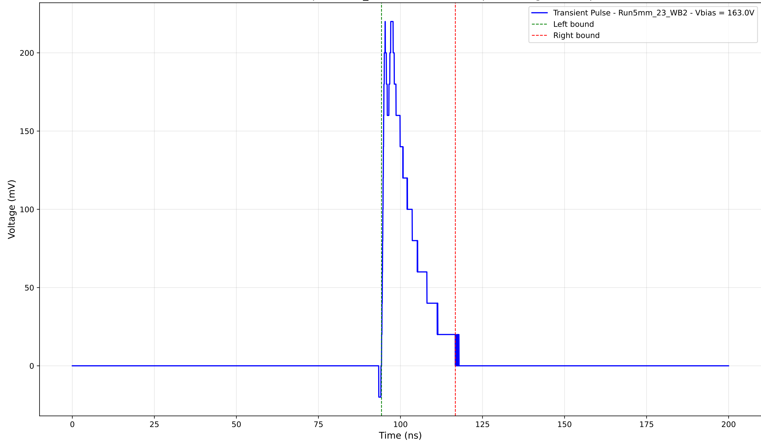
Transient Pulse - Sample: 5mm_23 - Position: 2000.0 \mu\text{m} - Charge: 38.82 pC
