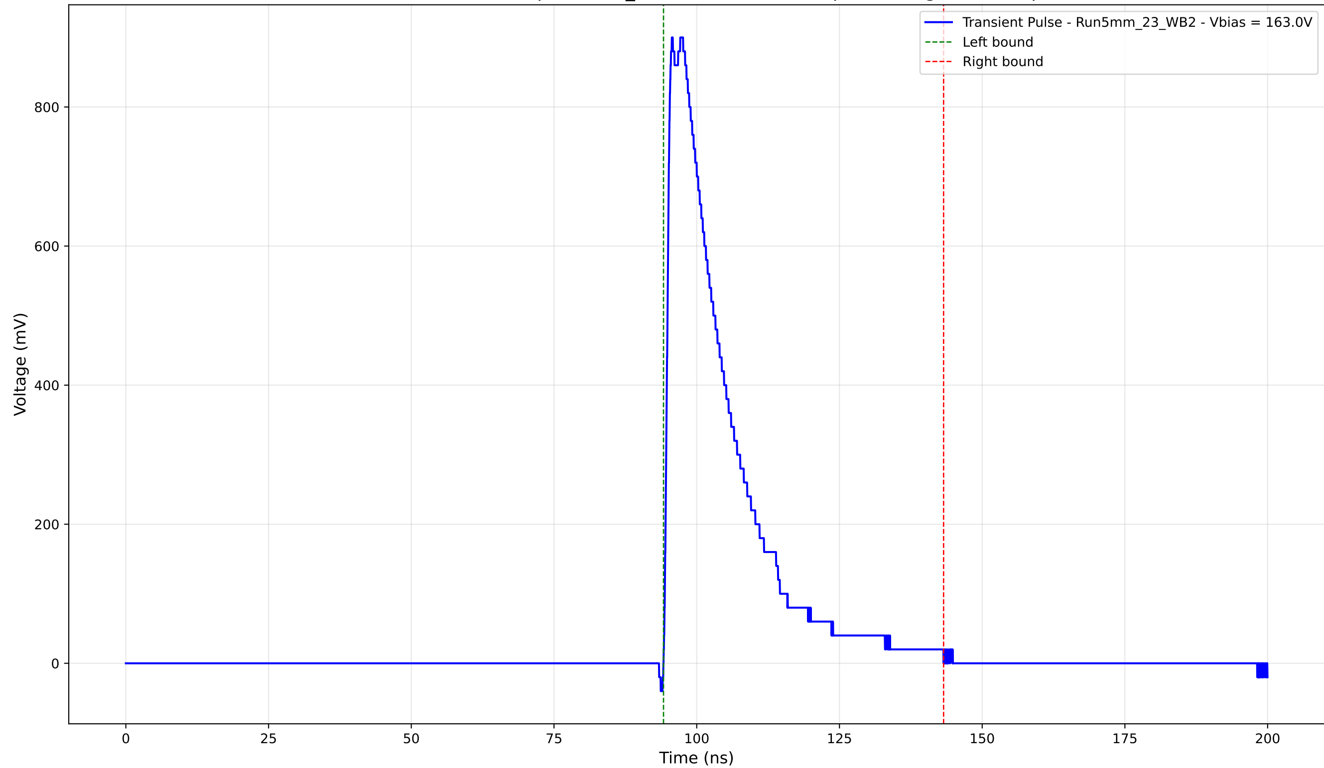
Transient Pulse - Sample: 5mm_23 - Position: 1730.0 \mu\text{m} - Charge: 212.06 pC
