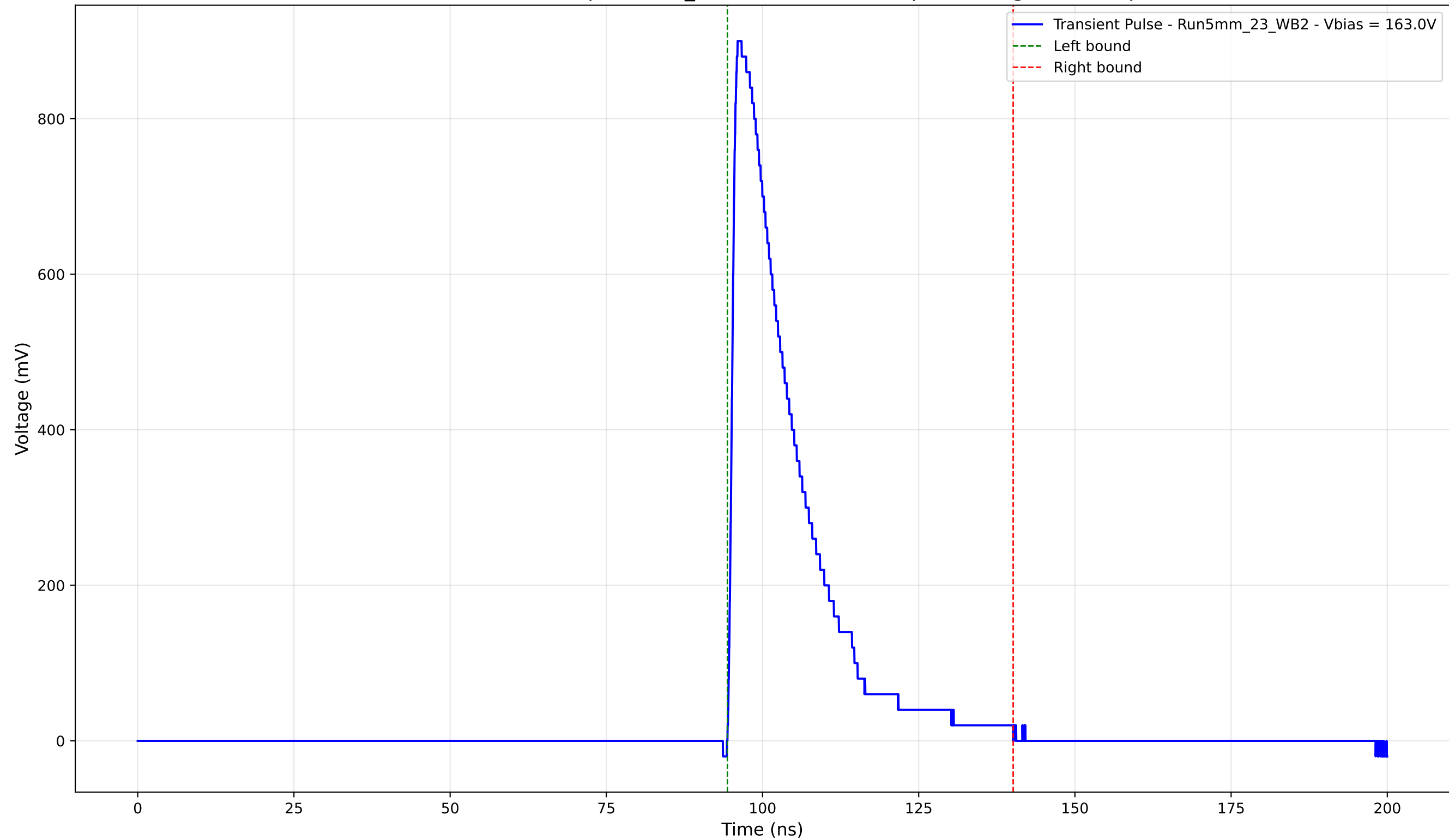
Transient Pulse - Sample: 5mm_23 - Position: 1245.0 \mu\text{m} - Charge: 199.61 pC
