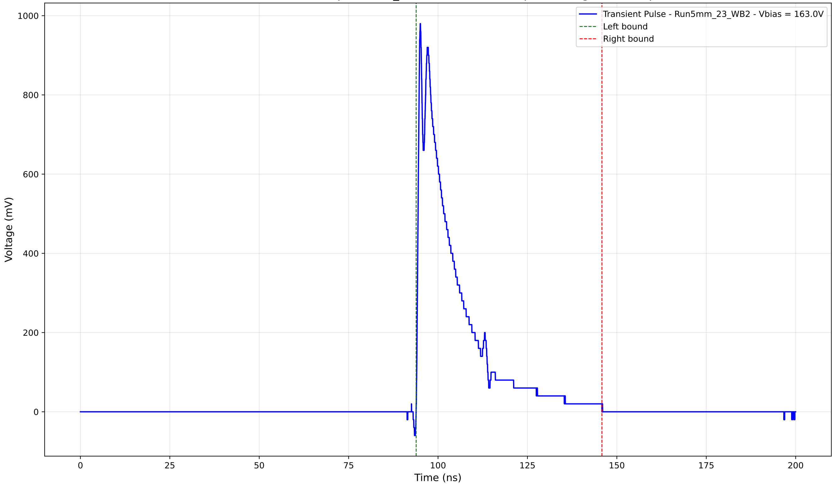
Transient Pulse - Sample: 5mm_23 - Position: 2295.0 \mu\text{m} - Charge: 205.38 pC
