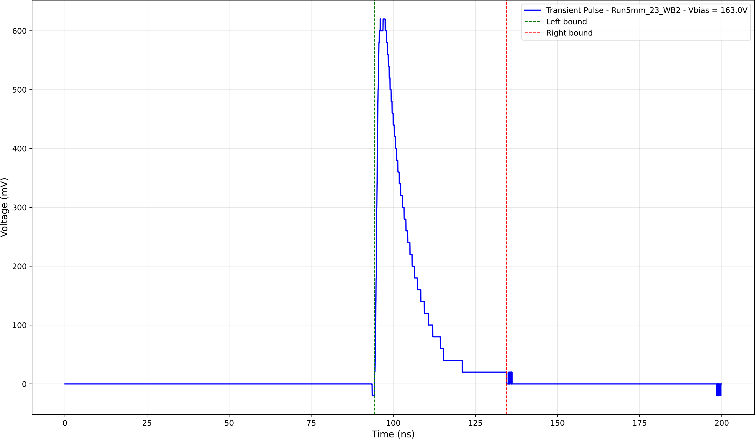
Transient Pulse - Sample: 5mm_23 - Position: 3465.0 \mu\text{m} - Charge: 125.53 pC
