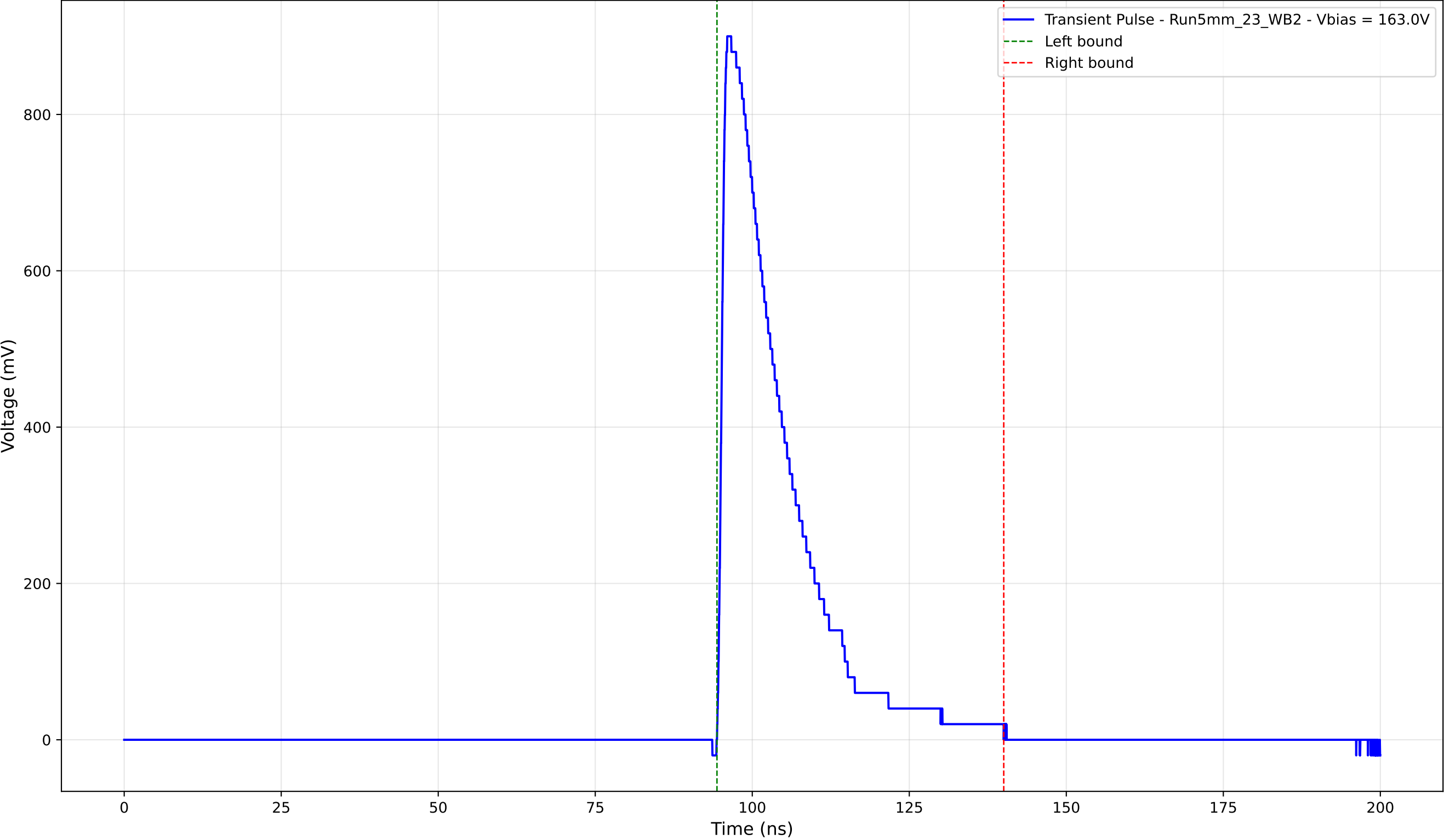
Transient Pulse - Sample: 5mm_23 - Position: 1260.0 \mu\text{m} - Charge: 199.87 pC
