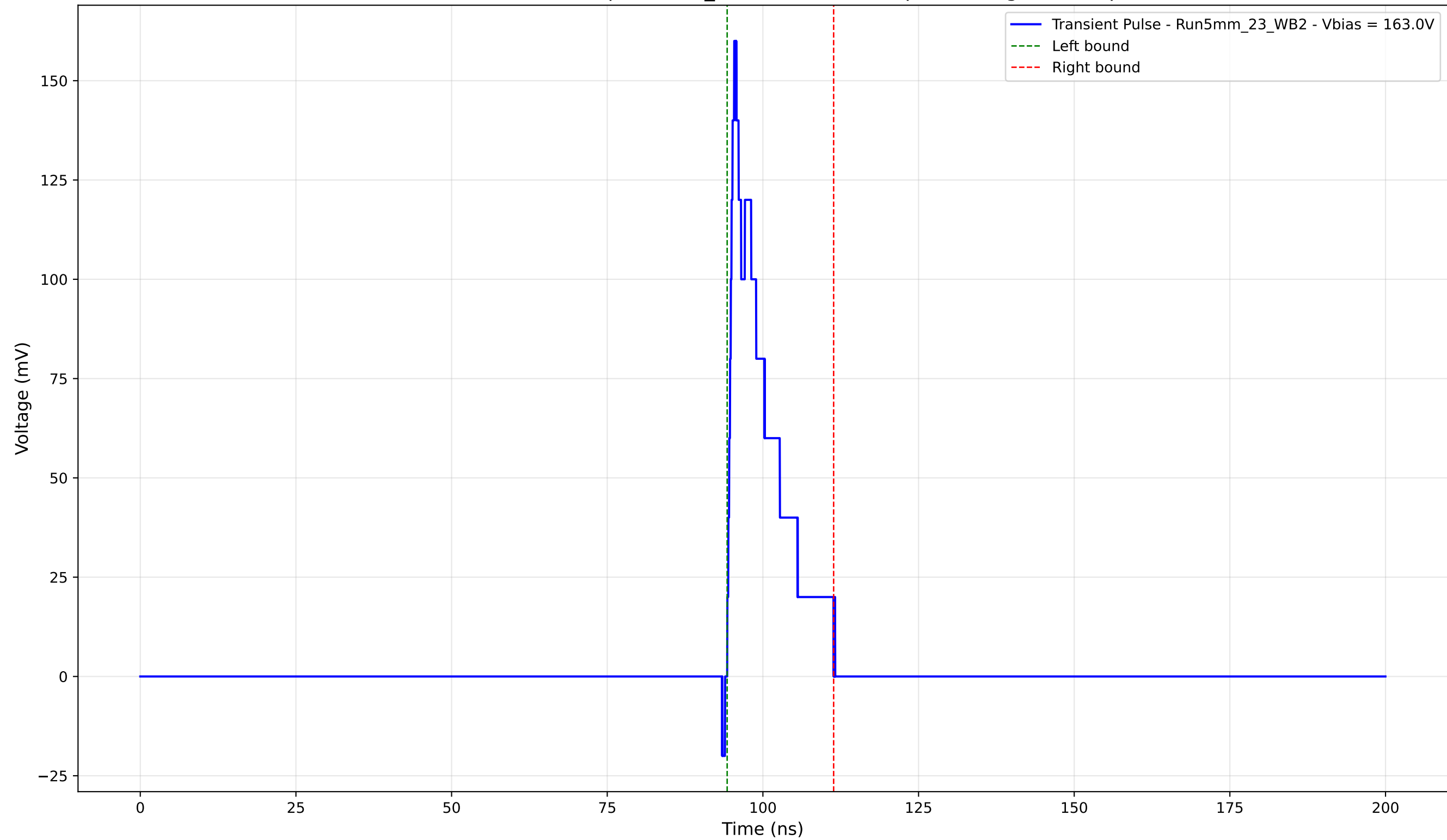
Transient Pulse - Sample: 5mm_23 - Position: 45.0 \mu\text{m} - Charge: 19.94 pC
