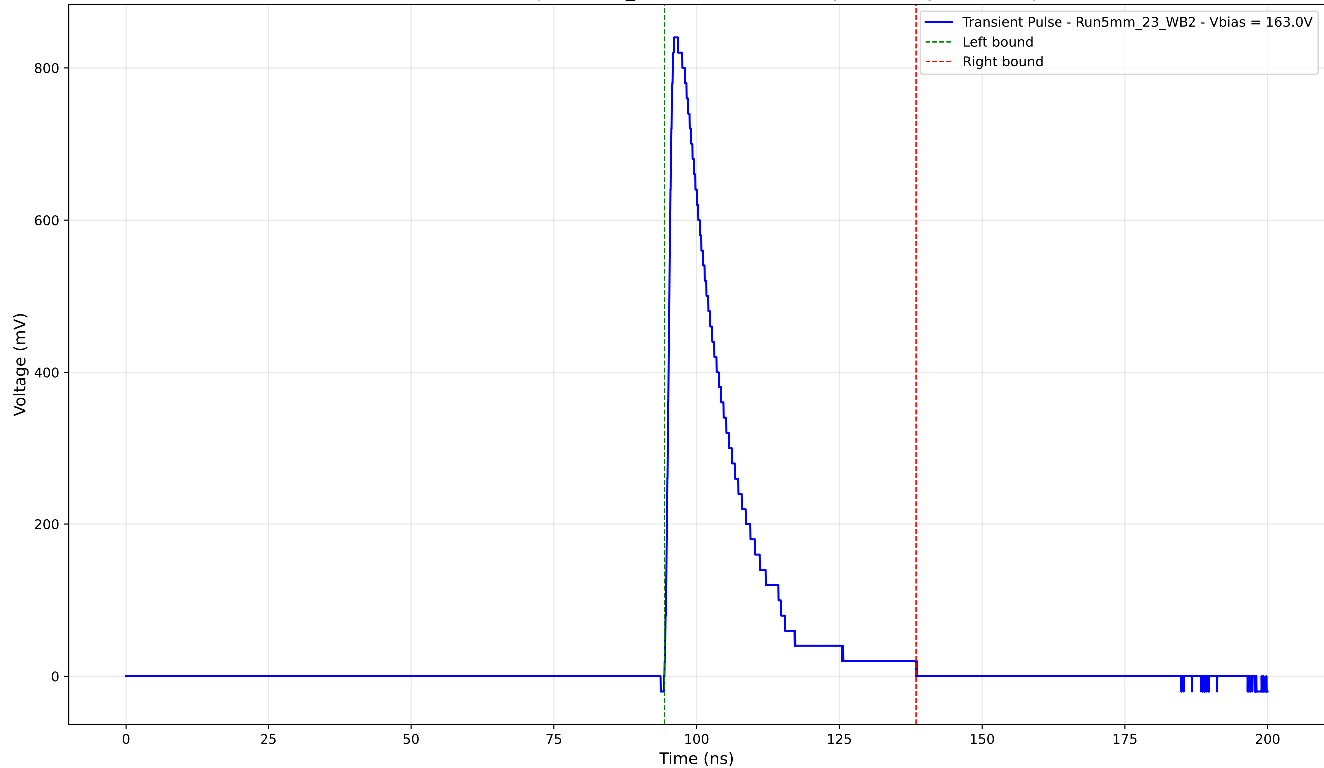
Transient Pulse - Sample: 5mm_23 - Position: 3700.0 \mu\text{m} - Charge: 174.76 pC
