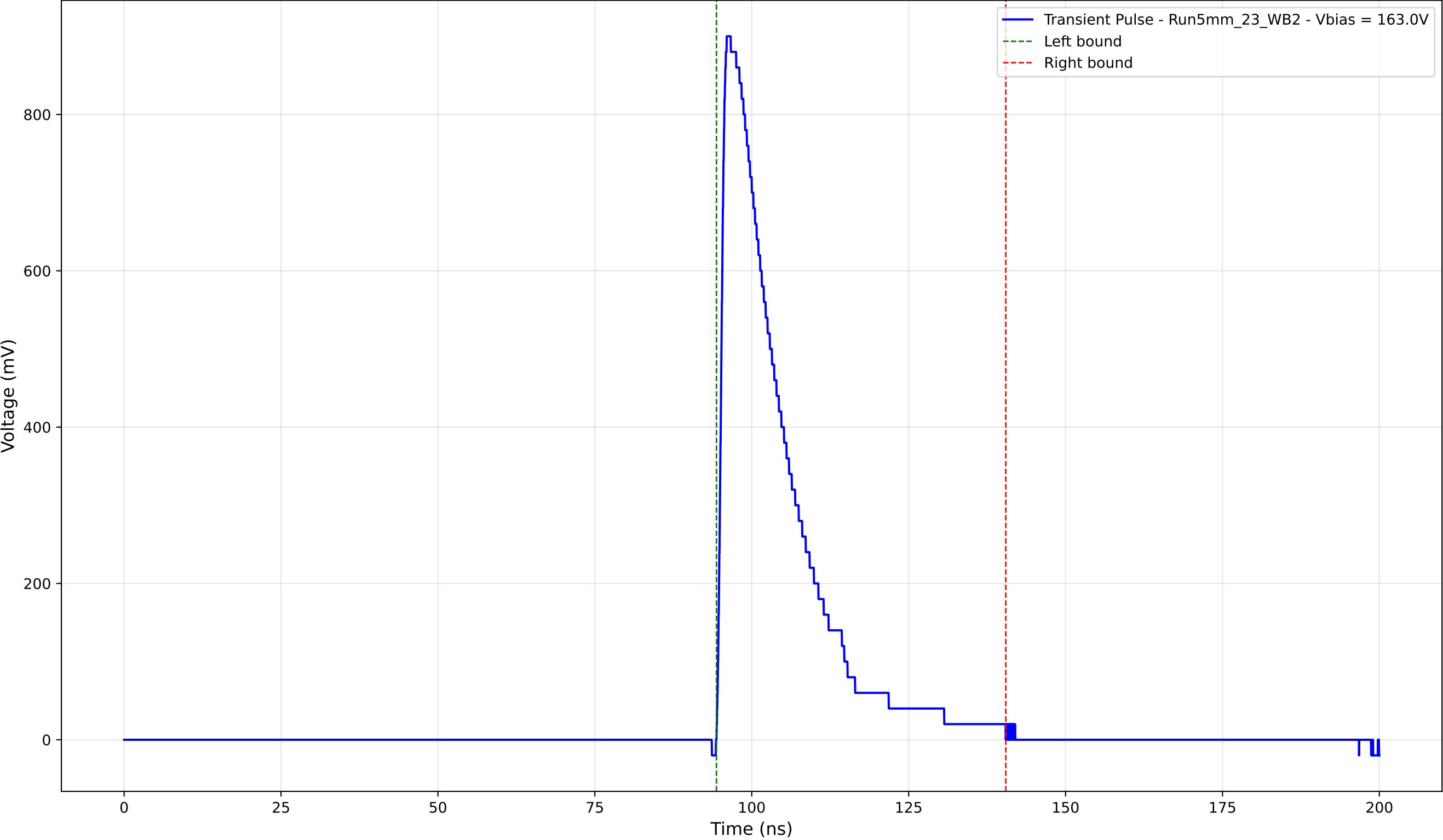
Transient Pulse - Sample: 5mm_23 - Position: 1265.0 \mu\text{m} - Charge: 200.68 pC
