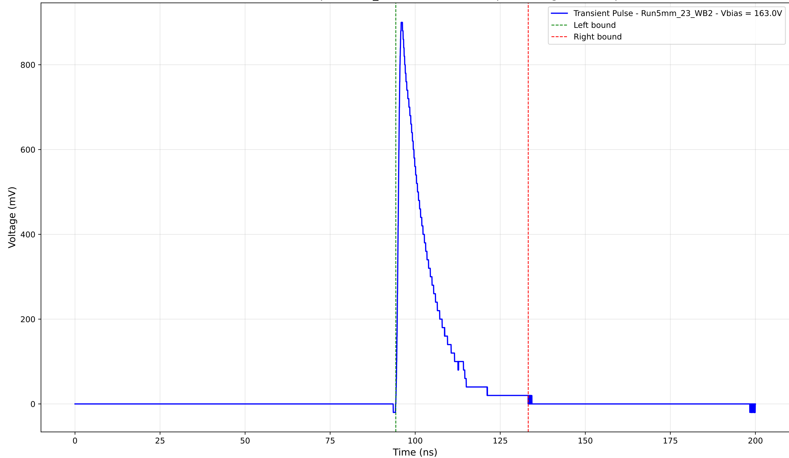
Transient Pulse - Sample: 5mm_23 - Position: 4400.0 \mu\text{m} - Charge: 156.42 pC
