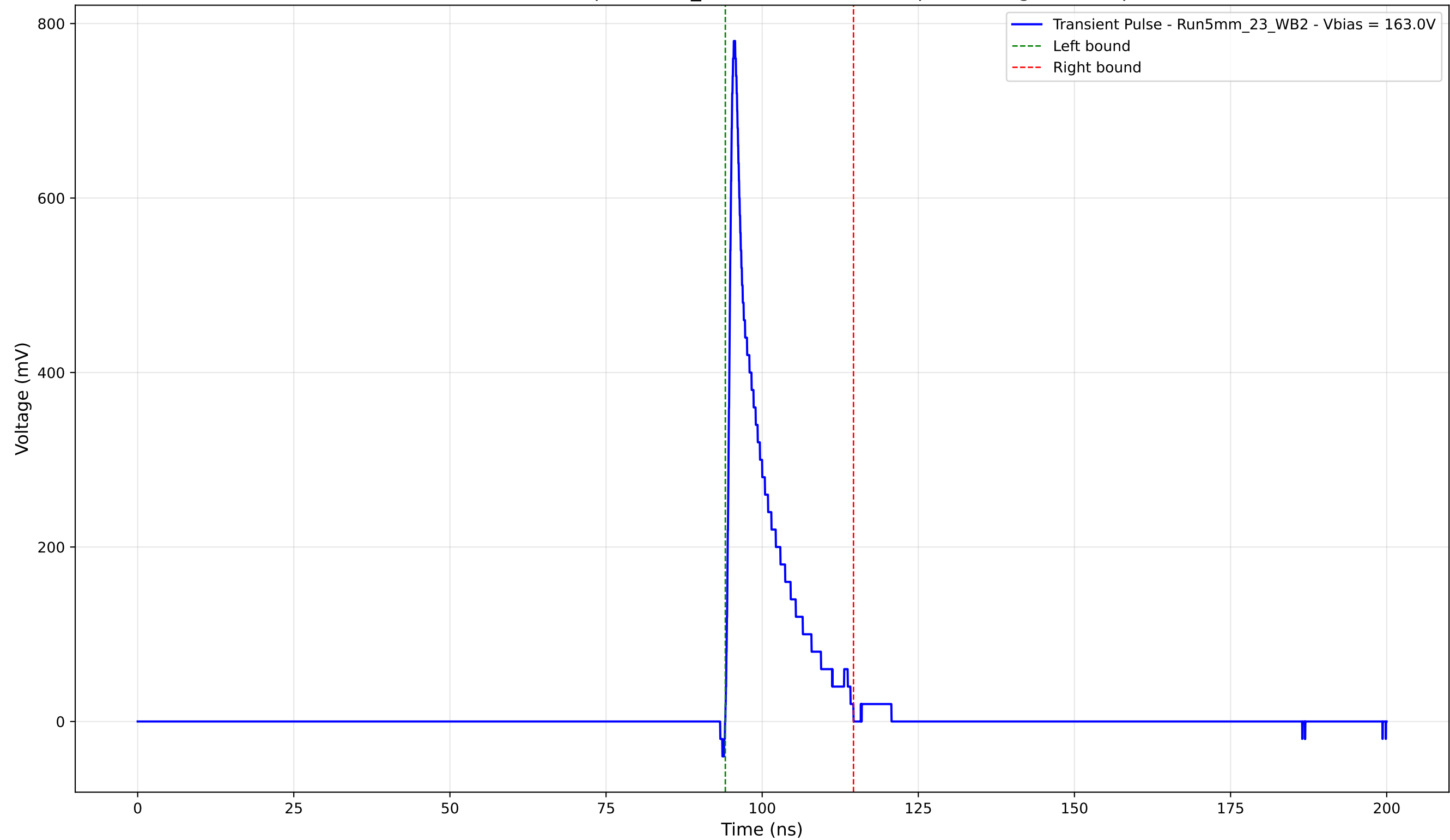
Transient Pulse - Sample: 5mm_23 - Position: 4915.0 \mu\text{m} - Charge: 87.90 pC
