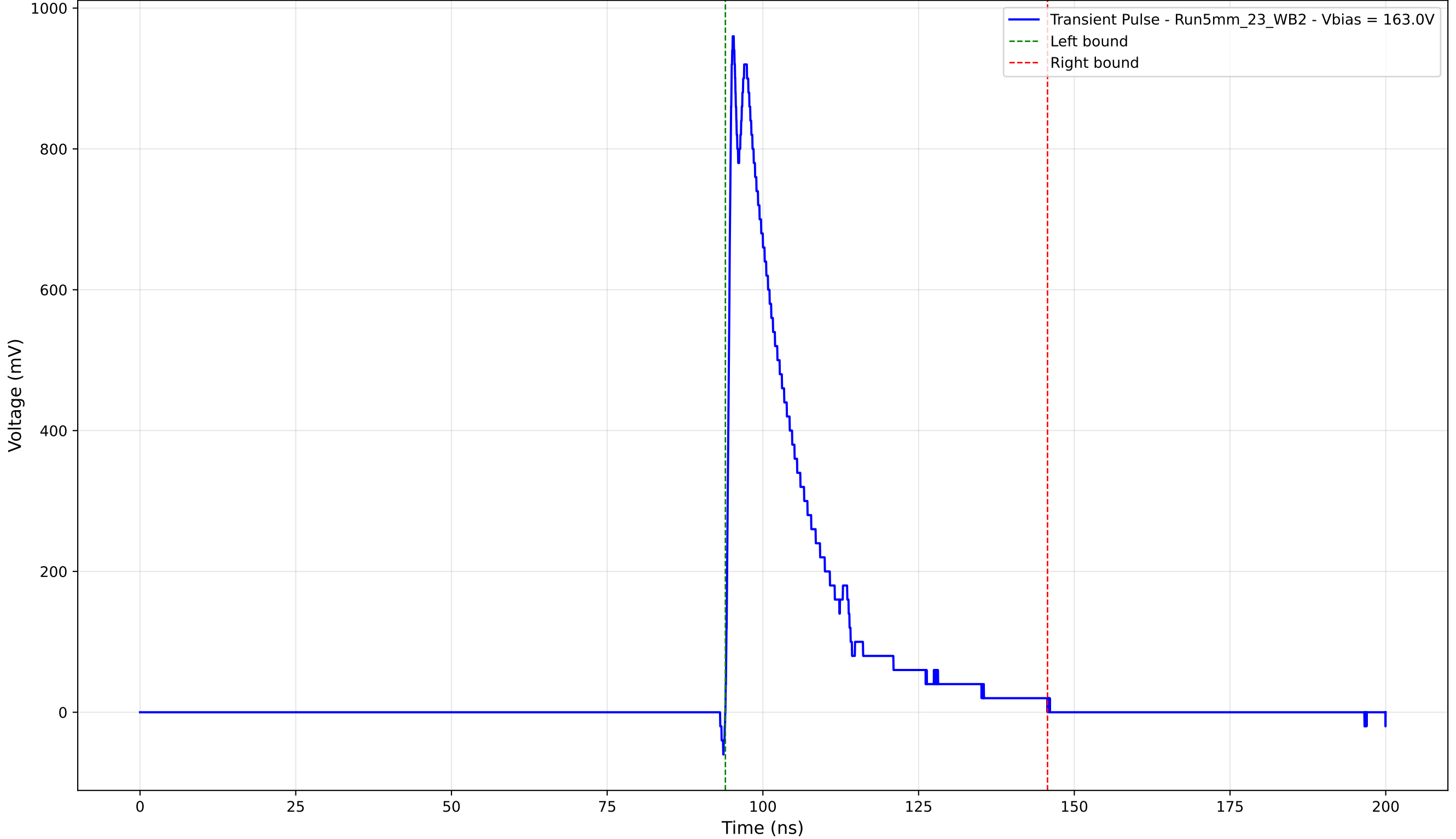
Transient Pulse - Sample: 5mm_23 - Position: 2925.0 \mu\text{m} - Charge: 214.14 pC
