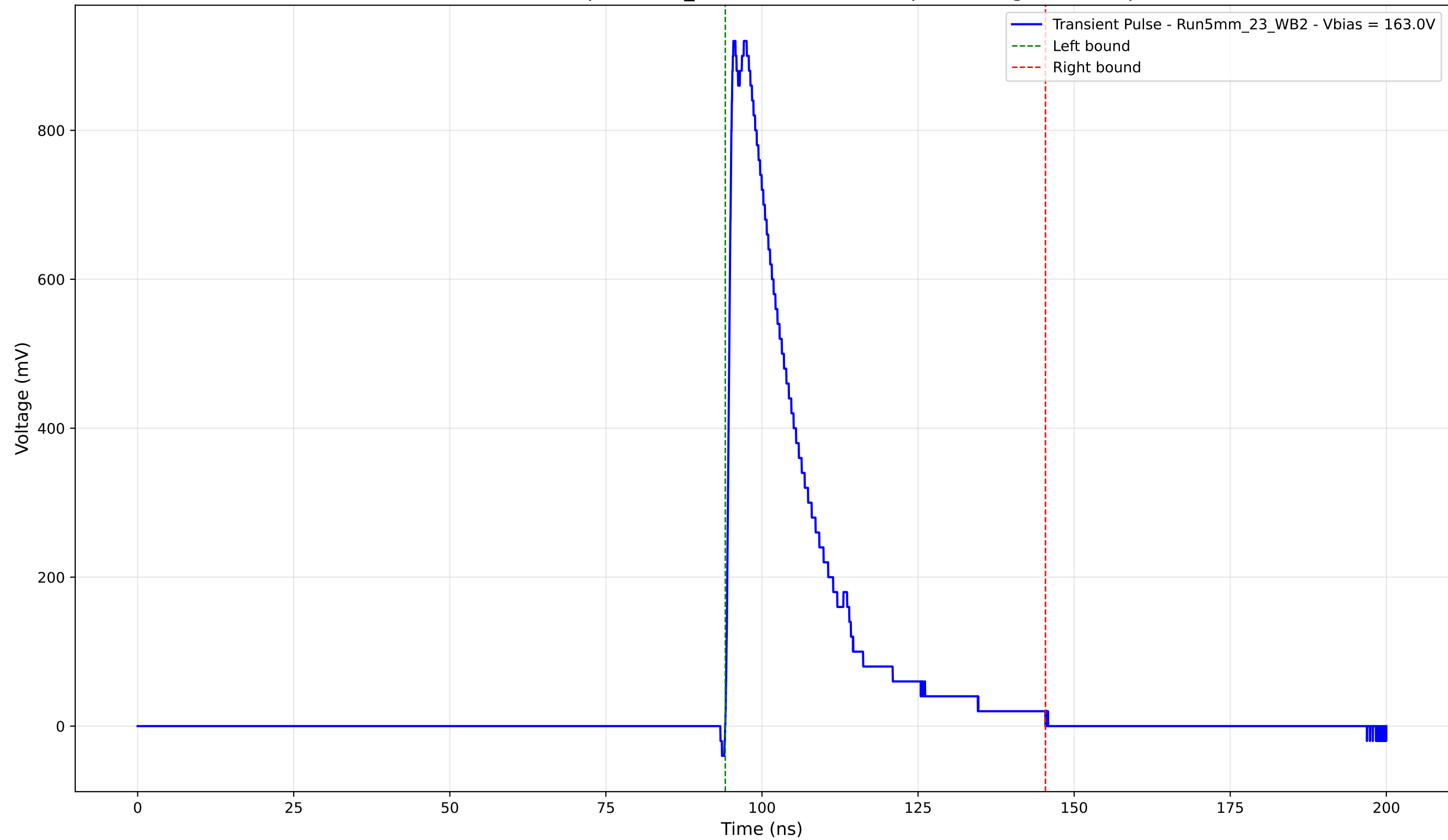
Transient Pulse - Sample: 5mm_23 - Position: 1830.0 \mu\text{m} - Charge: 221.84 pC
