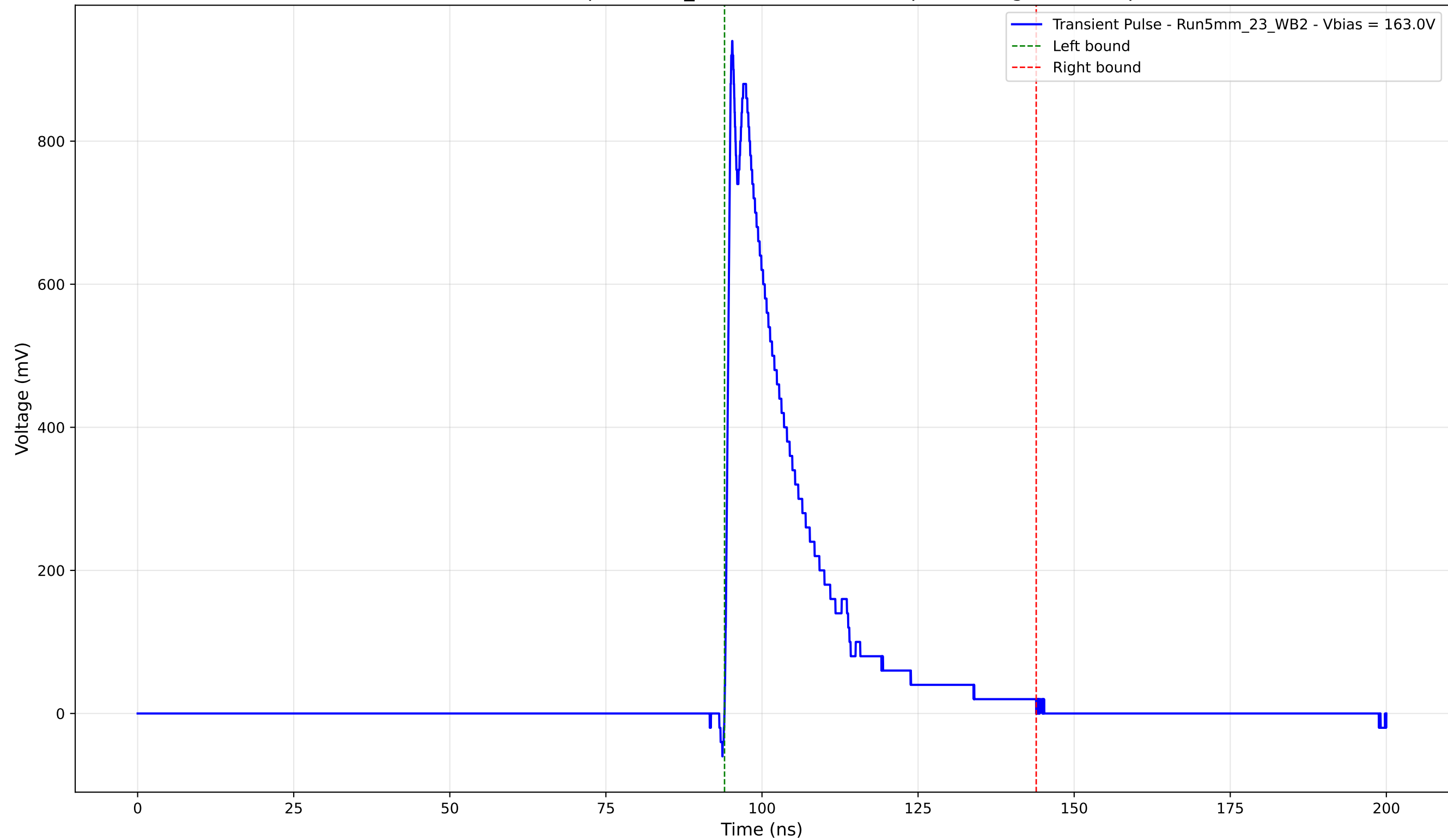
Transient Pulse - Sample: 5mm_23 - Position: 2940.0 \mu\text{m} - Charge: 198.69 pC
