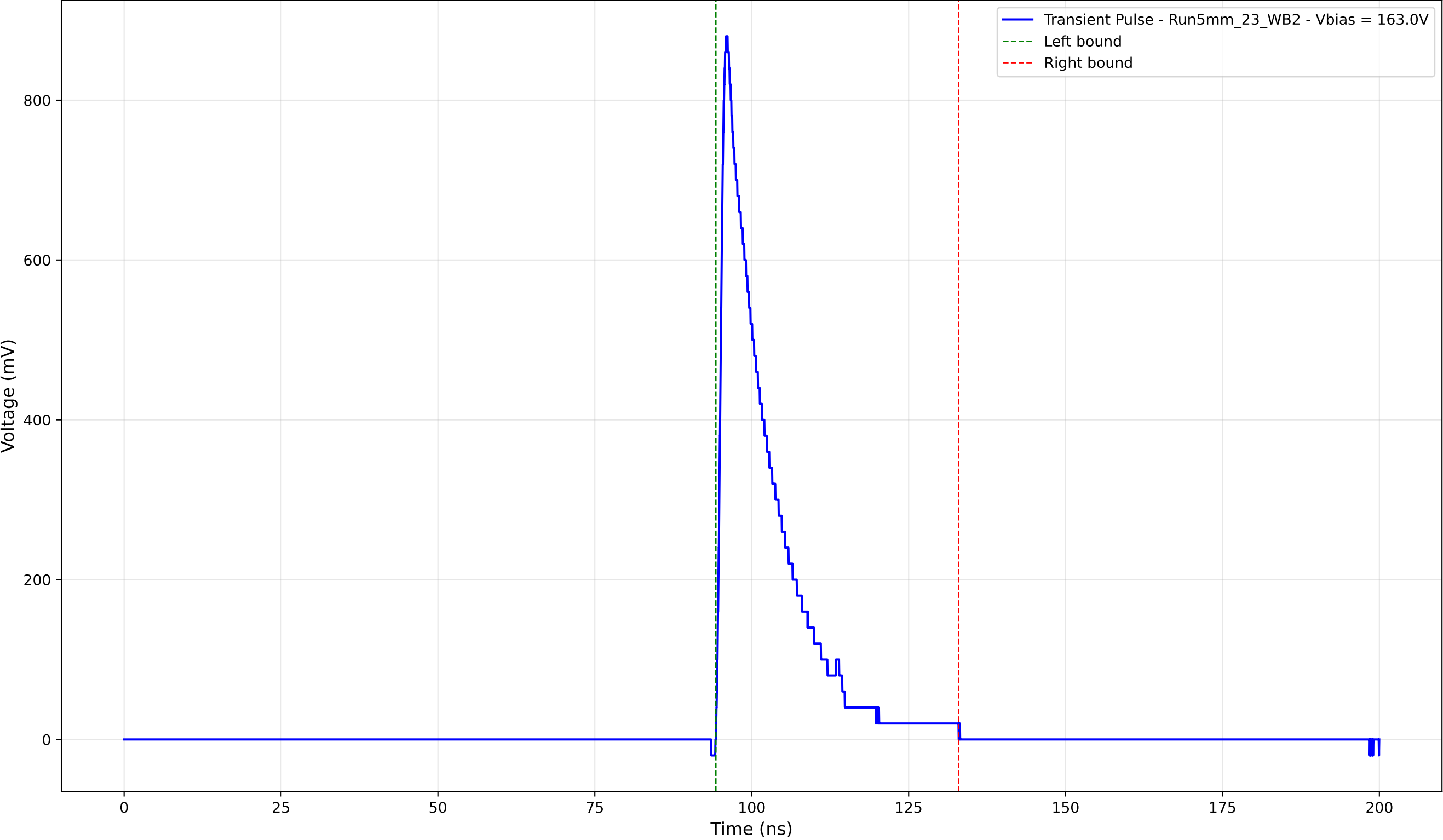
Transient Pulse - Sample: 5mm_23 - Position: 4450.0 \mu\text{m} - Charge: 145.97 pC
