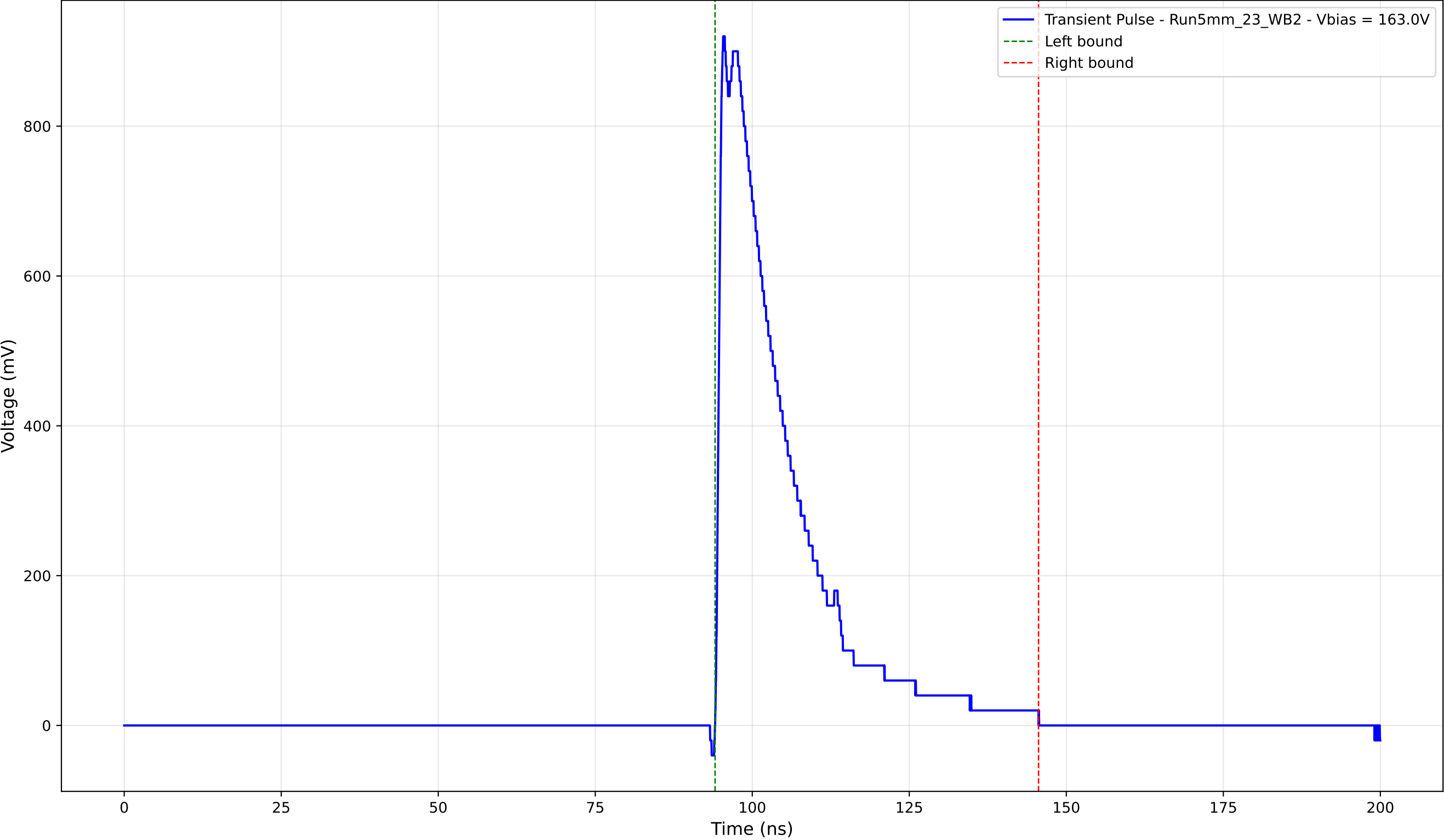
Transient Pulse - Sample: 5mm_23 - Position: 1895.0 \mu\text{m} - Charge: 218.56 pC
