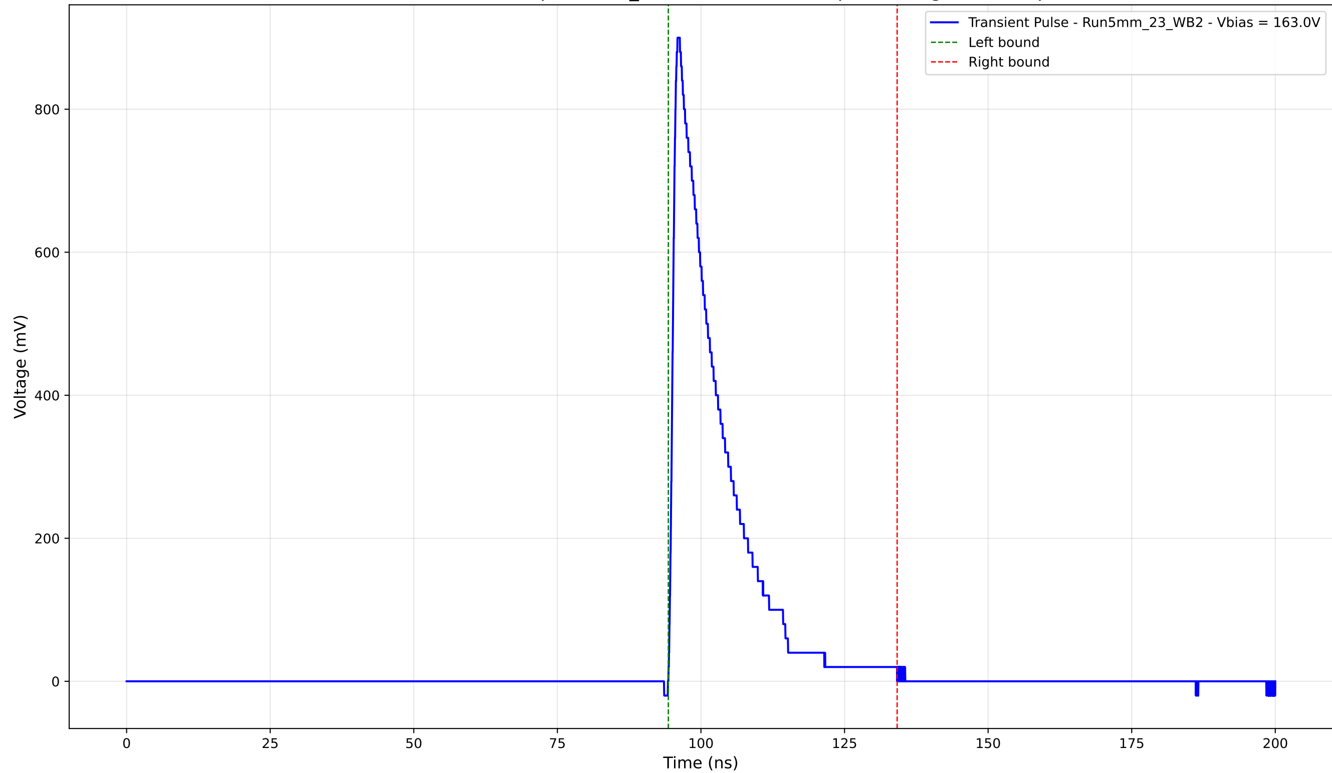
Transient Pulse - Sample: 5mm_23 - Position: 4345.0 \mu\text{m} - Charge: 160.54 pC
