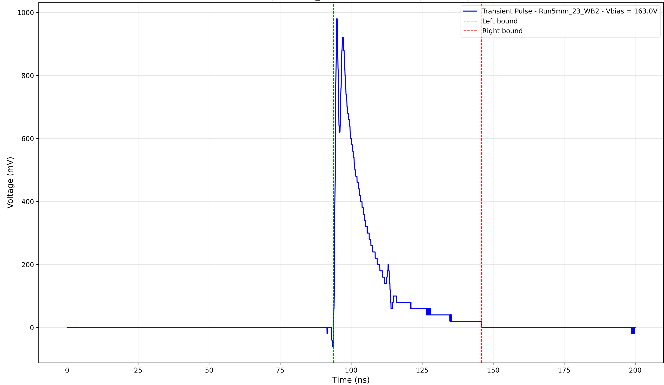
Transient Pulse - Sample: 5mm_23 - Position: 2690.0 \mu\text{m} - Charge: 201.29 pC
