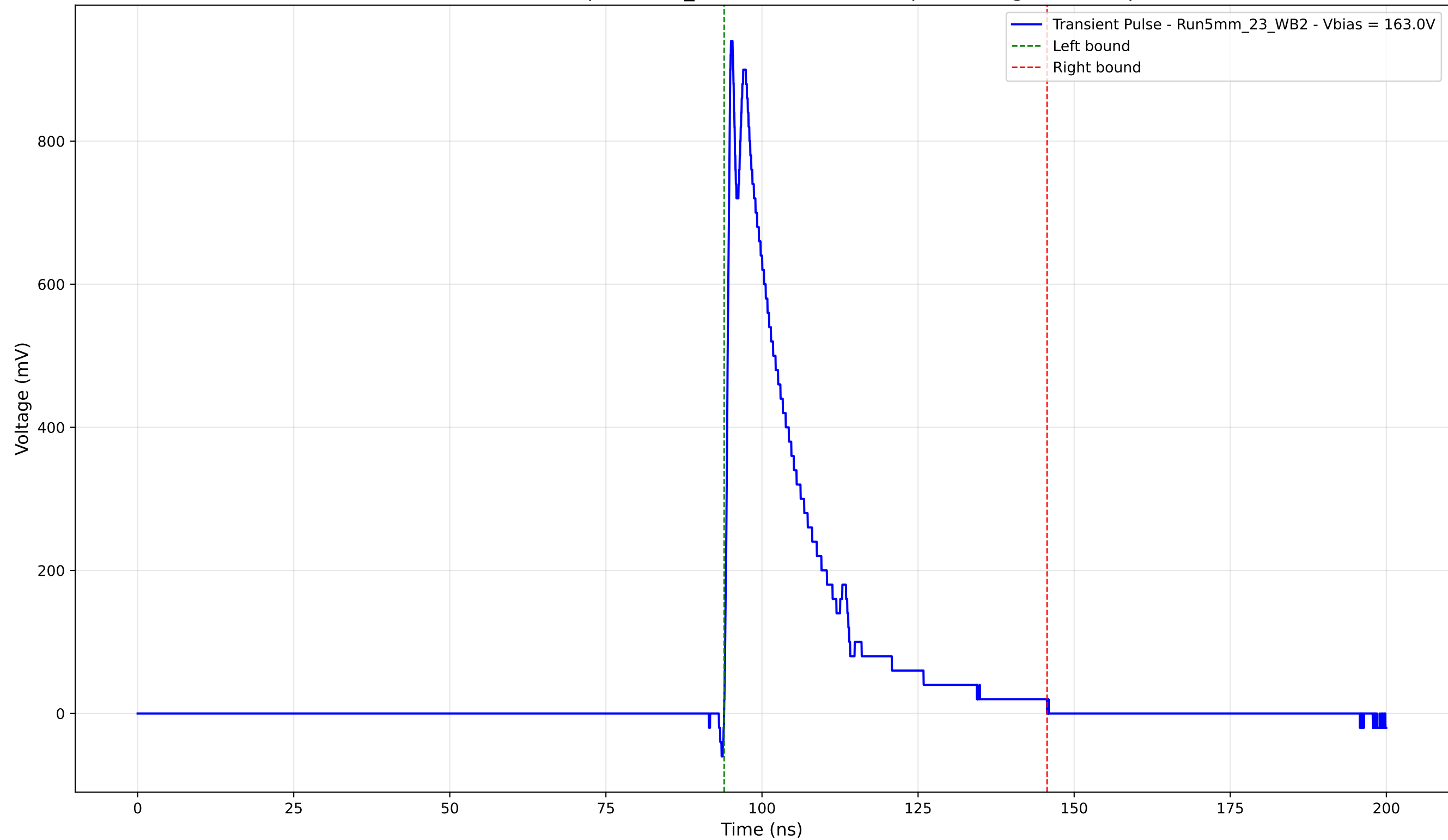
Transient Pulse - Sample: 5mm_23 - Position: 2185.0 \mu\text{m} - Charge: 205.40 pC
