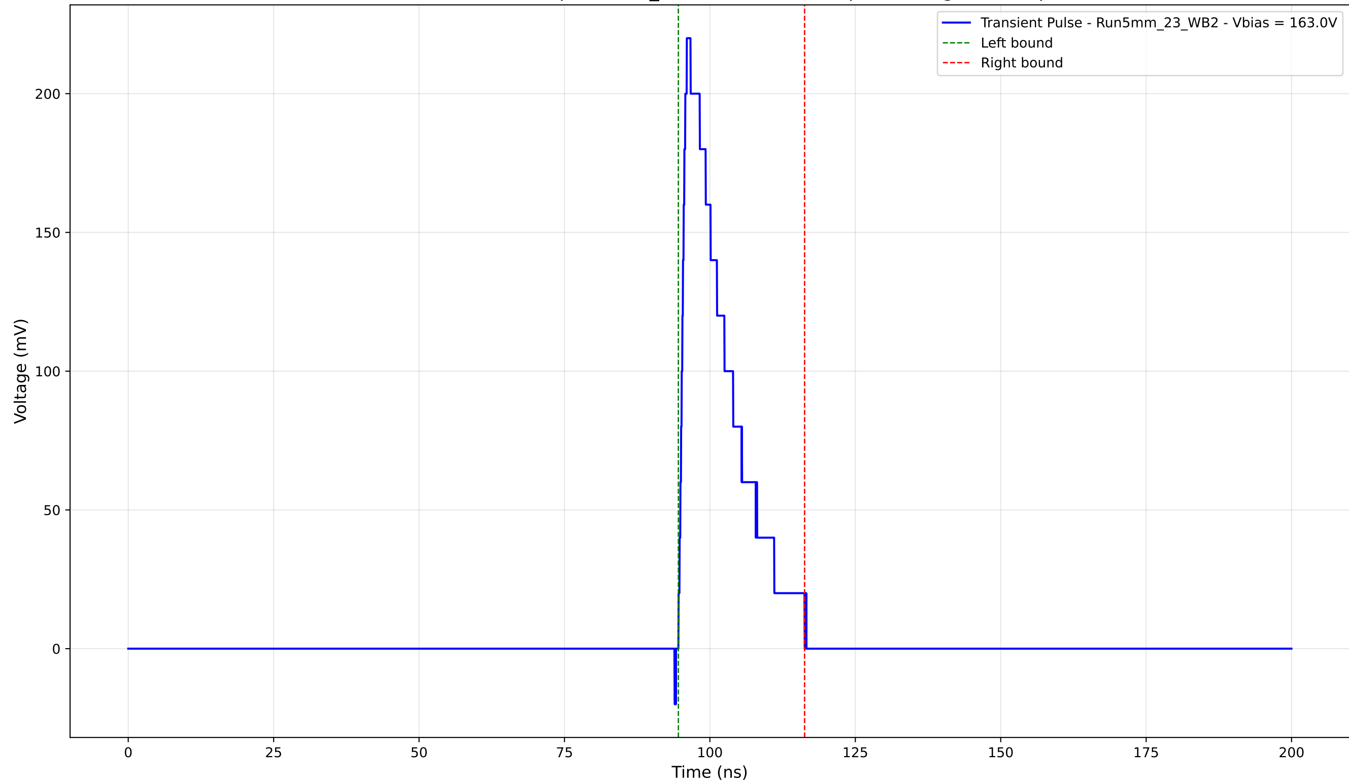
Transient Pulse - Sample: 5mm_23 - Position: 980.0 \mu\text{m} - Charge: 37.99 pC
