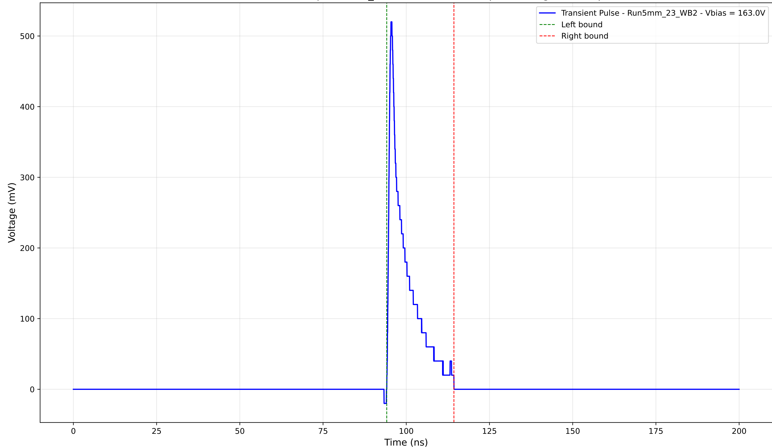
Transient Pulse - Sample: 5mm_23 - Position: 4935.0 \mu\text{m} - Charge: 54.69 pC
