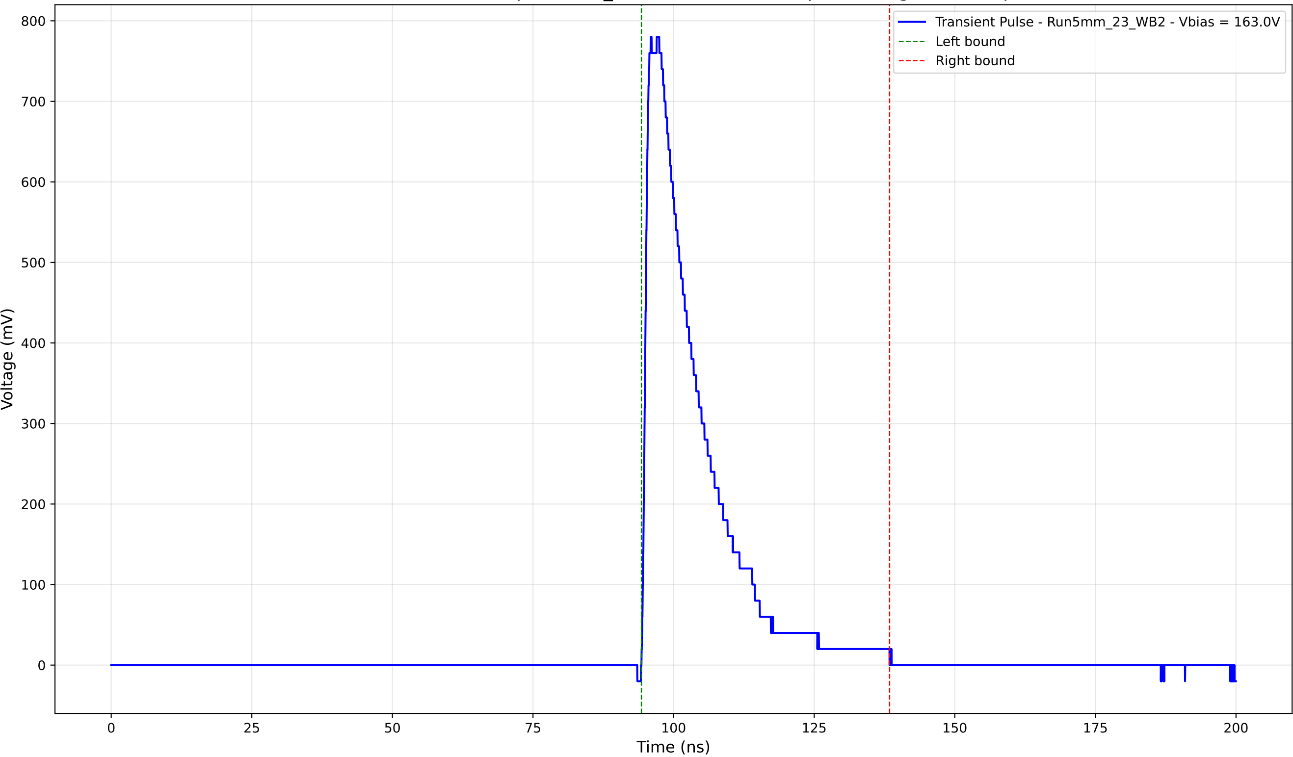
Transient Pulse - Sample: 5mm_23 - Position: 3440.0 \mu\text{m} - Charge: 165.32 pC
