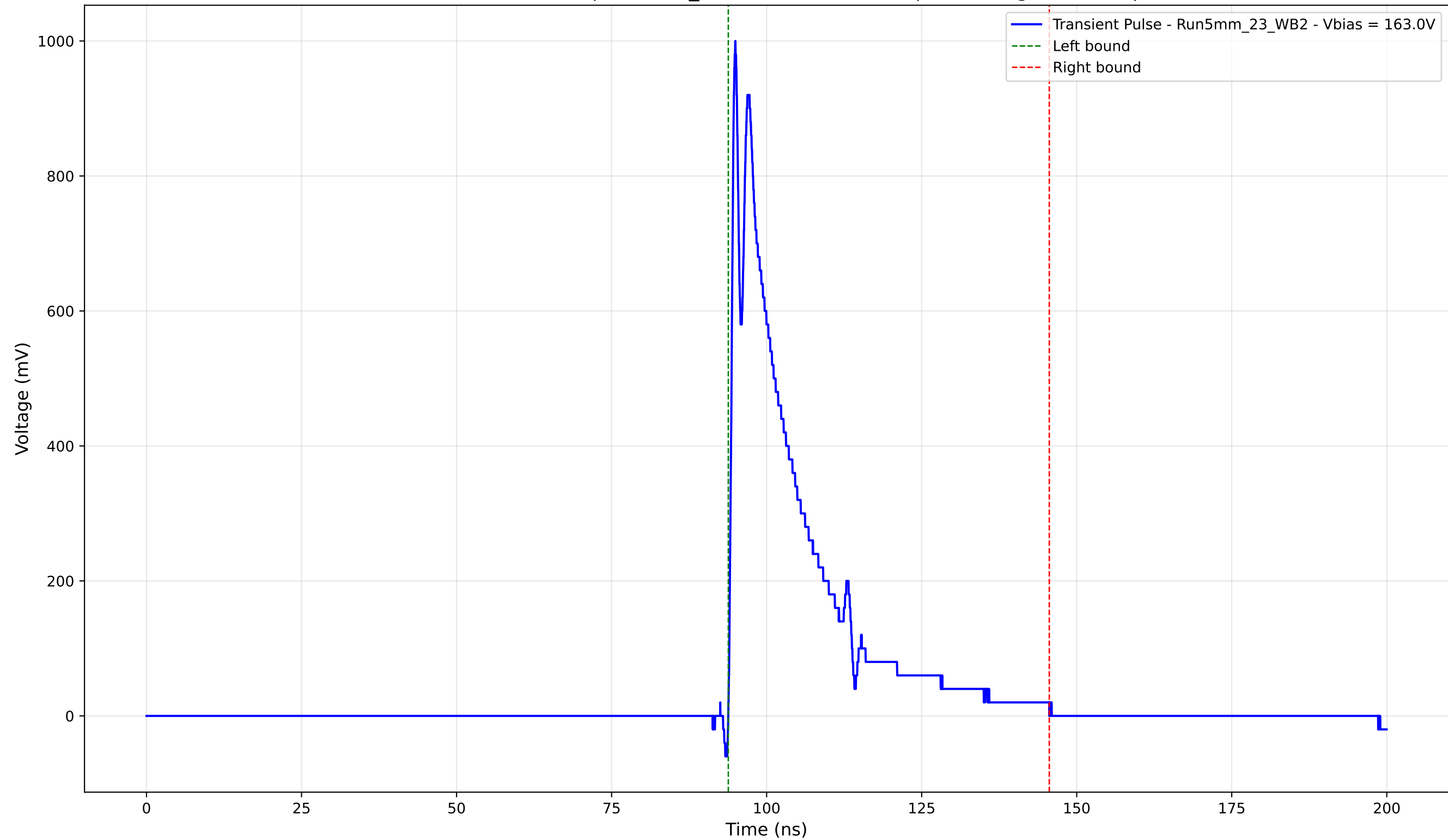
Transient Pulse - Sample: 5mm_23 - Position: 2390.0 \mu\text{m} - Charge: 199.74 pC
