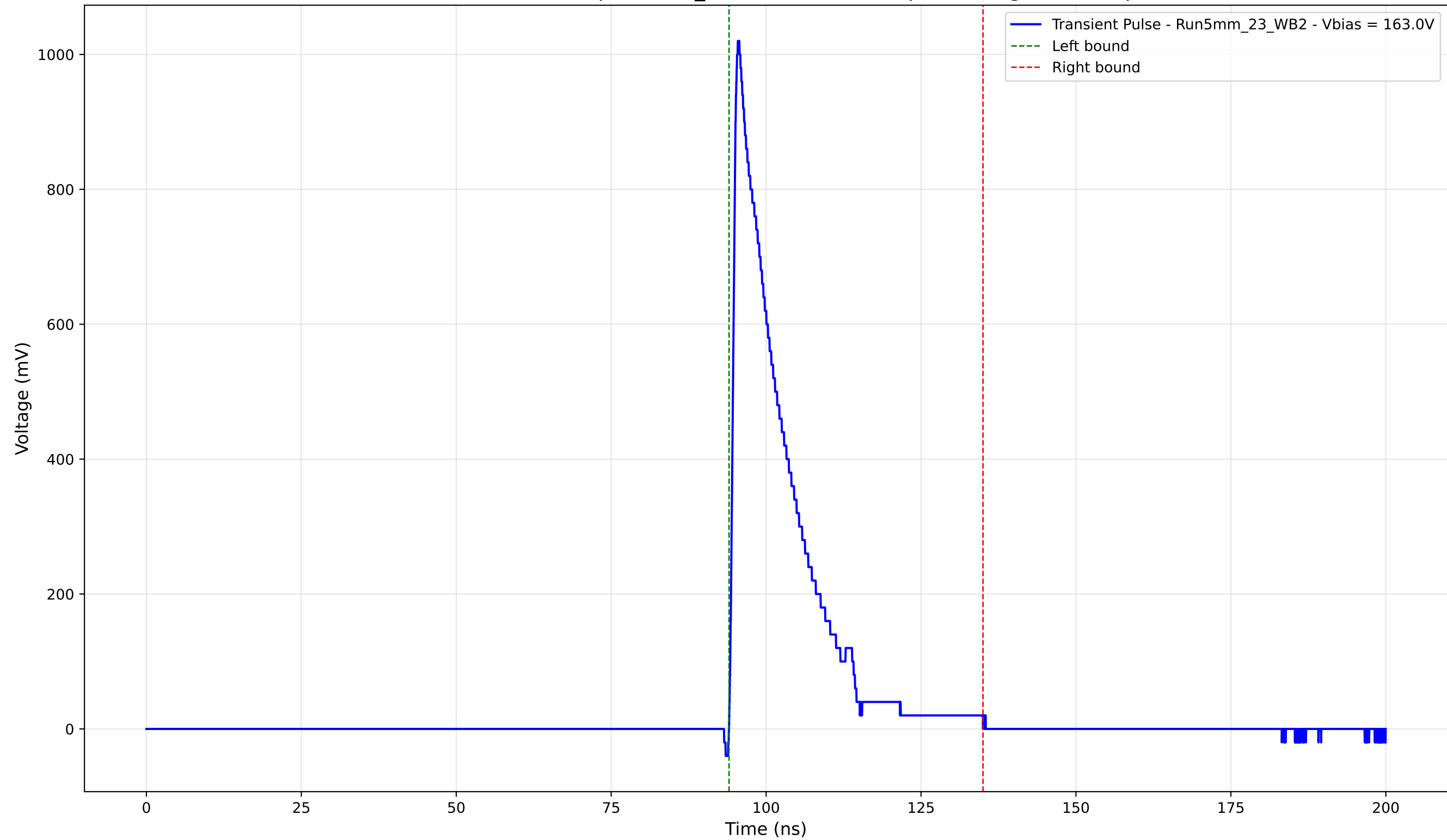
Transient Pulse - Sample: 5mm_23 - Position: 190.0 \mu\text{m} - Charge: 179.82 pC
