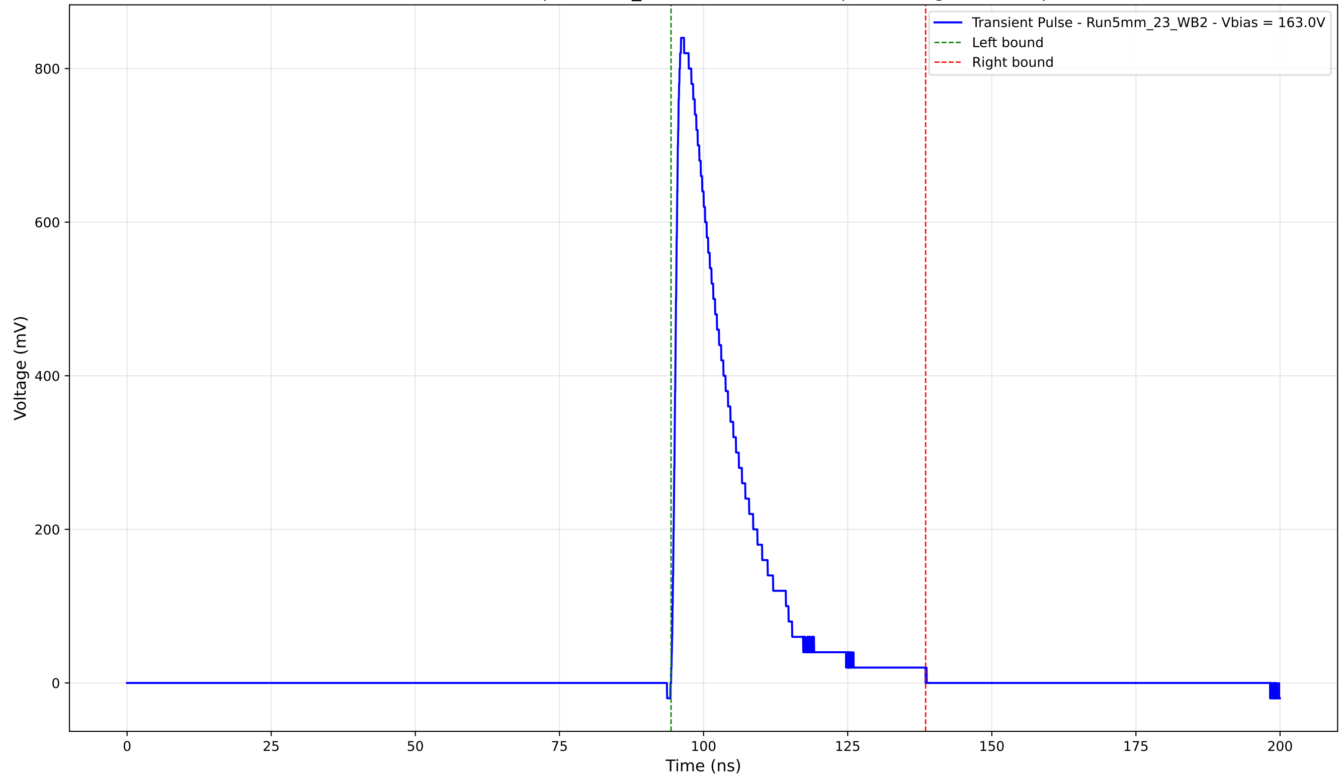
Transient Pulse - Sample: 5mm_23 - Position: 3685.0 \mu\text{m} - Charge: 174.62 pC
