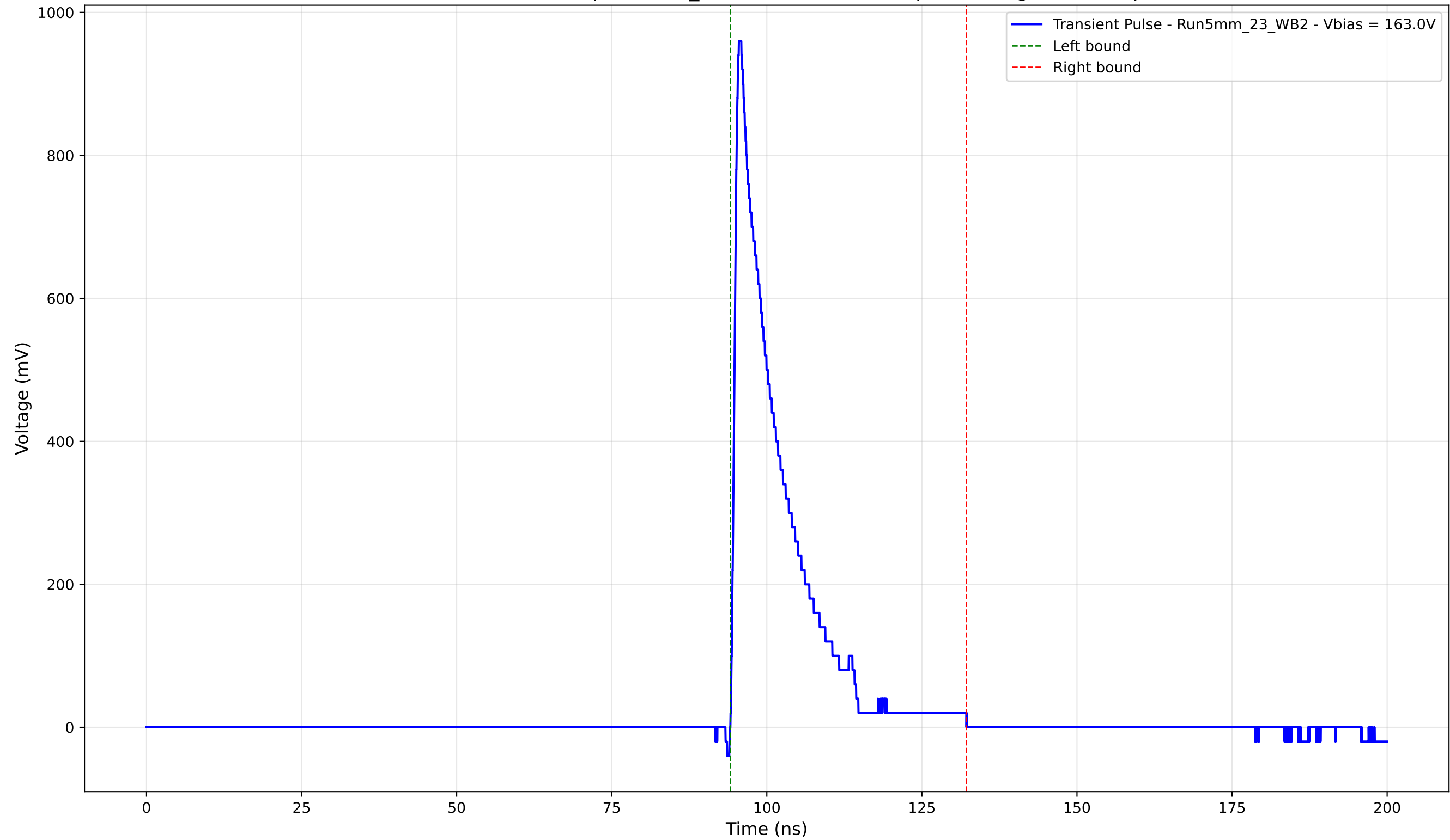
Transient Pulse - Sample: 5mm_23 - Position: 4765.0 \mu\text{m} - Charge: 147.83 pC
