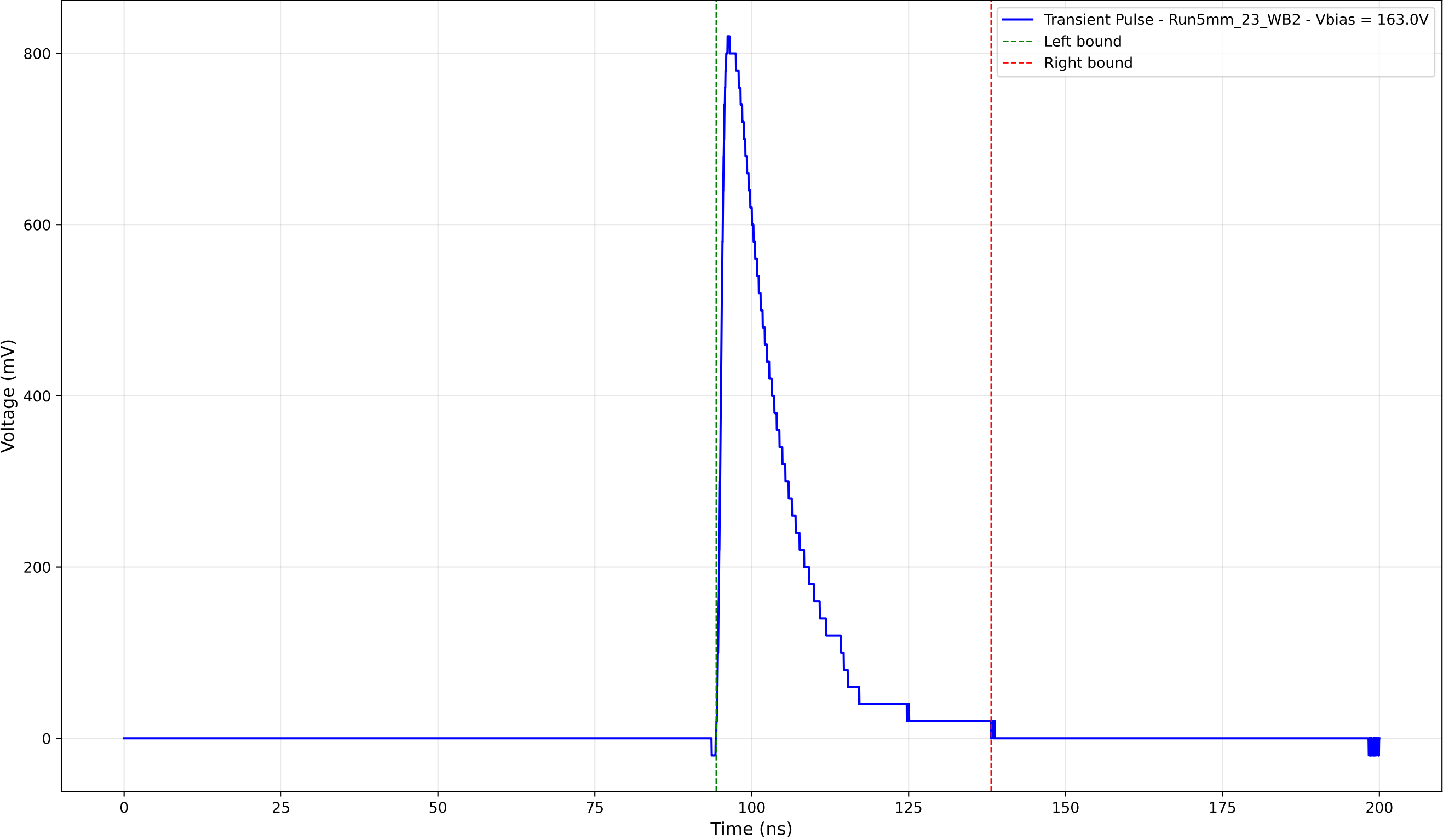
Transient Pulse - Sample: 5mm_23 - Position: 3635.0 \mu\text{m} - Charge: 169.80 pC
