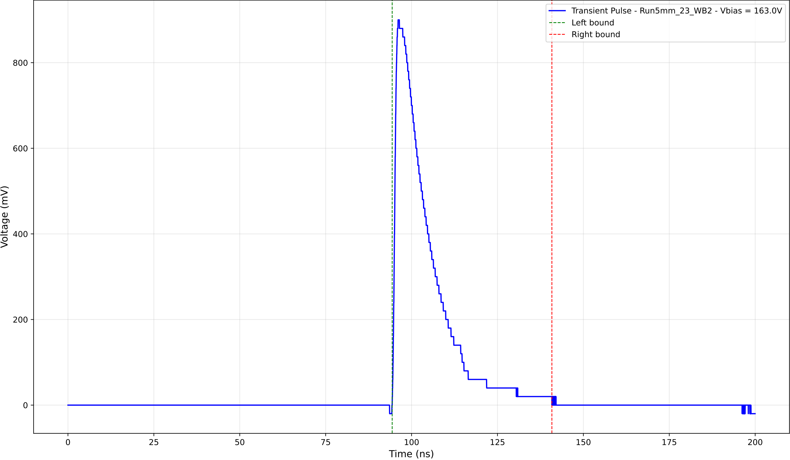
Transient Pulse - Sample: 5mm_23 - Position: 1340.0 \mu\text{m} - Charge: 200.26 pC
