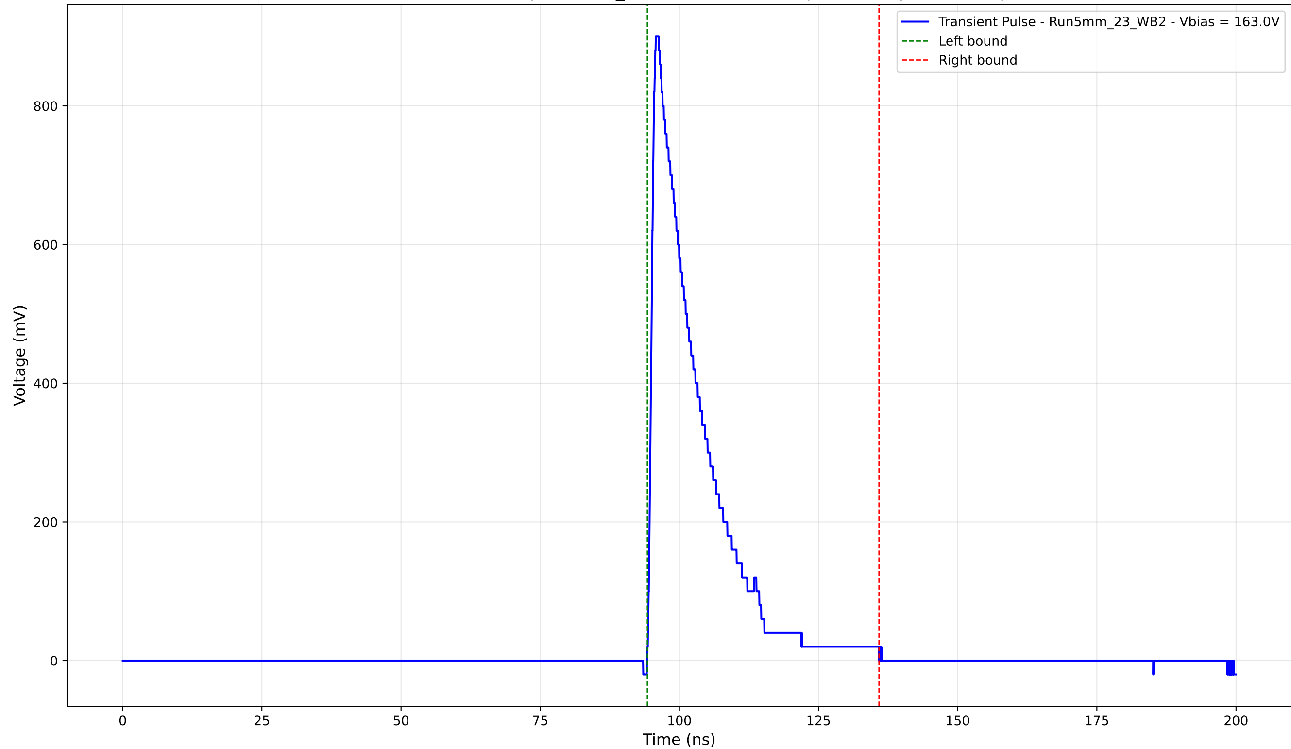
Transient Pulse - Sample: 5mm_23 - Position: 565.0 \mu\text{m} - Charge: 166.26 pC
