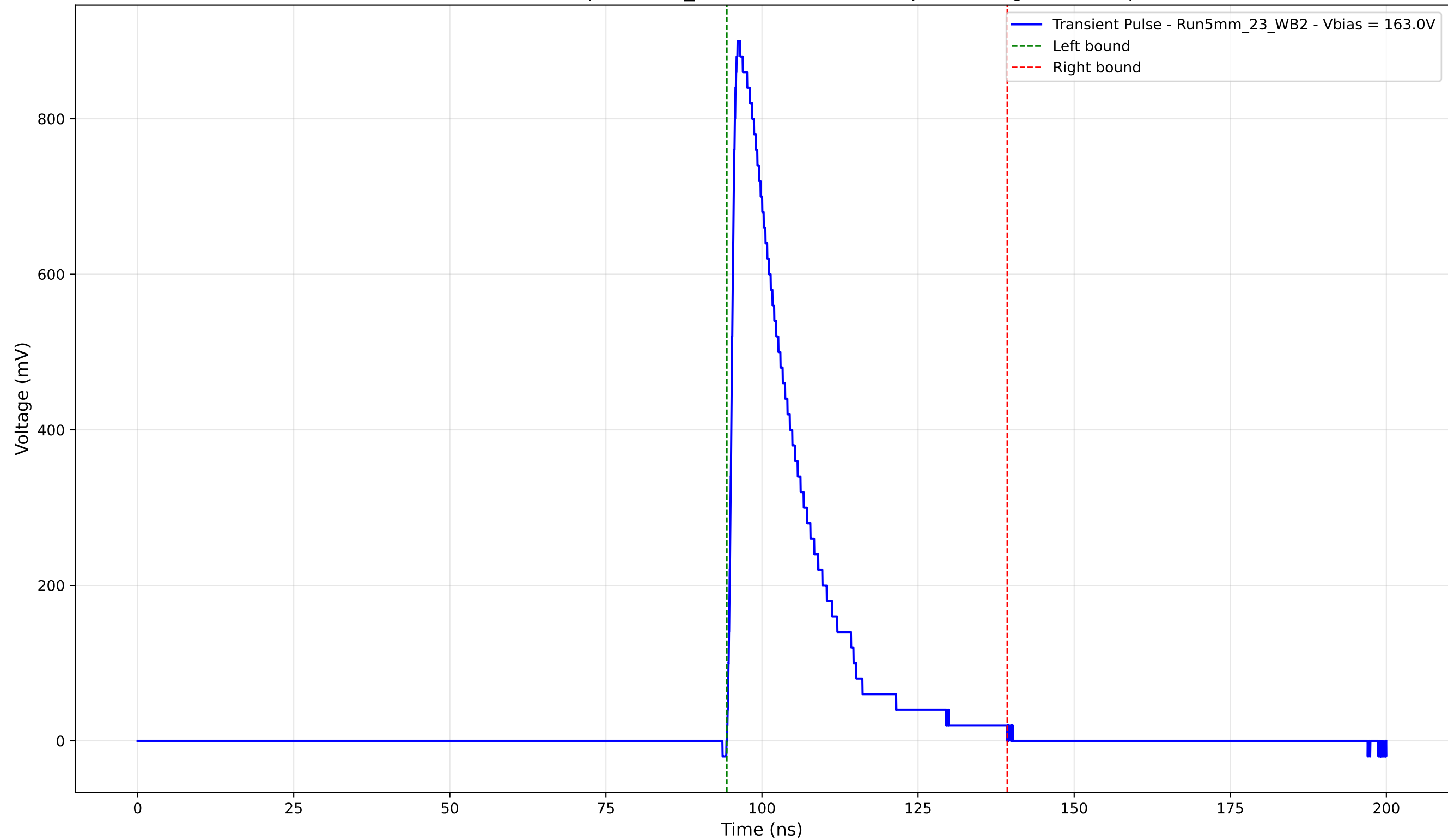
Transient Pulse - Sample: 5mm_23 - Position: 1185.0 \mu\text{m} - Charge: 195.02 pC
