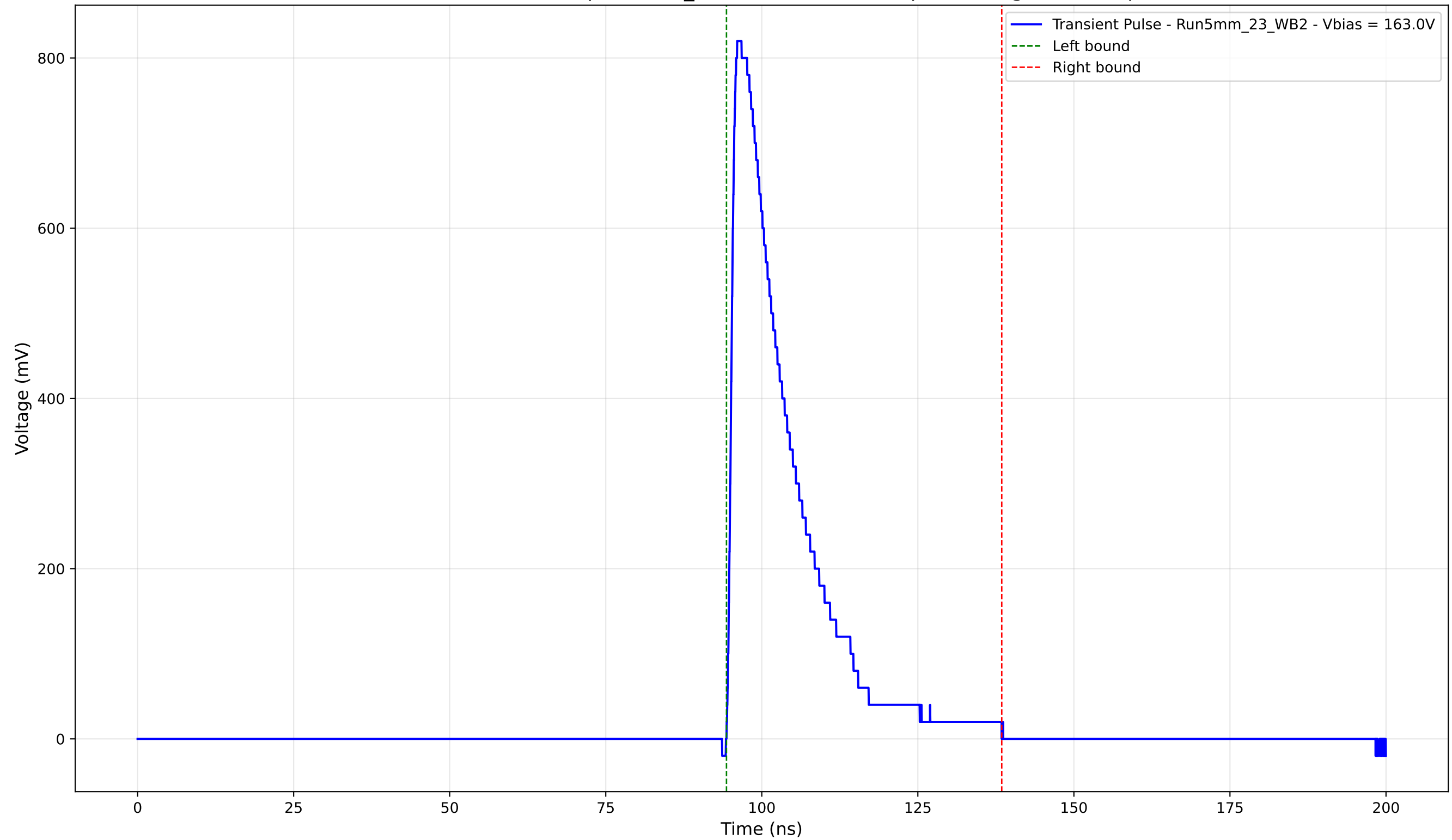
Transient Pulse - Sample: 5mm_23 - Position: 3645.0 \mu\text{m} - Charge: 171.59 pC
