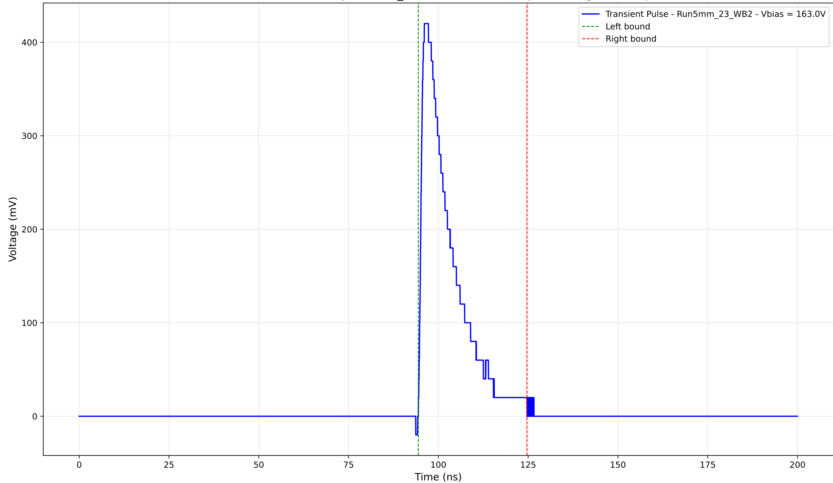
Transient Pulse - Sample: 5mm_23 - Position: 3565.0 \mu\text{m} - Charge: 79.37 pC
