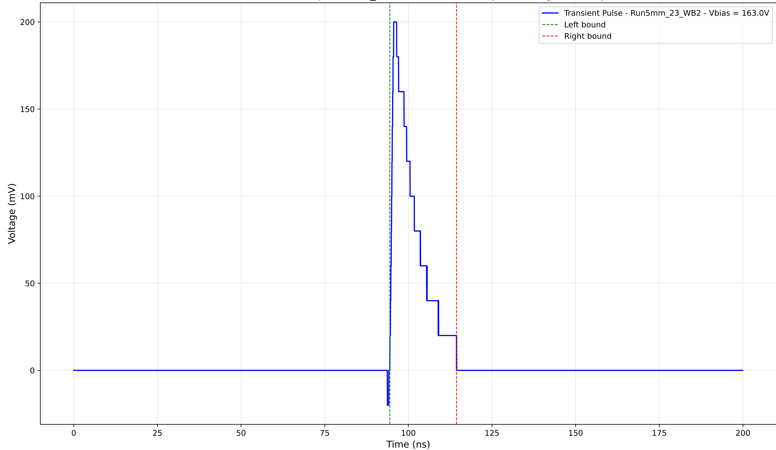
Transient Pulse - Sample: 5mm_23 - Position: 4530.0 \mu\text{m} - Charge: 30.47 pC
