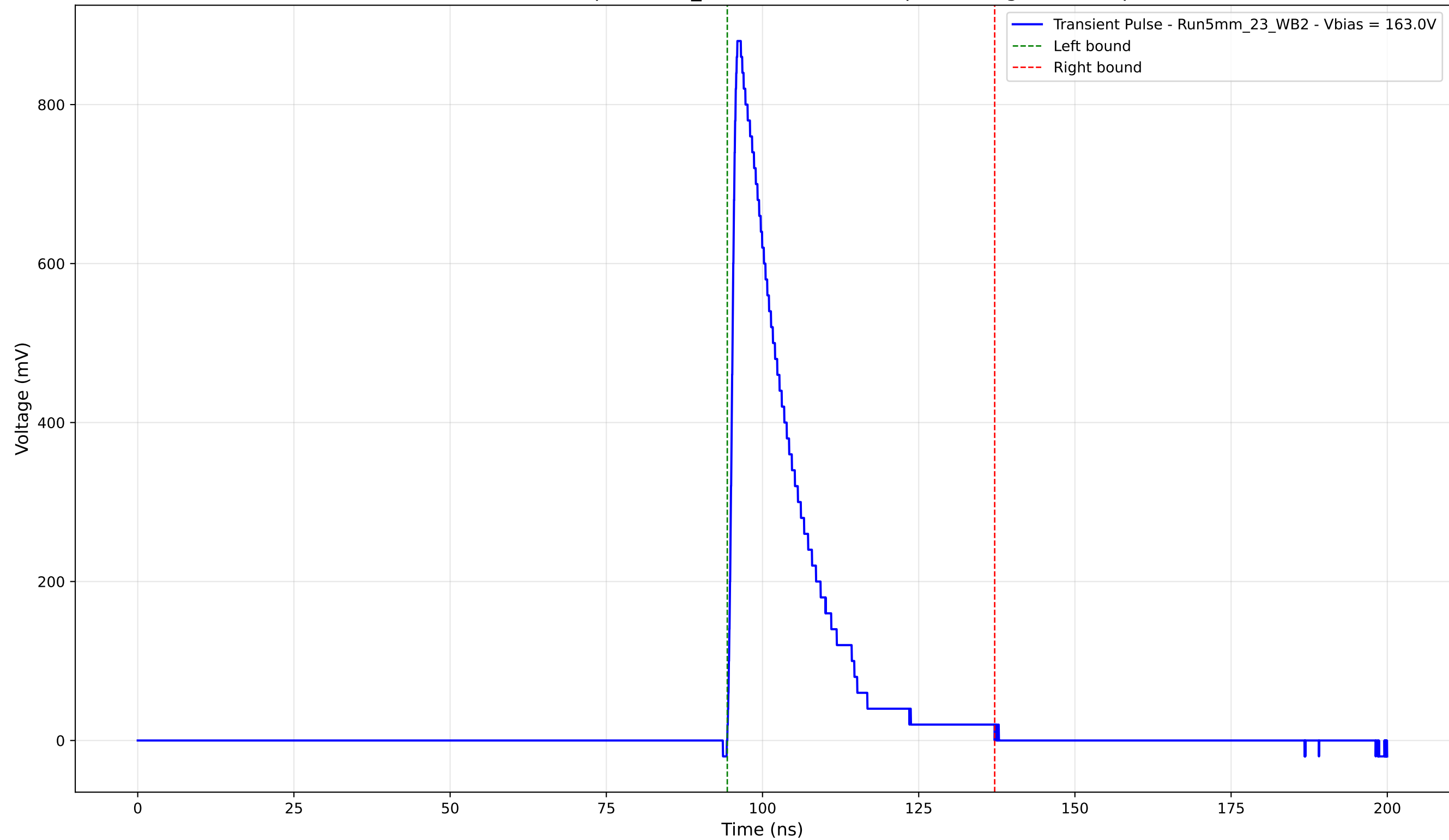
Transient Pulse - Sample: 5mm_23 - Position: 850.0 \mu\text{m} - Charge: 173.86 pC
