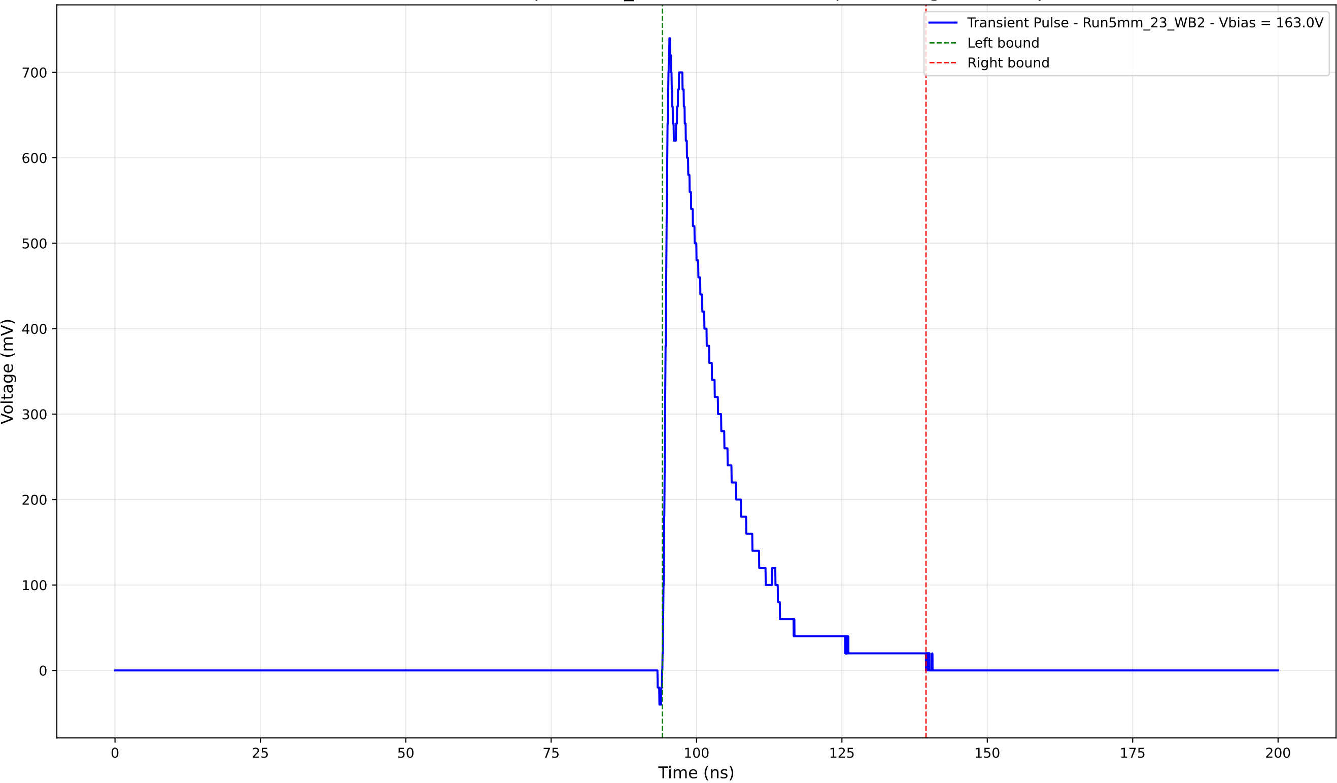
Transient Pulse - Sample: 5mm_23 - Position: 1950.0 \mu\text{m} - Charge: 149.02 pC
