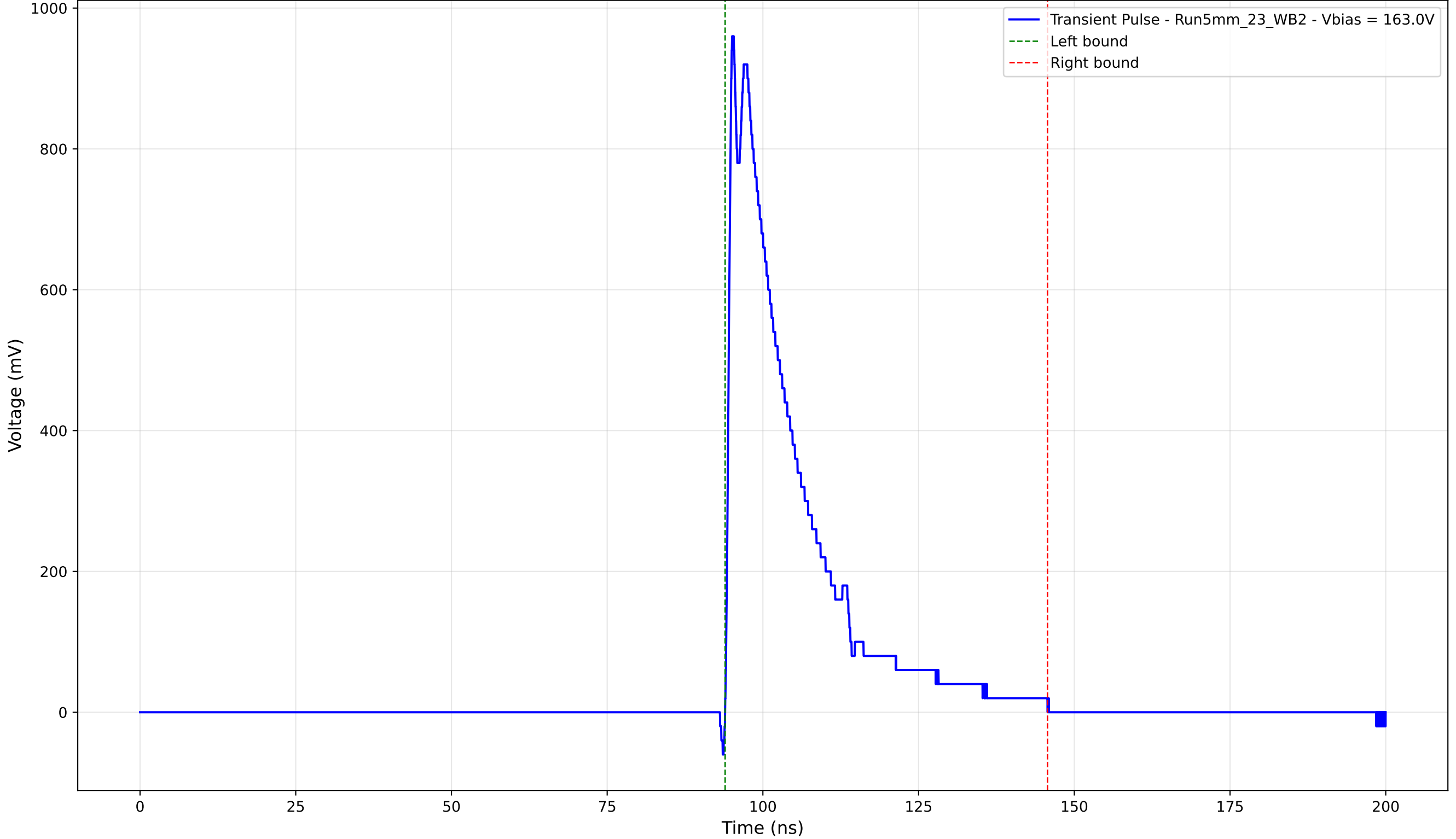
Transient Pulse - Sample: 5mm_23 - Position: 2875.0 \mu\text{m} - Charge: 216.60 pC
