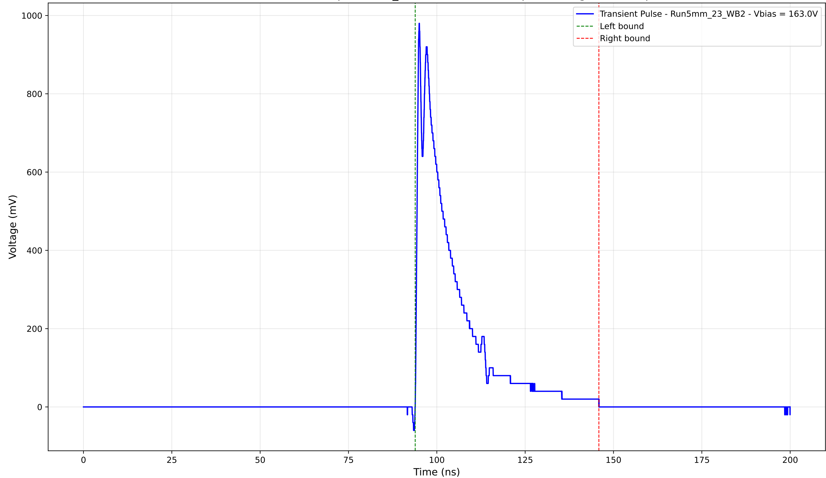
Transient Pulse - Sample: 5mm_23 - Position: 2725.0 \mu\text{m} - Charge: 202.44 pC
