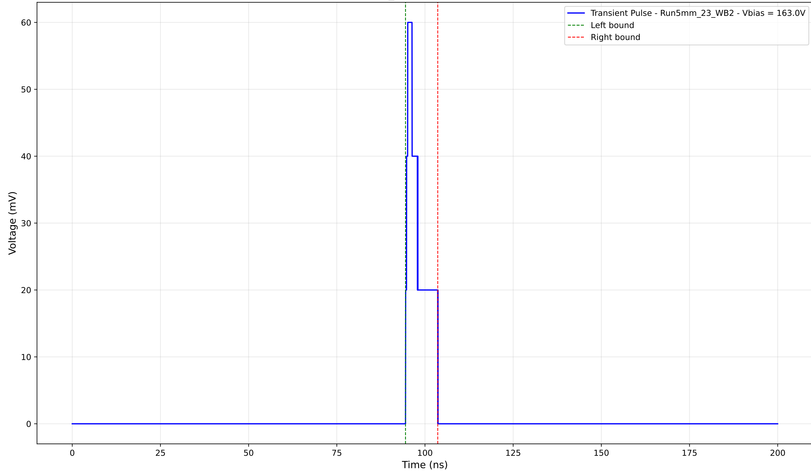
Transient Pulse - Sample: 5mm_23 - Position: 4990.0 \mu\text{m} - Charge: 5.39 pC
