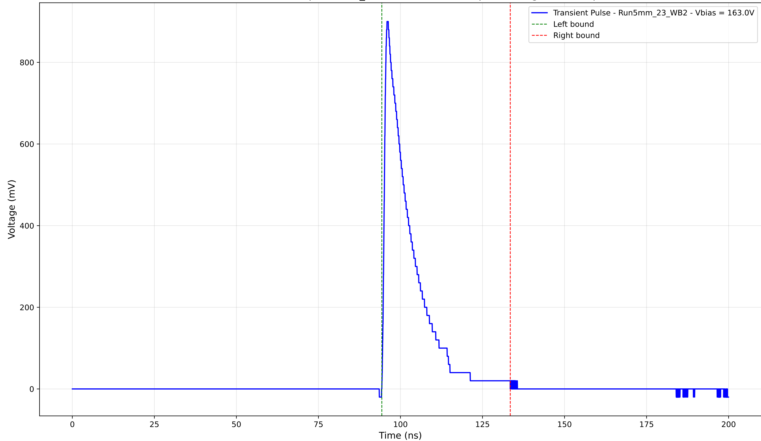
Transient Pulse - Sample: 5mm_23 - Position: 4375.0 \mu\text{m} - Charge: 158.50 pC
