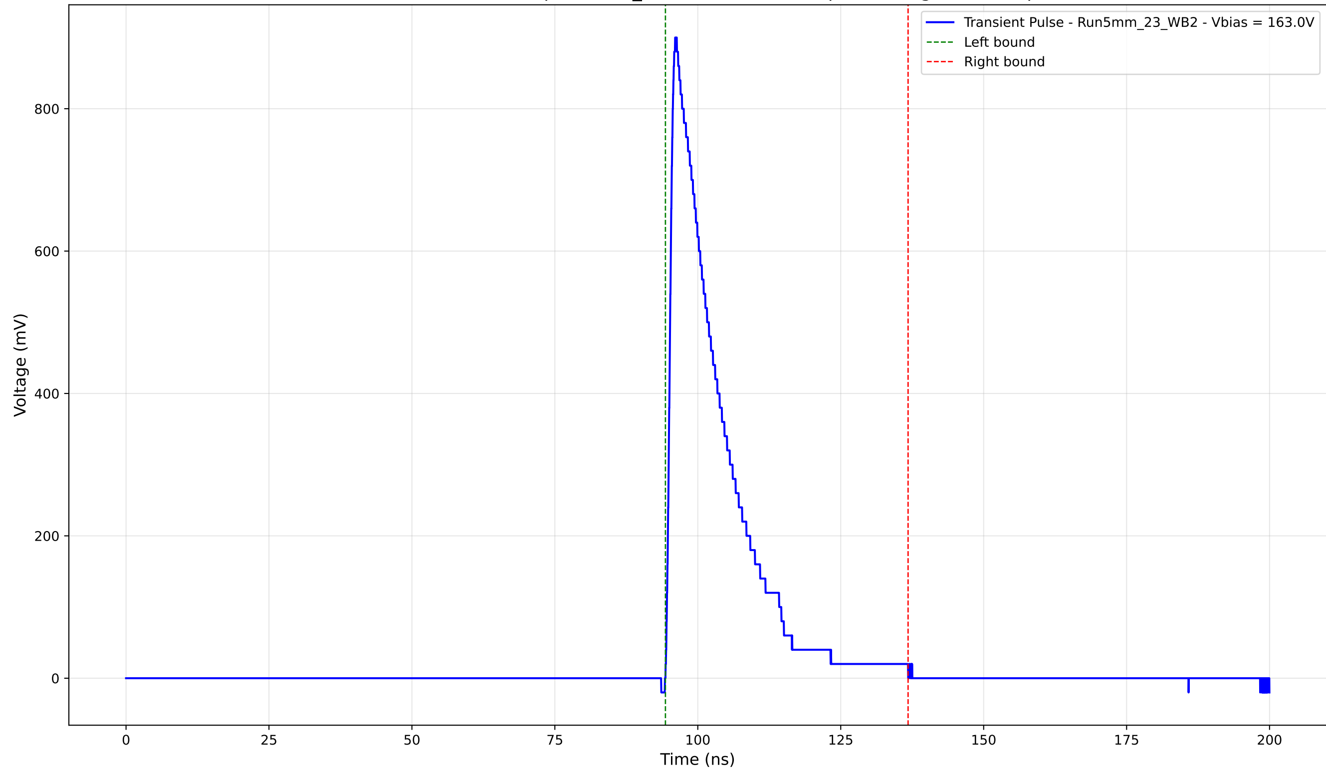
Transient Pulse - Sample: 5mm_23 - Position: 765.0 \mu\text{m} - Charge: 173.40 pC
