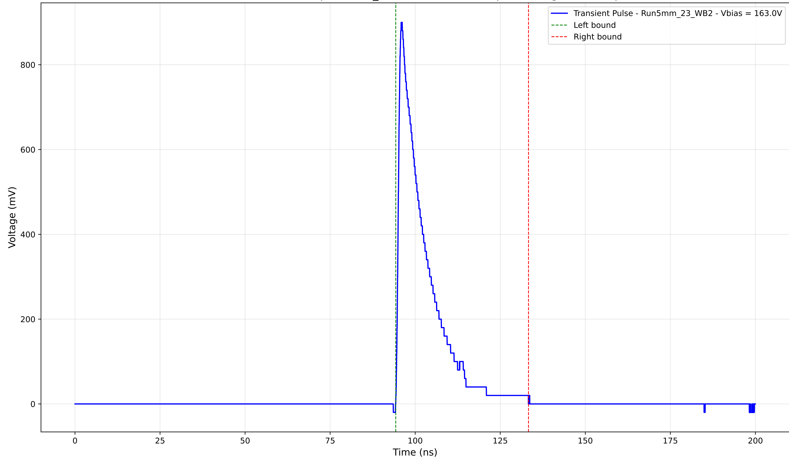
Transient Pulse - Sample: 5mm_23 - Position: 4425.0 \mu\text{m} - Charge: 153.78 pC
