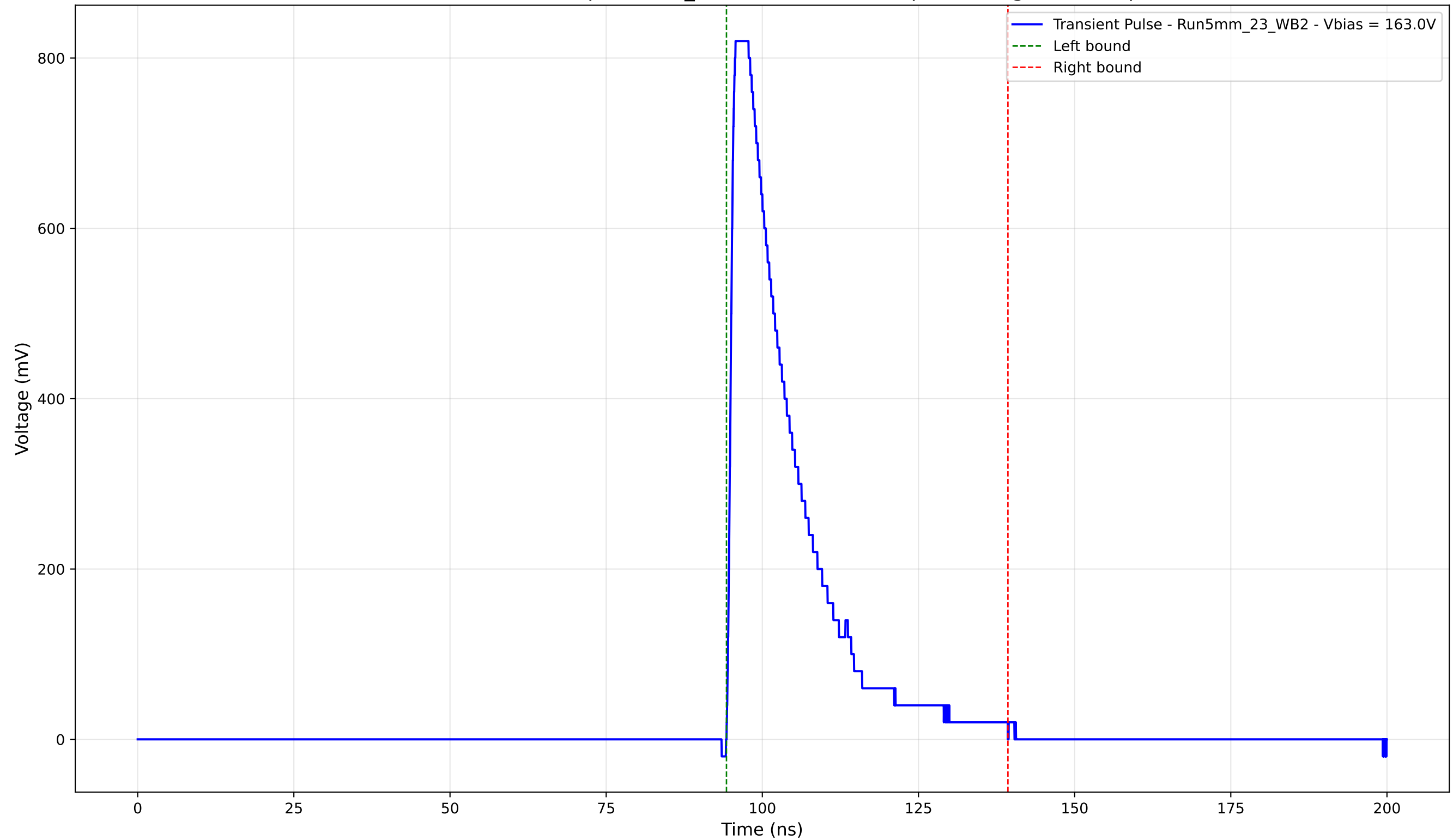
Transient Pulse - Sample: 5mm_23 - Position: 3410.0 \mu\text{m} - Charge: 182.87 pC
