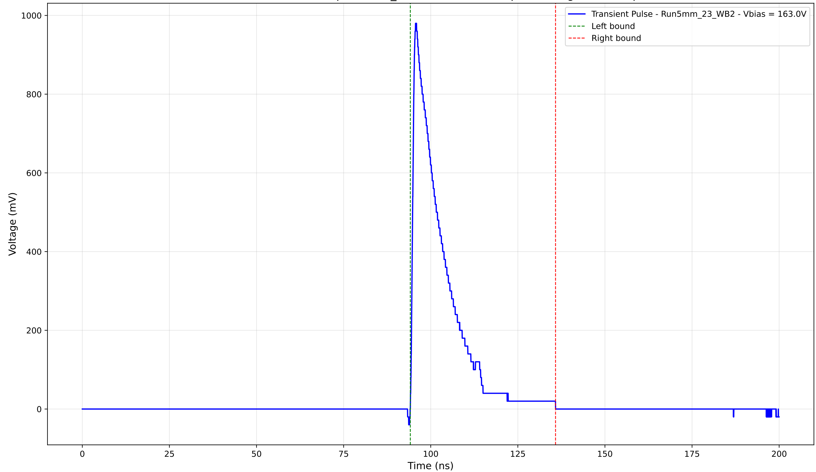
Transient Pulse - Sample: 5mm_23 - Position: 385.0 \mu\text{m} - Charge: 179.09 pC
