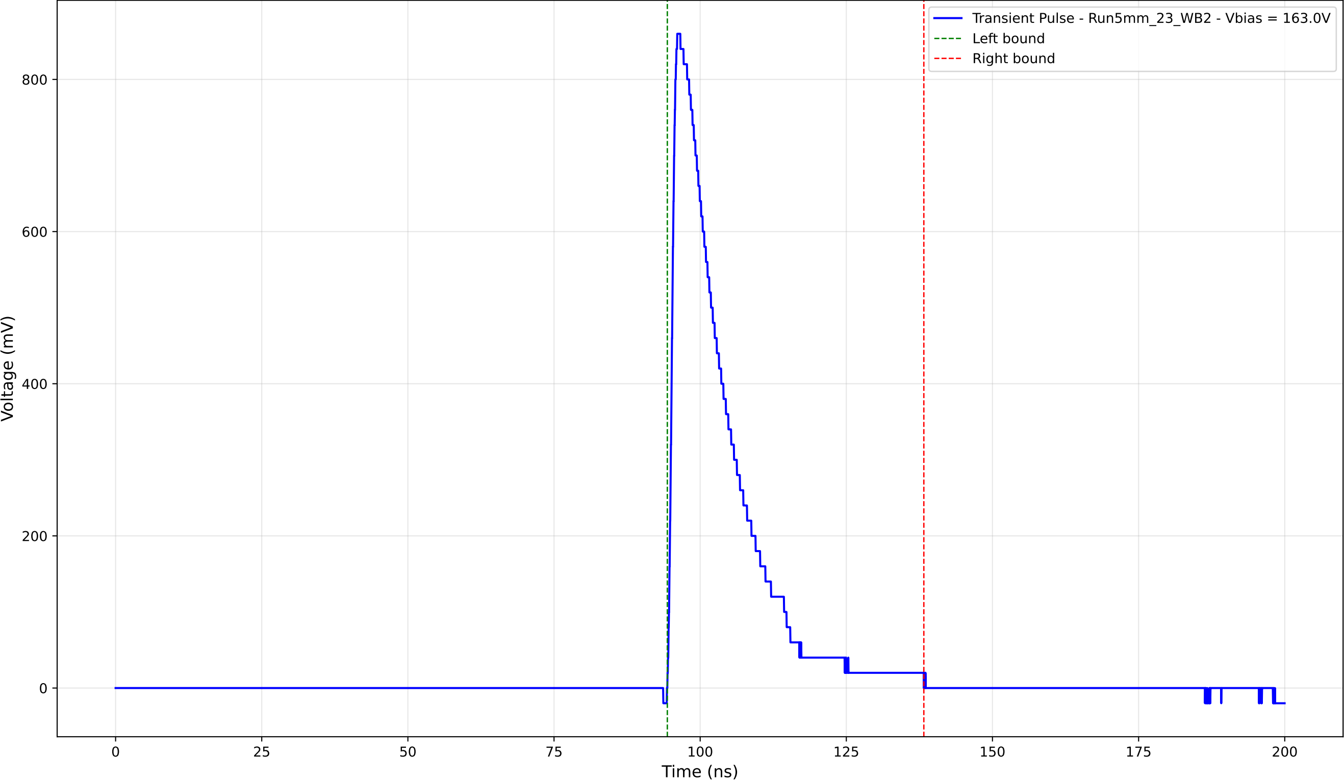
Transient Pulse - Sample: 5mm_23 - Position: 3765.0 \mu\text{m} - Charge: 176.82 pC
