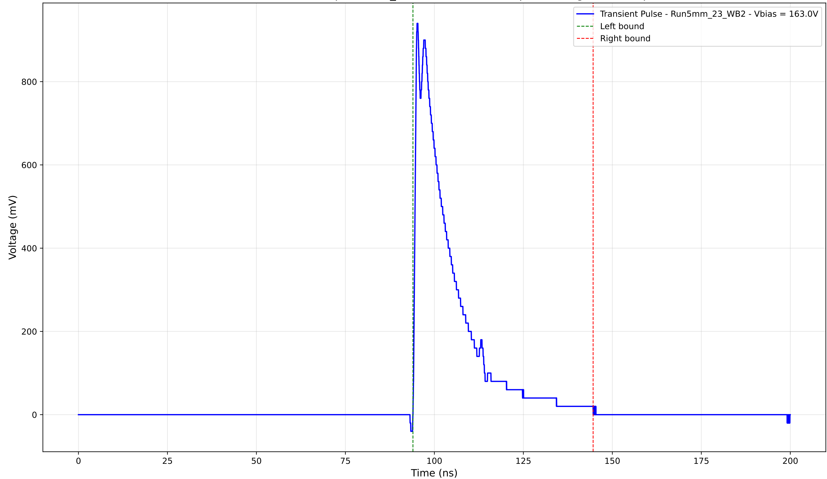
Transient Pulse - Sample: 5mm_23 - Position: 2935.0 \mu\text{m} - Charge: 205.58 pC
