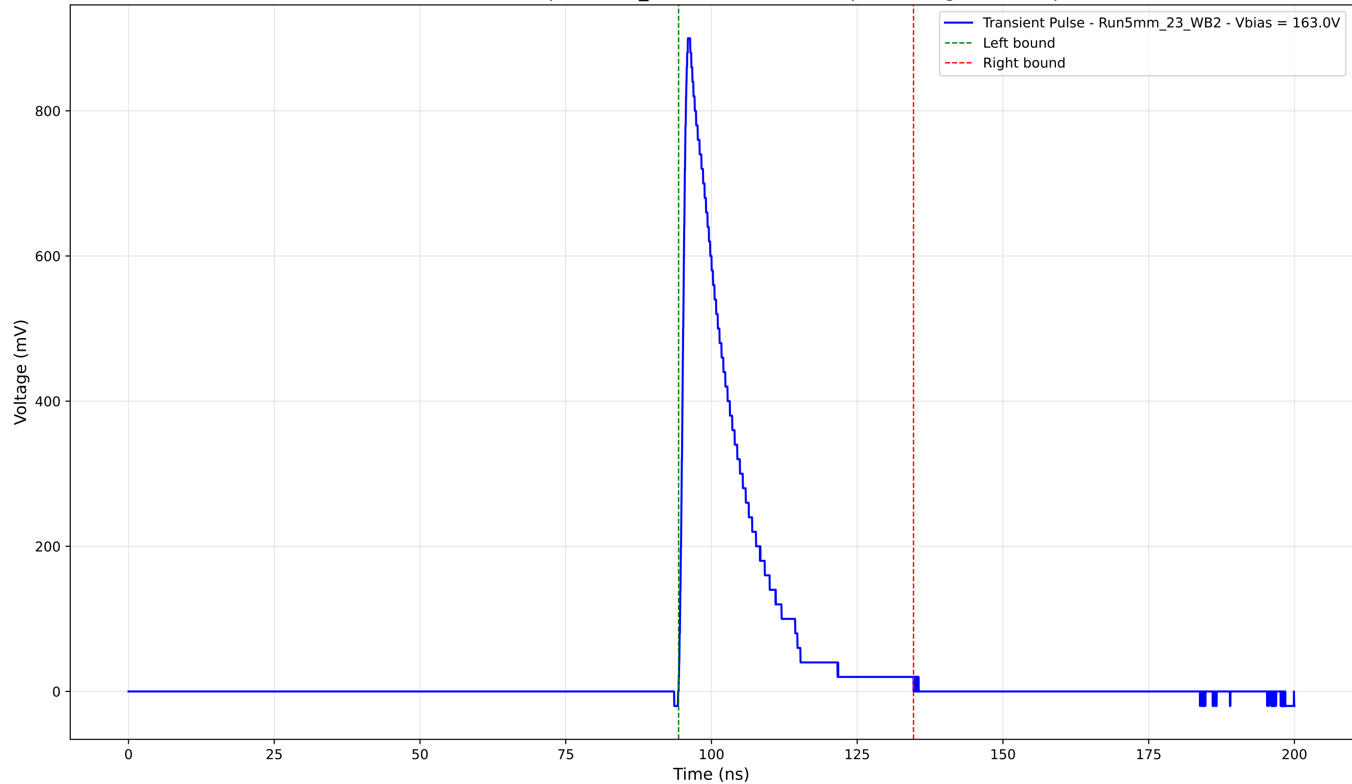
Transient Pulse - Sample: 5mm_23 - Position: 4290.0 \mu\text{m} - Charge: 162.60 pC
