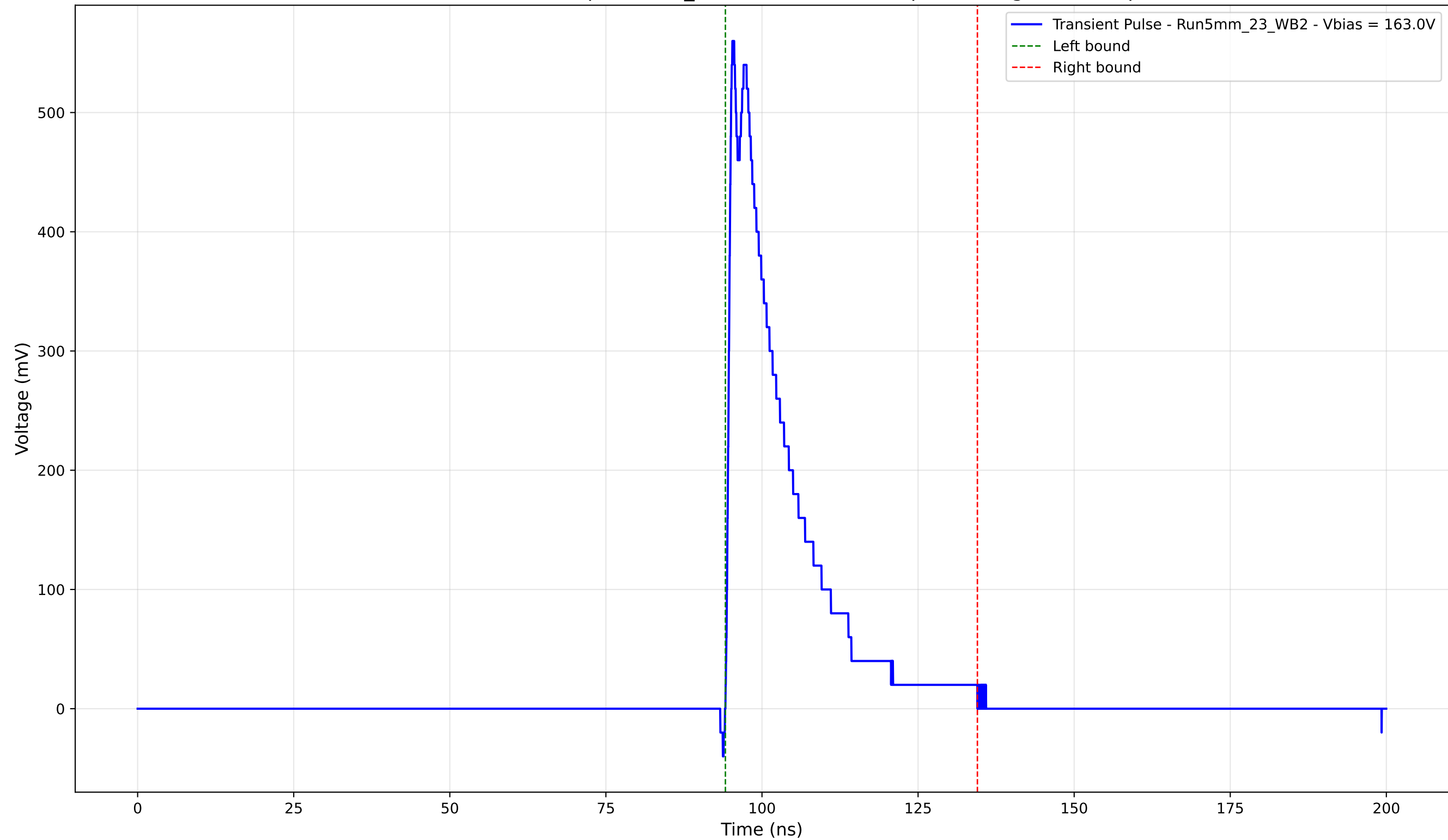
Transient Pulse - Sample: 5mm_23 - Position: 1965.0 \mu\text{m} - Charge: 110.00 pC
