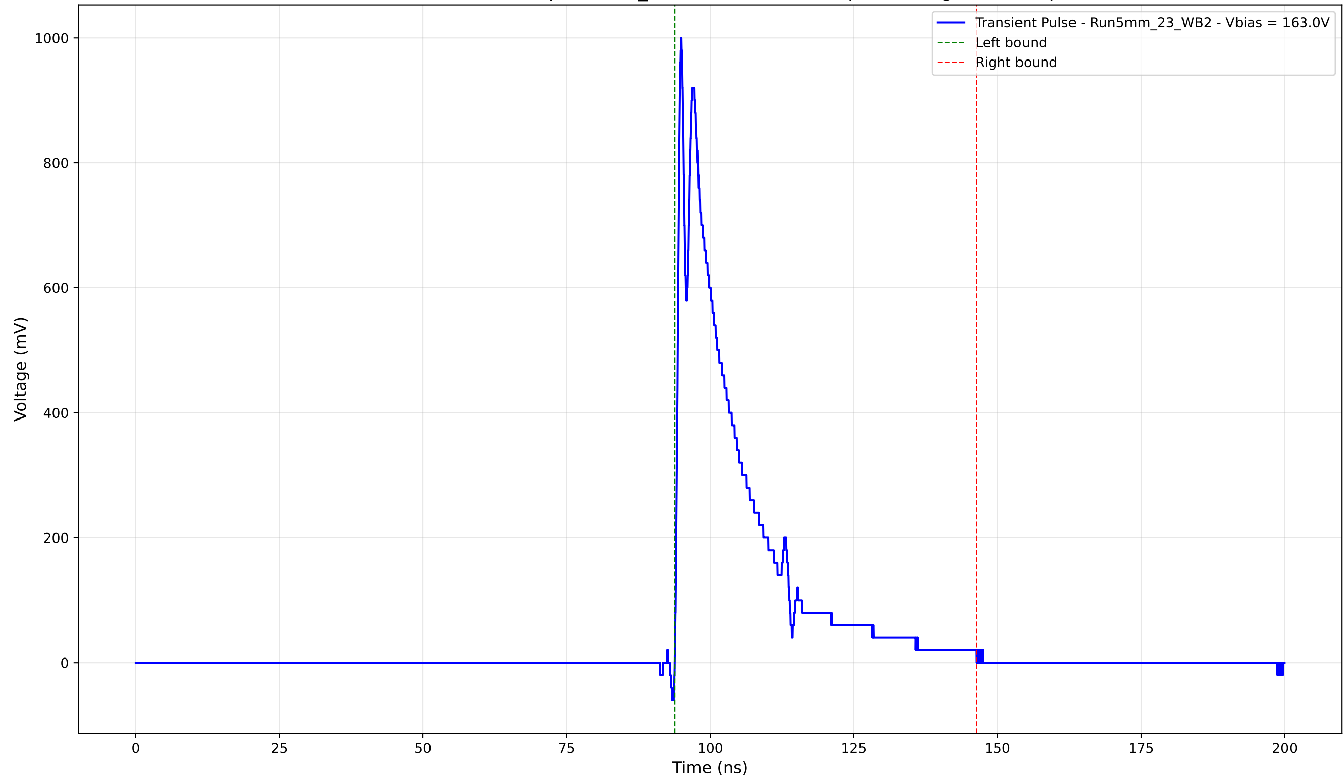
Transient Pulse - Sample: 5mm_23 - Position: 2650.0 \mu\text{m} - Charge: 201.94 pC
