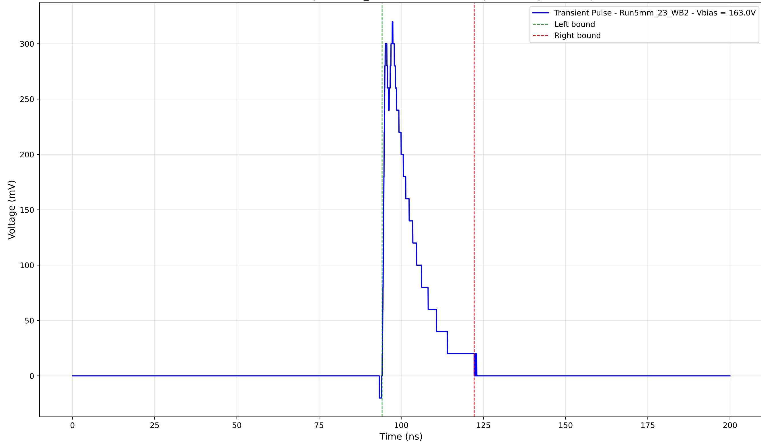
Transient Pulse - Sample: 5mm_23 - Position: 3045.0 \mu\text{m} - Charge: 58.34 pC
