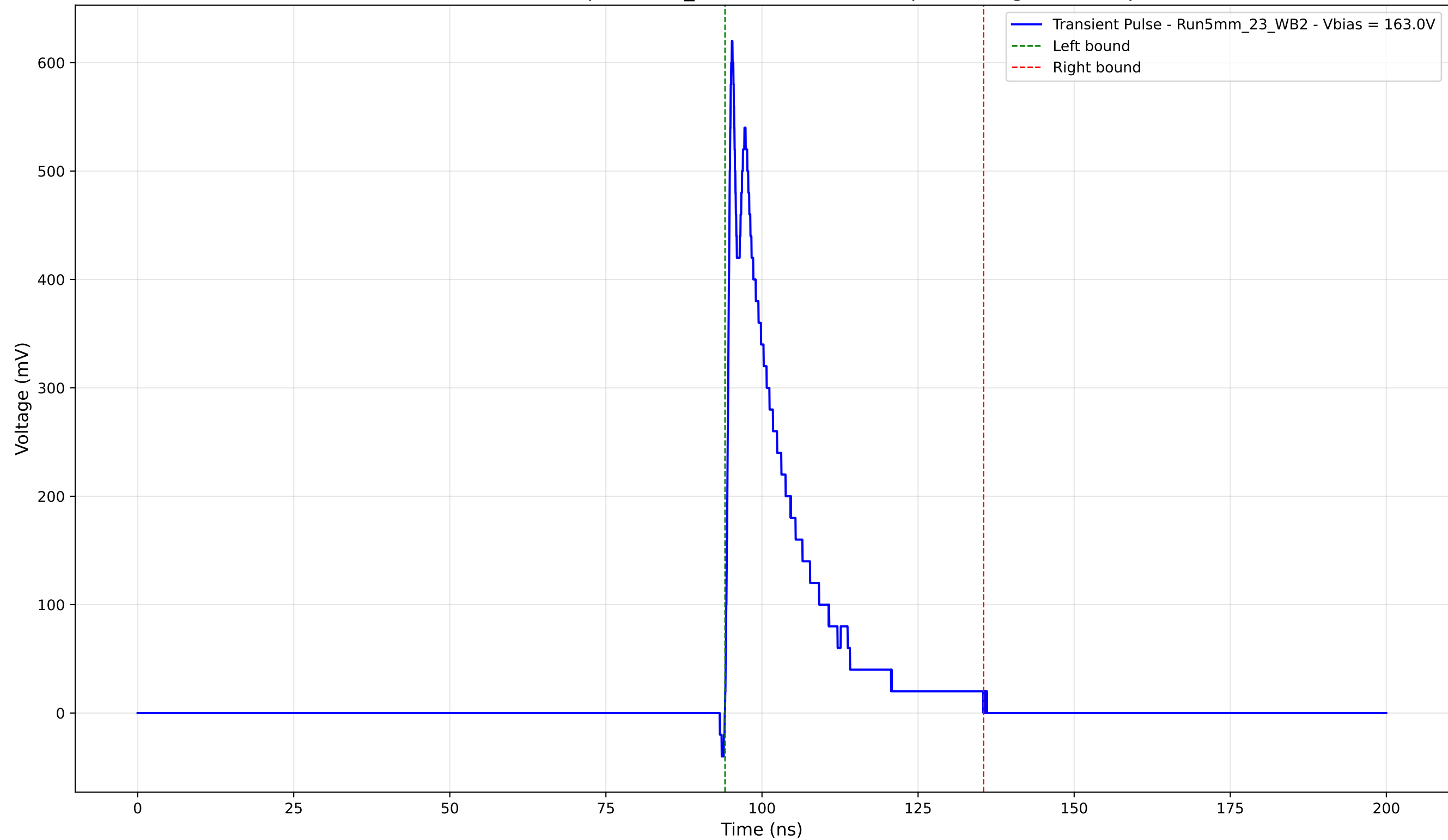
Transient Pulse - Sample: 5mm_23 - Position: 2055.0 \mu\text{m} - Charge: 107.18 pC
