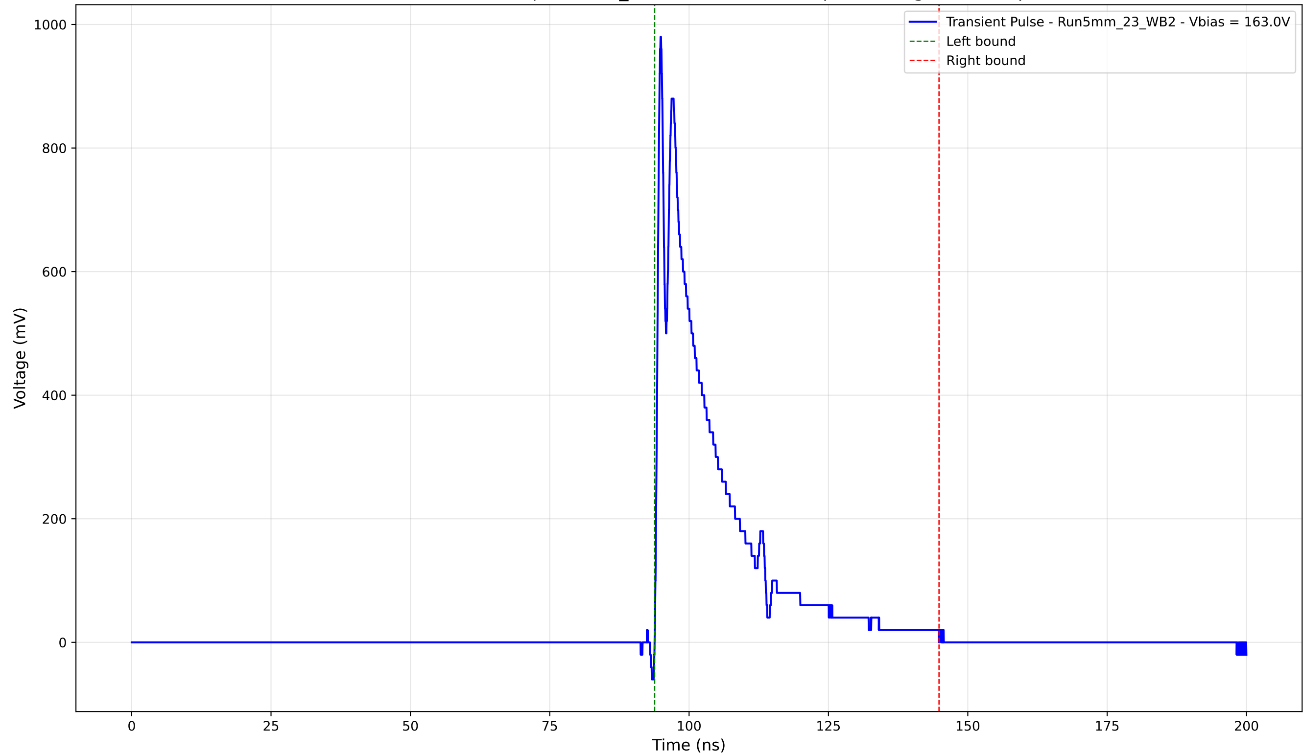
Transient Pulse - Sample: 5mm_23 - Position: 2430.0 \mu\text{m} - Charge: 183.95 pC
