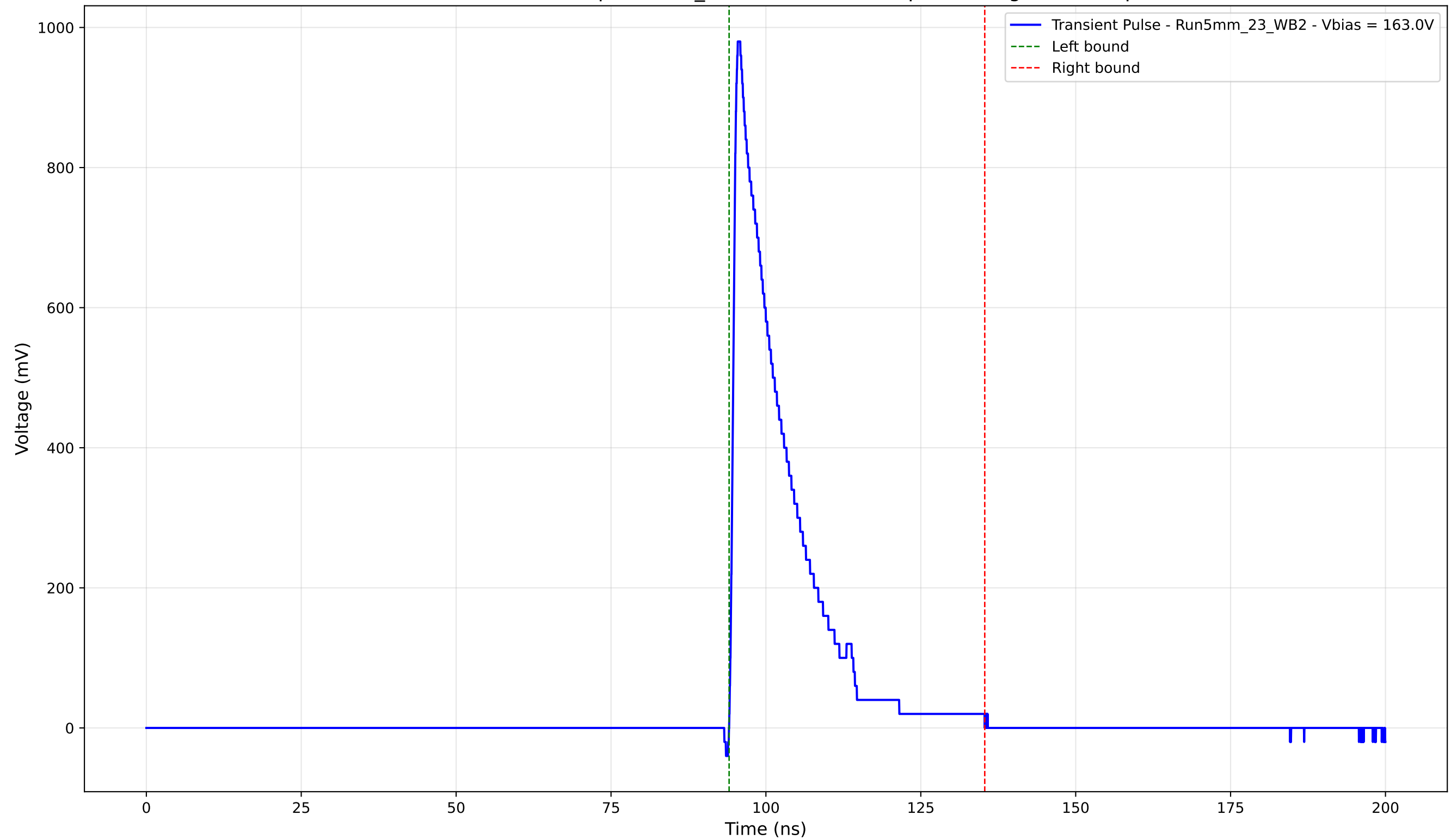
Transient Pulse - Sample: 5mm_23 - Position: 260.0 \mu\text{m} - Charge: 172.51 pC
