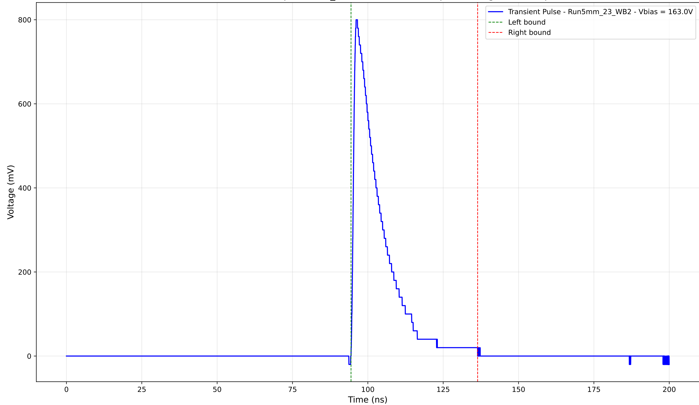
Transient Pulse - Sample: 5mm_23 - Position: 1070.0 \mu\text{m} - Charge: 157.54 pC
