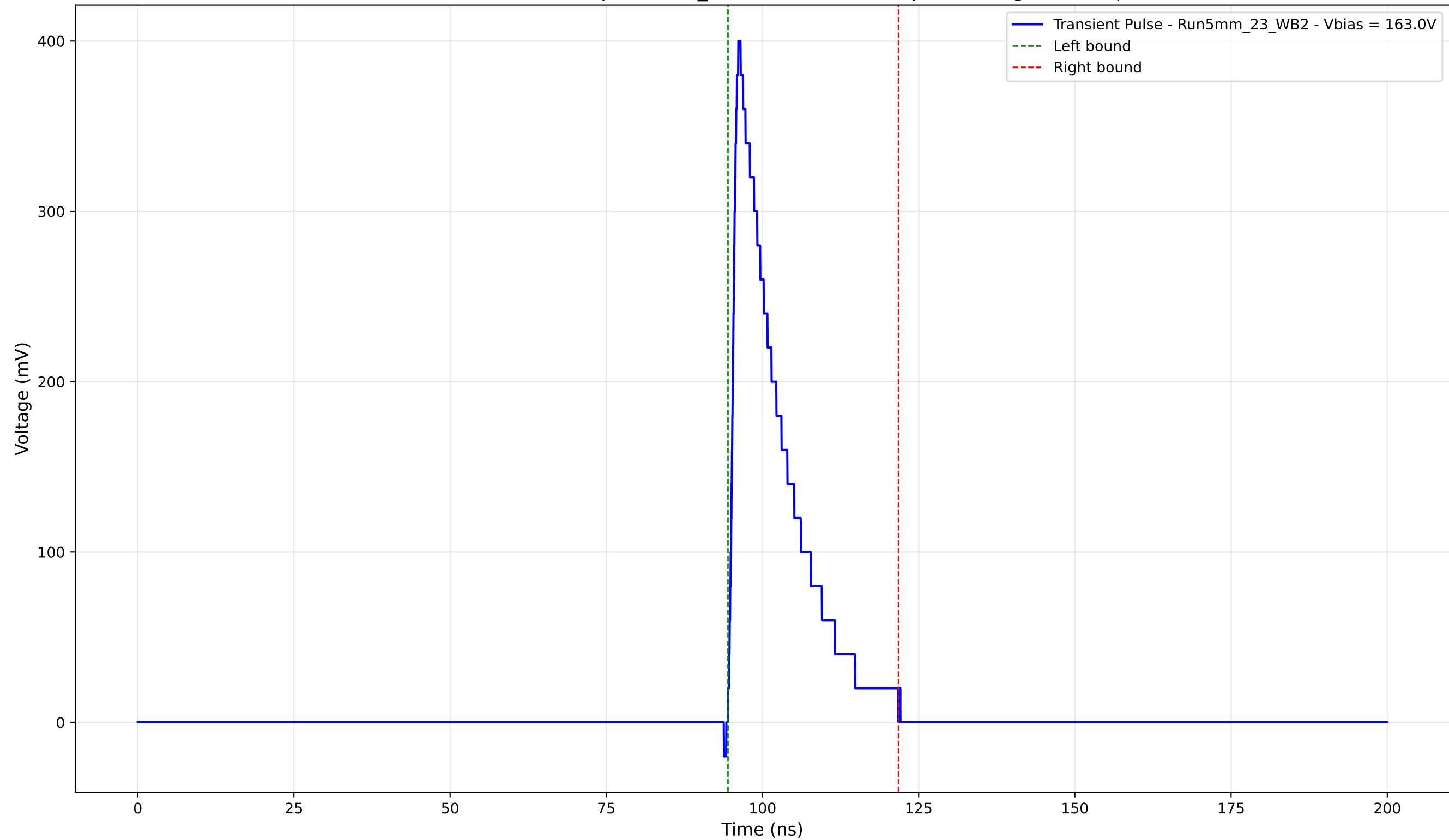
Transient Pulse - Sample: 5mm_23 - Position: 960.0 \mu\text{m} - Charge: 67.66 pC
