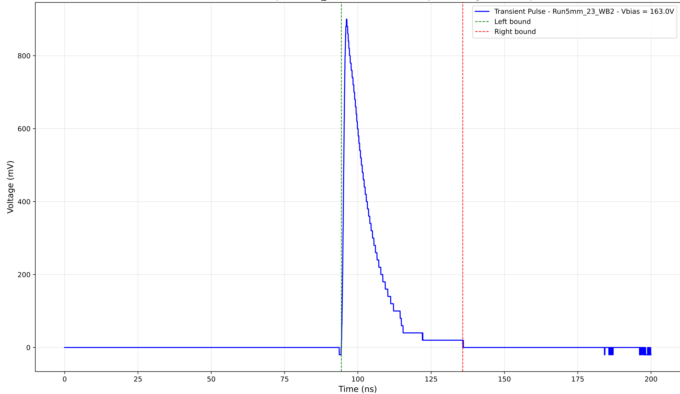
Transient Pulse - Sample: 5mm_23 - Position: 4220.0 \mu\text{m} - Charge: 164.12 pC
