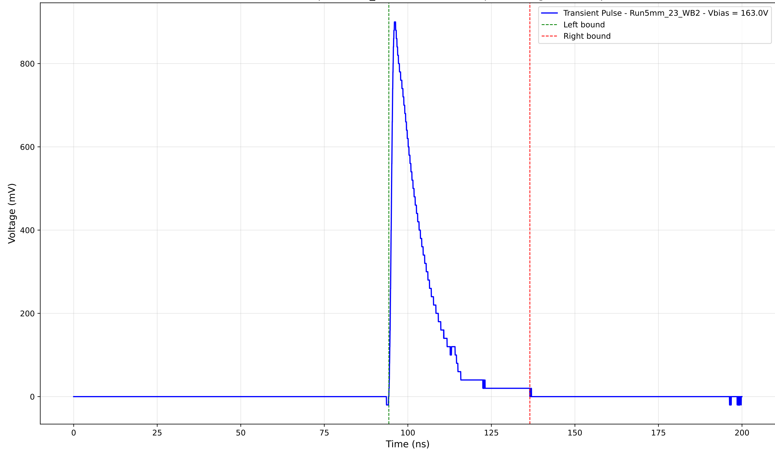
Transient Pulse - Sample: 5mm_23 - Position: 720.0 \mu\text{m} - Charge: 171.75 pC
