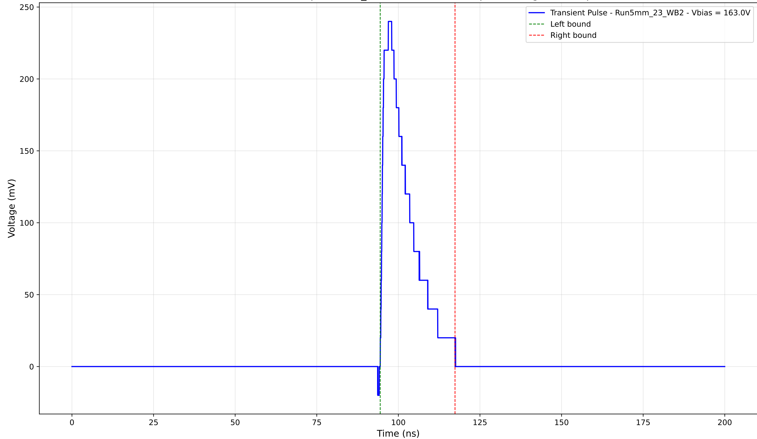
Transient Pulse - Sample: 5mm_23 - Position: 3505.0 \mu\text{m} - Charge: 44.11 pC
