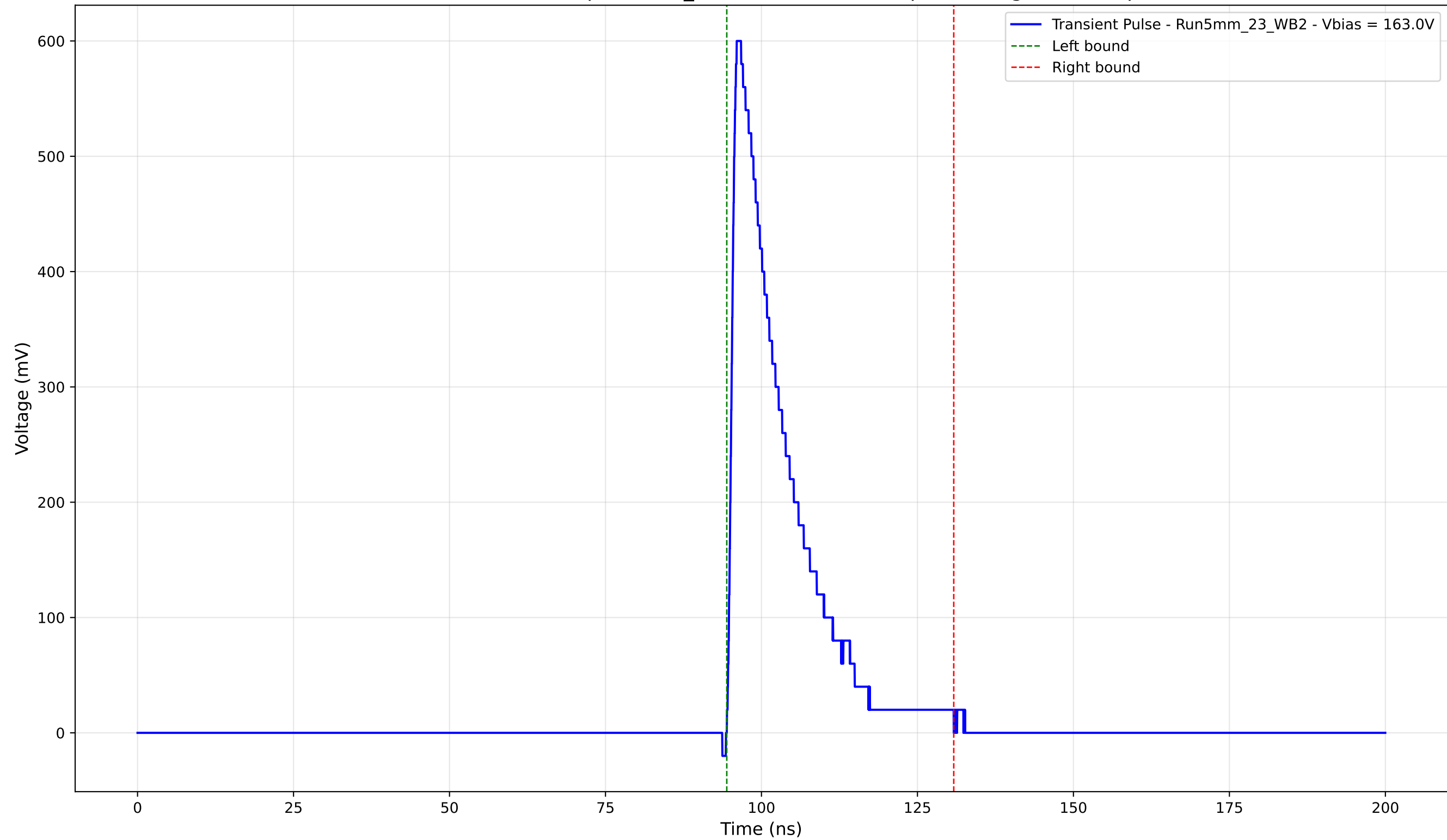
Transient Pulse - Sample: 5mm_23 - Position: 1045.0 \mu\text{m} - Charge: 112.76 pC
