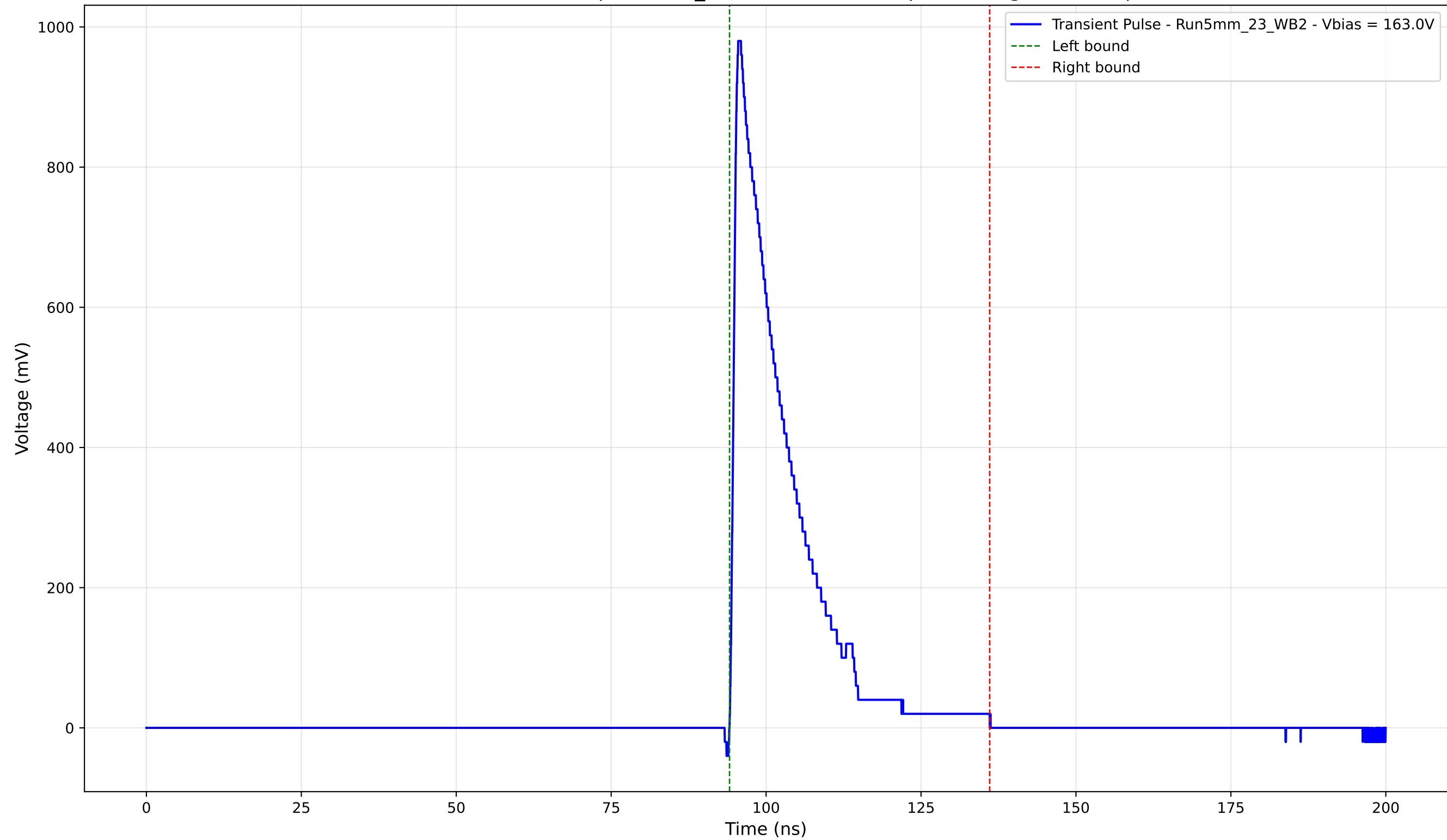
Transient Pulse - Sample: 5mm_23 - Position: 315.0 \mu\text{m} - Charge: 178.31 pC
