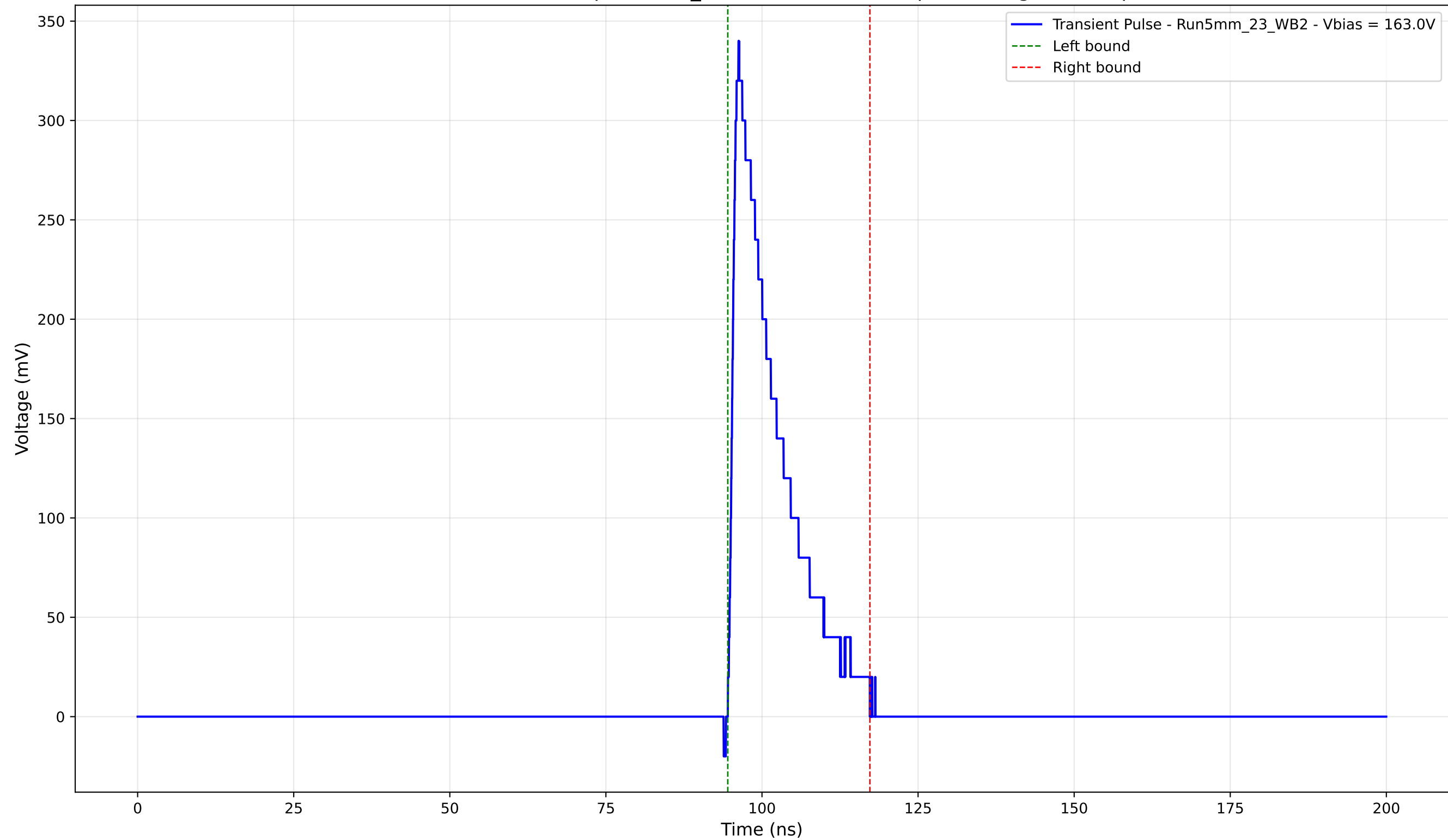
Transient Pulse - Sample: 5mm_23 - Position: 4065.0 \mu\text{m} - Charge: 53.53 pC
