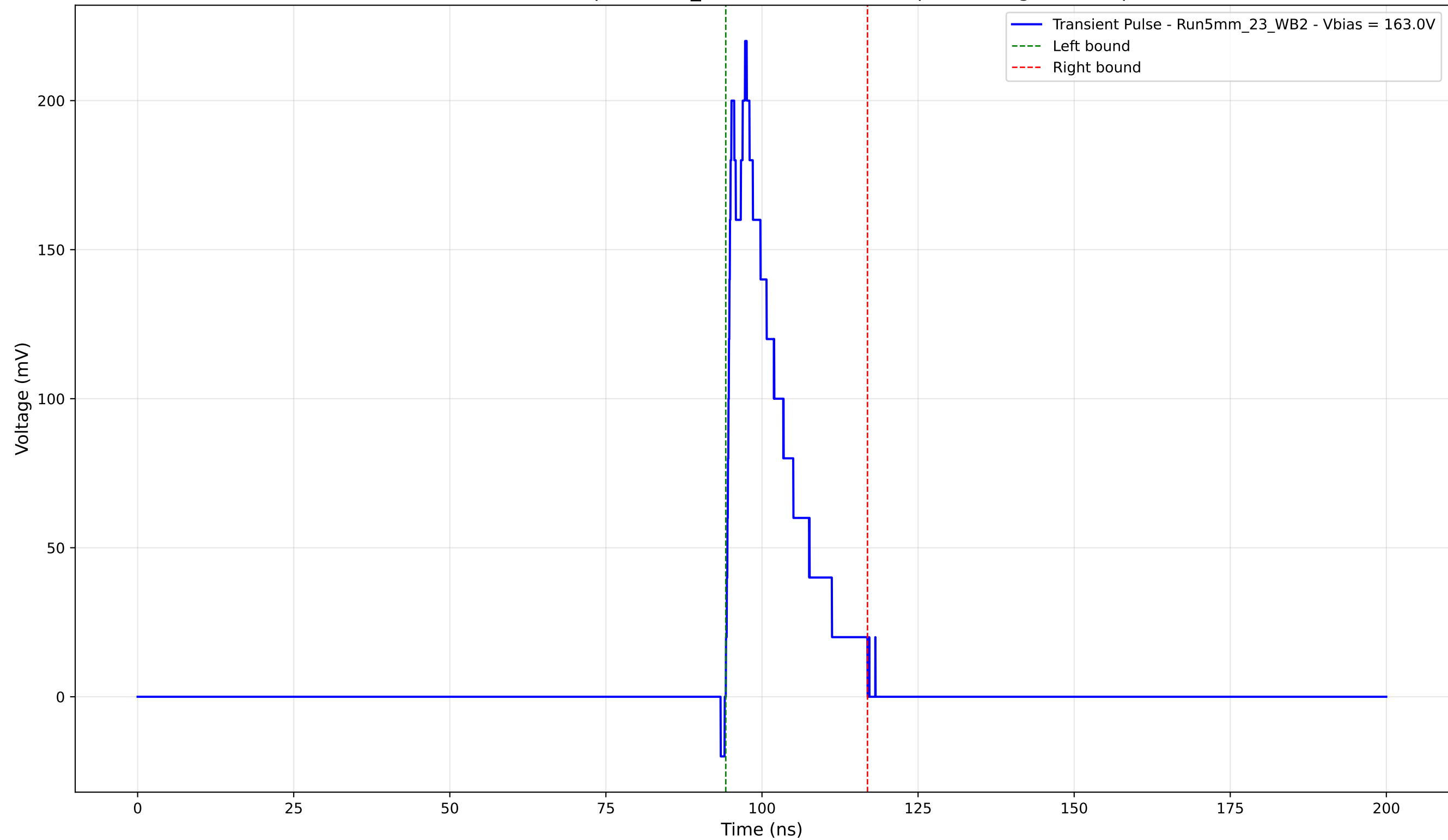
Transient Pulse - Sample: 5mm_23 - Position: 3030.0 \mu\text{m} - Charge: 37.86 pC
