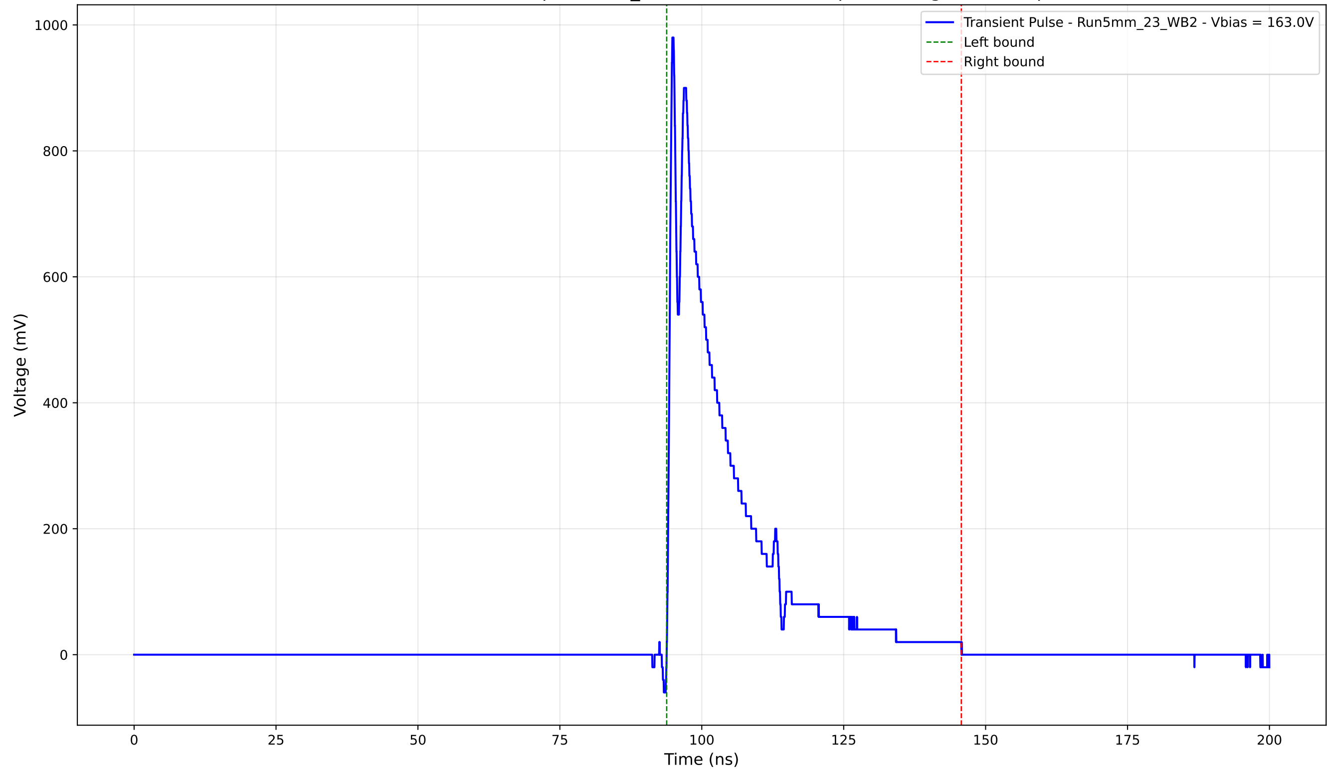
Transient Pulse - Sample: 5mm_23 - Position: 2420.0 \mu\text{m} - Charge: 191.67 pC
