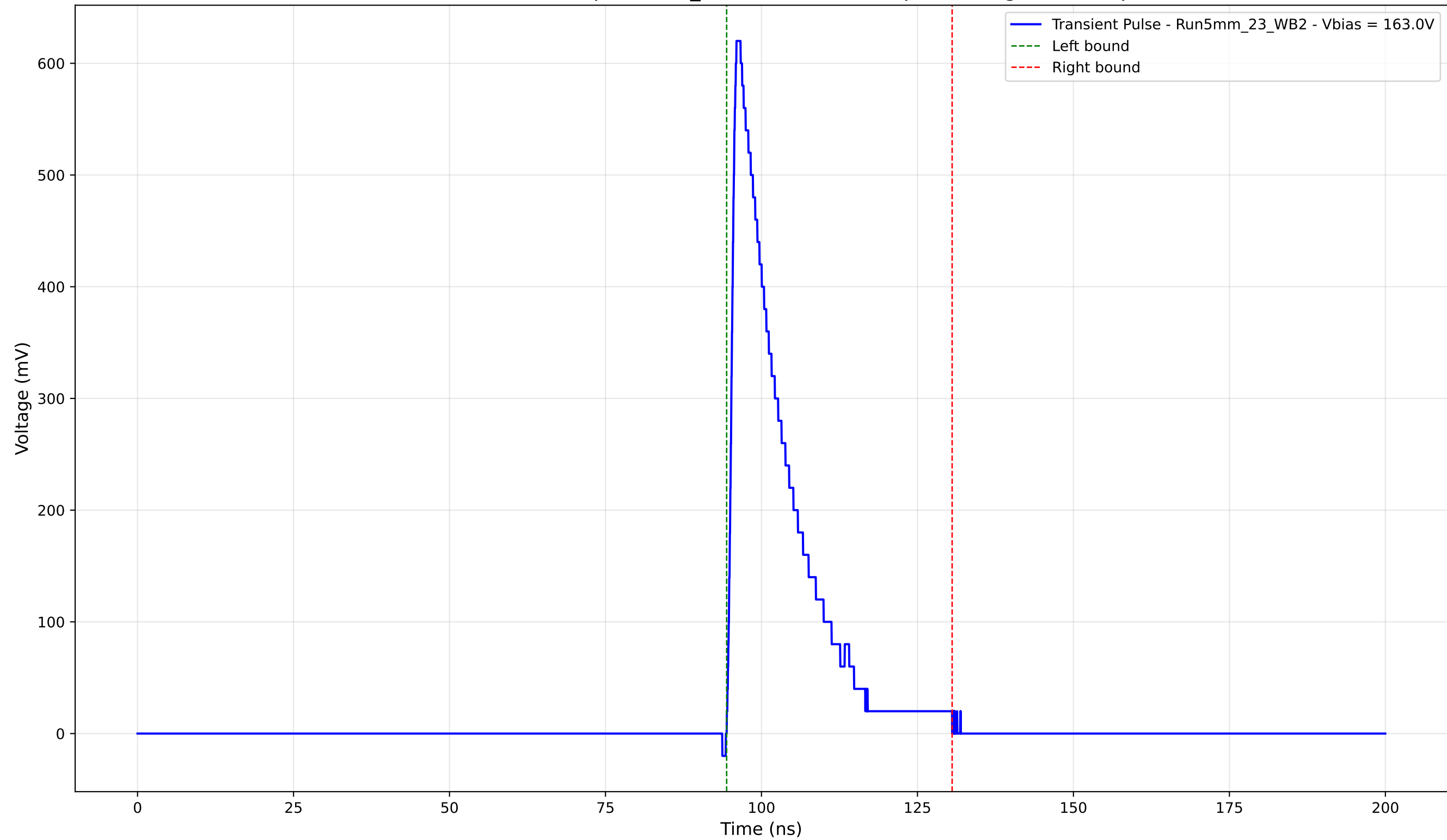
Transient Pulse - Sample: 5mm_23 - Position: 940.0 \mu\text{m} - Charge: 112.22 pC
