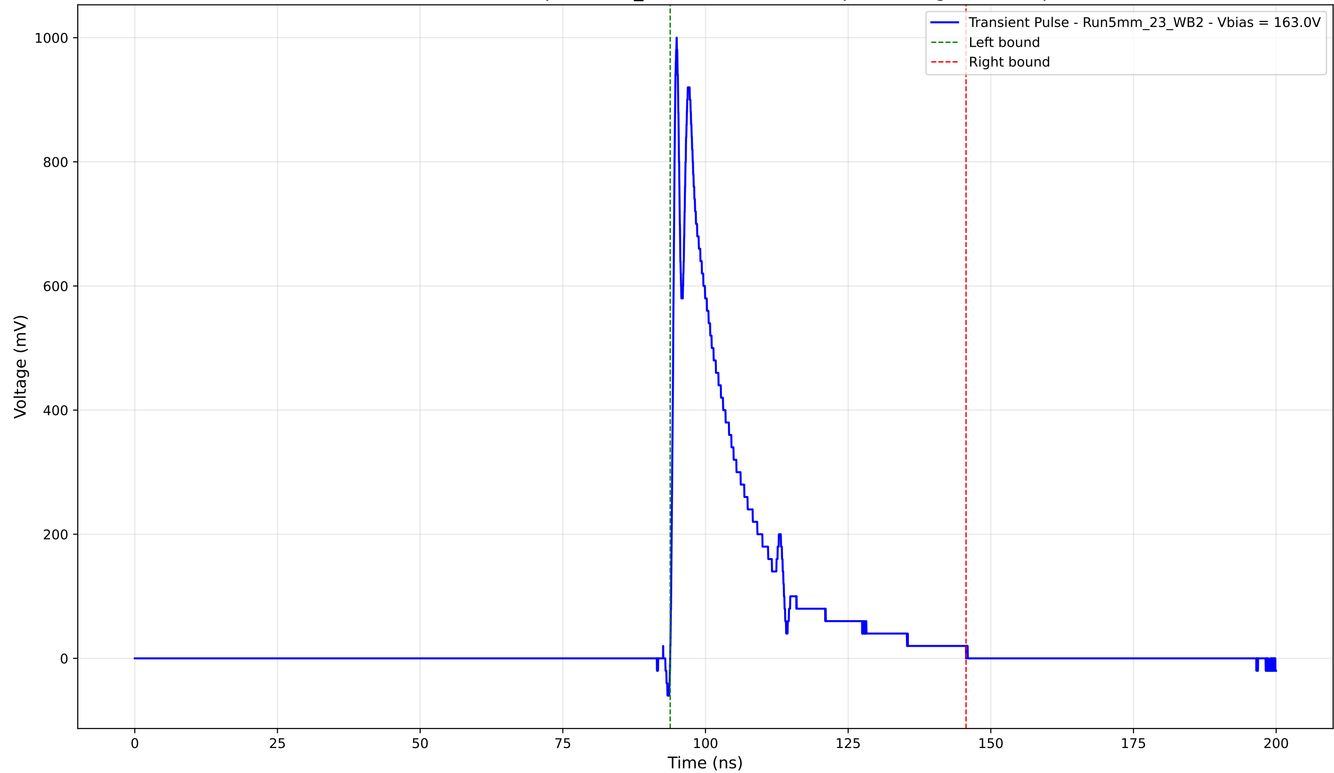
Transient Pulse - Sample: 5mm_23 - Position: 2395.0 \mu\text{m} - Charge: 198.91 pC
