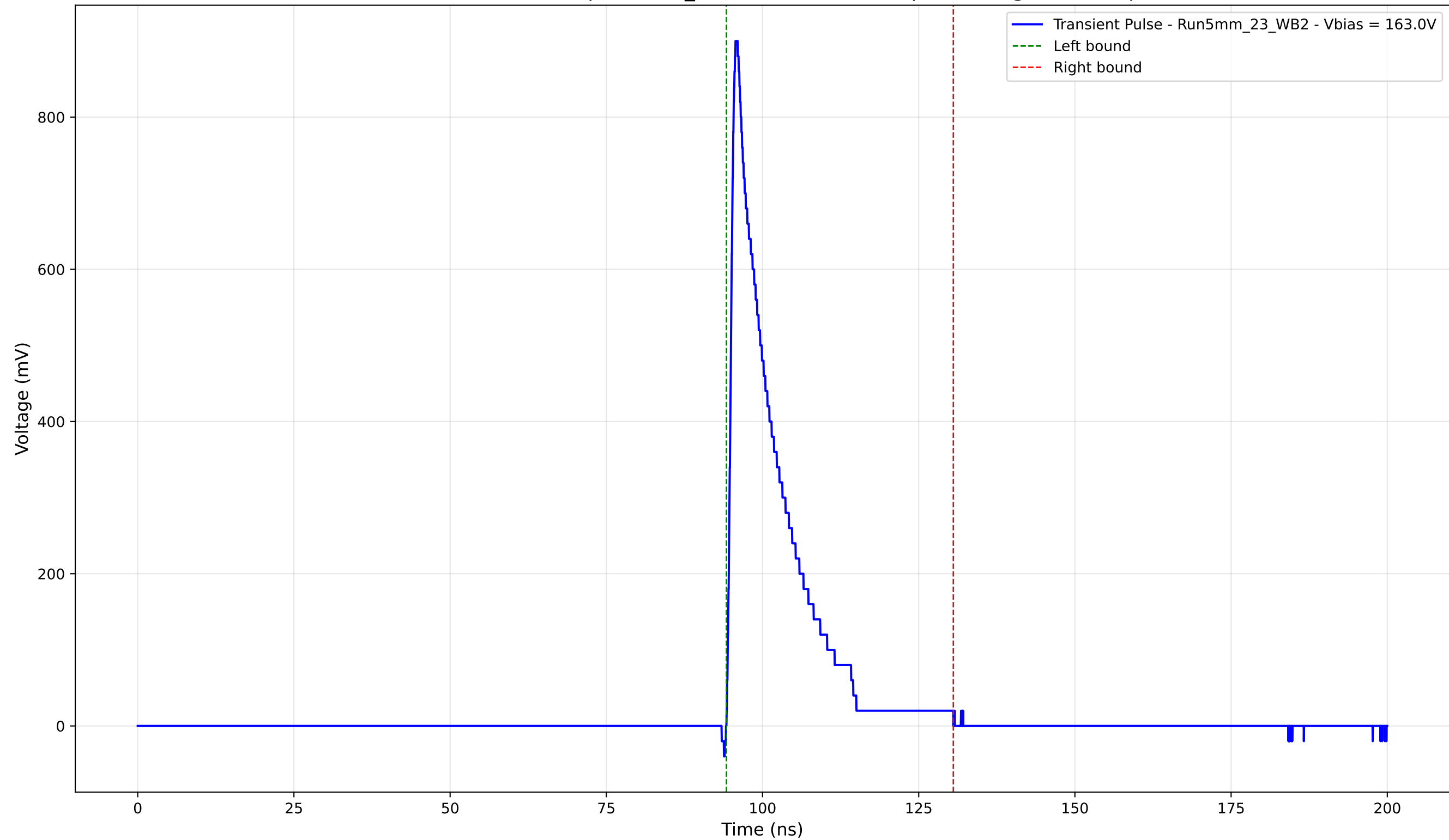
Transient Pulse - Sample: 5mm_23 - Position: 4615.0 \mu\text{m} - Charge: 137.92 pC
