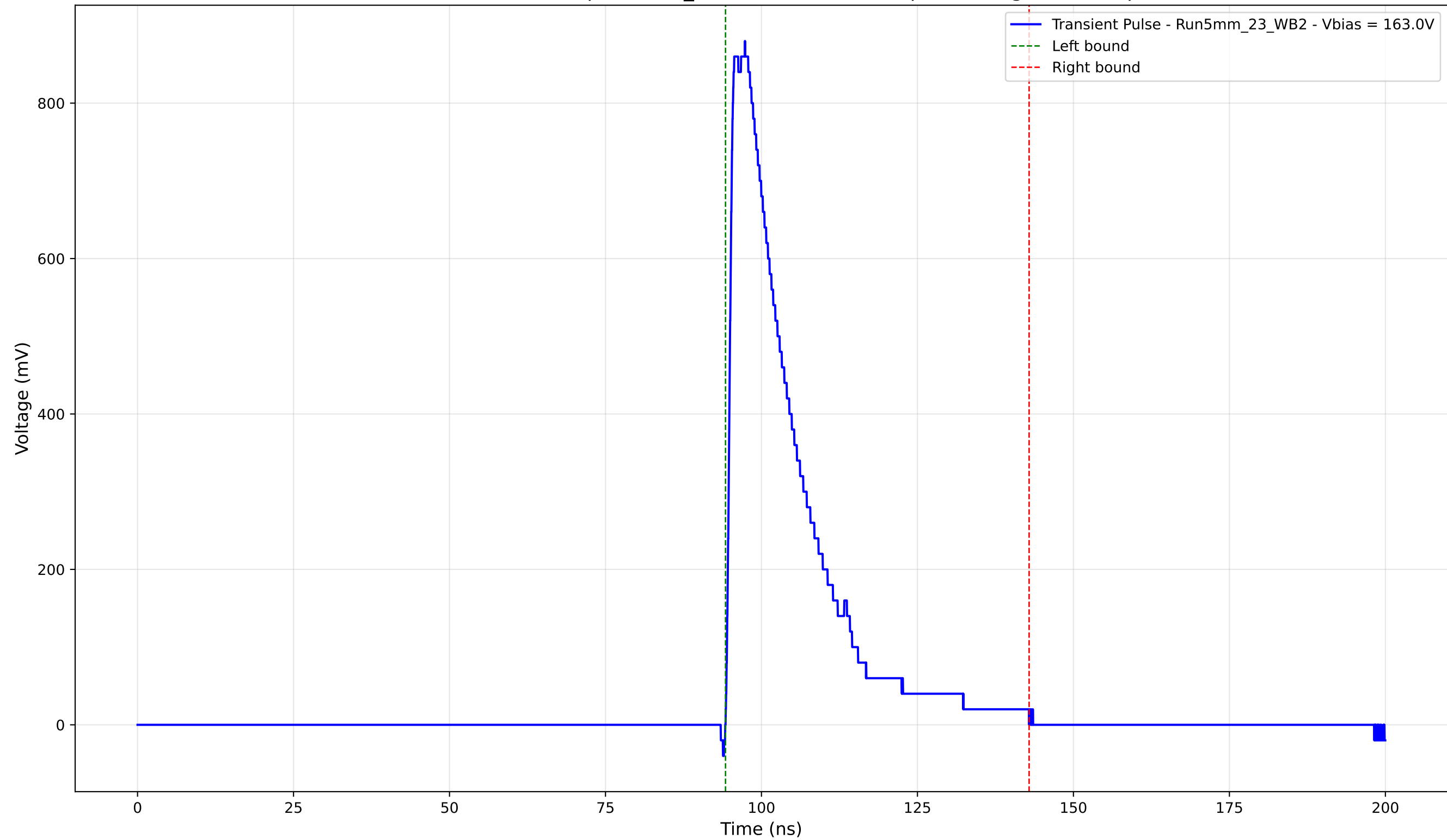
Transient Pulse - Sample: 5mm_23 - Position: 1645.0 \mu\text{m} - Charge: 201.63 pC
