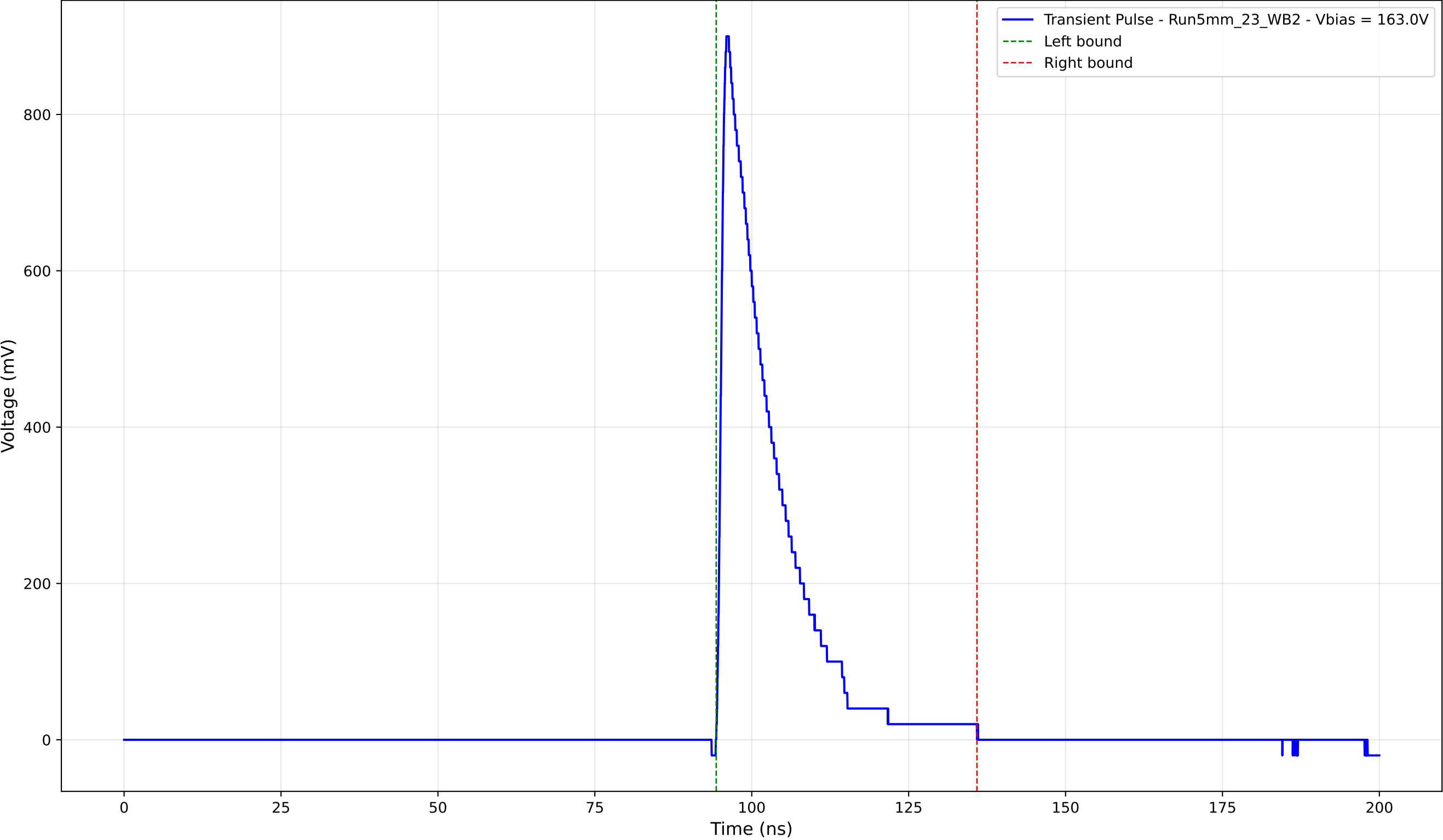
Transient Pulse - Sample: 5mm_23 - Position: 4300.0 \mu\text{m} - Charge: 163.05 pC
