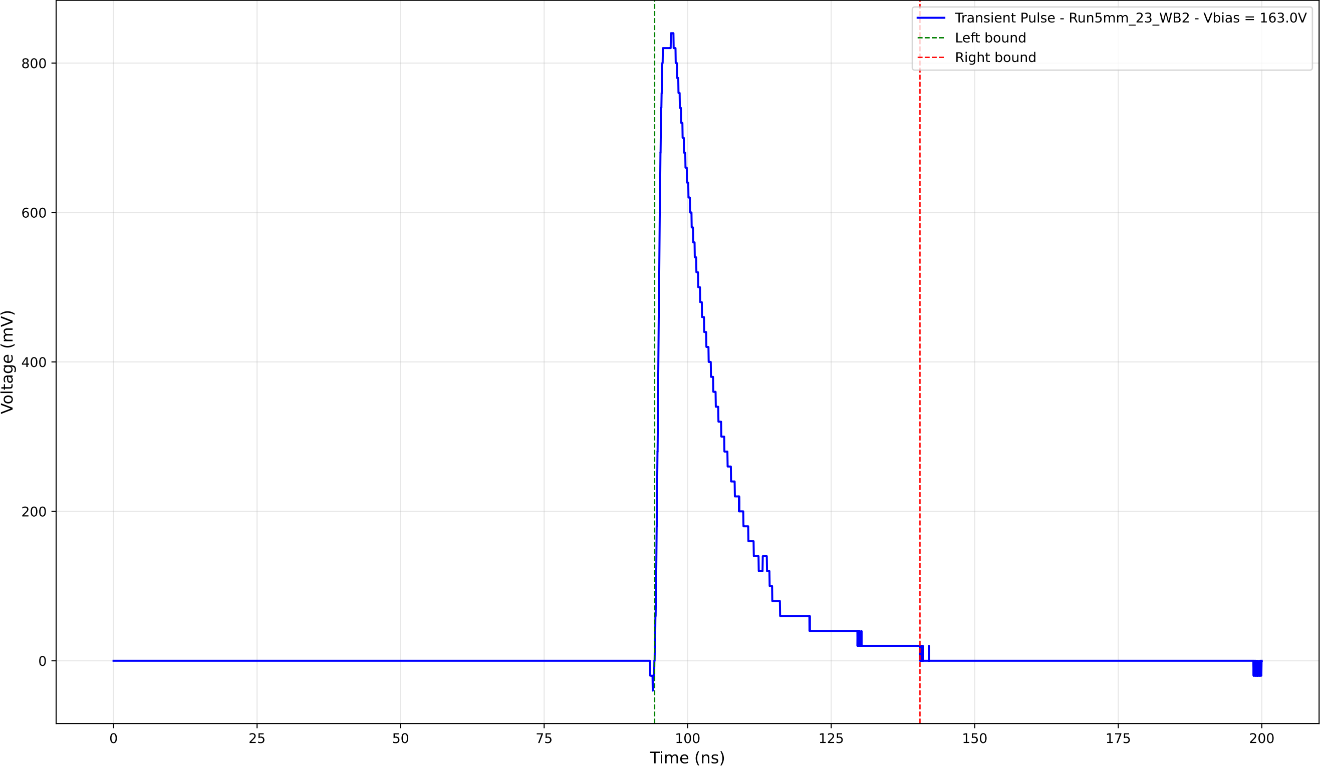
Transient Pulse - Sample: 5mm_23 - Position: 3400.0 \mu\text{m} - Charge: 185.34 pC
