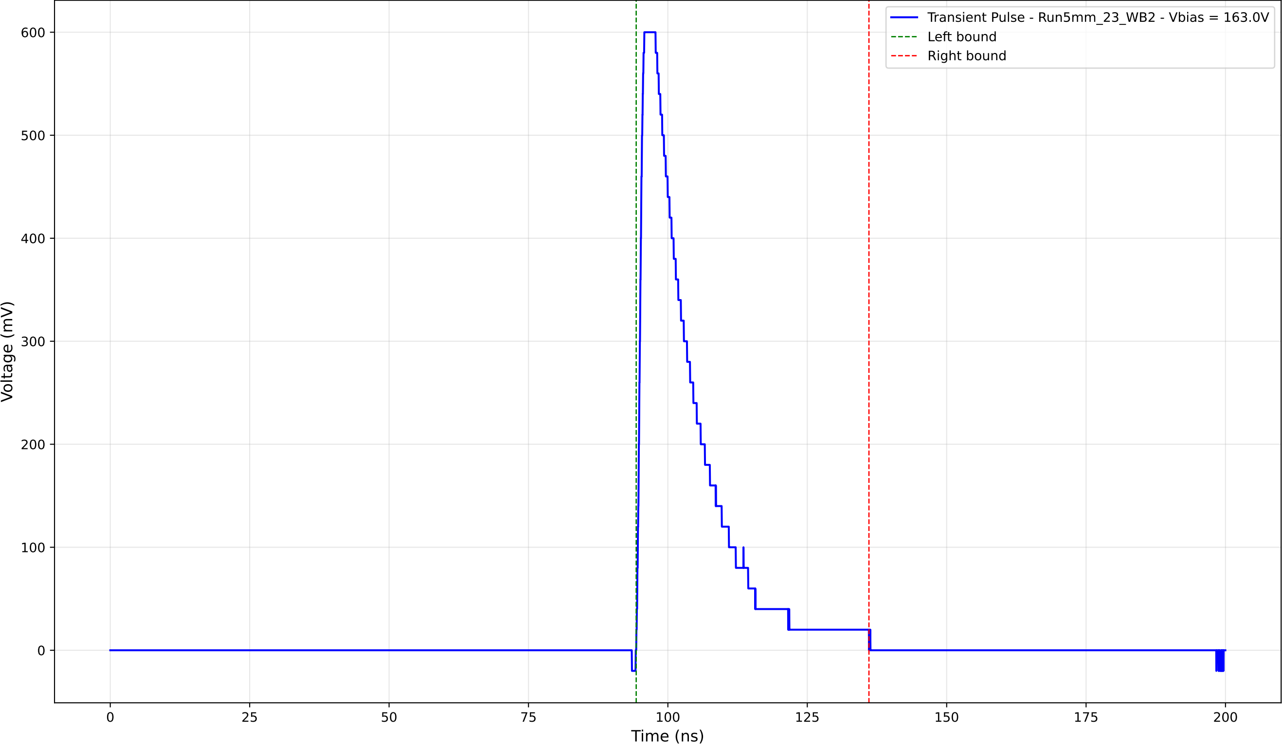
Transient Pulse - Sample: 5mm_23 - Position: 1555.0 \mu\text{m} - Charge: 126.99 pC
