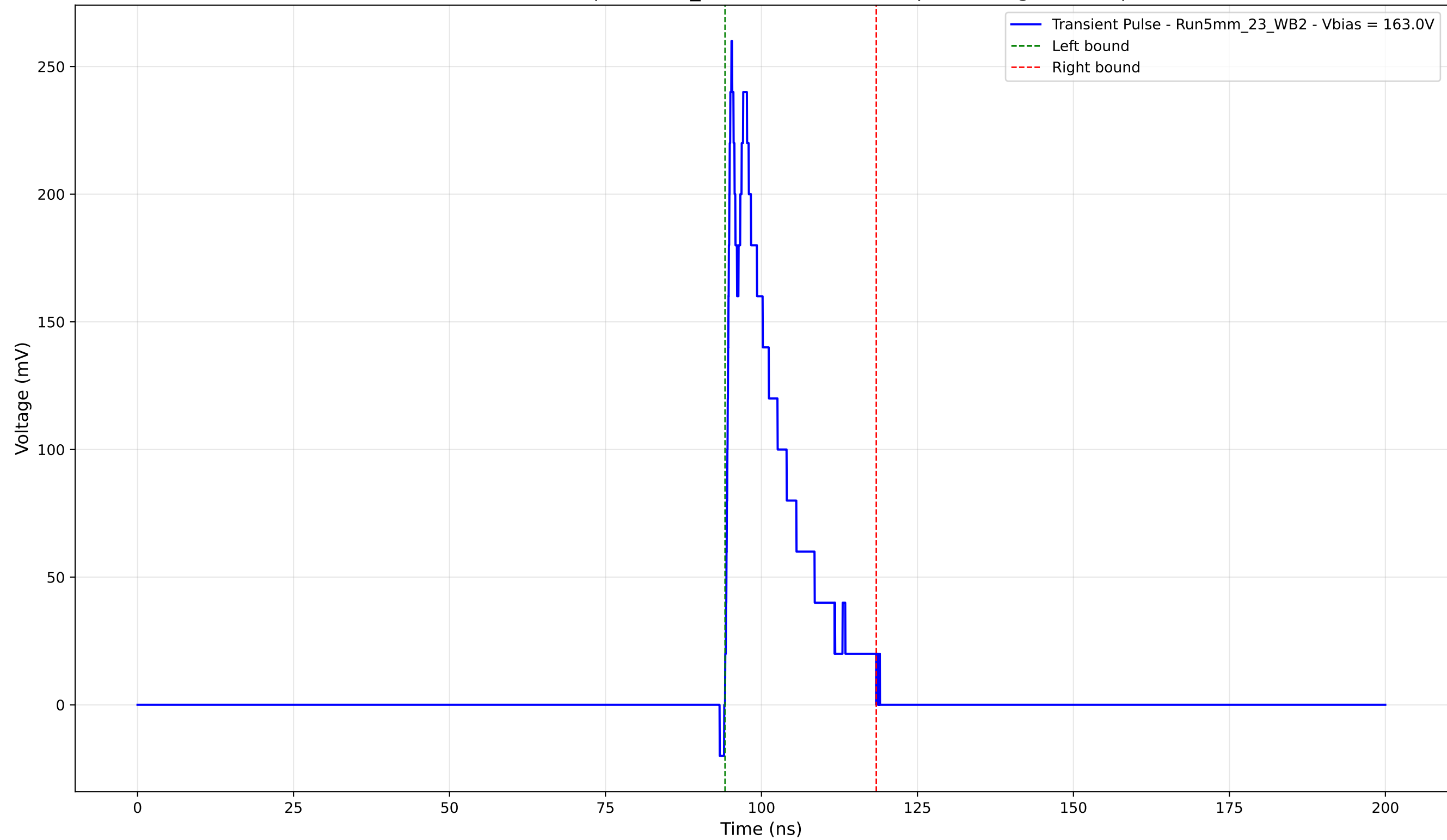
Transient Pulse - Sample: 5mm_23 - Position: 2025.0 \mu\text{m} - Charge: 42.86 pC
