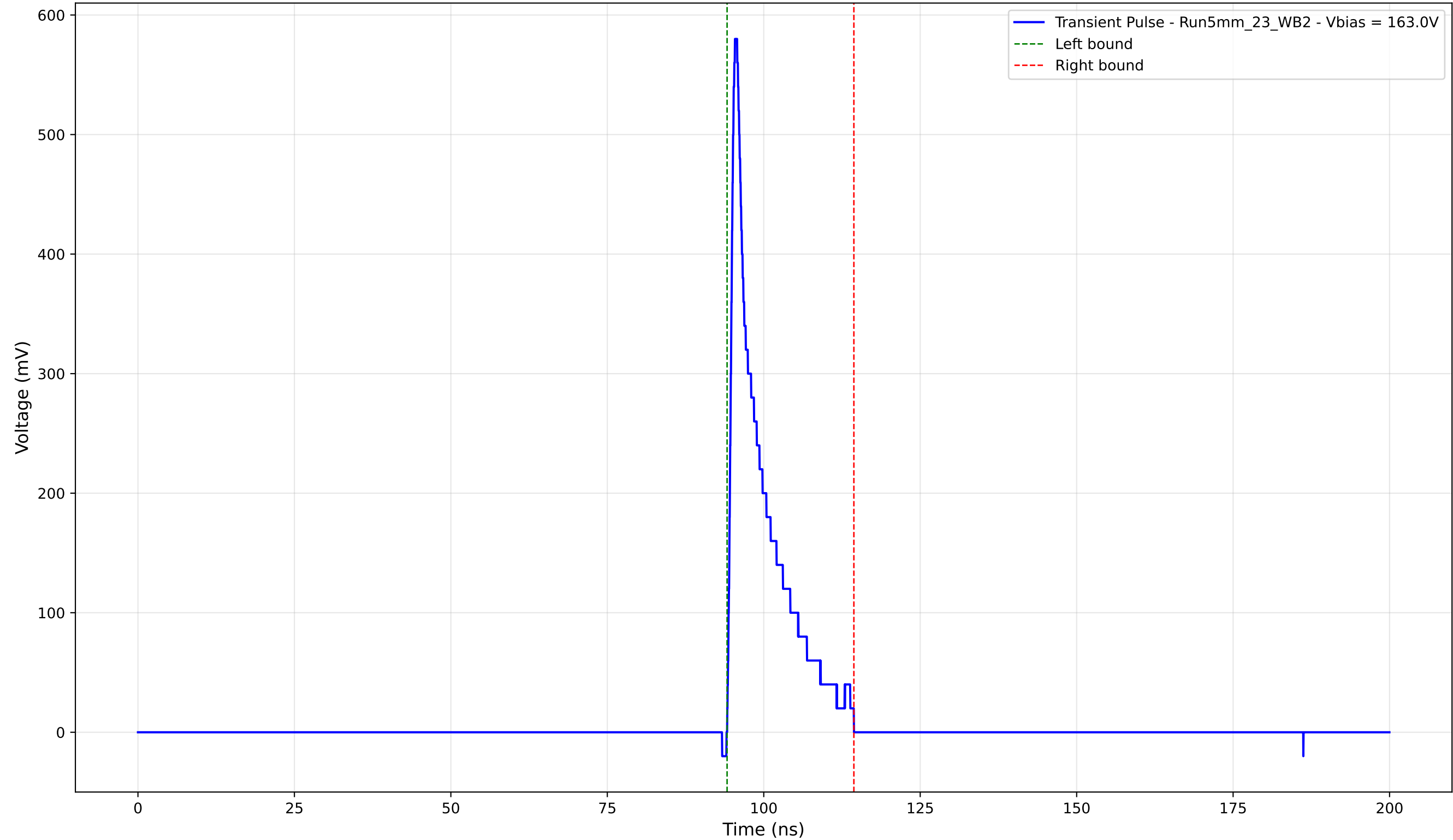
Transient Pulse - Sample: 5mm_23 - Position: 4930.0 \mu\text{m} - Charge: 62.47 pC
