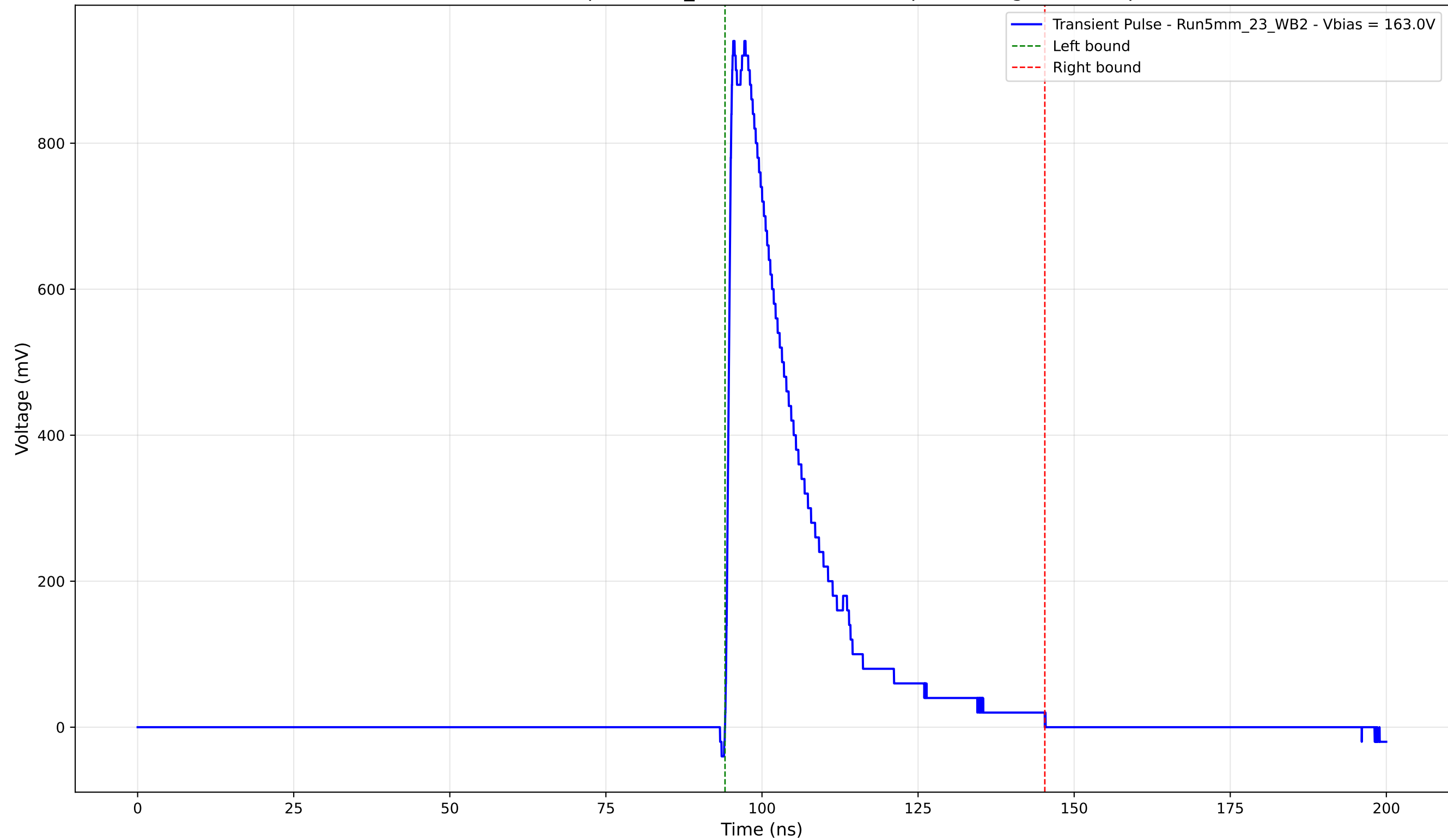
Transient Pulse - Sample: 5mm_23 - Position: 3165.0 \mu\text{m} - Charge: 224.13 pC
