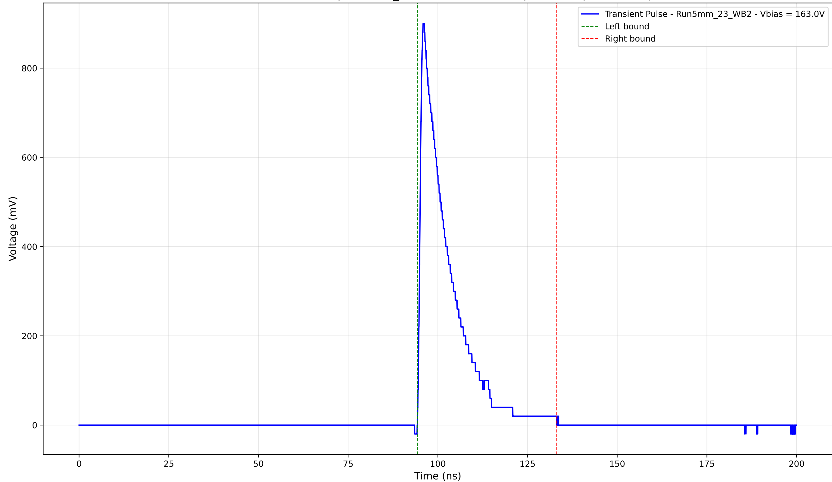
Transient Pulse - Sample: 5mm_23 - Position: 4410.0 \mu\text{m} - Charge: 155.24 pC
