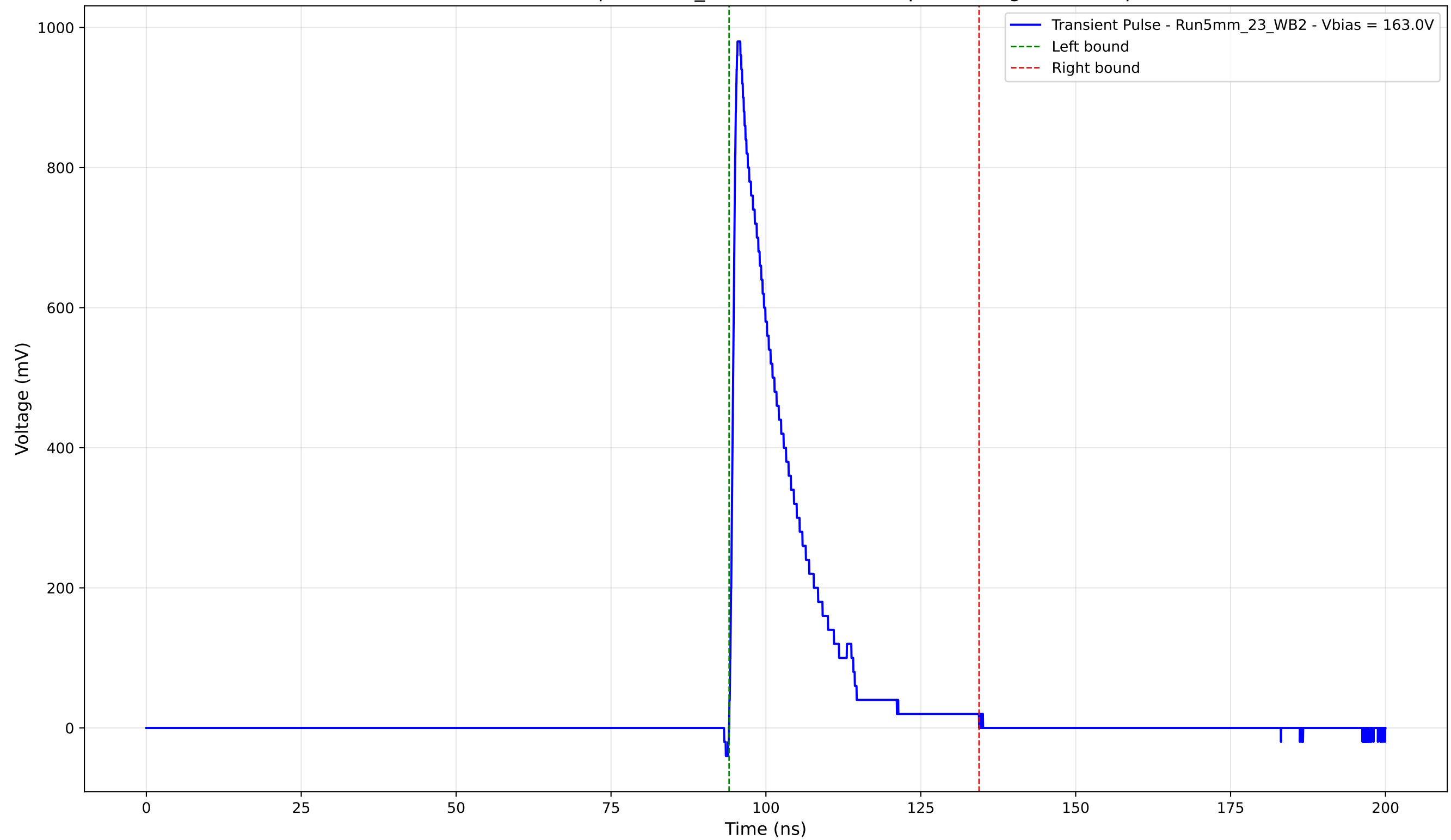
Transient Pulse - Sample: 5mm_23 - Position: 240.0 \mu\text{m} - Charge: 171.45 pC
