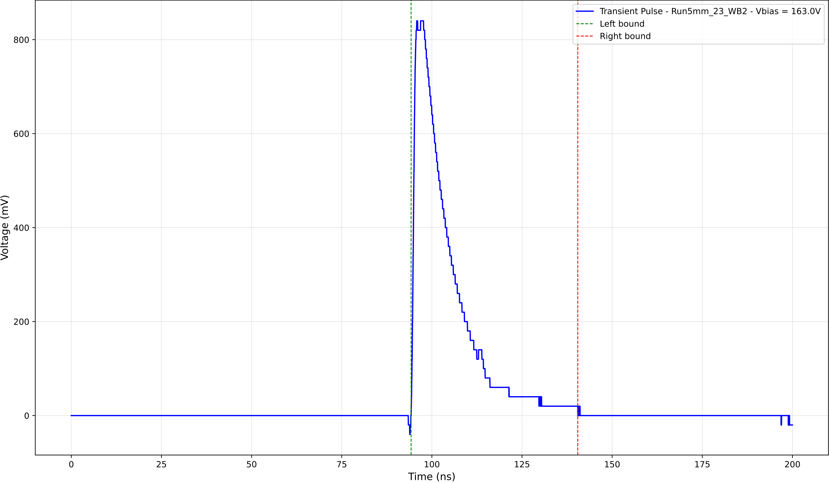
Transient Pulse - Sample: 5mm_23 - Position: 3390.0 \mu\text{m} - Charge: 187.46 pC
