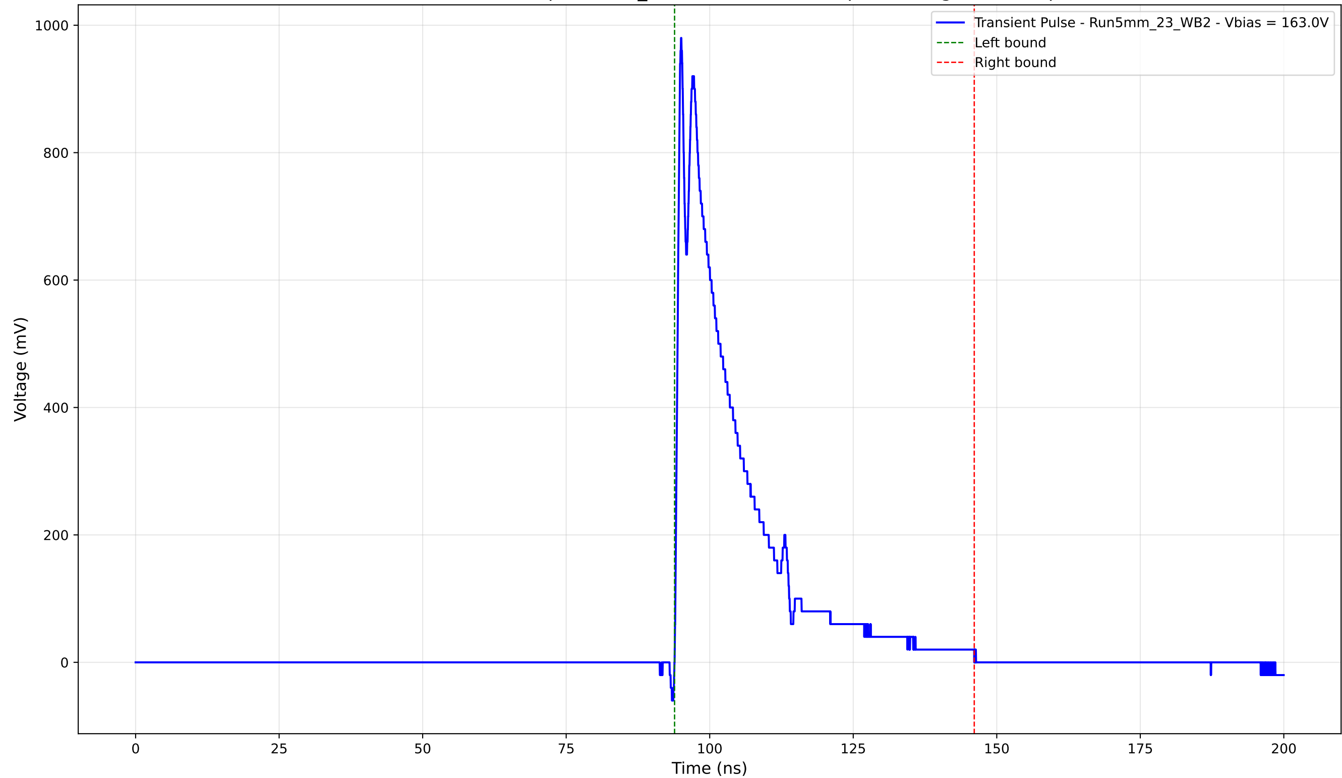
Transient Pulse - Sample: 5mm_23 - Position: 2310.0 \mu\text{m} - Charge: 204.16 pC
