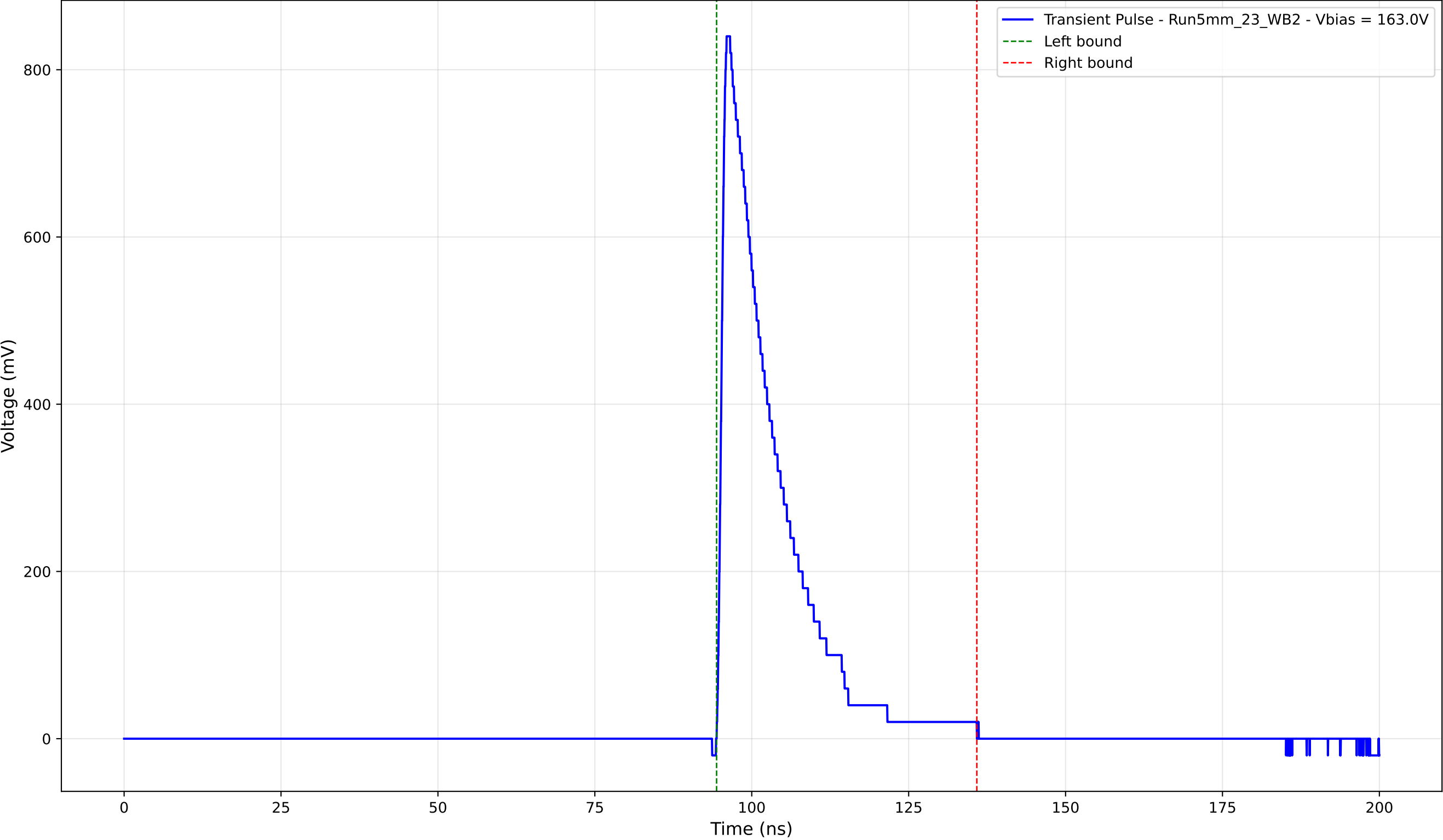
Transient Pulse - Sample: 5mm_23 - Position: 4135.0 \mu\text{m} - Charge: 155.62 pC
