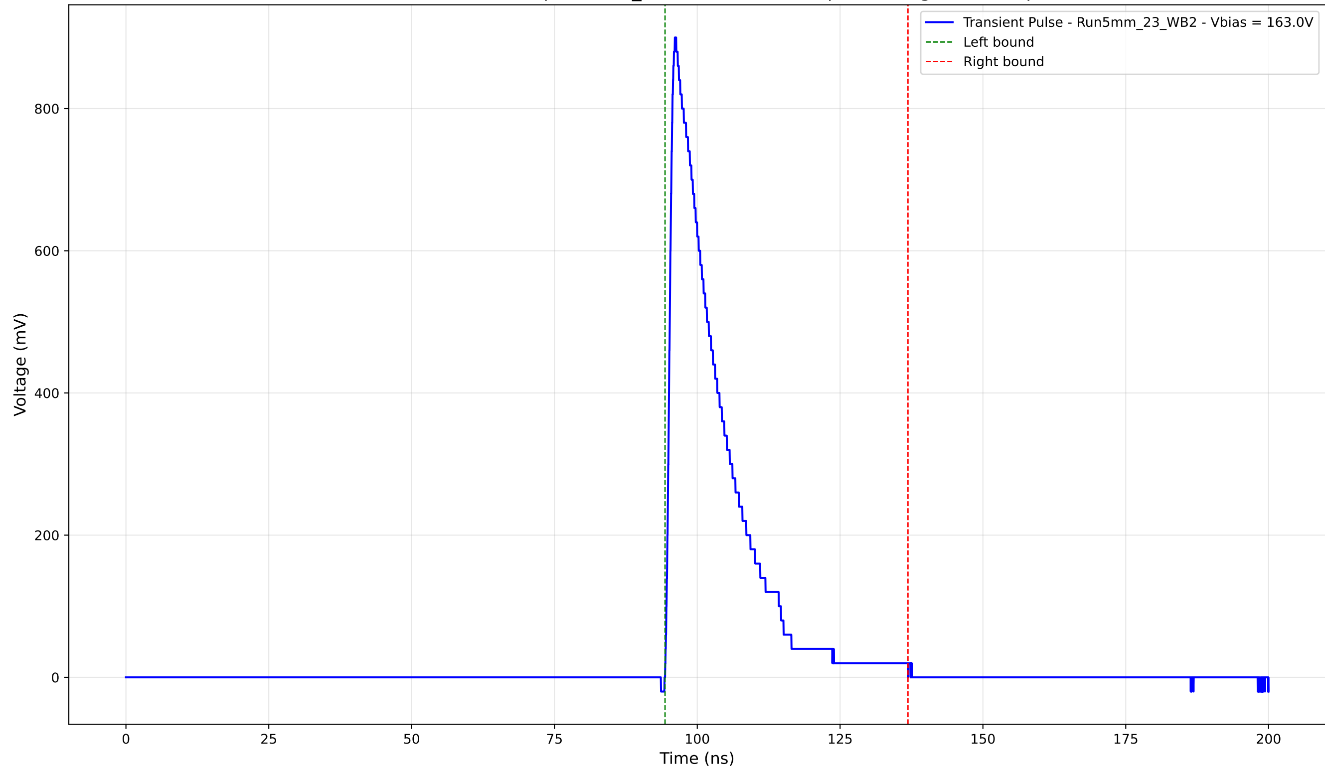
Transient Pulse - Sample: 5mm_23 - Position: 810.0 \mu\text{m} - Charge: 174.53 pC
