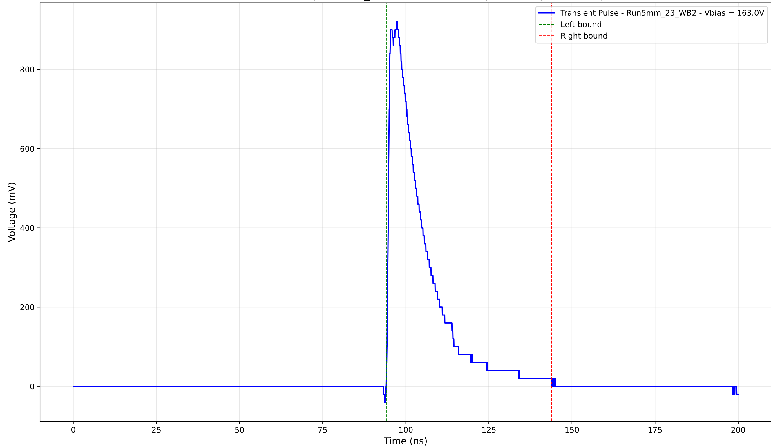
Transient Pulse - Sample: 5mm_23 - Position: 3250.0 \mu\text{m} - Charge: 215.50 pC
