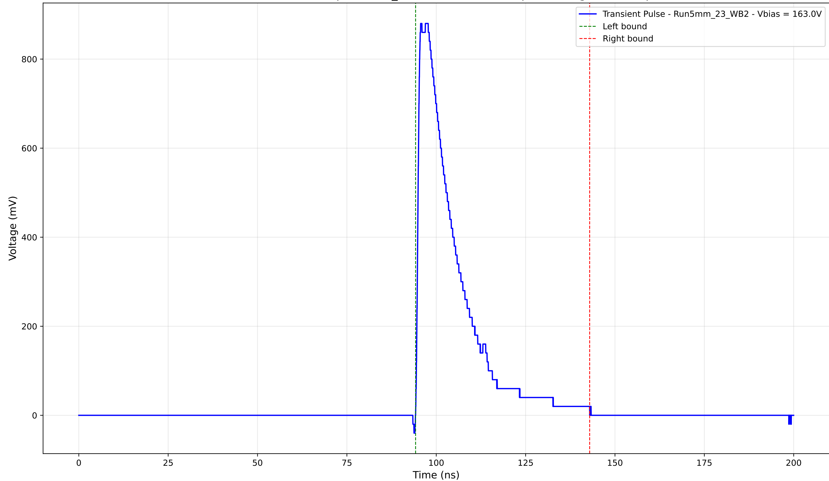
Transient Pulse - Sample: 5mm_23 - Position: 1685.0 \mu\text{m} - Charge: 206.15 pC
