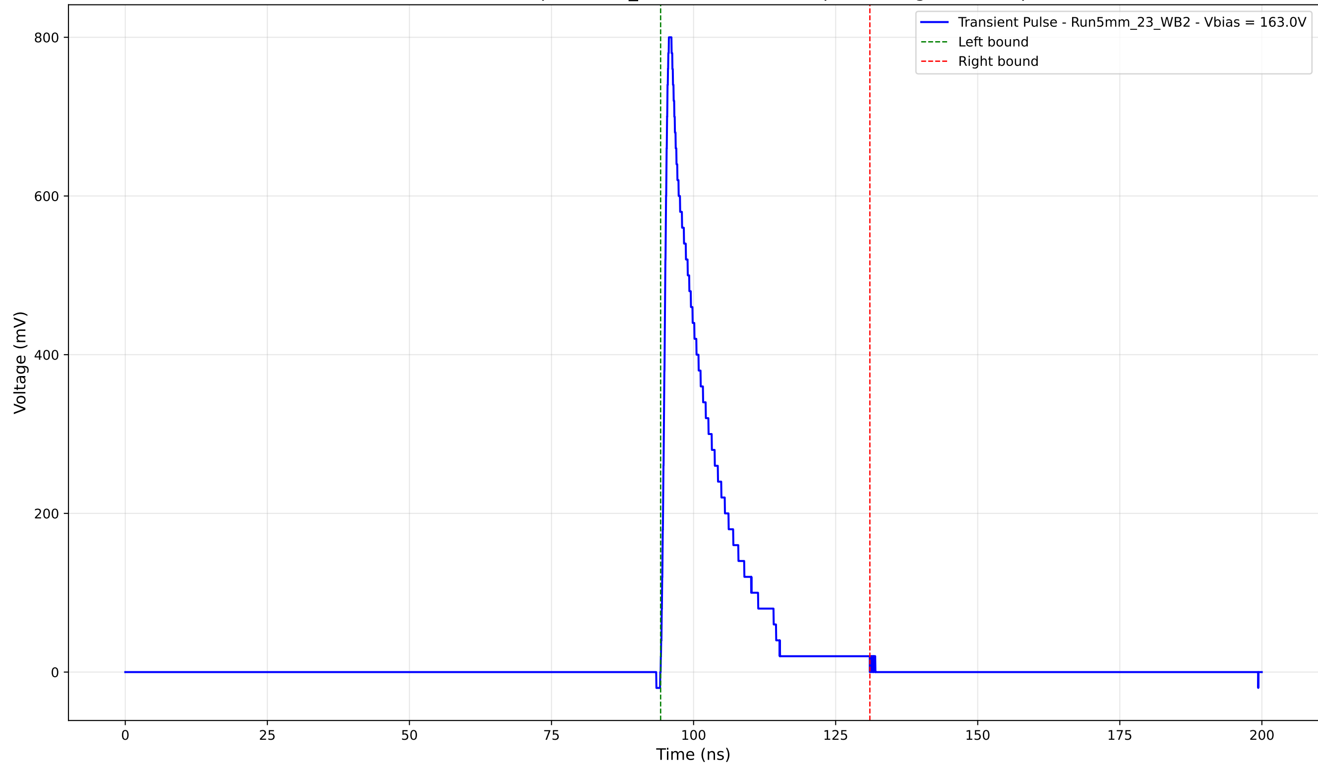
Transient Pulse - Sample: 5mm_23 - Position: 430.0 \mu\text{m} - Charge: 127.05 pC
