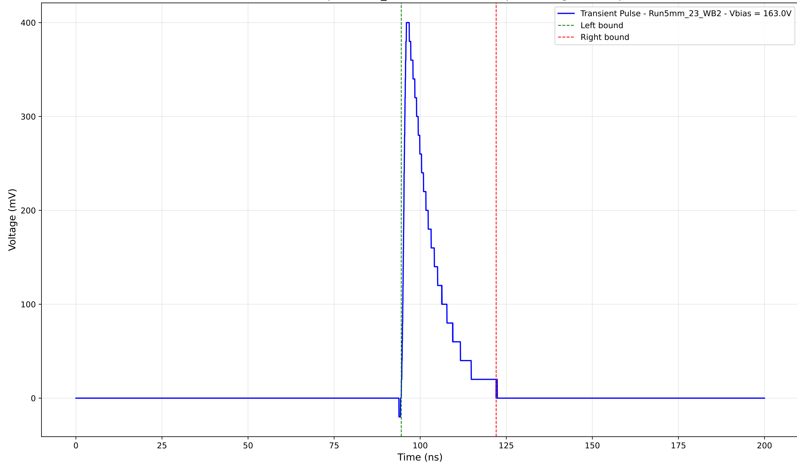
Transient Pulse - Sample: 5mm_23 - Position: 4000.0 \mu\text{m} - Charge: 69.39 pC
