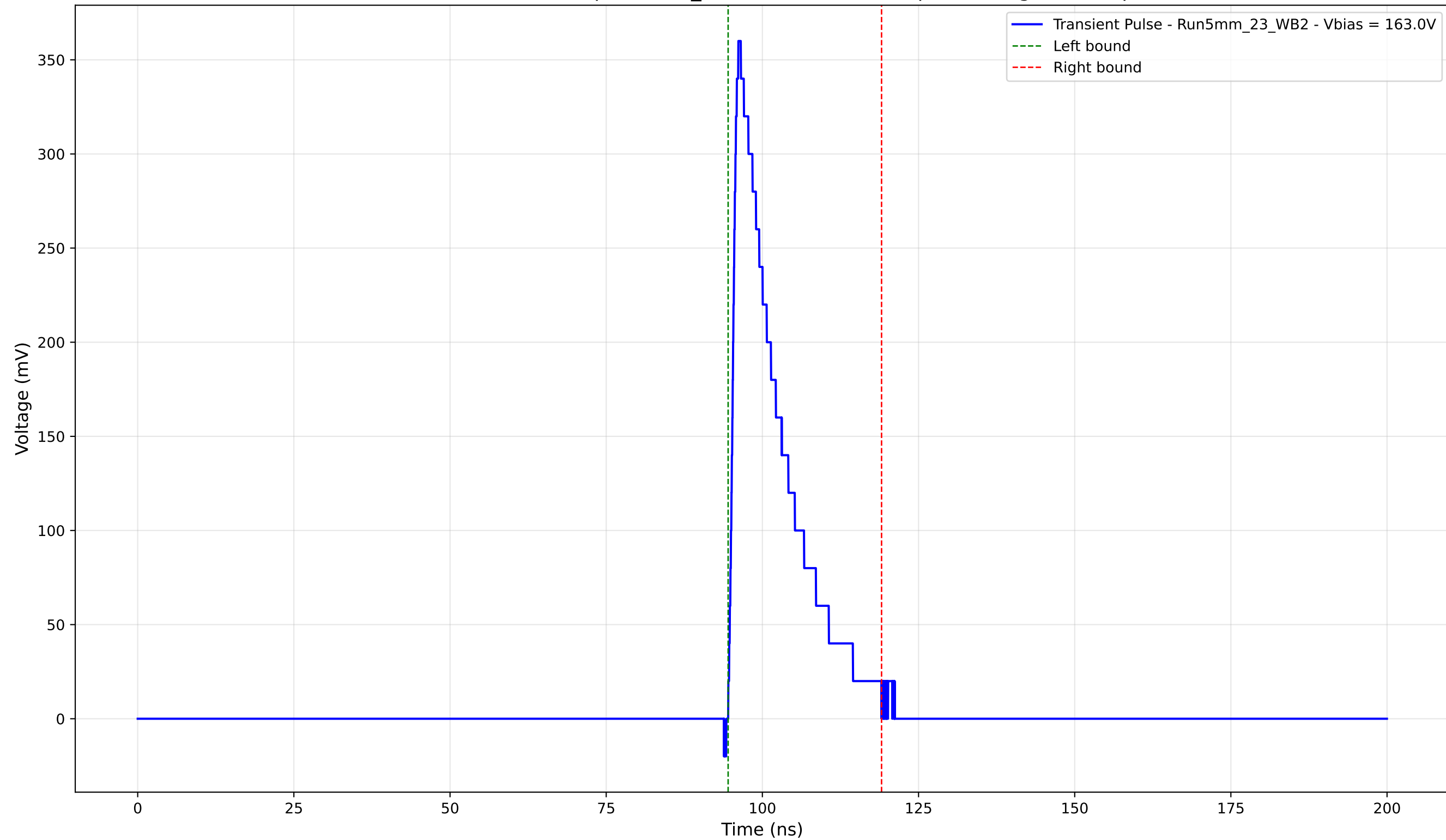
Transient Pulse - Sample: 5mm_23 - Position: 4005.0 \mu\text{m} - Charge: 59.77 pC
