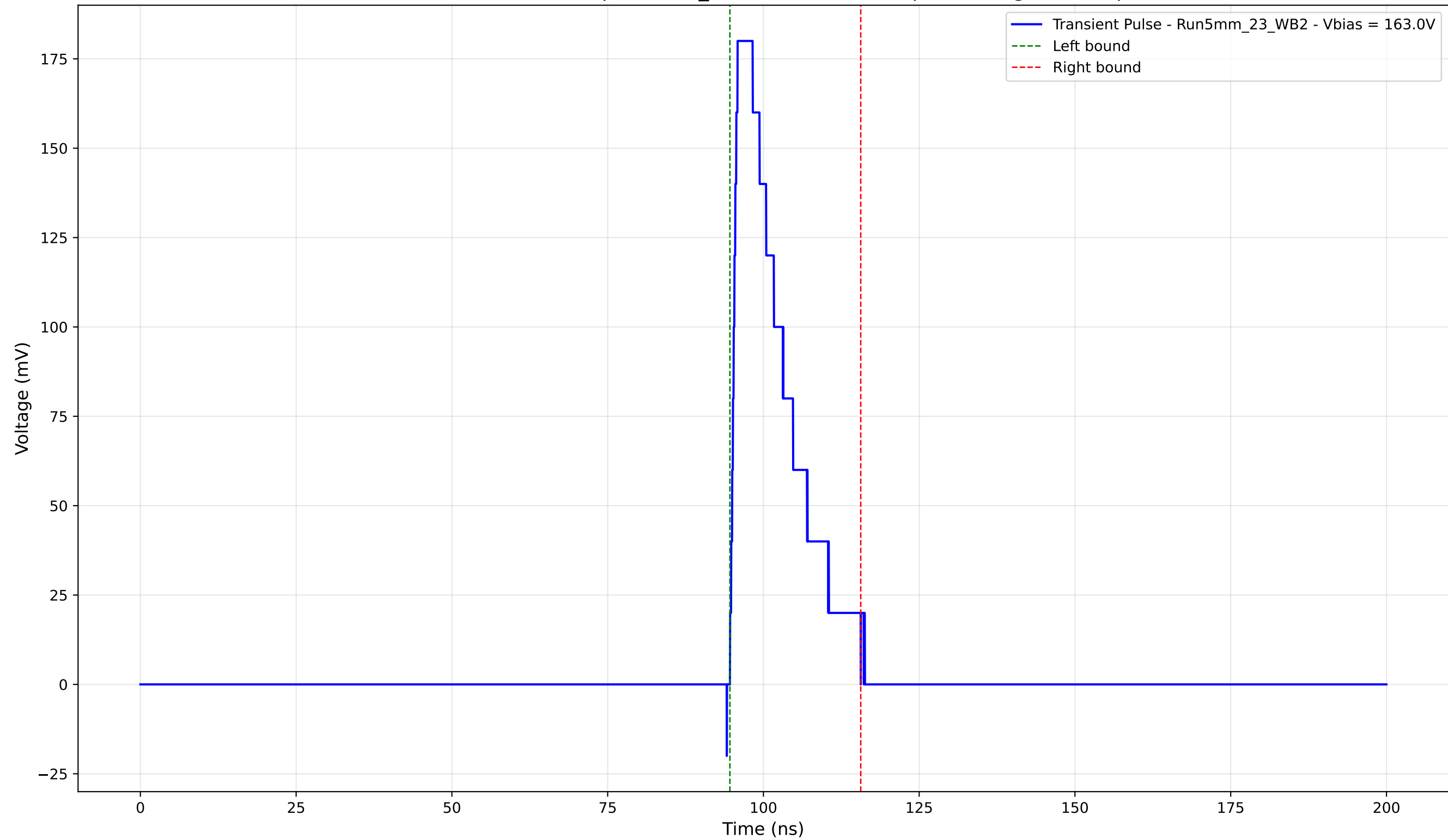
Transient Pulse - Sample: 5mm_23 - Position: 985.0 \mu\text{m} - Charge: 33.50 pC
