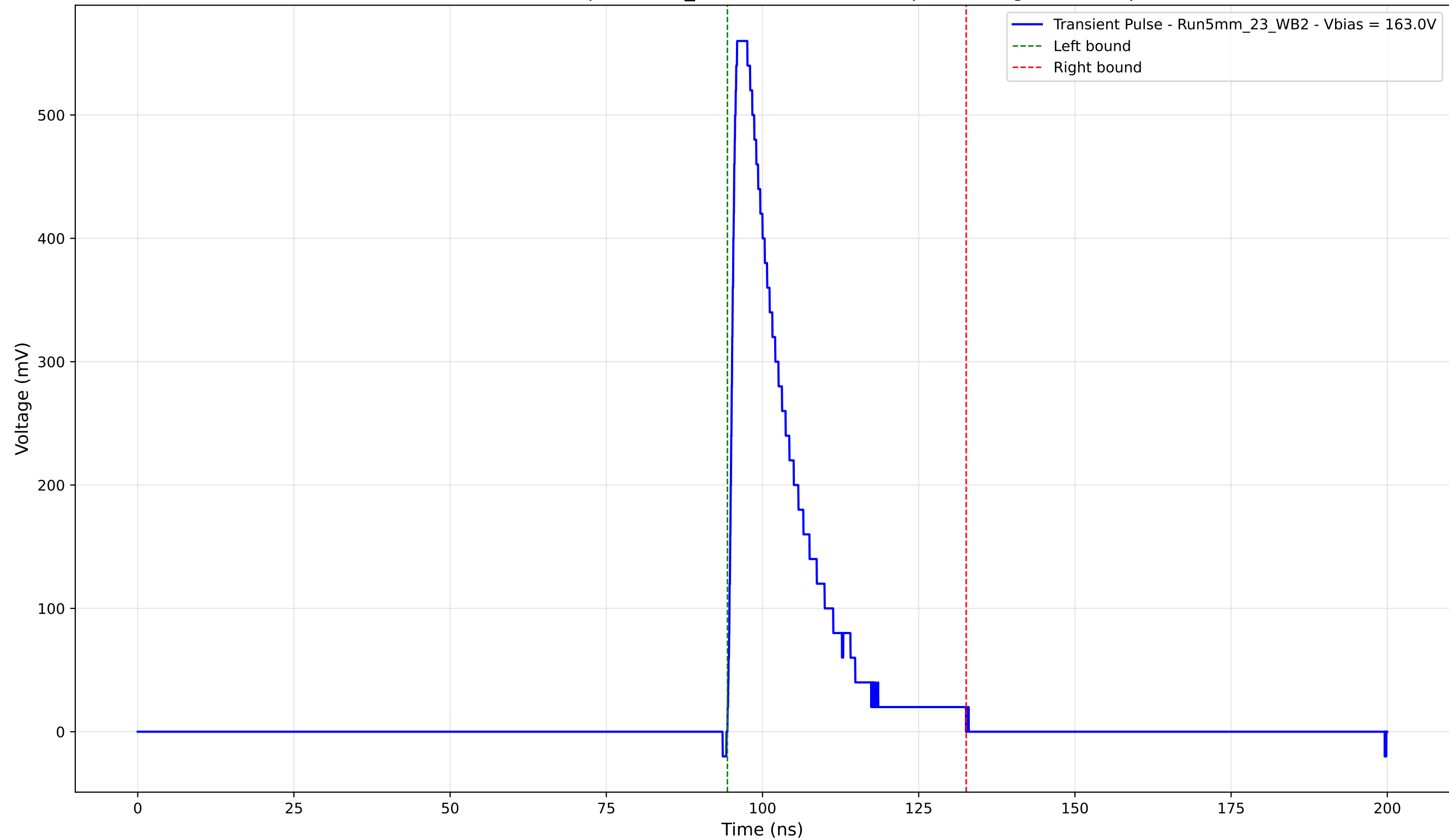
Transient Pulse - Sample: 5mm_23 - Position: 3580.0 \mu\text{m} - Charge: 112.31 pC
