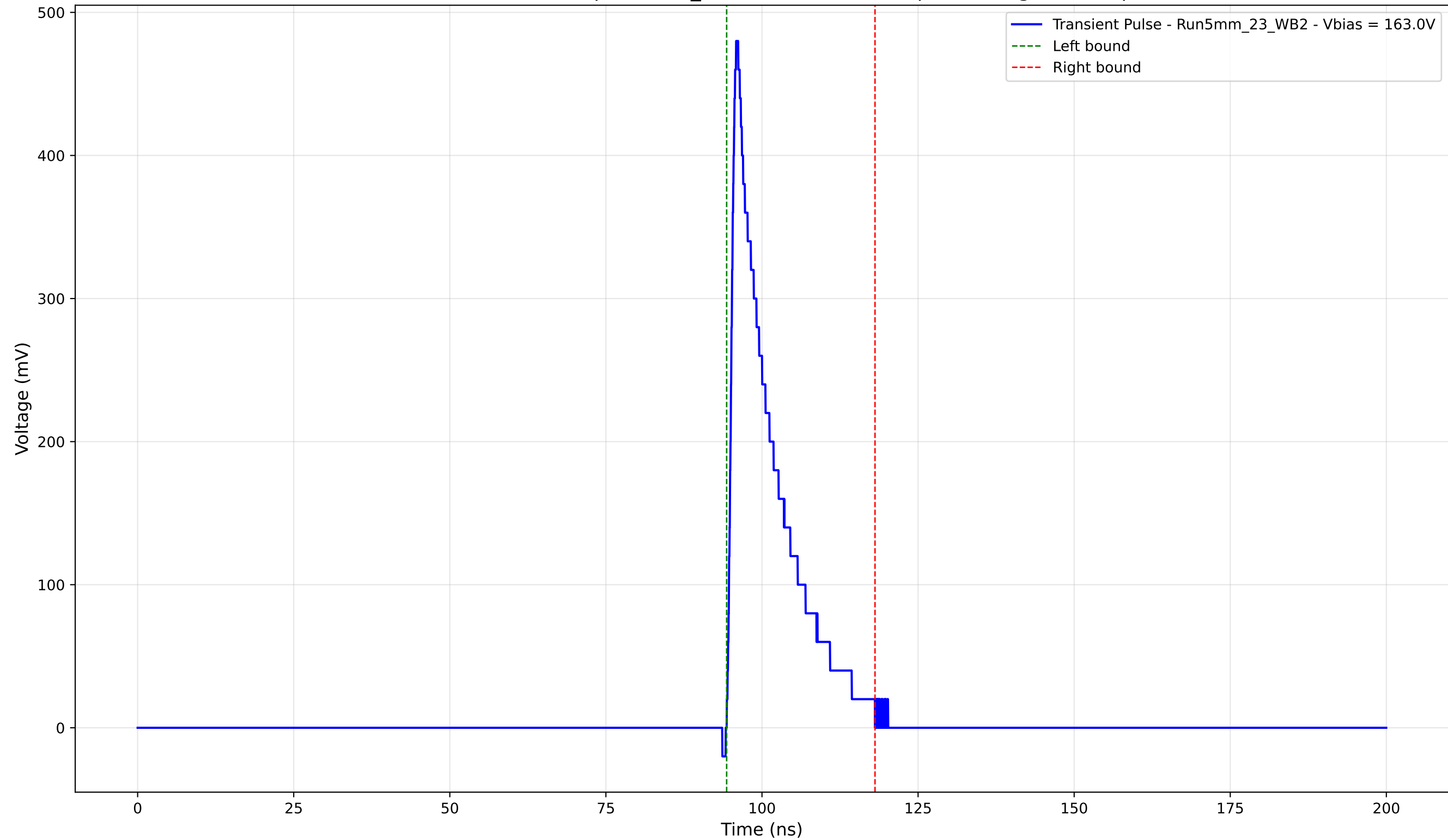
Transient Pulse - Sample: 5mm_23 - Position: 4500.0 \mu\text{m} - Charge: 68.46 pC
