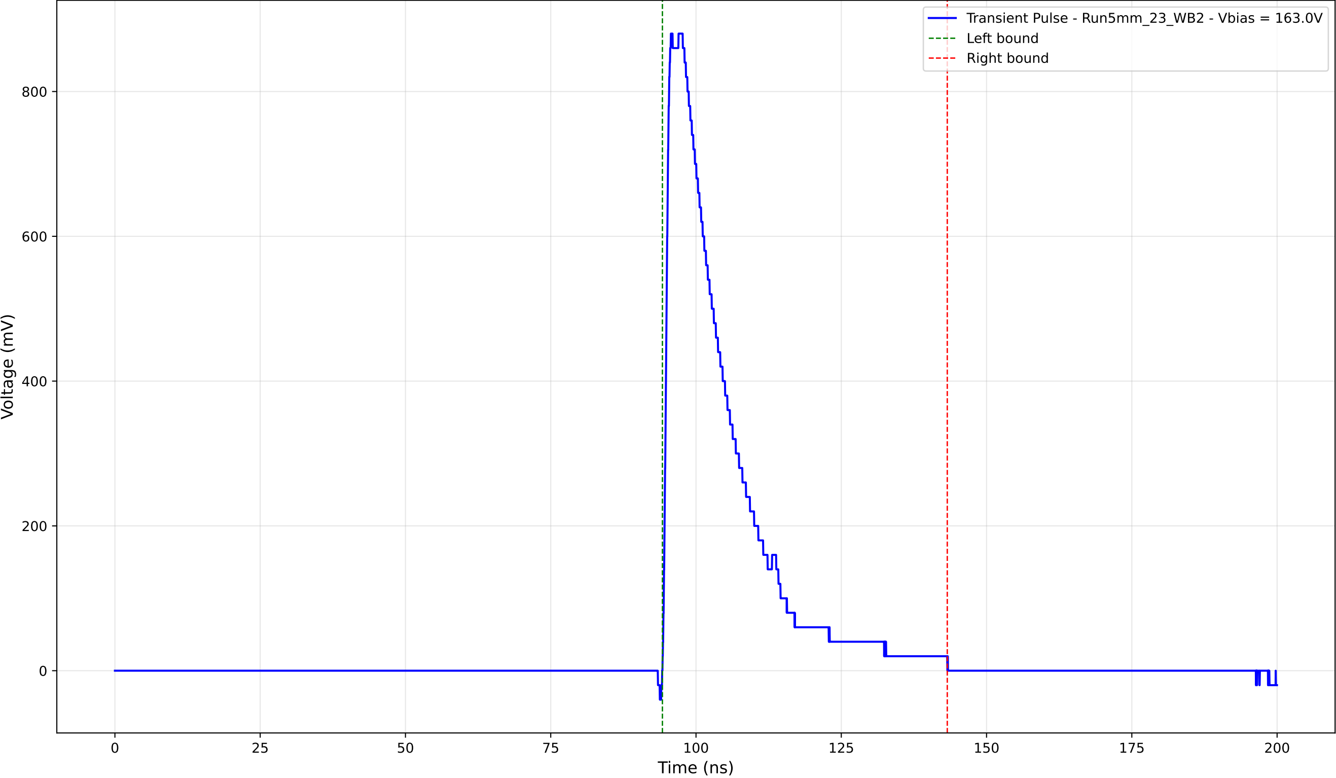
Transient Pulse - Sample: 5mm_23 - Position: 1675.0 \mu\text{m} - Charge: 205.26 pC
