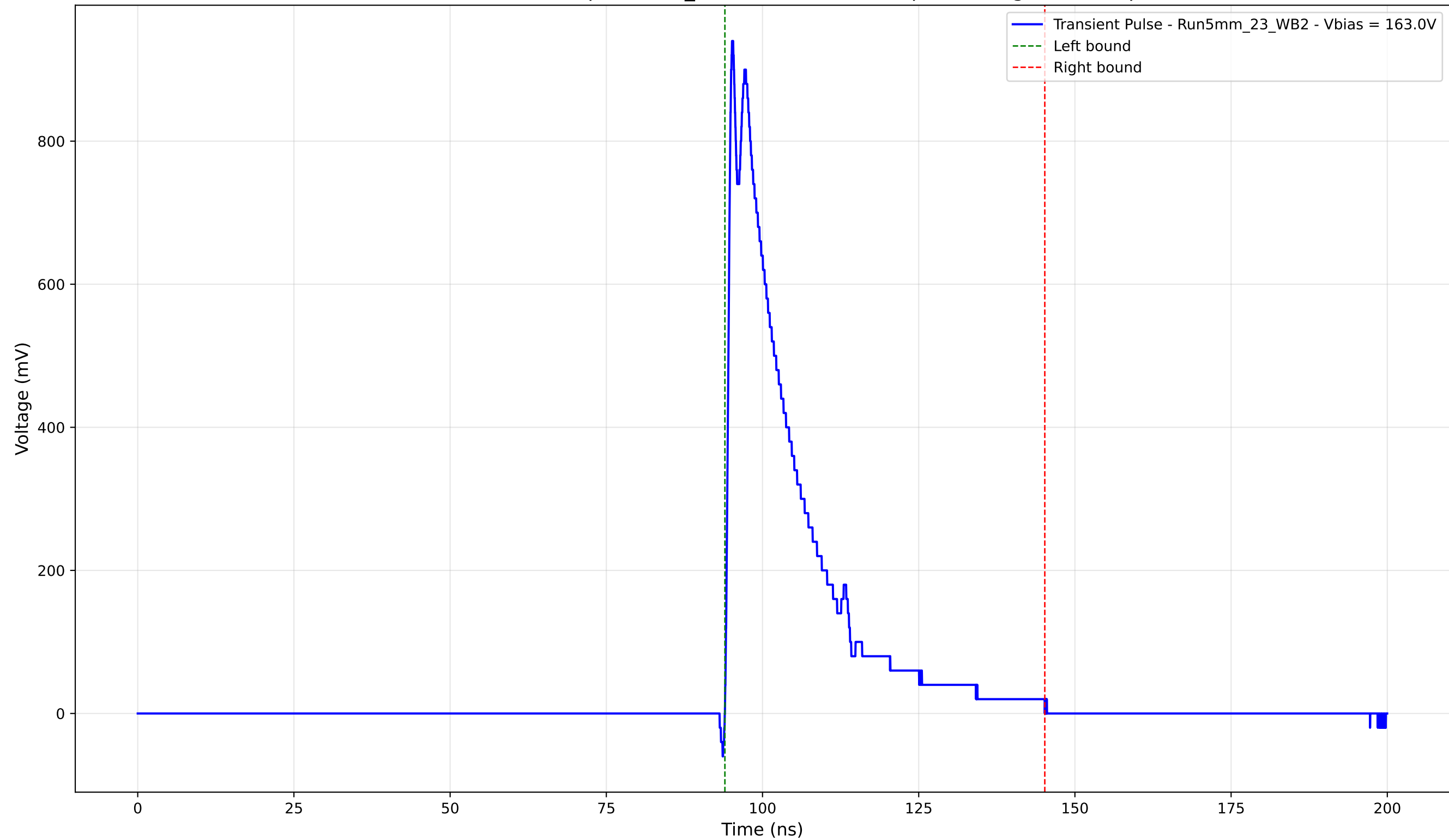
Transient Pulse - Sample: 5mm_23 - Position: 2135.0 \mu\text{m} - Charge: 204.13 pC
