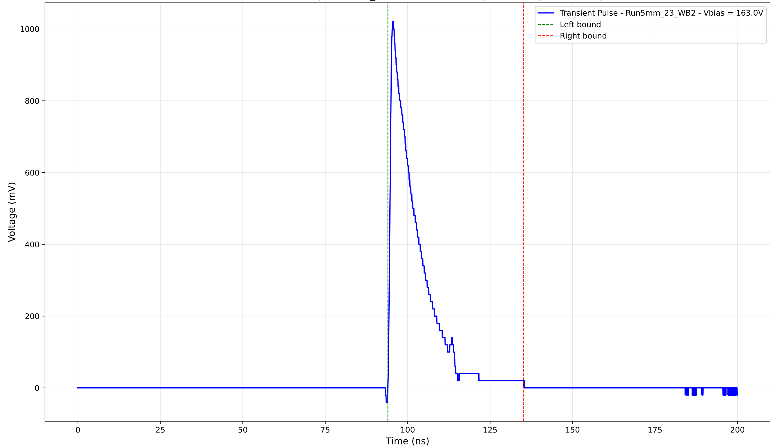
Transient Pulse - Sample: 5mm_23 - Position: 180.0 \mu\text{m} - Charge: 182.05 pC
