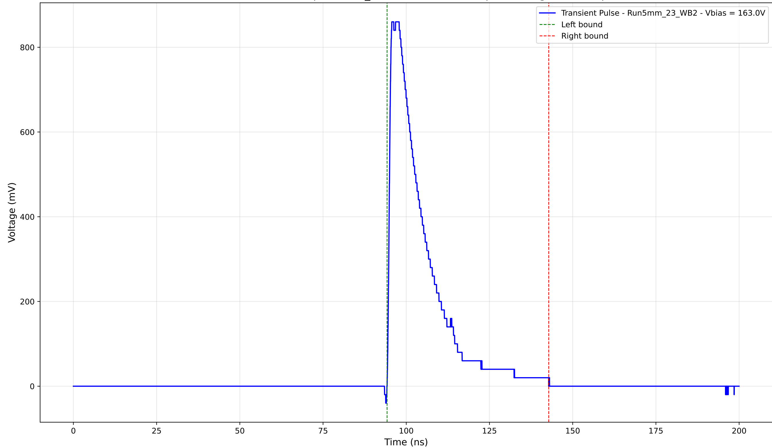
Transient Pulse - Sample: 5mm_23 - Position: 1640.0 \mu\text{m} - Charge: 201.02 pC
