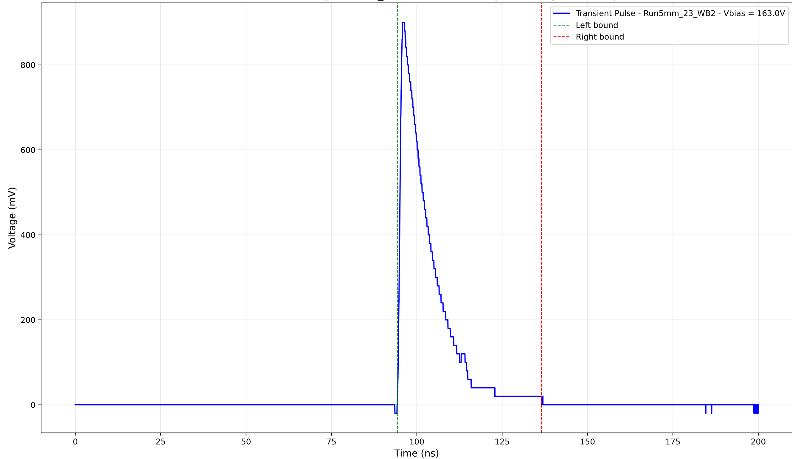
Transient Pulse - Sample: 5mm_23 - Position: 675.0 \mu\text{m} - Charge: 172.82 pC
