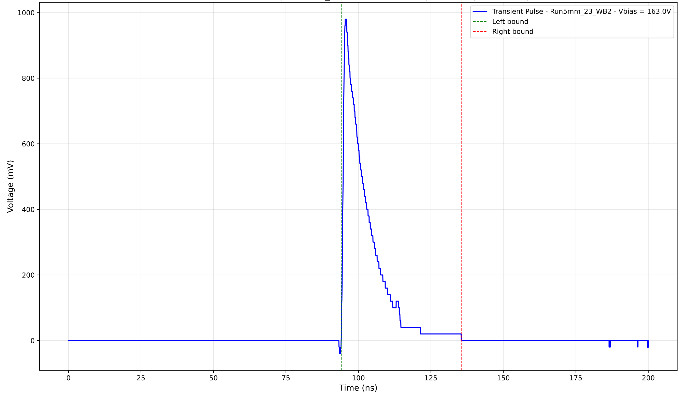
Transient Pulse - Sample: 5mm_23 - Position: 250.0 \mu\text{m} - Charge: 172.32 pC
