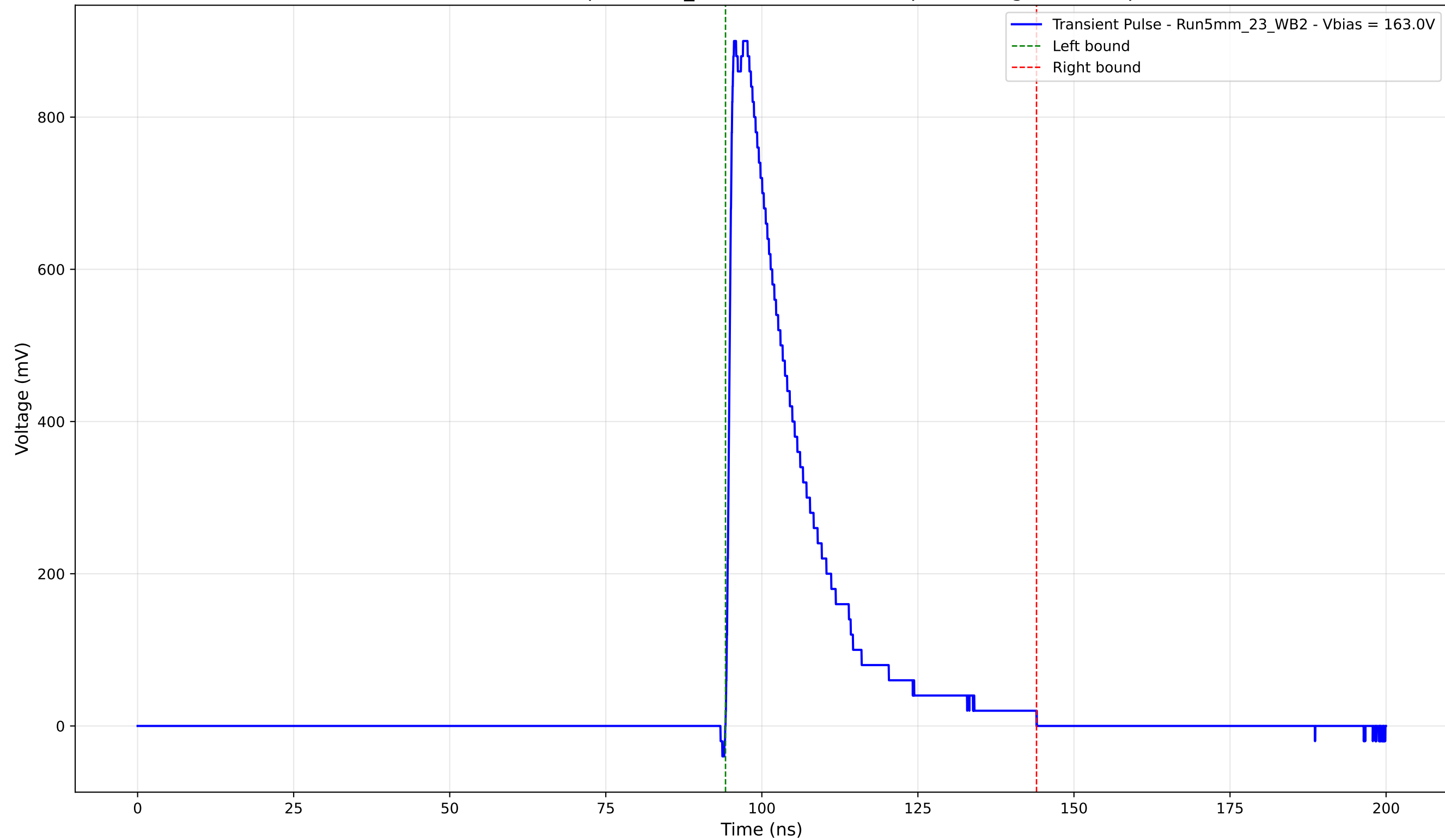
Transient Pulse - Sample: 5mm_23 - Position: 1750.0 \mu\text{m} - Charge: 214.78 pC
