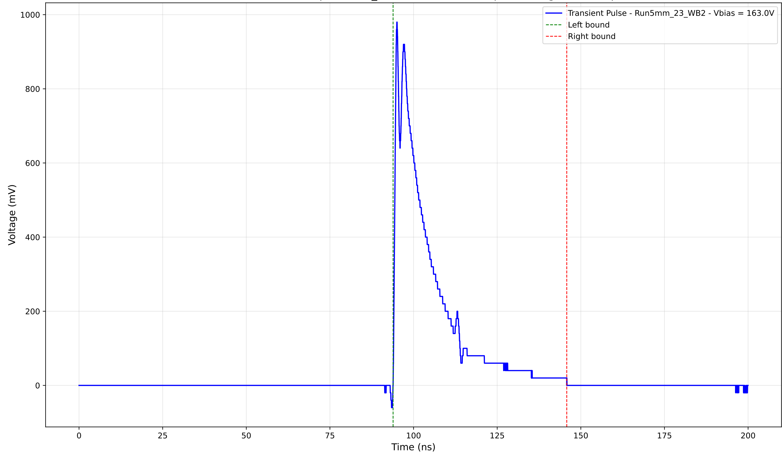
Transient Pulse - Sample: 5mm_23 - Position: 2305.0 \mu\text{m} - Charge: 204.84 pC
