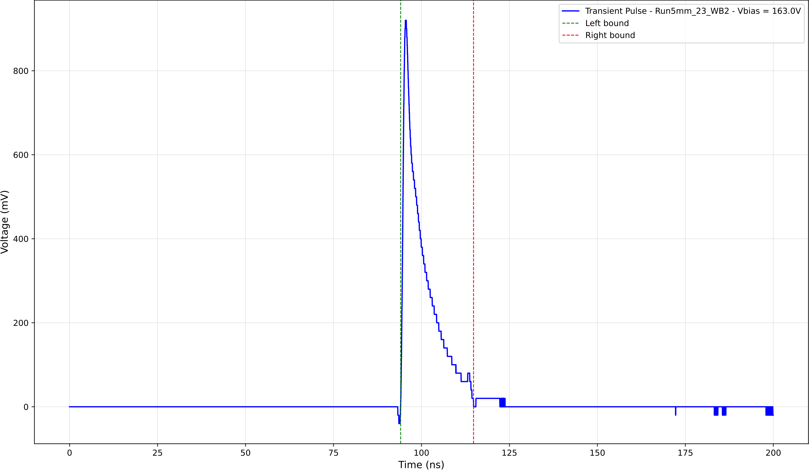
Transient Pulse - Sample: 5mm_23 - Position: 4895.0 \mu\text{m} - Charge: 114.04 pC
