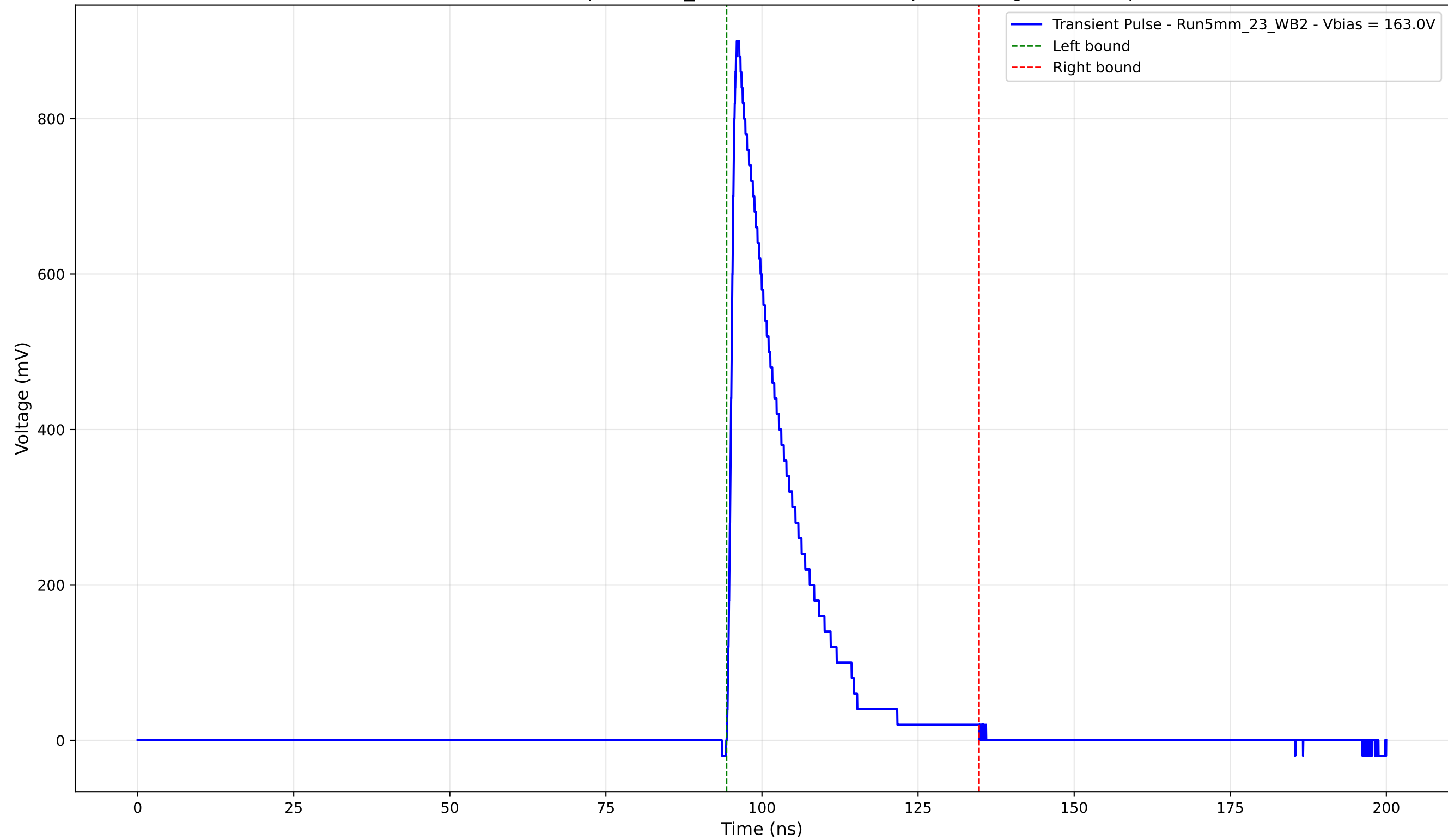
Transient Pulse - Sample: 5mm_23 - Position: 4305.0 \mu\text{m} - Charge: 162.32 pC
