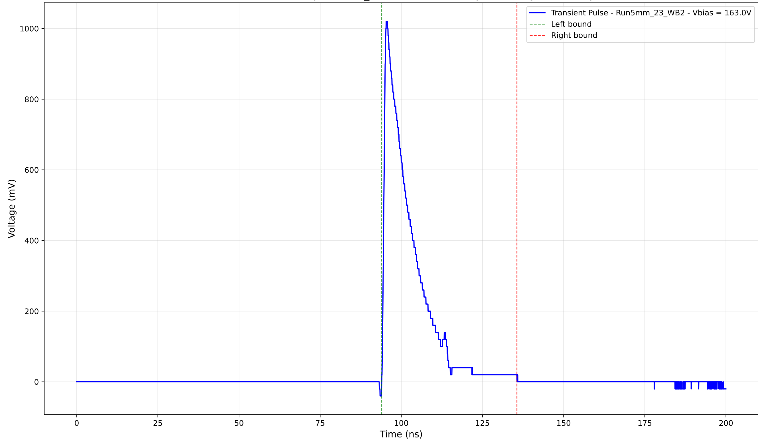
Transient Pulse - Sample: 5mm_23 - Position: 170.0 \mu\text{m} - Charge: 183.85 pC
