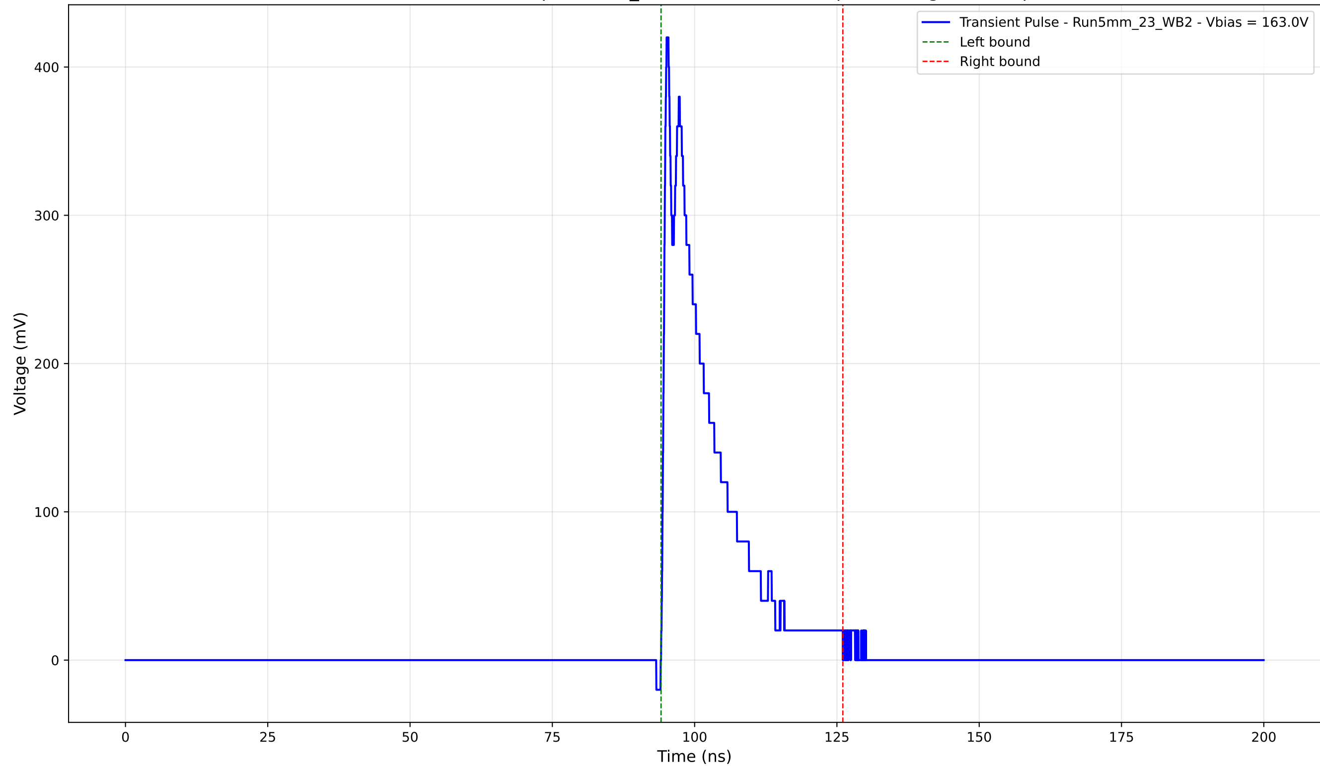
Transient Pulse - Sample: 5mm_23 - Position: 2995.0 \mu\text{m} - Charge: 71.02 pC
