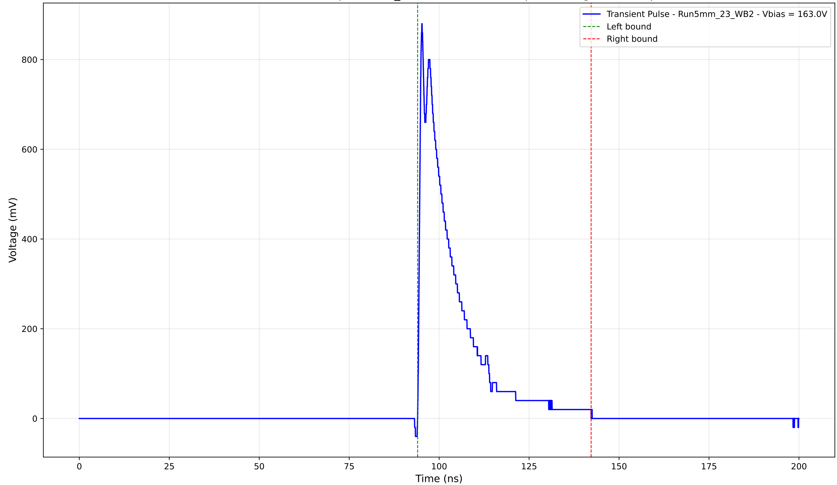
Transient Pulse - Sample: 5mm_23 - Position: 2955.0 \mu\text{m} - Charge: 172.52 pC
