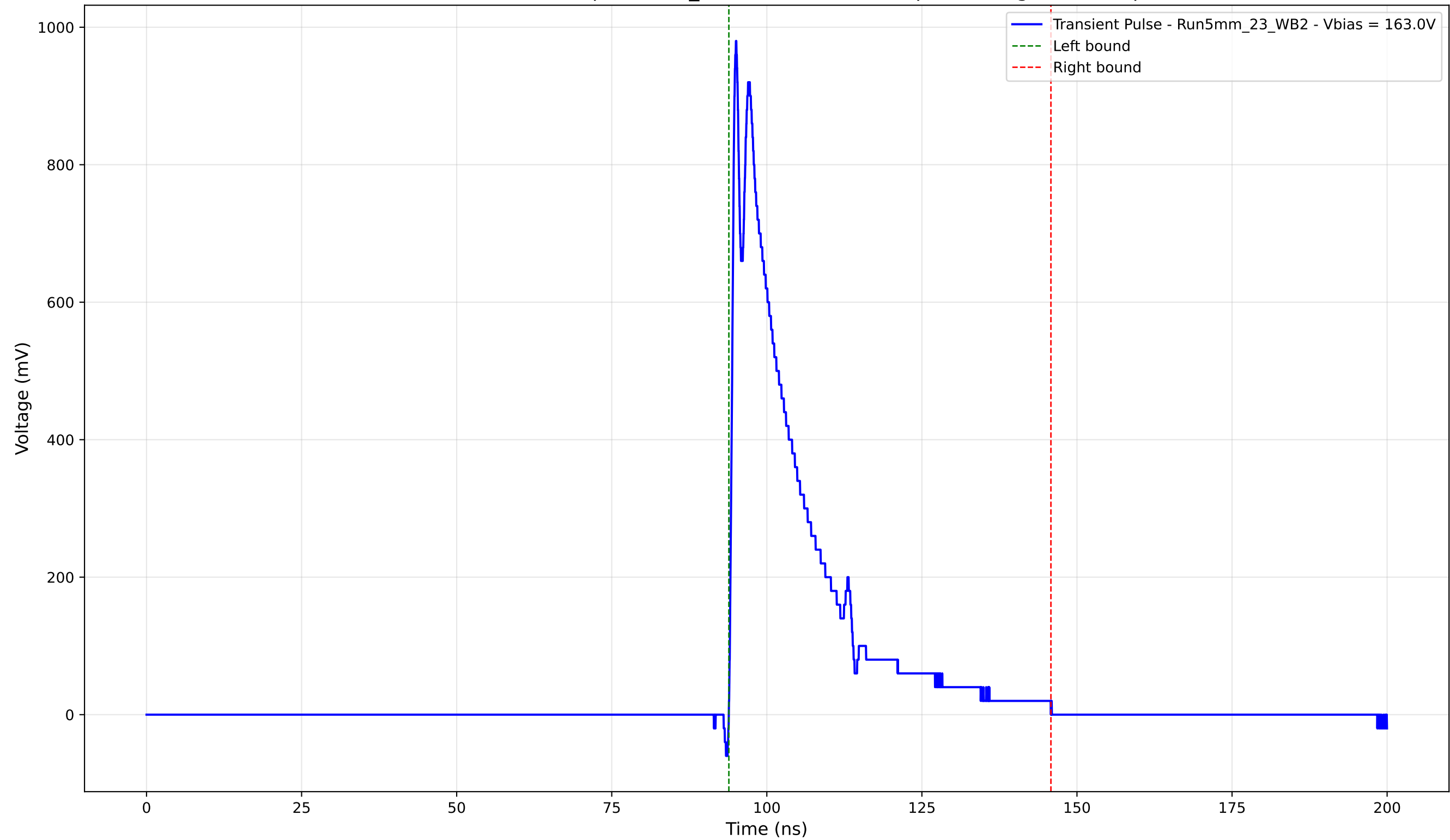
Transient Pulse - Sample: 5mm_23 - Position: 2300.0 \mu\text{m} - Charge: 204.71 pC
