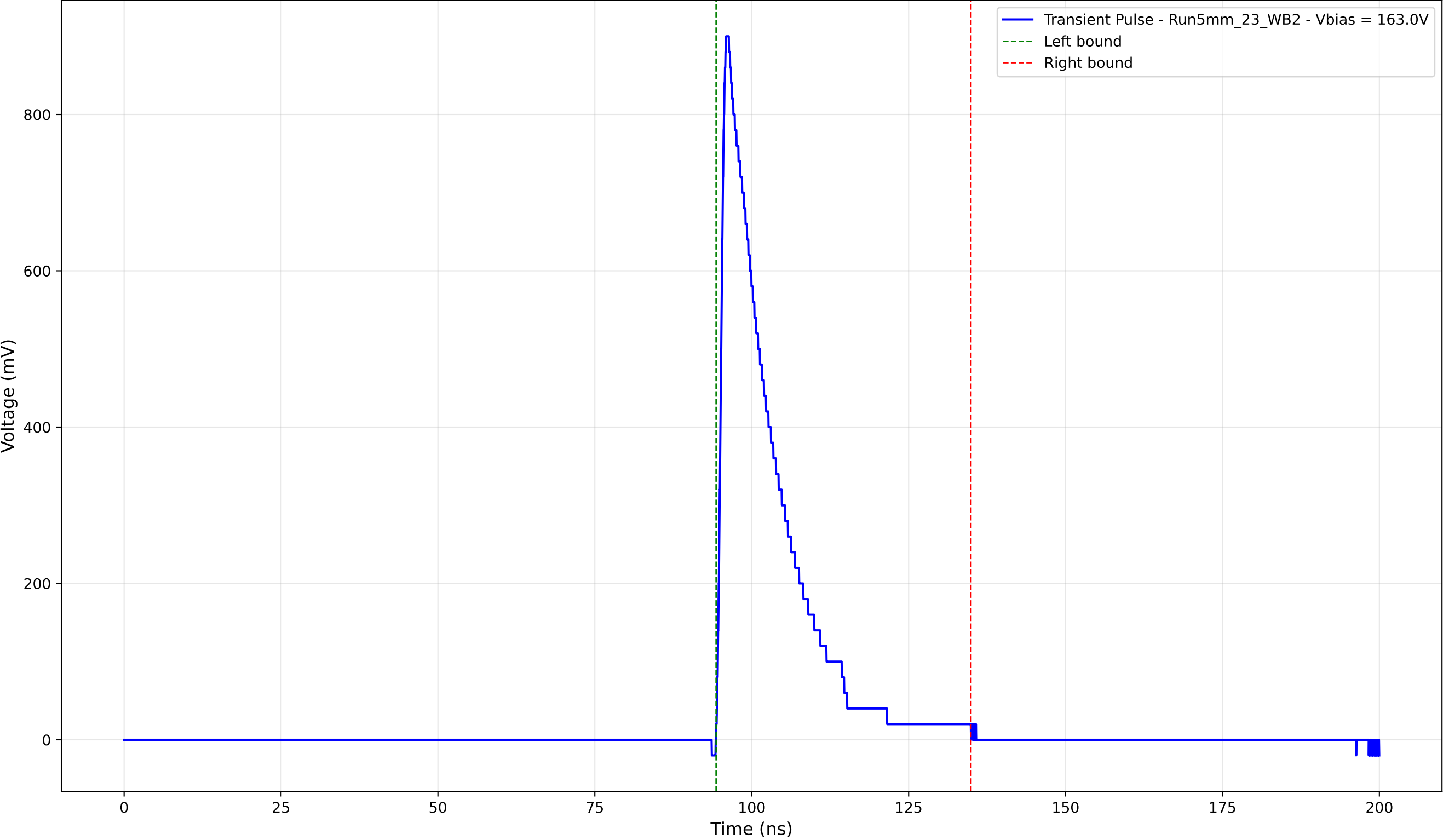
Transient Pulse - Sample: 5mm_23 - Position: 4325.0 \mu\text{m} - Charge: 161.64 pC
