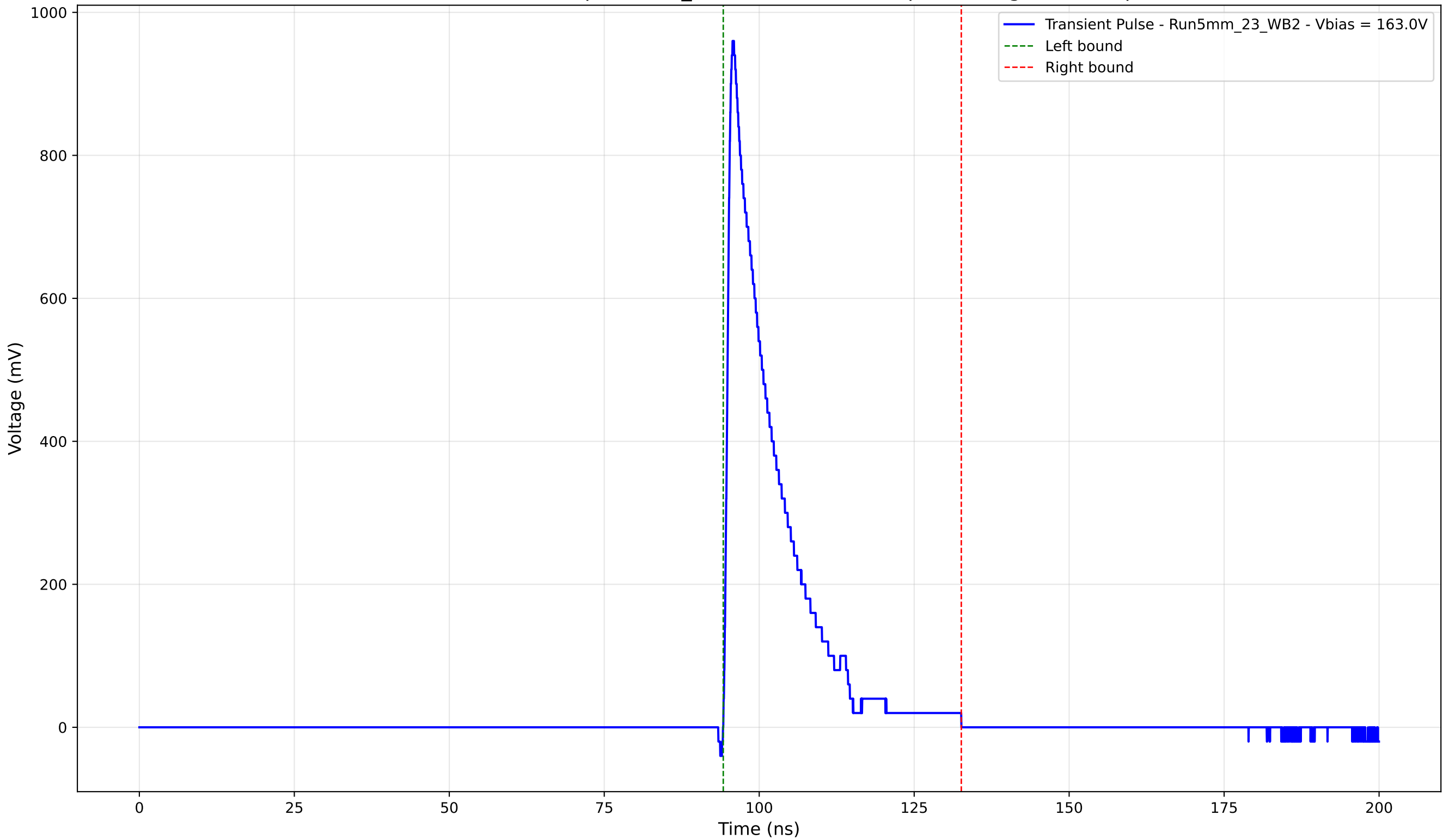
Transient Pulse - Sample: 5mm_23 - Position: 4640.0 \mu\text{m} - Charge: 155.42 pC
