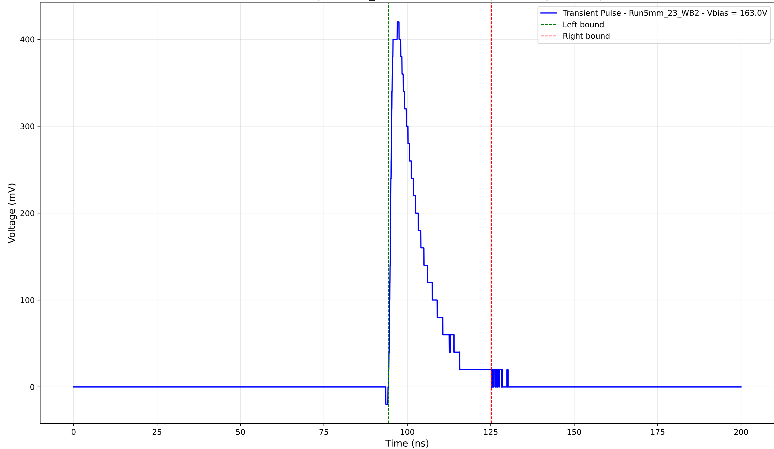
Transient Pulse - Sample: 5mm_23 - Position: 3485.0 \mu\text{m} - Charge: 80.30 pC
