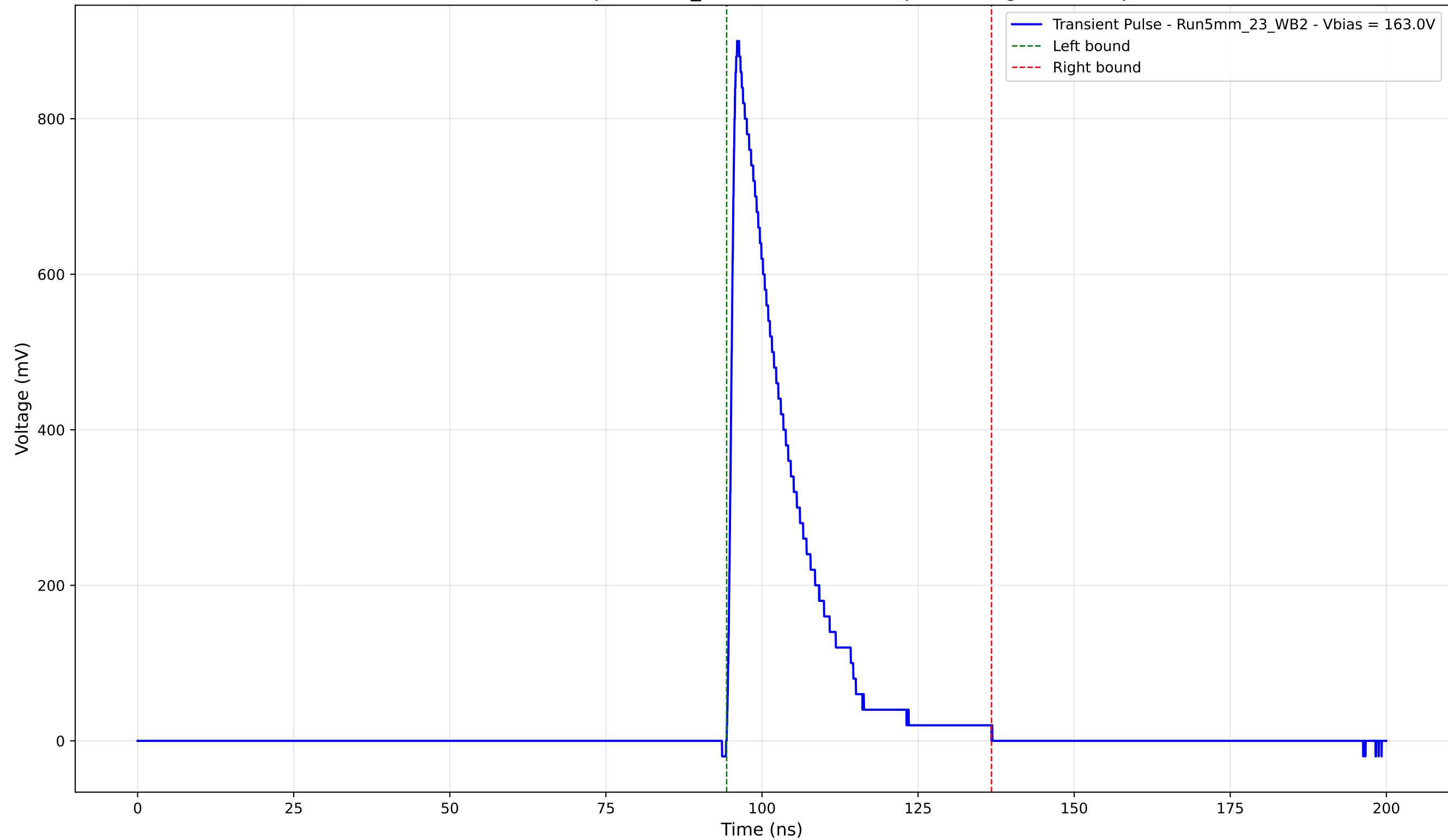
Transient Pulse - Sample: 5mm_23 - Position: 755.0 \mu\text{m} - Charge: 173.28 pC
