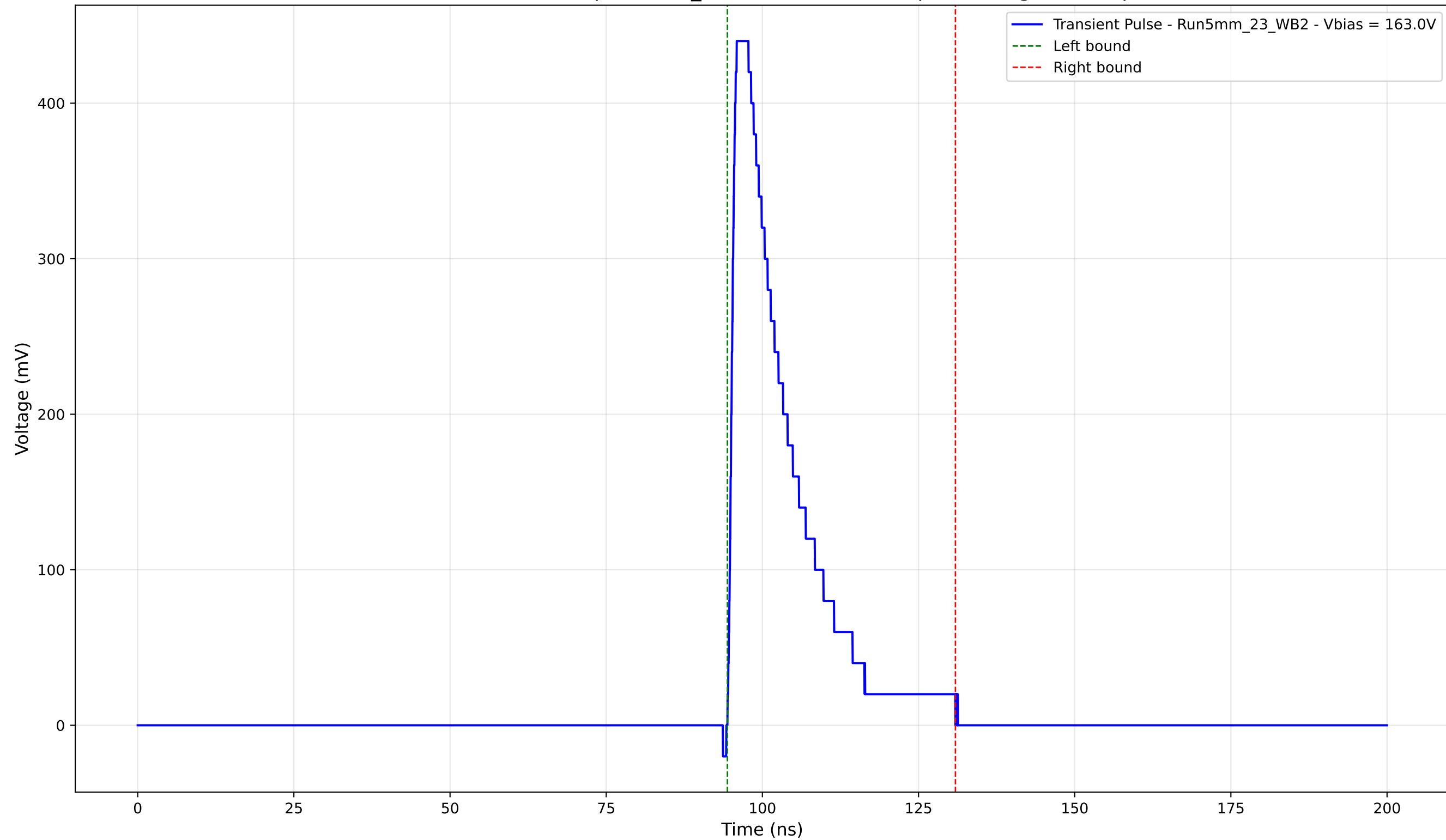
Transient Pulse - Sample: 5mm_23 - Position: 1460.0 \mu\text{m} - Charge: 89.54 pC
