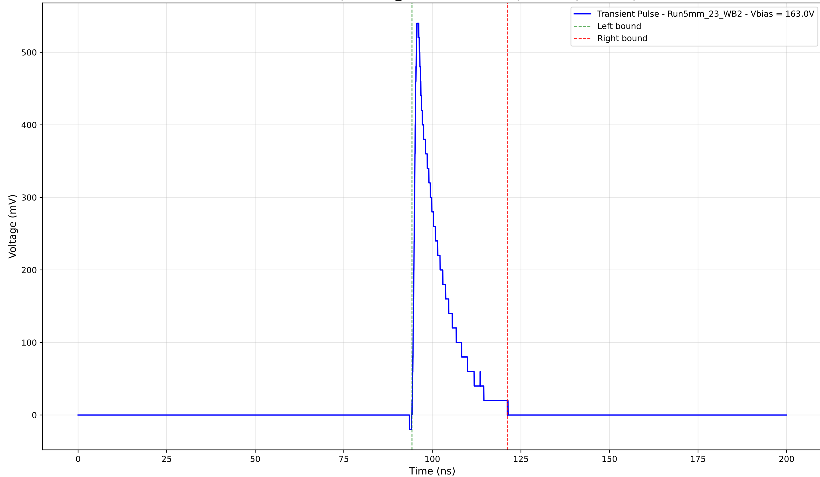
Transient Pulse - Sample: 5mm_23 - Position: 450.0 \mu\text{m} - Charge: 79.95 pC
