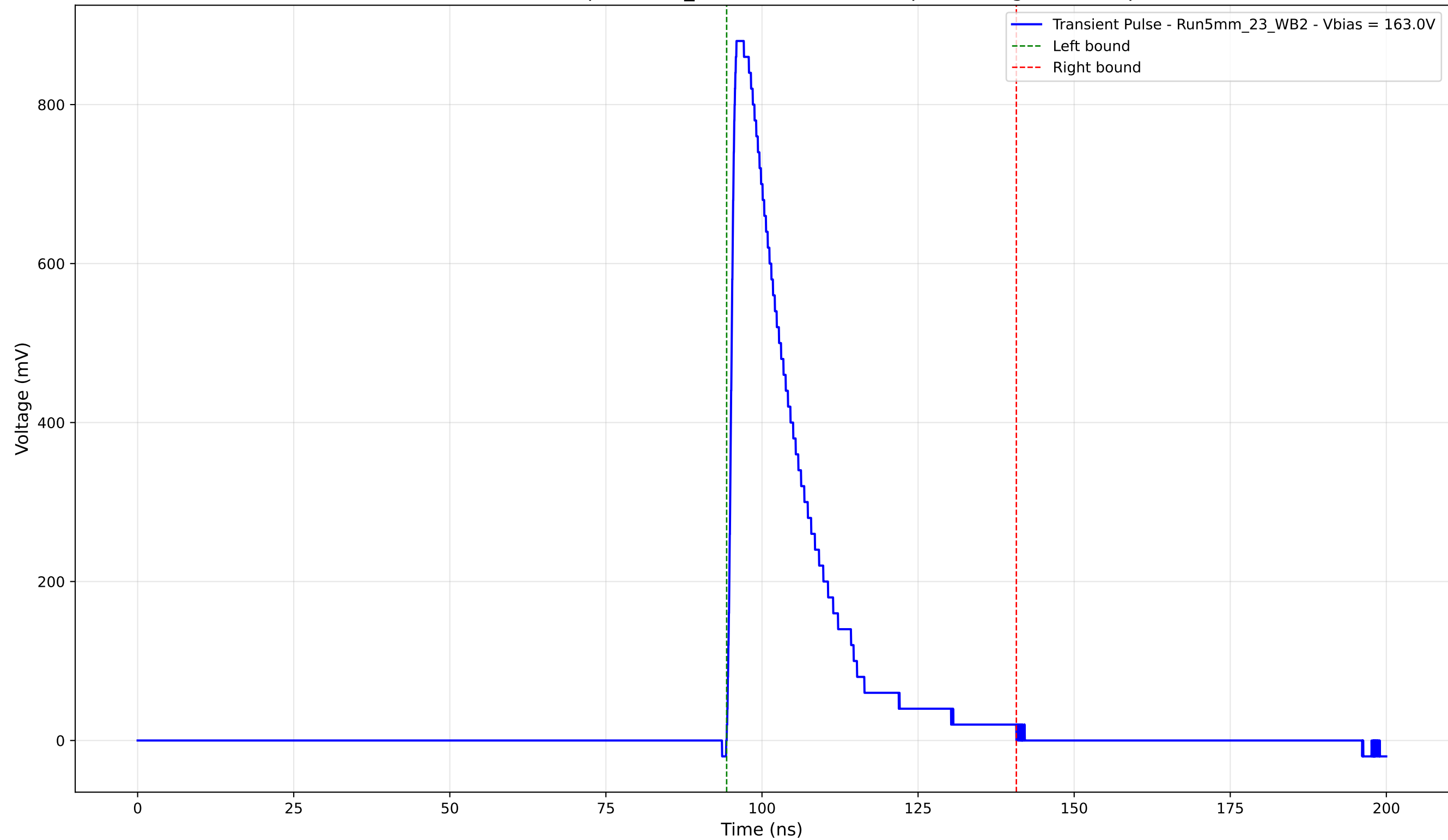
Transient Pulse - Sample: 5mm_23 - Position: 1360.0 \mu\text{m} - Charge: 198.73 pC
