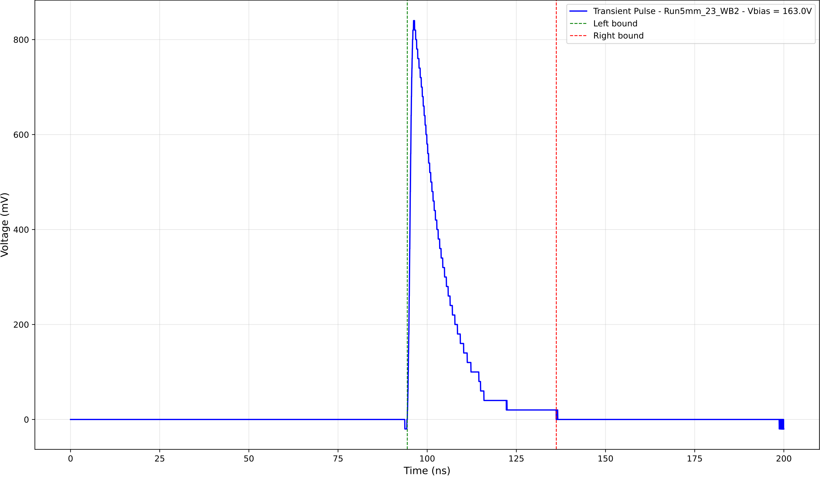
Transient Pulse - Sample: 5mm_23 - Position: 3945.0 \mu\text{m} - Charge: 159.16 pC
