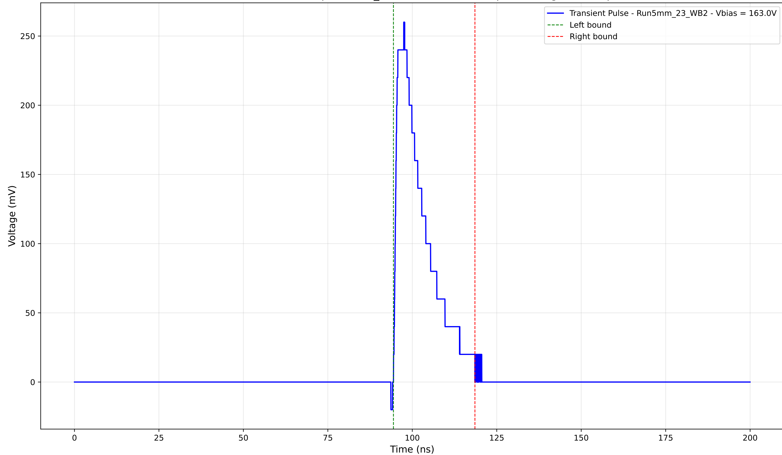
Transient Pulse - Sample: 5mm_23 - Position: 1520.0 \mu\text{m} - Charge: 48.45 pC
