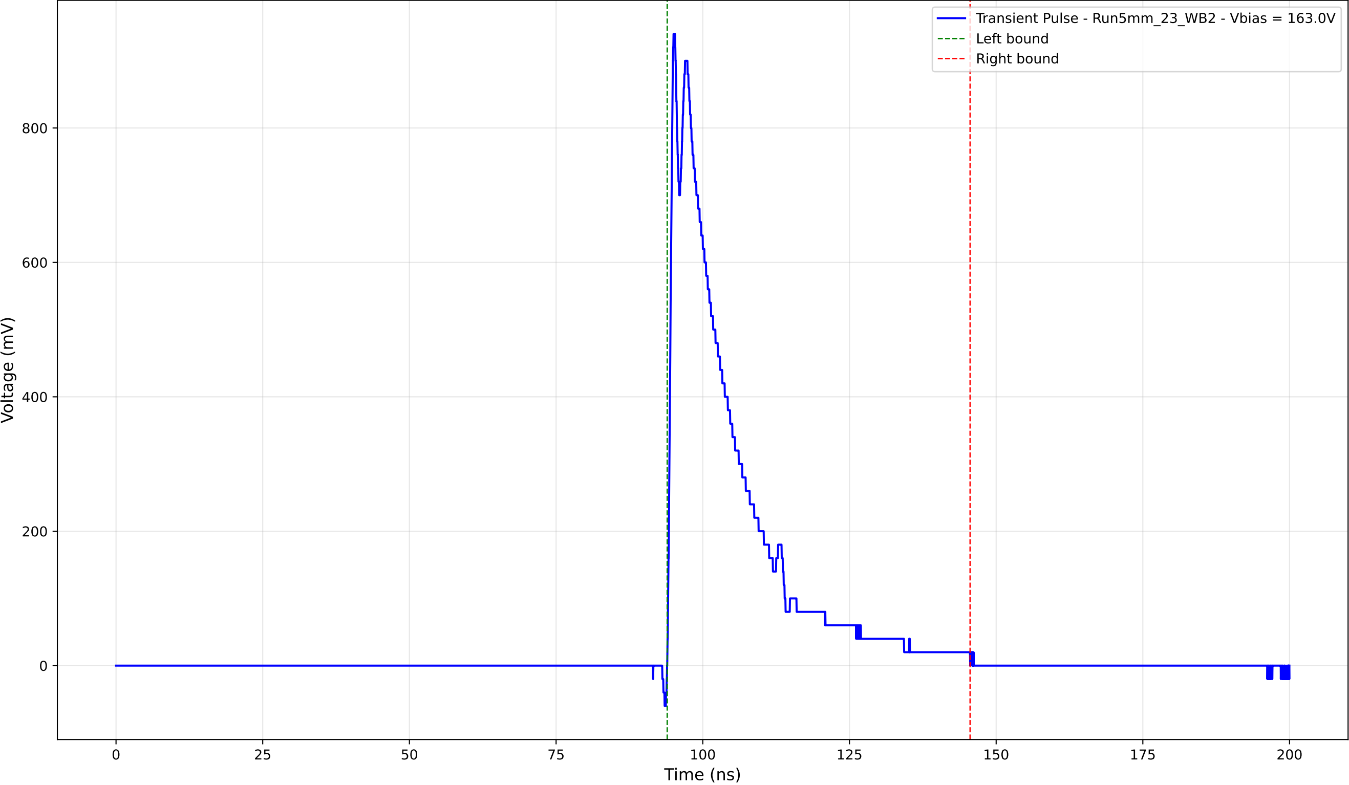
Transient Pulse - Sample: 5mm_23 - Position: 2205.0 \mu\text{m} - Charge: 205.12 pC
