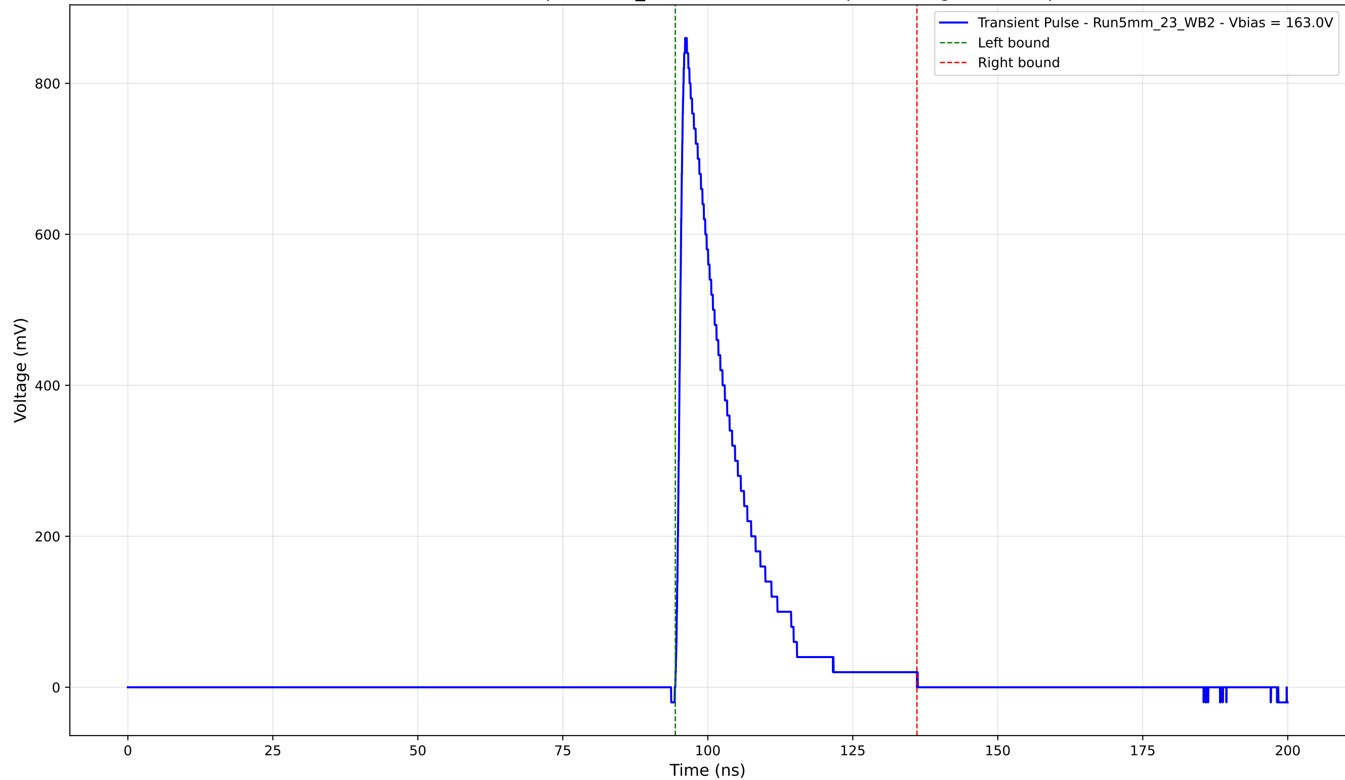
Transient Pulse - Sample: 5mm_23 - Position: 4140.0 \mu\text{m} - Charge: 157.61 pC
