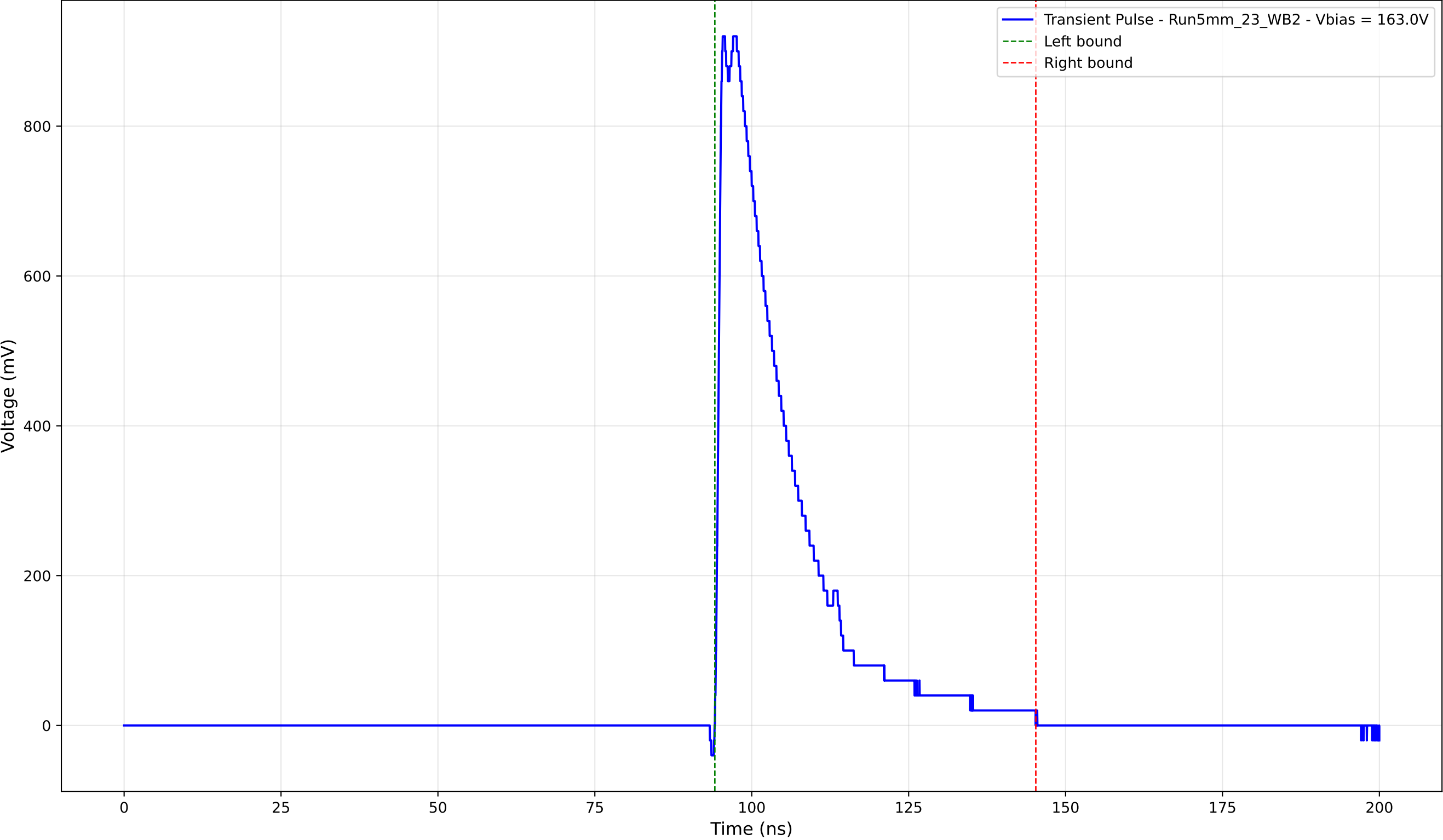
Transient Pulse - Sample: 5mm_23 - Position: 1845.0 \mu\text{m} - Charge: 222.77 pC
