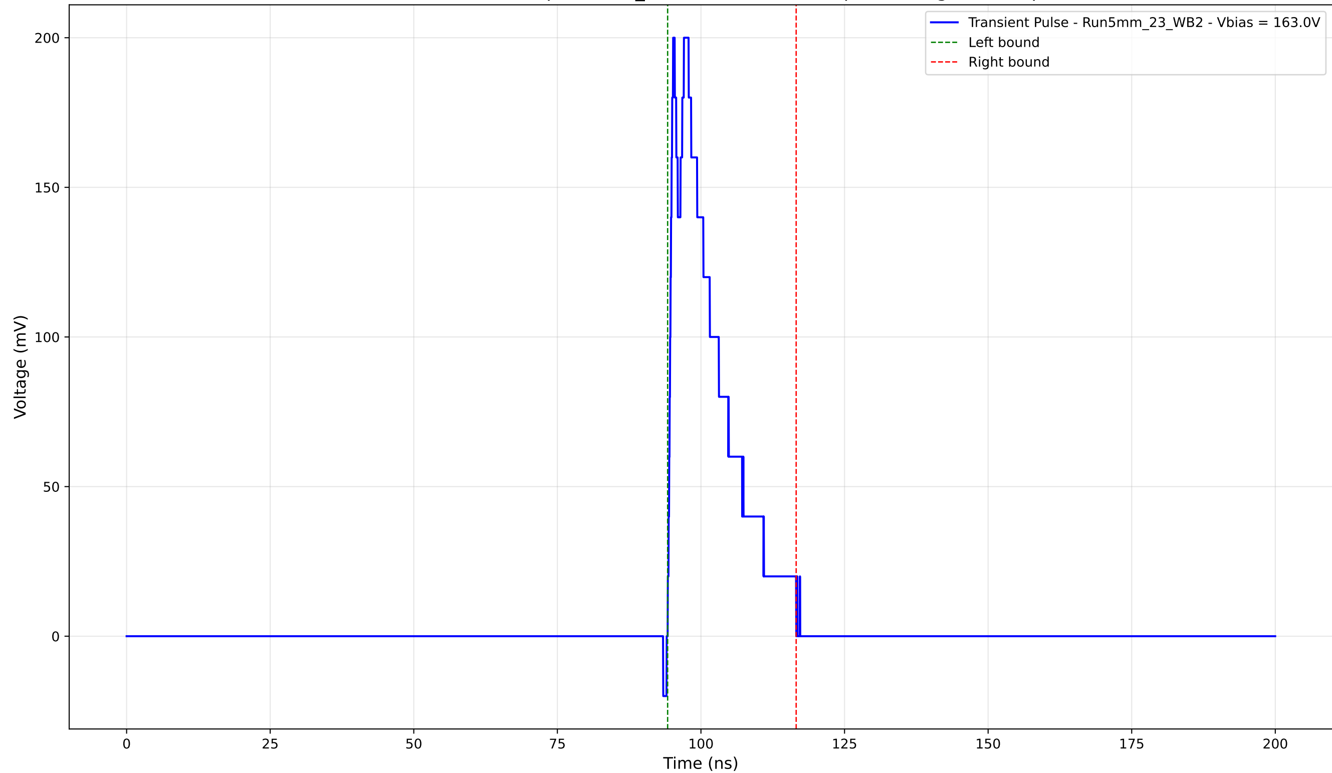
Transient Pulse - Sample: 5mm_23 - Position: 3025.0 \mu\text{m} - Charge: 36.19 pC
