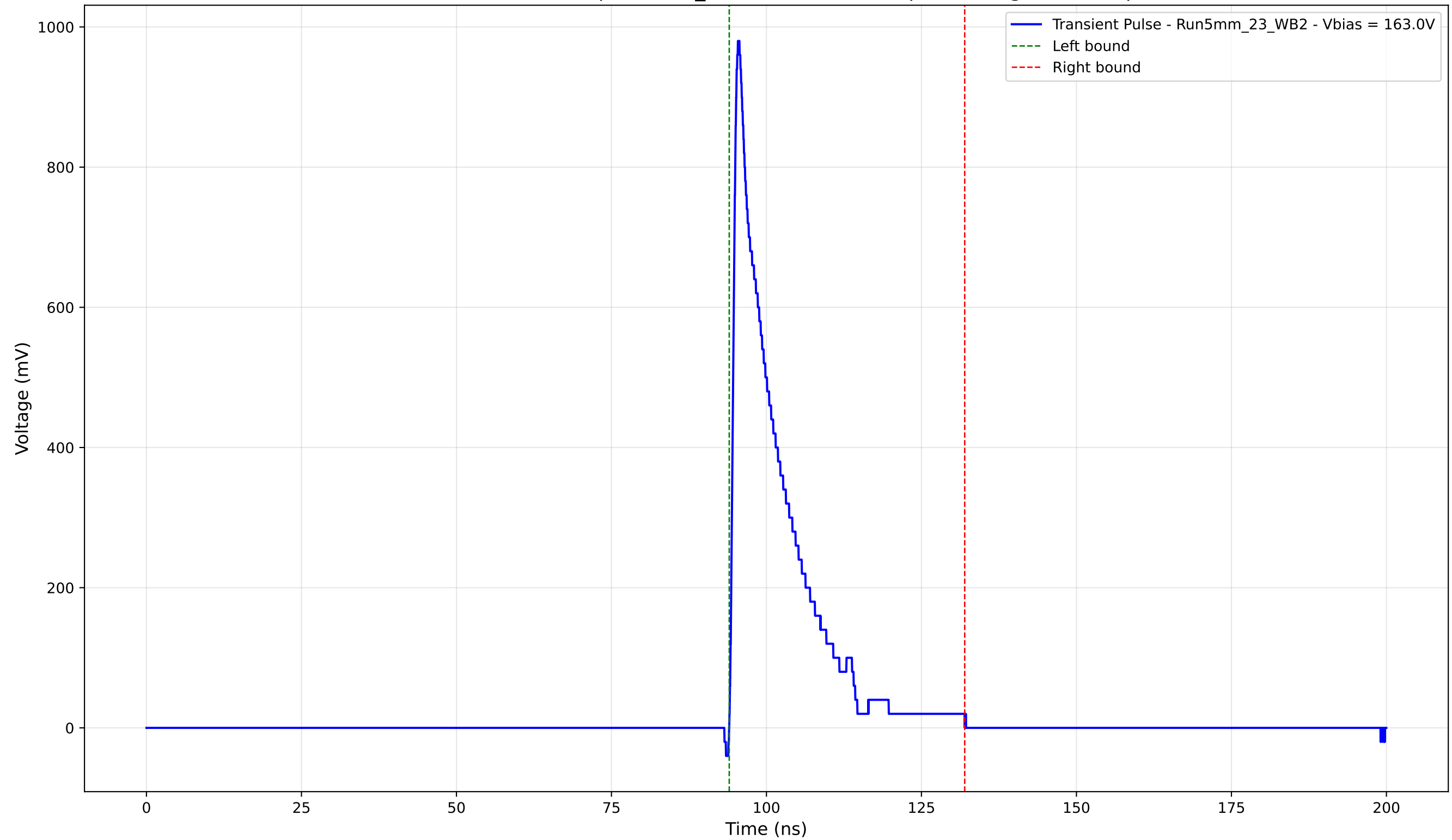
Transient Pulse - Sample: 5mm_23 - Position: 110.0 \mu\text{m} - Charge: 150.46 pC
