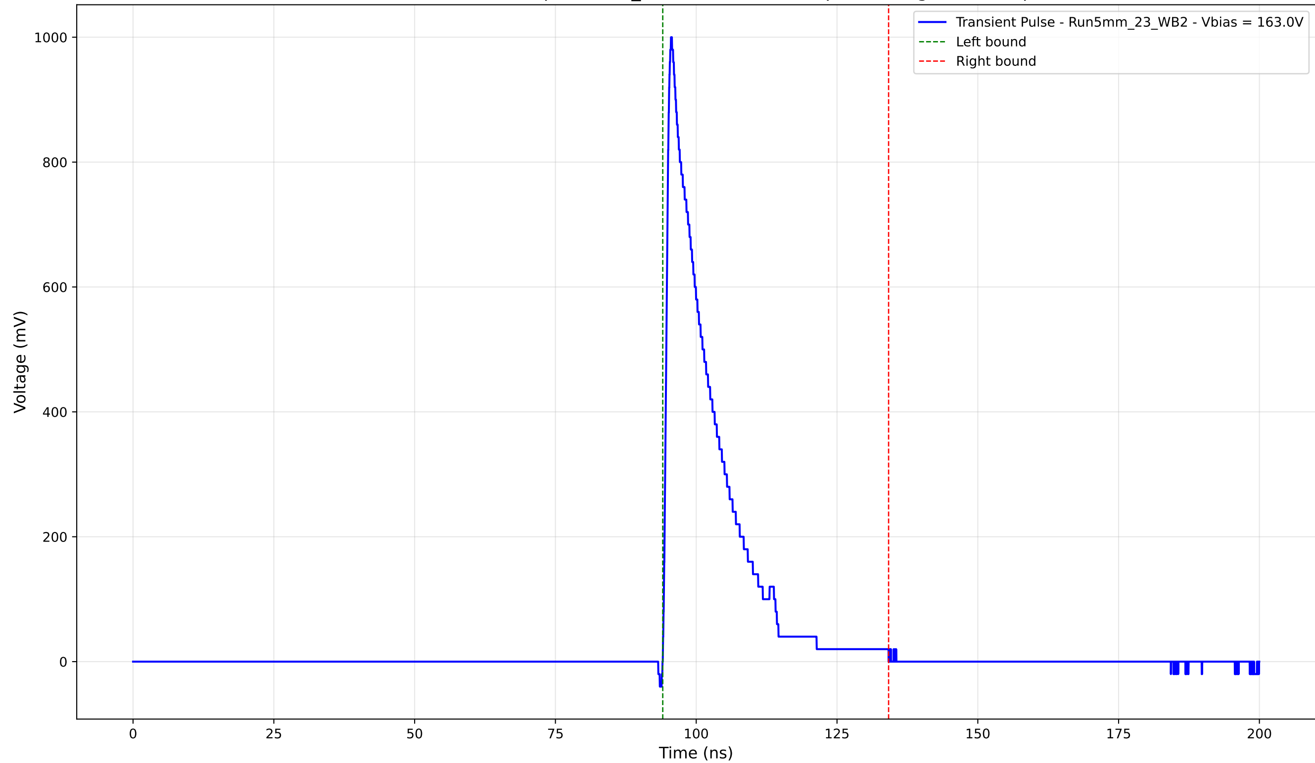
Transient Pulse - Sample: 5mm_23 - Position: 230.0 \mu\text{m} - Charge: 172.22 pC
