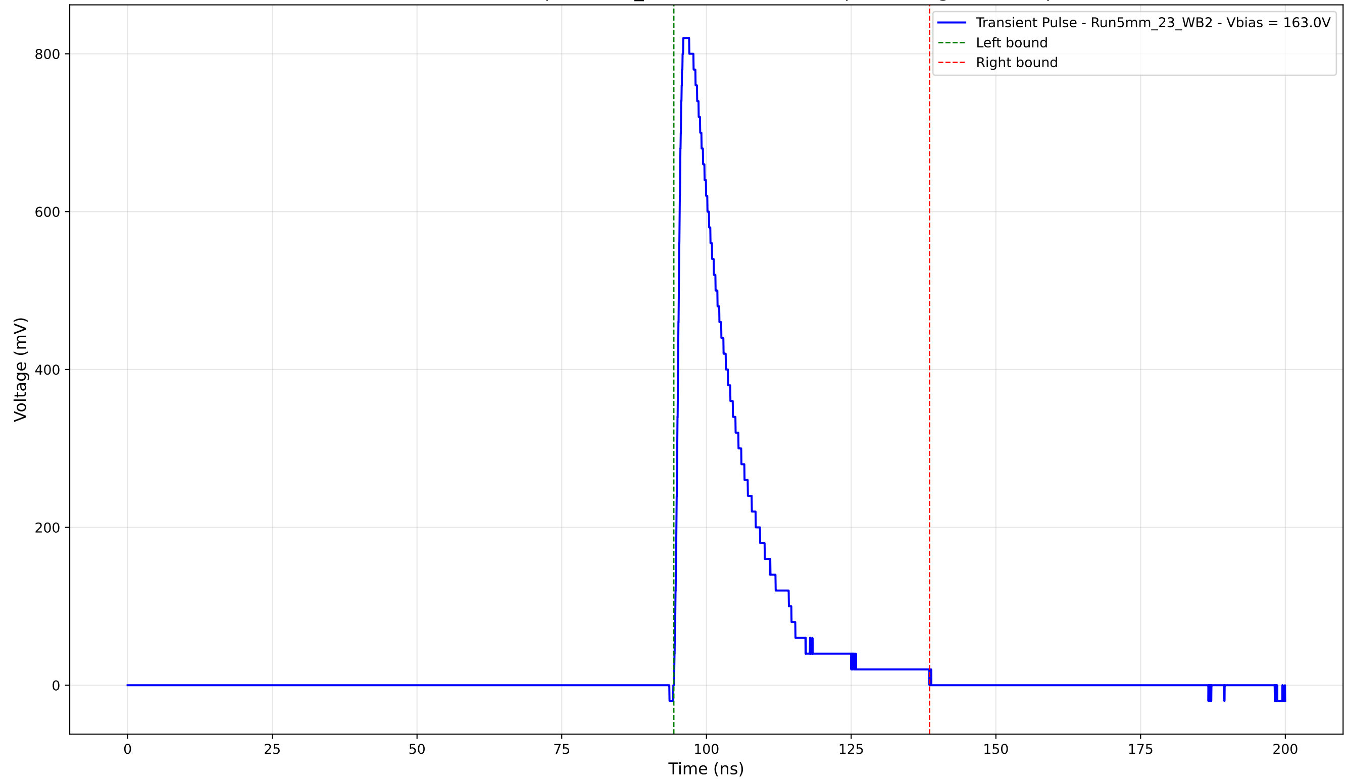
Transient Pulse - Sample: 5mm_23 - Position: 3655.0 \mu\text{m} - Charge: 172.67 pC
