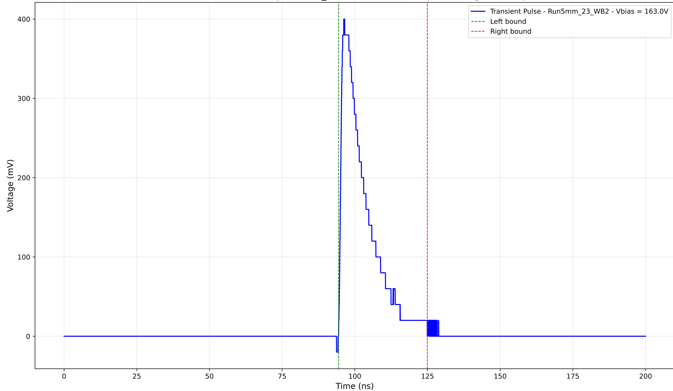
Transient Pulse - Sample: 5mm_23 - Position: 1465.0 \mu\text{m} - Charge: 76.22 pC
