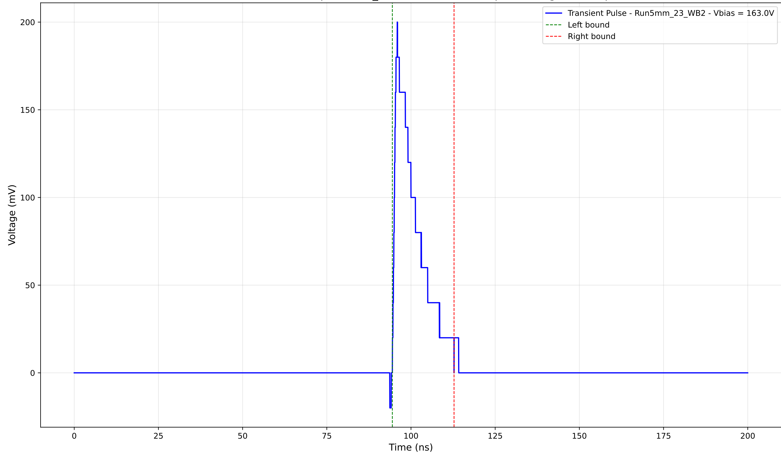
Transient Pulse - Sample: 5mm_23 - Position: 4540.0 \mu\text{m} - Charge: 27.79 pC
