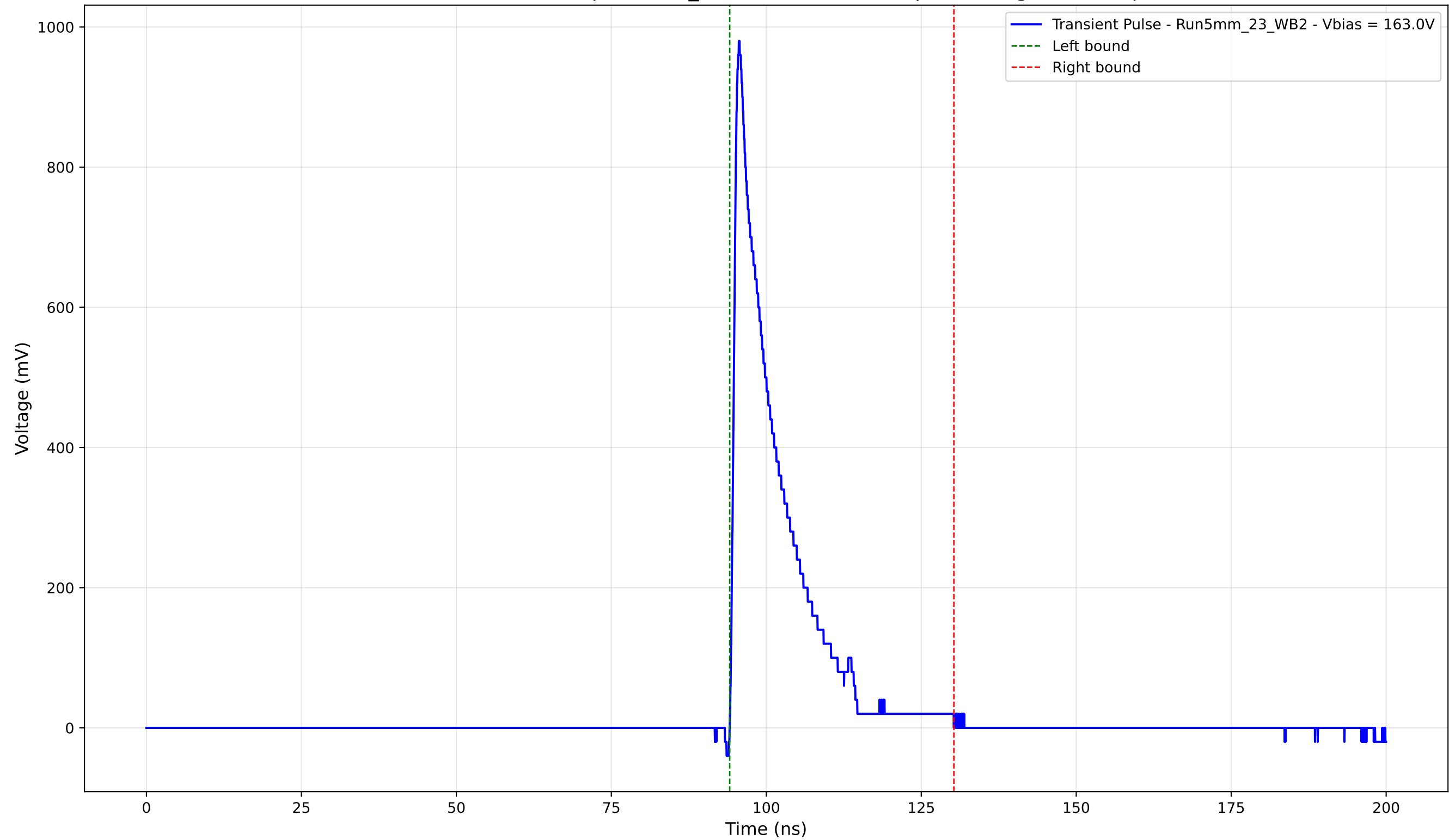
Transient Pulse - Sample: 5mm_23 - Position: 4805.0 \mu\text{m} - Charge: 145.12 pC
