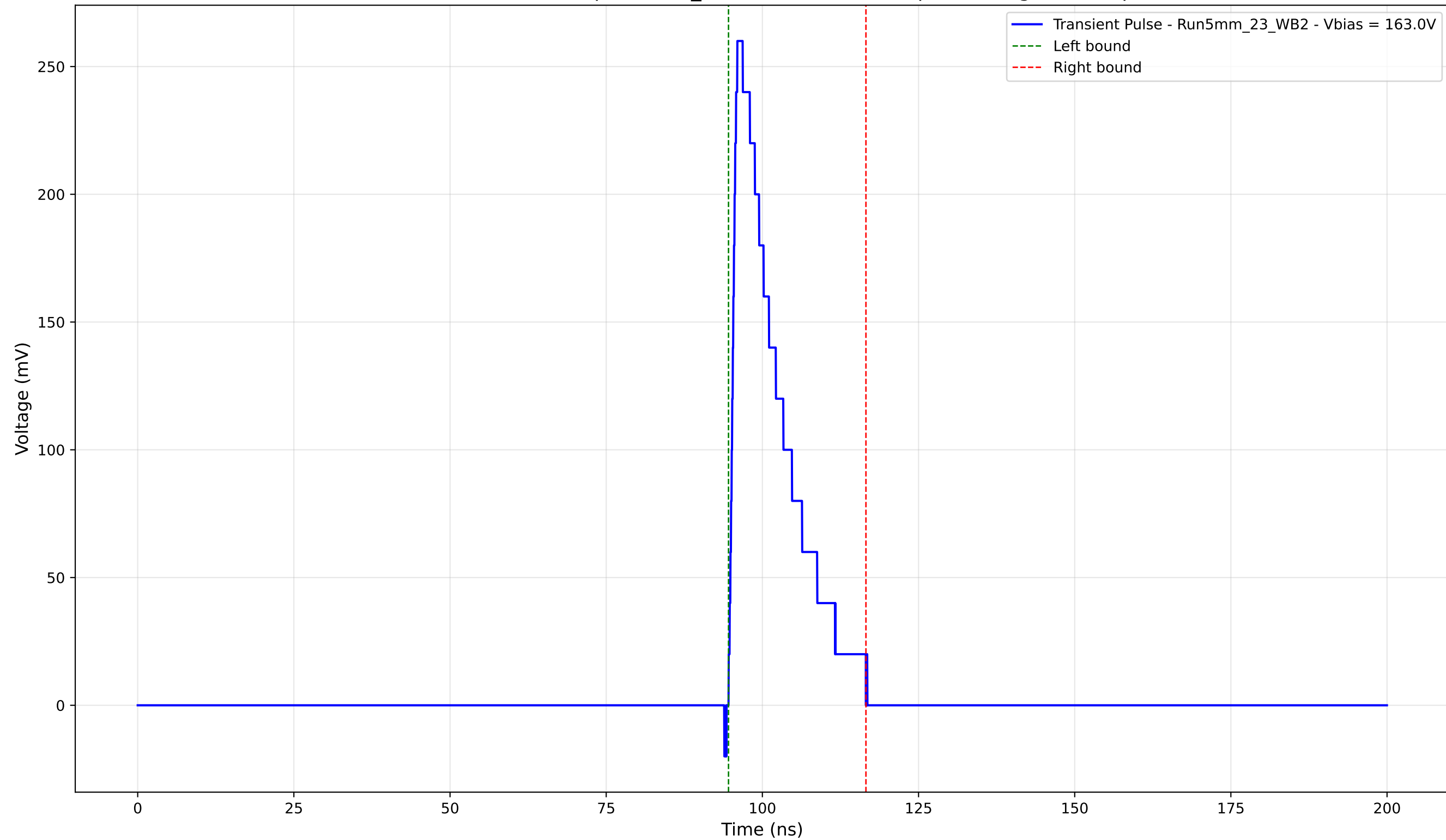
Transient Pulse - Sample: 5mm_23 - Position: 4015.0 \mu\text{m} - Charge: 43.85 pC
