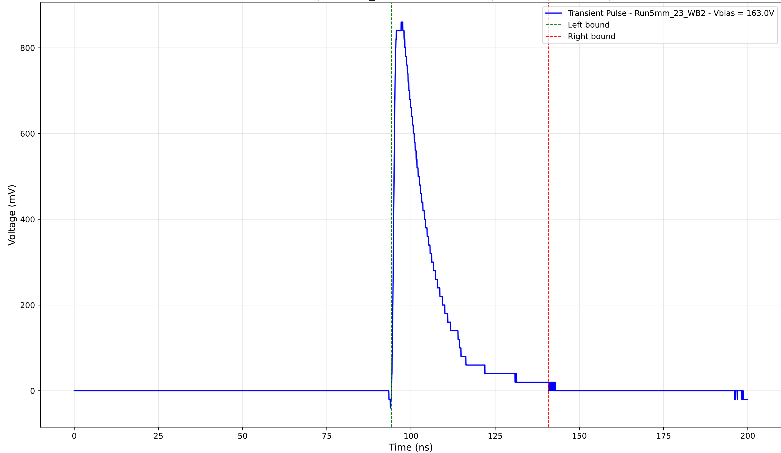
Transient Pulse - Sample: 5mm_23 - Position: 3365.0 \mu\text{m} - Charge: 192.72 pC
