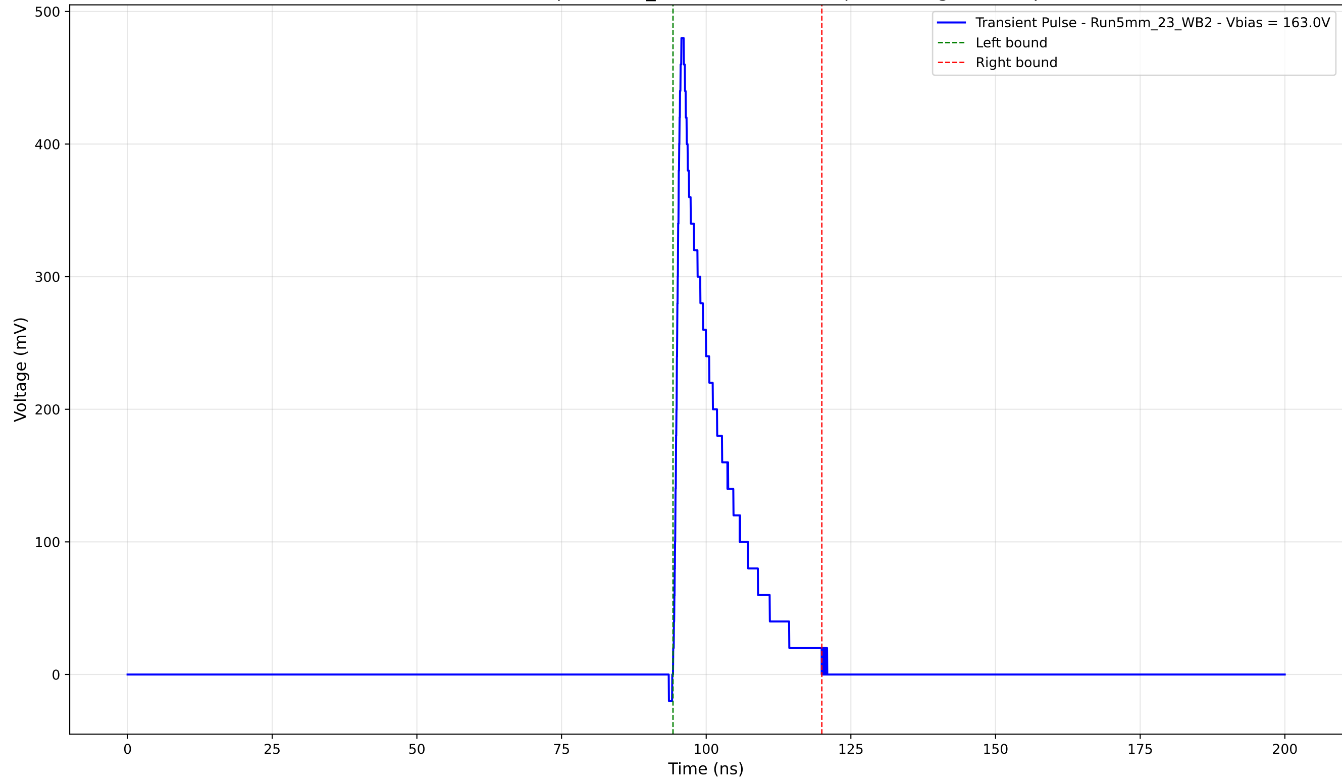
Transient Pulse - Sample: 5mm_23 - Position: 455.0 \mu\text{m} - Charge: 69.71 pC
