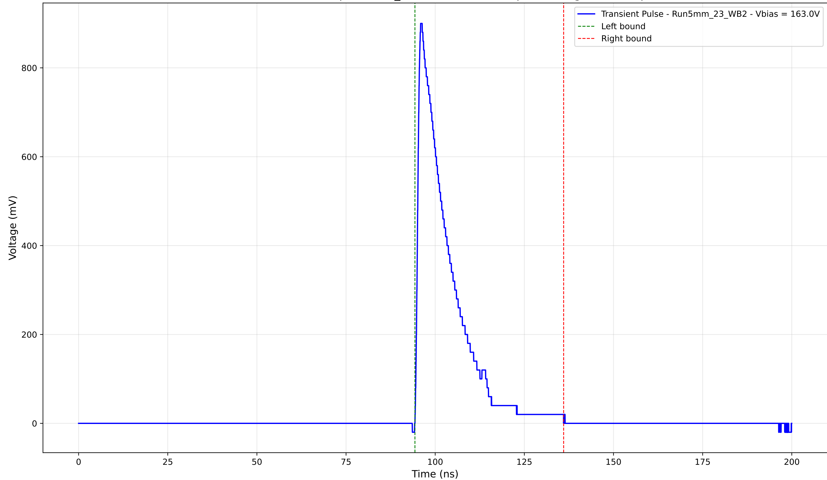
Transient Pulse - Sample: 5mm_23 - Position: 695.0 \mu\text{m} - Charge: 171.47 pC
