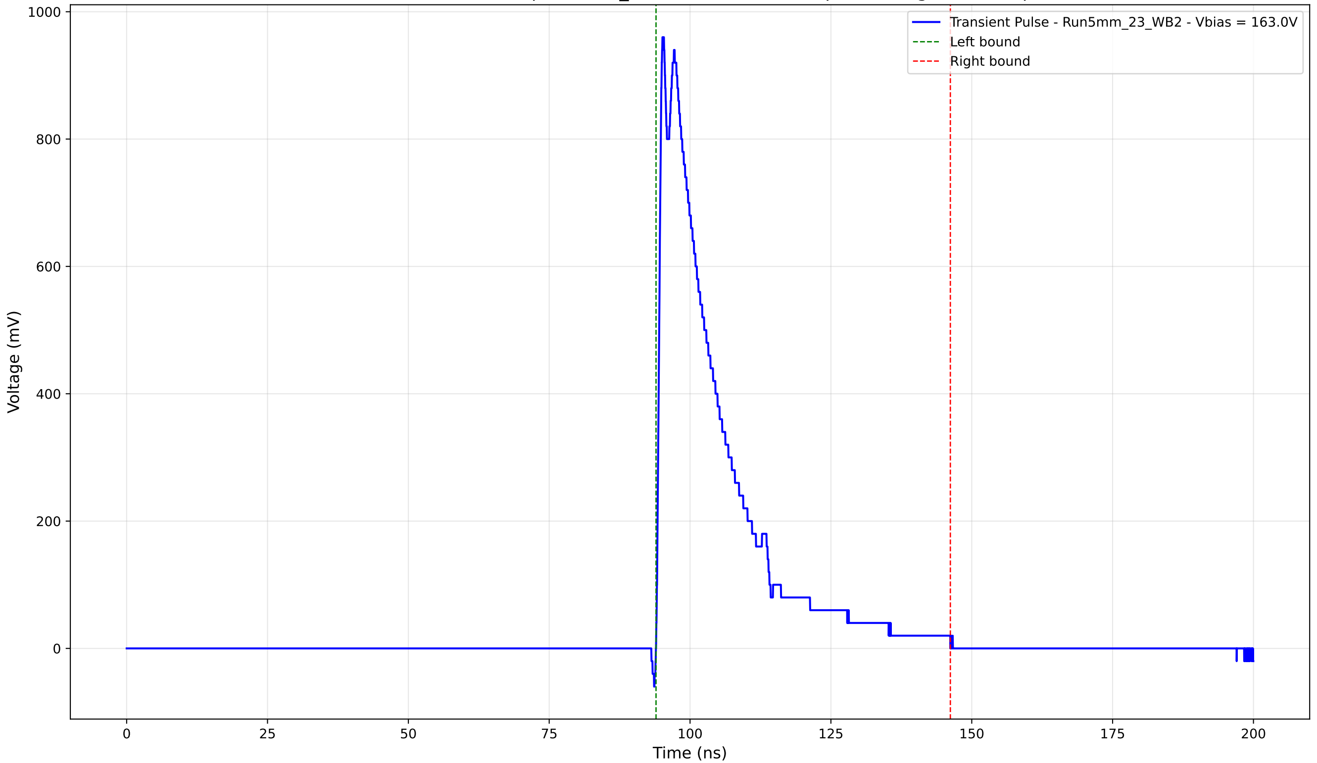
Transient Pulse - Sample: 5mm_23 - Position: 2900.0 \mu\text{m} - Charge: 218.62 pC
