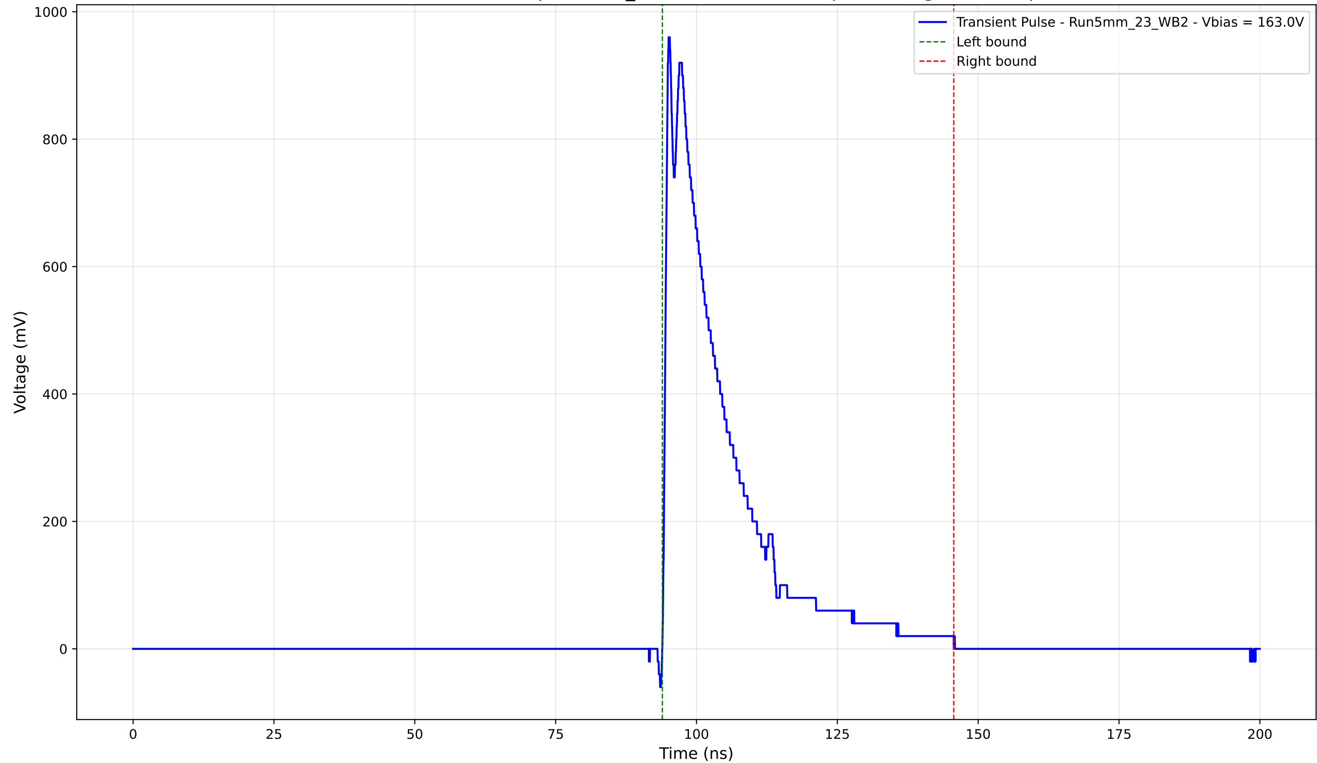
Transient Pulse - Sample: 5mm_23 - Position: 2845.0 \mu\text{m} - Charge: 213.13 pC
