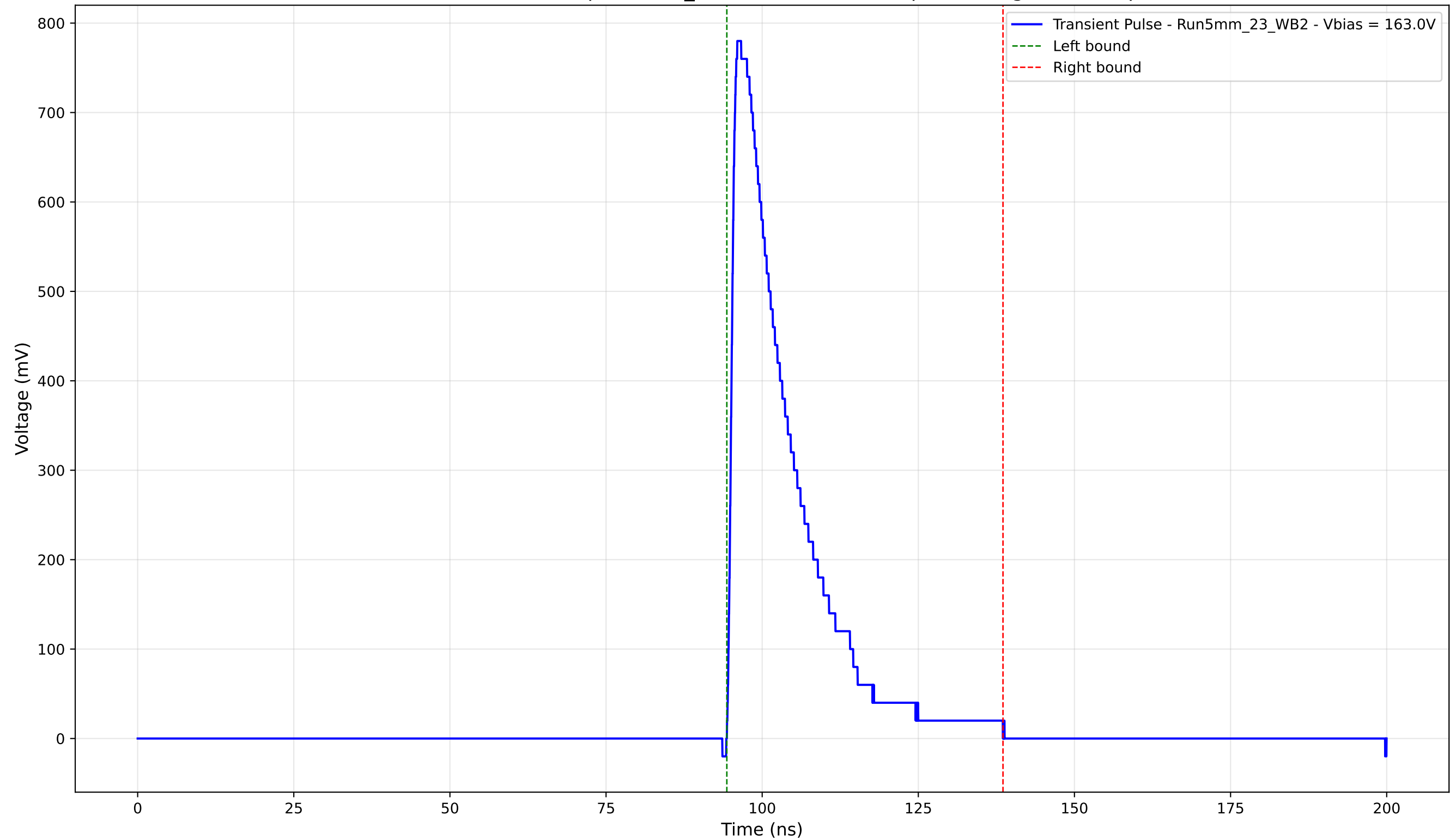
Transient Pulse - Sample: 5mm_23 - Position: 1425.0 \mu\text{m} - Charge: 164.08 pC
