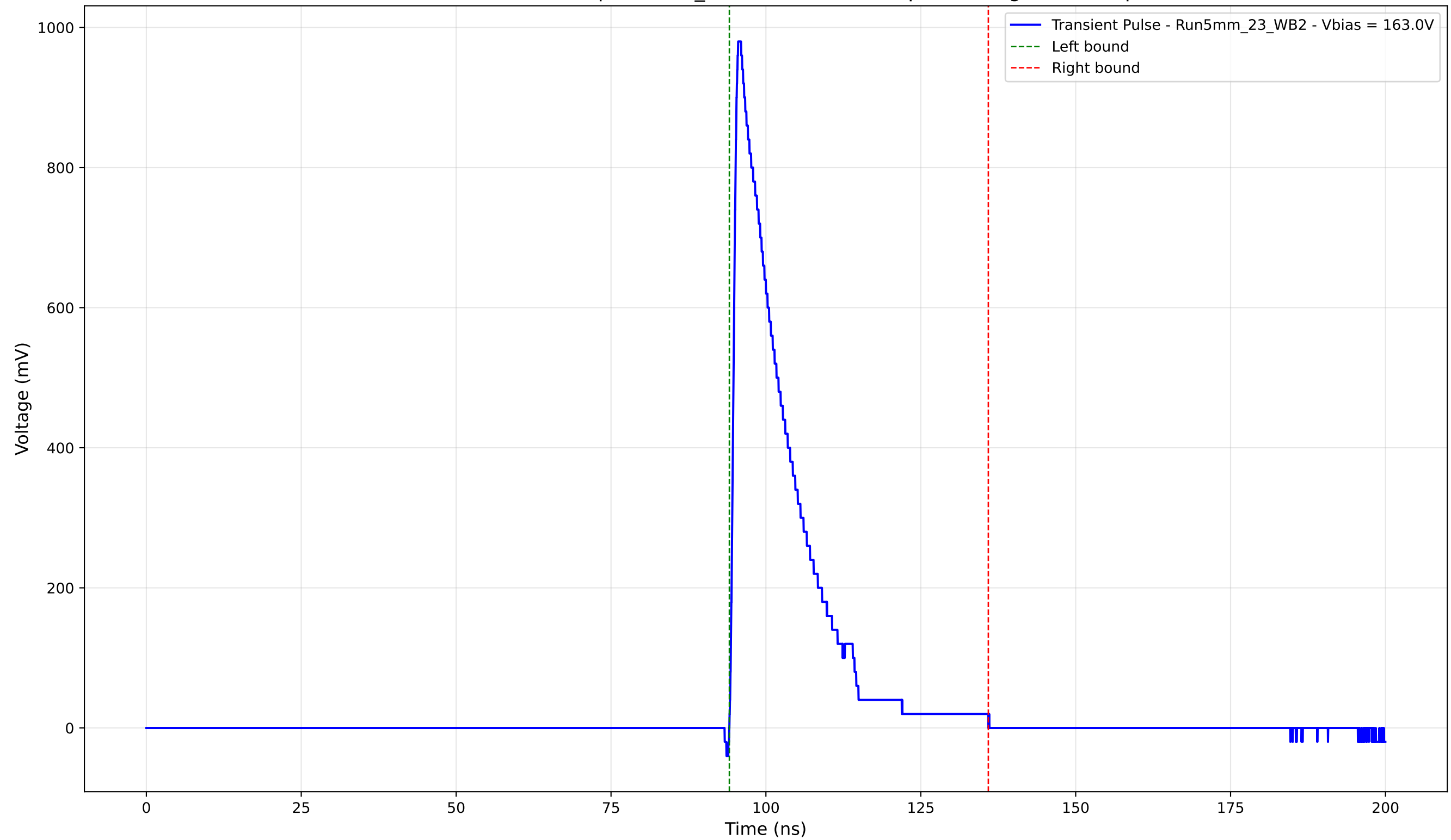
Transient Pulse - Sample: 5mm_23 - Position: 350.0 \mu\text{m} - Charge: 181.24 pC
