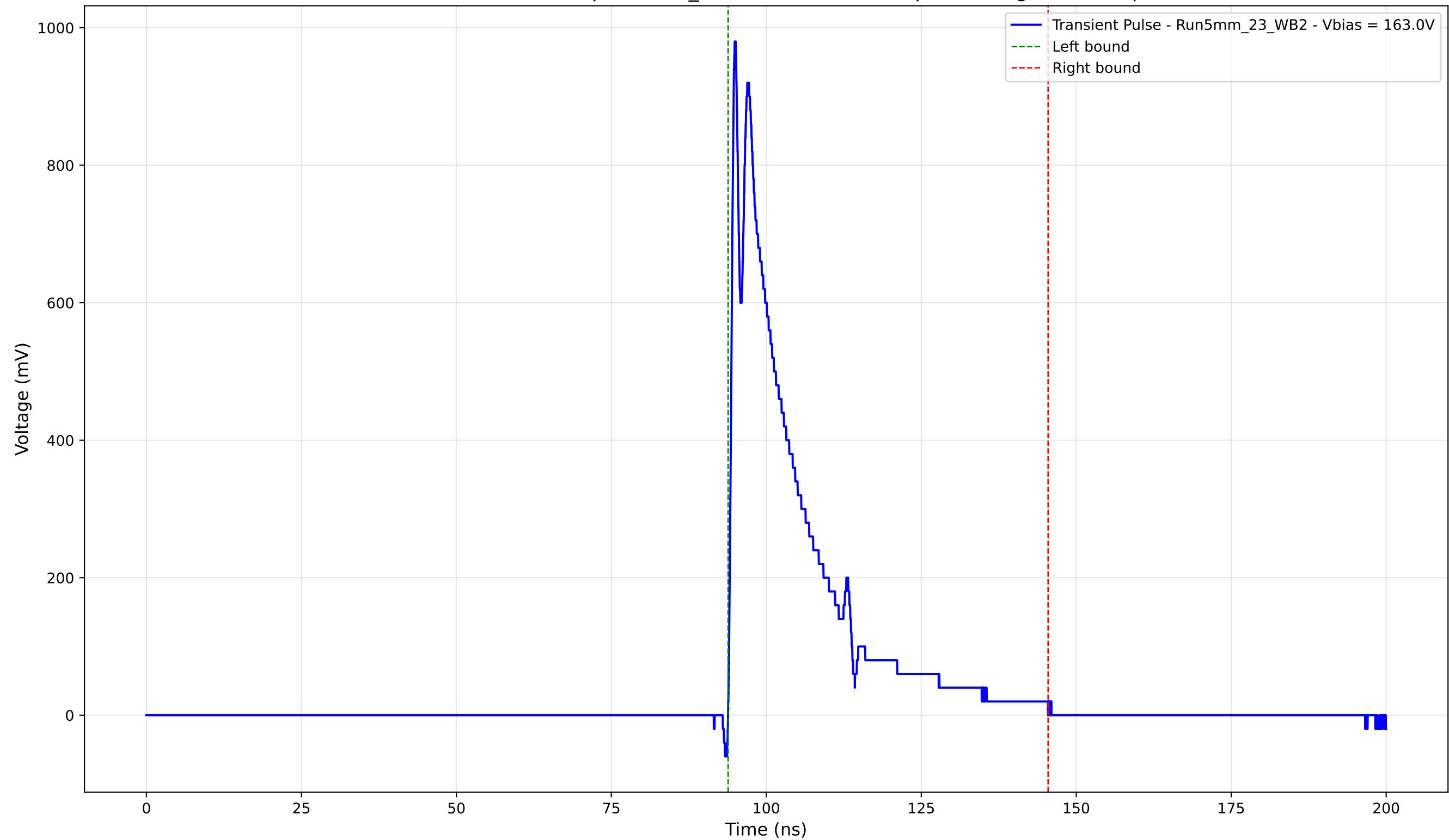
Transient Pulse - Sample: 5mm_23 - Position: 2365.0 \mu\text{m} - Charge: 200.82 pC
