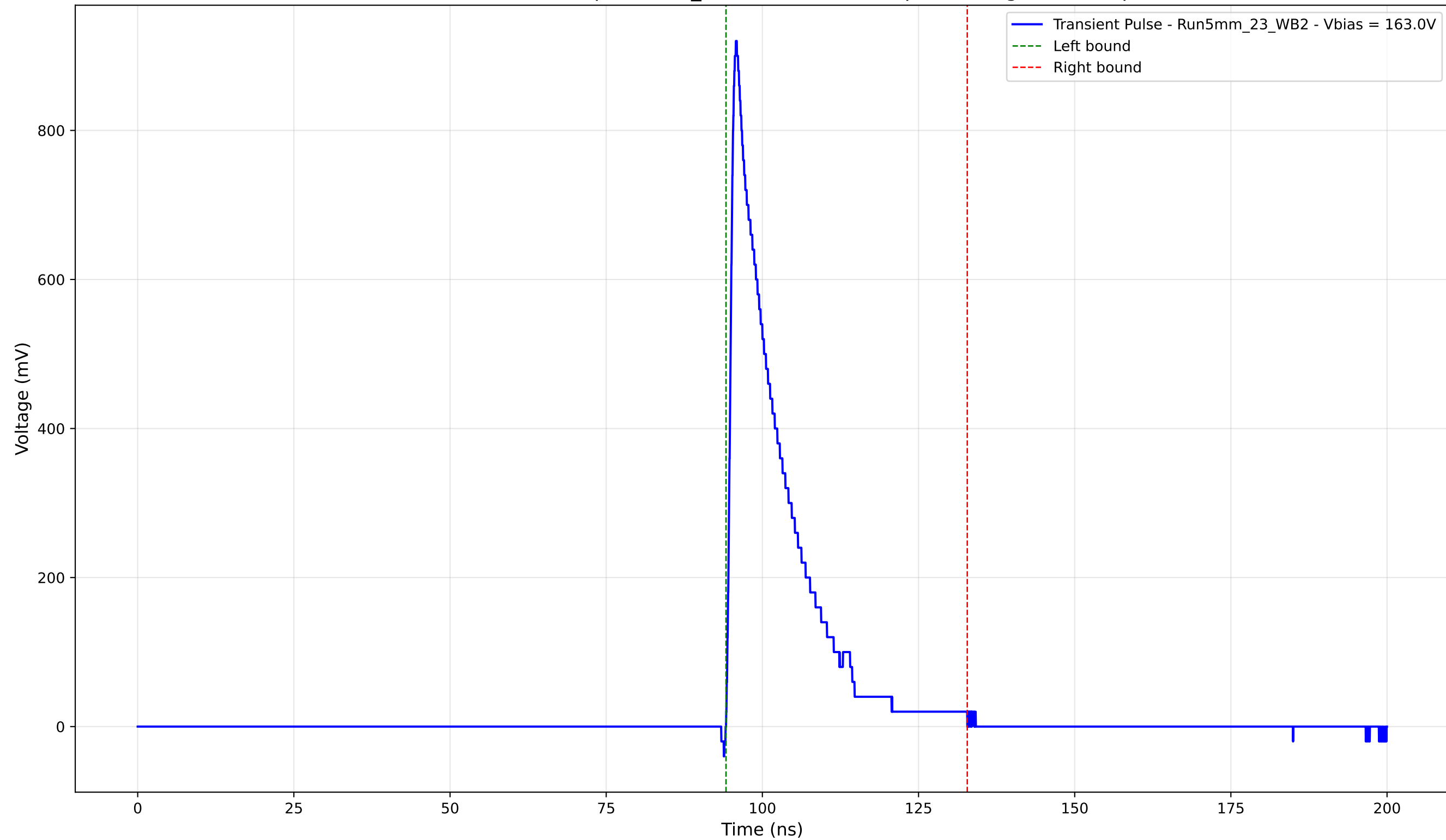
Transient Pulse - Sample: 5mm_23 - Position: 415.0 \mu\text{m} - Charge: 153.60 pC
