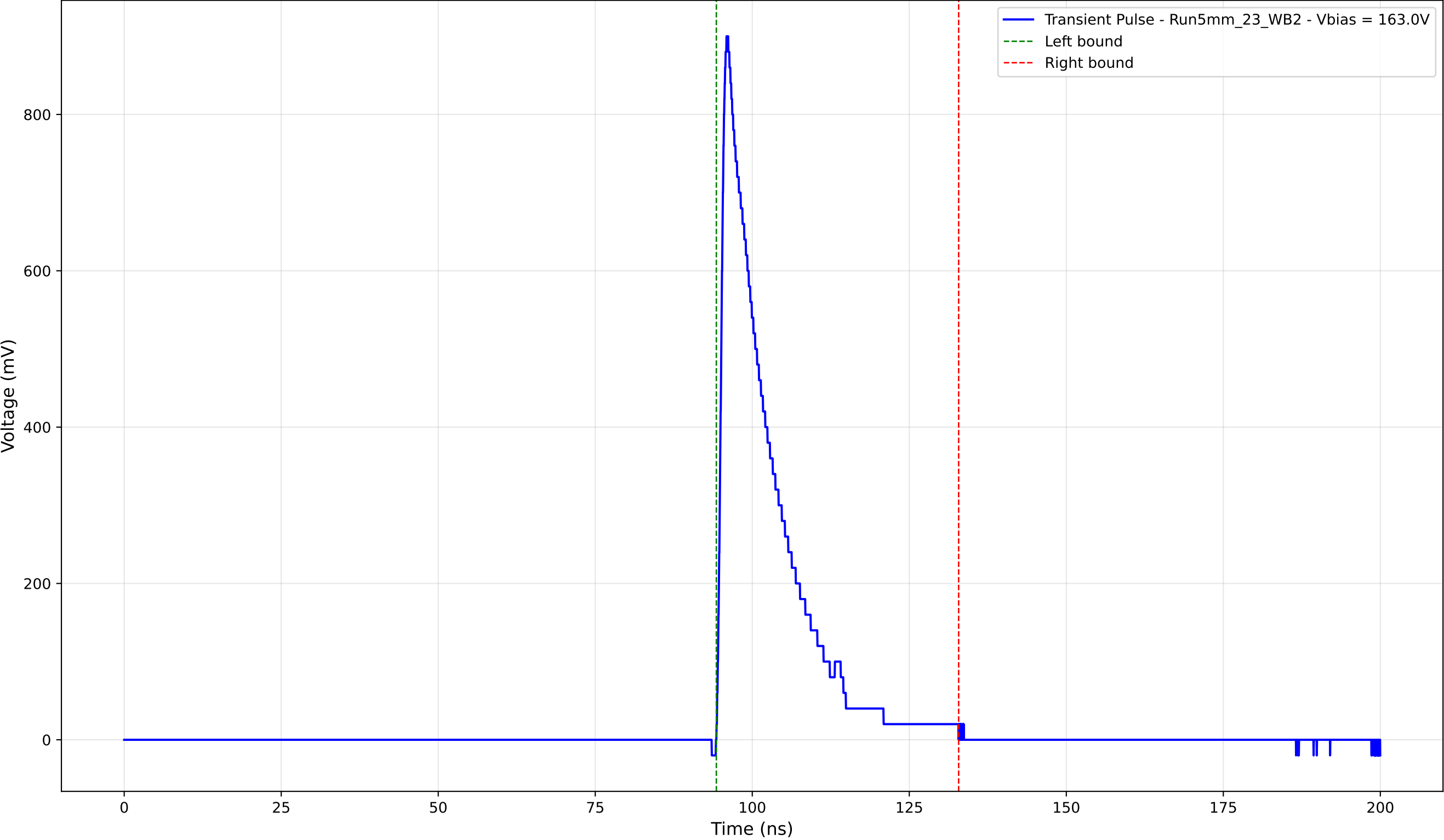
Transient Pulse - Sample: 5mm_23 - Position: 4430.0 \mu\text{m} - Charge: 152.80 pC
