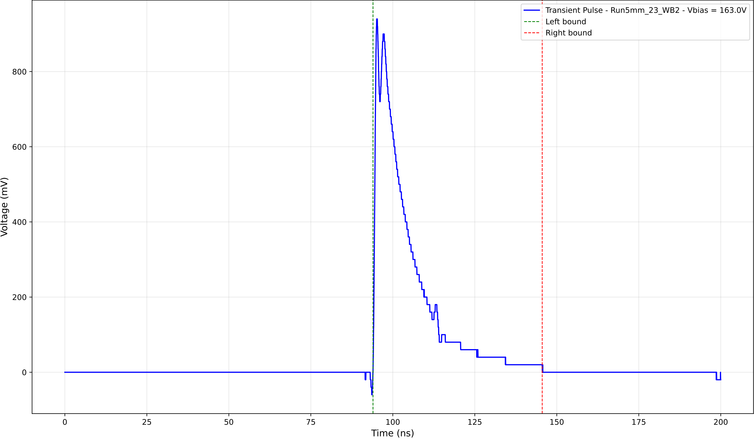
Transient Pulse - Sample: 5mm_23 - Position: 2160.0 \mu\text{m} - Charge: 205.24 pC
