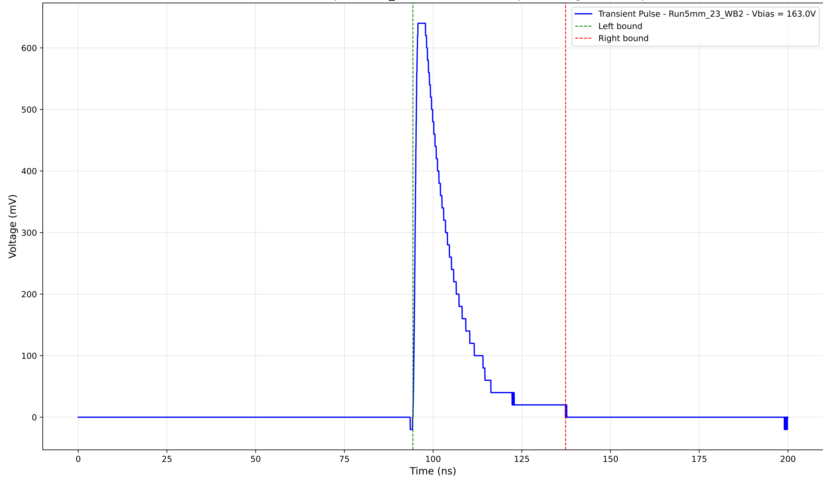
Transient Pulse - Sample: 5mm_23 - Position: 1560.0 \mu\text{m} - Charge: 137.62 pC
