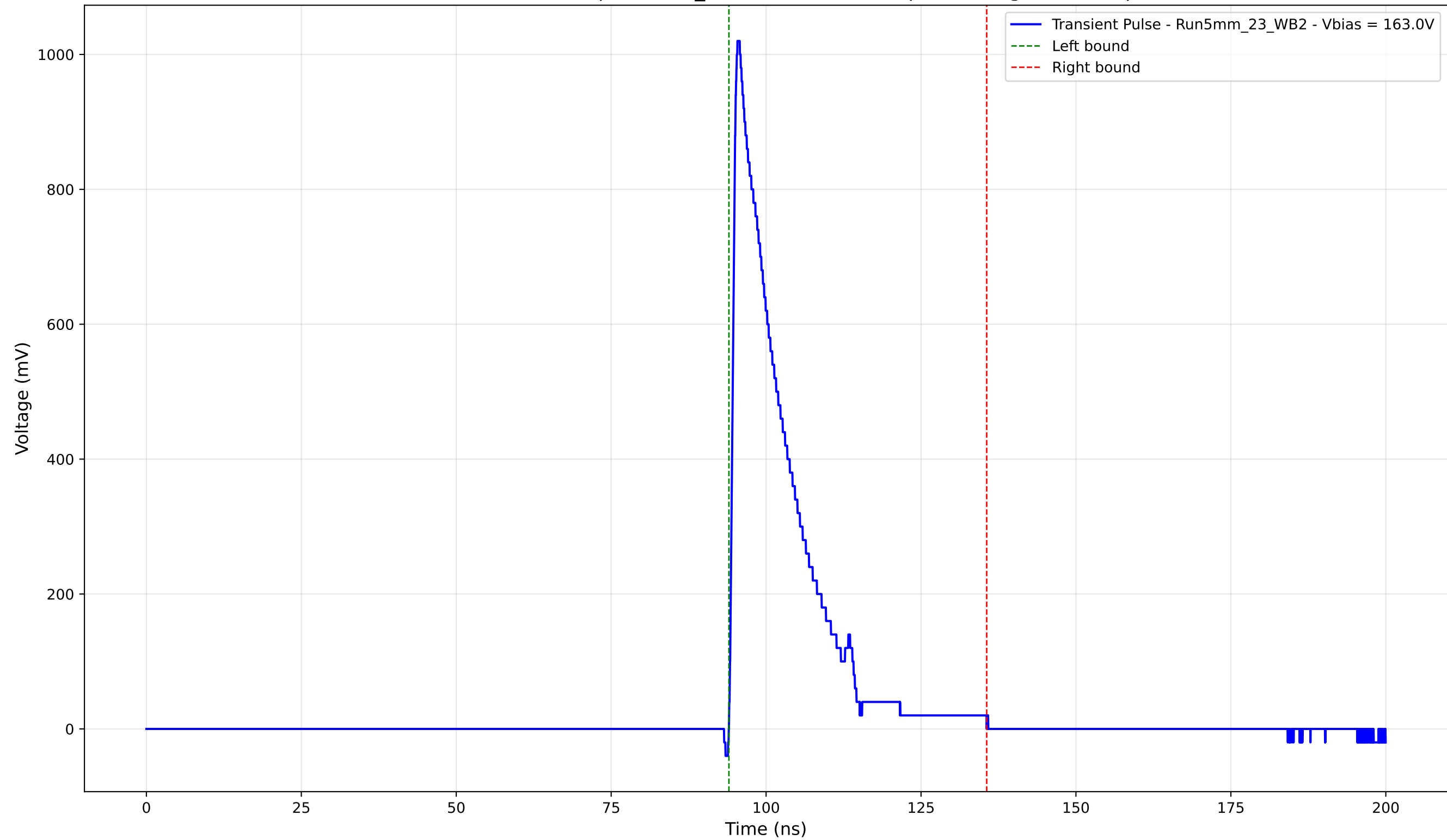
Transient Pulse - Sample: 5mm_23 - Position: 175.0 \mu\text{m} - Charge: 182.96 pC
