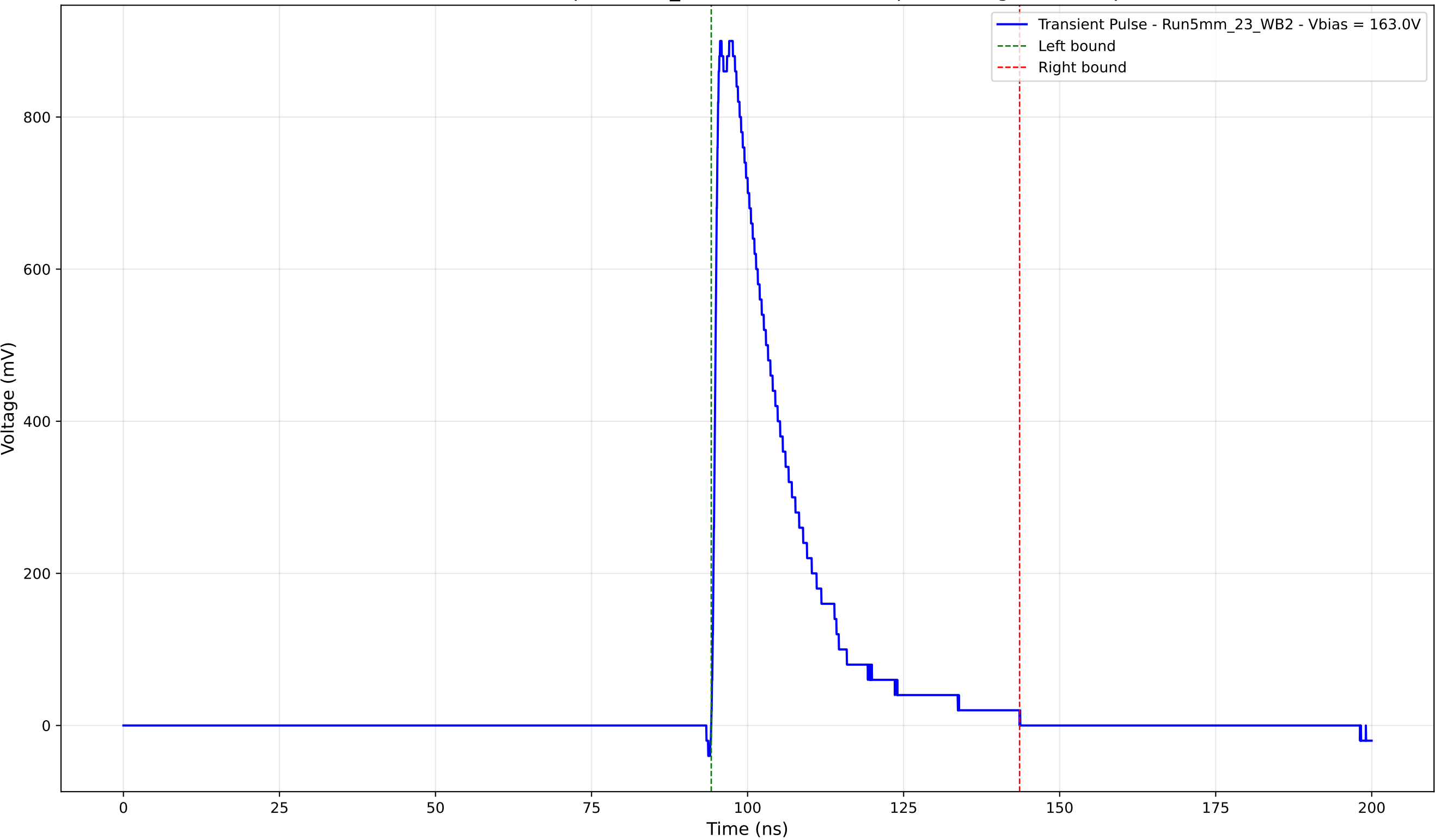
Transient Pulse - Sample: 5mm_23 - Position: 1735.0 \mu\text{m} - Charge: 213.06 pC
