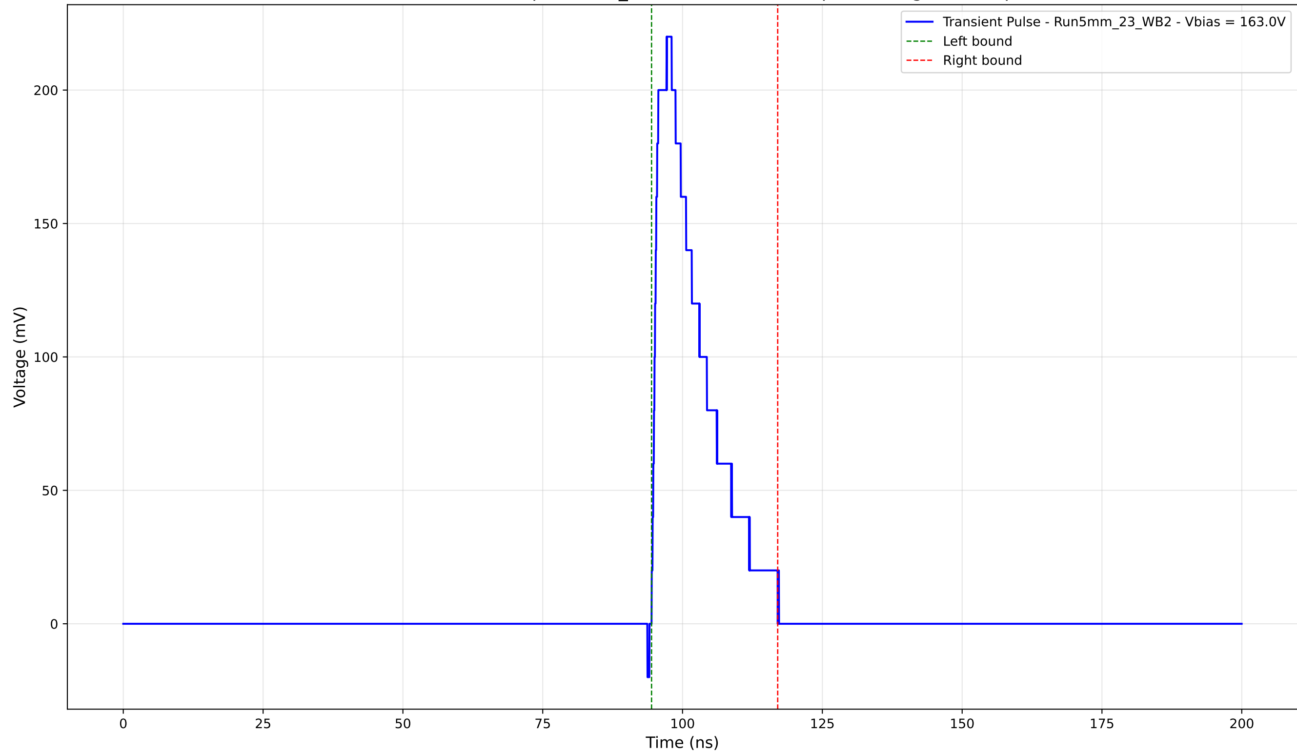
Transient Pulse - Sample: 5mm_23 - Position: 1515.0 \mu\text{m} - Charge: 40.98 pC
