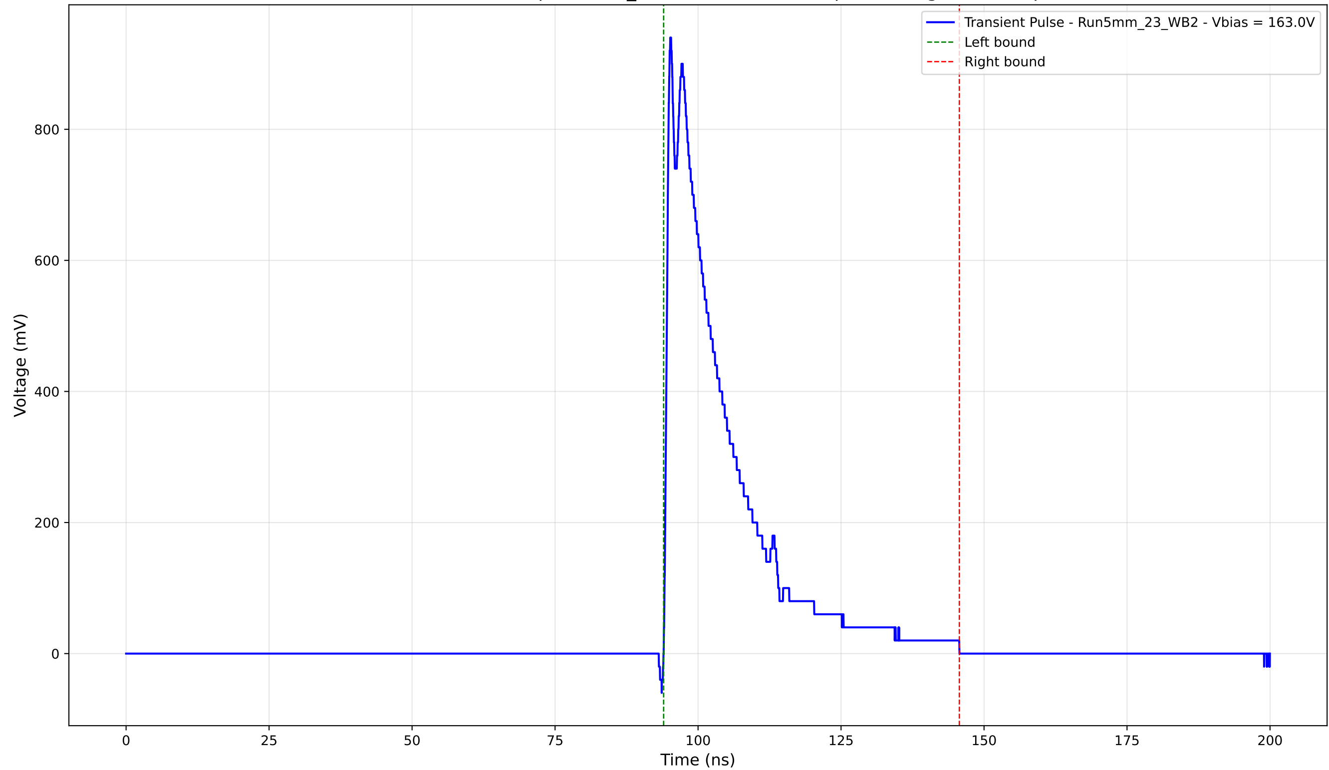
Transient Pulse - Sample: 5mm_23 - Position: 2130.0 \mu\text{m} - Charge: 204.17 pC
