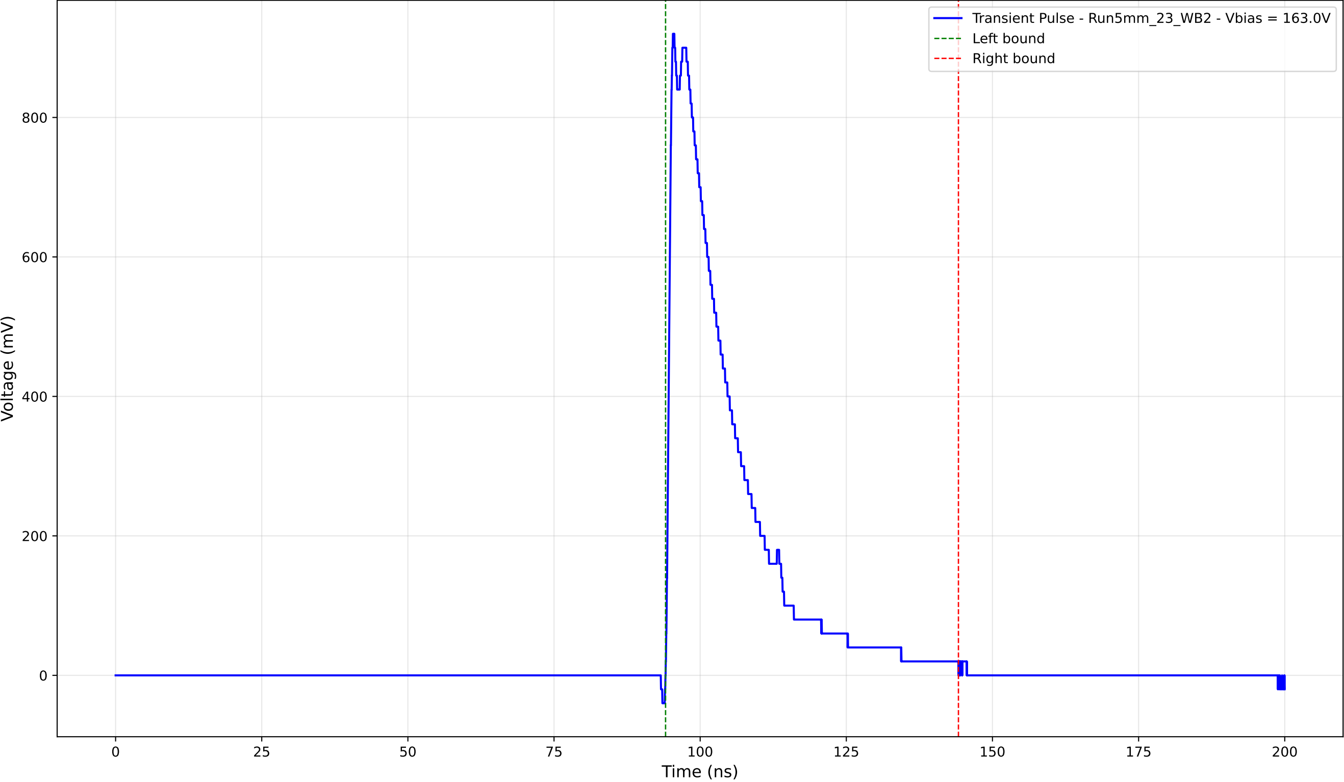
Transient Pulse - Sample: 5mm_23 - Position: 1905.0 \mu\text{m} - Charge: 215.09 pC
