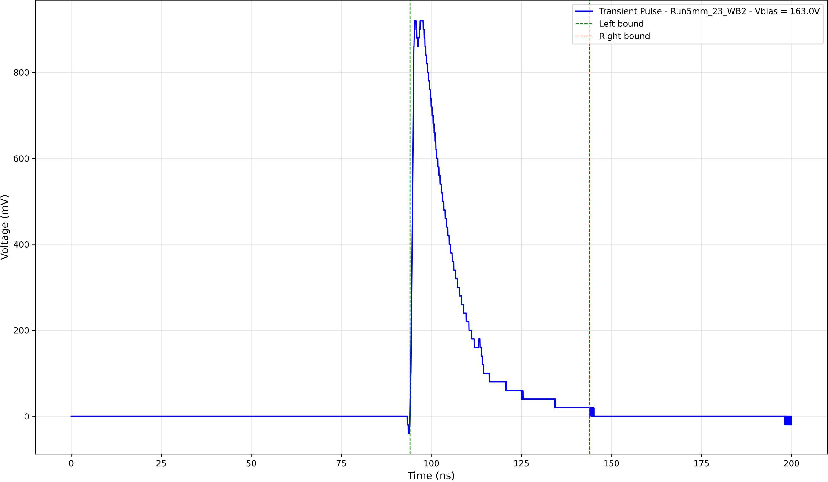
Transient Pulse - Sample: 5mm_23 - Position: 3180.0 \mu\text{m} - Charge: 220.53 pC
