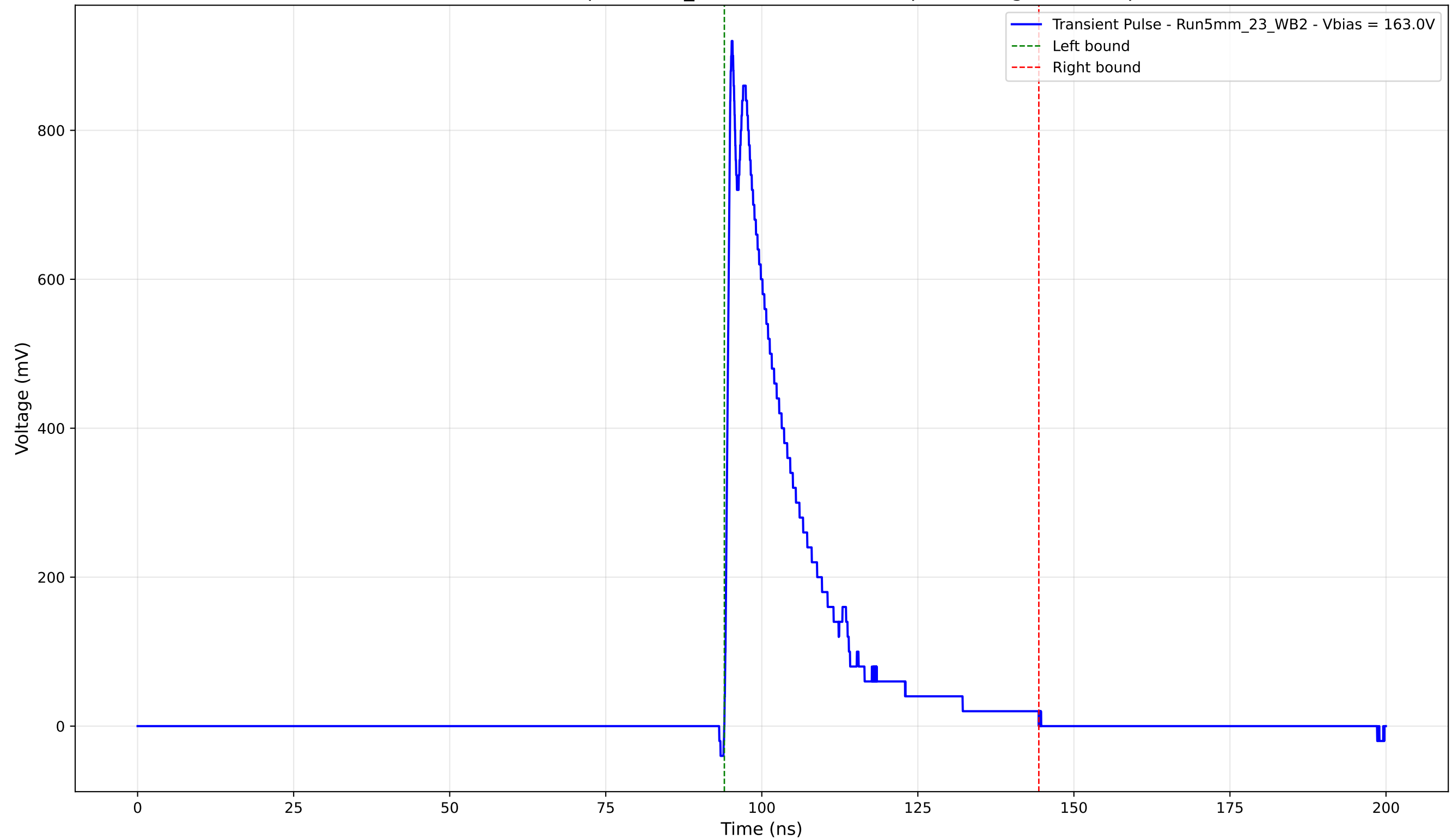
Transient Pulse - Sample: 5mm_23 - Position: 2945.0 \mu\text{m} - Charge: 190.65 pC
