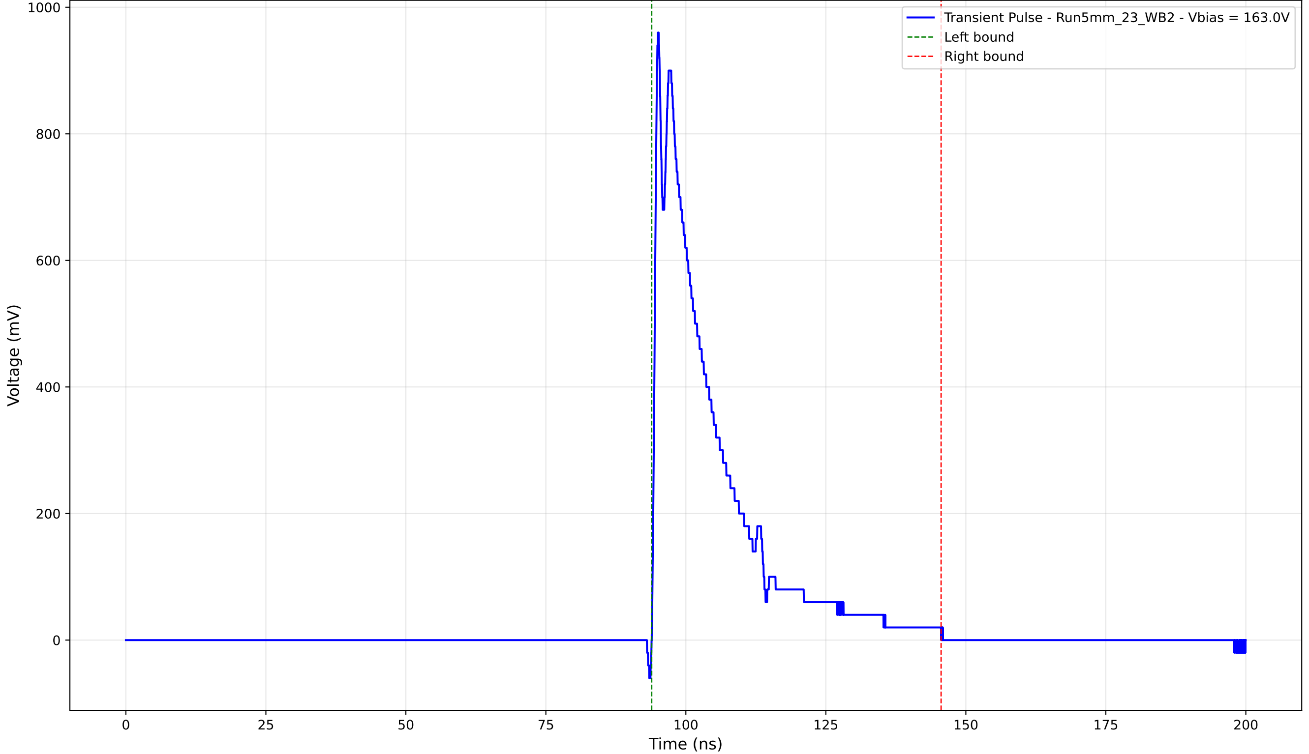
Transient Pulse - Sample: 5mm_23 - Position: 2260.0 \mu\text{m} - Charge: 205.06 pC
