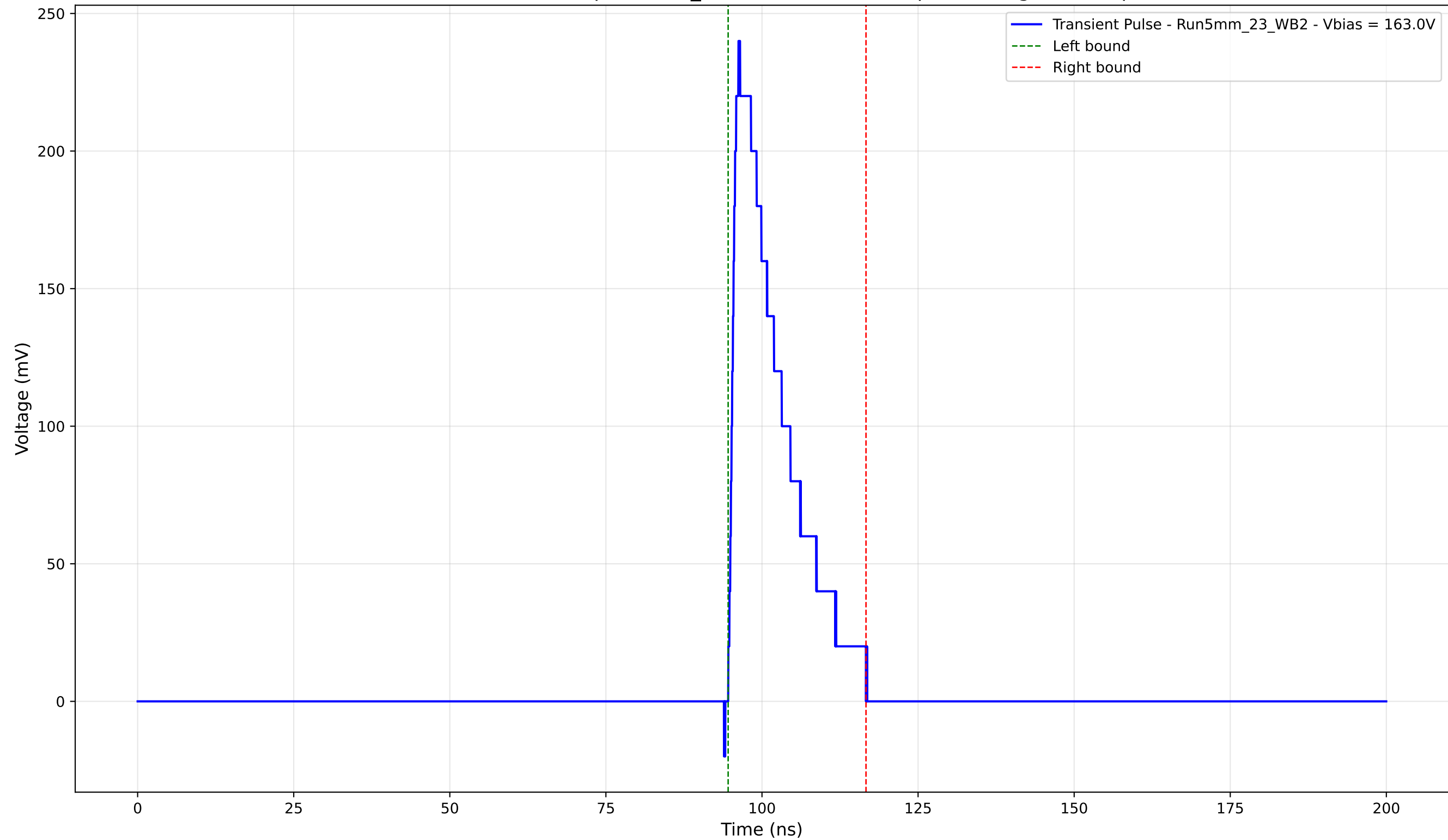
Transient Pulse - Sample: 5mm_23 - Position: 1010.0 \mu\text{m} - Charge: 41.54 pC
