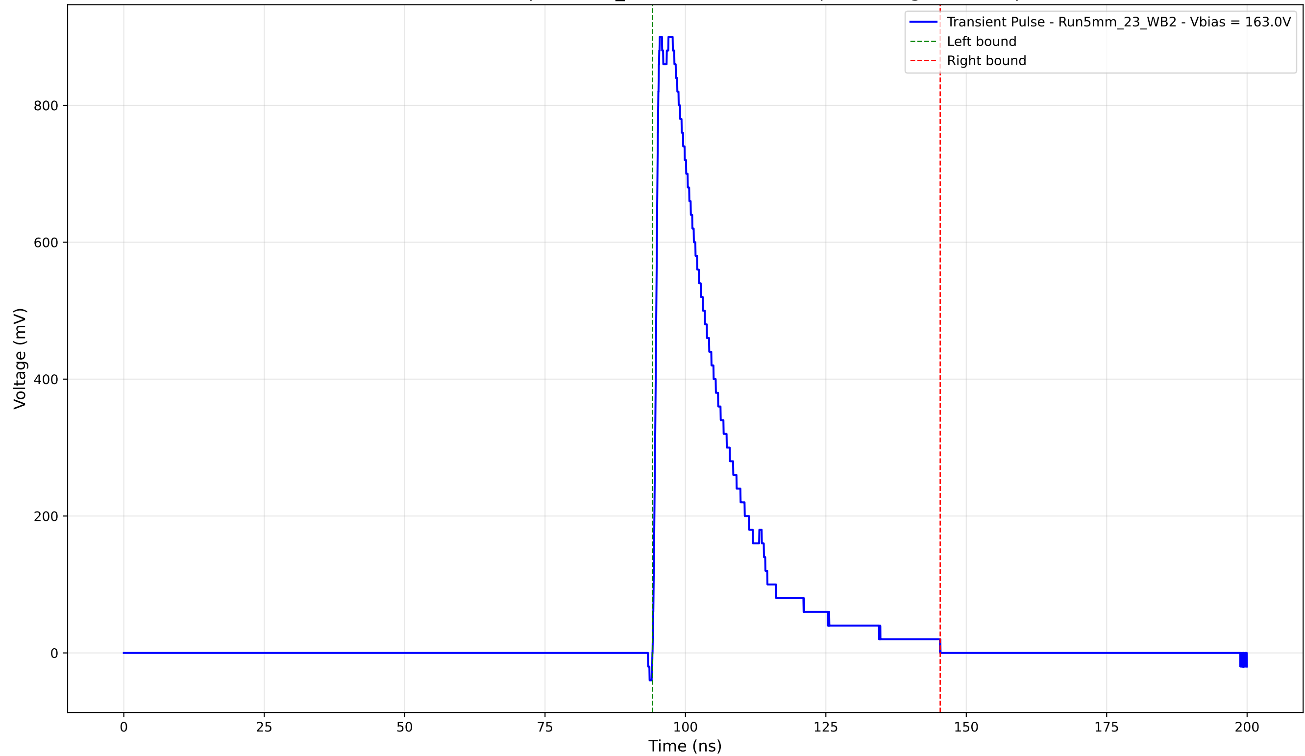
Transient Pulse - Sample: 5mm_23 - Position: 1810.0 \mu\text{m} - Charge: 219.18 pC
