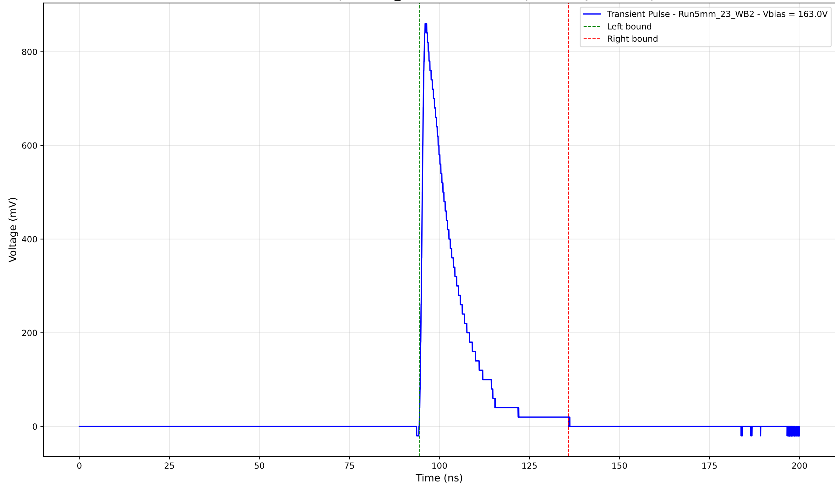
Transient Pulse - Sample: 5mm_23 - Position: 4145.0 \mu\text{m} - Charge: 159.15 pC
