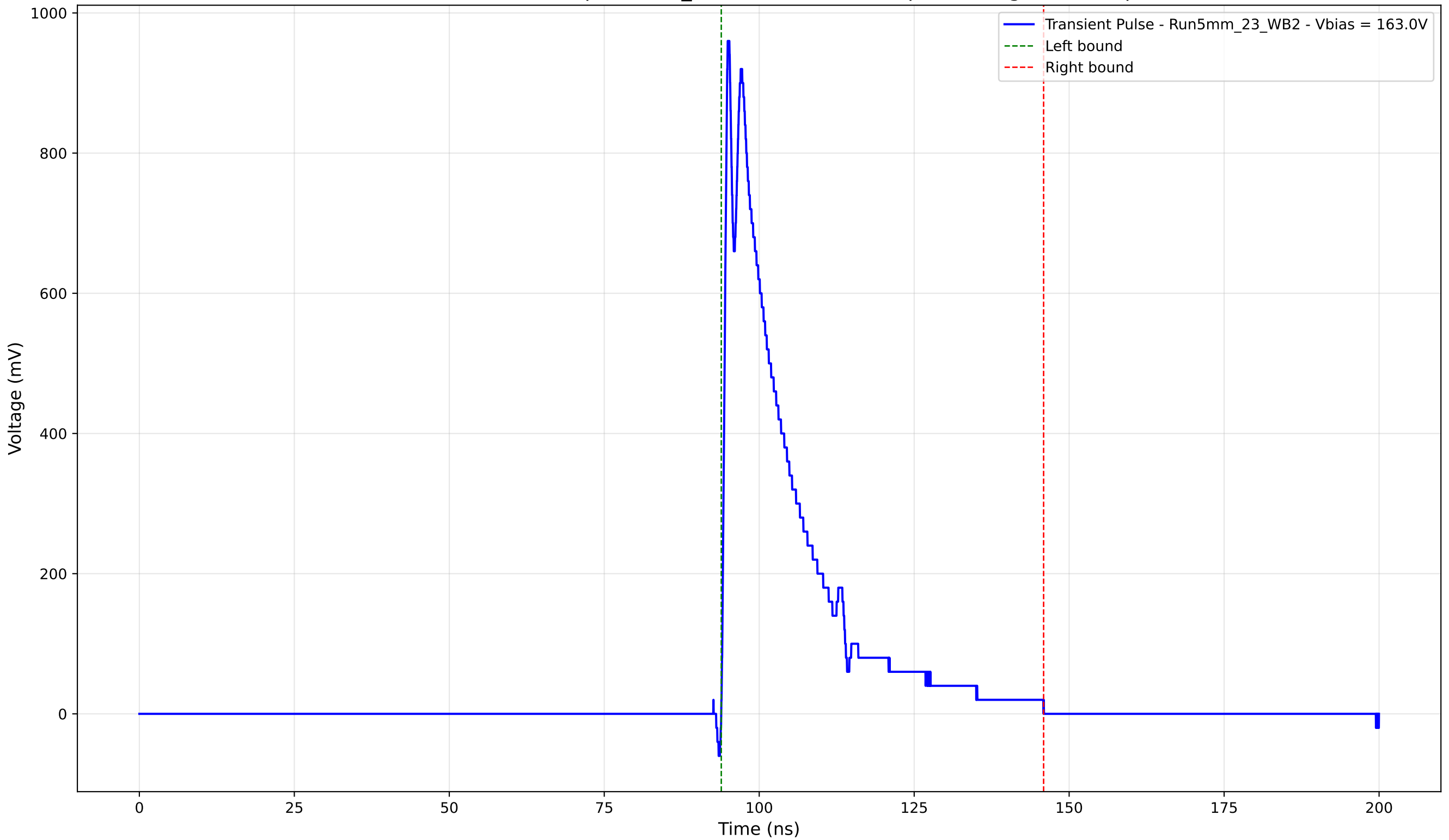
Transient Pulse - Sample: 5mm_23 - Position: 2755.0 \mu\text{m} - Charge: 204.28 pC
