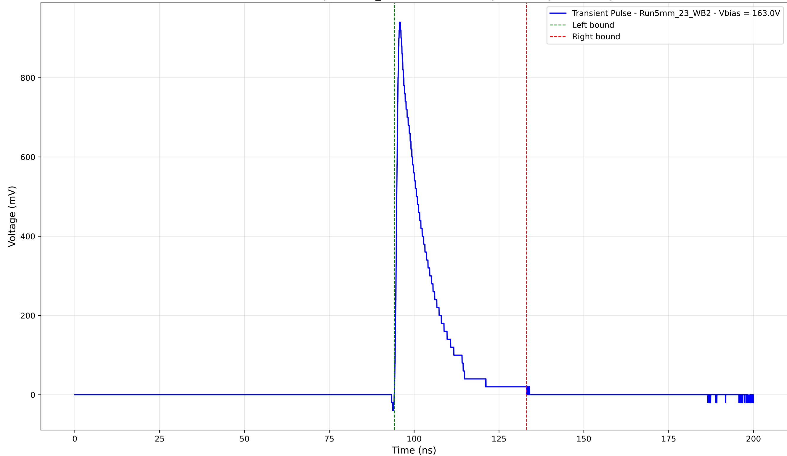
Transient Pulse - Sample: 5mm_23 - Position: 410.0 \mu\text{m} - Charge: 160.41 pC
