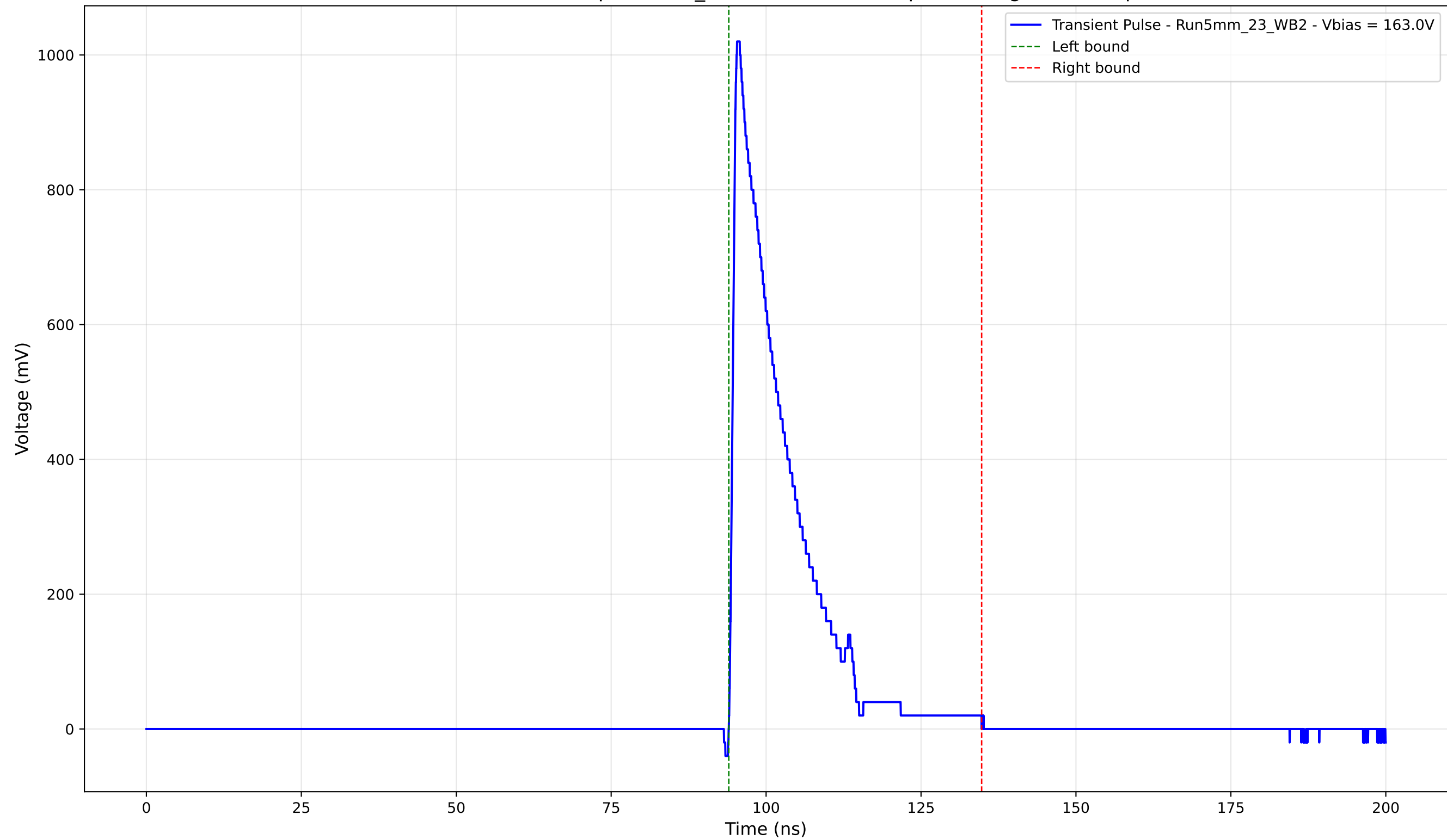
Transient Pulse - Sample: 5mm_23 - Position: 150.0 \mu\text{m} - Charge: 182.95 pC
