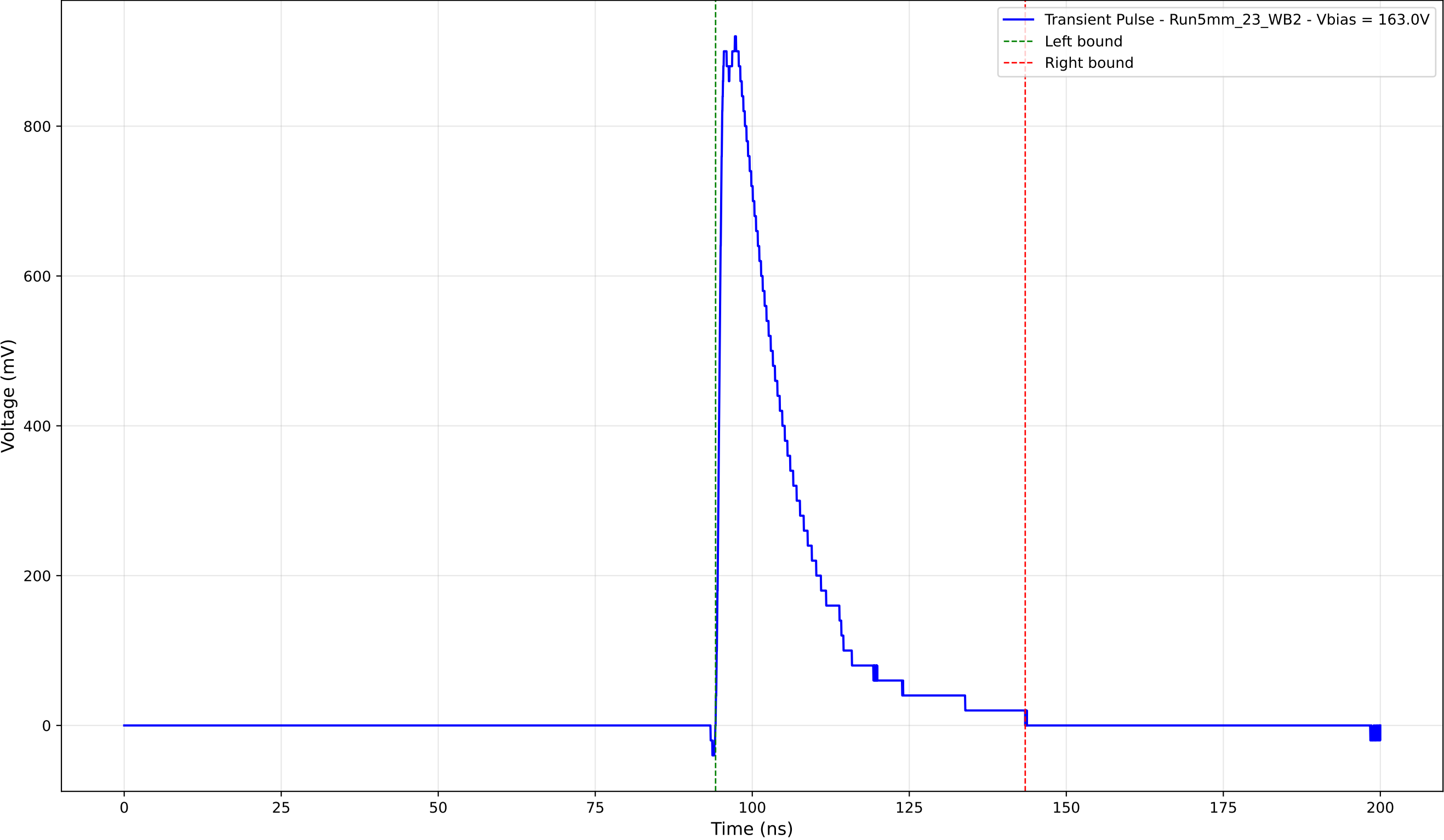
Transient Pulse - Sample: 5mm_23 - Position: 3260.0 \mu\text{m} - Charge: 214.36 pC
