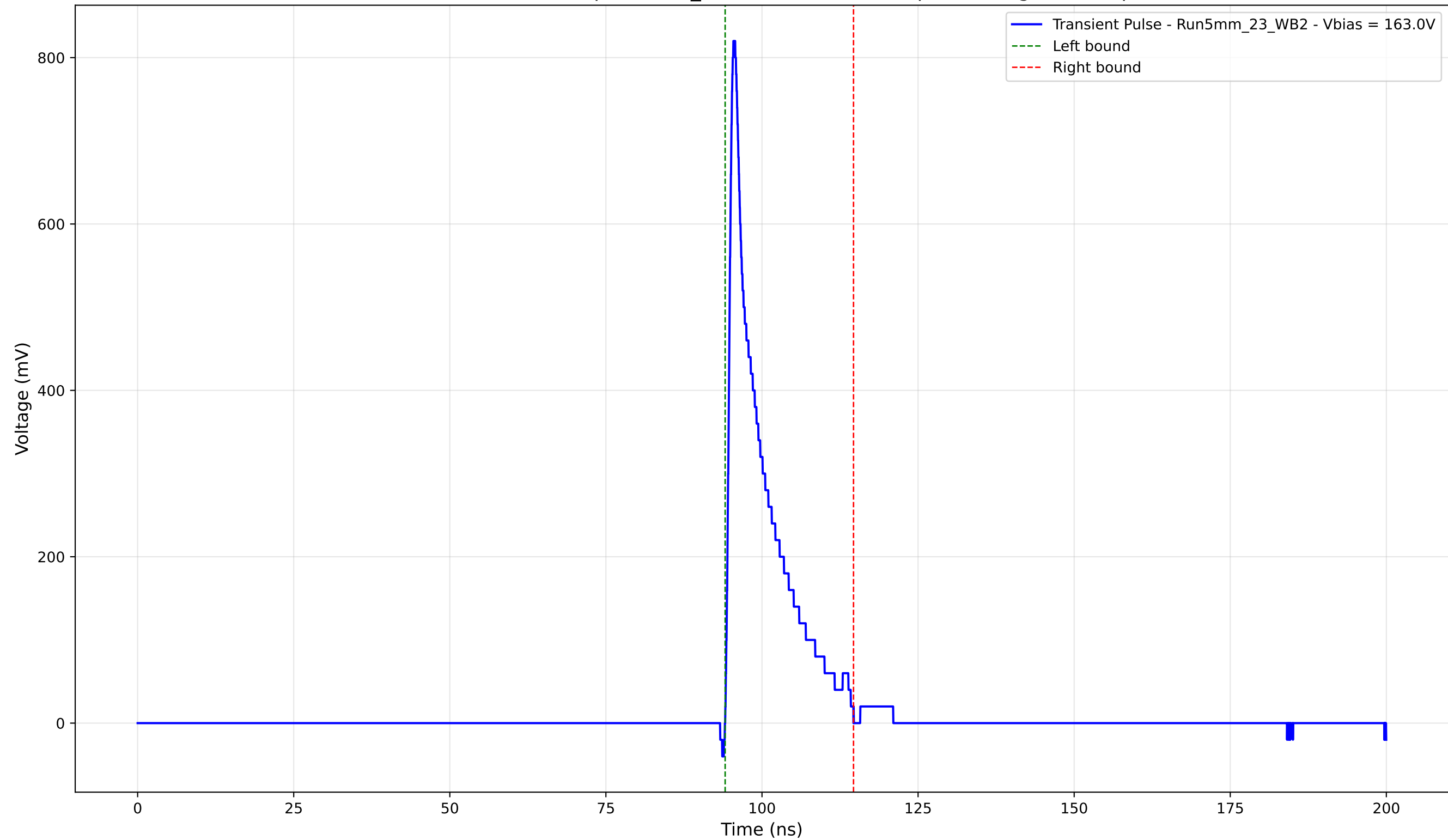
Transient Pulse - Sample: 5mm_23 - Position: 4910.0 \mu\text{m} - Charge: 95.12 pC
