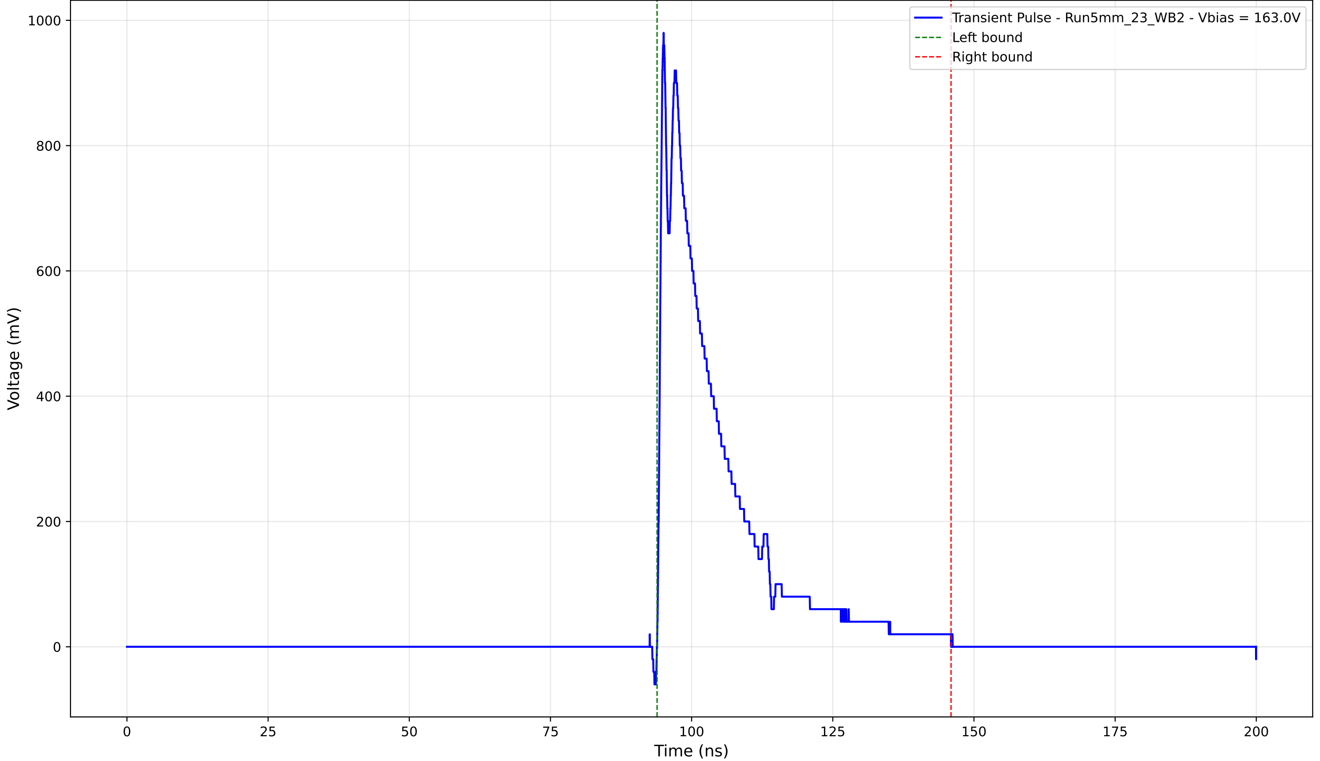
Transient Pulse - Sample: 5mm_23 - Position: 2740.0 \mu\text{m} - Charge: 203.19 pC
