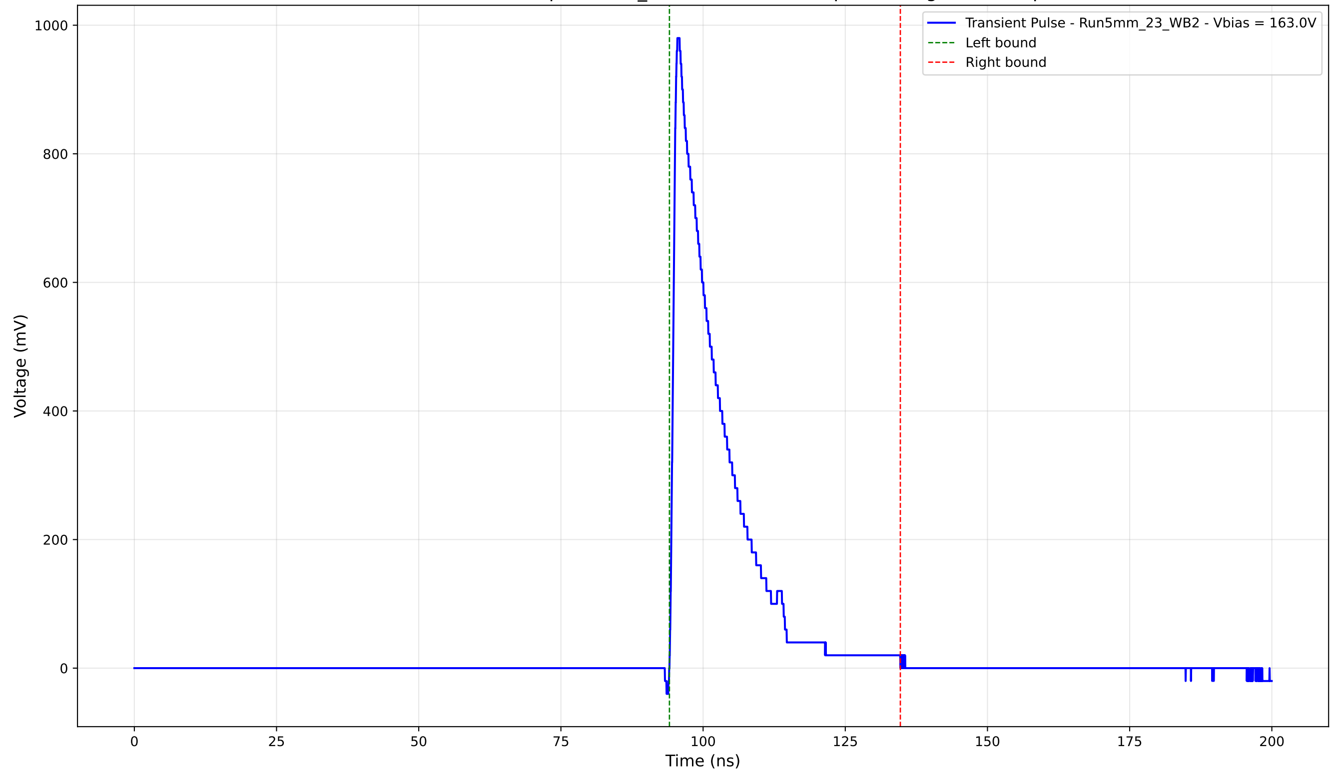
Transient Pulse - Sample: 5mm_23 - Position: 275.0 \mu\text{m} - Charge: 173.26 pC
