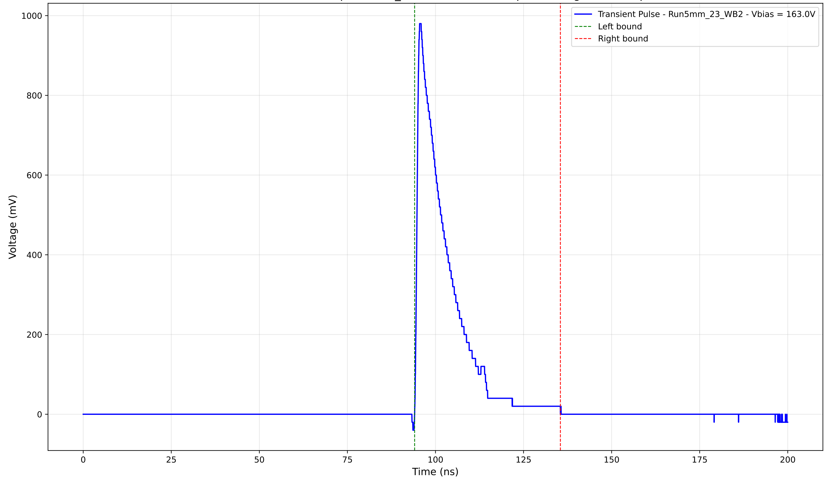
Transient Pulse - Sample: 5mm_23 - Position: 305.0 \mu\text{m} - Charge: 177.20 pC
