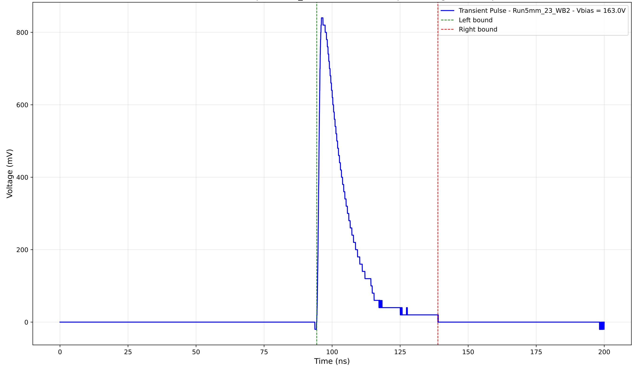
Transient Pulse - Sample: 5mm_23 - Position: 3690.0 \mu\text{m} - Charge: 174.75 pC
