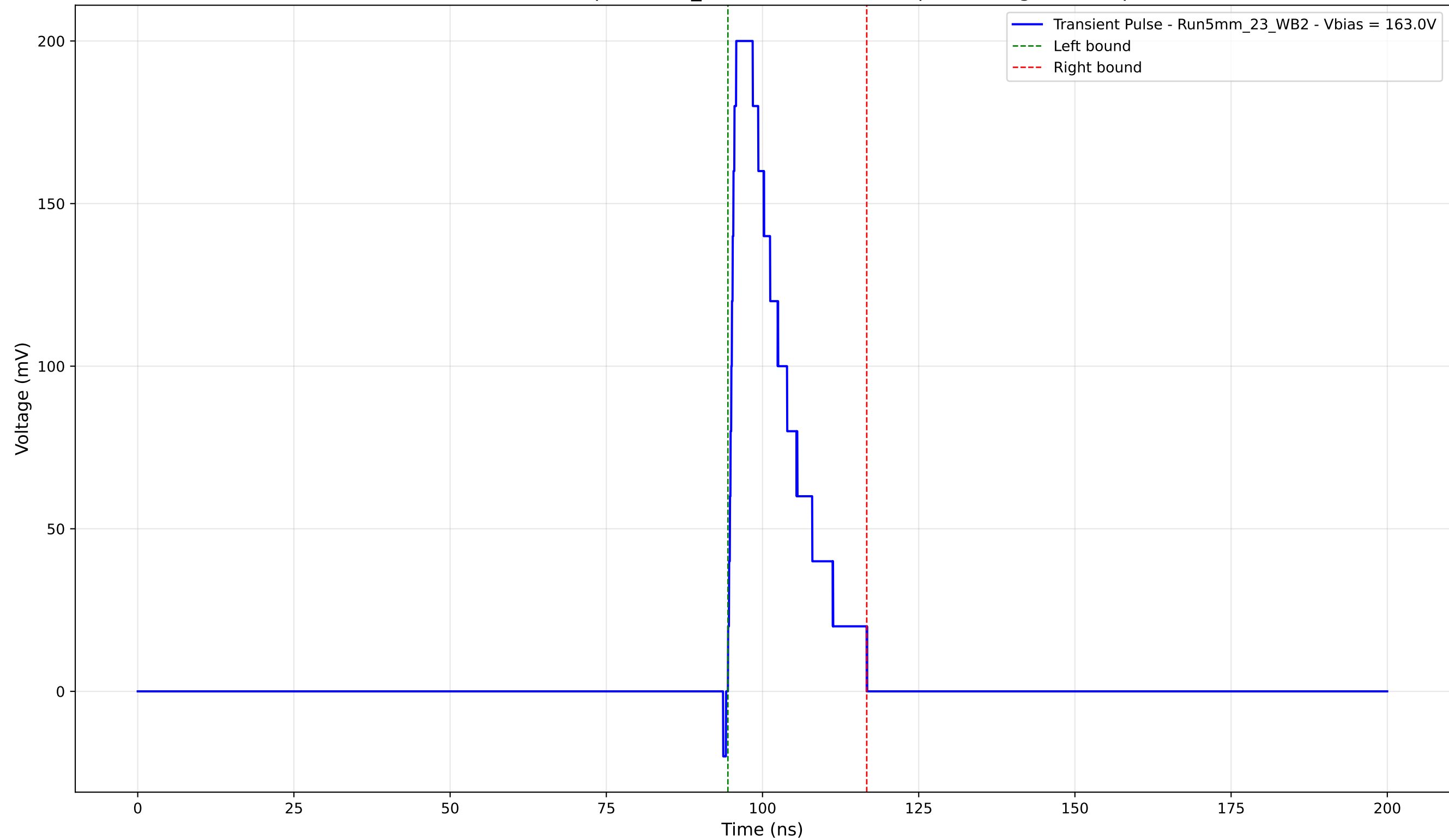
Transient Pulse - Sample: 5mm_23 - Position: 3510.0 \mu\text{m} - Charge: 38.54 pC
