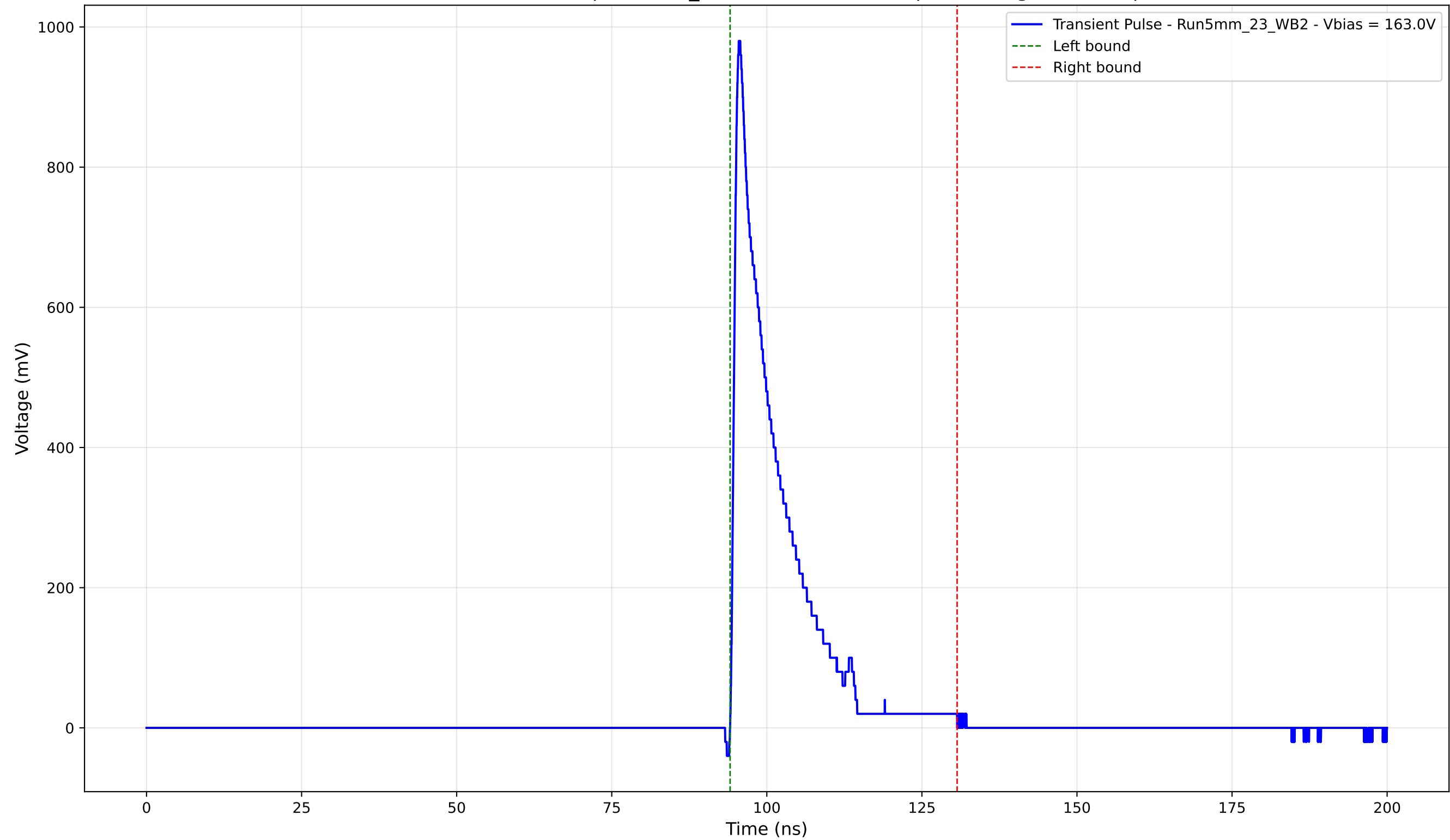
Transient Pulse - Sample: 5mm_23 - Position: 4840.0 \mu\text{m} - Charge: 142.80 pC
