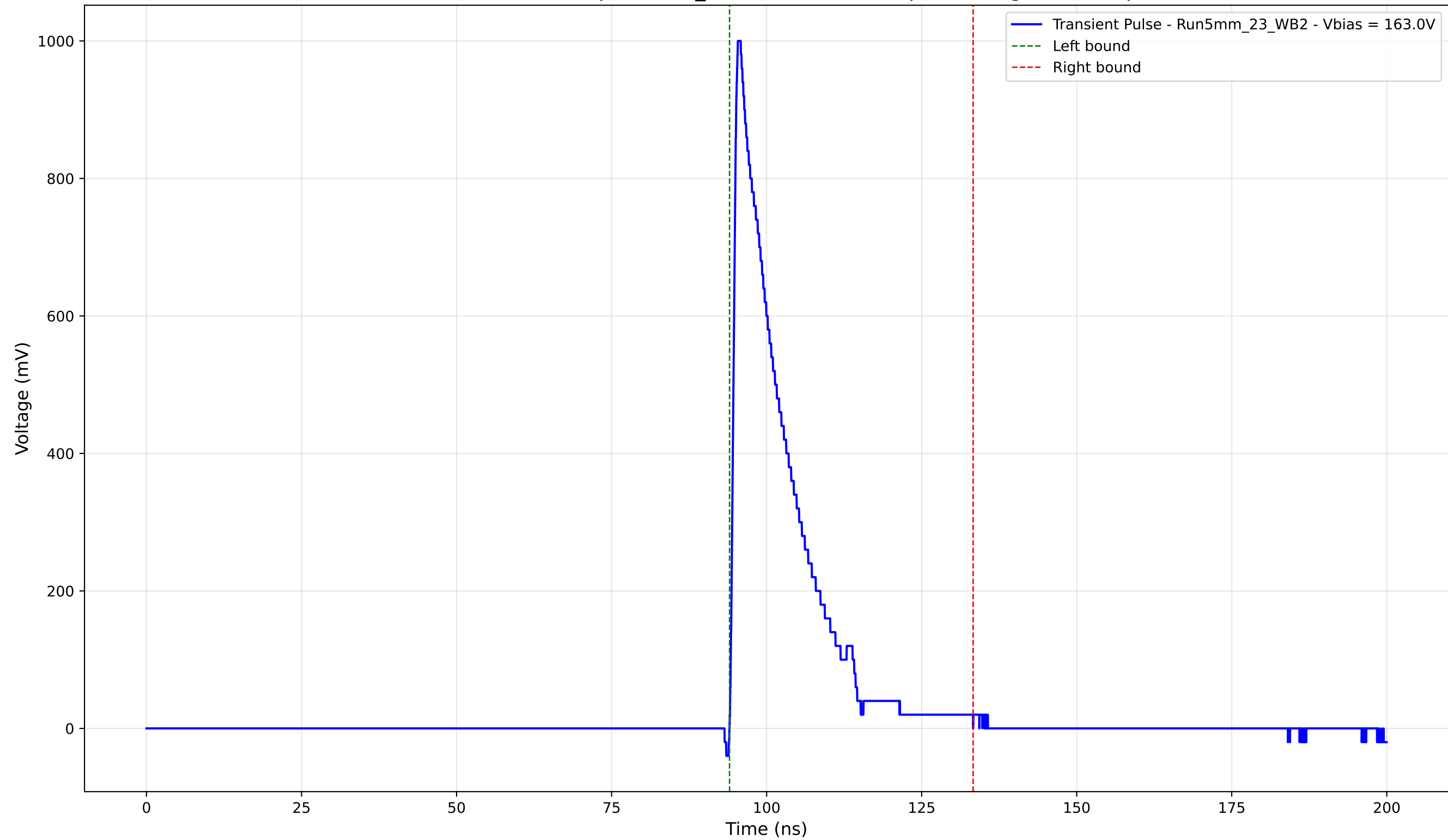
Transient Pulse - Sample: 5mm_23 - Position: 200.0 \mu\text{m} - Charge: 176.66 pC
