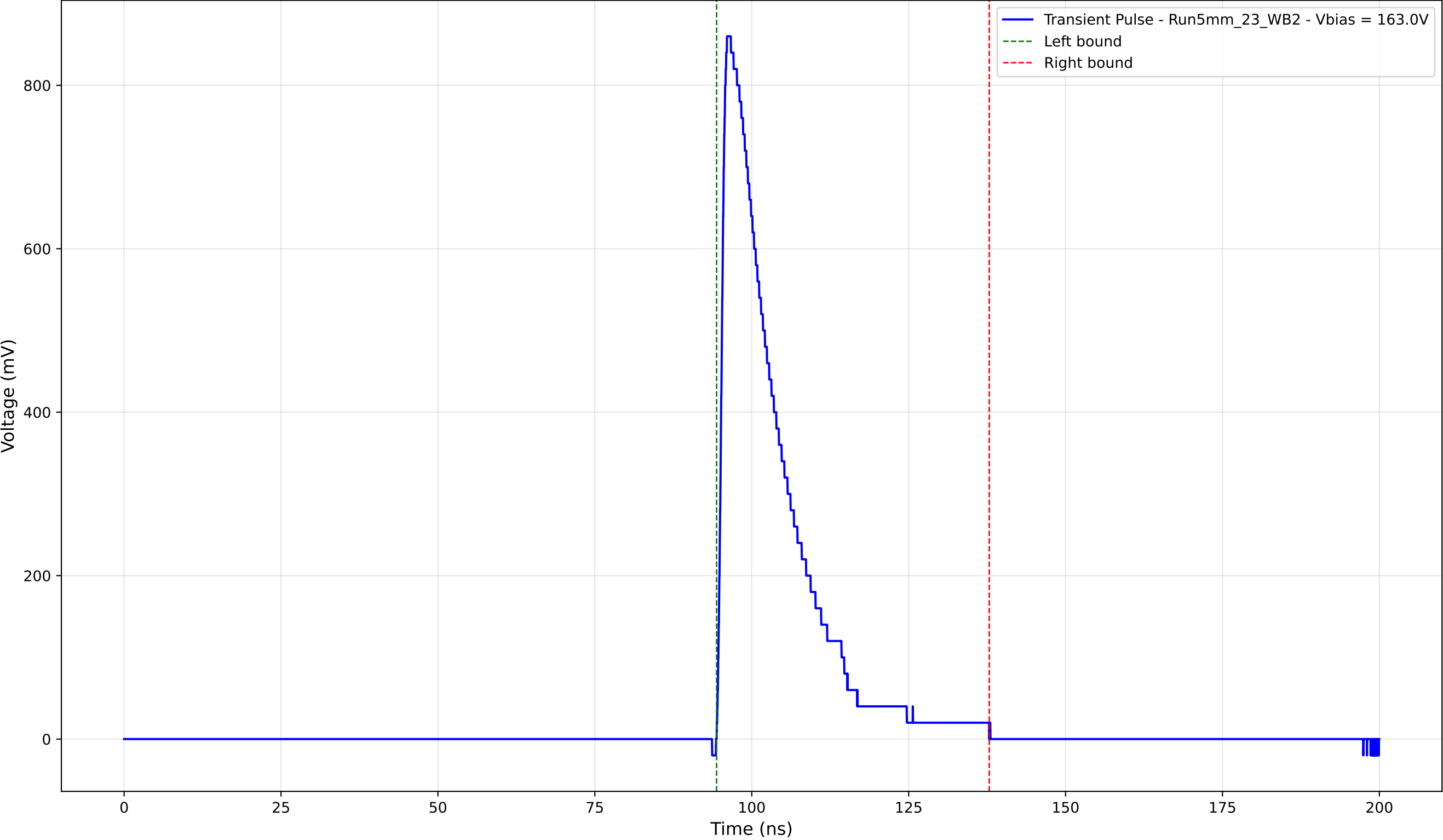
Transient Pulse - Sample: 5mm_23 - Position: 3825.0 \mu\text{m} - Charge: 175.15 pC
