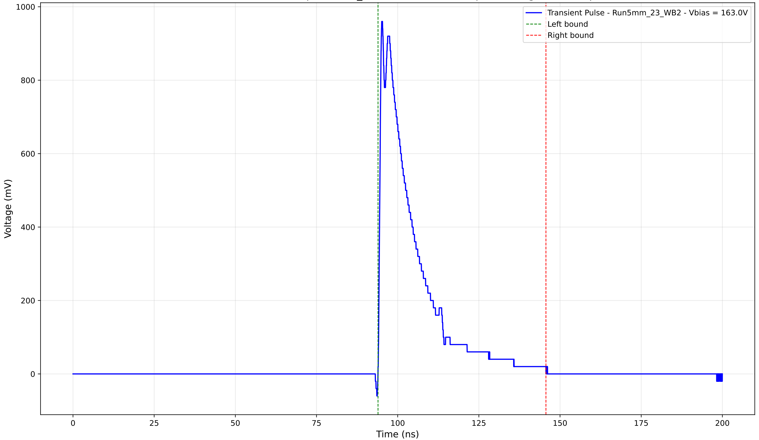
Transient Pulse - Sample: 5mm_23 - Position: 2880.0 \mu\text{m} - Charge: 217.18 pC
