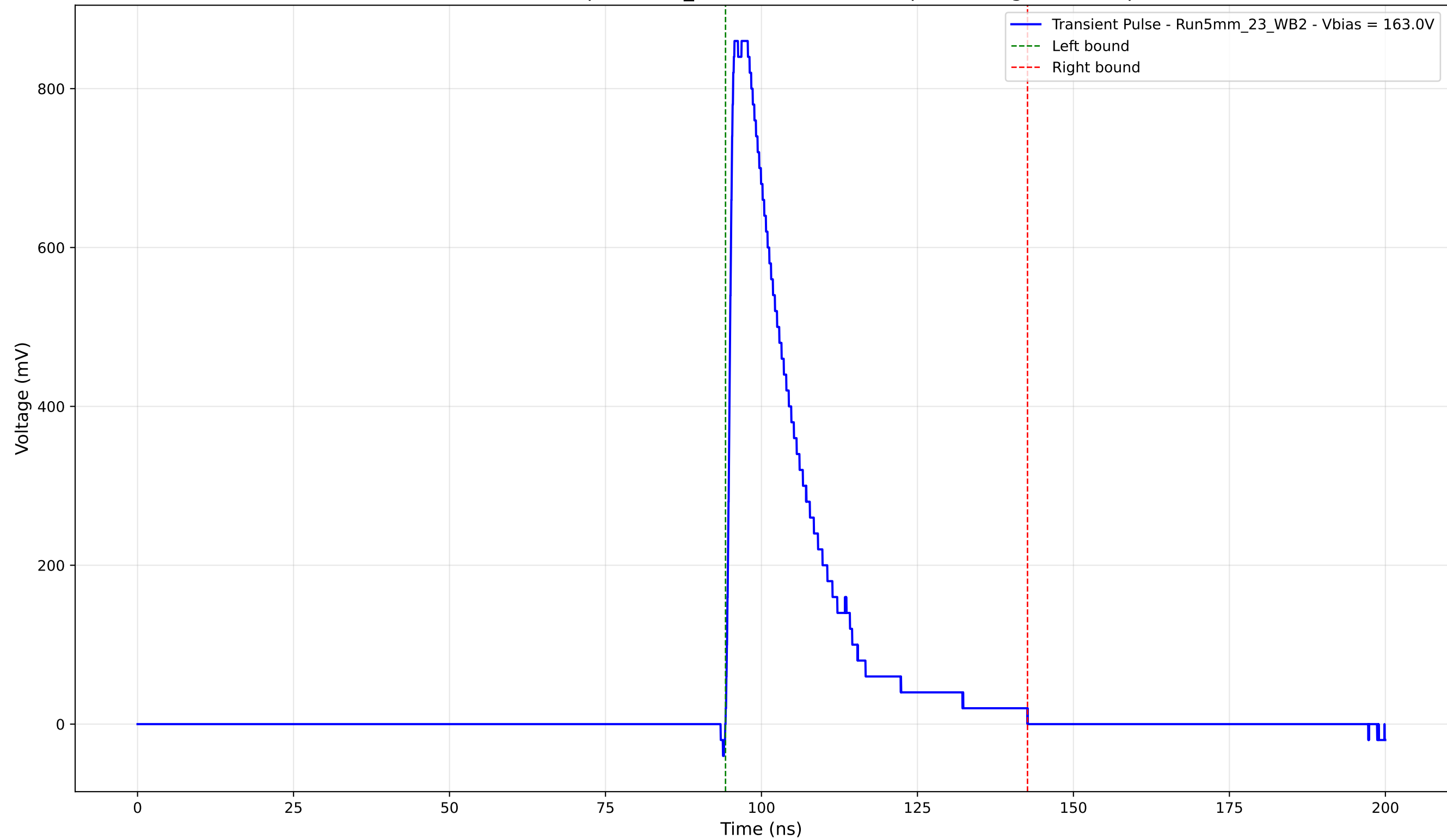
Transient Pulse - Sample: 5mm_23 - Position: 1630.0 \mu\text{m} - Charge: 200.05 pC
