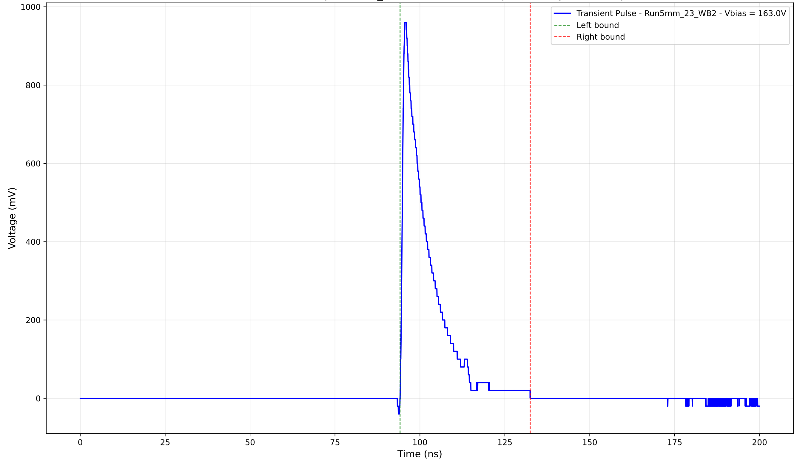
Transient Pulse - Sample: 5mm_23 - Position: 4695.0 \mu\text{m} - Charge: 154.66 pC
