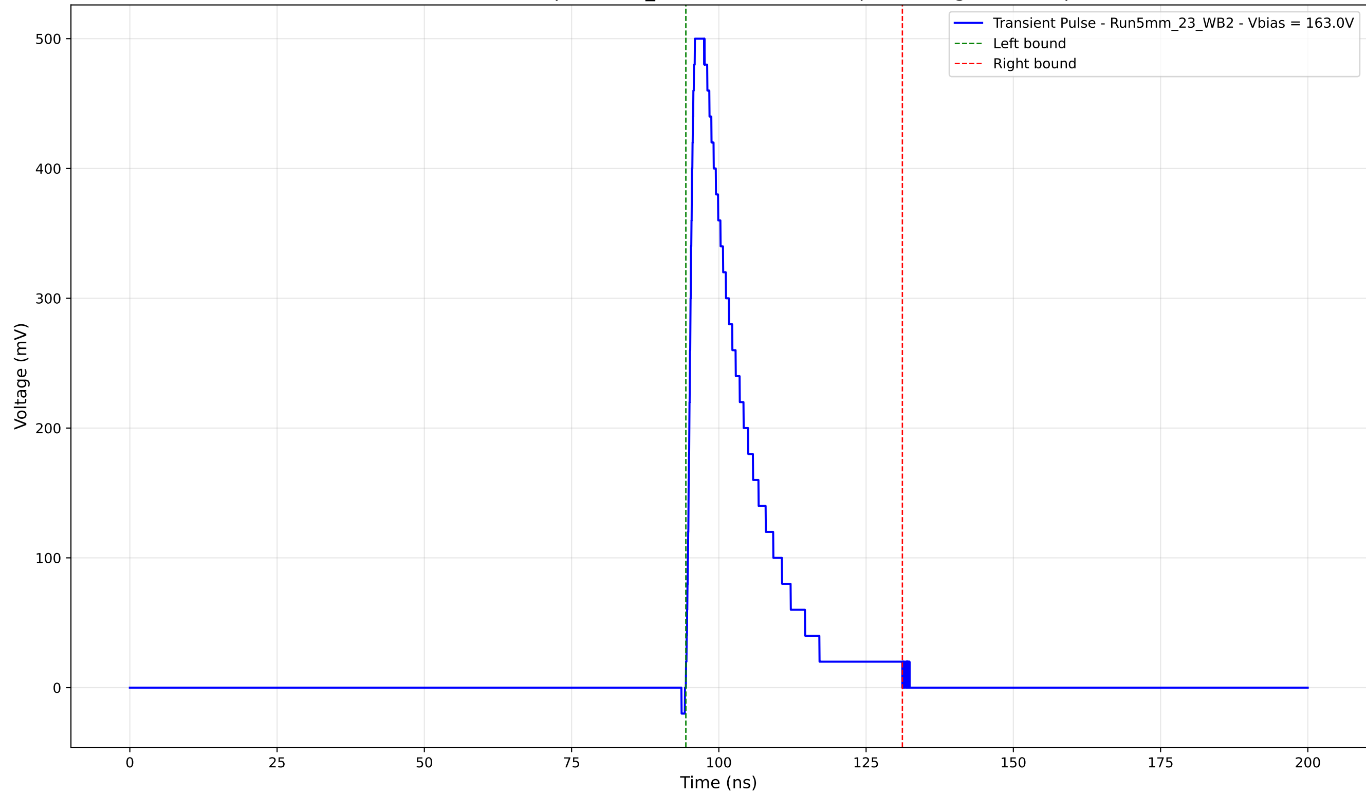
Transient Pulse - Sample: 5mm_23 - Position: 1455.0 \mu\text{m} - Charge: 100.22 pC
