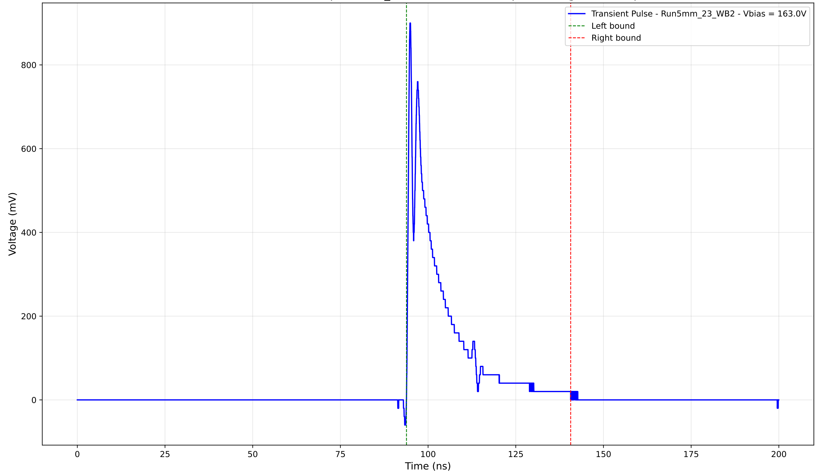
Transient Pulse - Sample: 5mm_23 - Position: 2455.0 \mu\text{m} - Charge: 145.30 pC
