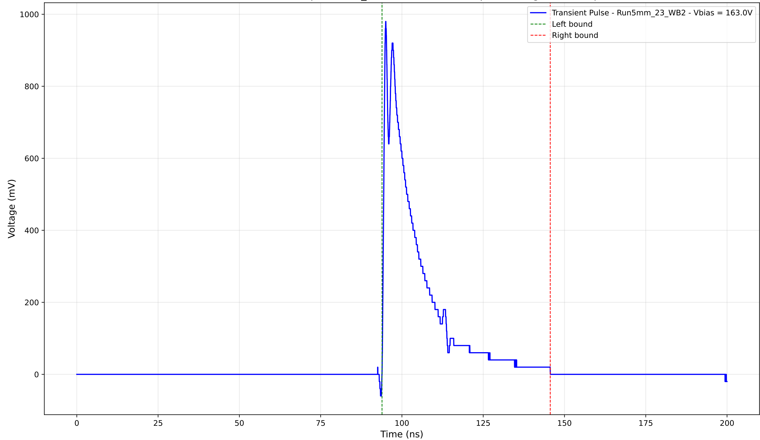
Transient Pulse - Sample: 5mm_23 - Position: 2730.0 \mu\text{m} - Charge: 202.39 pC
