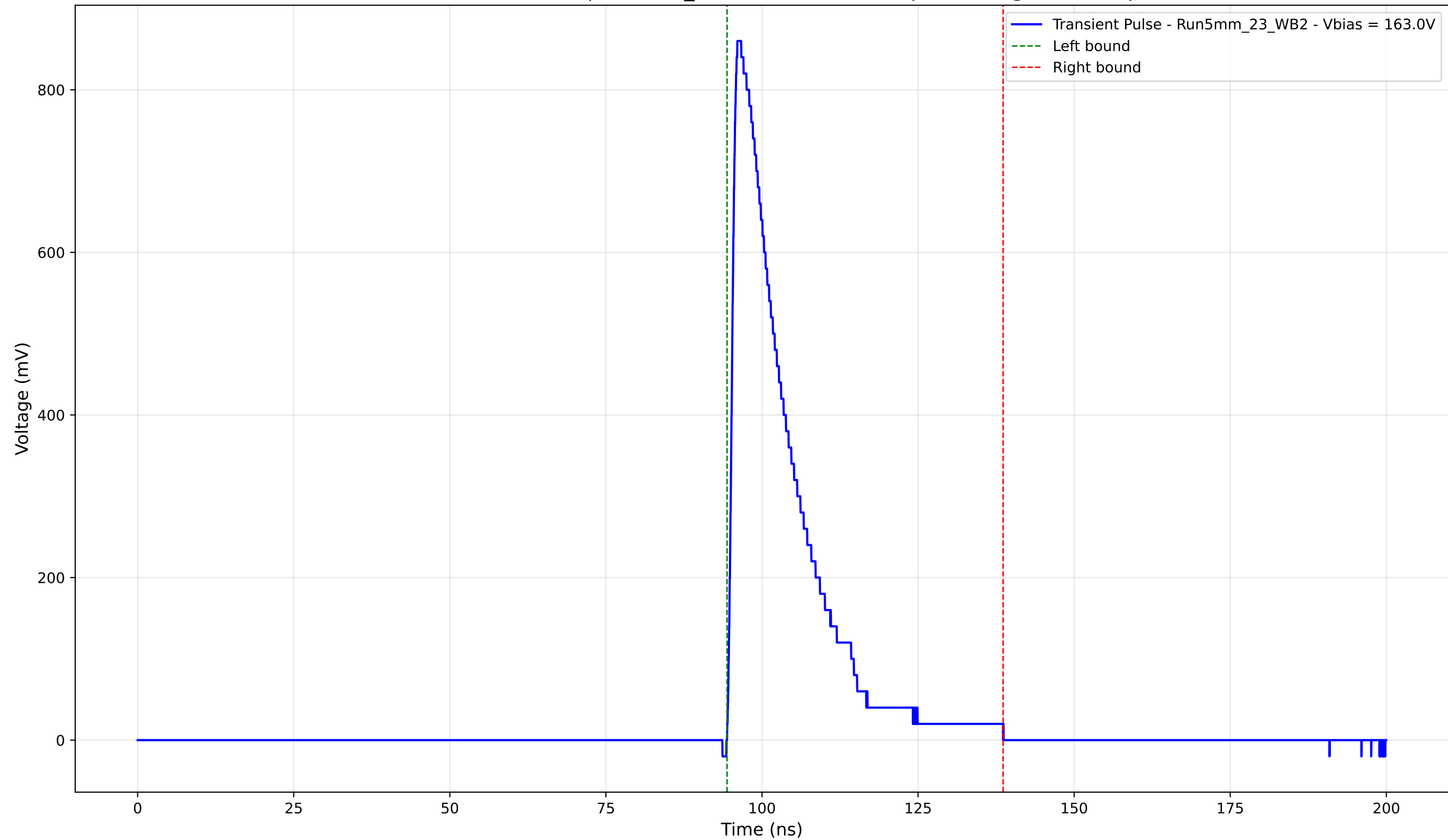
Transient Pulse - Sample: 5mm_23 - Position: 3845.0 \mu\text{m} - Charge: 174.34 pC
