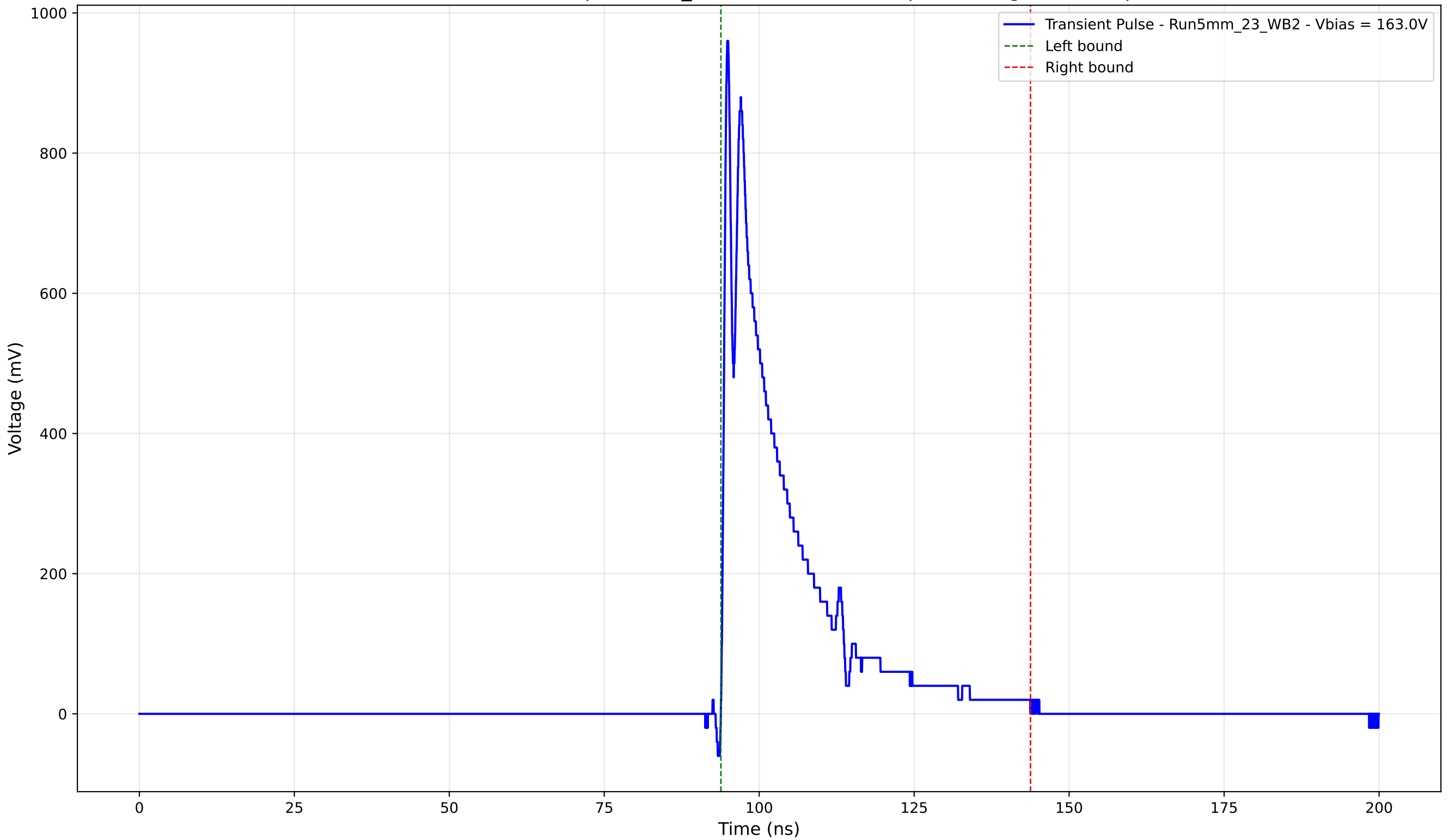
Transient Pulse - Sample: 5mm_23 - Position: 2435.0 \mu\text{m} - Charge: 178.37 pC
