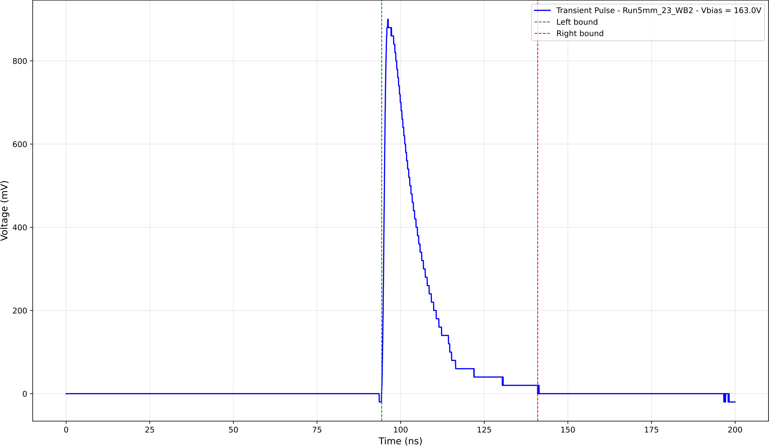
Transient Pulse - Sample: 5mm_23 - Position: 1355.0 \mu\text{m} - Charge: 199.52 pC
