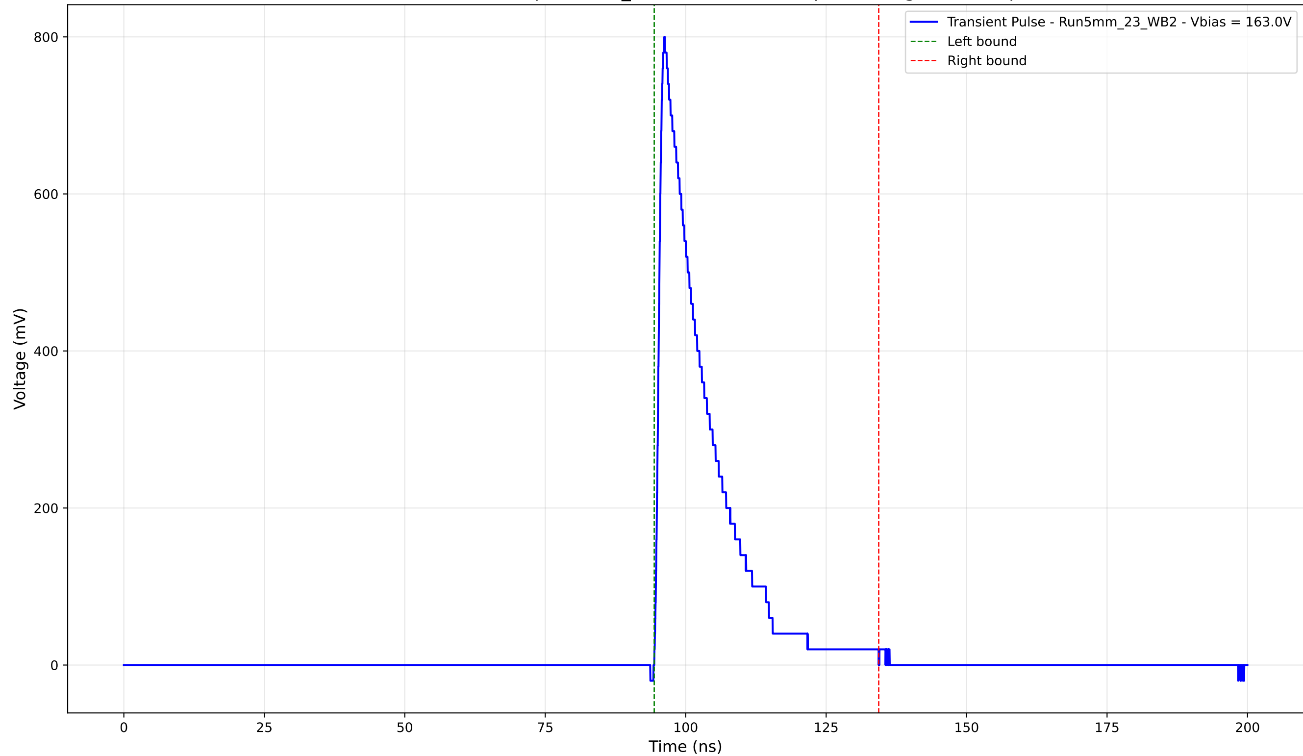
Transient Pulse - Sample: 5mm_23 - Position: 920.0 \mu\text{m} - Charge: 147.53 pC
