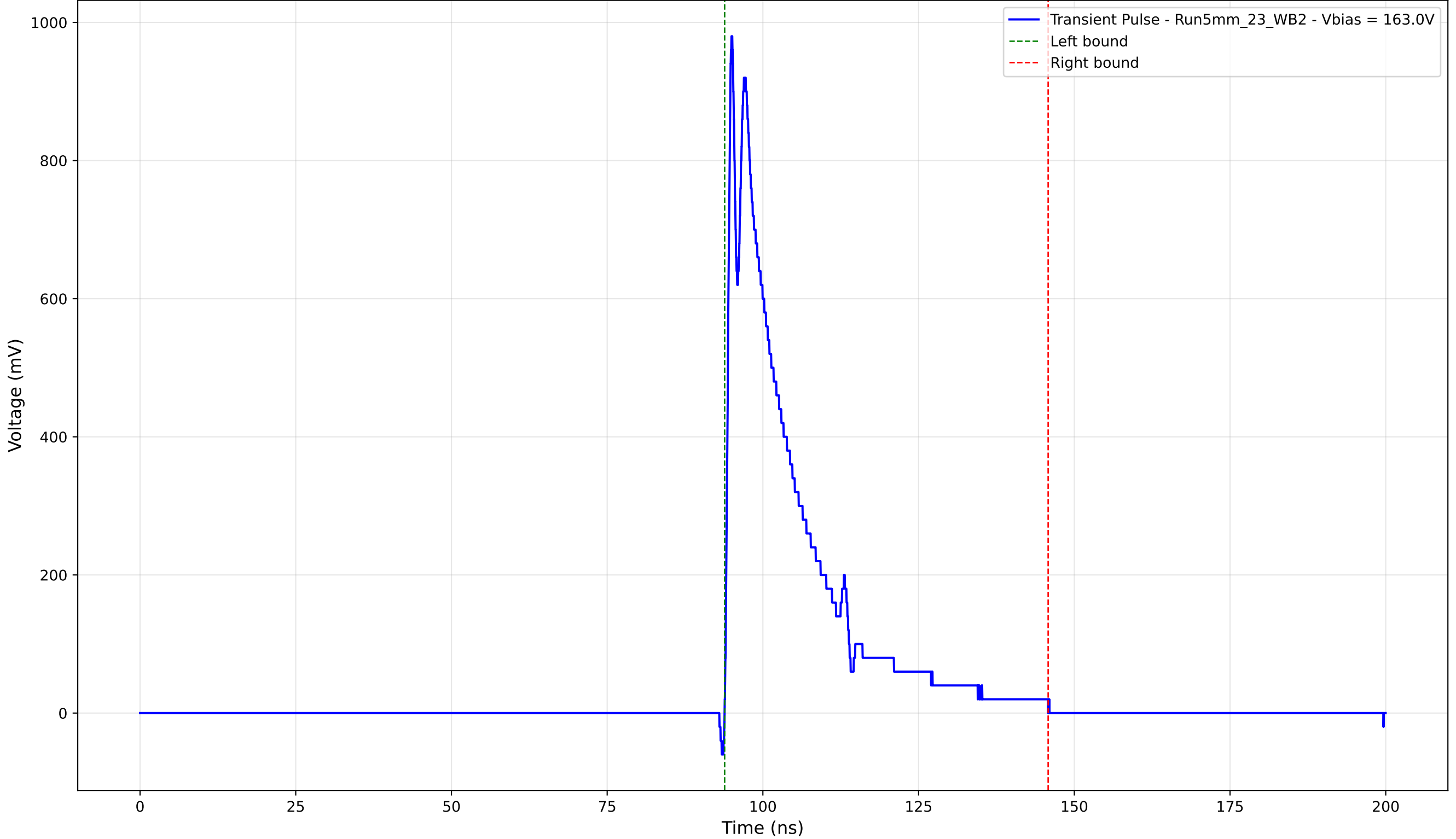
Transient Pulse - Sample: 5mm_23 - Position: 2705.0 \mu\text{m} - Charge: 201.95 pC
