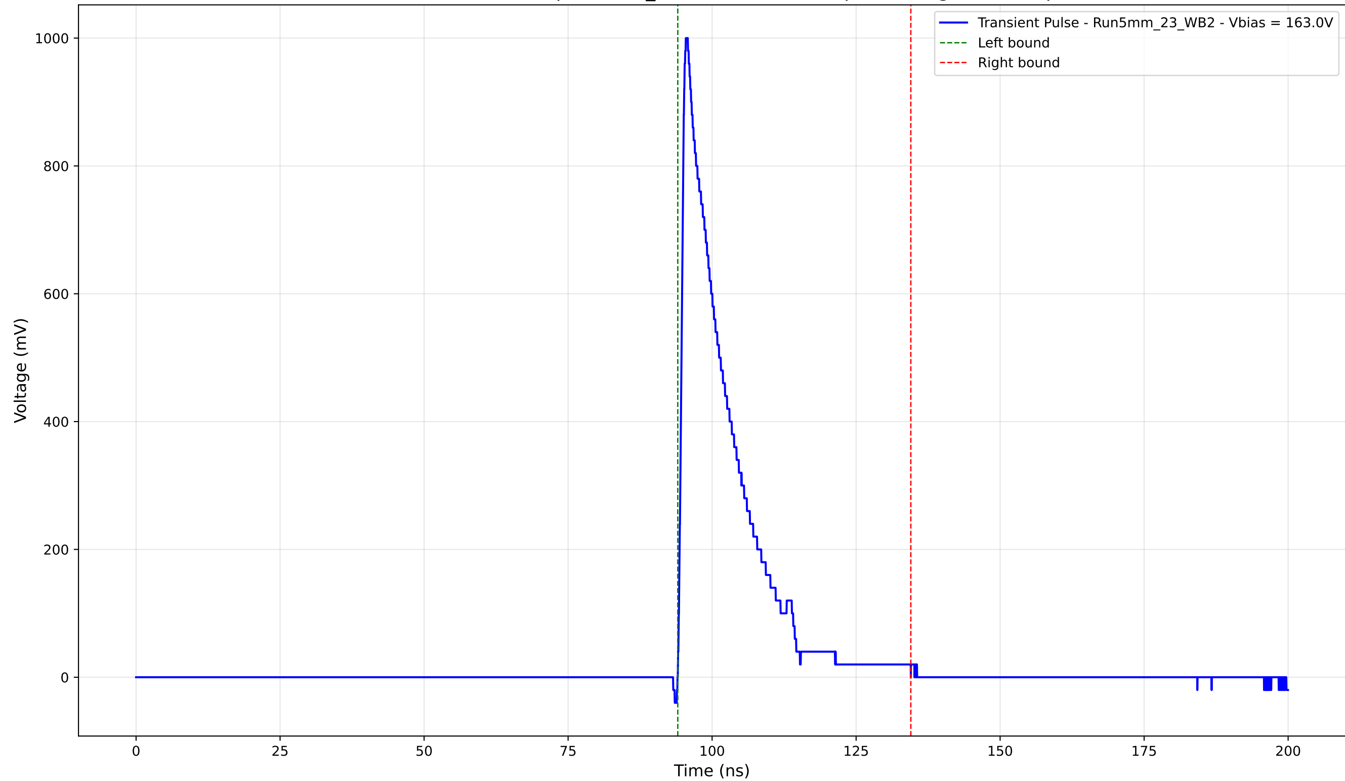
Transient Pulse - Sample: 5mm_23 - Position: 215.0 \mu\text{m} - Charge: 174.60 pC
