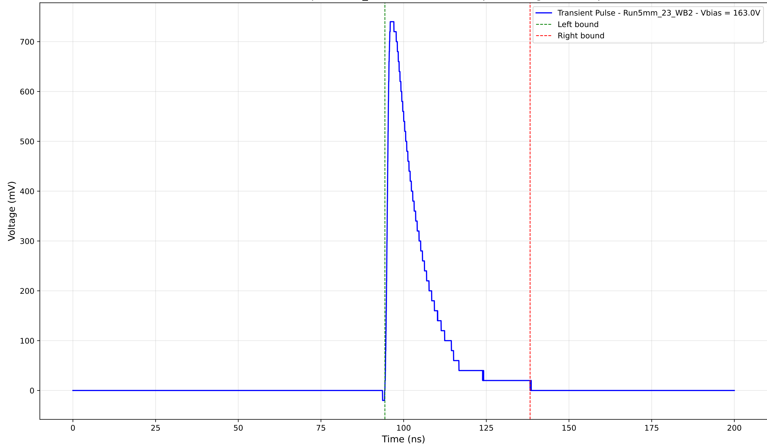
Transient Pulse - Sample: 5mm_23 - Position: 1430.0 \mu\text{m} - Charge: 155.27 pC
