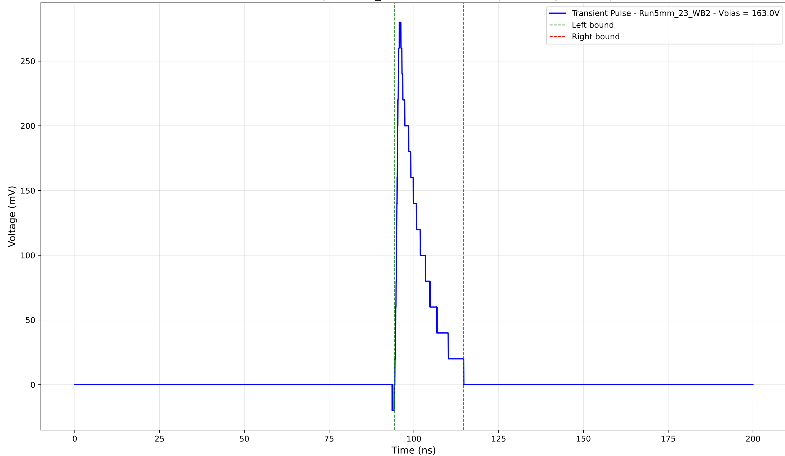
Transient Pulse - Sample: 5mm_23 - Position: 4555.0 \mu\text{m} - Charge: 38.54 pC
