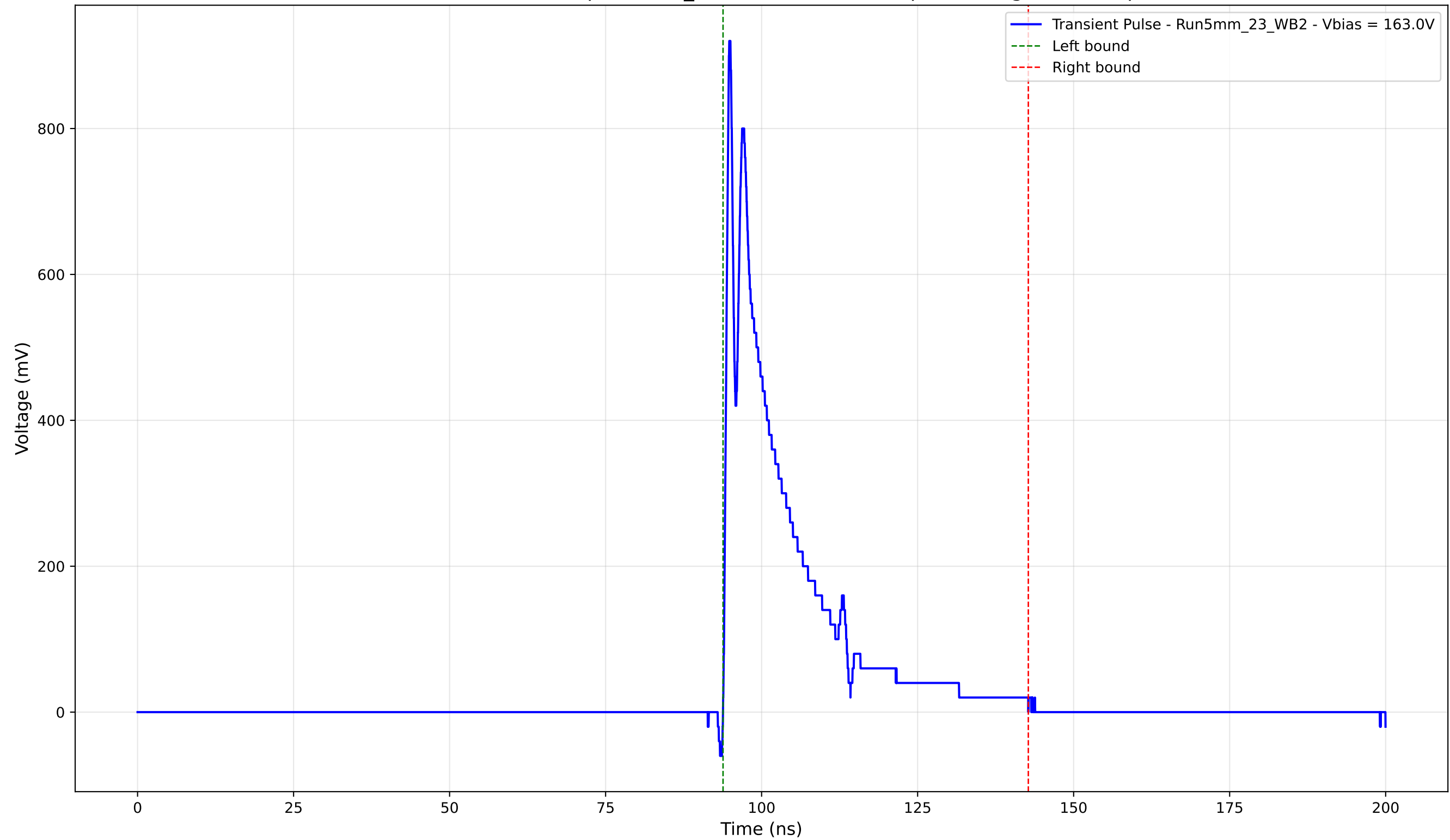
Transient Pulse - Sample: 5mm_23 - Position: 2585.0 \mu\text{m} - Charge: 158.03 pC
