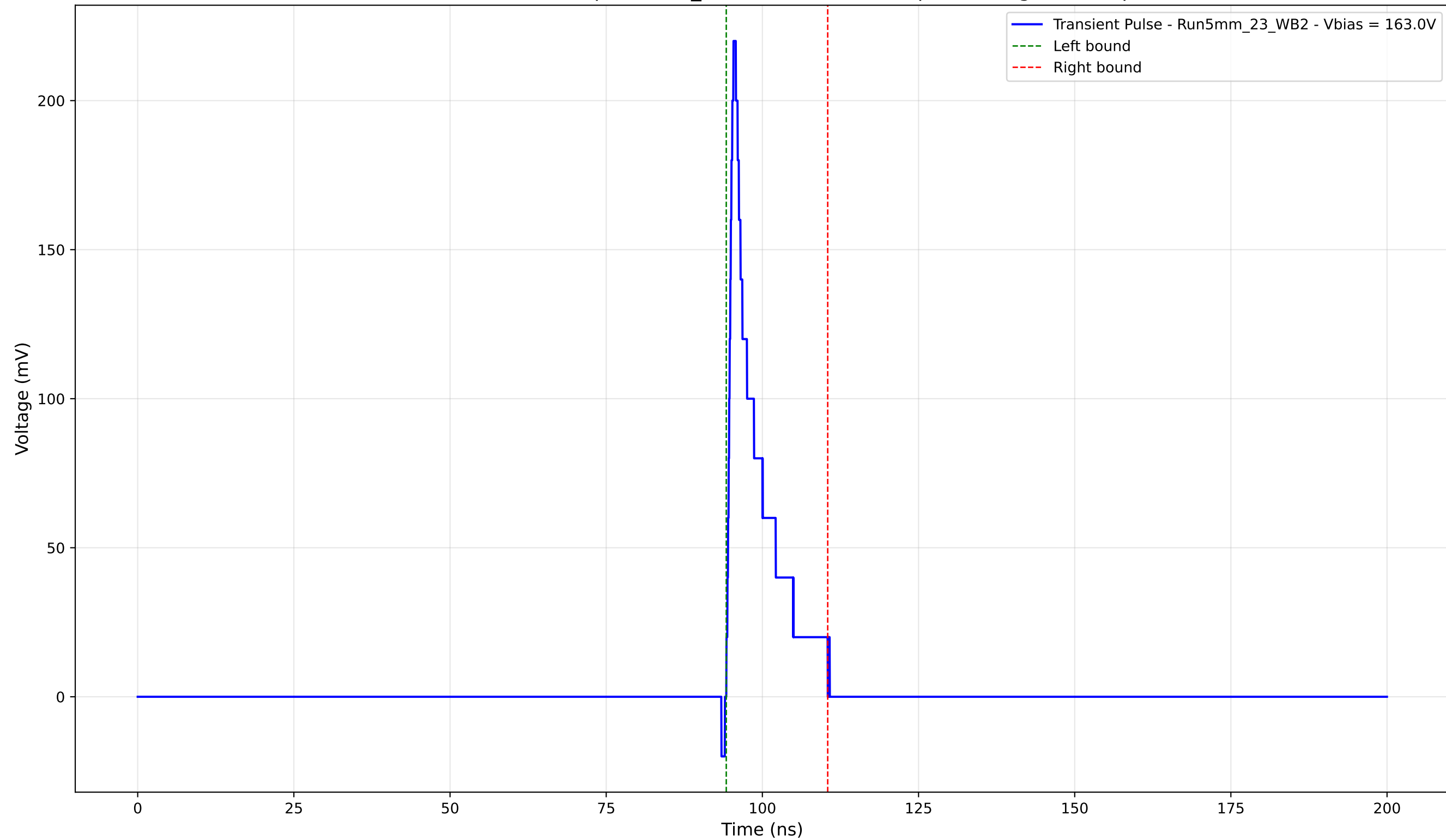
Transient Pulse - Sample: 5mm_23 - Position: 4960.0 \mu\text{m} - Charge: 21.03 pC
