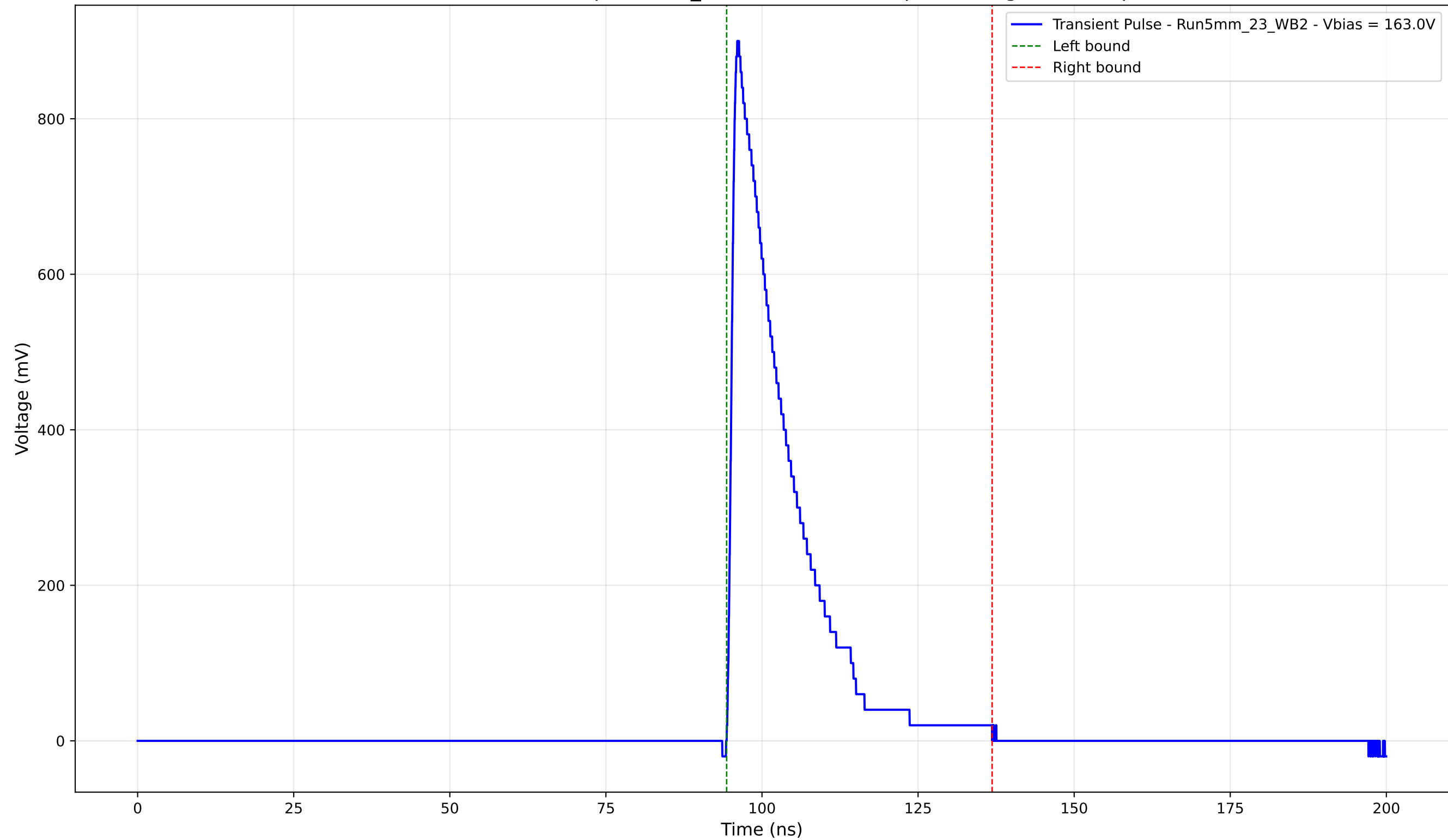
Transient Pulse - Sample: 5mm_23 - Position: 770.0 \mu\text{m} - Charge: 173.78 pC
