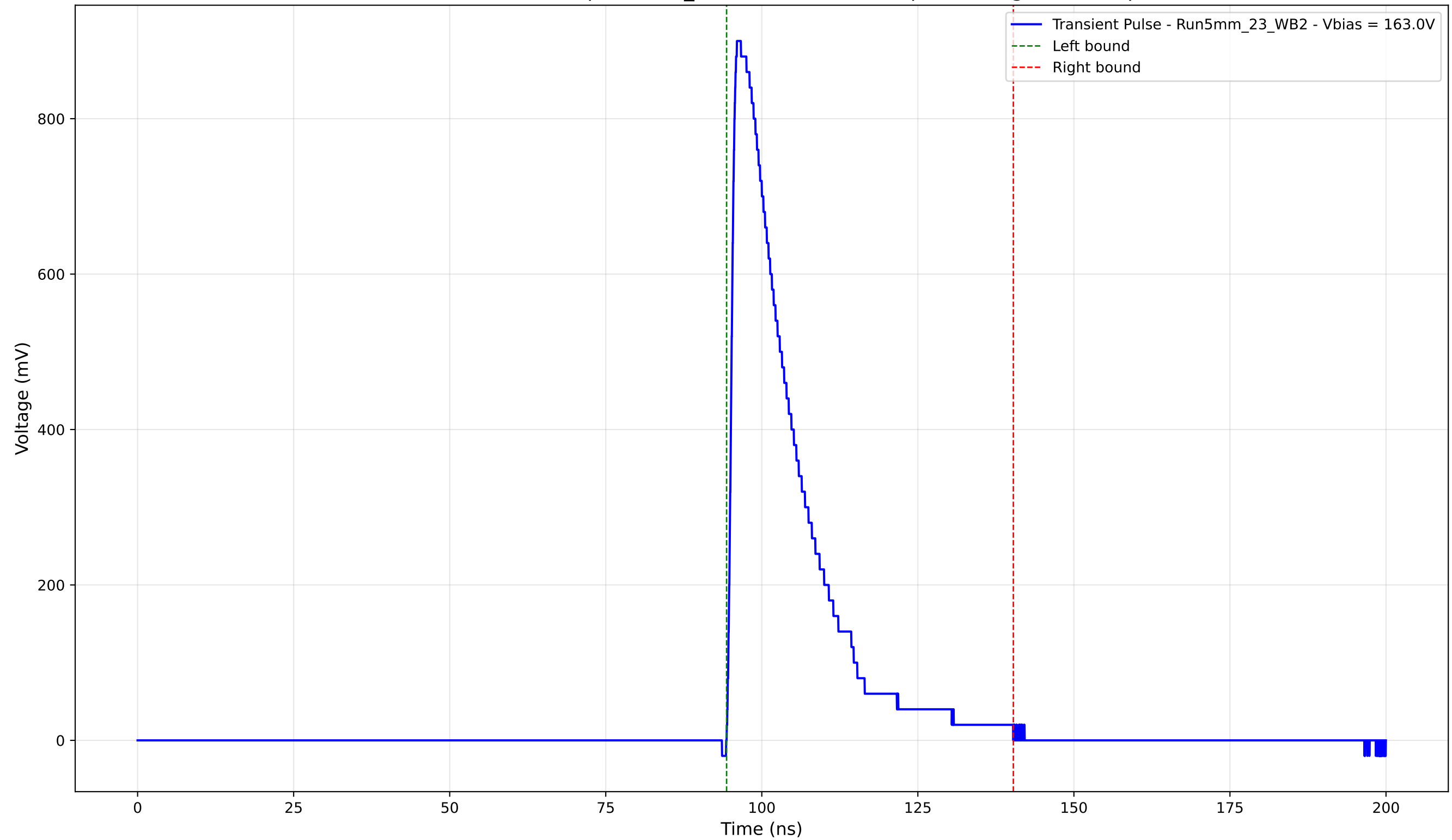
Transient Pulse - Sample: 5mm_23 - Position: 1290.0 \mu\text{m} - Charge: 200.81 pC
