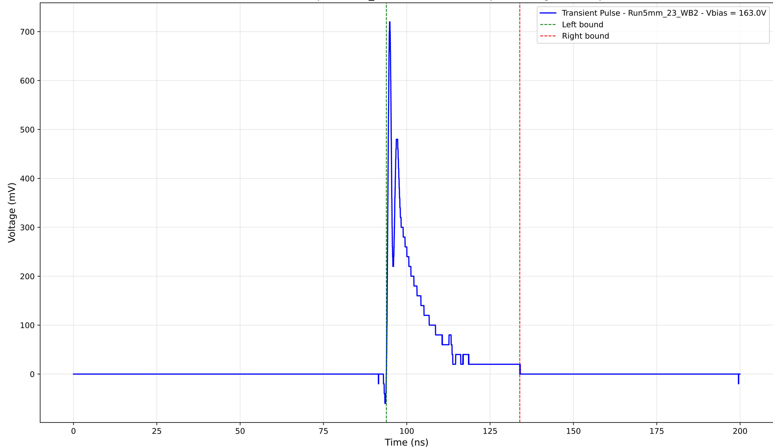
Transient Pulse - Sample: 5mm_23 - Position: 2480.0 \mu\text{m} - Charge: 87.90 pC
