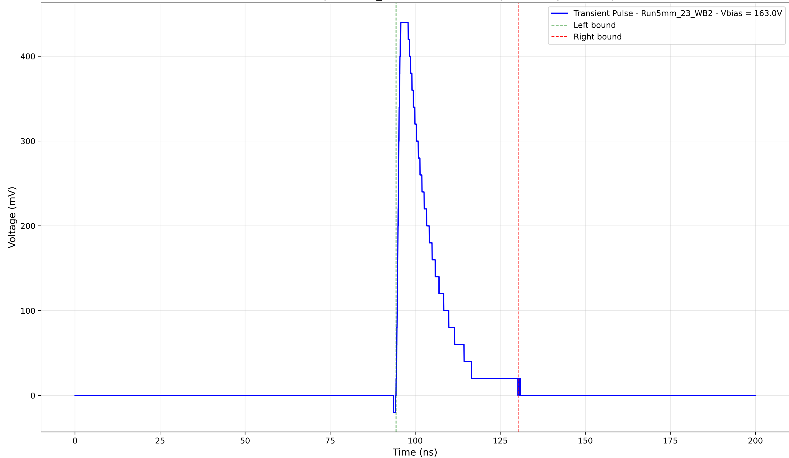
Transient Pulse - Sample: 5mm_23 - Position: 1540.0 \mu\text{m} - Charge: 90.54 pC
