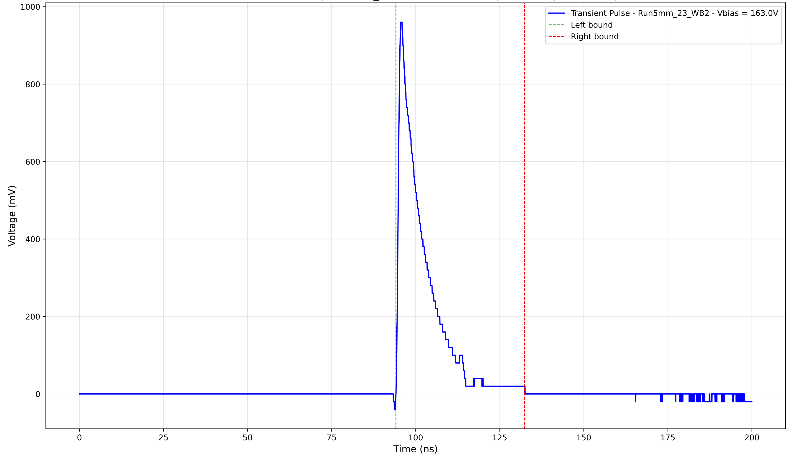
Transient Pulse - Sample: 5mm_23 - Position: 4715.0 \mu\text{m} - Charge: 152.70 pC
