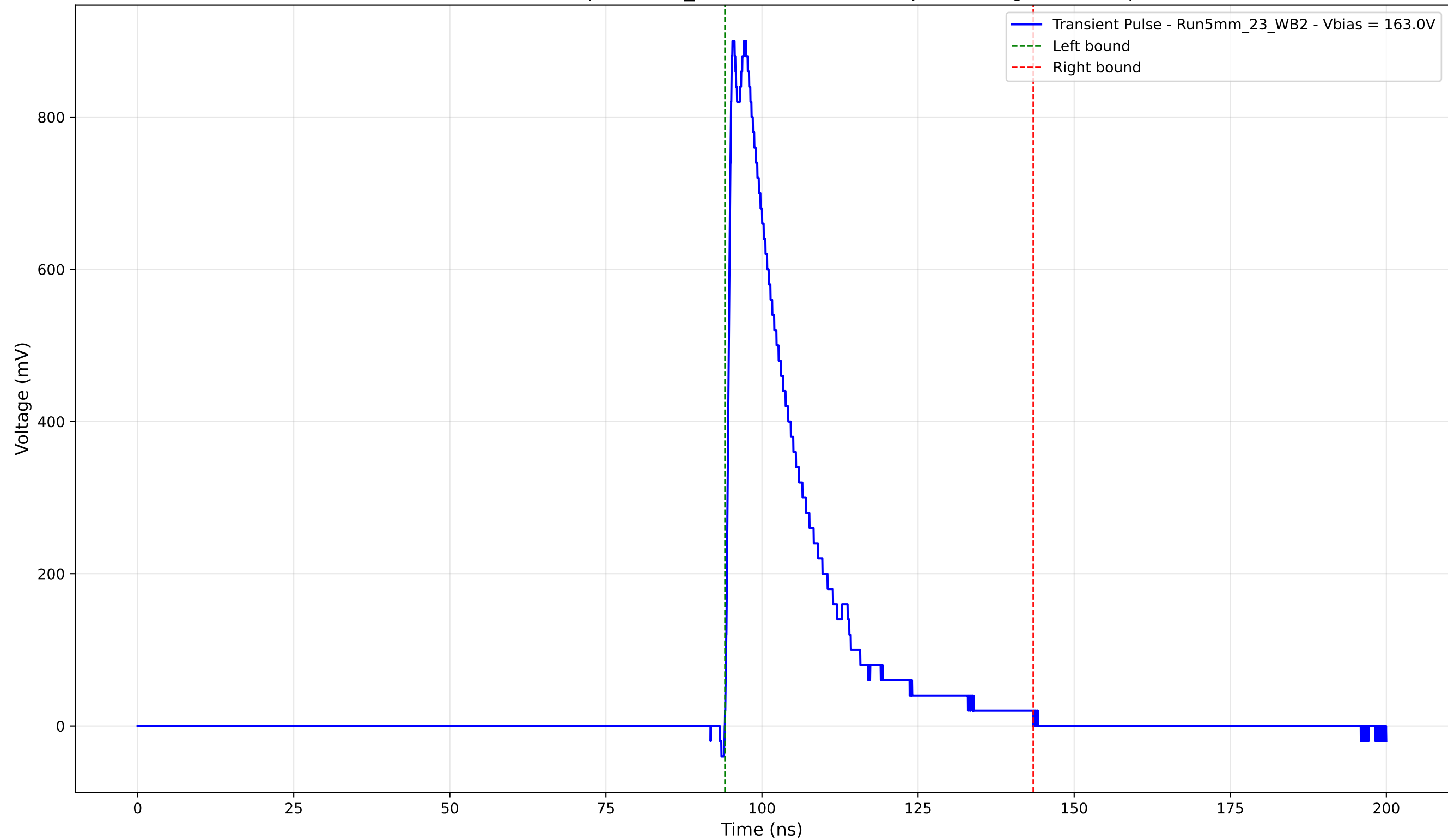
Transient Pulse - Sample: 5mm_23 - Position: 3105.0 \mu\text{m} - Charge: 206.38 pC
