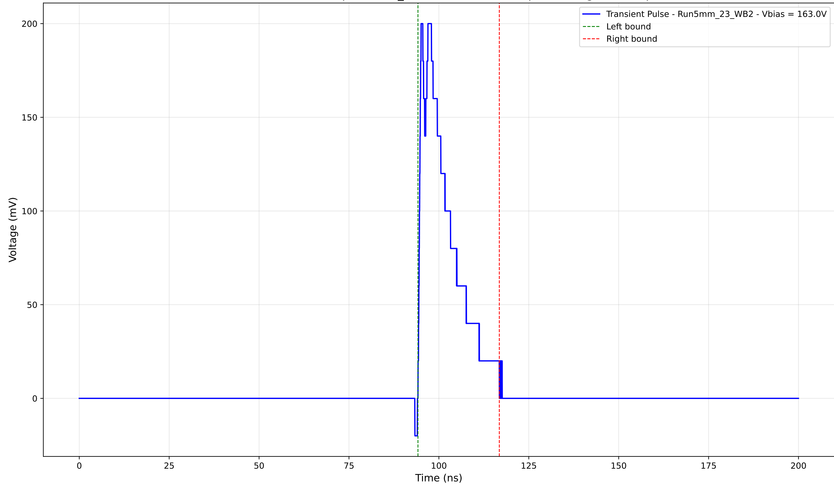
Transient Pulse - Sample: 5mm_23 - Position: 3020.0 \mu\text{m} - Charge: 37.25 pC
