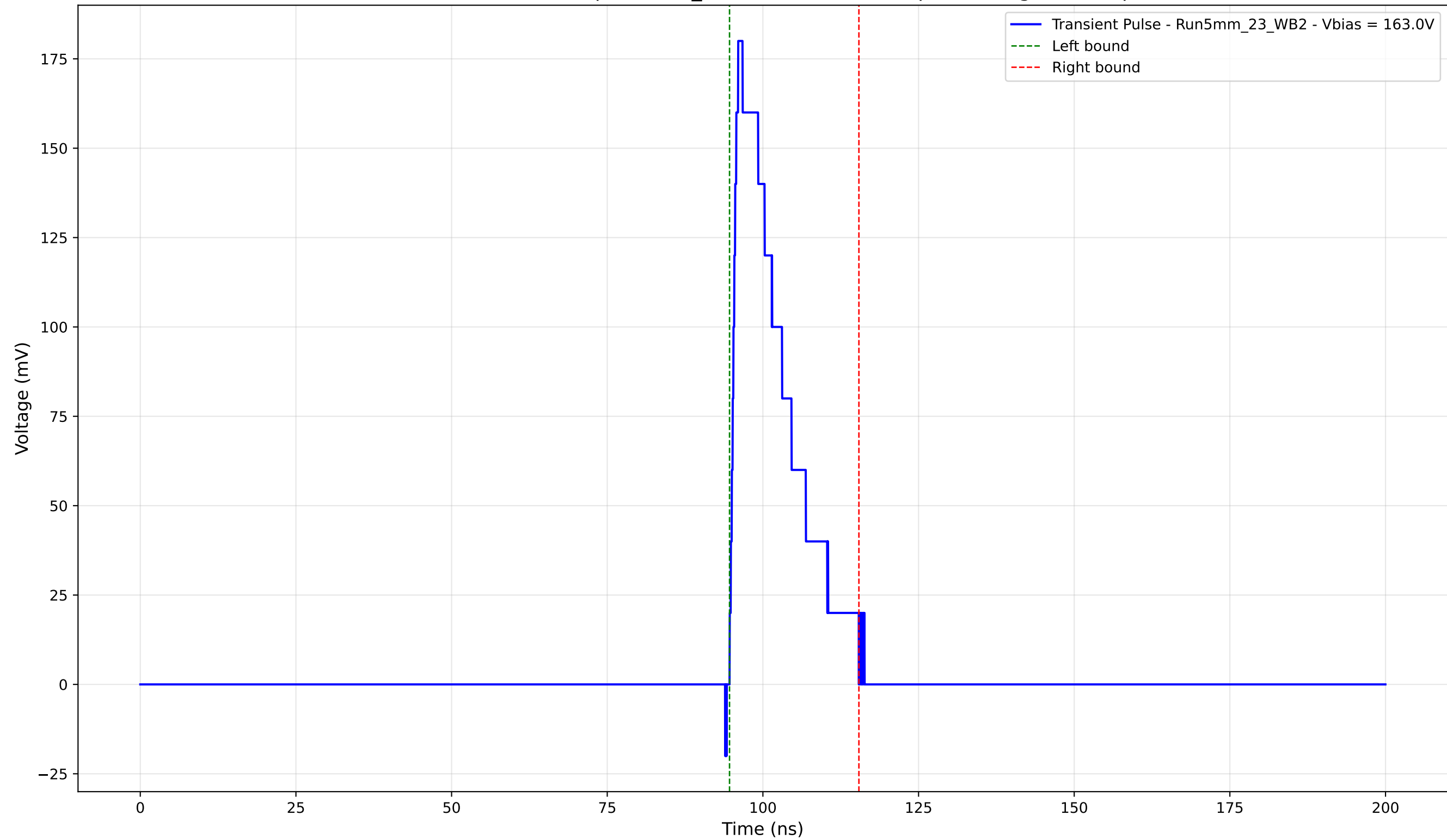
Transient Pulse - Sample: 5mm_23 -Position: 1000.0 \mu\text{m} - Charge: 32.22 pC
