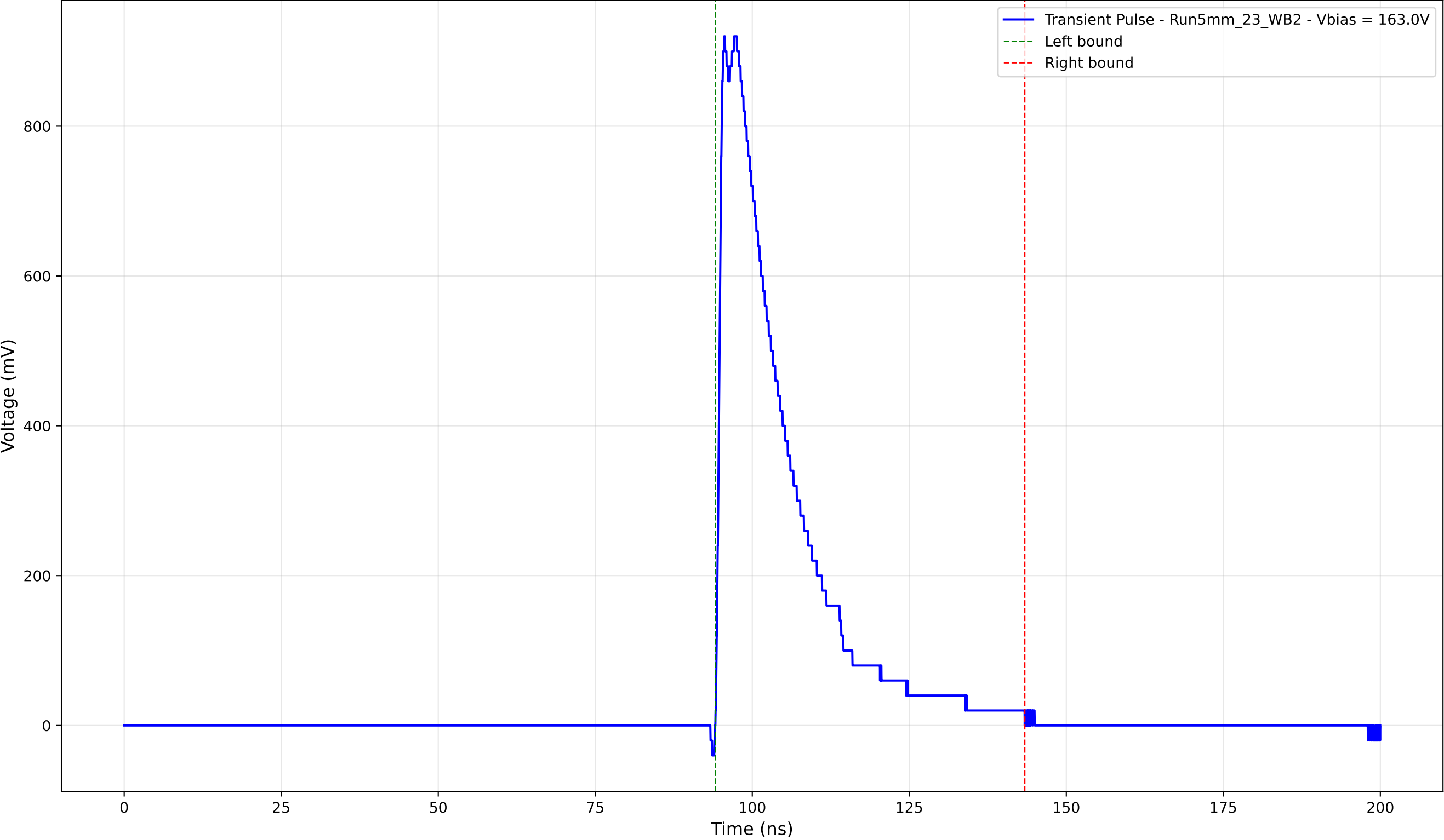
Transient Pulse - Sample: 5mm_23 - Position: 3220.0 \mu\text{m} - Charge: 216.52 pC
