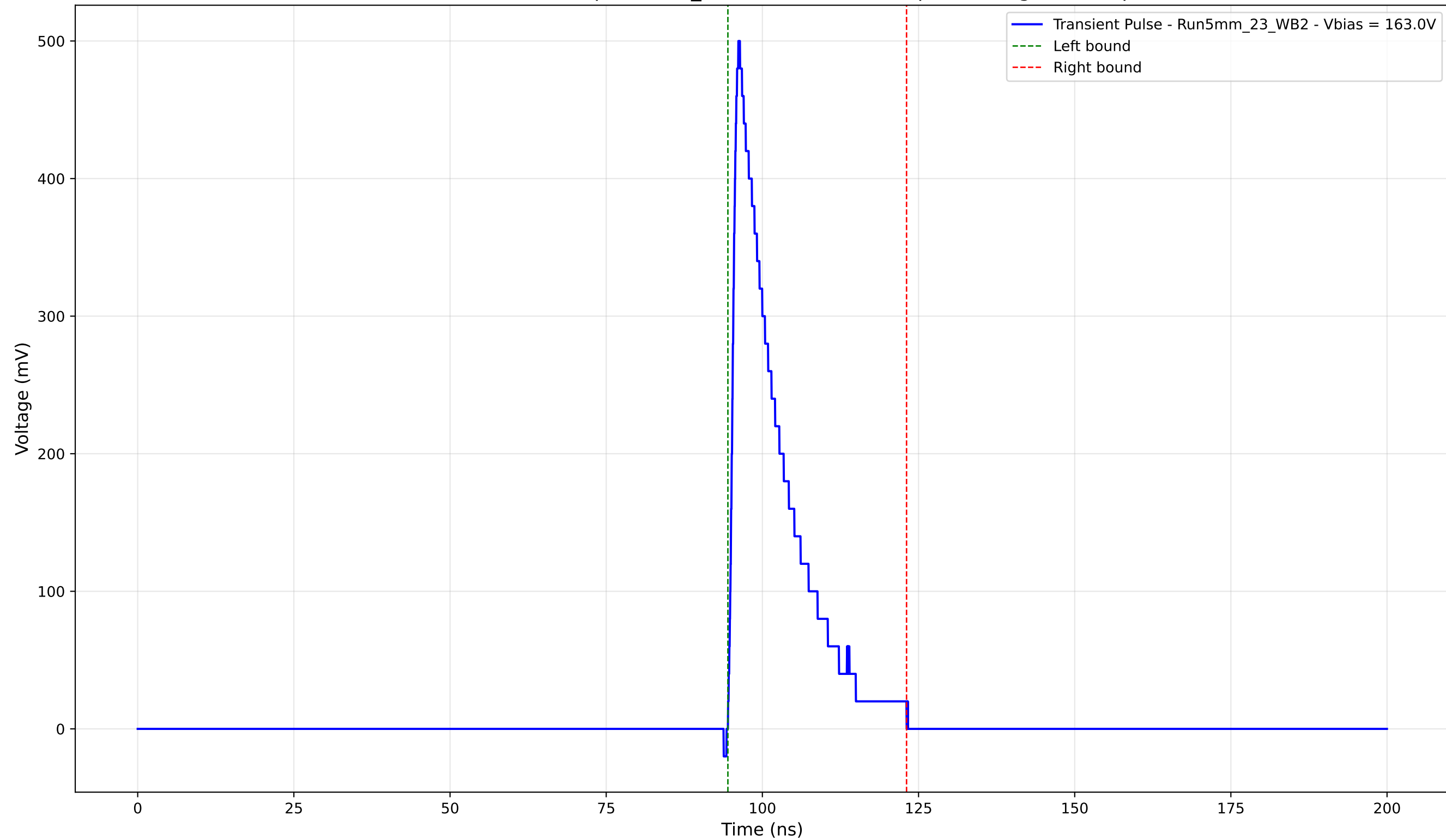
Transient Pulse - Sample: 5mm_23 - Position: 4080.0 \mu\text{m} - Charge: 81.34 pC
