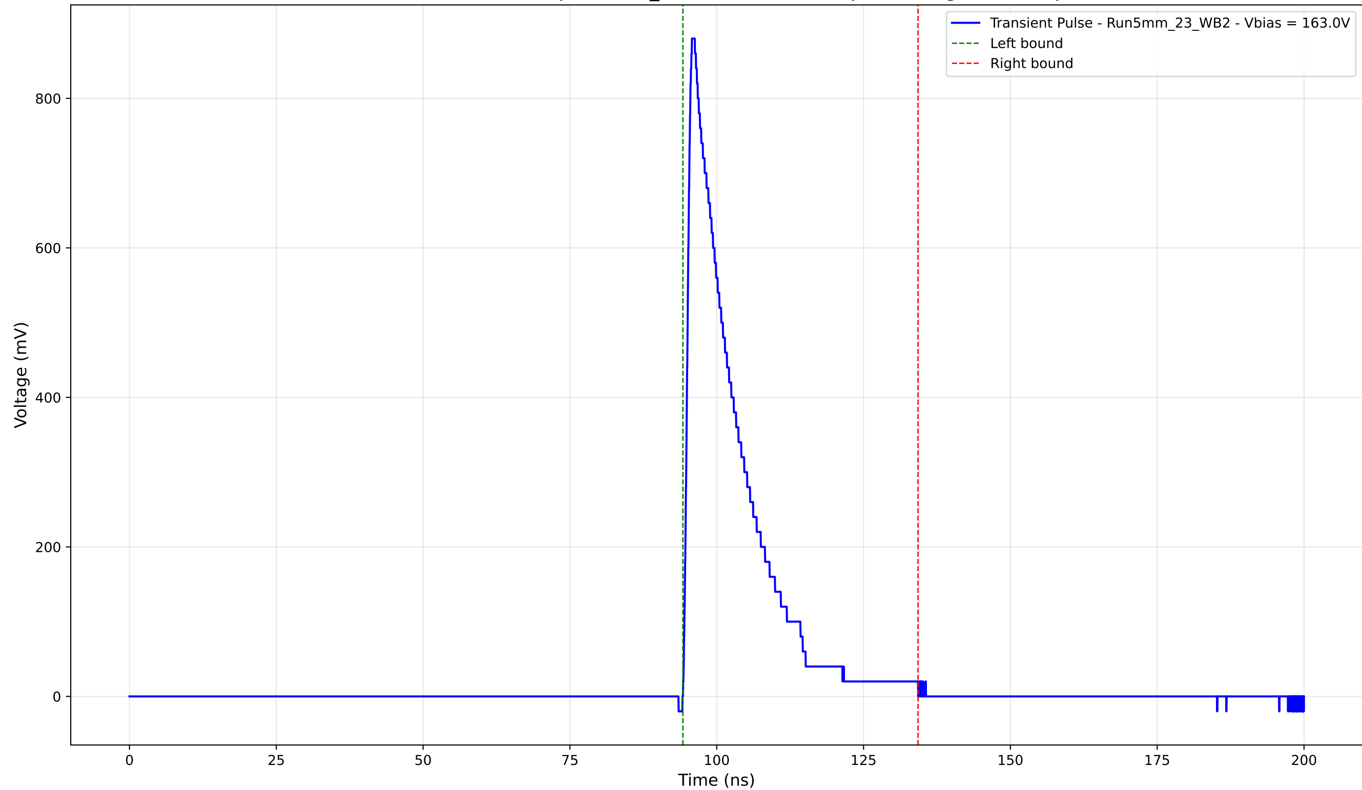
Transient Pulse - Sample: 5mm_23 - Position: 560.0 \mu\text{m} - Charge: 159.02 pC
