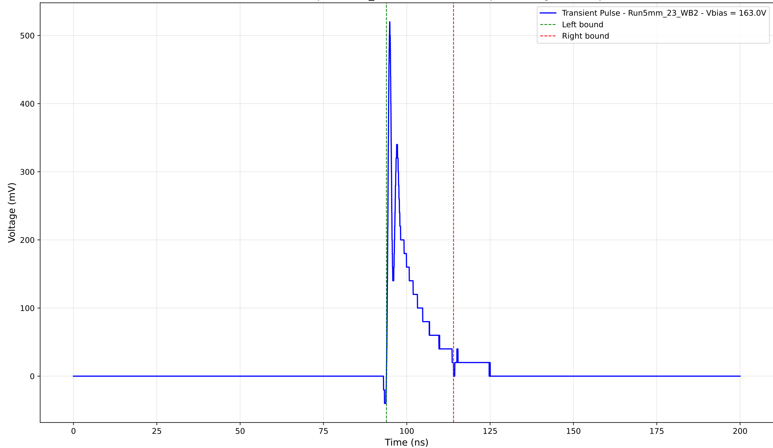
Transient Pulse - Sample: 5mm_23 - Position: 2495.0 \mu\text{m} - Charge: 52.30 pC
