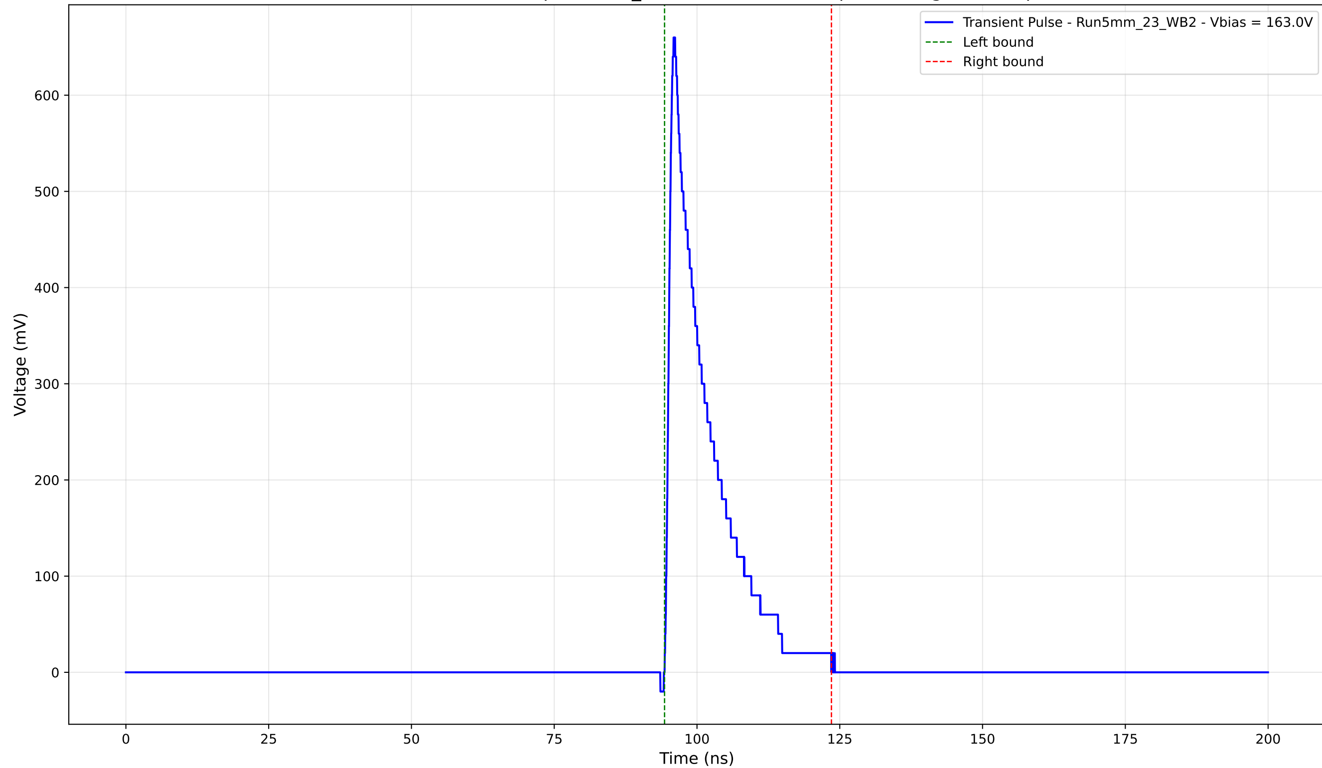
Transient Pulse - Sample: 5mm_23 - Position: 4485.0 \mu\text{m} - Charge: 97.98 pC
