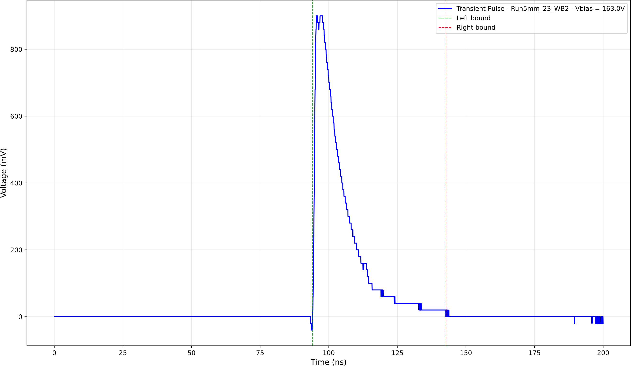
Transient Pulse - Sample: 5mm_23 - Position: 3270.0 \mu\text{m} - Charge: 212.82 pC
