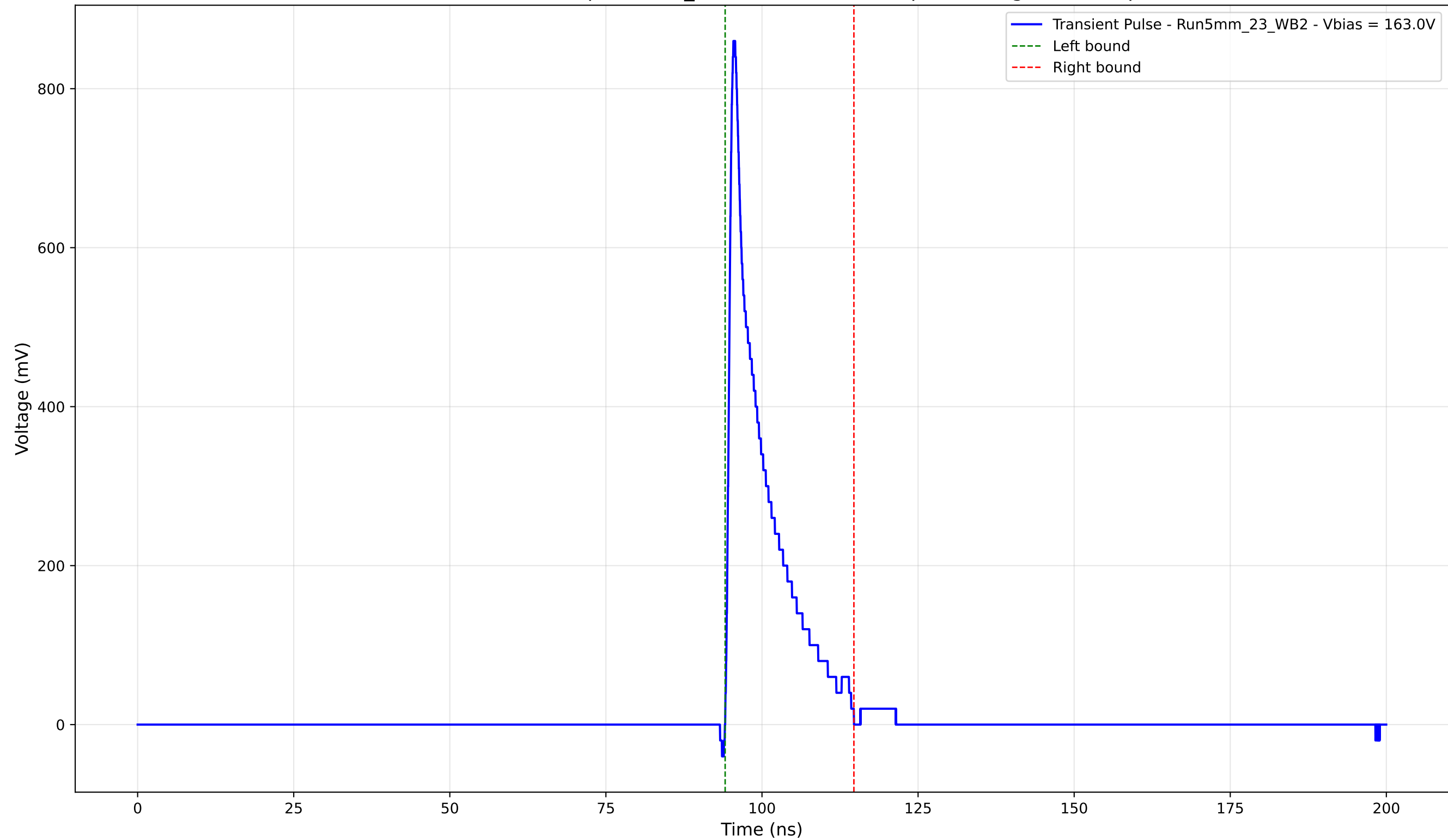
Transient Pulse - Sample: 5mm_23 - Position: 4905.0 \mu\text{m} - Charge: 101.87 pC
