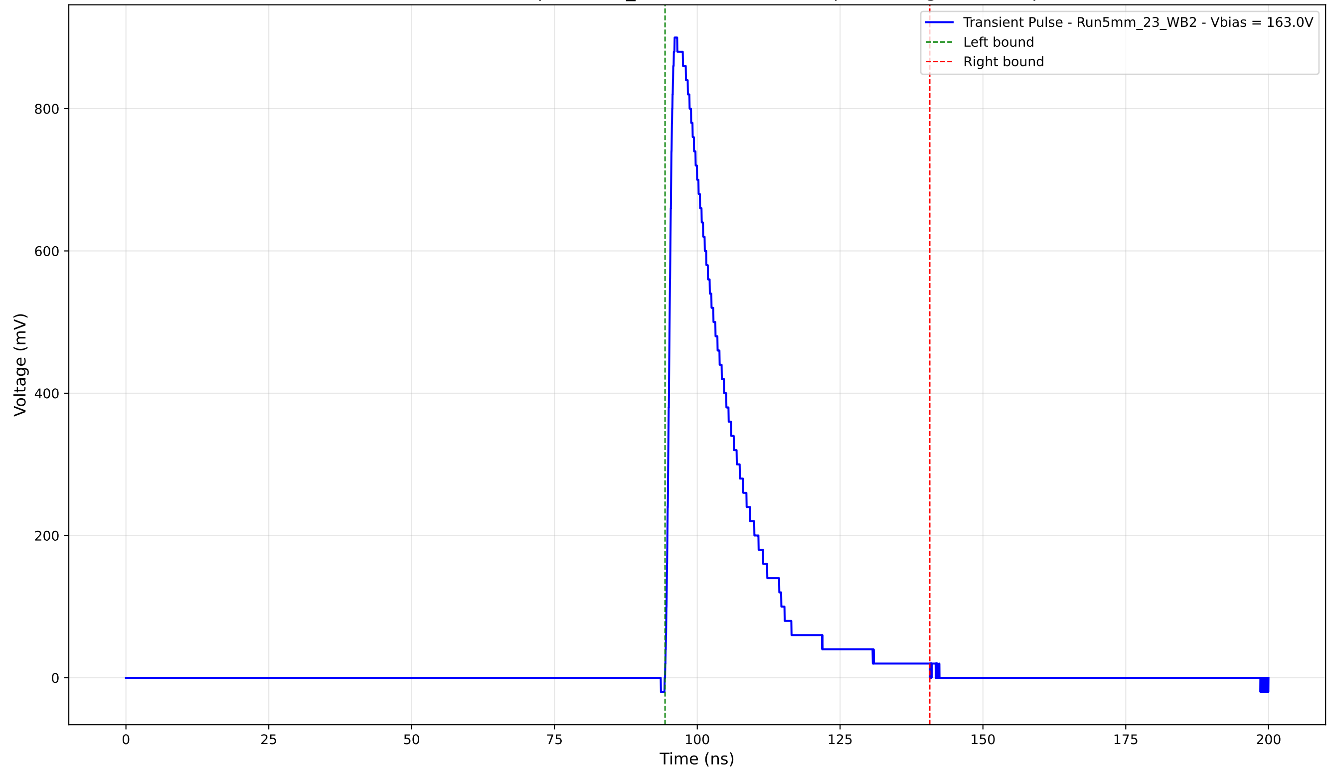
Transient Pulse - Sample: 5mm_23 - Position: 1325.0 \mu\text{m} - Charge: 200.68 pC
