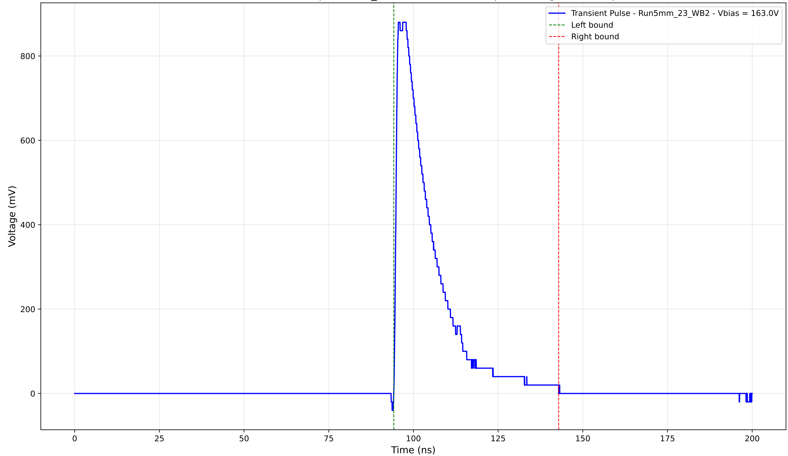
Transient Pulse - Sample: 5mm_23 - Position: 1705.0 \mu\text{m} - Charge: 208.72 pC
