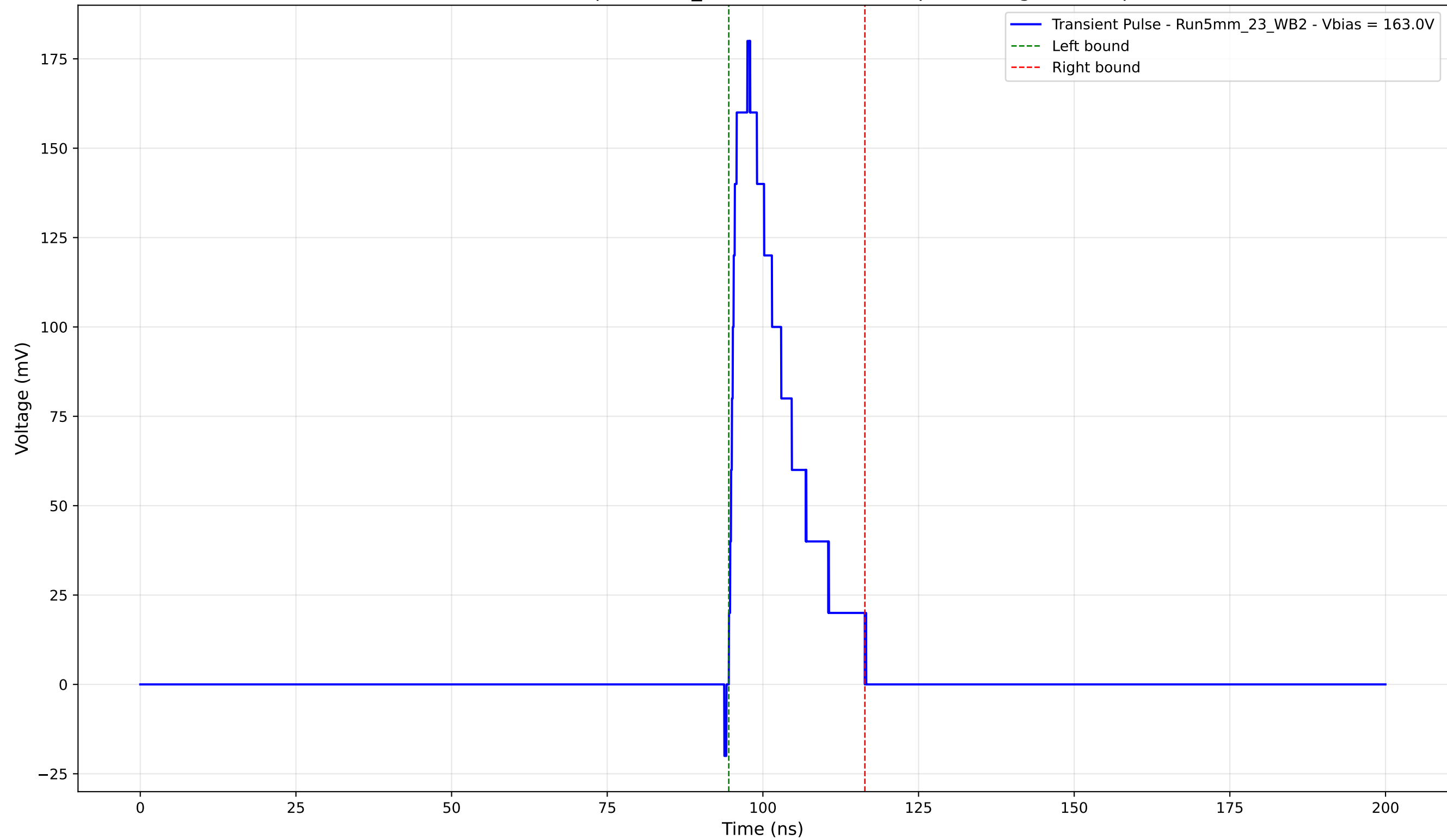
Transient Pulse - Sample: 5mm_23 -Position: 1500.0 \mu\text{m} - Charge: 32.68 pC
