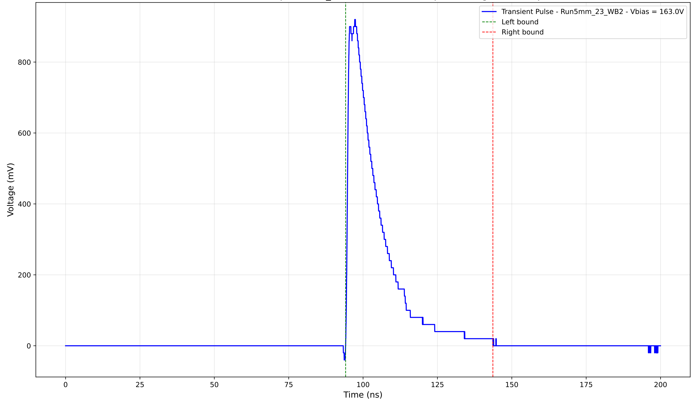
Transient Pulse - Sample: 5mm_23 - Position: 3255.0 \mu\text{m} - Charge: 215.25 pC
