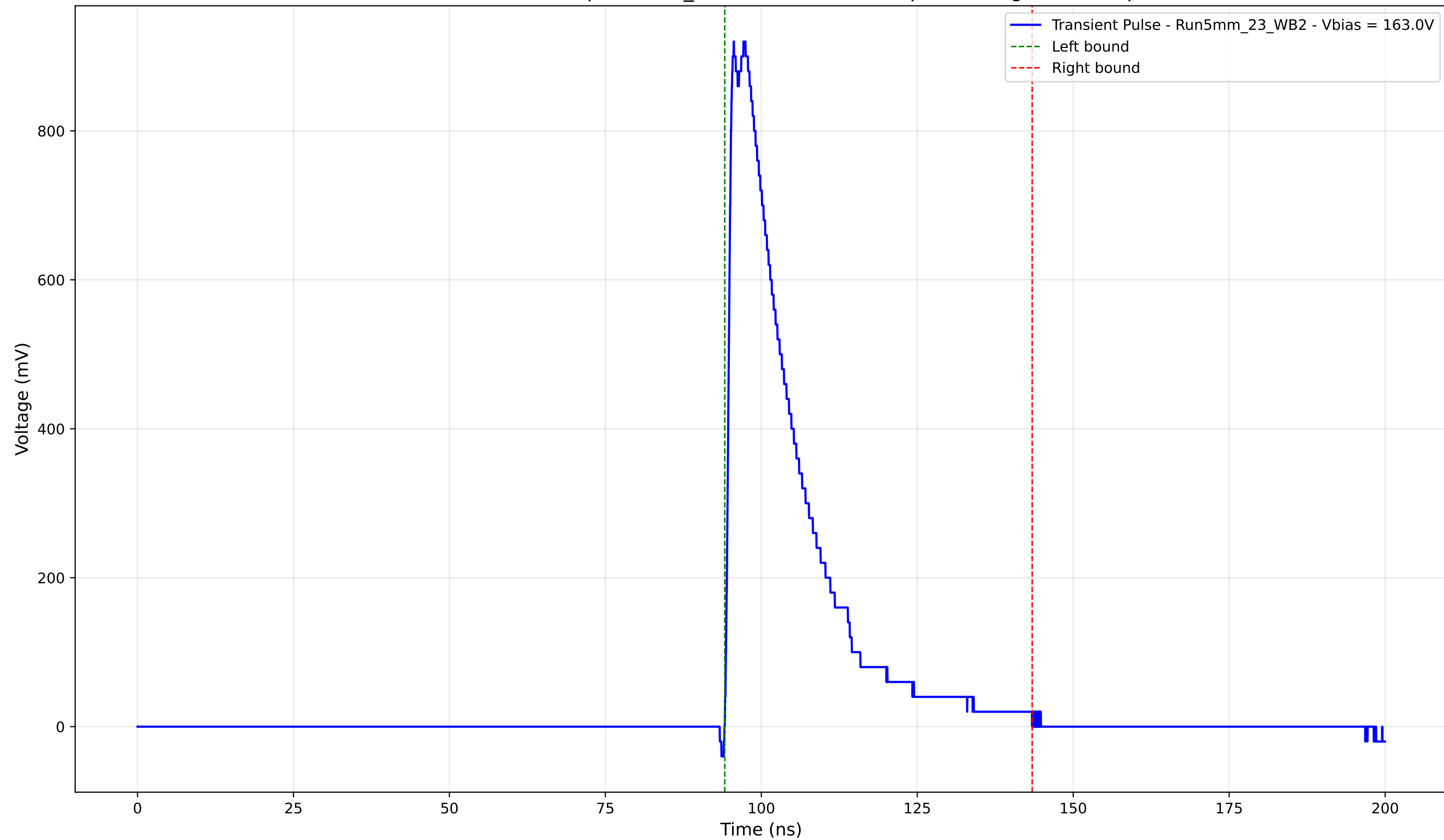
Transient Pulse - Sample: 5mm_23 - Position: 3235.0 \mu\text{m} - Charge: 215.80 pC
