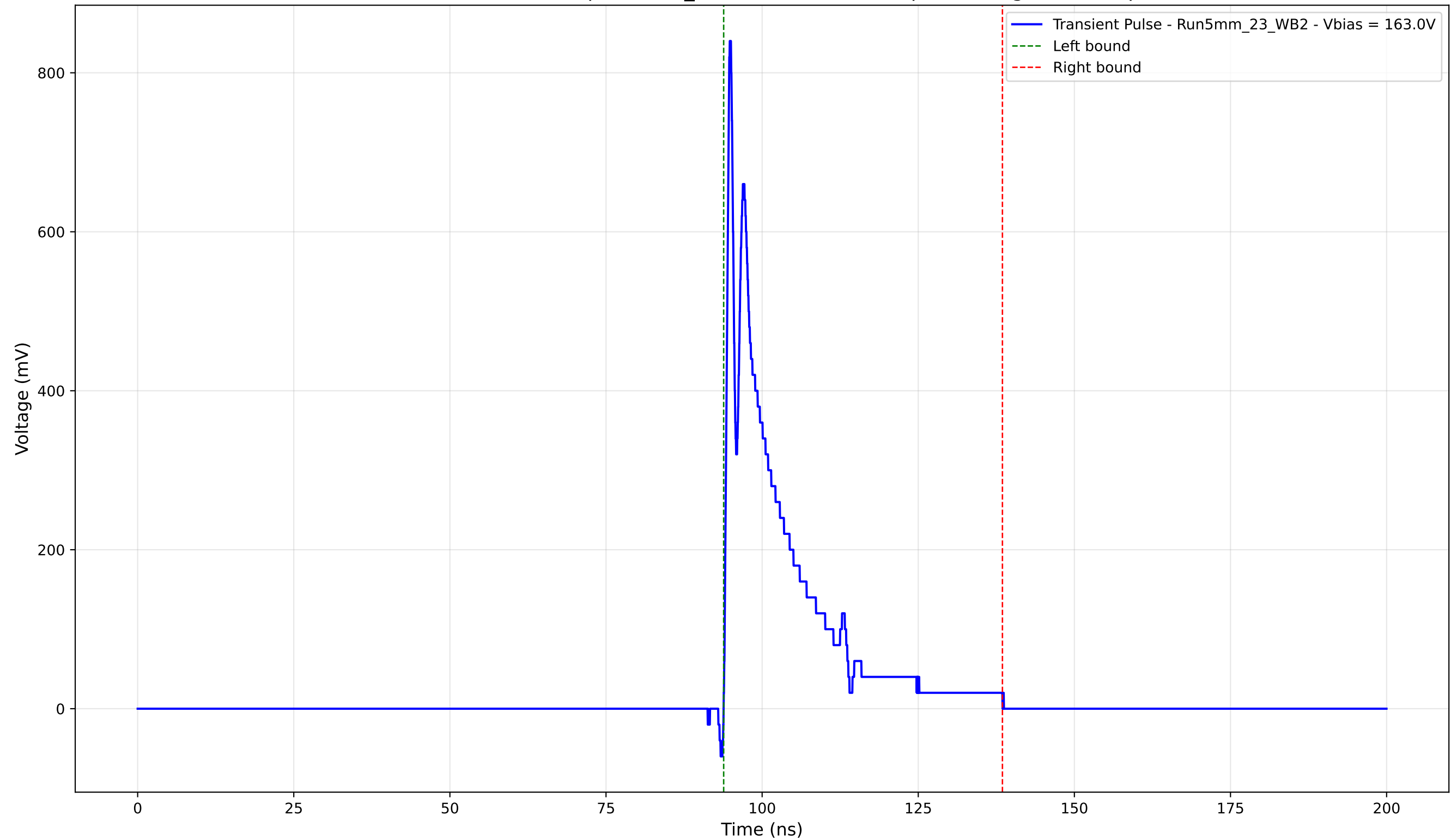
Transient Pulse - Sample: 5mm_23 - Position: 2465.0 \mu\text{m} - Charge: 122.70 pC
