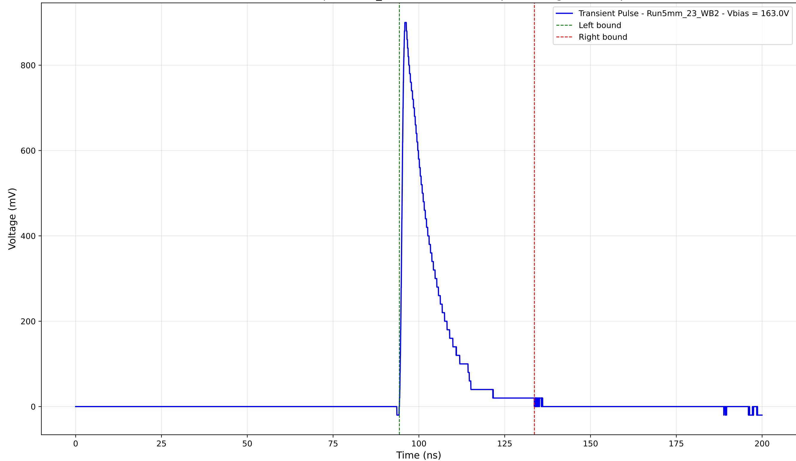
Transient Pulse - Sample: 5mm_23 - Position: 4340.0 \mu\text{m} - Charge: 160.53 pC
