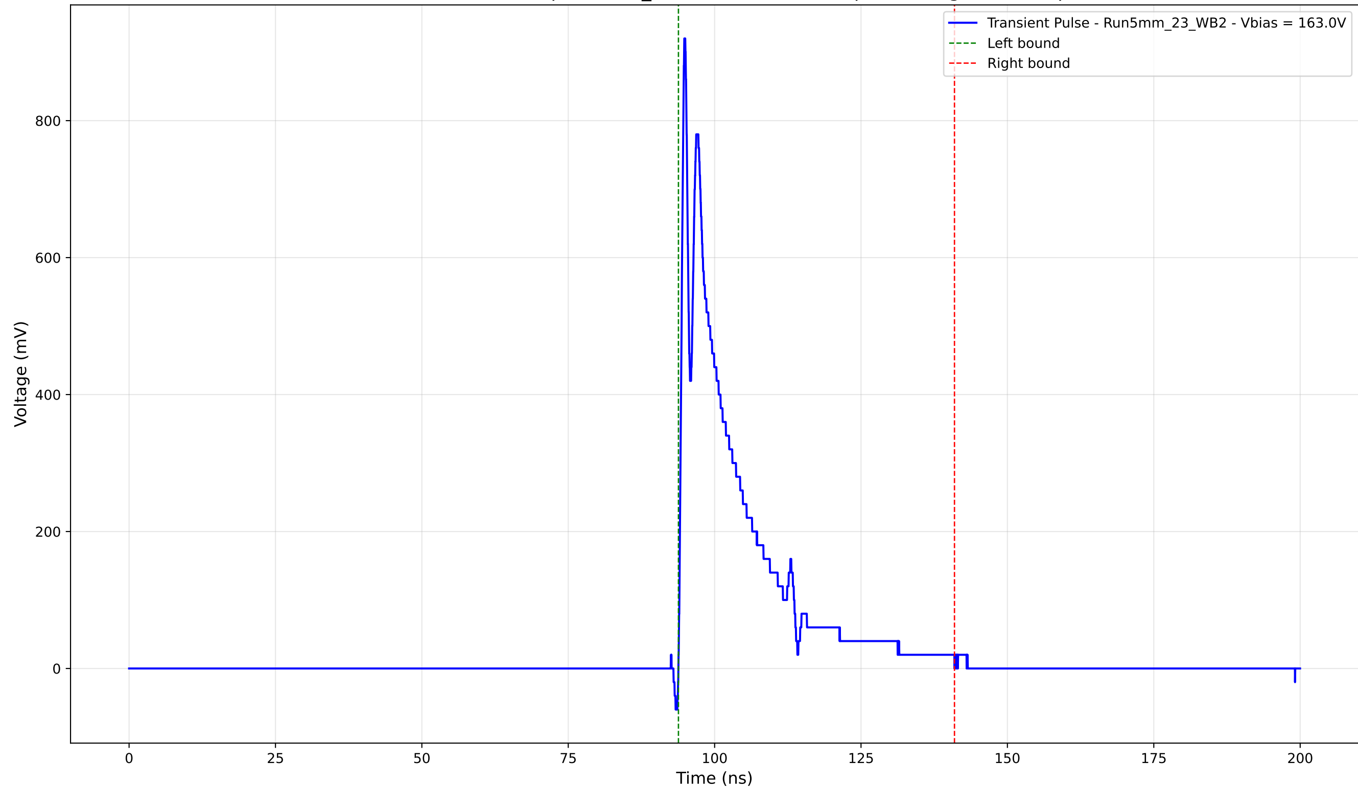
Transient Pulse - Sample: 5mm_23 - Position: 2450.0 \mu\text{m} - Charge: 154.20 pC
