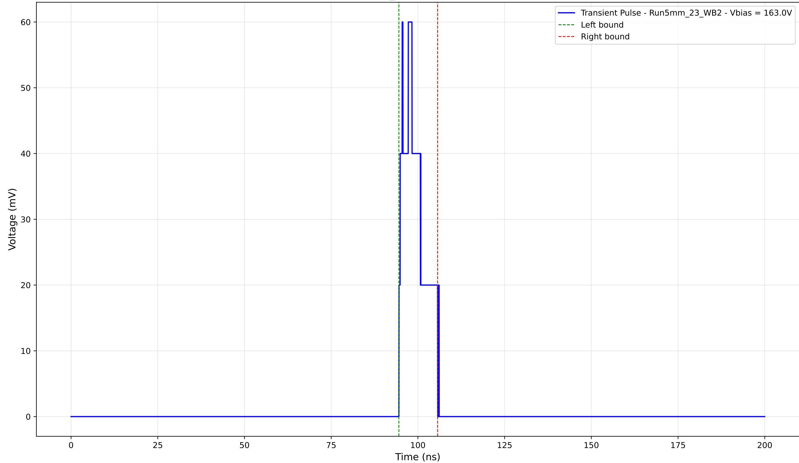
Transient Pulse - Sample: 5mm_23 - Position: 25.0 \mu\text{m} - Charge: 7.33 pC
