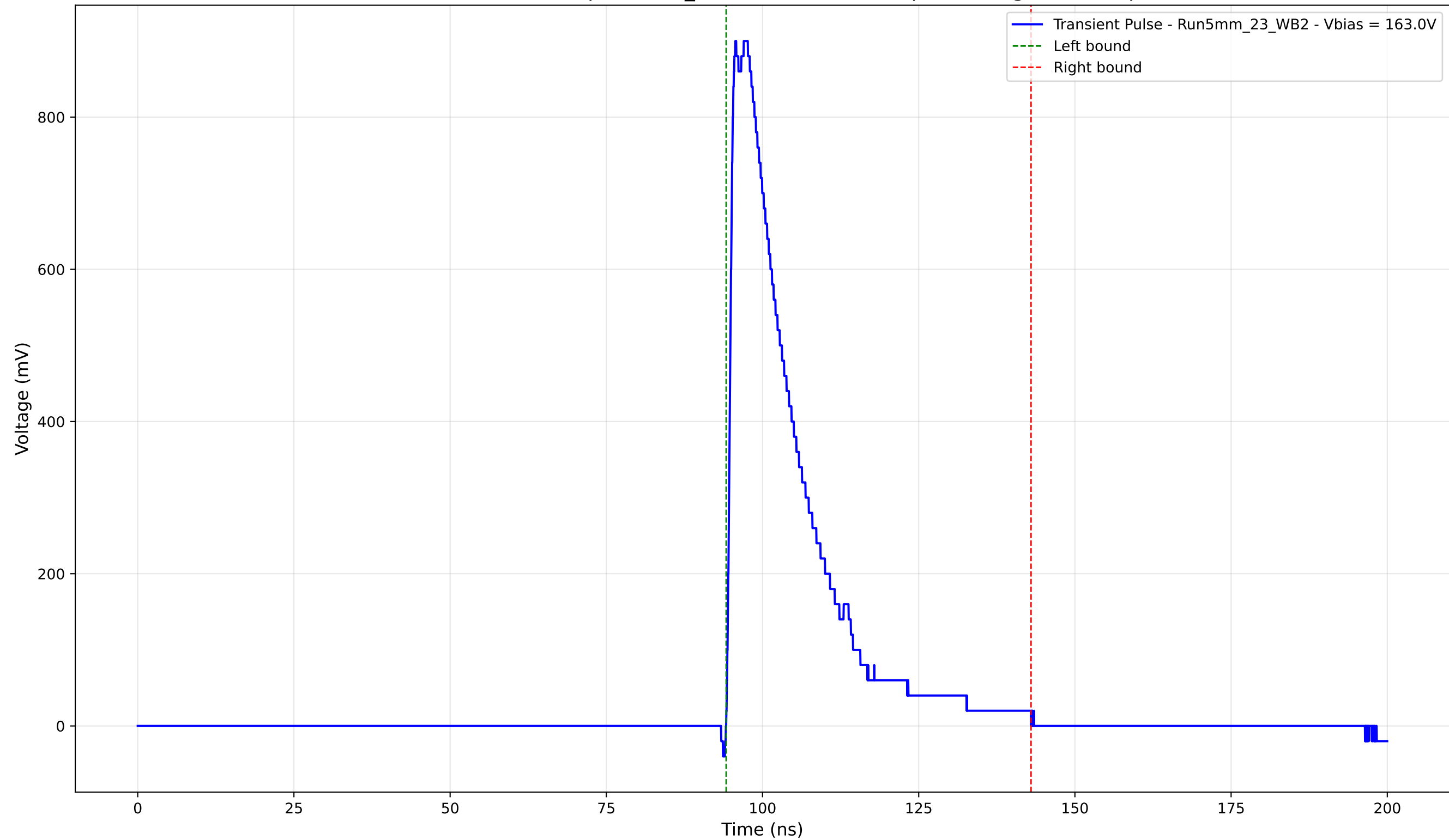
Transient Pulse - Sample: 5mm_23 - Position: 3295.0 \mu\text{m} - Charge: 208.38 pC
