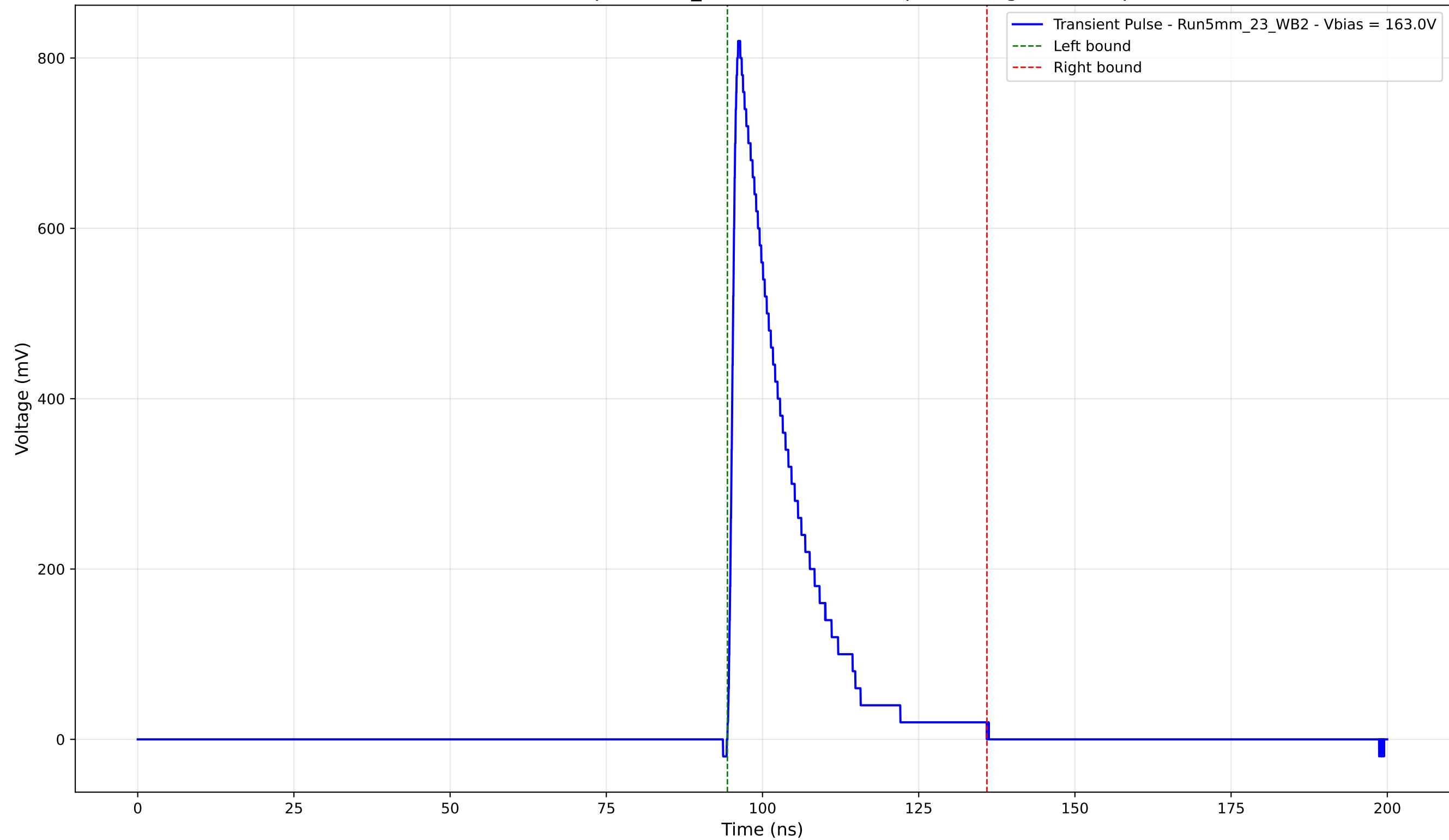
Transient Pulse - Sample: 5mm_23 - Position: 915.0 \mu\text{m} - Charge: 154.22 pC
