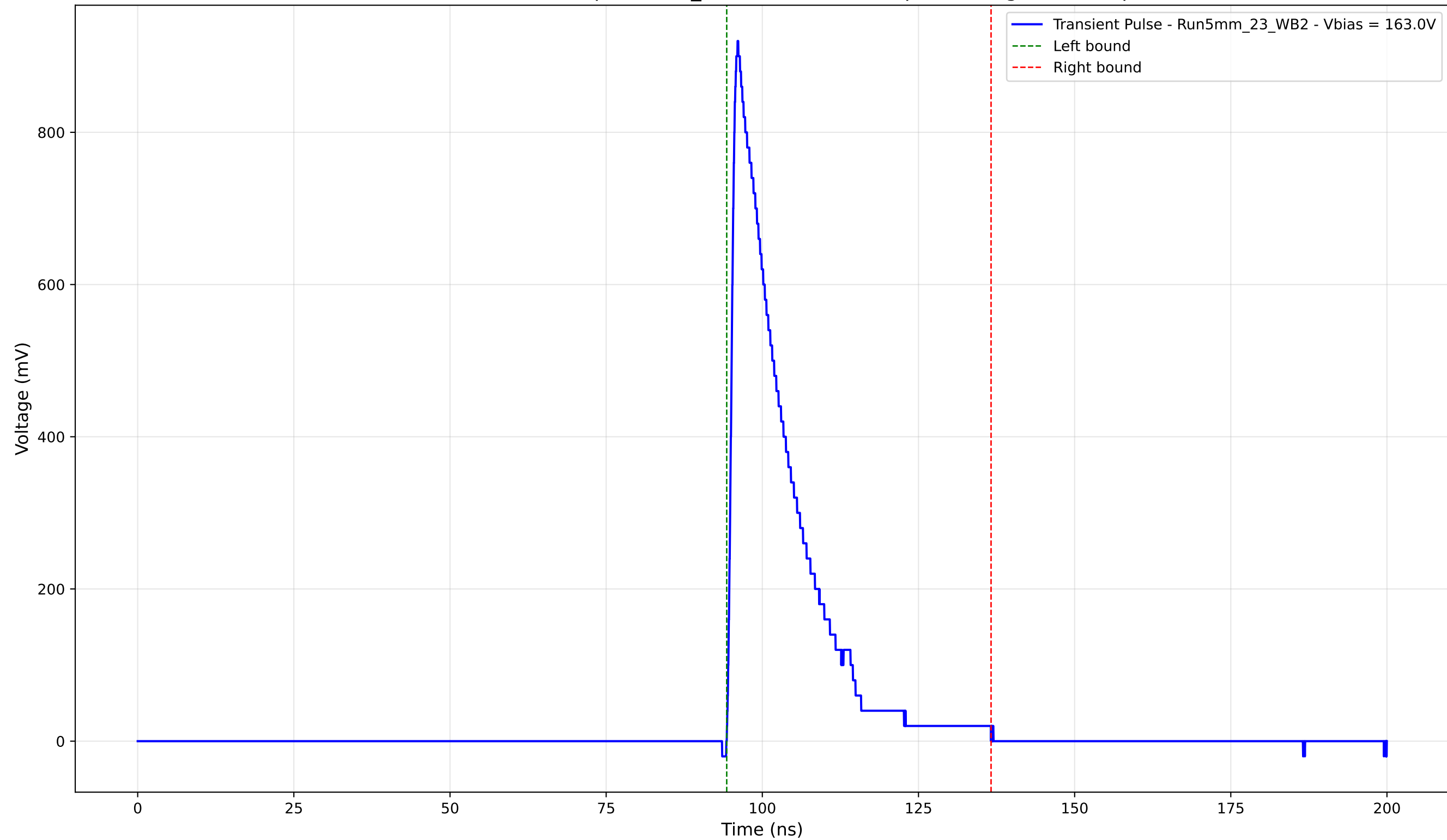
Transient Pulse - Sample: 5mm_23 - Position: 670.0 \mu\text{m} - Charge: 173.46 pC
