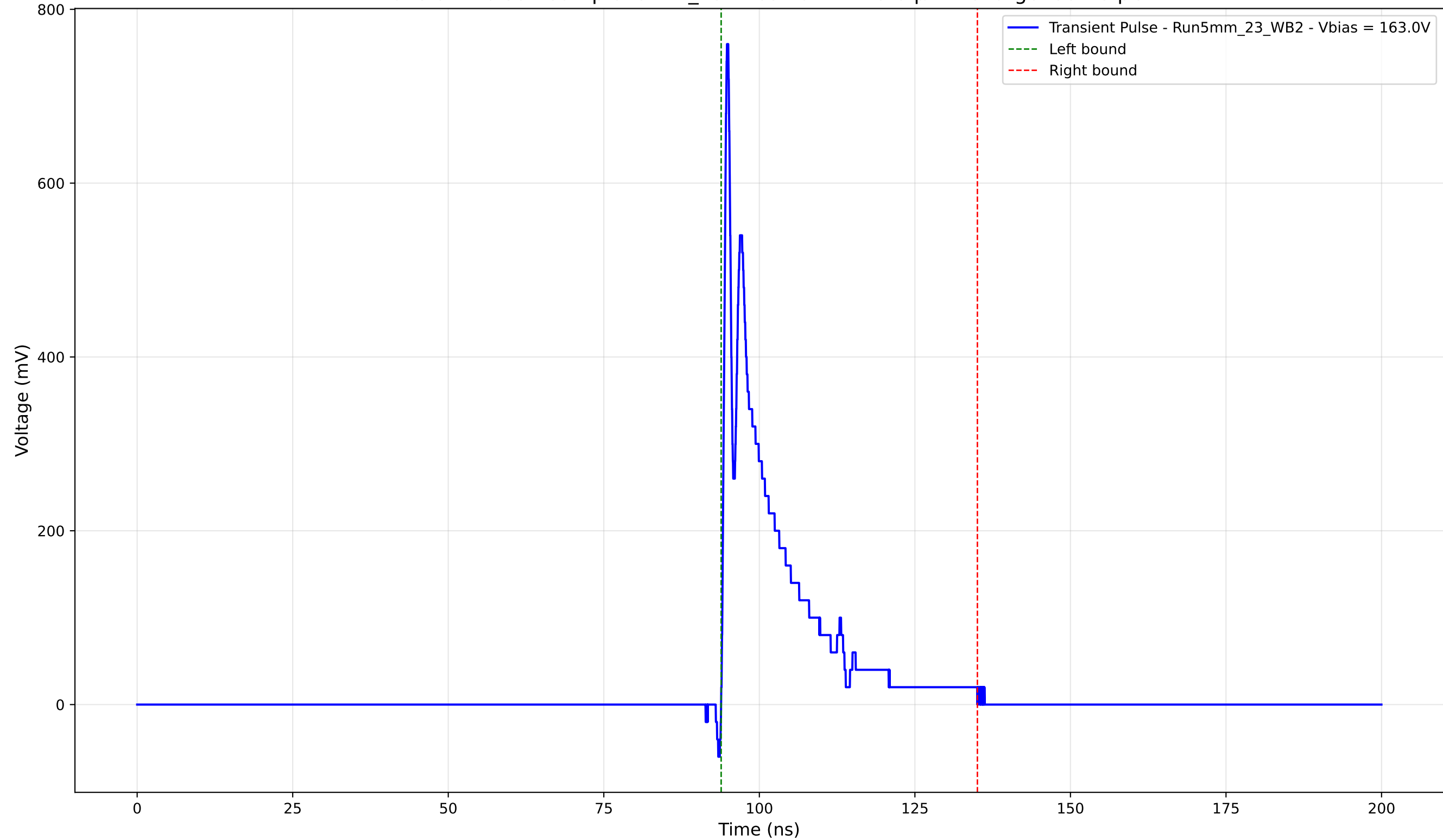
Transient Pulse - Sample: 5mm_23 - Position: 2475.0 \mu\text{m} - Charge: 99.48 pC
