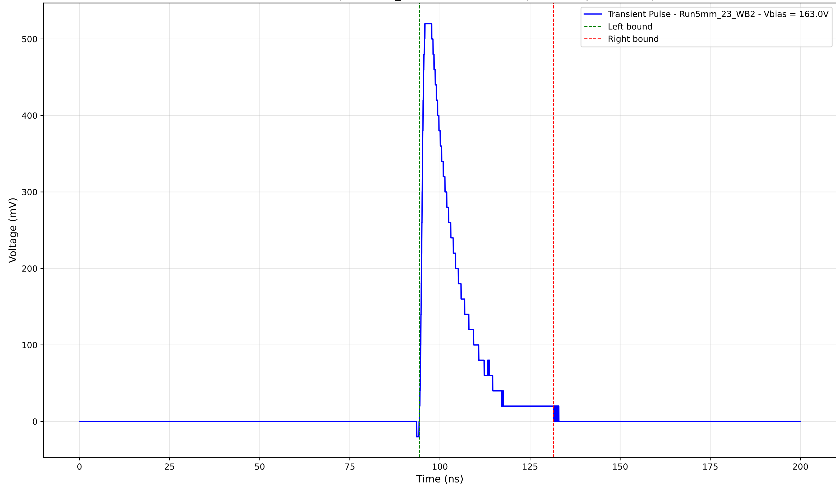
Transient Pulse - Sample: 5mm_23 - Position: 3475.0 \mu\text{m} - Charge: 104.25 pC
