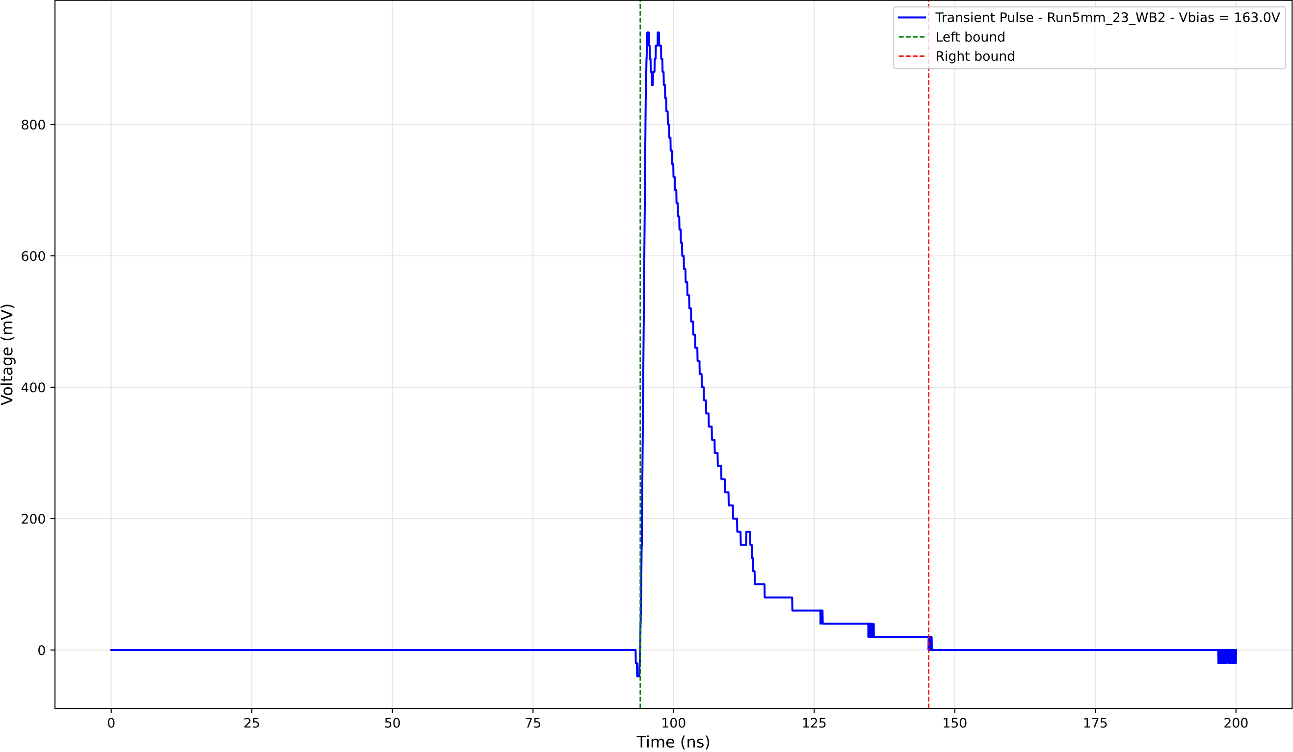
Transient Pulse - Sample: 5mm_23 - Position: 3125.0 \mu\text{m} - Charge: 223.92 pC
