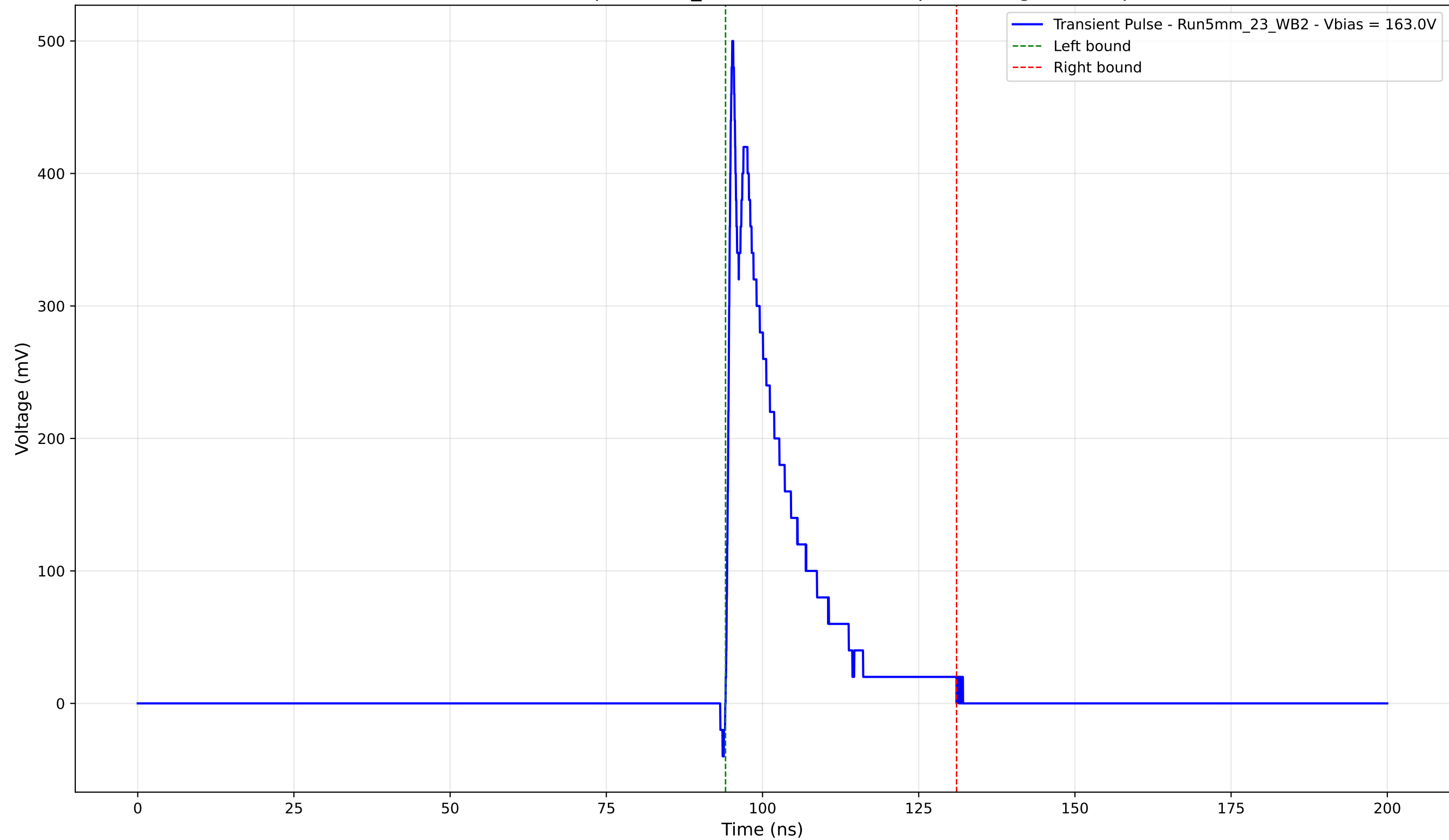
Transient Pulse - Sample: 5mm_23 - Position: 2990.0 \mu\text{m} - Charge: 83.62 pC
