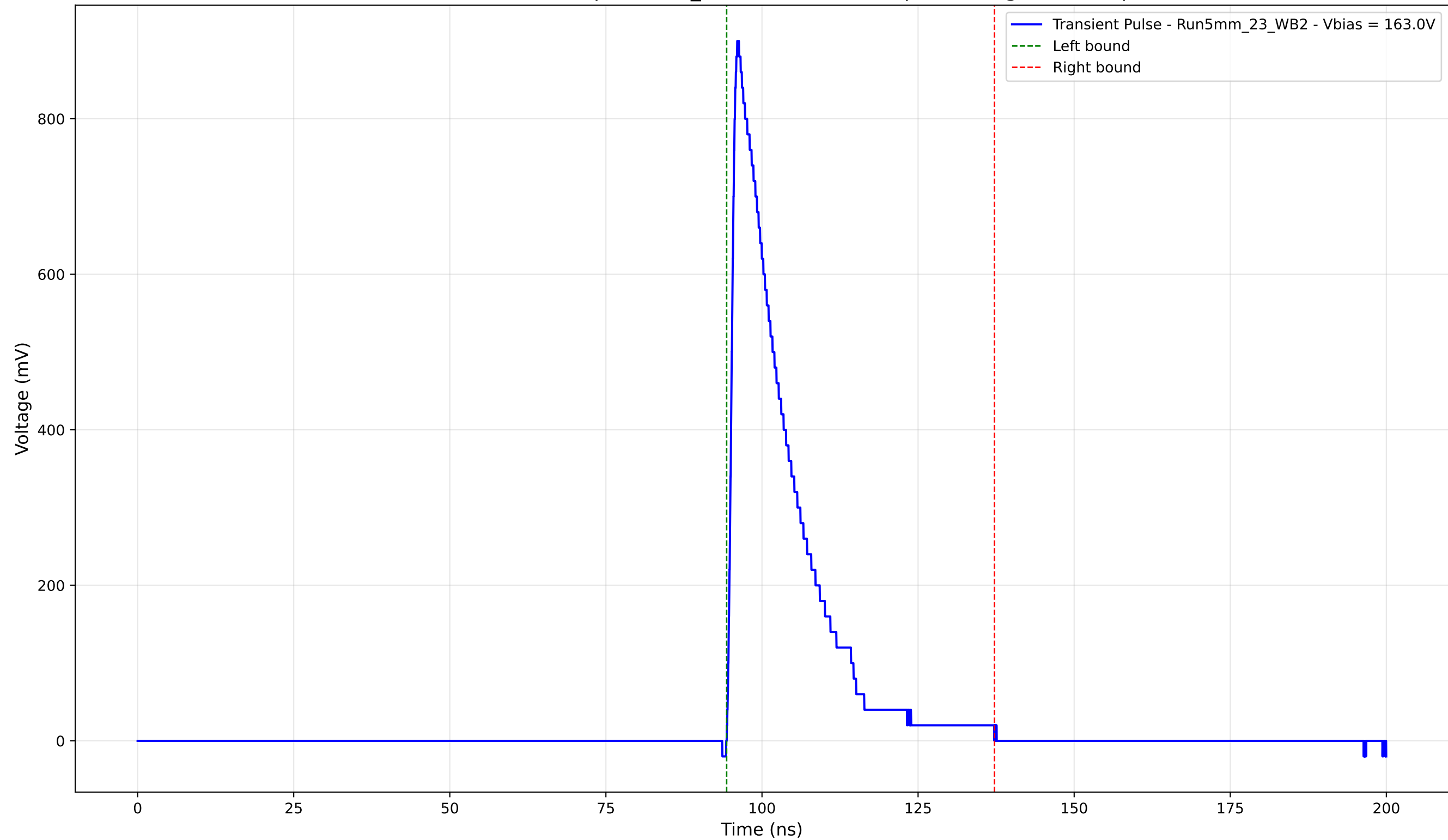
Transient Pulse - Sample: 5mm_23 - Position: 790.0 \mu\text{m} - Charge: 174.33 pC
