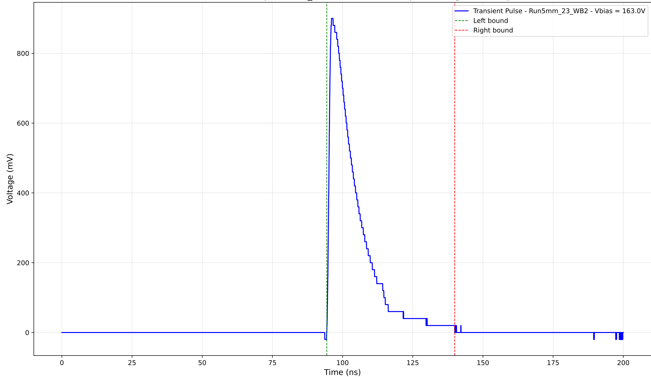
Transient Pulse - Sample: 5mm_23 - Position: 1225.0 \mu\text{m} - Charge: 198.24 pC
