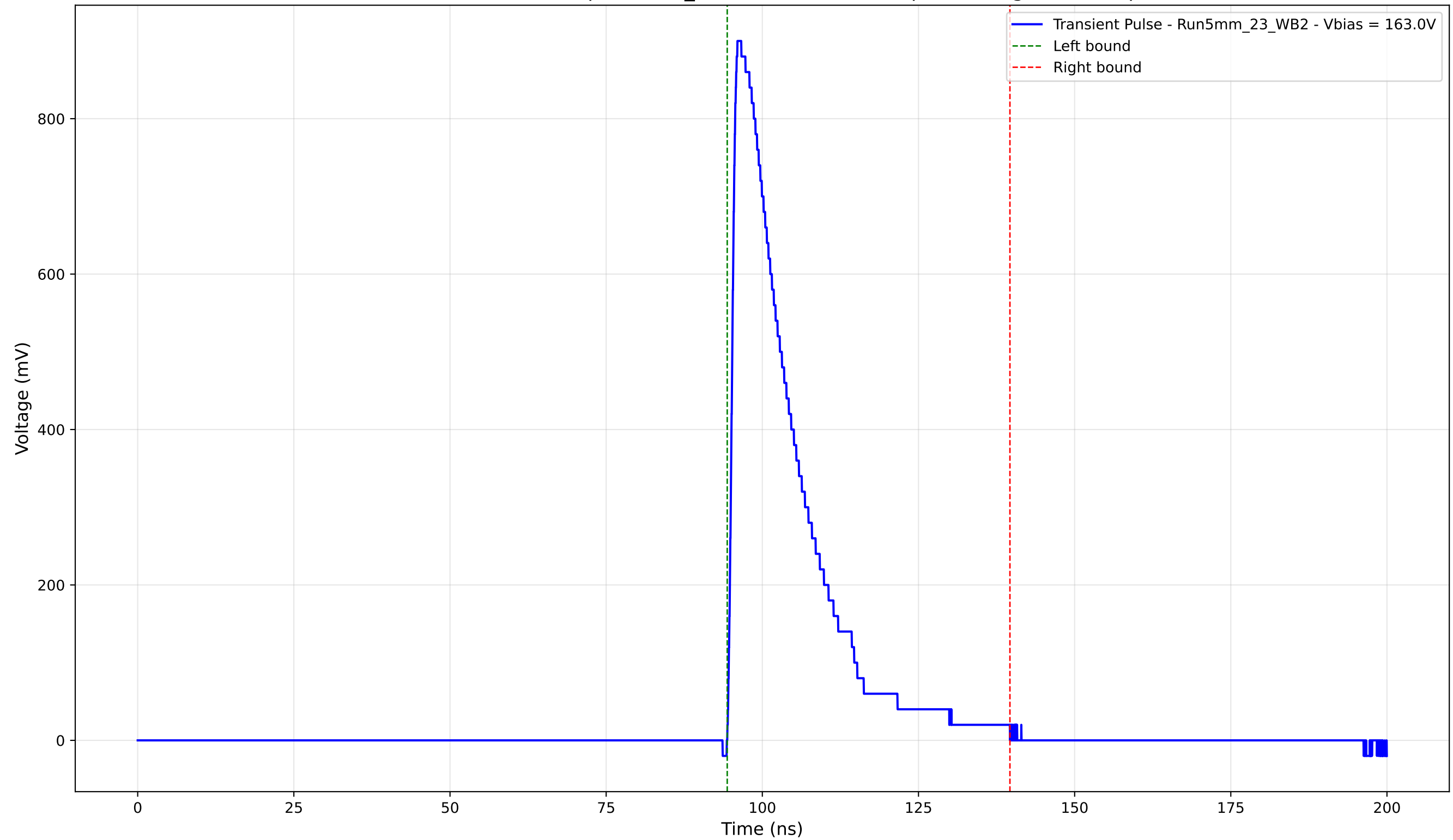
Transient Pulse - Sample: 5mm_23 - Position: 1230.0 \mu\text{m} - Charge: 198.57 pC
