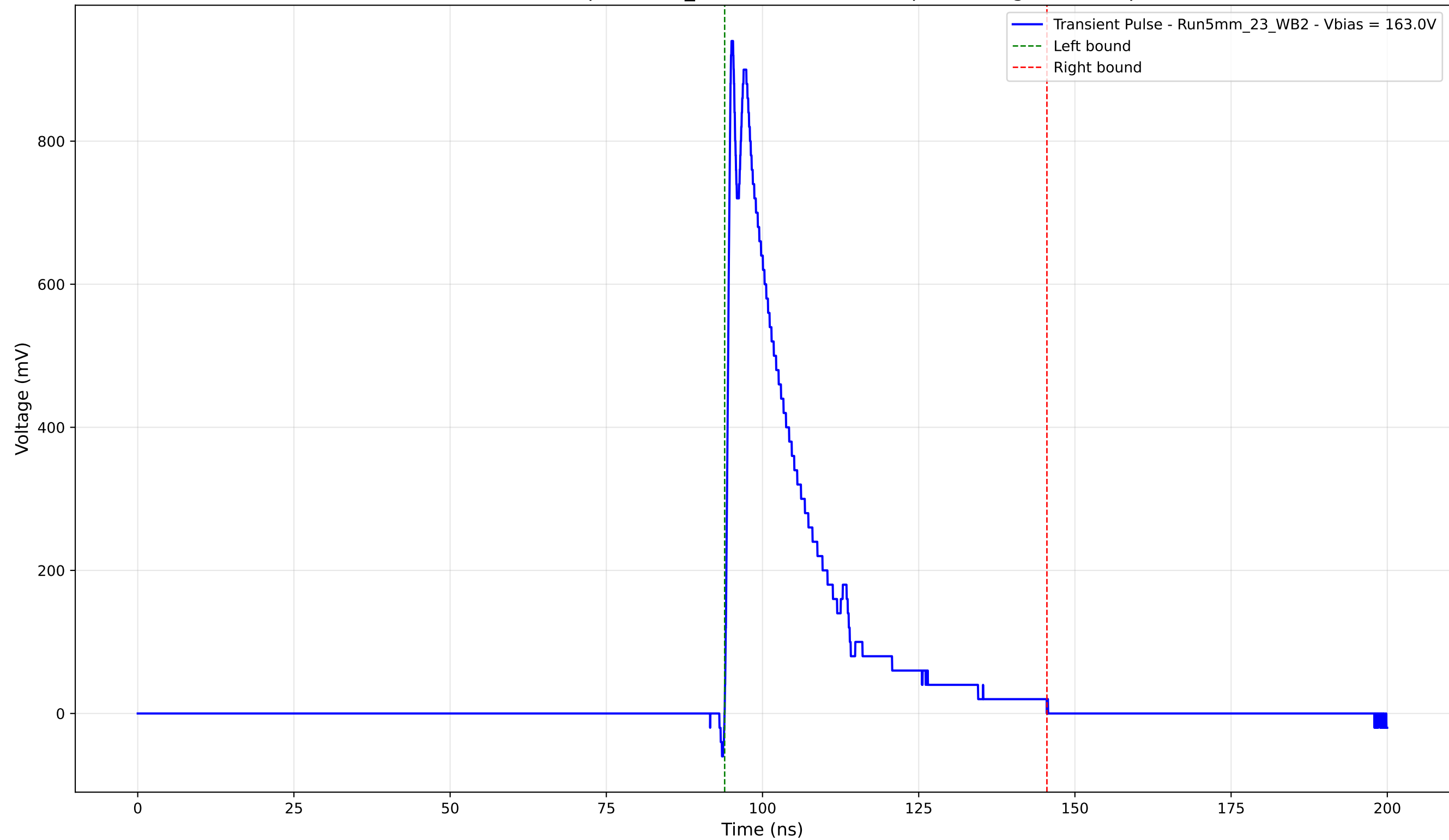
Transient Pulse - Sample: 5mm_23 - Position: 2190.0 \mu\text{m} - Charge: 205.54 pC
