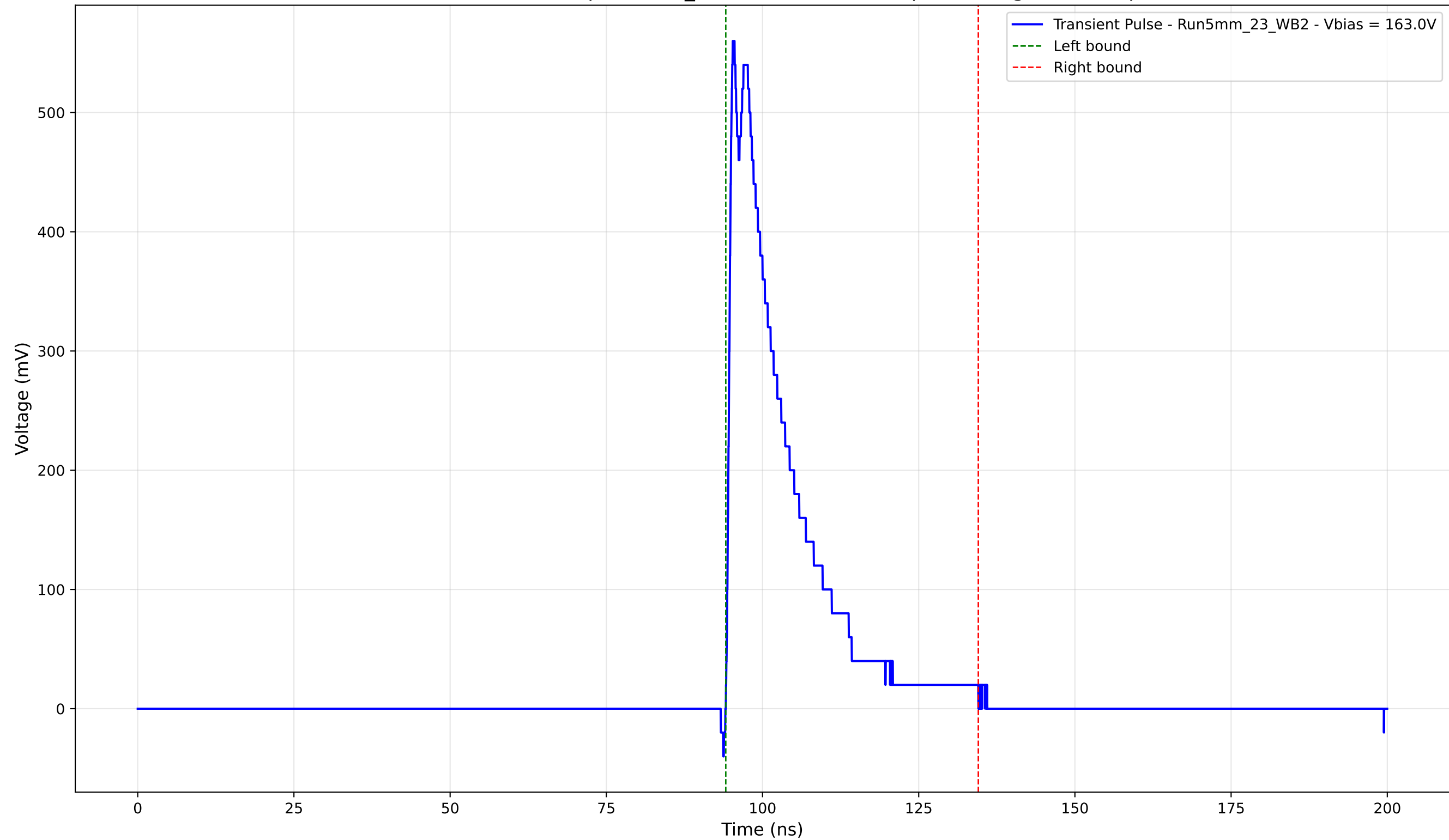
Transient Pulse - Sample: 5mm_23 - Position: 3065.0 \mu\text{m} - Charge: 111.04 pC
