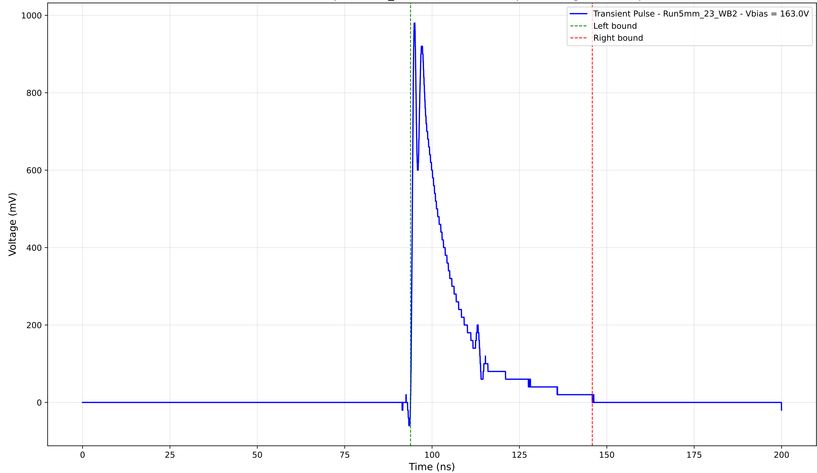
Transient Pulse - Sample: 5mm_23 - Position: 2670.0 \mu\text{m} - Charge: 201.65 pC
