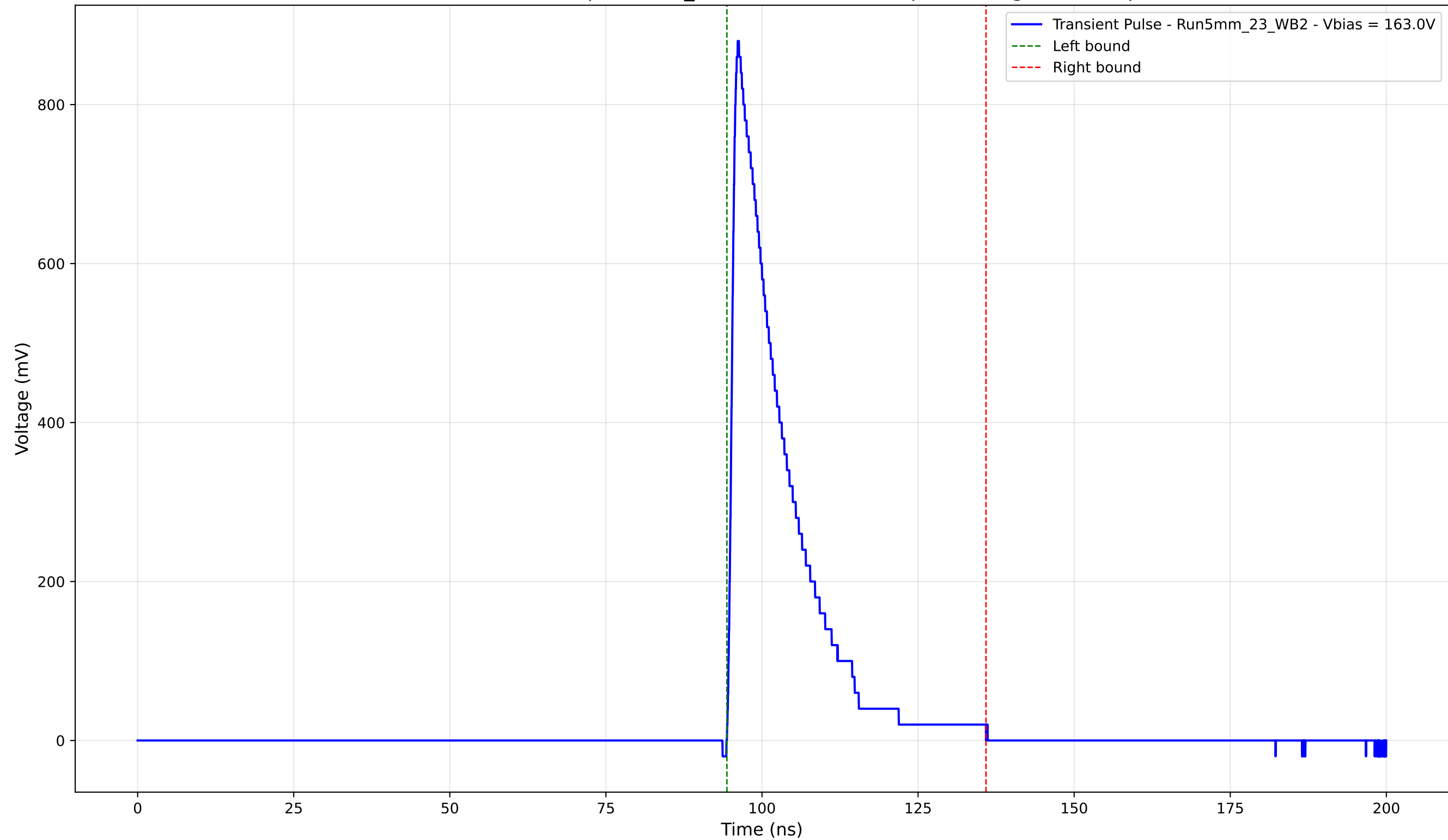
Transient Pulse - Sample: 5mm_23 - Position: 4160.0 \mu\text{m} - Charge: 161.54 pC
