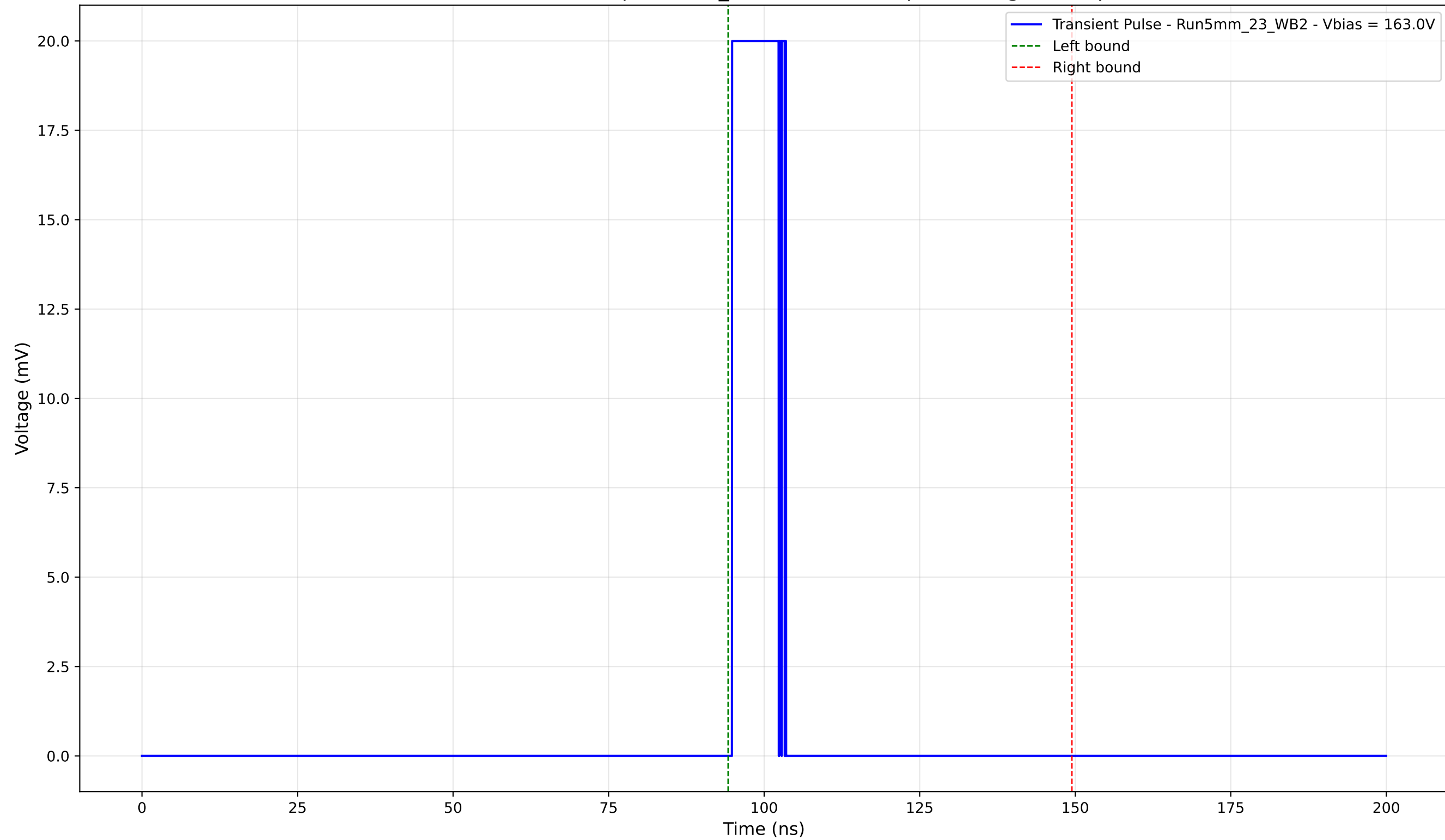
Transient Pulse - Sample: 5mm_23 - Position: 5.0 \mu\text{m} - Charge: 3.38 pC
