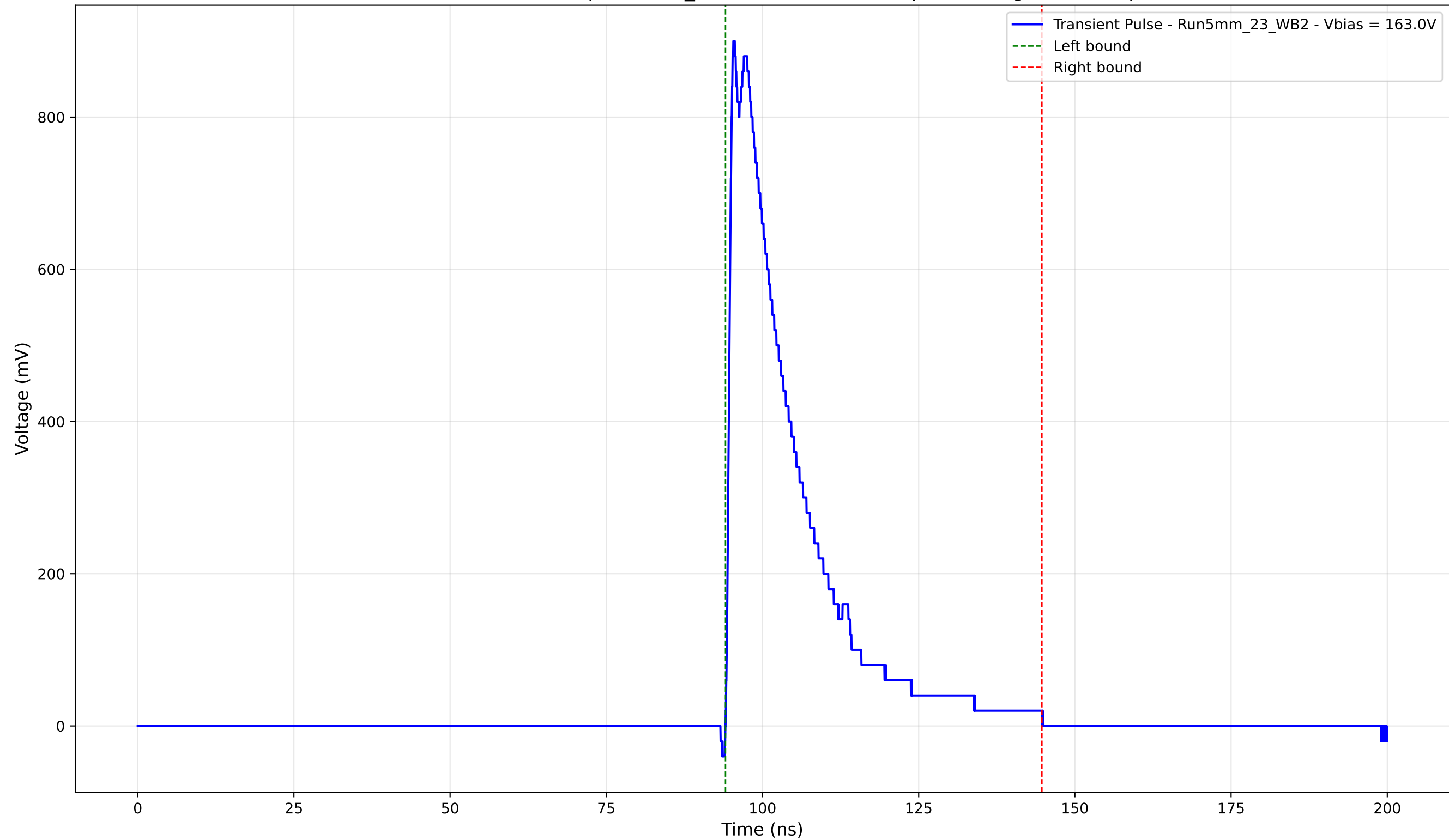
Transient Pulse - Sample: 5mm_23 - Position: 1920.0 \mu\text{m} - Charge: 205.51 pC
