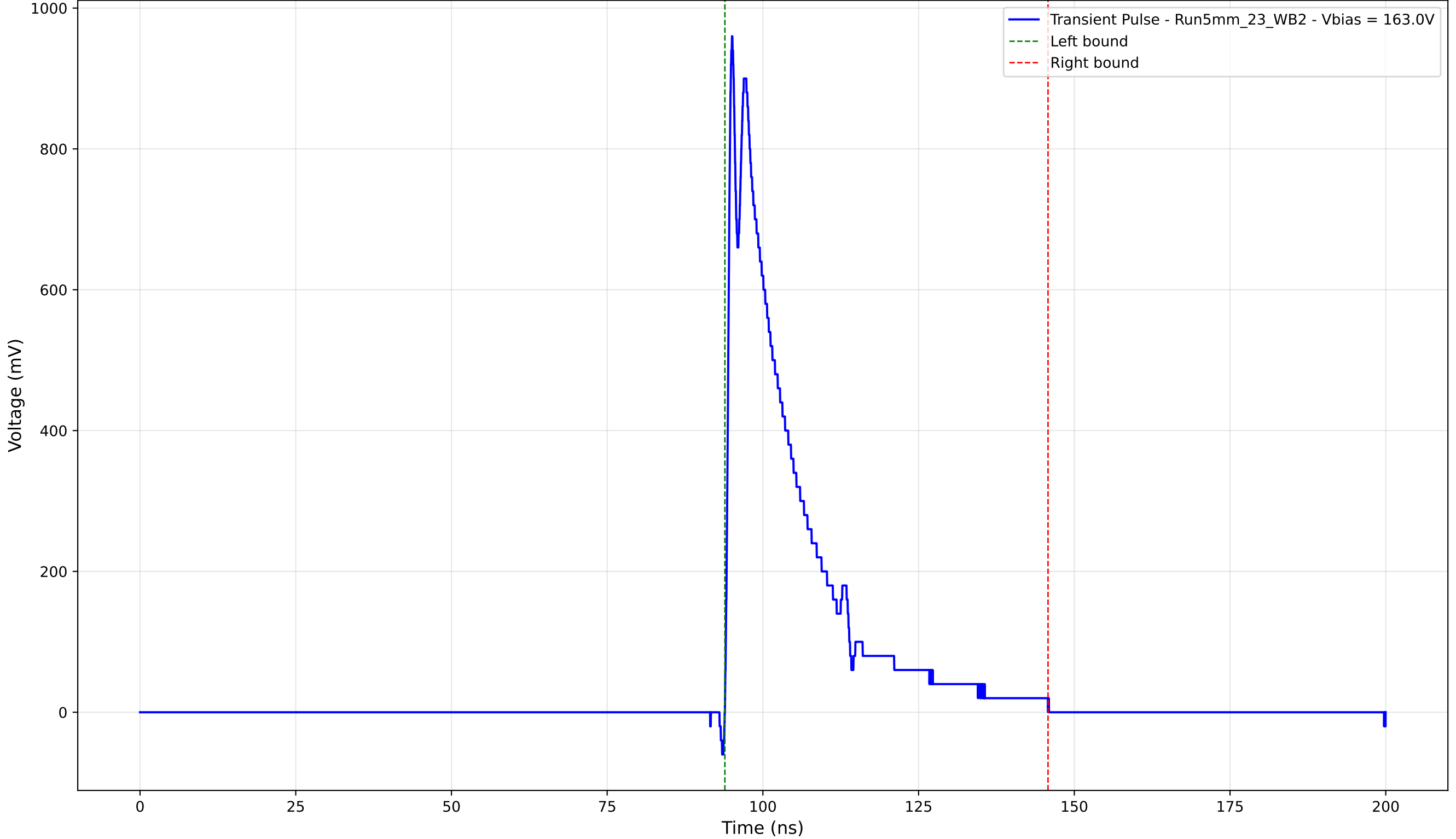
Transient Pulse - Sample: 5mm_23 - Position: 2270.0 \mu\text{m} - Charge: 203.62 pC
