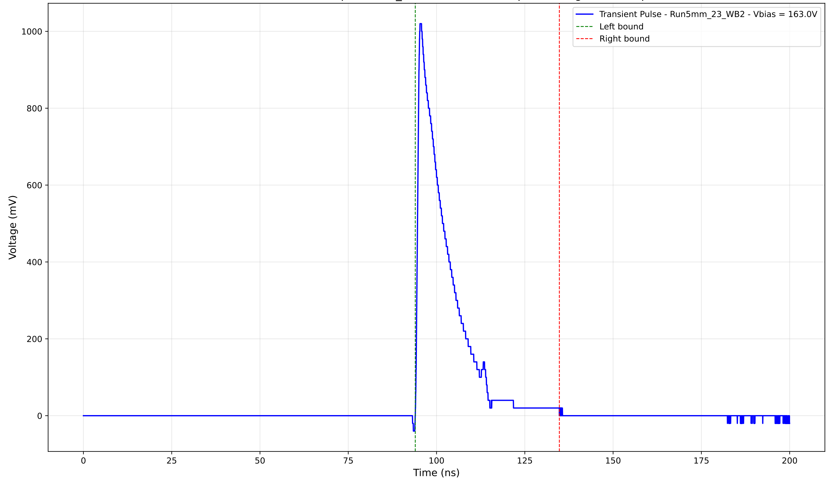
Transient Pulse - Sample: 5mm_23 - Position: 165.0 \mu\text{m} - Charge: 183.86 pC
