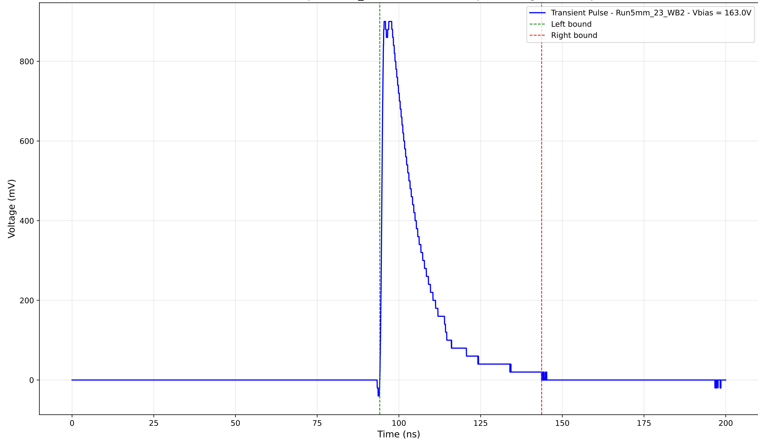
Transient Pulse - Sample: 5mm_23 - Position: 1770.0 \mu\text{m} - Charge: 216.70 pC
