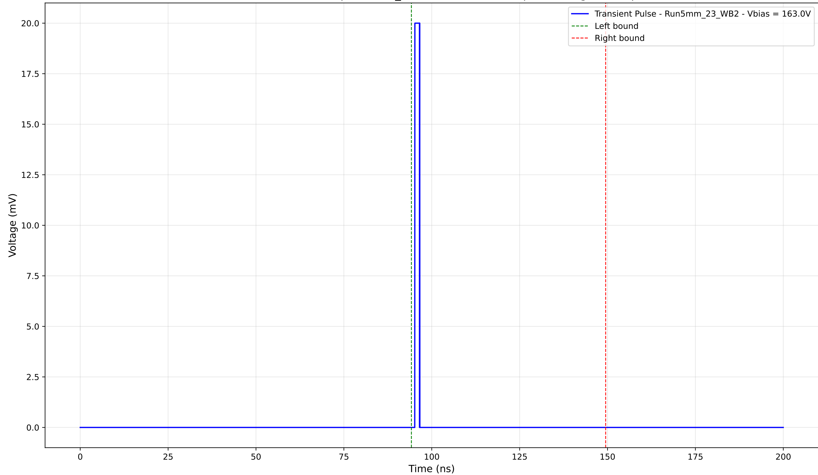
Transient Pulse - Sample: 5mm_23 - Position: 5045.0 \mu\text{m} - Charge: 0.56 pC
