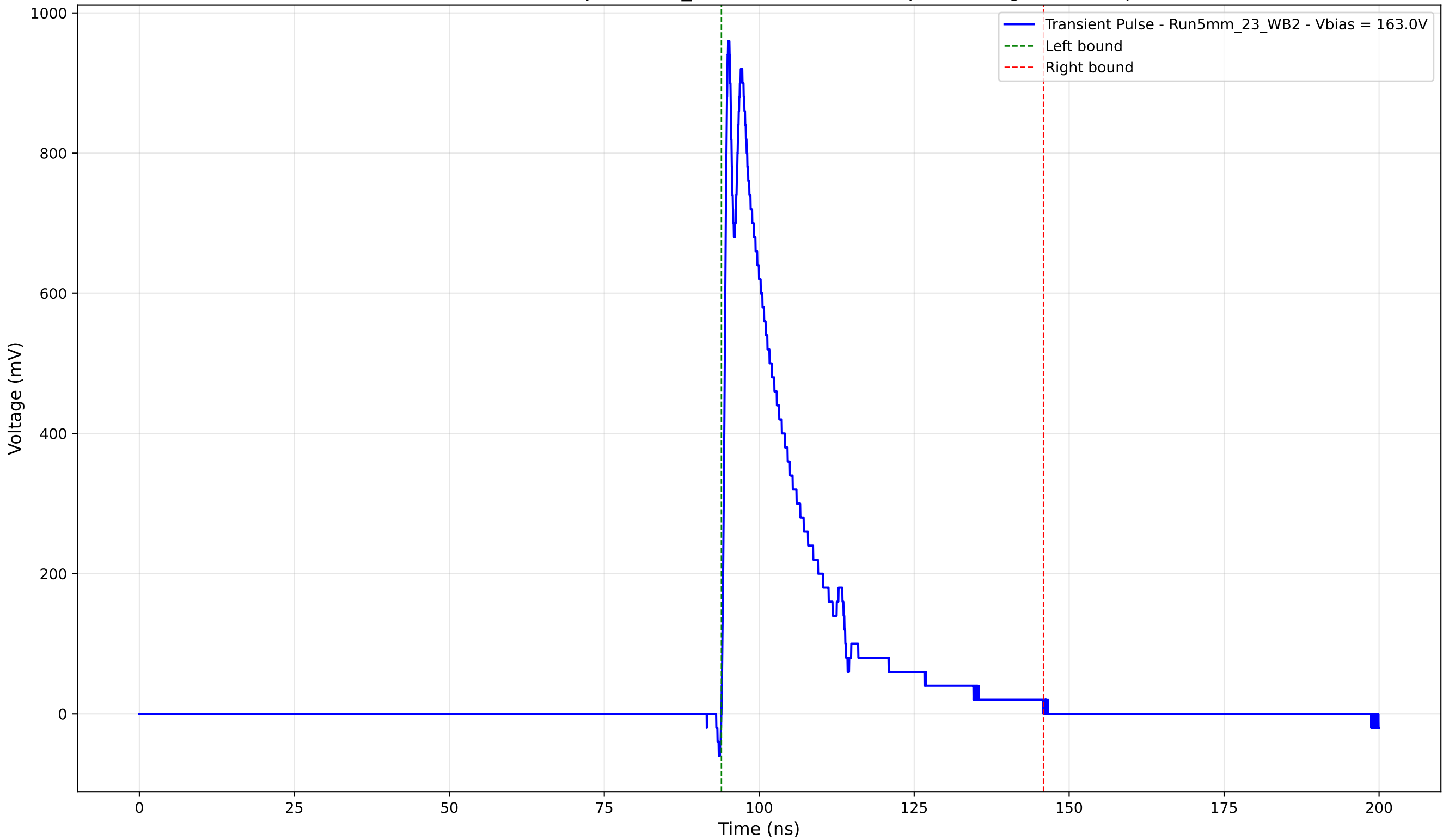
Transient Pulse - Sample: 5mm_23 - Position: 2780.0 \mu\text{m} - Charge: 205.54 pC
