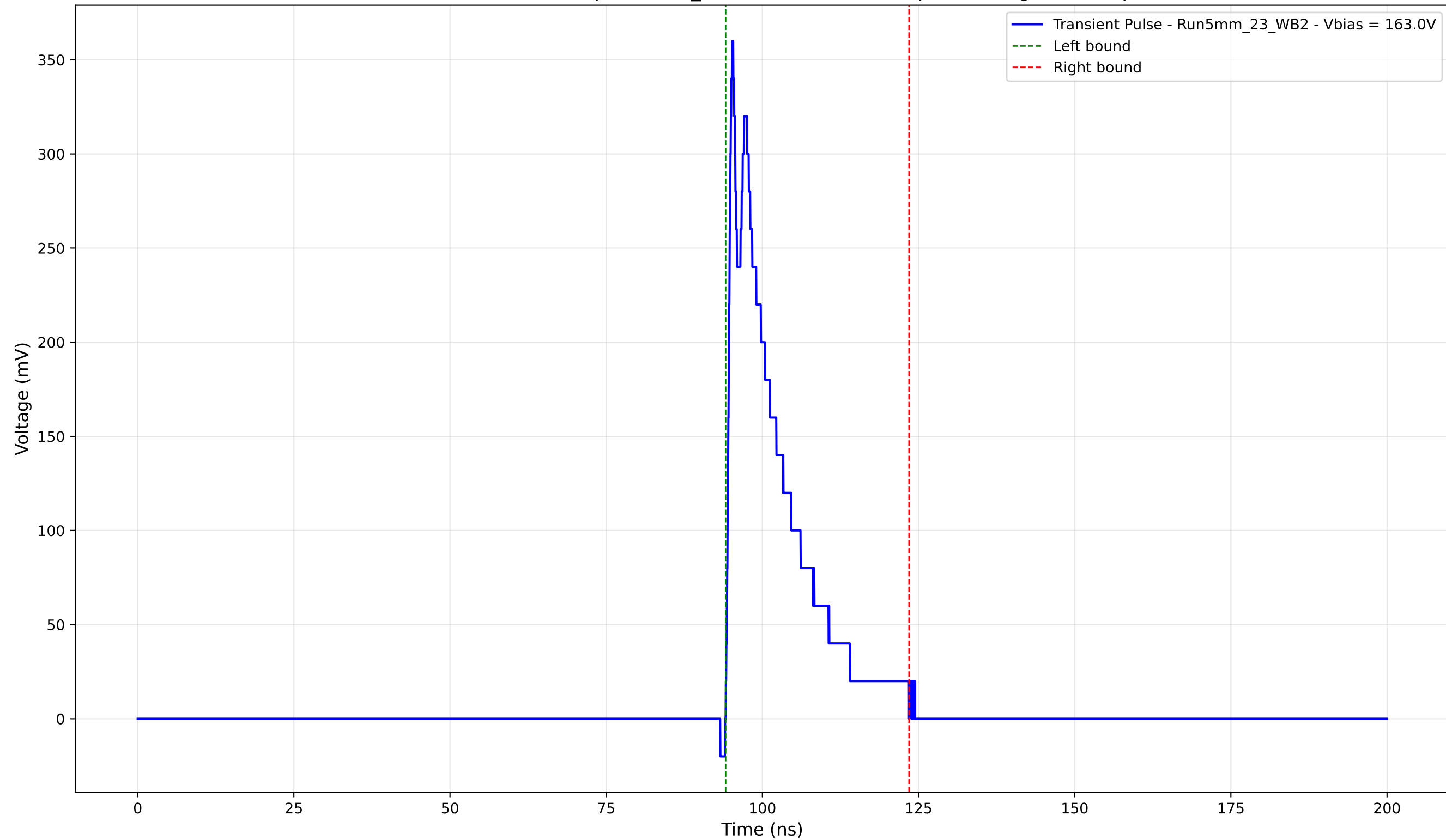
Transient Pulse - Sample: 5mm_23 - Position: 2035.0 \mu\text{m} - Charge: 59.33 pC
