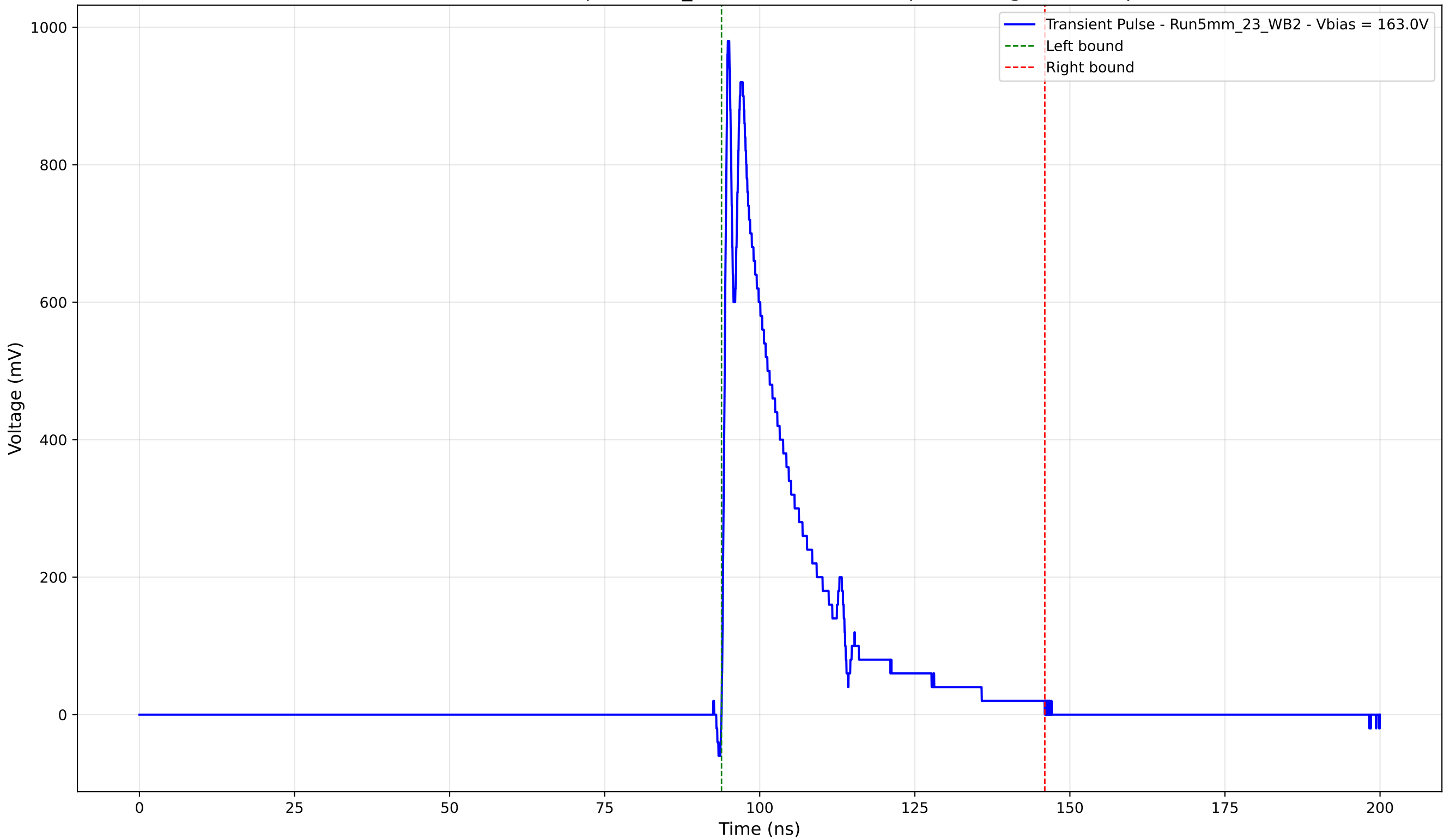
Transient Pulse - Sample: 5mm_23 - Position: 2660.0 \mu\text{m} - Charge: 201.76 pC
