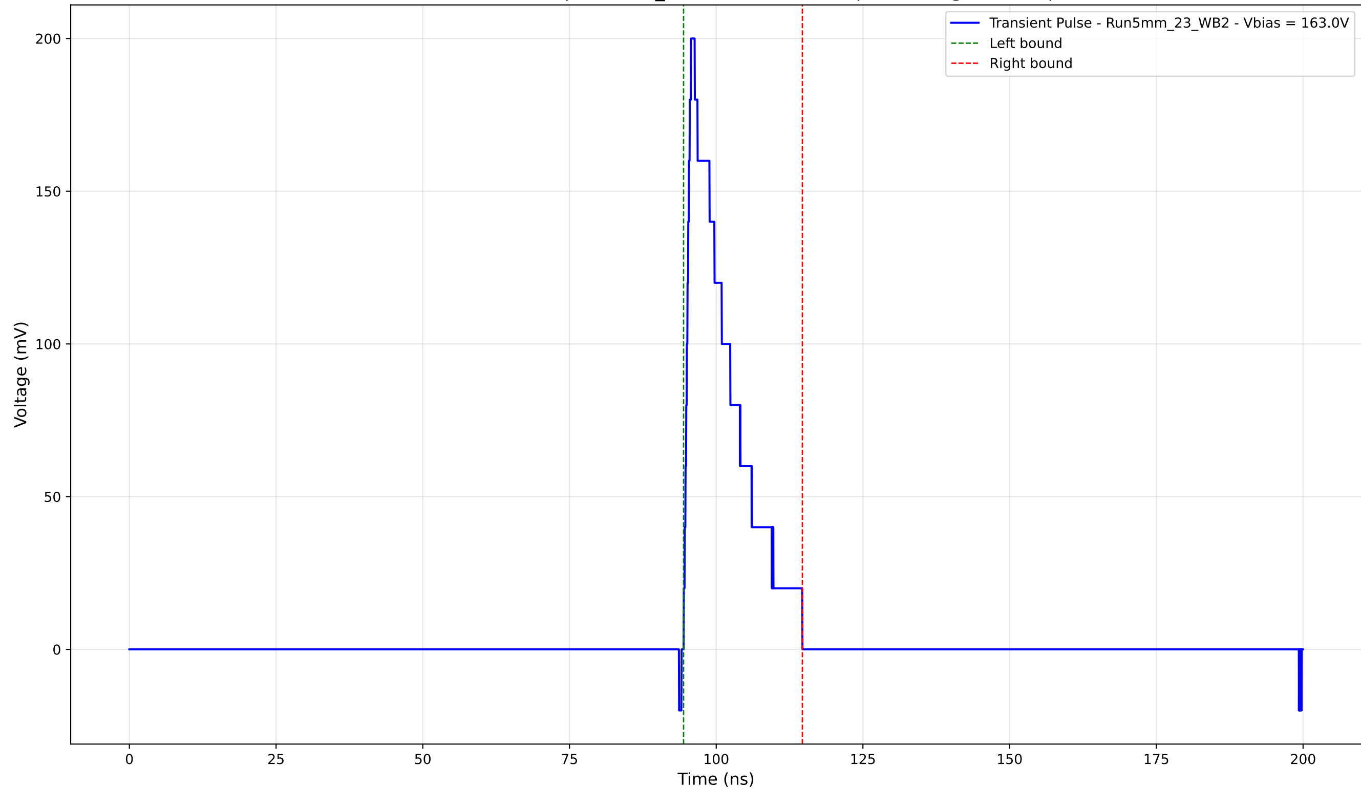
Transient Pulse - Sample: 5mm_23 - Position: 495.0 \mu\text{m} - Charge: 31.58 pC
