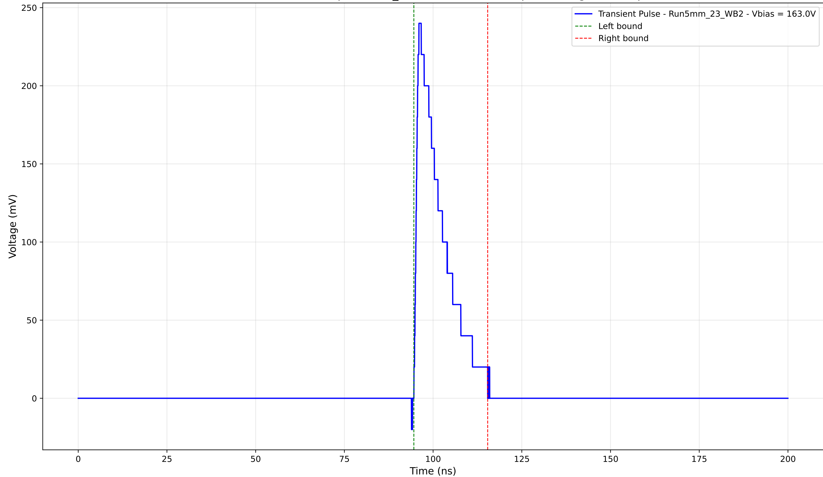
Transient Pulse - Sample: 5mm_23 - Position: 4055.0 \mu\text{m} - Charge: 38.98 pC
