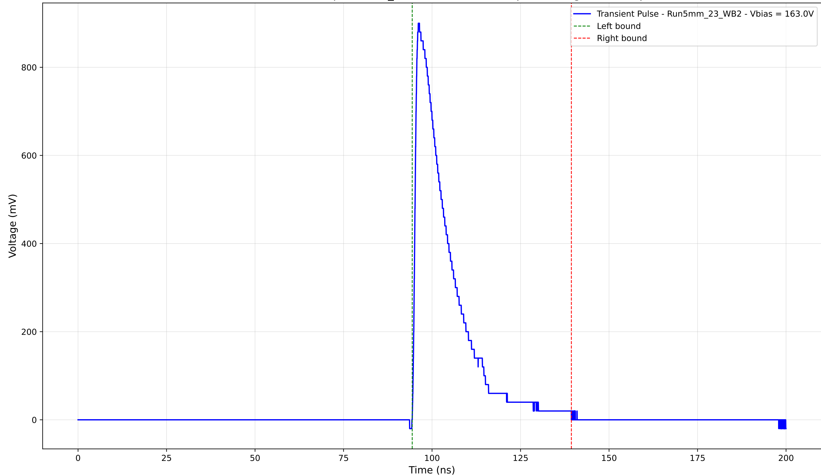
Transient Pulse - Sample: 5mm_23 - Position: 1165.0 \mu\text{m} - Charge: 193.46 pC
