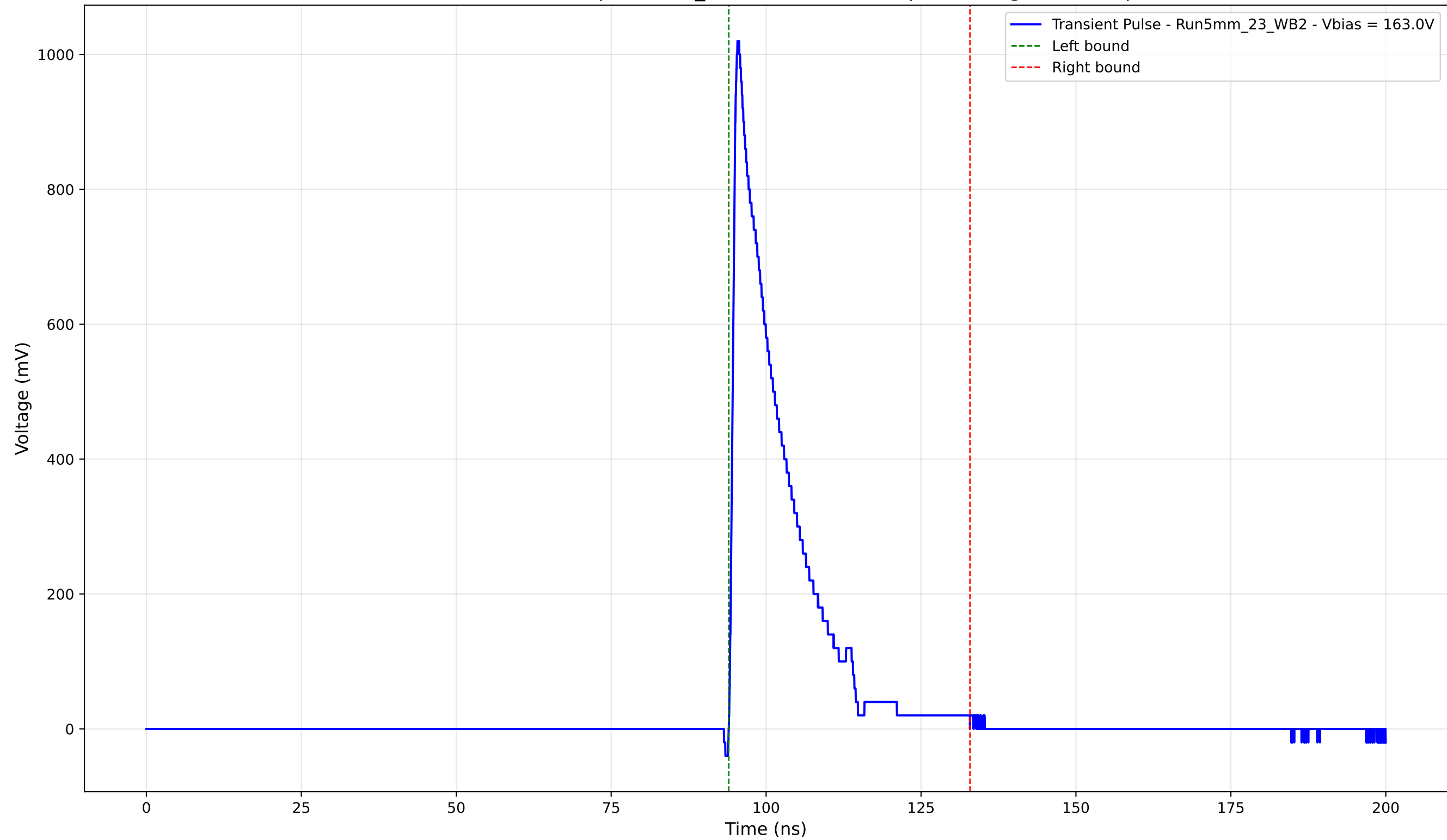
Transient Pulse - Sample: 5mm_23 - Position: 130.0 \mu\text{m} - Charge: 173.34 pC
