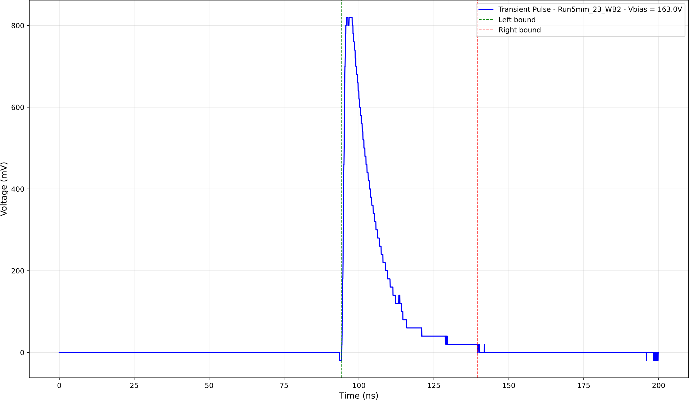
Transient Pulse - Sample: 5mm_23 - Position: 3415.0 \mu\text{m} - Charge: 181.38 pC
