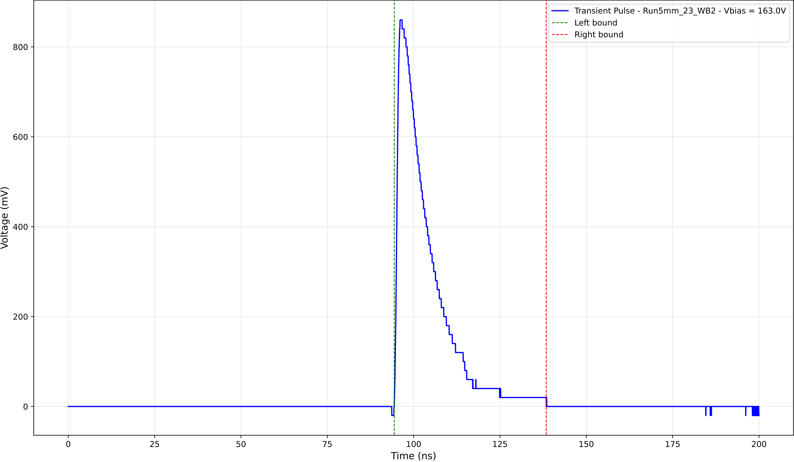
Transient Pulse - Sample: 5mm_23 - Position: 3760.0 \mu\text{m} - Charge: 177.26 pC
