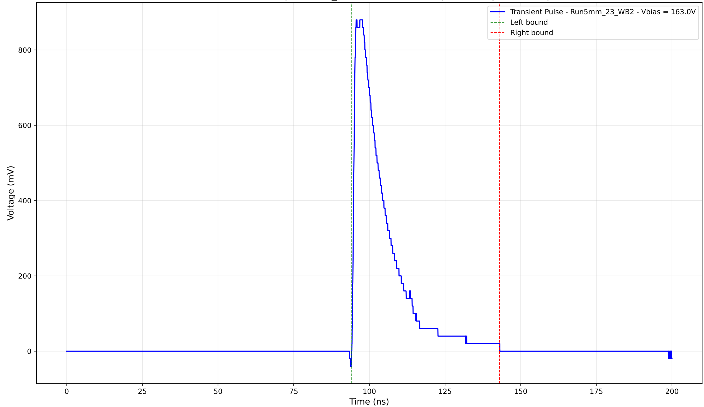
Transient Pulse - Sample: 5mm_23 - Position: 3320.0 \mu\text{m} - Charge: 203.14 pC
