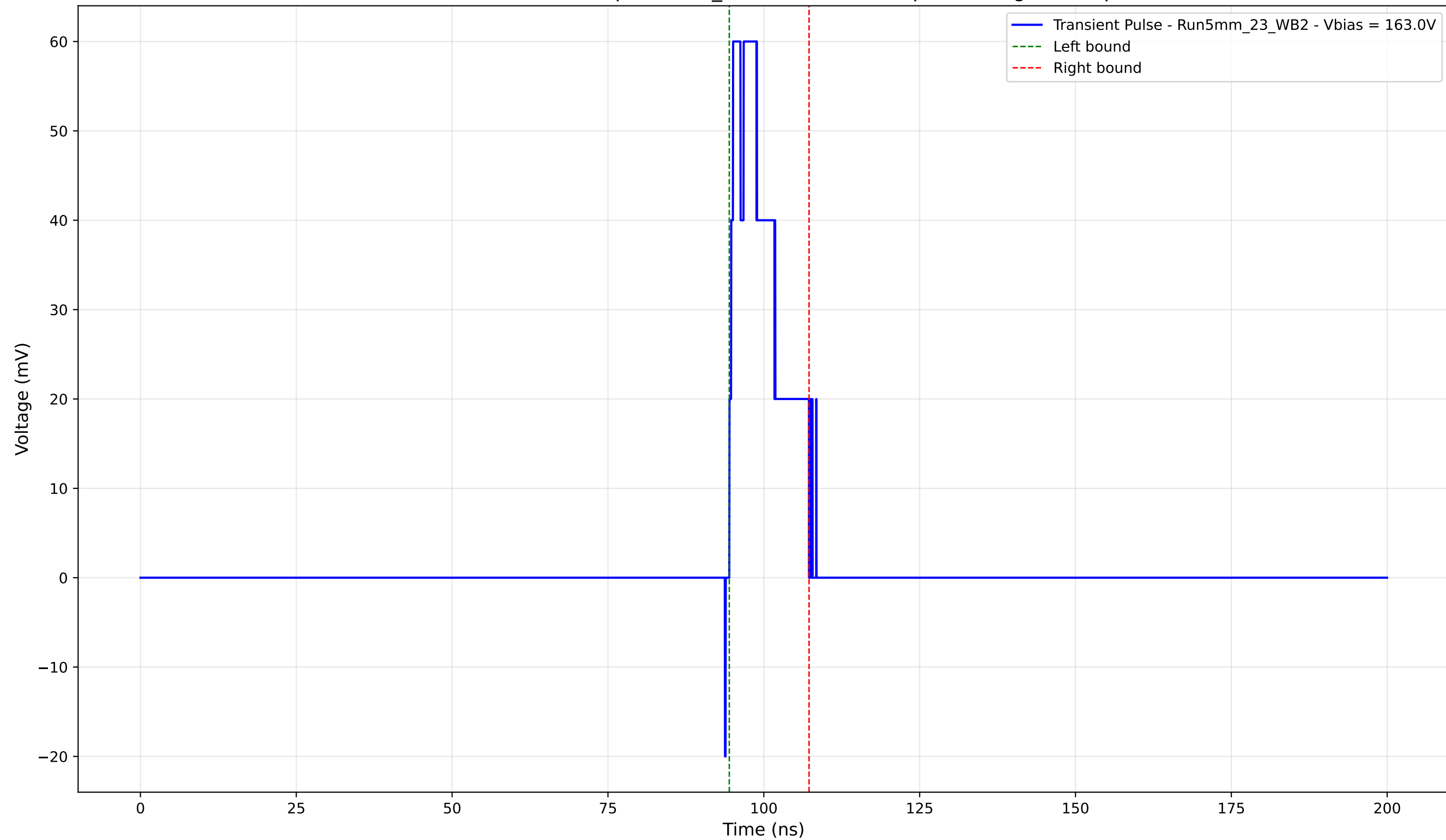
Transient Pulse - Sample: 5mm_23 - Position: 30.0 \mu\text{m} - Charge: 9.26 pC
