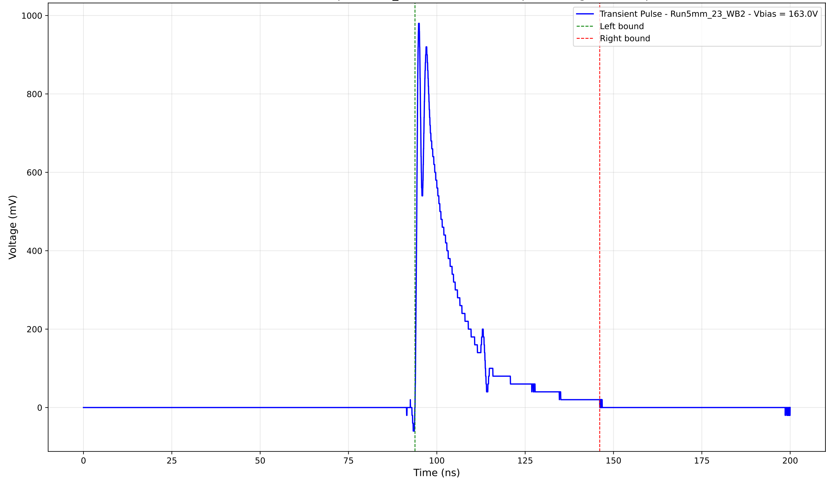
Transient Pulse - Sample: 5mm_23 - Position: 2615.0 \mu\text{m} - Charge: 194.72 pC
