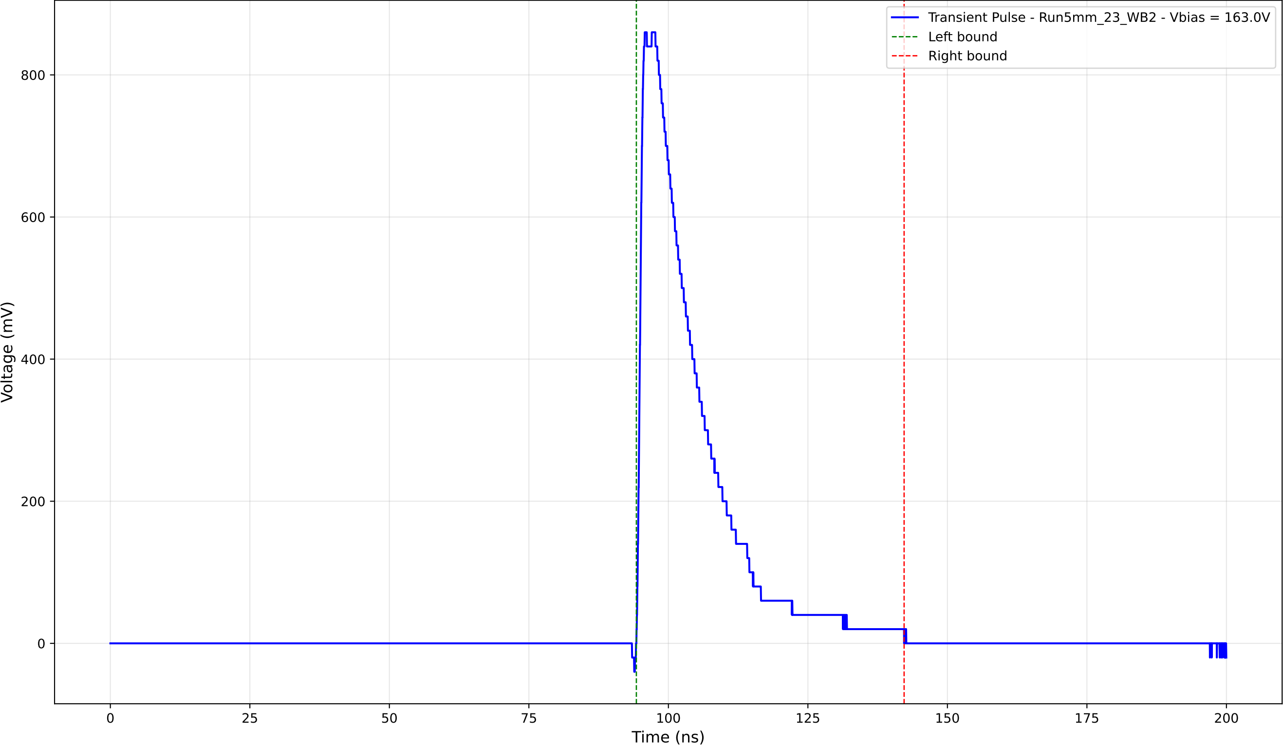
Transient Pulse - Sample: 5mm_23 - Position: 1615.0 \mu\text{m} - Charge: 197.39 pC
