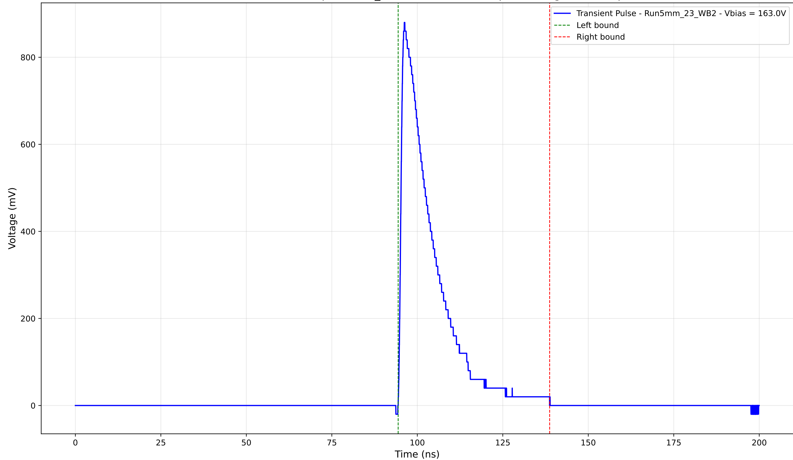
Transient Pulse - Sample: 5mm_23 - Position: 1095.0 \mu\text{m} - Charge: 180.65 pC
