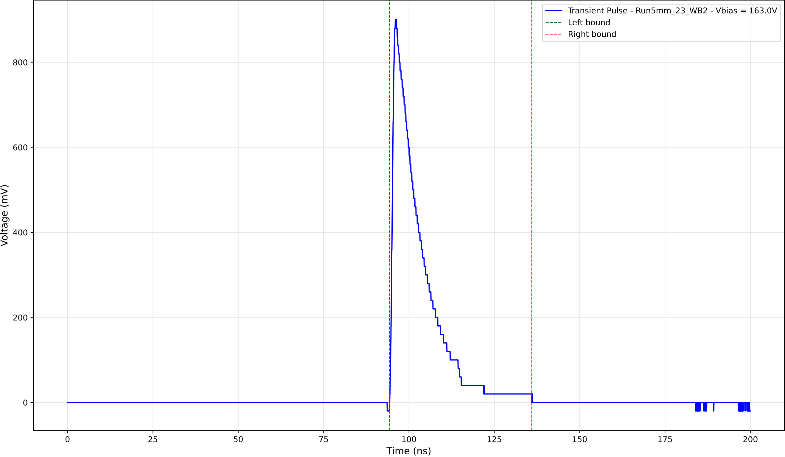
Transient Pulse - Sample: 5mm_23 - Position: 4270.0 \mu\text{m} - Charge: 163.70 pC
