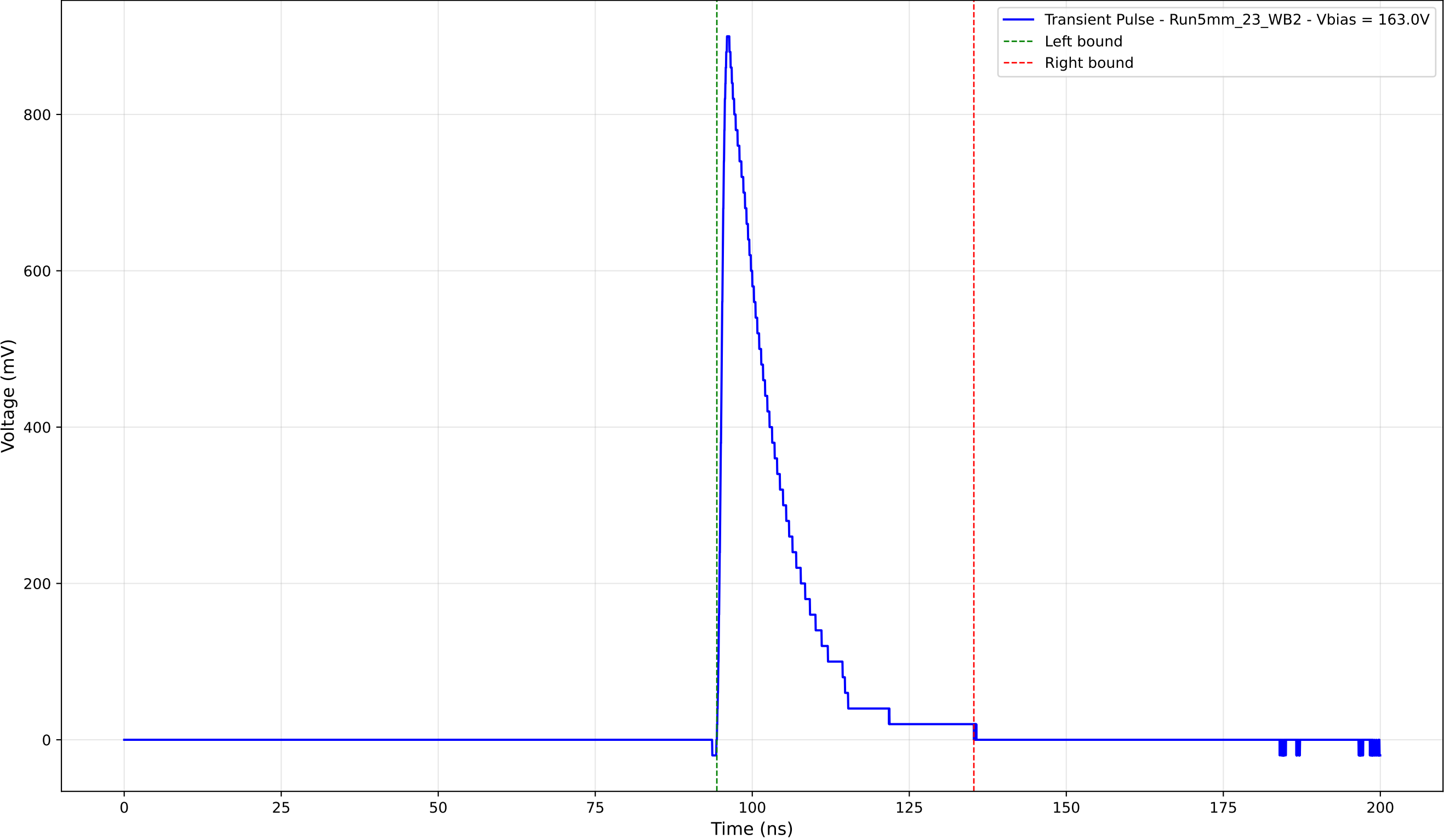
Transient Pulse - Sample: 5mm_23 - Position: 4285.0 \mu\text{m} - Charge: 163.02 pC
