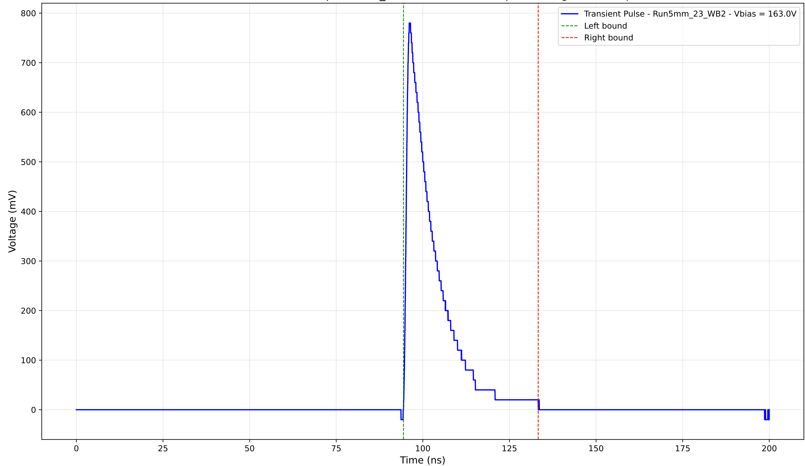
Transient Pulse - Sample: 5mm_23 - Position: 4115.0 \mu\text{m} - Charge: 139.11 pC
