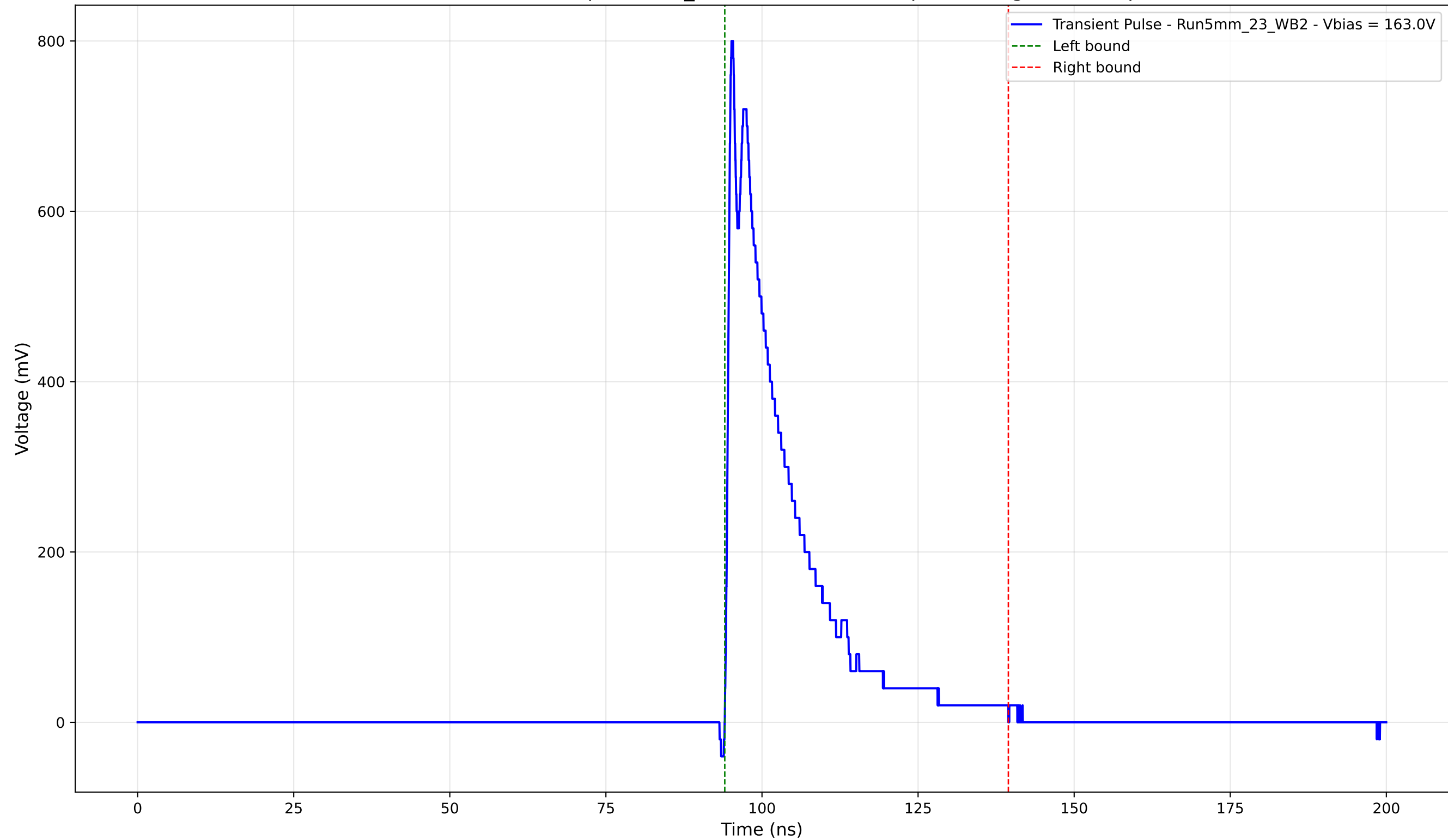
Transient Pulse - Sample: 5mm_23 - Position: 2075.0 \mu\text{m} - Charge: 153.46 pC
