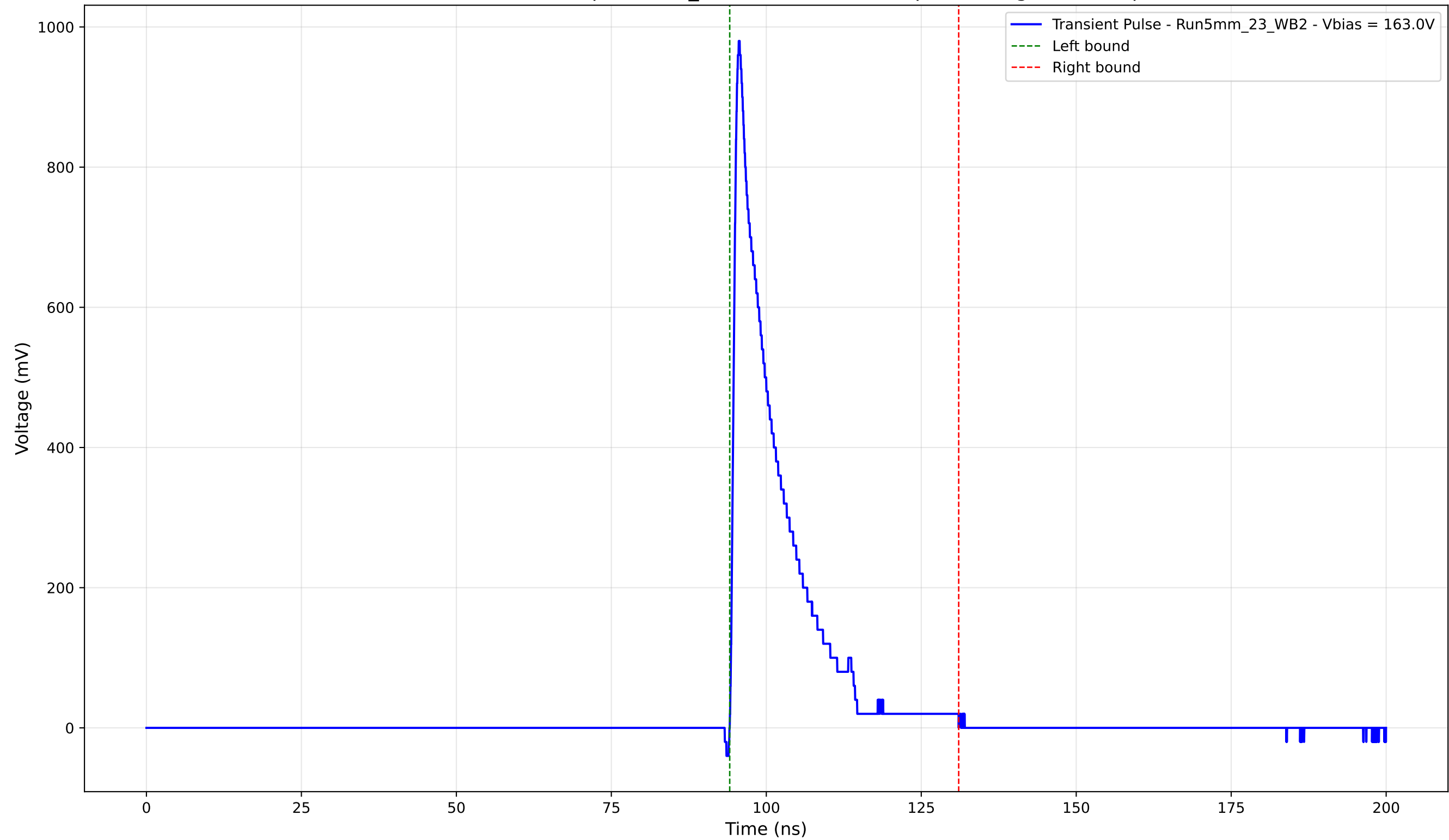
Transient Pulse - Sample: 5mm_23 - Position: 4815.0 \mu\text{m} - Charge: 144.86 pC
