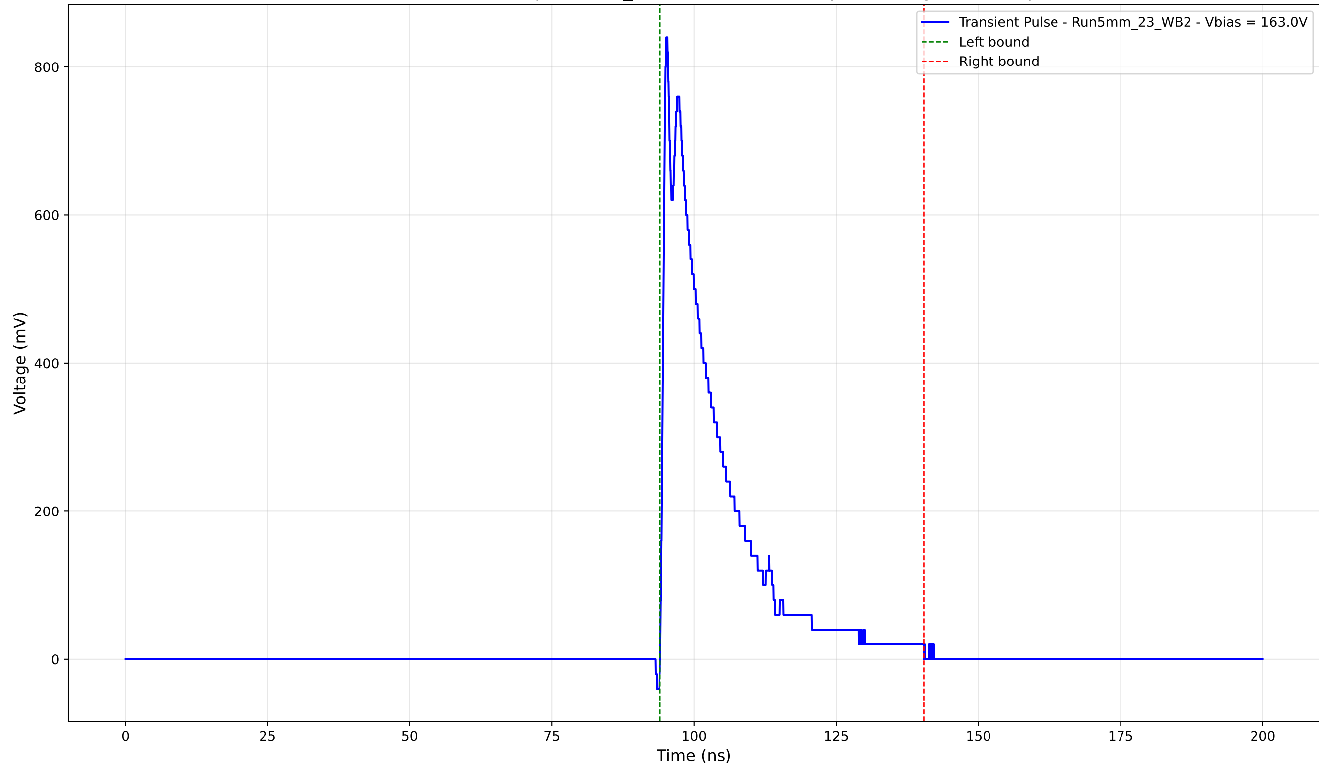
Transient Pulse - Sample: 5mm_23 - Position: 2960.0 \mu\text{m} - Charge: 161.46 pC
