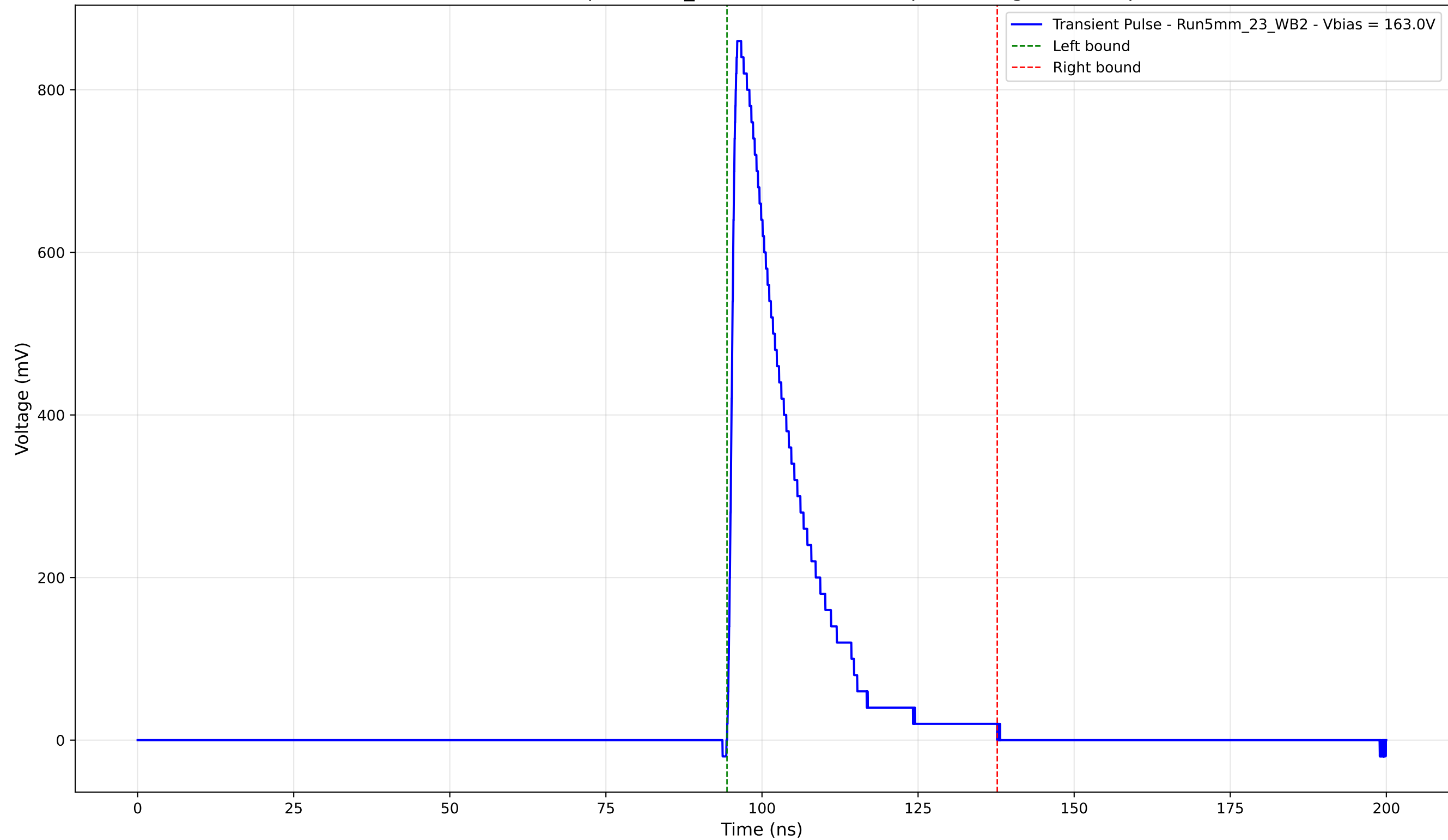
Transient Pulse - Sample: 5mm_23 - Position: 3840.0 \mu\text{m} - Charge: 174.54 pC
