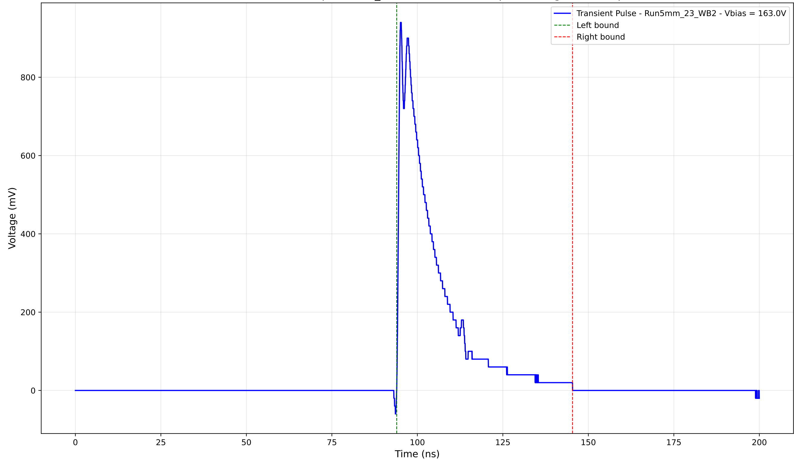
Transient Pulse - Sample: 5mm_23 - Position: 2170.0 \mu\text{m} - Charge: 205.54 pC
