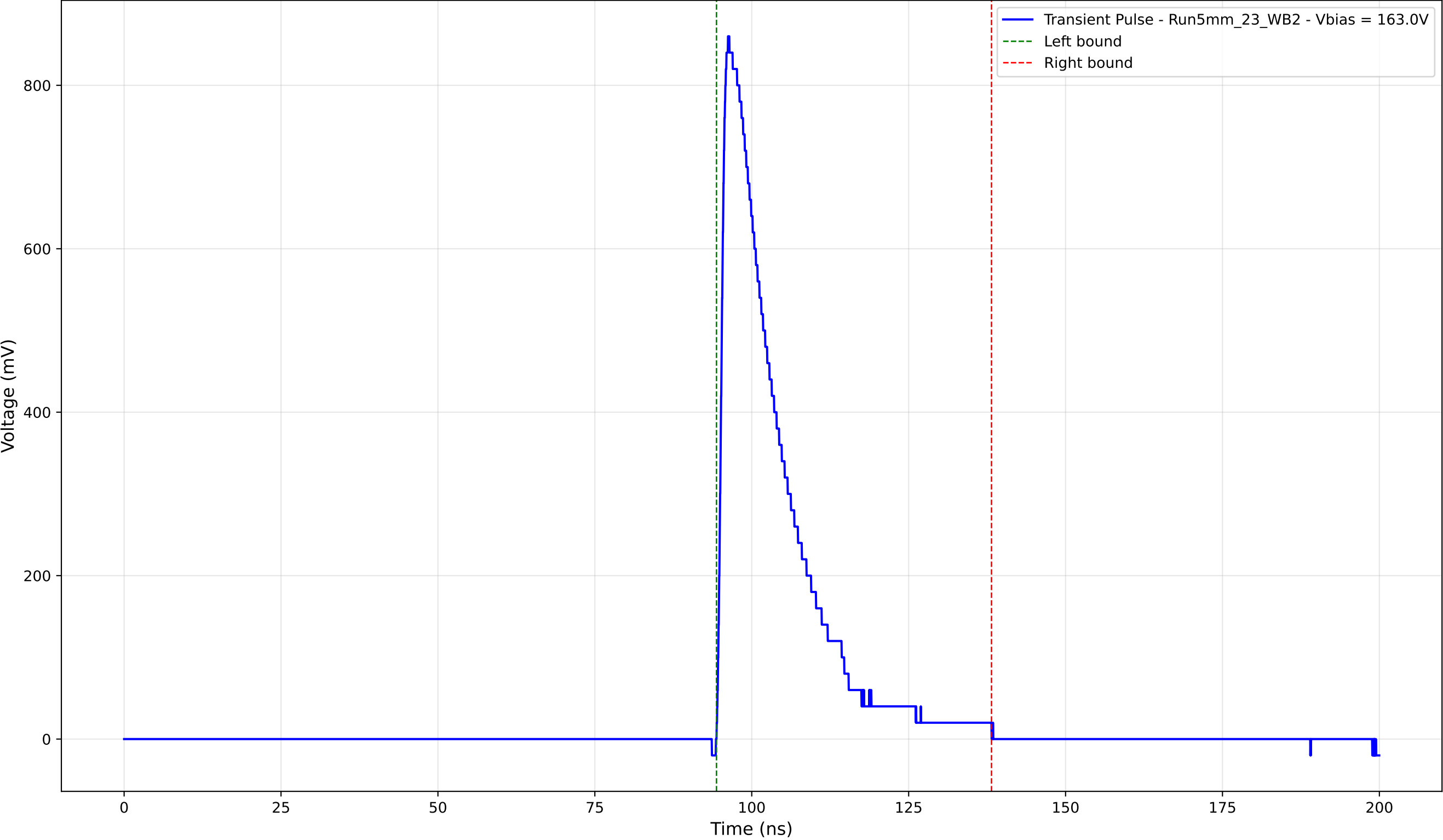
Transient Pulse - Sample: 5mm_23 - Position: 3725.0 \mu\text{m} - Charge: 176.80 pC
