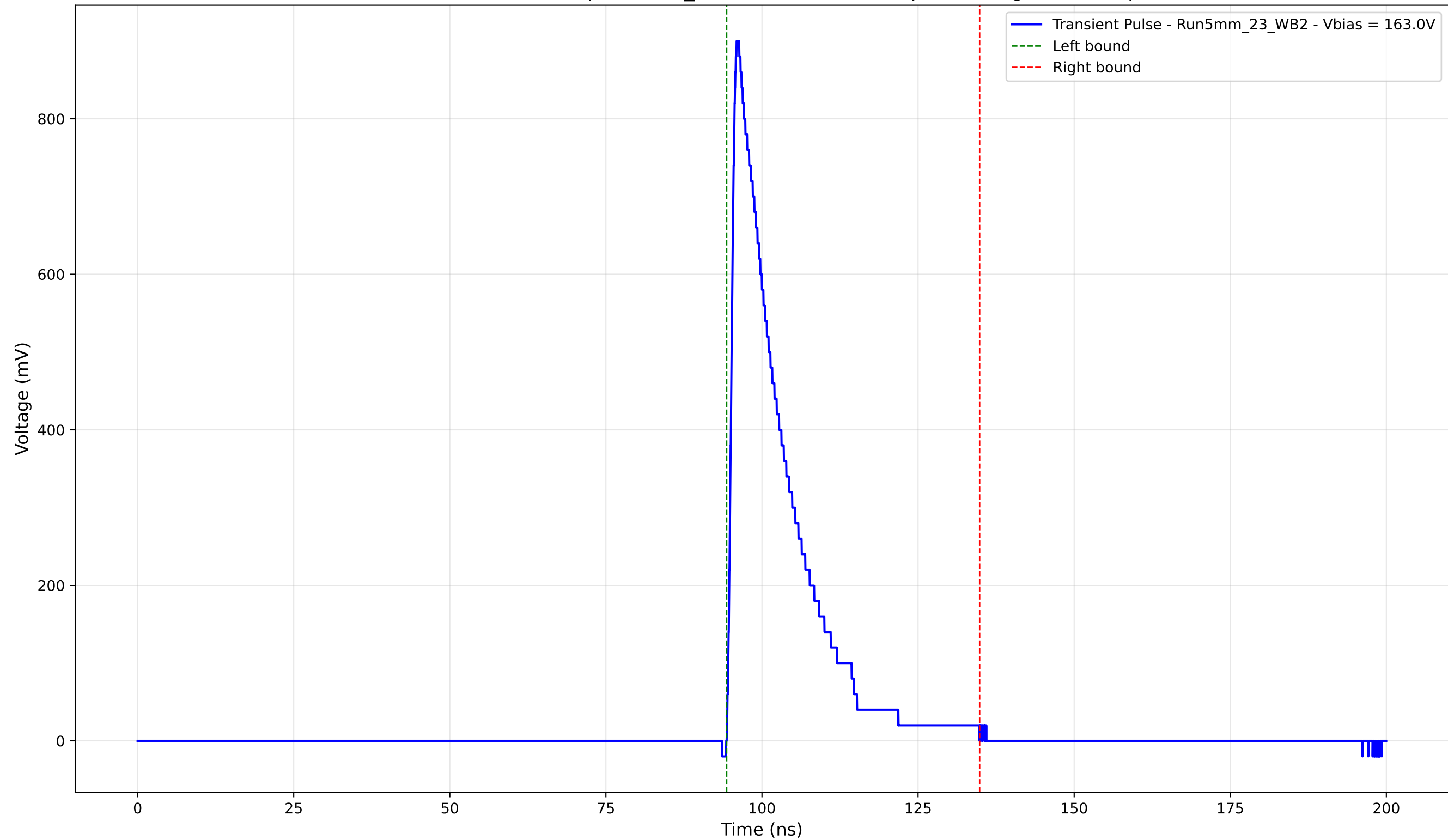
Transient Pulse - Sample: 5mm_23 - Position: 4310.0 \mu\text{m} - Charge: 162.54 pC
