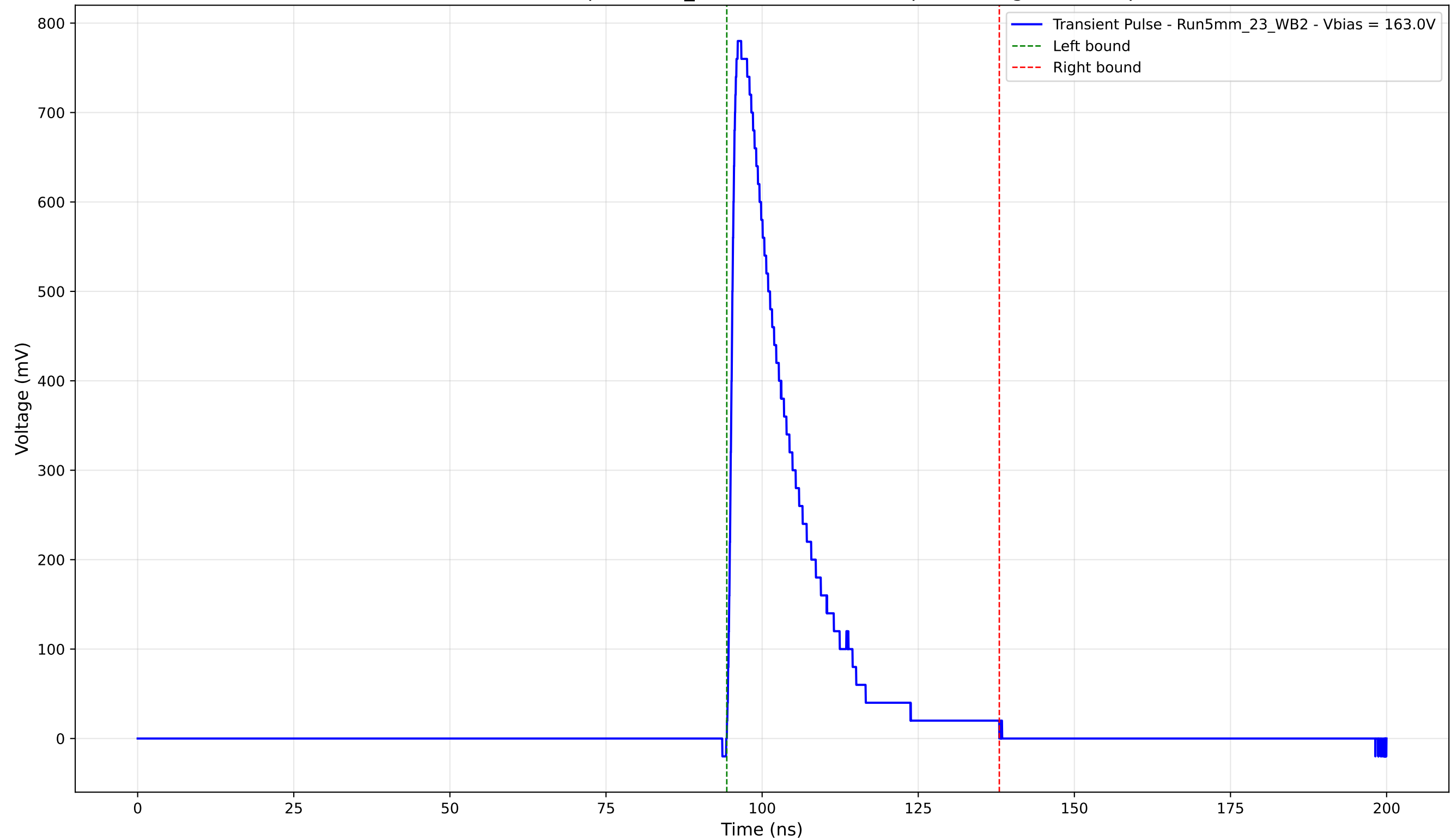
Transient Pulse - Sample: 5mm_23 - Position: 3615.0 \mu\text{m} - Charge: 160.22 pC
