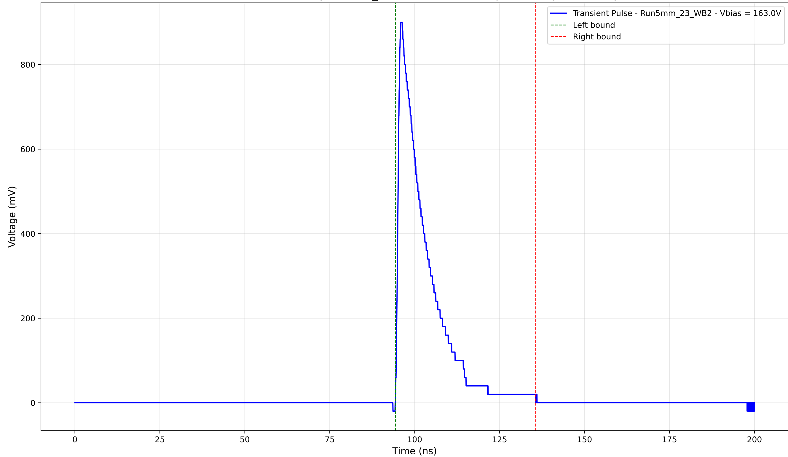
Transient Pulse - Sample: 5mm_23 - Position: 4350.0 \mu\text{m} - Charge: 161.26 pC
