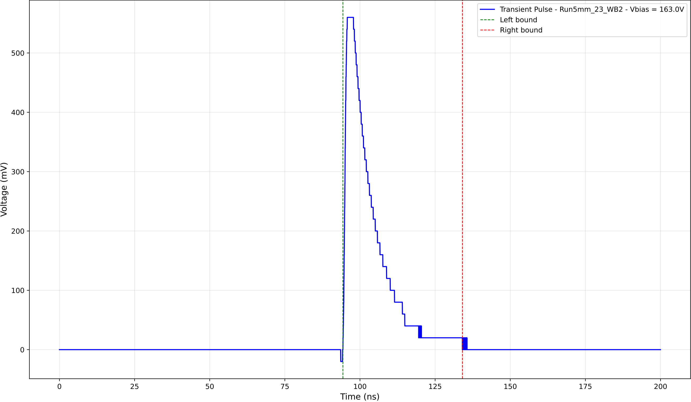
Transient Pulse - Sample: 5mm_23 - Position: 3470.0 \mu\text{m} - Charge: 115.93 pC
