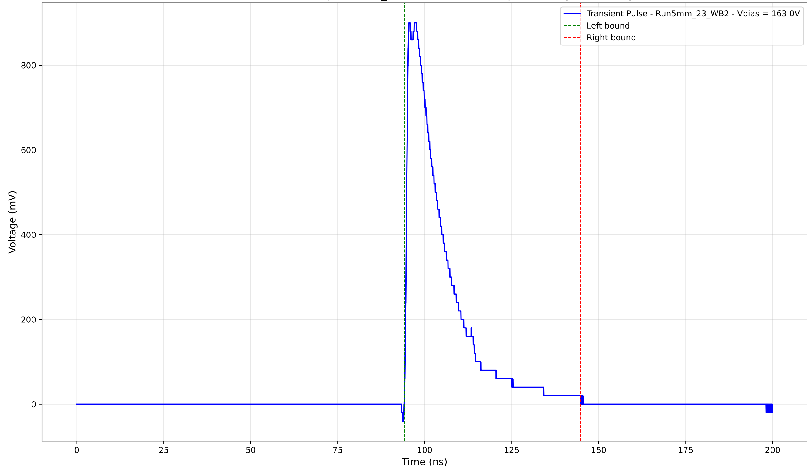
Transient Pulse - Sample: 5mm_23 - Position: 1780.0 \mu\text{m} - Charge: 217.22 pC
