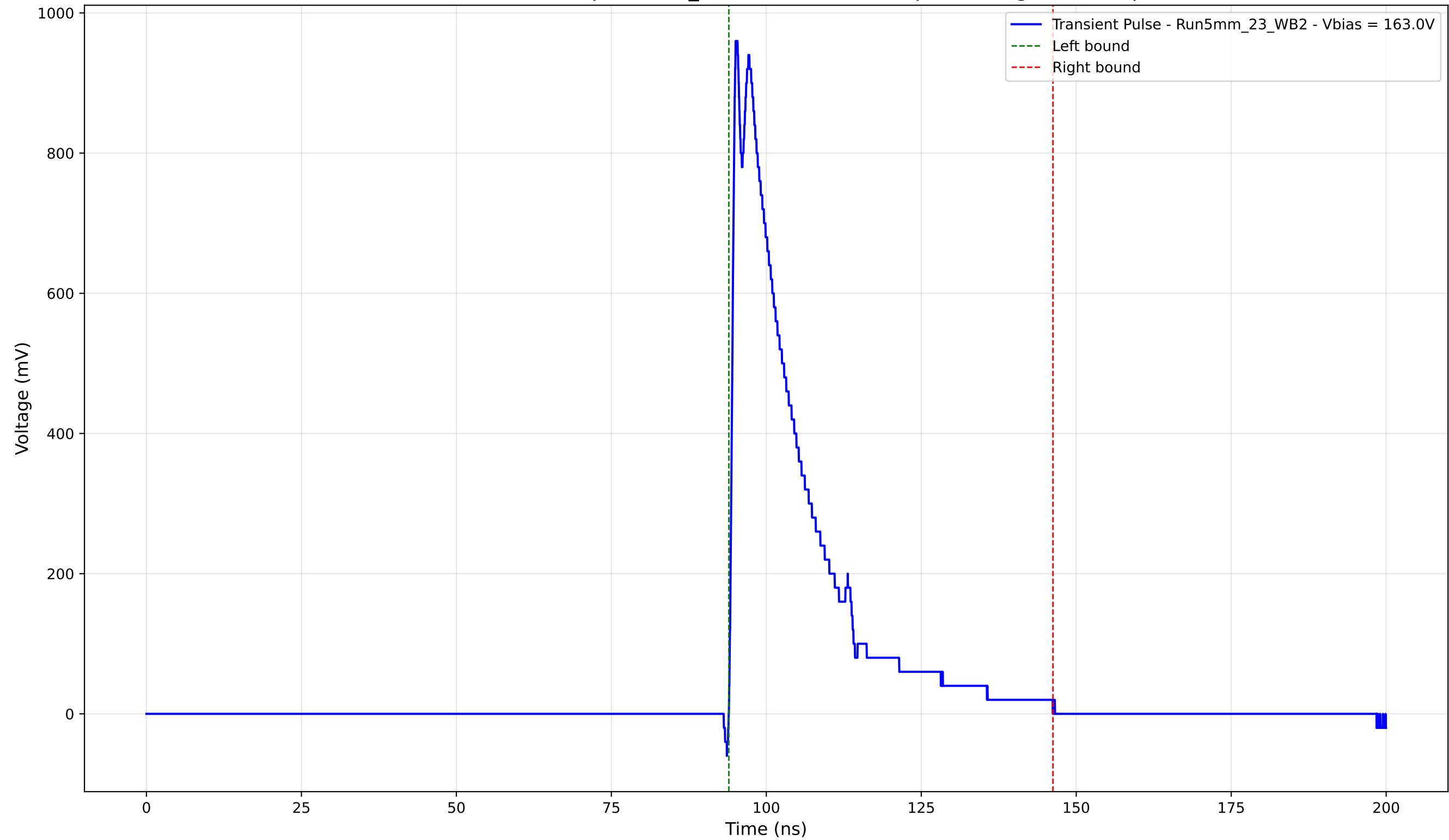
Transient Pulse - Sample: 5mm_23 - Position: 2895.0 \mu\text{m} - Charge: 218.90 pC
