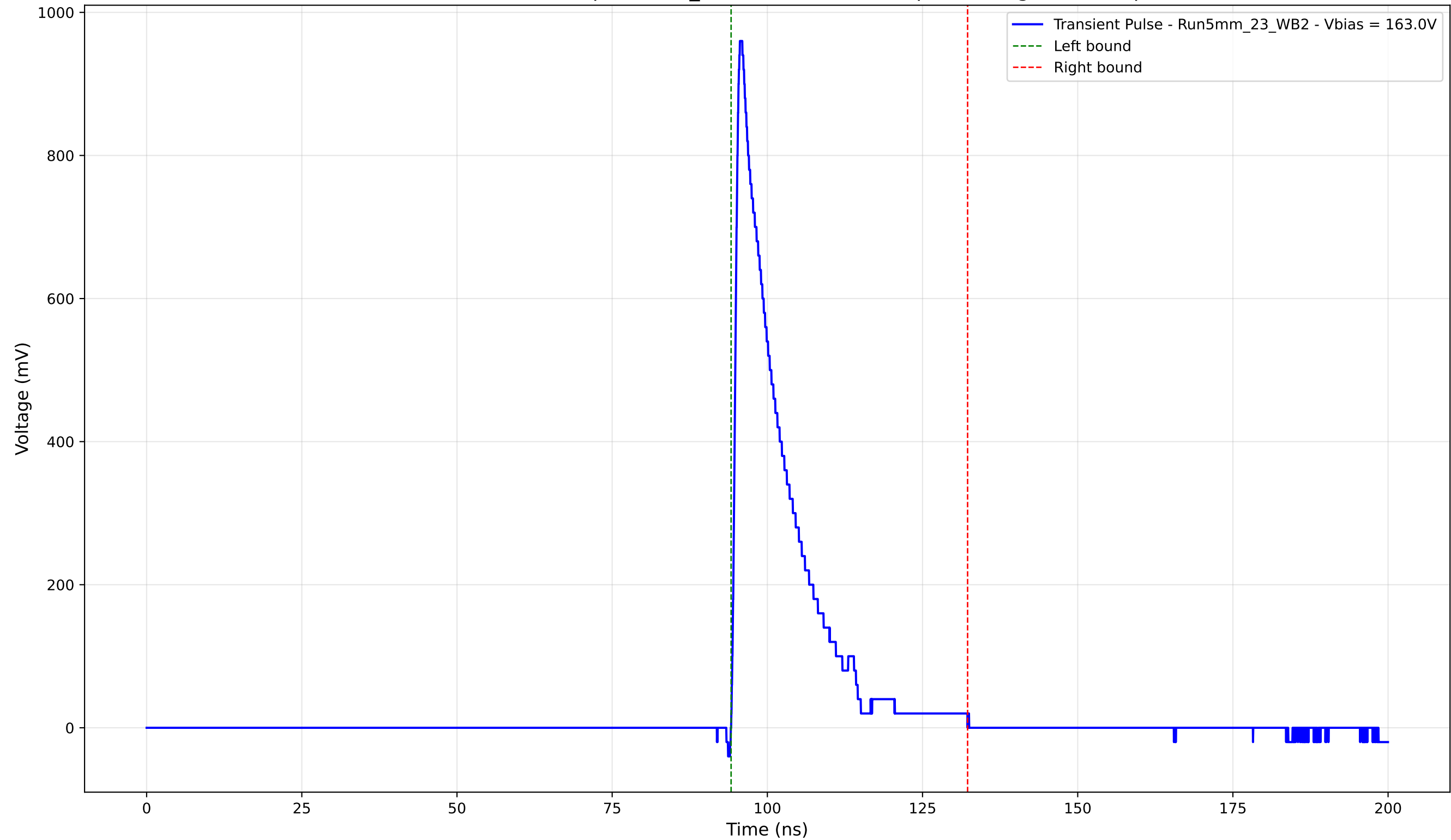
Transient Pulse - Sample: 5mm_23 - Position: 4685.0 \mu\text{m} - Charge: 155.59 pC
