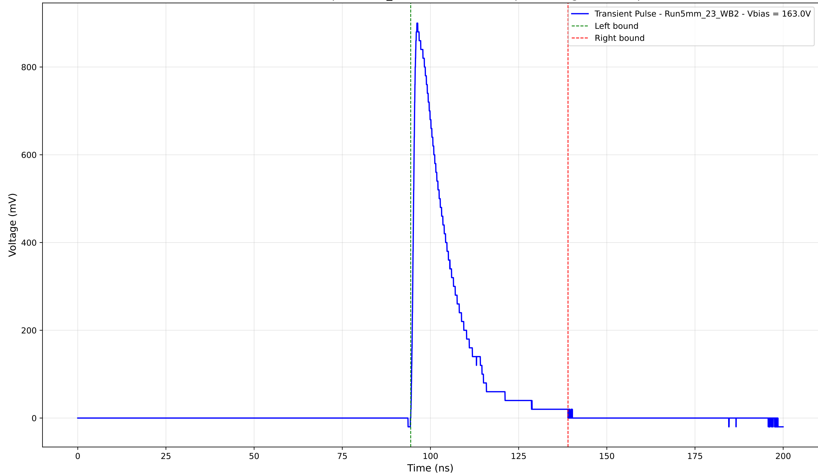
Transient Pulse - Sample: 5mm_23 - Position: 1145.0 \mu\text{m} - Charge: 191.13 pC
