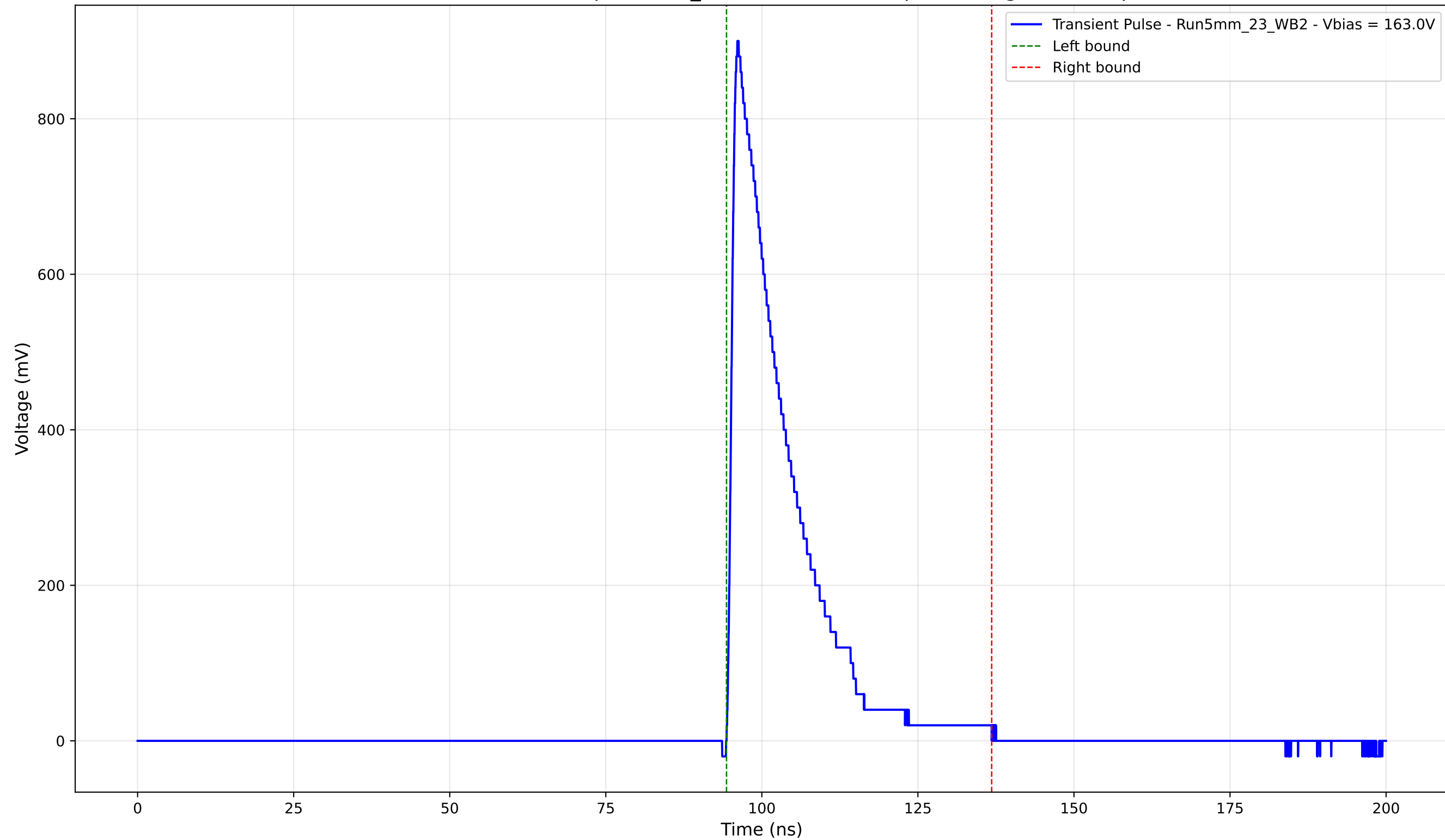
Transient Pulse - Sample: 5mm_23 - Position: 800.0 \mu\text{m} - Charge: 173.78 pC
