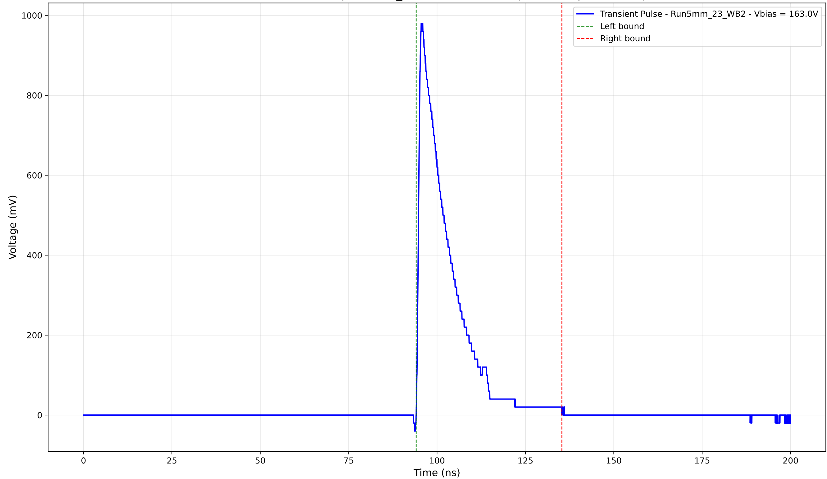
Transient Pulse - Sample: 5mm_23 - Position: 340.0 \mu\text{m} - Charge: 180.54 pC
