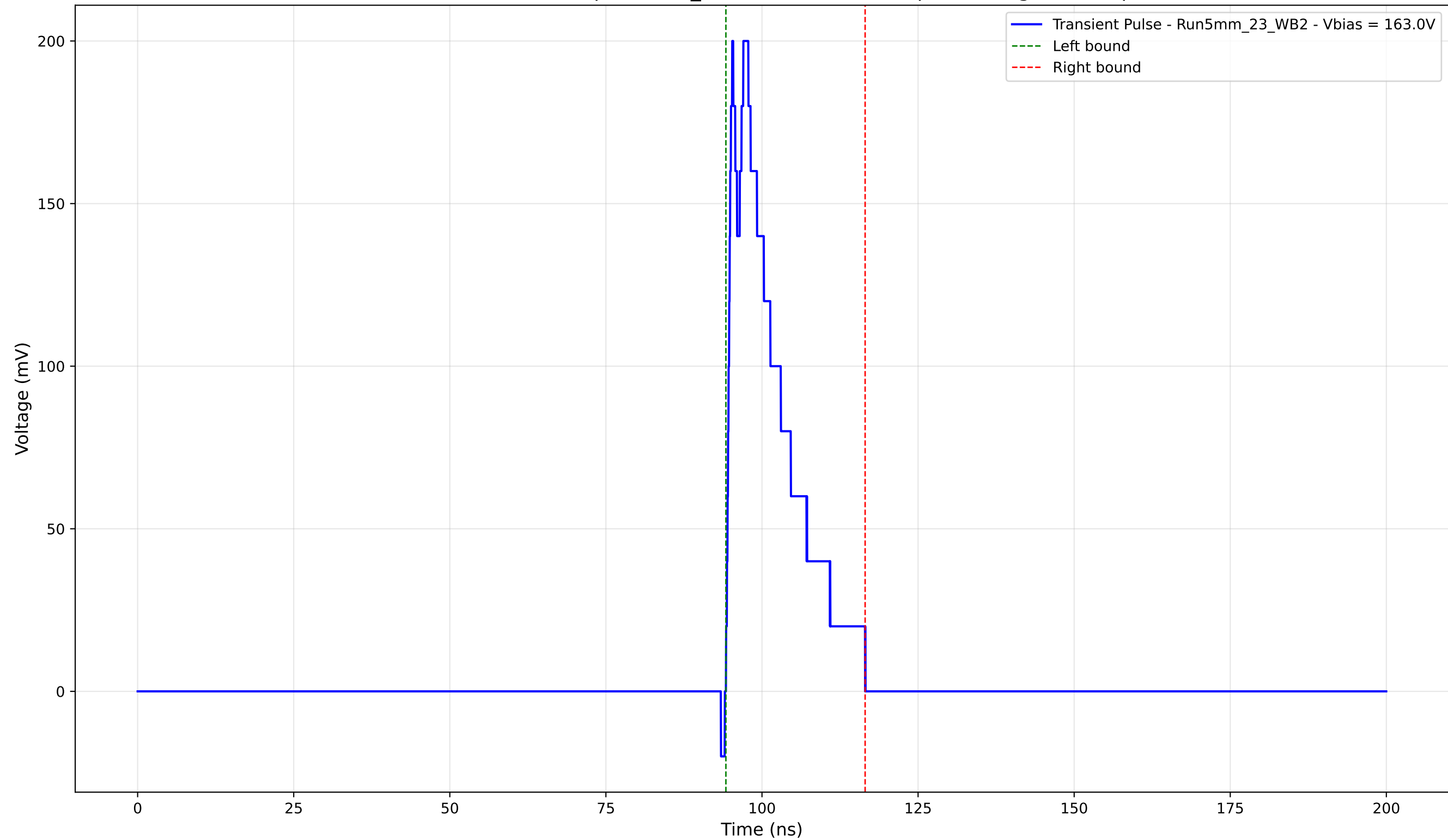
Transient Pulse - Sample: 5mm_23 - Position: 2005.0 \mu\text{m} - Charge: 35.62 pC
