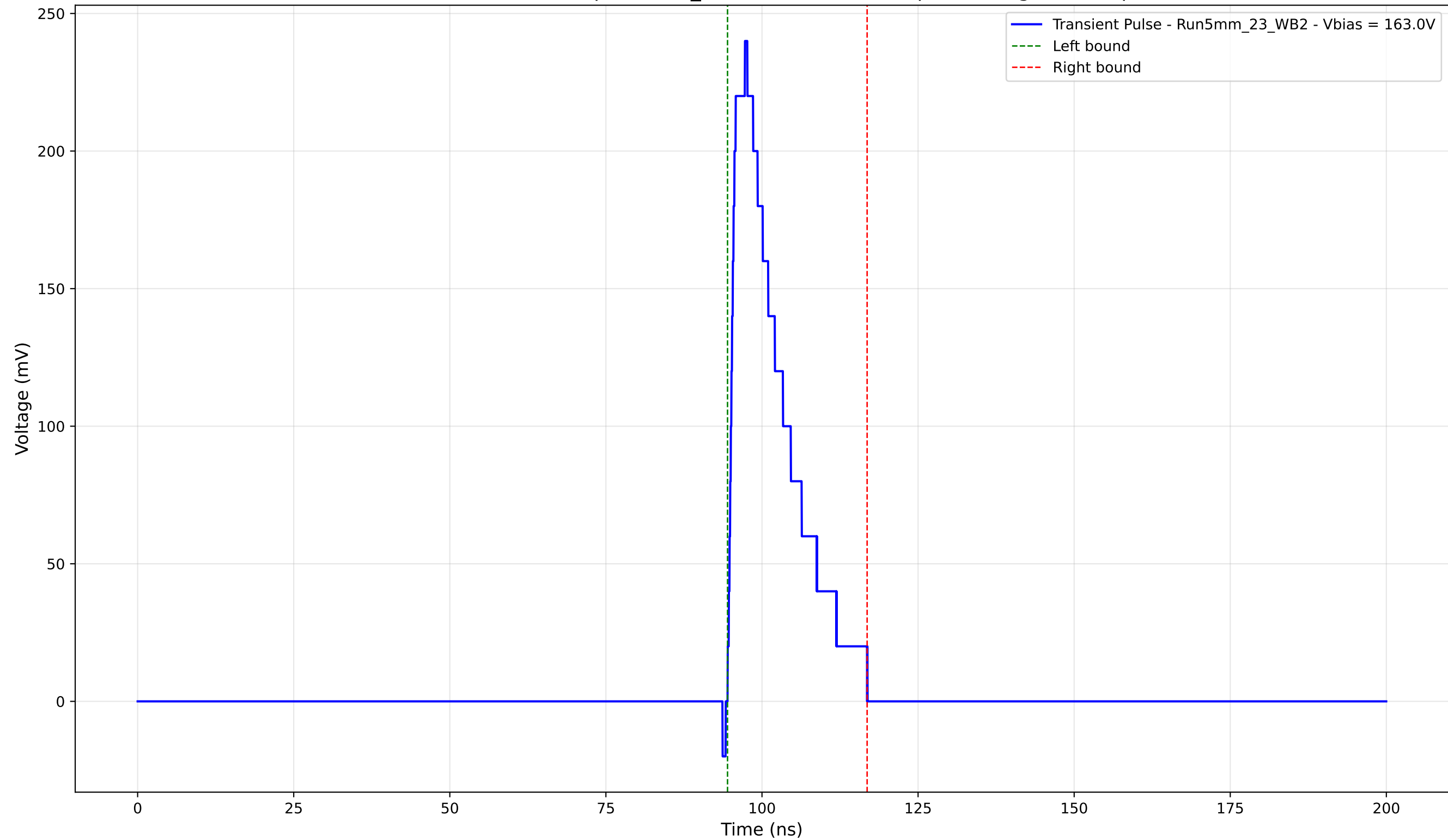
Transient Pulse - Sample: 5mm_23 - Position: 3545.0 \mu\text{m} - Charge: 42.83 pC
