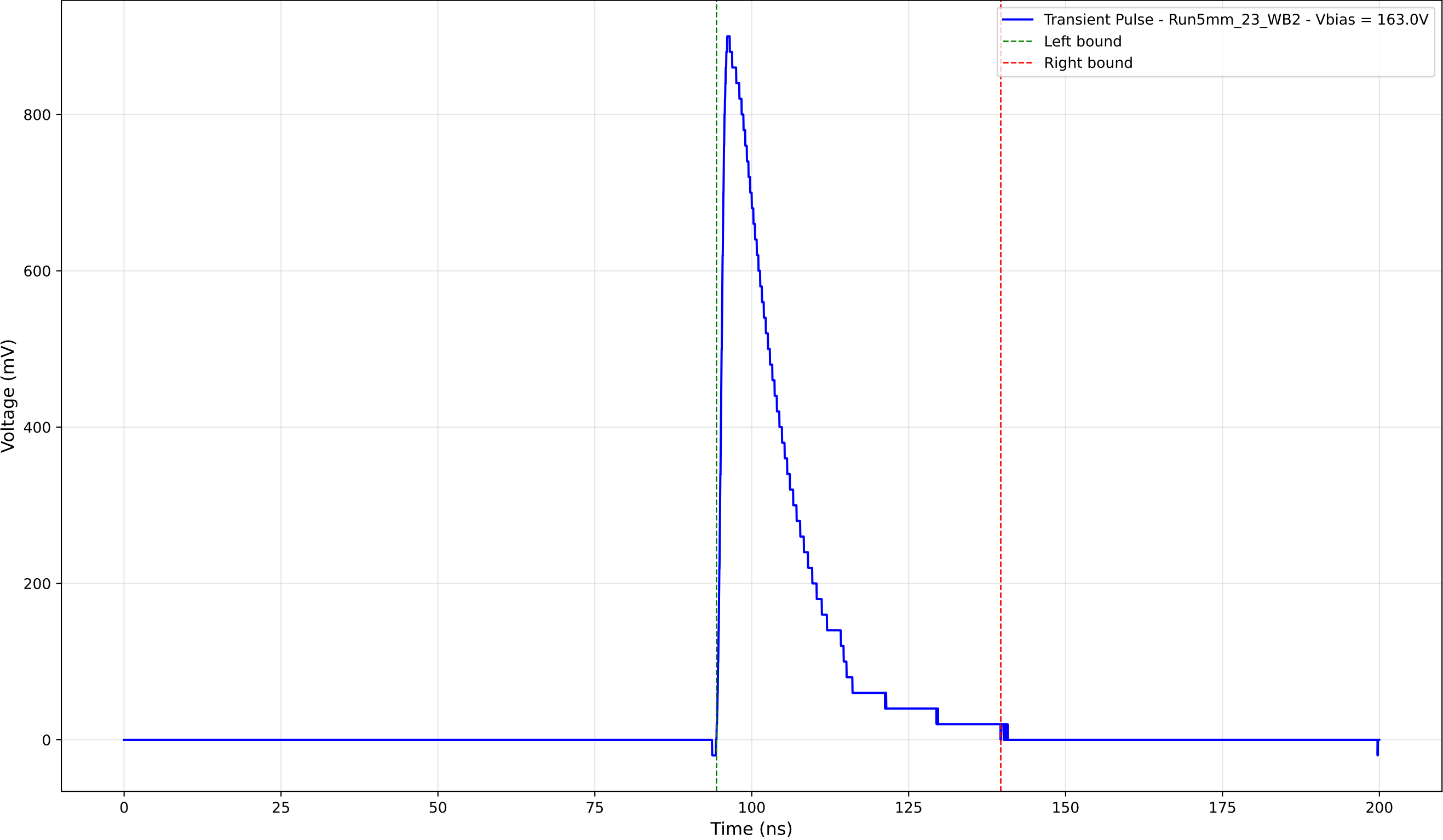
Transient Pulse - Sample: 5mm_23 - Position: 1170.0 \mu\text{m} - Charge: 194.18 pC
