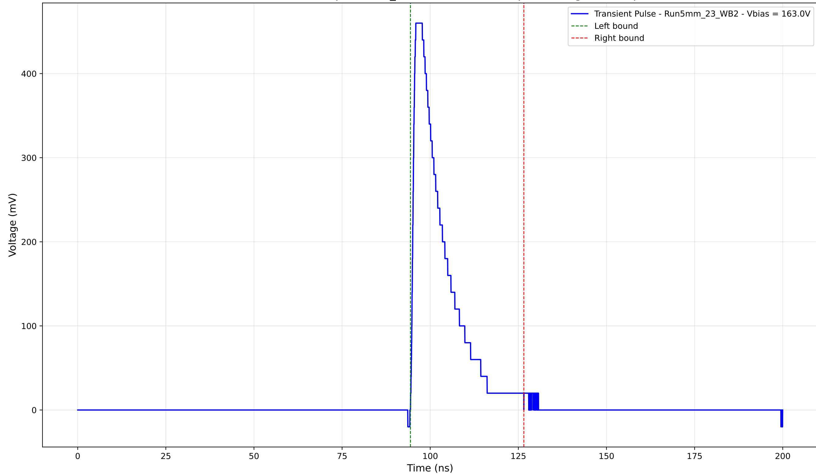
Transient Pulse - Sample: 5mm_23 - Position: 3570.0 \mu\text{m} - Charge: 89.88 pC
