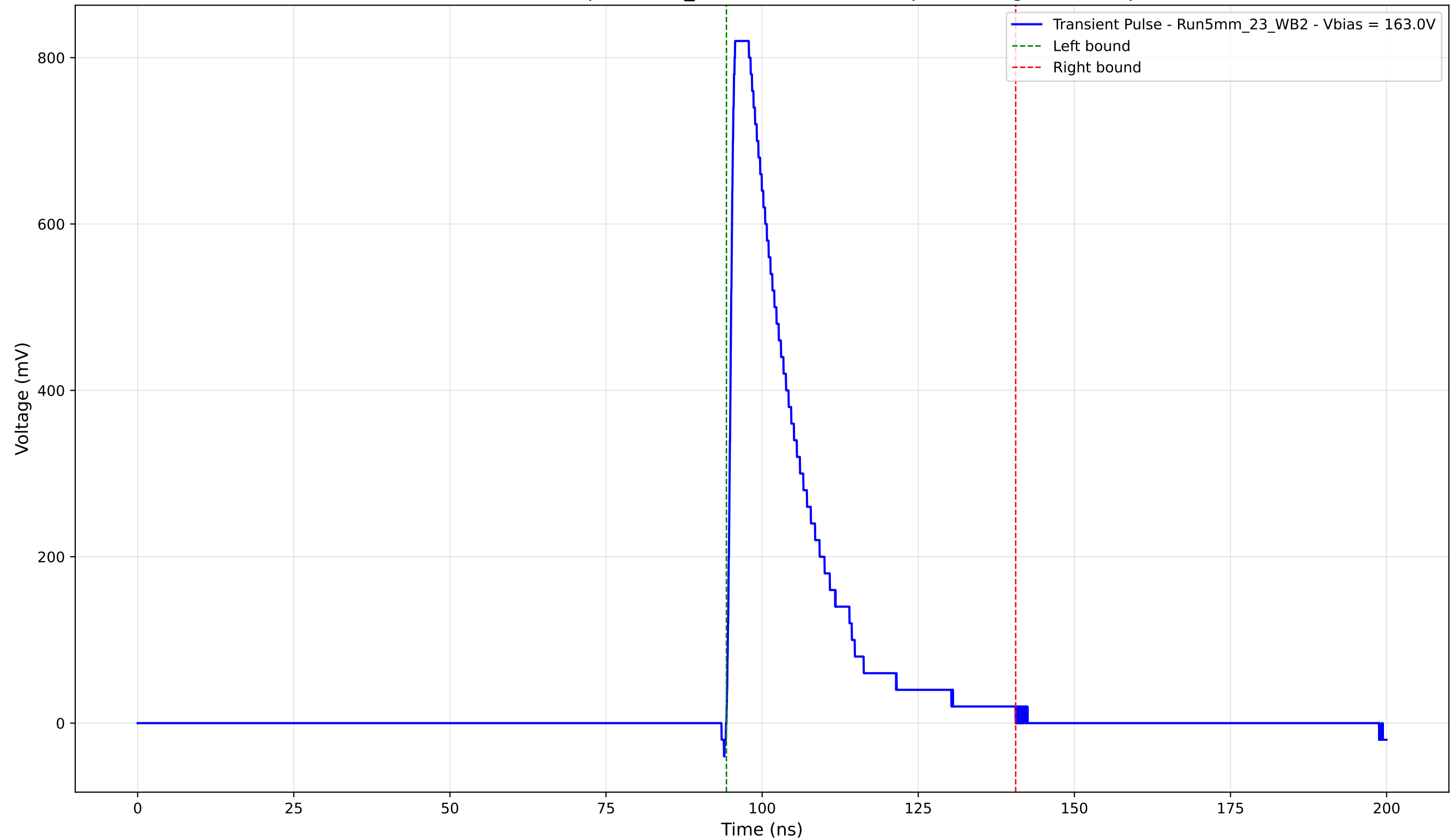
Transient Pulse - Sample: 5mm_23 - Position: 1595.0 \mu\text{m} - Charge: 187.66 pC
