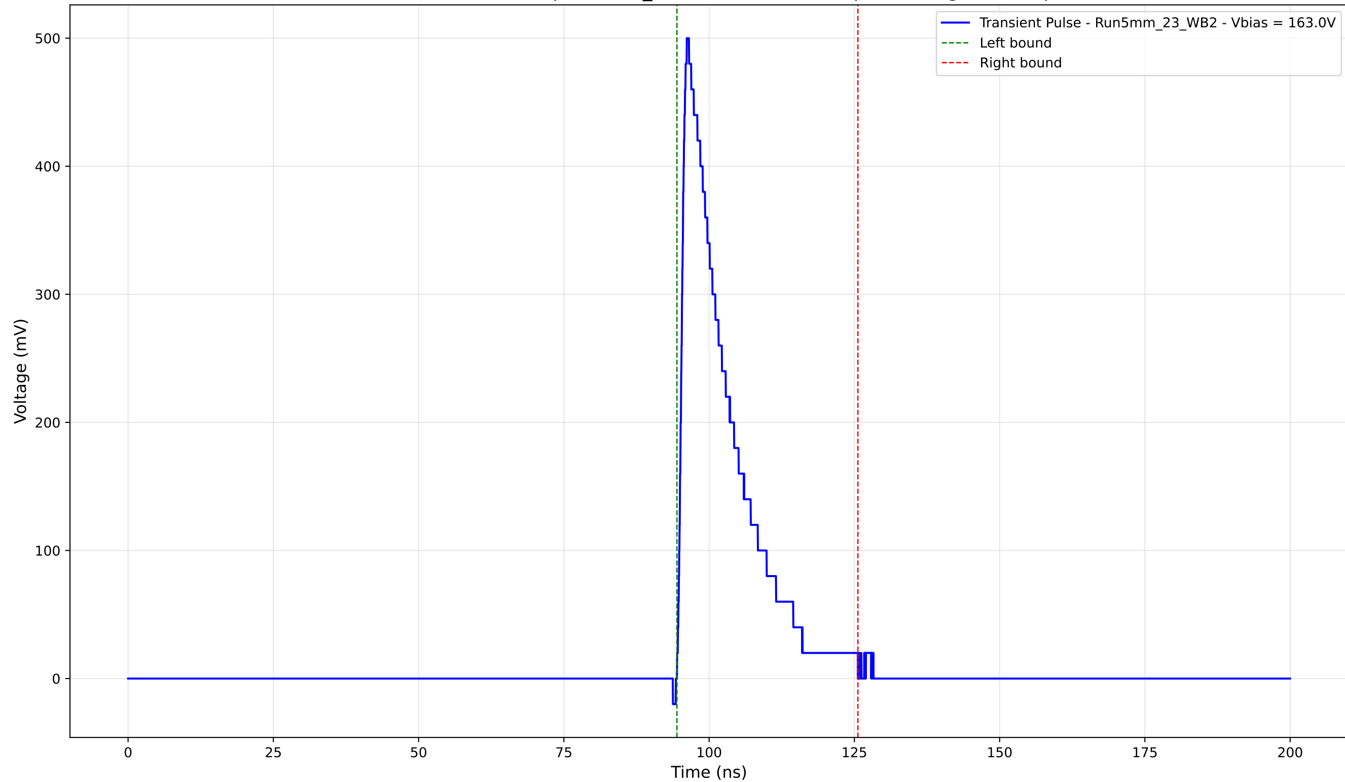
Transient Pulse - Sample: 5mm_23 - Position: 1035.0 \mu\text{m} - Charge: 89.66 pC
