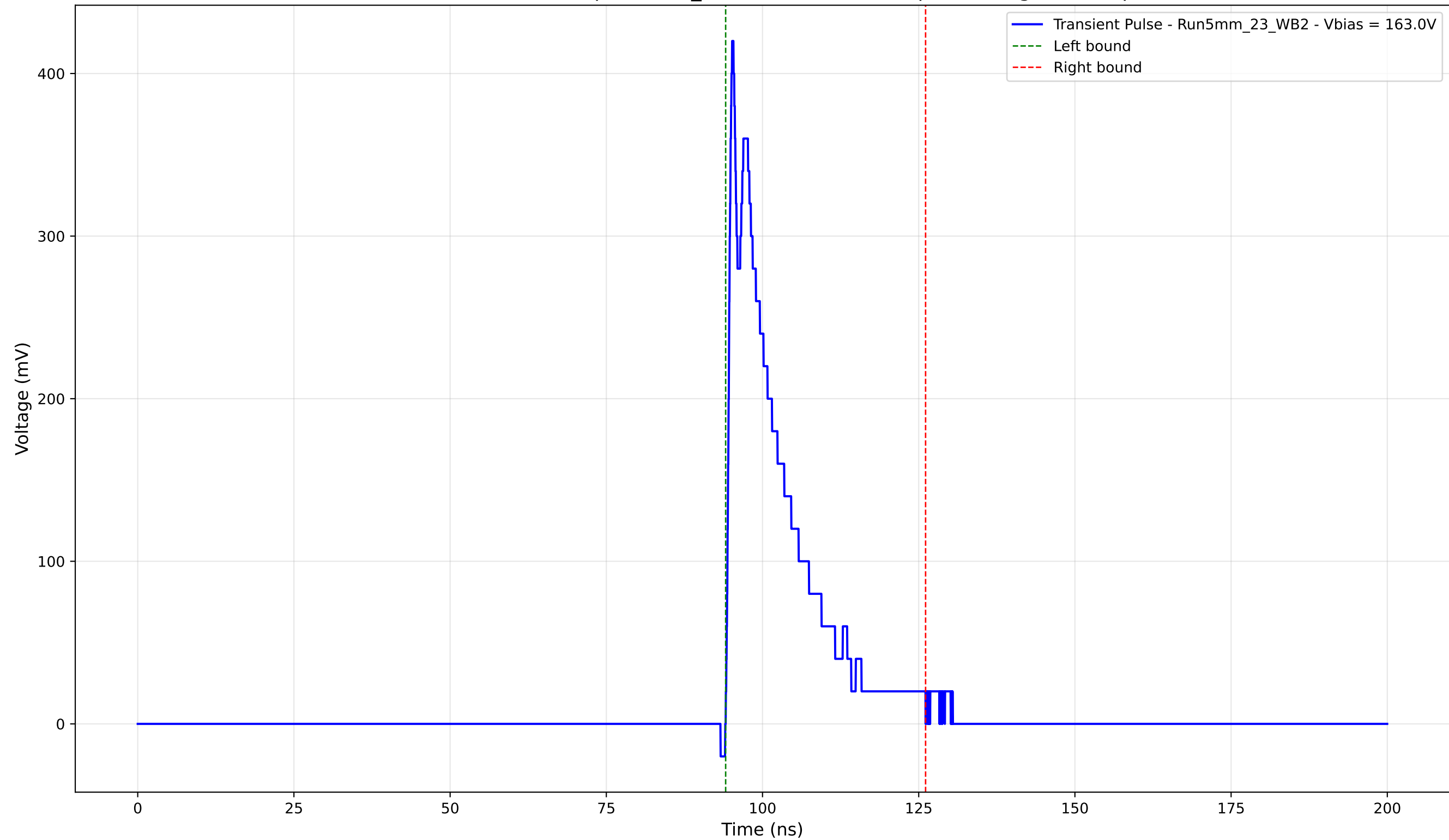
Transient Pulse - Sample: 5mm_23 - Position: 2040.0 \mu\text{m} - Charge: 70.35 pC
