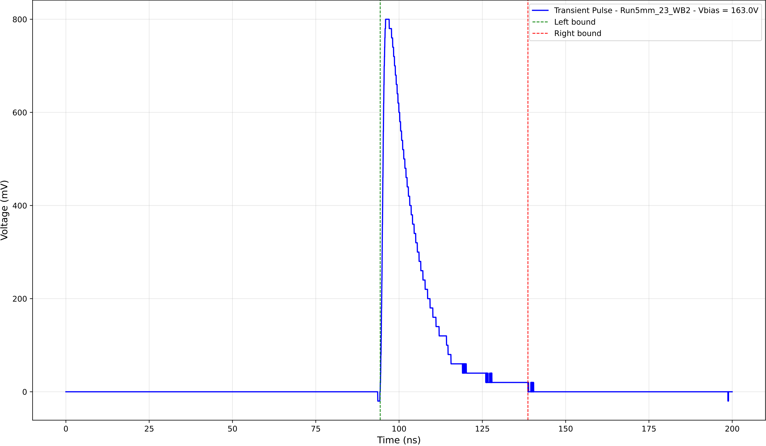
Transient Pulse - Sample: 5mm_23 - Position: 1420.0 \mu\text{m} - Charge: 172.10 pC
