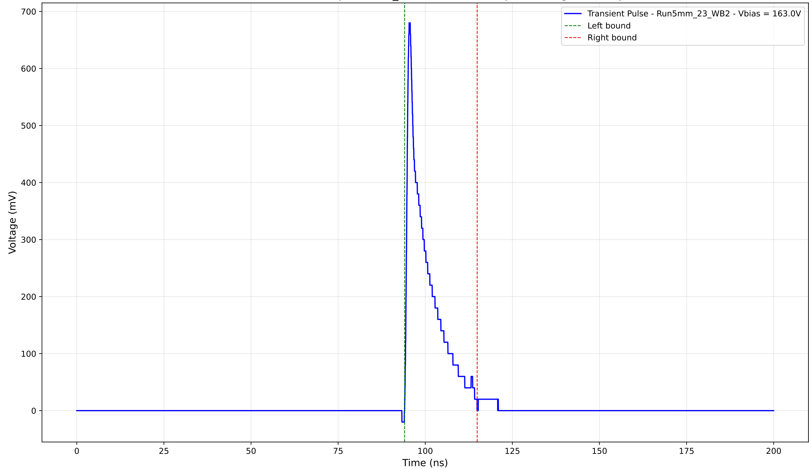
Transient Pulse - Sample: 5mm_23 - Position: 80.0 \mu\text{m} - Charge: 82.39 pC
