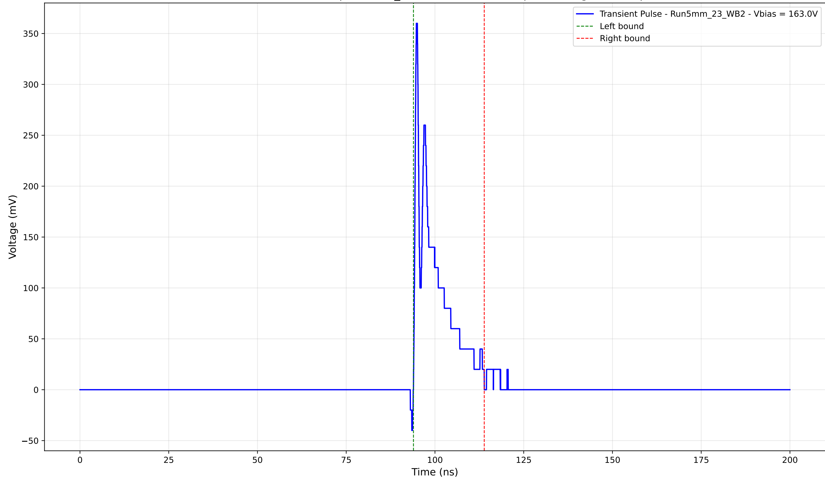
Transient Pulse - Sample: 5mm_23 -Position: 2530.0 \mu\text{m} - Charge: 38.55 pC
