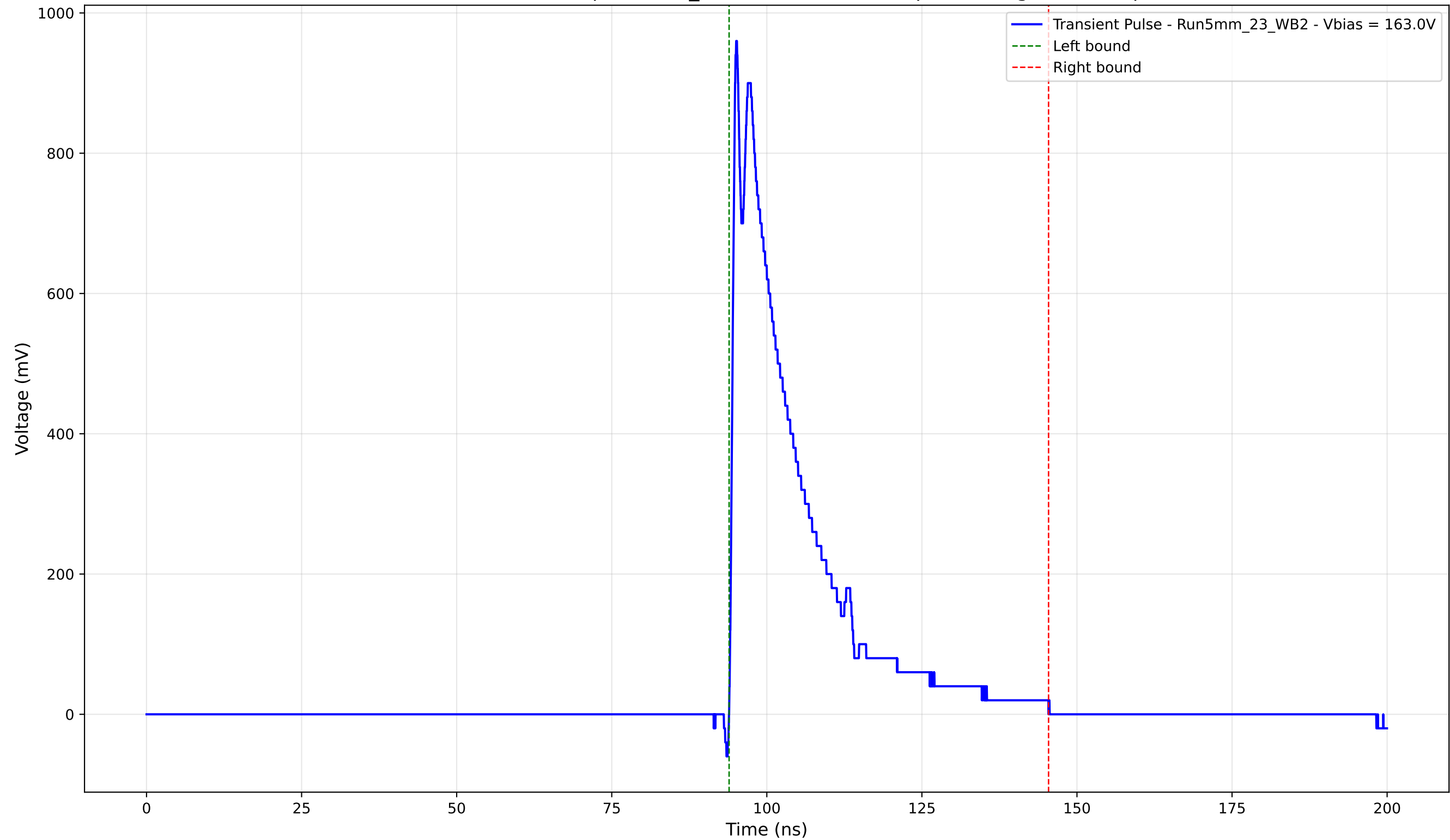
Transient Pulse - Sample: 5mm_23 - Position: 2225.0 \mu\text{m} - Charge: 205.90 pC
