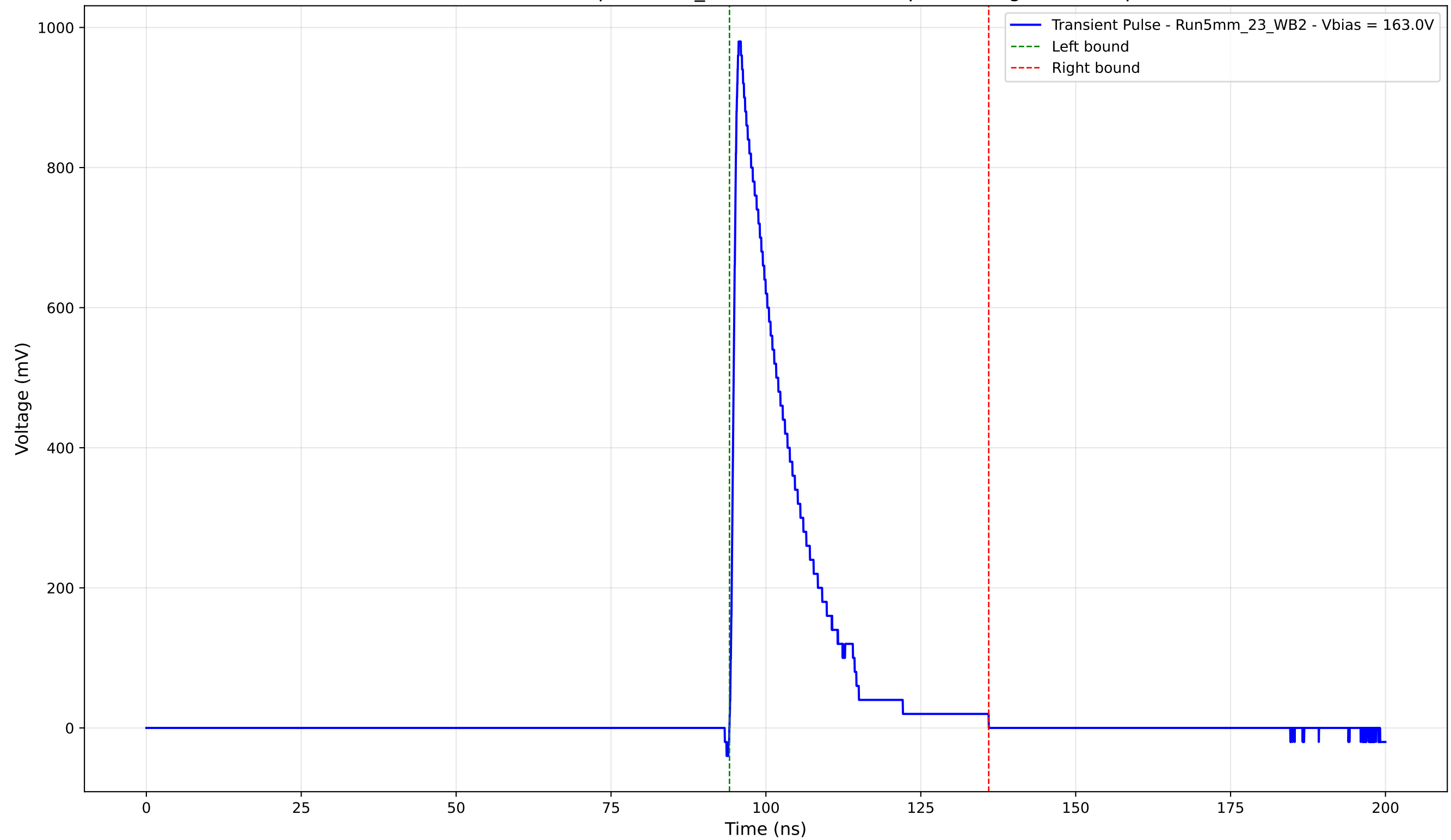
Transient Pulse - Sample: 5mm_23 - Position: 380.0 \mu\text{m} - Charge: 180.24 pC
