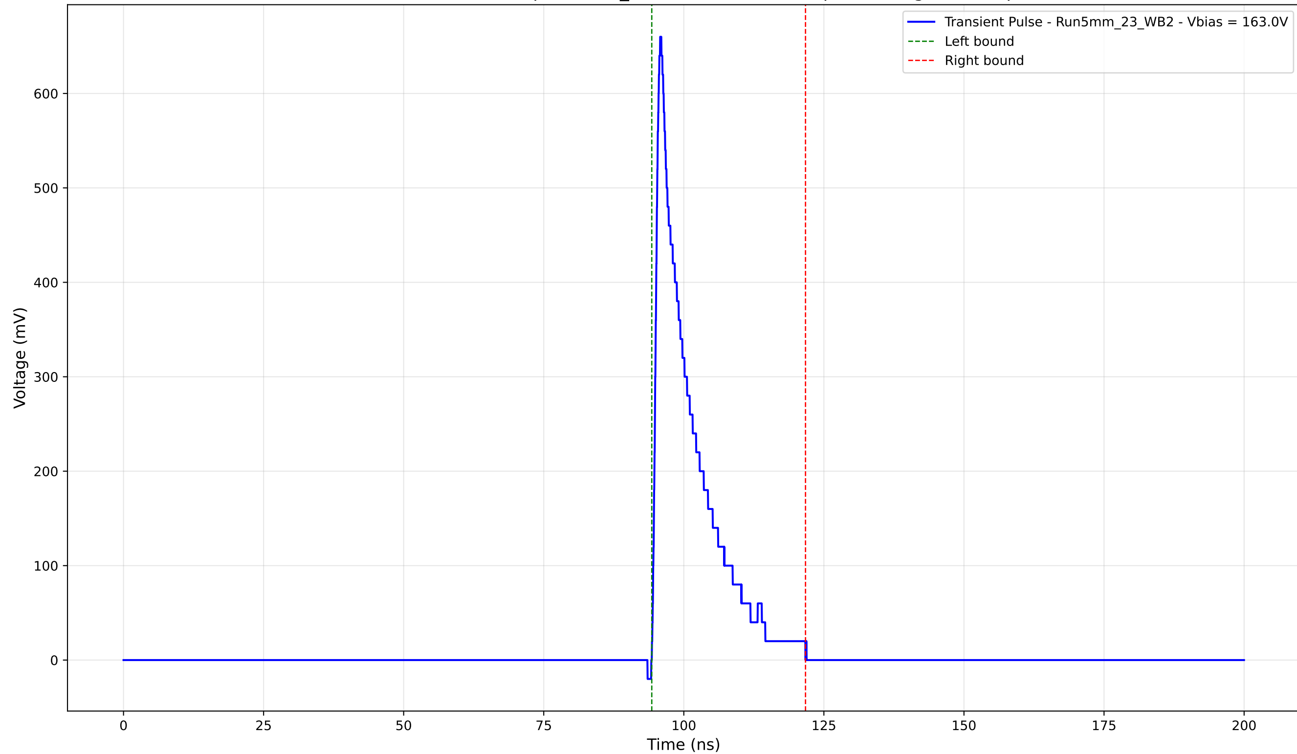
Transient Pulse - Sample: 5mm_23 - Position: 4585.0 \mu\text{m} - Charge: 90.21 pC
