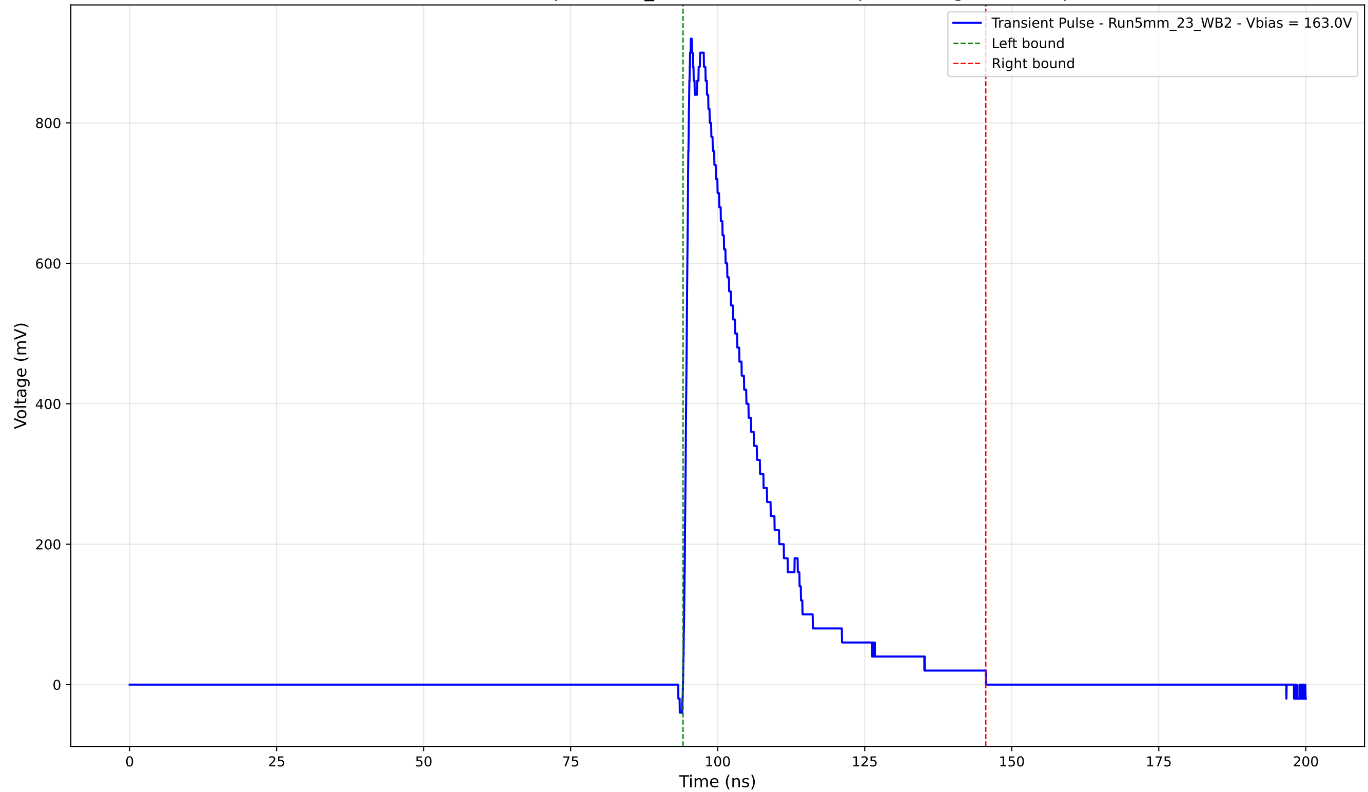
Transient Pulse - Sample: 5mm_23 - Position: 1885.0 \mu\text{m} - Charge: 218.78 pC
