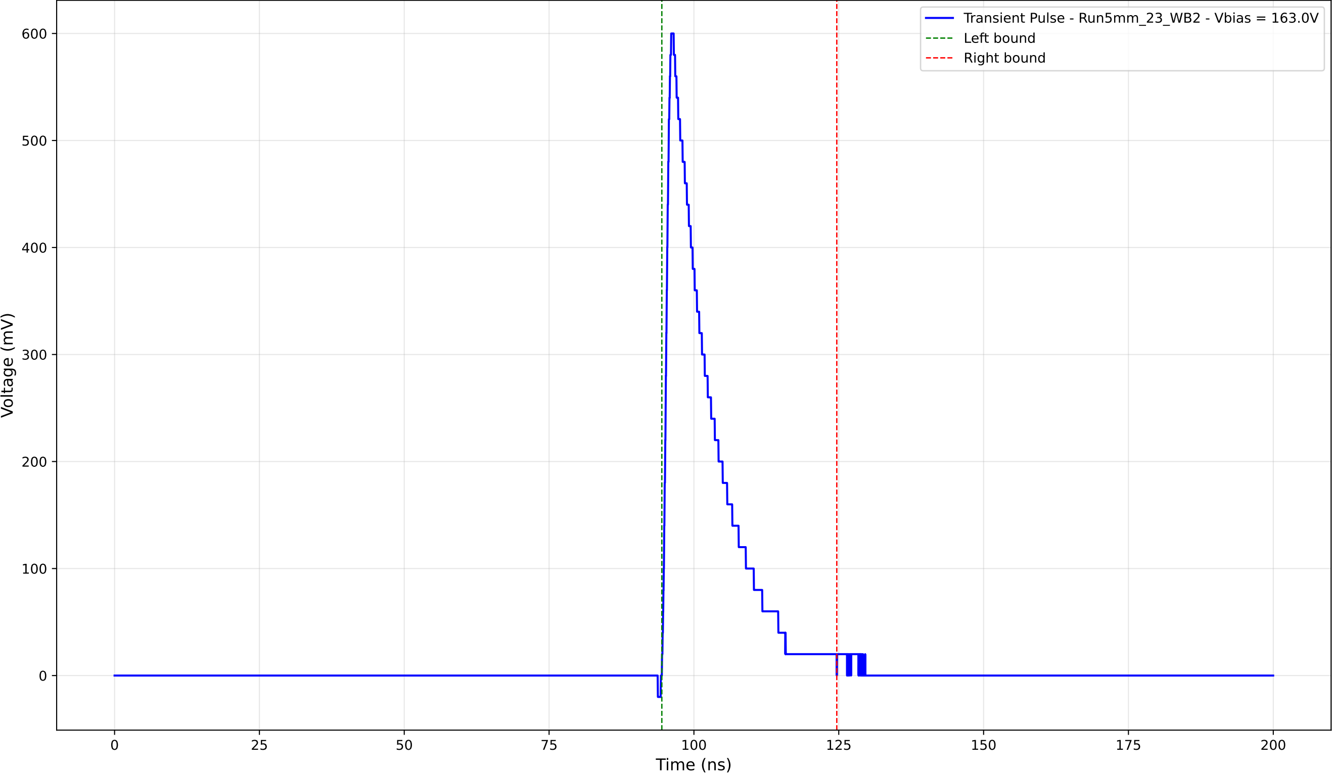
Transient Pulse - Sample: 5mm_23 - Position: 4090.0 \mu\text{m} - Charge: 100.36 pC
