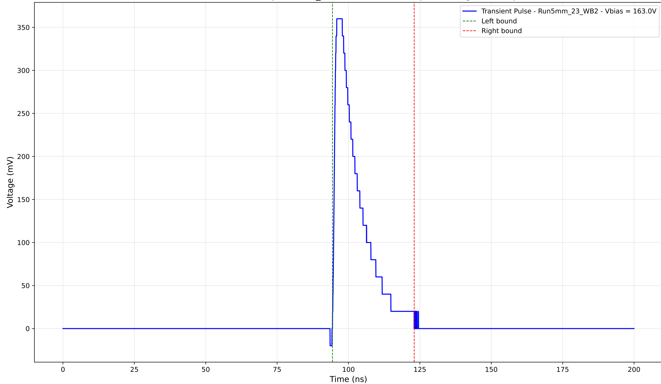
Transient Pulse - Sample: 5mm_23 - Position: 3490.0 \mu\text{m} - Charge: 69.31 pC
