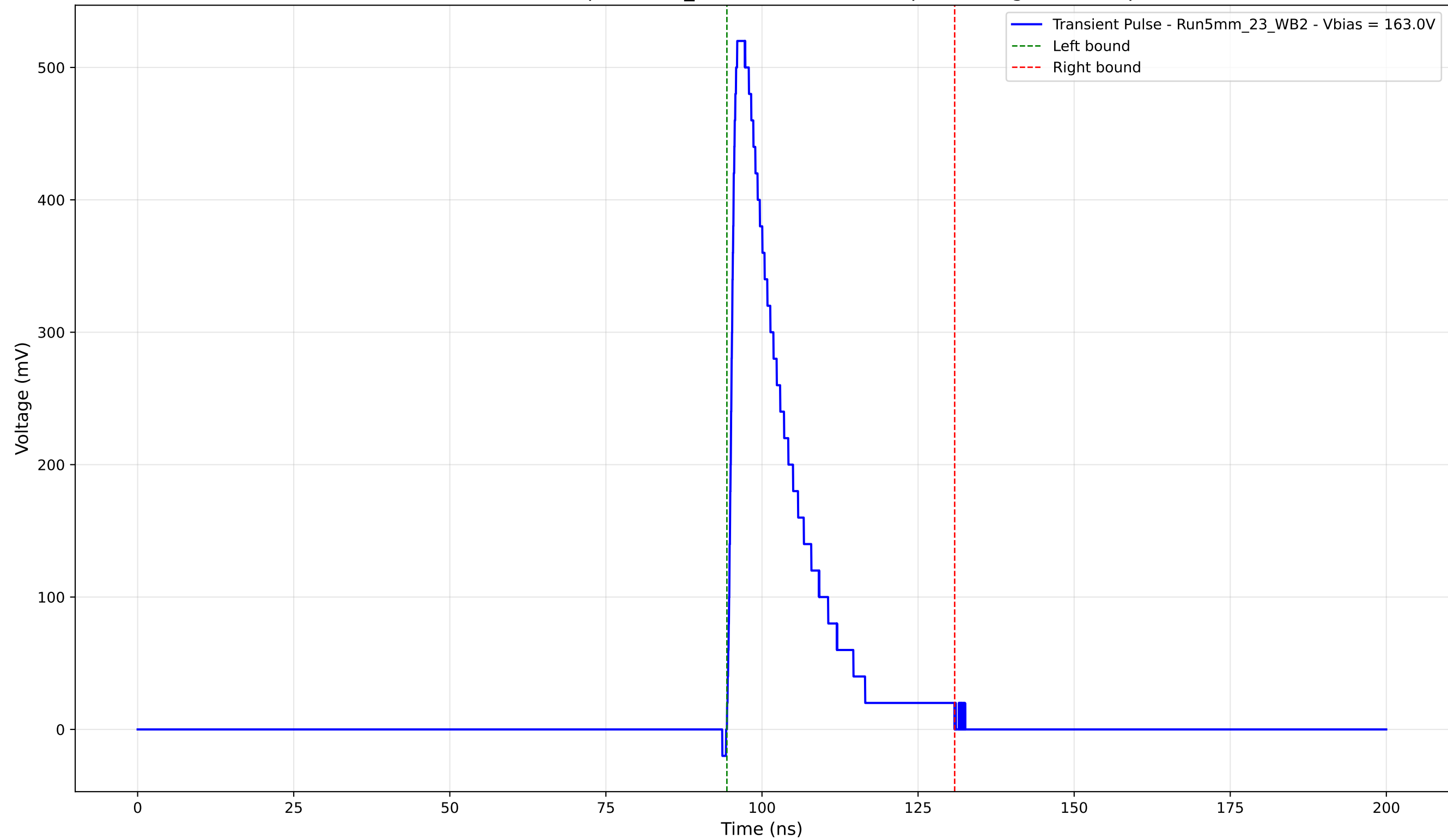
Transient Pulse - Sample: 5mm_23 - Position: 3575.0 \mu\text{m} - Charge: 101.24 pC
