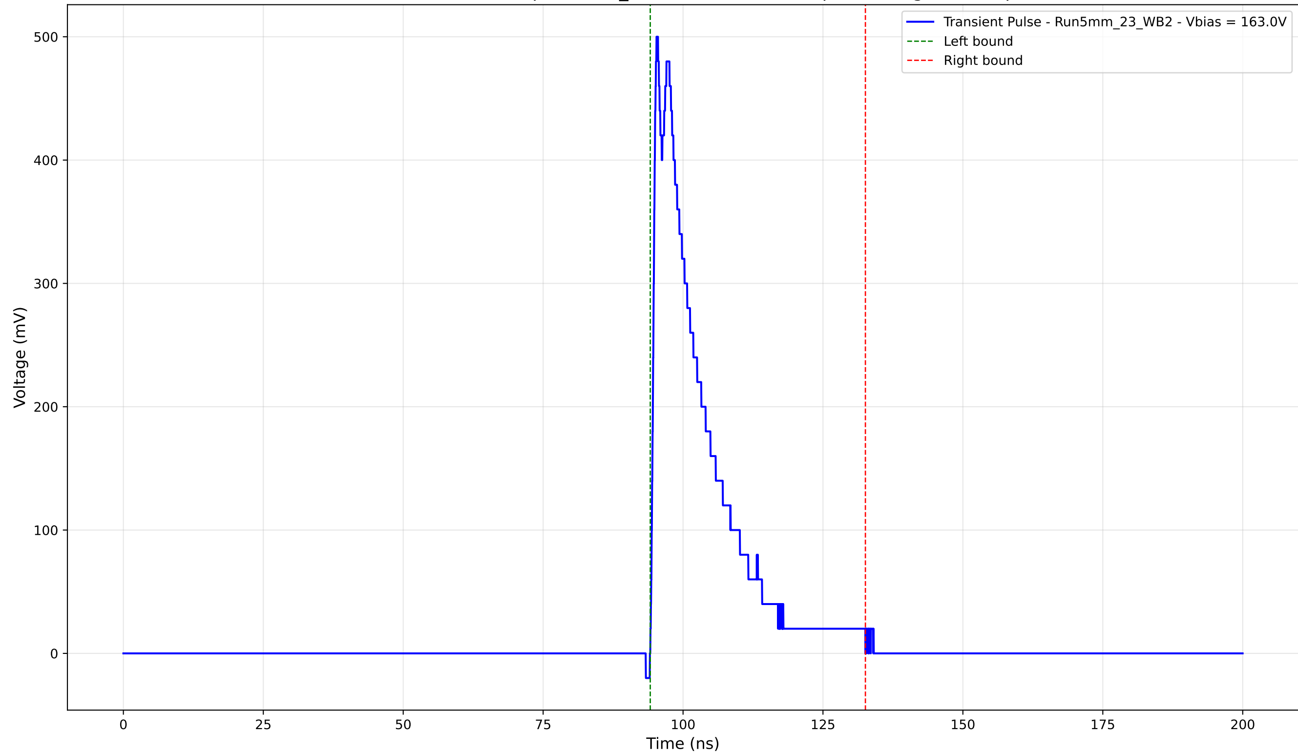
Transient Pulse - Sample: 5mm_23 - Position: 1970.0 \mu\text{m} - Charge: 96.01 pC
