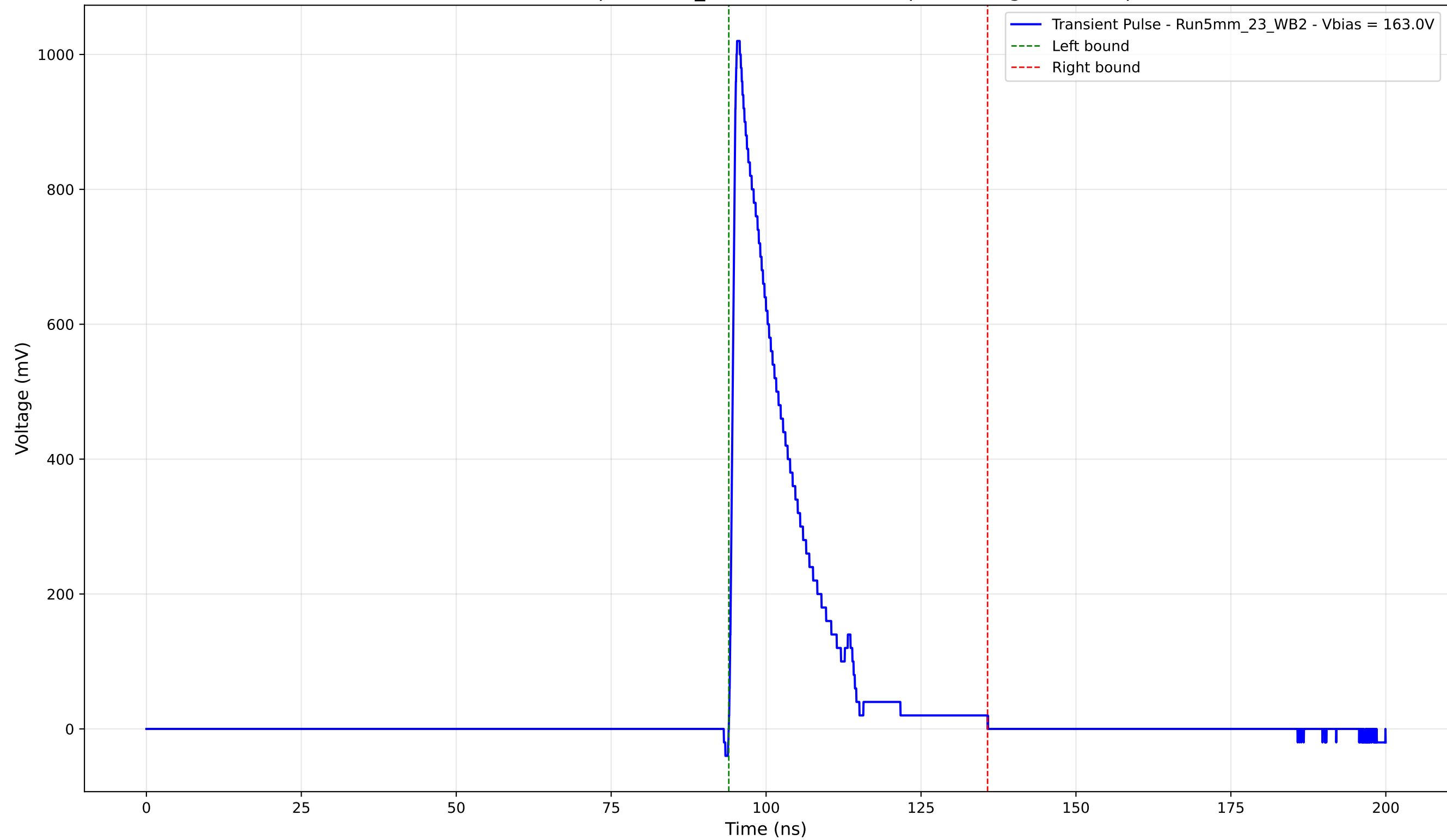
Transient Pulse - Sample: 5mm_23 - Position: 155.0 \mu\text{m} - Charge: 184.18 pC
