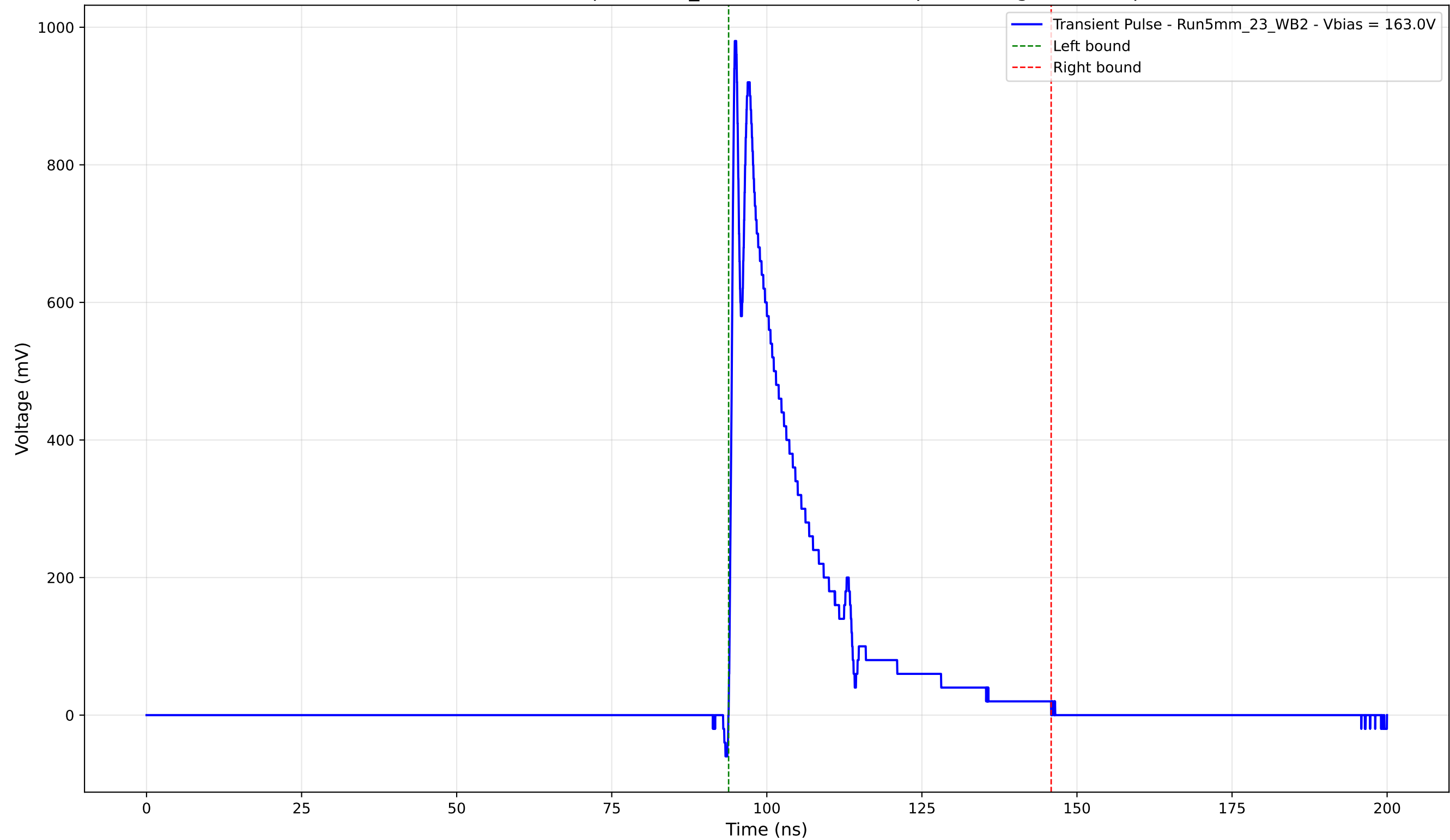
Transient Pulse - Sample: 5mm_23 - Position: 2385.0 \mu\text{m} - Charge: 199.91 pC
