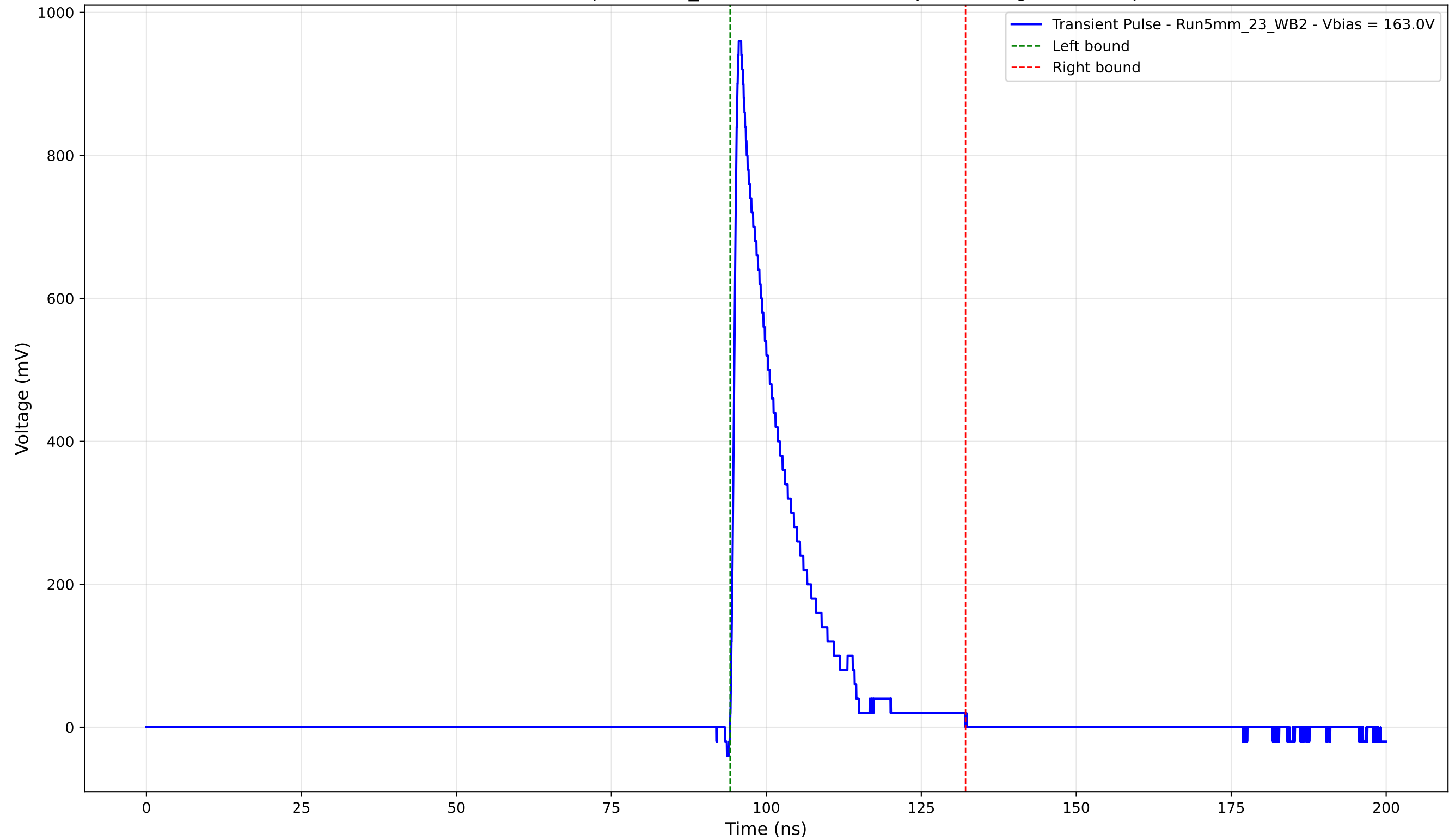
Transient Pulse - Sample: 5mm_23 - Position: 4705.0 \mu\text{m} - Charge: 153.59 pC
