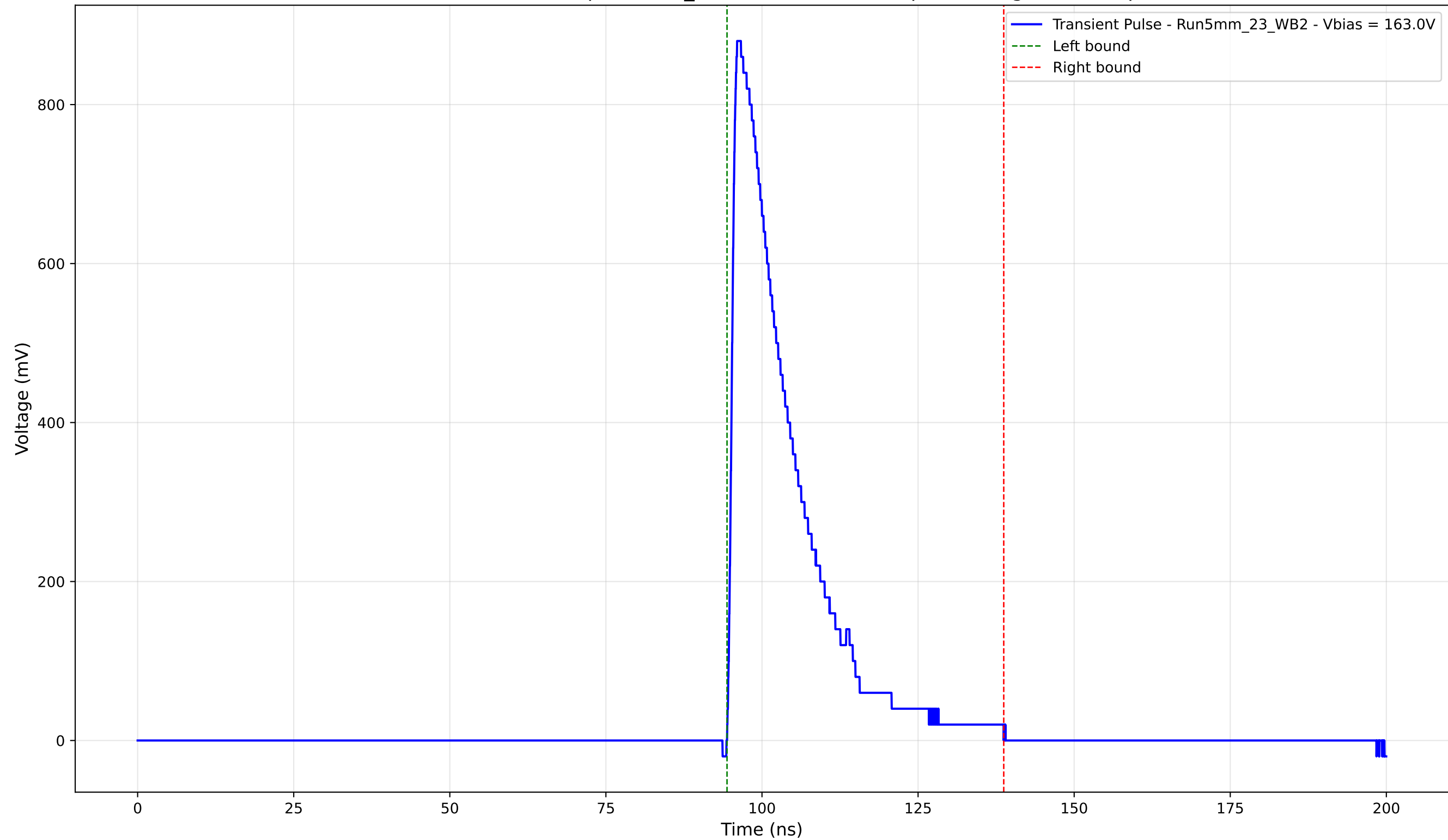
Transient Pulse - Sample: 5mm_23 - Position: 1115.0 \mu\text{m} - Charge: 186.94 pC
