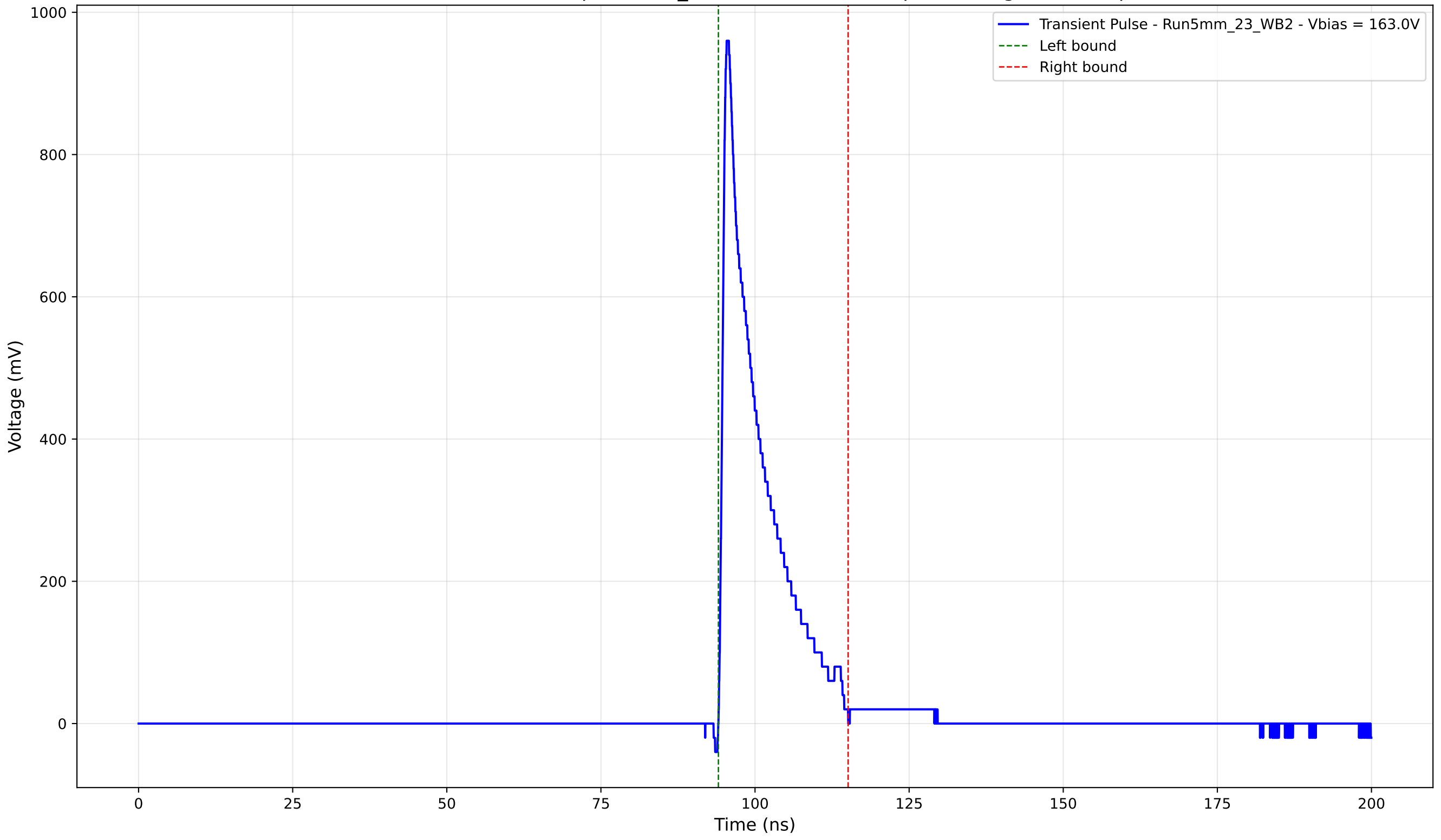
Transient Pulse - Sample: 5mm_23 - Position: 4875.0 \mu\text{m} - Charge: 128.86 pC
