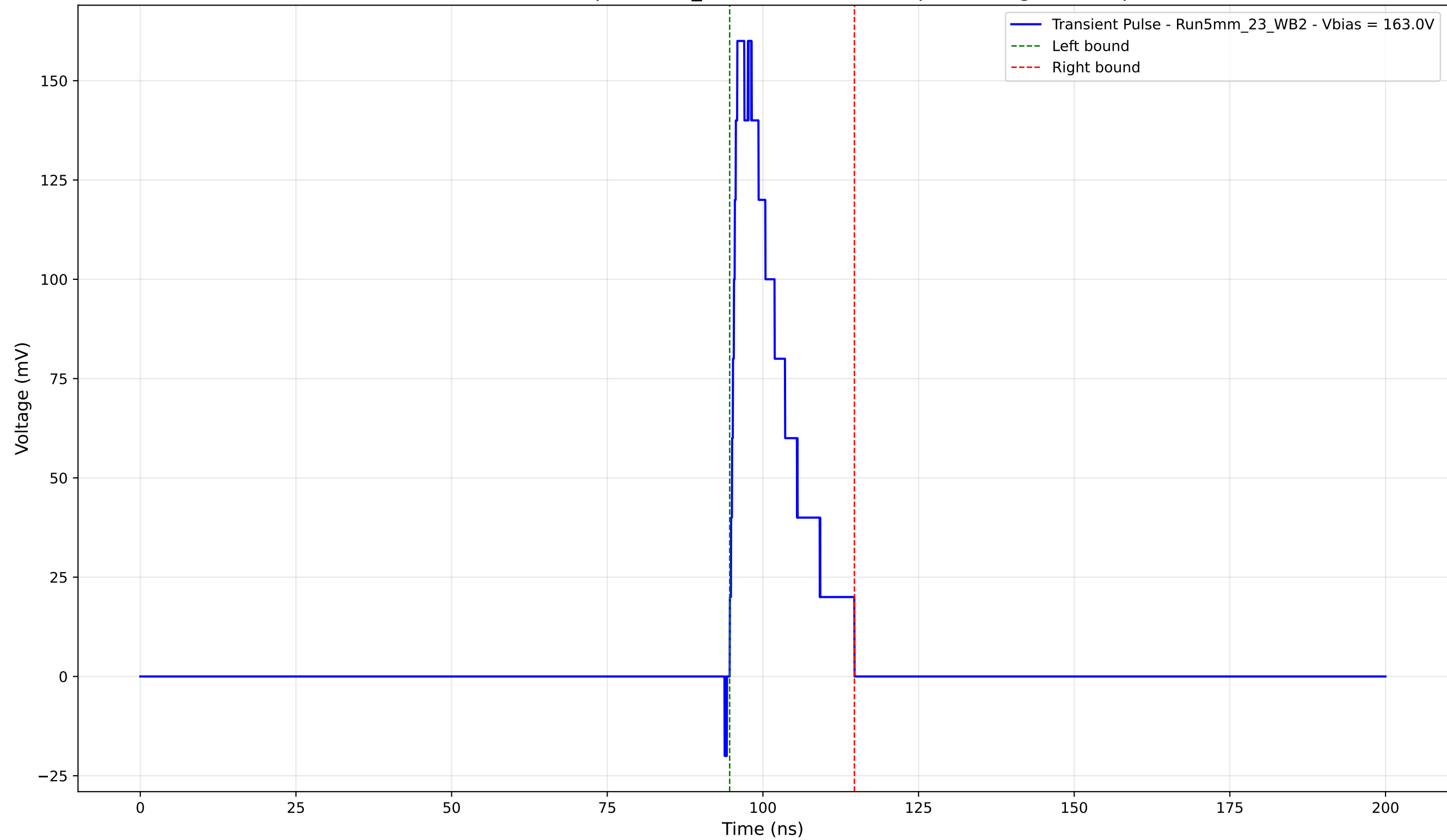
Transient Pulse - Sample: 5mm_23 -Position: 4040.0 \mu\text{m} - Charge: 27.99 pC
