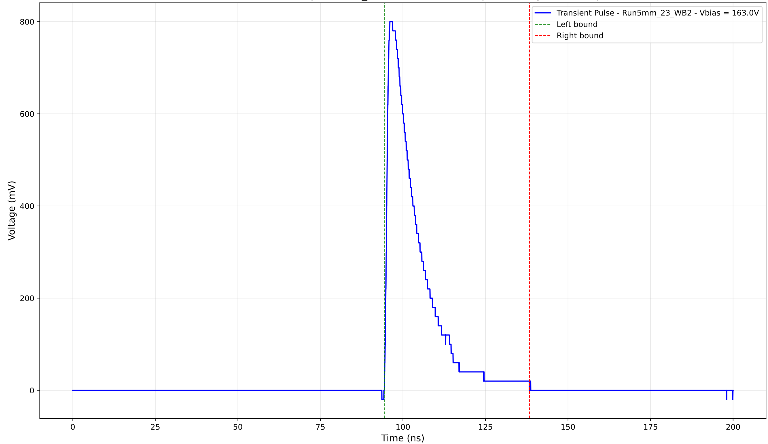
Transient Pulse - Sample: 5mm_23 - Position: 3625.0 \mu\text{m} - Charge: 166.76 pC
