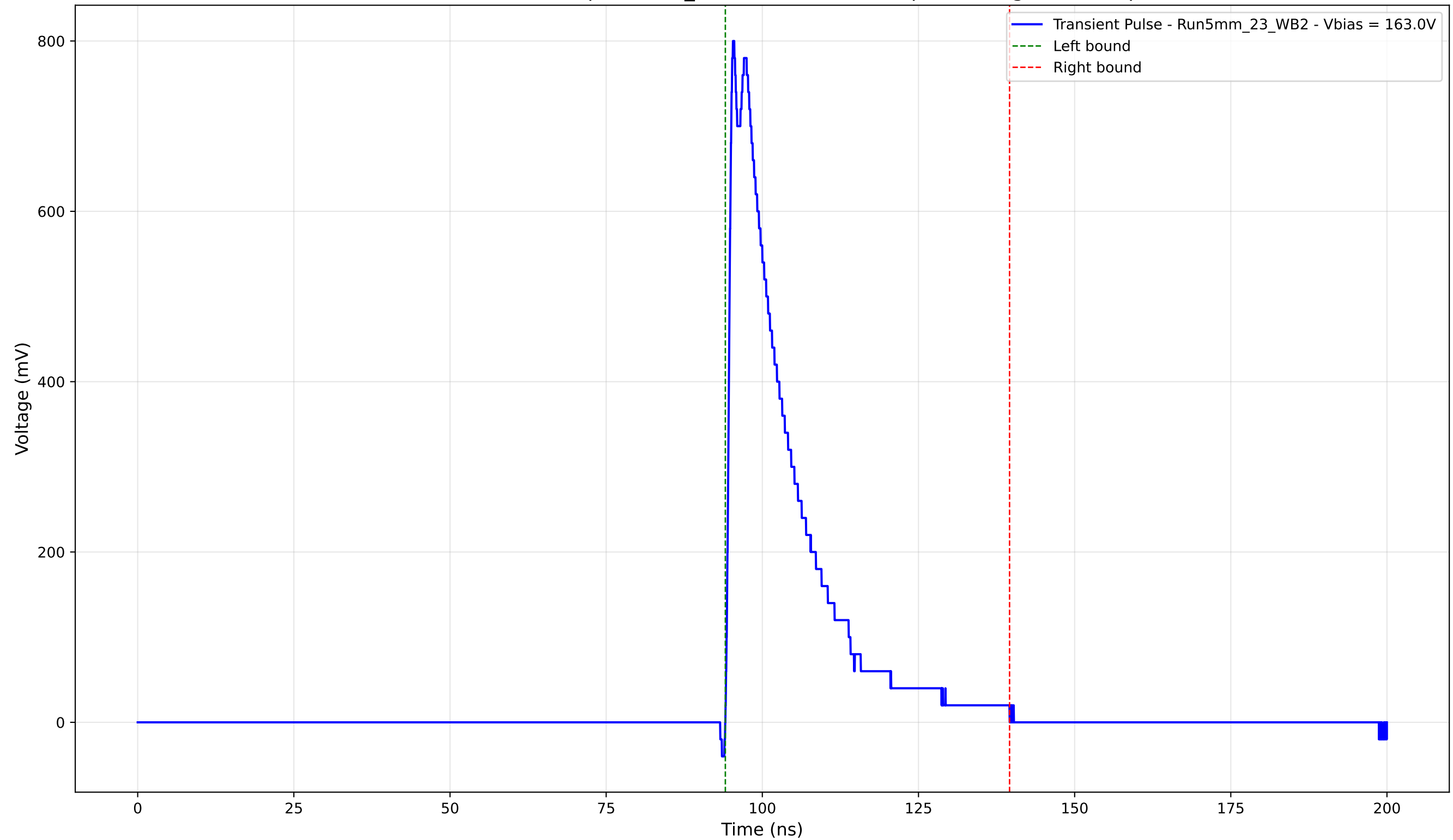
Transient Pulse - Sample: 5mm_23 - Position: 3085.0 \mu\text{m} - Charge: 168.25 pC
