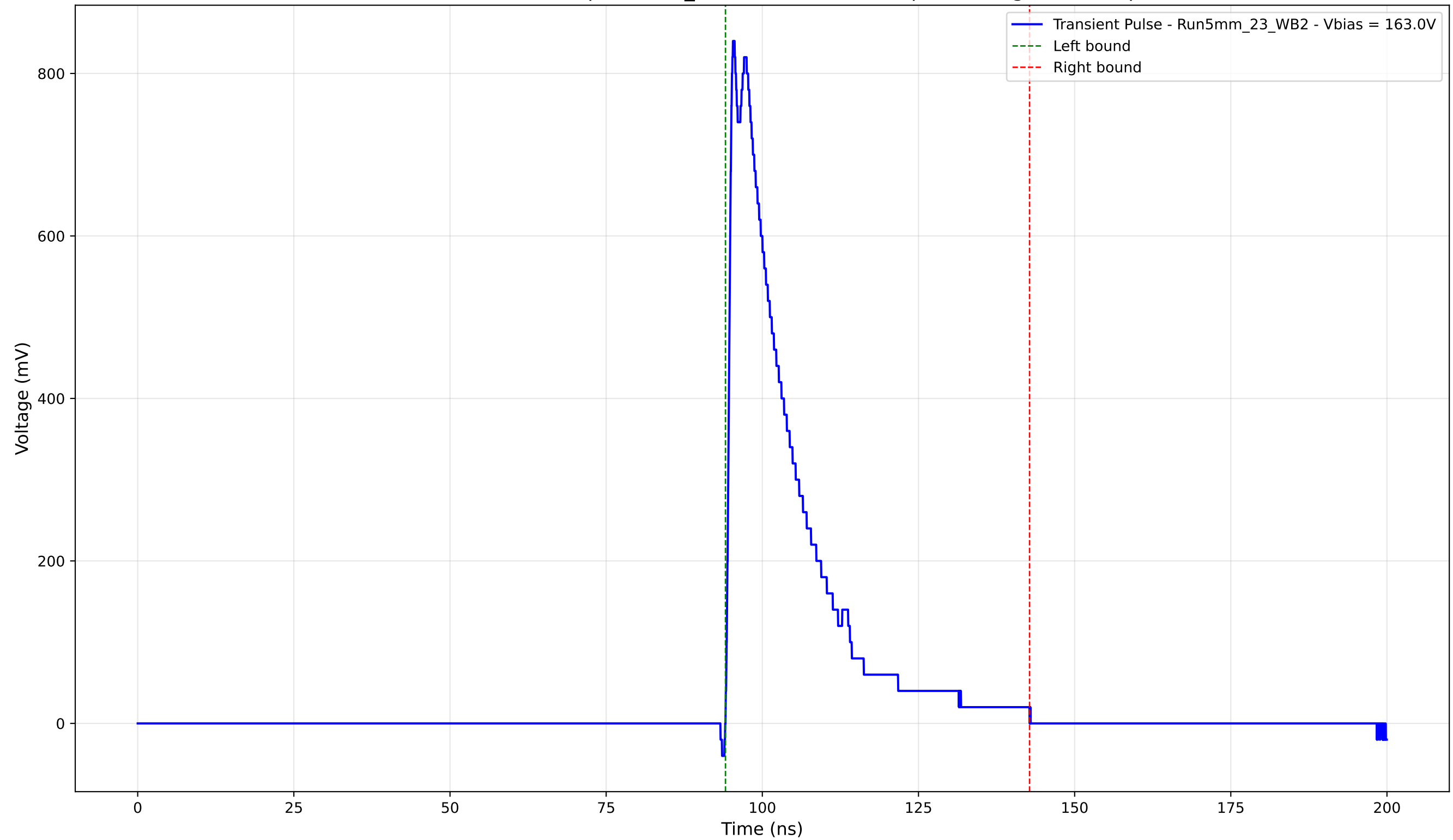
Transient Pulse - Sample: 5mm_23 - Position: 1935.0 \mu\text{m} - Charge: 182.67 pC
