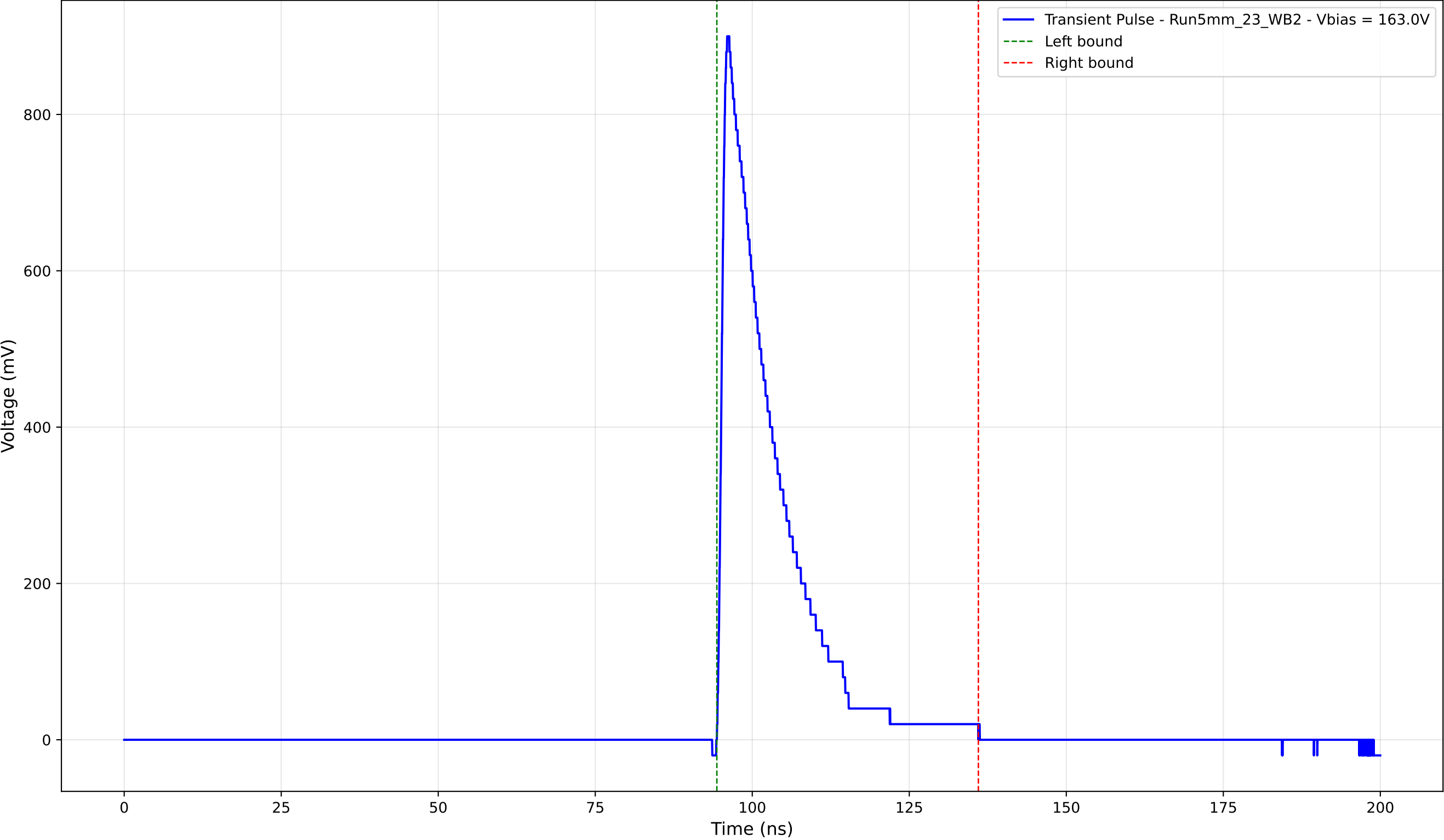
Transient Pulse - Sample: 5mm_23 - Position: 4265.0 \mu\text{m} - Charge: 163.81 pC
