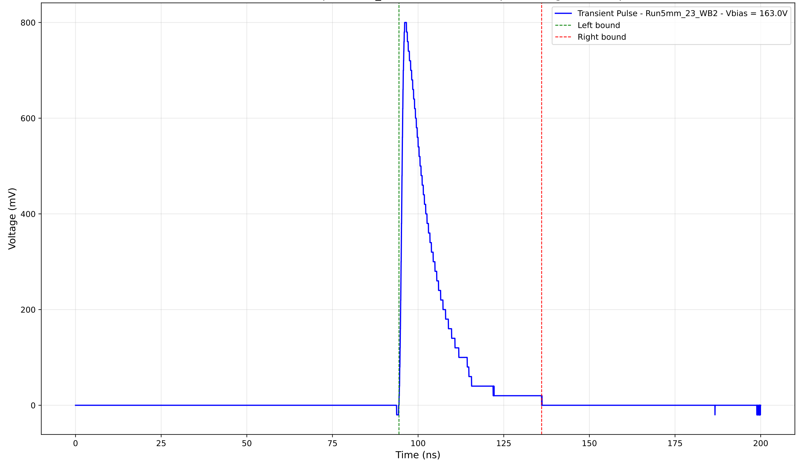
Transient Pulse - Sample: 5mm_23 - Position: 3955.0 \mu\text{m} - Charge: 151.22 pC
