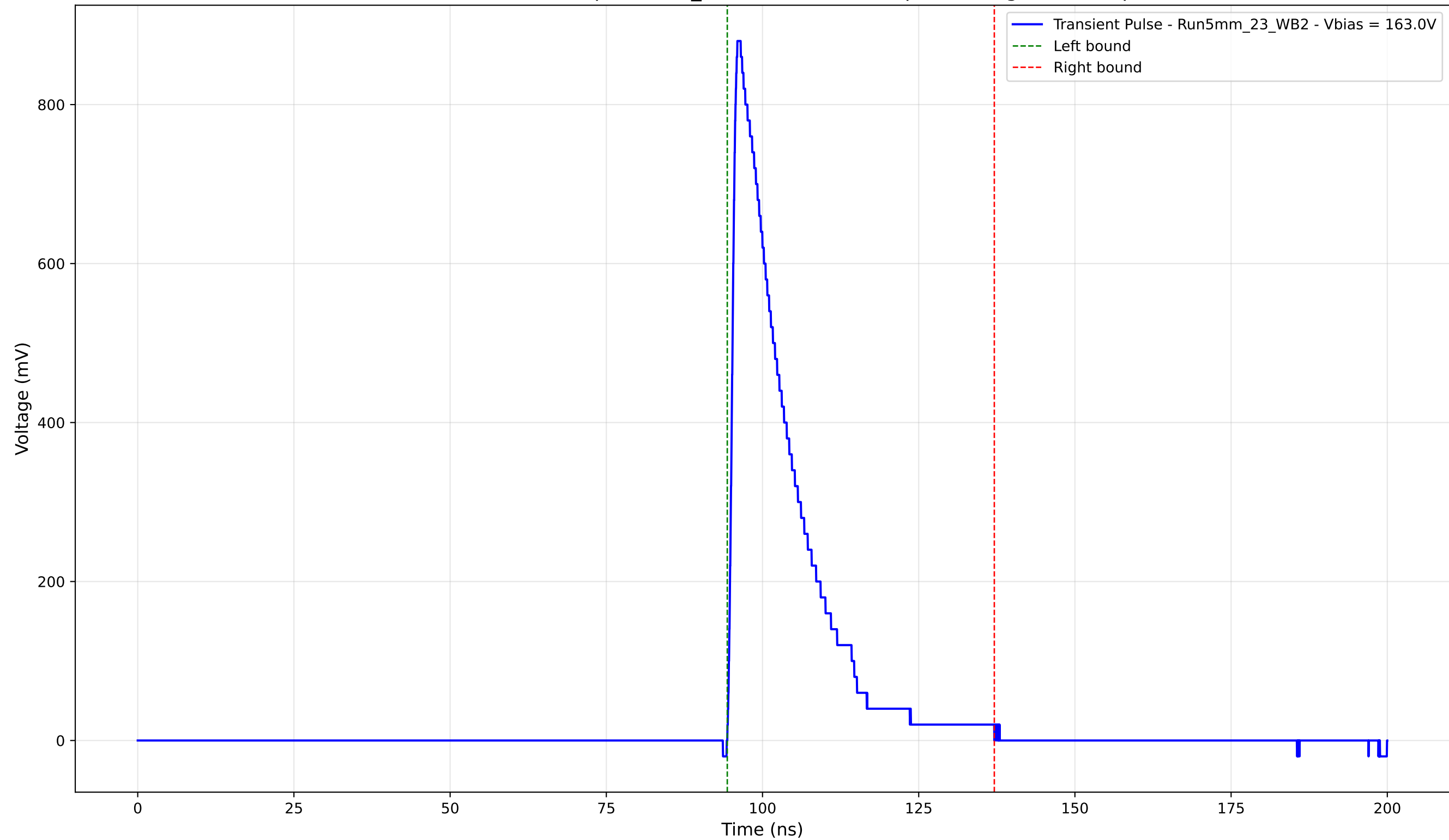
Transient Pulse - Sample: 5mm_23 - Position: 845.0 \mu\text{m} - Charge: 173.74 pC
