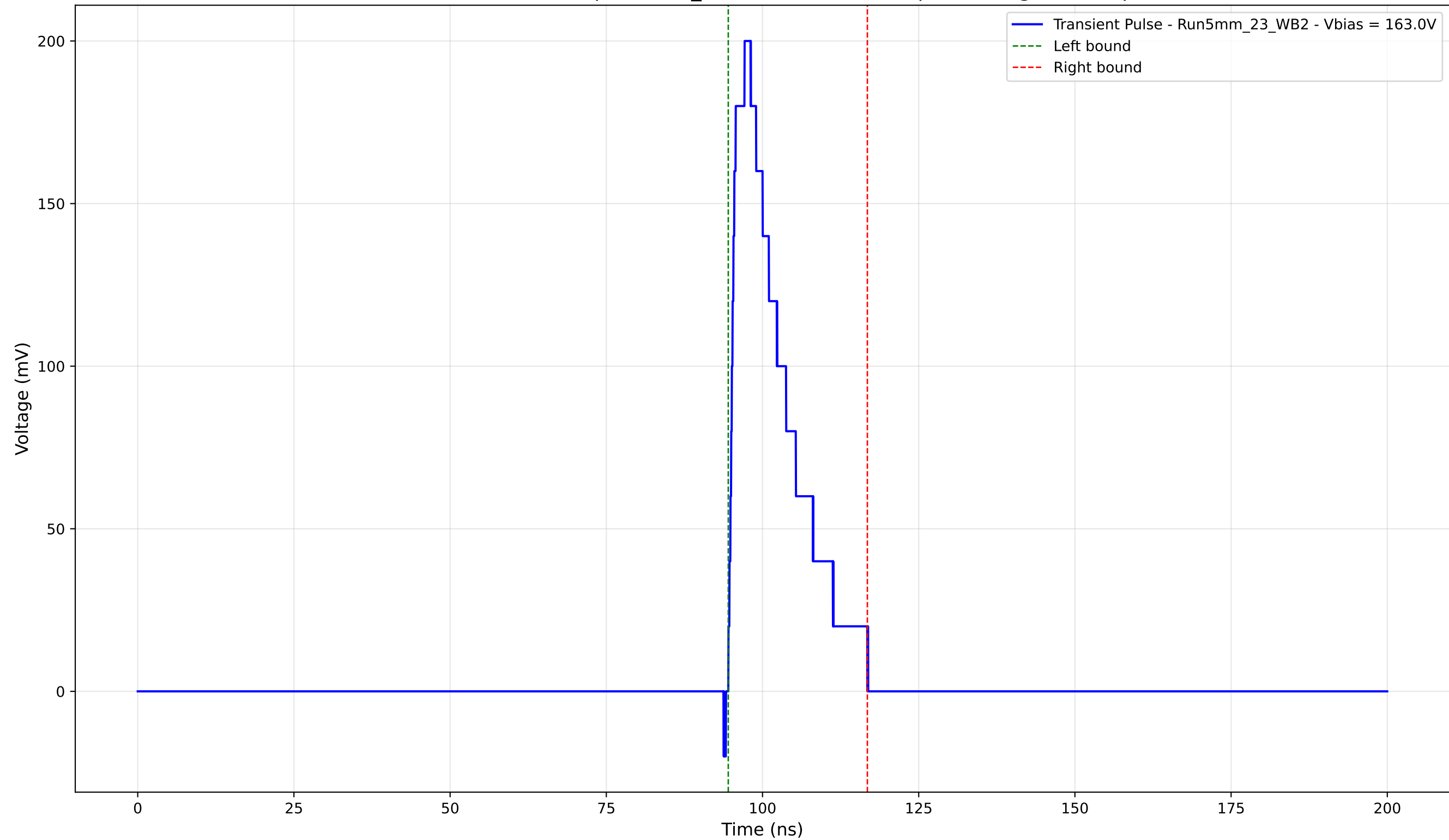
Transient Pulse - Sample: 5mm_23 - Position: 1490.0 \mu\text{m} - Charge: 37.10 pC
