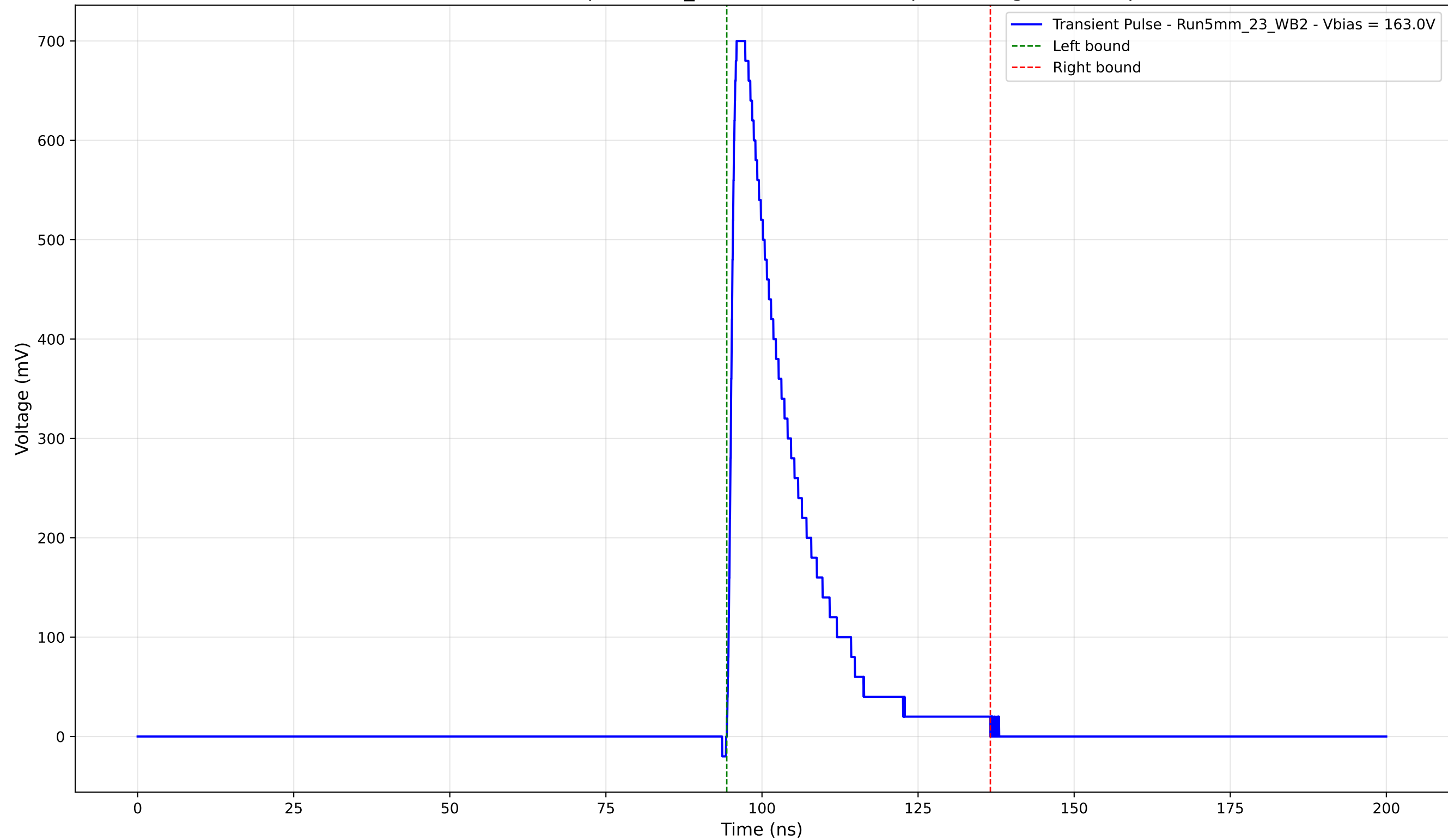
Transient Pulse - Sample: 5mm_23 - Position: 1435.0 \mu\text{m} - Charge: 145.65 pC
