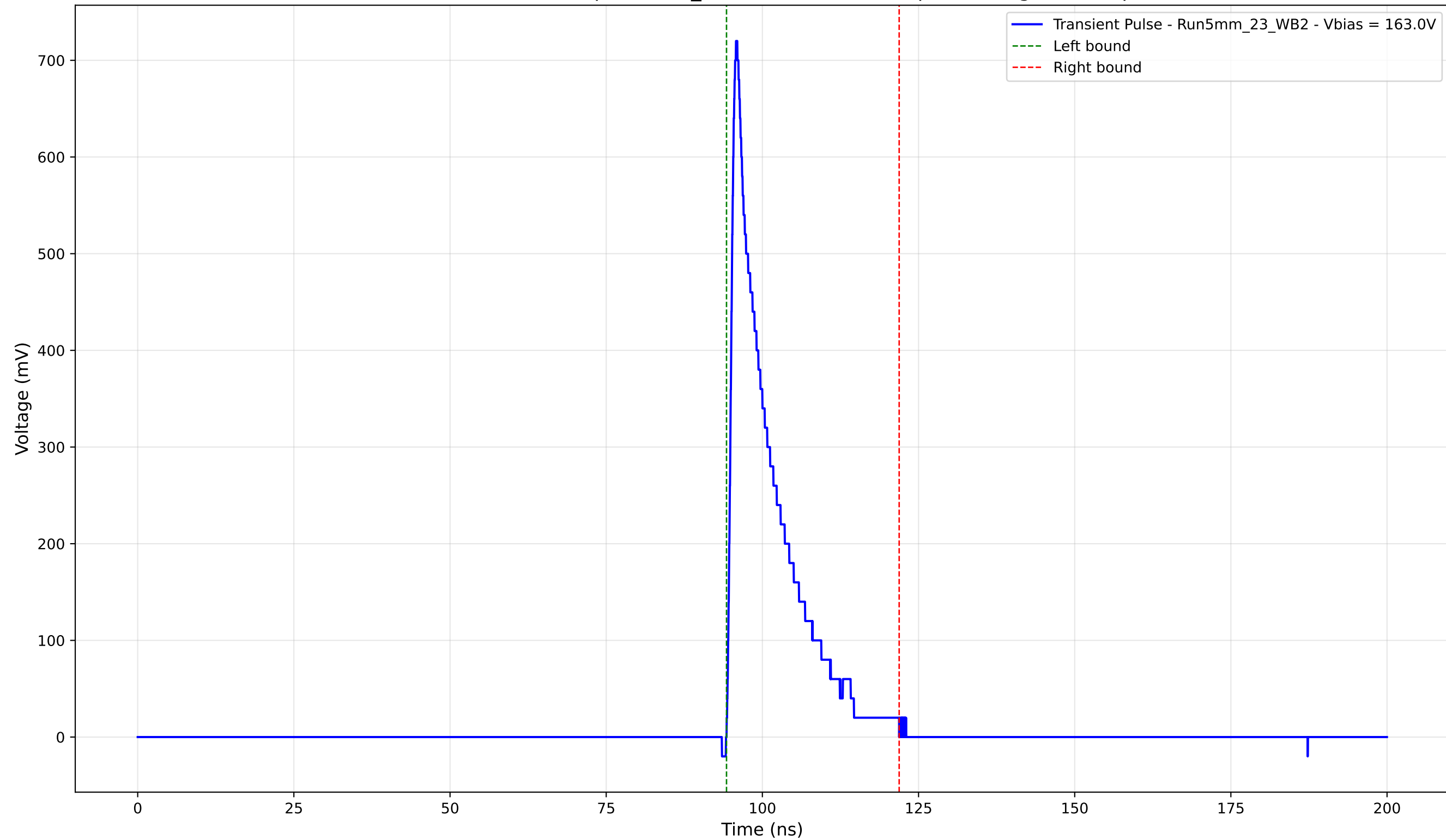
Transient Pulse - Sample: 5mm_23 - Position: 4590.0 \mu\text{m} - Charge: 99.54 pC
