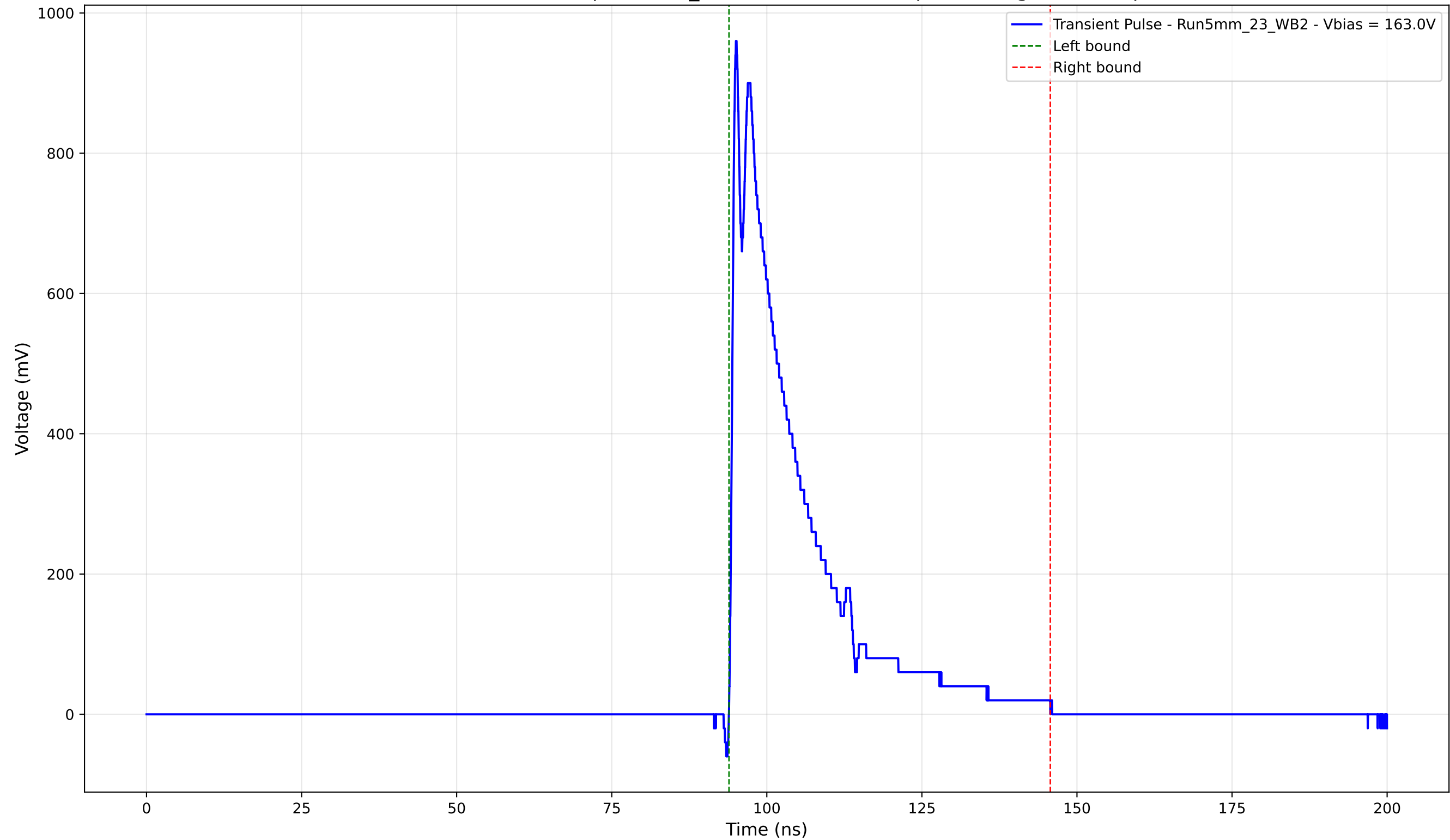
Transient Pulse - Sample: 5mm_23 - Position: 2265.0 \mu\text{m} - Charge: 204.85 pC
