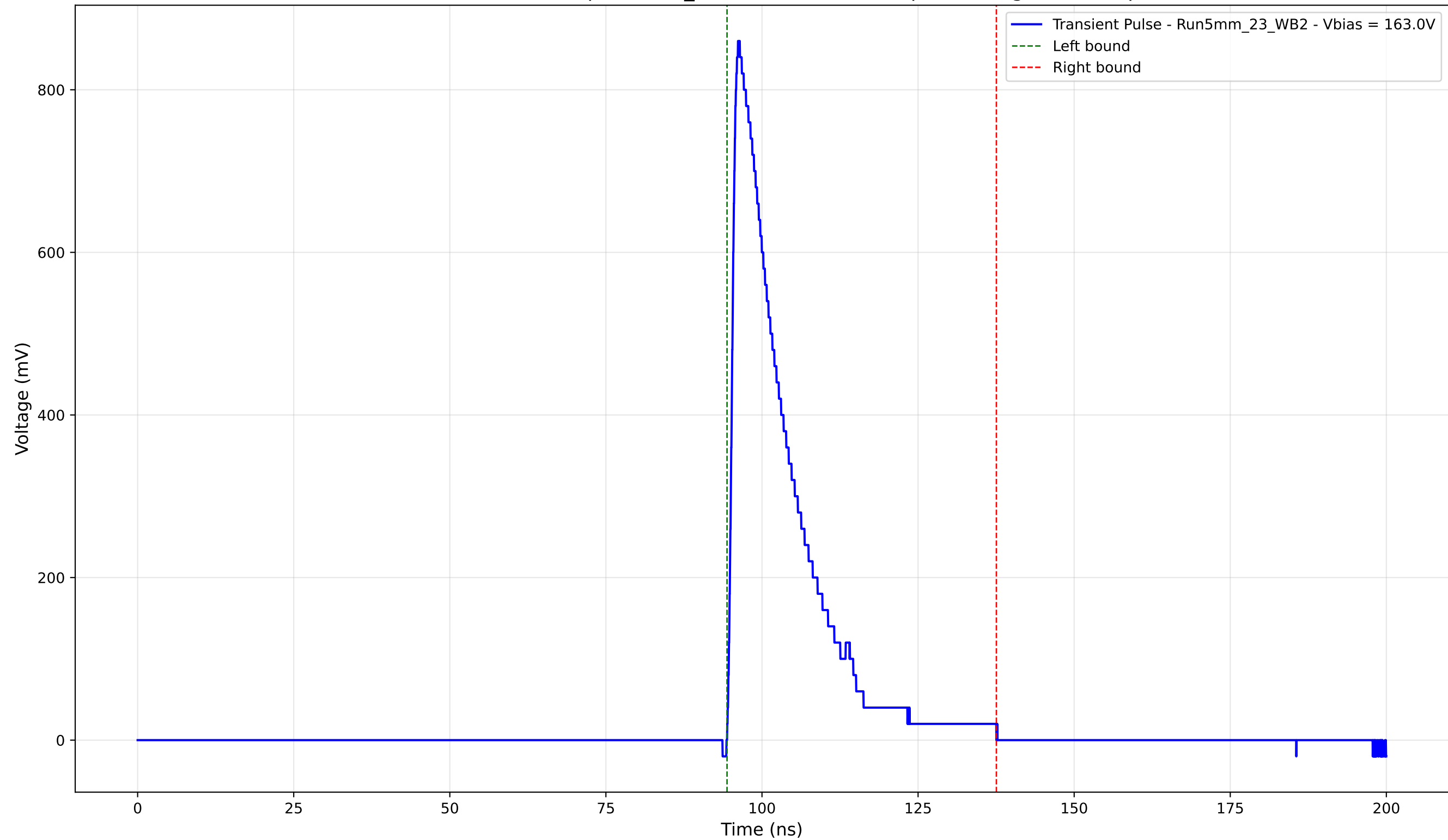
Transient Pulse - Sample: 5mm_23 - Position: 3925.0 \mu\text{m} - Charge: 166.78 pC
