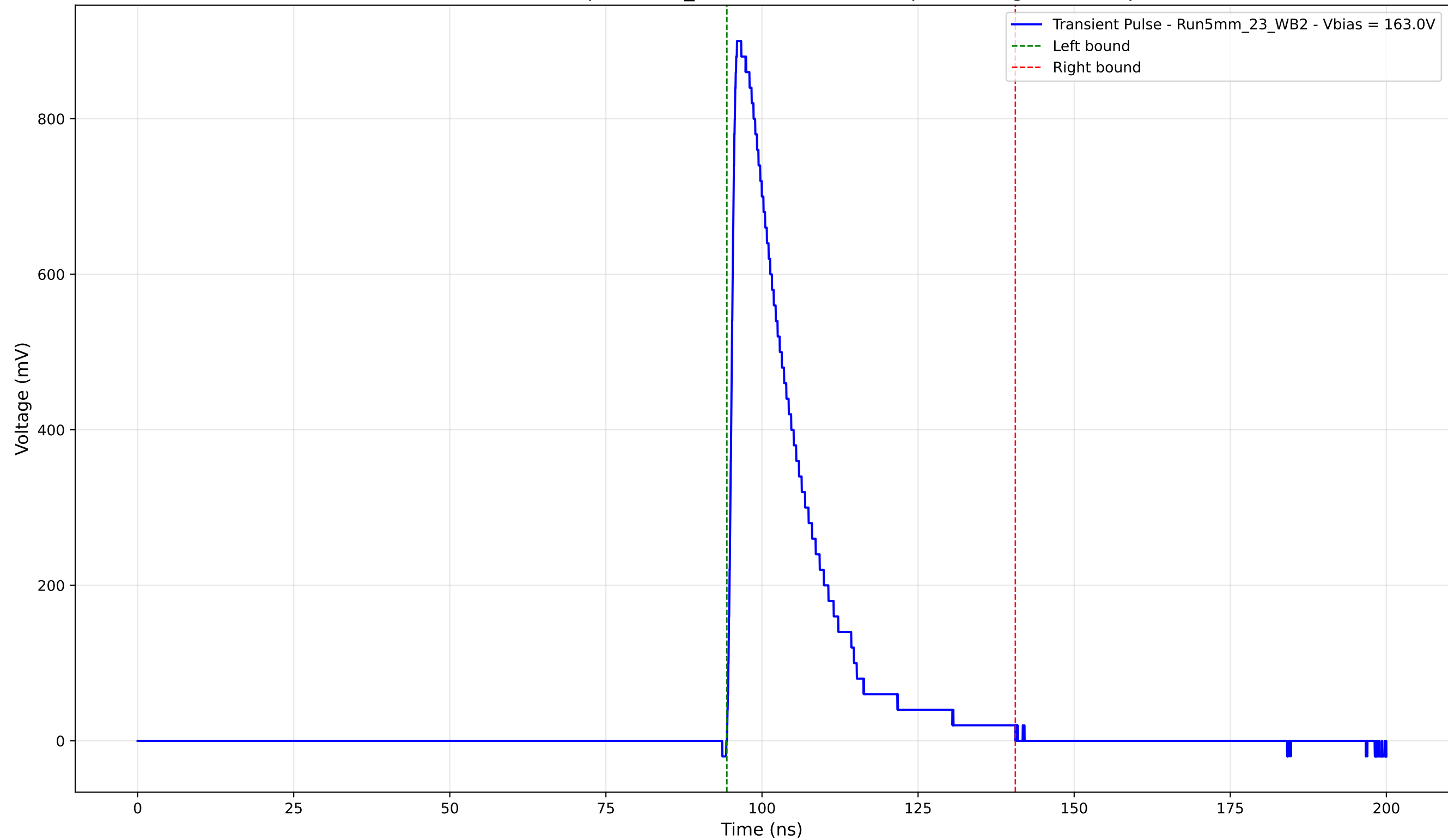
Transient Pulse - Sample: 5mm_23 - Position: 1255.0 \mu\text{m} - Charge: 200.14 pC
