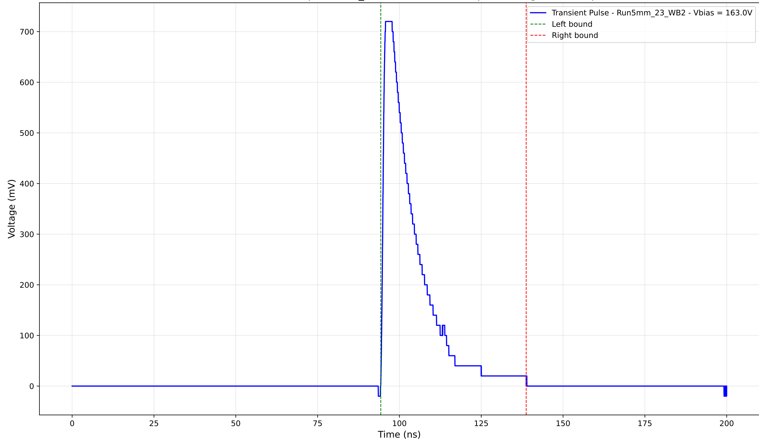
Transient Pulse - Sample: 5mm_23 - Position: 1570.0 \mu\text{m} - Charge: 156.54 pC
