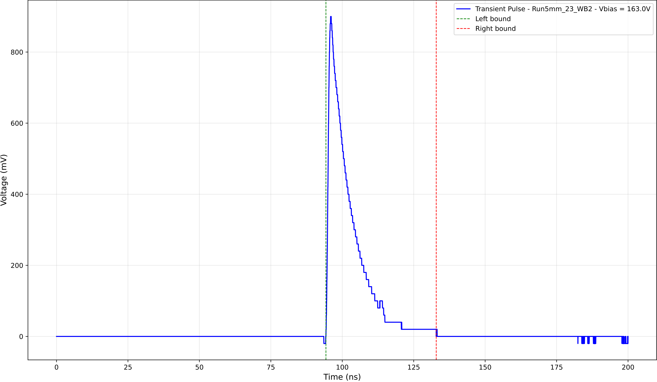
Transient Pulse - Sample: 5mm_23 - Position: 4435.0 \mu\text{m} - Charge: 151.74 pC
