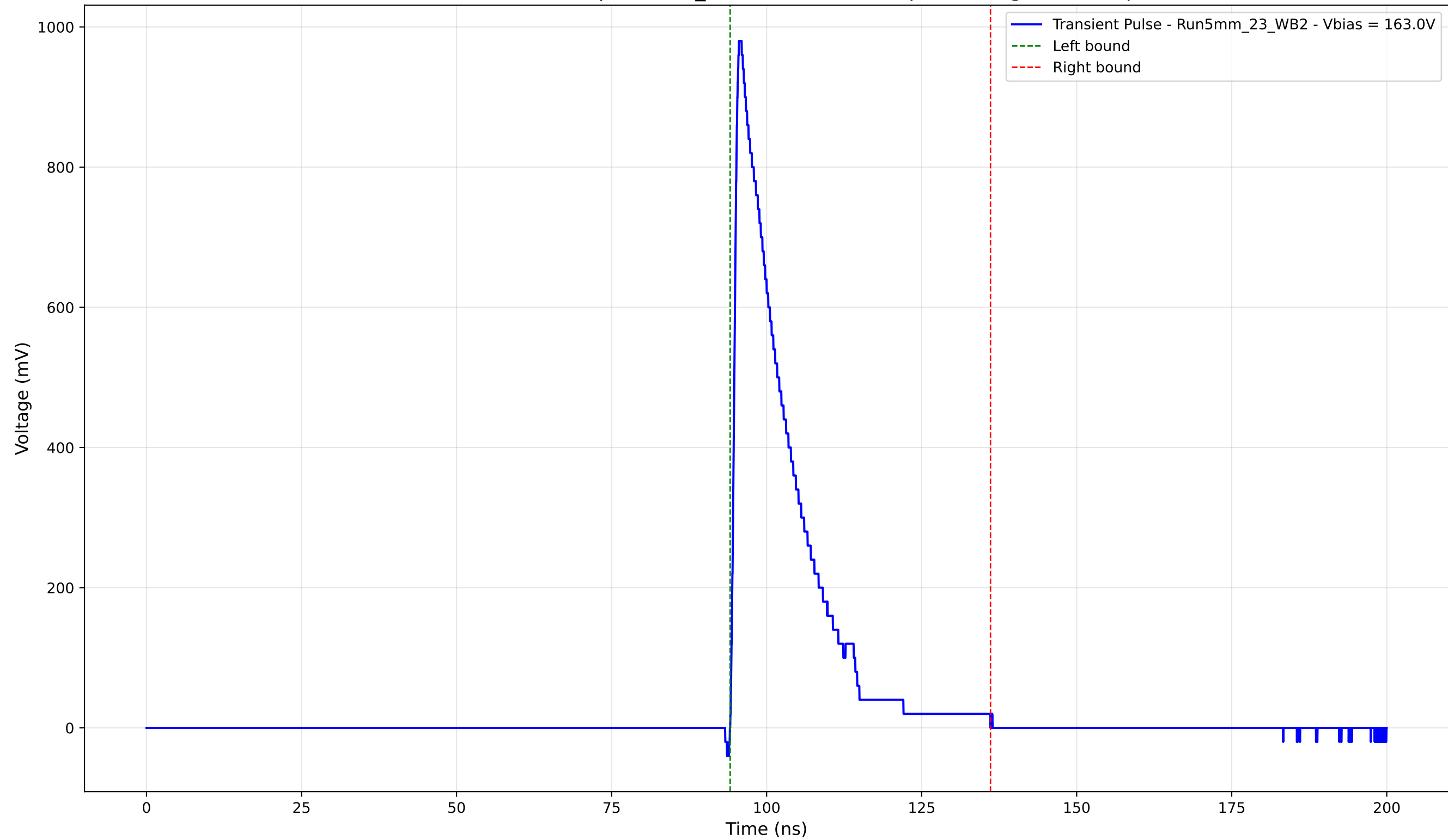
Transient Pulse - Sample: 5mm_23 - Position: 360.0 \mu\text{m} - Charge: 181.21 pC
