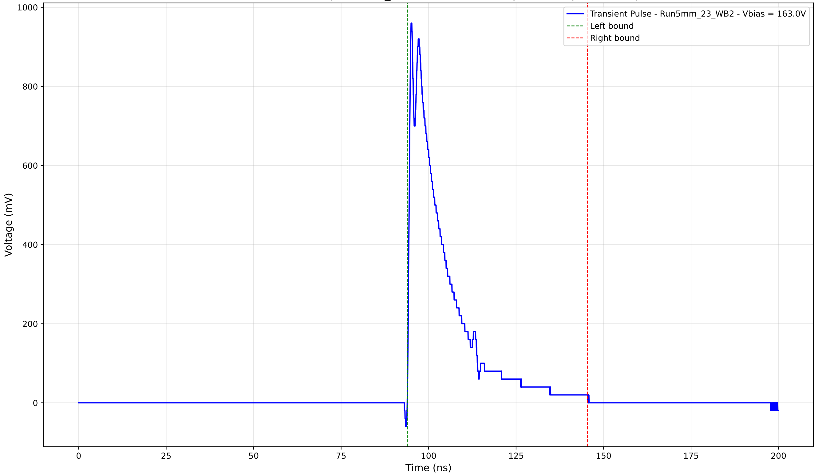
Transient Pulse - Sample: 5mm_23 - Position: 2795.0 \mu\text{m} - Charge: 206.06 pC
