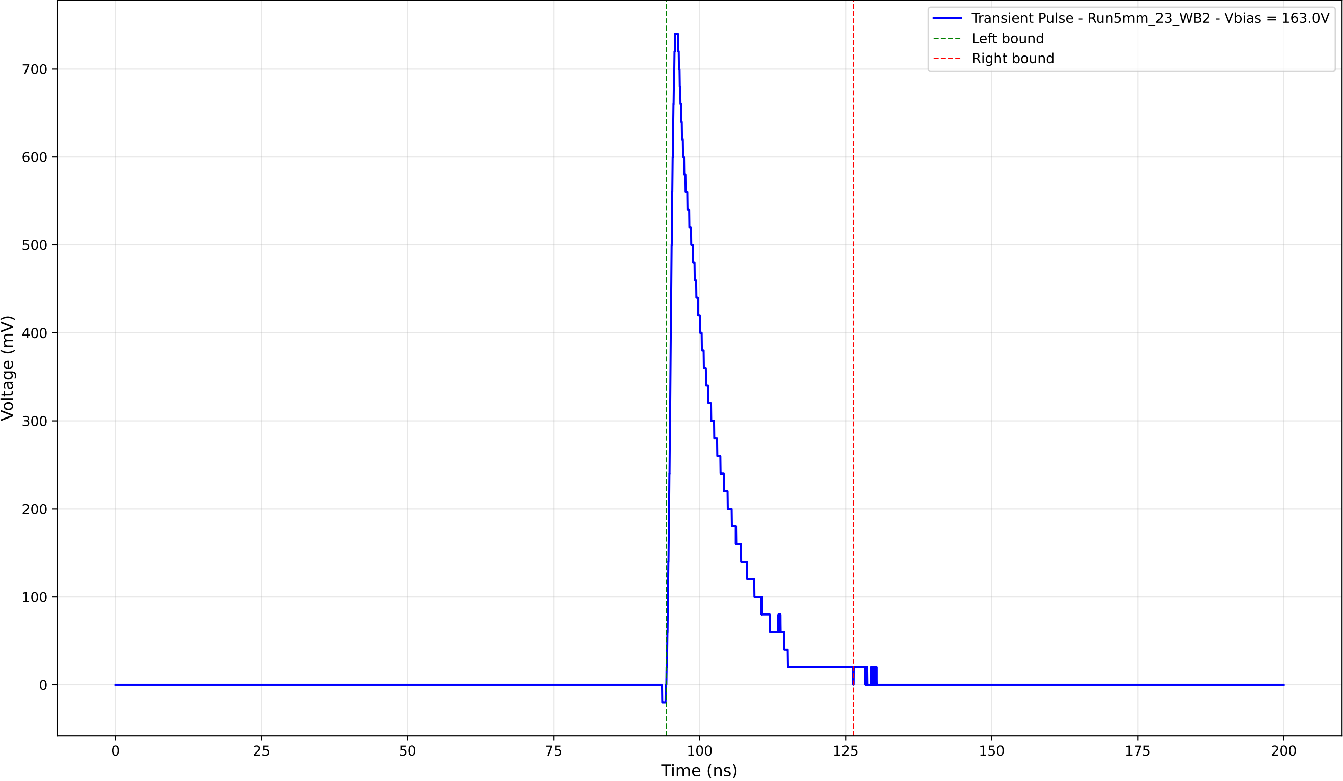
Transient Pulse - Sample: 5mm_23 - Position: 4475.0 \mu\text{m} - Charge: 114.42 pC
