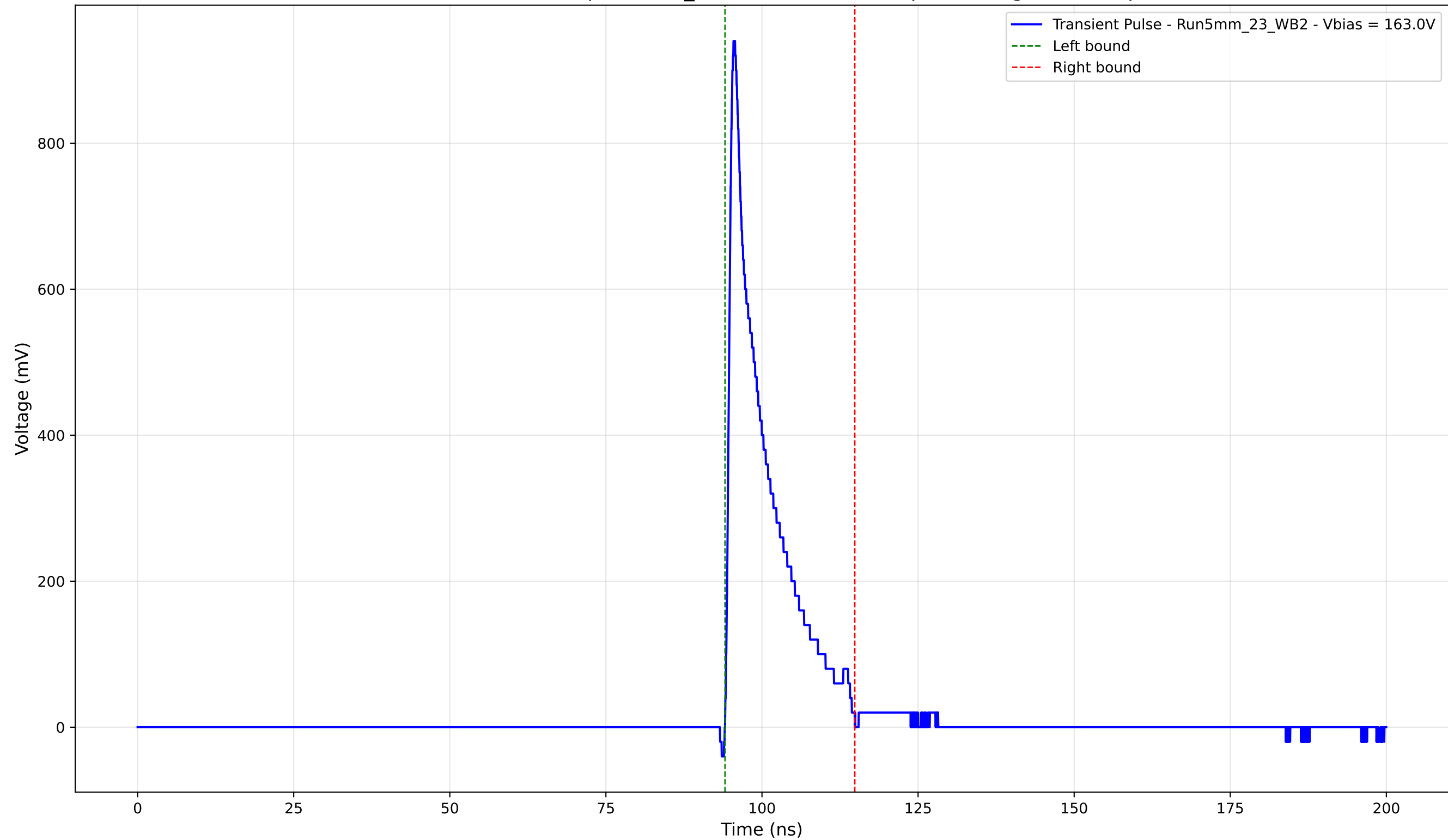
Transient Pulse - Sample: 5mm_23 - Position: 4890.0 \mu\text{m} - Charge: 119.12 pC
