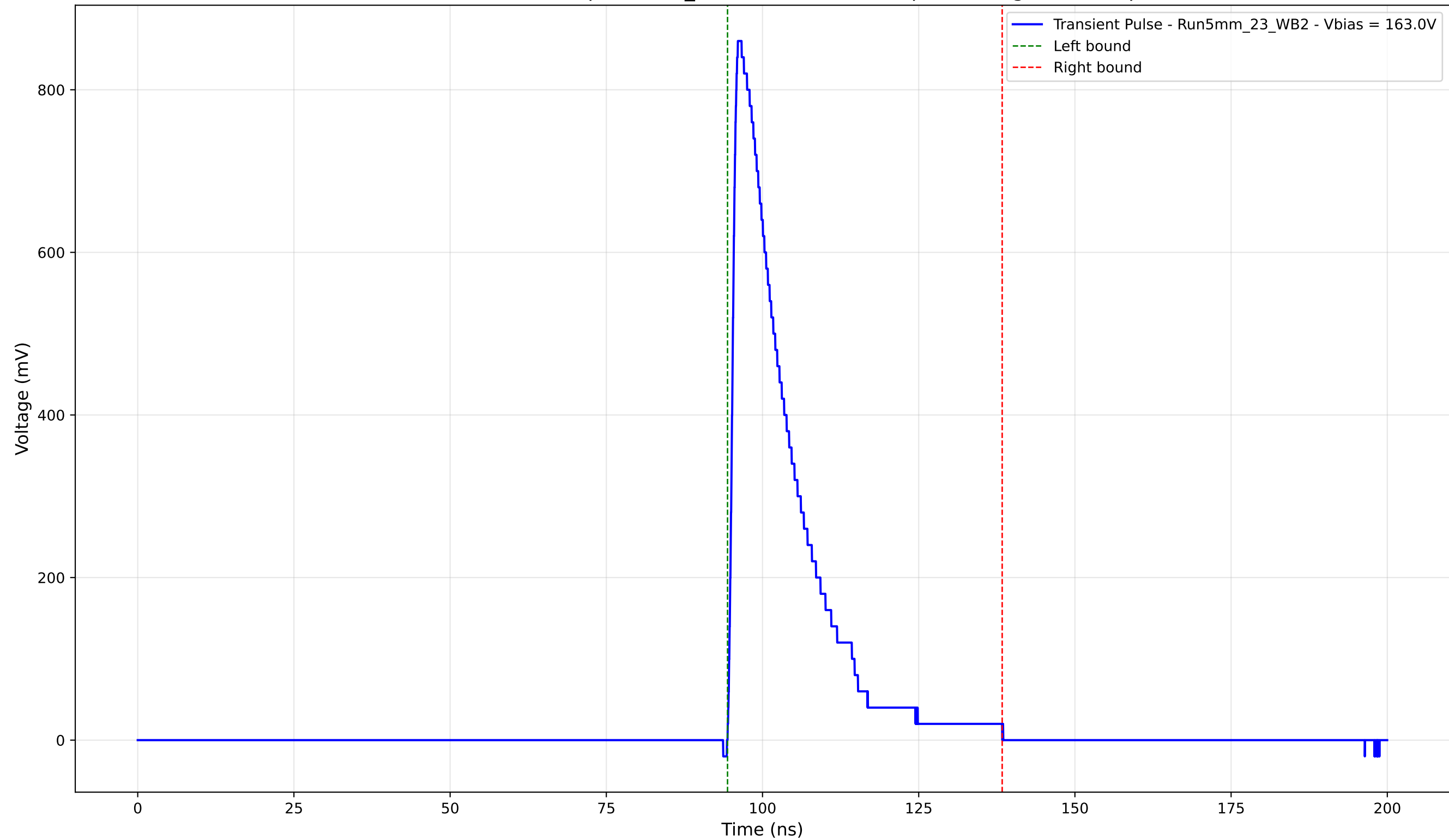
Transient Pulse - Sample: 5mm_23 - Position: 3850.0 \mu\text{m} - Charge: 174.19 pC
