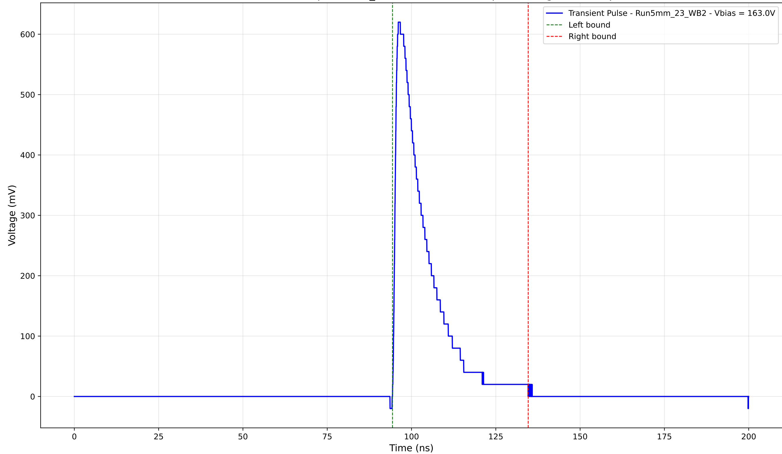
Transient Pulse - Sample: 5mm_23 - Position: 1445.0 \mu\text{m} - Charge: 125.16 pC
