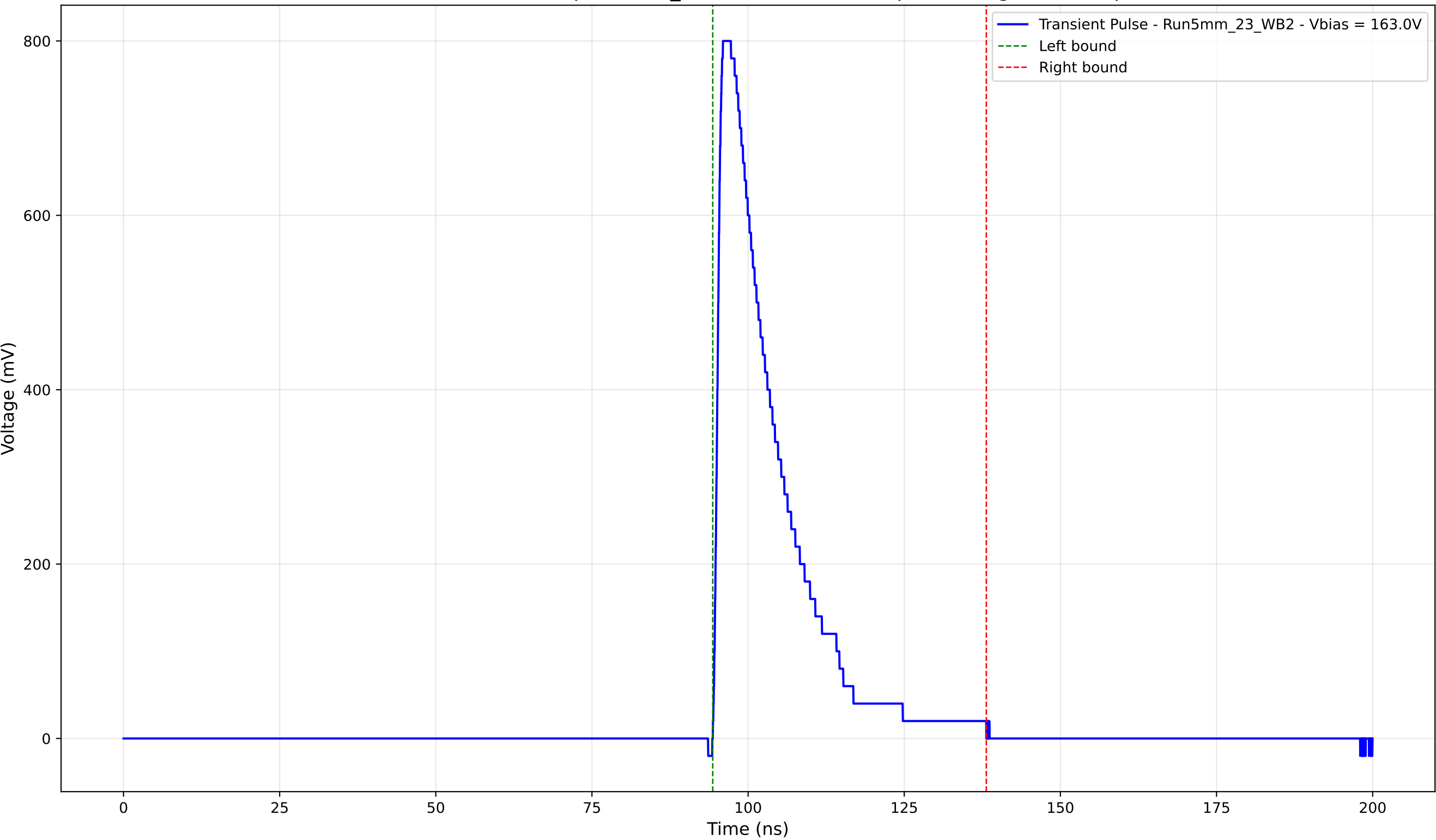
Transient Pulse - Sample: 5mm_23 - Position: 3630.0 \mu\text{m} - Charge: 168.29 pC
