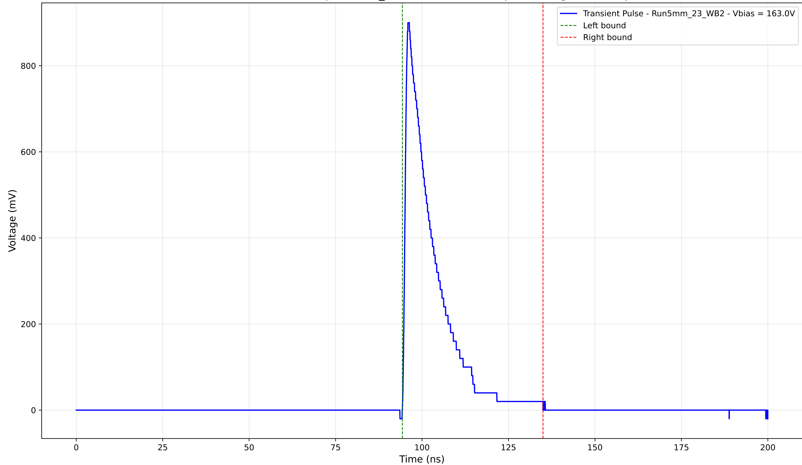
Transient Pulse - Sample: 5mm_23 - Position: 4335.0 \mu\text{m} - Charge: 161.28 pC
