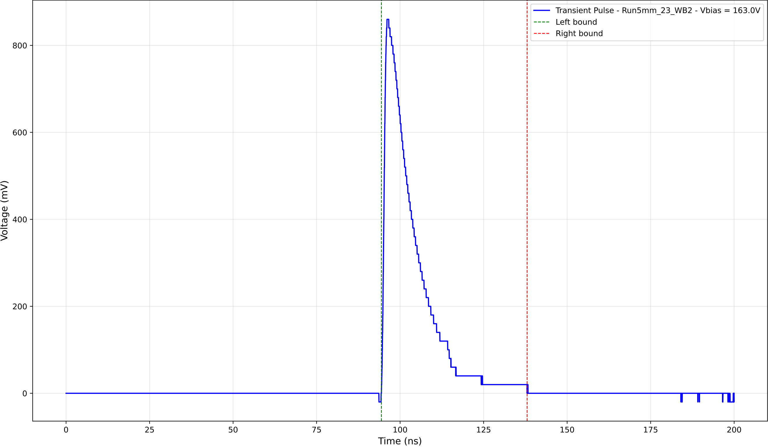
Transient Pulse - Sample: 5mm_23 - Position: 3865.0 \mu\text{m} - Charge: 172.95 pC
