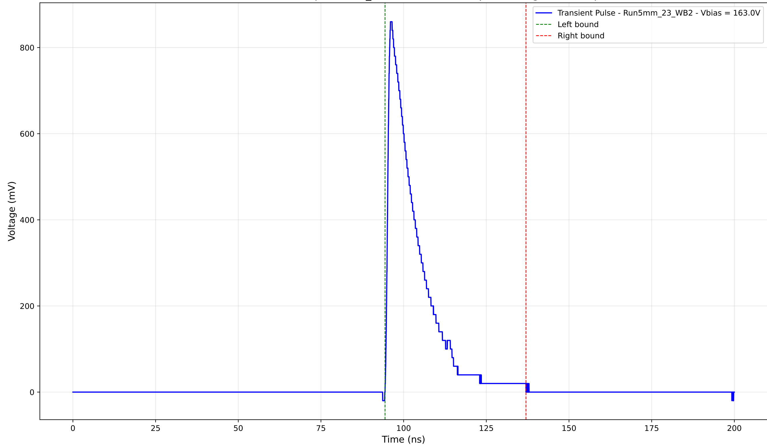
Transient Pulse - Sample: 5mm_23 - Position: 900.0 \mu\text{m} - Charge: 167.14 pC
