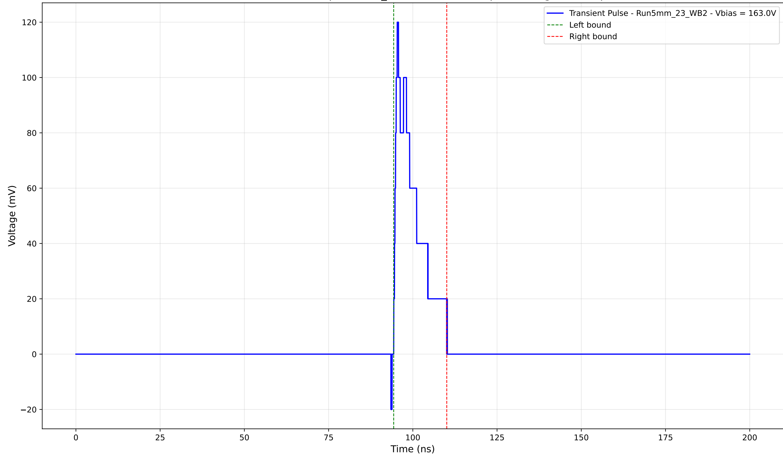
Transient Pulse - Sample: 5mm_23 - Position: 40.0 \mu\text{m} - Charge: 15.50 pC
