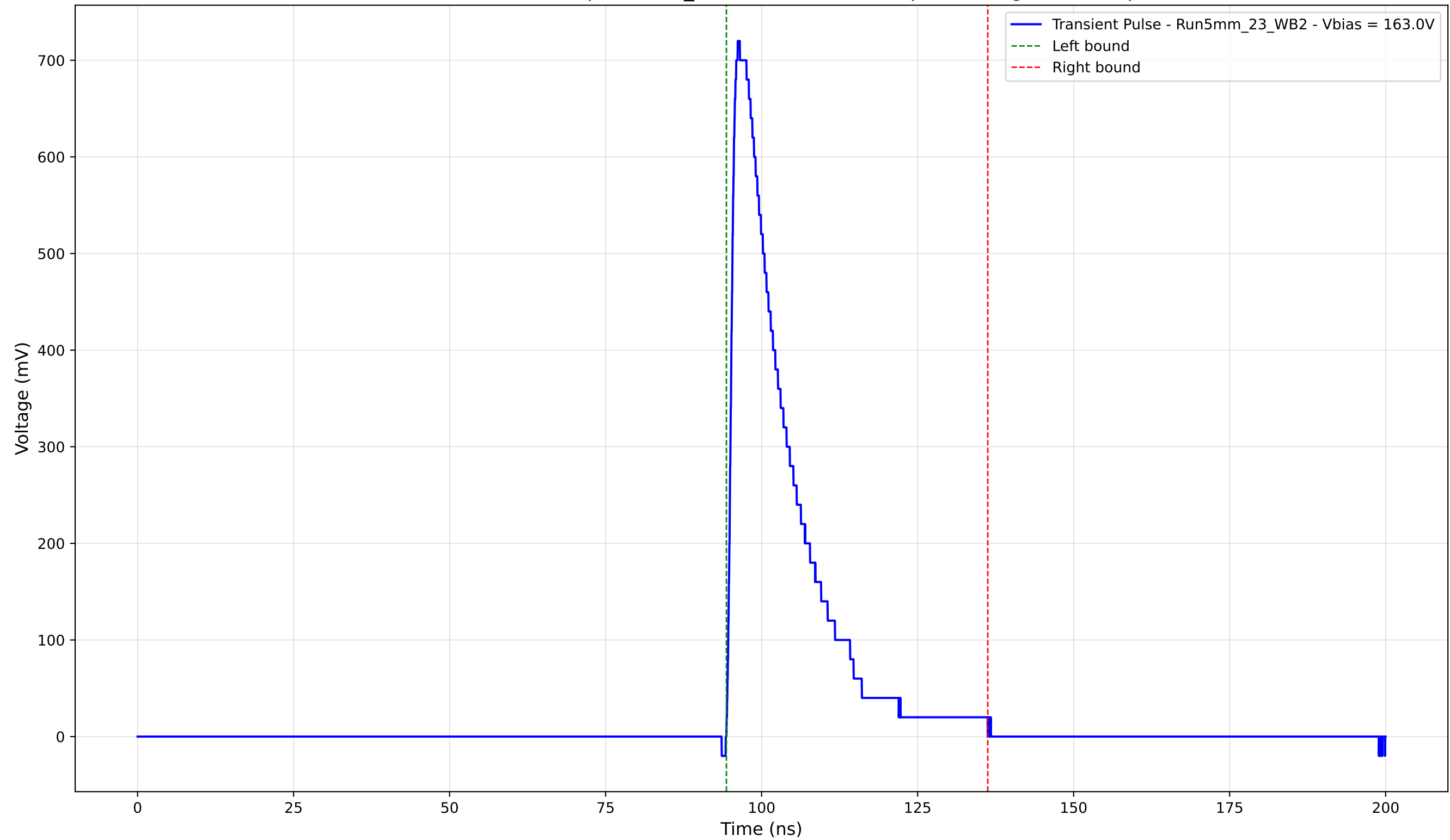
Transient Pulse - Sample: 5mm_23 - Position: 3600.0 \mu\text{m} - Charge: 144.75 pC
