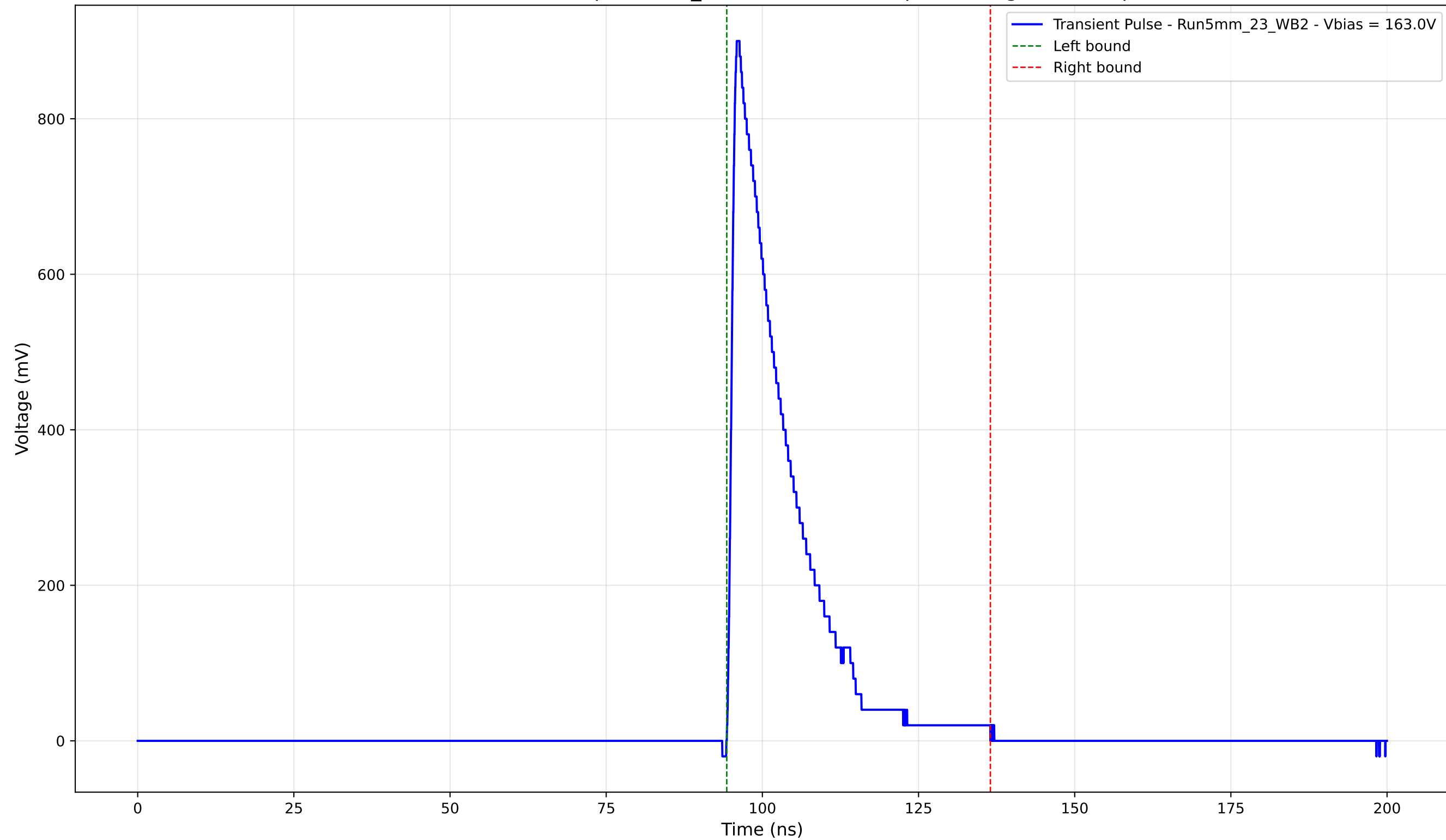
Transient Pulse - Sample: 5mm_23 - Position: 690.0 \mu\text{m} - Charge: 172.15 pC
