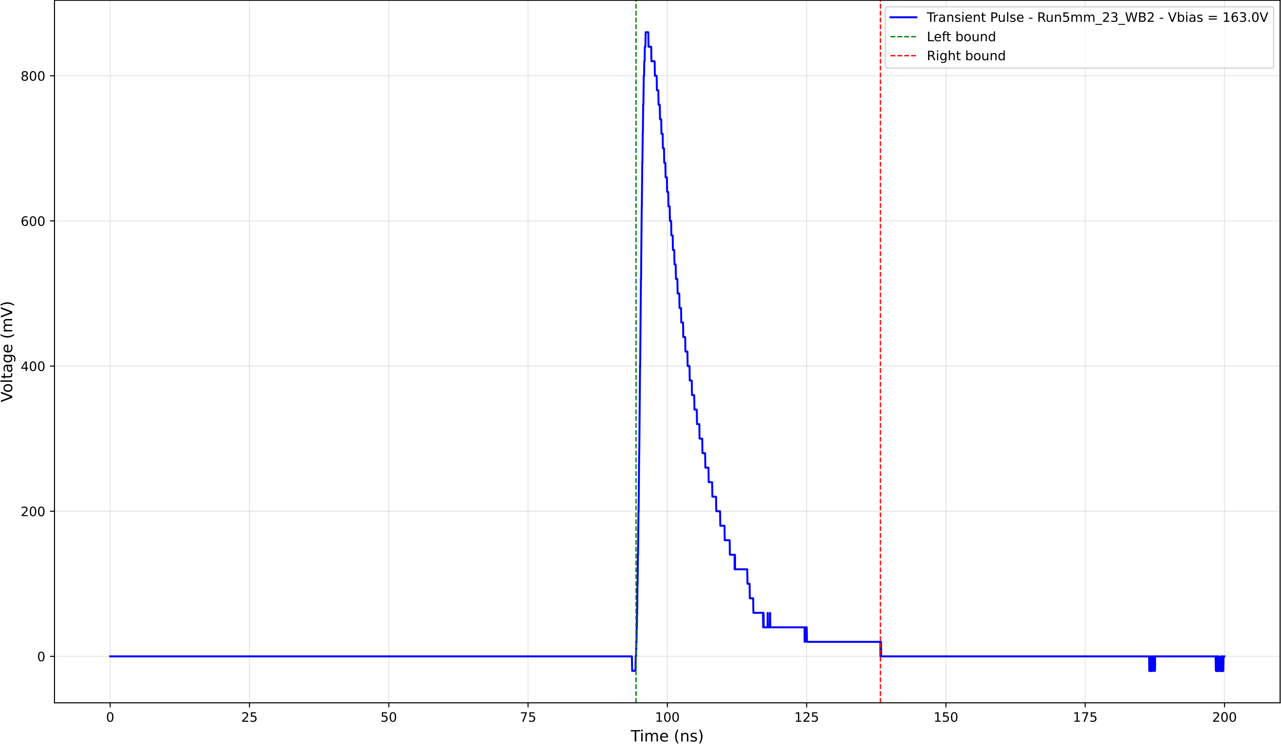
Transient Pulse - Sample: 5mm_23 - Position: 3750.0 \mu\text{m} - Charge: 176.93 pC
