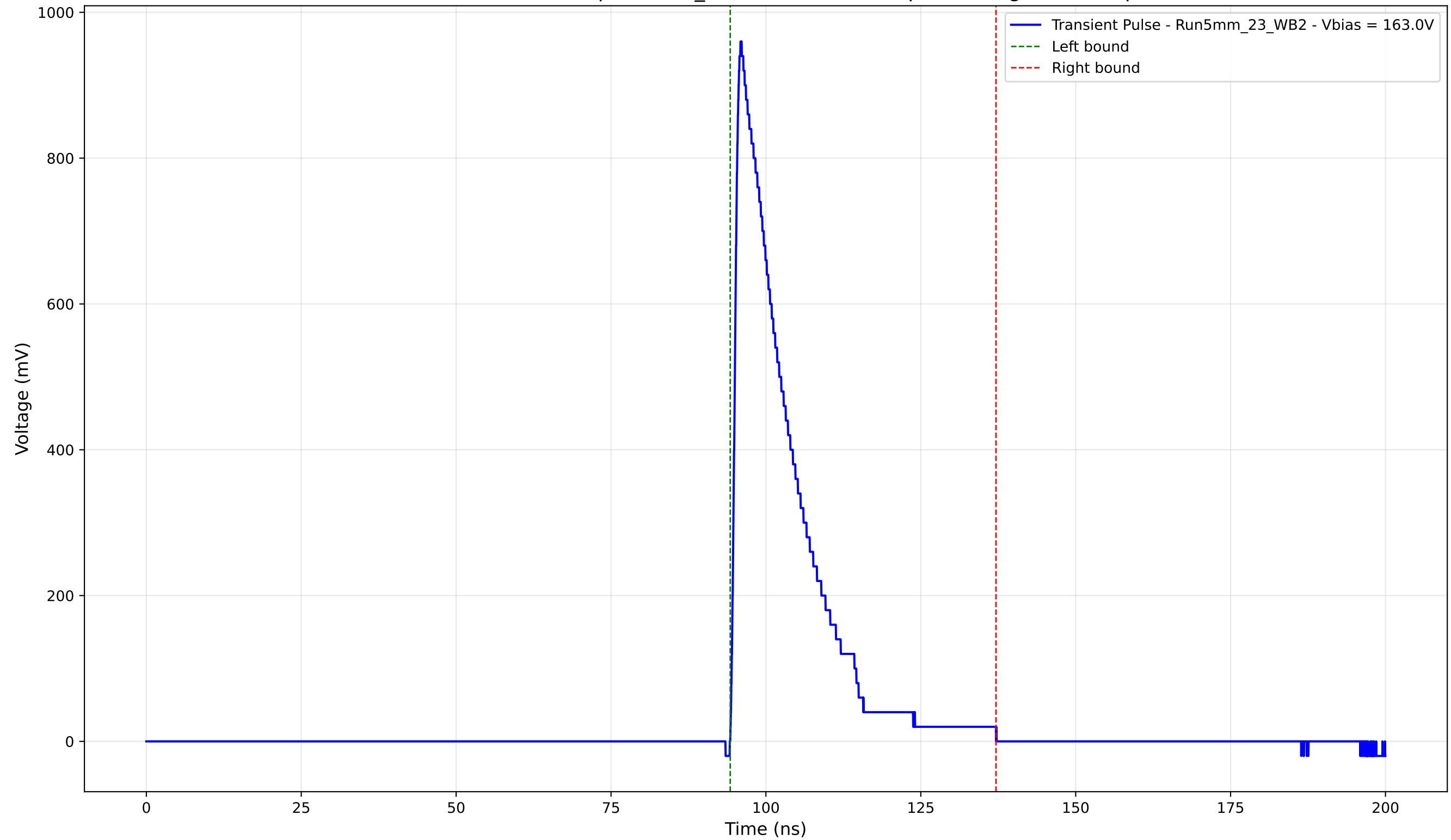
Transient Pulse - Sample: 5mm_23 - Position: 600.0 \mu\text{m} - Charge: 185.55 pC
