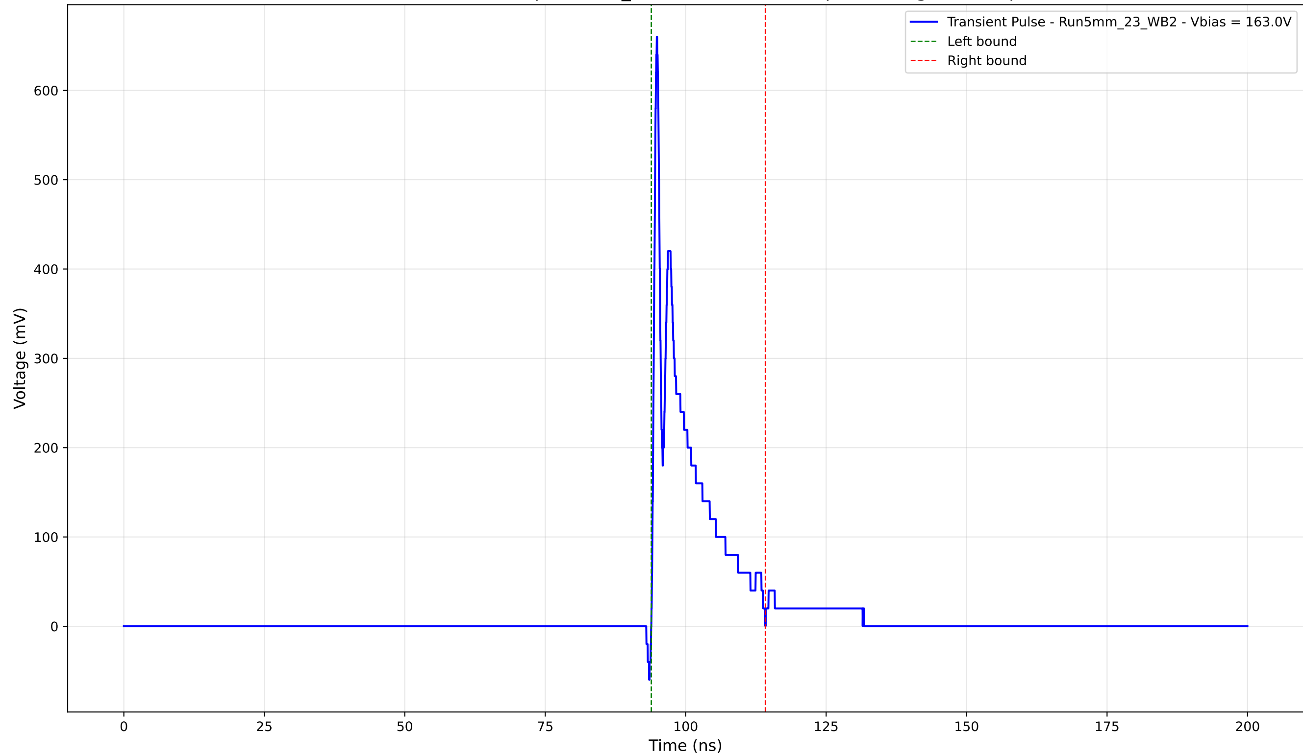
Transient Pulse - Sample: 5mm_23 - Position: 2485.0 \mu\text{m} - Charge: 68.64 pC
