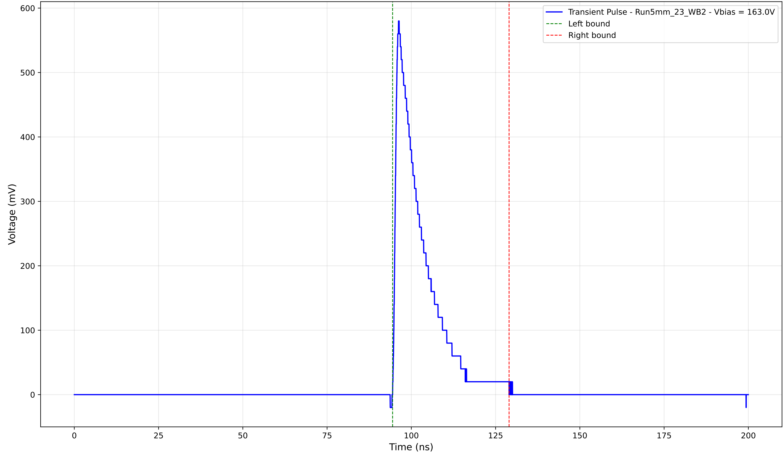
Transient Pulse - Sample: 5mm_23 - Position: 945.0 \mu\text{m} - Charge: 101.36 pC
