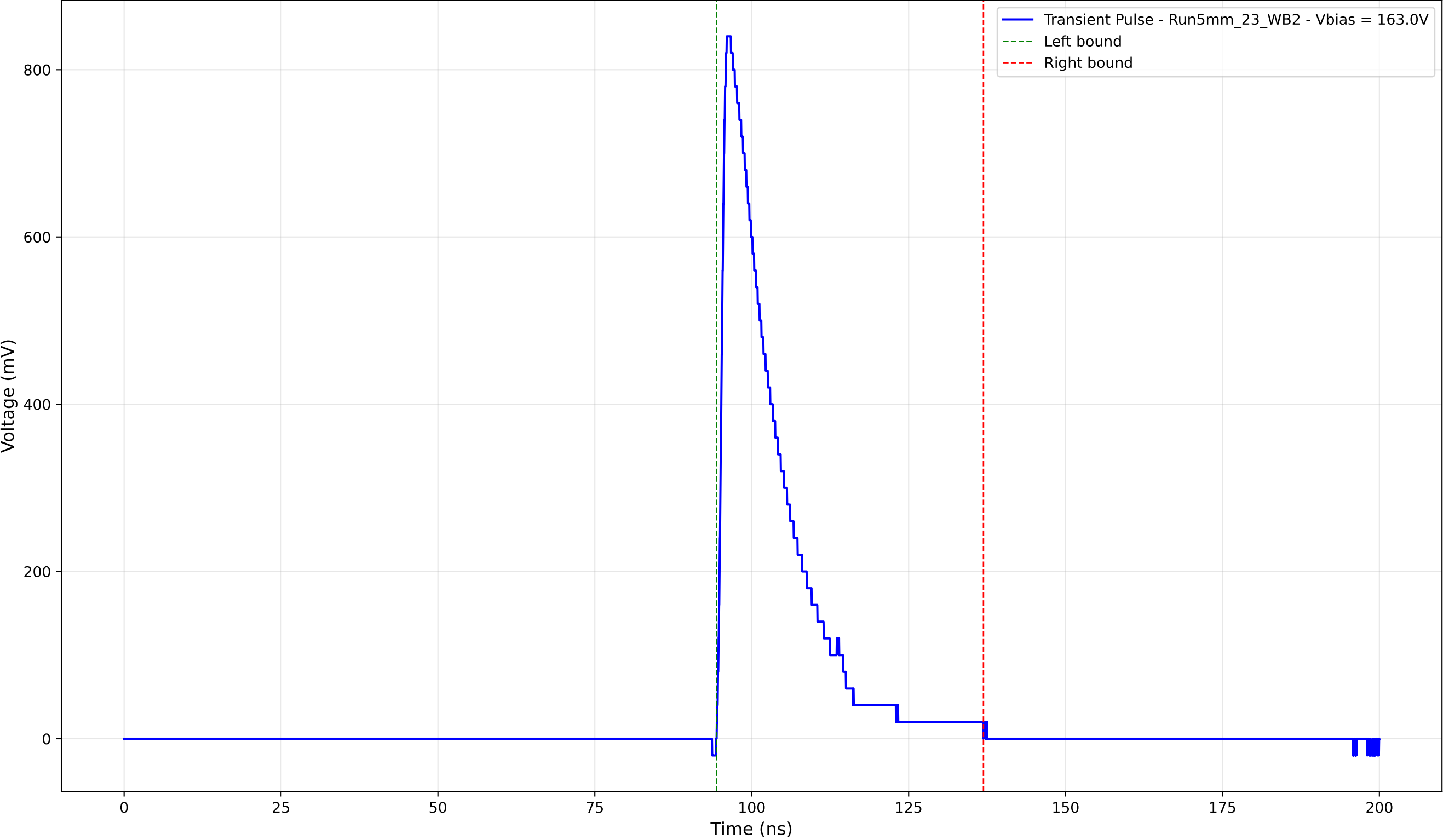
Transient Pulse - Sample: 5mm_23 - Position: 3935.0 \mu\text{m} - Charge: 164.19 pC
