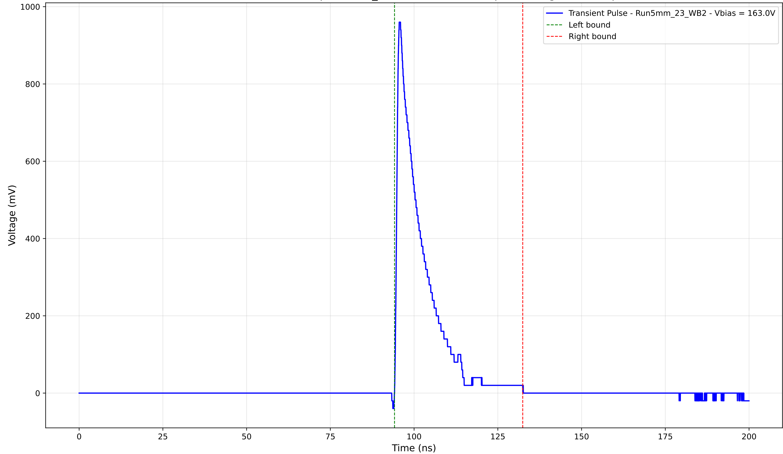
Transient Pulse - Sample: 5mm_23 - Position: 4700.0 \mu\text{m} - Charge: 153.92 pC
