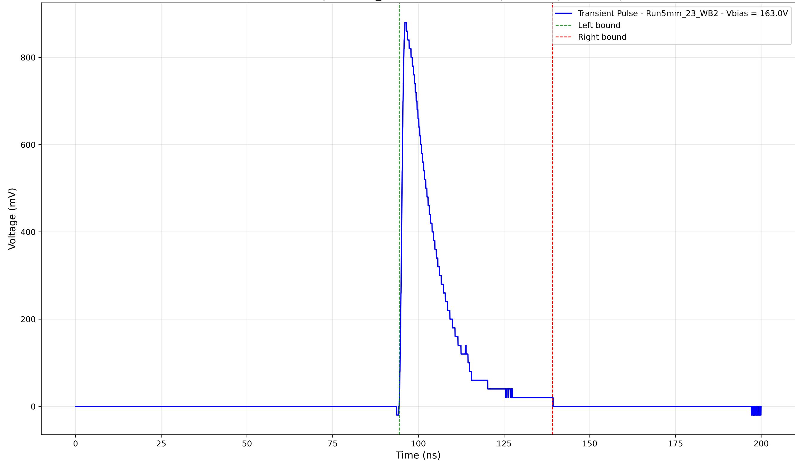
Transient Pulse - Sample: 5mm_23 - Position: 1105.0 \mu\text{m} - Charge: 184.44 pC
