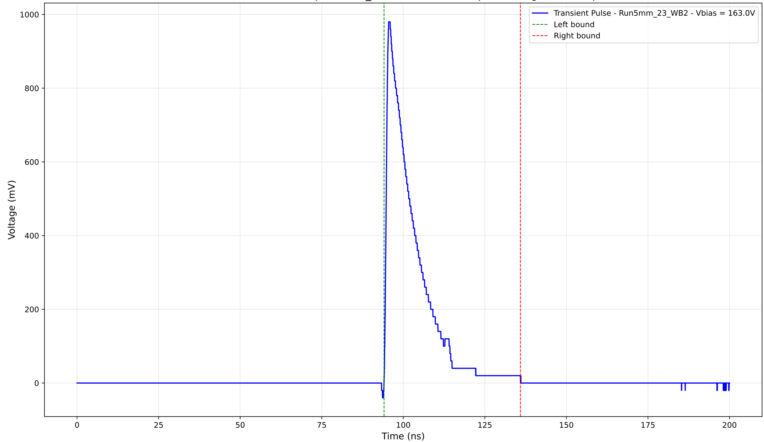
Transient Pulse - Sample: 5mm_23 - Position: 345.0 \mu\text{m} - Charge: 180.87 pC
