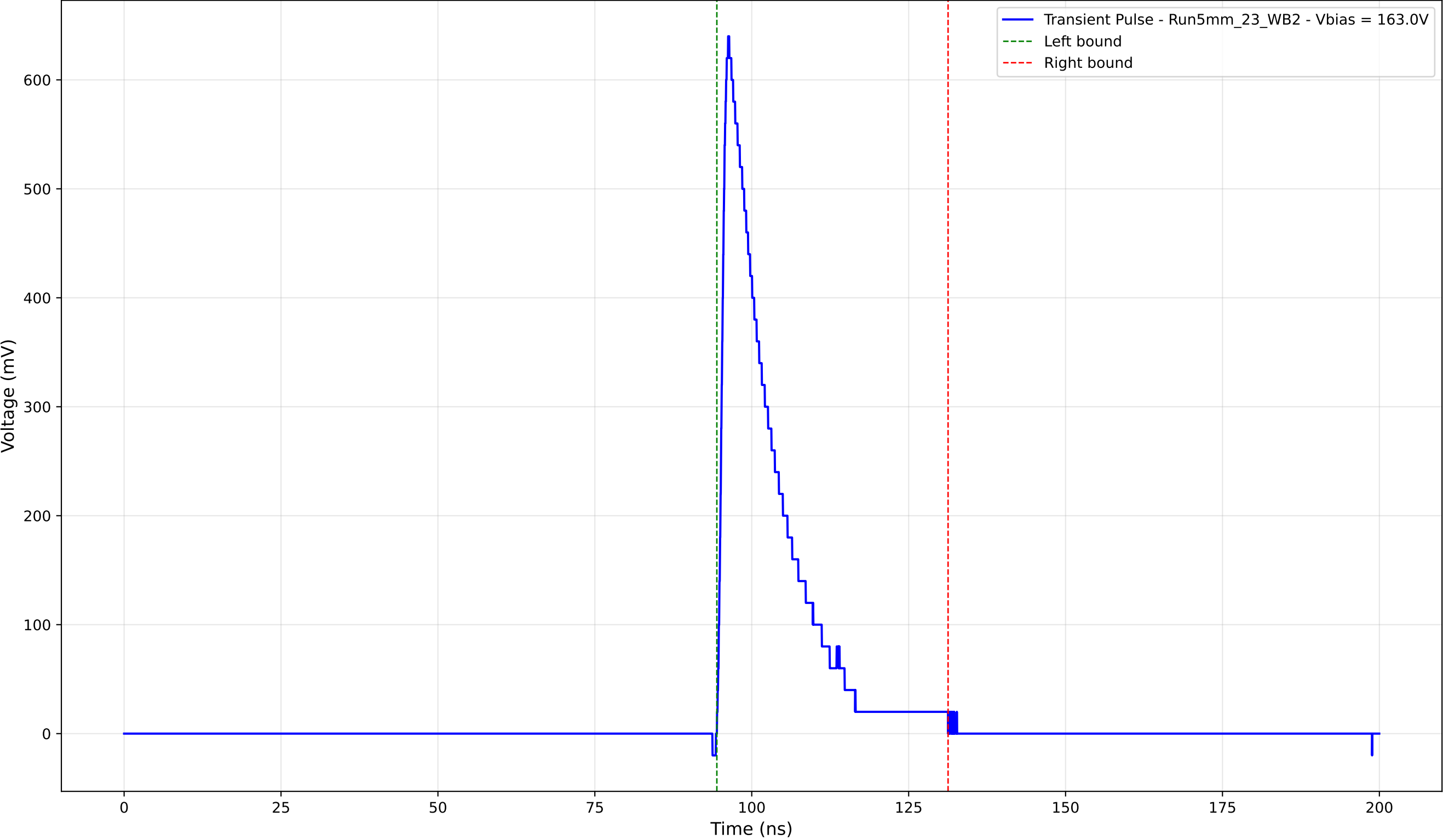
Transient Pulse - Sample: 5mm_23 - Position: 3980.0 \mu\text{m} - Charge: 112.02 pC
