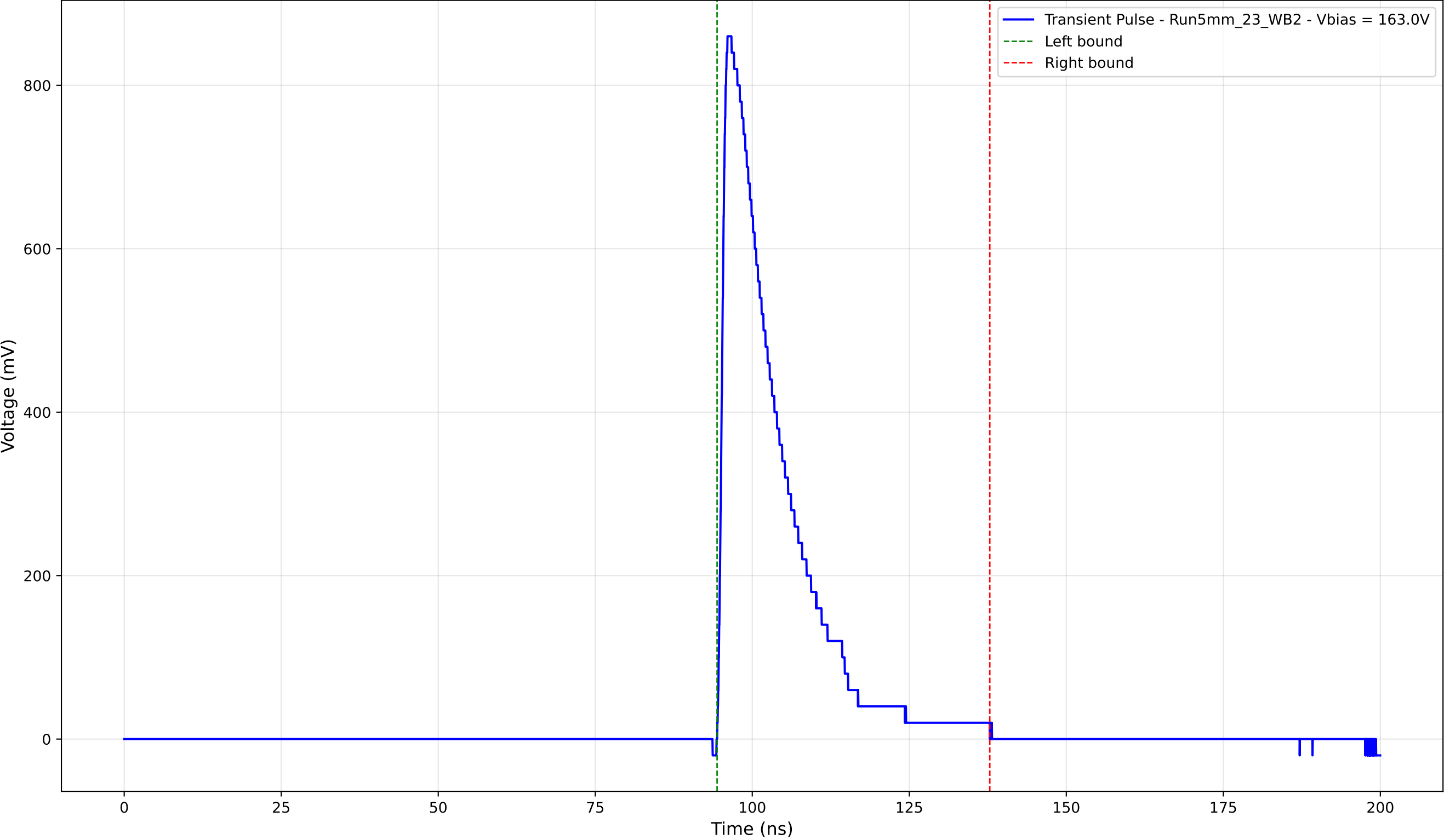
Transient Pulse - Sample: 5mm_23 - Position: 3830.0 \mu\text{m} - Charge: 175.01 pC
