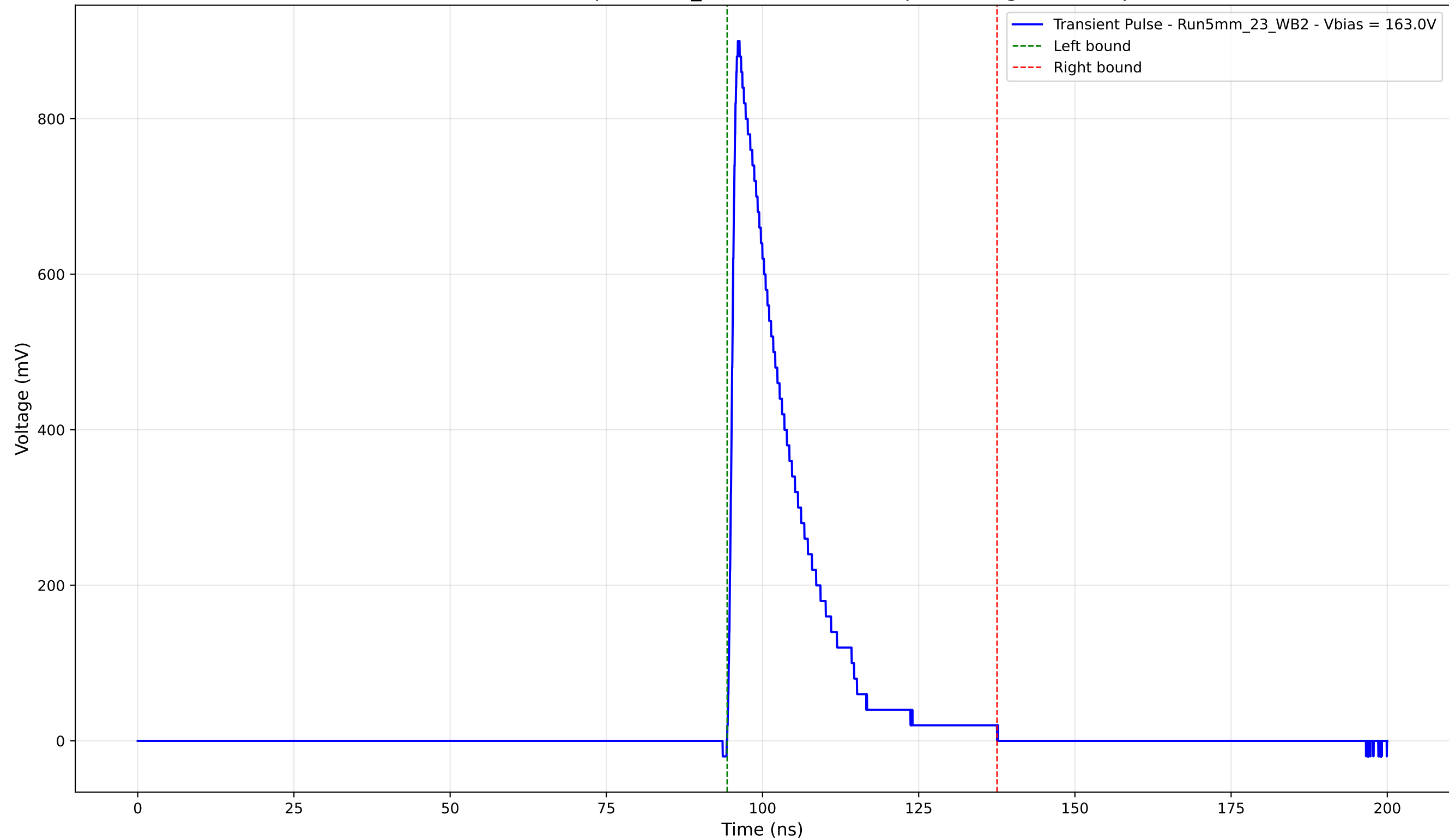
Transient Pulse - Sample: 5mm_23 - Position: 805.0 \mu\text{m} - Charge: 174.97 pC
