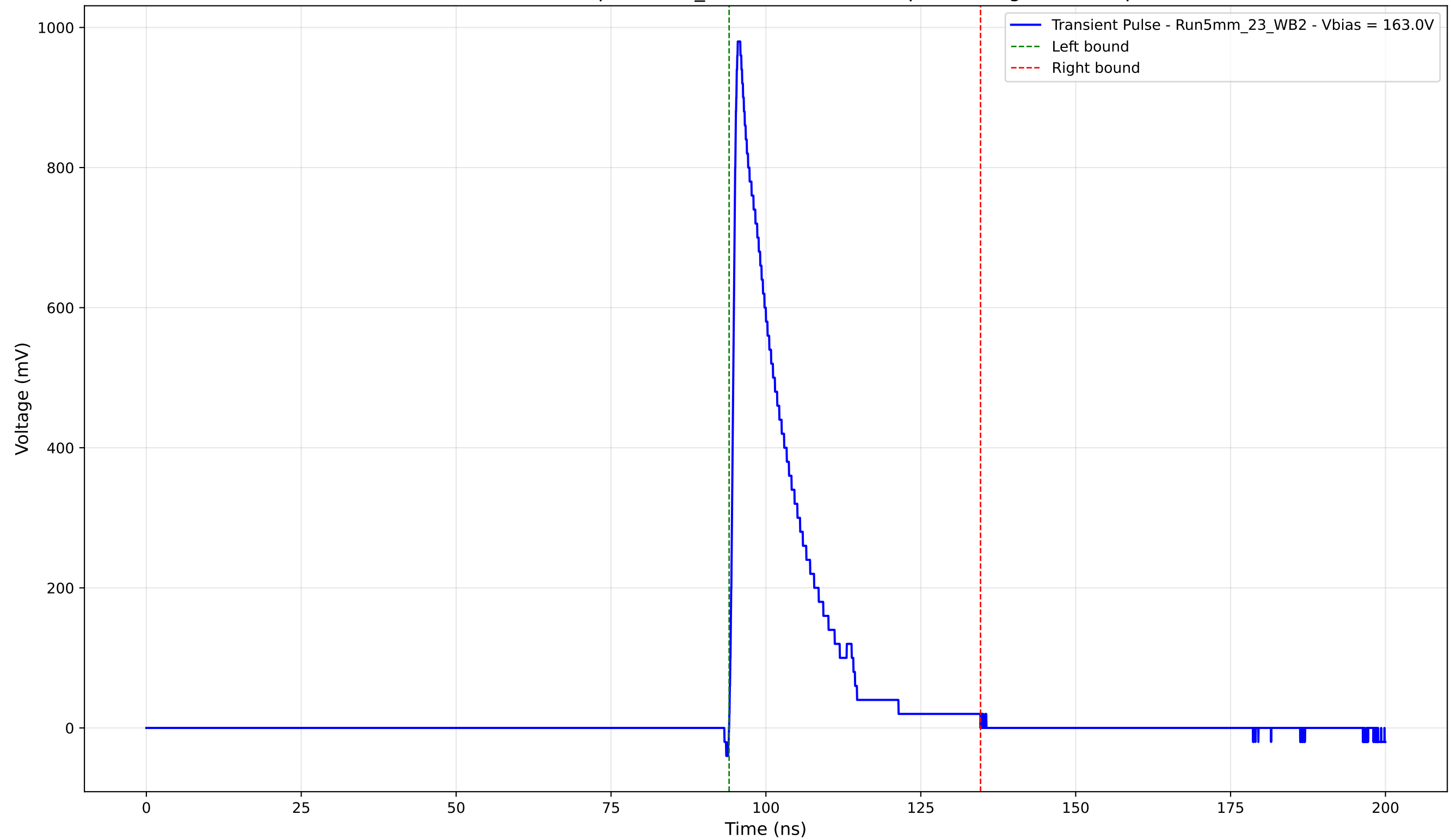
Transient Pulse - Sample: 5mm_23 - Position: 265.0 \mu\text{m} - Charge: 172.58 pC
