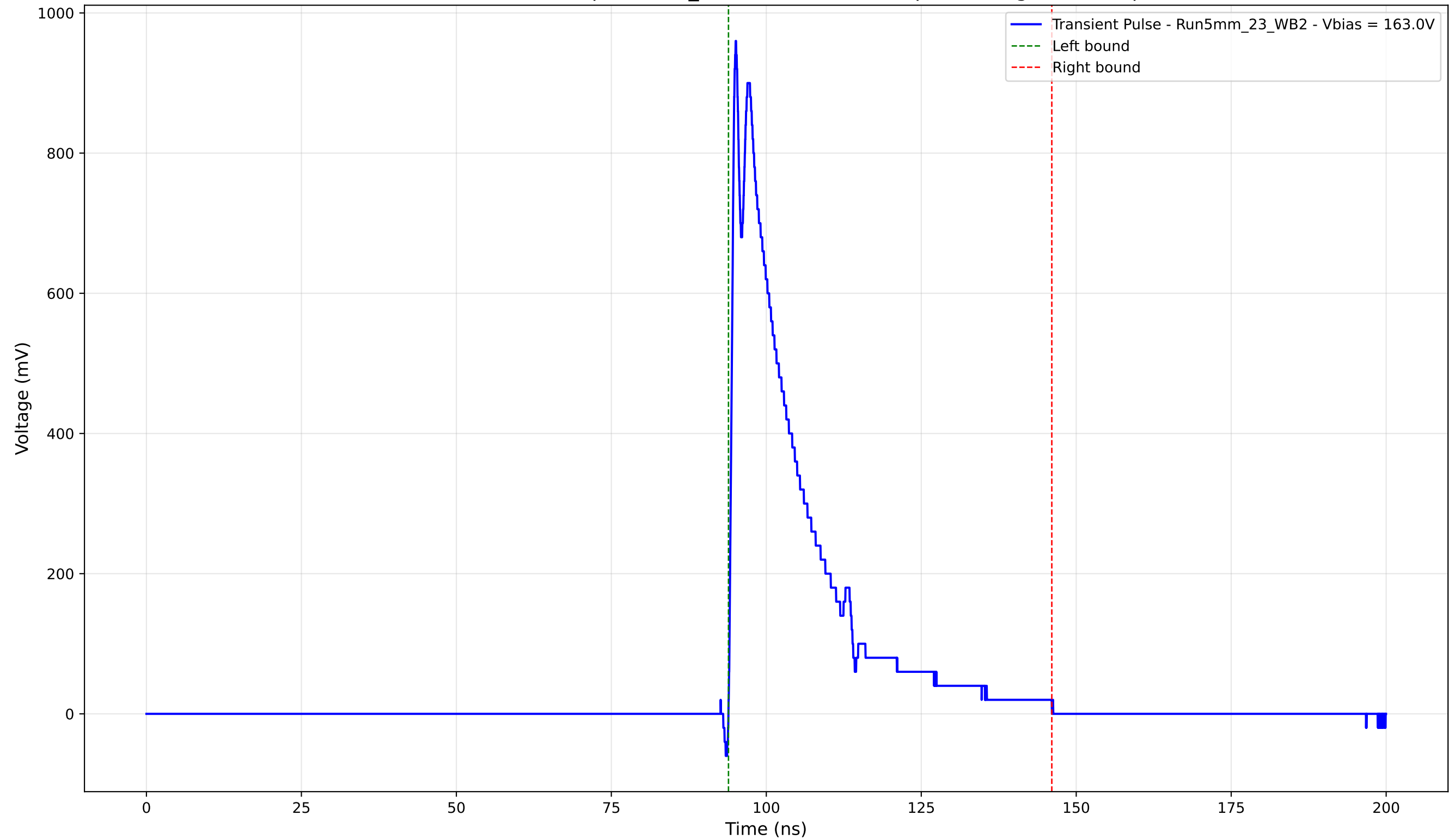
Transient Pulse - Sample: 5mm_23 - Position: 2245.0 \mu\text{m} - Charge: 205.19 pC
