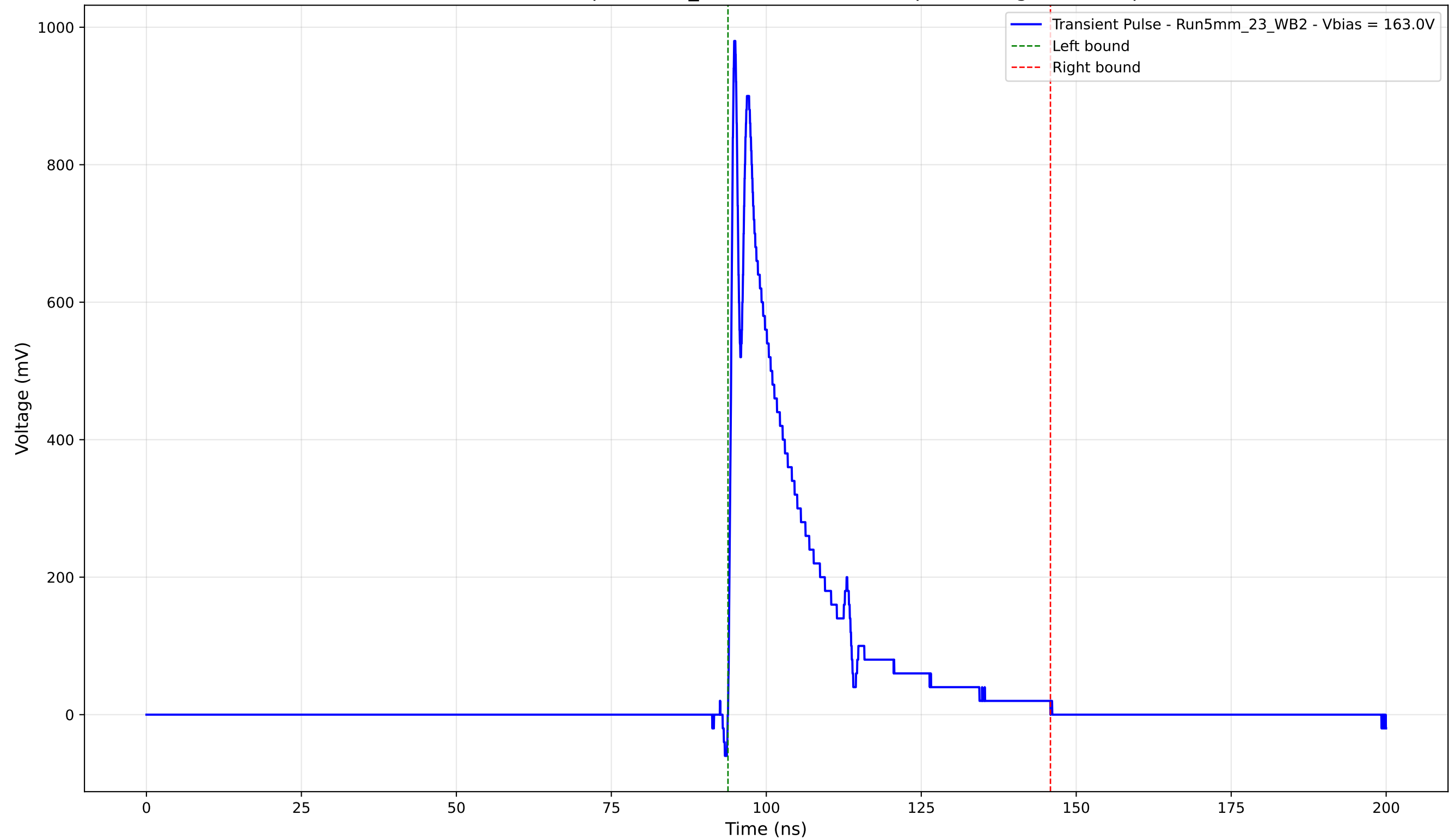
Transient Pulse - Sample: 5mm_23 - Position: 2610.0 \mu\text{m} - Charge: 190.56 pC
