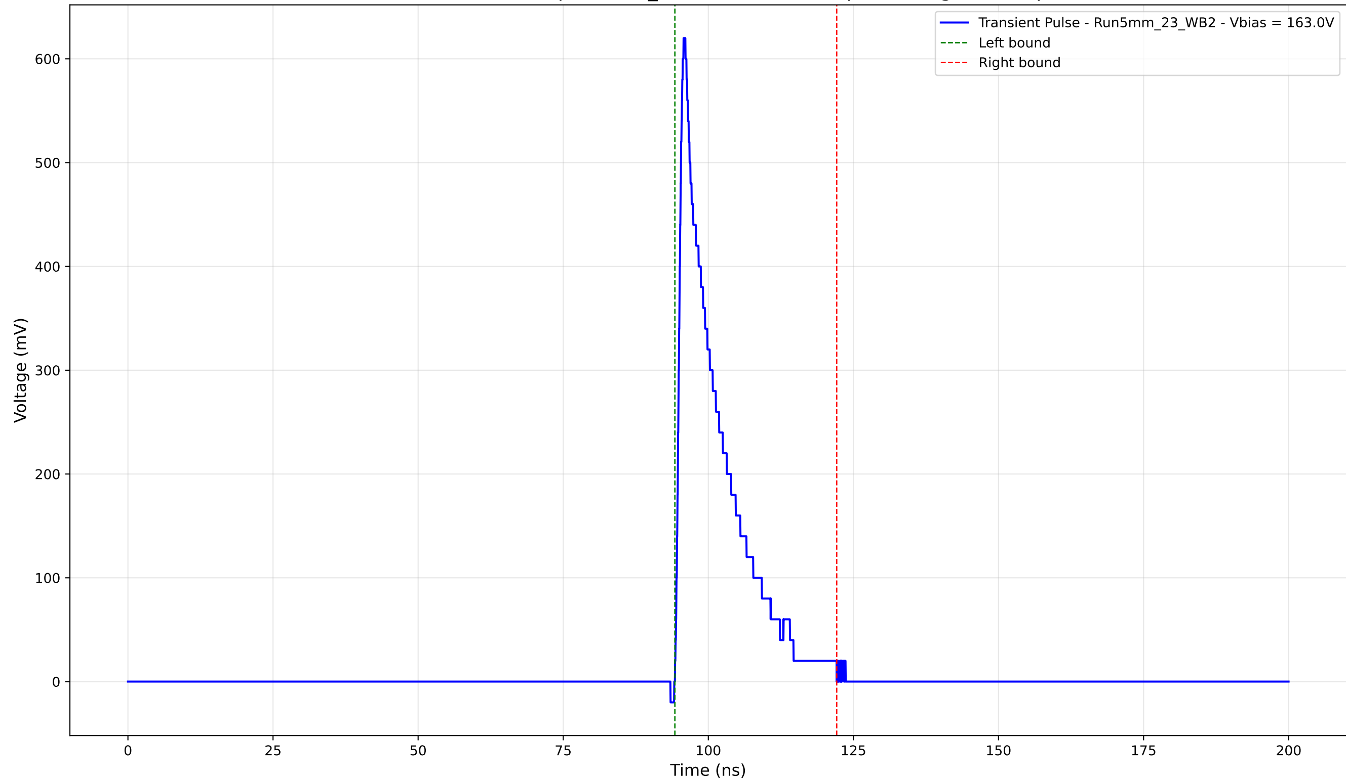
Transient Pulse - Sample: 5mm_23 - Position: 445.0 \mu\text{m} - Charge: 91.34 pC
