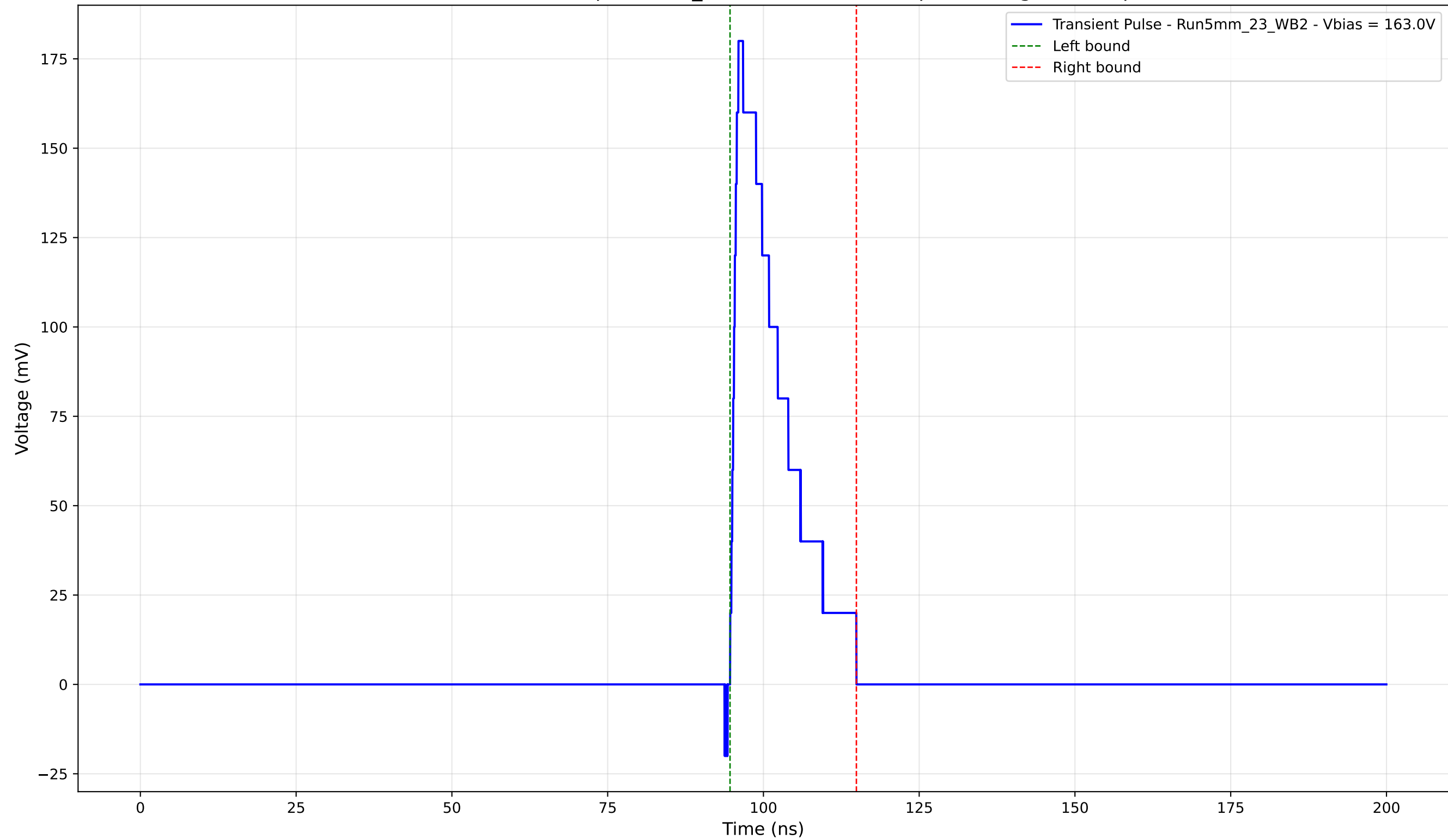
Transient Pulse - Sample: 5mm_23 -Position: 4045.0 \mu\text{m} - Charge: 30.14 pC
