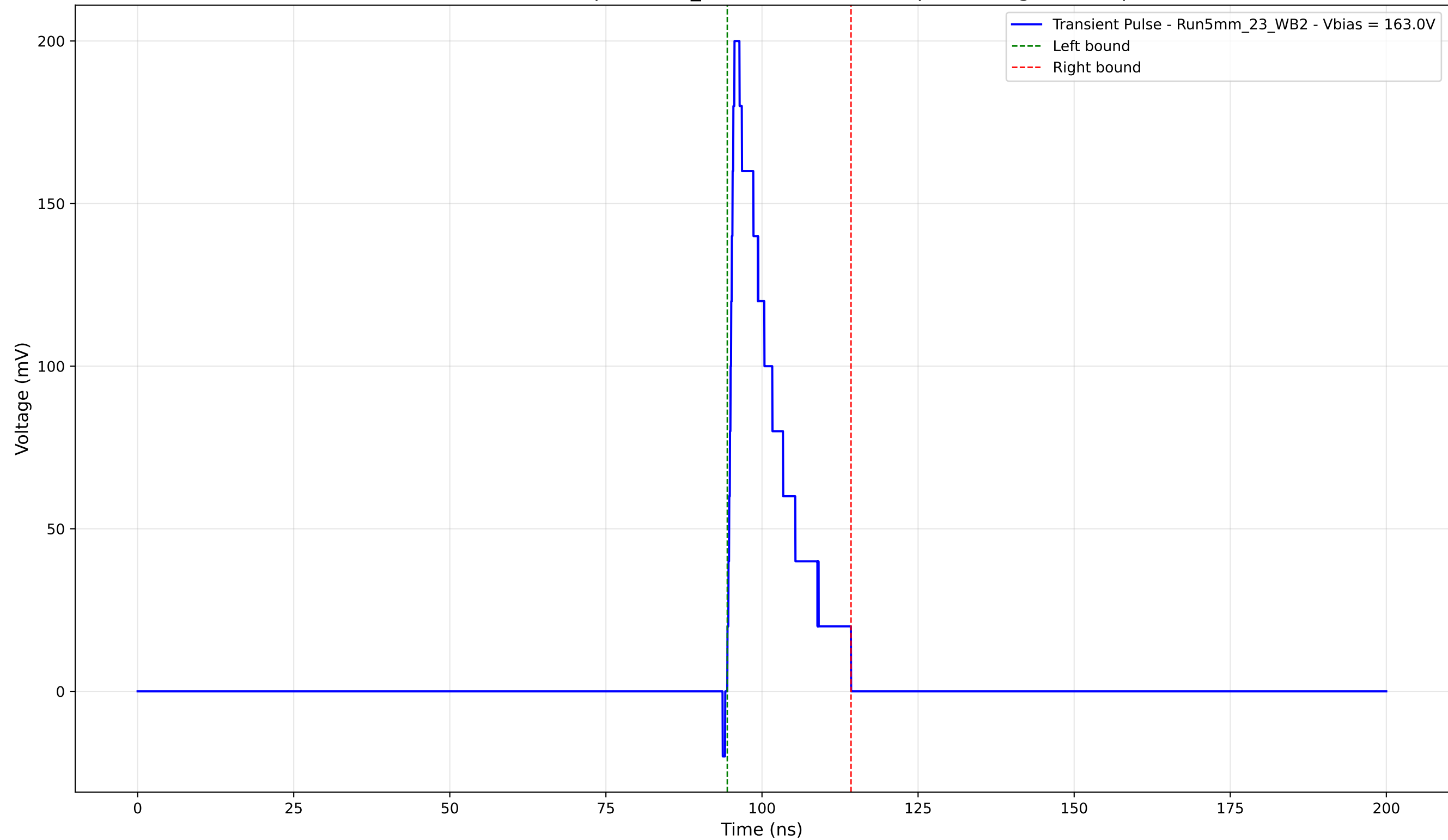
Transient Pulse - Sample: 5mm_23 - Position: 4545.0 \mu\text{m} - Charge: 30.01 pC
