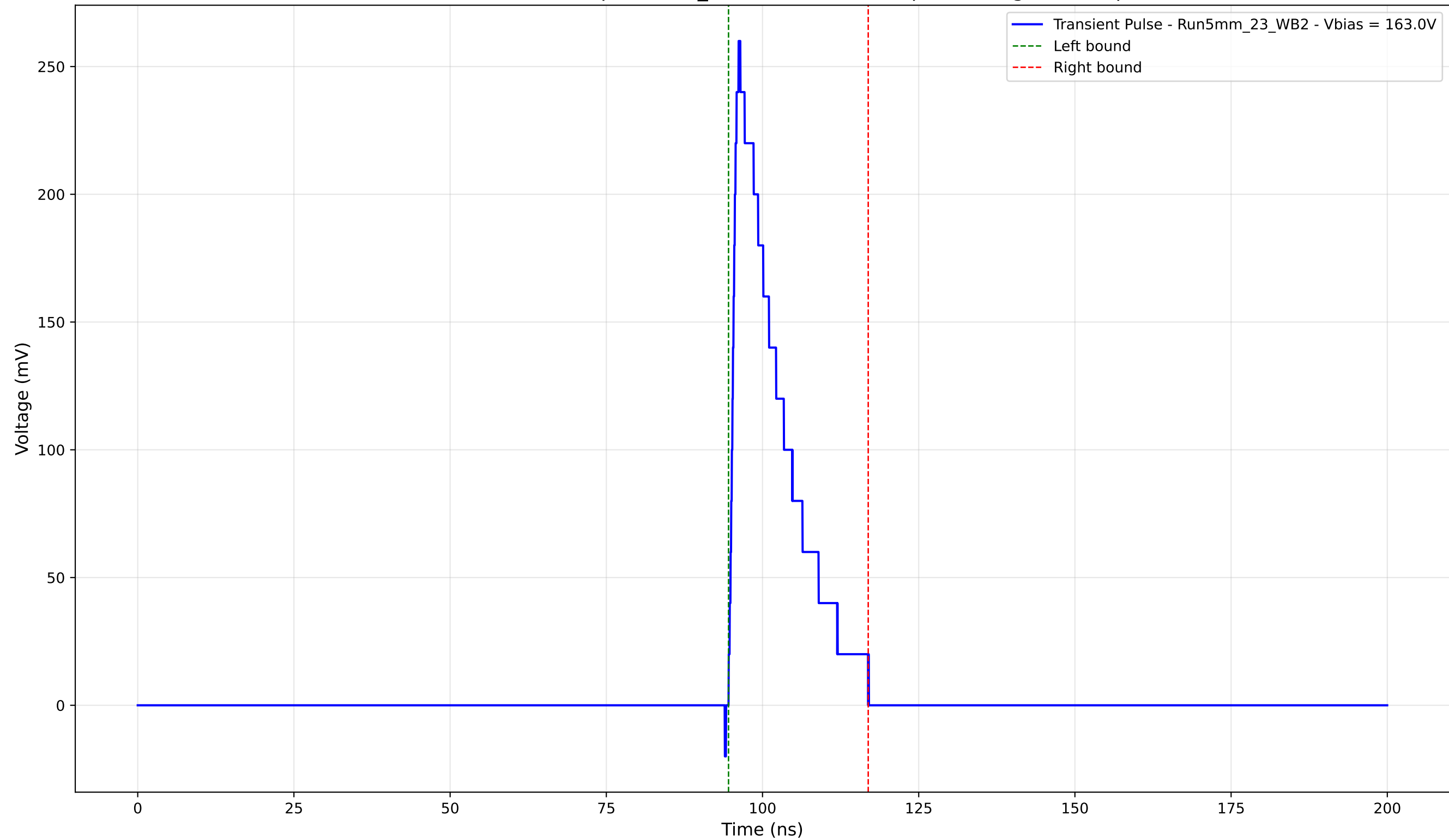
Transient Pulse - Sample: 5mm_23 - Position: 975.0 \mu\text{m} - Charge: 43.42 pC
