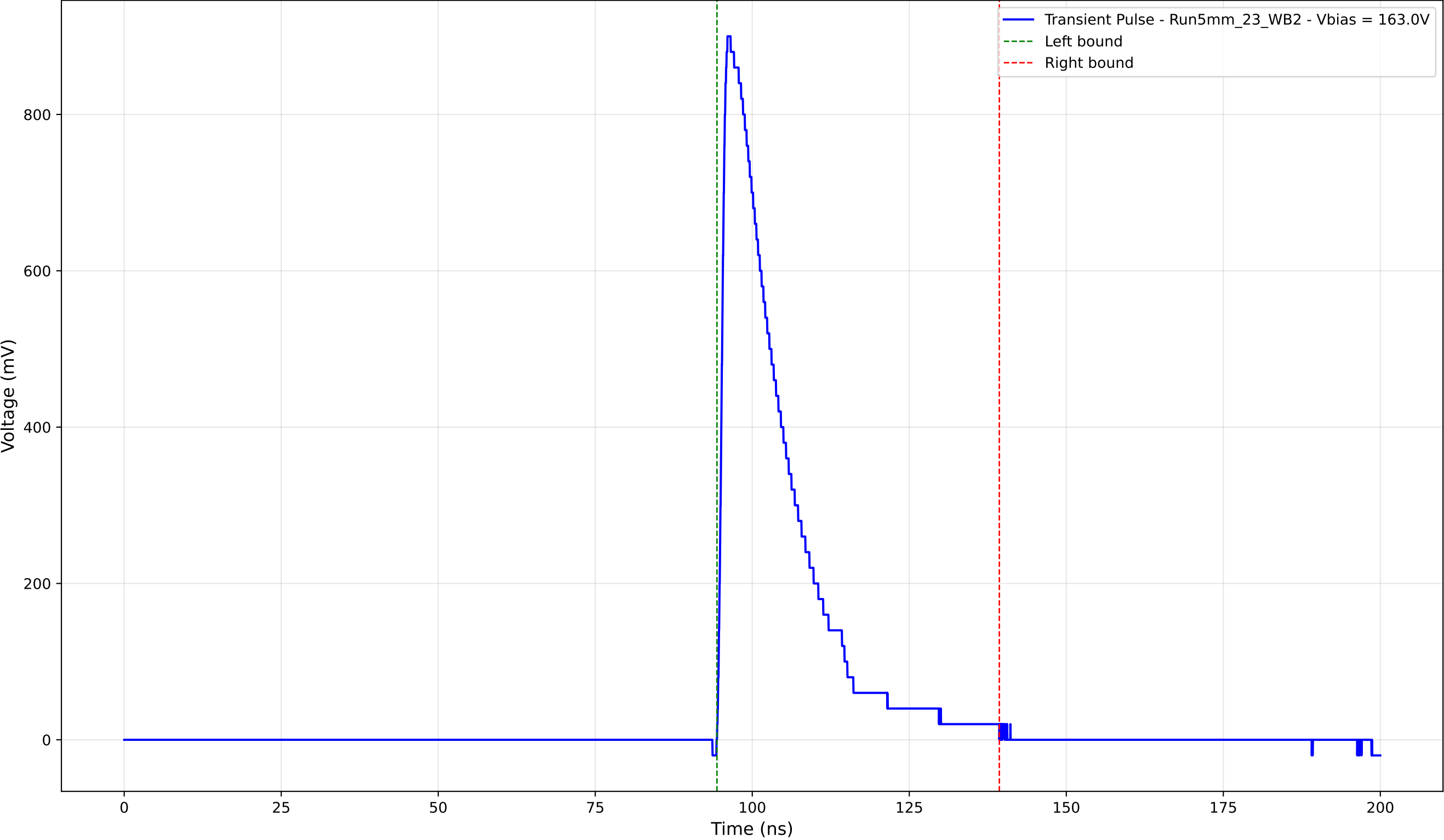
Transient Pulse - Sample: 5mm_23 - Position: 1215.0 \mu\text{m} - Charge: 196.84 pC
