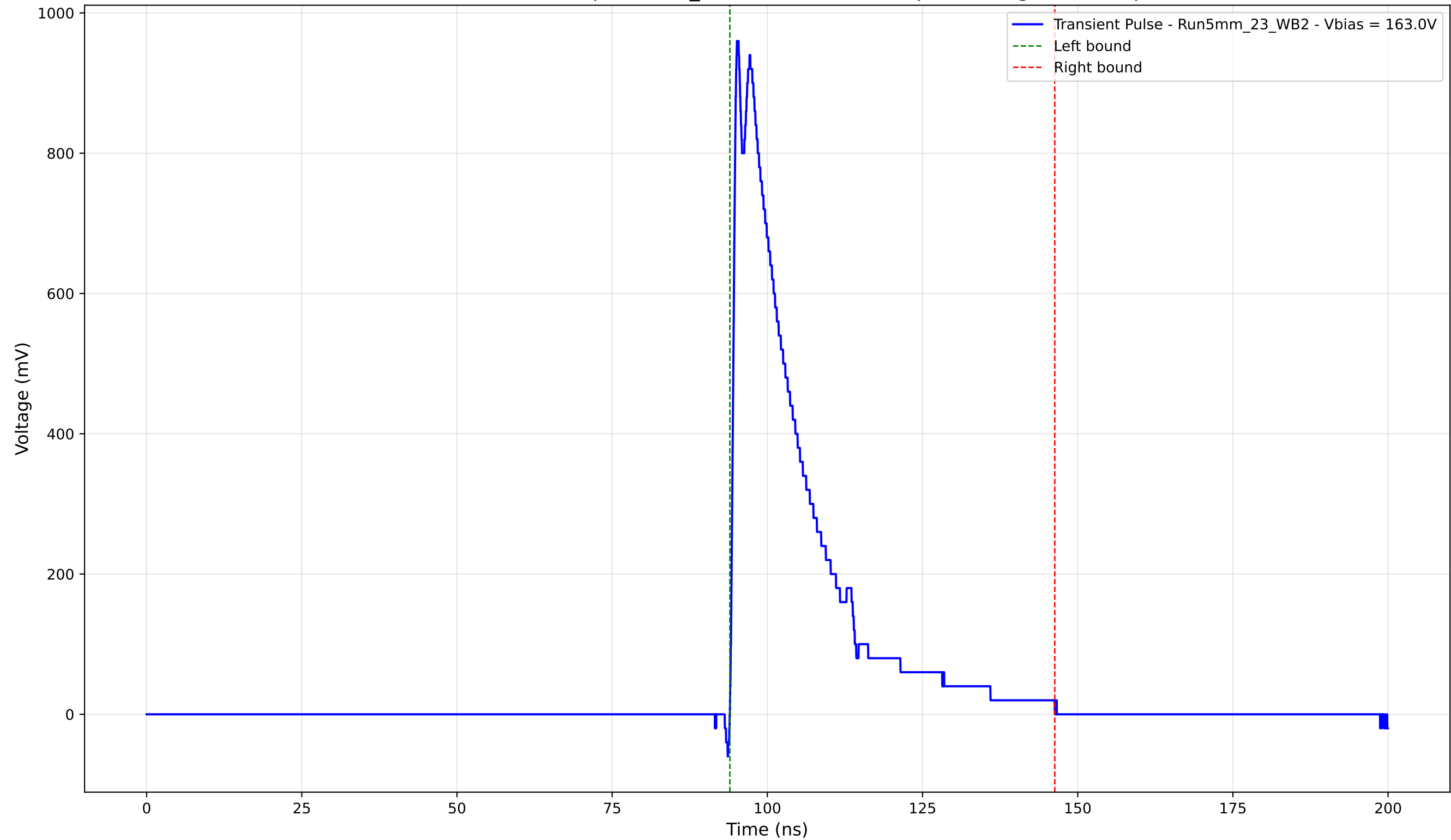
Transient Pulse - Sample: 5mm_23 - Position: 2910.0 \mu\text{m} - Charge: 219.36 pC
