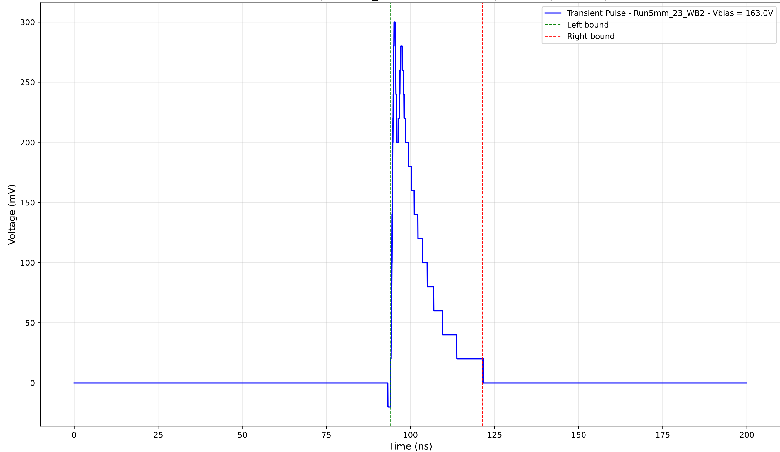
Transient Pulse - Sample: 5mm_23 - Position: 2030.0 \mu\text{m} - Charge: 50.98 pC
