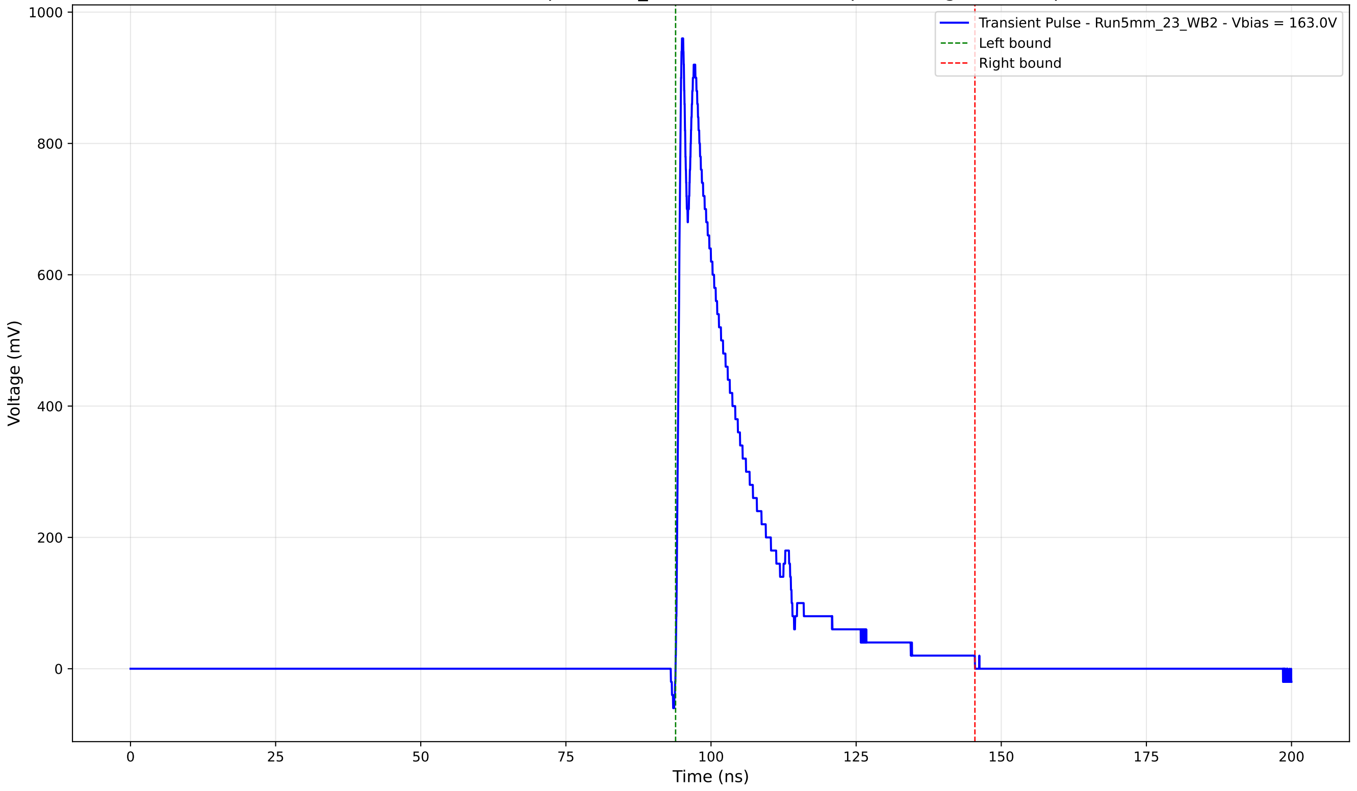
Transient Pulse - Sample: 5mm_23 - Position: 2785.0 \mu\text{m} - Charge: 205.29 pC
