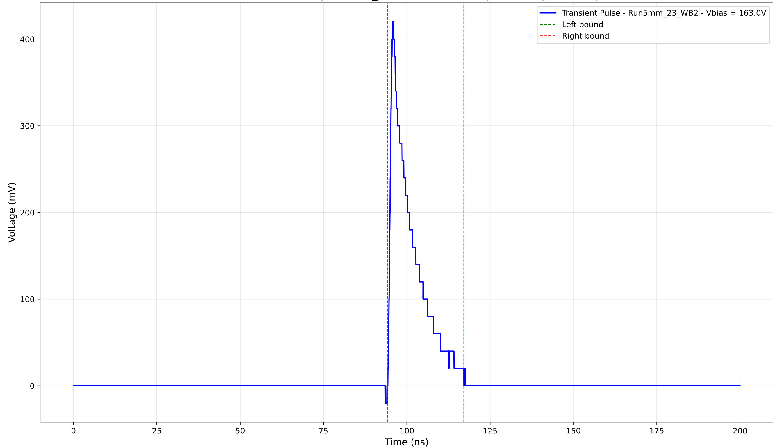
Transient Pulse - Sample: 5mm_23 - Position: 460.0 \mu\text{m} - Charge: 60.05 pC
