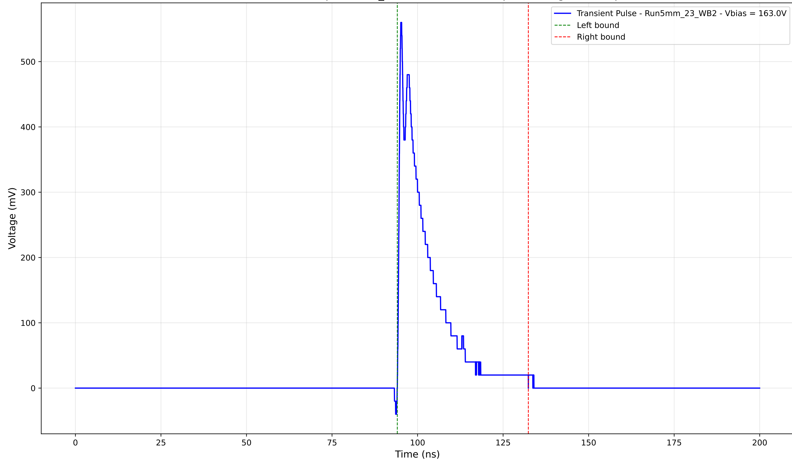
Transient Pulse - Sample: 5mm_23 - Position: 2985.0 \mu\text{m} - Charge: 95.74 pC
