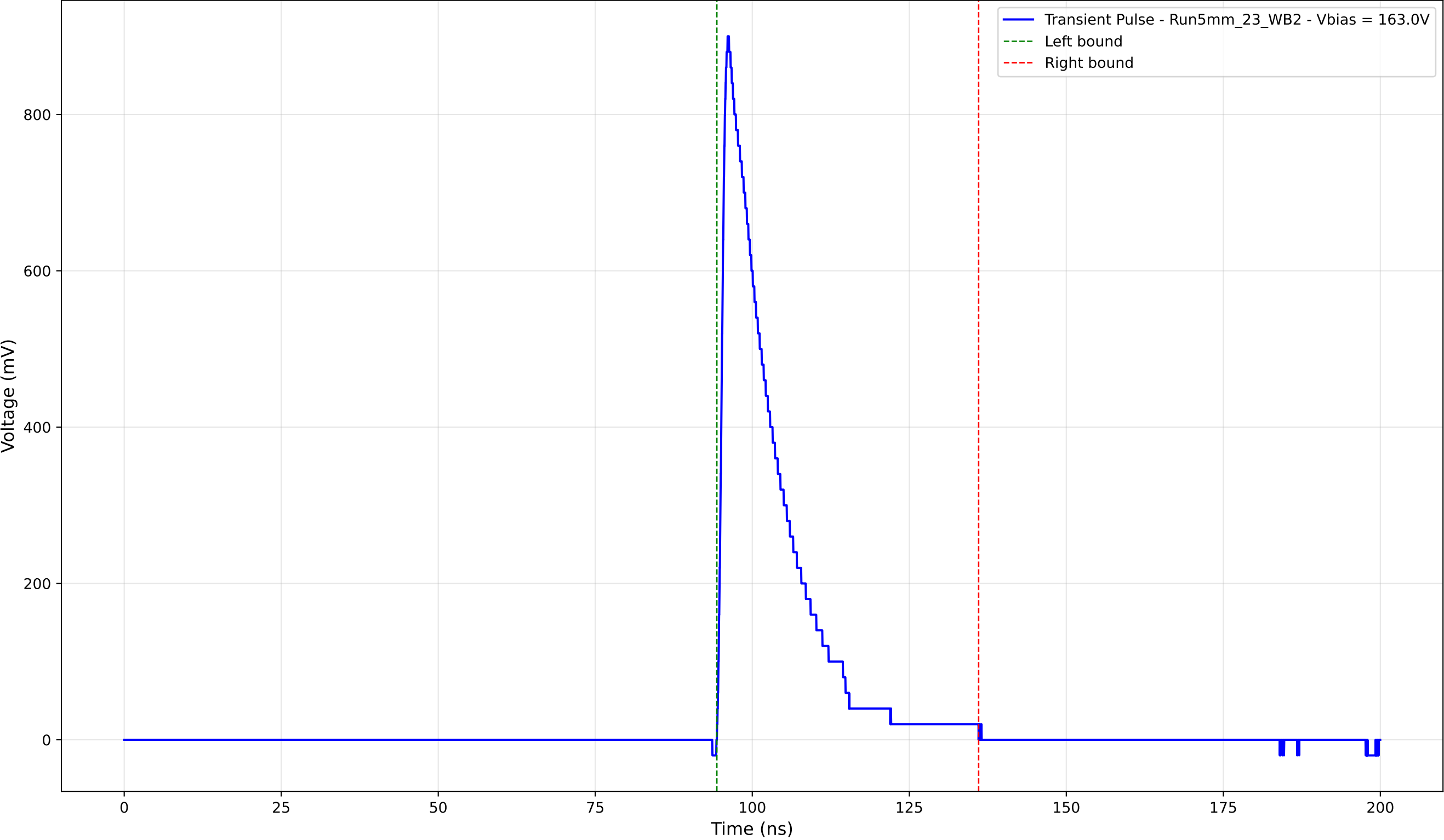
Transient Pulse - Sample: 5mm_23 - Position: 4230.0 \mu\text{m} - Charge: 164.14 pC
