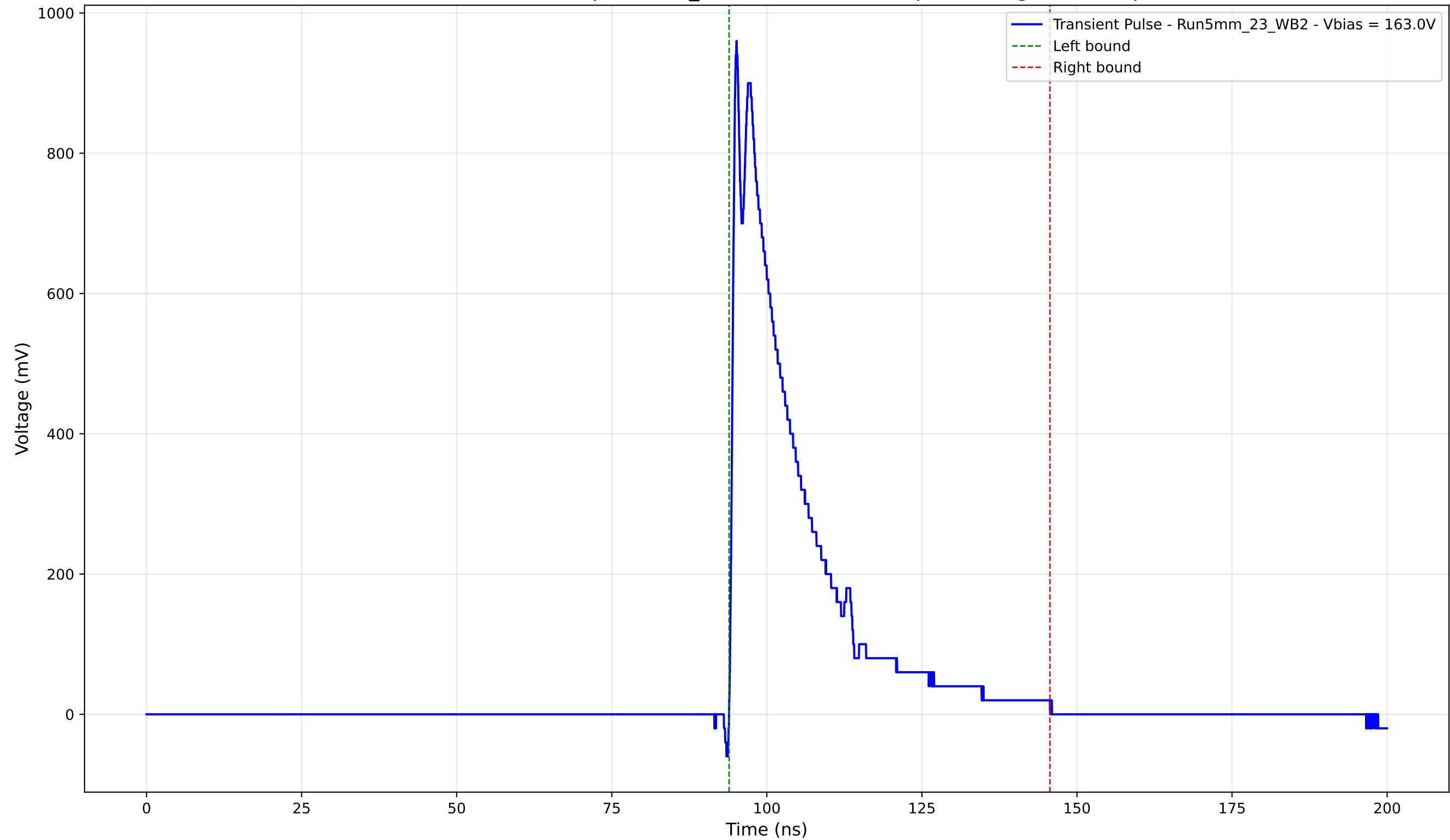
Transient Pulse - Sample: 5mm_23 - Position: 2215.0 \mu\text{m} - Charge: 205.48 pC
