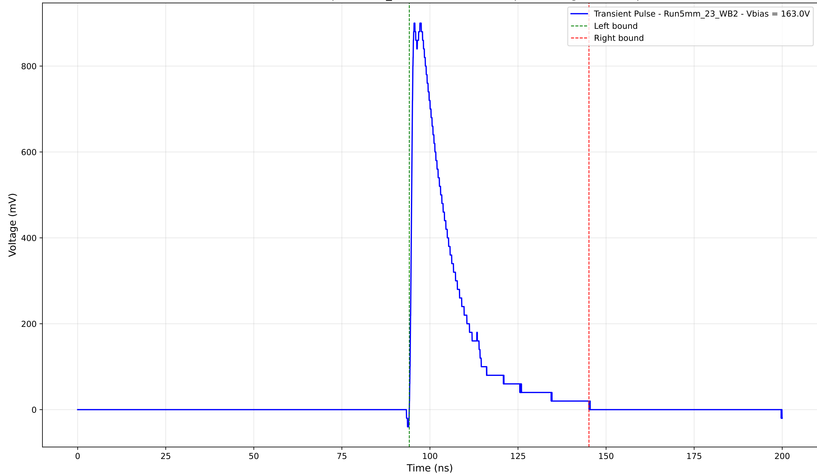
Transient Pulse - Sample: 5mm_23 - Position: 1800.0 \mu\text{m} - Charge: 217.14 pC
