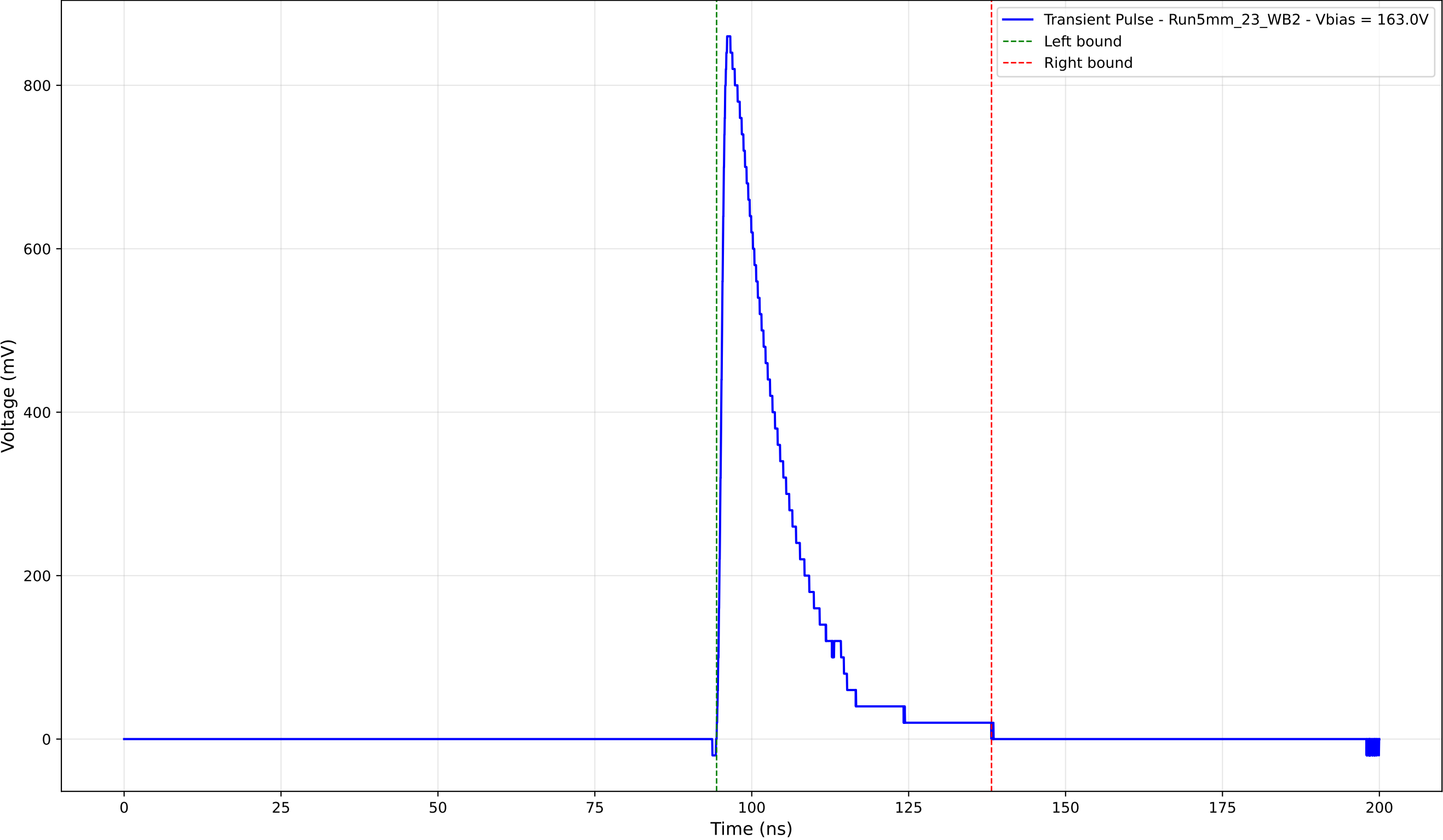
Transient Pulse - Sample: 5mm_23 - Position: 3895.0 \mu\text{m} - Charge: 171.38 pC
