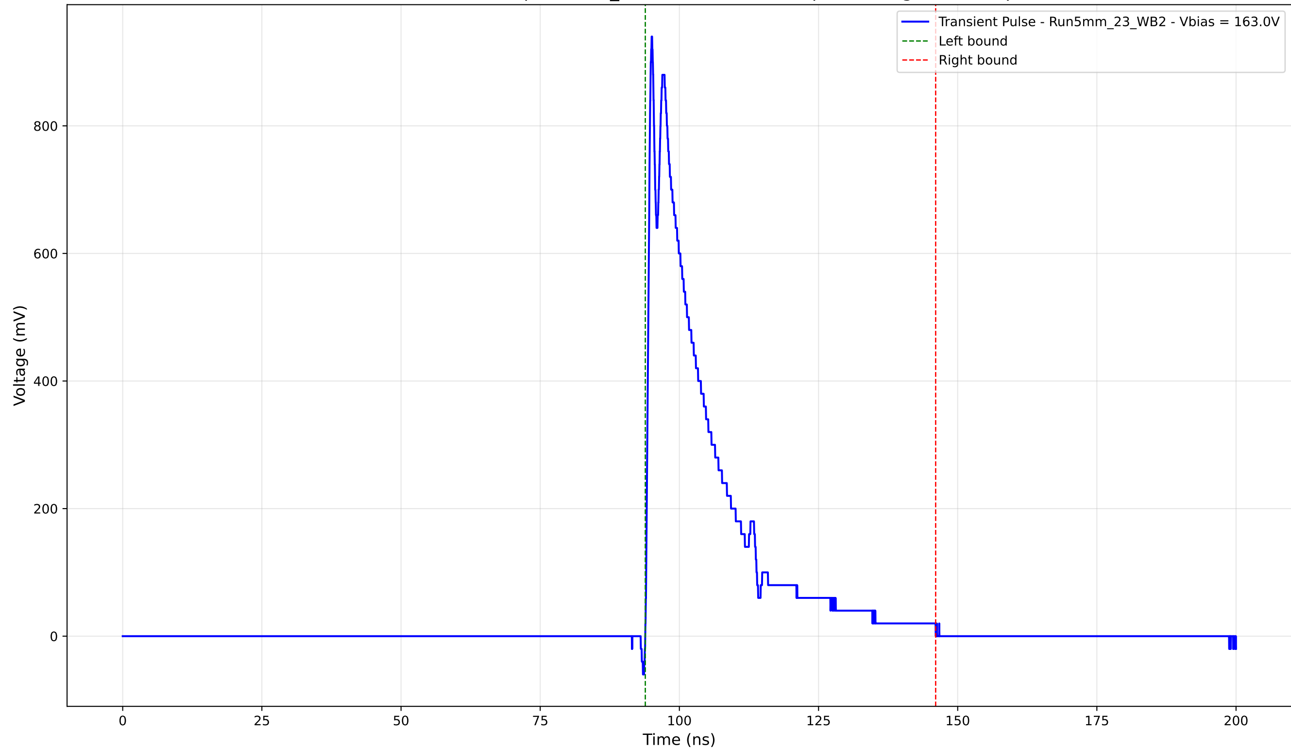
Transient Pulse - Sample: 5mm_23 - Position: 2285.0 \mu\text{m} - Charge: 200.24 pC
