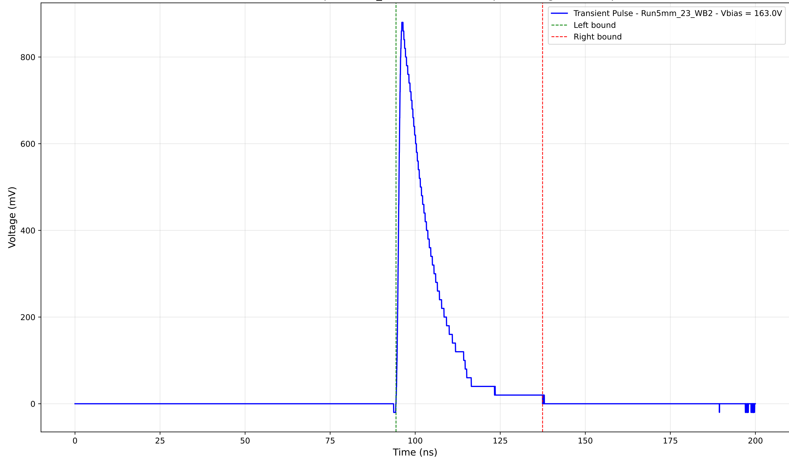
Transient Pulse - Sample: 5mm_23 - Position: 885.0 \mu\text{m} - Charge: 171.23 pC
