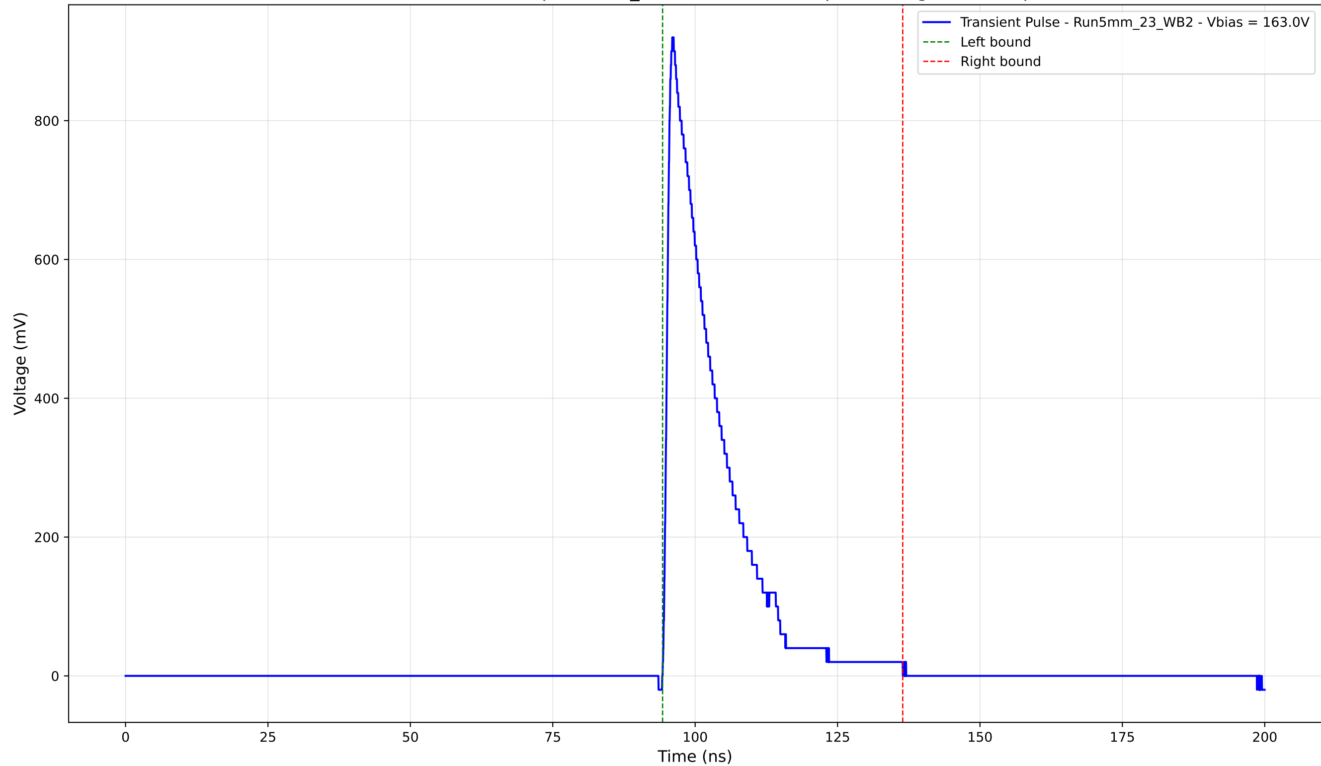
Transient Pulse - Sample: 5mm_23 - Position: 665.0 \mu\text{m} - Charge: 174.58 pC
