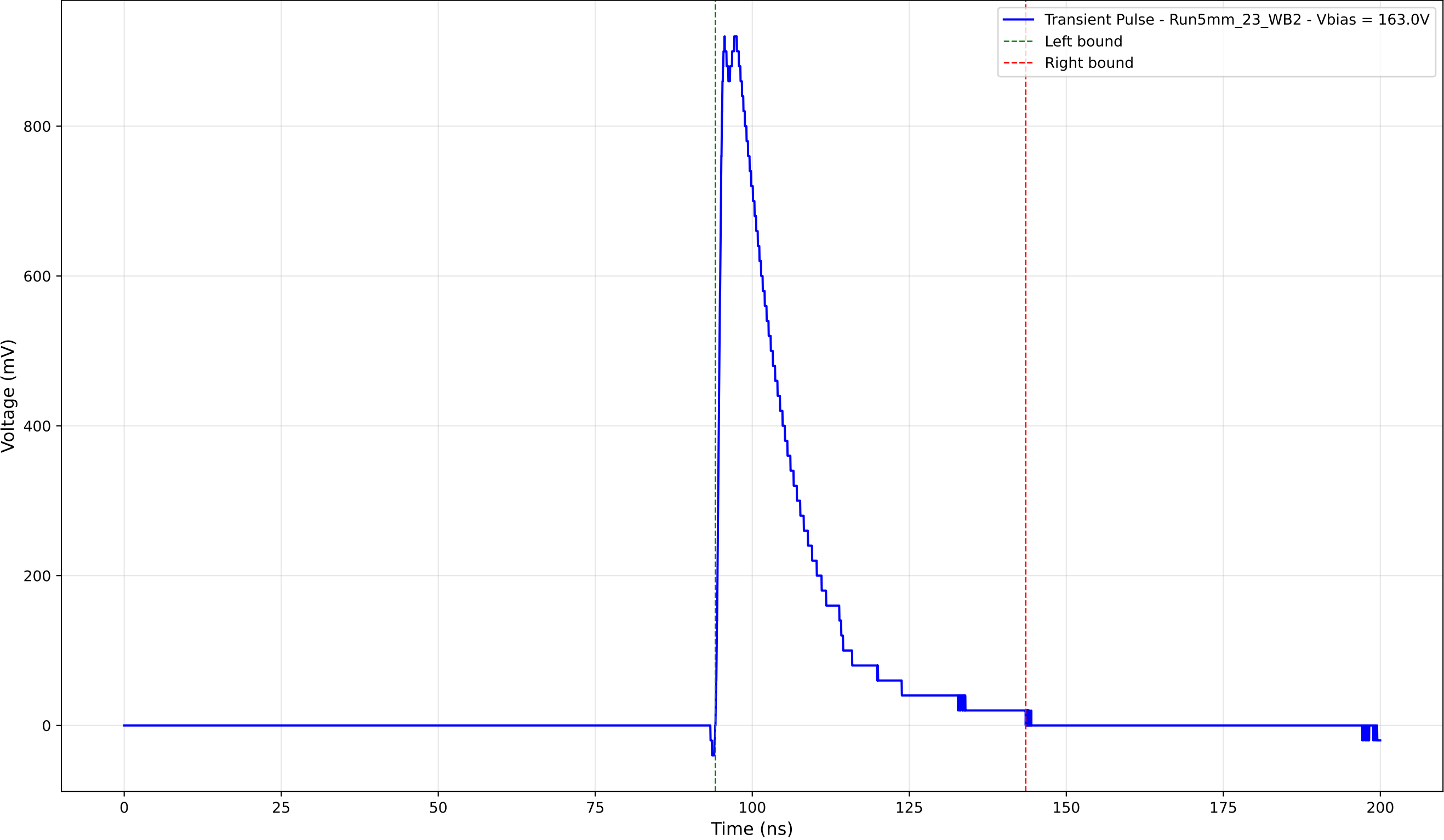
Transient Pulse - Sample: 5mm_23 - Position: 3230.0 \mu\text{m} - Charge: 215.30 pC
