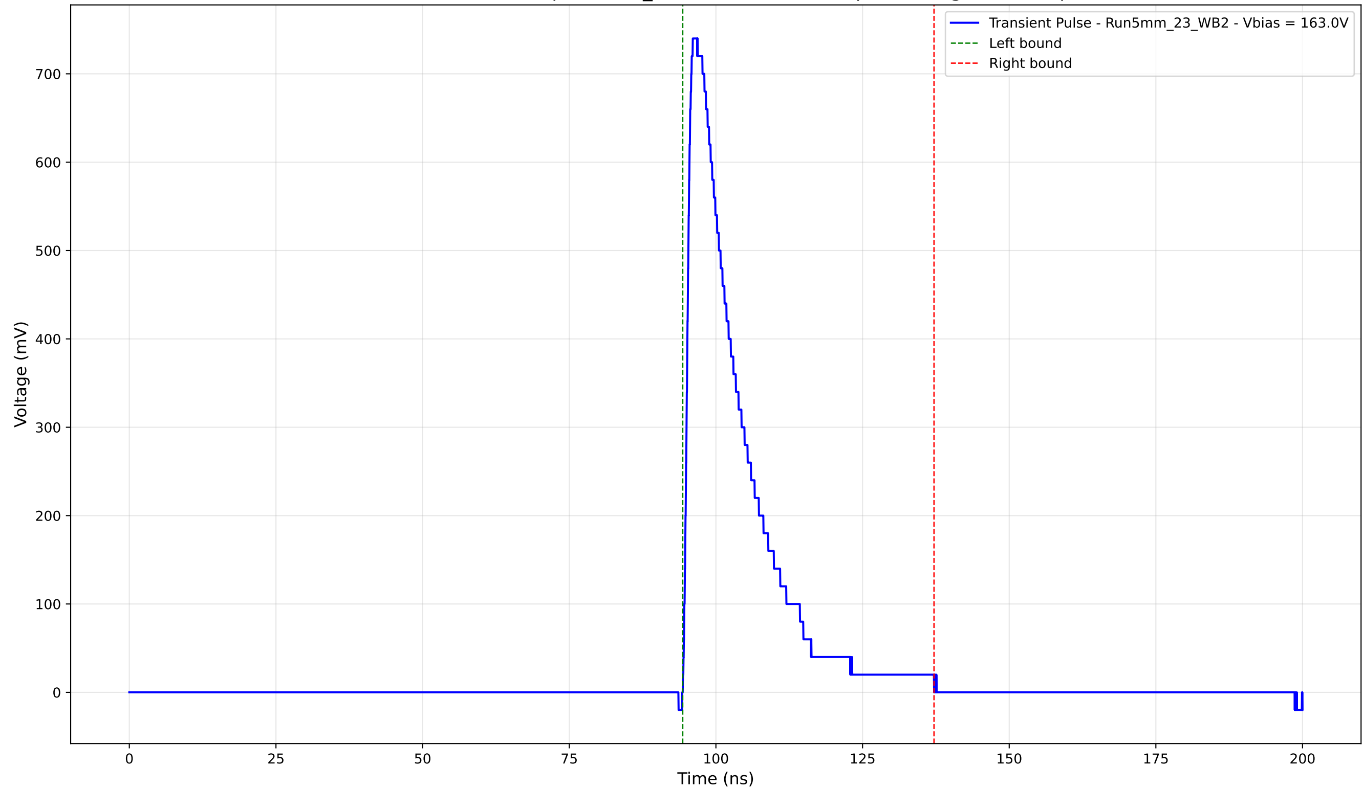
Transient Pulse - Sample: 5mm_23 - Position: 3605.0 \mu\text{m} - Charge: 151.07 pC
