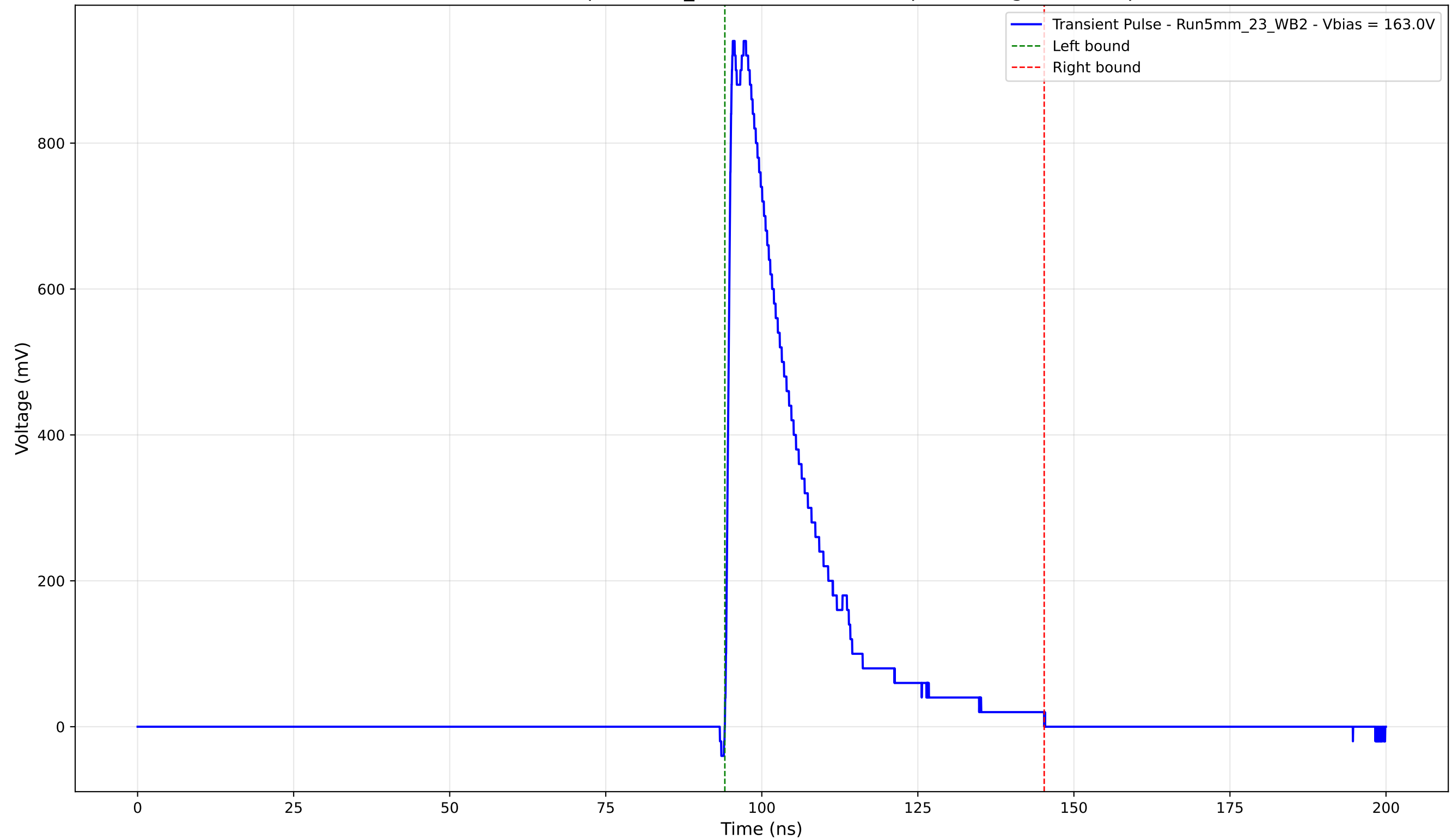
Transient Pulse - Sample: 5mm_23 - Position: 3155.0 \mu\text{m} - Charge: 225.34 pC
