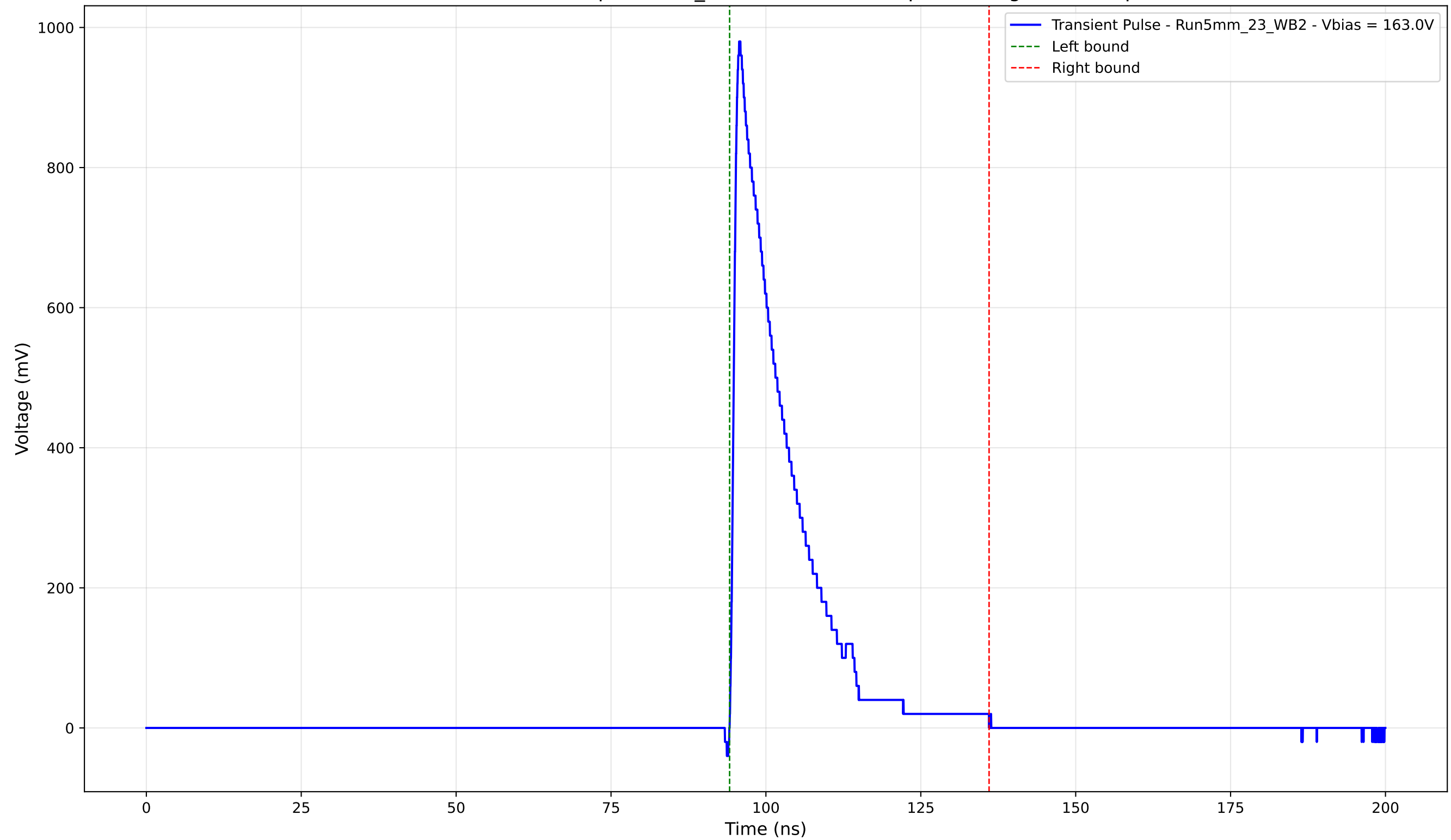
Transient Pulse - Sample: 5mm_23 - Position: 390.0 \mu\text{m} - Charge: 177.81 pC
