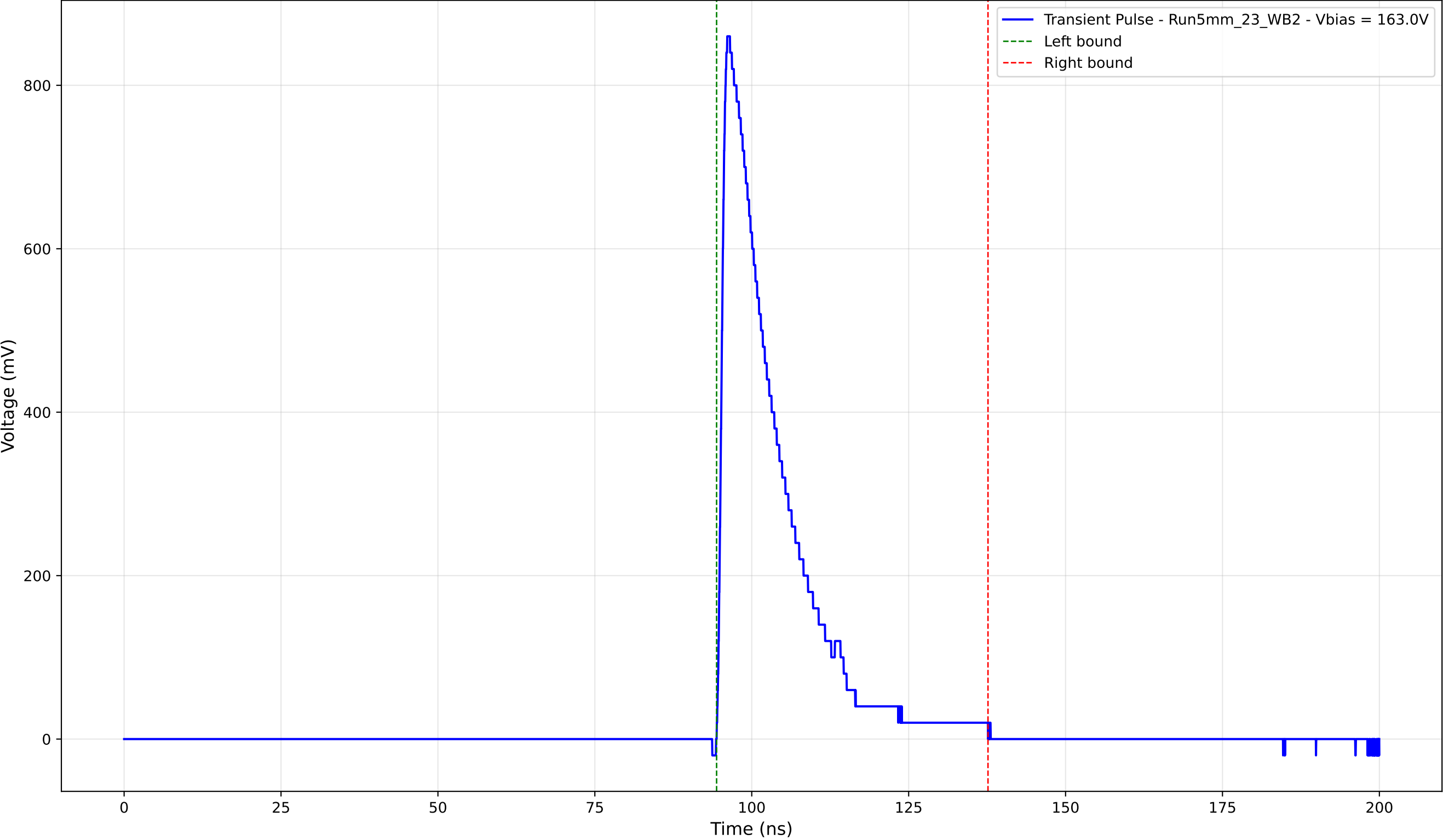
Transient Pulse - Sample: 5mm_23 - Position: 3915.0 \mu\text{m} - Charge: 168.75 pC
