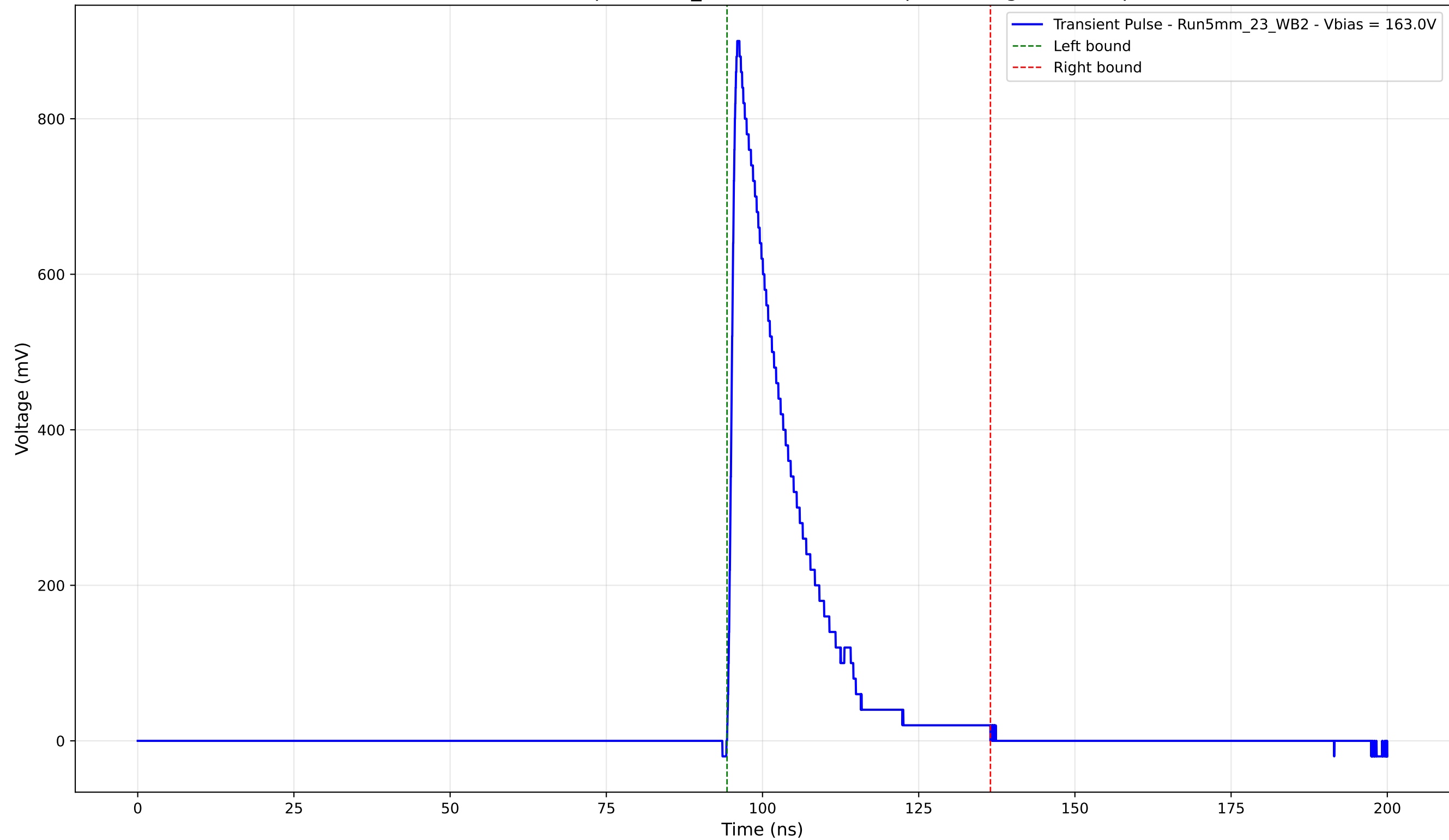
Transient Pulse - Sample: 5mm_23 - Position: 705.0 \mu\text{m} - Charge: 171.21 pC
