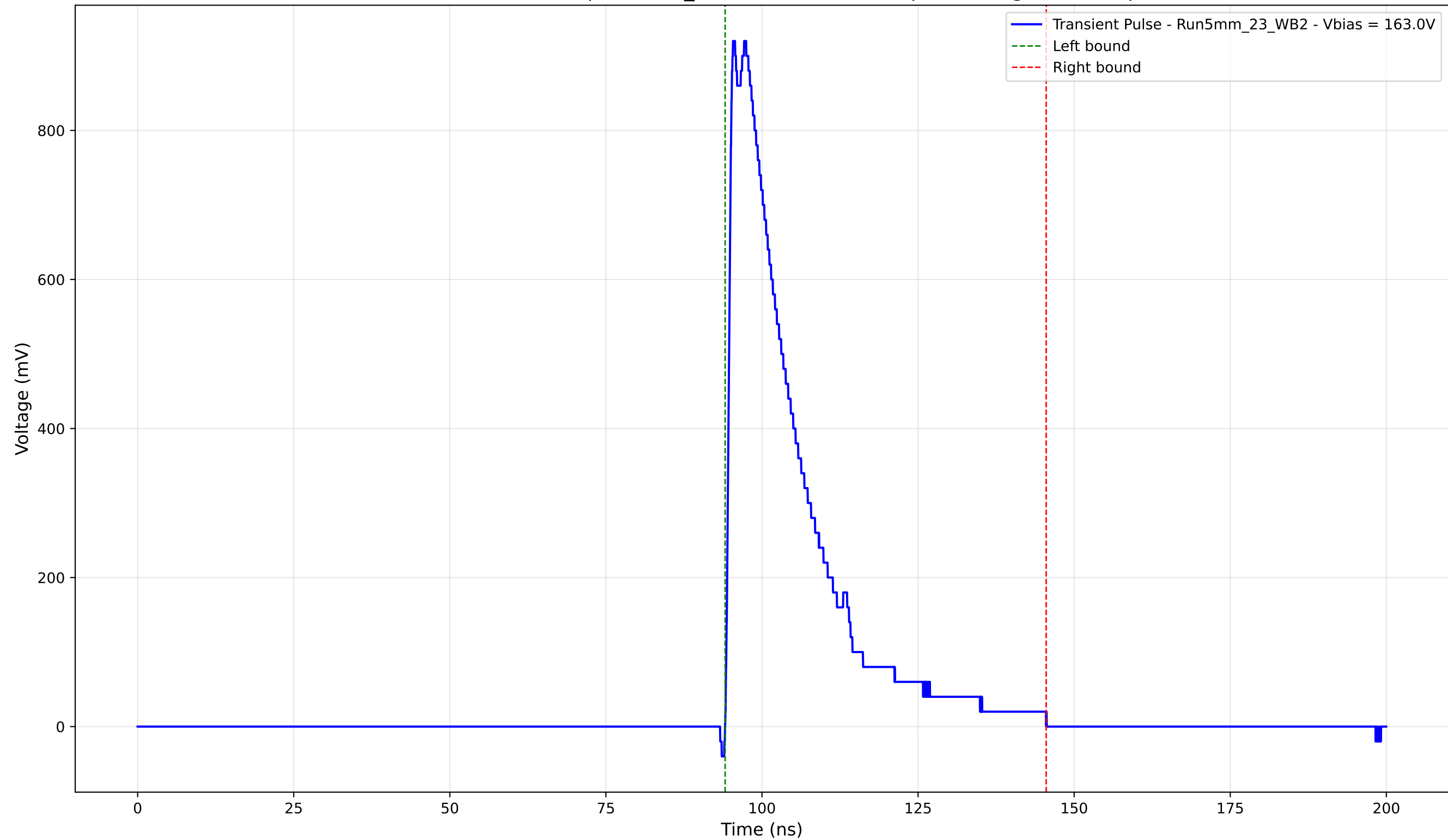
Transient Pulse - Sample: 5mm_23 - Position: 1875.0 \mu\text{m} - Charge: 221.46 pC
