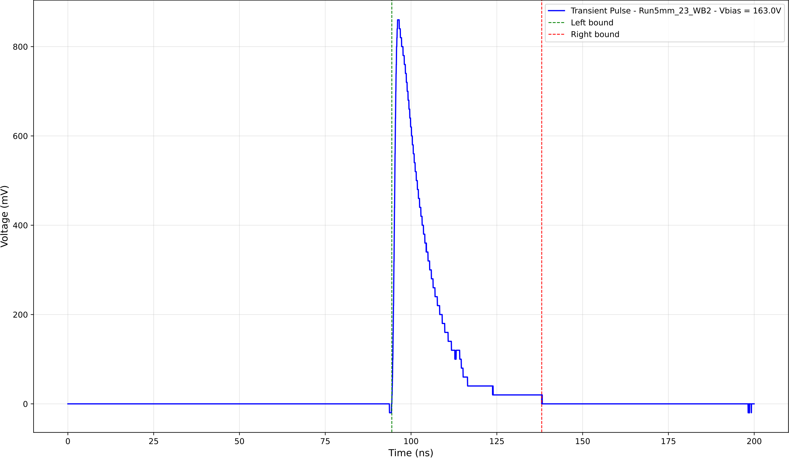
Transient Pulse - Sample: 5mm_23 - Position: 3905.0 \mu\text{m} - Charge: 170.17 pC
