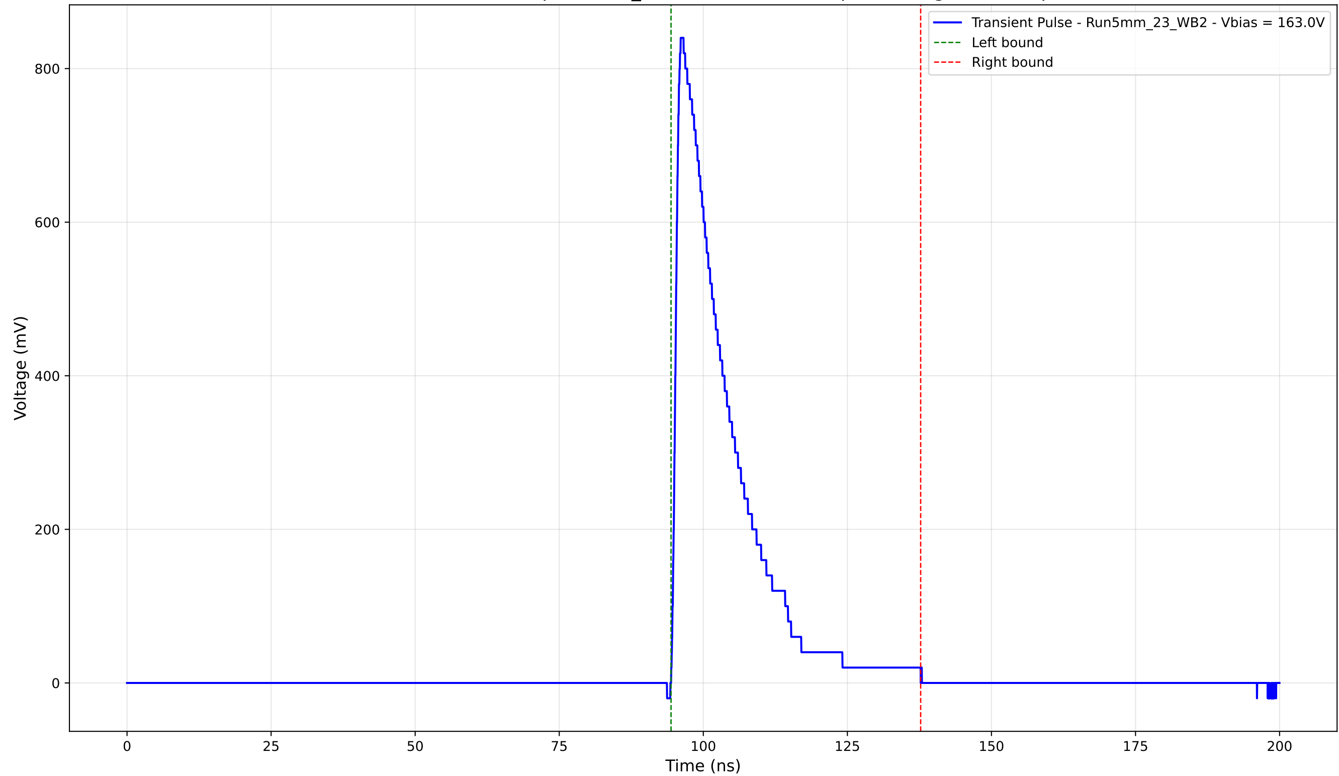
Transient Pulse - Sample: 5mm_23 - Position: 1080.0 \mu\text{m} - Charge: 169.50 pC
