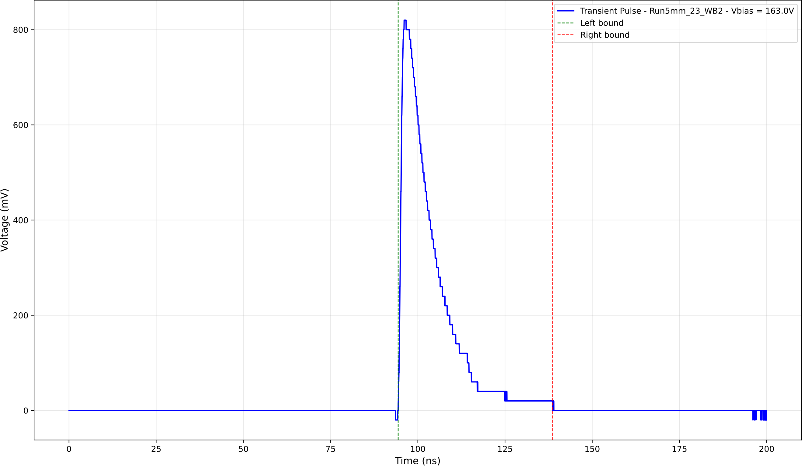
Transient Pulse - Sample: 5mm_23 - Position: 3640.0 \mu\text{m} - Charge: 170.98 pC
