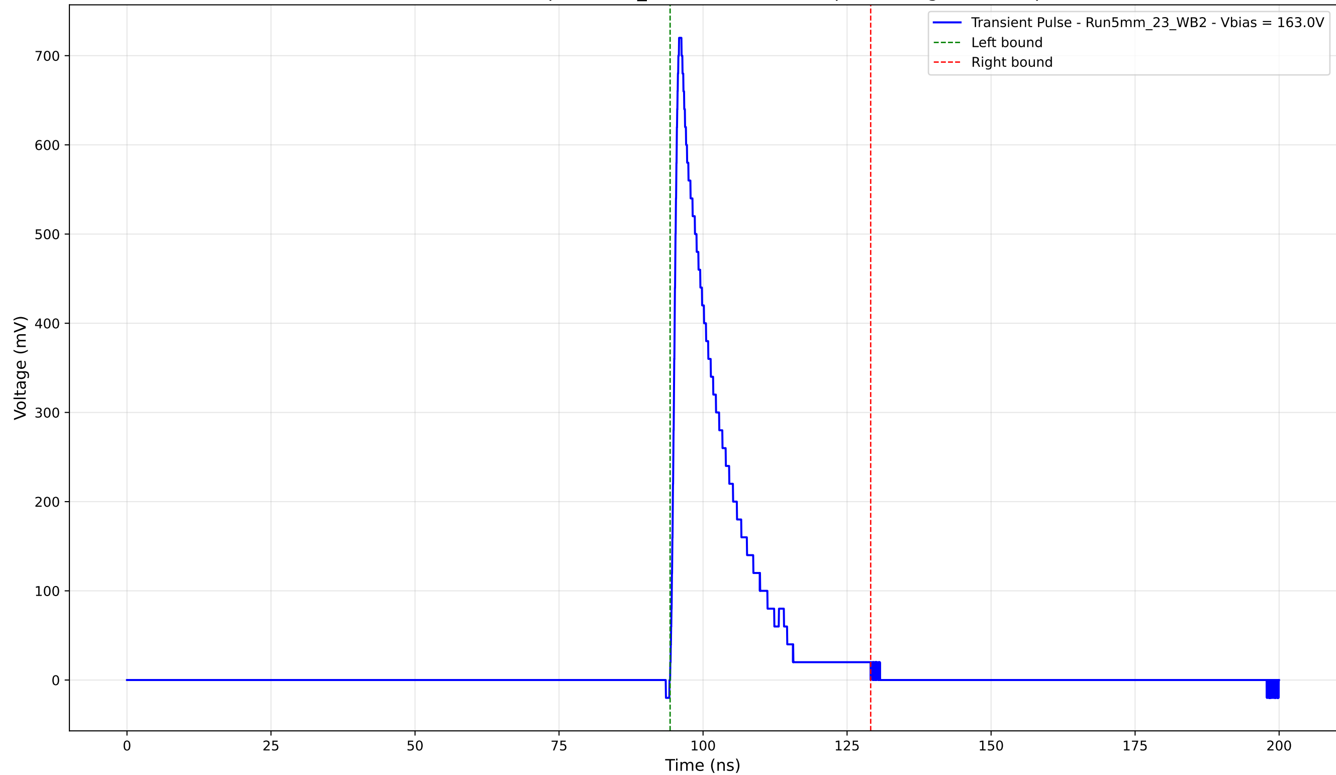
Transient Pulse - Sample: 5mm_23 - Position: 540.0 \mu\text{m} - Charge: 117.93 pC
