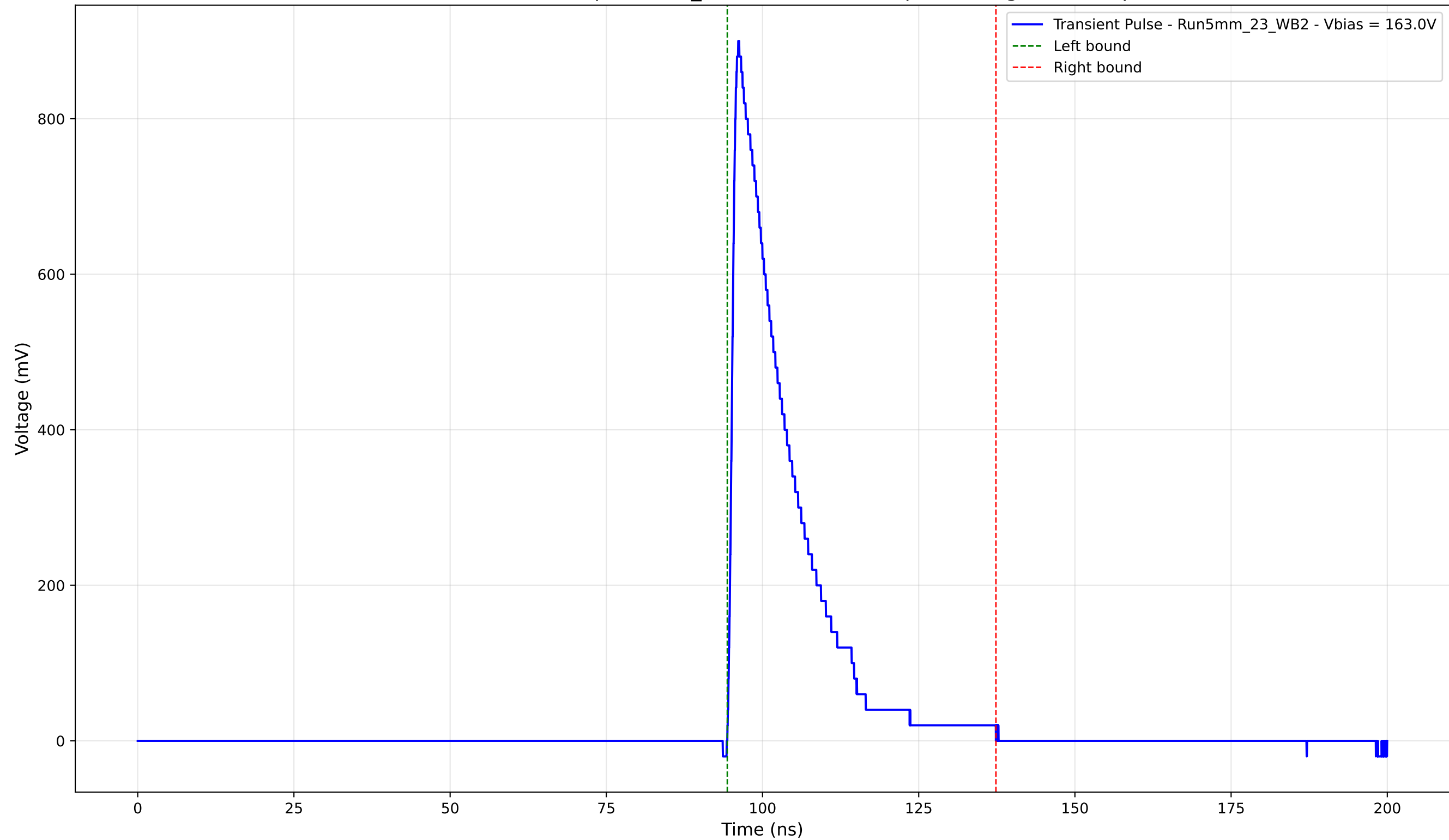
Transient Pulse - Sample: 5mm_23 - Position: 820.0 \mu\text{m} - Charge: 174.83 pC
