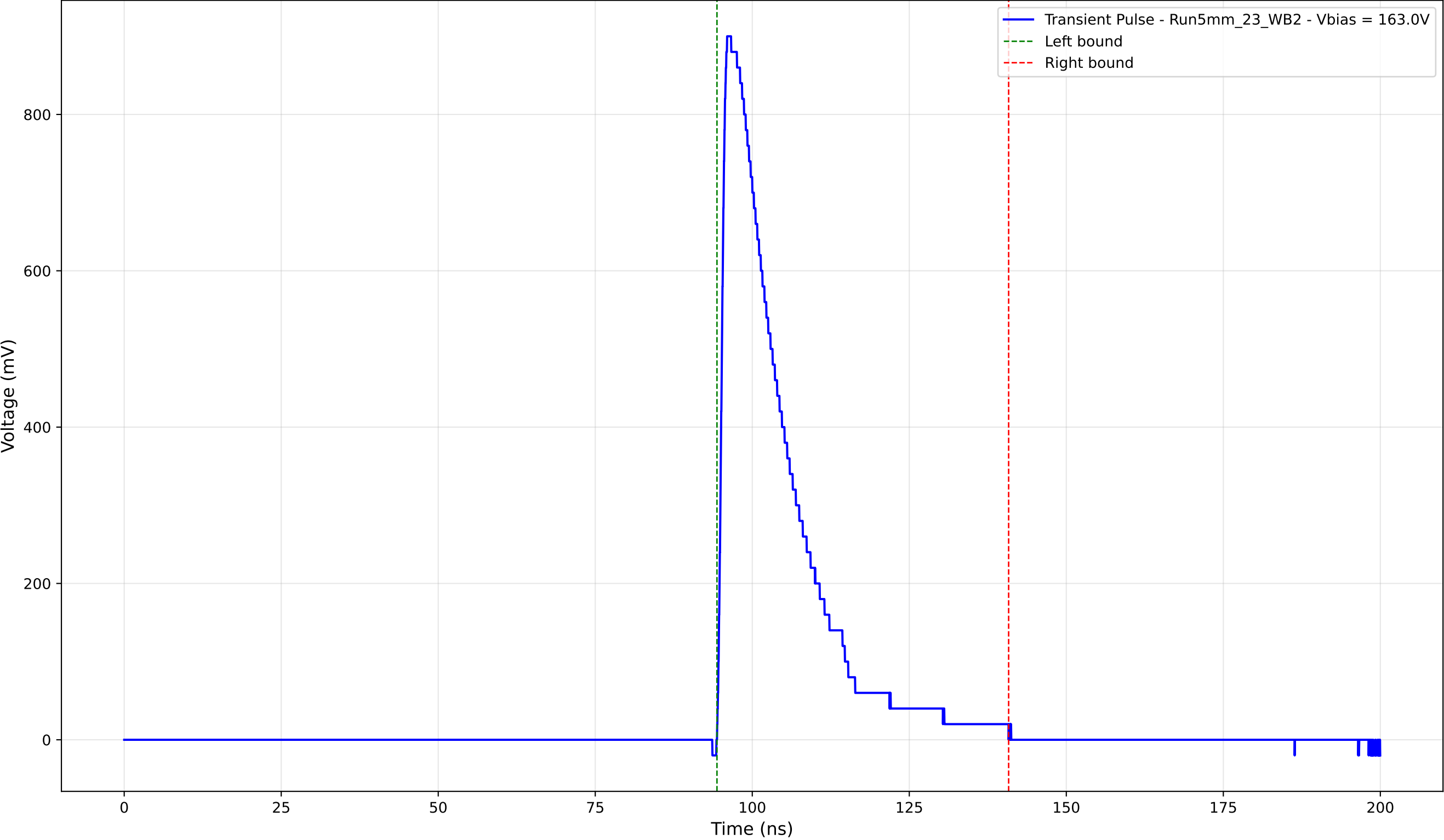
Transient Pulse - Sample: 5mm_23 - Position: 1285.0 \mu\text{m} - Charge: 201.22 pC
