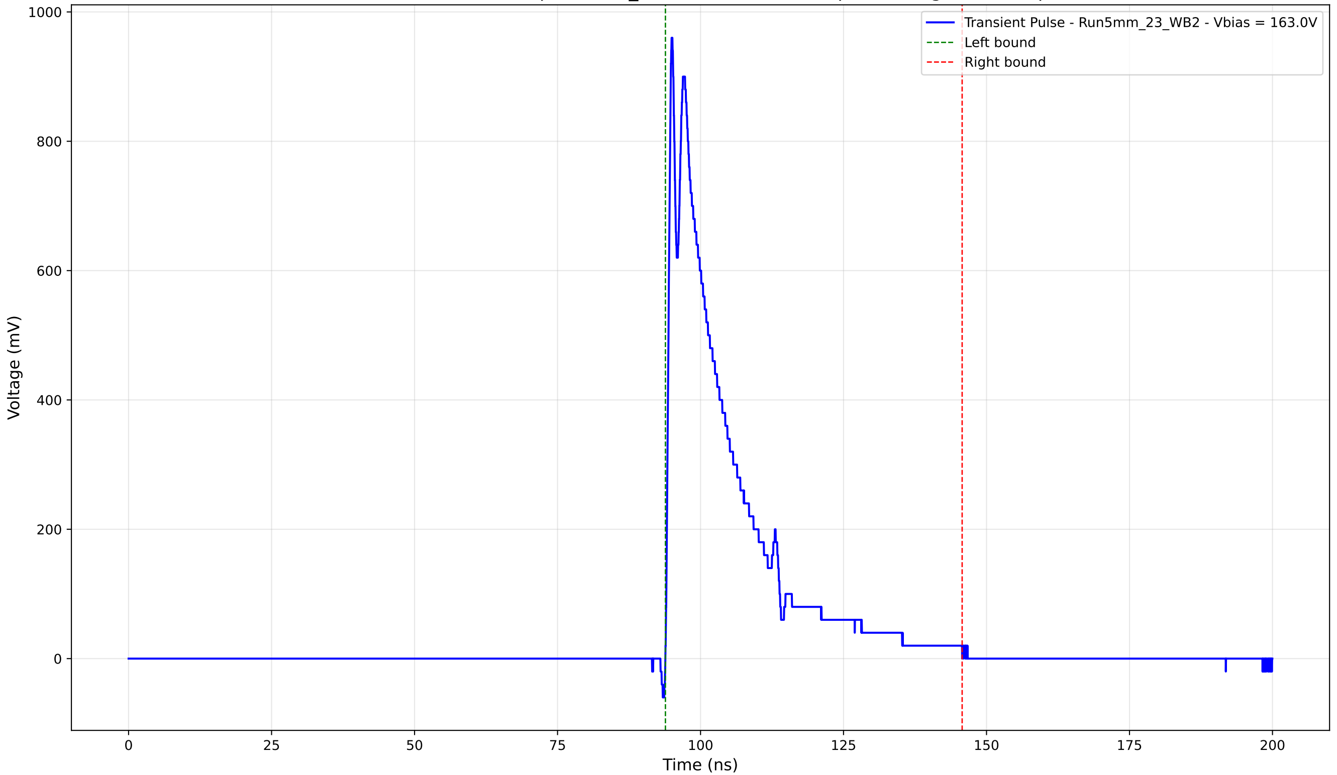
Transient Pulse - Sample: 5mm_23 - Position: 2330.0 \mu\text{m} - Charge: 200.79 pC
