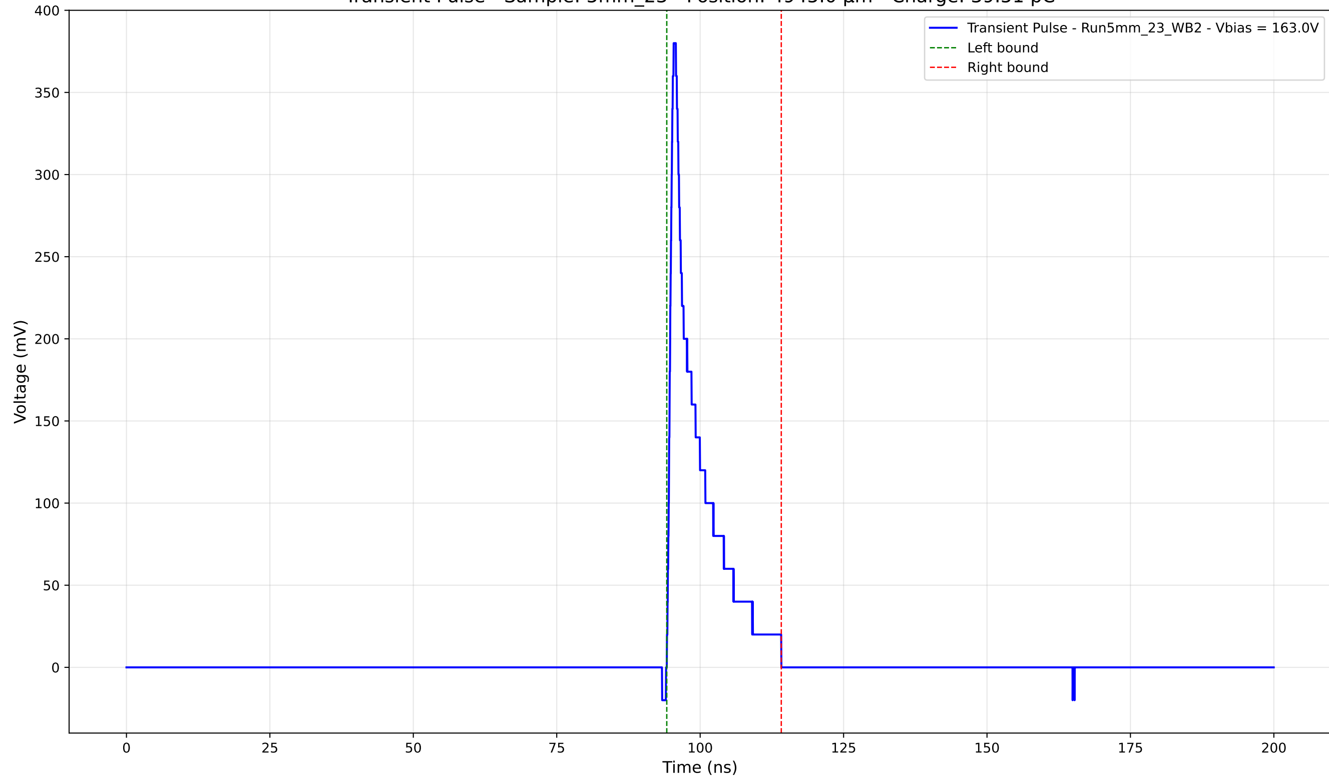
Transient Pulse - Sample: 5mm_23 - Position: 4945.0 \mu\text{m} - Charge: 39.51 pC
