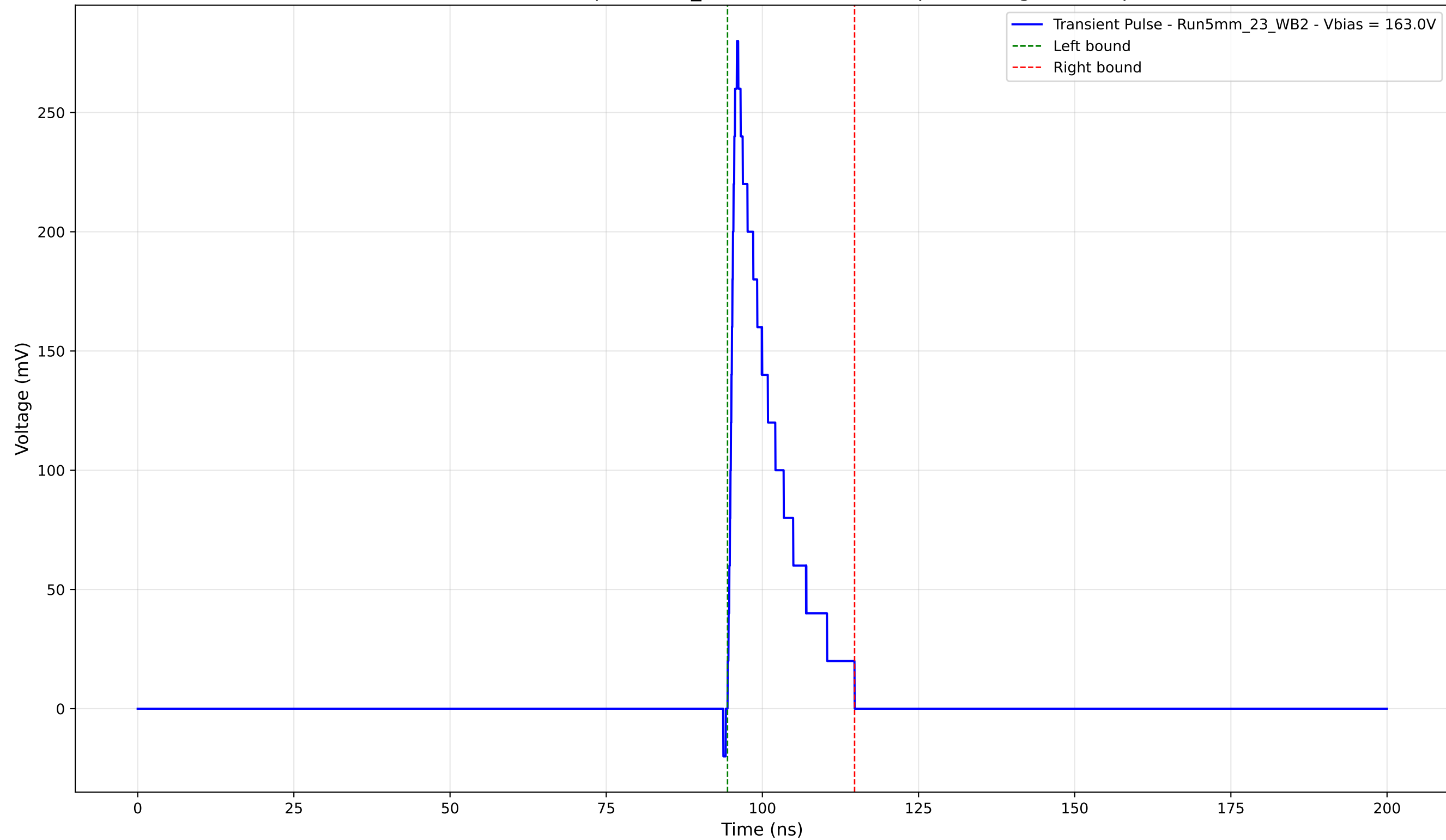
Transient Pulse - Sample: 5mm_23 - Position: 4520.0 \mu\text{m} - Charge: 38.74 pC
