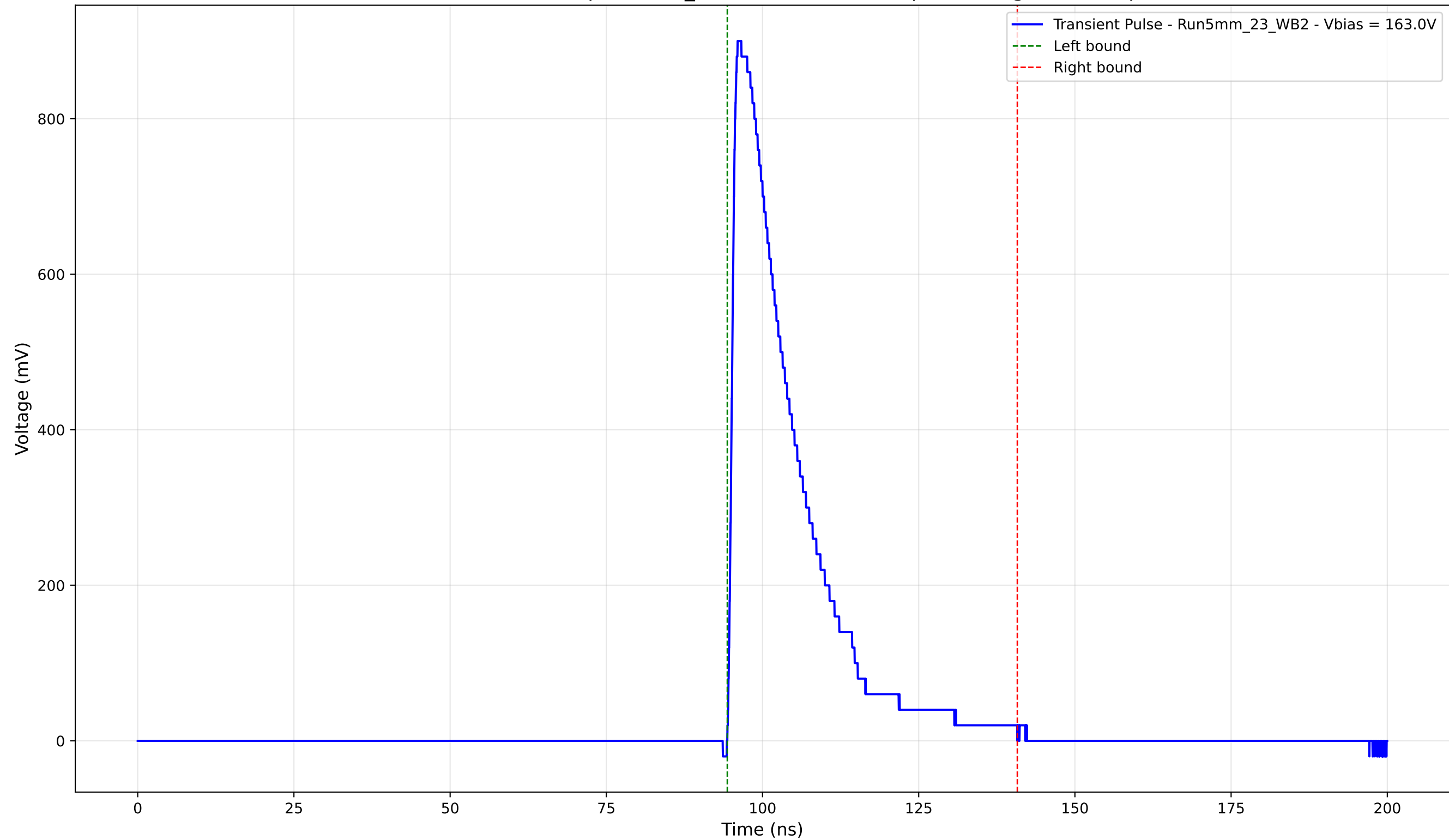
Transient Pulse - Sample: 5mm_23 - Position: 1305.0 \mu\text{m} - Charge: 201.33 pC
