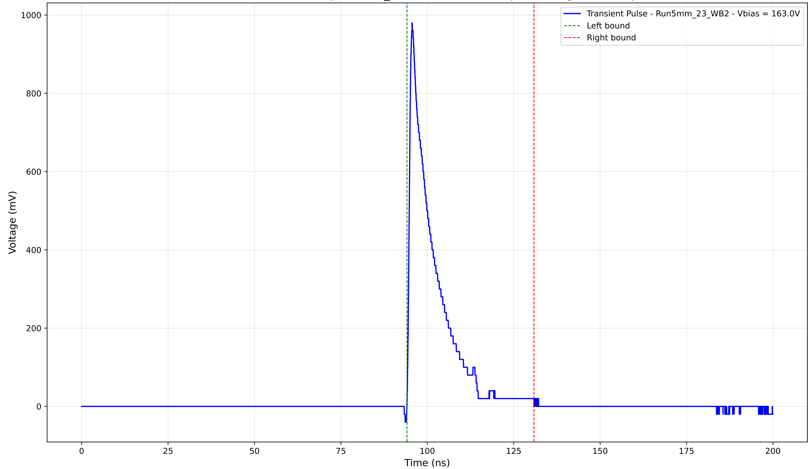
Transient Pulse - Sample: 5mm_23 - Position: 4785.0 \mu\text{m} - Charge: 146.81 pC
