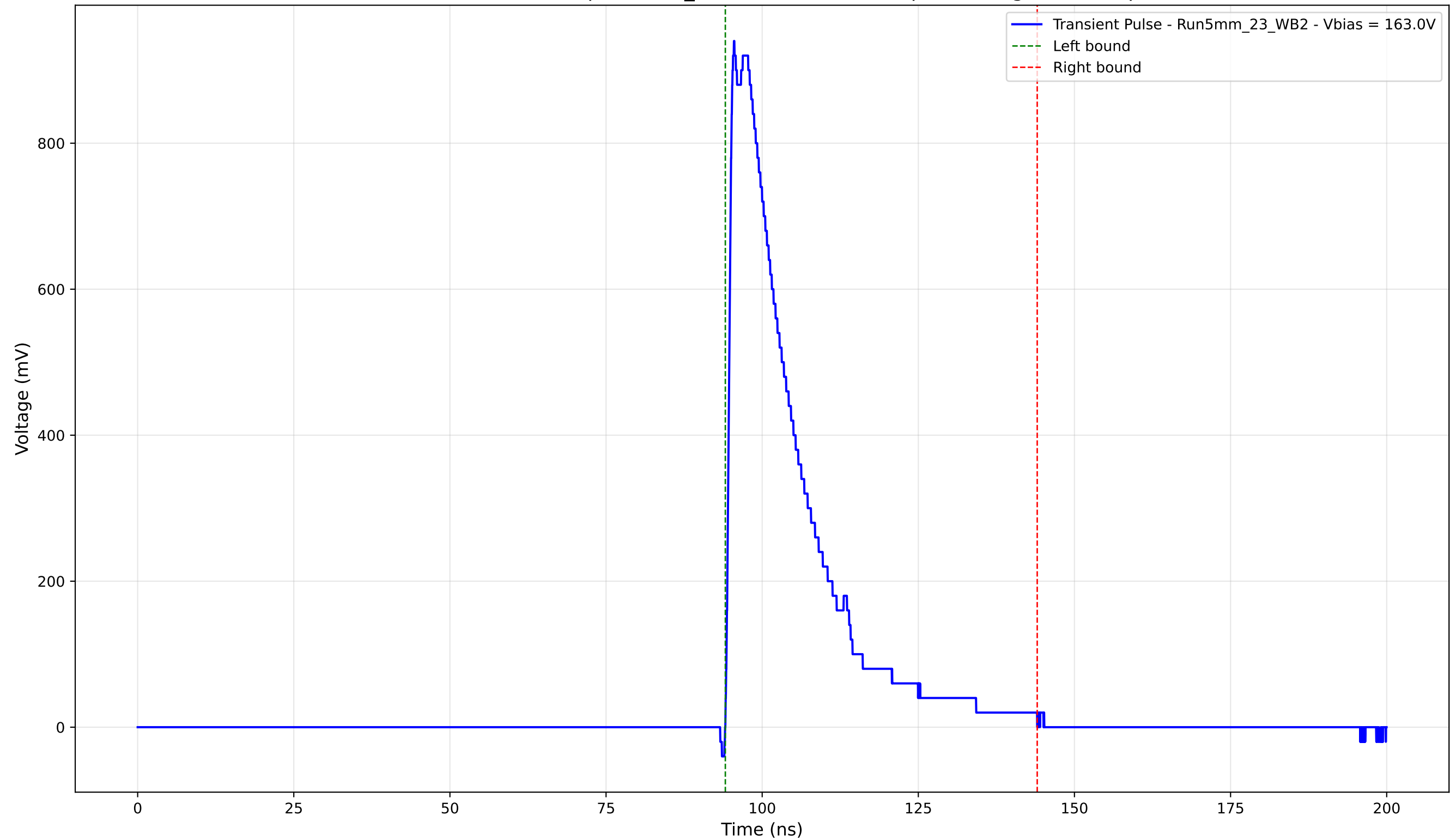
Transient Pulse - Sample: 5mm_23 - Position: 3175.0 \mu\text{m} - Charge: 221.30 pC
