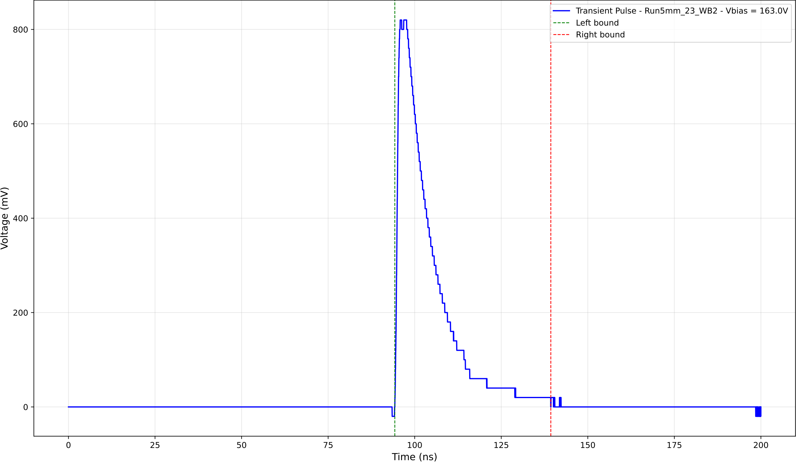
Transient Pulse - Sample: 5mm_23 - Position: 3420.0 \mu\text{m} - Charge: 180.01 pC
