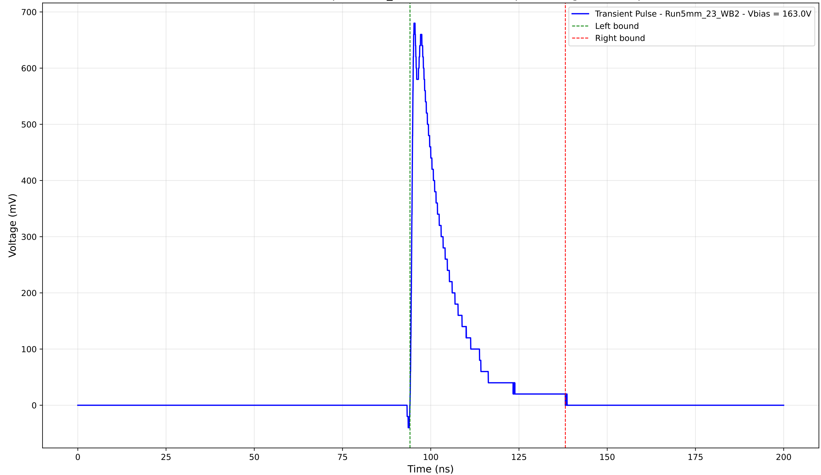
Transient Pulse - Sample: 5mm_23 - Position: 1955.0 \mu\text{m} - Charge: 137.12 pC
