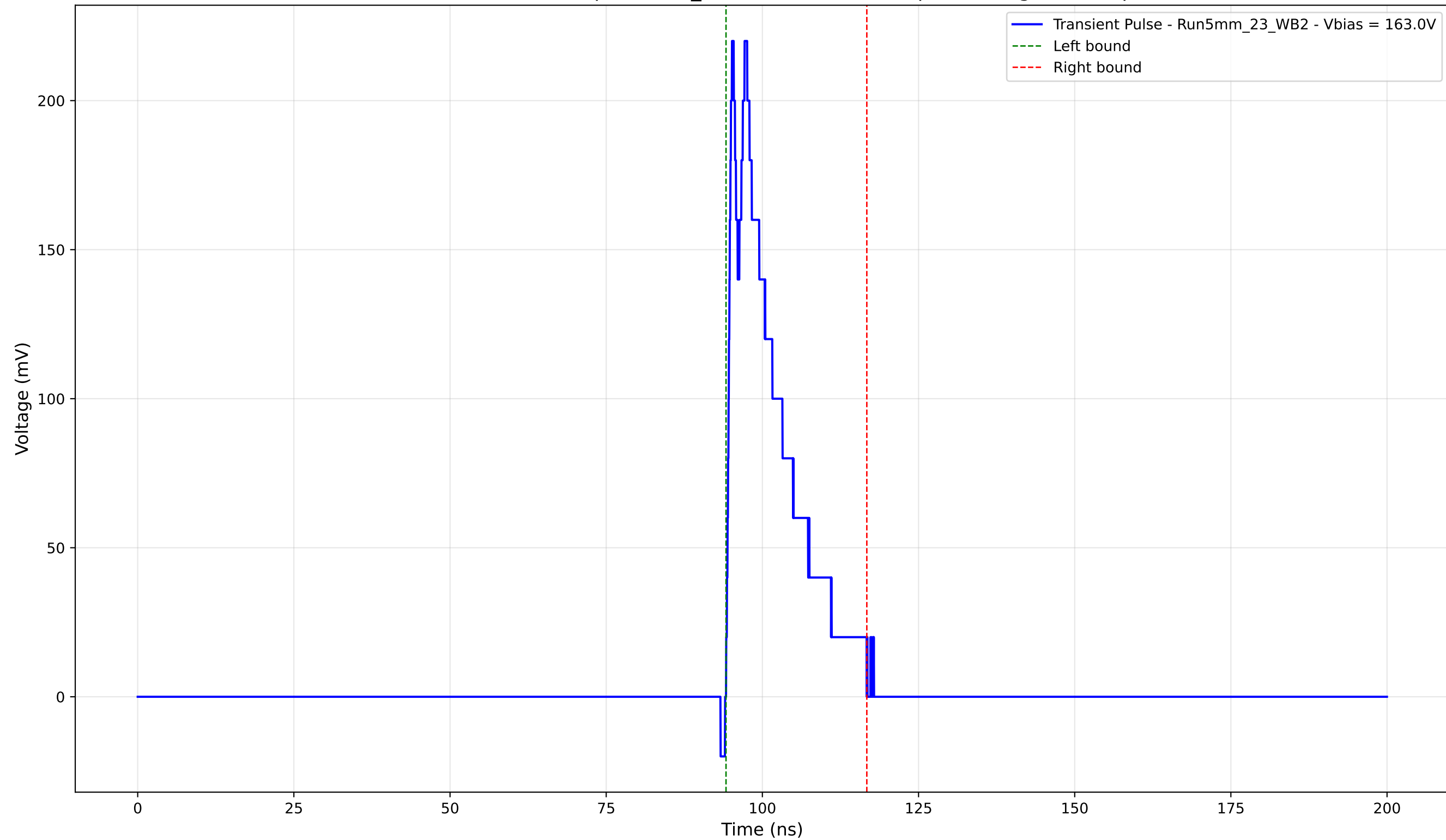
Transient Pulse - Sample: 5mm_23 - Position: 2020.0 \mu\text{m} - Charge: 37.38 pC
