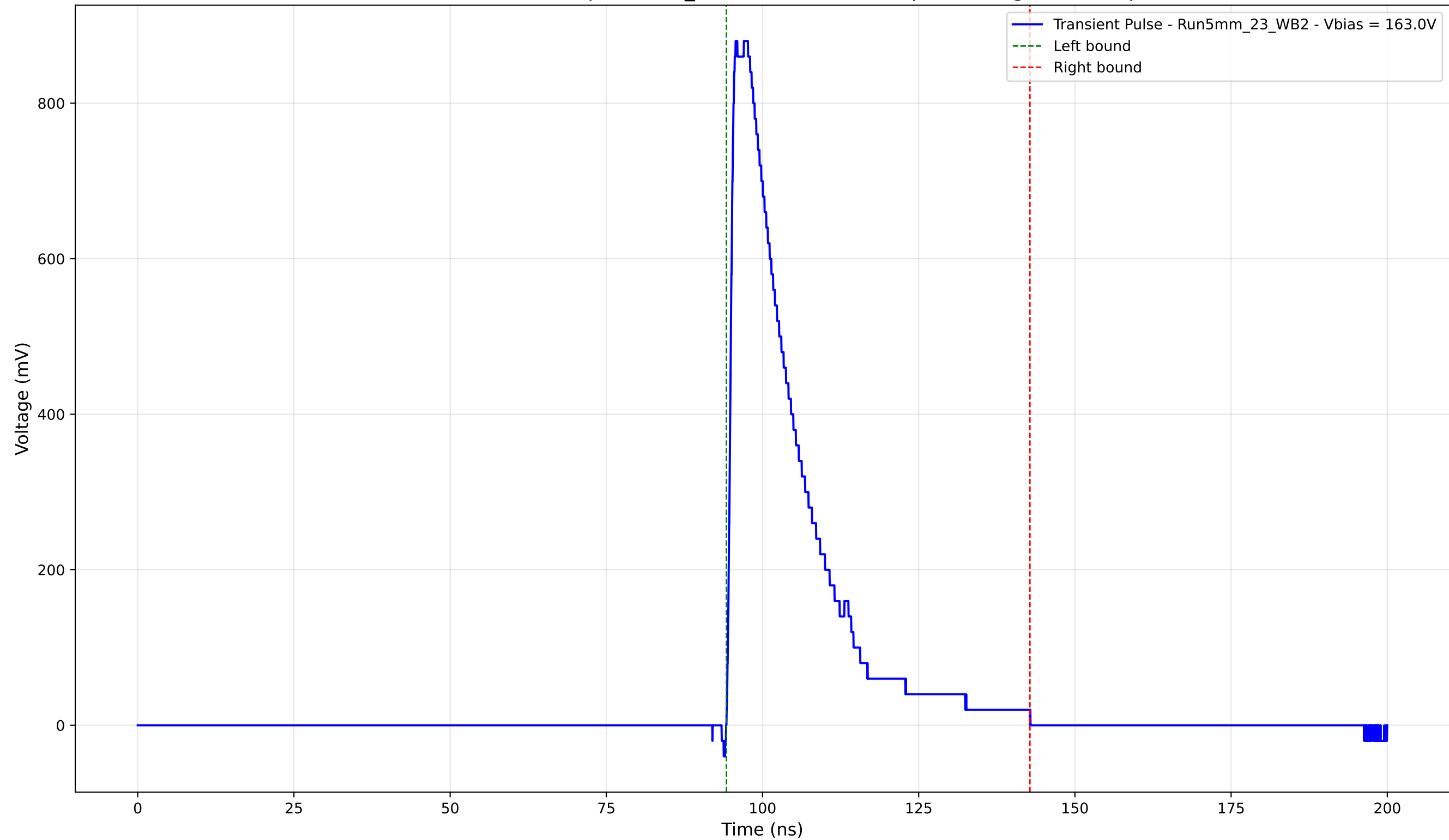
Transient Pulse - Sample: 5mm_23 - Position: 1670.0 \mu\text{m} - Charge: 204.50 pC
