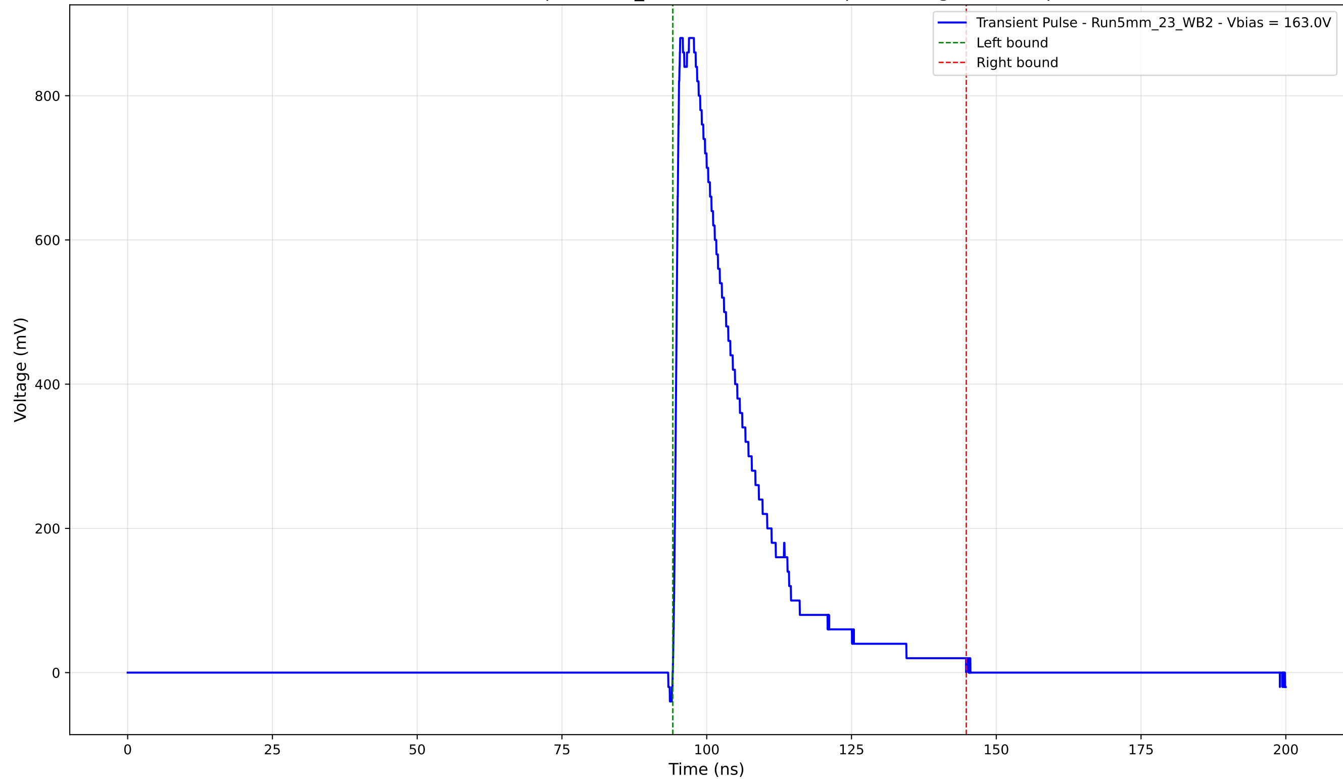
Transient Pulse - Sample: 5mm_23 - Position: 1795.0 \mu\text{m} - Charge: 215.54 pC
