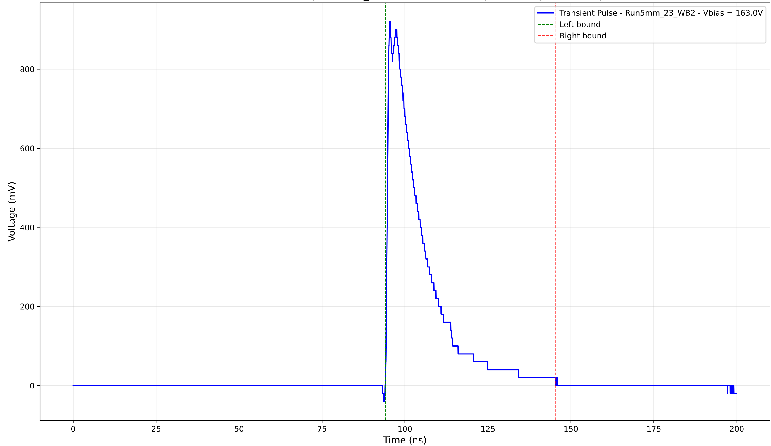
Transient Pulse - Sample: 5mm_23 - Position: 1910.0 \mu\text{m} - Charge: 213.03 pC
