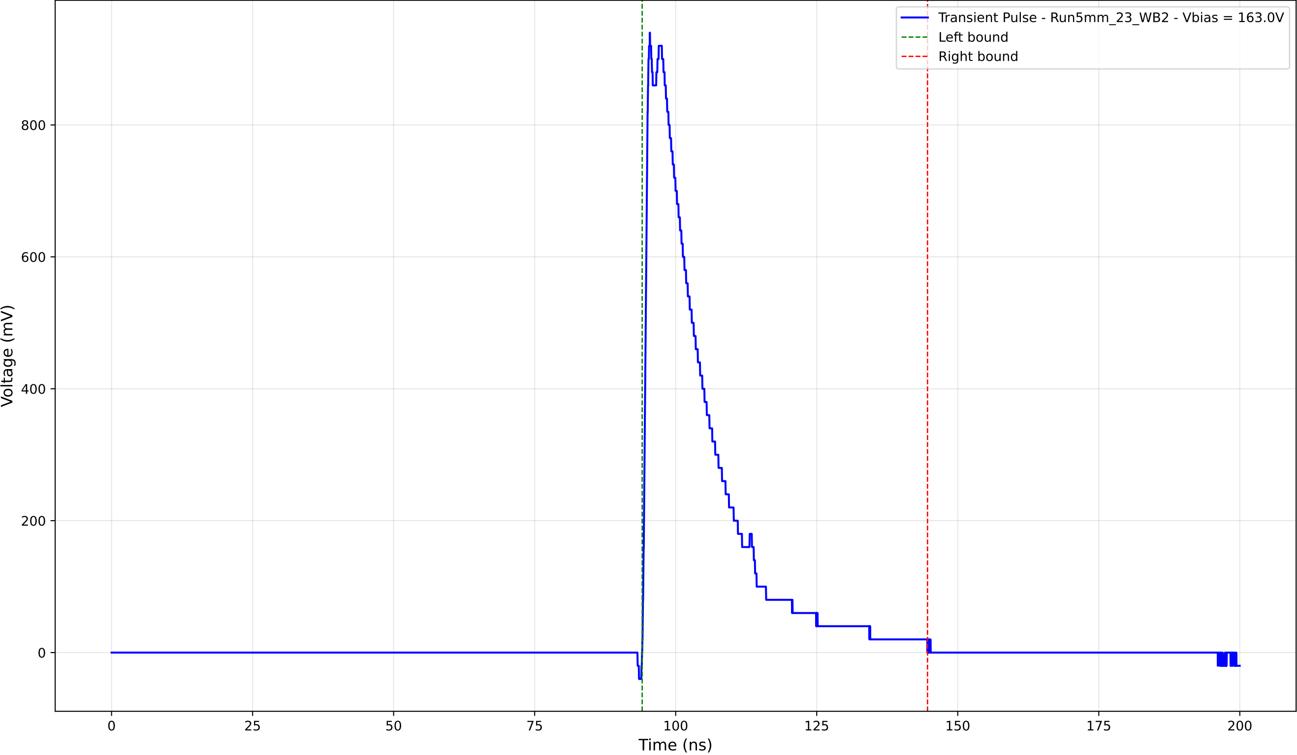
Transient Pulse - Sample: 5mm_23 - Position: 3115.0 \mu\text{m} - Charge: 217.65 pC
