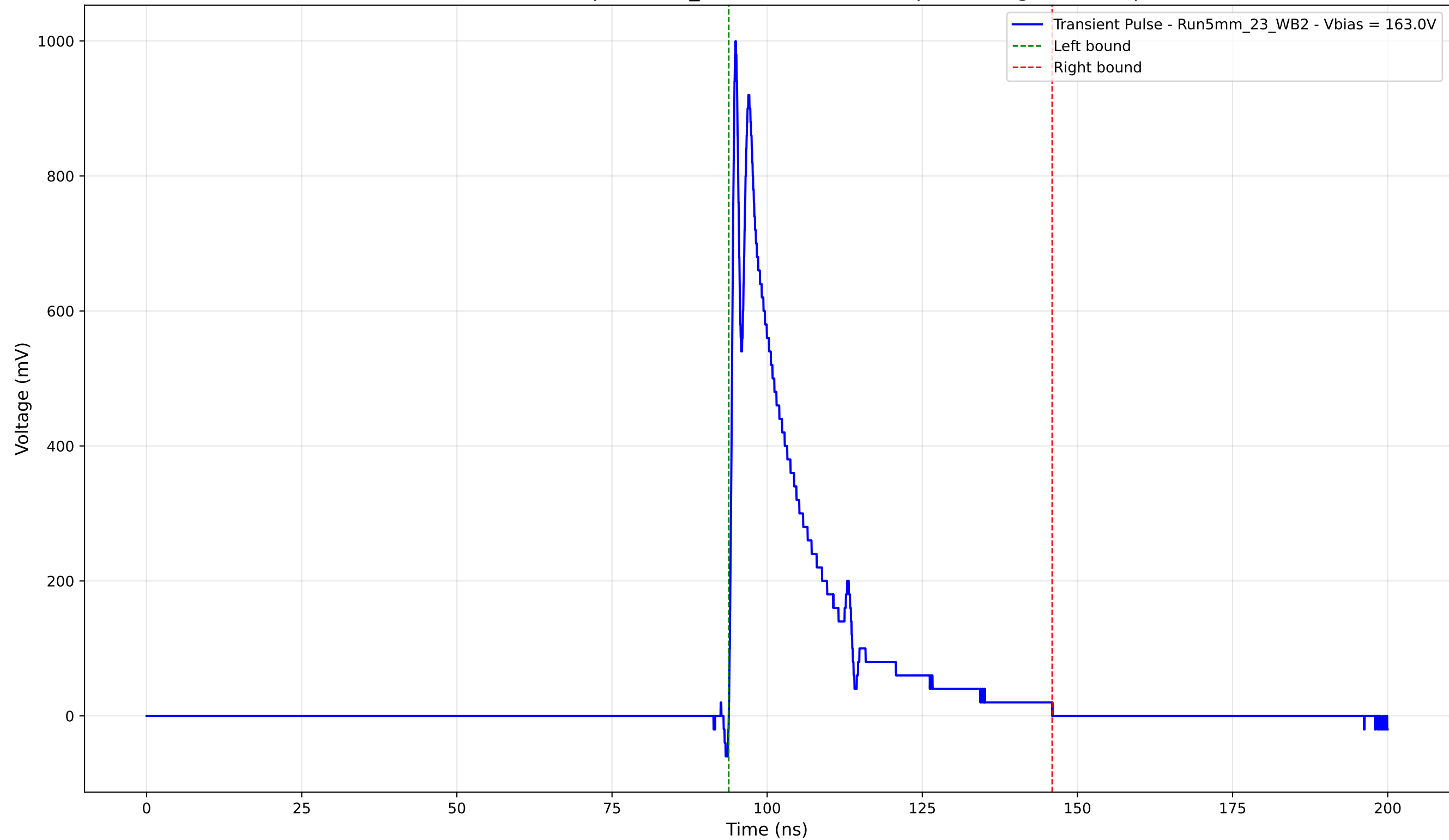
Transient Pulse - Sample: 5mm_23 - Position: 2415.0 \mu\text{m} - Charge: 193.89 pC
