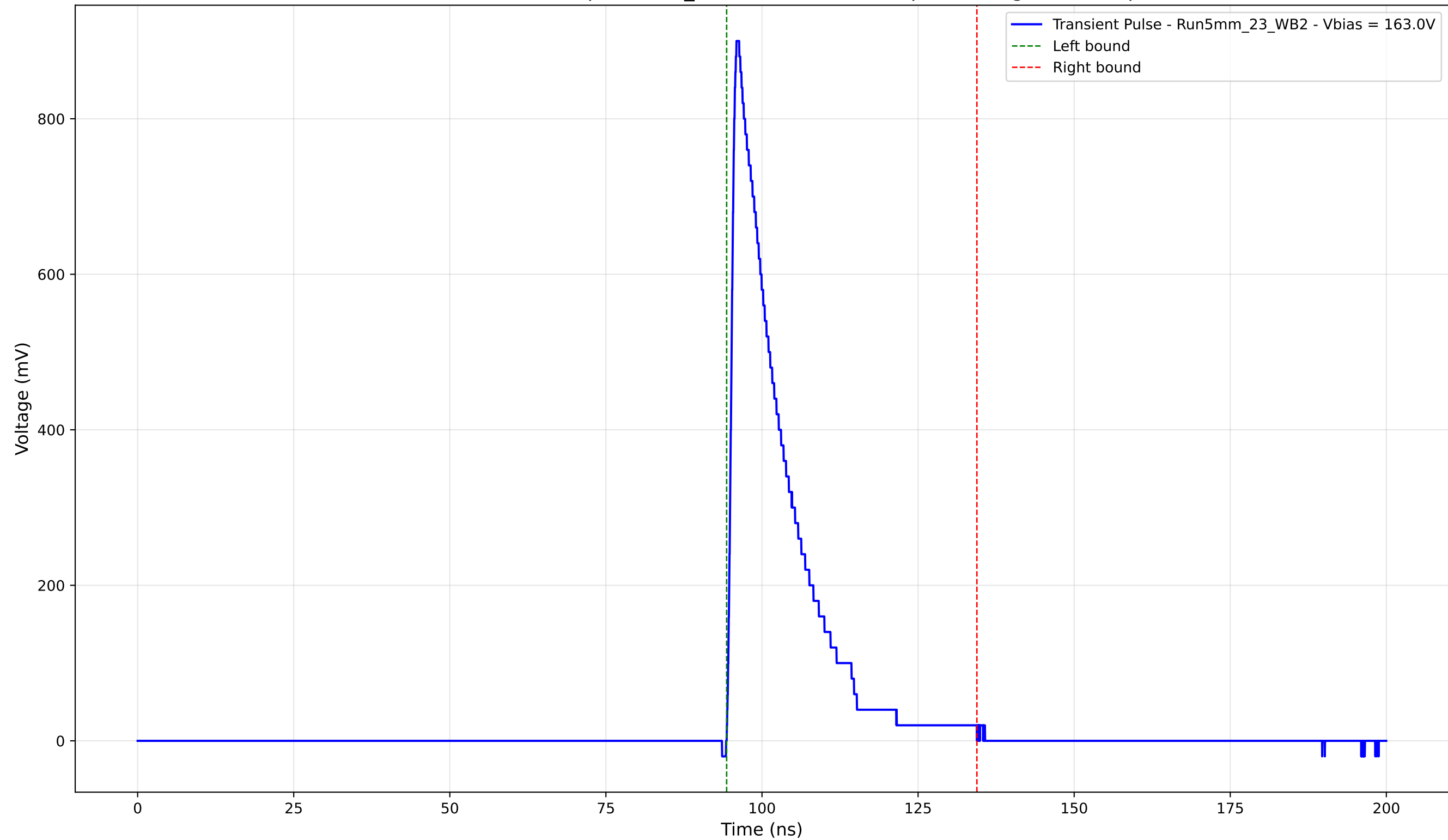
Transient Pulse - Sample: 5mm_23 - Position: 4320.0 \mu\text{m} - Charge: 161.78 pC
