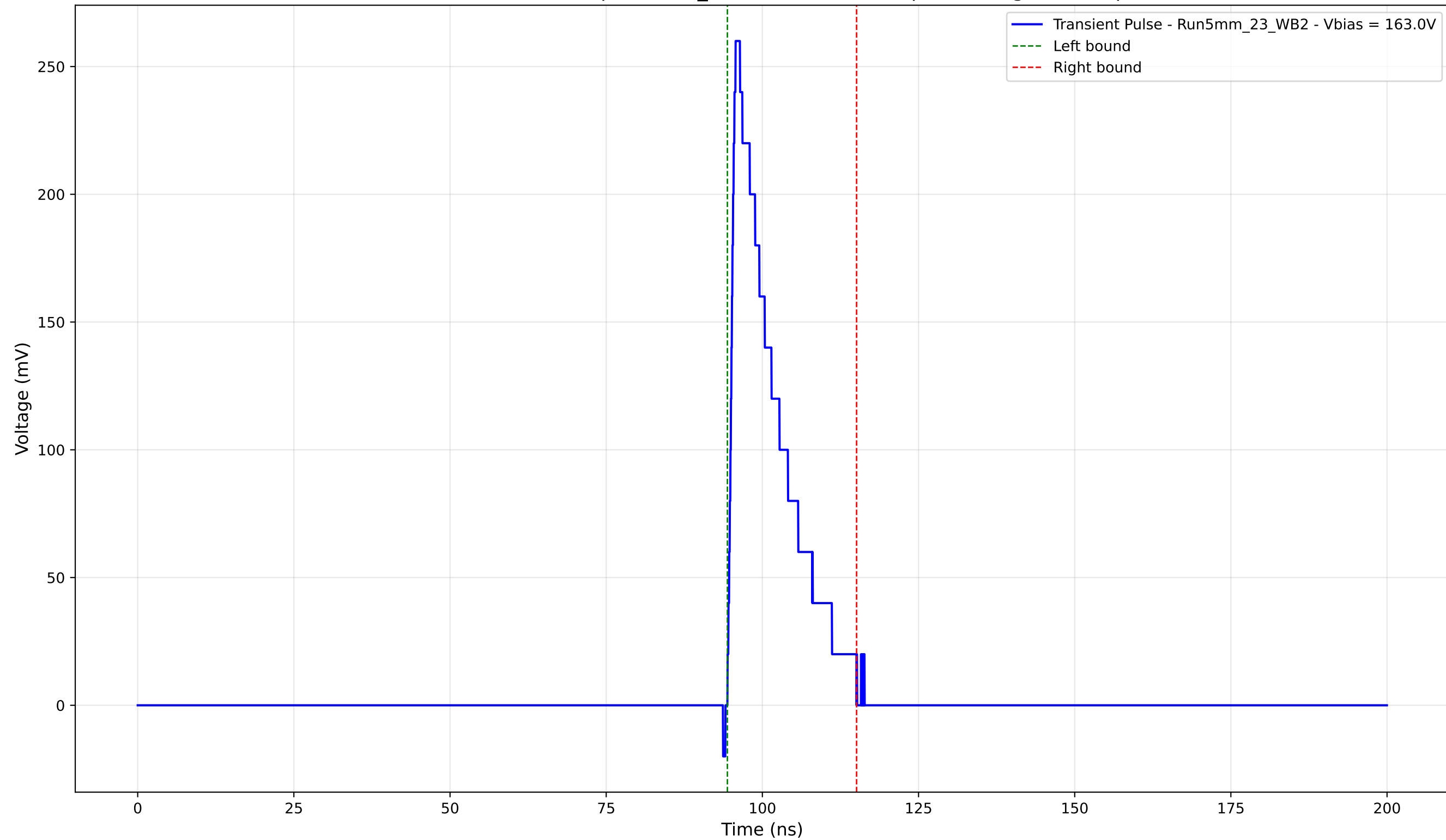
Transient Pulse - Sample: 5mm_23 - Position: 505.0 \mu\text{m} - Charge: 41.07 pC
