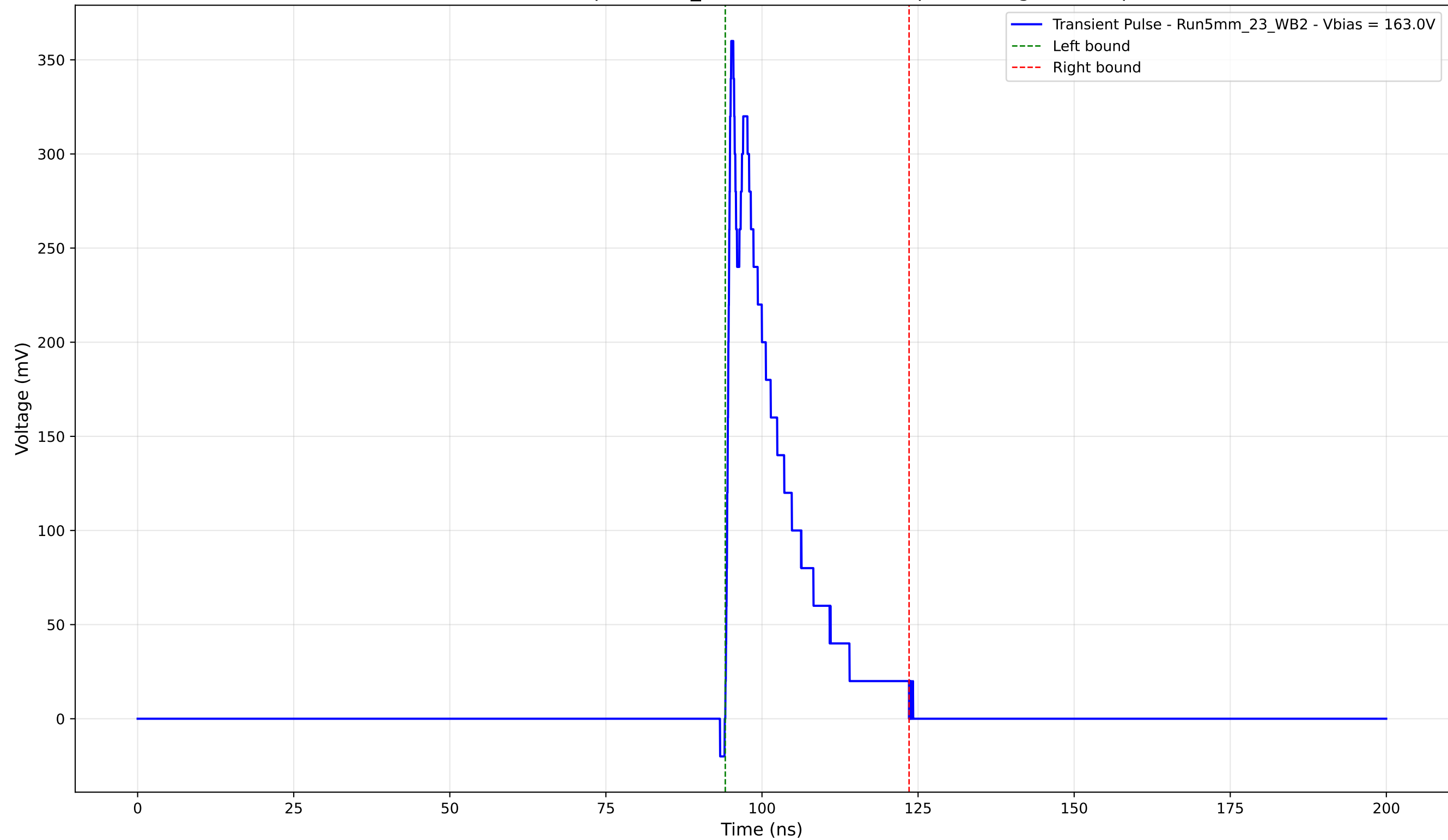
Transient Pulse - Sample: 5mm_23 - Position: 3000.0 \mu\text{m} - Charge: 60.88 pC
