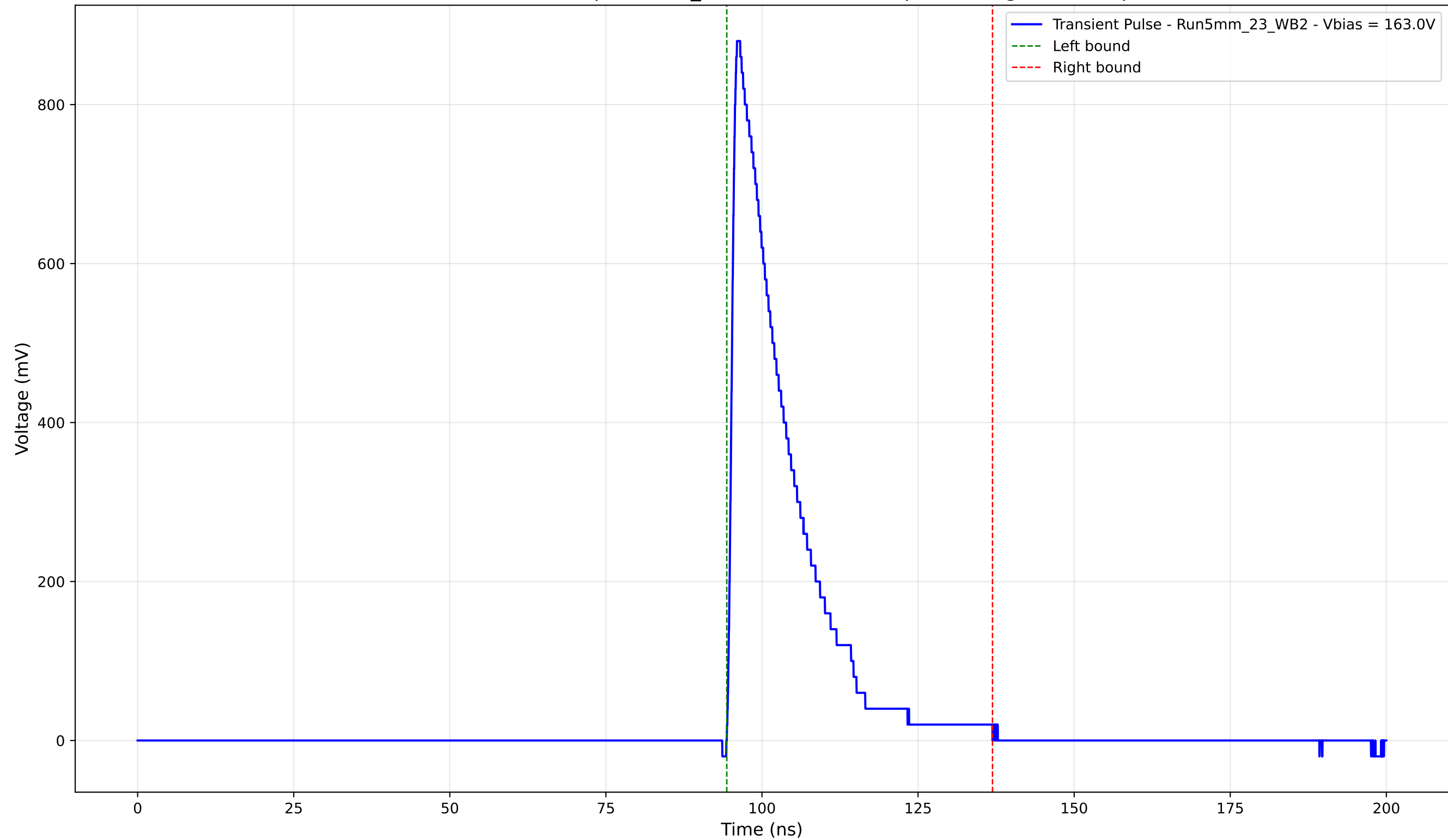
Transient Pulse - Sample: 5mm_23 - Position: 860.0 \mu\text{m} - Charge: 173.12 pC
