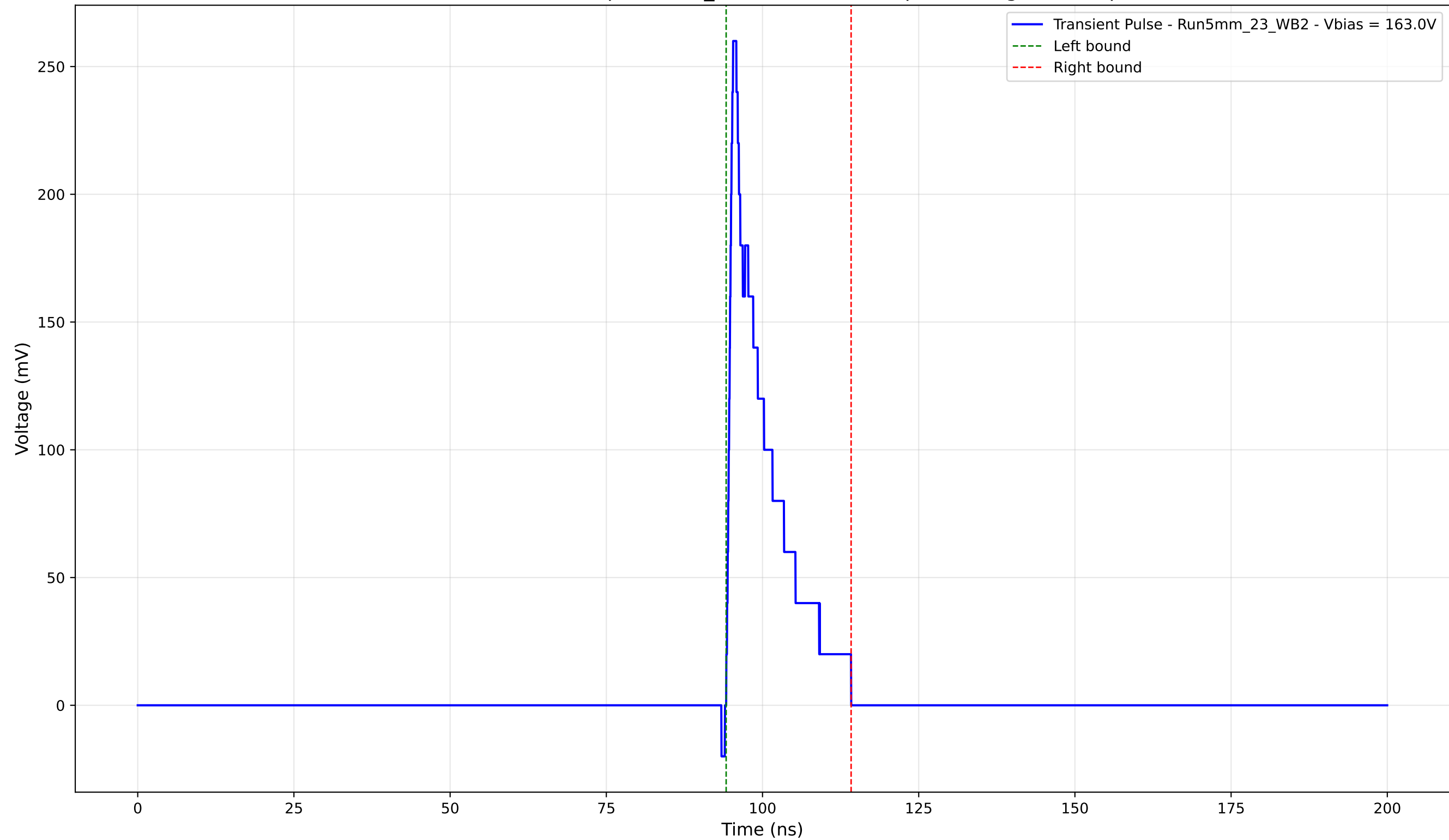
Transient Pulse - Sample: 5mm_23 - Position: 55.0 \mu\text{m} - Charge: 32.77 pC
