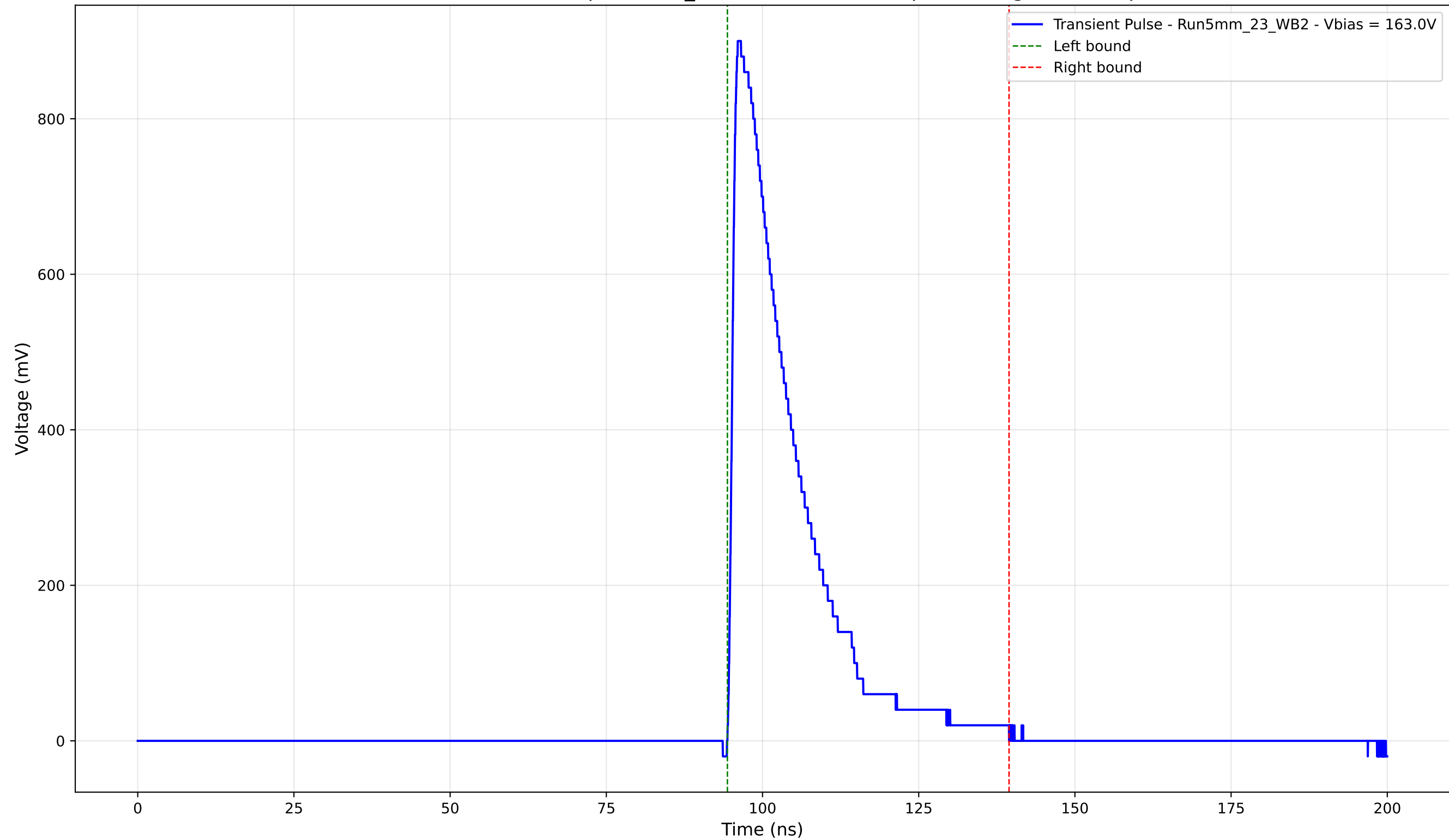
Transient Pulse - Sample: 5mm_23 - Position: 1200.0 \mu\text{m} - Charge: 196.18 pC
