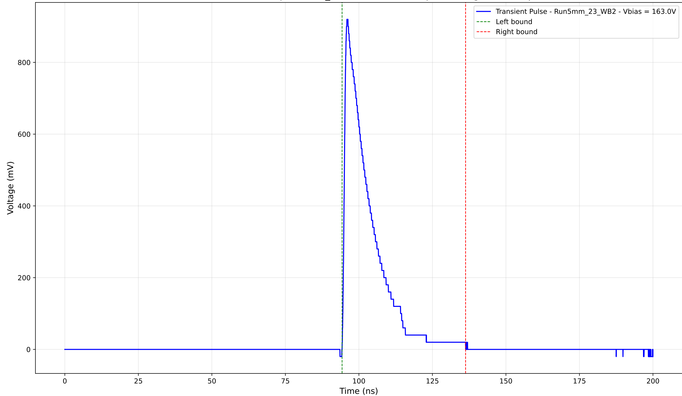
Transient Pulse - Sample: 5mm_23 - Position: 655.0 \mu\text{m} - Charge: 175.60 pC
