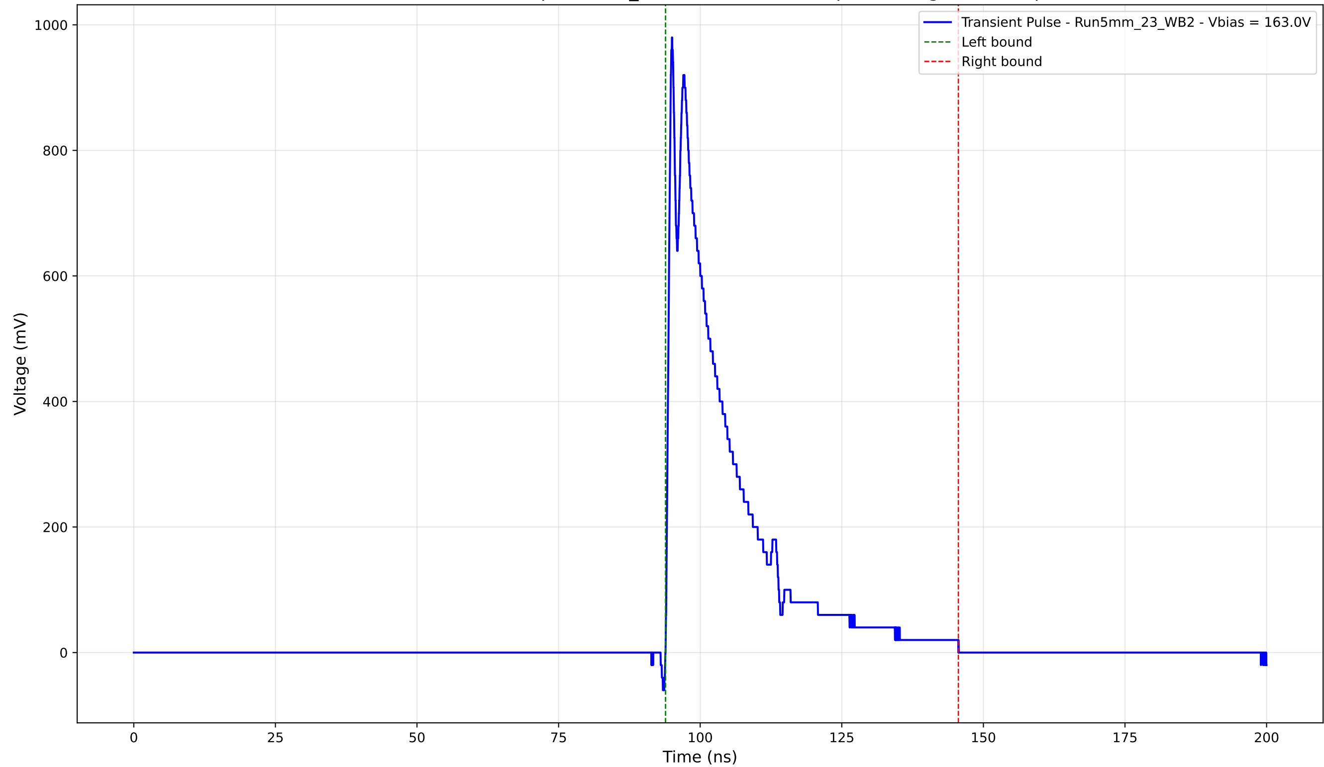
Transient Pulse - Sample: 5mm_23 - Position: 2735.0 \mu\text{m} - Charge: 202.15 pC
