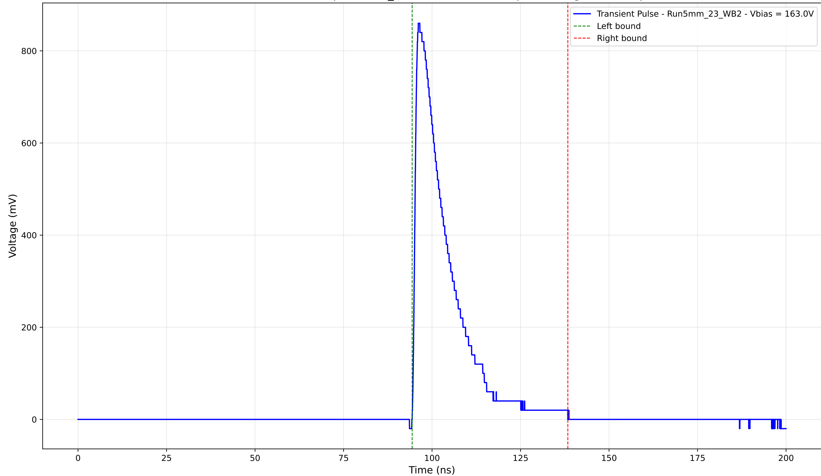
Transient Pulse - Sample: 5mm_23 - Position: 3740.0 \mu\text{m} - Charge: 176.93 pC
