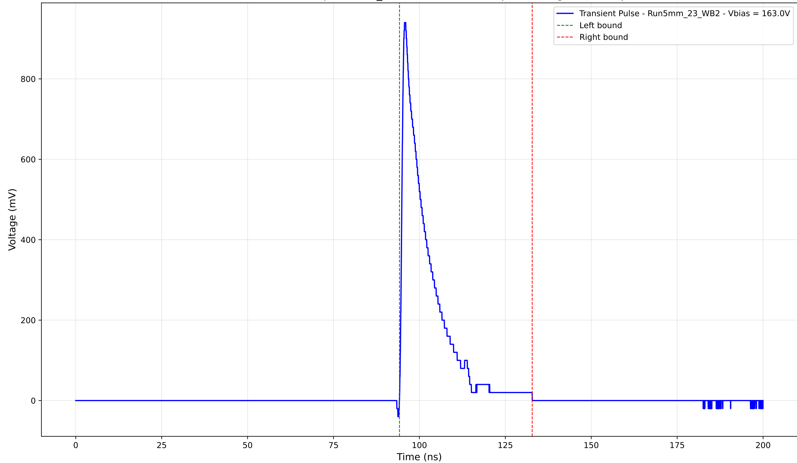
Transient Pulse - Sample: 5mm_23 - Position: 4630.0 \mu\text{m} - Charge: 151.70 pC
