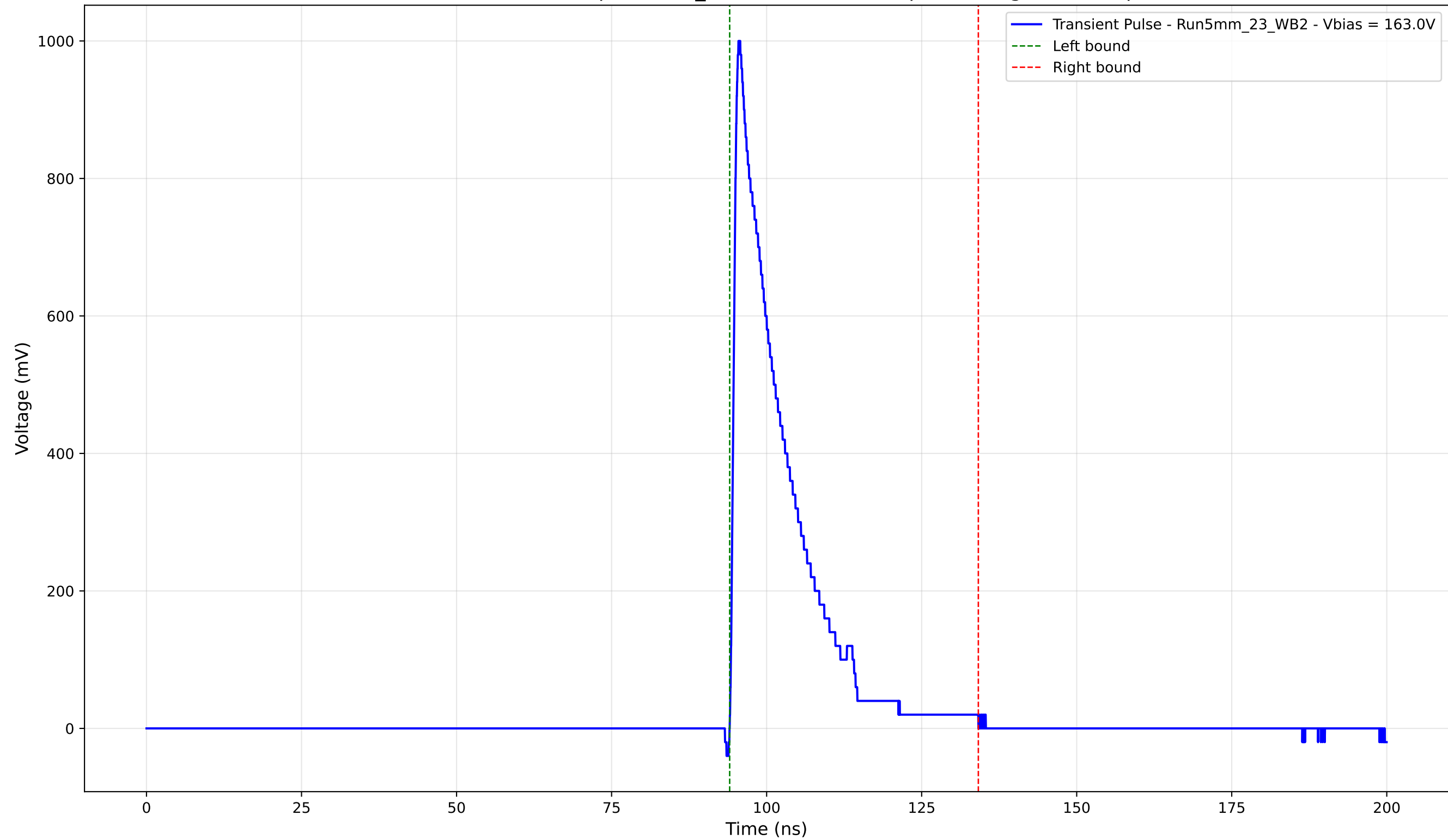
Transient Pulse - Sample: 5mm_23 - Position: 220.0 \mu\text{m} - Charge: 173.63 pC
