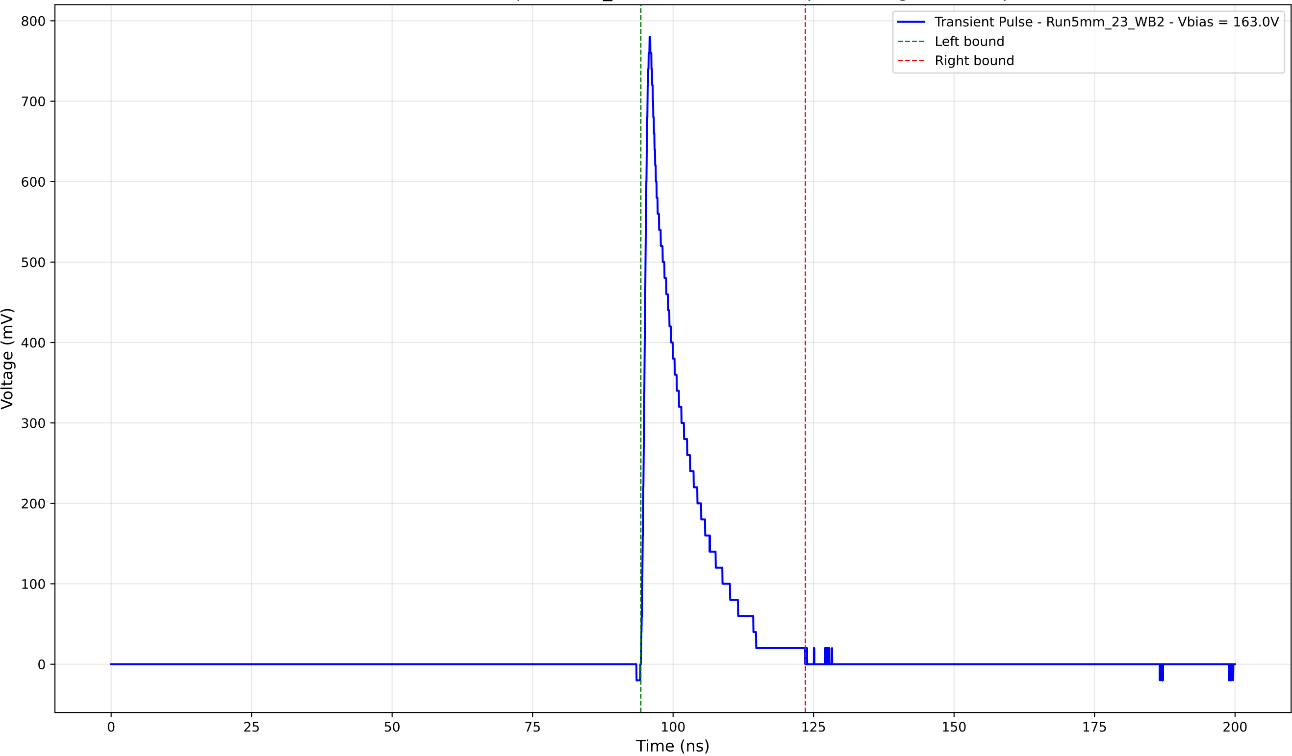
Transient Pulse - Sample: 5mm_23 - Position: 4595.0 \mu\text{m} - Charge: 109.73 pC
