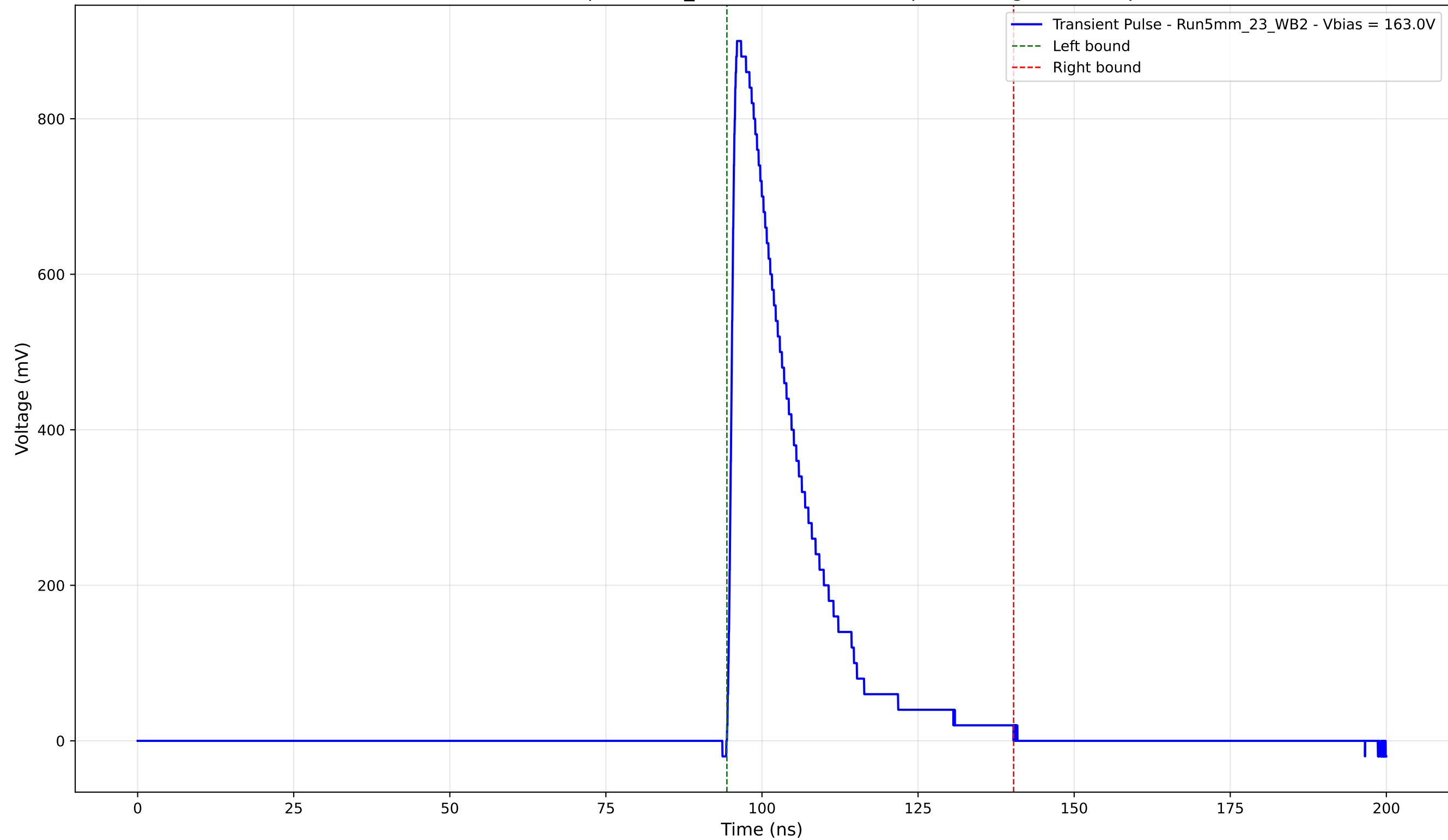
Transient Pulse - Sample: 5mm_23 - Position: 1250.0 \mu\text{m} - Charge: 200.19 pC
