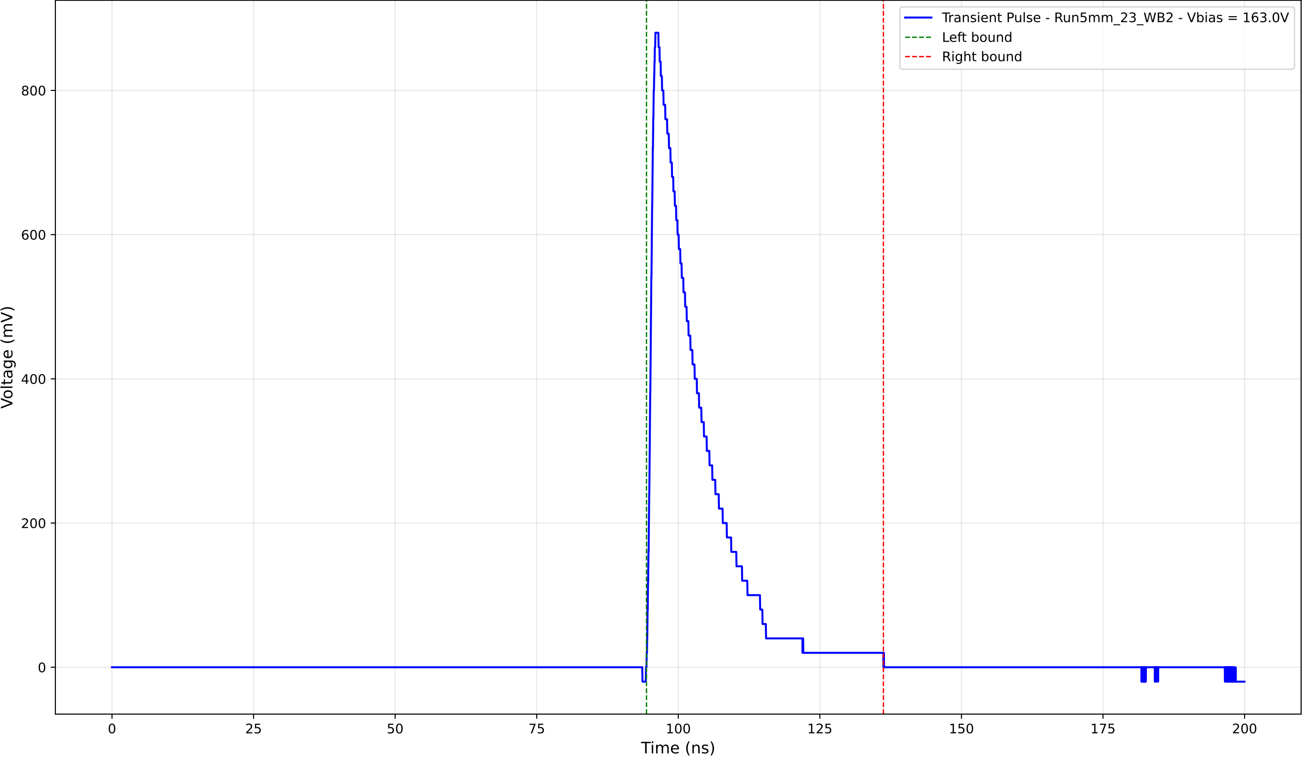
Transient Pulse - Sample: 5mm_23 - Position: 4205.0 \mu\text{m} - Charge: 164.05 pC
