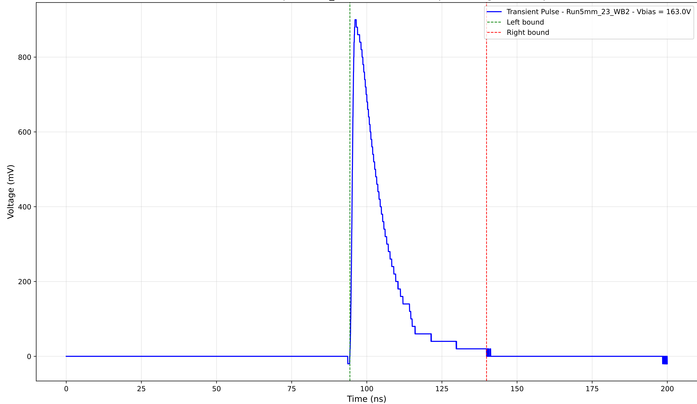
Transient Pulse - Sample: 5mm_23 - Position: 1180.0 \mu\text{m} - Charge: 194.91 pC
