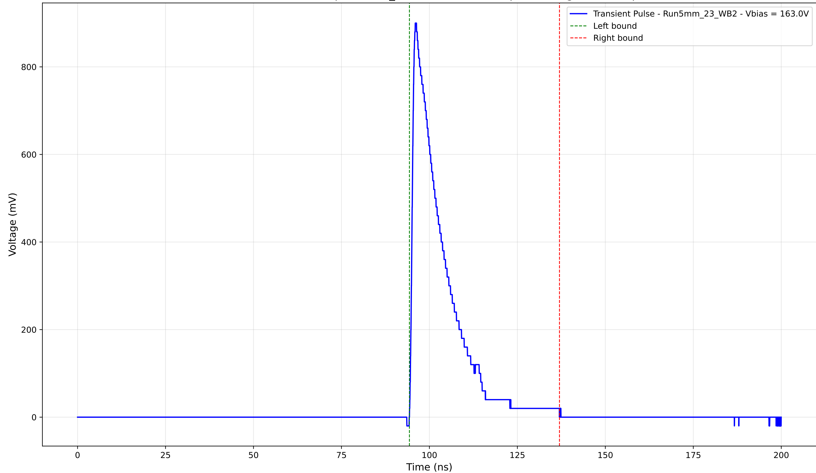
Transient Pulse - Sample: 5mm_23 - Position: 725.0 \mu\text{m} - Charge: 172.20 pC
