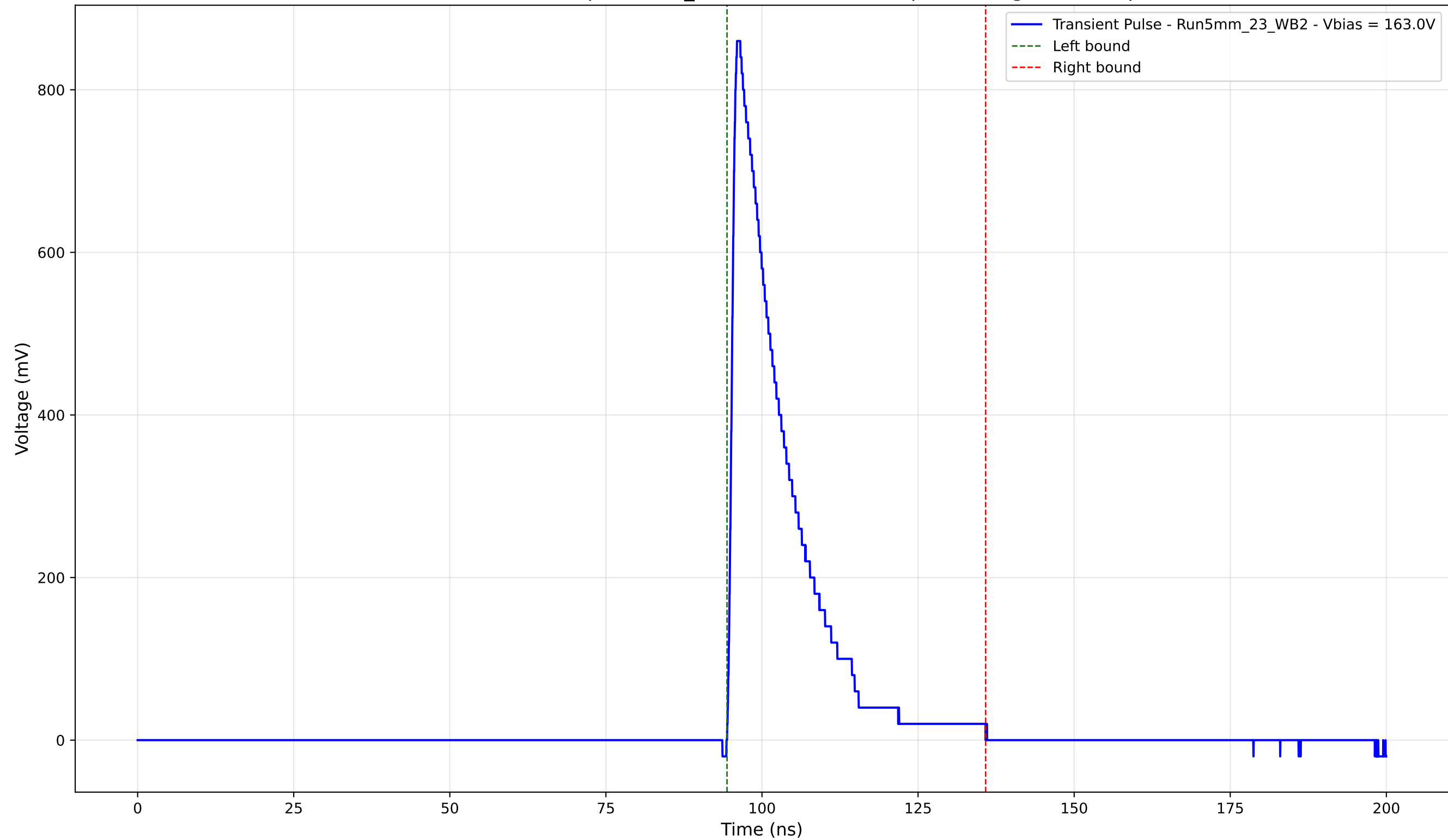
Transient Pulse - Sample: 5mm_23 - Position: 4150.0 \mu\text{m} - Charge: 160.14 pC
