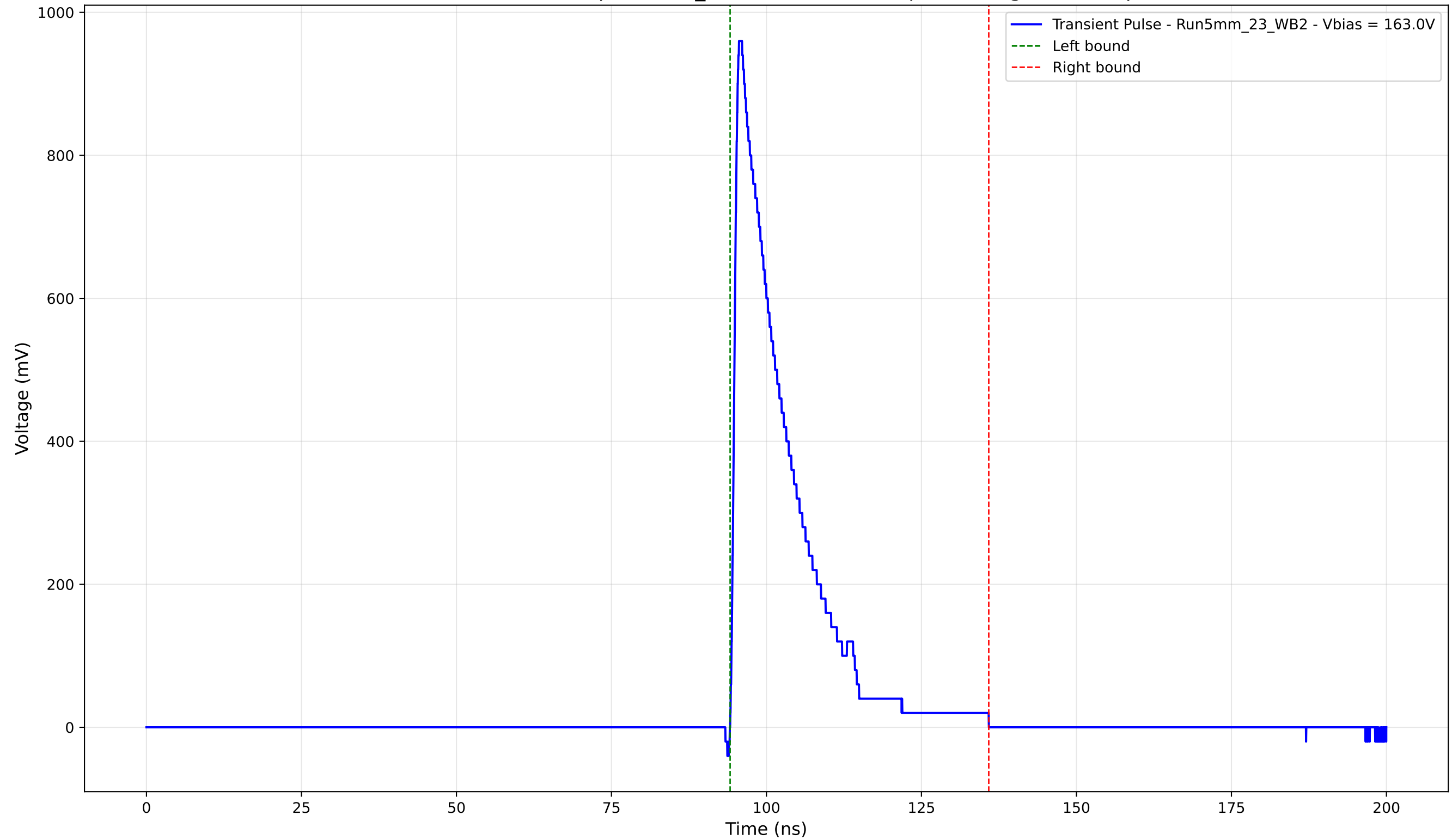
Transient Pulse - Sample: 5mm_23 - Position: 395.0 \mu\text{m} - Charge: 175.13 pC
