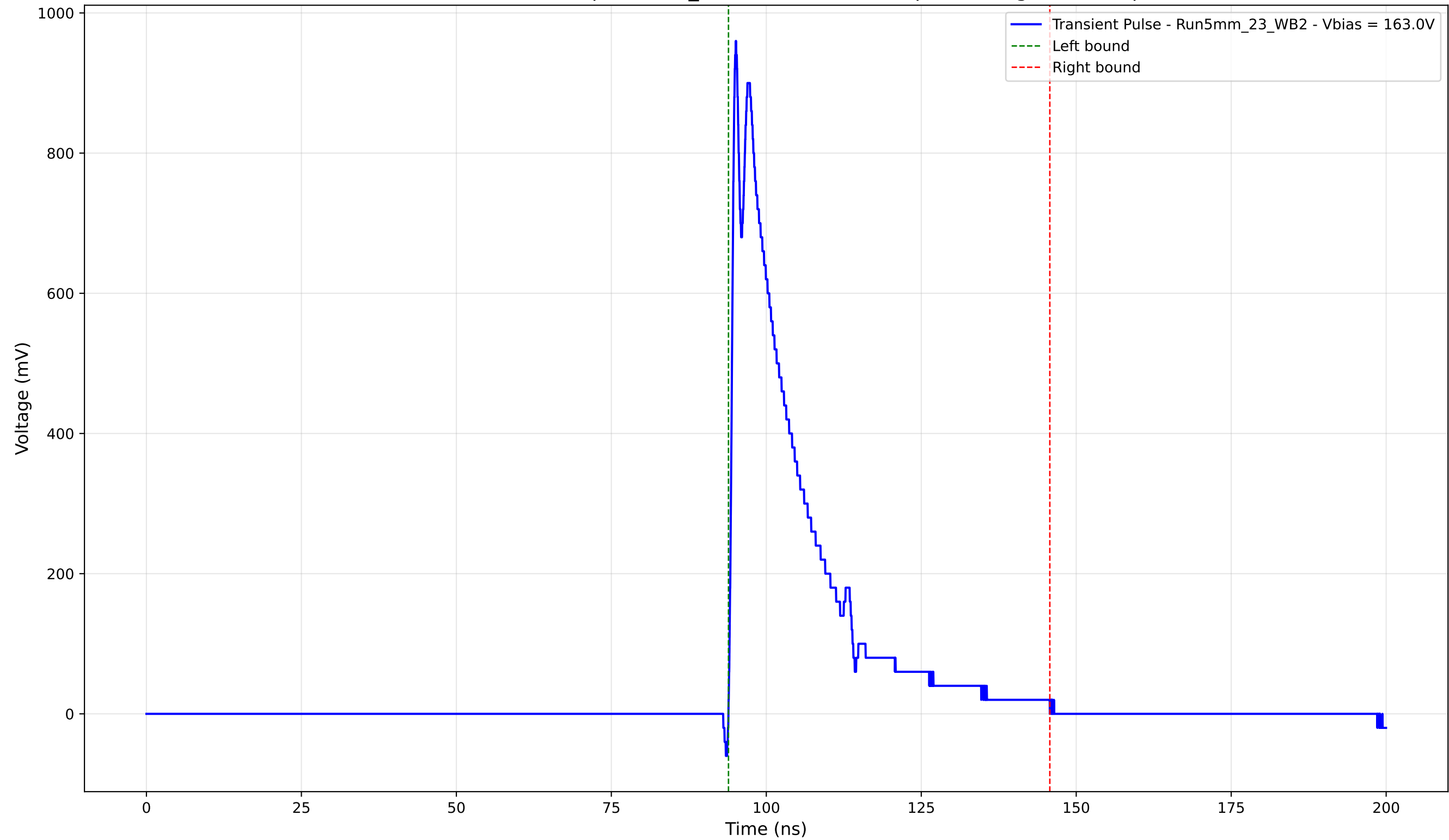
Transient Pulse - Sample: 5mm_23 - Position: 2240.0 \mu\text{m} - Charge: 204.64 pC
