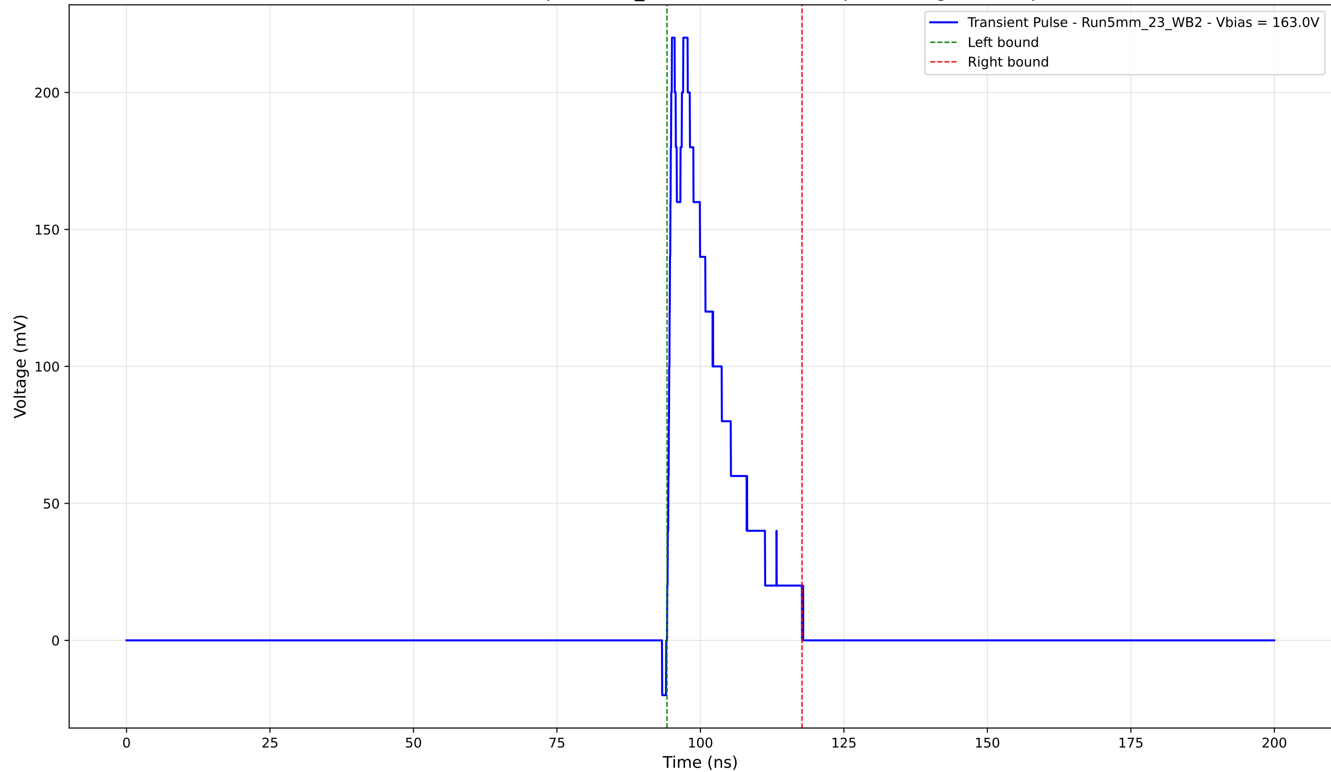
Transient Pulse - Sample: 5mm_23 - Position: 3015.0 \mu\text{m} - Charge: 39.94 pC
