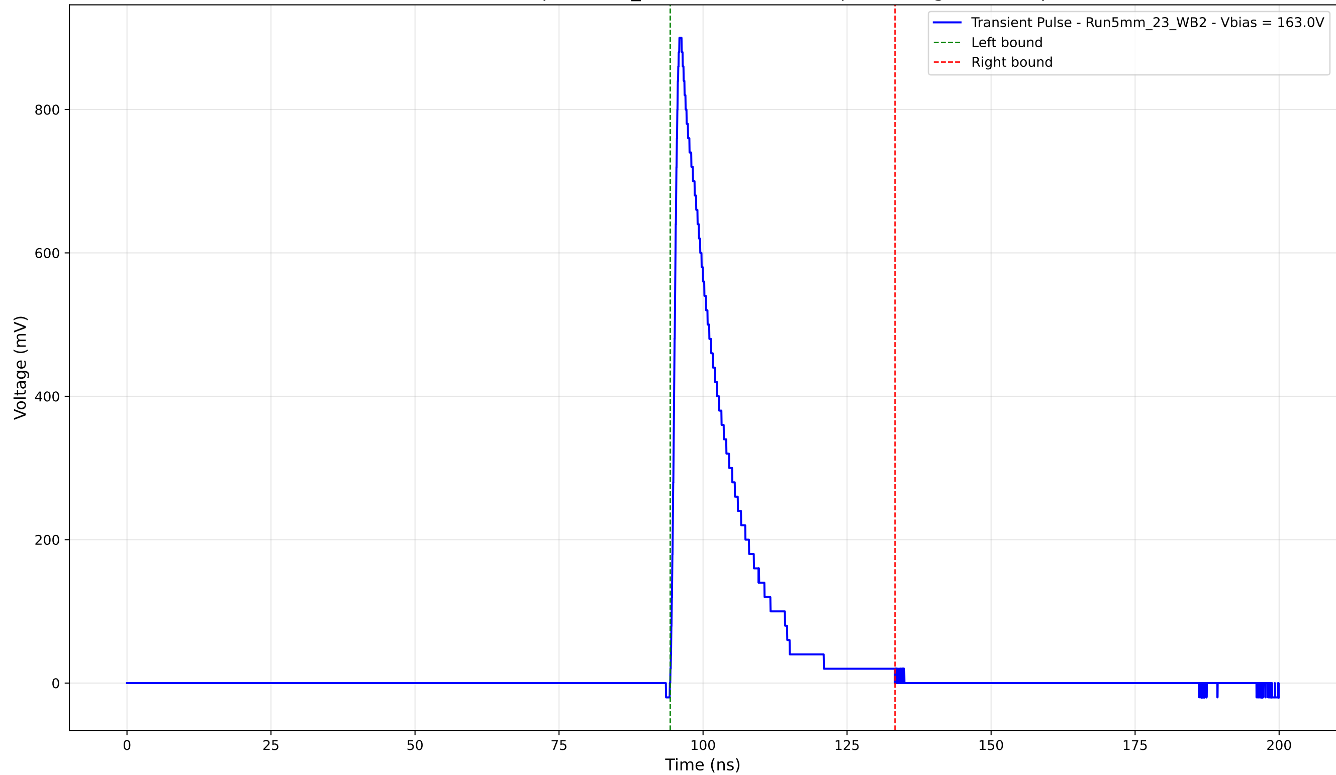
Transient Pulse - Sample: 5mm_23 - Position: 4380.0 \mu\text{m} - Charge: 157.89 pC
