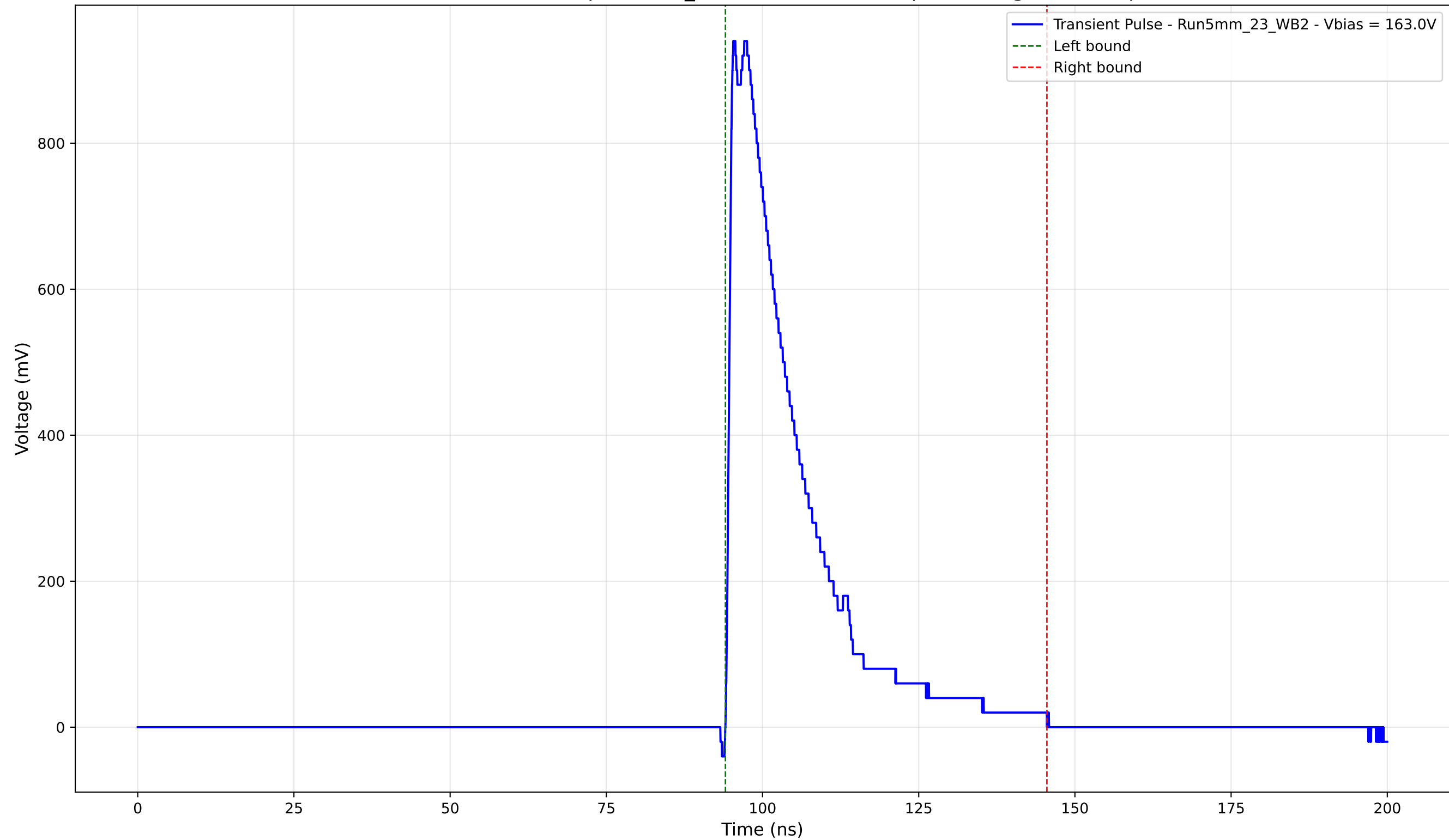
Transient Pulse - Sample: 5mm_23 - Position: 3135.0 \mu\text{m} - Charge: 225.89 pC
