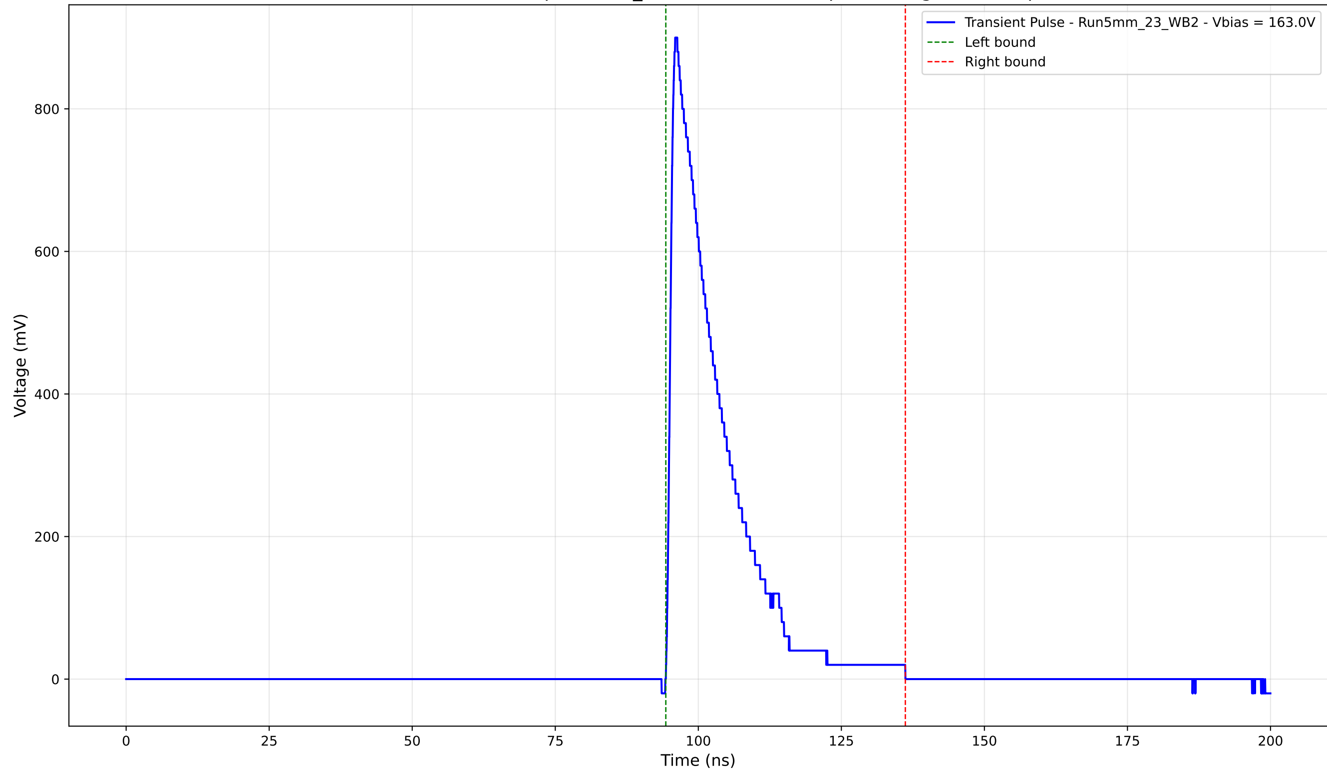
Transient Pulse - Sample: 5mm_23 - Position: 710.0 \mu\text{m} - Charge: 171.45 pC
