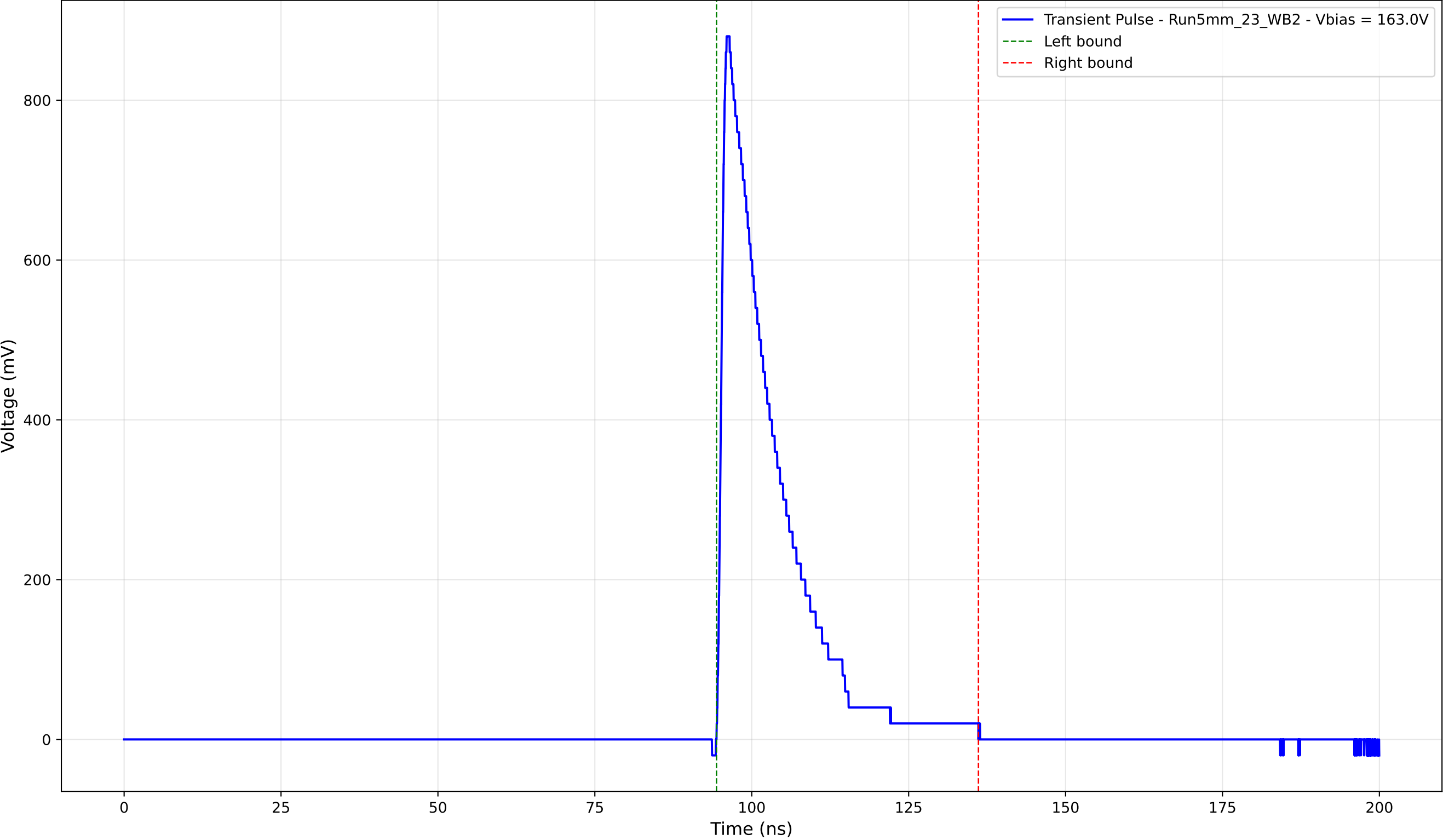
Transient Pulse - Sample: 5mm_23 - Position: 4195.0 \mu\text{m} - Charge: 163.40 pC
