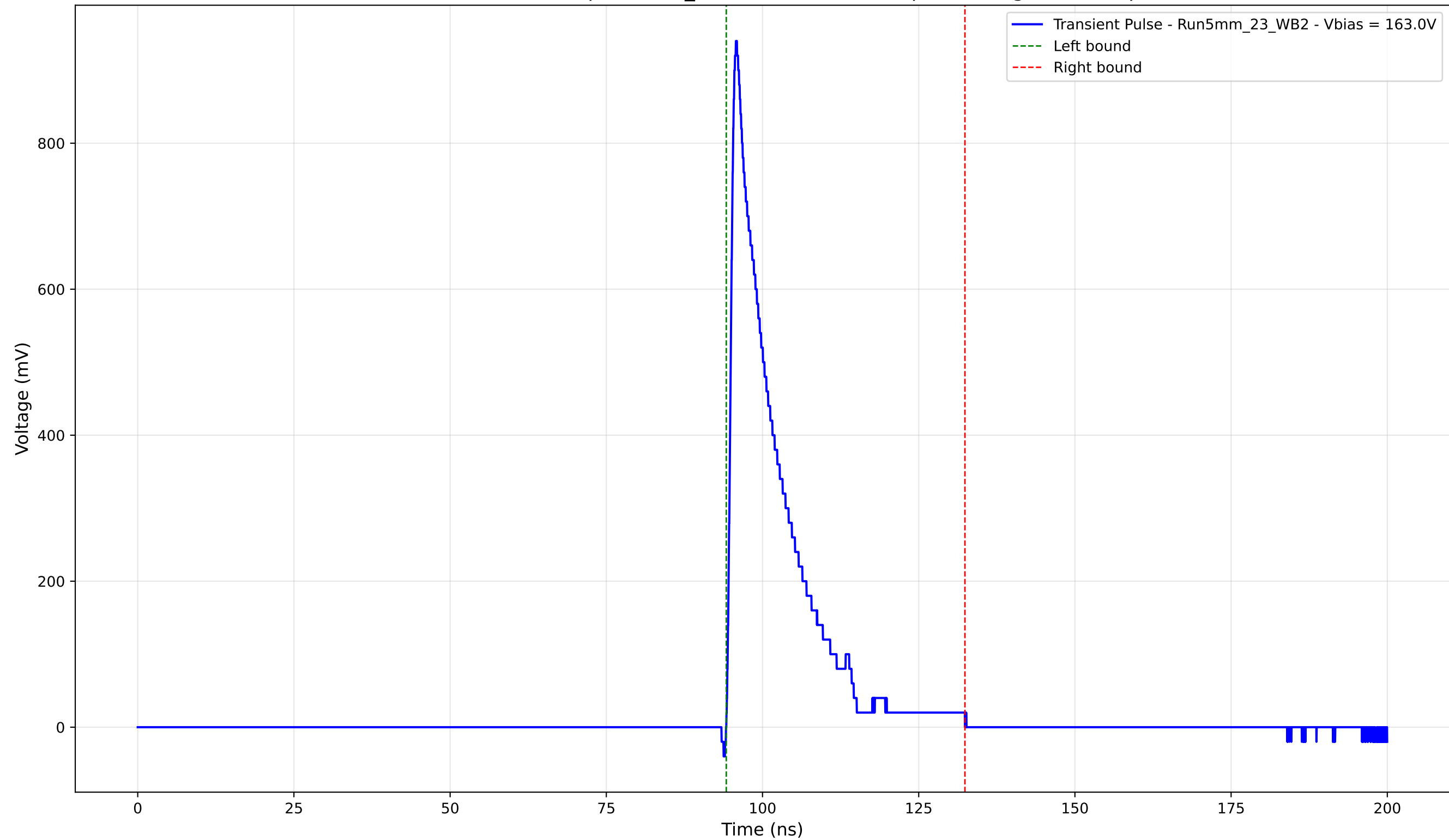
Transient Pulse - Sample: 5mm_23 - Position: 4625.0 \mu\text{m} - Charge: 147.55 pC
