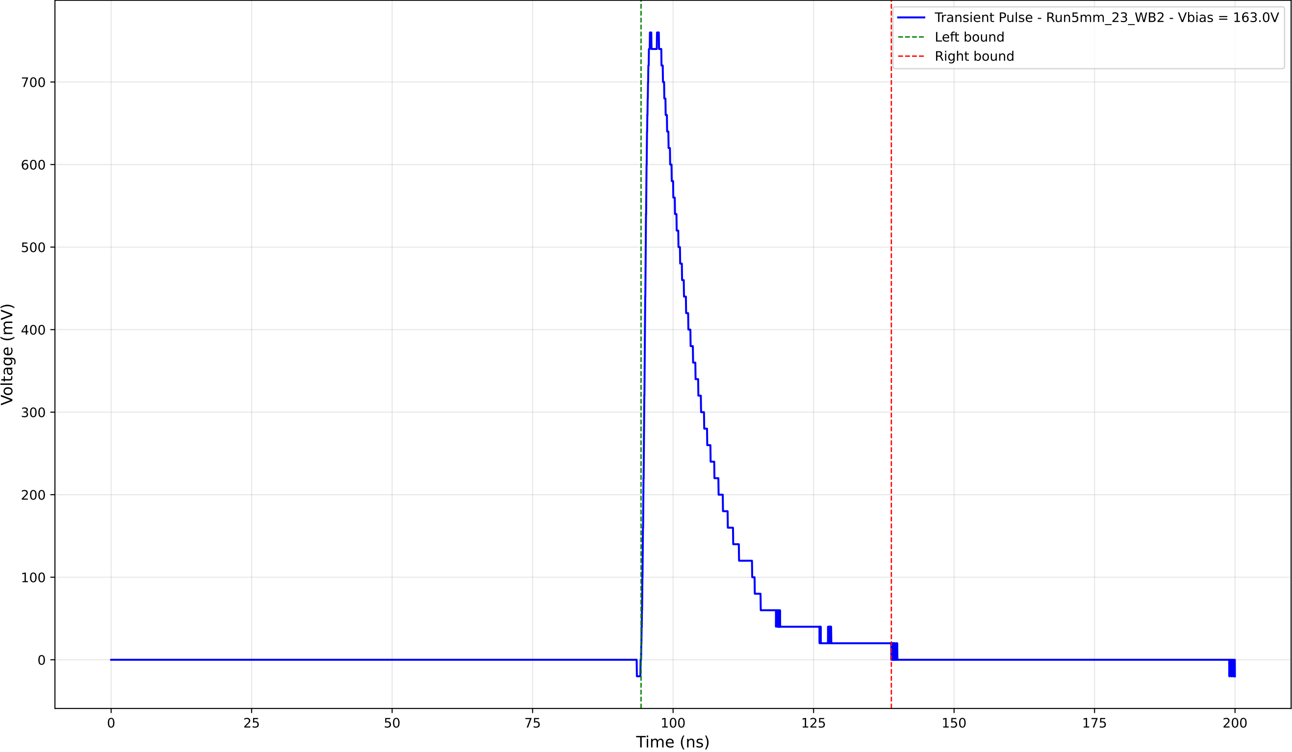
Transient Pulse - Sample: 5mm_23 - Position: 1575.0 \mu\text{m} - Charge: 164.68 pC
