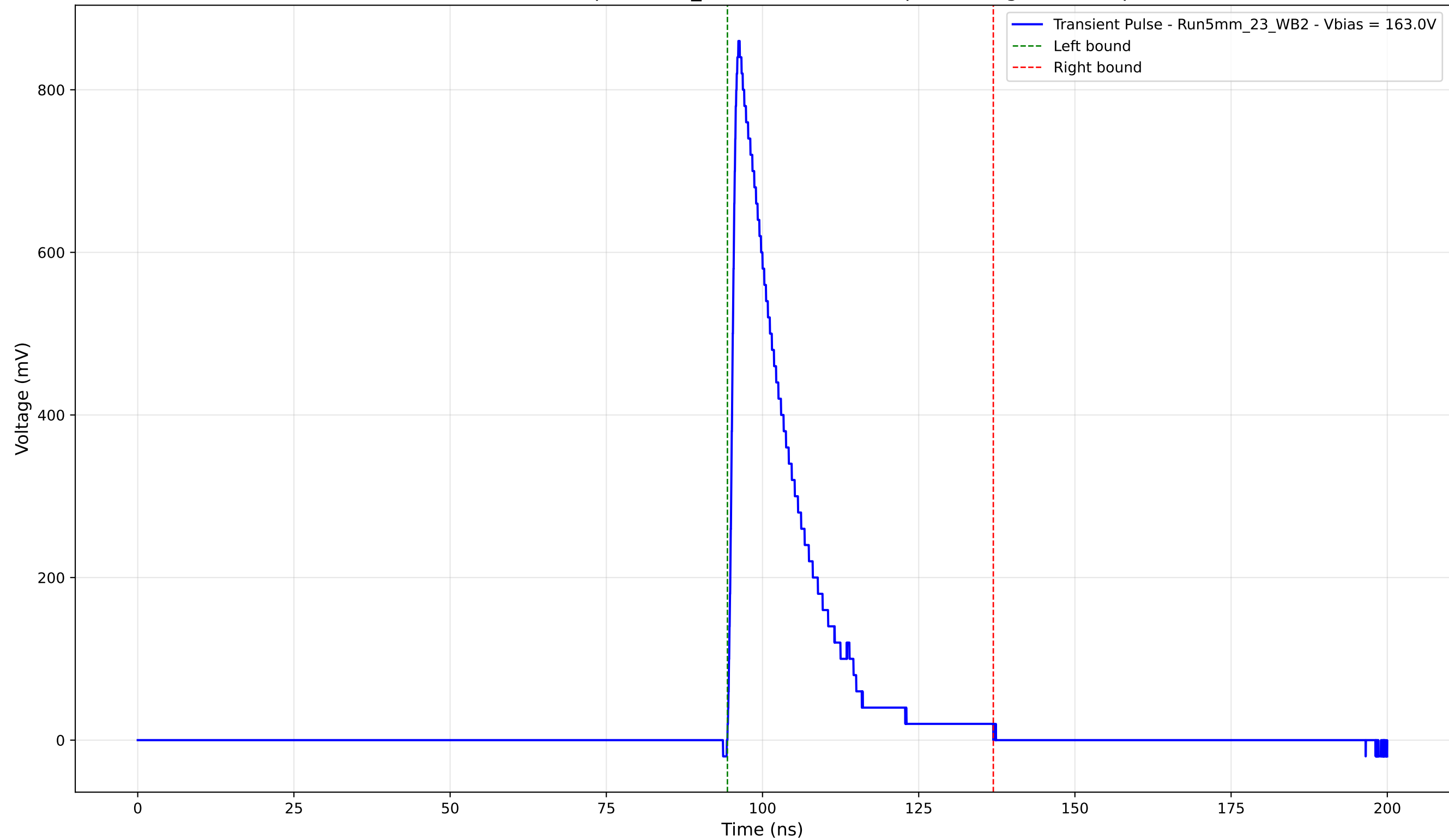
Transient Pulse - Sample: 5mm_23 - Position: 905.0 \mu\text{m} - Charge: 163.86 pC
