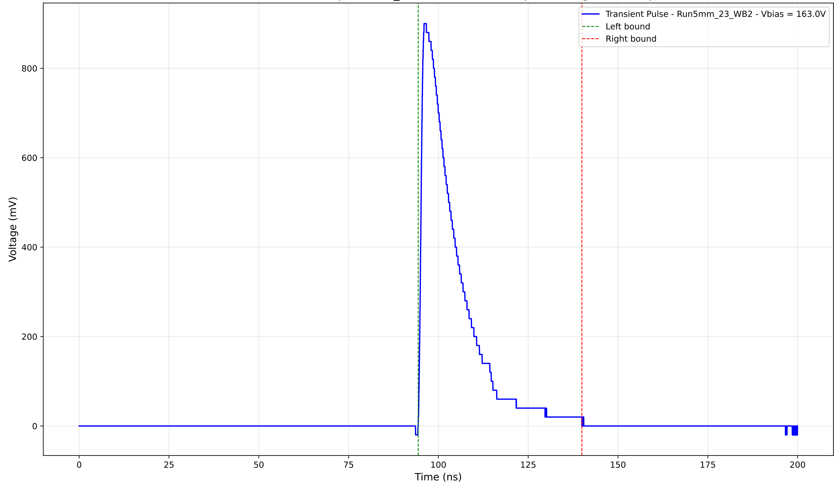
Transient Pulse - Sample: 5mm_23 - Position: 1235.0 \mu\text{m} - Charge: 198.99 pC
