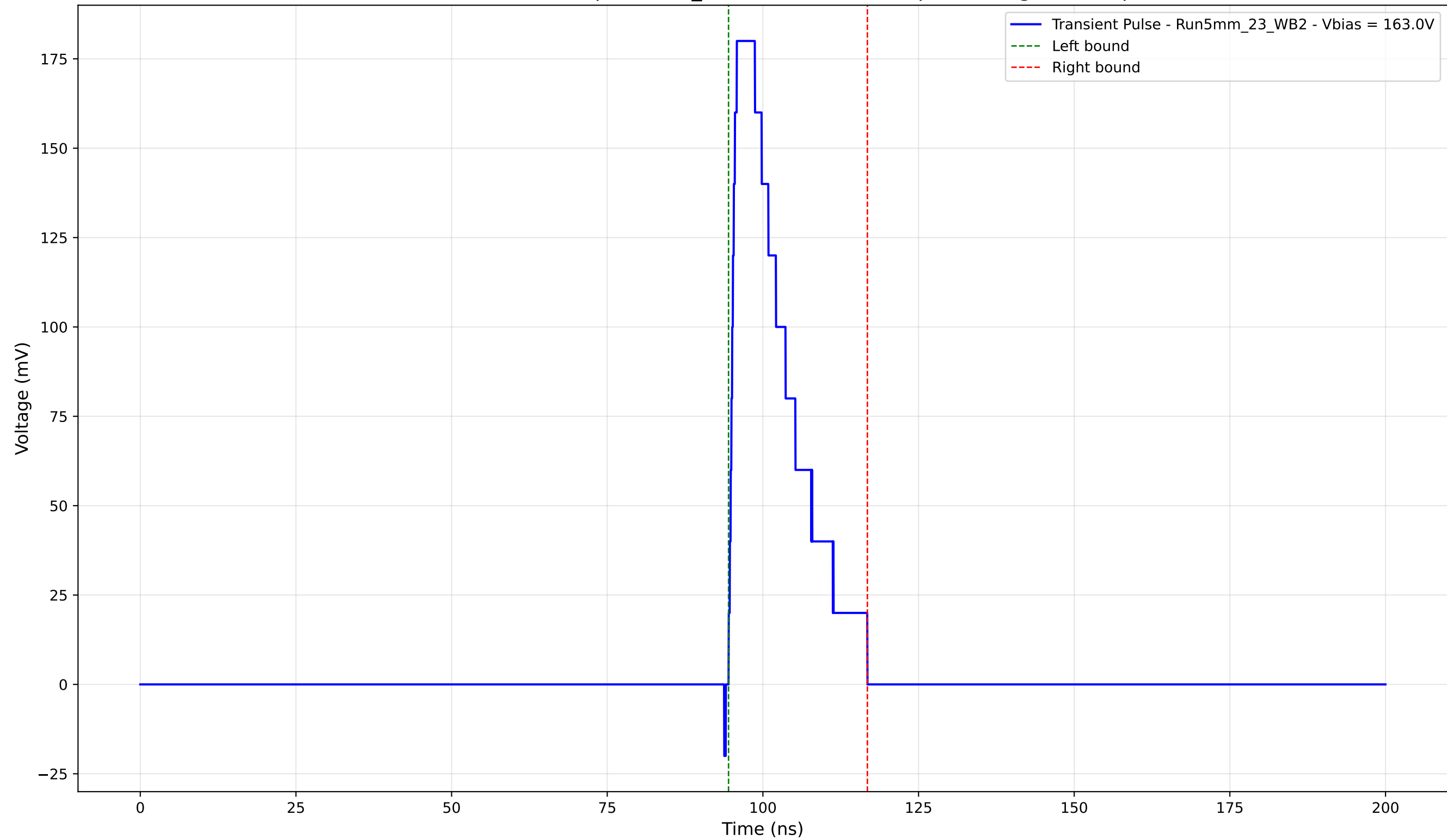
Transient Pulse - Sample: 5mm_23 -Position: 1510.0 \mu\text{m} - Charge: 36.19 pC
