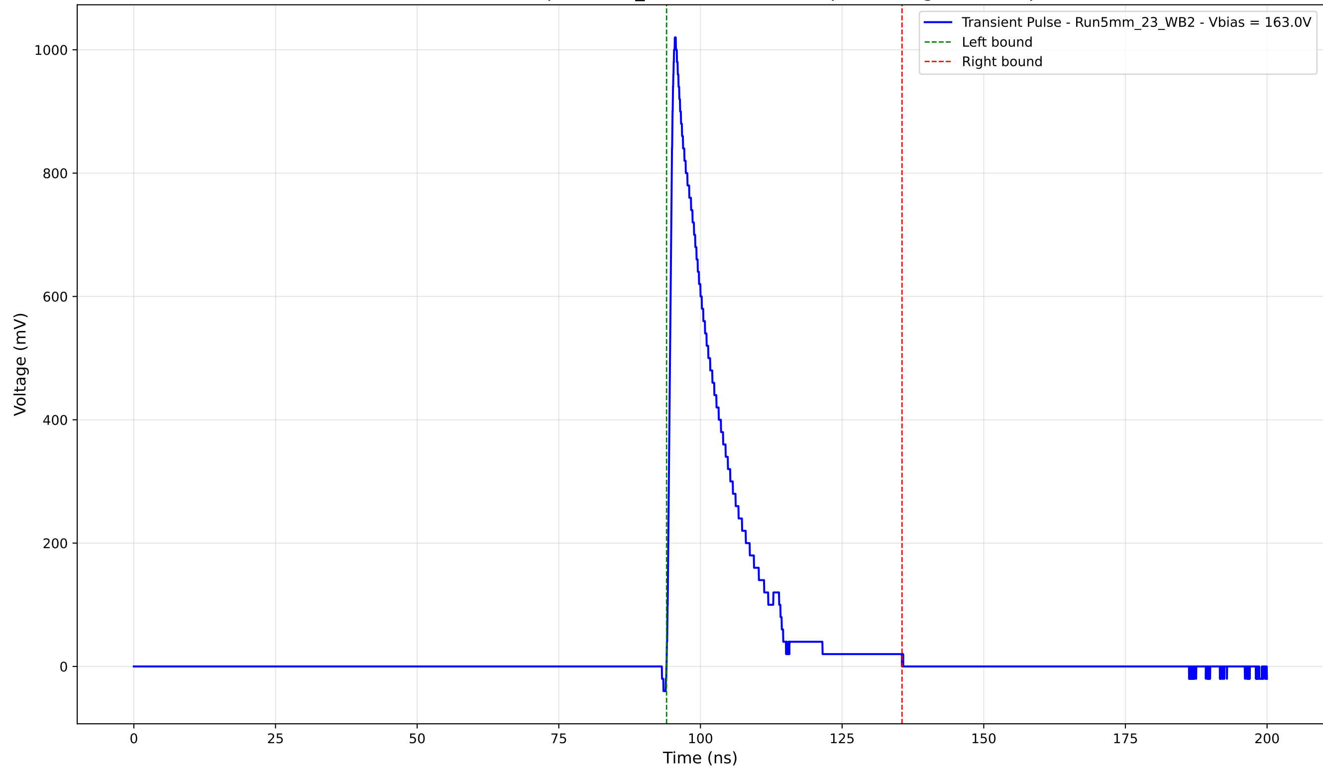
Transient Pulse - Sample: 5mm_23 - Position: 195.0 \mu\text{m} - Charge: 178.77 pC
