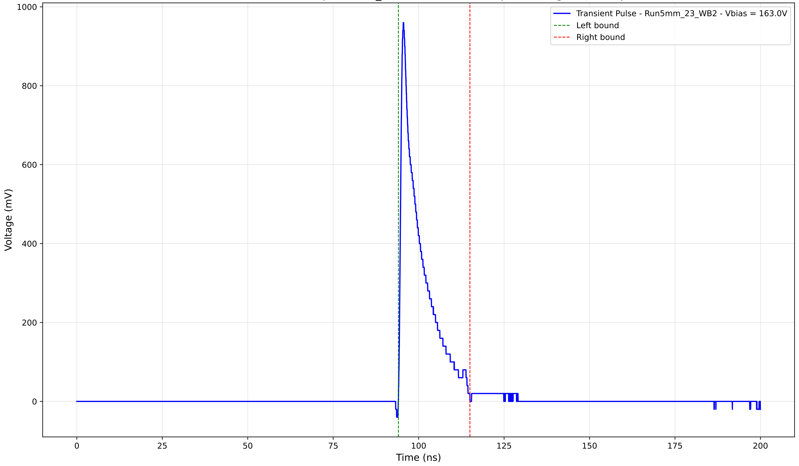
Transient Pulse - Sample: 5mm_23 - Position: 4885.0 \mu\text{m} - Charge: 123.22 pC
