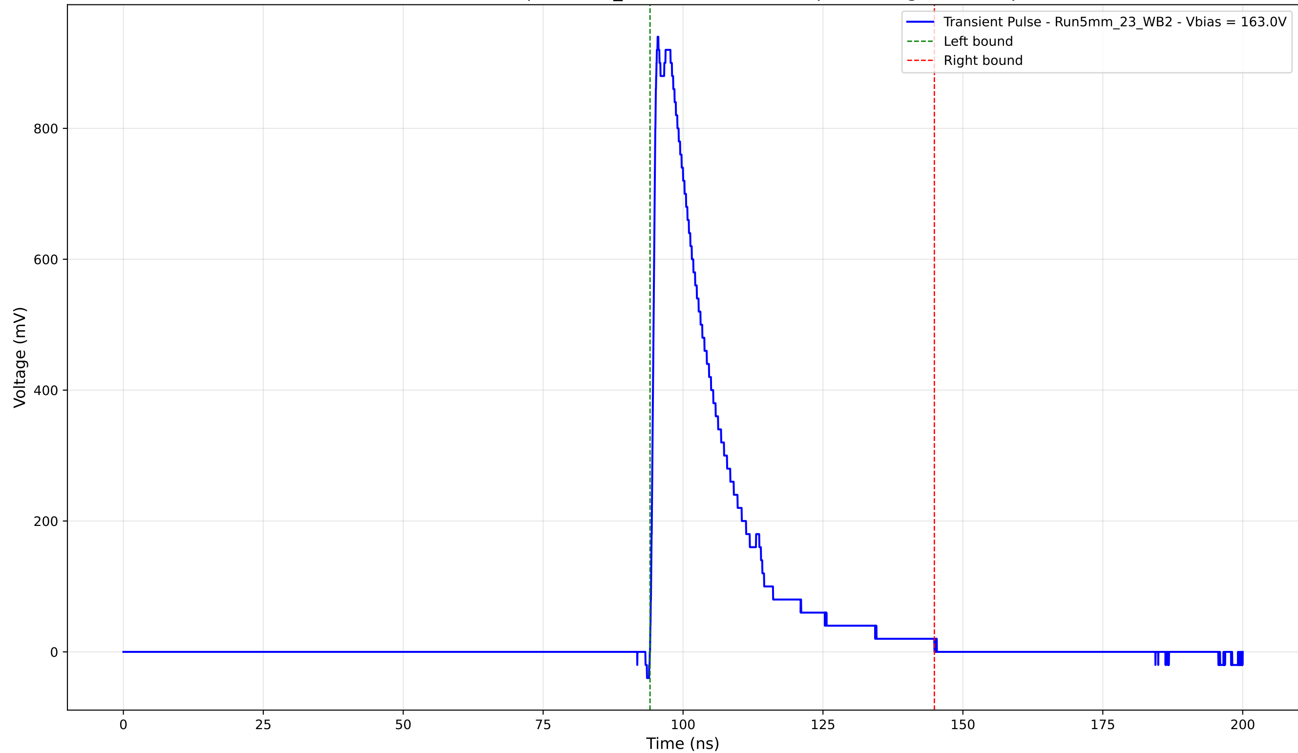
Transient Pulse - Sample: 5mm_23 - Position: 3170.0 \mu\text{m} - Charge: 222.29 pC
