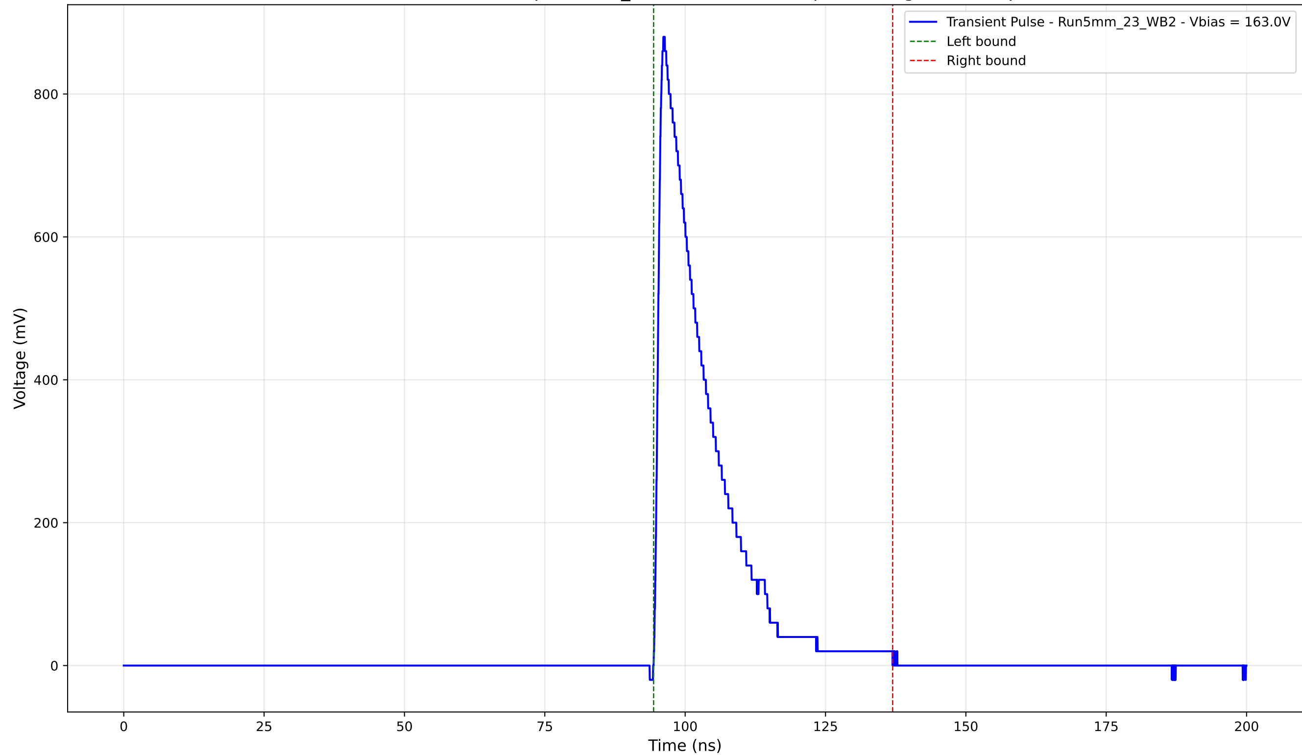
Transient Pulse - Sample: 5mm_23 - Position: 890.0 \mu\text{m} - Charge: 170.12 pC
