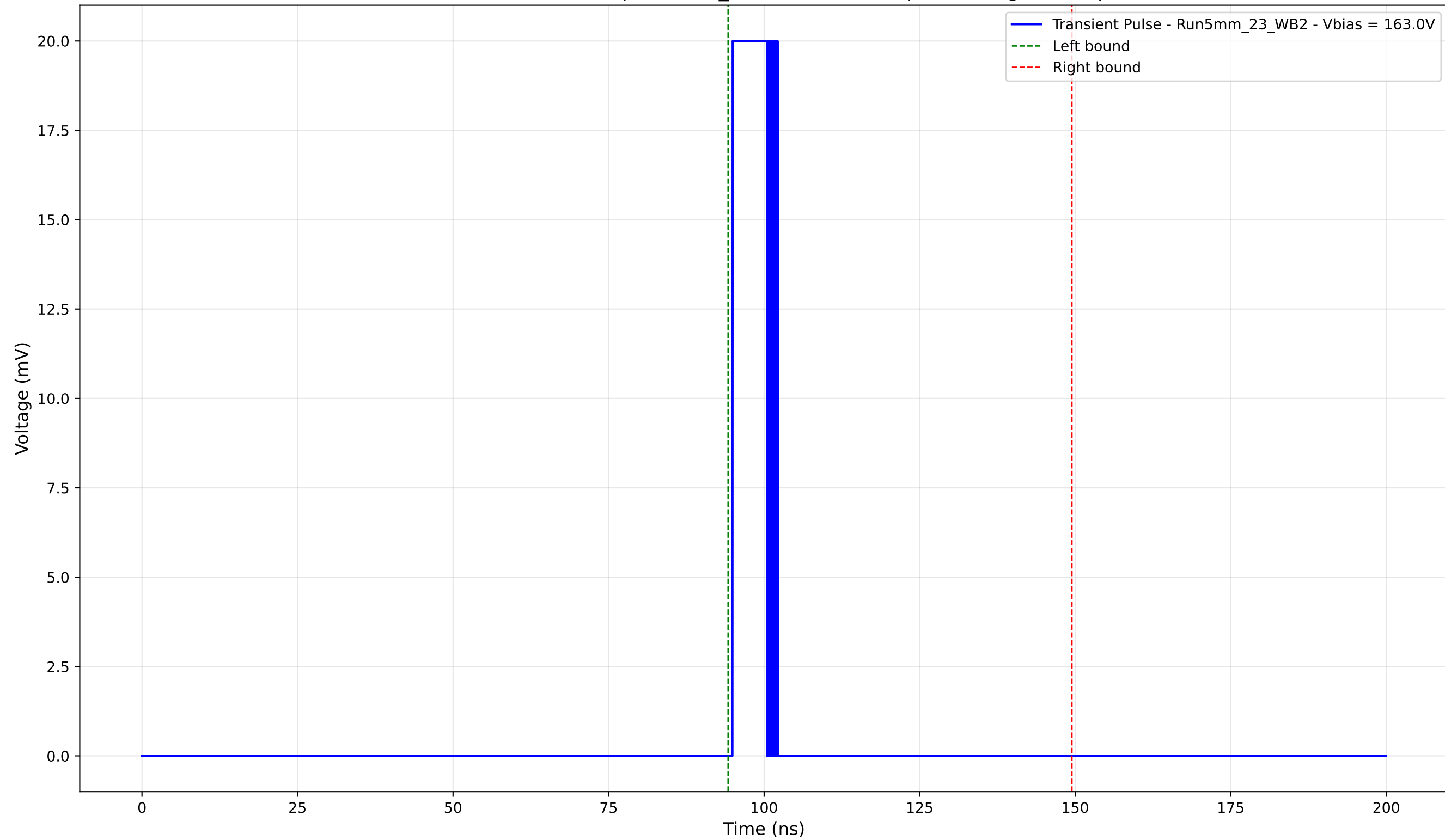
Transient Pulse - Sample: 5mm_23 - Position: 0.0 \mu\text{m} - Charge: 2.32 pC
