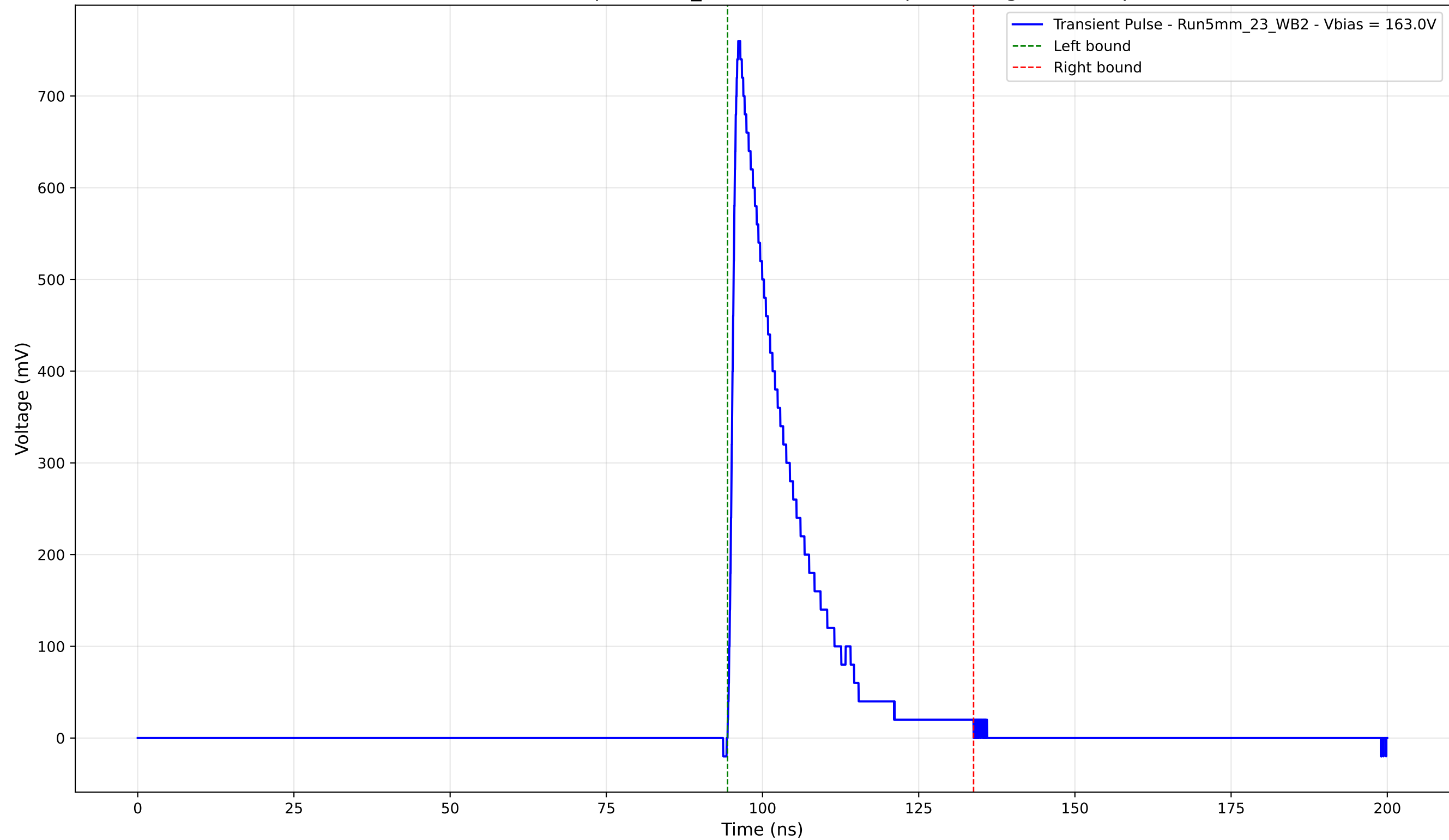
Transient Pulse - Sample: 5mm_23 - Position: 925.0 \mu\text{m} - Charge: 139.85 pC
