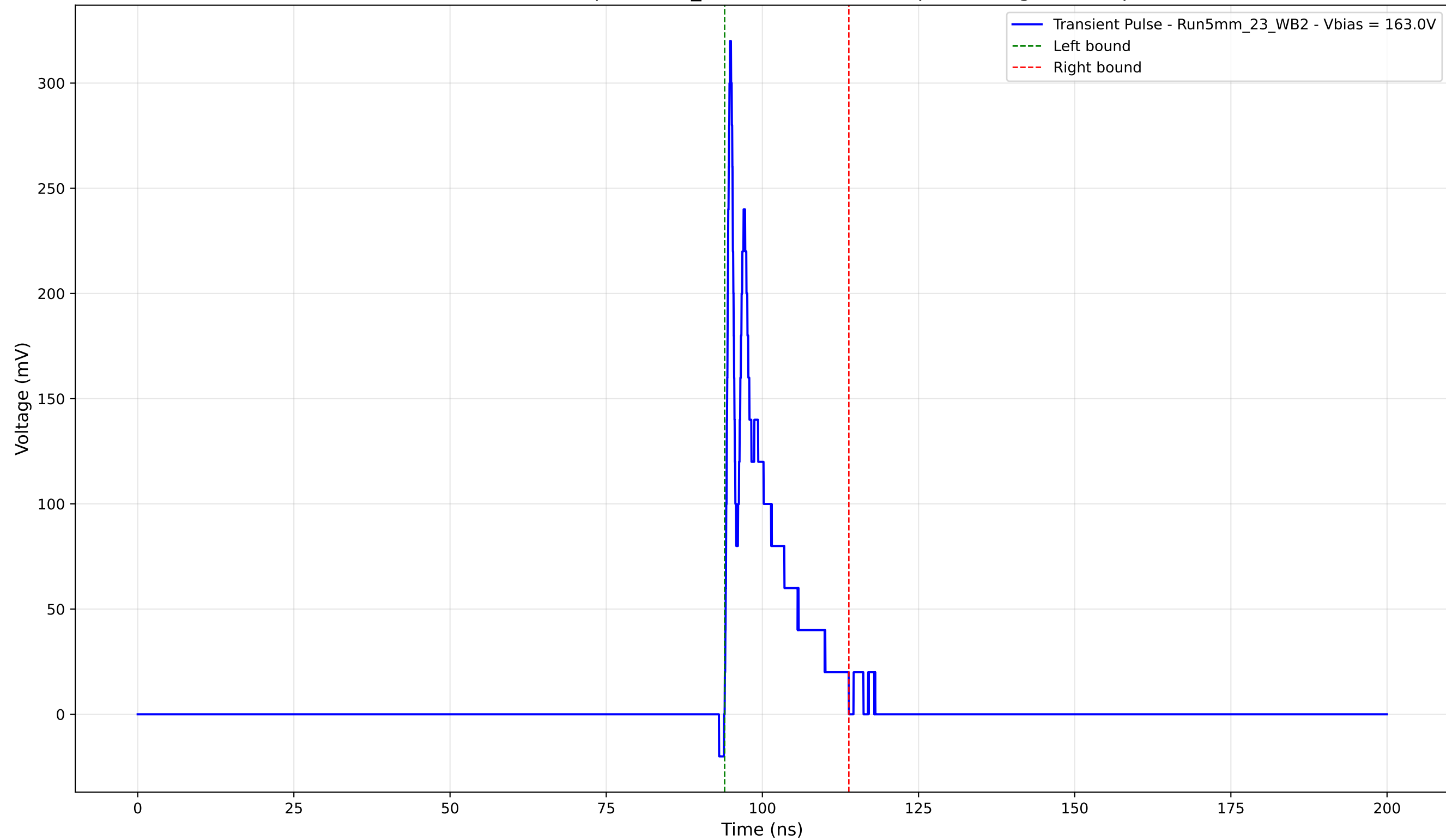
Transient Pulse - Sample: 5mm_23 - Position: 2515.0 \mu\text{m} - Charge: 33.49 pC
