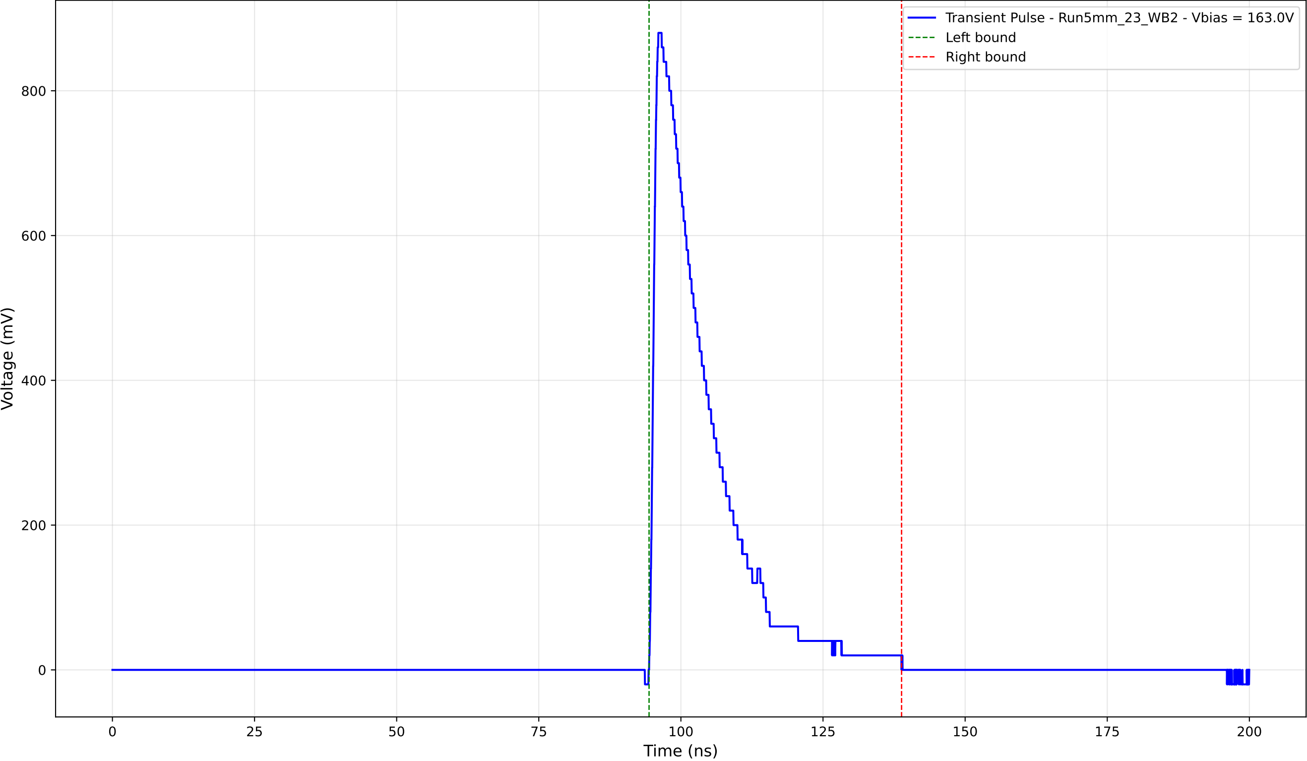
Transient Pulse - Sample: 5mm_23 - Position: 1110.0 \mu\text{m} - Charge: 186.30 pC
