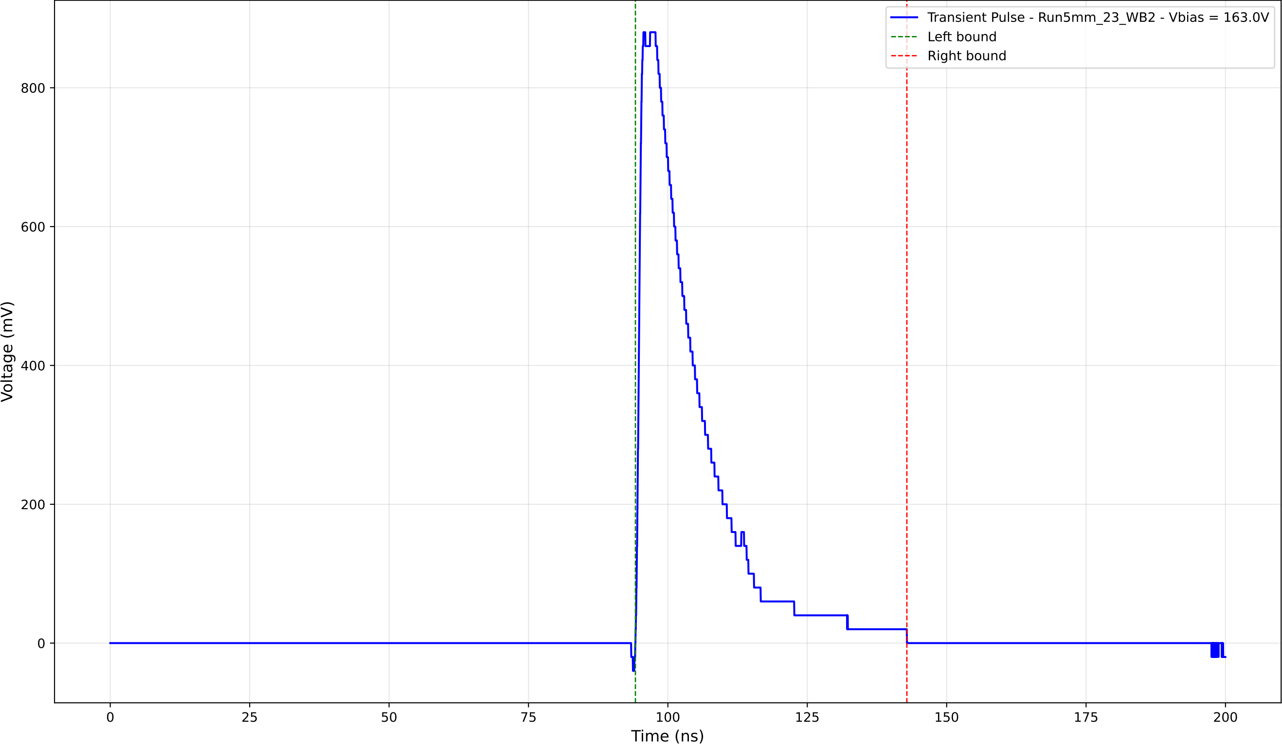
Transient Pulse - Sample: 5mm_23 - Position: 3315.0 \mu\text{m} - Charge: 203.90 pC
