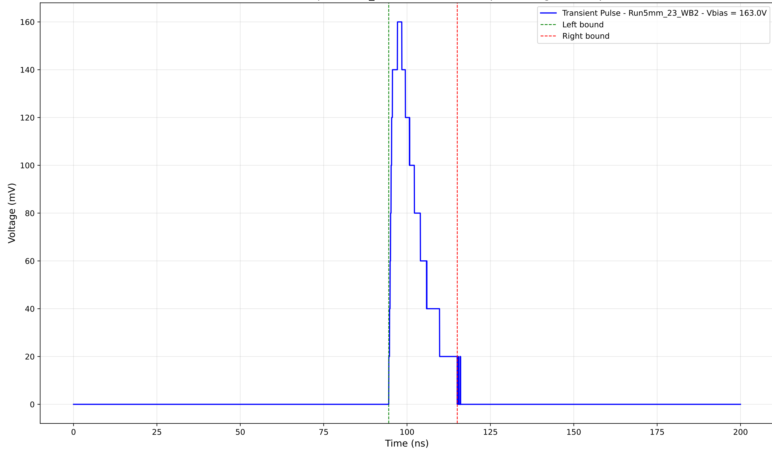
Transient Pulse - Sample: 5mm_23 - Position: 3525.0 \mu\text{m} - Charge: 29.19 pC
