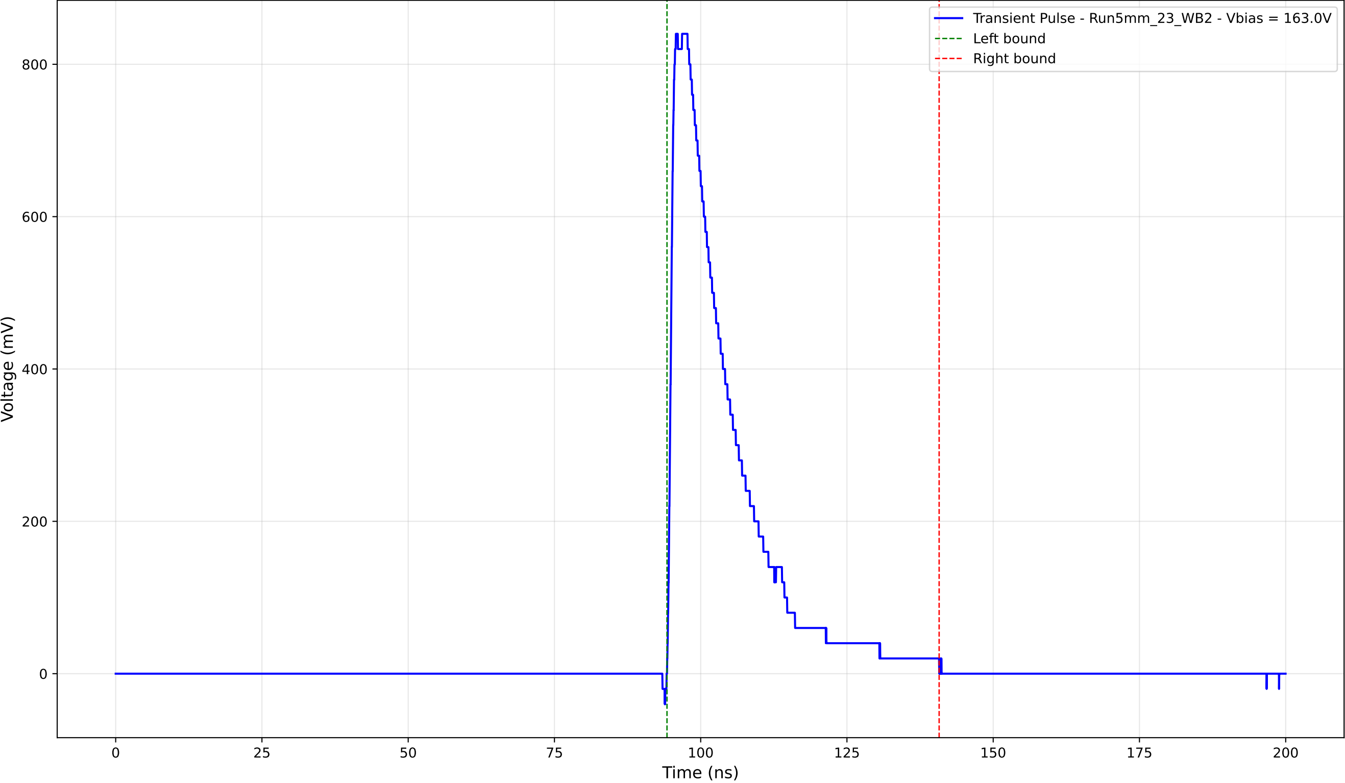
Transient Pulse - Sample: 5mm_23 - Position: 3385.0 \mu\text{m} - Charge: 188.73 pC
