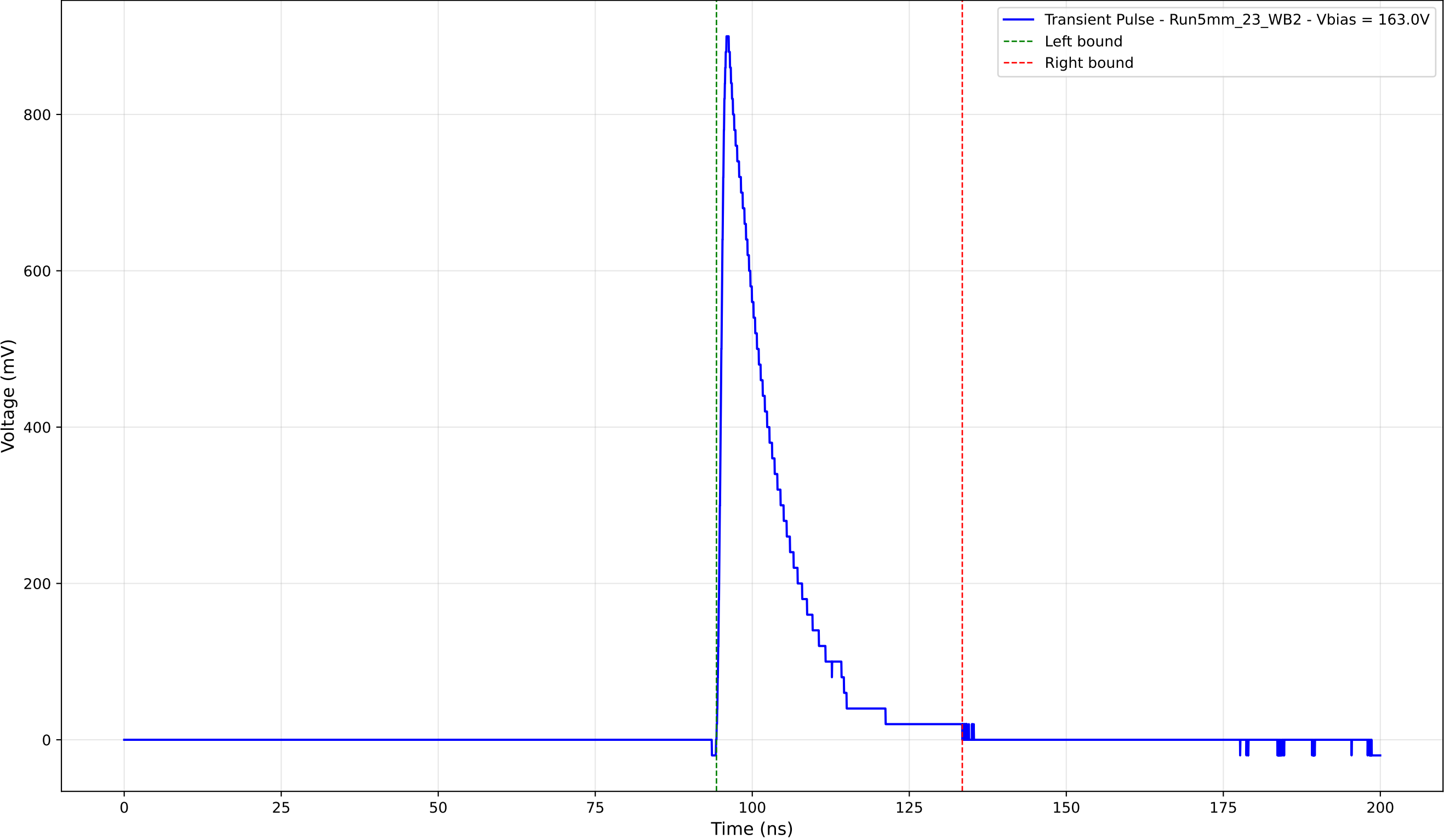
Transient Pulse - Sample: 5mm_23 - Position: 4390.0 \mu\text{m} - Charge: 157.40 pC
