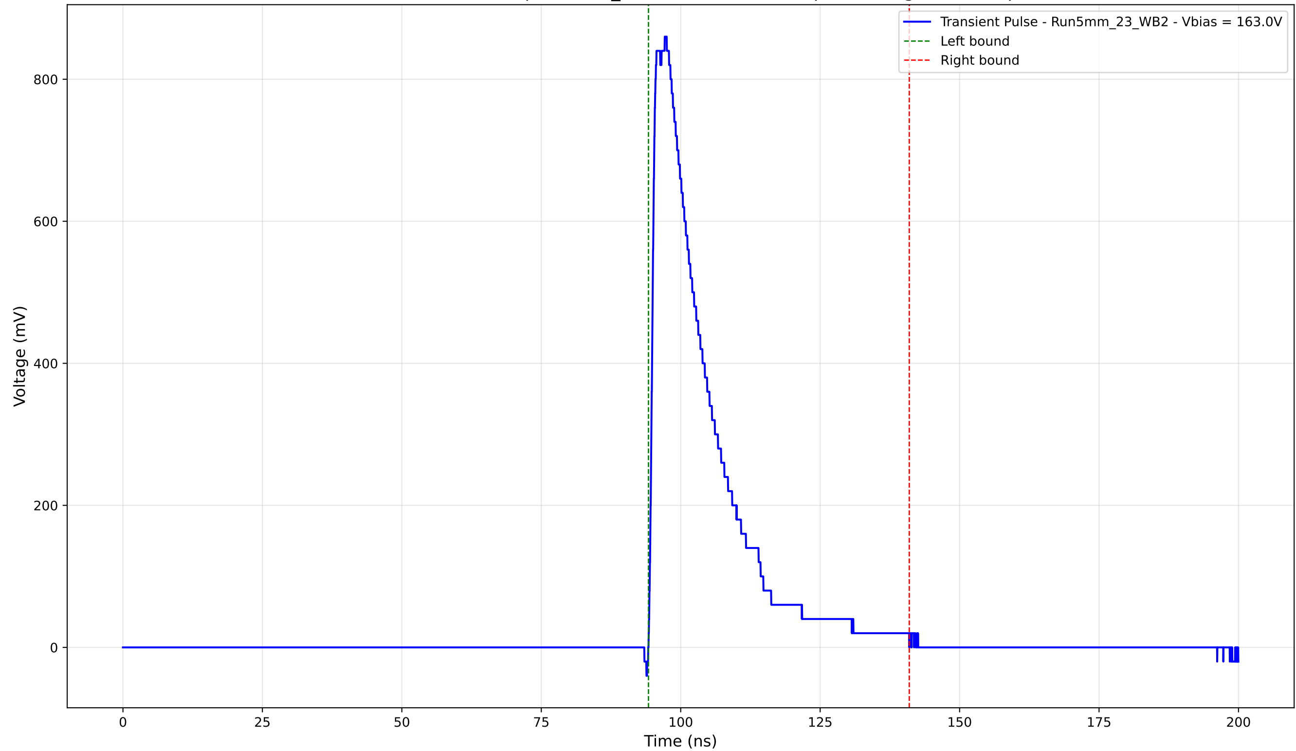
Transient Pulse - Sample: 5mm_23 - Position: 3370.0 \mu\text{m} - Charge: 191.72 pC
