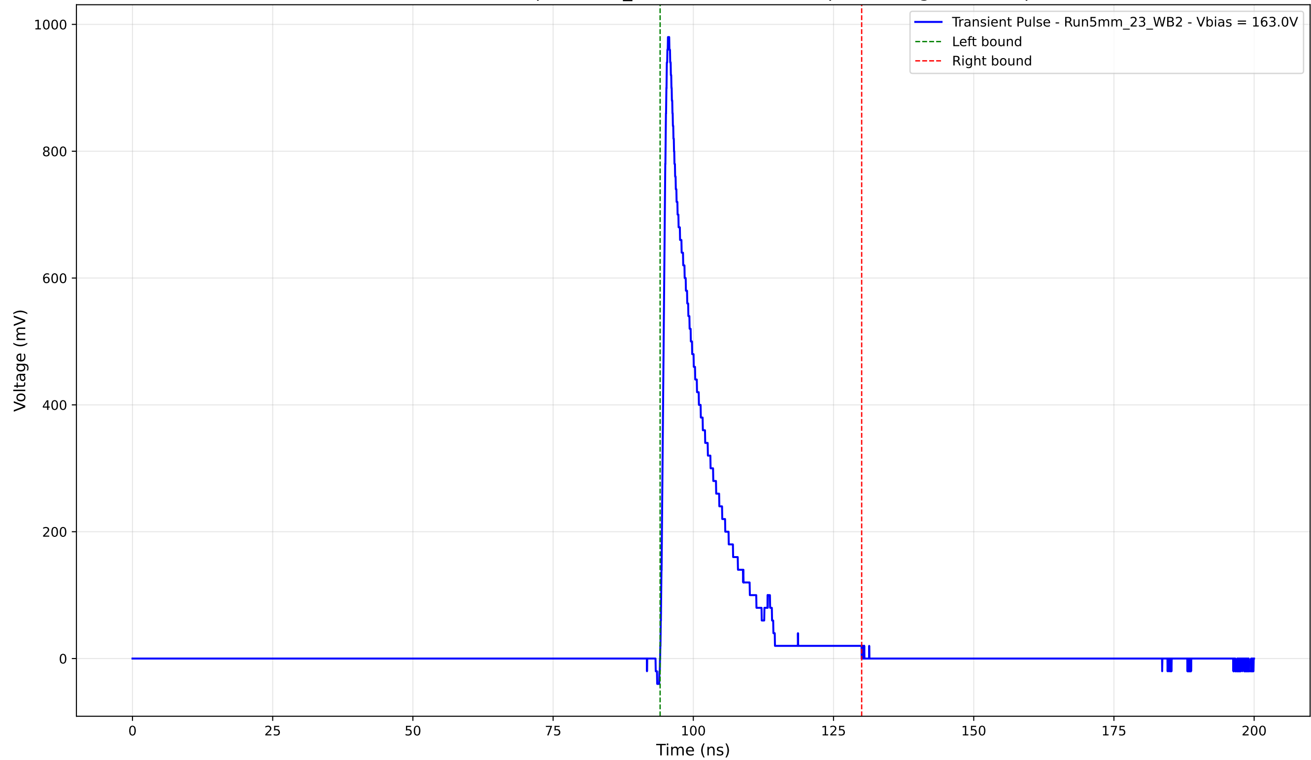
Transient Pulse - Sample: 5mm_23 - Position: 4850.0 \mu\text{m} - Charge: 141.26 pC
