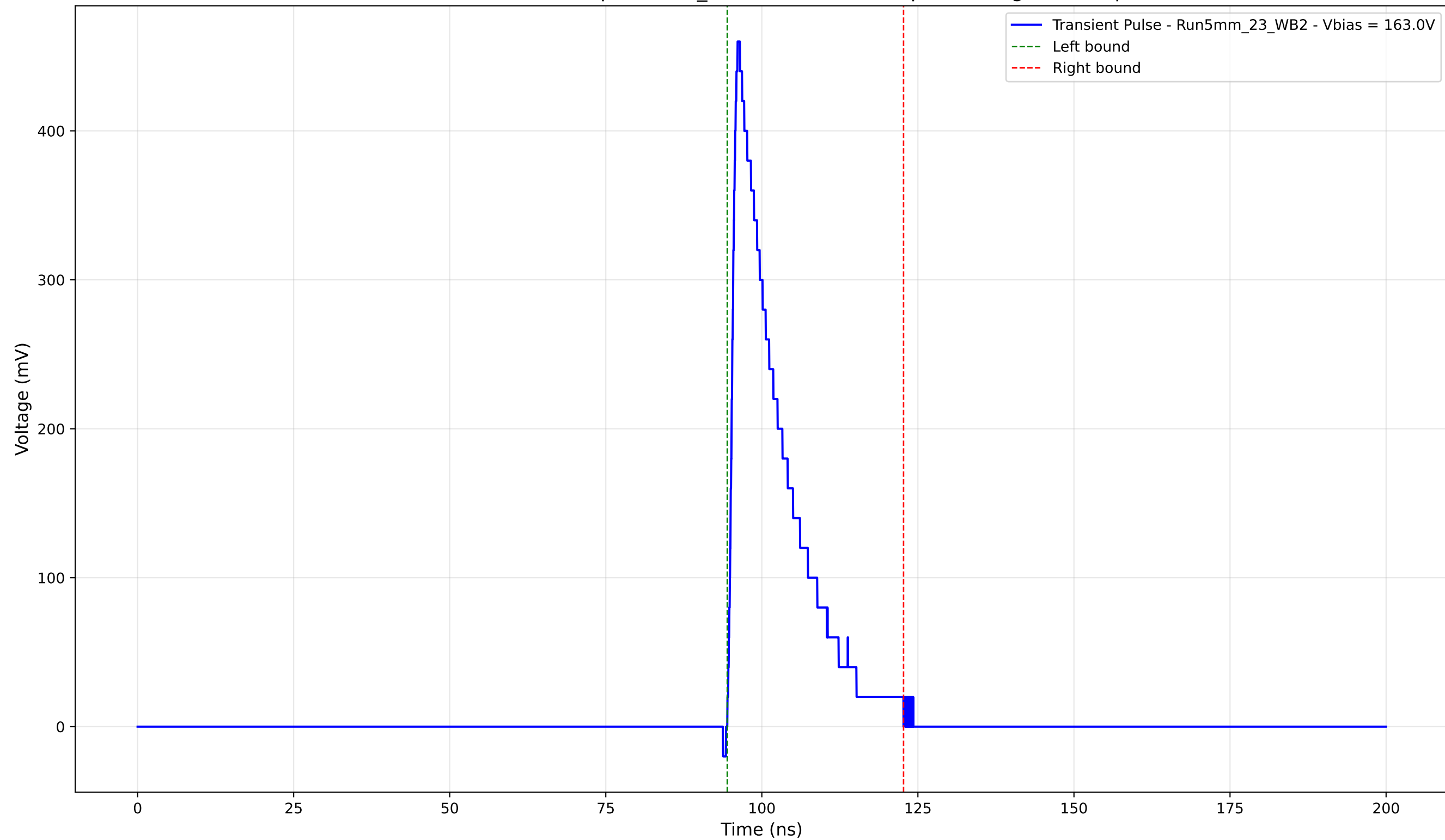
Transient Pulse - Sample: 5mm_23 - Position: 955.0 \mu\text{m} - Charge: 78.06 pC
