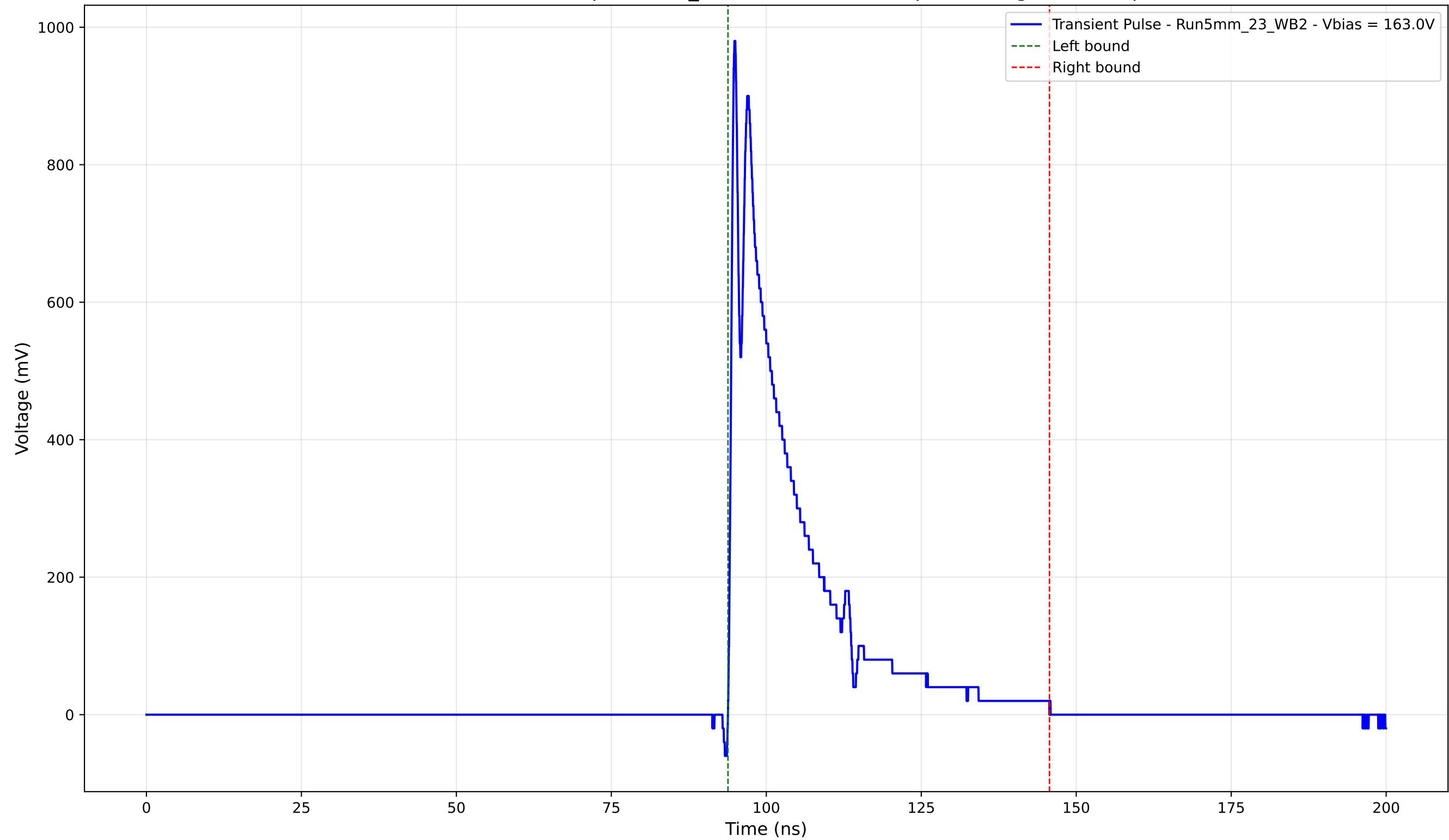
Transient Pulse - Sample: 5mm_23 - Position: 2425.0 \mu\text{m} - Charge: 188.36 pC
