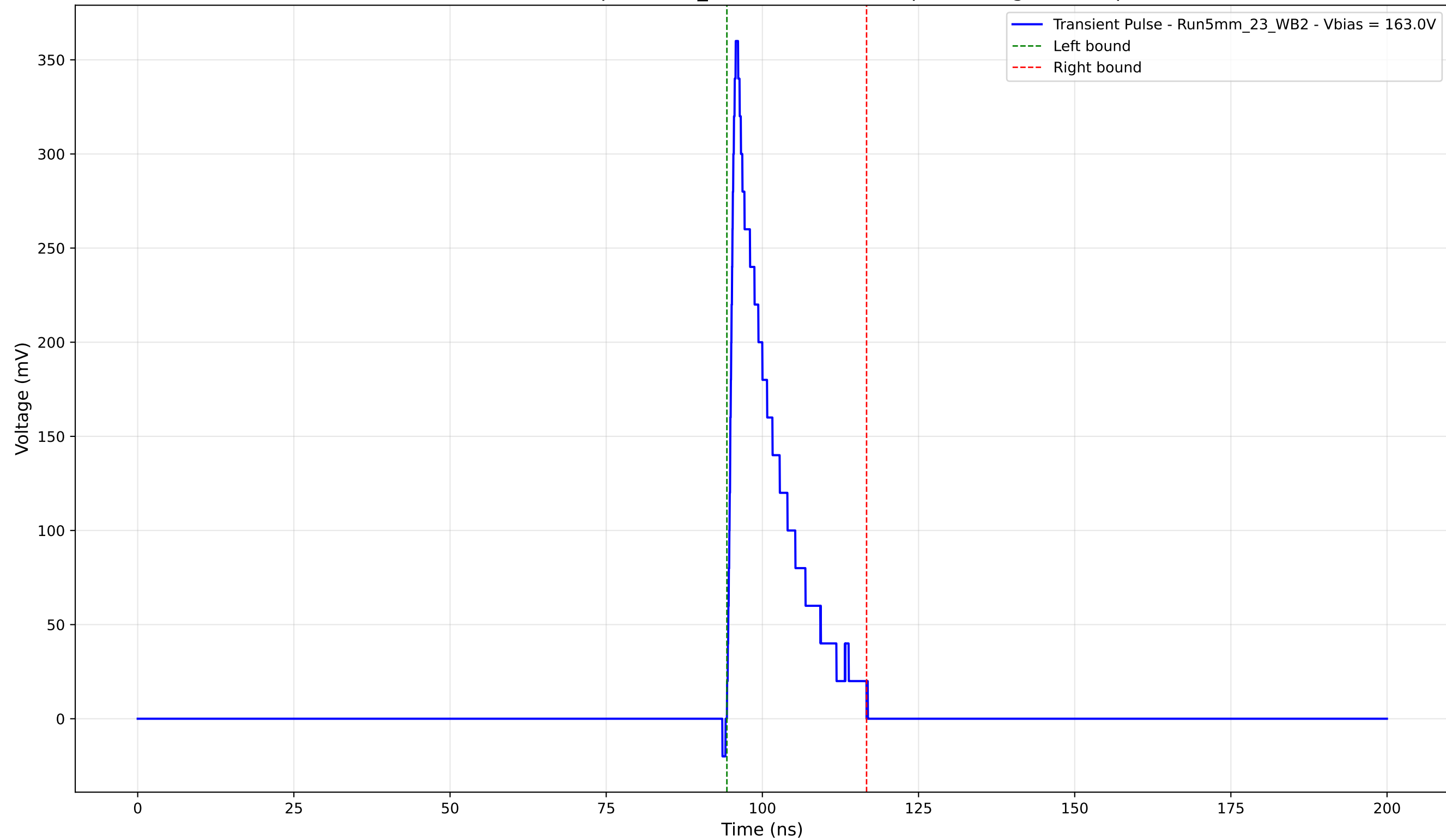
Transient Pulse - Sample: 5mm_23 - Position: 465.0 \mu\text{m} - Charge: 51.64 pC
