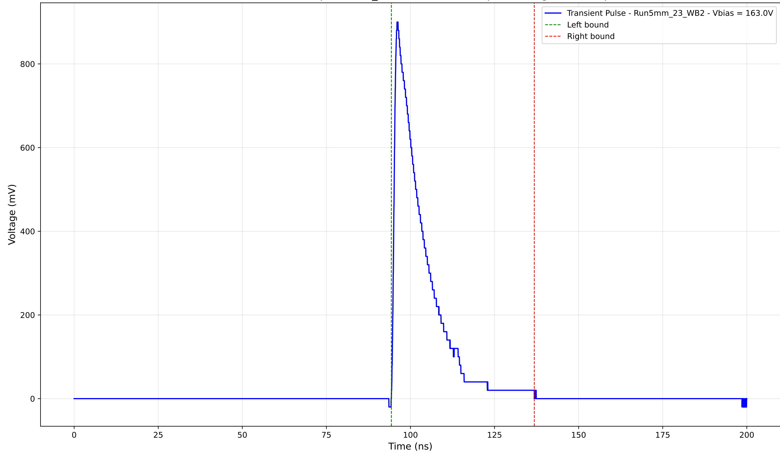
Transient Pulse - Sample: 5mm_23 - Position: 730.0 \mu\text{m} - Charge: 172.06 pC
