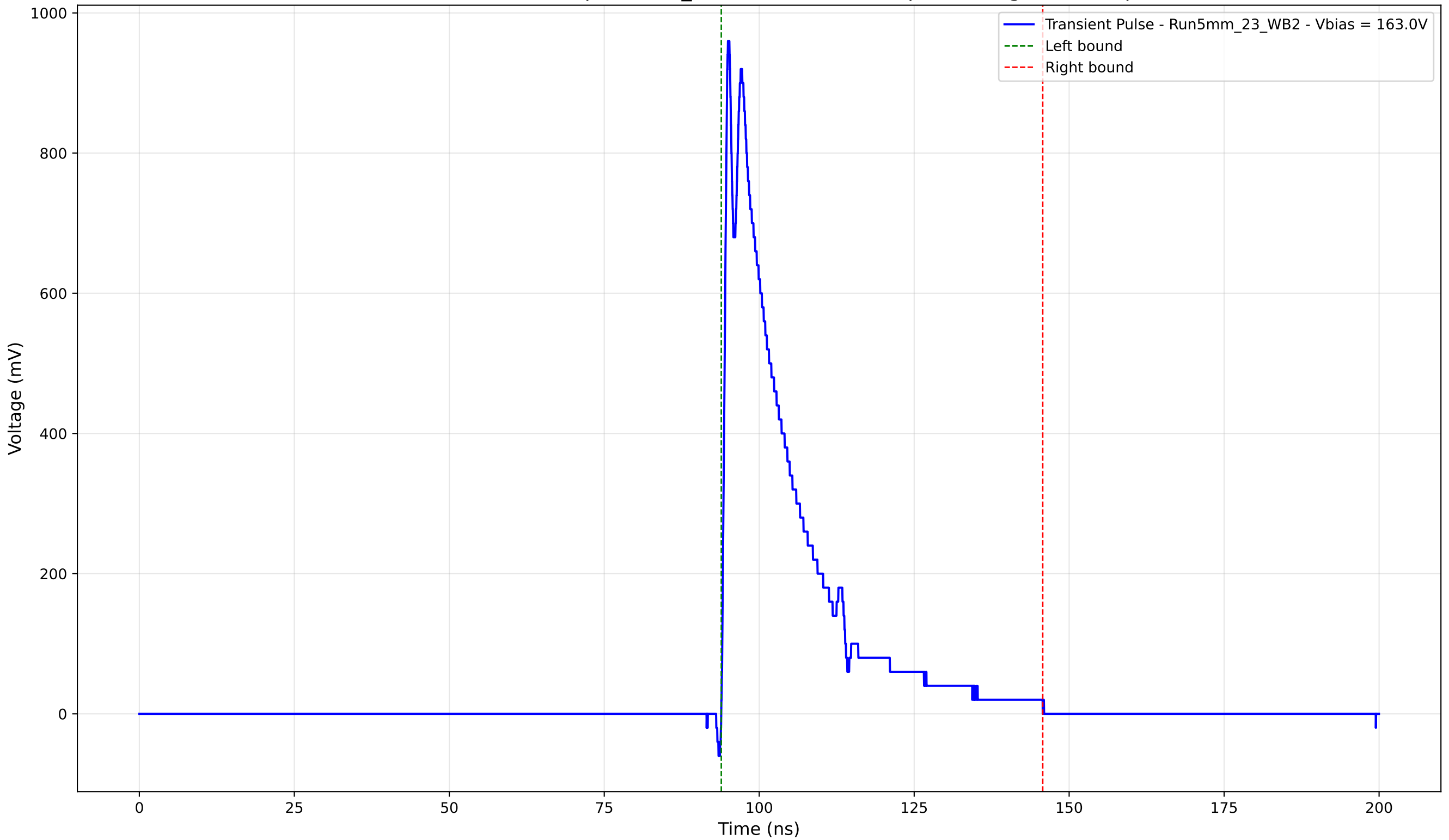
Transient Pulse - Sample: 5mm_23 - Position: 2765.0 \mu\text{m} - Charge: 204.57 pC
