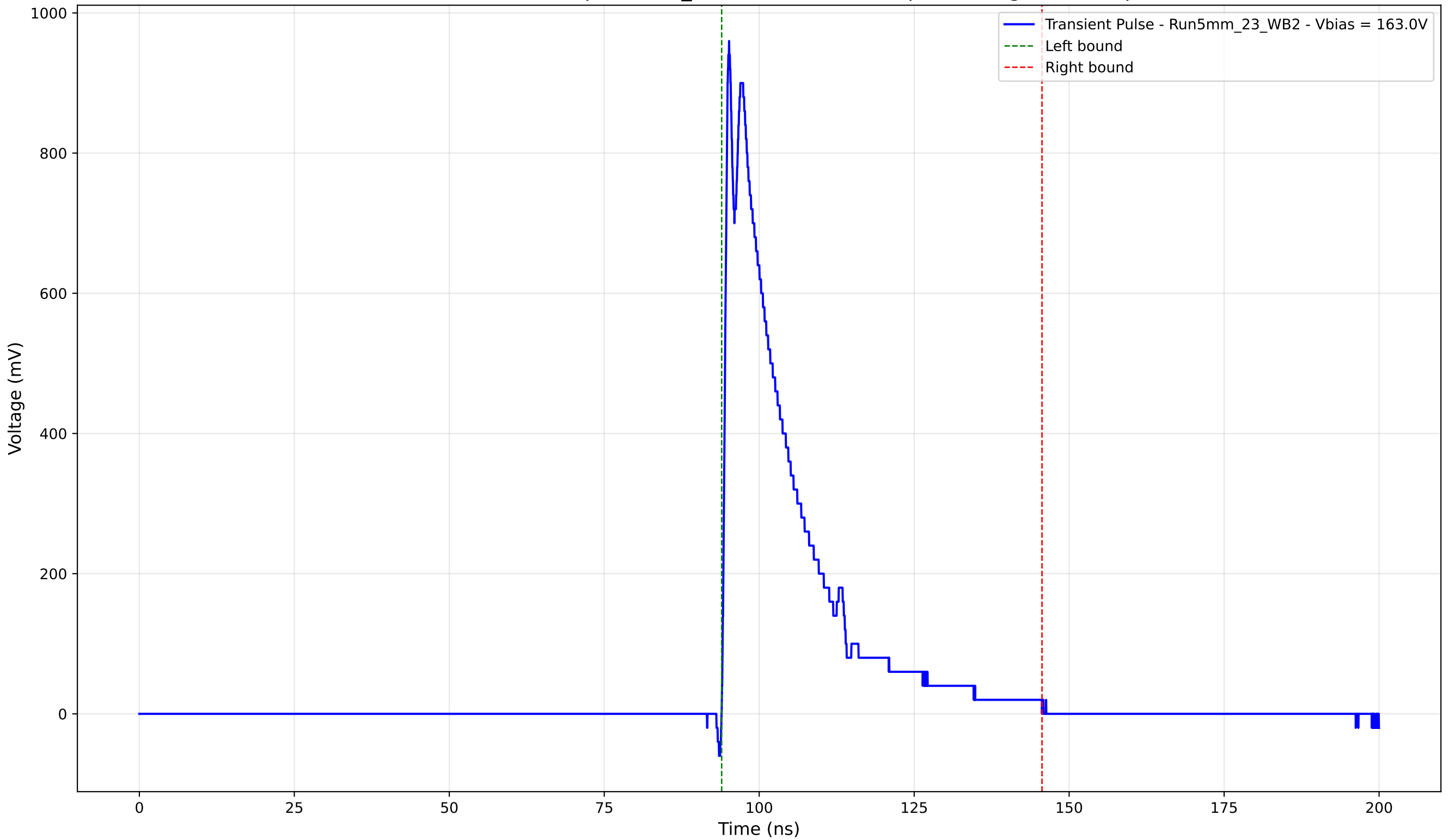
Transient Pulse - Sample: 5mm_23 - Position: 2200.0 \mu\text{m} - Charge: 206.02 pC
