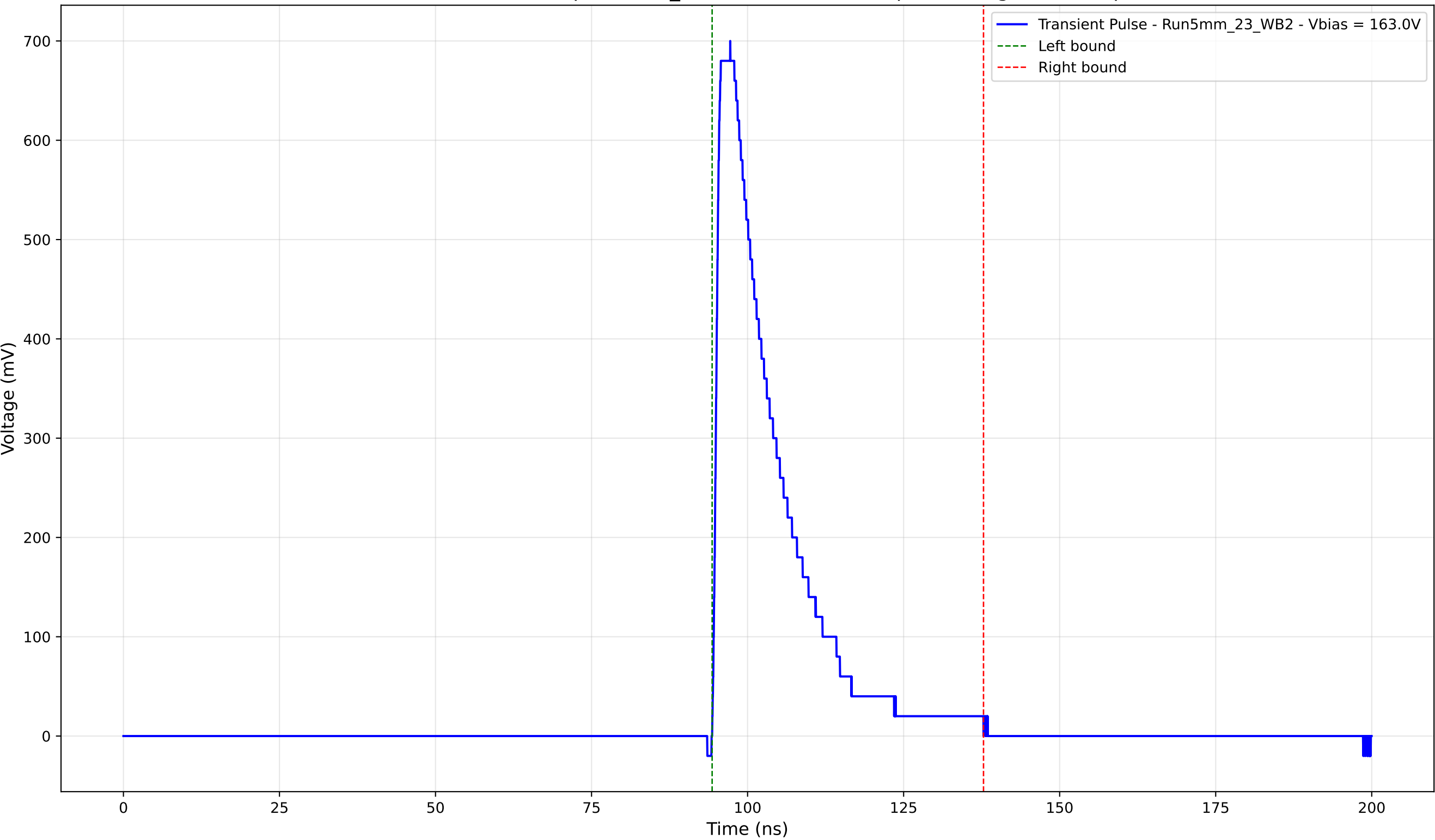
Transient Pulse - Sample: 5mm_23 - Position: 1565.0 \mu\text{m} - Charge: 147.11 pC
