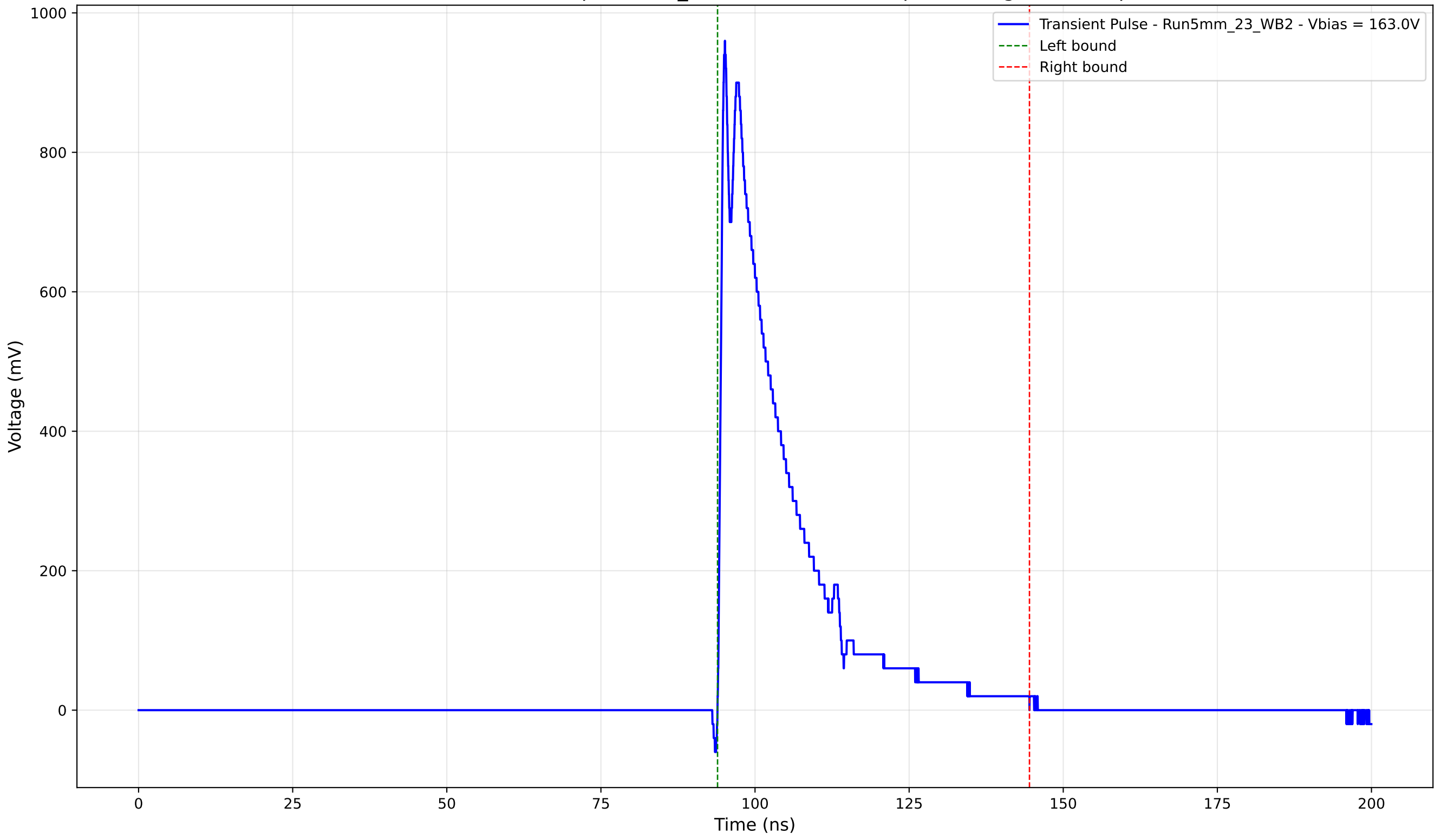
Transient Pulse - Sample: 5mm_23 - Position: 2220.0 \mu\text{m} - Charge: 204.53 pC
