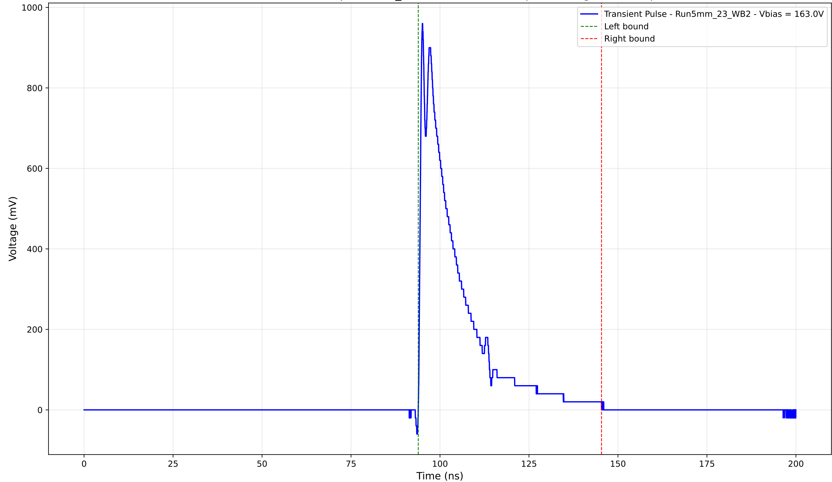
Transient Pulse - Sample: 5mm_23 - Position: 2250.0 \mu\text{m} - Charge: 204.39 pC
