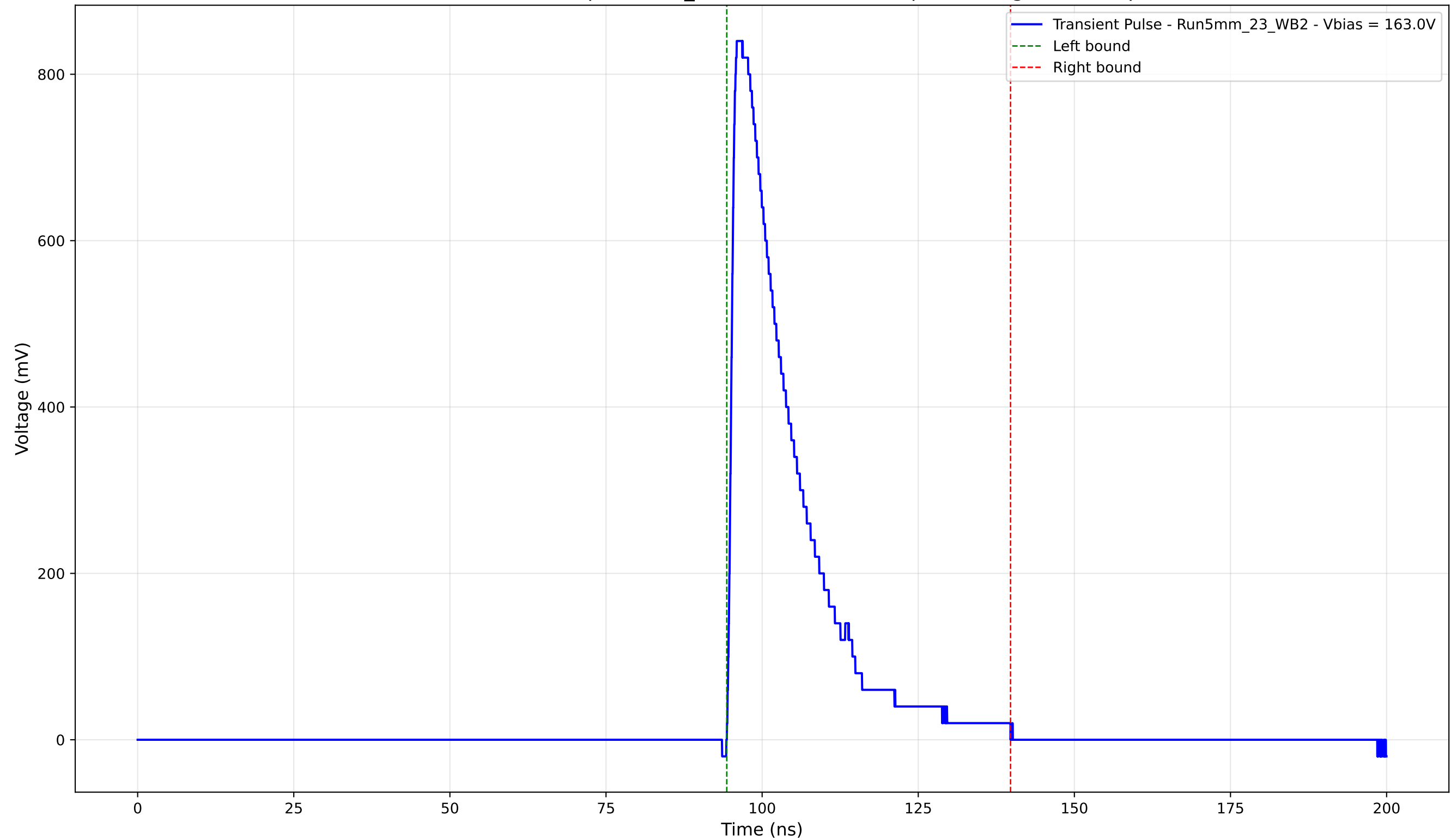
Transient Pulse - Sample: 5mm_23 - Position: 1410.0 \mu\text{m} - Charge: 184.70 pC
