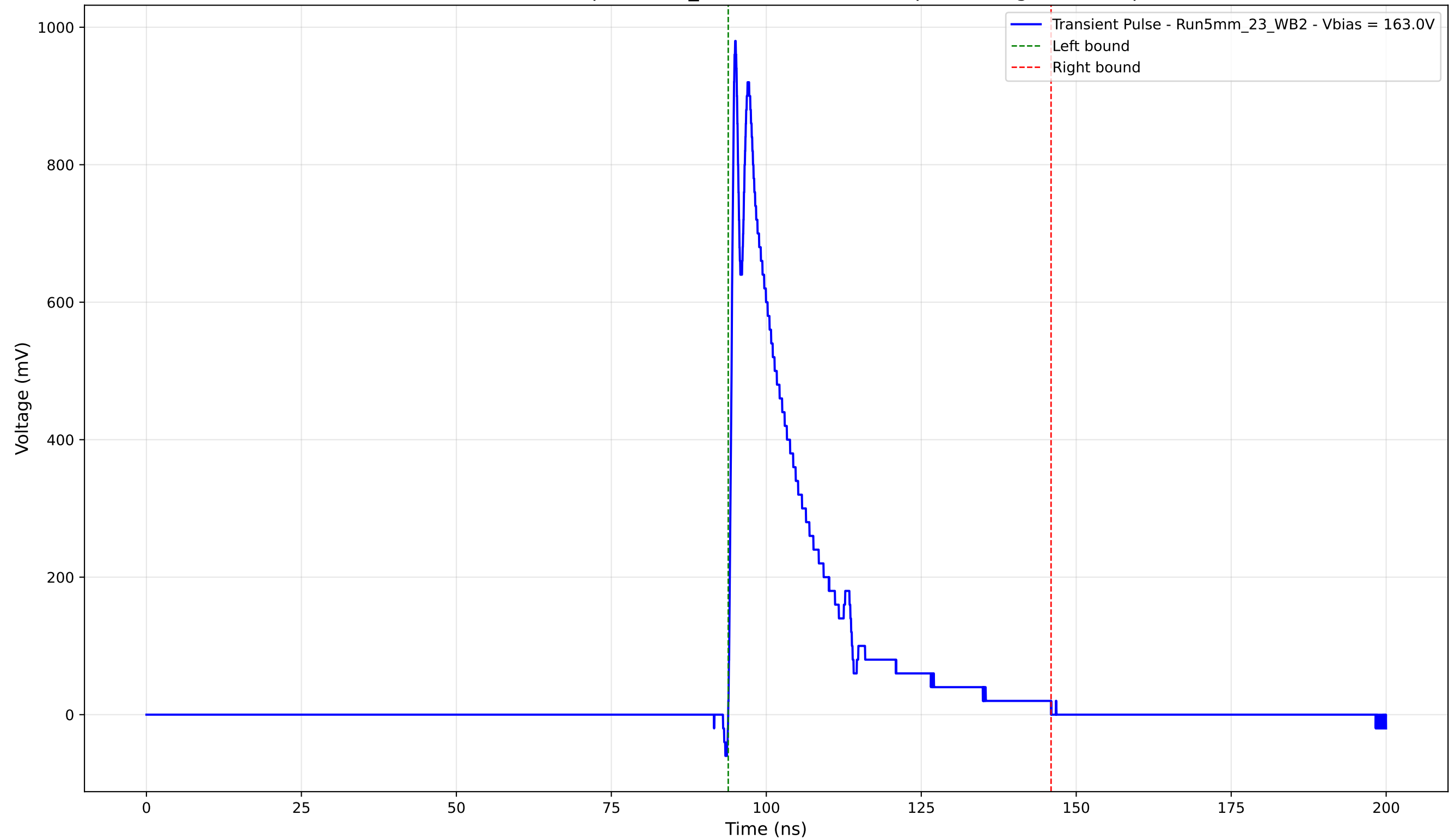
Transient Pulse - Sample: 5mm_23 - Position: 2715.0 \mu\text{m} - Charge: 201.69 pC
