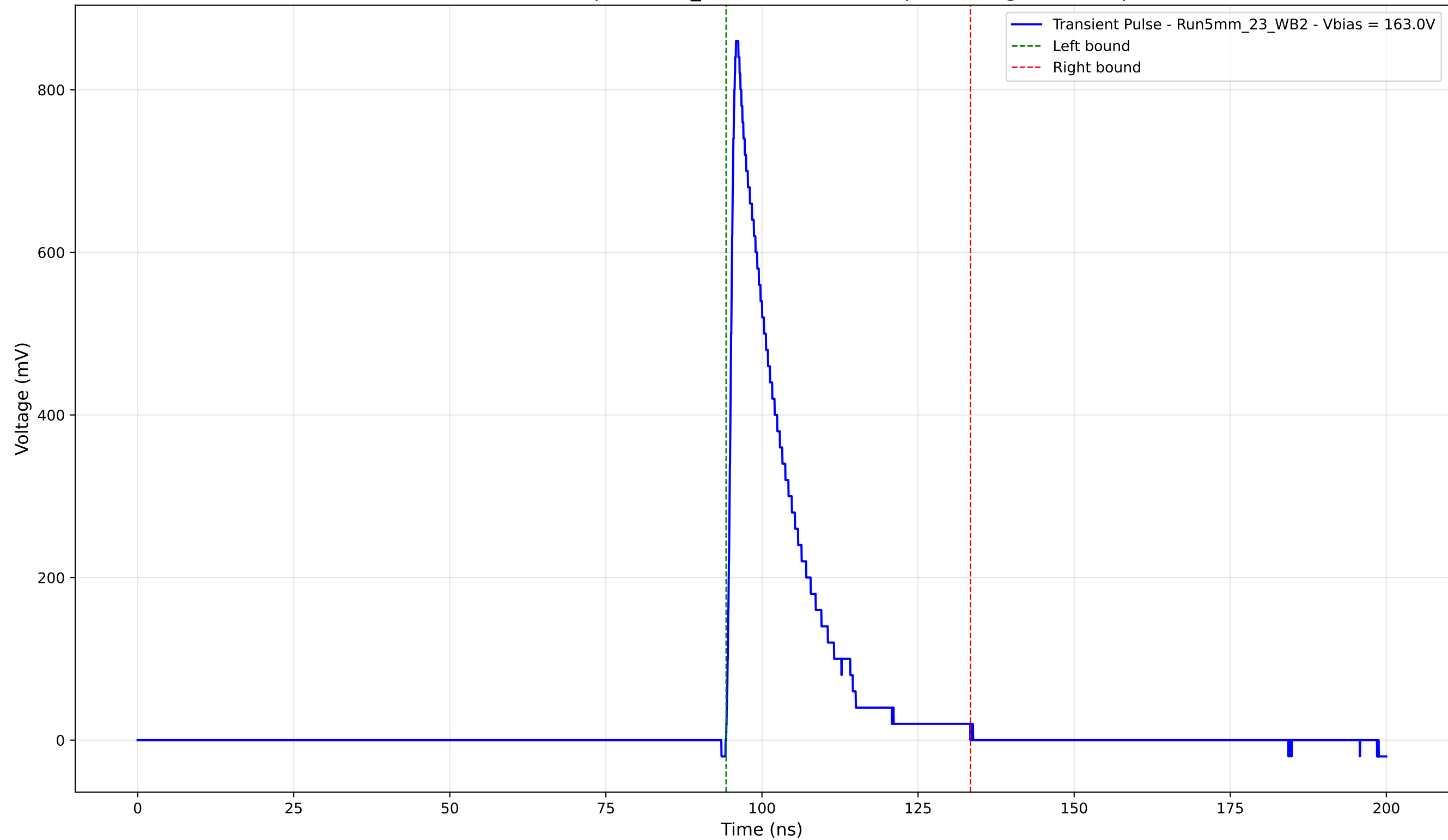
Transient Pulse - Sample: 5mm_23 - Position: 555.0 \mu\text{m} - Charge: 151.36 pC
