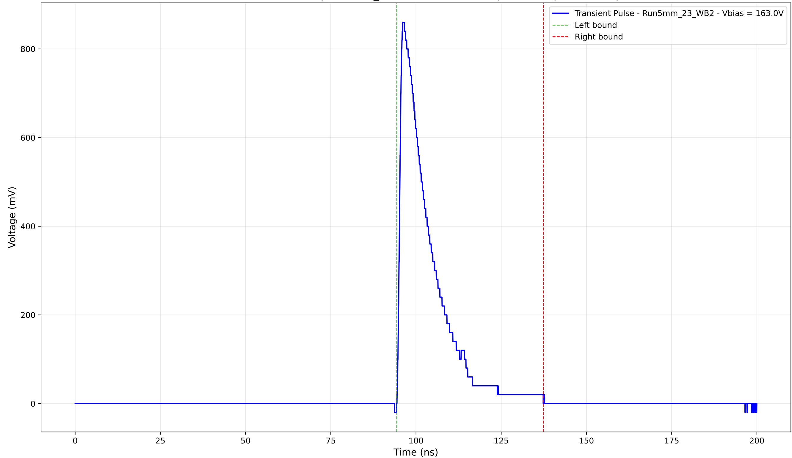
Transient Pulse - Sample: 5mm_23 - Position: 3900.0 \mu\text{m} - Charge: 170.26 pC
