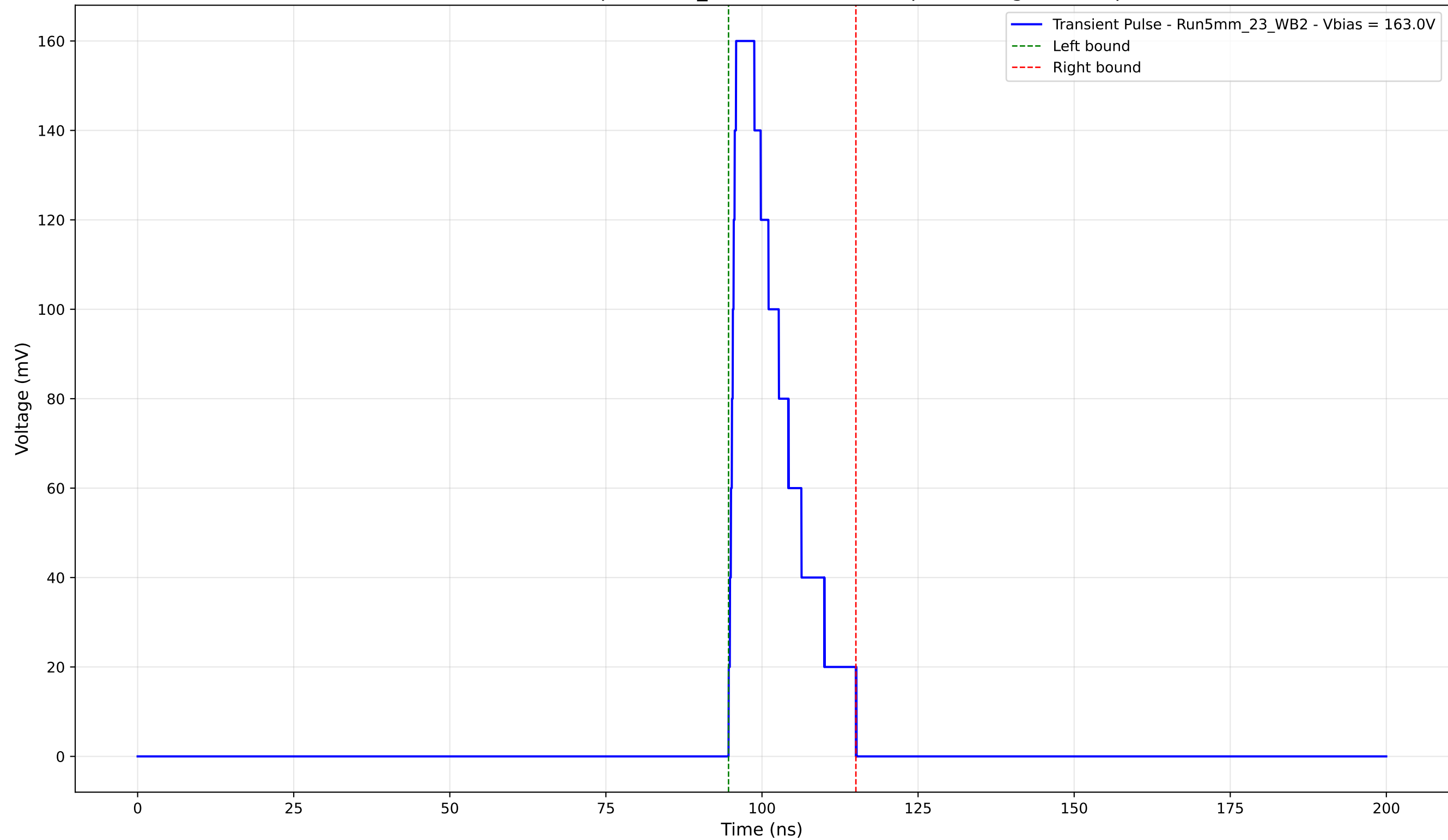
Transient Pulse - Sample: 5mm_23 - Position: 995.0 \mu\text{m} - Charge: 30.38 pC
