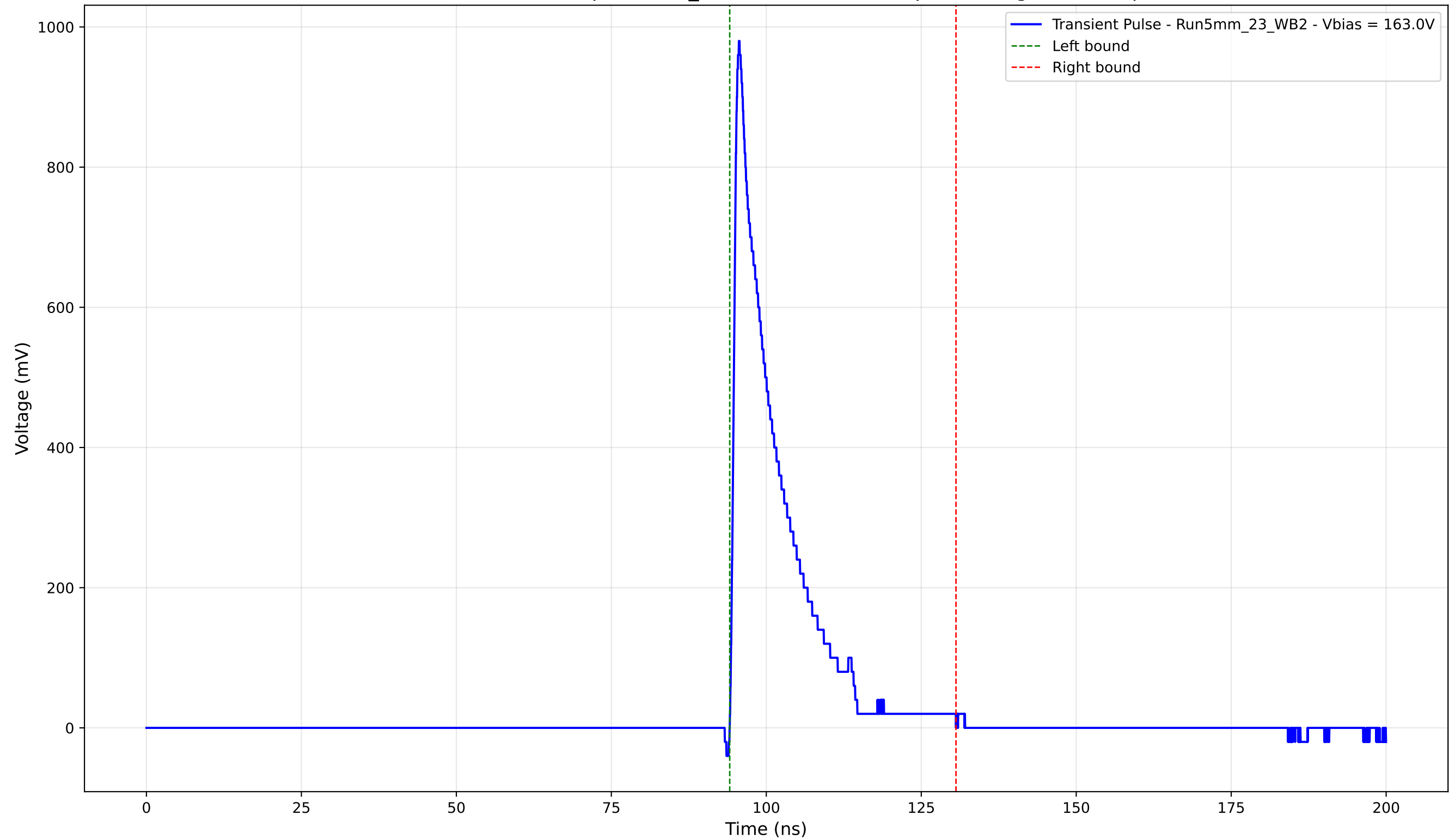
Transient Pulse - Sample: 5mm_23 - Position: 4800.0 \mu\text{m} - Charge: 145.29 pC
