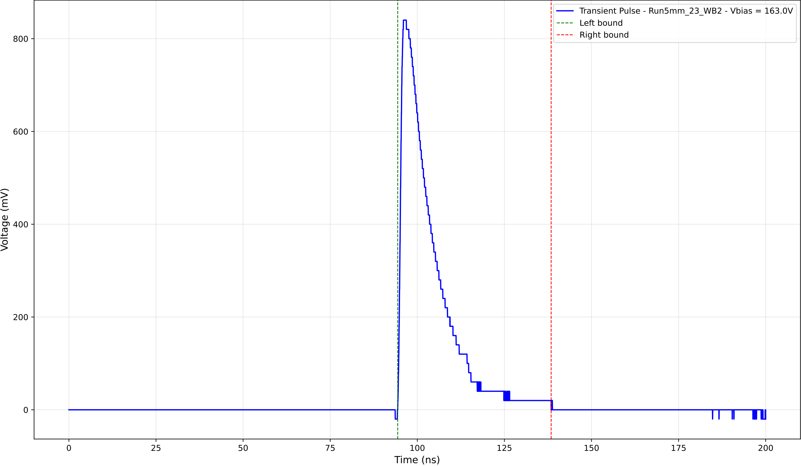
Transient Pulse - Sample: 5mm_23 - Position: 3710.0 \mu\text{m} - Charge: 175.63 pC
