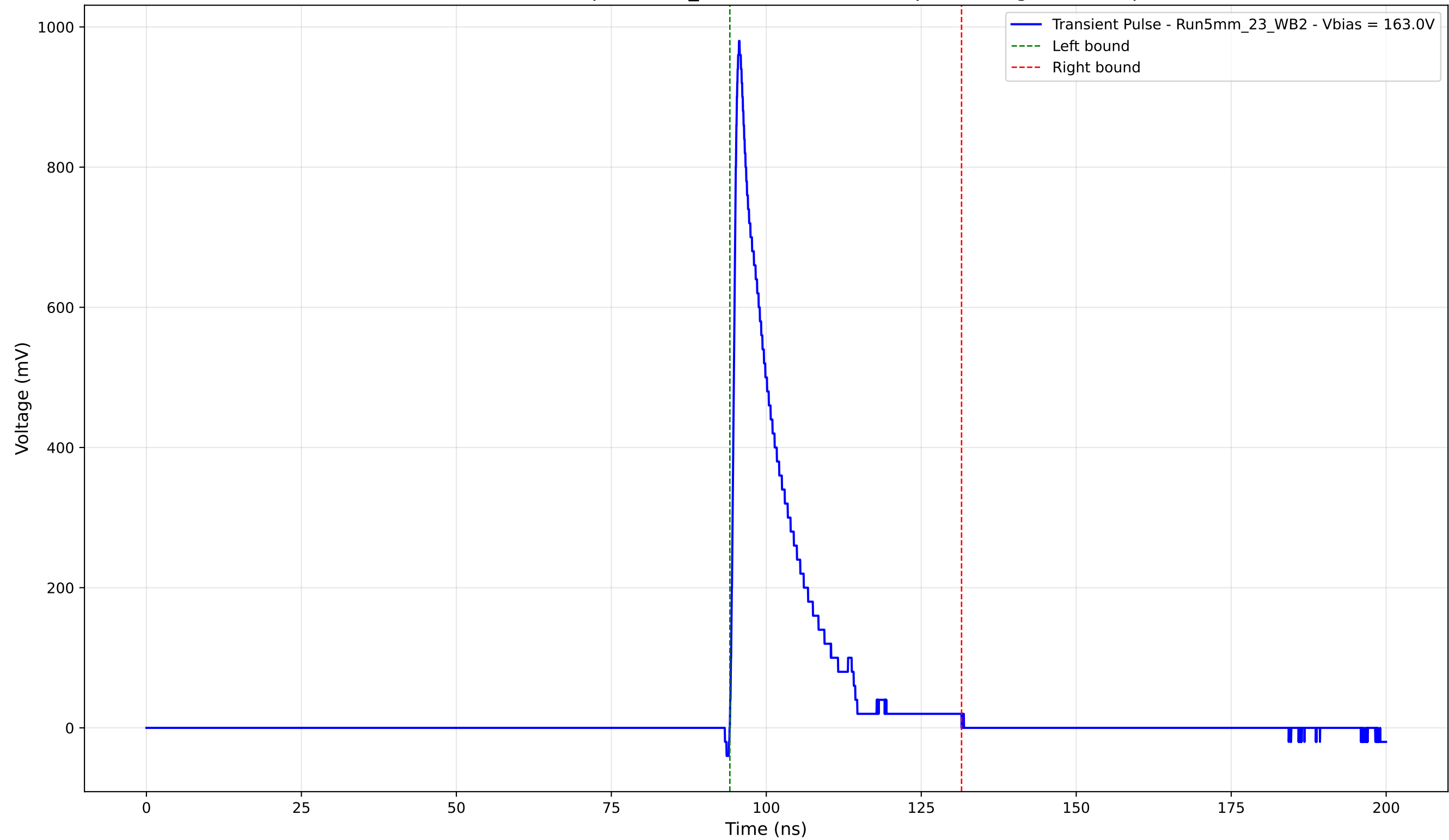
Transient Pulse - Sample: 5mm_23 - Position: 4790.0 \mu\text{m} - Charge: 146.95 pC
