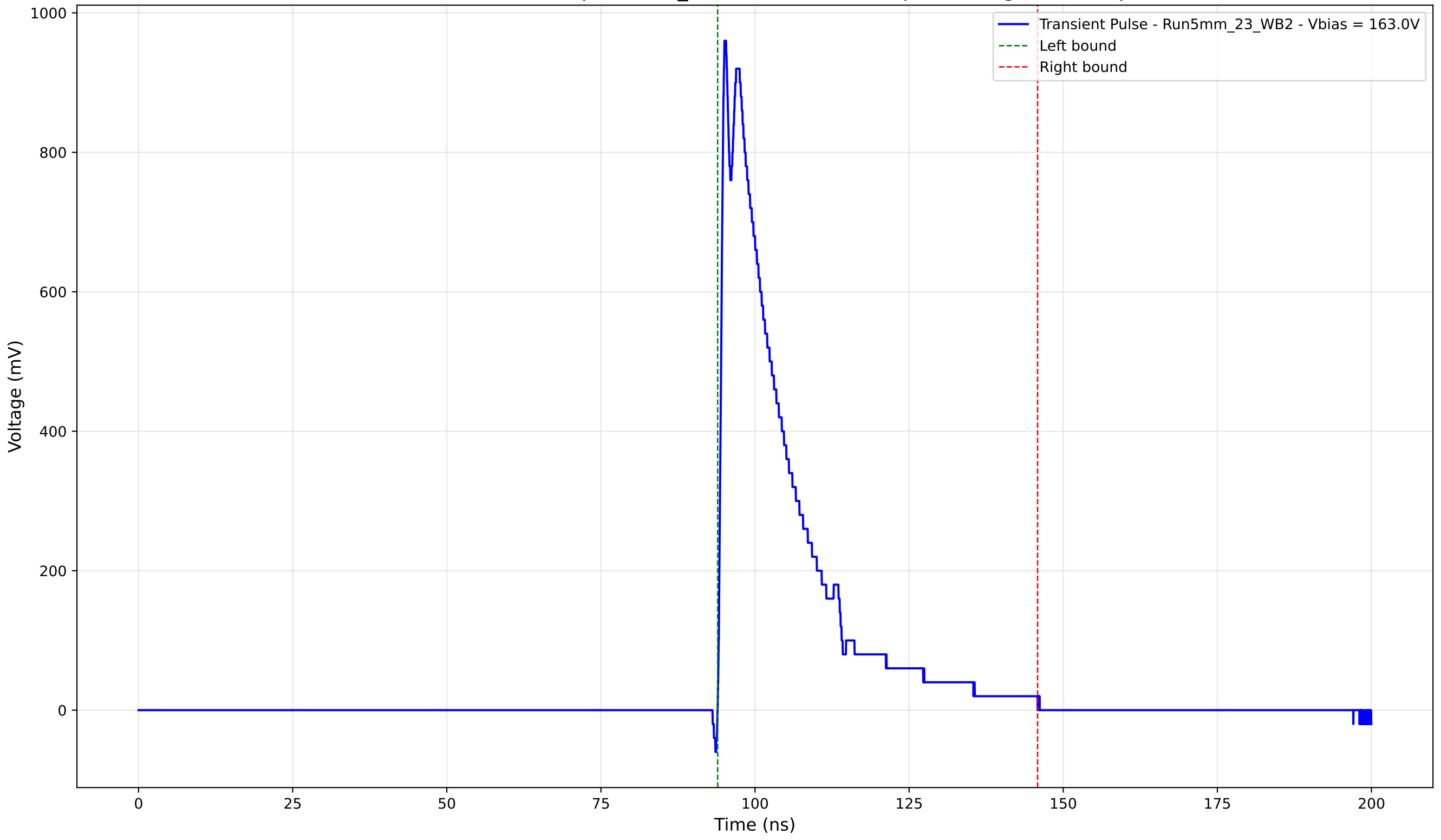
Transient Pulse - Sample: 5mm_23 - Position: 2870.0 \mu\text{m} - Charge: 215.52 pC
