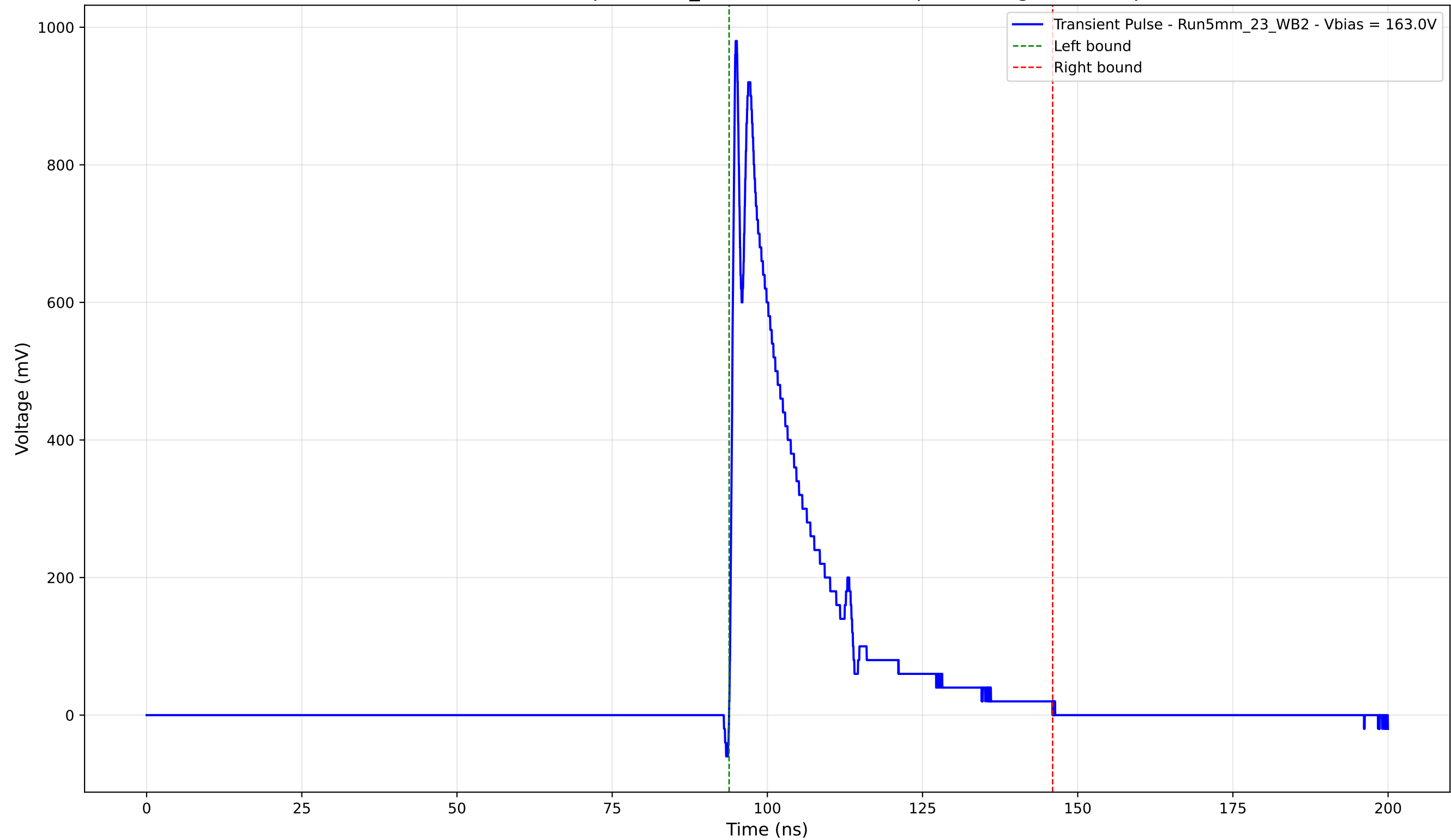
Transient Pulse - Sample: 5mm_23 - Position: 2675.0 \mu\text{m} - Charge: 202.11 pC
