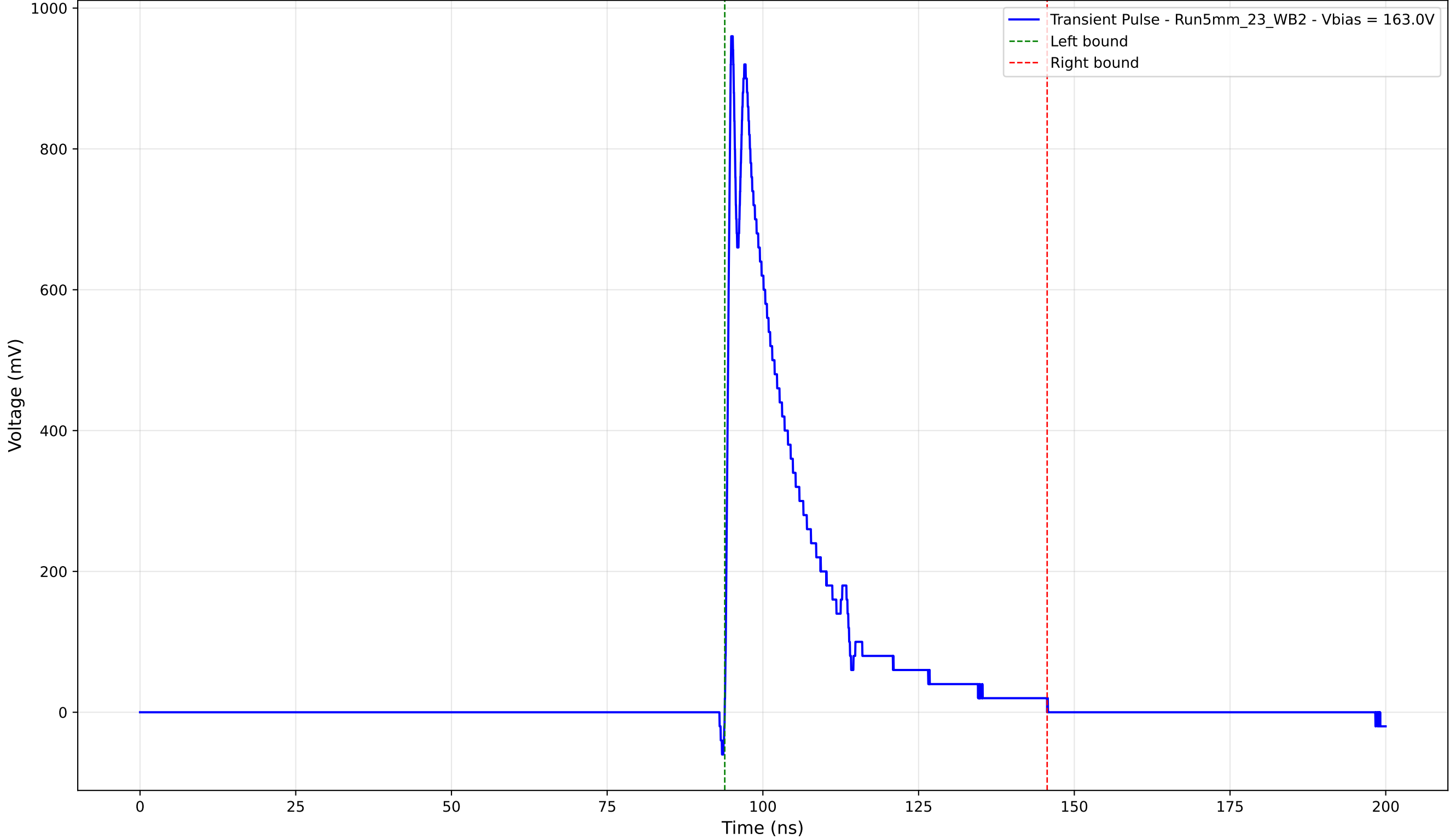
Transient Pulse - Sample: 5mm_23 - Position: 2750.0 \mu\text{m} - Charge: 203.12 pC
