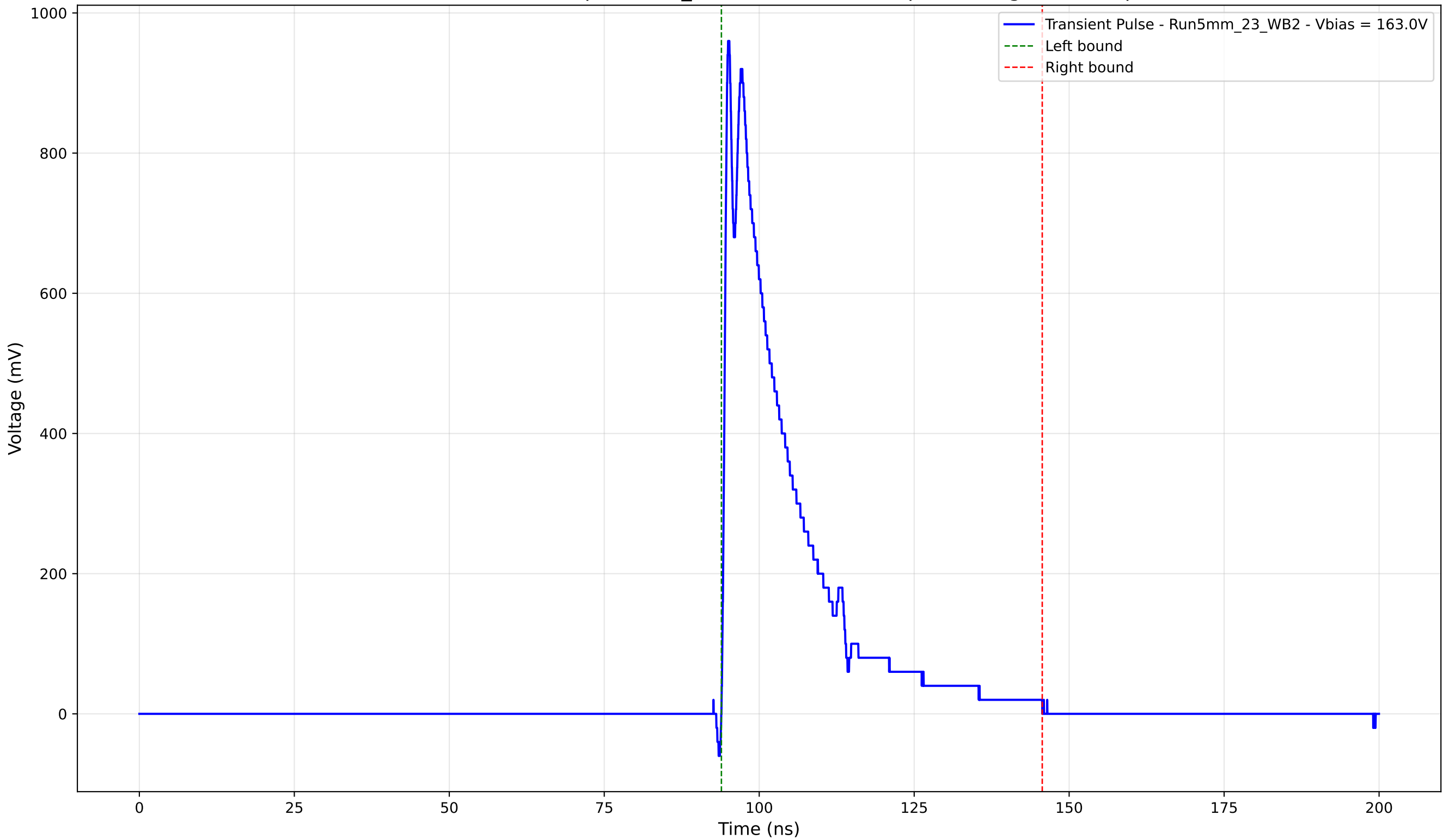
Transient Pulse - Sample: 5mm_23 - Position: 2775.0 \mu\text{m} - Charge: 205.46 pC
