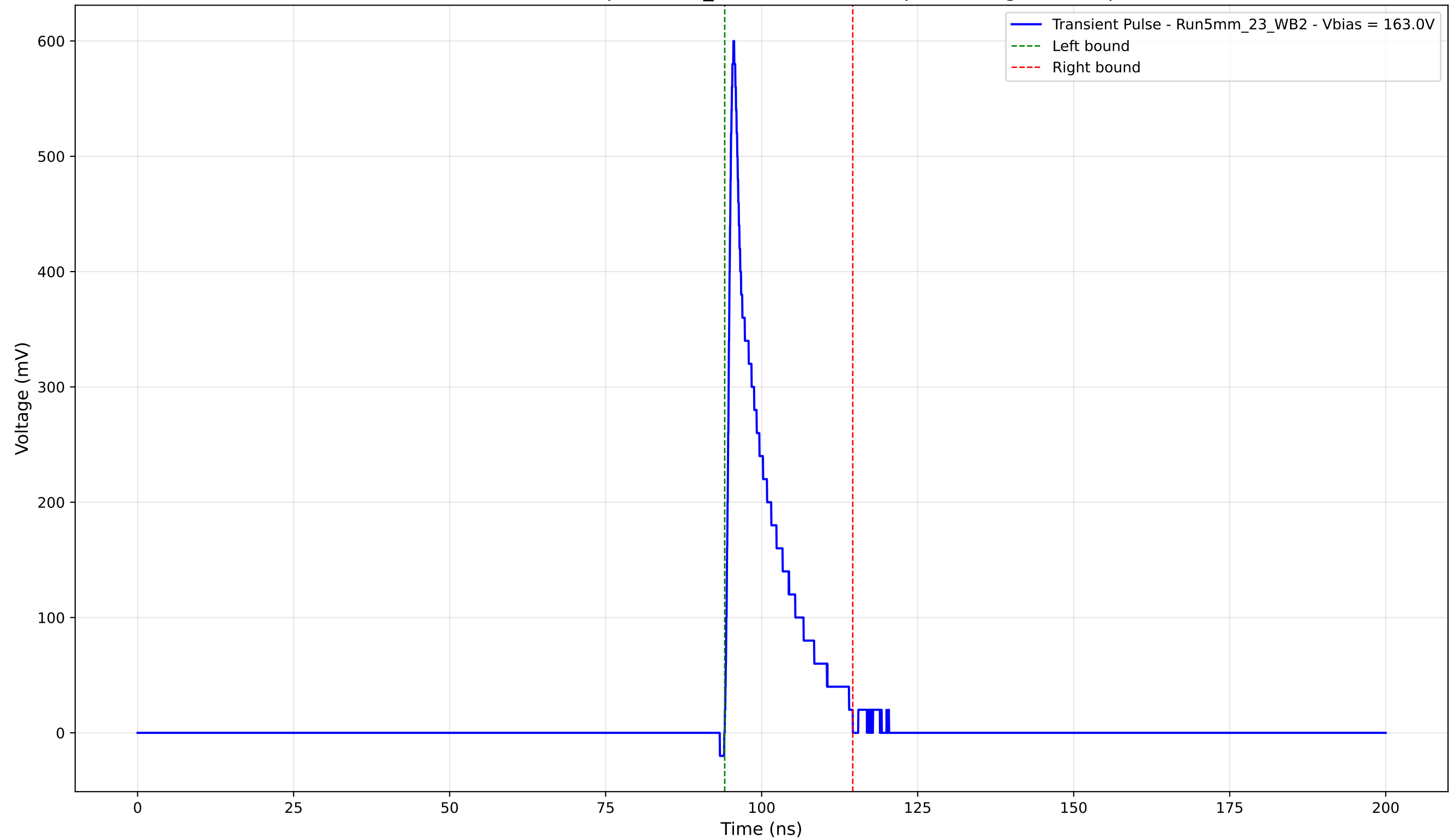
Transient Pulse - Sample: 5mm_23 - Position: 75.0 \mu\text{m} - Charge: 70.57 pC
