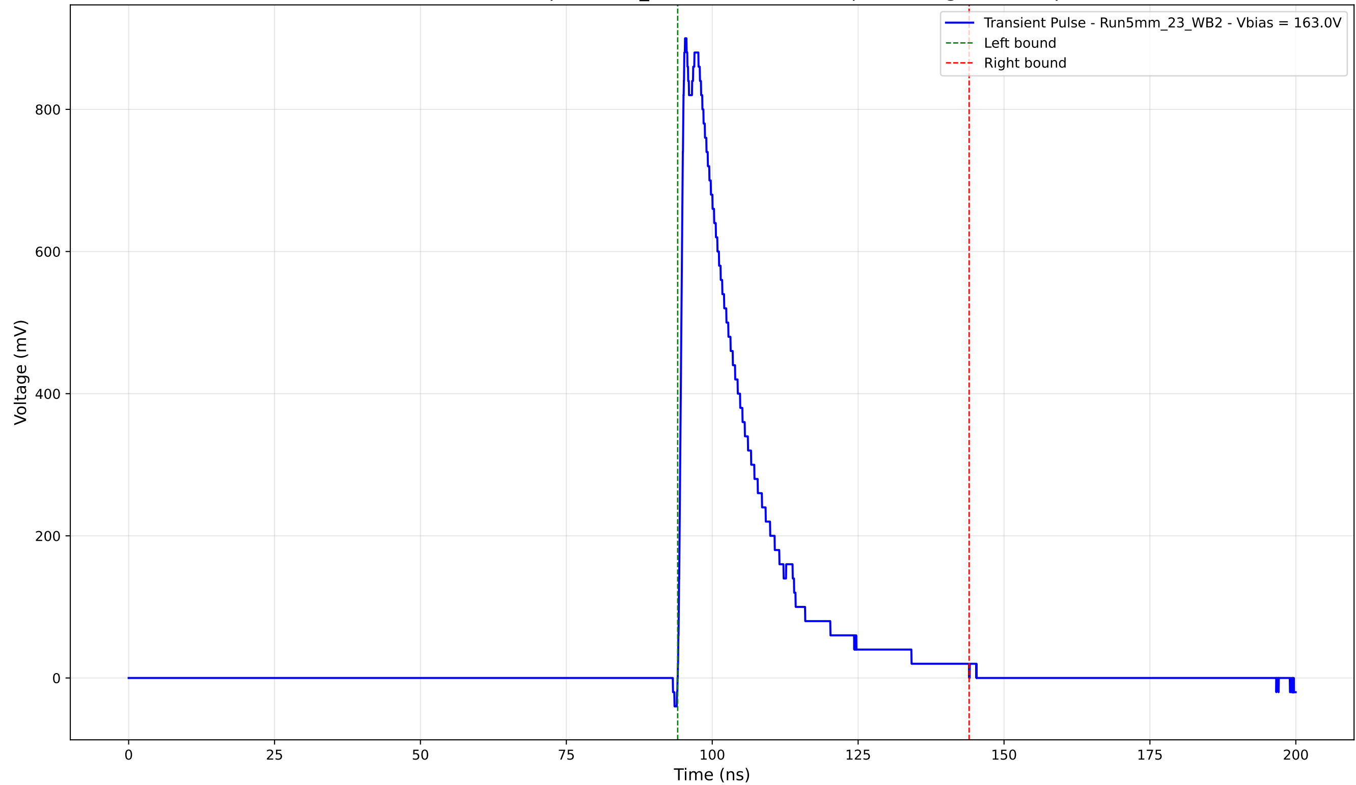
Transient Pulse - Sample: 5mm_23 - Position: 1915.0 \mu\text{m} - Charge: 208.40 pC
