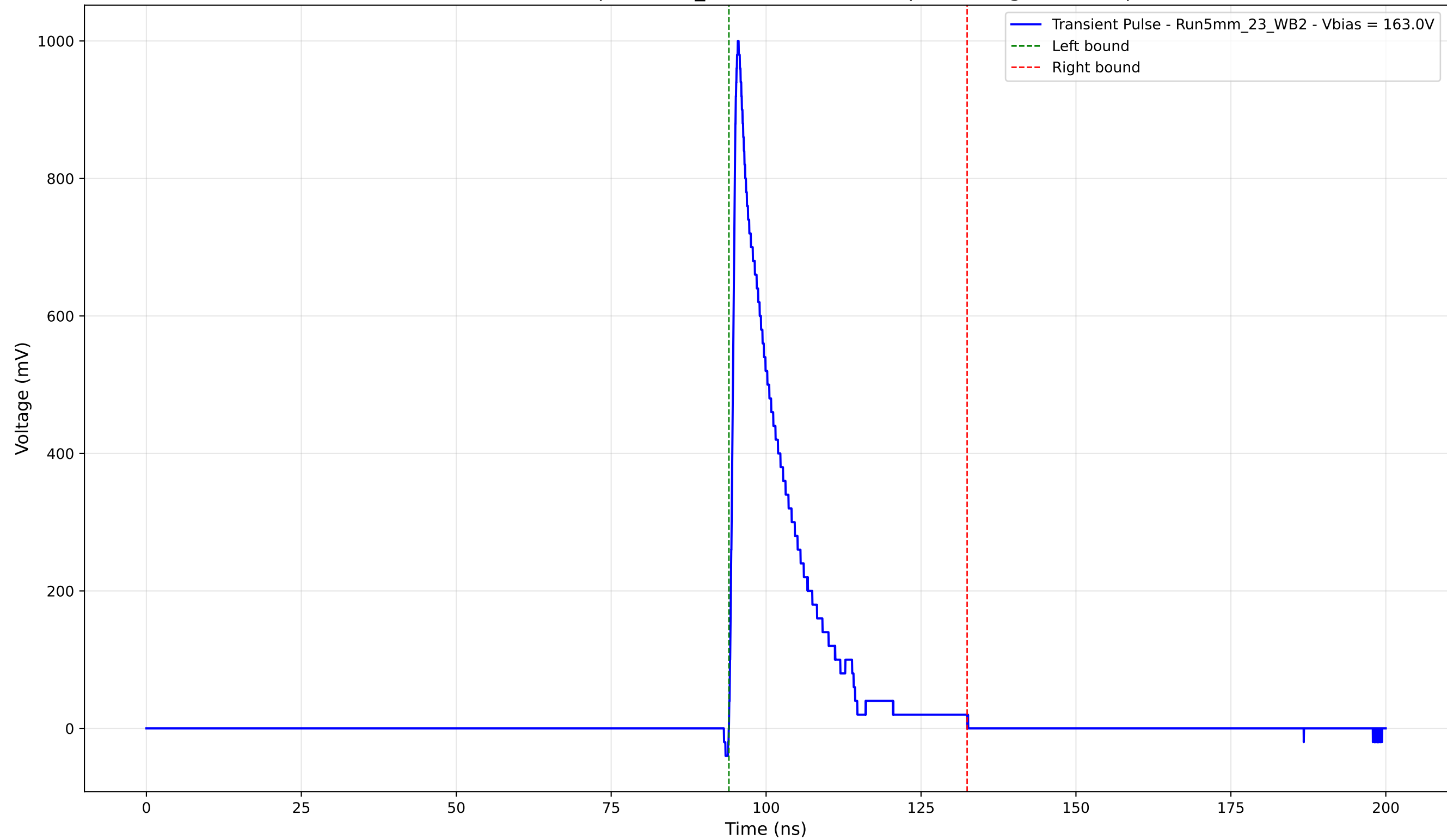
Transient Pulse - Sample: 5mm_23 - Position: 115.0 \mu\text{m} - Charge: 157.71 pC
