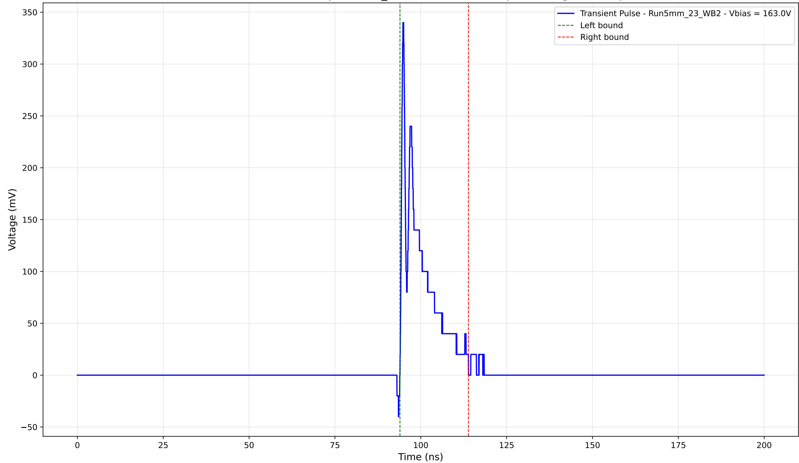
Transient Pulse - Sample: 5mm_23 -Position: 2510.0 \mu\text{m} - Charge: 35.73 pC
