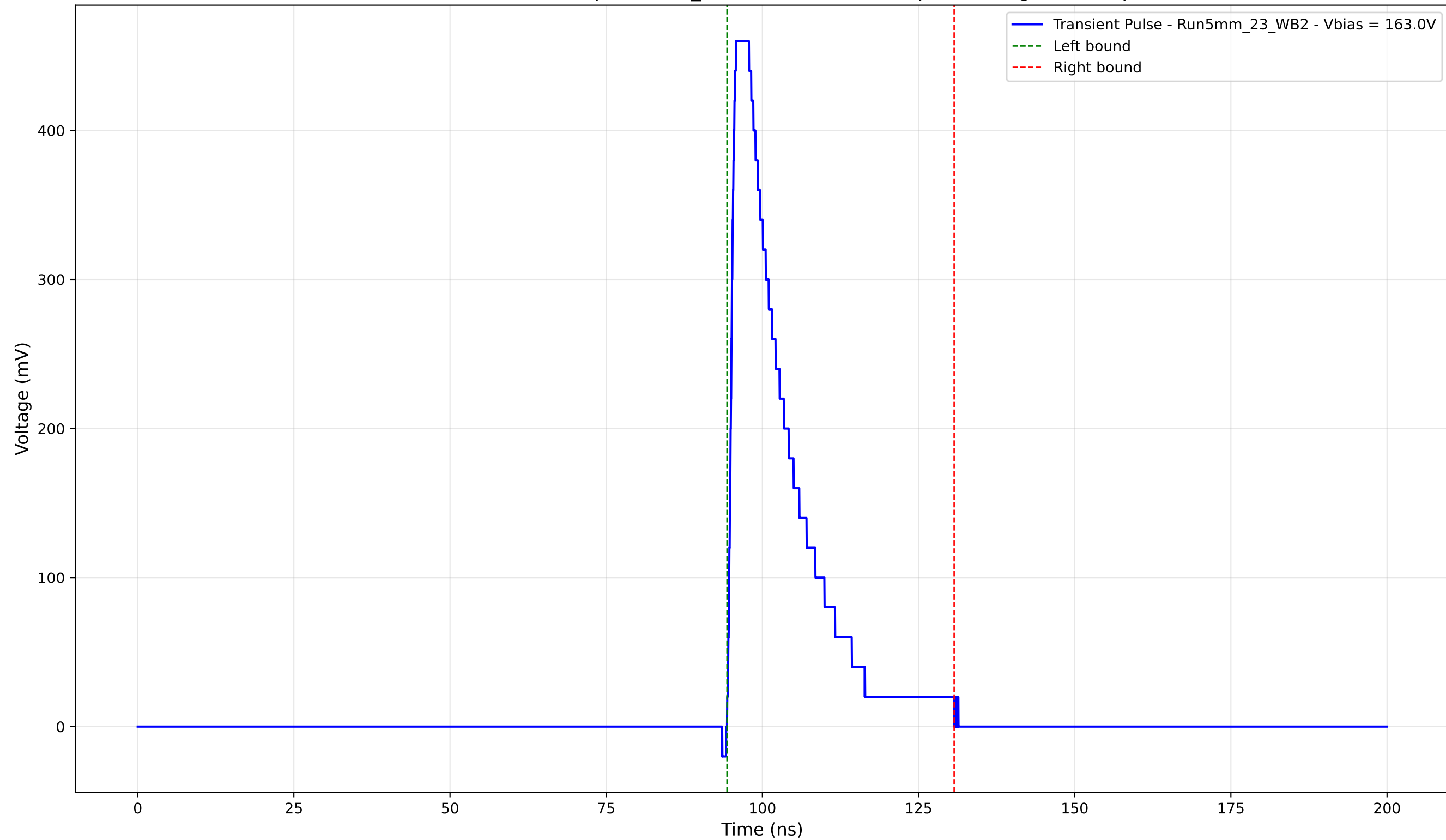
Transient Pulse - Sample: 5mm_23 - Position: 3480.0 \mu\text{m} - Charge: 92.89 pC
