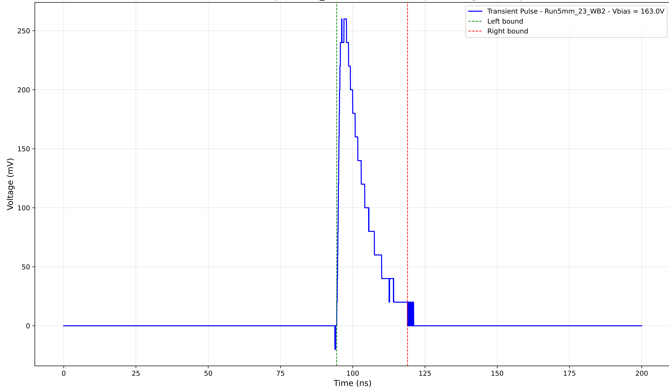
Transient Pulse - Sample: 5mm_23 - Position: 1480.0 \mu\text{m} - Charge: 49.34 pC
