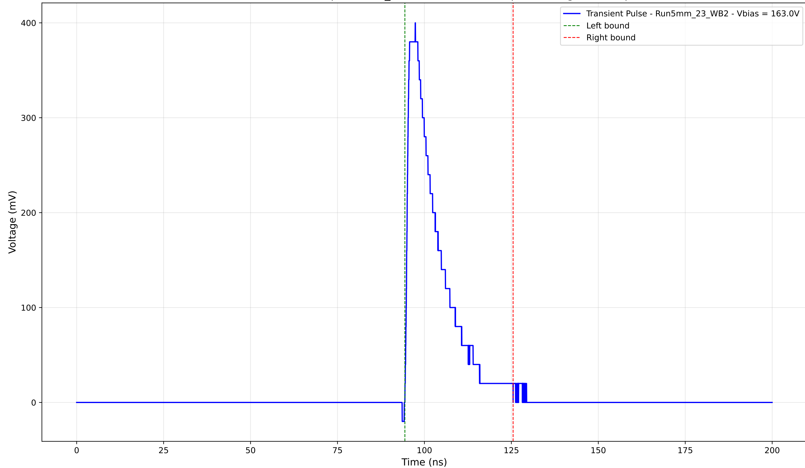
Transient Pulse - Sample: 5mm_23 - Position: 1535.0 \mu\text{m} - Charge: 78.06 pC
