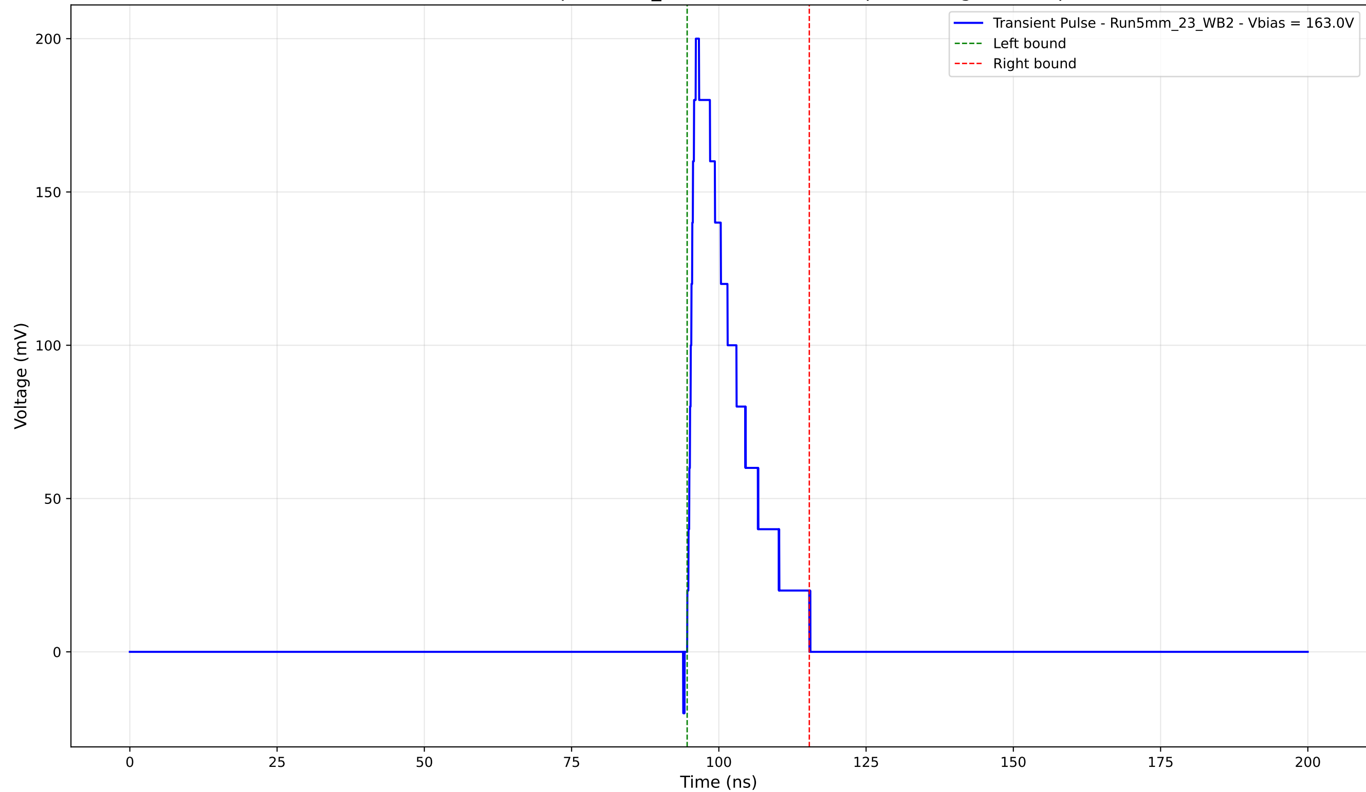
Transient Pulse - Sample: 5mm_23 - Position: 4025.0 \mu\text{m} - Charge: 33.21 pC
