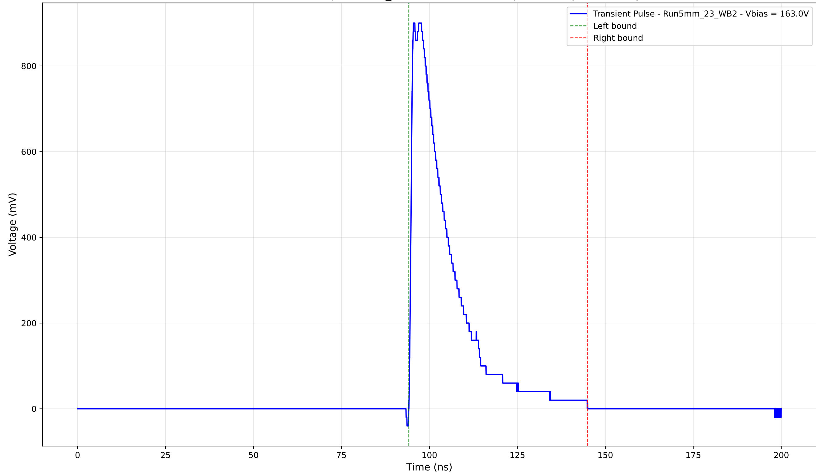
Transient Pulse - Sample: 5mm_23 - Position: 1785.0 \mu\text{m} - Charge: 217.86 pC
