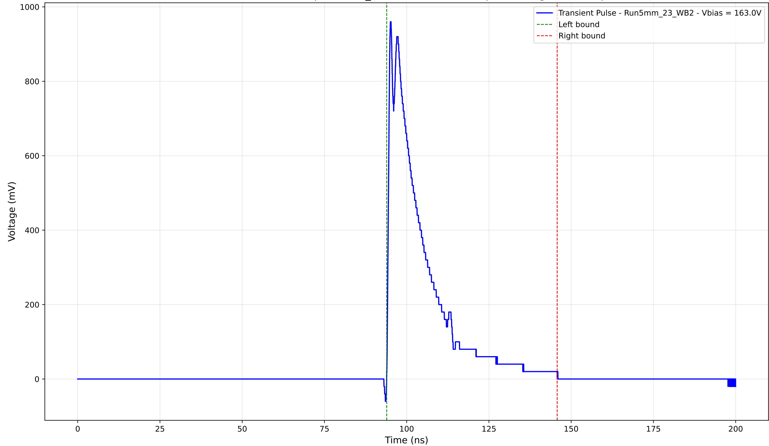
Transient Pulse - Sample: 5mm_23 - Position: 2830.0 \mu\text{m} - Charge: 211.04 pC
