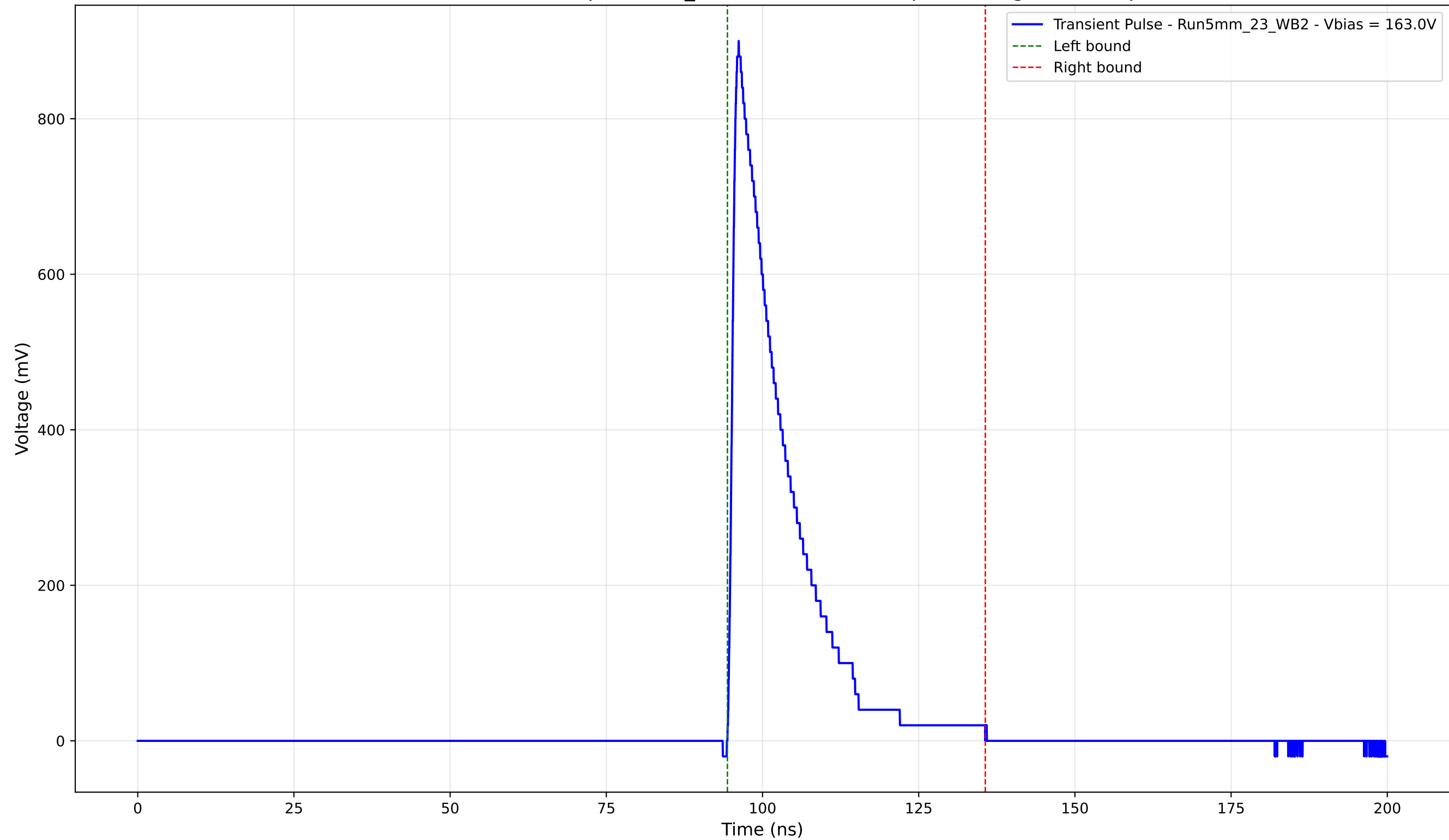
Transient Pulse - Sample: 5mm_23 - Position: 4215.0 \mu\text{m} - Charge: 163.60 pC
