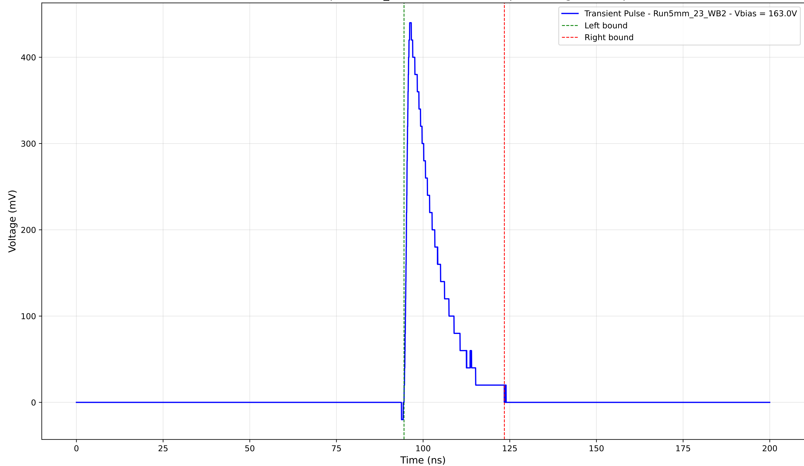
Transient Pulse - Sample: 5mm_23 - Position: 1030.0 \mu\text{m} - Charge: 78.17 pC
