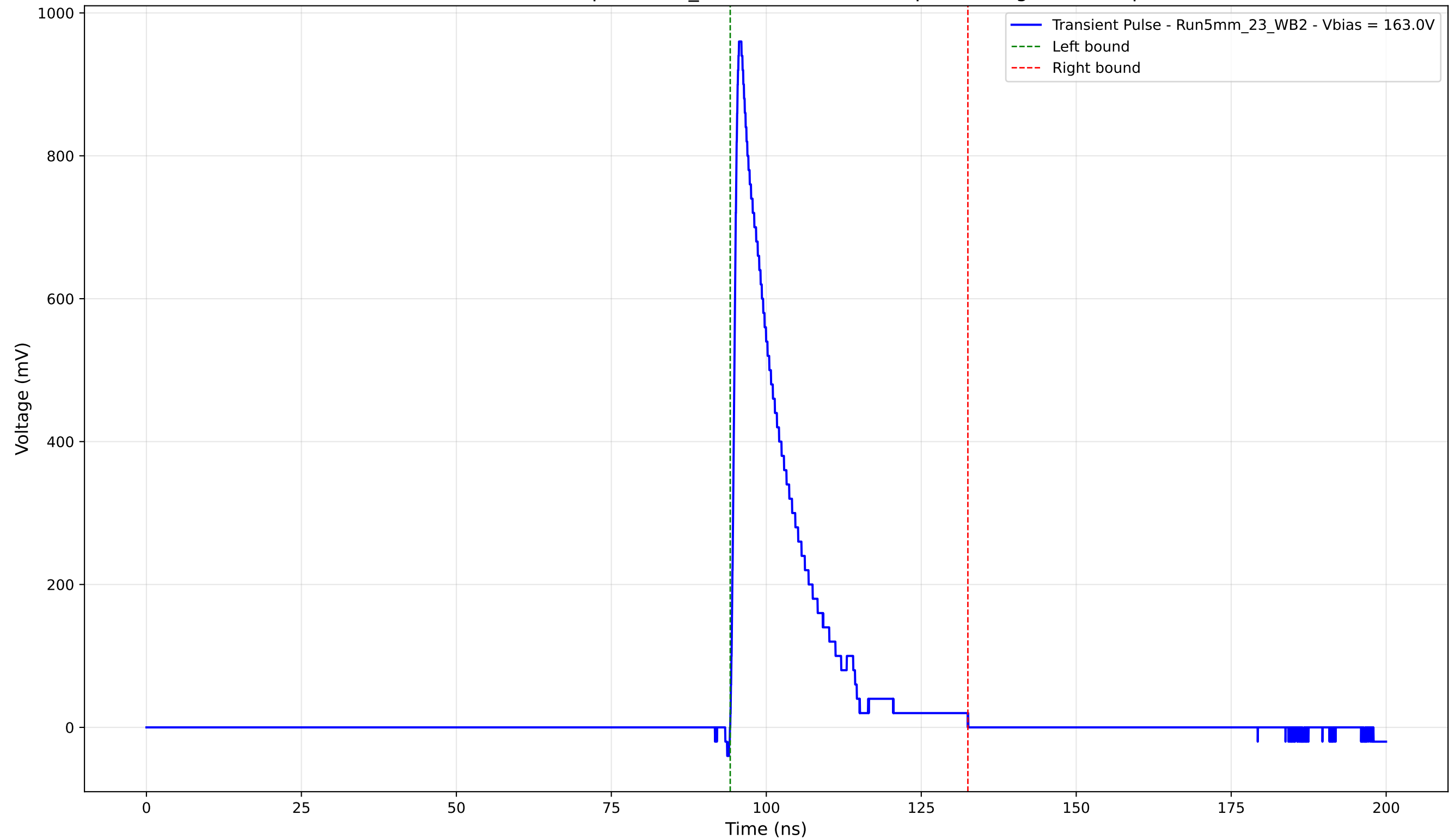
Transient Pulse - Sample: 5mm_23 - Position: 4665.0 \mu\text{m} - Charge: 157.11 pC
