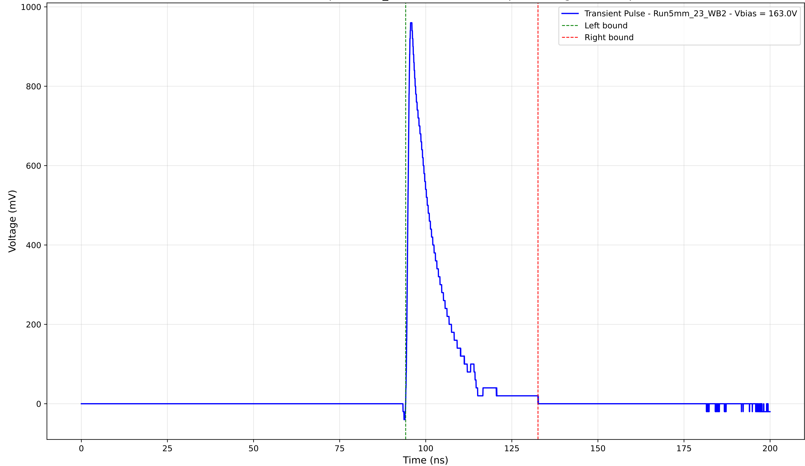
Transient Pulse - Sample: 5mm_23 - Position: 4670.0 \mu\text{m} - Charge: 156.71 pC
