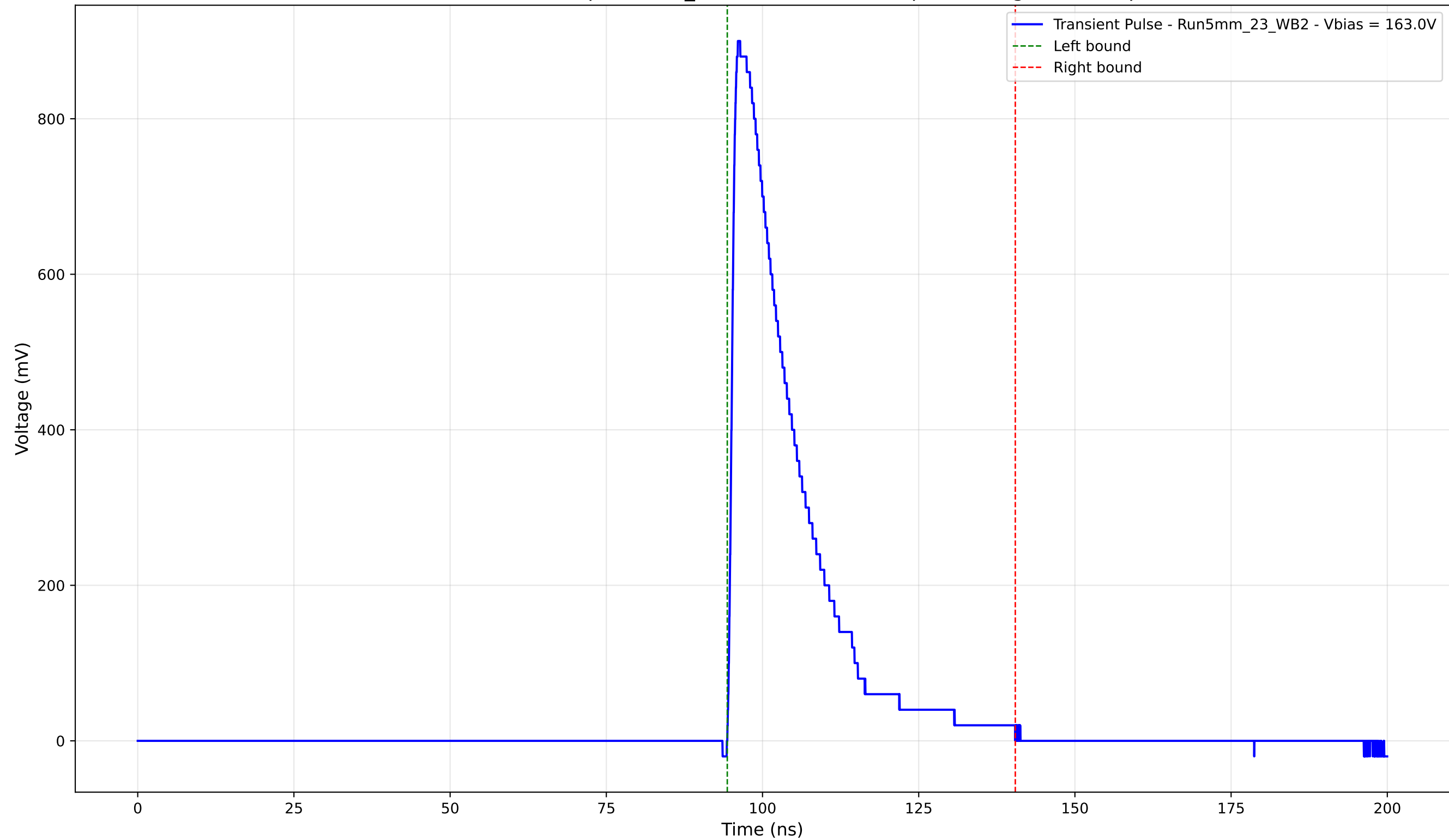
Transient Pulse - Sample: 5mm_23 - Position: 1335.0 \mu\text{m} - Charge: 200.38 pC
