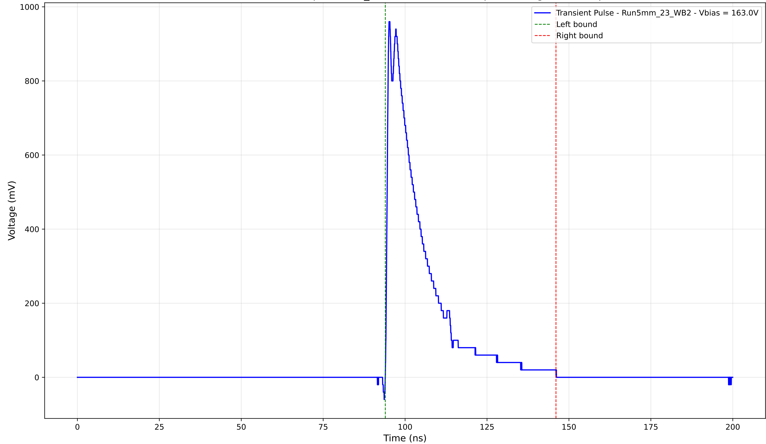
Transient Pulse - Sample: 5mm_23 - Position: 2905.0 \mu\text{m} - Charge: 218.86 pC
