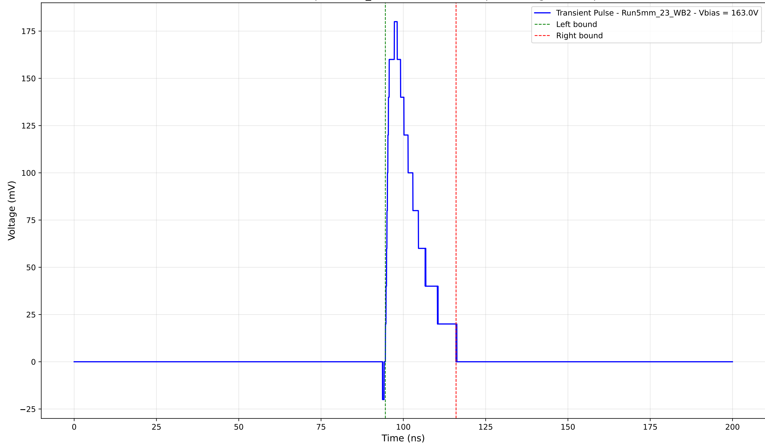
Transient Pulse - Sample: 5mm_23 -Position: 3535.0 \mu\text{m} - Charge: 32.60 pC
