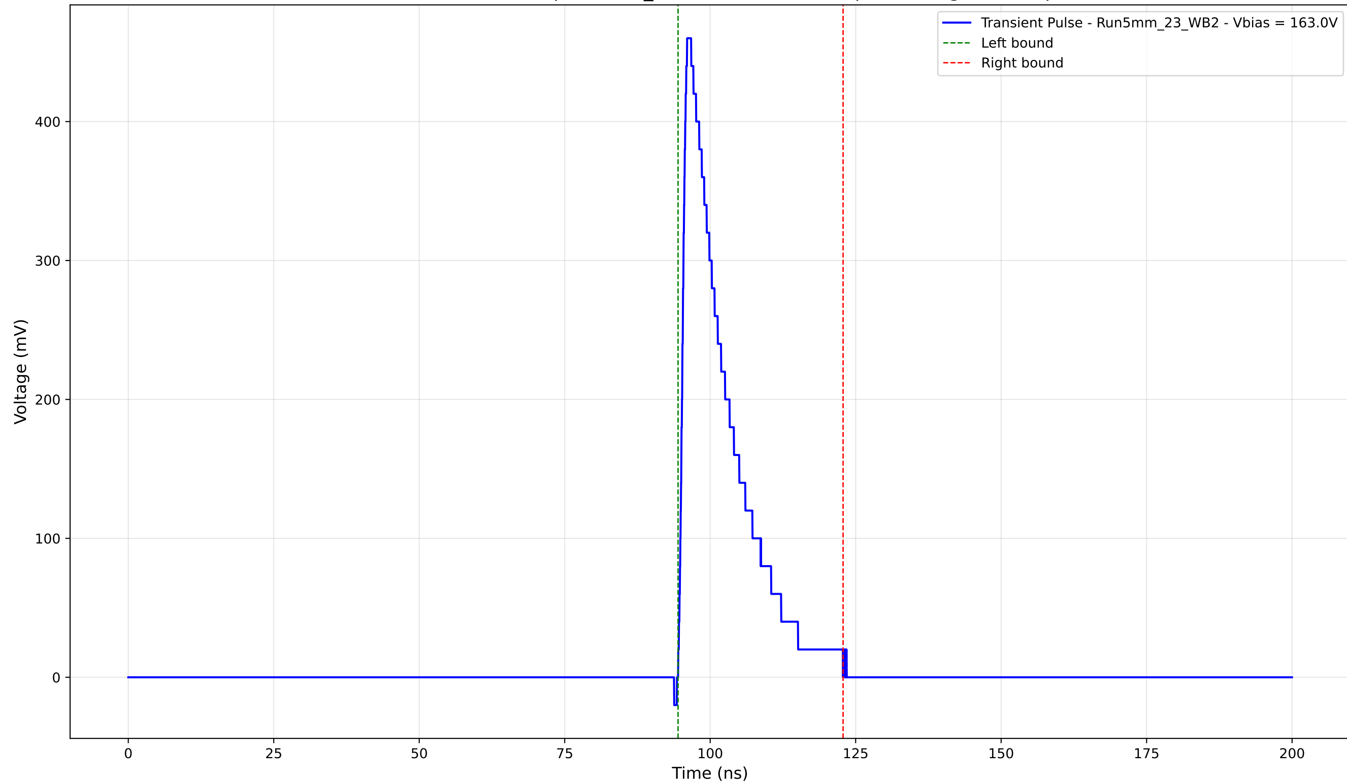
Transient Pulse - Sample: 5mm_23 - Position: 3995.0 \mu\text{m} - Charge: 79.02 pC
