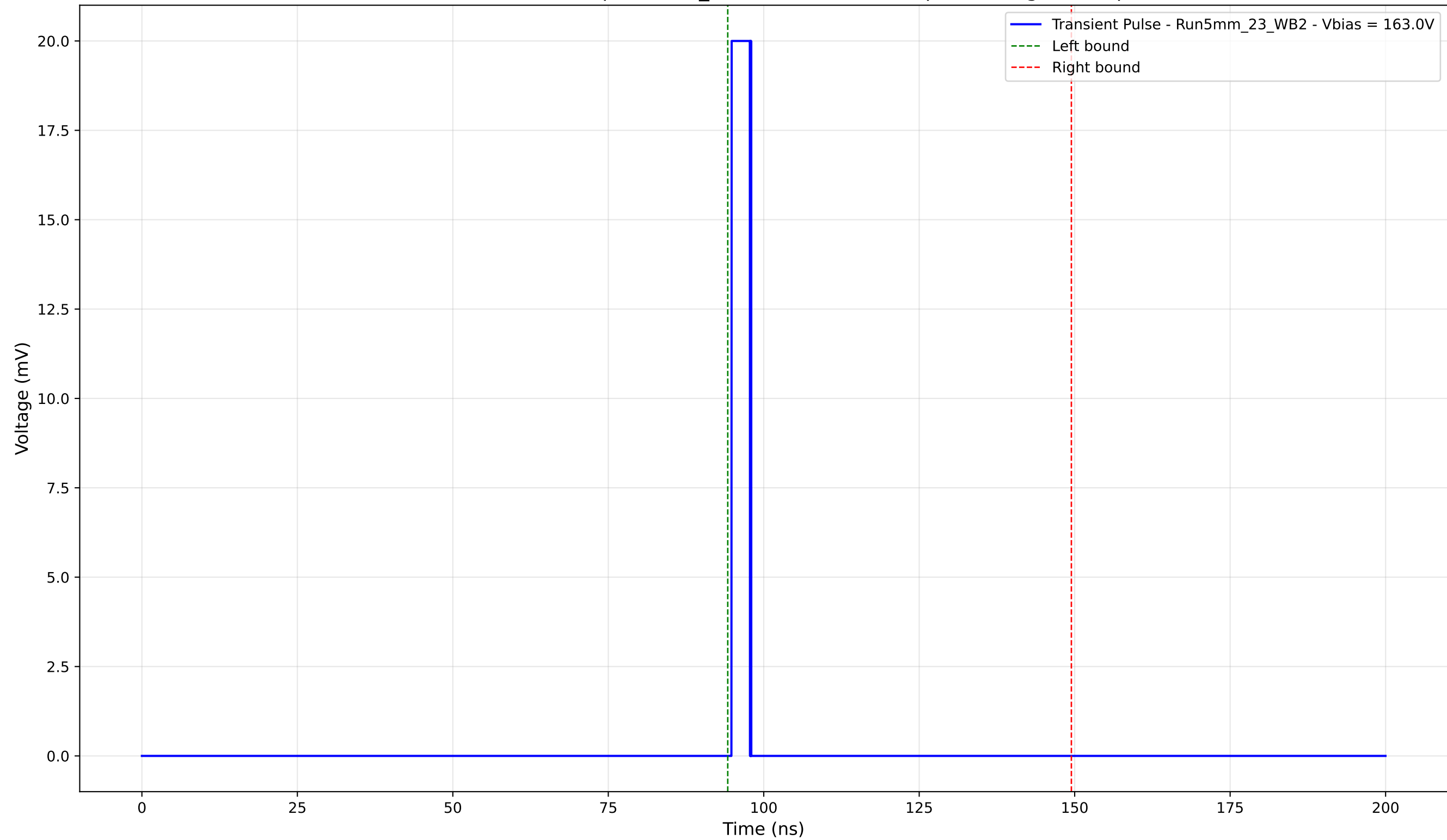
Transient Pulse - Sample: 5mm_23 - Position: 5030.0 \mu\text{m} - Charge: 1.22 pC
