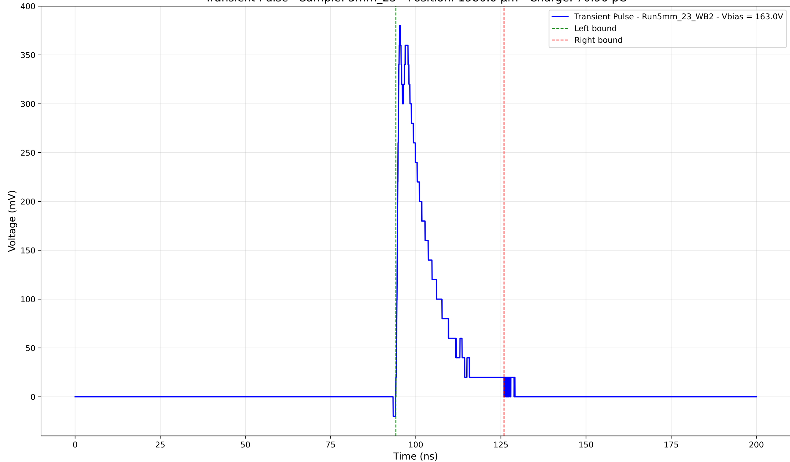
Transient Pulse - Sample: 5mm_23 - Position: 1980.0 \mu\text{m} - Charge: 70.90 pC
