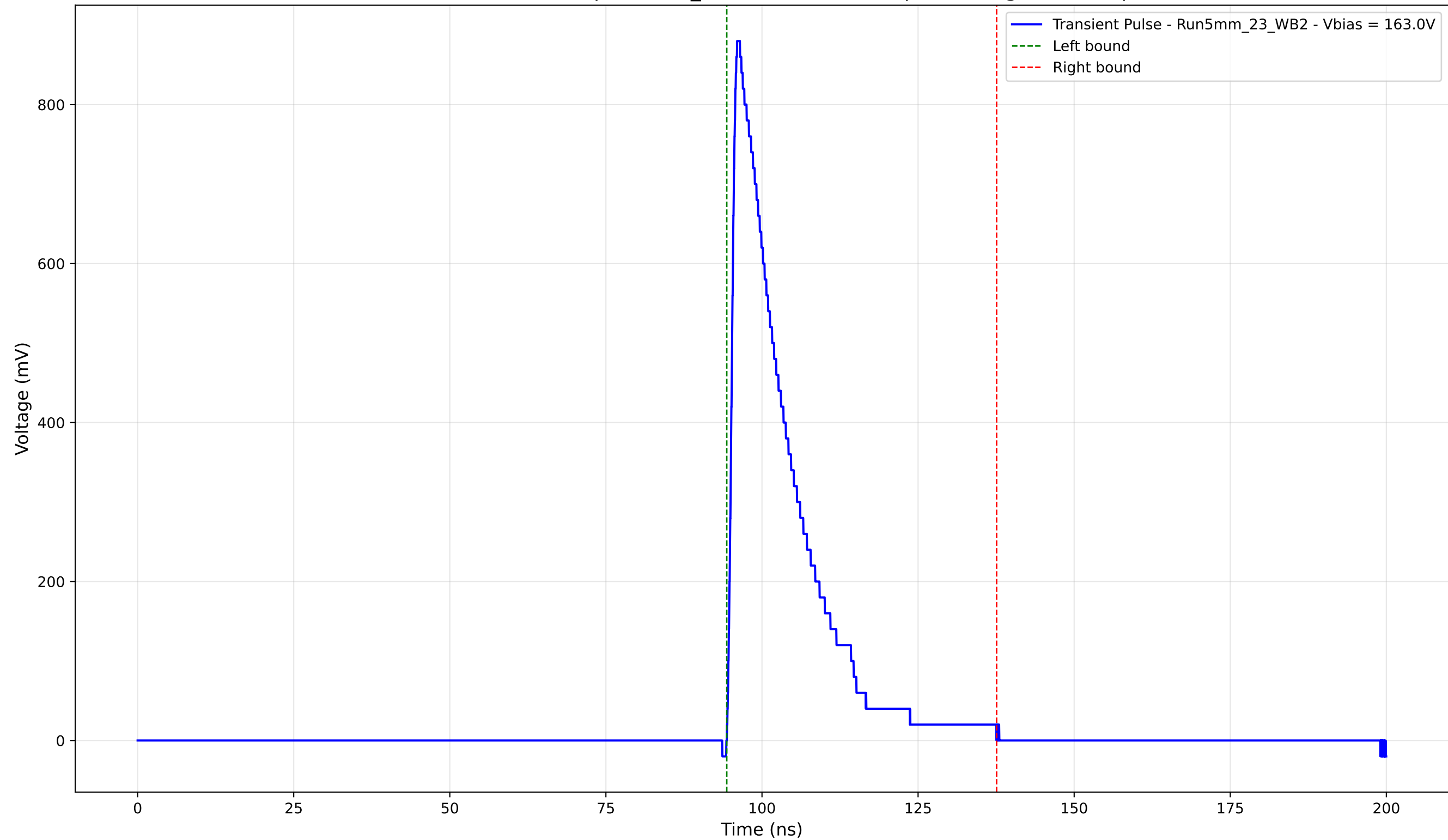
Transient Pulse - Sample: 5mm_23 - Position: 875.0 \mu\text{m} - Charge: 172.82 pC
