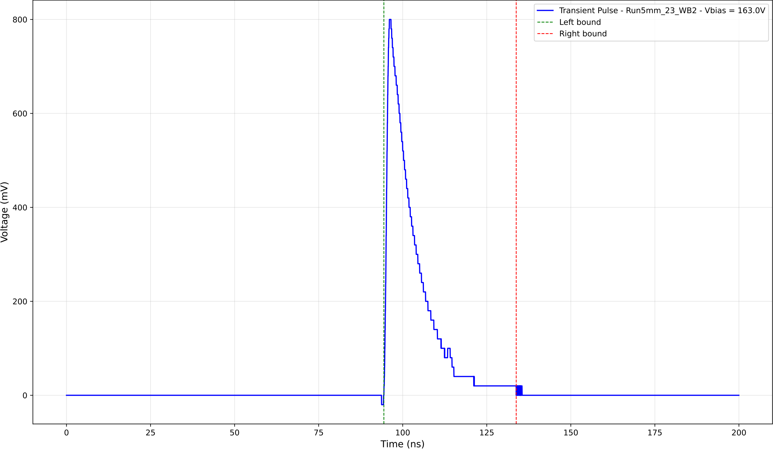
Transient Pulse - Sample: 5mm_23 - Position: 4120.0 \mu\text{m} - Charge: 144.64 pC
