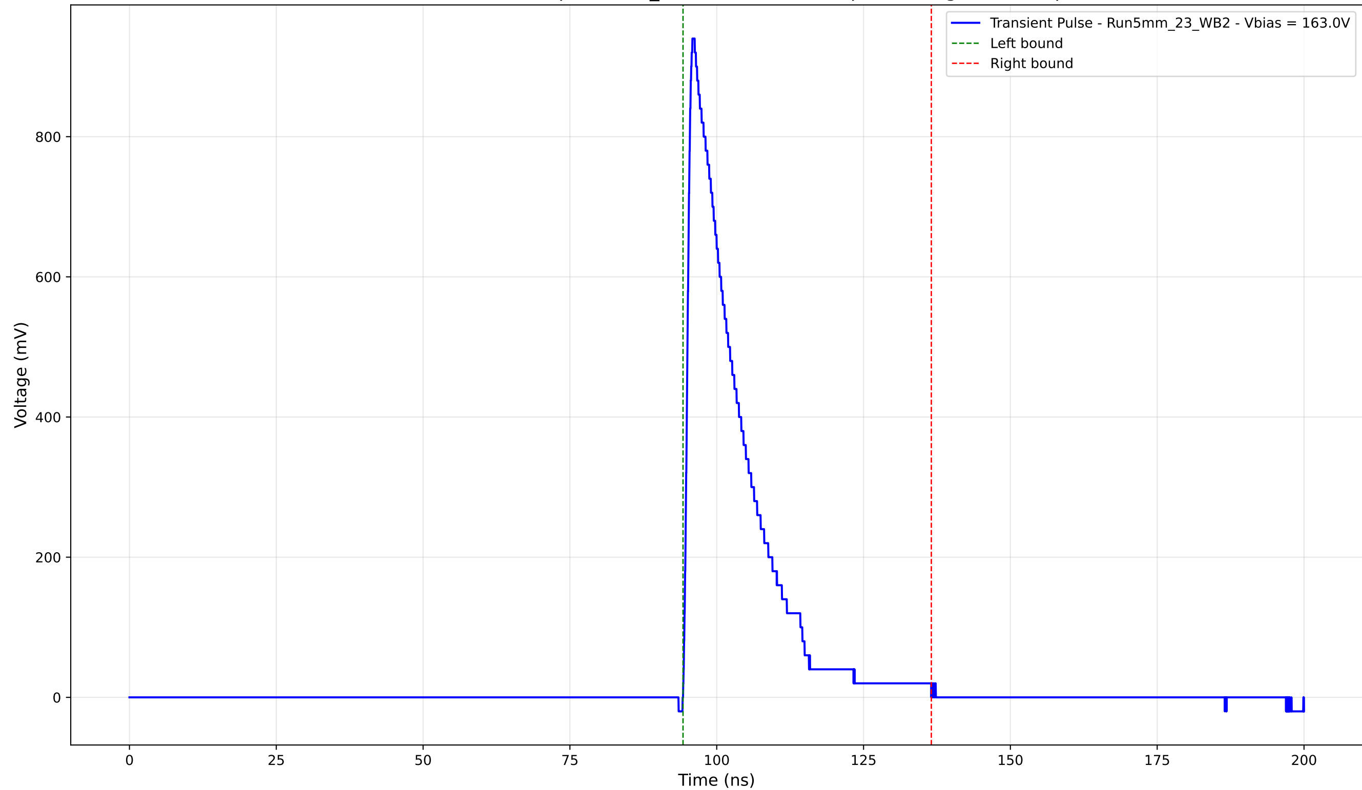
Transient Pulse - Sample: 5mm_23 - Position: 625.0 \mu\text{m} - Charge: 181.36 pC
