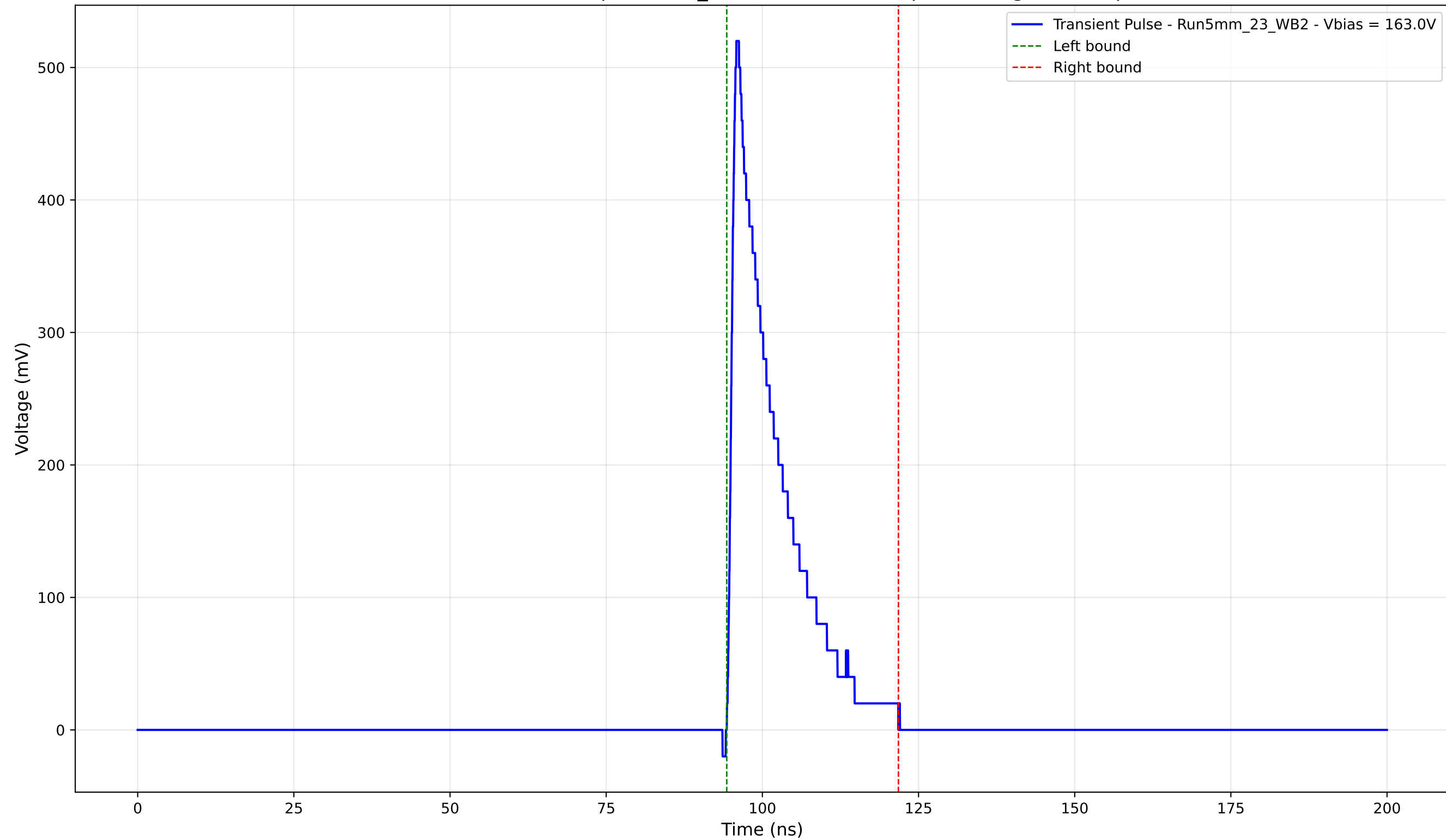
Transient Pulse - Sample: 5mm_23 - Position: 525.0 \mu\text{m} - Charge: 81.22 pC
