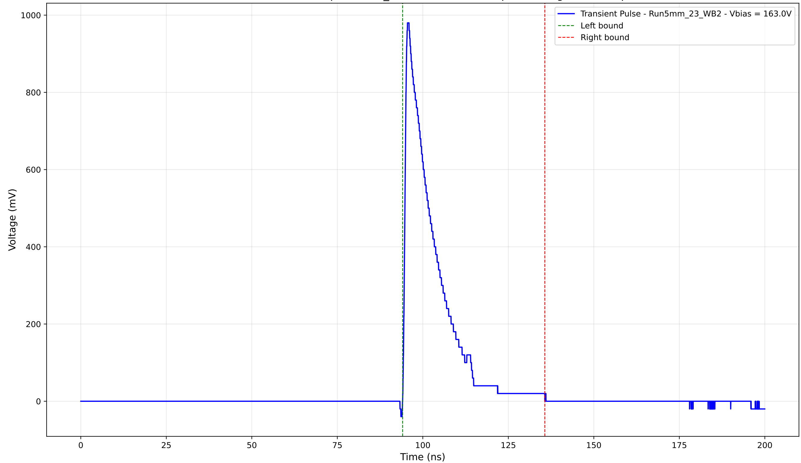
Transient Pulse - Sample: 5mm_23 - Position: 325.0 \mu\text{m} - Charge: 179.14 pC
