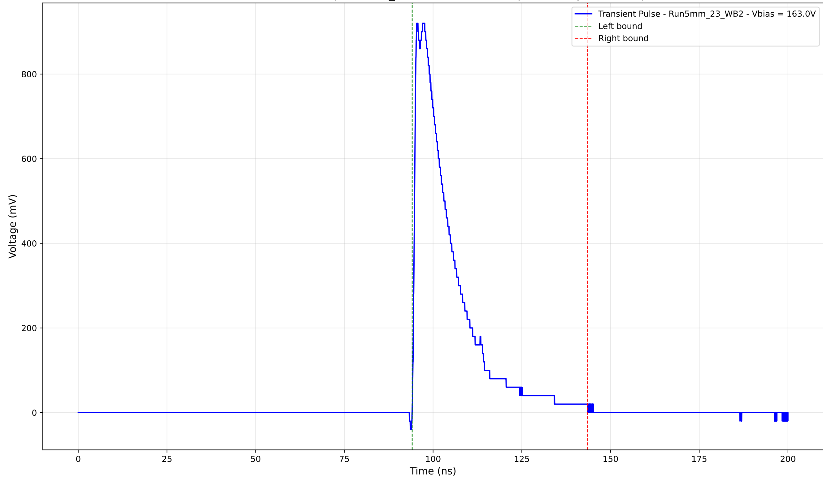
Transient Pulse - Sample: 5mm_23 - Position: 3195.0 \mu\text{m} - Charge: 218.58 pC
