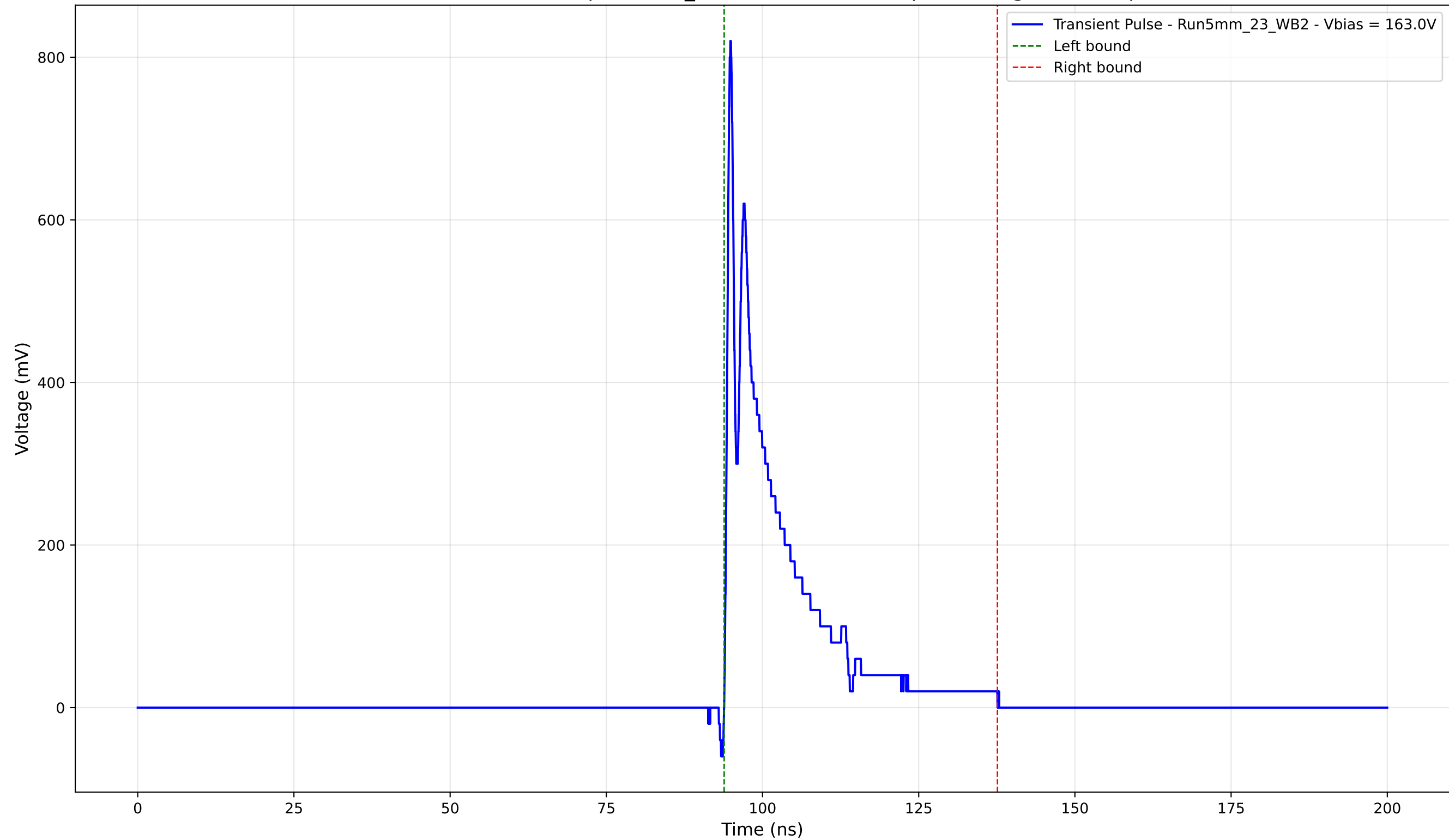
Transient Pulse - Sample: 5mm_23 - Position: 2565.0 \mu\text{m} - Charge: 113.50 pC
