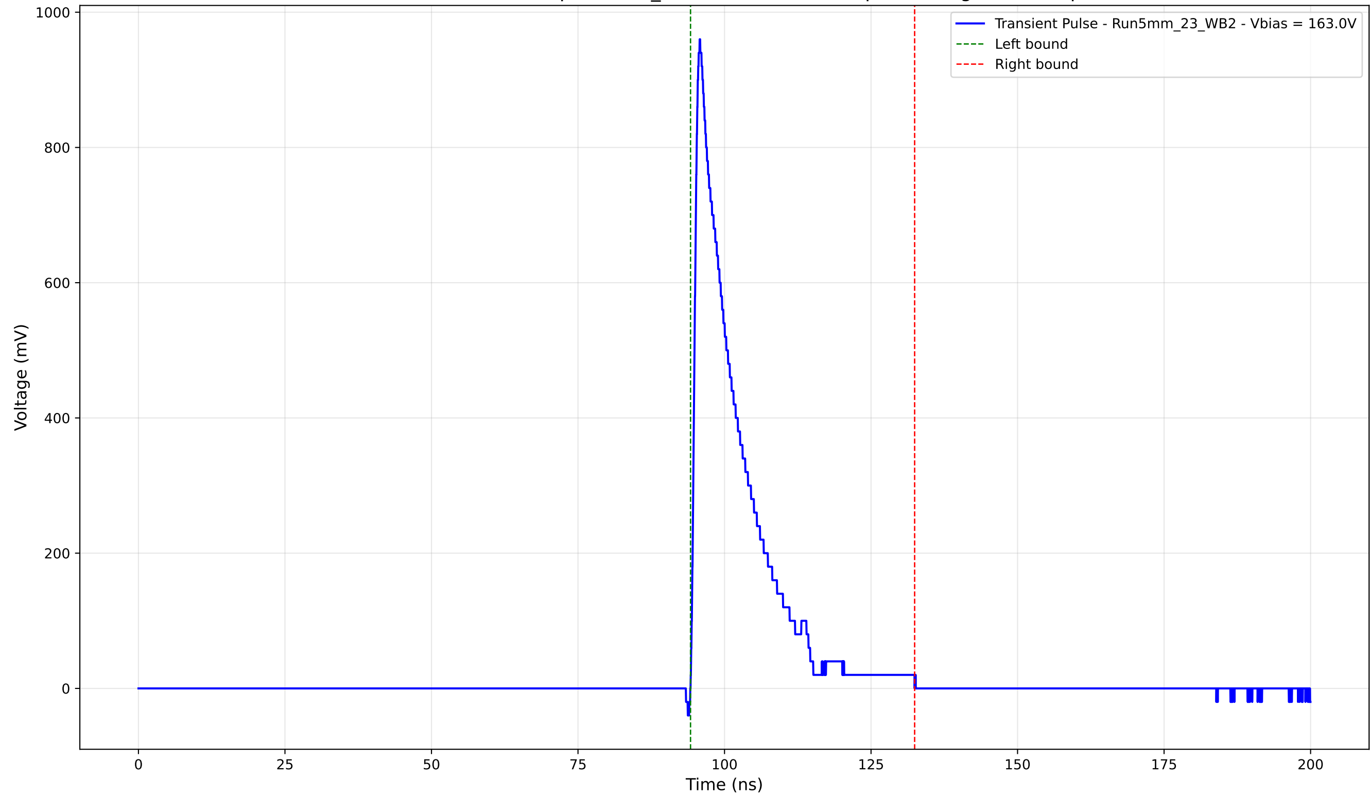
Transient Pulse - Sample: 5mm_23 - Position: 4635.0 \mu\text{m} - Charge: 153.39 pC
