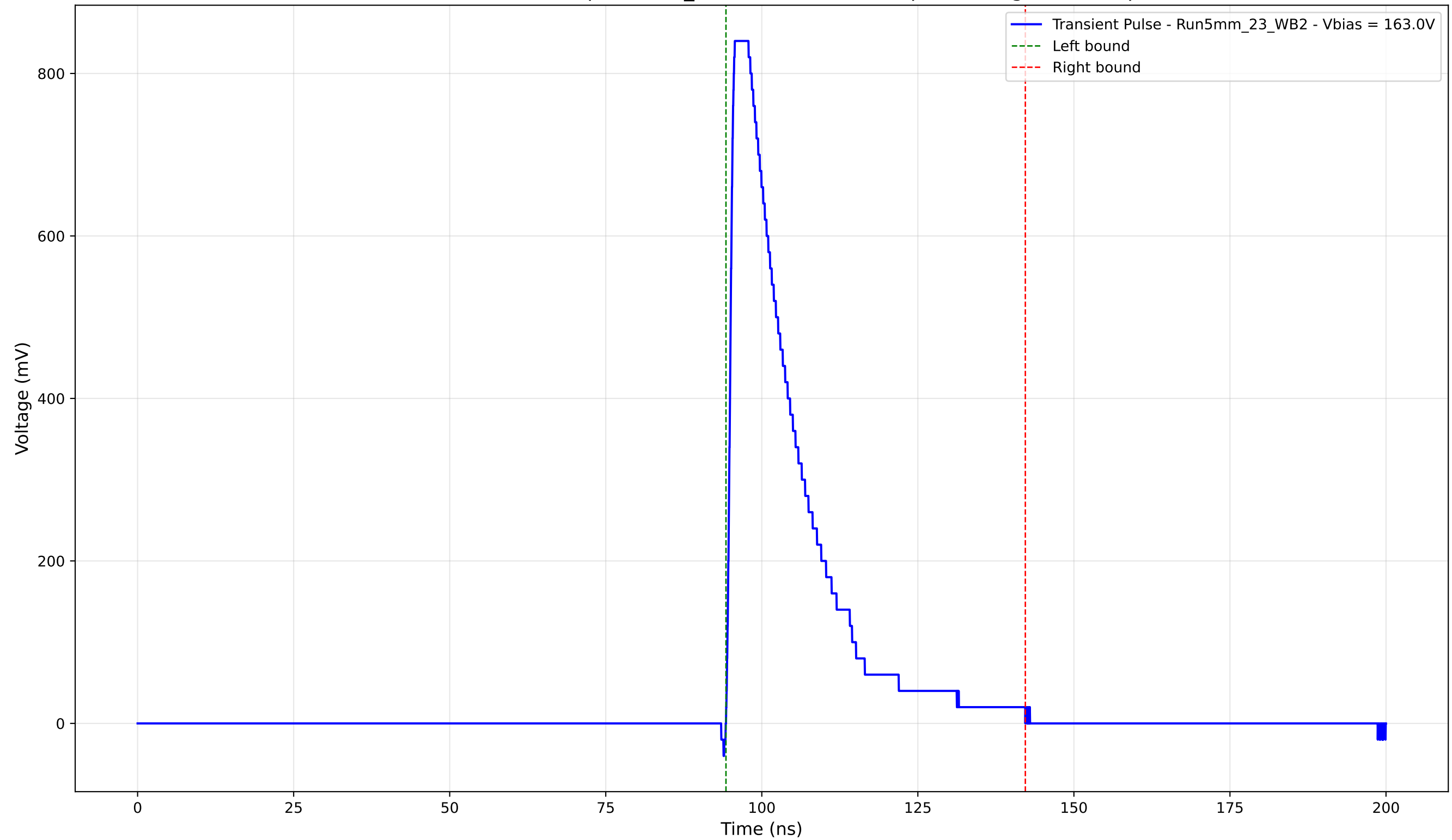
Transient Pulse - Sample: 5mm_23 - Position: 1605.0 \mu\text{m} - Charge: 194.55 pC
