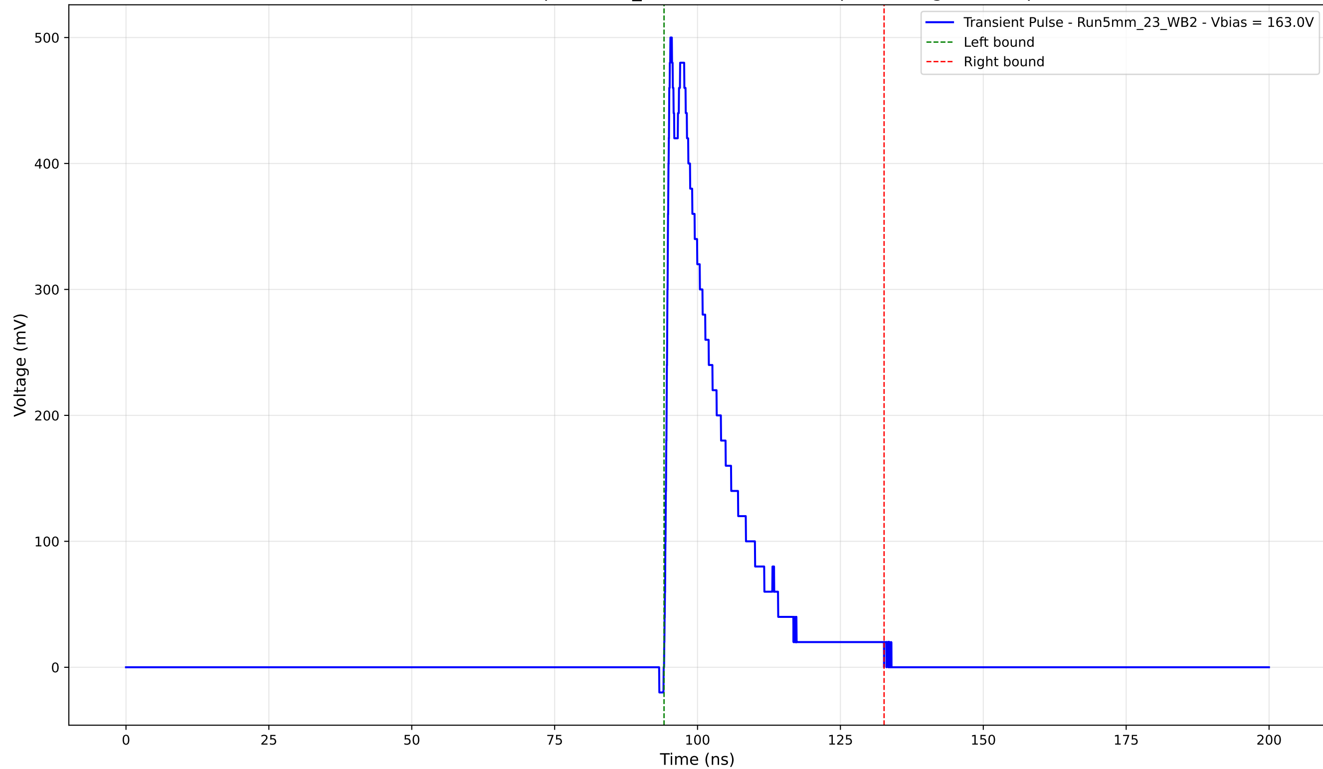
Transient Pulse - Sample: 5mm_23 - Position: 3060.0 \mu\text{m} - Charge: 96.70 pC
