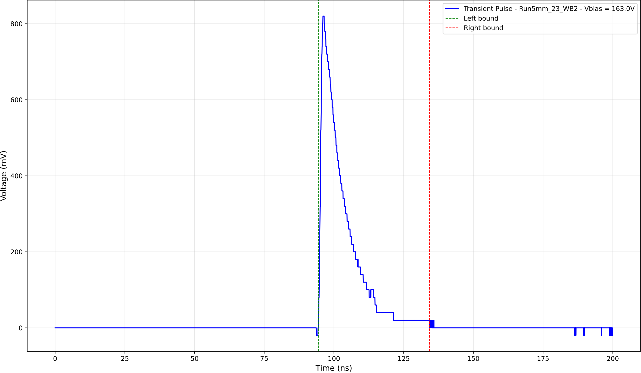
Transient Pulse - Sample: 5mm_23 - Position: 4125.0 \mu\text{m} - Charge: 148.66 pC
