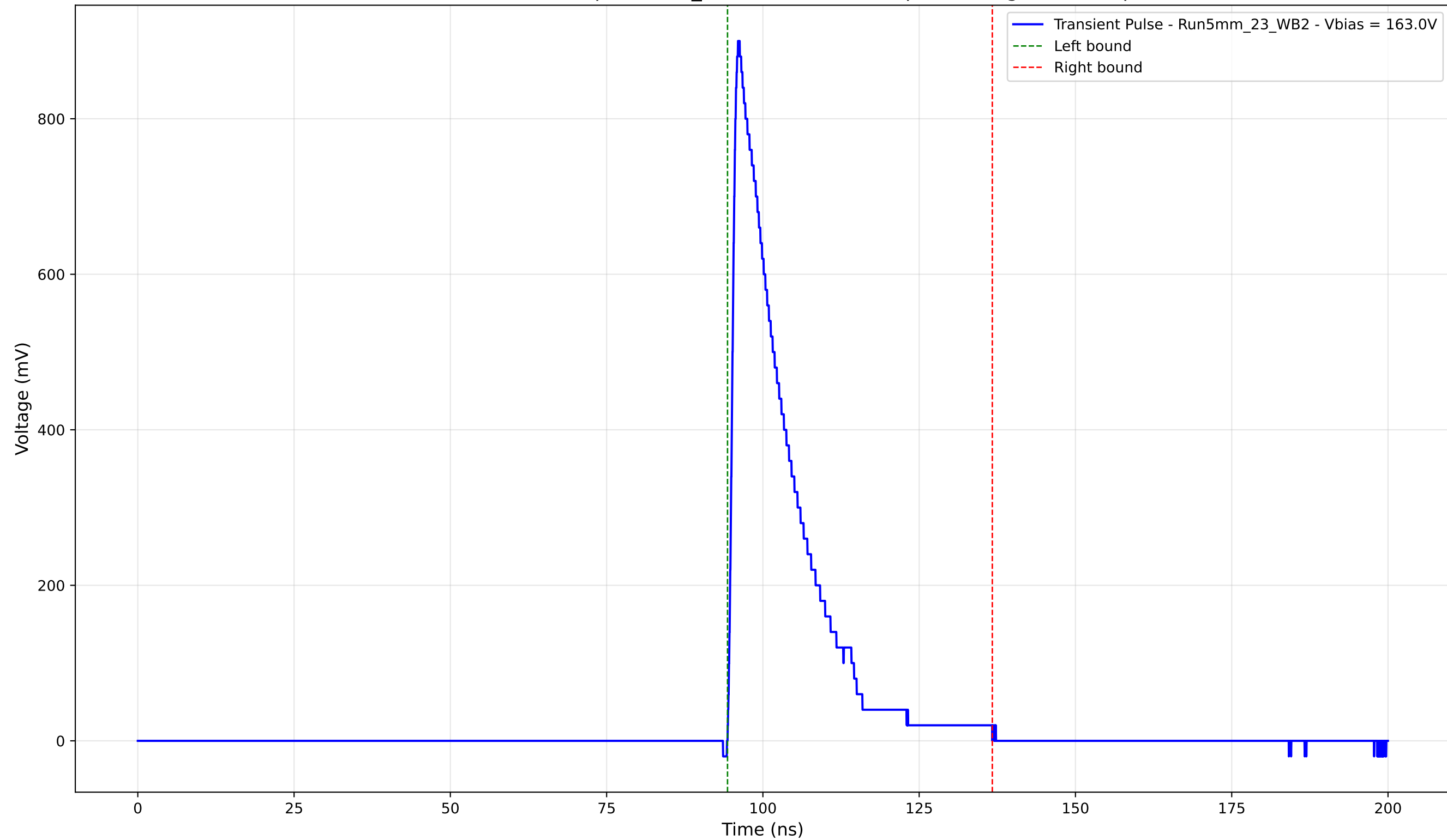
Transient Pulse - Sample: 5mm_23 - Position: 745.0 \mu\text{m} - Charge: 172.32 pC
