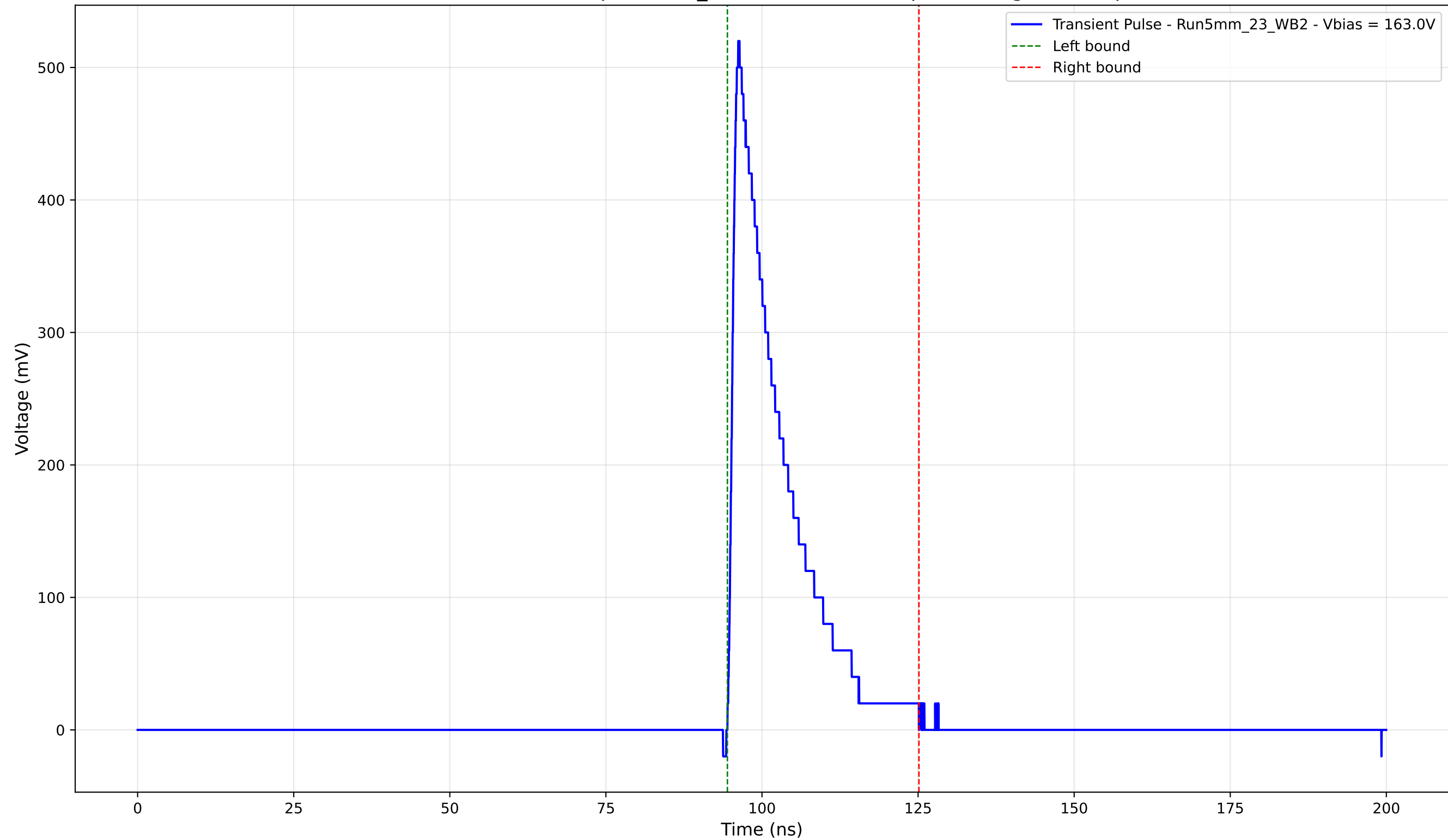
Transient Pulse - Sample: 5mm_23 - Position: 950.0 \mu\text{m} - Charge: 89.16 pC
