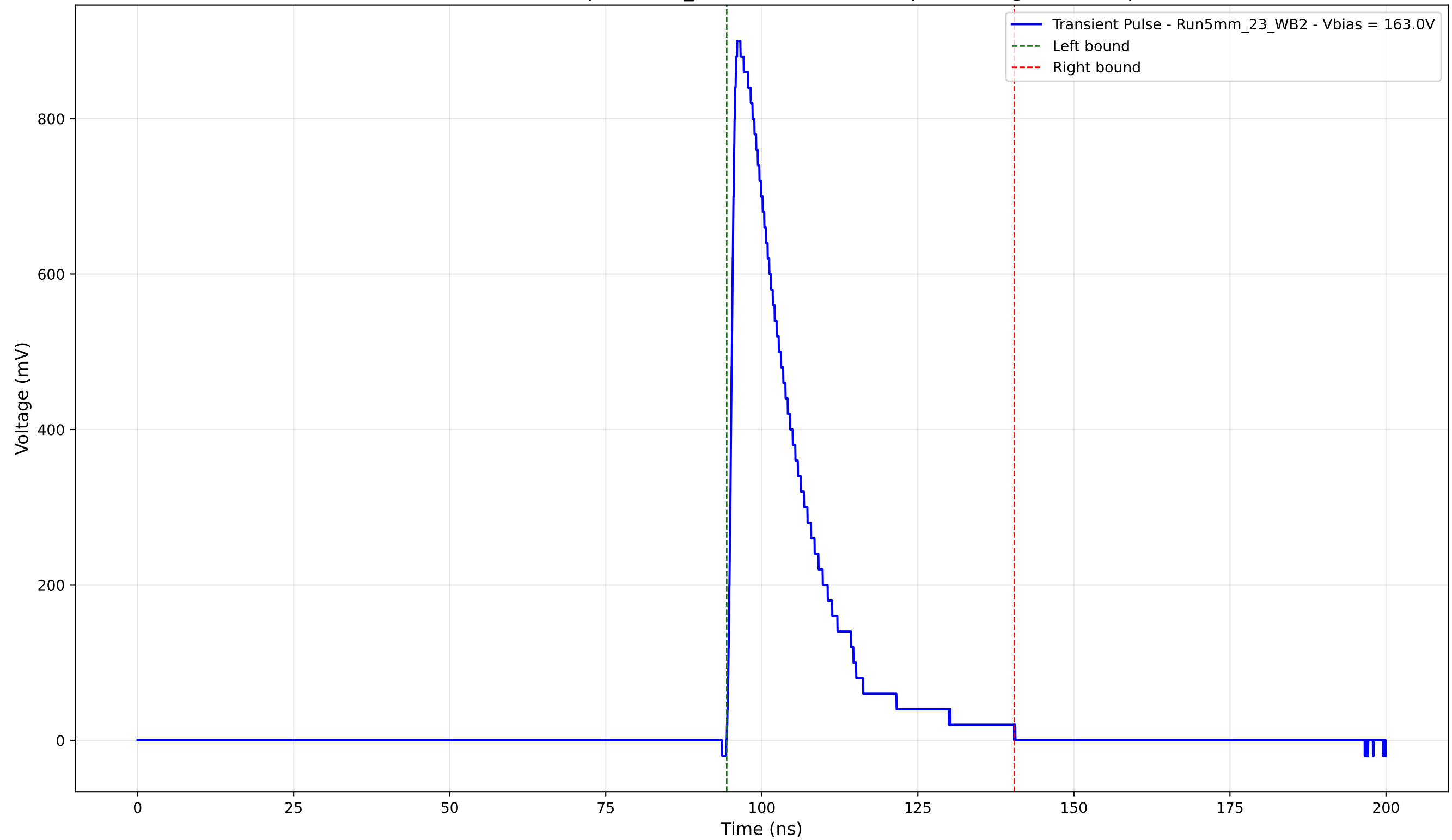
Transient Pulse - Sample: 5mm_23 - Position: 1210.0 \mu\text{m} - Charge: 197.51 pC
