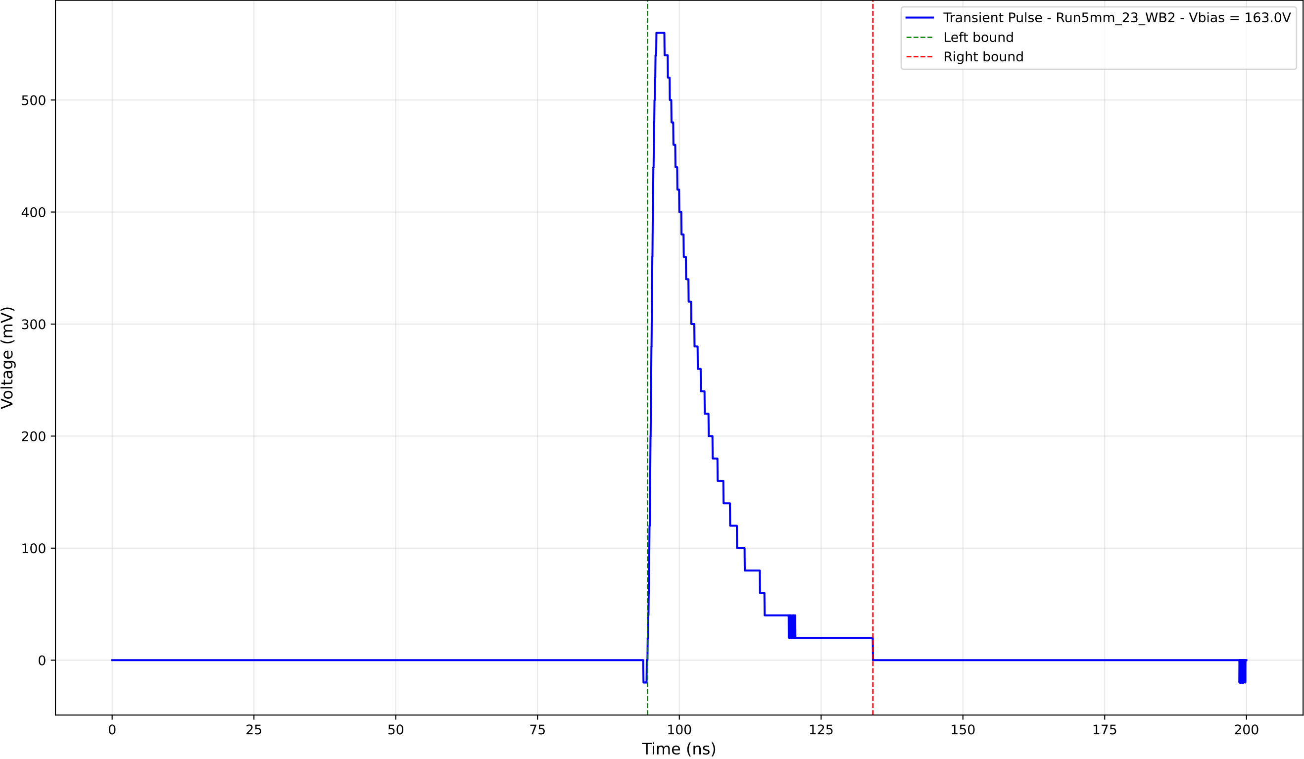
Transient Pulse - Sample: 5mm_23 - Position: 1450.0 \mu\text{m} - Charge: 114.62 pC
