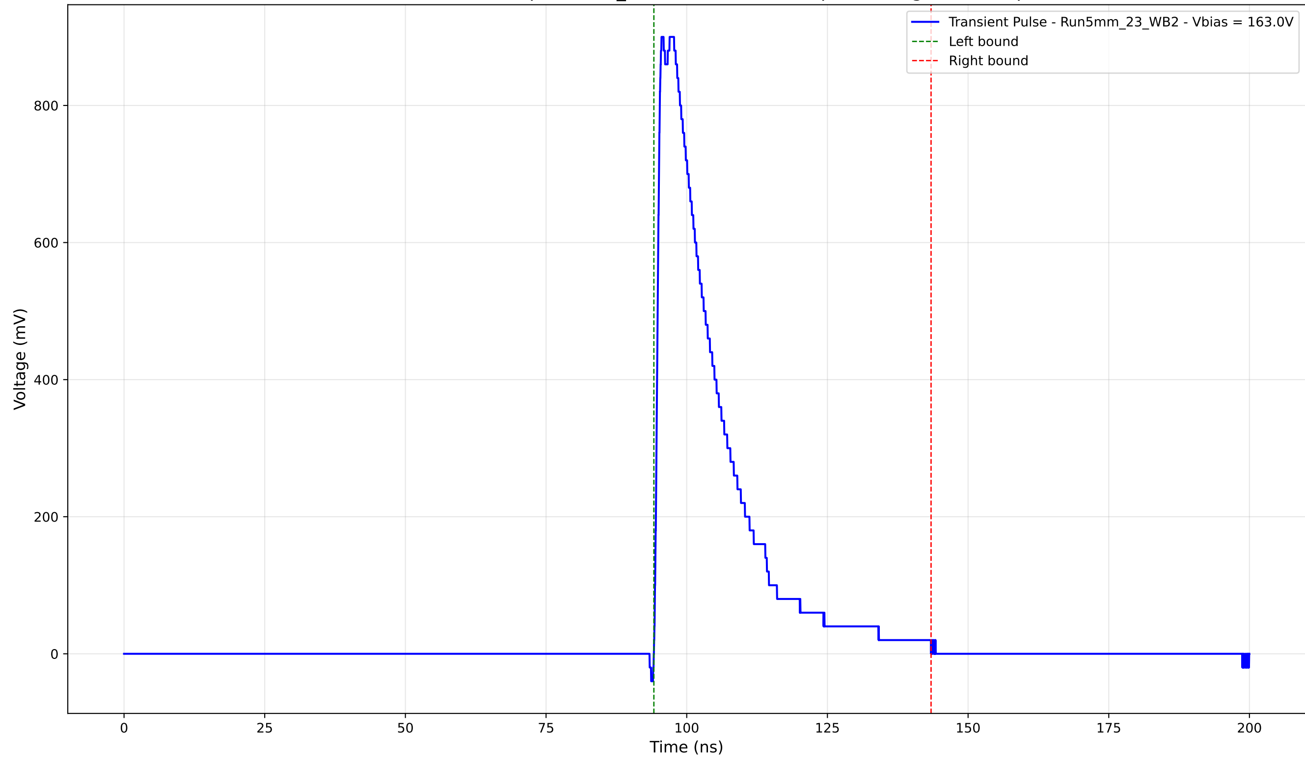
Transient Pulse - Sample: 5mm_23 - Position: 1760.0 \mu\text{m} - Charge: 215.38 pC
