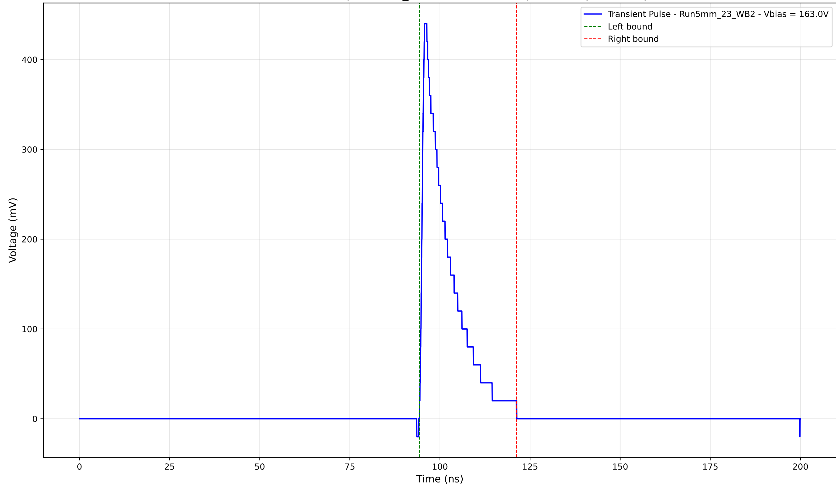
Transient Pulse - Sample: 5mm_23 - Position: 520.0 \mu\text{m} - Charge: 70.12 pC
