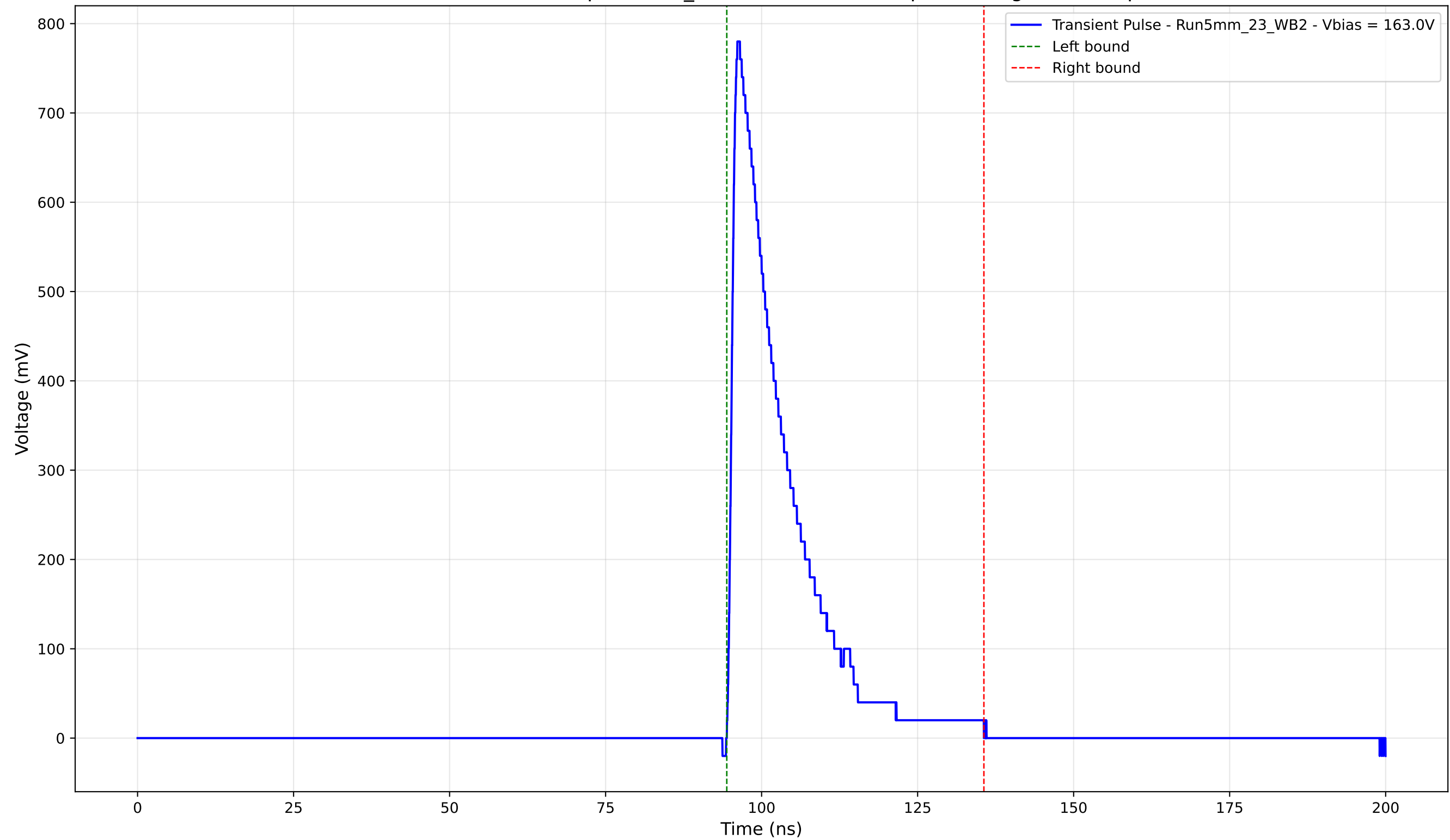
Transient Pulse - Sample: 5mm_23 - Position: 3960.0 \mu\text{m} - Charge: 145.58 pC
