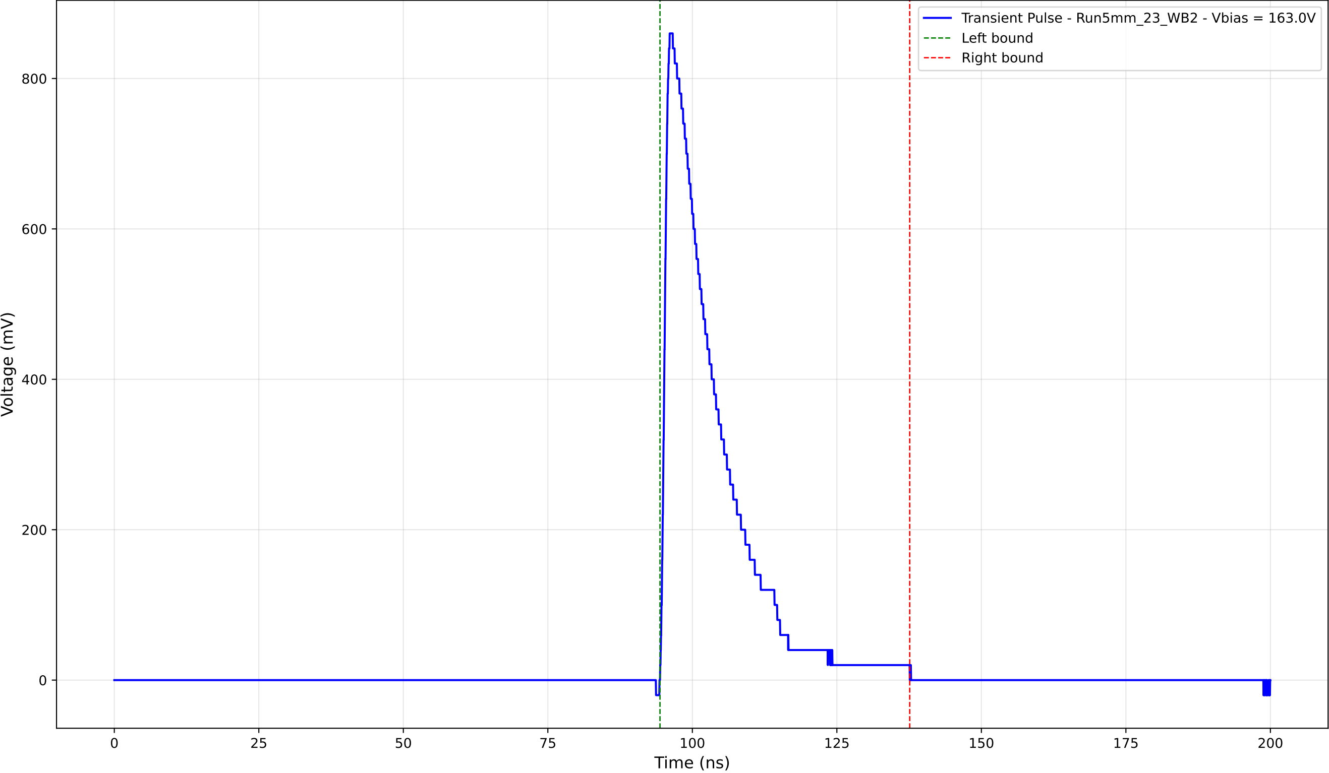
Transient Pulse - Sample: 5mm_23 - Position: 3890.0 \mu\text{m} - Charge: 171.33 pC
