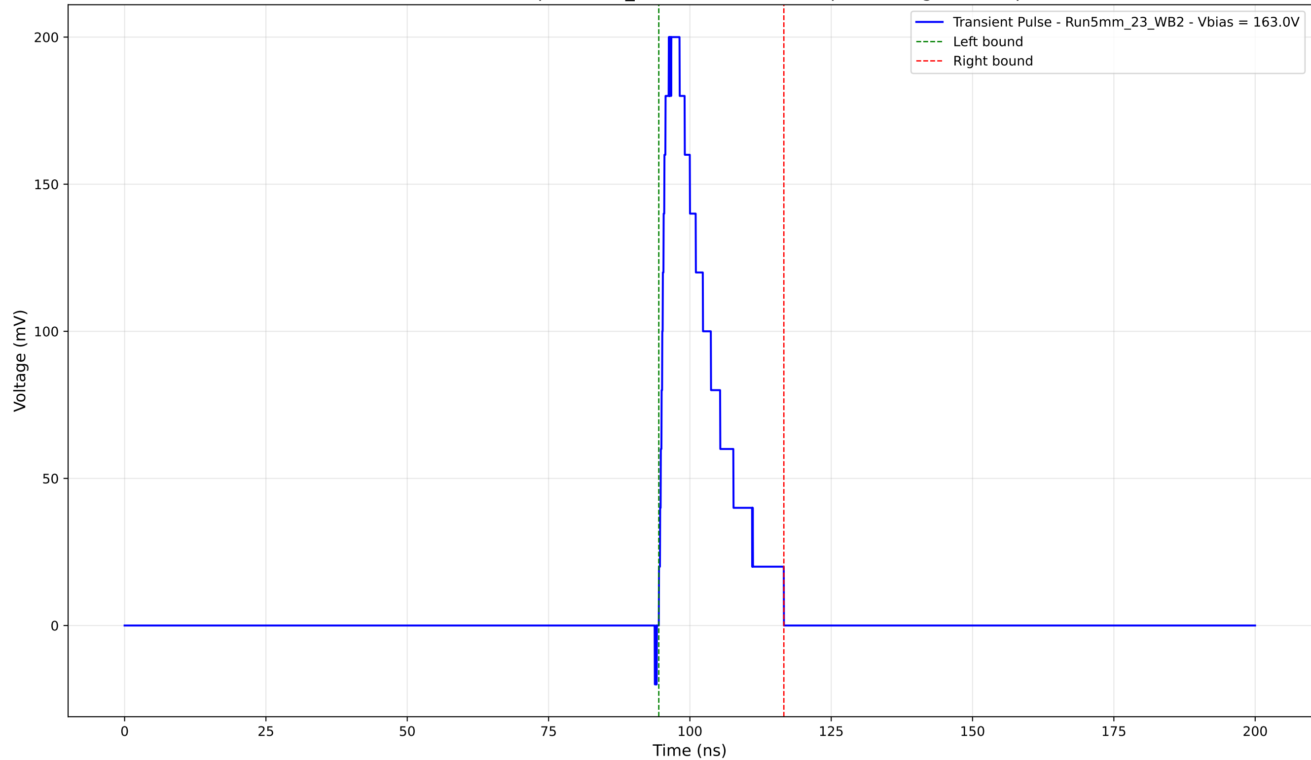
Transient Pulse - Sample: 5mm_23 - Position: 3540.0 \mu\text{m} - Charge: 37.14 pC
