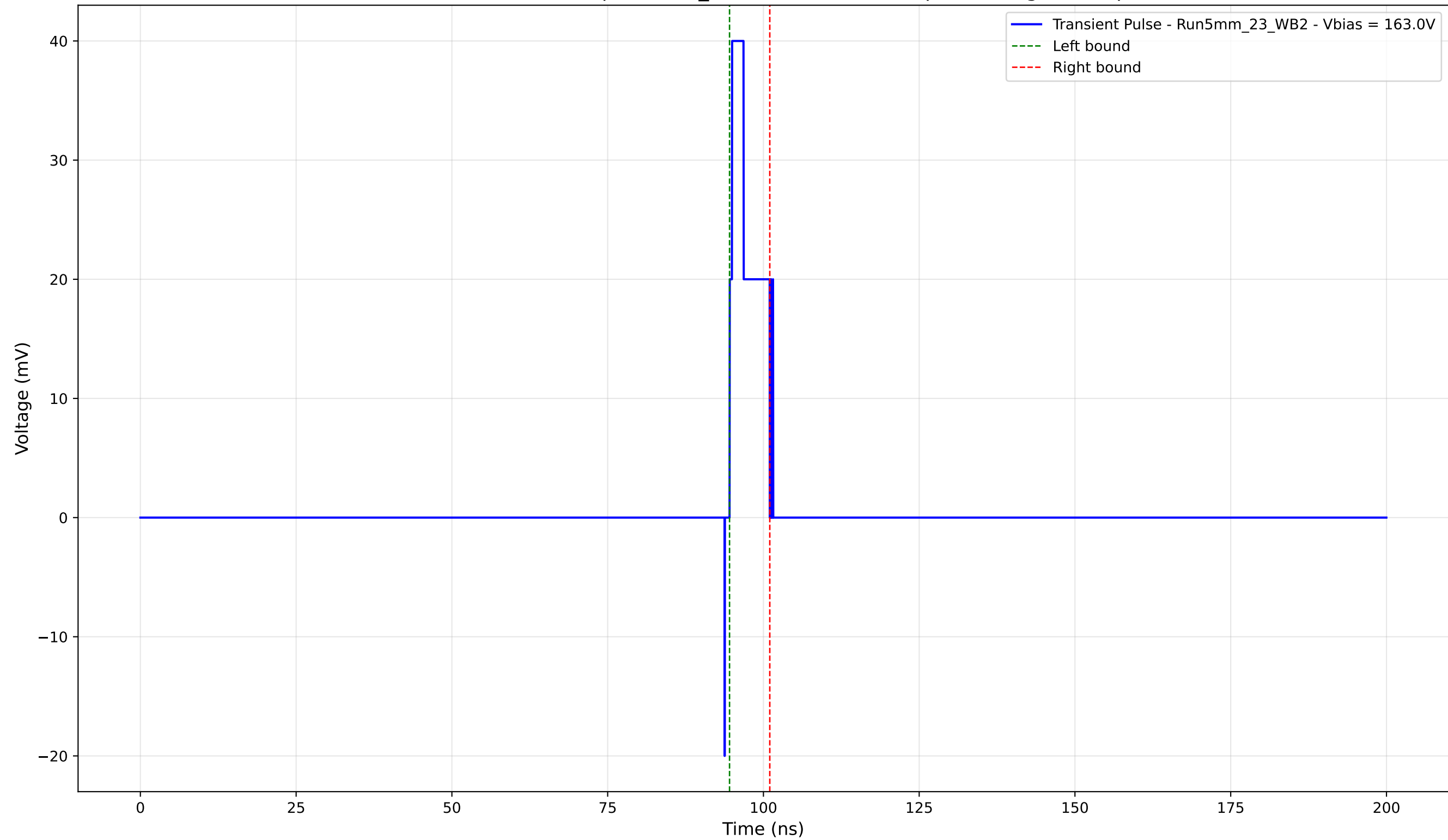
Transient Pulse - Sample: 5mm_23 - Position: 5000.0 \mu\text{m} - Charge: 3.32 pC
