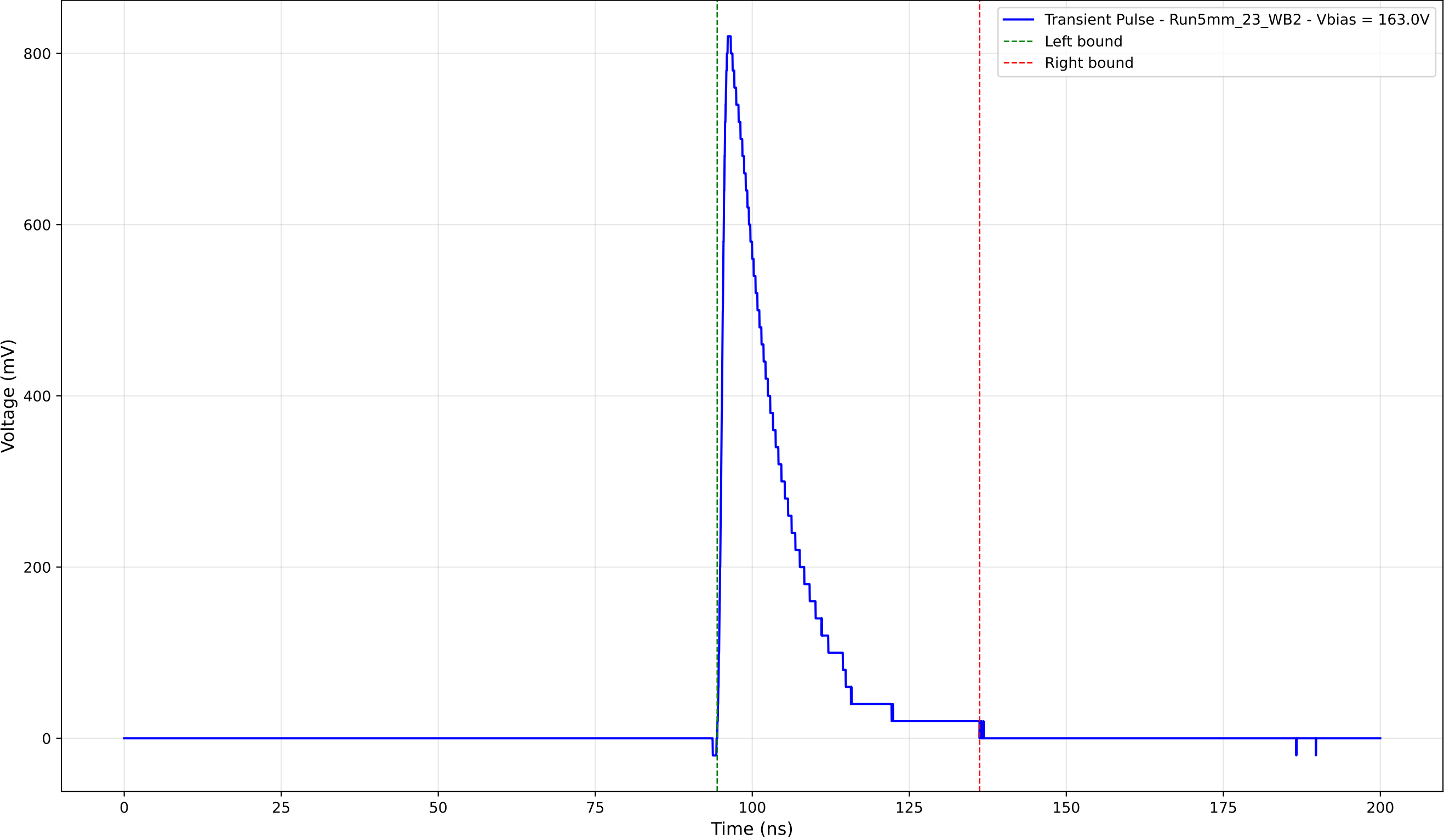
Transient Pulse - Sample: 5mm_23 - Position: 3950.0 \mu\text{m} - Charge: 155.93 pC
