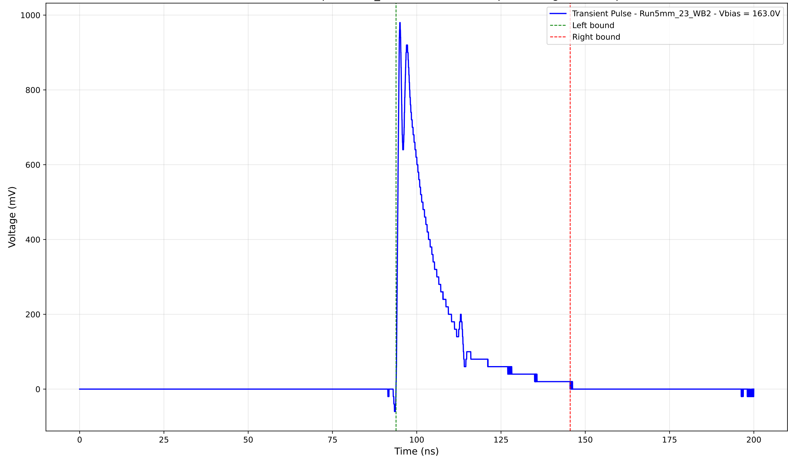
Transient Pulse - Sample: 5mm_23 - Position: 2315.0 \mu\text{m} - Charge: 203.96 pC
