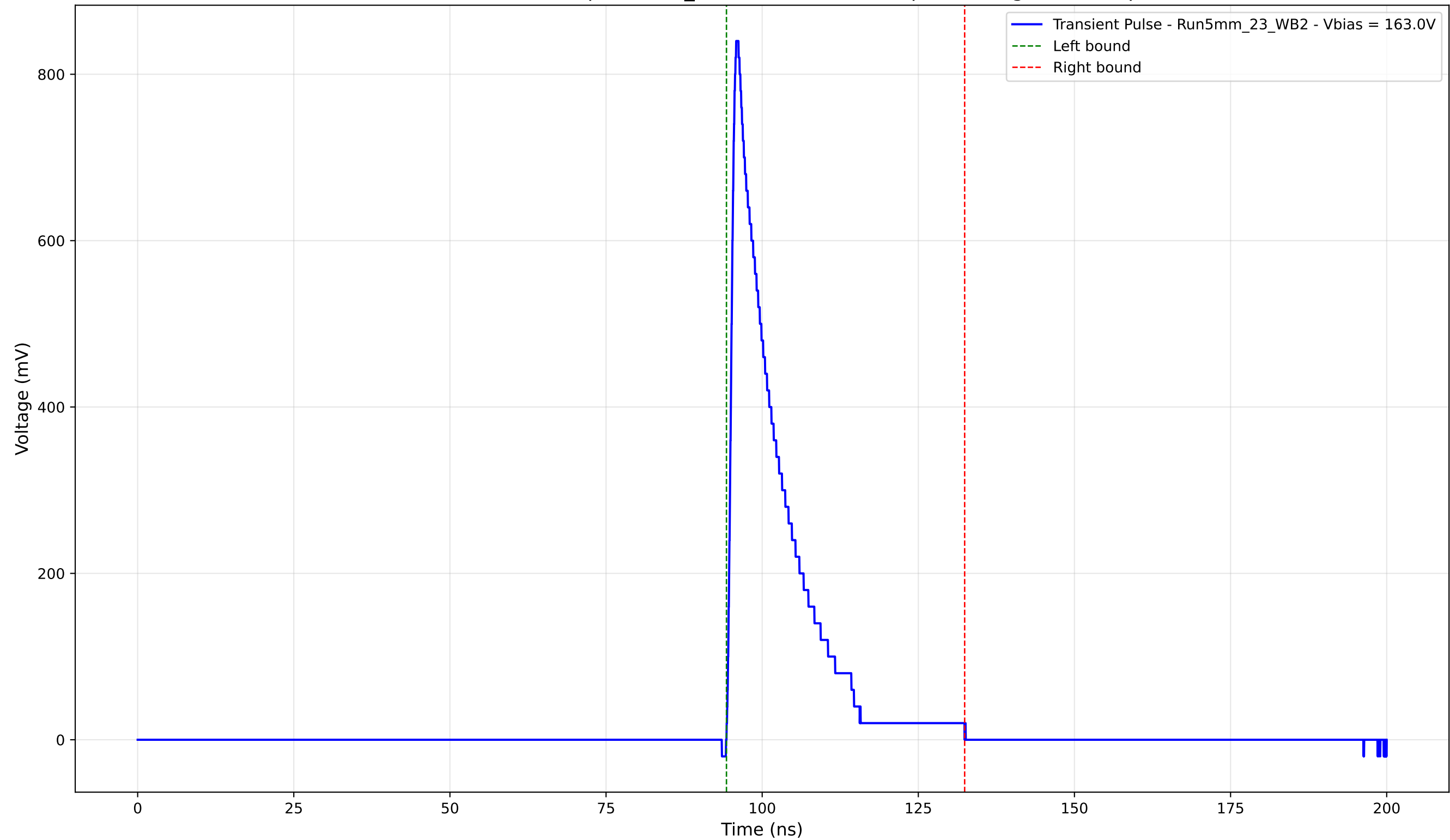
Transient Pulse - Sample: 5mm_23 - Position: 4460.0 \mu\text{m} - Charge: 135.34 pC
