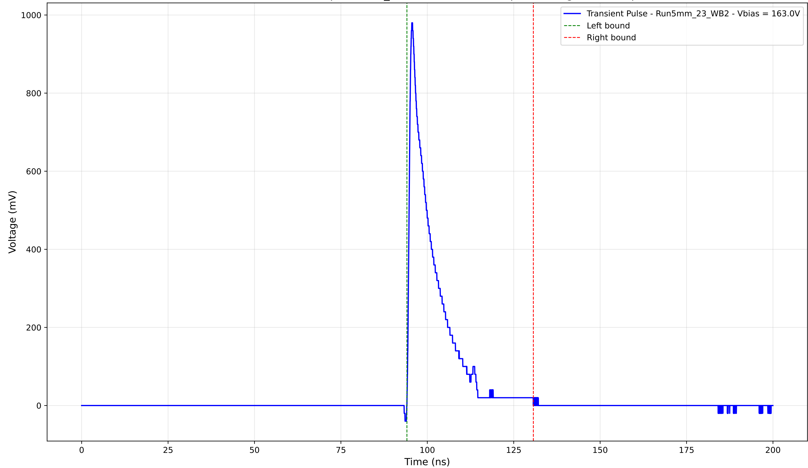
Transient Pulse - Sample: 5mm_23 - Position: 4825.0 \mu\text{m} - Charge: 144.14 pC
