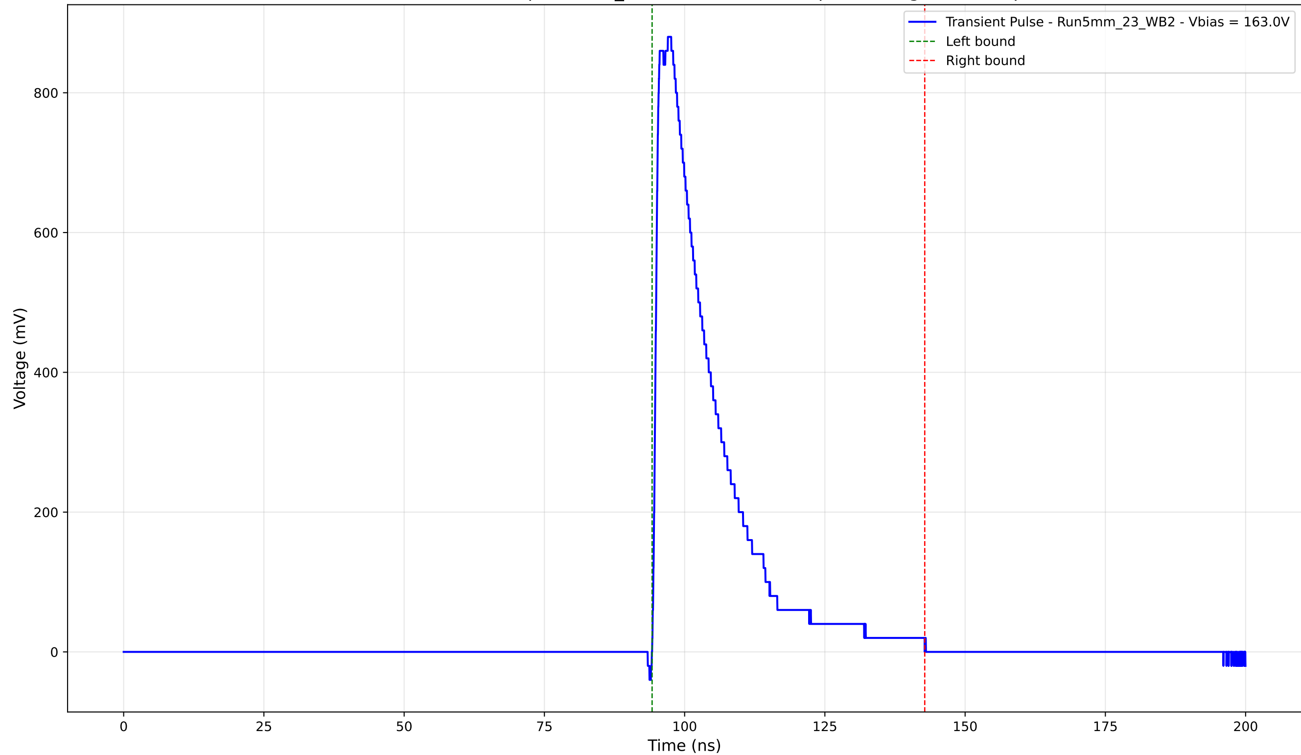
Transient Pulse - Sample: 5mm_23 - Position: 3330.0 \mu\text{m} - Charge: 200.45 pC
