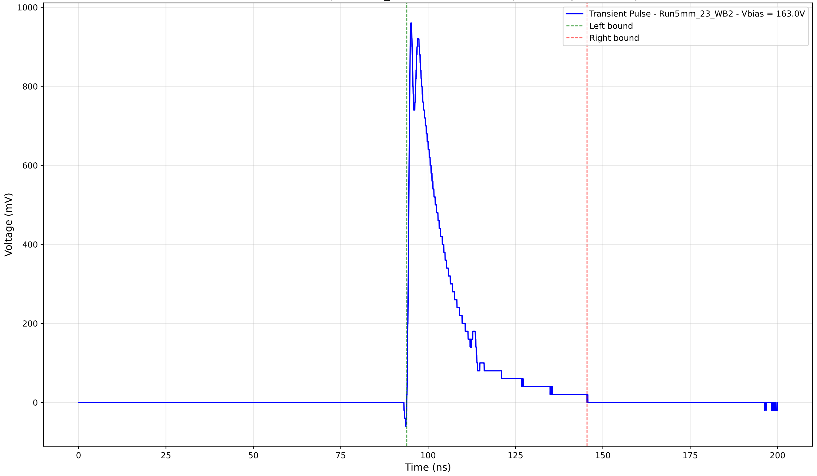
Transient Pulse - Sample: 5mm_23 - Position: 2835.0 \mu\text{m} - Charge: 210.94 pC
