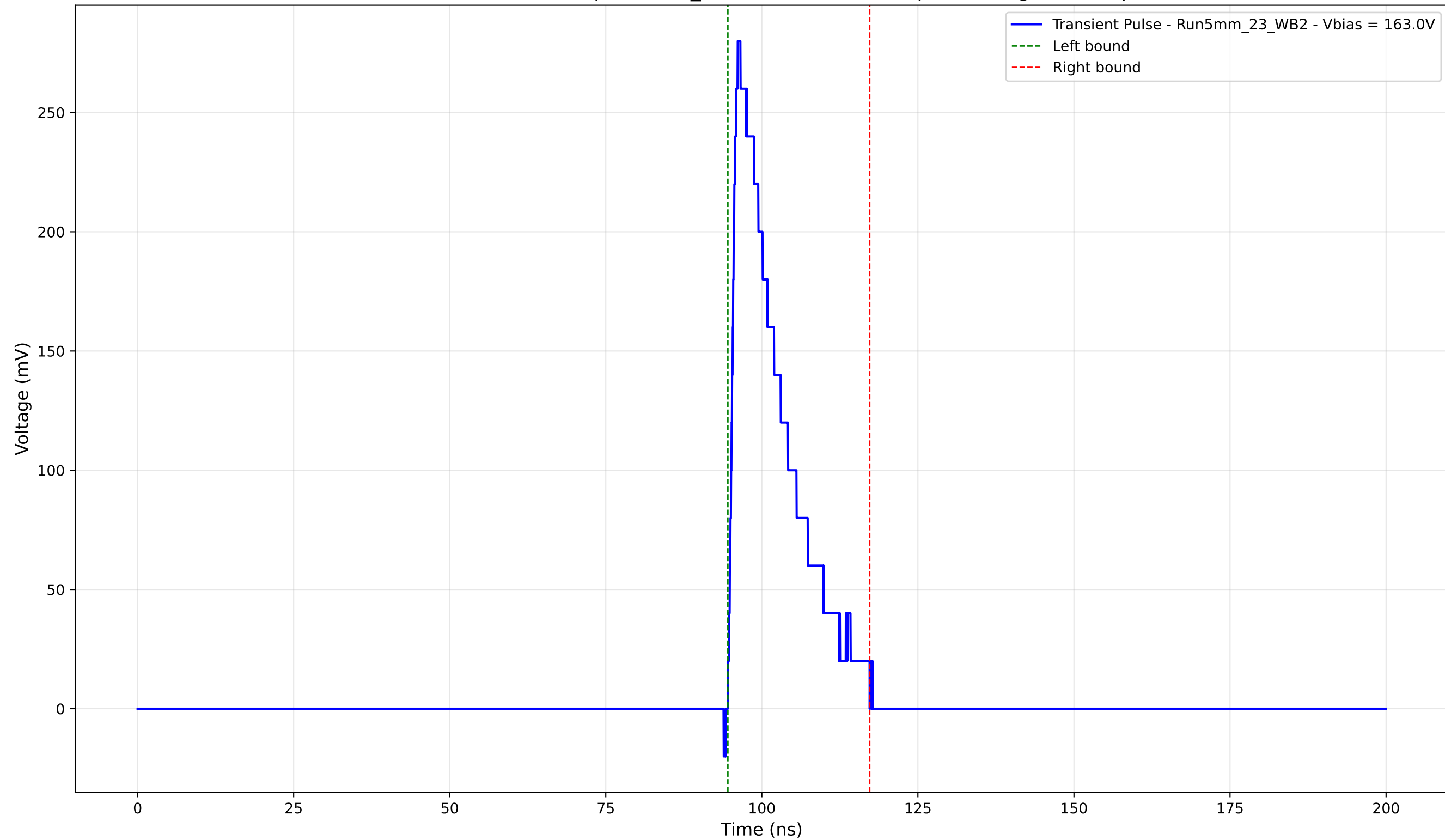
Transient Pulse - Sample: 5mm_23 - Position: 1015.0 \mu\text{m} - Charge: 48.66 pC
