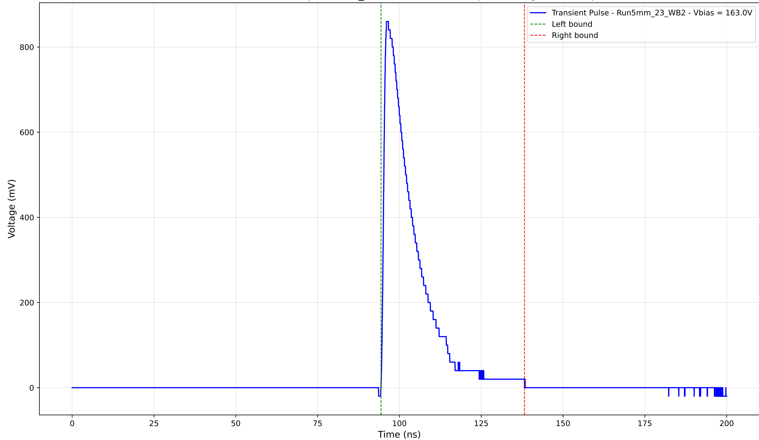
Transient Pulse - Sample: 5mm_23 - Position: 3770.0 \mu\text{m} - Charge: 176.97 pC
