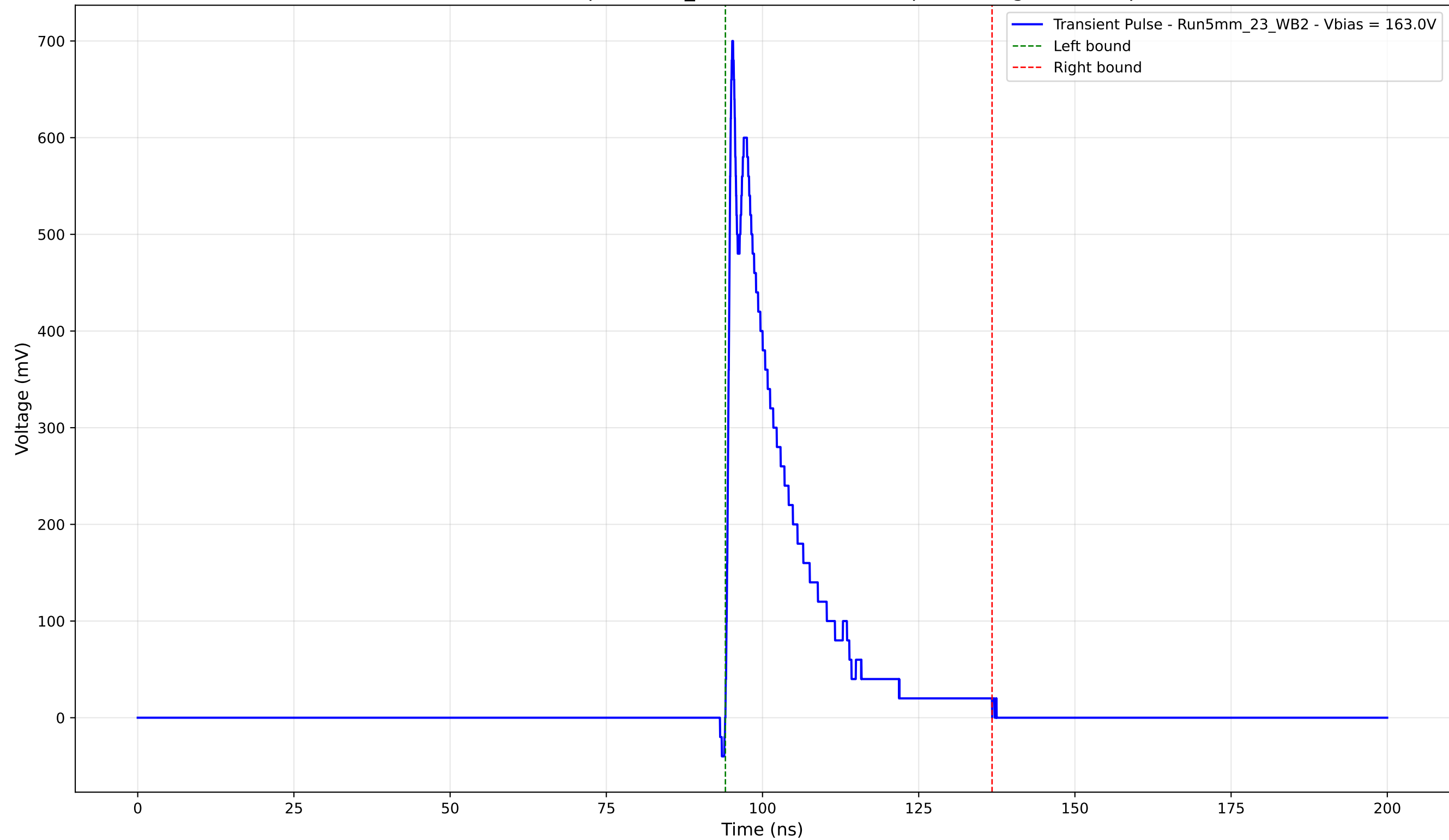
Transient Pulse - Sample: 5mm_23 - Position: 2975.0 \mu\text{m} - Charge: 122.63 pC
