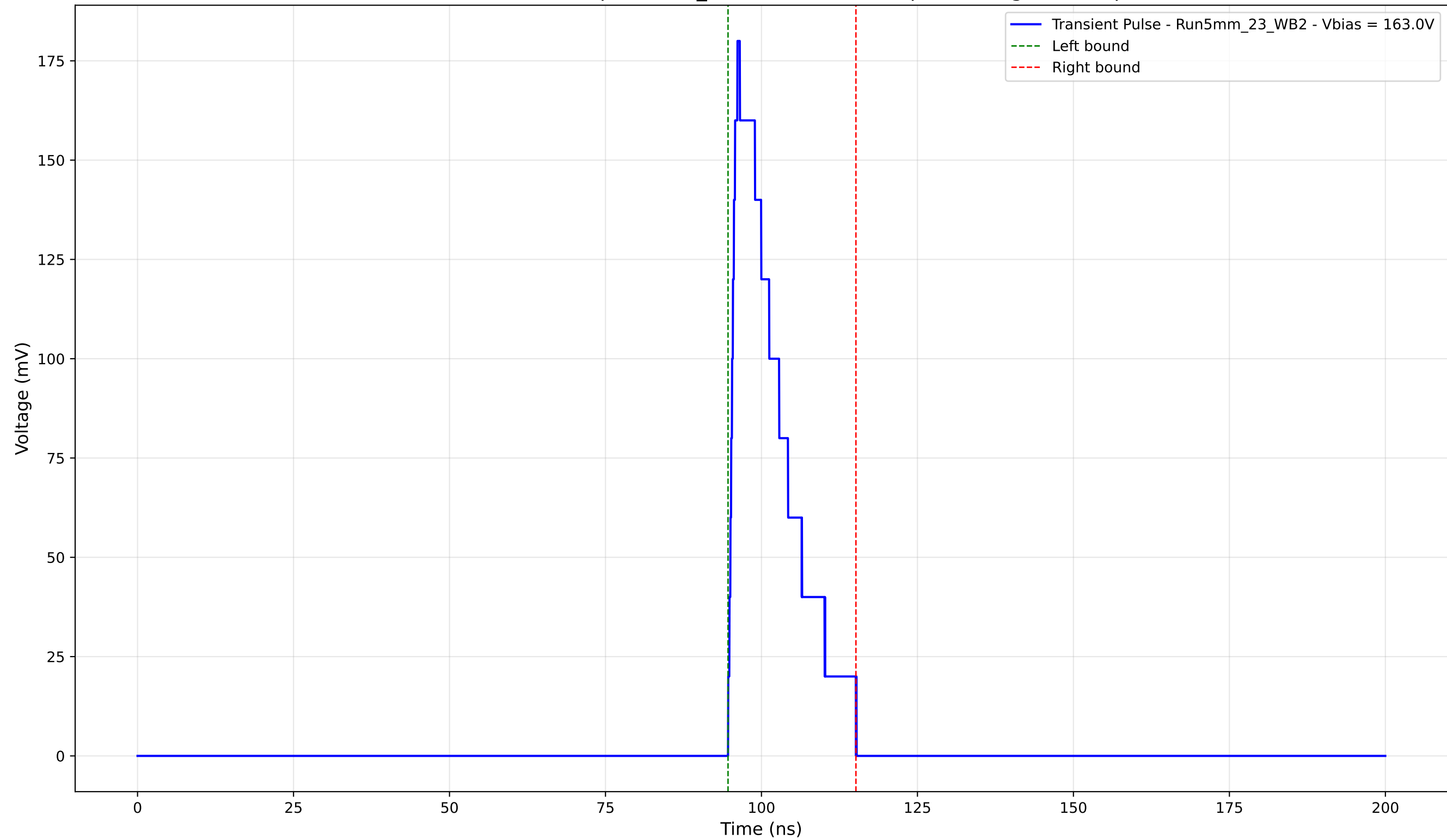
Transient Pulse - Sample: 5mm_23 - Position: 990.0 \mu\text{m} - Charge: 31.09 pC
