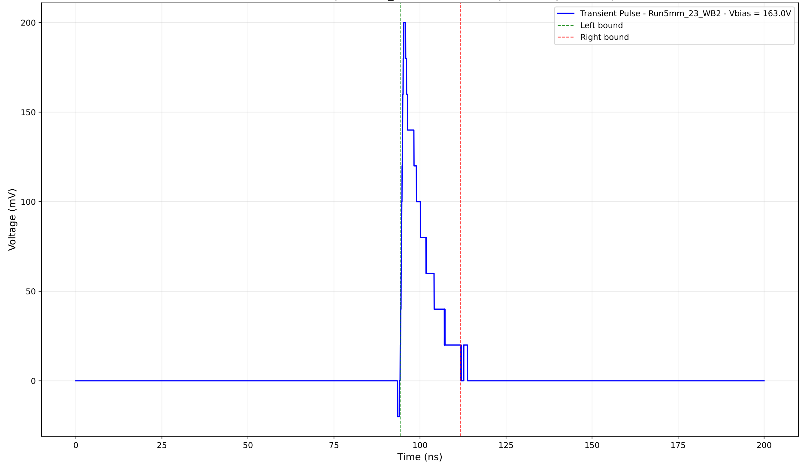
Transient Pulse - Sample: 5mm_23 - Position: 50.0 \mu\text{m} - Charge: 25.26 pC
