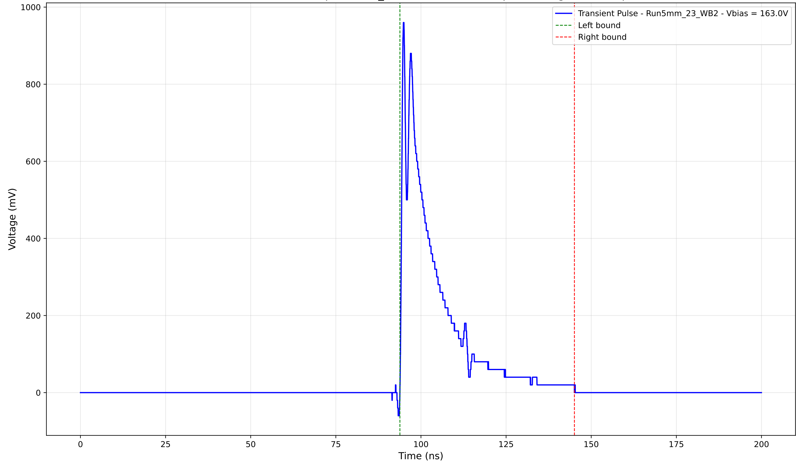
Transient Pulse - Sample: 5mm_23 - Position: 2600.0 \mu\text{m} - Charge: 180.62 pC
