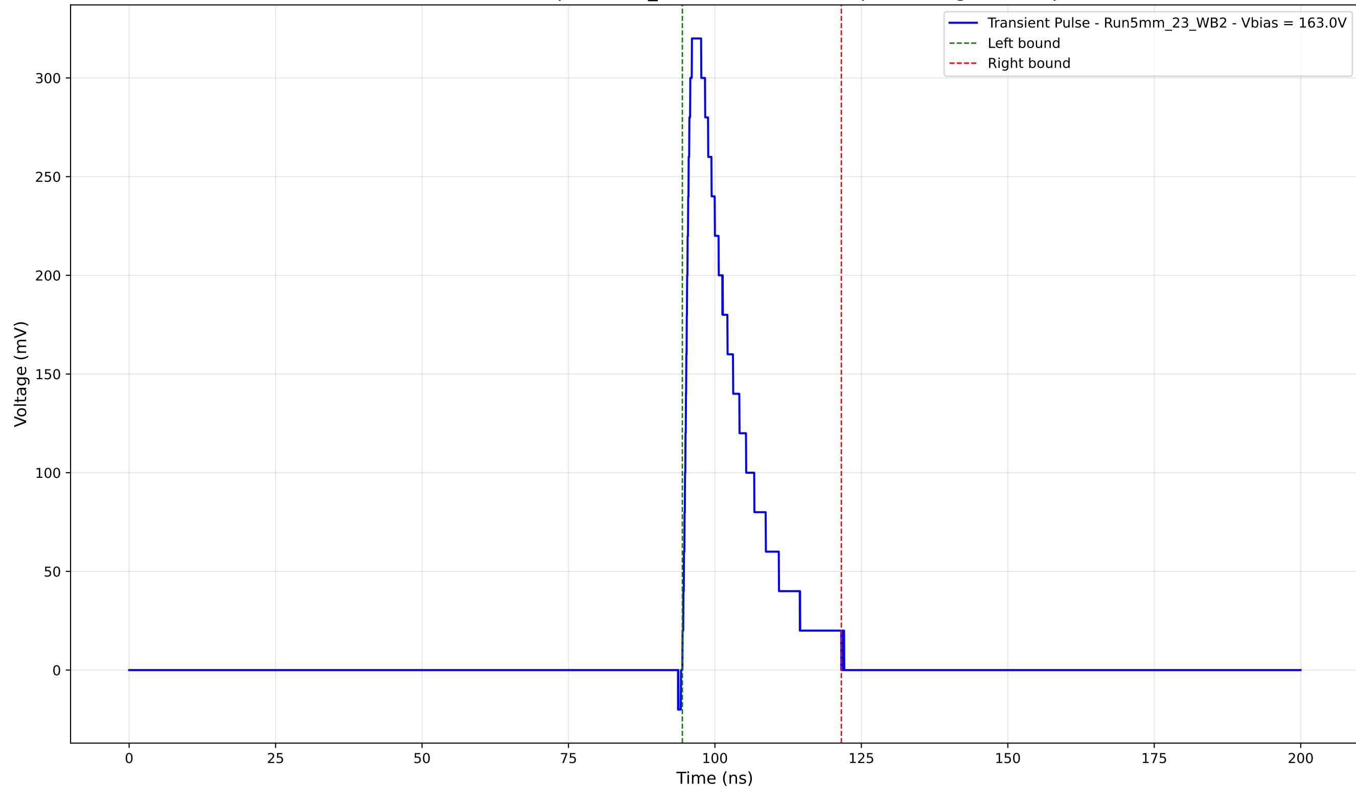
Transient Pulse - Sample: 5mm_23 - Position: 3555.0 \mu\text{m} - Charge: 60.27 pC
