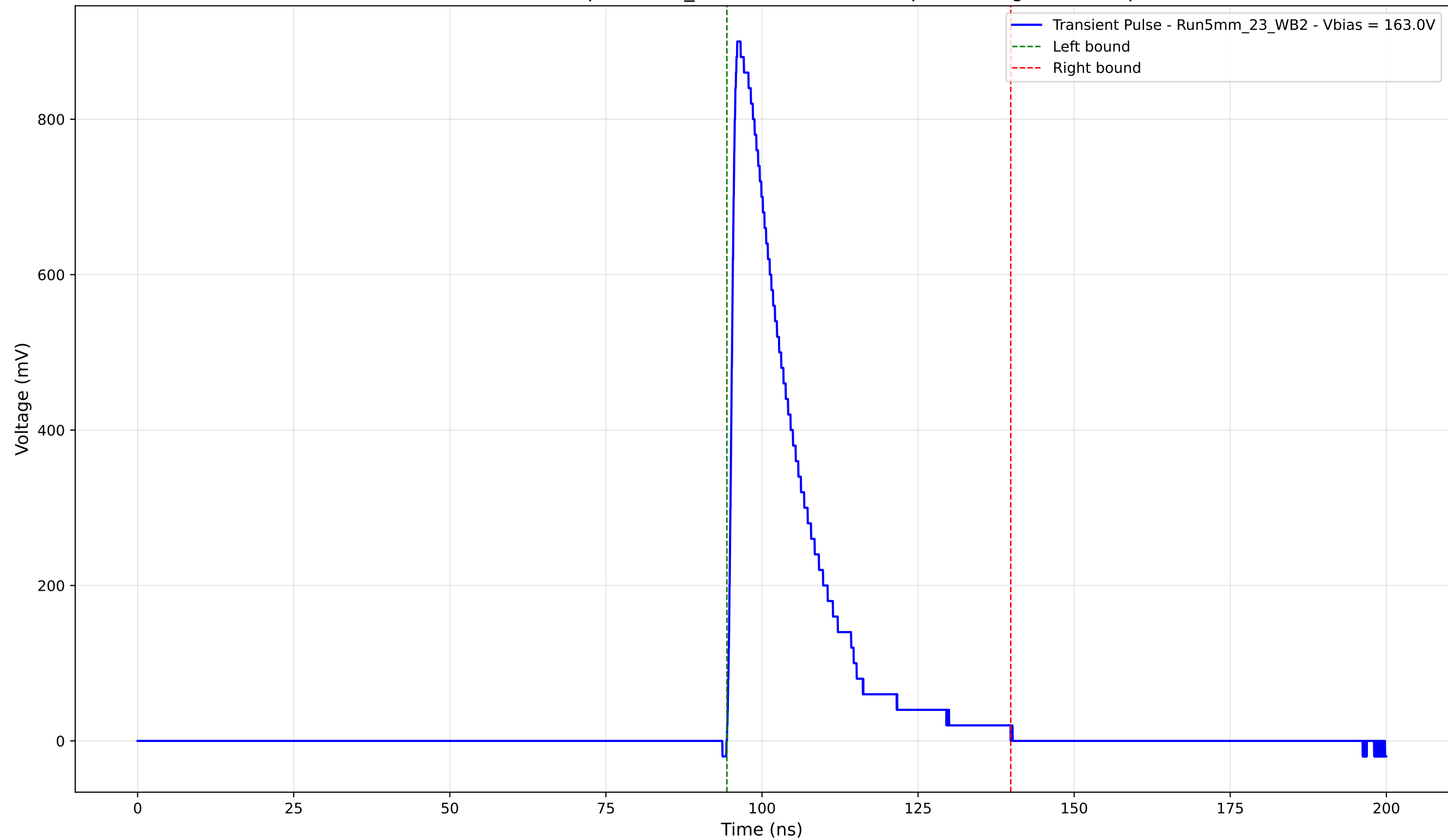
Transient Pulse - Sample: 5mm_23 - Position: 1220.0 \mu\text{m} - Charge: 197.34 pC
