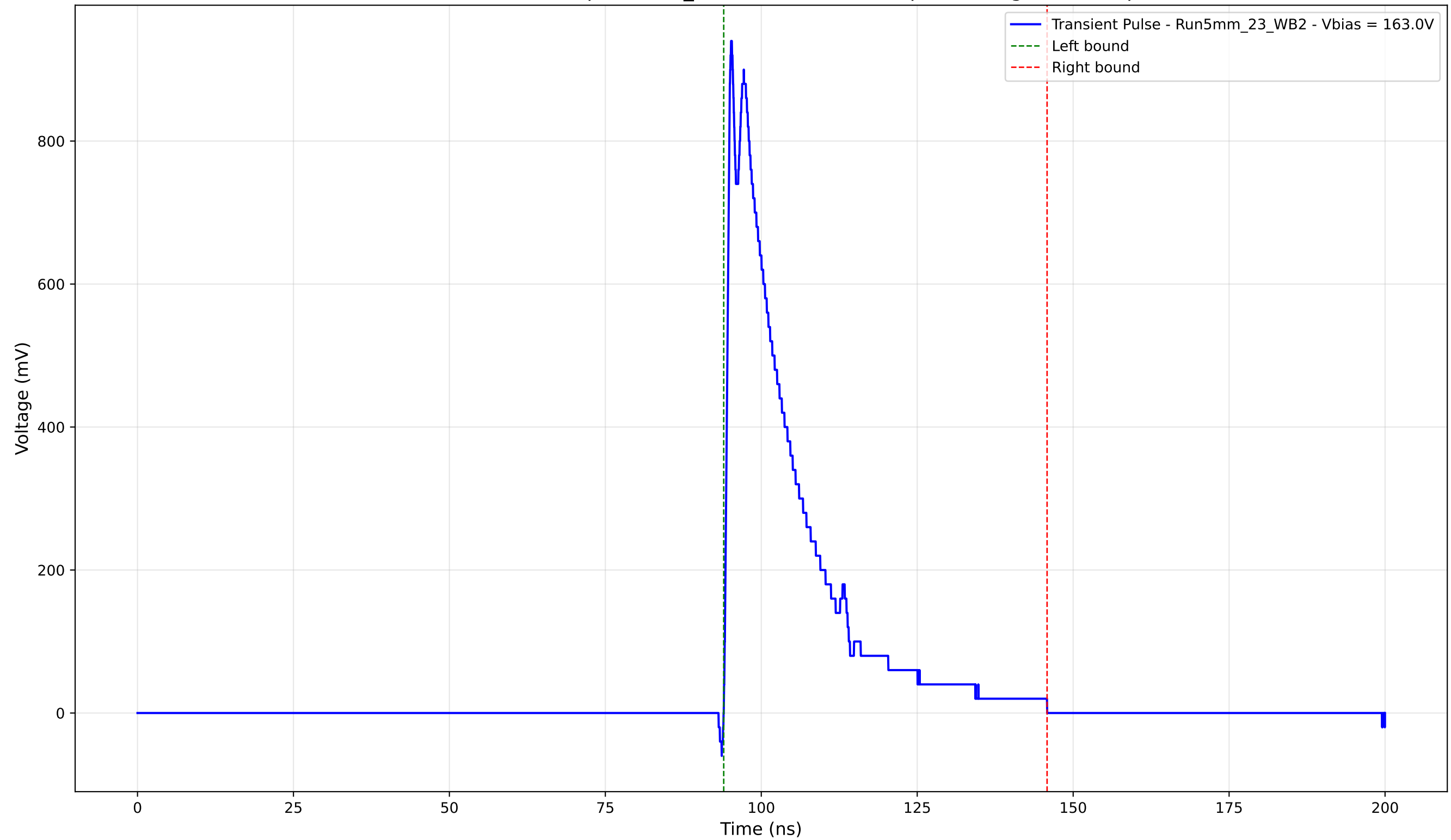
Transient Pulse - Sample: 5mm_23 - Position: 2125.0 \mu\text{m} - Charge: 203.38 pC
