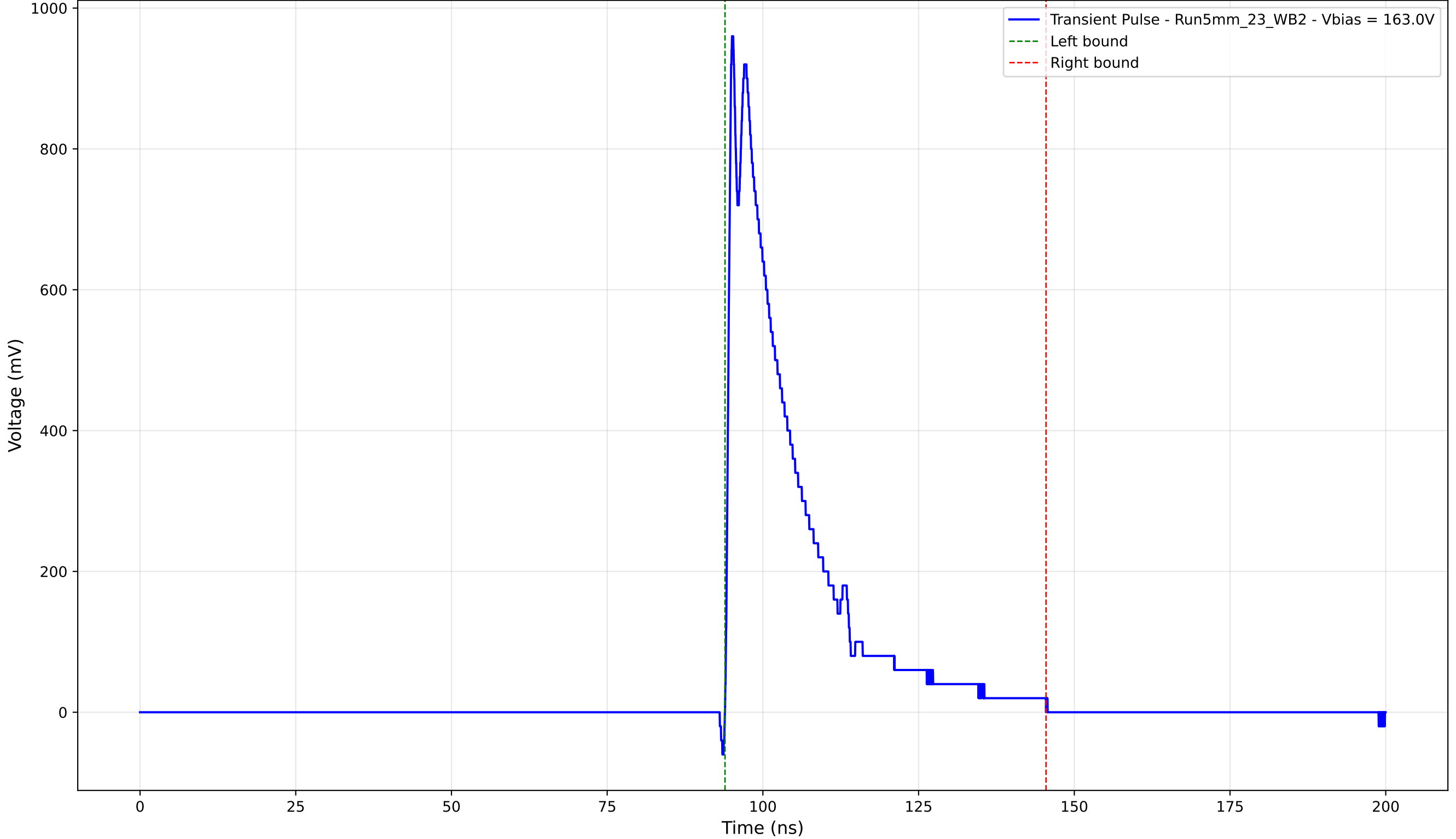
Transient Pulse - Sample: 5mm_23 - Position: 2820.0 \mu\text{m} - Charge: 209.18 pC
