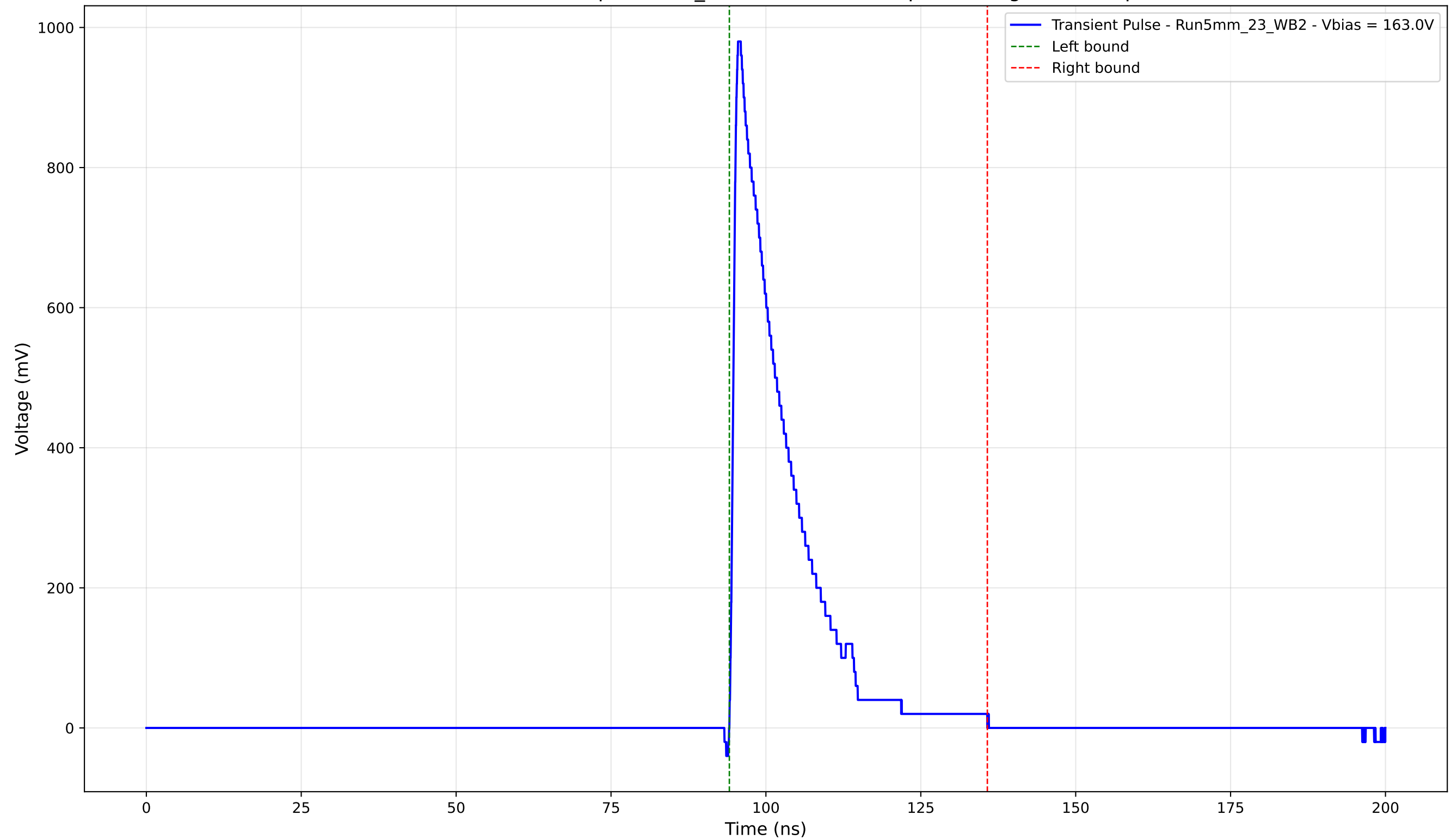
Transient Pulse - Sample: 5mm_23 - Position: 310.0 \mu\text{m} - Charge: 177.85 pC
