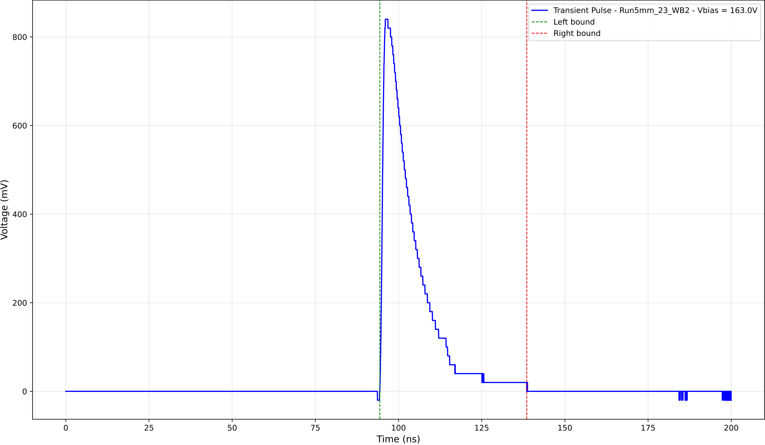
Transient Pulse - Sample: 5mm_23 - Position: 3705.0 \mu\text{m} - Charge: 175.11 pC
