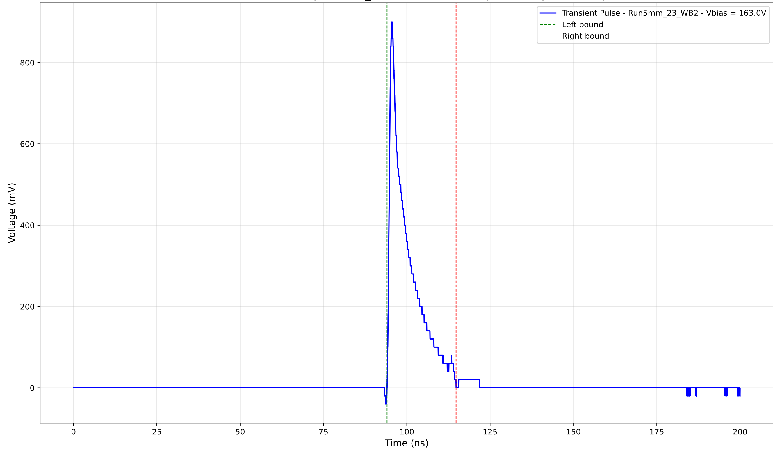
Transient Pulse - Sample: 5mm_23 - Position: 4900.0 \mu\text{m} - Charge: 108.02 pC
