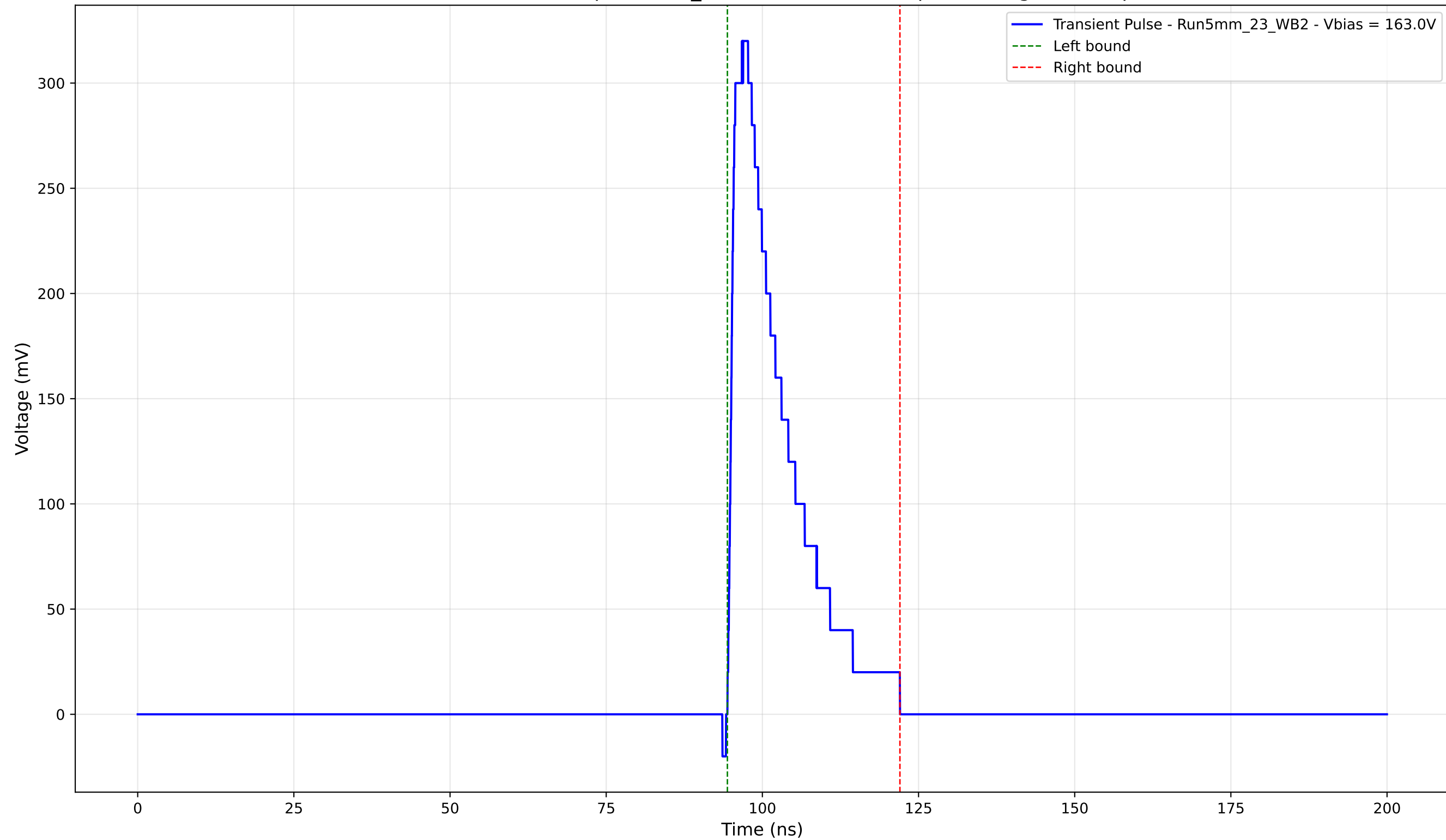
Transient Pulse - Sample: 5mm_23 - Position: 3495.0 \mu\text{m} - Charge: 60.50 pC
