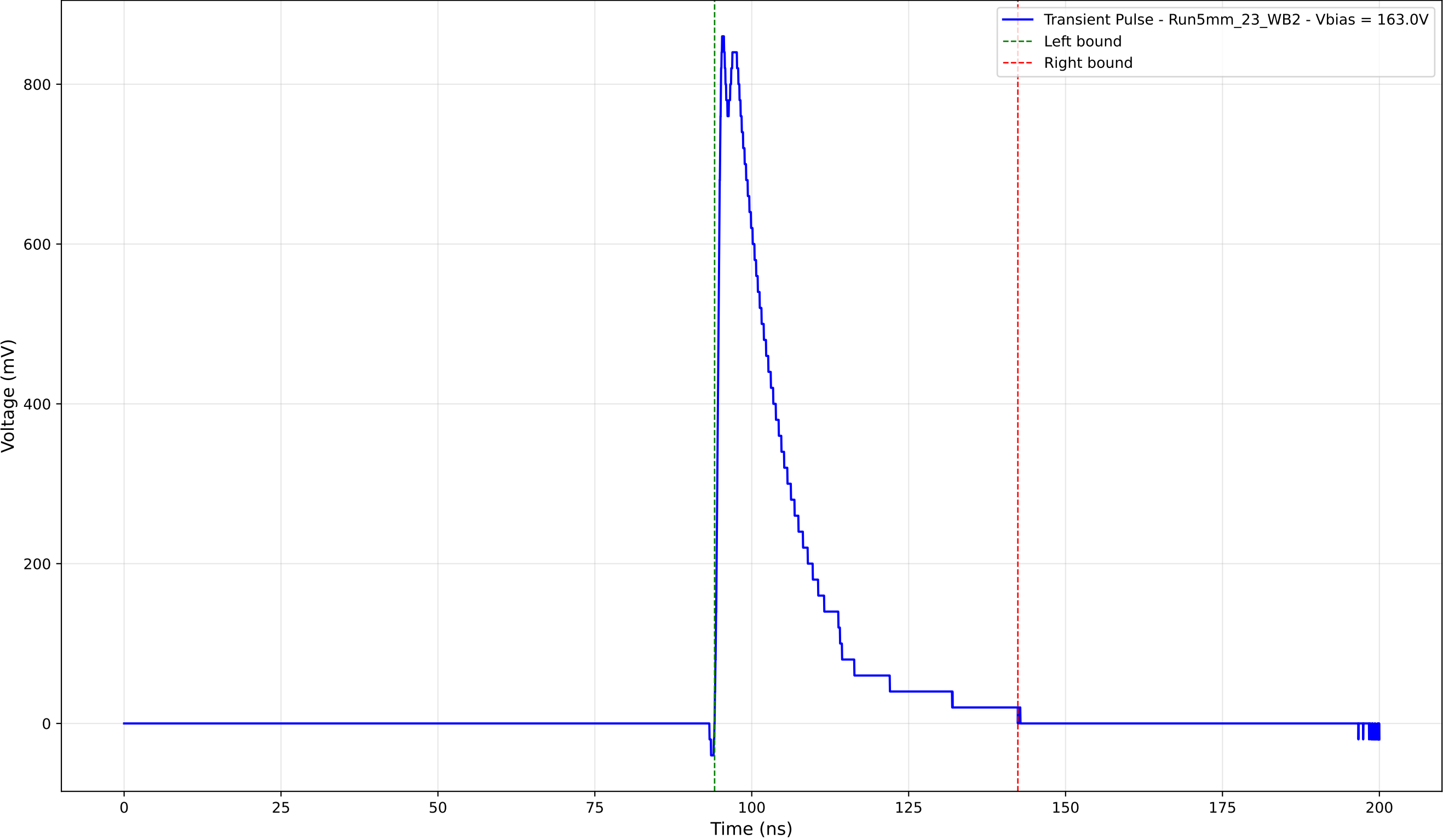
Transient Pulse - Sample: 5mm_23 - Position: 3095.0 \mu\text{m} - Charge: 189.72 pC
