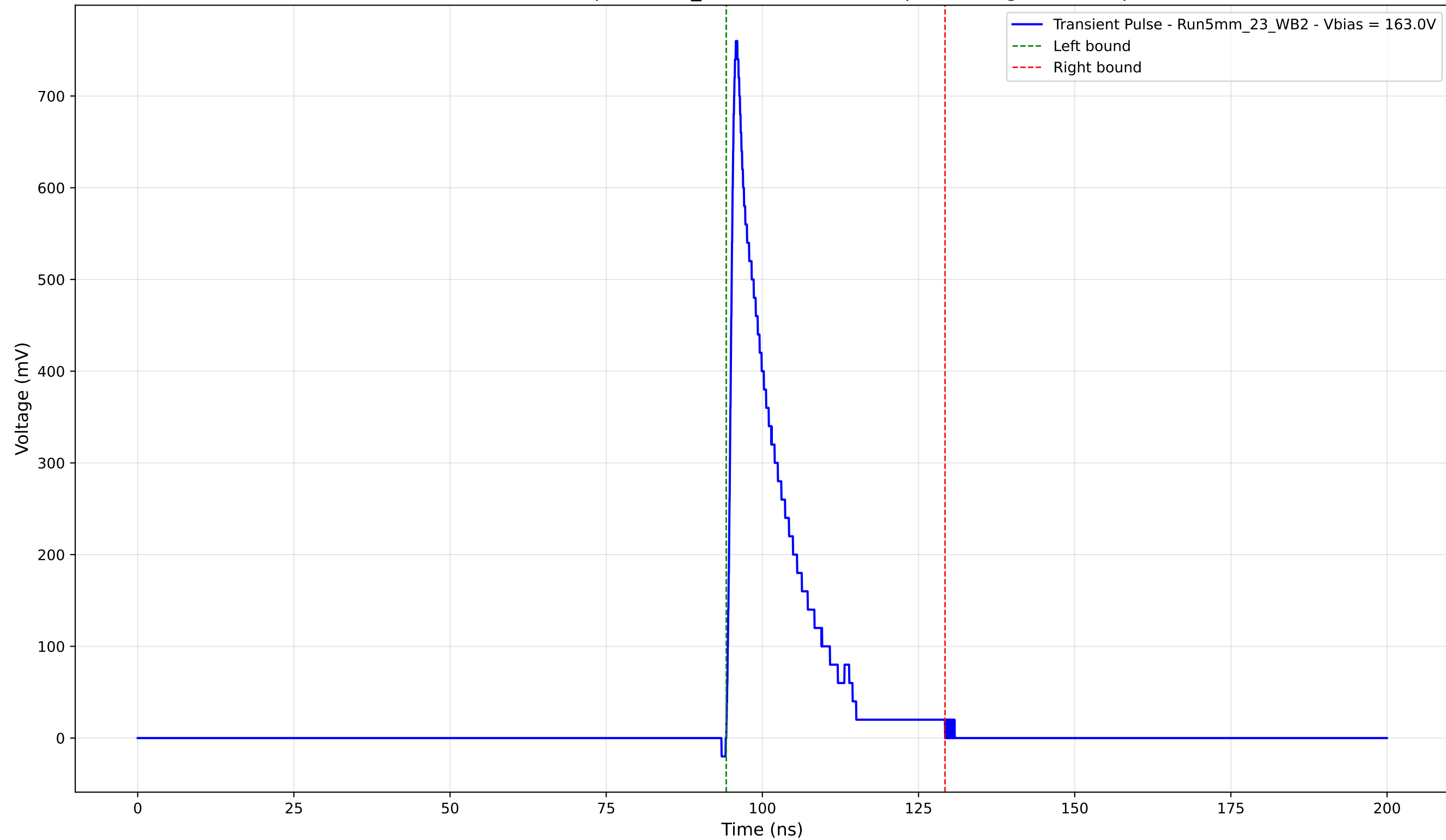
Transient Pulse - Sample: 5mm_23 - Position: 435.0 \mu\text{m} - Charge: 116.58 pC
