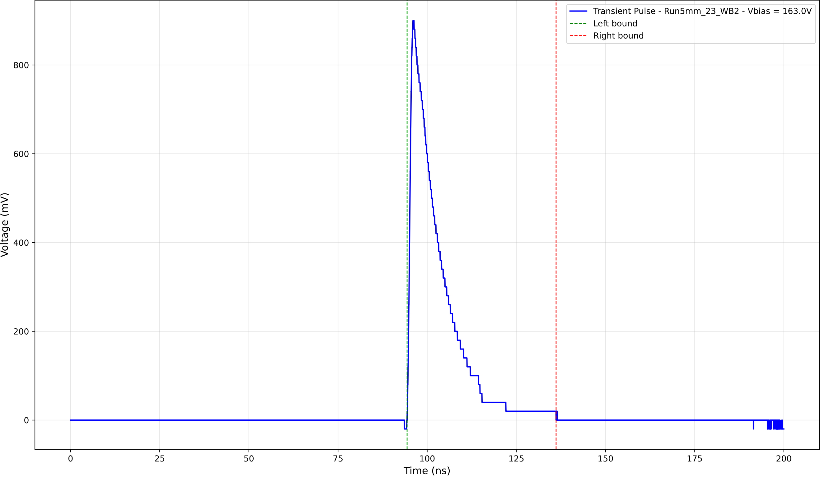
Transient Pulse - Sample: 5mm_23 - Position: 4250.0 \mu\text{m} - Charge: 164.19 pC
