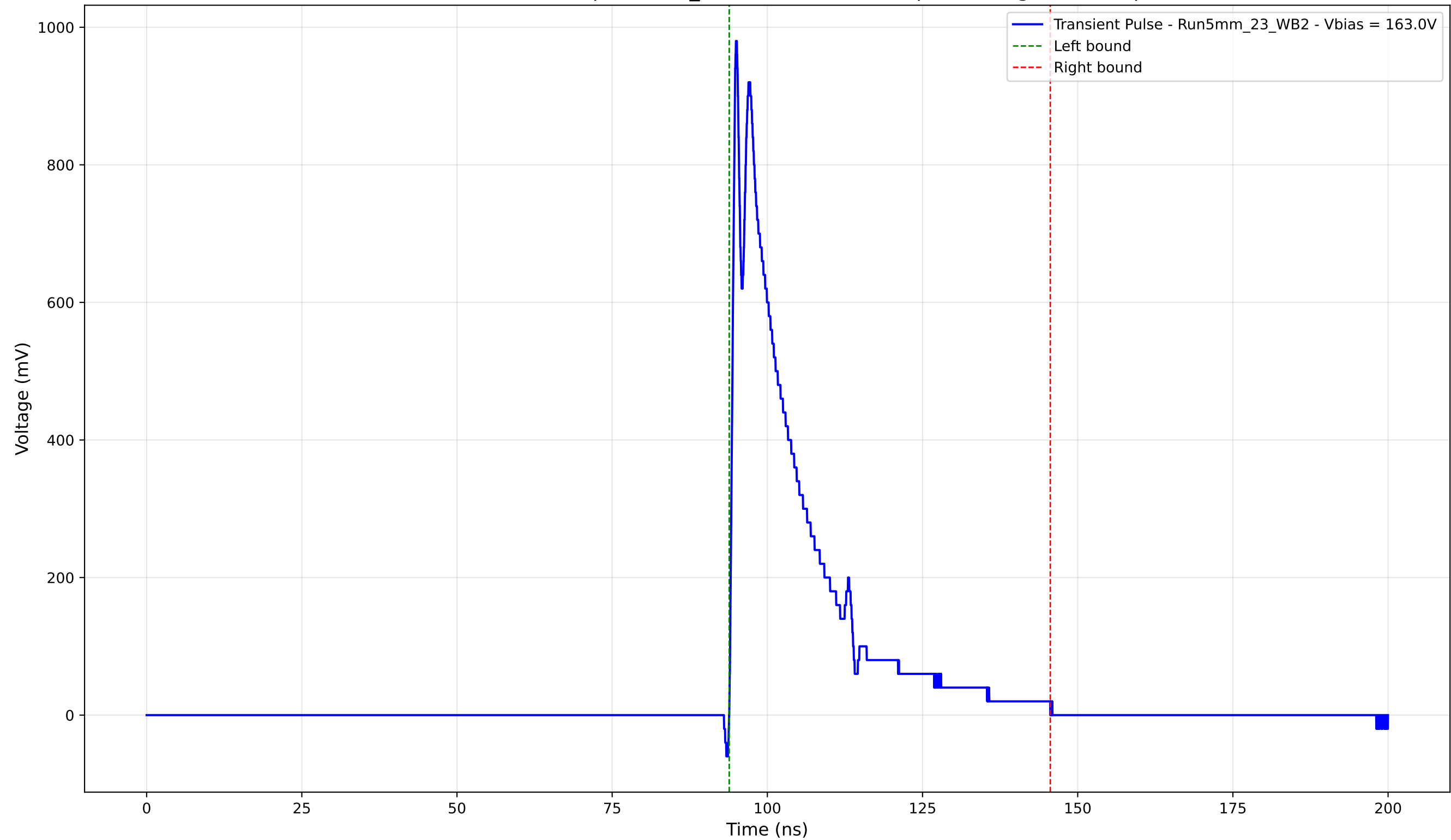
Transient Pulse - Sample: 5mm_23 - Position: 2700.0 \mu\text{m} - Charge: 202.06 pC
