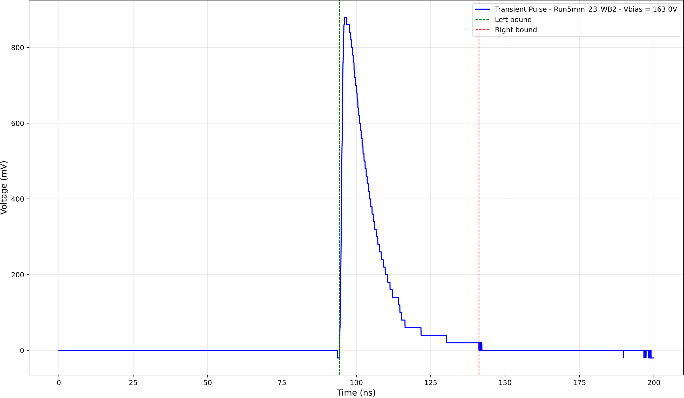
Transient Pulse - Sample: 5mm_23 - Position: 1380.0 \mu\text{m} - Charge: 196.83 pC
