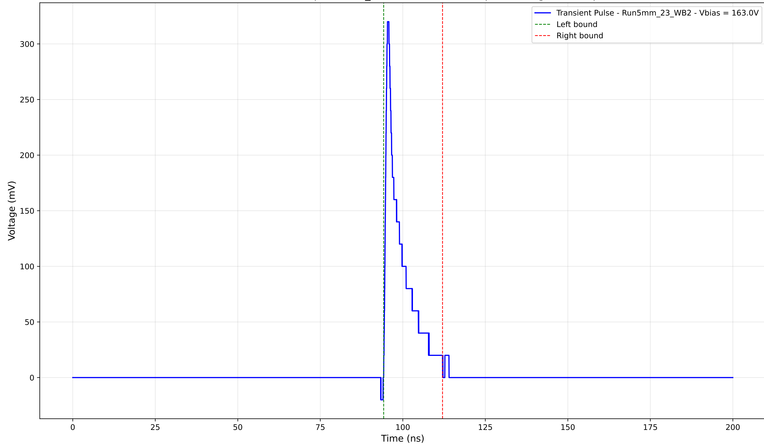
Transient Pulse - Sample: 5mm_23 - Position: 4950.0 \mu\text{m} - Charge: 32.24 pC
