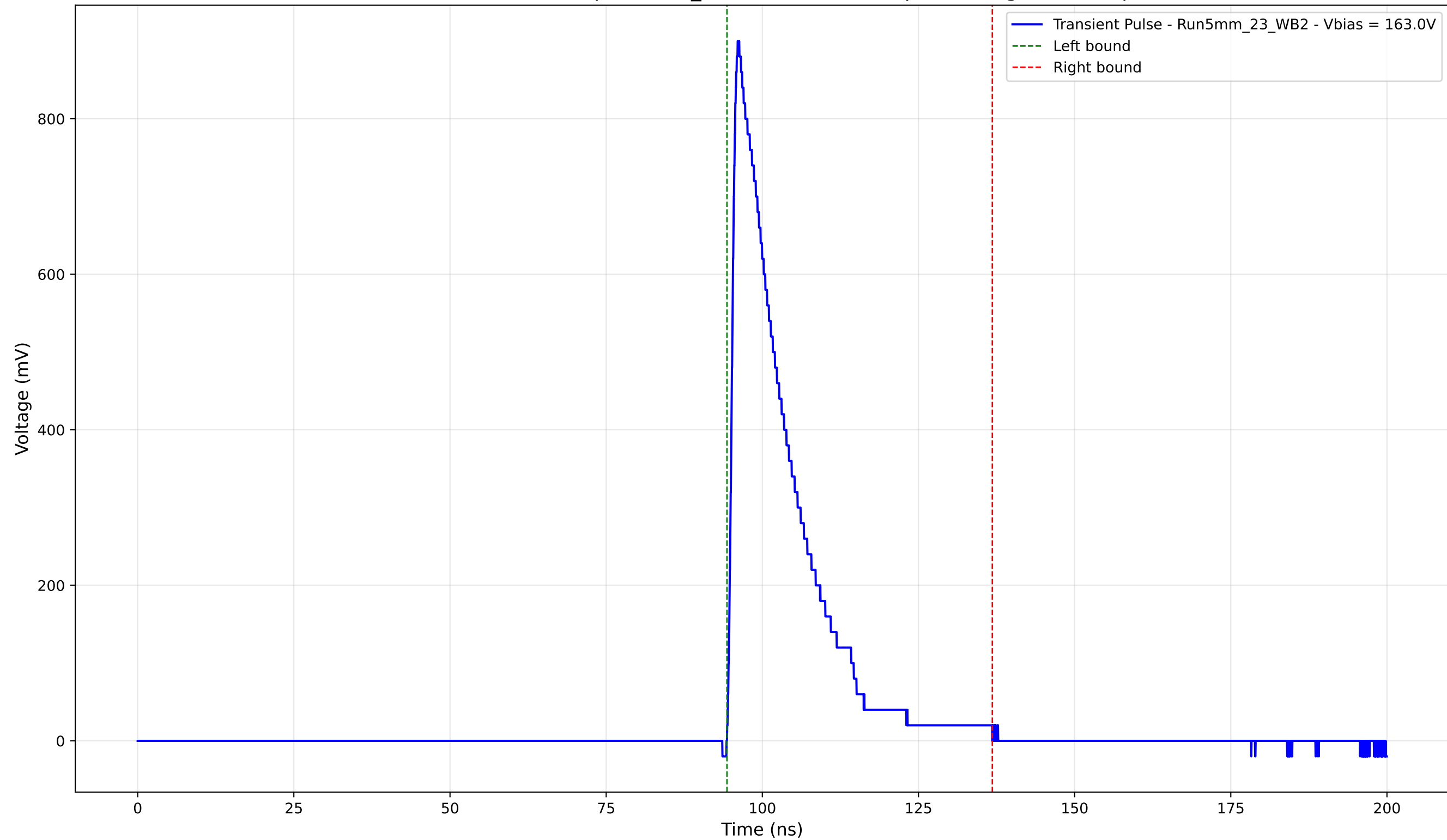
Transient Pulse - Sample: 5mm_23 - Position: 795.0 \mu\text{m} - Charge: 173.81 pC
