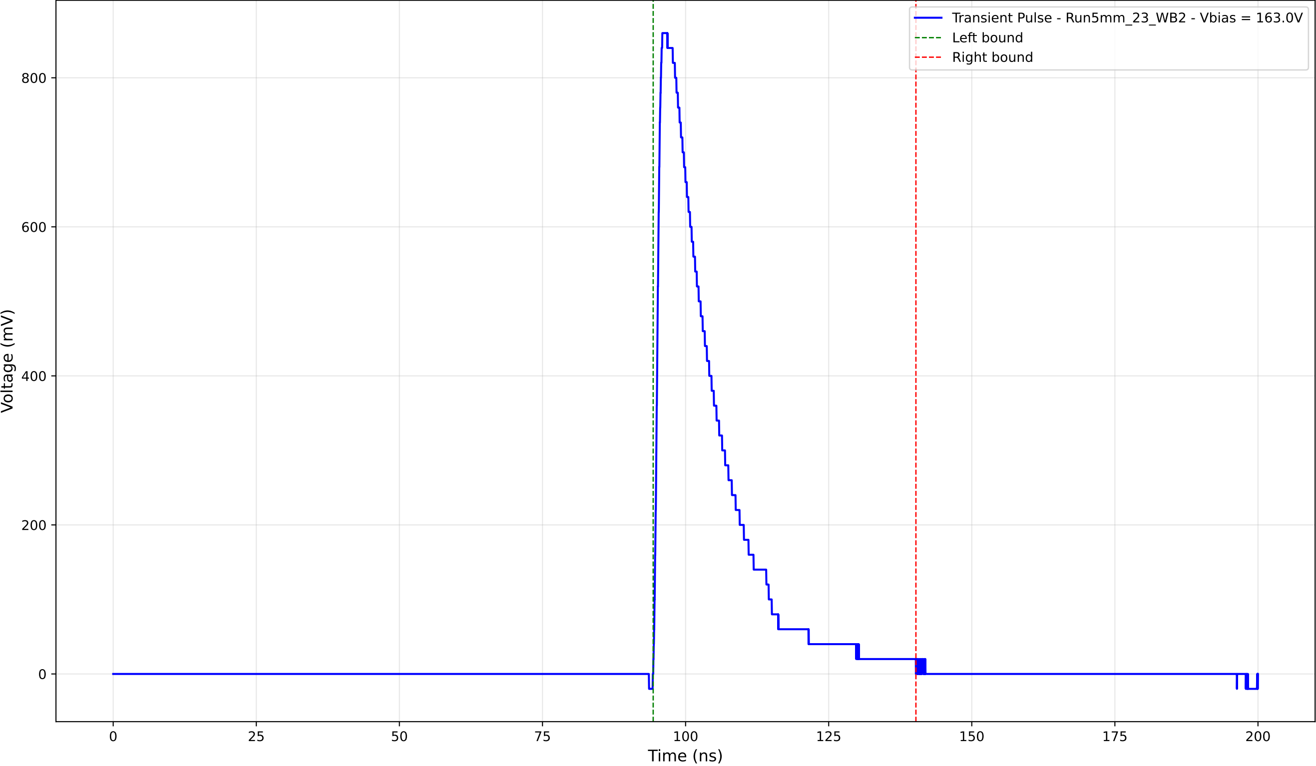
Transient Pulse - Sample: 5mm_23 - Position: 1400.0 \mu\text{m} - Charge: 191.08 pC
