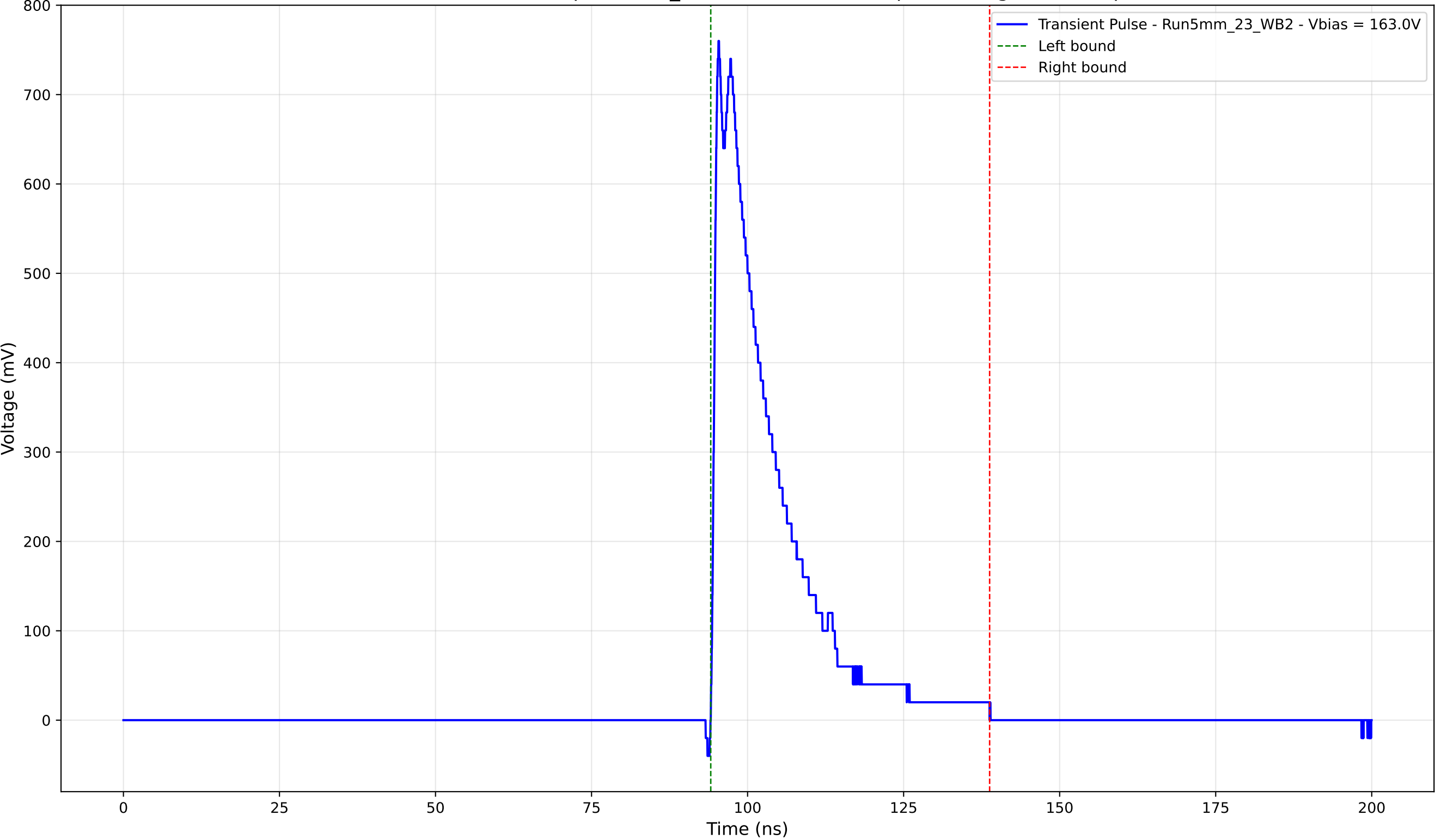
Transient Pulse - Sample: 5mm_23 - Position: 3080.0 \mu\text{m} - Charge: 154.18 pC
