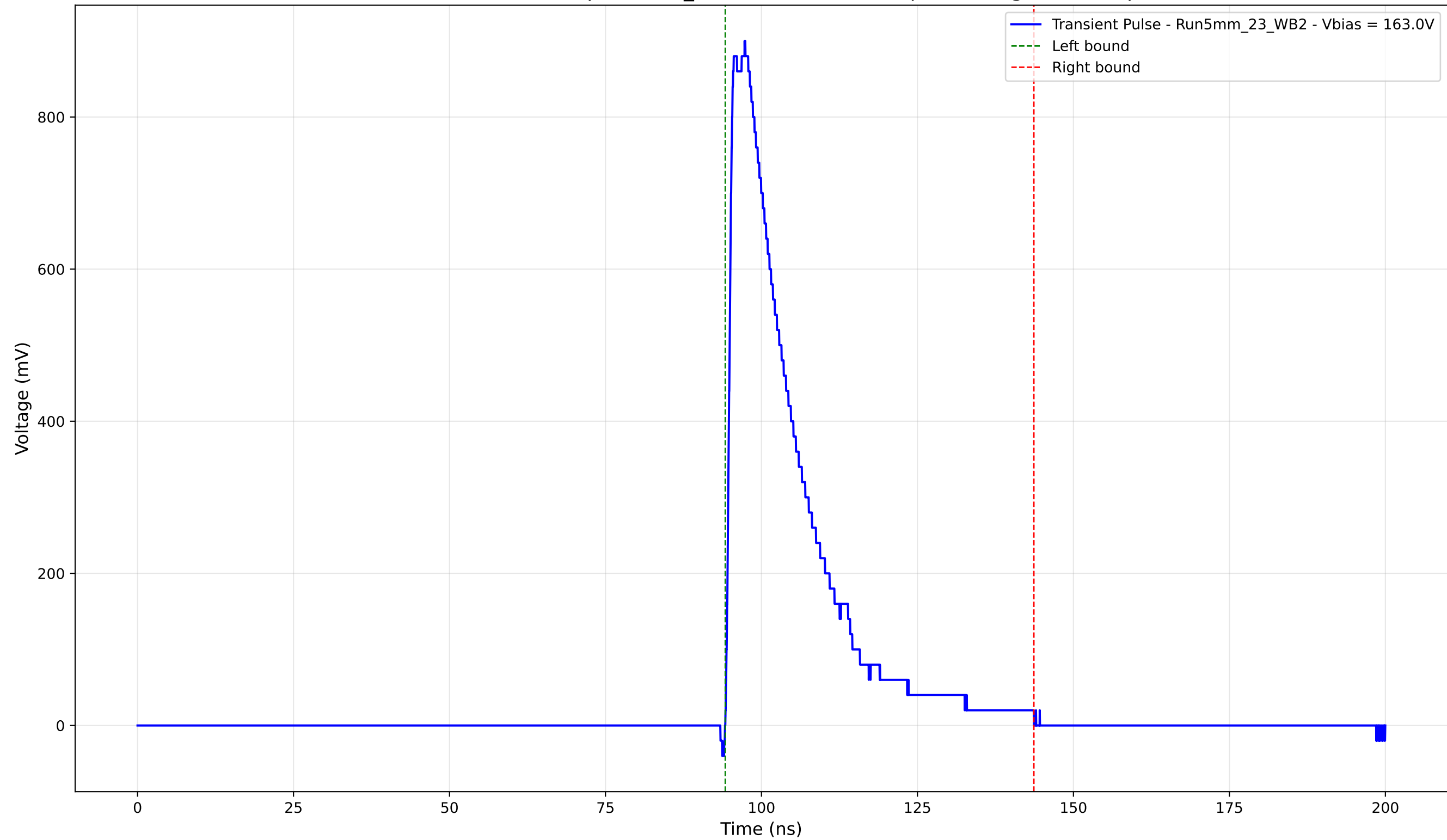
Transient Pulse - Sample: 5mm_23 - Position: 1710.0 \mu\text{m} - Charge: 209.74 pC
