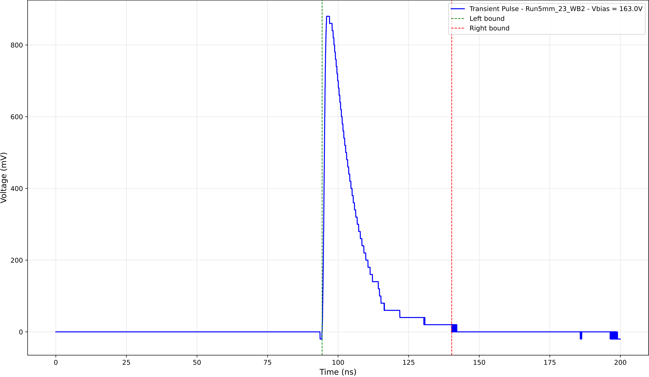
Transient Pulse - Sample: 5mm_23 - Position: 1365.0 \mu\text{m} - Charge: 198.07 pC
