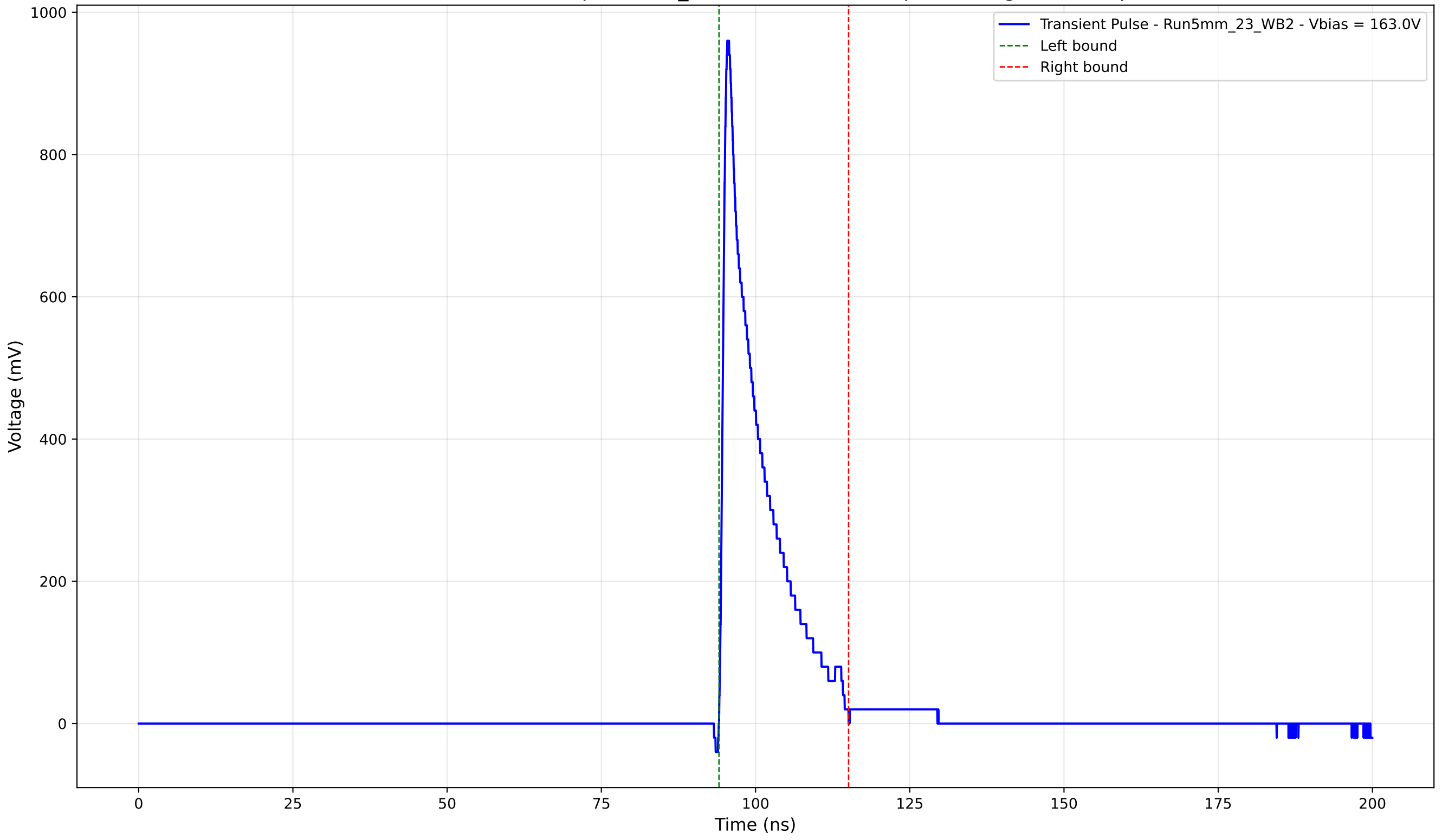
Transient Pulse - Sample: 5mm_23 - Position: 4880.0 \mu\text{m} - Charge: 126.30 pC
