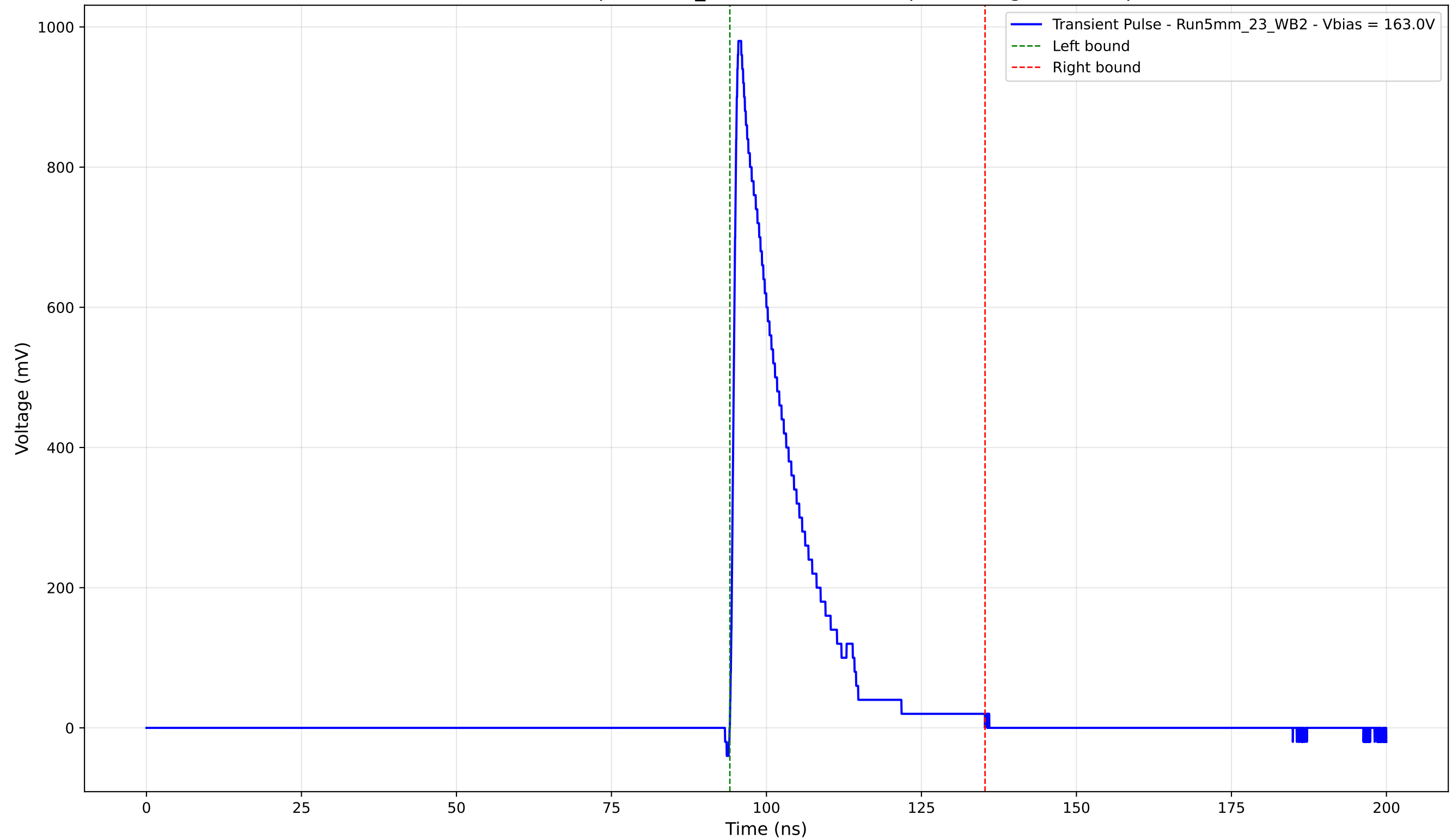
Transient Pulse - Sample: 5mm_23 - Position: 300.0 \mu\text{m} - Charge: 176.56 pC
