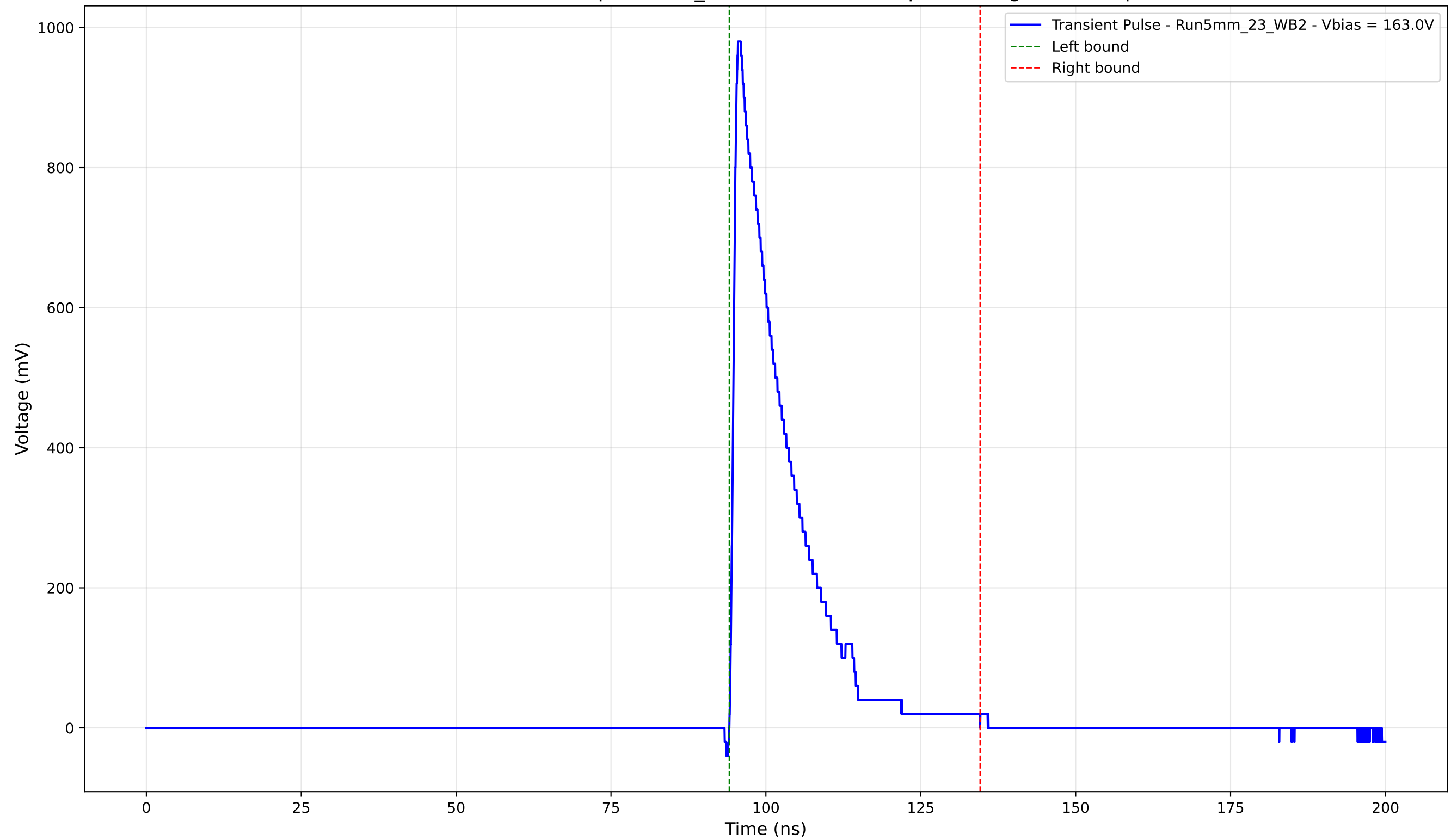
Transient Pulse - Sample: 5mm_23 - Position: 320.0 \mu\text{m} - Charge: 178.18 pC
