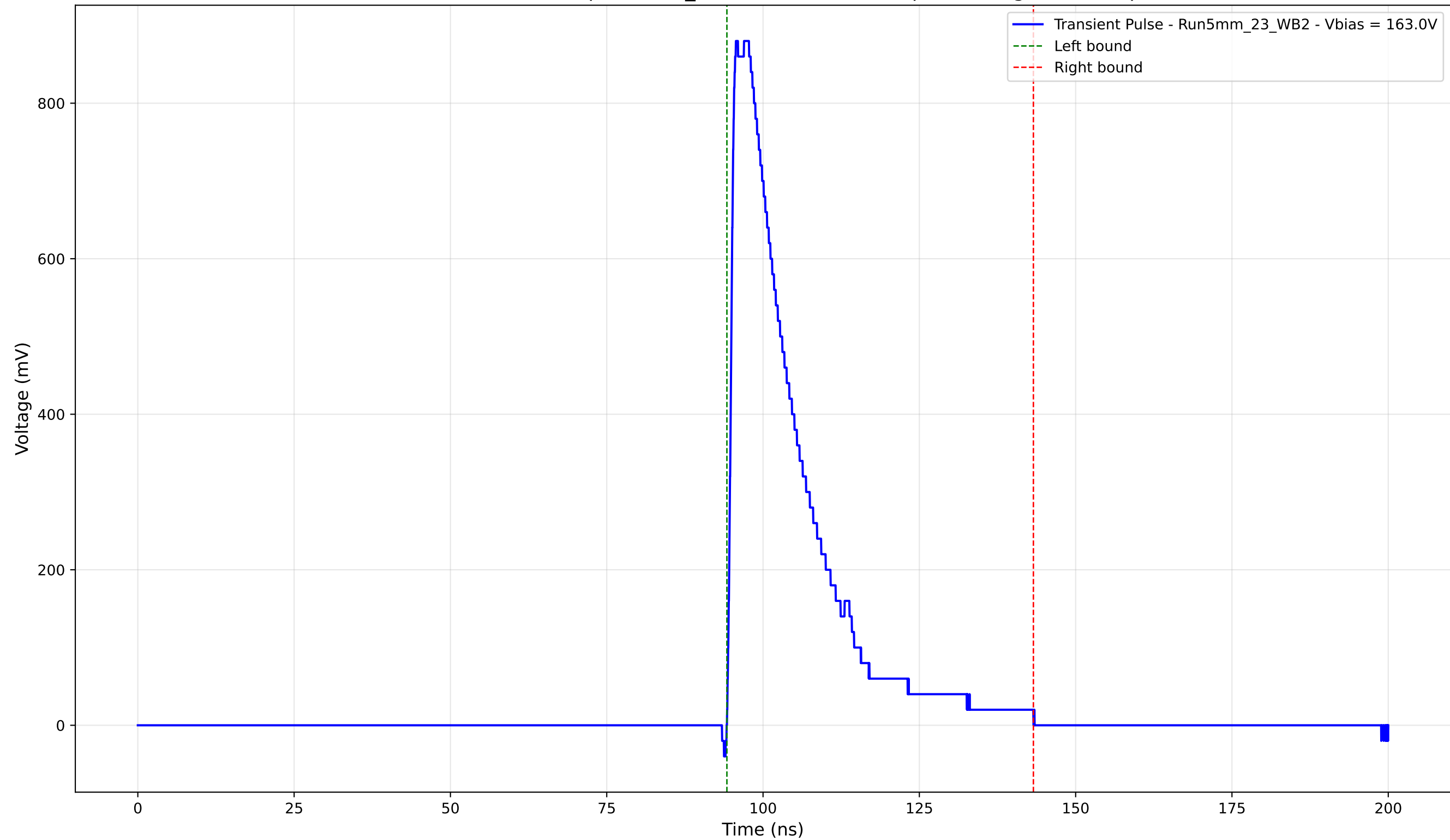
Transient Pulse - Sample: 5mm_23 - Position: 1680.0 \mu\text{m} - Charge: 206.14 pC
