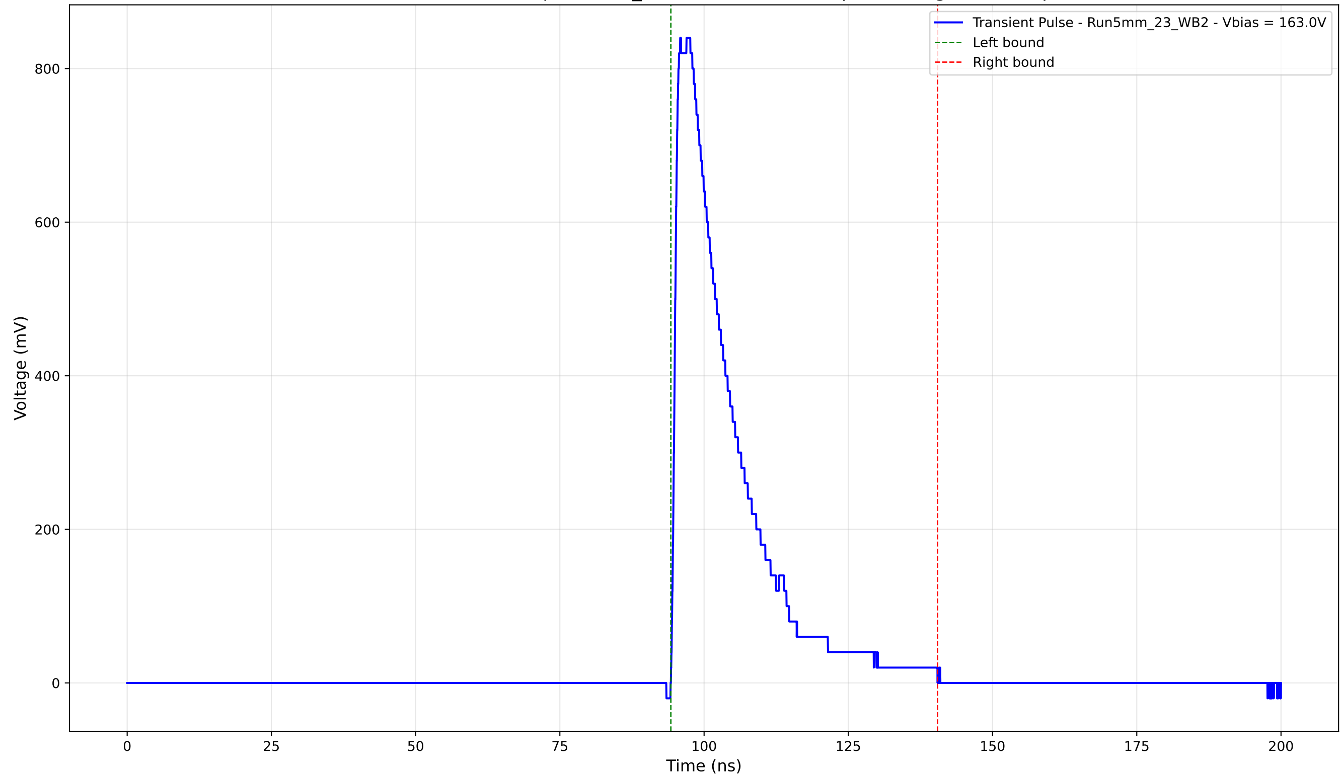
Transient Pulse - Sample: 5mm_23 - Position: 3395.0 \mu\text{m} - Charge: 186.59 pC
