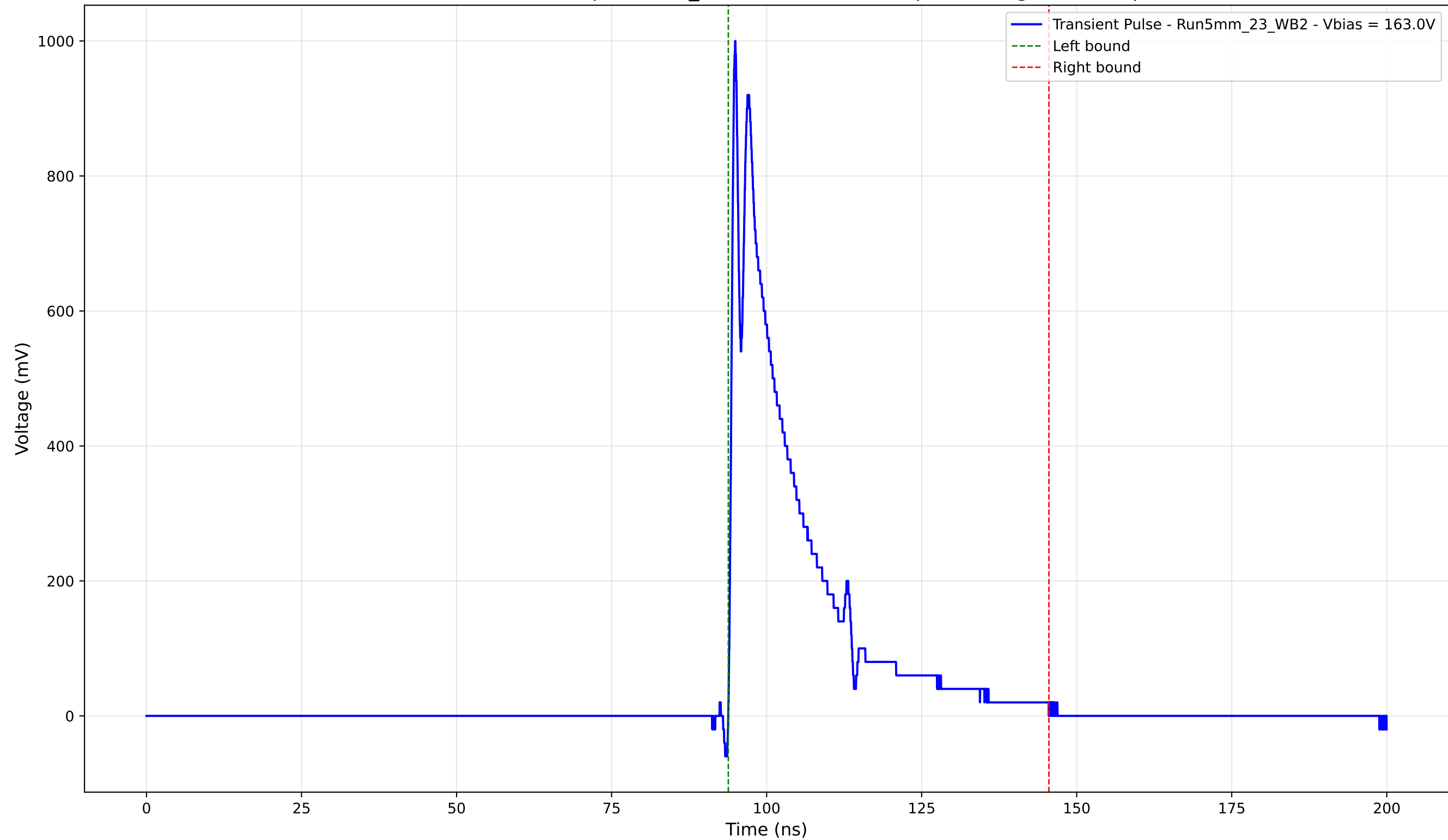
Transient Pulse - Sample: 5mm_23 - Position: 2620.0 \mu\text{m} - Charge: 196.30 pC
