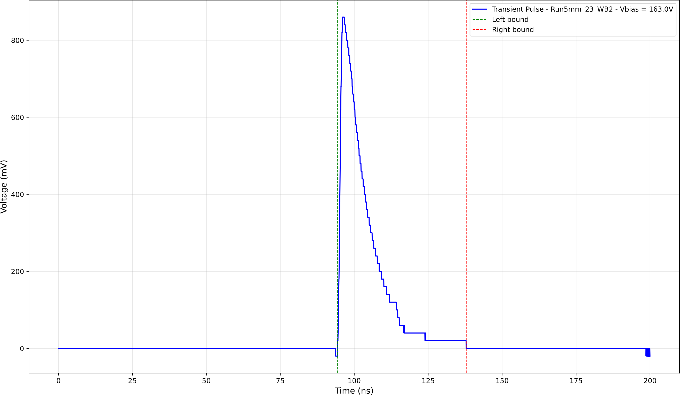
Transient Pulse - Sample: 5mm_23 - Position: 3875.0 \mu\text{m} - Charge: 172.50 pC
