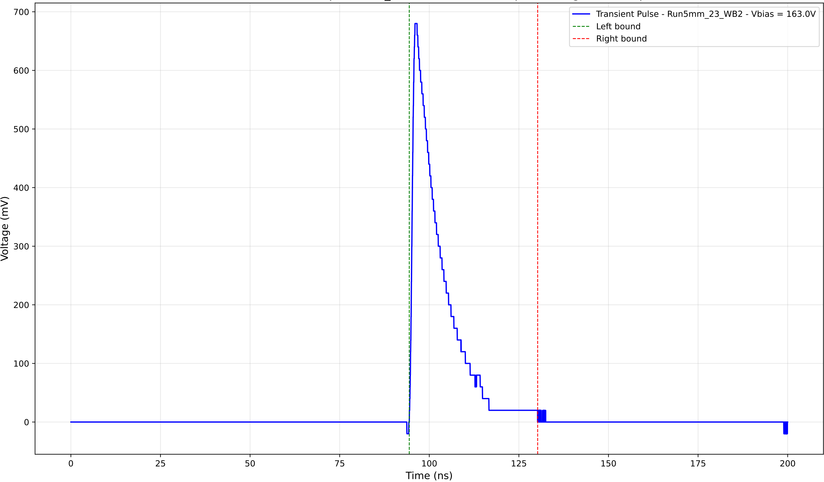
Transient Pulse - Sample: 5mm_23 - Position: 4100.0 \mu\text{m} - Charge: 118.57 pC
