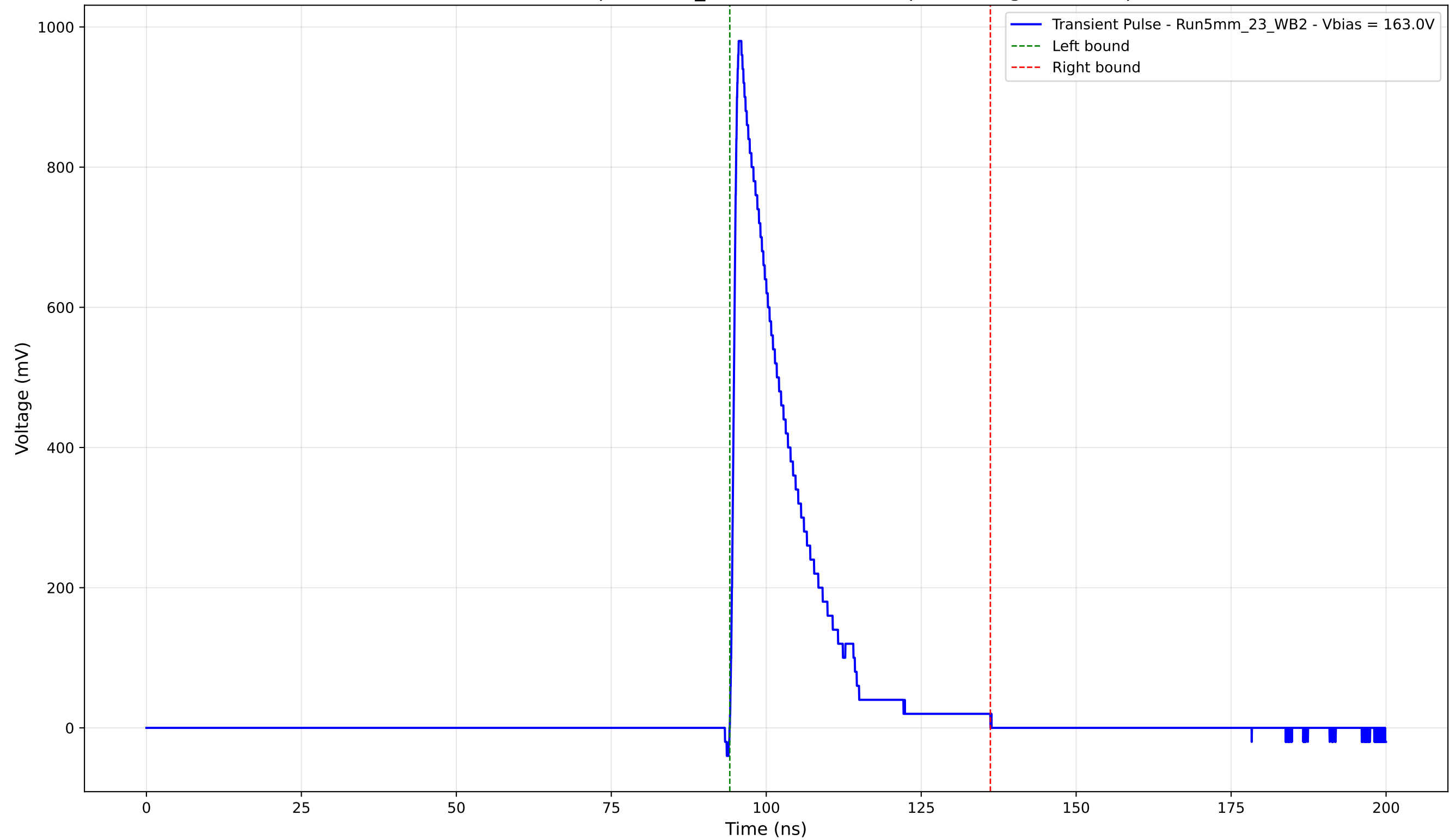
Transient Pulse - Sample: 5mm_23 - Position: 365.0 \mu\text{m} - Charge: 181.32 pC
