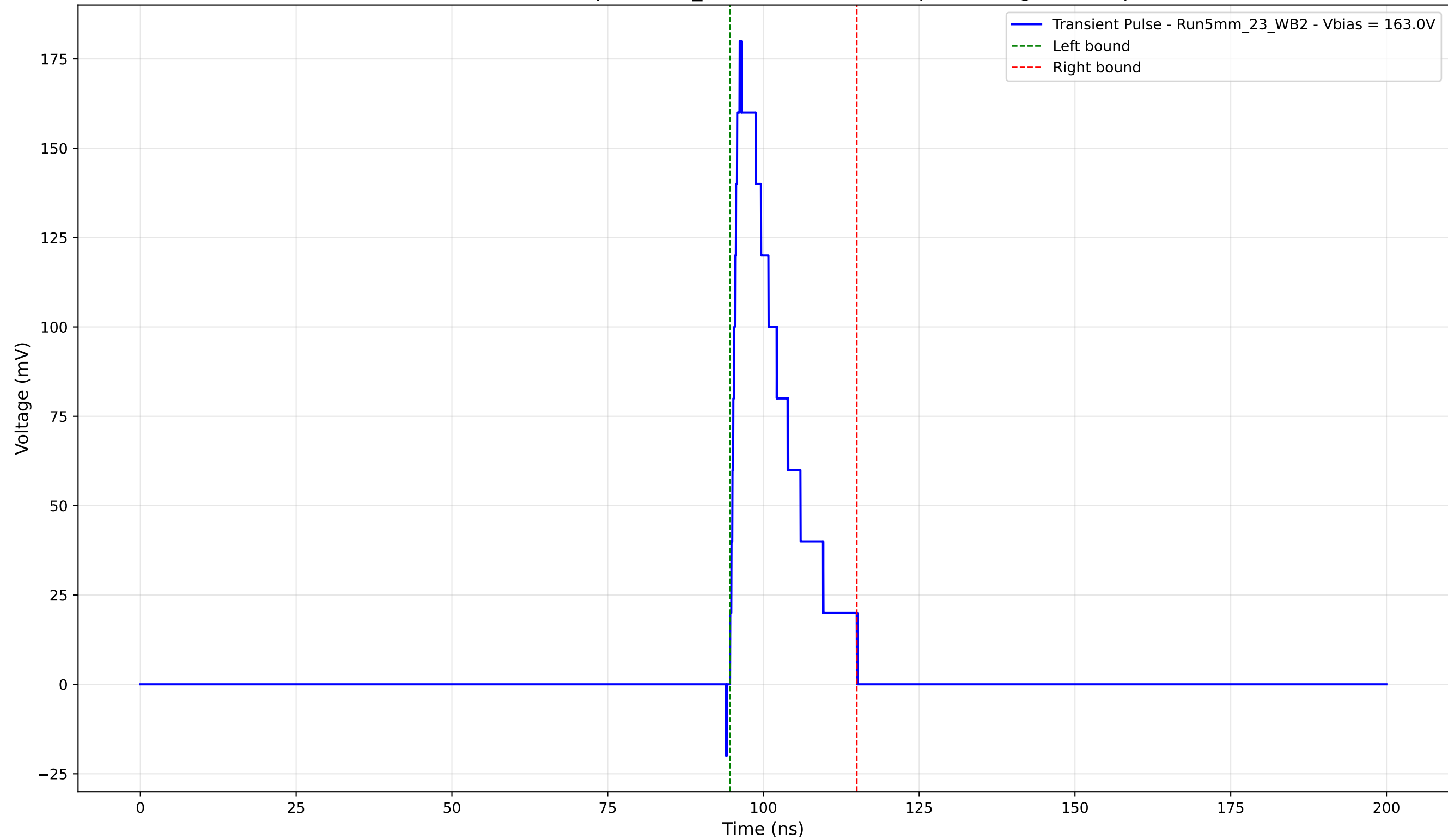
Transient Pulse - Sample: 5mm_23 -Position: 4030.0 \mu\text{m} - Charge: 29.74 pC
