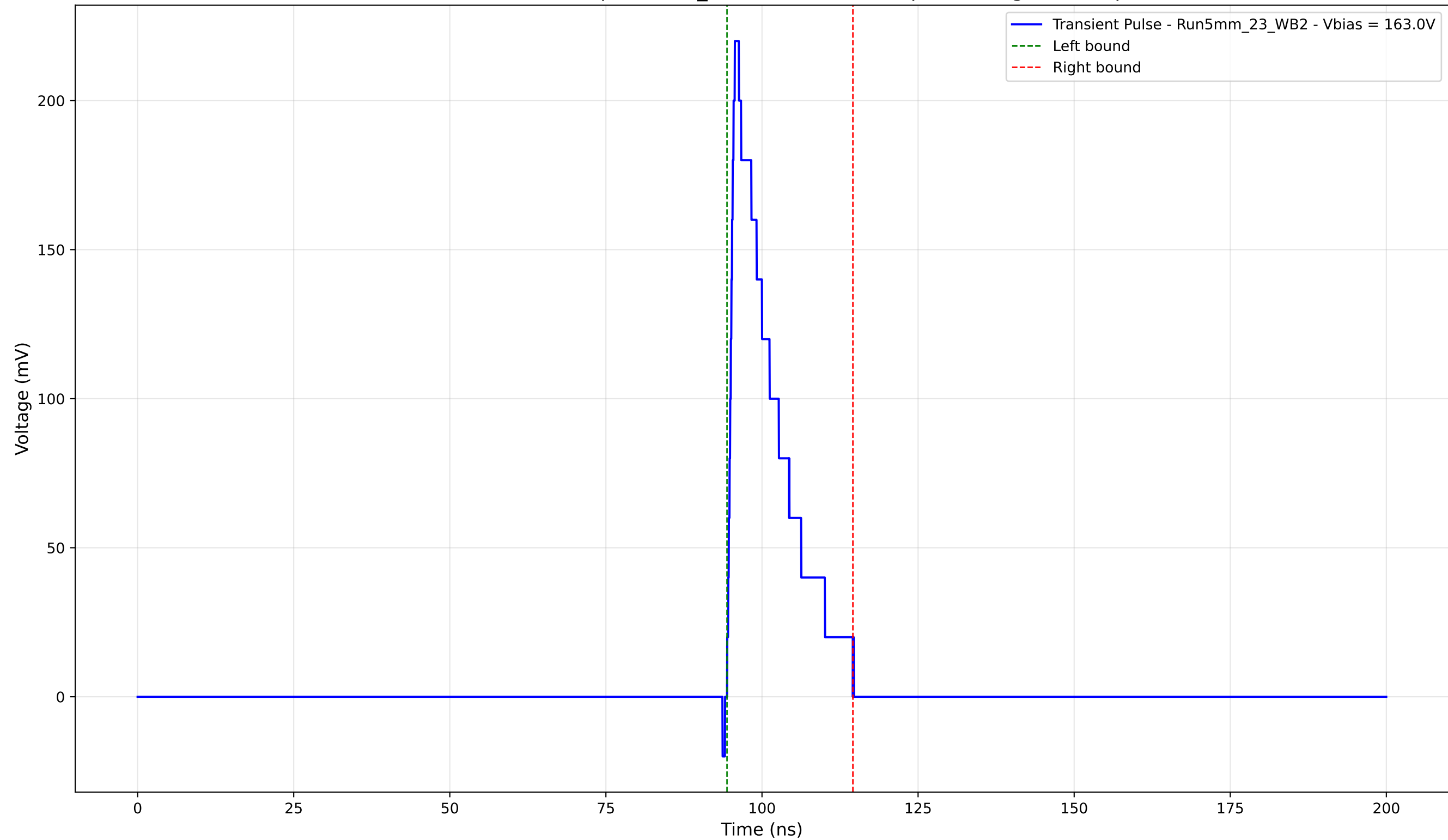
Transient Pulse - Sample: 5mm_23 - Position: 480.0 \mu\text{m} - Charge: 33.82 pC
