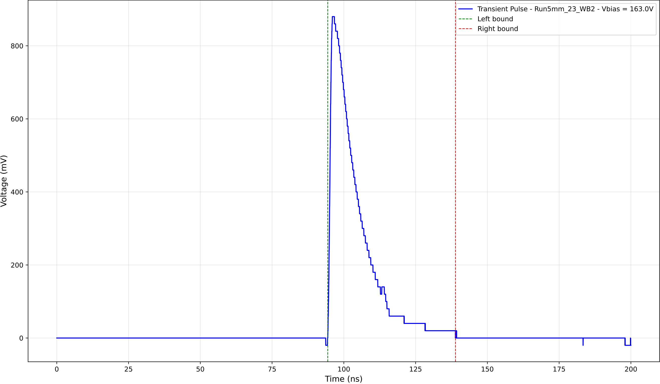
Transient Pulse - Sample: 5mm_23 - Position: 1135.0 \mu\text{m} - Charge: 189.66 pC
