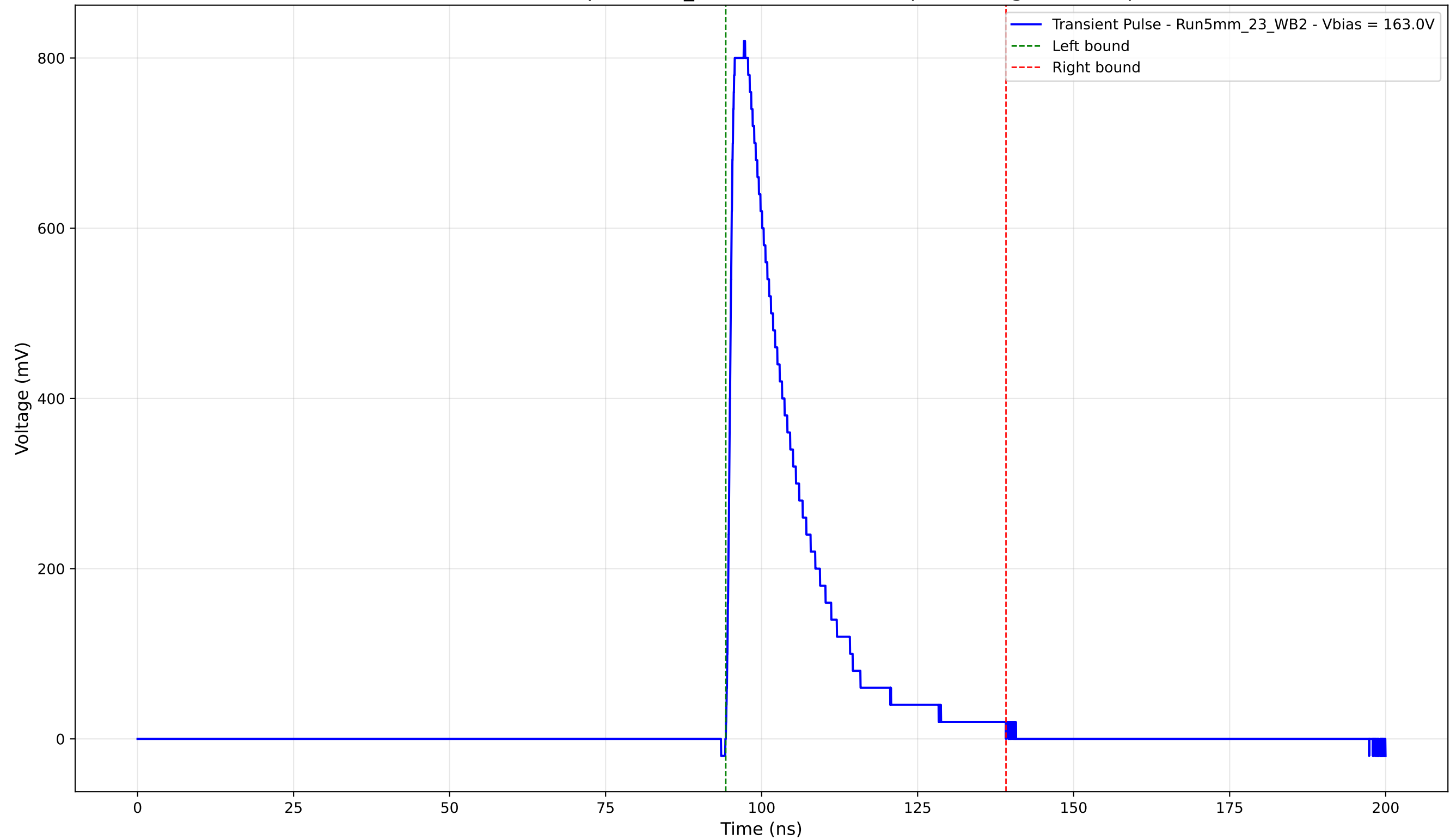
Transient Pulse - Sample: 5mm_23 - Position: 3425.0 \mu\text{m} - Charge: 177.63 pC
