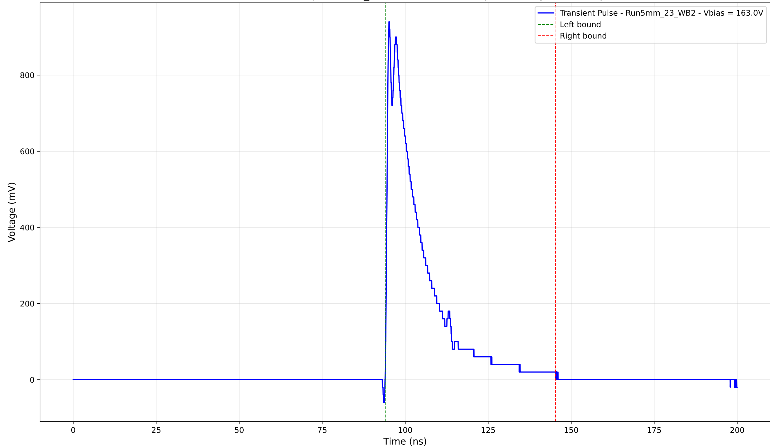
Transient Pulse - Sample: 5mm_23 - Position: 2155.0 \mu\text{m} - Charge: 204.94 pC
