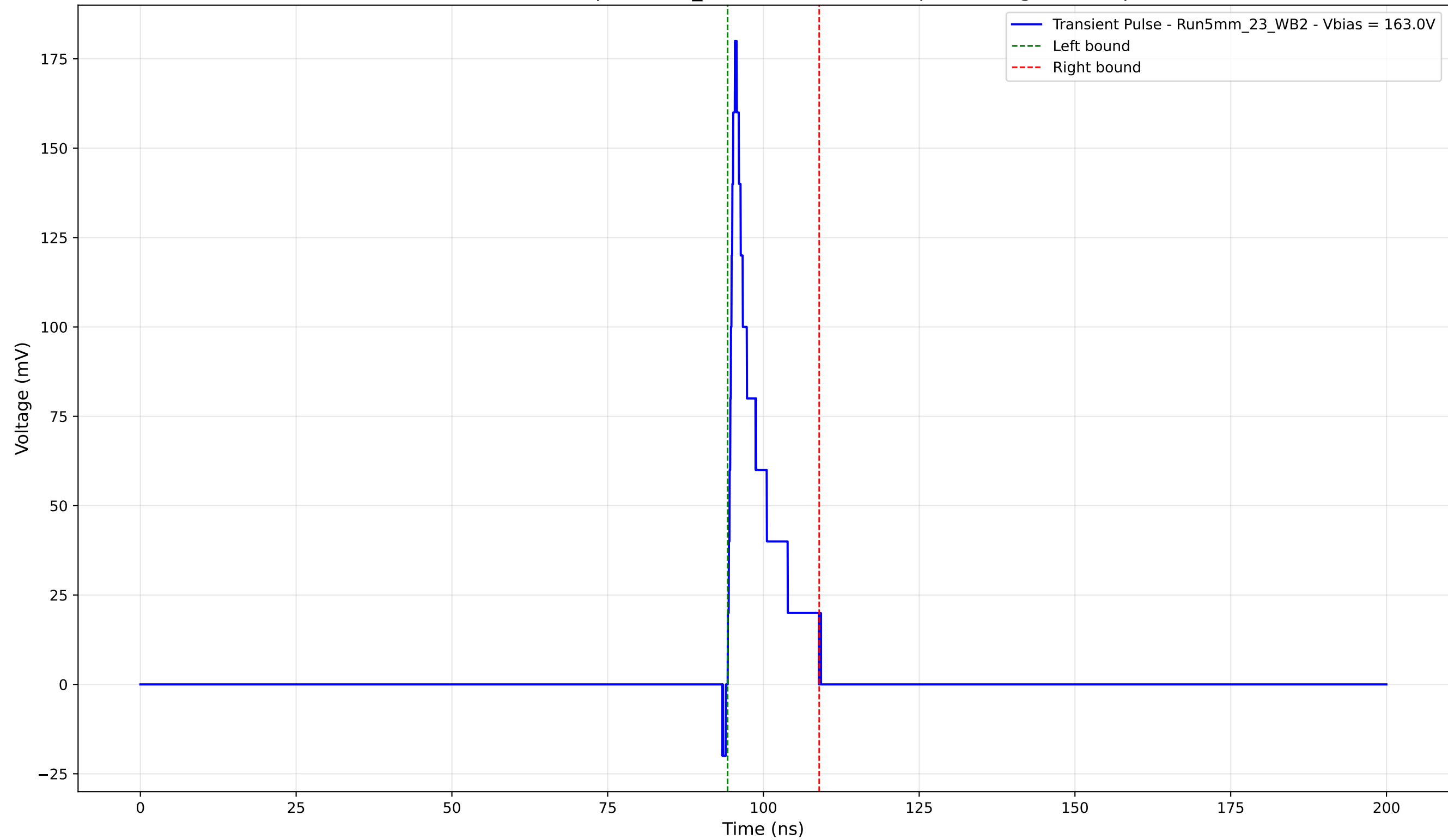
Transient Pulse - Sample: 5mm_23 -Position: 4965.0 \mu\text{m} - Charge: 16.44 pC
