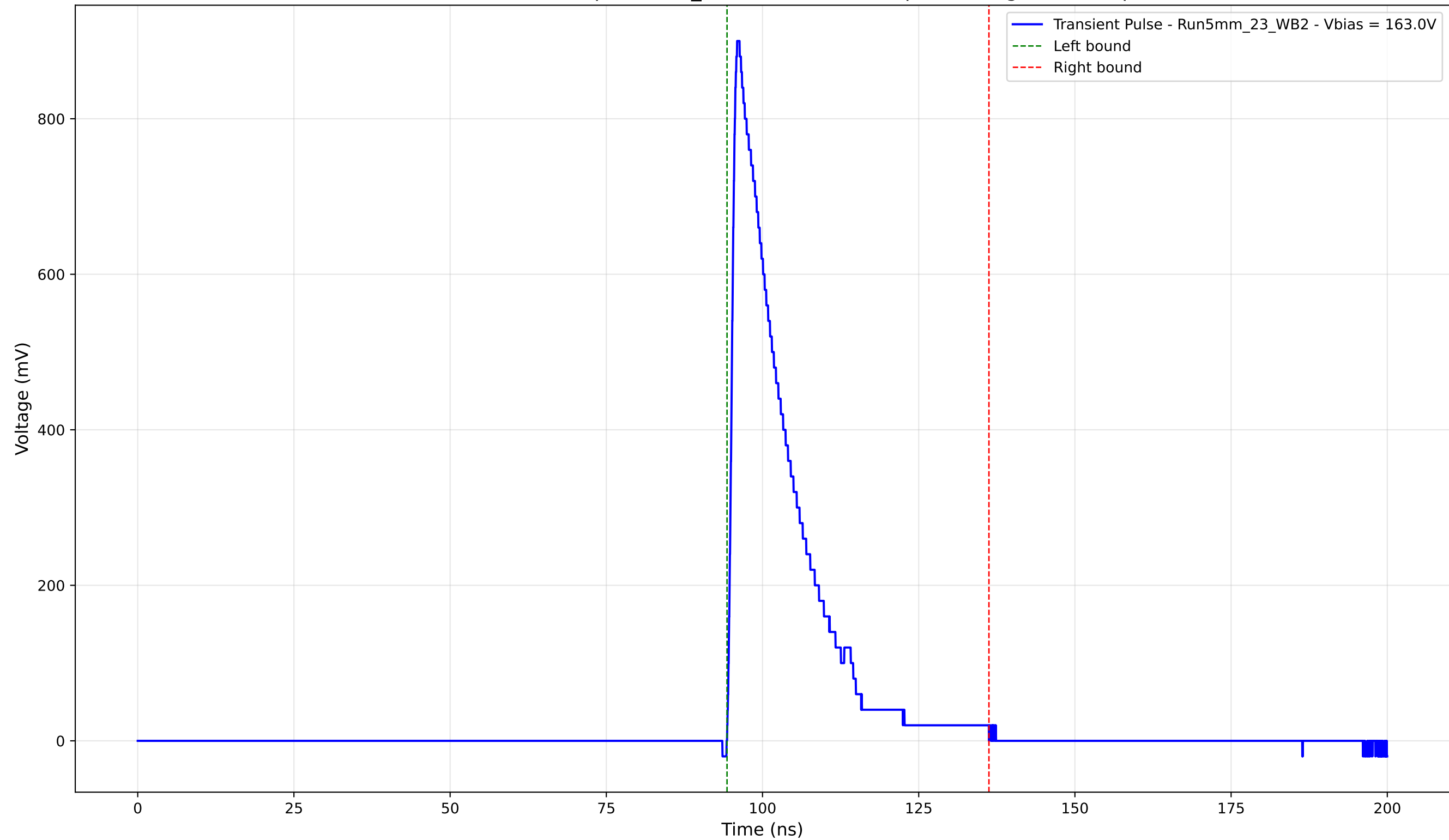
Transient Pulse - Sample: 5mm_23 - Position: 700.0 \mu\text{m} - Charge: 171.30 pC
