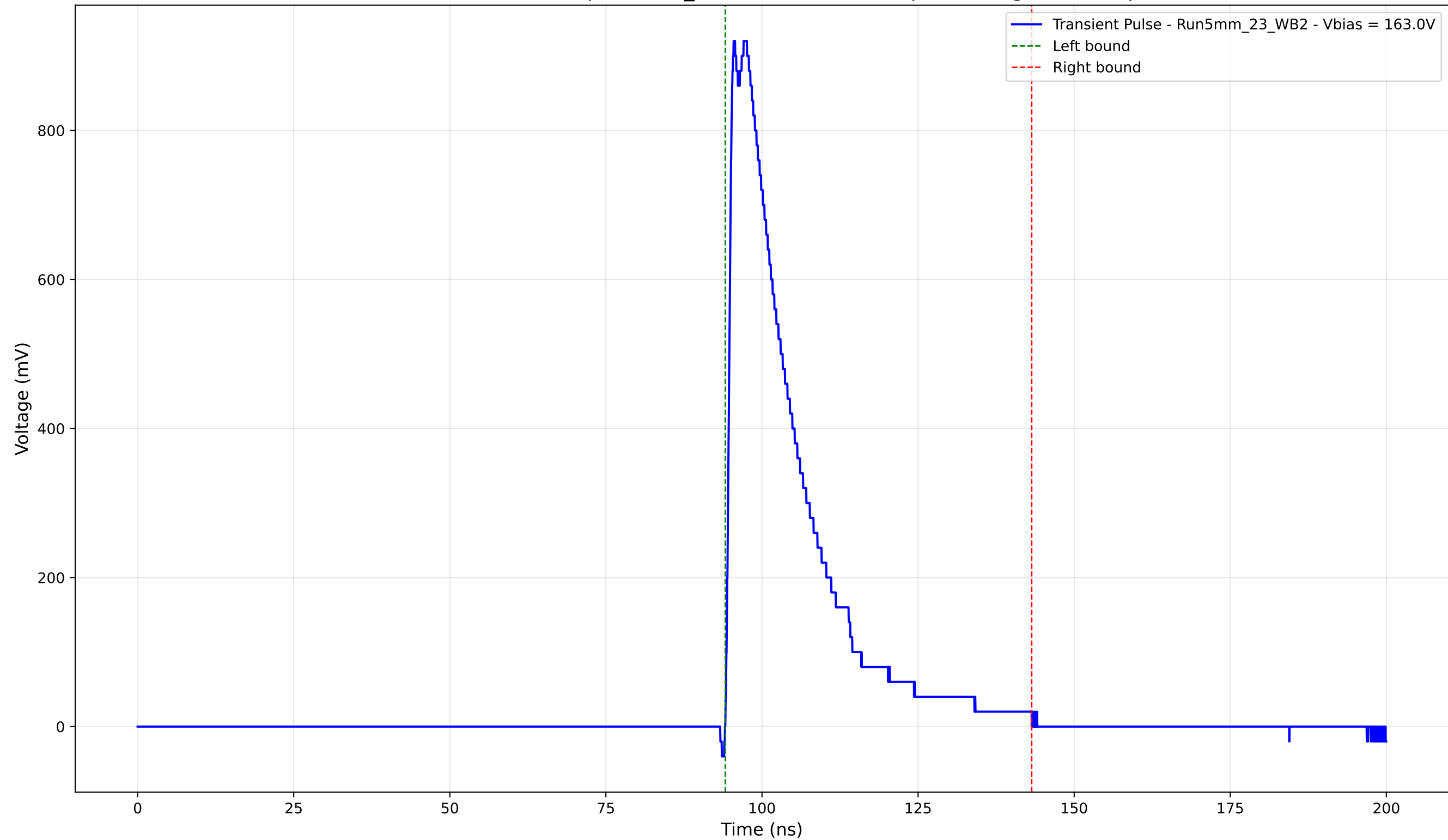
Transient Pulse - Sample: 5mm_23 - Position: 3205.0 \mu\text{m} - Charge: 216.94 pC
