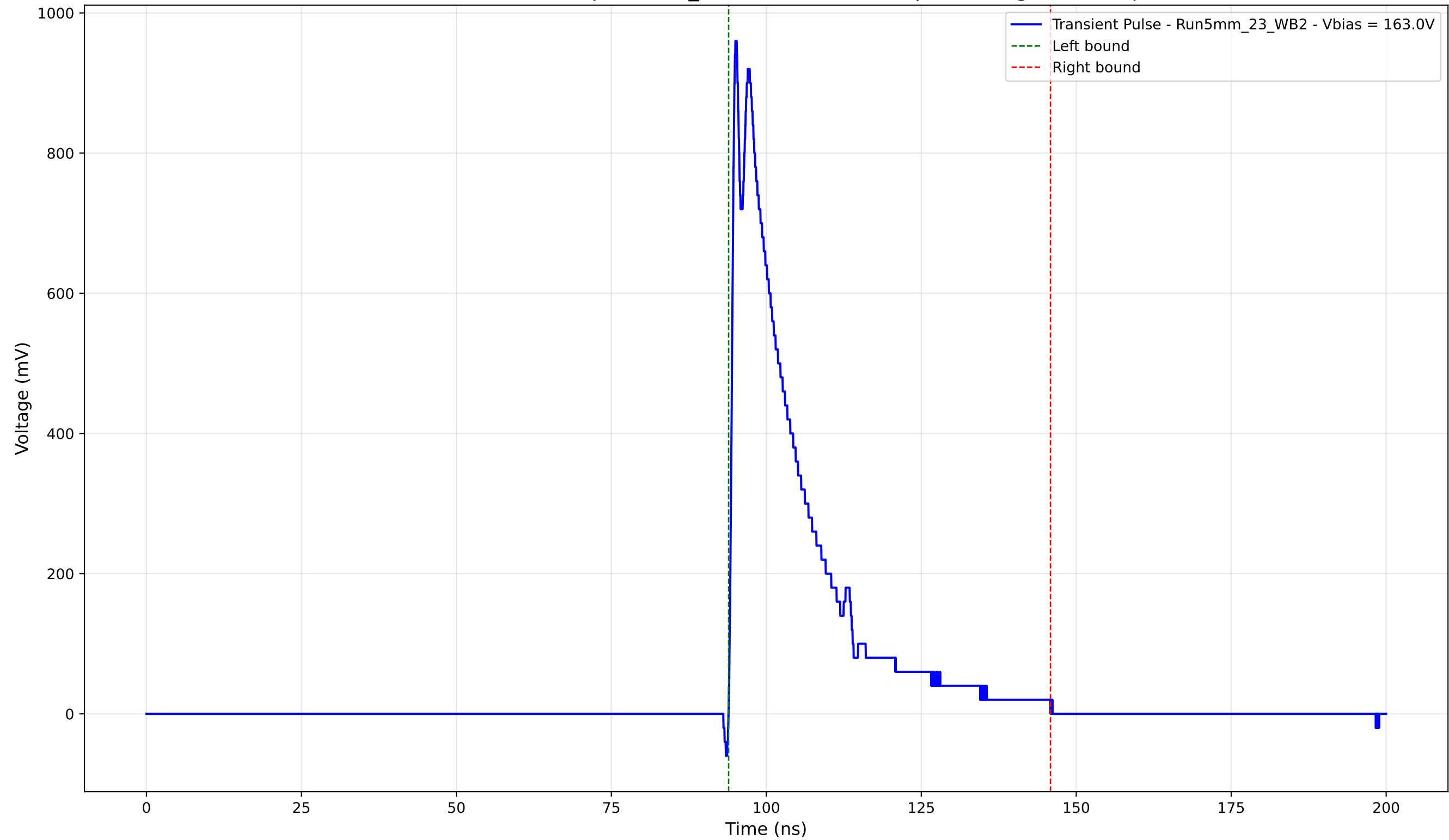
Transient Pulse - Sample: 5mm_23 - Position: 2810.0 \mu\text{m} - Charge: 208.28 pC
