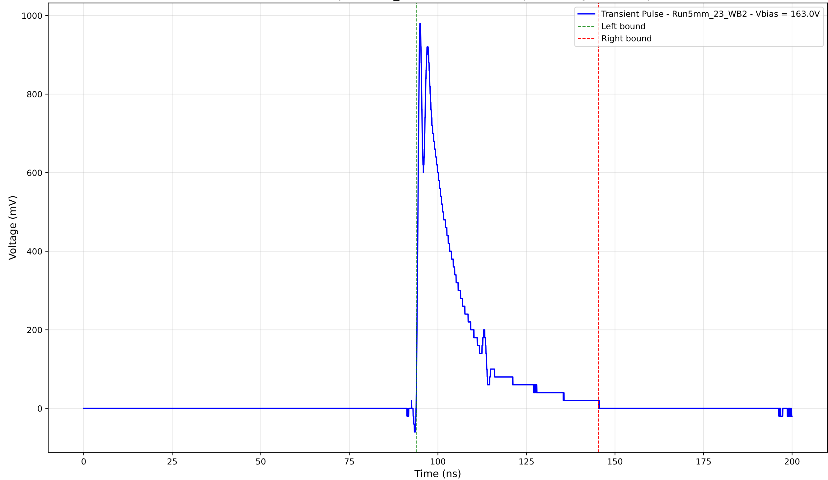
Transient Pulse - Sample: 5mm_23 - Position: 2350.0 \mu\text{m} - Charge: 201.96 pC
