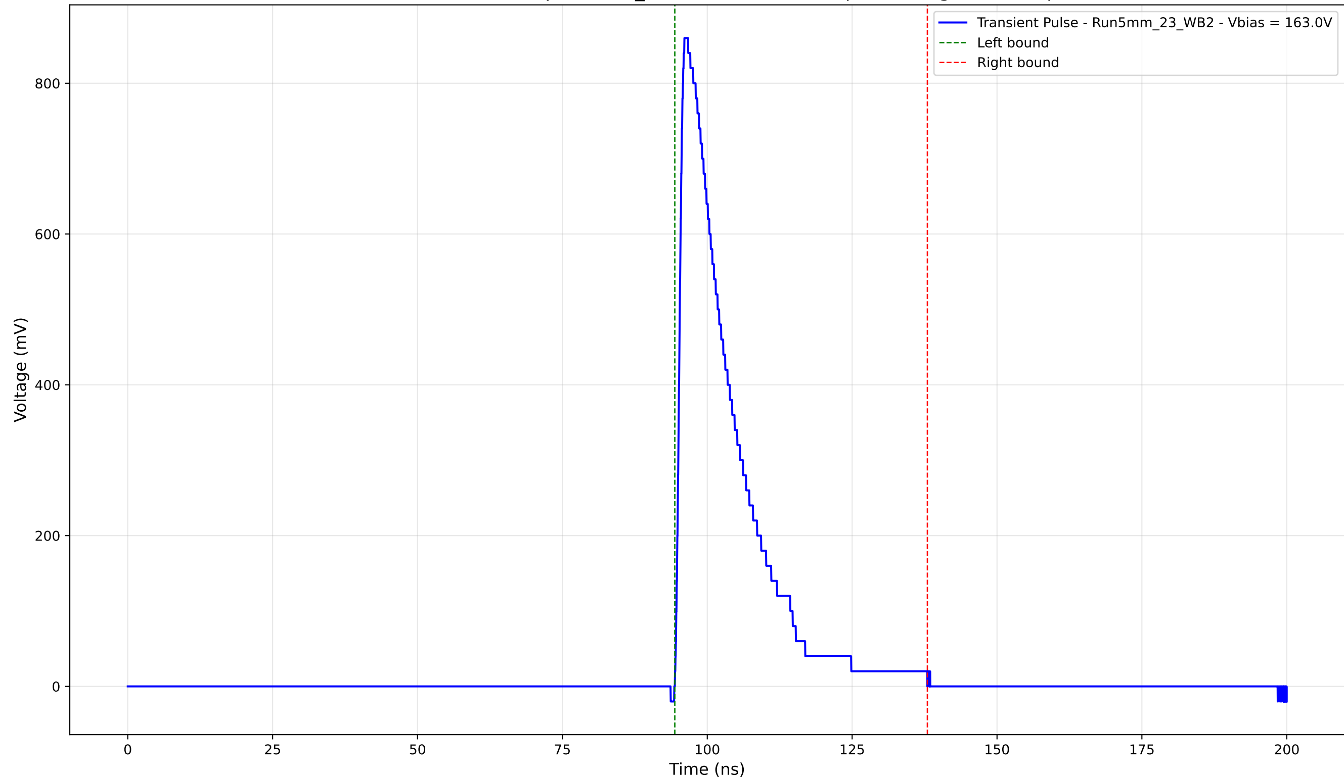
Transient Pulse - Sample: 5mm_23 - Position: 3835.0 \mu\text{m} - Charge: 174.87 pC
