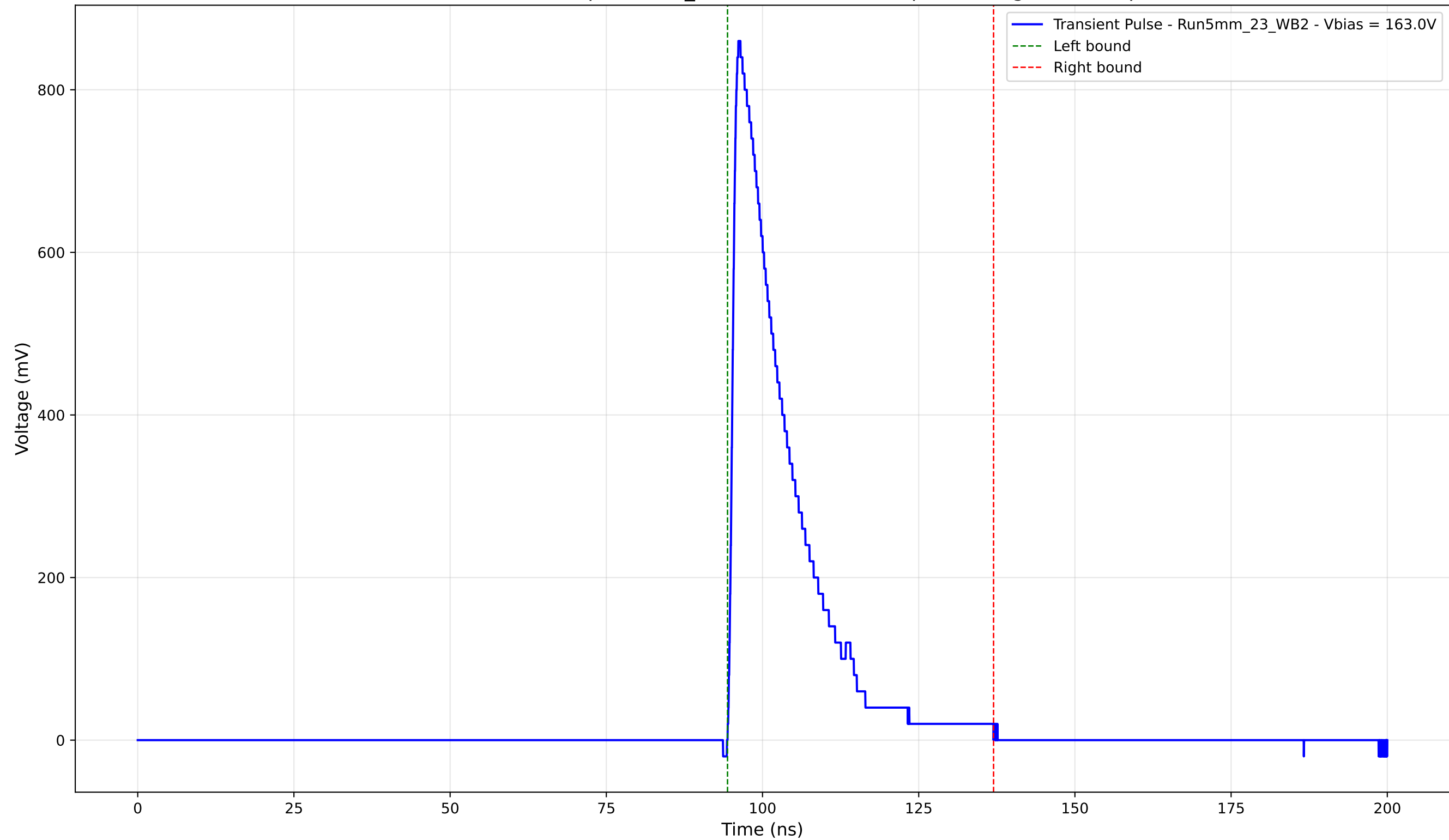
Transient Pulse - Sample: 5mm_23 - Position: 3920.0 \mu\text{m} - Charge: 167.29 pC
