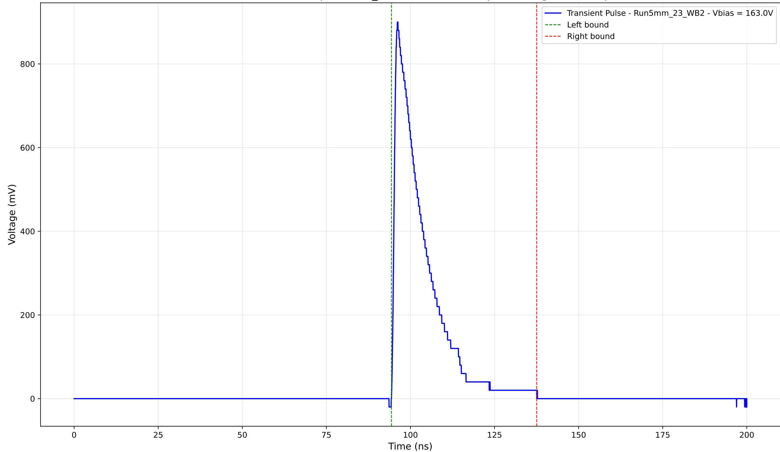
Transient Pulse - Sample: 5mm_23 - Position: 815.0 \mu\text{m} - Charge: 174.82 pC
