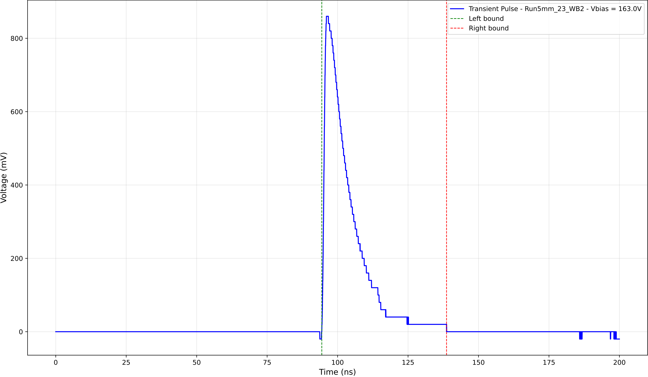
Transient Pulse - Sample: 5mm_23 - Position: 3810.0 \mu\text{m} - Charge: 176.37 pC
