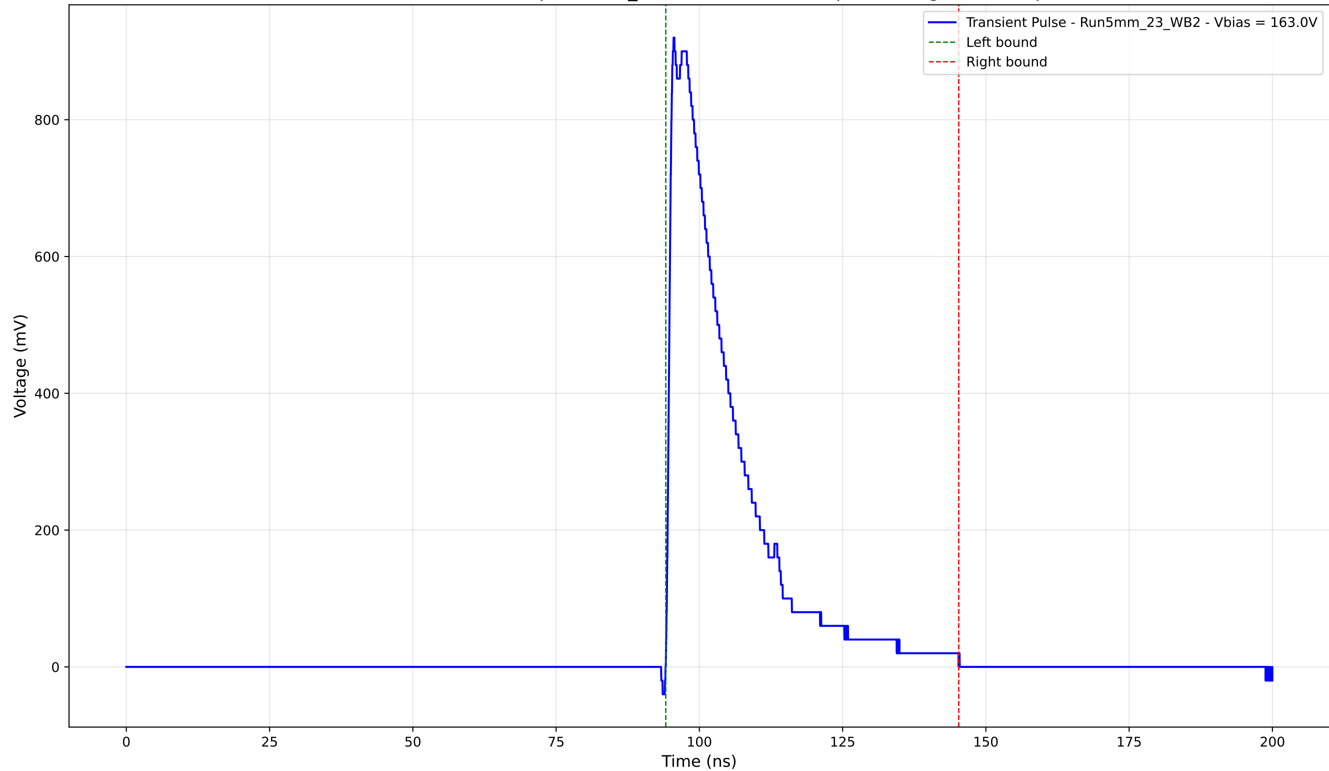
Transient Pulse - Sample: 5mm_23 - Position: 1825.0 \mu\text{m} - Charge: 220.30 pC
