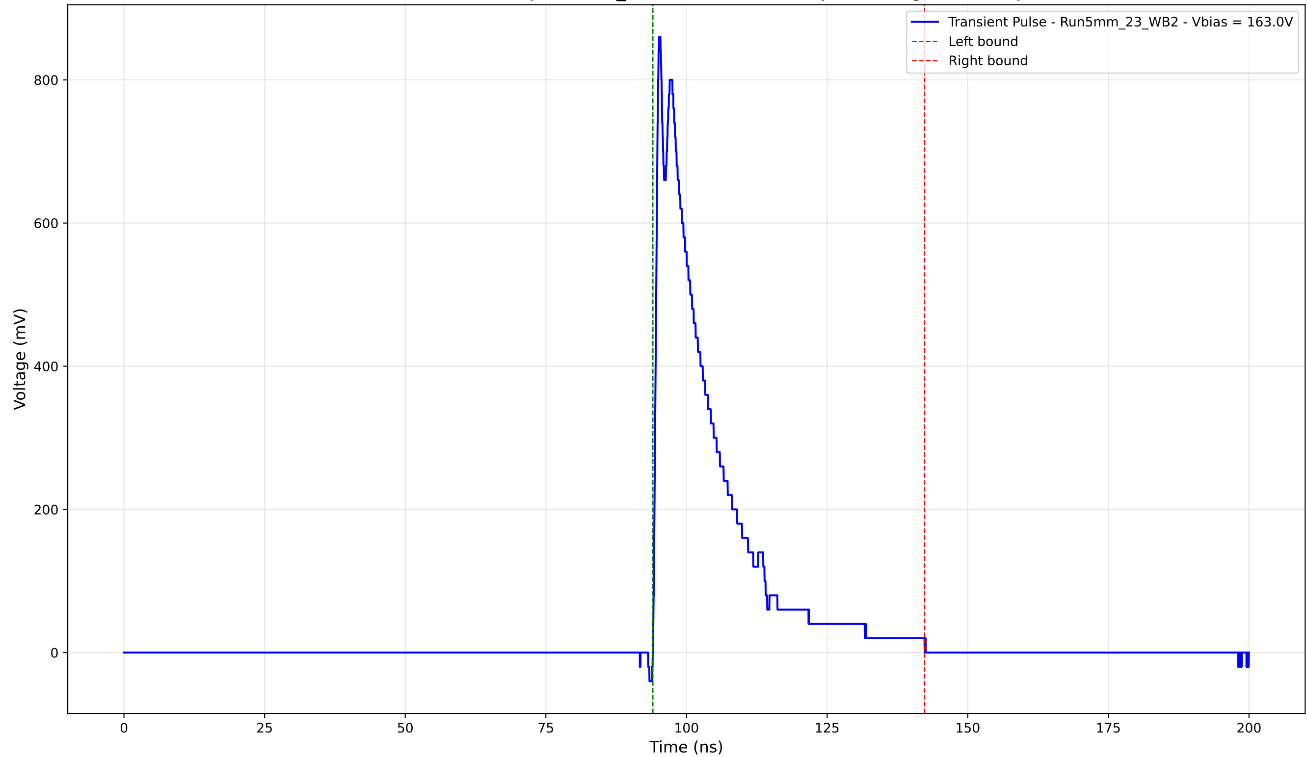
Transient Pulse - Sample: 5mm_23 - Position: 2090.0 \mu\text{m} - Charge: 175.86 pC
