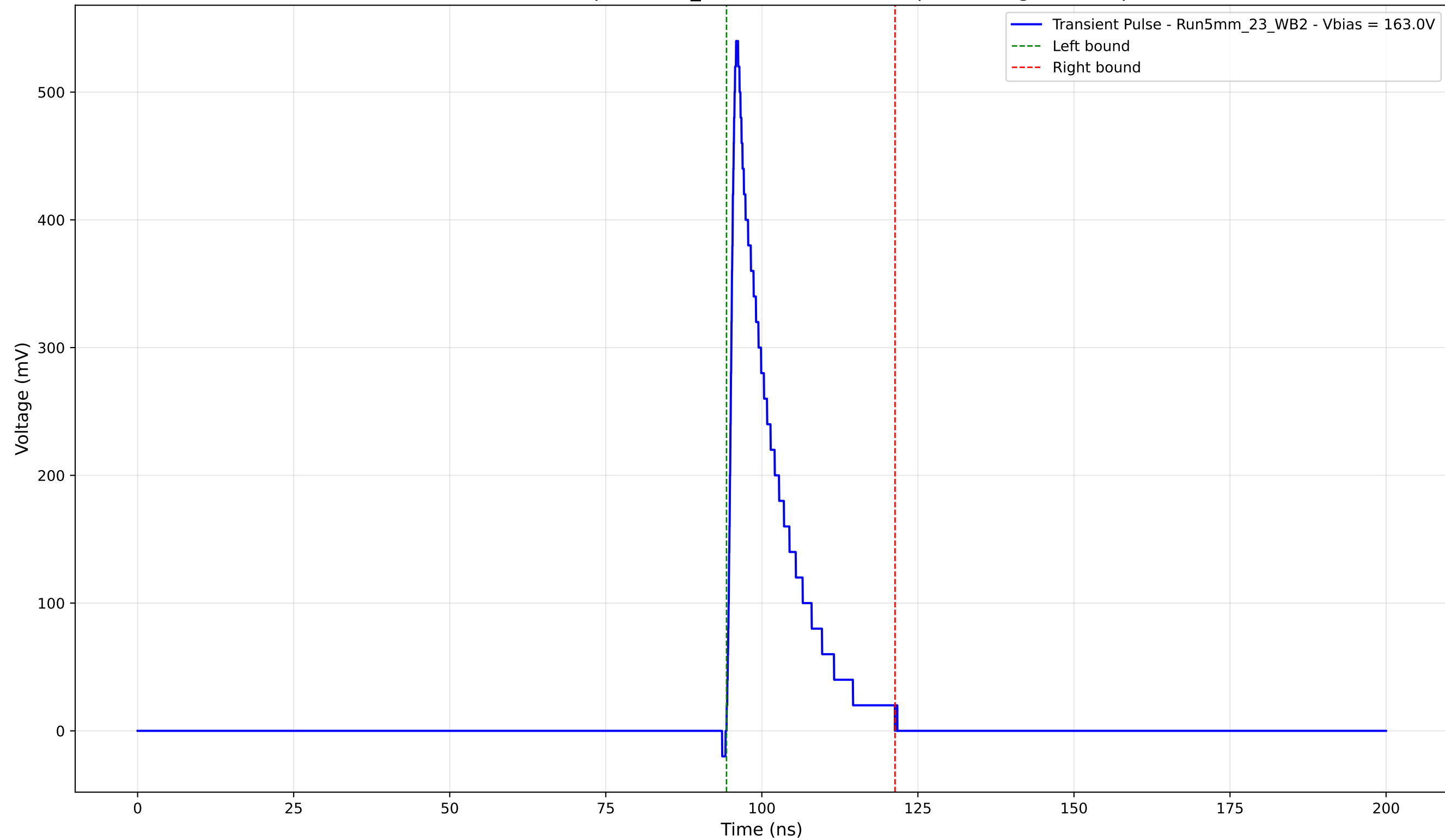
Transient Pulse - Sample: 5mm_23 - Position: 4495.0 \mu\text{m} - Charge: 78.42 pC
