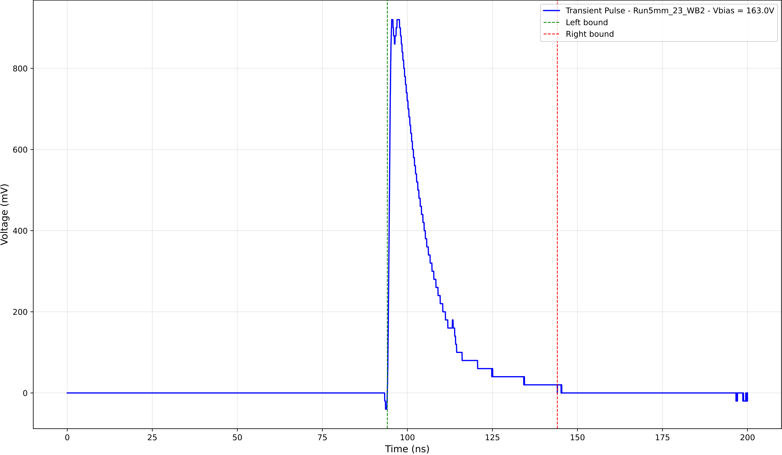
Transient Pulse - Sample: 5mm_23 - Position: 3185.0 \mu\text{m} - Charge: 219.58 pC
