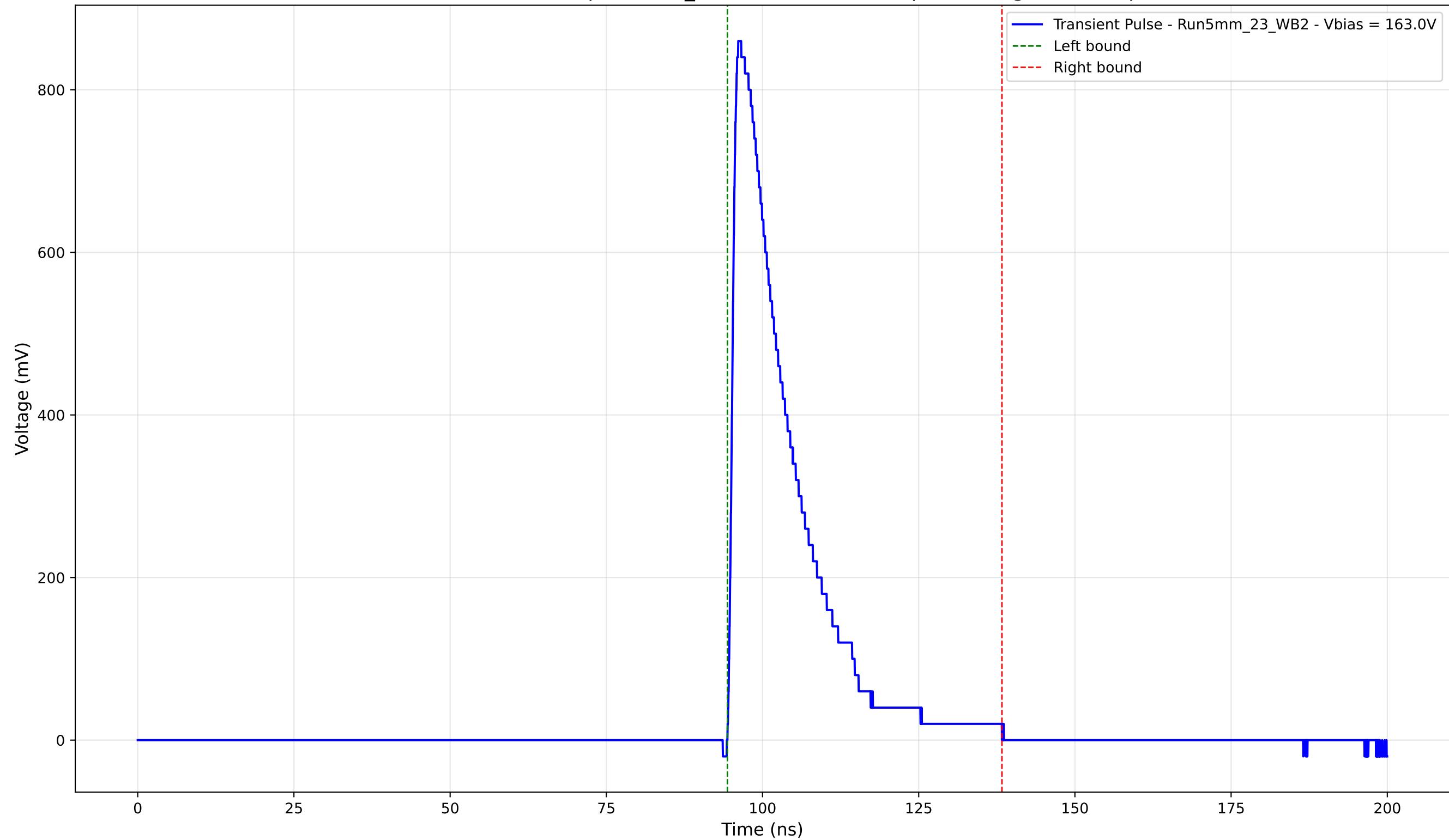
Transient Pulse - Sample: 5mm_23 - Position: 3745.0 \mu\text{m} - Charge: 177.11 pC
