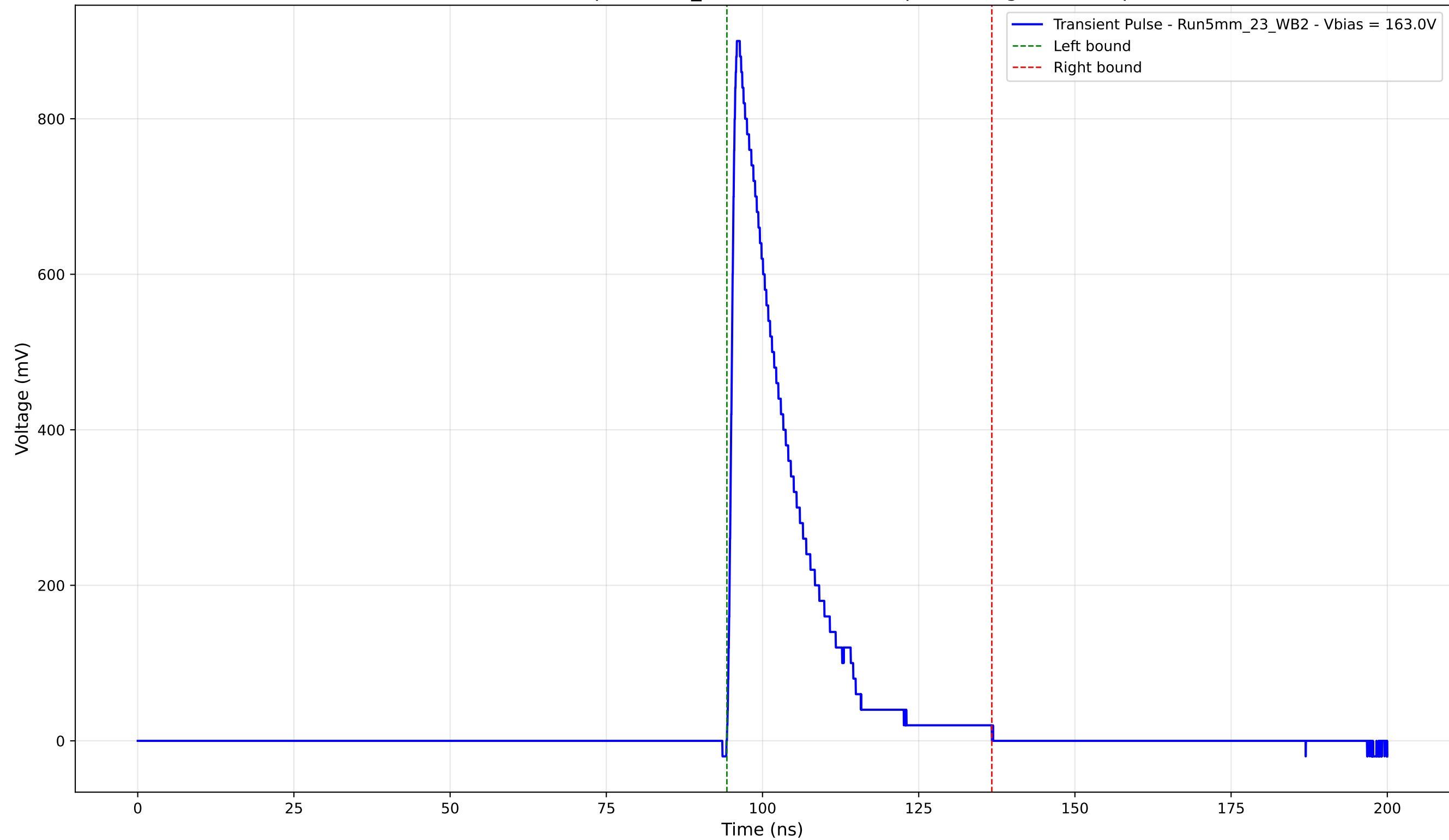
Transient Pulse - Sample: 5mm_23 - Position: 685.0 \mu\text{m} - Charge: 172.38 pC
