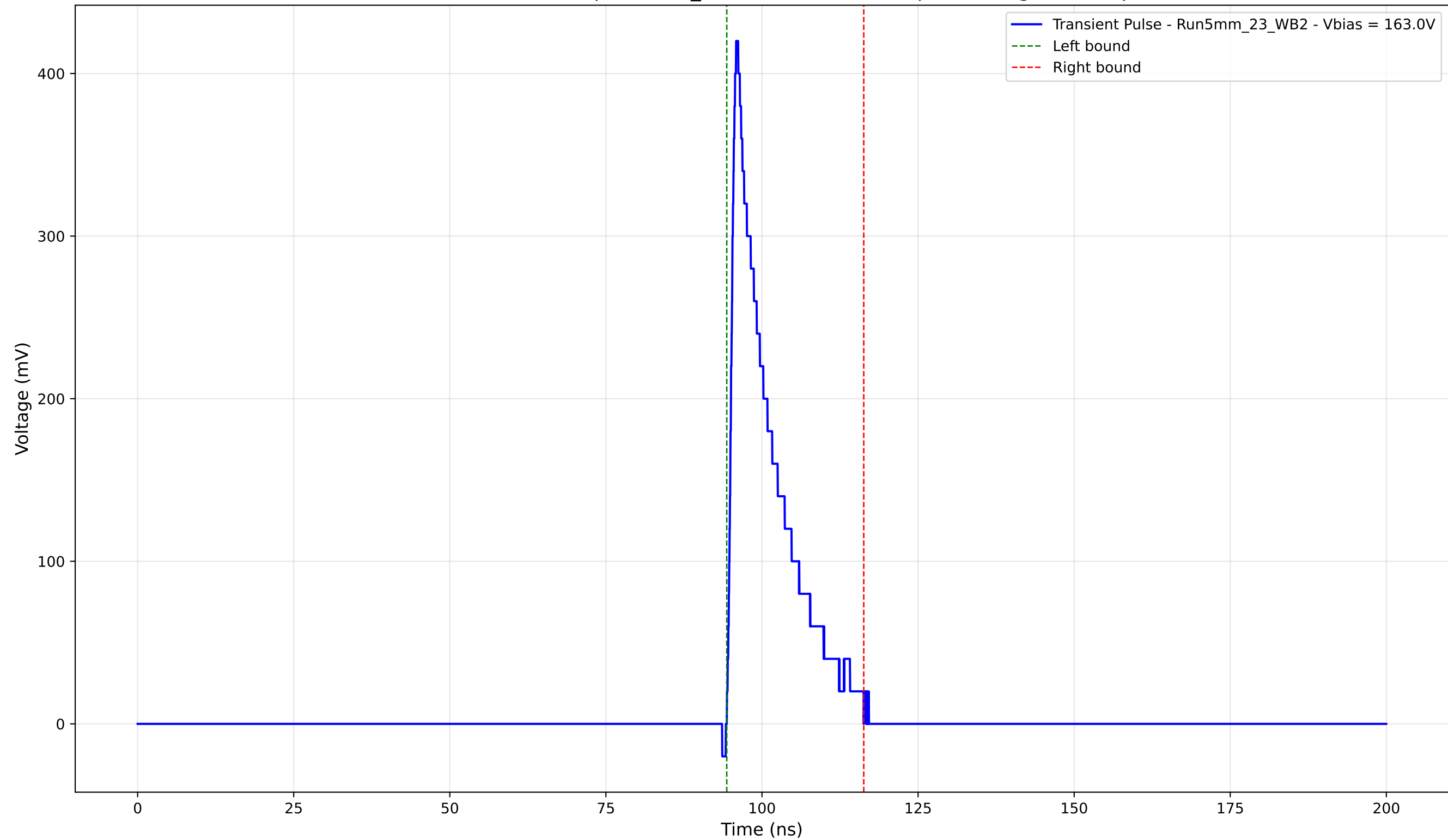
Transient Pulse - Sample: 5mm_23 - Position: 4505.0 \mu\text{m} - Charge: 58.70 pC
