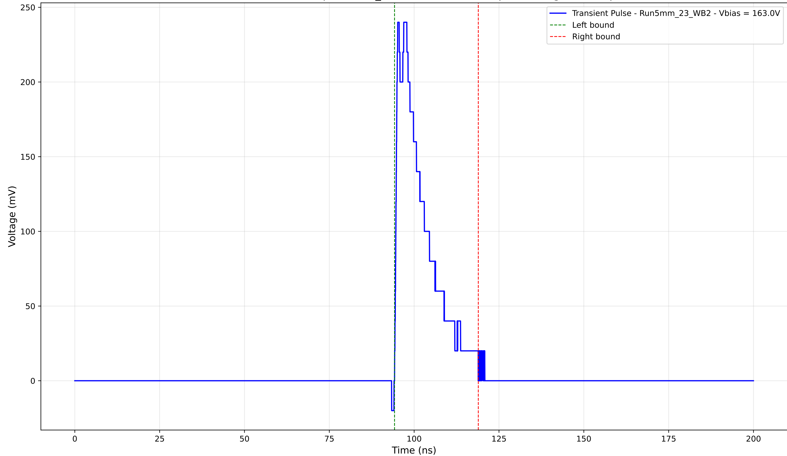
Transient Pulse - Sample: 5mm_23 - Position: 1995.0 \mu\text{m} - Charge: 45.23 pC
