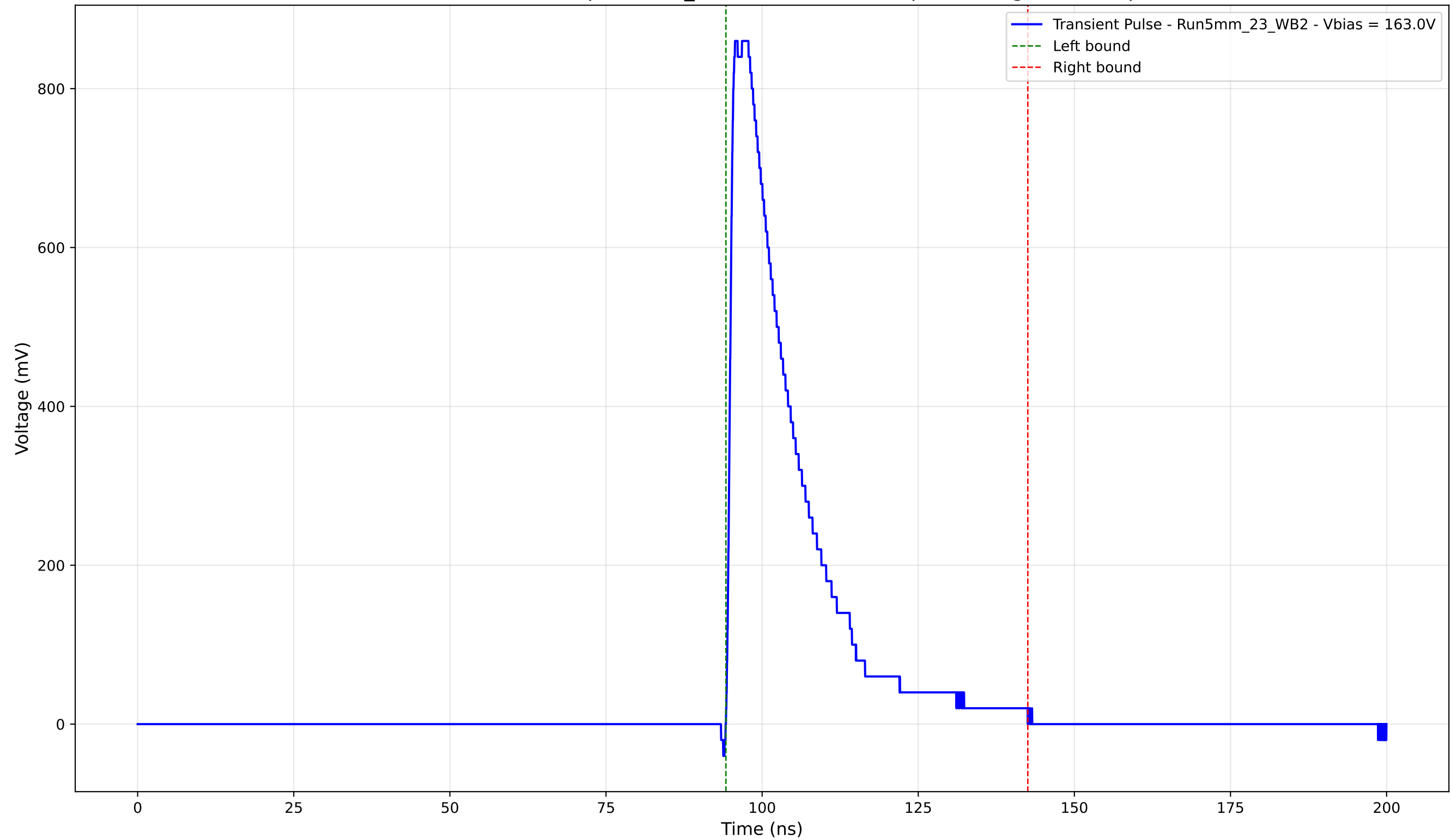
Transient Pulse - Sample: 5mm_23 - Position: 3345.0 \mu\text{m} - Charge: 197.48 pC
