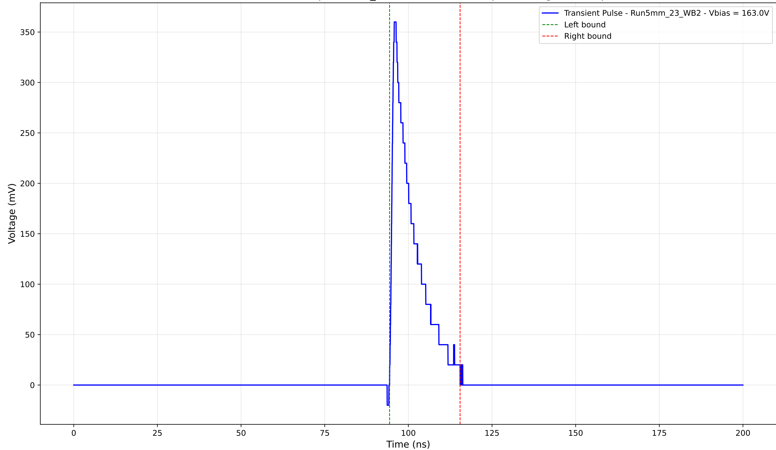
Transient Pulse - Sample: 5mm_23 - Position: 4510.0 \mu\text{m} - Charge: 51.25 pC
