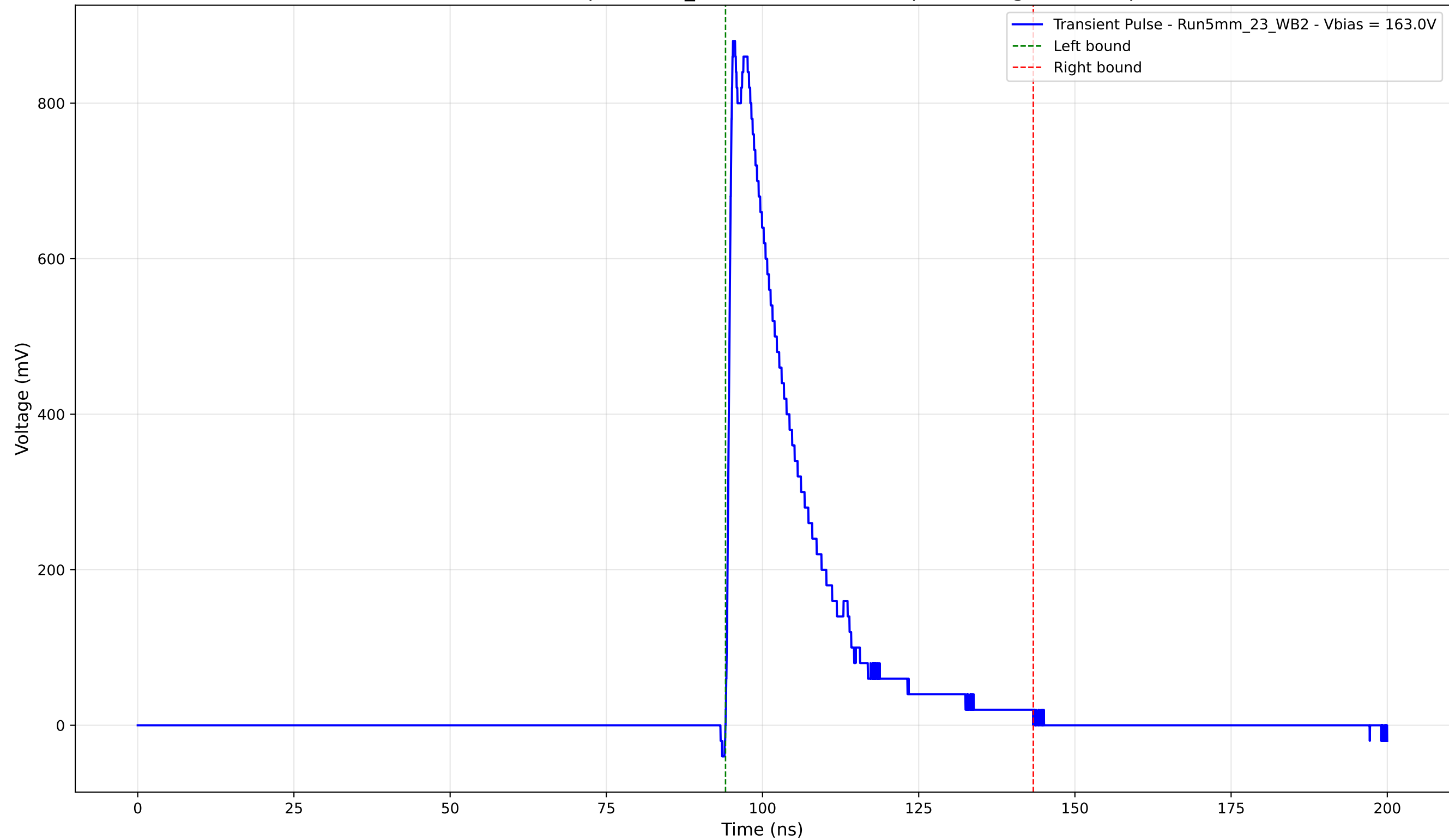
Transient Pulse - Sample: 5mm_23 - Position: 1925.0 \mu\text{m} - Charge: 198.32 pC
