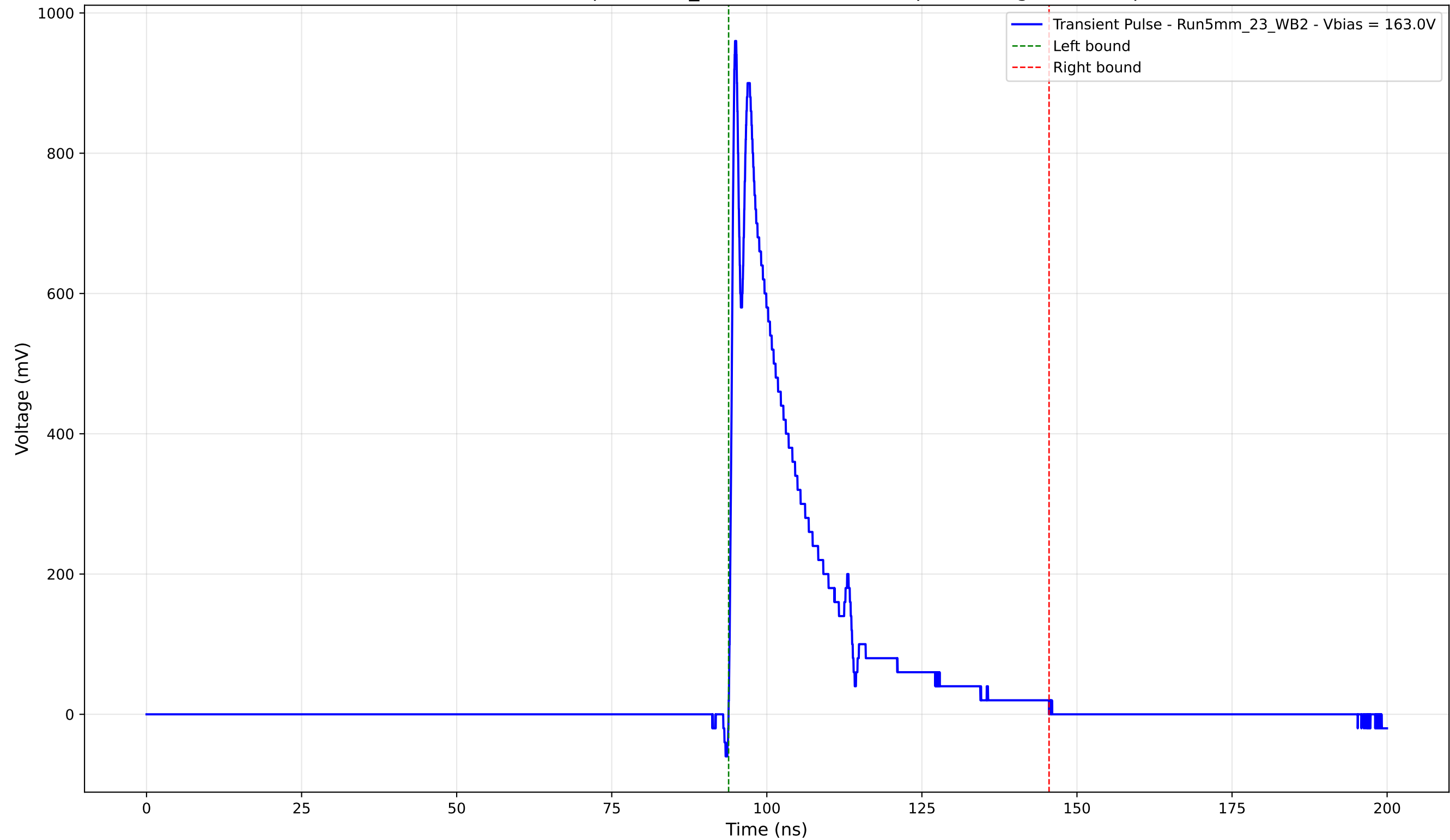
Transient Pulse - Sample: 5mm_23 - Position: 2375.0 \mu\text{m} - Charge: 197.15 pC
