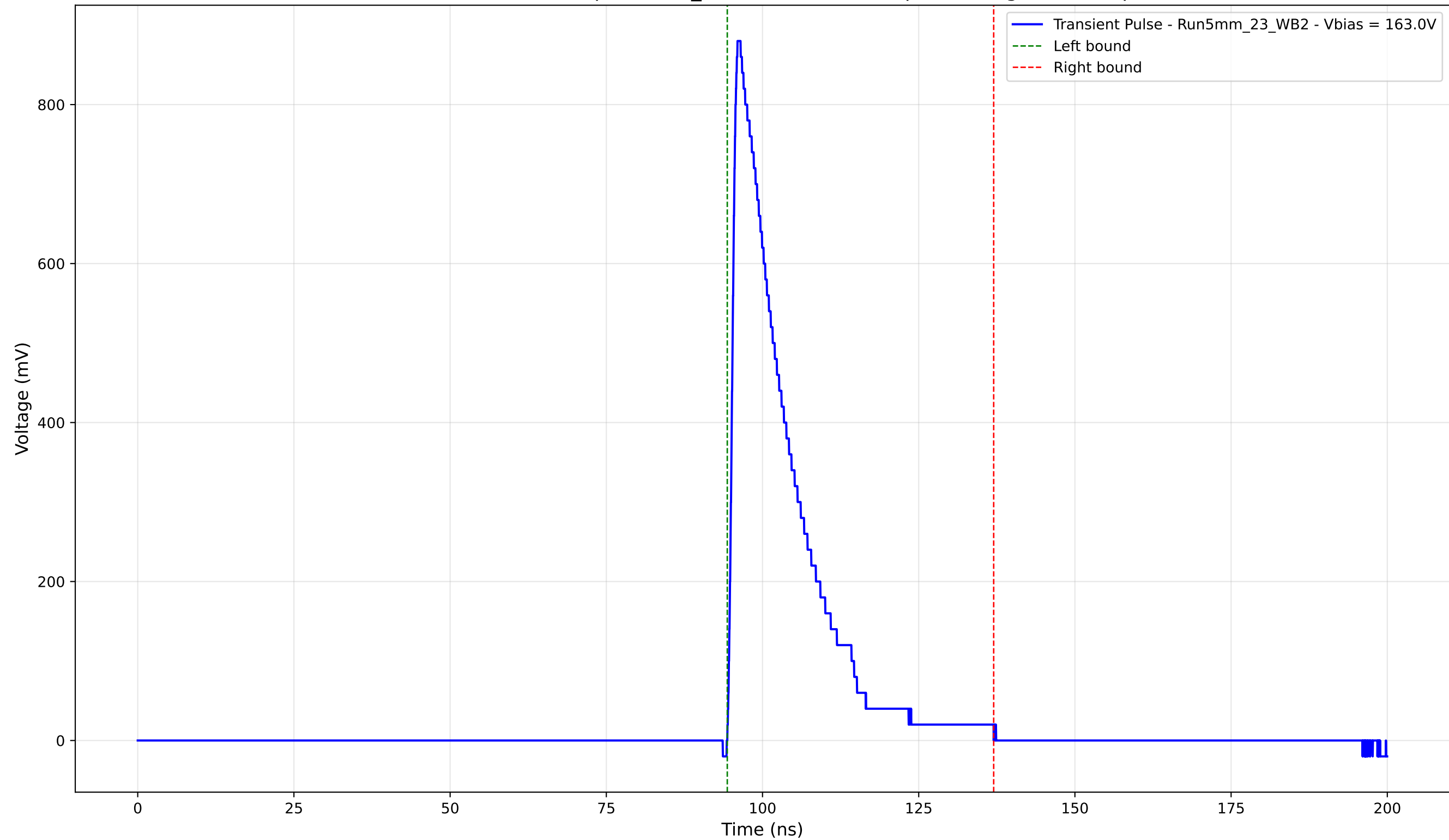
Transient Pulse - Sample: 5mm_23 - Position: 865.0 \mu\text{m} - Charge: 172.79 pC
