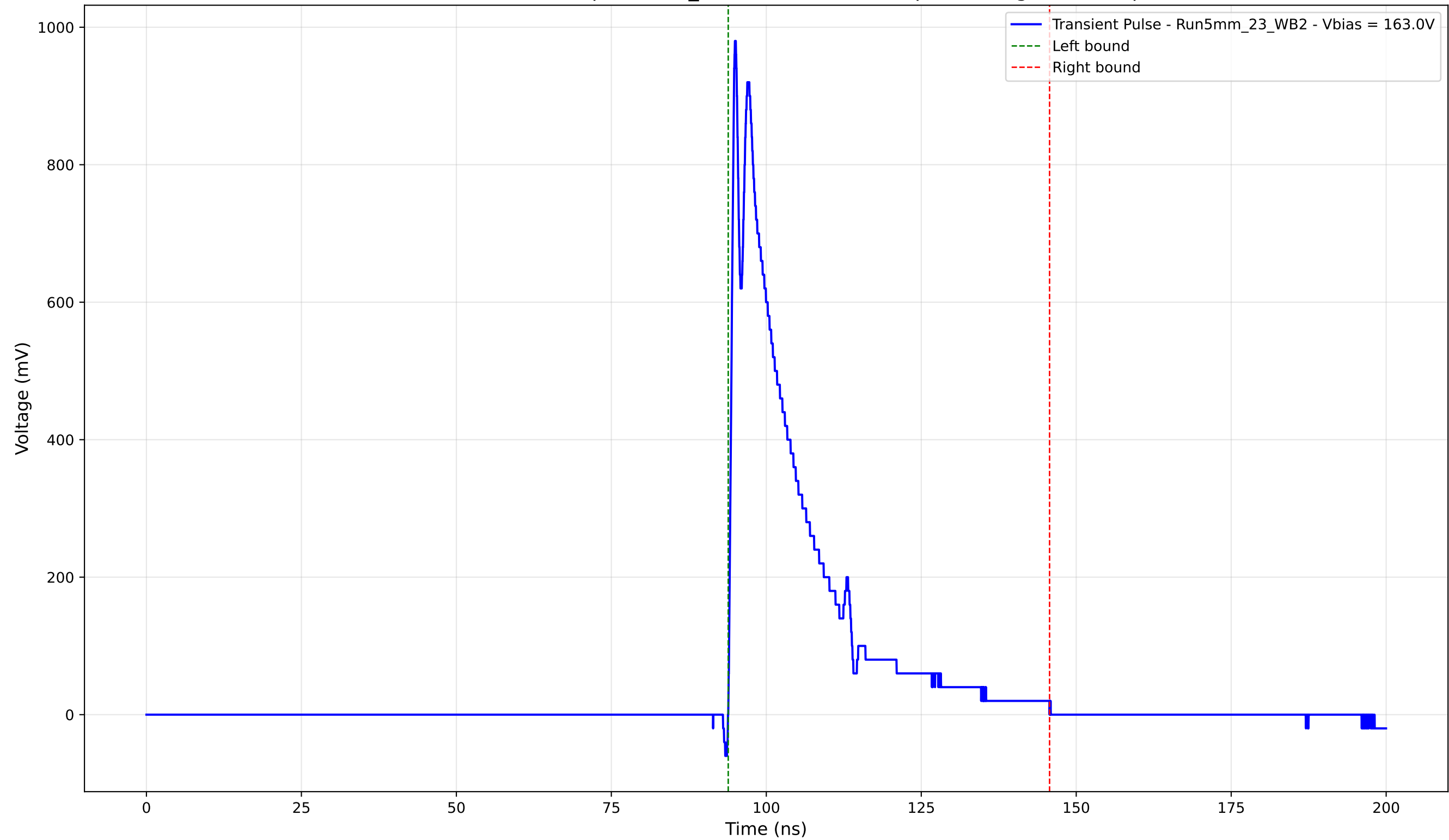
Transient Pulse - Sample: 5mm_23 - Position: 2340.0 \mu\text{m} - Charge: 202.66 pC
