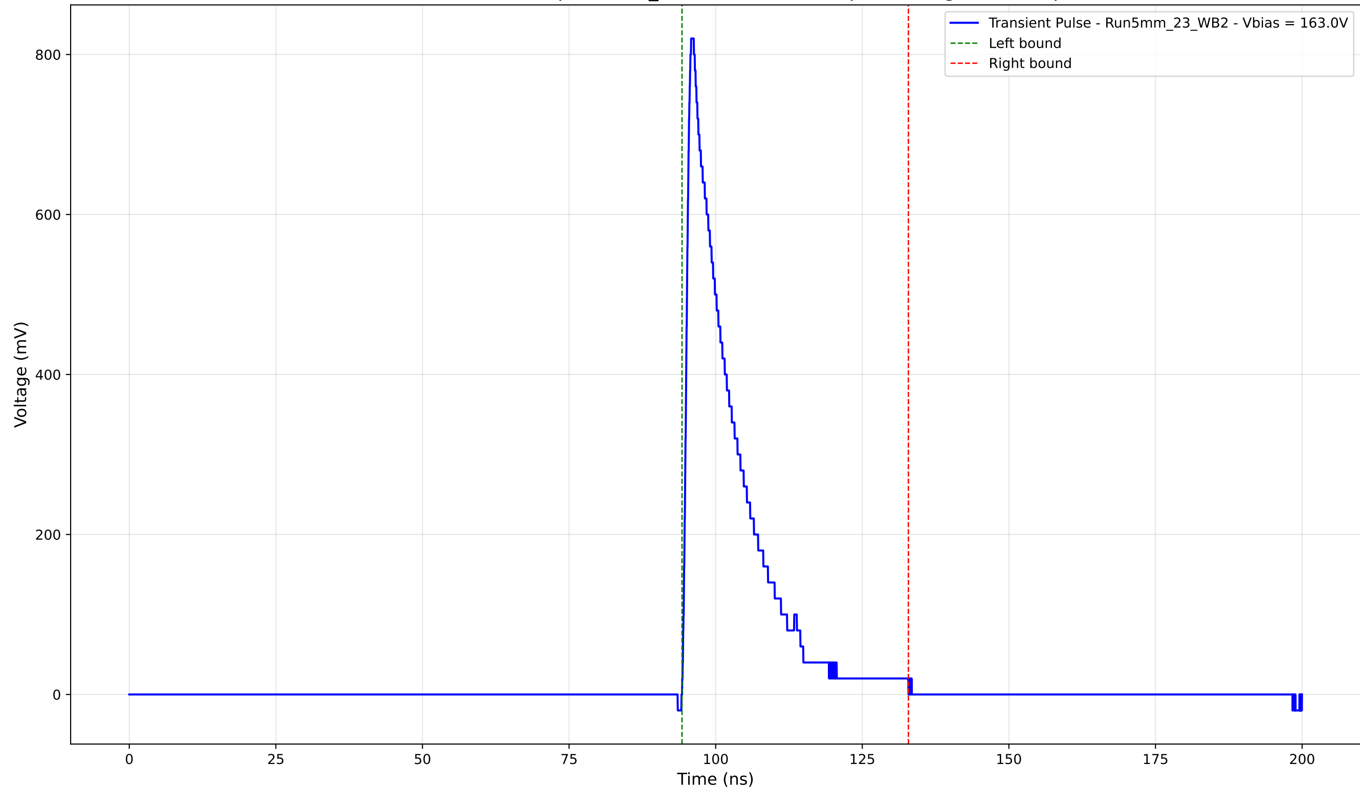
Transient Pulse - Sample: 5mm_23 - Position: 550.0 \mu\text{m} - Charge: 142.09 pC
