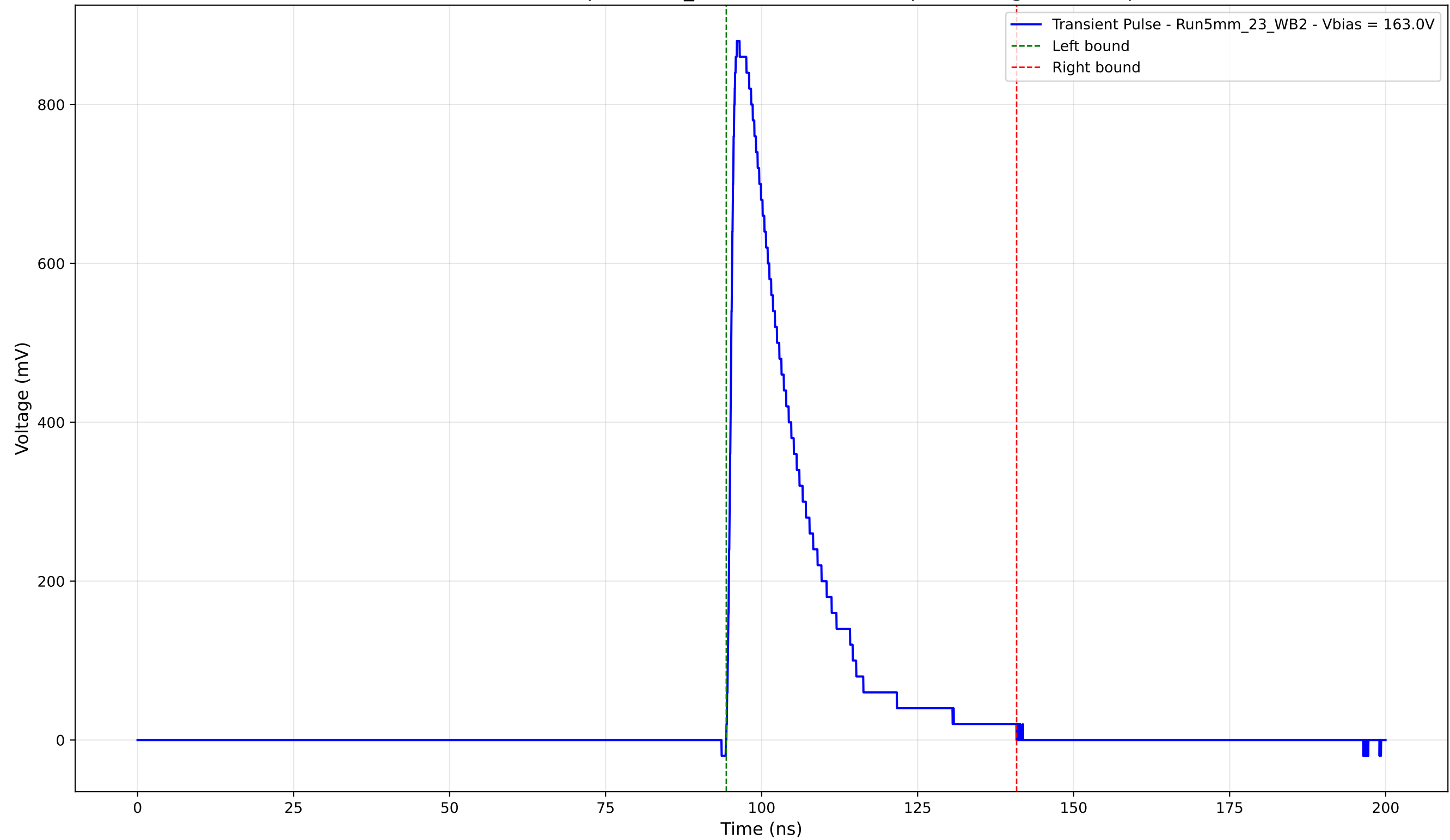
Transient Pulse - Sample: 5mm_23 - Position: 1390.0 \mu\text{m} - Charge: 195.14 pC
