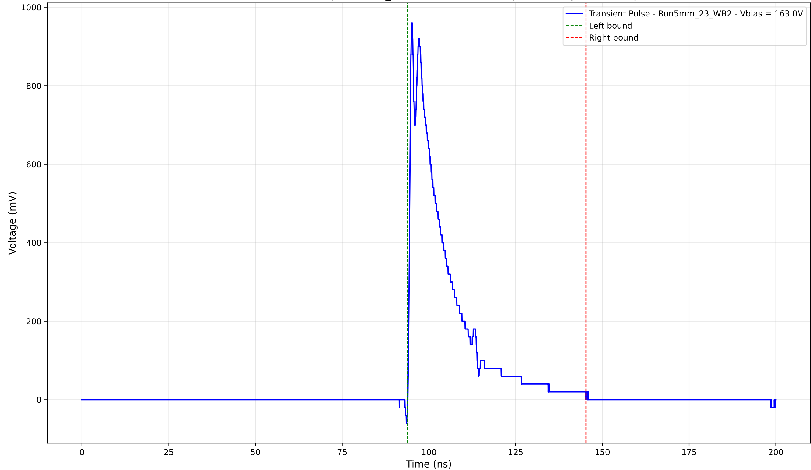
Transient Pulse - Sample: 5mm_23 - Position: 2800.0 \mu\text{m} - Charge: 206.82 pC
