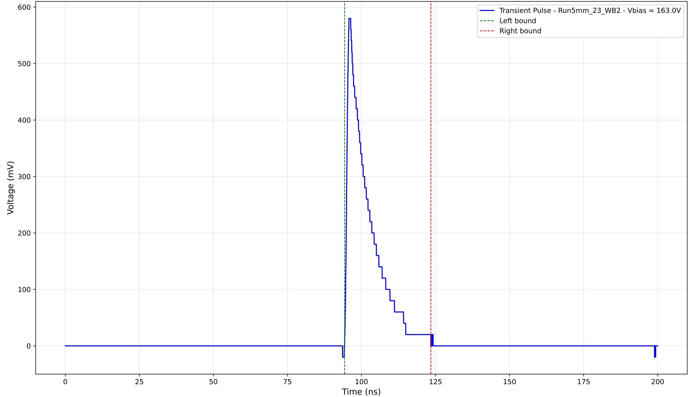
Transient Pulse - Sample: 5mm_23 - Position: 530.0 \mu\text{m} - Charge: 93.18 pC
