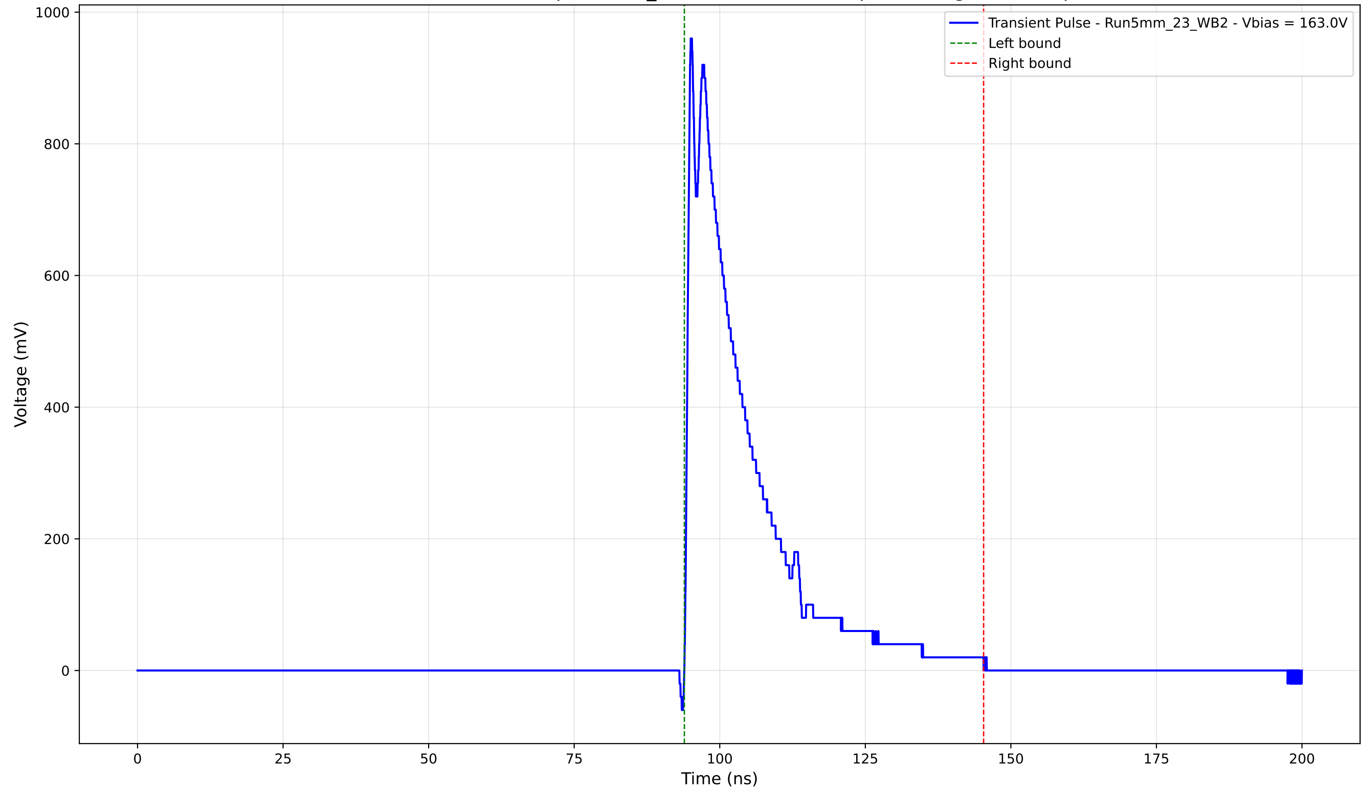
Transient Pulse - Sample: 5mm_23 - Position: 2815.0 \mu\text{m} - Charge: 208.26 pC
