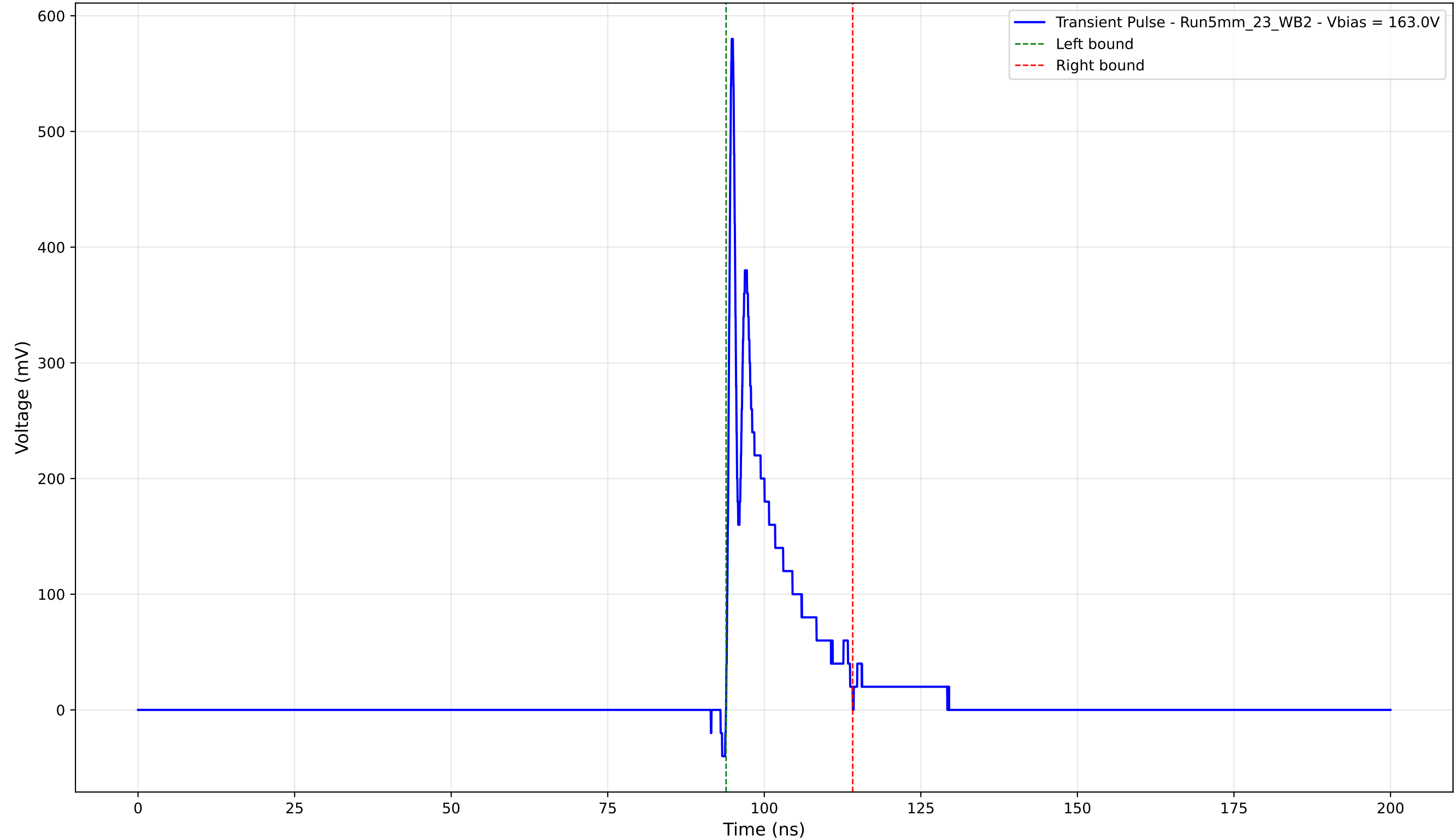
Transient Pulse - Sample: 5mm_23 - Position: 2490.0 \mu\text{m} - Charge: 60.26 pC
