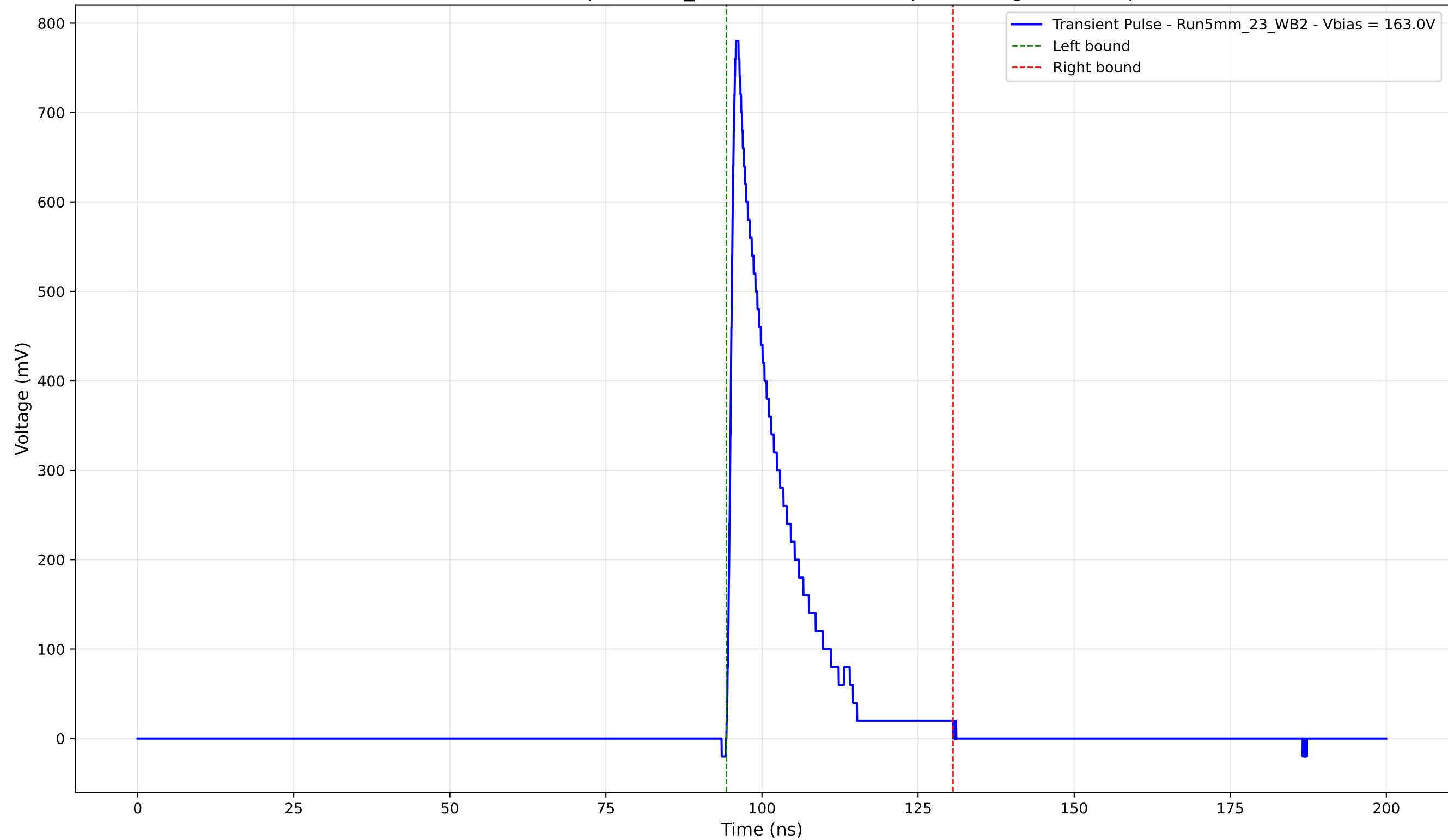
Transient Pulse - Sample: 5mm_23 - Position: 4470.0 \mu\text{m} - Charge: 122.68 pC
