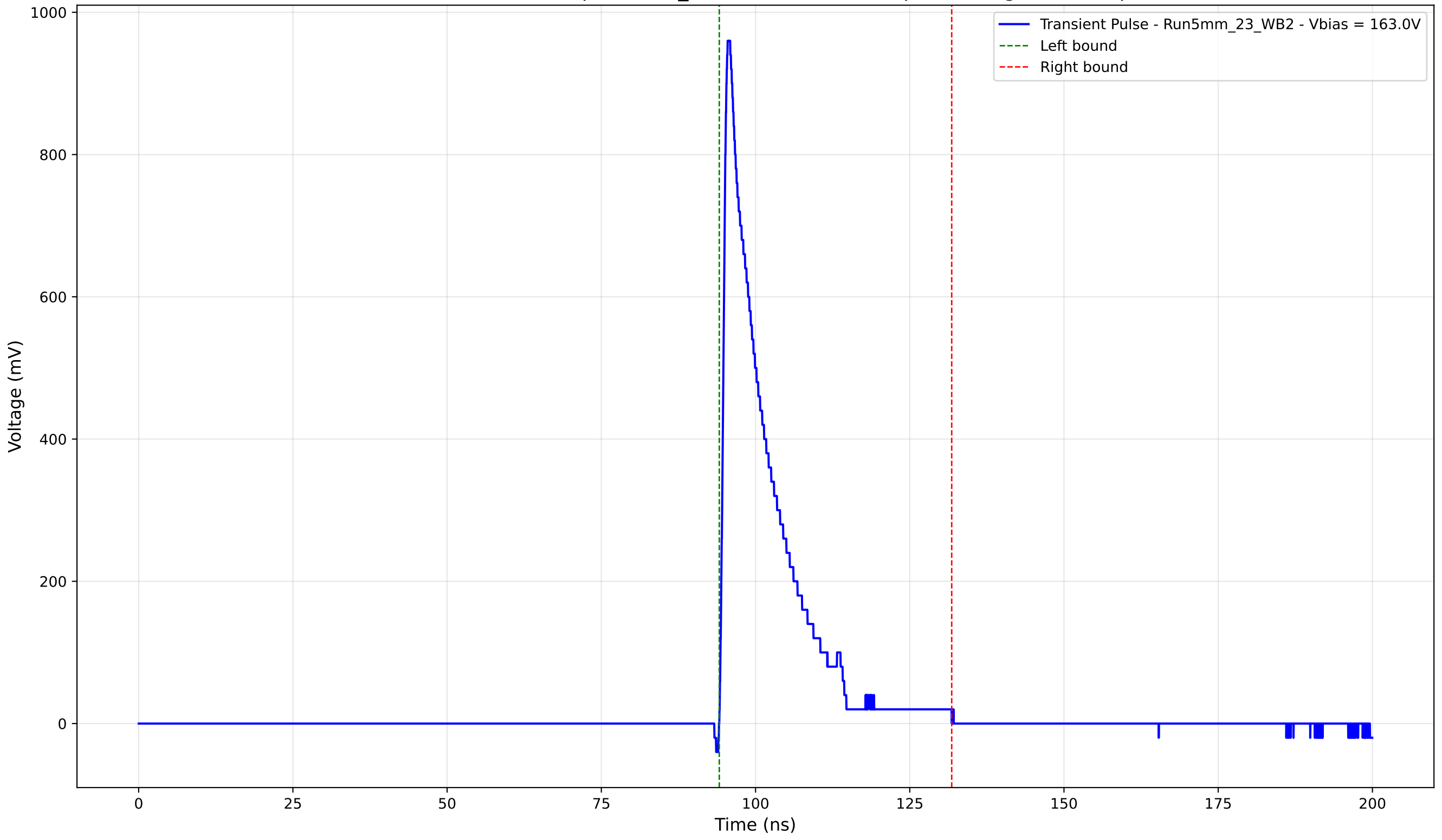
Transient Pulse - Sample: 5mm_23 - Position: 4775.0 \mu\text{m} - Charge: 147.13 pC
