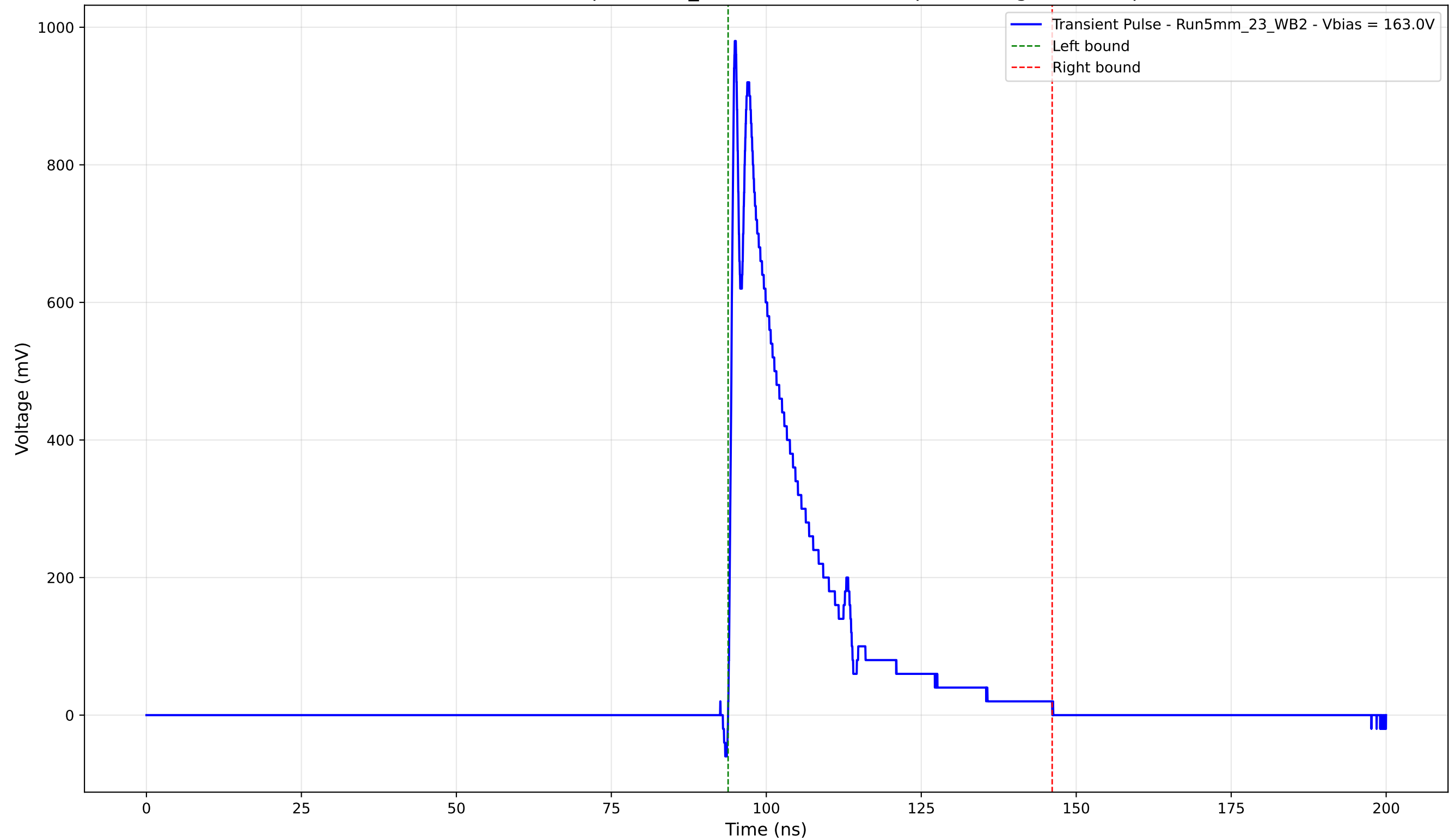
Transient Pulse - Sample: 5mm_23 - Position: 2685.0 \mu\text{m} - Charge: 201.98 pC
