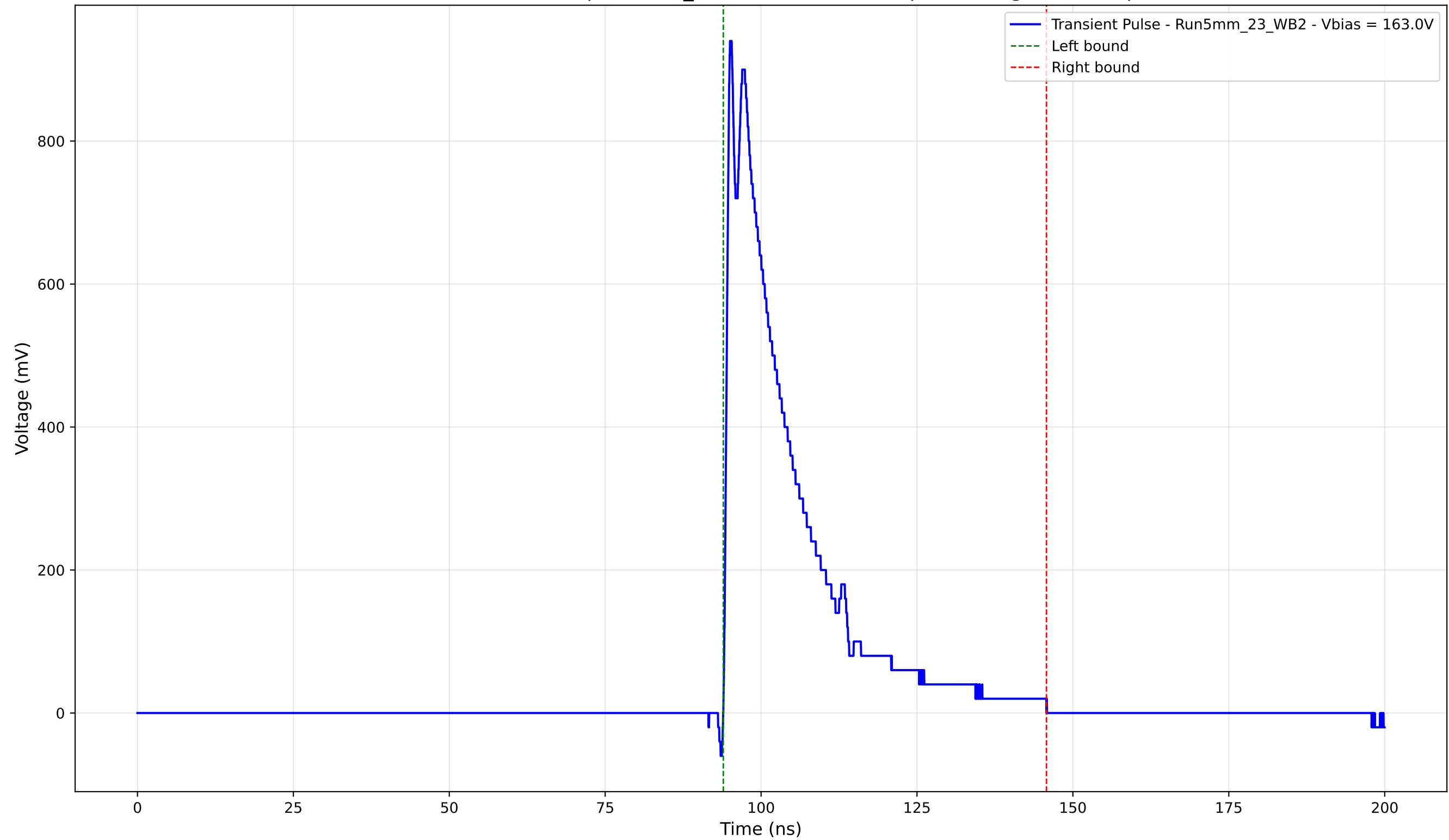
Transient Pulse - Sample: 5mm_23 - Position: 2195.0 \mu\text{m} - Charge: 205.46 pC
