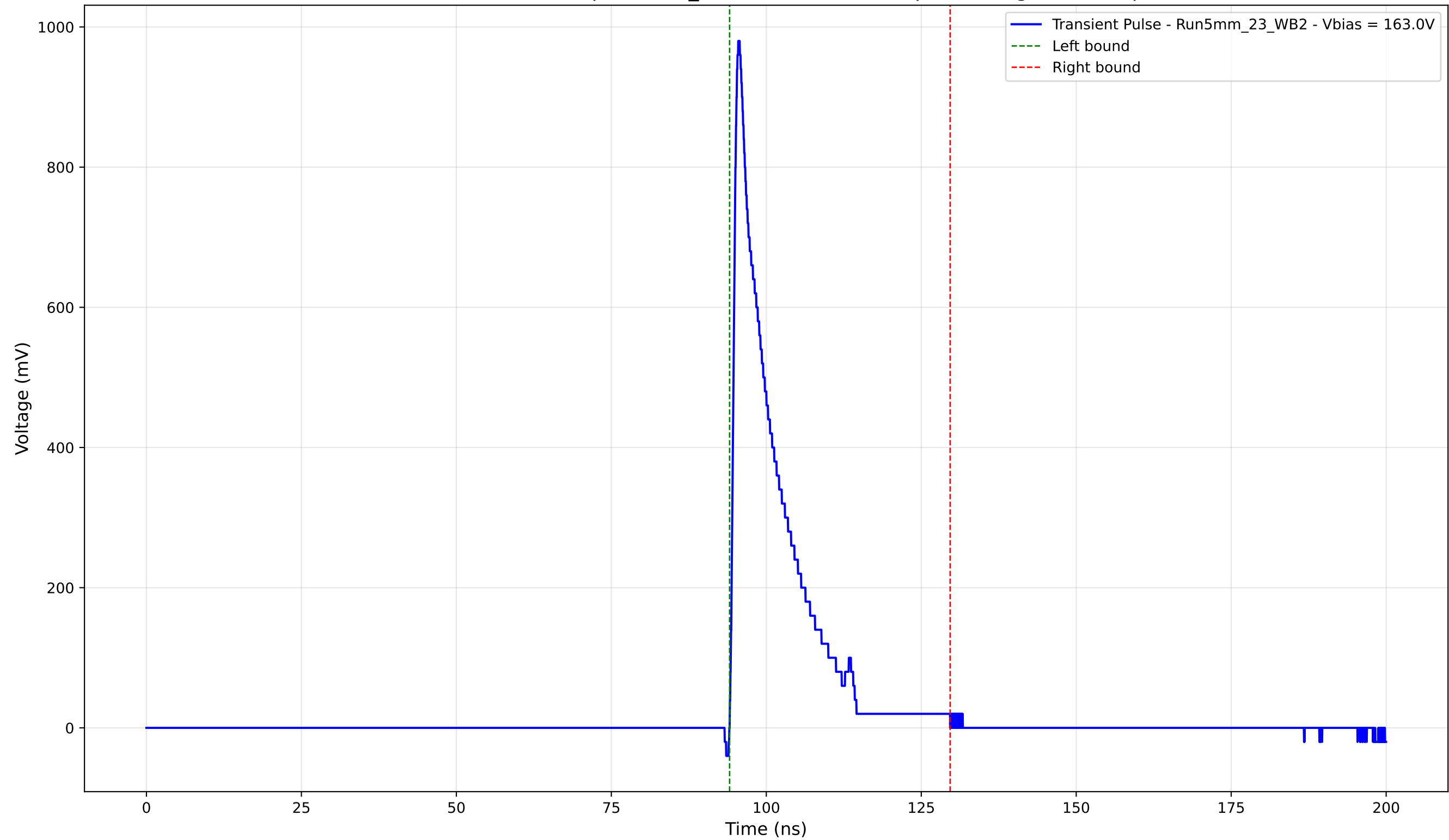
Transient Pulse - Sample: 5mm_23 - Position: 4855.0 \mu\text{m} - Charge: 140.57 pC
