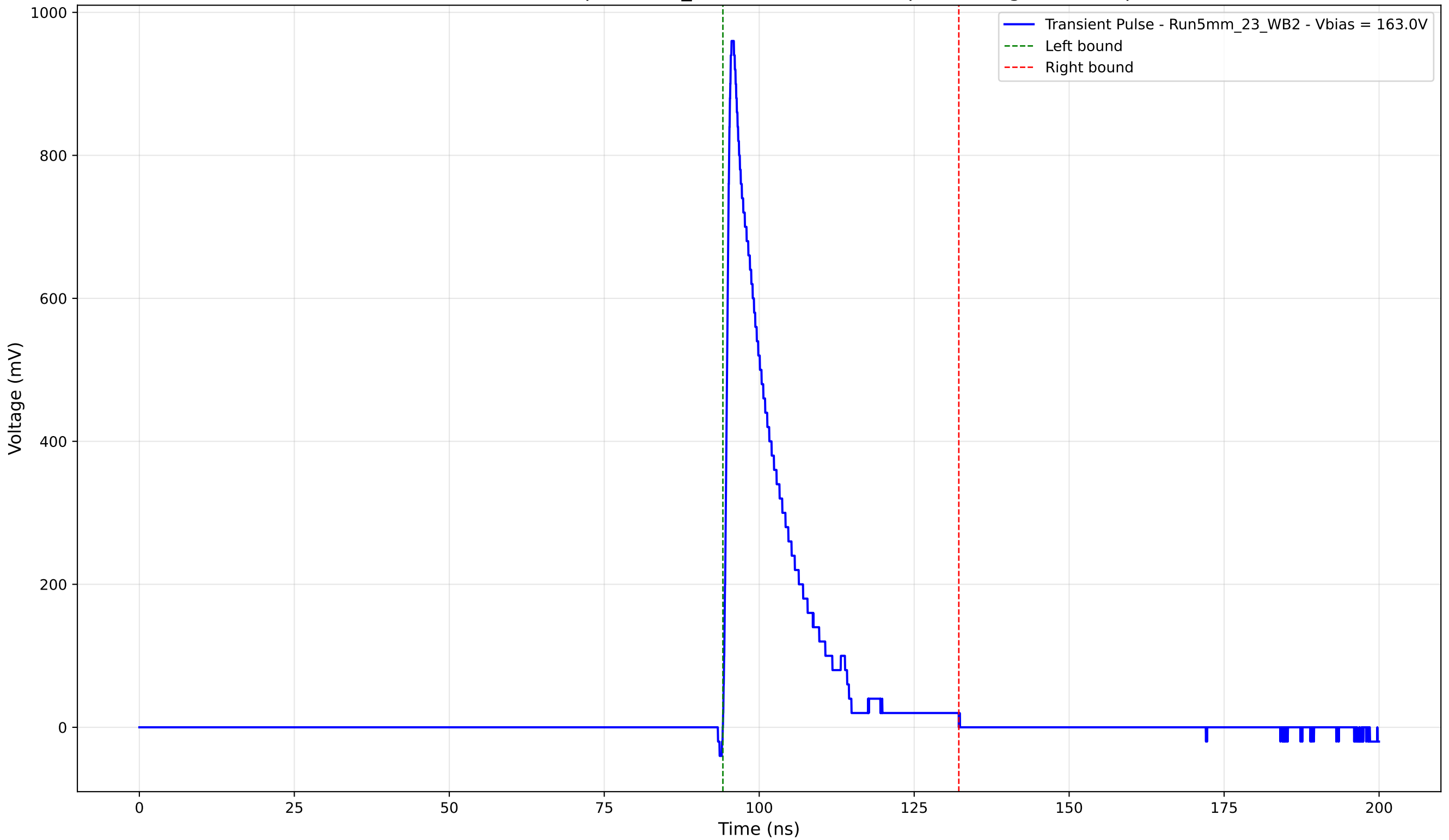
Transient Pulse - Sample: 5mm_23 - Position: 4735.0 \mu\text{m} - Charge: 150.54 pC
