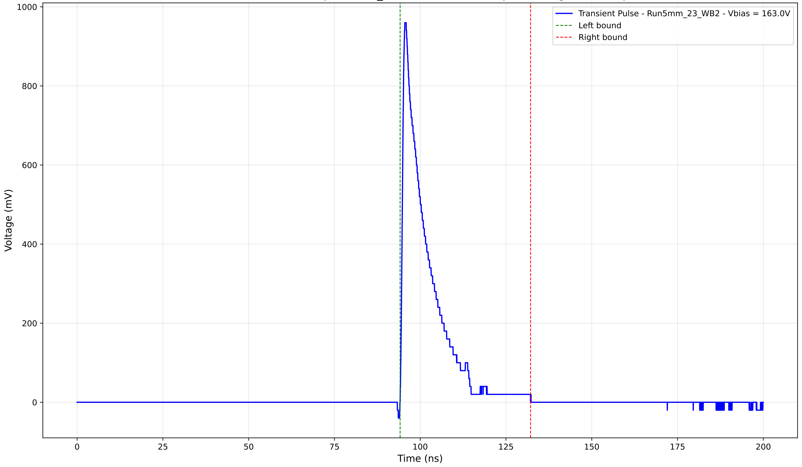
Transient Pulse - Sample: 5mm_23 - Position: 4750.0 \mu\text{m} - Charge: 149.54 pC
