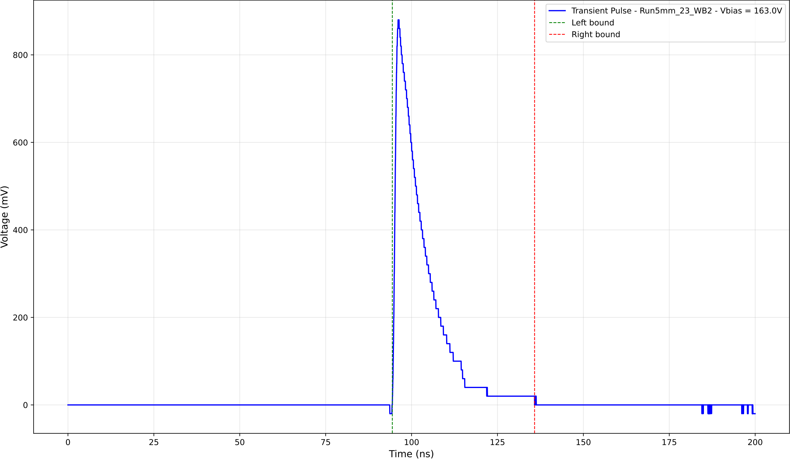
Transient Pulse - Sample: 5mm_23 - Position: 4165.0 \mu\text{m} - Charge: 162.07 pC
