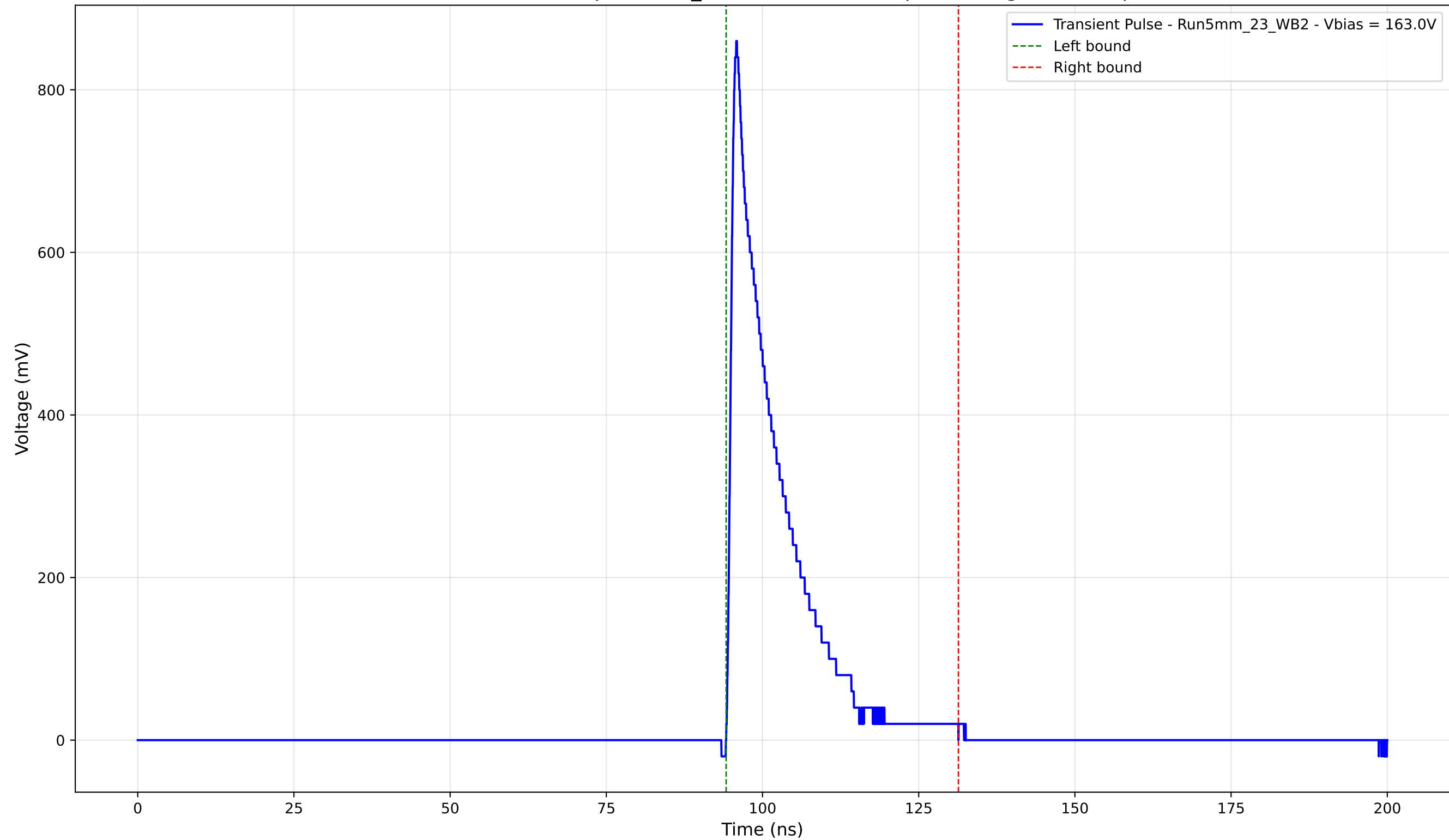
Transient Pulse - Sample: 5mm_23 - Position: 425.0 \mu\text{m} - Charge: 136.79 pC
