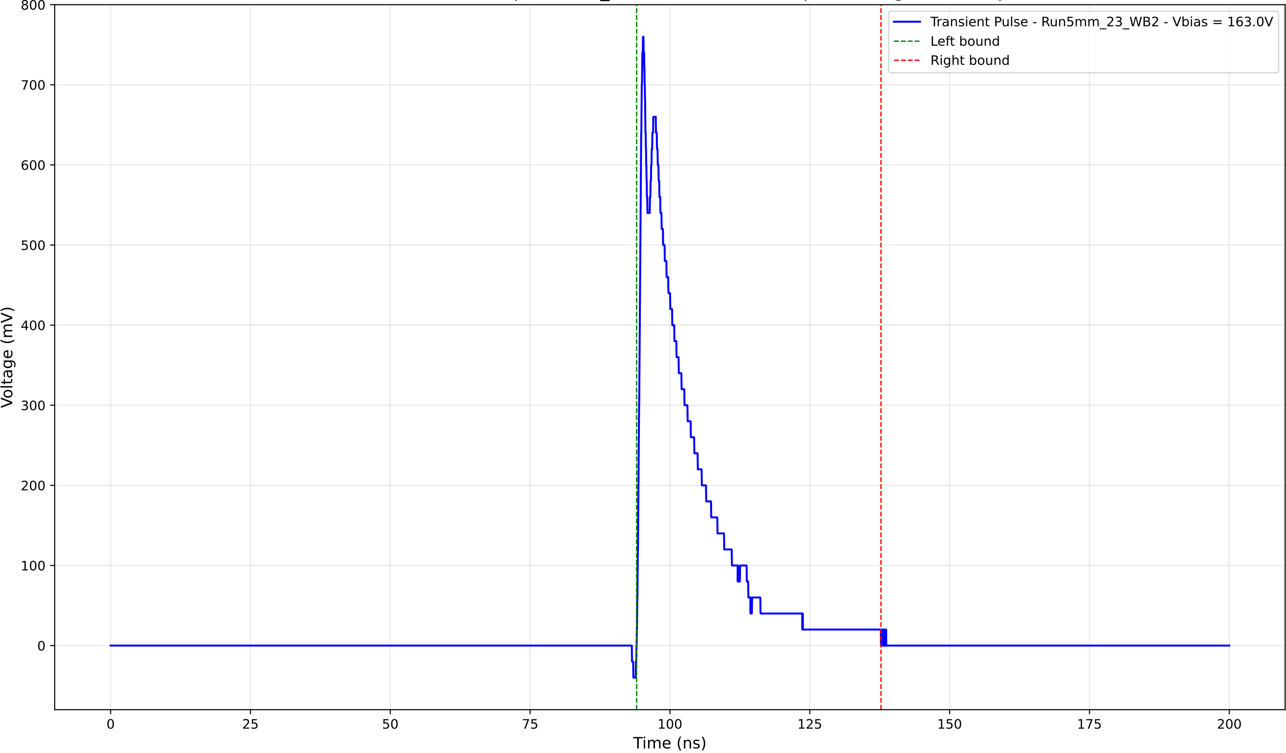
Transient Pulse - Sample: 5mm_23 - Position: 2970.0 \mu\text{m} - Charge: 135.38 pC
