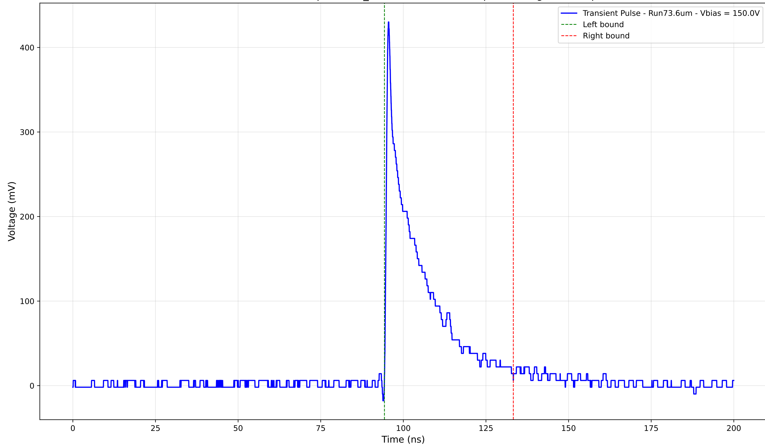
Transient Pulse - Sample: 1cm_42 - Position: 2505.0 \mu\text{m} - Charge: 80.85 pC
