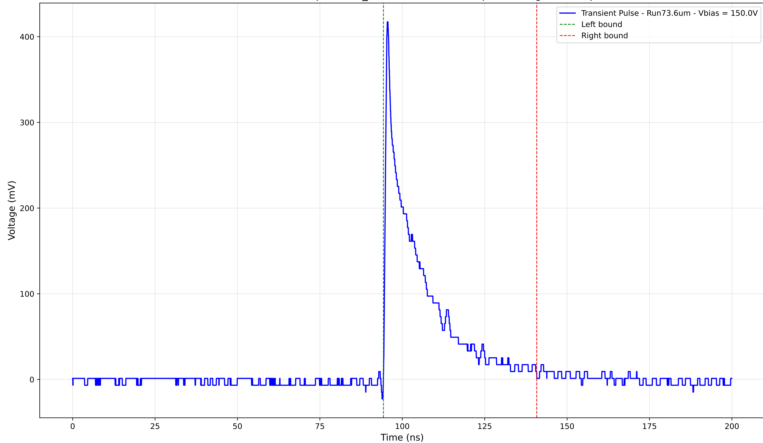
Transient Pulse - Sample: 1cm_42 - Position: 2710.0 \mu\text{m} - Charge: 77.96 pC
