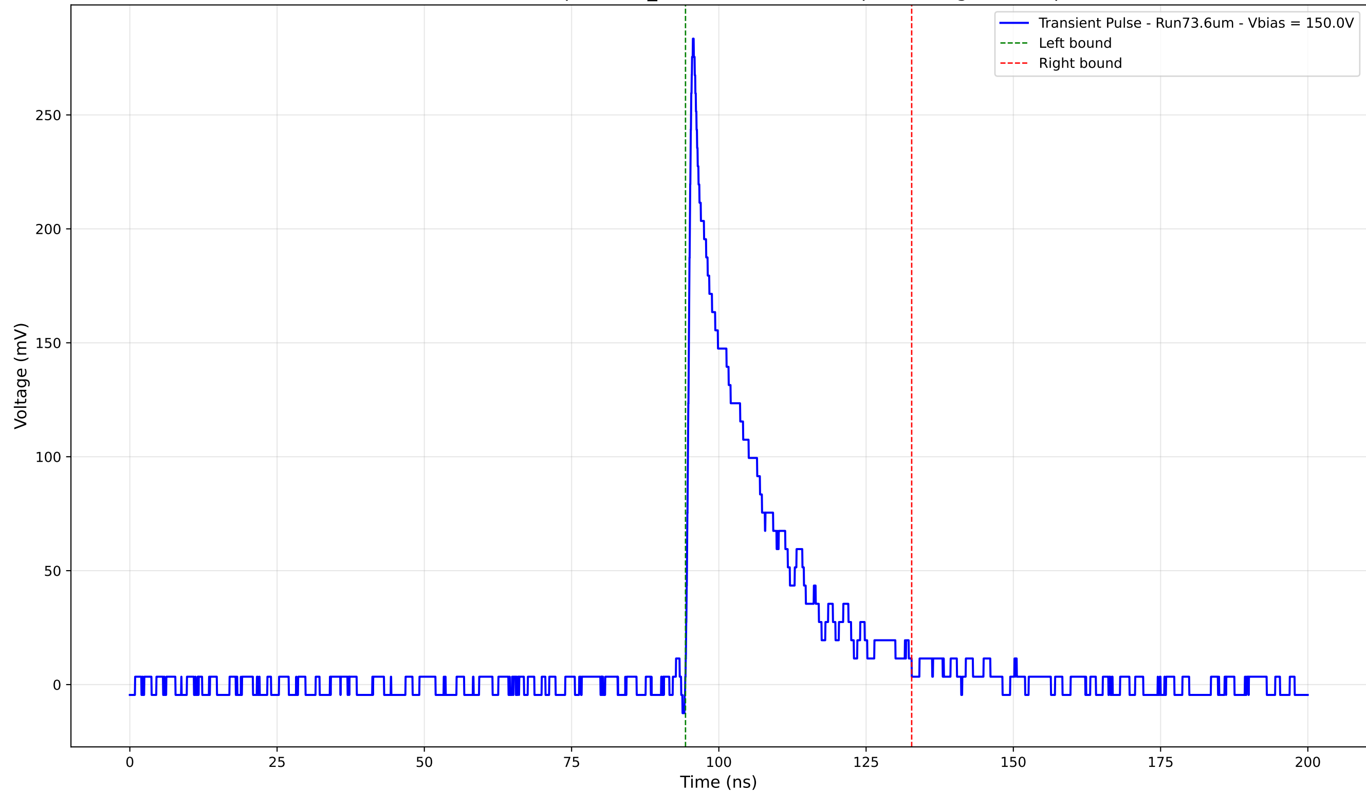
Transient Pulse - Sample: 1cm_42 - Position: 3405.0 \mu\text{m} - Charge: 55.95 pC
