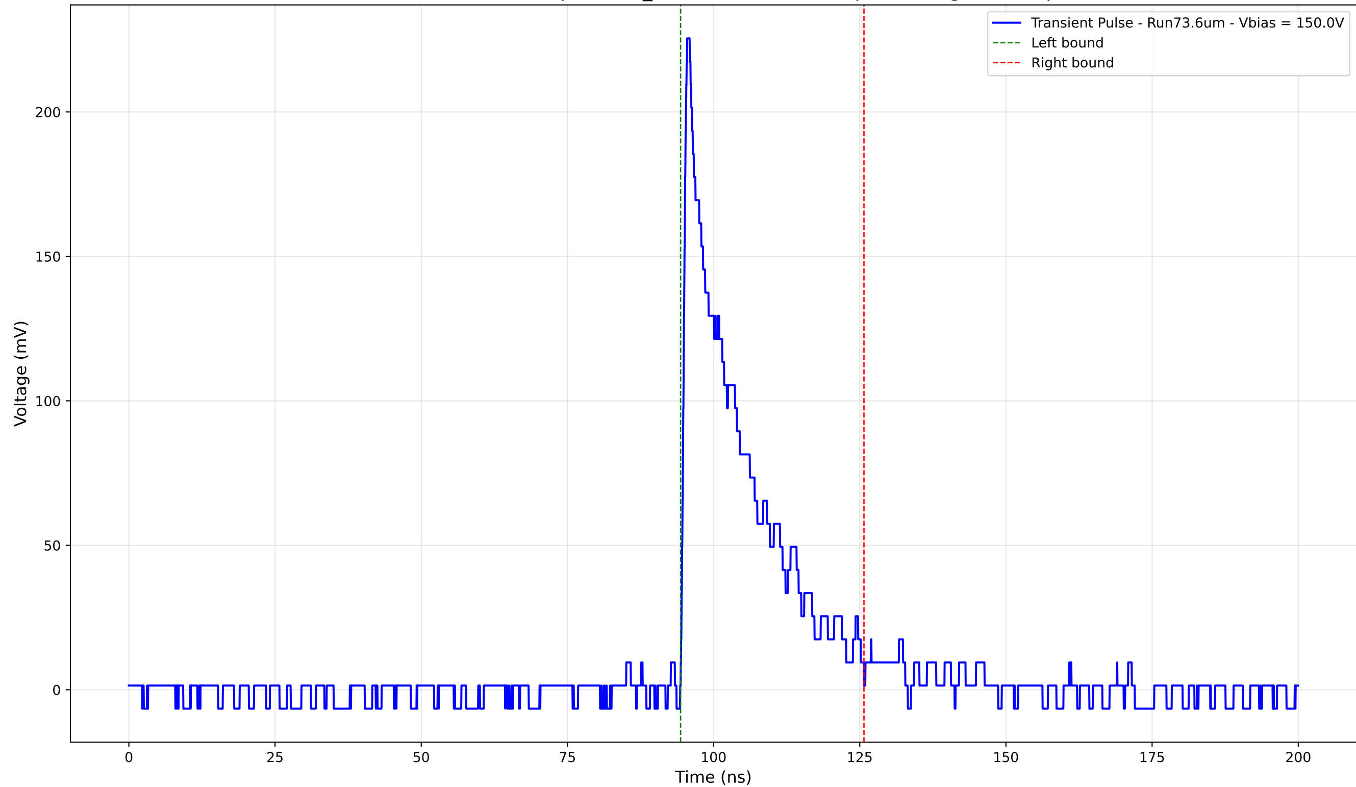
Transient Pulse - Sample: 1cm_42 - Position: 3740.0 \mu\text{m} - Charge: 43.99 pC
