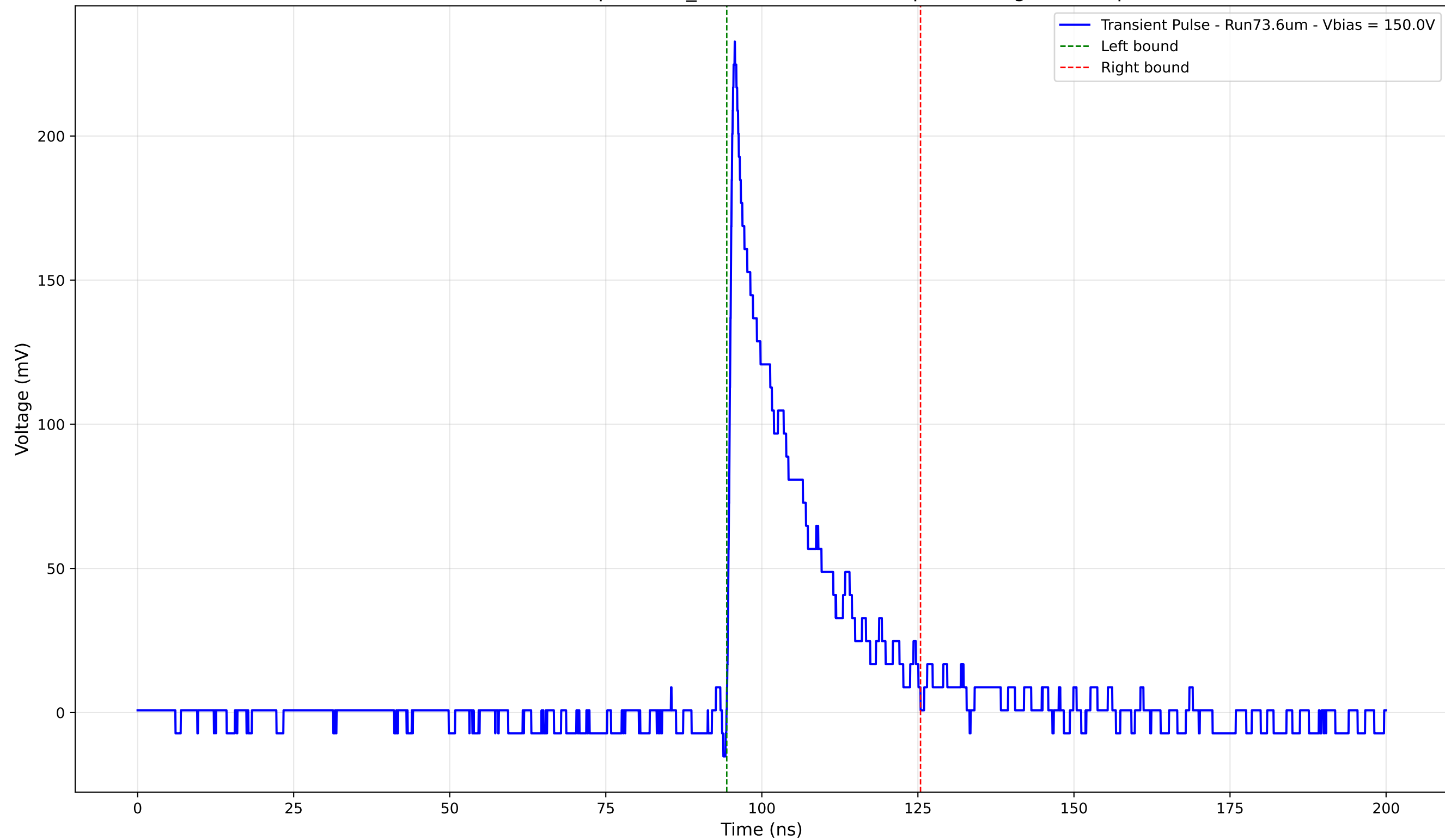
Transient Pulse - Sample: 1cm_42 - Position: 3720.0 \mu\text{m} - Charge: 42.67 pC
