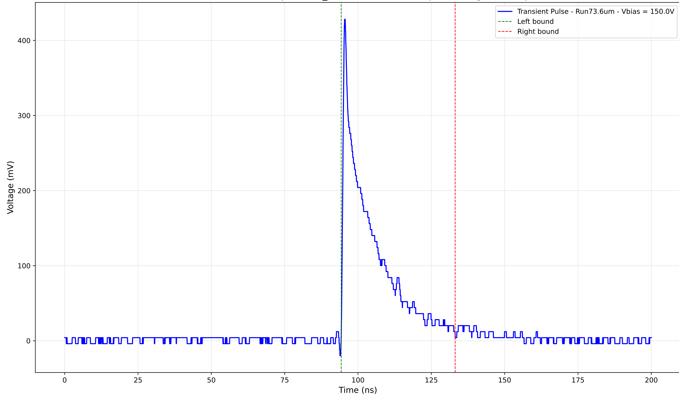
Transient Pulse - Sample: 1cm_42 - Position: 2555.0 \mu\text{m} - Charge: 78.66 pC
