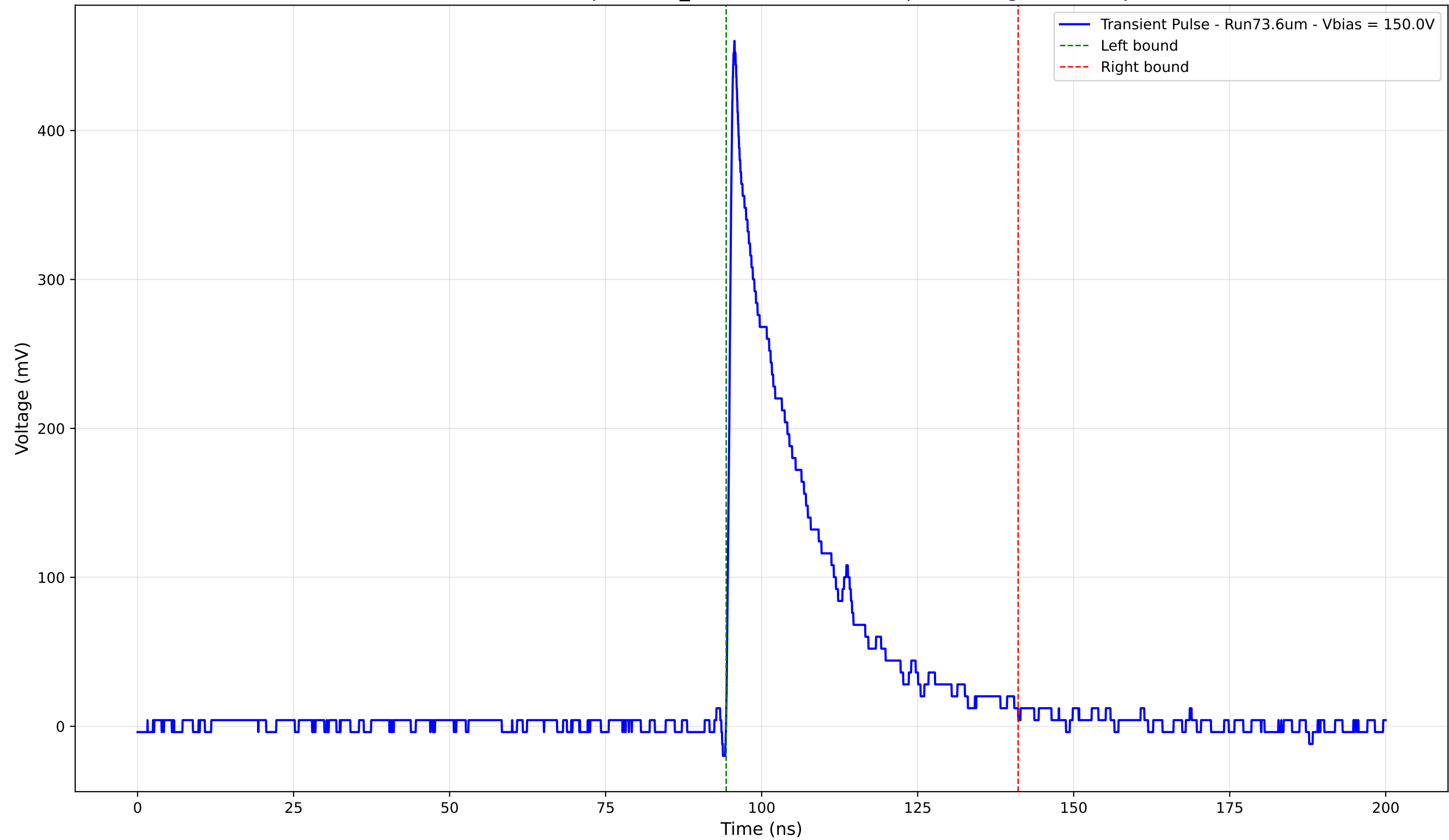
Transient Pulse - Sample: 1cm_42 - Position: 1445.0 \mu\text{m} - Charge: 100.76 pC
