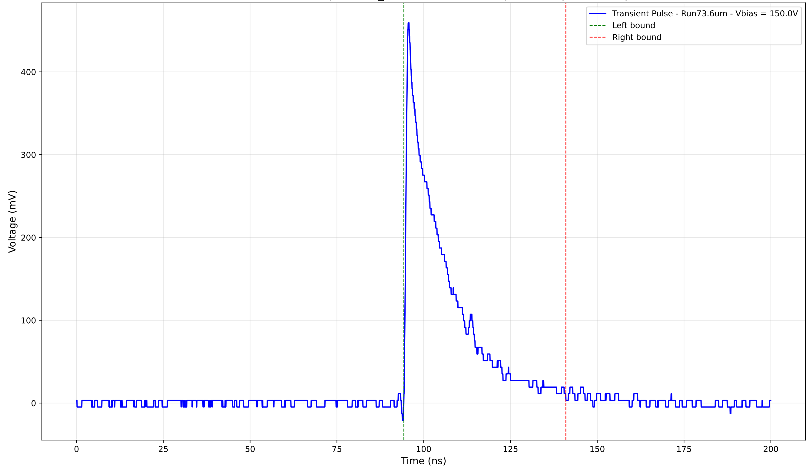
Transient Pulse - Sample: 1cm_42 - Position: 1295.0 \mu\text{m} - Charge: 101.39 pC
