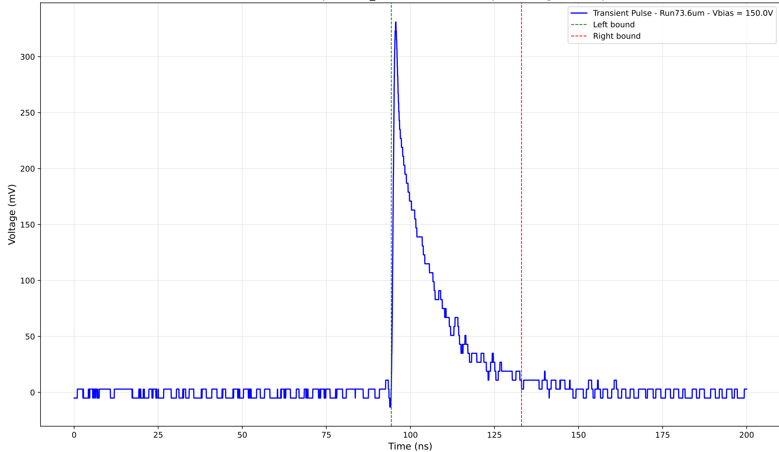
Transient Pulse - Sample: 1cm_42 - Position: 3125.0 \mu\text{m} - Charge: 62.99 pC
