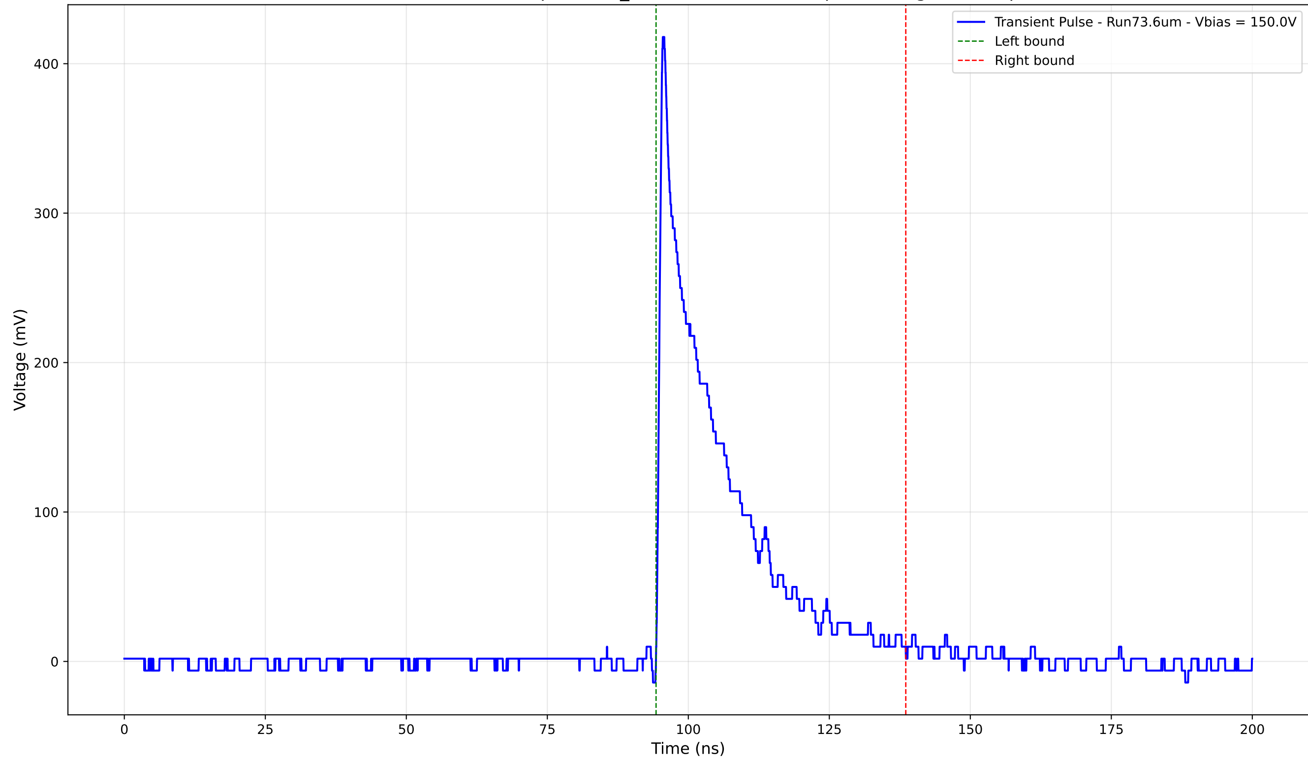
Transient Pulse - Sample: 1cm_42 - Position: 2135.0 \mu\text{m} - Charge: 83.96 pC
