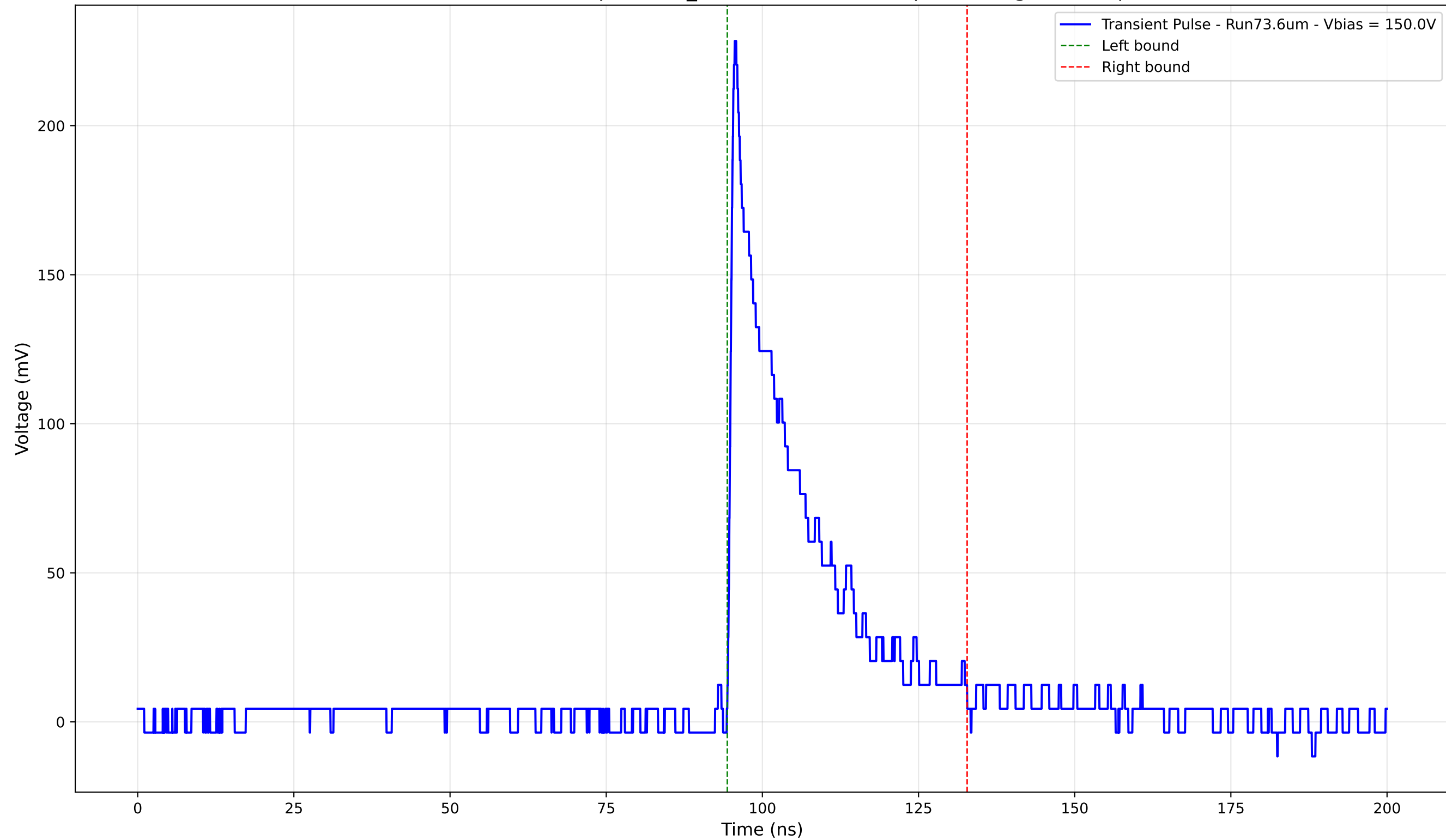
Transient Pulse - Sample: 1cm_42 - Position: 3790.0 \mu\text{m} - Charge: 46.59 pC
