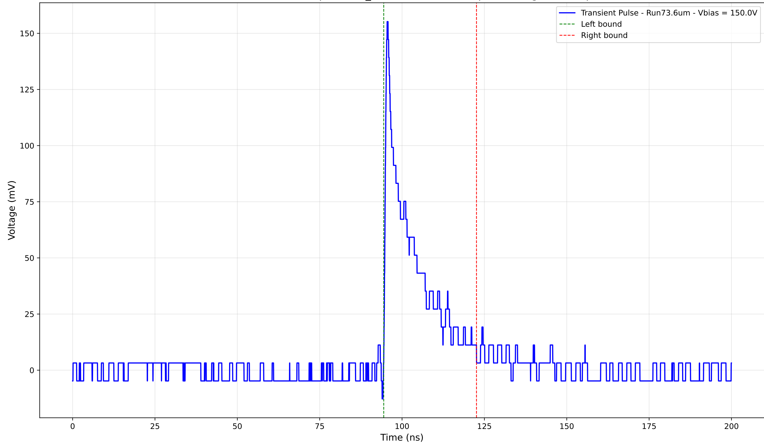
Transient Pulse - Sample: 1cm_42 -Position: 130.0 \mu\text{m} - Charge: 24.79 pC
