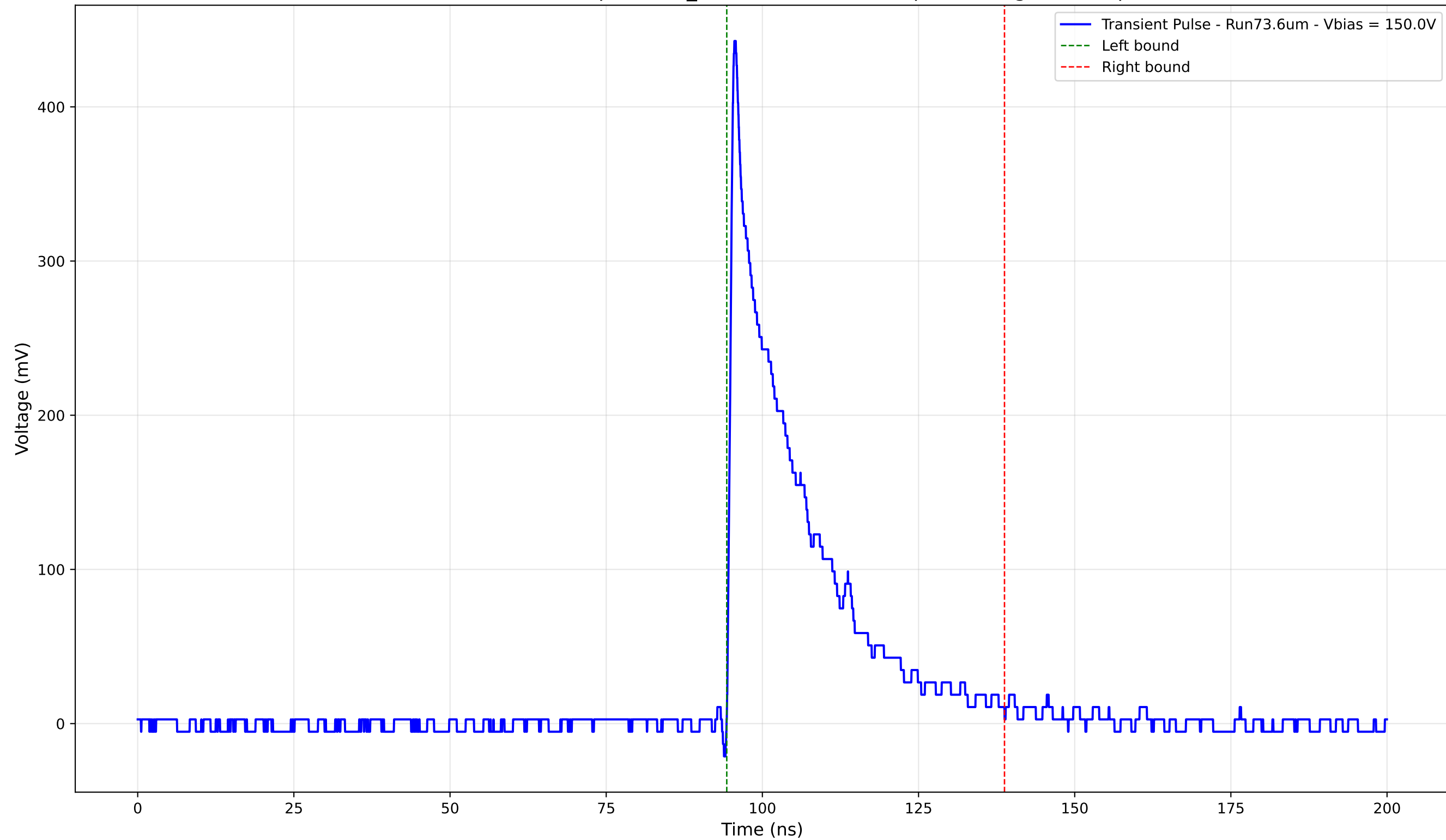
Transient Pulse - Sample: 1cm_42 - Position: 1925.0 \mu\text{m} - Charge: 91.50 pC
