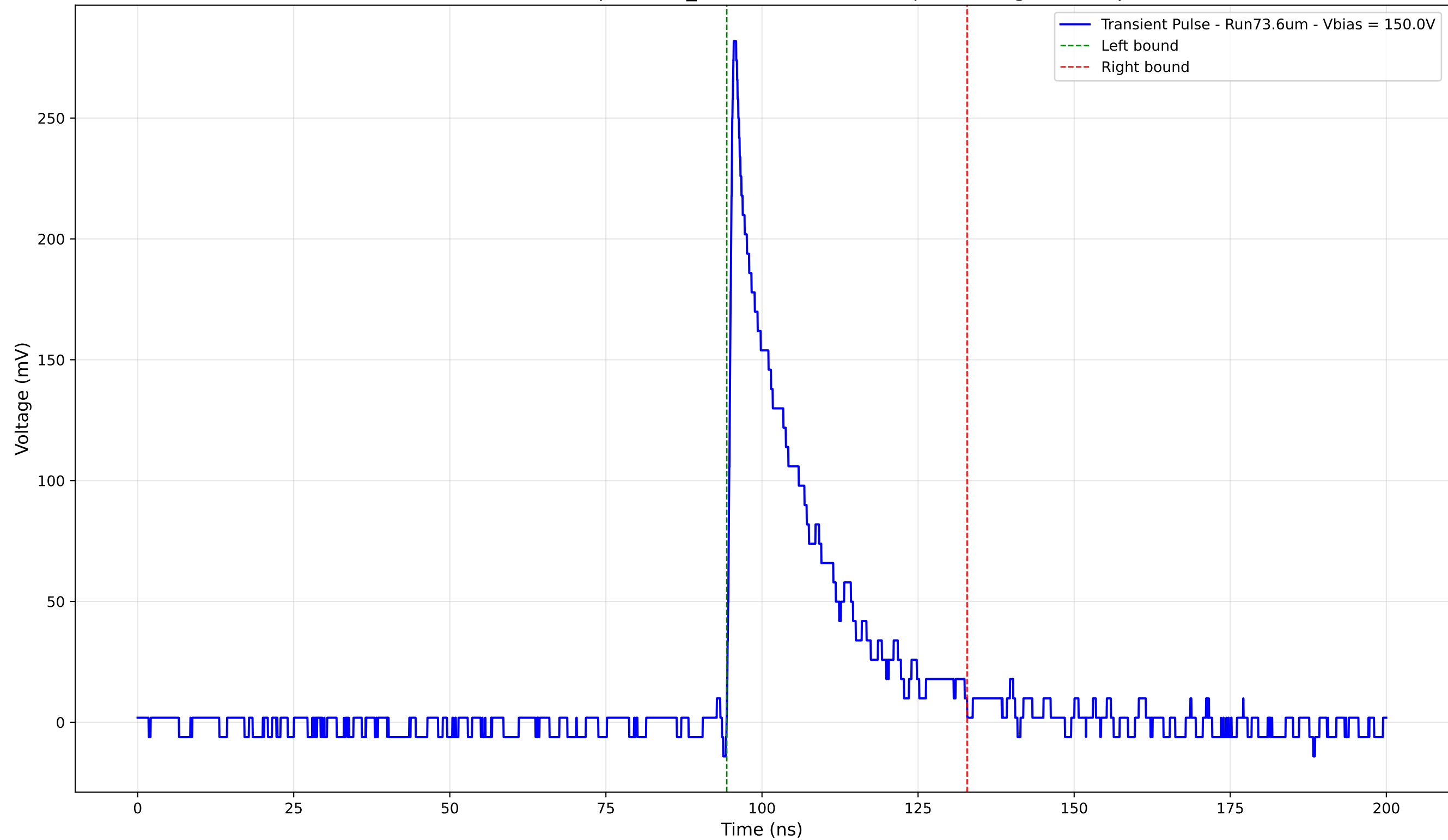
Transient Pulse - Sample: 1cm_42 - Position: 3365.0 \mu\text{m} - Charge: 56.98 pC
