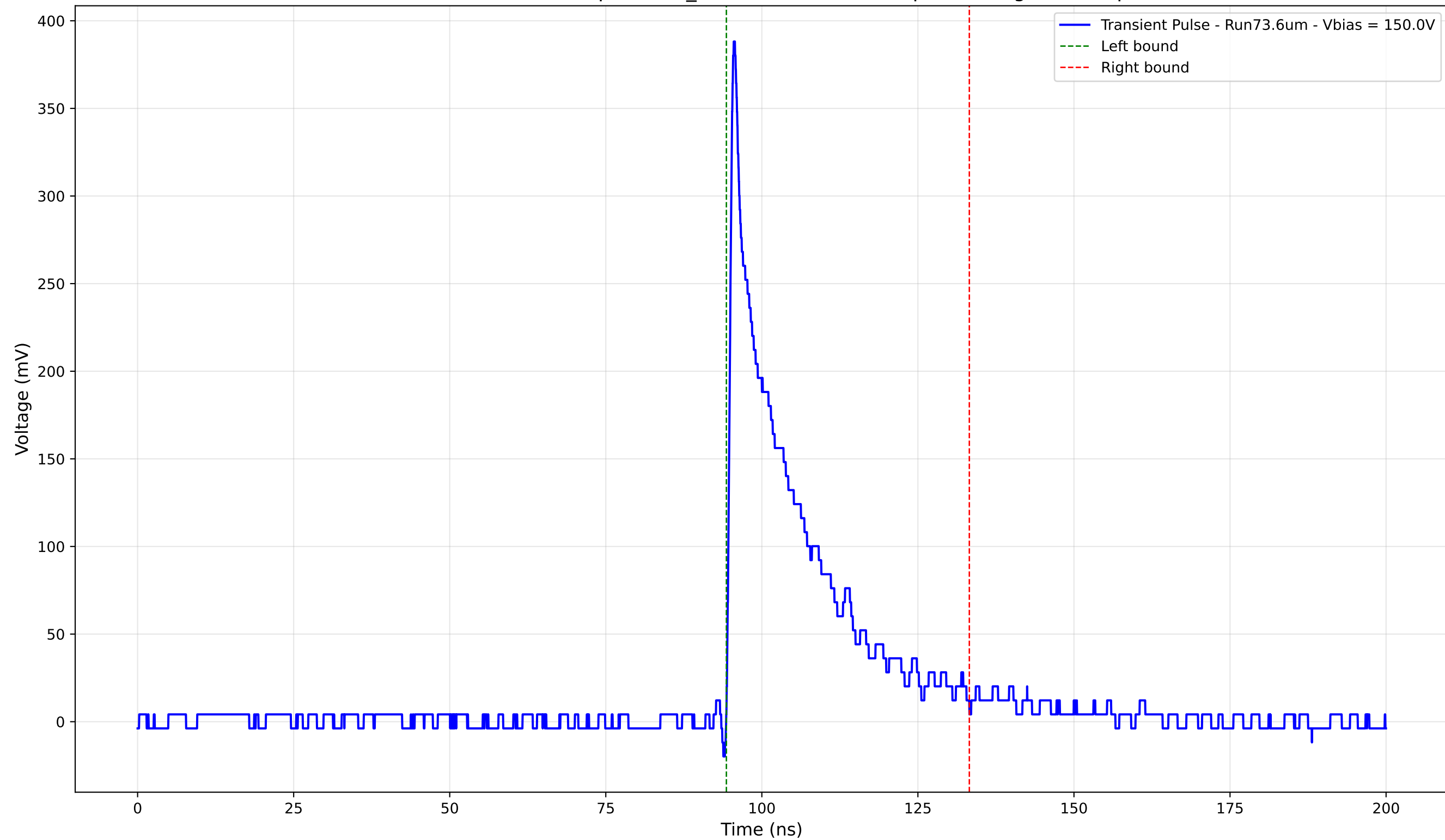
Transient Pulse - Sample: 1cm_42 - Position: 2870.0 \mu\text{m} - Charge: 72.73 pC
