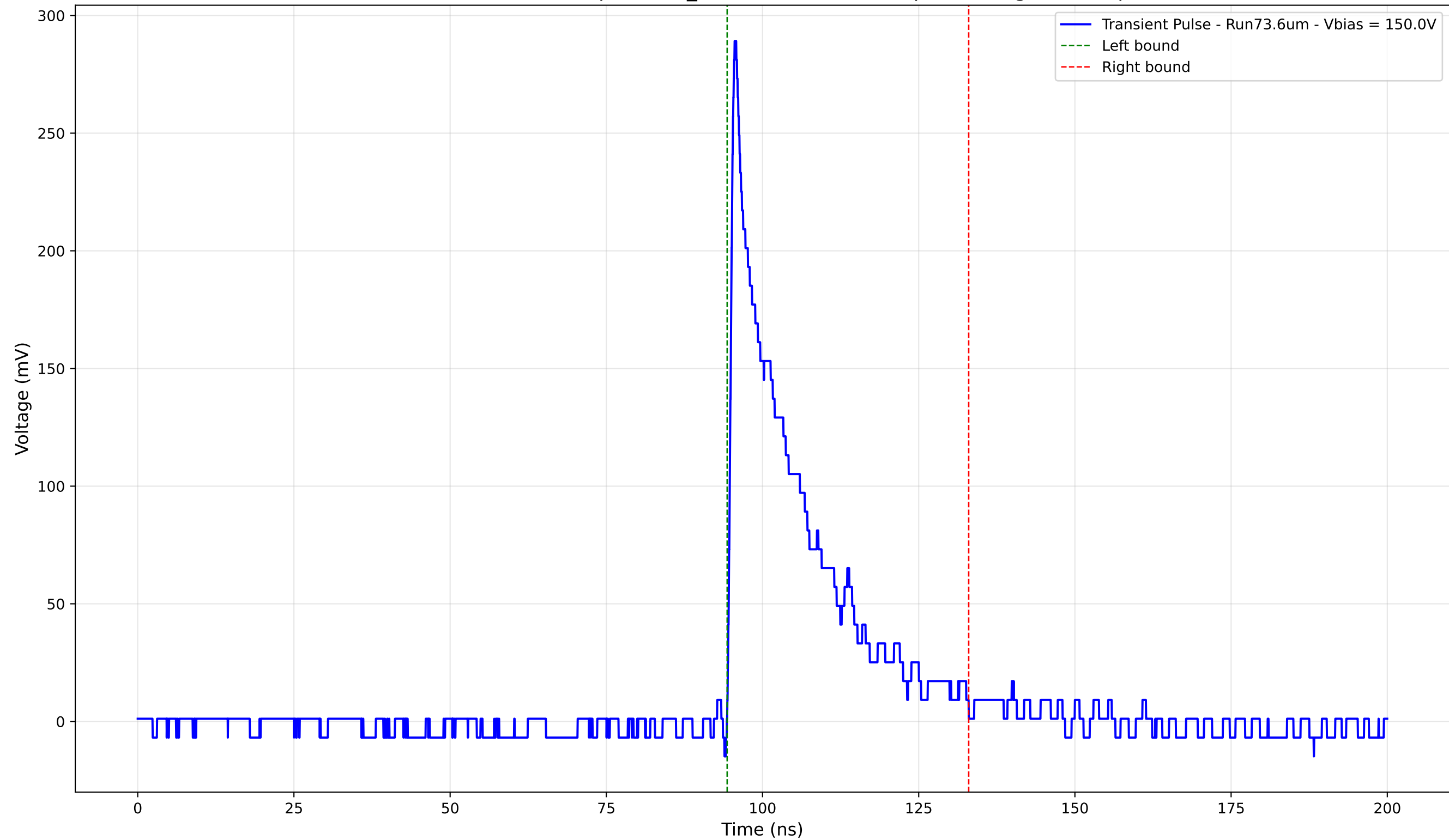
Transient Pulse - Sample: 1cm_42 - Position: 3285.0 \mu\text{m} - Charge: 56.83 pC
