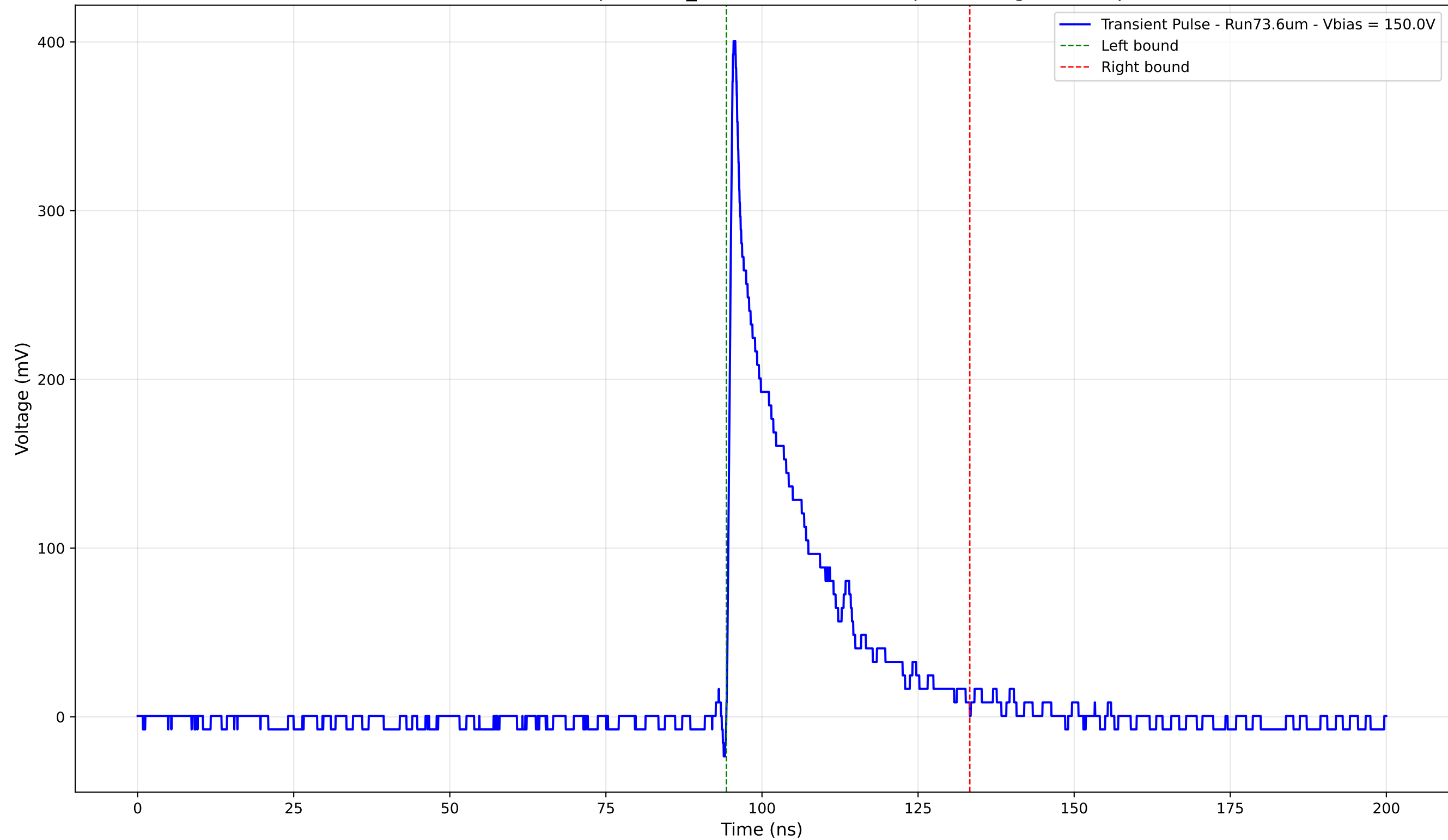
Transient Pulse - Sample: 1cm_42 - Position: 2815.0 \mu\text{m} - Charge: 73.08 pC
