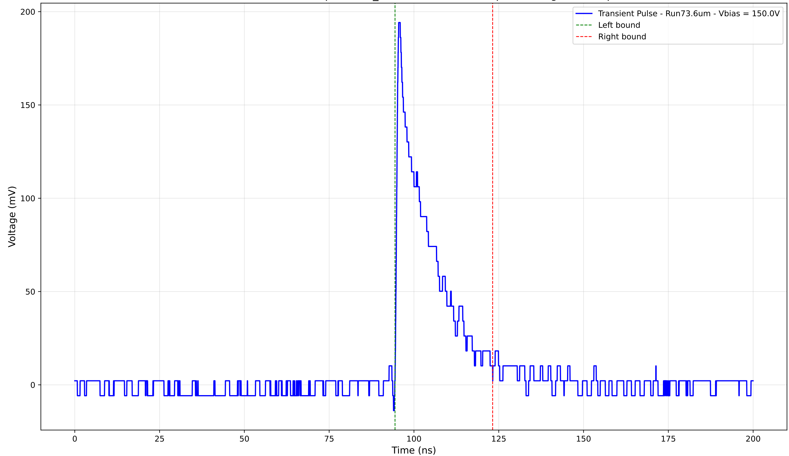
Transient Pulse - Sample: 1cm_42 - Position: 4020.0 \mu\text{m} - Charge: 37.33 pC
