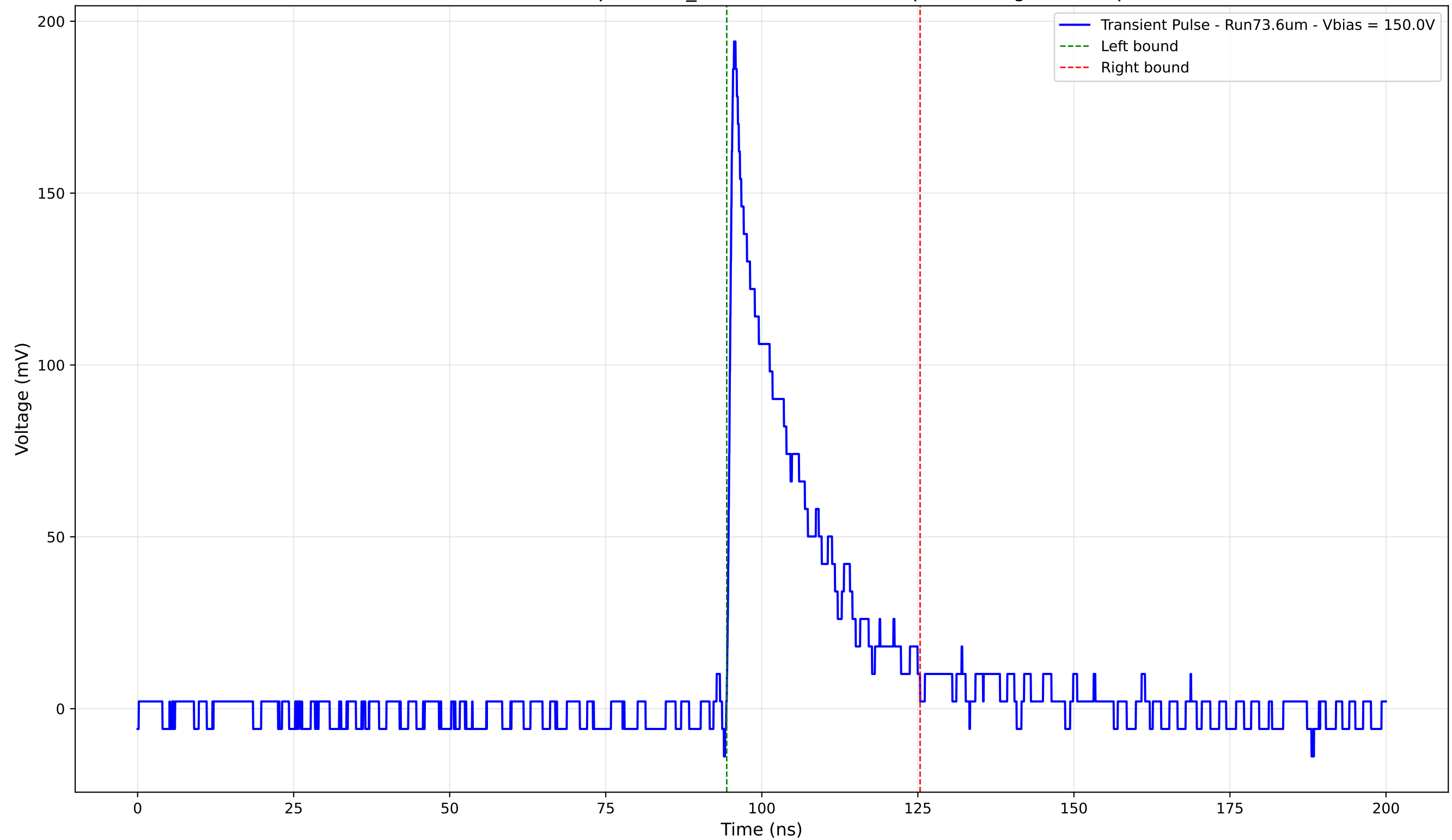
Transient Pulse - Sample: 1cm_42 - Position: 3990.0 \mu\text{m} - Charge: 37.09 pC
