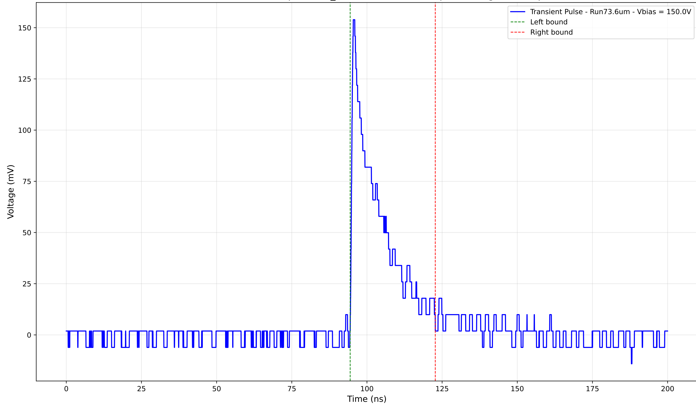
Transient Pulse - Sample: 1cm_42 - Position: 4425.0 \mu\text{m} - Charge: 28.51 pC
