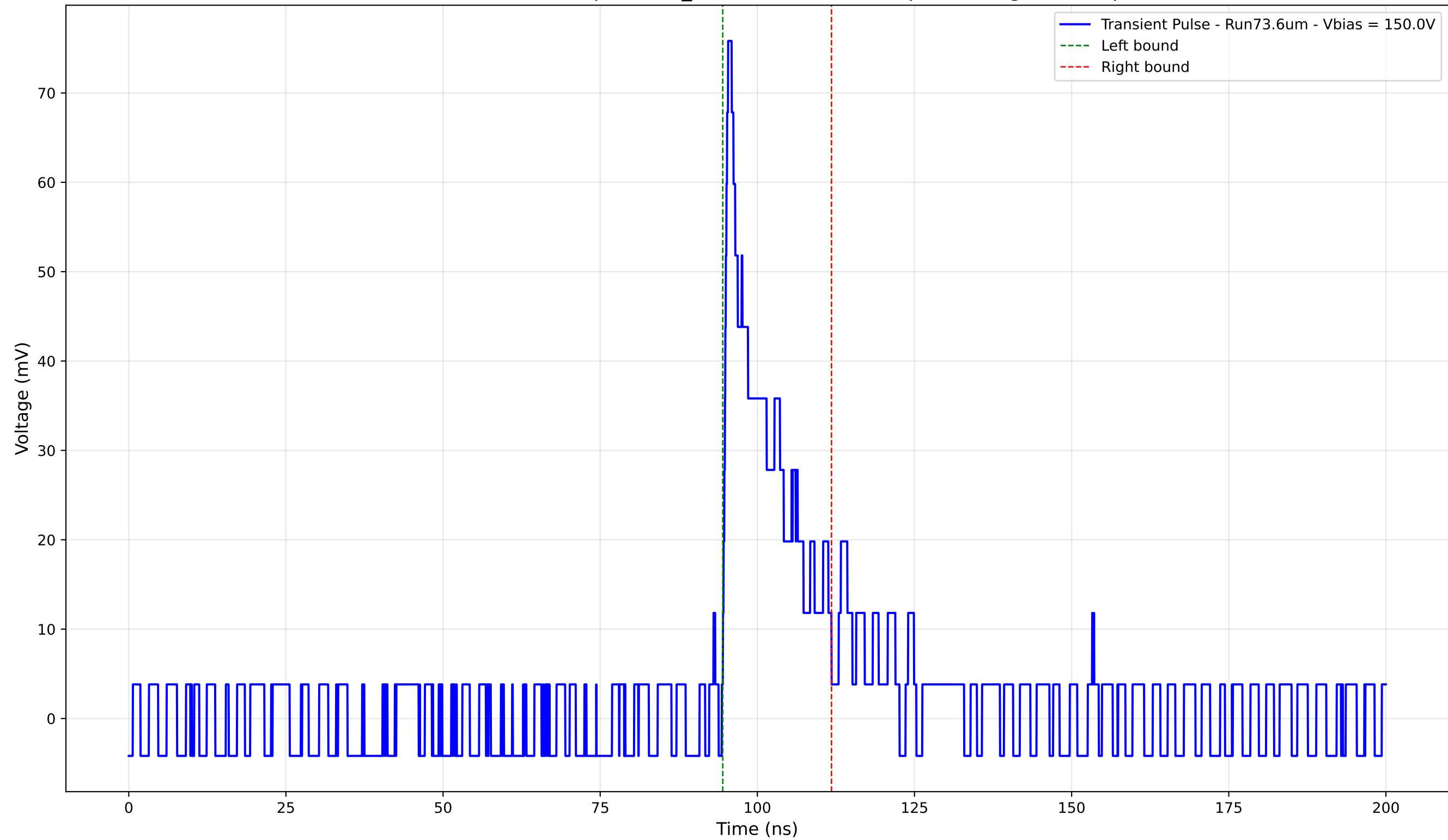
Transient Pulse - Sample: 1cm_42 - Position: 4905.0 \mu\text{m} - Charge: 10.58 pC
