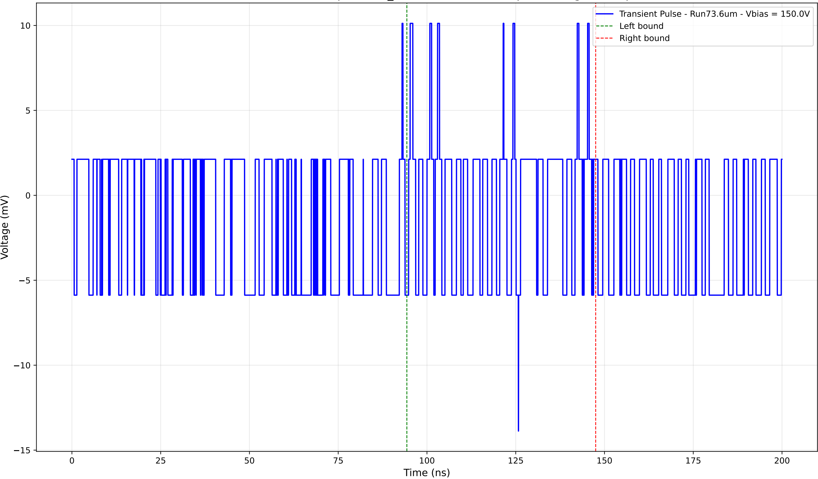
Transient Pulse - Sample: 1cm_42 - Position: 5050.0 \mu\text{m} - Charge: 0.05 pC
