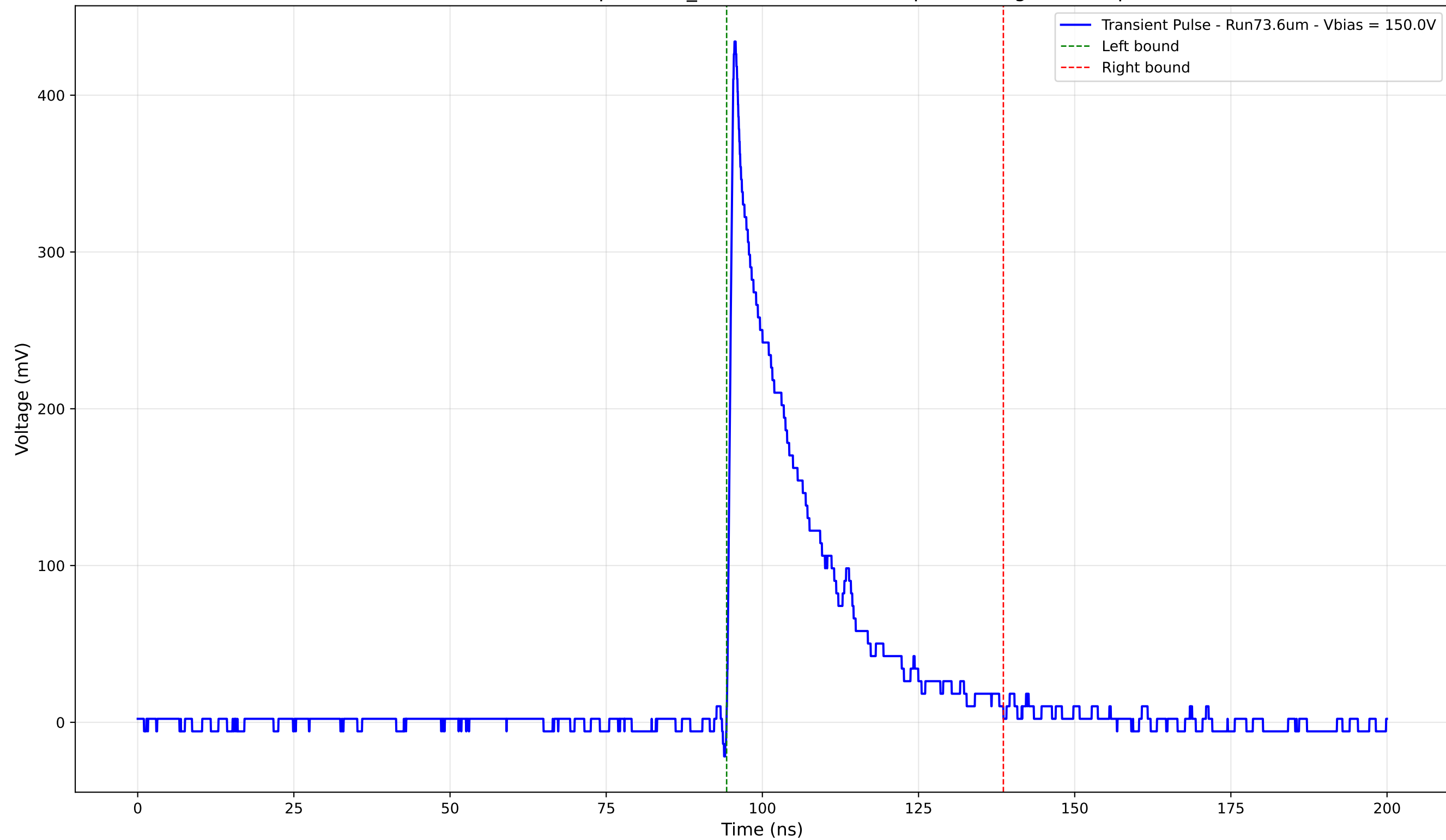
Transient Pulse - Sample: 1cm_42 - Position: 1780.0 \mu\text{m} - Charge: 91.40 pC
