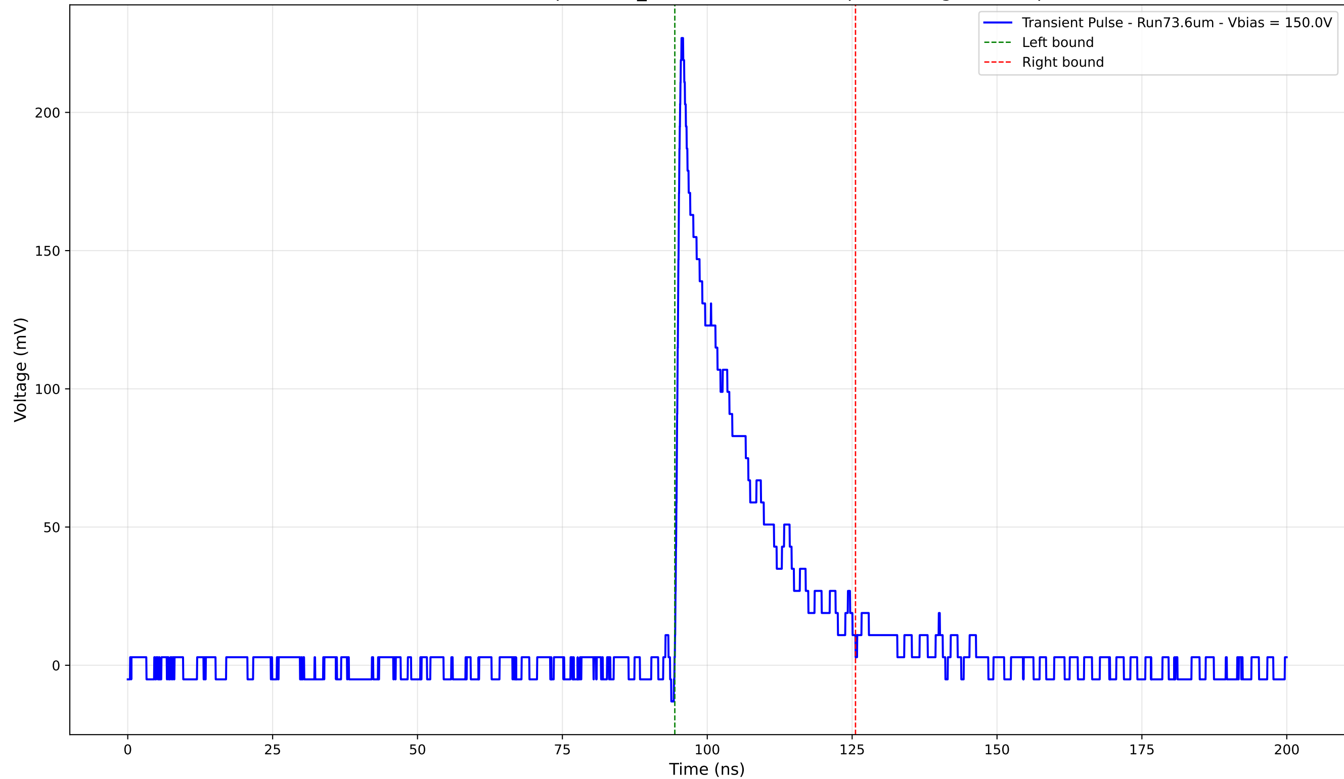
Transient Pulse - Sample: 1cm_42 - Position: 3770.0 \mu\text{m} - Charge: 44.06 pC
