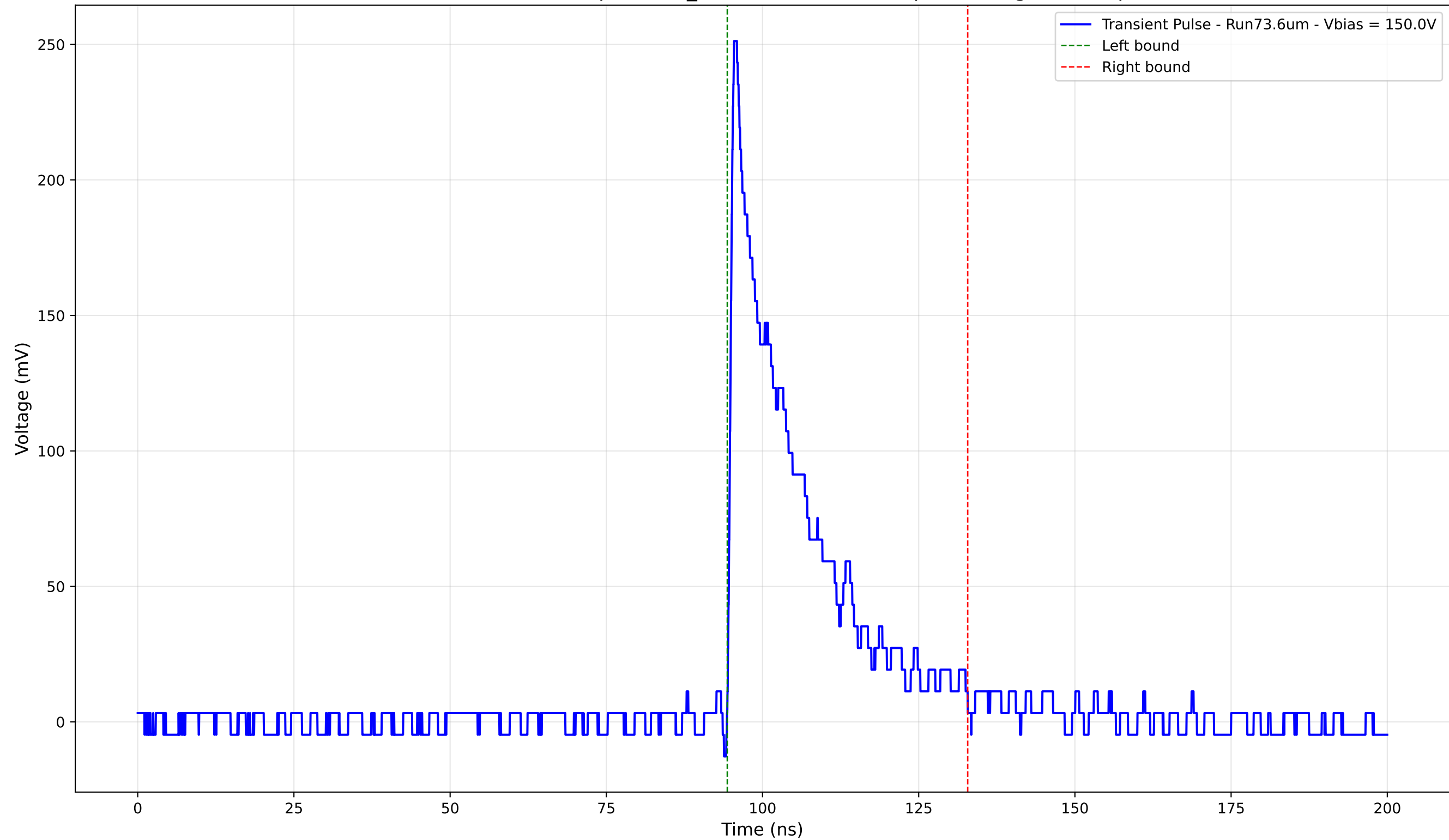
Transient Pulse - Sample: 1cm_42 - Position: 3575.0 \mu\text{m} - Charge: 52.26 pC
