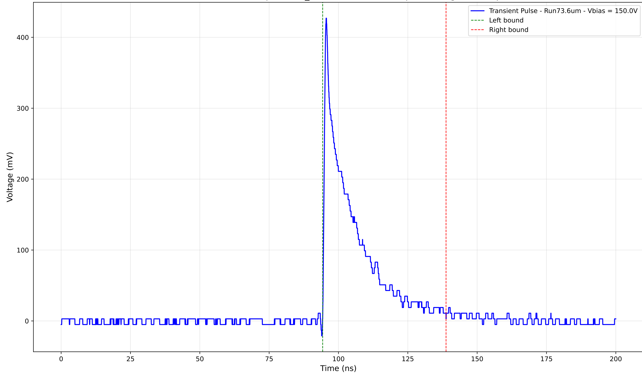
Transient Pulse - Sample: 1cm_42 - Position: 2275.0 \mu\text{m} - Charge: 82.88 pC
