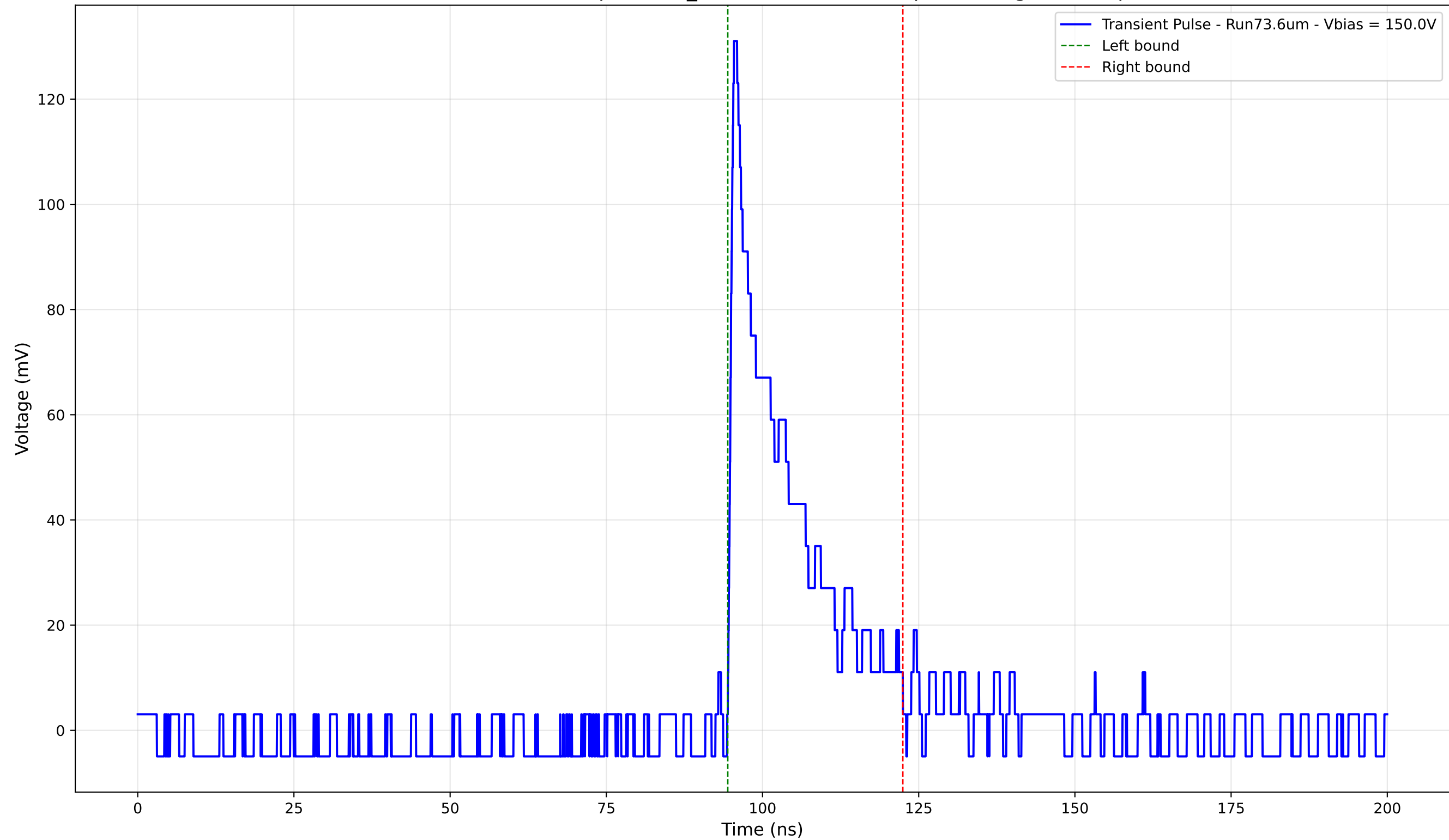
Transient Pulse - Sample: 1cm_42 - Position: 4635.0 \mu\text{m} - Charge: 23.07 pC
