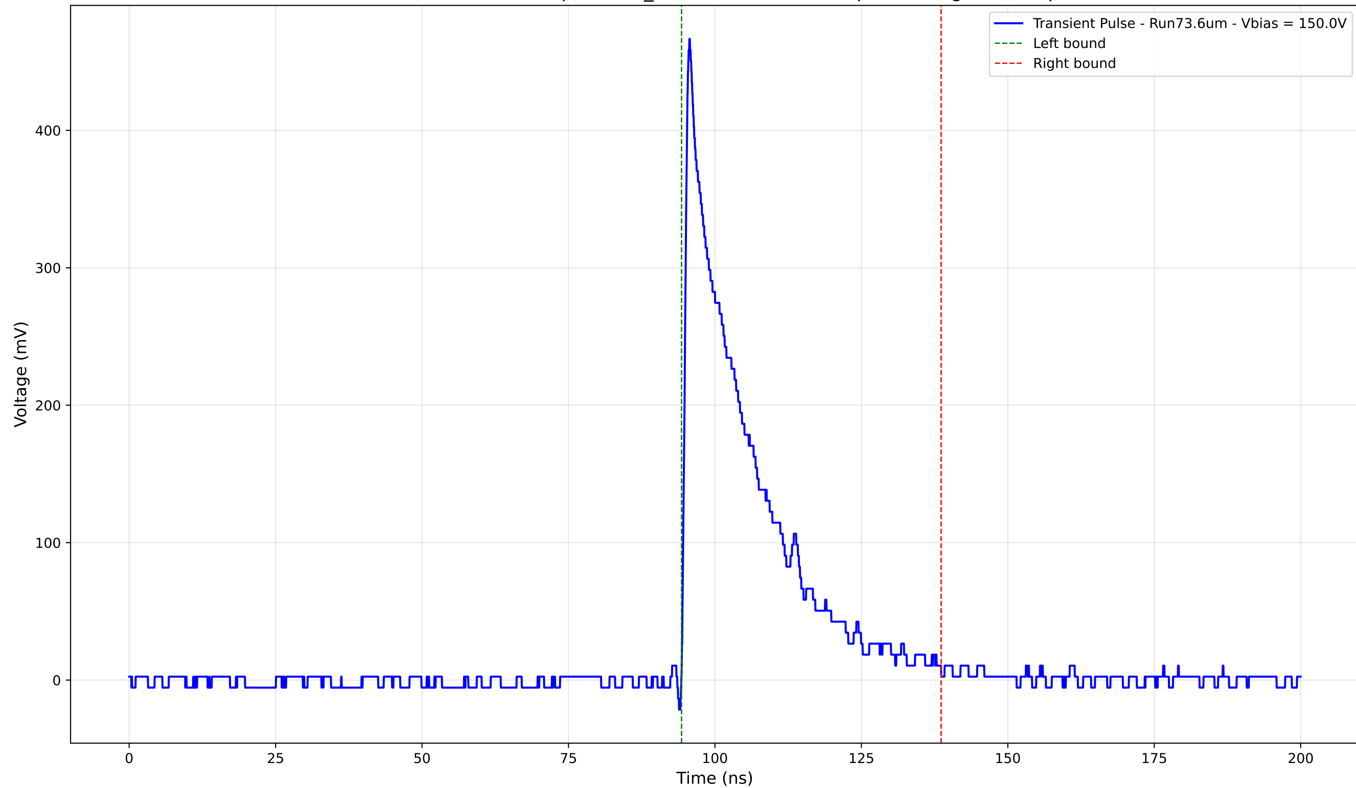
Transient Pulse - Sample: 1cm_42 - Position: 1110.0 \mu\text{m} - Charge: 99.93 pC
