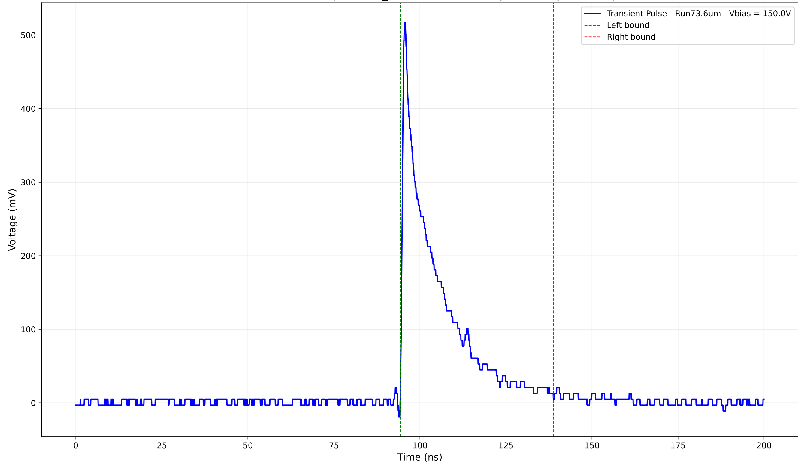
Transient Pulse - Sample: 1cm_42 - Position: 195.0 \mu\text{m} - Charge: 98.58 pC
