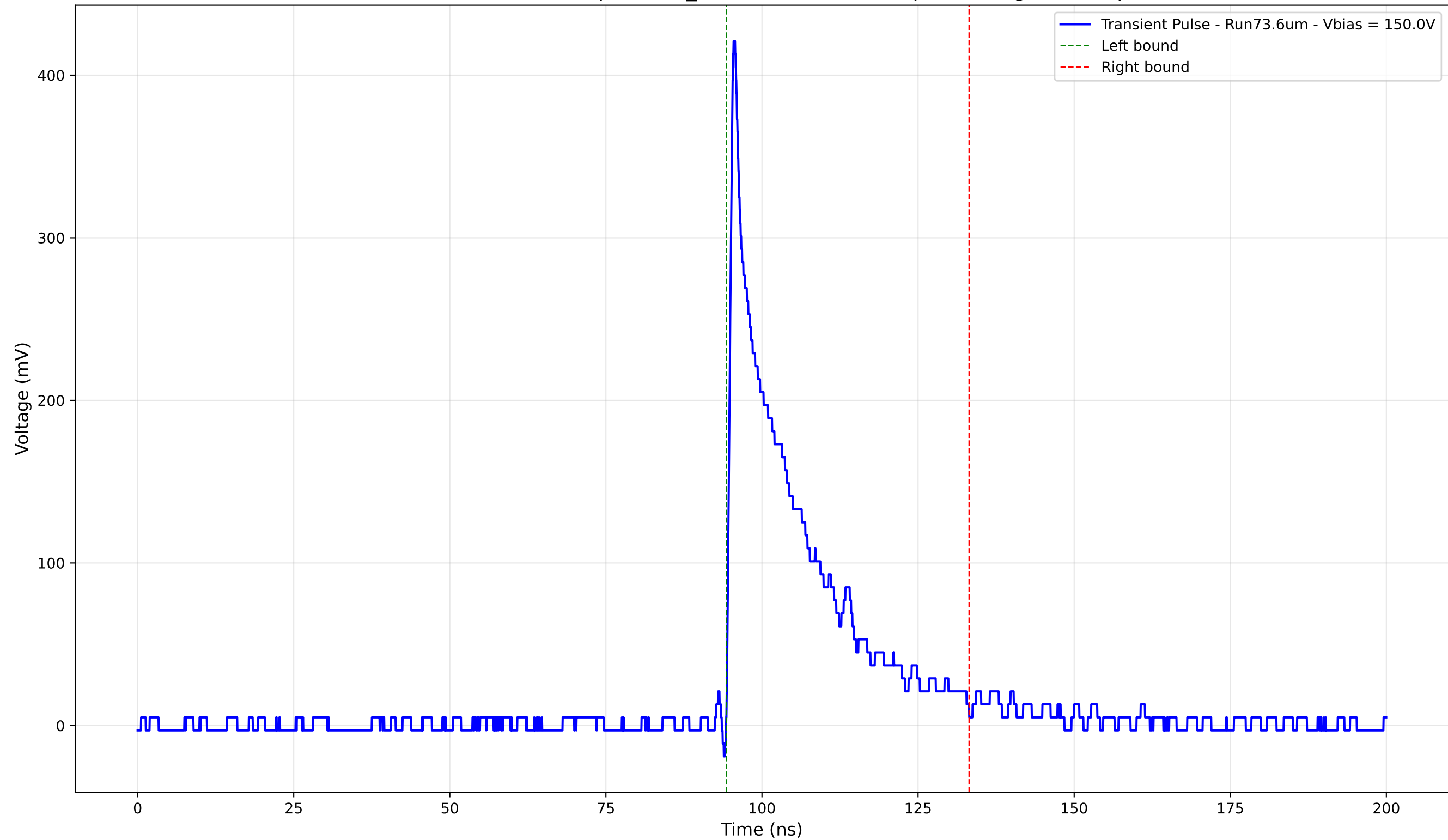
Transient Pulse - Sample: 1cm_42 - Position: 2780.0 \mu\text{m} - Charge: 78.09 pC
