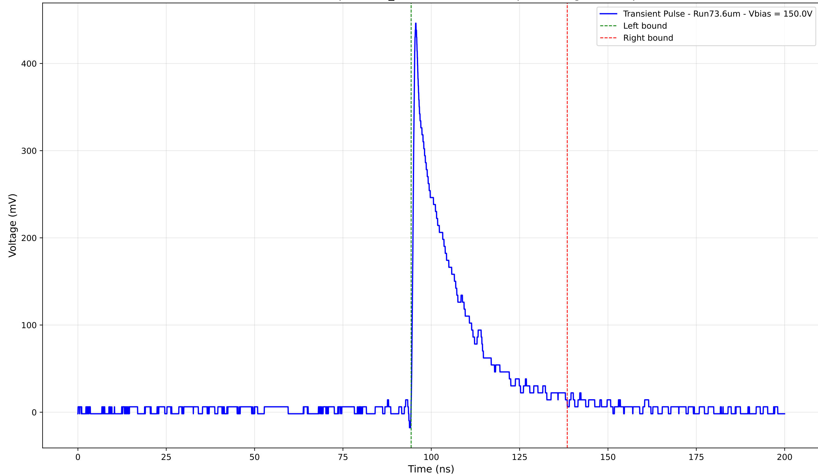
Transient Pulse - Sample: 1cm_42 - Position: 1880.0 \mu\text{m} - Charge: 94.29 pC
