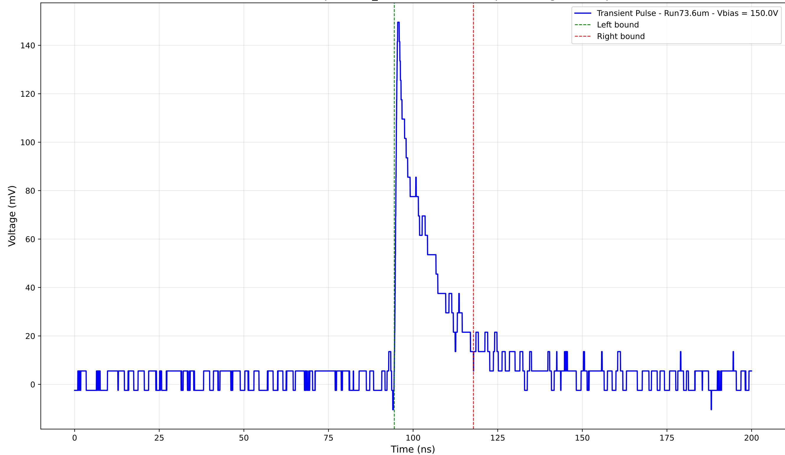
Transient Pulse - Sample: 1cm_42 - Position: 4500.0 \mu\text{m} - Charge: 26.11 pC
