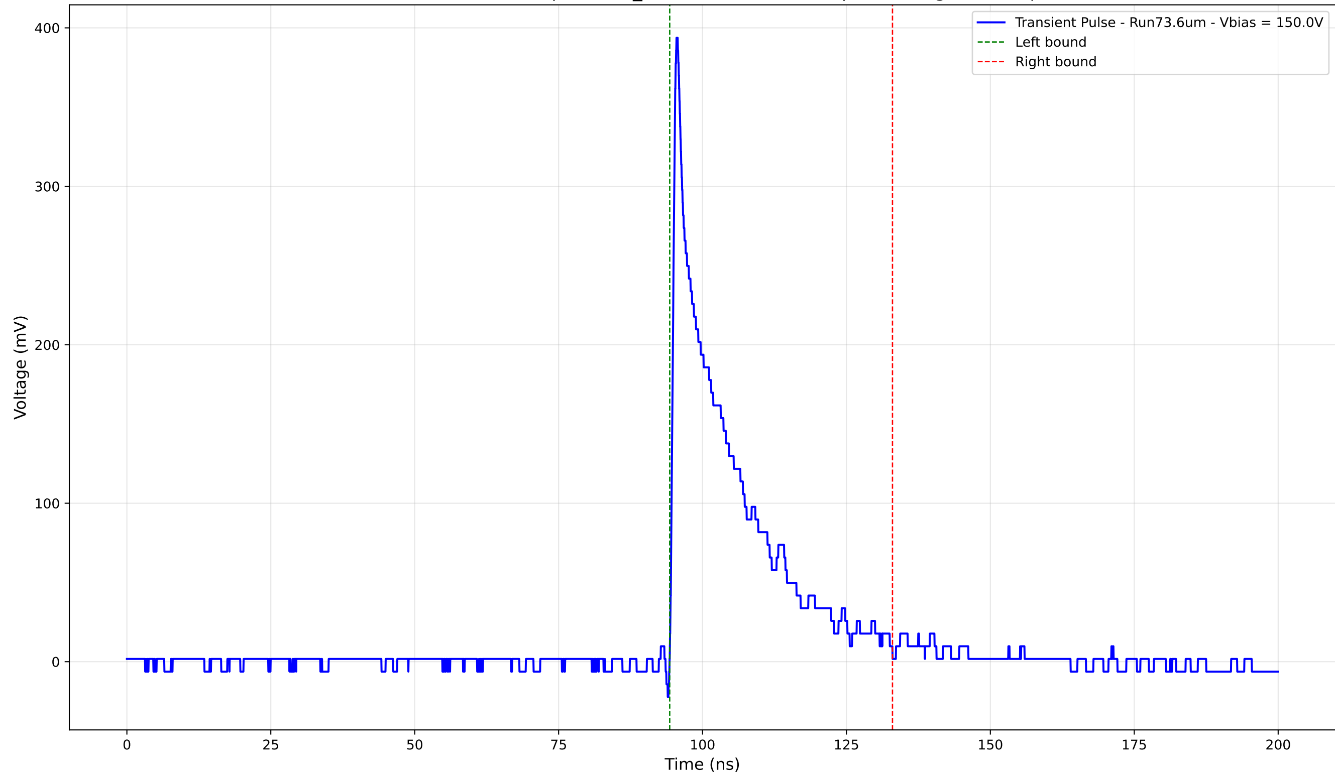
Transient Pulse - Sample: 1cm_42 - Position: 2855.0 \mu\text{m} - Charge: 71.75 pC
