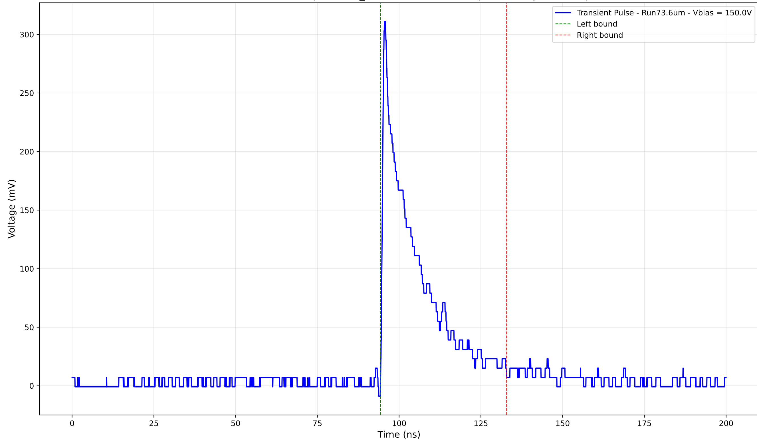
Transient Pulse - Sample: 1cm_42 - Position: 3230.0 \mu\text{m} - Charge: 63.13 pC
