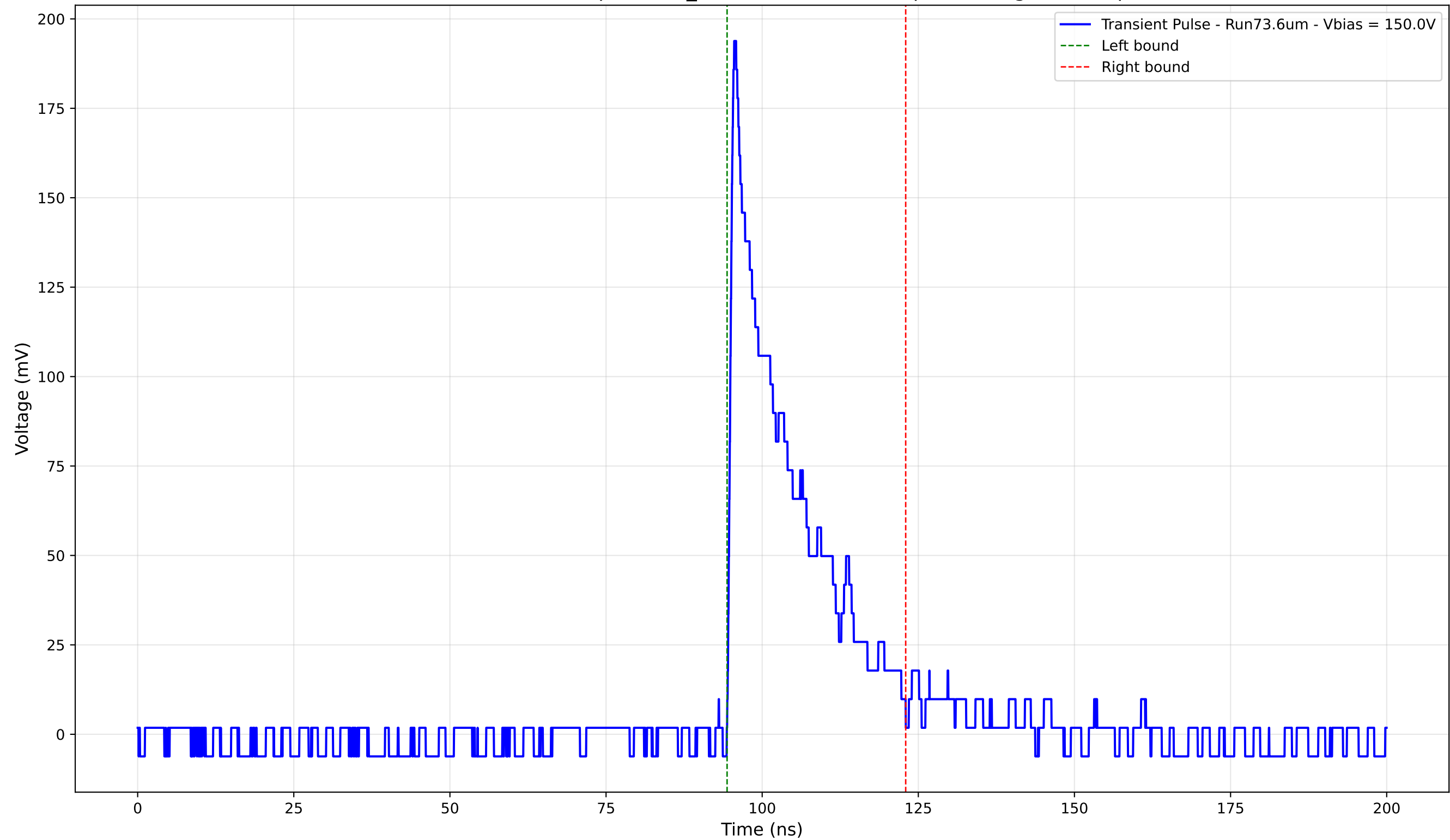
Transient Pulse - Sample: 1cm_42 - Position: 3980.0 \mu\text{m} - Charge: 36.91 pC
