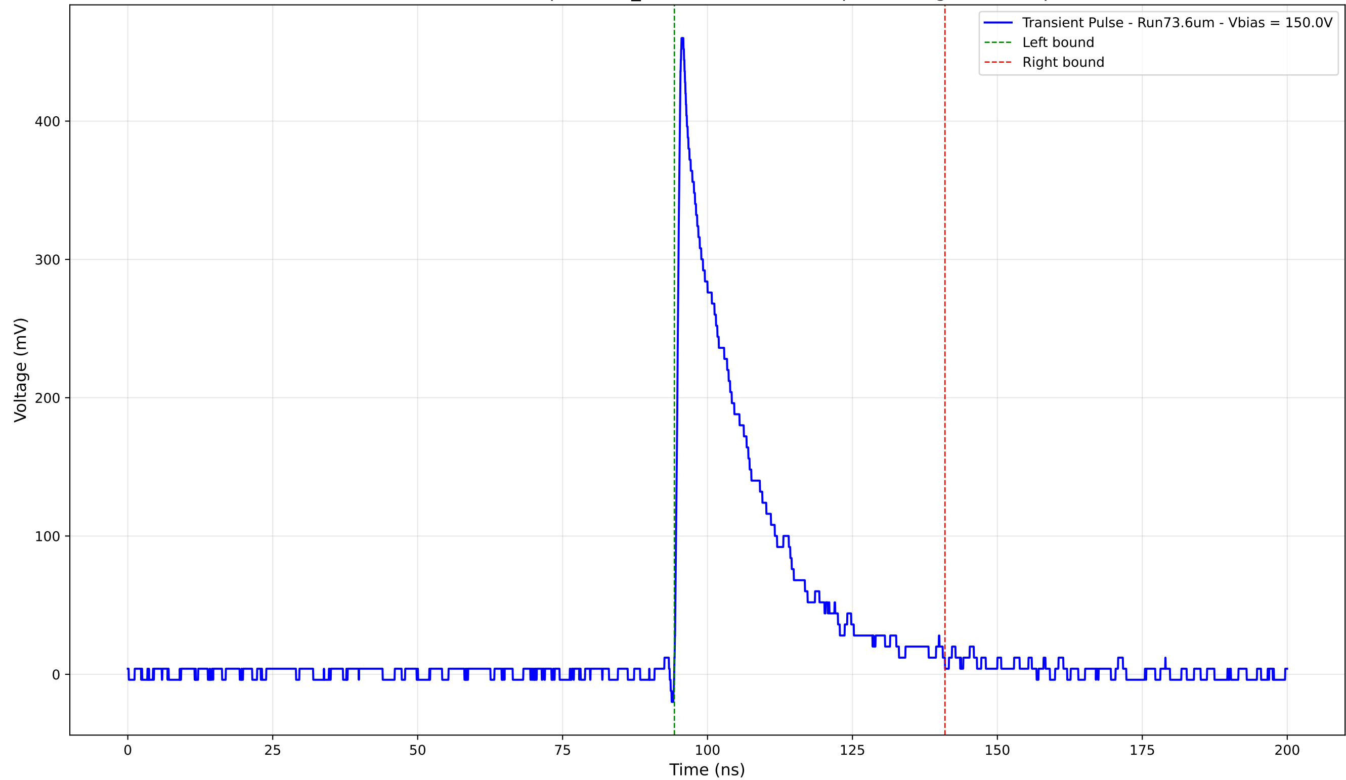
Transient Pulse - Sample: 1cm_42 - Position: 1130.0 \mu\text{m} - Charge: 103.63 pC
