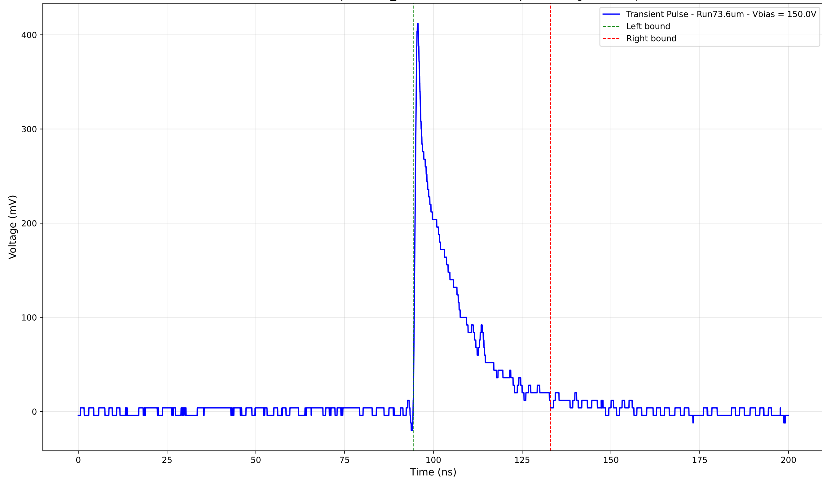
Transient Pulse - Sample: 1cm_42 - Position: 2400.0 \mu\text{m} - Charge: 77.30 pC
