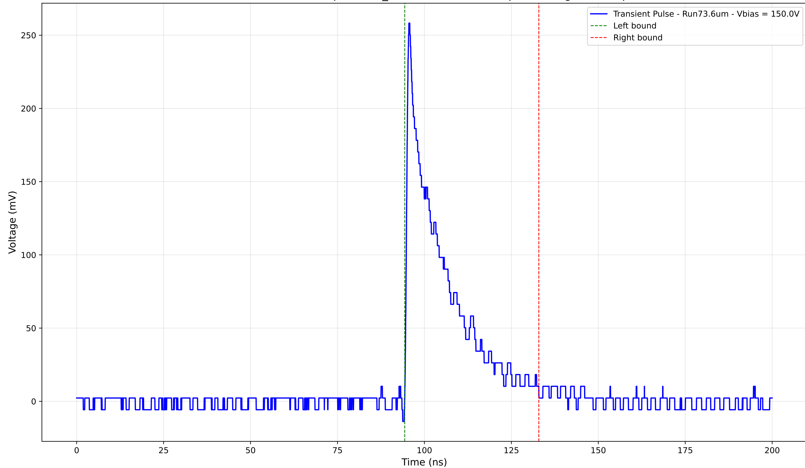
Transient Pulse - Sample: 1cm_42 - Position: 3555.0 \mu\text{m} - Charge: 52.44 pC
