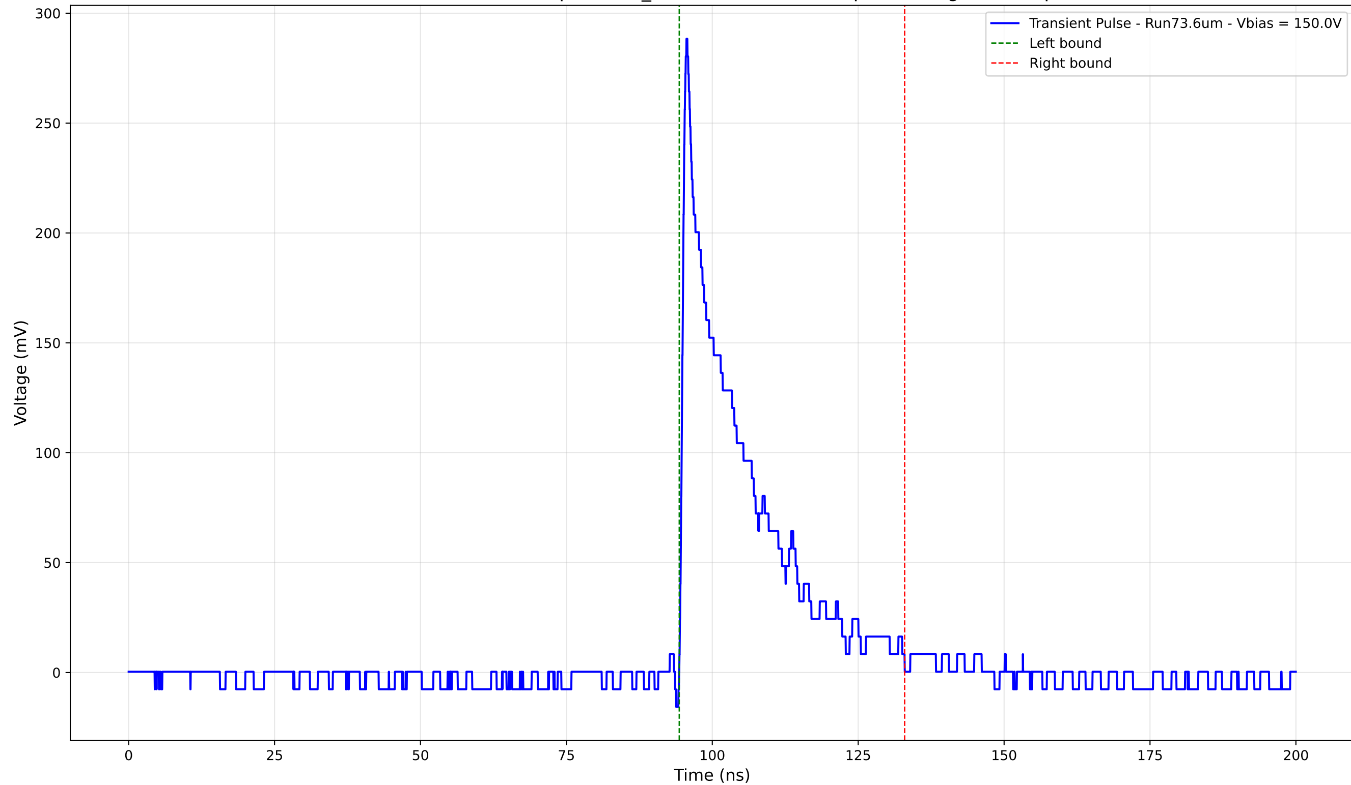
Transient Pulse - Sample: 1cm_42 - Position: 3380.0 \mu\text{m} - Charge: 55.43 pC
