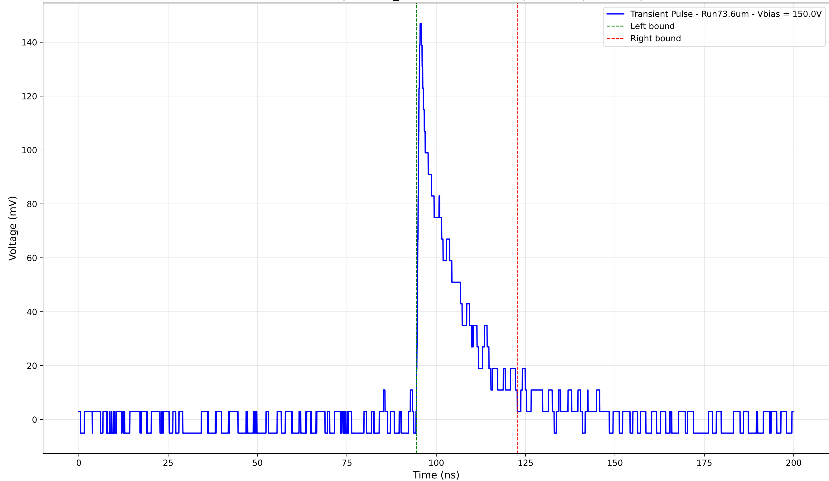
Transient Pulse - Sample: 1cm_42 - Position: 4510.0 \mu\text{m} - Charge: 26.53 pC
