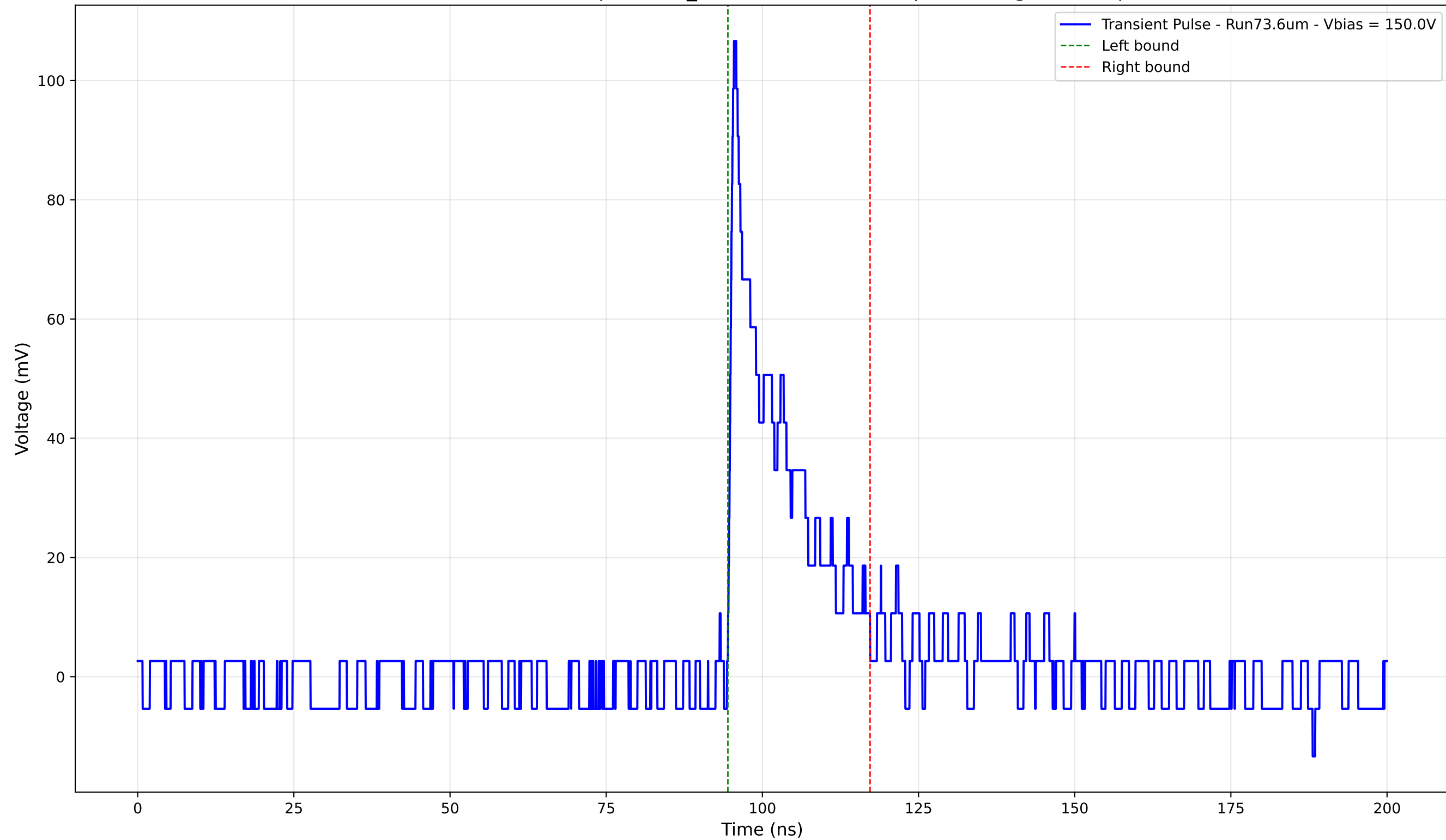
Transient Pulse - Sample: 1cm_42 - Position: 4825.0 \mu\text{m} - Charge: 16.43 pC
