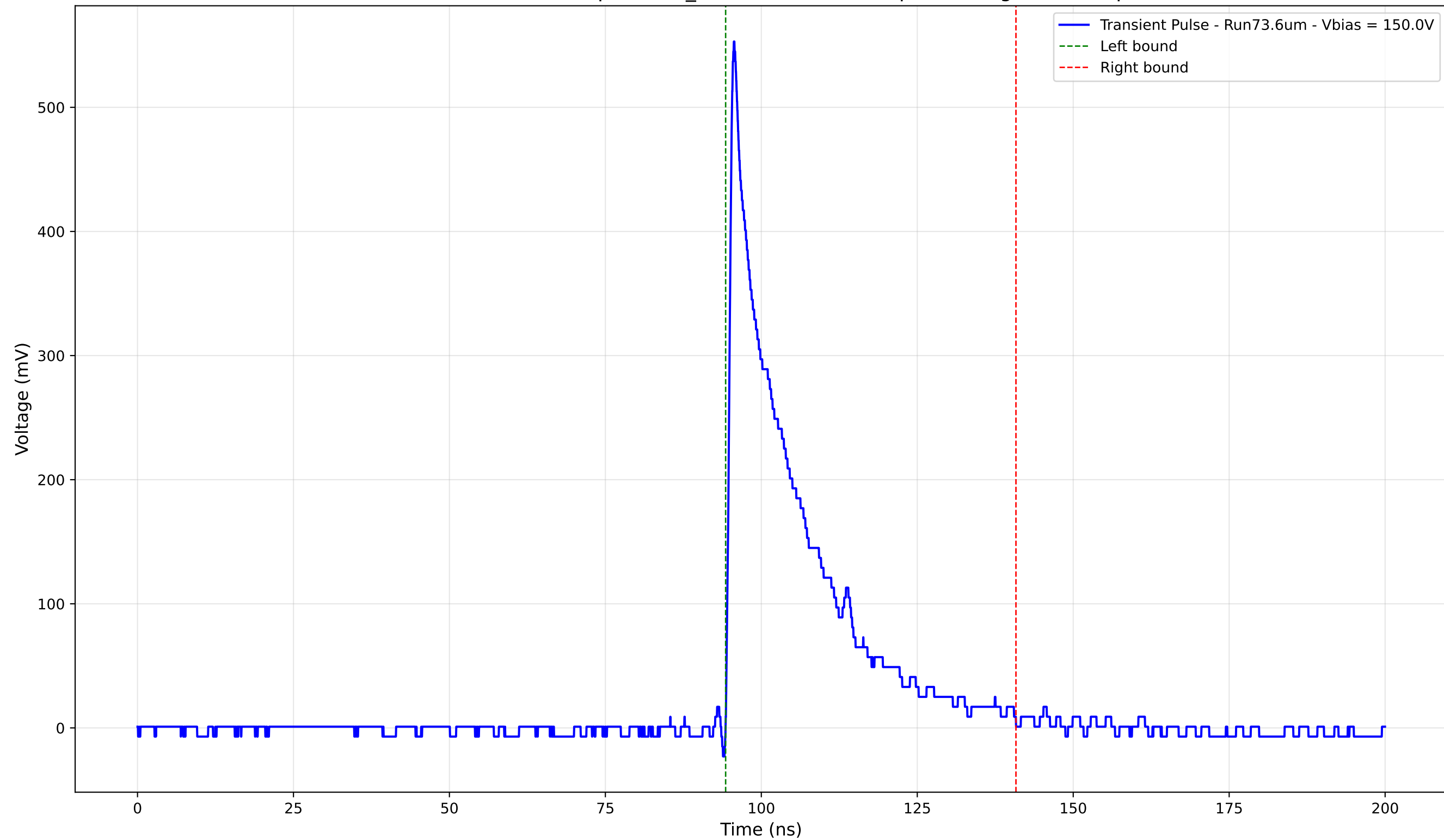
Transient Pulse - Sample: 1cm_42 - Position: 435.0 \mu\text{m} - Charge: 110.50 pC
