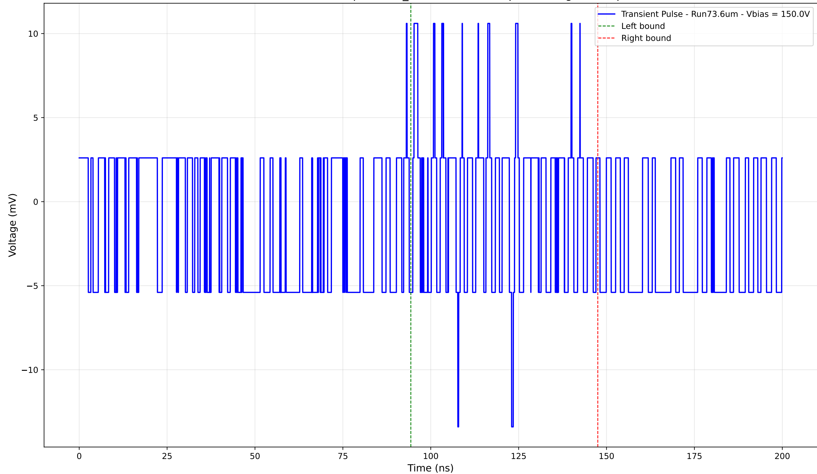
Transient Pulse - Sample: 1cm_42 - Position: 5.0 \mu\text{m} - Charge: 0.13 pC
