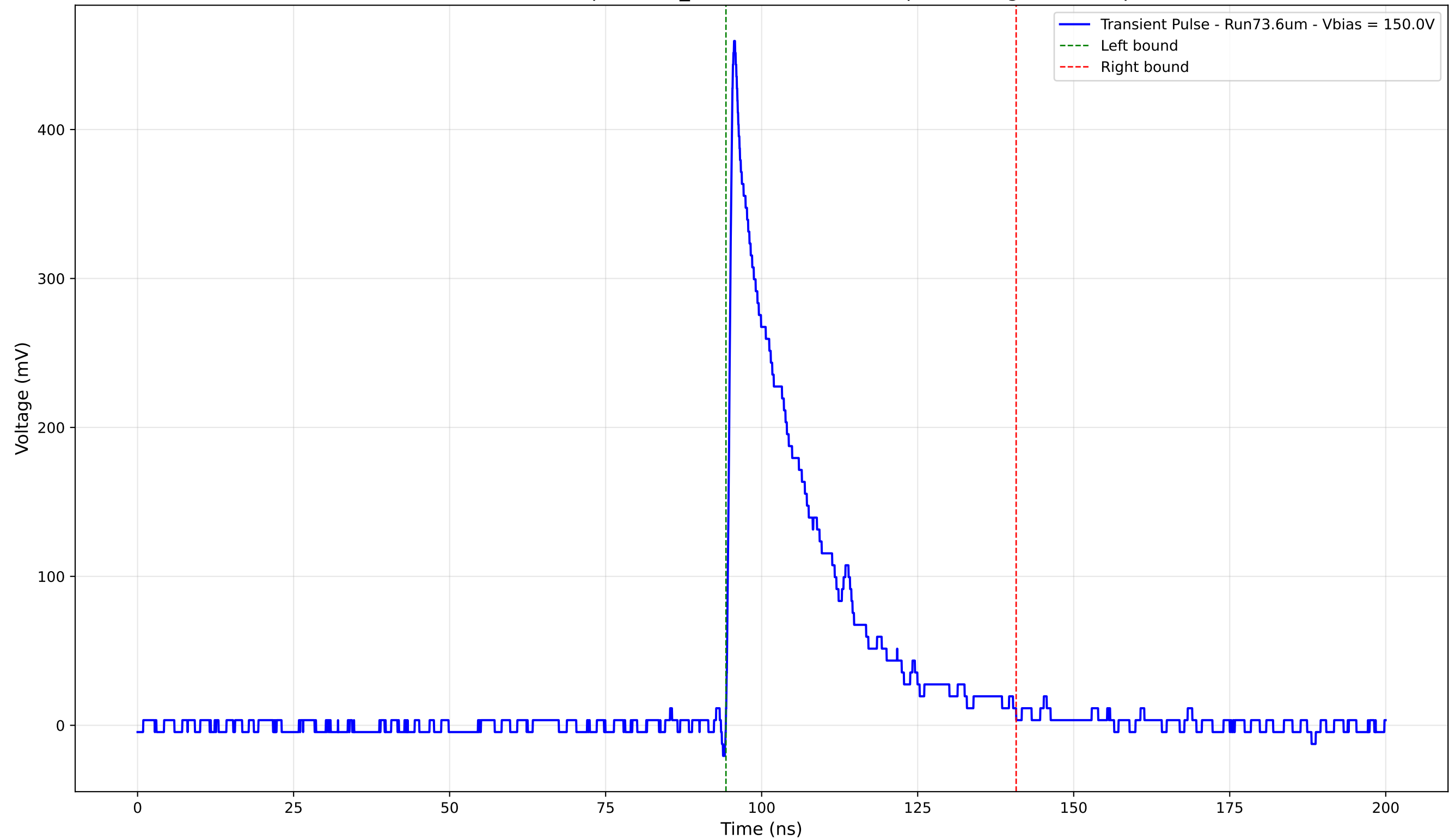
Transient Pulse - Sample: 1cm_42 - Position: 1280.0 \mu\text{m} - Charge: 101.04 pC
