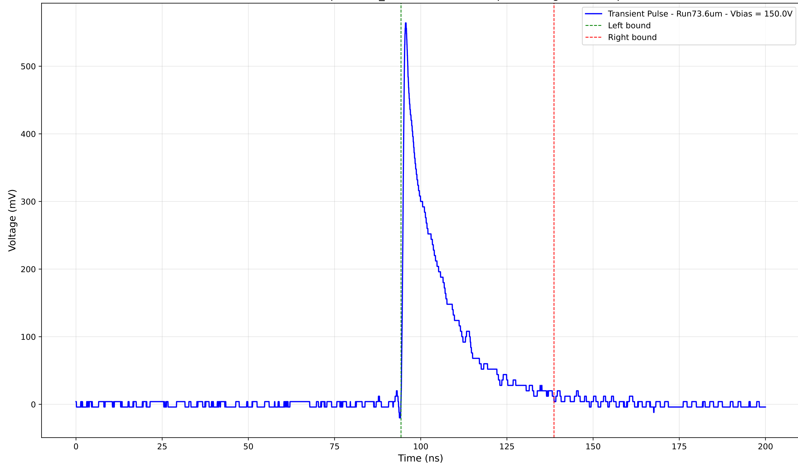
Transient Pulse - Sample: 1cm_42 - Position: 385.0 \mu\text{m} - Charge: 112.79 pC
