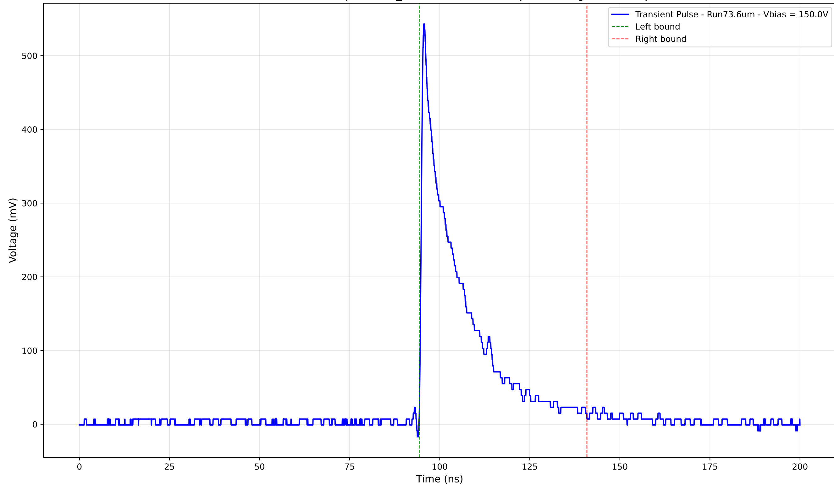
Transient Pulse - Sample: 1cm_42 - Position: 480.0 \mu\text{m} - Charge: 114.54 pC
