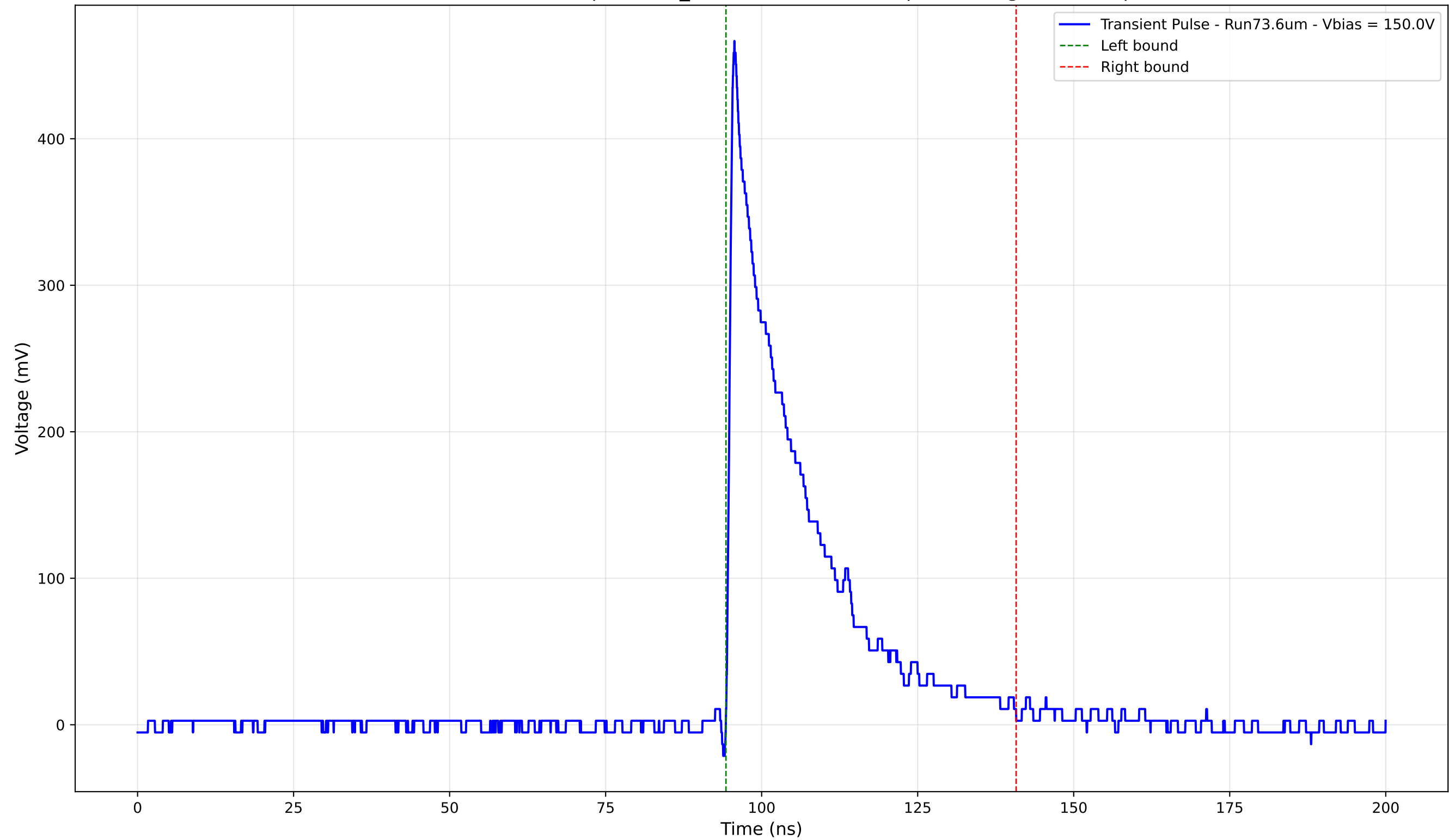
Transient Pulse - Sample: 1cm_42 - Position: 1075.0 \mu\text{m} - Charge: 103.00 pC
