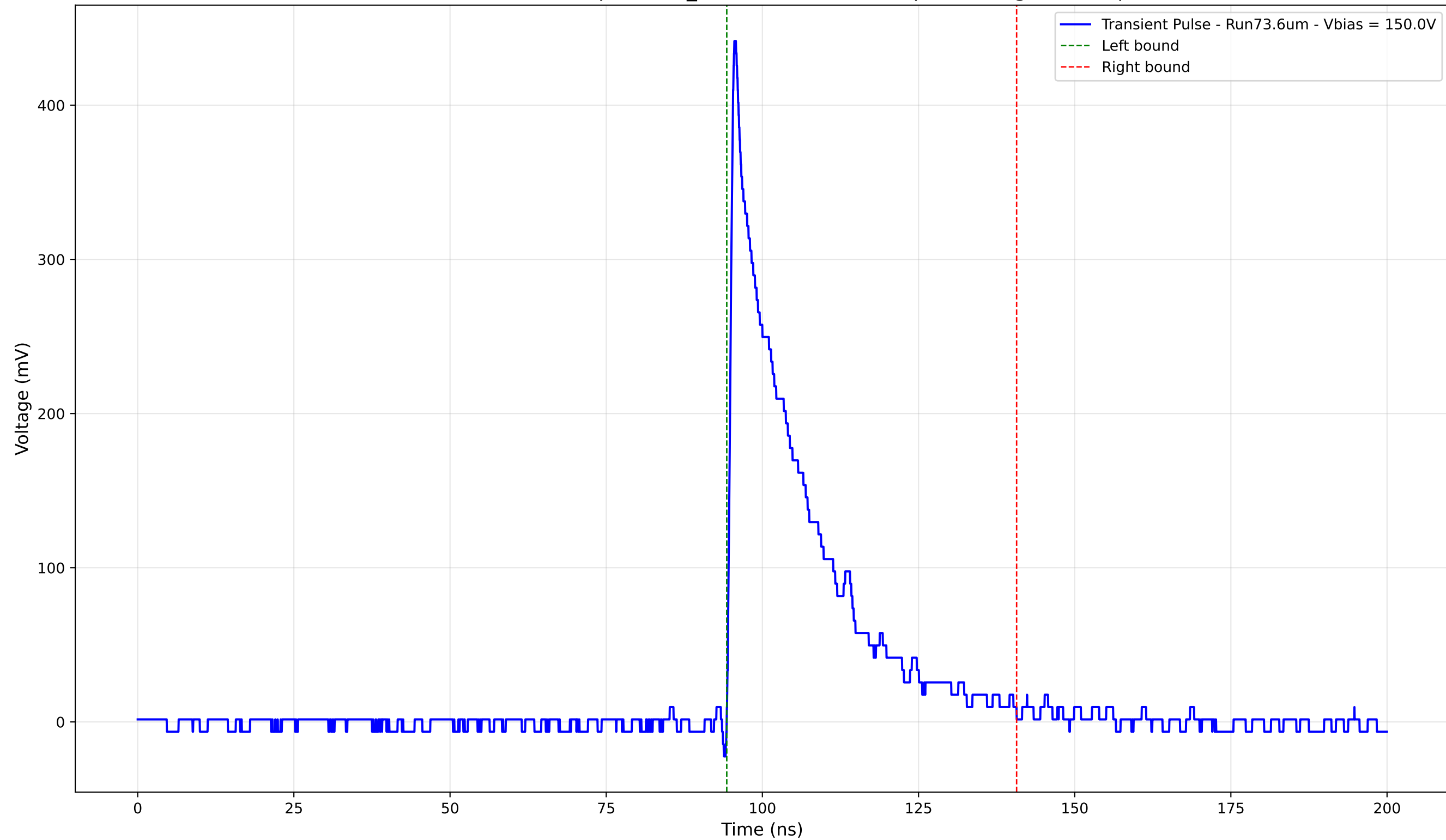
Transient Pulse - Sample: 1cm_42 - Position: 1645.0 \mu\text{m} - Charge: 94.67 pC
