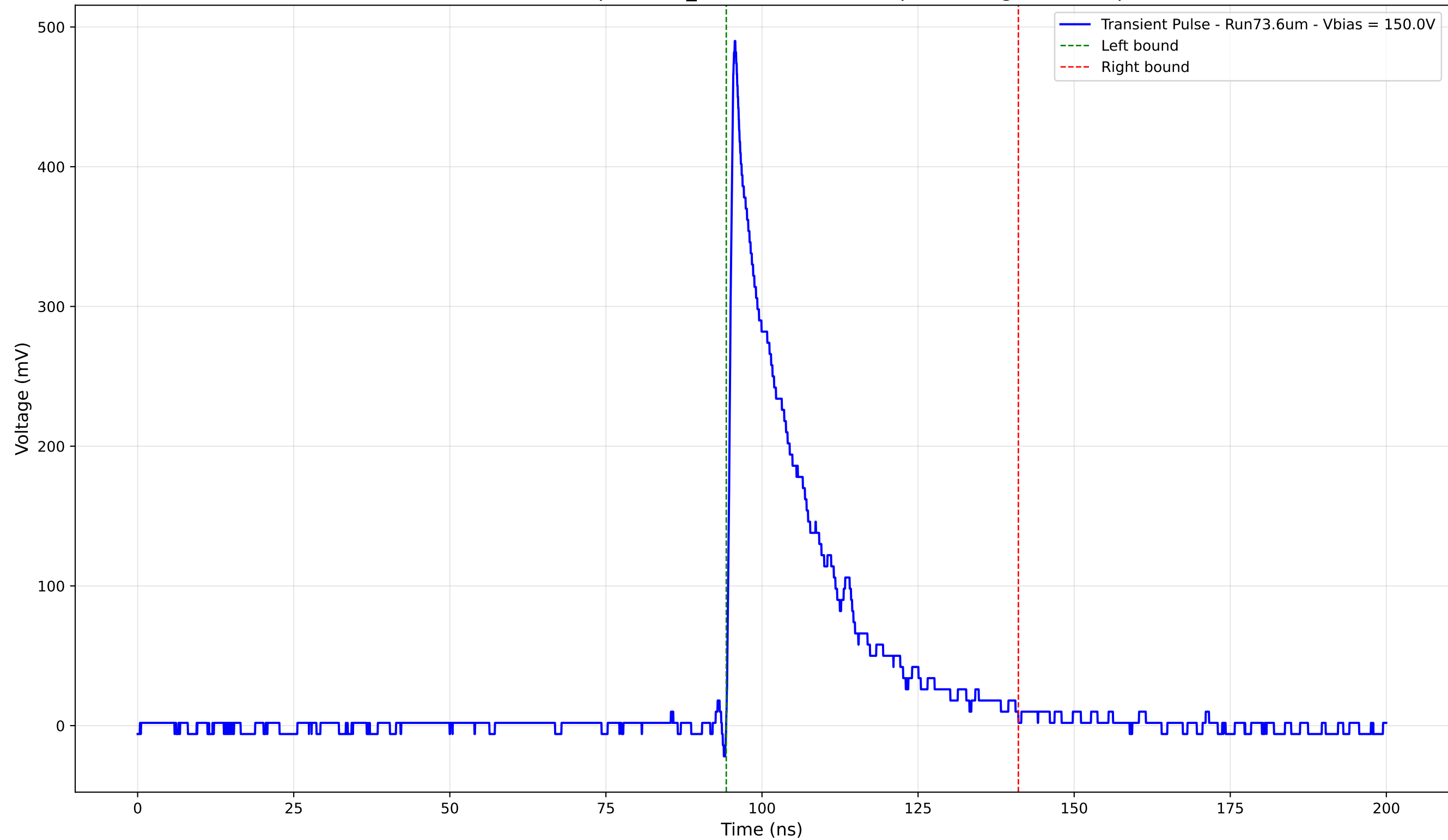
Transient Pulse - Sample: 1cm_42 - Position: 870.0 \mu\text{m} - Charge: 105.35 pC
