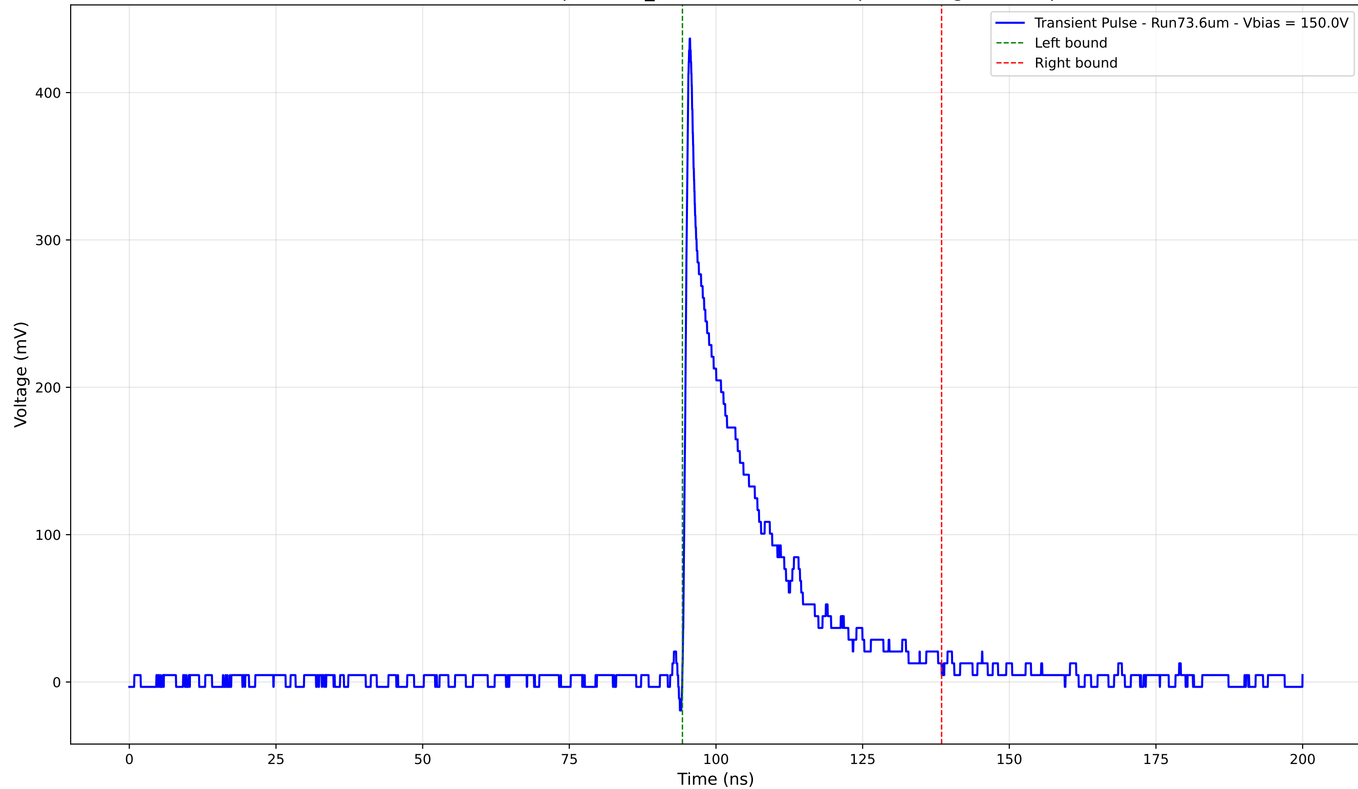
Transient Pulse - Sample: 1cm_42 - Position: 2685.0 \mu\text{m} - Charge: 81.48 pC
