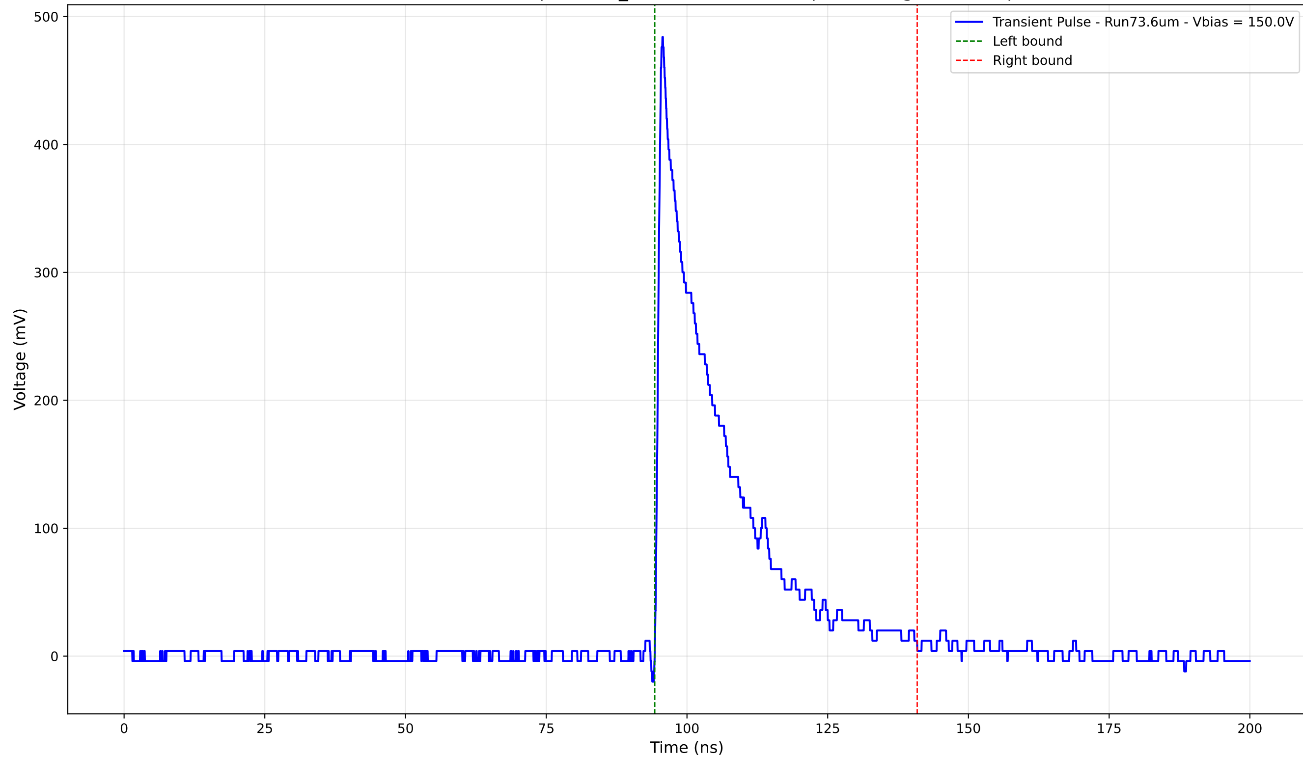
Transient Pulse - Sample: 1cm_42 - Position: 905.0 \mu\text{m} - Charge: 106.01 pC
