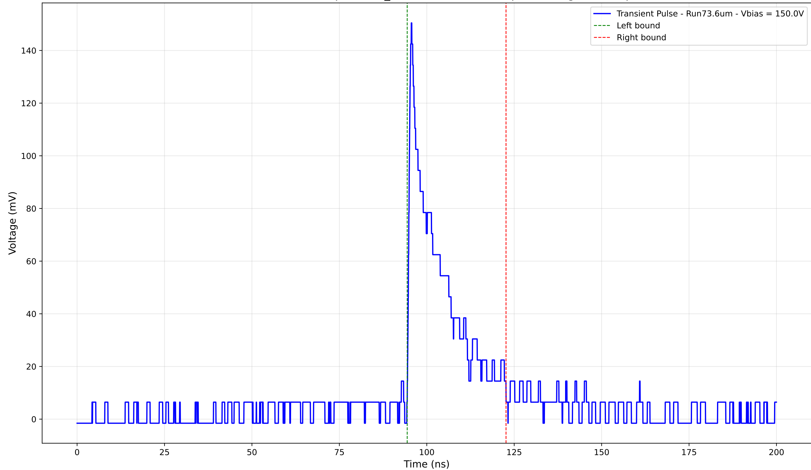
Transient Pulse - Sample: 1cm_42 - Position: 4555.0 \mu\text{m} - Charge: 27.15 pC
