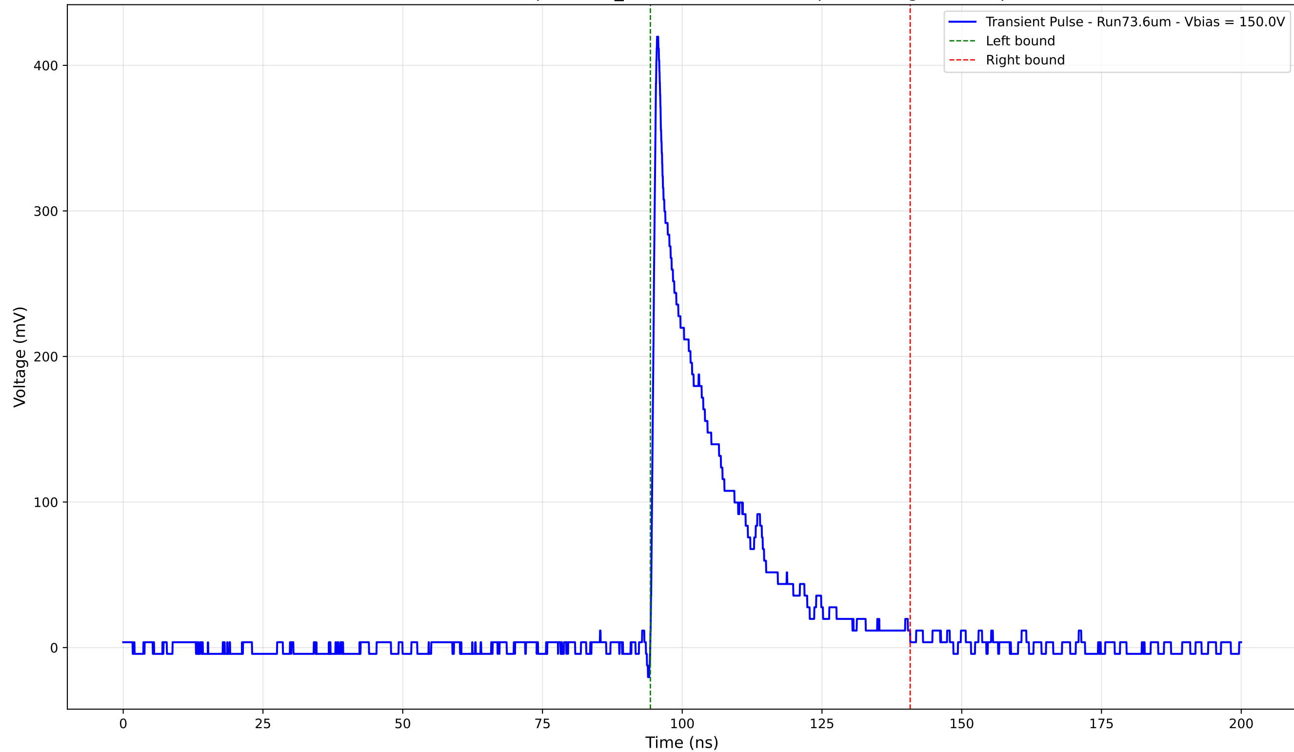
Transient Pulse - Sample: 1cm_42 - Position: 2210.0 \mu\text{m} - Charge: 82.95 pC
