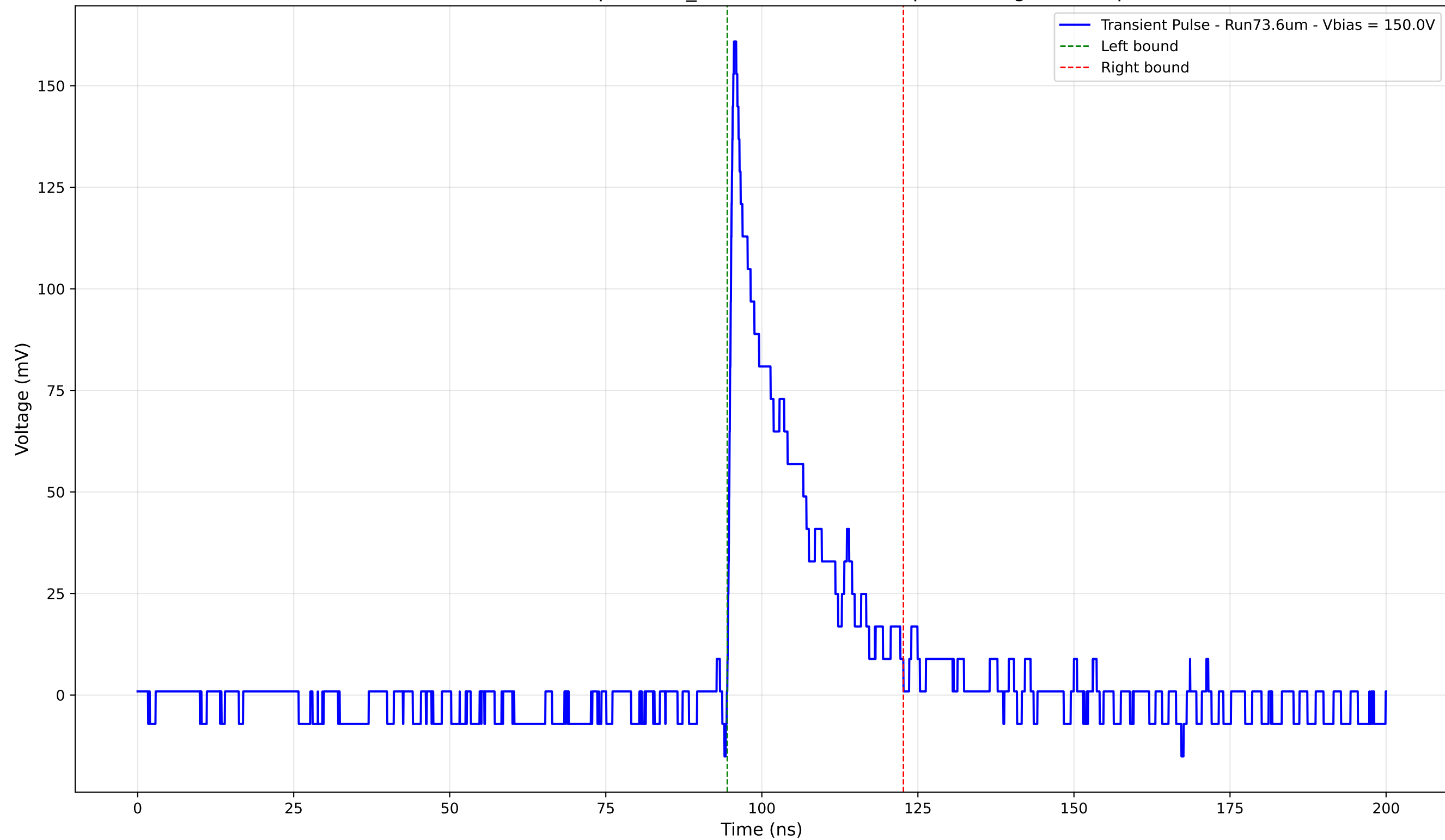
Transient Pulse - Sample: 1cm_42 - Position: 4365.0 \mu\text{m} - Charge: 28.48 pC
