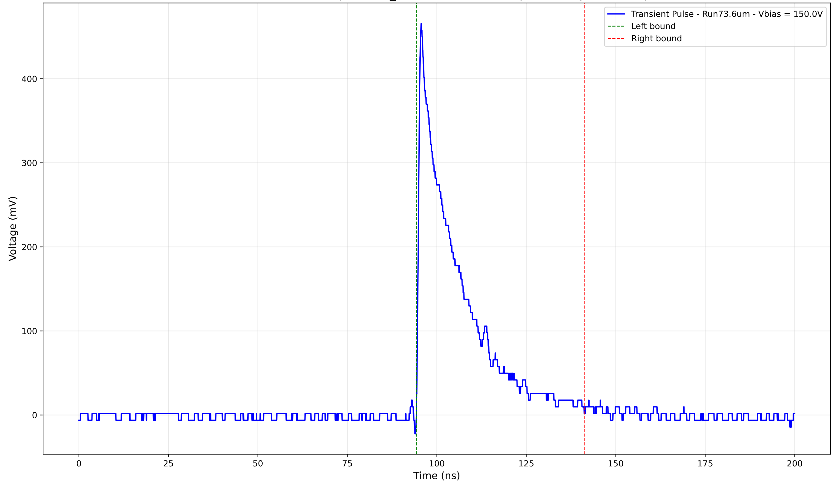
Transient Pulse - Sample: 1cm_42 - Position: 1070.0 \mu\text{m} - Charge: 101.57 pC
