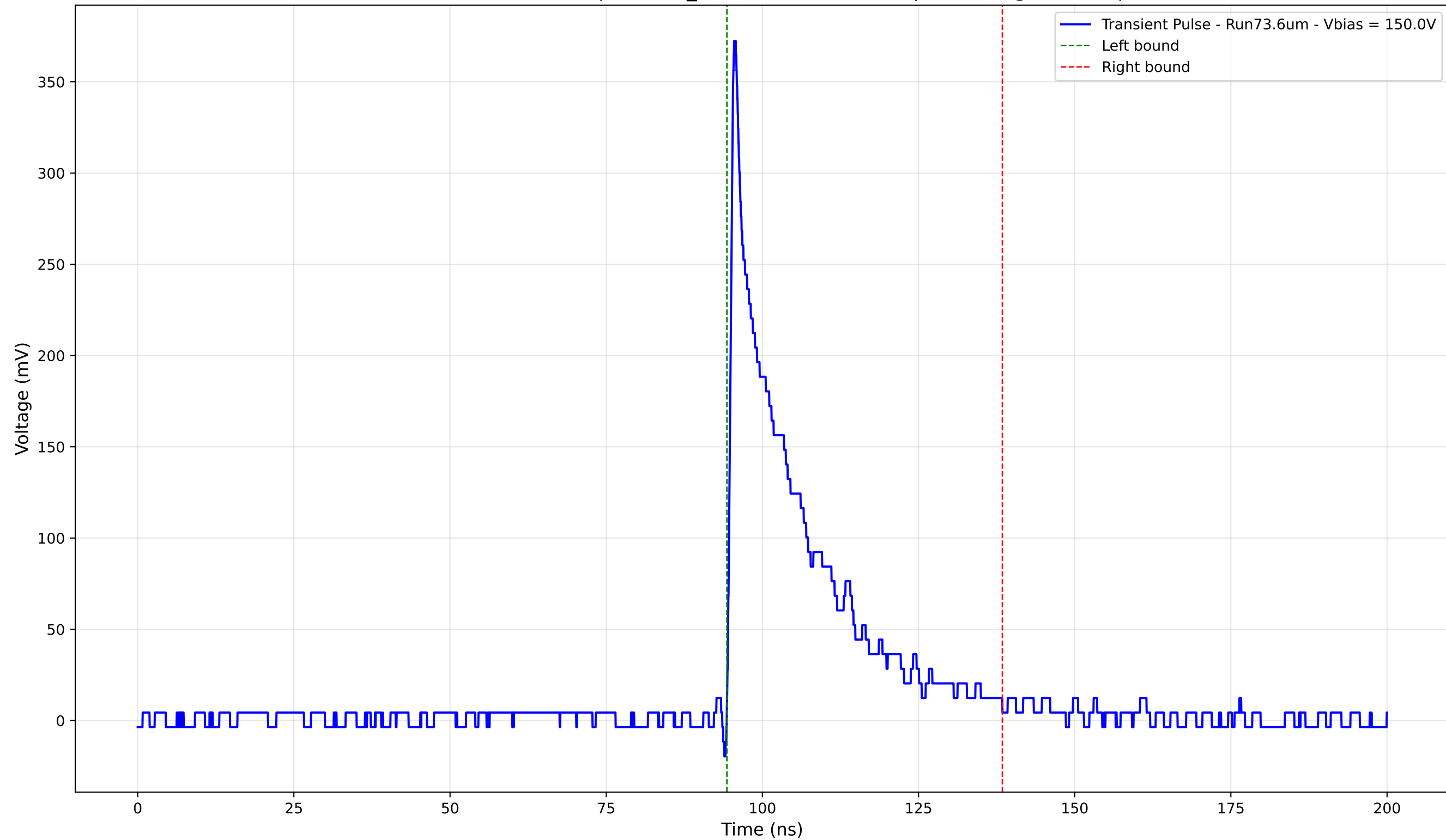
Transient Pulse - Sample: 1cm_42 - Position: 2895.0 \mu\text{m} - Charge: 71.90 pC
