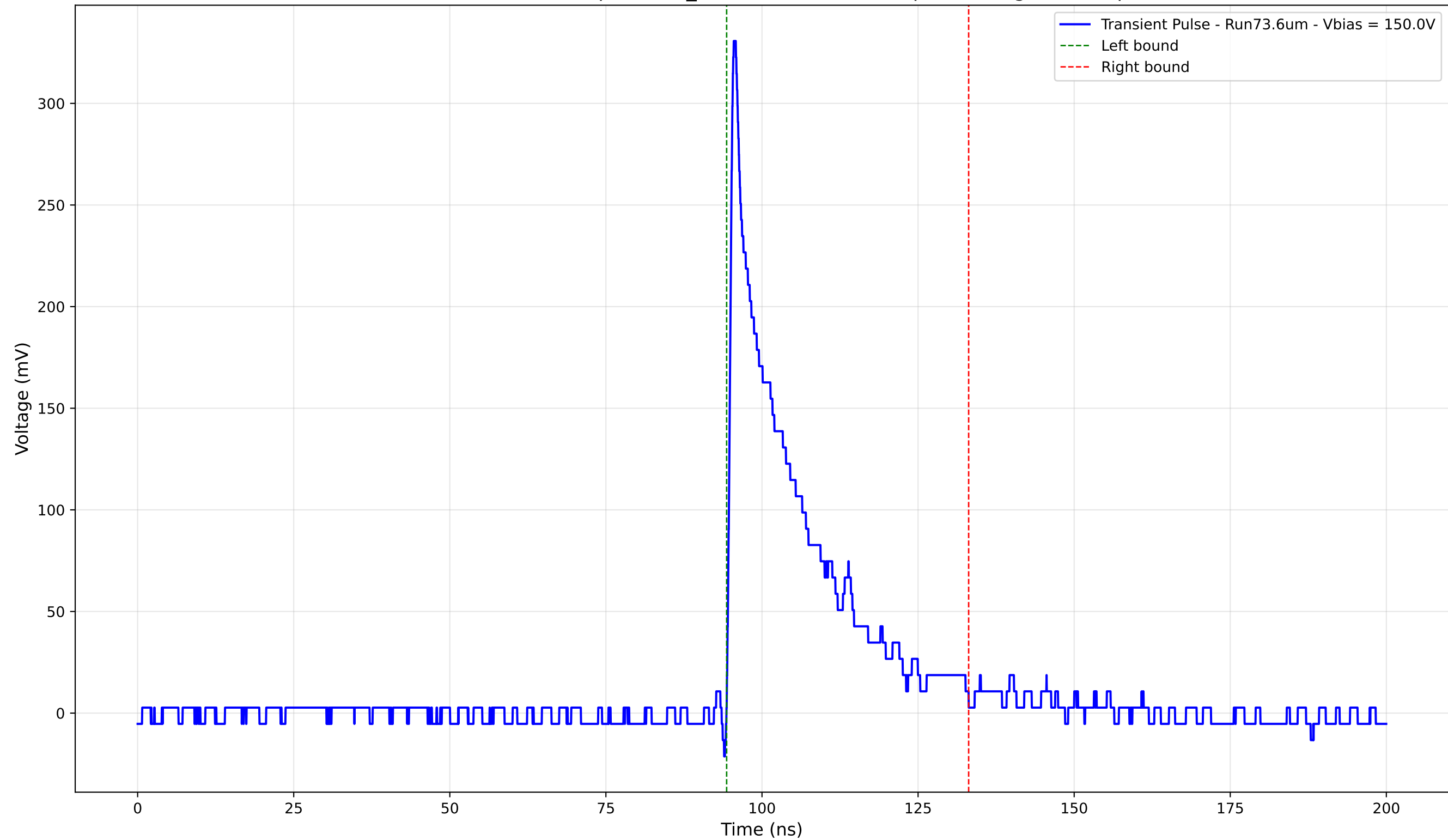
Transient Pulse - Sample: 1cm_42 - Position: 3025.0 \mu\text{m} - Charge: 63.14 pC
