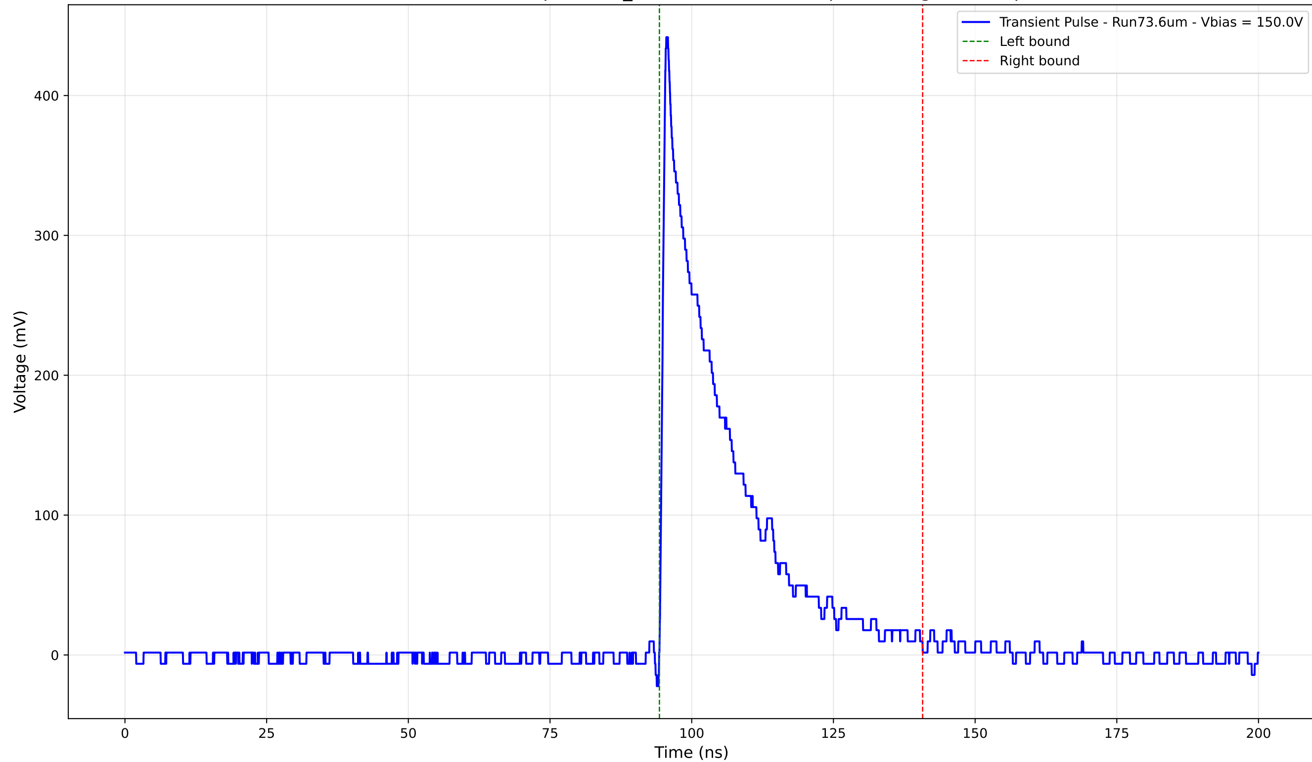
Transient Pulse - Sample: 1cm_42 - Position: 1500.0 \mu\text{m} - Charge: 96.81 pC
