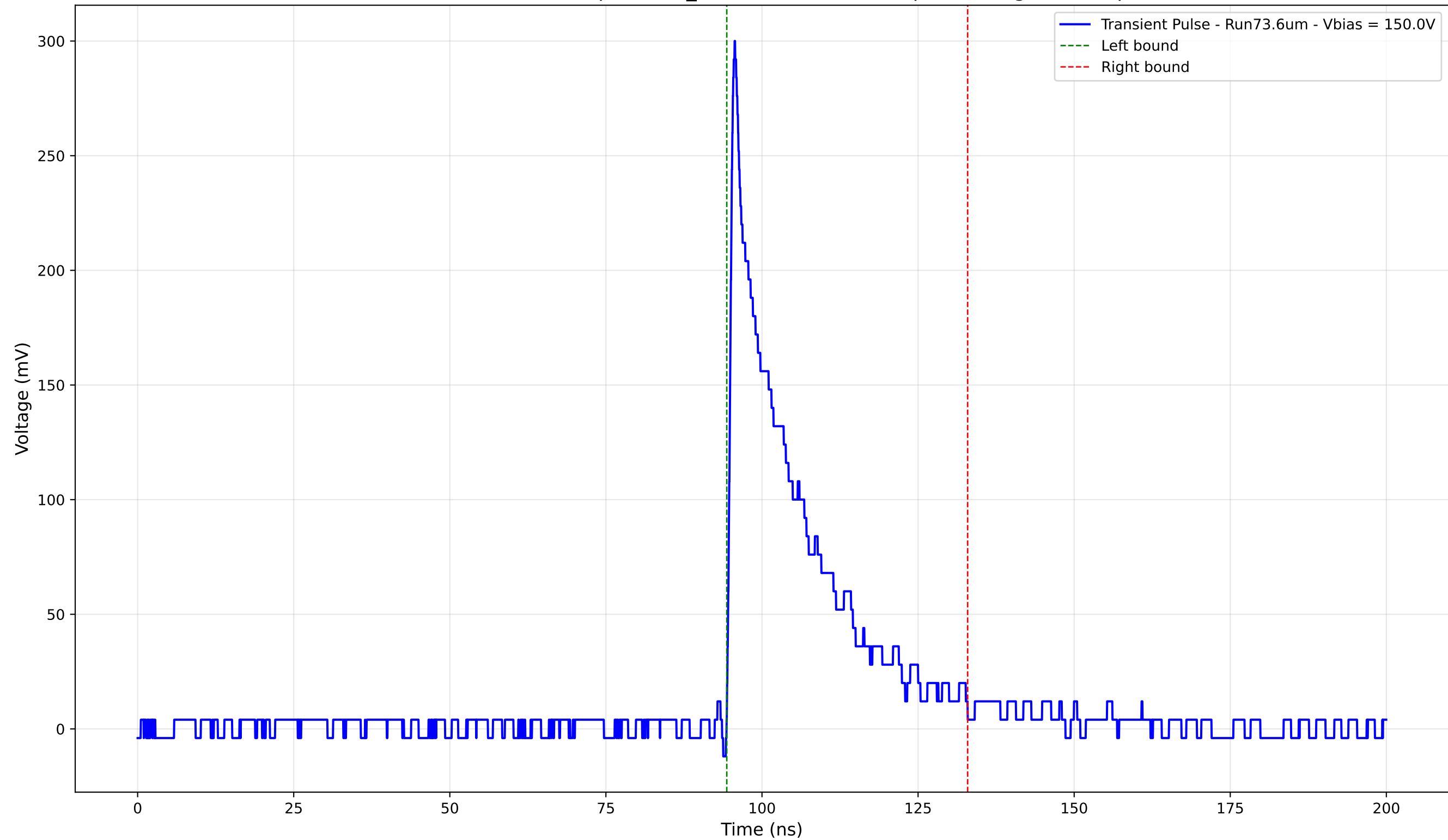
Transient Pulse - Sample: 1cm_42 - Position: 3280.0 \mu\text{m} - Charge: 58.91 pC
