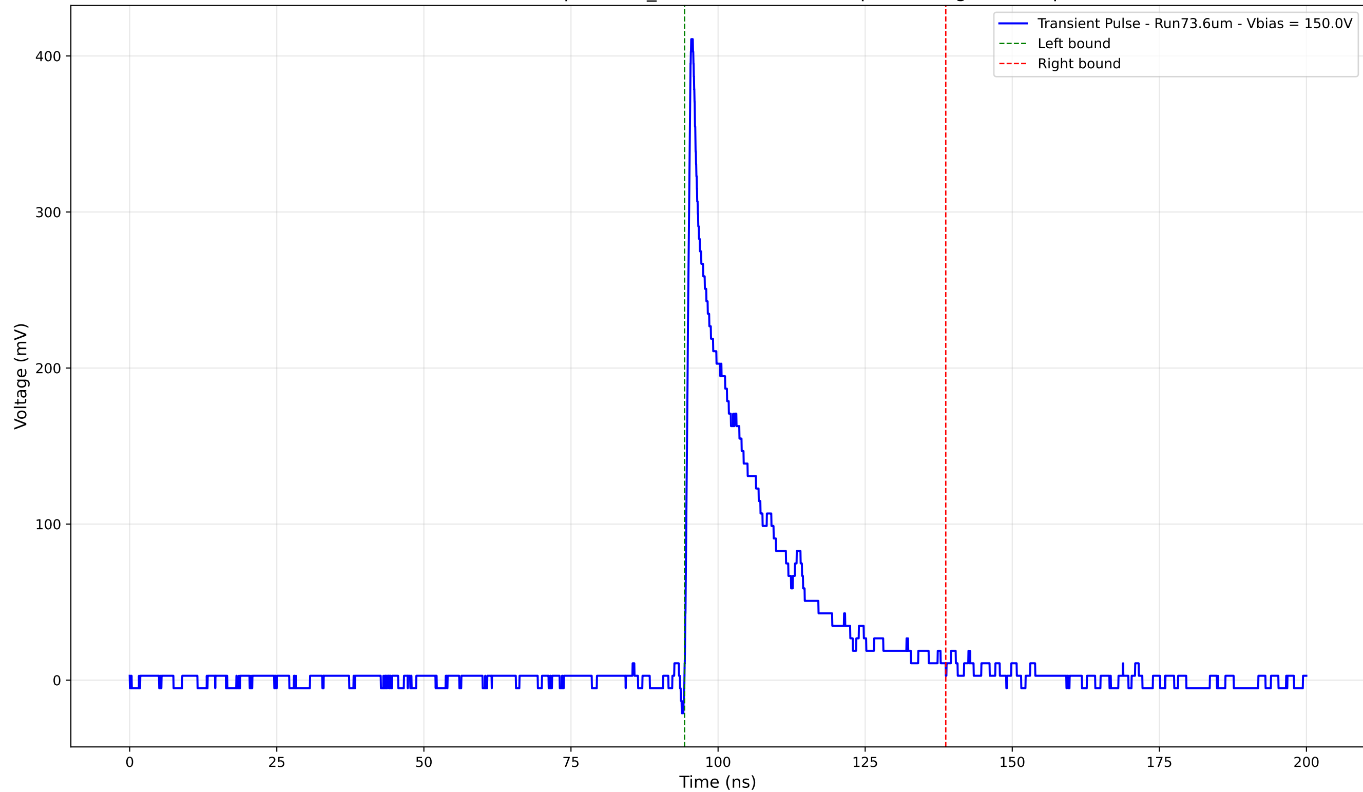
Transient Pulse - Sample: 1cm_42 - Position: 2790.0 \mu\text{m} - Charge: 77.69 pC
