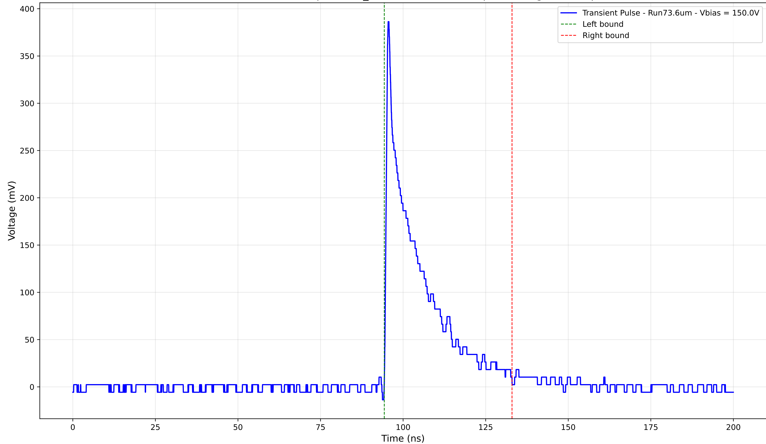
Transient Pulse - Sample: 1cm_42 - Position: 2875.0 \mu\text{m} - Charge: 71.43 pC
