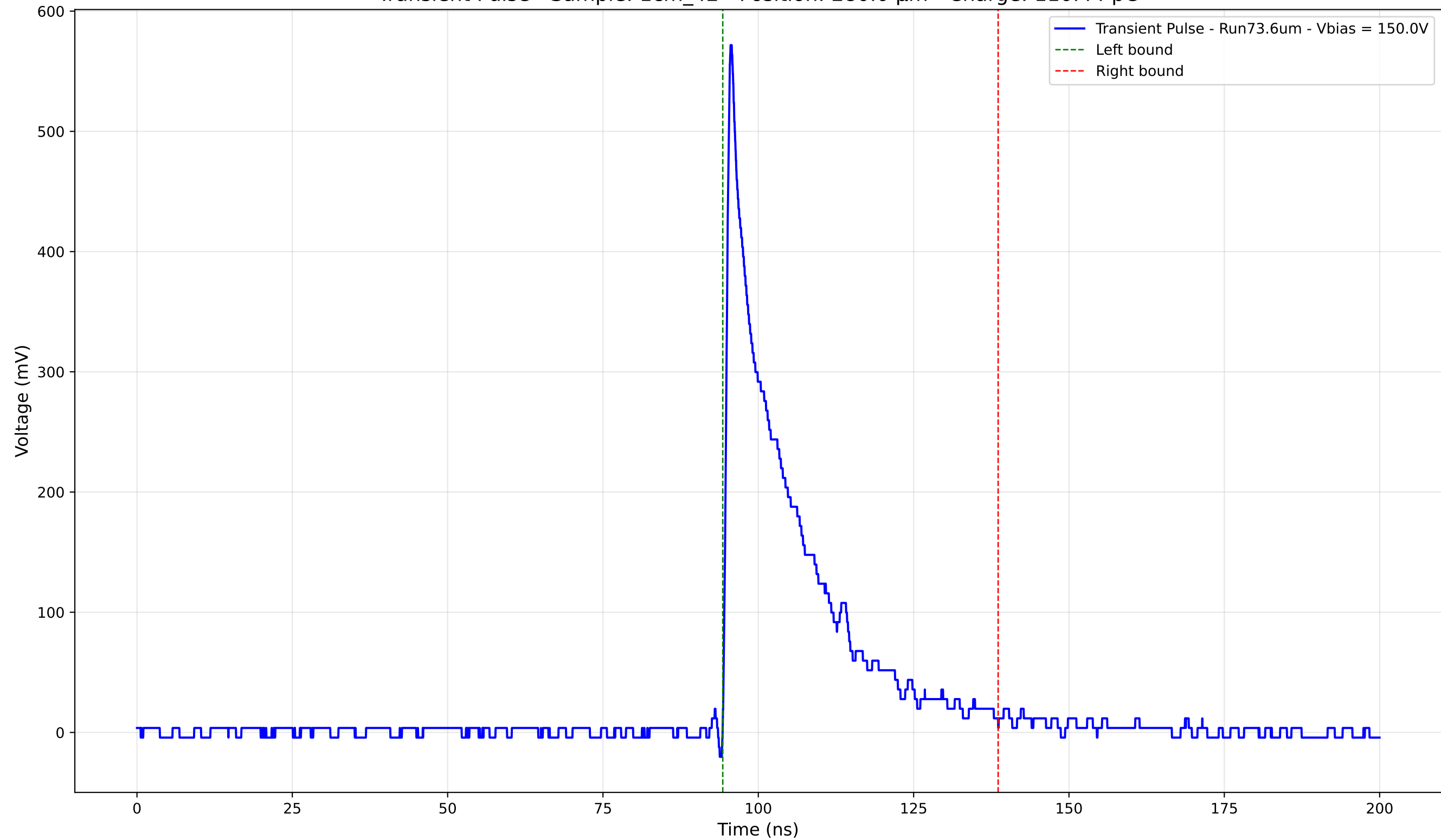
Transient Pulse - Sample: 1cm_42 - Position: 280.0 \mu\text{m} - Charge: 110.44 pC
