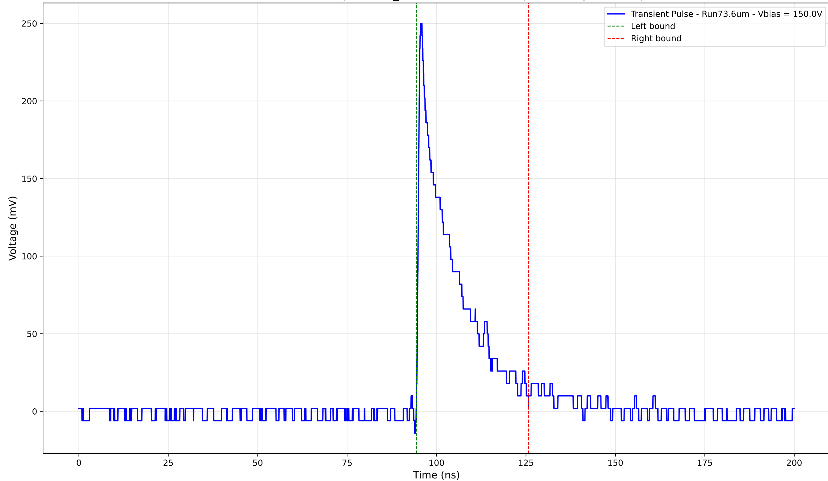
Transient Pulse - Sample: 1cm_42 - Position: 3600.0 \mu\text{m} - Charge: 48.48 pC
