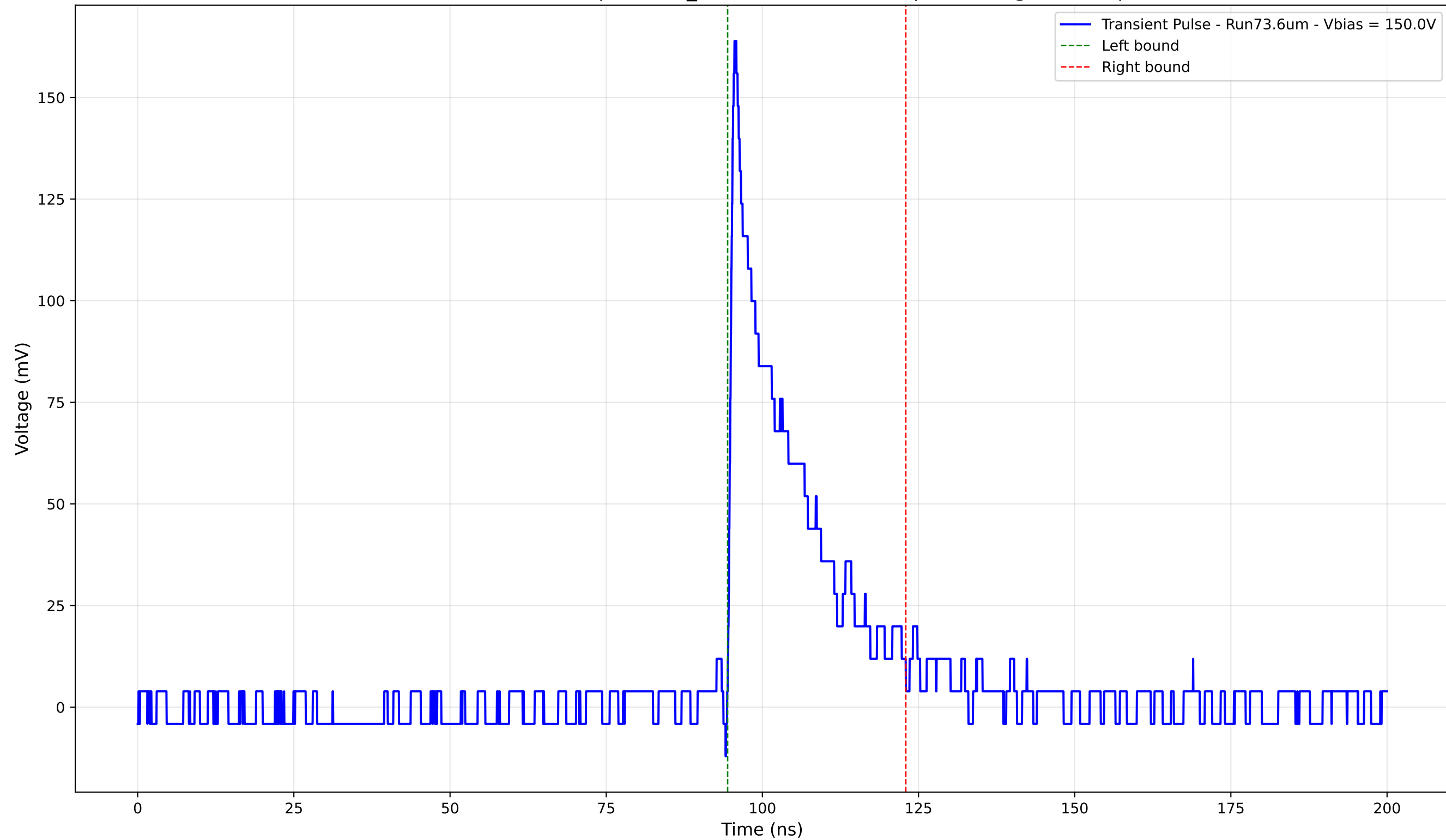
Transient Pulse - Sample: 1cm_42 - Position: 4380.0 \mu\text{m} - Charge: 30.07 pC
