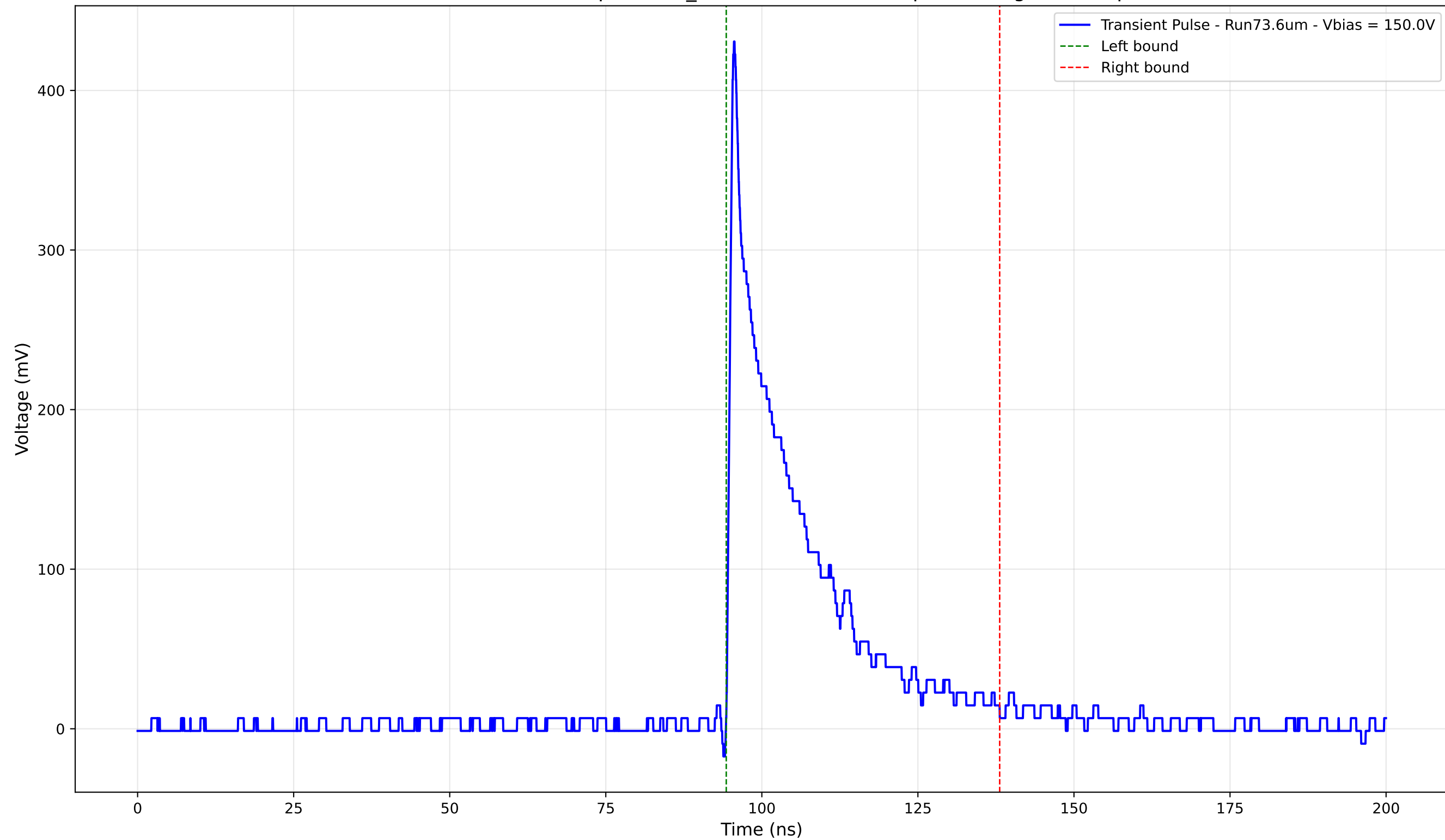
Transient Pulse - Sample: 1cm_42 - Position: 2330.0 \mu\text{m} - Charge: 83.83 pC
