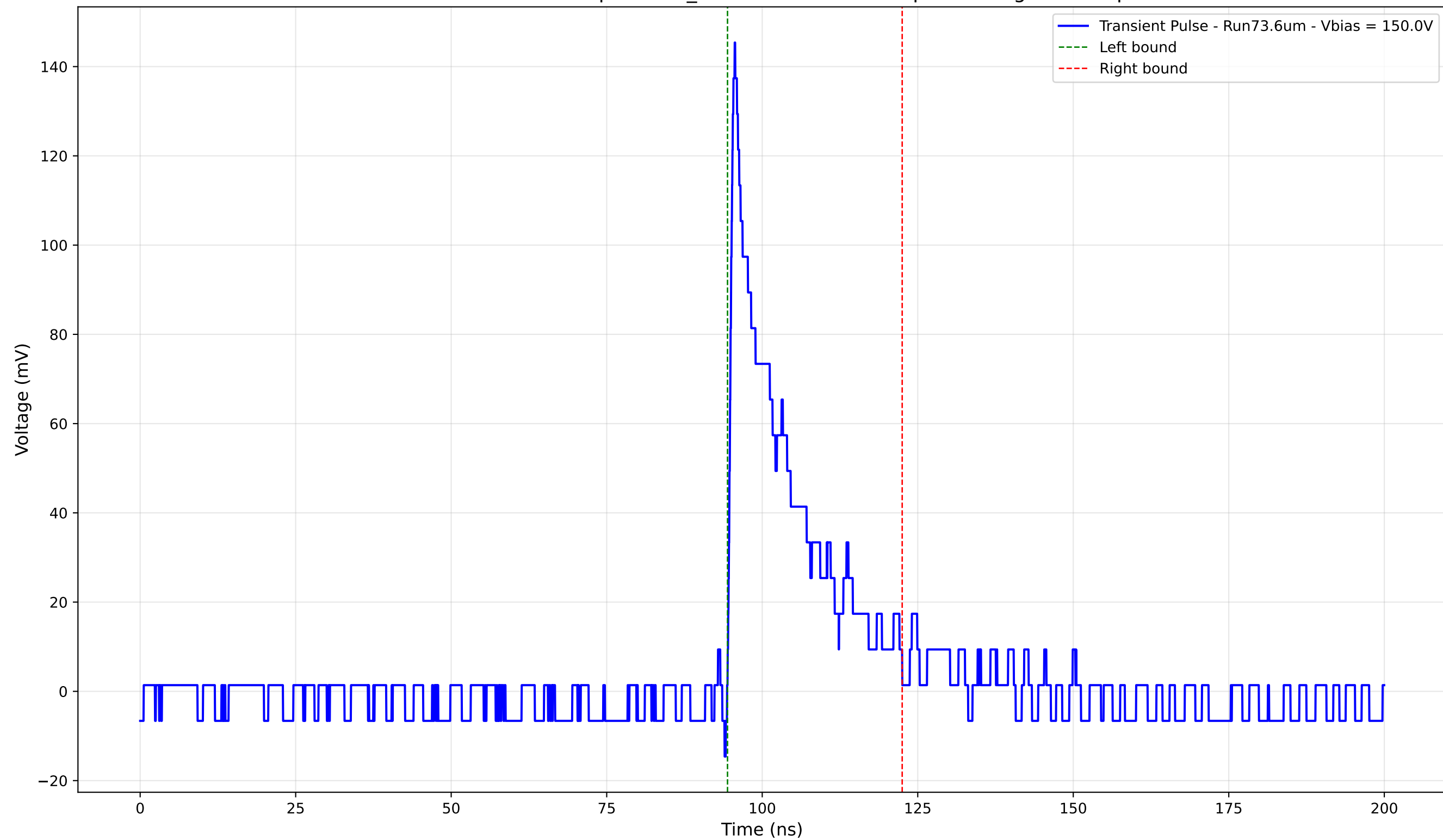
Transient Pulse - Sample: 1cm_42 - Position: 4575.0 \mu\text{m} - Charge: 24.24 pC
