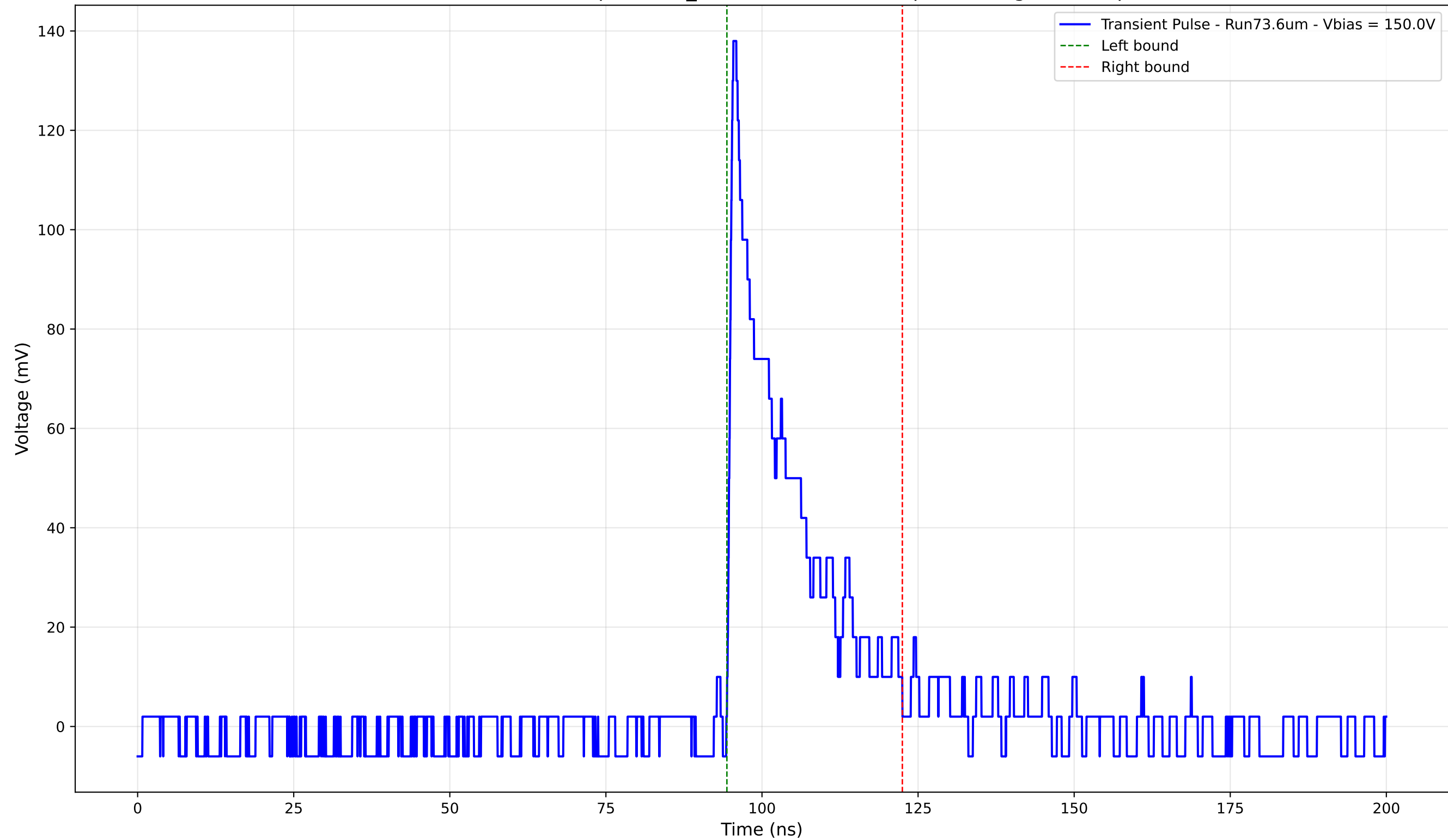
Transient Pulse - Sample: 1cm_42 - Position: 4590.0 \mu\text{m} - Charge: 24.67 pC
