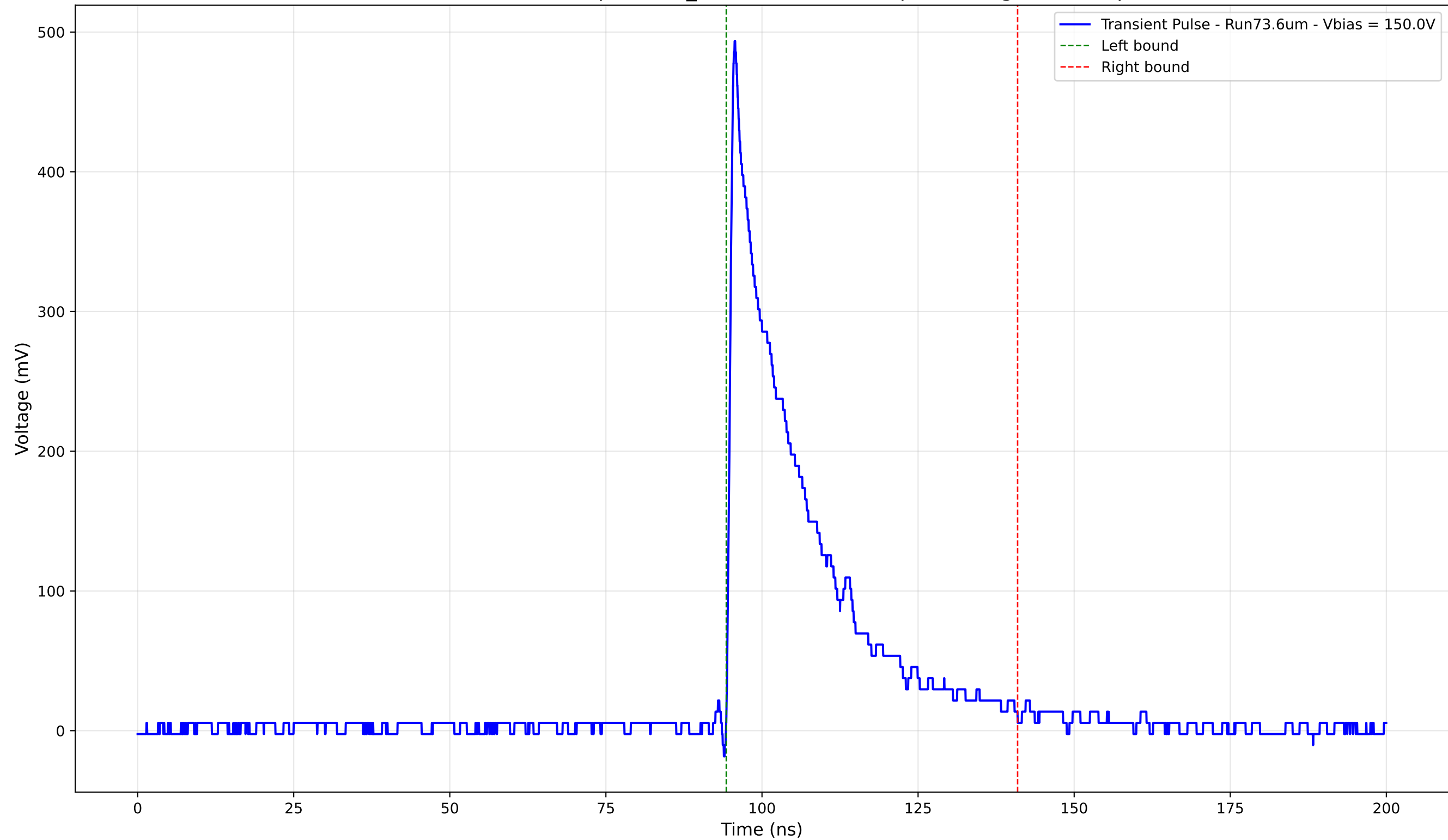
Transient Pulse - Sample: 1cm_42 - Position: 880.0 \mu\text{m} - Charge: 109.60 pC
