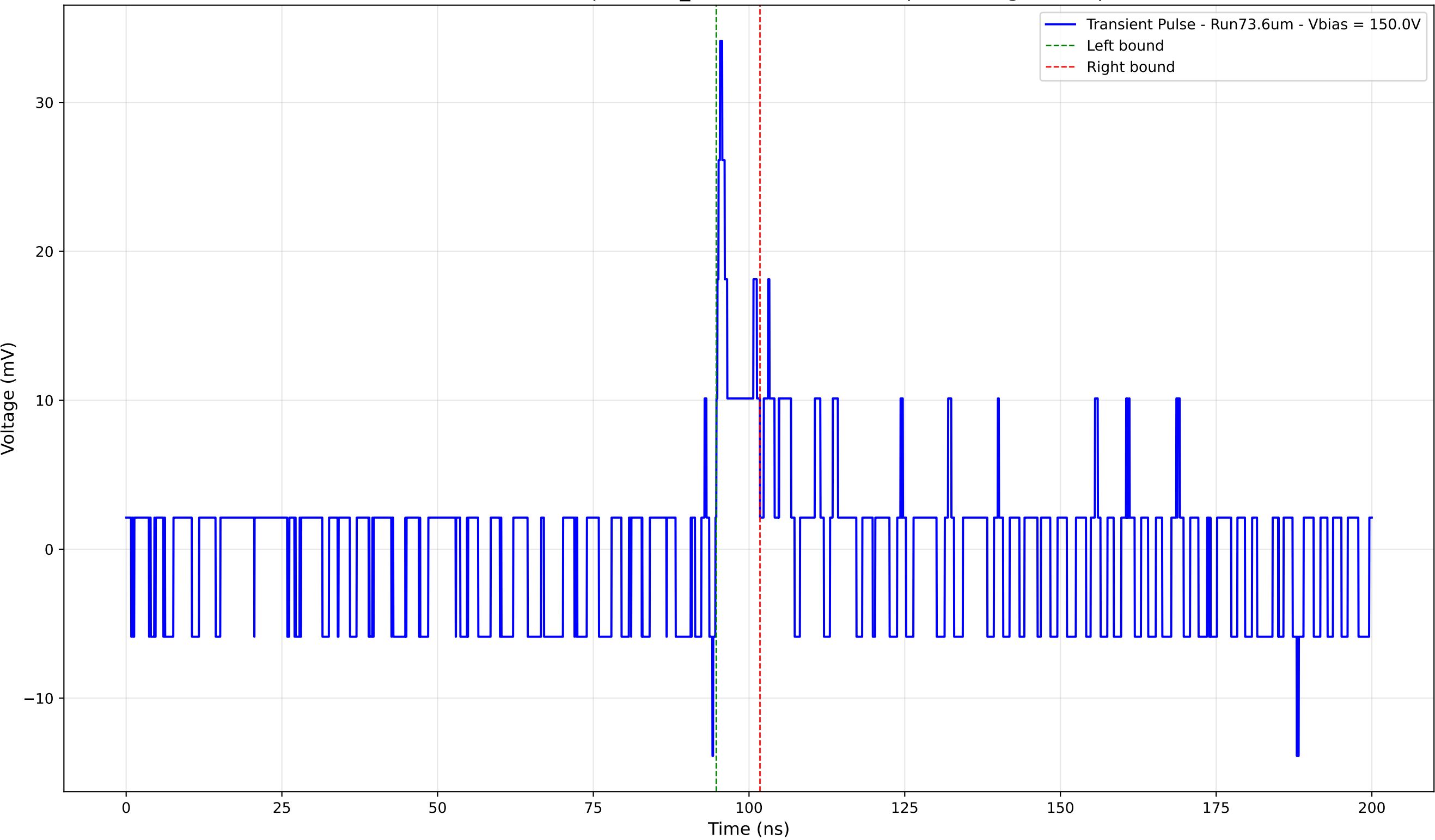
Transient Pulse - Sample: 1cm_42 - Position: 4950.0 \mu\text{m} - Charge: 1.98 pC
