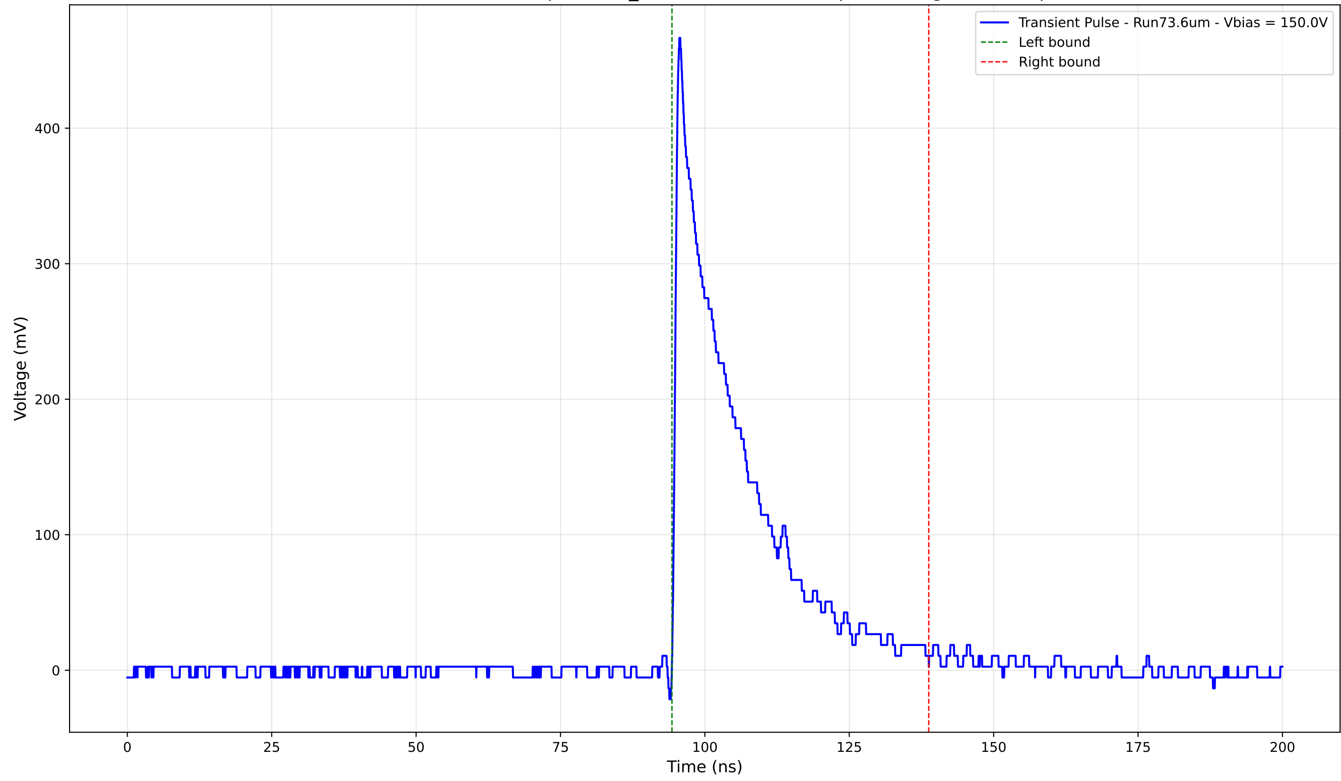
Transient Pulse - Sample: 1cm_42 - Position: 1040.0 \mu\text{m} - Charge: 101.88 pC
