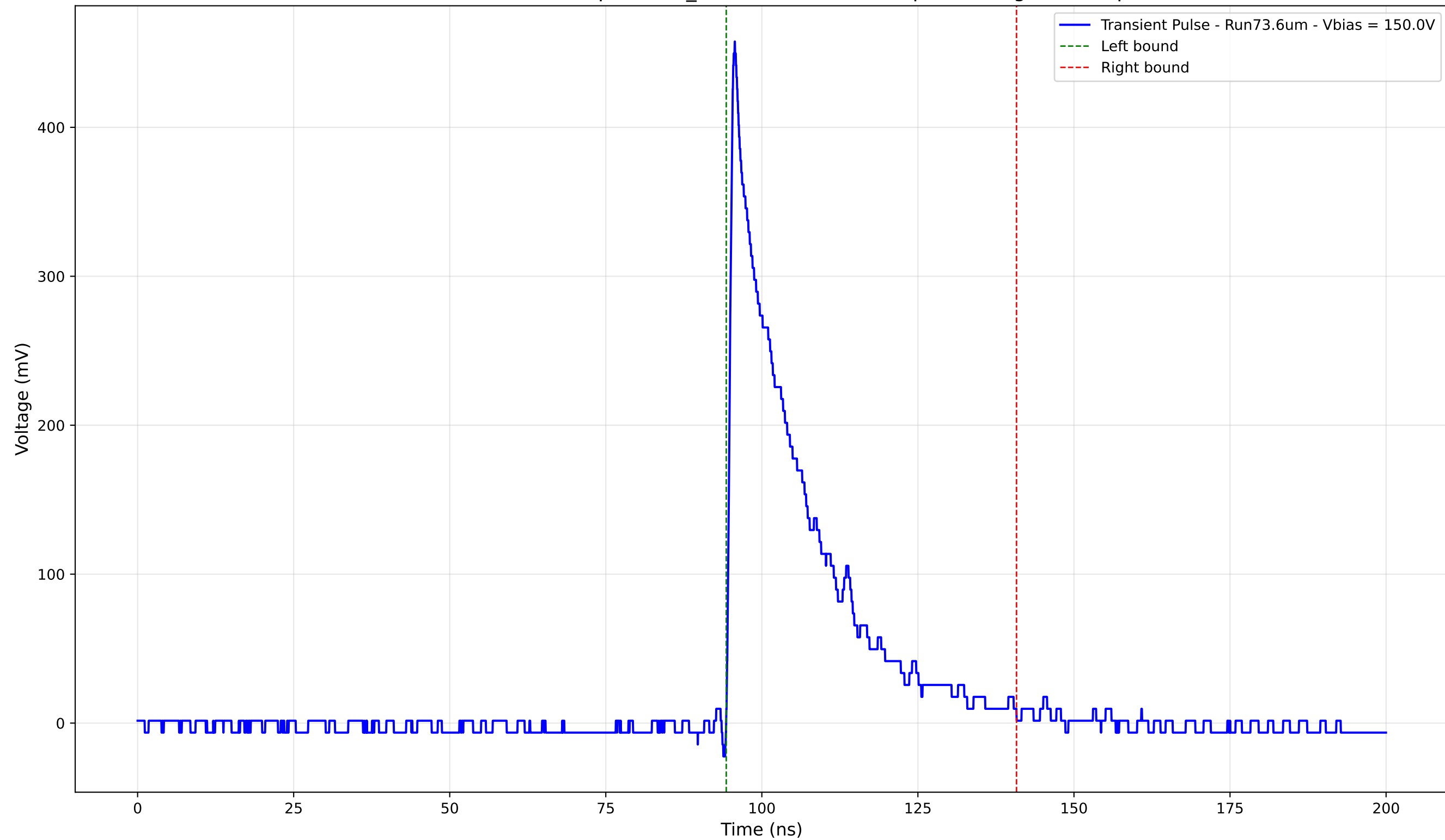
Transient Pulse - Sample: 1cm_42 - Position: 1265.0 \mu\text{m} - Charge: 98.69 pC
