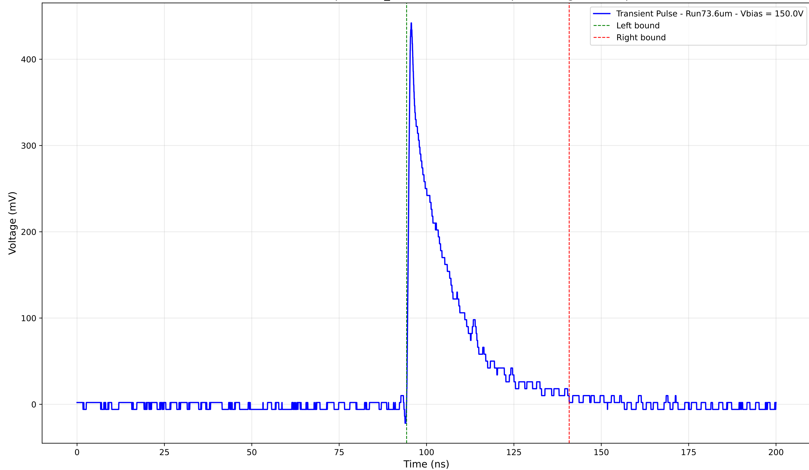
Transient Pulse - Sample: 1cm_42 - Position: 1835.0 \mu\text{m} - Charge: 92.24 pC
