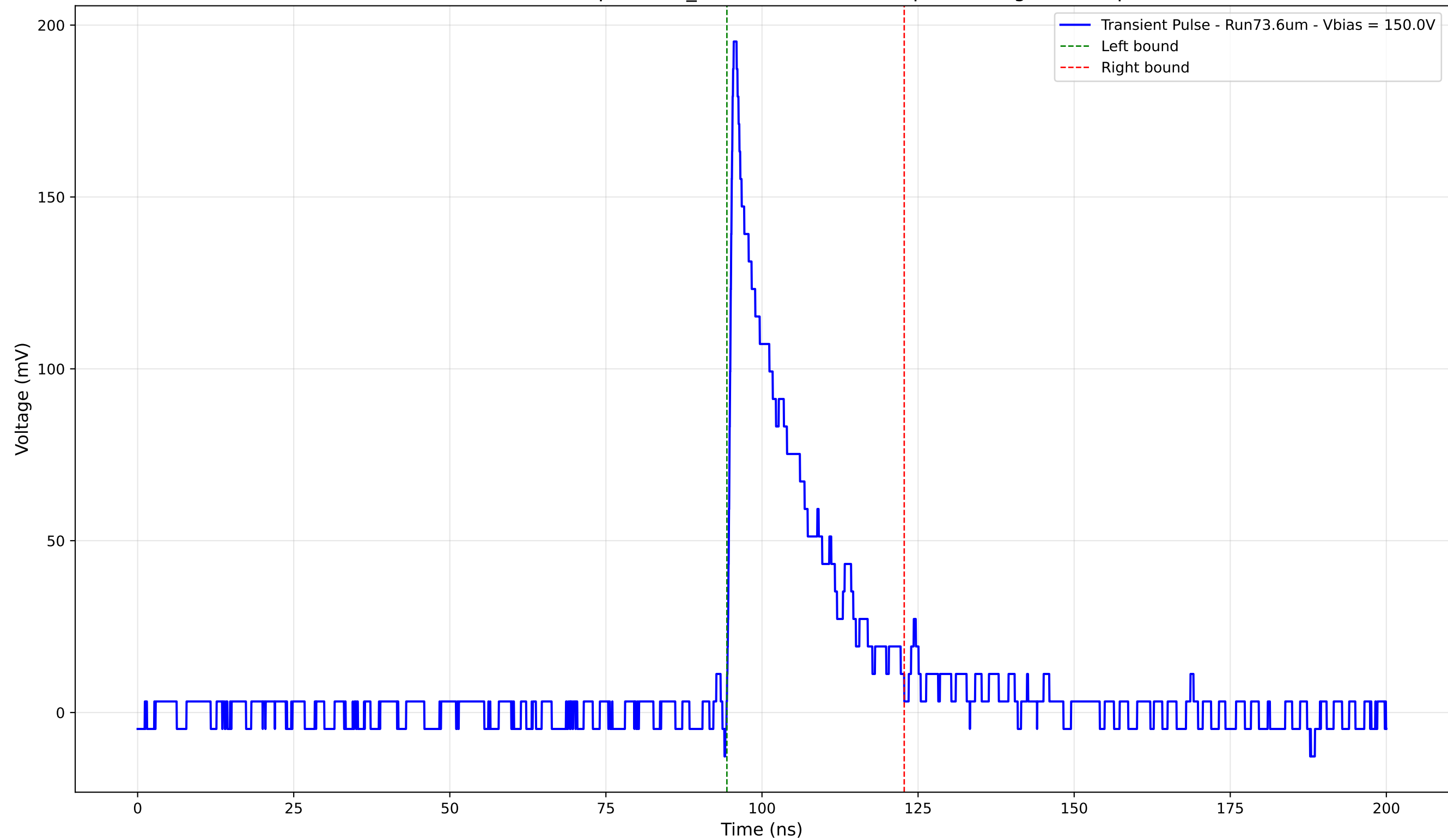
Transient Pulse - Sample: 1cm_42 - Position: 4000.0 \mu\text{m} - Charge: 36.88 pC
