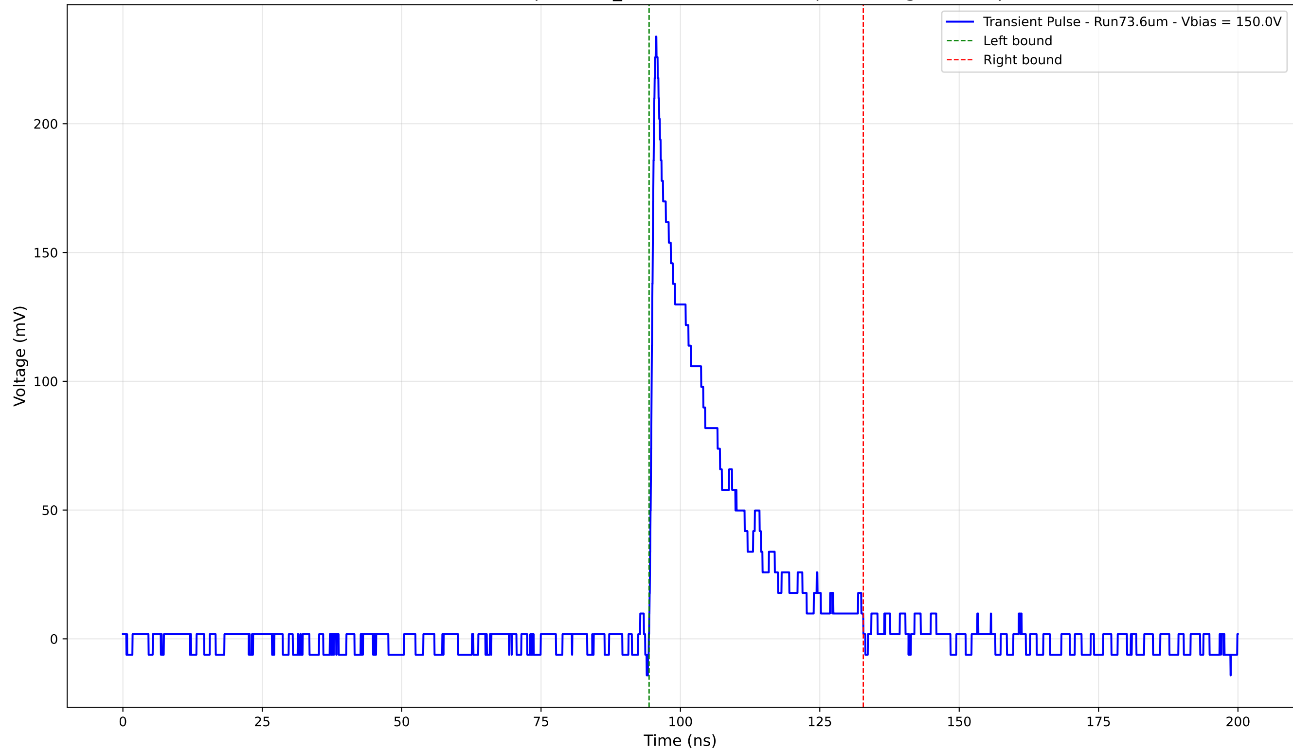
Transient Pulse - Sample: 1cm_42 - Position: 3710.0 \mu\text{m} - Charge: 45.54 pC
