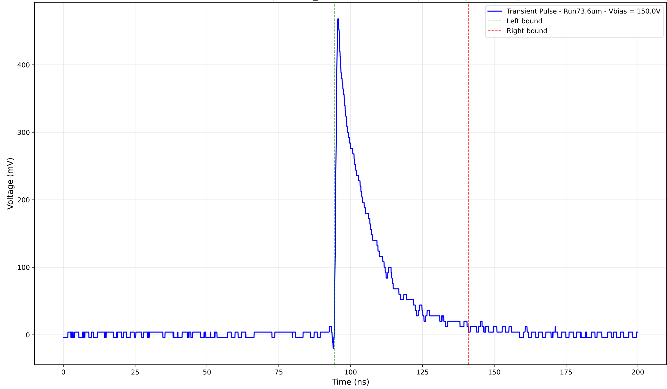
Transient Pulse - Sample: 1cm_42 - Position: 1025.0 \mu\text{m} - Charge: 104.25 pC
