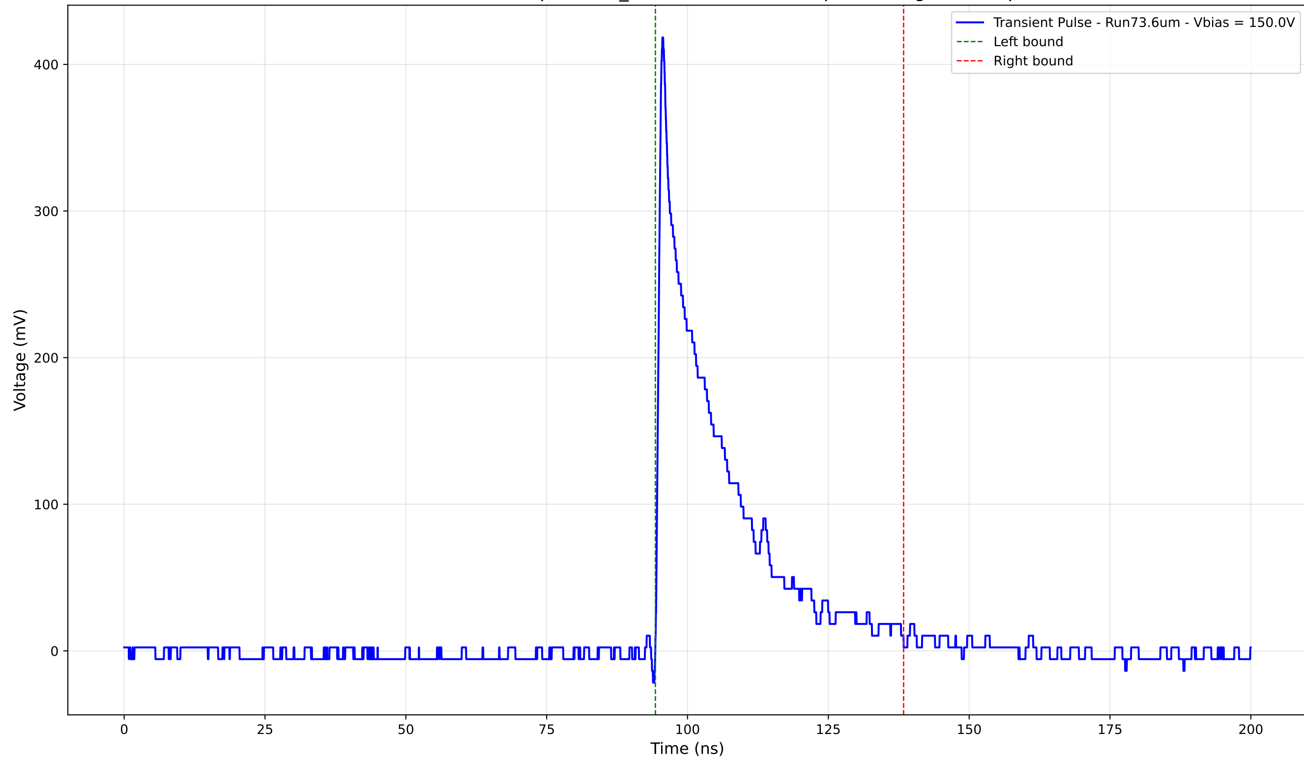
Transient Pulse - Sample: 1cm_42 - Position: 2170.0 \mu\text{m} - Charge: 83.35 pC
