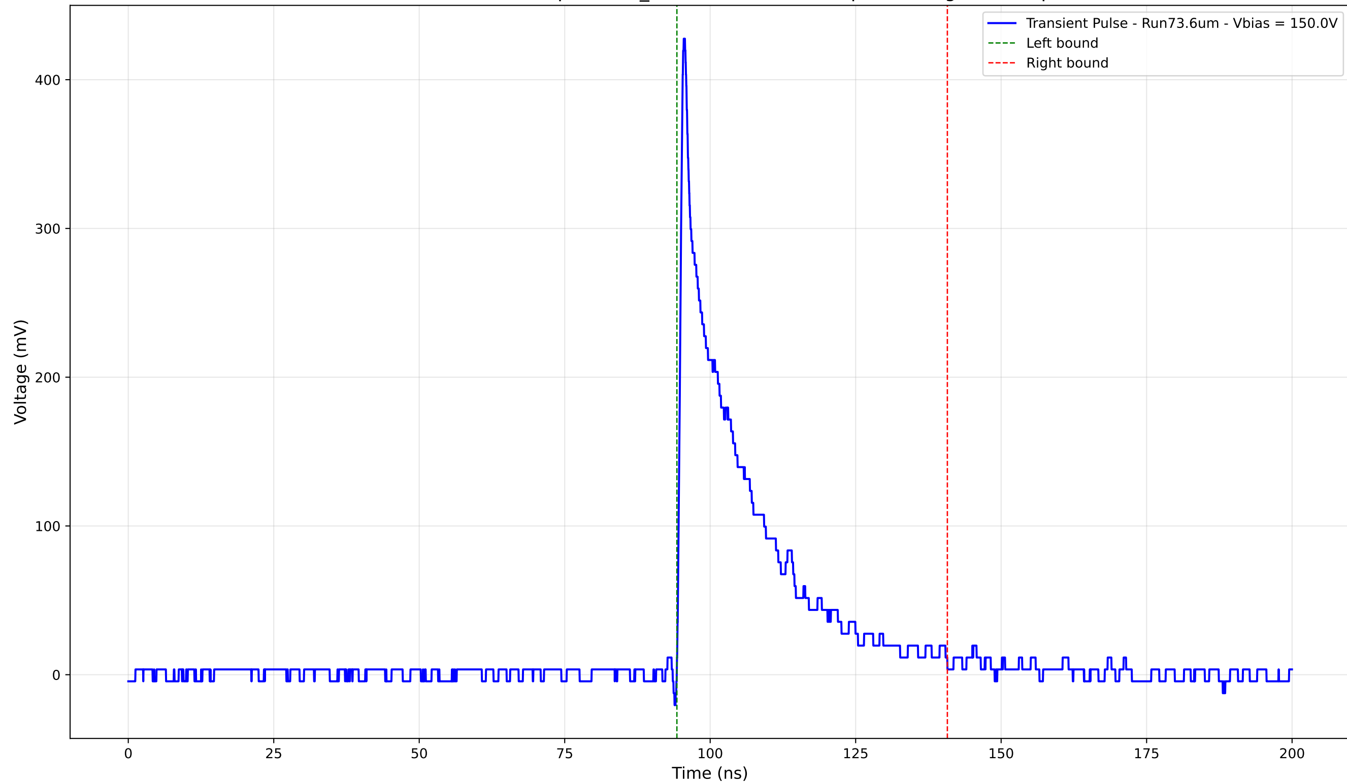
Transient Pulse - Sample: 1cm_42 - Position: 2520.0 \mu\text{m} - Charge: 82.67 pC
