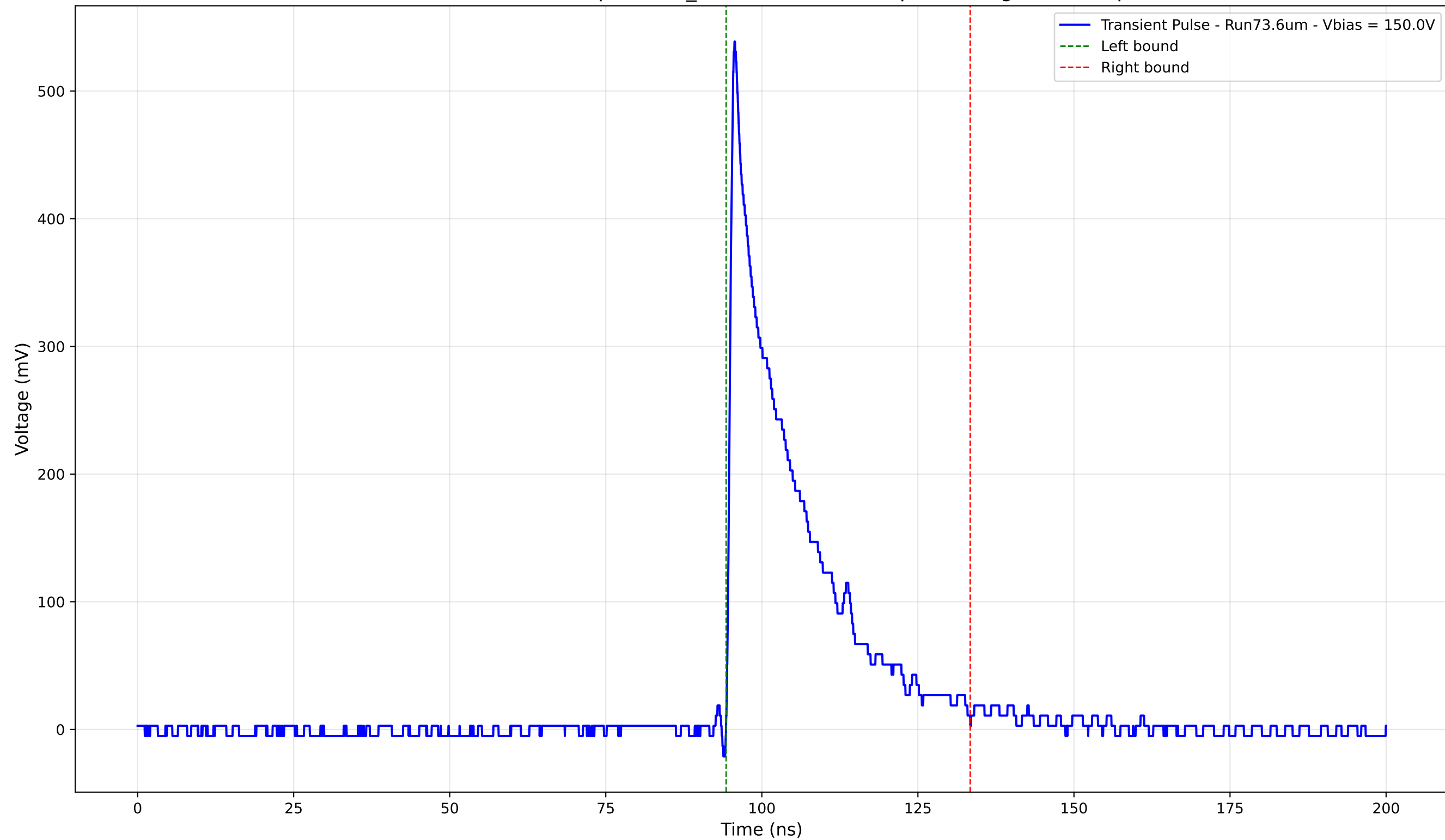
Transient Pulse - Sample: 1cm_42 - Position: 510.0 \mu\text{m} - Charge: 107.70 pC
