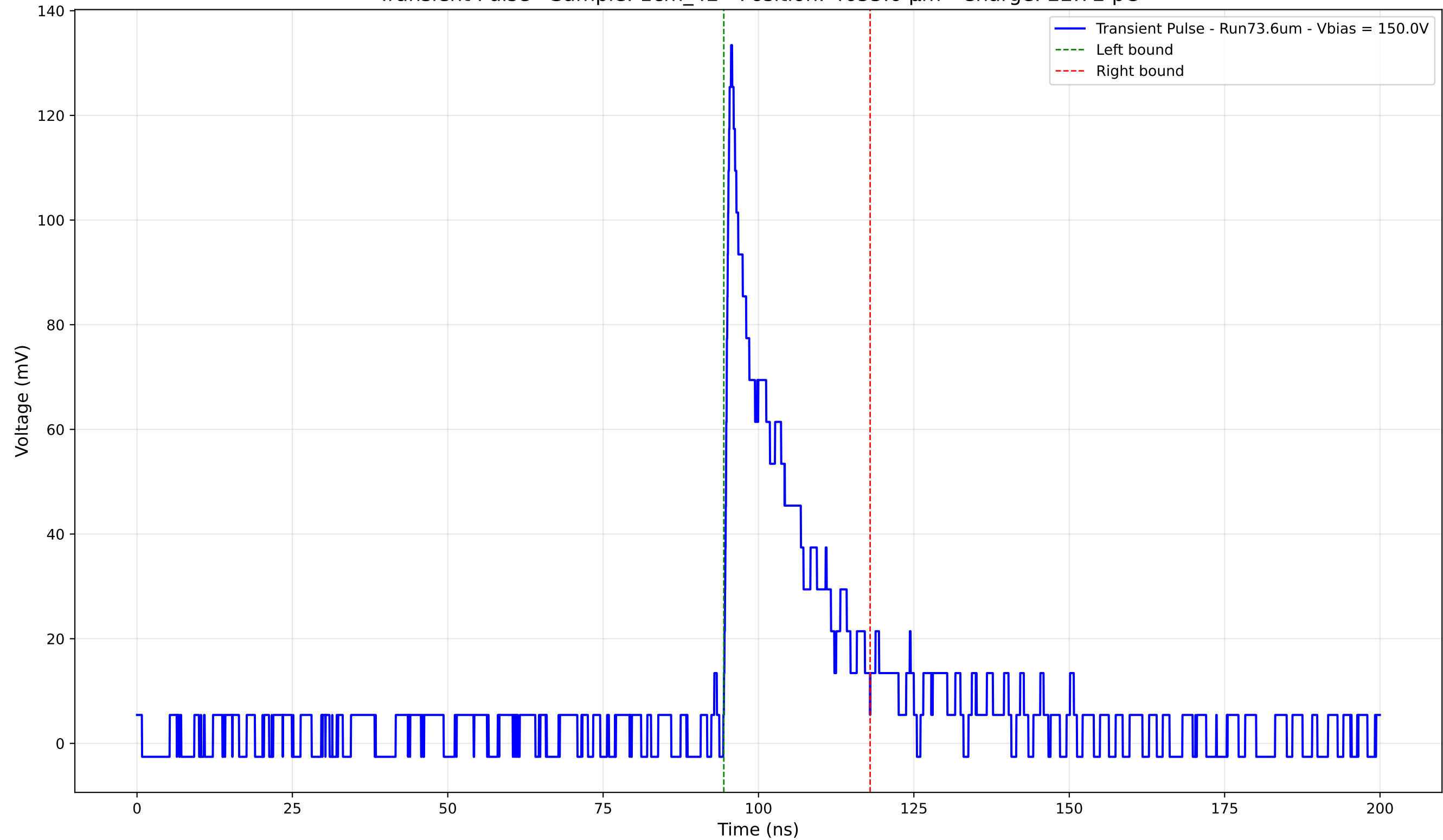
Transient Pulse - Sample: 1cm_42 - Position: 4655.0 \mu\text{m} - Charge: 22.72 pC
