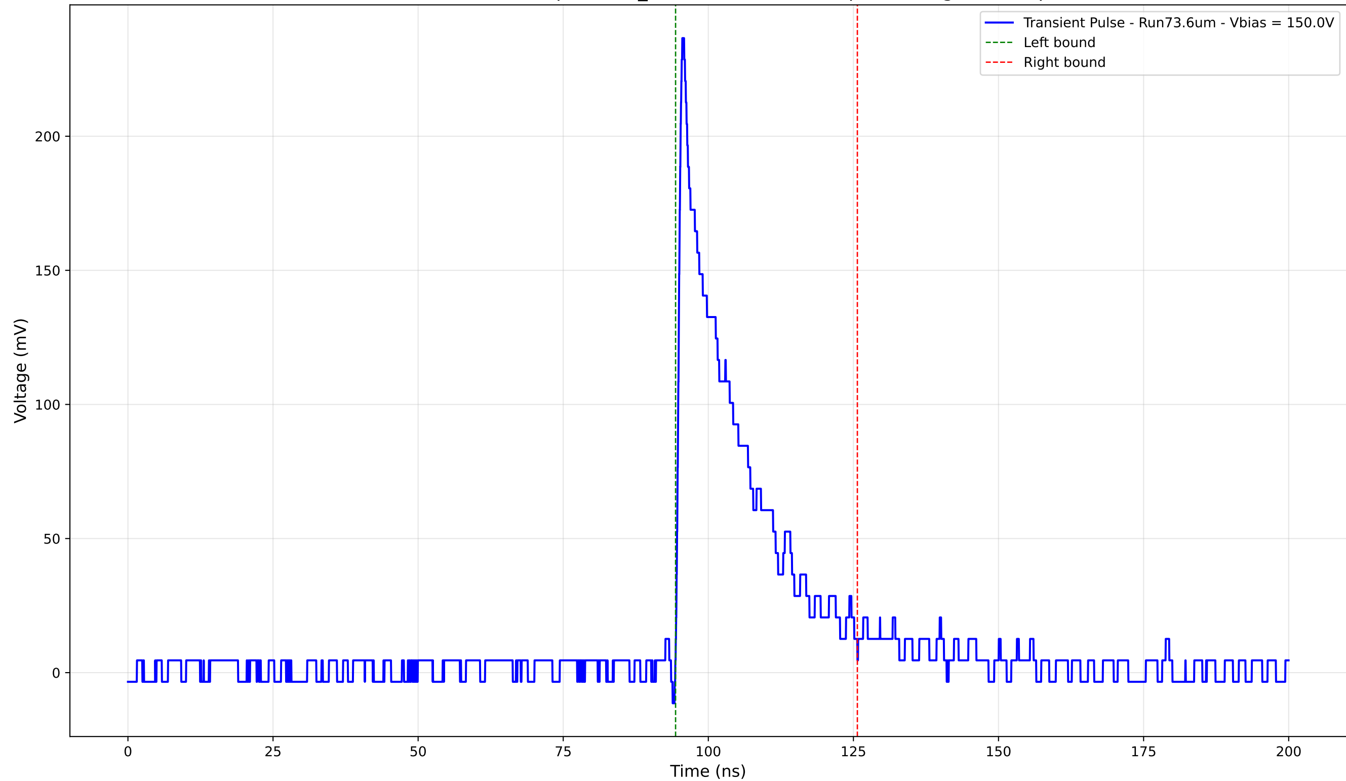
Transient Pulse - Sample: 1cm_42 - Position: 3680.0 \mu\text{m} - Charge: 46.83 pC
