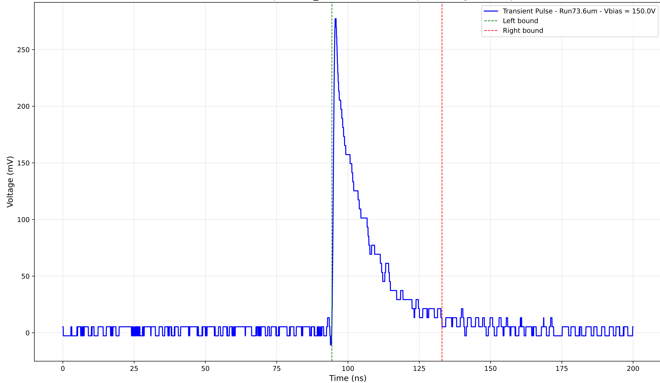
Transient Pulse - Sample: 1cm_42 - Position: 3420.0 \mu\text{m} - Charge: 57.61 pC
