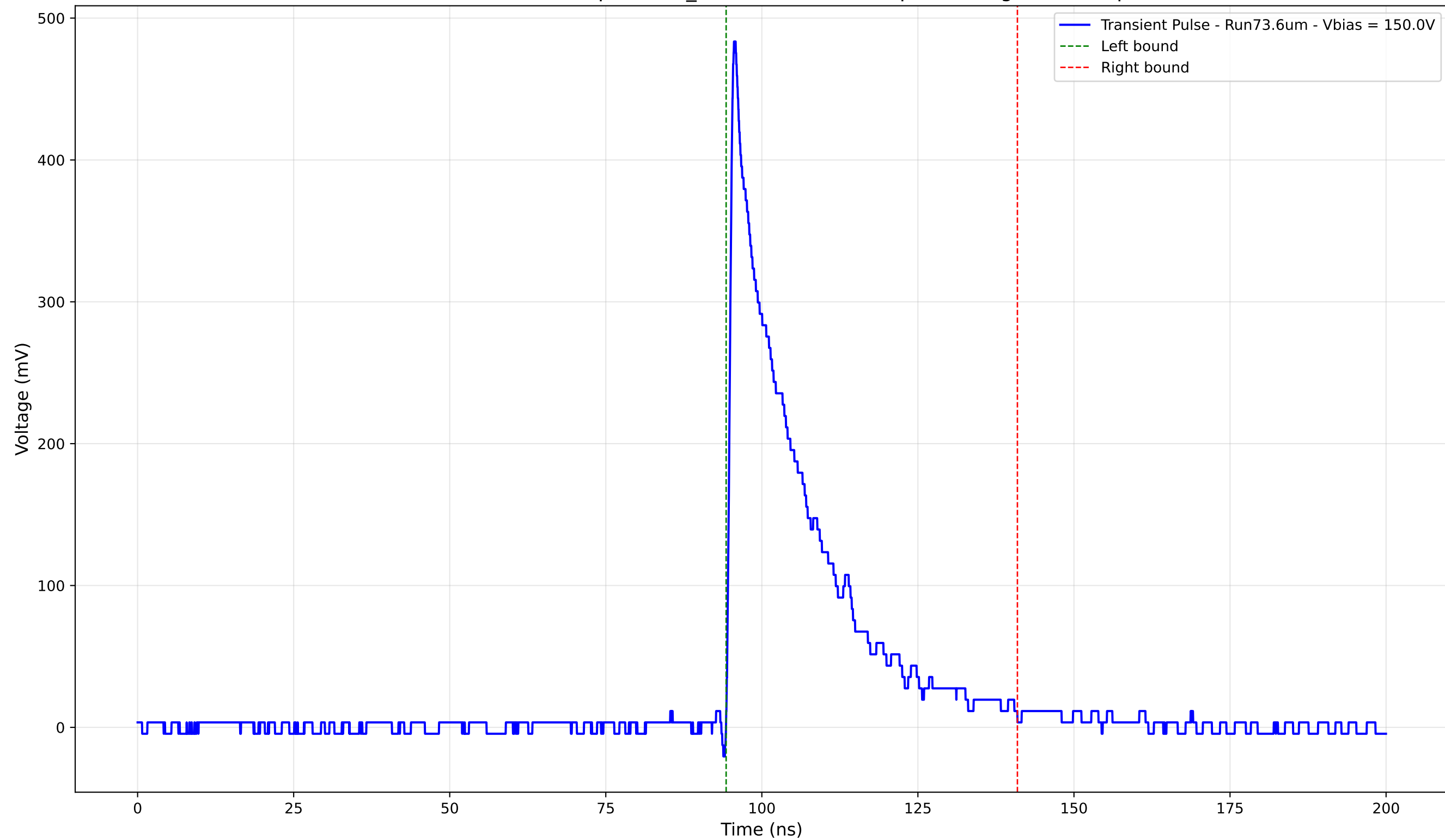
Transient Pulse - Sample: 1cm_42 - Position: 925.0 \mu\text{m} - Charge: 106.59 pC
