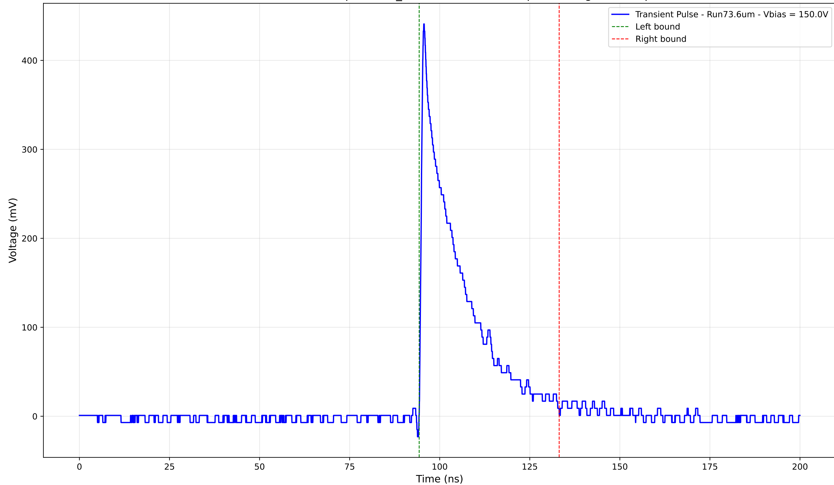
Transient Pulse - Sample: 1cm_42 - Position: 1570.0 \mu\text{m} - Charge: 92.23 pC
