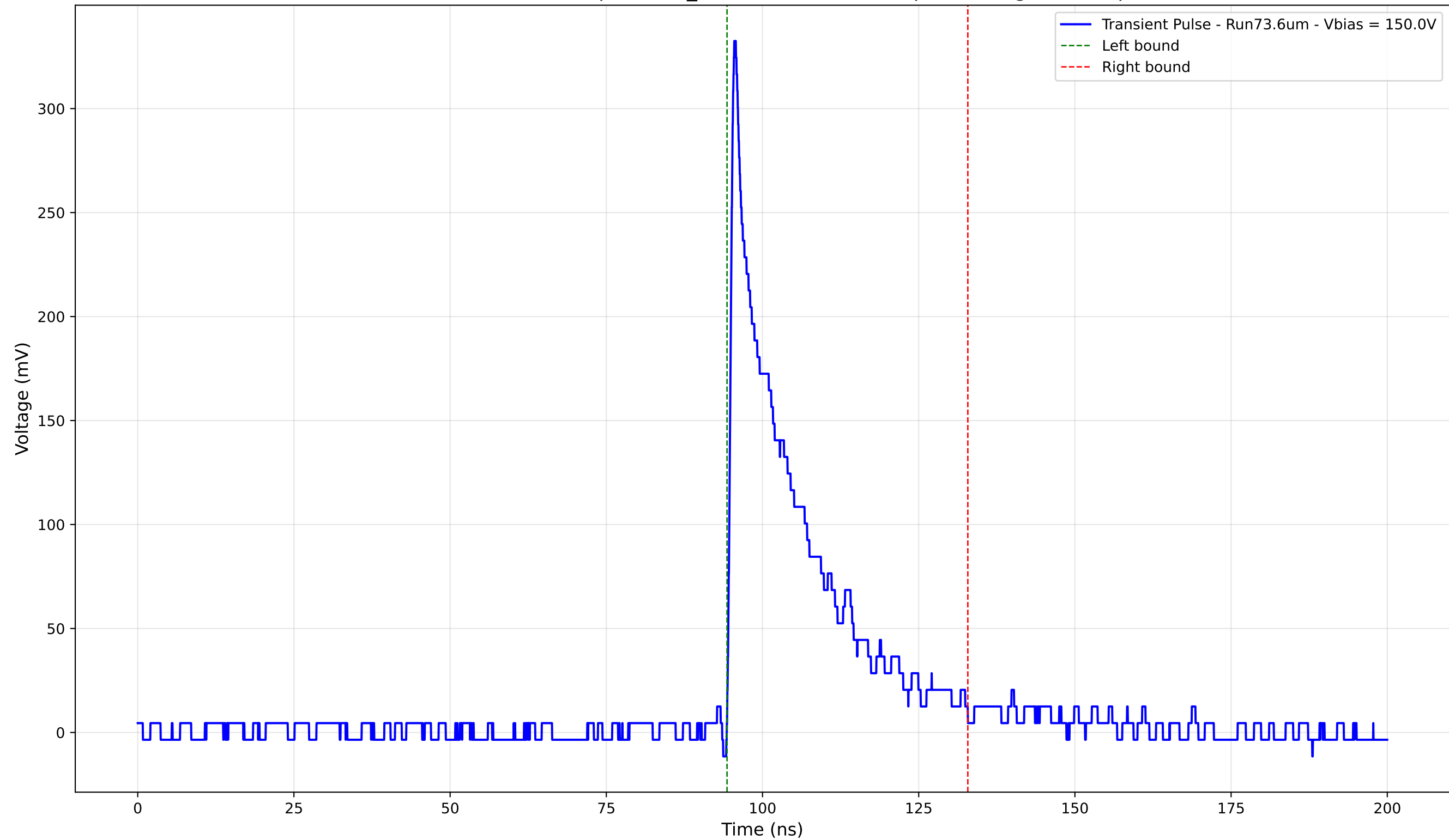
Transient Pulse - Sample: 1cm_42 - Position: 3055.0 \mu\text{m} - Charge: 64.14 pC
