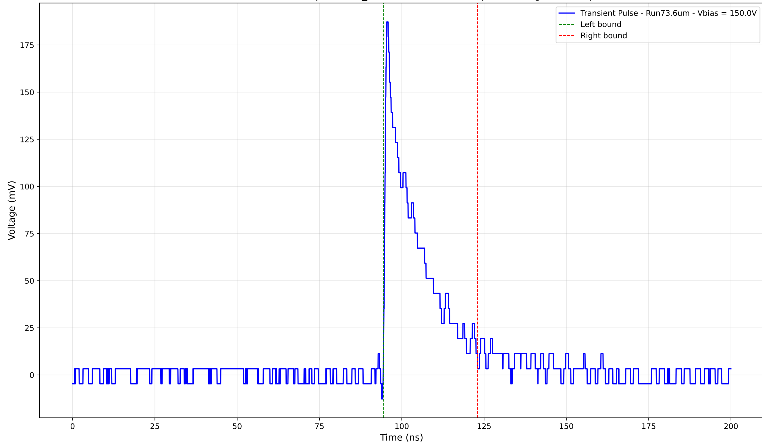
Transient Pulse - Sample: 1cm_42 - Position: 4080.0 \mu\text{m} - Charge: 36.17 pC
