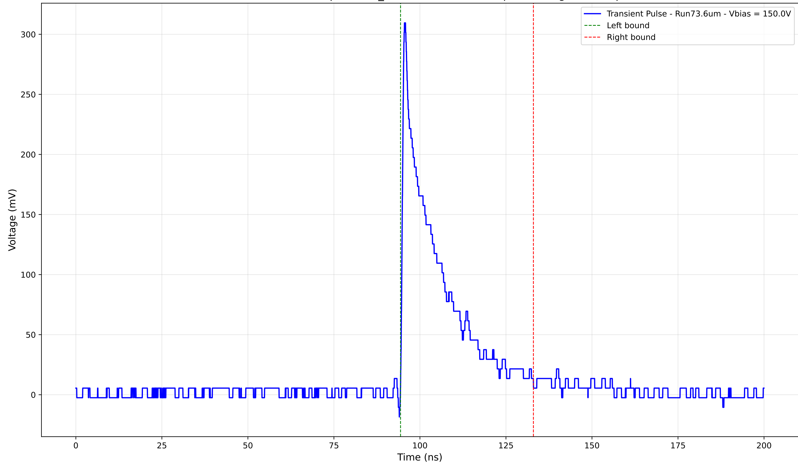
Transient Pulse - Sample: 1cm_42 - Position: 3225.0 \mu\text{m} - Charge: 62.17 pC
