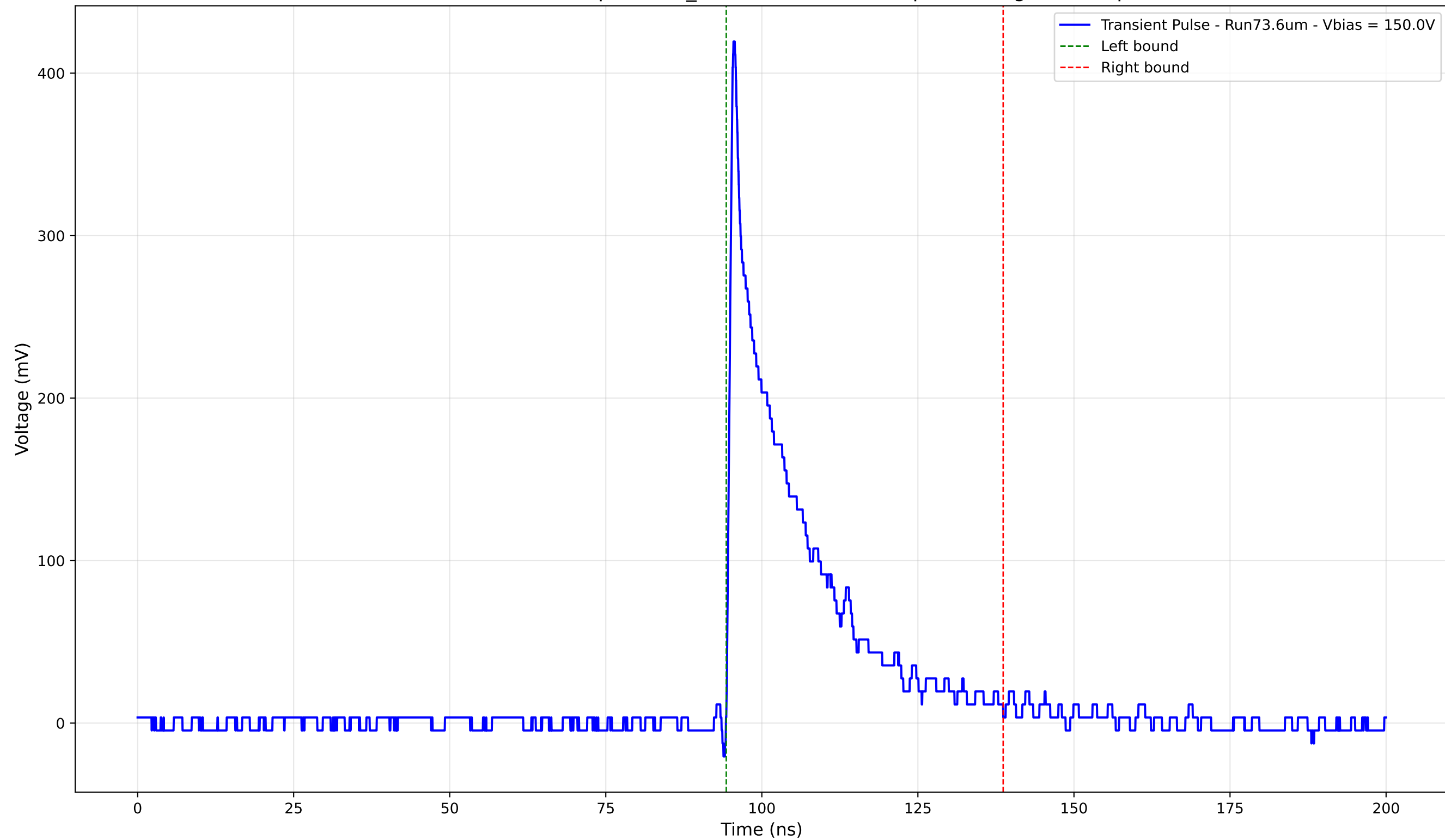
Transient Pulse - Sample: 1cm_42 - Position: 2490.0 \mu\text{m} - Charge: 79.36 pC
