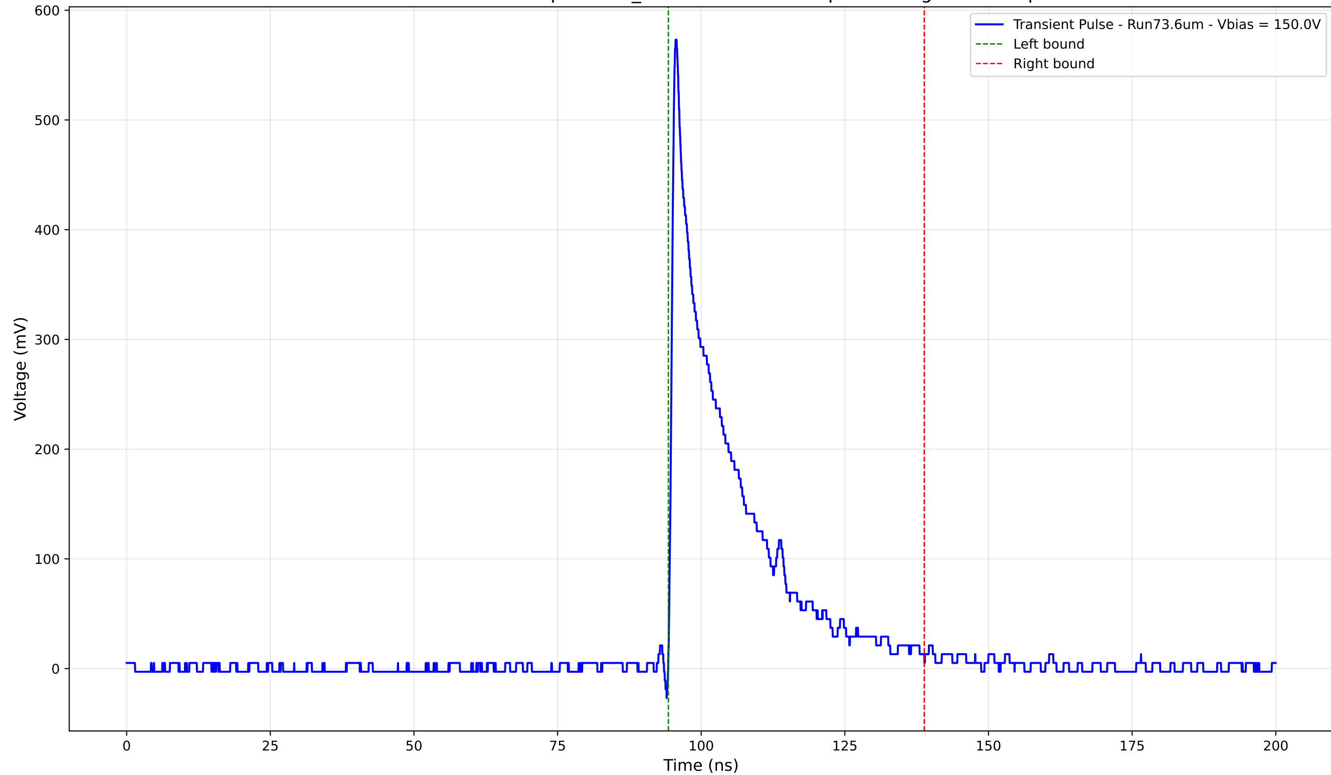
Transient Pulse - Sample: 1cm_42 - Position: 240.0 \mu\text{m} - Charge: 111.16 pC
