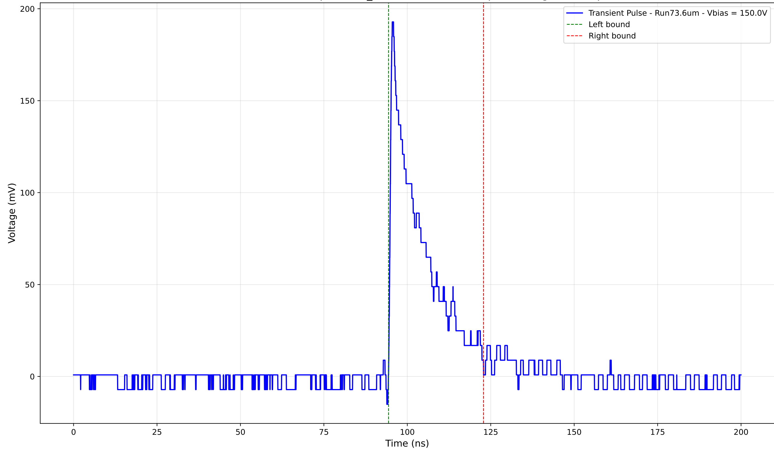
Transient Pulse - Sample: 1cm_42 - Position: 4045.0 \mu\text{m} - Charge: 36.16 pC
