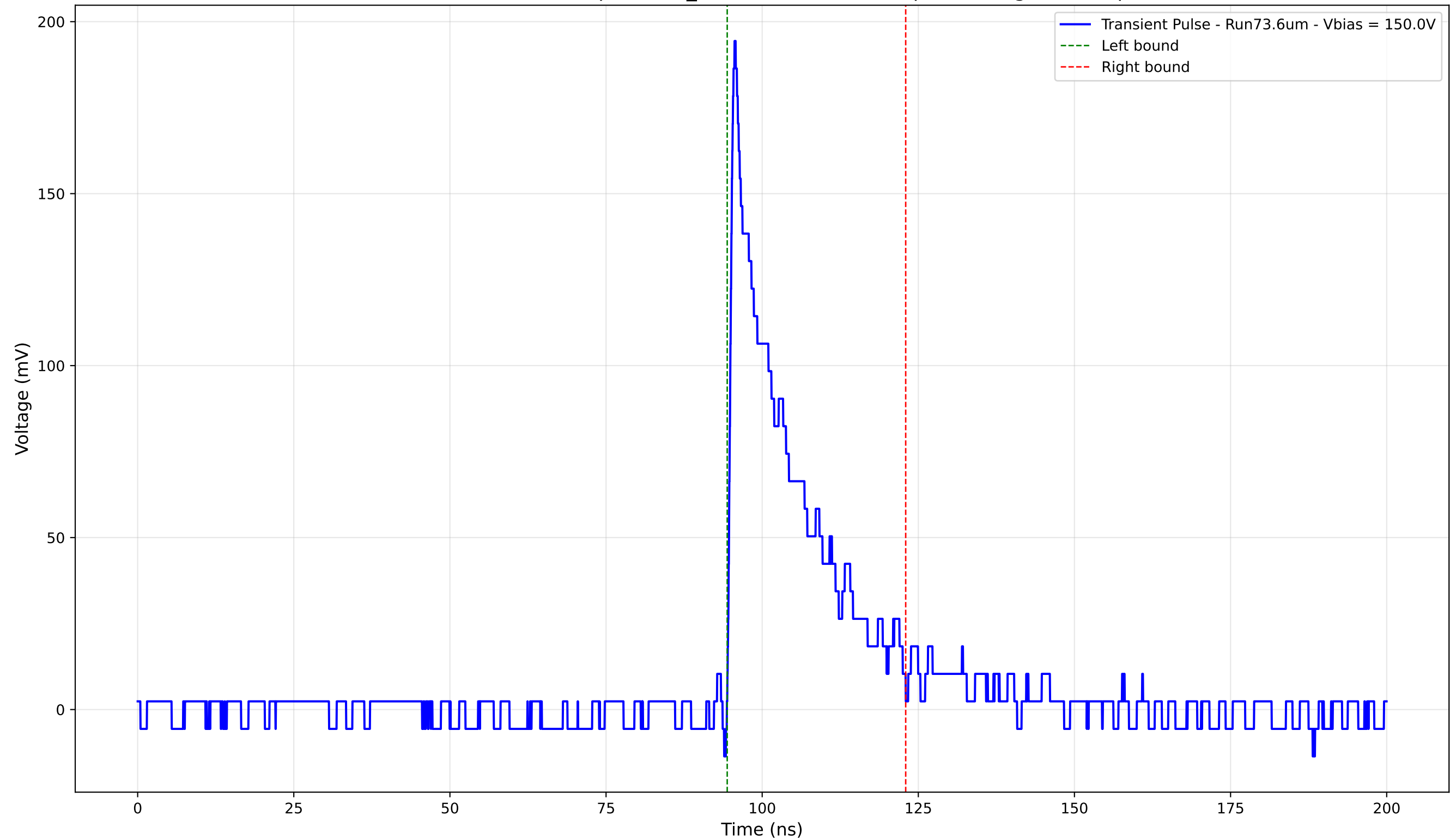
Transient Pulse - Sample: 1cm_42 - Position: 4075.0 \mu\text{m} - Charge: 36.23 pC
