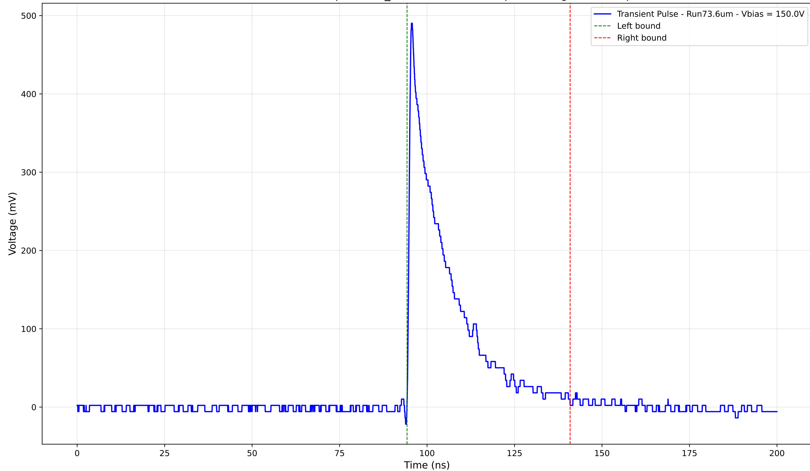
Transient Pulse - Sample: 1cm_42 - Position: 820.0 \mu\text{m} - Charge: 105.72 pC
