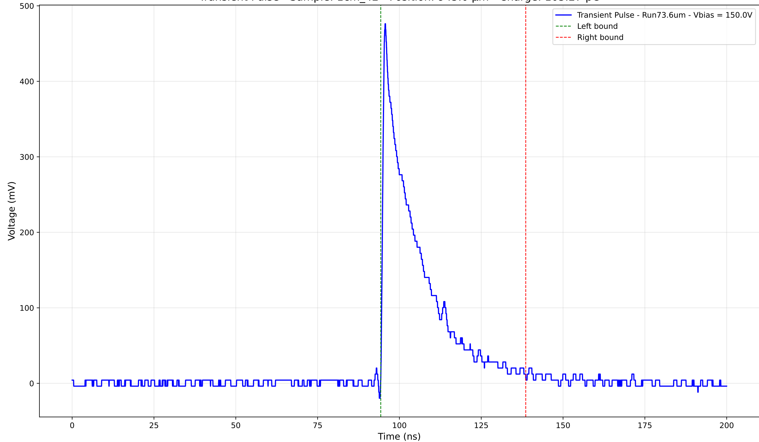
Transient Pulse - Sample: 1cm_42 - Position: 945.0 \mu\text{m} - Charge: 103.27 pC
