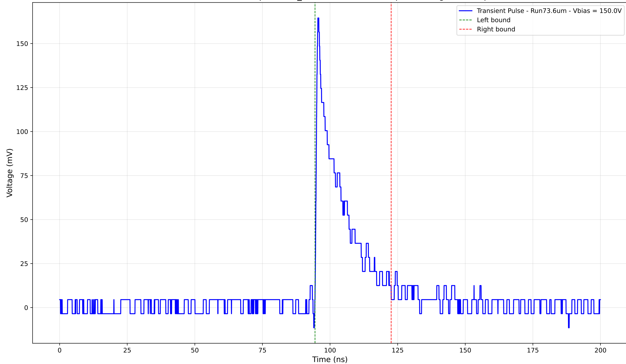
Transient Pulse - Sample: 1cm_42 - Position: 4385.0 \mu\text{m} - Charge: 30.03 pC
