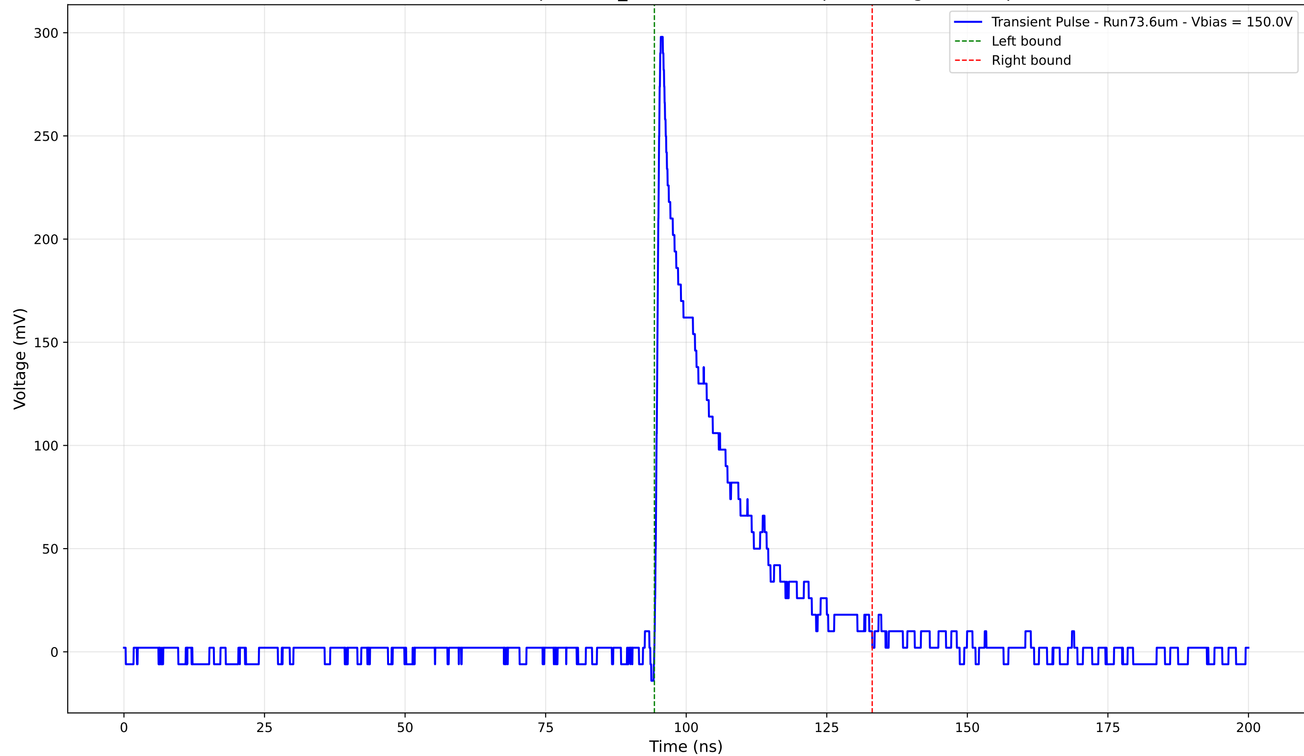
Transient Pulse - Sample: 1cm_42 - Position: 3245.0 \mu\text{m} - Charge: 59.25 pC
