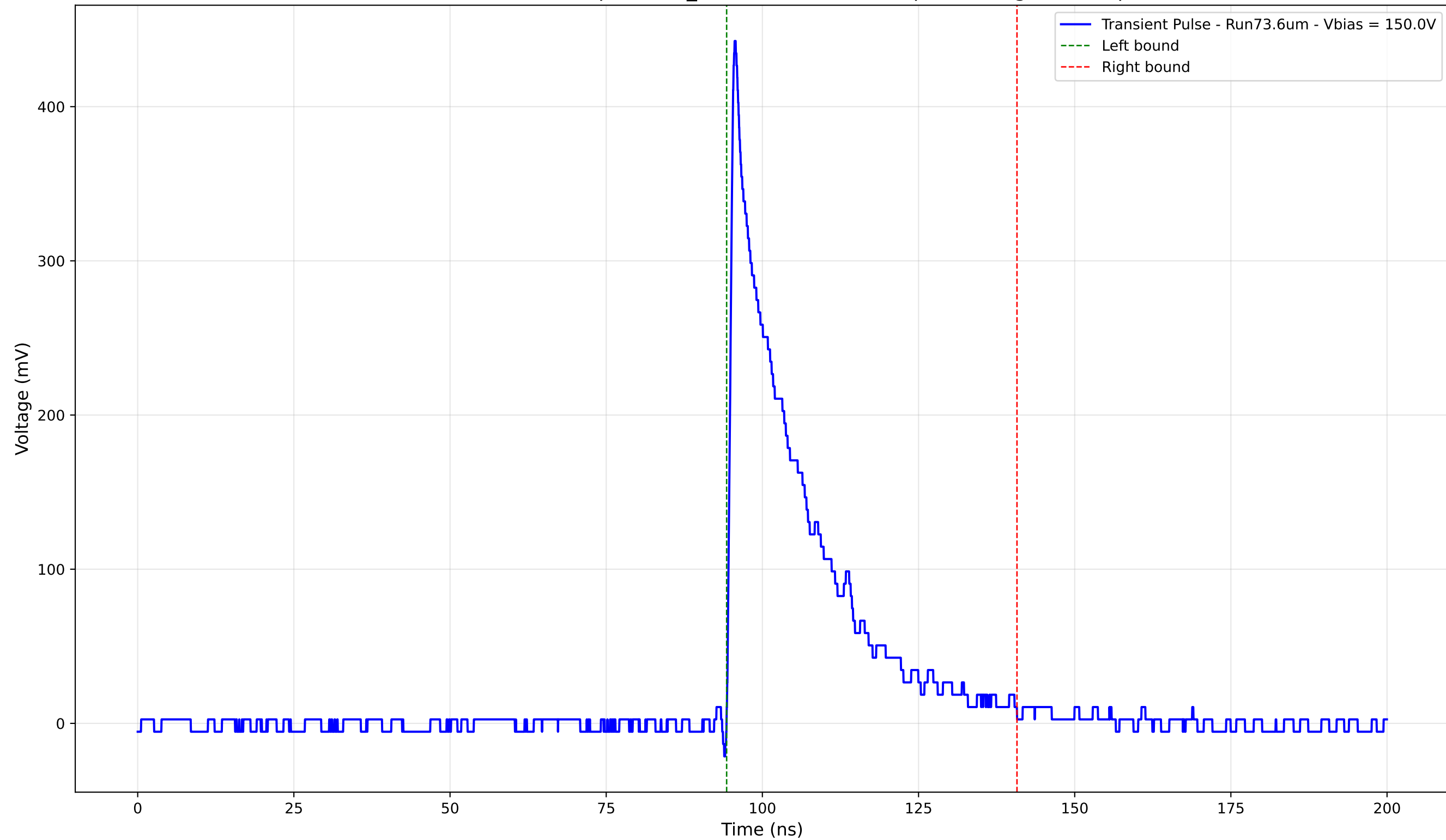
Transient Pulse - Sample: 1cm_42 - Position: 1665.0 \mu\text{m} - Charge: 94.18 pC
