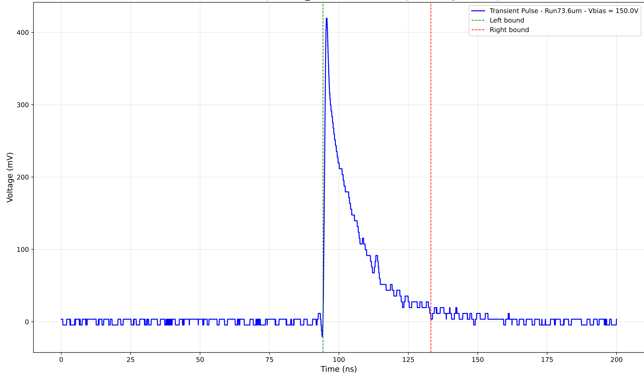
Transient Pulse - Sample: 1cm_42 - Position: 2255.0 \mu\text{m} - Charge: 82.08 pC
