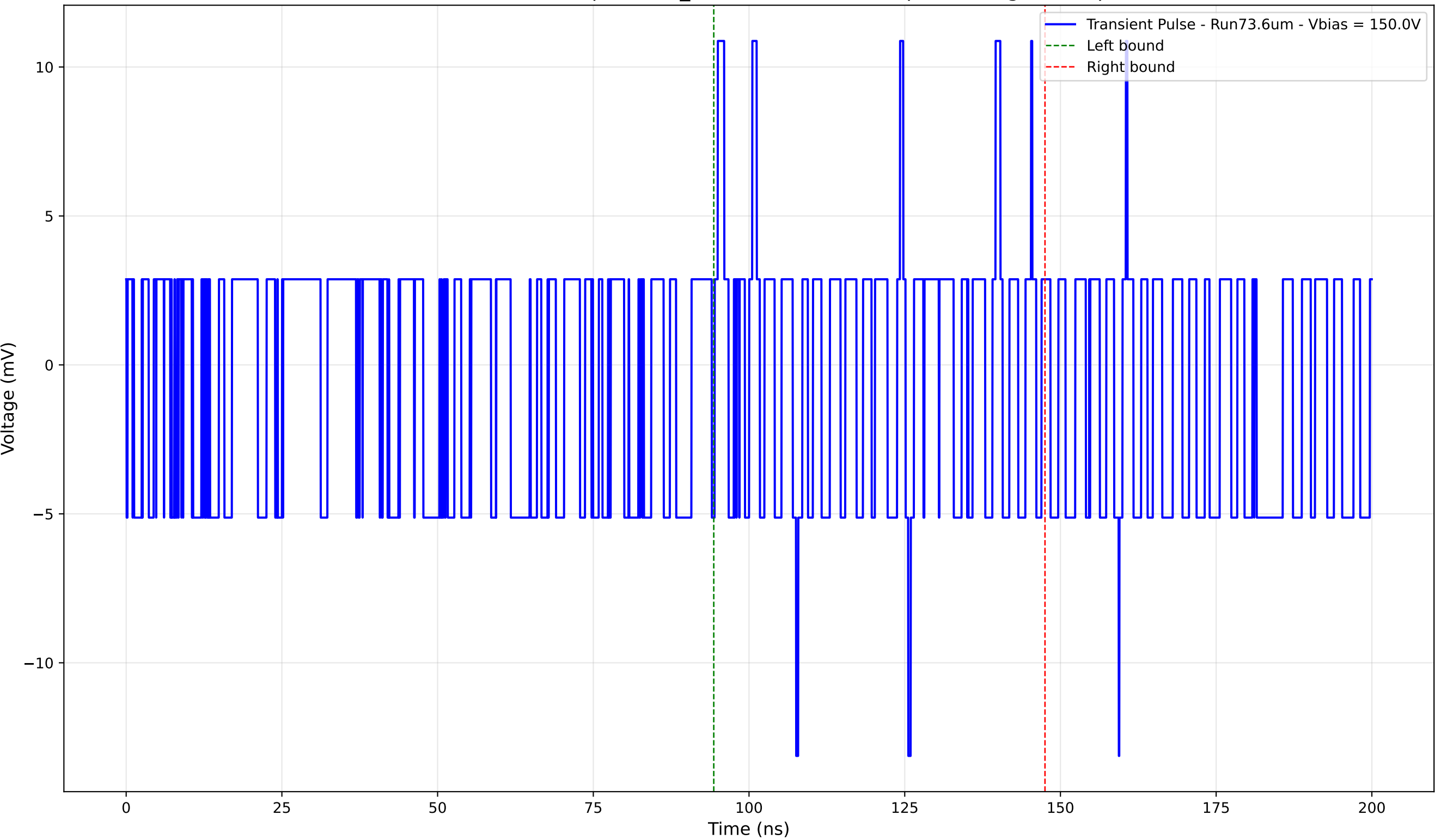
Transient Pulse - Sample: 1cm_42 - Position: 5035.0 \mu\text{m} - Charge: 0.42 pC
