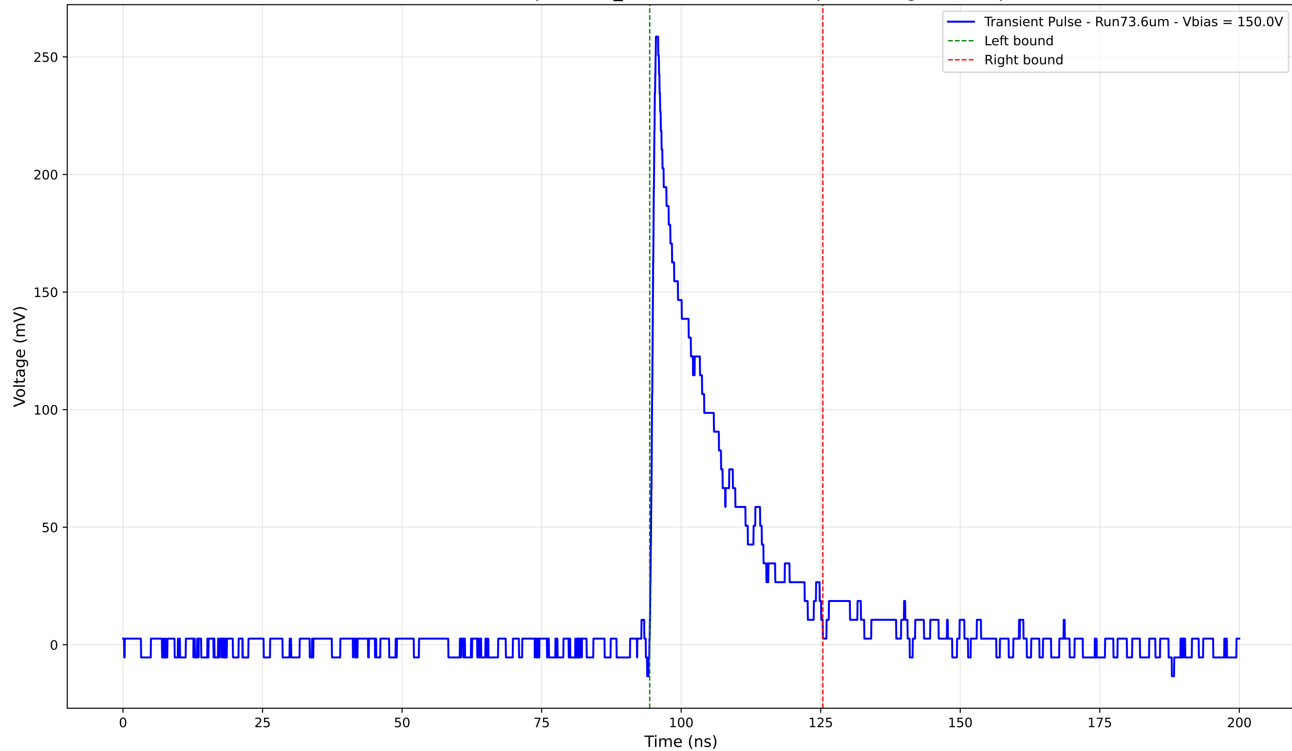
Transient Pulse - Sample: 1cm_42 - Position: 3545.0 \mu\text{m} - Charge: 50.47 pC
