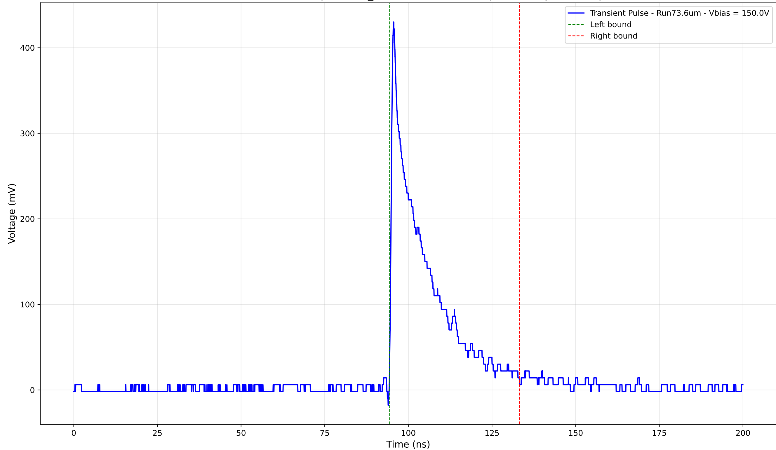
Transient Pulse - Sample: 1cm_42 - Position: 2180.0 \mu\text{m} - Charge: 84.02 pC
