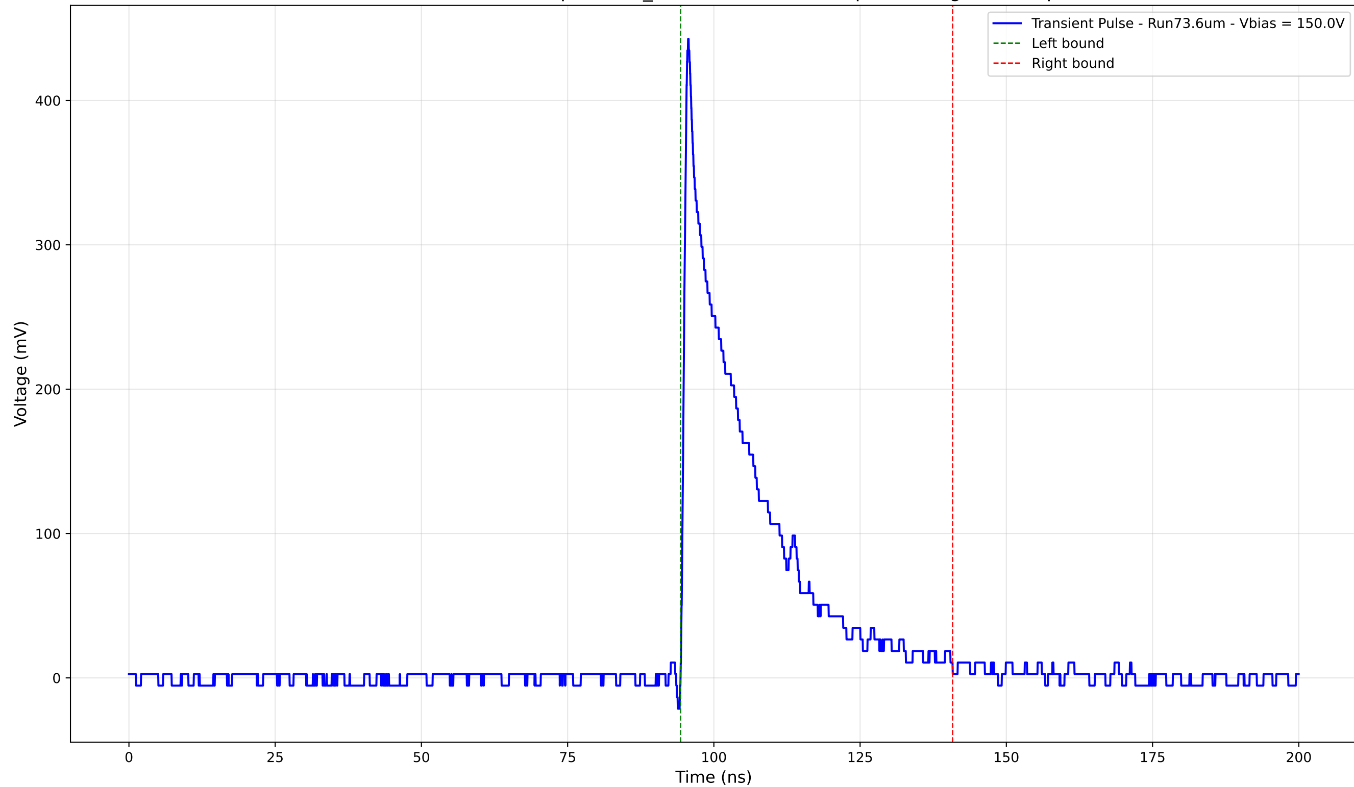
Transient Pulse - Sample: 1cm_42 - Position: 1805.0 \mu\text{m} - Charge: 92.76 pC
