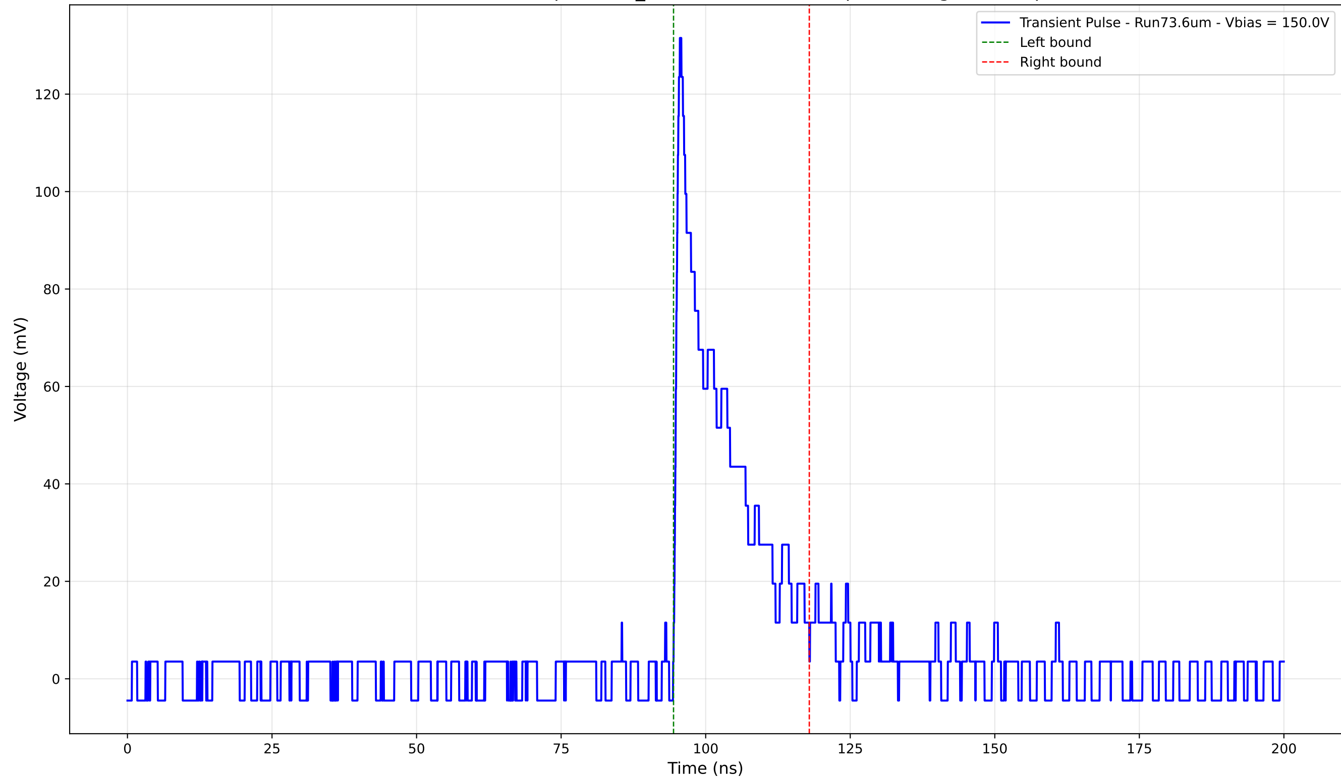
Transient Pulse - Sample: 1cm_42 - Position: 4660.0 \mu\text{m} - Charge: 21.72 pC
