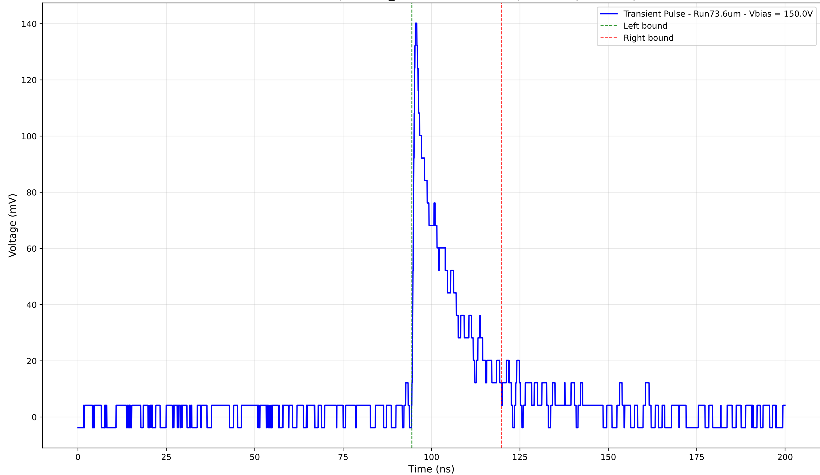
Transient Pulse - Sample: 1cm_42 - Position: 4615.0 \mu\text{m} - Charge: 24.23 pC
