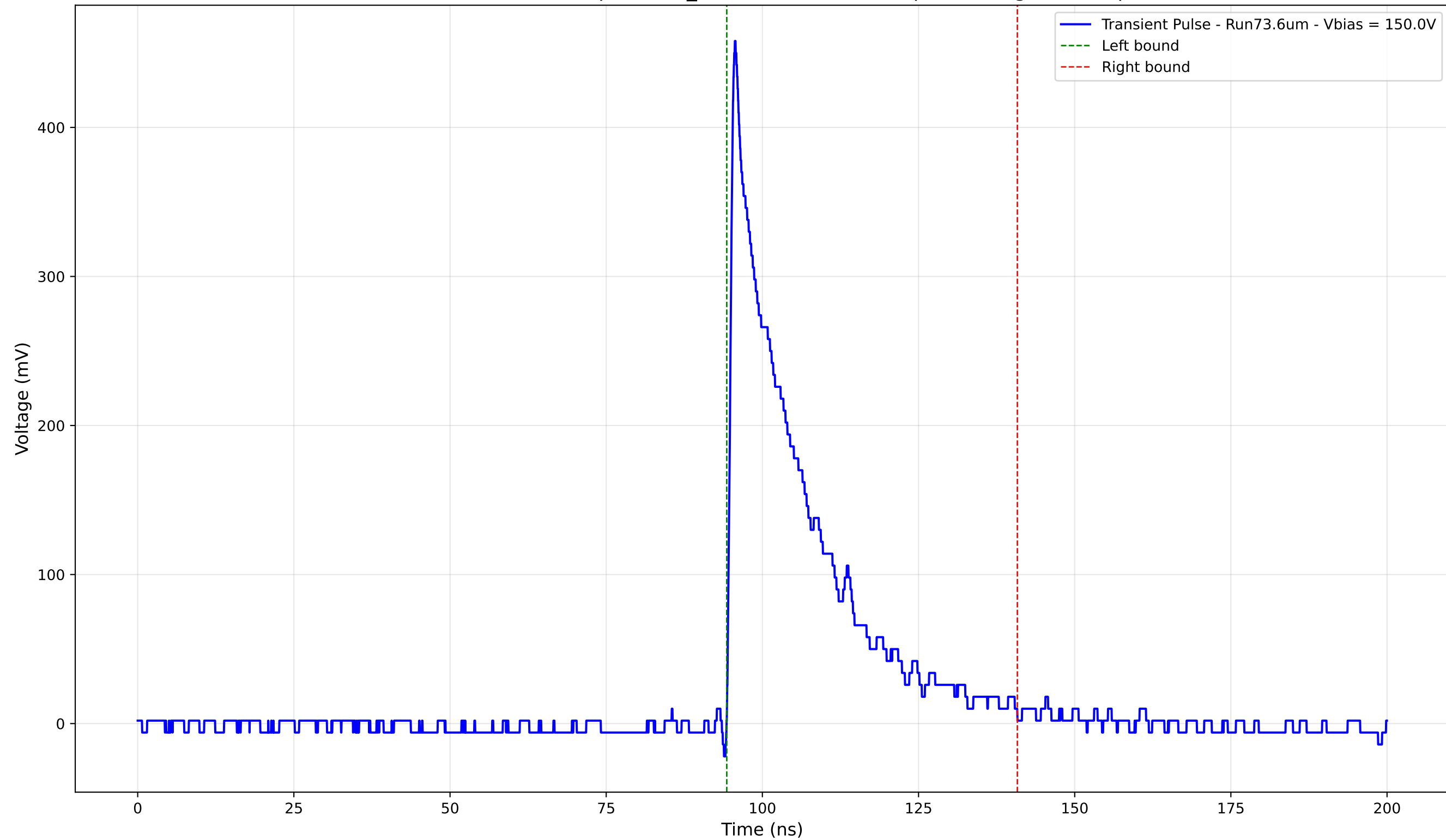
Transient Pulse - Sample: 1cm_42 - Position: 1380.0 \mu\text{m} - Charge: 99.74 pC
