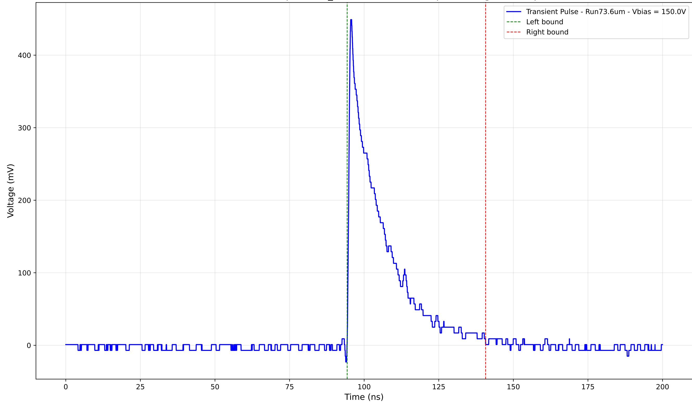
Transient Pulse - Sample: 1cm_42 - Position: 1410.0 \mu\text{m} - Charge: 97.58 pC
