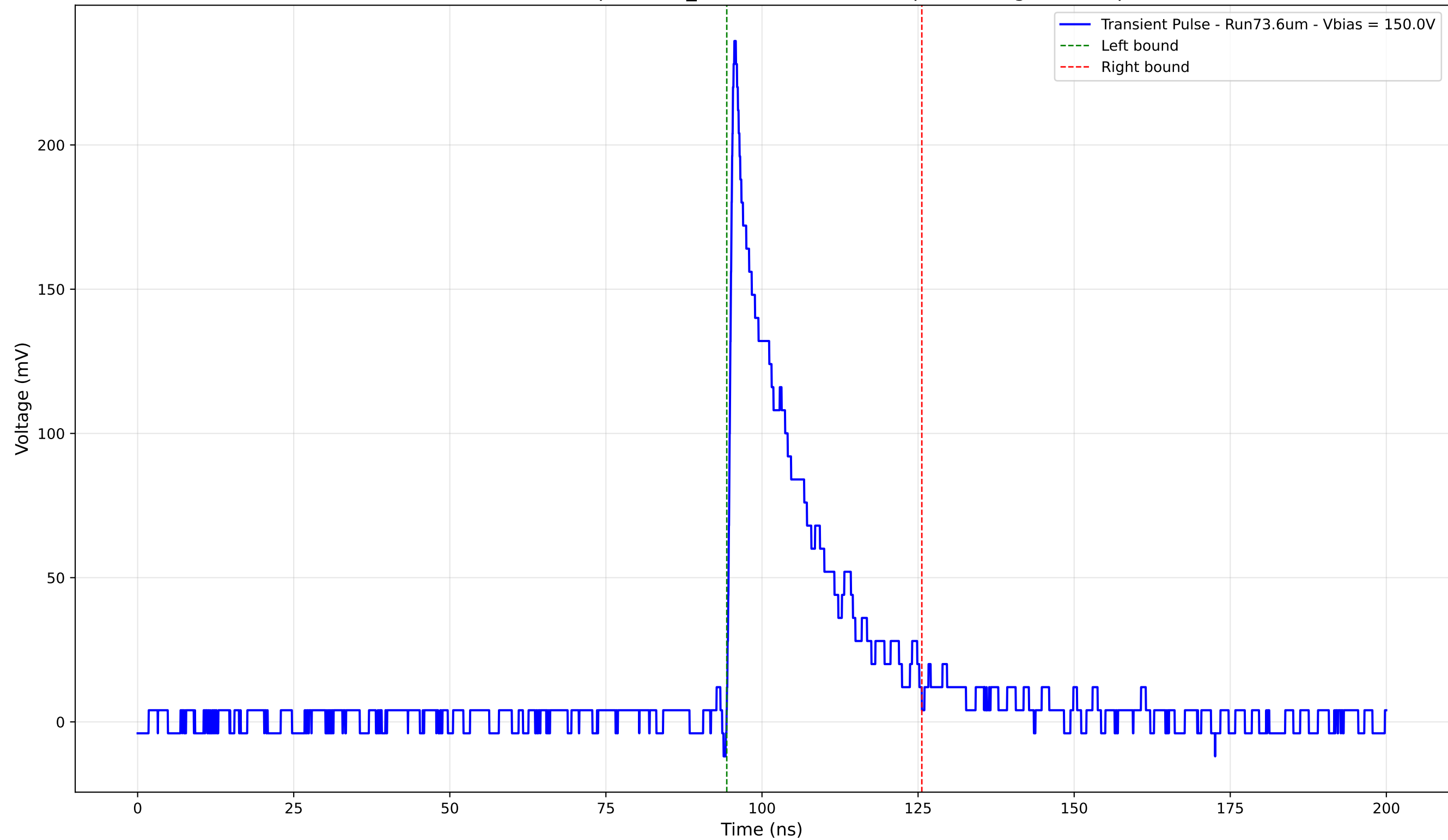
Transient Pulse - Sample: 1cm_42 - Position: 3690.0 \mu\text{m} - Charge: 46.21 pC
