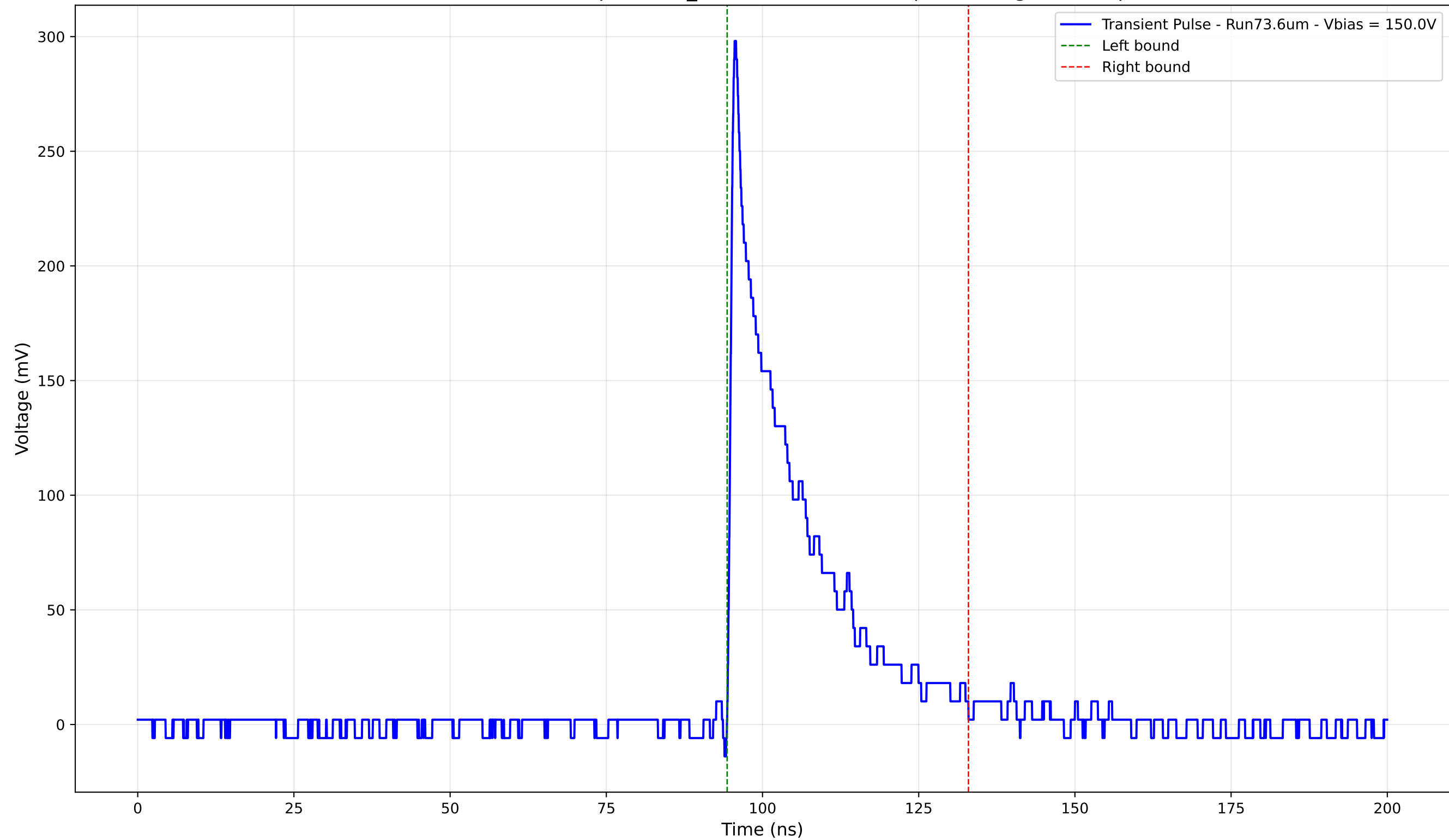
Transient Pulse - Sample: 1cm_42 - Position: 3295.0 \mu\text{m} - Charge: 57.96 pC
