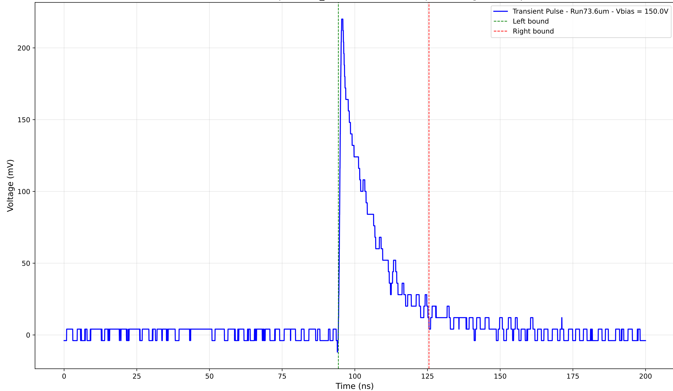
Transient Pulse - Sample: 1cm_42 - Position: 3800.0 \mu\text{m} - Charge: 44.21 pC
