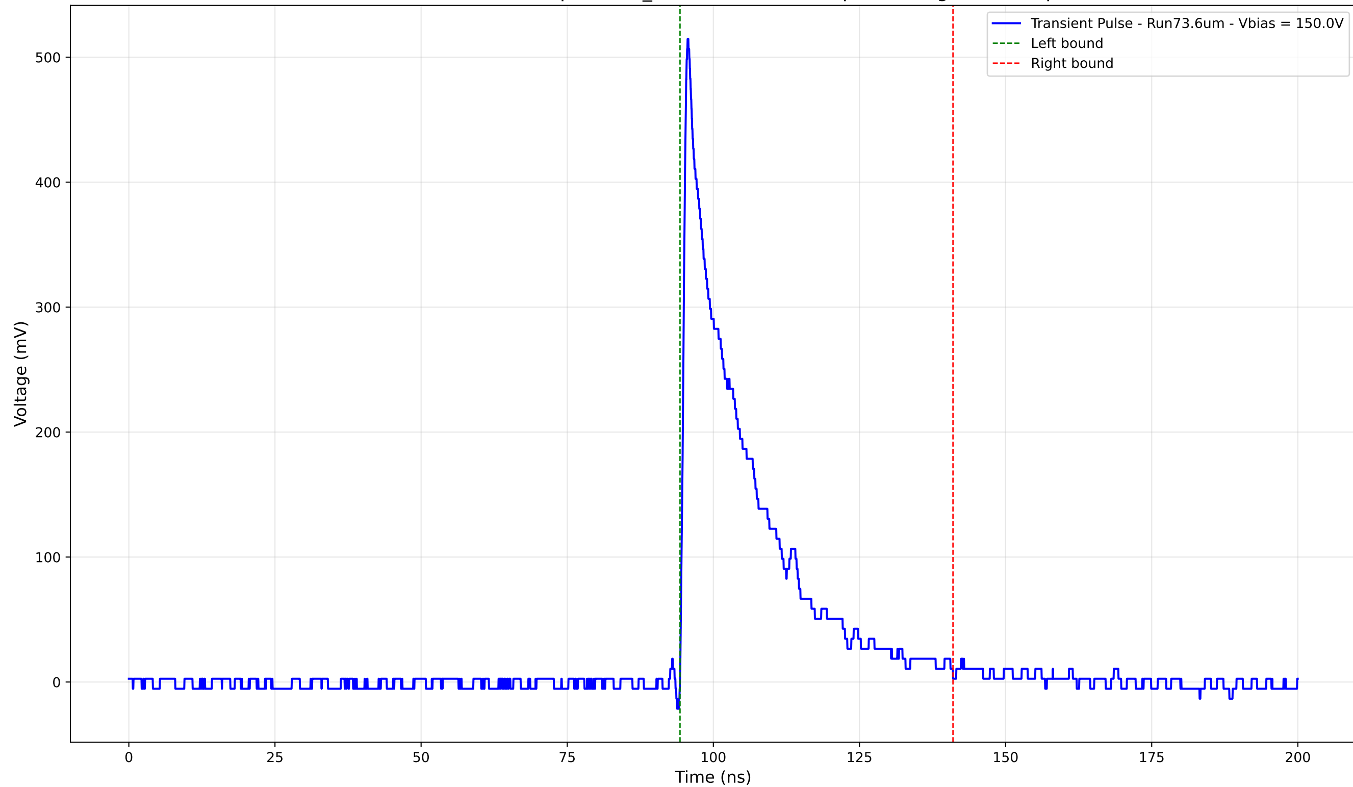
Transient Pulse - Sample: 1cm_42 - Position: 600.0 \mu\text{m} - Charge: 107.24 pC
