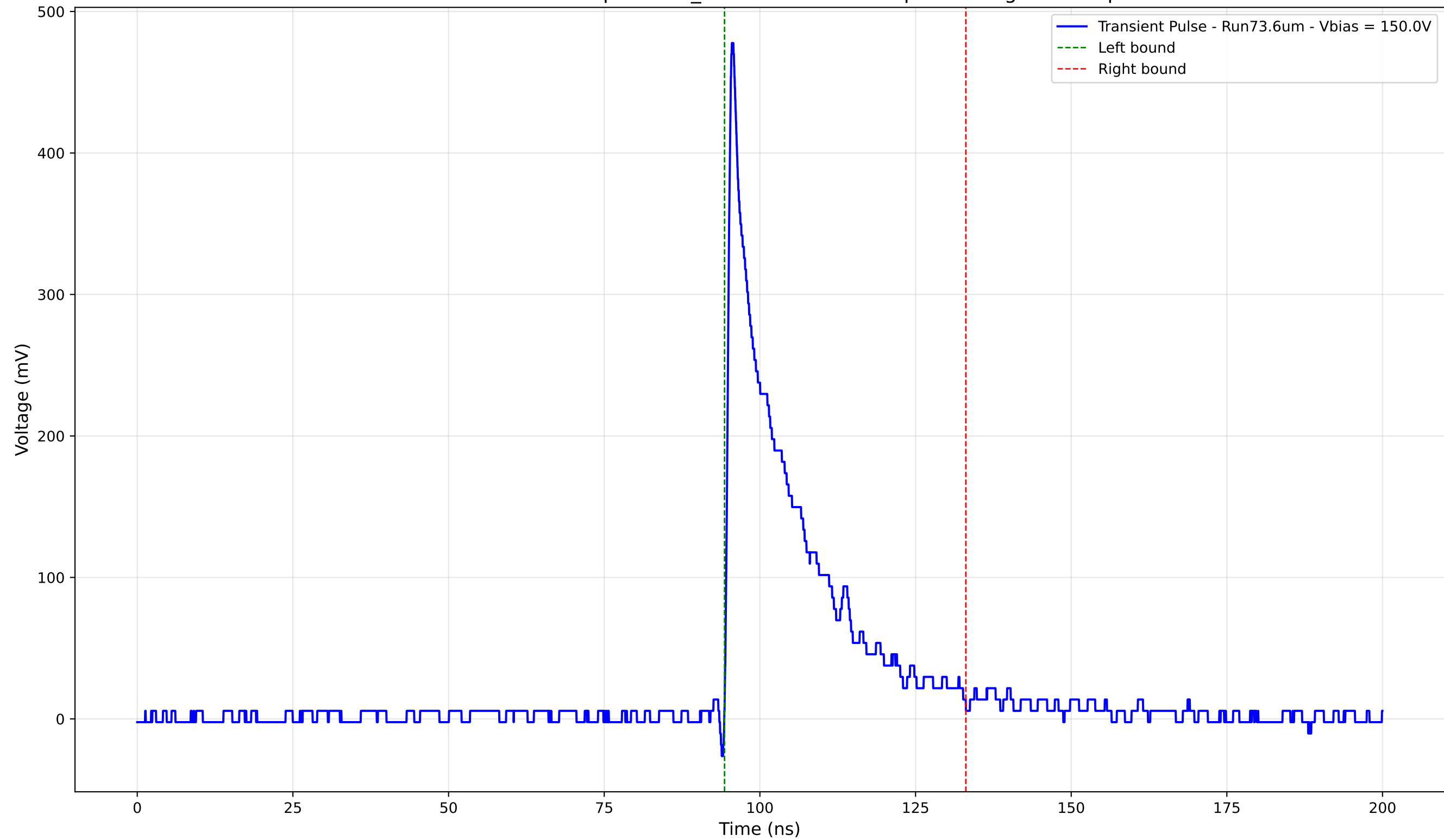
Transient Pulse - Sample: 1cm_42 - Position: 185.0 \mu\text{m} - Charge: 89.15 pC
