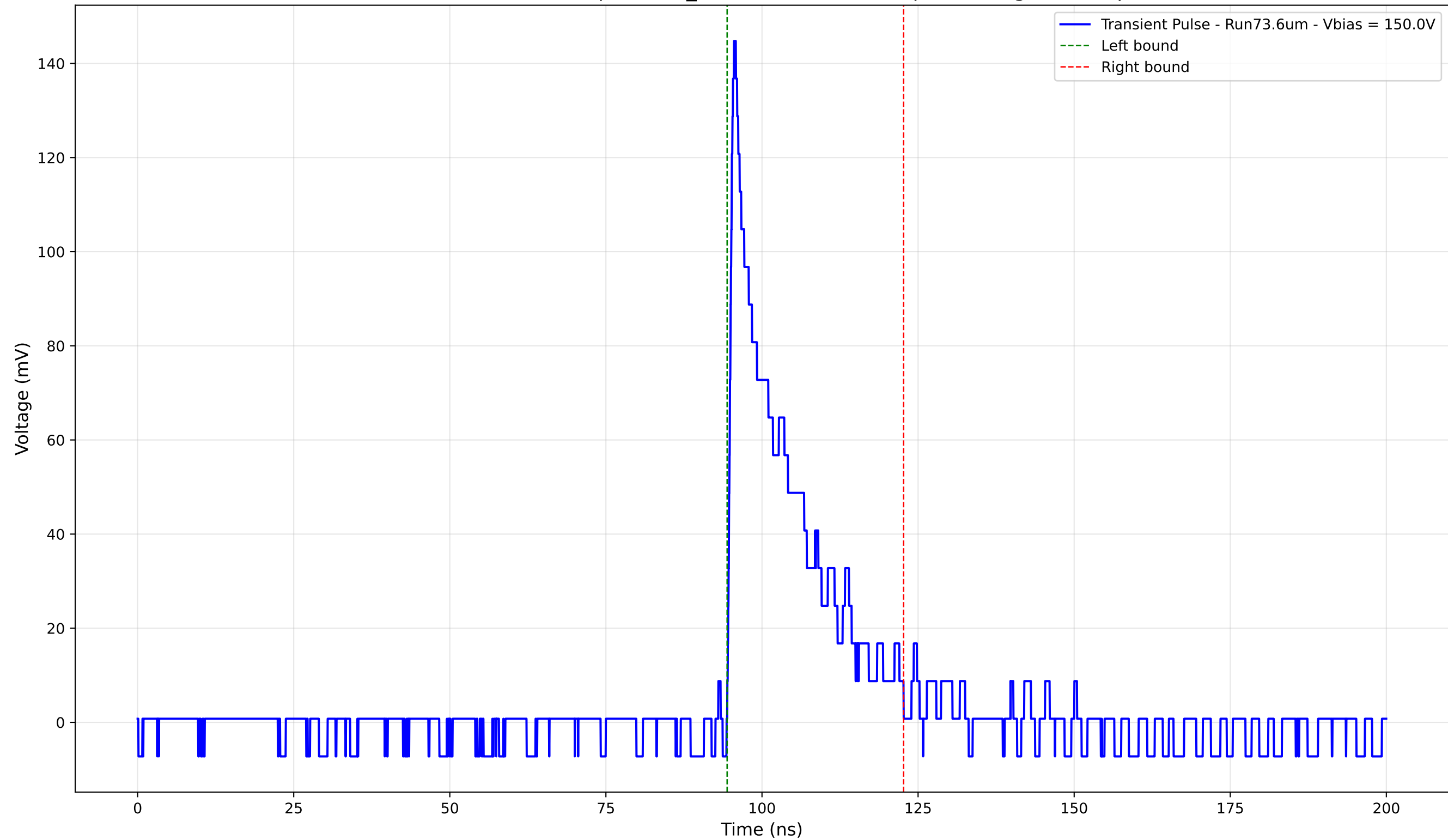
Transient Pulse - Sample: 1cm_42 - Position: 4540.0 \mu\text{m} - Charge: 24.99 pC
