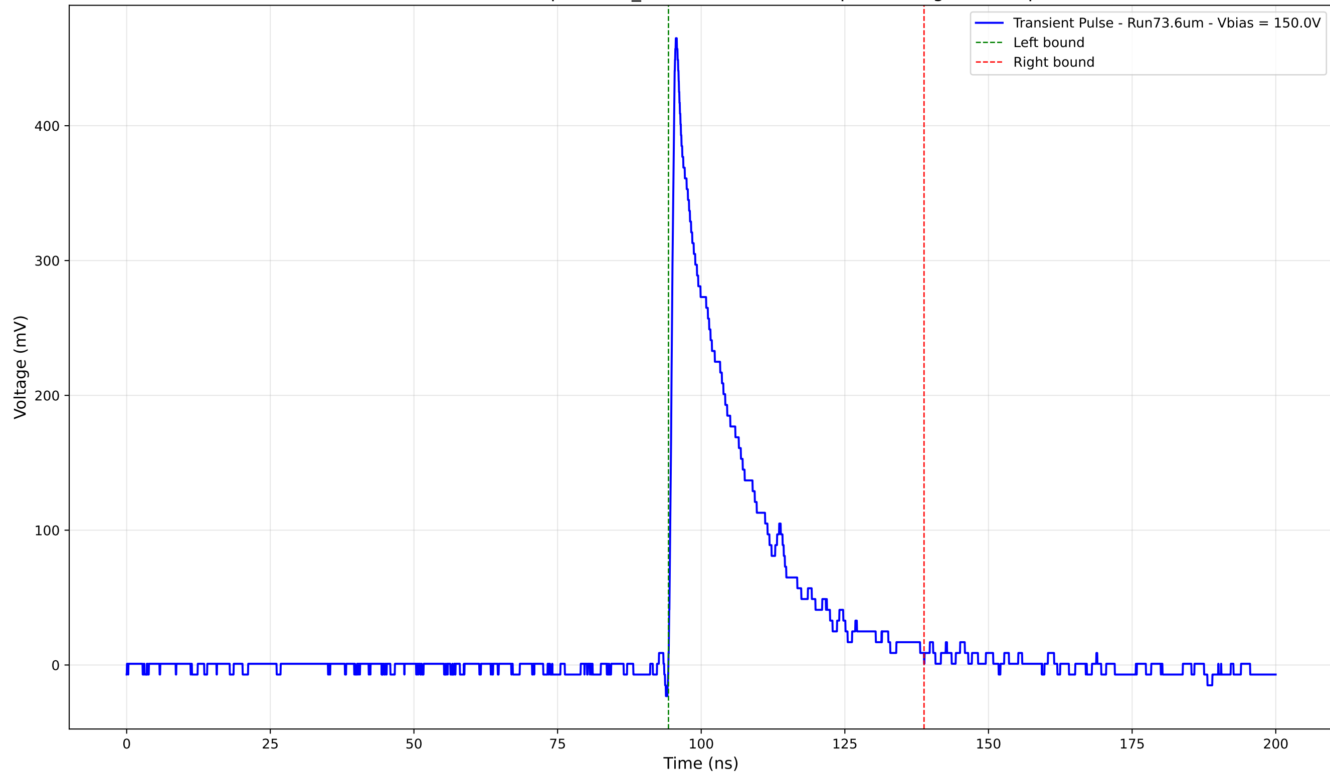
Transient Pulse - Sample: 1cm_42 - Position: 1015.0 \mu\text{m} - Charge: 99.55 pC
