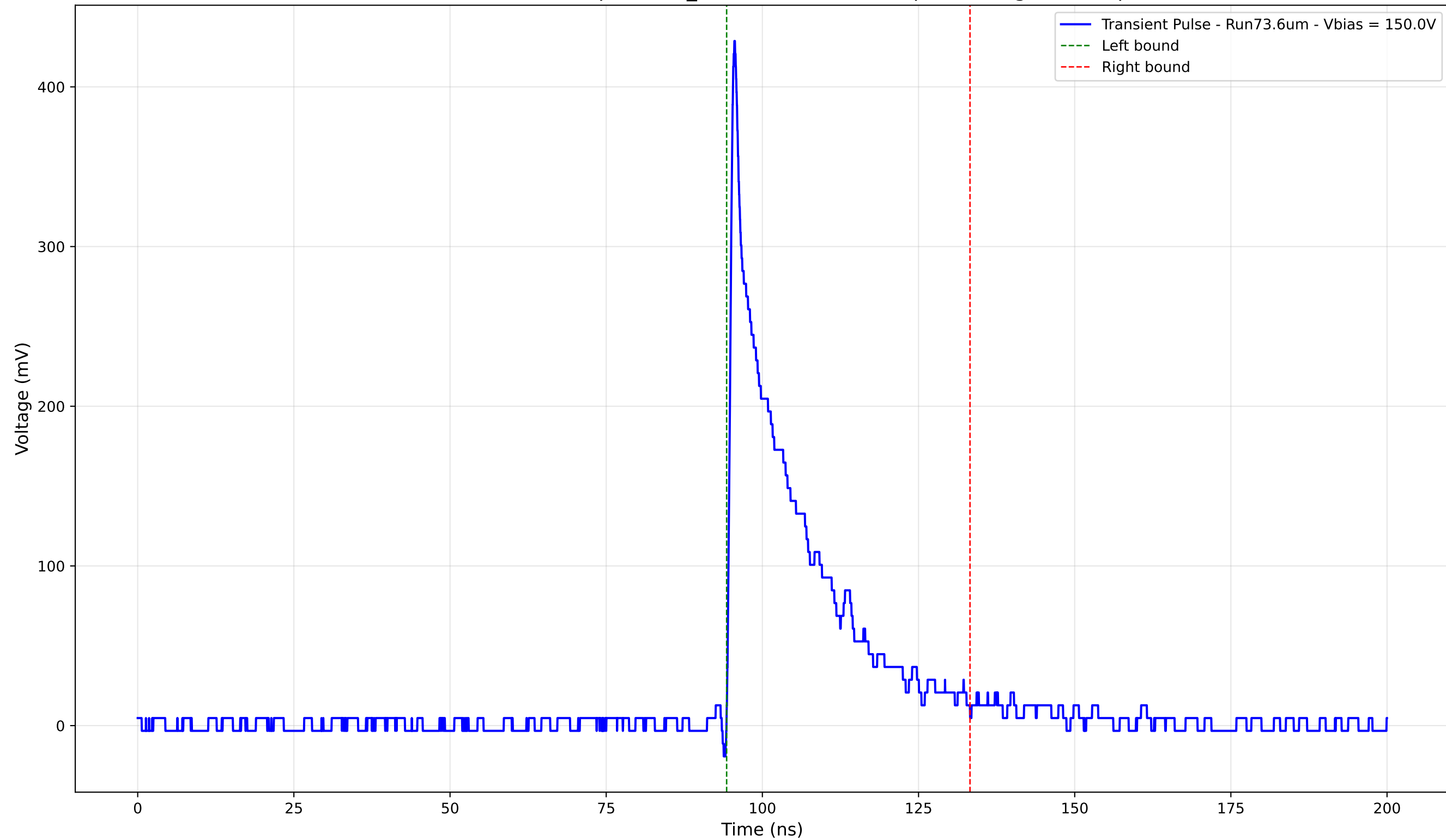
Transient Pulse - Sample: 1cm_42 - Position: 2550.0 \mu\text{m} - Charge: 78.85 pC
