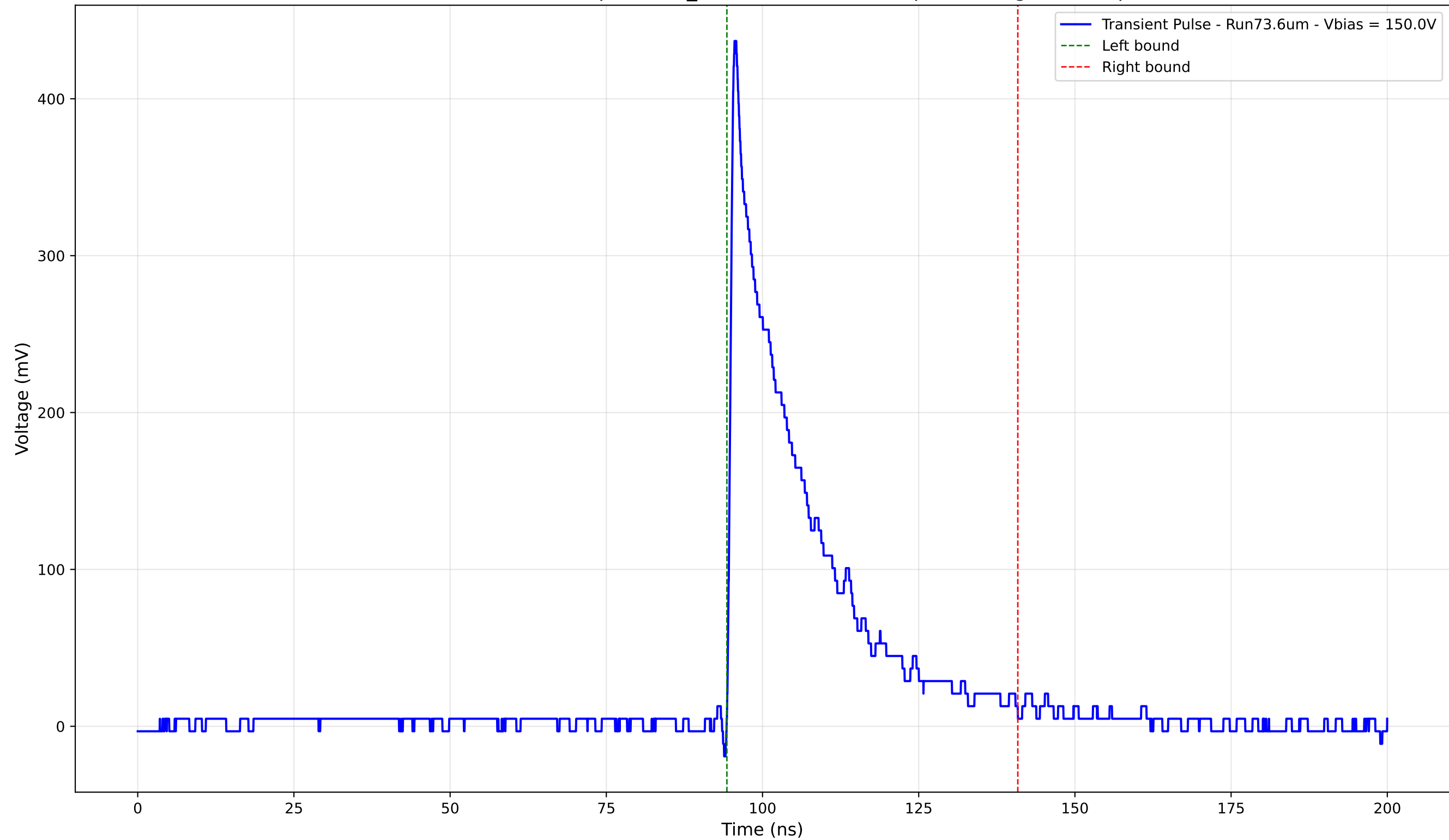
Transient Pulse - Sample: 1cm_42 - Position: 1690.0 \mu\text{m} - Charge: 96.75 pC
