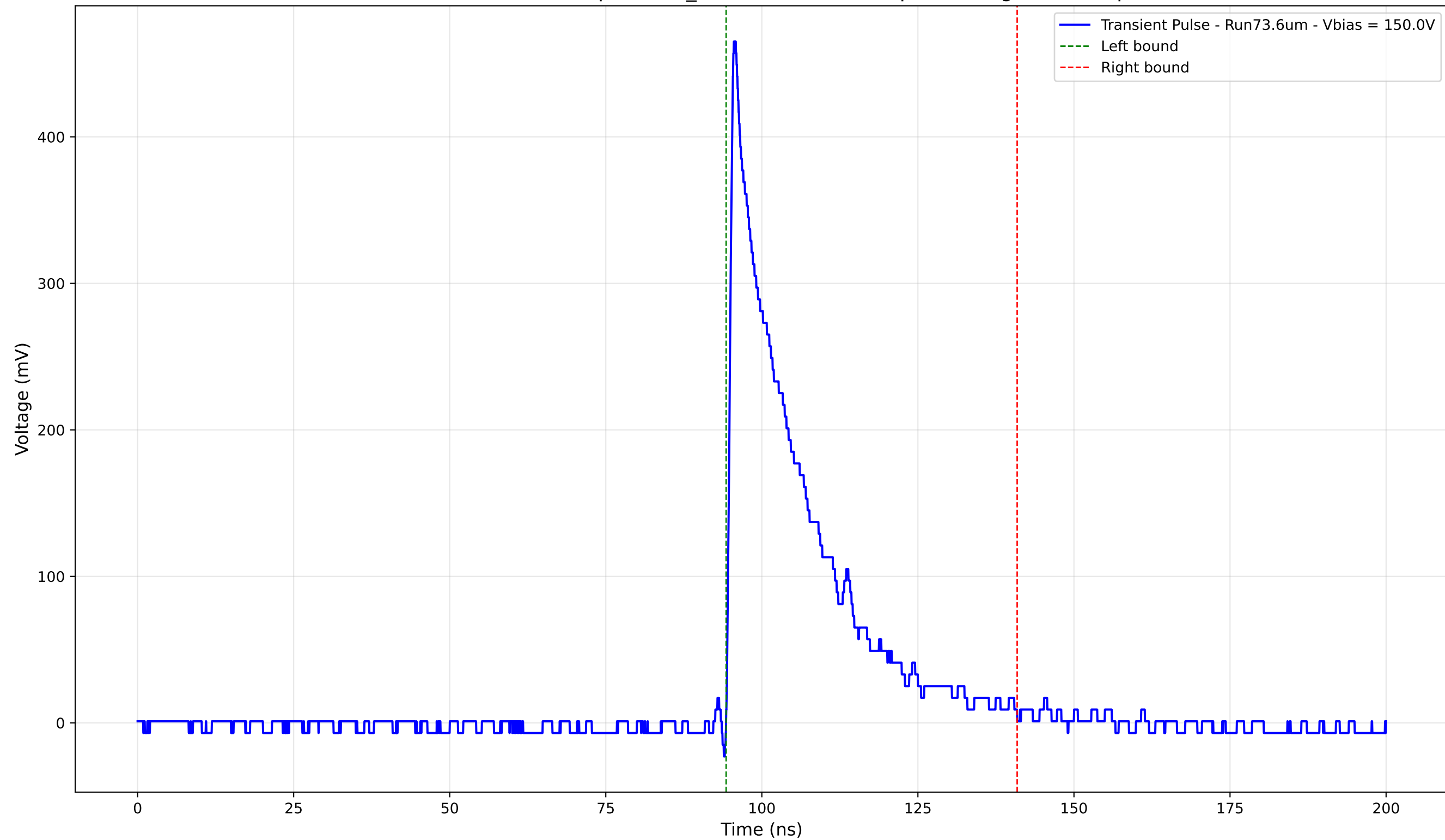
Transient Pulse - Sample: 1cm_42 - Position: 985.0 \mu\text{m} - Charge: 100.88 pC
