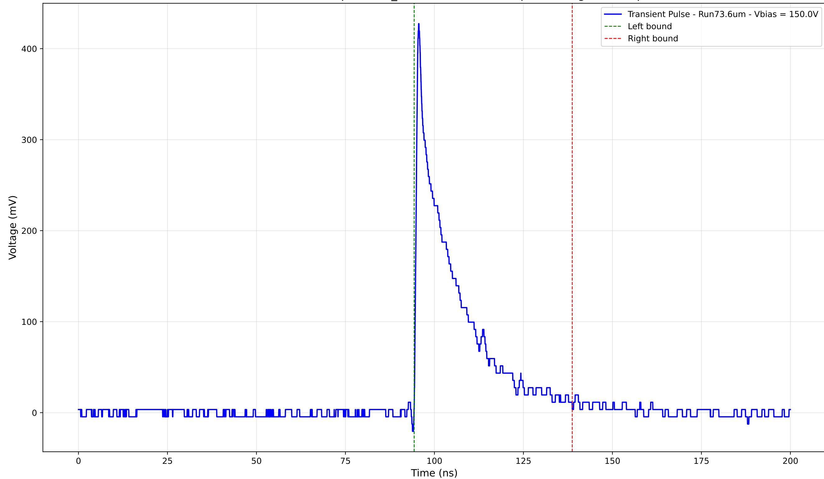
Transient Pulse - Sample: 1cm_42 - Position: 2120.0 \mu\text{m} - Charge: 86.39 pC
