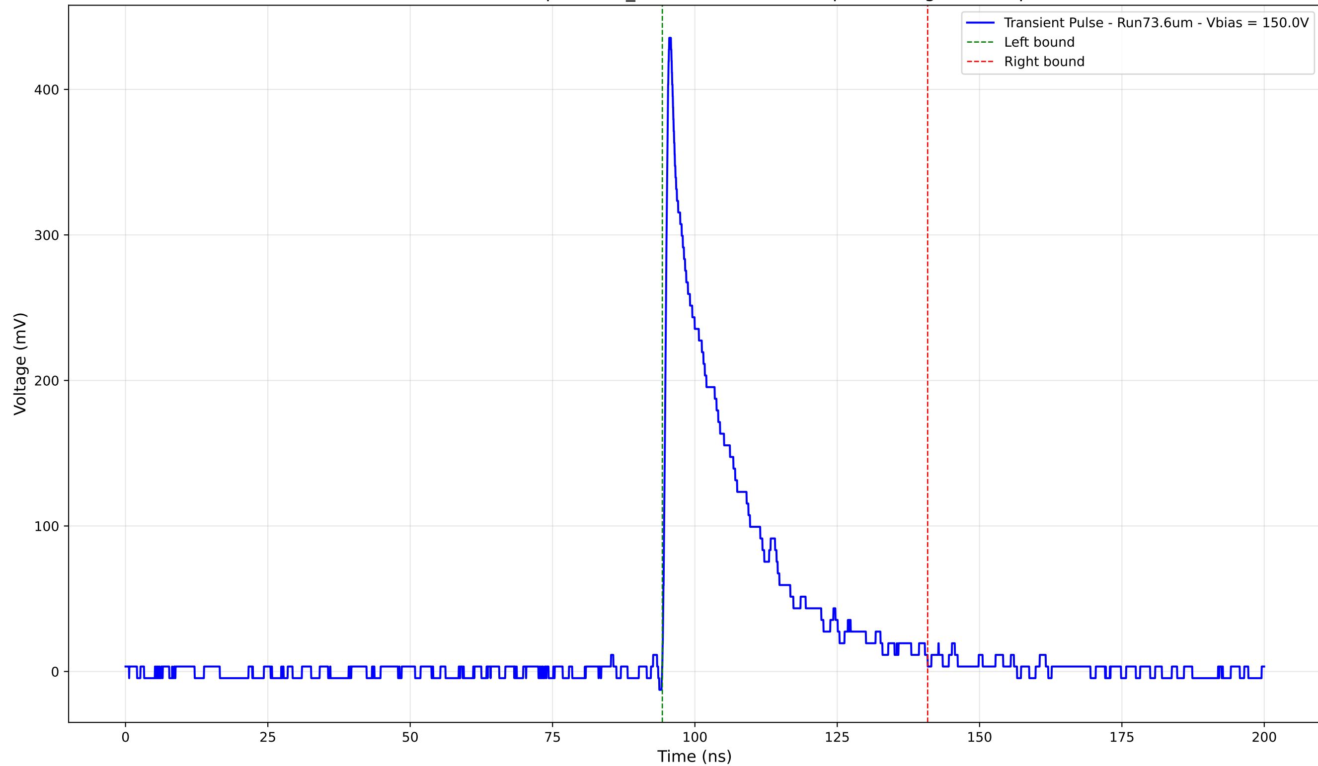
Transient Pulse - Sample: 1cm_42 - Position: 2020.0 \mu\text{m} - Charge: 90.82 pC
