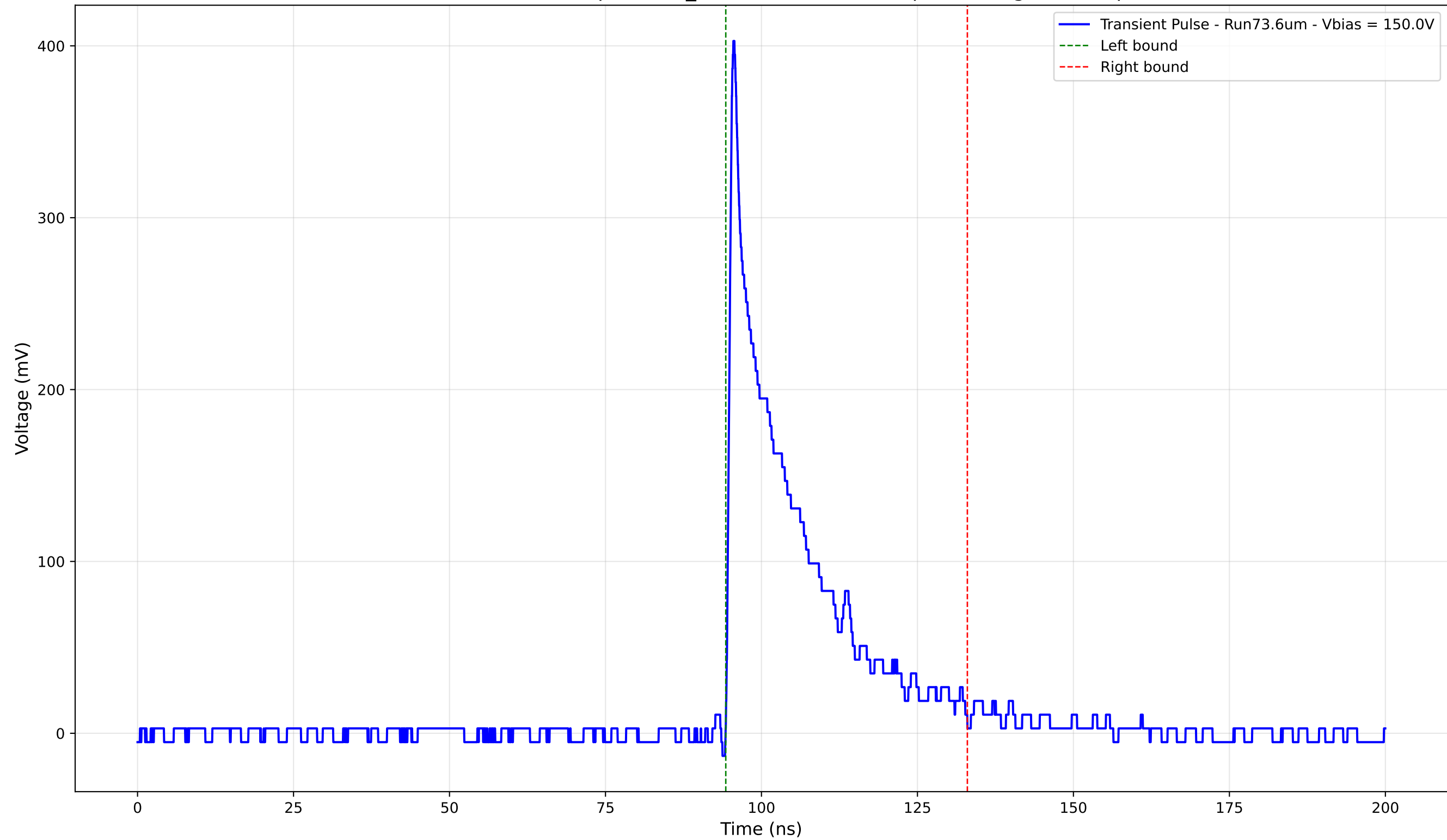
Transient Pulse - Sample: 1cm_42 - Position: 2830.0 \mu\text{m} - Charge: 74.62 pC
