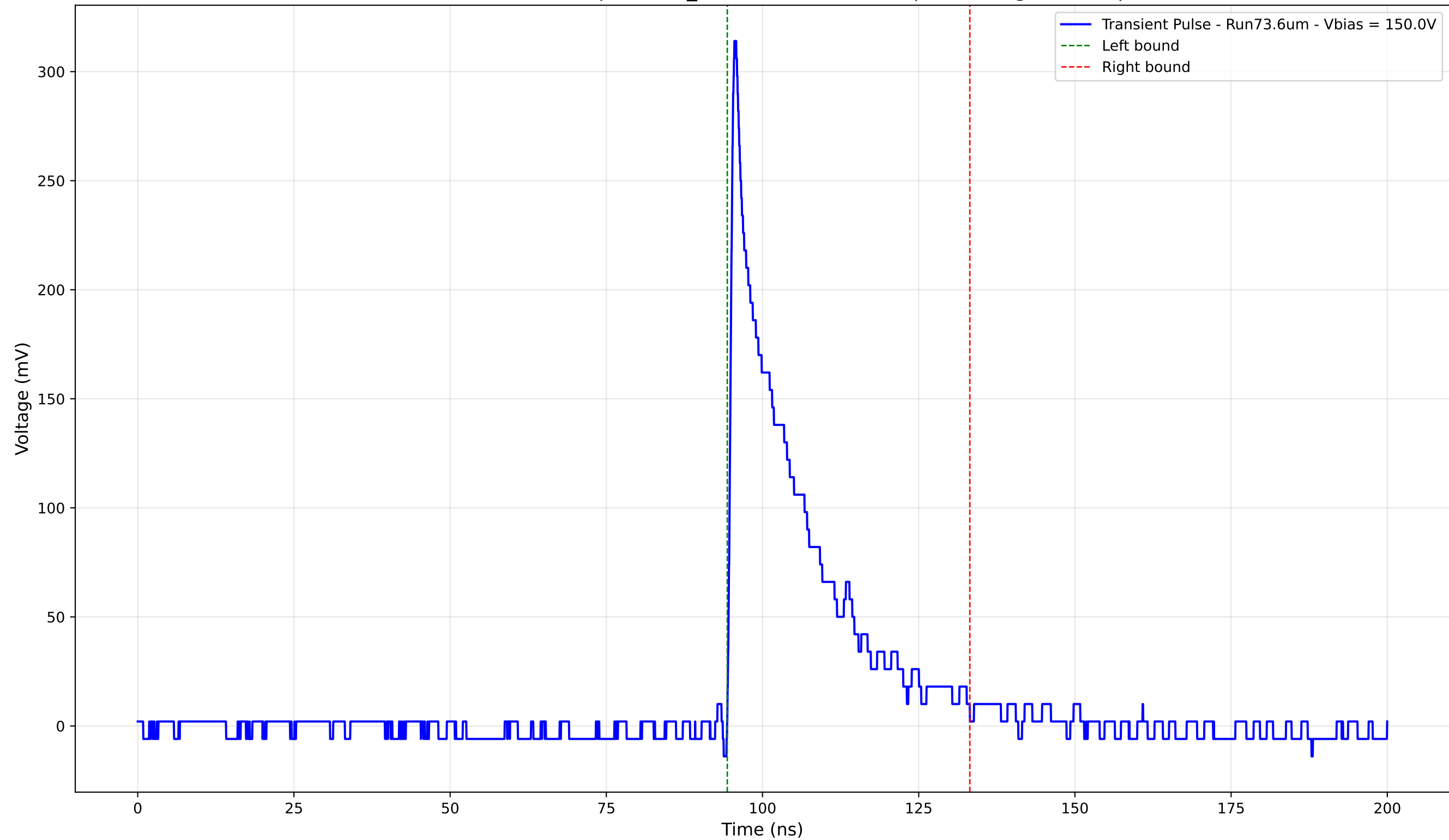
Transient Pulse - Sample: 1cm_42 - Position: 3175.0 \mu\text{m} - Charge: 60.71 pC
