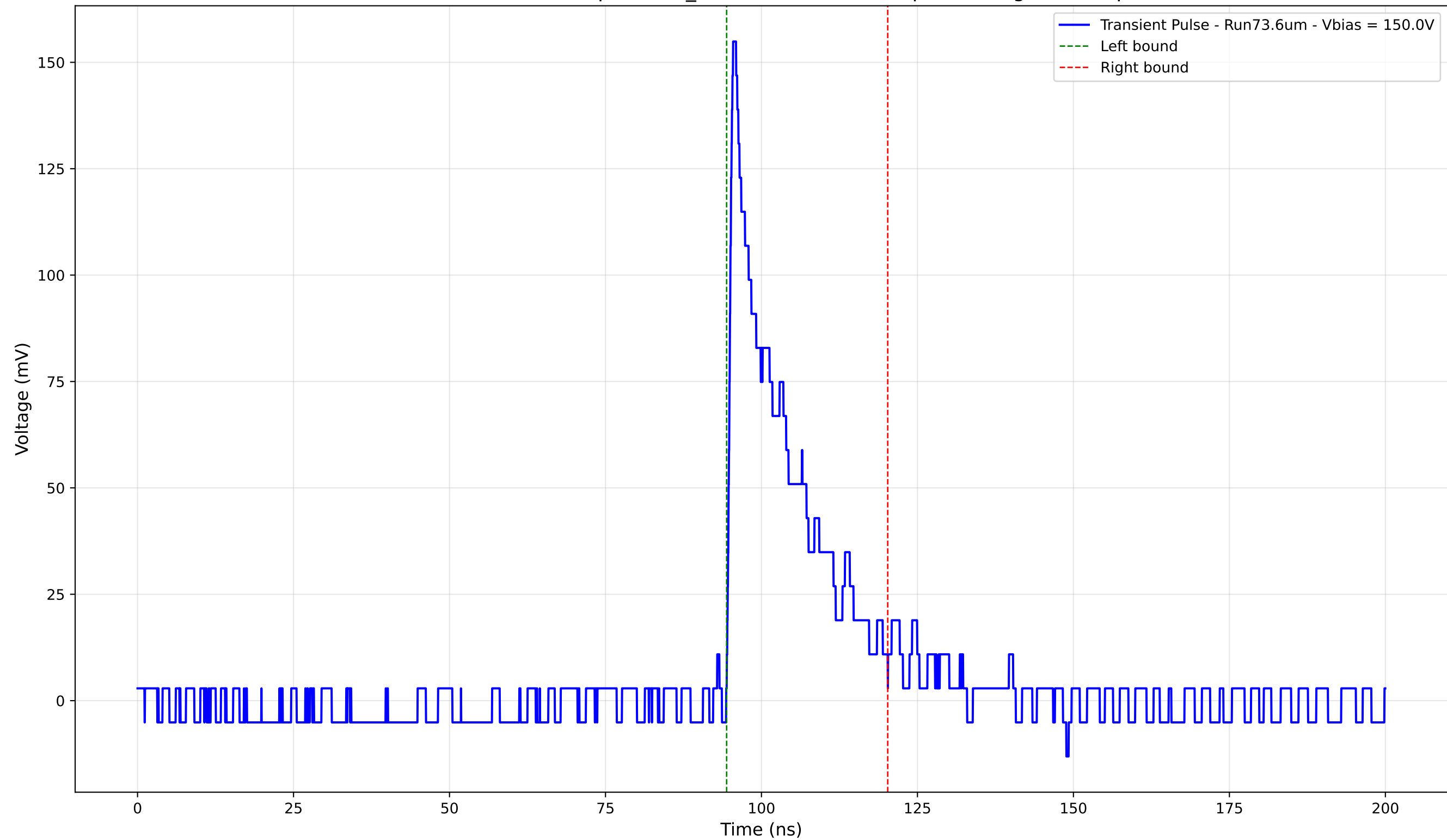
Transient Pulse - Sample: 1cm_42 - Position: 4420.0 \mu\text{m} - Charge: 27.54 pC
