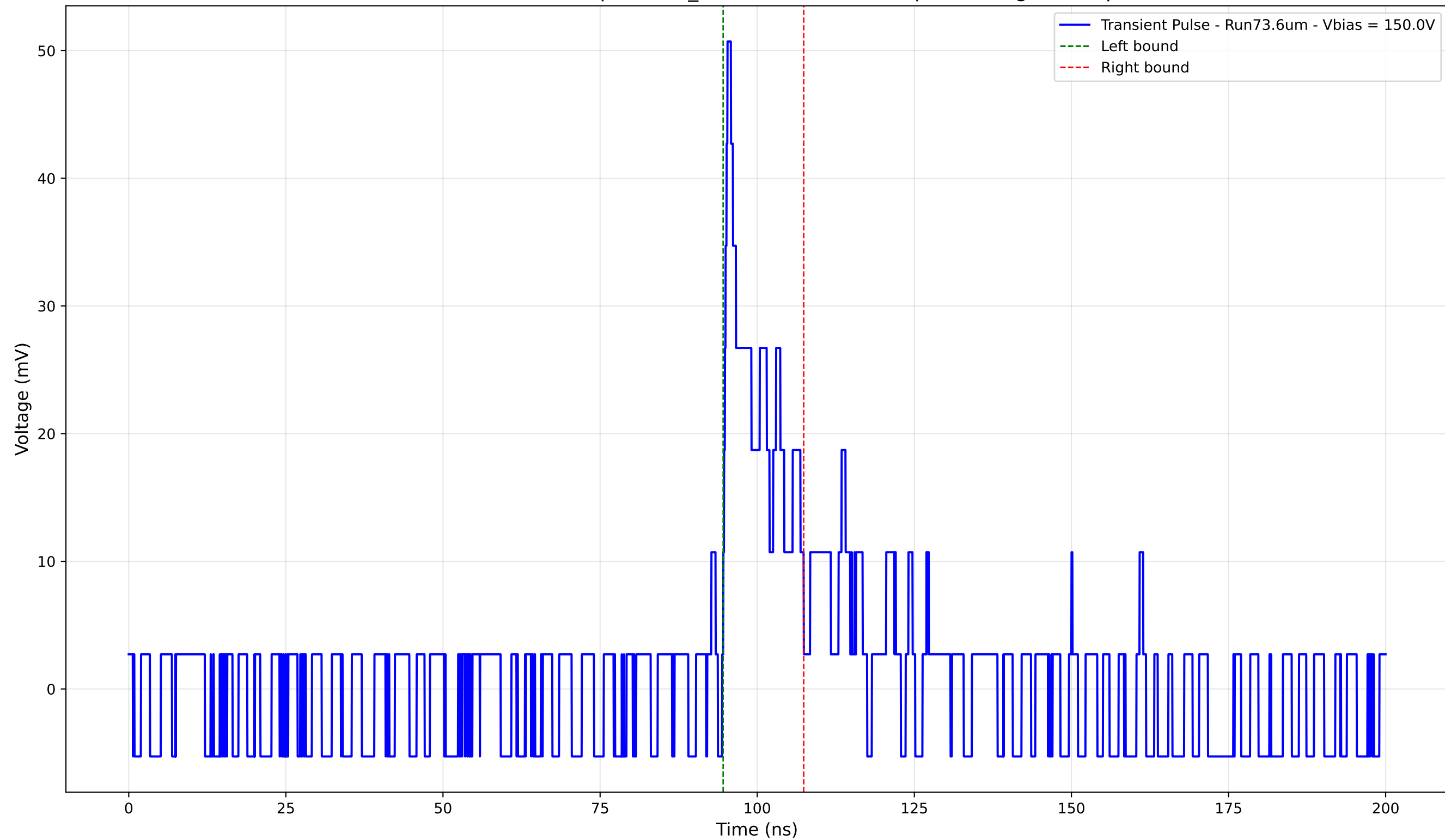
Transient Pulse - Sample: 1cm_42 - Position: 4930.0 \mu\text{m} - Charge: 5.86 pC
