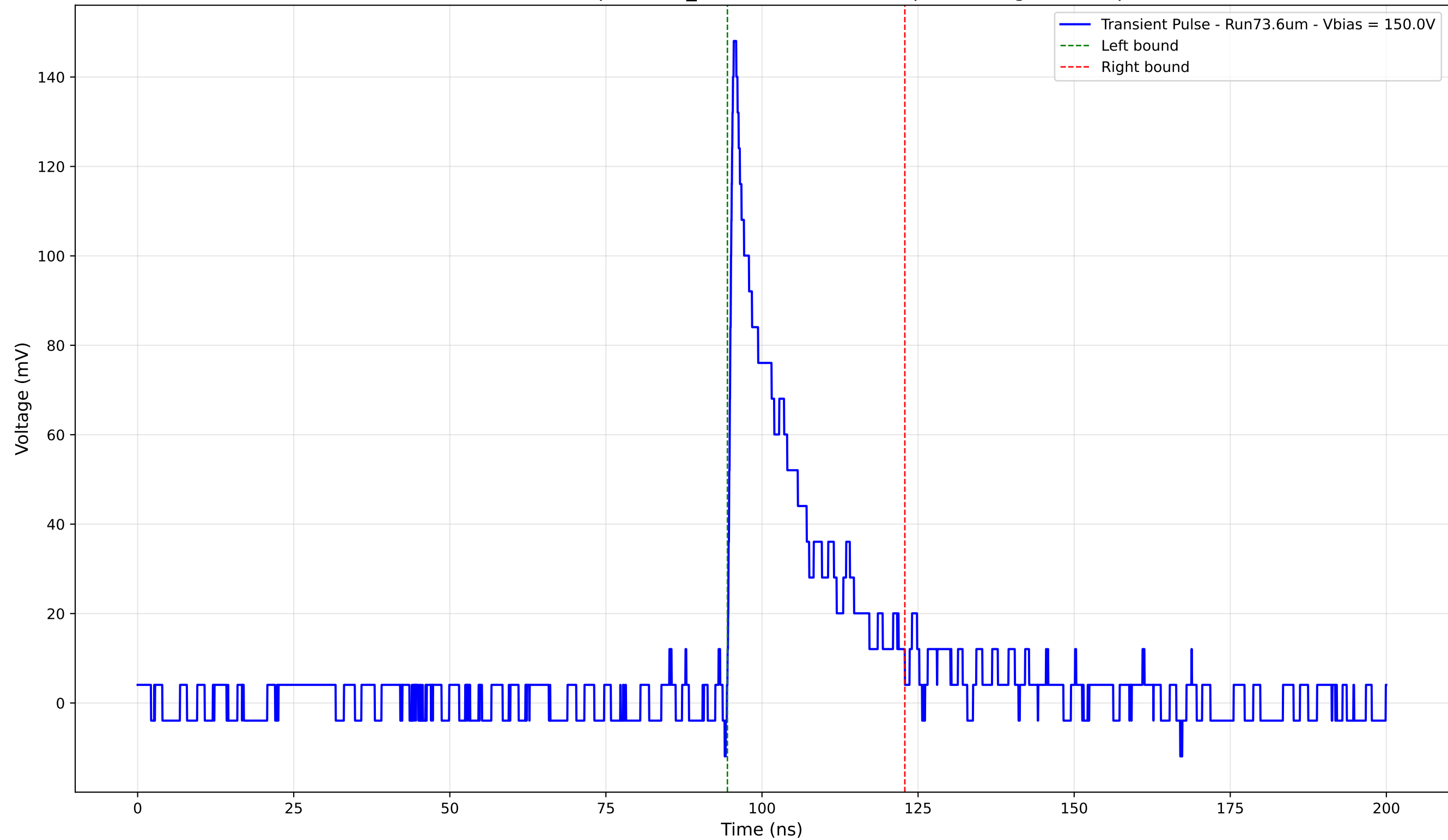
Transient Pulse - Sample: 1cm_42 - Position: 4485.0 \mu\text{m} - Charge: 26.67 pC
