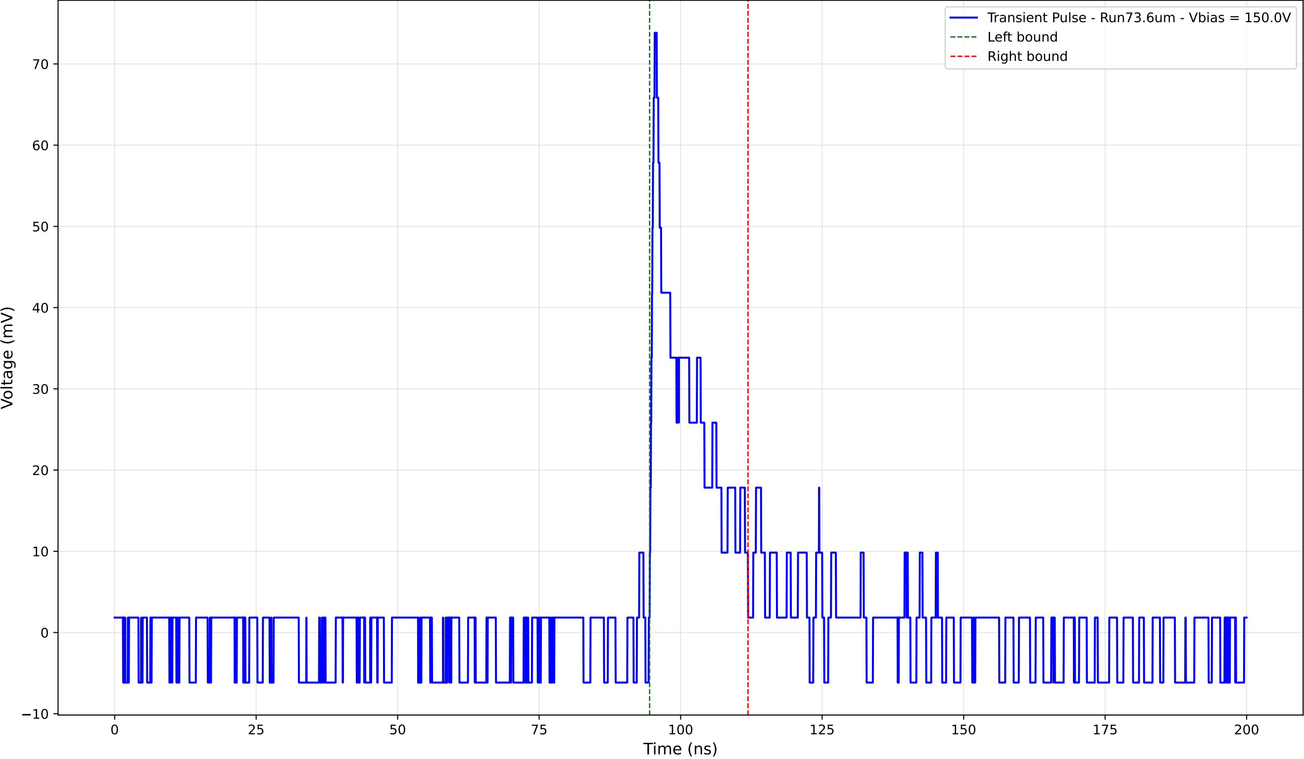
Transient Pulse - Sample: 1cm_42 - Position: 4910.0 \mu\text{m} - Charge: 9.70 pC
