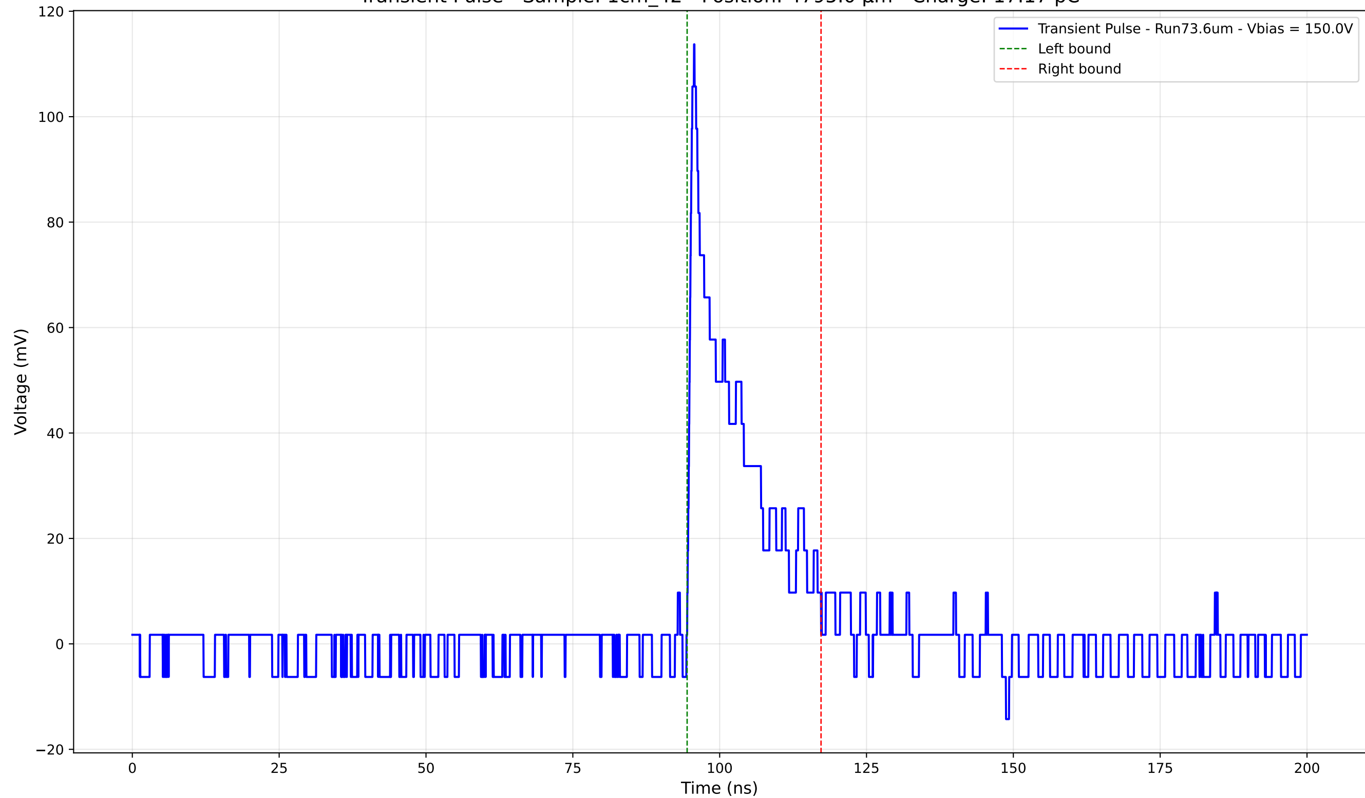
Transient Pulse - Sample: 1cm_42 - Position: 4795.0 \mu\text{m} - Charge: 17.17 pC
