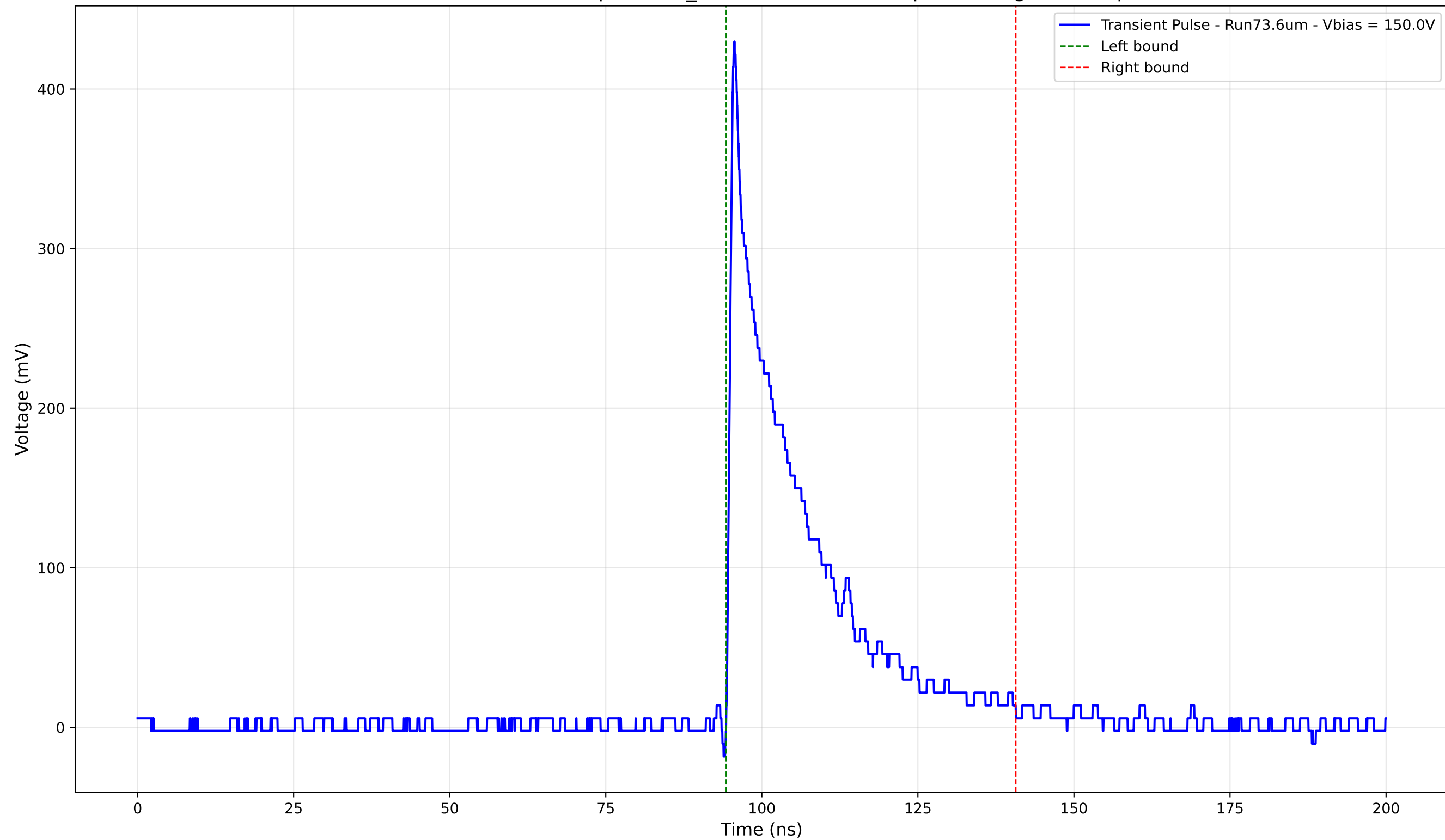
Transient Pulse - Sample: 1cm_42 - Position: 2100.0 \mu\text{m} - Charge: 88.51 pC
