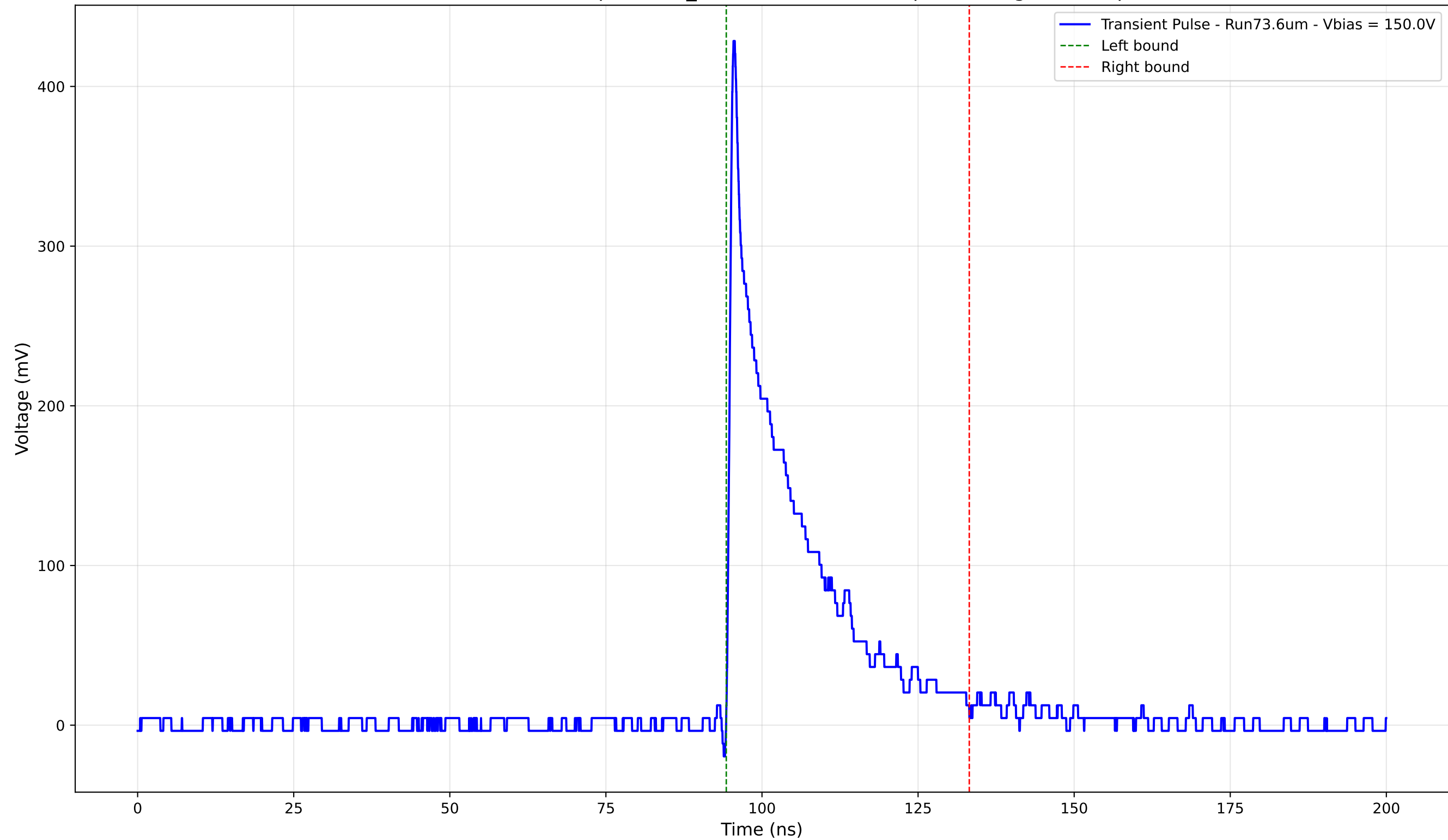
Transient Pulse - Sample: 1cm_42 - Position: 2640.0 \mu\text{m} - Charge: 78.84 pC
