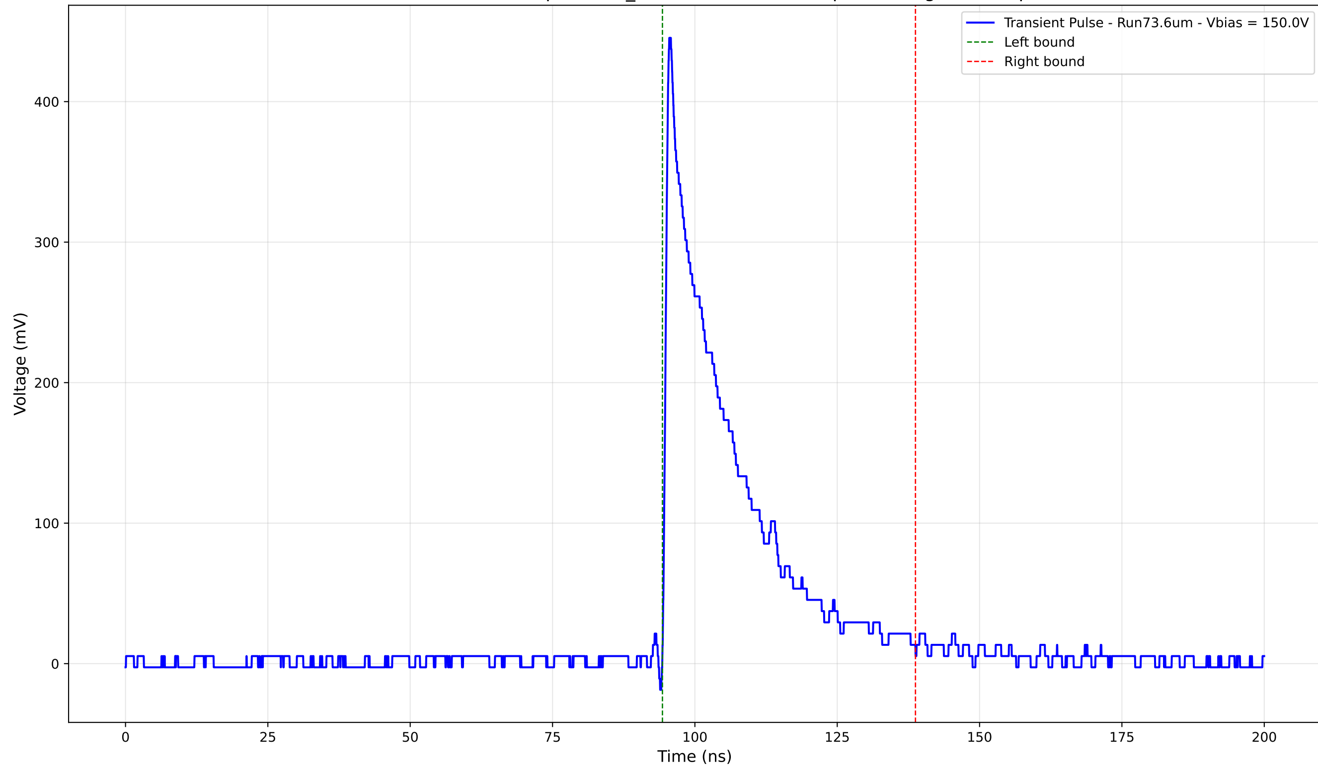
Transient Pulse - Sample: 1cm_42 - Position: 1520.0 \mu\text{m} - Charge: 98.58 pC
