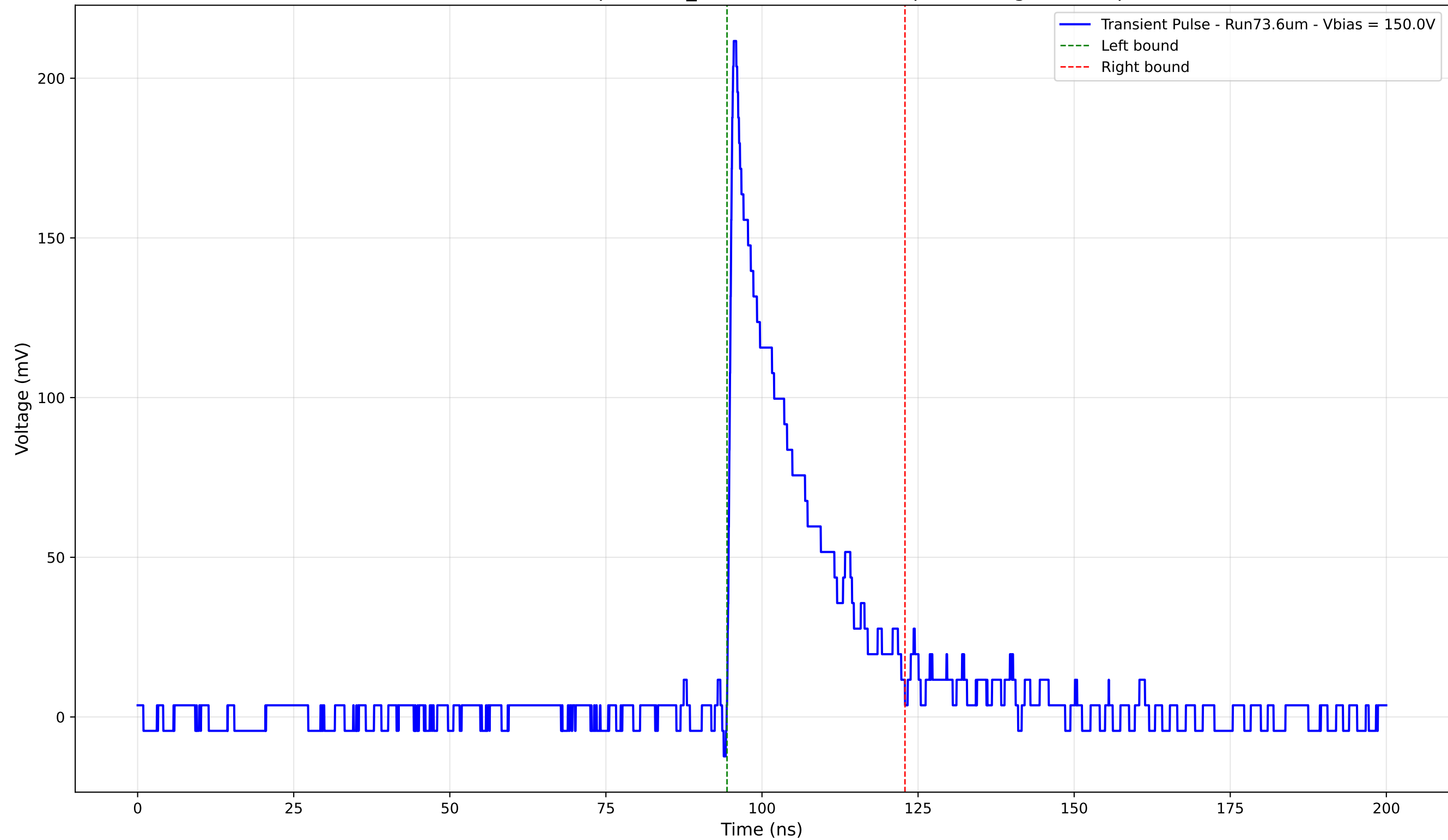
Transient Pulse - Sample: 1cm_42 - Position: 3885.0 \mu\text{m} - Charge: 41.29 pC
