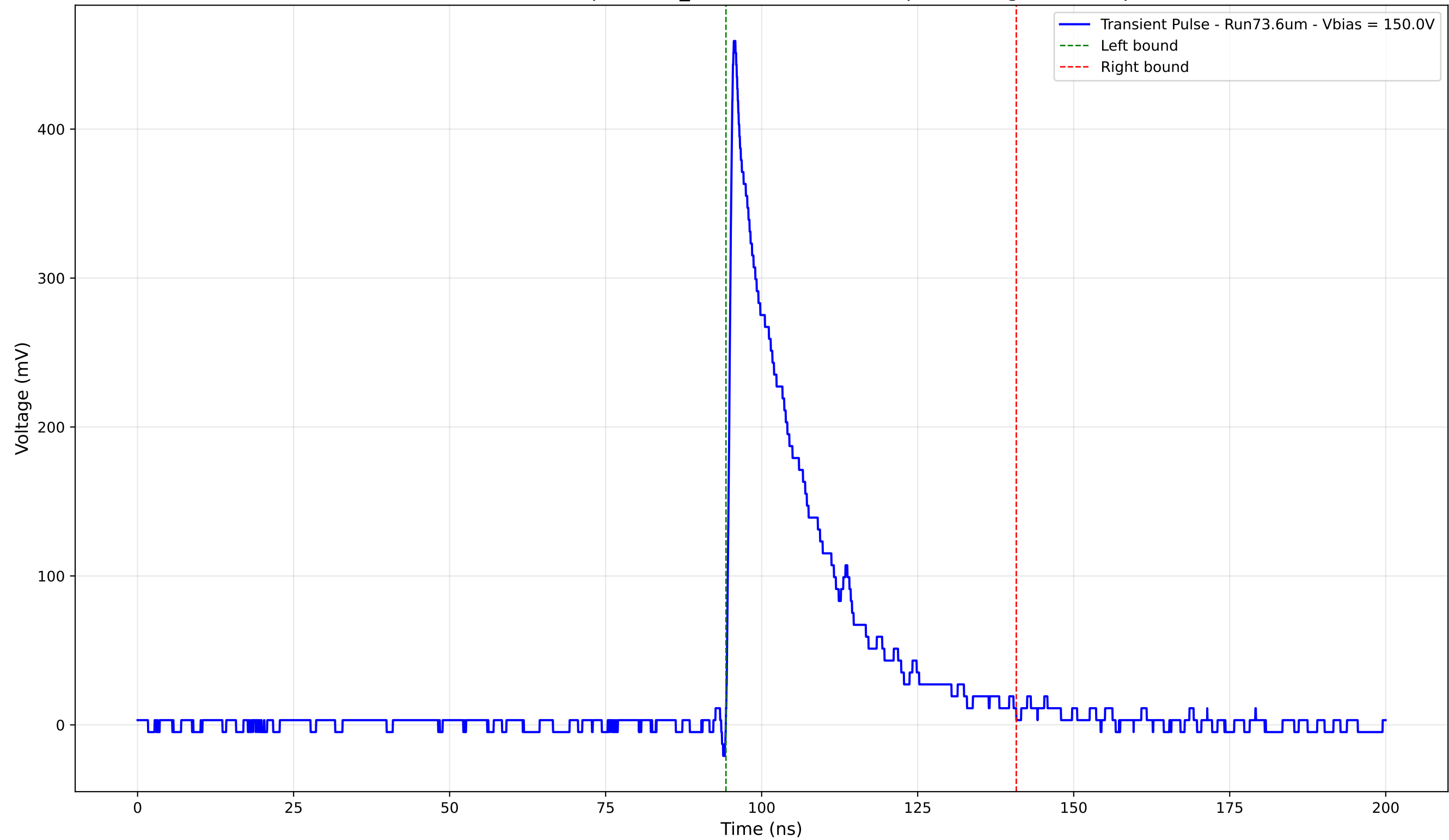
Transient Pulse - Sample: 1cm_42 - Position: 1105.0 \mu\text{m} - Charge: 102.05 pC
