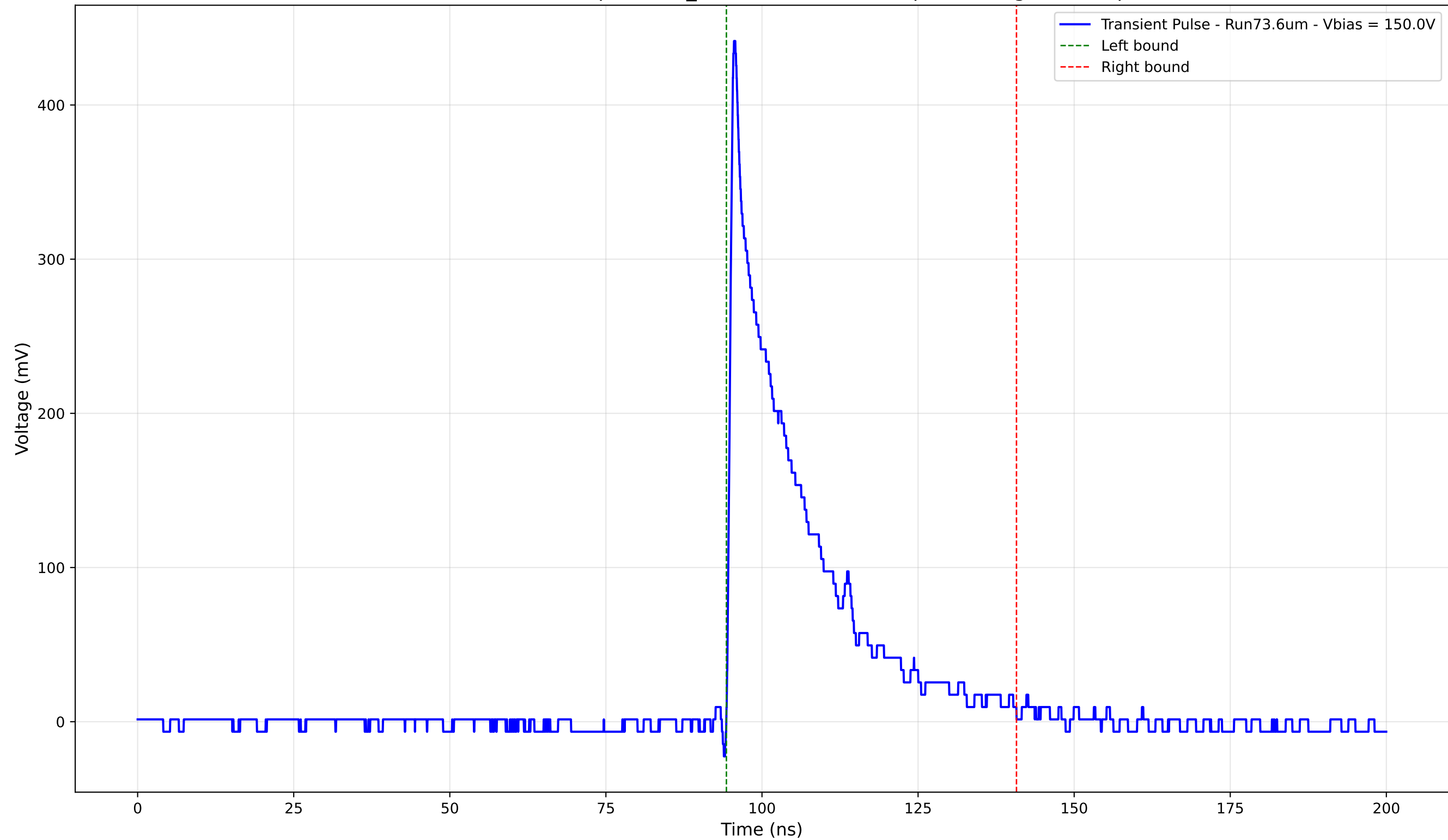
Transient Pulse - Sample: 1cm_42 - Position: 2005.0 \mu\text{m} - Charge: 89.87 pC
