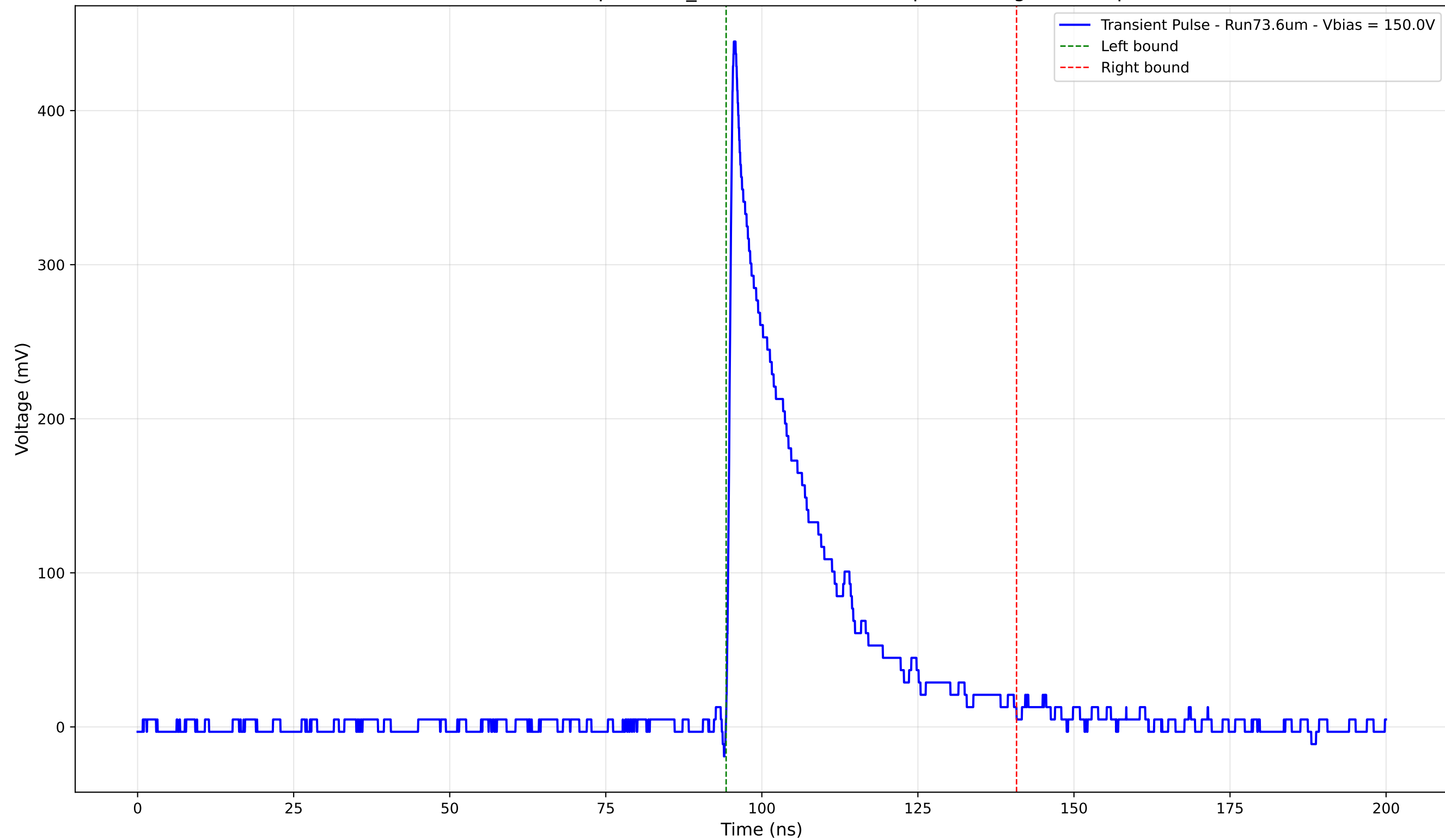
Transient Pulse - Sample: 1cm_42 - Position: 1655.0 \mu\text{m} - Charge: 97.84 pC
