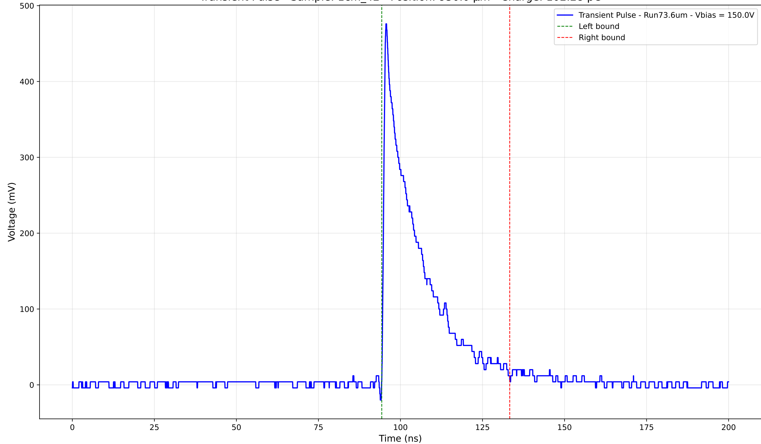
Transient Pulse - Sample: 1cm_42 - Position: 950.0 \mu\text{m} - Charge: 102.28 pC
