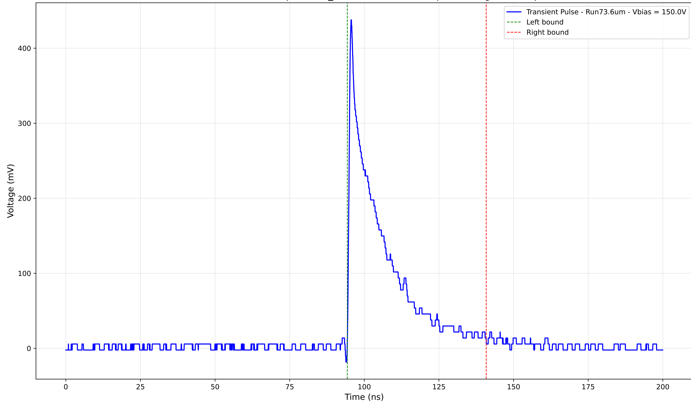
Transient Pulse - Sample: 1cm_42 - Position: 2050.0 \mu\text{m} - Charge: 91.36 pC
