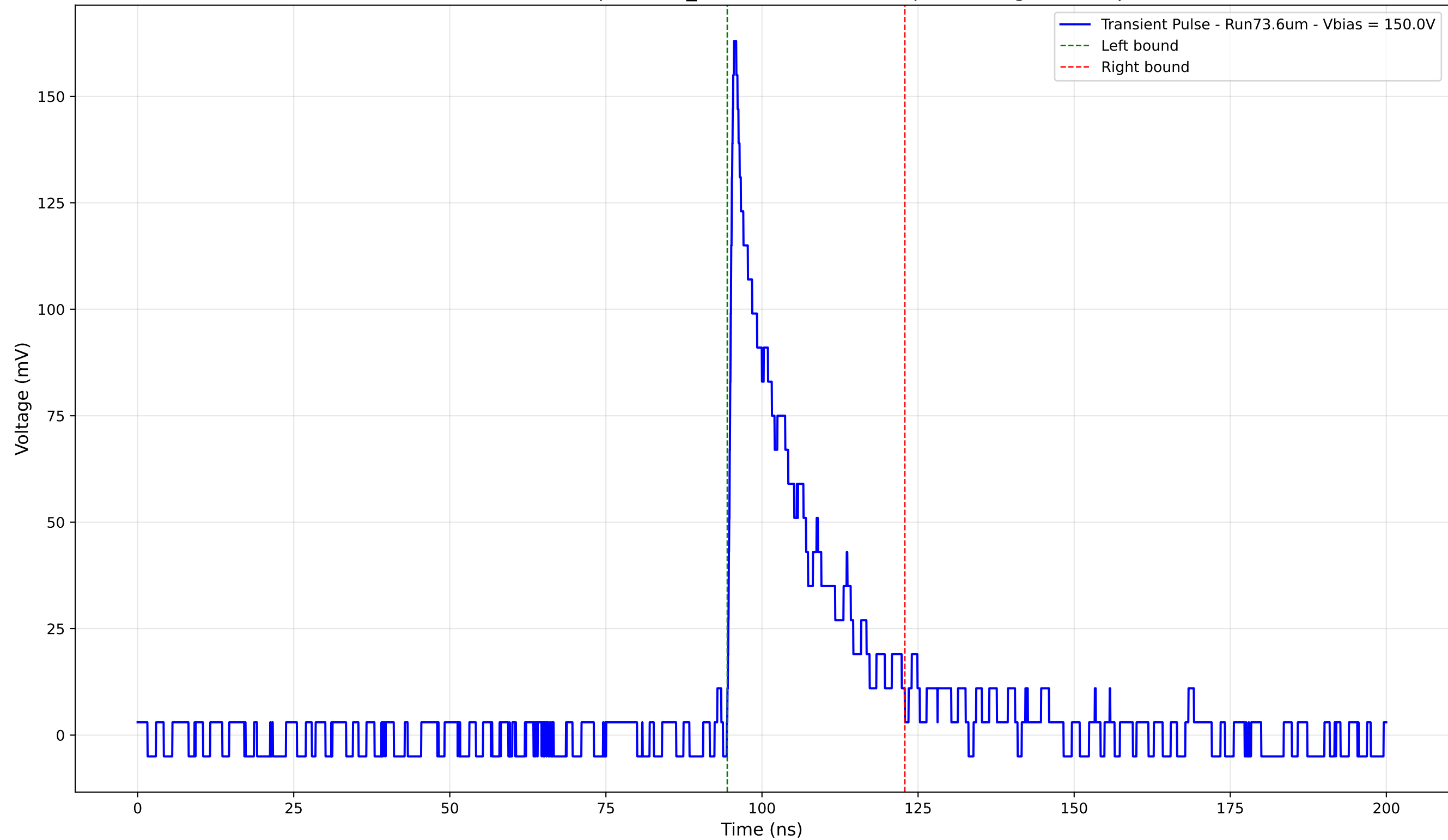
Transient Pulse - Sample: 1cm_42 - Position: 4330.0 \mu\text{m} - Charge: 30.19 pC
