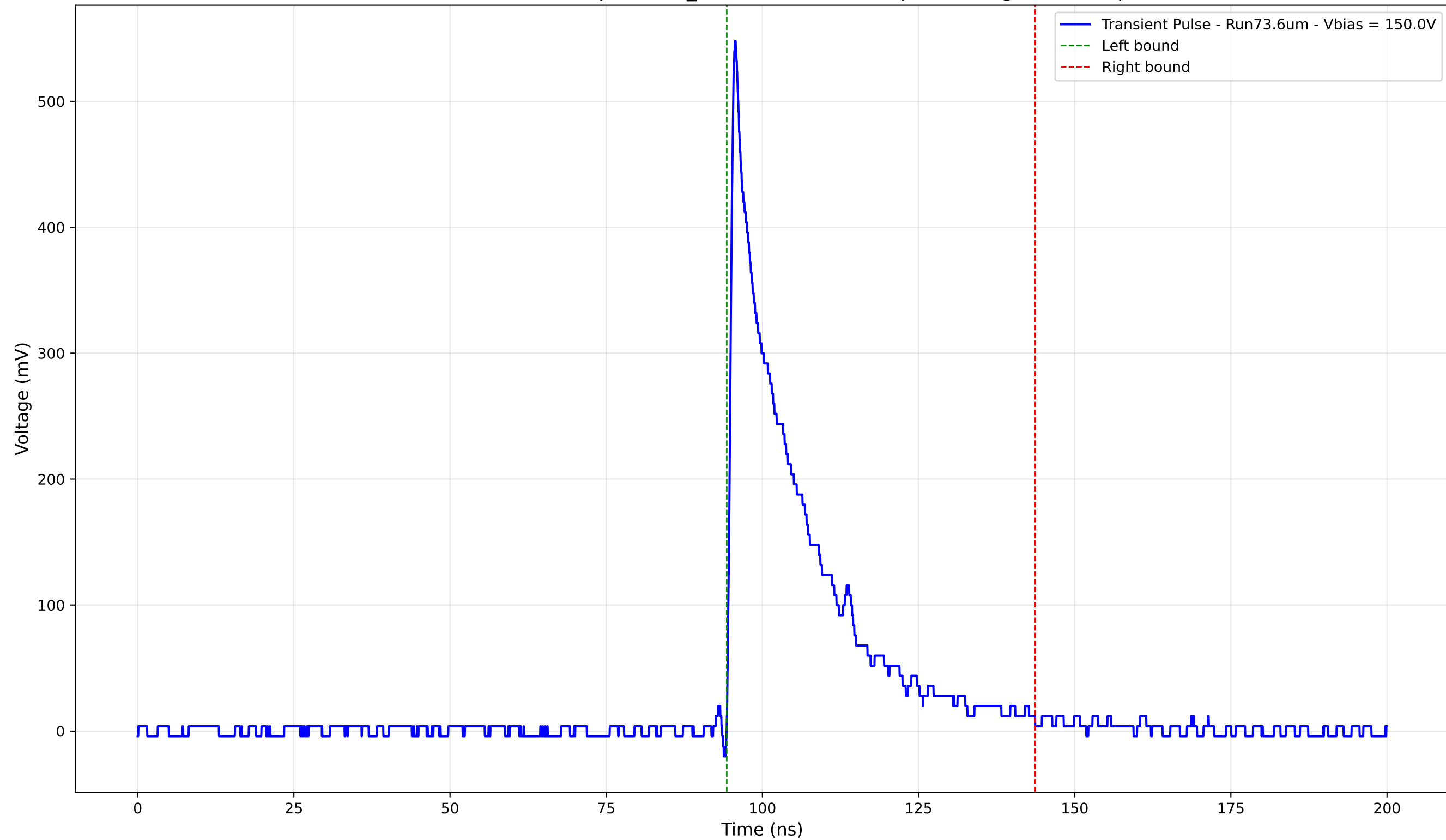
Transient Pulse - Sample: 1cm_42 - Position: 455.0 \mu\text{m} - Charge: 112.71 pC
