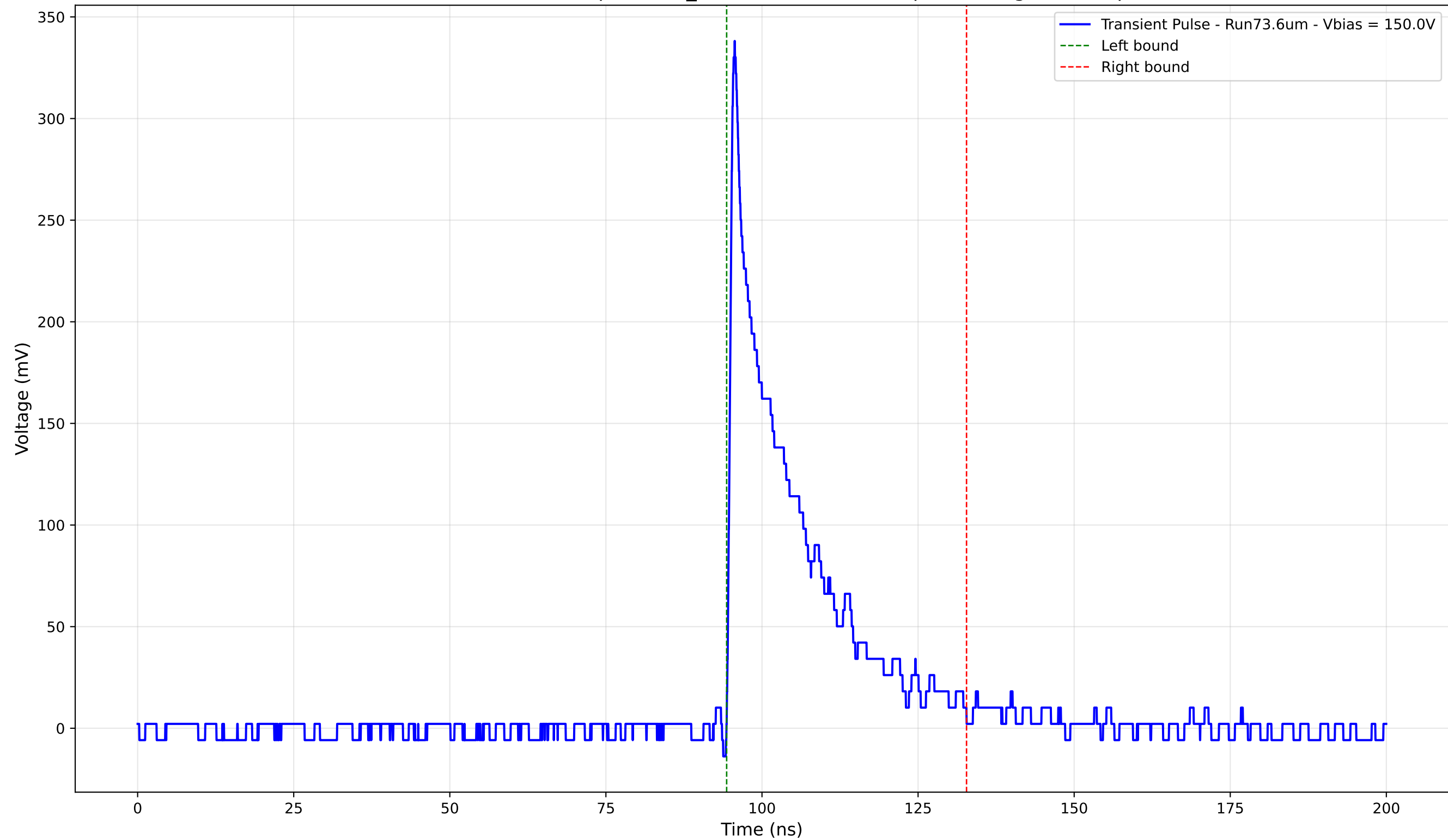
Transient Pulse - Sample: 1cm_42 - Position: 3035.0 \mu\text{m} - Charge: 62.44 pC
