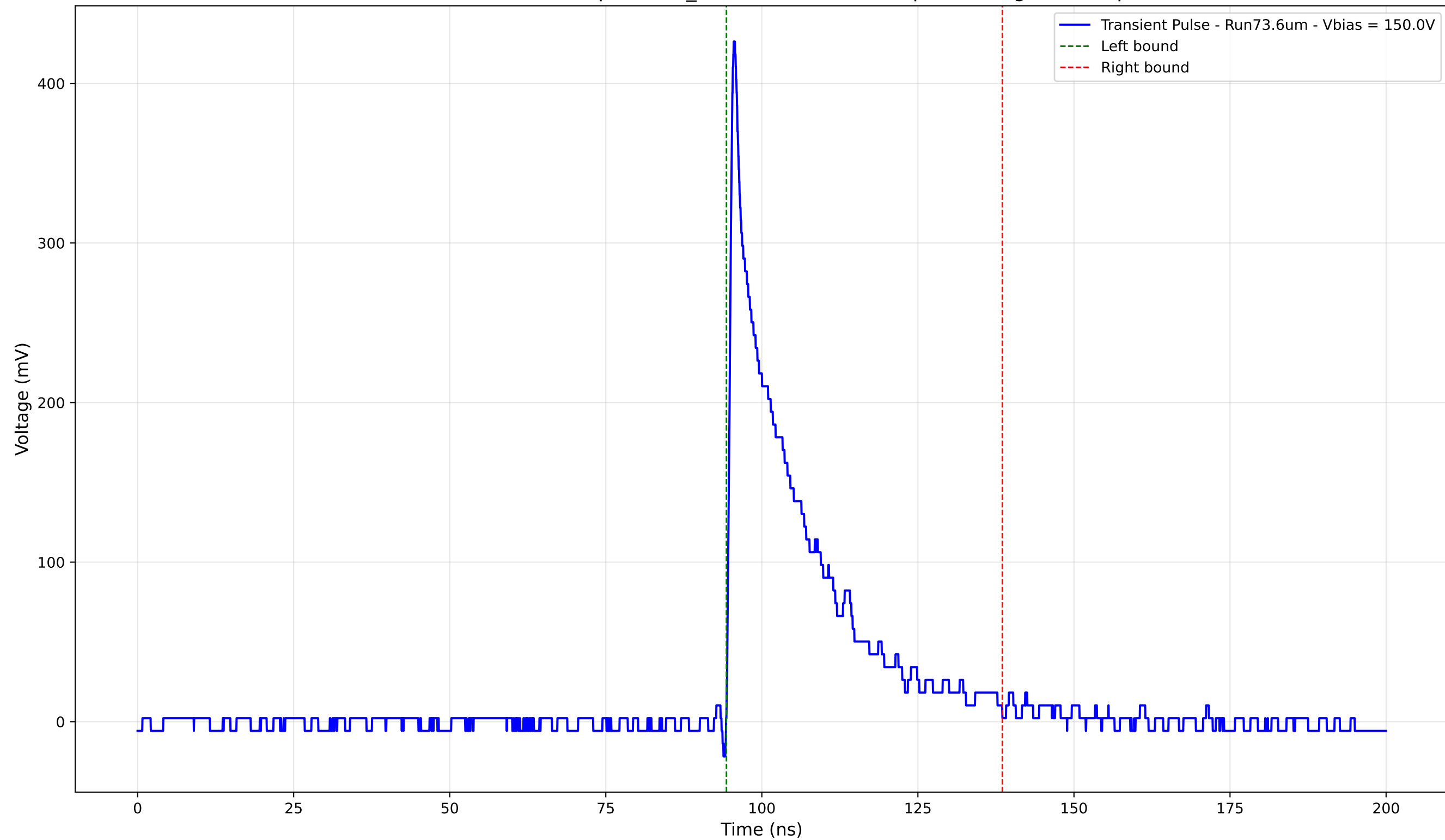
Transient Pulse - Sample: 1cm_42 - Position: 2300.0 \mu\text{m} - Charge: 81.87 pC
