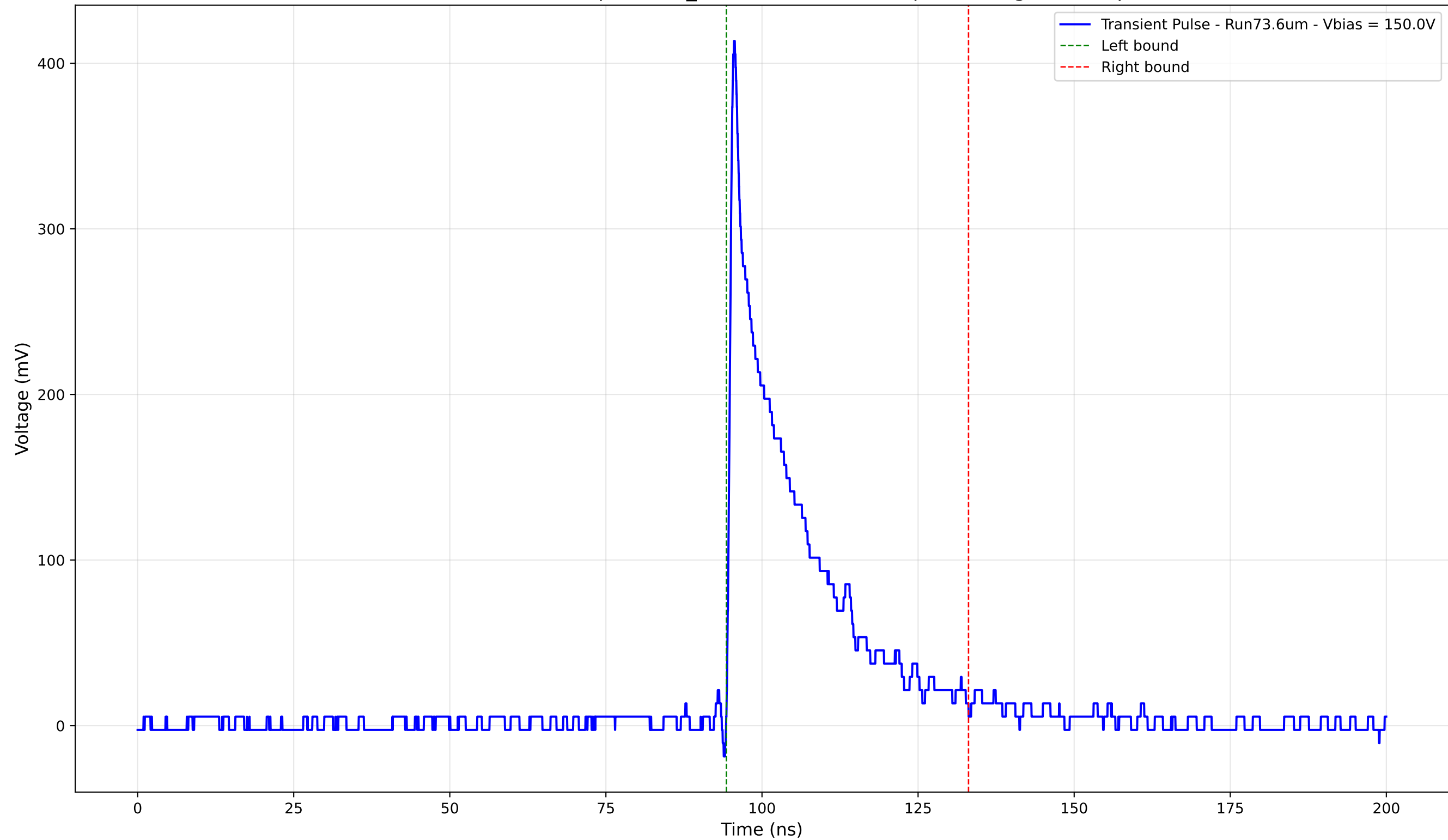
Transient Pulse - Sample: 1cm_42 - Position: 2420.0 \mu\text{m} - Charge: 77.84 pC
