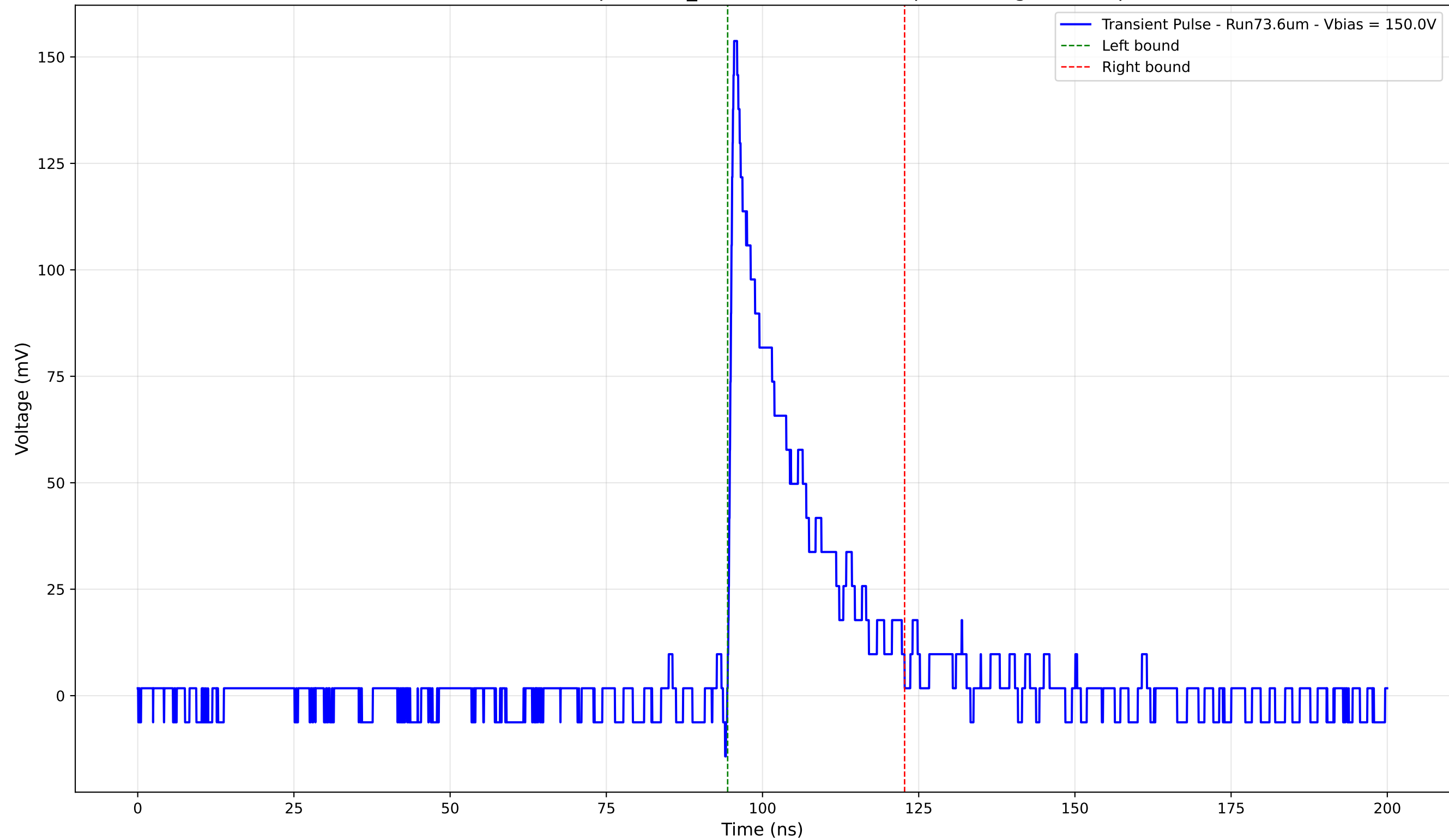
Transient Pulse - Sample: 1cm_42 - Position: 4390.0 \mu\text{m} - Charge: 28.16 pC
