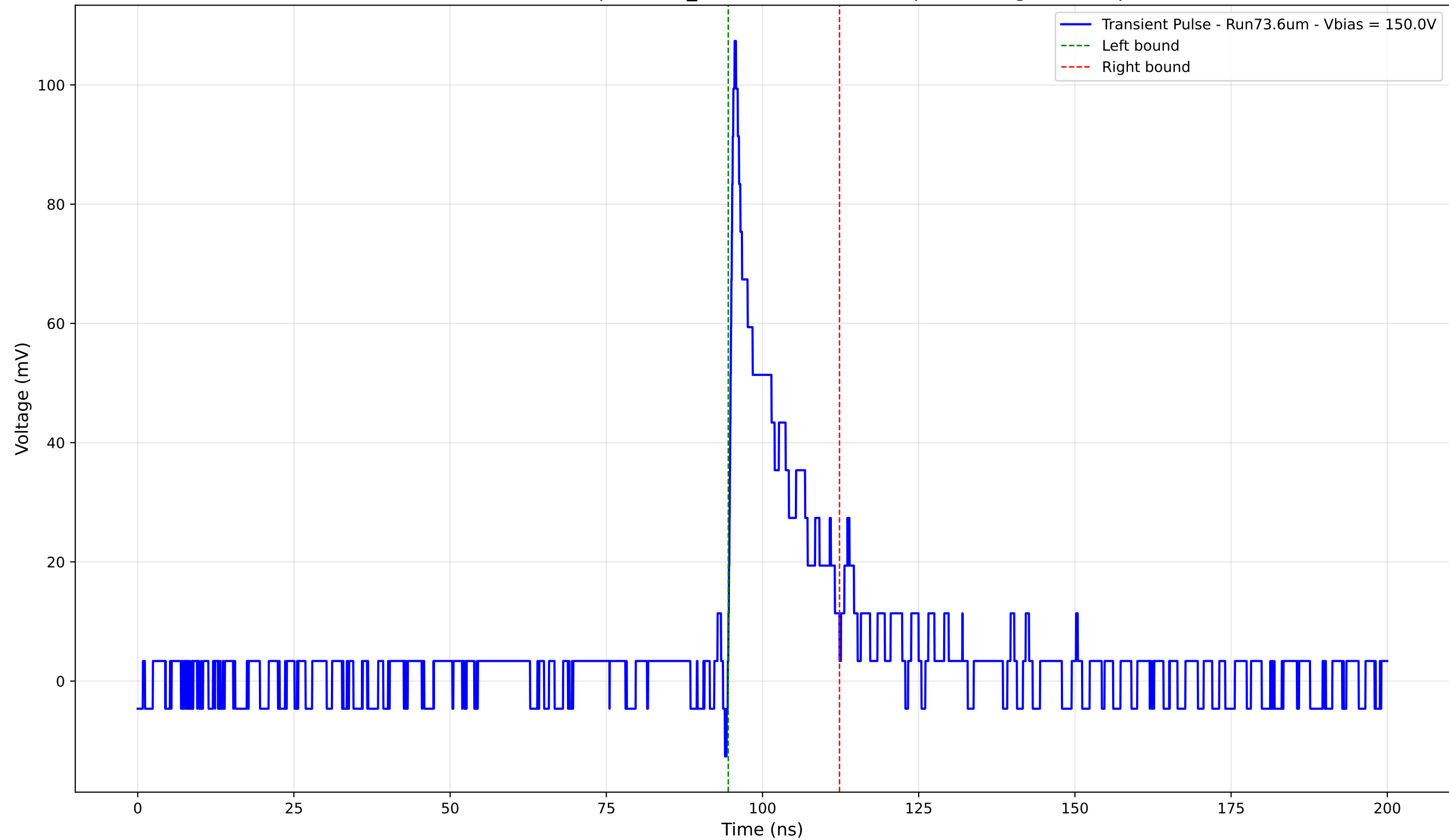
Transient Pulse - Sample: 1cm_42 - Position: 4840.0 \mu\text{m} - Charge: 14.77 pC
