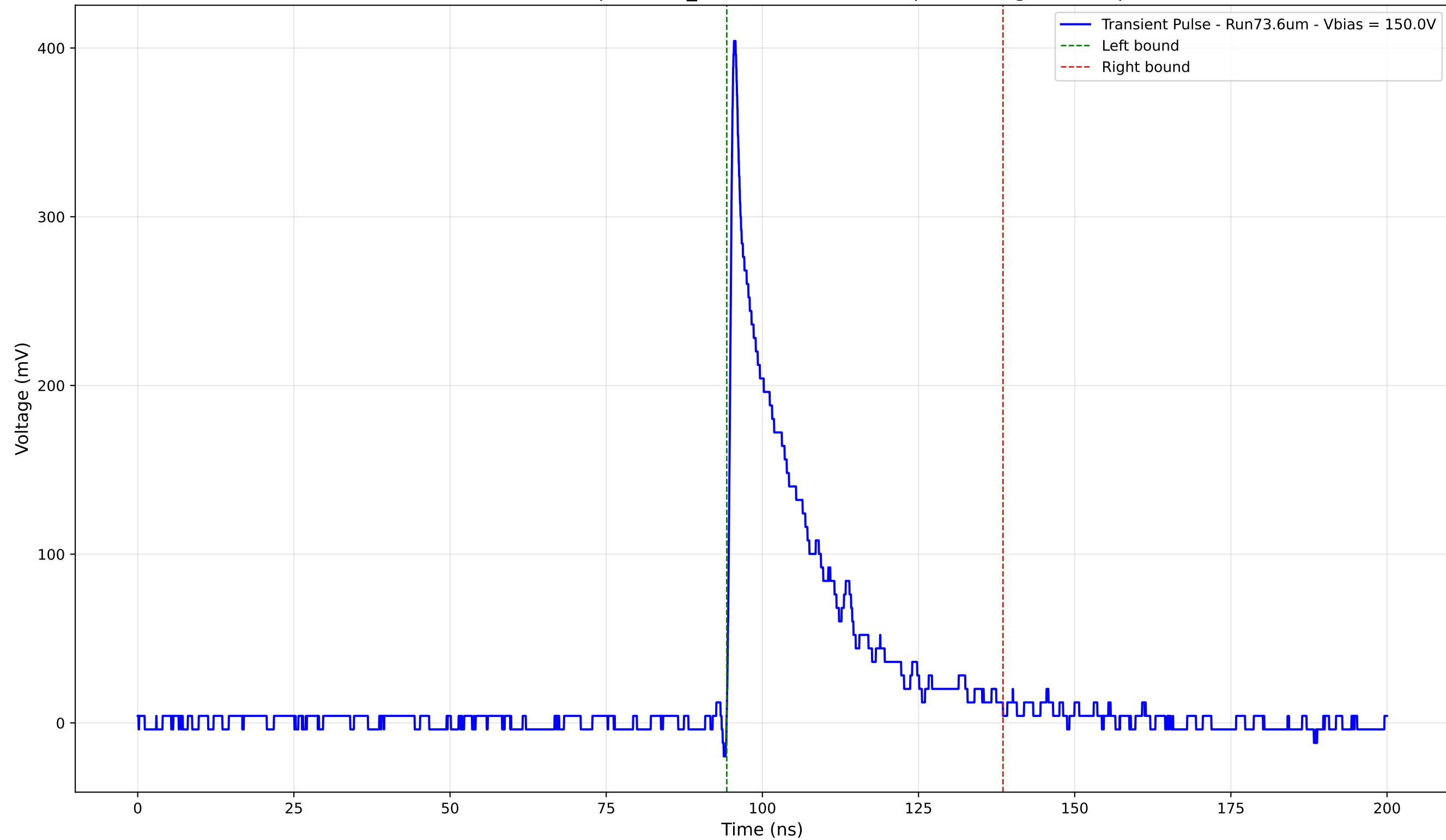
Transient Pulse - Sample: 1cm_42 - Position: 2415.0 \mu\text{m} - Charge: 78.14 pC
