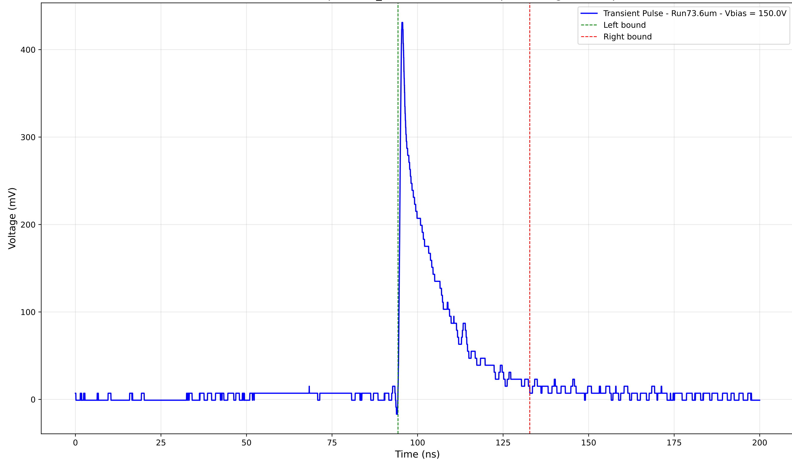
Transient Pulse - Sample: 1cm_42 - Position: 2675.0 \mu\text{m} - Charge: 79.37 pC
