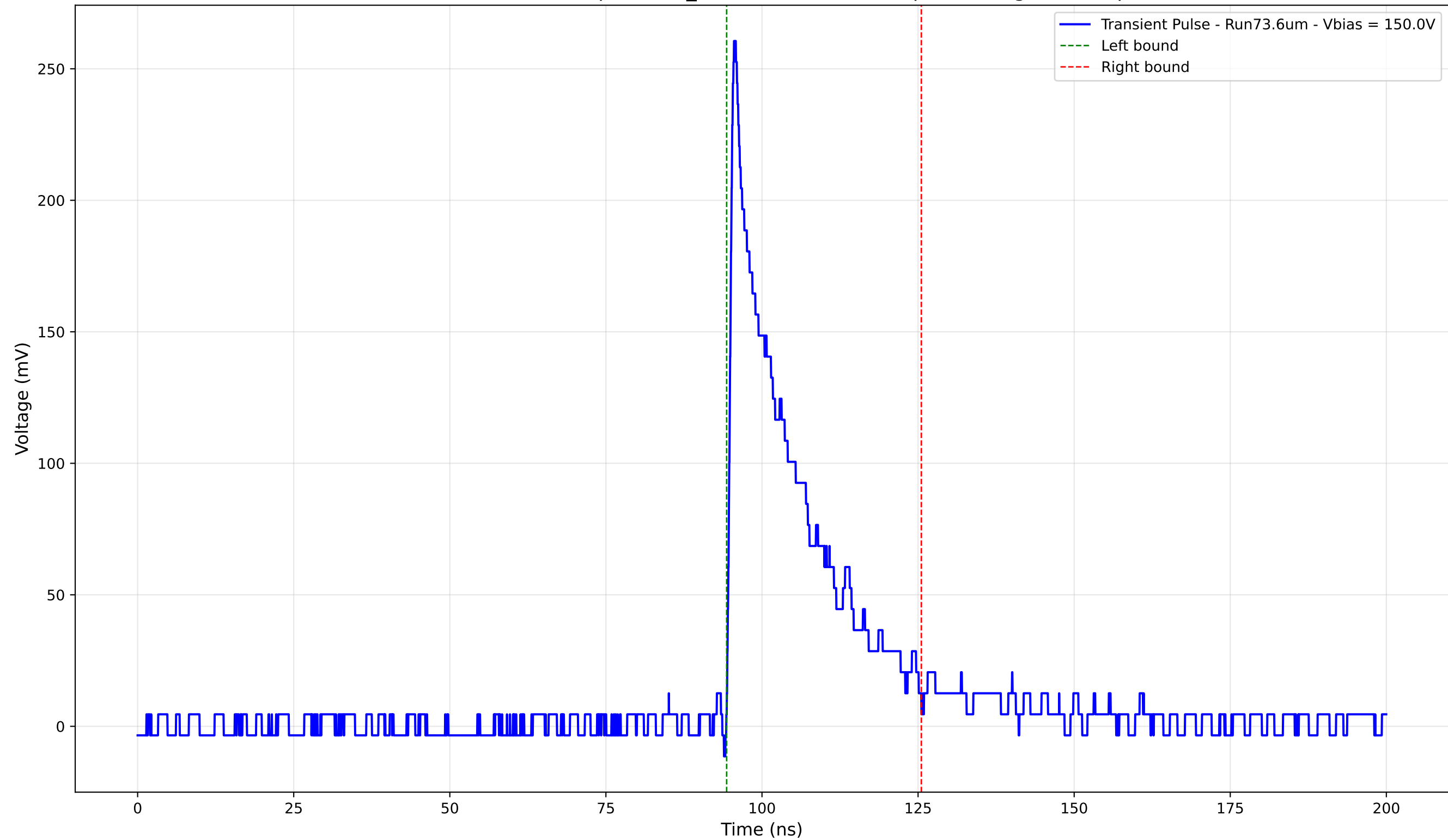
Transient Pulse - Sample: 1cm_42 - Position: 3530.0 \mu\text{m} - Charge: 51.88 pC
