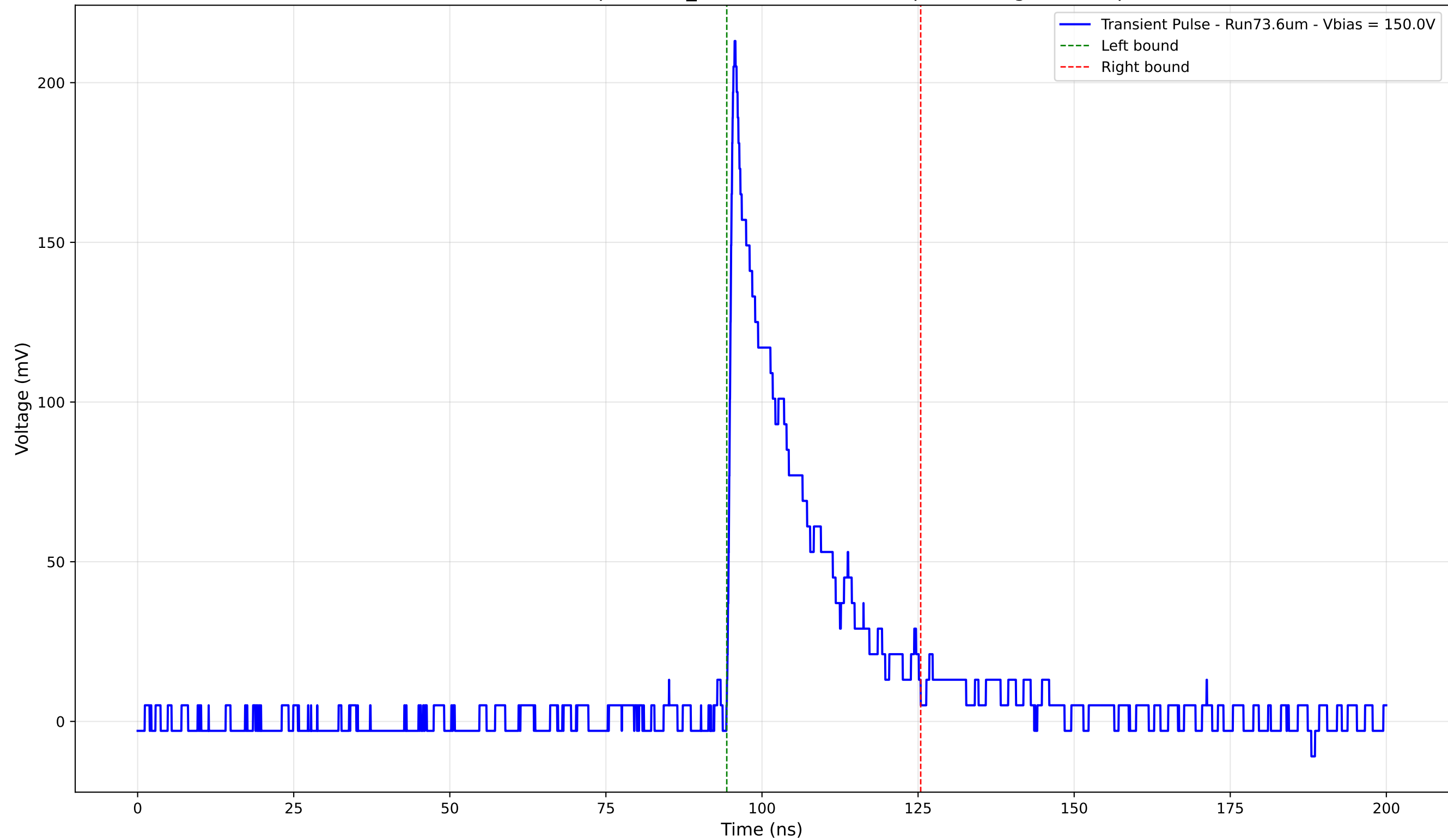
Transient Pulse - Sample: 1cm_42 - Position: 3900.0 \mu\text{m} - Charge: 41.65 pC
