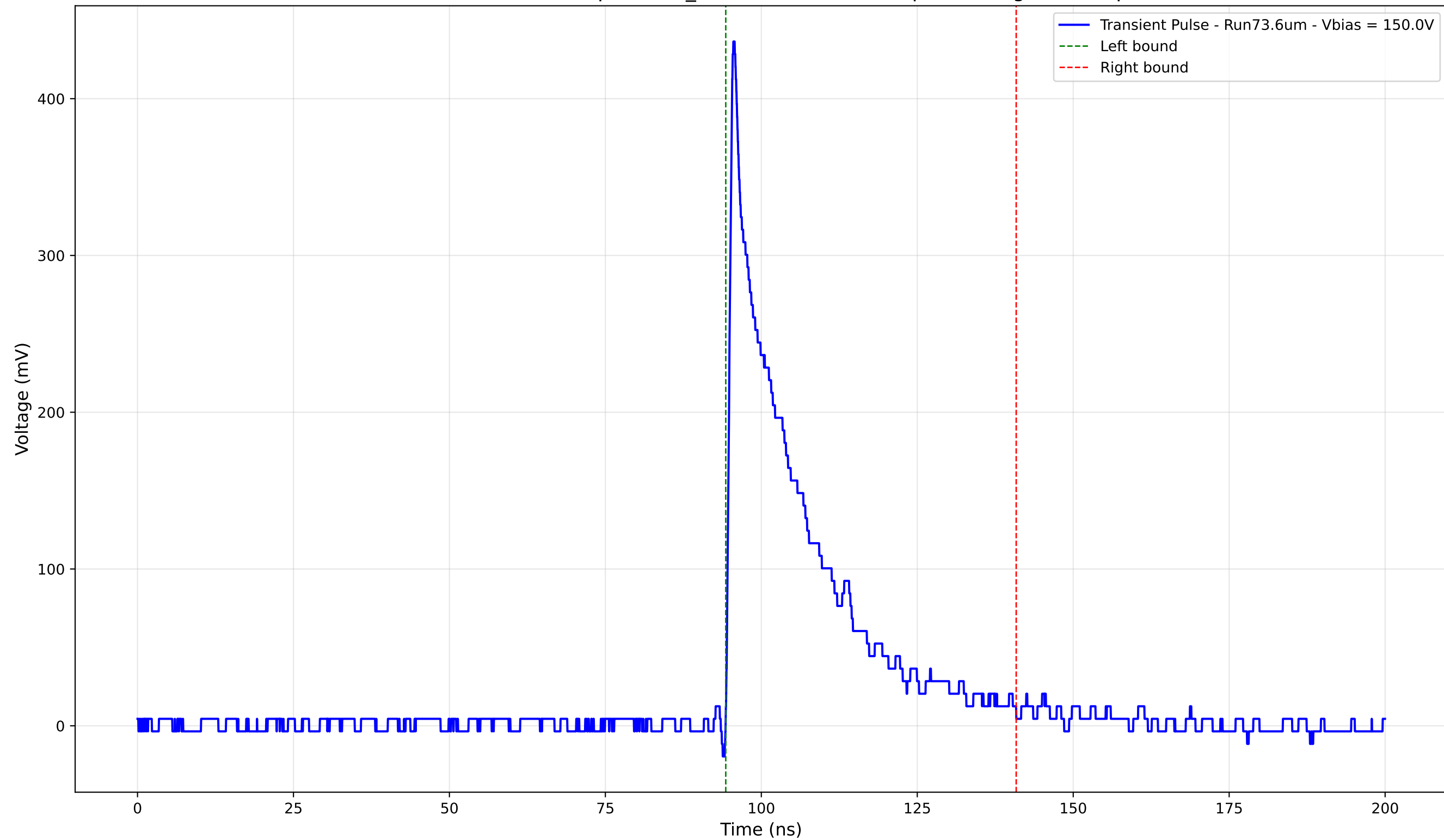
Transient Pulse - Sample: 1cm_42 - Position: 2025.0 \mu\text{m} - Charge: 90.35 pC
