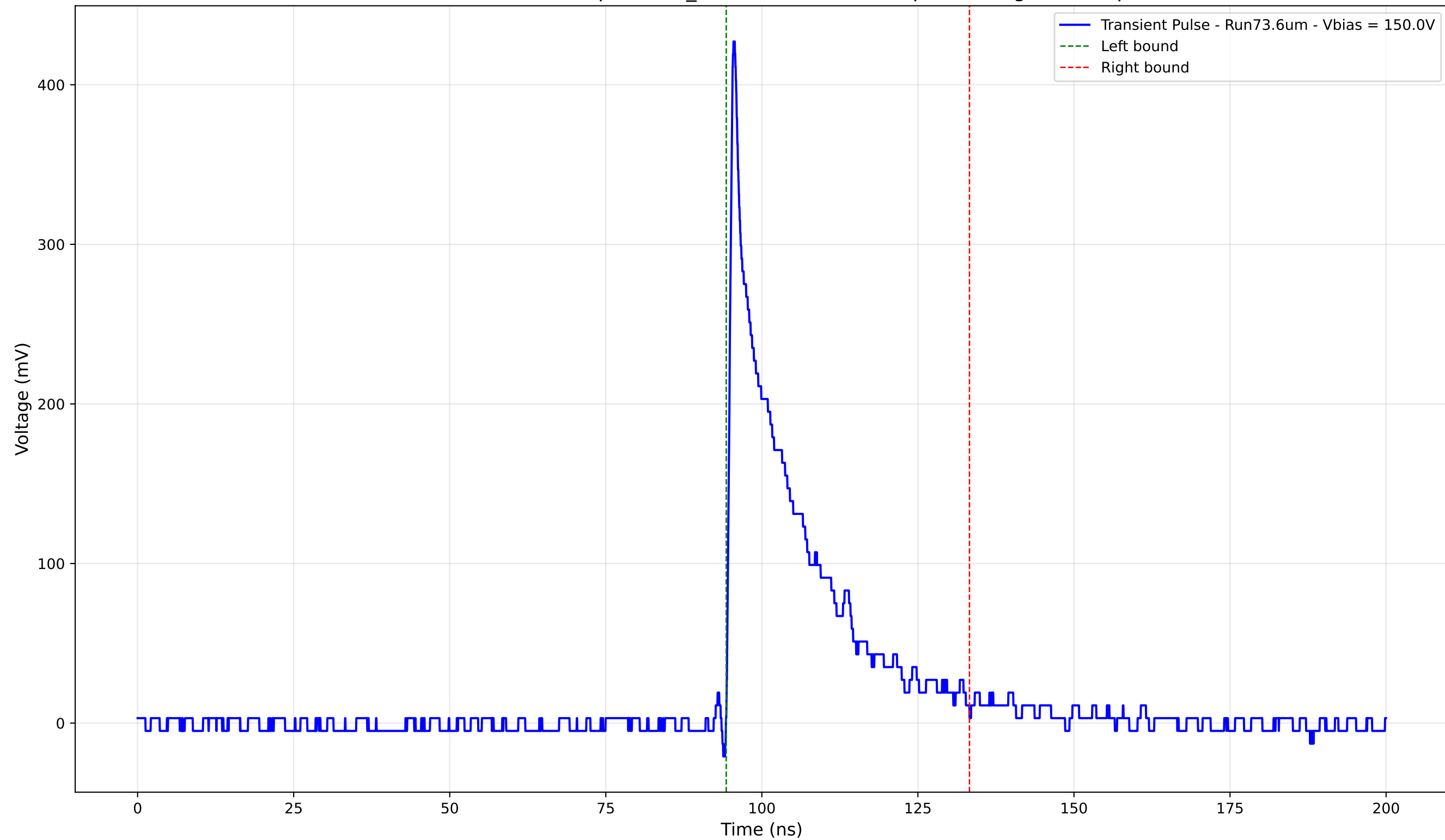
Transient Pulse - Sample: 1cm_42 - Position: 2650.0 \mu\text{m} - Charge: 77.82 pC
