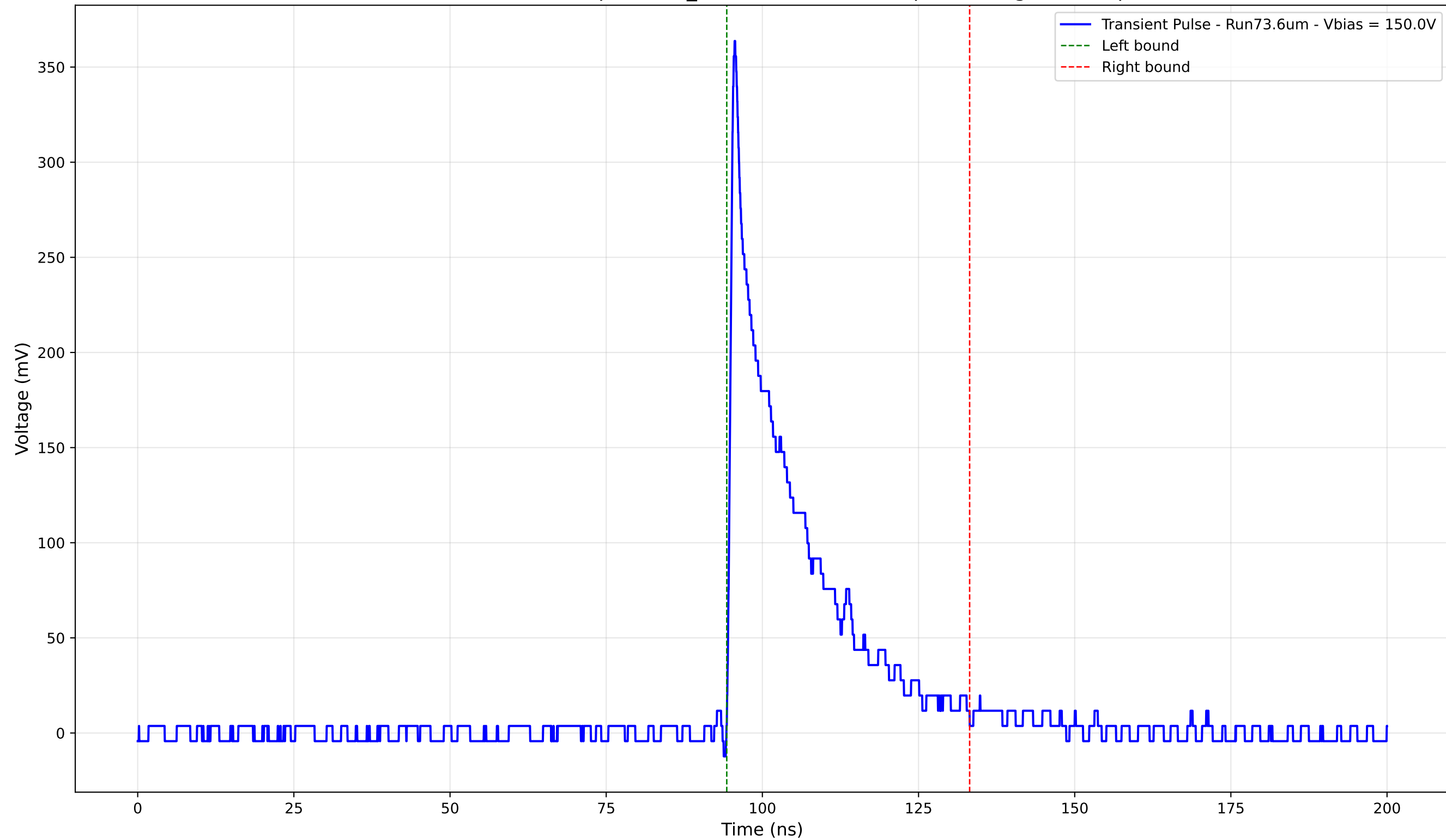
Transient Pulse - Sample: 1cm_42 - Position: 2925.0 \mu\text{m} - Charge: 68.02 pC
