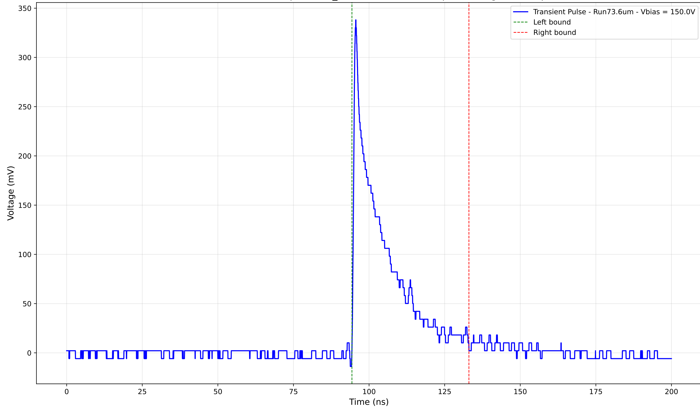
Transient Pulse - Sample: 1cm_42 - Position: 3020.0 \mu\text{m} - Charge: 62.50 pC
