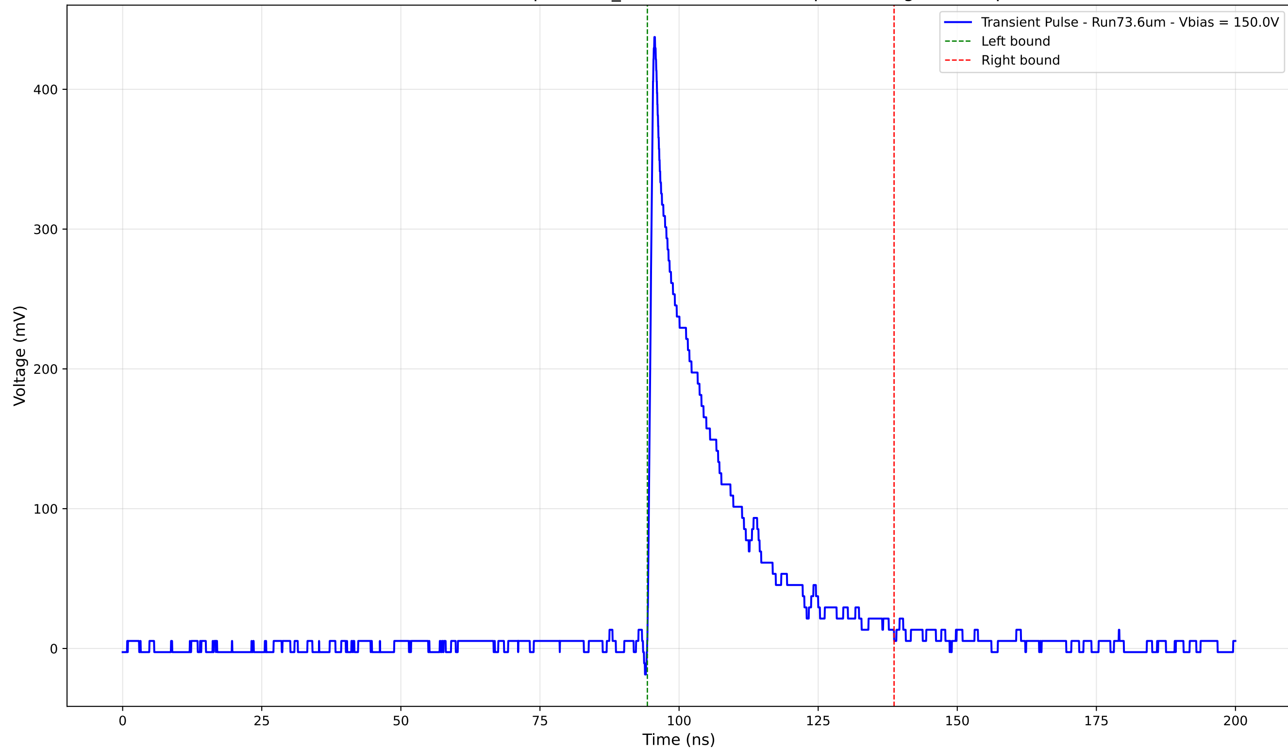
Transient Pulse - Sample: 1cm_42 - Position: 2055.0 \mu\text{m} - Charge: 90.37 pC
