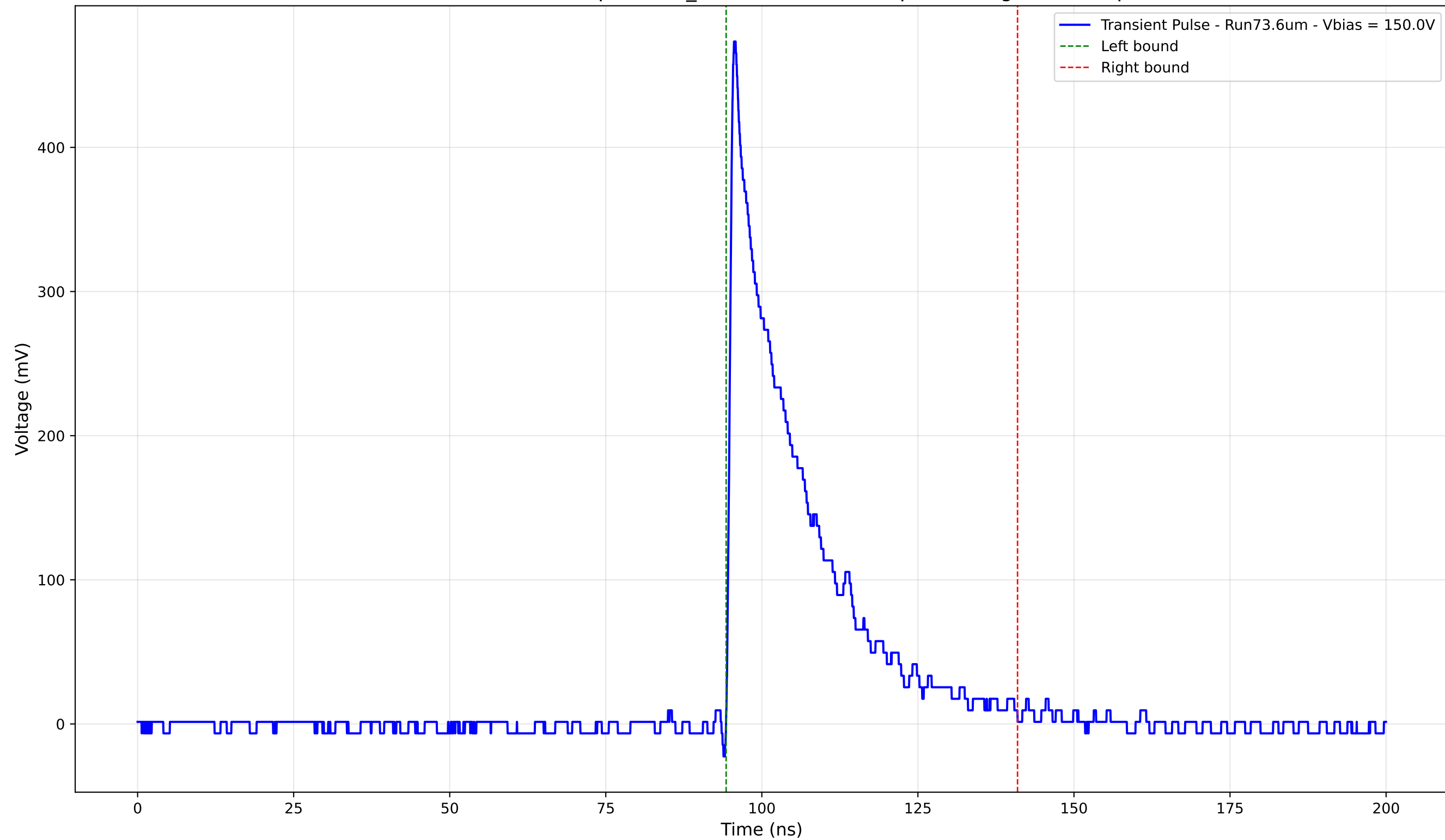
Transient Pulse - Sample: 1cm_42 - Position: 940.0 \mu\text{m} - Charge: 103.22 pC
