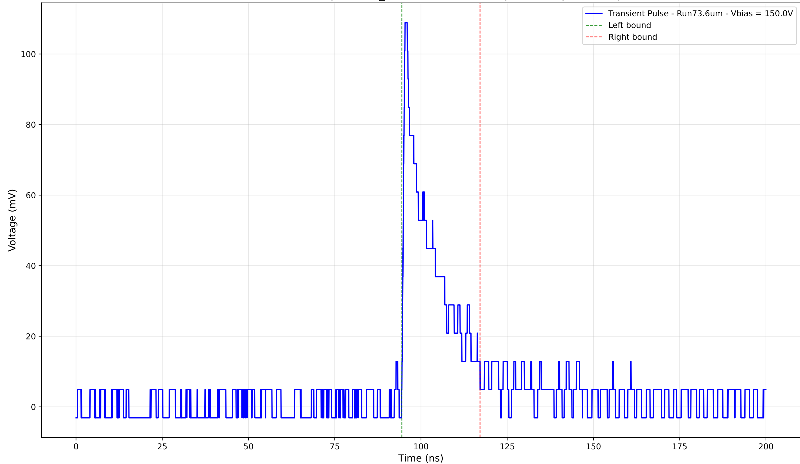
Transient Pulse - Sample: 1cm_42 - Position: 4775.0 \mu\text{m} - Charge: 18.43 pC
