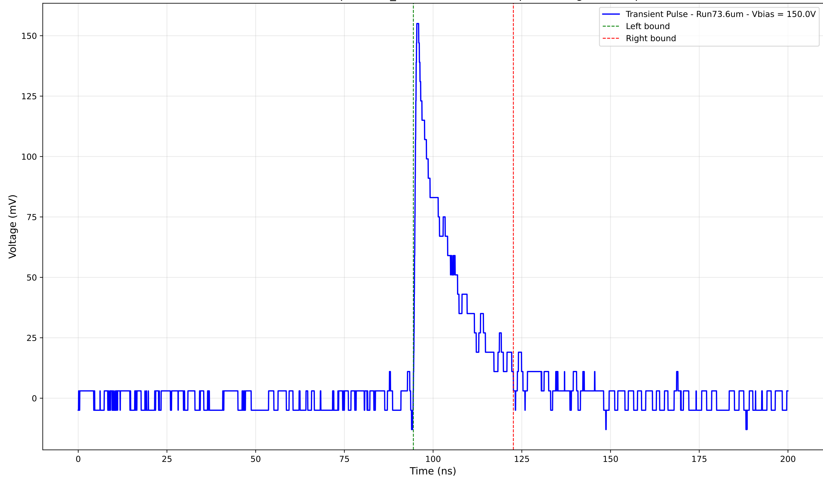
Transient Pulse - Sample: 1cm_42 - Position: 4415.0 \mu\text{m} - Charge: 28.98 pC
