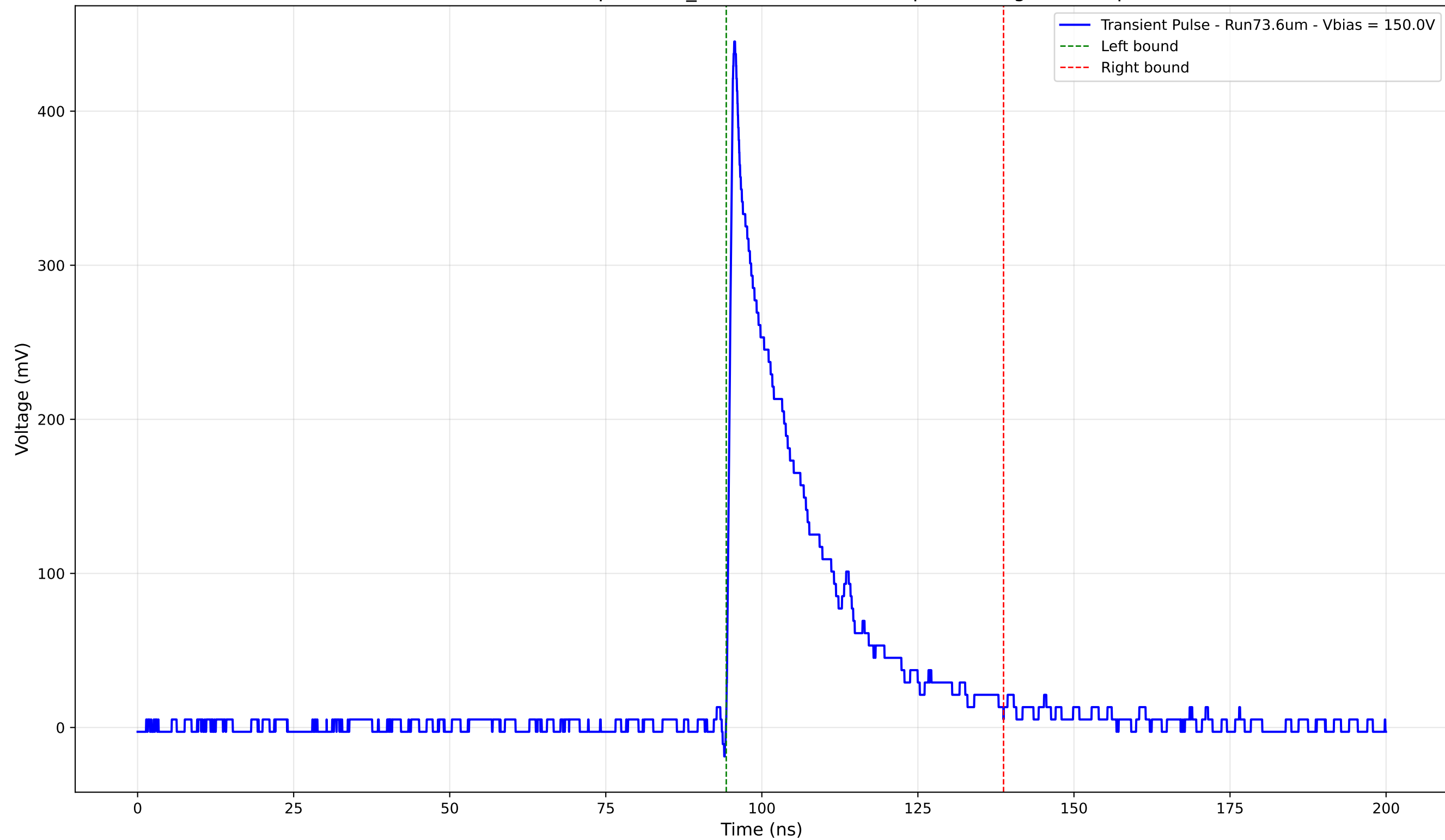
Transient Pulse - Sample: 1cm_42 - Position: 1715.0 \mu\text{m} - Charge: 95.53 pC
