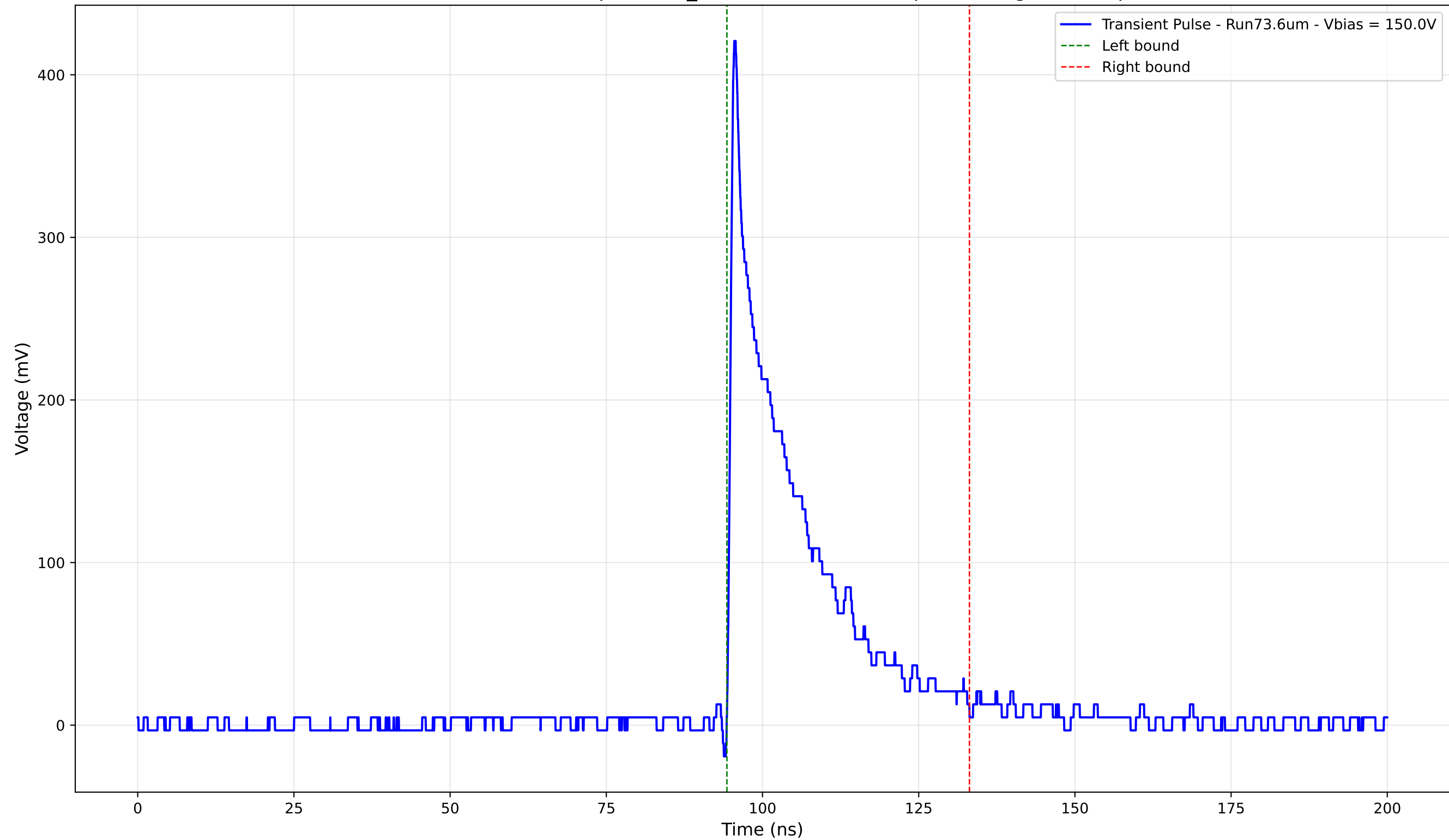
Transient Pulse - Sample: 1cm_42 - Position: 2335.0 \mu\text{m} - Charge: 80.28 pC
