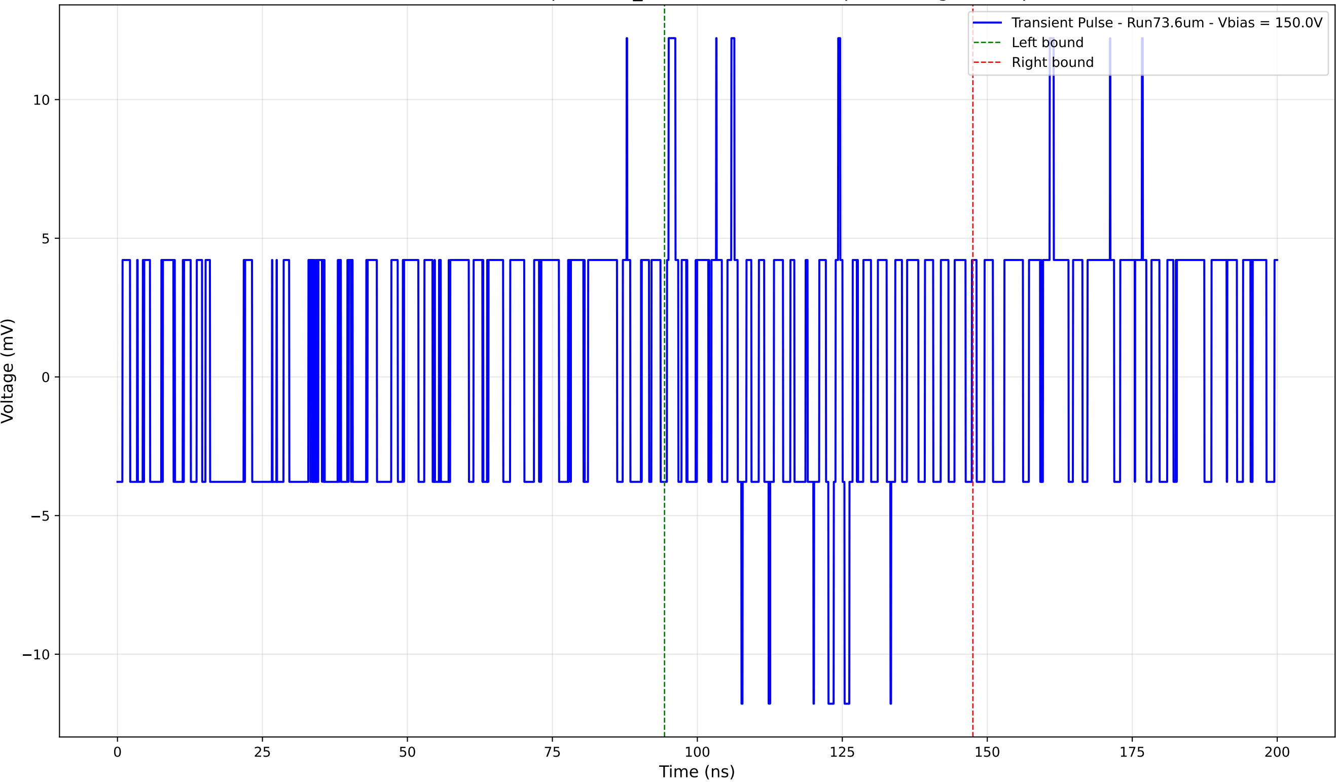
Transient Pulse - Sample: 1cm_42 - Position: 5025.0 \mu\text{m} - Charge: 0.30 pC
