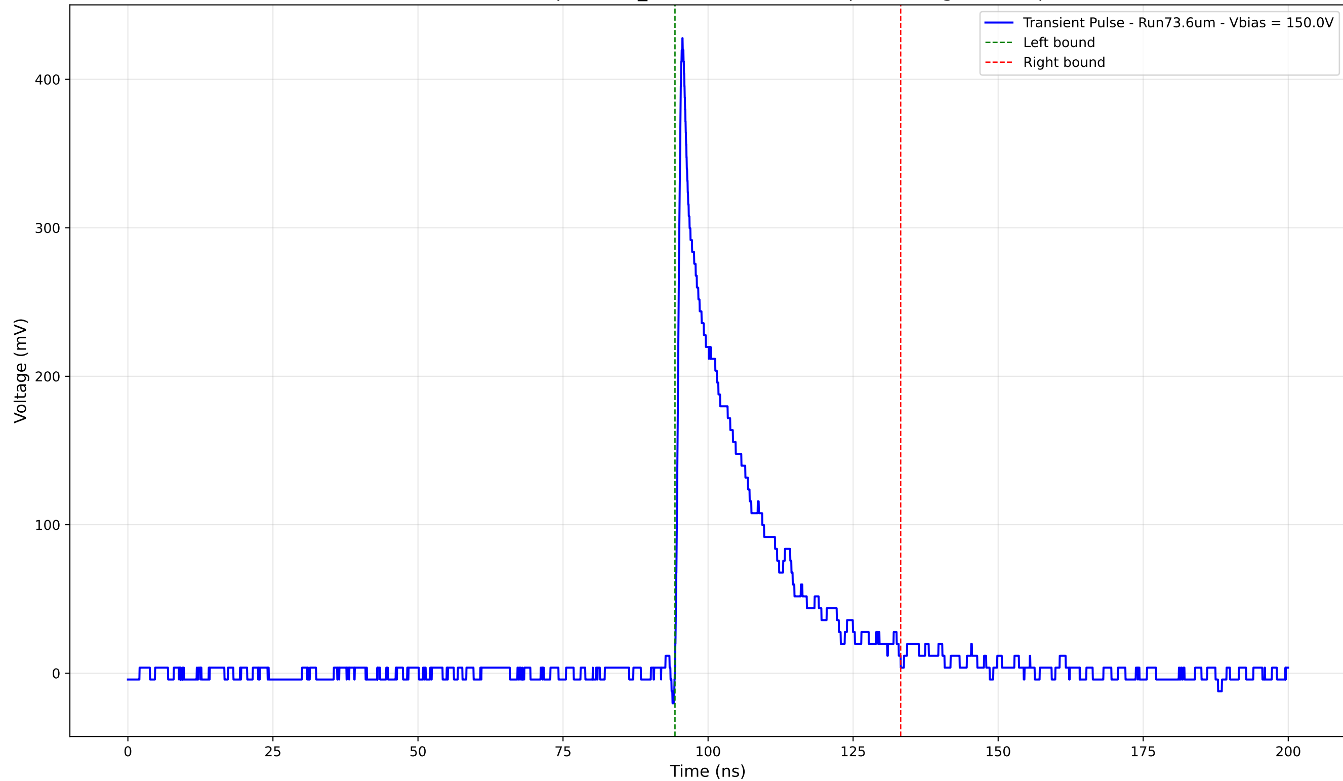
Transient Pulse - Sample: 1cm_42 - Position: 2305.0 \mu\text{m} - Charge: 81.67 pC
