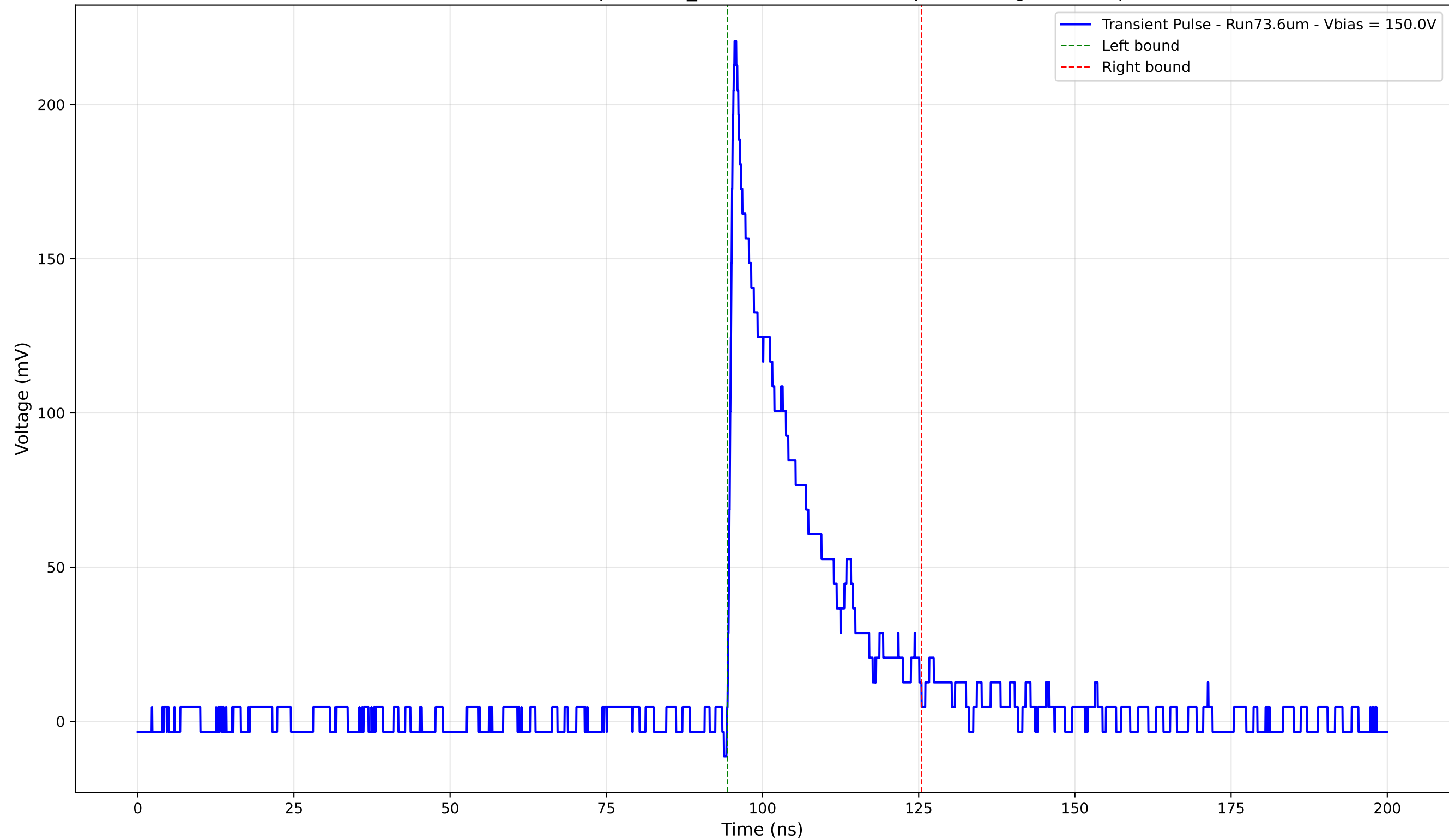
Transient Pulse - Sample: 1cm_42 - Position: 3835.0 \mu\text{m} - Charge: 43.00 pC
