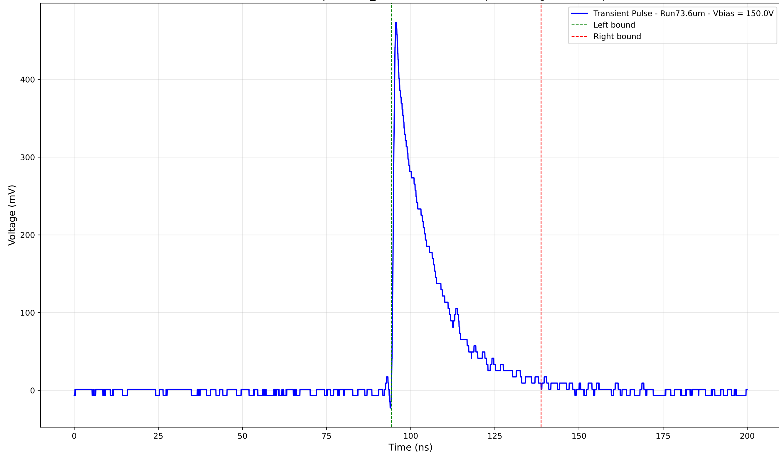
Transient Pulse - Sample: 1cm_42 - Position: 960.0 \mu\text{m} - Charge: 101.71 pC
