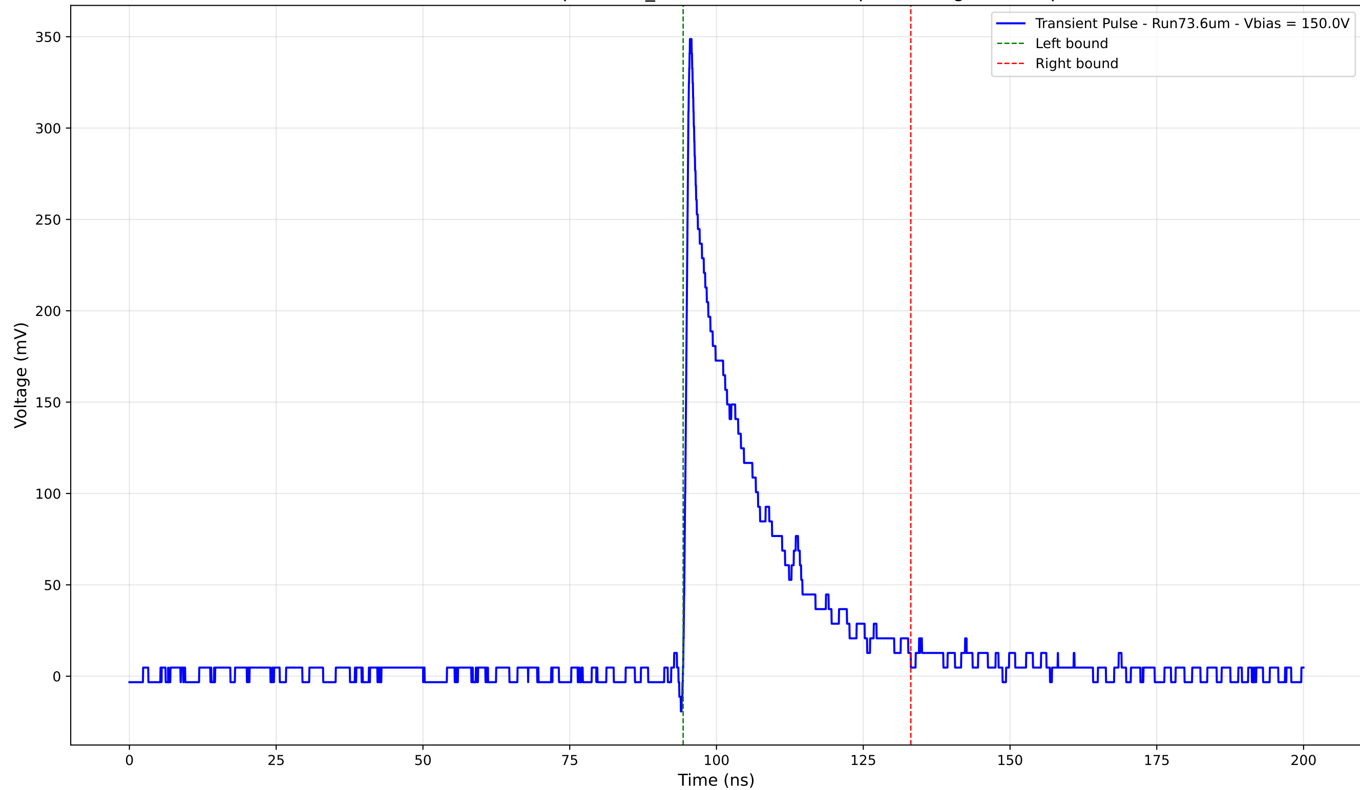
Transient Pulse - Sample: 1cm_42 - Position: 2955.0 \mu\text{m} - Charge: 66.73 pC
