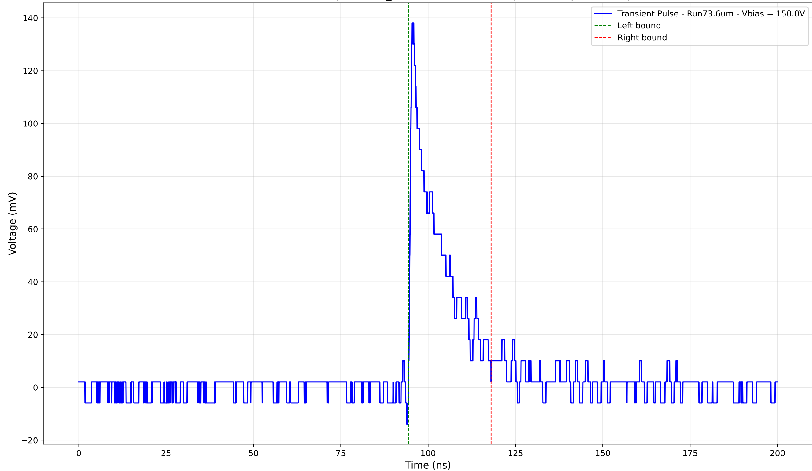
Transient Pulse - Sample: 1cm_42 - Position: 4600.0 \mu\text{m} - Charge: 23.02 pC
