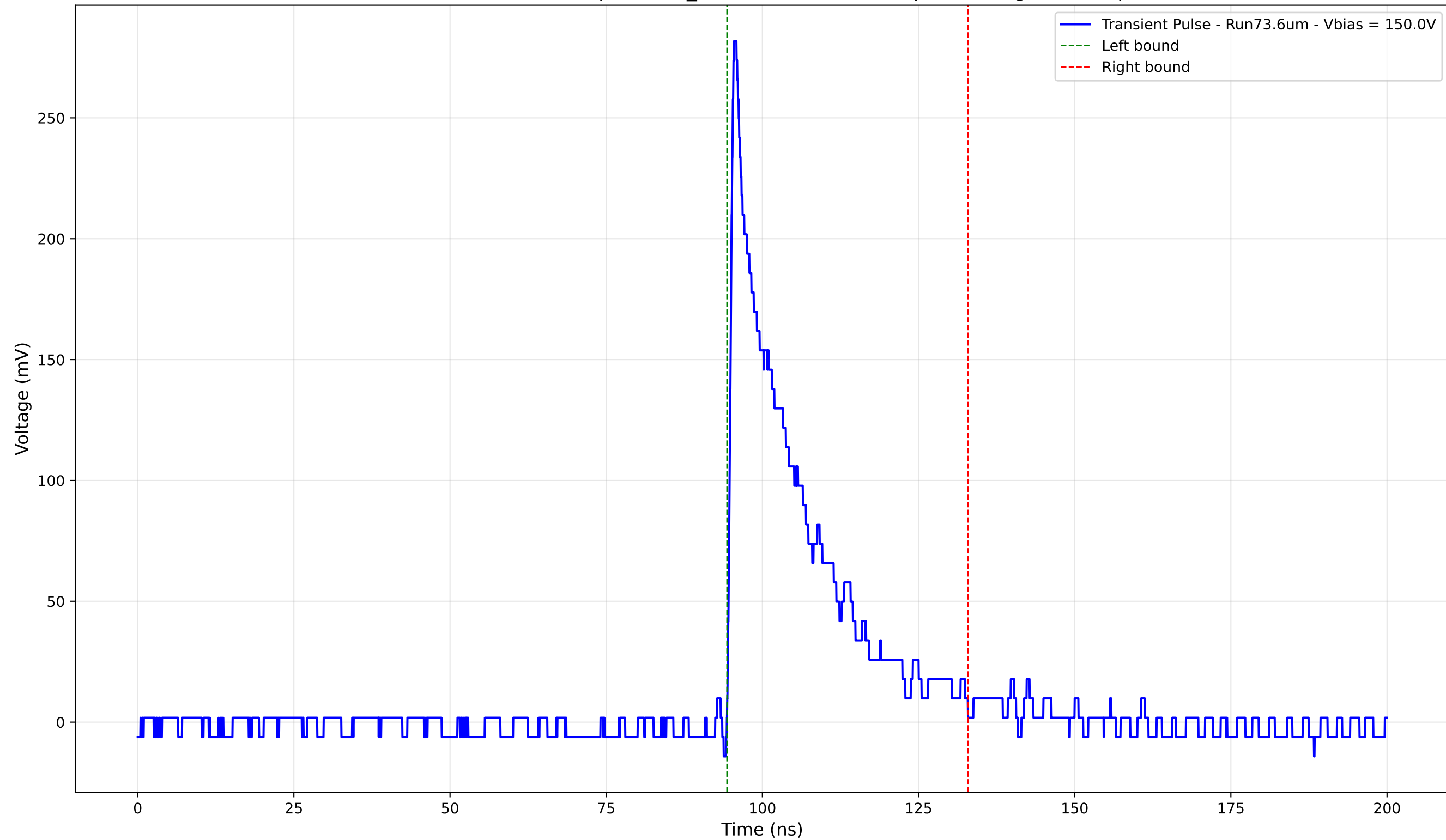
Transient Pulse - Sample: 1cm_42 - Position: 3370.0 \mu\text{m} - Charge: 56.08 pC
