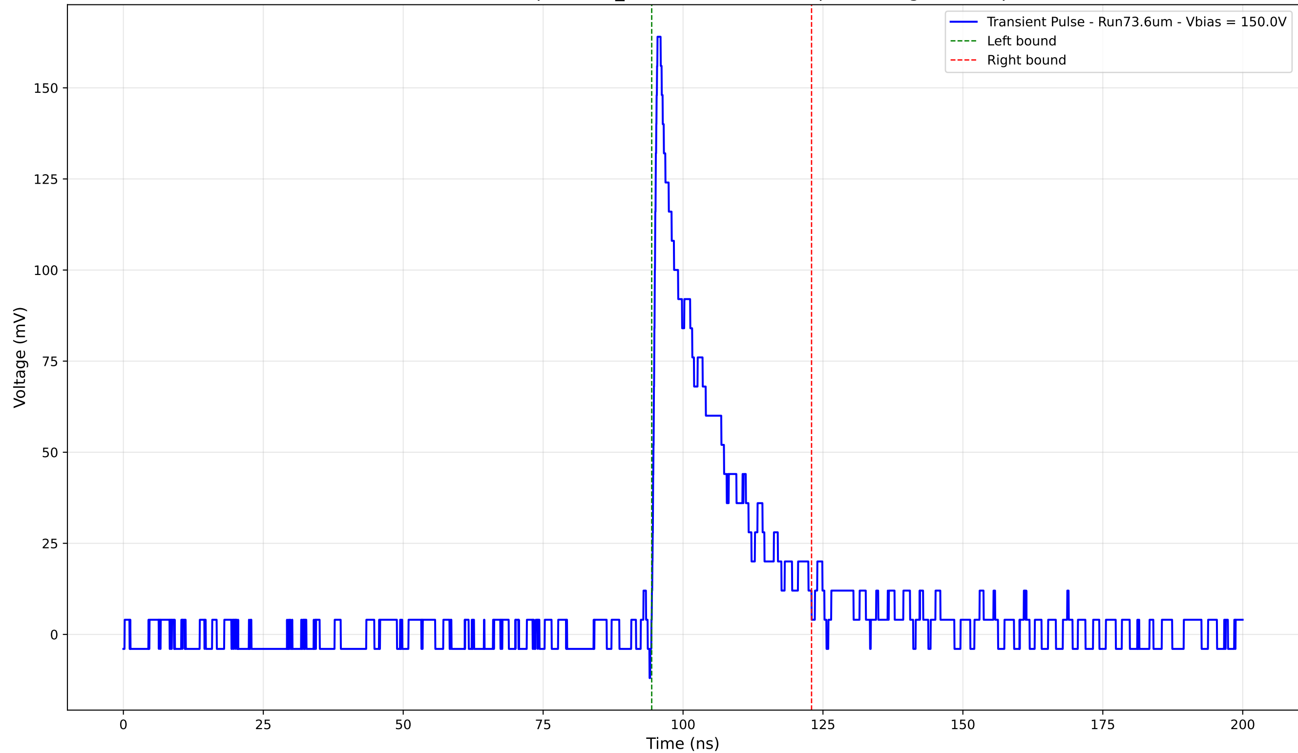
Transient Pulse - Sample: 1cm_42 - Position: 4310.0 \mu\text{m} - Charge: 31.27 pC
