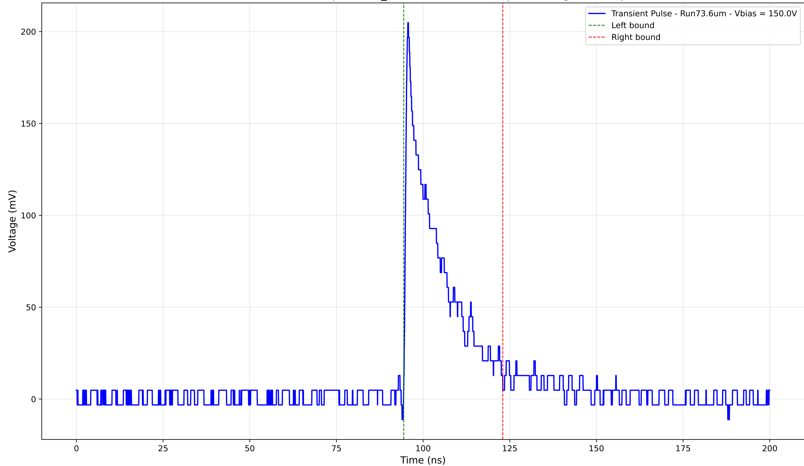
Transient Pulse - Sample: 1cm_42 - Position: 3945.0 \mu\text{m} - Charge: 39.06 pC
