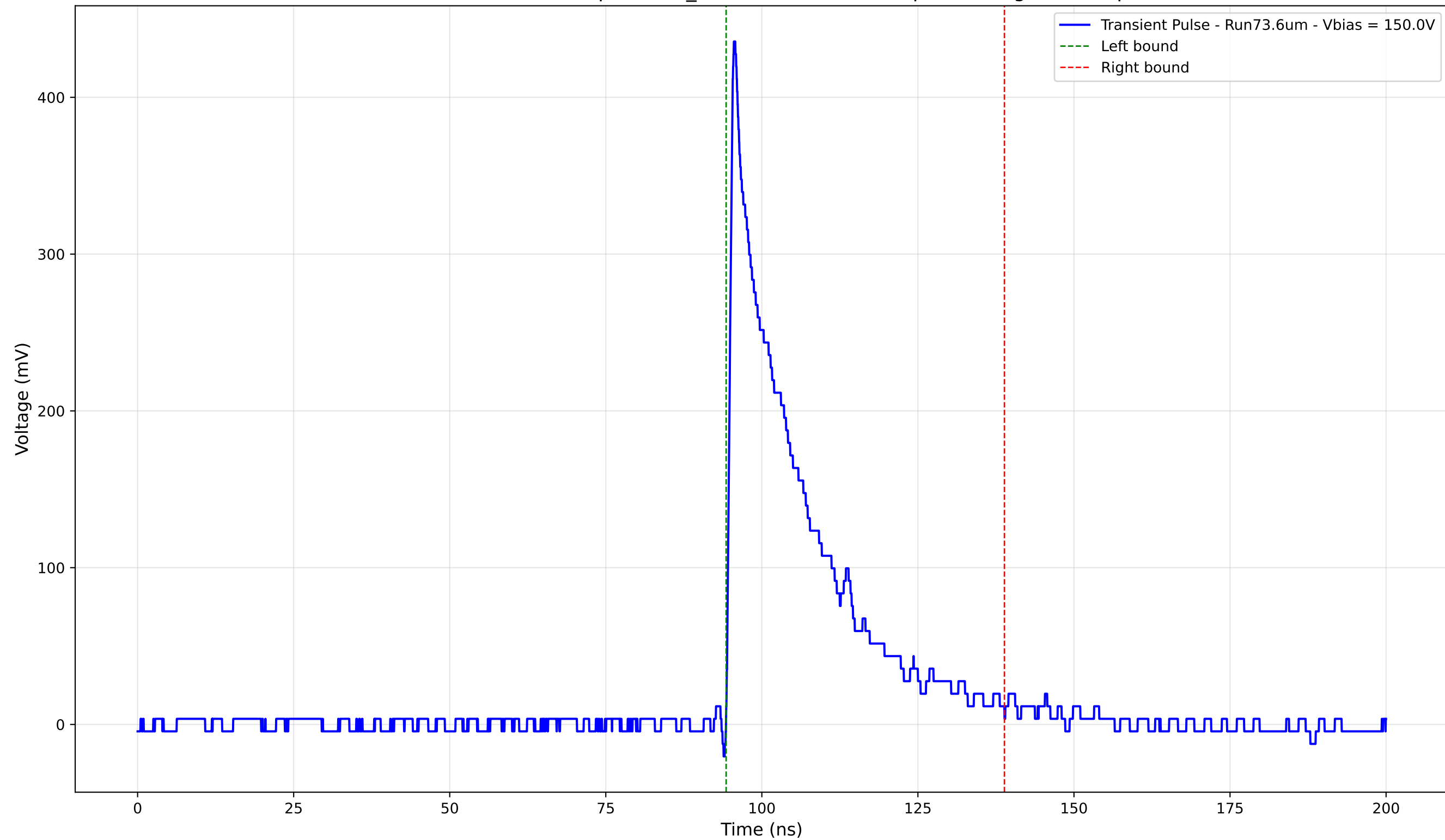
Transient Pulse - Sample: 1cm_42 - Position: 1730.0 \mu\text{m} - Charge: 93.78 pC
