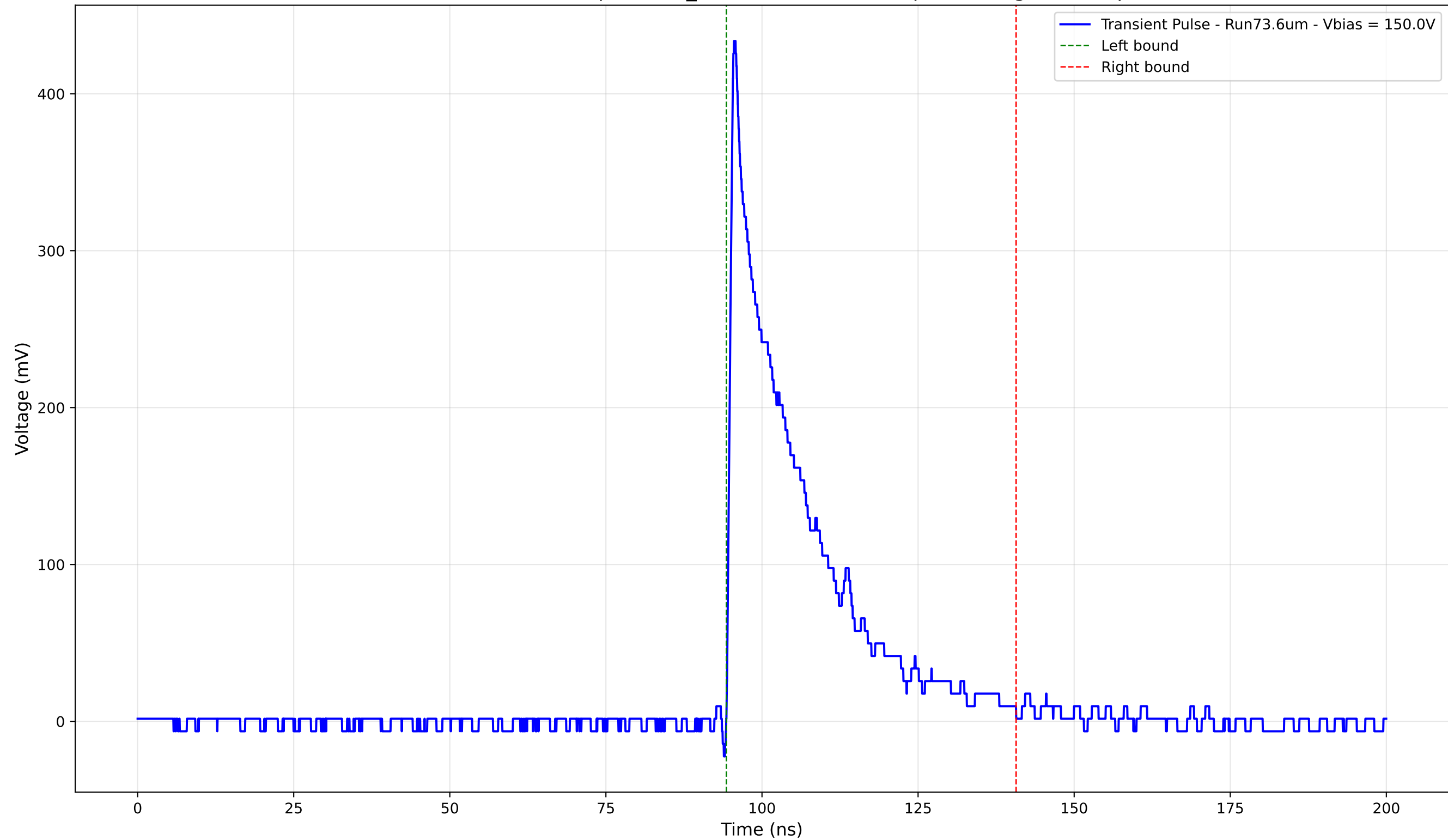
Transient Pulse - Sample: 1cm_42 - Position: 1770.0 \mu\text{m} - Charge: 91.78 pC
