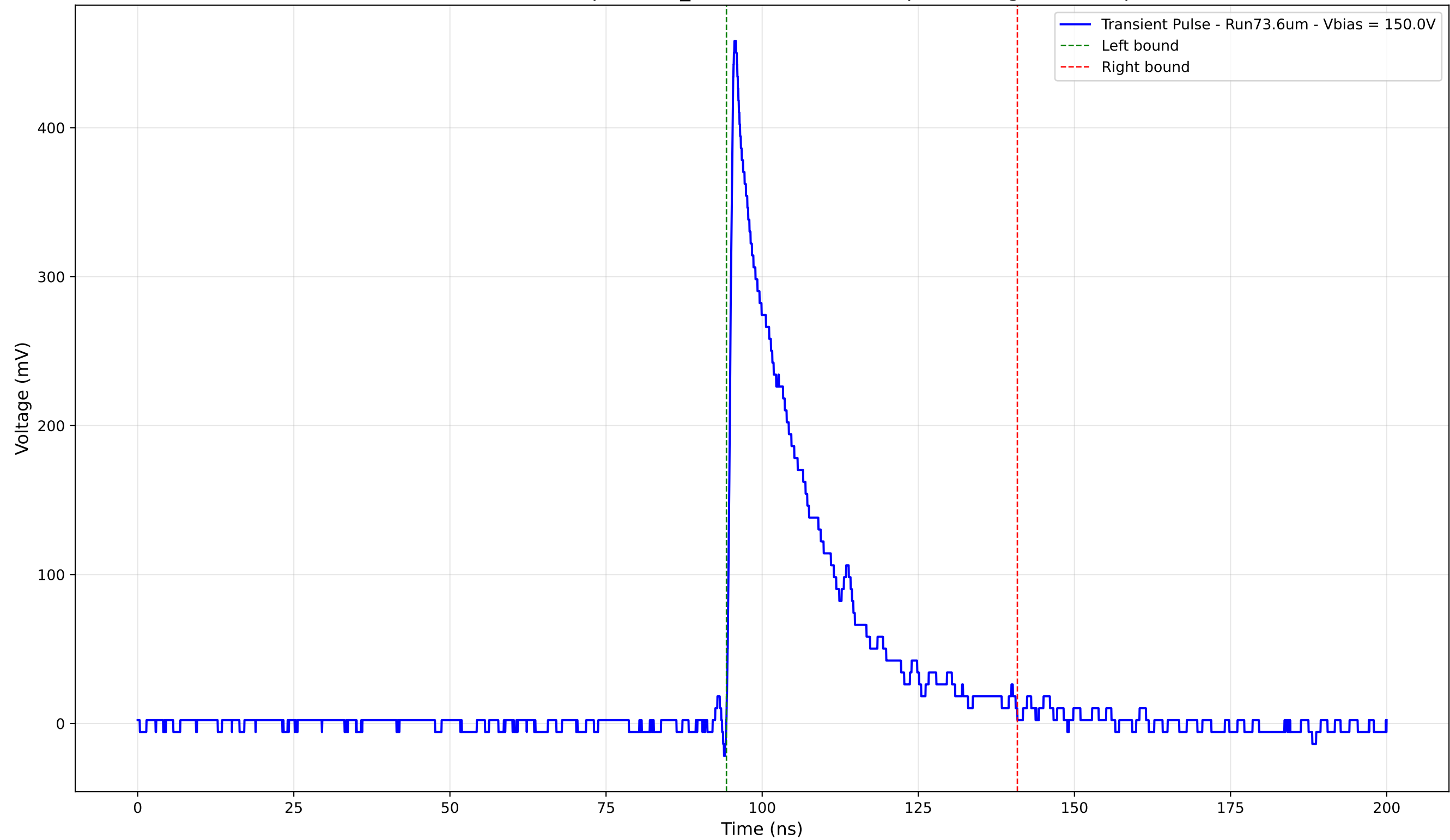
Transient Pulse - Sample: 1cm_42 - Position: 1035.0 \mu\text{m} - Charge: 101.49 pC
