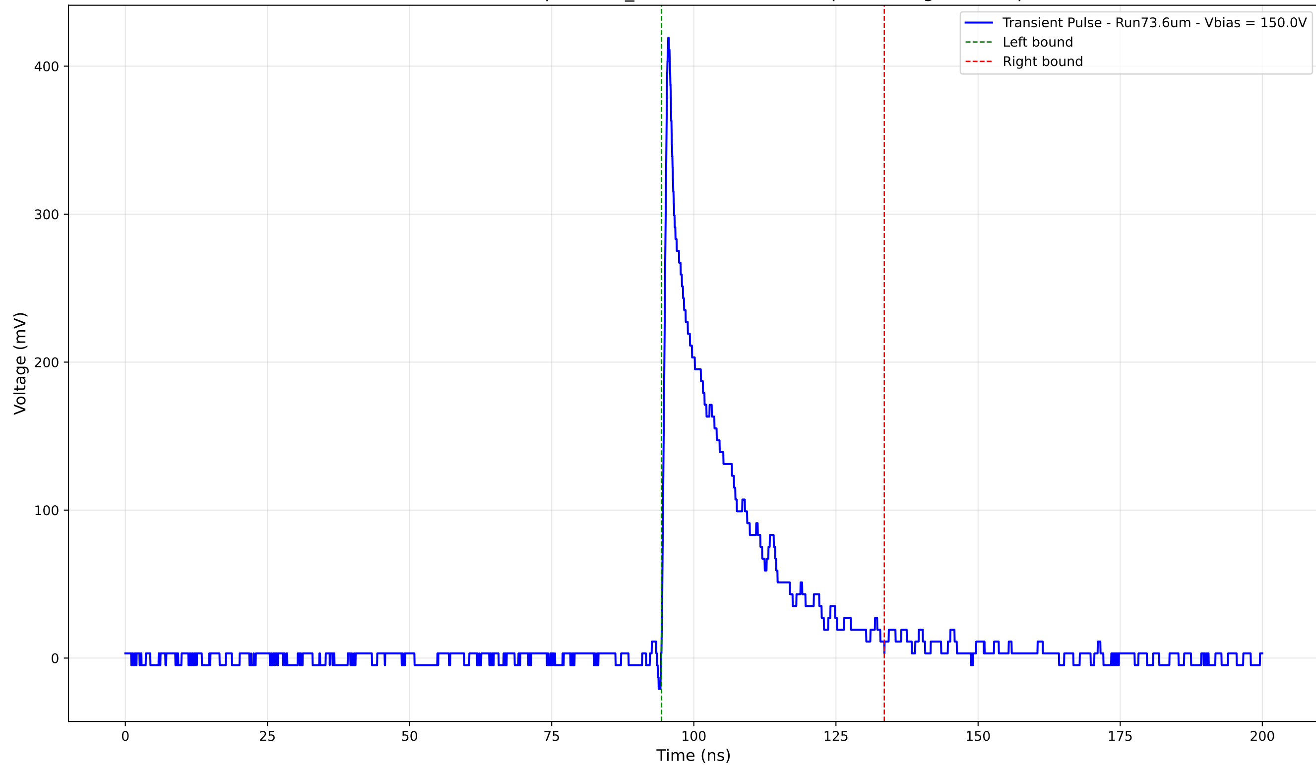
Transient Pulse - Sample: 1cm_42 - Position: 2470.0 \mu\text{m} - Charge: 76.87 pC
