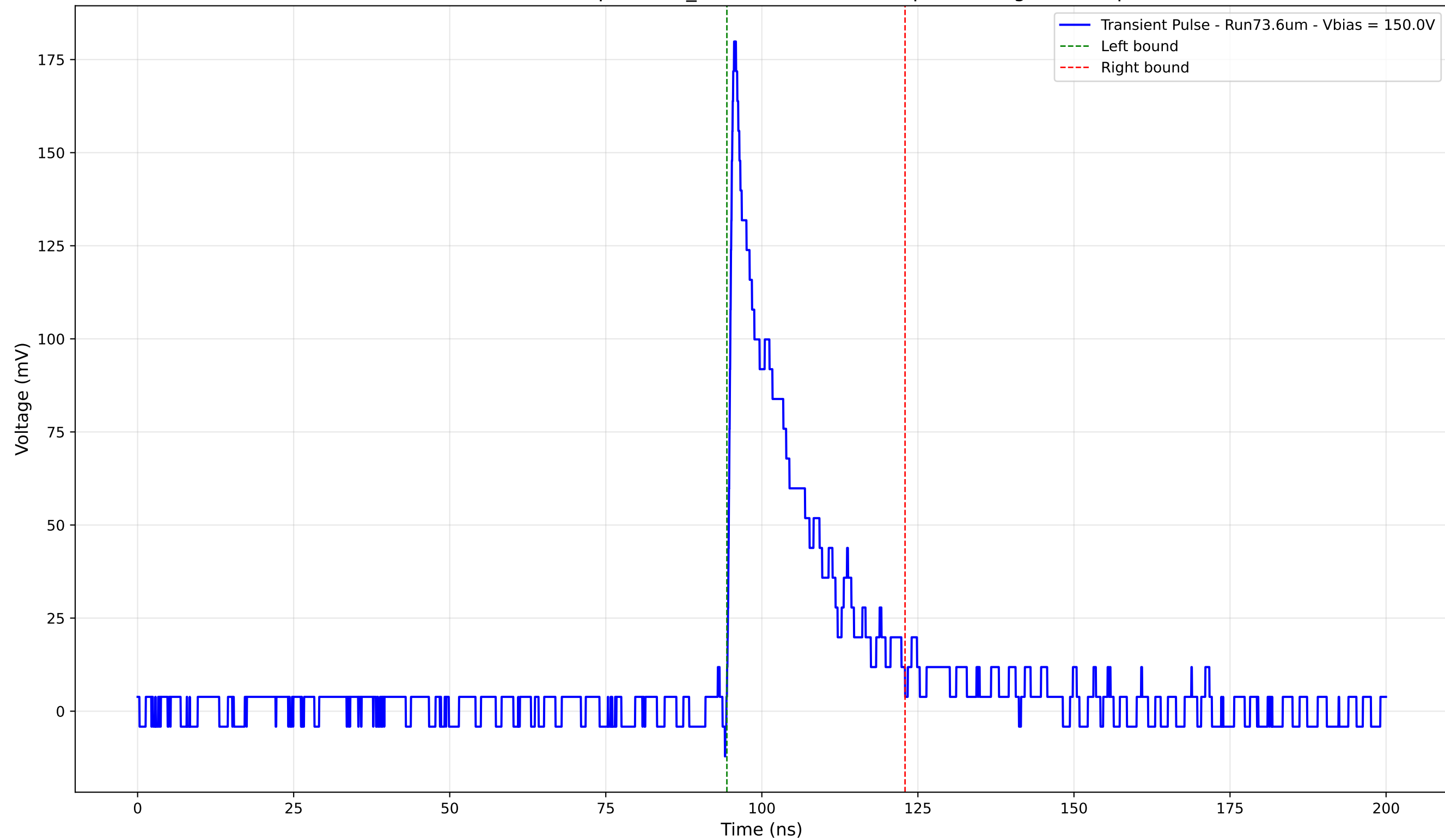
Transient Pulse - Sample: 1cm_42 - Position: 4170.0 \mu\text{m} - Charge: 33.17 pC
