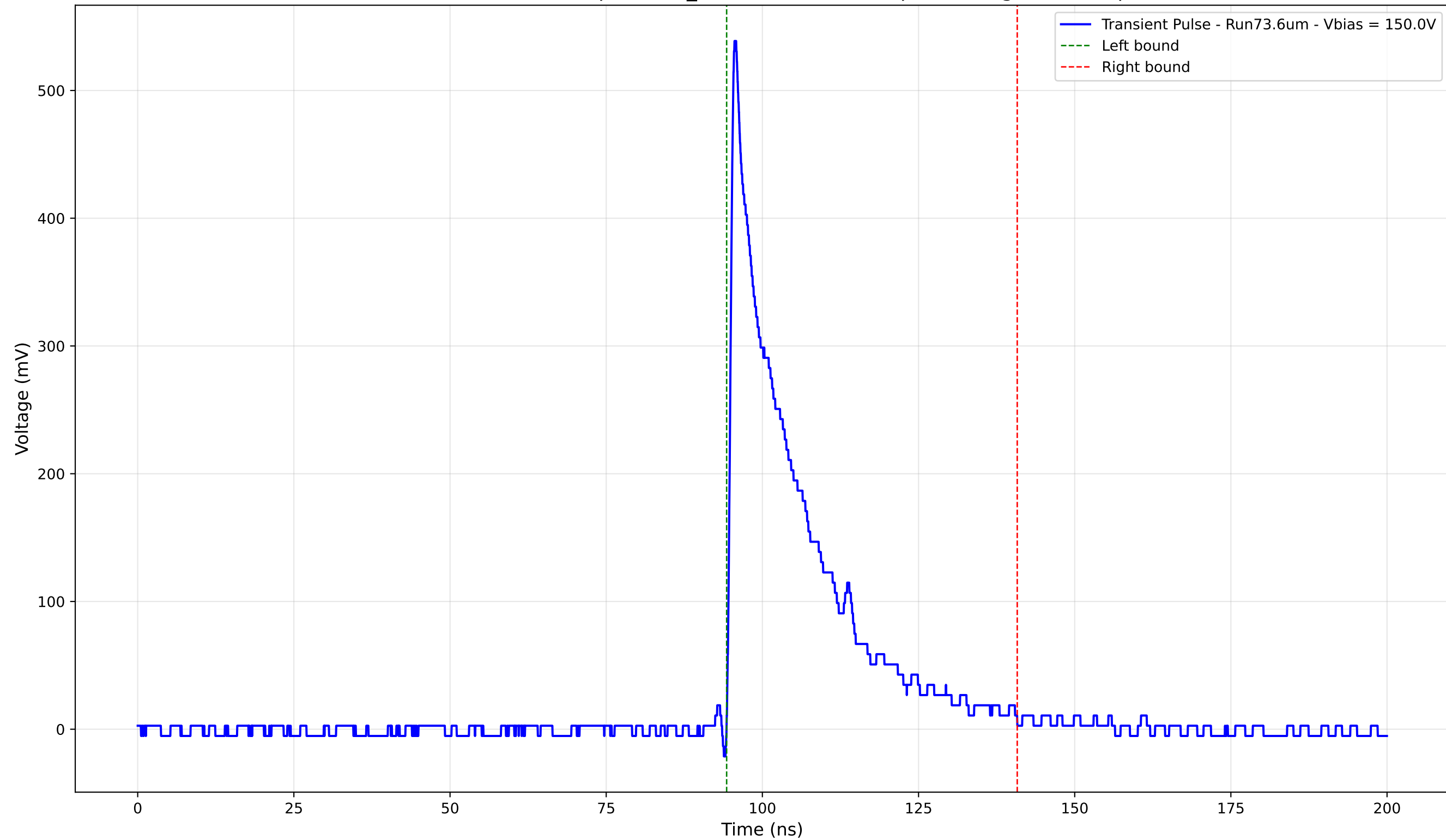
Transient Pulse - Sample: 1cm_42 - Position: 490.0 \mu\text{m} - Charge: 110.96 pC
