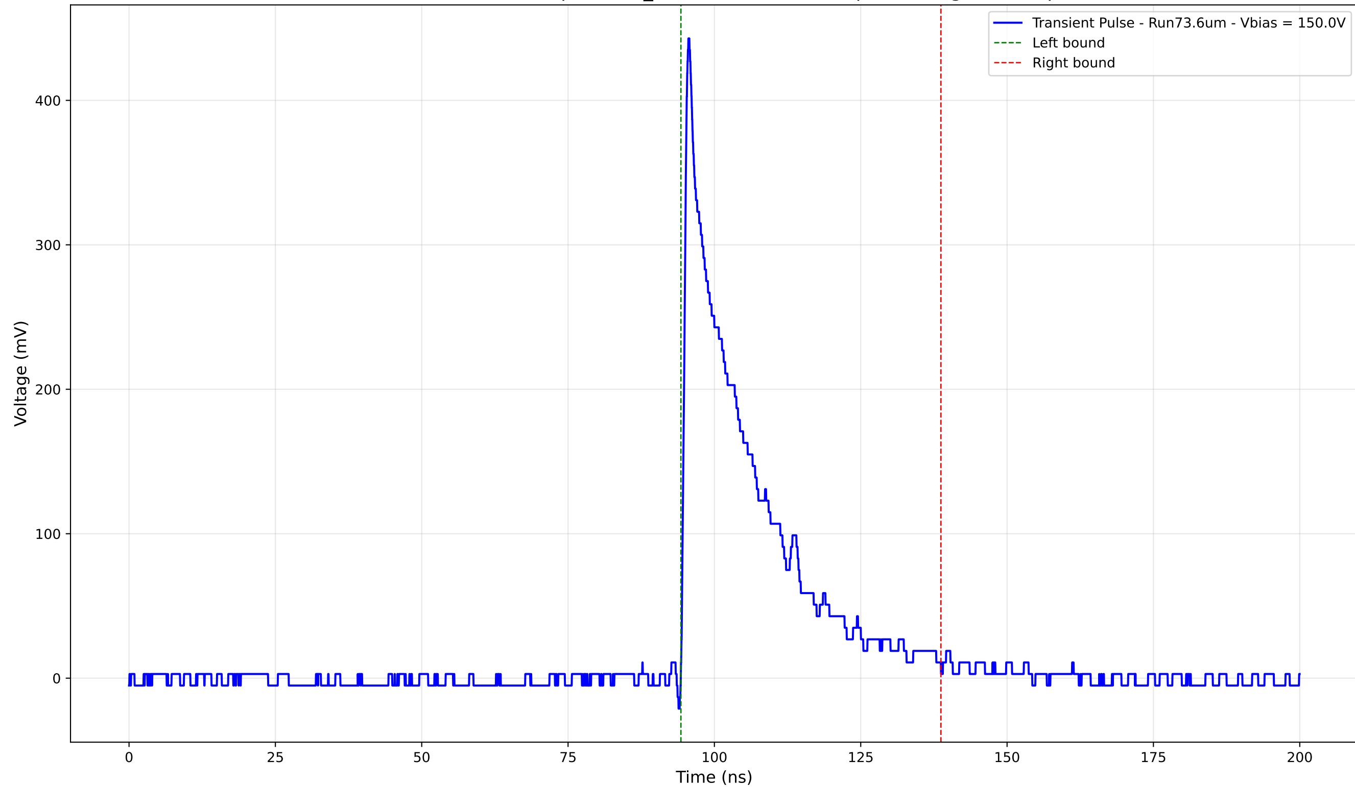
Transient Pulse - Sample: 1cm_42 - Position: 1900.0 \mu\text{m} - Charge: 92.31 pC
