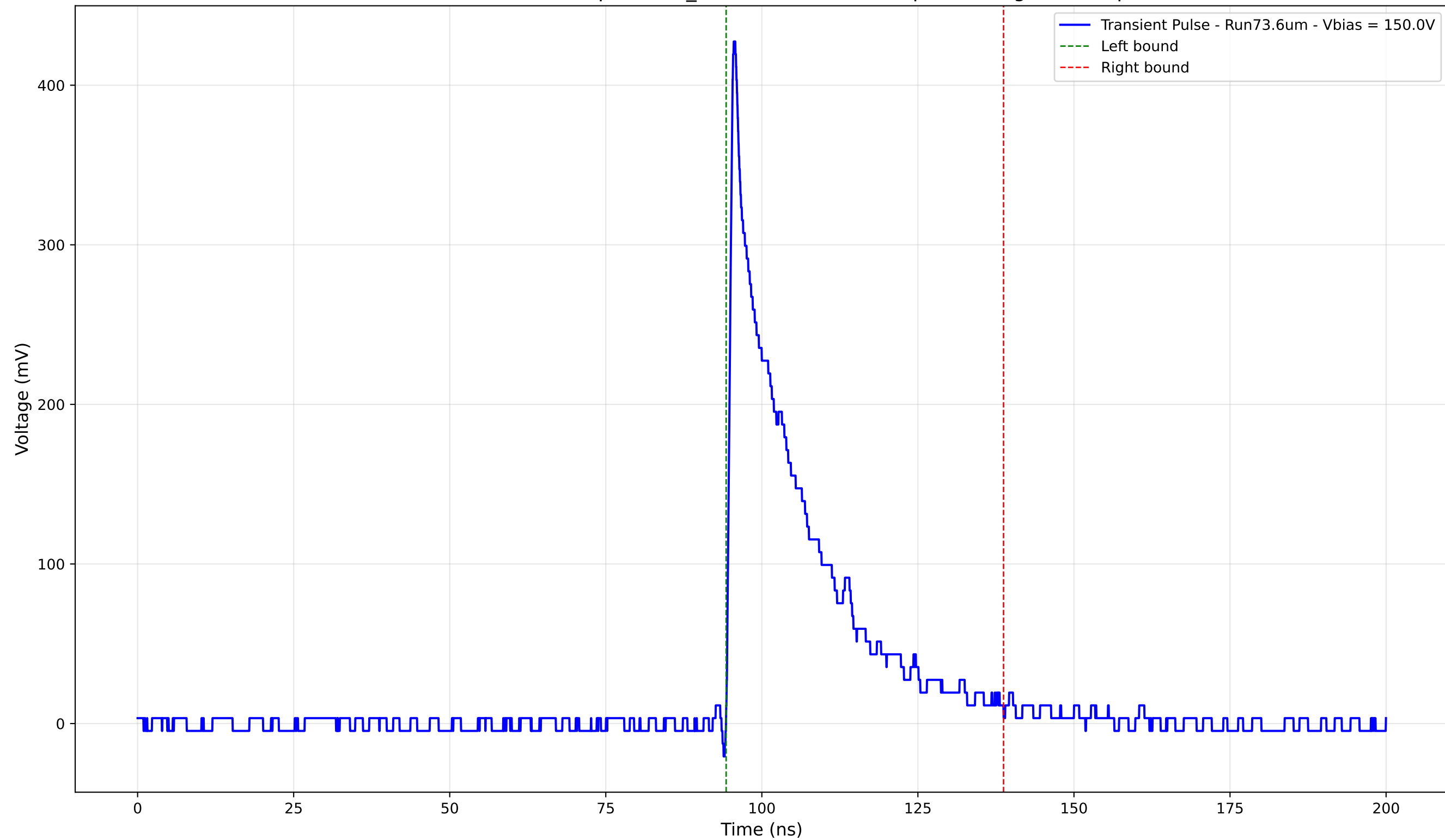
Transient Pulse - Sample: 1cm_42 - Position: 2085.0 \mu\text{m} - Charge: 87.55 pC
