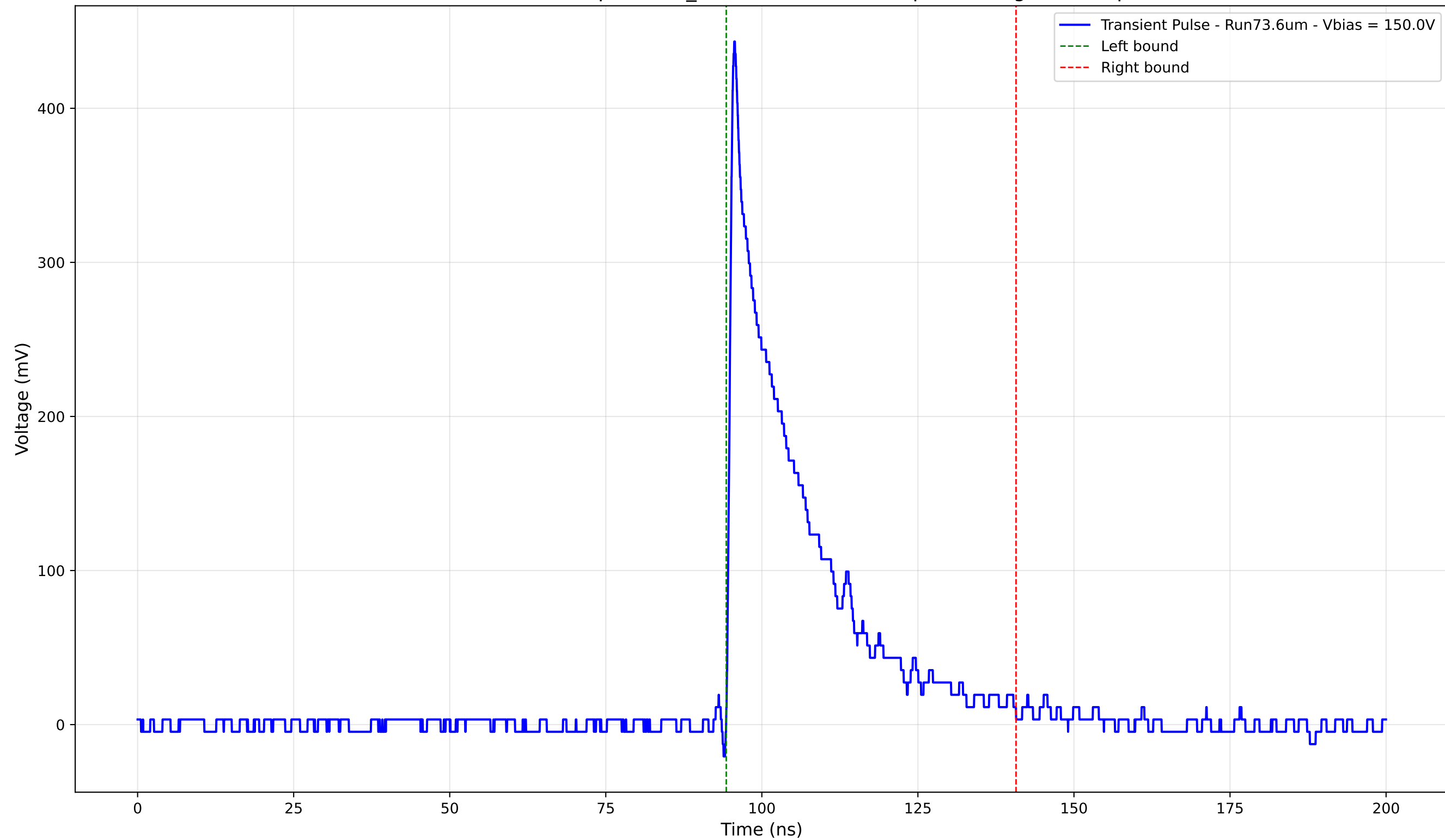
Transient Pulse - Sample: 1cm_42 - Position: 1885.0 \mu\text{m} - Charge: 93.12 pC
