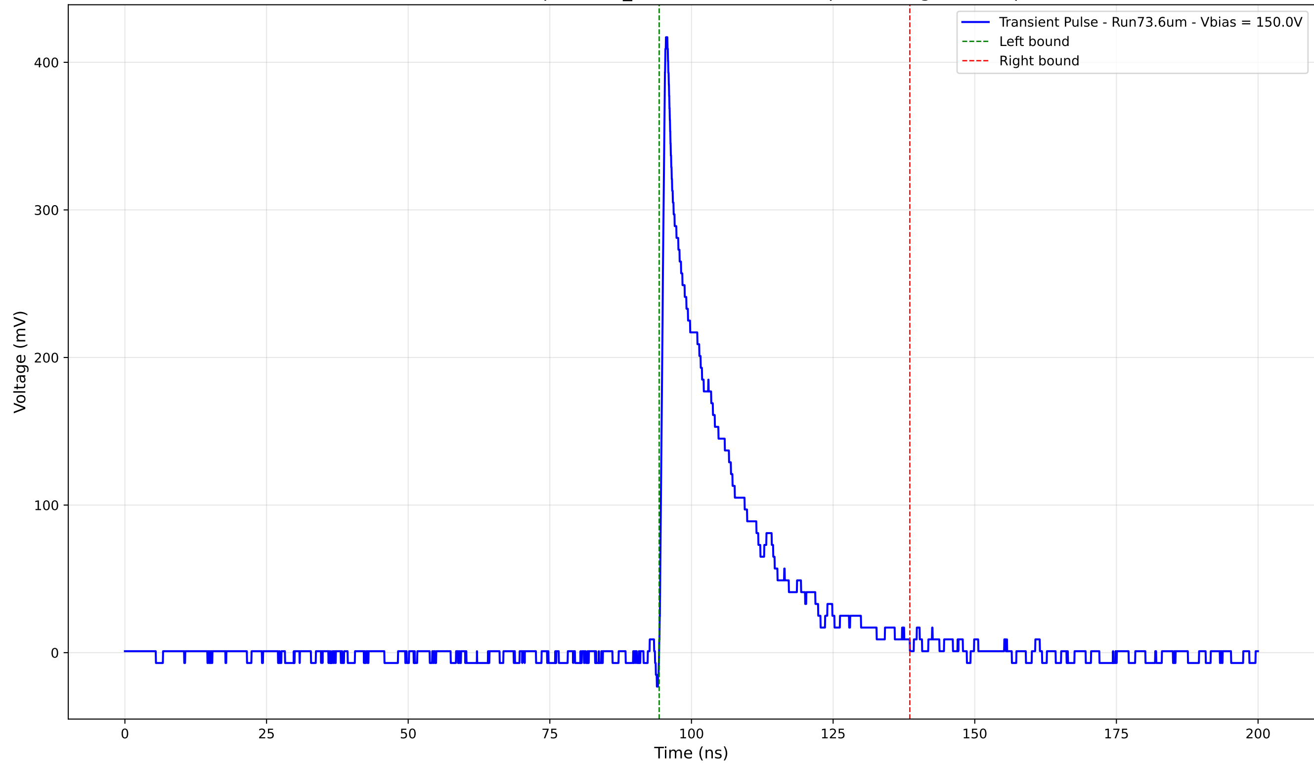
Transient Pulse - Sample: 1cm_42 - Position: 2235.0 \mu\text{m} - Charge: 81.44 pC
