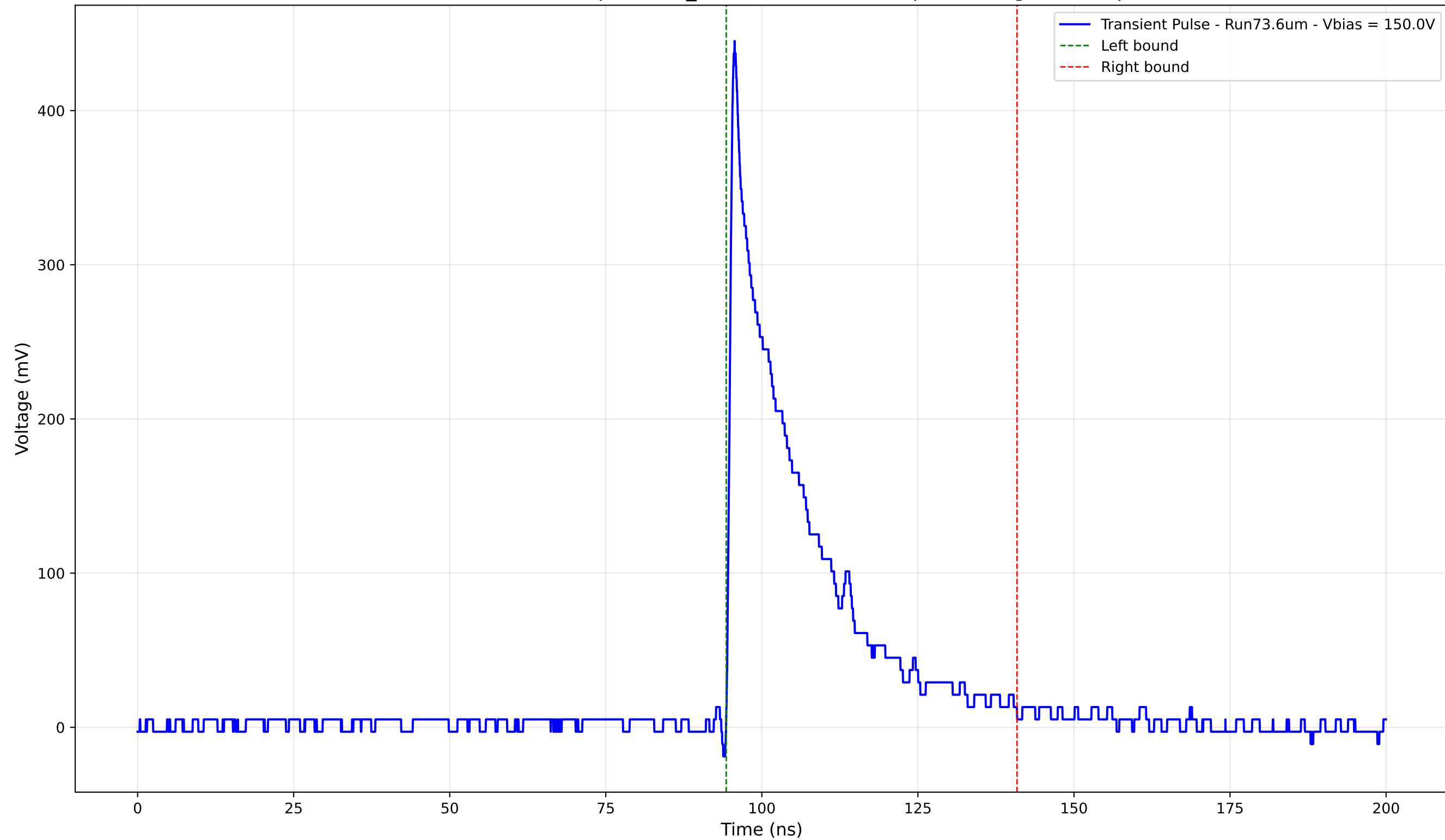
Transient Pulse - Sample: 1cm_42 - Position: 1790.0 \mu\text{m} - Charge: 95.11 pC
