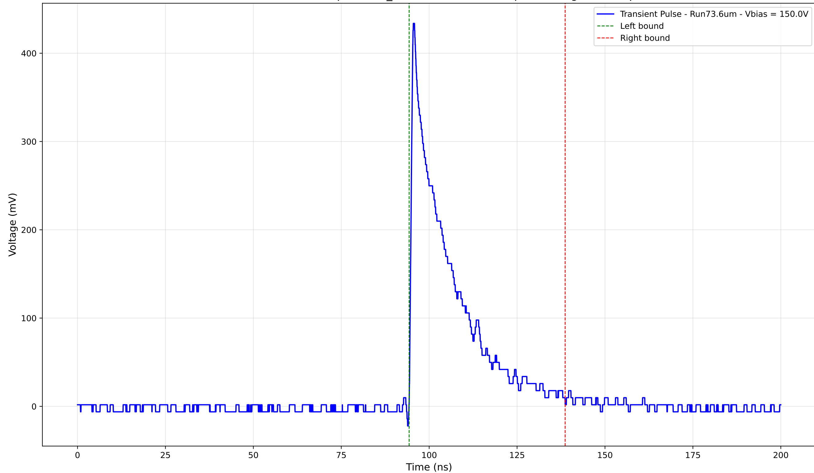
Transient Pulse - Sample: 1cm_42 - Position: 1605.0 \mu\text{m} - Charge: 94.08 pC
