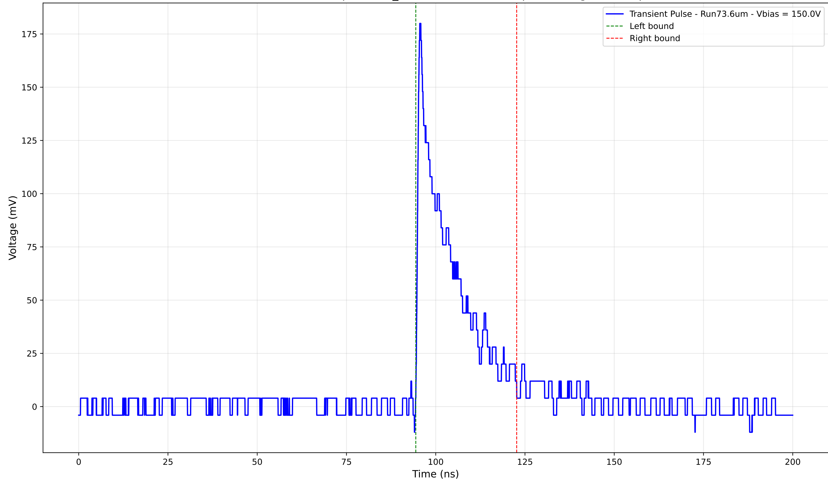
Transient Pulse - Sample: 1cm_42 - Position: 4160.0 \mu\text{m} - Charge: 33.17 pC
