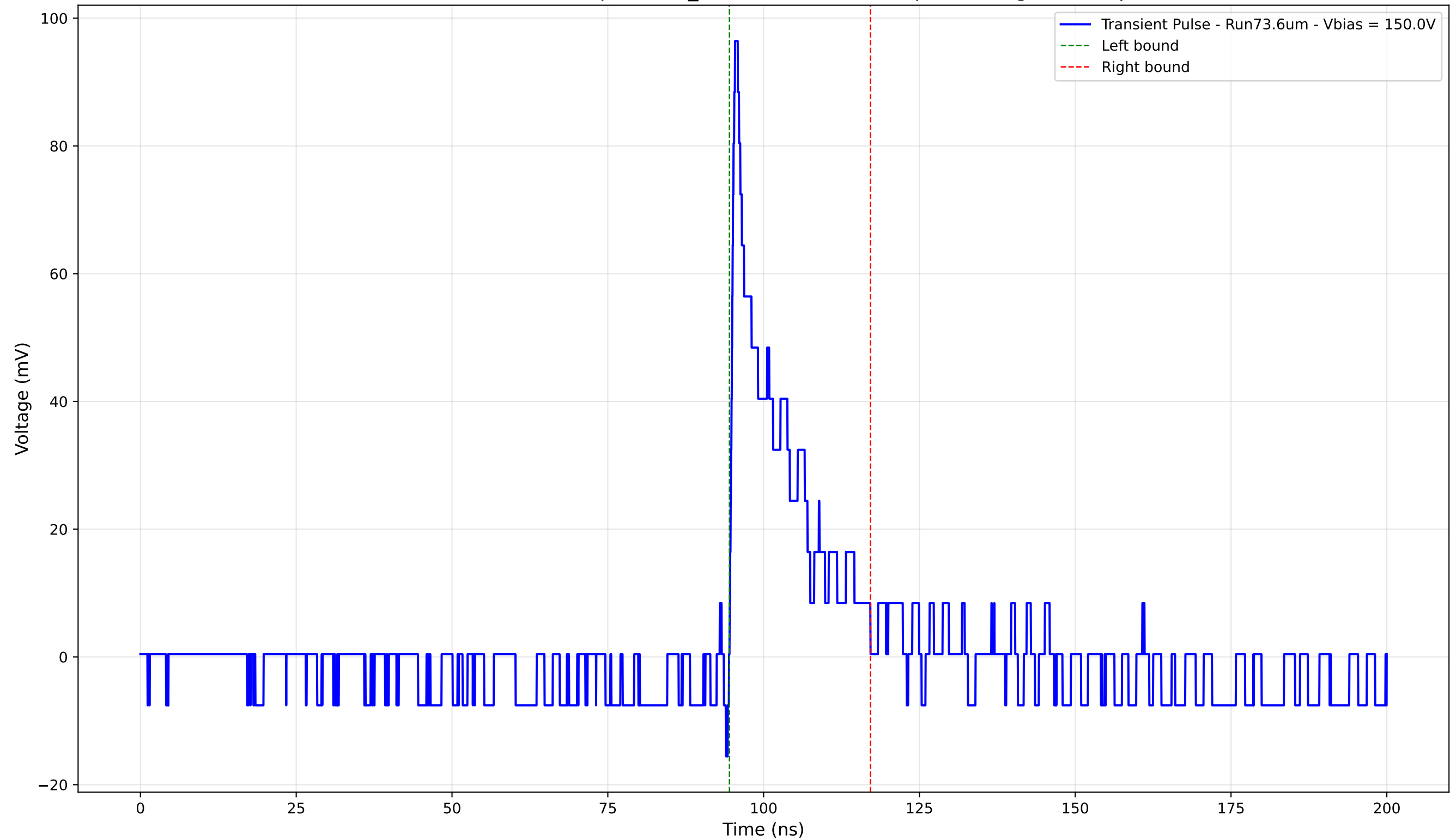
Transient Pulse - Sample: 1cm_42 - Position: 4865.0 \mu\text{m} - Charge: 13.63 pC
