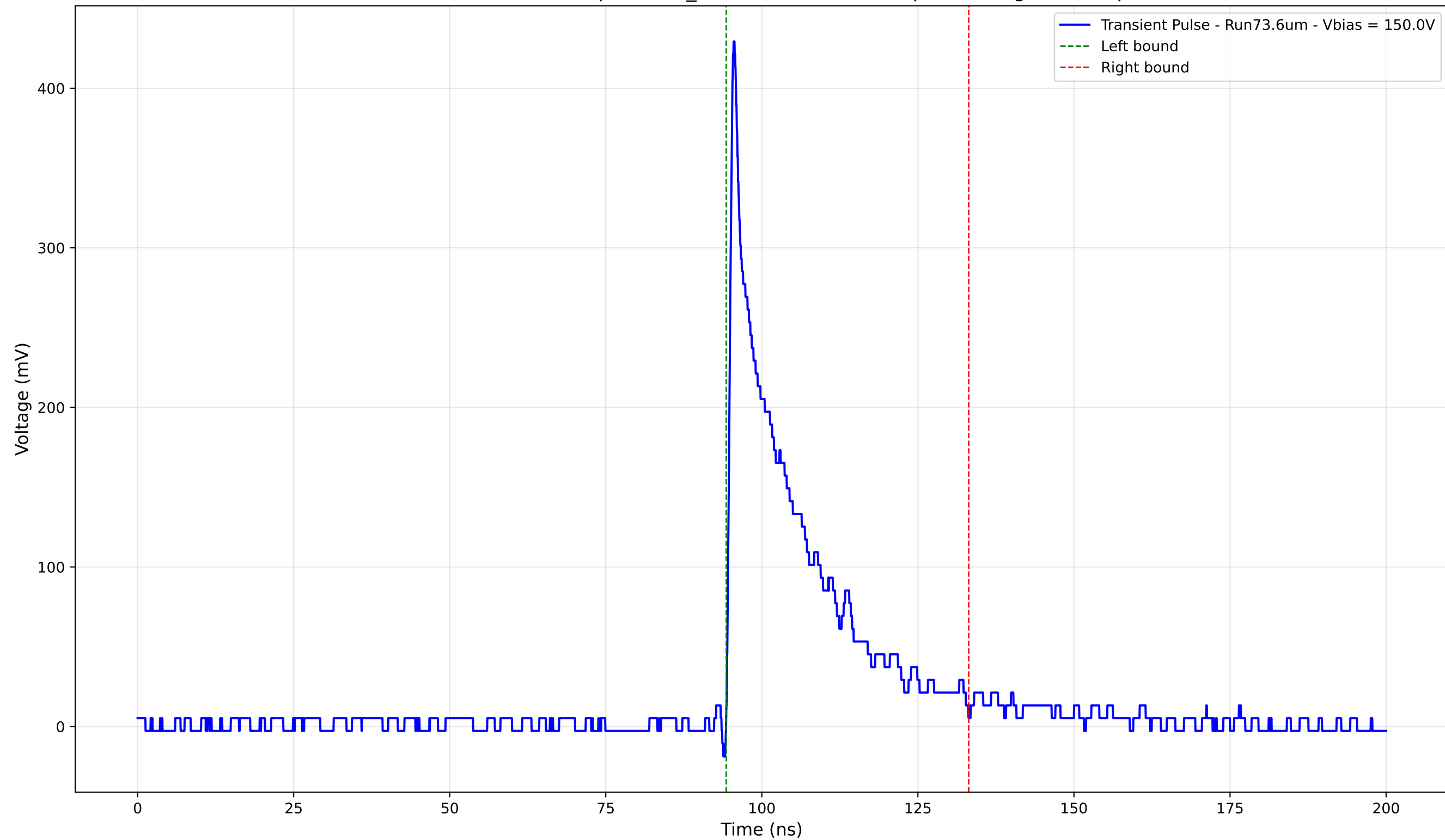
Transient Pulse - Sample: 1cm_42 - Position: 2695.0 \mu\text{m} - Charge: 78.86 pC
