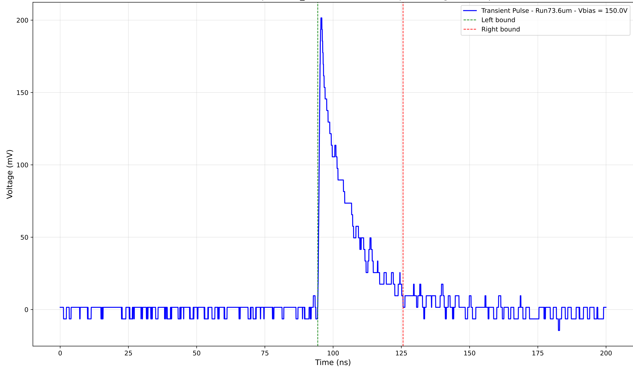
Transient Pulse - Sample: 1cm_42 - Position: 3940.0 \mu\text{m} - Charge: 38.70 pC
