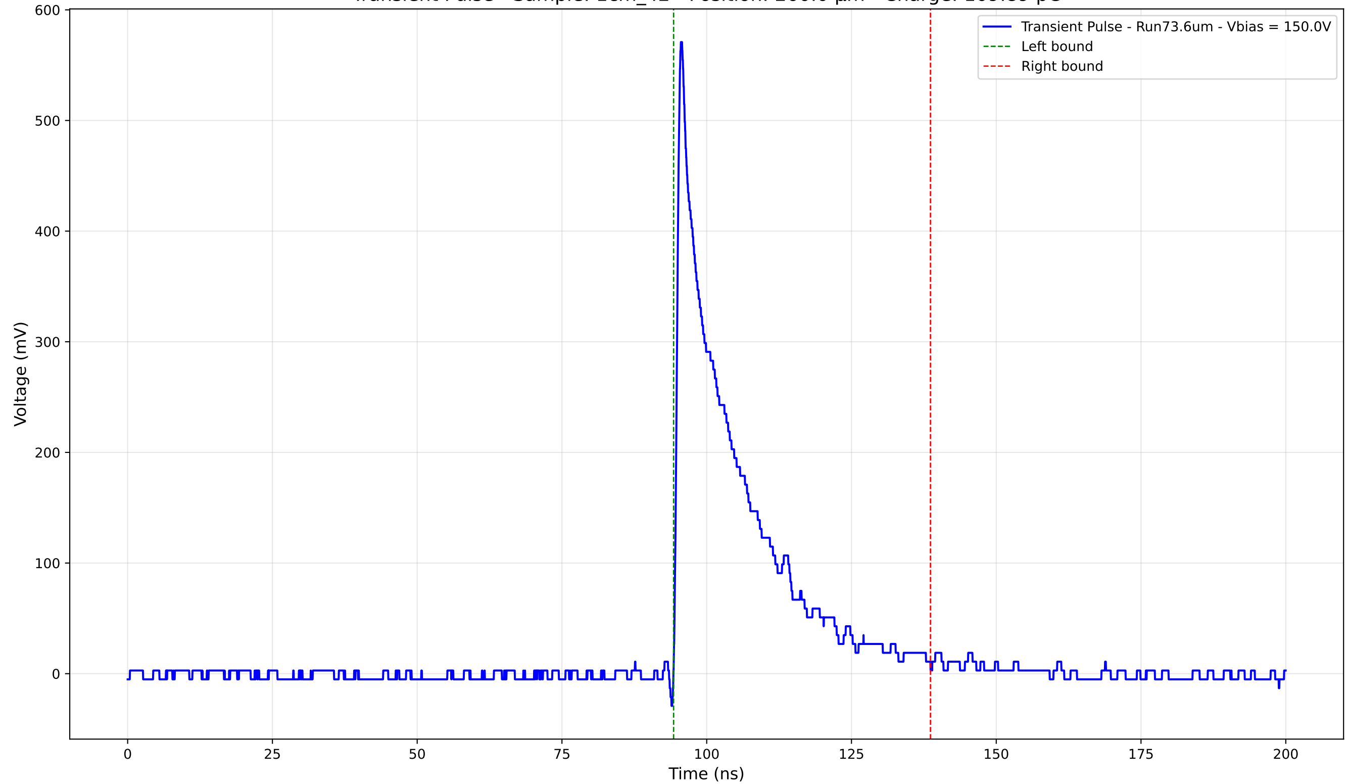
Transient Pulse - Sample: 1cm_42 - Position: 260.0 \mu\text{m} - Charge: 109.89 pC
