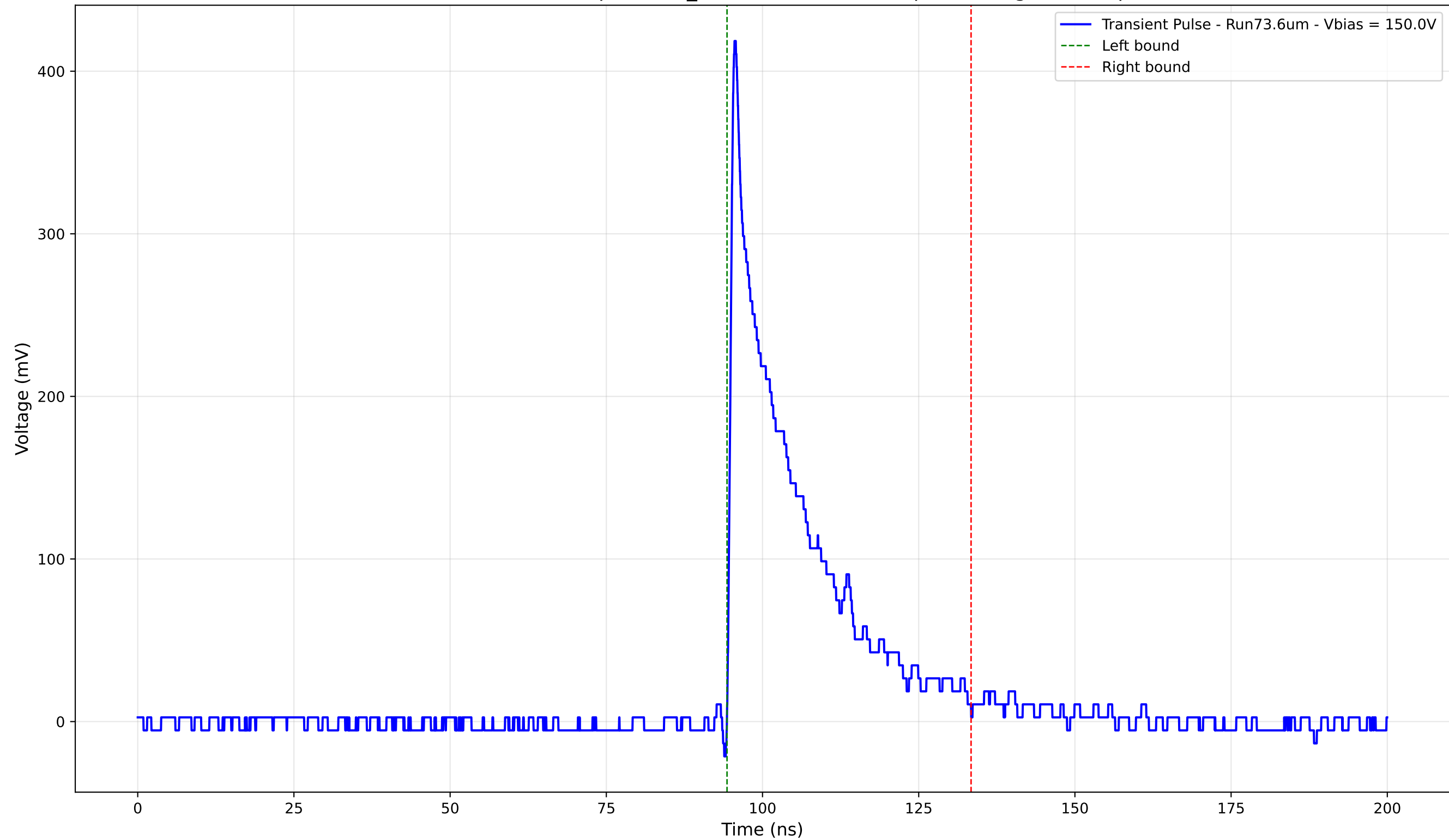
Transient Pulse - Sample: 1cm_42 - Position: 2195.0 \mu\text{m} - Charge: 81.50 pC
