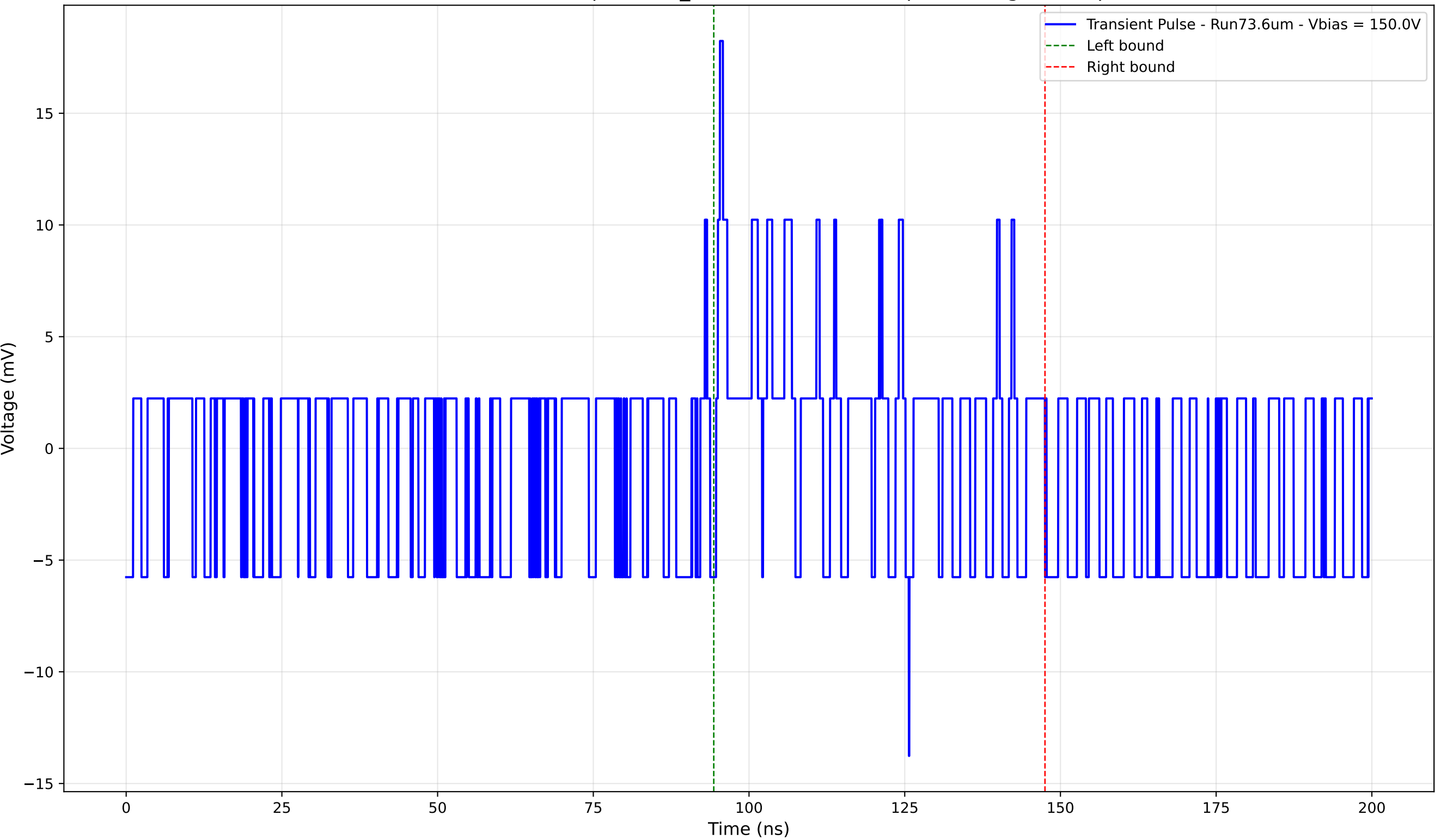
Transient Pulse - Sample: 1cm_42 - Position: 4975.0 \mu\text{m} - Charge: 1.58 pC
