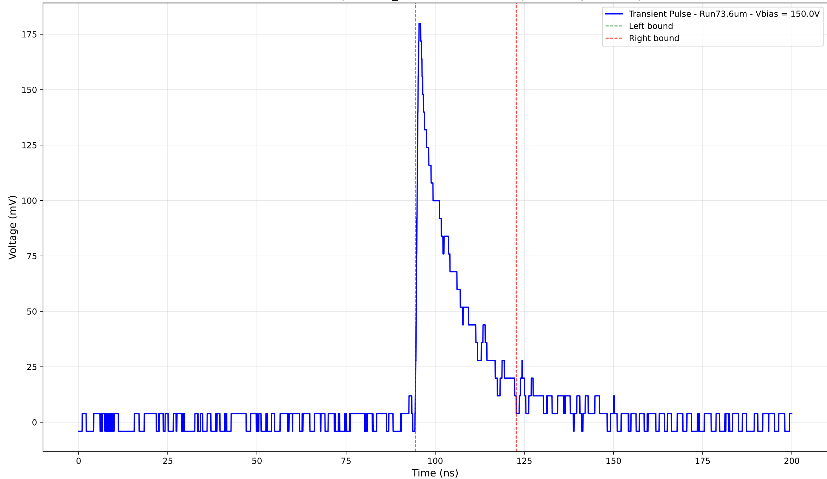
Transient Pulse - Sample: 1cm_42 - Position: 4125.0 \mu\text{m} - Charge: 34.92 pC
