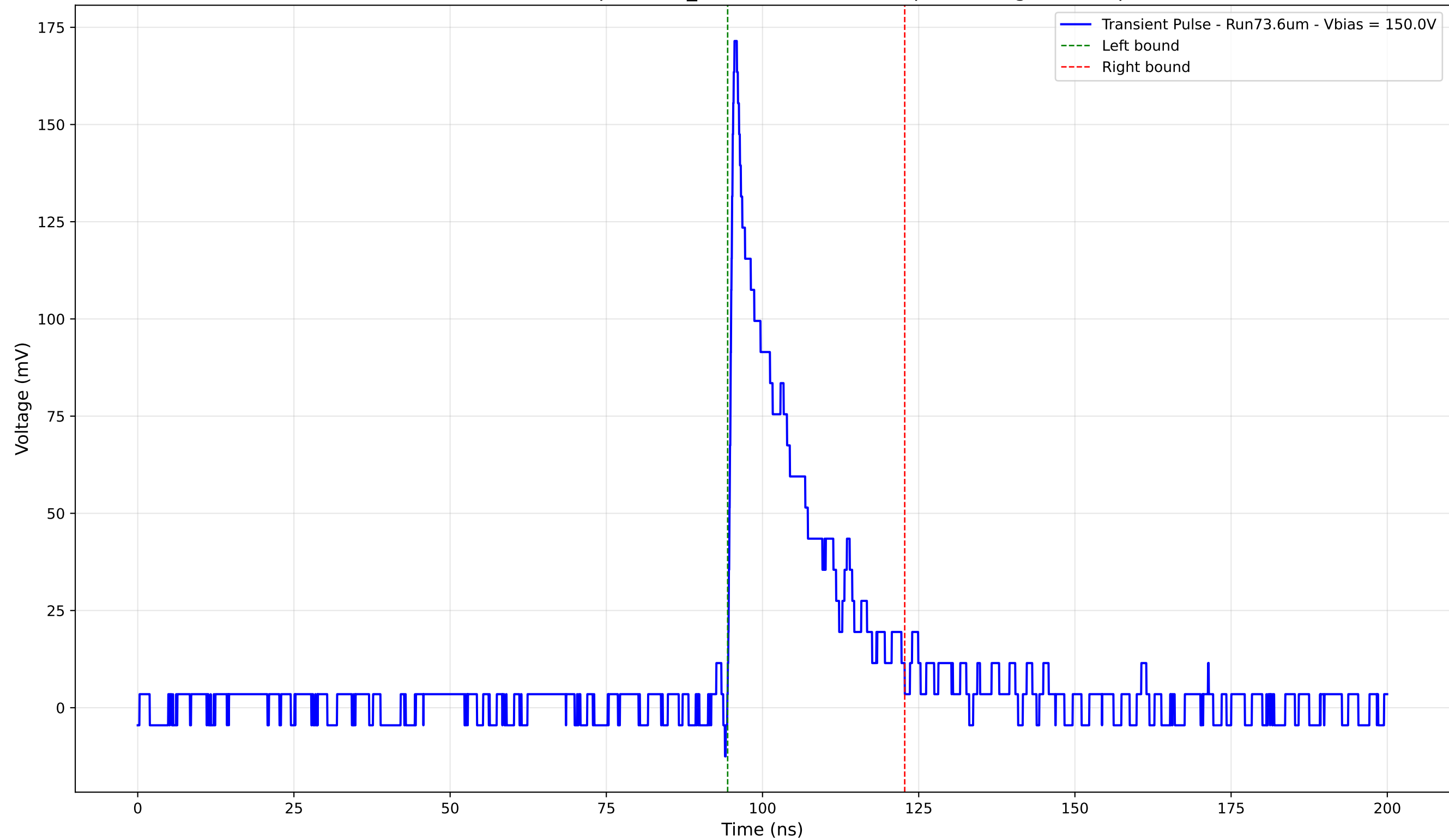
Transient Pulse - Sample: 1cm_42 - Position: 4290.0 \mu\text{m} - Charge: 31.77 pC
