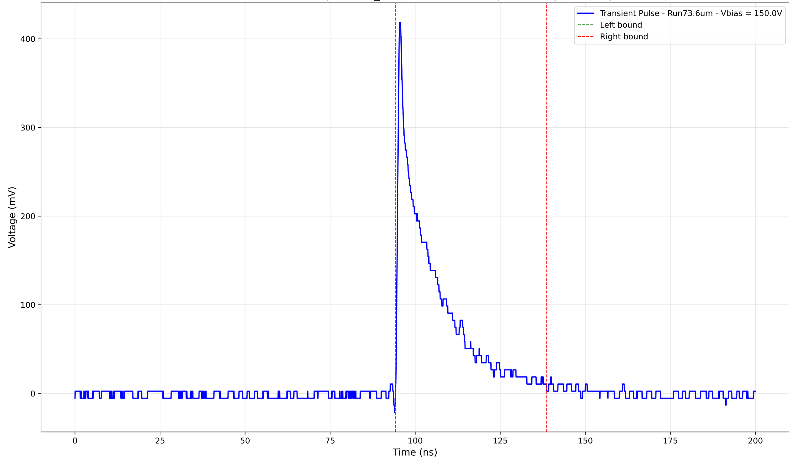
Transient Pulse - Sample: 1cm_42 - Position: 2705.0 \mu\text{m} - Charge: 79.13 pC
