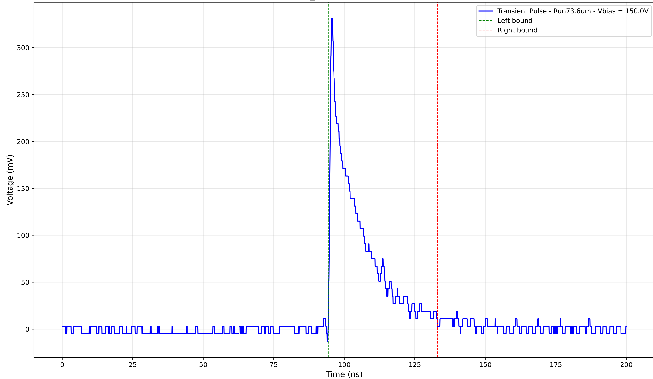
Transient Pulse - Sample: 1cm_42 - Position: 3100.0 \mu\text{m} - Charge: 63.67 pC
