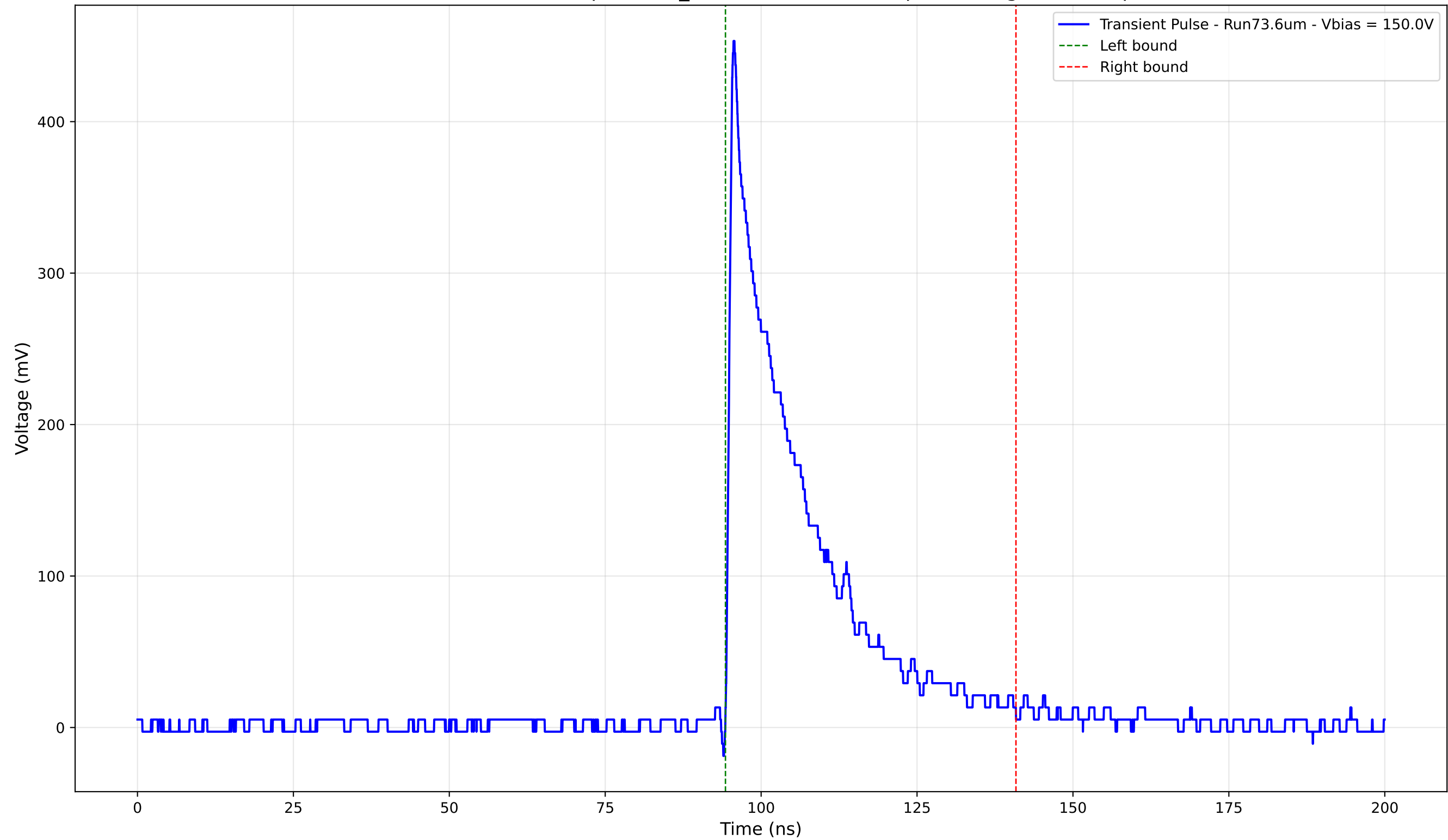
Transient Pulse - Sample: 1cm_42 - Position: 1495.0 \mu\text{m} - Charge: 100.13 pC
