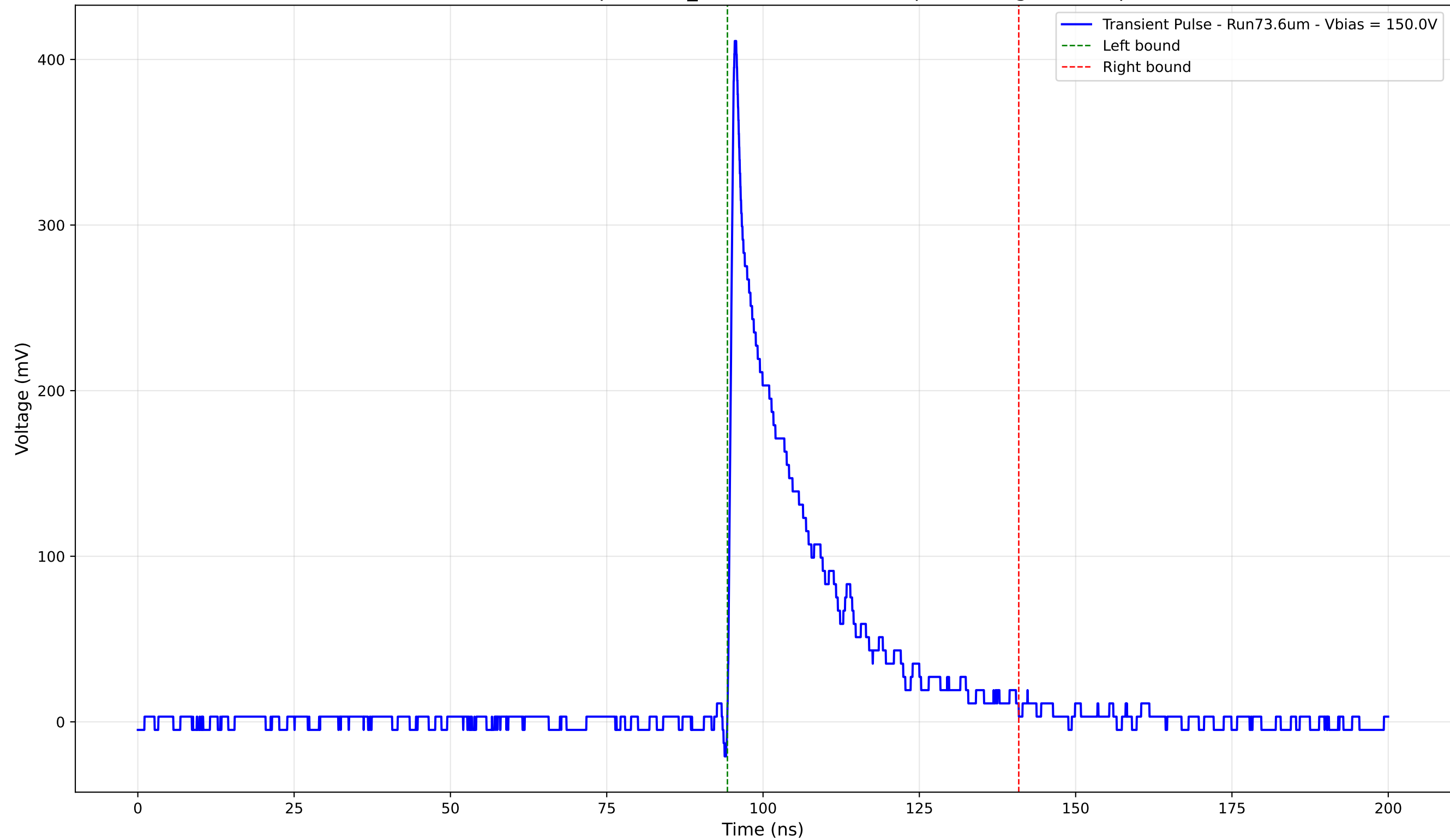
Transient Pulse - Sample: 1cm_42 - Position: 2375.0 \mu\text{m} - Charge: 80.38 pC
