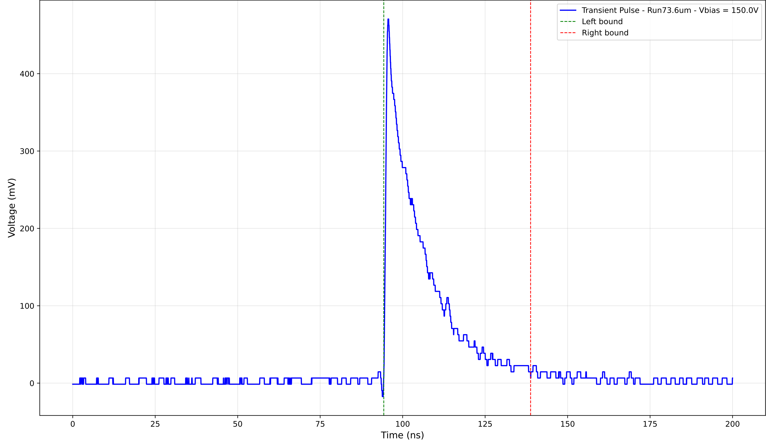
Transient Pulse - Sample: 1cm_42 - Position: 1010.0 \mu\text{m} - Charge: 105.24 pC
