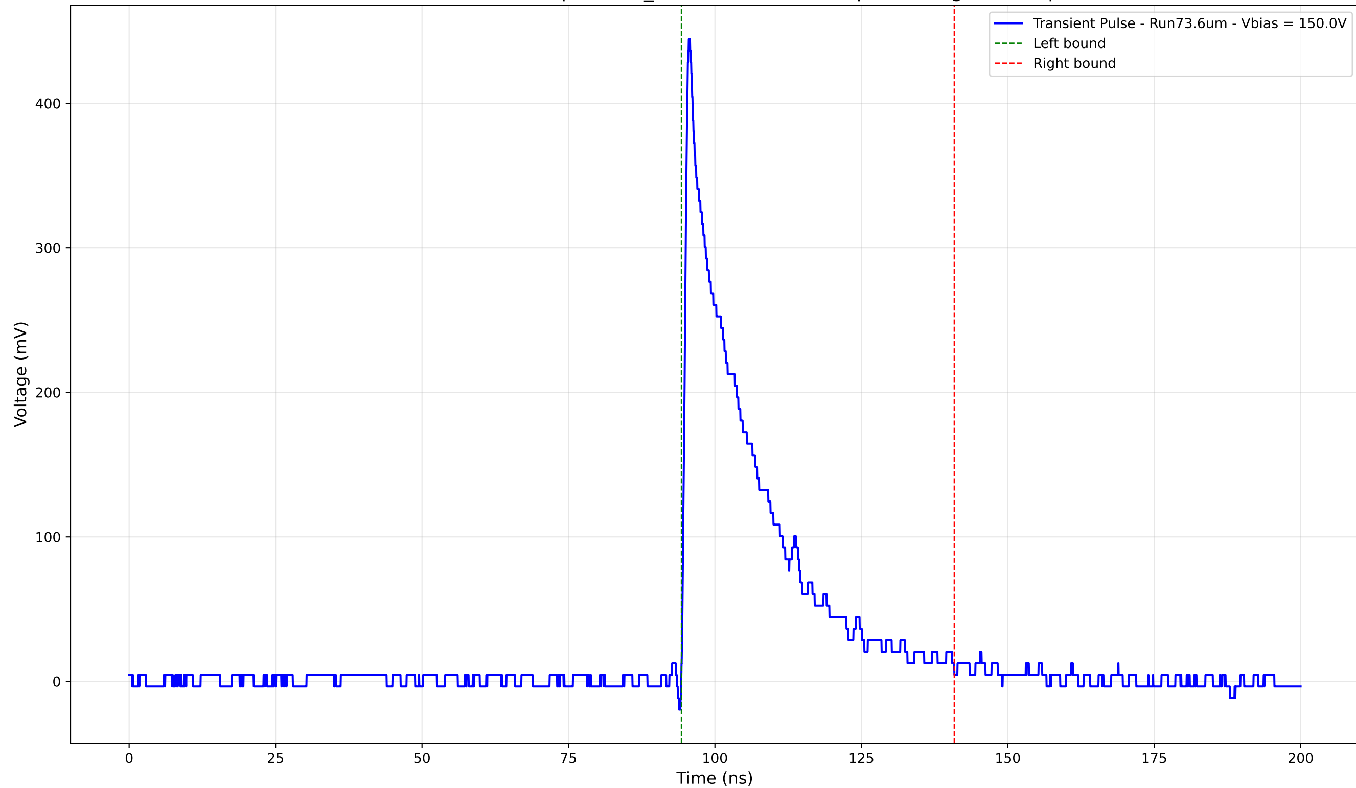
Transient Pulse - Sample: 1cm_42 - Position: 1660.0 \mu\text{m} - Charge: 97.02 pC
