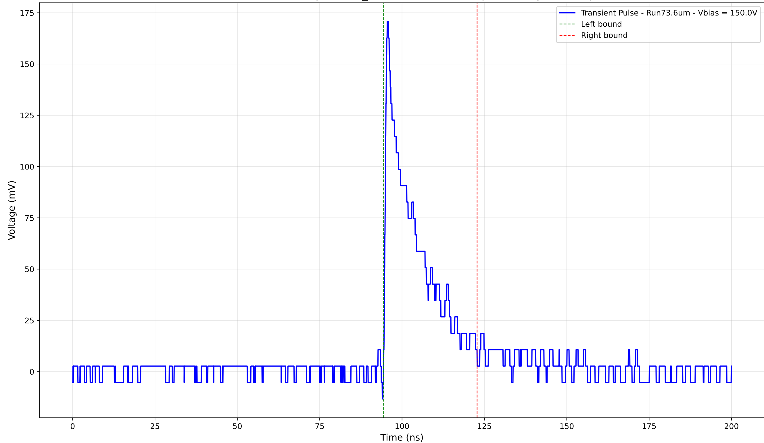
Transient Pulse - Sample: 1cm_42 - Position: 4265.0 \mu\text{m} - Charge: 31.95 pC
