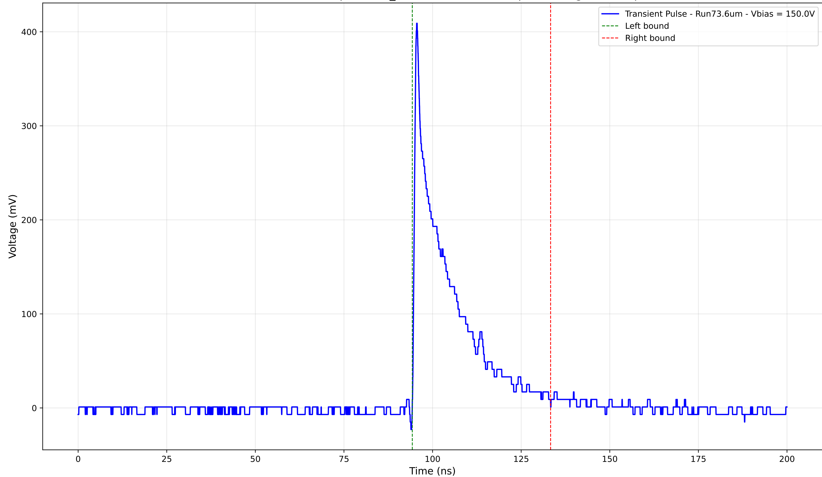
Transient Pulse - Sample: 1cm_42 - Position: 2445.0 \mu\text{m} - Charge: 73.57 pC
