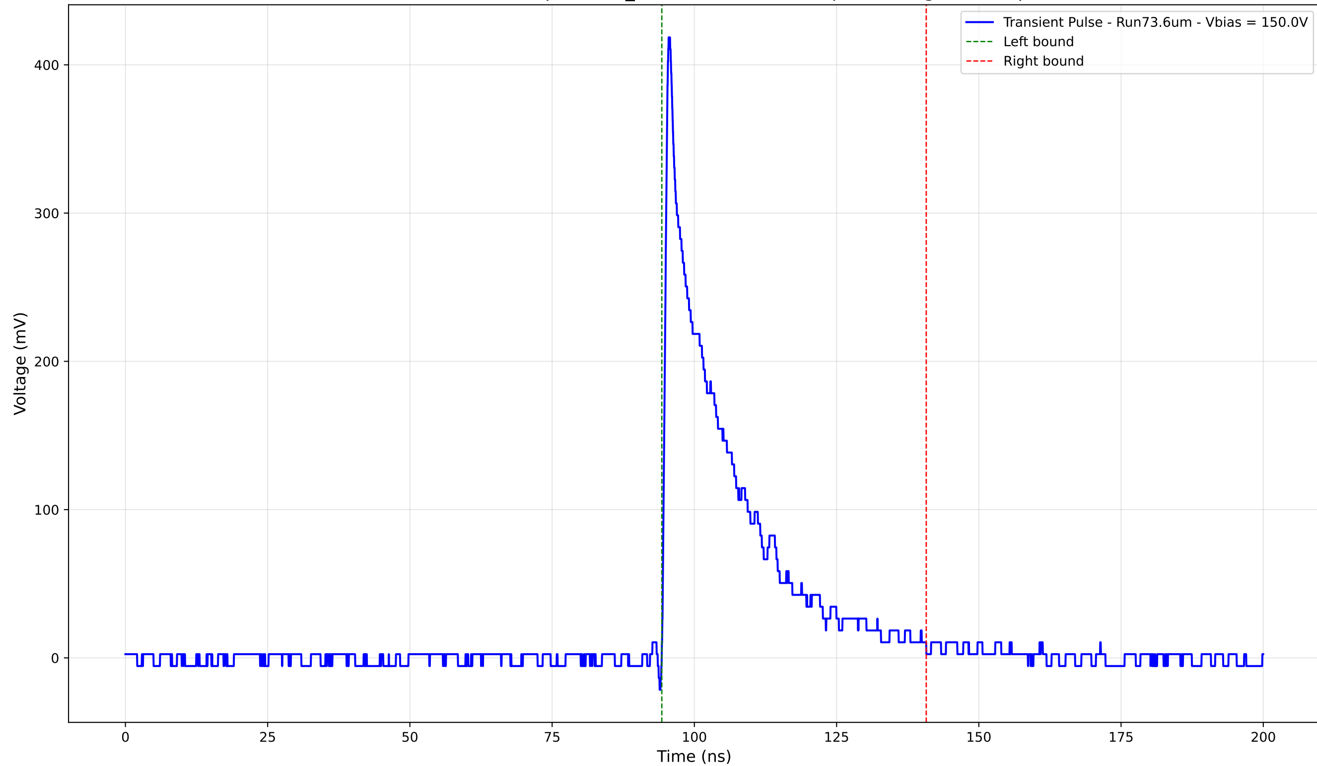
Transient Pulse - Sample: 1cm_42 - Position: 2215.0 \mu\text{m} - Charge: 84.02 pC
