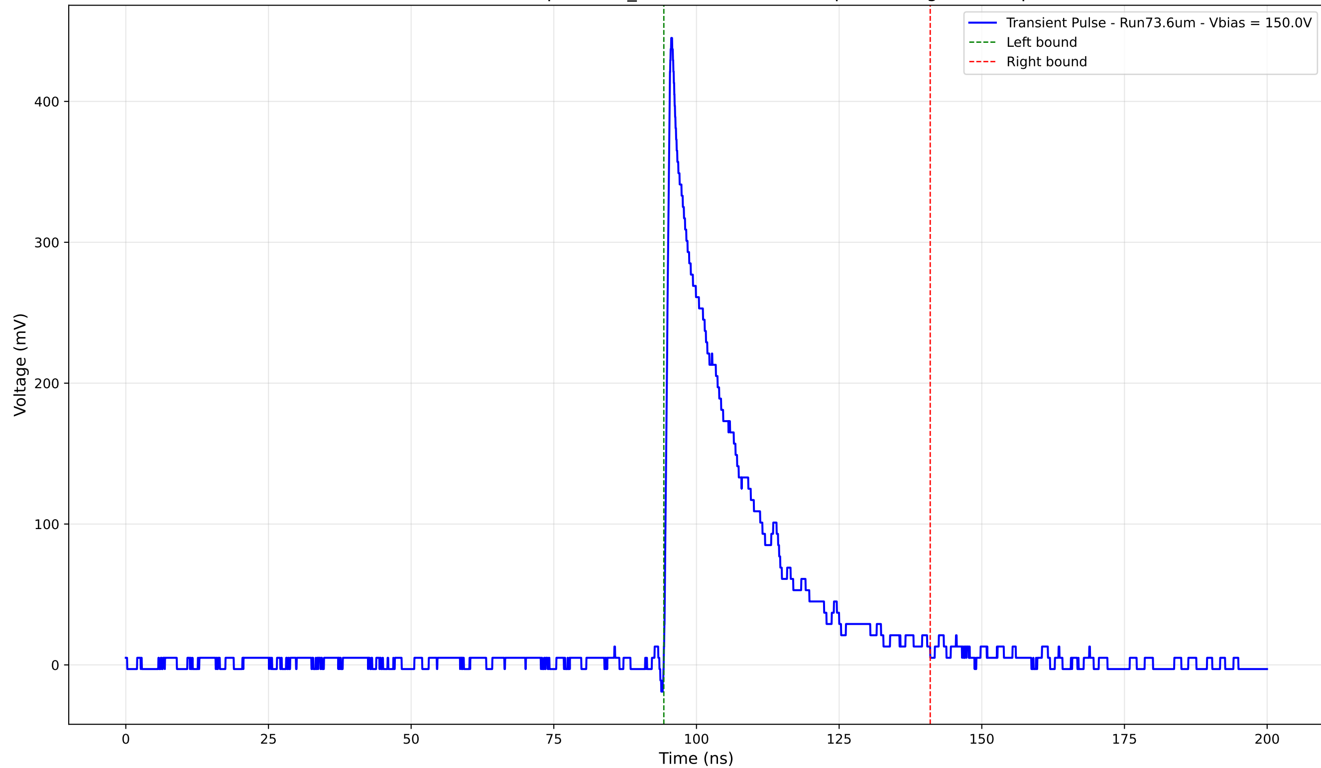
Transient Pulse - Sample: 1cm_42 - Position: 1620.0 \mu\text{m} - Charge: 97.99 pC
