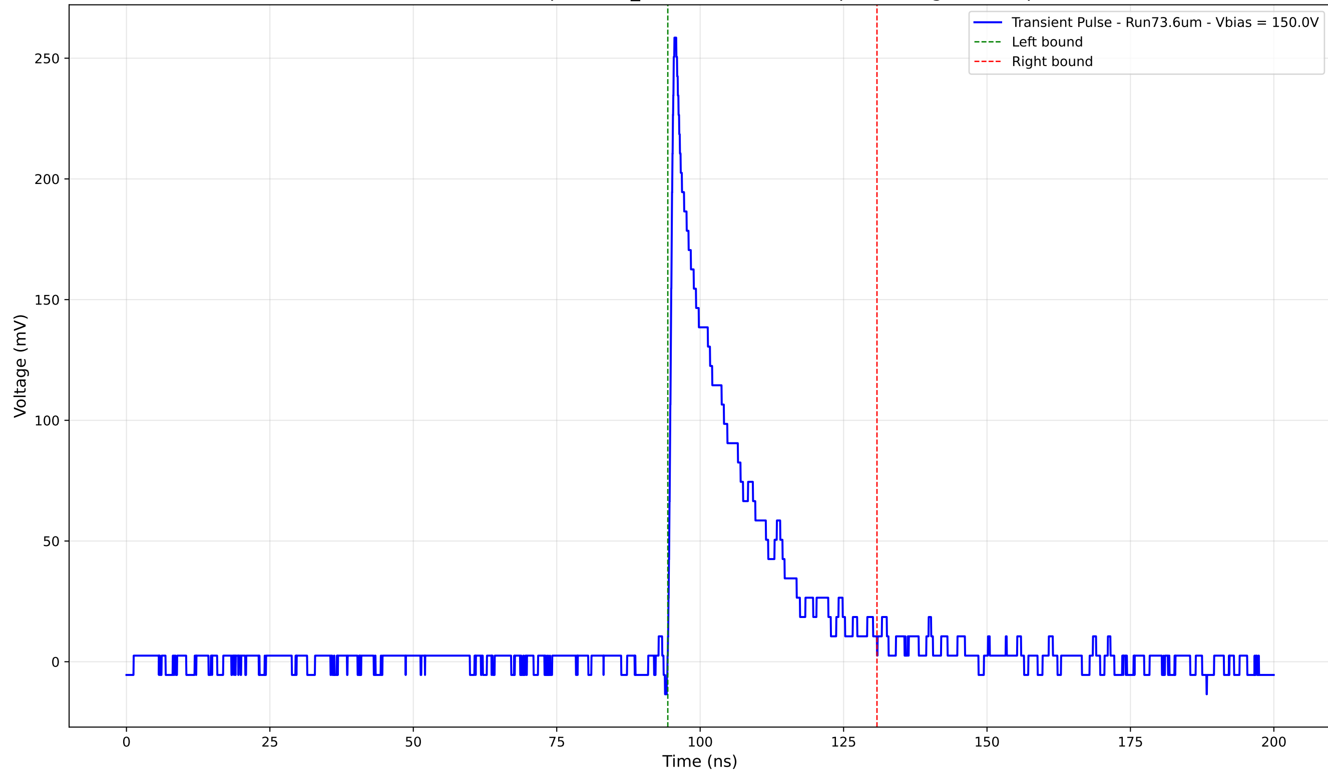
Transient Pulse - Sample: 1cm_42 - Position: 3550.0 \mu\text{m} - Charge: 50.99 pC
