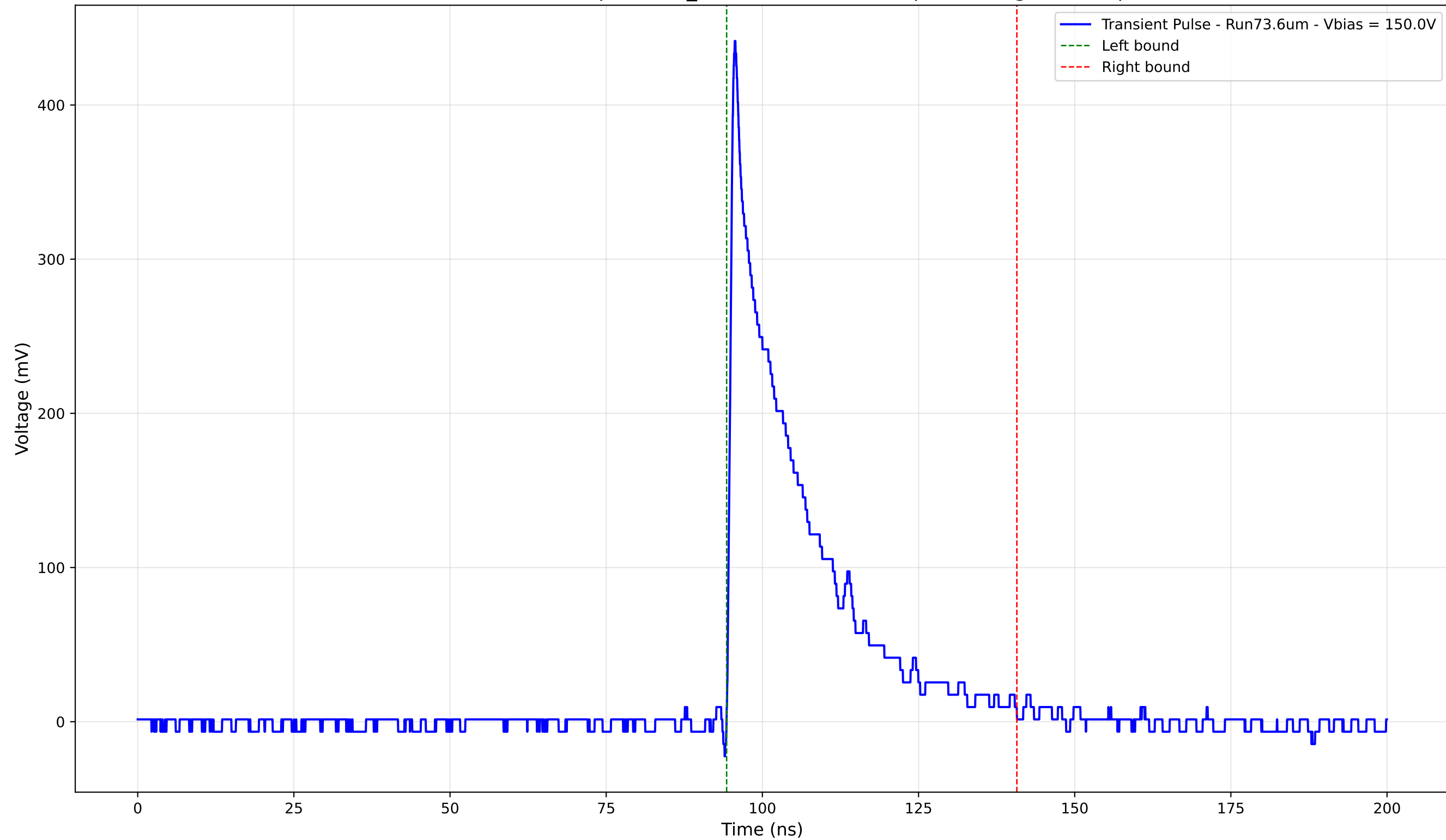
Transient Pulse - Sample: 1cm_42 - Position: 1875.0 \mu\text{m} - Charge: 91.37 pC
