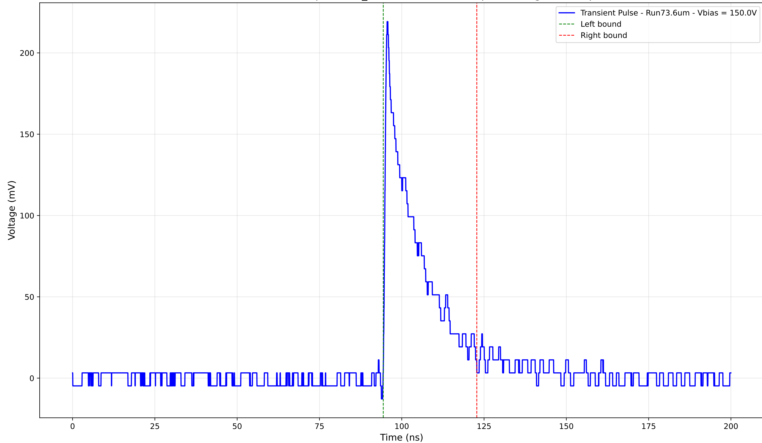
Transient Pulse - Sample: 1cm_42 - Position: 3840.0 \mu\text{m} - Charge: 41.53 pC
