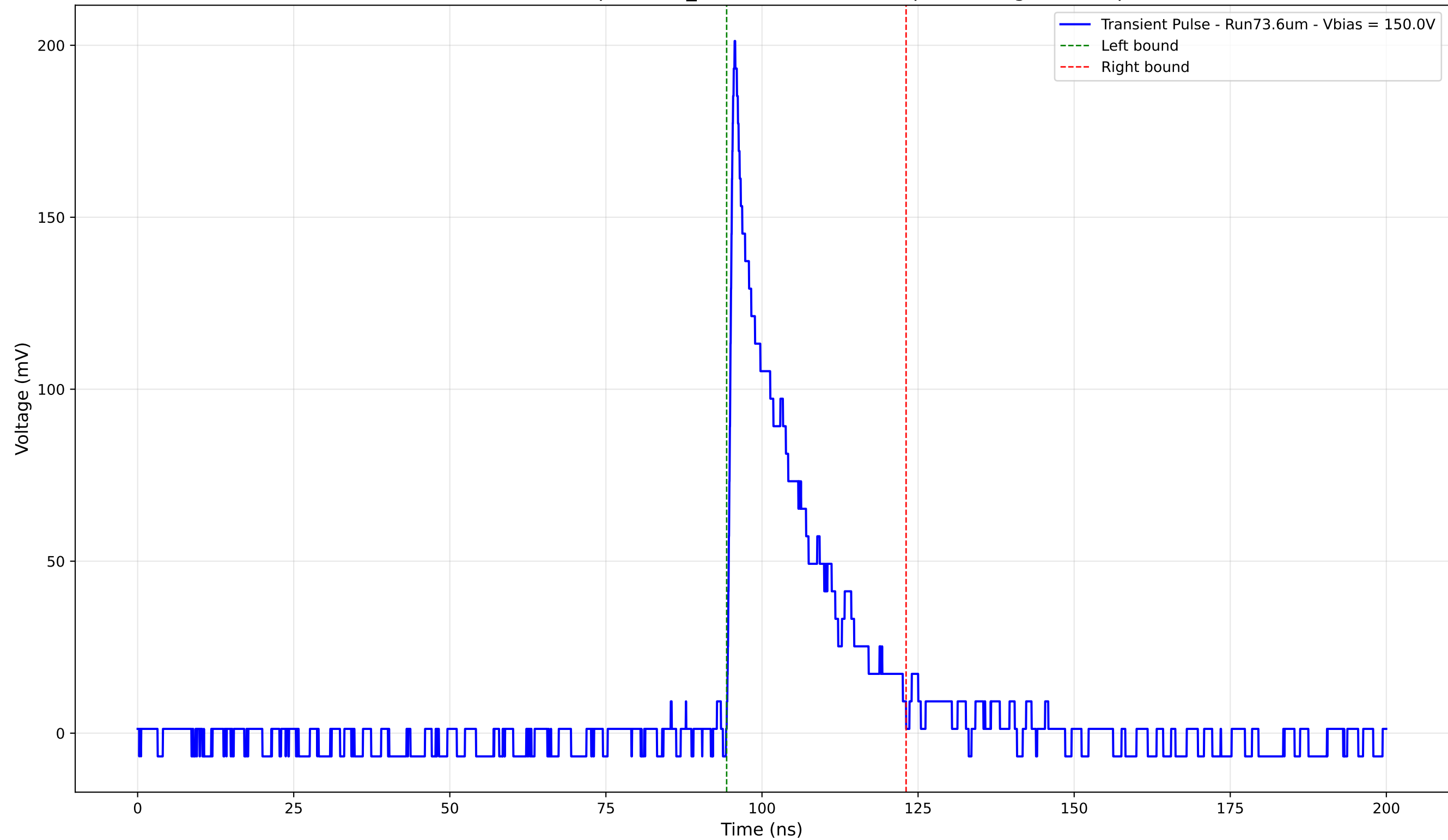
Transient Pulse - Sample: 1cm_42 - Position: 3960.0 \mu\text{m} - Charge: 36.85 pC
