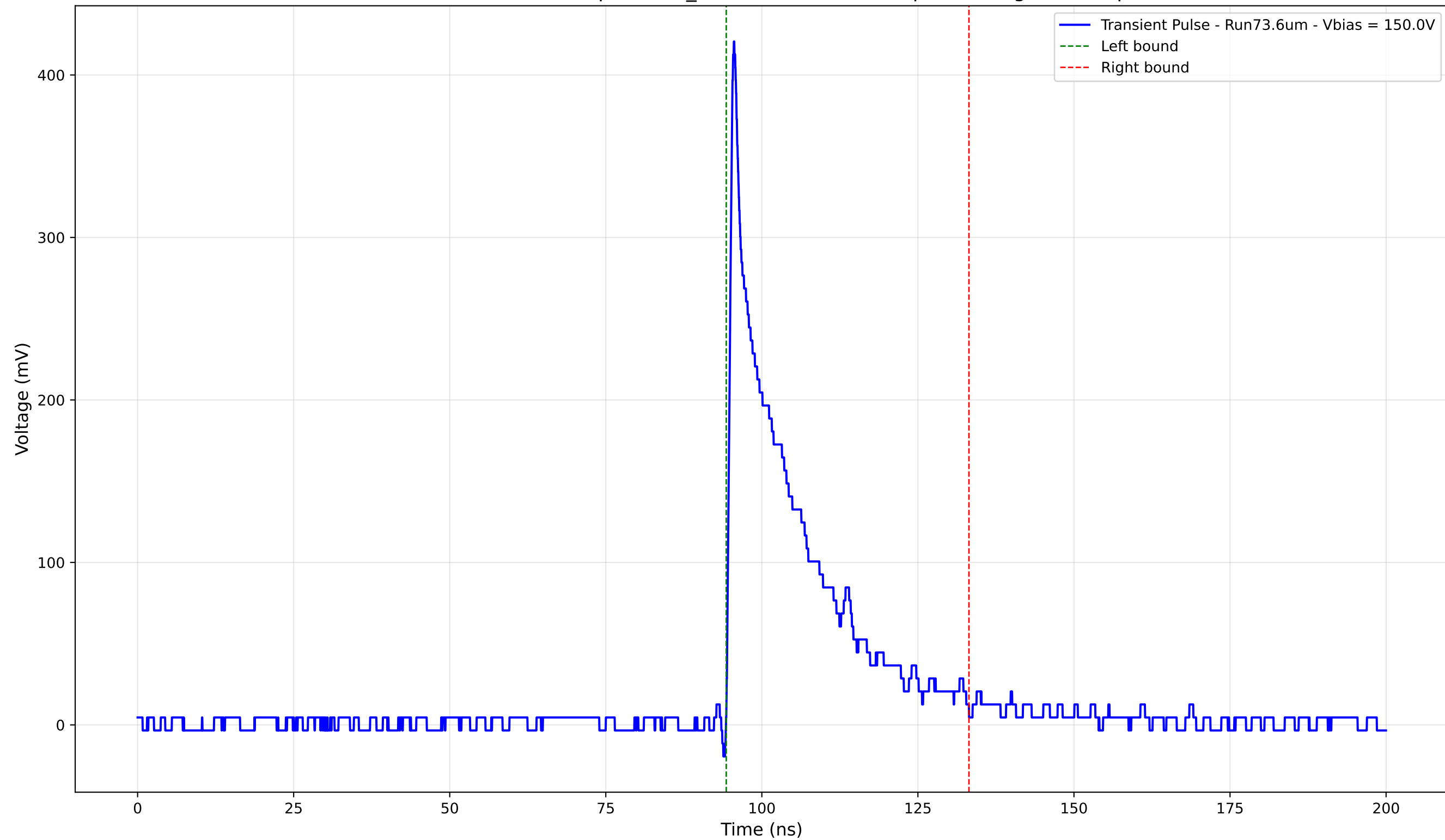
Transient Pulse - Sample: 1cm_42 - Position: 2785.0 \mu\text{m} - Charge: 76.91 pC
