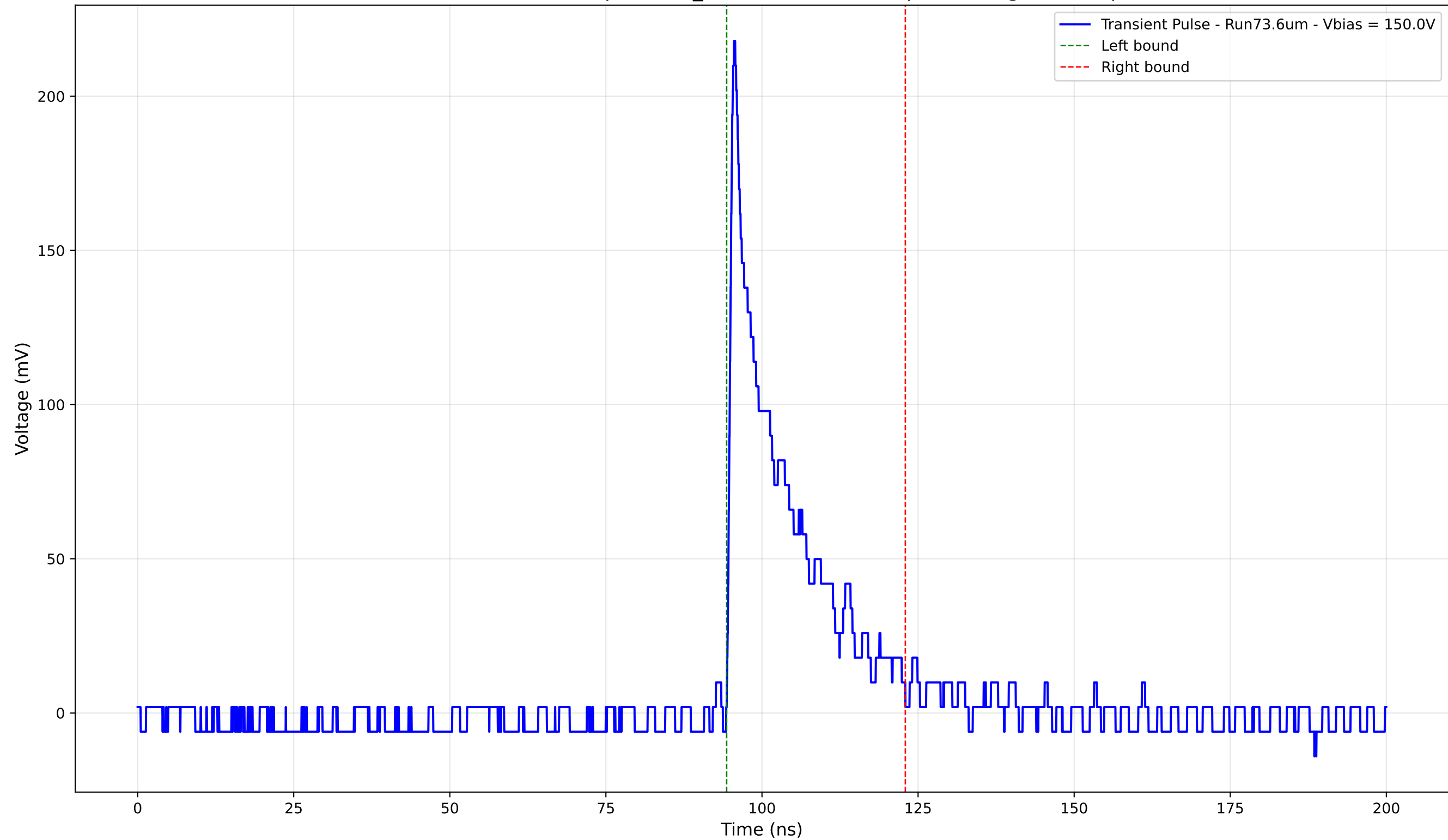
Transient Pulse - Sample: 1cm_42 - Position: 140.0 \mu\text{m} - Charge: 34.92 pC
