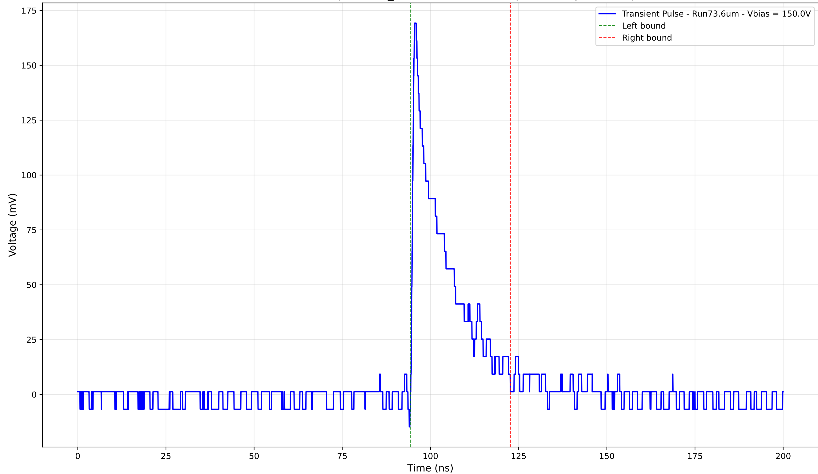
Transient Pulse - Sample: 1cm_42 - Position: 4270.0 \mu\text{m} - Charge: 30.64 pC
