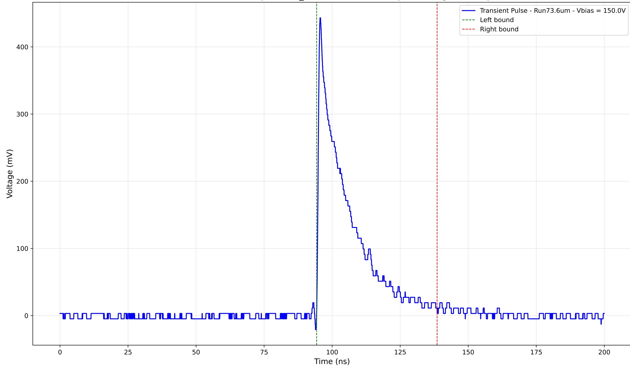
Transient Pulse - Sample: 1cm_42 - Position: 1595.0 \mu\text{m} - Charge: 96.08 pC
