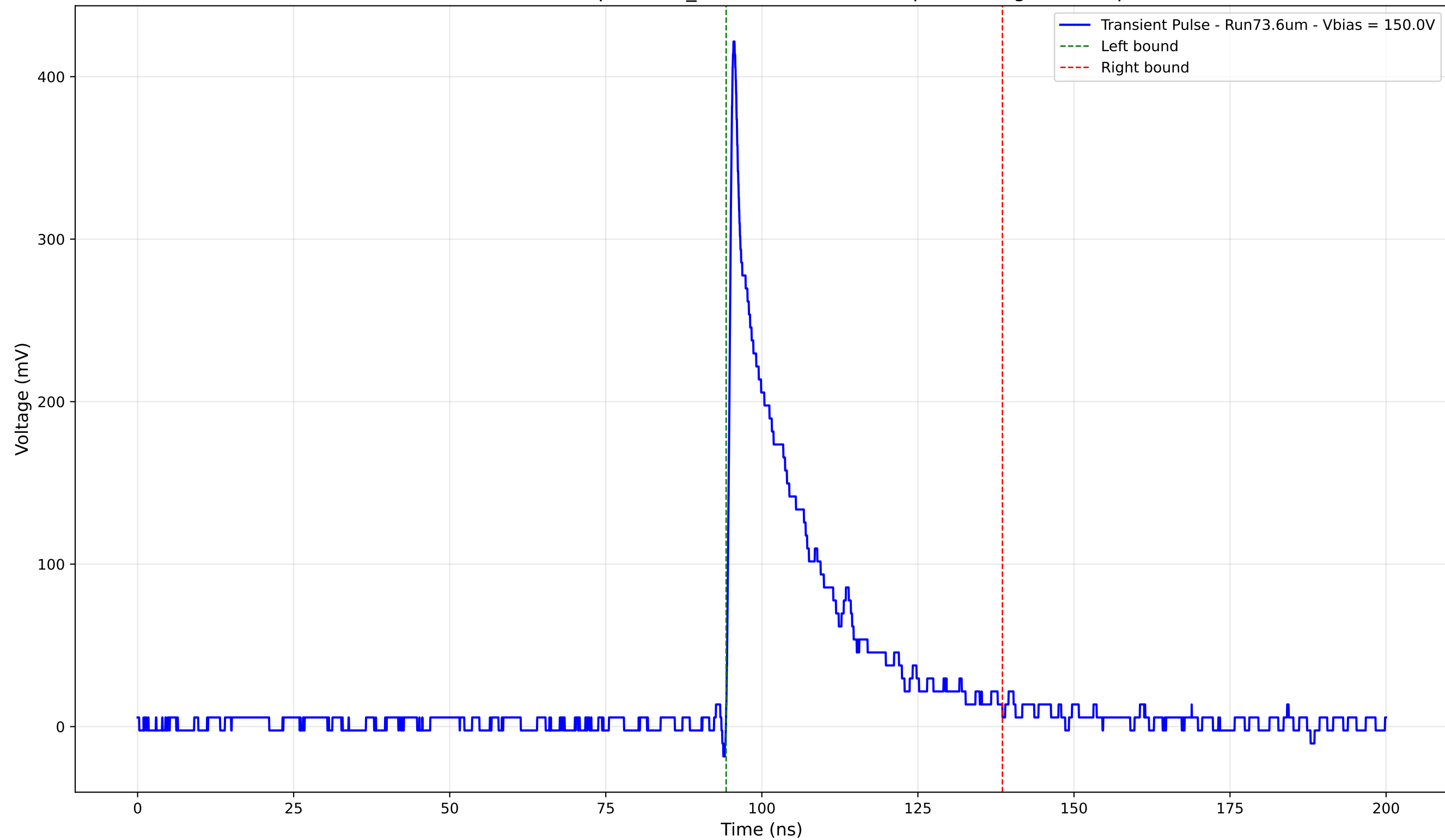
Transient Pulse - Sample: 1cm_42 - Position: 2575.0 \mu\text{m} - Charge: 80.78 pC
