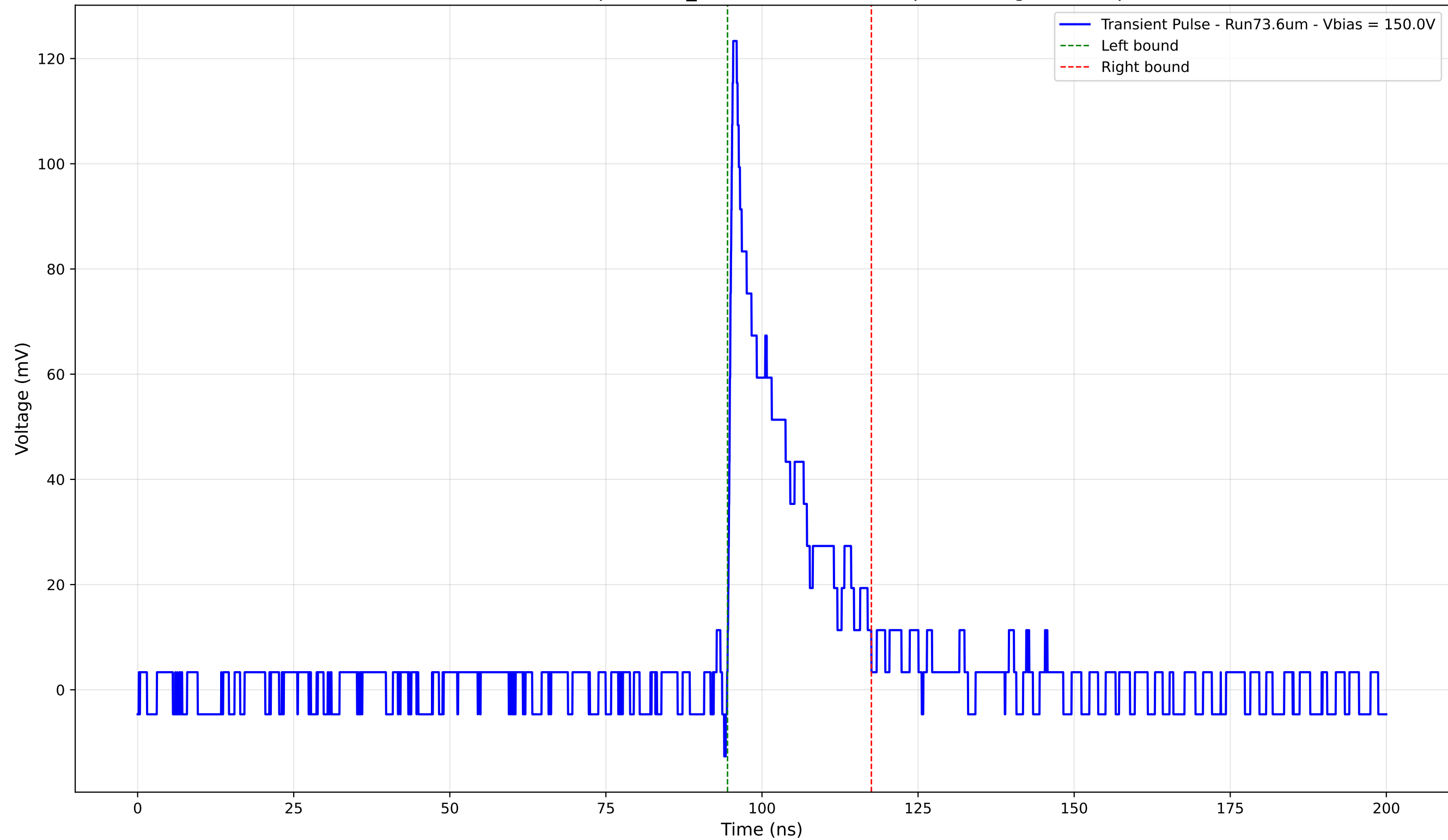
Transient Pulse - Sample: 1cm_42 - Position: 4685.0 \mu\text{m} - Charge: 20.15 pC
