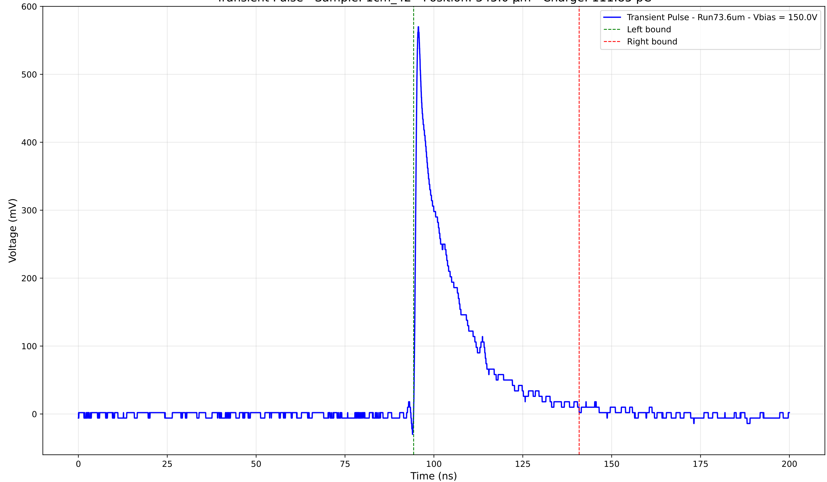
Transient Pulse - Sample: 1cm_42 - Position: 345.0 \mu\text{m} - Charge: 111.85 pC
