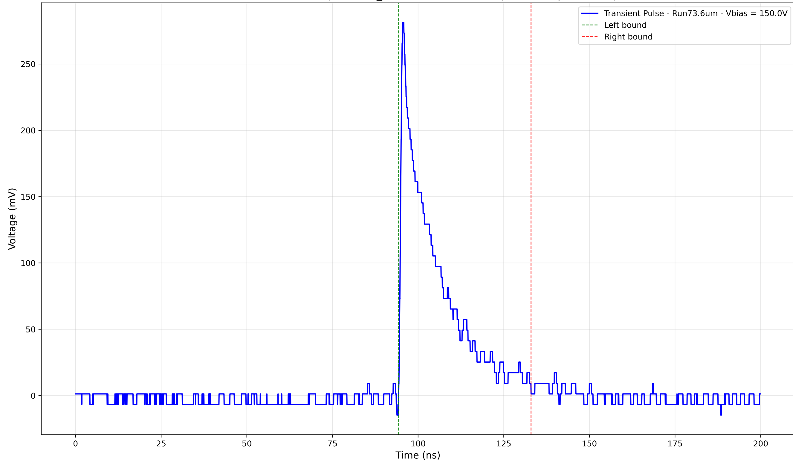
Transient Pulse - Sample: 1cm_42 - Position: 3375.0 \mu\text{m} - Charge: 56.21 pC
