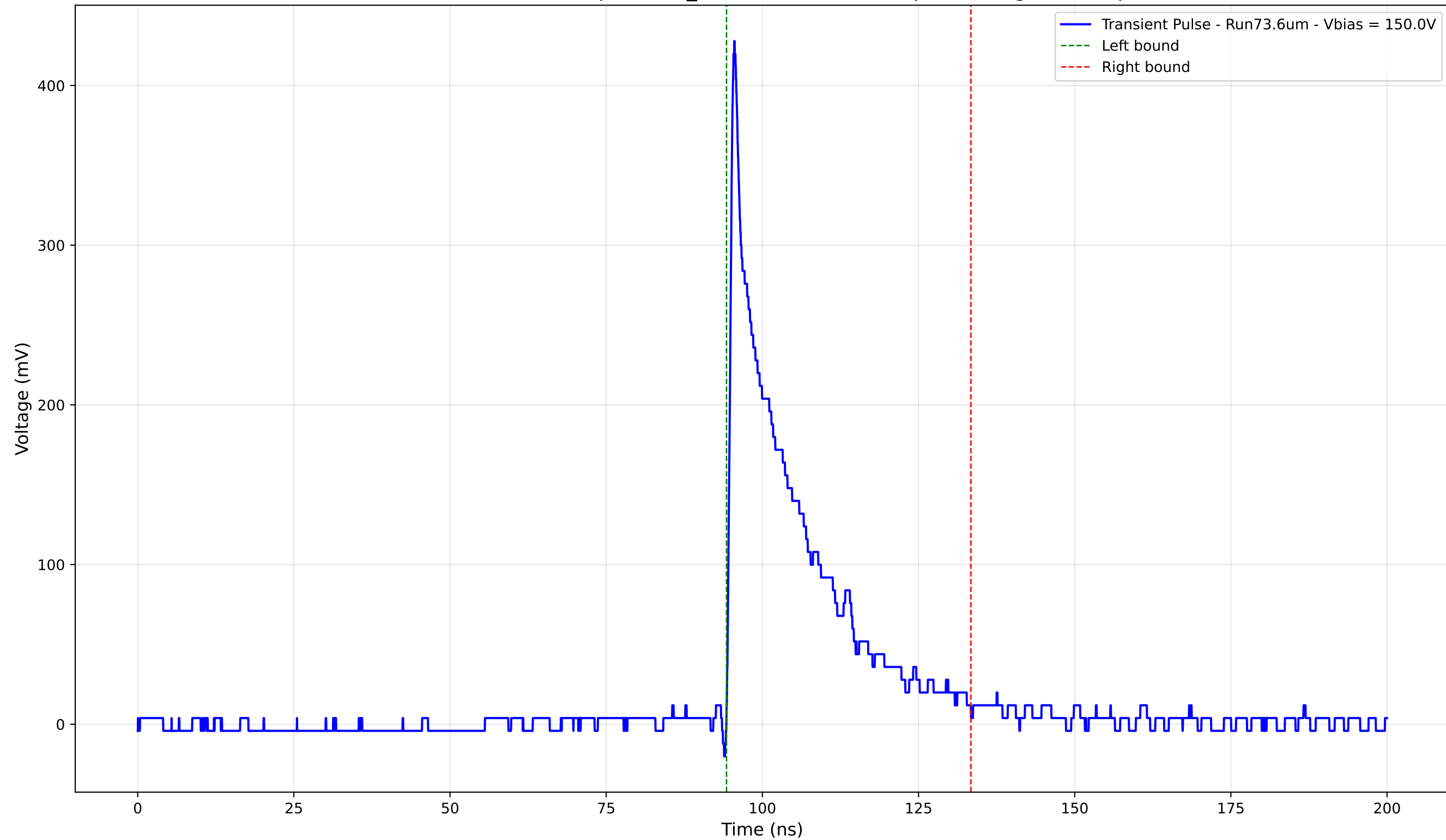
Transient Pulse - Sample: 1cm_42 - Position: 2560.0 \mu\text{m} - Charge: 78.48 pC
