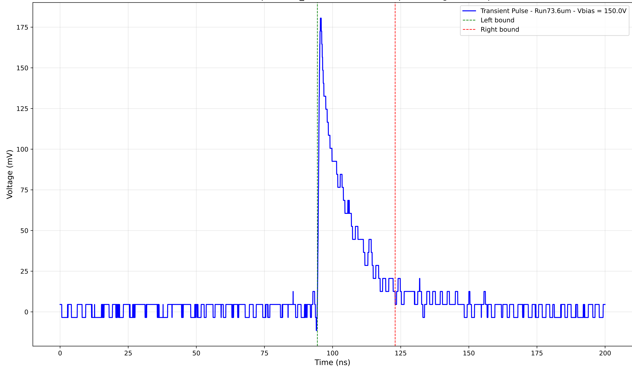
Transient Pulse - Sample: 1cm_42 - Position: 4175.0 \mu\text{m} - Charge: 33.77 pC
