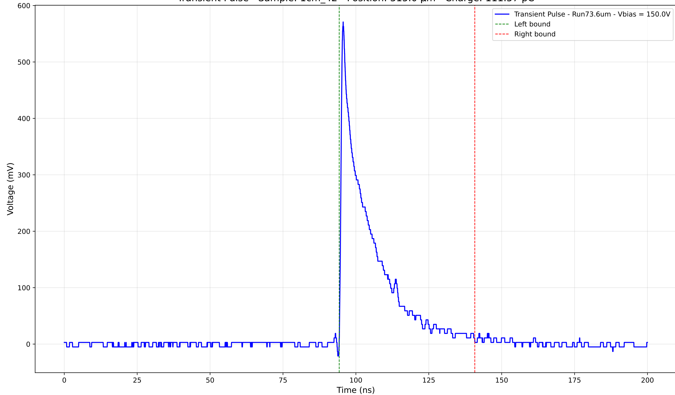
Transient Pulse - Sample: 1cm_42 - Position: 315.0 \mu\text{m} - Charge: 111.57 pC
