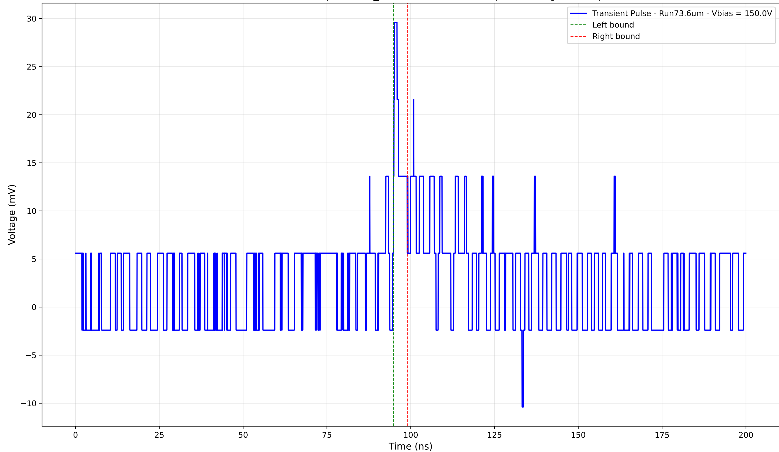
Transient Pulse - Sample: 1cm_42 - Position: 4960.0 \mu\text{m} - Charge: 1.45 pC
