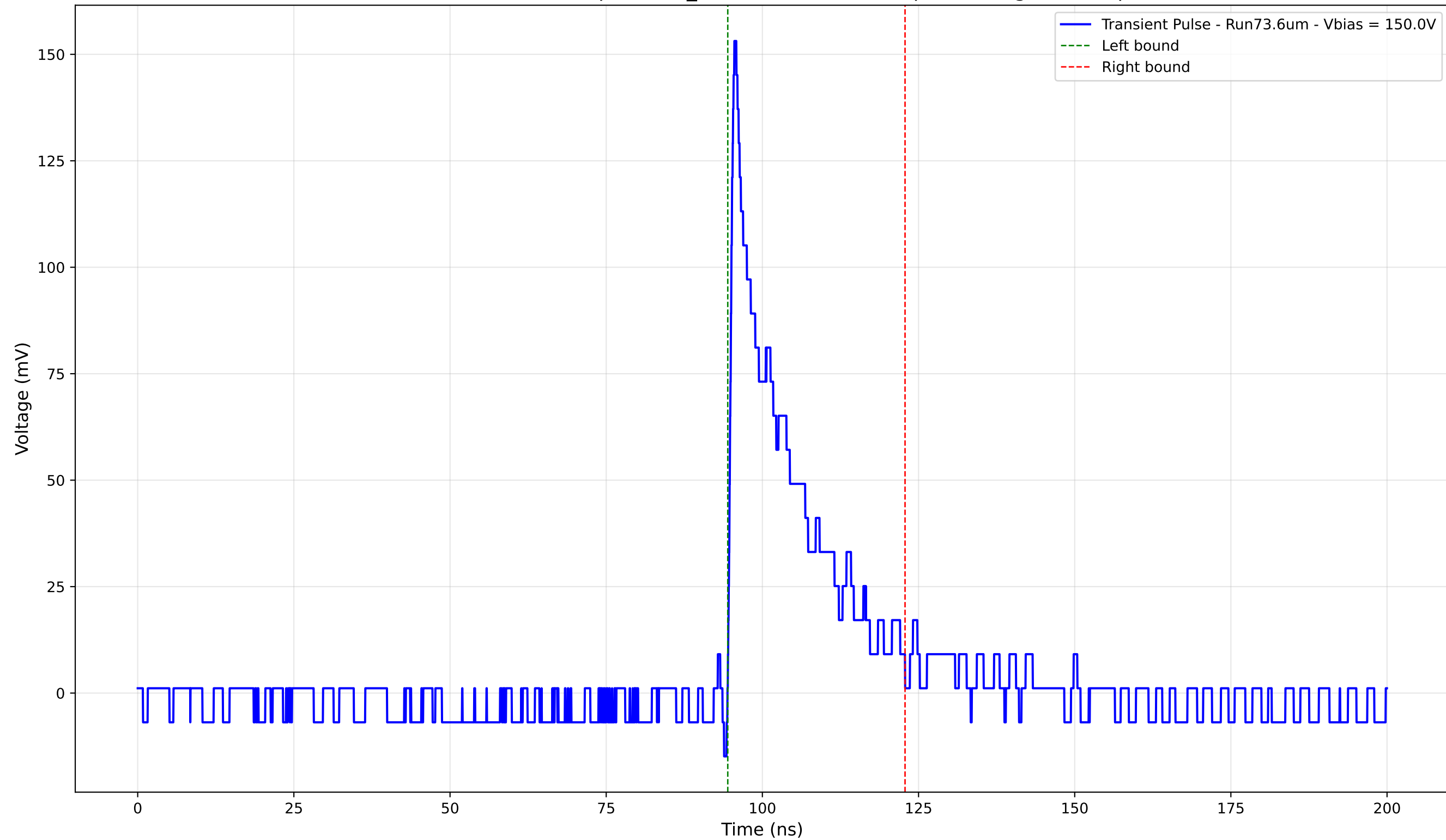
Transient Pulse - Sample: 1cm_42 - Position: 4465.0 \mu\text{m} - Charge: 26.57 pC
