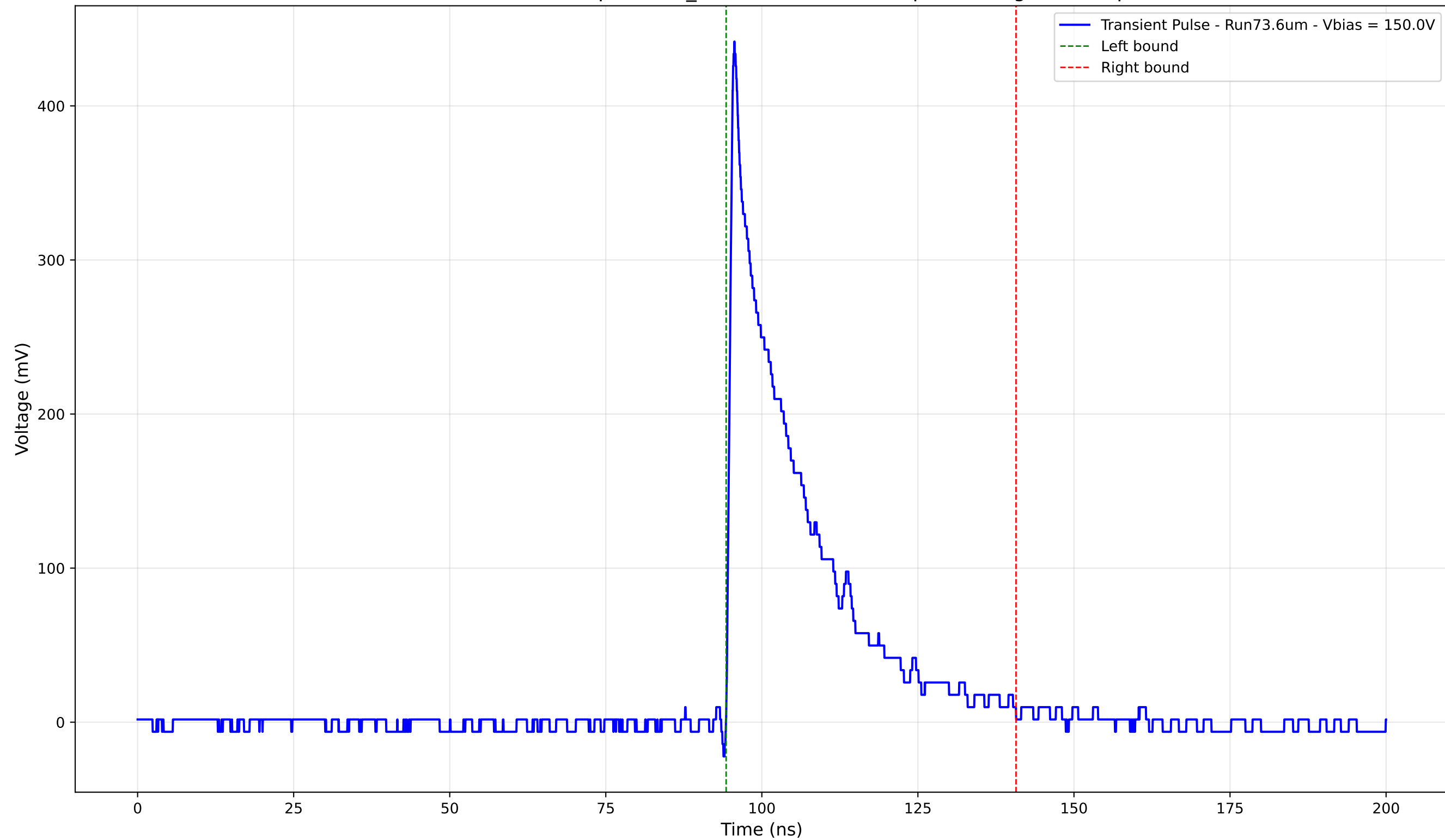
Transient Pulse - Sample: 1cm_42 - Position: 1765.0 \mu\text{m} - Charge: 93.14 pC
