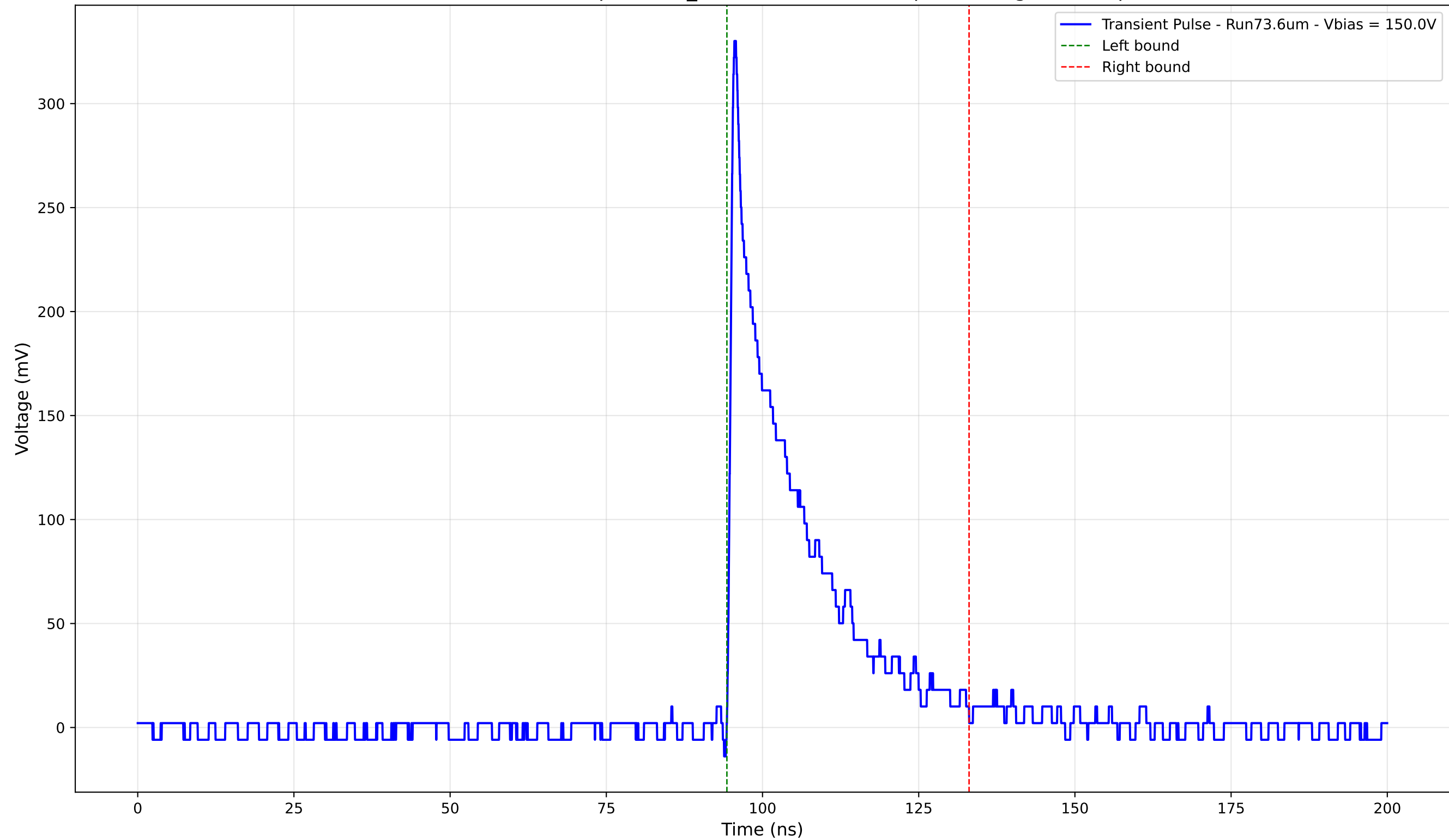
Transient Pulse - Sample: 1cm_42 - Position: 3040.0 \mu\text{m} - Charge: 62.88 pC
