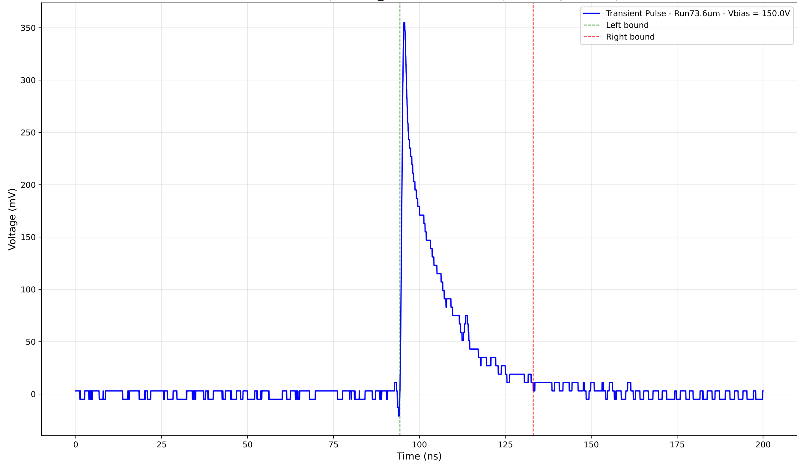
Transient Pulse - Sample: 1cm_42 - Position: 2945.0 \mu\text{m} - Charge: 66.02 pC
