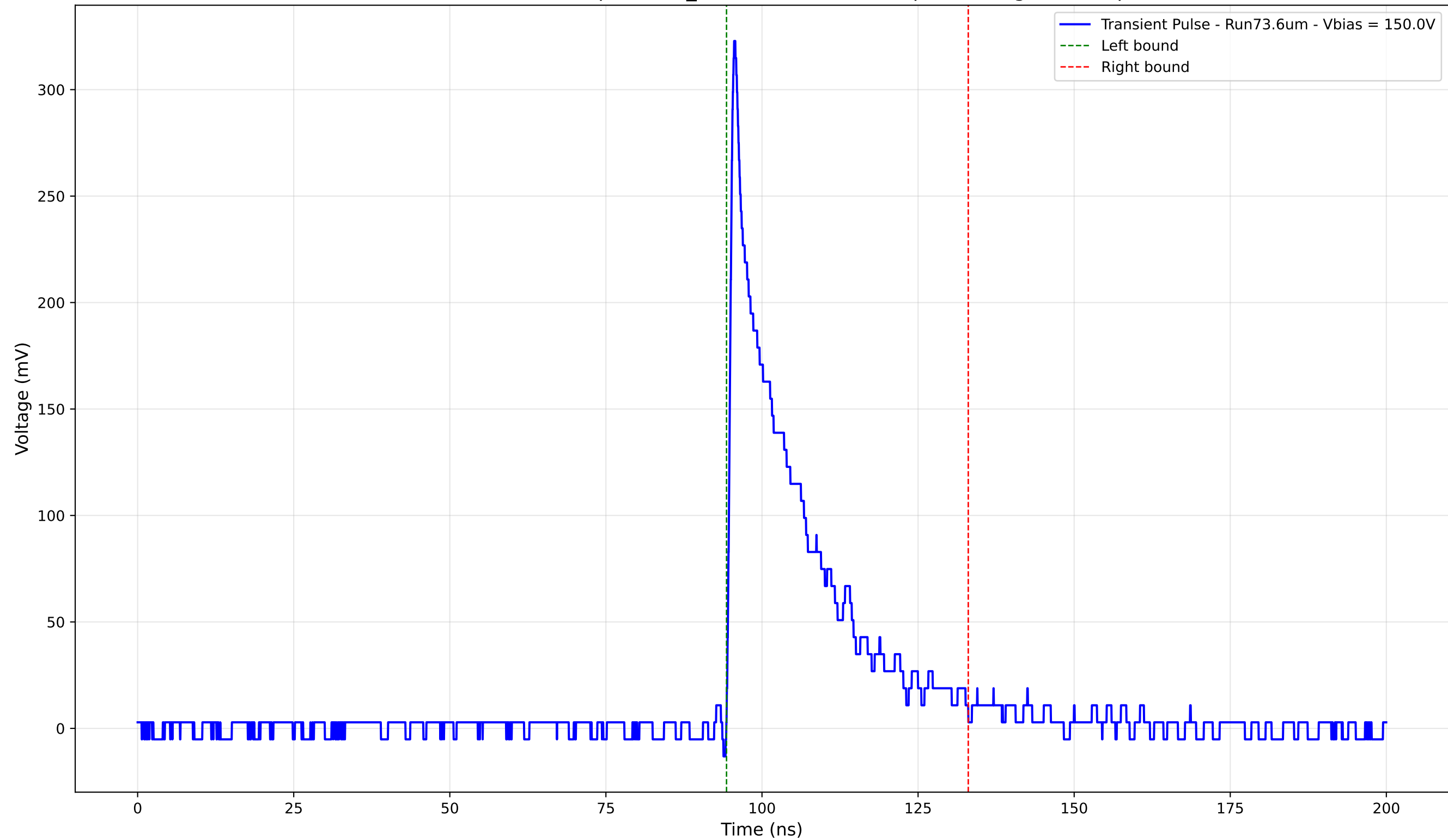
Transient Pulse - Sample: 1cm_42 - Position: 3155.0 \mu\text{m} - Charge: 62.65 pC
