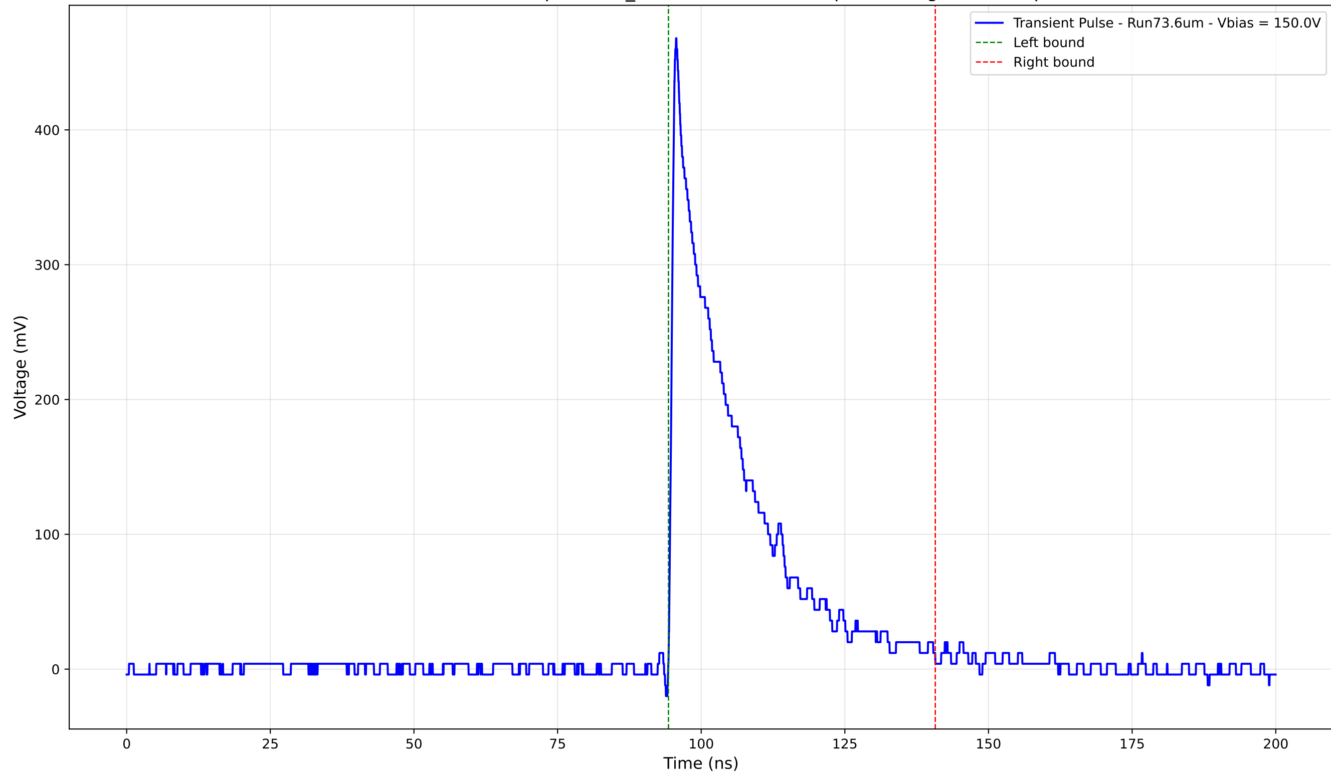
Transient Pulse - Sample: 1cm_42 - Position: 1165.0 \mu\text{m} - Charge: 103.11 pC
