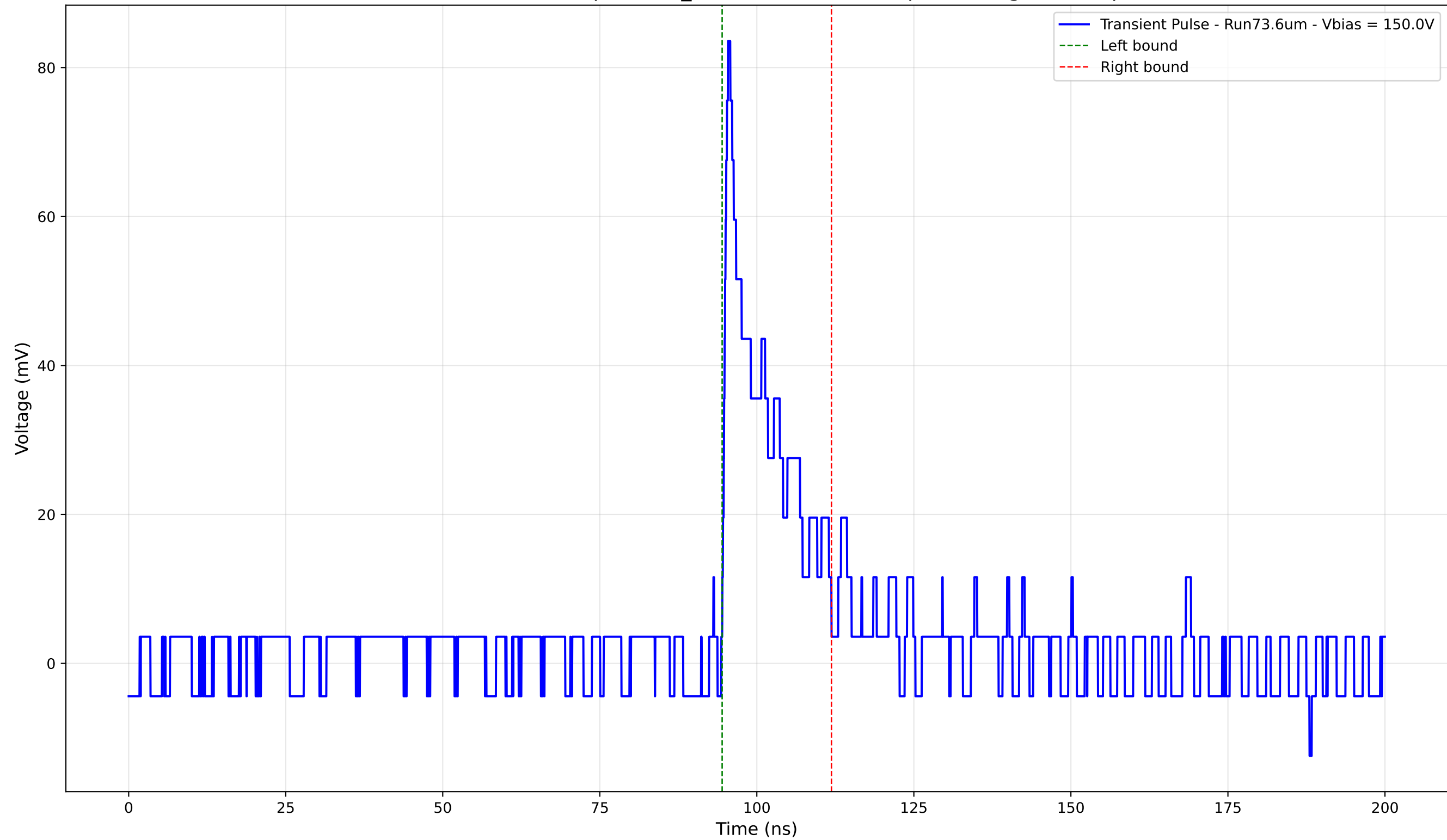
Transient Pulse - Sample: 1cm_42 - Position: 4900.0 \mu\text{m} - Charge: 11.40 pC
