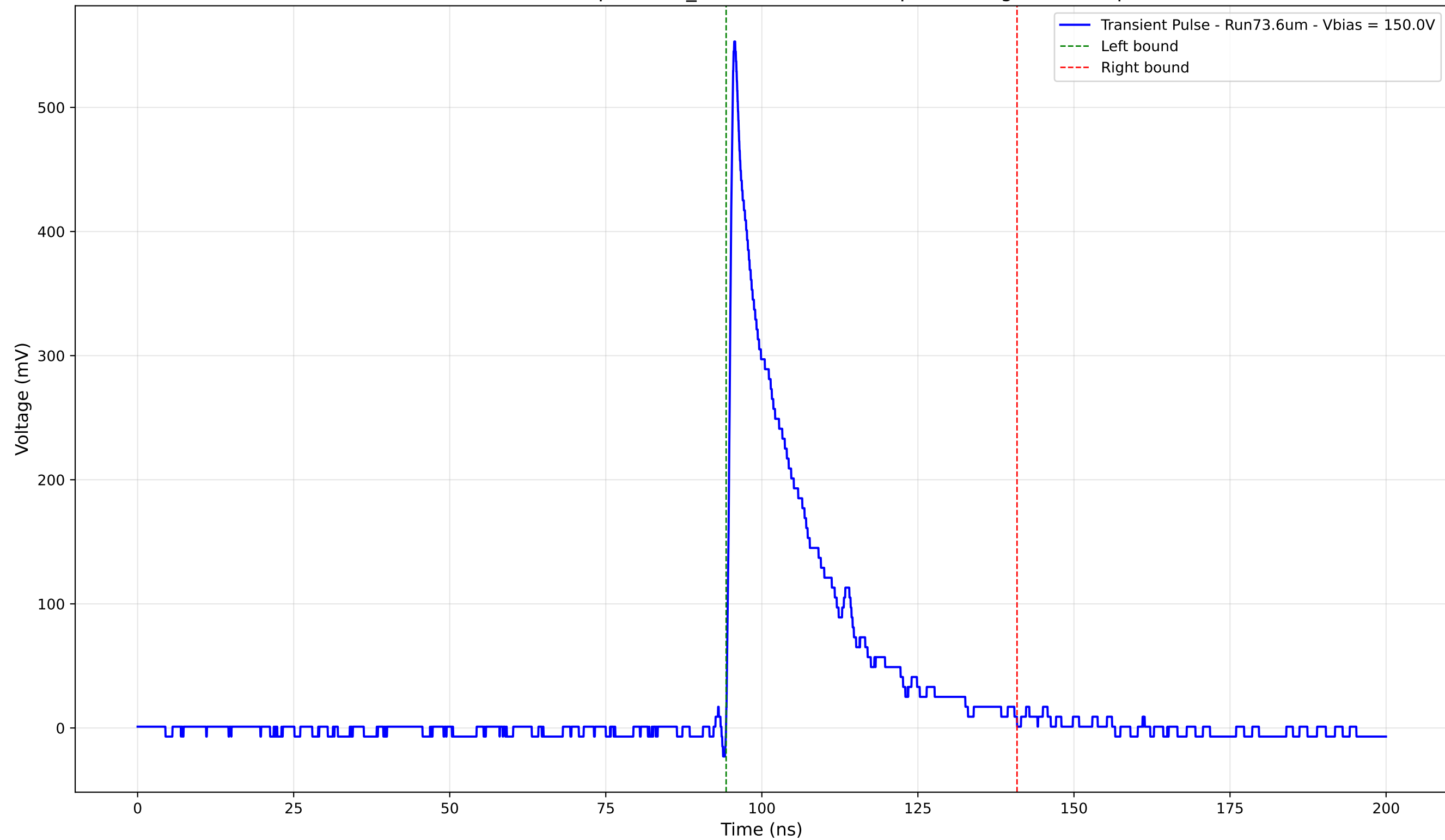
Transient Pulse - Sample: 1cm_42 - Position: 430.0 \mu\text{m} - Charge: 111.28 pC
