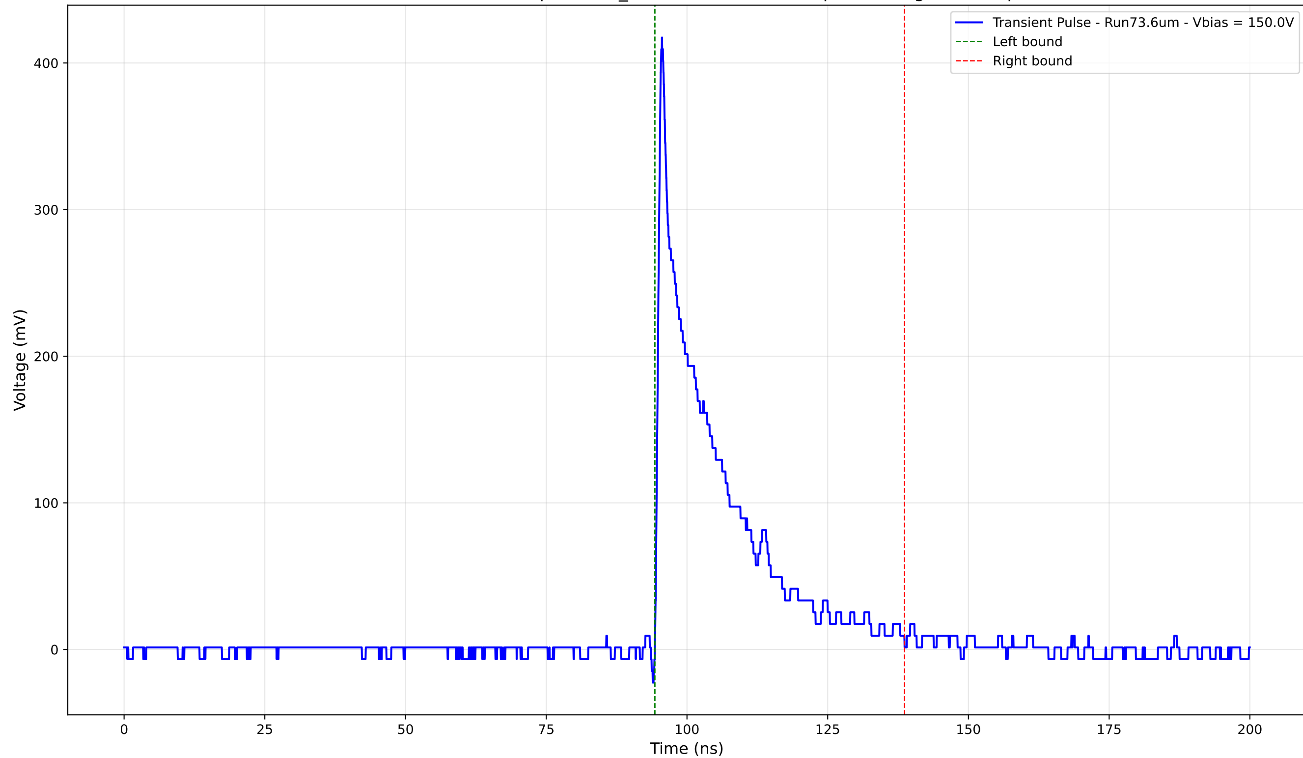
Transient Pulse - Sample: 1cm_42 - Position: 2805.0 \mu\text{m} - Charge: 76.34 pC
