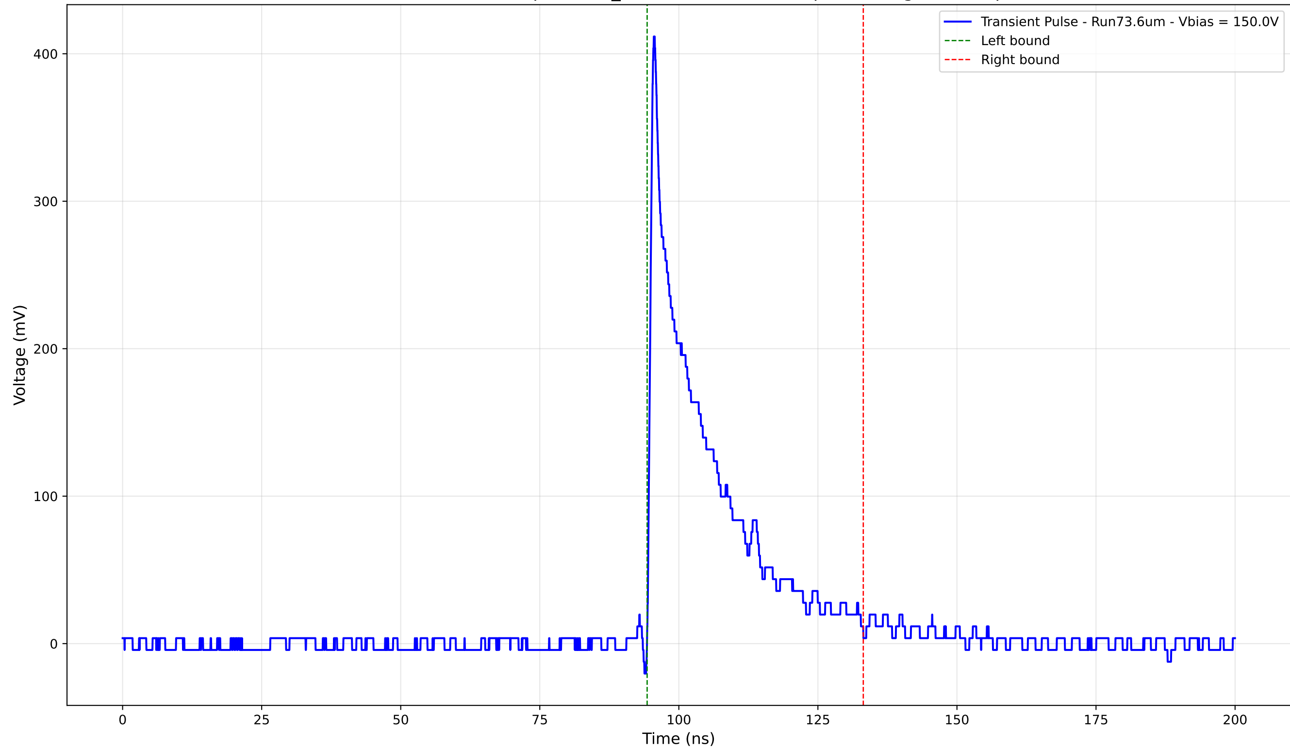
Transient Pulse - Sample: 1cm_42 - Position: 2435.0 \mu\text{m} - Charge: 76.49 pC
