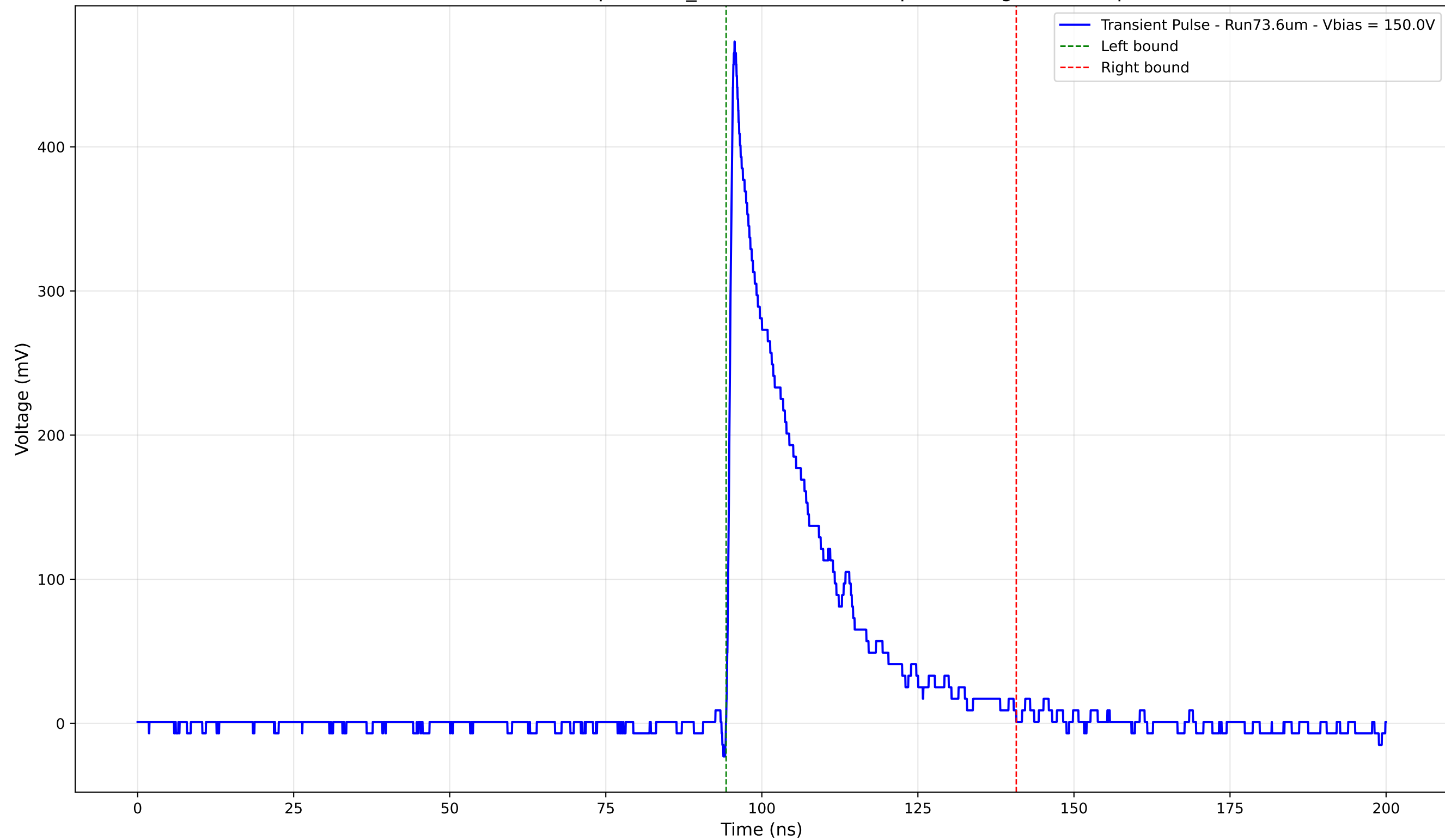
Transient Pulse - Sample: 1cm_42 - Position: 955.0 \mu\text{m} - Charge: 102.22 pC
