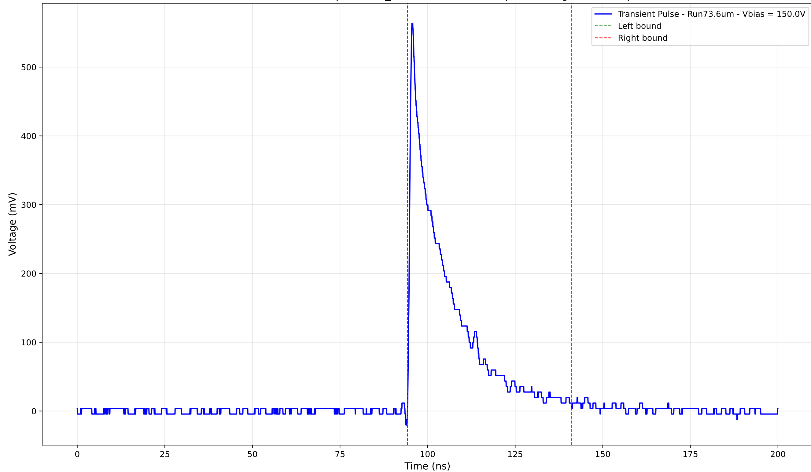
Transient Pulse - Sample: 1cm_42 - Position: 355.0 \mu\text{m} - Charge: 112.76 pC
