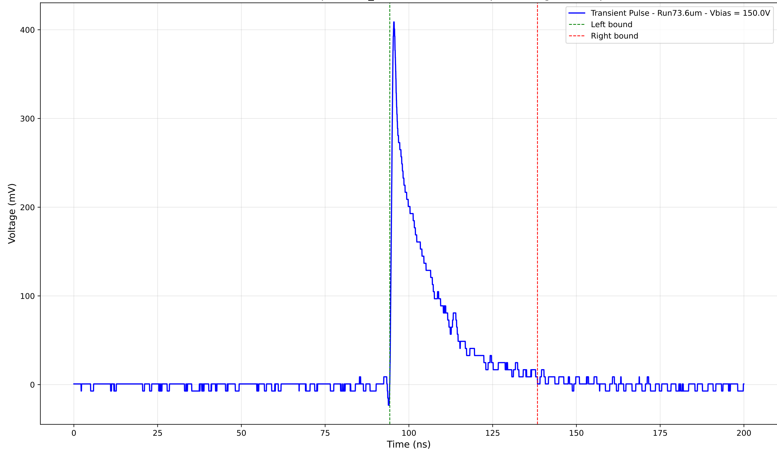
Transient Pulse - Sample: 1cm_42 - Position: 2455.0 \mu\text{m} - Charge: 75.75 pC
