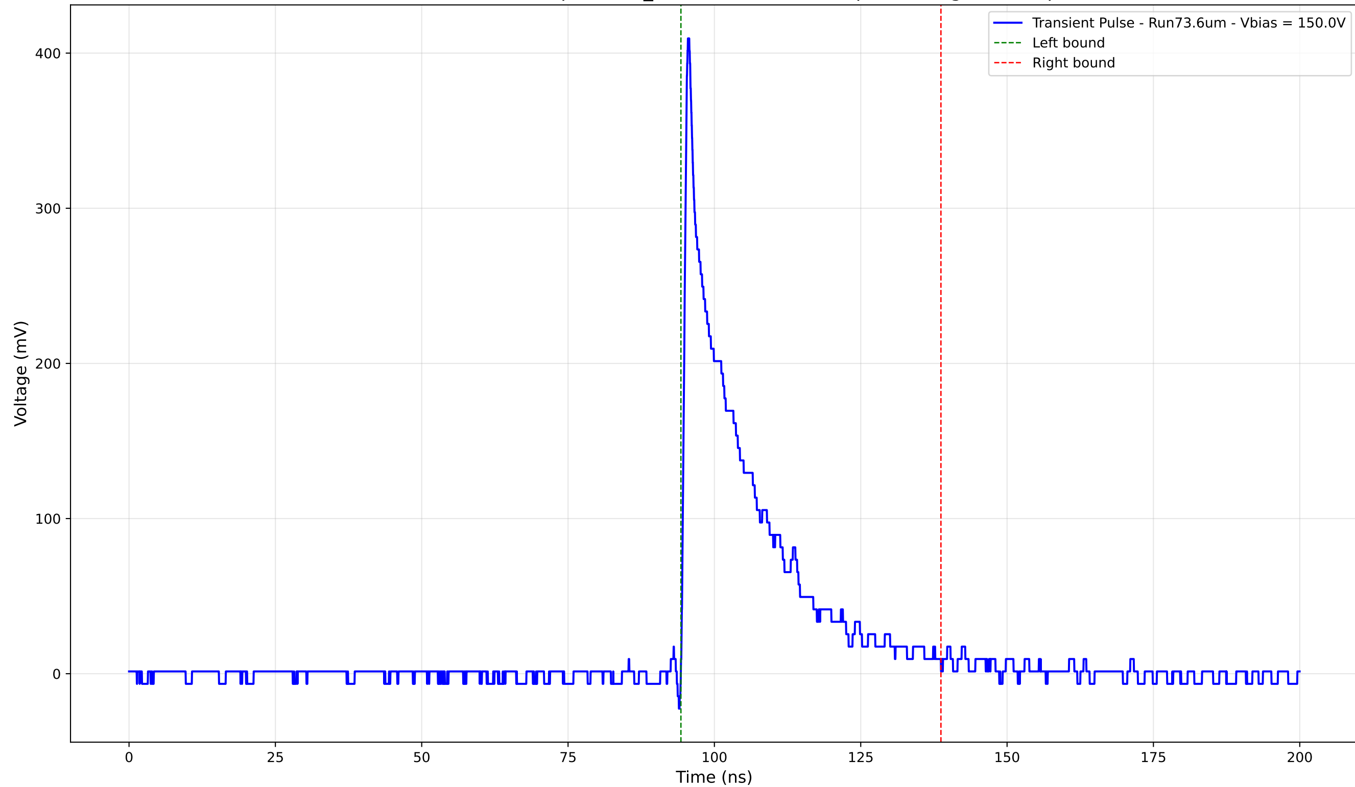
Transient Pulse - Sample: 1cm_42 - Position: 2385.0 \mu\text{m} - Charge: 77.53 pC
