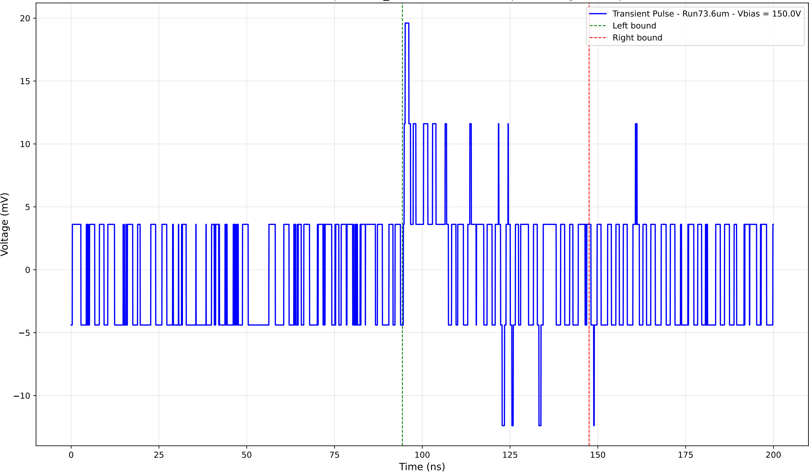
Transient Pulse - Sample: 1cm_42 - Position: 4970.0 \mu\text{m} - Charge: 2.12 pC
