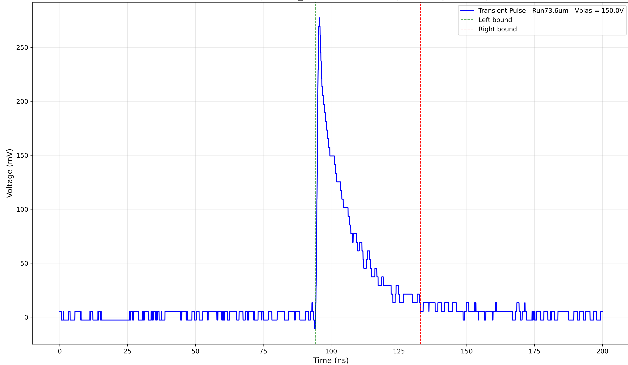
Transient Pulse - Sample: 1cm_42 - Position: 3470.0 \mu\text{m} - Charge: 56.70 pC
