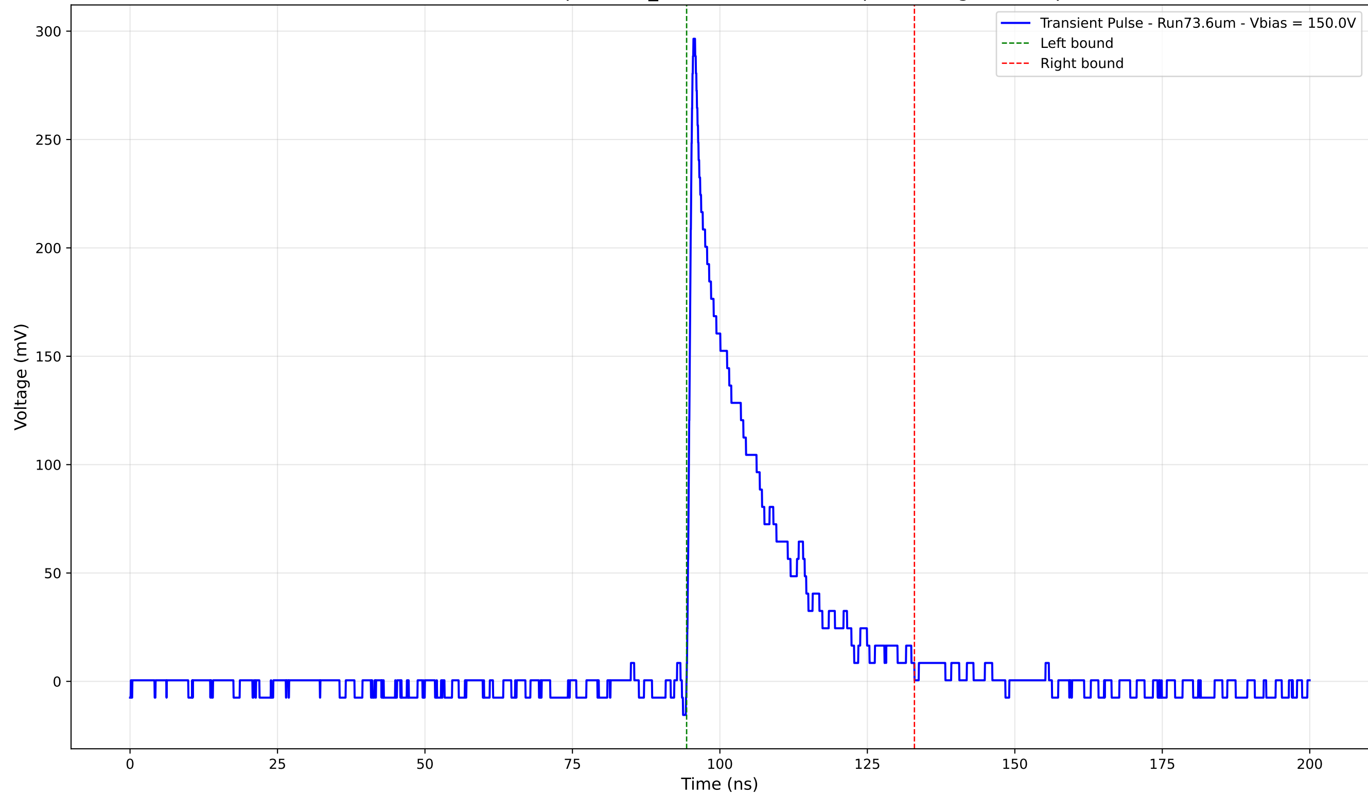
Transient Pulse - Sample: 1cm_42 - Position: 3270.0 \mu\text{m} - Charge: 57.06 pC
