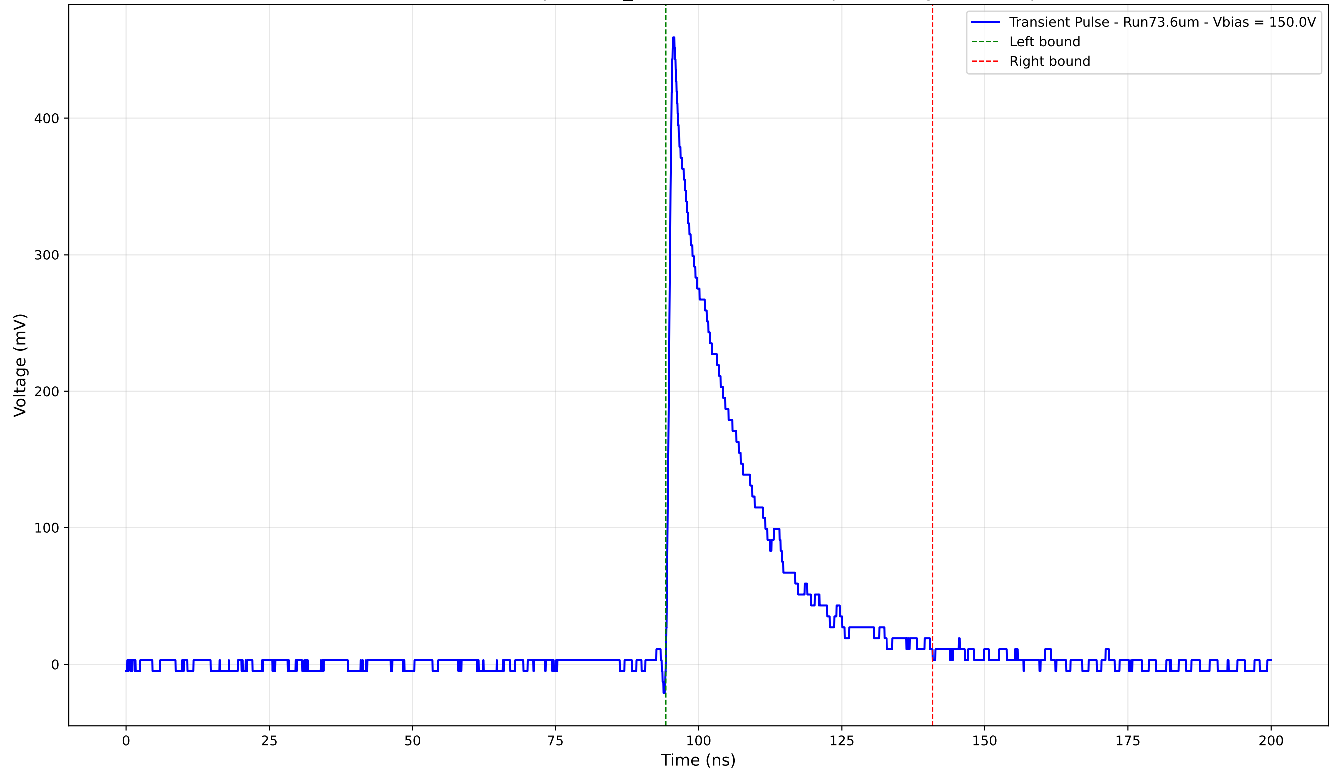
Transient Pulse - Sample: 1cm_42 - Position: 1160.0 \mu\text{m} - Charge: 101.69 pC
