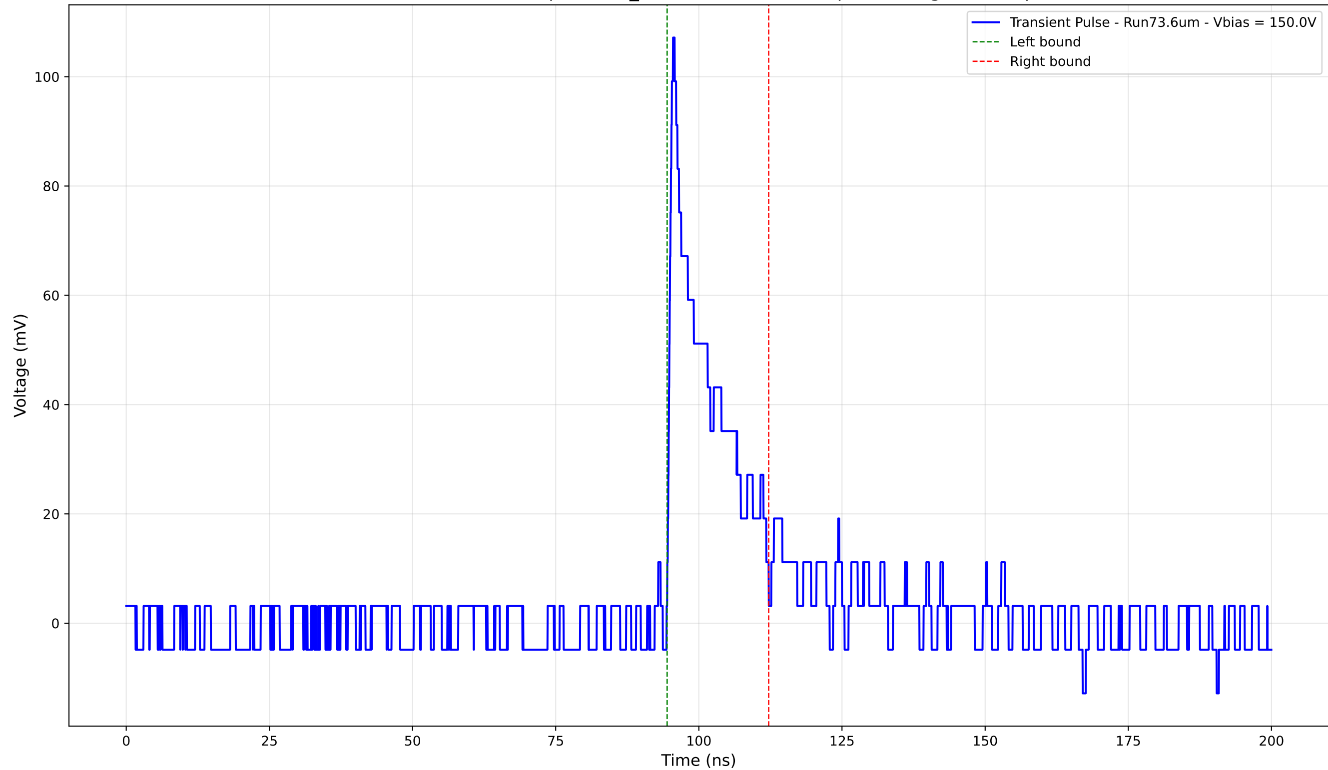
Transient Pulse - Sample: 1cm_42 - Position: 4810.0 \mu\text{m} - Charge: 15.37 pC
