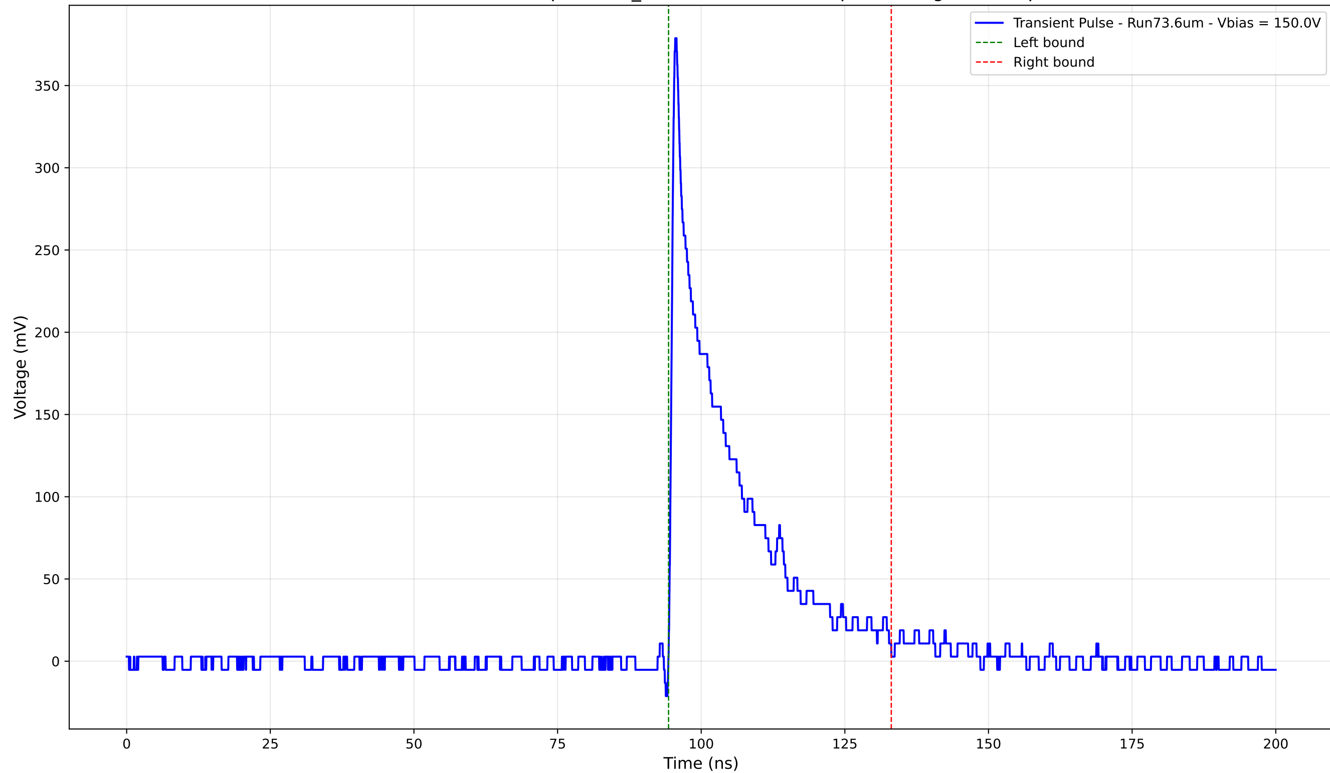
Transient Pulse - Sample: 1cm_42 - Position: 2885.0 \mu\text{m} - Charge: 71.22 pC
