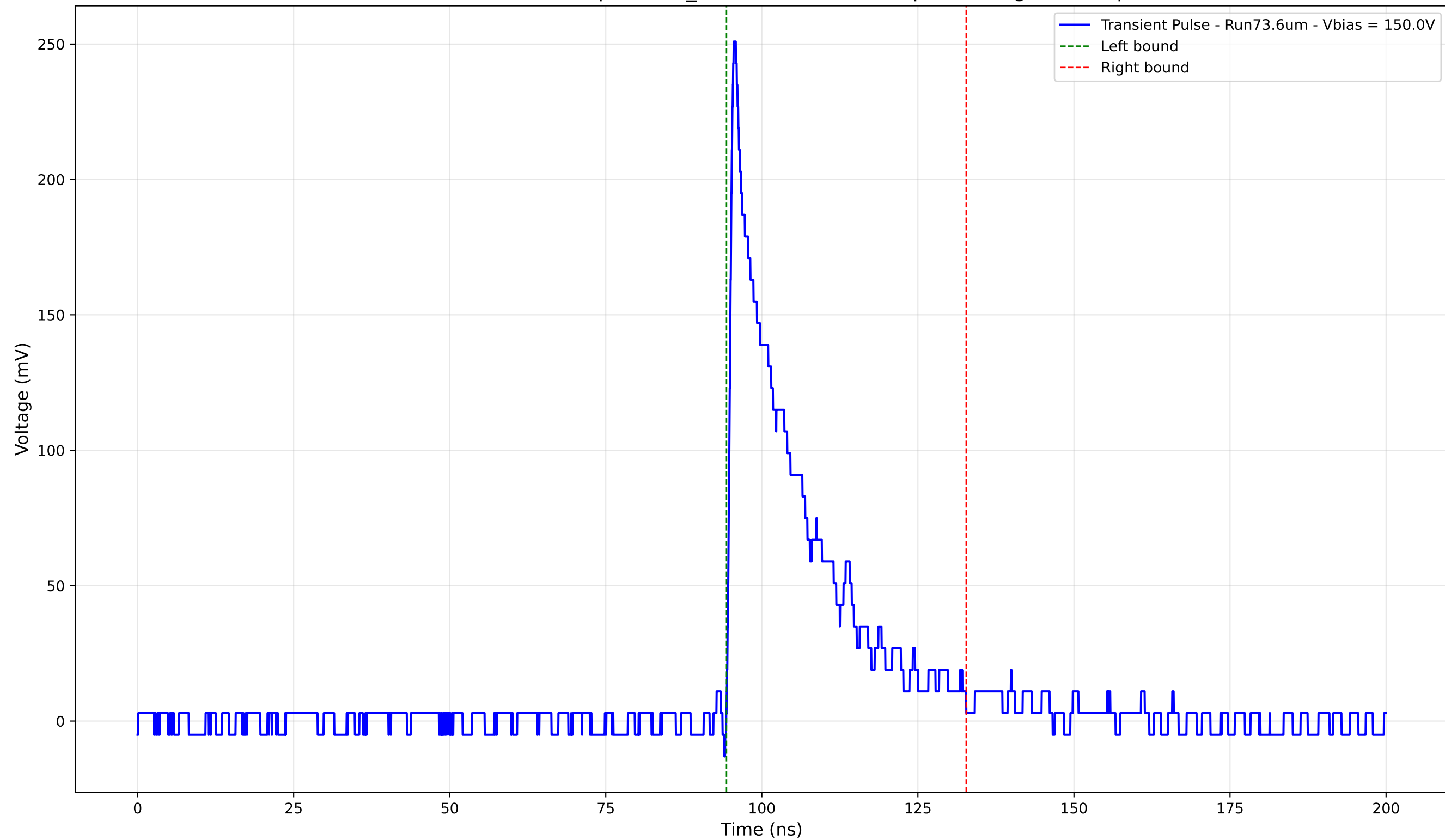
Transient Pulse - Sample: 1cm_42 - Position: 3595.0 \mu\text{m} - Charge: 50.86 pC
