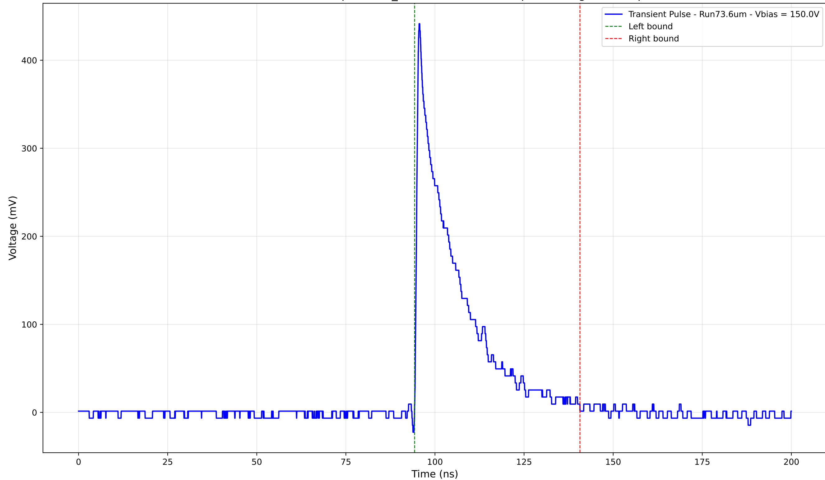
Transient Pulse - Sample: 1cm_42 - Position: 1560.0 \mu\text{m} - Charge: 95.22 pC
