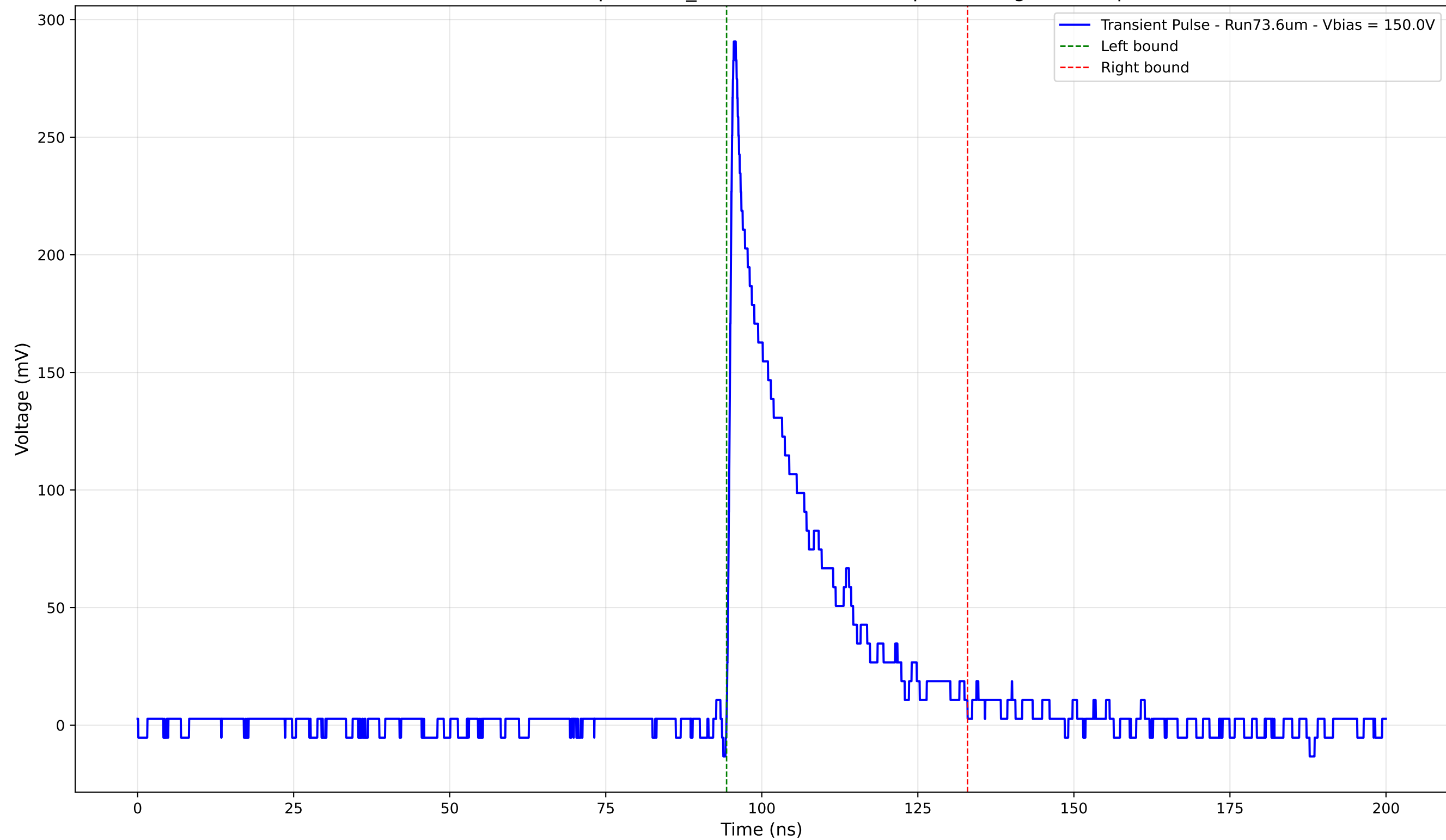
Transient Pulse - Sample: 1cm_42 - Position: 3290.0 \mu\text{m} - Charge: 57.98 pC
