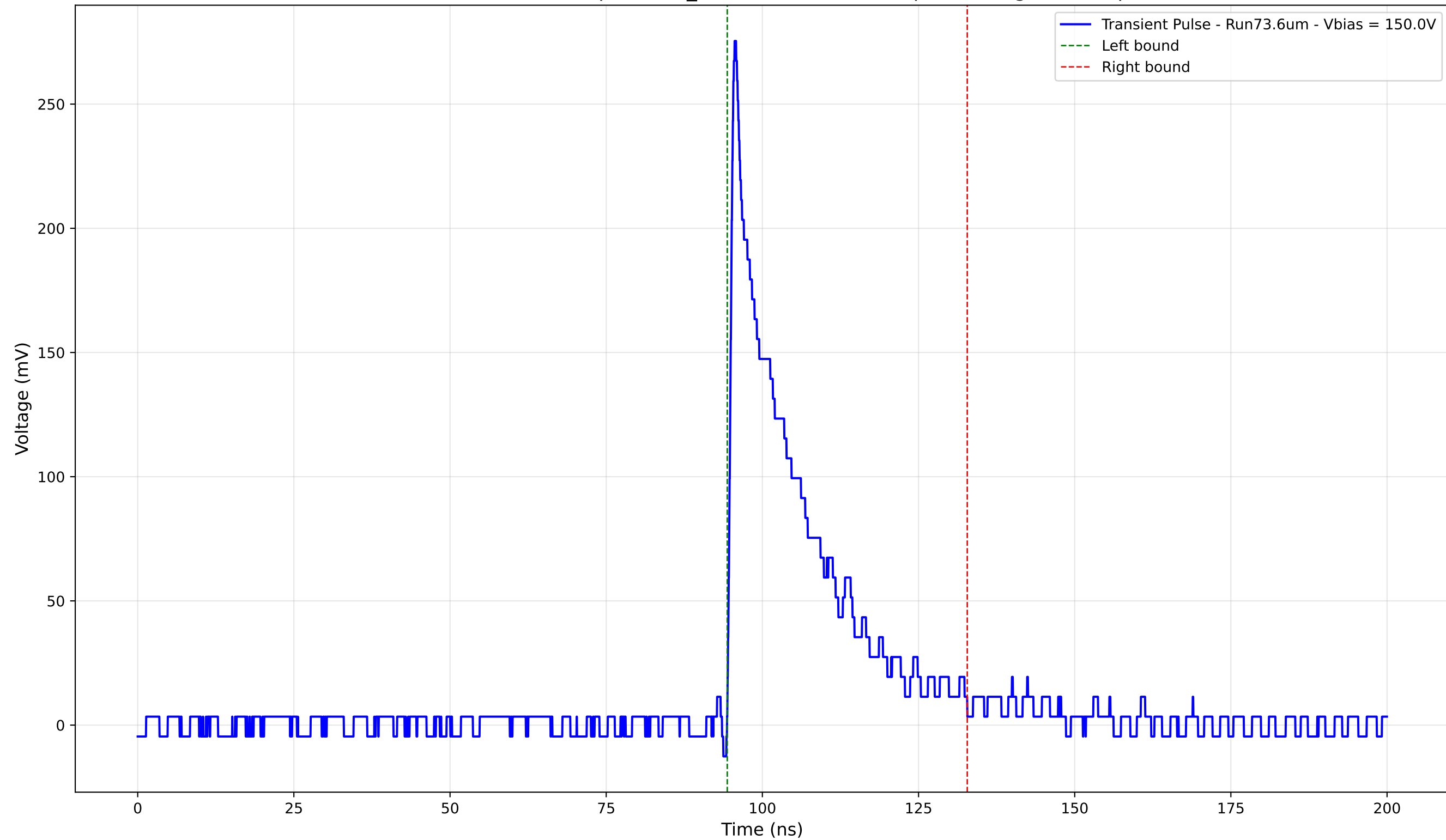
Transient Pulse - Sample: 1cm_42 - Position: 3480.0 \mu\text{m} - Charge: 54.95 pC
