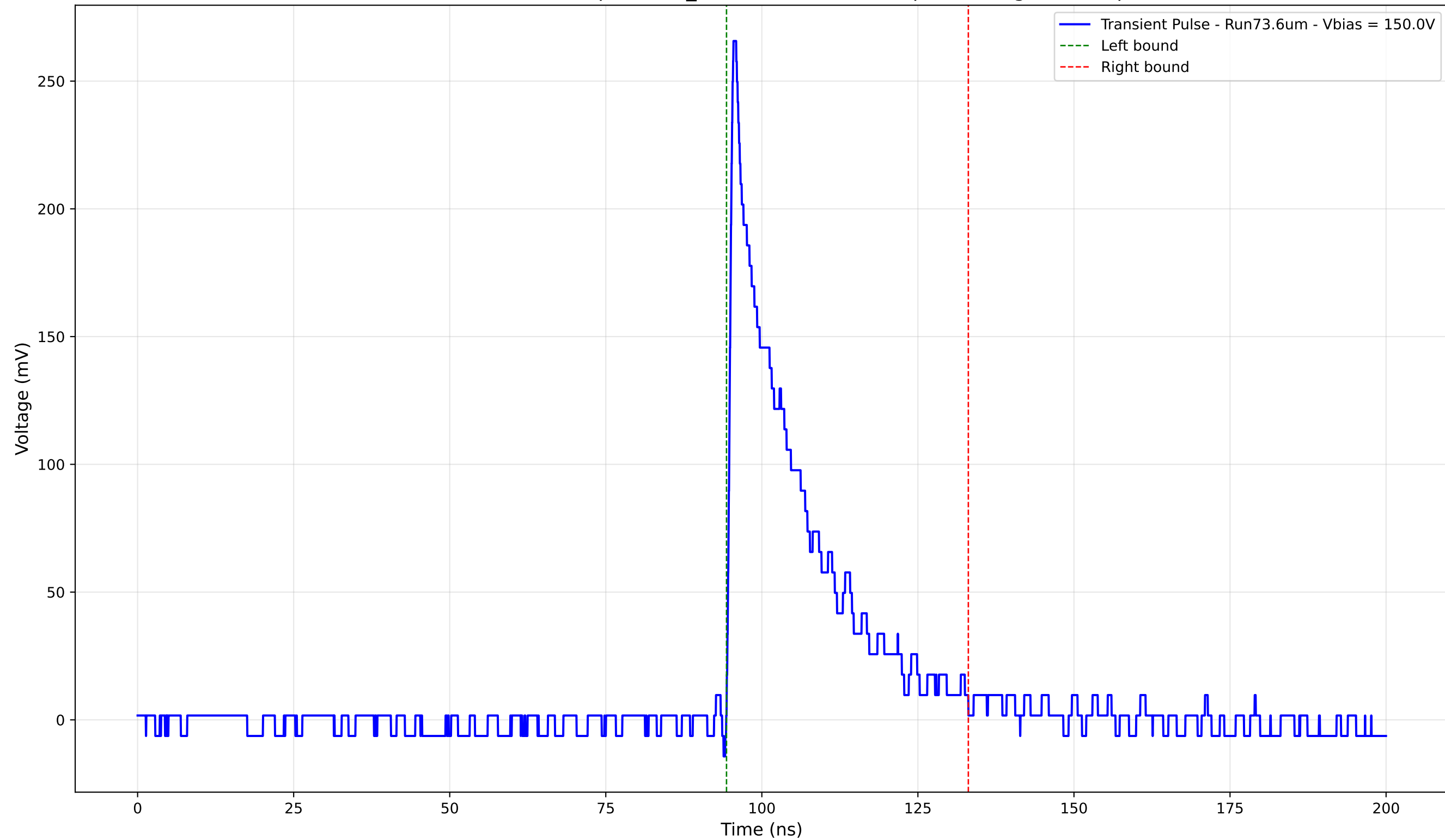
Transient Pulse - Sample: 1cm_42 - Position: 3475.0 \mu\text{m} - Charge: 53.90 pC
