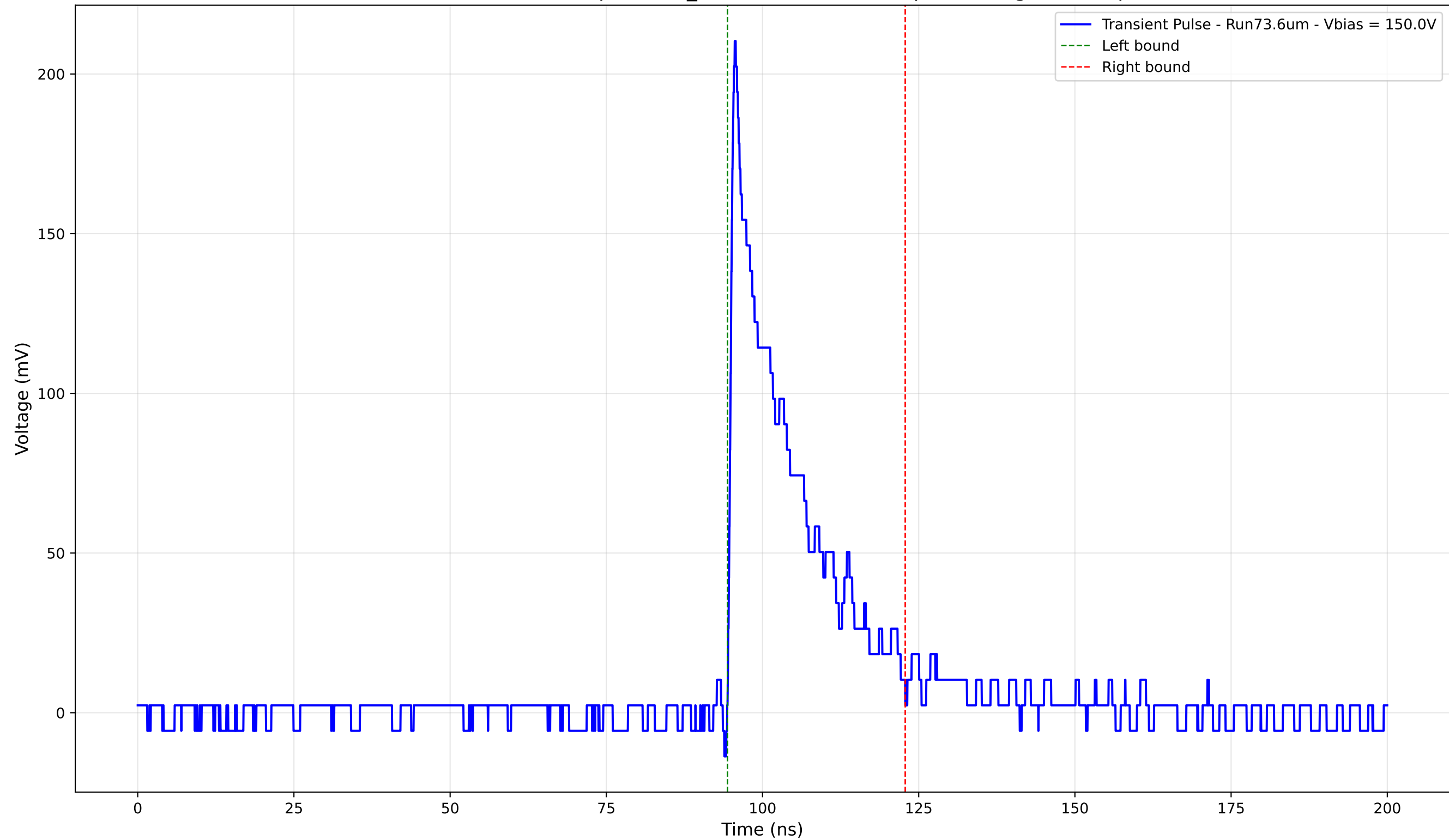
Transient Pulse - Sample: 1cm_42 - Position: 3905.0 \mu\text{m} - Charge: 38.96 pC
