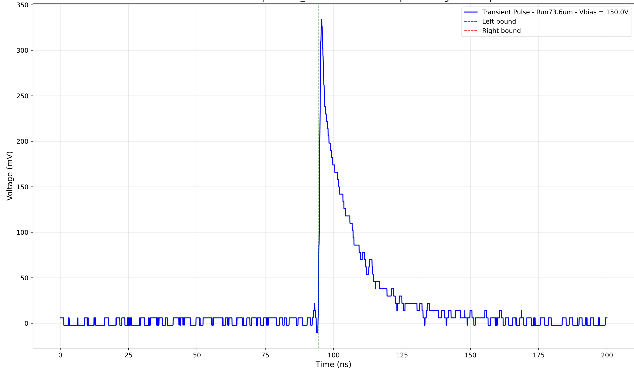
Transient Pulse - Sample: 1cm_42 - Position: 3115.0 \mu\text{m} - Charge: 65.14 pC
