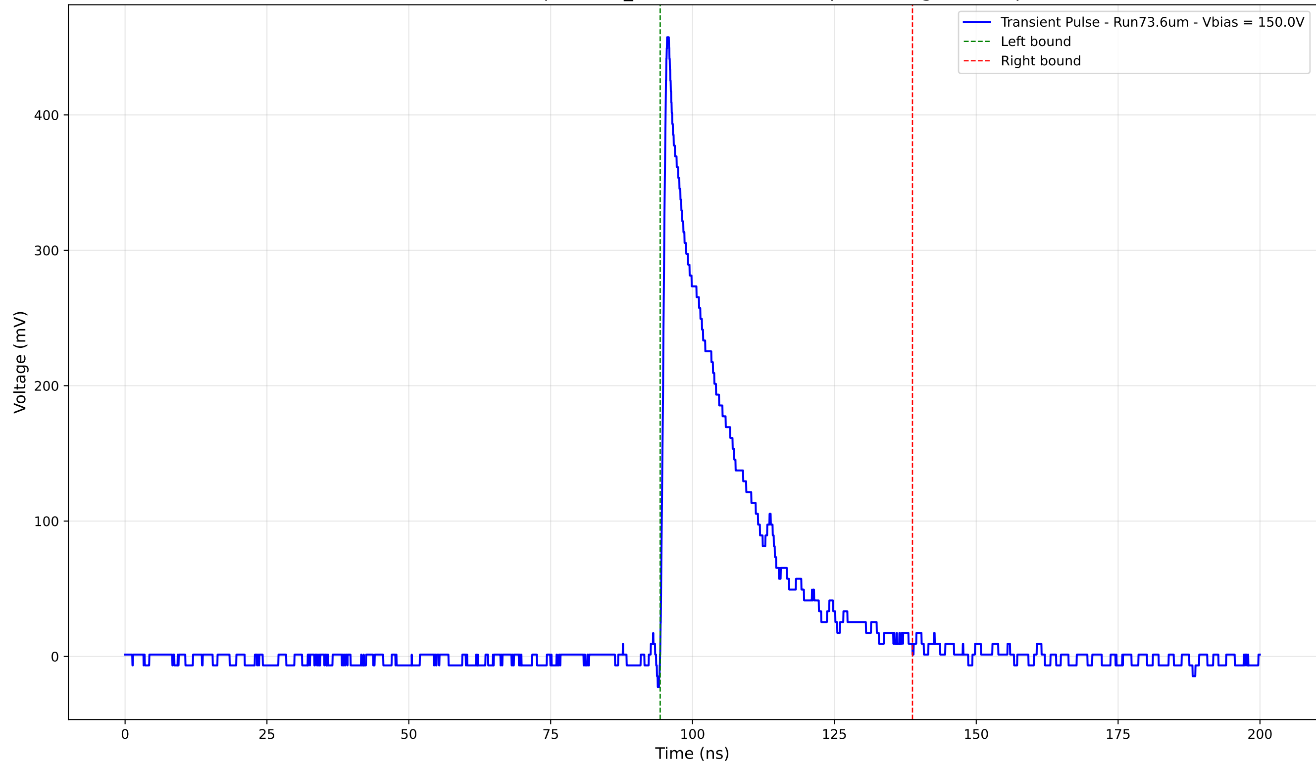
Transient Pulse - Sample: 1cm_42 - Position: 1055.0 \mu\text{m} - Charge: 99.70 pC
