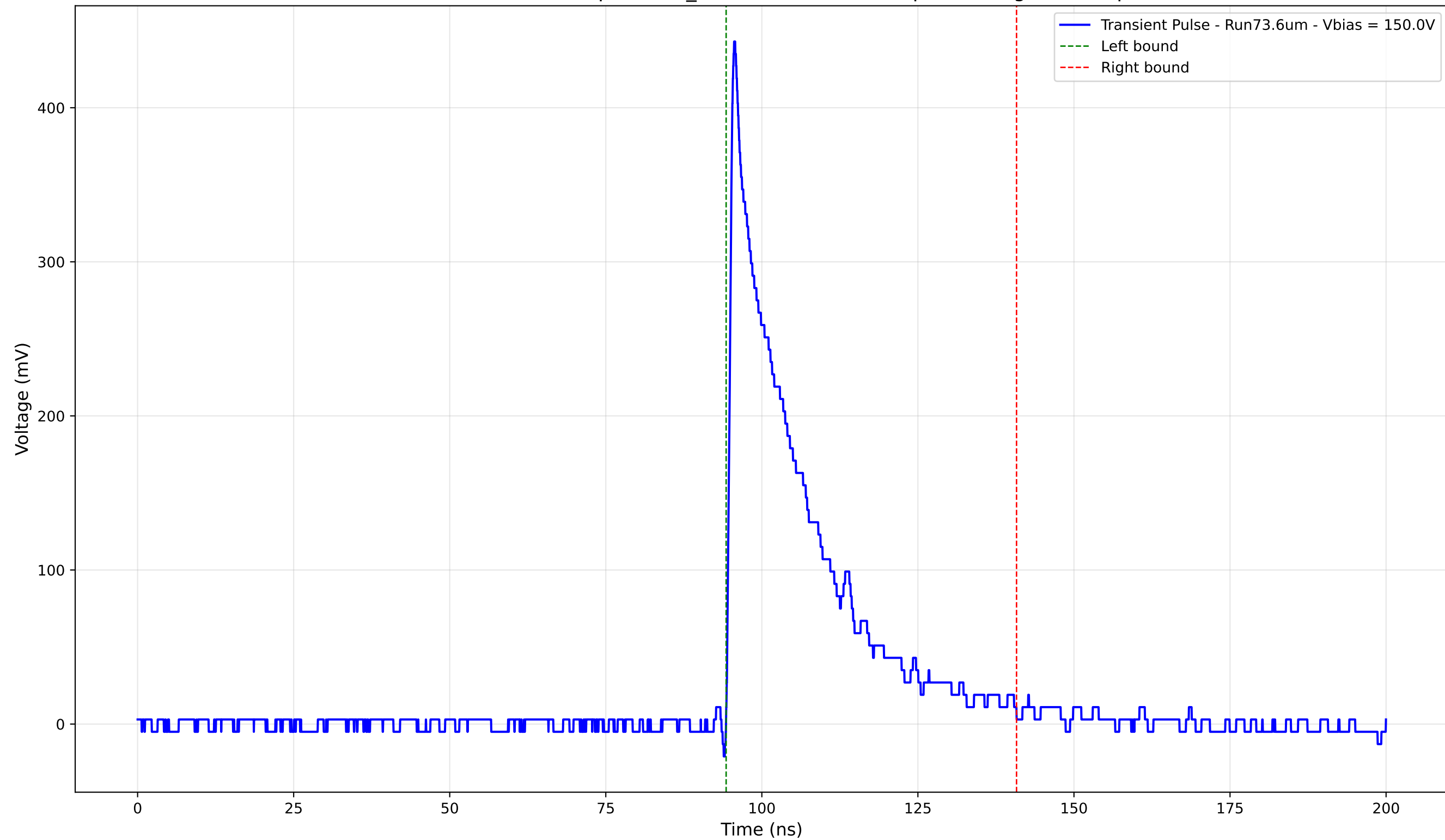
Transient Pulse - Sample: 1cm_42 - Position: 1540.0 \mu\text{m} - Charge: 96.24 pC
