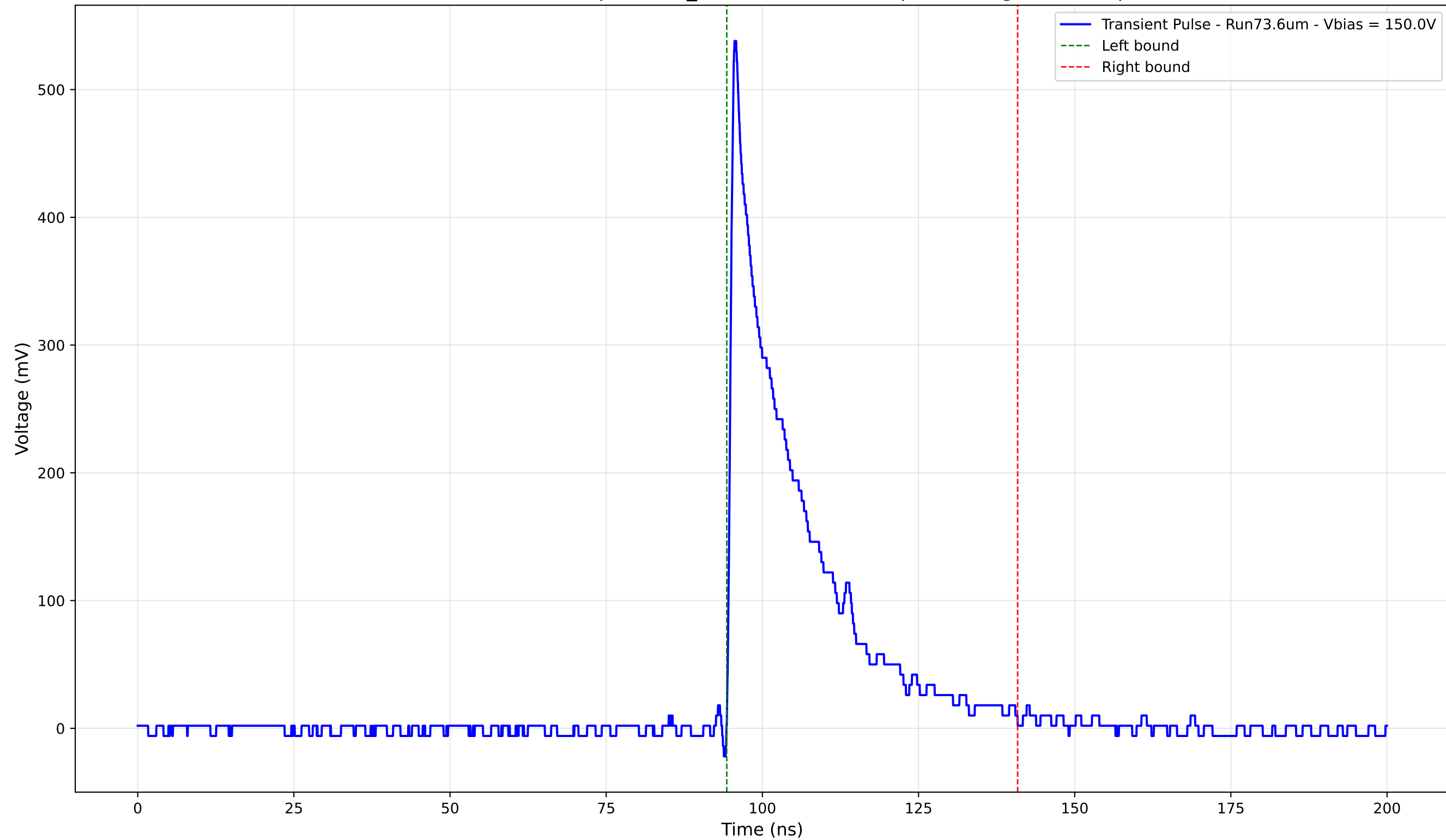
Transient Pulse - Sample: 1cm_42 - Position: 465.0 \mu\text{m} - Charge: 110.15 pC
