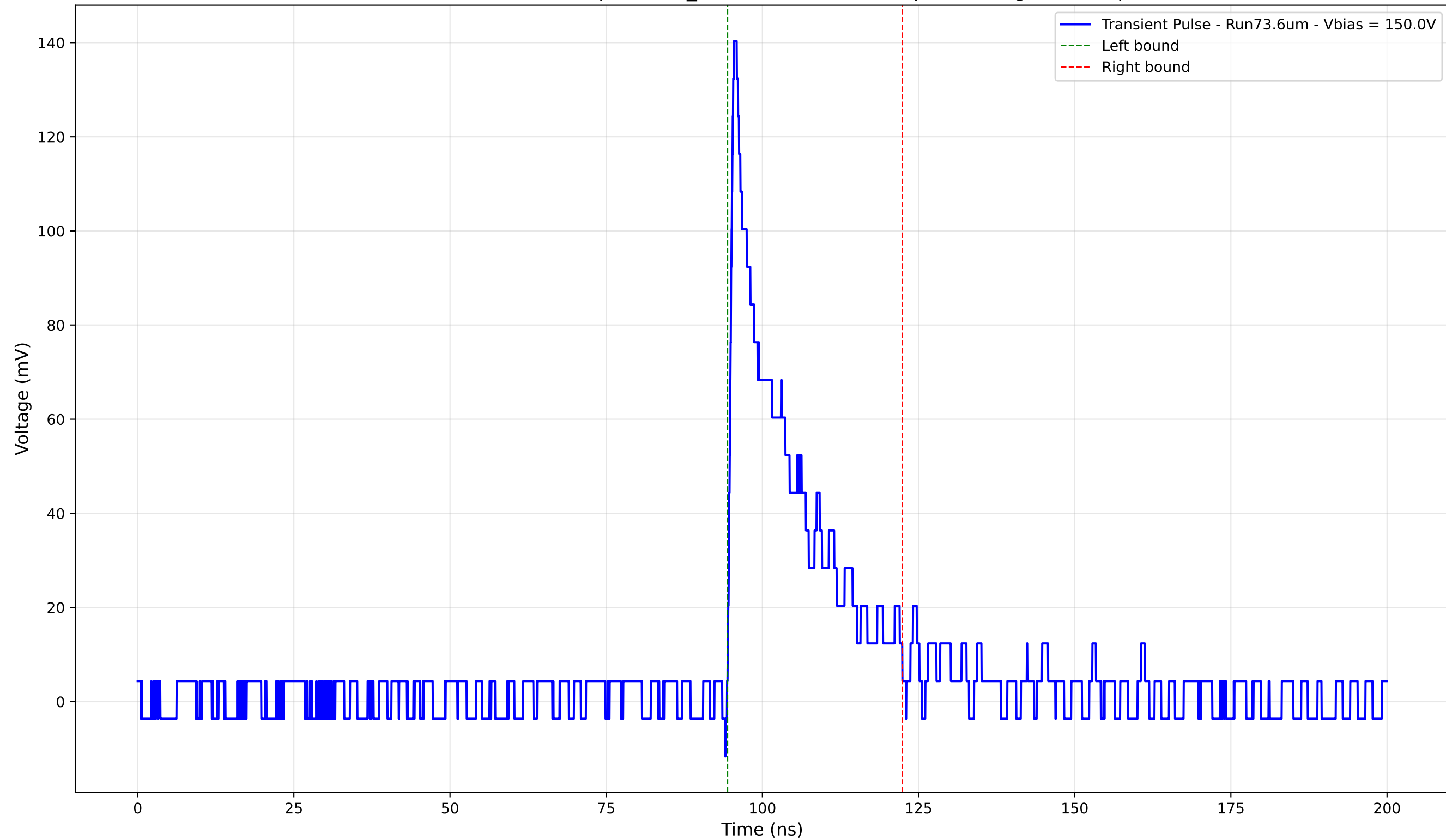
Transient Pulse - Sample: 1cm_42 - Position: 4595.0 \mu\text{m} - Charge: 25.16 pC
