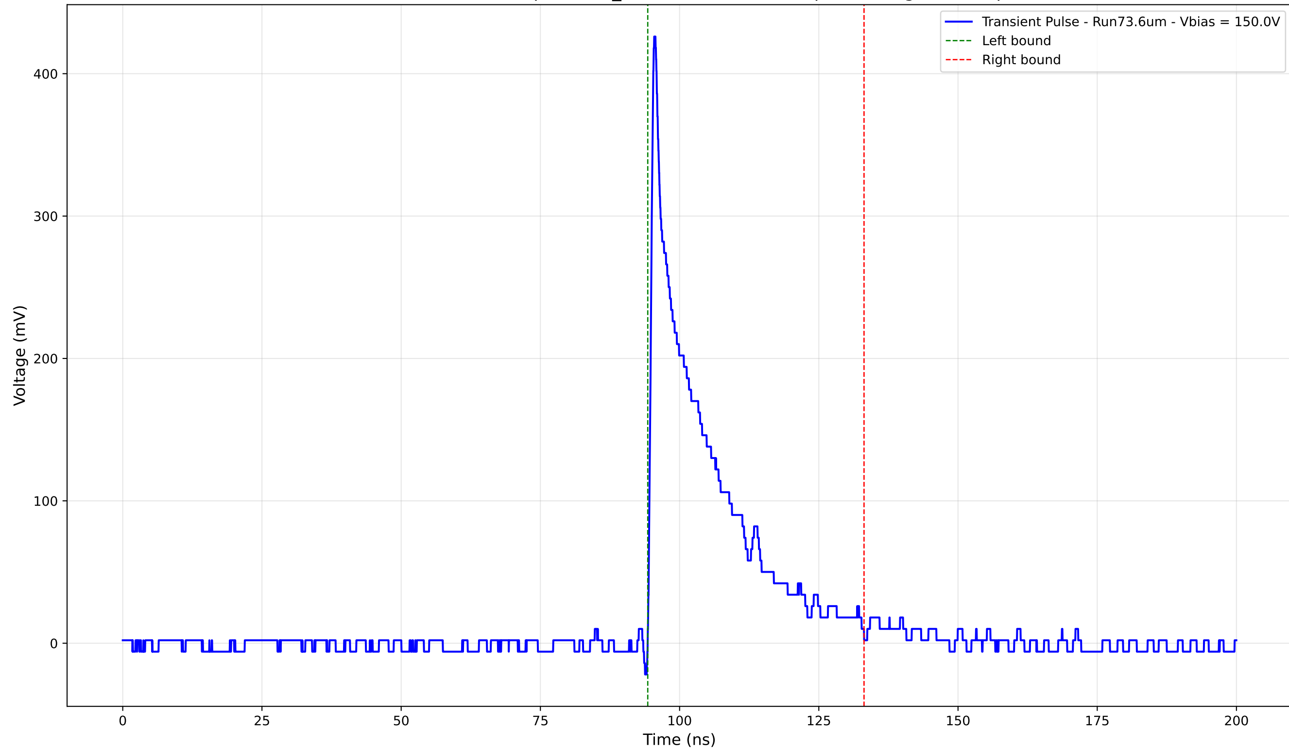
Transient Pulse - Sample: 1cm_42 - Position: 2665.0 \mu\text{m} - Charge: 77.33 pC
