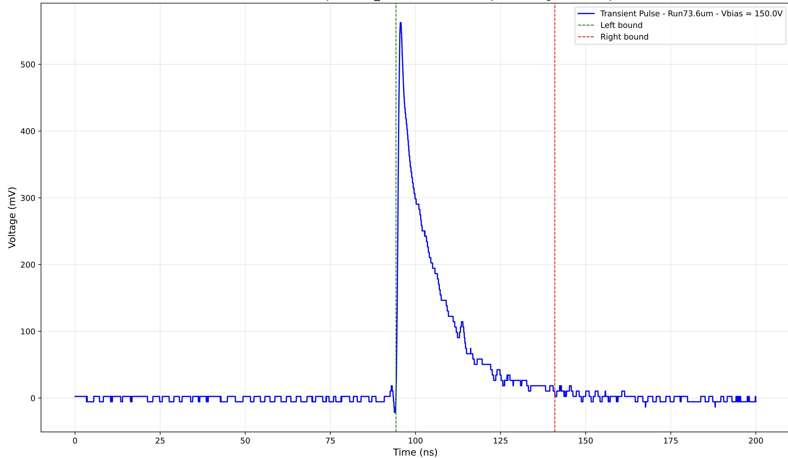
Transient Pulse - Sample: 1cm_42 - Position: 350.0 \mu\text{m} - Charge: 111.81 pC
