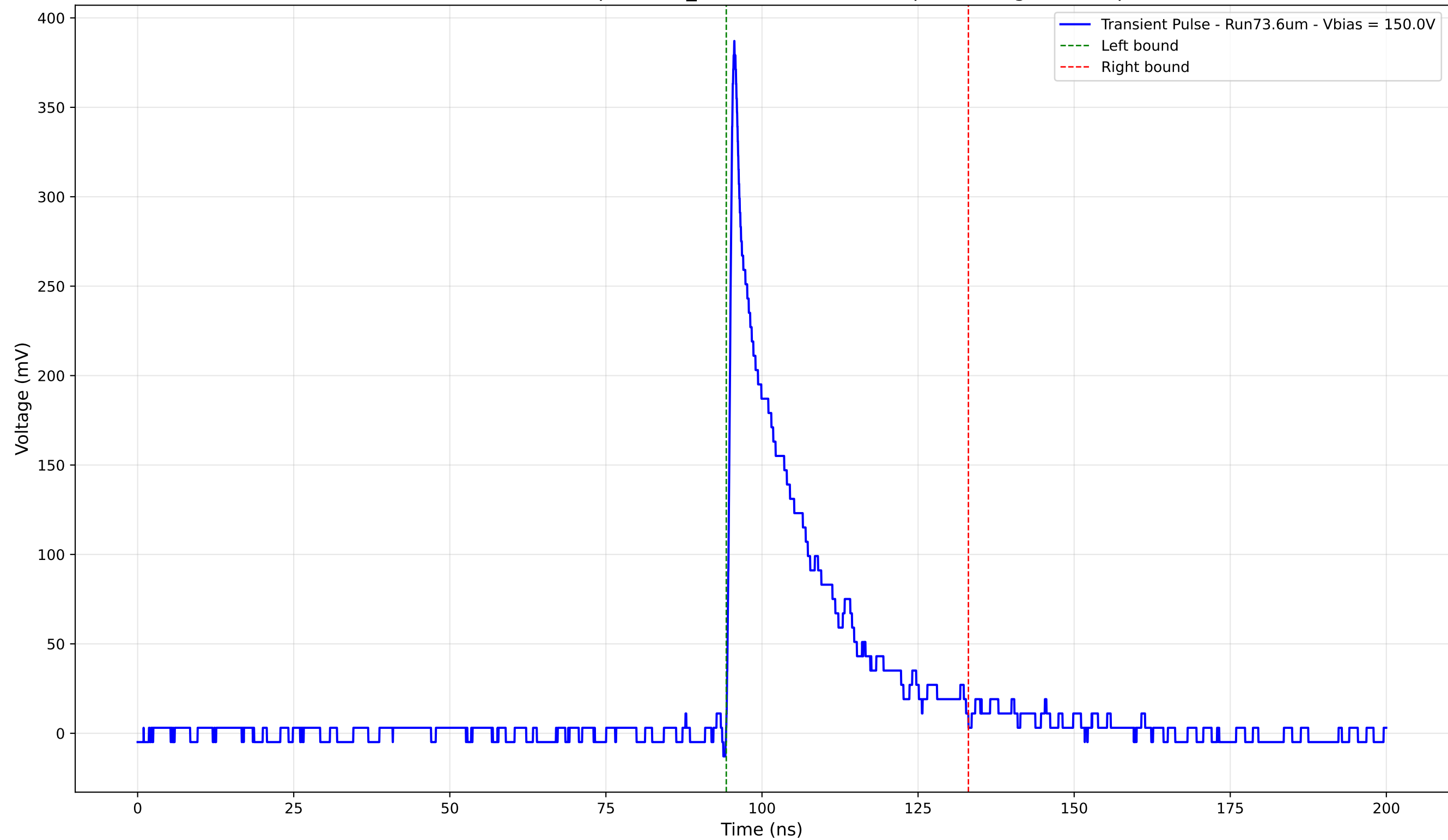
Transient Pulse - Sample: 1cm_42 - Position: 2880.0 \mu\text{m} - Charge: 72.10 pC
