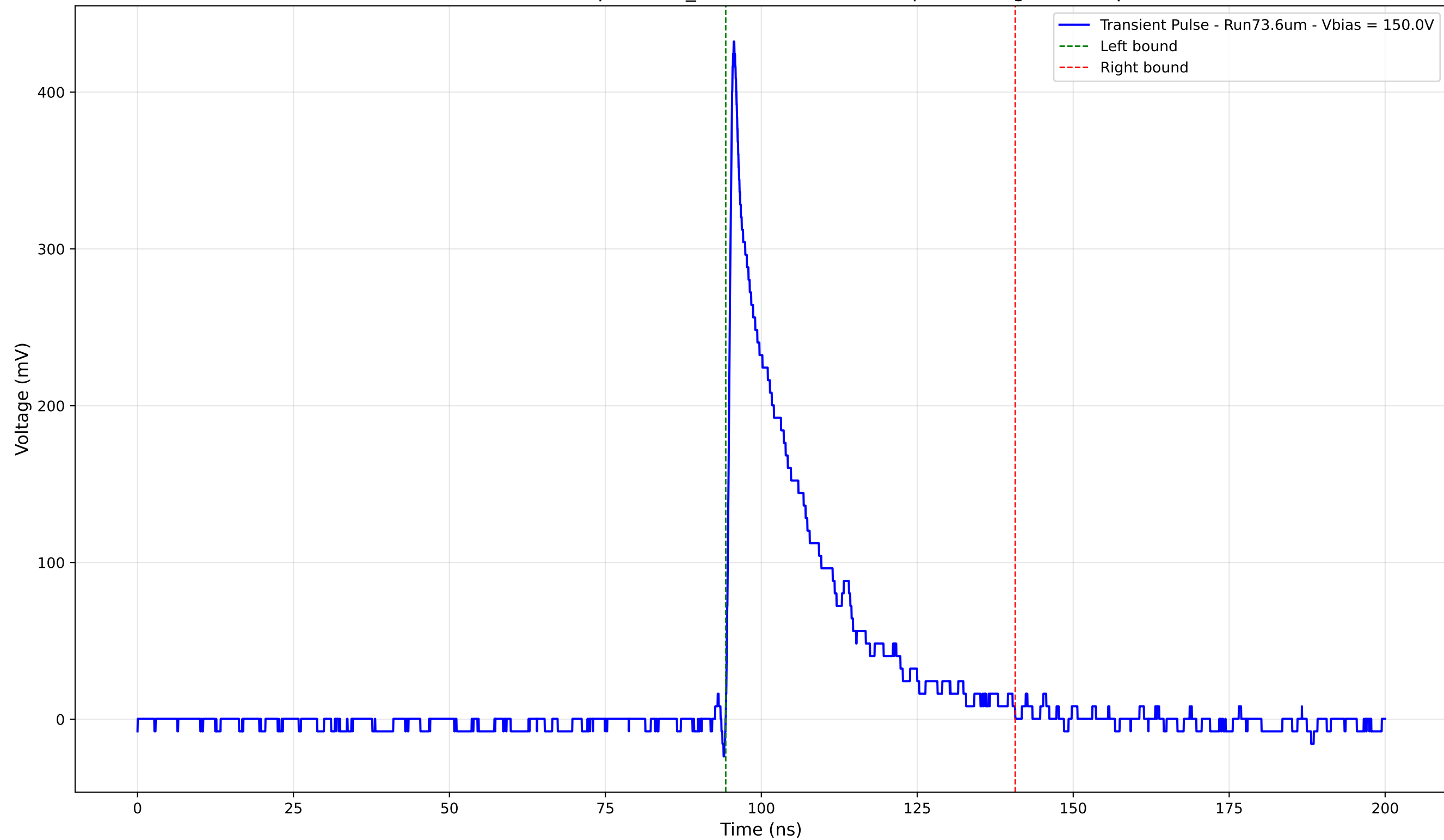
Transient Pulse - Sample: 1cm_42 - Position: 2080.0 \mu\text{m} - Charge: 86.37 pC
