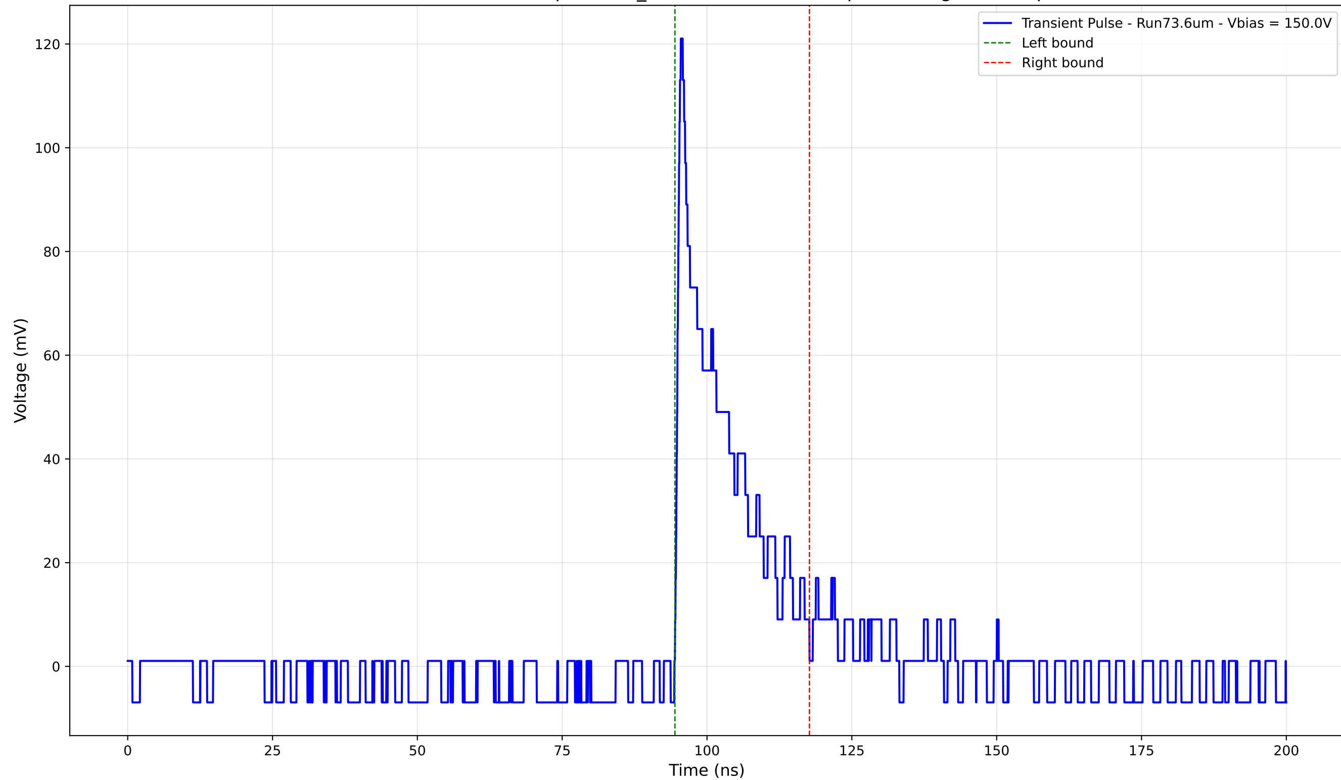
Transient Pulse - Sample: 1cm_42 - Position: 4705.0 \mu\text{m} - Charge: 18.97 pC
