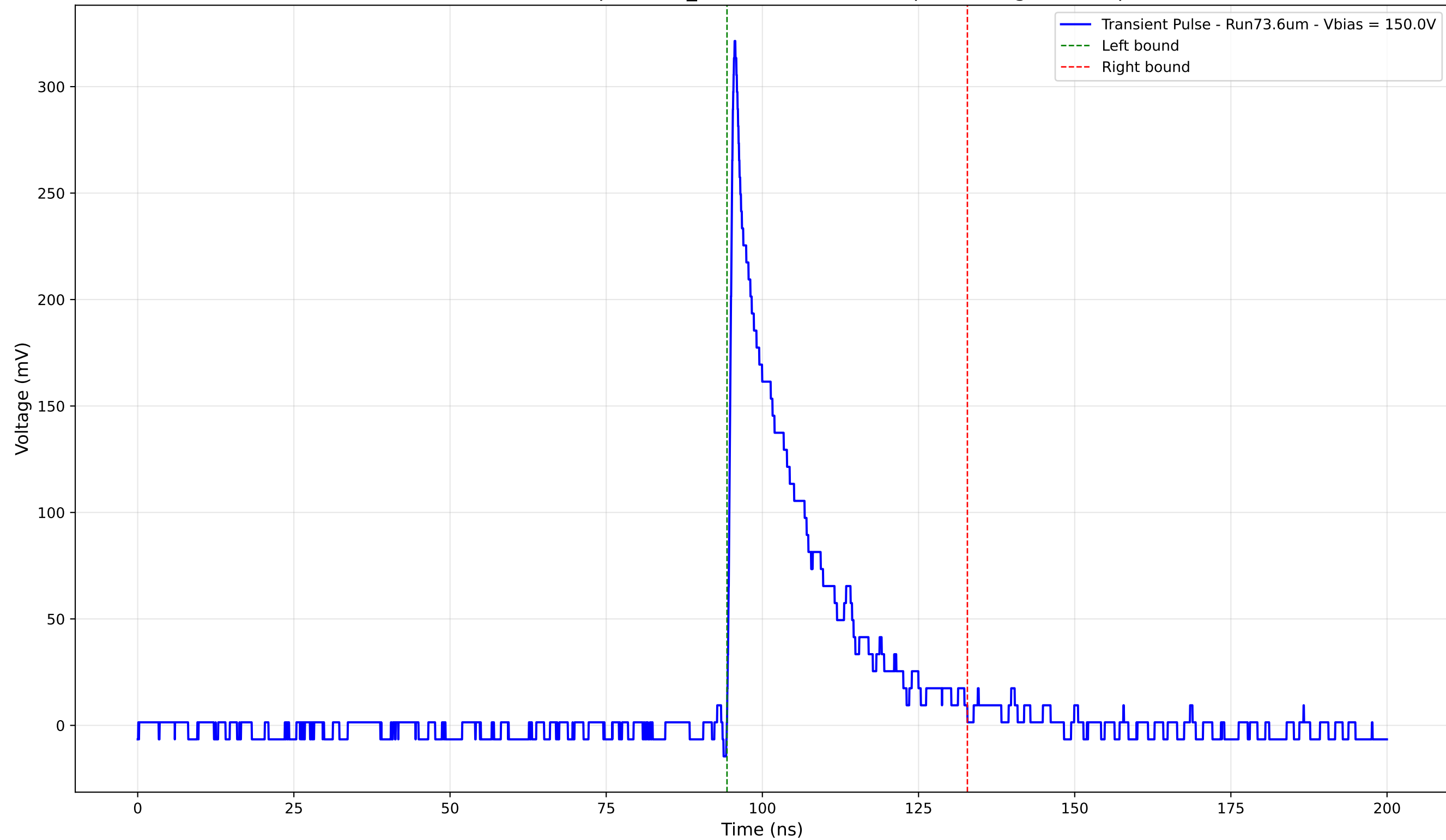
Transient Pulse - Sample: 1cm_42 - Position: 3150.0 \mu\text{m} - Charge: 60.61 pC
