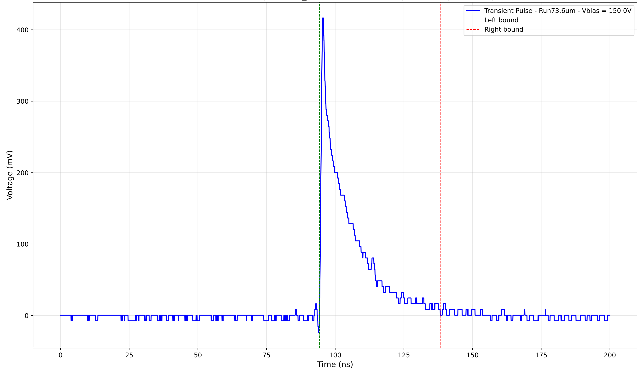
Transient Pulse - Sample: 1cm_42 - Position: 2610.0 \mu\text{m} - Charge: 76.67 pC
