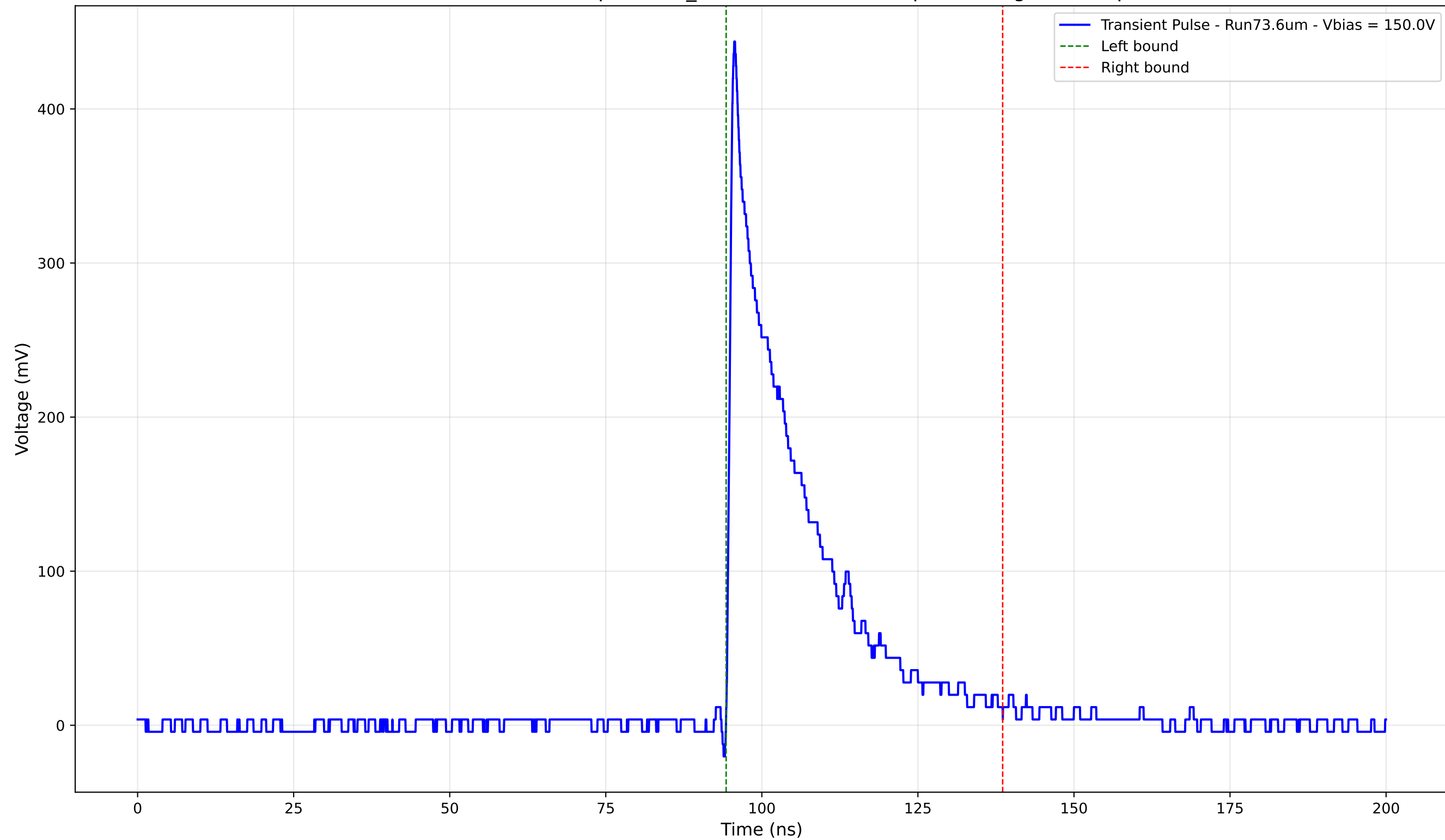
Transient Pulse - Sample: 1cm_42 - Position: 1670.0 \mu\text{m} - Charge: 95.02 pC
