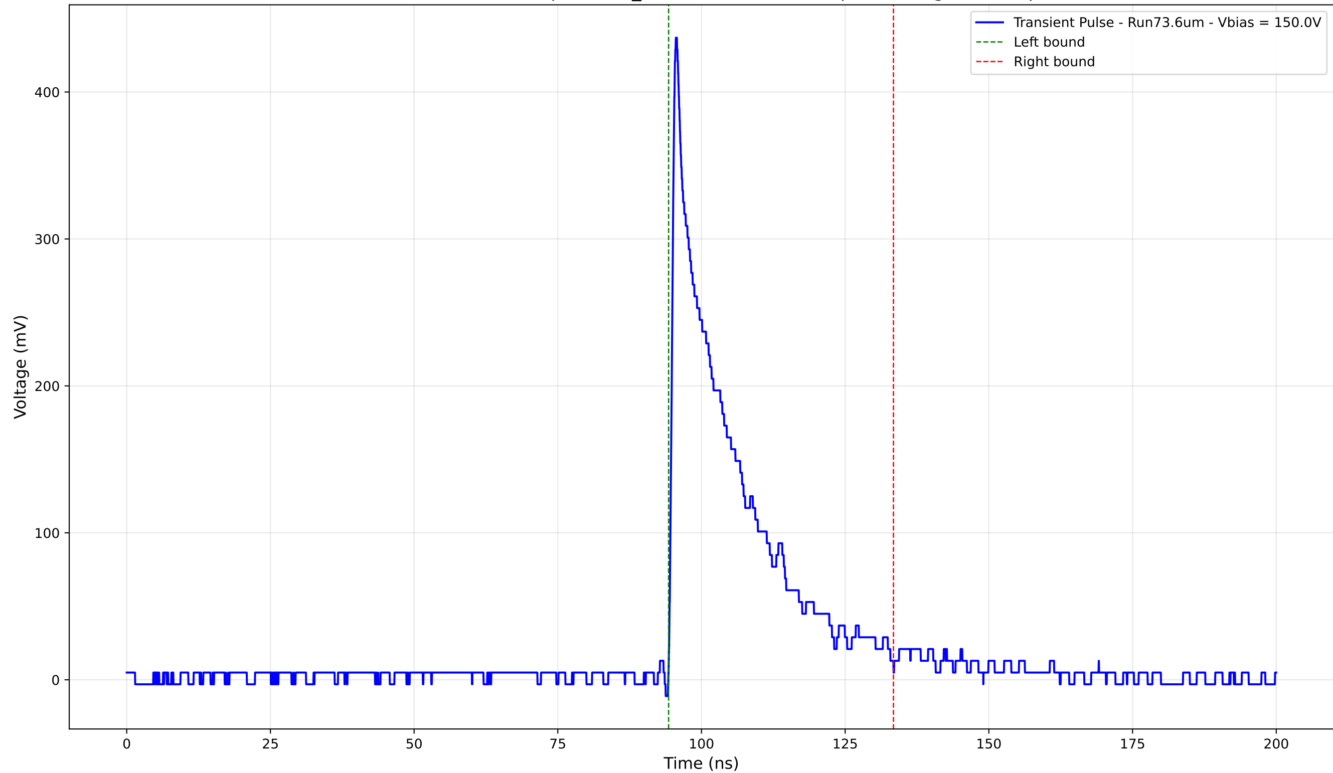
Transient Pulse - Sample: 1cm_42 - Position: 2030.0 \mu\text{m} - Charge: 89.18 pC
