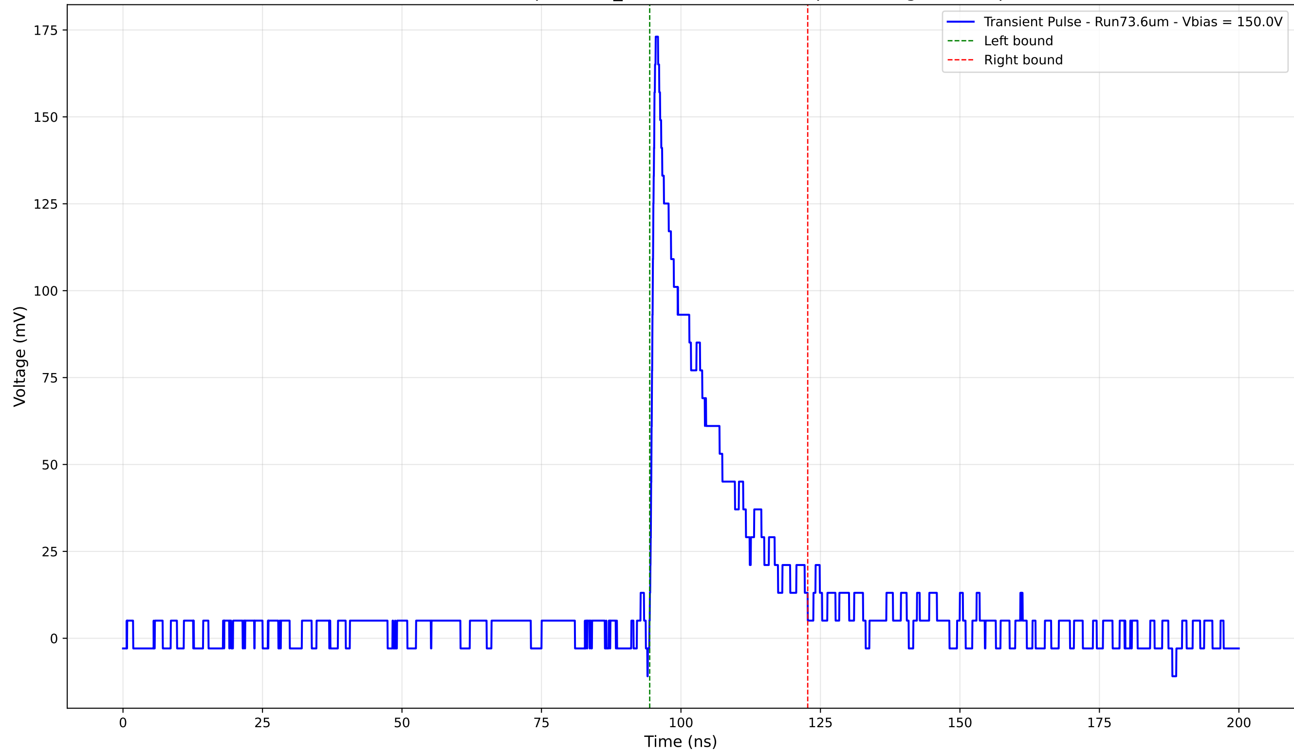
Transient Pulse - Sample: 1cm_42 - Position: 4220.0 \mu\text{m} - Charge: 32.98 pC
