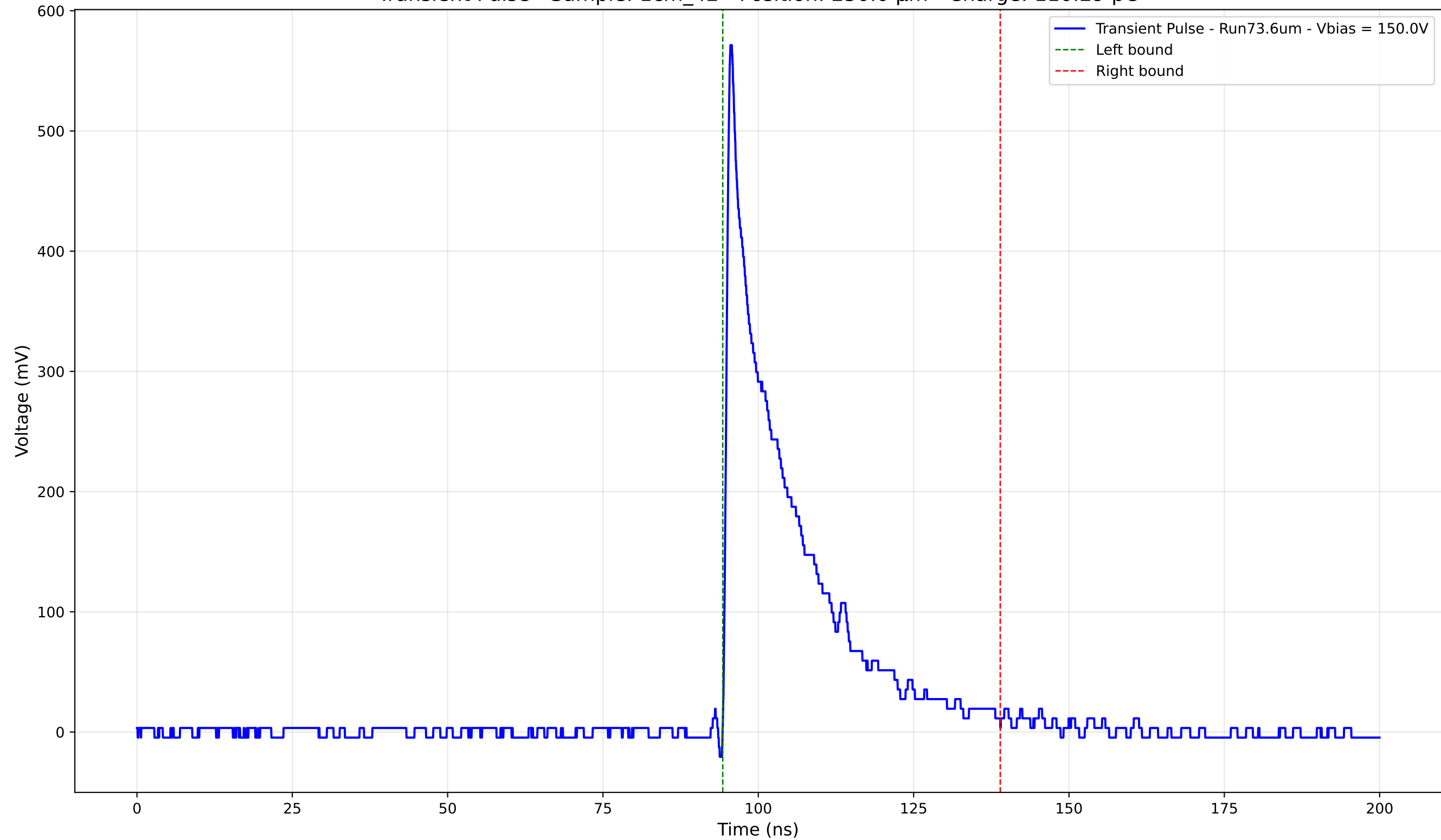
Transient Pulse - Sample: 1cm_42 - Position: 250.0 \mu\text{m} - Charge: 110.29 pC
