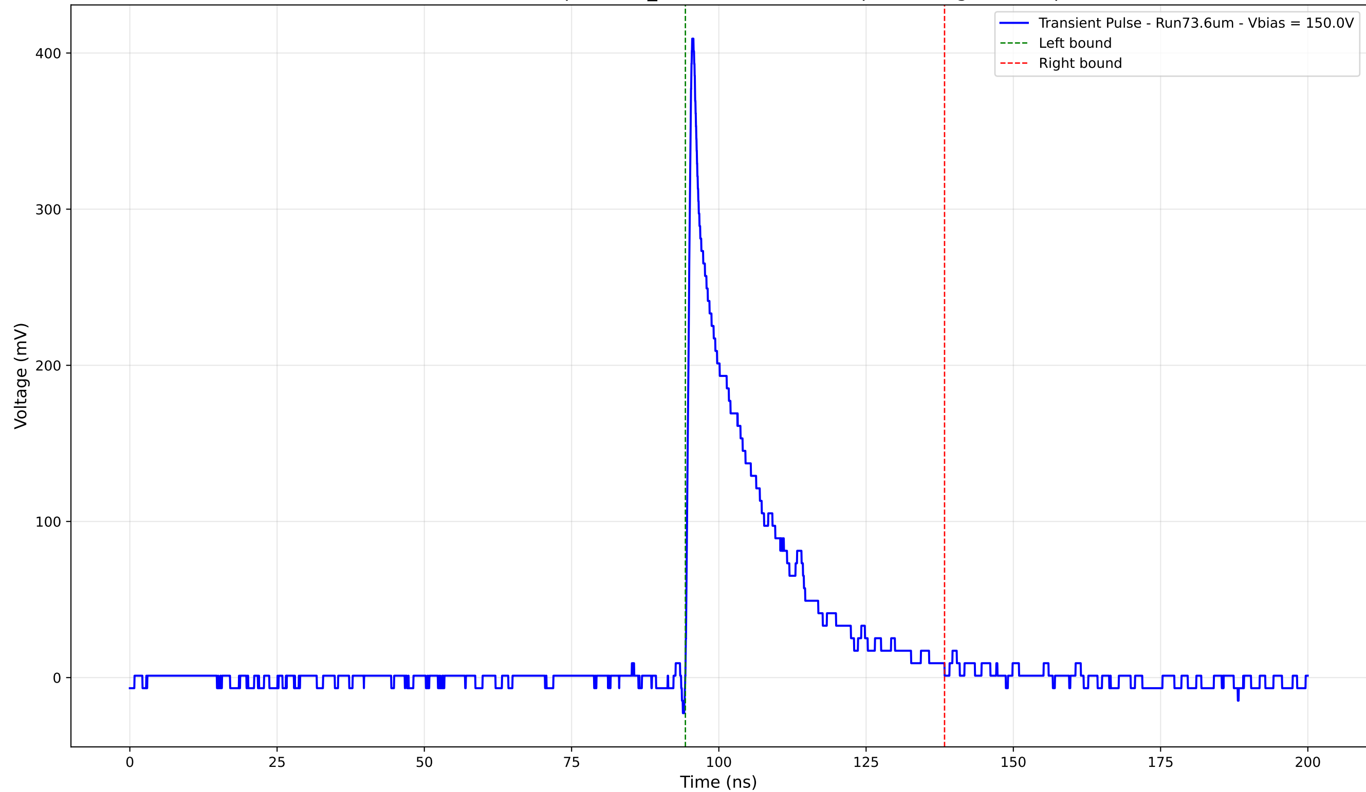
Transient Pulse - Sample: 1cm_42 - Position: 2390.0 \mu\text{m} - Charge: 76.63 pC
