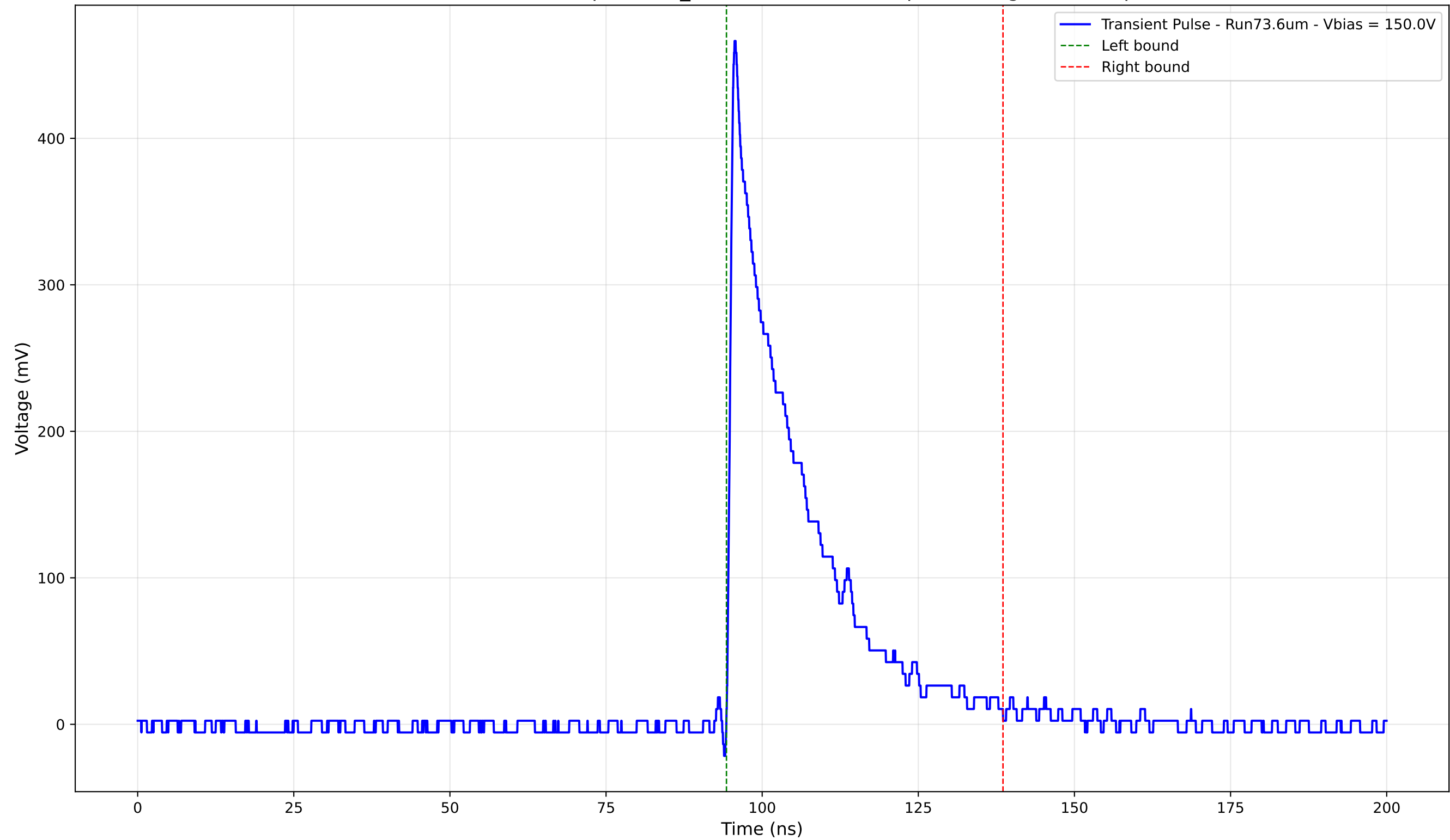
Transient Pulse - Sample: 1cm_42 - Position: 1115.0 \mu\text{m} - Charge: 100.58 pC
