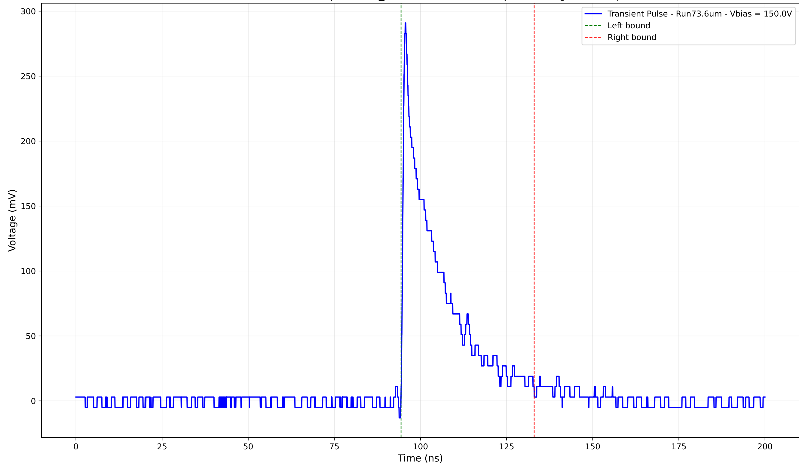
Transient Pulse - Sample: 1cm_42 - Position: 3325.0 \mu\text{m} - Charge: 57.82 pC
