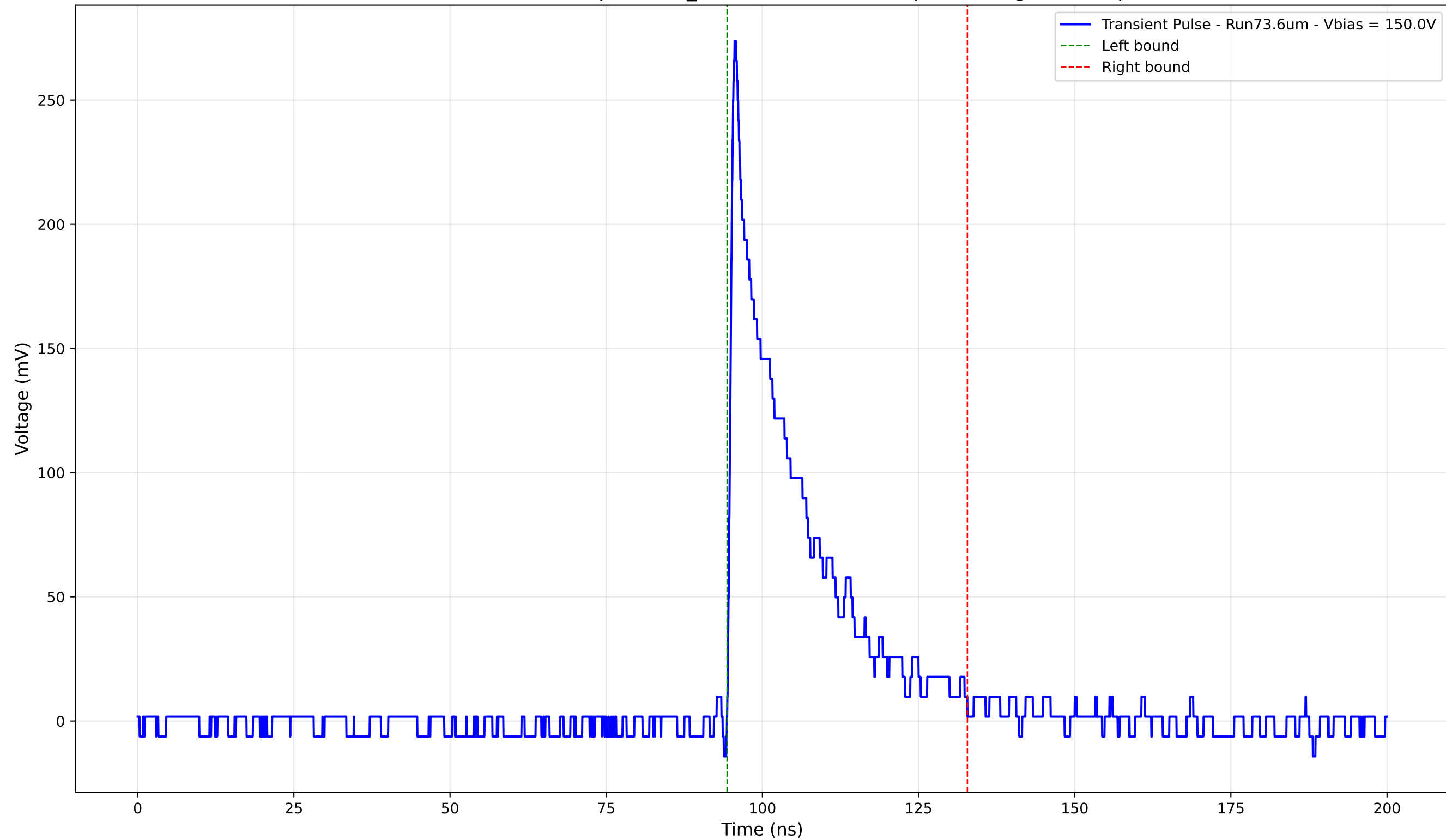
Transient Pulse - Sample: 1cm_42 - Position: 3485.0 \mu\text{m} - Charge: 53.79 pC
