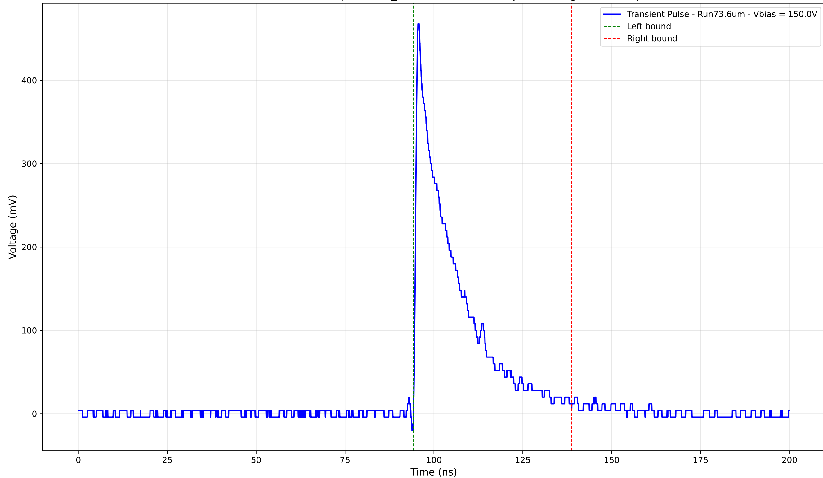
Transient Pulse - Sample: 1cm_42 - Position: 990.0 \mu\text{m} - Charge: 103.33 pC
