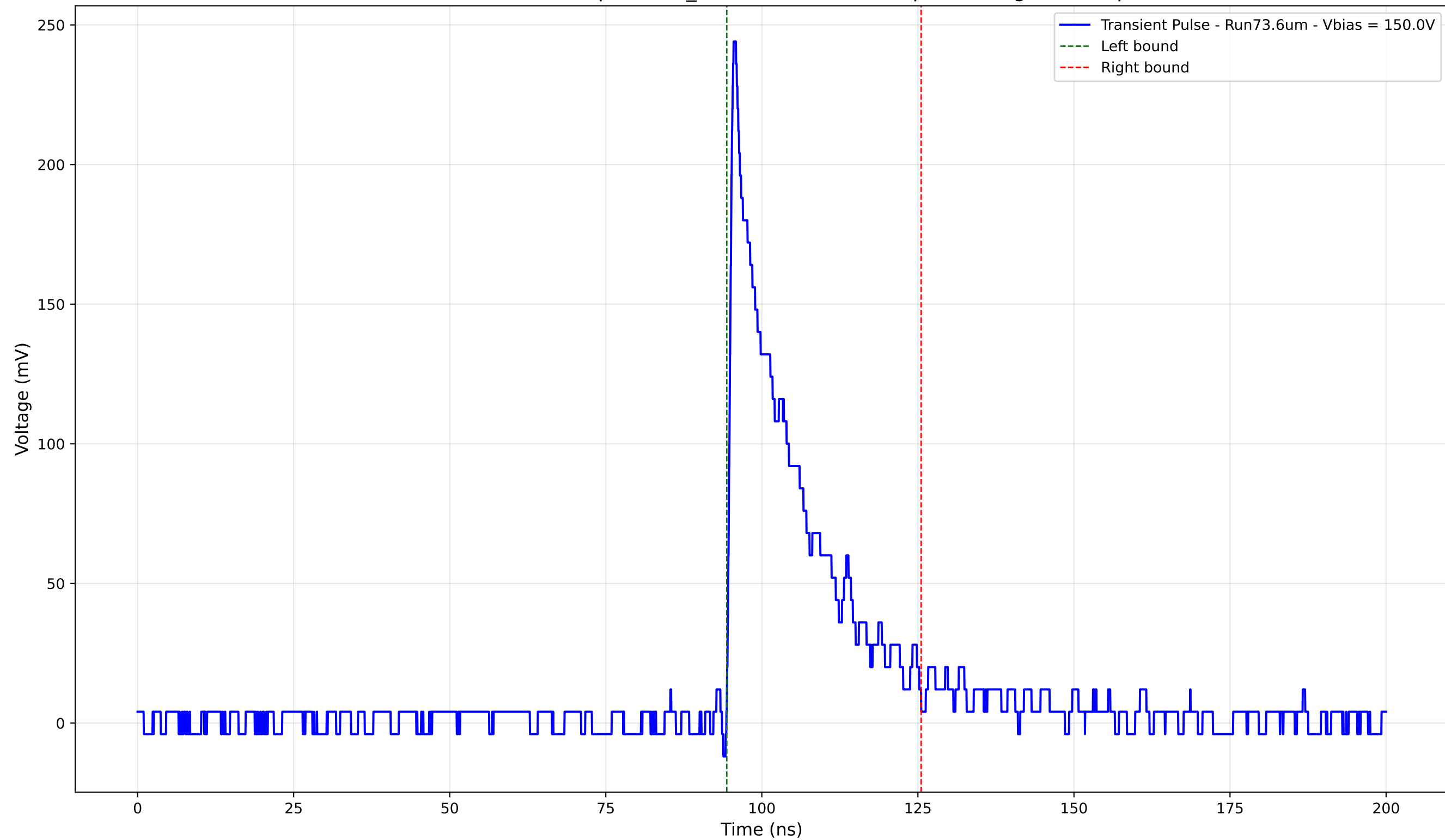
Transient Pulse - Sample: 1cm_42 - Position: 3640.0 \mu\text{m} - Charge: 48.21 pC
