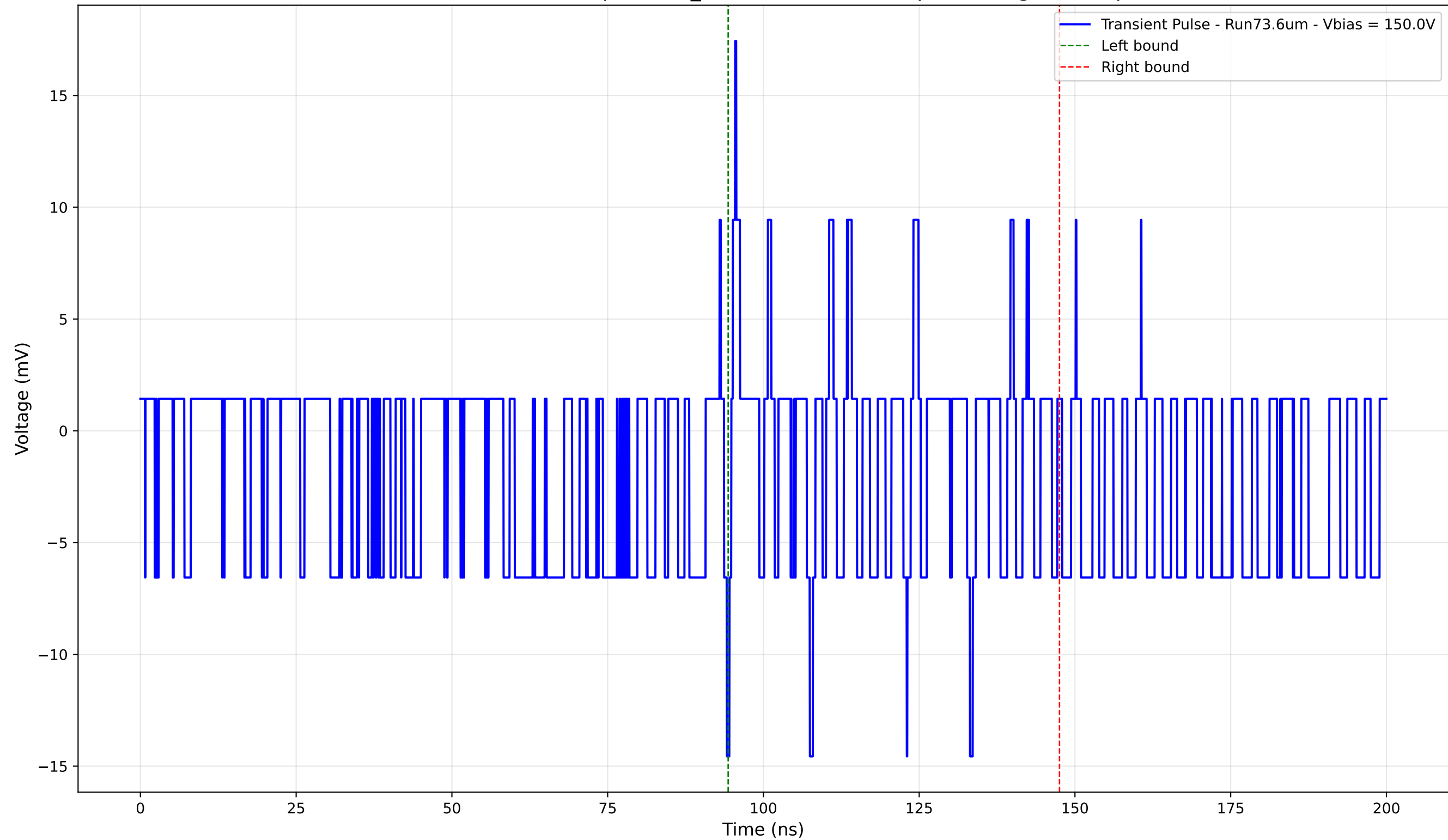
Transient Pulse - Sample: 1cm_42 - Position: 4990.0 \mu\text{m} - Charge: -0.54 pC
