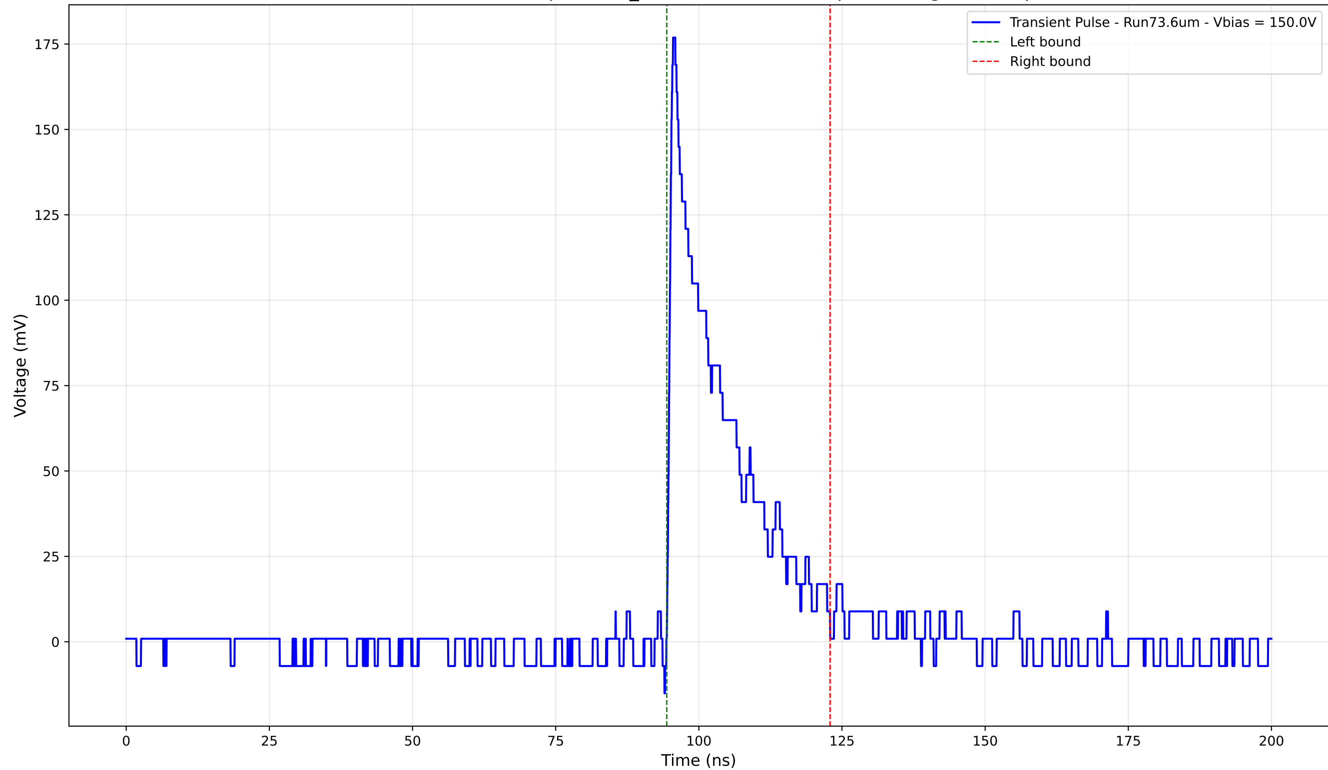
Transient Pulse - Sample: 1cm_42 - Position: 4115.0 \mu\text{m} - Charge: 33.40 pC
