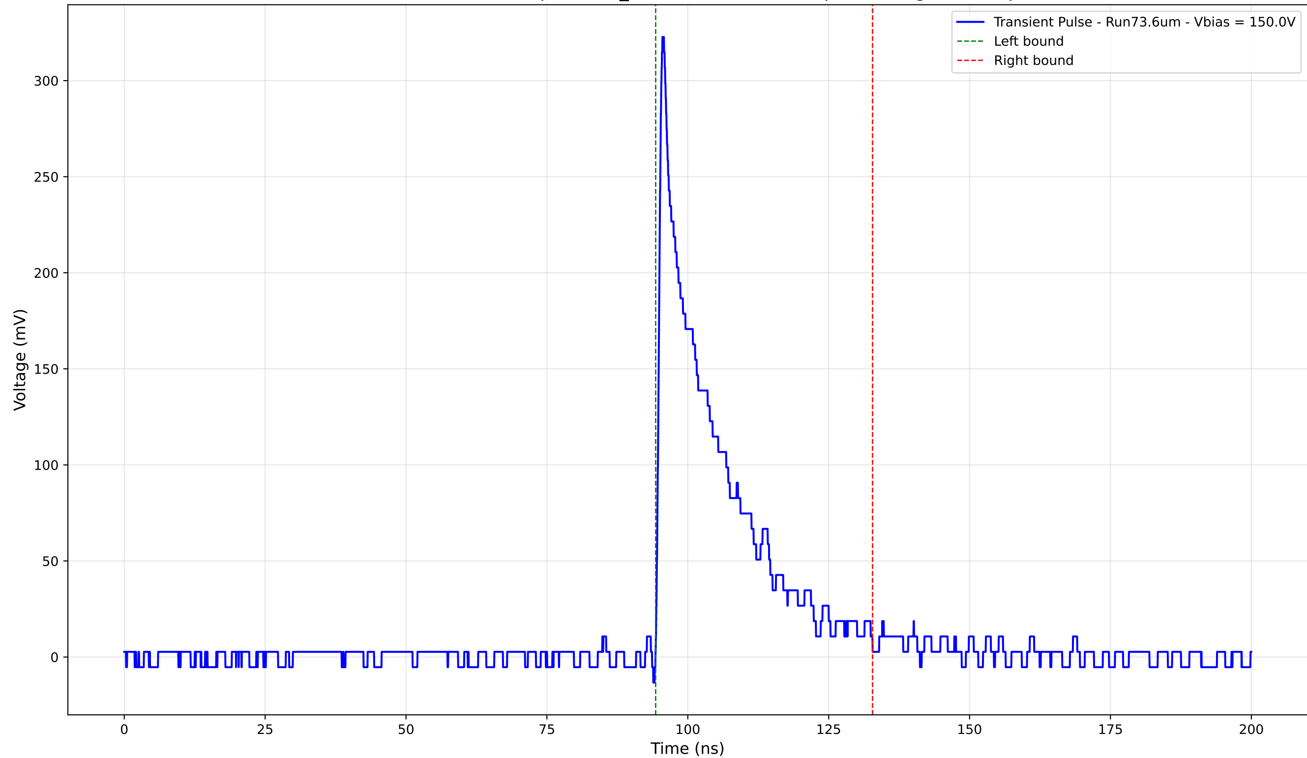
Transient Pulse - Sample: 1cm_42 - Position: 3120.0 \mu\text{m} - Charge: 62.54 pC
