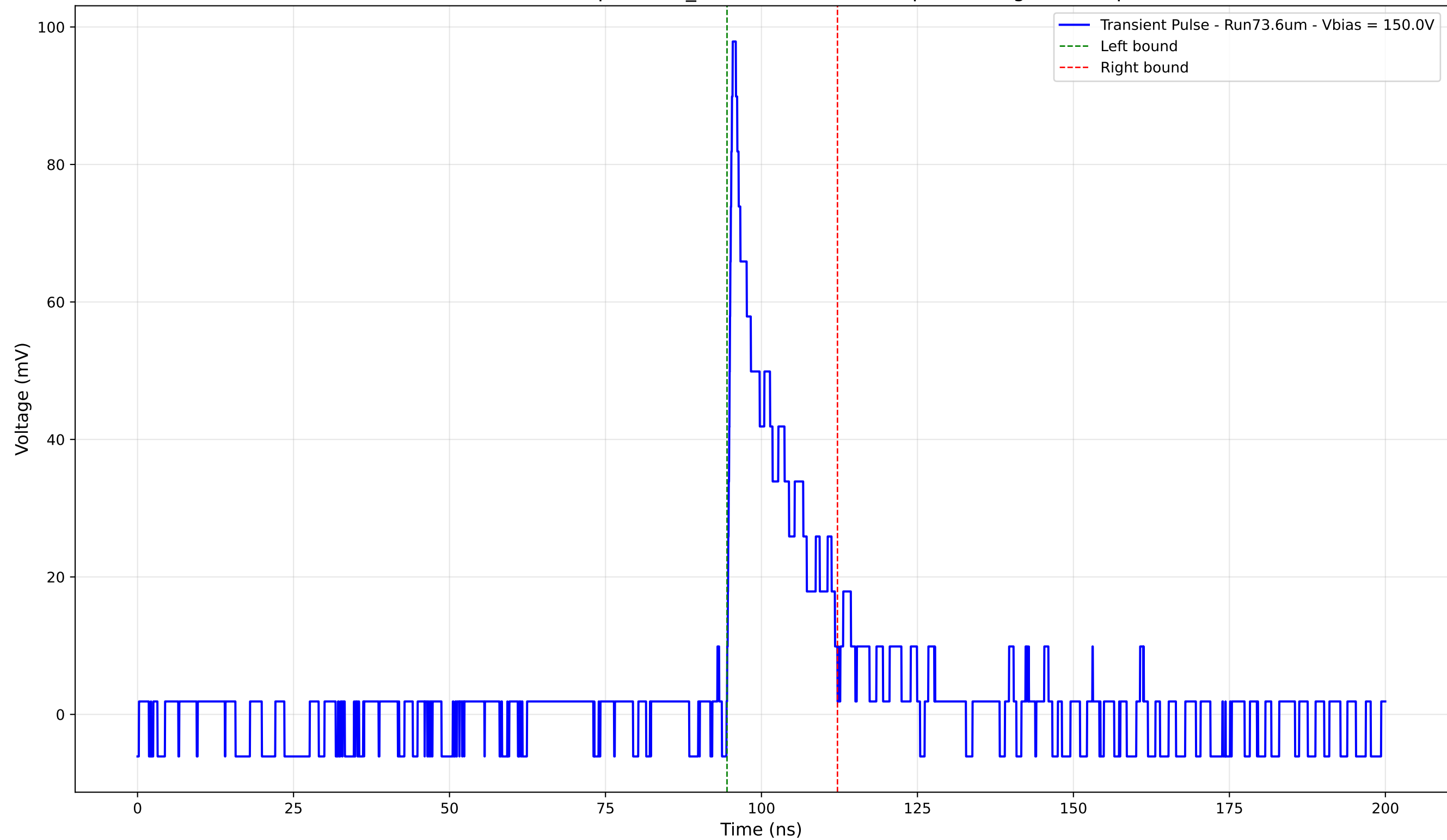
Transient Pulse - Sample: 1cm_42 - Position: 4860.0 \mu\text{m} - Charge: 14.05 pC
