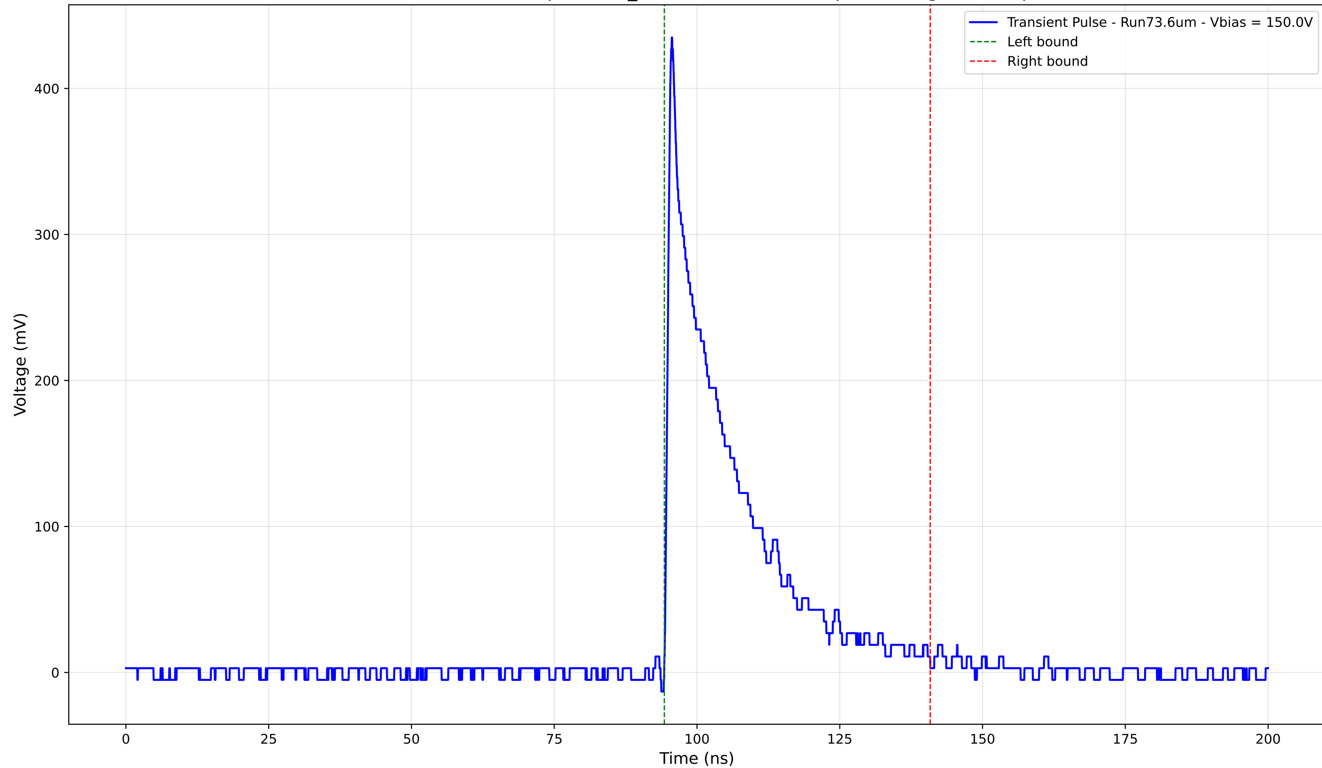
Transient Pulse - Sample: 1cm_42 - Position: 2045.0 \mu\text{m} - Charge: 89.61 pC
