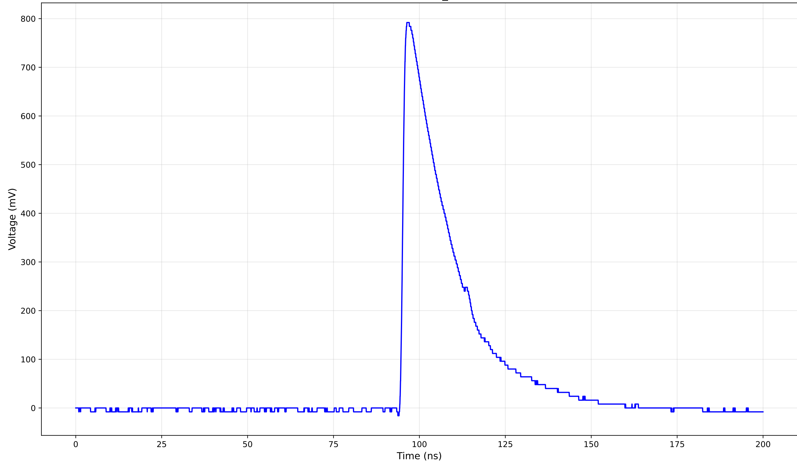
TCT Pulse Waveform - Run GainCalib: 1cm_42 (150.0 V) - Rise Time: 1.25 ns
