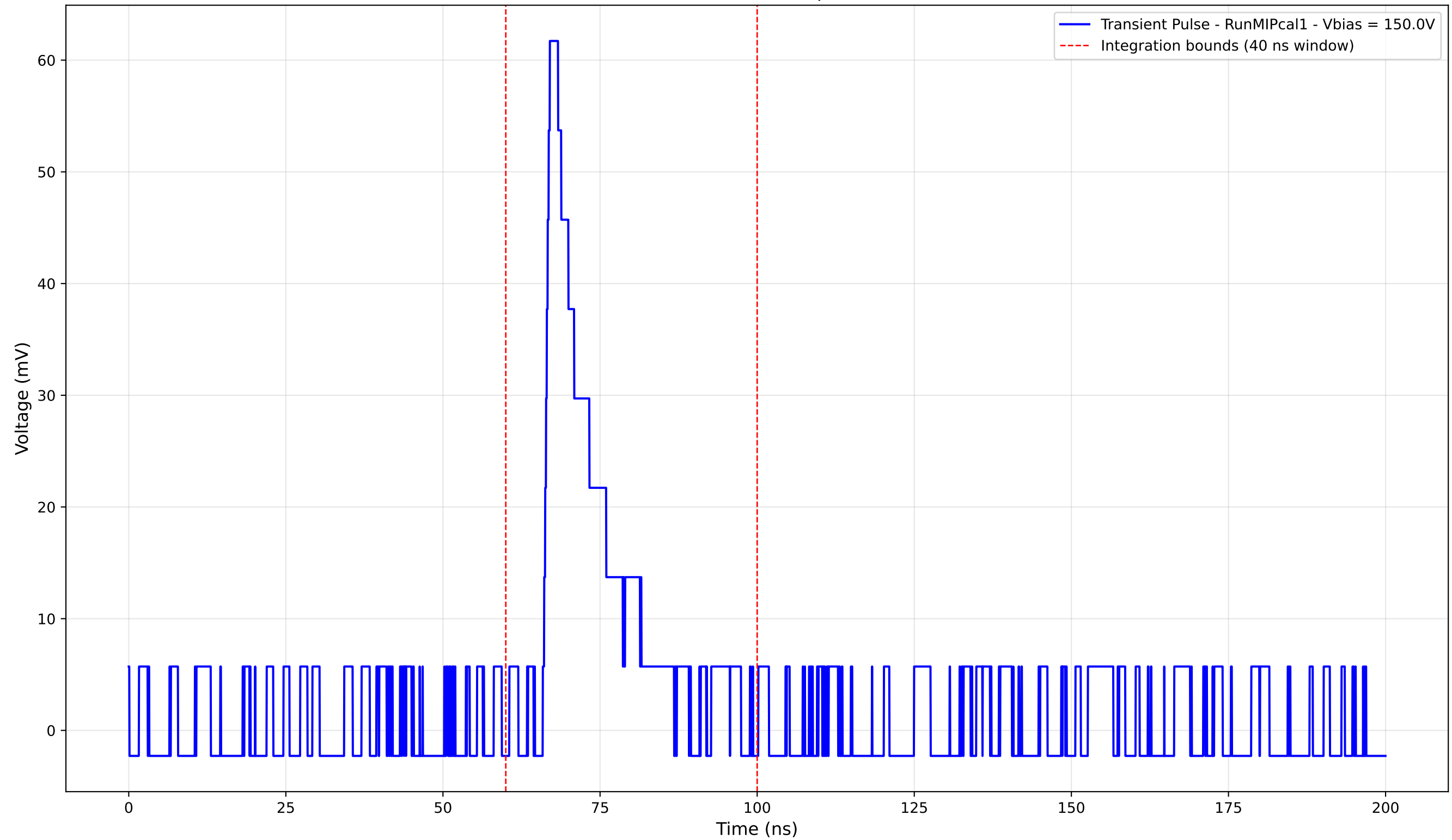
Transient Pulse - Sample: new5
