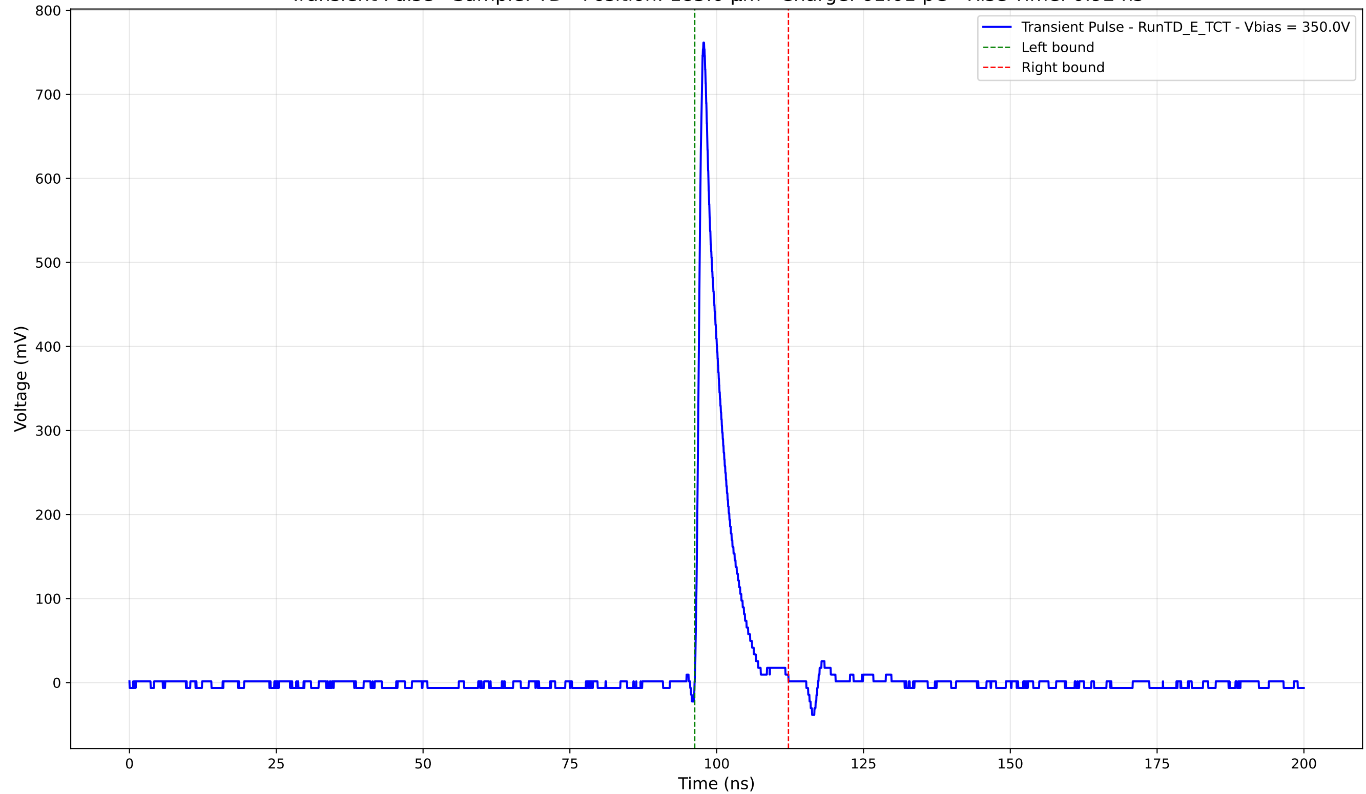
Transient Pulse - Sample: TD - Position: 185.0 \mu\text{m} - Charge: 61.01 pC - Rise Time: 0.92 ns
