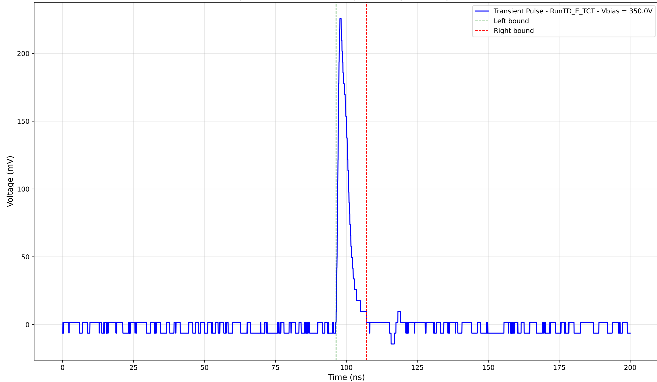
Transient Pulse - Sample: TD - Position: 475.0 \mu\text{m} - Charge: 17.48 pC - Rise Time: 0.99 ns
