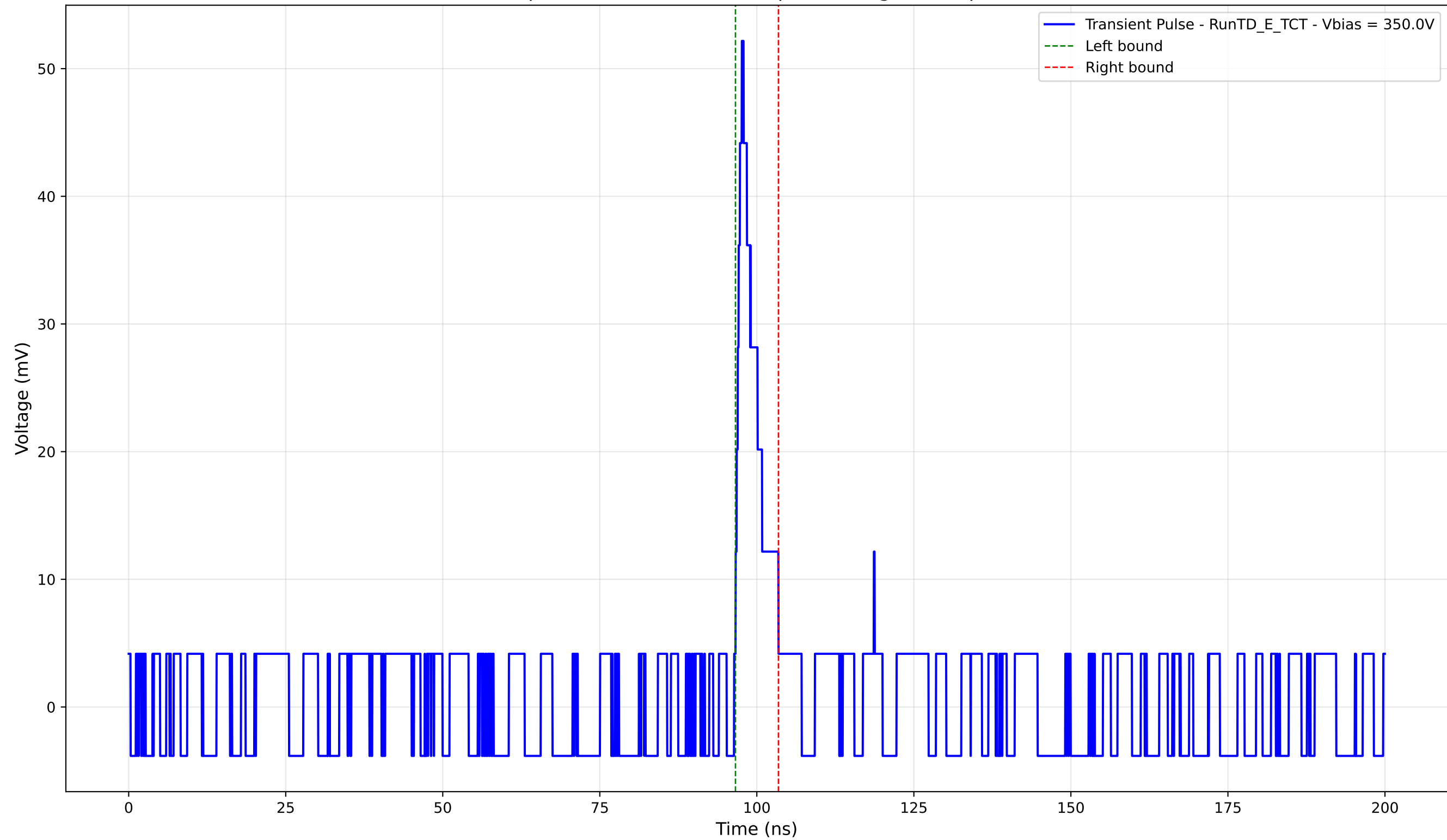
Transient Pulse - Sample: TD - Position: 680.0 \mu\text{m} - Charge: 3.34 pC - Rise Time: 1.00 ns
