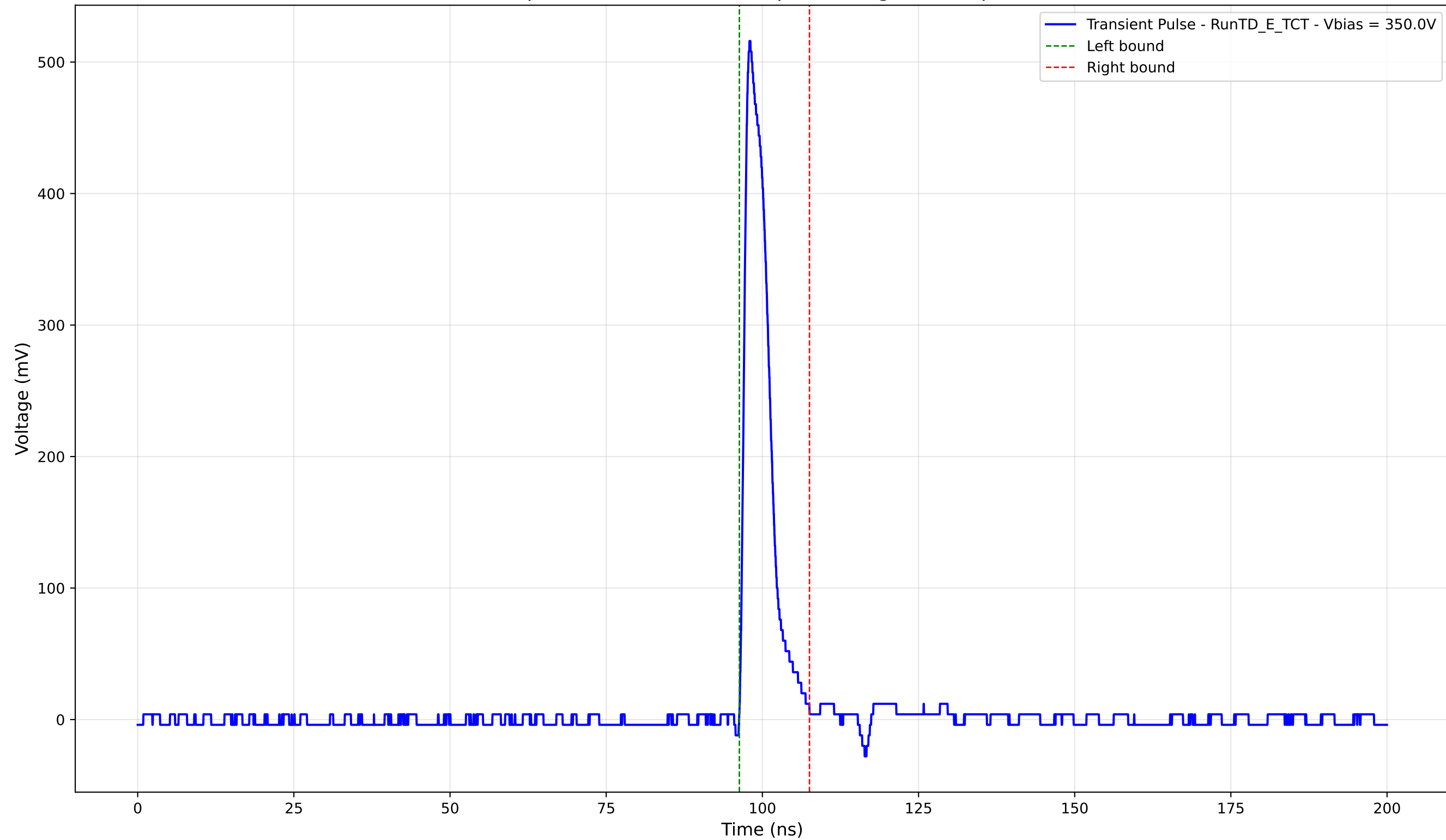
Transient Pulse - Sample: TD - Position: 355.0 \mu\text{m} - Charge: 44.75 pC - Rise Time: 1.02 ns
