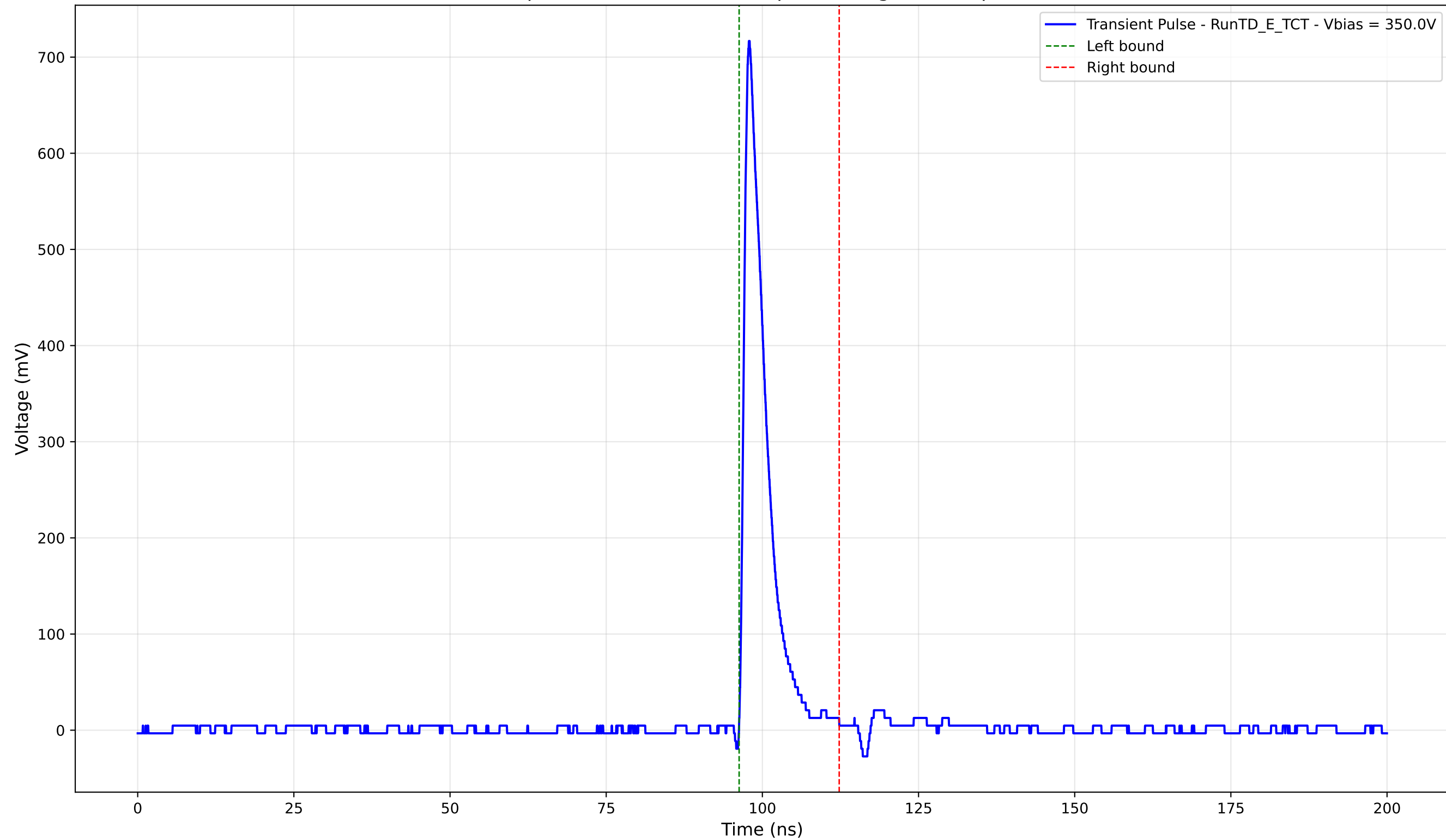
Transient Pulse - Sample: TD - Position: 270.0 \mu\text{m} - Charge: 57.28 pC - Rise Time: 0.97 ns
