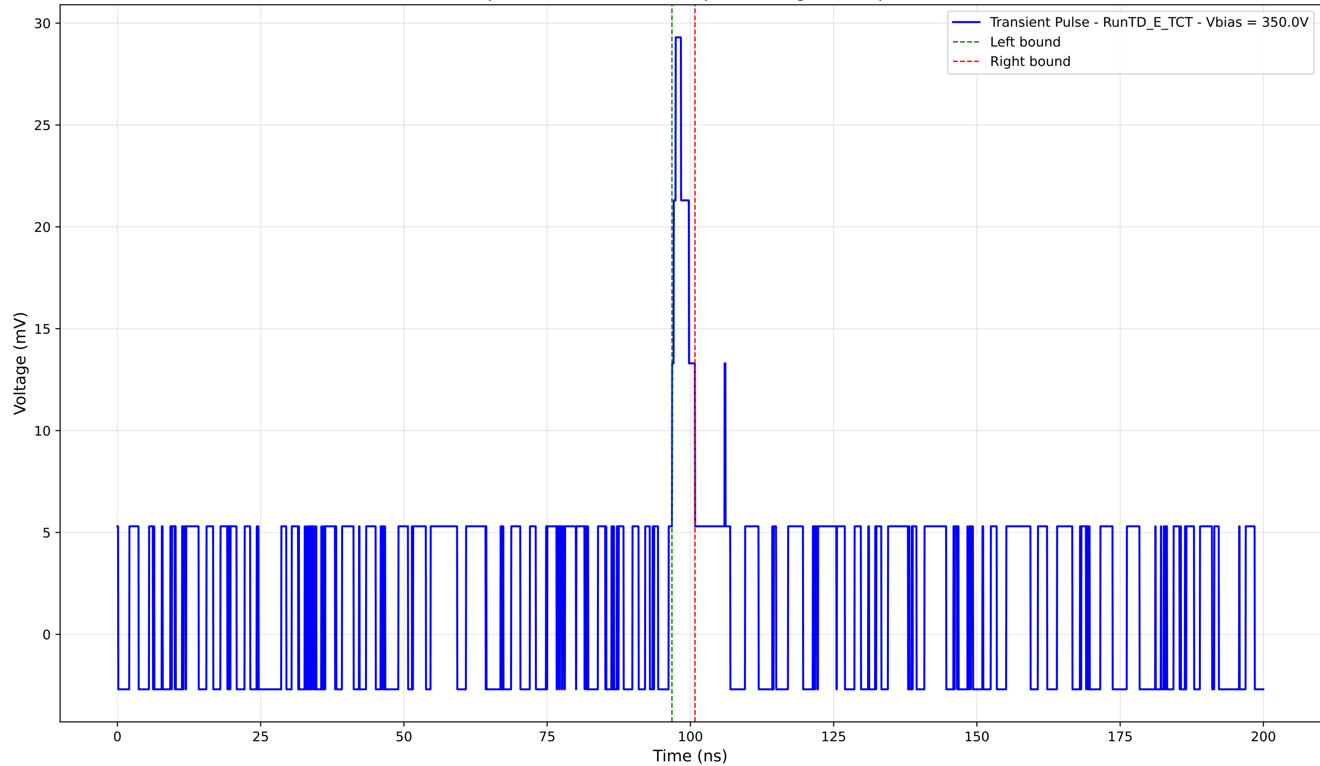
Transient Pulse - Sample: TD - Position: 20.0 \mu\text{m} - Charge: 1.64 pC - Rise Time: 1.24 ns
