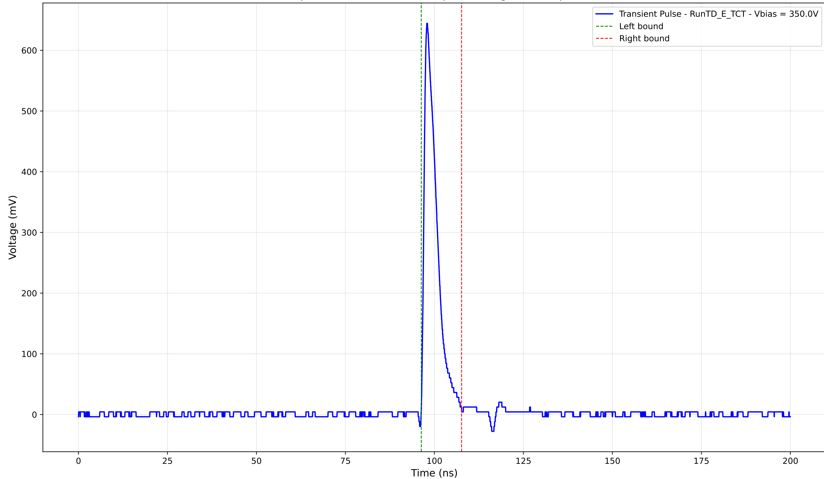
Transient Pulse - Sample: TD - Position: 305.0 \mu\text{m} - Charge: 52.30 pC - Rise Time: 0.99 ns
