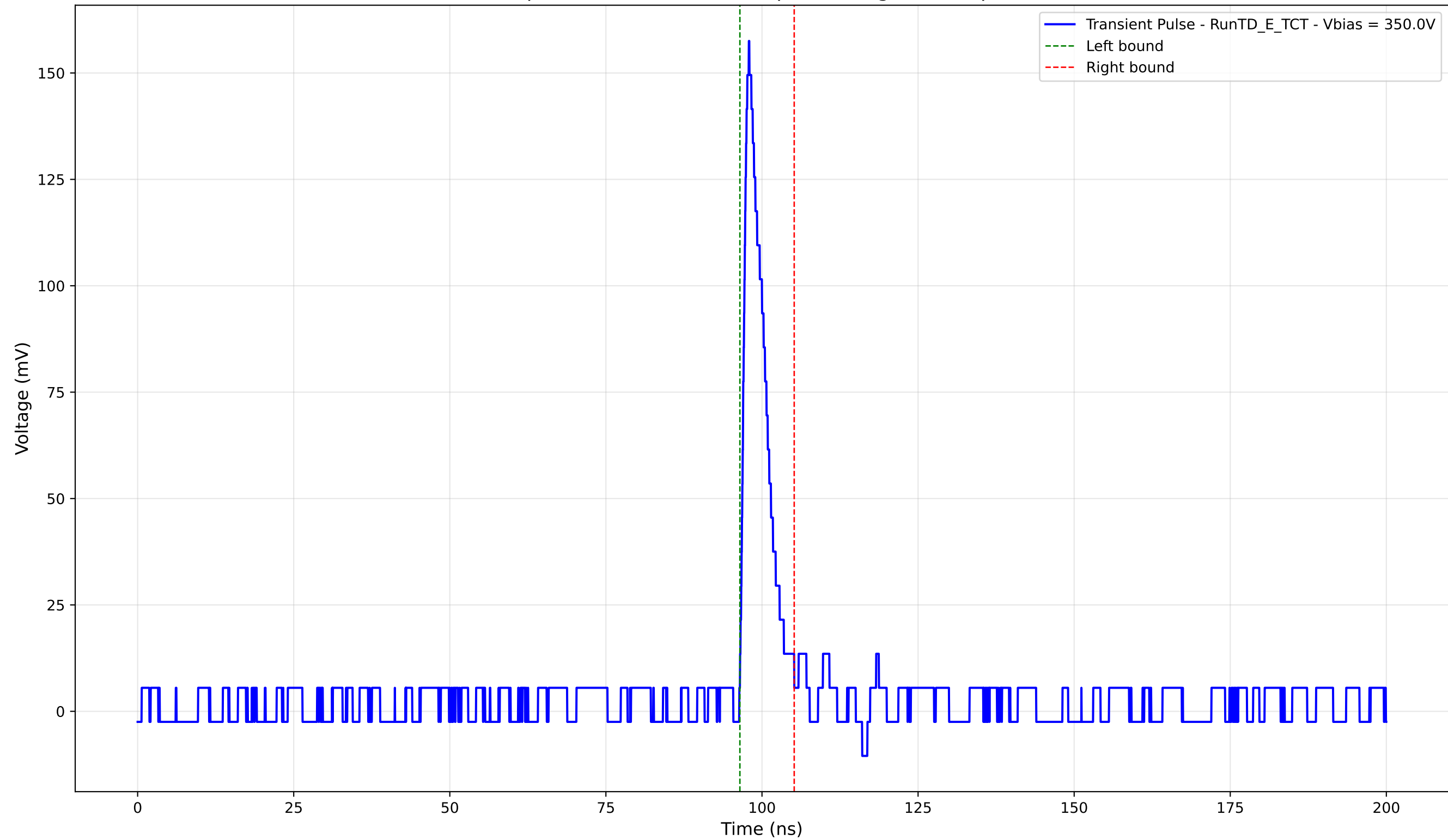
Transient Pulse - Sample: TD - Position: 395.0 \mu\text{m} - Charge: 11.70 pC - Rise Time: 1.09 ns
