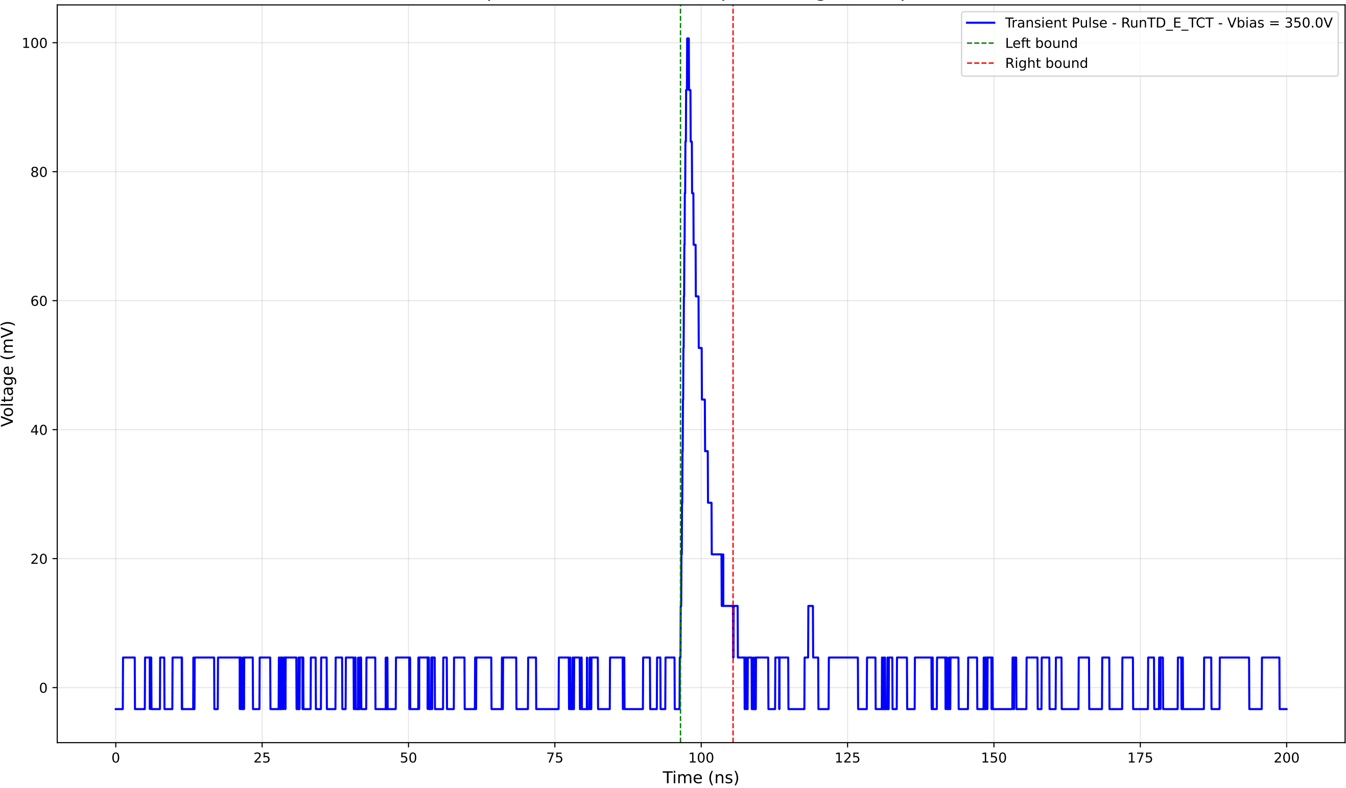
Transient Pulse - Sample: TD - Position: 615.0 \mu\text{m} - Charge: 7.32 pC - Rise Time: 0.93 ns
