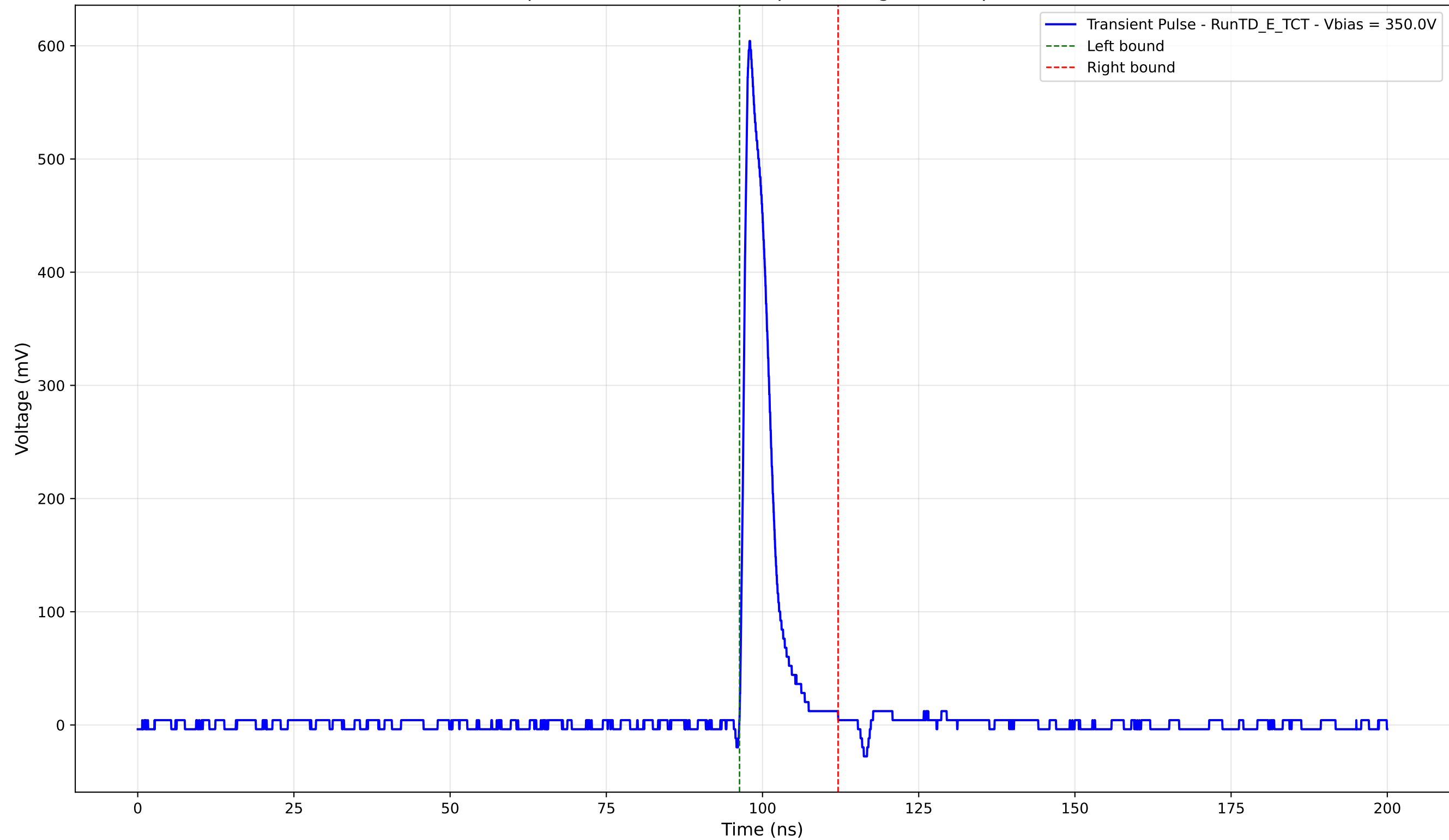
Transient Pulse - Sample: TD - Position: 330.0 \mu\text{m} - Charge: 52.60 pC - Rise Time: 1.01 ns
