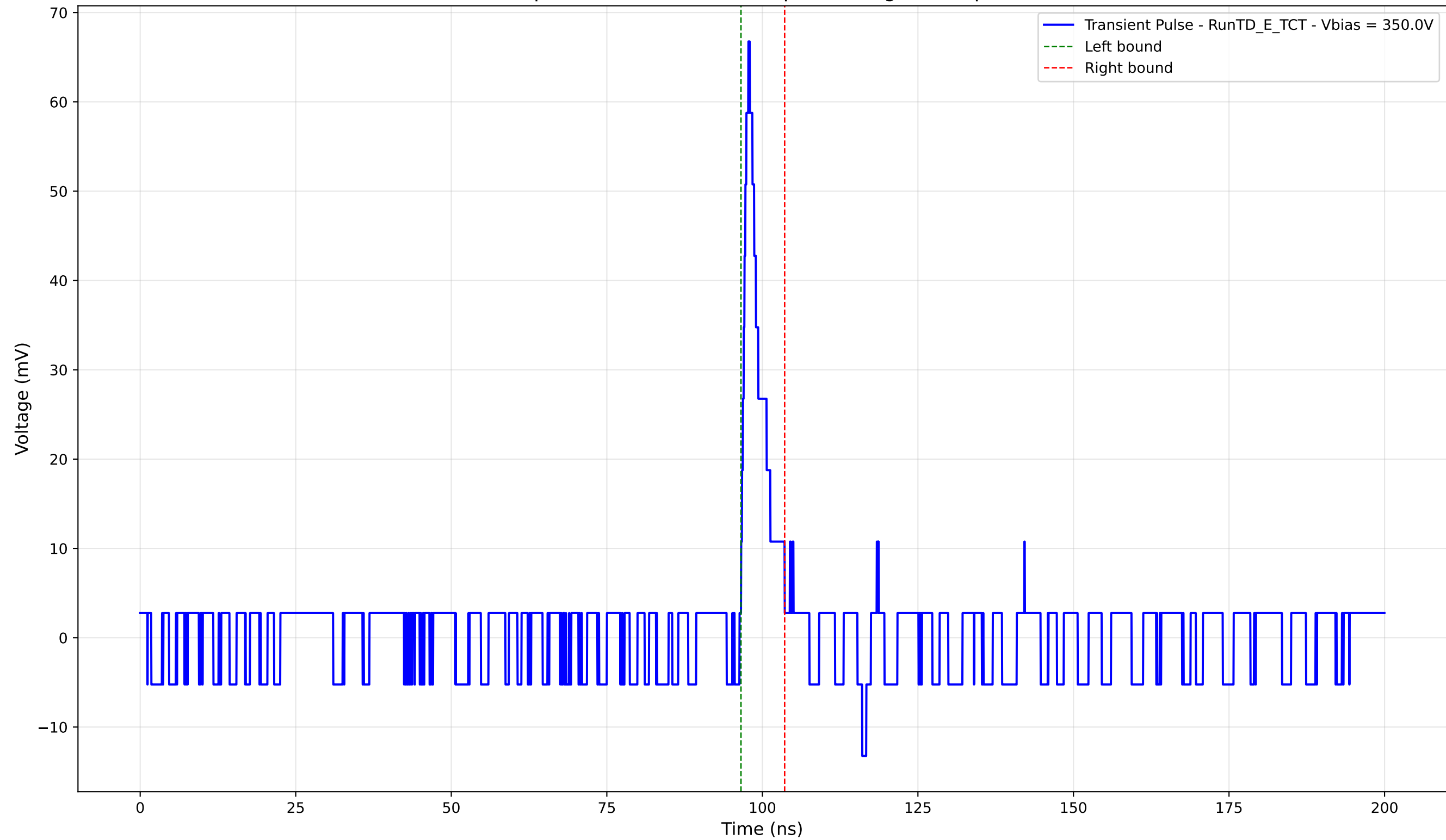
Transient Pulse - Sample: TD - Position: 670.0 \mu\text{m} - Charge: 3.94 pC - Rise Time: 1.17 ns
