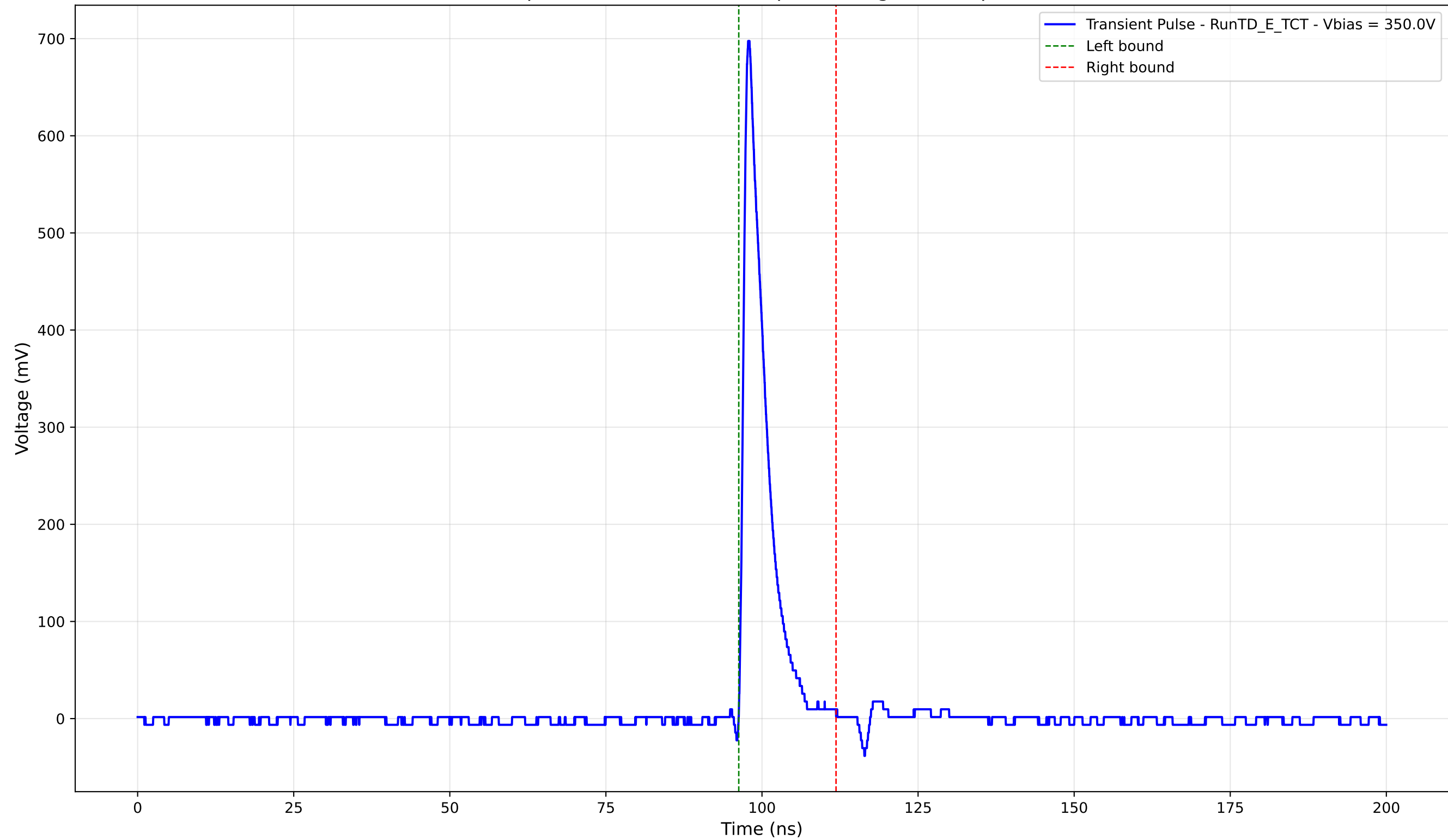
Transient Pulse - Sample: TD - Position: 245.0 \mu\text{m} - Charge: 55.43 pC - Rise Time: 0.96 ns
