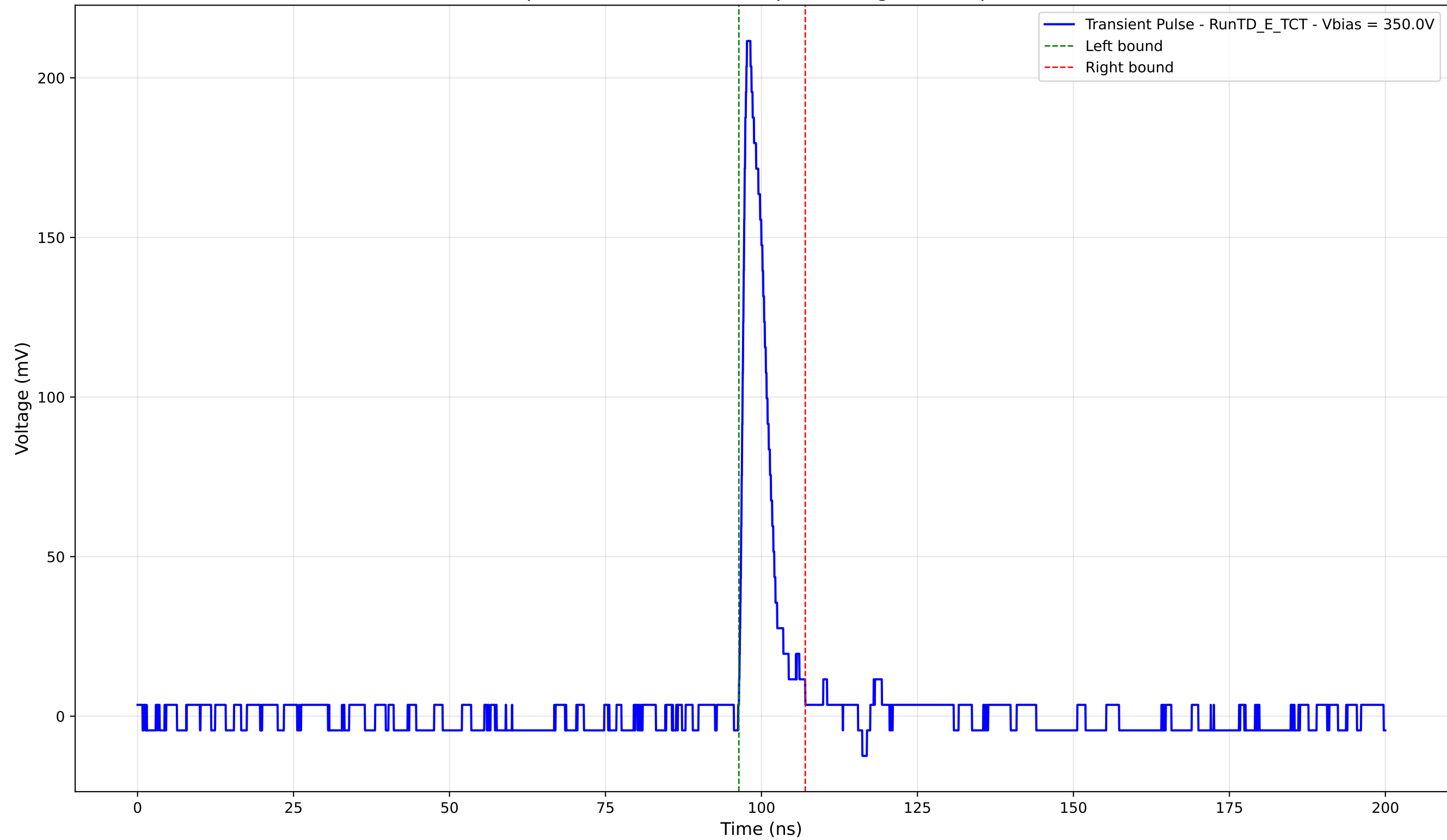
Transient Pulse - Sample: TD - Position: 485.0 \mu\text{m} - Charge: 17.33 pC - Rise Time: 0.98 ns
