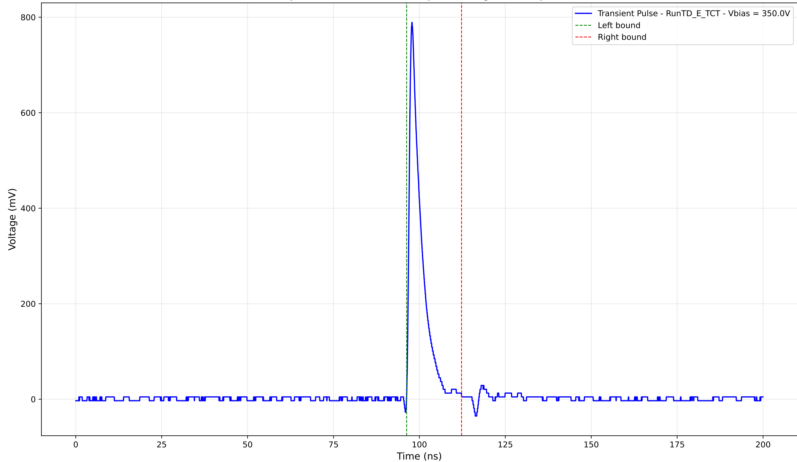
Transient Pulse - Sample: TD - Position: 140.0 \mu\text{m} - Charge: 62.07 pC - Rise Time: 0.96 ns
