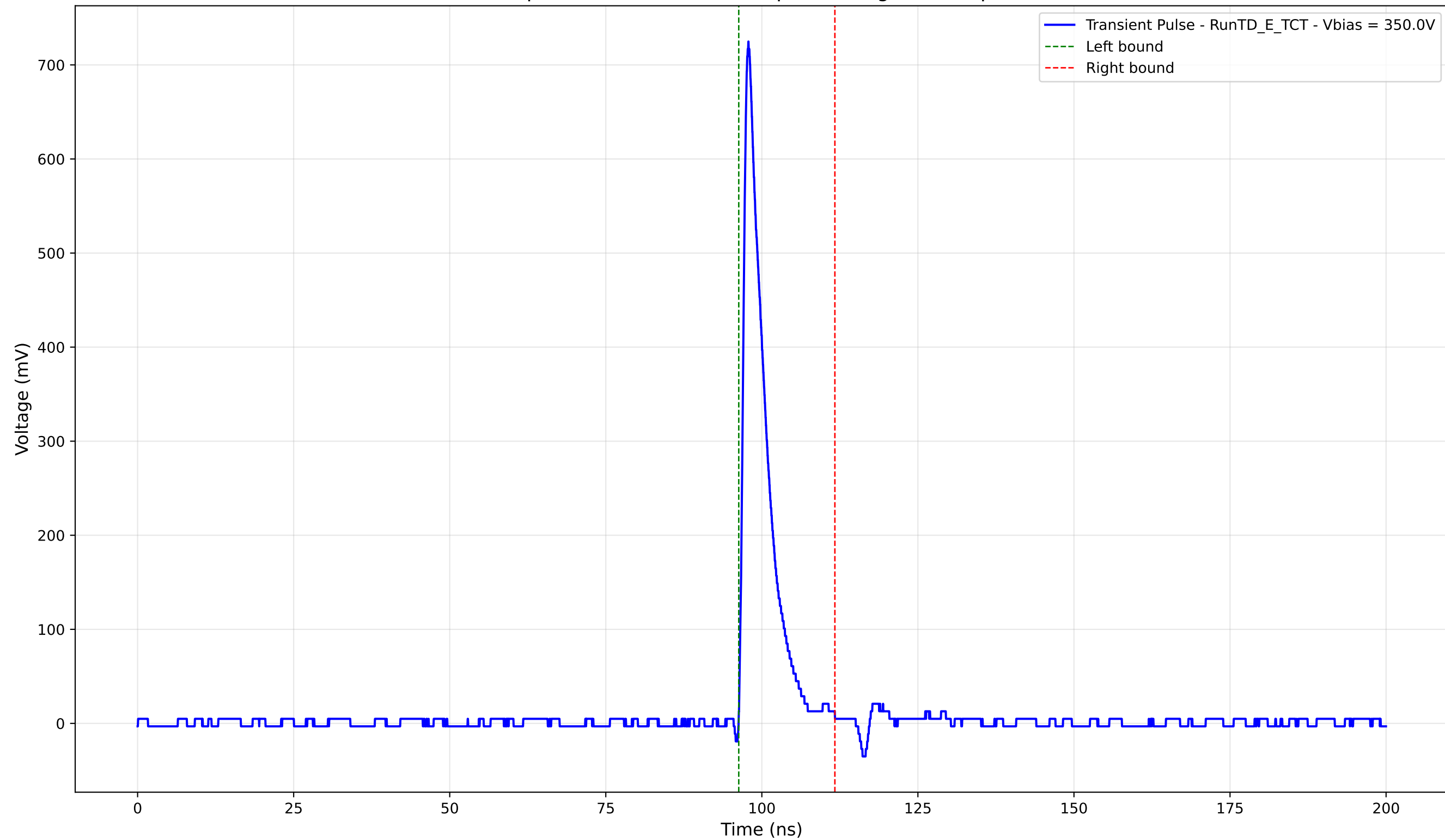
Transient Pulse - Sample: TD - Position: 230.0 \mu\text{m} - Charge: 57.43 pC - Rise Time: 0.95 ns
