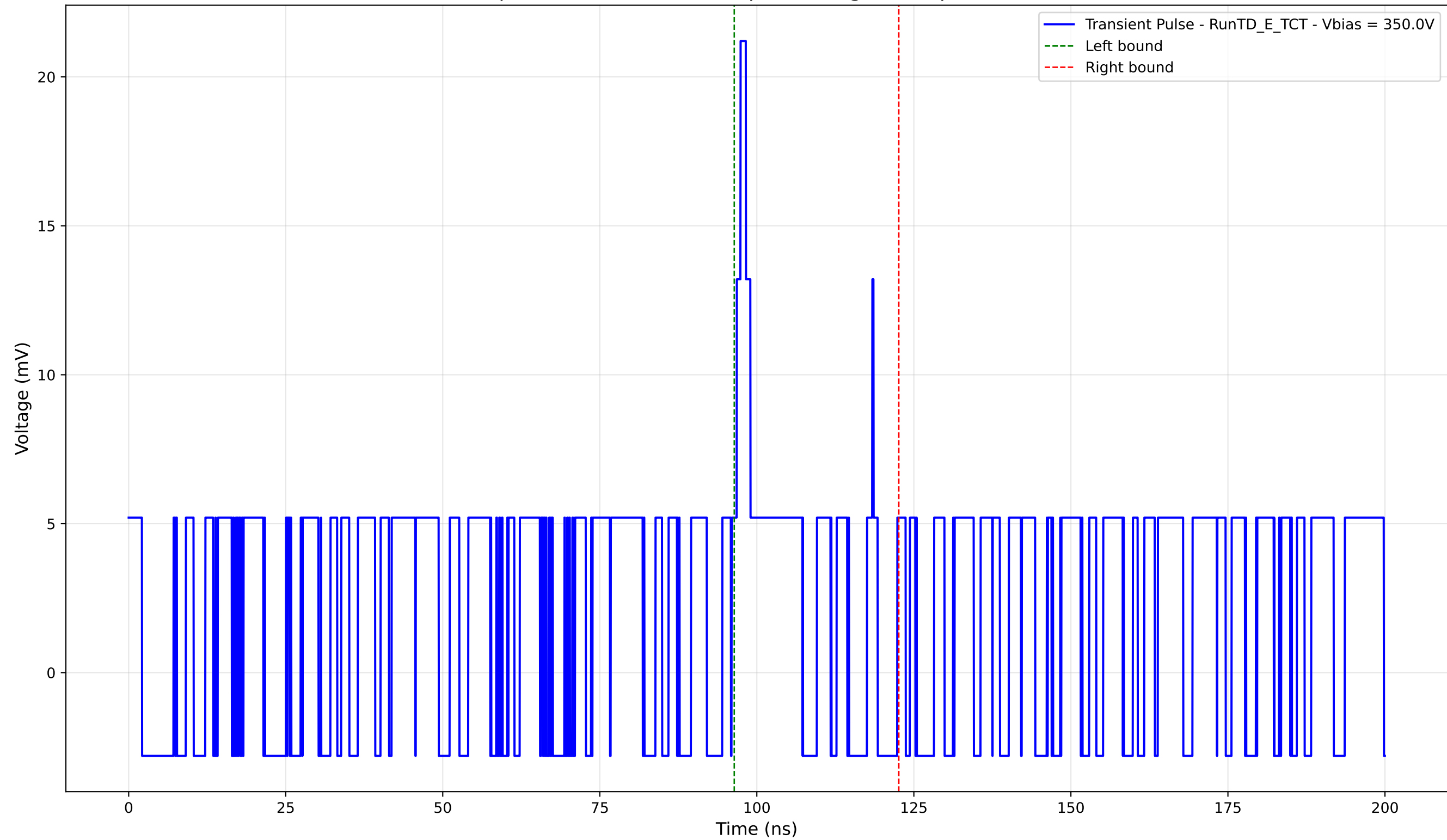
Transient Pulse - Sample: TD - Position: 720.0 \mu\text{m} - Charge: 1.75 pC - Rise Time: 0.00 ns (N/A)
