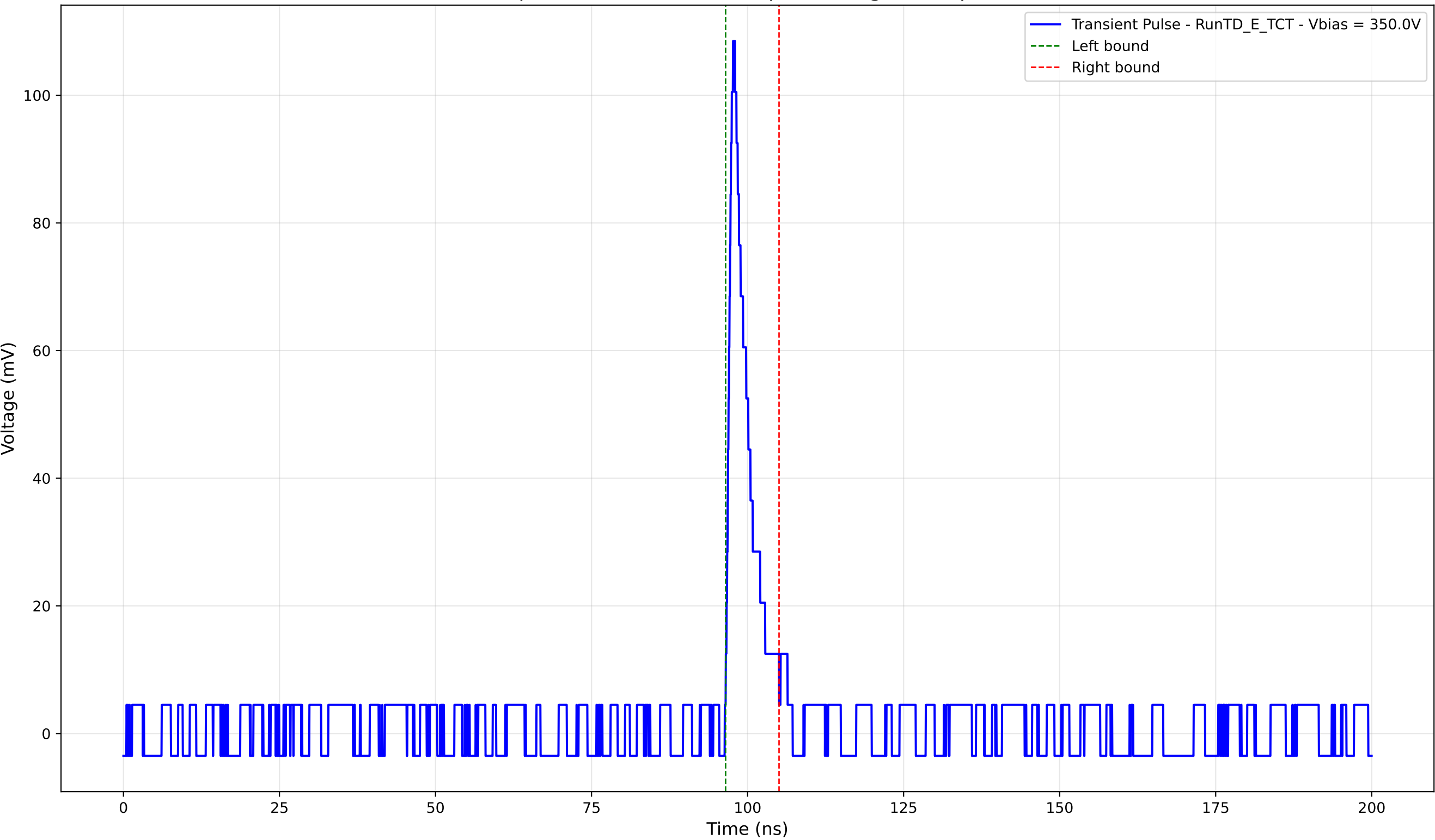
Transient Pulse - Sample: TD - Position: 590.0 \mu\text{m} - Charge: 7.33 pC - Rise Time: 0.96 ns
