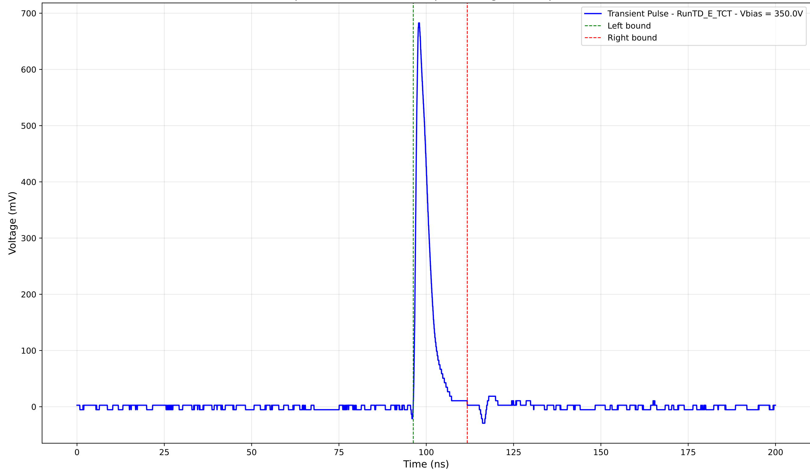
Transient Pulse - Sample: TD - Position: 295.0 \mu\text{m} - Charge: 55.20 pC - Rise Time: 0.99 ns
