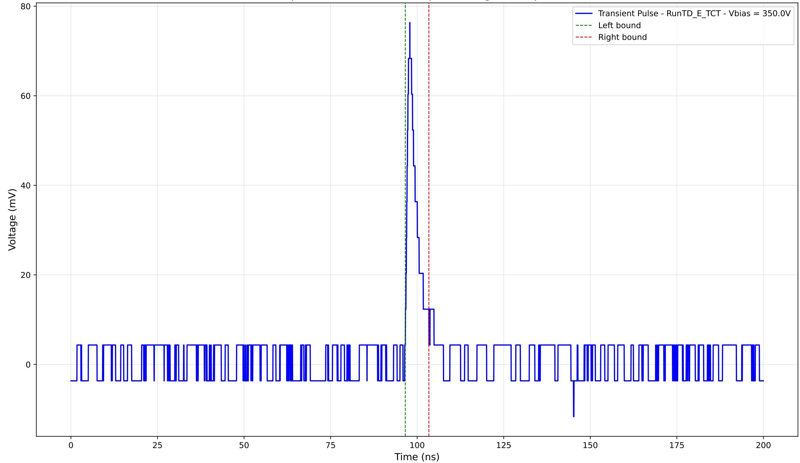
Transient Pulse - Sample: TD - Position: 665.0 \mu\text{m} - Charge: 4.57 pC - Rise Time: 1.29 ns
