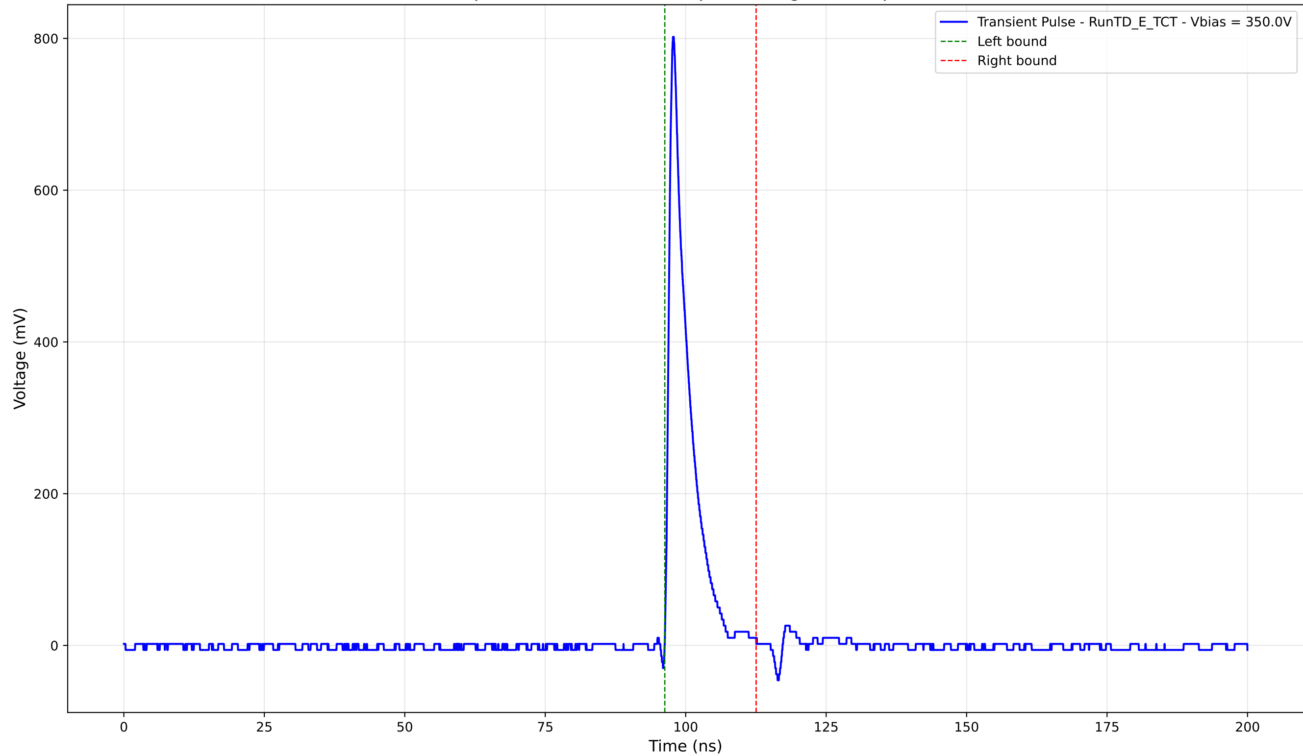
Transient Pulse - Sample: TD - Position: 155.0 \mu\text{m} - Charge: 63.09 pC - Rise Time: 0.92 ns
