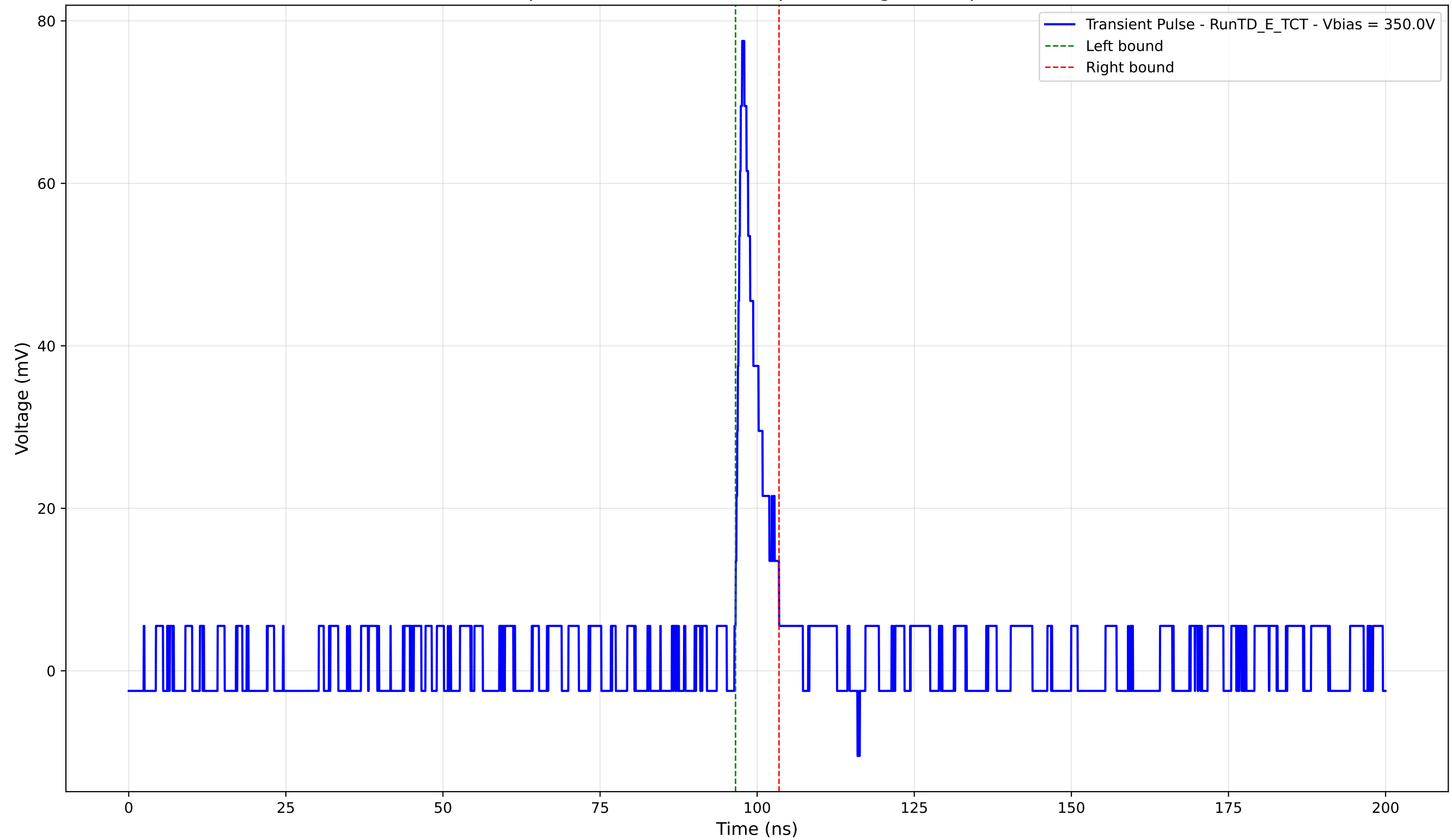
Transient Pulse - Sample: TD - Position: 660.0 \mu\text{m} - Charge: 4.99 pC - Rise Time: 1.03 ns
