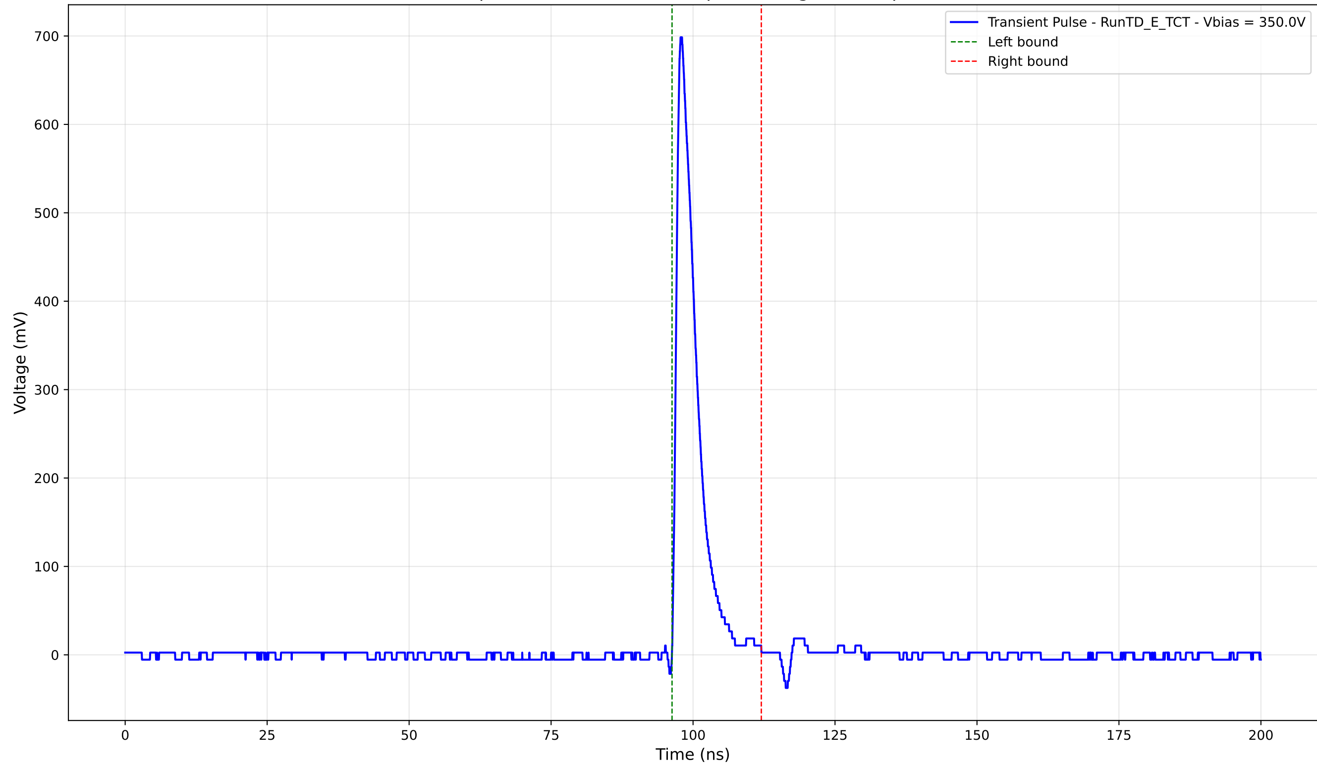
Transient Pulse - Sample: TD - Position: 285.0 \mu\text{m} - Charge: 56.25 pC - Rise Time: 0.98 ns
