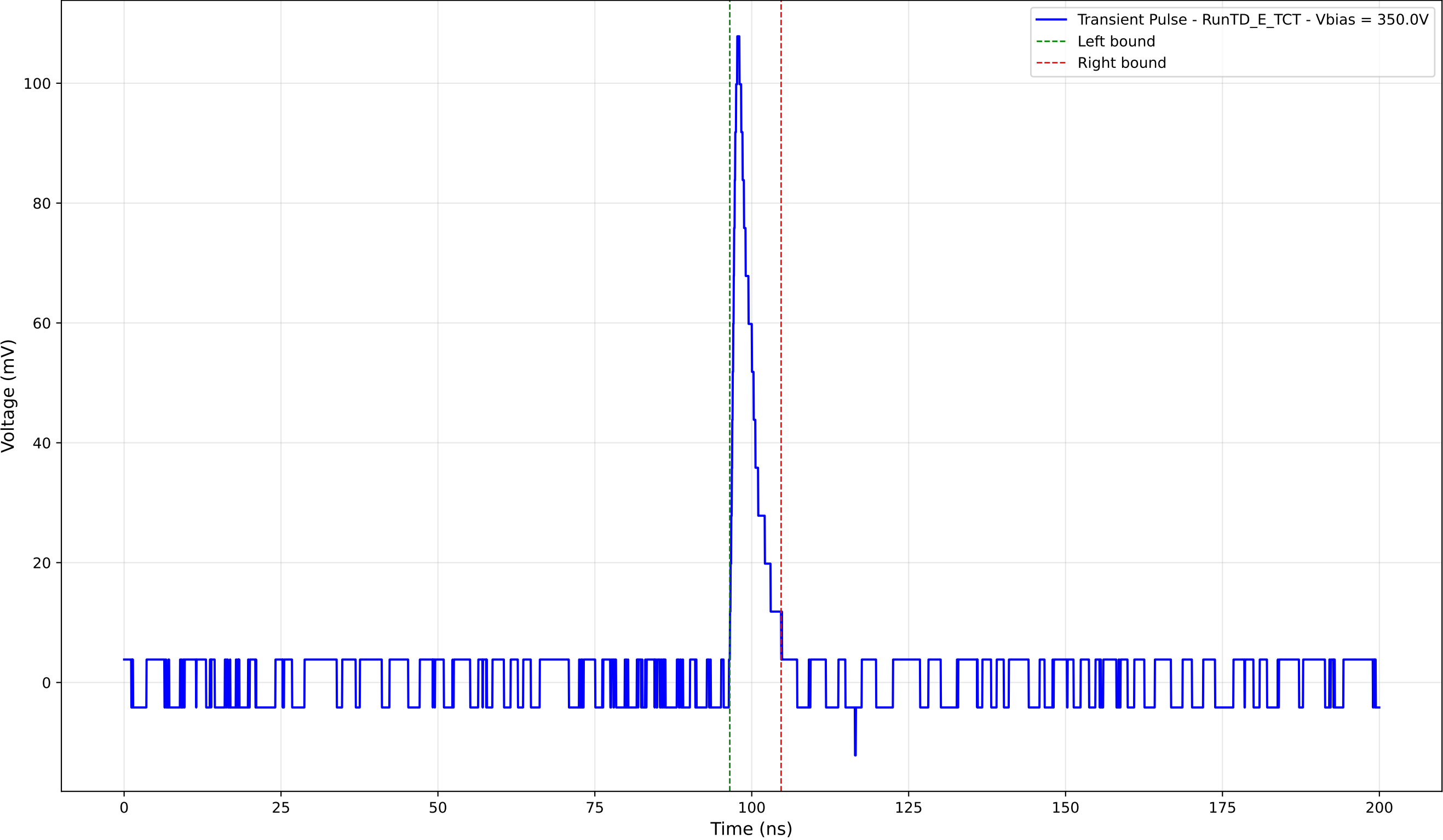
Transient Pulse - Sample: TD - Position: 585.0 \mu\text{m} - Charge: 7.37 pC - Rise Time: 0.98 ns
