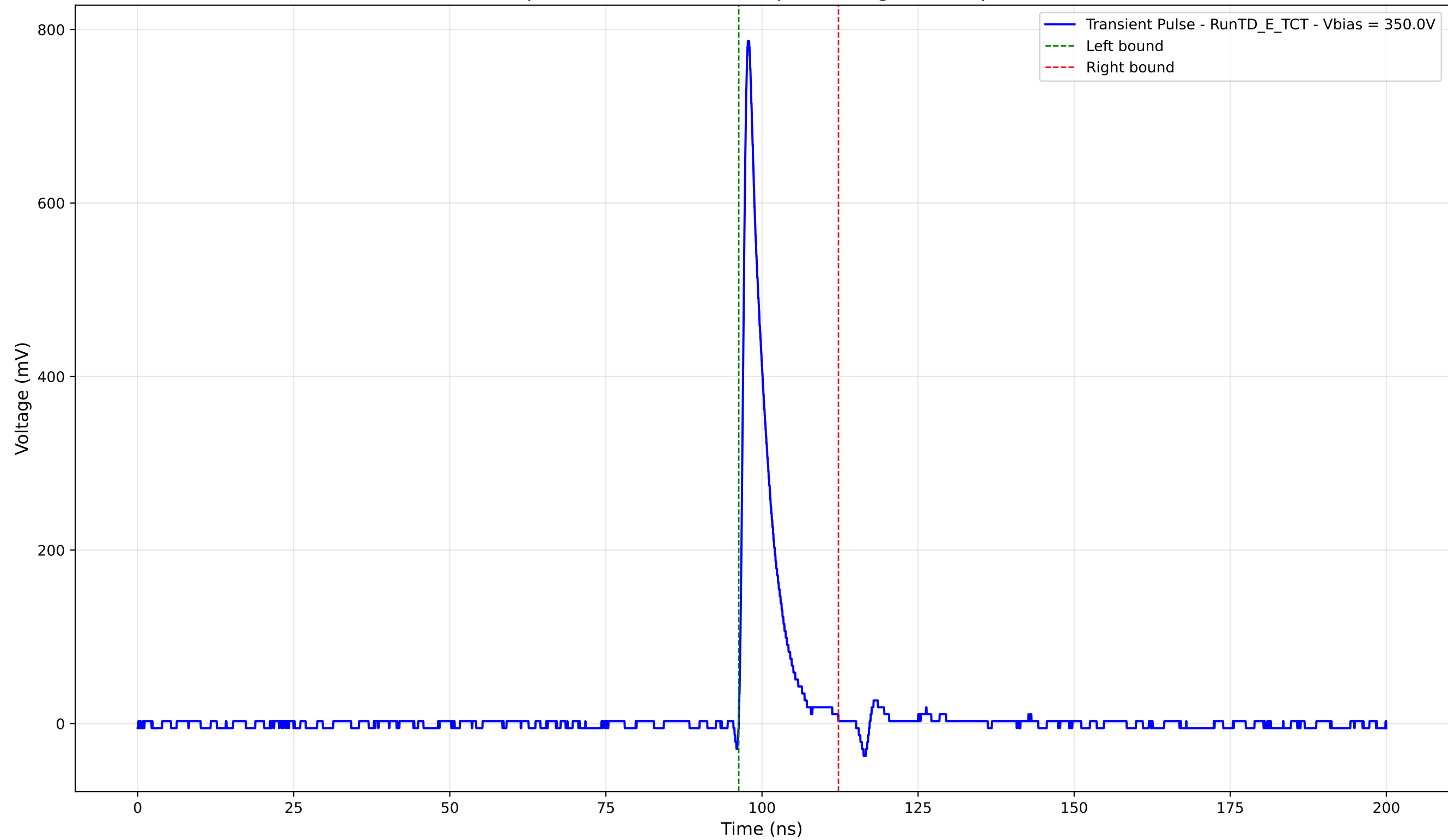
Transient Pulse - Sample: TD - Position: 145.0 \mu\text{m} - Charge: 62.02 pC - Rise Time: 0.92 ns
