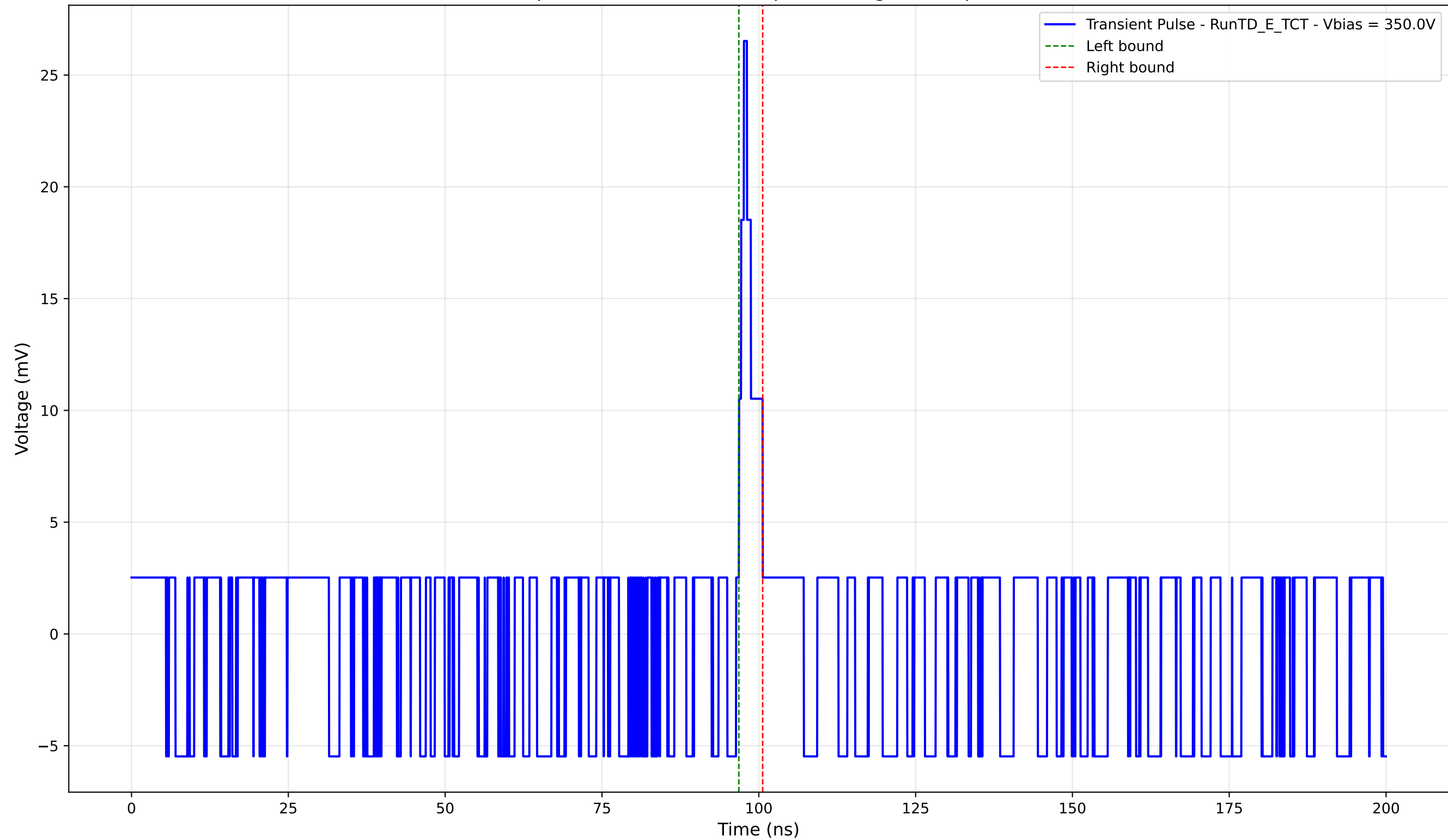
Transient Pulse - Sample: TD - Position: 10.0 \mu\text{m} - Charge: 1.13 pC - Rise Time: 0.80 ns
