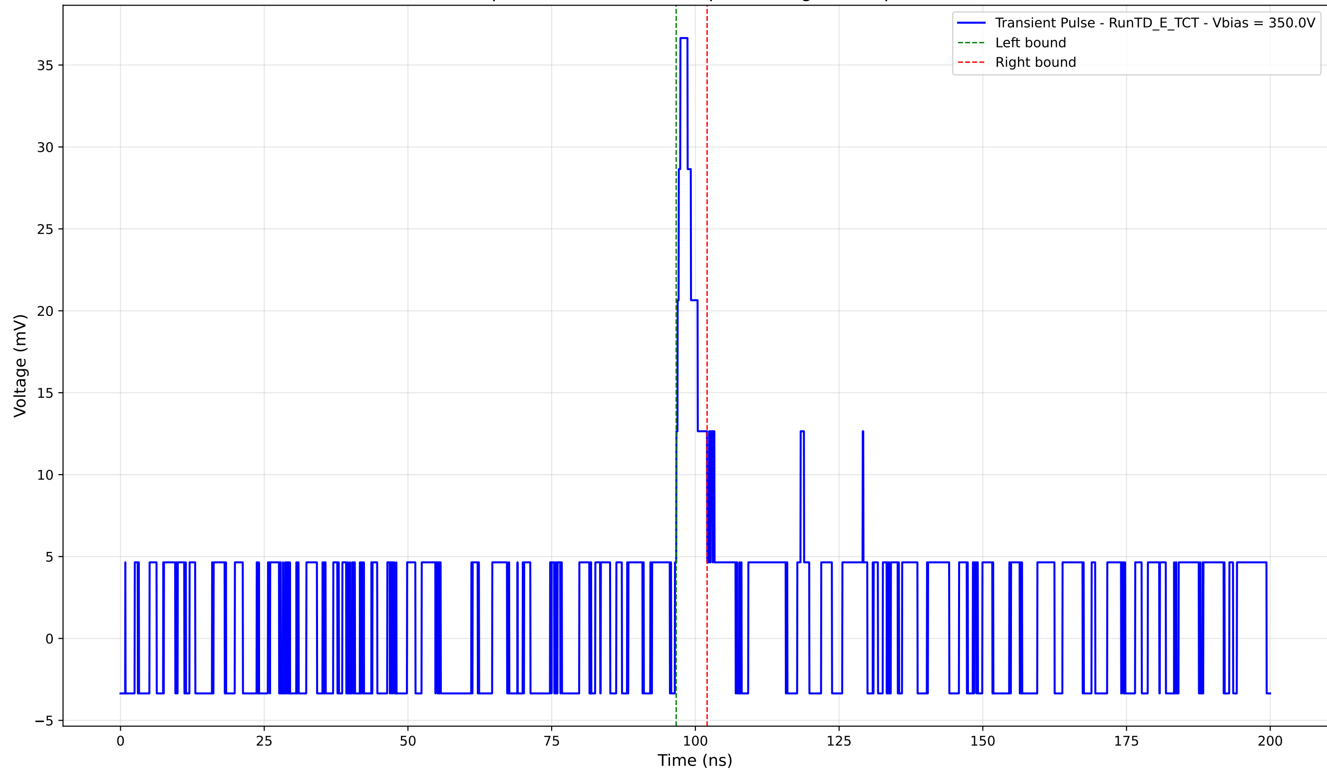
Transient Pulse - Sample: TD - Position: 35.0 \mu\text{m} - Charge: 2.46 pC - Rise Time: 0.96 ns
