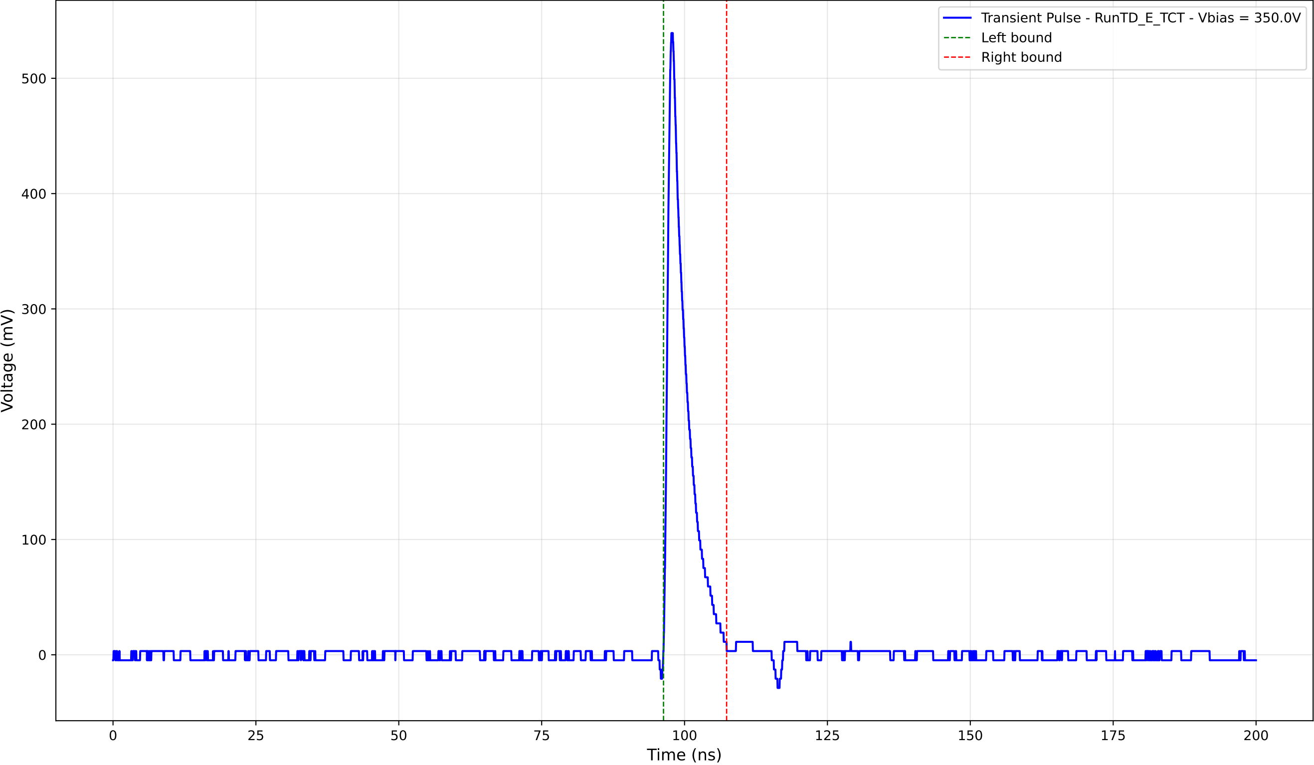
Transient Pulse - Sample: TD - Position: 85.0 \mu\text{m} - Charge: 39.88 pC - Rise Time: 0.93 ns
