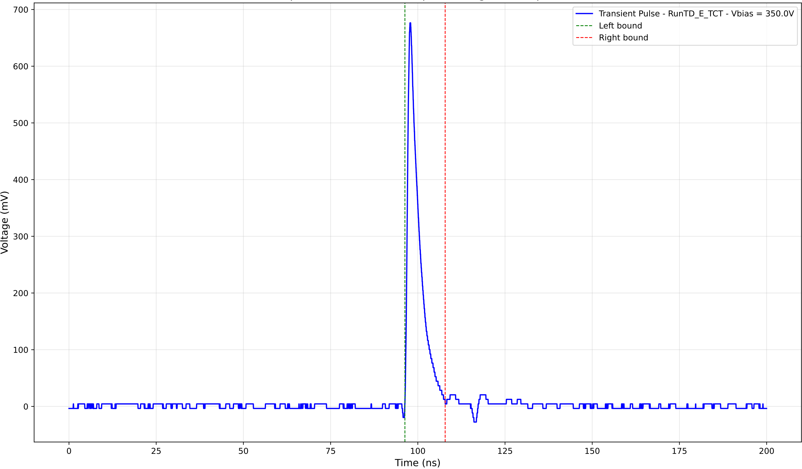
Transient Pulse - Sample: TD - Position: 95.0 \mu\text{m} - Charge: 51.42 pC - Rise Time: 0.95 ns
