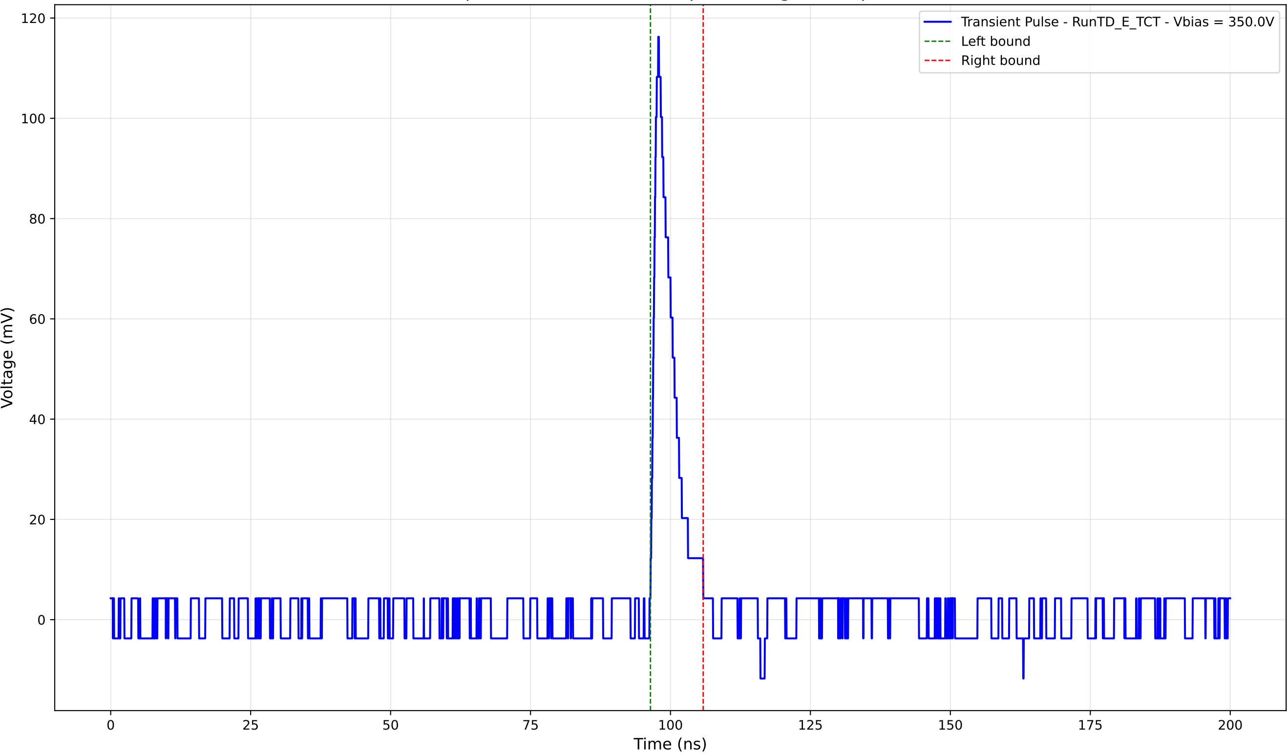
Transient Pulse - Sample: TD - Position: 420.0 \mu\text{m} - Charge: 8.54 pC - Rise Time: 1.10 ns
