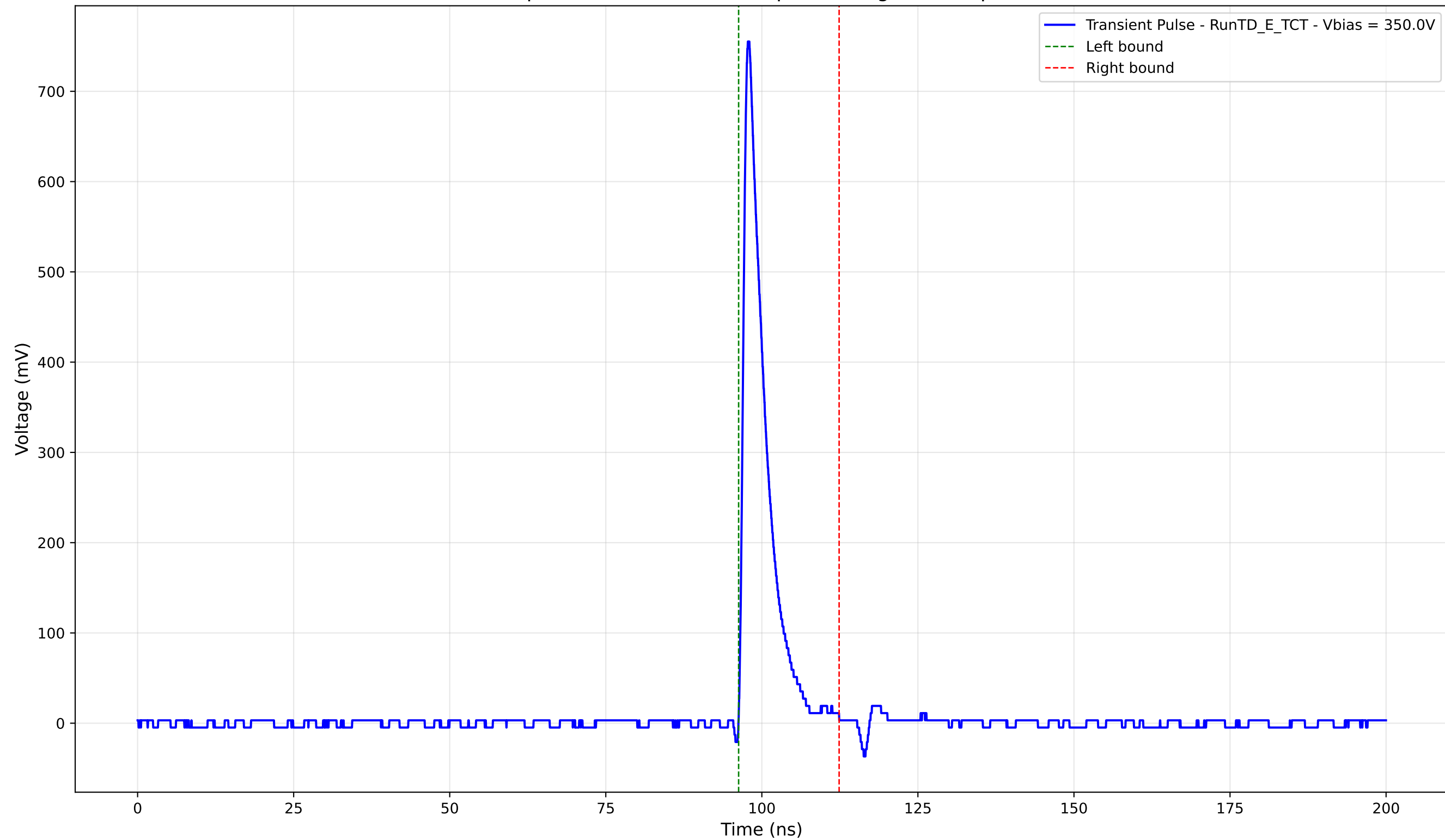
Transient Pulse - Sample: TD - Position: 115.0 \mu\text{m} - Charge: 59.79 pC - Rise Time: 0.95 ns
