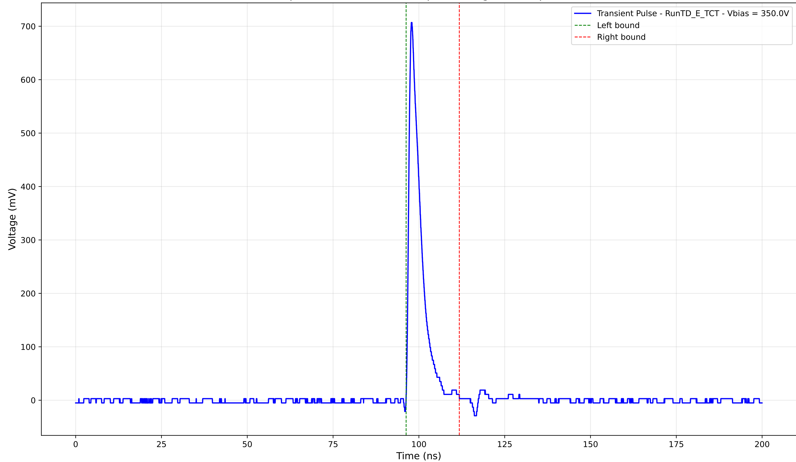
Transient Pulse - Sample: TD - Position: 255.0 \mu\text{m} - Charge: 56.13 pC - Rise Time: 0.97 ns
