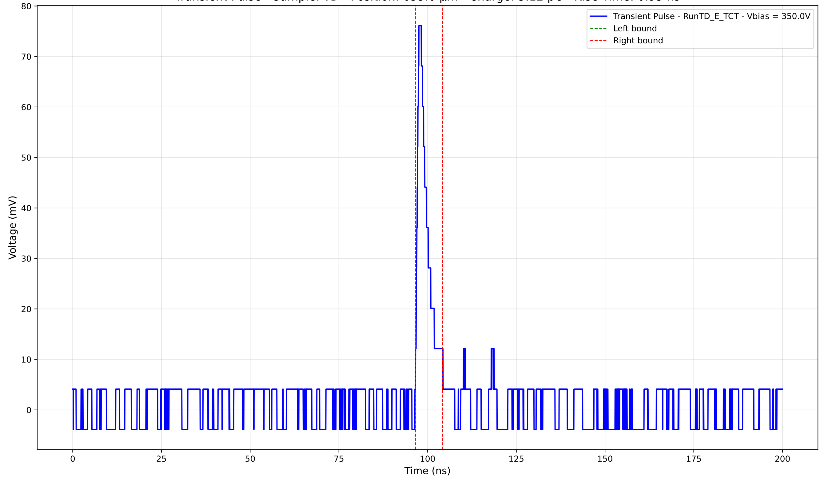
Transient Pulse - Sample: TD - Position: 655.0 \mu\text{m} - Charge: 5.12 pC - Rise Time: 0.95 ns
