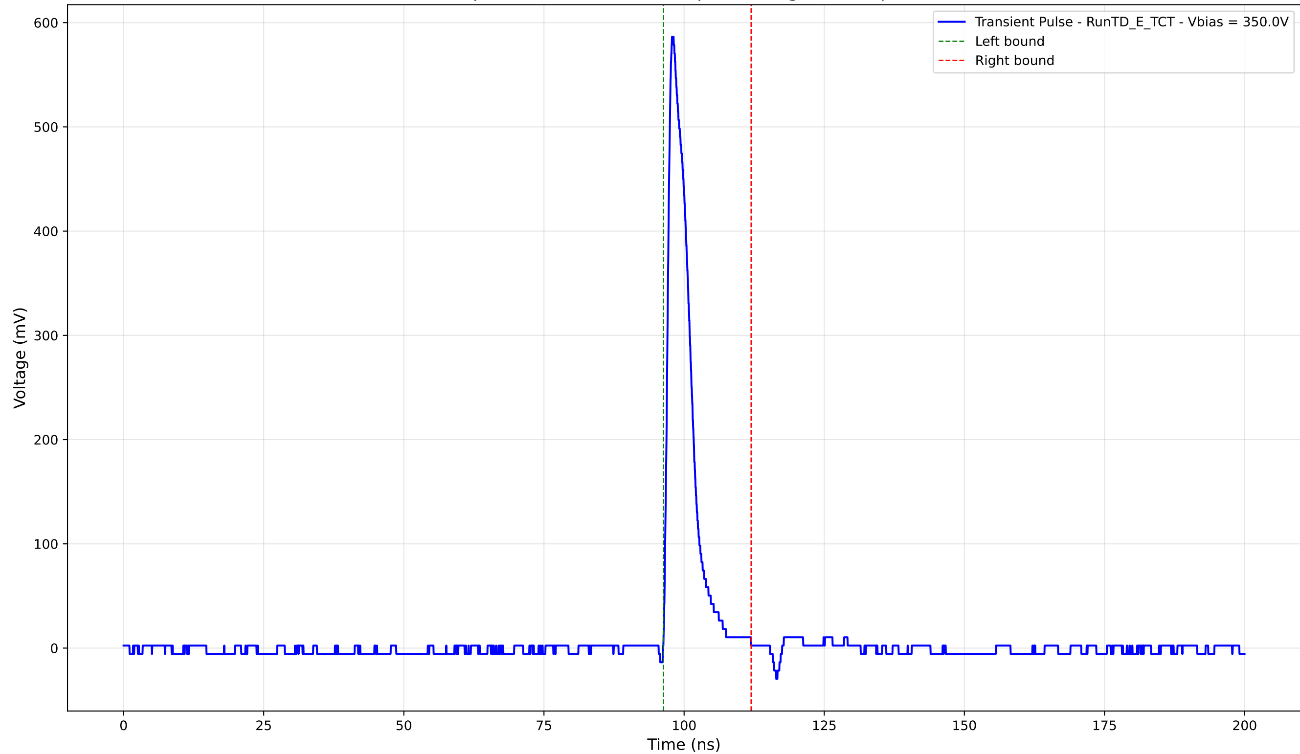
Transient Pulse - Sample: TD - Position: 325.0 \mu\text{m} - Charge: 51.20 pC - Rise Time: 1.00 ns
