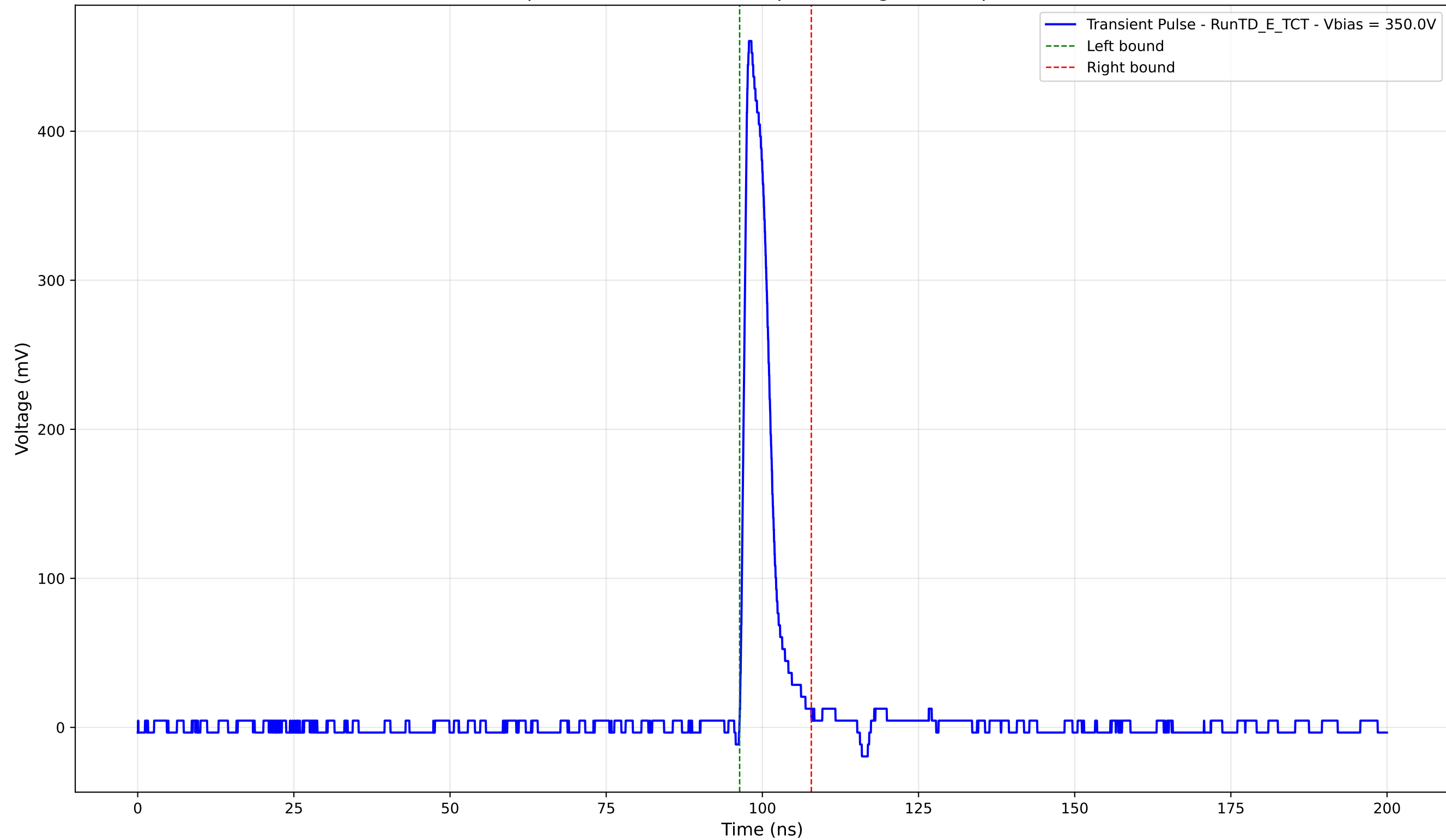
Transient Pulse - Sample: TD - Position: 365.0 \mu\text{m} - Charge: 40.11 pC - Rise Time: 1.00 ns
