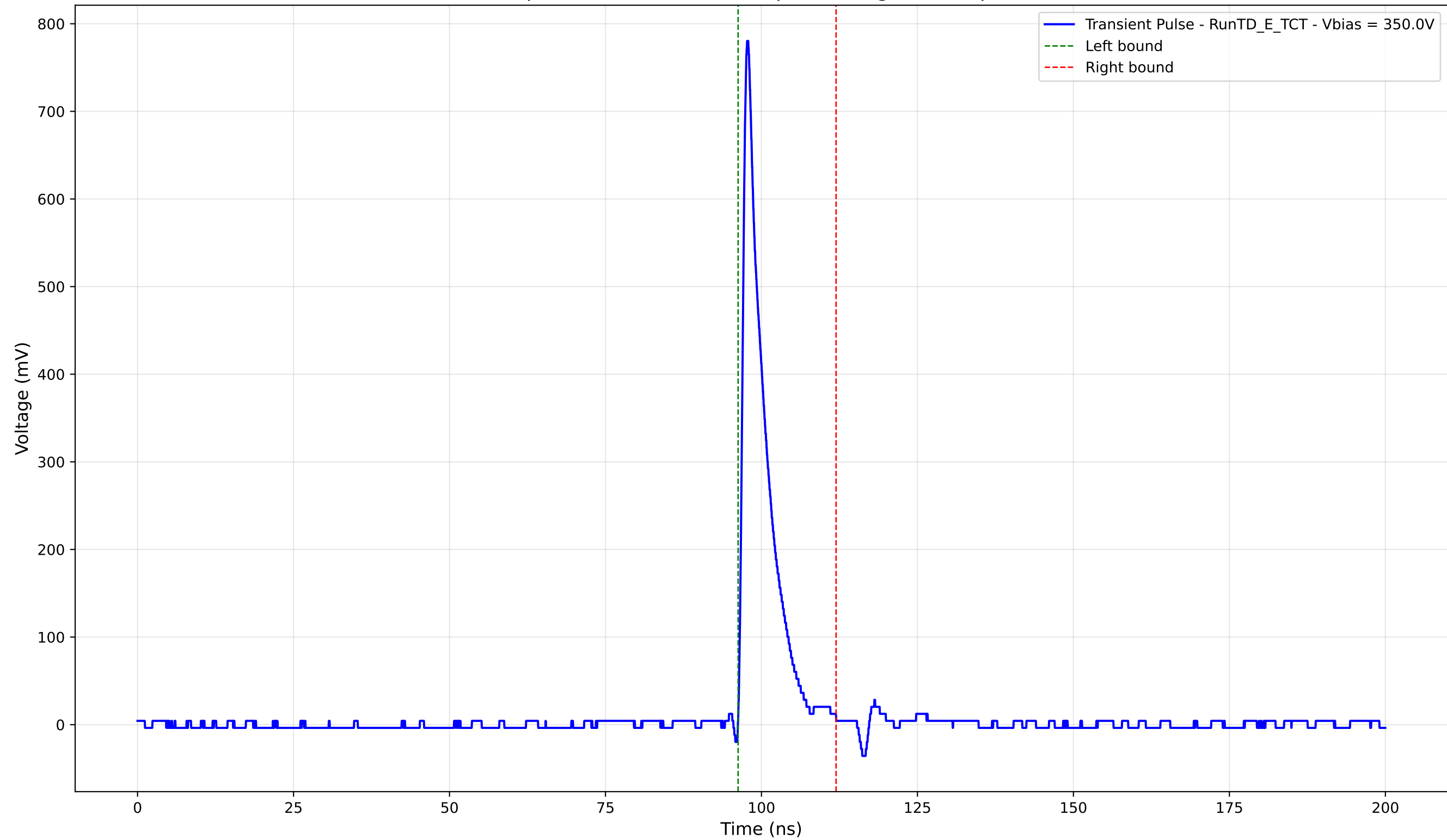
Transient Pulse - Sample: TD - Position: 170.0 \mu\text{m} - Charge: 62.56 pC - Rise Time: 0.92 ns
