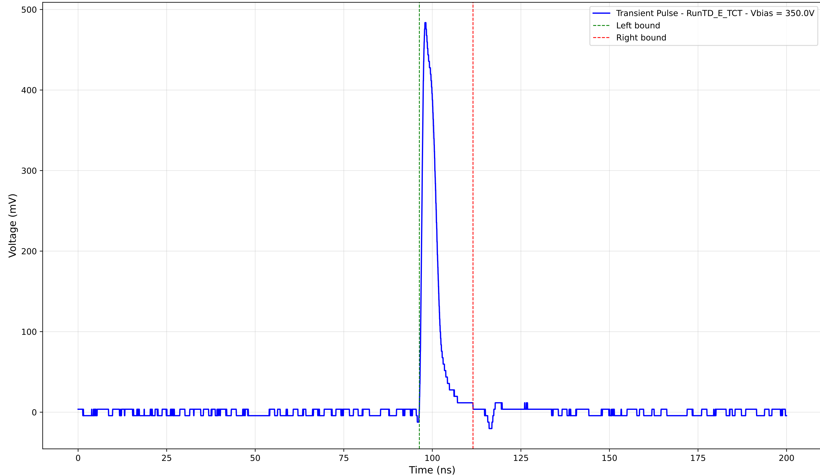
Transient Pulse - Sample: TD - Position: 360.0 \mu\text{m} - Charge: 42.80 pC - Rise Time: 1.03 ns
