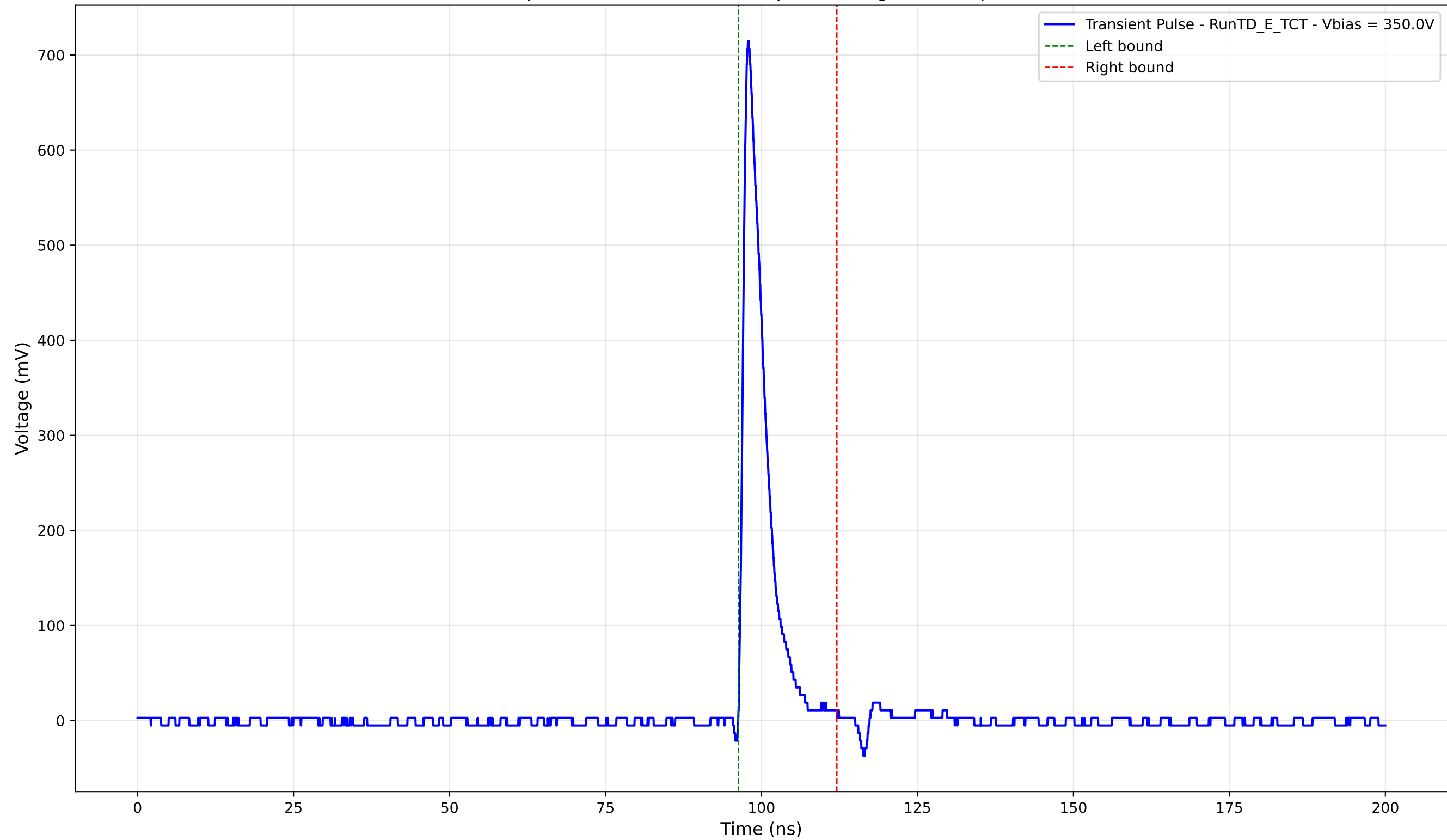
Transient Pulse - Sample: TD - Position: 275.0 \mu\text{m} - Charge: 56.61 pC - Rise Time: 0.97 ns
