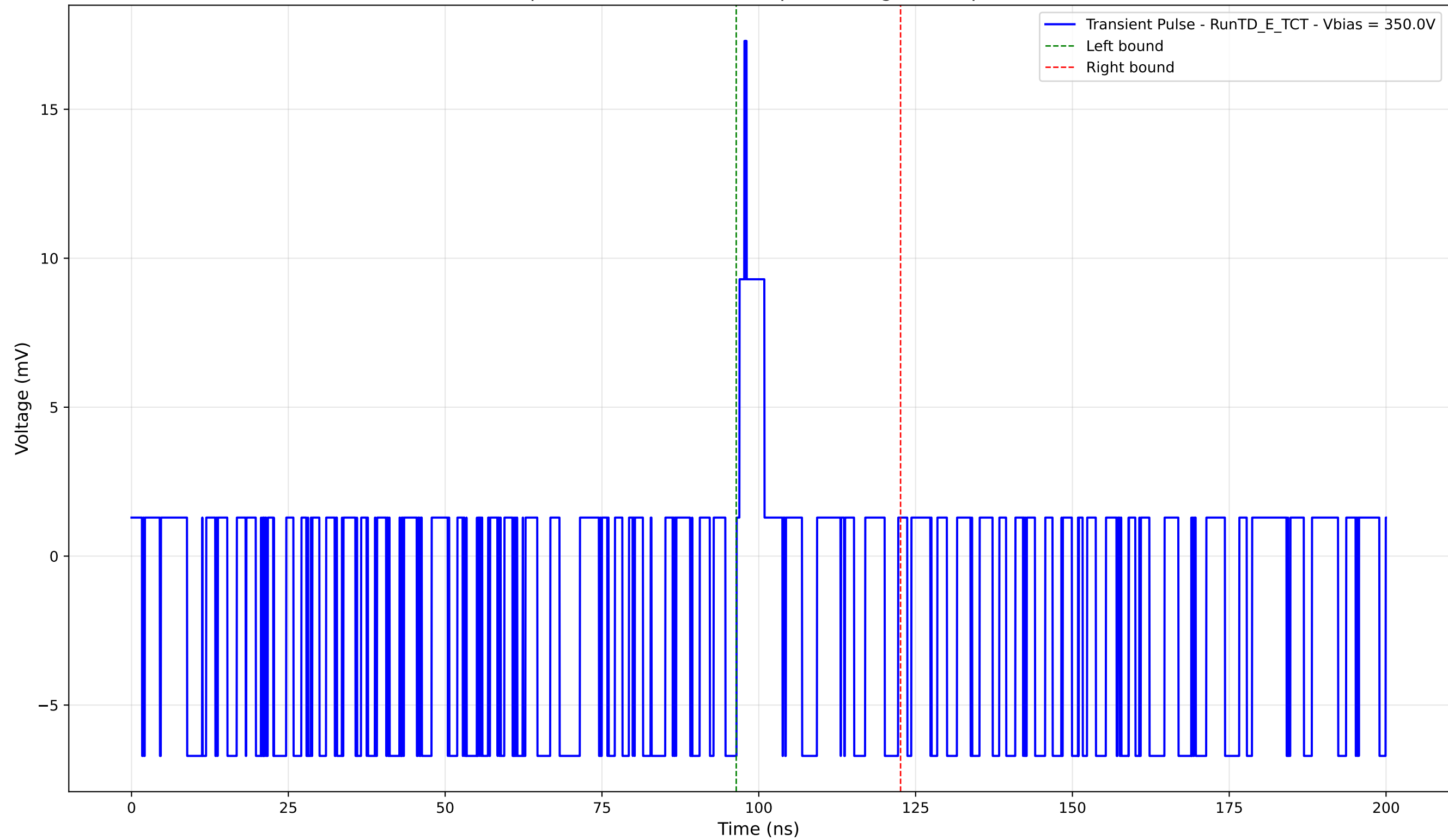
Transient Pulse - Sample: TD - Position: 725.0 \mu\text{m} - Charge: 0.29 pC - Rise Time: 0.80 ns
