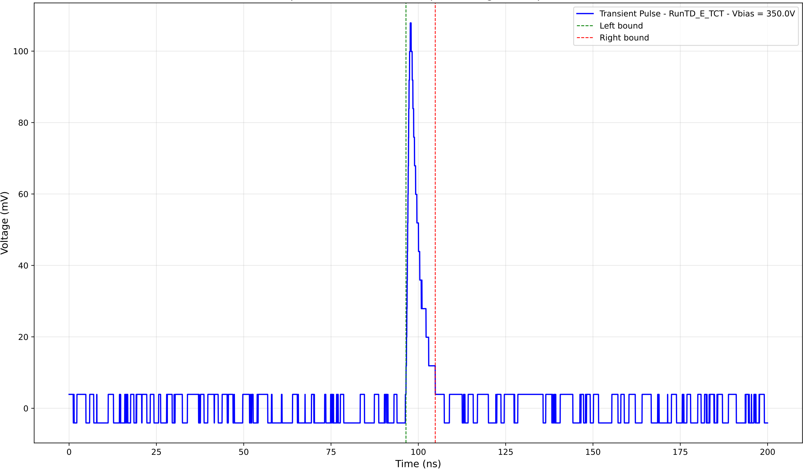
Transient Pulse - Sample: TD - Position: 600.0 \mu\text{m} - Charge: 7.20 pC - Rise Time: 1.00 ns
