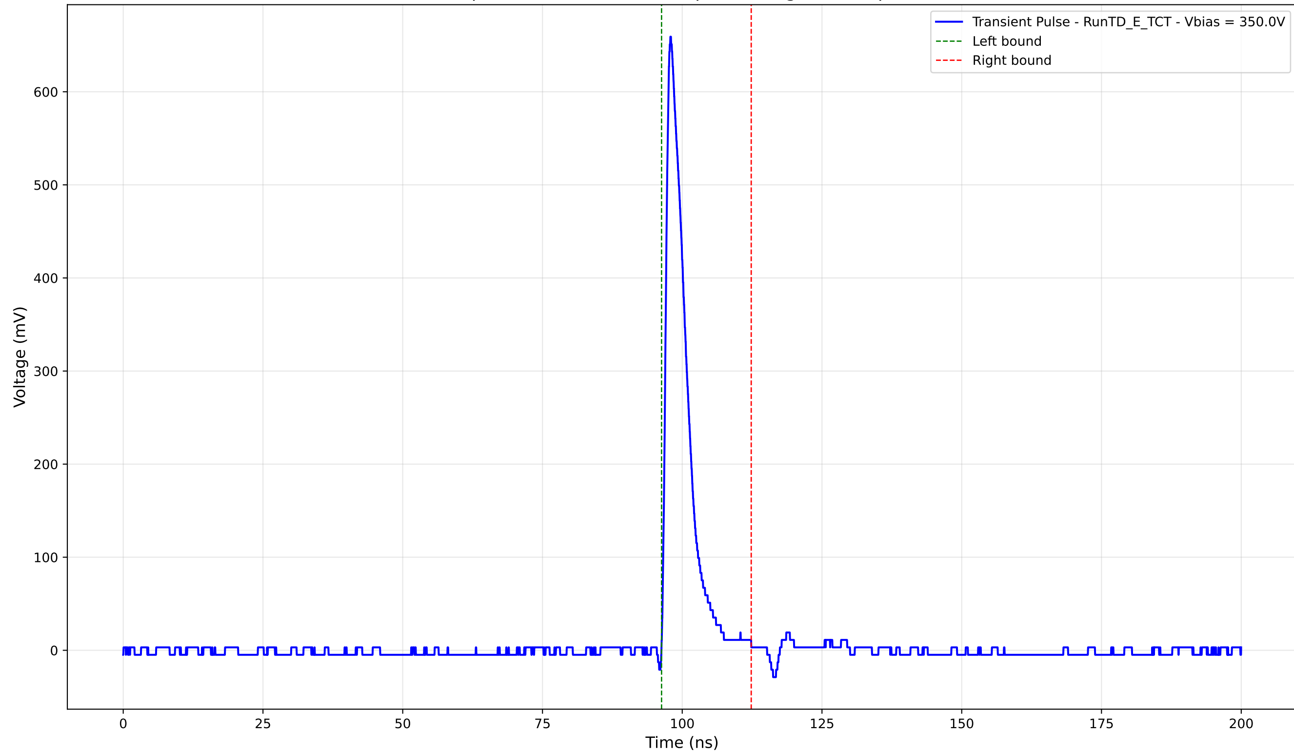
Transient Pulse - Sample: TD - Position: 300.0 \mu\text{m} - Charge: 53.77 pC - Rise Time: 0.98 ns
