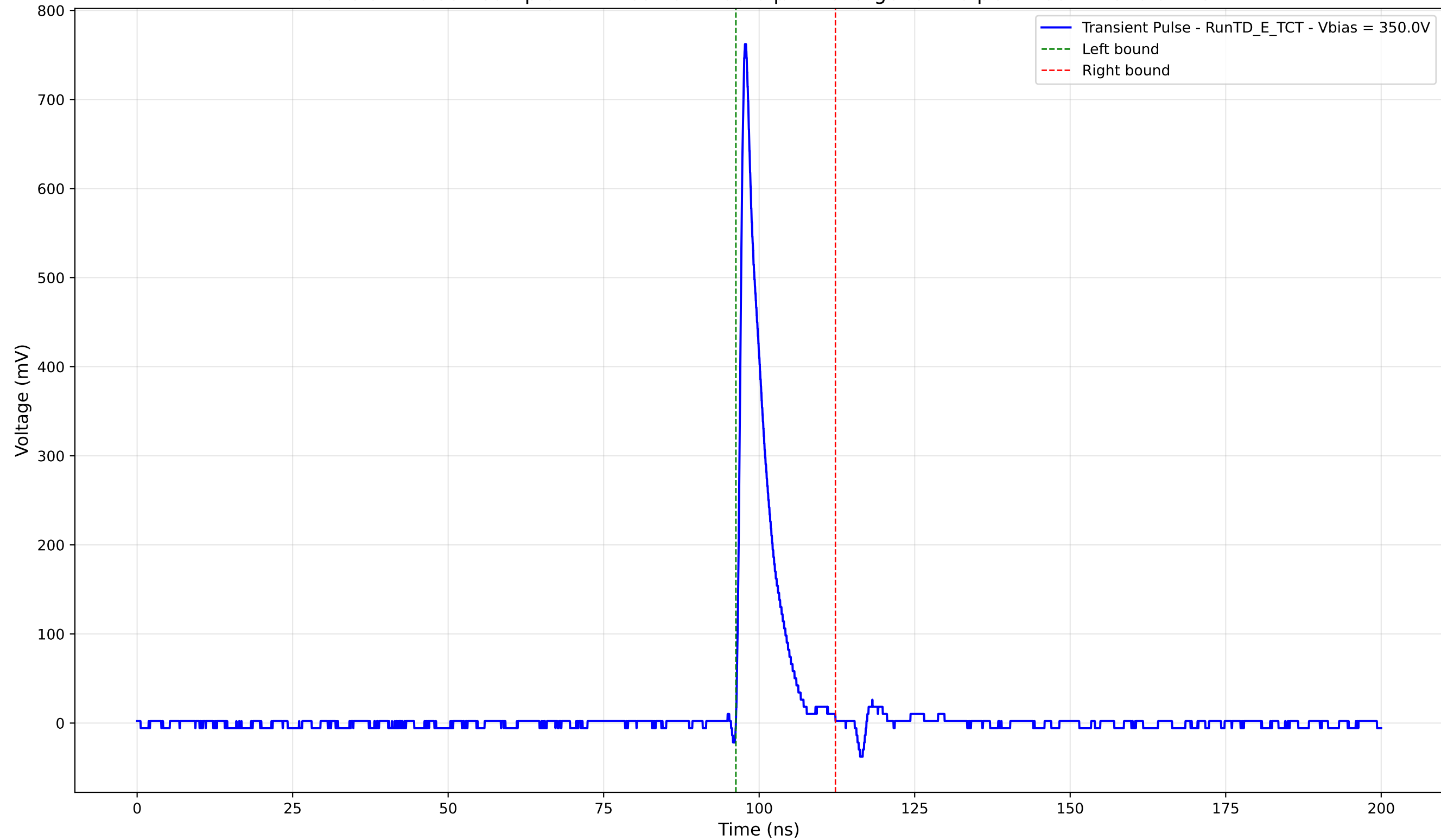
Transient Pulse - Sample: TD - Position: 195.0 \mu\text{m} - Charge: 61.46 pC - Rise Time: 0.92 ns
