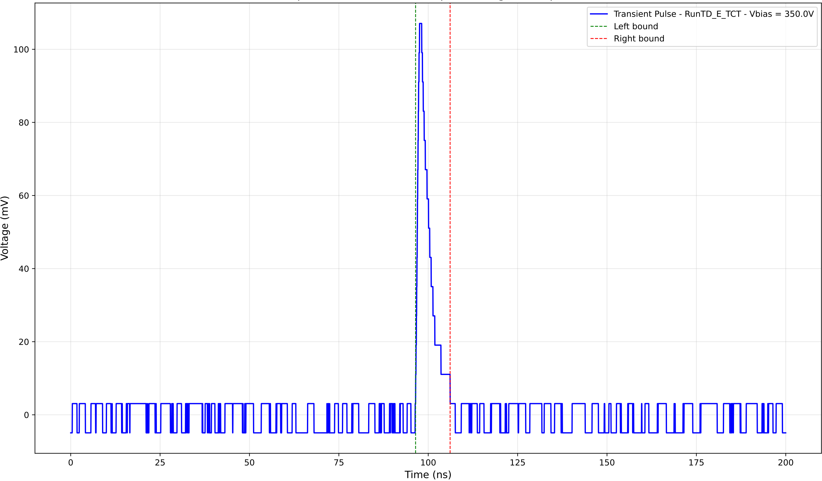
Transient Pulse - Sample: TD - Position: 580.0 \mu\text{m} - Charge: 7.97 pC - Rise Time: 0.94 ns
