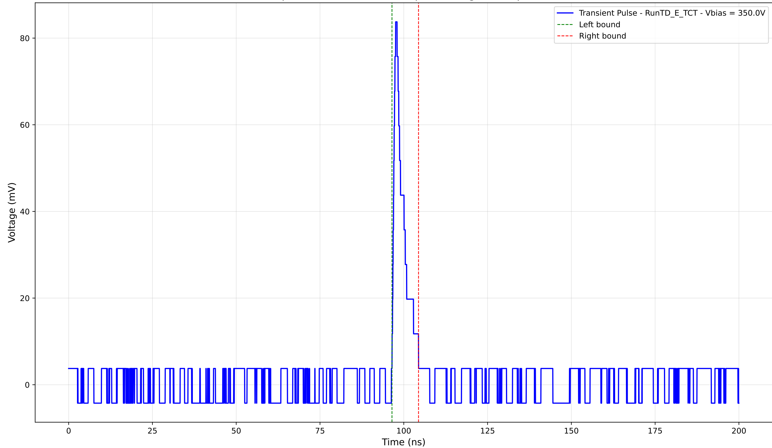
Transient Pulse - Sample: TD - Position: 635.0 \mu\text{m} - Charge: 5.60 pC - Rise Time: 0.87 ns
