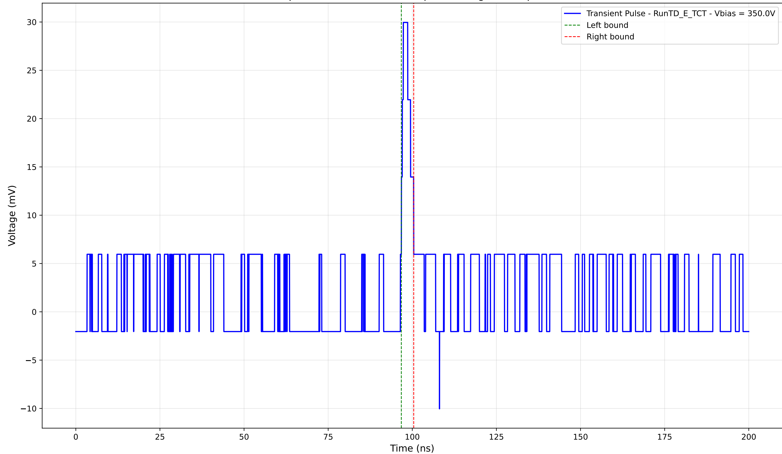
Transient Pulse - Sample: TD - Position: 705.0 \mu\text{m} - Charge: 1.63 pC - Rise Time: 0.88 ns
