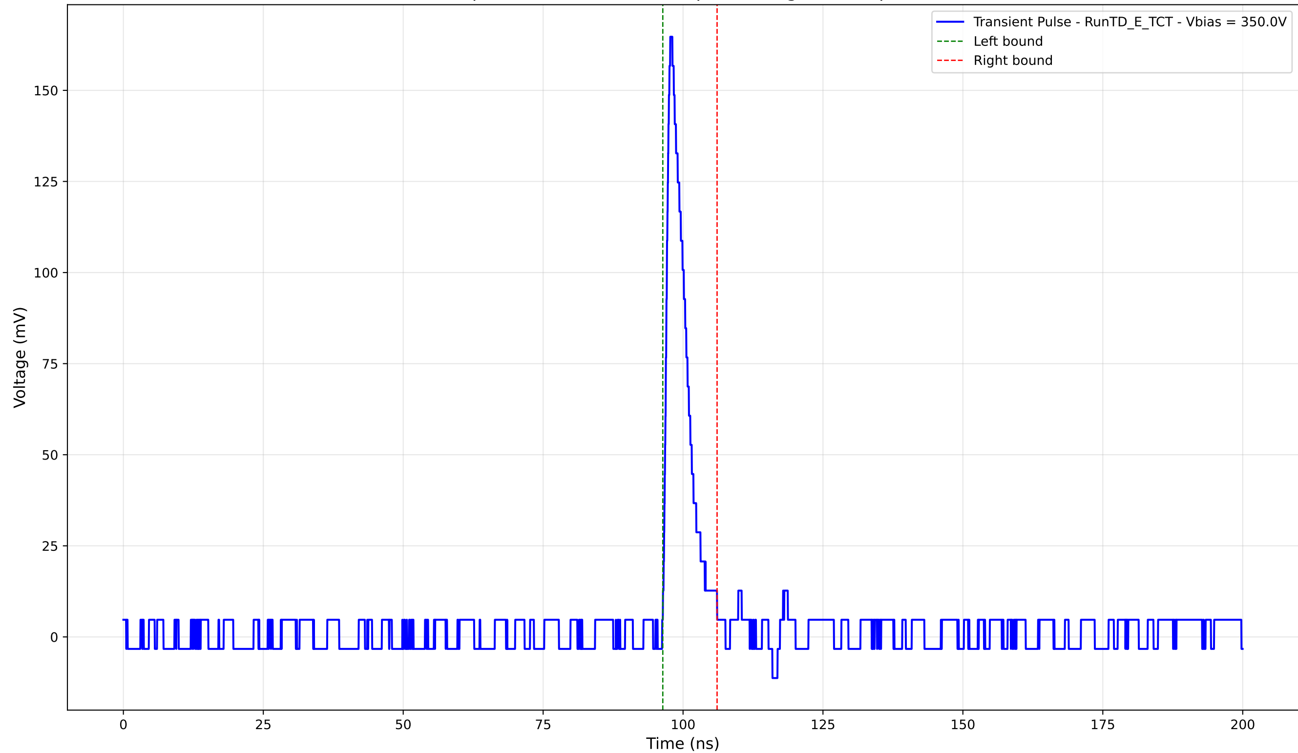
Transient Pulse - Sample: TD - Position: 520.0 \mu\text{m} - Charge: 12.78 pC - Rise Time: 0.95 ns
