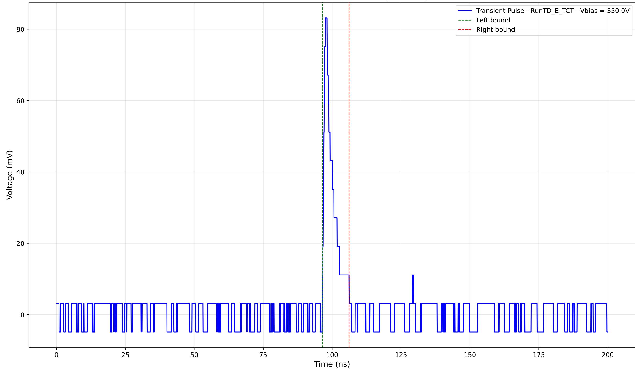
Transient Pulse - Sample: TD - Position: 630.0 \mu\text{m} - Charge: 6.13 pC - Rise Time: 0.83 ns
