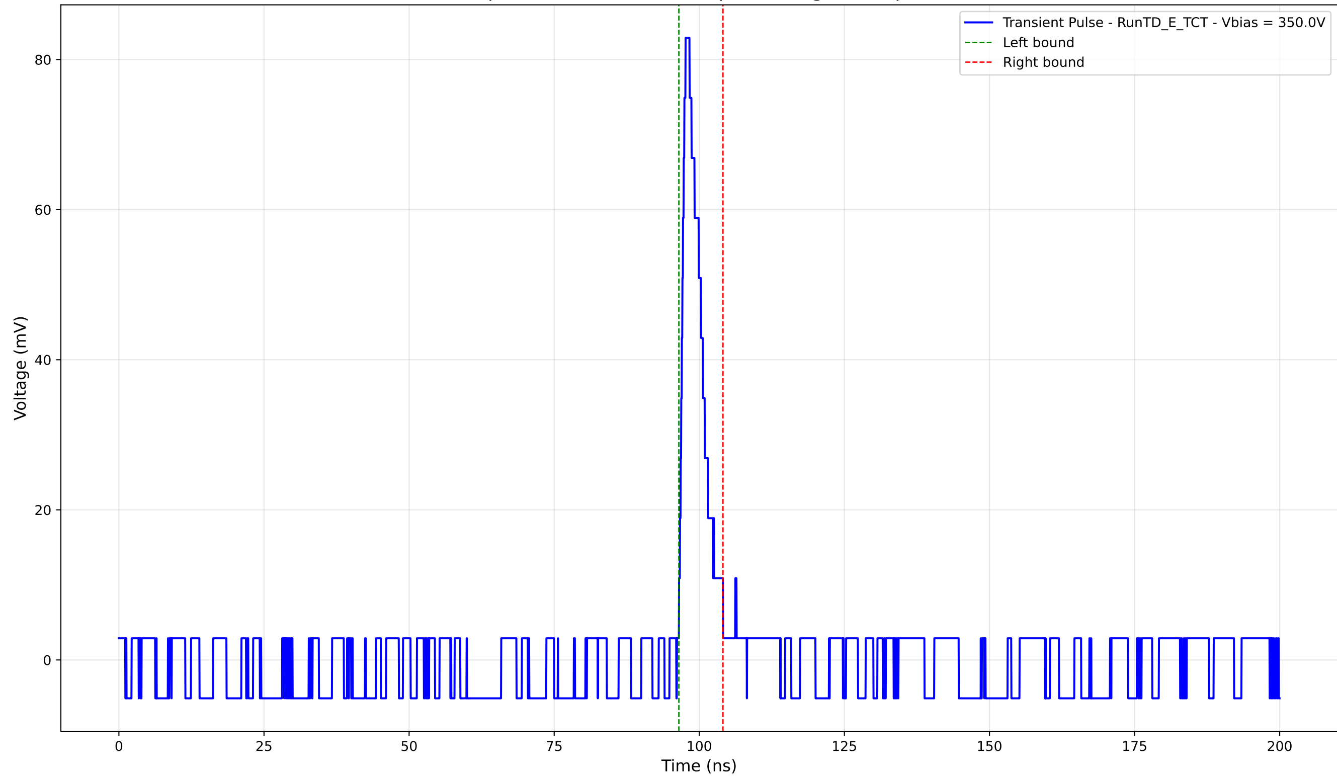
Transient Pulse - Sample: TD - Position: 410.0 \mu\text{m} - Charge: 6.14 pC - Rise Time: 0.93 ns
