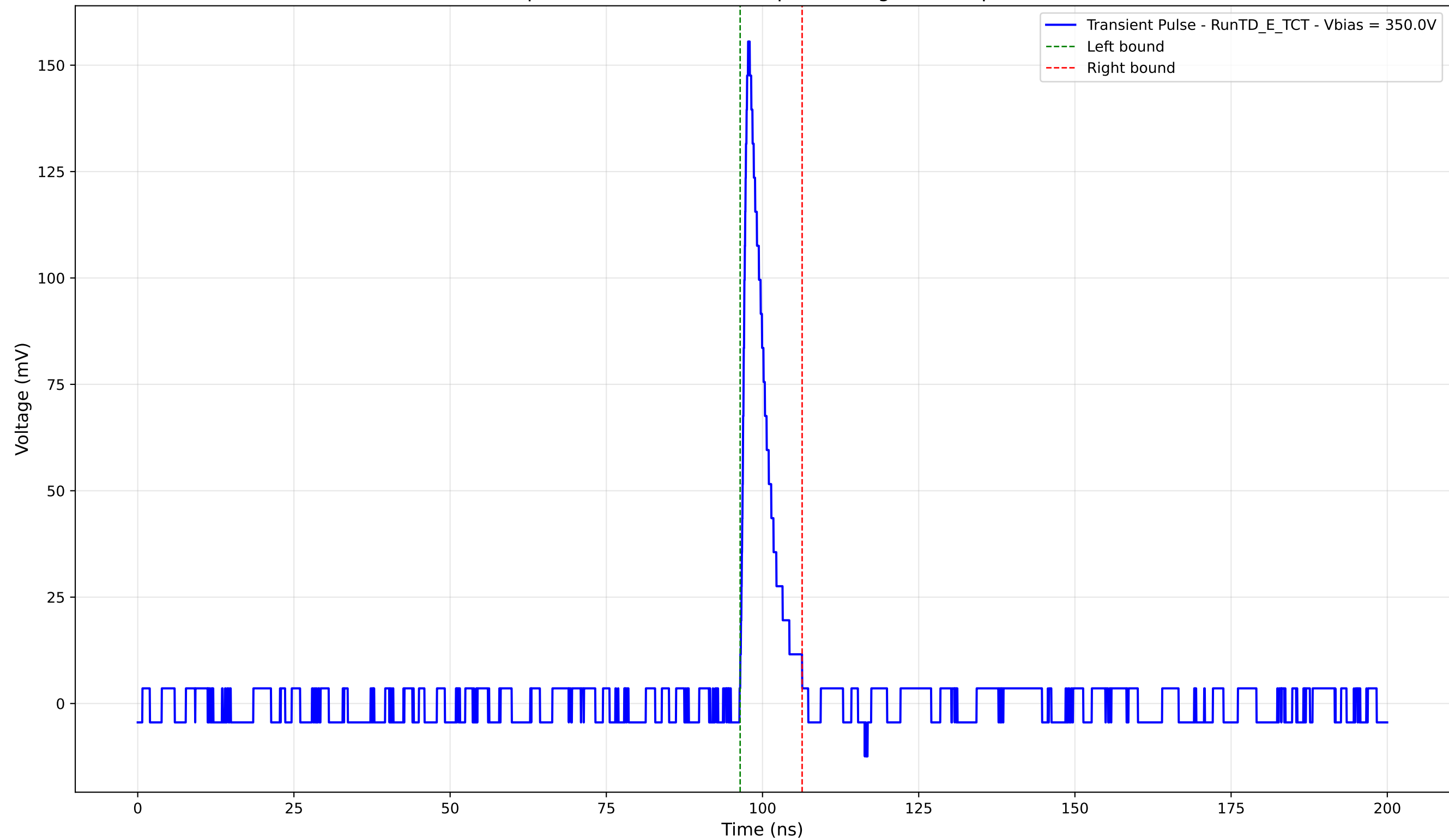
Transient Pulse - Sample: TD - Position: 445.0 \mu\text{m} - Charge: 11.62 pC - Rise Time: 0.99 ns
