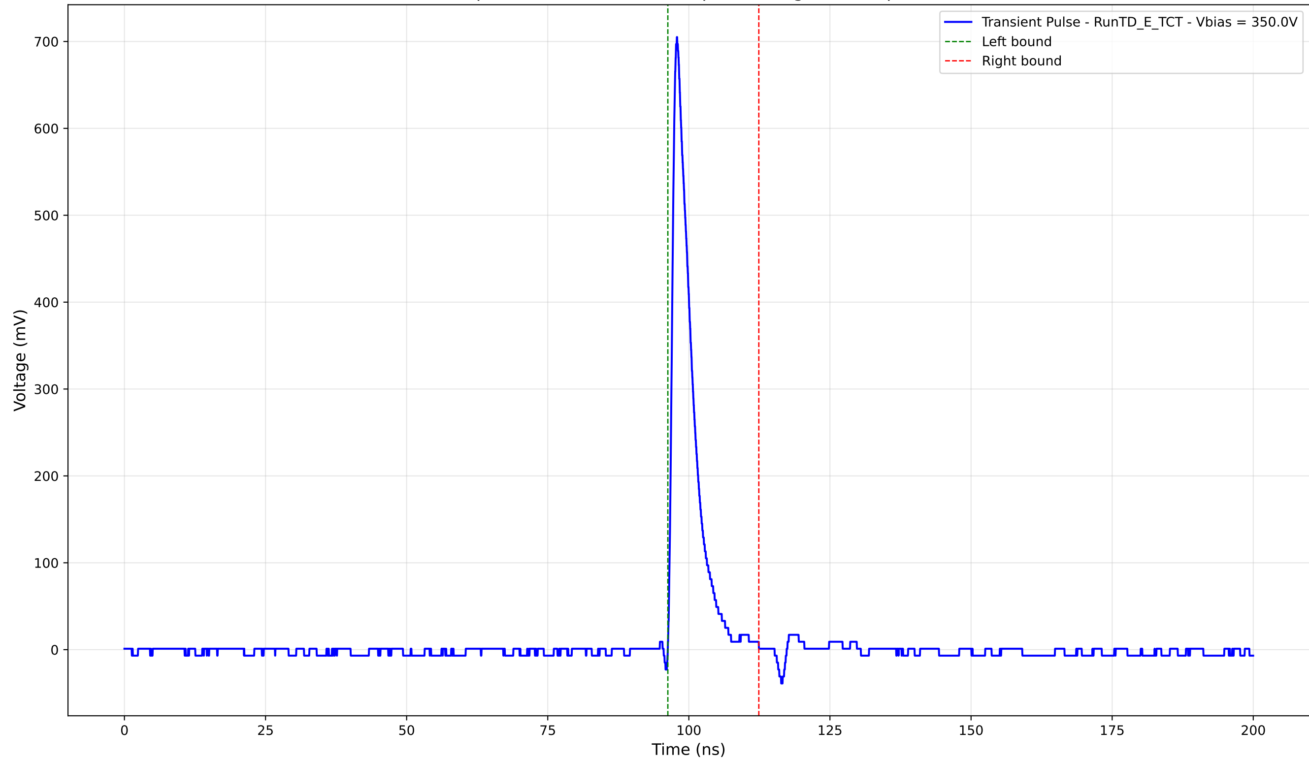
Transient Pulse - Sample: TD - Position: 250.0 \mu\text{m} - Charge: 55.56 pC - Rise Time: 0.97 ns
