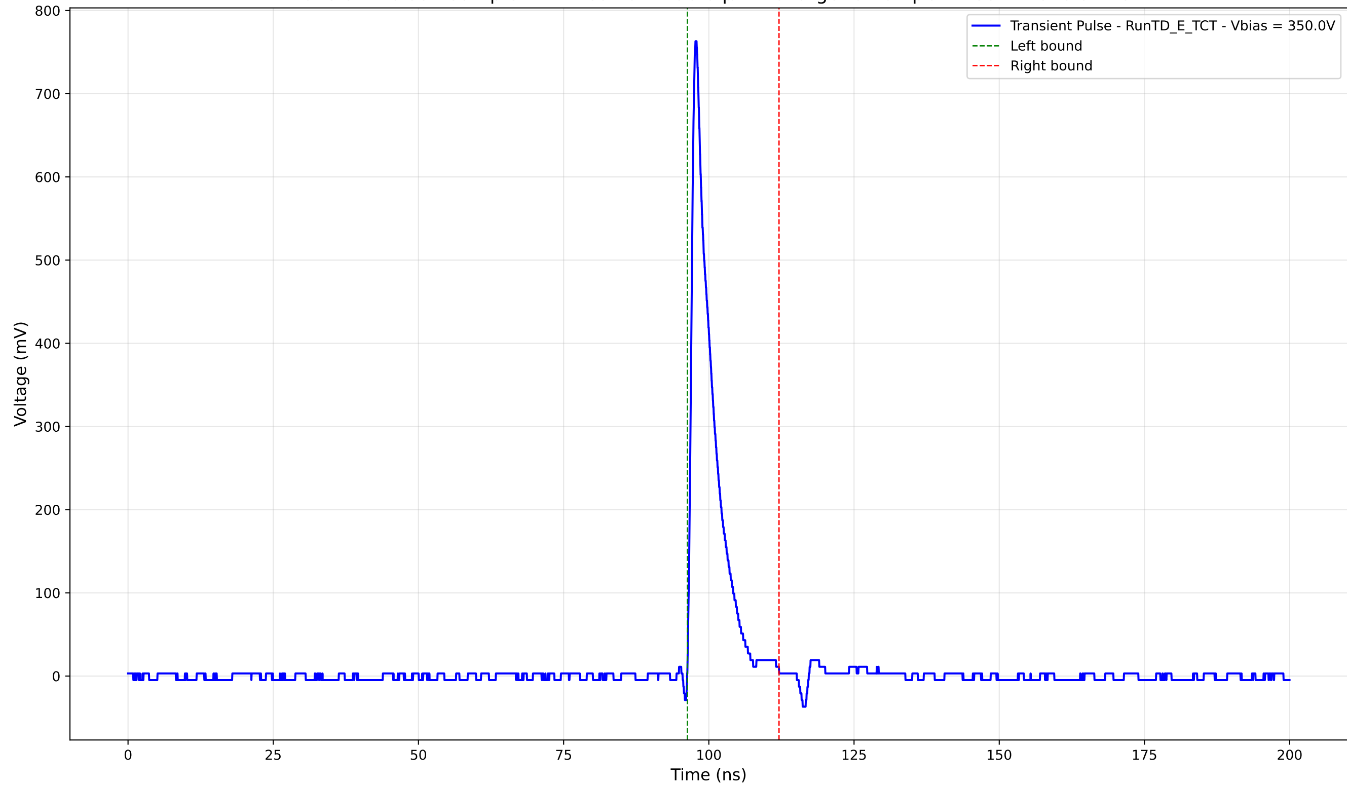
Transient Pulse - Sample: TD - Position: 190.0 \mu\text{m} - Charge: 61.82 pC - Rise Time: 0.91 ns
