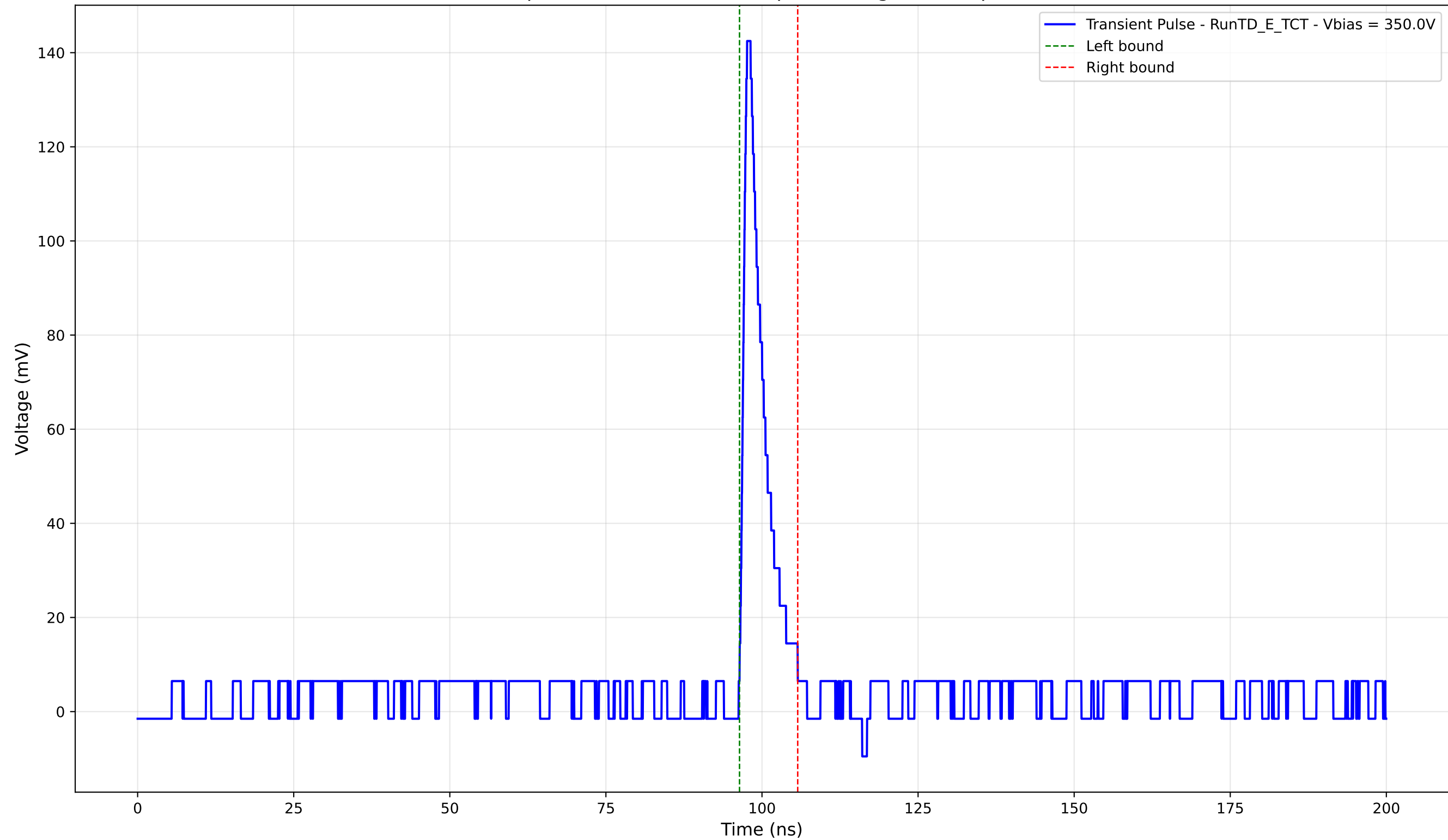
Transient Pulse - Sample: TD - Position: 555.0 \mu\text{m} - Charge: 10.71 pC - Rise Time: 1.06 ns
