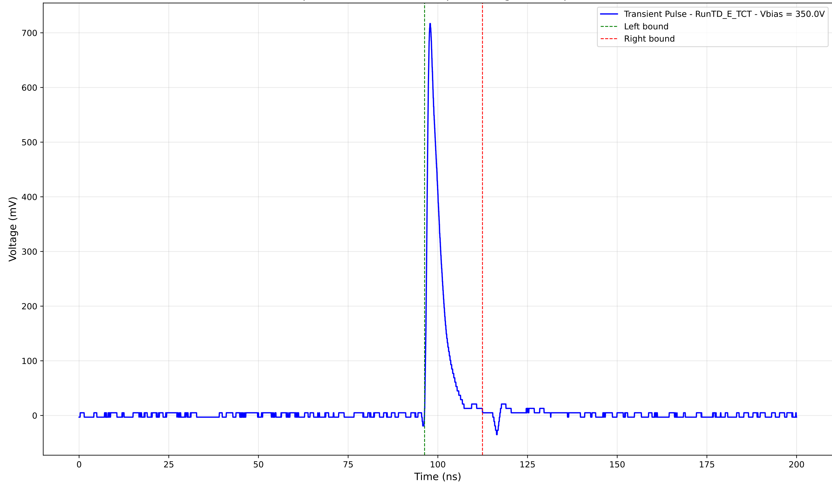
Transient Pulse - Sample: TD - Position: 235.0 \mu\text{m} - Charge: 57.43 pC - Rise Time: 0.95 ns
