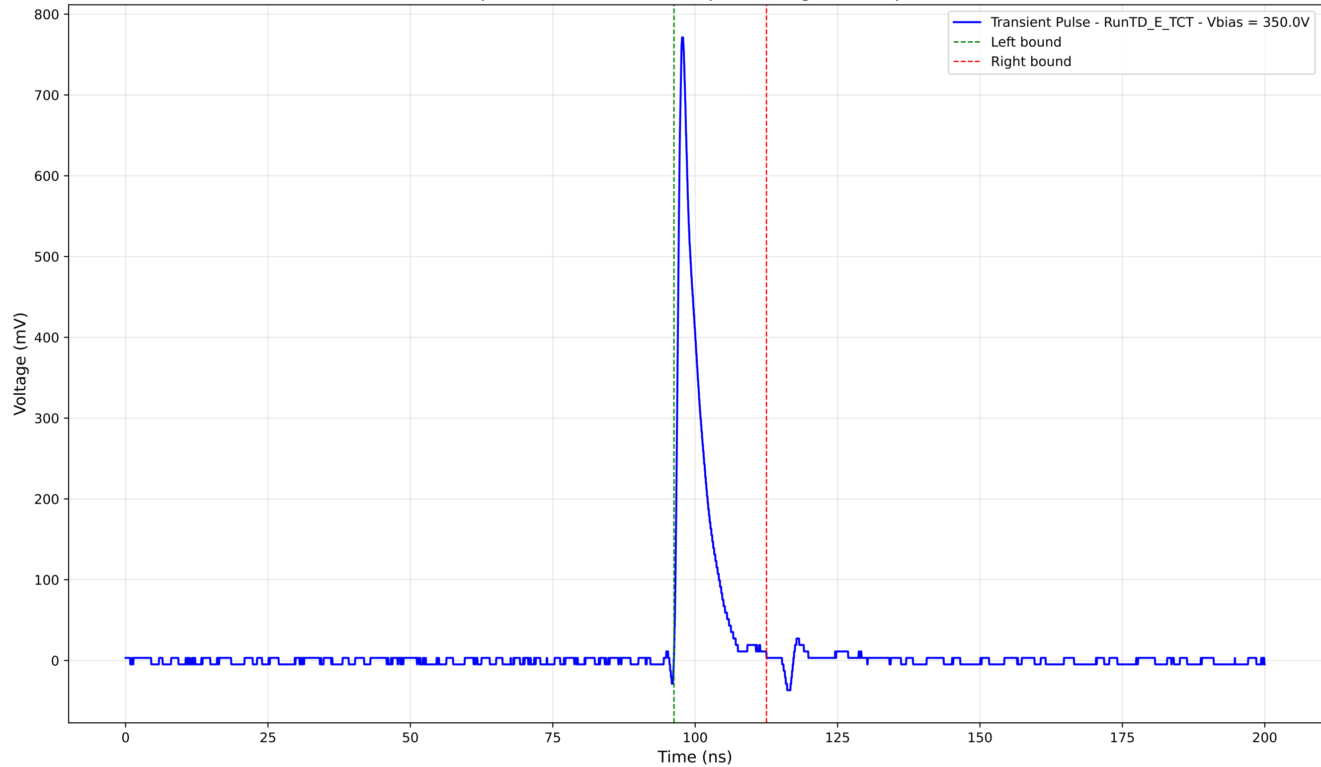
Transient Pulse - Sample: TD - Position: 175.0 \mu\text{m} - Charge: 61.43 pC - Rise Time: 0.92 ns
