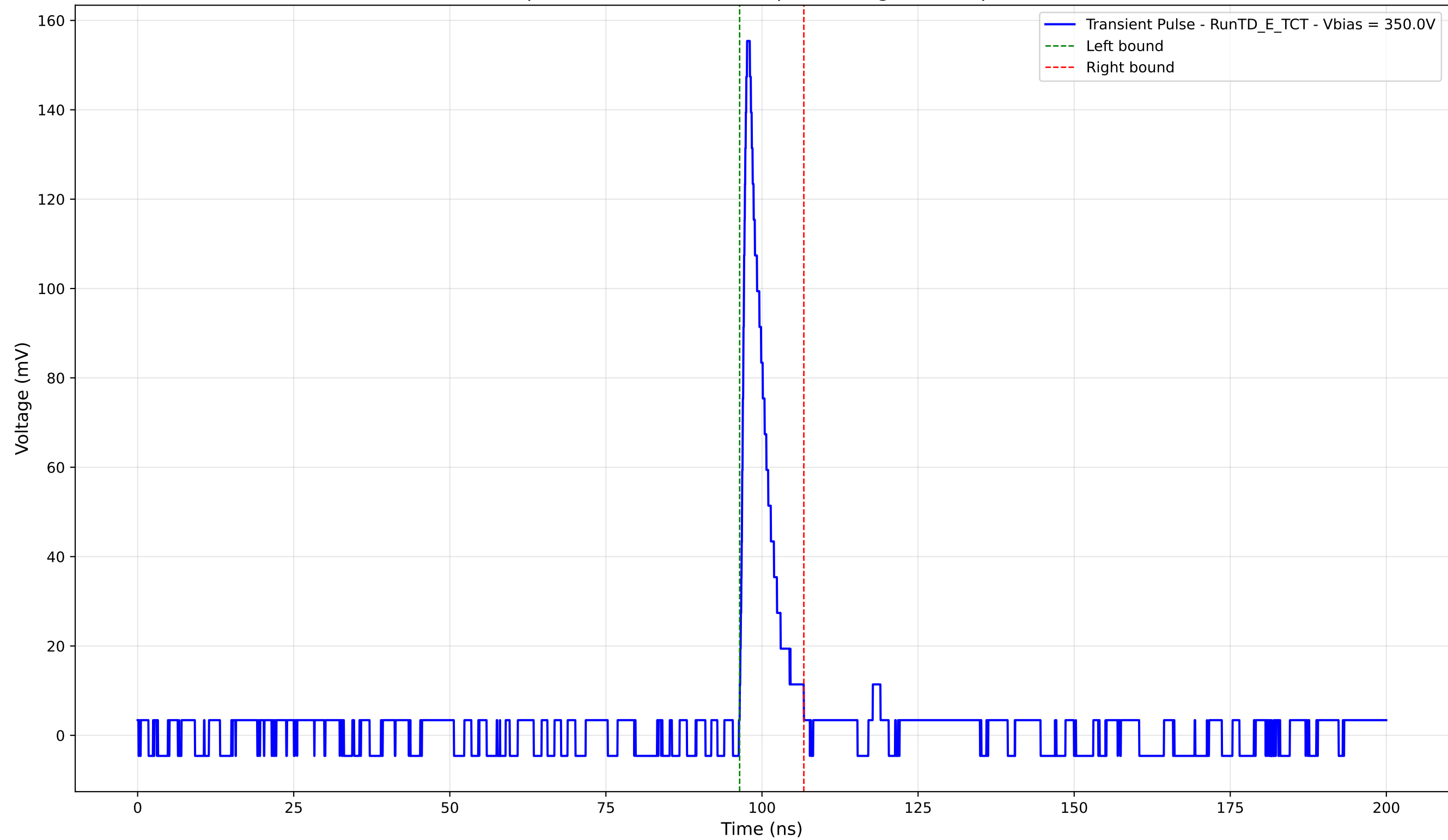
Transient Pulse - Sample: TD - Position: 450.0 \mu\text{m} - Charge: 11.64 pC - Rise Time: 0.97 ns
