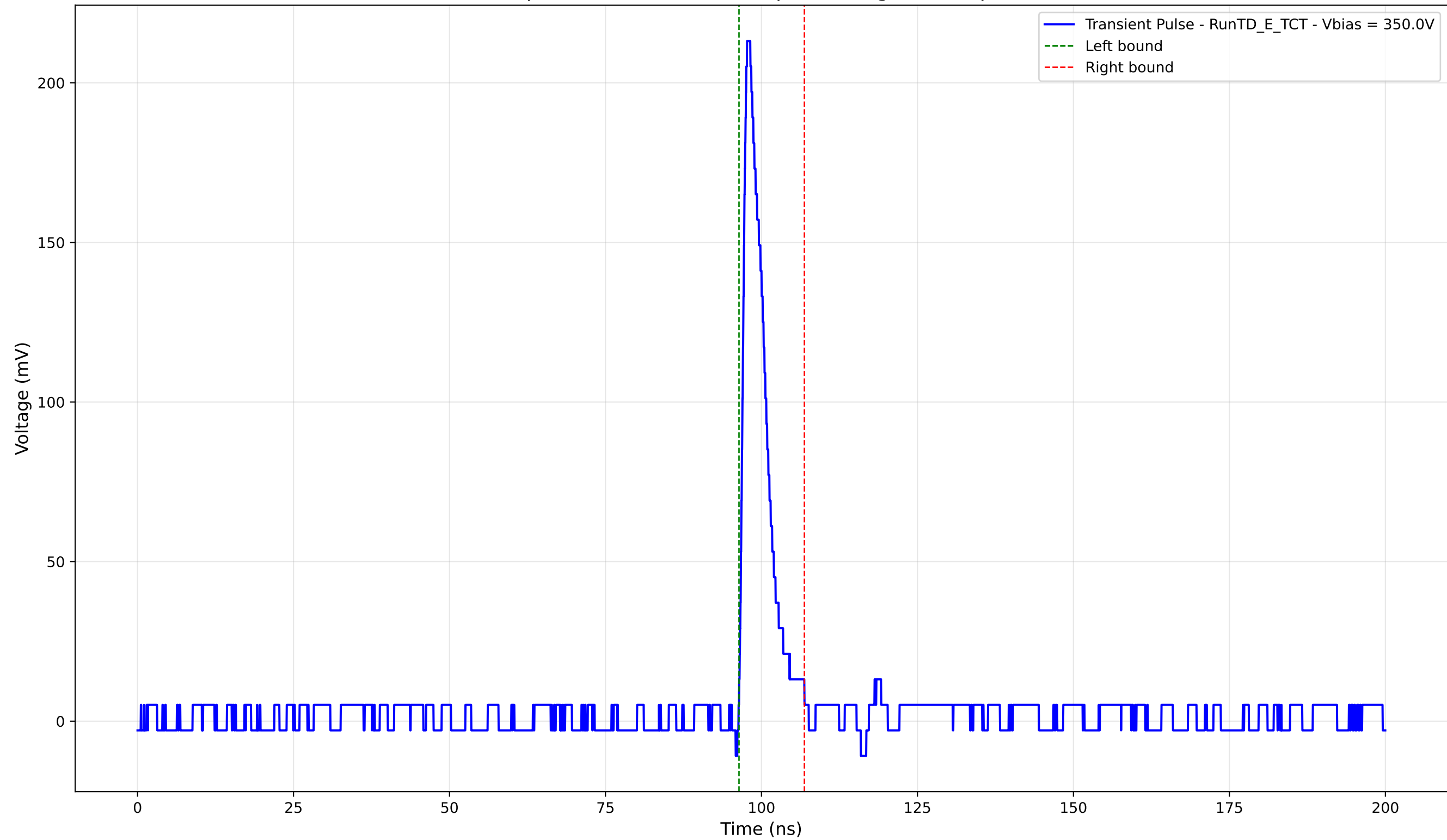
Transient Pulse - Sample: TD - Position: 470.0 \mu\text{m} - Charge: 16.86 pC - Rise Time: 0.96 ns
