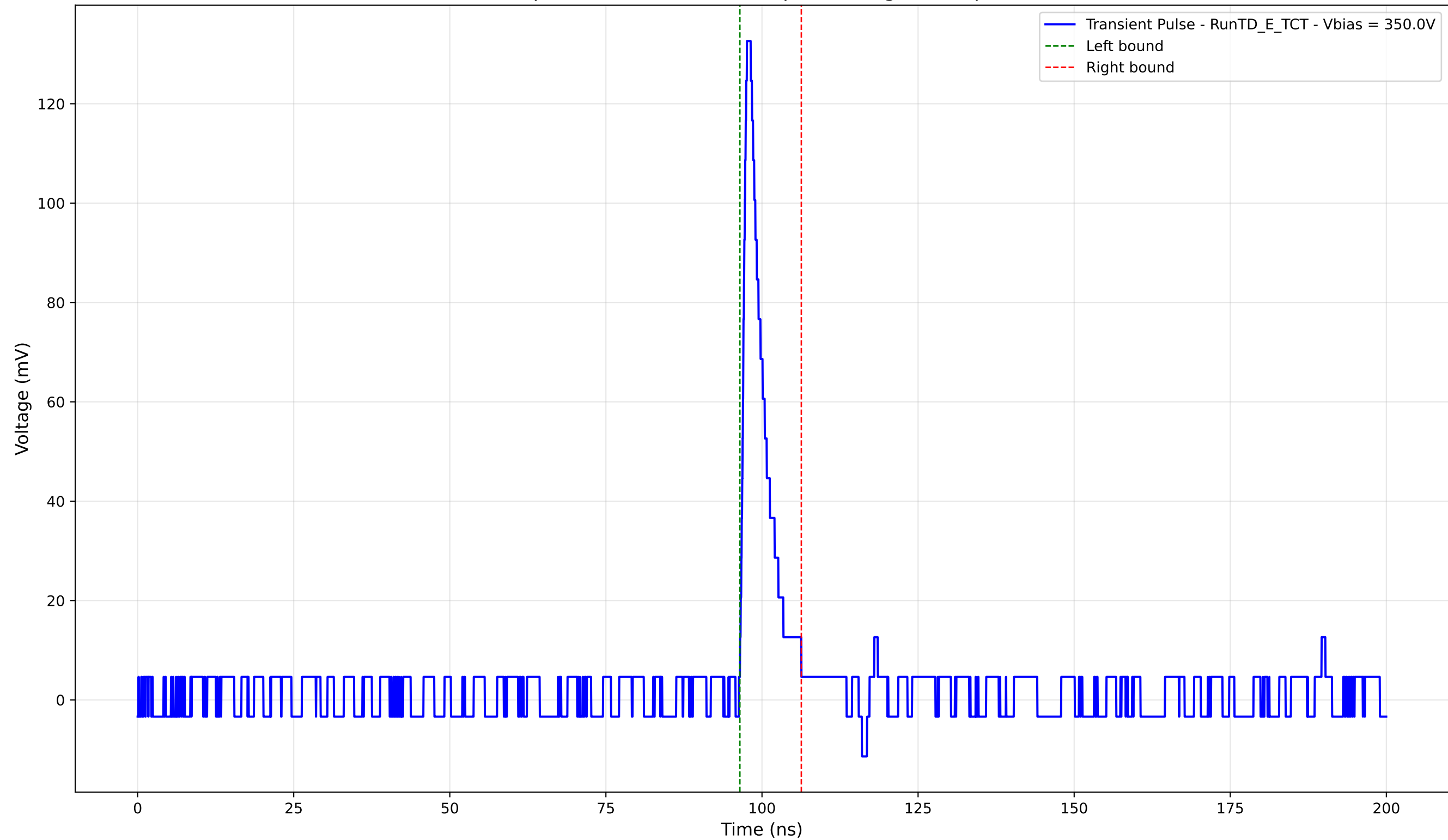
Transient Pulse - Sample: TD - Position: 560.0 \mu\text{m} - Charge: 9.84 pC - Rise Time: 0.90 ns
