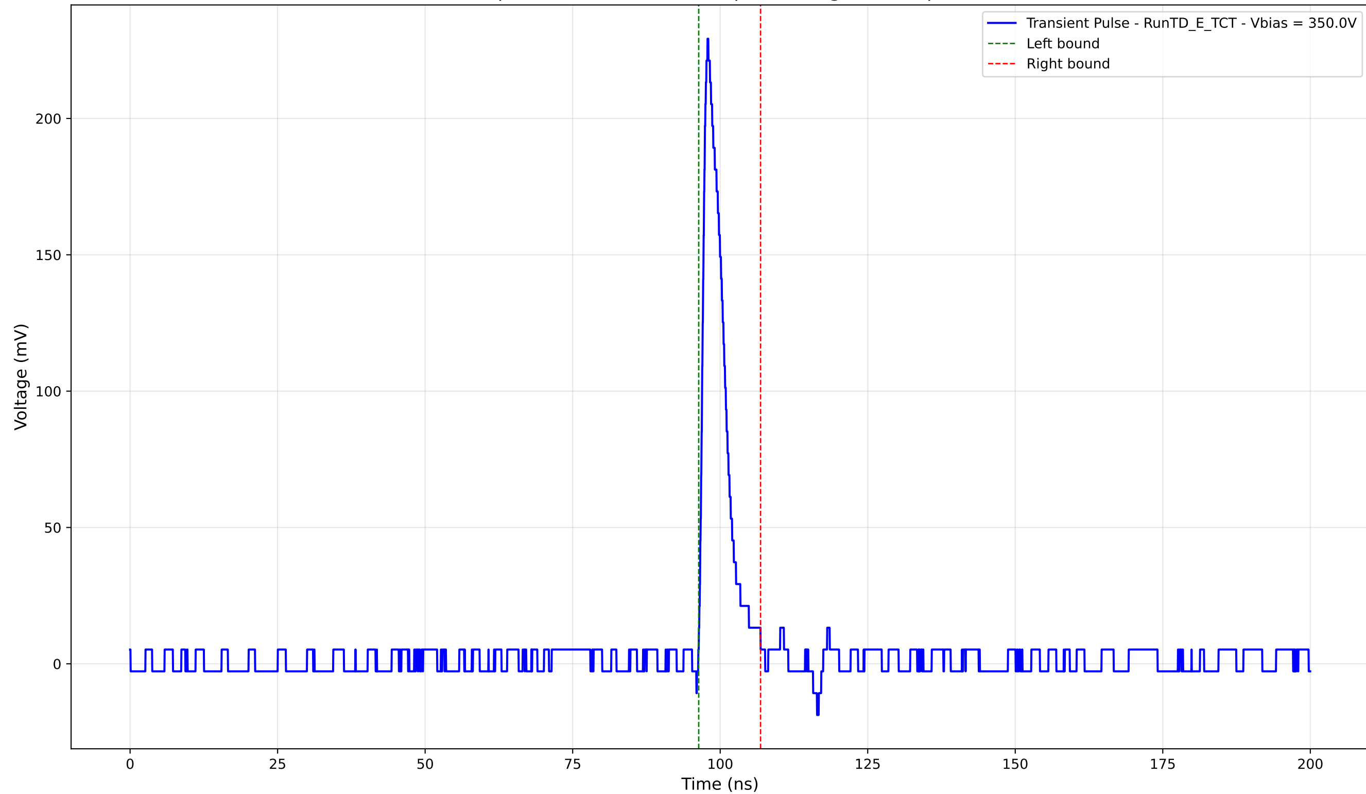
Transient Pulse - Sample: TD - Position: 480.0 \mu\text{m} - Charge: 18.05 pC - Rise Time: 1.04 ns
