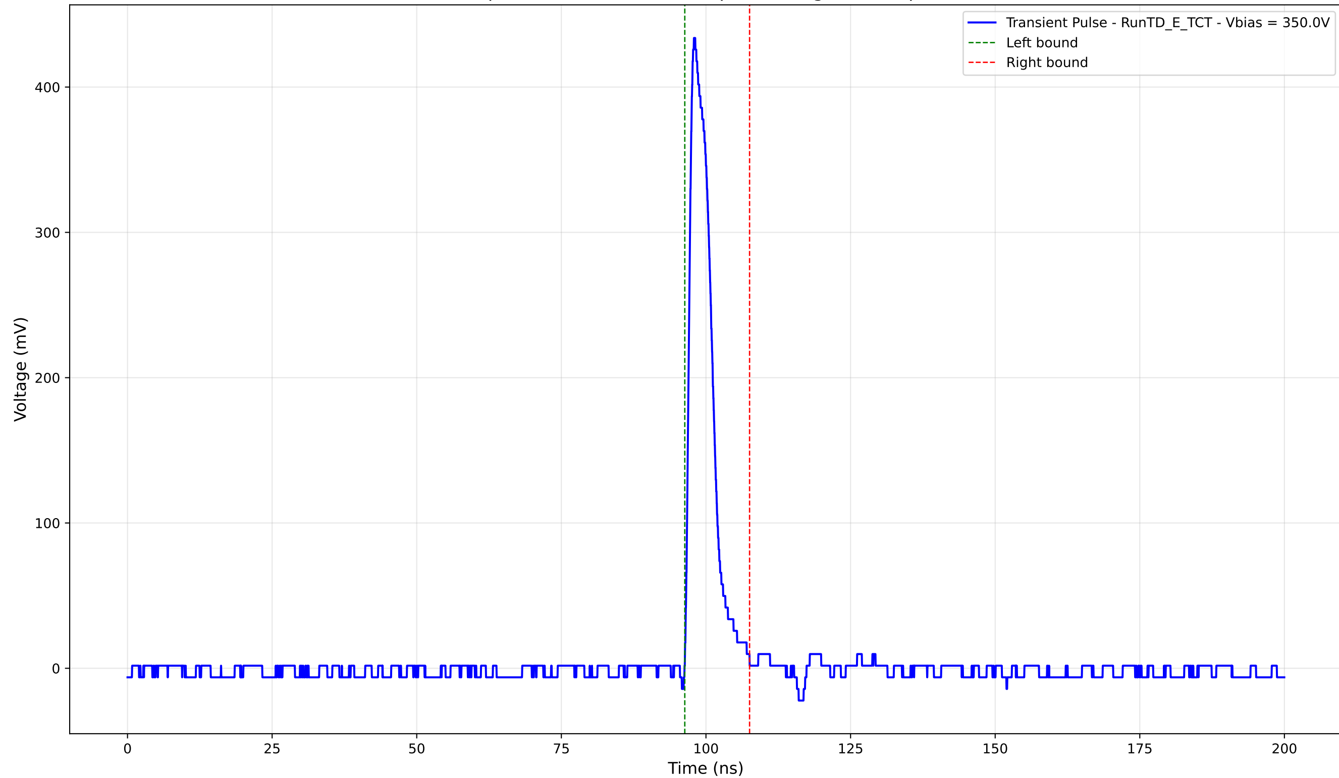
Transient Pulse - Sample: TD - Position: 370.0 \mu\text{m} - Charge: 36.81 pC - Rise Time: 1.02 ns
