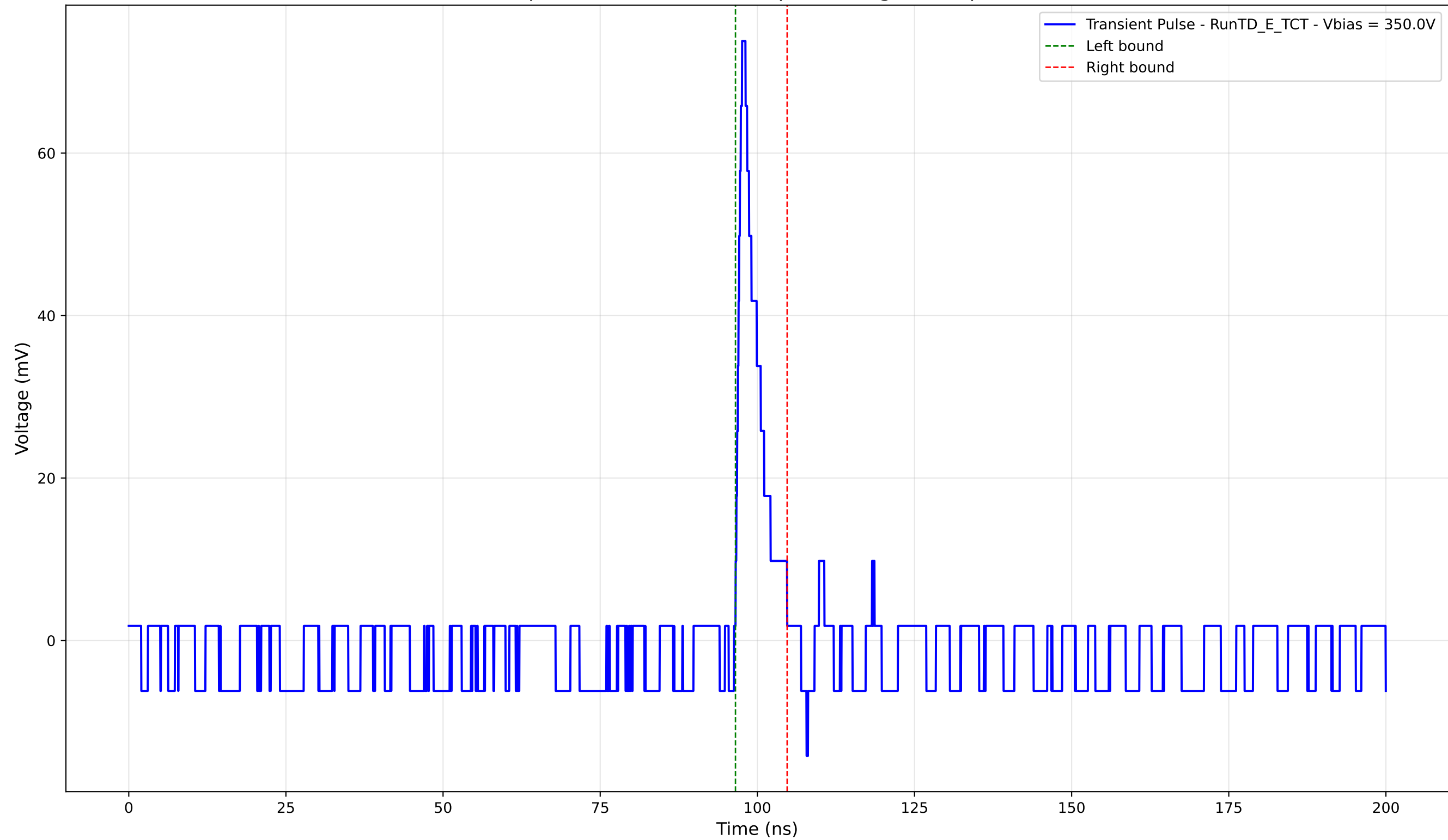
Transient Pulse - Sample: TD - Position: 650.0 \mu\text{m} - Charge: 5.01 pC - Rise Time: 1.03 ns
