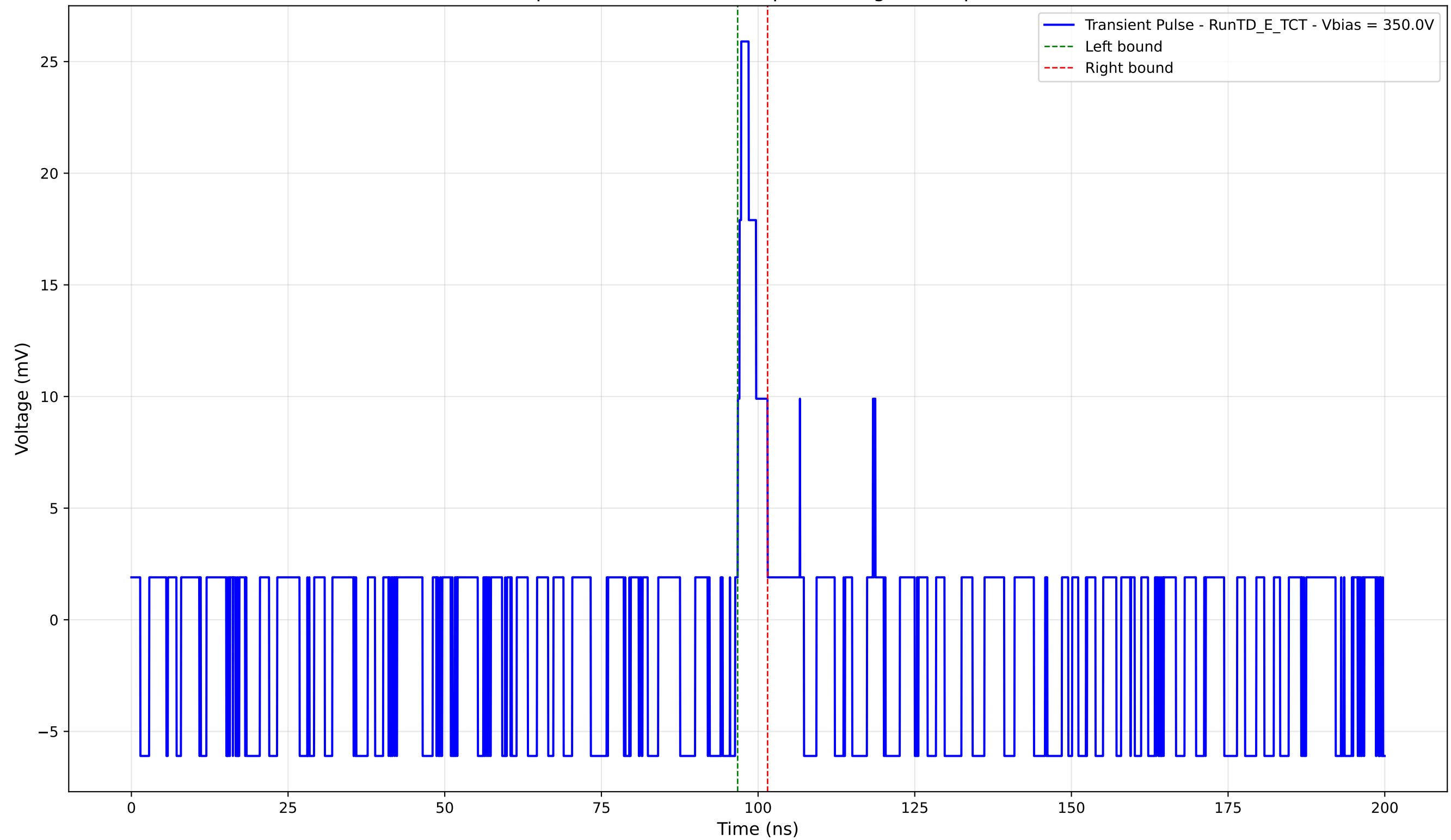
Transient Pulse - Sample: TD - Position: 25.0 \mu\text{m} - Charge: 1.56 pC - Rise Time: 0.56 ns
