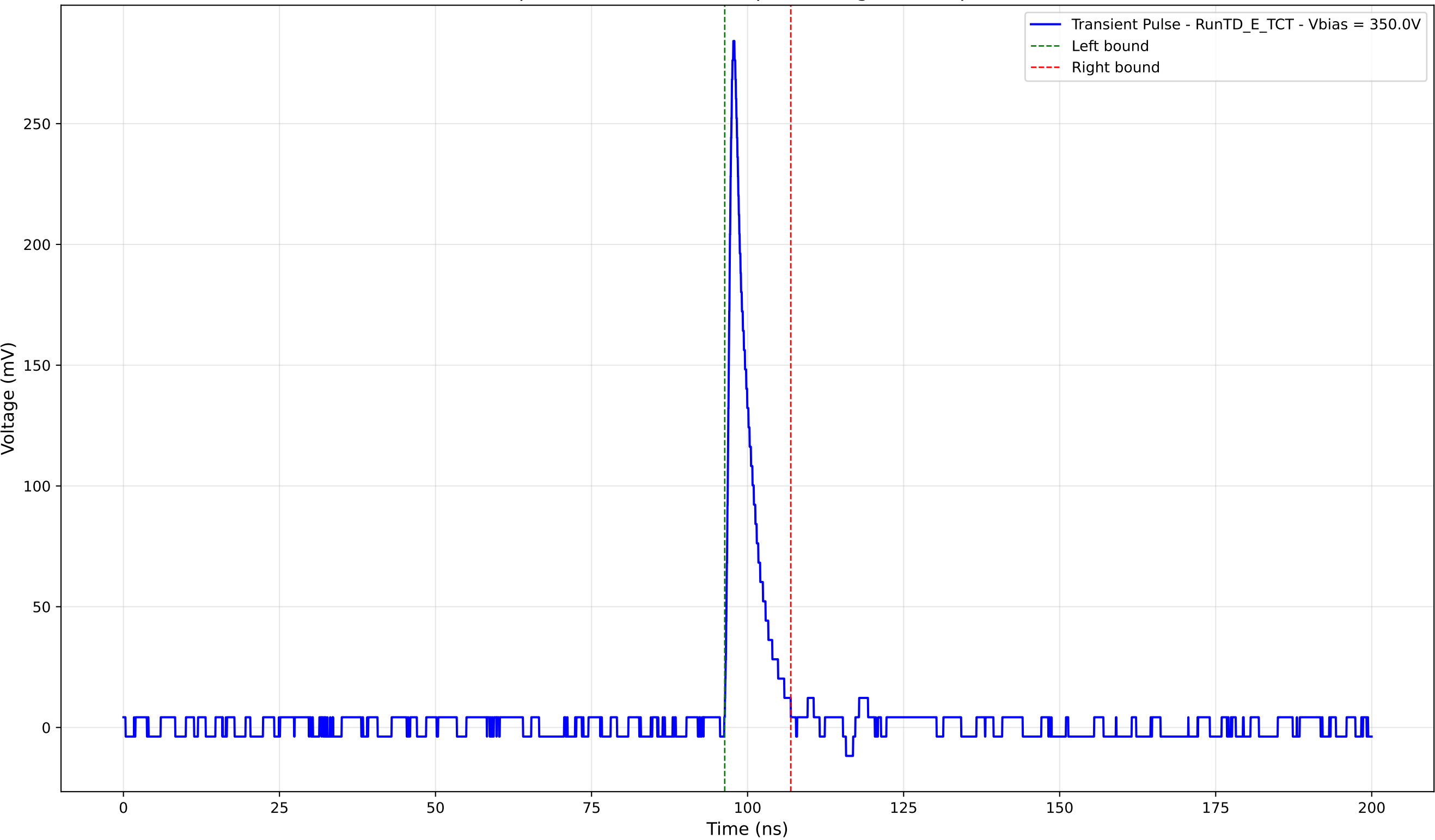
Transient Pulse - Sample: TD - Position: 70.0 \mu\text{m} - Charge: 20.34 pC - Rise Time: 0.94 ns
