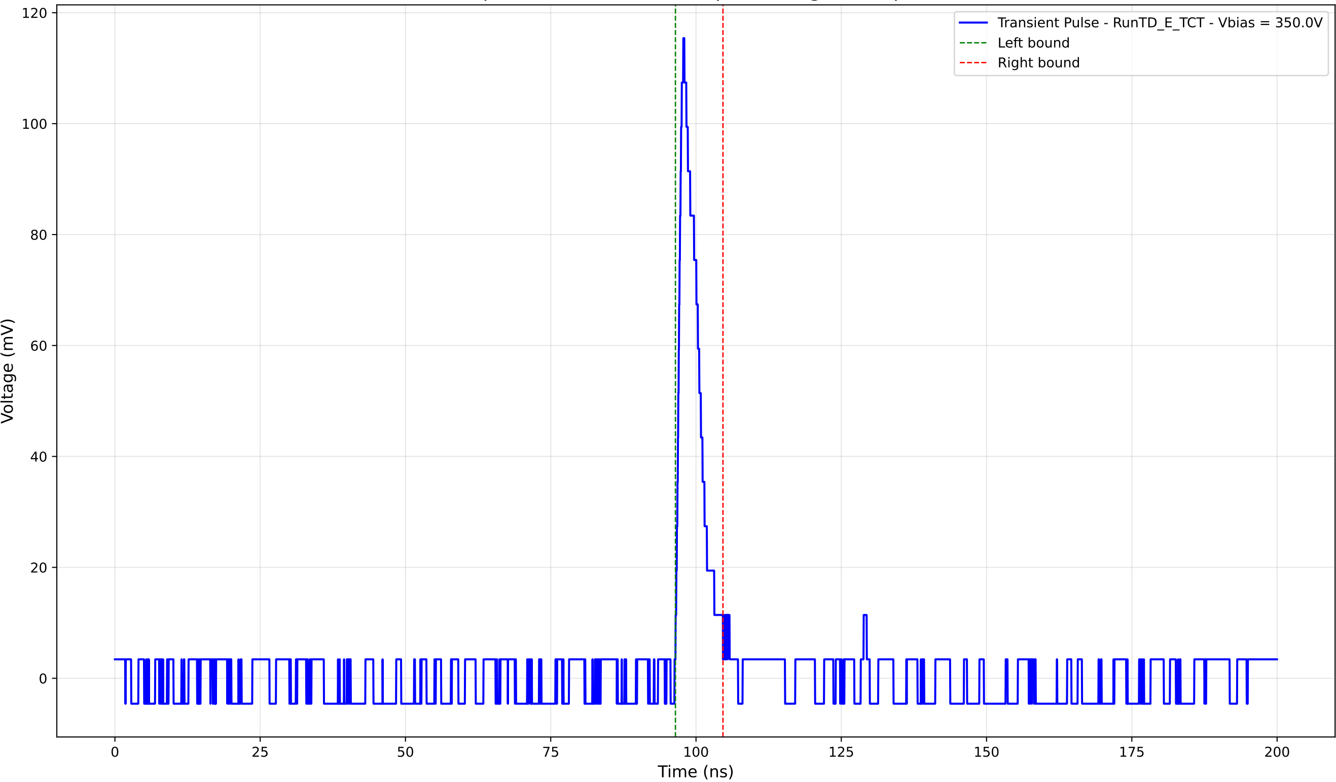
Transient Pulse - Sample: TD - Position: 400.0 \mu\text{m} - Charge: 8.34 pC - Rise Time: 0.96 ns
