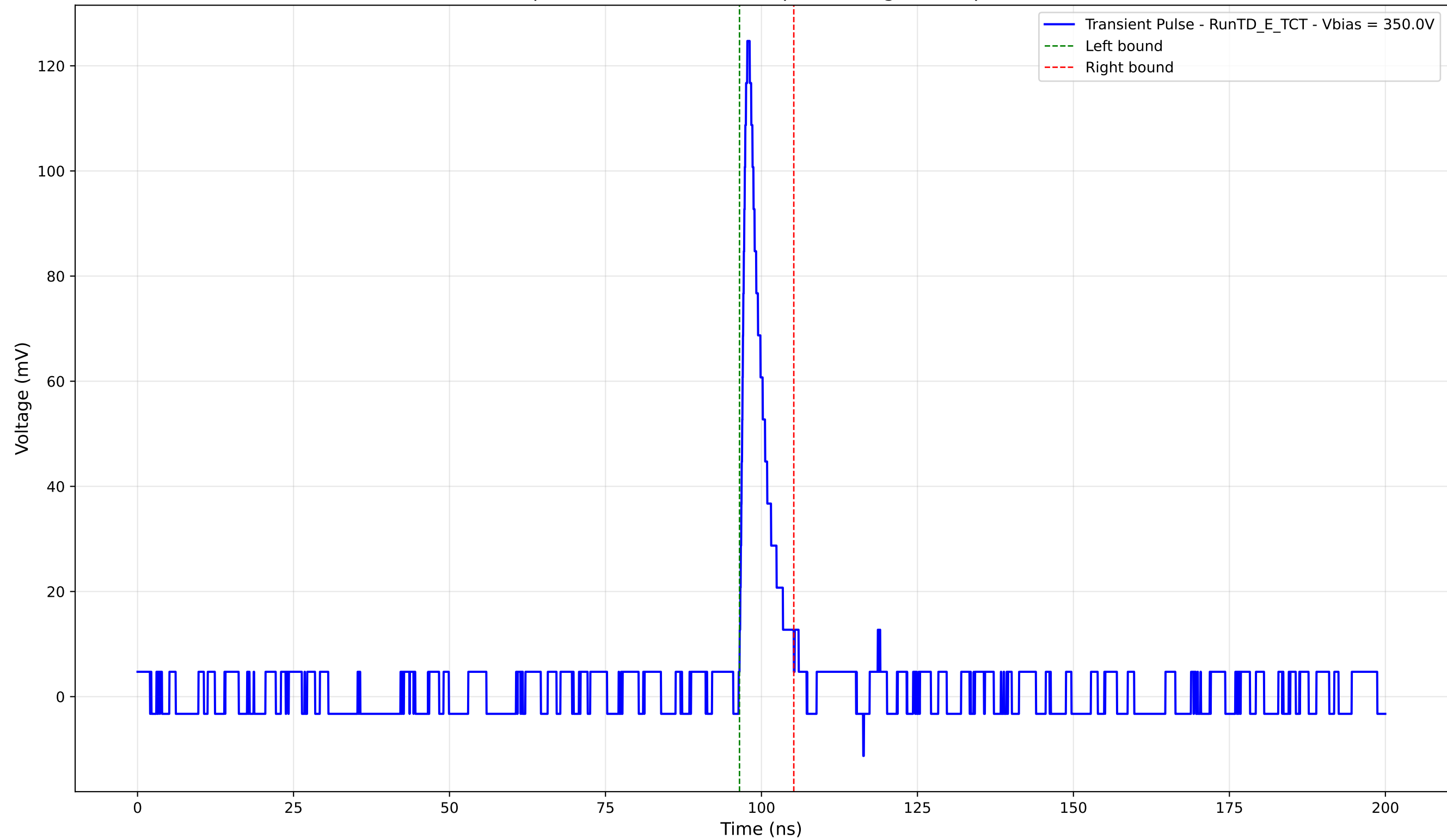
Transient Pulse - Sample: TD - Position: 570.0 \mu\text{m} - Charge: 8.77 pC - Rise Time: 1.02 ns
