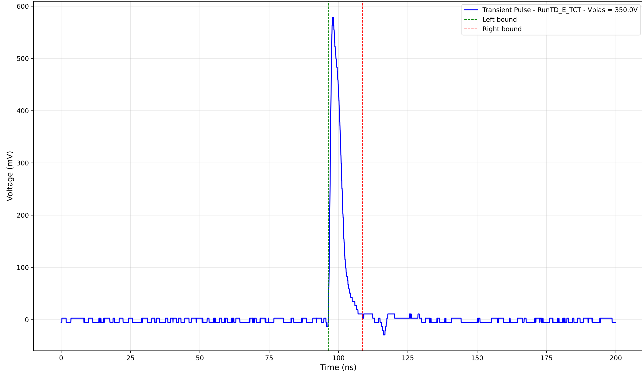
Transient Pulse - Sample: TD - Position: 340.0 \mu\text{m} - Charge: 49.45 pC - Rise Time: 0.98 ns
