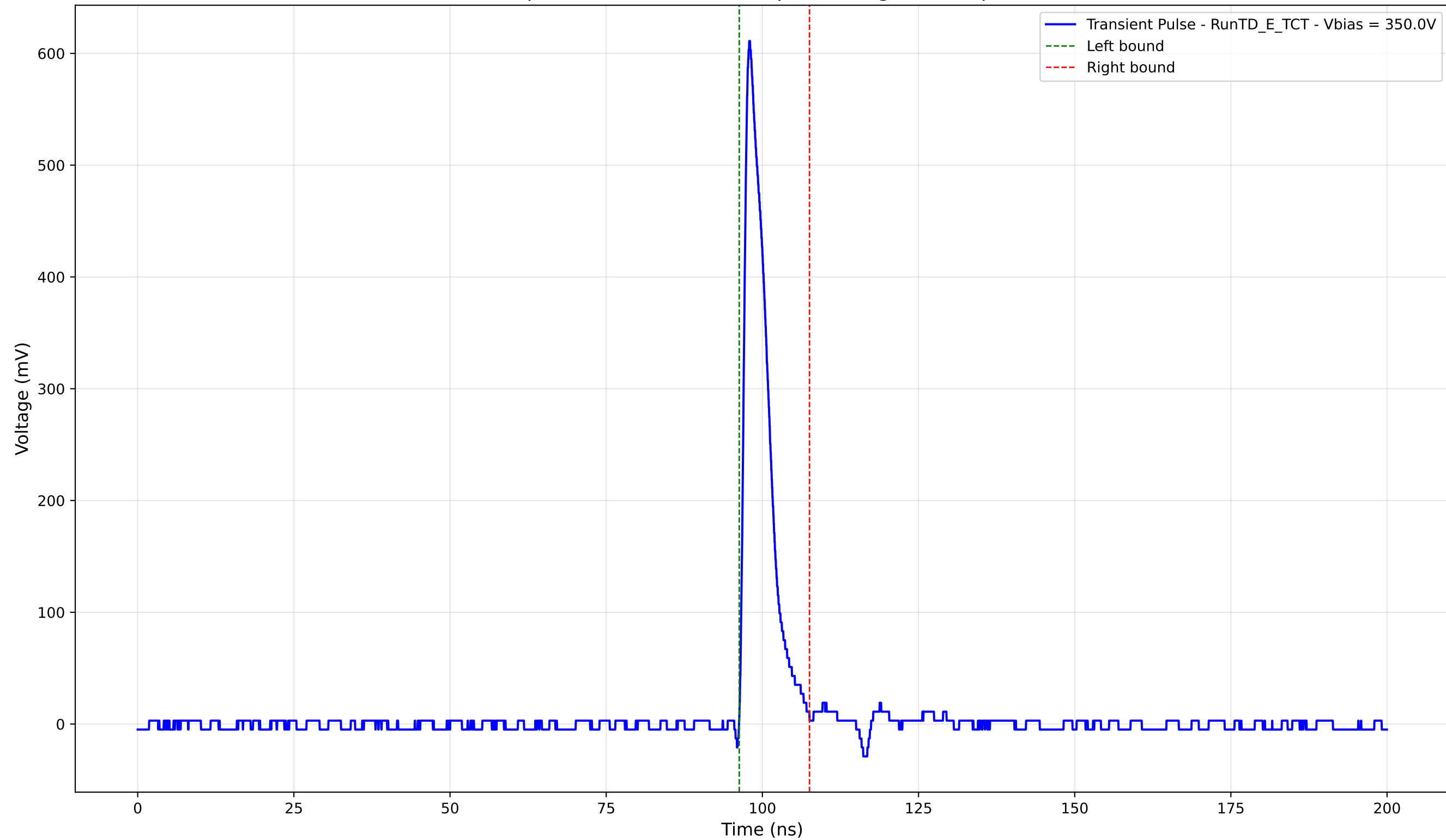
Transient Pulse - Sample: TD - Position: 315.0 \mu\text{m} - Charge: 50.39 pC - Rise Time: 1.00 ns
