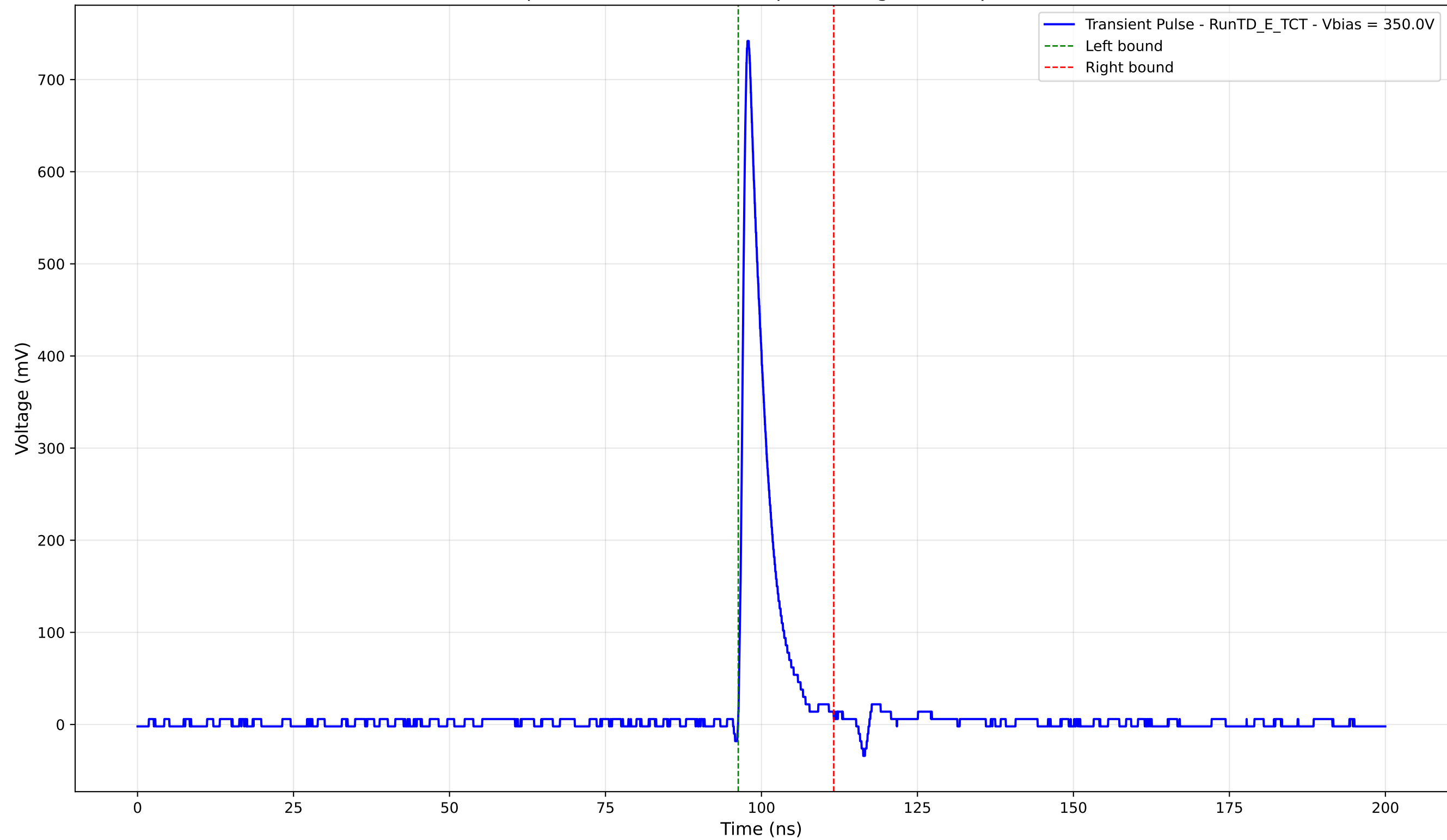
Transient Pulse - Sample: TD - Position: 105.0 \mu\text{m} - Charge: 59.03 pC - Rise Time: 0.96 ns
