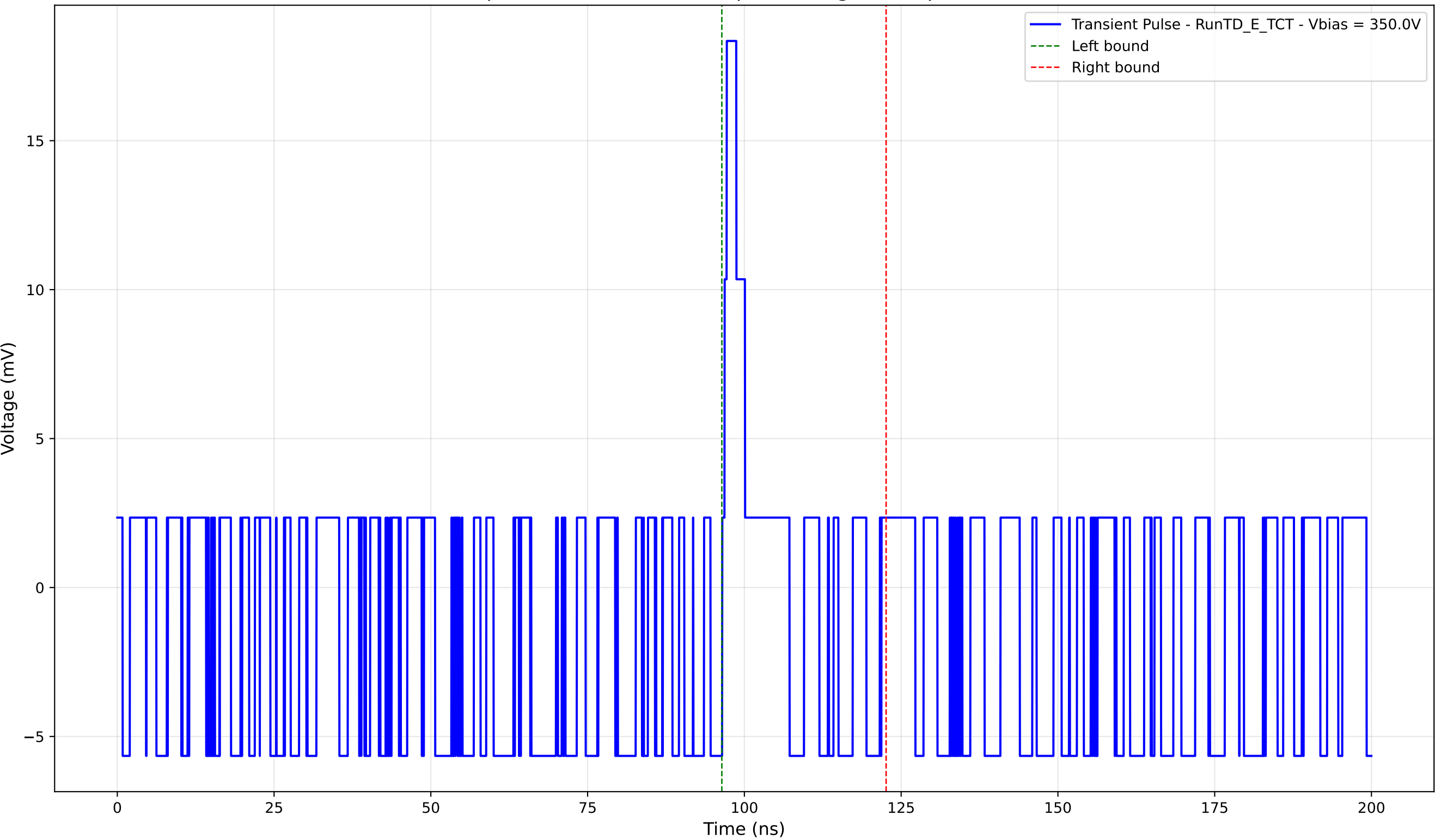
Transient Pulse - Sample: TD - Position: 715.0 \mu\text{m} - Charge: 0.56 pC - Rise Time: 0.00 ns (N/A)
