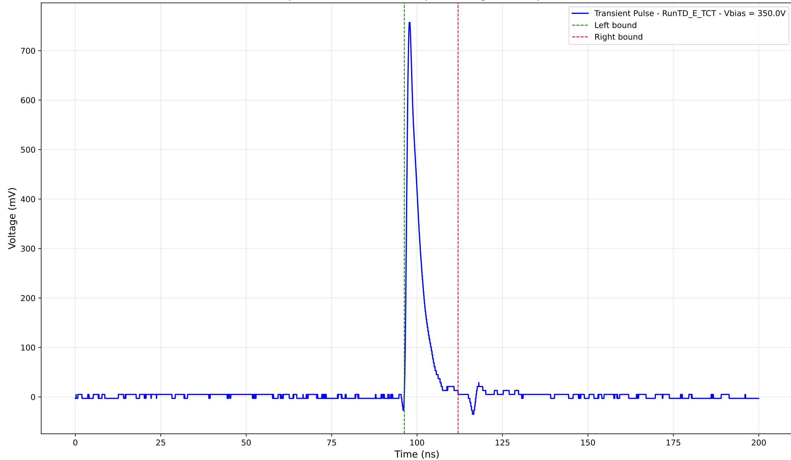
Transient Pulse - Sample: TD - Position: 210.0 \mu\text{m} - Charge: 61.18 pC - Rise Time: 0.91 ns
