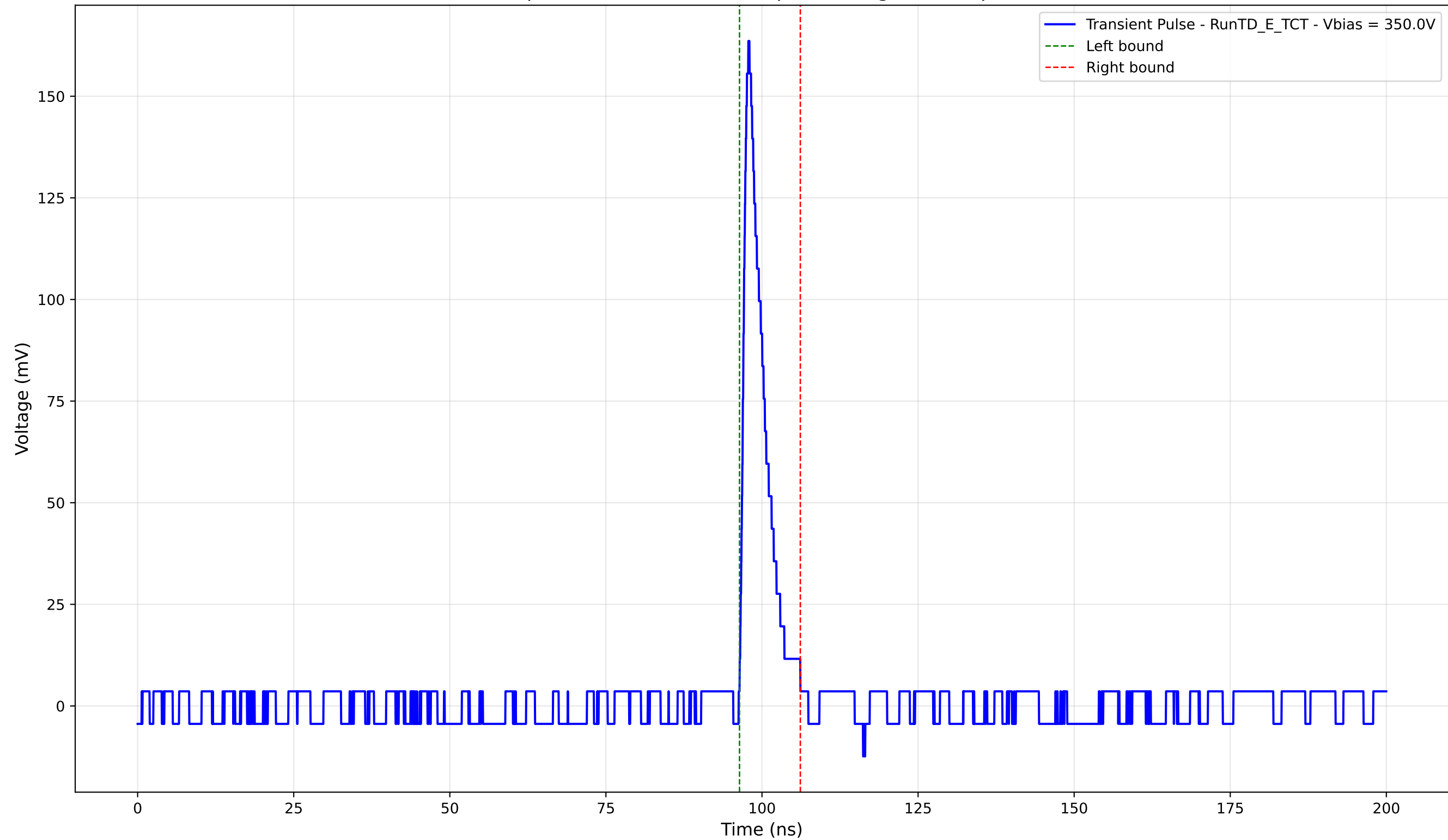
Transient Pulse - Sample: TD - Position: 535.0 \mu\text{m} - Charge: 11.85 pC - Rise Time: 0.97 ns
