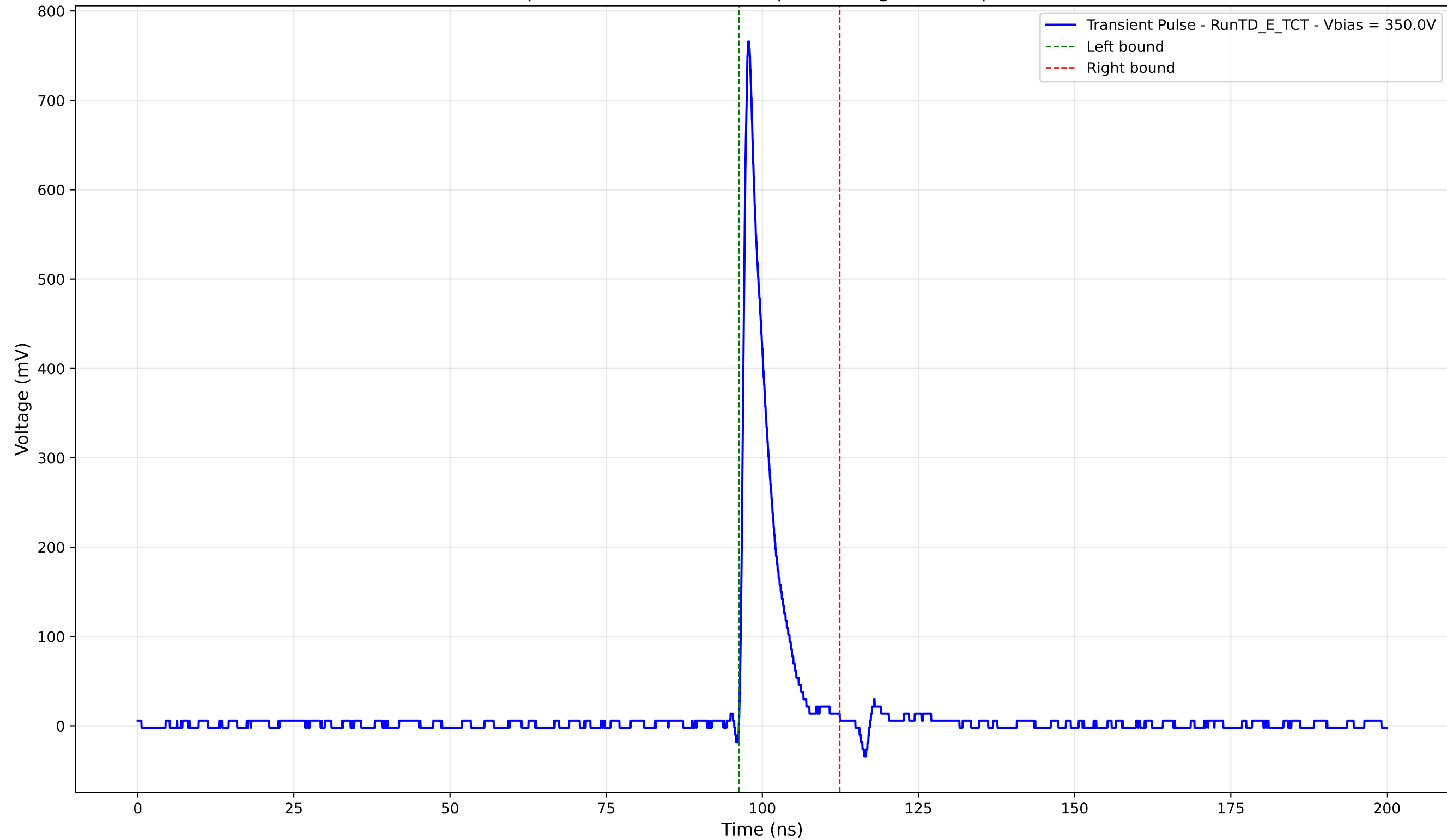
Transient Pulse - Sample: TD - Position: 205.0 \mu\text{m} - Charge: 62.46 pC - Rise Time: 0.94 ns
