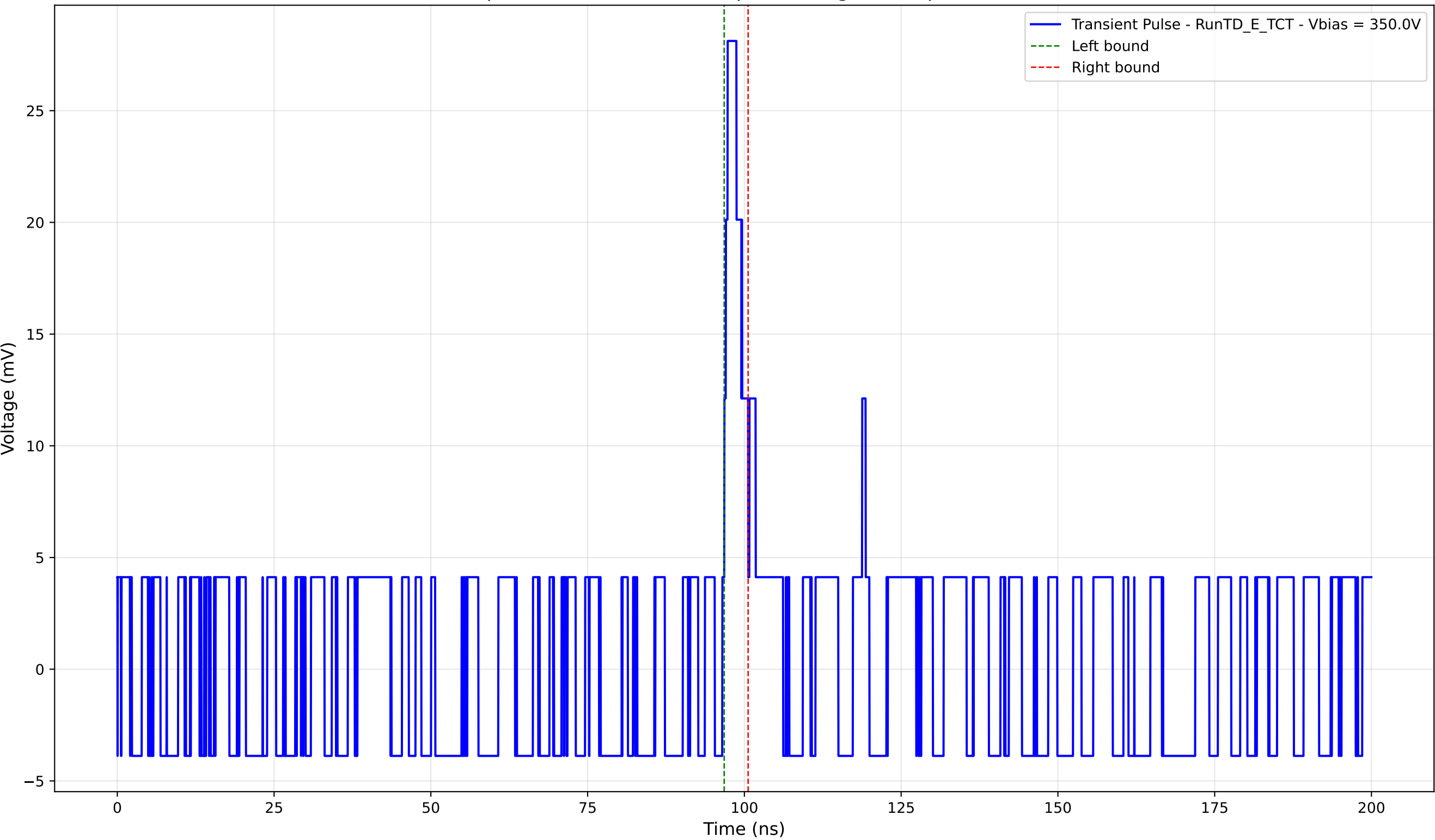
Transient Pulse - Sample: TD - Position: 700.0 \mu\text{m} - Charge: 1.56 pC - Rise Time: 0.00 ns (N/A)
