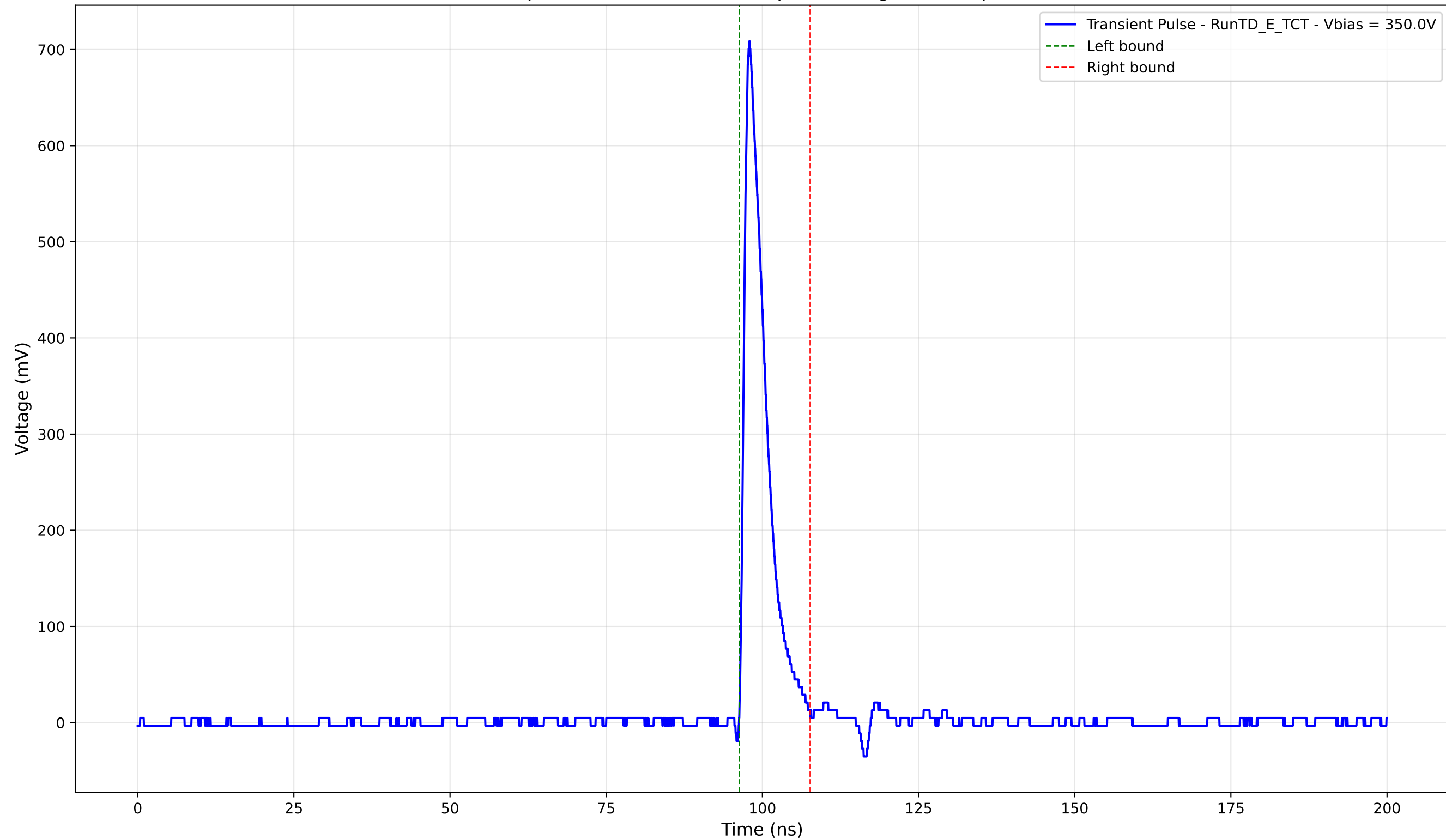
Transient Pulse - Sample: TD - Position: 280.0 \mu\text{m} - Charge: 55.76 pC - Rise Time: 1.00 ns
