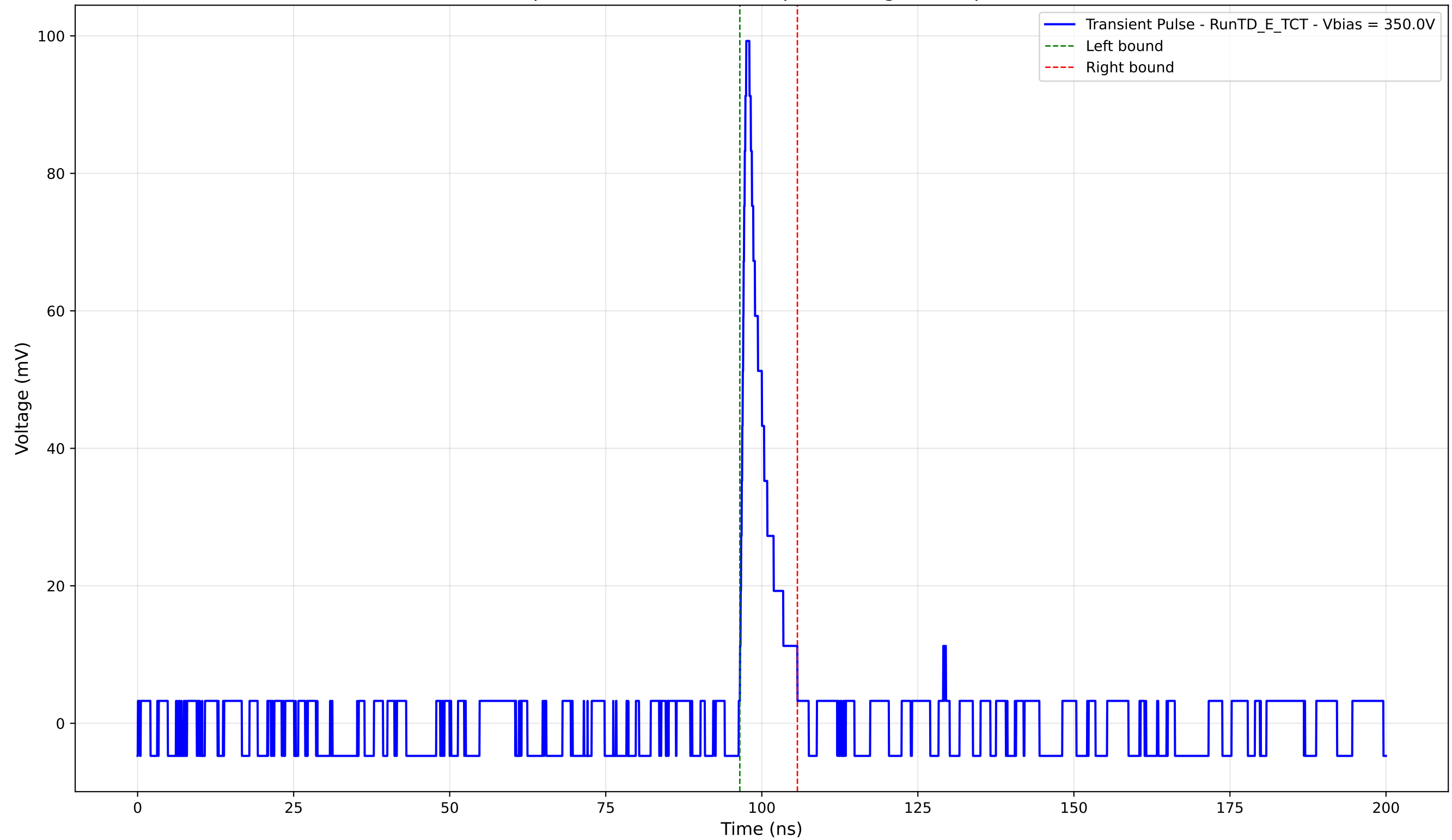
Transient Pulse - Sample: TD - Position: 610.0 \mu\text{m} - Charge: 7.03 pC - Rise Time: 0.86 ns
