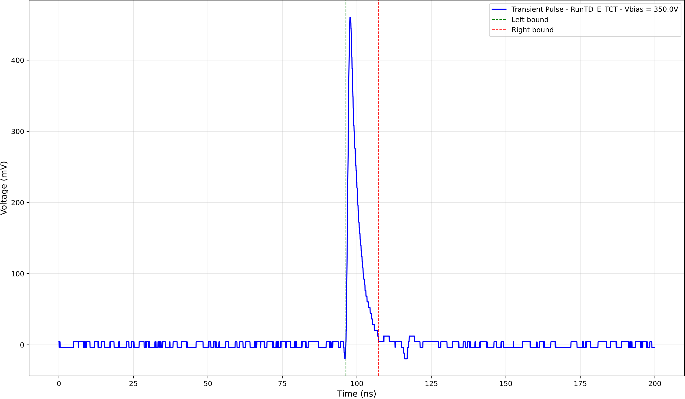
Transient Pulse - Sample: TD - Position: 80.0 \mu\text{m} - Charge: 33.62 pC - Rise Time: 0.92 ns
