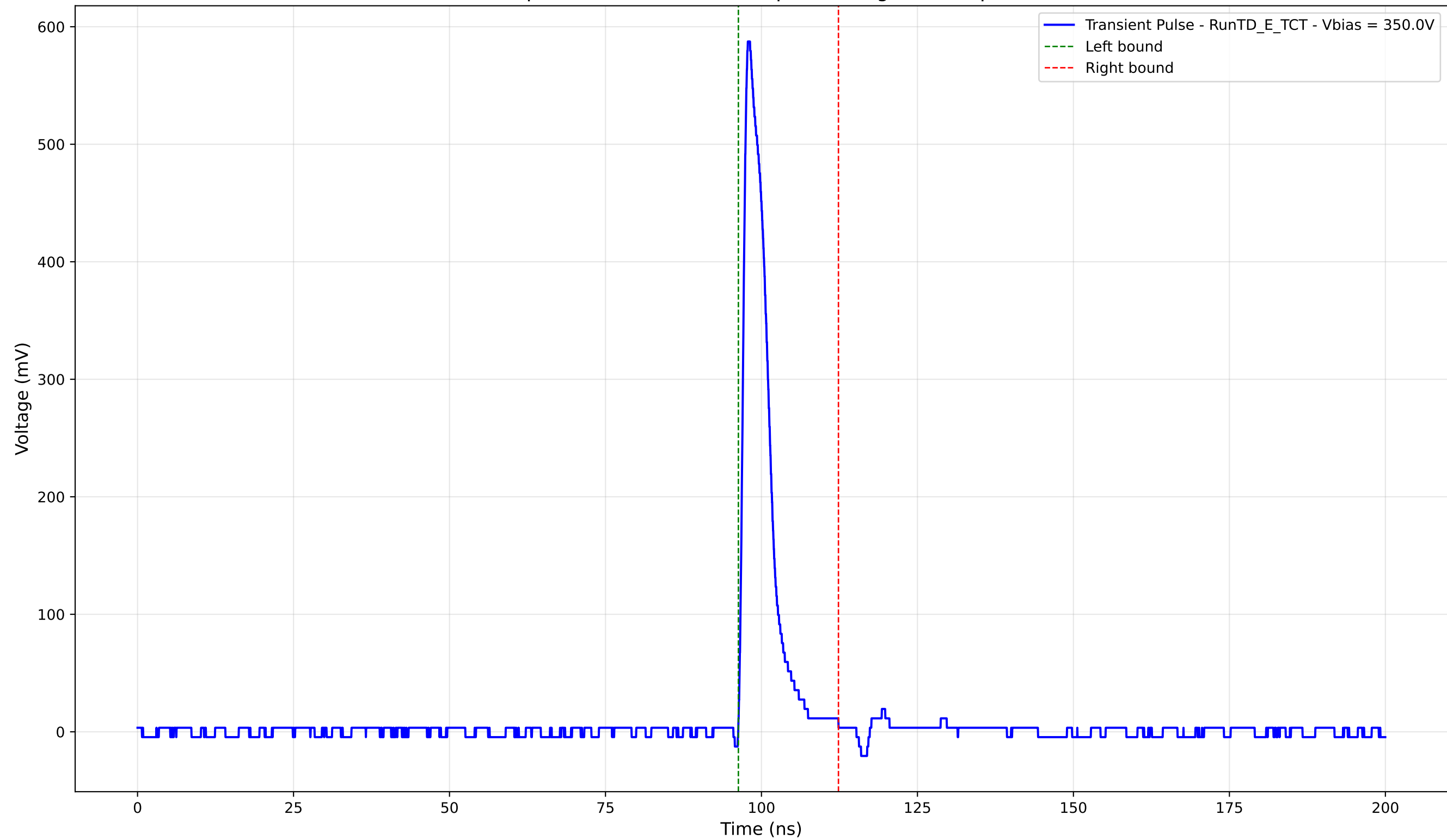
Transient Pulse - Sample: TD - Position: 335.0 \mu\text{m} - Charge: 51.91 pC - Rise Time: 1.00 ns
