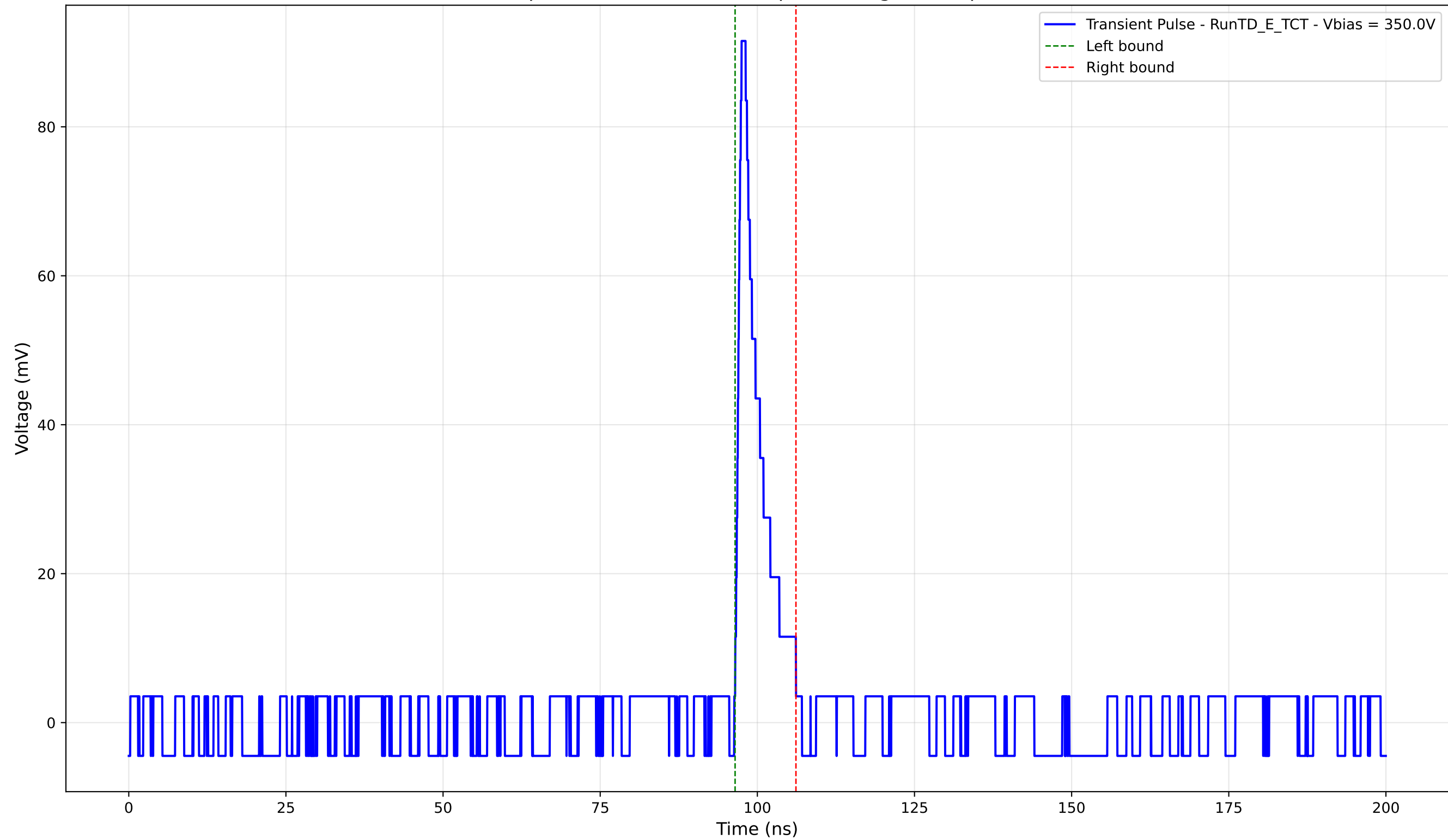
Transient Pulse - Sample: TD - Position: 620.0 \mu\text{m} - Charge: 6.93 pC - Rise Time: 0.89 ns
