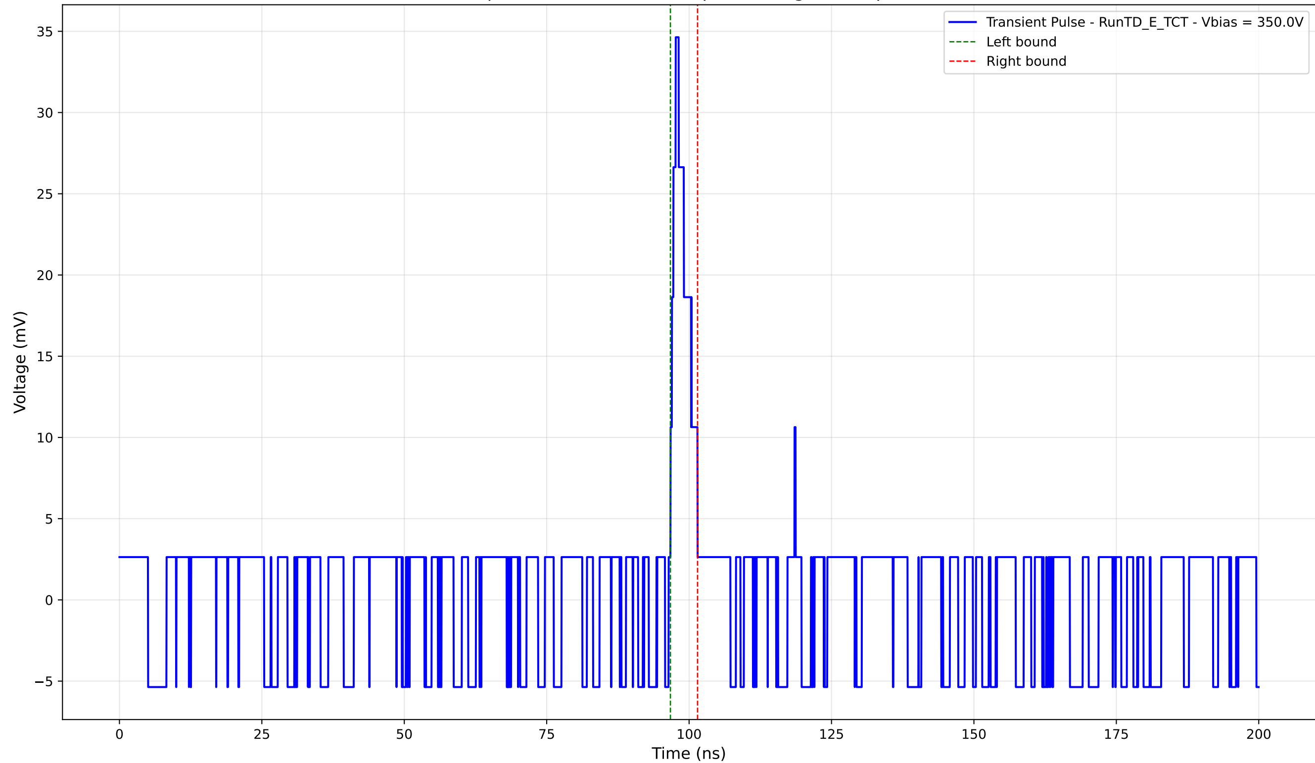
Transient Pulse - Sample: TD - Position: 30.0 \mu\text{m} - Charge: 1.94 pC - Rise Time: 0.92 ns
