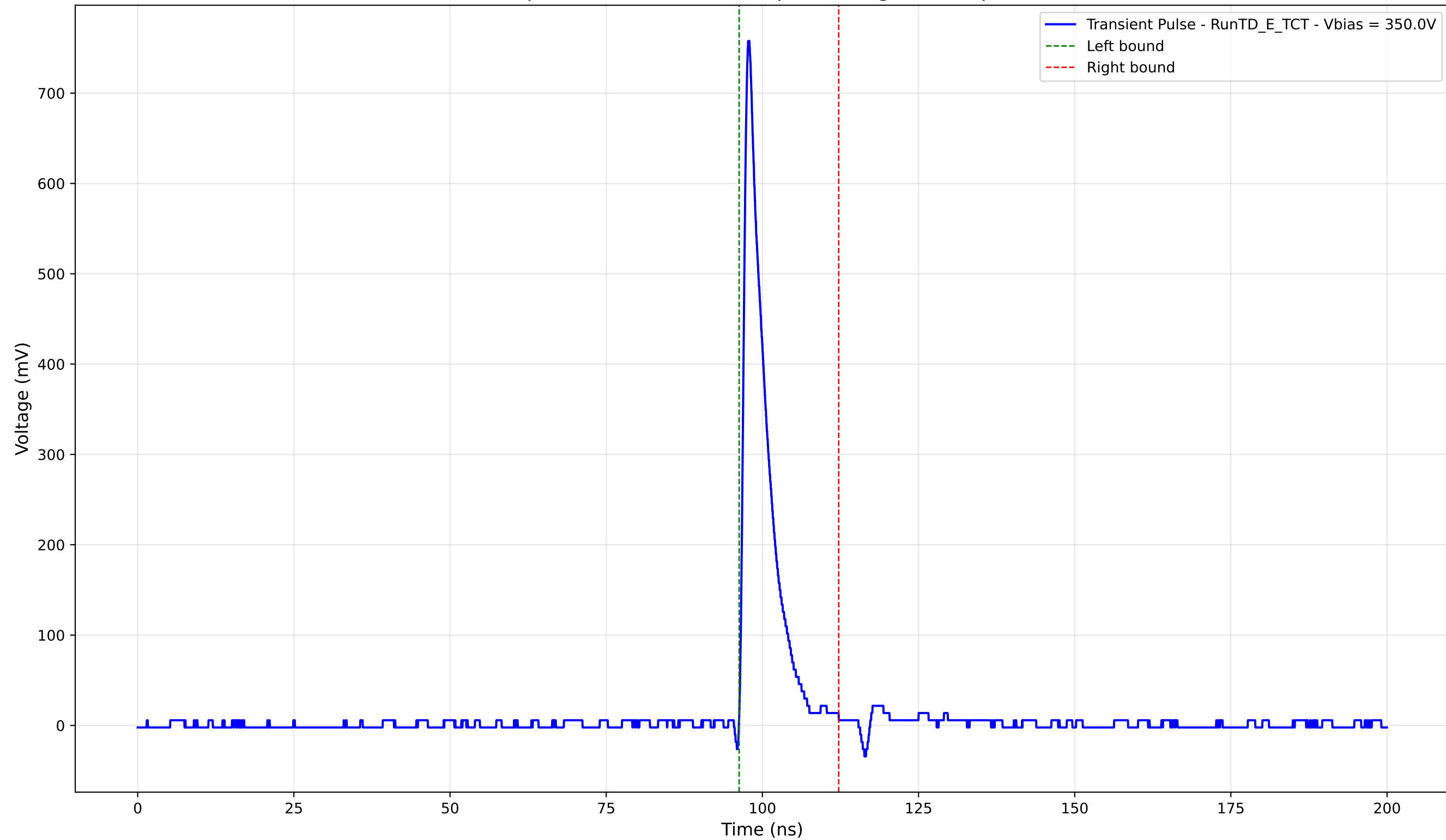
Transient Pulse - Sample: TD - Position: 215.0 \mu\text{m} - Charge: 61.47 pC - Rise Time: 0.94 ns
