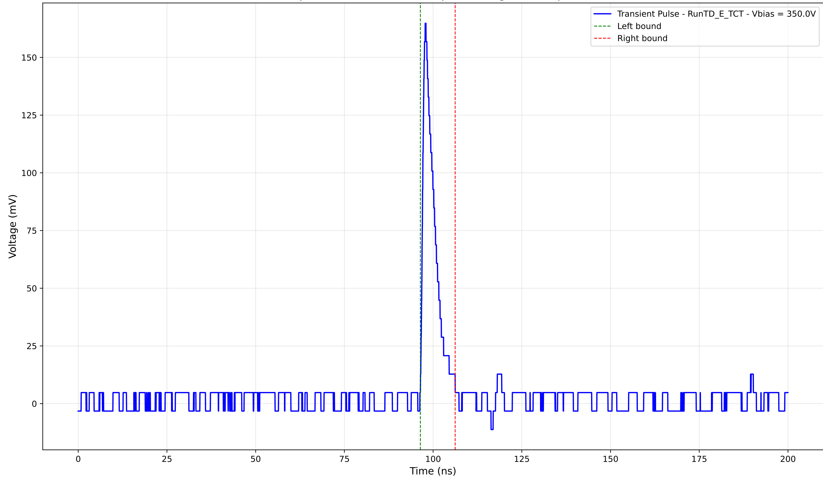
Transient Pulse - Sample: TD - Position: 460.0 \mu\text{m} - Charge: 12.54 pC - Rise Time: 0.93 ns
