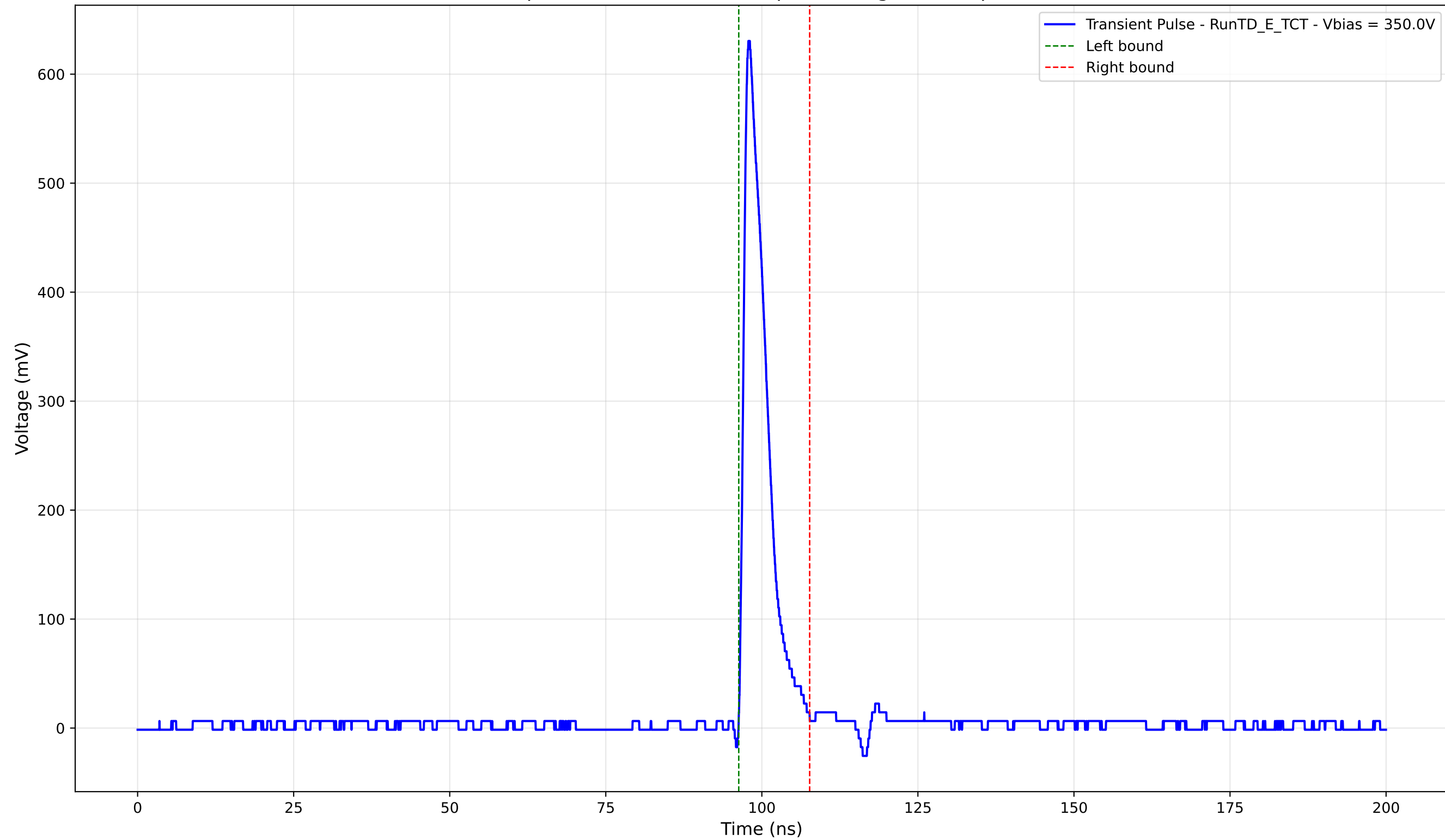
Transient Pulse - Sample: TD - Position: 310.0 \mu\text{m} - Charge: 51.79 pC - Rise Time: 1.00 ns
