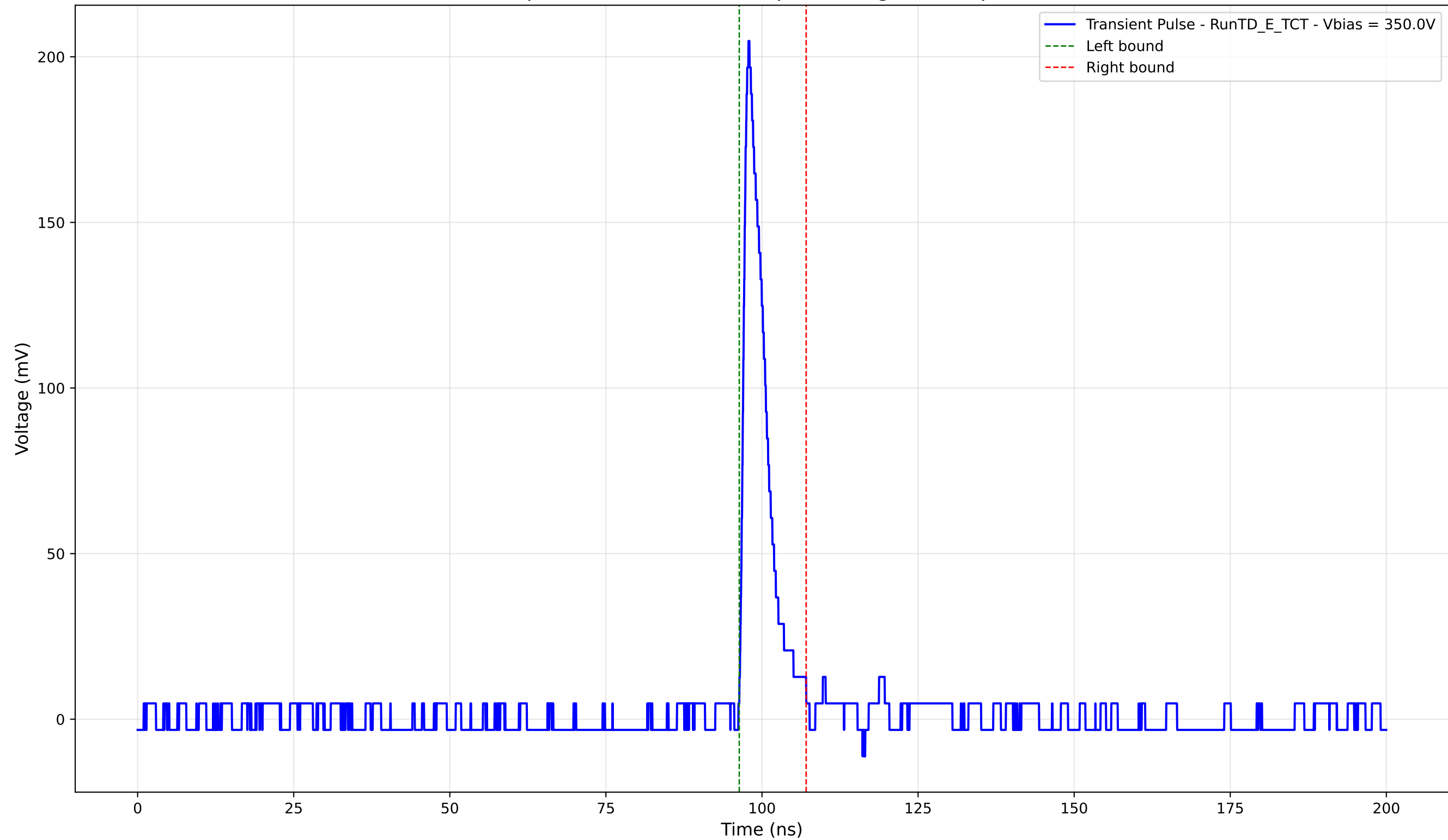
Transient Pulse - Sample: TD - Position: 500.0 \mu\text{m} - Charge: 15.99 pC - Rise Time: 1.04 ns
