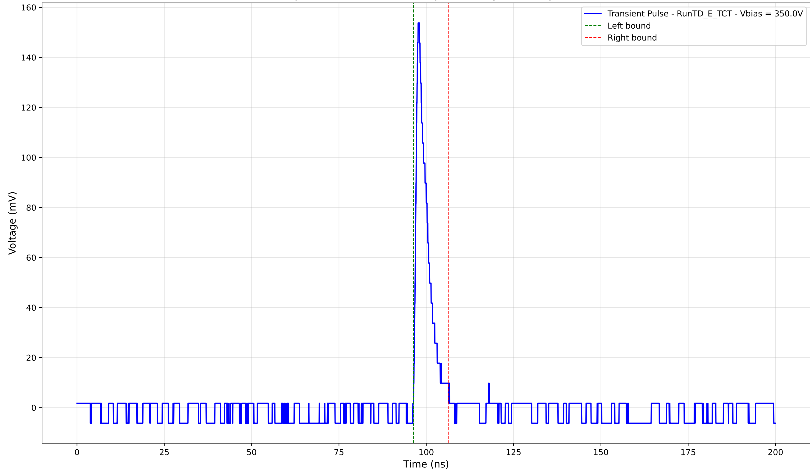
Transient Pulse - Sample: TD - Position: 440.0 \mu\text{m} - Charge: 11.26 pC - Rise Time: 1.05 ns
