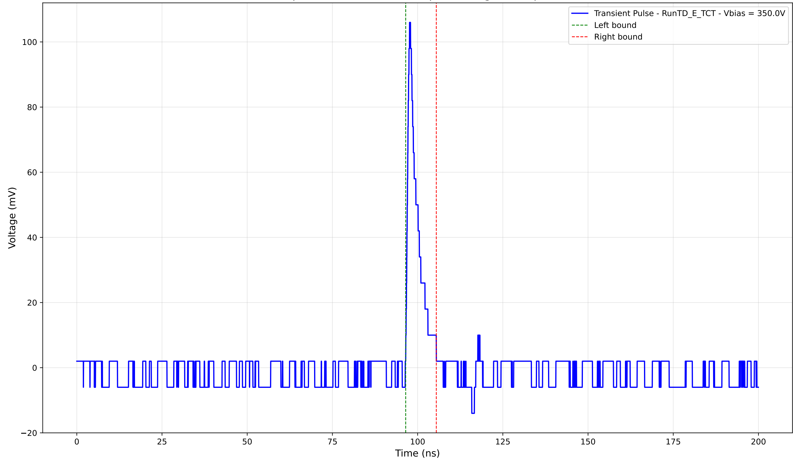
Transient Pulse - Sample: TD - Position: 605.0 \mu\text{m} - Charge: 6.92 pC - Rise Time: 0.86 ns
