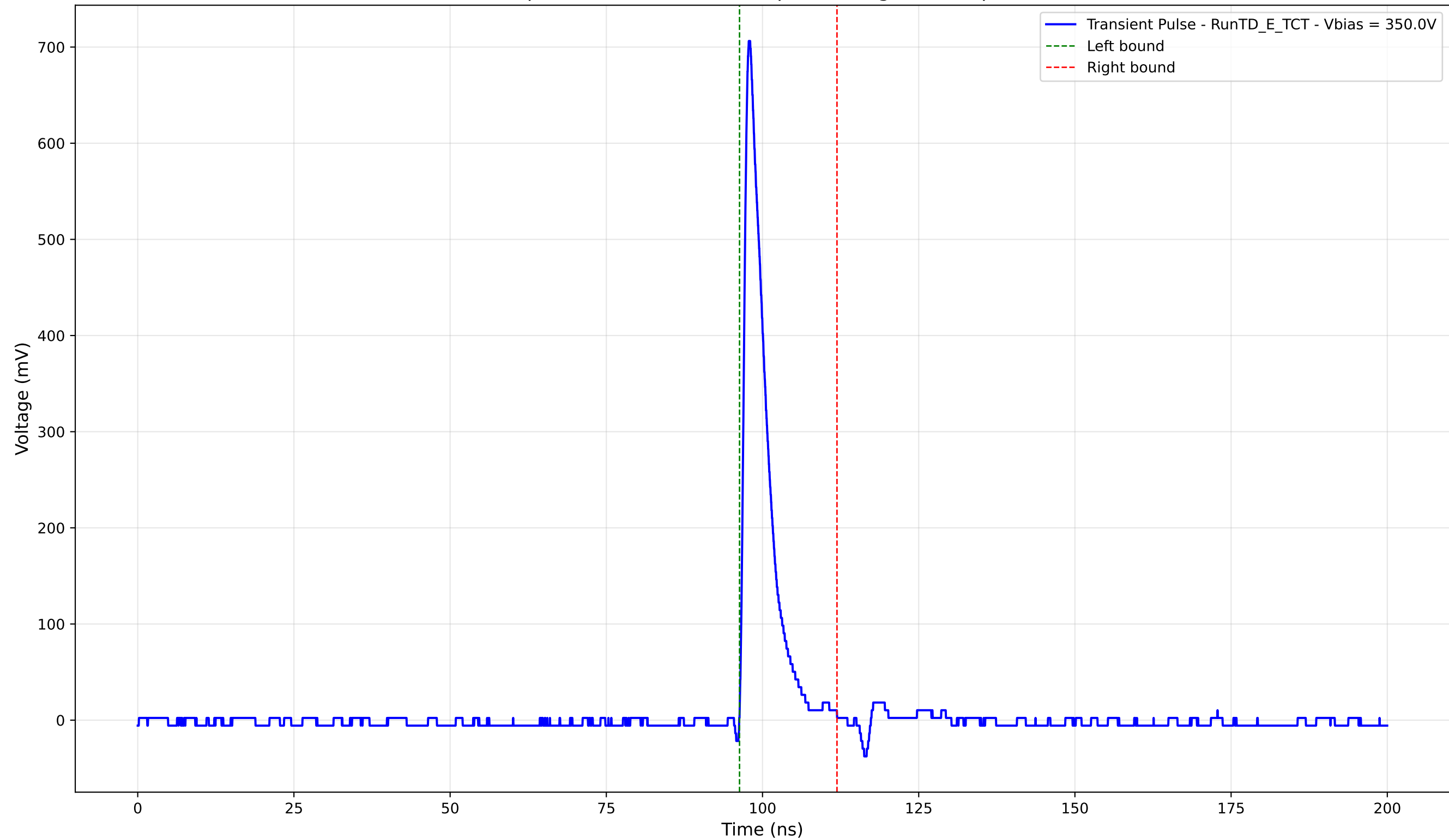
Transient Pulse - Sample: TD - Position: 265.0 \mu\text{m} - Charge: 55.65 pC - Rise Time: 0.95 ns
