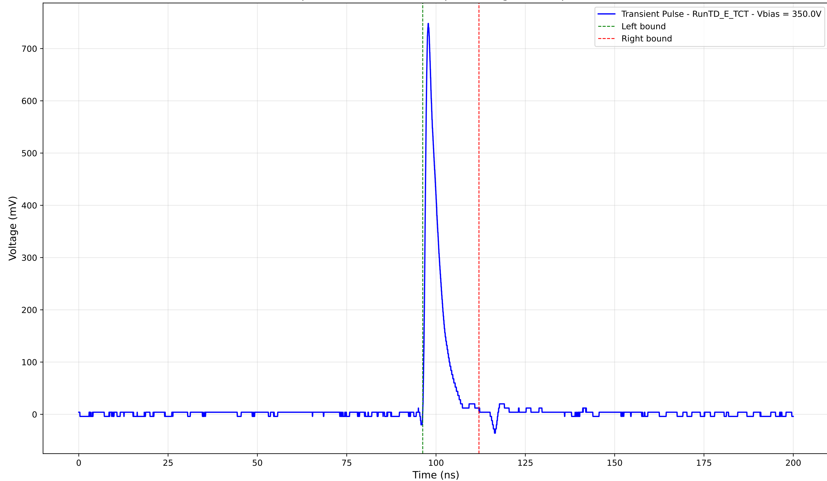
Transient Pulse - Sample: TD - Position: 220.0 \mu\text{m} - Charge: 59.74 pC - Rise Time: 0.96 ns
