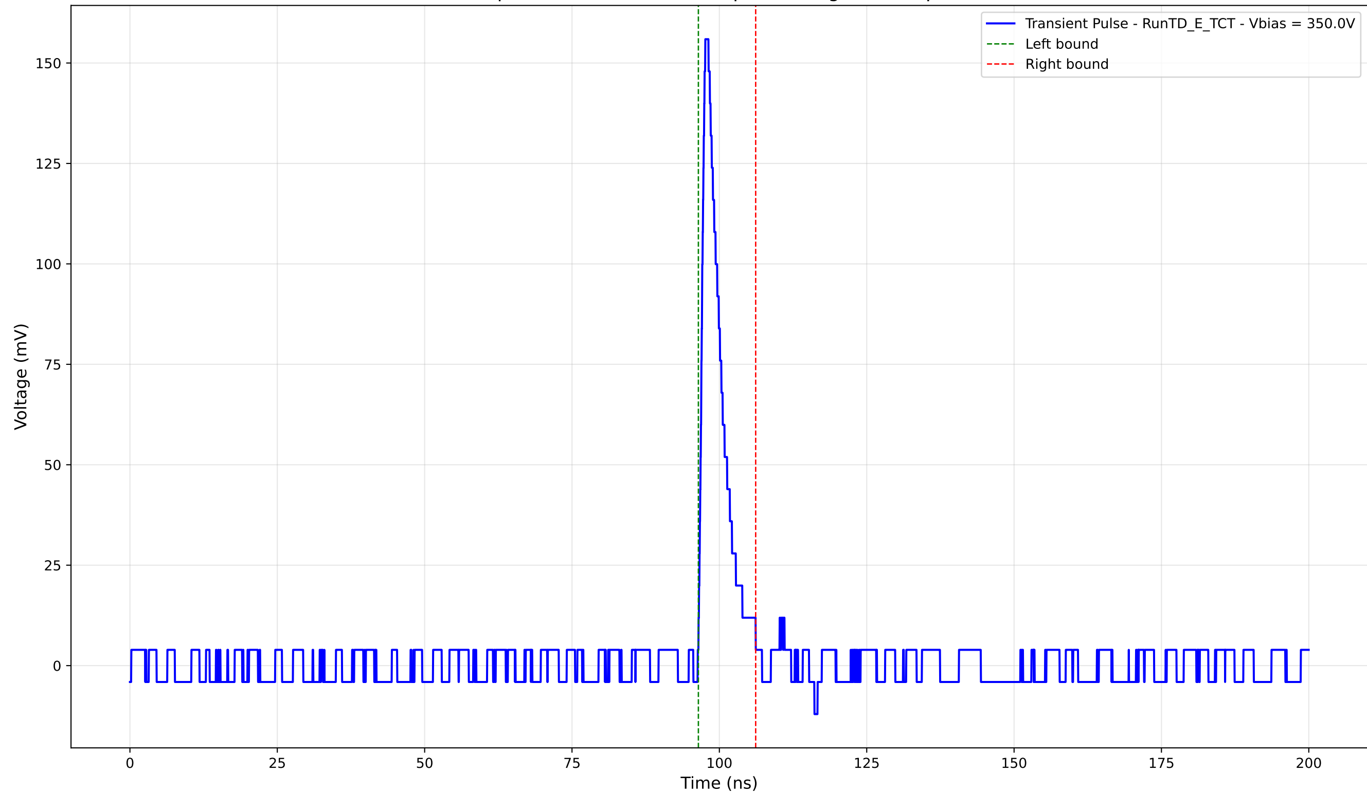
Transient Pulse - Sample: TD - Position: 540.0 \mu\text{m} - Charge: 11.55 pC - Rise Time: 0.95 ns
