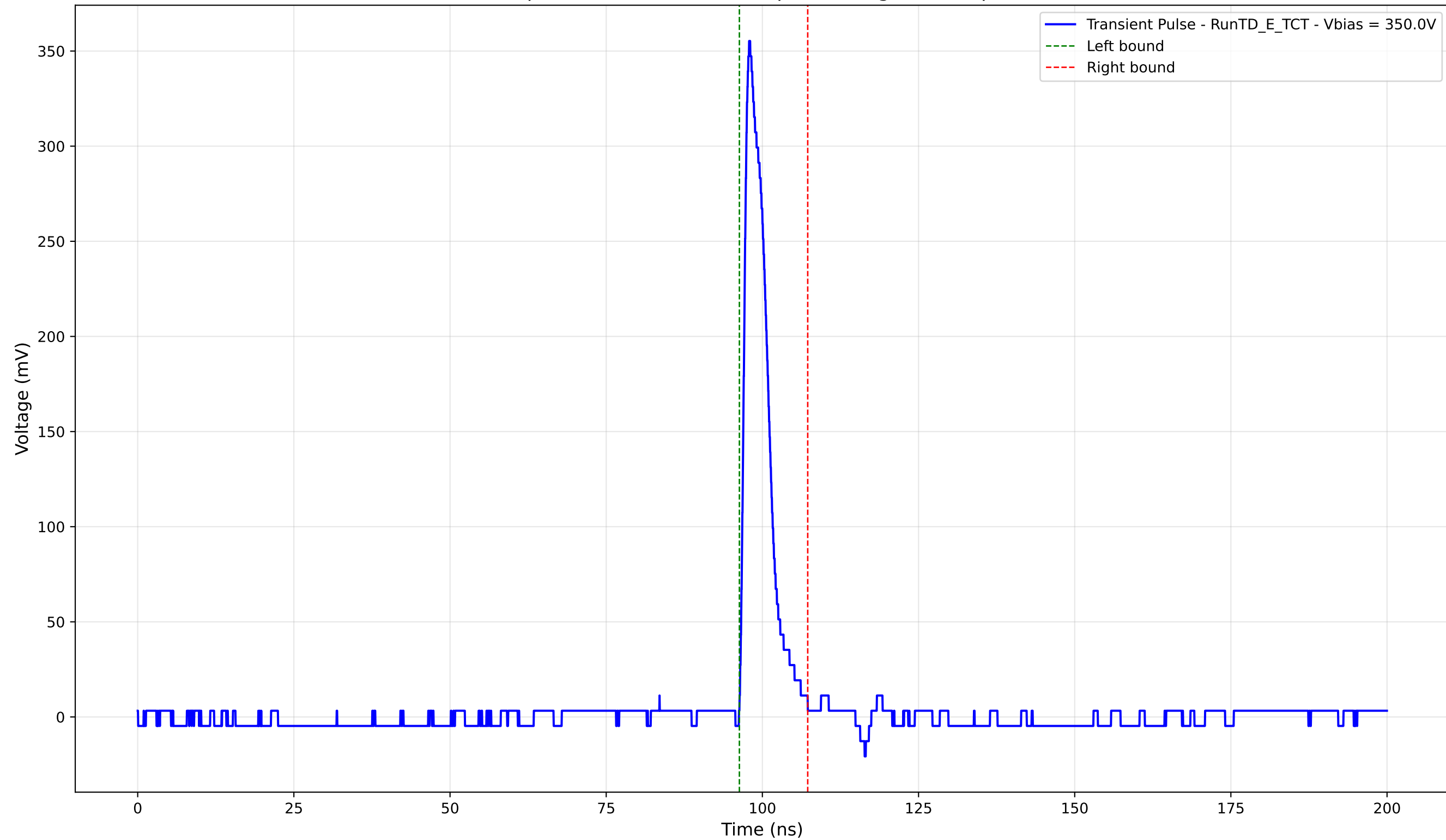
Transient Pulse - Sample: TD - Position: 380.0 \mu\text{m} - Charge: 29.07 pC - Rise Time: 1.00 ns
