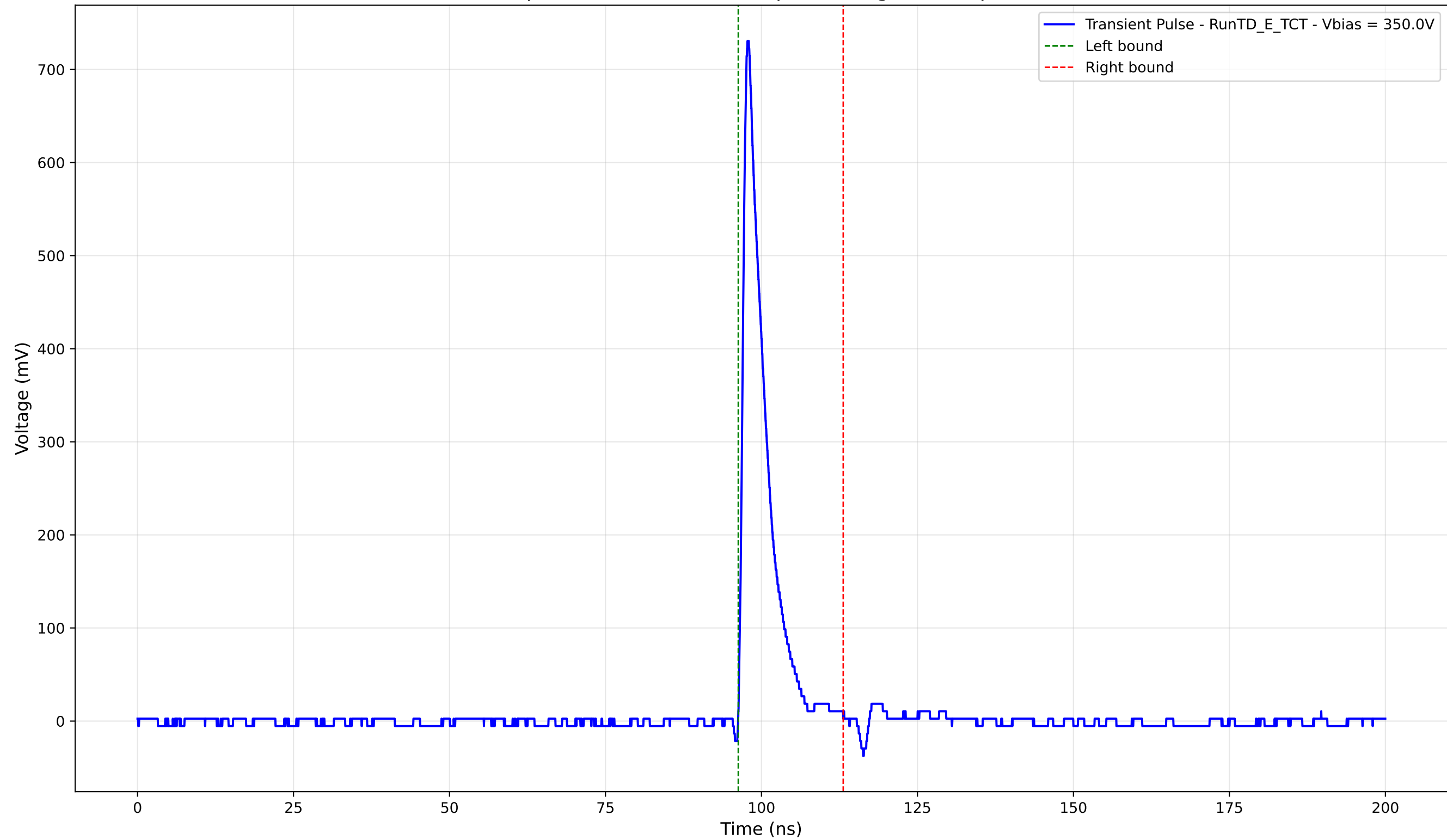
Transient Pulse - Sample: TD - Position: 225.0 \mu\text{m} - Charge: 58.83 pC - Rise Time: 0.94 ns
