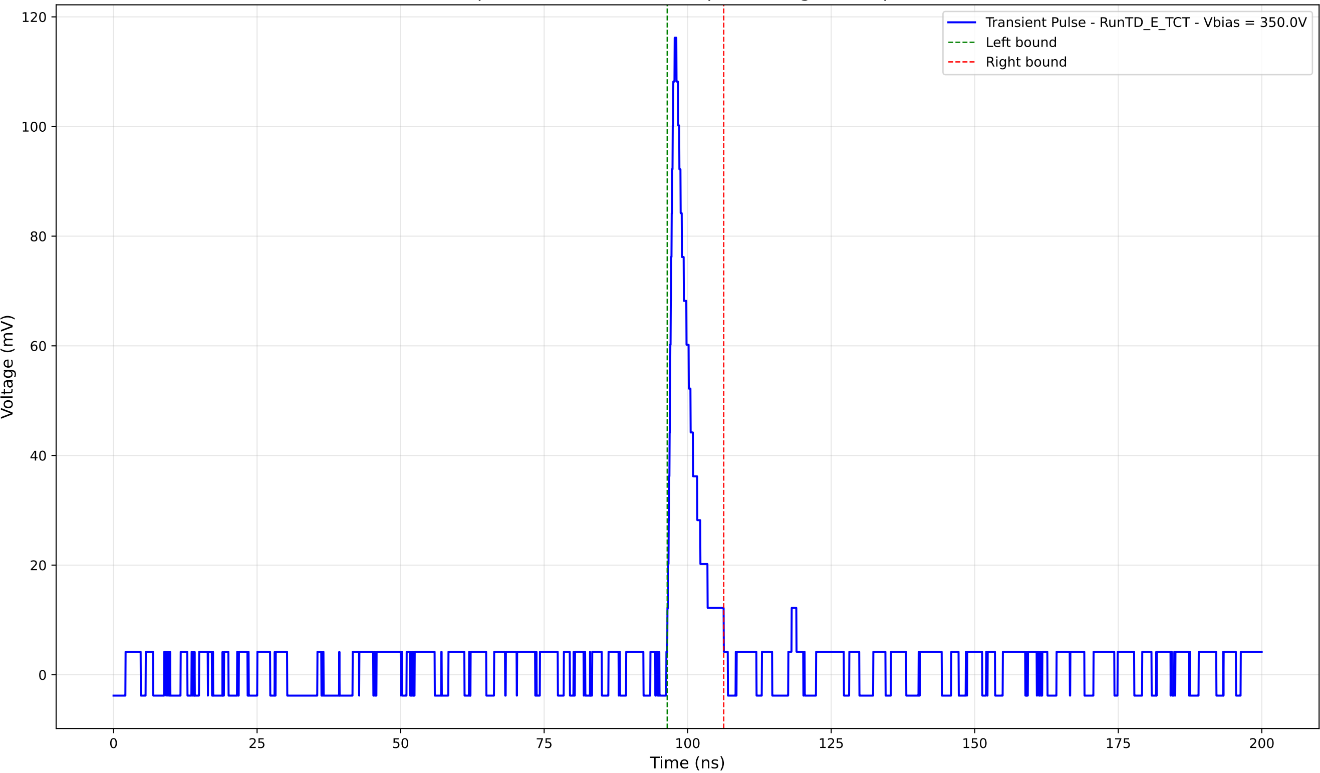
Transient Pulse - Sample: TD - Position: 575.0 \mu\text{m} - Charge: 8.59 pC - Rise Time: 1.02 ns
