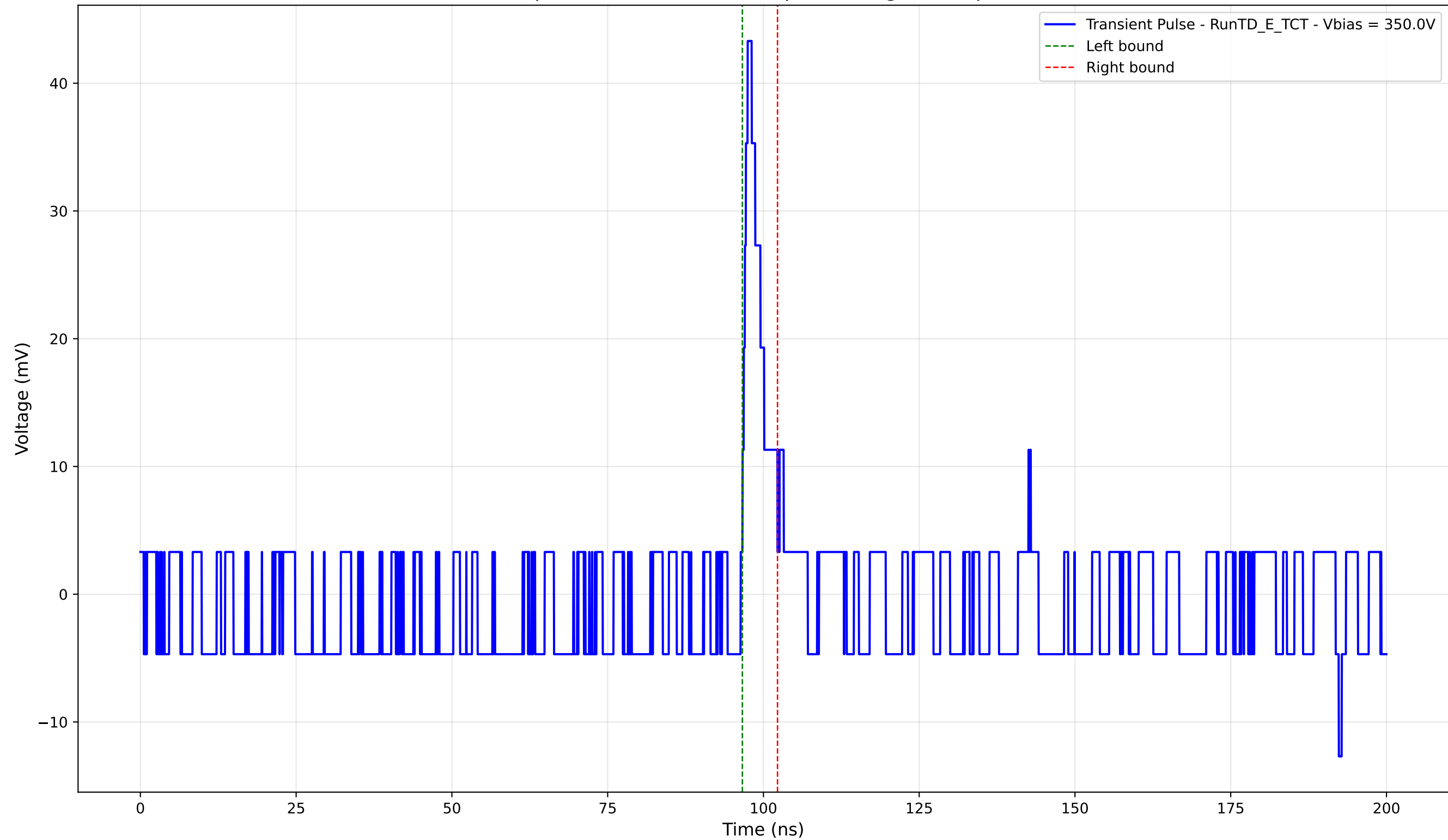
Transient Pulse - Sample: TD - Position: 685.0 \mu\text{m} - Charge: 2.54 pC - Rise Time: 0.84 ns
