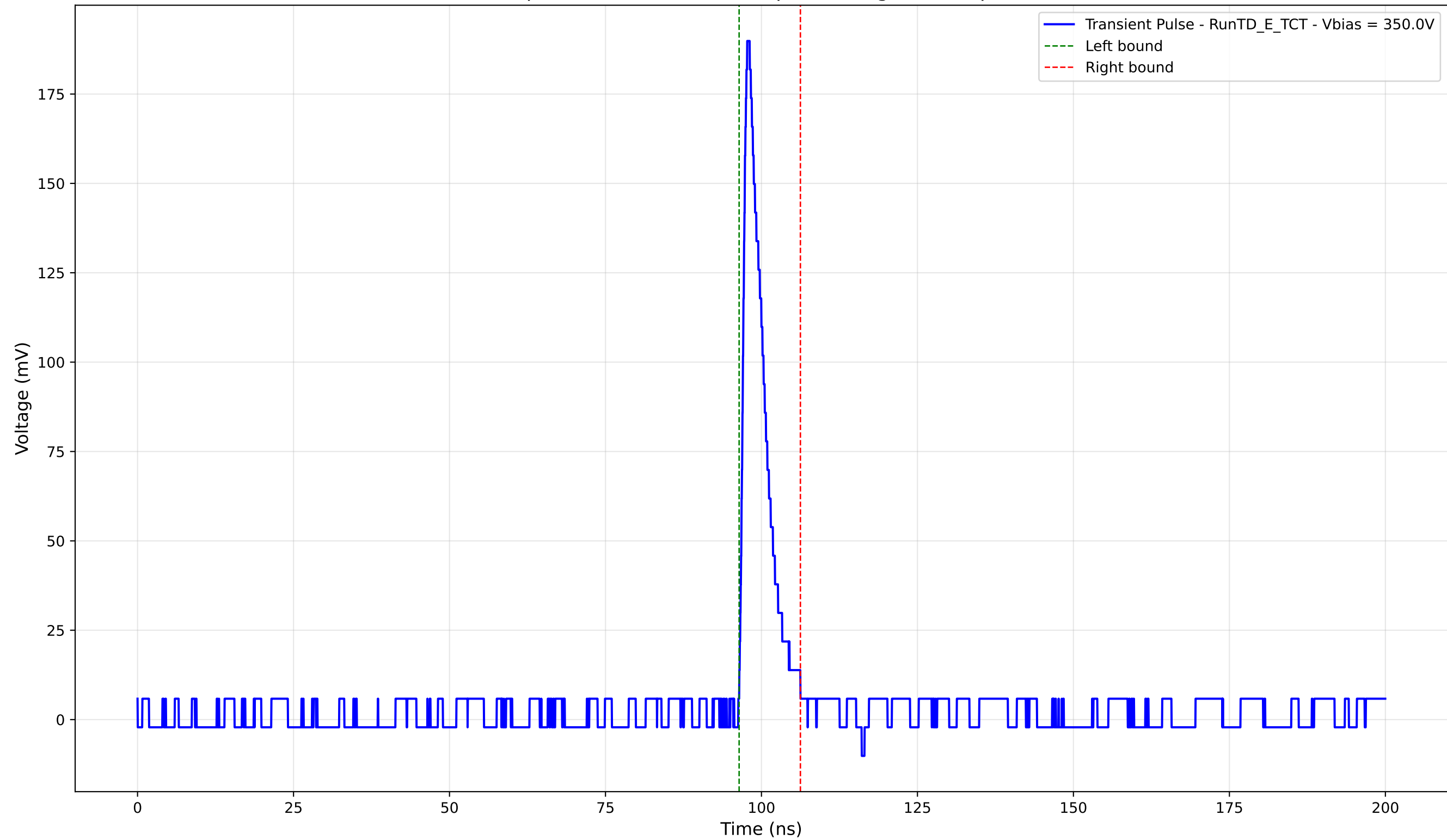
Transient Pulse - Sample: TD - Position: 510.0 \mu\text{m} - Charge: 14.52 pC - Rise Time: 0.99 ns
