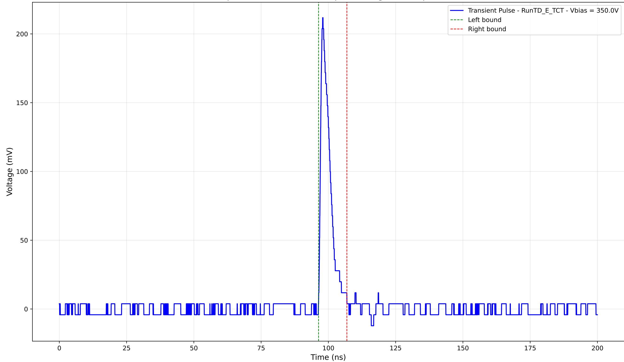
Transient Pulse - Sample: TD - Position: 495.0 \mu\text{m} - Charge: 16.52 pC - Rise Time: 1.02 ns
