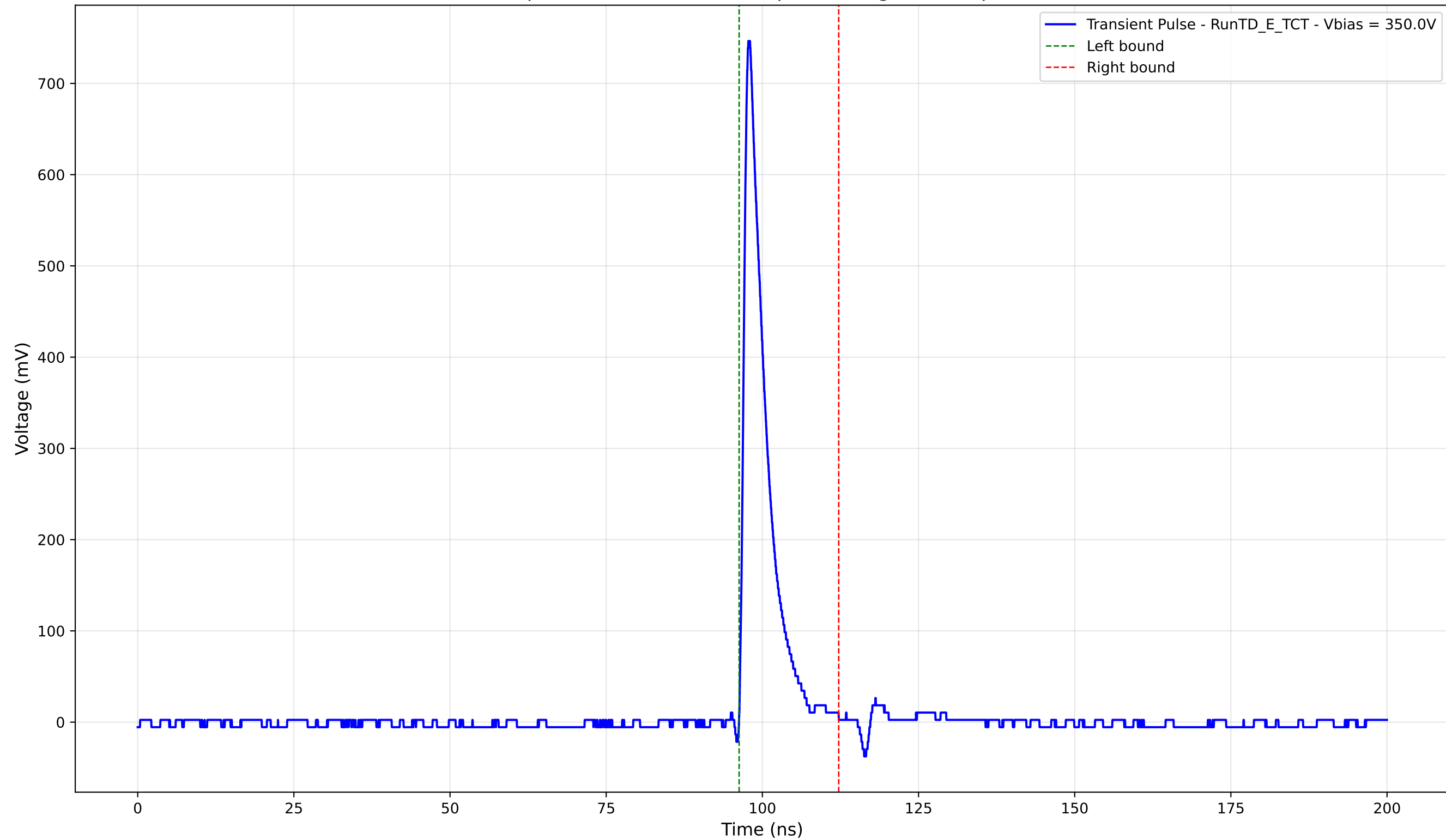
Transient Pulse - Sample: TD - Position: 110.0 \mu\text{m} - Charge: 59.32 pC - Rise Time: 0.95 ns
