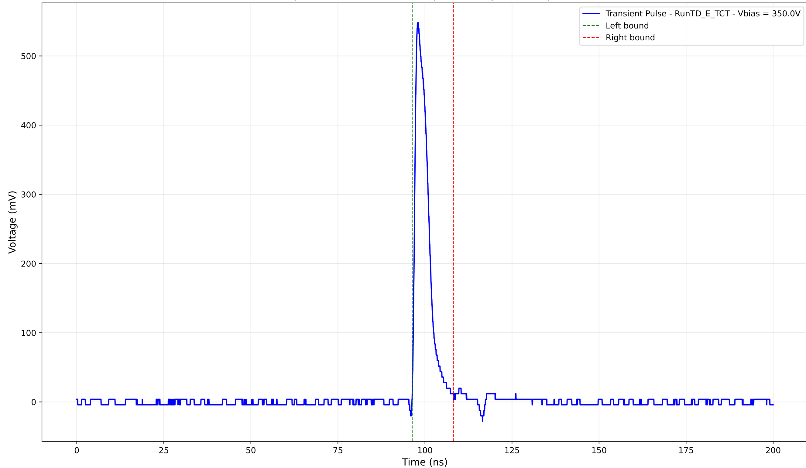
Transient Pulse - Sample: TD - Position: 350.0 \mu\text{m} - Charge: 47.41 pC - Rise Time: 1.00 ns
