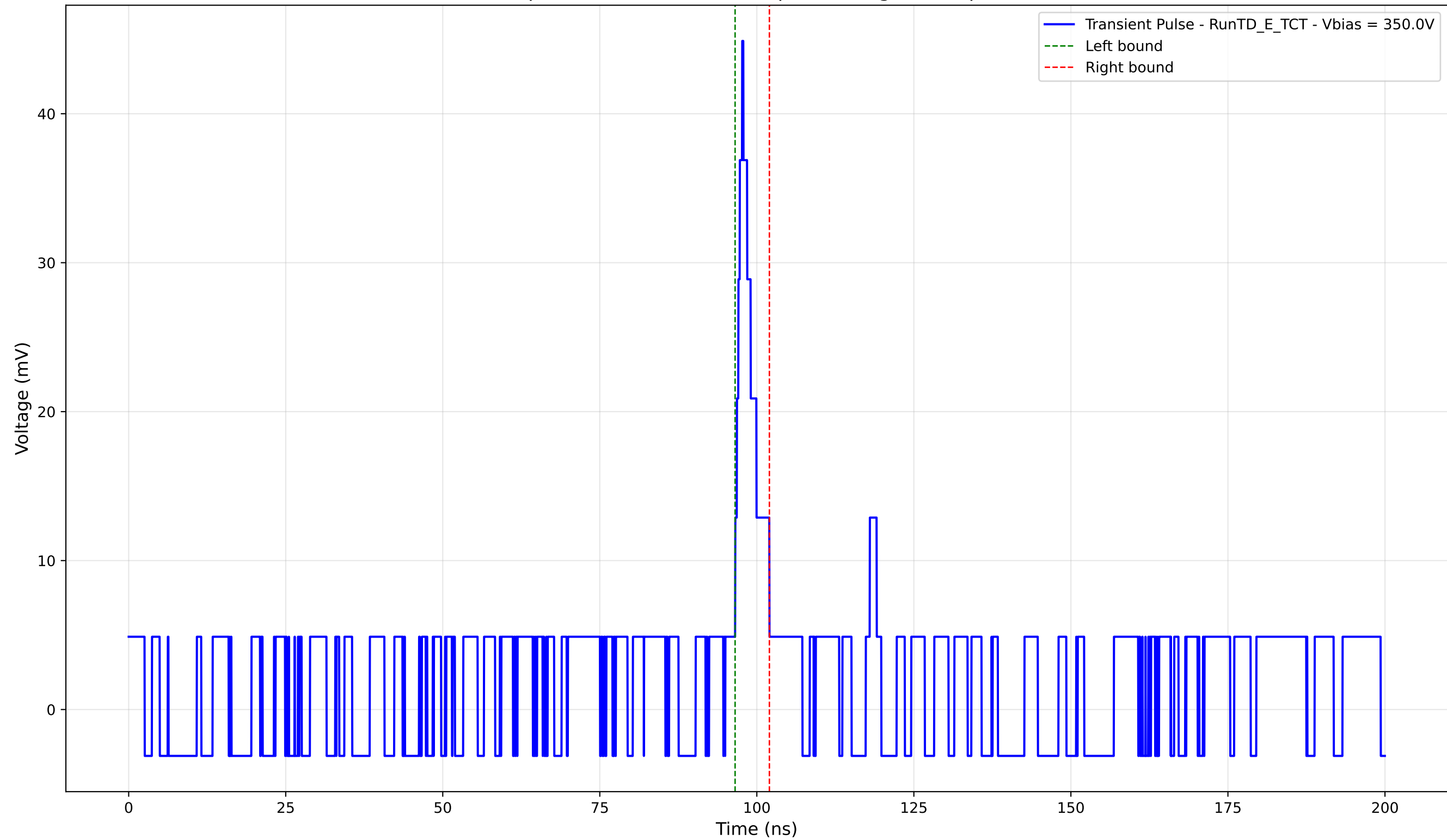
Transient Pulse - Sample: TD - Position: 690.0 \mu\text{m} - Charge: 2.44 pC - Rise Time: 2.68 ns
