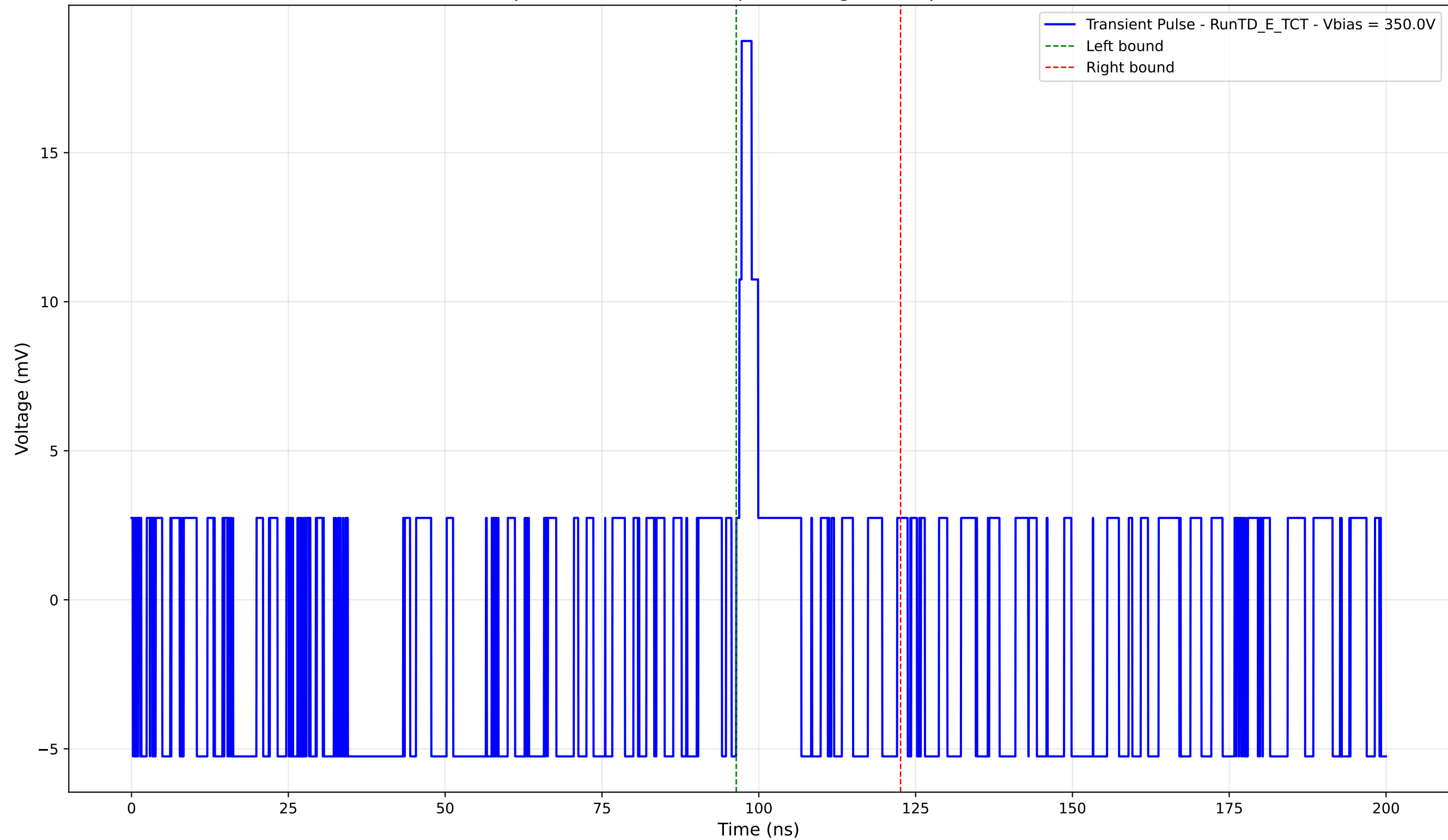
Transient Pulse - Sample: TD - Position: 5.0 \mu\text{m} - Charge: 0.66 pC - Rise Time: 0.00 ns (N/A)
