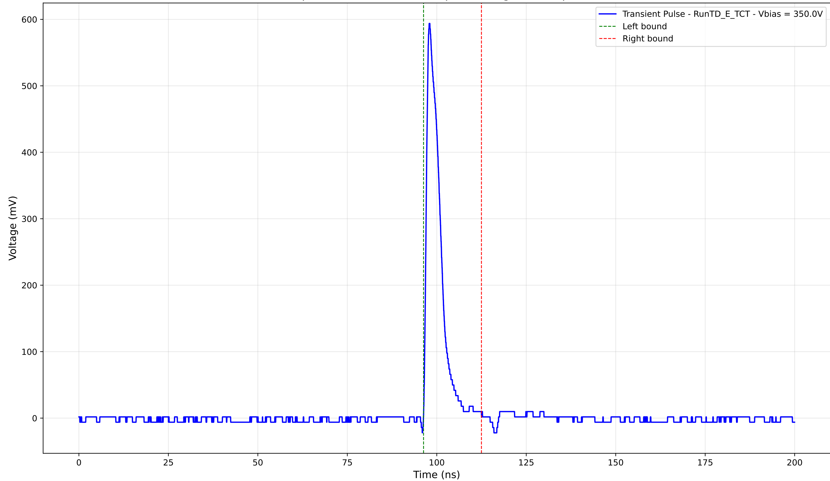
Transient Pulse - Sample: TD - Position: 320.0 \mu\text{m} - Charge: 51.35 pC - Rise Time: 1.00 ns
