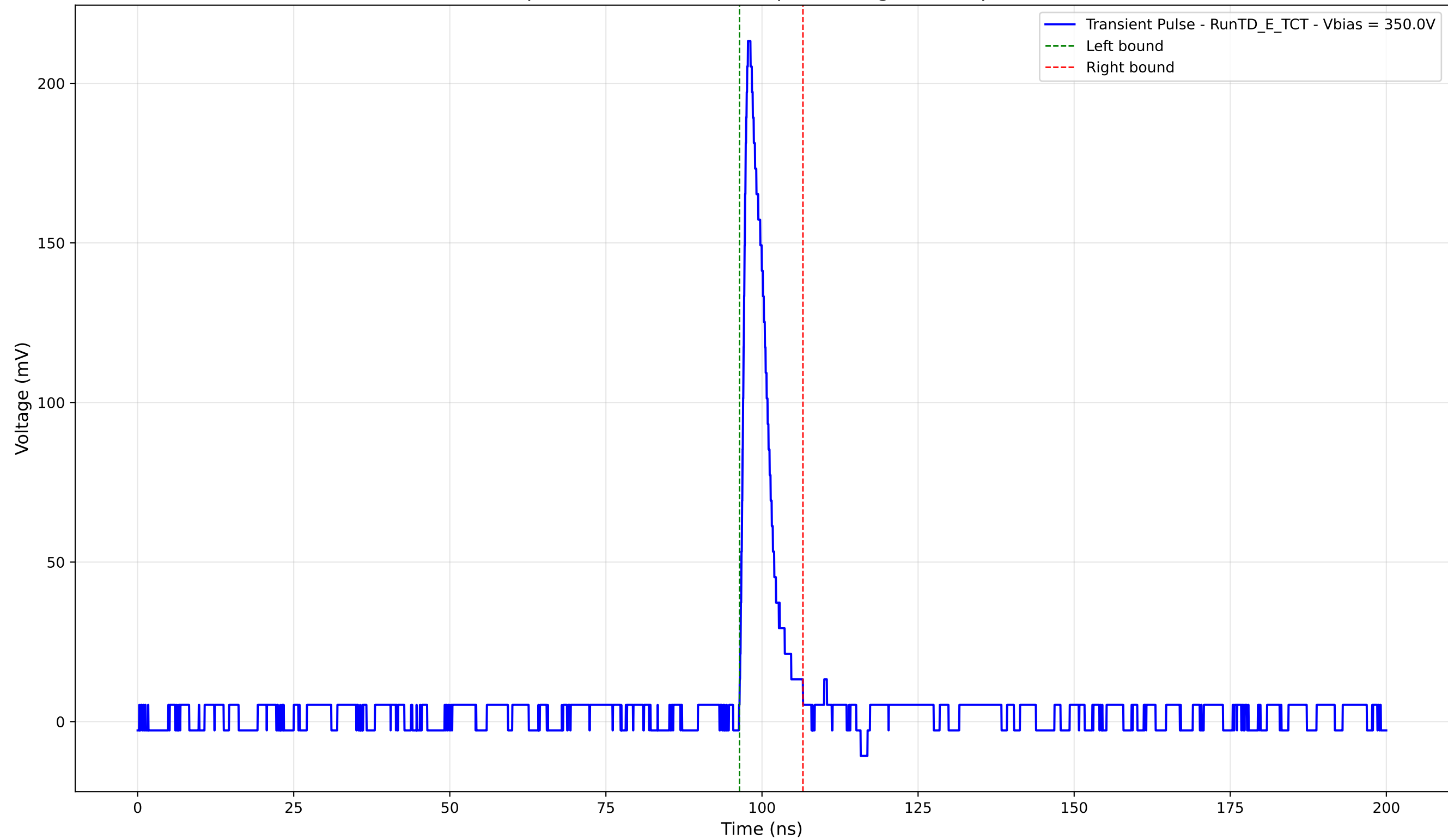
Transient Pulse - Sample: TD - Position: 490.0 \mu\text{m} - Charge: 16.99 pC - Rise Time: 0.98 ns
