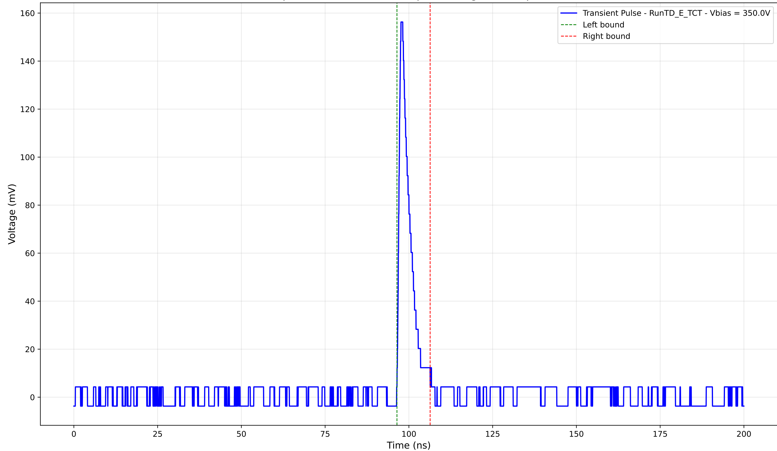
Transient Pulse - Sample: TD - Position: 545.0 \mu\text{m} - Charge: 11.46 pC - Rise Time: 0.95 ns
