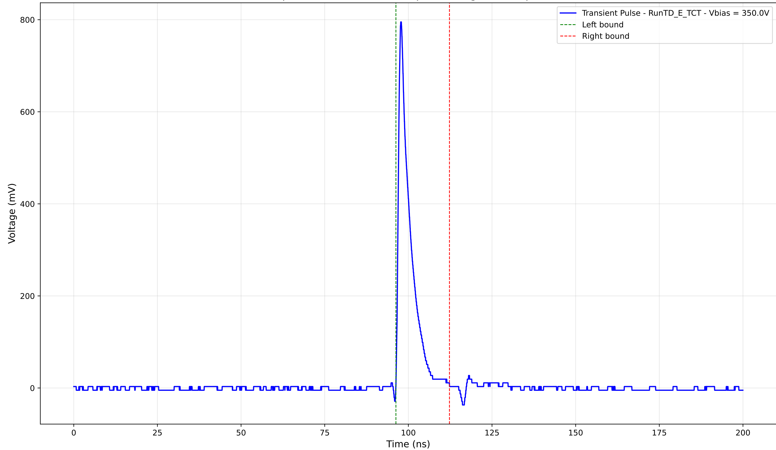
Transient Pulse - Sample: TD - Position: 160.0 \mu\text{m} - Charge: 63.02 pC - Rise Time: 0.93 ns
