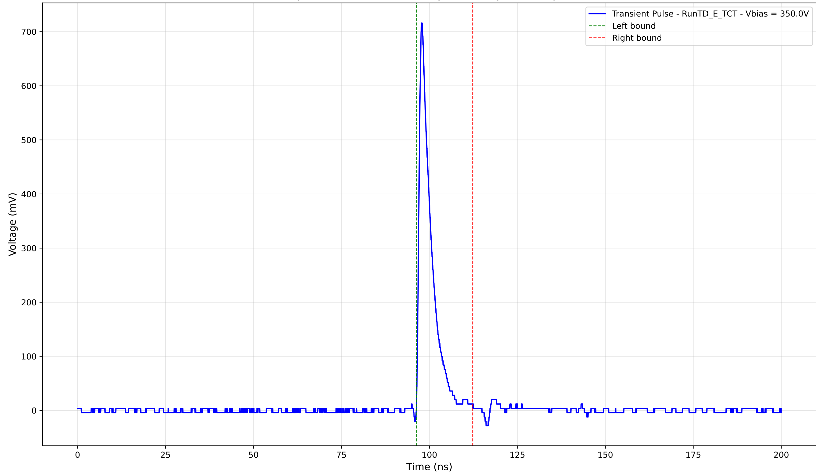
Transient Pulse - Sample: TD - Position: 100.0 \mu\text{m} - Charge: 56.12 pC - Rise Time: 0.95 ns
