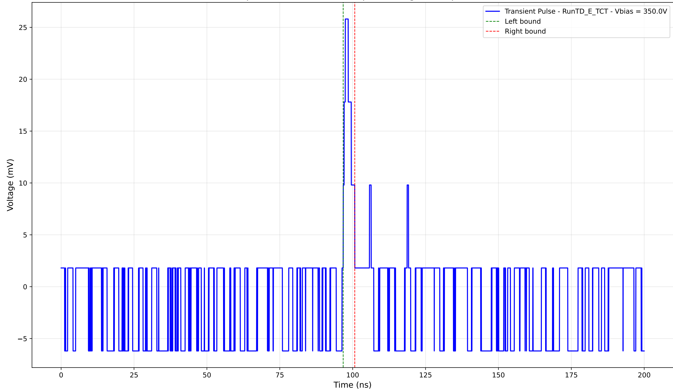
Transient Pulse - Sample: TD - Position: 710.0 \mu\text{m} - Charge: 1.33 pC - Rise Time: 0.72 ns
