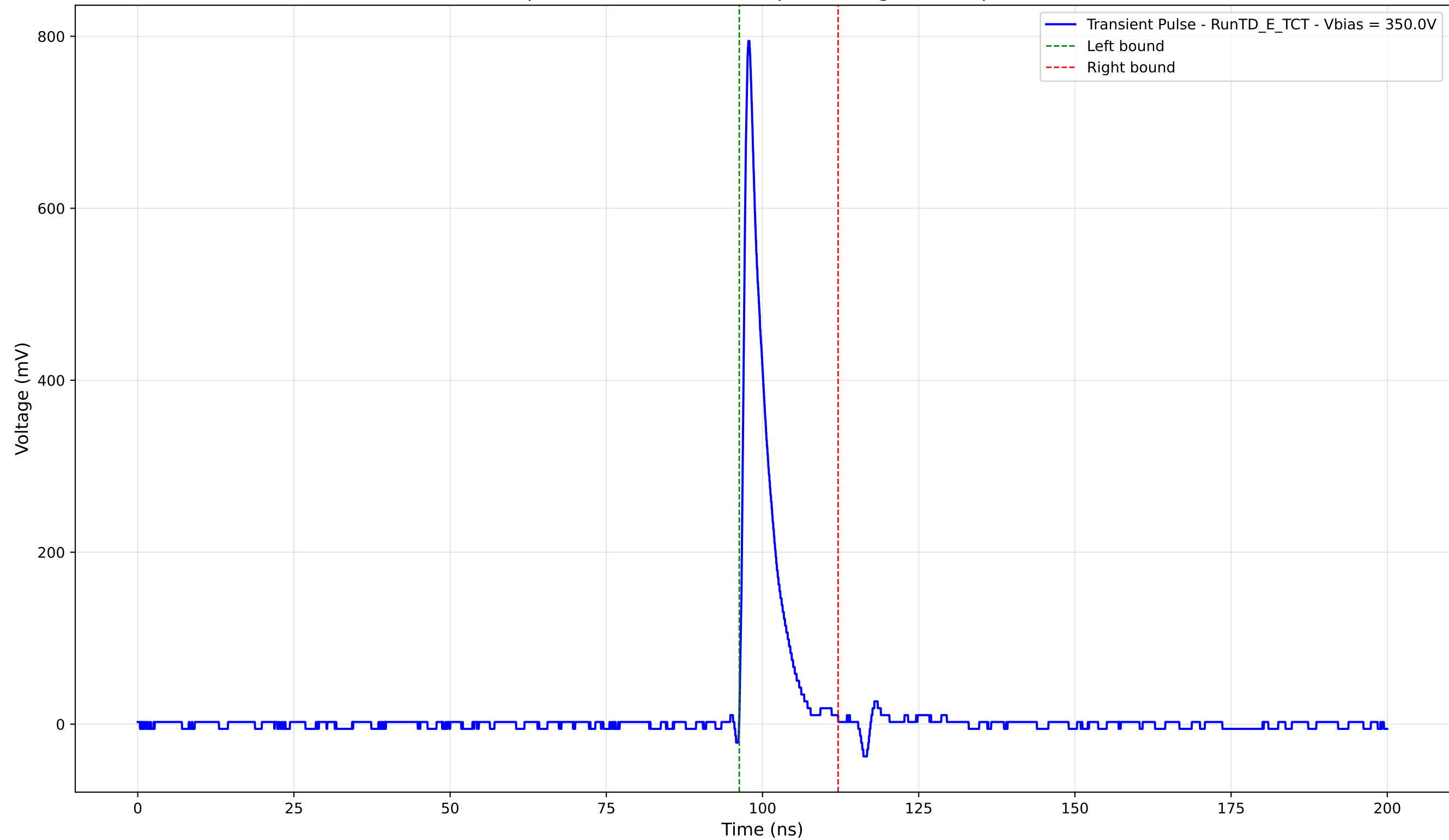
Transient Pulse - Sample: TD - Position: 150.0 \mu\text{m} - Charge: 62.25 pC - Rise Time: 0.93 ns
