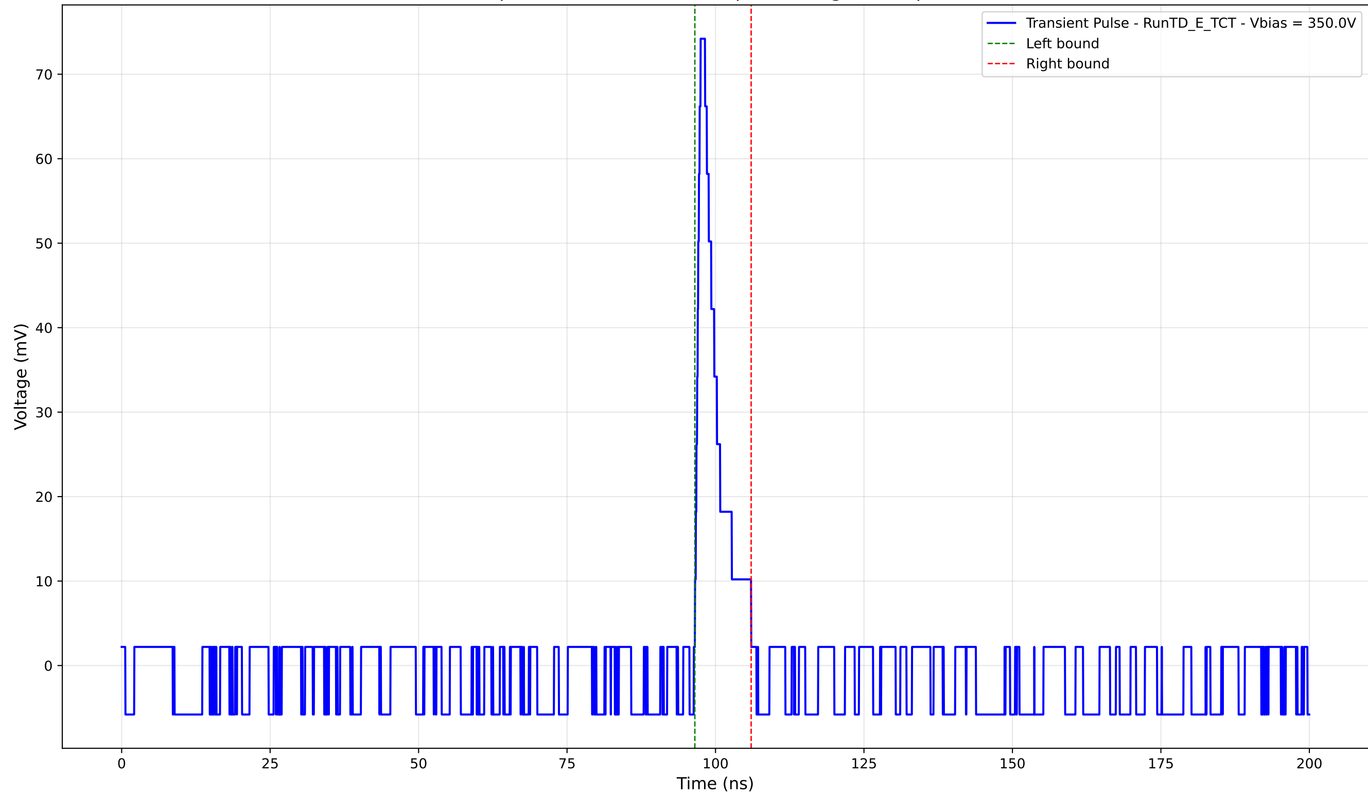
Transient Pulse - Sample: TD - Position: 640.0 \mu\text{m} - Charge: 5.45 pC - Rise Time: 0.95 ns
