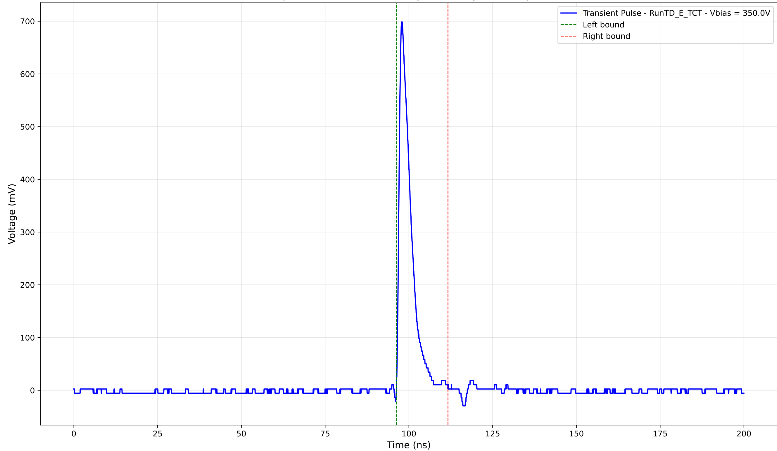
Transient Pulse - Sample: TD - Position: 290.0 \mu\text{m} - Charge: 55.97 pC - Rise Time: 0.98 ns
