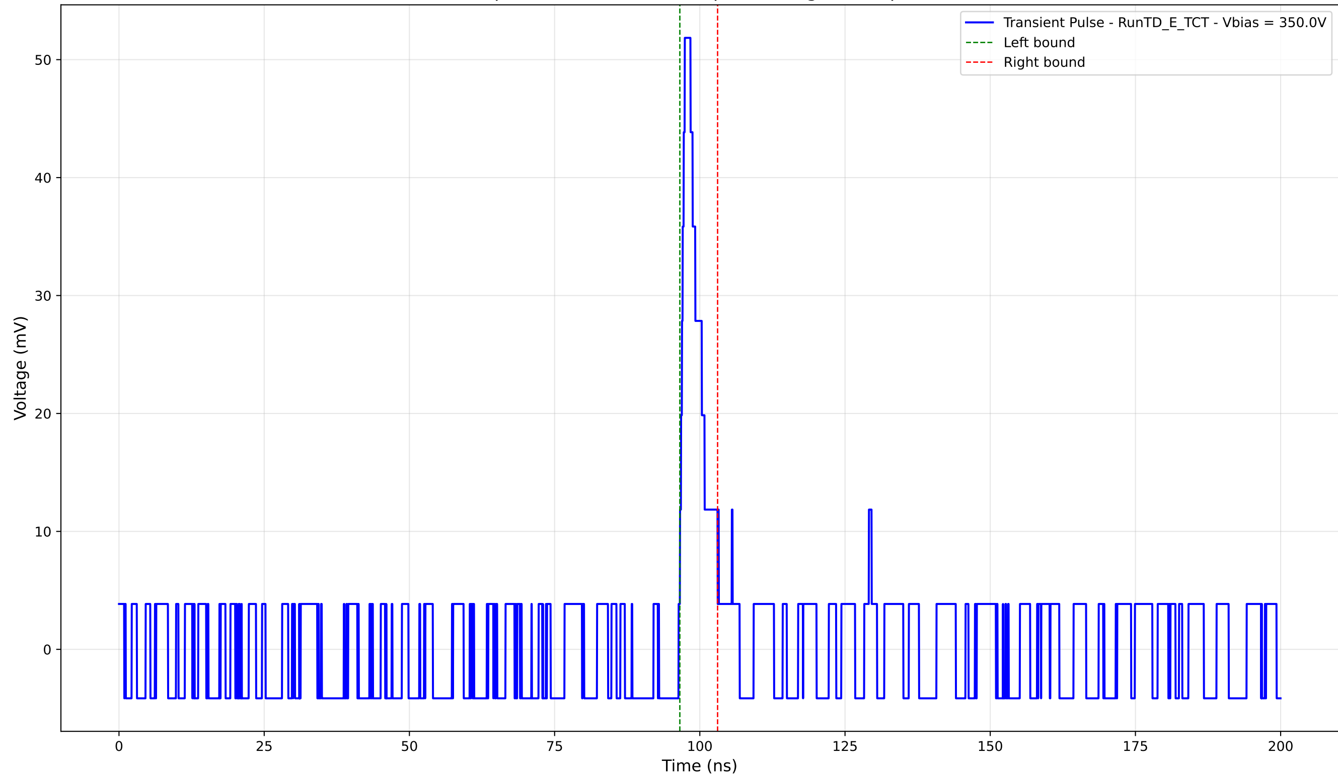
Transient Pulse - Sample: TD - Position: 45.0 \mu\text{m} - Charge: 3.49 pC - Rise Time: 0.84 ns
