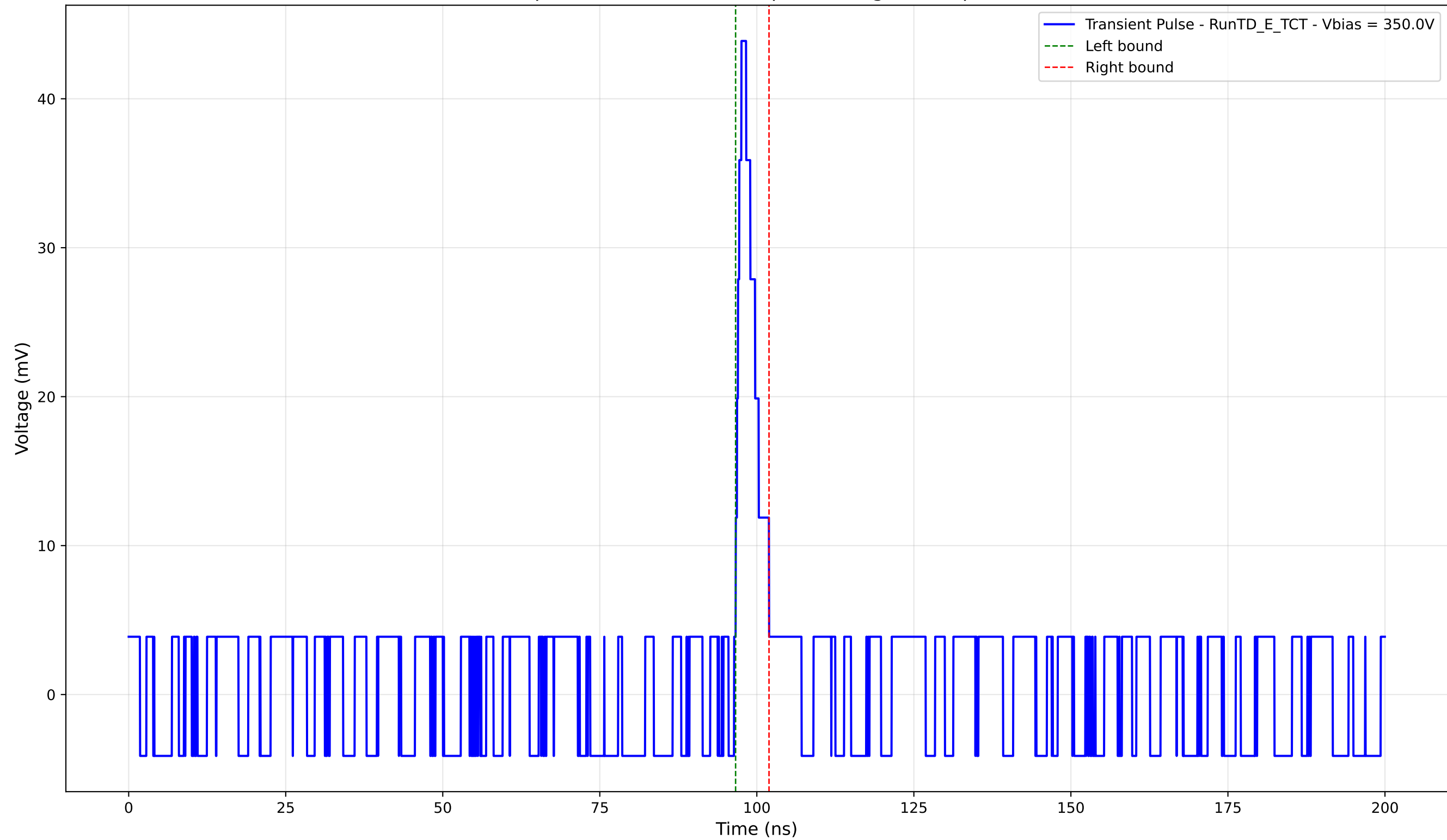
Transient Pulse - Sample: TD - Position: 40.0 \mu\text{m} - Charge: 2.65 pC - Rise Time: 0.92 ns
