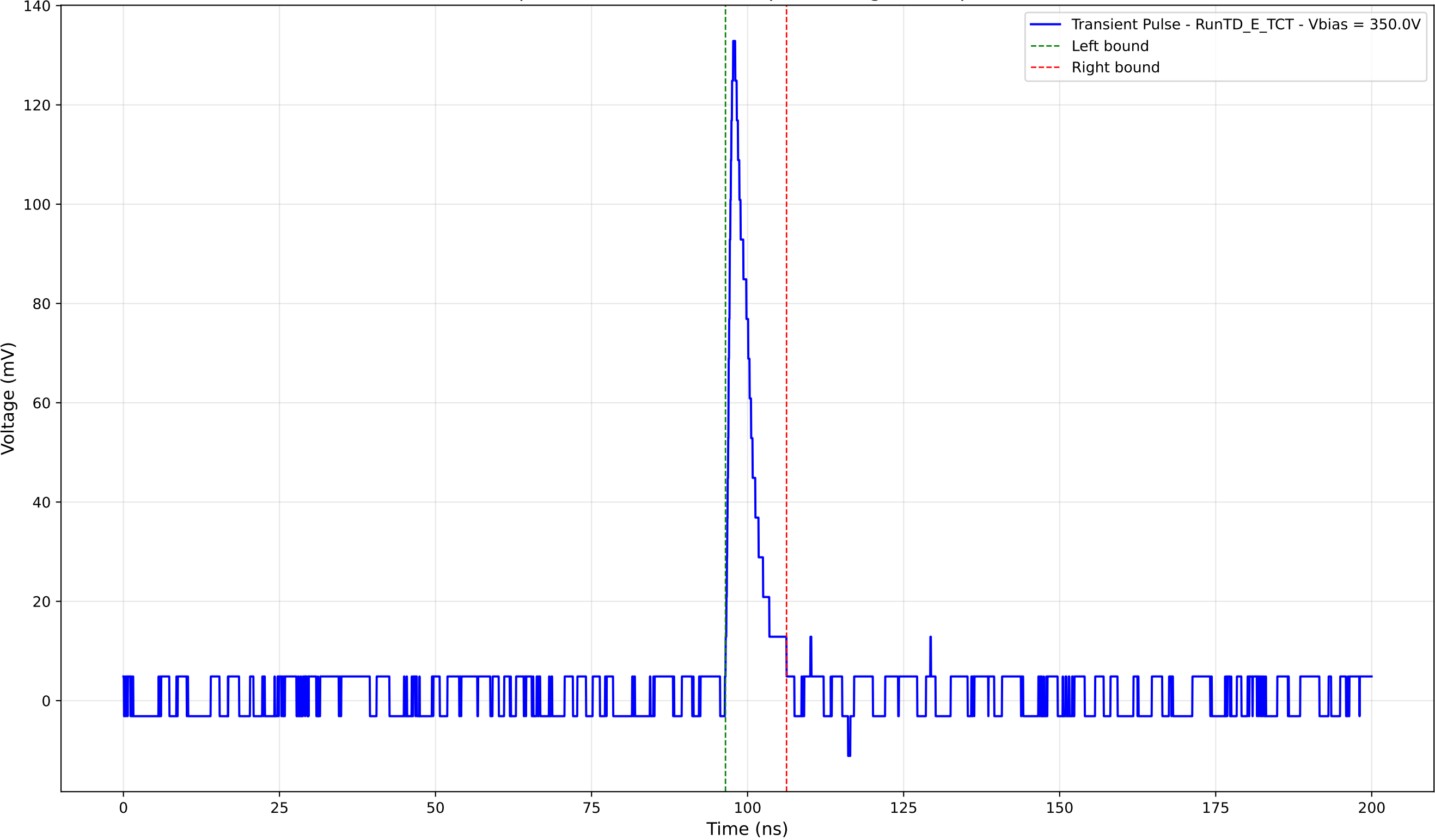
Transient Pulse - Sample: TD - Position: 425.0 \mu\text{m} - Charge: 9.89 pC - Rise Time: 0.92 ns
