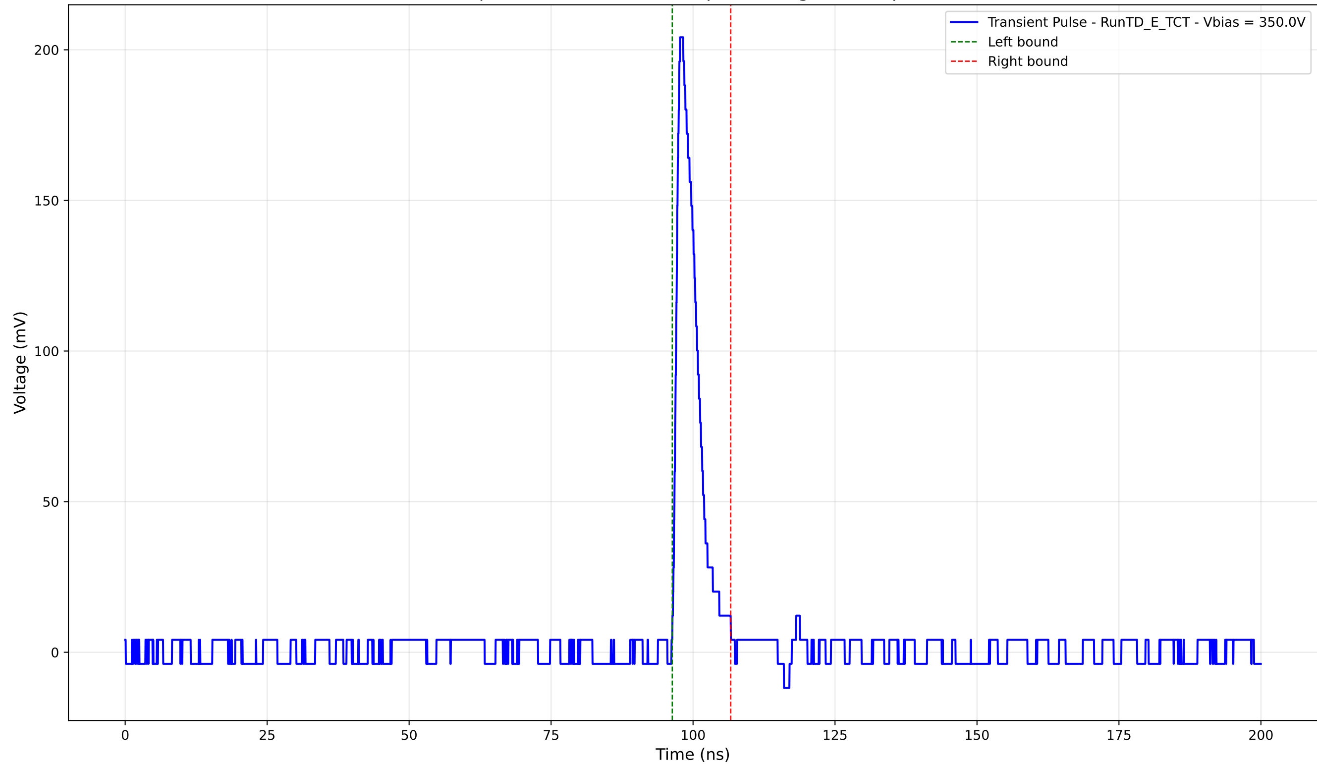
Transient Pulse - Sample: TD - Position: 390.0 \mu\text{m} - Charge: 16.51 pC - Rise Time: 1.00 ns
