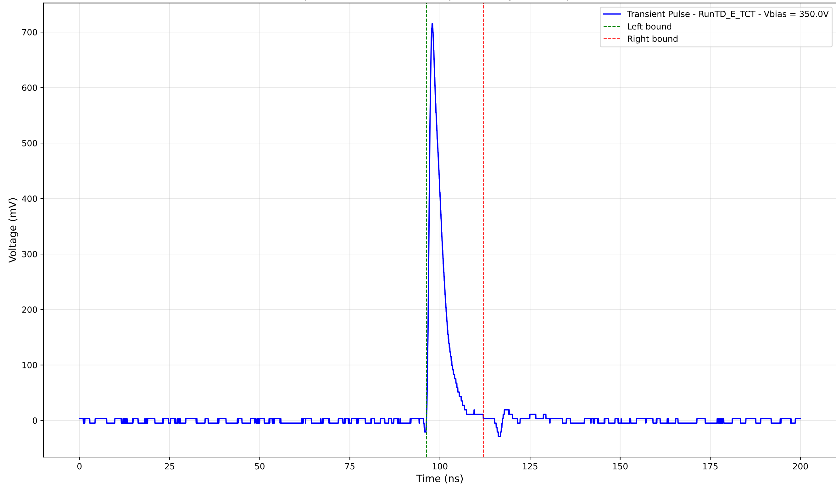
Transient Pulse - Sample: TD - Position: 240.0 \mu\text{m} - Charge: 56.57 pC - Rise Time: 0.97 ns
