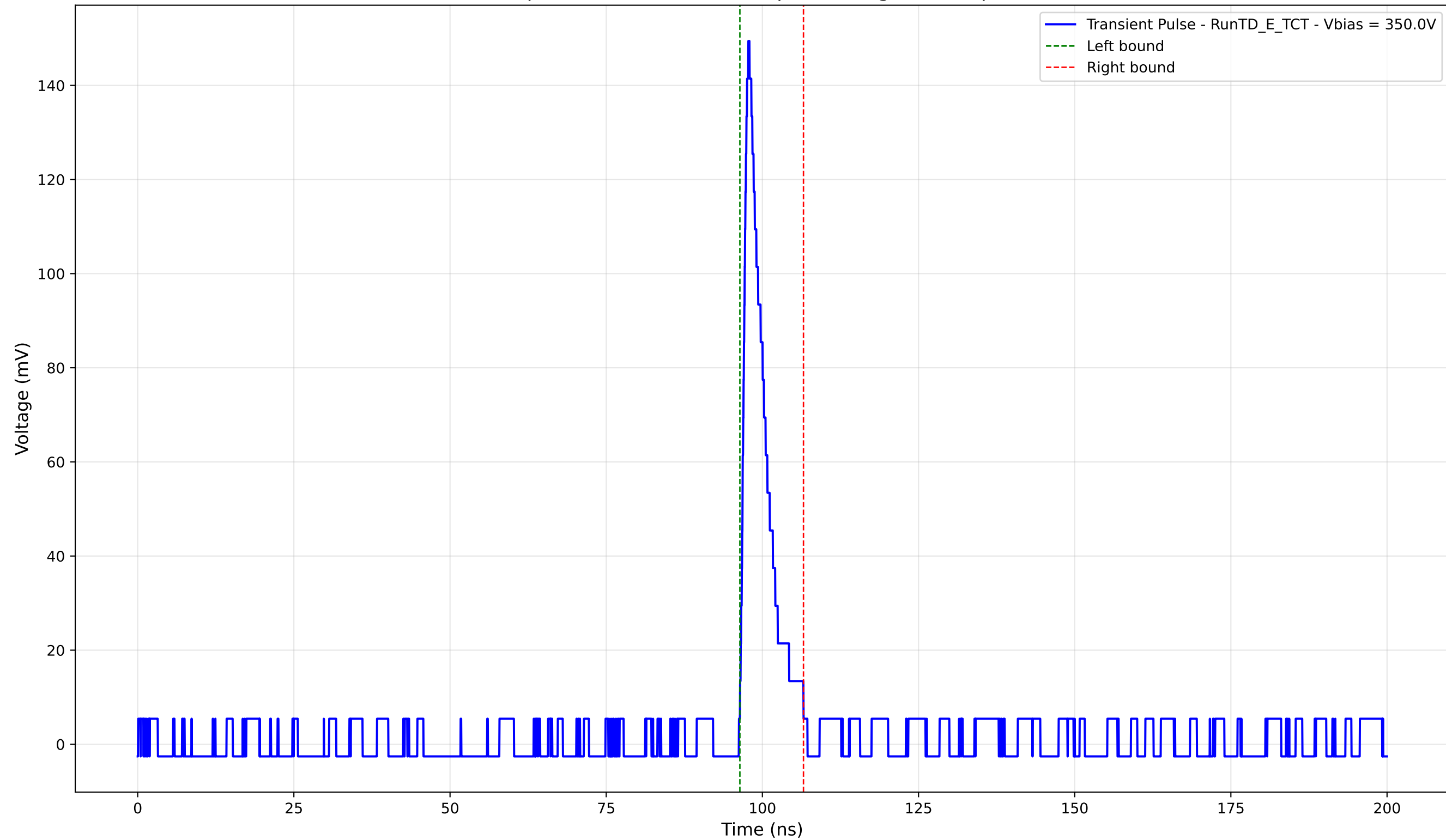
Transient Pulse - Sample: TD - Position: 435.0 \mu\text{m} - Charge: 11.26 pC - Rise Time: 1.04 ns
