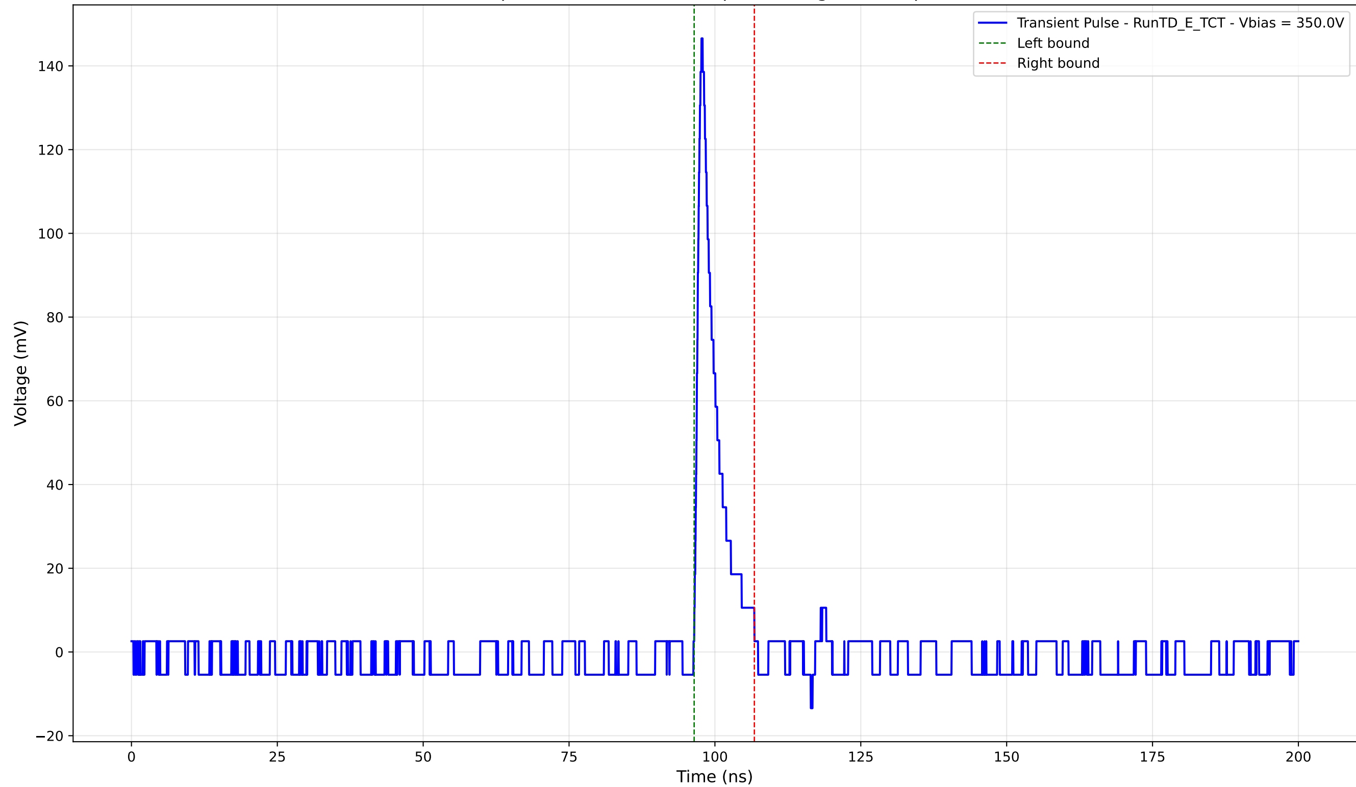
Transient Pulse - Sample: TD - Position: 60.0 \mu\text{m} - Charge: 10.06 pC - Rise Time: 0.99 ns
