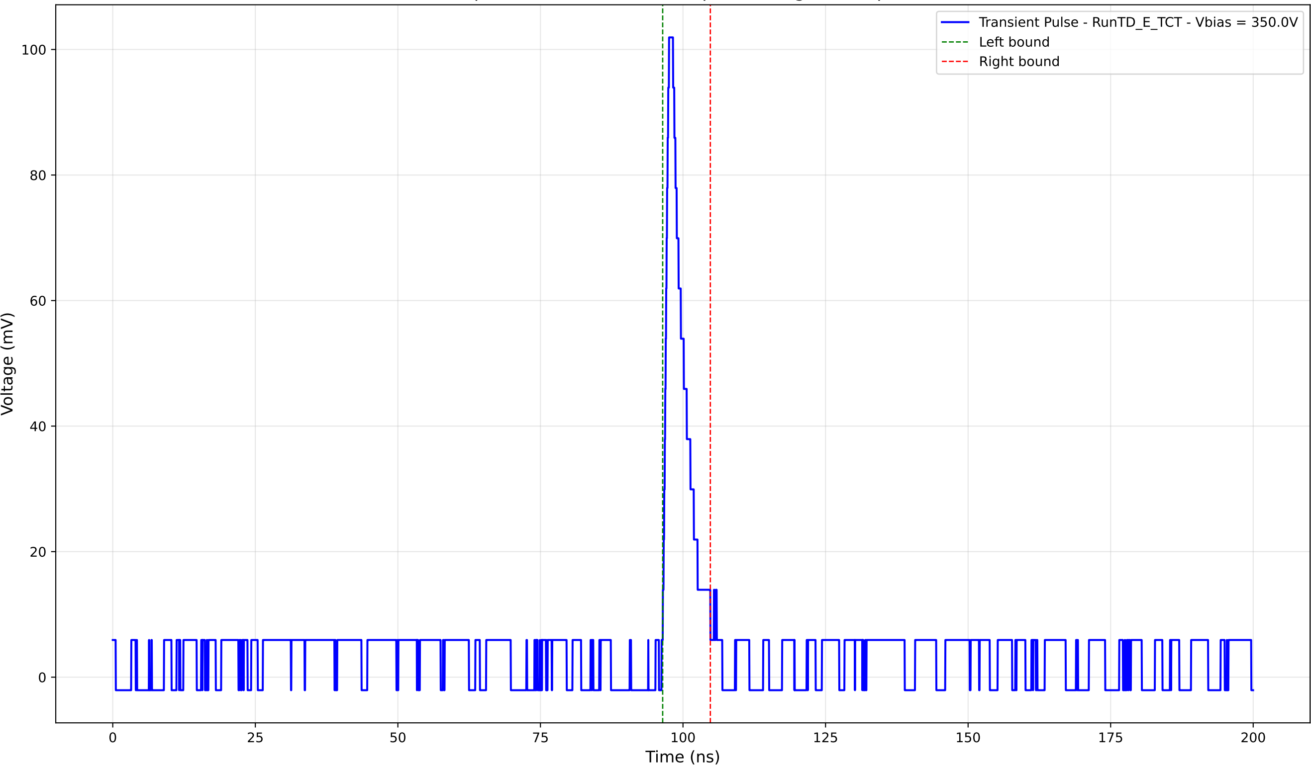
Transient Pulse - Sample: TD - Position: 595.0 \mu\text{m} - Charge: 7.47 pC - Rise Time: 0.95 ns
