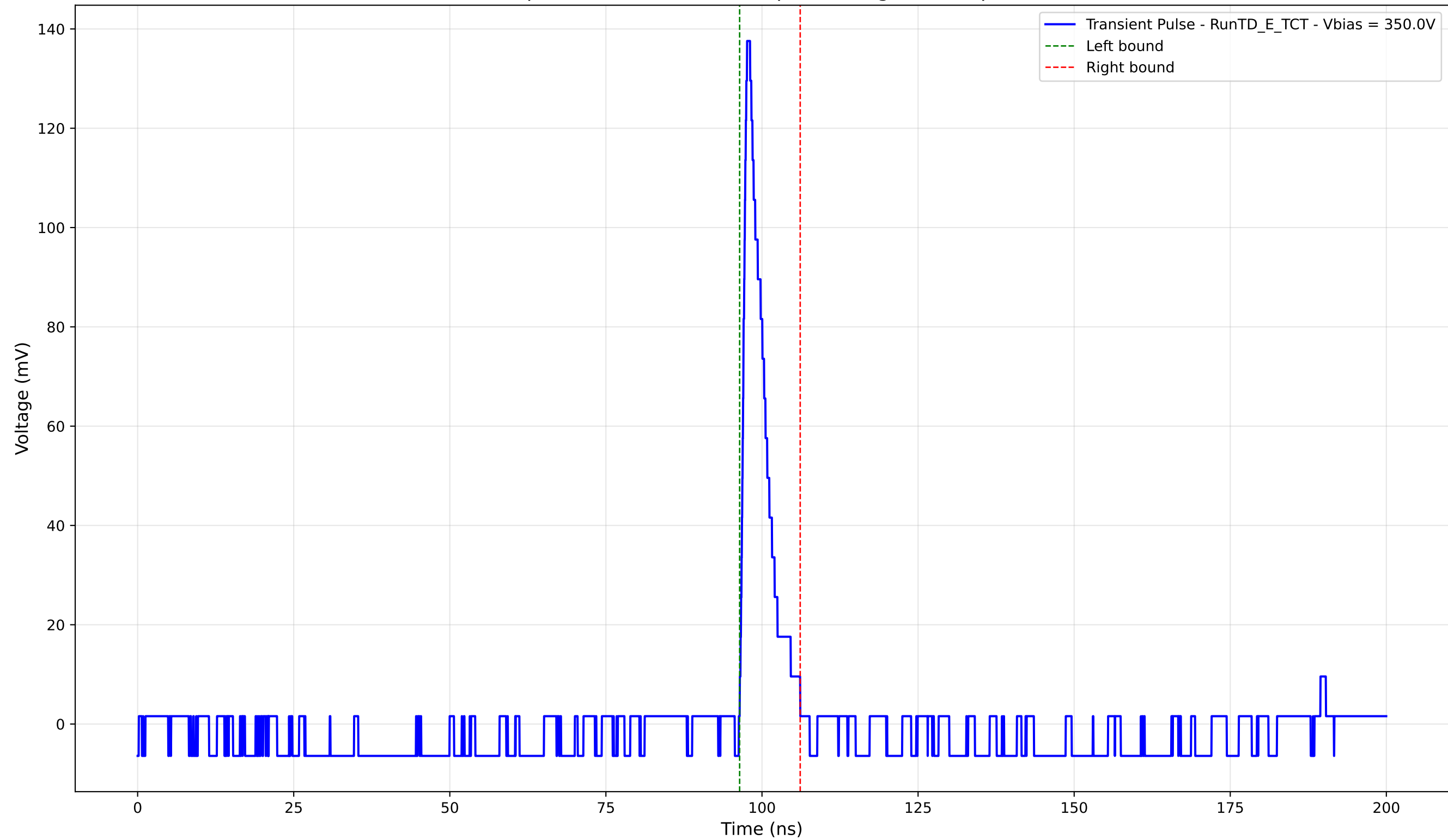
Transient Pulse - Sample: TD - Position: 430.0 \mu\text{m} - Charge: 10.23 pC - Rise Time: 0.93 ns
