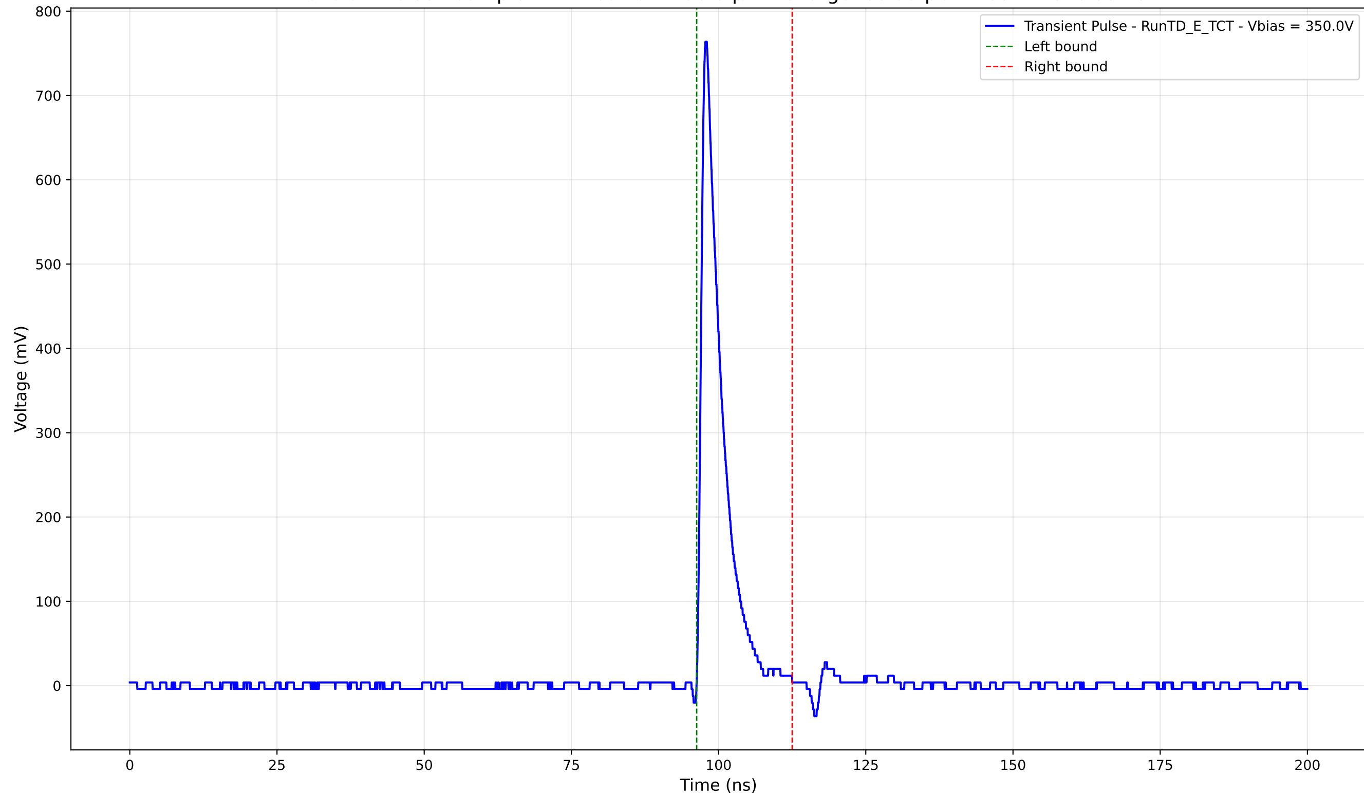
Transient Pulse - Sample: TD - Position: 130.0 \mu\text{m} - Charge: 60.93 pC - Rise Time: 0.95 ns
