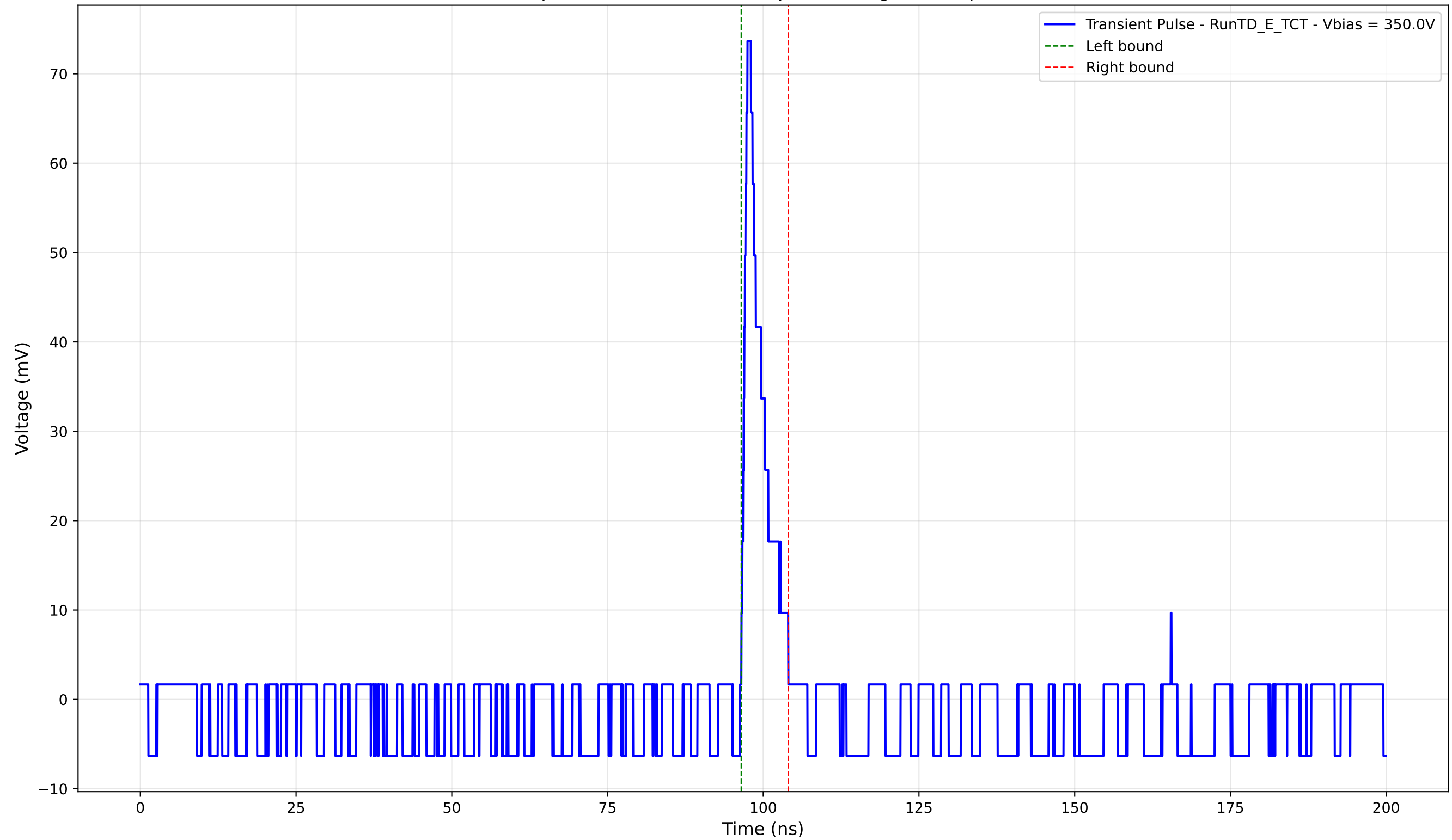
Transient Pulse - Sample: TD - Position: 50.0 \mu\text{m} - Charge: 4.77 pC - Rise Time: 0.97 ns
