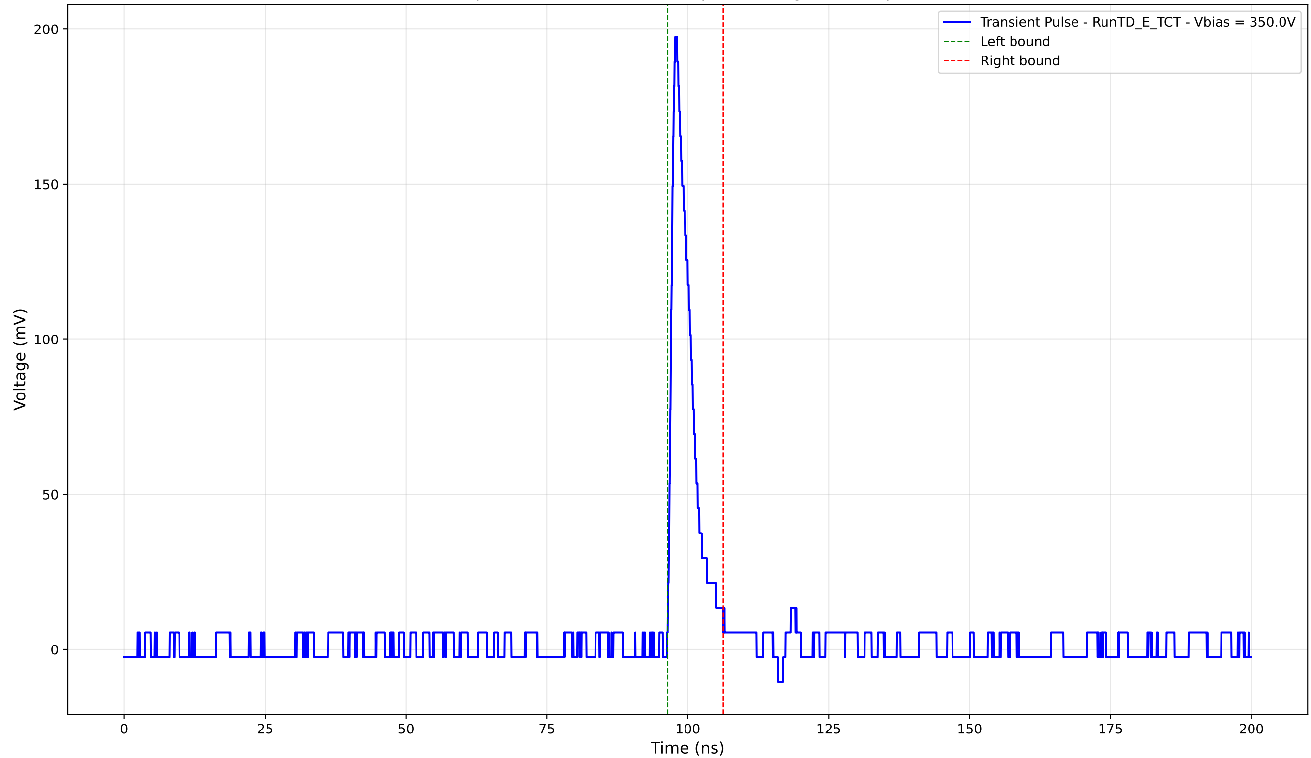
Transient Pulse - Sample: TD - Position: 505.0 \mu\text{m} - Charge: 15.14 pC - Rise Time: 1.00 ns
