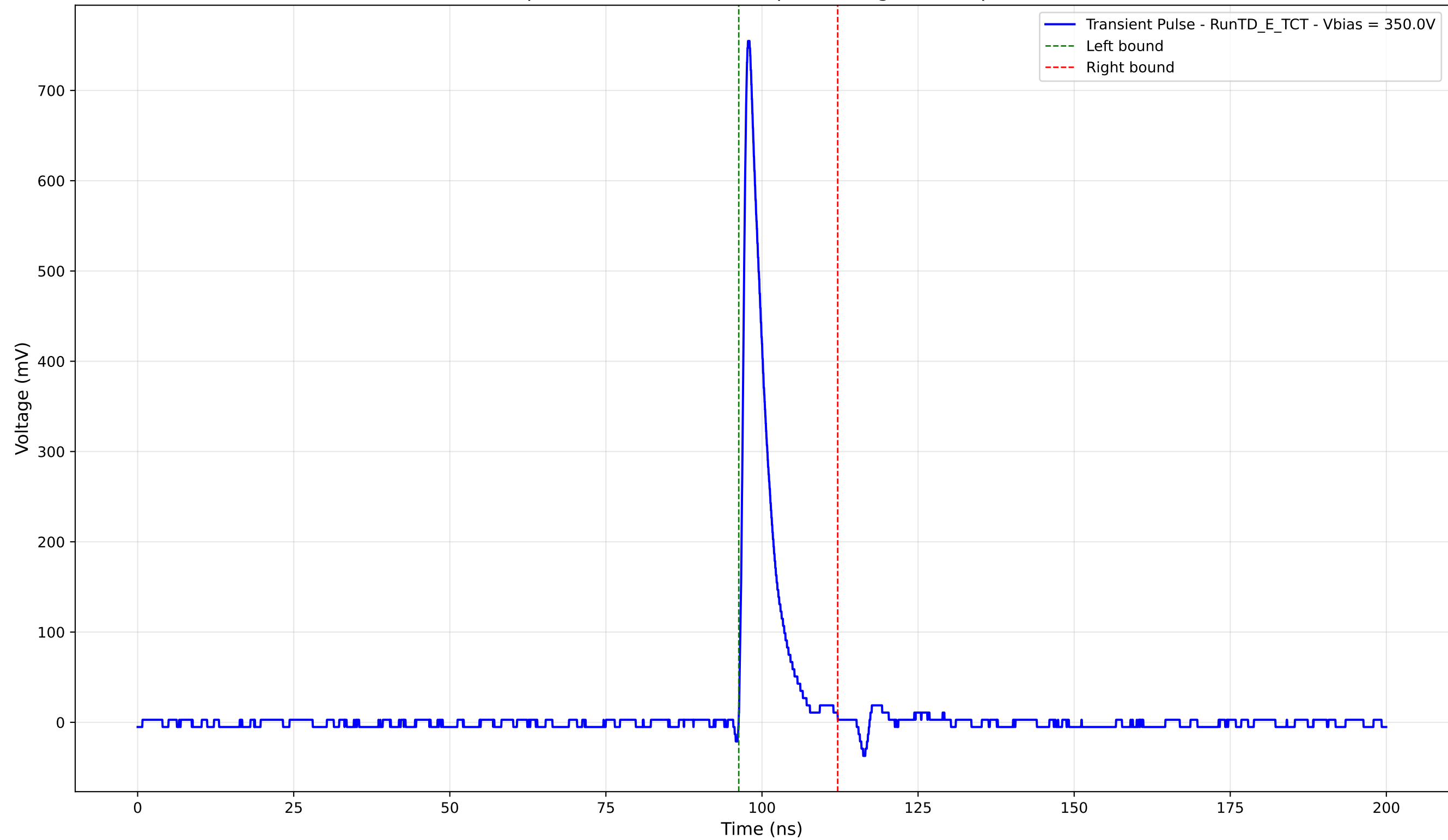
Transient Pulse - Sample: TD - Position: 120.0 \mu\text{m} - Charge: 60.00 pC - Rise Time: 0.95 ns
