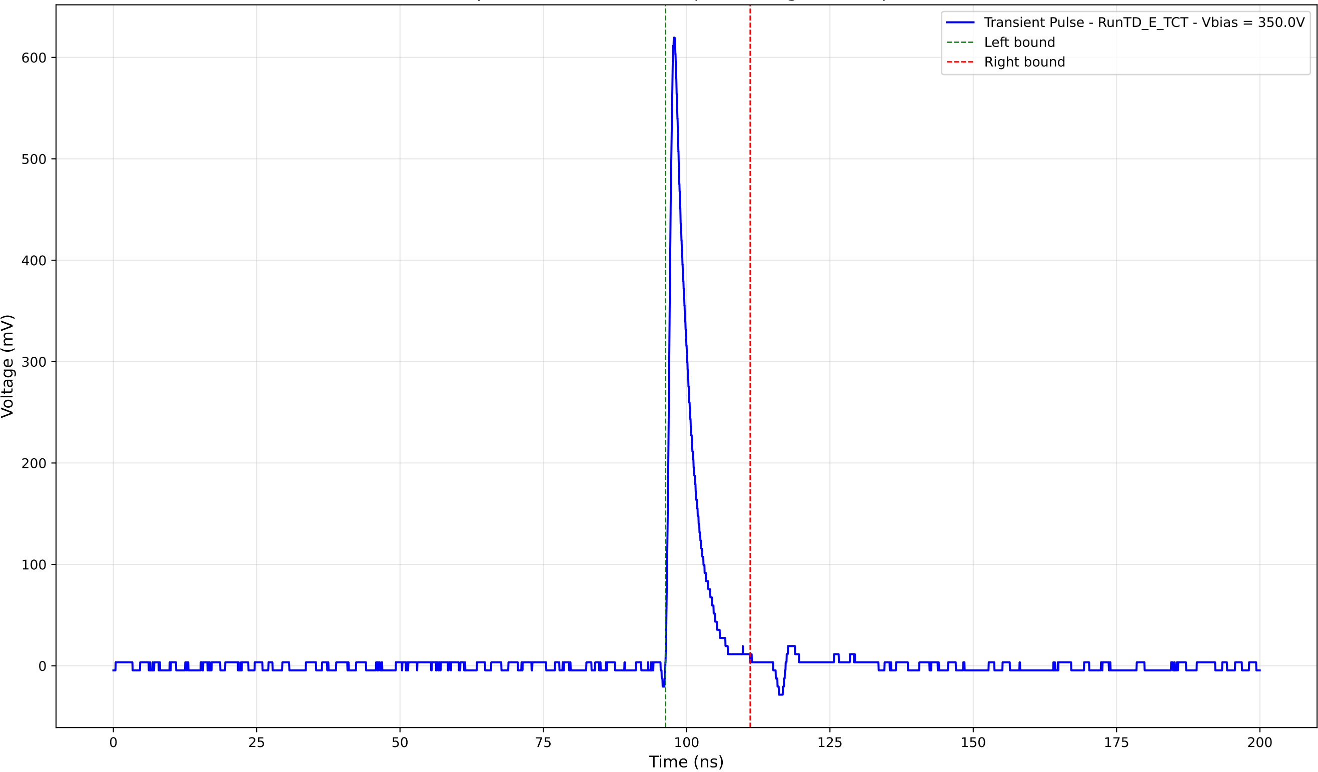
Transient Pulse - Sample: TD - Position: 90.0 \mu\text{m} - Charge: 46.75 pC - Rise Time: 0.93 ns
