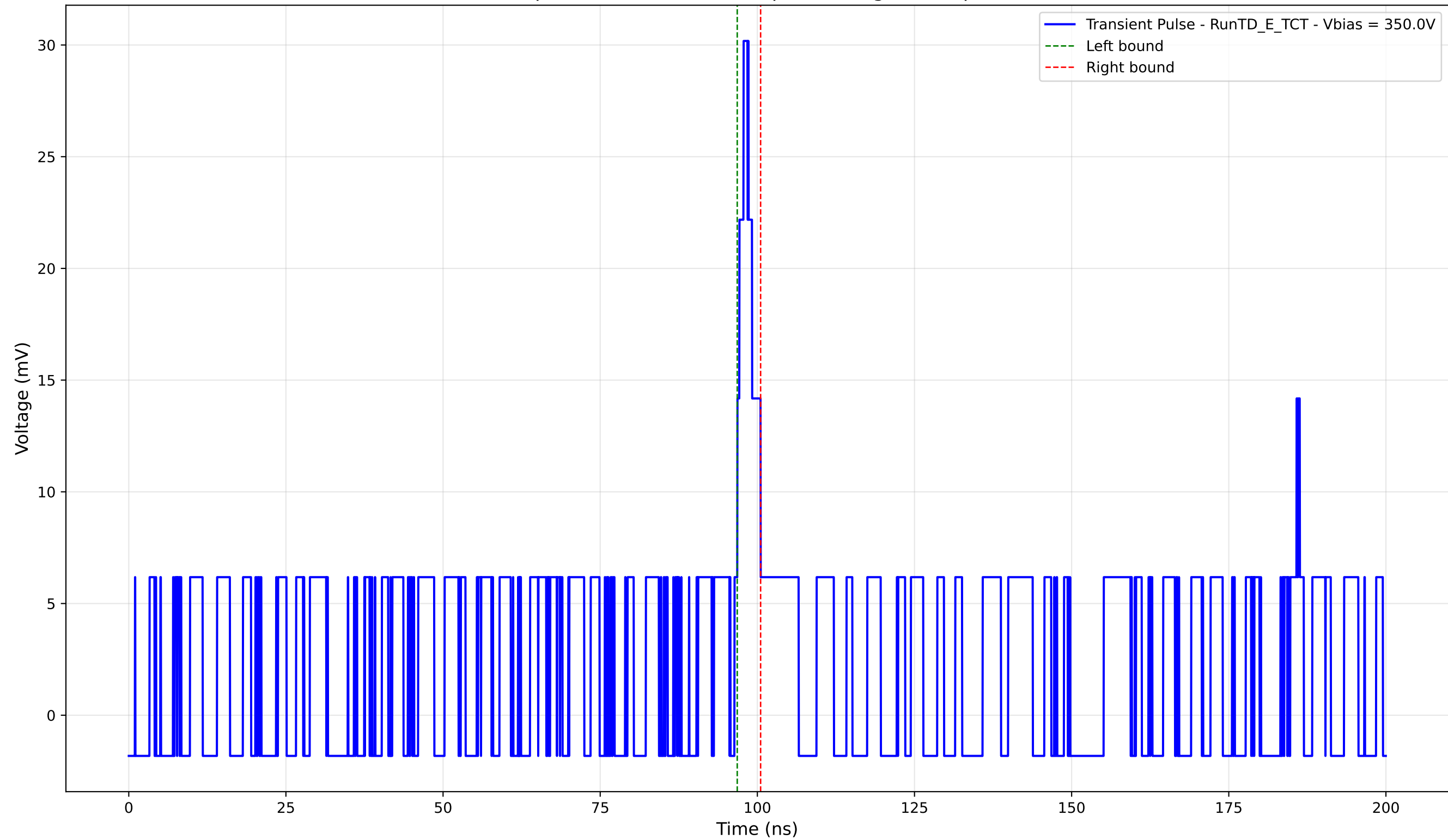
Transient Pulse - Sample: TD - Position: 15.0 \mu\text{m} - Charge: 1.49 pC - Rise Time: 1.45 ns
