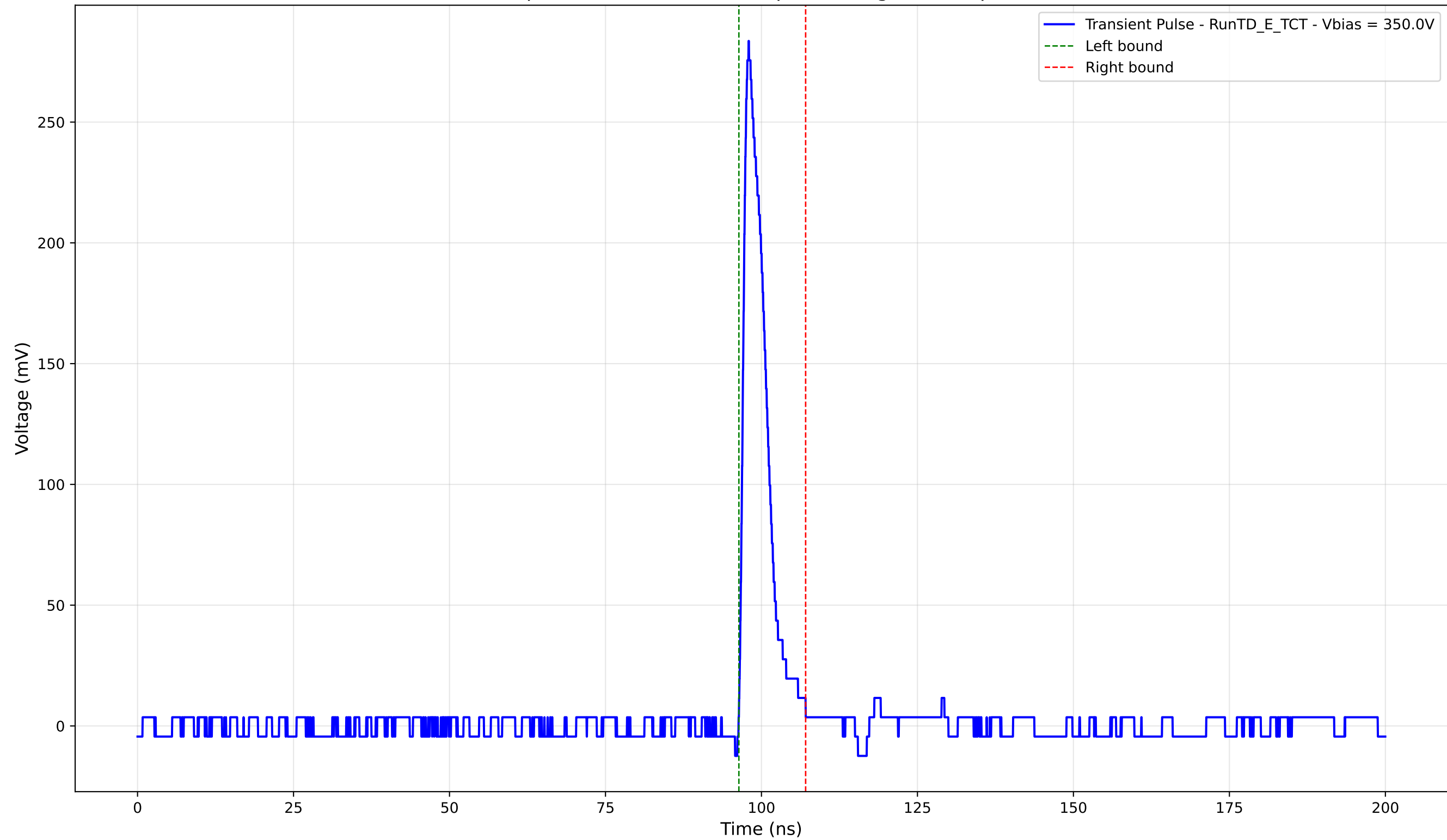
Transient Pulse - Sample: TD - Position: 385.0 \mu\text{m} - Charge: 22.38 pC - Rise Time: 1.00 ns
