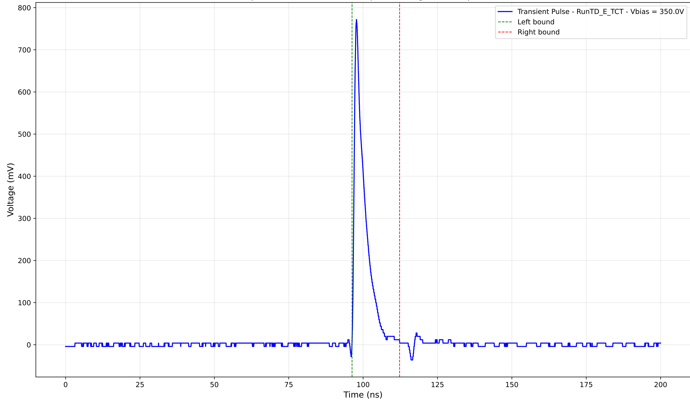
Transient Pulse - Sample: TD - Position: 180.0 \mu\text{m} - Charge: 61.72 pC - Rise Time: 0.92 ns
