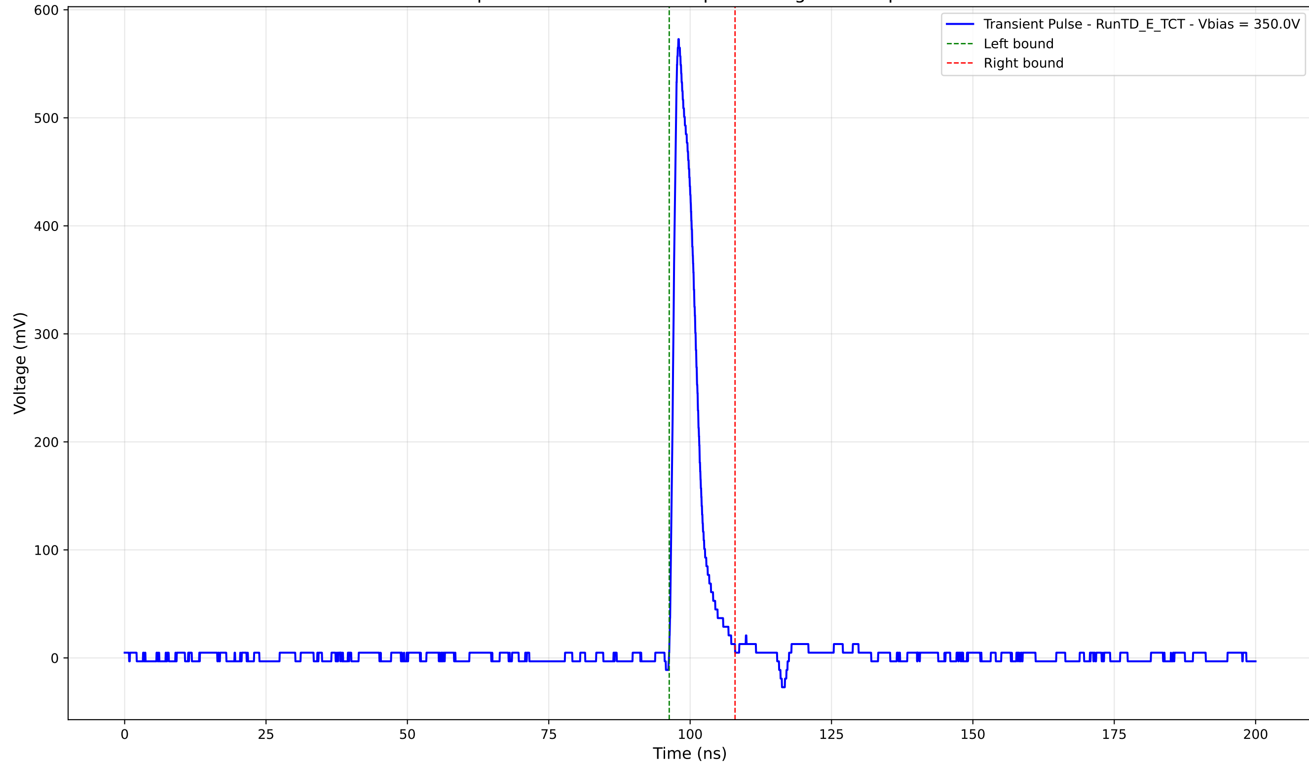
Transient Pulse - Sample: TD - Position: 345.0 \mu\text{m} - Charge: 48.93 pC - Rise Time: 1.03 ns
