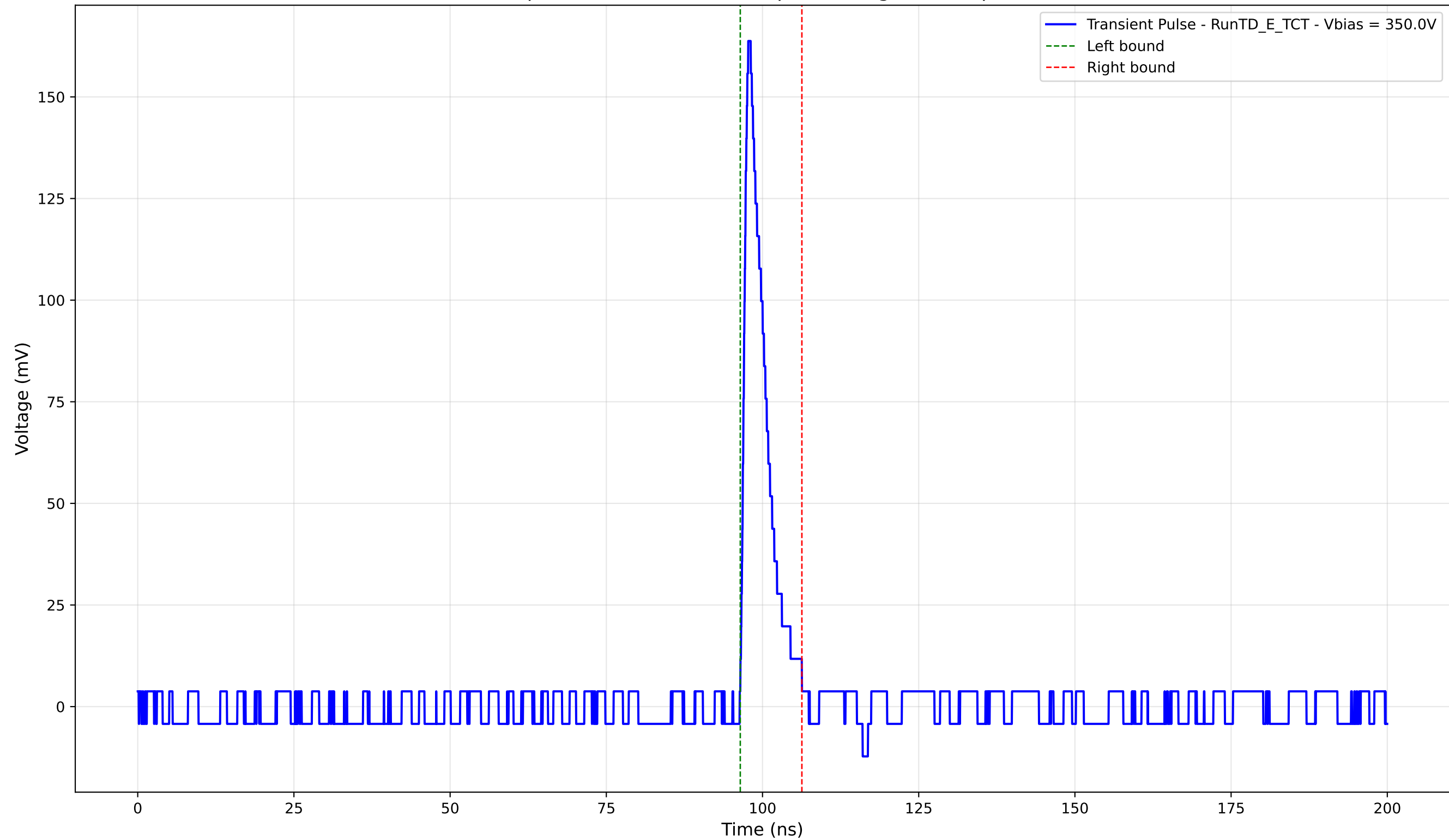
Transient Pulse - Sample: TD - Position: 525.0 \mu\text{m} - Charge: 12.41 pC - Rise Time: 0.93 ns
