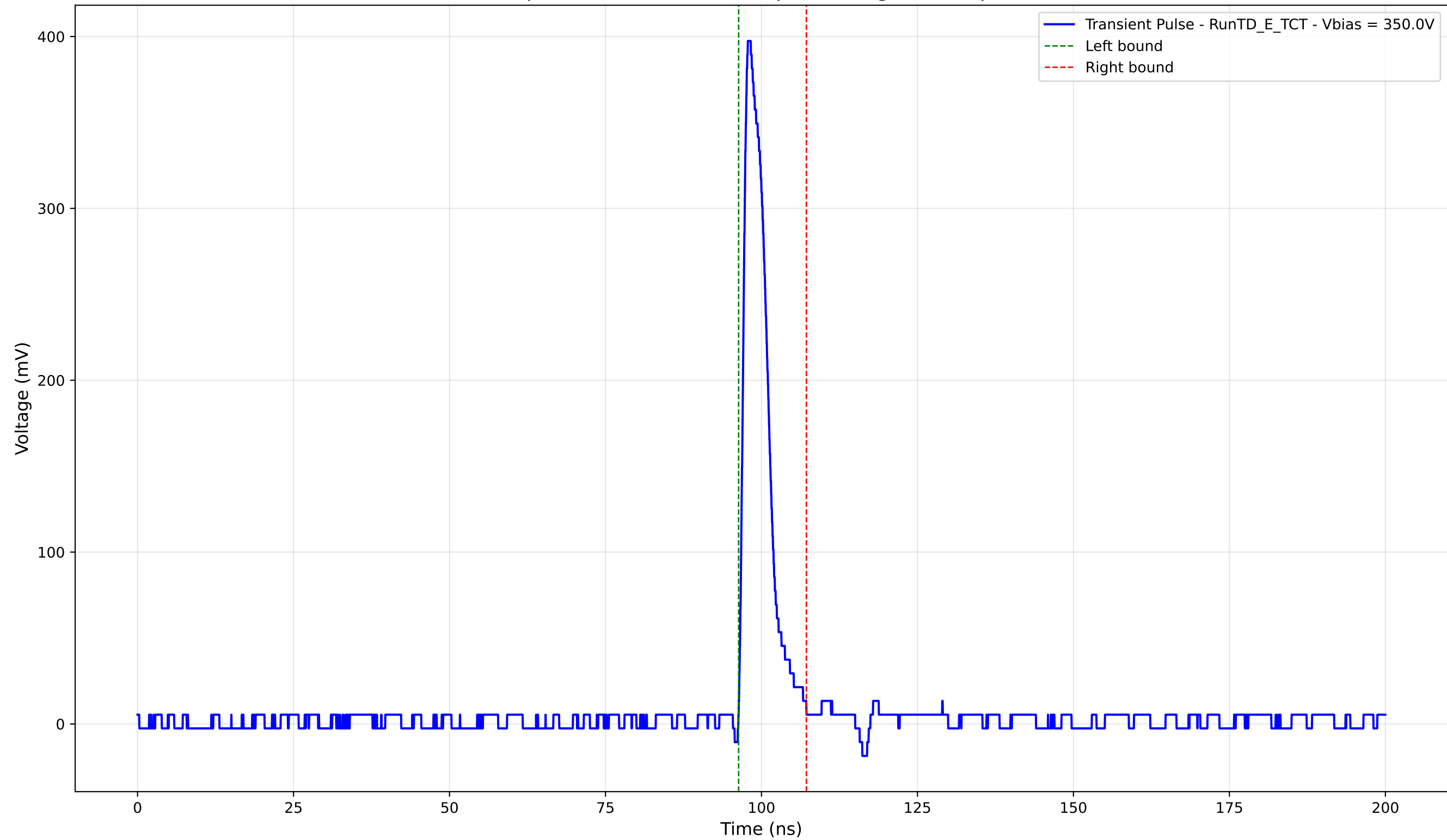
Transient Pulse - Sample: TD - Position: 375.0 \mu\text{m} - Charge: 33.94 pC - Rise Time: 1.05 ns
