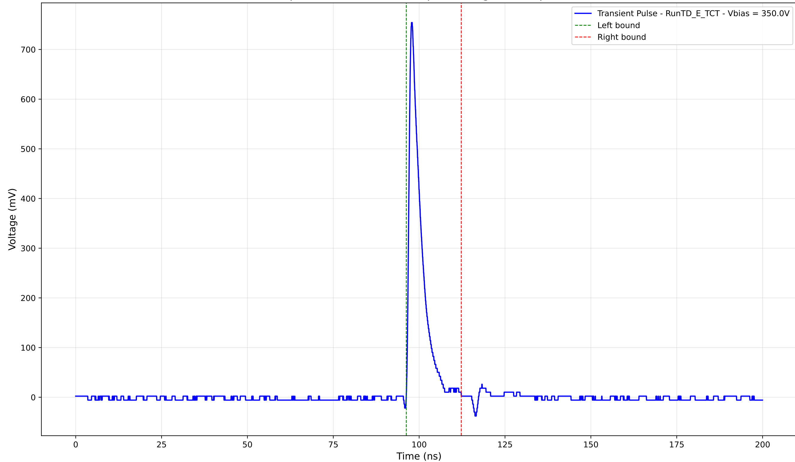
Transient Pulse - Sample: TD - Position: 125.0 \mu\text{m} - Charge: 59.83 pC - Rise Time: 0.95 ns
