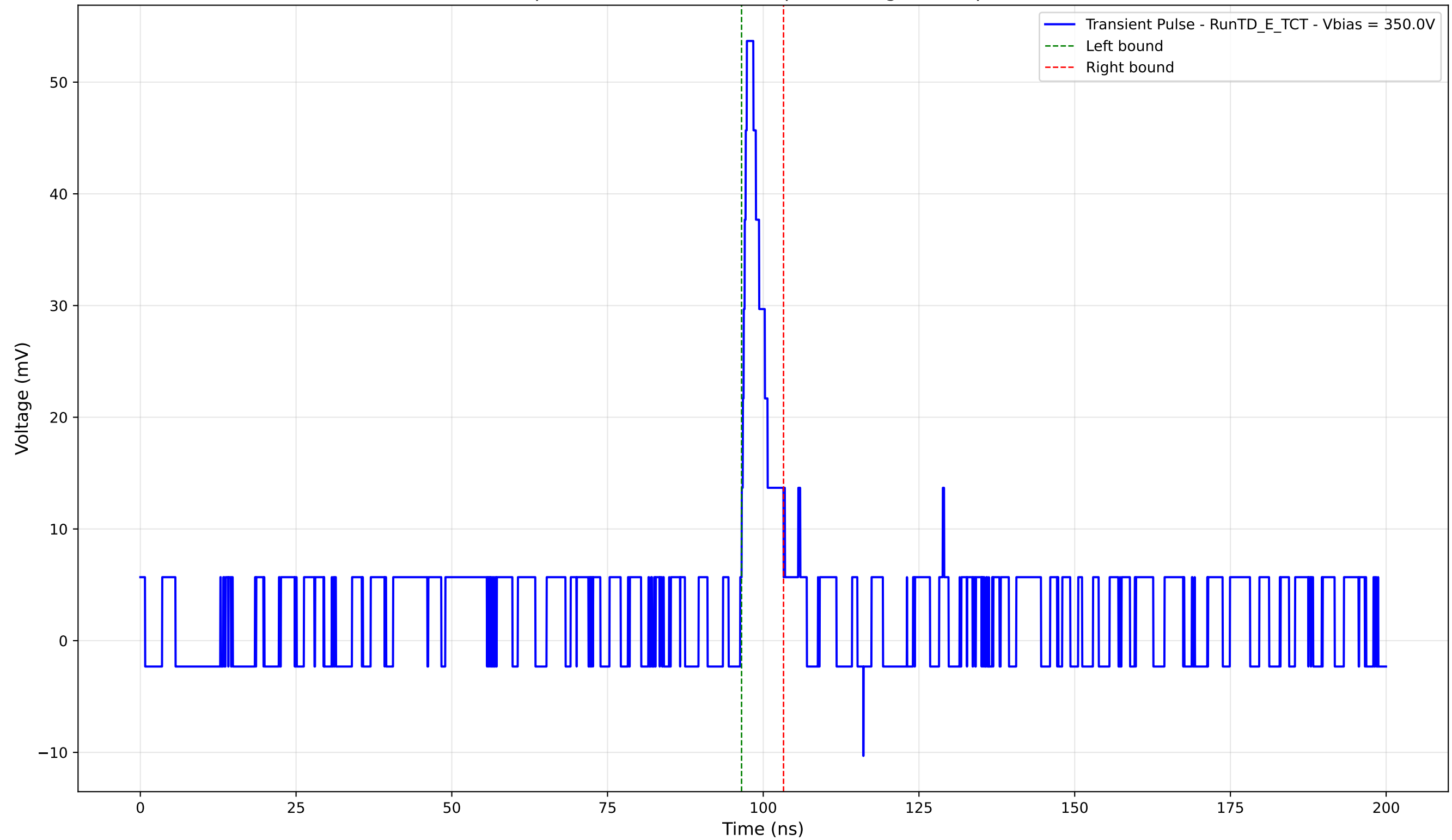
Transient Pulse - Sample: TD - Position: 675.0 \mu\text{m} - Charge: 3.83 pC - Rise Time: 1.06 ns
