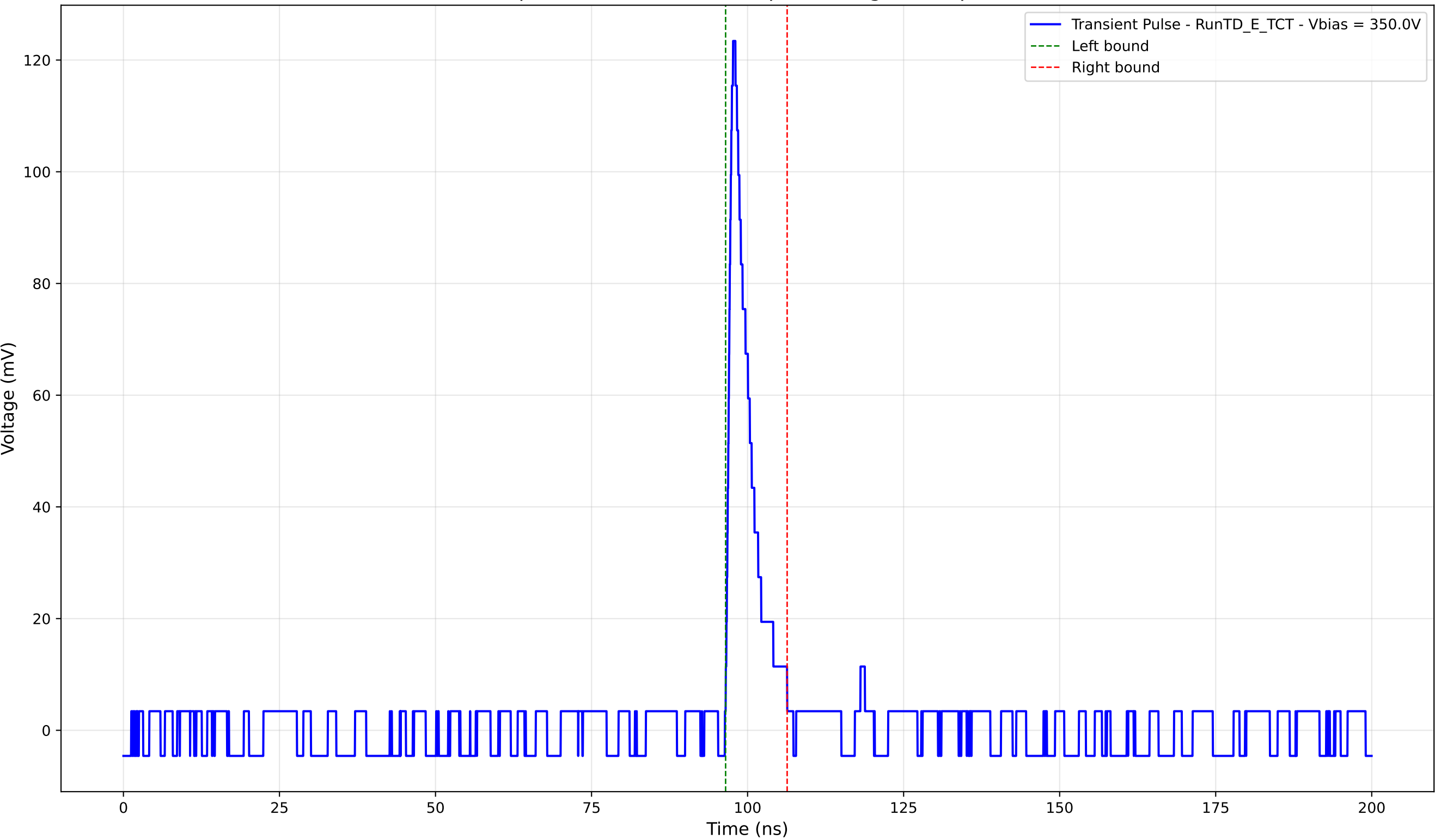
Transient Pulse - Sample: TD - Position: 565.0 \mu\text{m} - Charge: 9.05 pC - Rise Time: 0.90 ns
