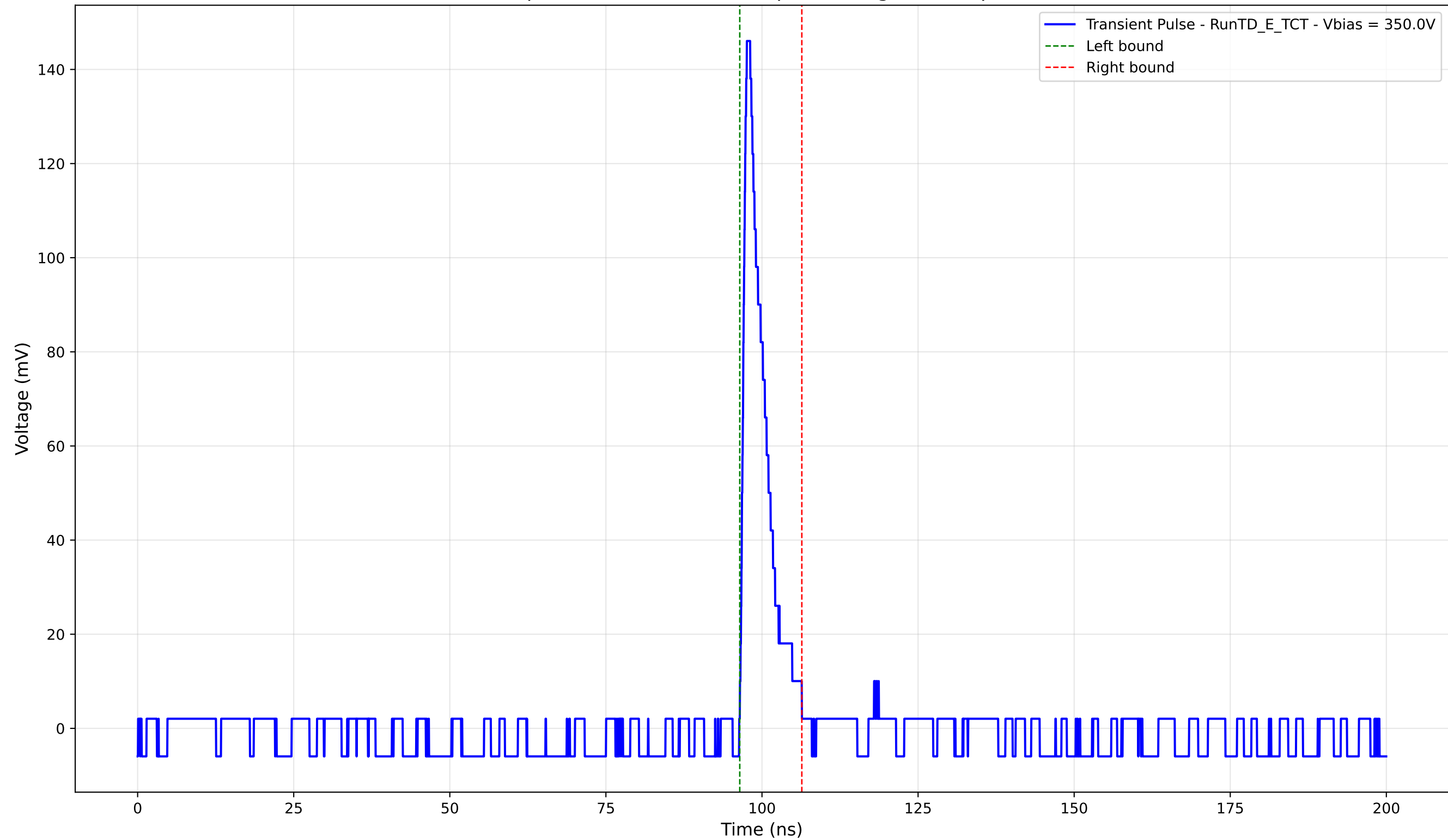
Transient Pulse - Sample: TD - Position: 455.0 \mu\text{m} - Charge: 10.97 pC - Rise Time: 0.91 ns
