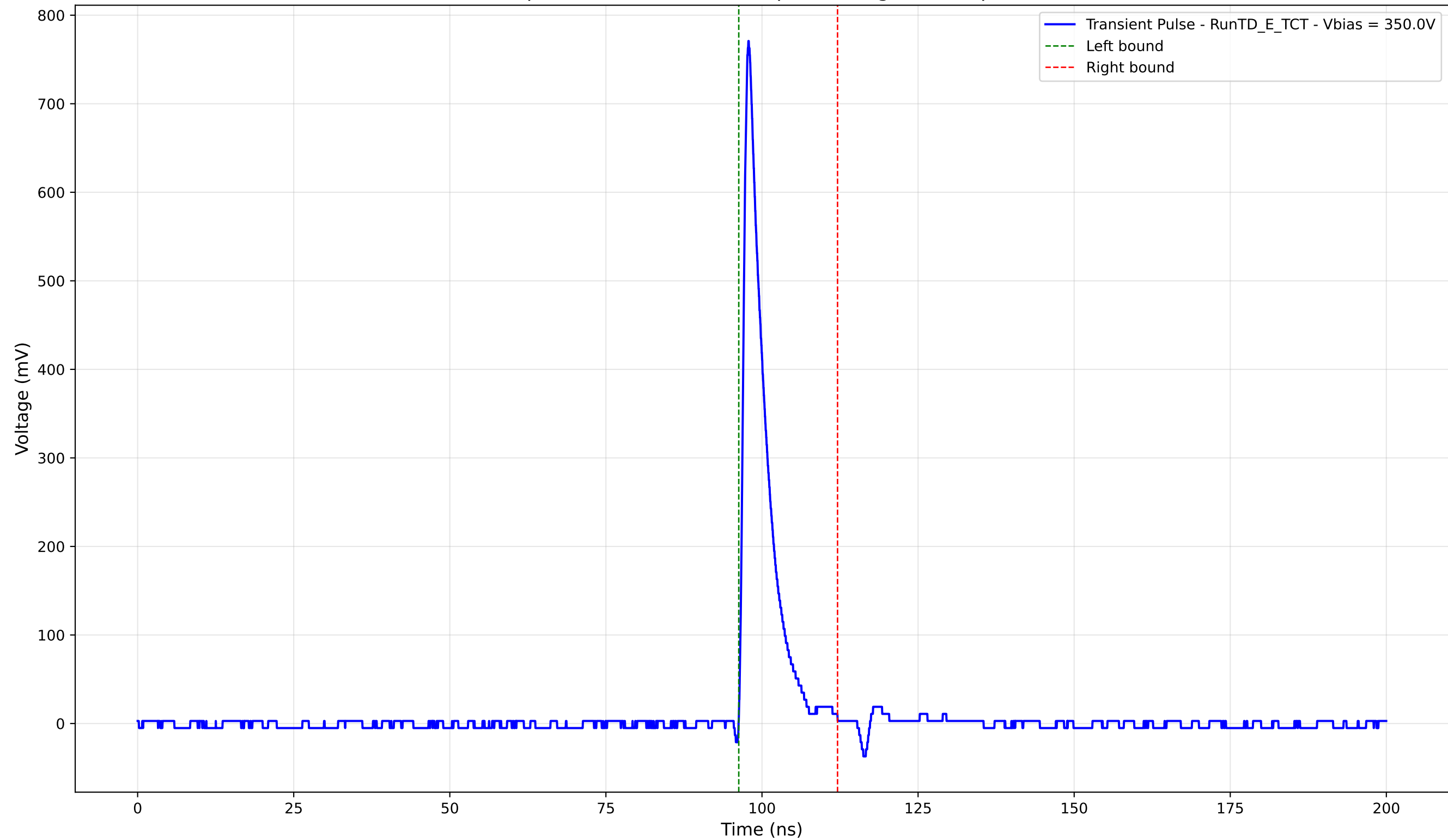
Transient Pulse - Sample: TD - Position: 135.0 \mu\text{m} - Charge: 60.61 pC - Rise Time: 0.96 ns
