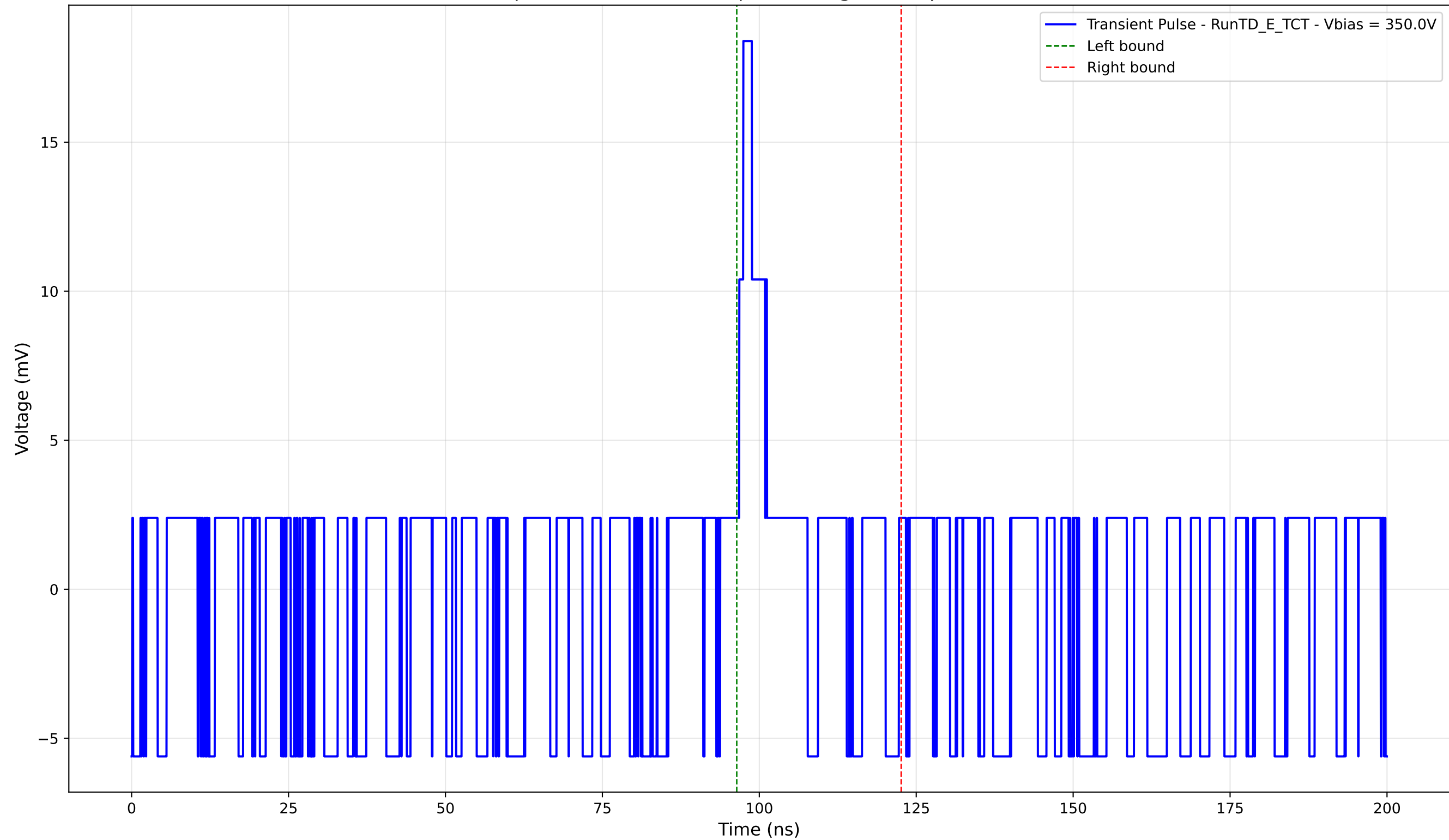
Transient Pulse - Sample: TD - Position: 0.0 \mu\text{m} - Charge: 1.20 pC - Rise Time: 0.00 ns (N/A)
