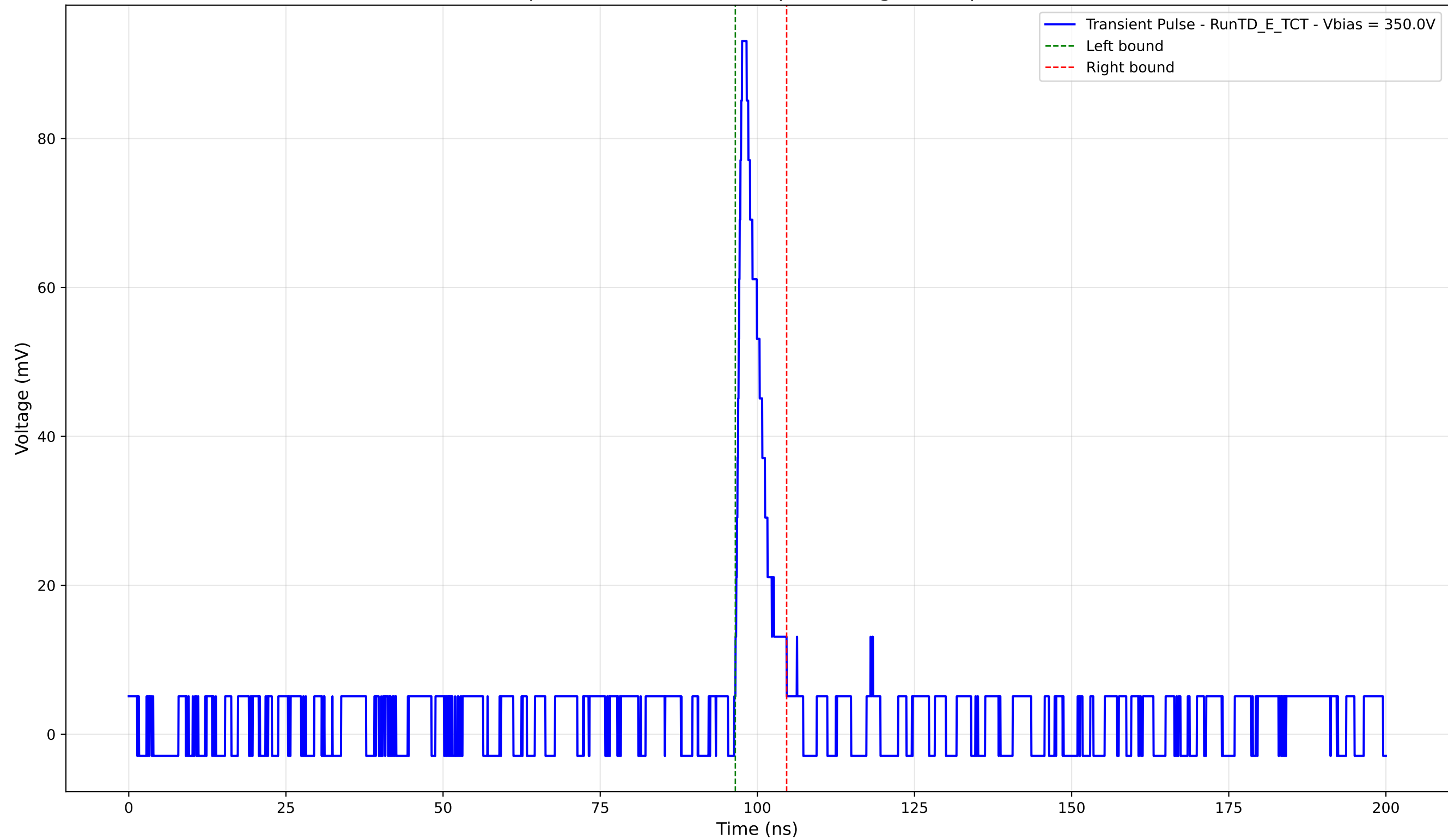
Transient Pulse - Sample: TD - Position: 415.0 \mu\text{m} - Charge: 7.04 pC - Rise Time: 0.91 ns
