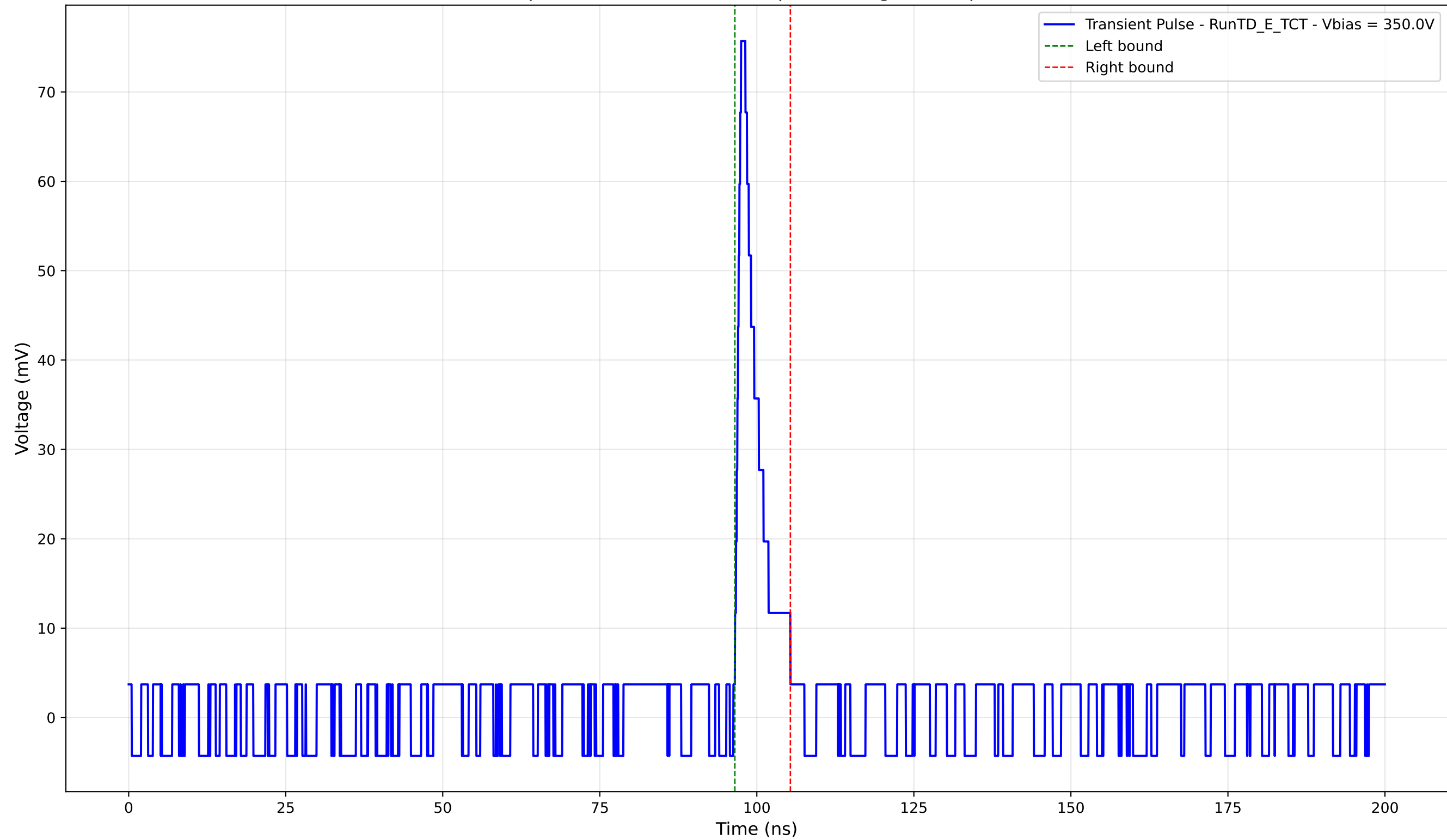
Transient Pulse - Sample: TD - Position: 645.0 \mu\text{m} - Charge: 5.38 pC - Rise Time: 0.97 ns
