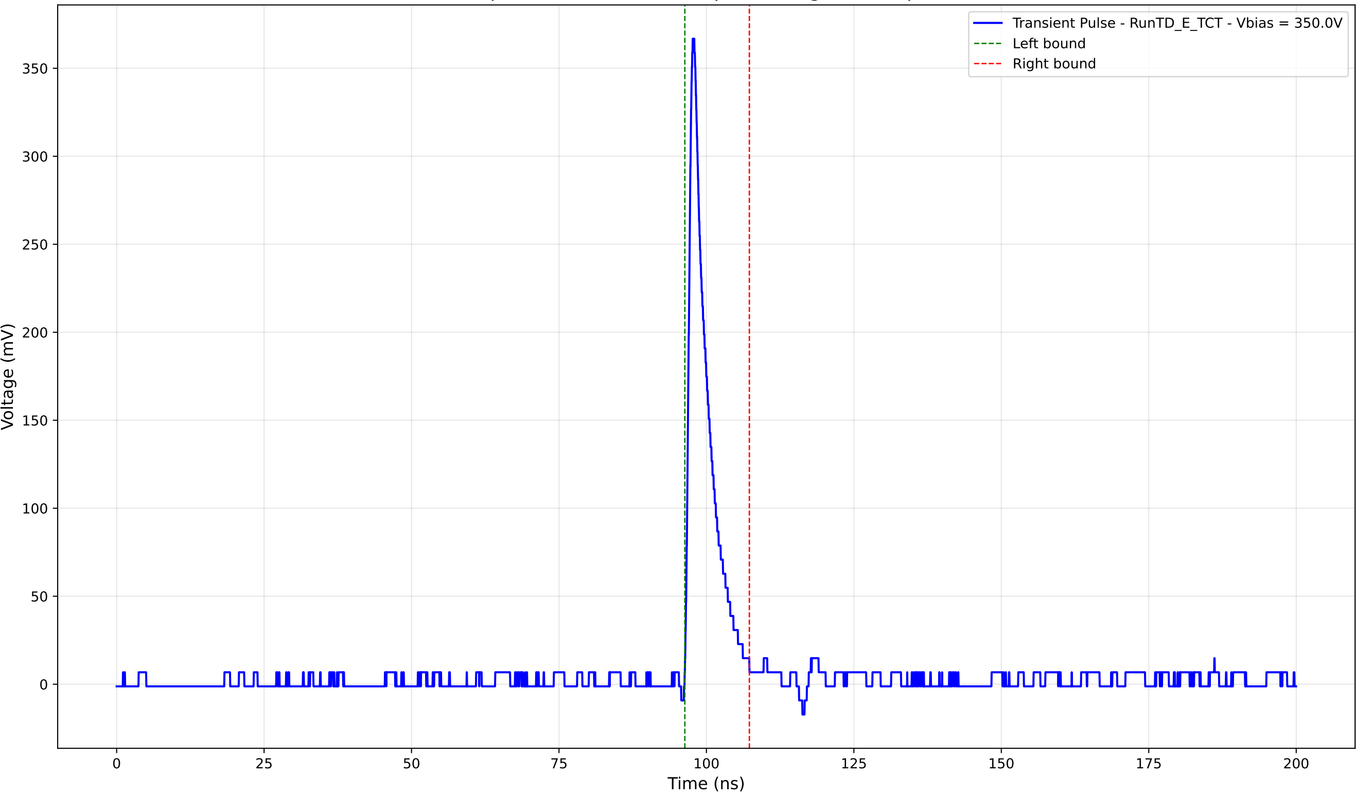
Transient Pulse - Sample: TD - Position: 75.0 \mu\text{m} - Charge: 26.83 pC - Rise Time: 0.95 ns
