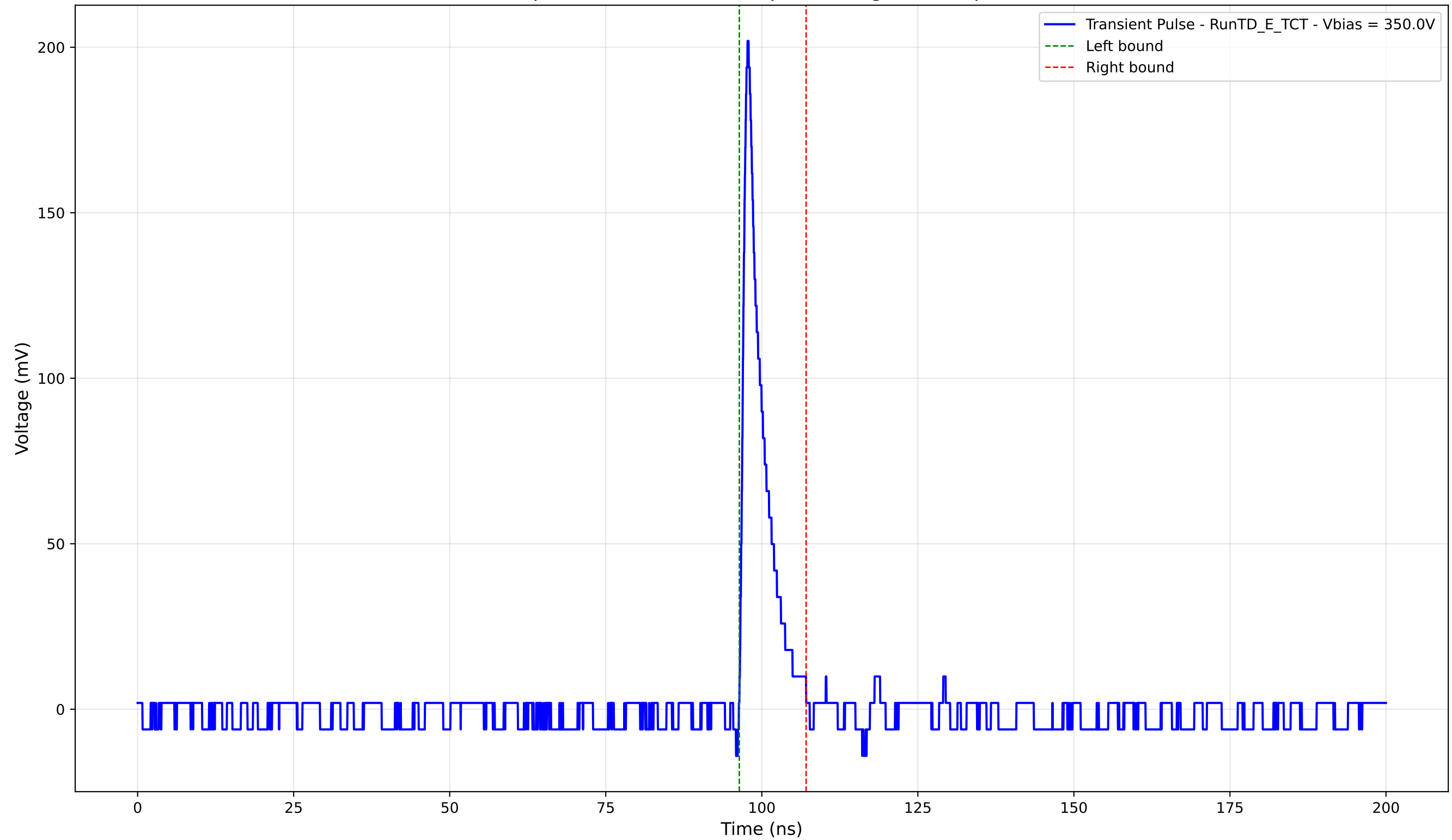
Transient Pulse - Sample: TD - Position: 65.0 \mu\text{m} - Charge: 14.00 pC - Rise Time: 0.91 ns
