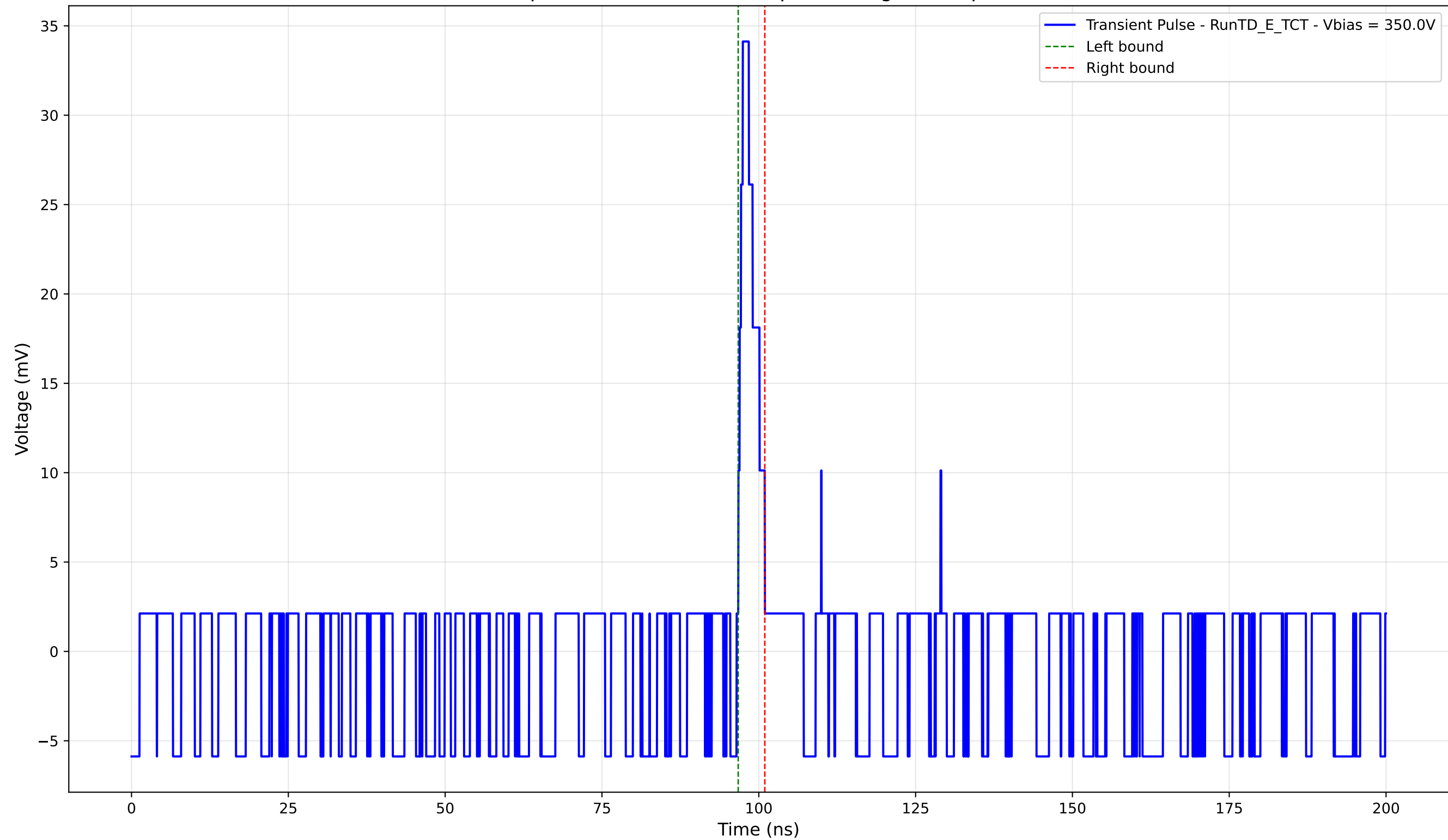
Transient Pulse - Sample: TD - Position: 695.0 \mu\text{m} - Charge: 1.82 pC - Rise Time: 0.72 ns
