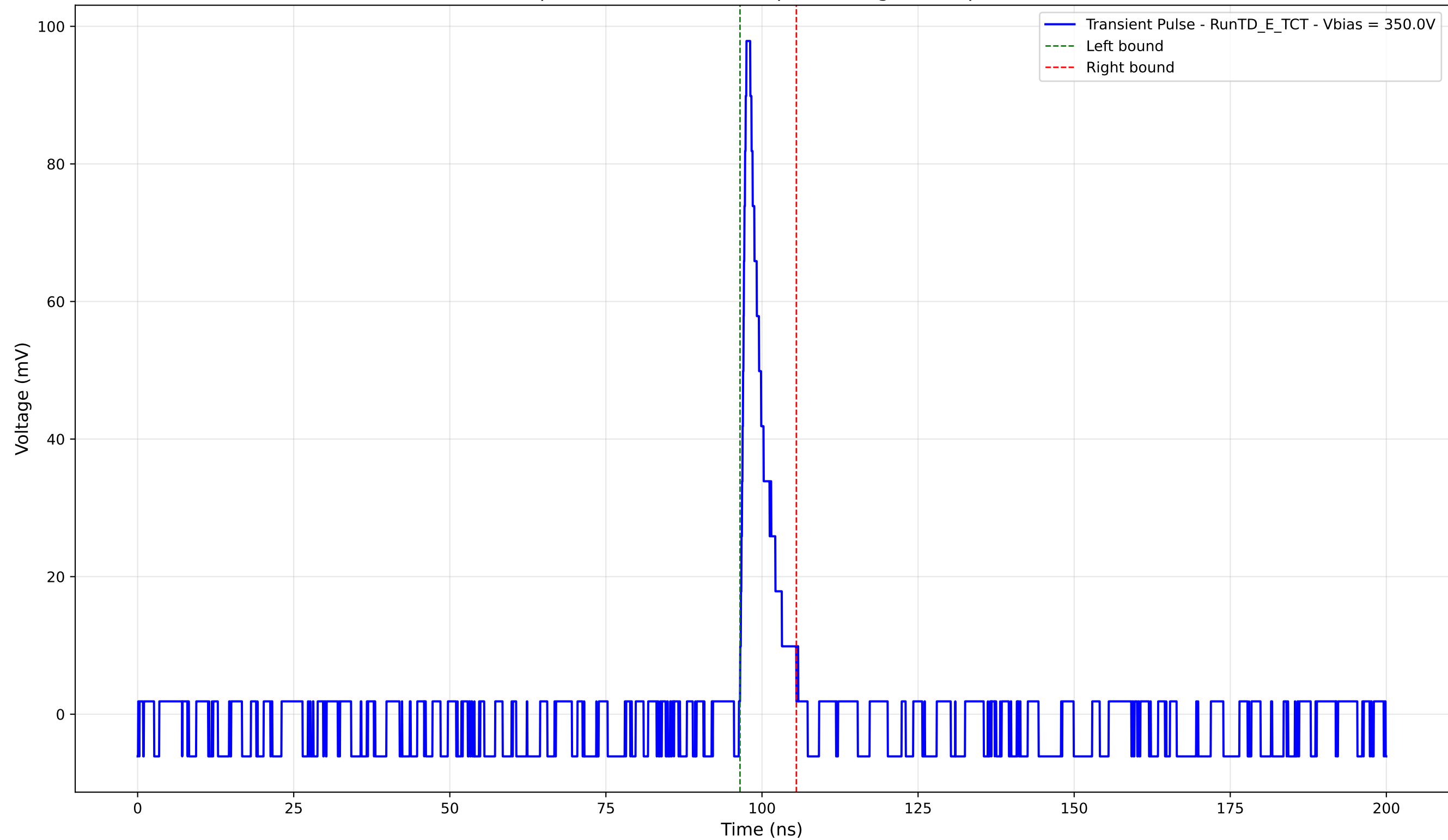
Transient Pulse - Sample: TD - Position: 55.0 \mu\text{m} - Charge: 6.86 pC - Rise Time: 0.88 ns
