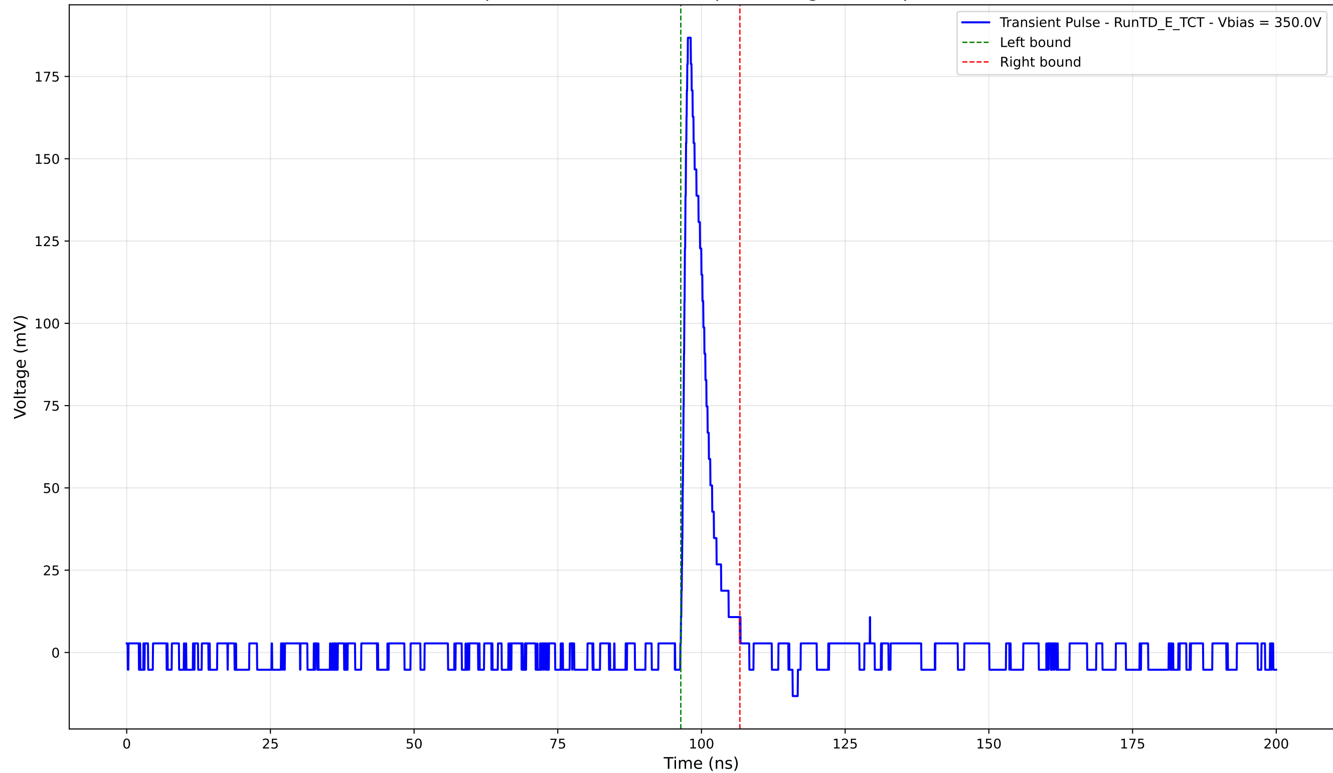
Transient Pulse - Sample: TD - Position: 465.0 \mu\text{m} - Charge: 14.54 pC - Rise Time: 0.94 ns
