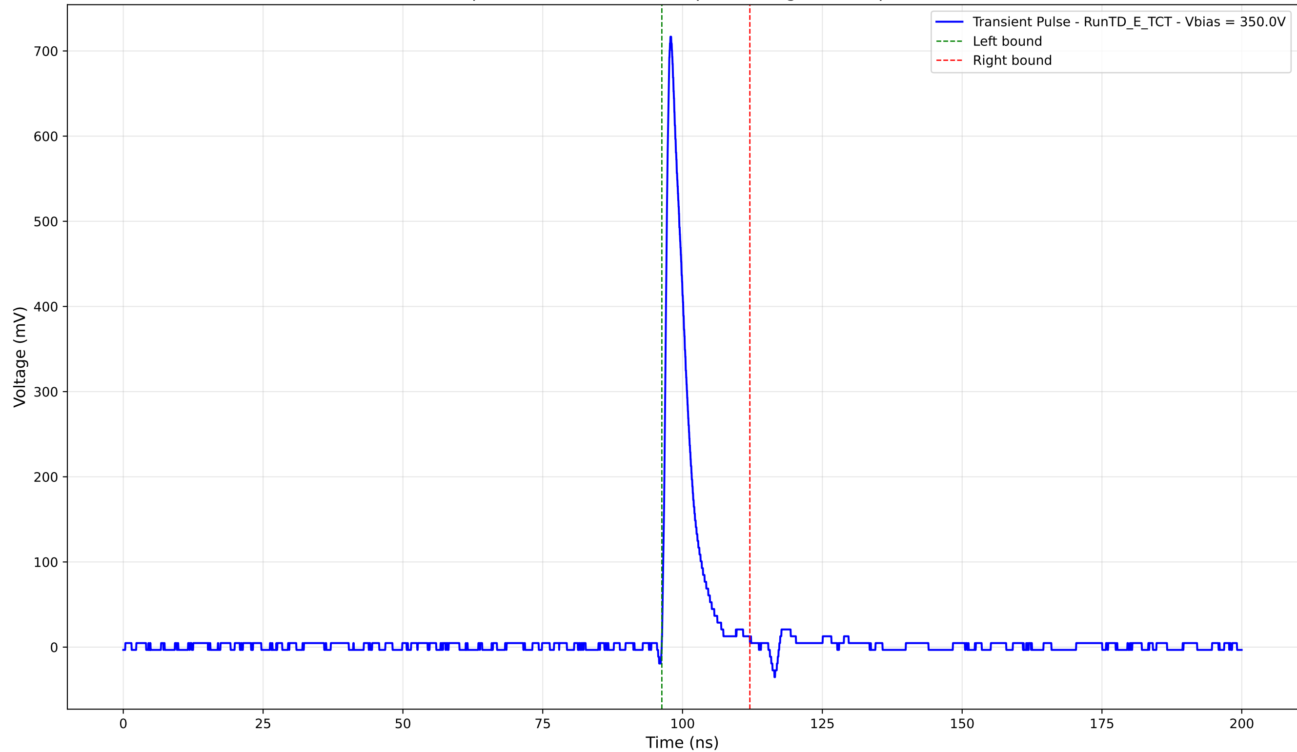
Transient Pulse - Sample: TD - Position: 260.0 \mu\text{m} - Charge: 57.04 pC - Rise Time: 0.97 ns
