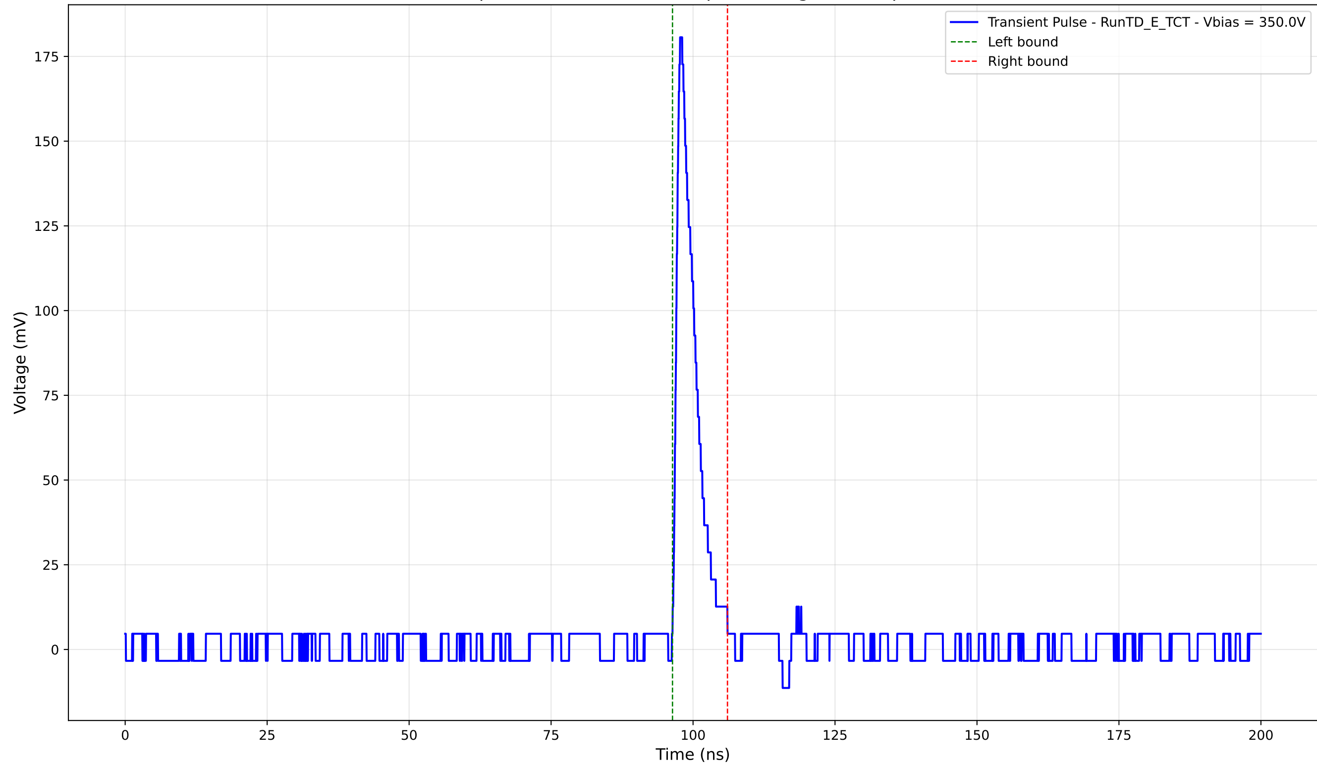
Transient Pulse - Sample: TD - Position: 515.0 \mu\text{m} - Charge: 13.51 pC - Rise Time: 0.97 ns
