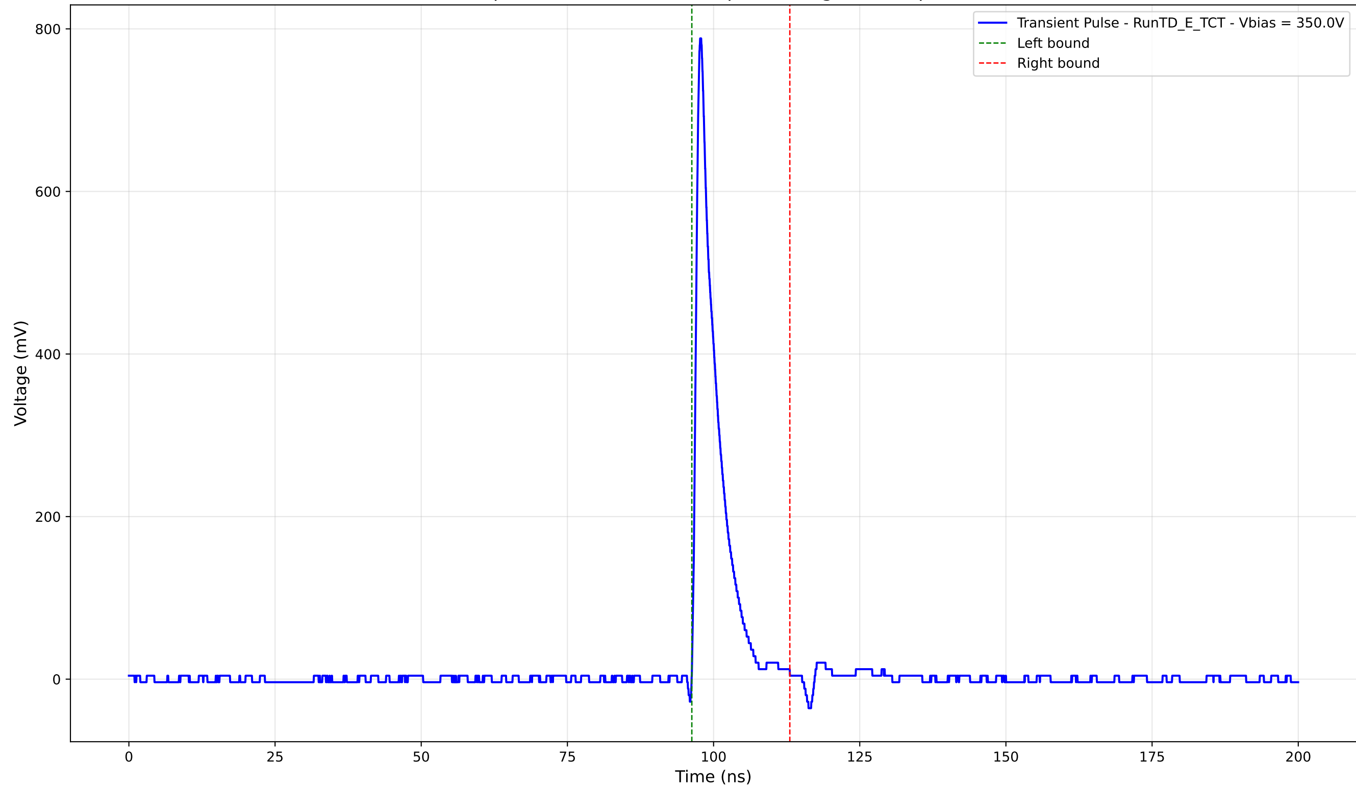
Transient Pulse - Sample: TD - Position: 165.0 \mu\text{m} - Charge: 62.98 pC - Rise Time: 0.92 ns
