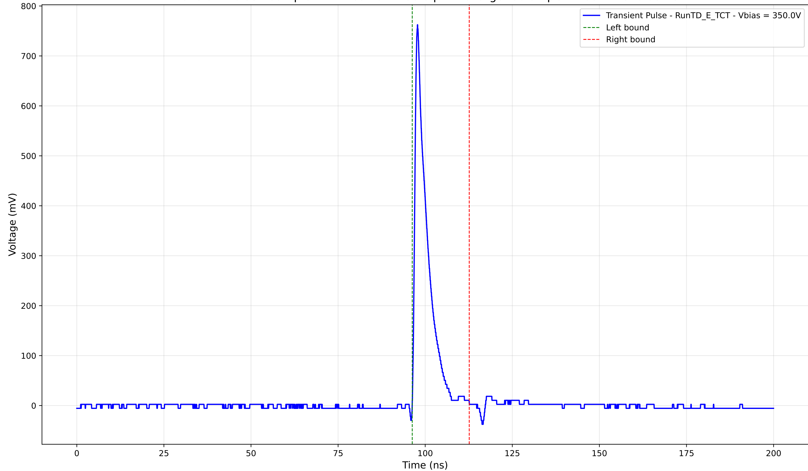
Transient Pulse - Sample: TD - Position: 200.0 \mu\text{m} - Charge: 60.91 pC - Rise Time: 0.93 ns
