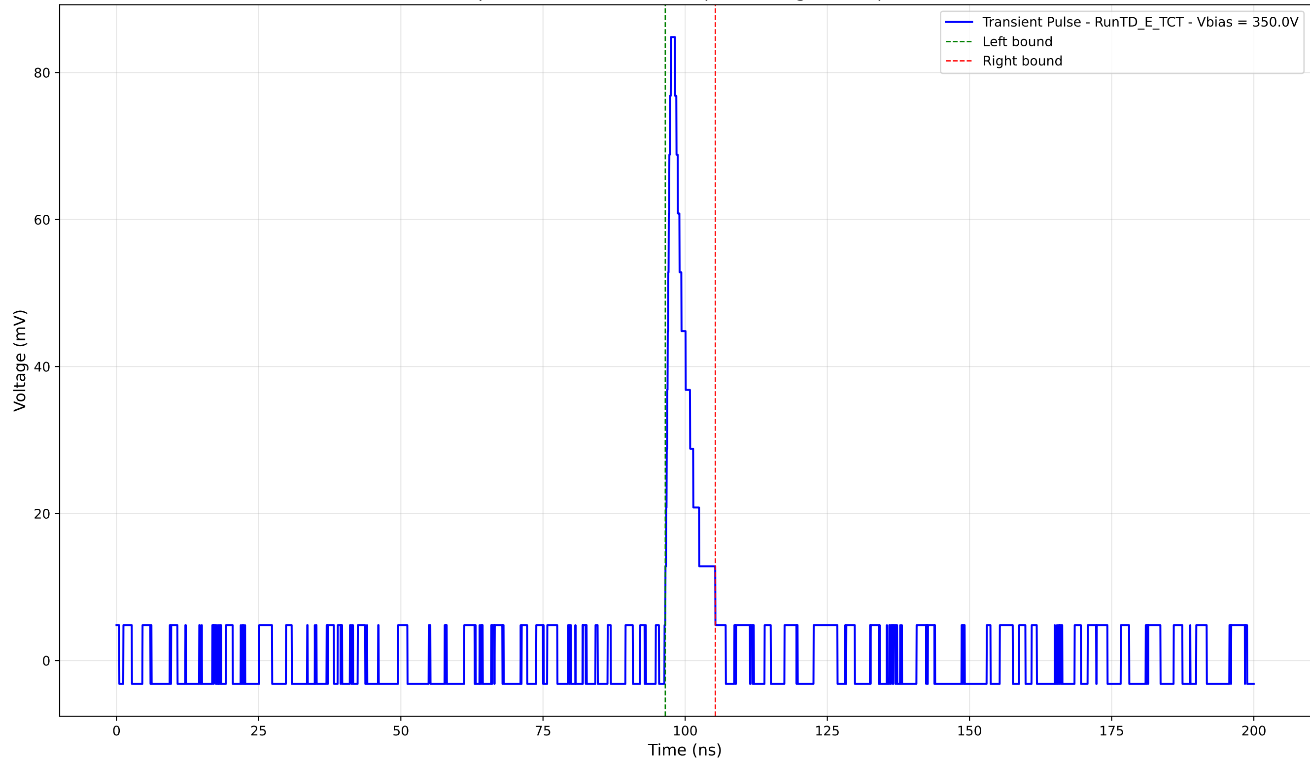
Transient Pulse - Sample: TD - Position: 625.0 \mu\text{m} - Charge: 6.30 pC - Rise Time: 0.81 ns
