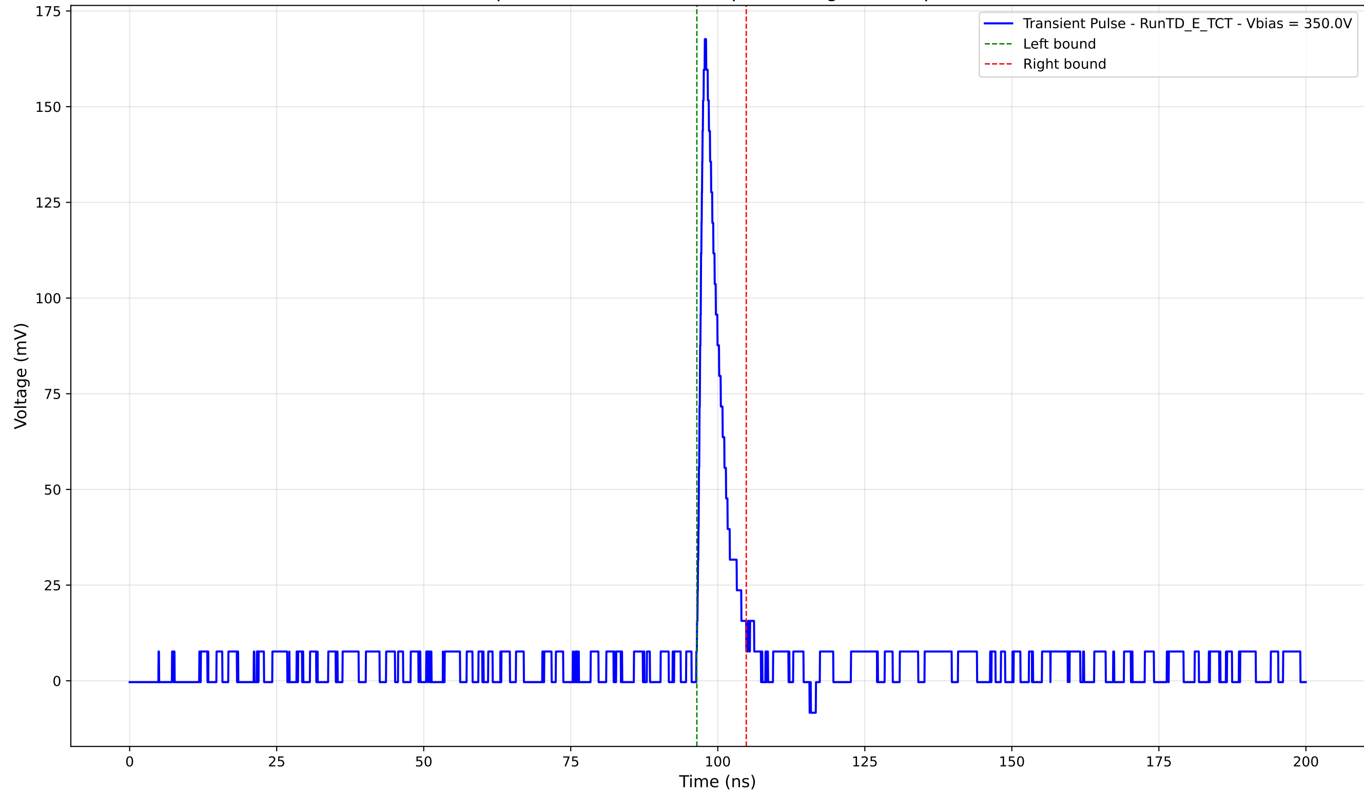
Transient Pulse - Sample: TD - Position: 530.0 \mu\text{m} - Charge: 12.24 pC - Rise Time: 0.94 ns
