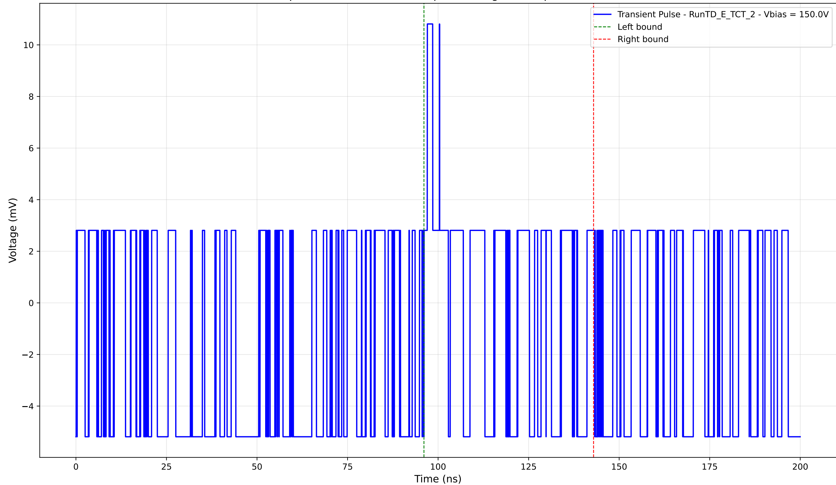
Transient Pulse - Sample: TD - Position: 165.0 \mu\text{m} - Charge: 0.39 pC - Rise Time: 0.00 ns (N/A)
