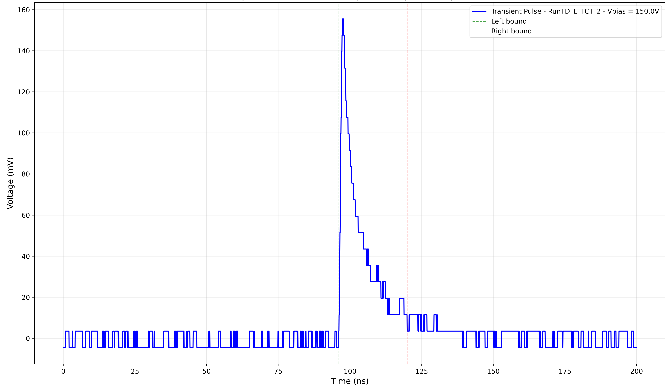
Transient Pulse - Sample: TD - Position: 335.0 \mu\text{m} - Charge: 21.26 pC - Rise Time: 0.97 ns
