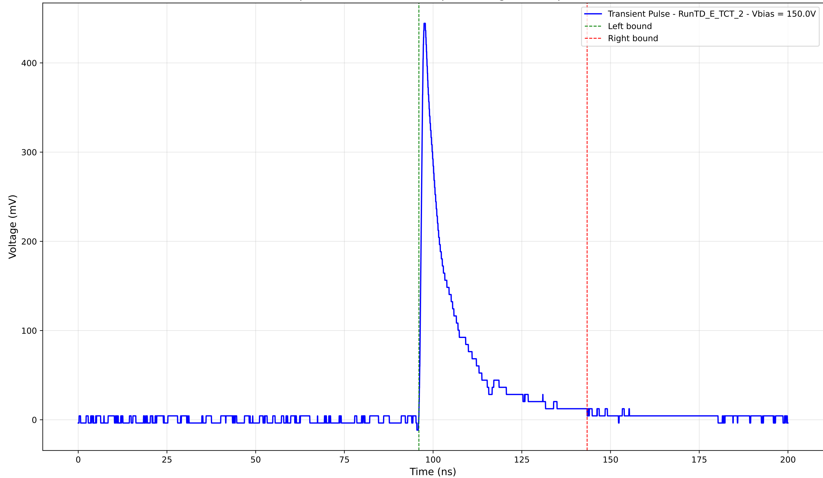
Transient Pulse - Sample: TD - Position: 490.0 \mu\text{m} - Charge: 73.61 pC - Rise Time: 0.98 ns
