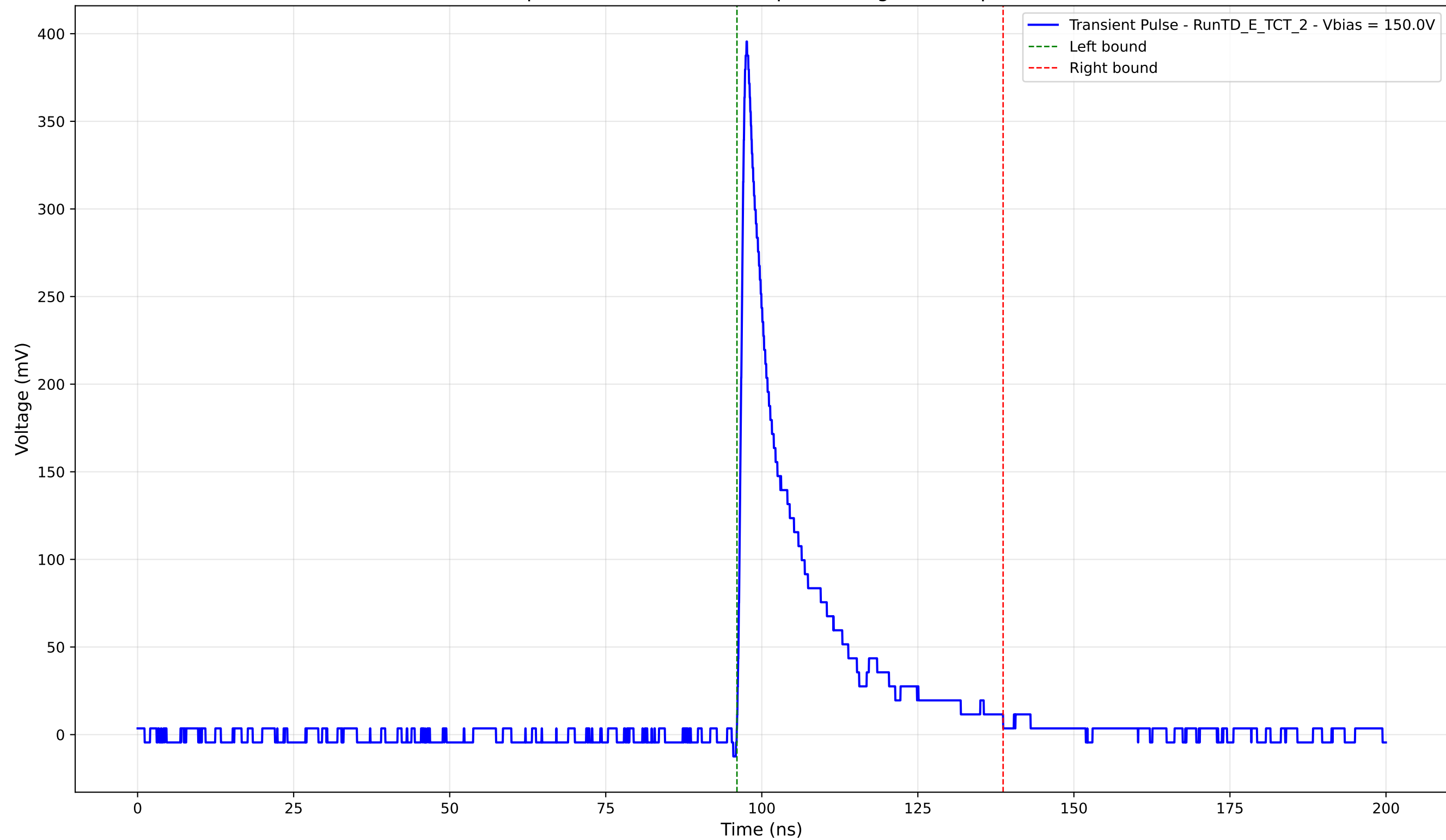
Transient Pulse - Sample: TD - Position: 355.0 \mu\text{m} - Charge: 64.25 pC - Rise Time: 1.01 ns
