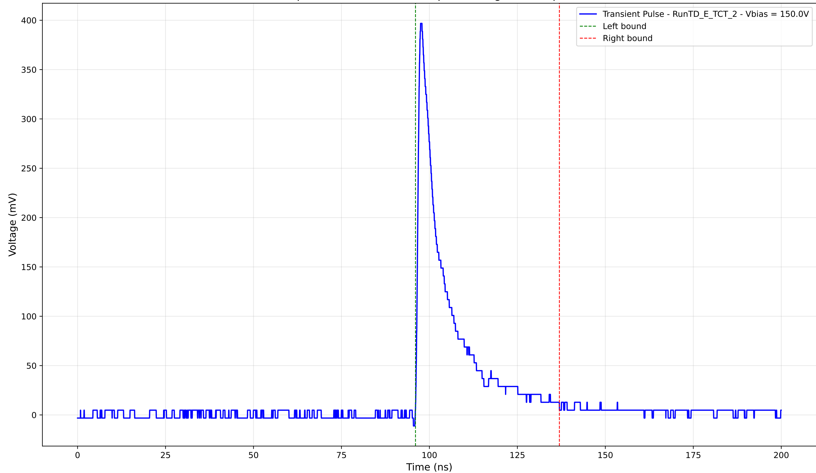
Transient Pulse - Sample: TD - Position: 510.0 \mu\text{m} - Charge: 66.35 pC - Rise Time: 0.99 ns
