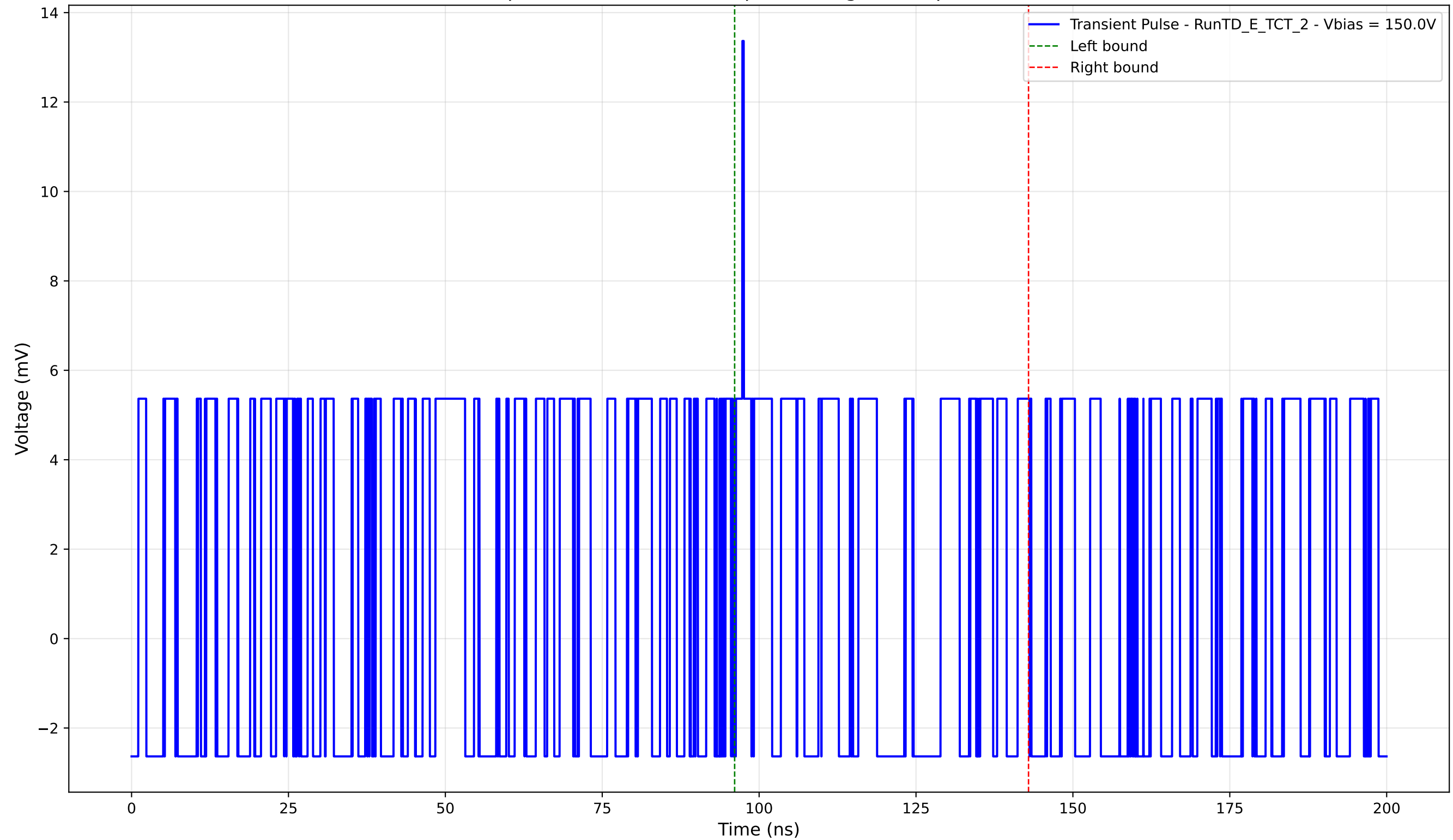
Transient Pulse - Sample: TD - Position: 25.0 \mu\text{m} - Charge: 1.80 pC - Rise Time: 0.00 ns (N/A)
