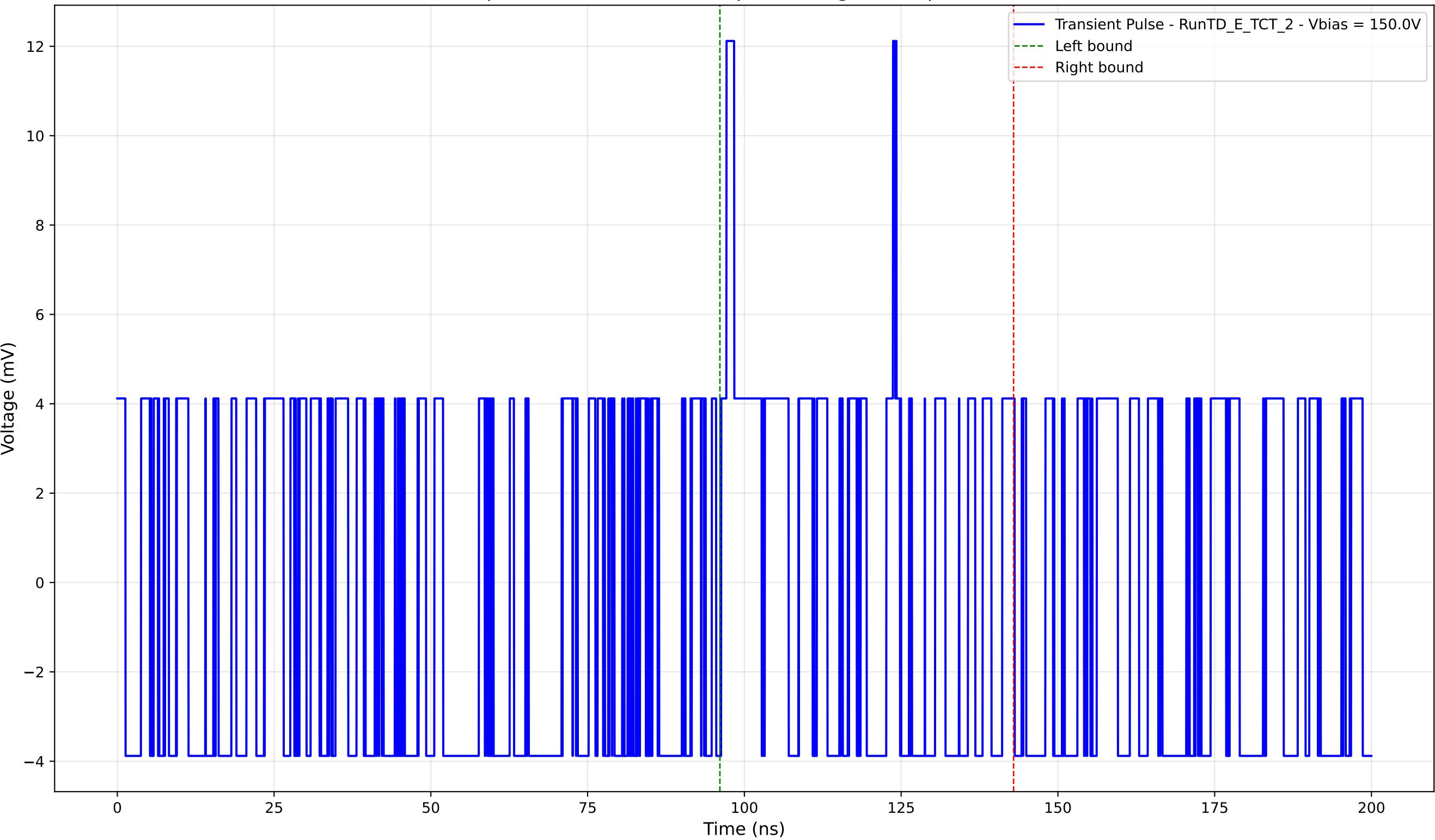
Transient Pulse - Sample: TD - Position: 215.0 \mu\text{m} - Charge: 0.78 pC - Rise Time: 0.00 ns (N/A)
