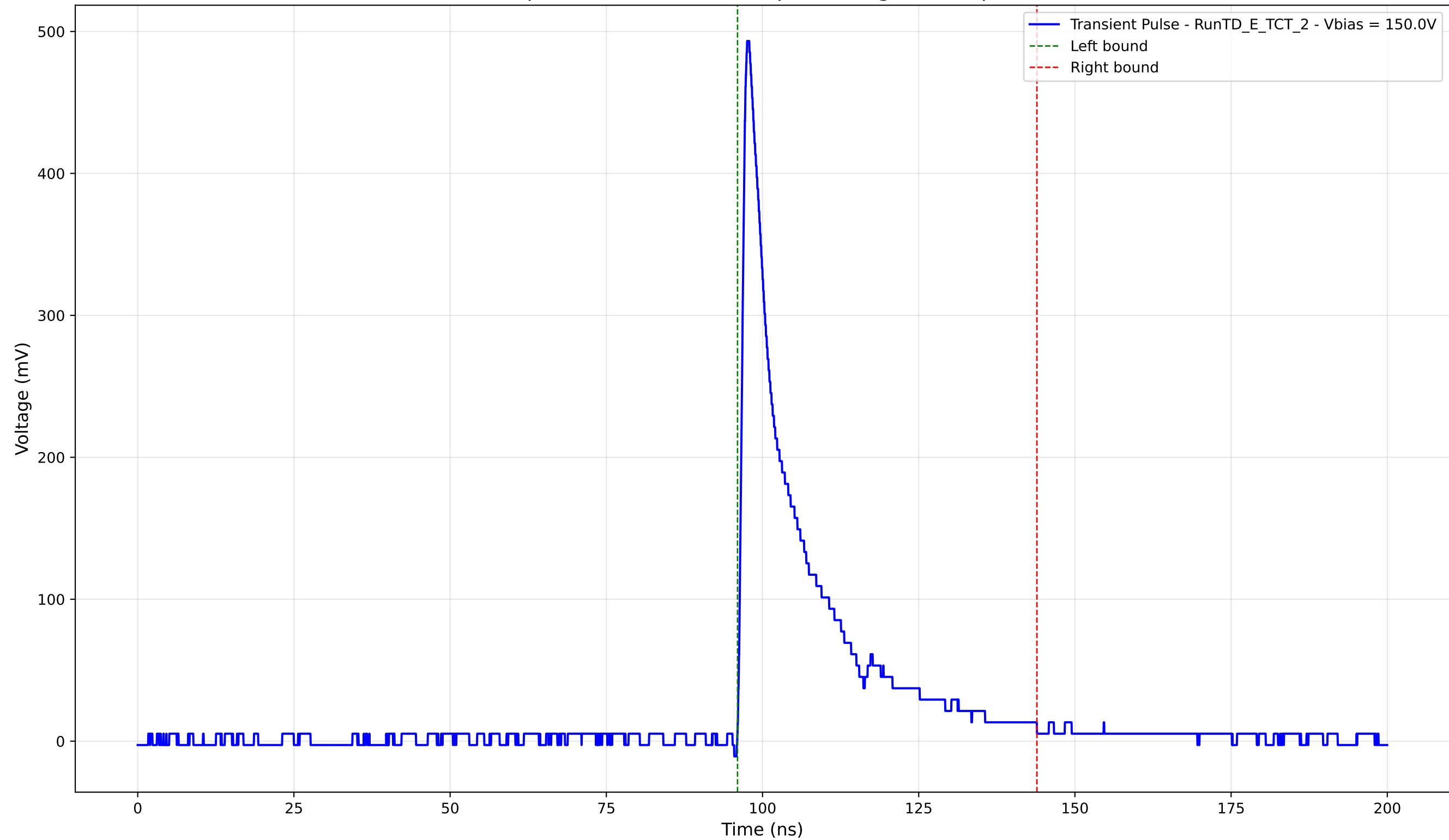
Transient Pulse - Sample: TD - Position: 375.0 \mu\text{m} - Charge: 87.91 pC - Rise Time: 1.01 ns
