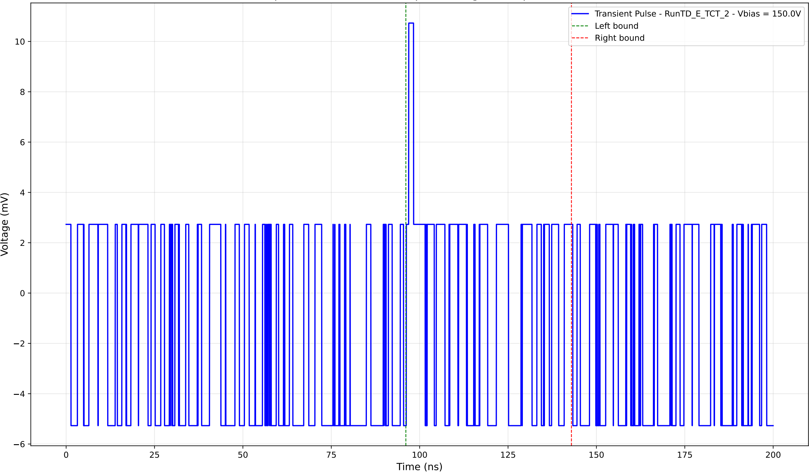
Transient Pulse - - Sample: TD - Position: 145.0 \mu\text{m} - Charge: 0.17 pC - Rise Time: 0.00 ns (N/A)
