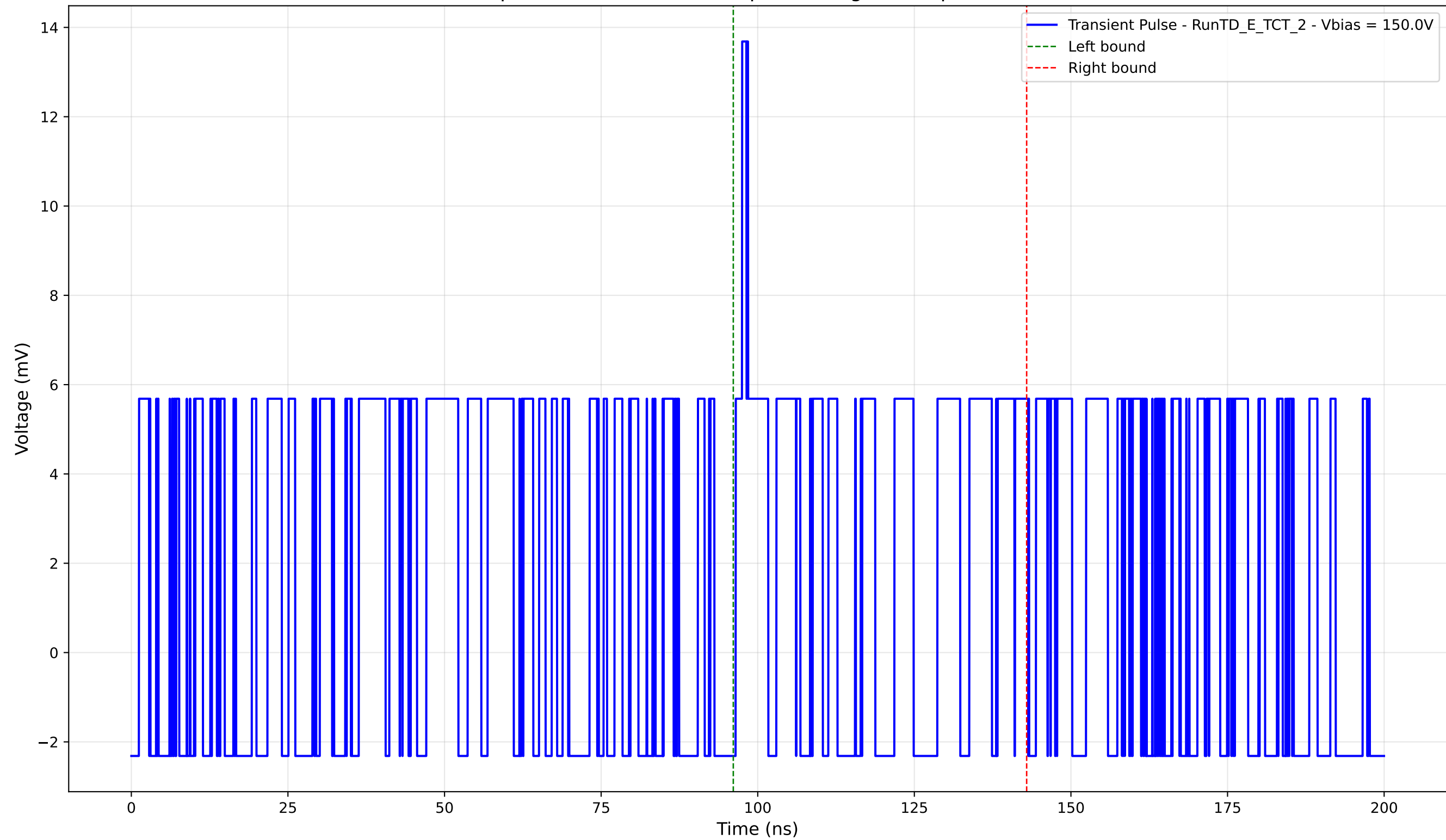
Transient Pulse - - Sample: TD - Position: 105.0 \mu\text{m} - Charge: 2.67 pC - Rise Time: 0.00 ns (N/A)
