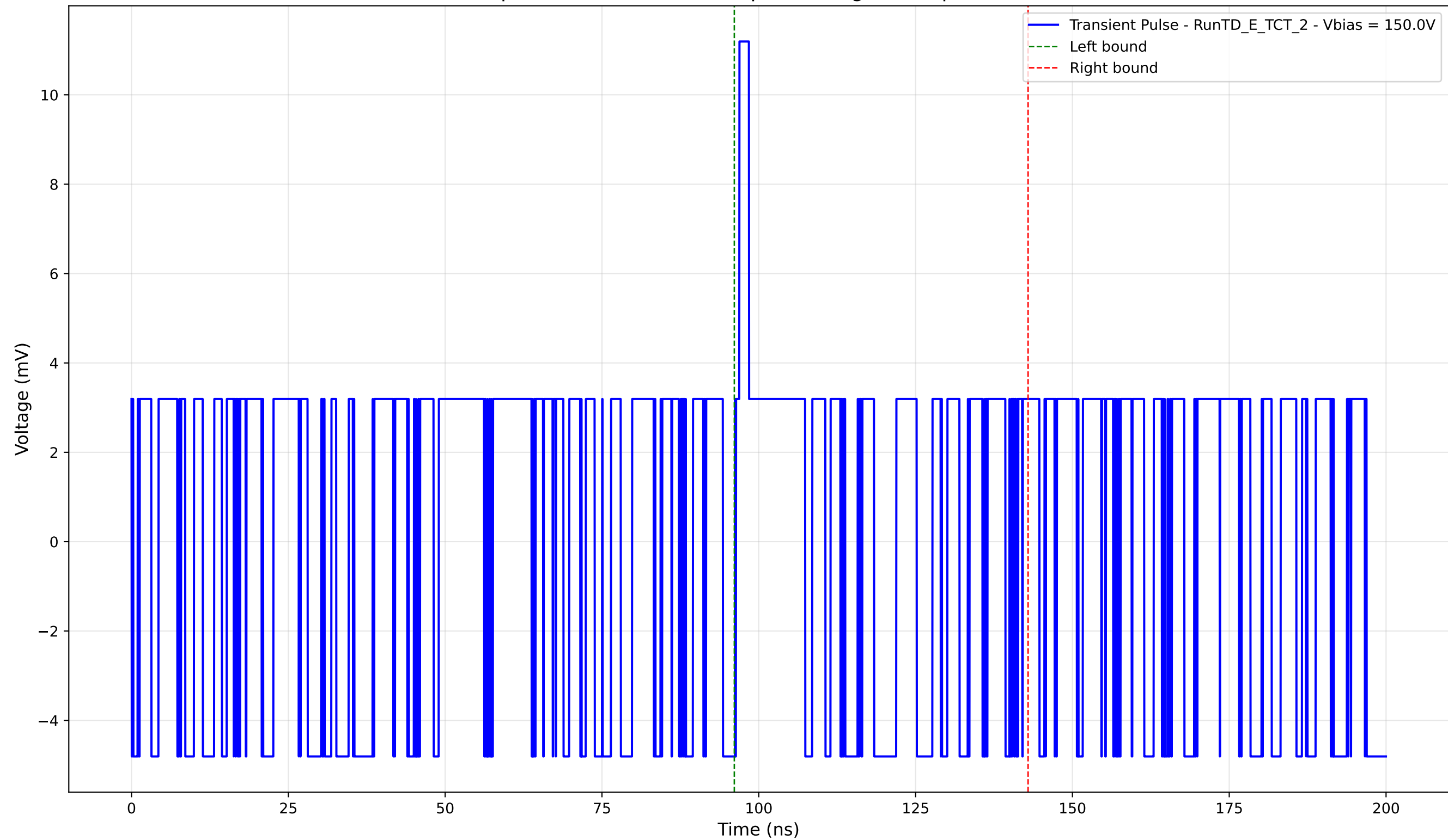
Transient Pulse - Sample: TD - Position: 100.0 \mu\text{m} - Charge: 0.76 pC - Rise Time: 0.00 ns (N/A)
