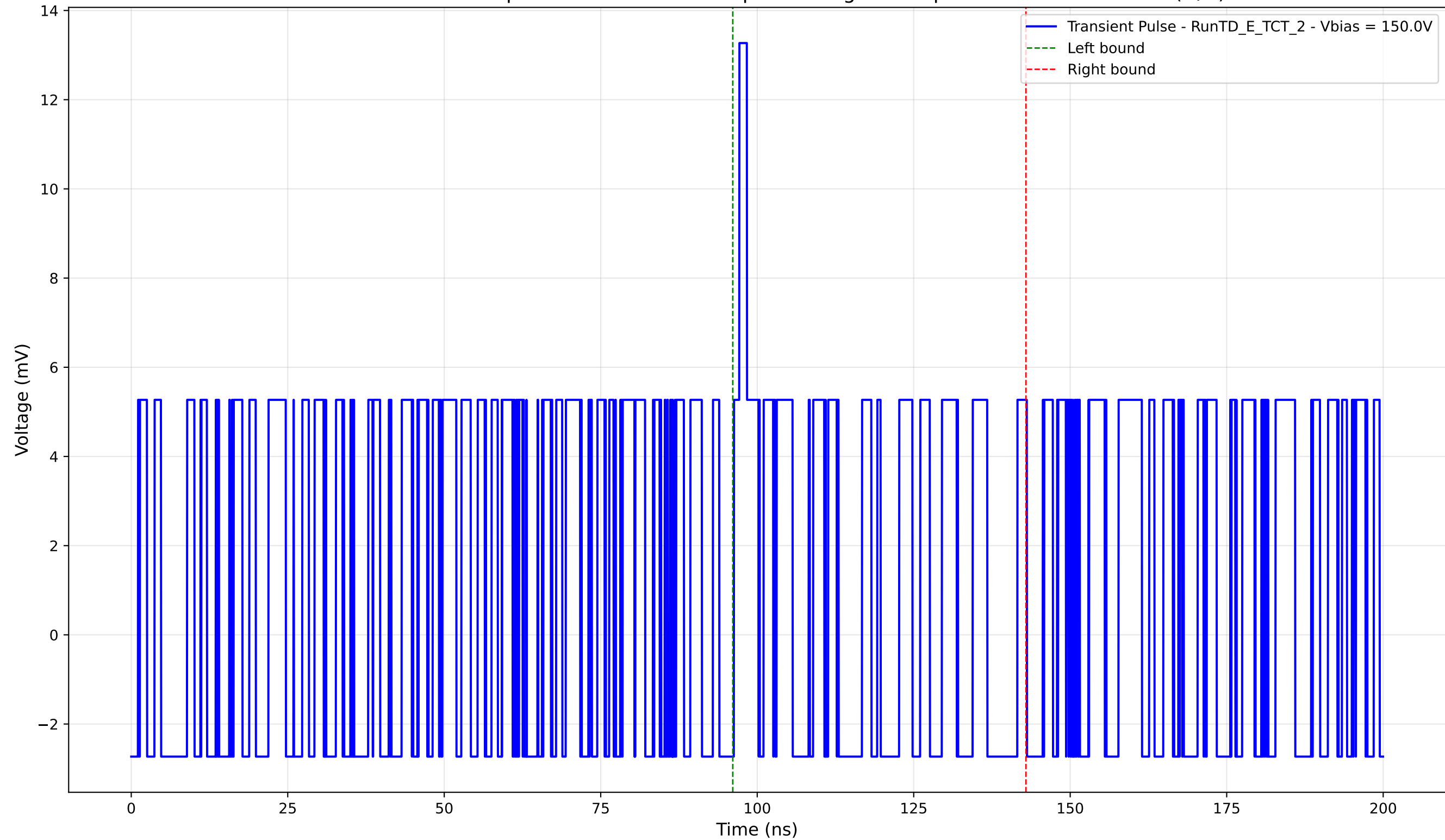
Transient Pulse - Sample: TD - Position: 90.0 \mu\text{m} - Charge: 1.47 pC - Rise Time: 0.00 ns (N/A)
