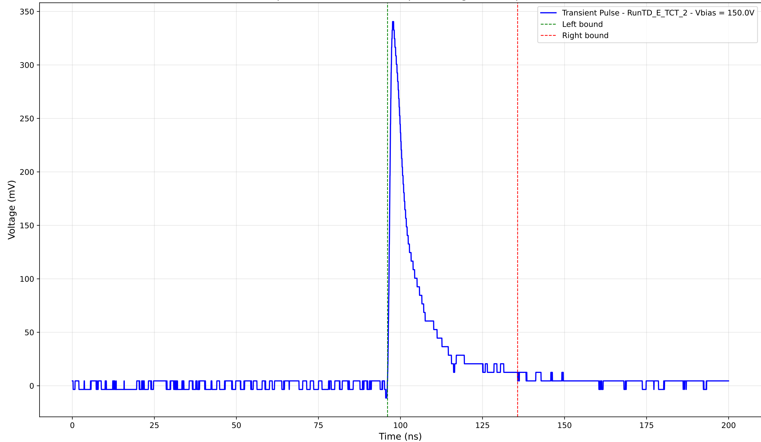
Transient Pulse - Sample: TD - Position: 565.0 \mu\text{m} - Charge: 53.68 pC - Rise Time: 1.03 ns
