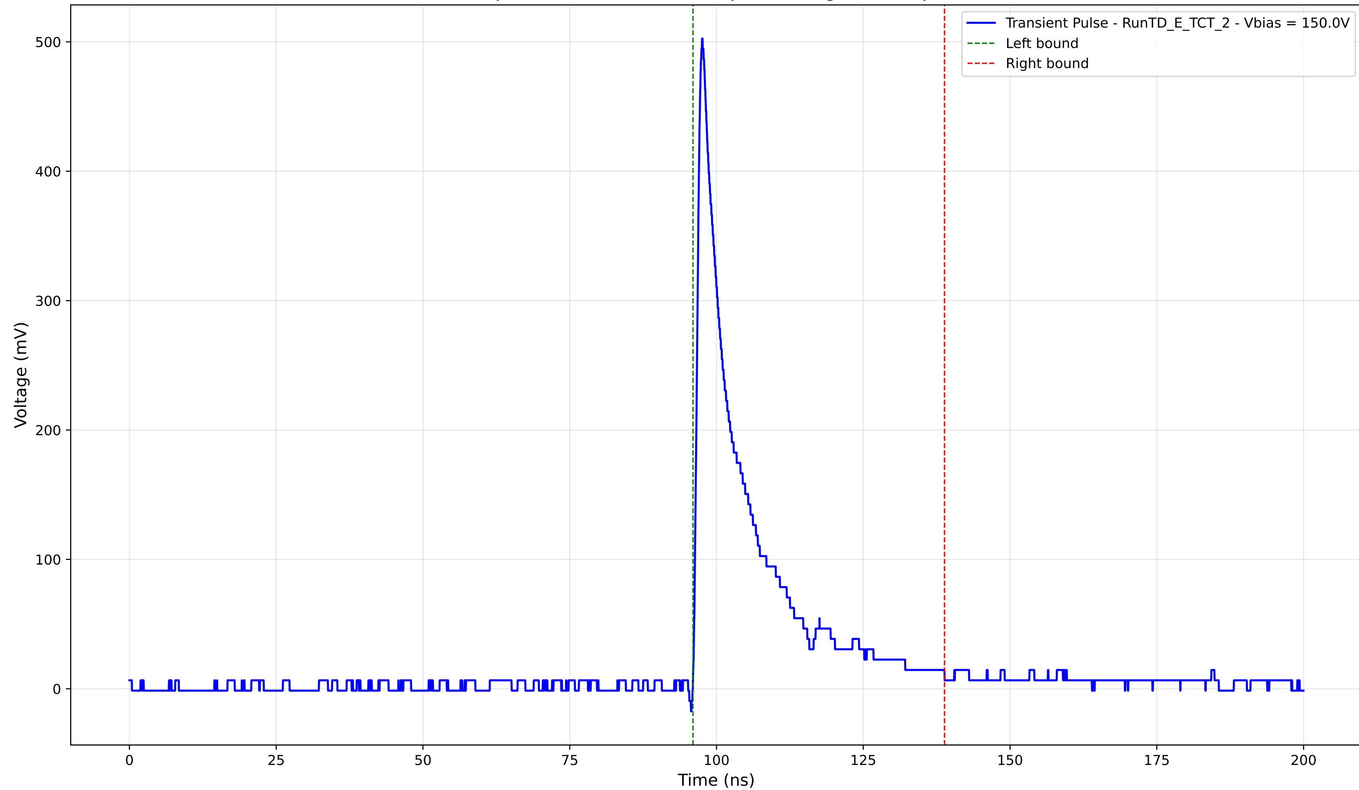
Transient Pulse - Sample: TD - Position: 480.0 \mu\text{m} - Charge: 80.37 pC - Rise Time: 0.99 ns
