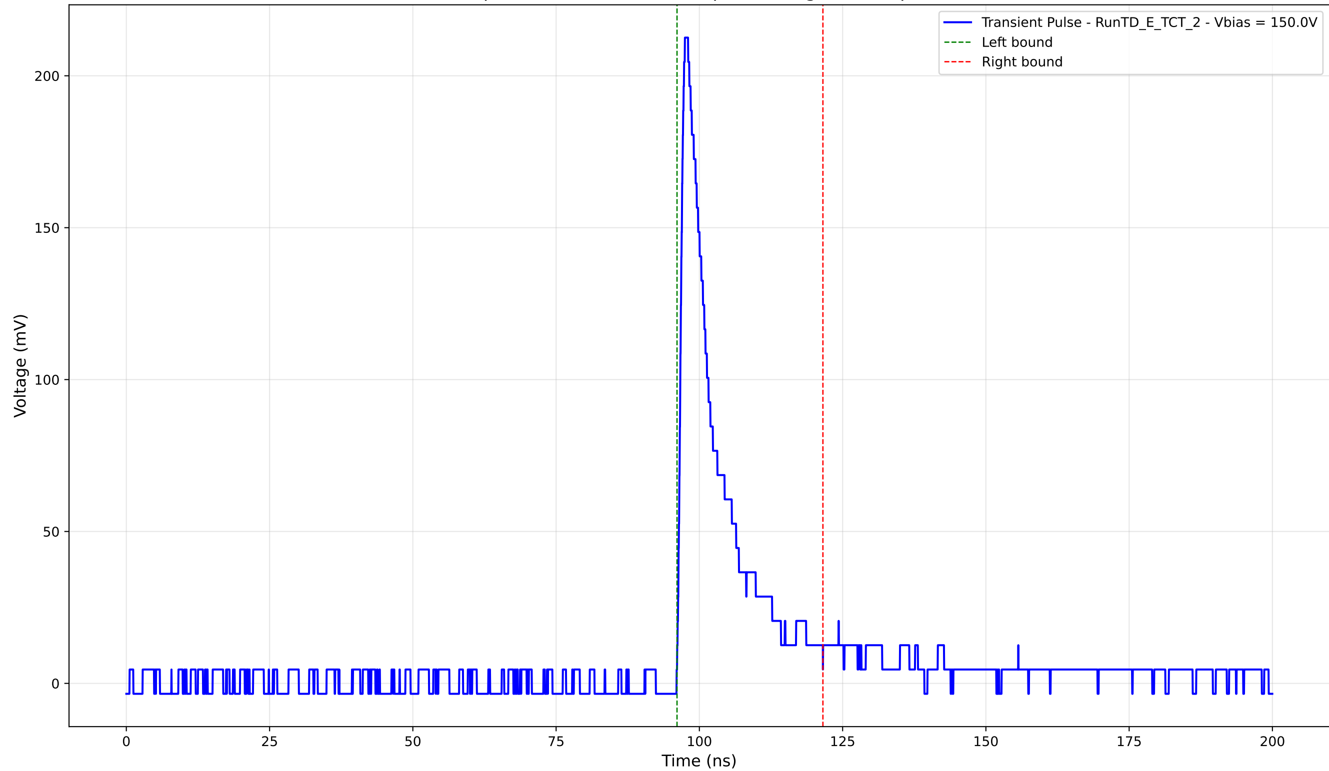
Transient Pulse - Sample: TD - Position: 615.0 \mu\text{m} - Charge: 29.94 pC - Rise Time: 0.98 ns
