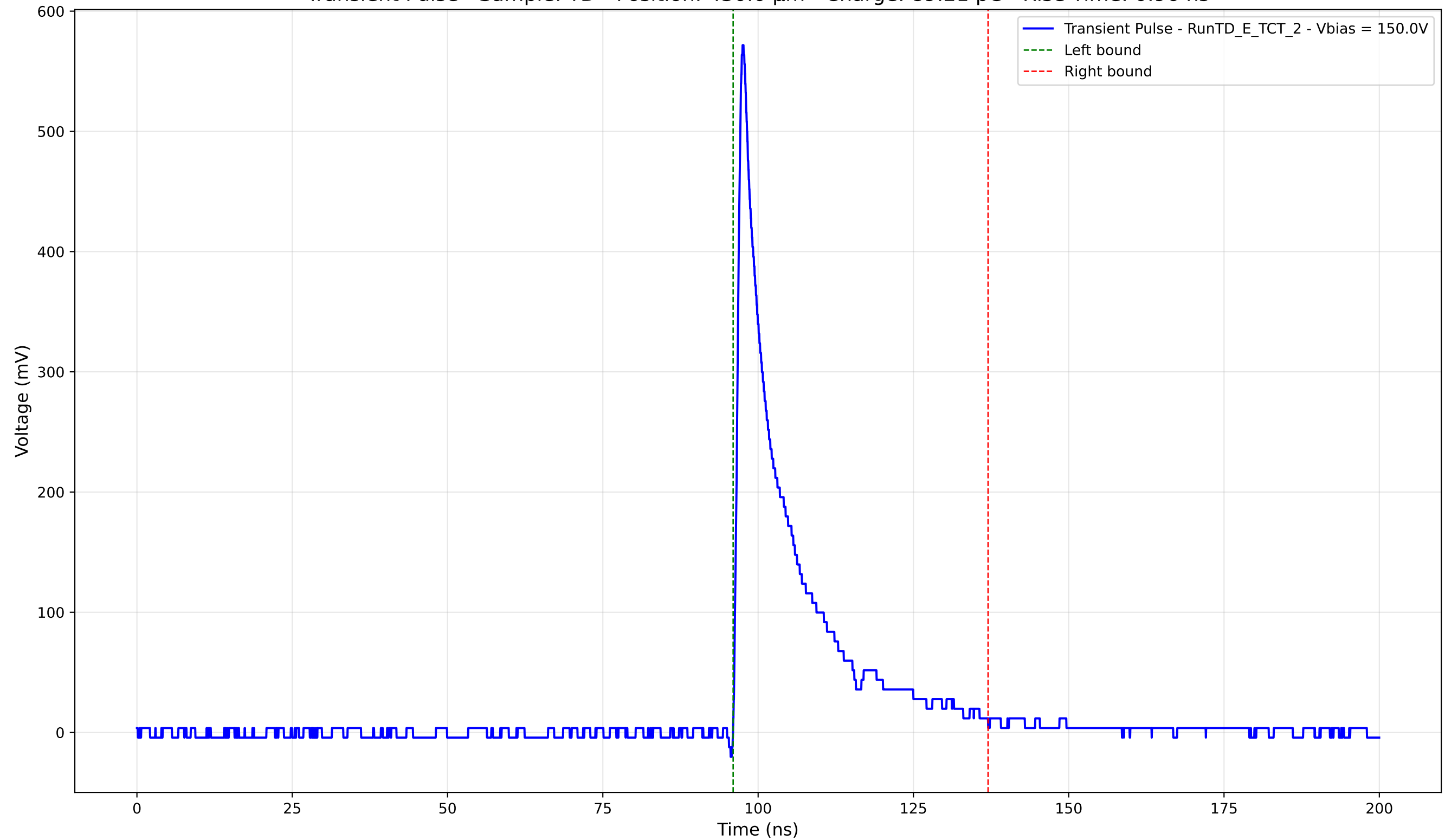
Transient Pulse - Sample: TD - Position: 430.0 \mu\text{m} - Charge: 89.21 pC - Rise Time: 0.96 ns
