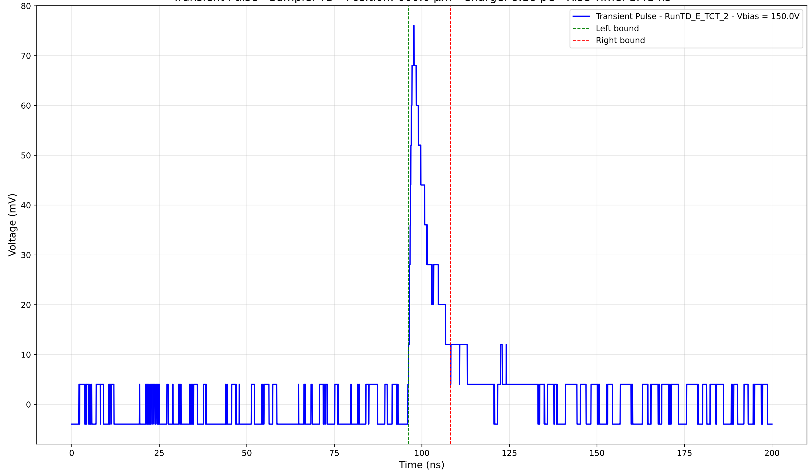
Transient Pulse - Sample: TD - Position: 660.0 \mu\text{m} - Charge: 8.18 pC - Rise Time: 1.41 ns
