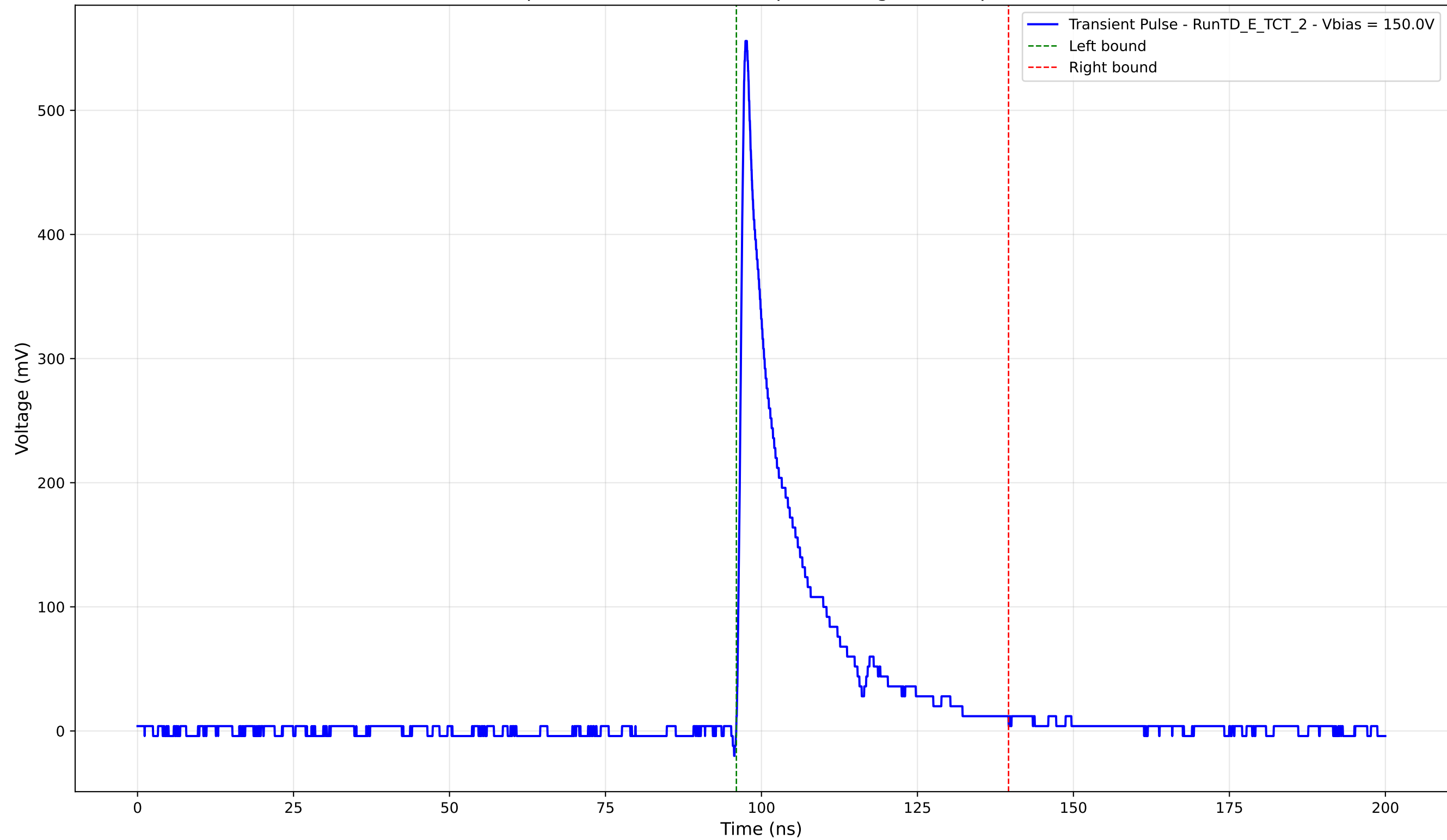
Transient Pulse - Sample: TD - Position: 440.0 \mu\text{m} - Charge: 87.20 pC - Rise Time: 0.97 ns
