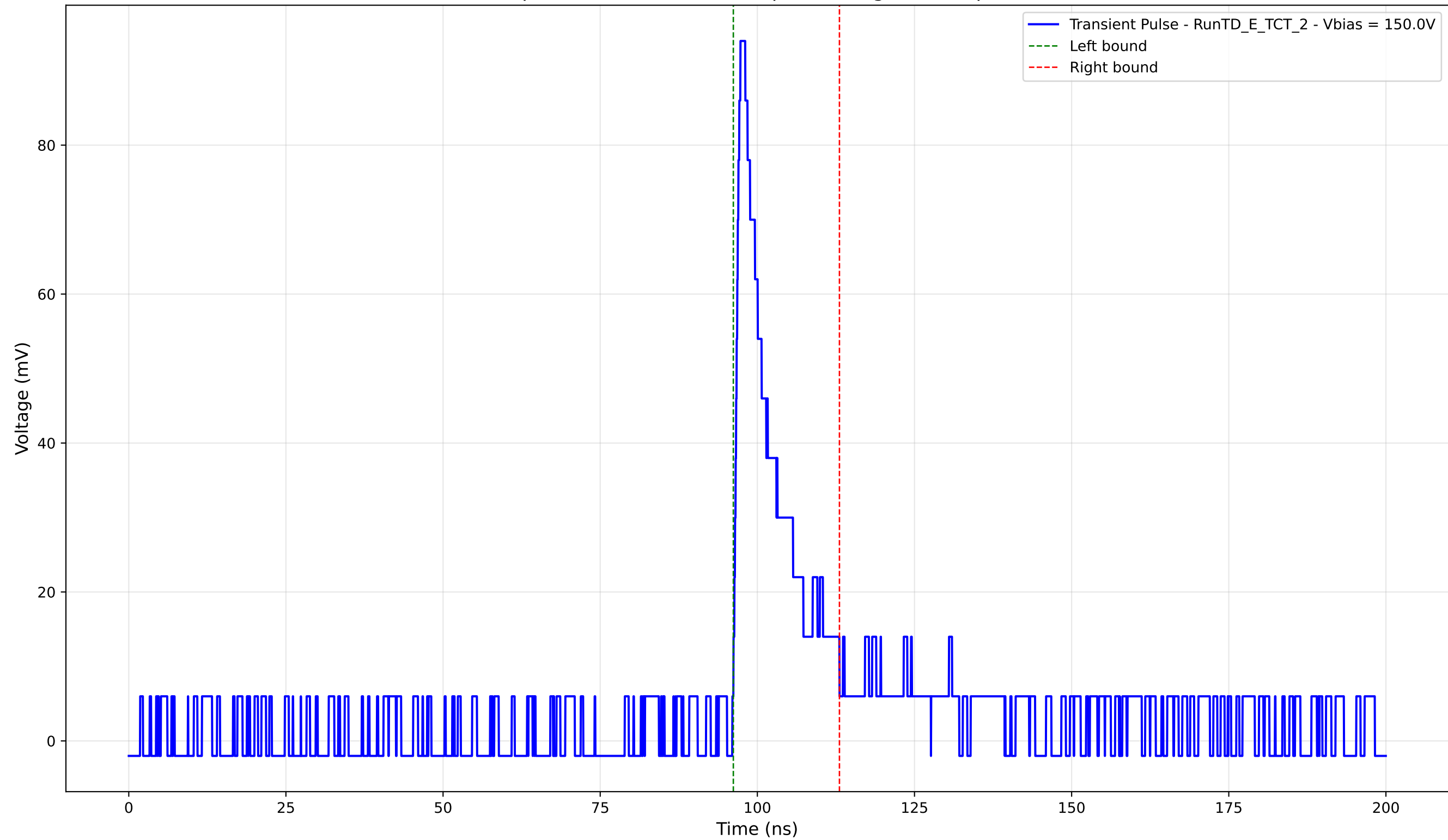
Transient Pulse - Sample: TD - Position: 725.0 \mu\text{m} - Charge: 12.23 pC - Rise Time: 0.93 ns
