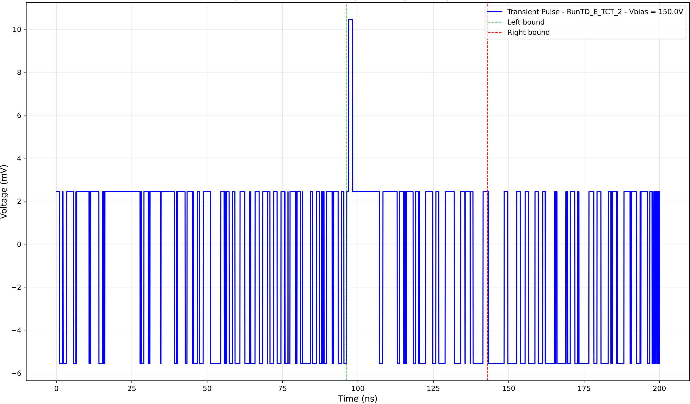
Transient Pulse - Sample: TD - Position: 130.0 \mu\text{m} - Charge: 0.22 pC - Rise Time: 0.00 ns (N/A)
