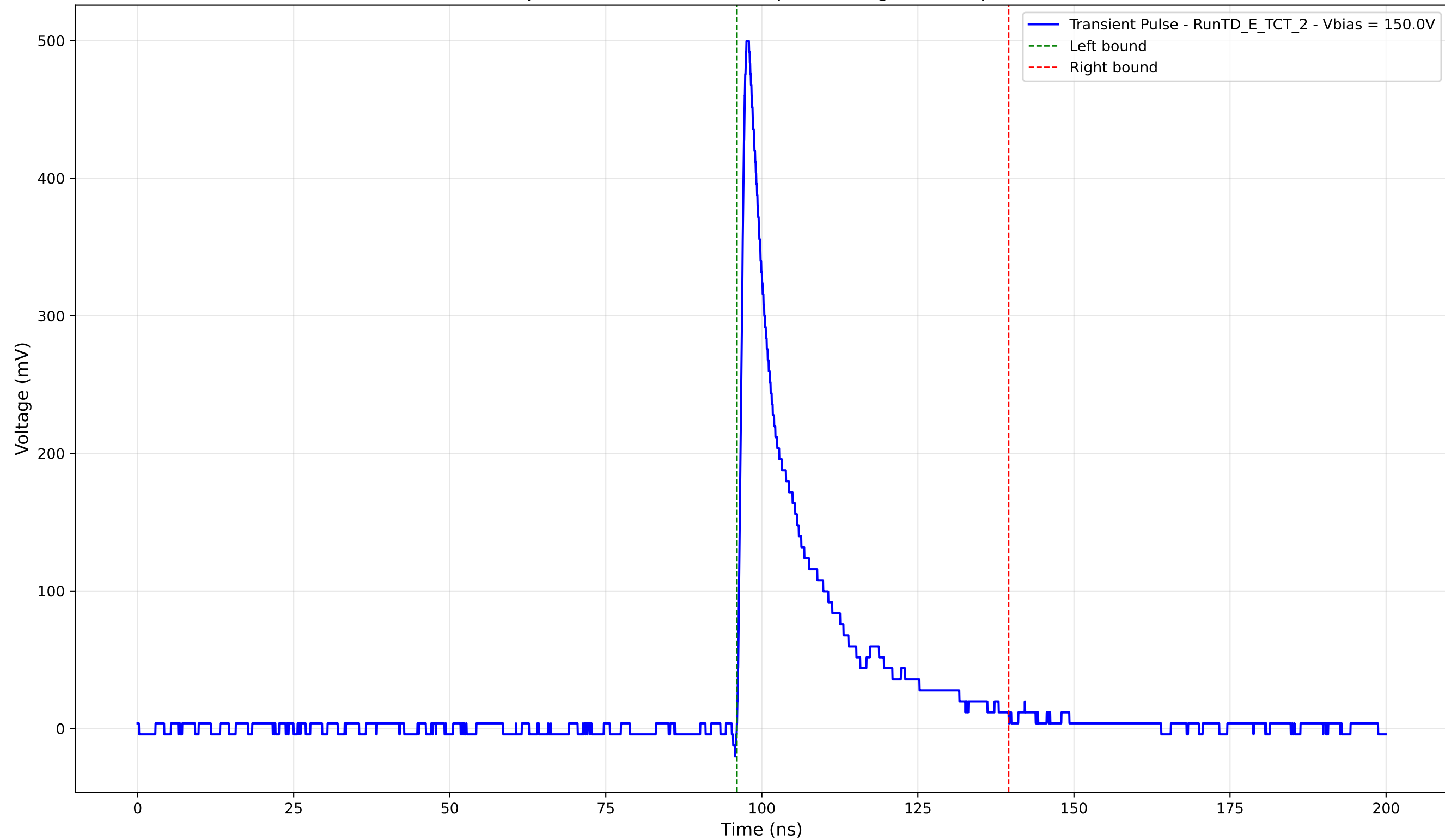
Transient Pulse - Sample: TD - Position: 380.0 \mu\text{m} - Charge: 87.06 pC - Rise Time: 1.02 ns
