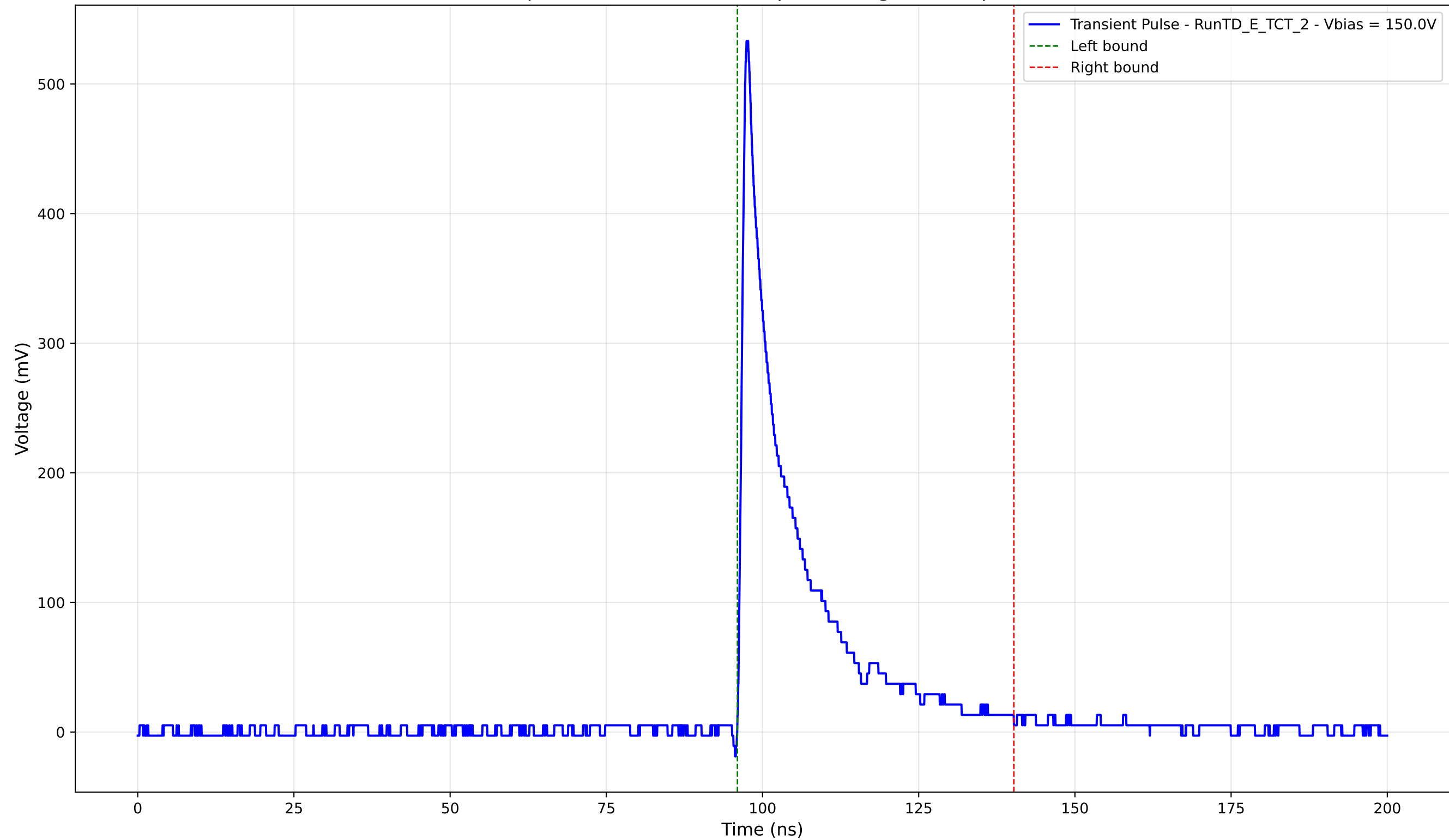
Transient Pulse - Sample: TD - Position: 460.0 \mu\text{m} - Charge: 86.23 pC - Rise Time: 0.97 ns
