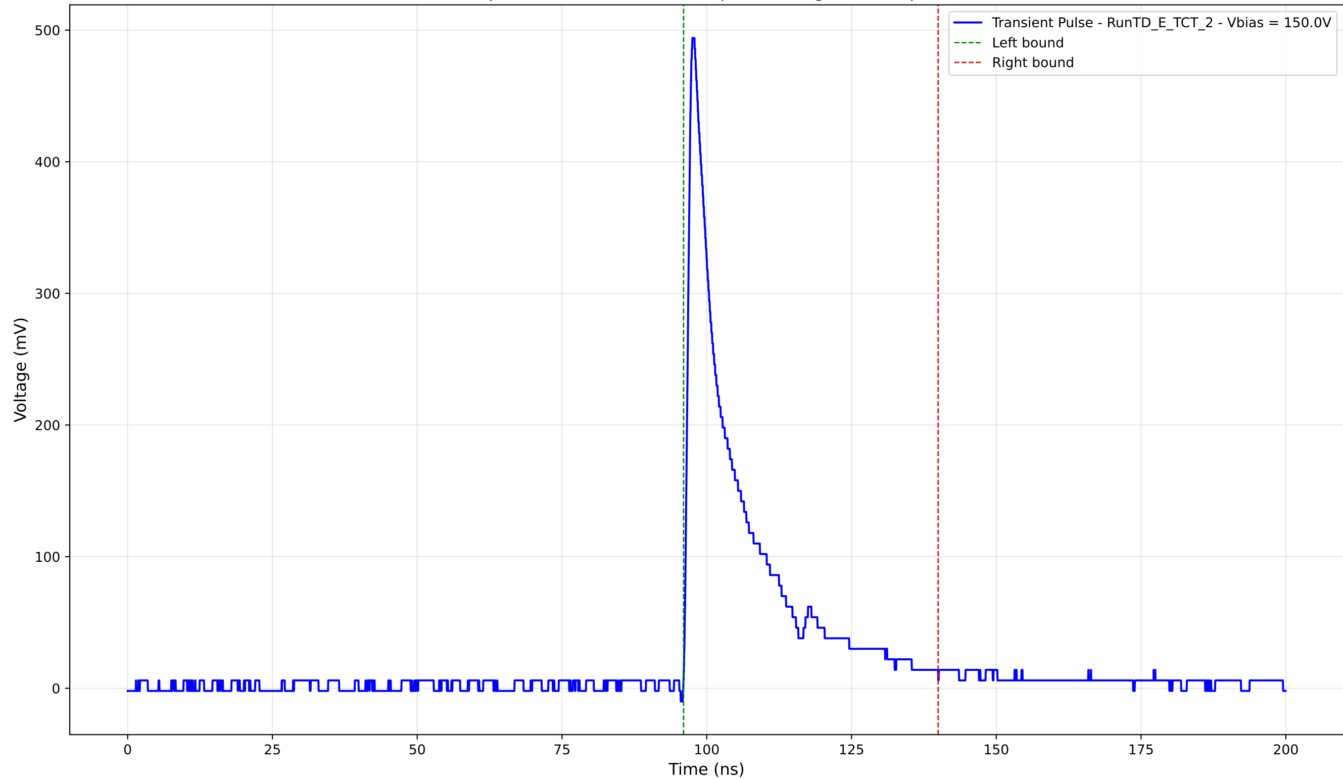
Transient Pulse - Sample: TD - Position: 390.0 \mu\text{m} - Charge: 86.49 pC - Rise Time: 1.01 ns
