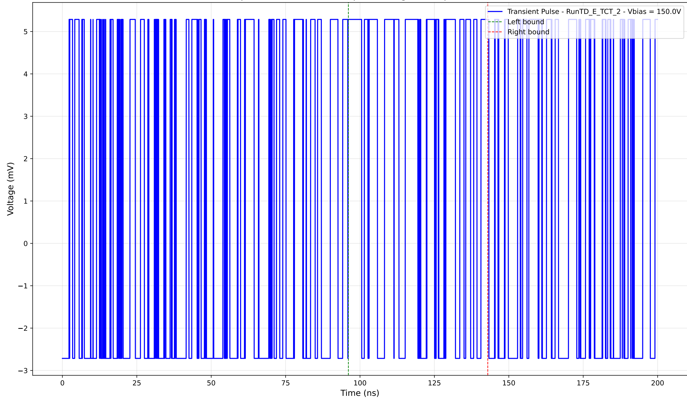
Transient Pulse - Sample: TD - Position: 45.0 \mu\text{m} - Charge: 2.51 pC - Rise Time: 0.00 ns (N/A)
