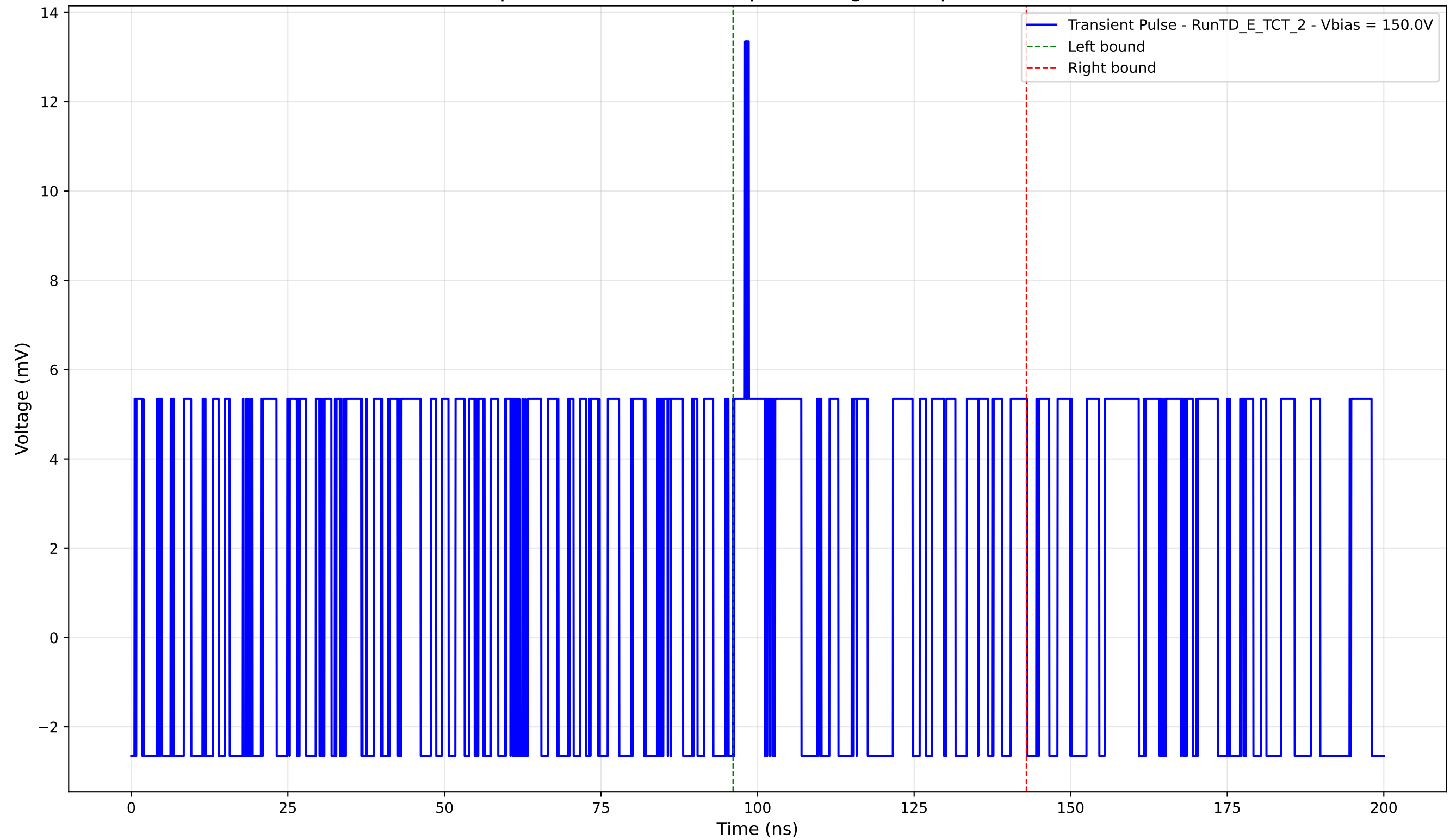
Transient Pulse - Sample: TD - Position: 170.0 \mu\text{m} - Charge: 2.32 pC - Rise Time: 0.00 ns (N/A)
