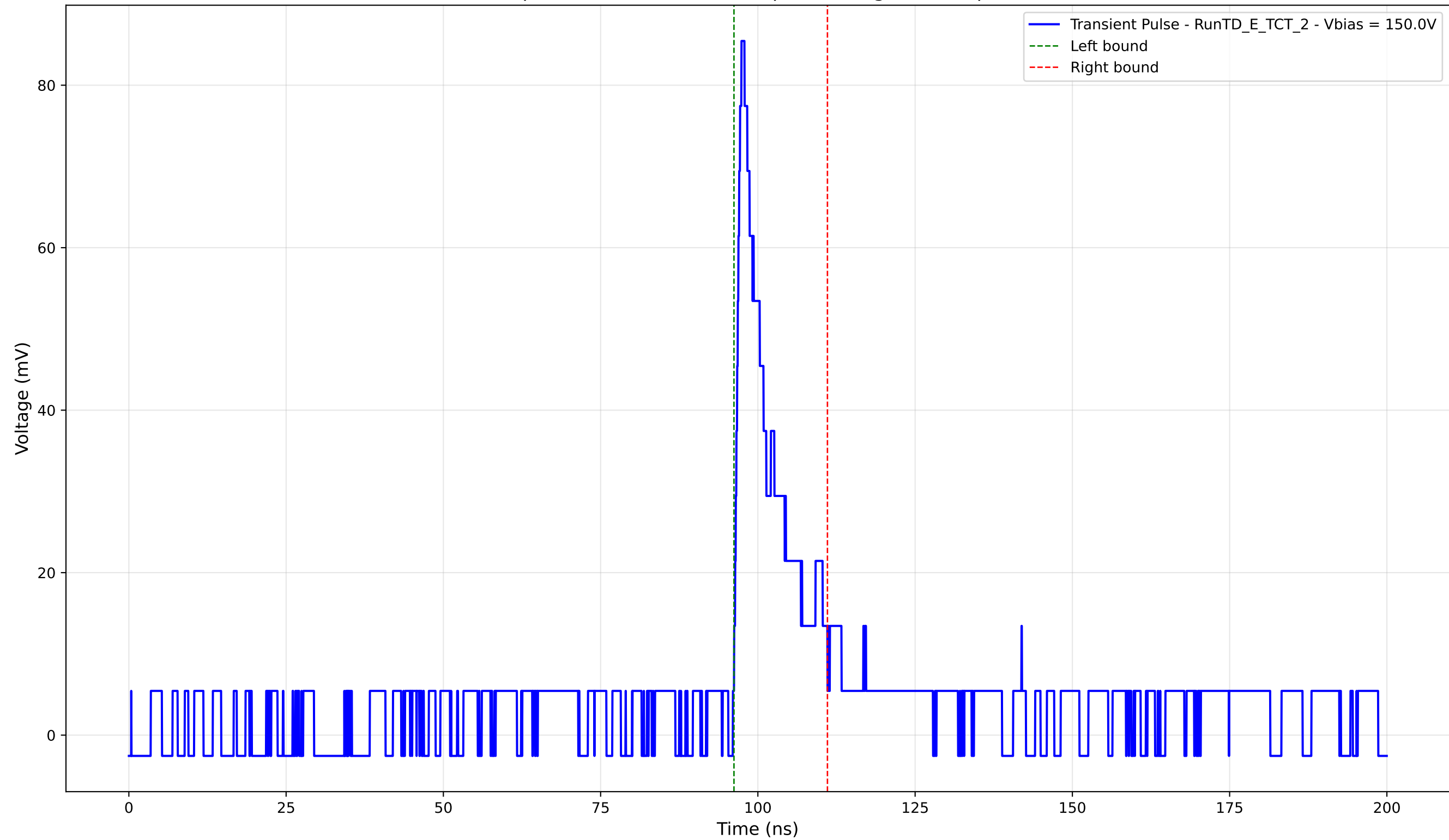
Transient Pulse - Sample: TD - Position: 690.0 \mu\text{m} - Charge: 10.13 pC - Rise Time: 0.95 ns
