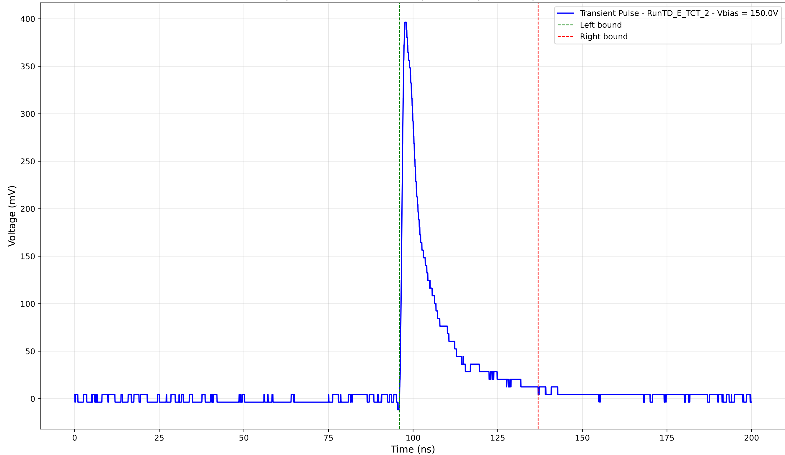
Transient Pulse - Sample: TD - Position: 545.0 \mu\text{m} - Charge: 65.92 pC - Rise Time: 1.05 ns
