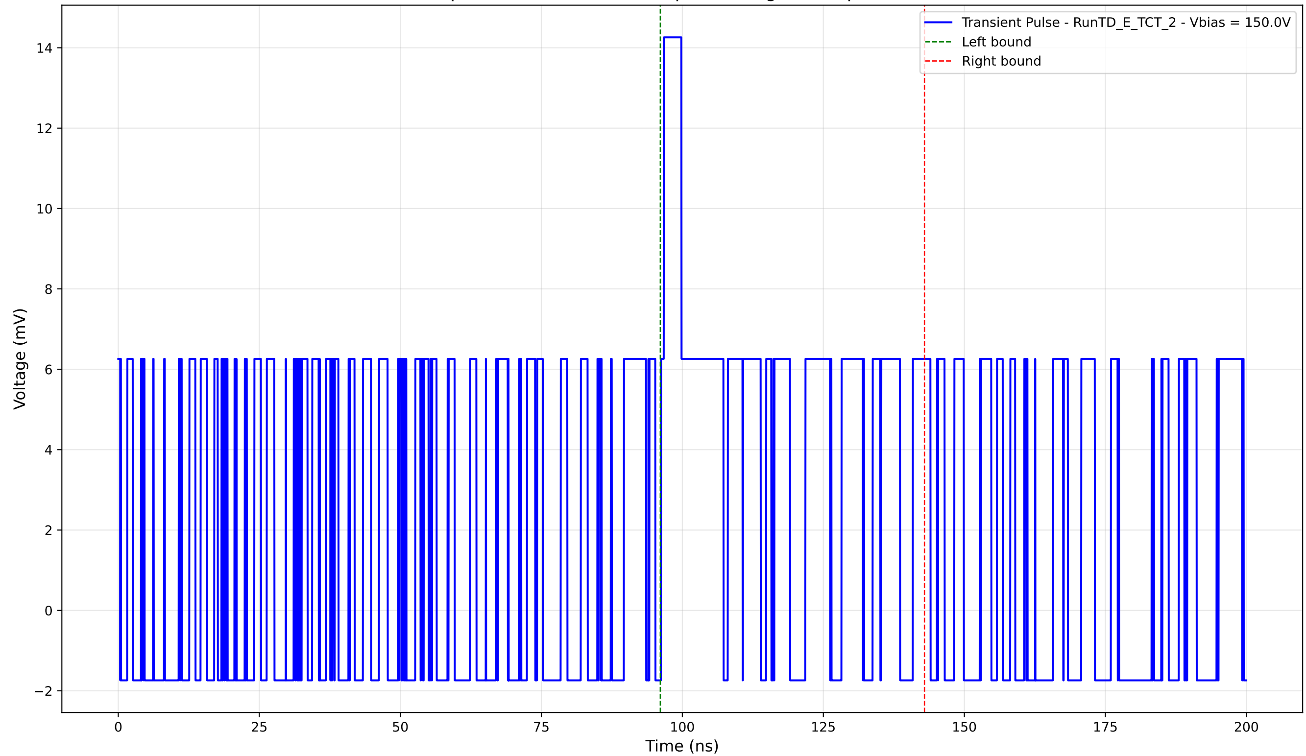
Transient Pulse - Sample: TD - Position: 265.0 \mu\text{m} - Charge: 4.60 pC - Rise Time: 0.00 ns (N/A)
