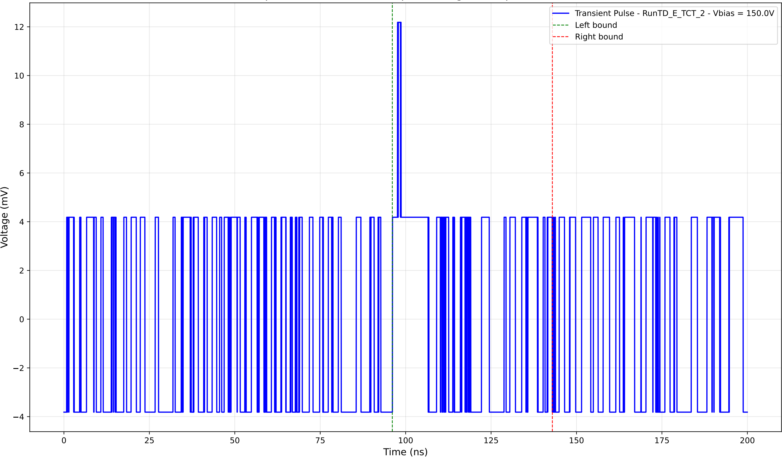
Transient Pulse - Sample: TD - Position: 200.0 \mu\text{m} - Charge: 0.94 pC - Rise Time: 0.00 ns (N/A)
