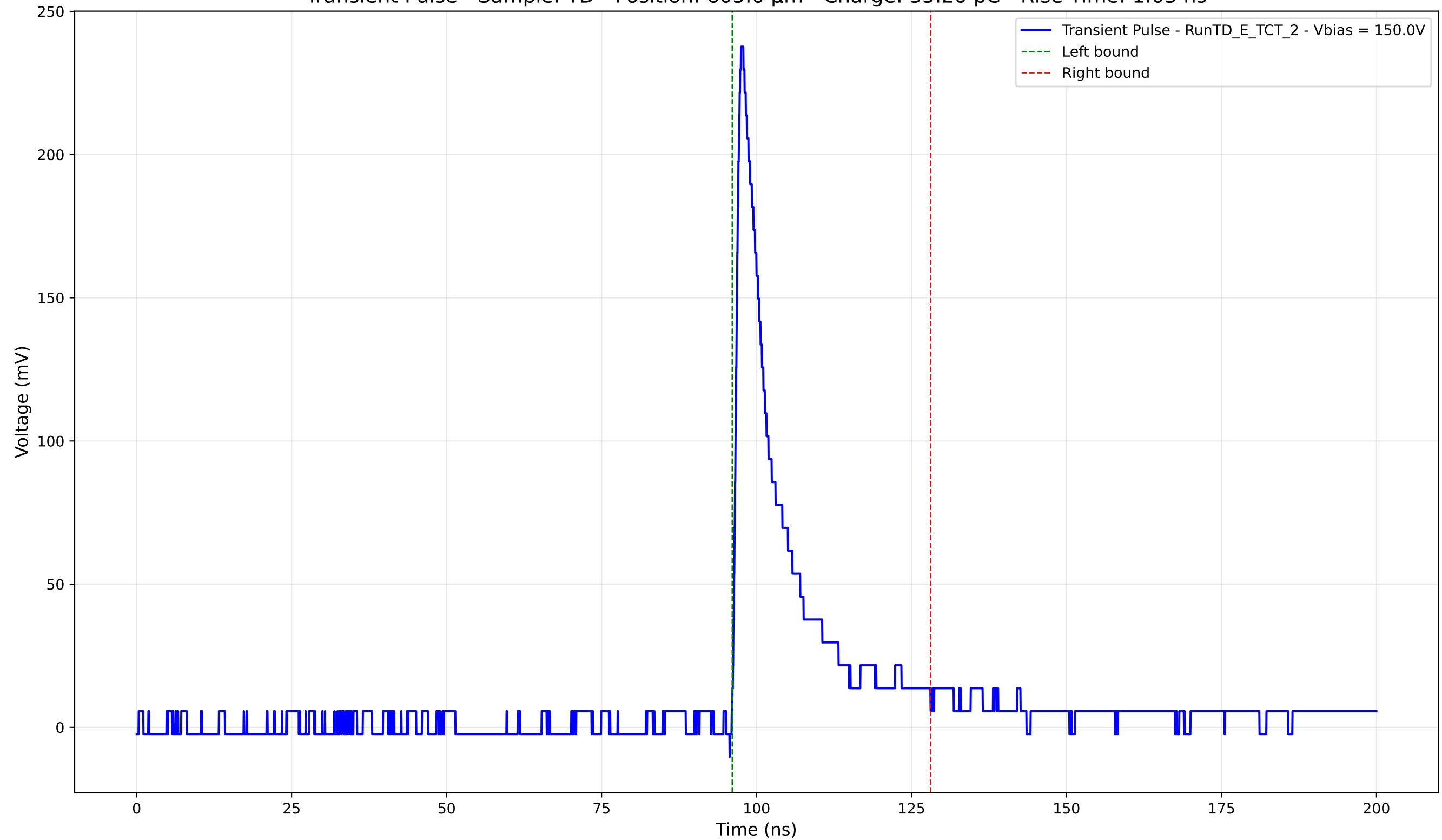
Transient Pulse - Sample: TD - Position: 605.0 \mu\text{m} - Charge: 35.20 pC - Rise Time: 1.03 ns
