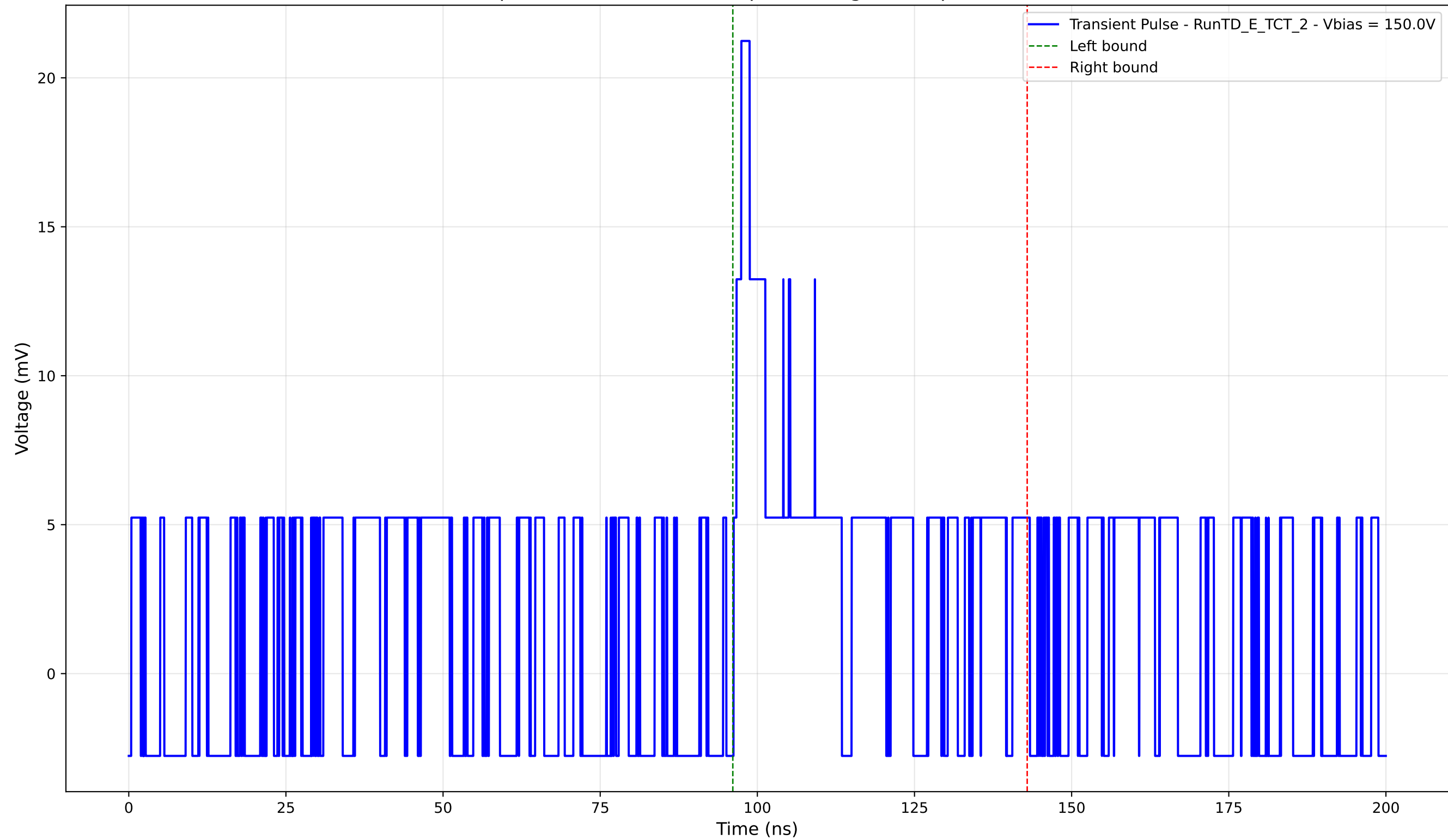
Transient Pulse - Sample: TD - Position: 285.0 \mu\text{m} - Charge: 4.62 pC - Rise Time: 0.00 ns (N/A)
