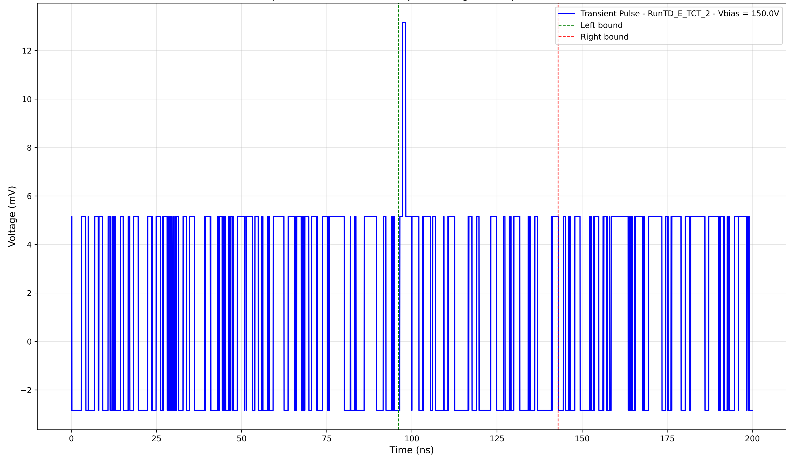
Transient Pulse - - Sample: TD - Position: 175.0 \mu\text{m} - Charge: 0.61 pC - Rise Time: 0.00 ns (N/A)
