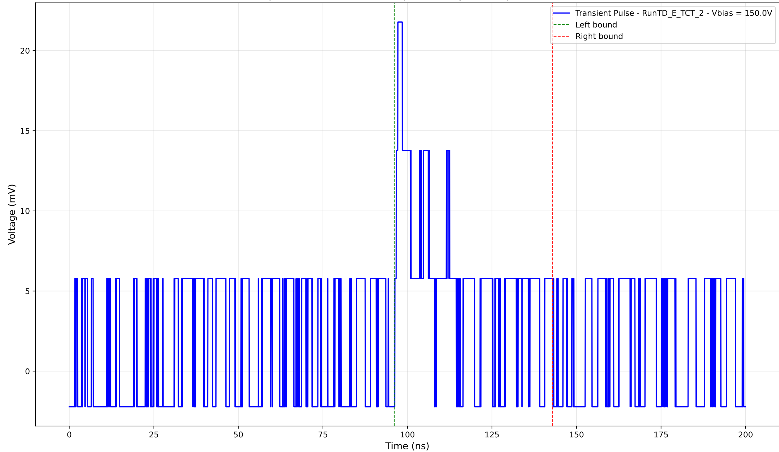
Transient Pulse - Sample: TD - Position: 280.0 \mu\text{m} - Charge: 5.48 pC - Rise Time: 0.00 ns (N/A)
