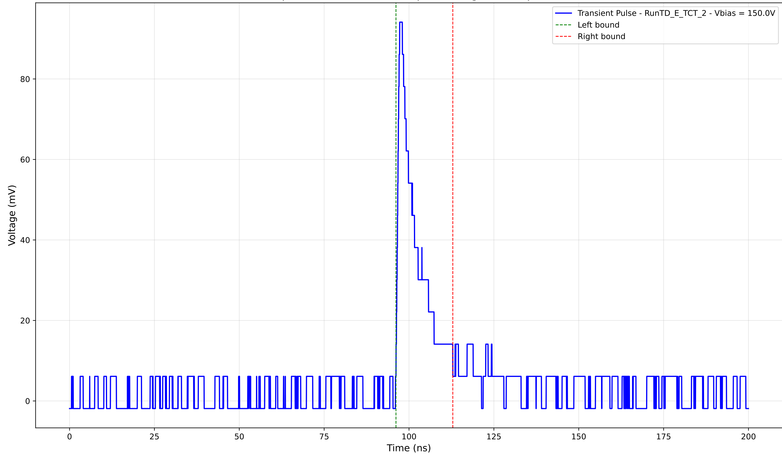
Transient Pulse - Sample: TD - Position: 705.0 \mu\text{m} - Charge: 11.95 pC - Rise Time: 0.91 ns
