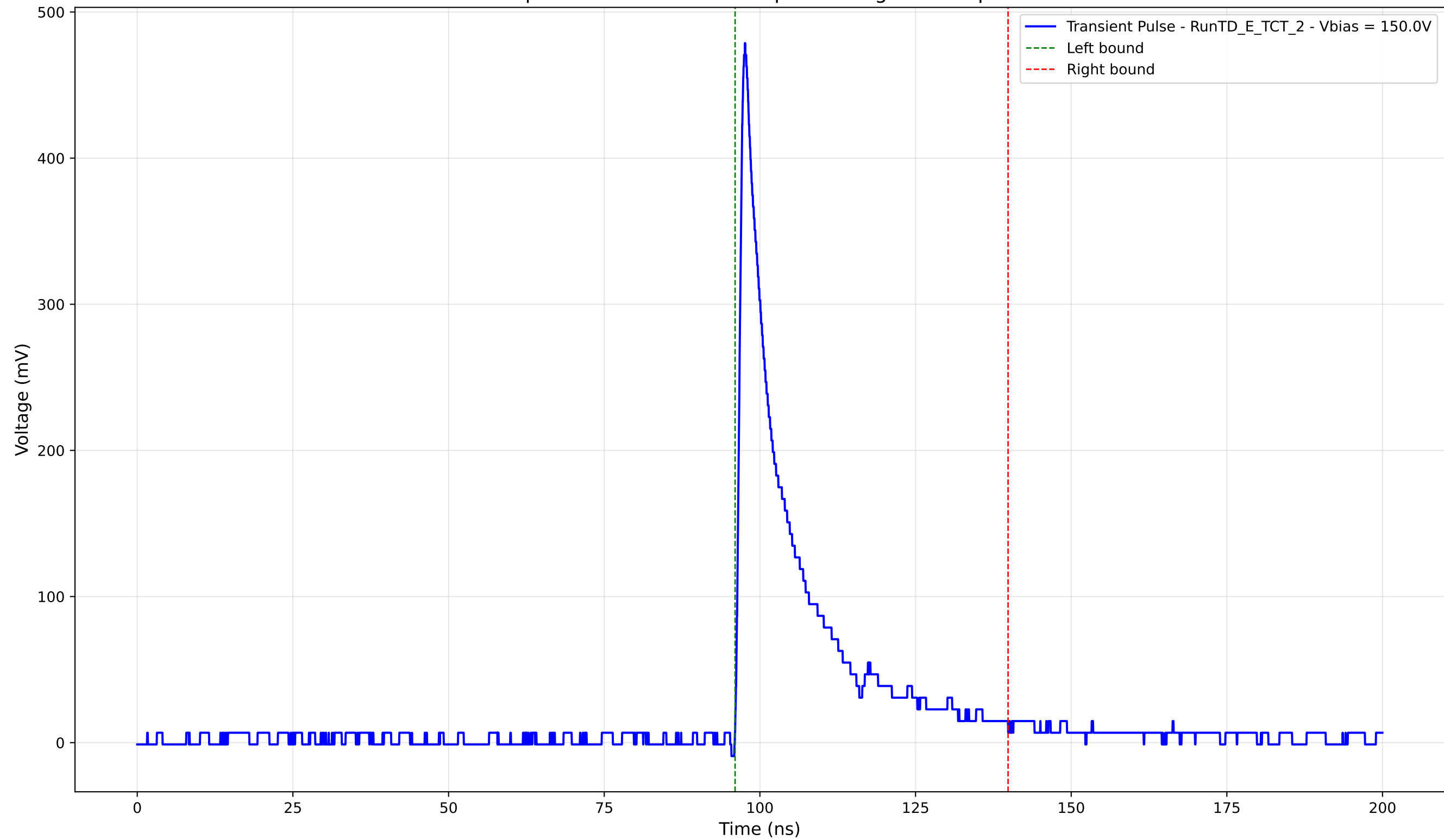
Transient Pulse - Sample: TD - Position: 485.0 \mu\text{m} - Charge: 78.40 pC - Rise Time: 1.04 ns
