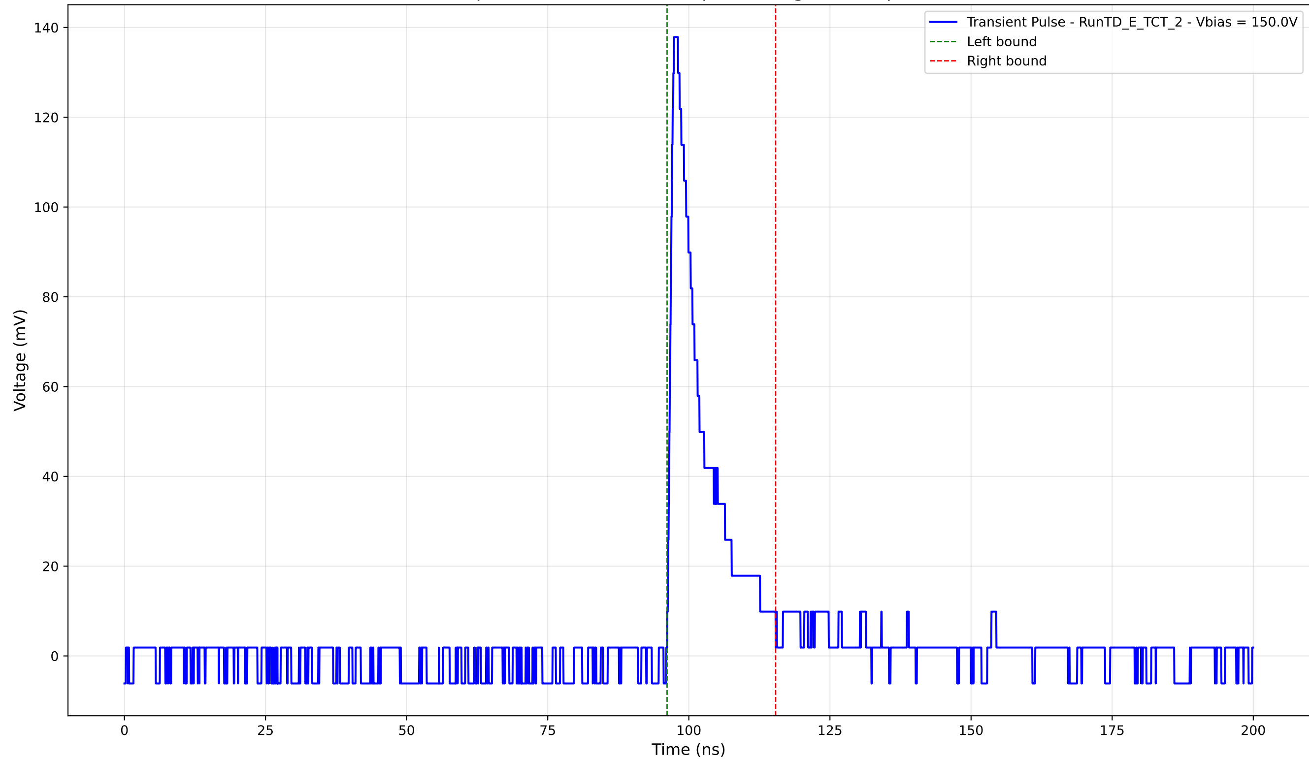
Transient Pulse - Sample: TD - Position: 645.0 \mu\text{m} - Charge: 17.38 pC - Rise Time: 0.97 ns
