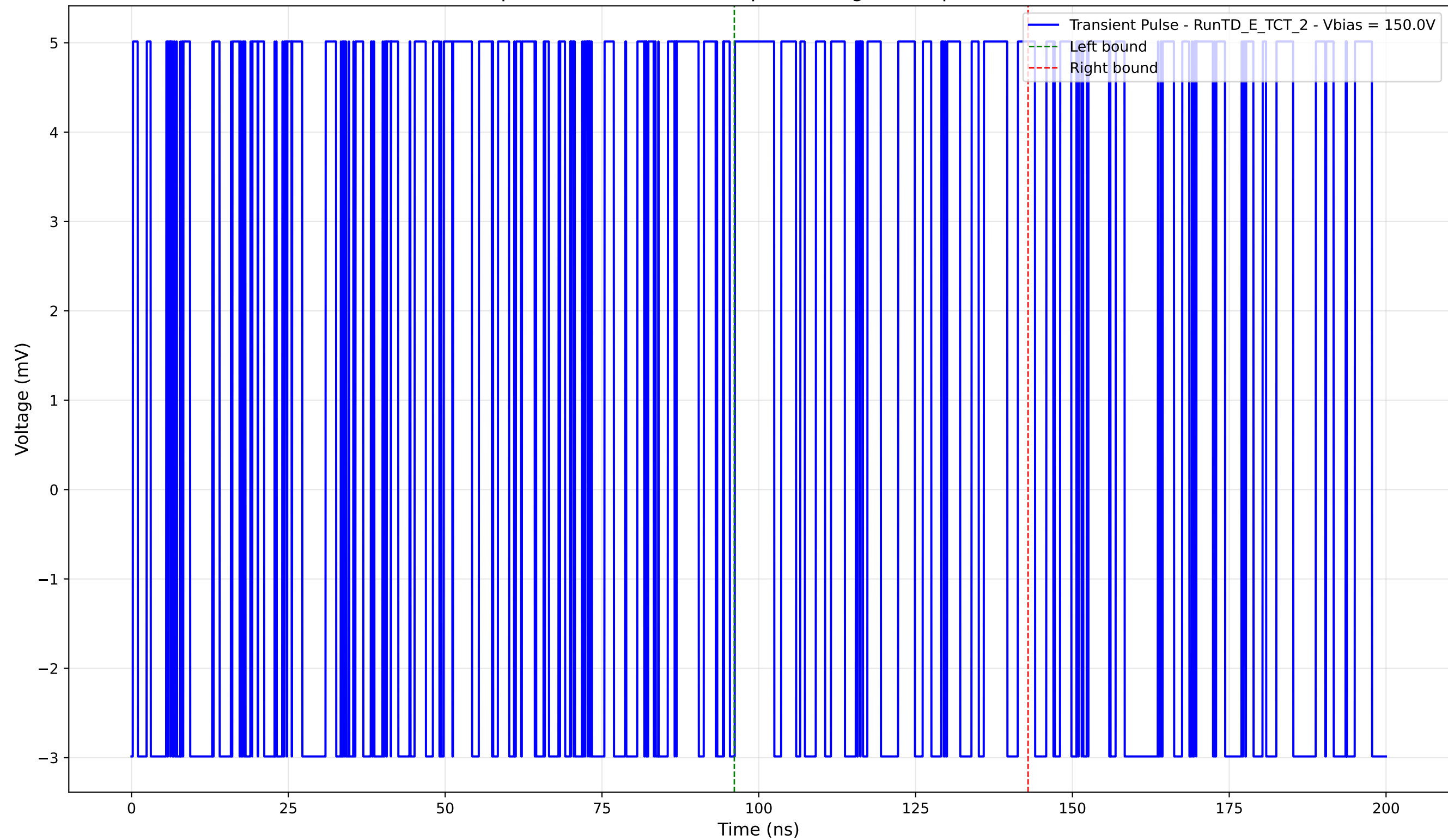
Transient Pulse - Sample: TD - Position: 210.0 \mu\text{m} - Charge: 1.89 pC - Rise Time: 0.00 ns (N/A)
