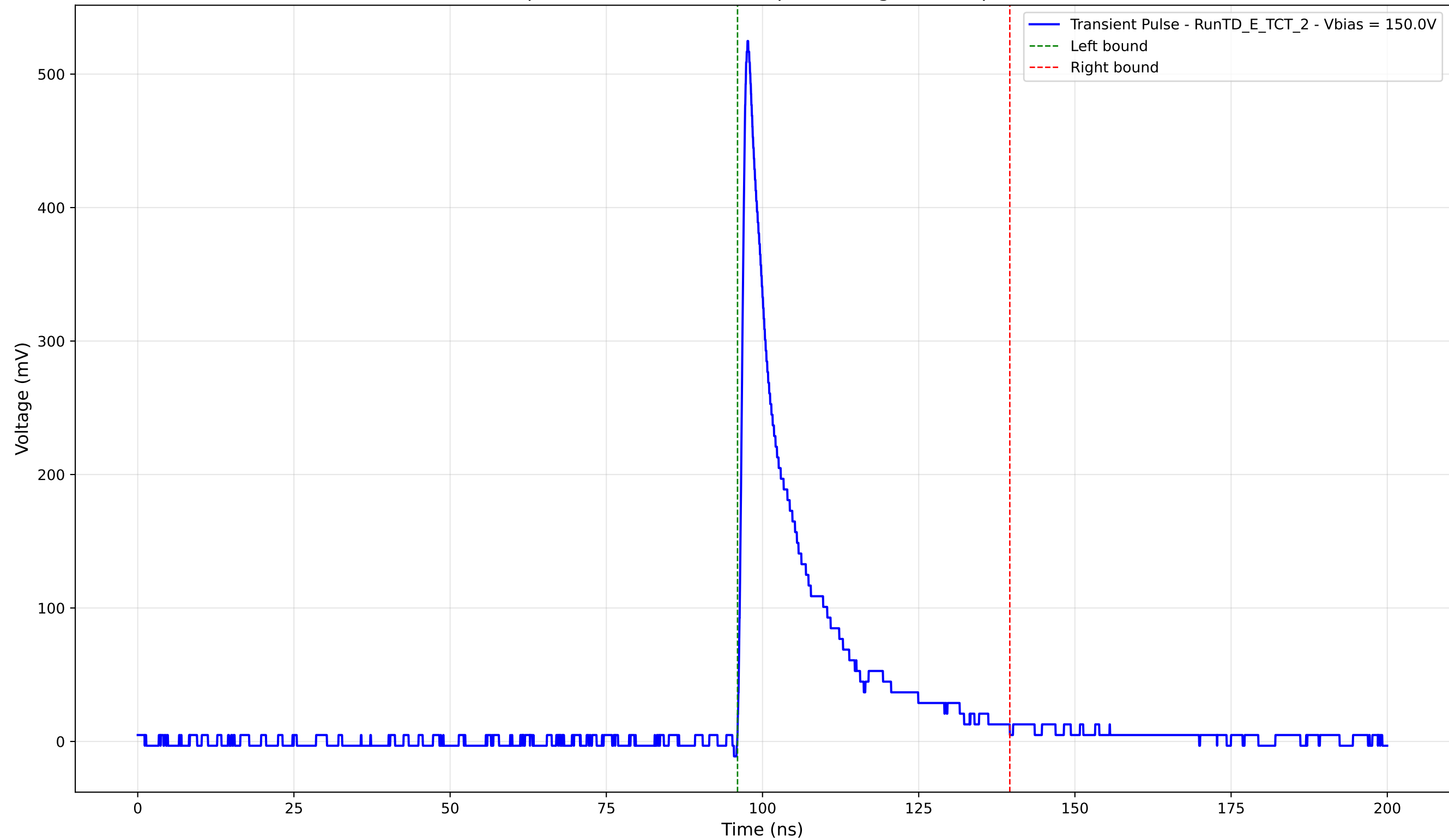
Transient Pulse - Sample: TD - Position: 405.0 \mu\text{m} - Charge: 87.31 pC - Rise Time: 1.02 ns
