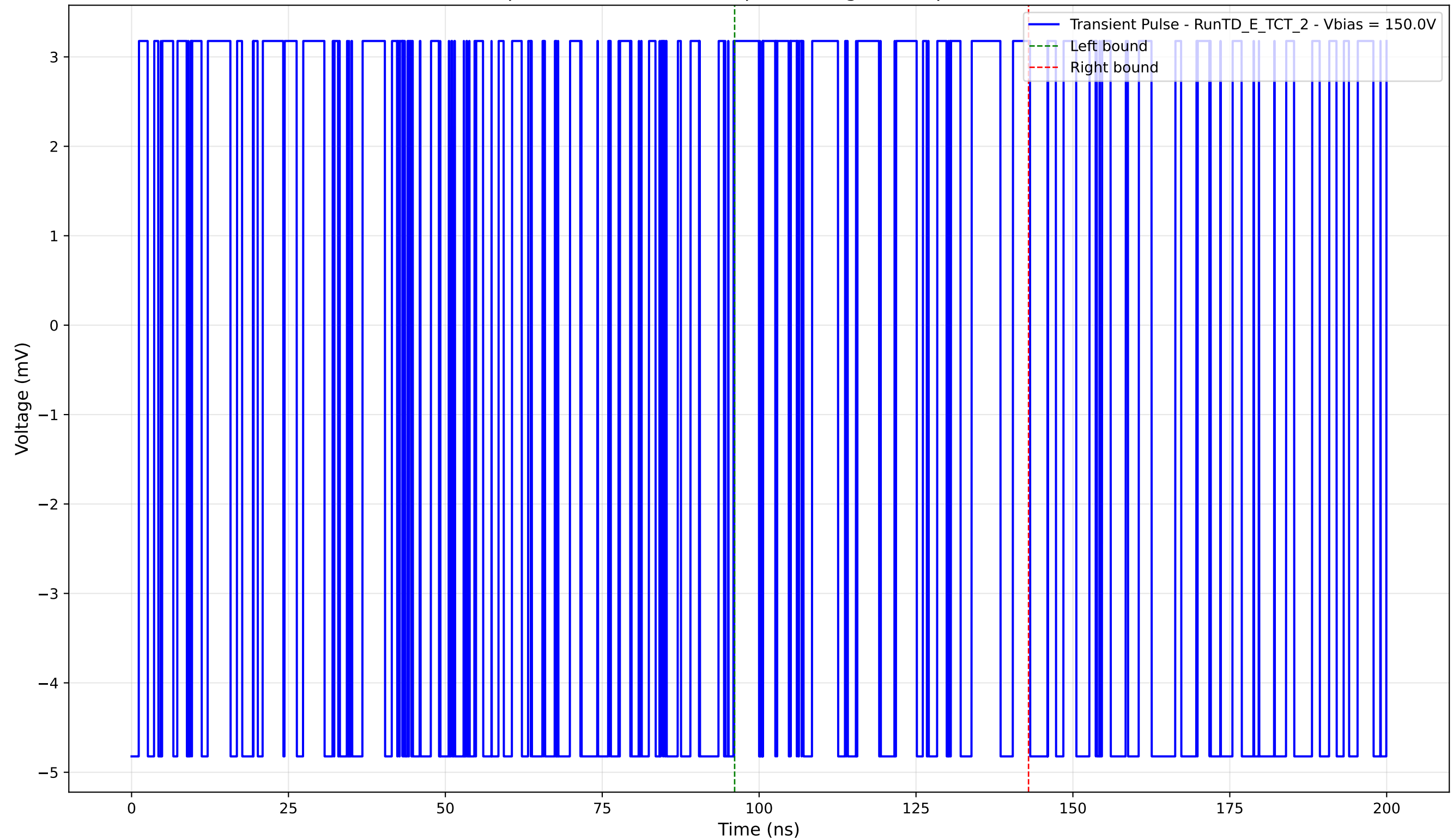
Transient Pulse - Sample: TD - Position: 40.0 \mu\text{m} - Charge: 0.66 pC - Rise Time: 0.00 ns (N/A)
