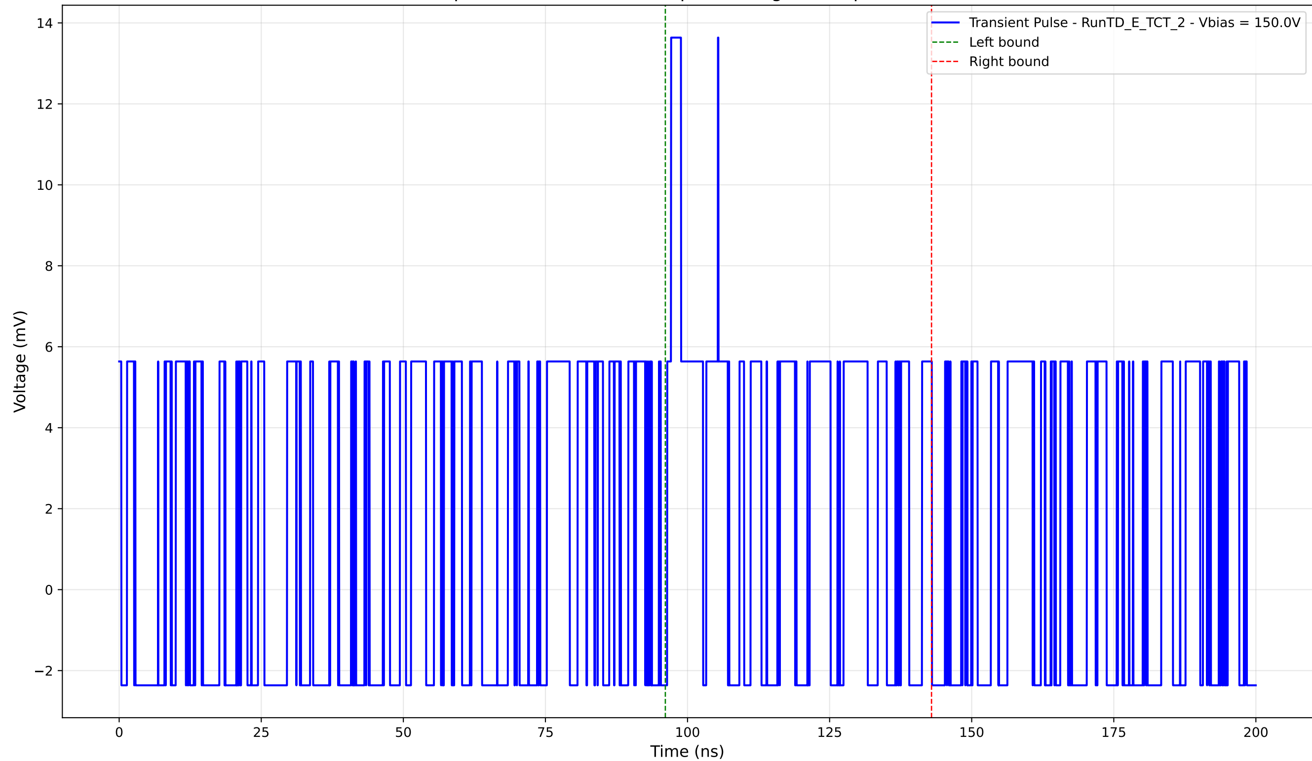
Transient Pulse - Sample: TD - Position: 120.0 \mu\text{m} - Charge: 2.77 pC - Rise Time: 0.00 ns (N/A)
