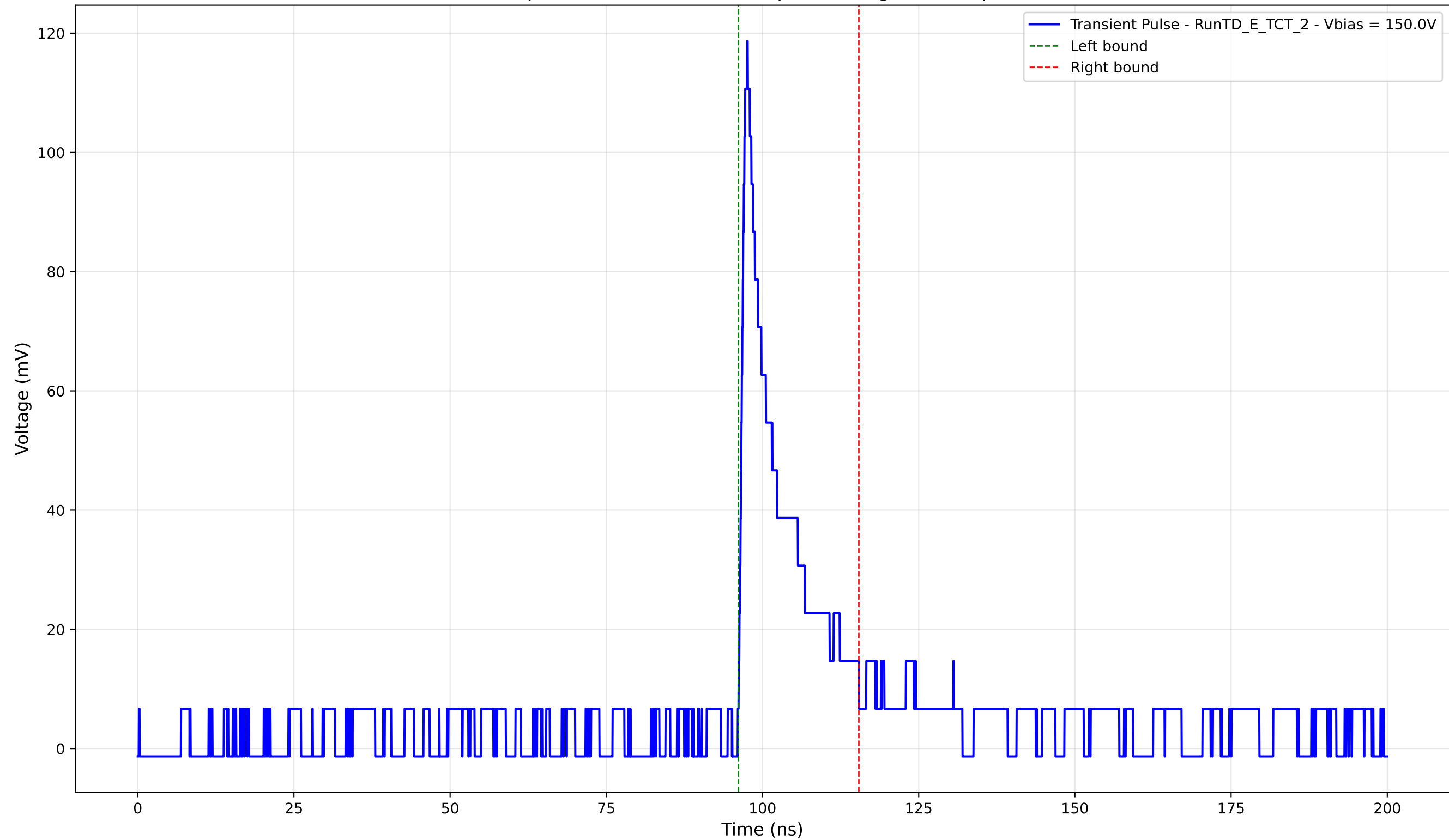
Transient Pulse - Sample: TD - Position: 330.0 \mu\text{m} - Charge: 15.31 pC - Rise Time: 1.05 ns
