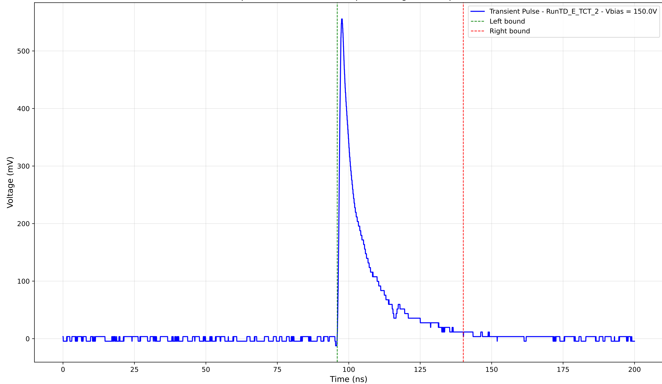
Transient Pulse - Sample: TD - Position: 415.0 \mu\text{m} - Charge: 89.59 pC - Rise Time: 1.01 ns
