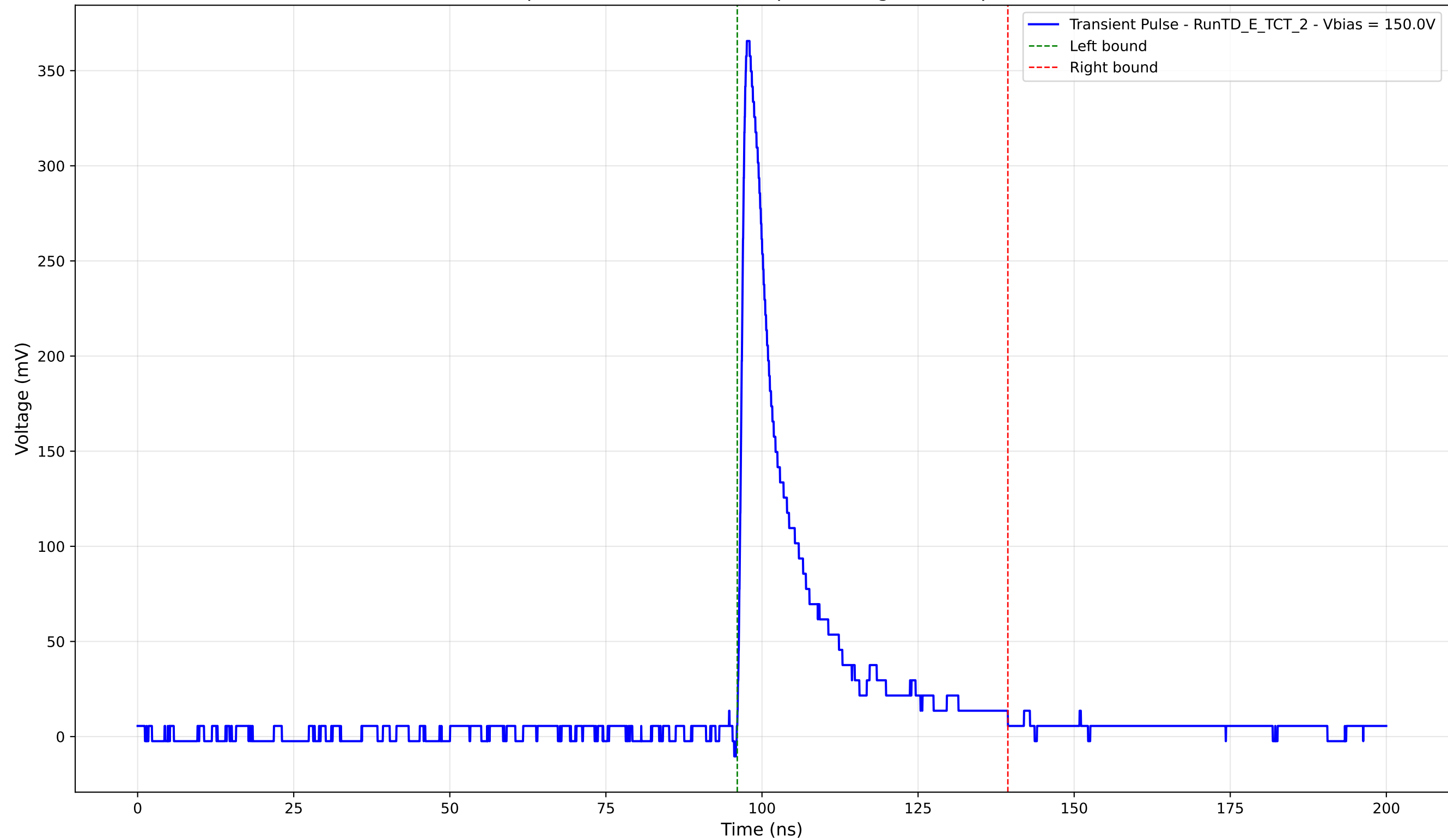
Transient Pulse - Sample: TD - Position: 560.0 \mu\text{m} - Charge: 60.14 pC - Rise Time: 1.06 ns
