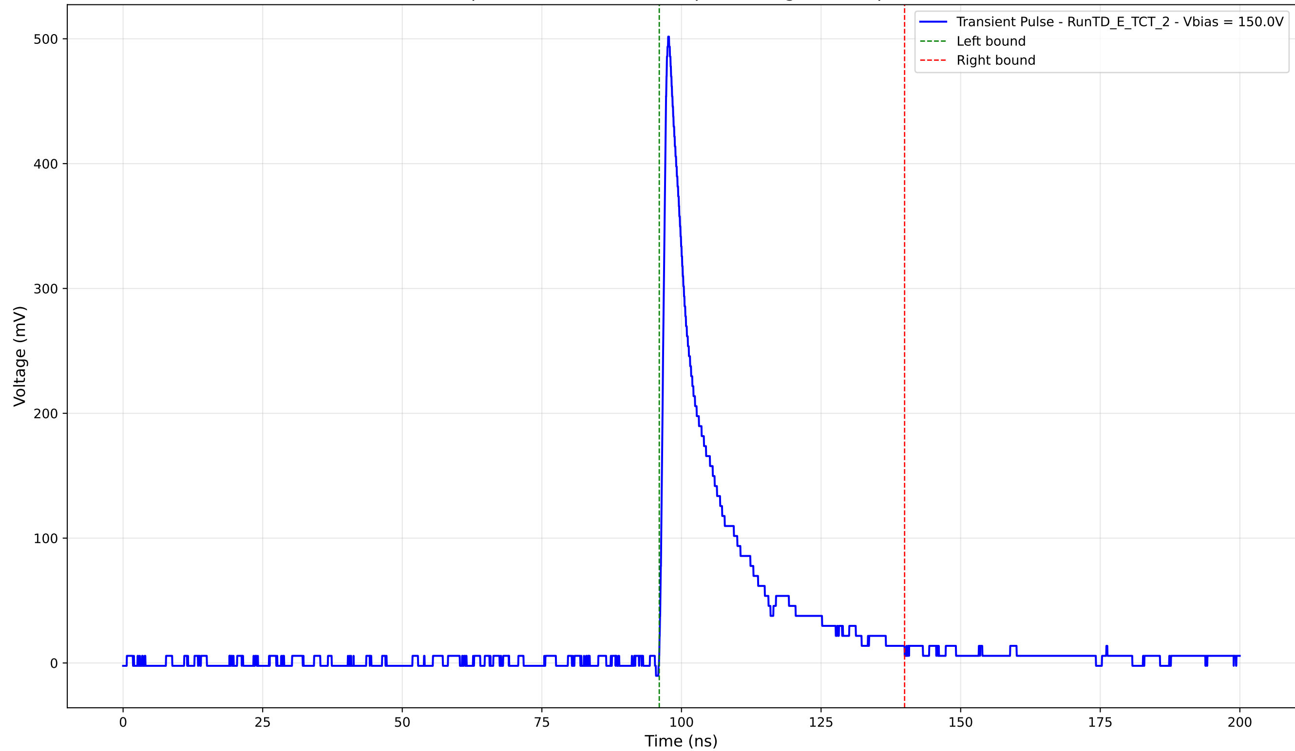
Transient Pulse - Sample: TD - Position: 395.0 \mu\text{m} - Charge: 86.39 pC - Rise Time: 1.03 ns
