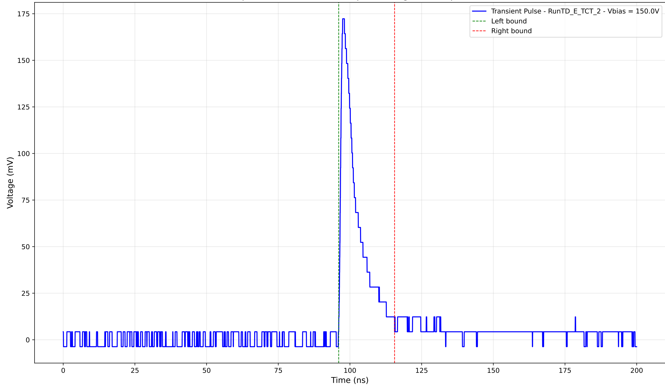
Transient Pulse - Sample: TD - Position: 625.0 \mu\text{m} - Charge: 22.74 pC - Rise Time: 1.01 ns
