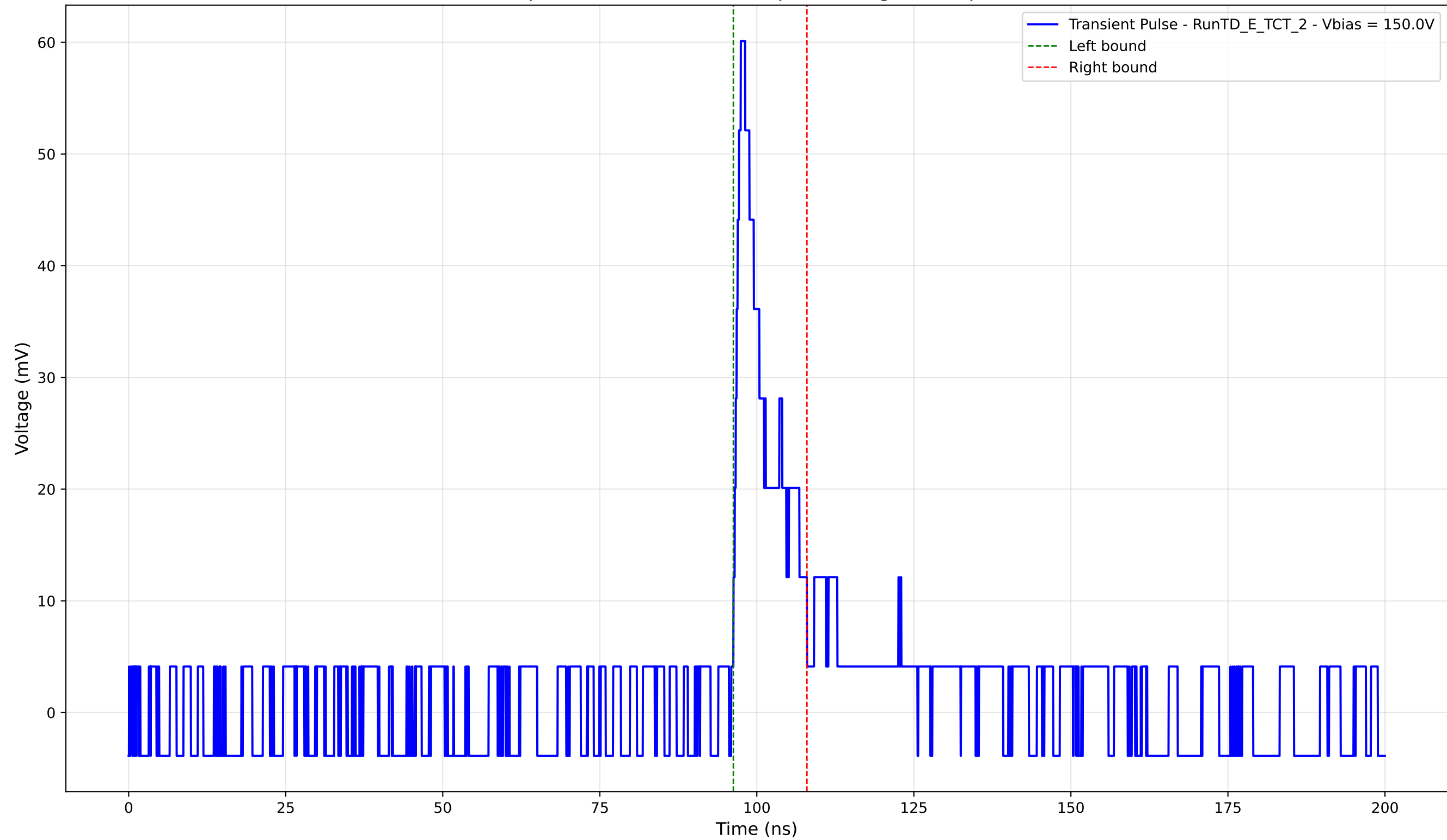
Transient Pulse - Sample: TD - Position: 665.0 \mu\text{m} - Charge: 6.62 pC - Rise Time: 1.18 ns
