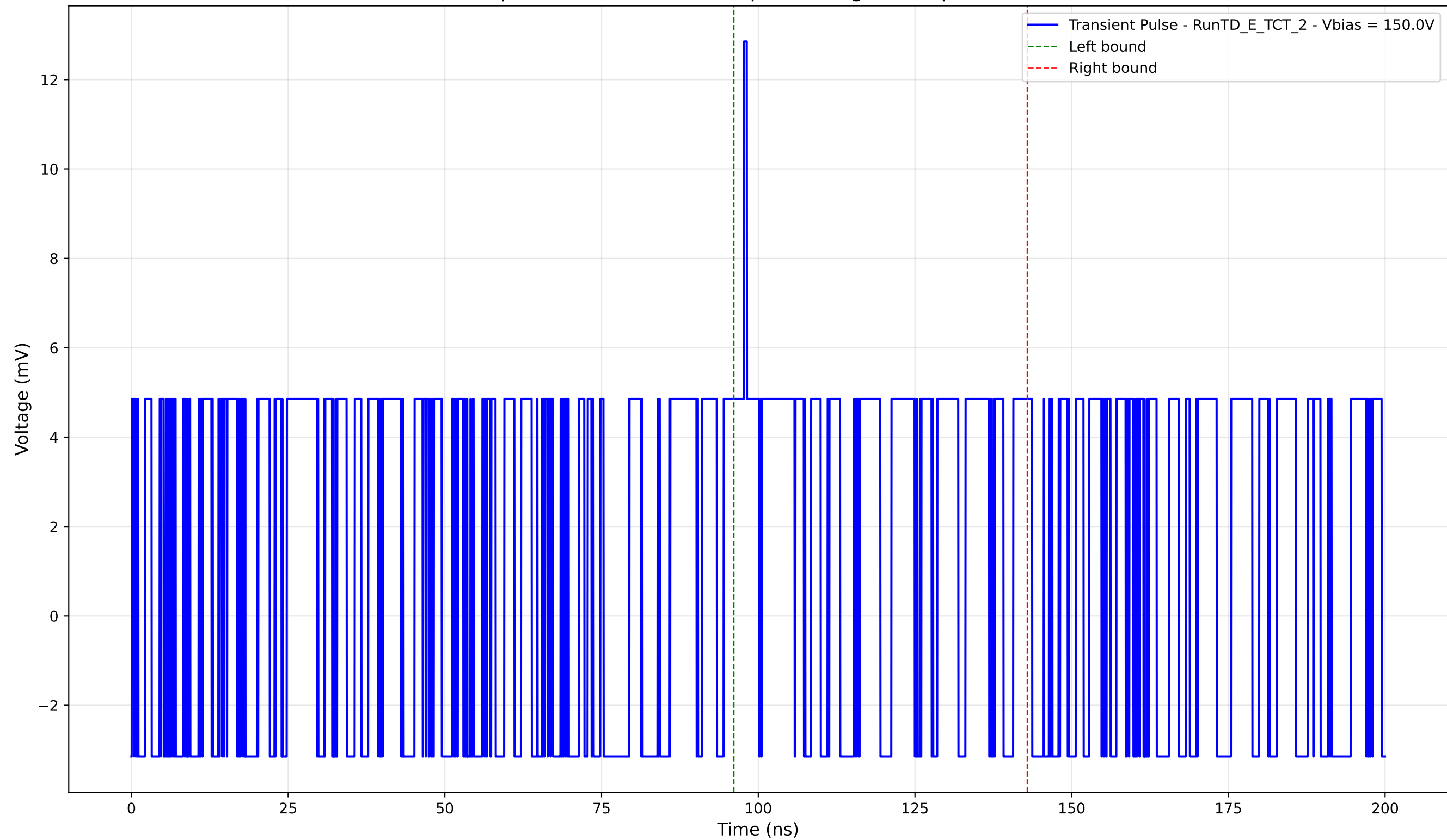
Transient Pulse - Sample: TD - Position: 190.0 \mu\text{m} - Charge: 2.70 pC - Rise Time: 0.00 ns (N/A)
