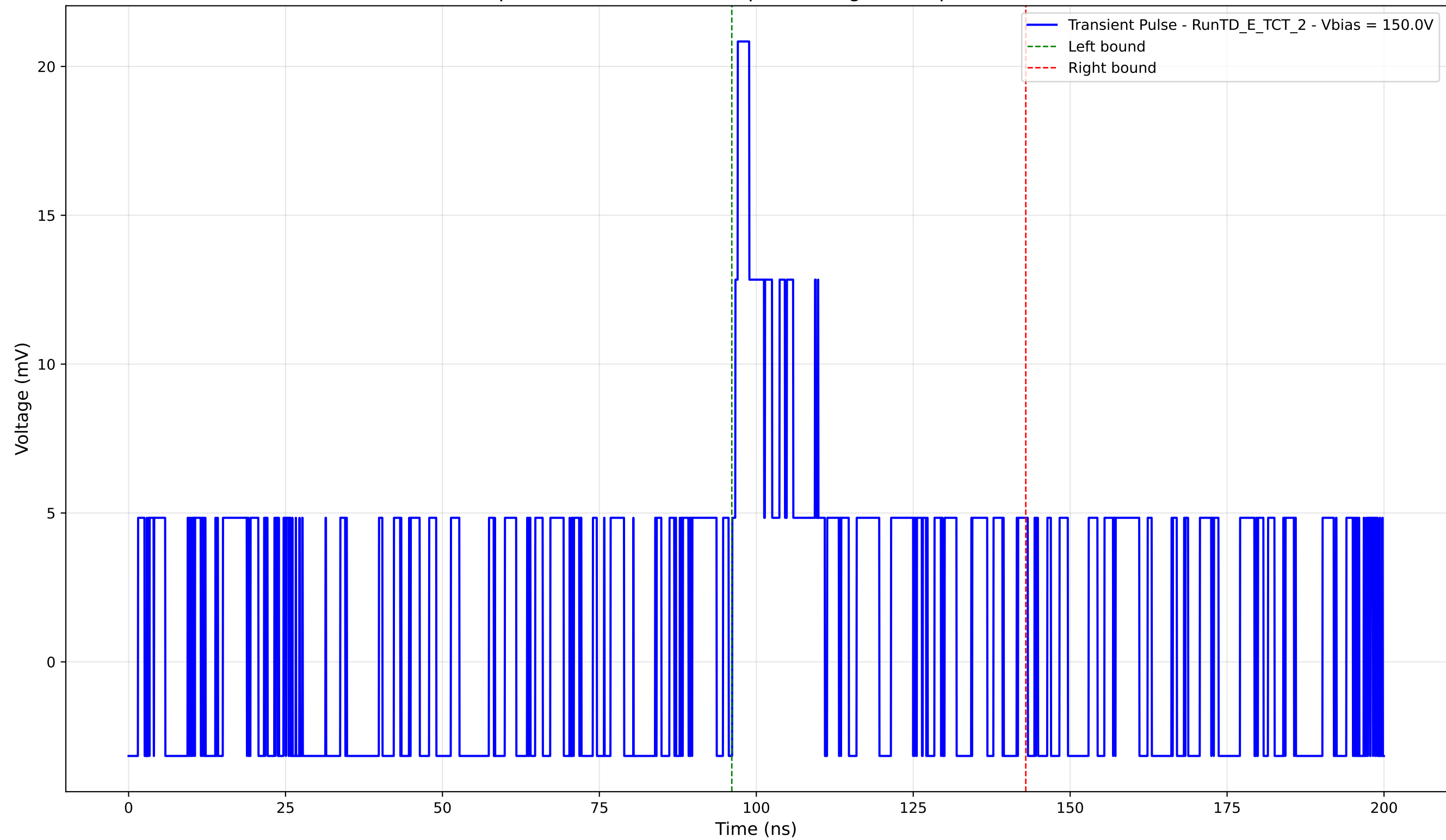
Transient Pulse - Sample: TD - Position: 290.0 \mu\text{m} - Charge: 4.30 pC - Rise Time: 0.00 ns (N/A)
