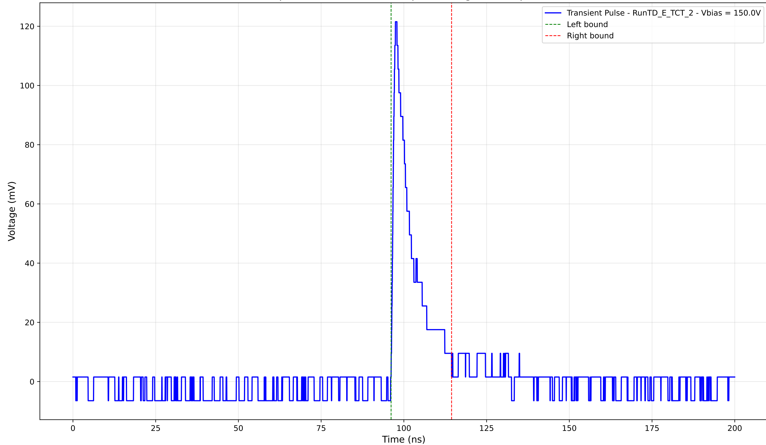
Transient Pulse - Sample: TD - Position: 650.0 \mu\text{m} - Charge: 15.01 pC - Rise Time: 0.99 ns
