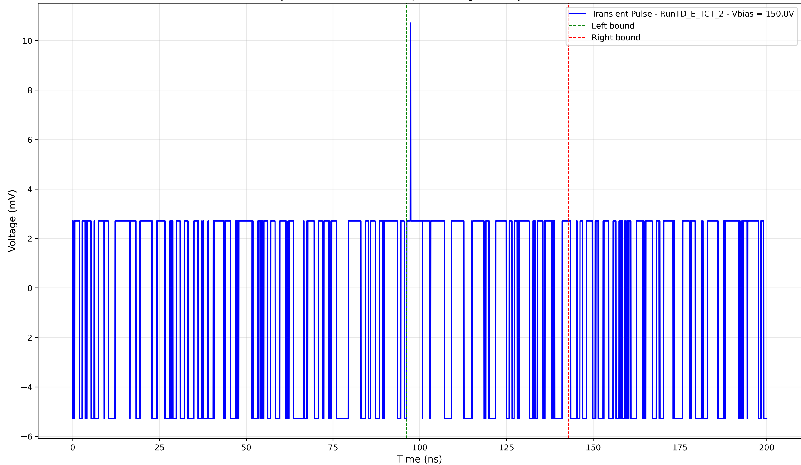
Transient Pulse - Sample: TD - Position: 85.0 \mu\text{m} - Charge: 0.35 pC - Rise Time: 0.00 ns (N/A)
