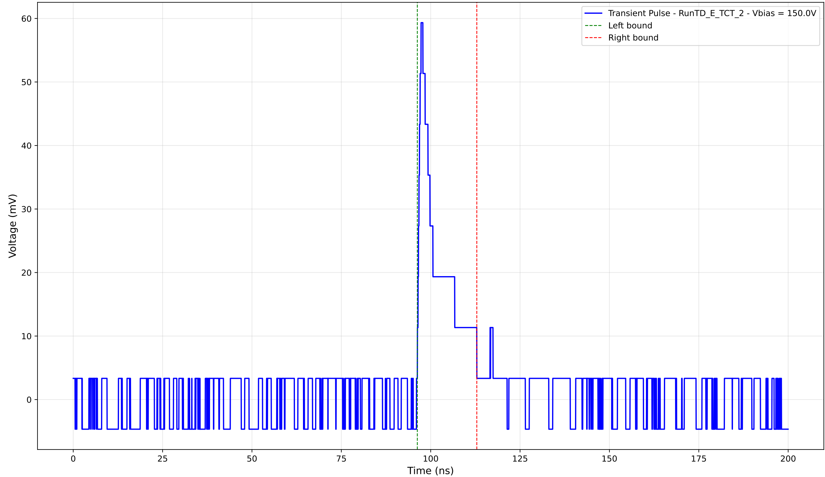
Transient Pulse - Sample: TD - Position: 320.0 \mu\text{m} - Charge: 7.24 pC - Rise Time: 1.03 ns
