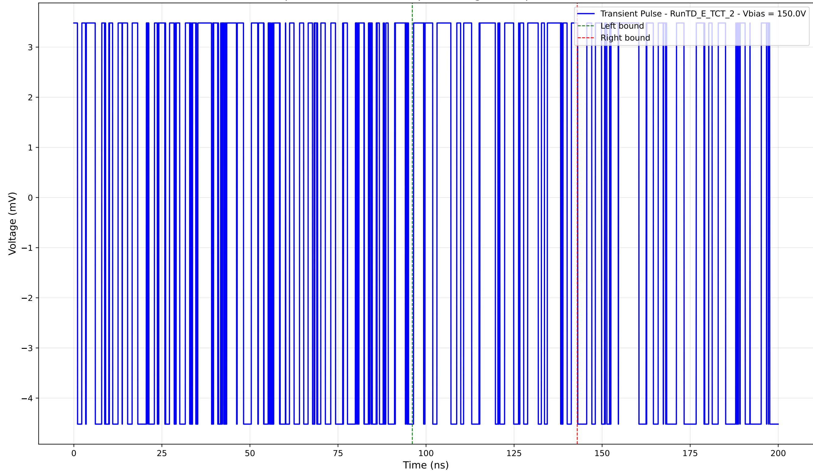
Transient Pulse - Sample: TD - Position: 50.0 \mu\text{m} - Charge: 0.87 pC - Rise Time: 0.00 ns (N/A)
