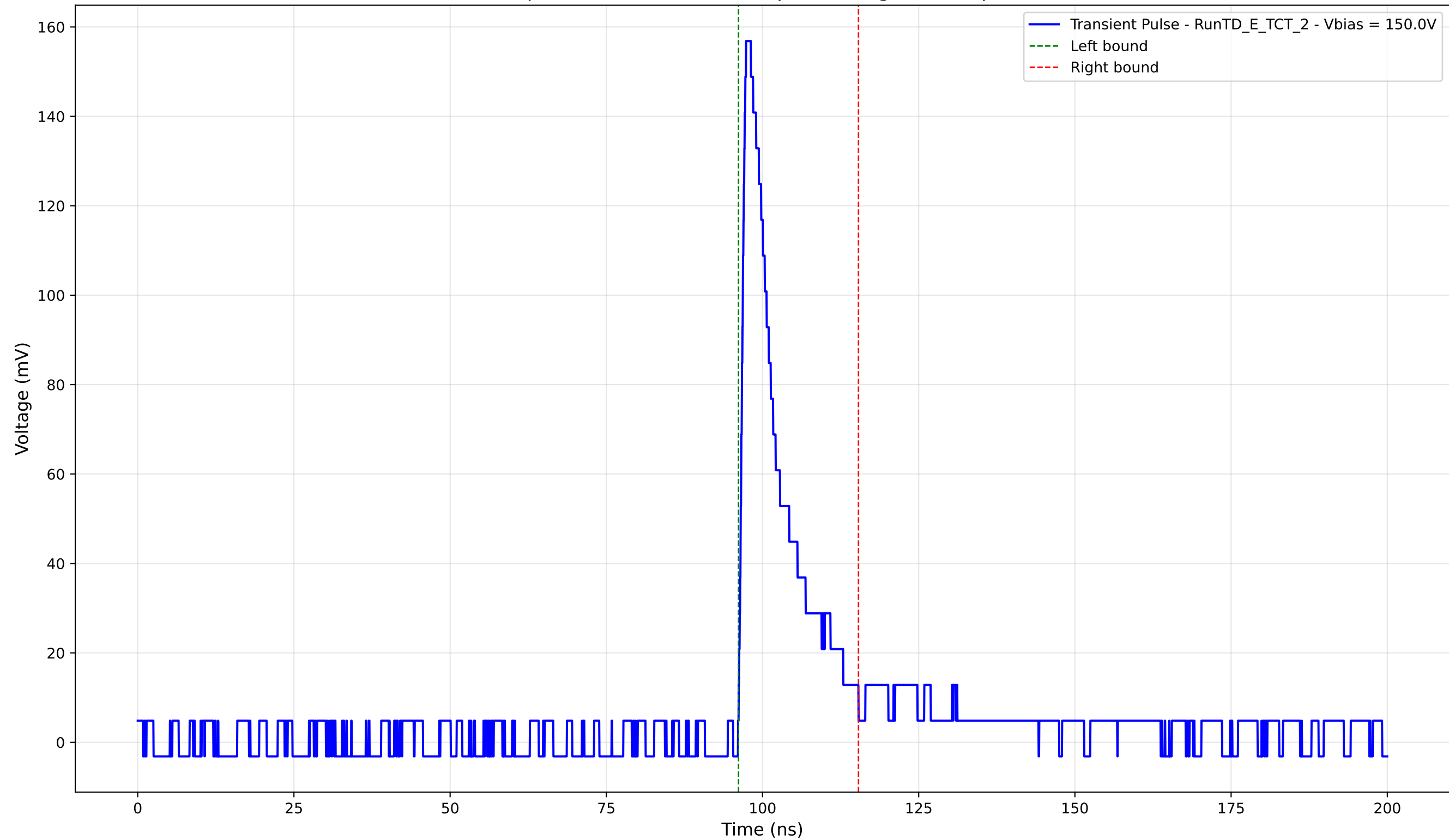
Transient Pulse - Sample: TD - Position: 635.0 \mu\text{m} - Charge: 21.46 pC - Rise Time: 0.99 ns
