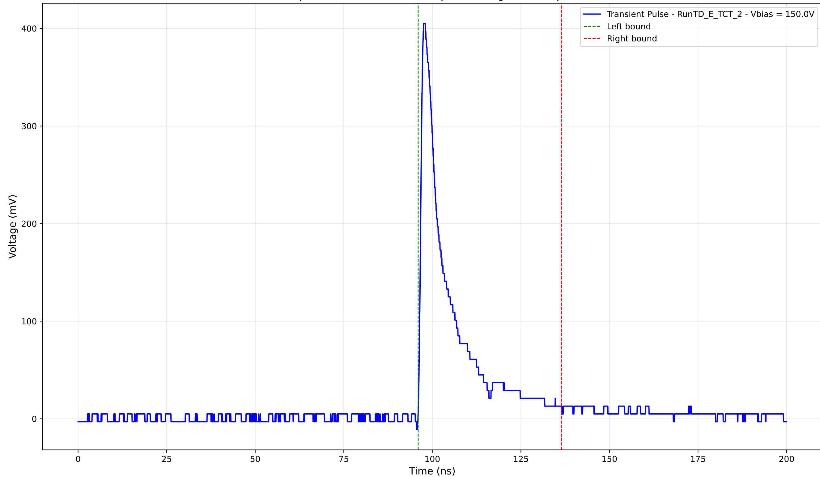
Transient Pulse - Sample: TD - Position: 540.0 \mu\text{m} - Charge: 67.12 pC - Rise Time: 1.01 ns
