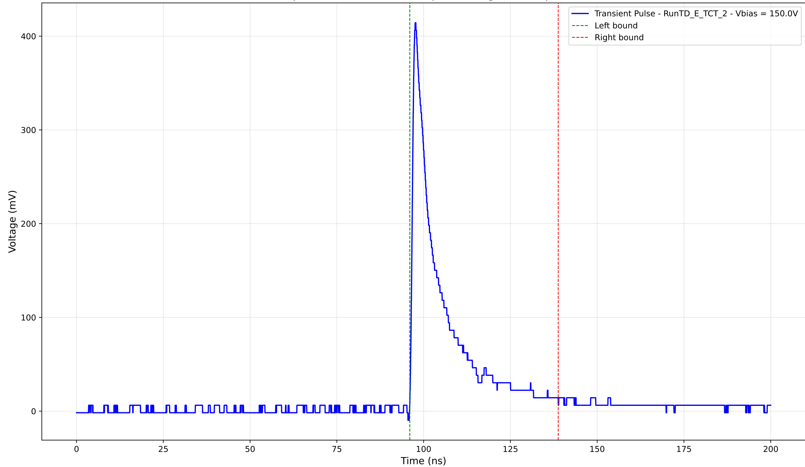
Transient Pulse - Sample: TD - Position: 500.0 \mu\text{m} - Charge: 69.39 pC - Rise Time: 1.01 ns
