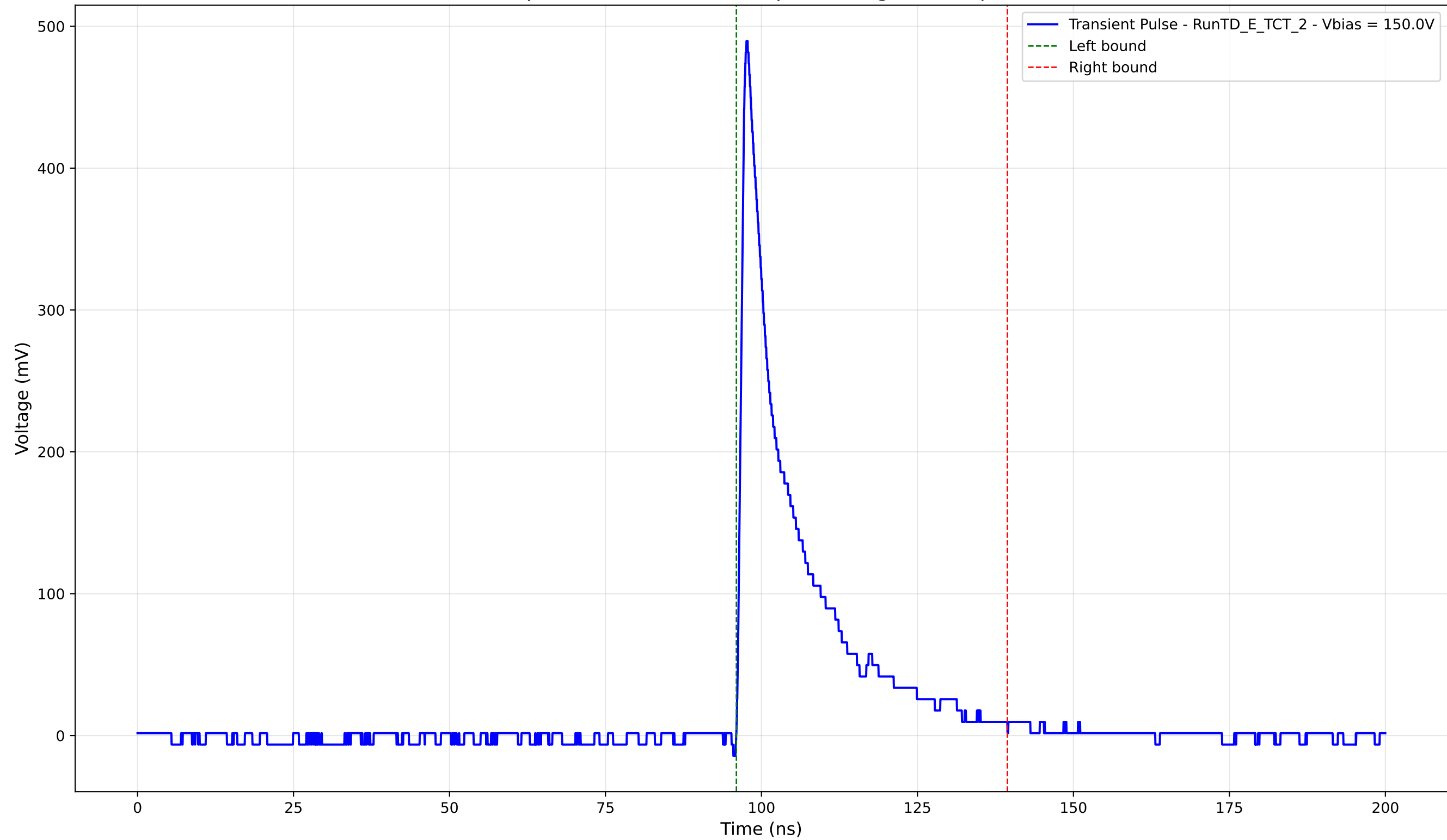
Transient Pulse - Sample: TD - Position: 370.0 \mu\text{m} - Charge: 82.80 pC - Rise Time: 1.02 ns
