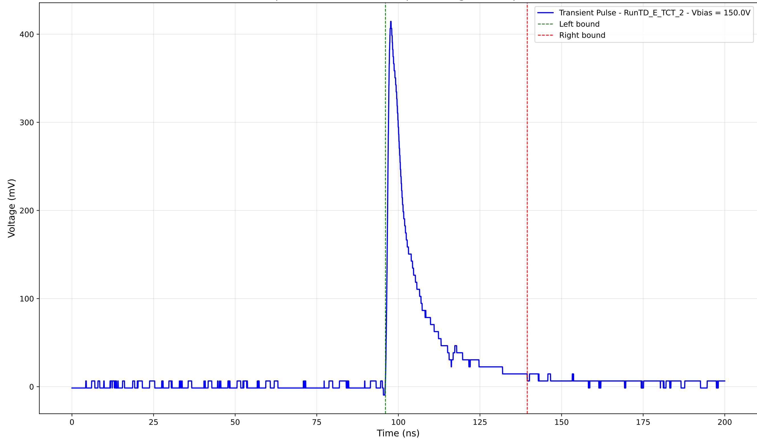
Transient Pulse - Sample: TD - Position: 530.0 \mu\text{m} - Charge: 69.72 pC - Rise Time: 1.01 ns
