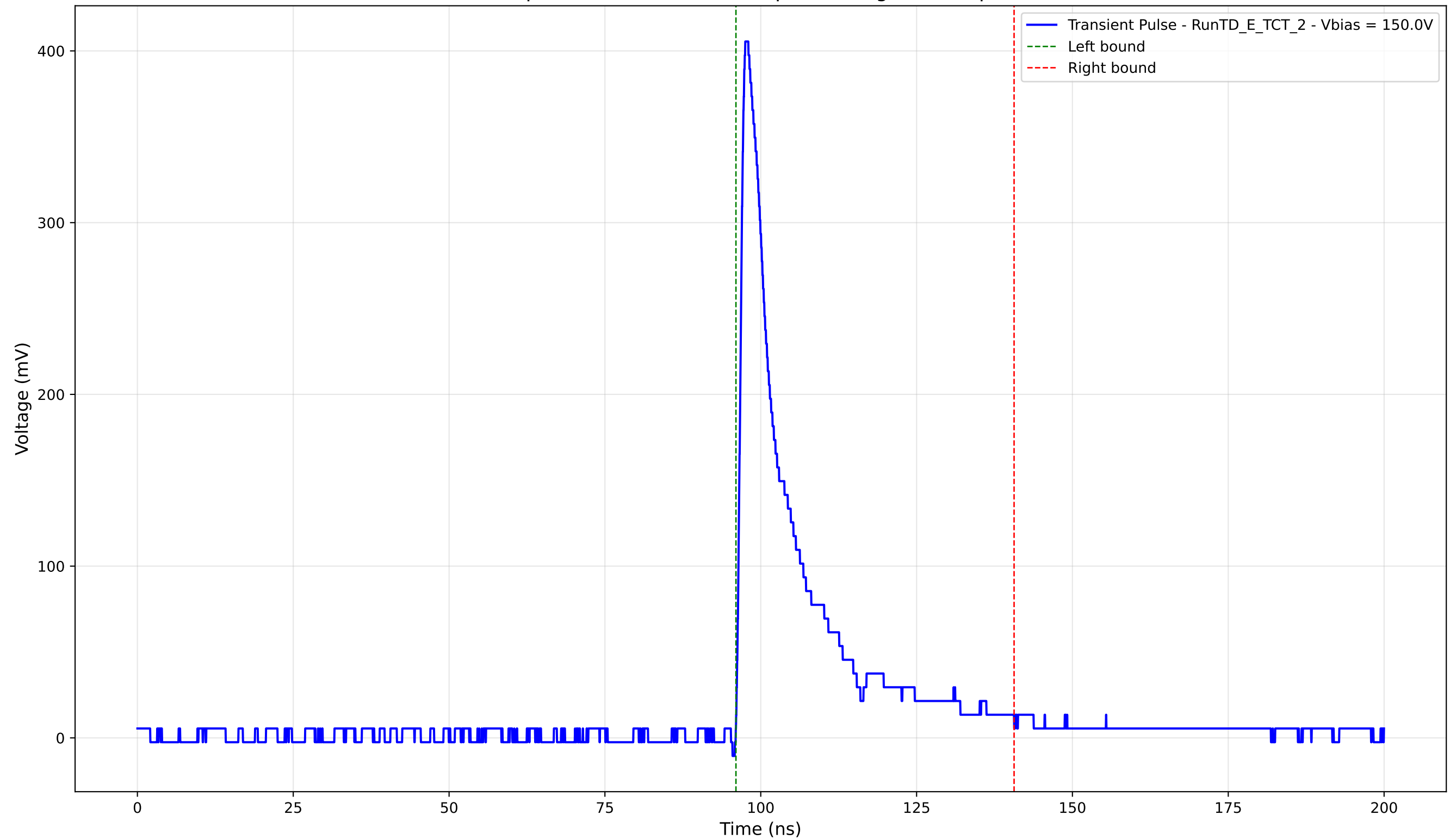
Transient Pulse - Sample: TD - Position: 535.0 \mu\text{m} - Charge: 69.13 pC - Rise Time: 1.01 ns
