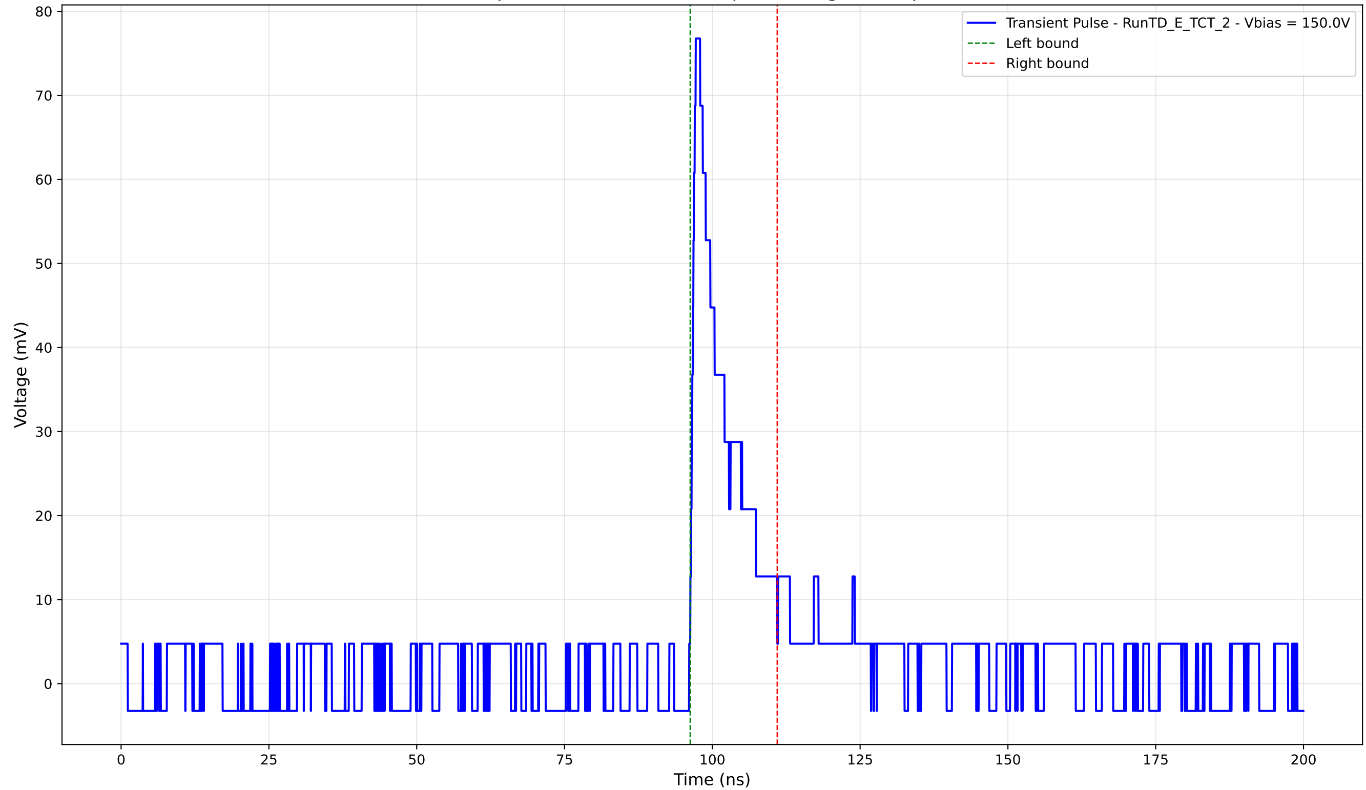
Transient Pulse - Sample: TD - Position: 325.0 \mu\text{m} - Charge: 9.38 pC - Rise Time: 0.91 ns
