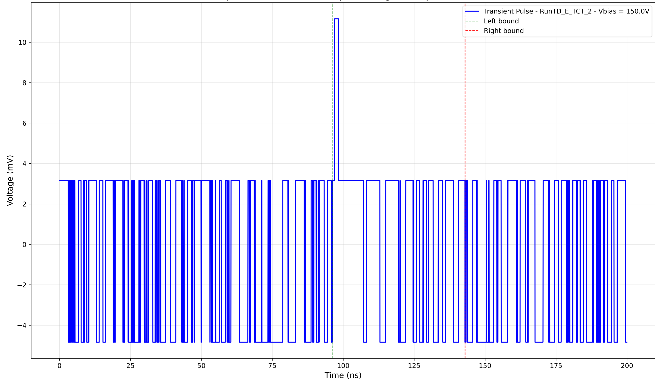
Transient Pulse - - Sample: TD - Position: 225.0 \mu\text{m} - Charge: 1.06 pC - Rise Time: 0.00 ns (N/A)
