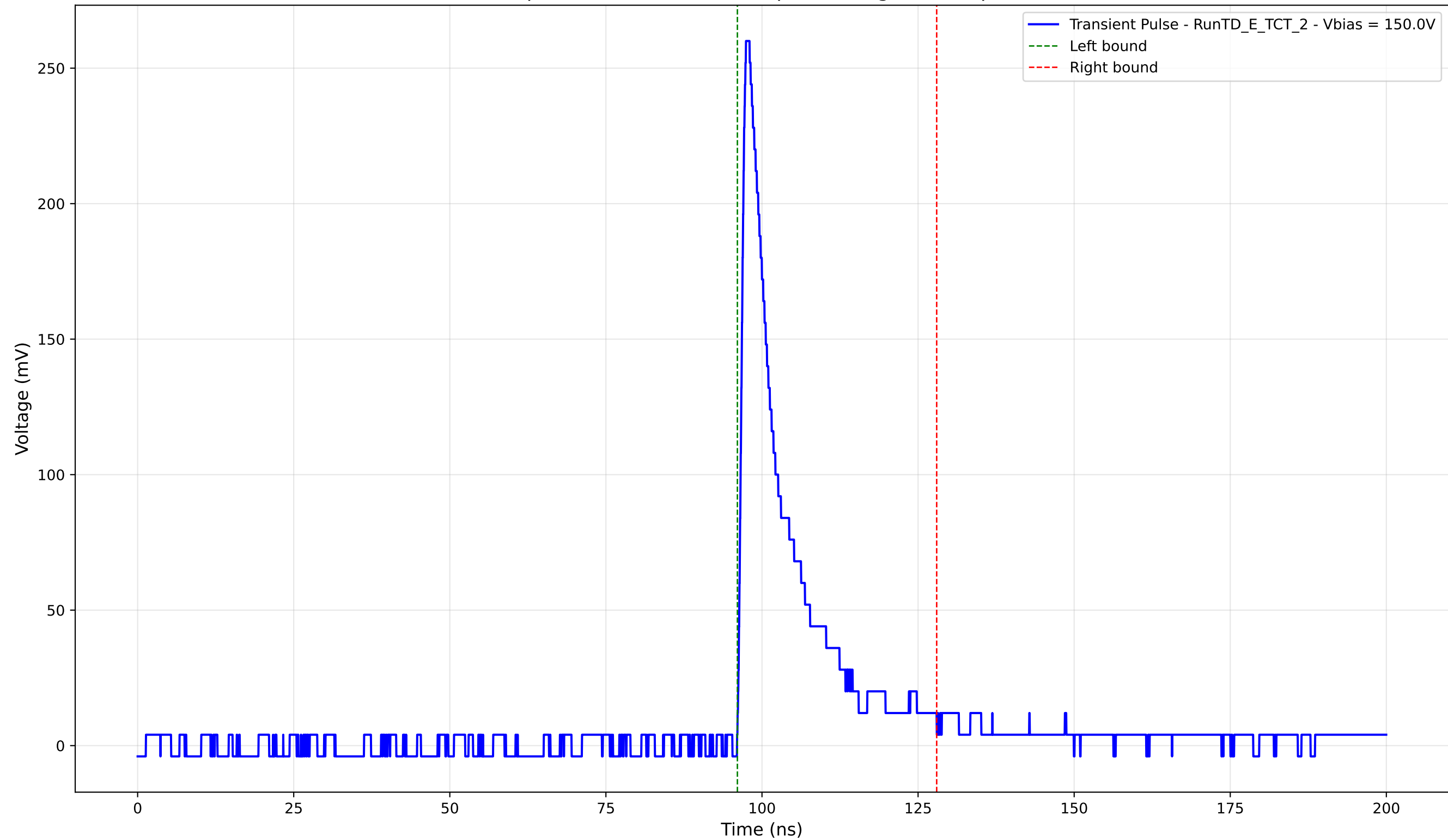
Transient Pulse - Sample: TD - Position: 590.0 \mu\text{m} - Charge: 38.35 pC - Rise Time: 0.99 ns
