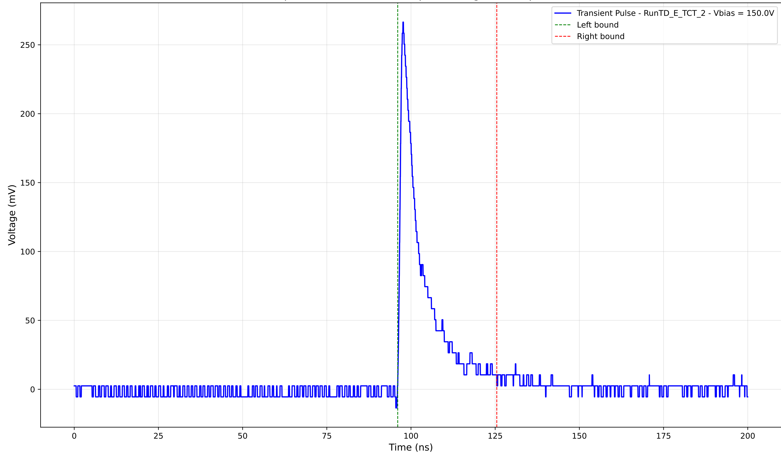
Transient Pulse - Sample: TD - Position: 595.0 \mu\text{m} - Charge: 36.68 pC - Rise Time: 1.00 ns
