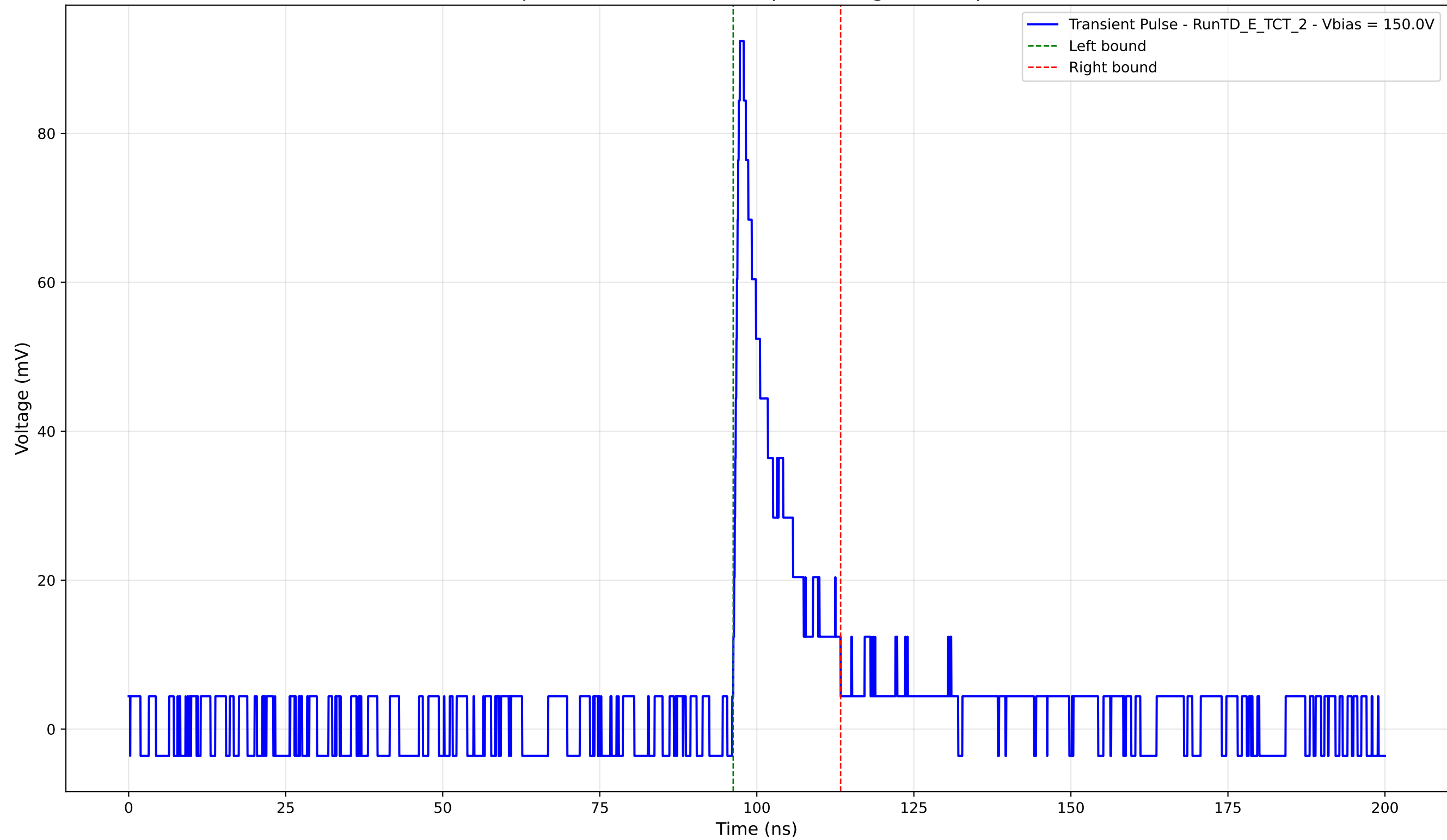
Transient Pulse - Sample: TD - Position: 720.0 \mu\text{m} - Charge: 11.57 pC - Rise Time: 0.87 ns
