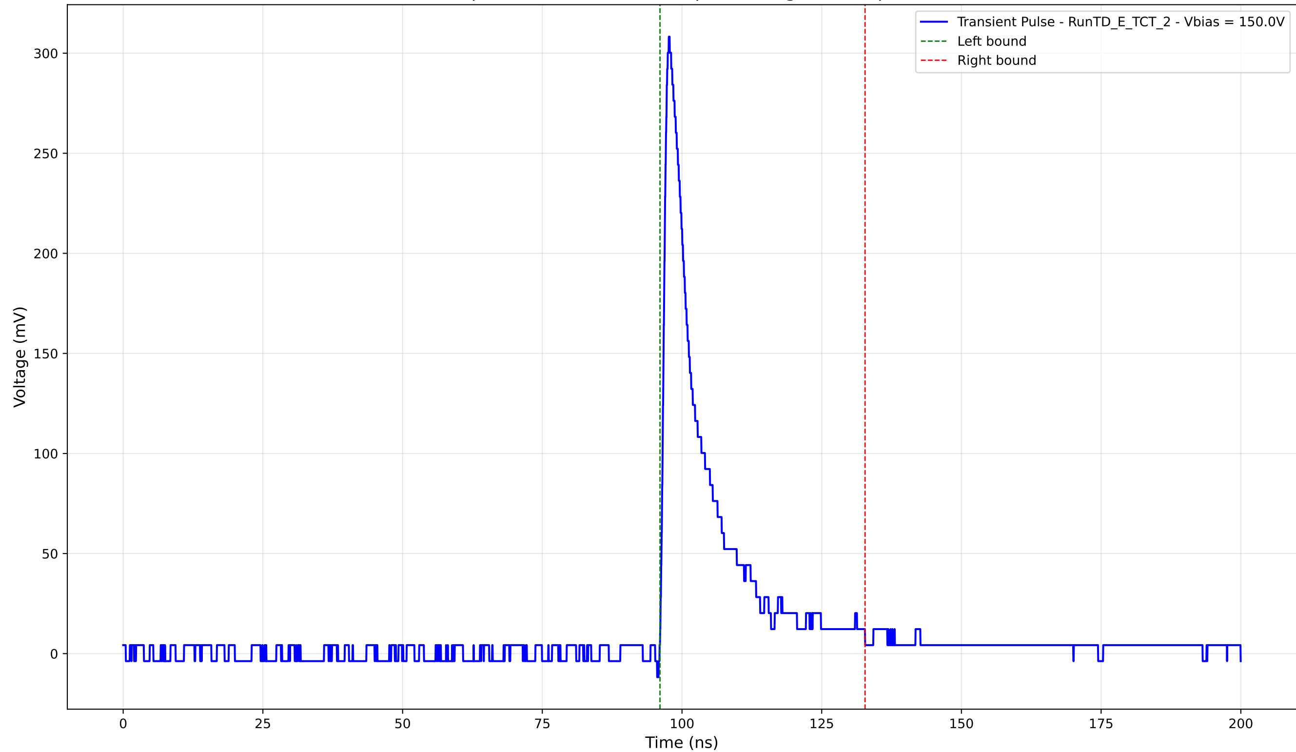
Transient Pulse - Sample: TD - Position: 575.0 \mu\text{m} - Charge: 46.35 pC - Rise Time: 1.05 ns
