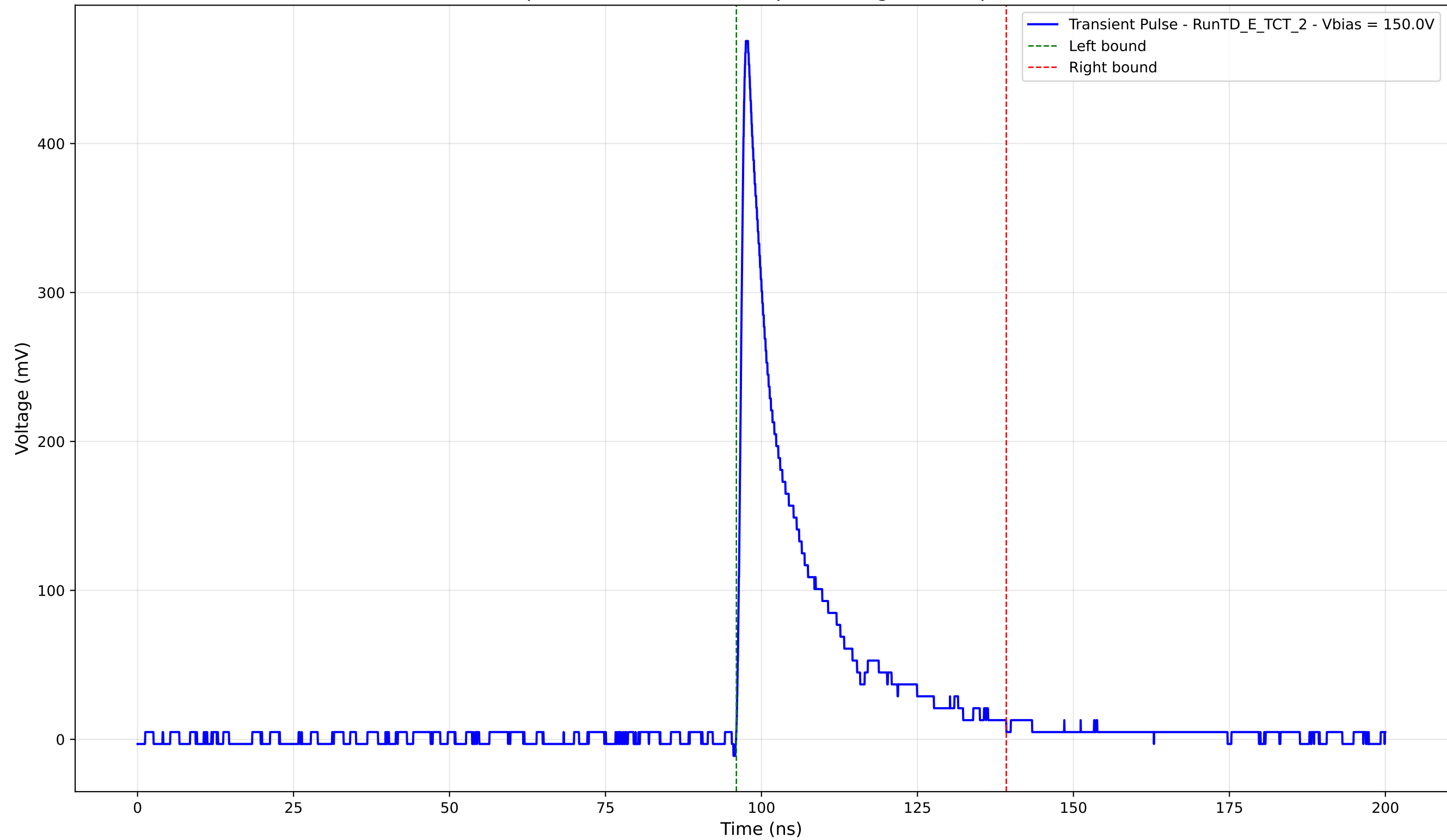
Transient Pulse - Sample: TD - Position: 365.0 \mu\text{m} - Charge: 81.12 pC - Rise Time: 1.03 ns
