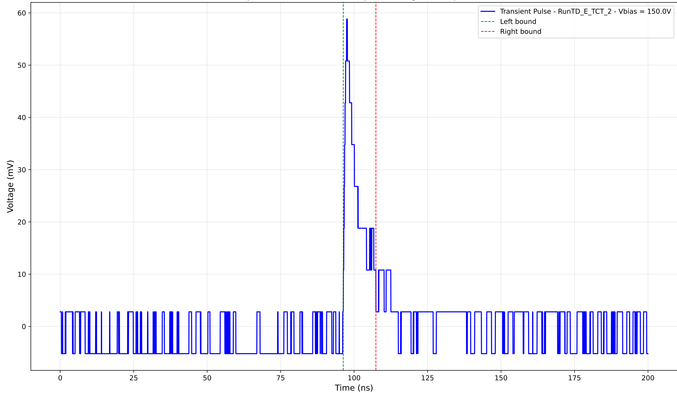
Transient Pulse - Sample: TD - Position: 680.0 \mu\text{m} - Charge: 5.72 pC - Rise Time: 1.11 ns
