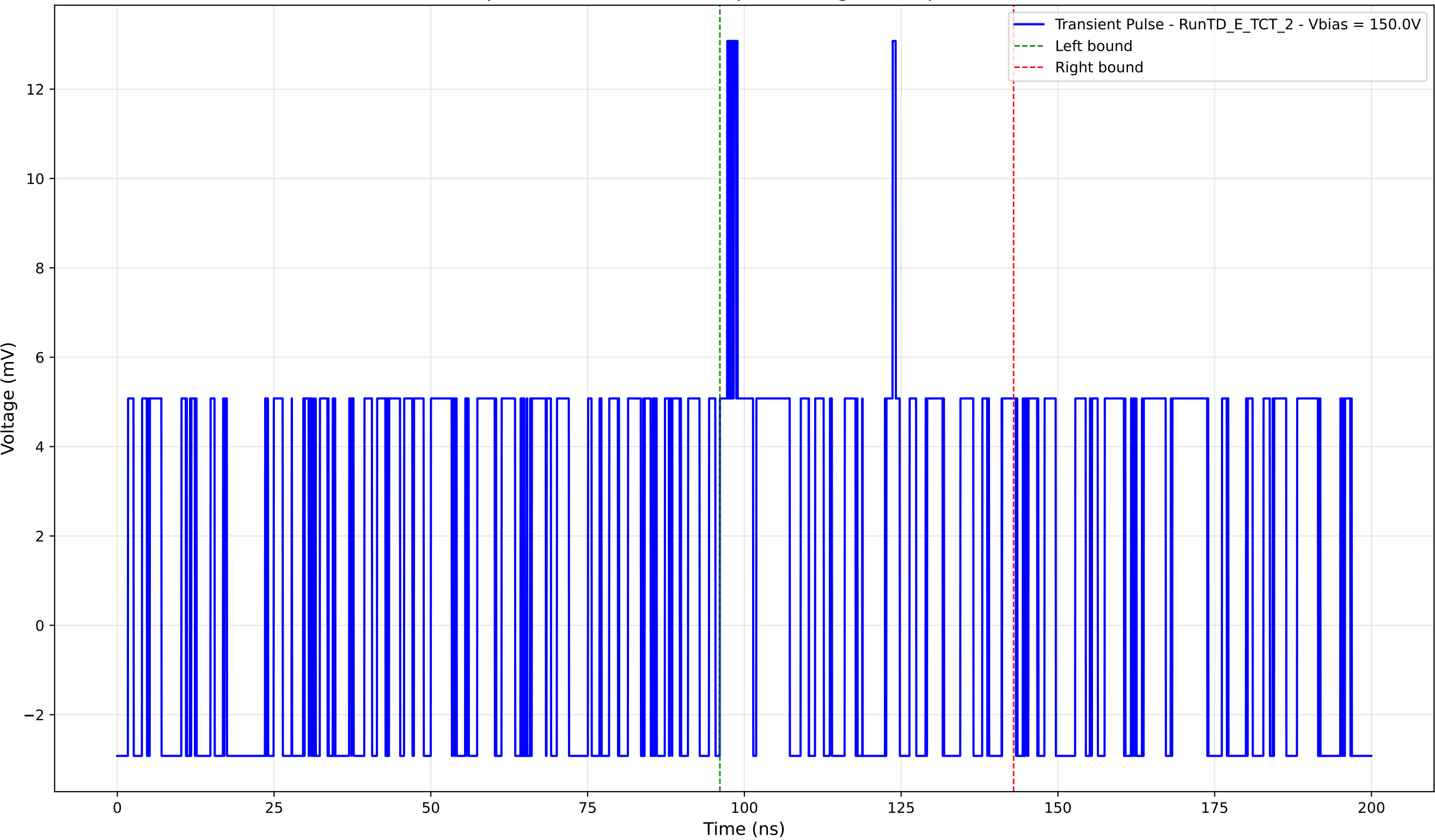
Transient Pulse - Sample: TD - Position: 125.0 \mu\text{m} - Charge: 1.73 pC - Rise Time: 0.00 ns (N/A)
