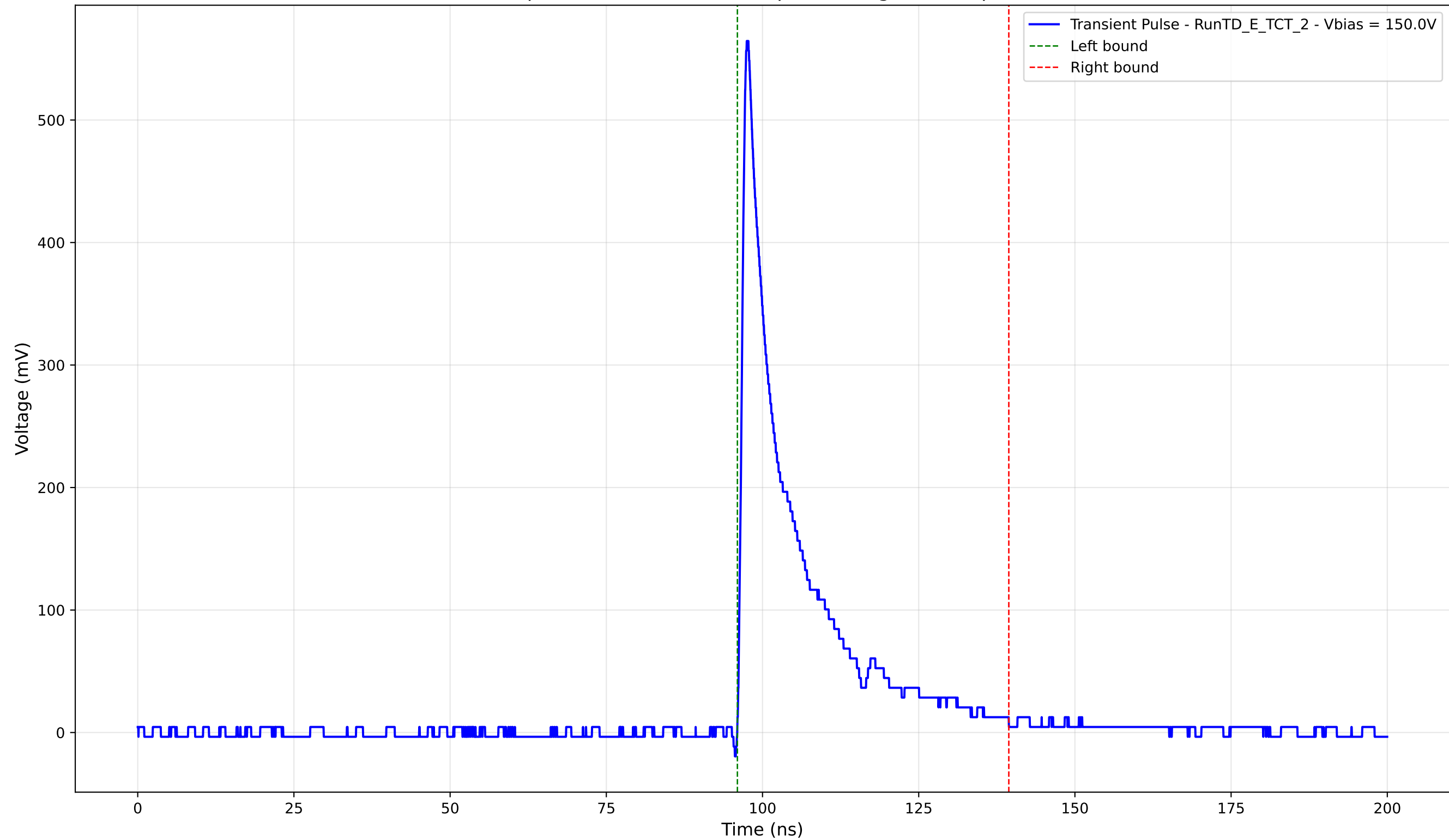
Transient Pulse - Sample: TD - Position: 420.0 \mu\text{m} - Charge: 90.83 pC - Rise Time: 0.97 ns
