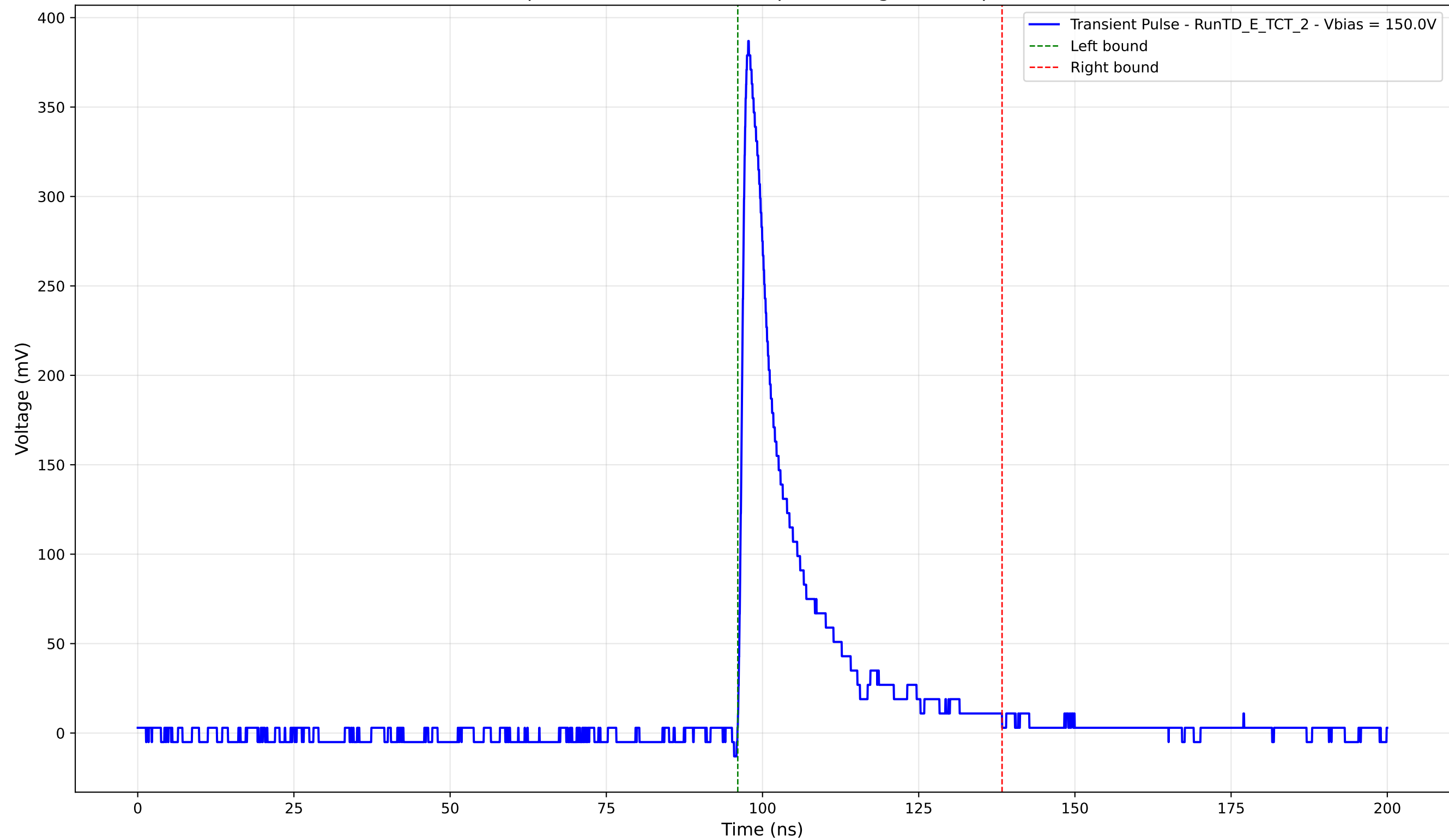
Transient Pulse - Sample: TD - Position: 555.0 \mu\text{m} - Charge: 60.90 pC - Rise Time: 1.07 ns
