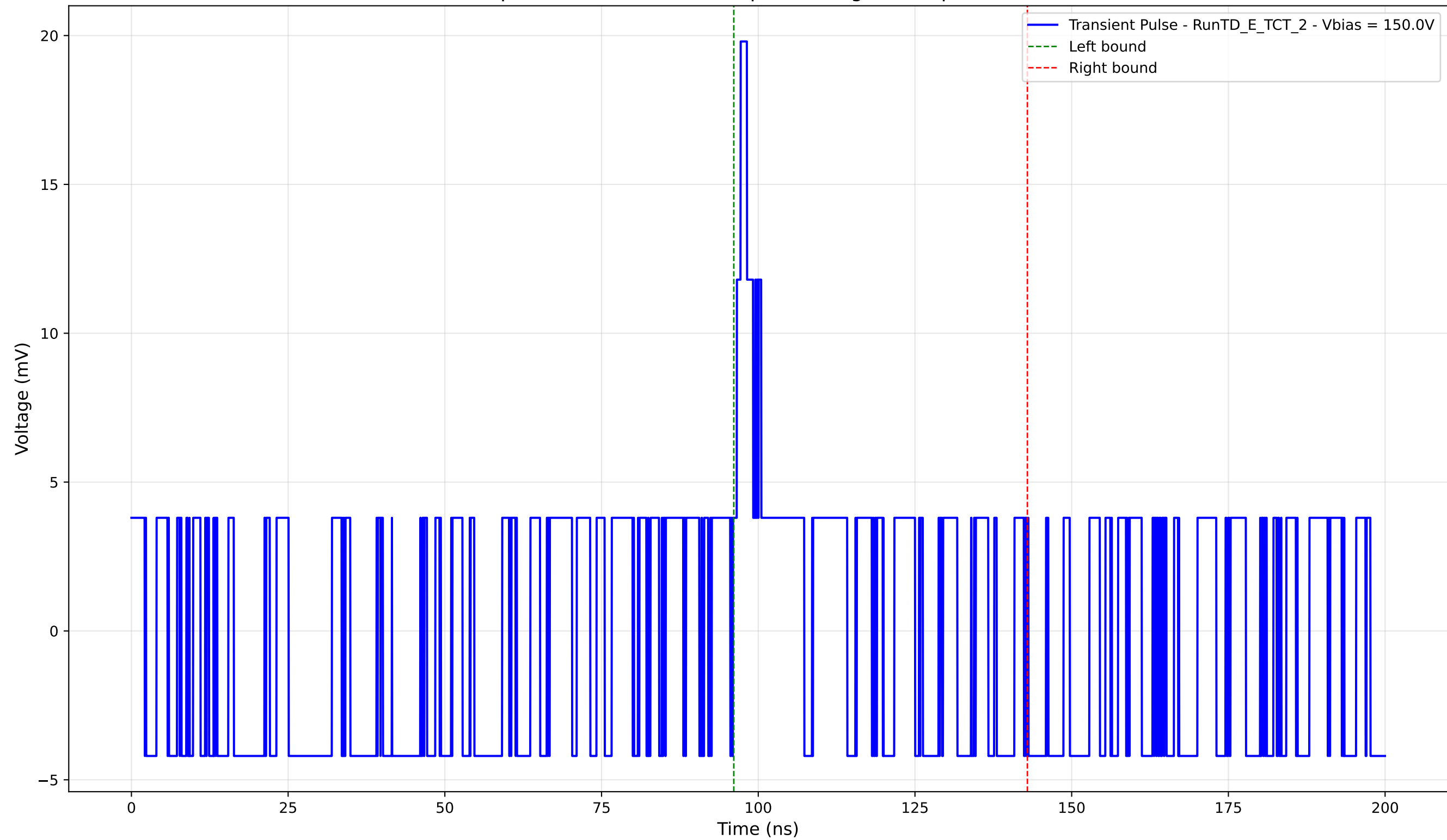
Transient Pulse - Sample: TD - Position: 260.0 \mu\text{m} - Charge: 1.82 pC - Rise Time: 0.00 ns (N/A)
