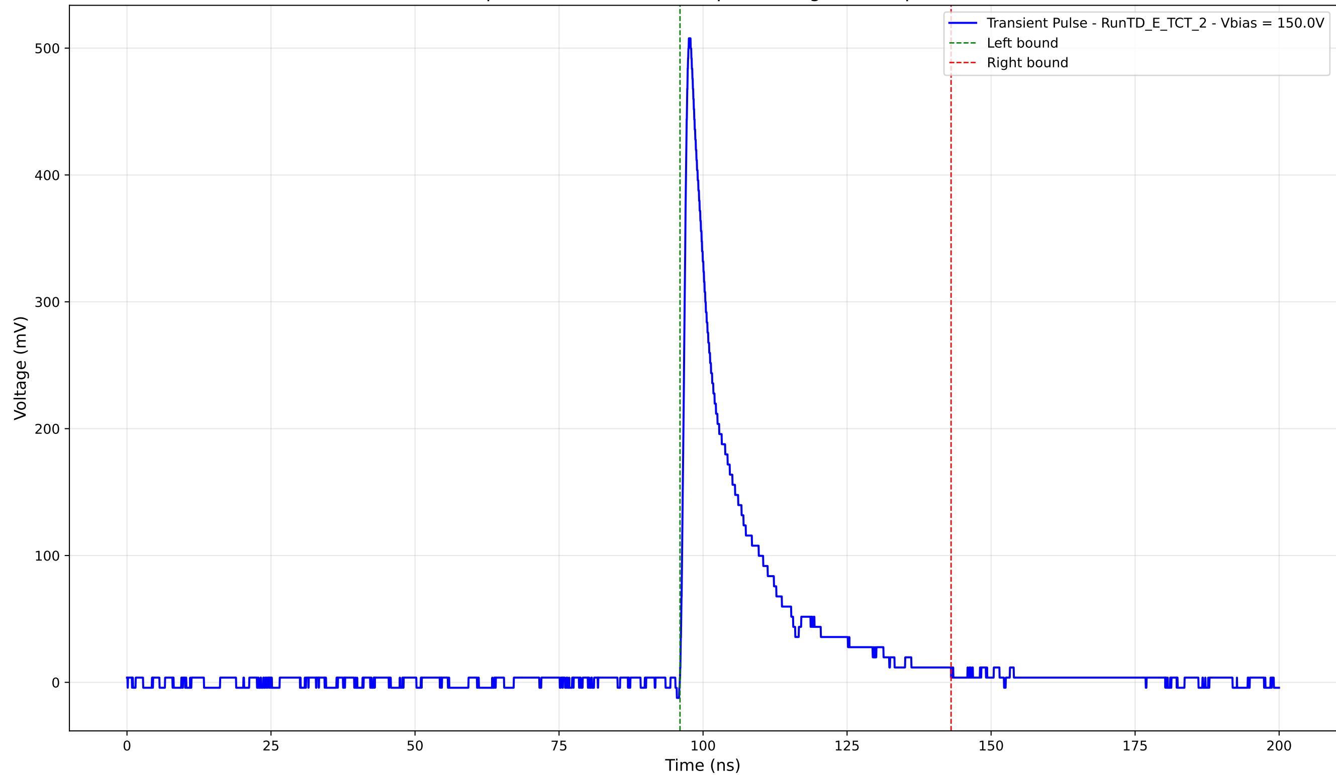
Transient Pulse - Sample: TD - Position: 400.0 \mu\text{m} - Charge: 86.59 pC - Rise Time: 1.00 ns
