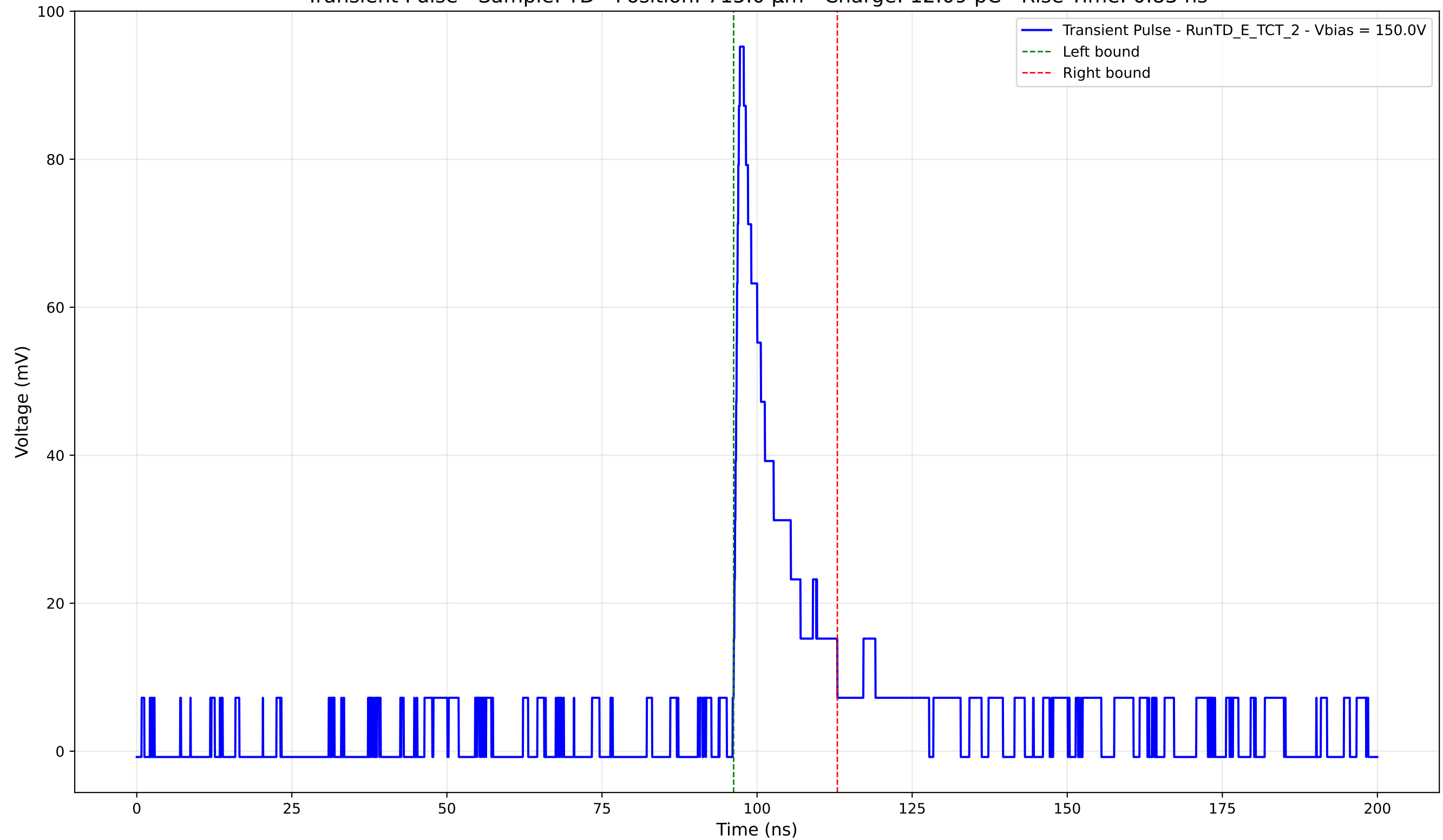
Transient Pulse - Sample: TD - Position: 715.0 \mu\text{m} - Charge: 12.09 pC - Rise Time: 0.83 ns
