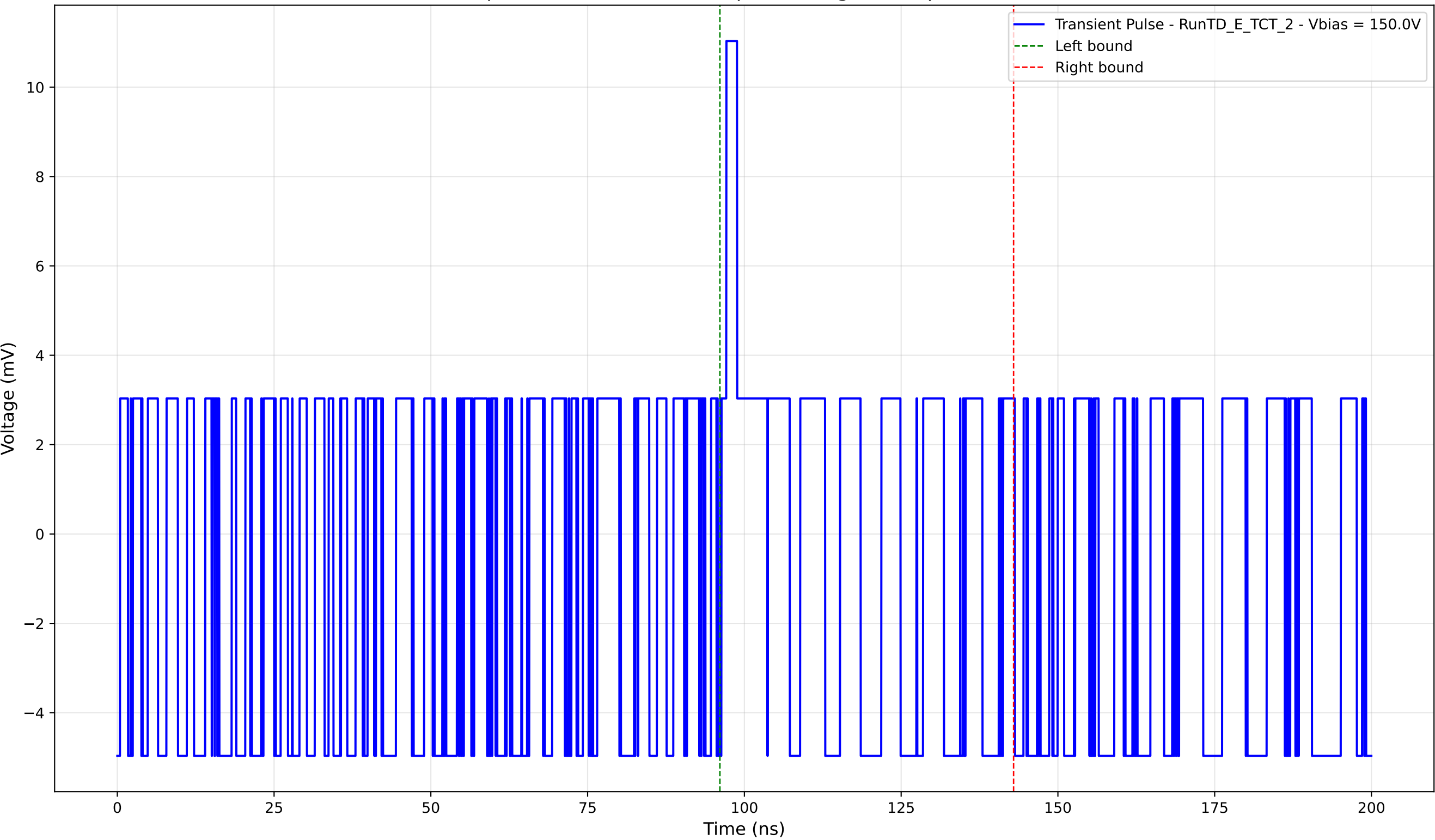
Transient Pulse - Sample: TD - Position: 230.0 \mu\text{m} - Charge: 0.36 pC - Rise Time: 0.00 ns (N/A)
