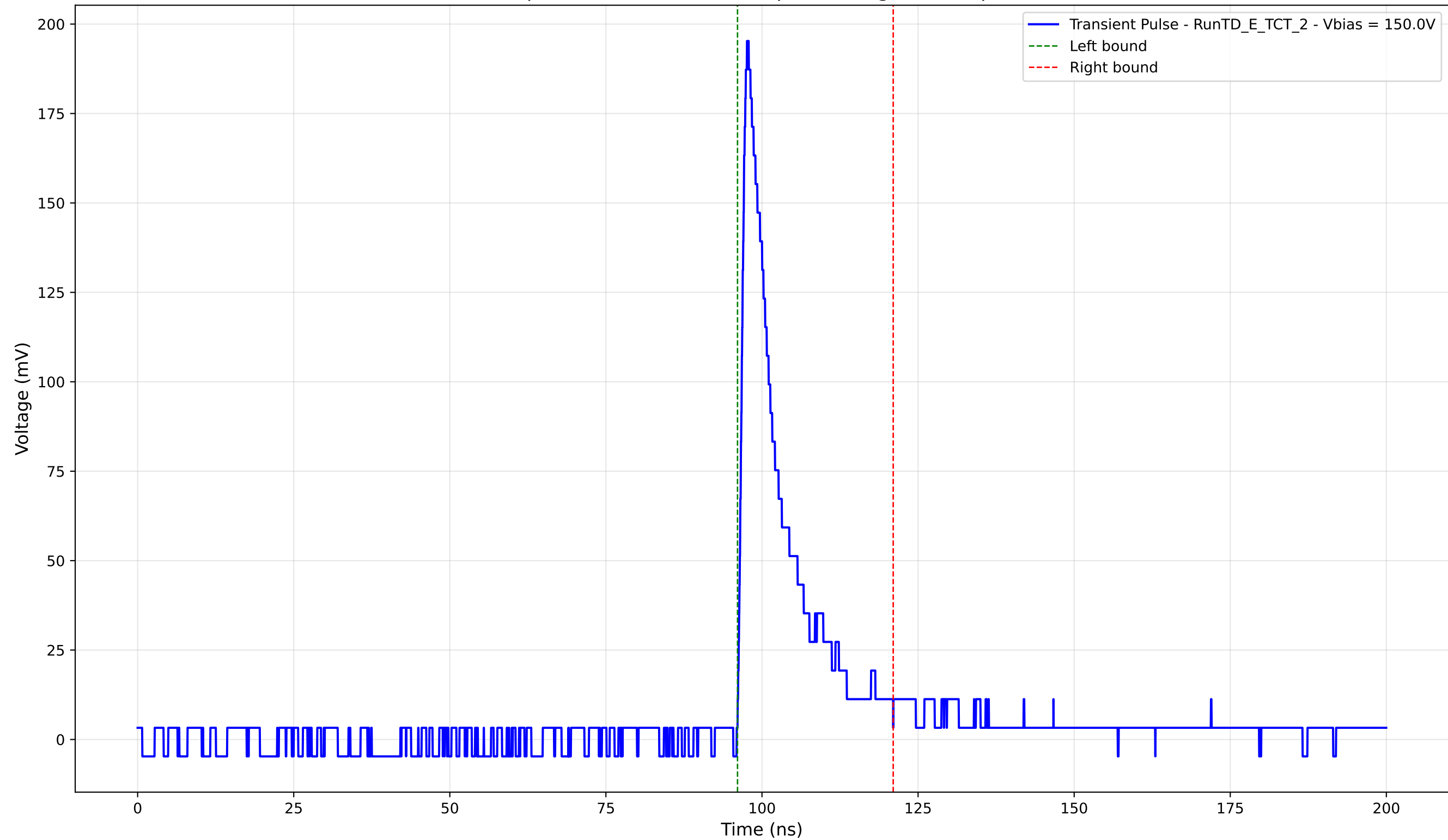
Transient Pulse - Sample: TD - Position: 620.0 \mu\text{m} - Charge: 26.34 pC - Rise Time: 1.08 ns
