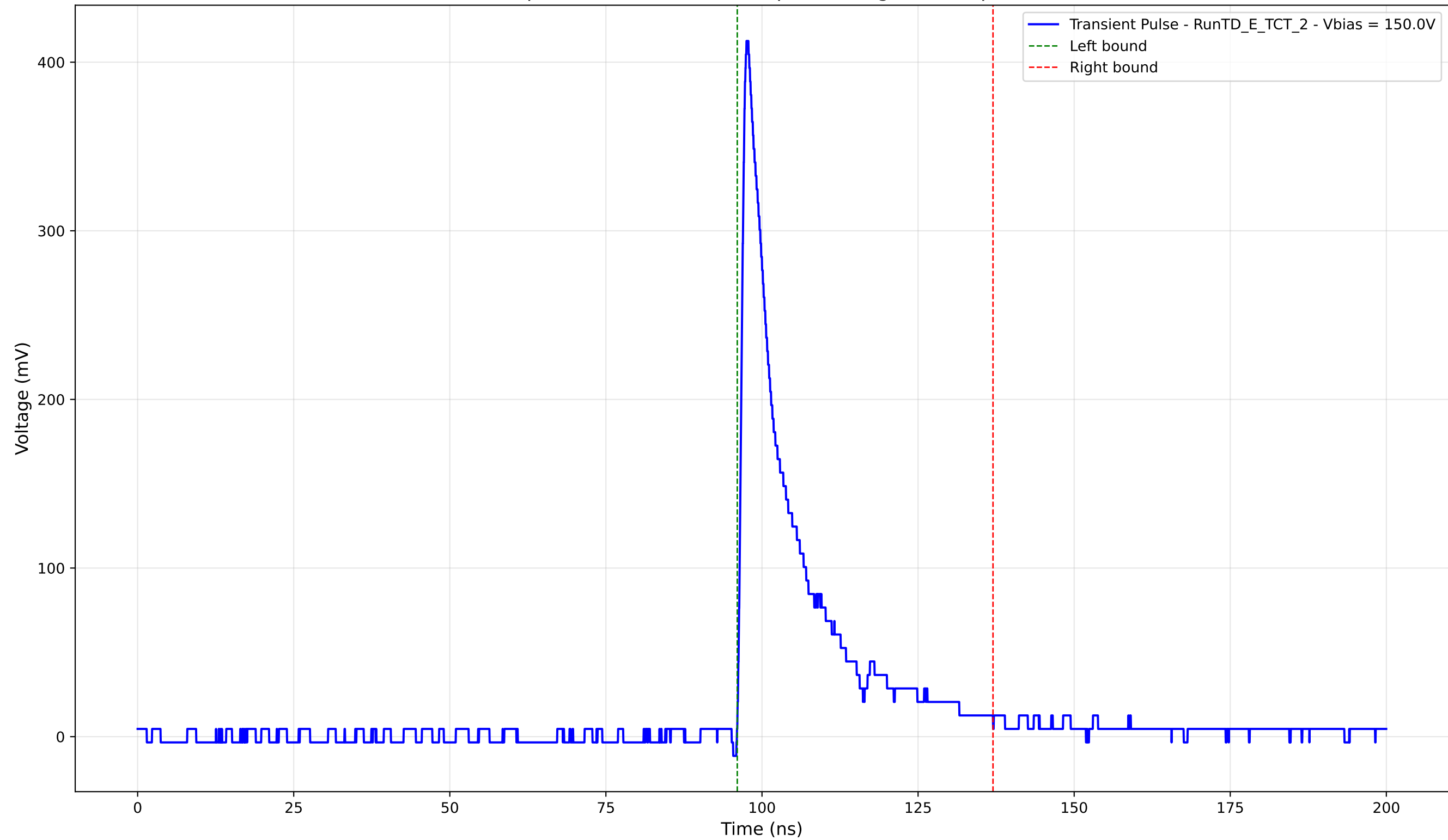
Transient Pulse - Sample: TD - Position: 505.0 \mu\text{m} - Charge: 67.78 pC - Rise Time: 0.99 ns
