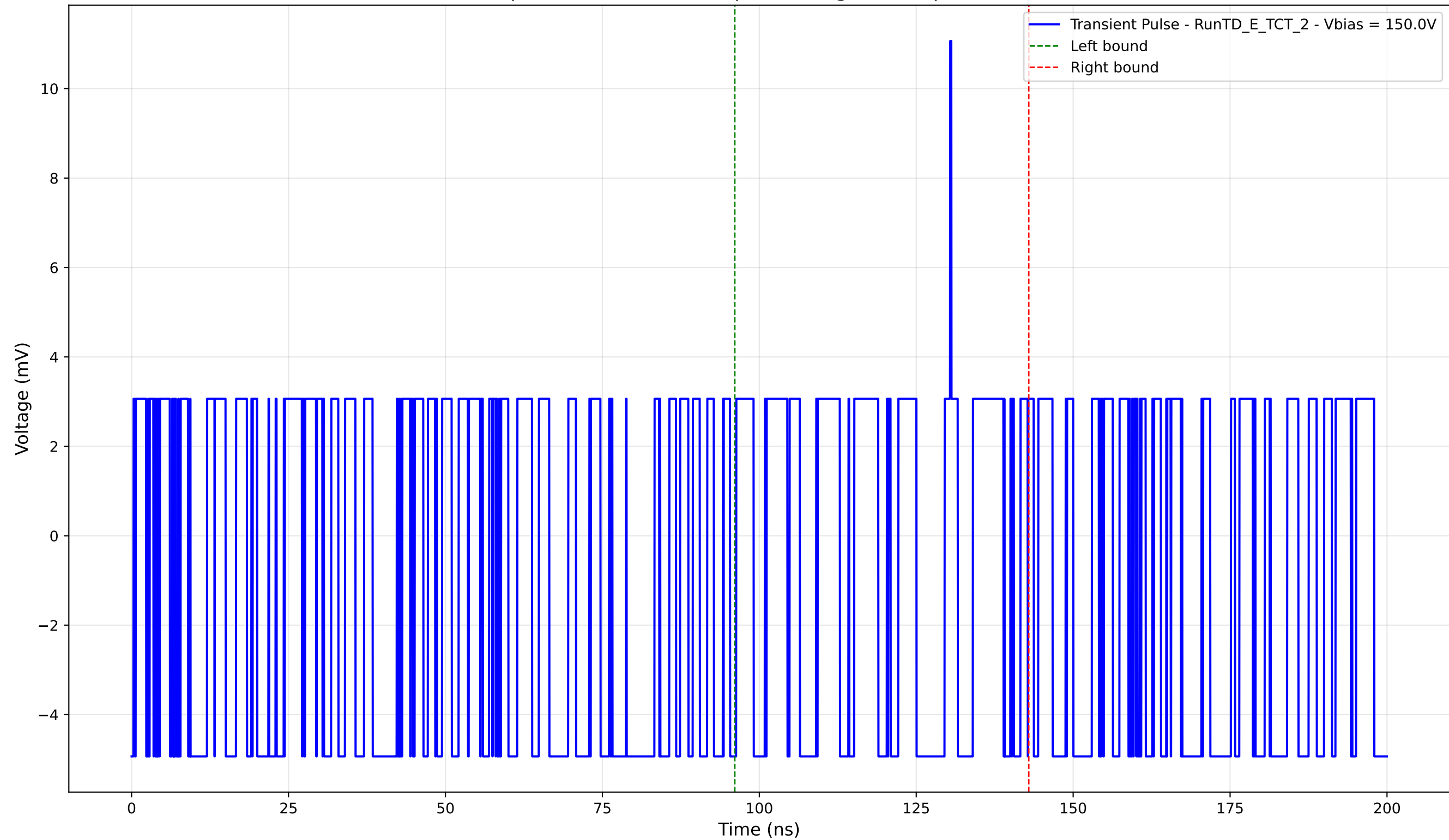
Transient Pulse - Sample: TD - Position: 0.0 \mu\text{m} - Charge: -0.18 pC - Rise Time: 0.00 ns (N/A)
