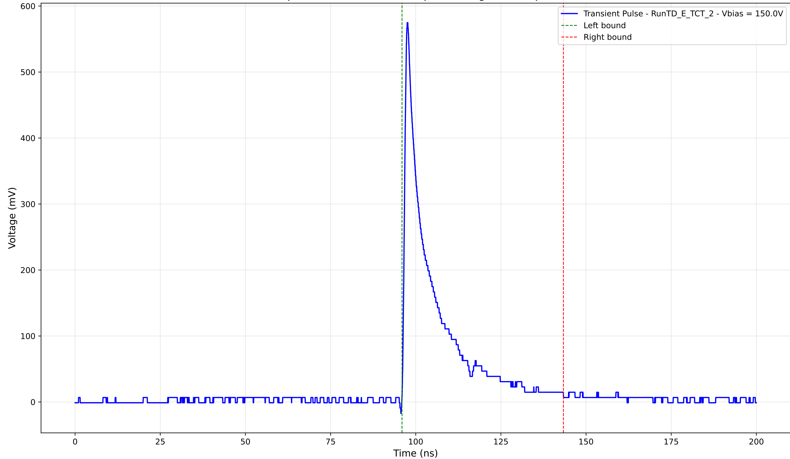
Transient Pulse - Sample: TD - Position: 425.0 \mu\text{m} - Charge: 93.65 pC - Rise Time: 0.99 ns
