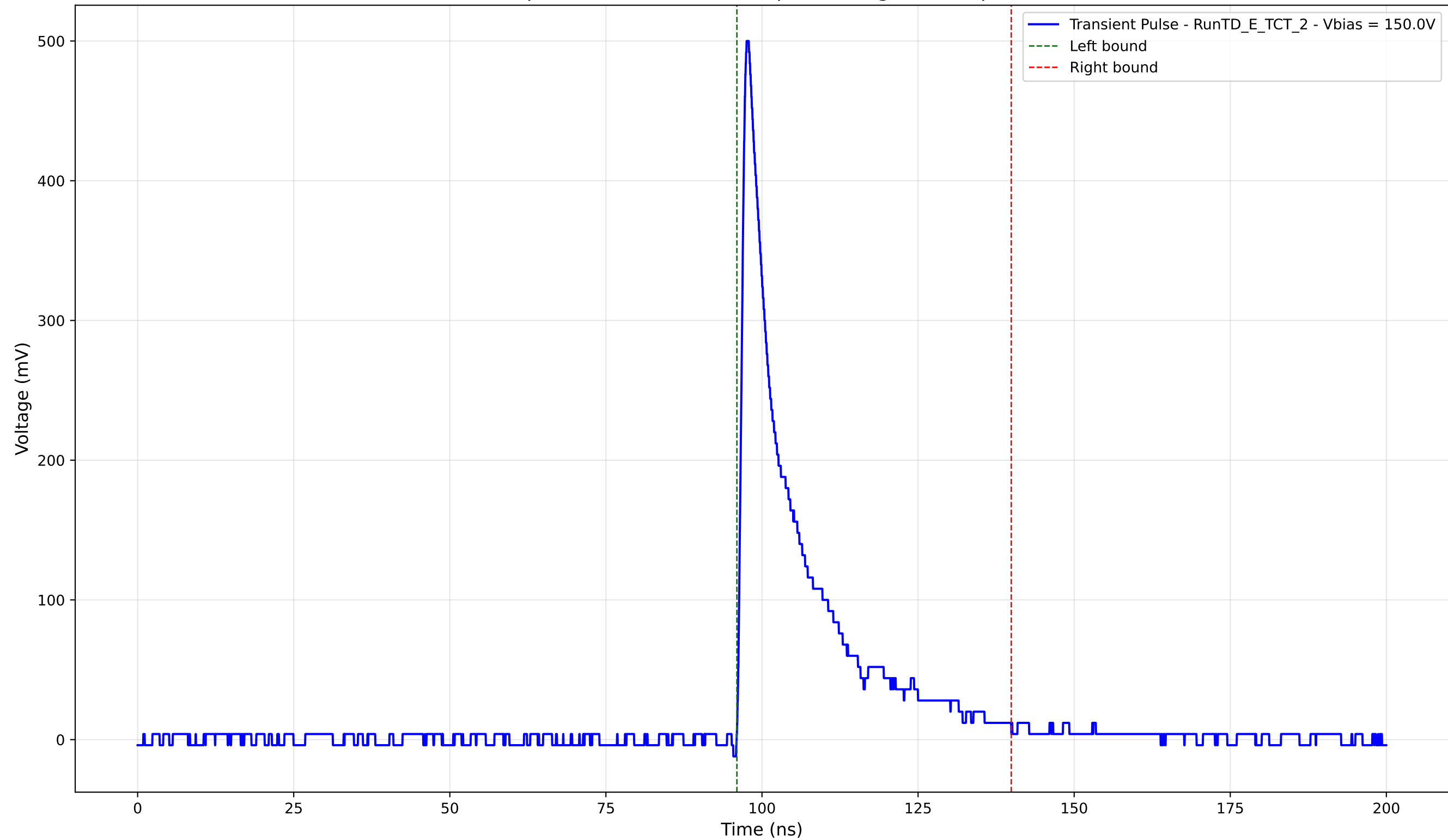
Transient Pulse - Sample: TD - Position: 385.0 \mu\text{m} - Charge: 86.13 pC - Rise Time: 1.04 ns
