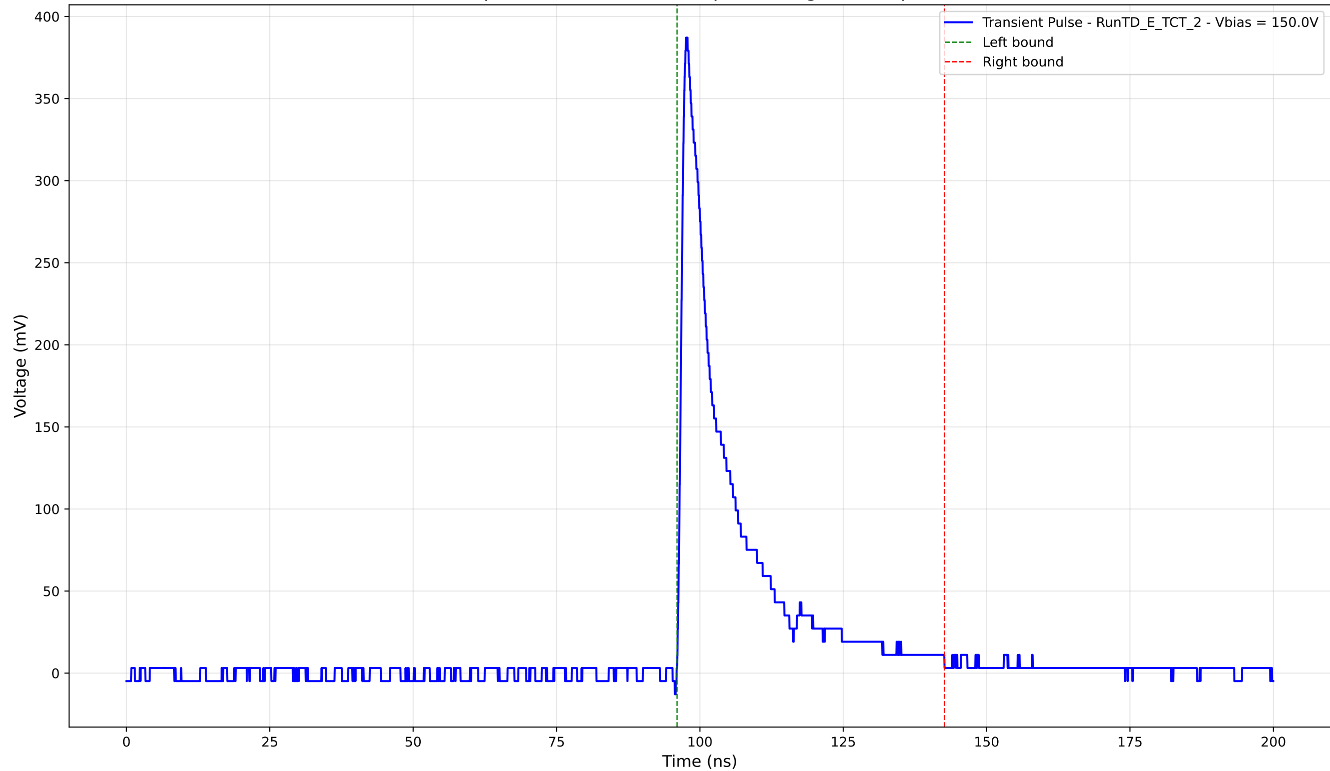
Transient Pulse - Sample: TD - Position: 515.0 \mu\text{m} - Charge: 65.48 pC - Rise Time: 1.07 ns
