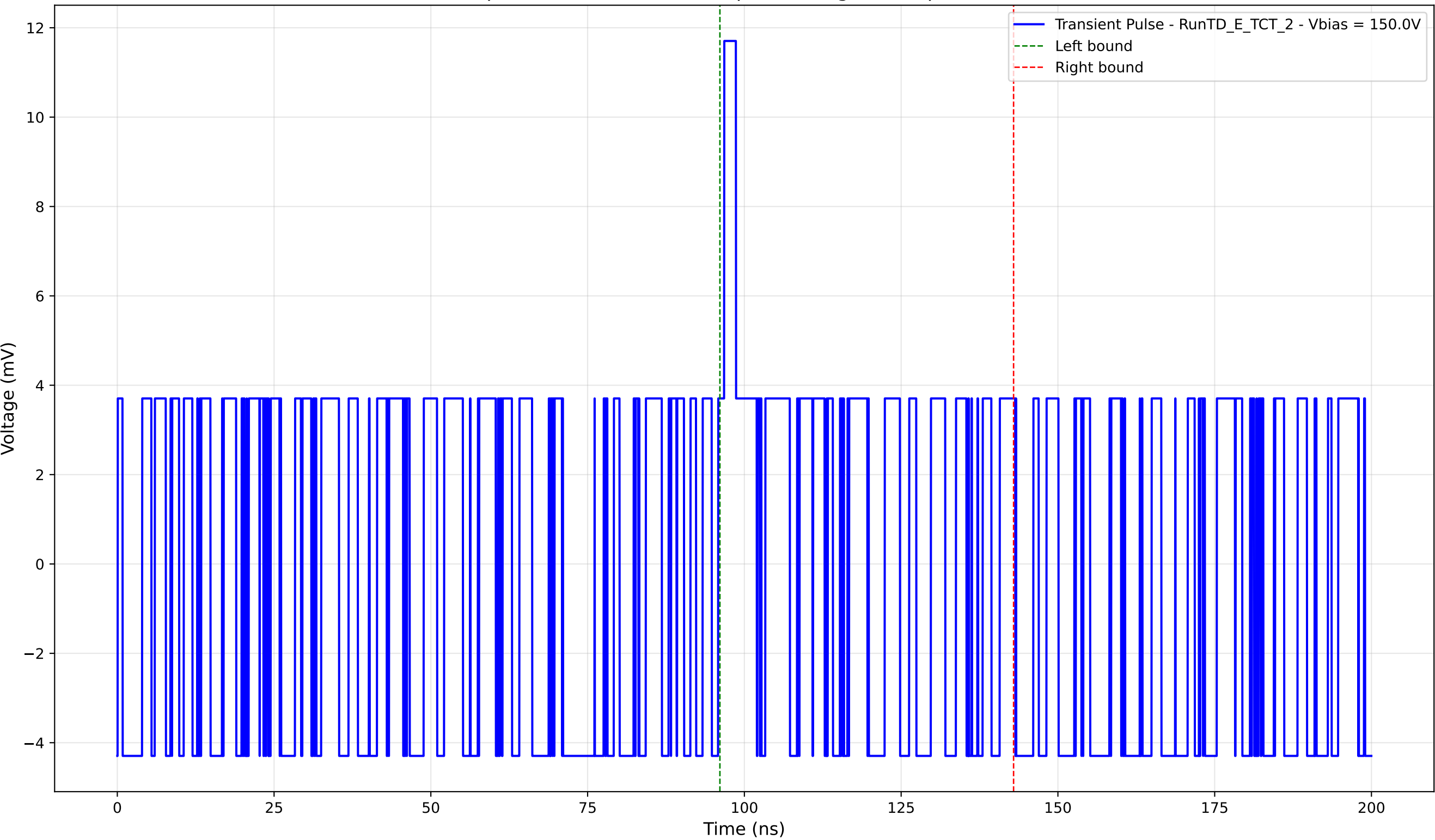
Transient Pulse - - Sample: TD - Position: 205.0 \mu\text{m} - Charge: 1.12 pC - Rise Time: 0.00 ns (N/A)
