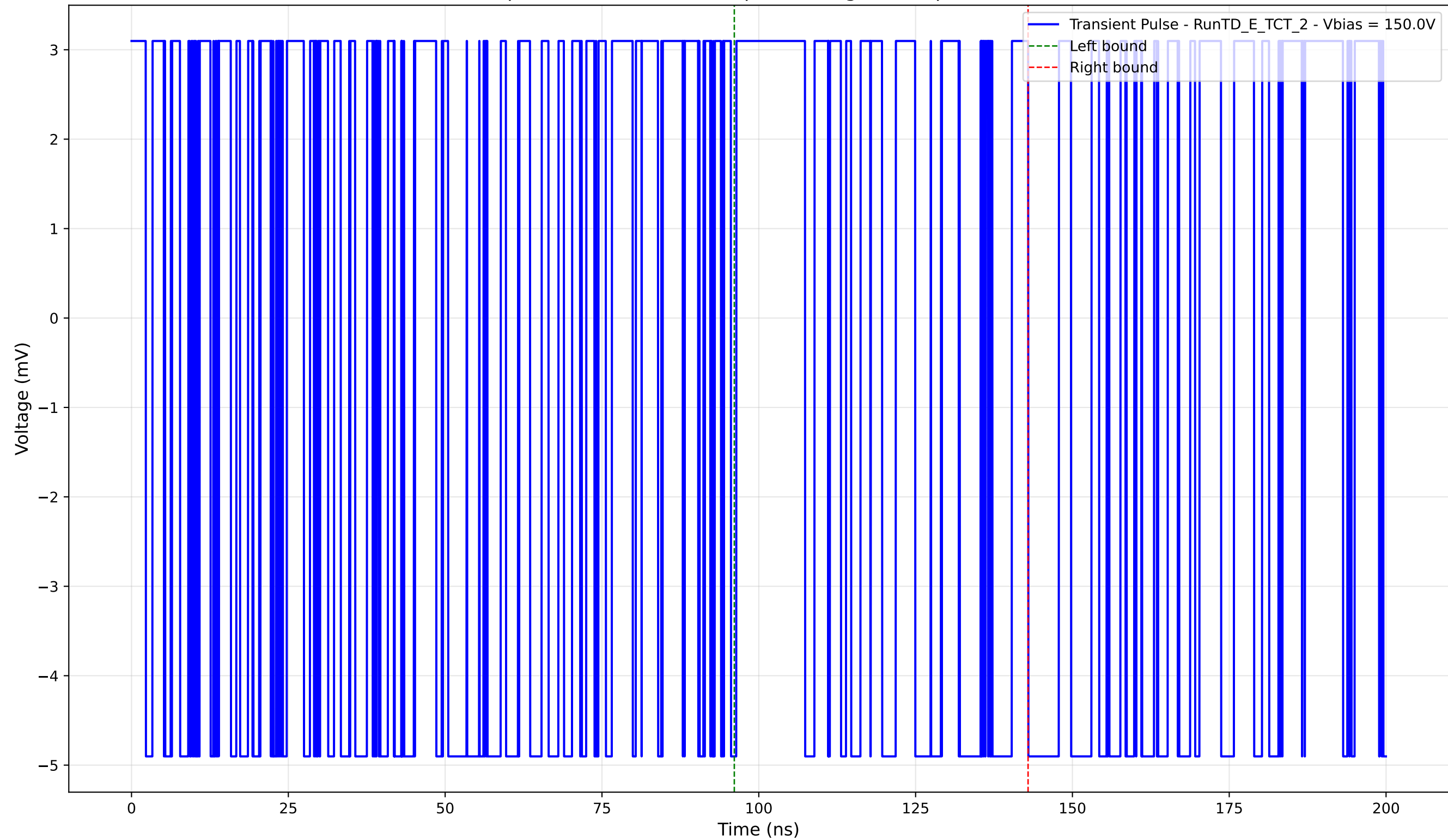
Transient Pulse - Sample: TD - Position: 70.0 \mu\text{m} - Charge: 0.04 pC - Rise Time: 0.00 ns (N/A)
