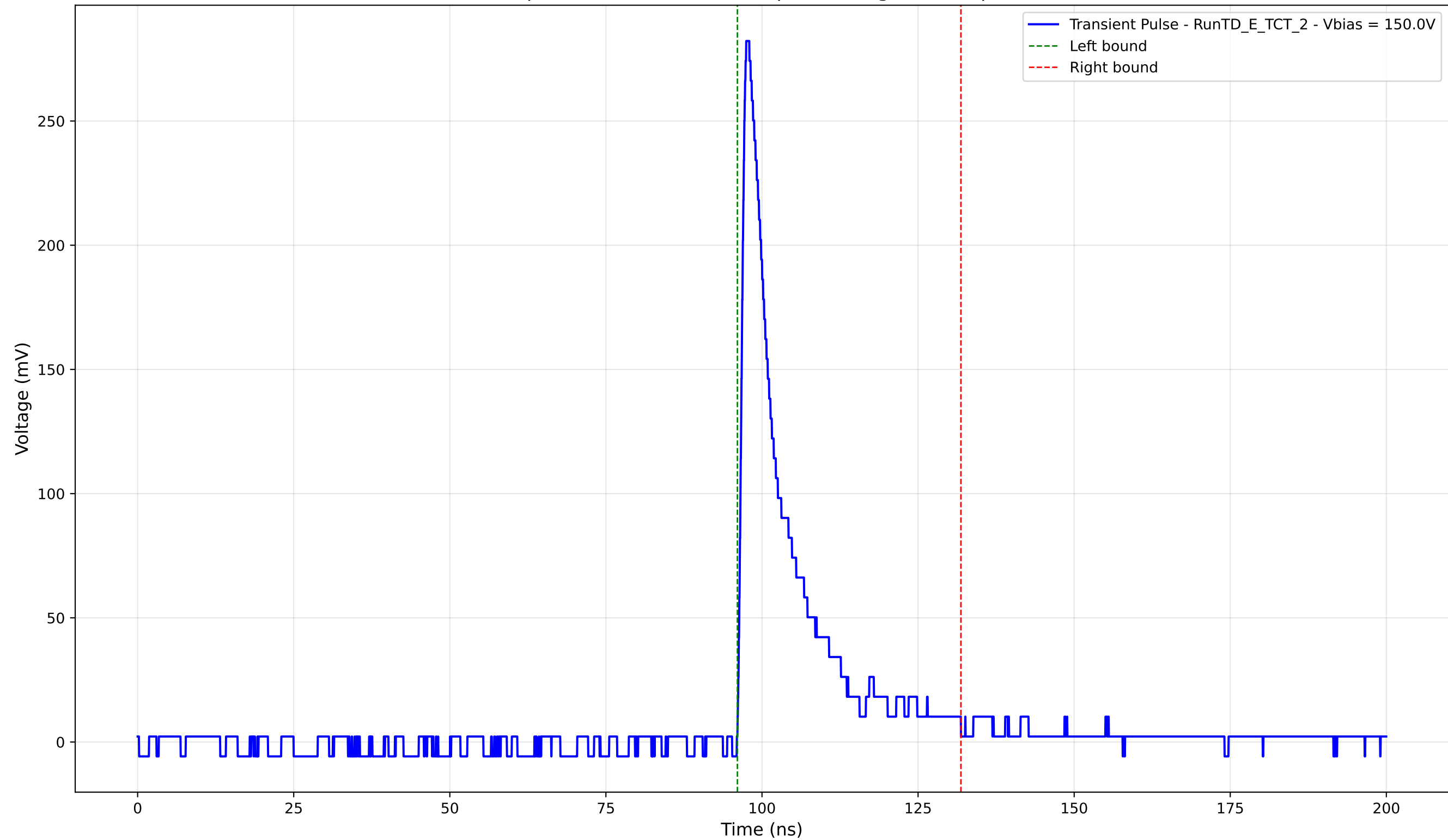
Transient Pulse - Sample: TD - Position: 580.0 \mu\text{m} - Charge: 41.24 pC - Rise Time: 0.97 ns
