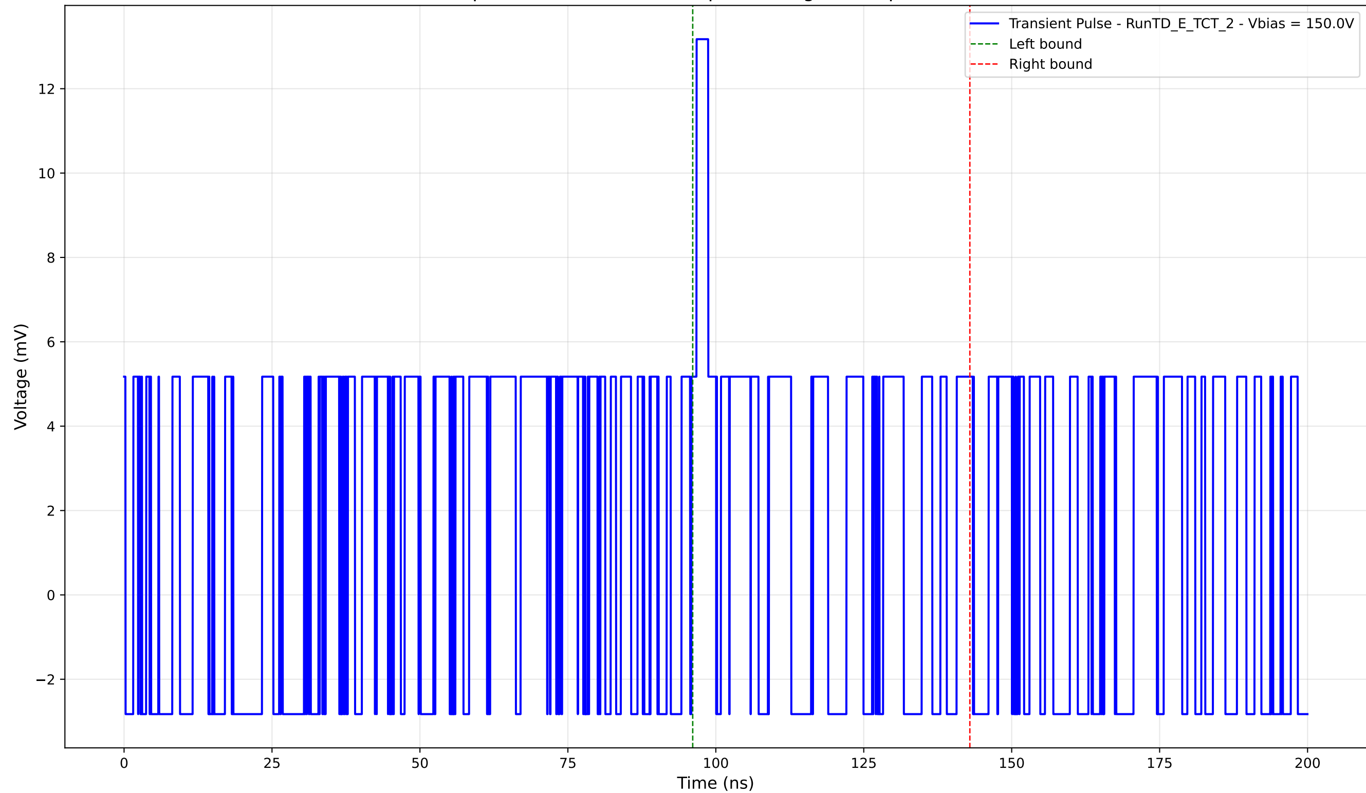
Transient Pulse - Sample: TD - Position: 185.0 \mu\text{m} - Charge: 2.29 pC - Rise Time: 0.00 ns (N/A)
