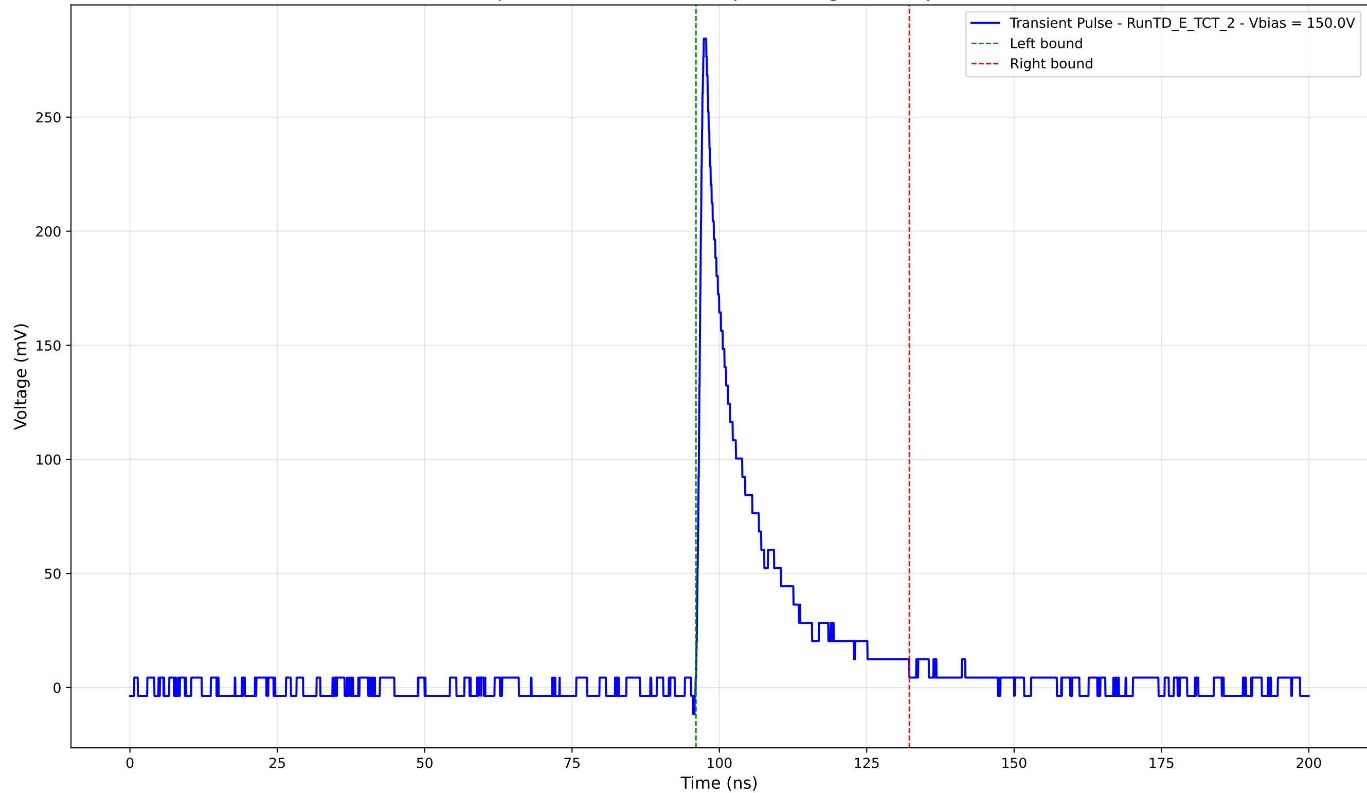
Transient Pulse - Sample: TD - Position: 345.0 \mu\text{m} - Charge: 43.99 pC - Rise Time: 0.94 ns
