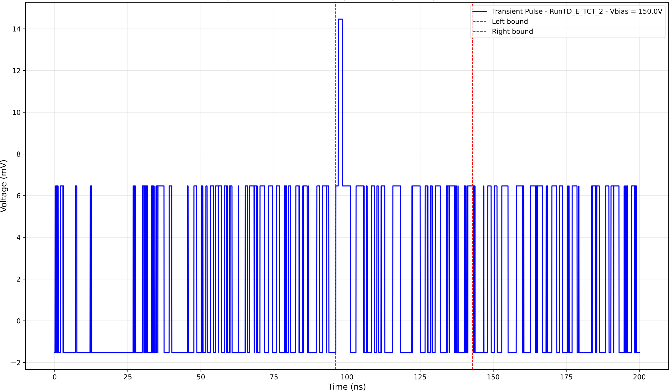
Transient Pulse - - Sample: TD - Position: 220.0 \mu\text{m} - Charge: 2.69 pC - Rise Time: 0.00 ns (N/A)
