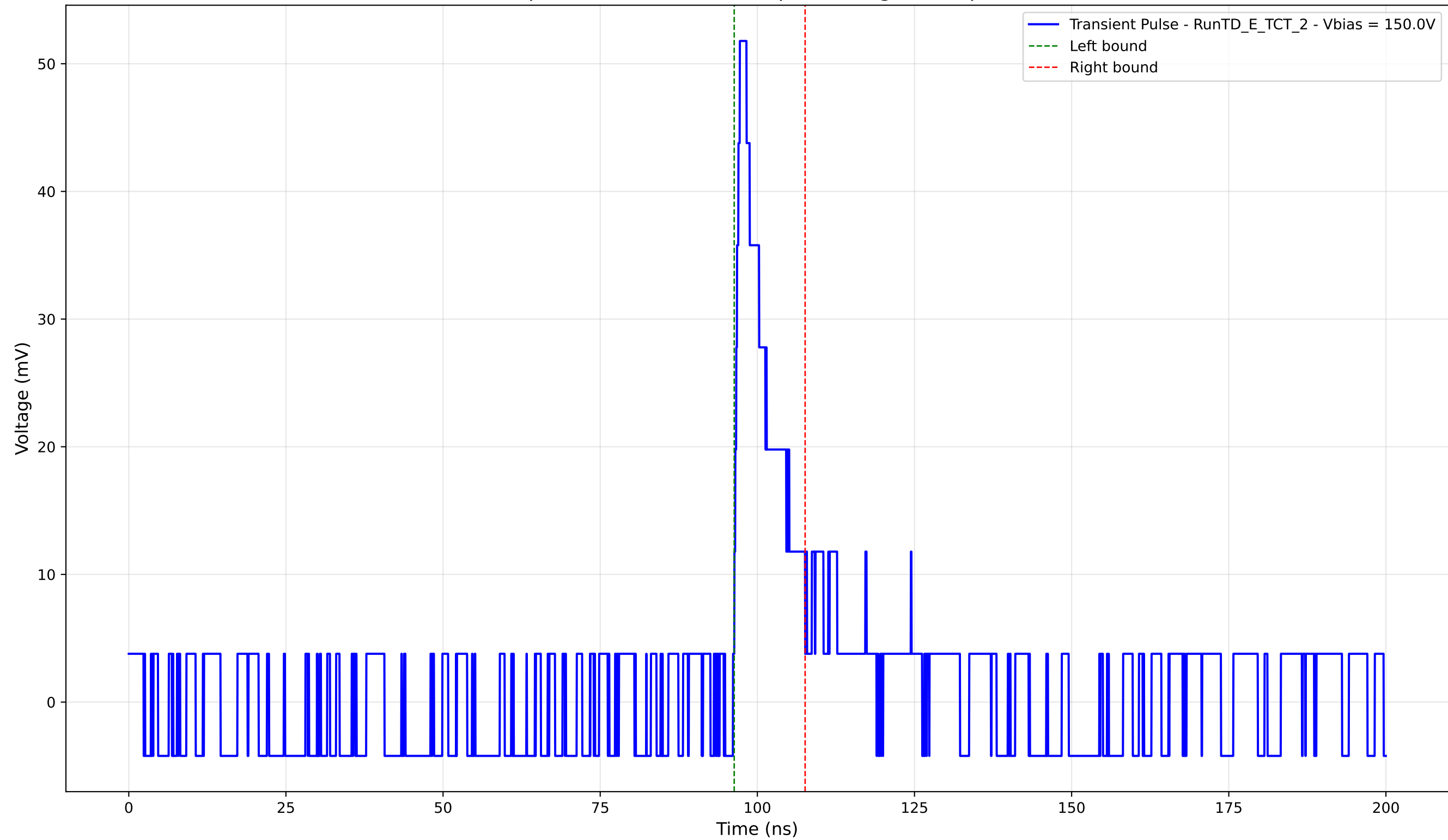
Transient Pulse - Sample: TD - Position: 670.0 \mu\text{m} - Charge: 5.77 pC - Rise Time: 0.88 ns
