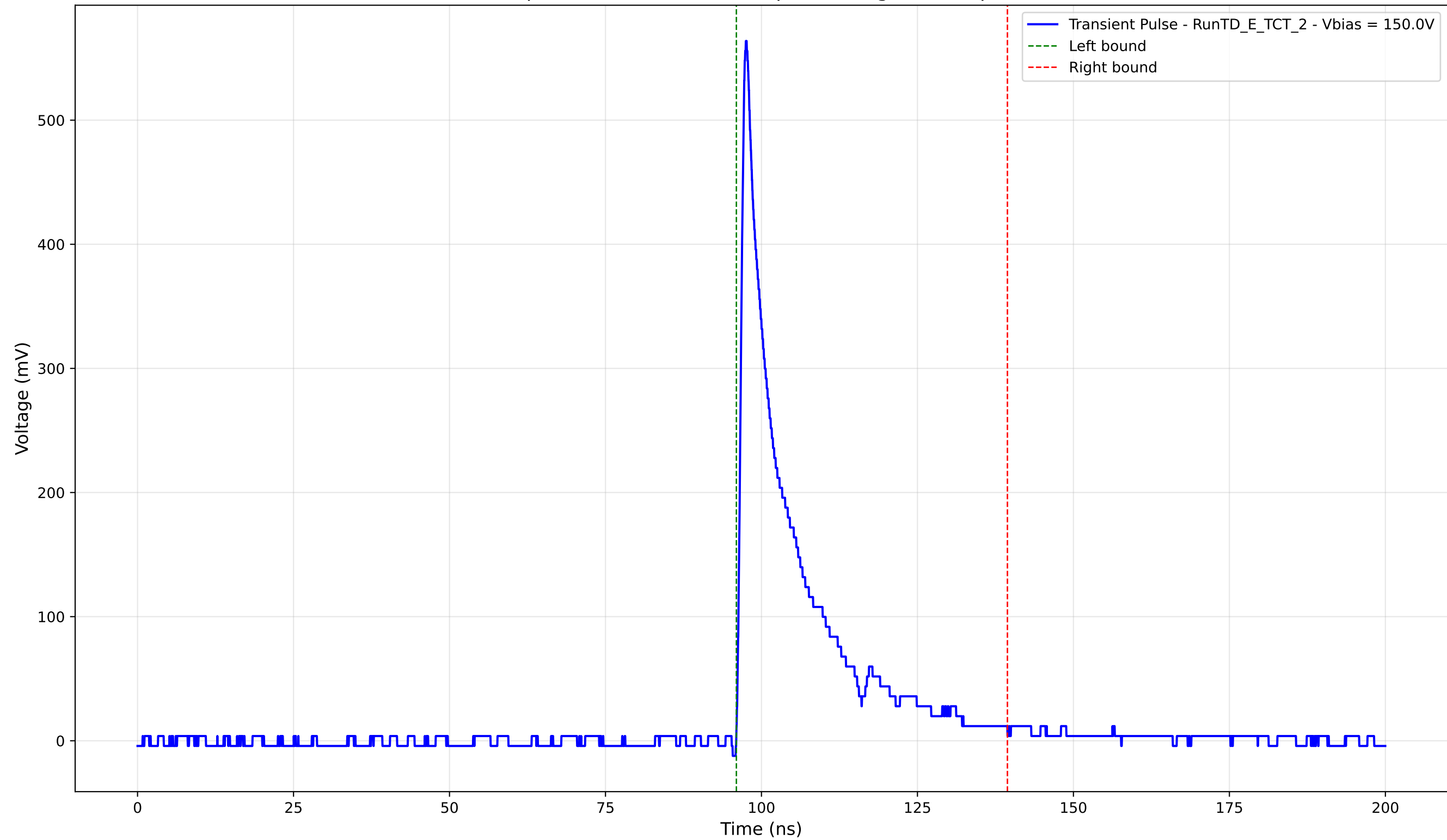
Transient Pulse - Sample: TD - Position: 435.0 \mu\text{m} - Charge: 87.90 pC - Rise Time: 0.97 ns
