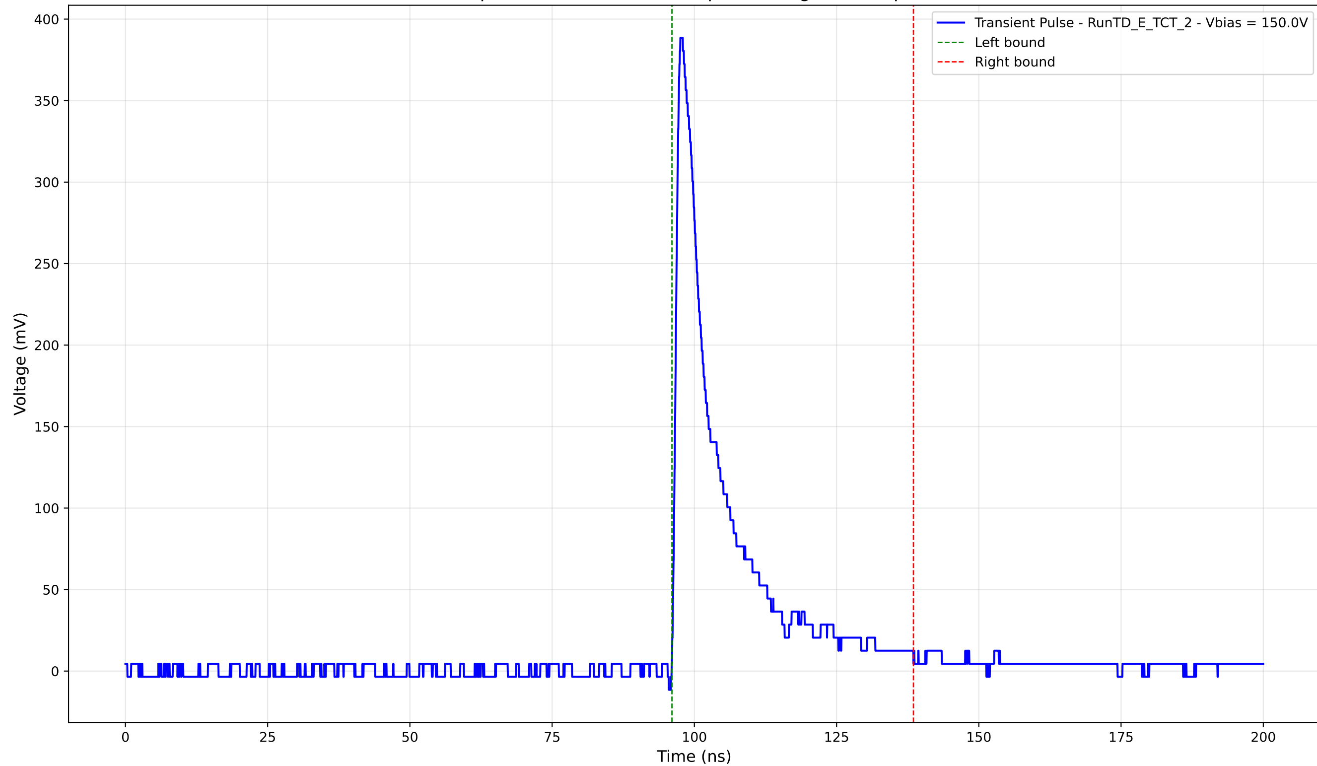
Transient Pulse - Sample: TD - Position: 550.0 \mu\text{m} - Charge: 63.52 pC - Rise Time: 1.05 ns
