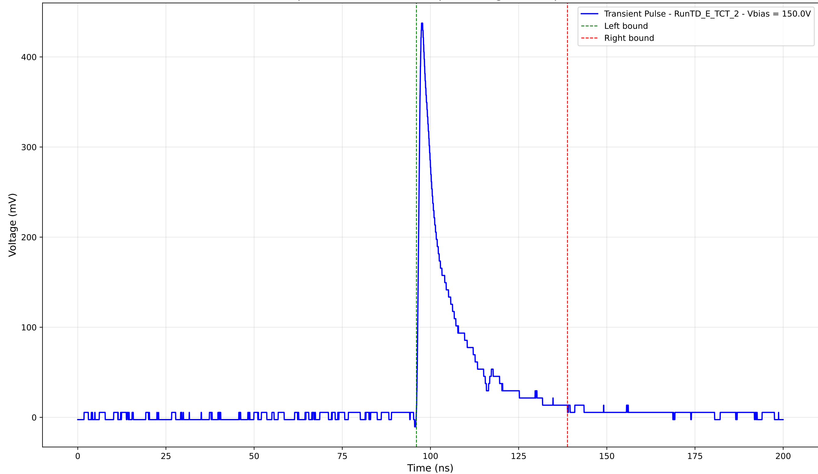
Transient Pulse - Sample: TD - Position: 360.0 \mu\text{m} - Charge: 73.55 pC - Rise Time: 1.00 ns
