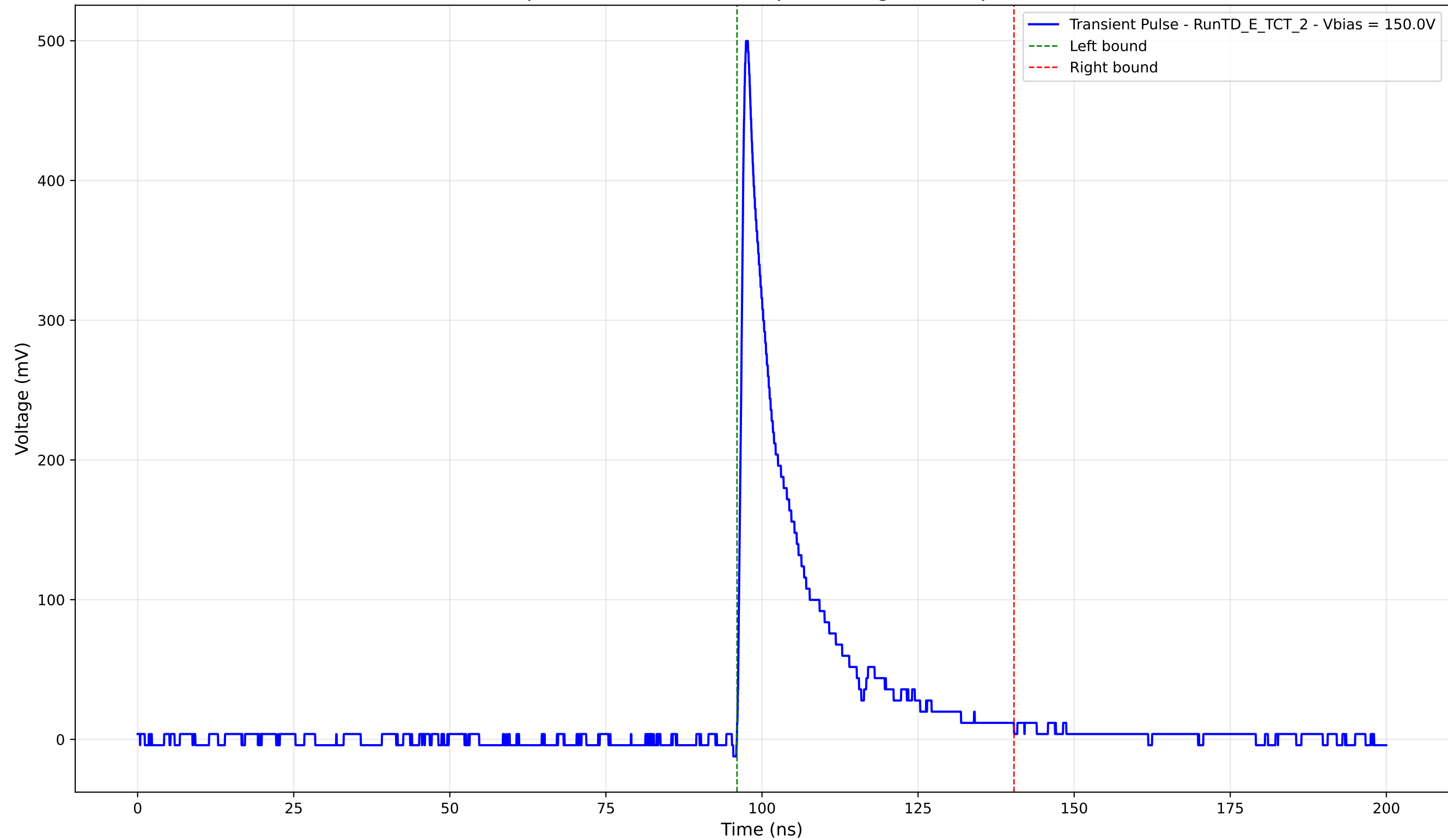
Transient Pulse - Sample: TD - Position: 475.0 \mu\text{m} - Charge: 80.24 pC - Rise Time: 0.96 ns
