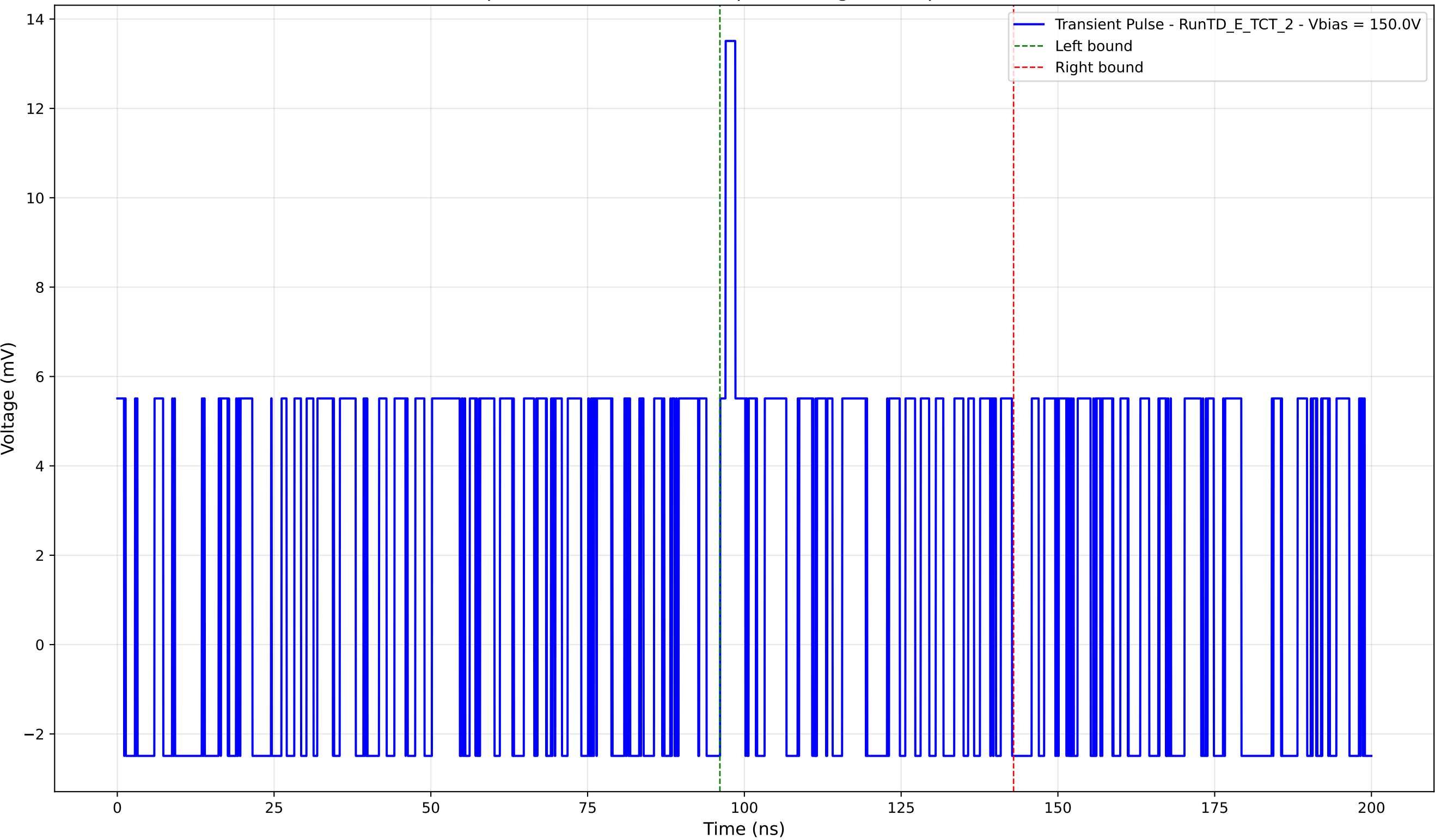
Transient Pulse - Sample: TD - Position: 110.0 \mu\text{m} - Charge: 2.69 pC - Rise Time: 0.00 ns (N/A)
