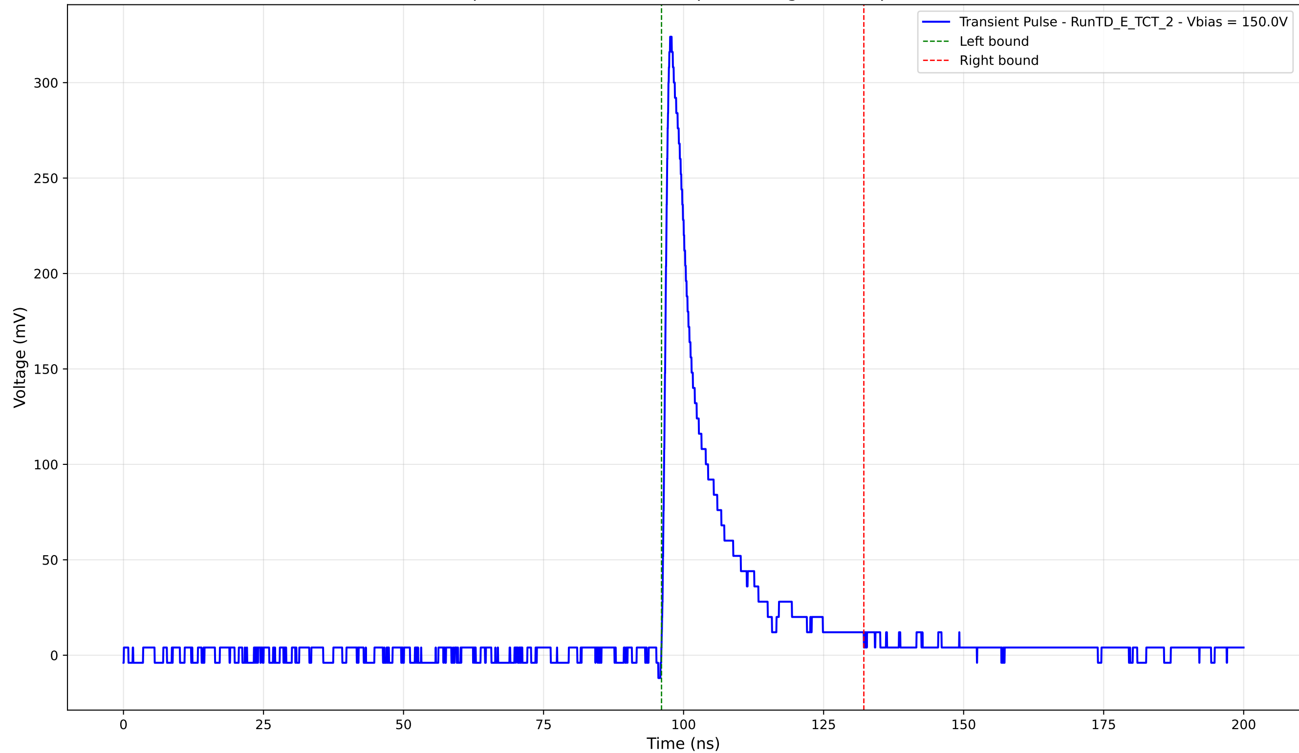
Transient Pulse - Sample: TD - Position: 570.0 \mu\text{m} - Charge: 48.84 pC - Rise Time: 1.01 ns
