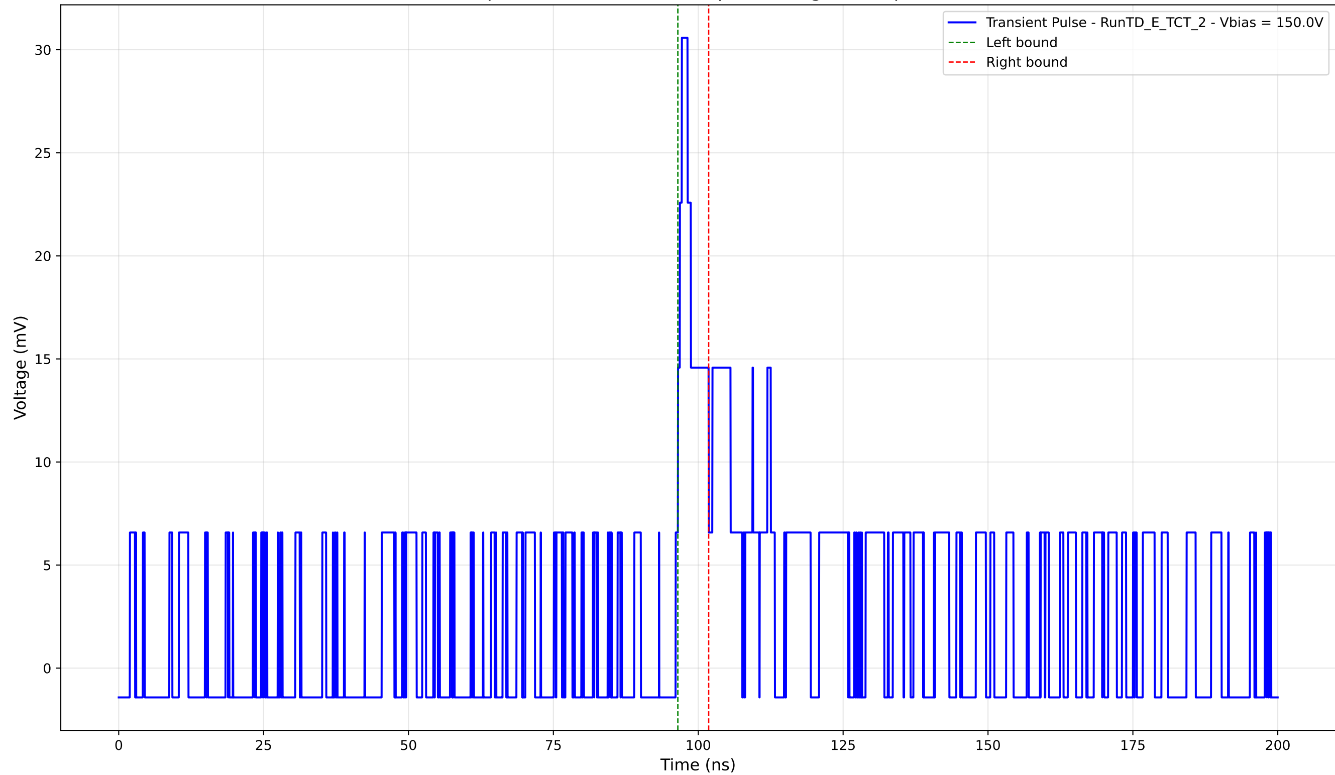
Transient Pulse - Sample: TD - Position: 300.0 \mu\text{m} - Charge: 2.01 pC - Rise Time: 1.07 ns
