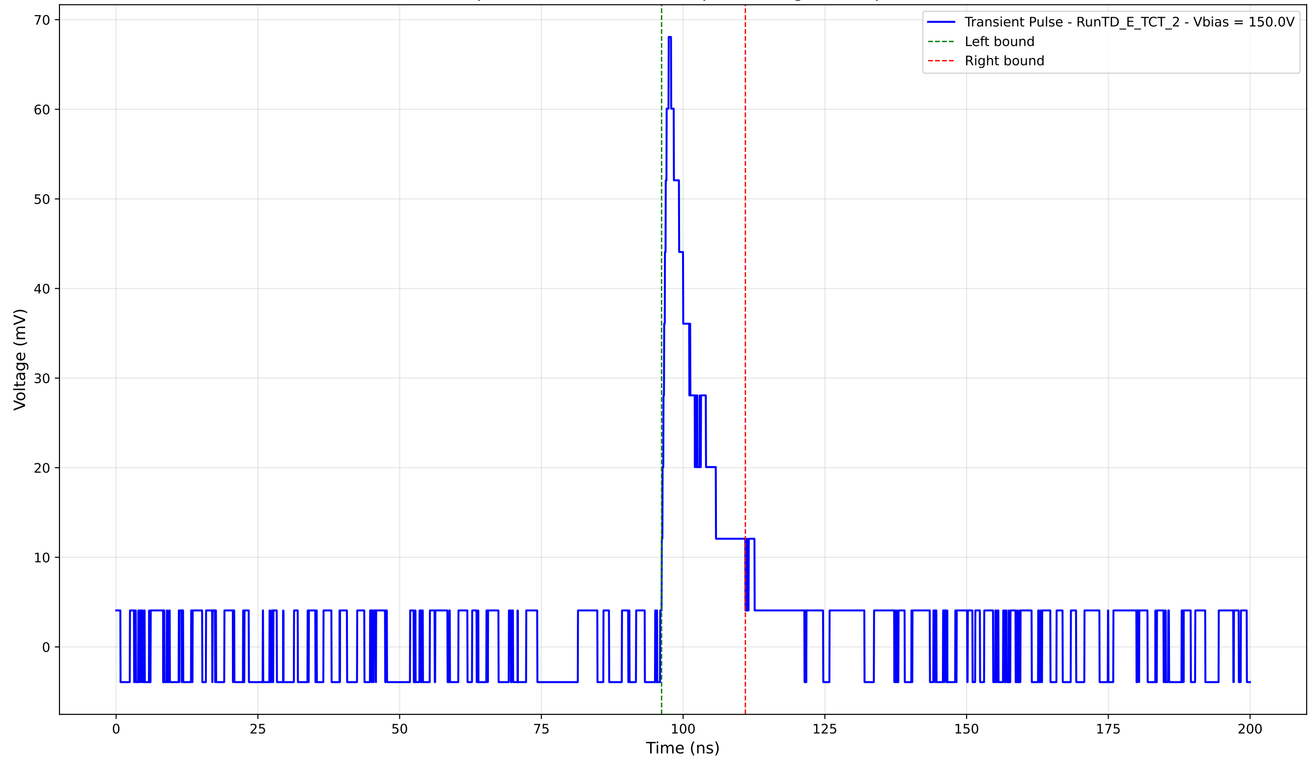
Transient Pulse - Sample: TD - Position: 685.0 \mu\text{m} - Charge: 8.03 pC - Rise Time: 1.23 ns
