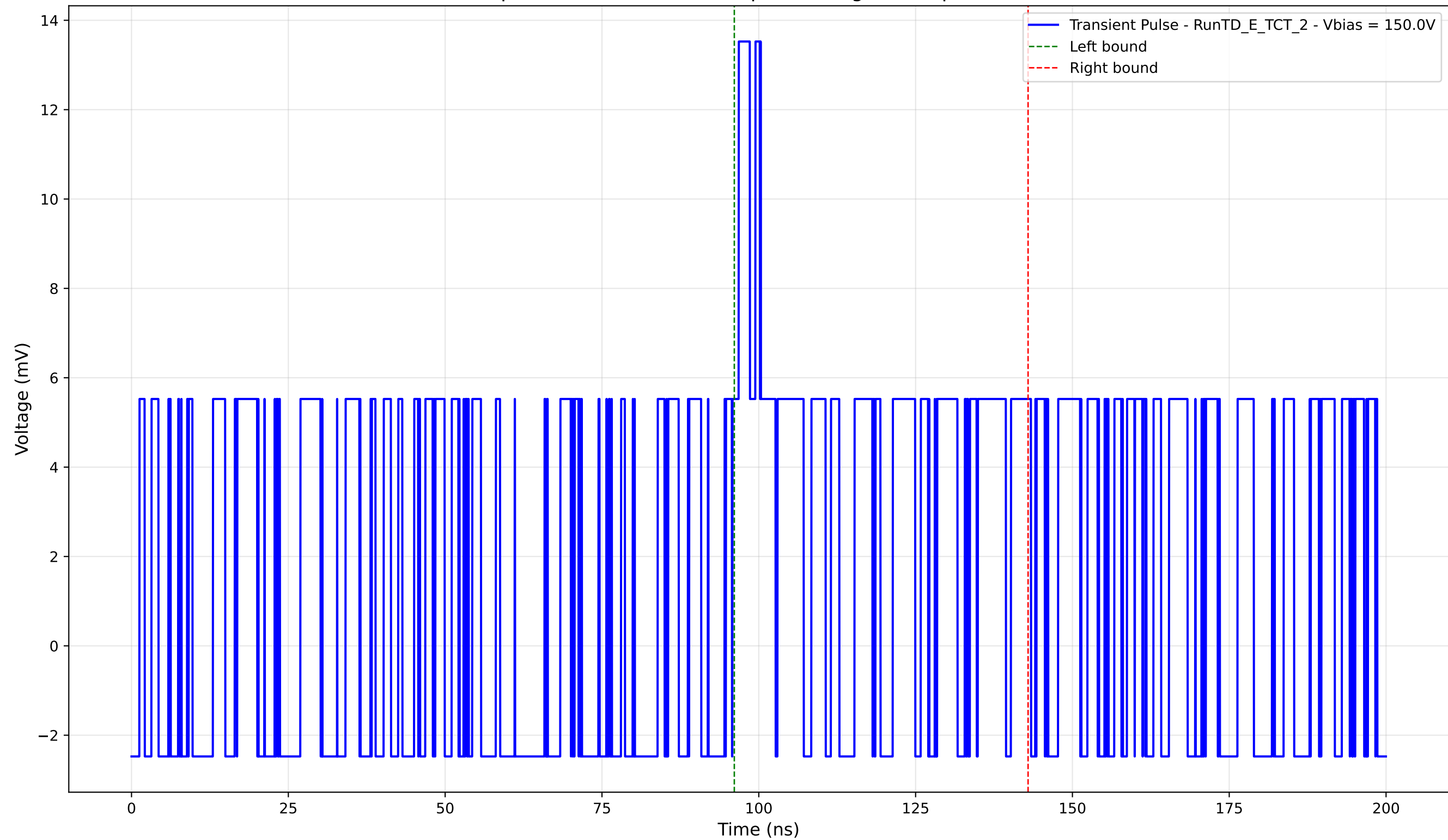
Transient Pulse - Sample: TD - Position: 250.0 \mu\text{m} - Charge: 3.69 pC - Rise Time: 0.00 ns (N/A)
