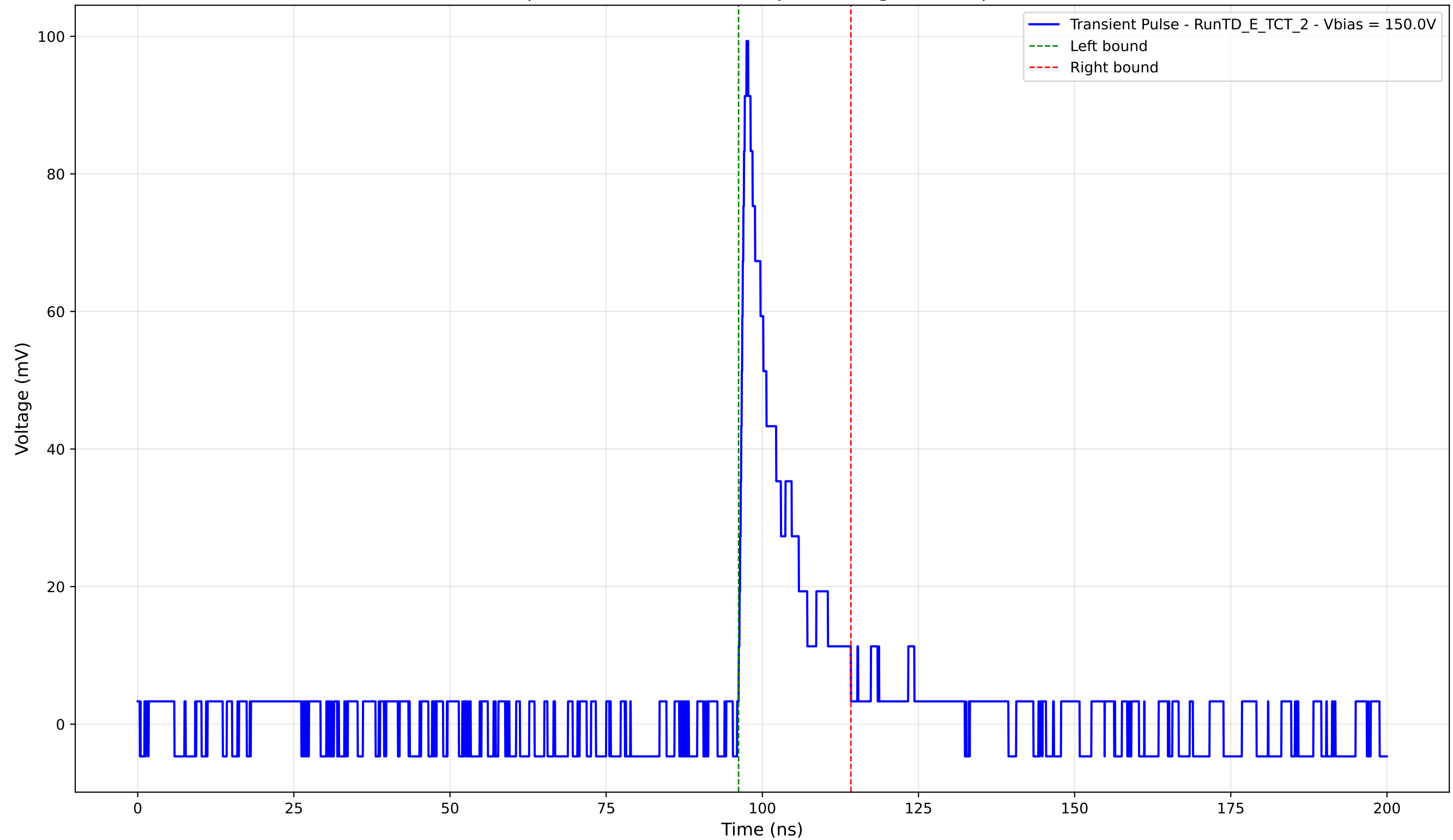
Transient Pulse - Sample: TD - Position: 710.0 \mu\text{m} - Charge: 12.04 pC - Rise Time: 0.96 ns
