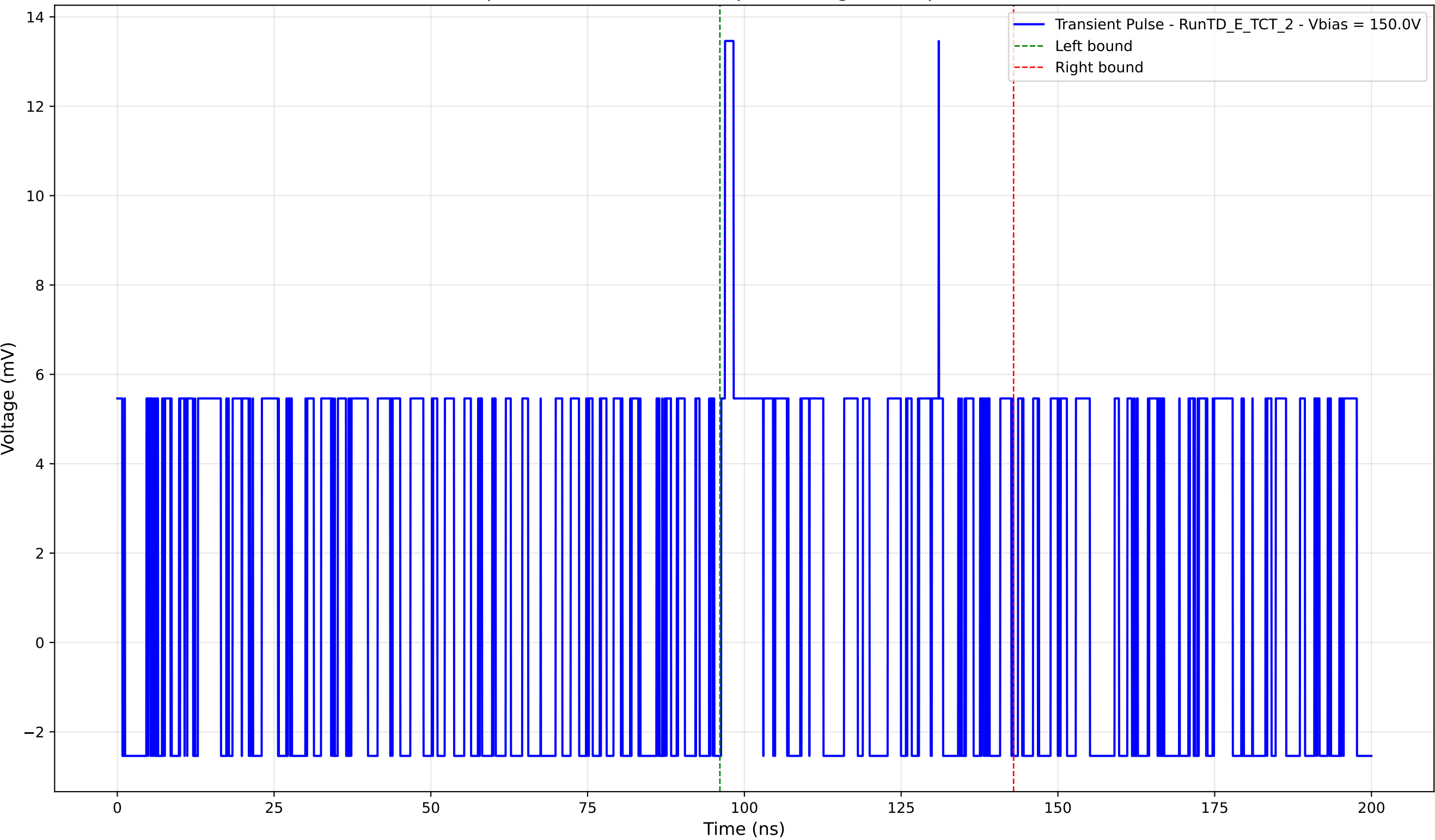
Transient Pulse - - Sample: TD - Position: 180.0 \mu\text{m} - Charge: 2.35 pC - Rise Time: 0.00 ns (N/A)
