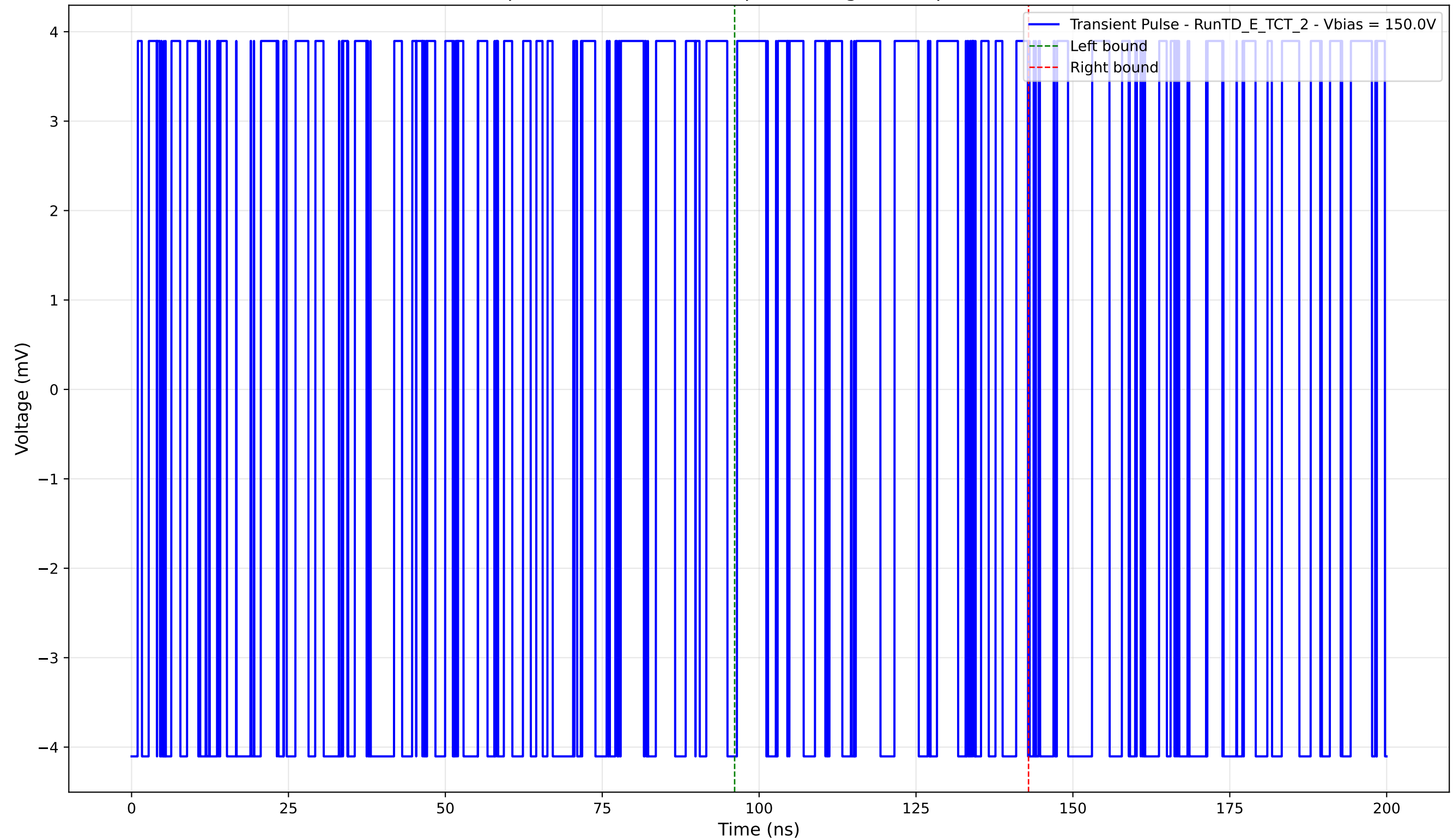
Transient Pulse - Sample: TD - Position: 15.0 \mu\text{m} - Charge: 0.81 pC - Rise Time: 0.00 ns (N/A)
