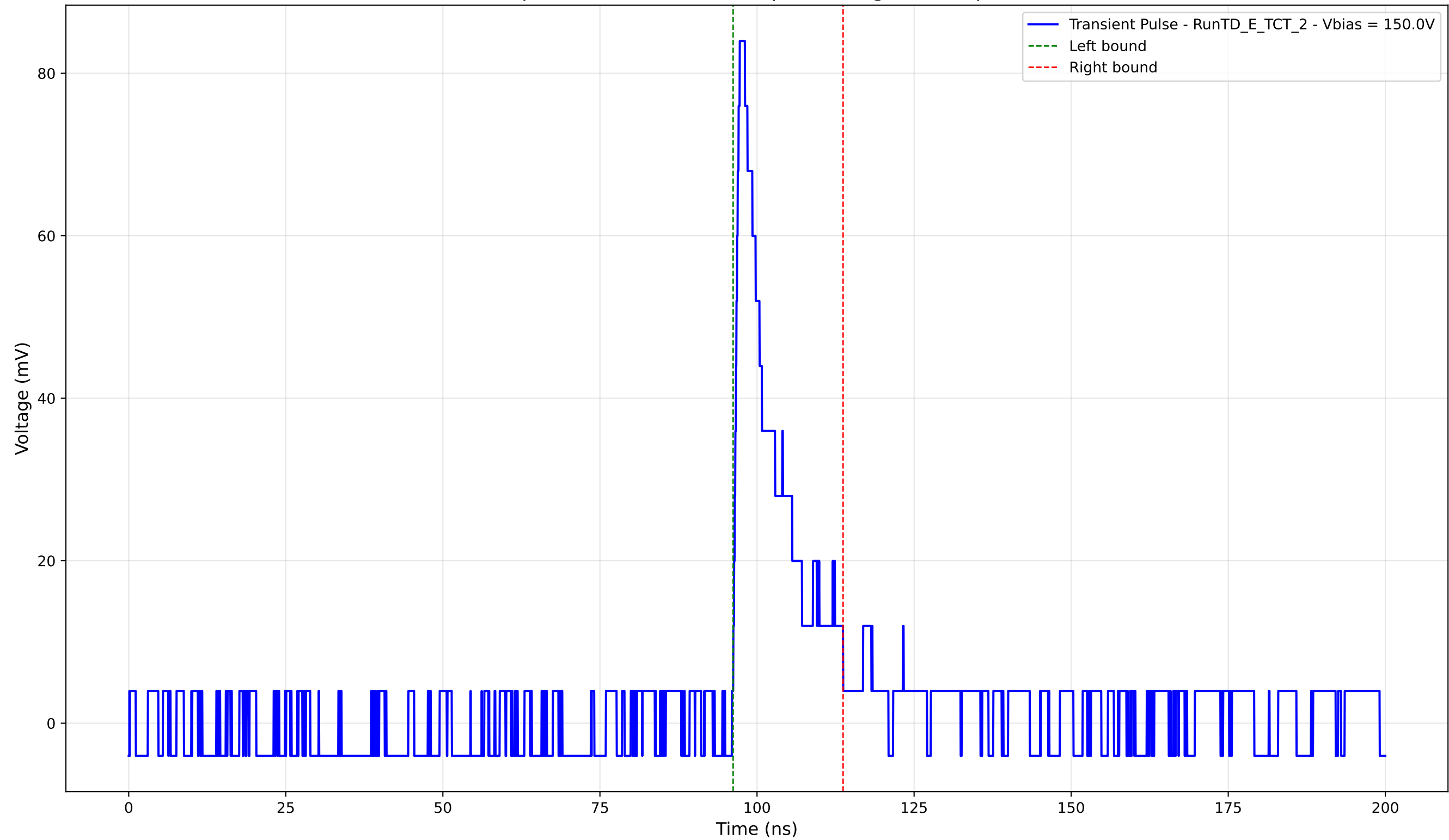
Transient Pulse - Sample: TD - Position: 695.0 \mu\text{m} - Charge: 11.05 pC - Rise Time: 0.85 ns
