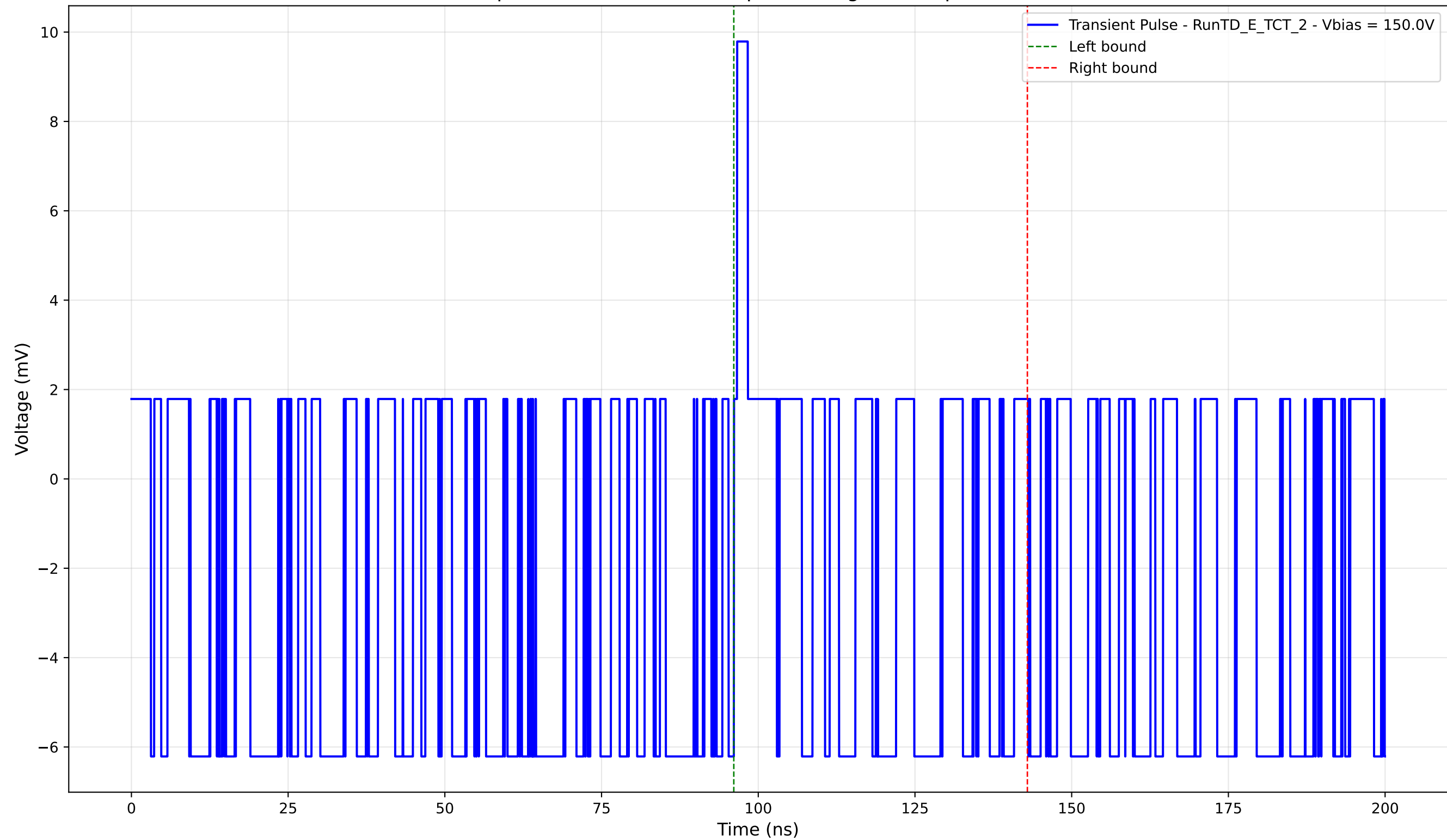
Transient Pulse - Sample: TD - Position: 140.0 \mu\text{m} - Charge: -1.03 pC - Rise Time: 0.00 ns (N/A)
