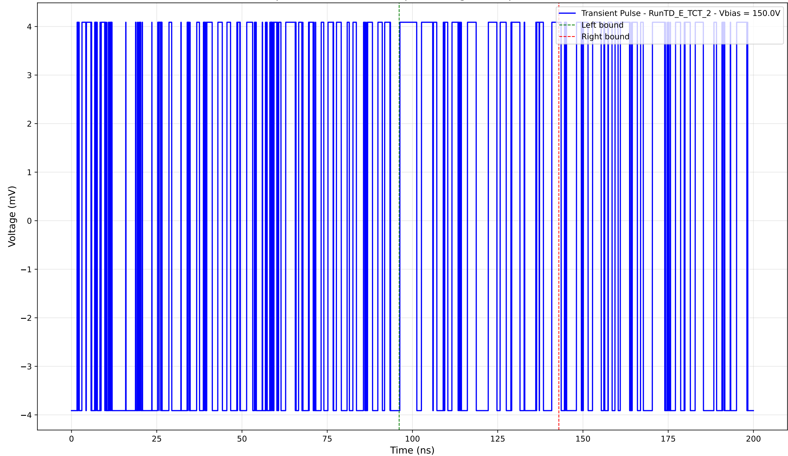
Transient Pulse - Sample: TD - Position: 80.0 \mu\text{m} - Charge: 0.56 pC - Rise Time: 0.00 ns (N/A)
