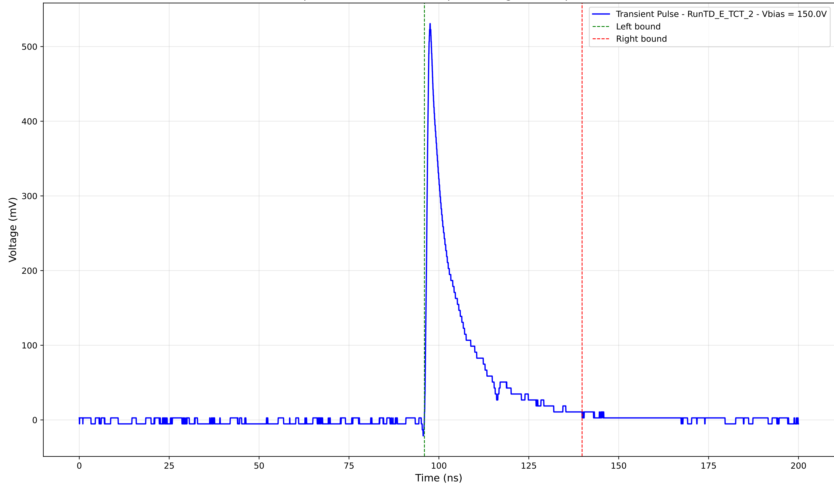
Transient Pulse - Sample: TD - Position: 465.0 \mu\text{m} - Charge: 83.65 pC - Rise Time: 0.98 ns
