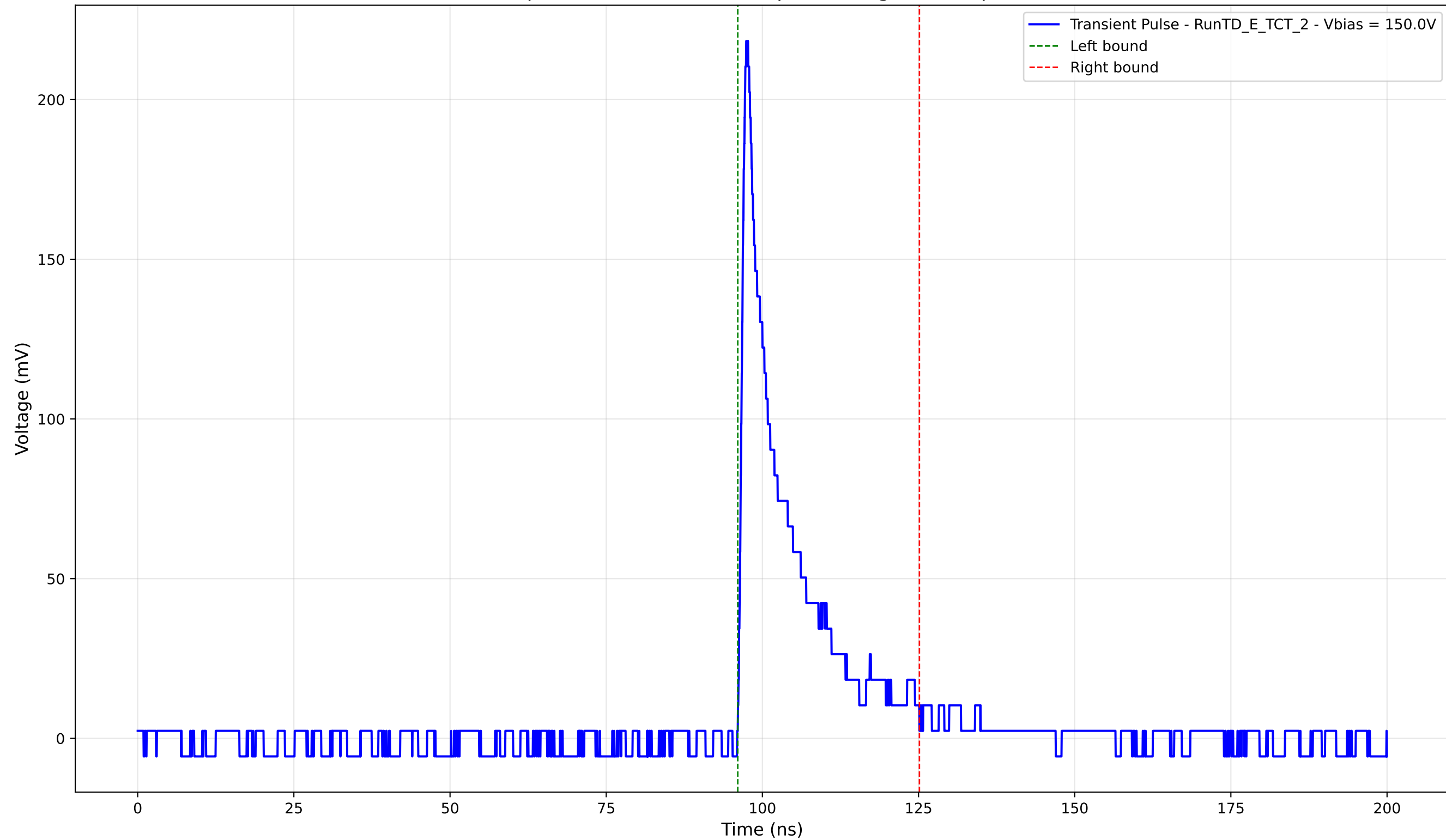
Transient Pulse - Sample: TD - Position: 340.0 \mu\text{m} - Charge: 30.41 pC - Rise Time: 0.97 ns
