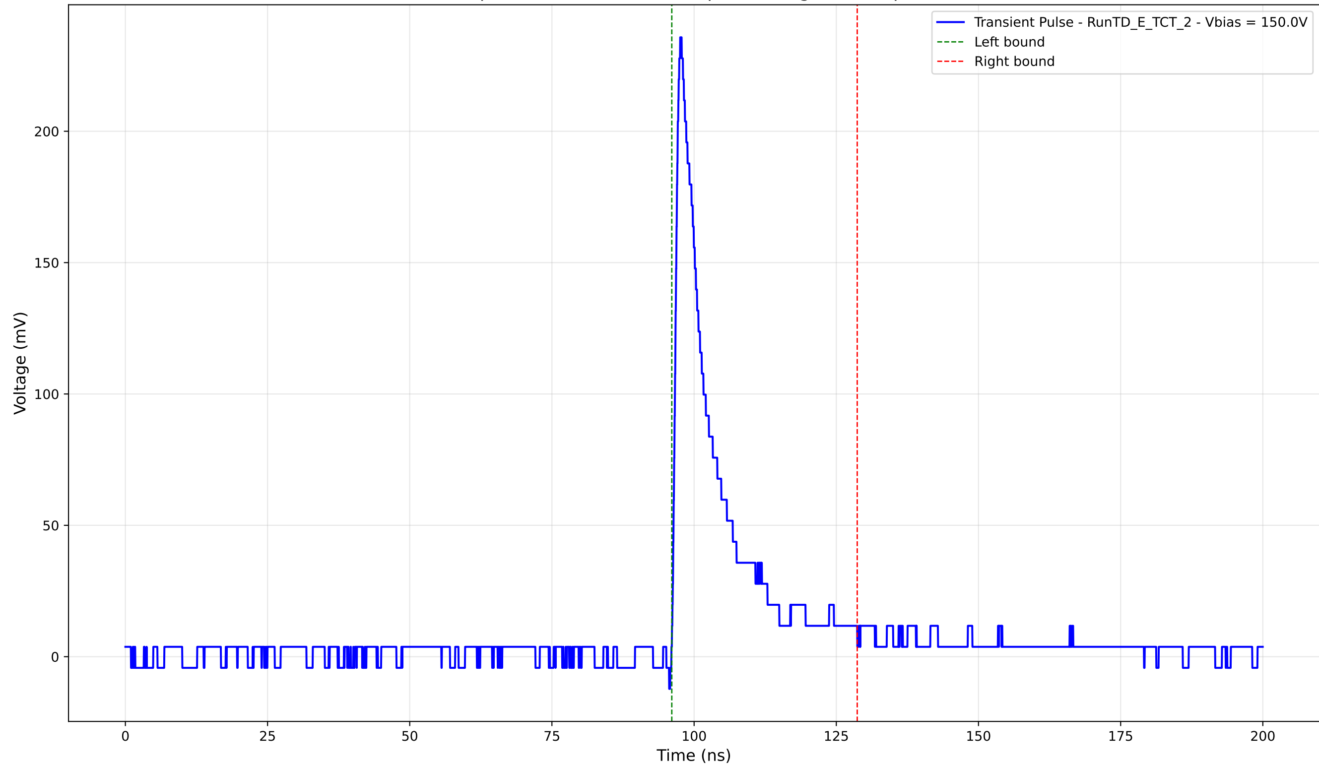
Transient Pulse - Sample: TD - Position: 610.0 \mu\text{m} - Charge: 33.90 pC - Rise Time: 1.05 ns
