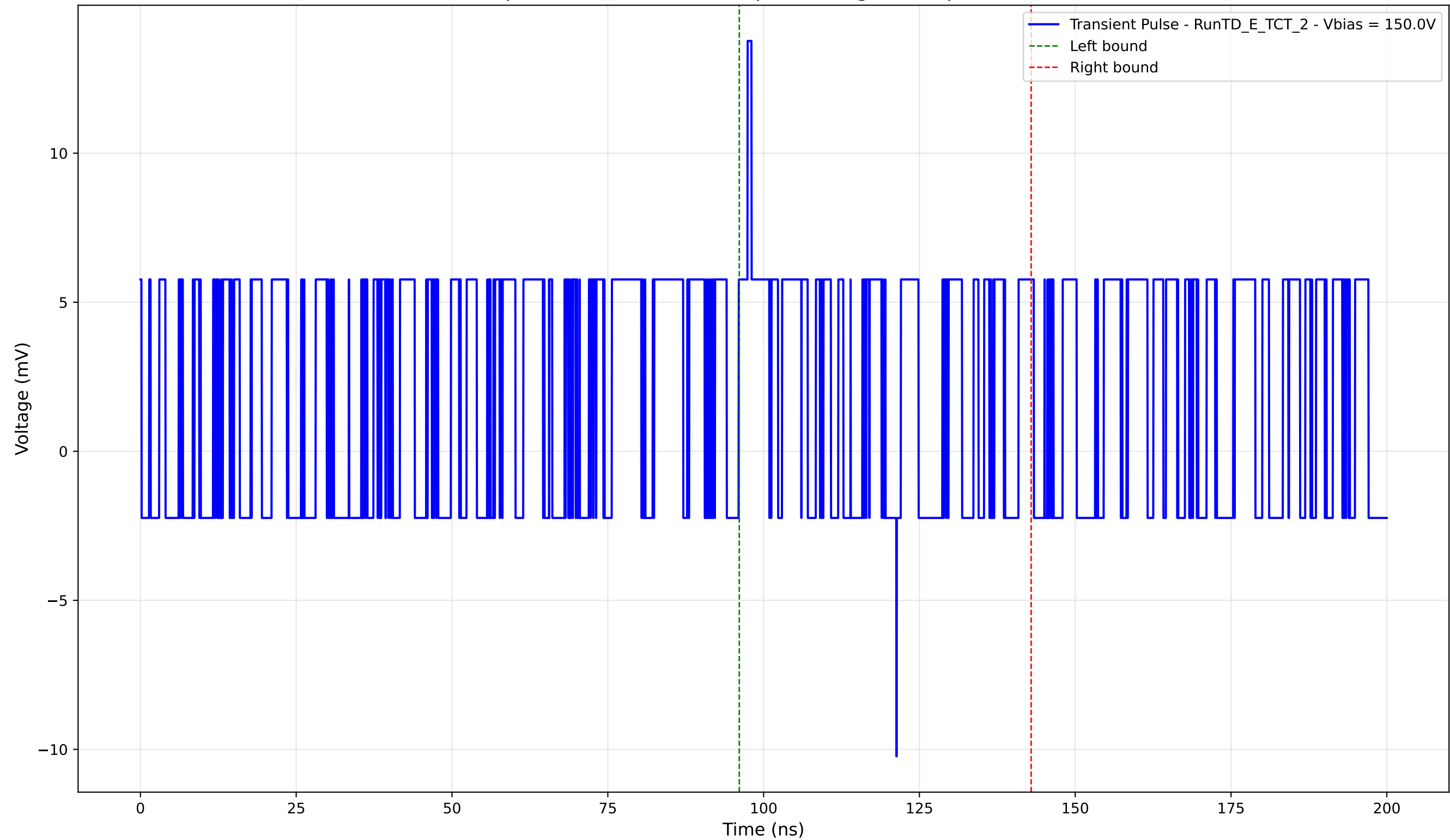
Transient Pulse - Sample: TD - Position: 195.0 \mu\text{m} - Charge: 2.35 pC - Rise Time: 0.00 ns (N/A)
