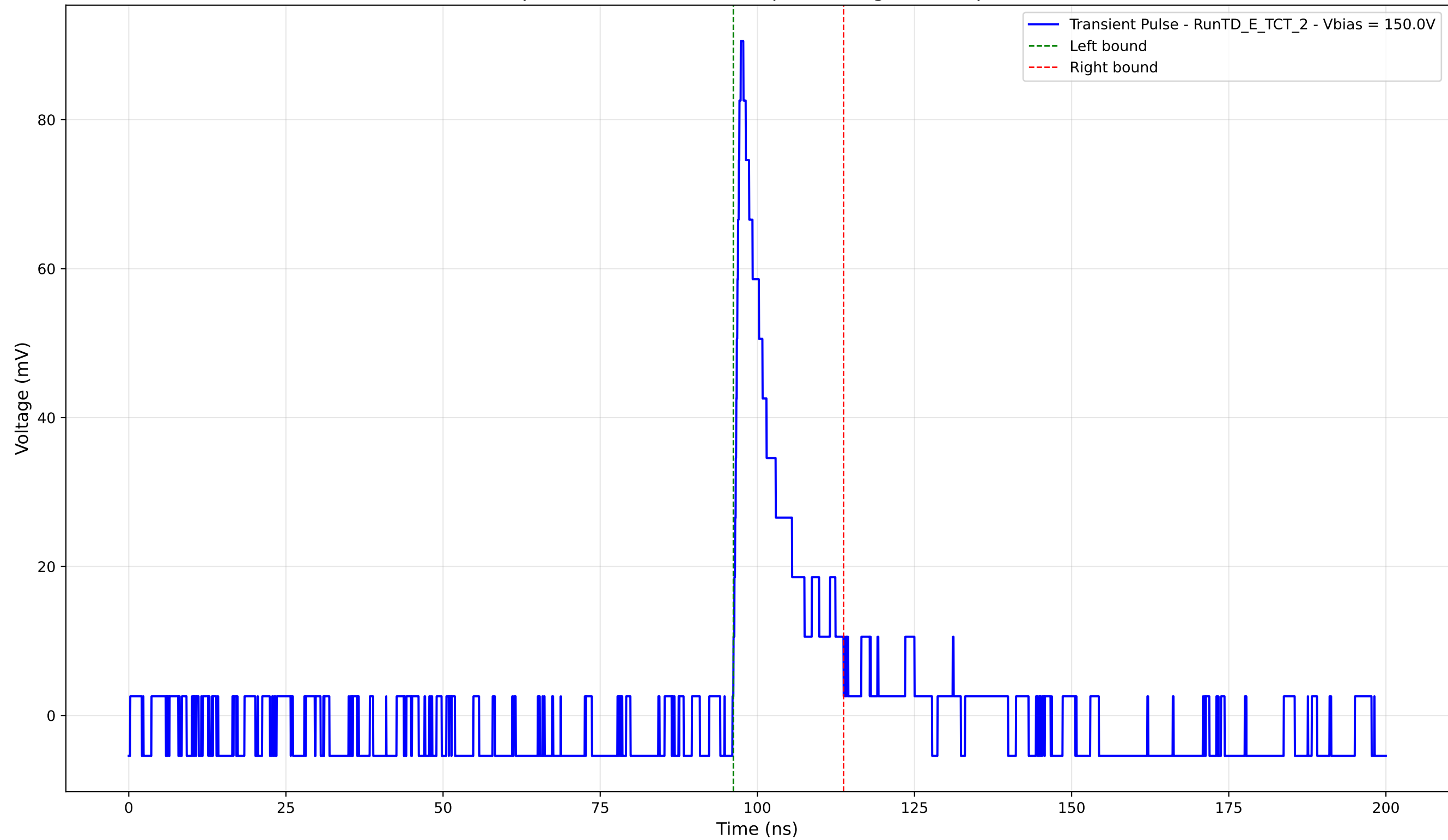
Transient Pulse - Sample: TD - Position: 700.0 \mu\text{m} - Charge: 11.13 pC - Rise Time: 0.94 ns
