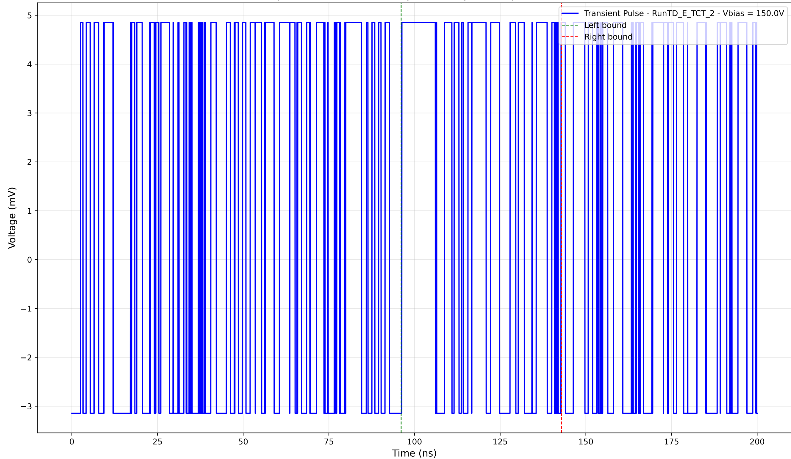
Transient Pulse - Sample: TD - Position: 65.0 \mu\text{m} - Charge: 1.84 pC - Rise Time: 0.00 ns (N/A)
