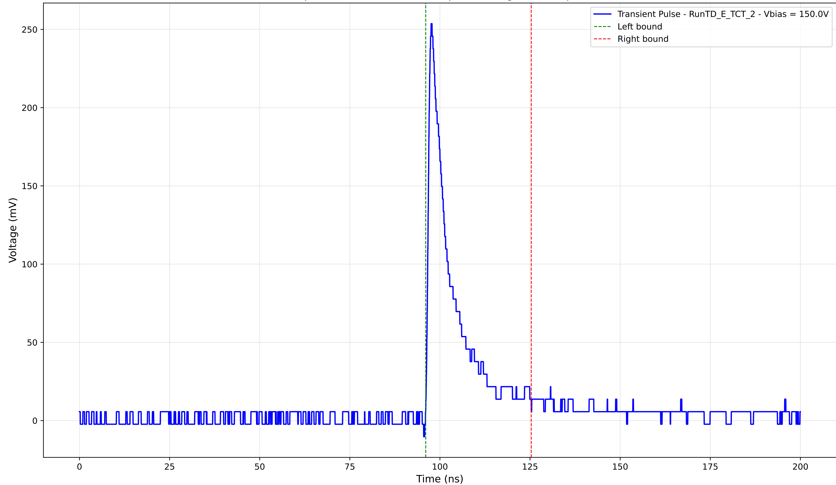
Transient Pulse - Sample: TD - Position: 600.0 \mu\text{m} - Charge: 36.53 pC - Rise Time: 1.01 ns
