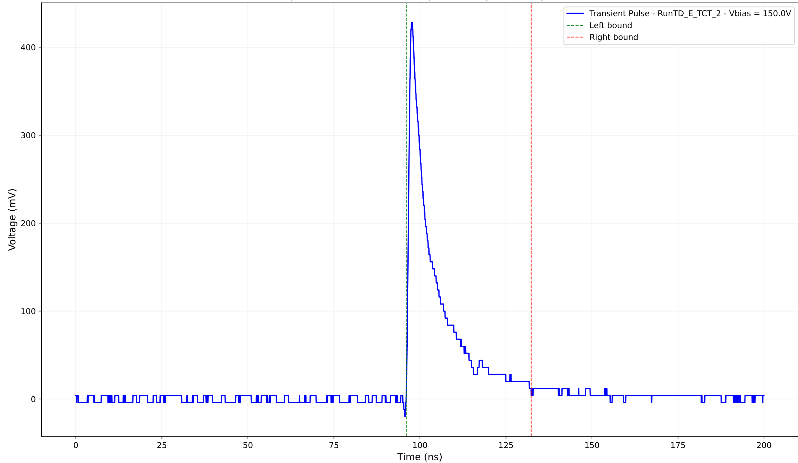
Transient Pulse - Sample: TD - Position: 495.0 \mu\text{m} - Charge: 68.13 pC - Rise Time: 1.00 ns
