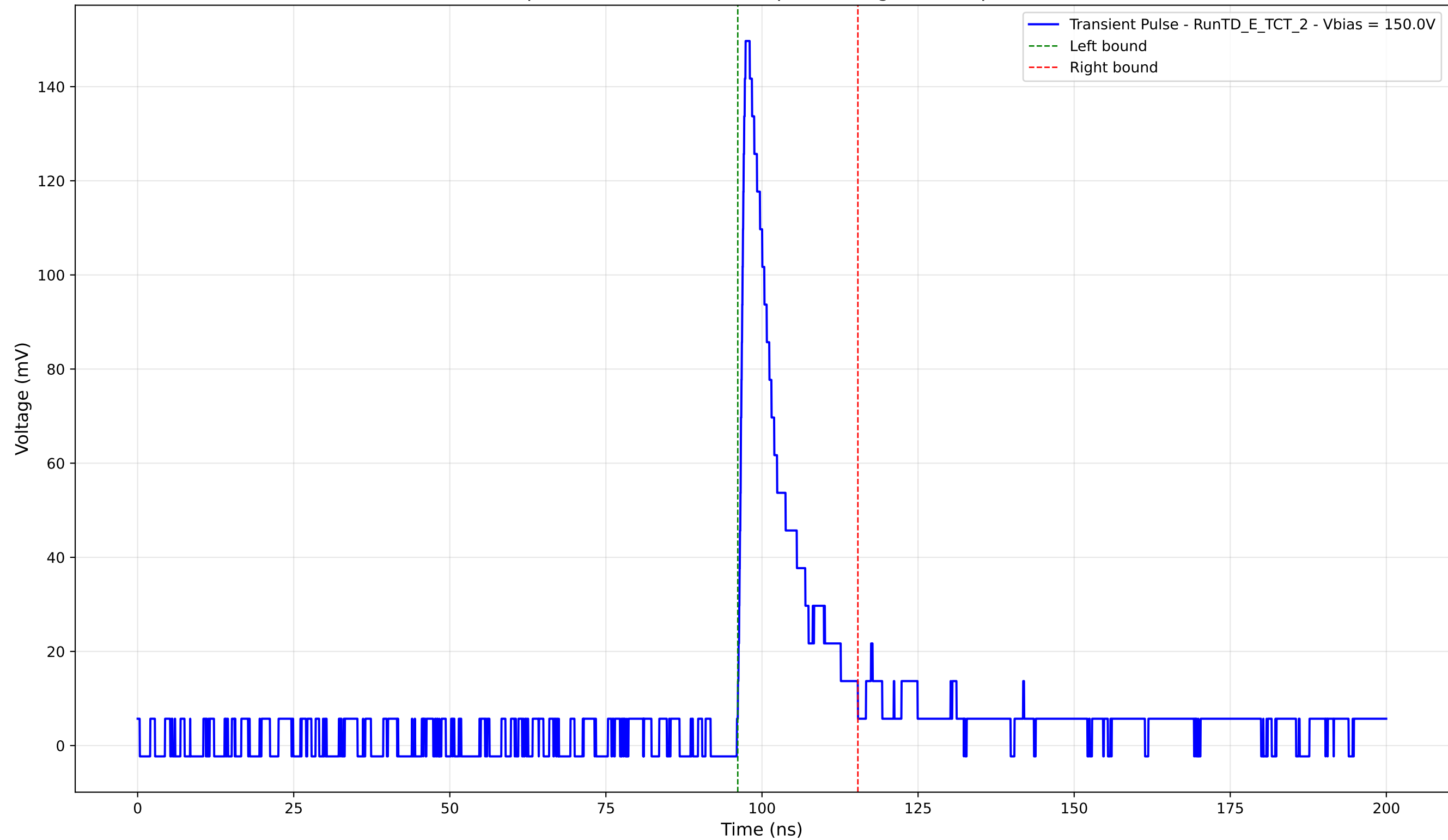
Transient Pulse - Sample: TD - Position: 640.0 \mu\text{m} - Charge: 20.53 pC - Rise Time: 1.02 ns
