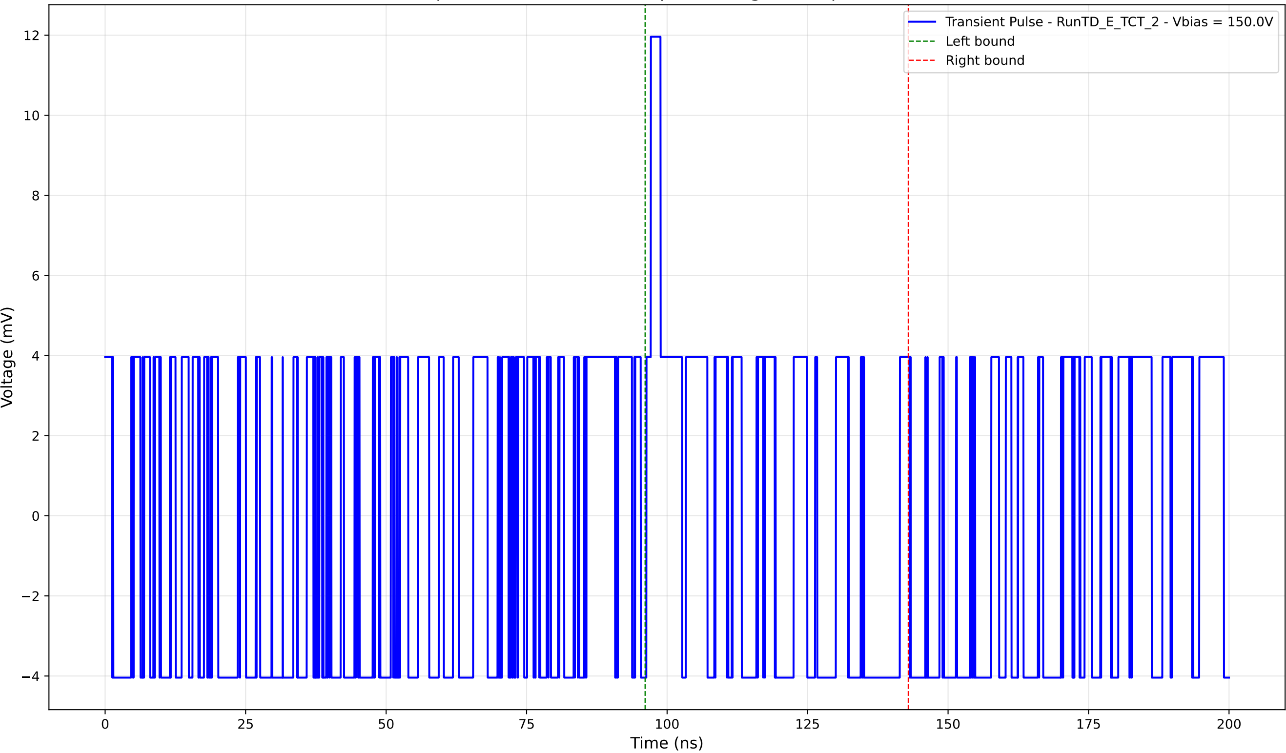
Transient Pulse - Sample: TD - Position: 135.0 \mu\text{m} - Charge: 0.40 pC - Rise Time: 0.00 ns (N/A)
