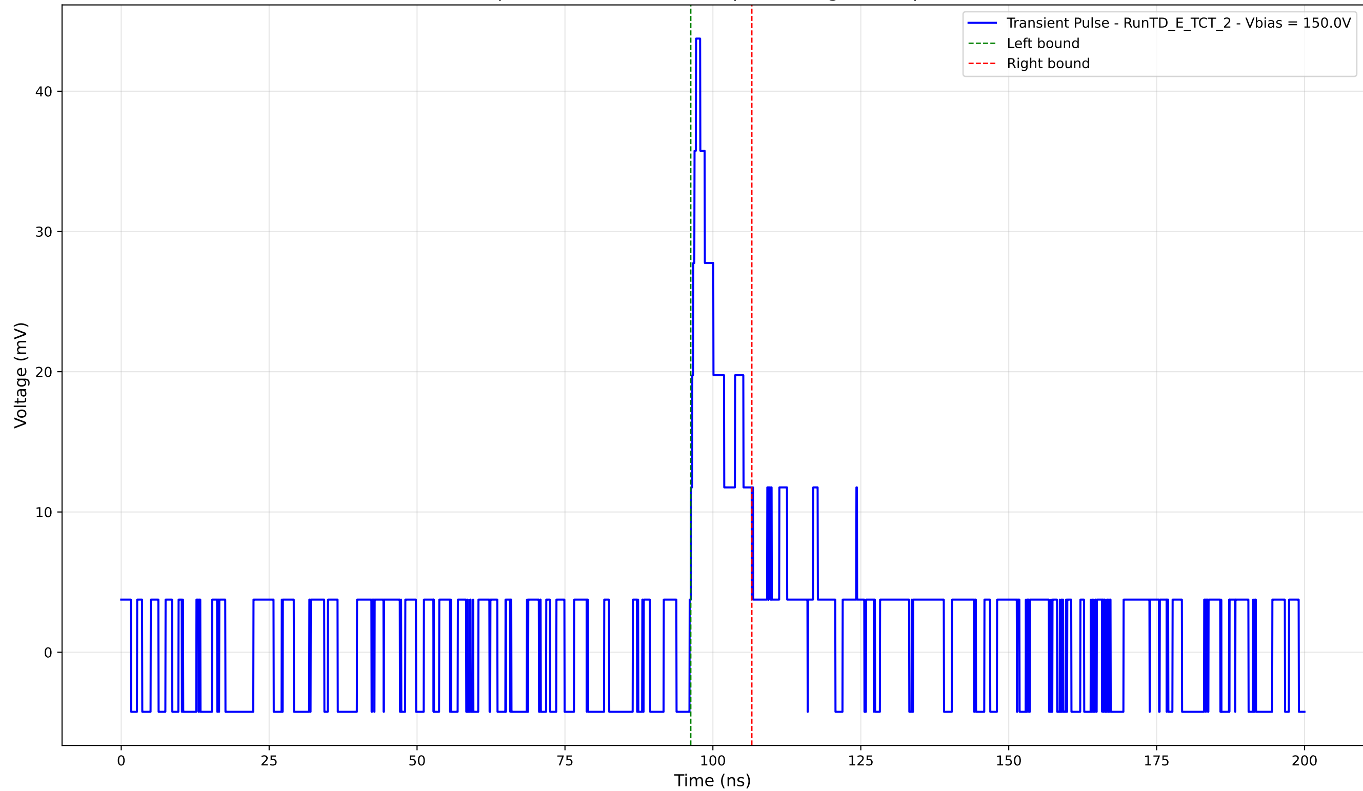
Transient Pulse - Sample: TD - Position: 315.0 \mu\text{m} - Charge: 4.45 pC - Rise Time: 0.88 ns
