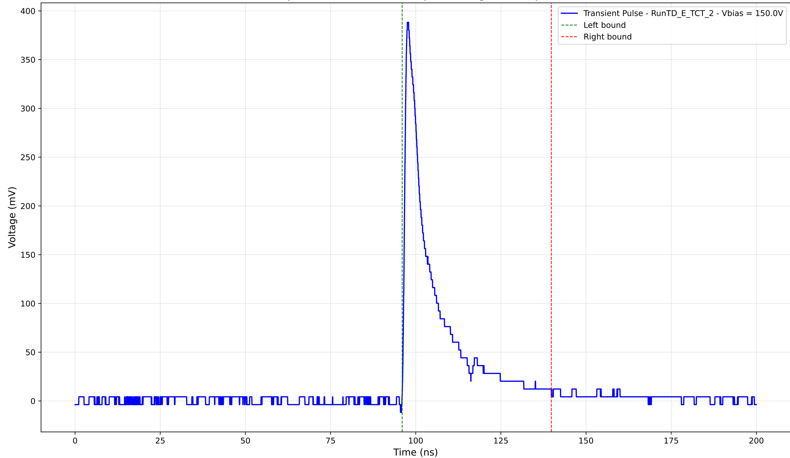
Transient Pulse - Sample: TD - Position: 520.0 \mu\text{m} - Charge: 66.51 pC - Rise Time: 1.01 ns
