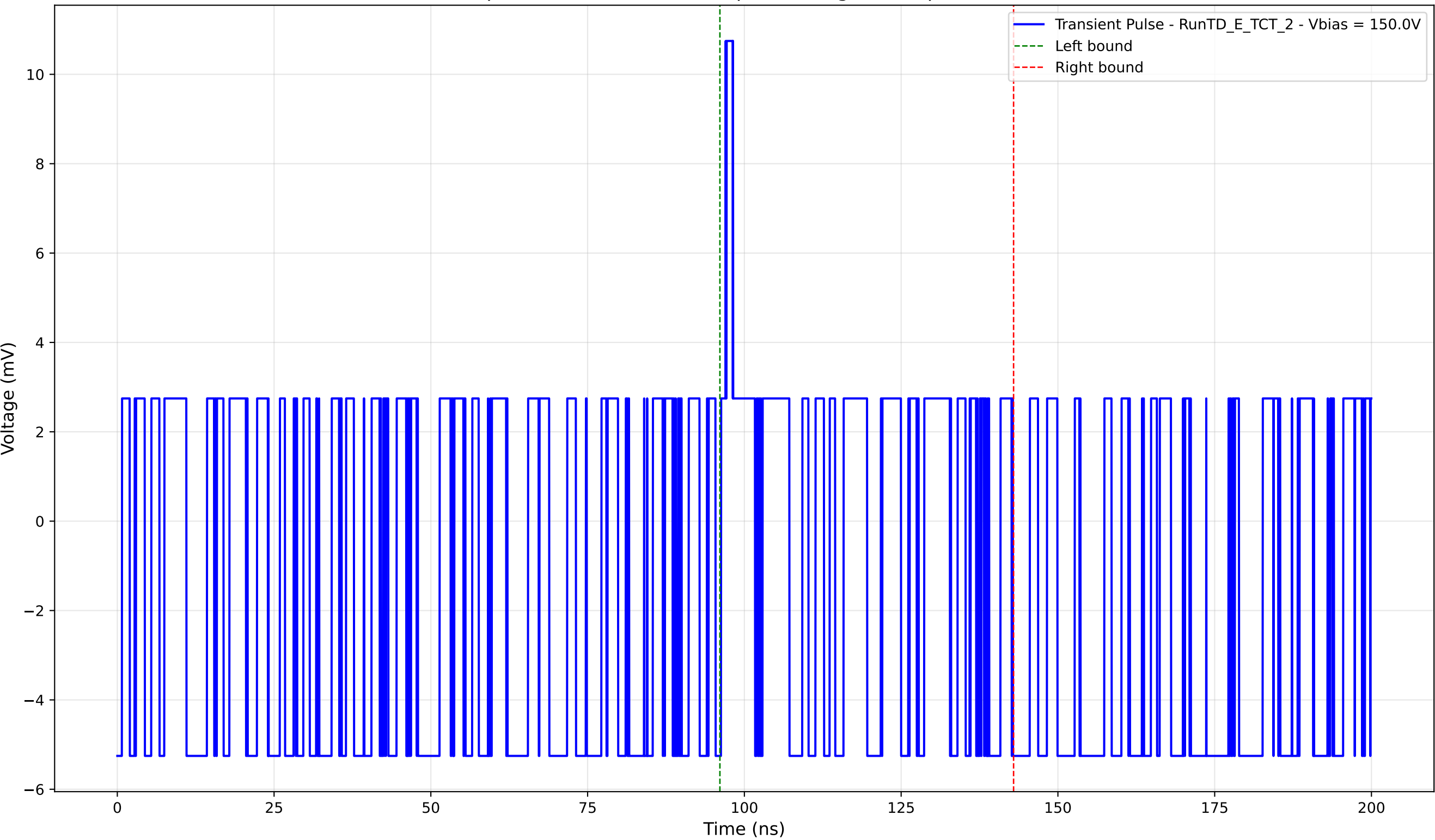
Transient Pulse - - Sample: TD - Position: 150.0 \mu\text{m} - Charge: 0.19 pC - Rise Time: 0.00 ns (N/A)
