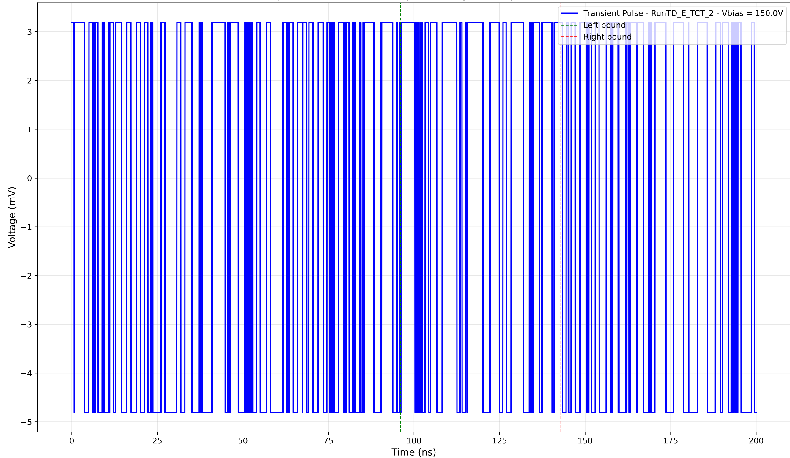
Transient Pulse - Sample: TD - Position: 20.0 \mu\text{m} - Charge: 0.67 pC - Rise Time: 0.00 ns (N/A)
