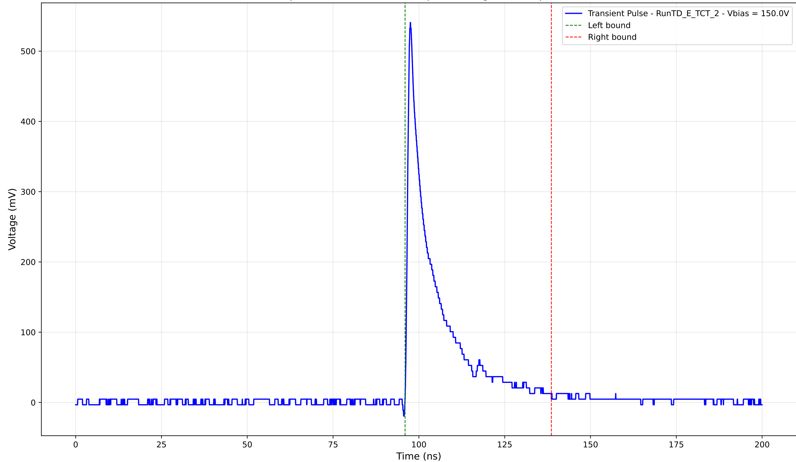
Transient Pulse - Sample: TD - Position: 455.0 \mu\text{m} - Charge: 86.32 pC - Rise Time: 0.98 ns
