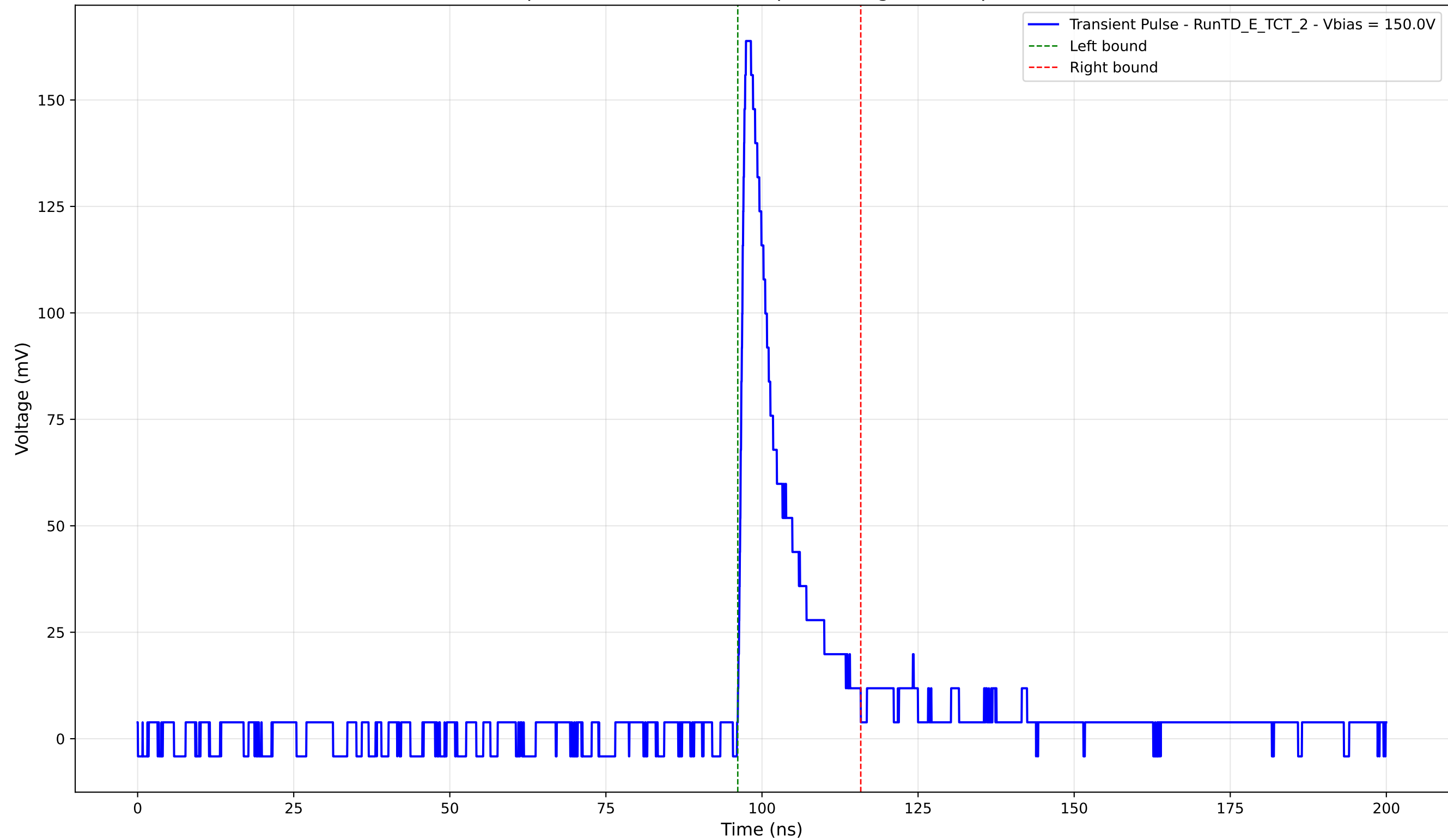
Transient Pulse - Sample: TD - Position: 630.0 \mu\text{m} - Charge: 22.09 pC - Rise Time: 0.97 ns
