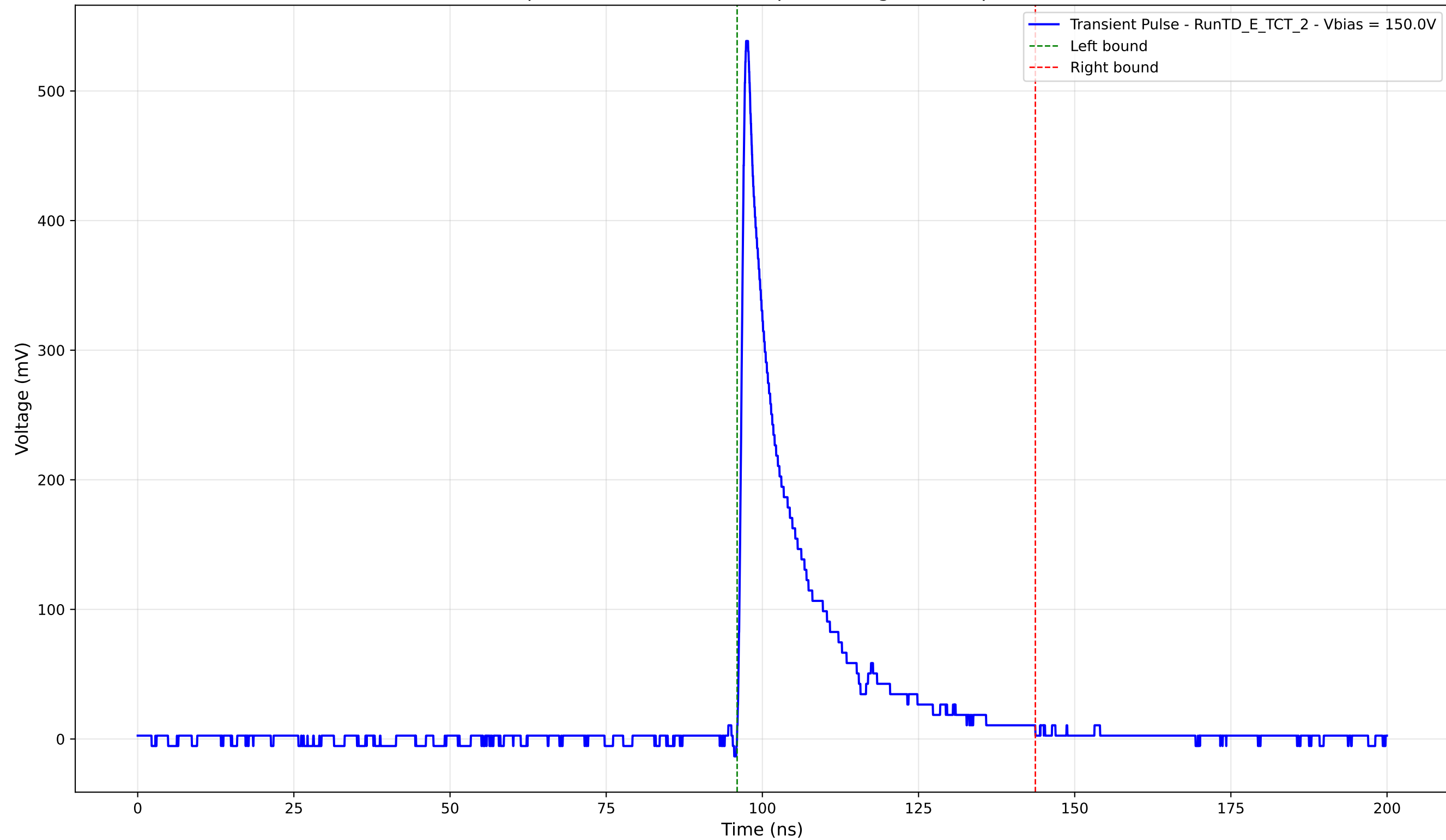
Transient Pulse - Sample: TD - Position: 445.0 \mu\text{m} - Charge: 86.63 pC - Rise Time: 0.96 ns
