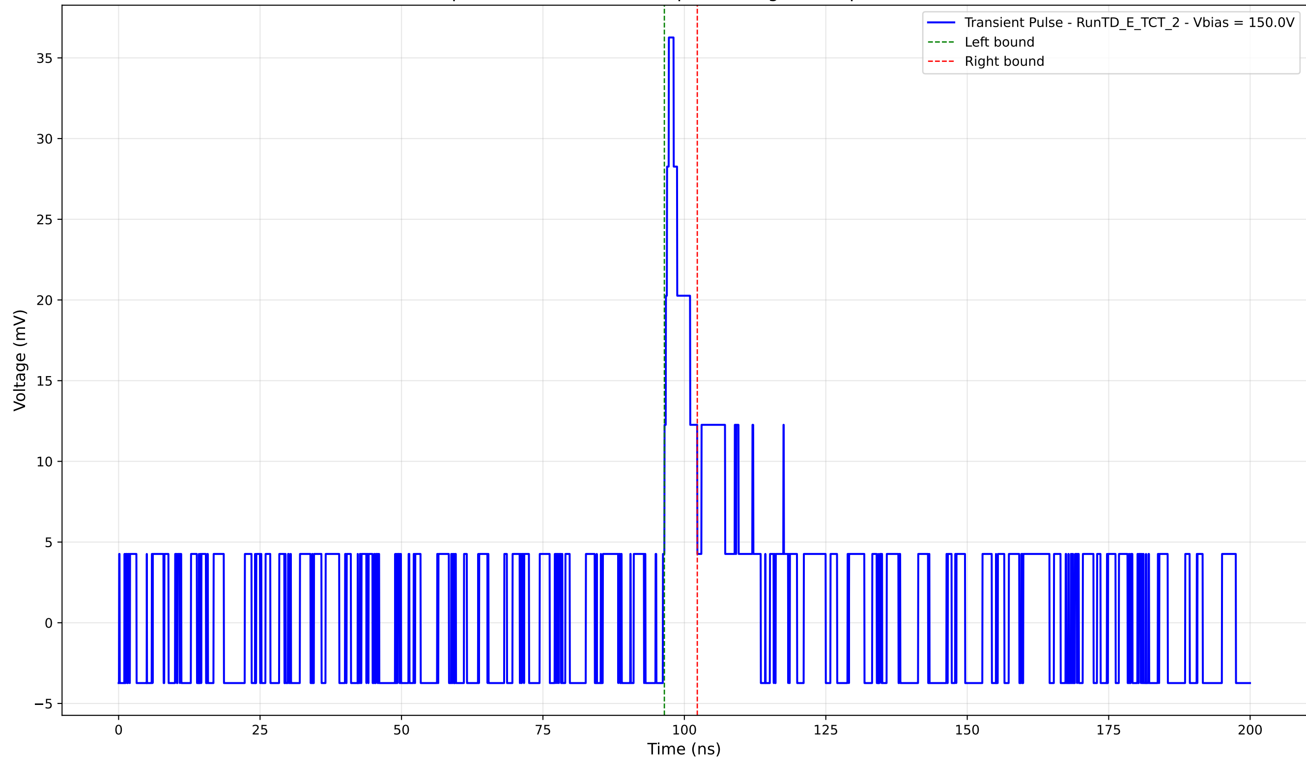
Transient Pulse - Sample: TD - Position: 310.0 \mu\text{m} - Charge: 2.54 pC - Rise Time: 0.00 ns (N/A)
