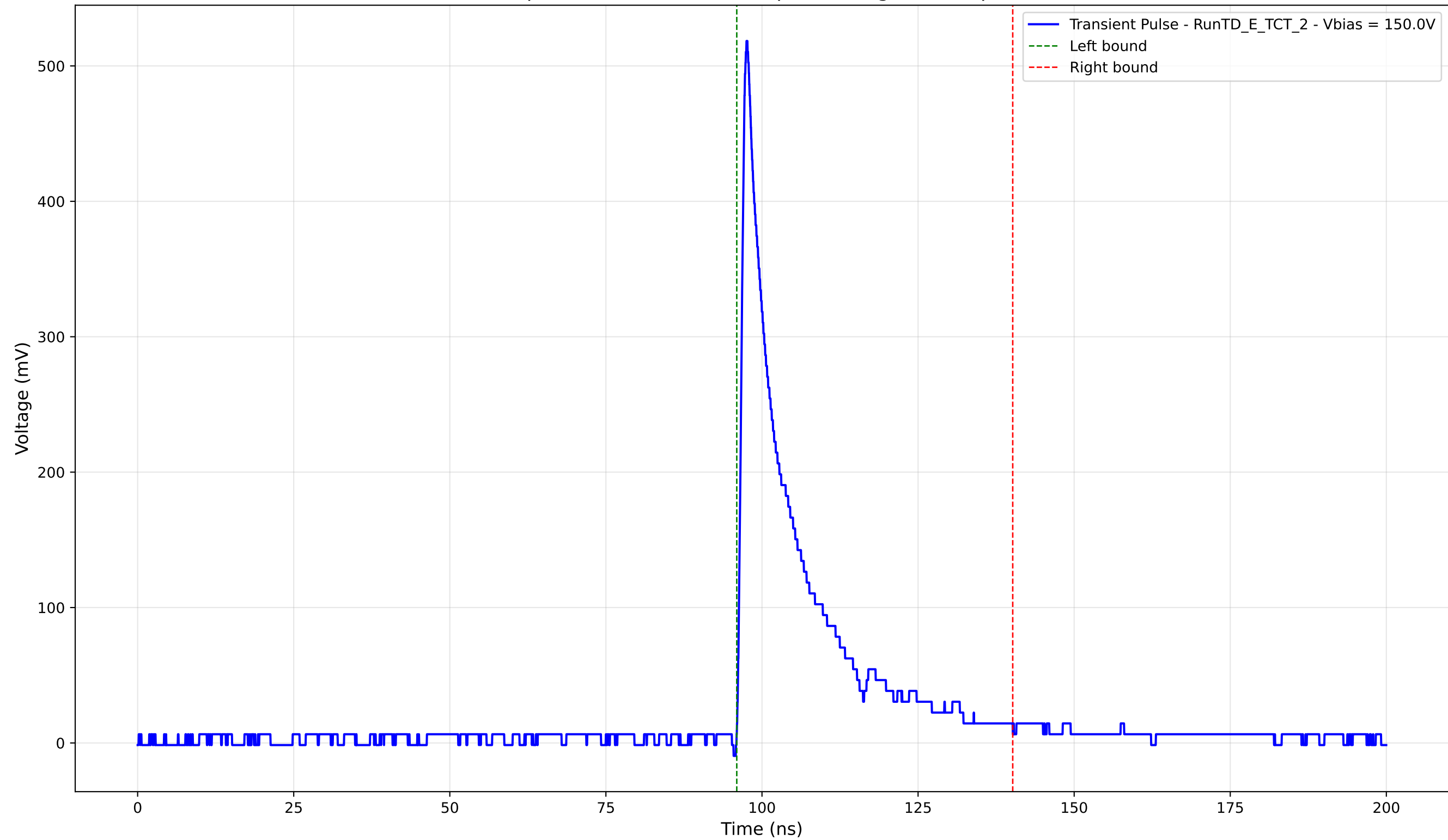
Transient Pulse - Sample: TD - Position: 470.0 \mu\text{m} - Charge: 85.21 pC - Rise Time: 1.00 ns
