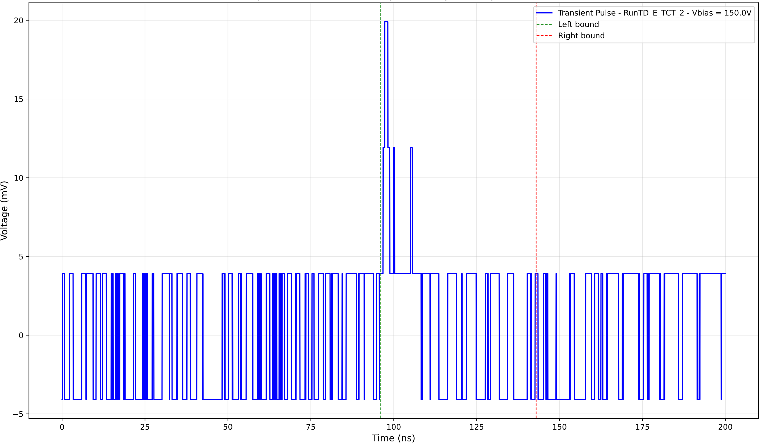
Transient Pulse - Sample: TD - Position: 255.0 \mu\text{m} - Charge: 1.52 pC - Rise Time: 0.00 ns (N/A)
