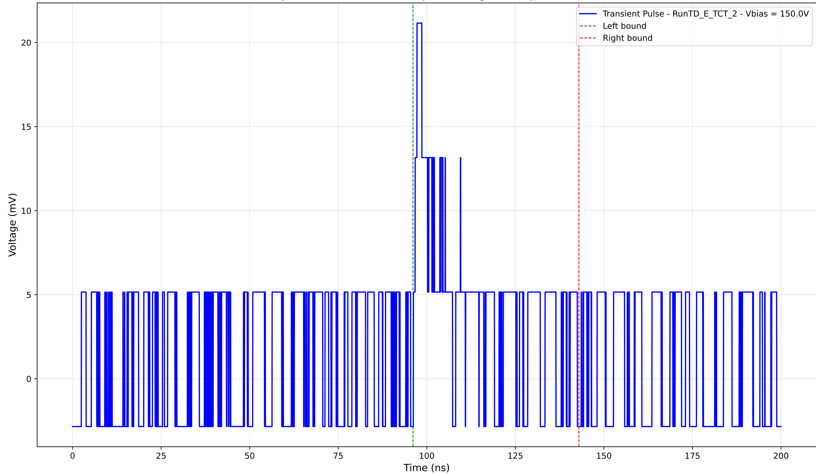
Transient Pulse - Sample: TD - Position: 275.0 \mu\text{m} - Charge: 4.33 pC - Rise Time: 0.00 ns (N/A)
