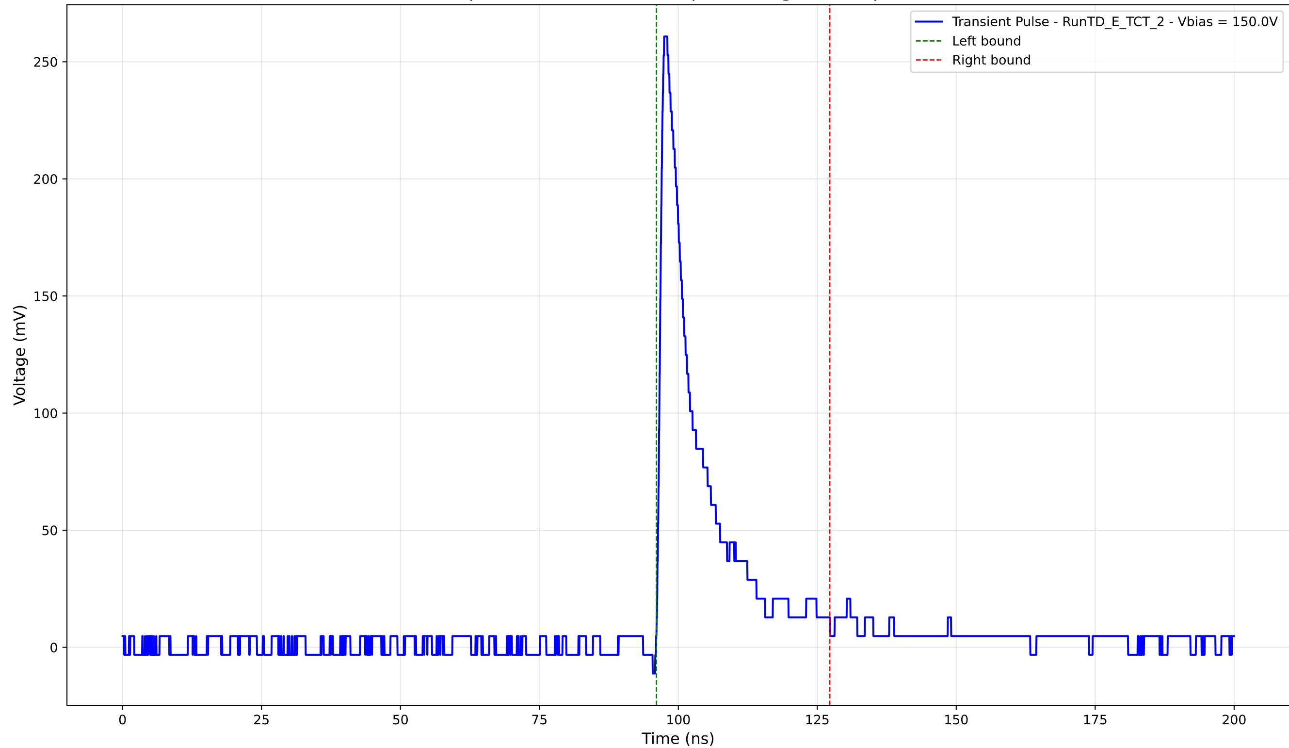
Transient Pulse - Sample: TD - Position: 585.0 \mu\text{m} - Charge: 38.82 pC - Rise Time: 0.99 ns
