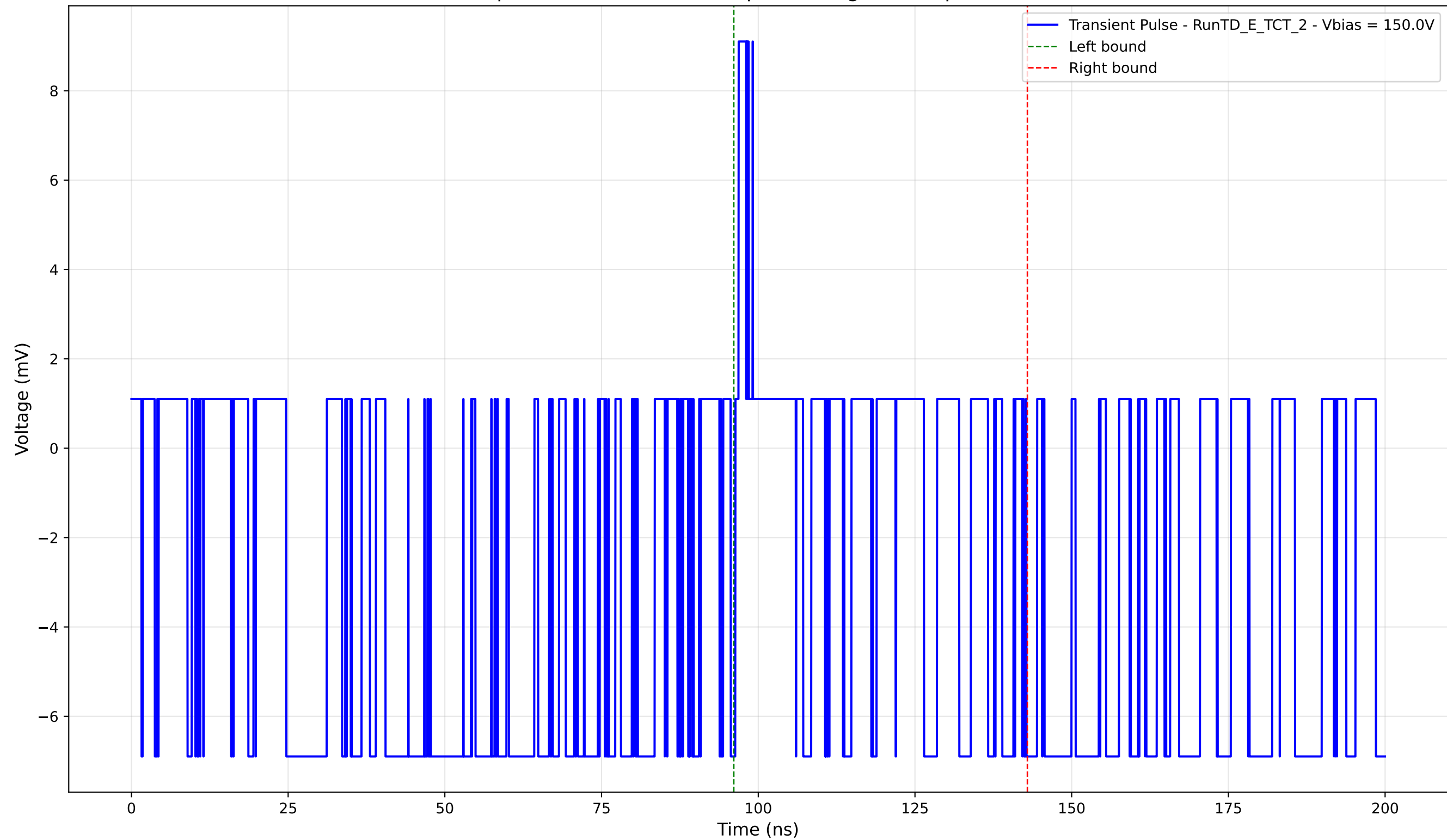
Transient Pulse - Sample: TD - Position: 235.0 \mu\text{m} - Charge: -0.58 pC - Rise Time: 0.00 ns (N/A)
