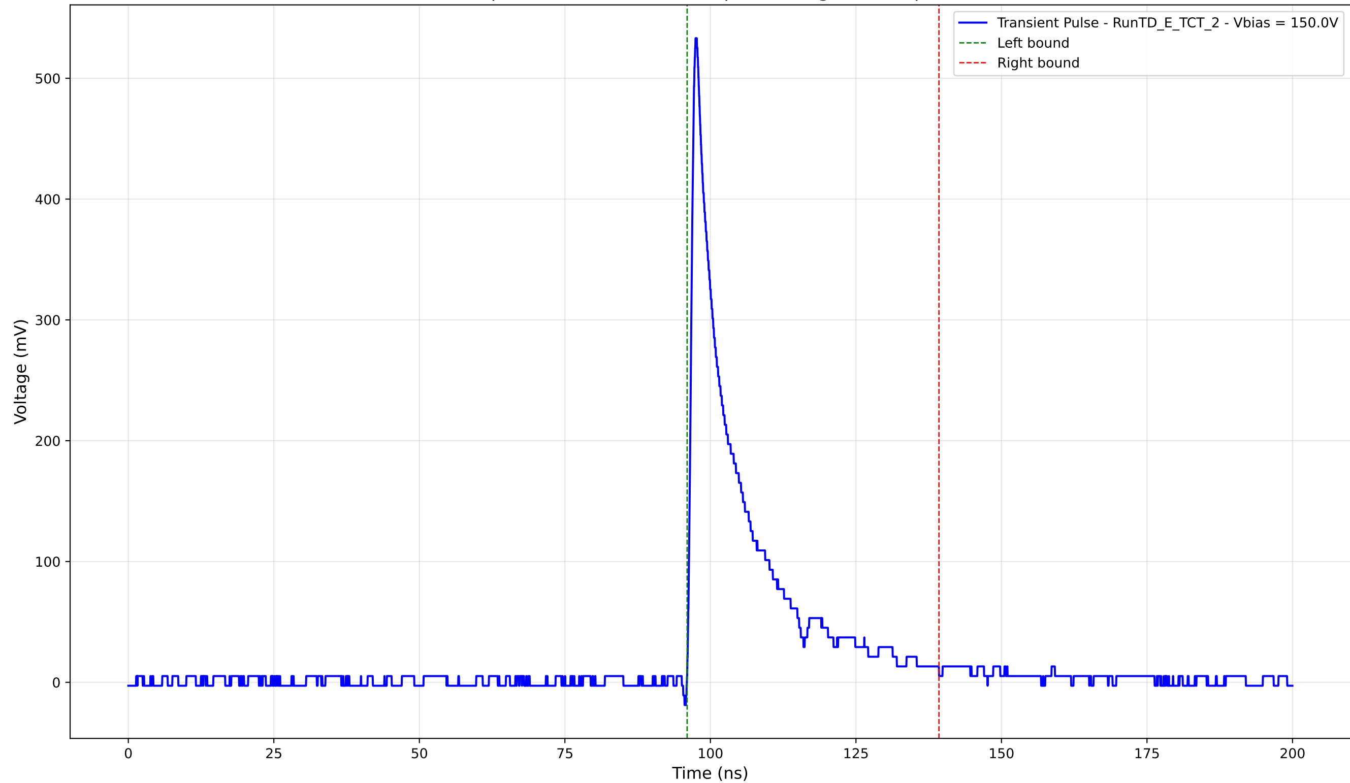
Transient Pulse - Sample: TD - Position: 450.0 \mu\text{m} - Charge: 86.74 pC - Rise Time: 0.97 ns
