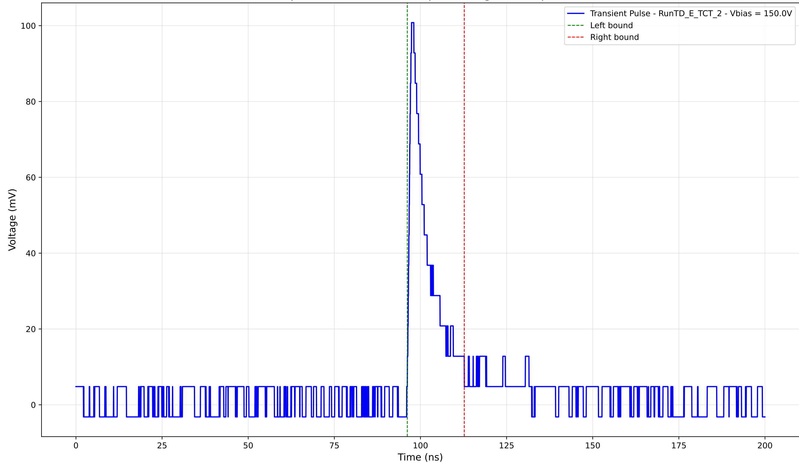
Transient Pulse - Sample: TD - Position: 655.0 \mu\text{m} - Charge: 12.35 pC - Rise Time: 1.03 ns
