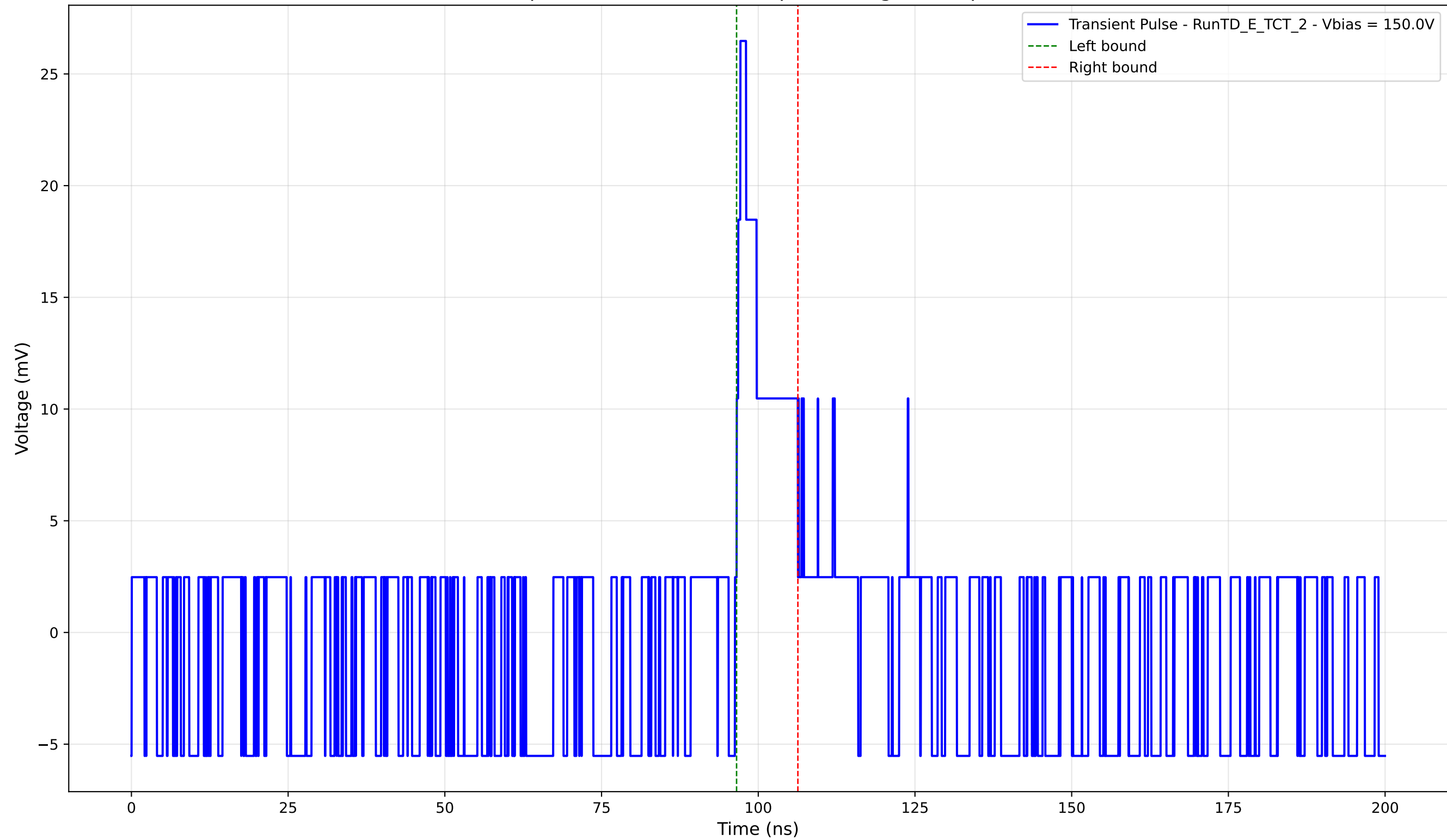
Transient Pulse - Sample: TD - Position: 305.0 \mu\text{m} - Charge: 2.66 pC - Rise Time: 0.60 ns
