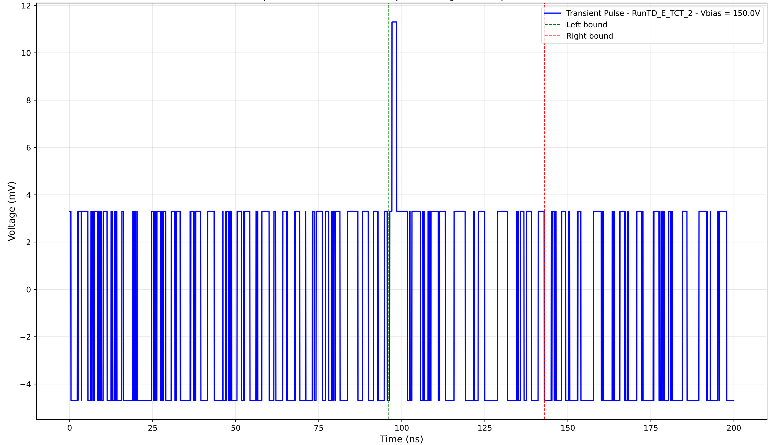
Transient Pulse - Sample: TD - Position: 115.0 \mu\text{m} - Charge: -0.03 pC - Rise Time: 0.00 ns (N/A)
