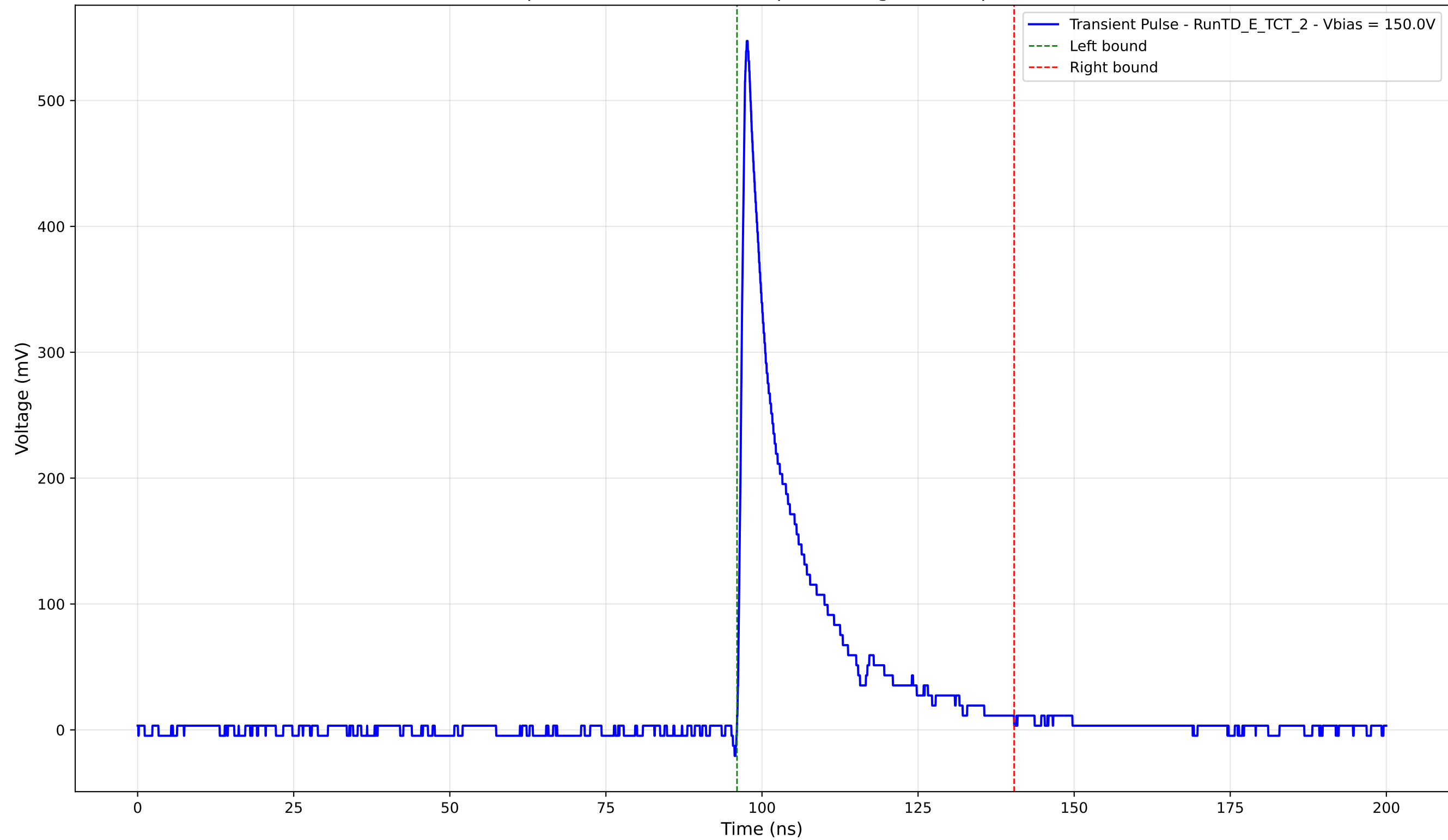
Transient Pulse - Sample: TD - Position: 410.0 \mu\text{m} - Charge: 89.00 pC - Rise Time: 1.01 ns
