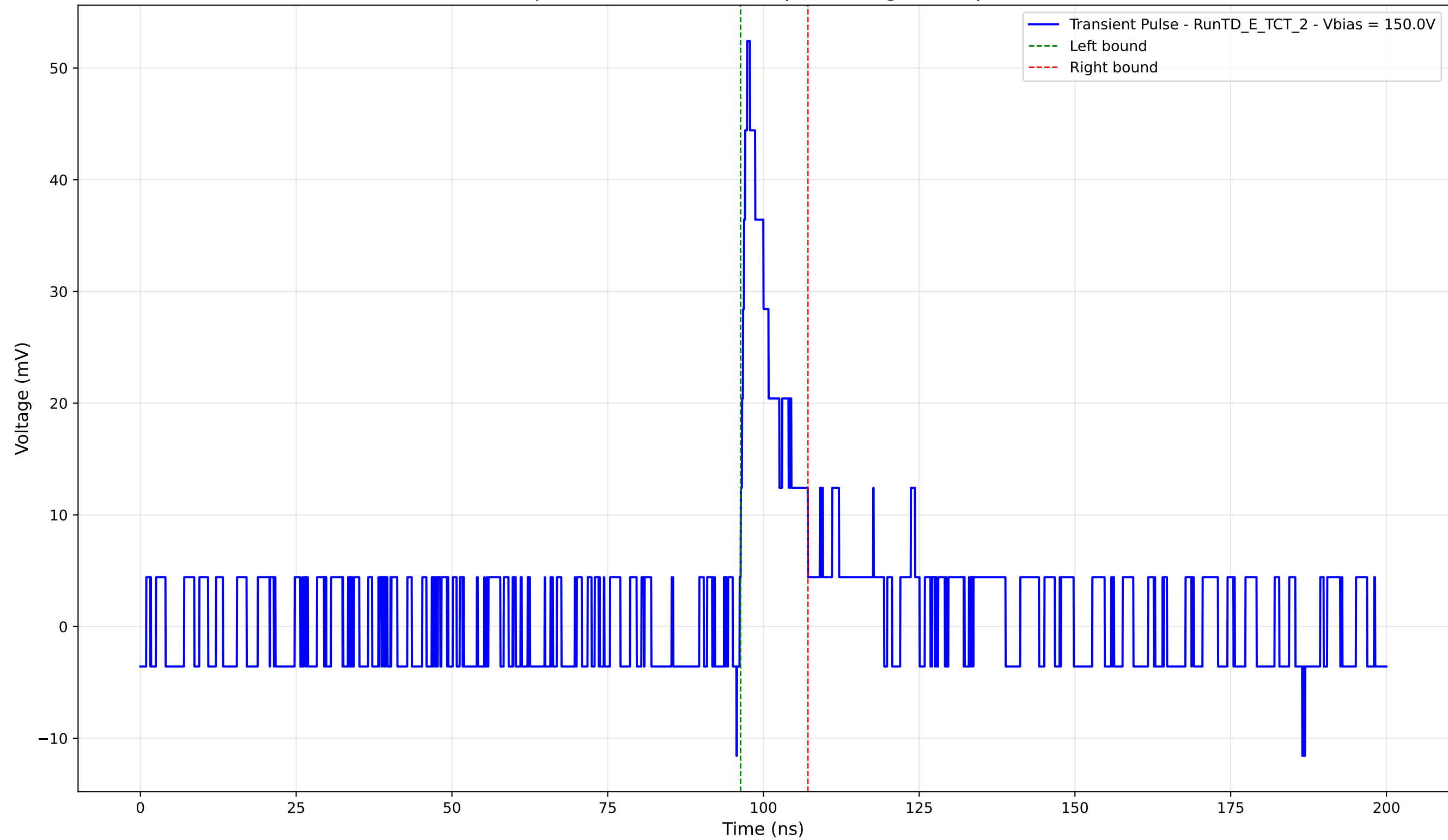
Transient Pulse - Sample: TD - Position: 675.0 \mu\text{m} - Charge: 5.34 pC - Rise Time: 1.04 ns
