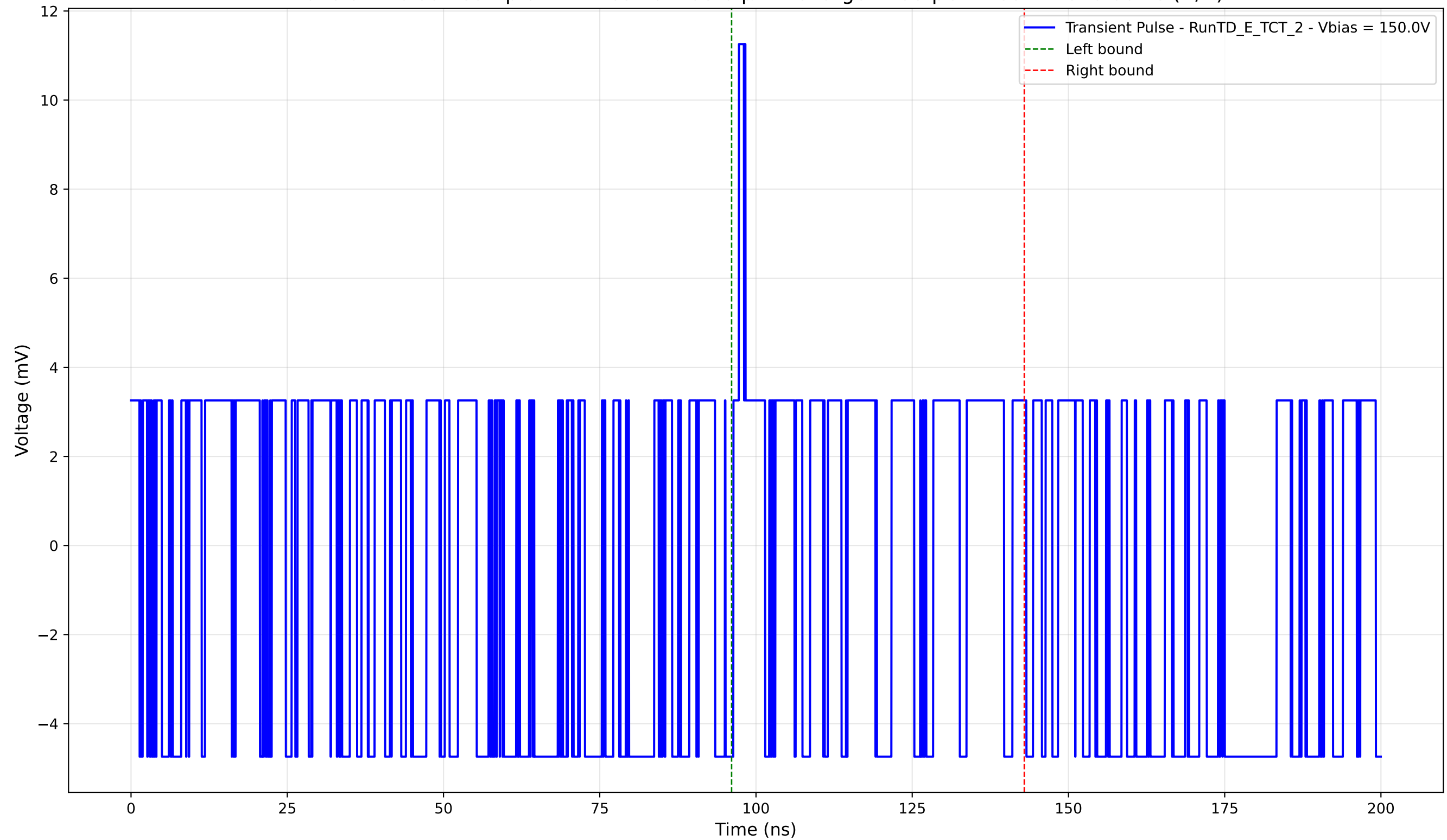
Transient Pulse - Sample: TD - Position: 95.0 \mu\text{m} - Charge: 1.33 pC - Rise Time: 0.00 ns (N/A)
