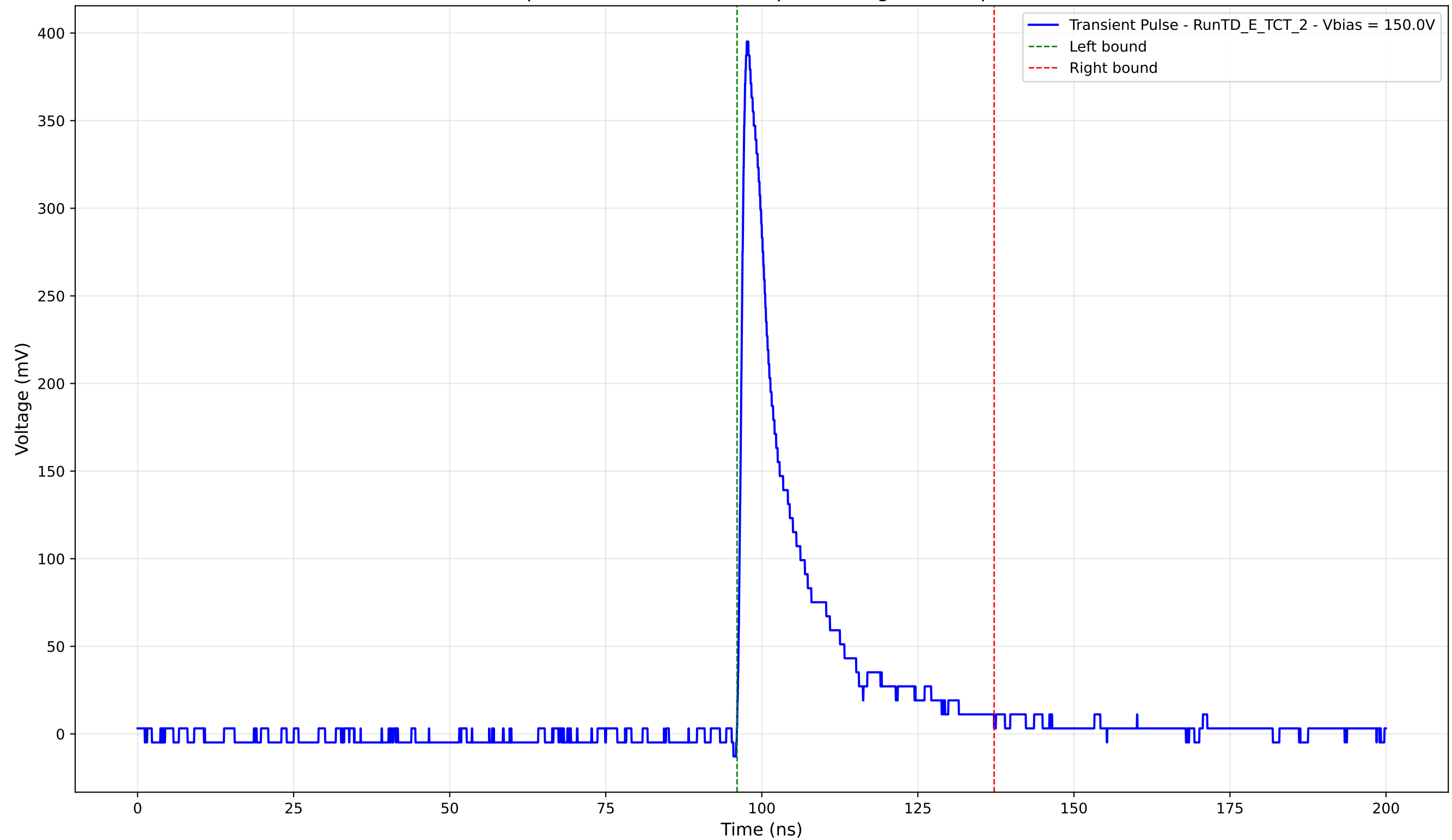
Transient Pulse - Sample: TD - Position: 525.0 \mu\text{m} - Charge: 65.10 pC - Rise Time: 1.05 ns
