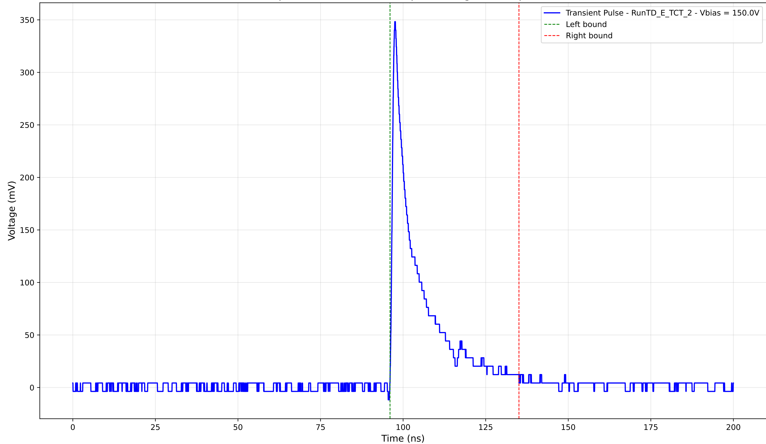
Transient Pulse - Sample: TD - Position: 350.0 \mu\text{m} - Charge: 54.62 pC - Rise Time: 0.98 ns
