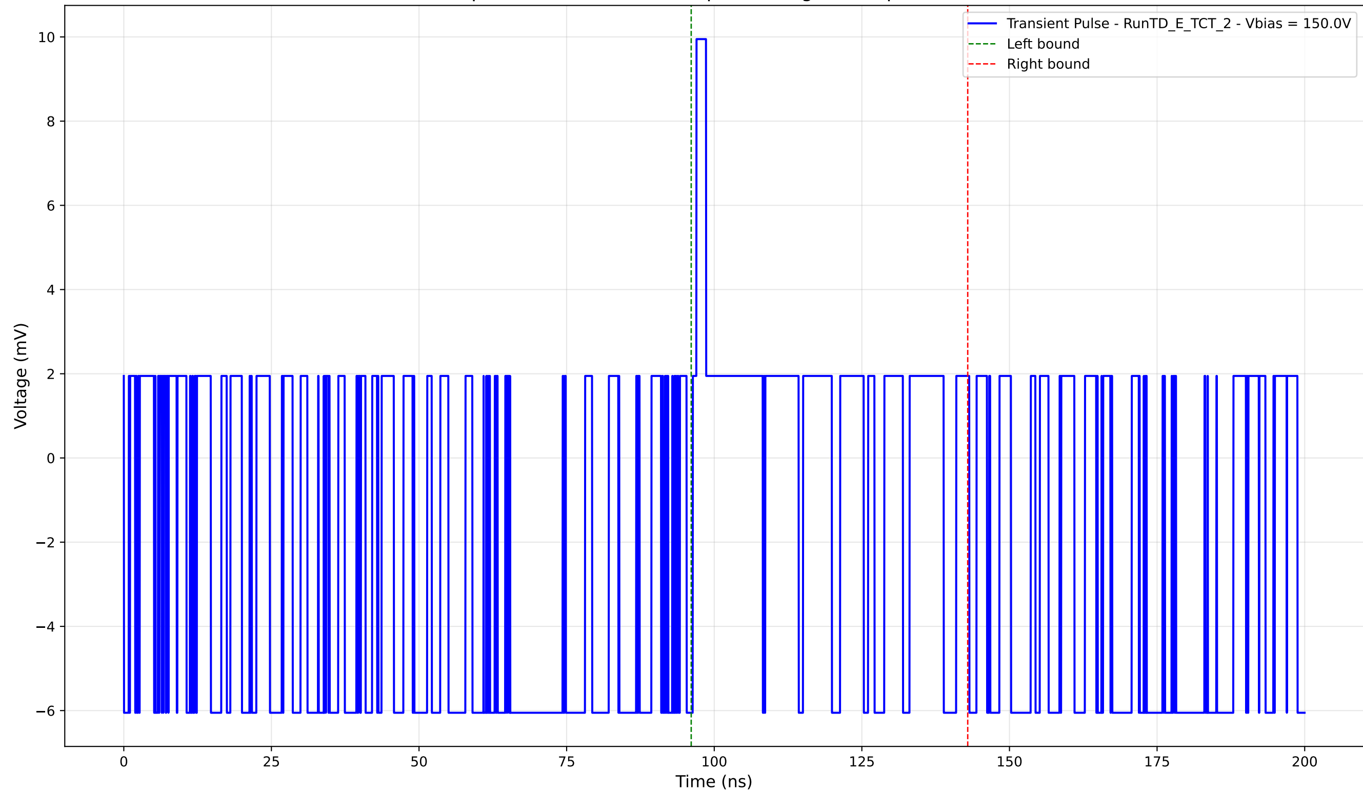
Transient Pulse - - Sample: TD - Position: 245.0 \mu\text{m} - Charge: 0.76 pC - Rise Time: 0.00 ns (N/A)
