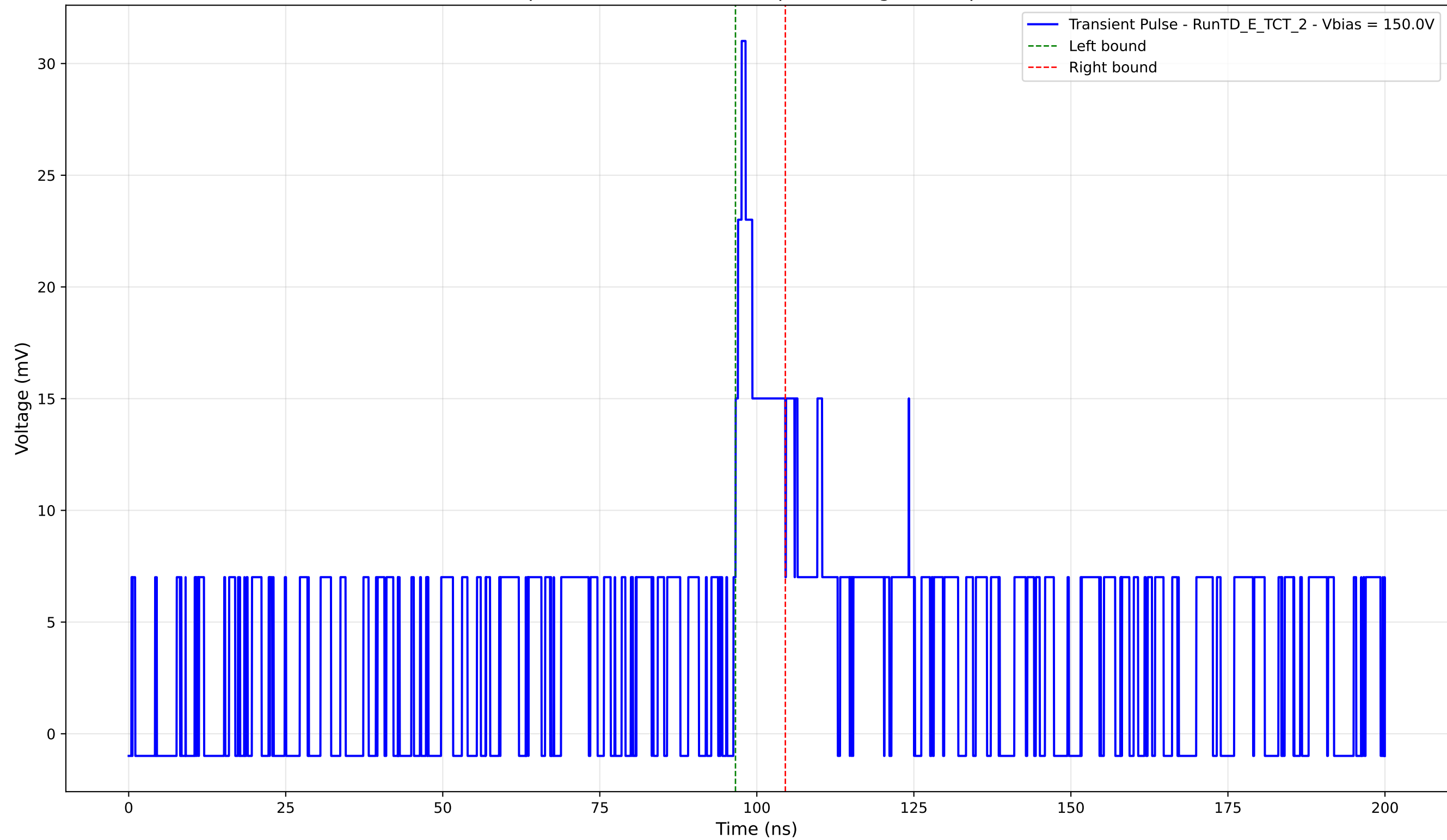
Transient Pulse - Sample: TD - Position: 295.0 \mu\text{m} - Charge: 2.85 pC - Rise Time: 1.31 ns
