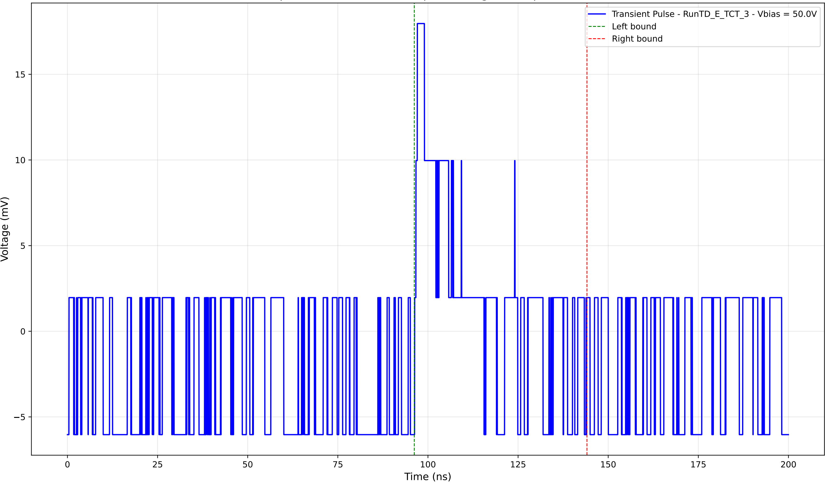
Transient Pulse - Sample: TD - Position: 670.0 \mu\text{m} - Charge: 2.14 pC - Rise Time: 0.00 ns (N/A)
