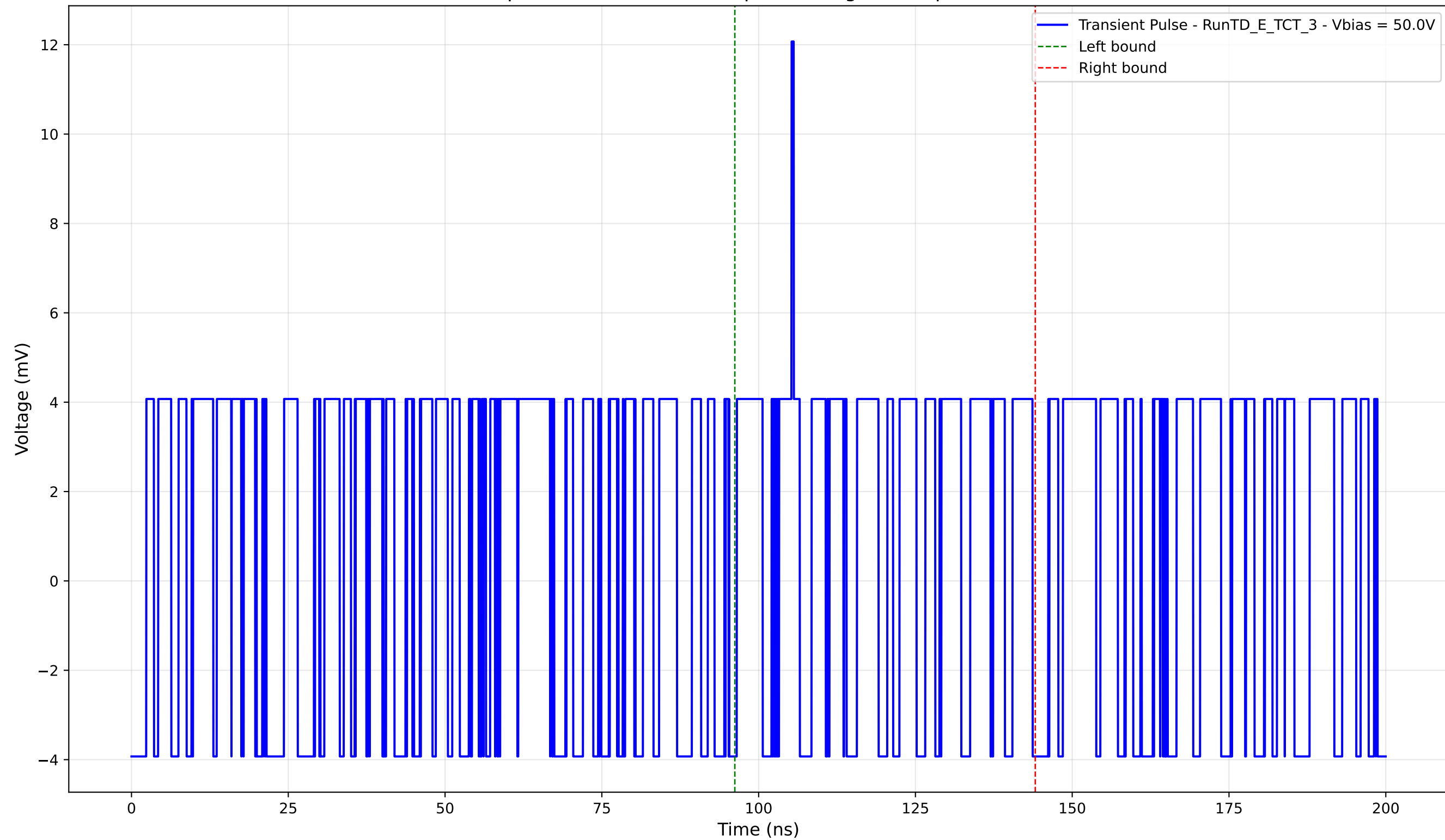
Transient Pulse - Sample: TD - Position: 85.0 \mu\text{m} - Charge: 1.67 pC - Rise Time: 0.00 ns (N/A)
