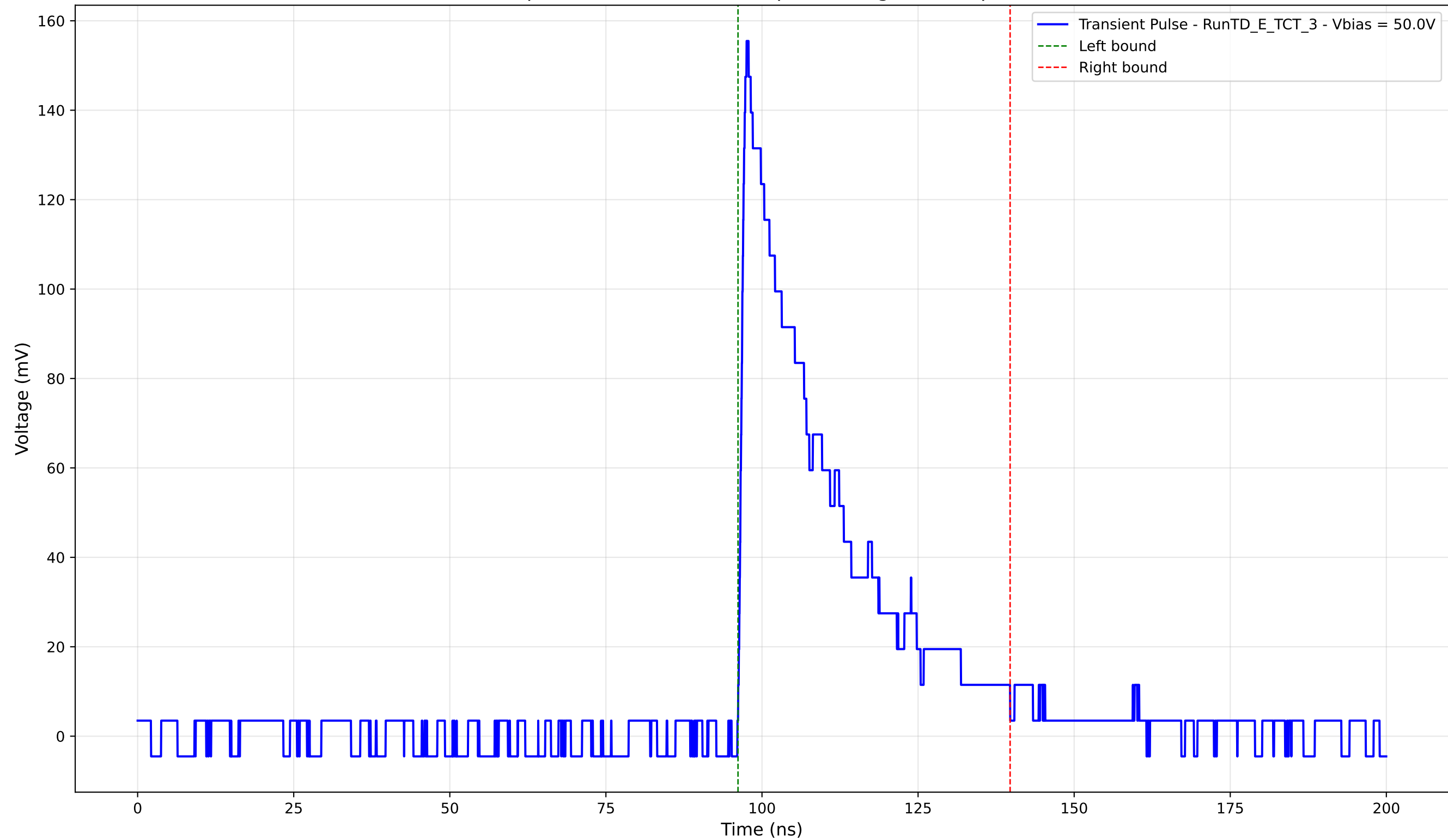
Transient Pulse - Sample: TD - Position: 350.0 \mu\text{m} - Charge: 42.05 pC - Rise Time: 1.05 ns
