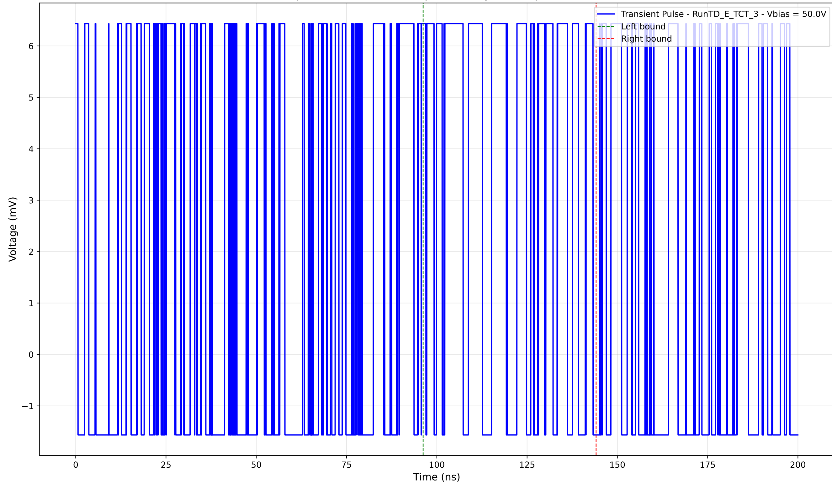
Transient Pulse - Sample: TD - Position: 0.0 \mu\text{m} - Charge: 3.56 pC - Rise Time: 0.00 ns (N/A)
