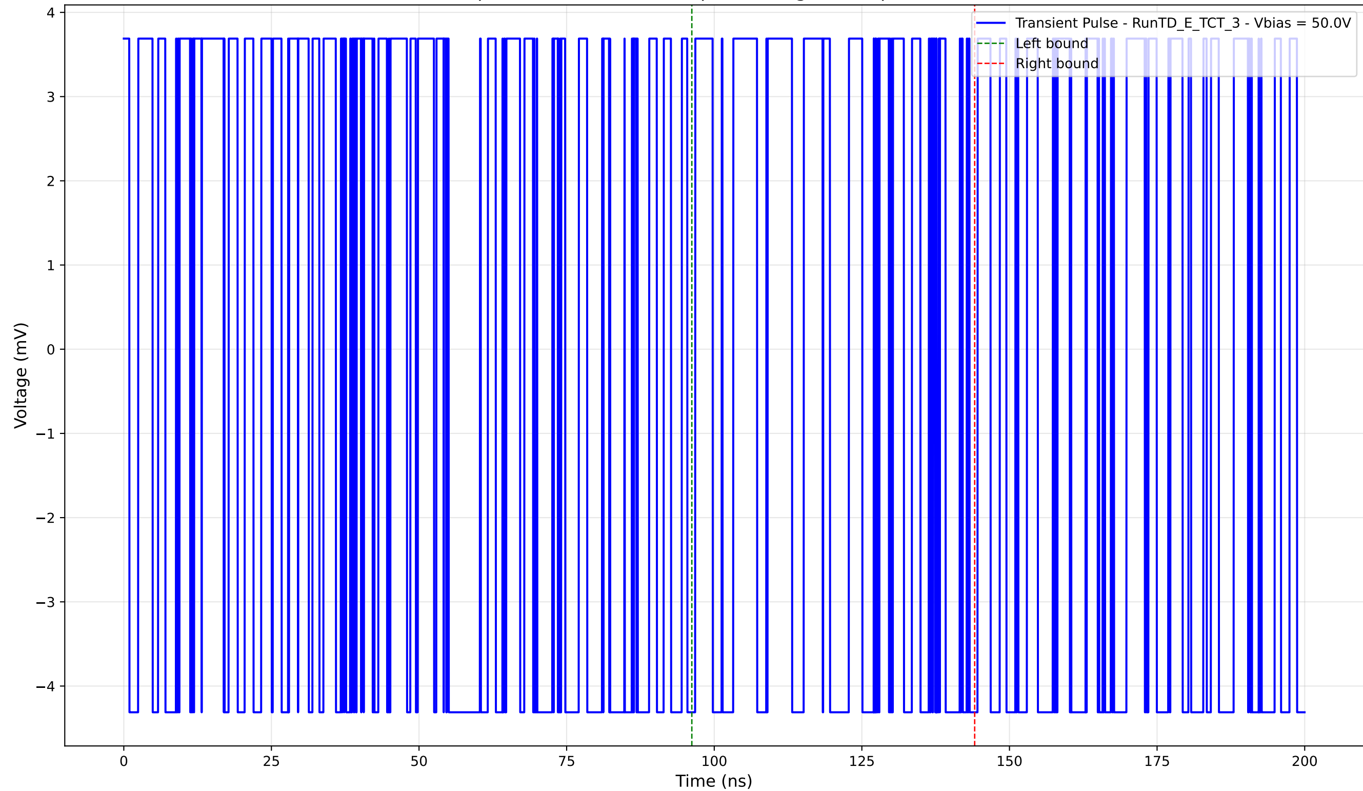
Transient Pulse - Sample: TD - Position: 70.0 \mu\text{m} - Charge: 0.02 pC - Rise Time: 0.00 ns (N/A)
