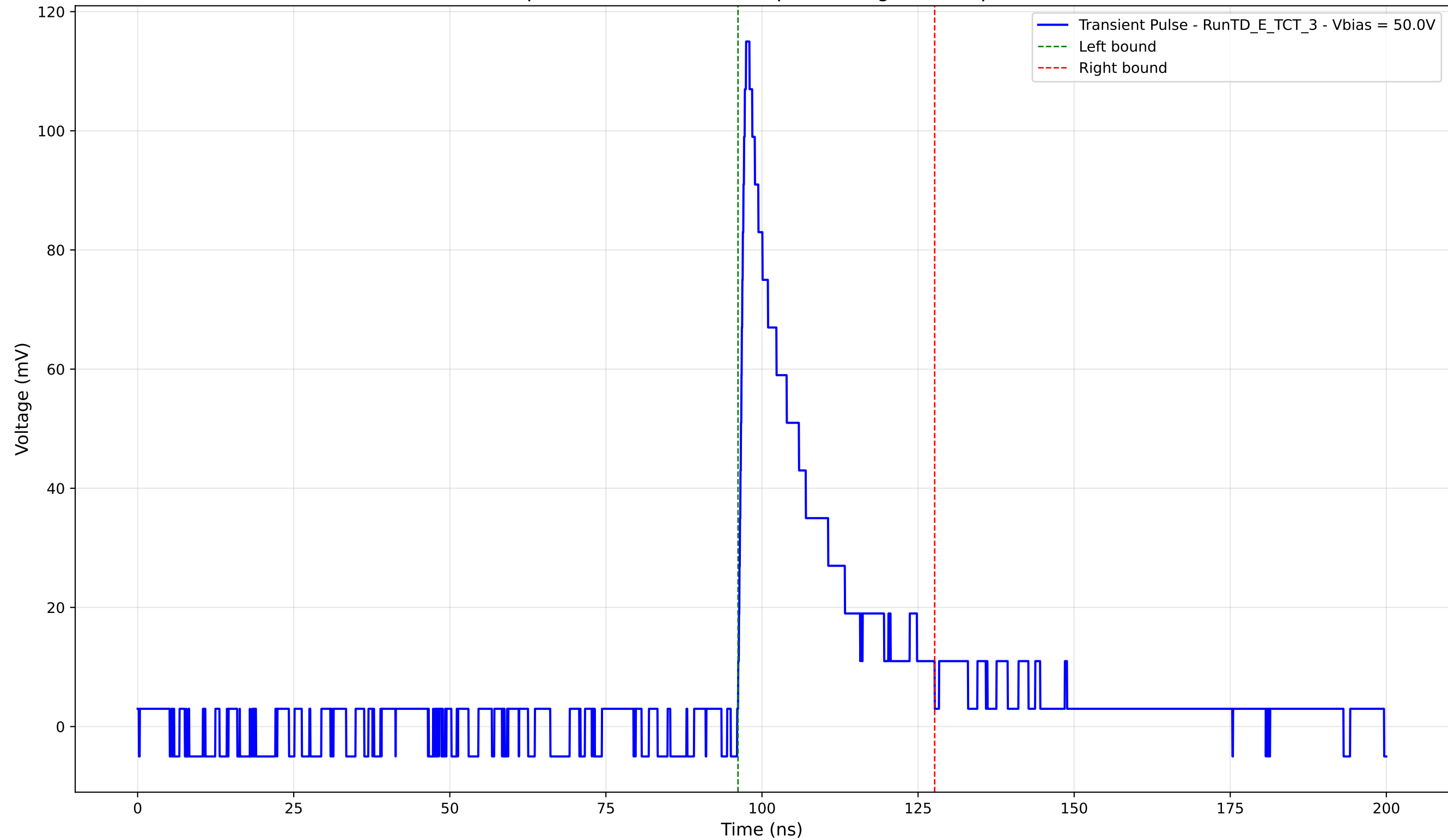
Transient Pulse - Sample: TD - Position: 550.0 \mu\text{m} - Charge: 23.14 pC - Rise Time: 0.96 ns
