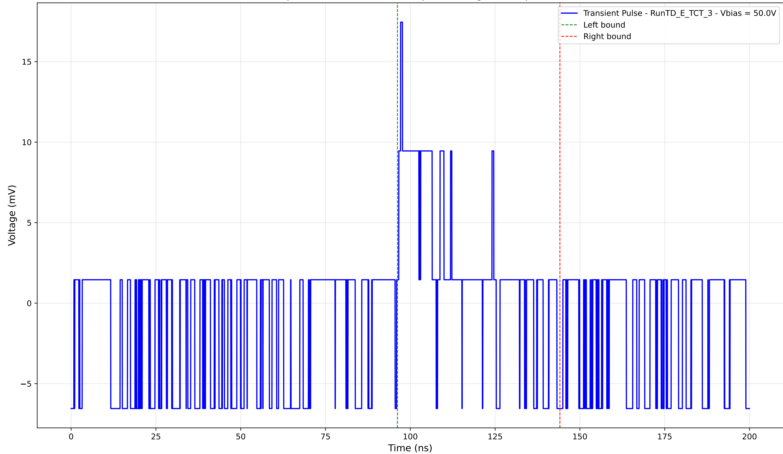
Transient Pulse - Sample: TD - Position: 305.0 \mu\text{m} - Charge: 2.42 pC - Rise Time: 0.56 ns
