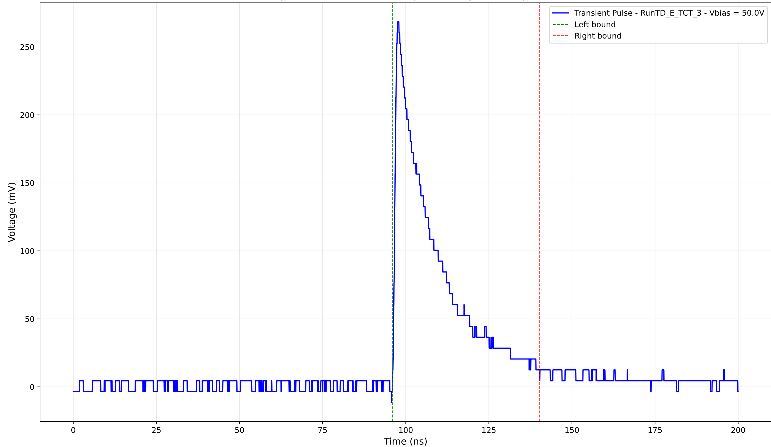
Transient Pulse - Sample: TD - Position: 435.0 \mu\text{m} - Charge: 68.43 pC - Rise Time: 1.04 ns
