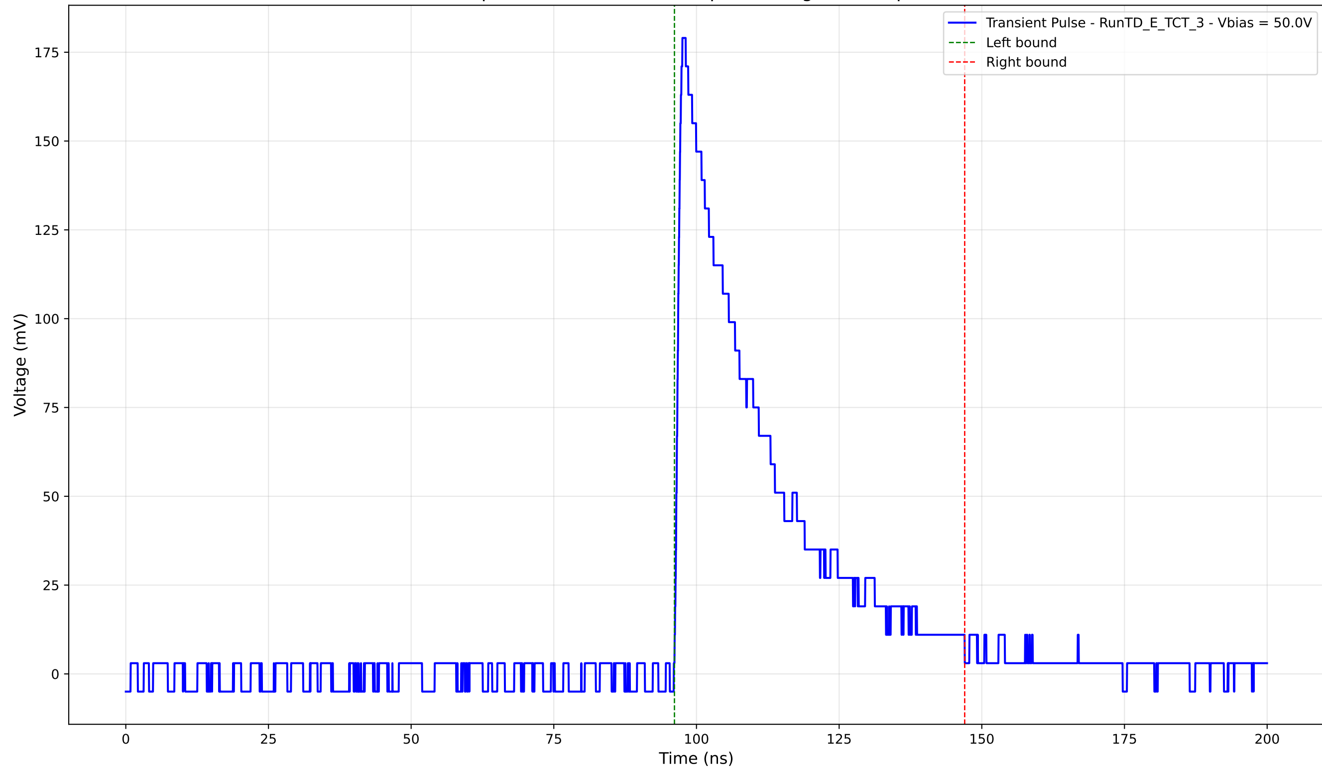
Transient Pulse - Sample: TD - Position: 360.0 \mu\text{m} - Charge: 54.12 pC - Rise Time: 1.02 ns
