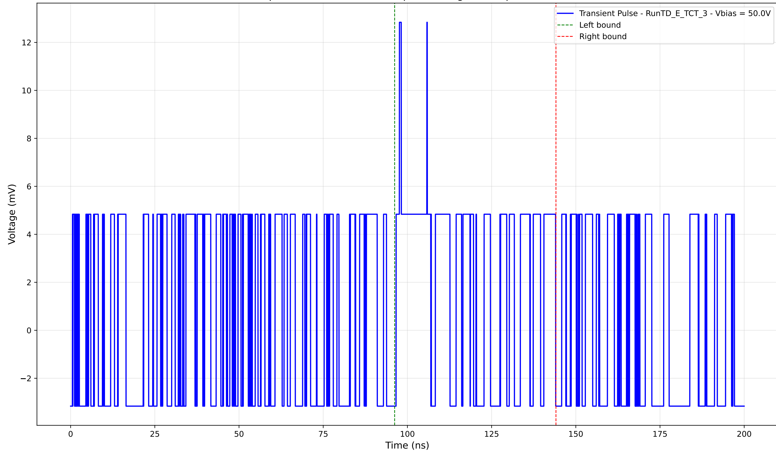
Transient Pulse - Sample: TD - Position: 270.0 \mu\text{m} - Charge: 2.43 pC - Rise Time: 0.00 ns (N/A)
