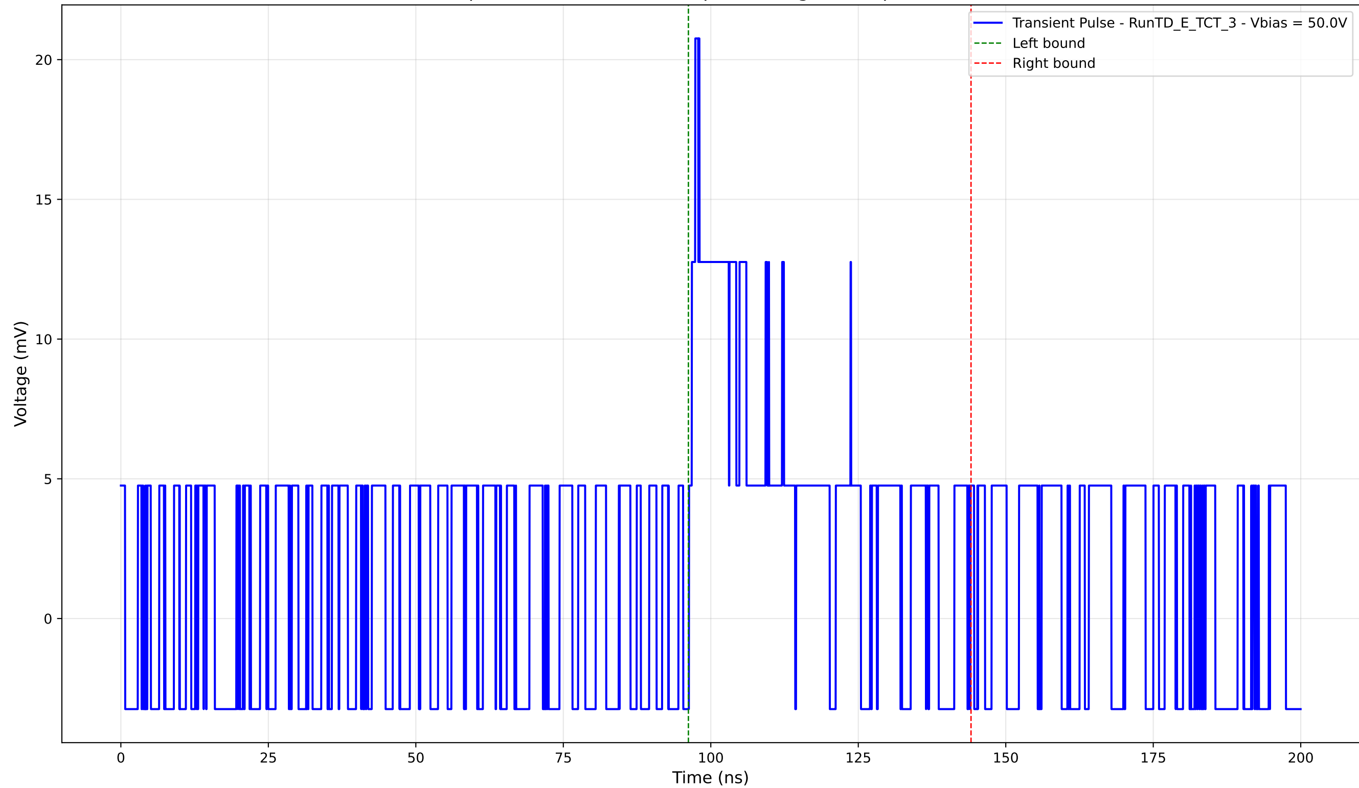
Transient Pulse - Sample: TD - Position: 310.0 \mu\text{m} - Charge: 4.89 pC - Rise Time: 0.00 ns (N/A)
