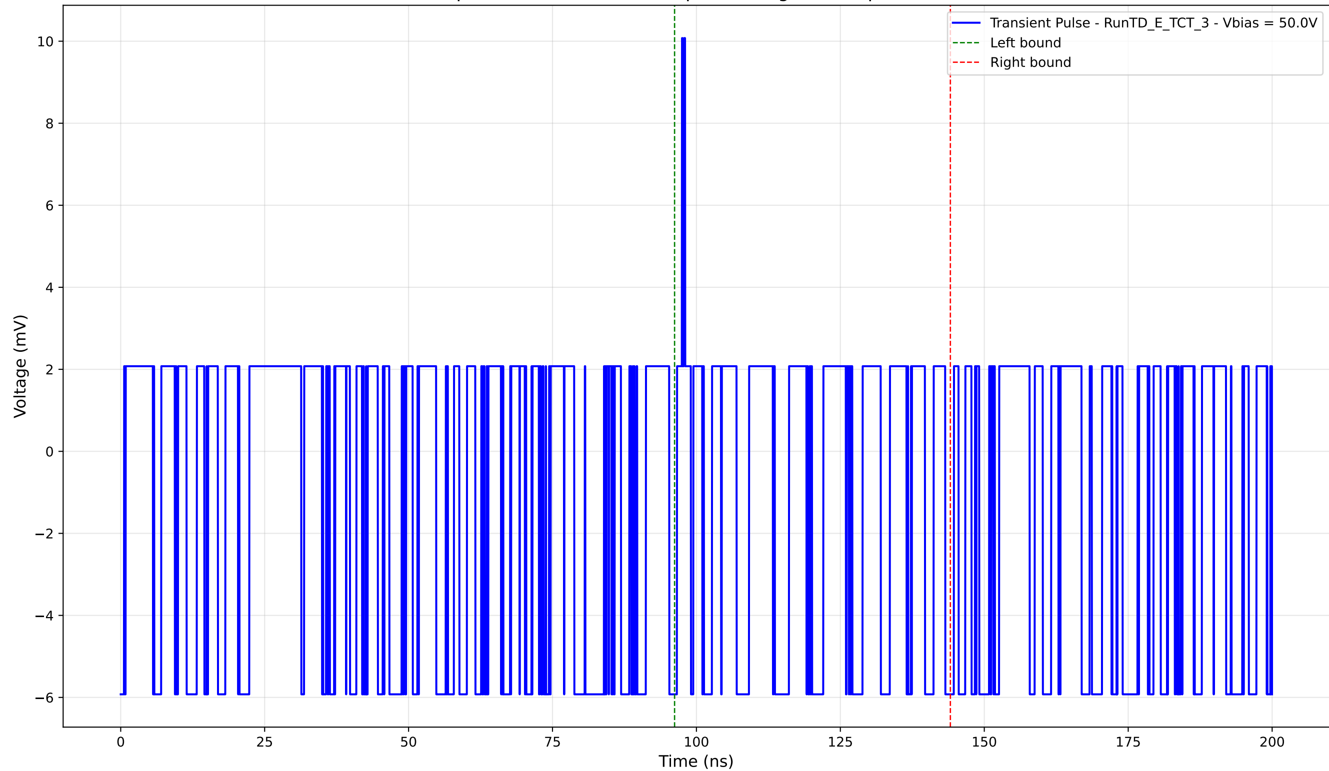
Transient Pulse - Sample: TD - Position: 200.0 \mu\text{m} - Charge: -0.60 pC - Rise Time: 0.00 ns (N/A)
