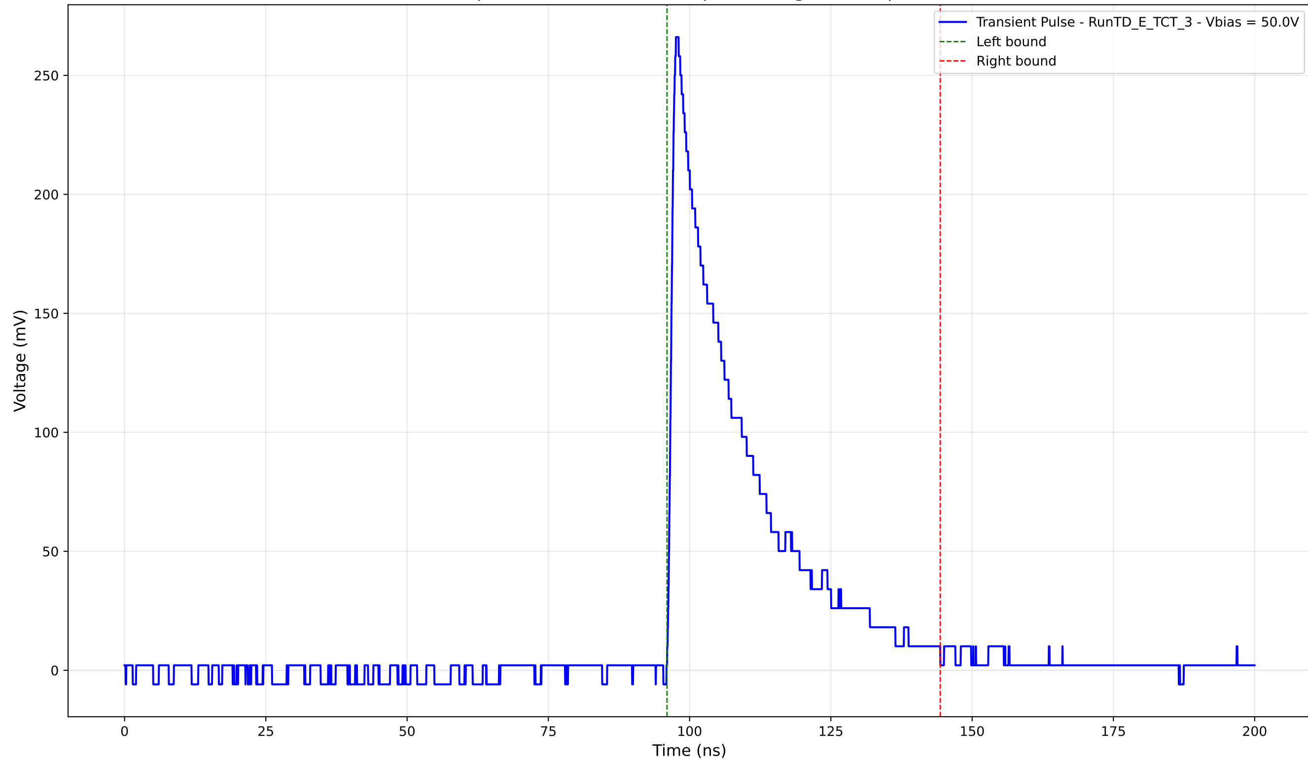
Transient Pulse - Sample: TD - Position: 430.0 \mu\text{m} - Charge: 68.20 pC - Rise Time: 1.04 ns
