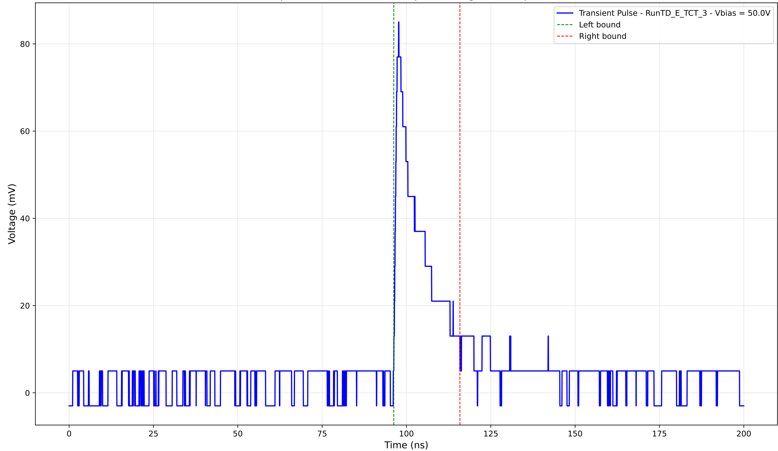
Transient Pulse - Sample: TD - Position: 605.0 \mu\text{m} - Charge: 13.37 pC - Rise Time: 0.97 ns
