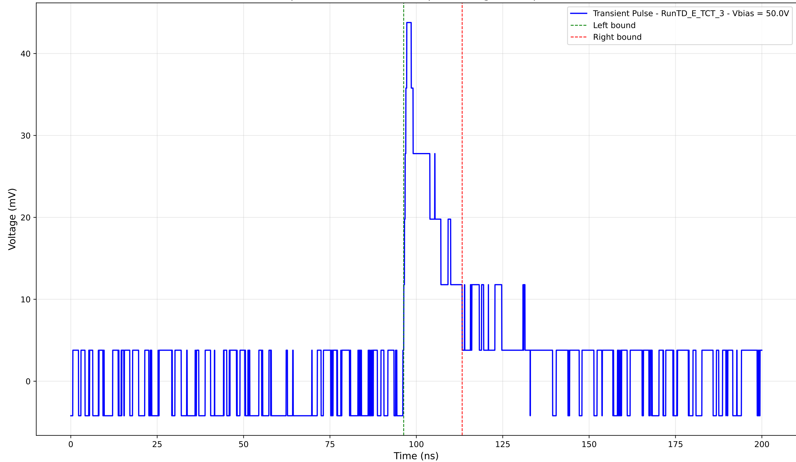
Transient Pulse - Sample: TD - Position: 710.0 \mu\text{m} - Charge: 7.50 pC - Rise Time: 0.88 ns
