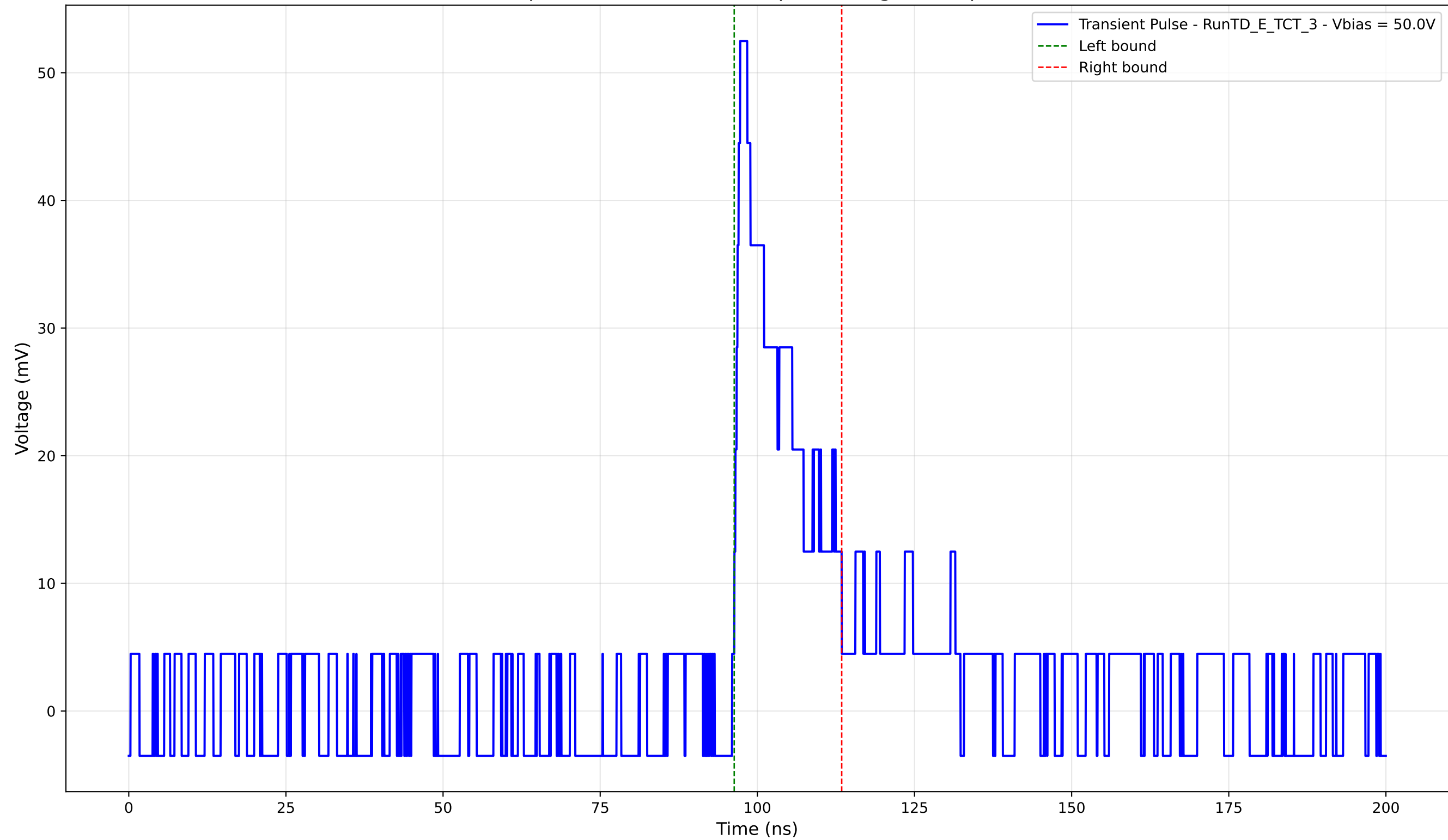
Transient Pulse - Sample: TD - Position: 625.0 \mu\text{m} - Charge: 8.79 pC - Rise Time: 0.94 ns
