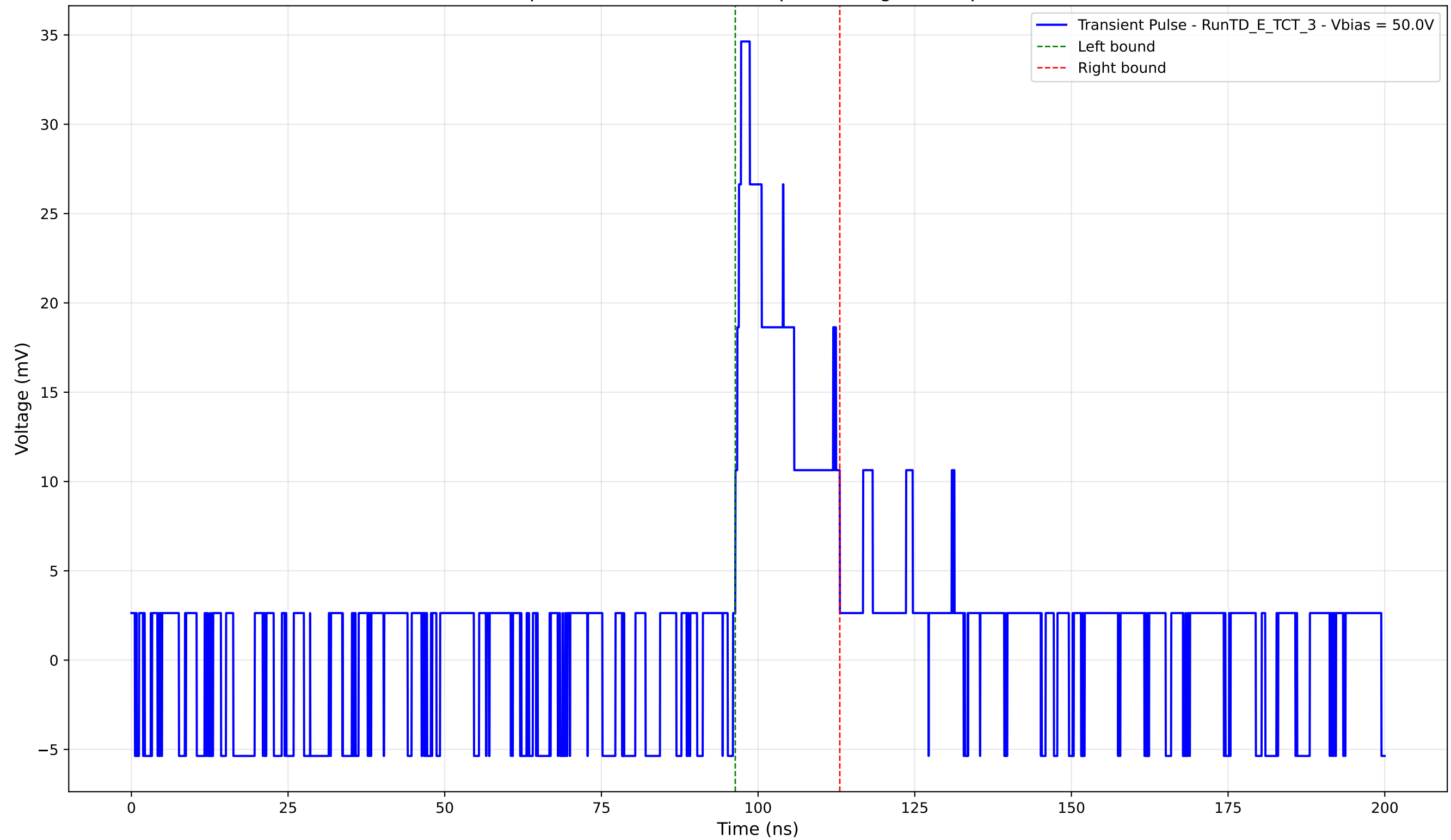
Transient Pulse - Sample: TD - Position: 690.0 \mu\text{m} - Charge: 5.88 pC - Rise Time: 0.92 ns
