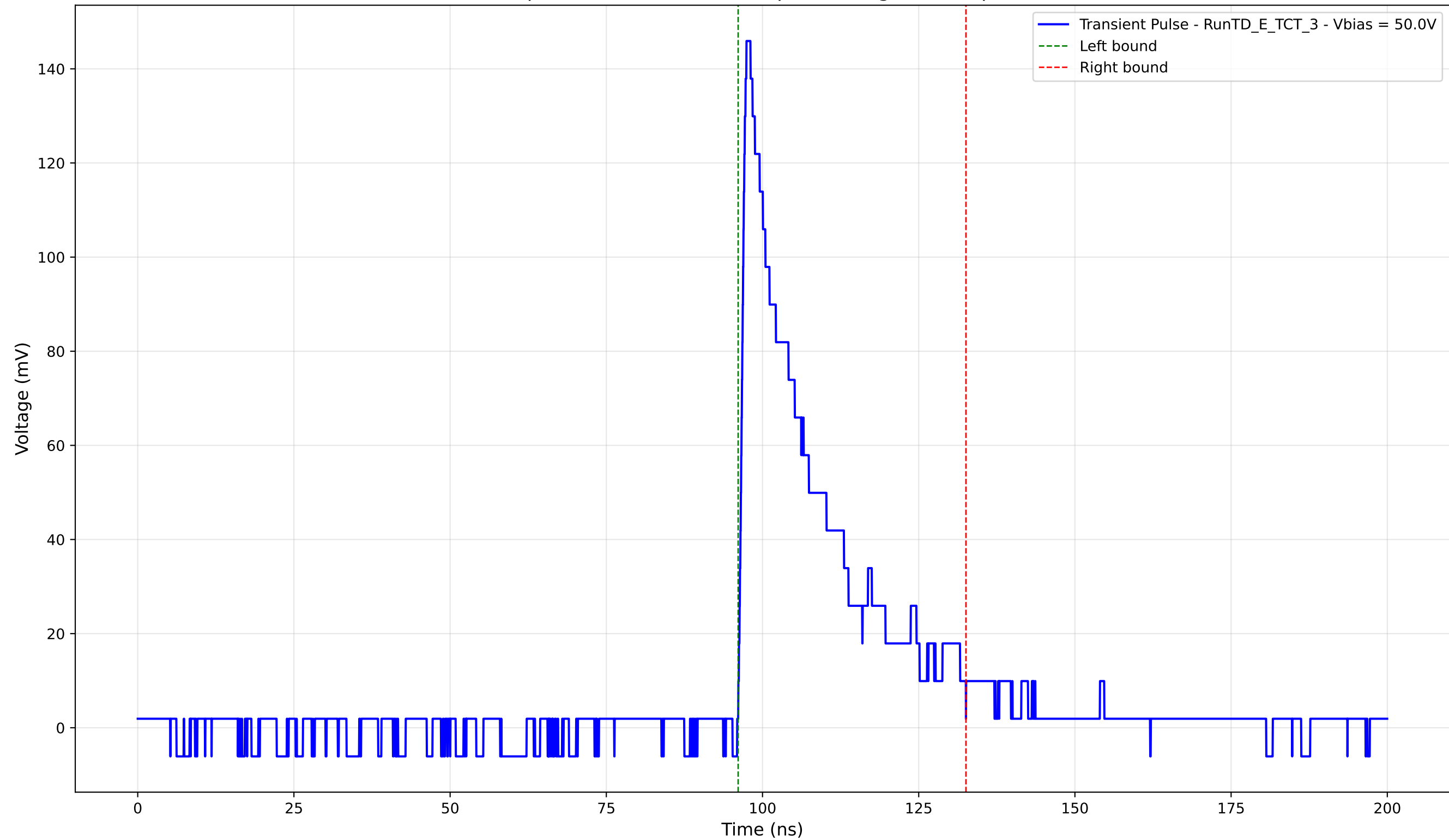
Transient Pulse - Sample: TD - Position: 500.0 \mu\text{m} - Charge: 33.45 pC - Rise Time: 1.07 ns
