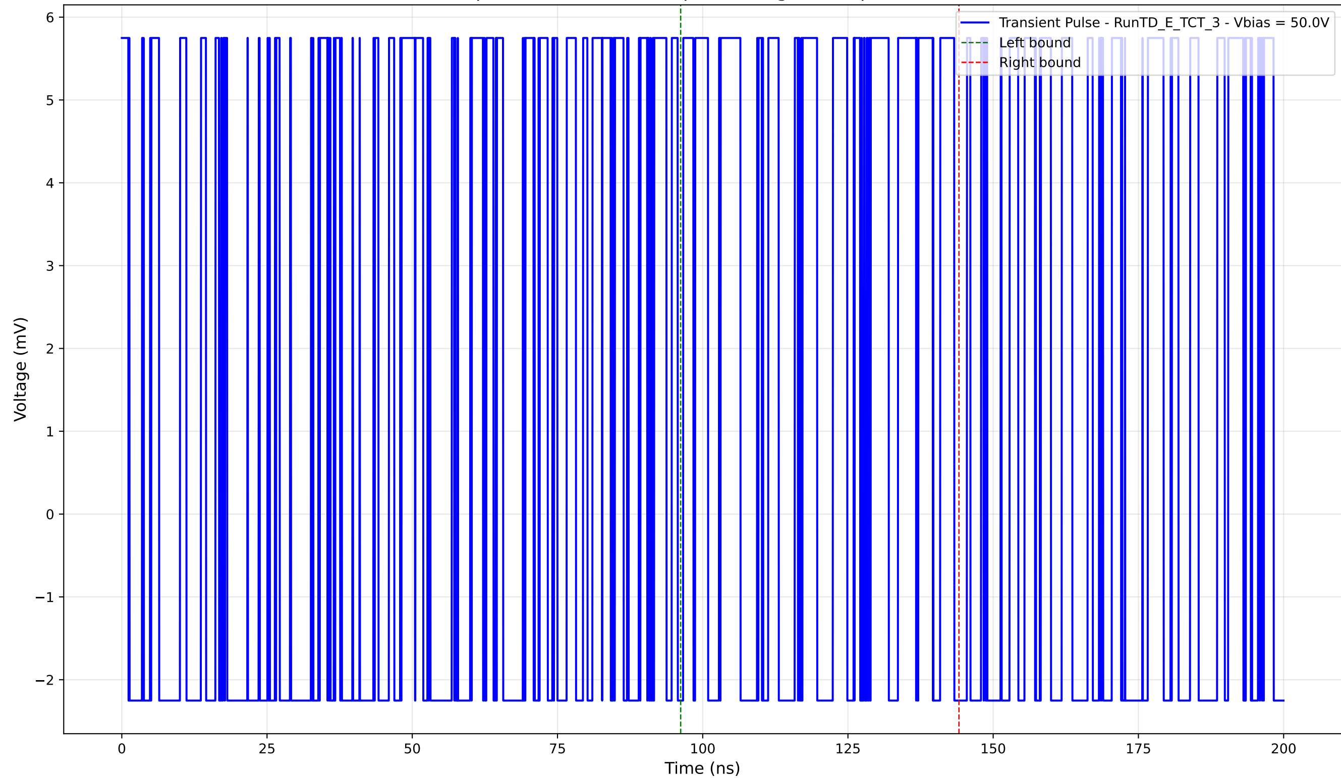
Transient Pulse - Sample: TD - Position: 5.0 \mu\text{m} - Charge: 2.48 pC - Rise Time: 0.00 ns (N/A)
