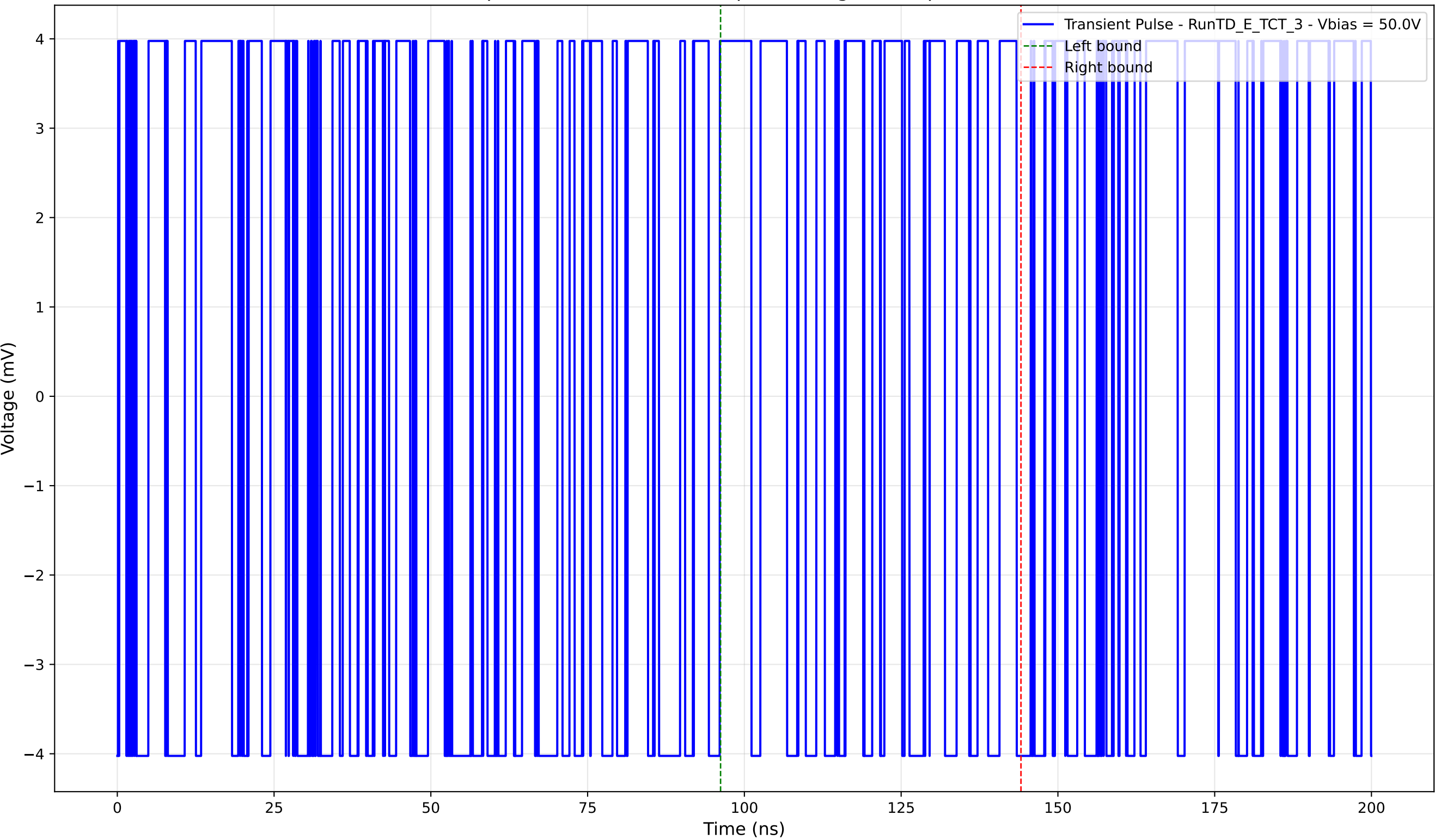
Transient Pulse - Sample: TD - Position: 160.0 \mu\text{m} - Charge: 0.90 pC - Rise Time: 0.00 ns (N/A)
