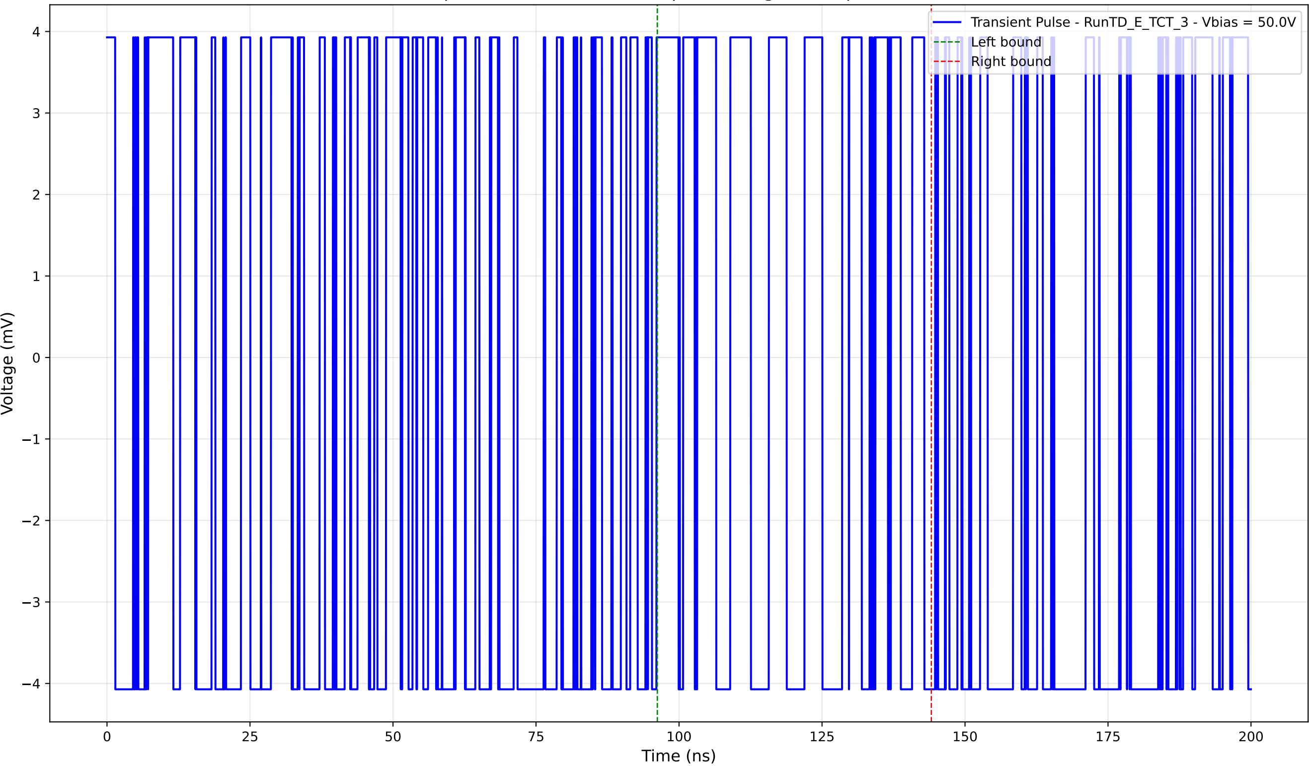
Transient Pulse - Sample: TD - Position: 115.0 \mu\text{m} - Charge: 0.75 pC - Rise Time: 0.00 ns (N/A)
