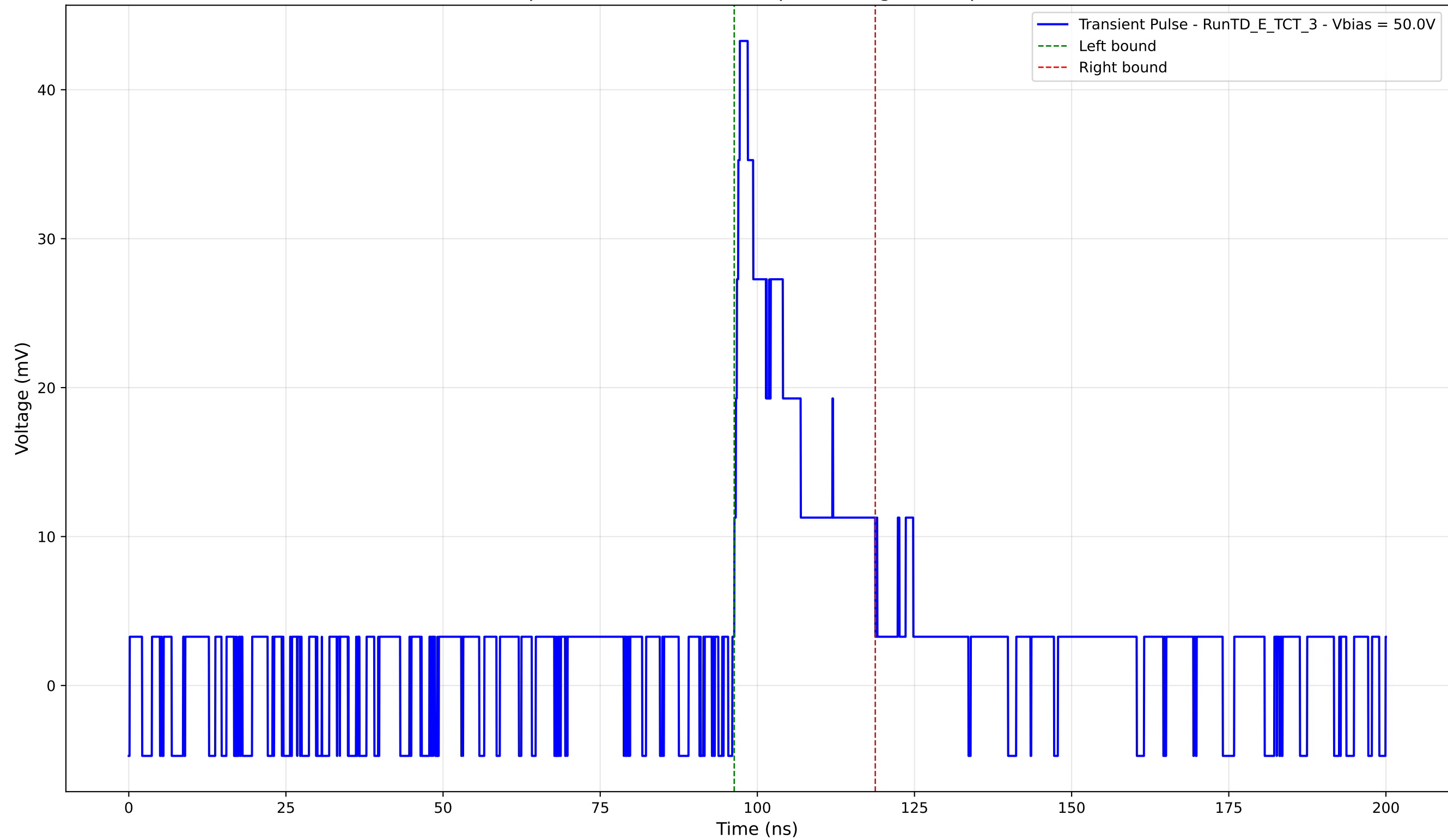
Transient Pulse - Sample: TD - Position: 715.0 \mu\text{m} - Charge: 8.38 pC - Rise Time: 0.88 ns
