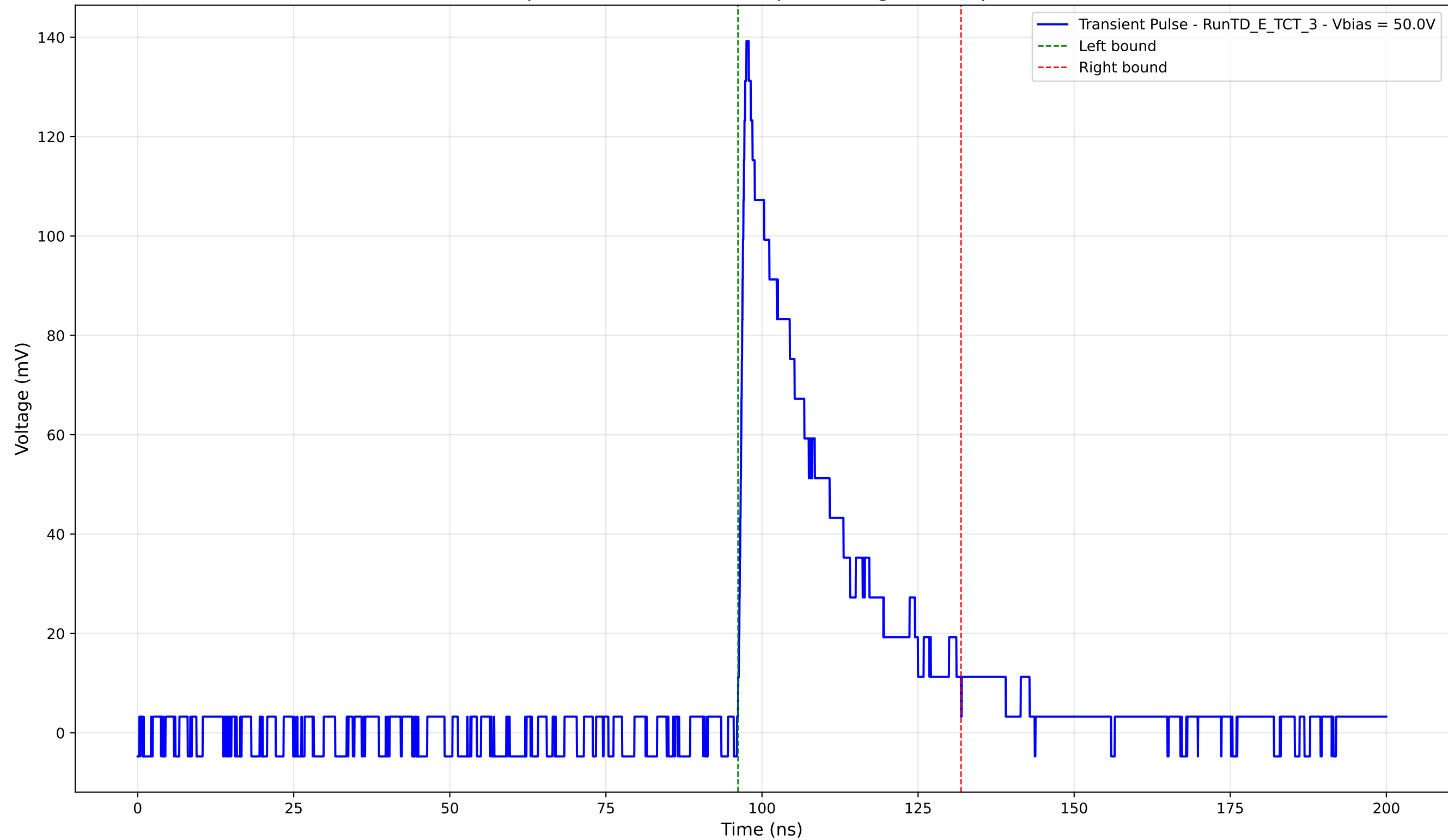
Transient Pulse - Sample: TD - Position: 345.0 \mu\text{m} - Charge: 33.73 pC - Rise Time: 1.01 ns
