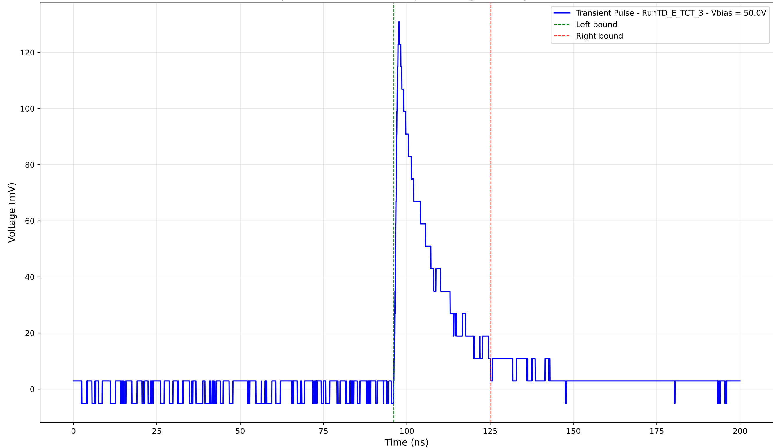
Transient Pulse - Sample: TD - Position: 535.0 \mu\text{m} - Charge: 25.83 pC - Rise Time: 1.09 ns
