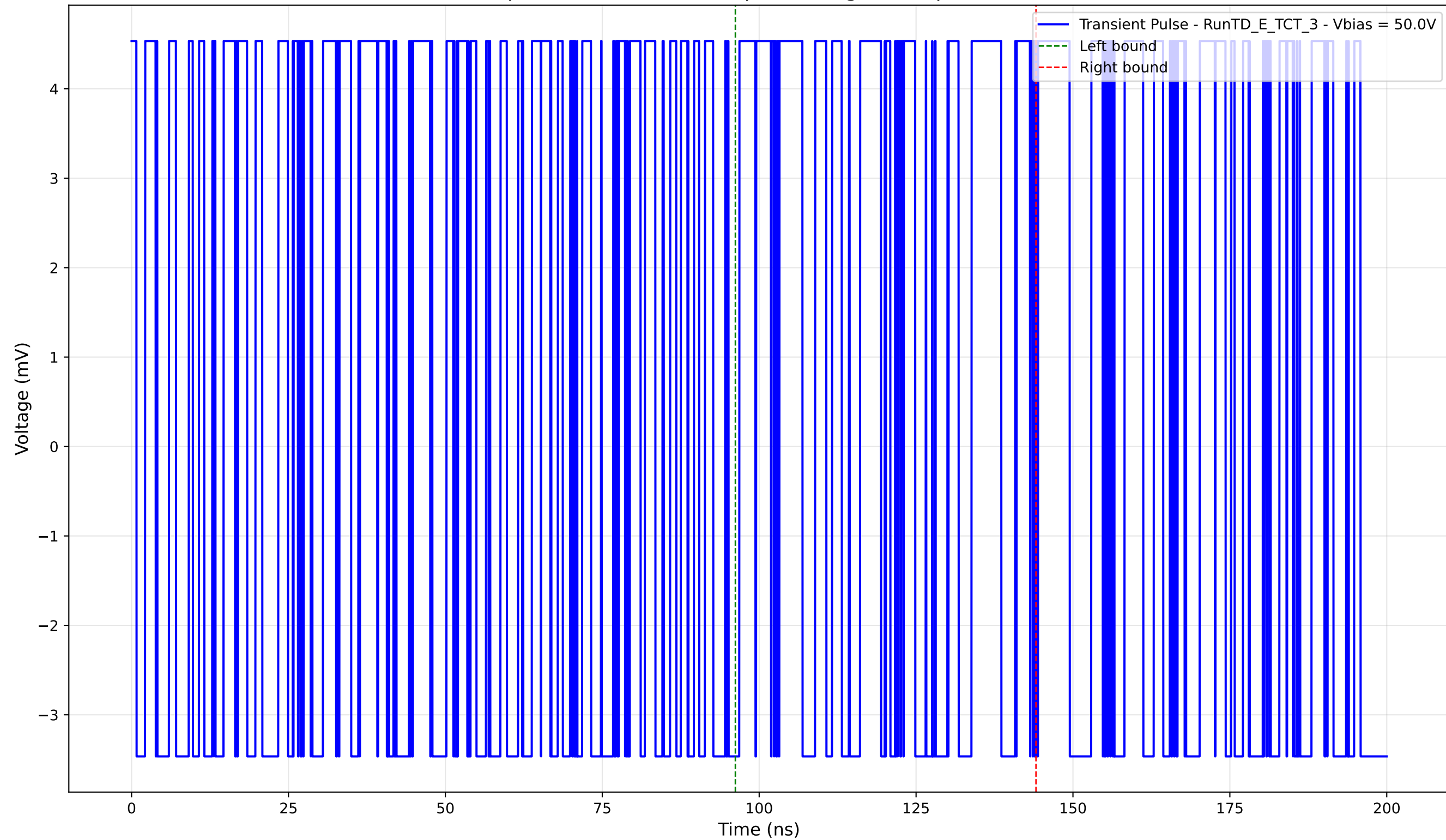
Transient Pulse - Sample: TD - Position: 65.0 \mu\text{m} - Charge: 1.36 pC - Rise Time: 0.00 ns (N/A)
