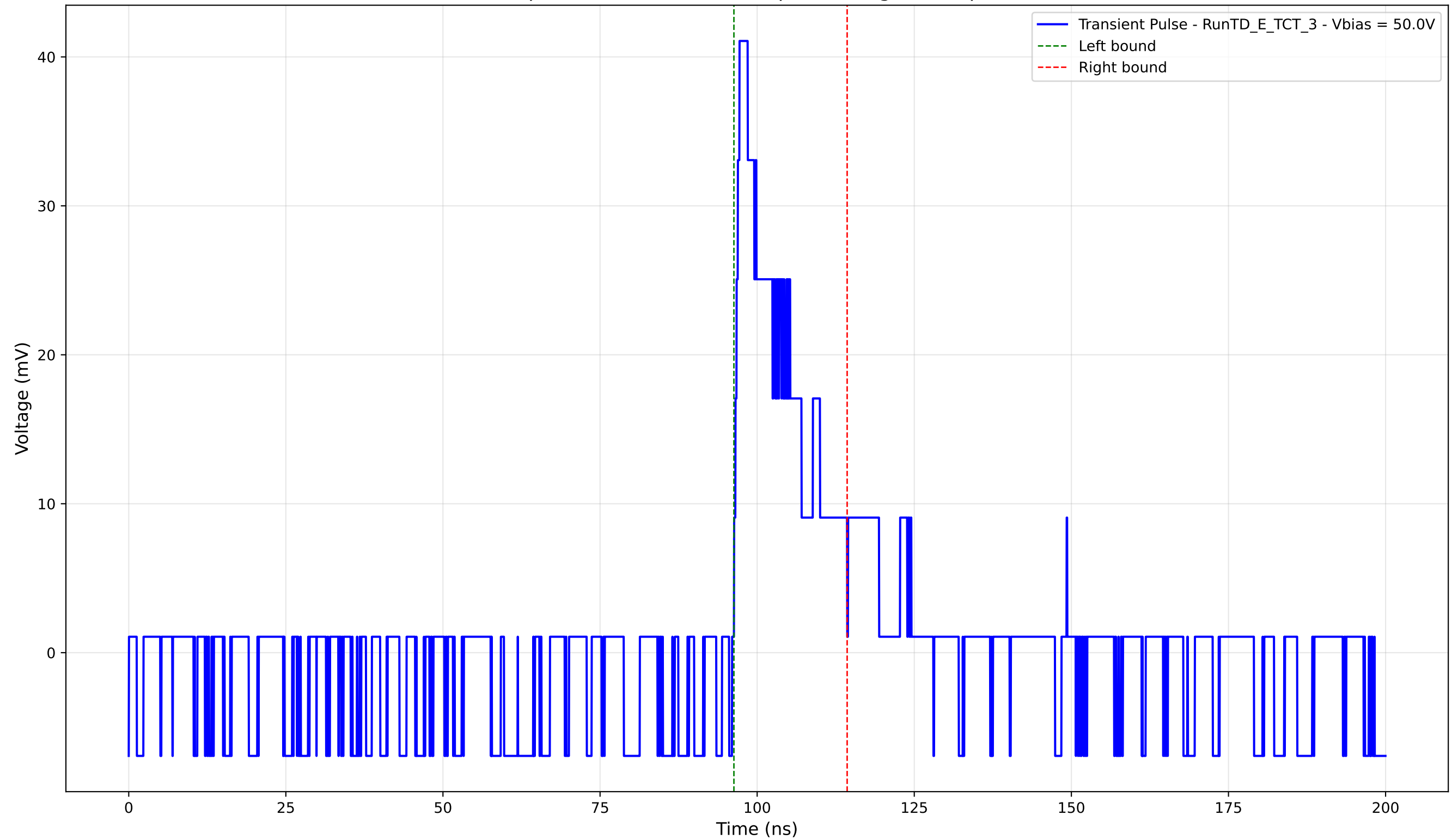
Transient Pulse - Sample: TD - Position: 705.0 \mu\text{m} - Charge: 6.95 pC - Rise Time: 0.87 ns
