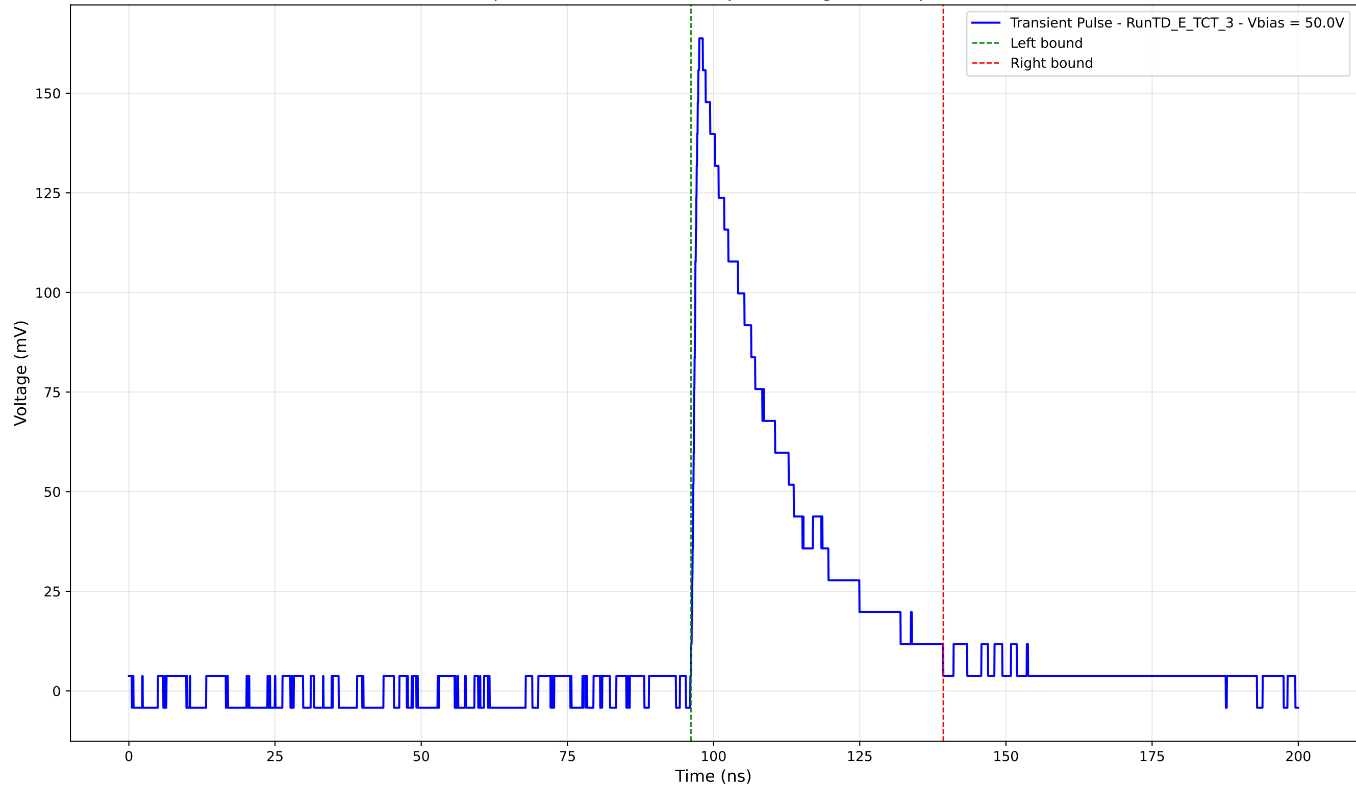
Transient Pulse - Sample: TD - Position: 355.0 \mu\text{m} - Charge: 46.00 pC - Rise Time: 1.03 ns
