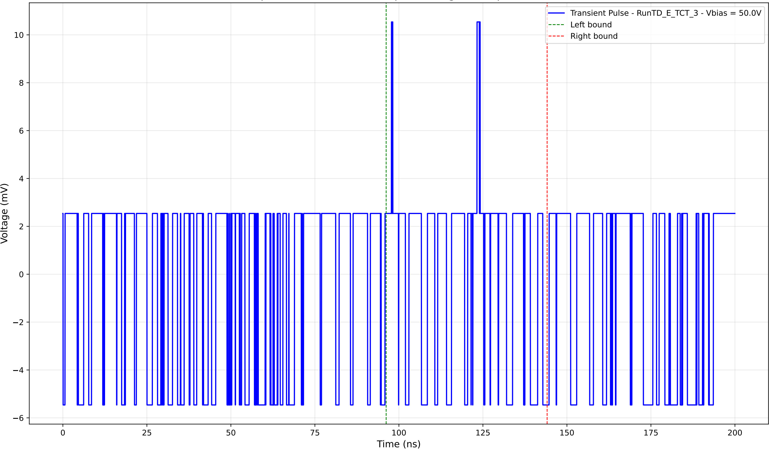
Transient Pulse - Sample: TD - Position: 230.0 \mu\text{m} - Charge: 0.63 pC - Rise Time: 0.00 ns (N/A)
