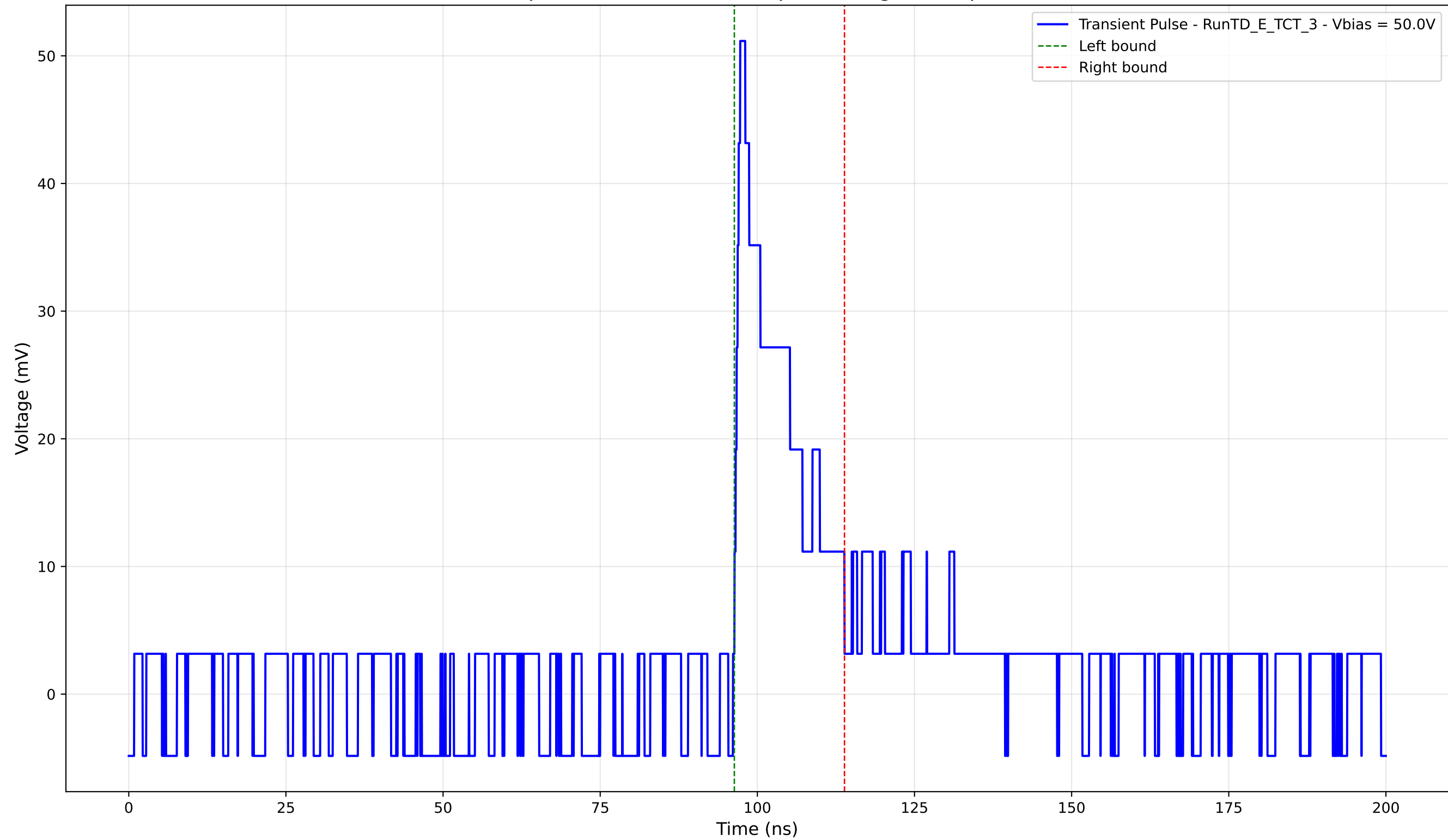
Transient Pulse - Sample: TD - Position: 635.0 \mu\text{m} - Charge: 8.14 pC - Rise Time: 0.92 ns
