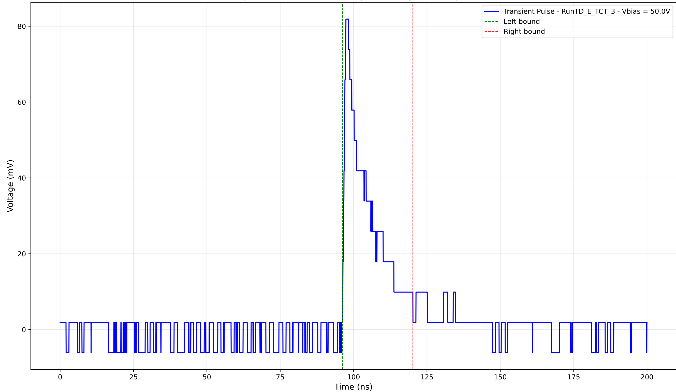
Transient Pulse - Sample: TD - Position: 585.0 \mu\text{m} - Charge: 14.40 pC - Rise Time: 0.96 ns
