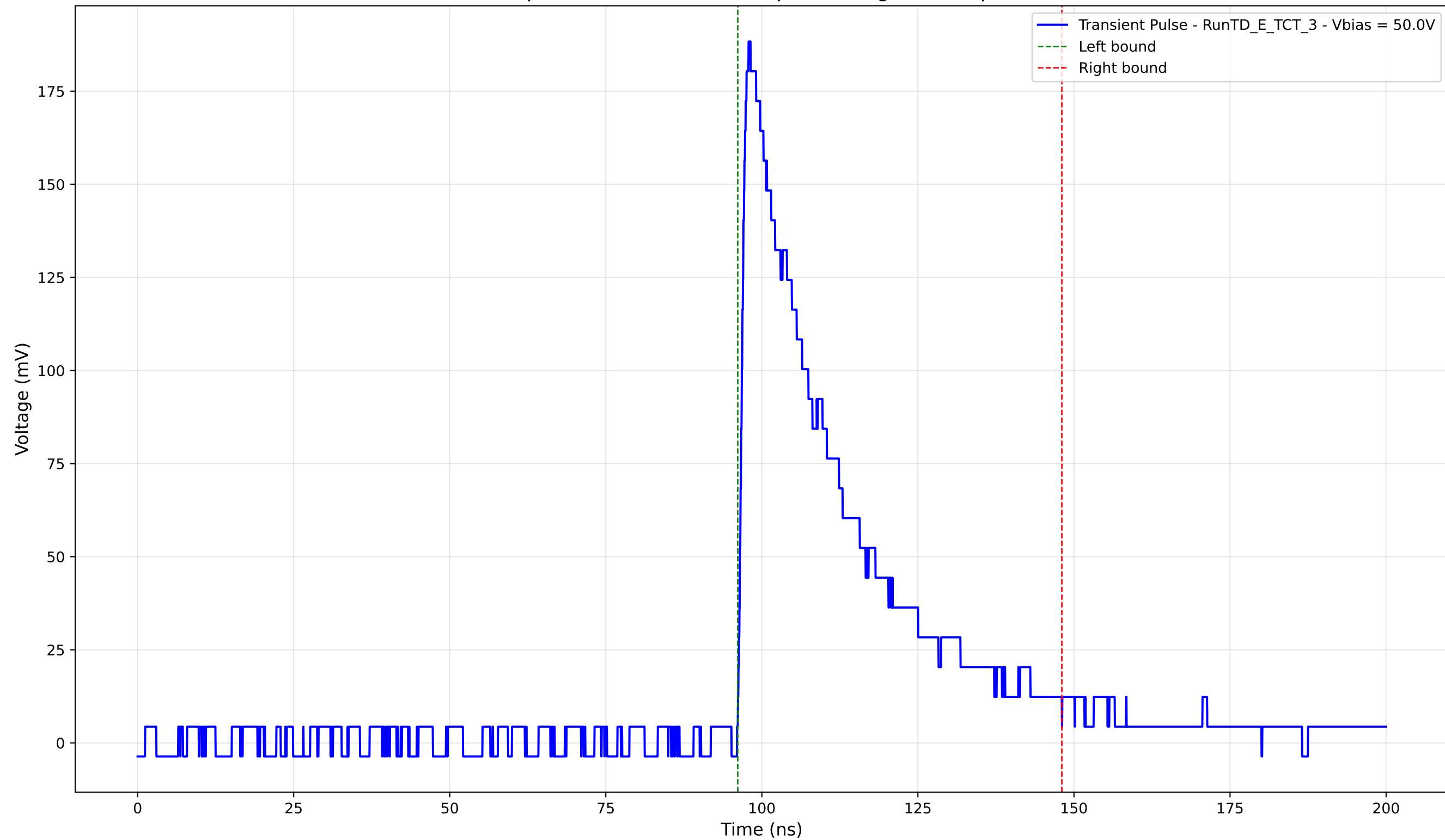
Transient Pulse - Sample: TD - Position: 385.0 \mu\text{m} - Charge: 59.82 pC - Rise Time: 1.16 ns
