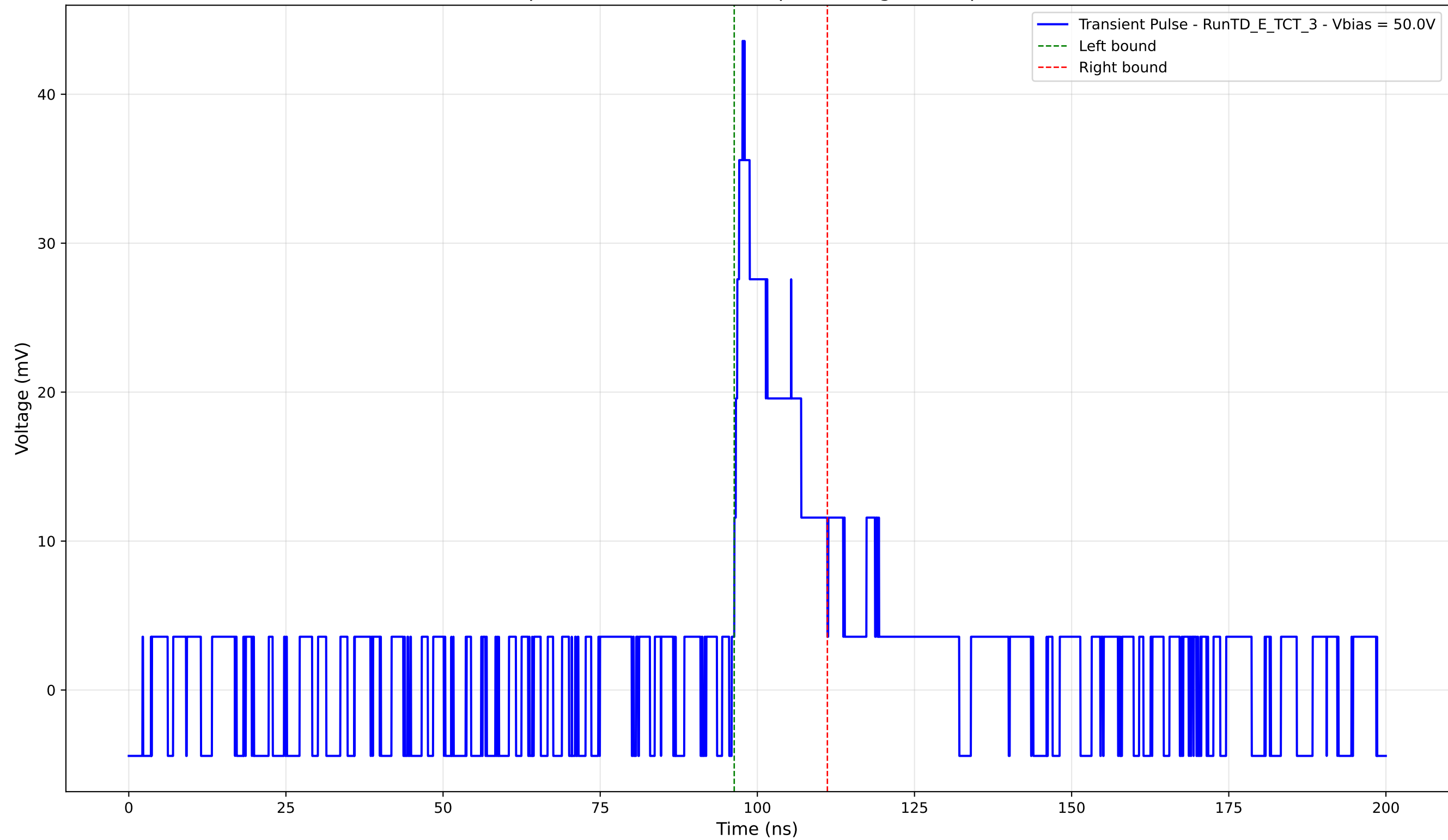
Transient Pulse - Sample: TD - Position: 700.0 \mu\text{m} - Charge: 6.16 pC - Rise Time: 1.32 ns
