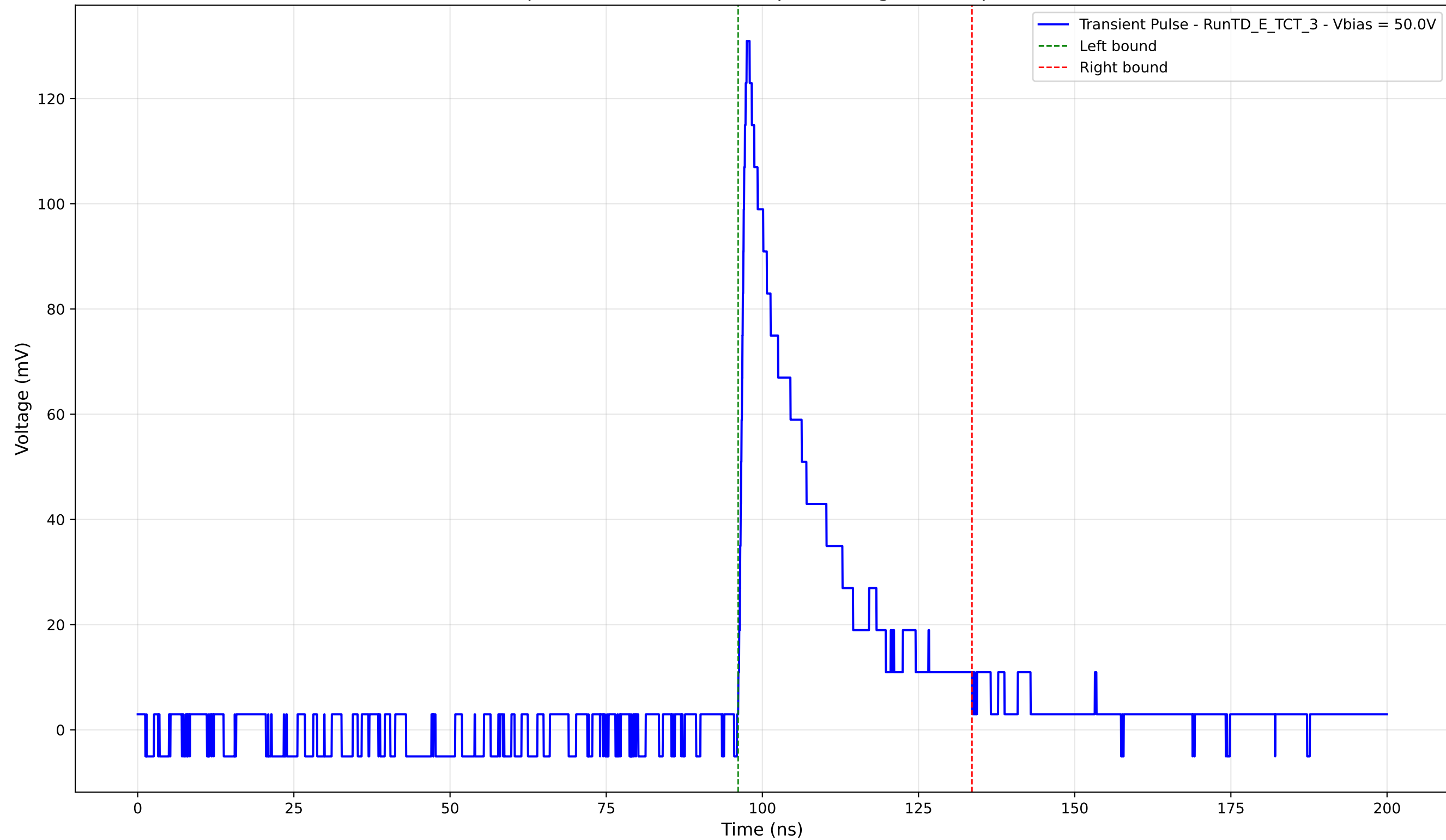
Transient Pulse - Sample: TD - Position: 530.0 \mu\text{m} - Charge: 28.29 pC - Rise Time: 1.05 ns
