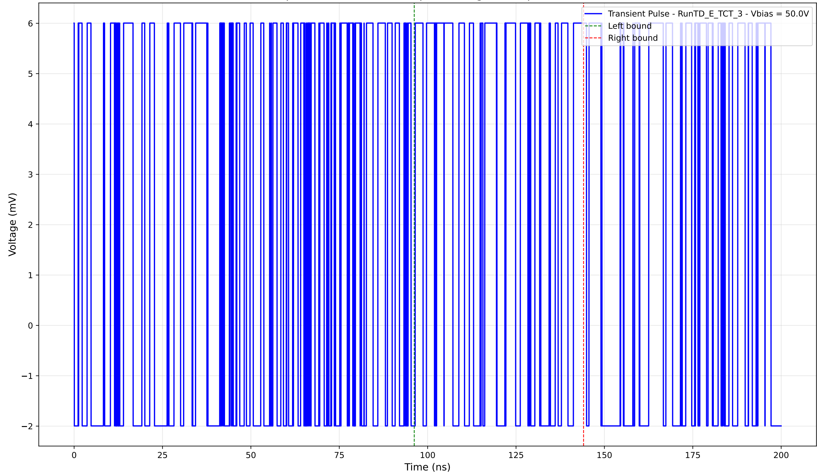
Transient Pulse - Sample: TD - Position: 40.0 \mu\text{m} - Charge: 2.73 pC - Rise Time: 0.00 ns (N/A)
