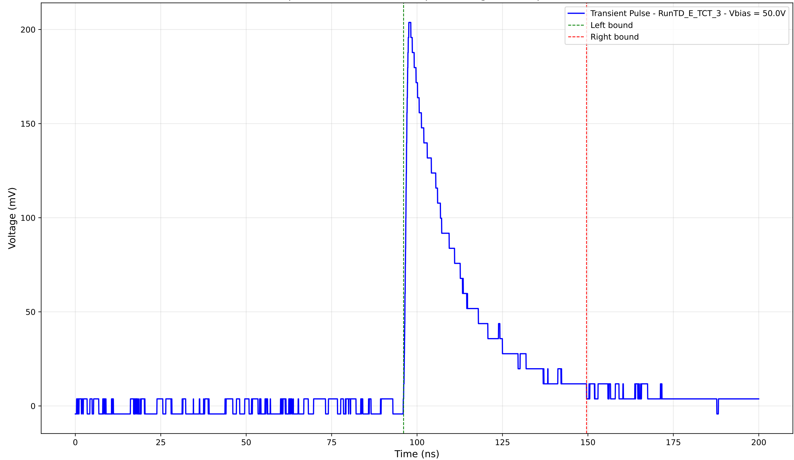
Transient Pulse - Sample: TD - Position: 405.0 \mu\text{m} - Charge: 61.14 pC - Rise Time: 1.08 ns
