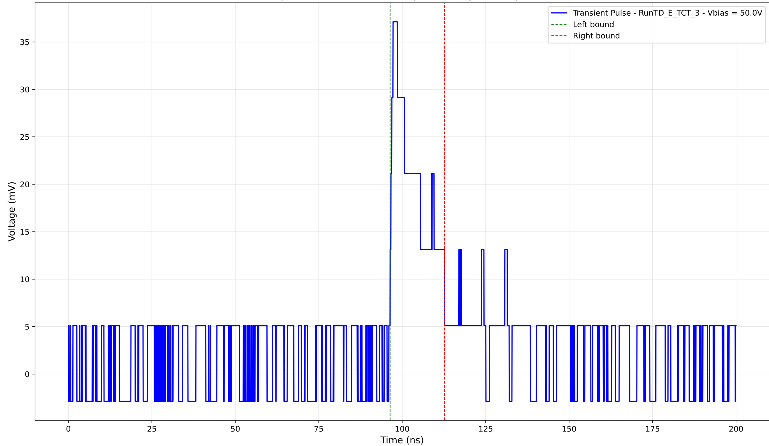
Transient Pulse - Sample: TD - Position: 655.0 \mu\text{m} - Charge: 6.62 pC - Rise Time: 1.25 ns
