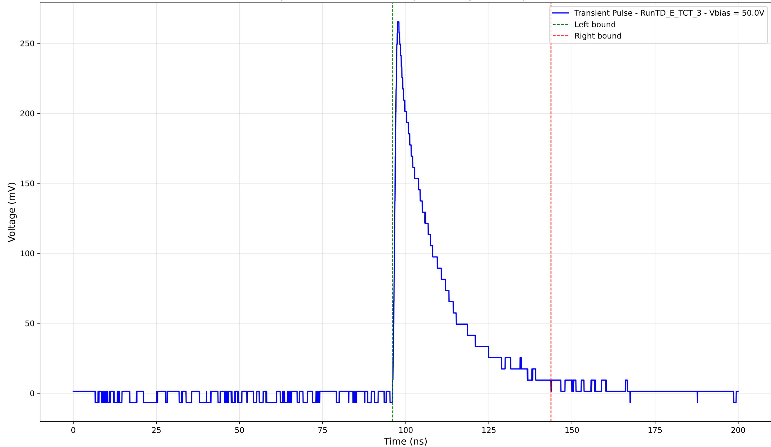
Transient Pulse - Sample: TD - Position: 440.0 \mu\text{m} - Charge: 65.10 pC - Rise Time: 1.02 ns
