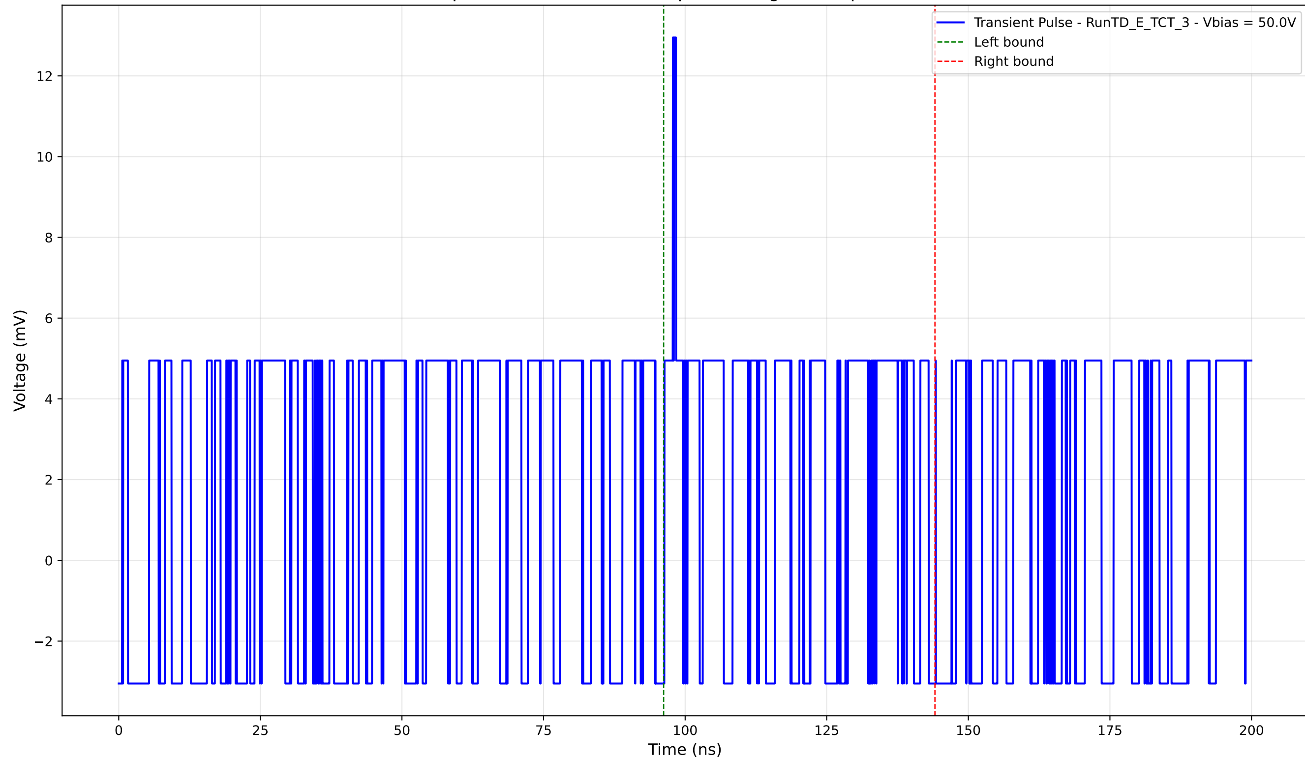
Transient Pulse - Sample: TD - Position: 140.0 \mu\text{m} - Charge: 2.59 pC - Rise Time: 0.00 ns (N/A)
