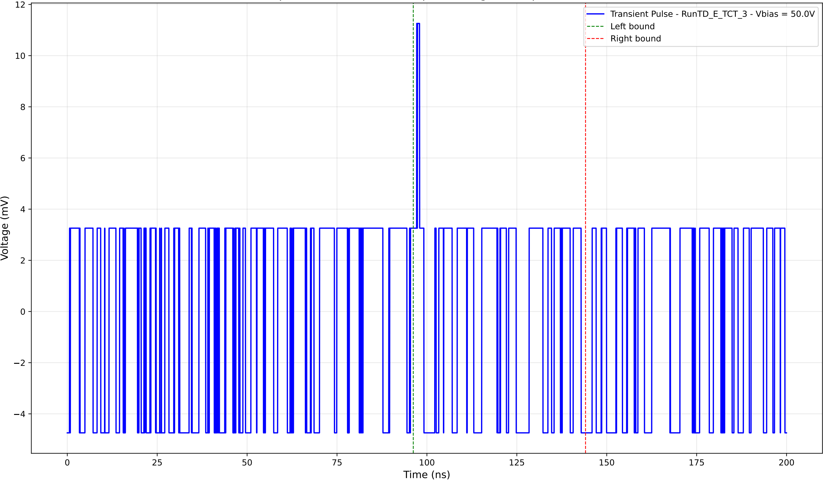
Transient Pulse - Sample: TD - Position: 190.0 \mu\text{m} - Charge: 0.51 pC - Rise Time: 0.00 ns (N/A)
