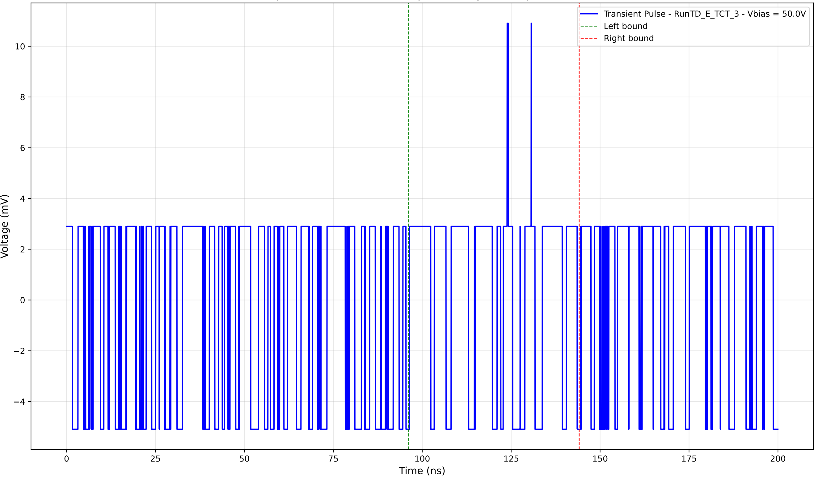
Transient Pulse - Sample: TD - Position: 255.0 \mu\text{m} - Charge: 0.70 pC - Rise Time: 0.00 ns (N/A)
