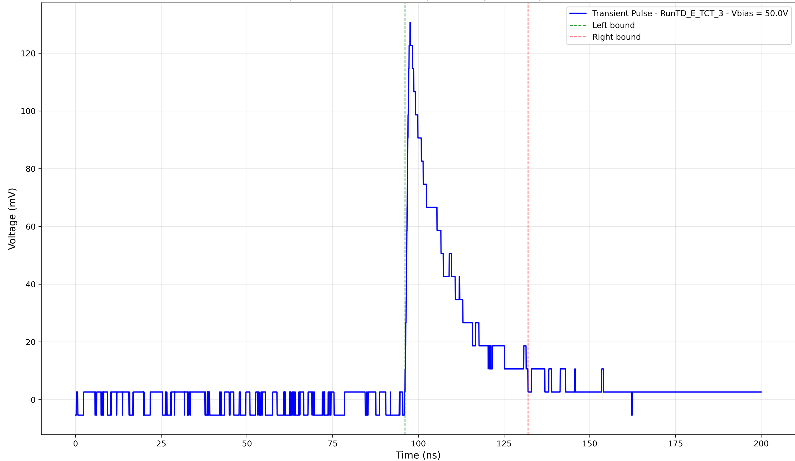
Transient Pulse - Sample: TD - Position: 525.0 \mu\text{m} - Charge: 28.78 pC - Rise Time: 1.05 ns
