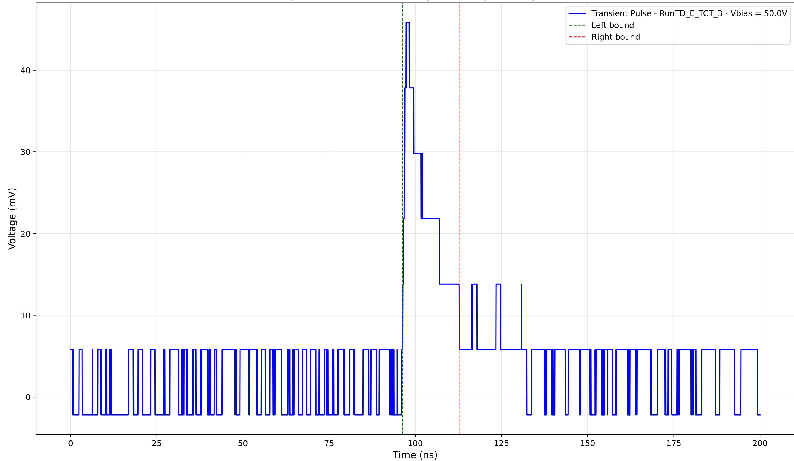
Transient Pulse - Sample: TD - Position: 725.0 \mu\text{m} - Charge: 7.56 pC - Rise Time: 1.29 ns
