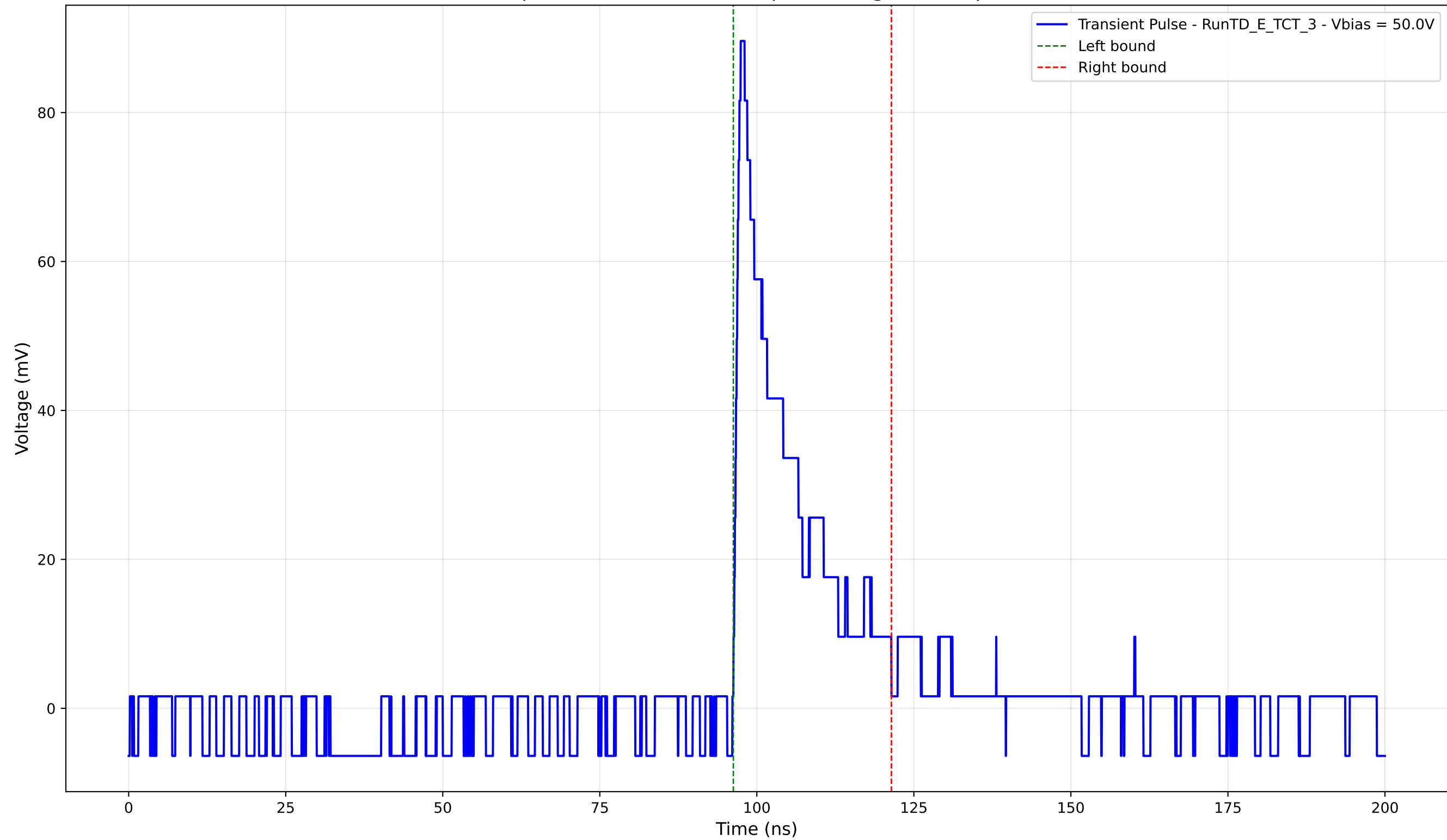
Transient Pulse - Sample: TD - Position: 595.0 \mu\text{m} - Charge: 15.05 pC - Rise Time: 0.94 ns
