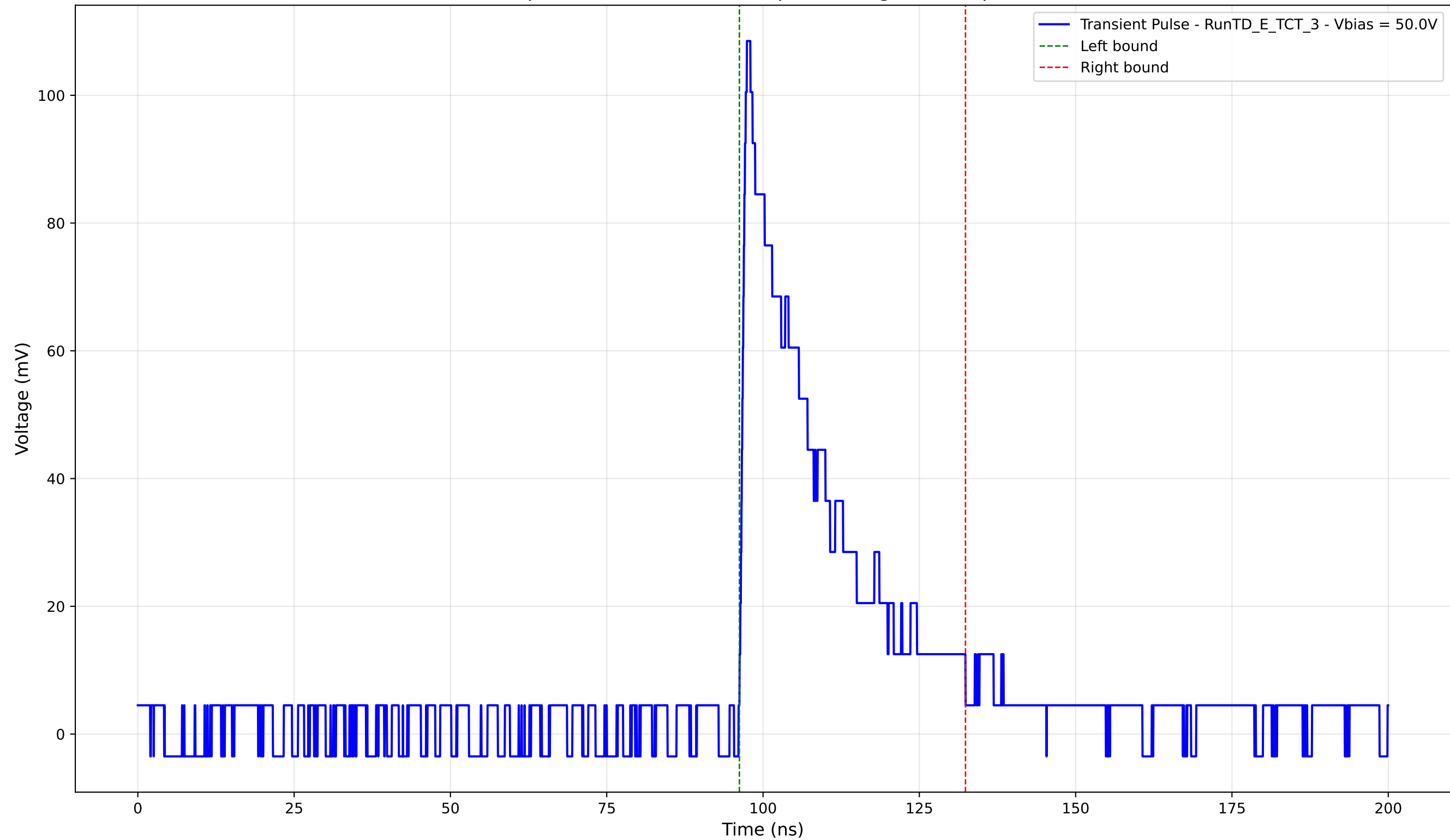
Transient Pulse - Sample: TD - Position: 340.0 \mu\text{m} - Charge: 26.71 pC - Rise Time: 0.98 ns
