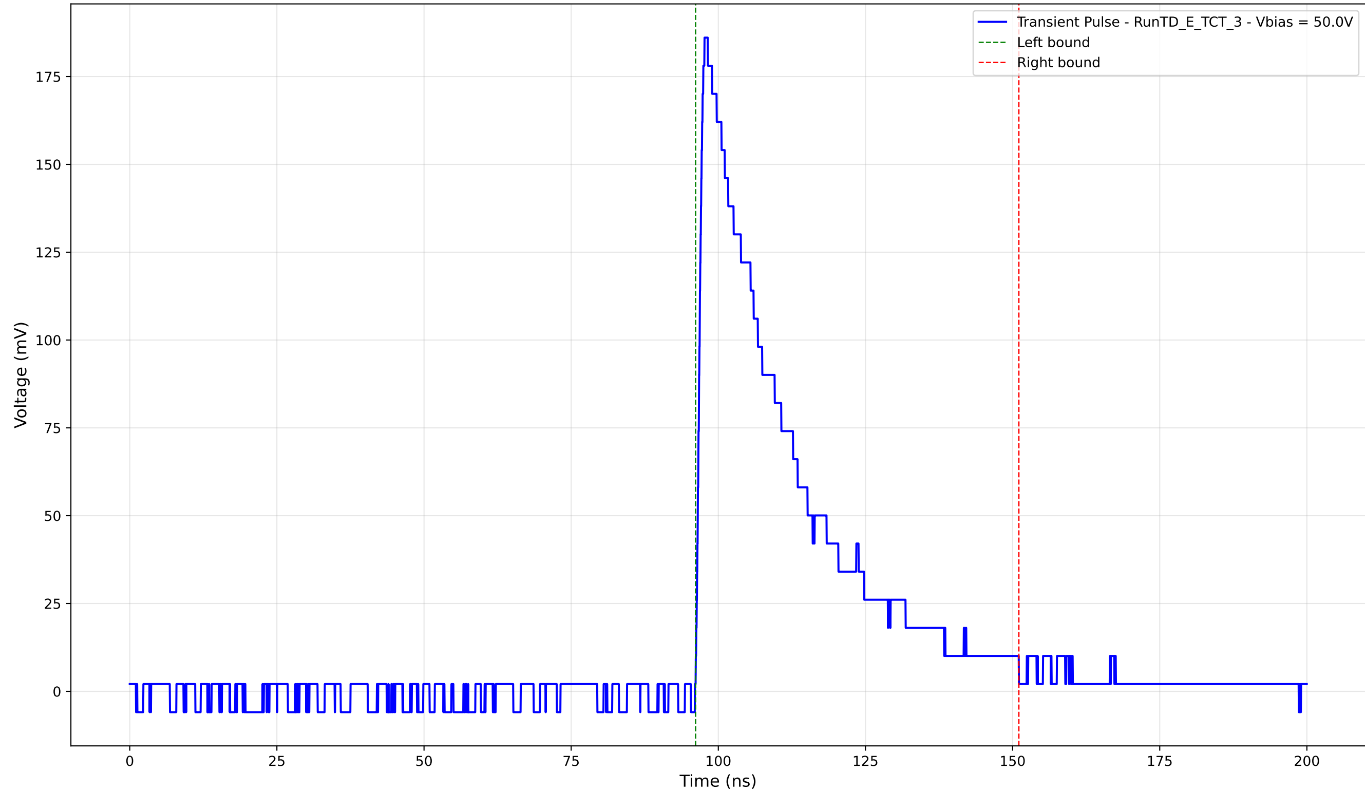
Transient Pulse - Sample: TD - Position: 370.0 \mu\text{m} - Charge: 58.68 pC - Rise Time: 1.02 ns
