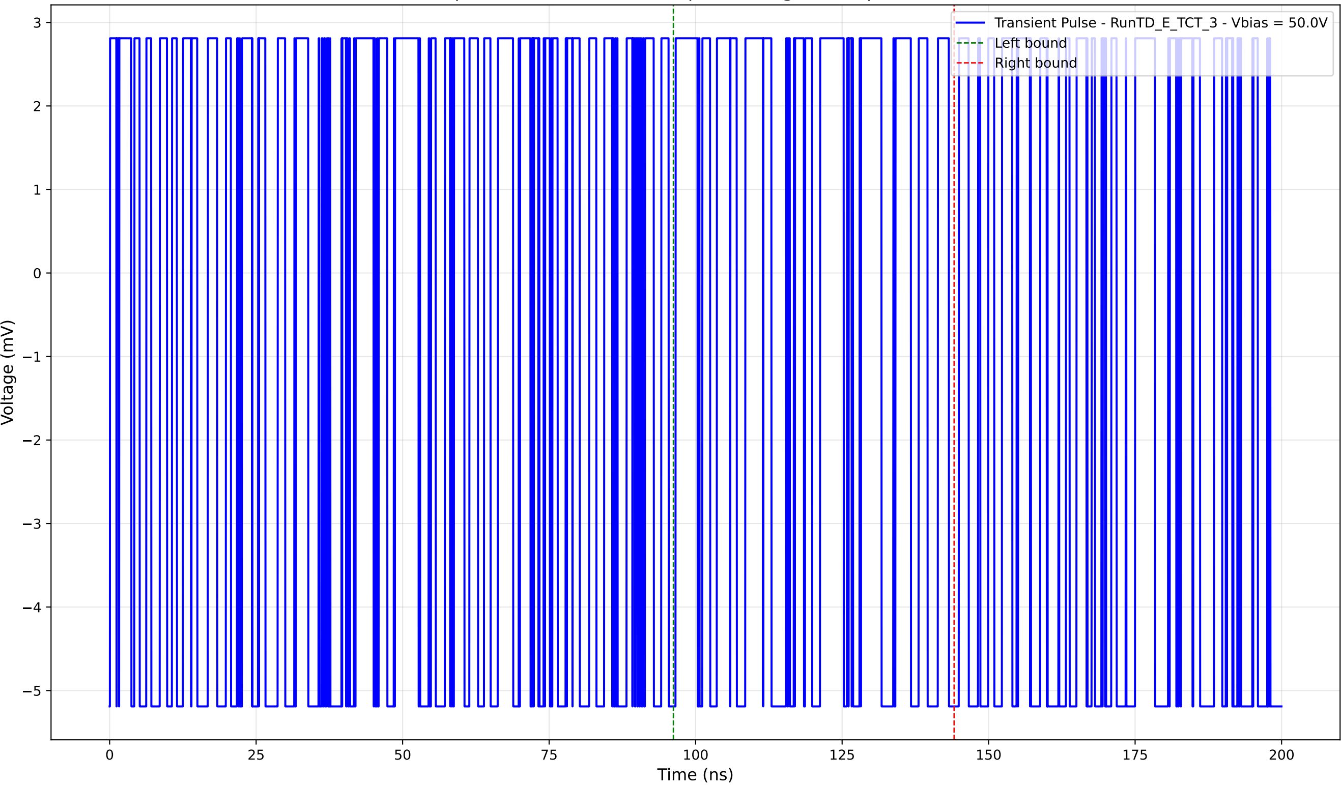
Transient Pulse - Sample: TD - Position: 180.0 \mu\text{m} - Charge: 0.03 pC - Rise Time: 0.00 ns (N/A)
