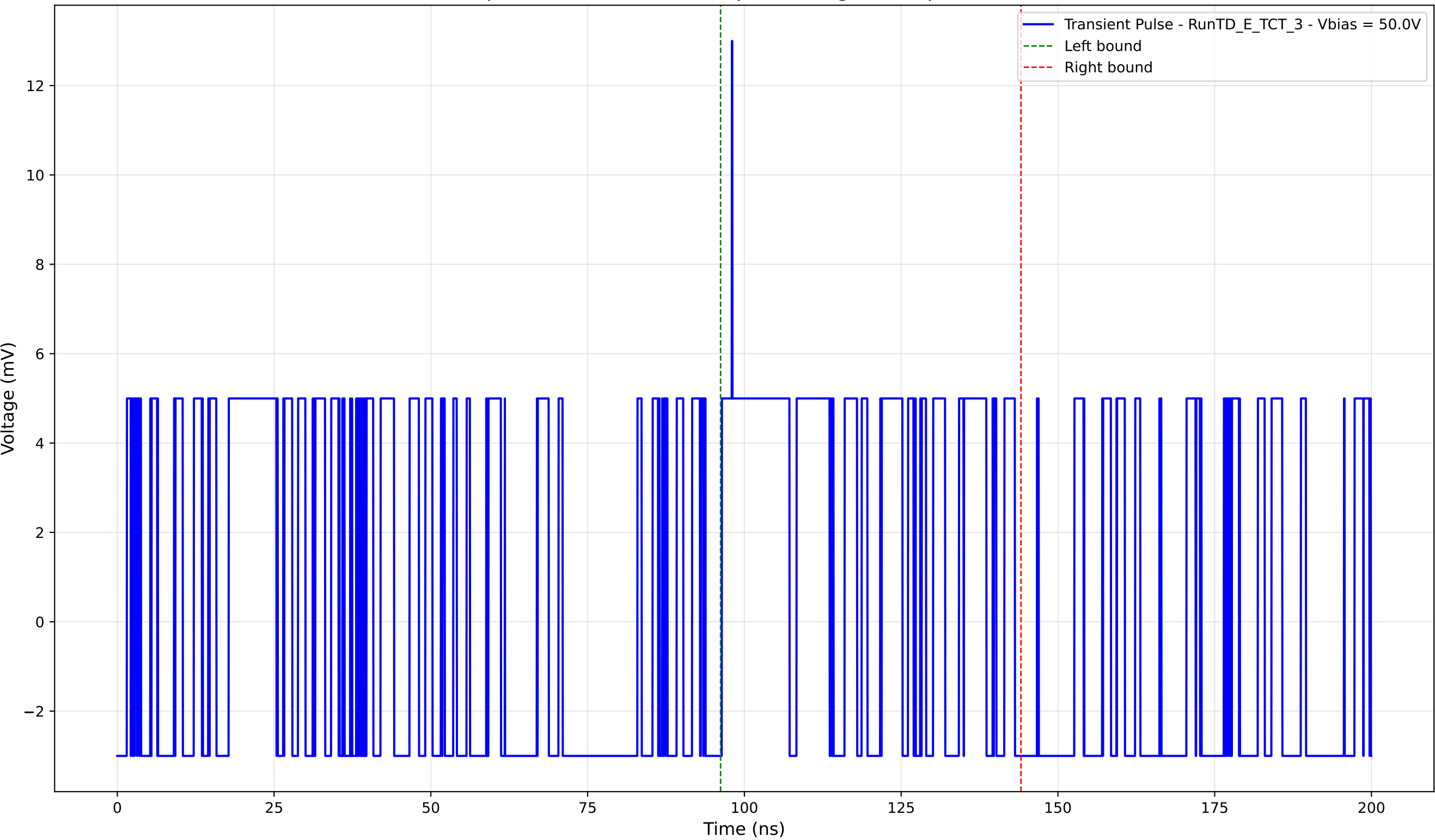
Transient Pulse - Sample: TD - Position: 280.0 \mu\text{m} - Charge: 2.39 pC - Rise Time: 0.00 ns (N/A)
