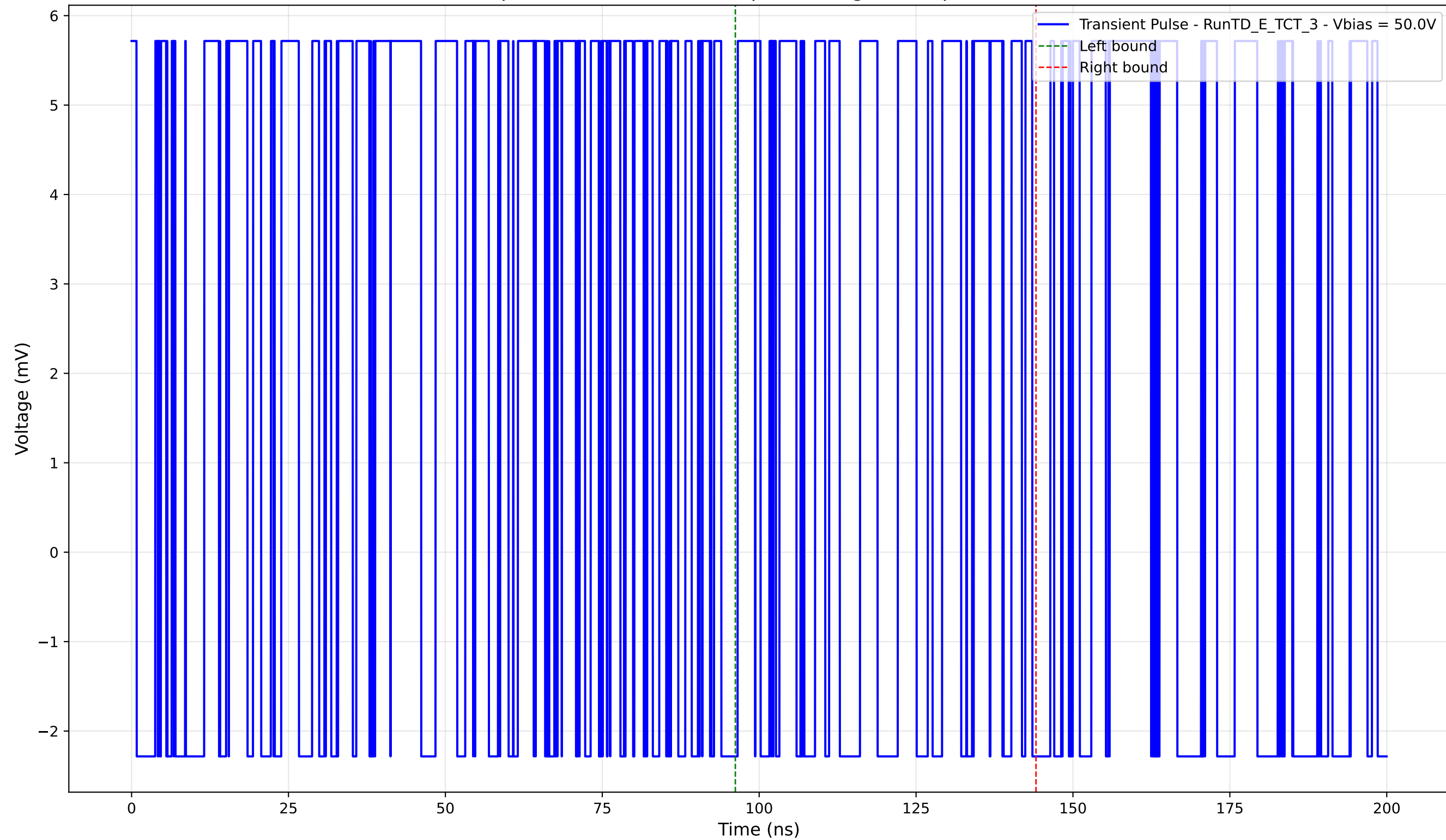
Transient Pulse - Sample: TD - Position: 175.0 \mu\text{m} - Charge: 2.25 pC - Rise Time: 0.00 ns (N/A)
