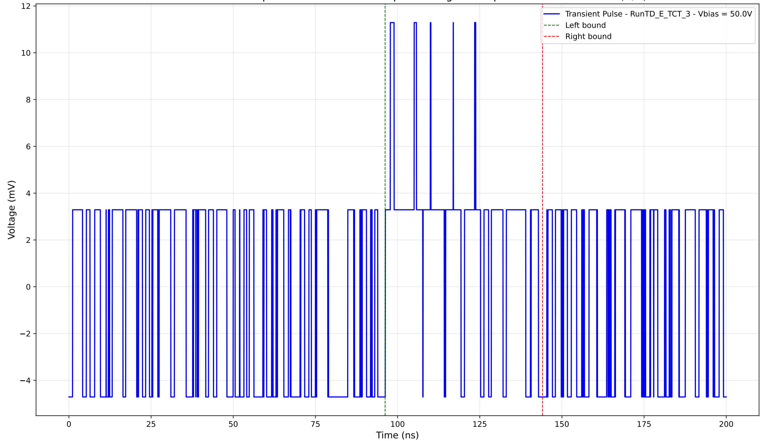
Transient Pulse - Sample: TD - Position: 285.0 \mu\text{m} - Charge: 2.41 pC - Rise Time: 0.00 ns (N/A)
