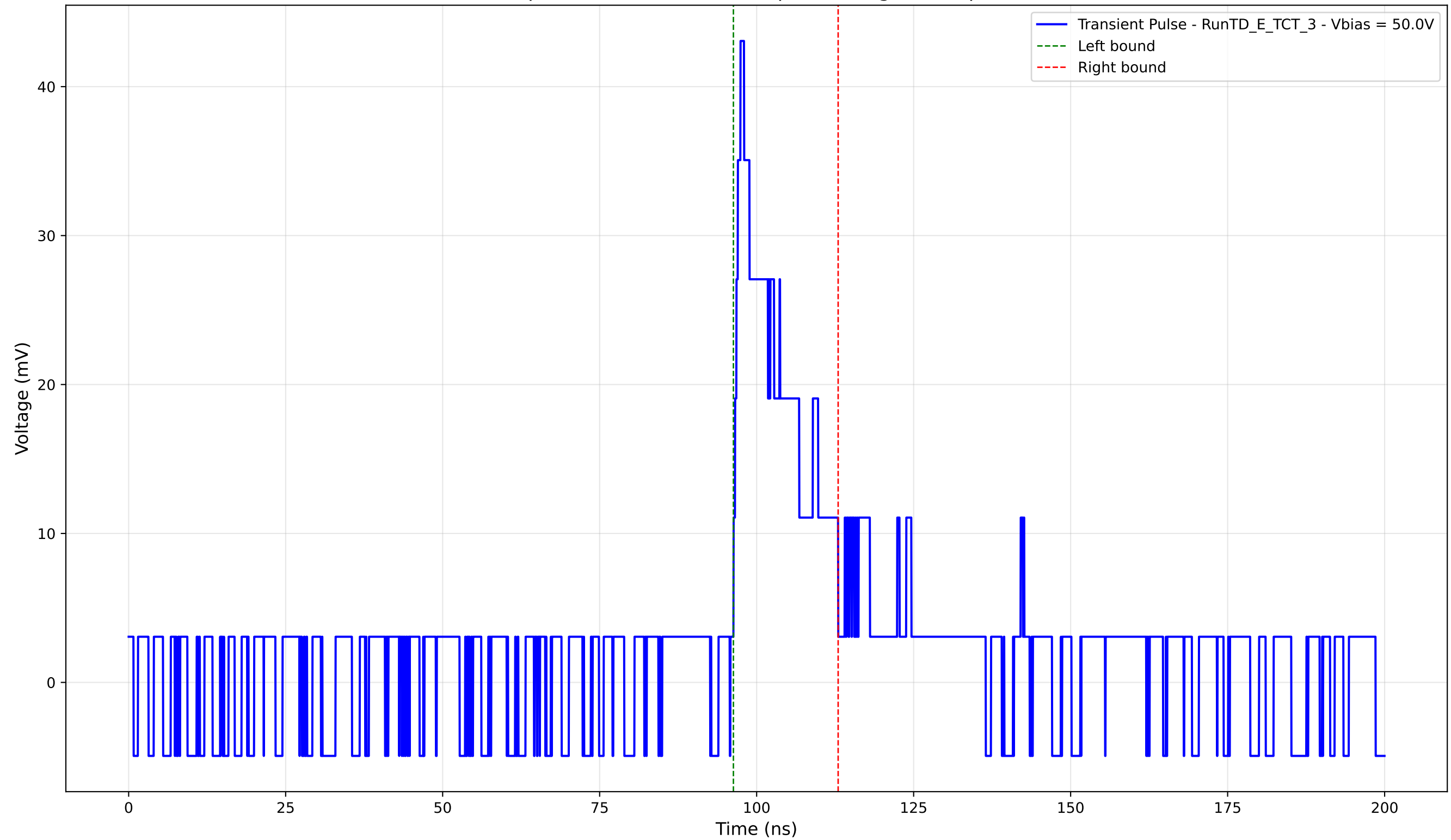
Transient Pulse - Sample: TD - Position: 720.0 \mu\text{m} - Charge: 6.78 pC - Rise Time: 1.12 ns
