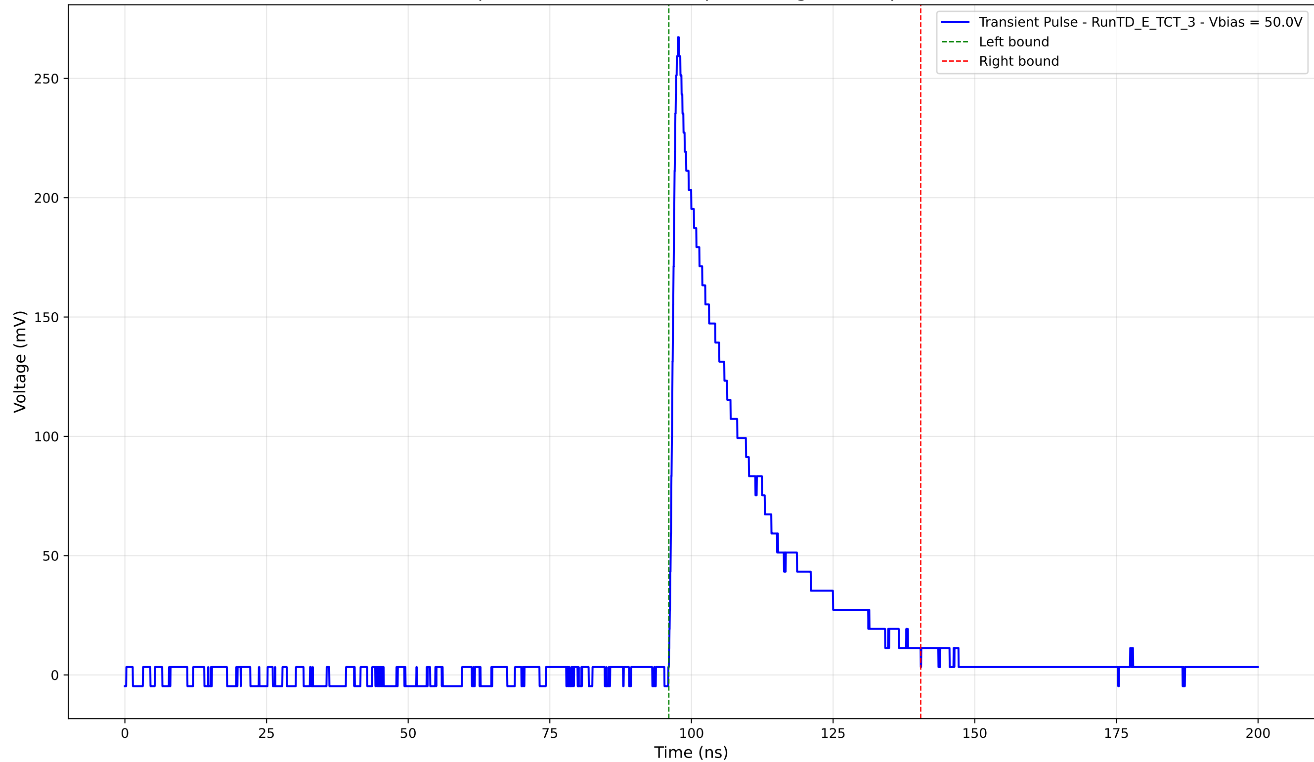
Transient Pulse - Sample: TD - Position: 450.0 \mu\text{m} - Charge: 65.25 pC - Rise Time: 1.06 ns
