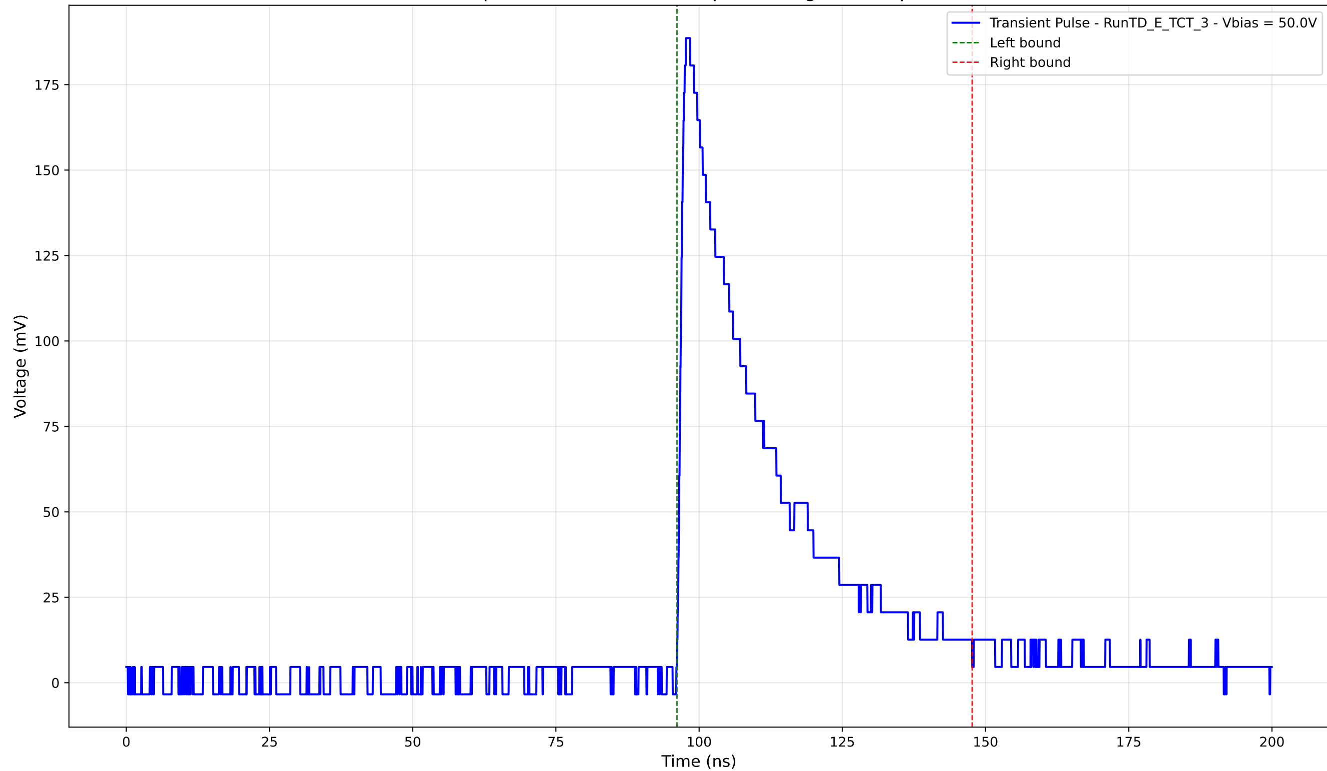
Transient Pulse - Sample: TD - Position: 395.0 \mu\text{m} - Charge: 58.61 pC - Rise Time: 1.10 ns
