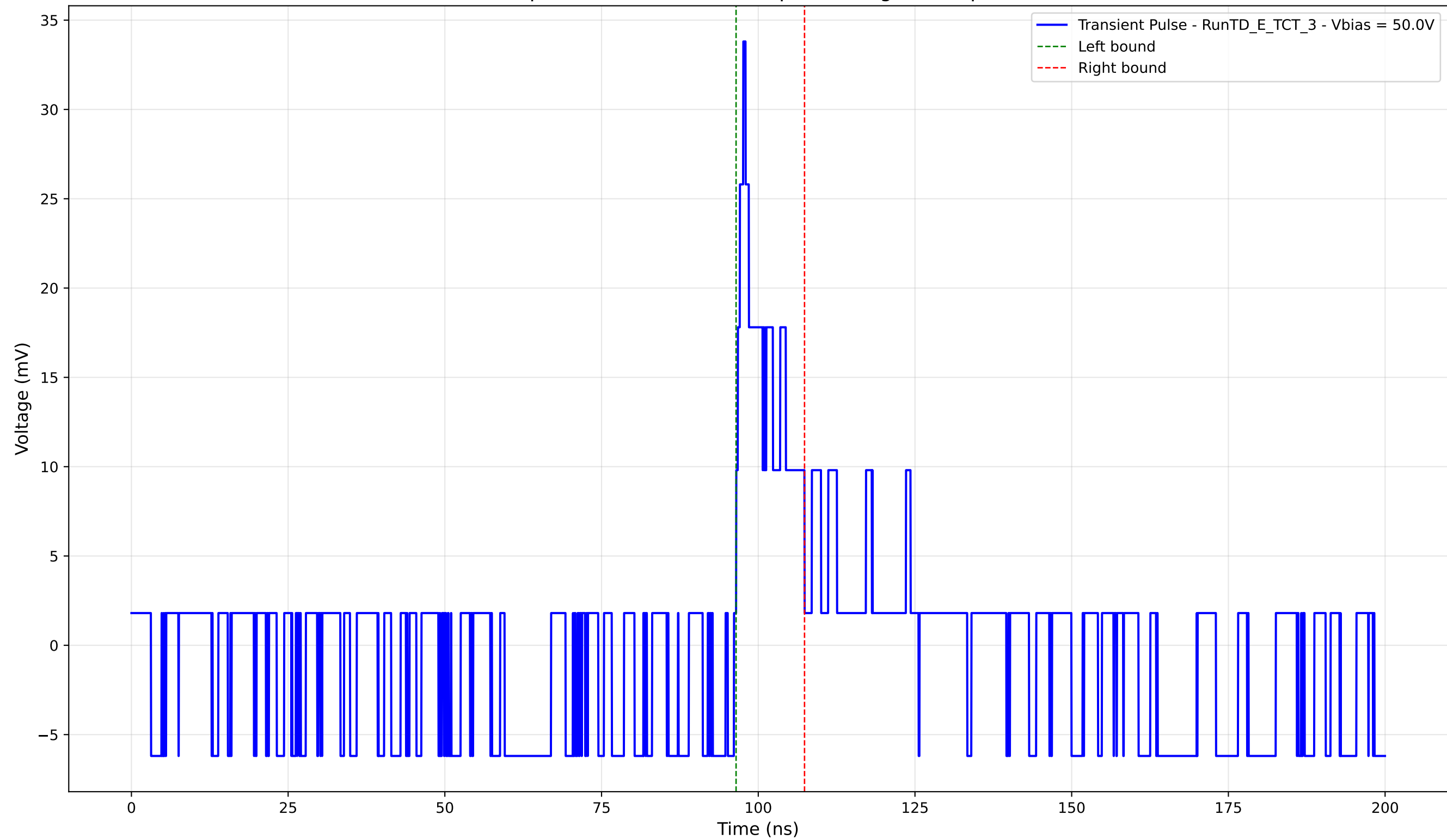
Transient Pulse - Sample: TD - Position: 660.0 \mu\text{m} - Charge: 3.41 pC - Rise Time: 1.14 ns
