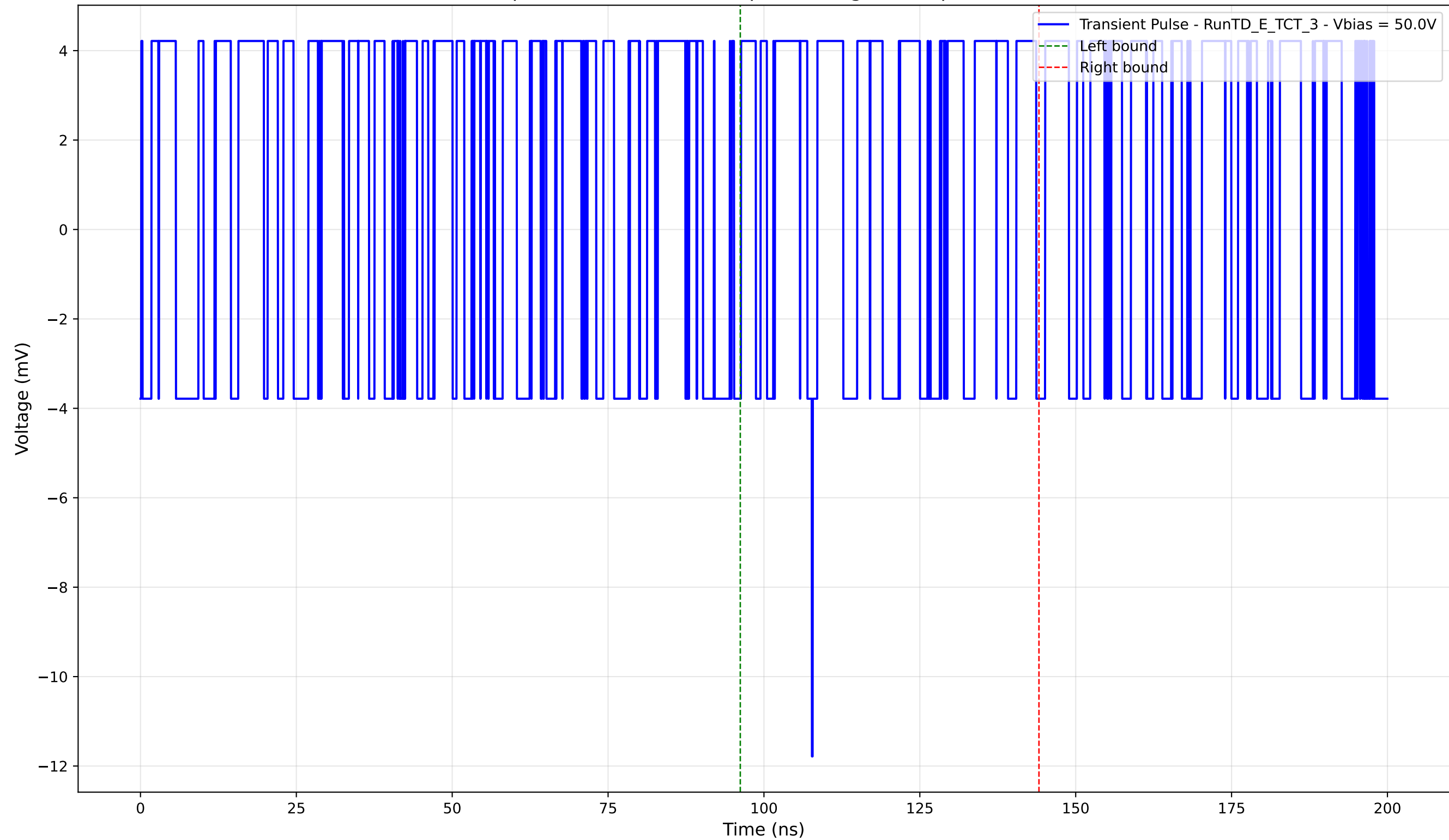
Transient Pulse - Sample: TD - Position: 45.0 \mu m - Charge: 1.50 pC - Rise Time: 0.00 ns (N/A)
