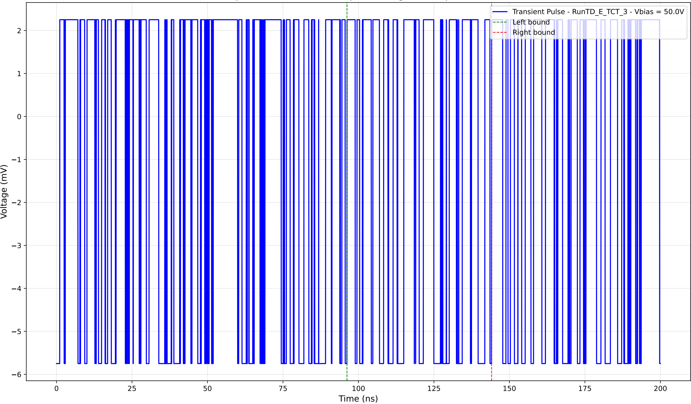
Transient Pulse - Sample: TD - Position: 90.0 \mu\text{m} - Charge: -0.73 pC - Rise Time: 0.00 ns (N/A)
