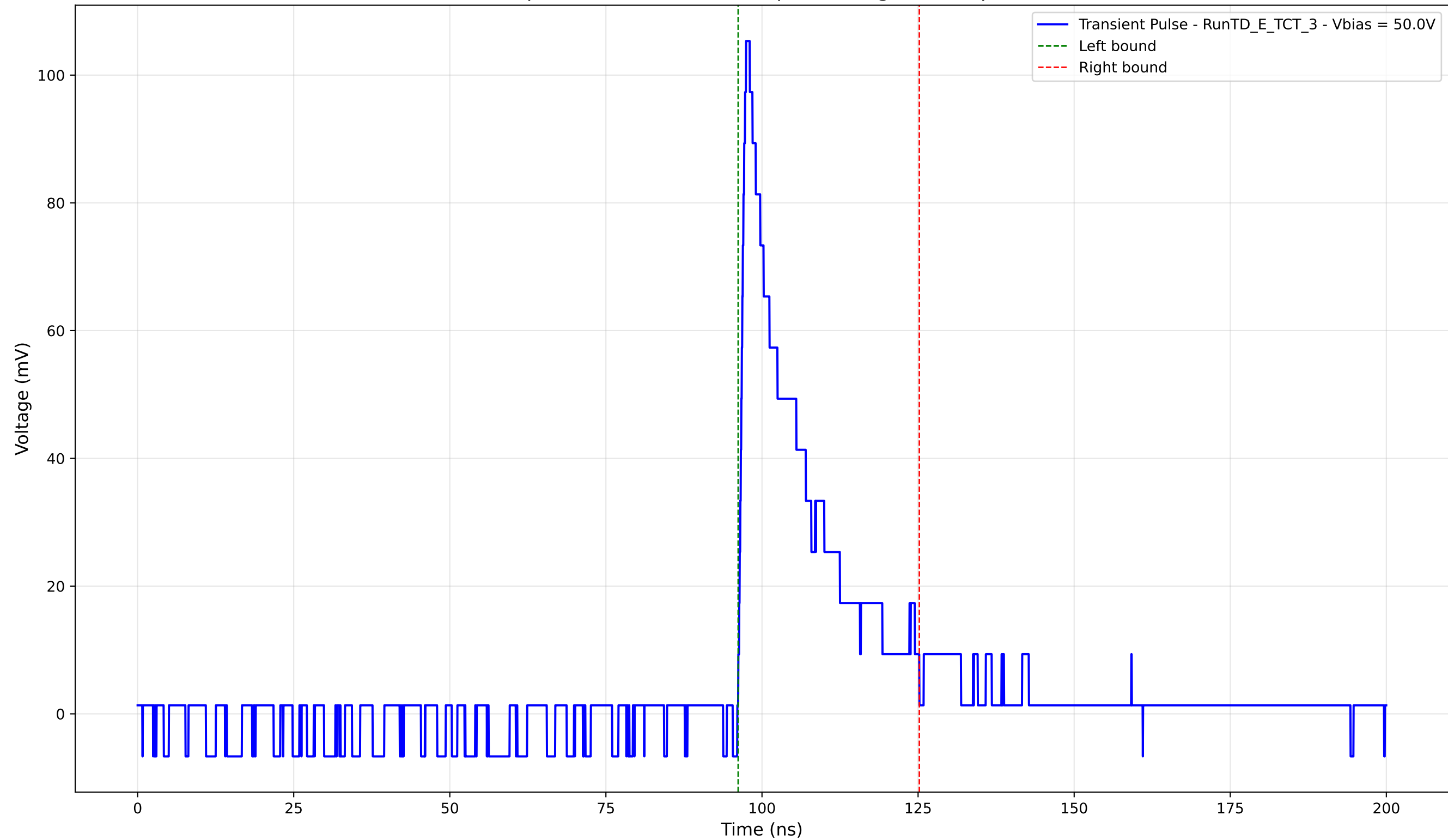
Transient Pulse - Sample: TD - Position: 560.0 \mu\text{m} - Charge: 20.06 pC - Rise Time: 0.96 ns
