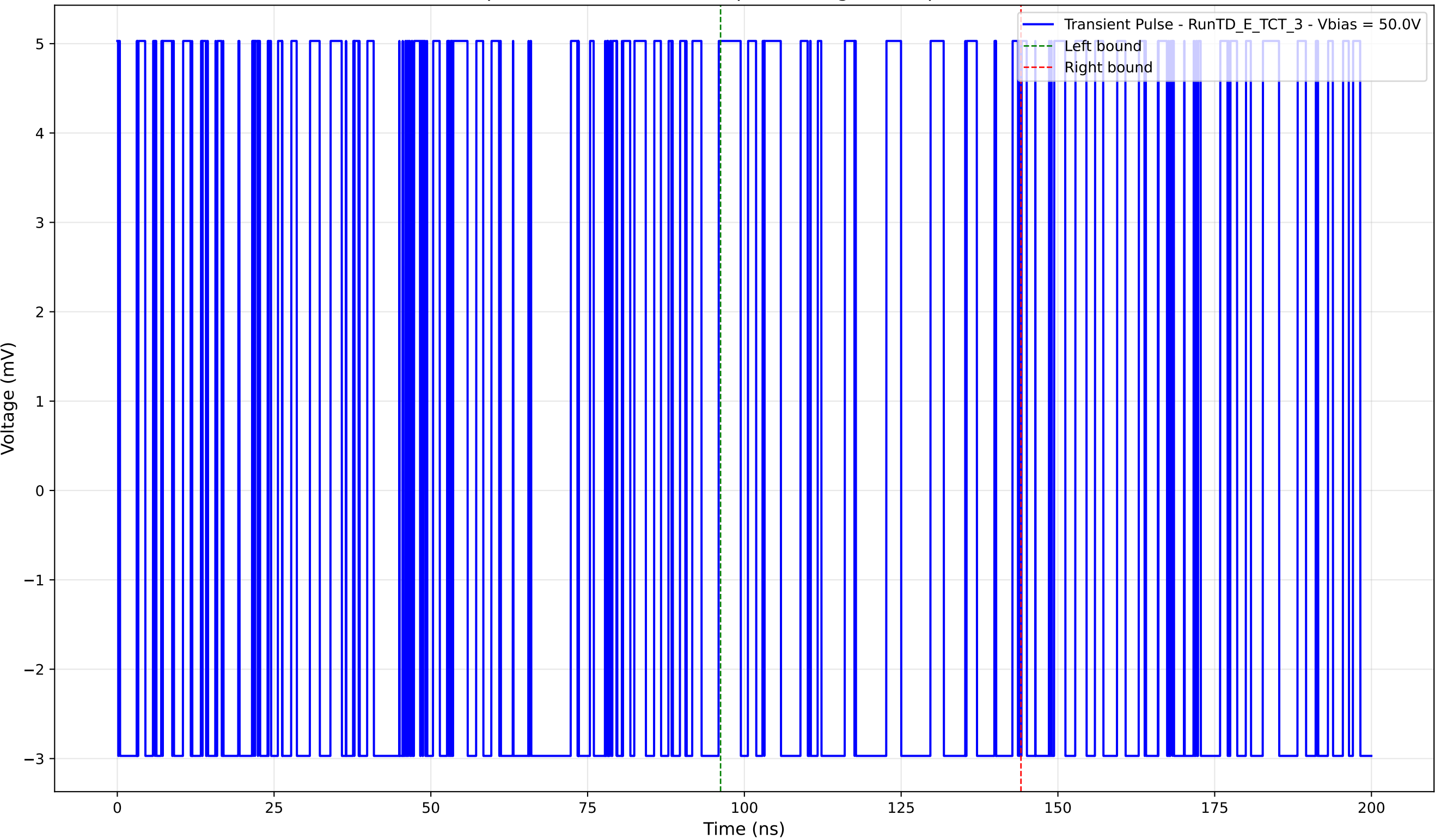
Transient Pulse - Sample: TD - Position: 155.0 \mu\text{m} - Charge: 0.13 pC - Rise Time: 0.00 ns (N/A)
