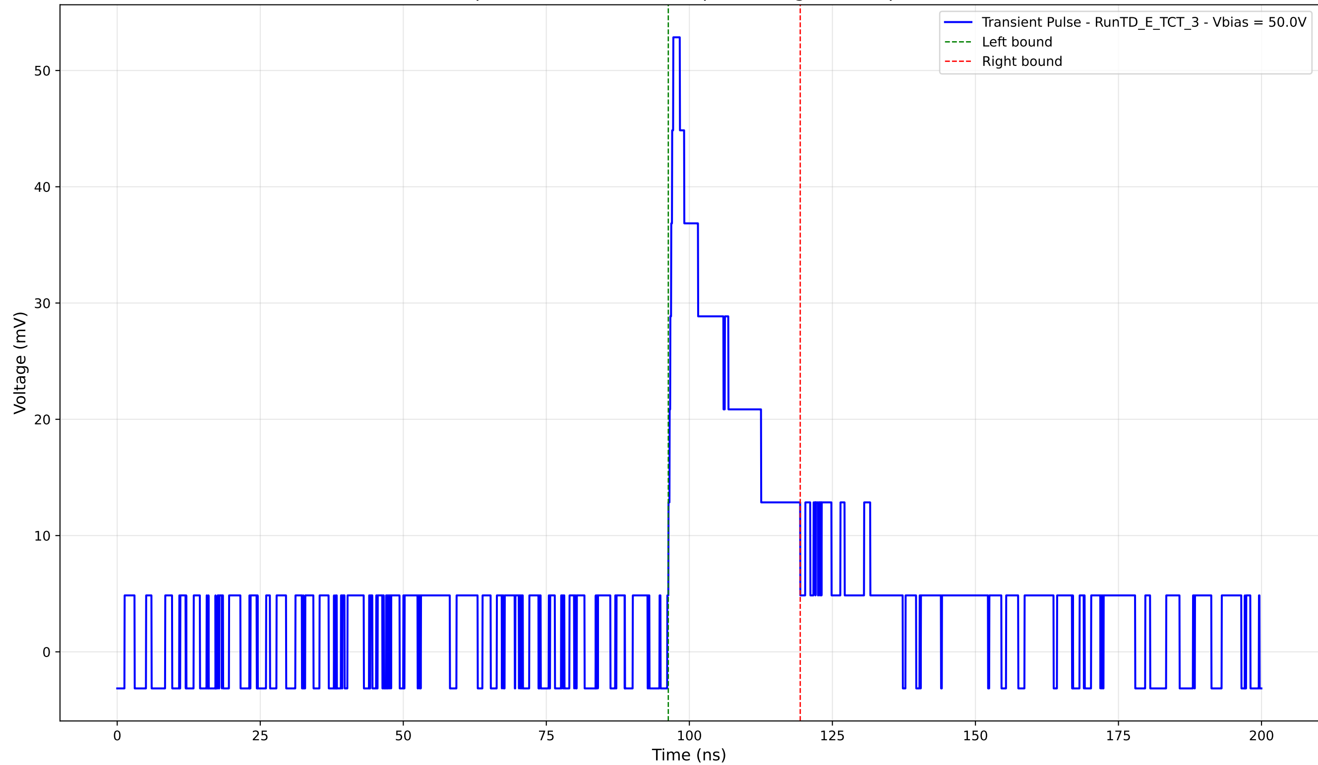
Transient Pulse - Sample: TD - Position: 330.0 \mu\text{m} - Charge: 11.35 pC - Rise Time: 0.86 ns
