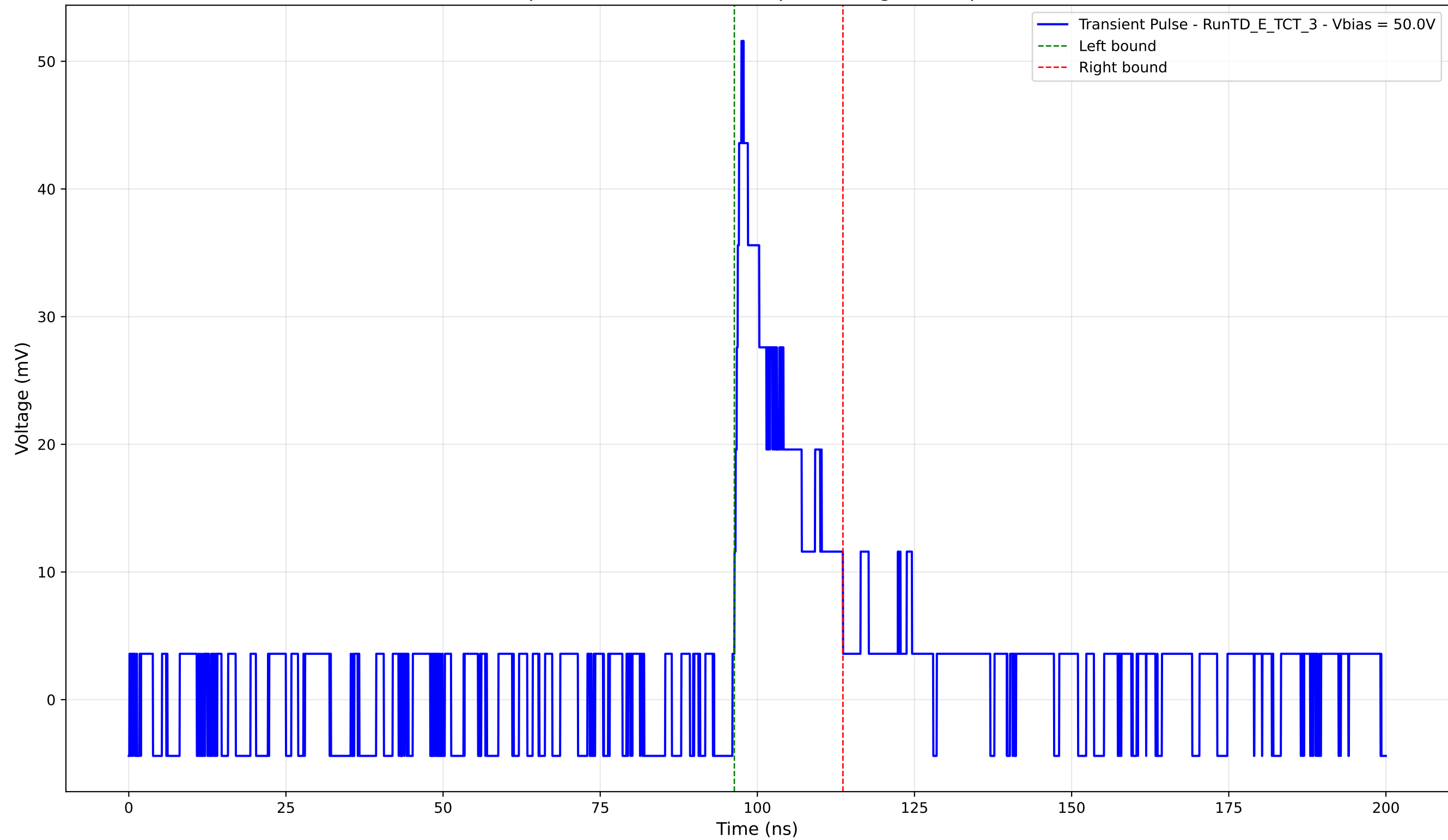
Transient Pulse - Sample: TD - Position: 645.0 \mu\text{m} - Charge: 7.66 pC - Rise Time: 1.12 ns
