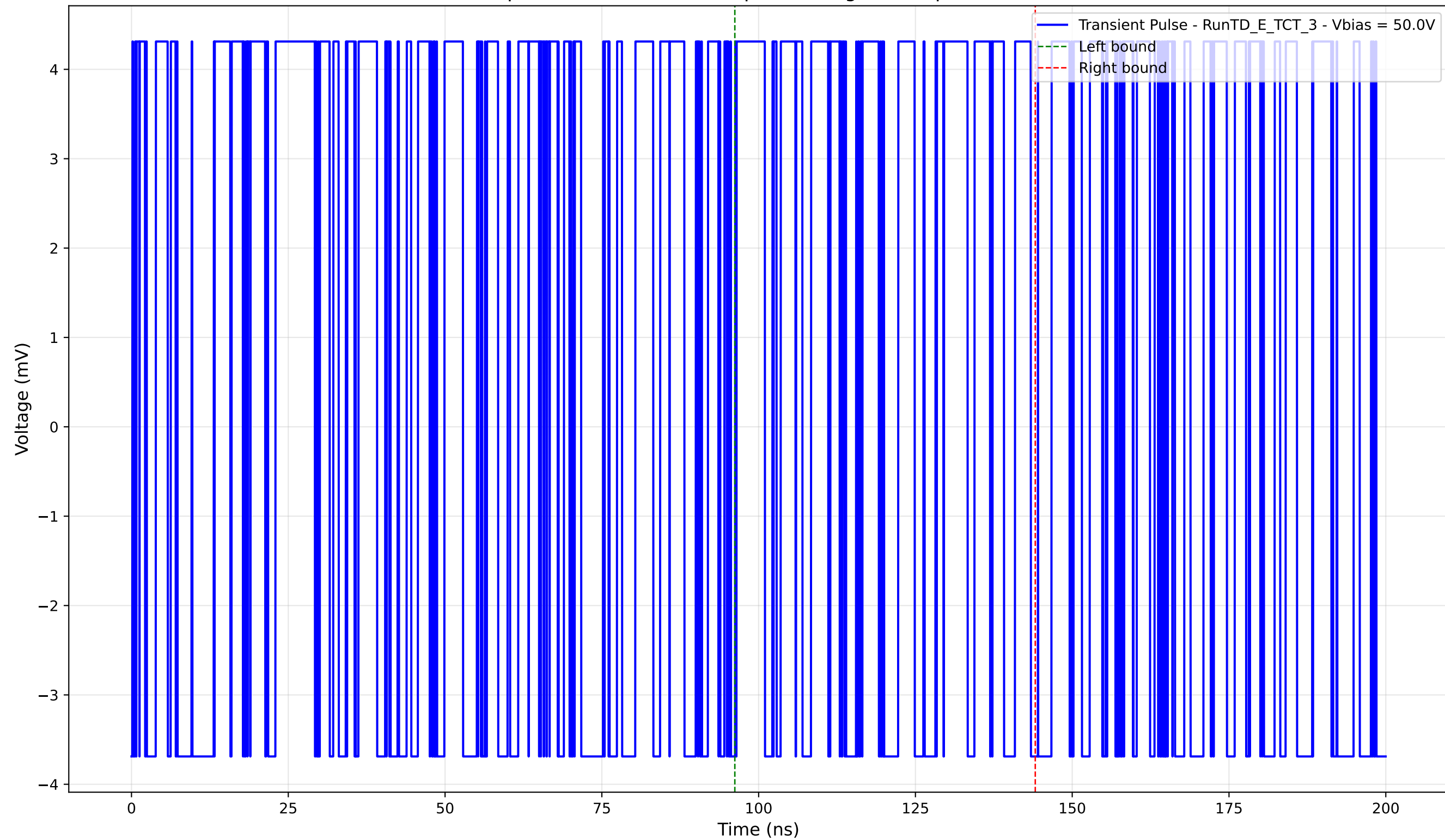
Transient Pulse - Sample: TD - Position: 50.0 \mu\text{m} - Charge: 1.52 pC - Rise Time: 0.00 ns (N/A)
