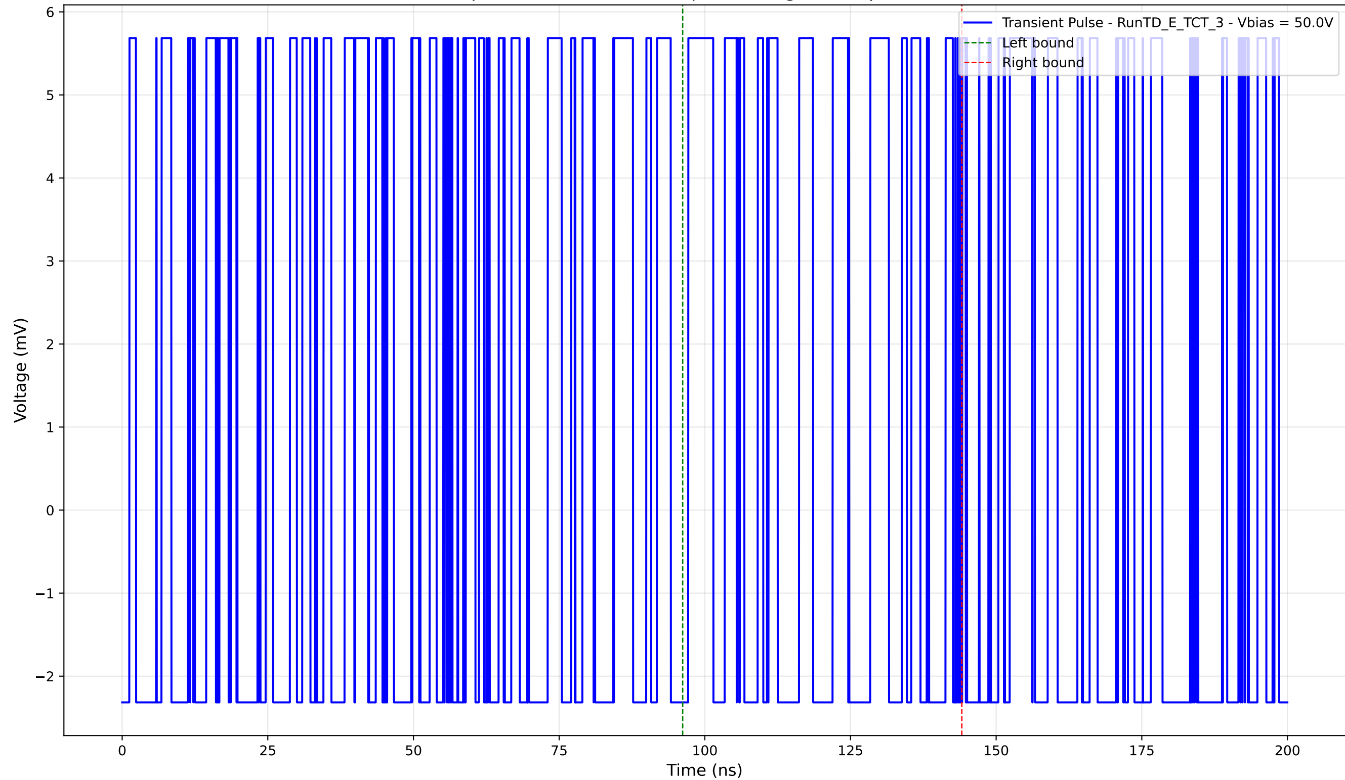
Transient Pulse - Sample: TD - Position: 35.0 \mu\text{m} - Charge: 1.42 pC - Rise Time: 0.00 ns (N/A)
