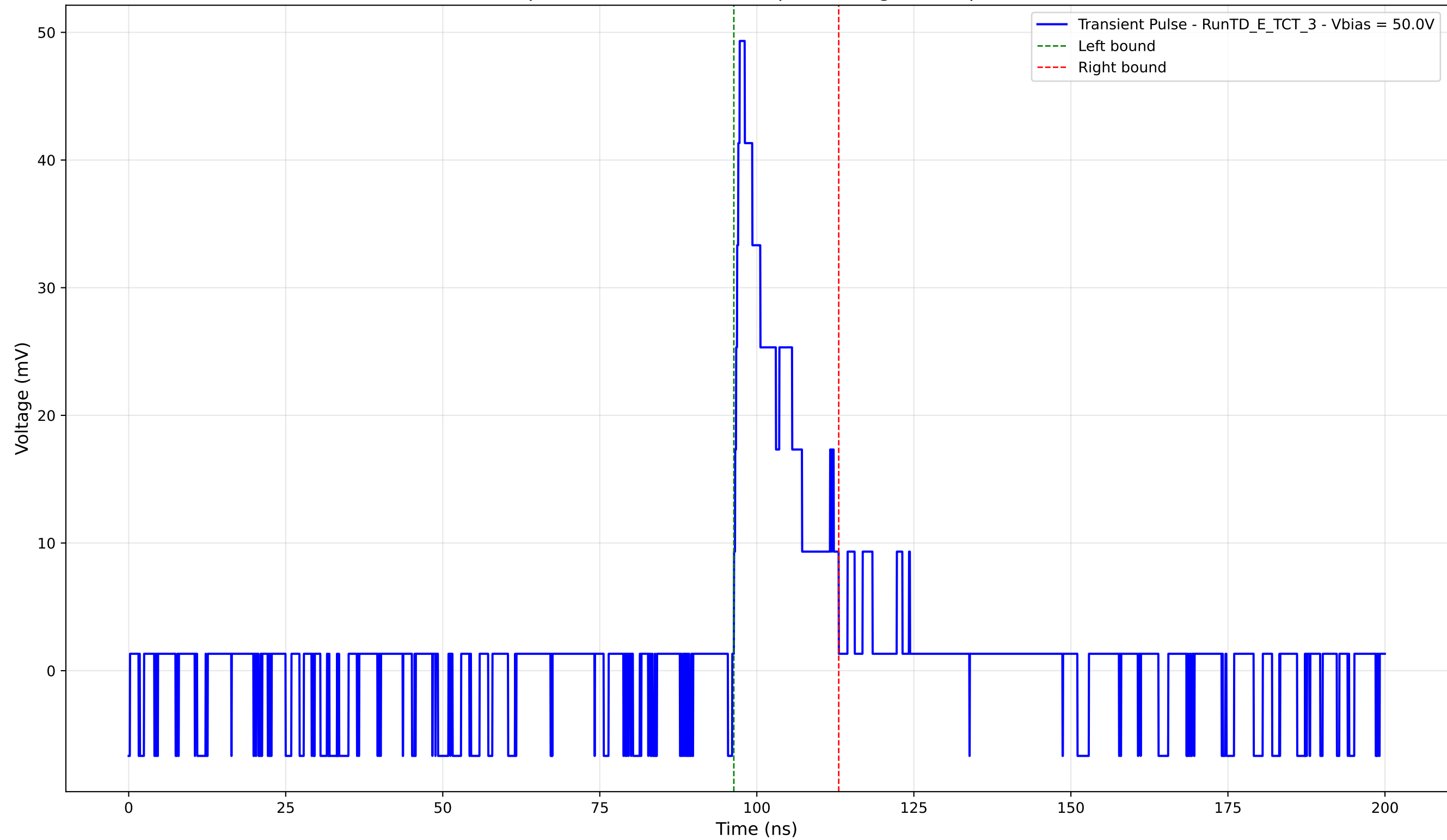
Transient Pulse - Sample: TD - Position: 630.0 \mu\text{m} - Charge: 7.32 pC - Rise Time: 0.91 ns
