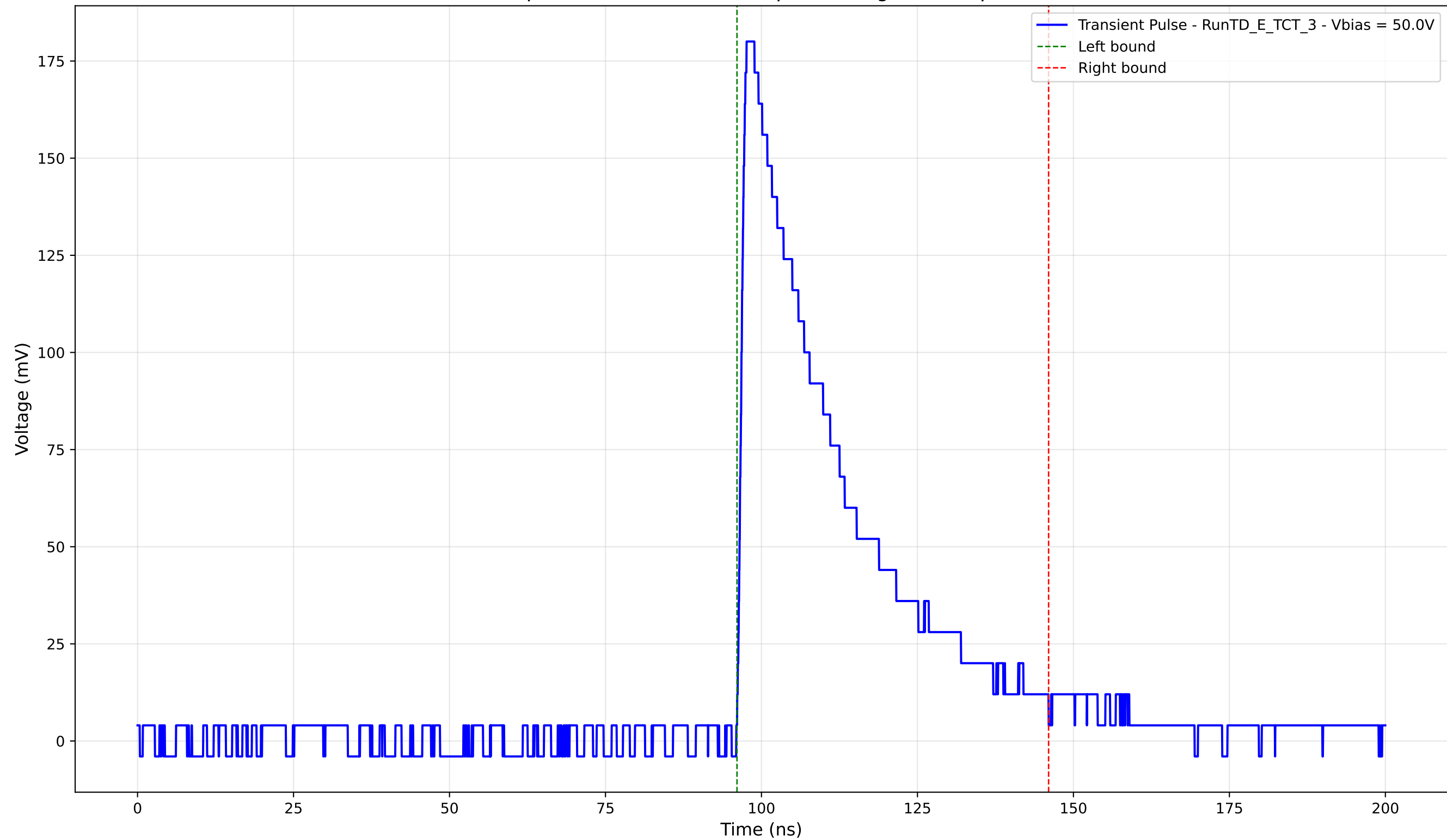
Transient Pulse - Sample: TD - Position: 375.0 \mu\text{m} - Charge: 59.78 pC - Rise Time: 1.13 ns
