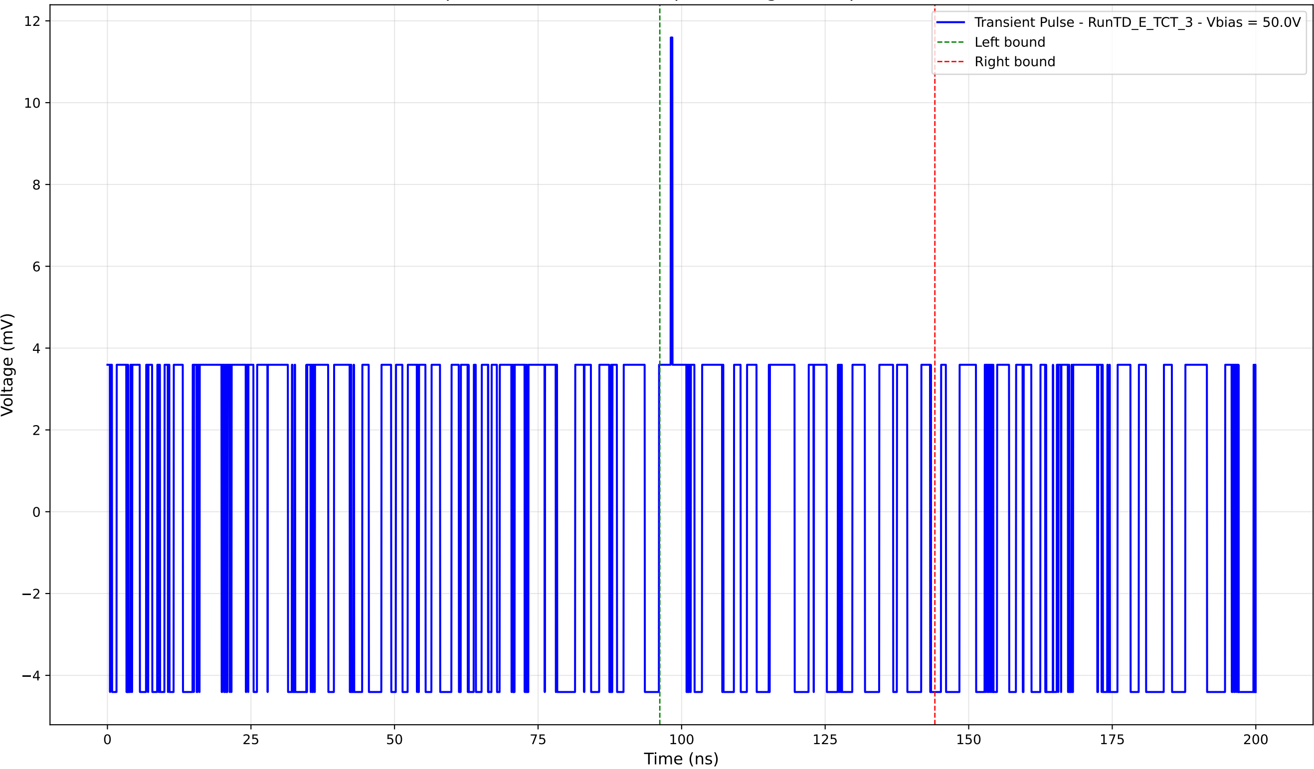
Transient Pulse - Sample: TD - Position: 235.0 \mu\text{m} - Charge: 0.30 pC - Rise Time: 0.00 ns (N/A)
