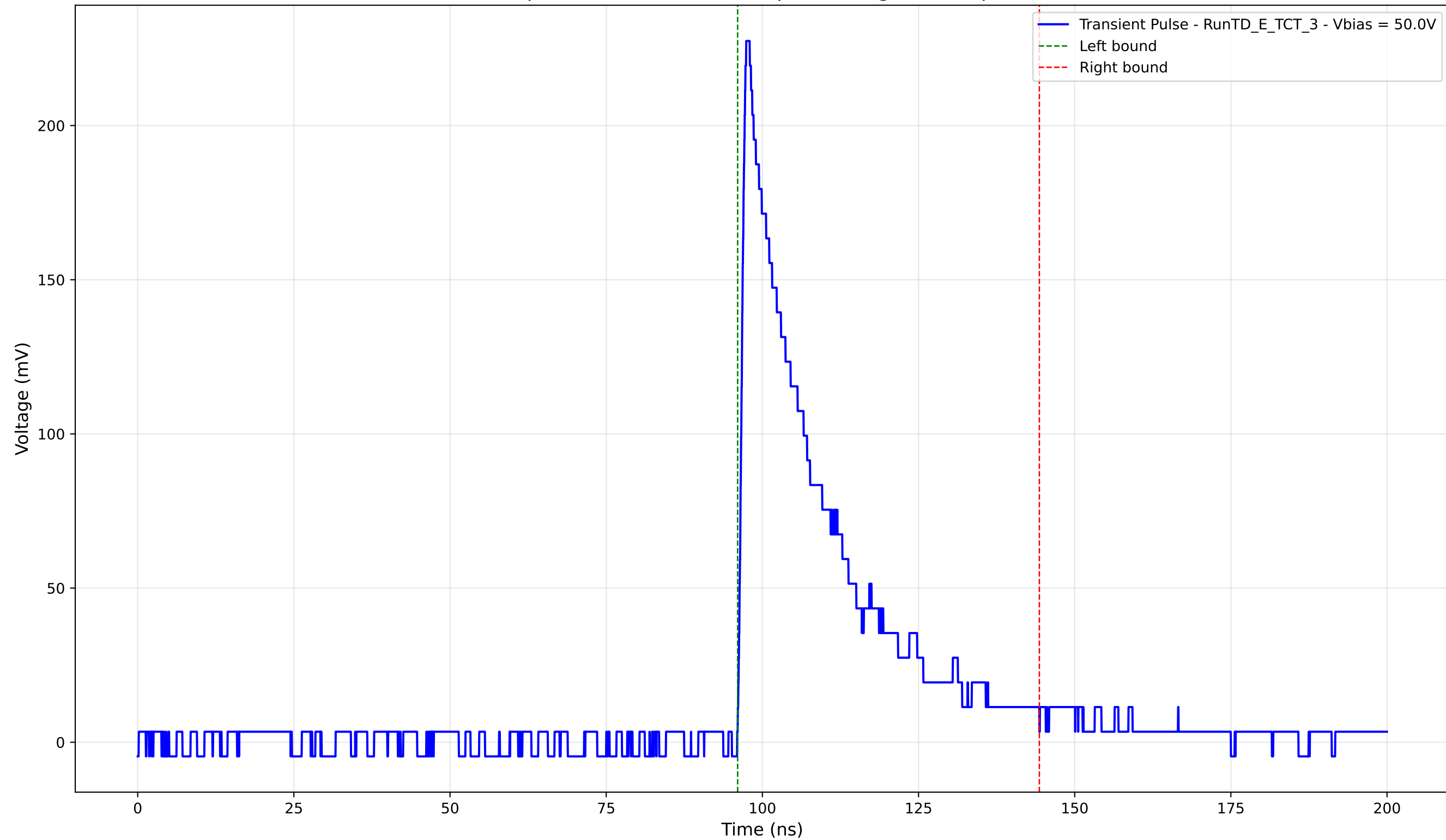
Transient Pulse - Sample: TD - Position: 470.0 \mu\text{m} - Charge: 57.29 pC - Rise Time: 1.03 ns
