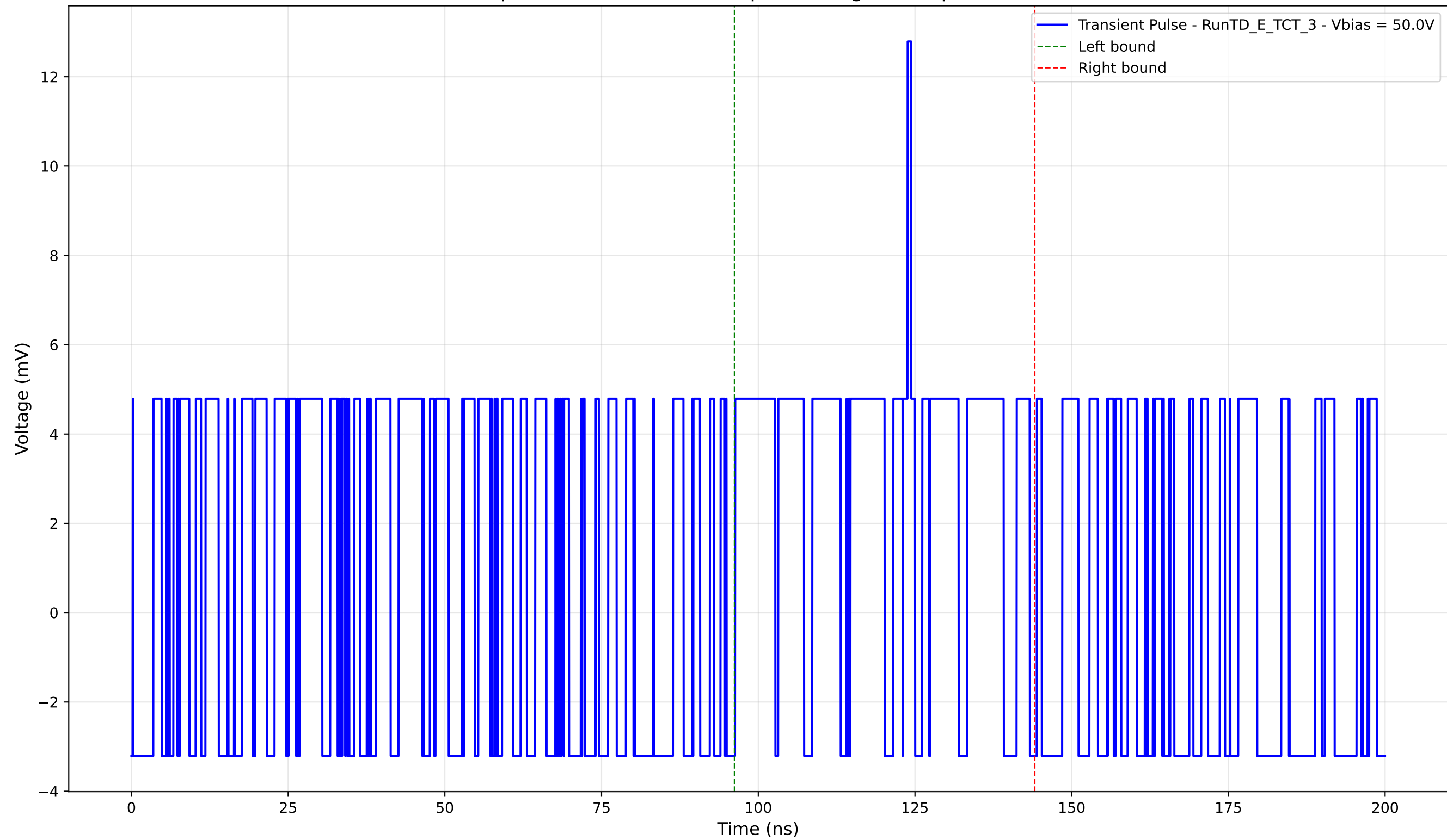
Transient Pulse - Sample: TD - Position: 260.0 \mu\text{m} - Charge: 3.07 pC - Rise Time: 0.00 ns (N/A)
