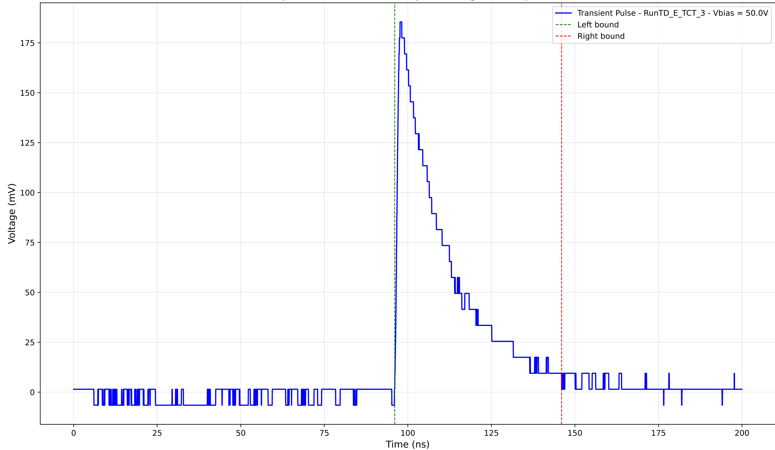
Transient Pulse - Sample: TD - Position: 390.0 \mu\text{m} - Charge: 55.91 pC - Rise Time: 1.08 ns
