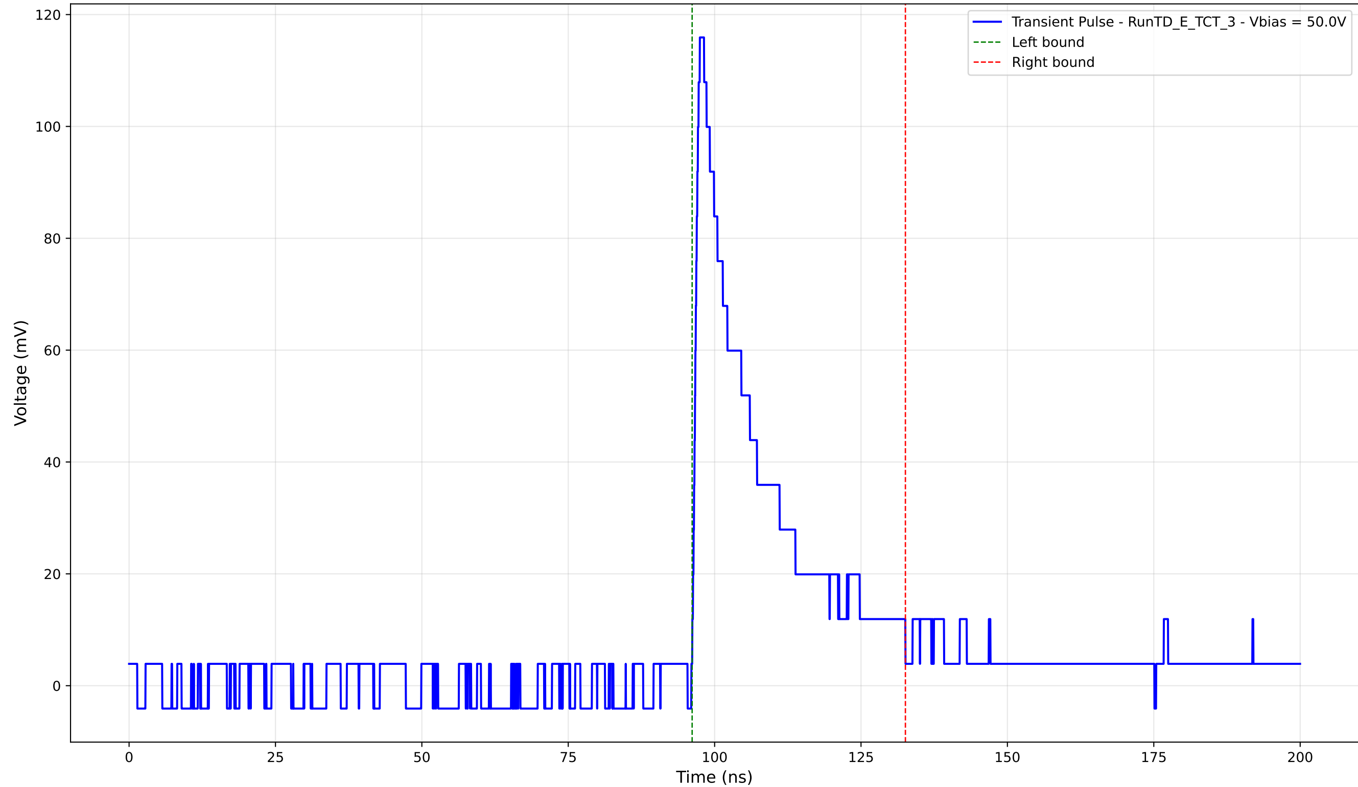
Transient Pulse - Sample: TD - Position: 545.0 \mu\text{m} - Charge: 25.83 pC - Rise Time: 1.08 ns
