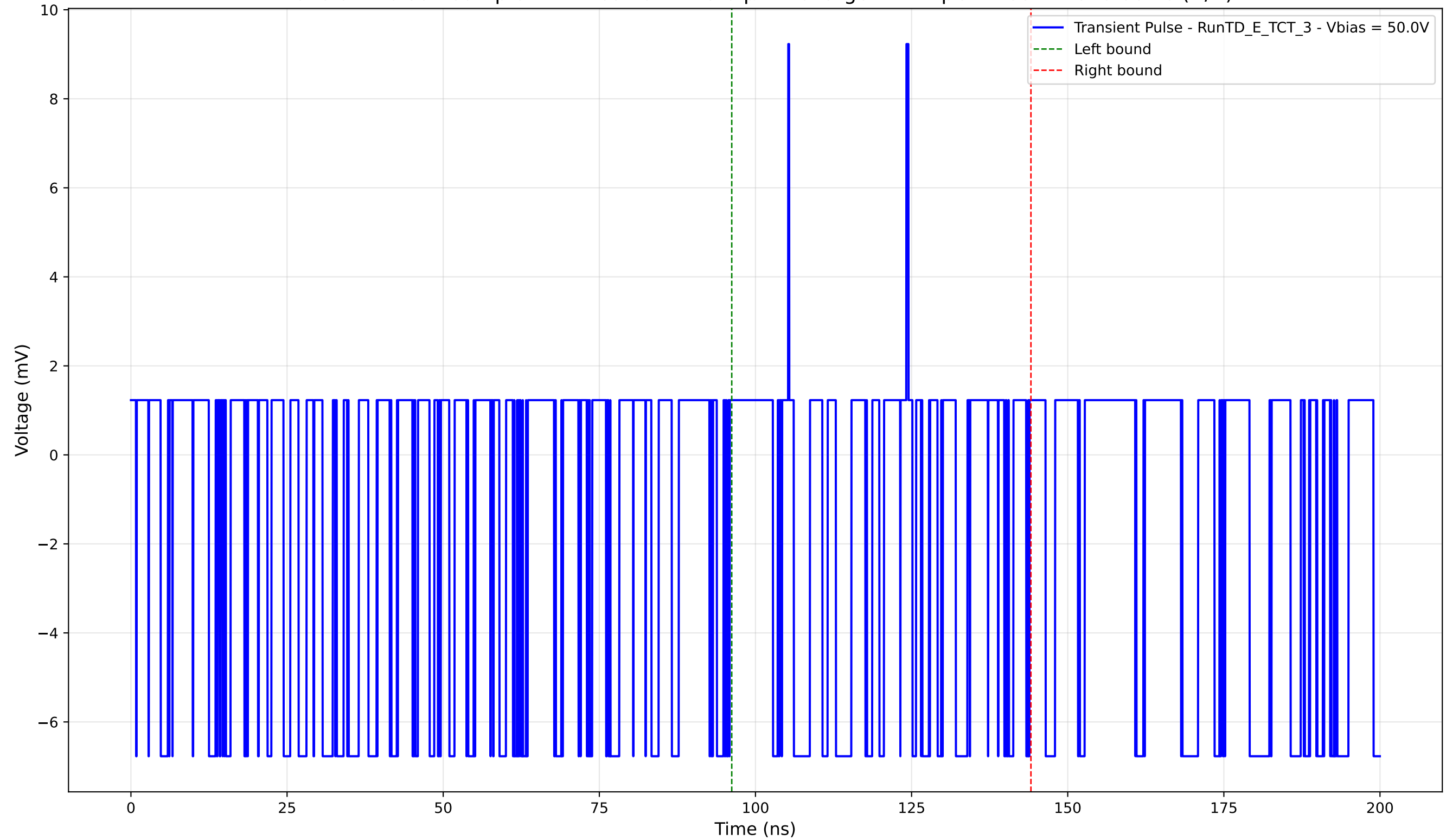
Transient Pulse - Sample: TD - Position: 145.0 \mu\text{m} - Charge: -1.14 pC - Rise Time: 0.00 ns (N/A)
