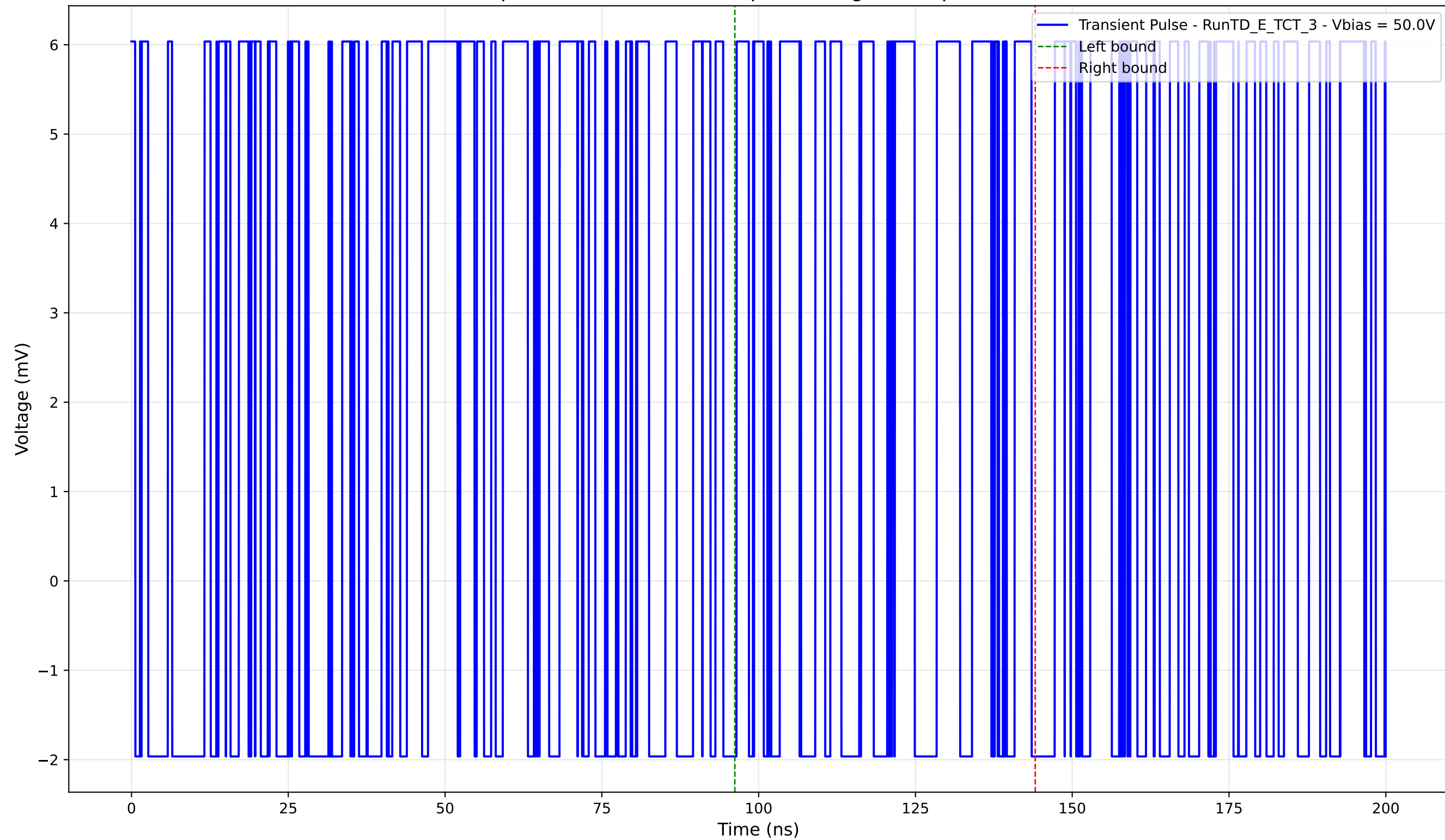
Transient Pulse - Sample: TD - Position: 105.0 \mu\text{m} - Charge: 2.46 pC - Rise Time: 0.00 ns (N/A)
