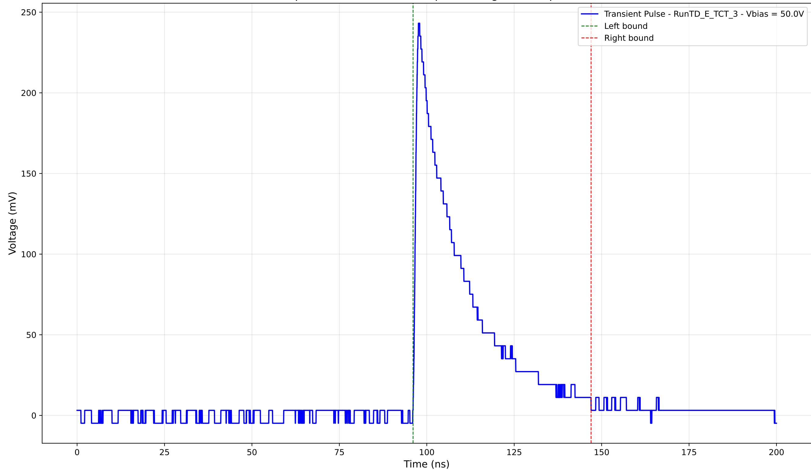
Transient Pulse - Sample: TD - Position: 415.0 \mu\text{m} - Charge: 66.62 pC - Rise Time: 1.05 ns
