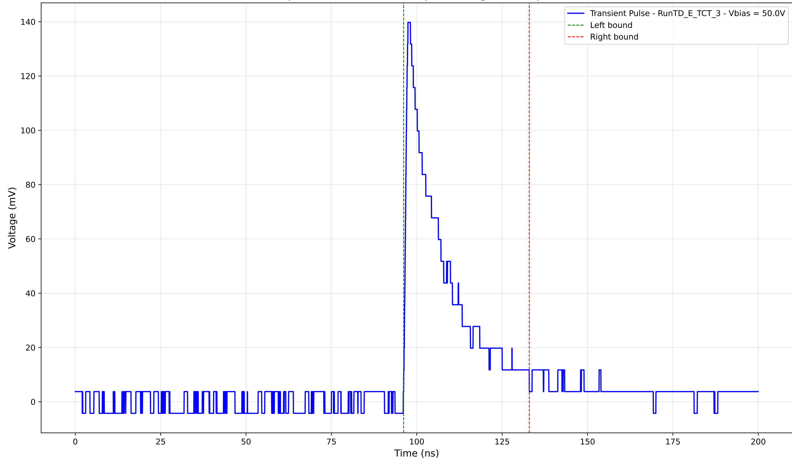
Transient Pulse - Sample: TD - Position: 510.0 \mu\text{m} - Charge: 31.73 pC - Rise Time: 1.01 ns
