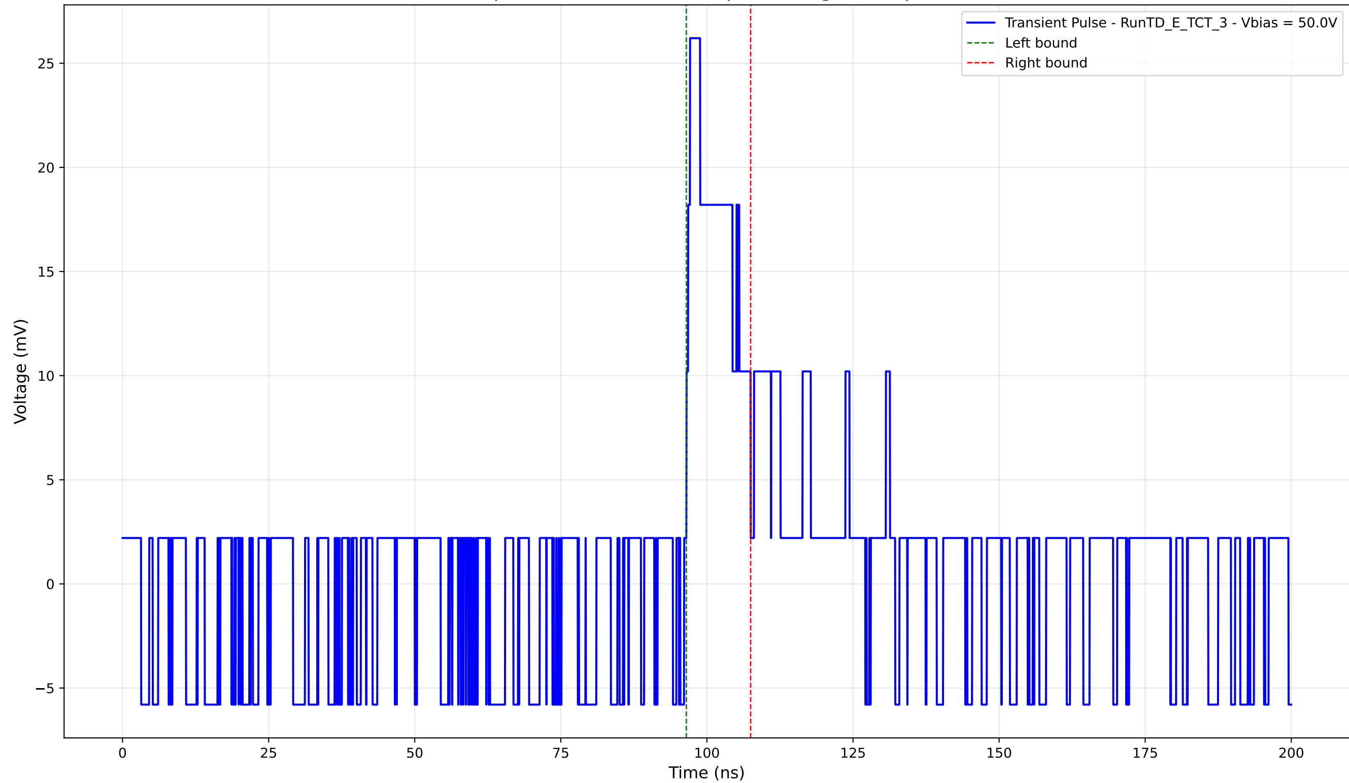
Transient Pulse - Sample: TD - Position: 320.0 \mu\text{m} - Charge: 3.81 pC - Rise Time: 0.62 ns
