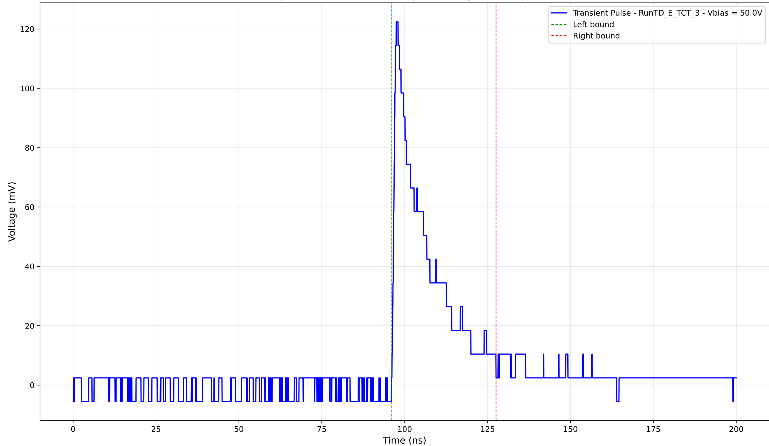
Transient Pulse - Sample: TD - Position: 540.0 \mu\text{m} - Charge: 24.66 pC - Rise Time: 1.02 ns
