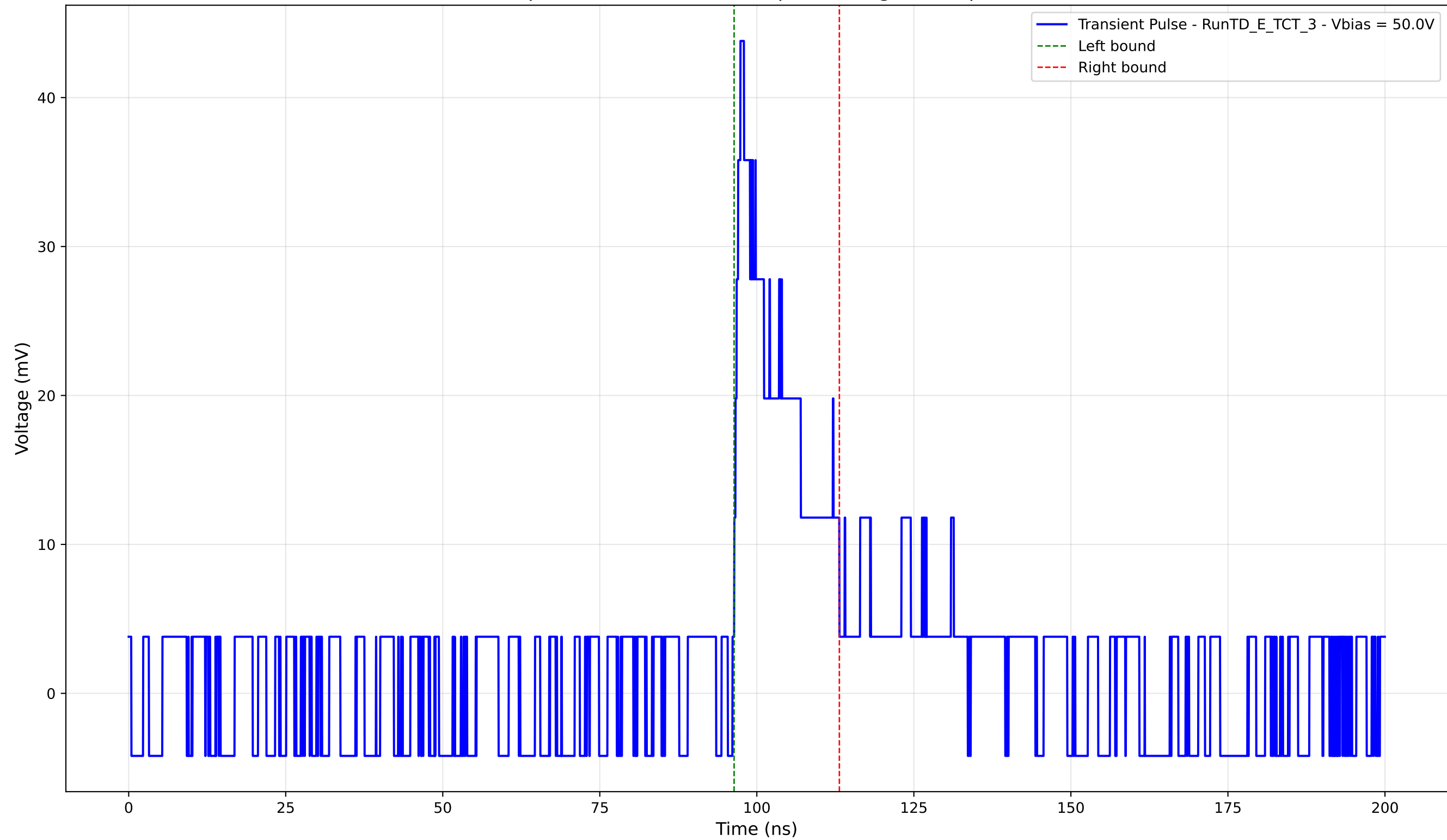
Transient Pulse - Sample: TD - Position: 695.0 \mu\text{m} - Charge: 6.83 pC - Rise Time: 1.00 ns
