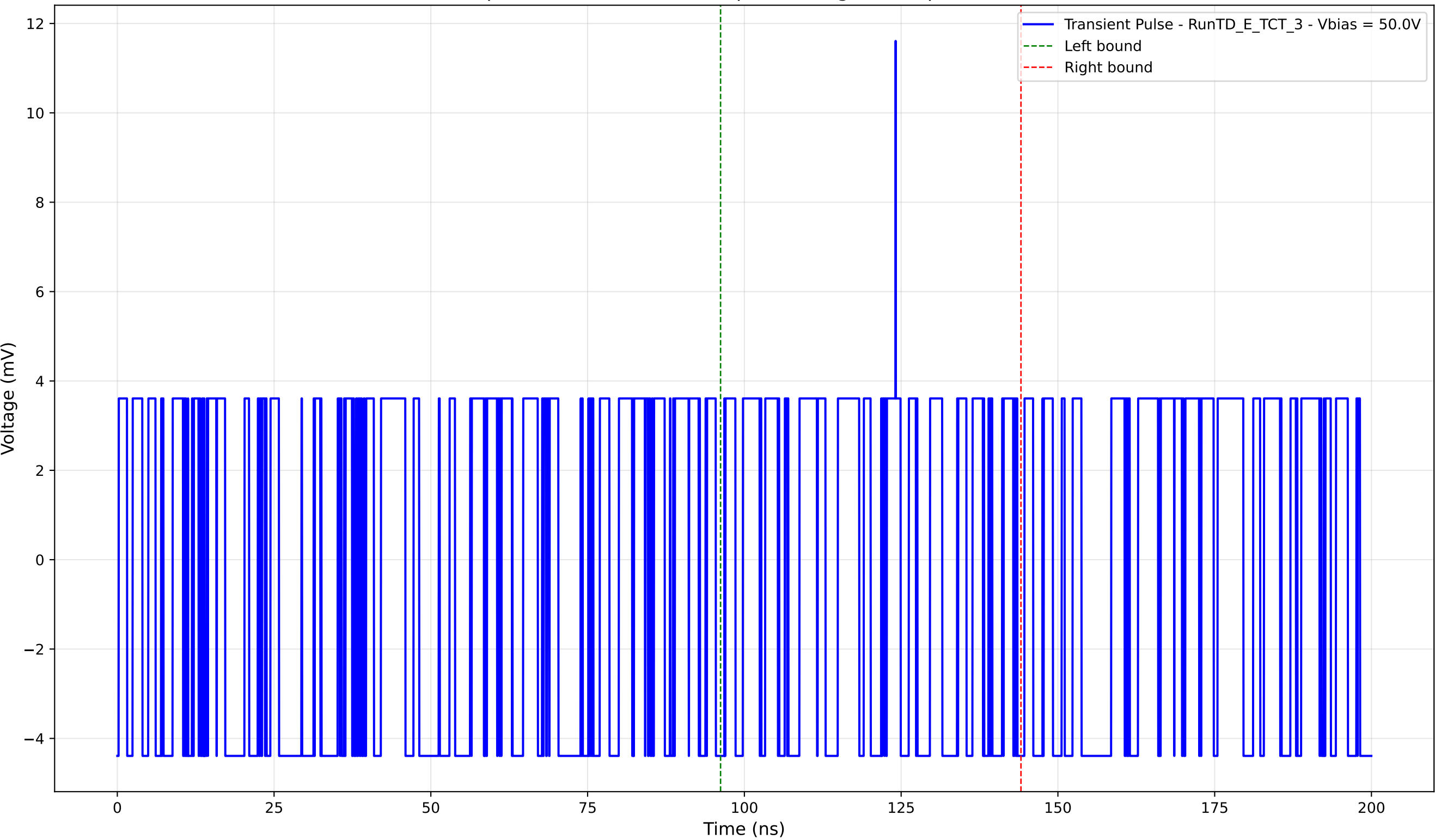
Transient Pulse - Sample: TD - Position: 210.0 \mu\text{m} - Charge: 0.17 pC - Rise Time: 0.00 ns (N/A)
