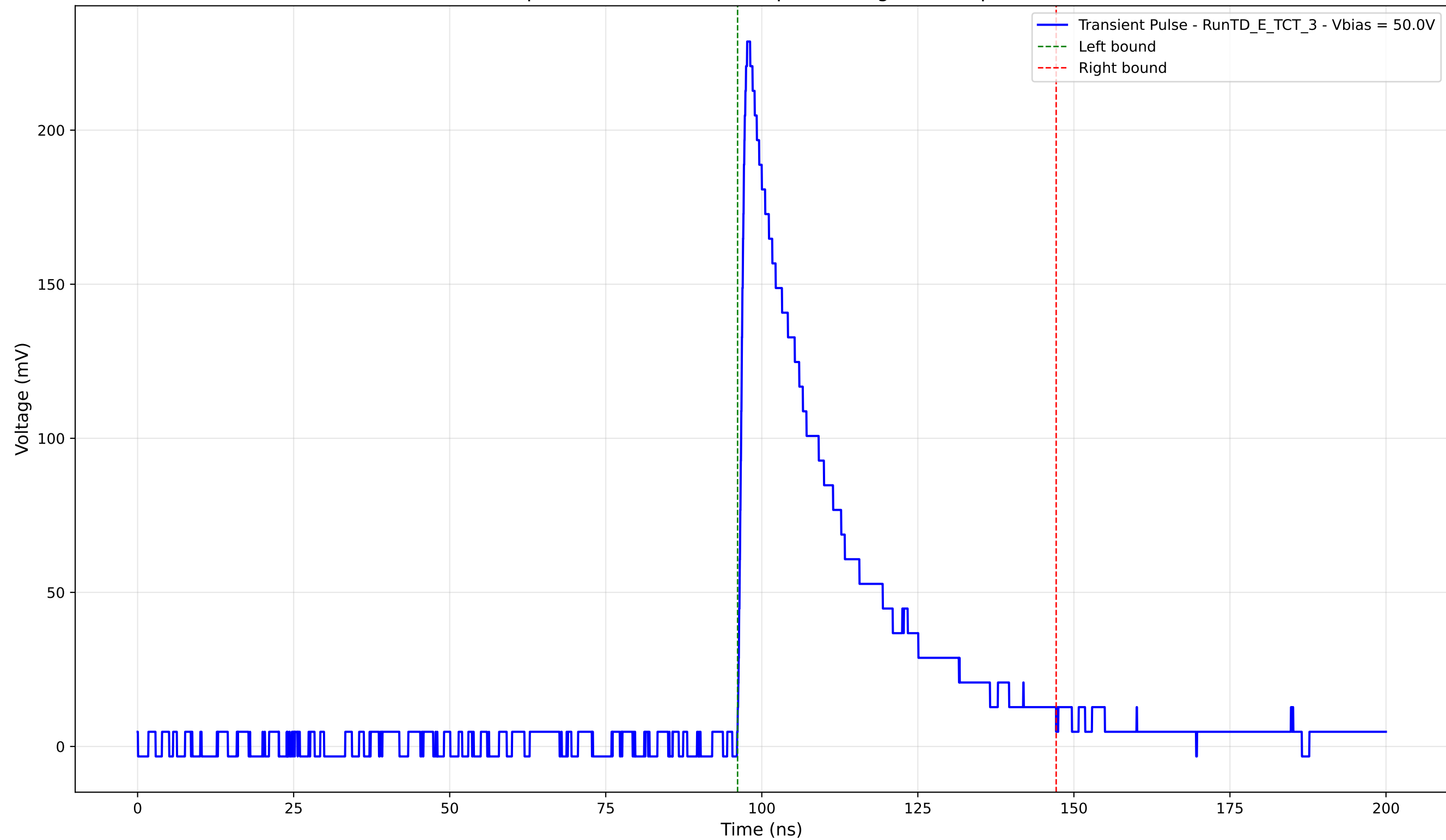
Transient Pulse - Sample: TD - Position: 410.0 \mu\text{m} - Charge: 65.29 pC - Rise Time: 1.09 ns
