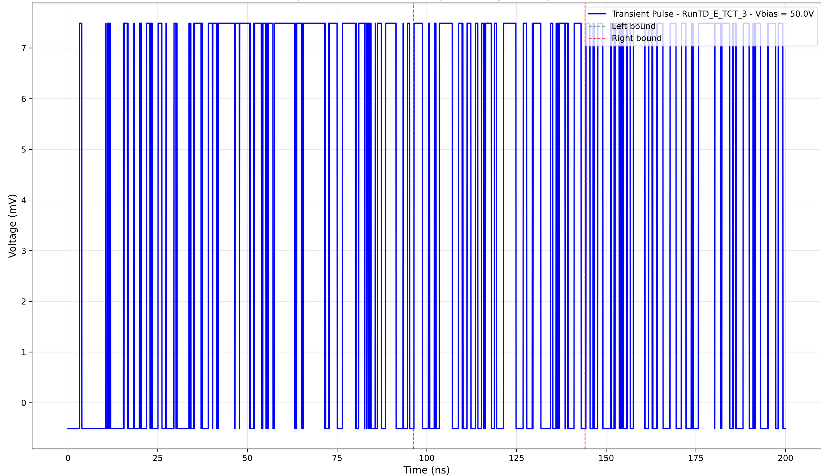
Transient Pulse - Sample: TD - Position: 135.0 \mu\text{m} - Charge: 3.46 pC - Rise Time: 0.02 ns
