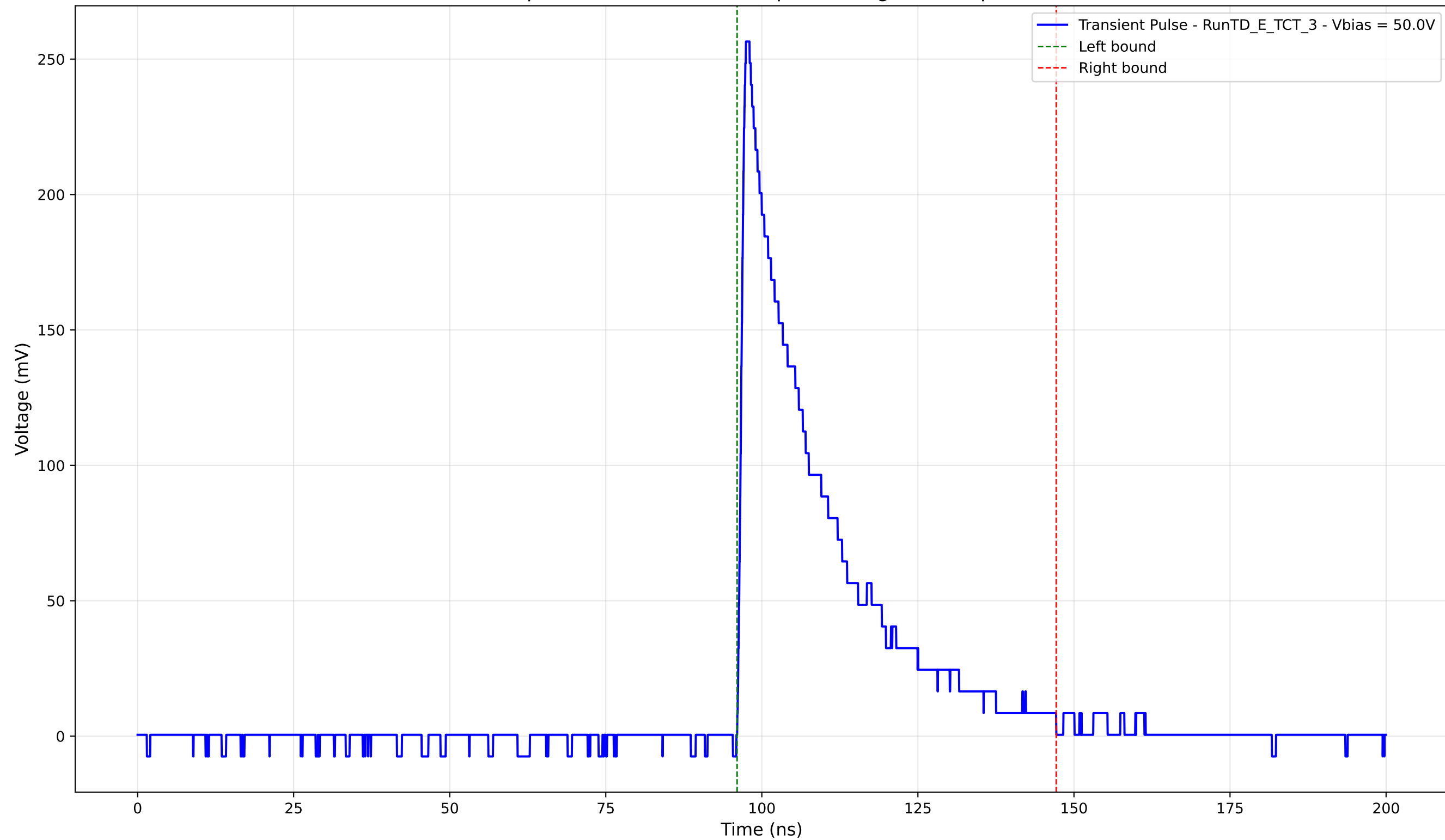
Transient Pulse - Sample: TD - Position: 445.0 \mu\text{m} - Charge: 64.51 pC - Rise Time: 0.98 ns
