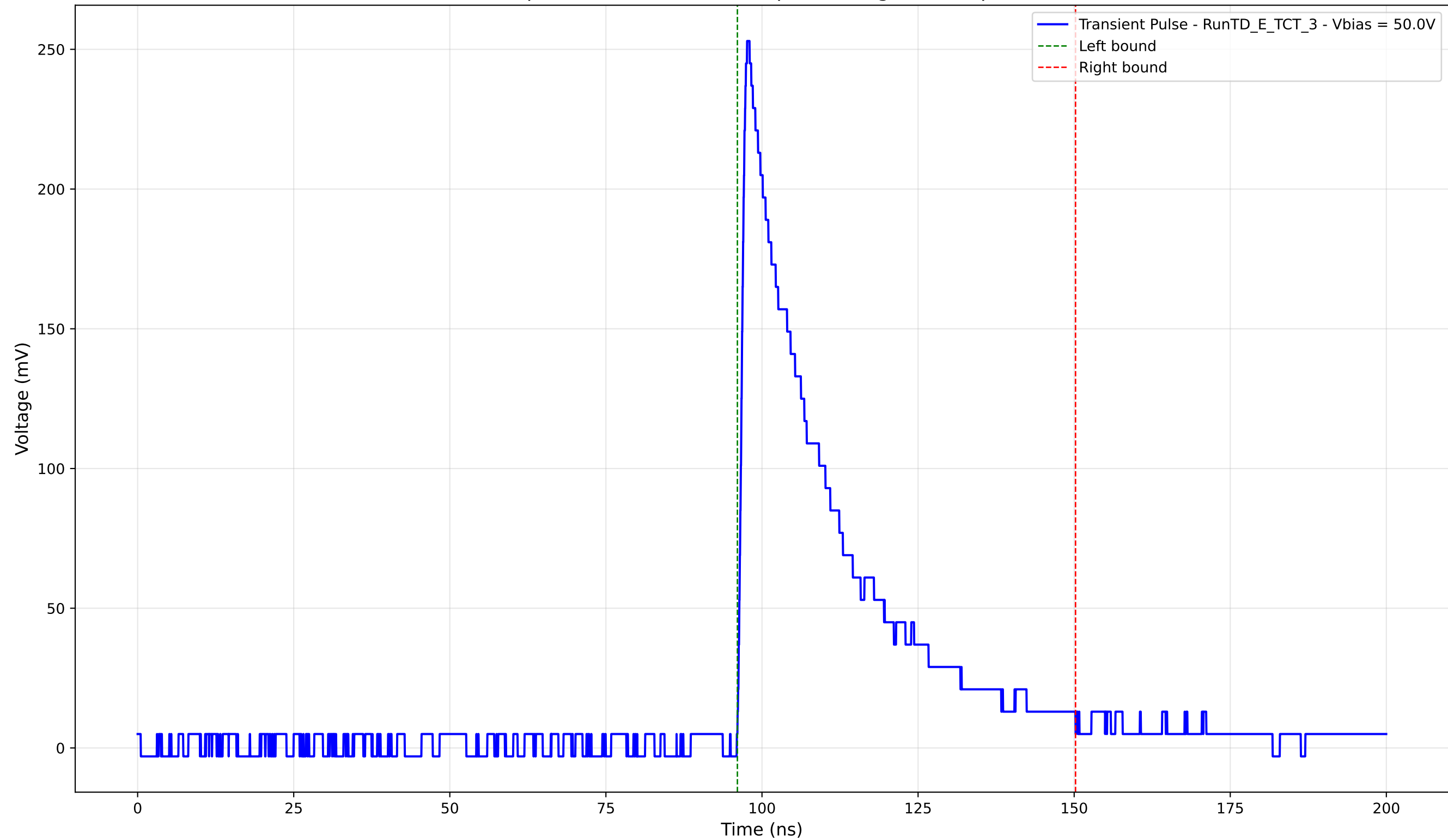
Transient Pulse - Sample: TD - Position: 420.0 \mu\text{m} - Charge: 71.67 pC - Rise Time: 1.05 ns
