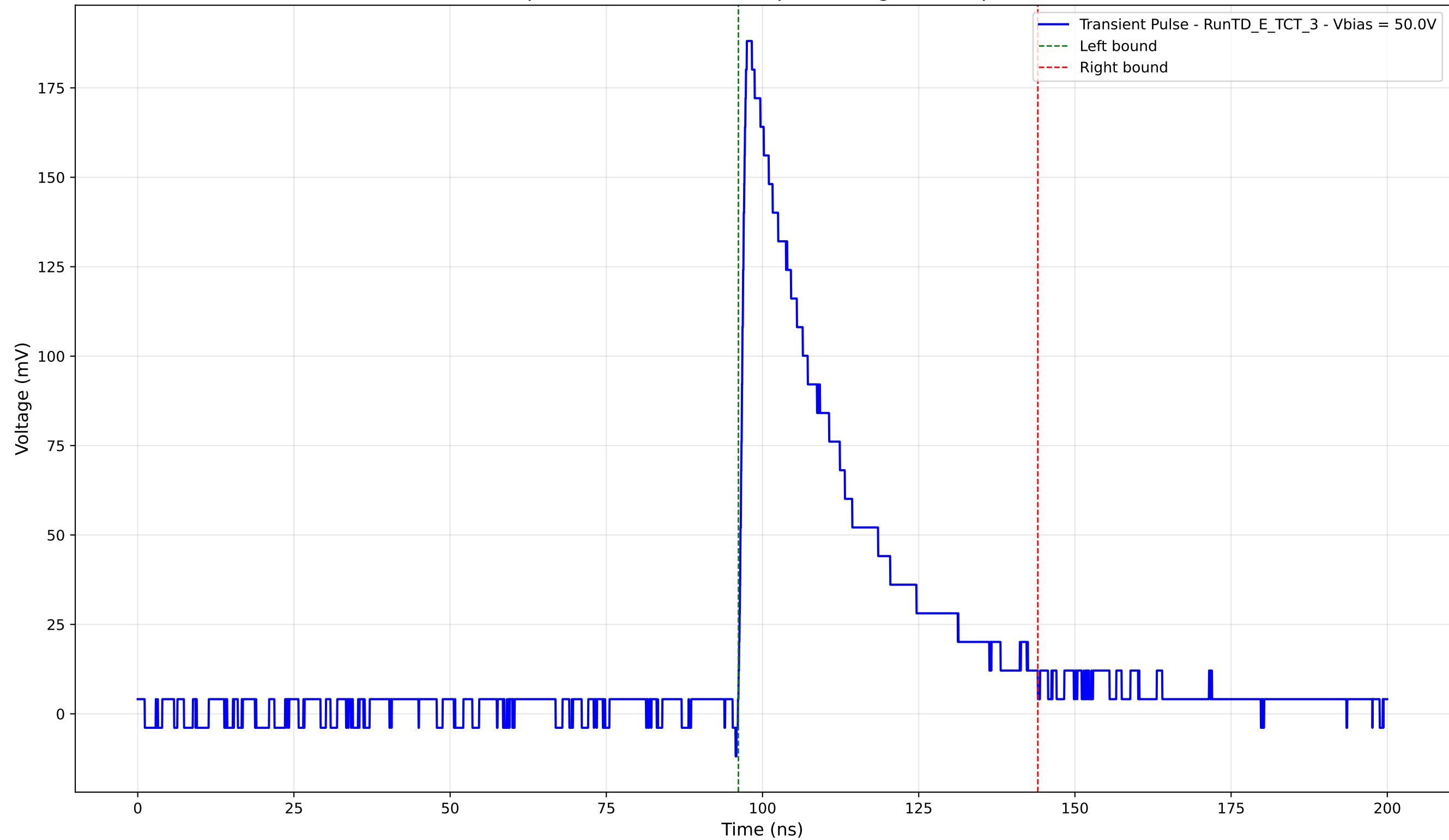
Transient Pulse - Sample: TD - Position: 365.0 \mu\text{m} - Charge: 58.51 pC - Rise Time: 1.02 ns
