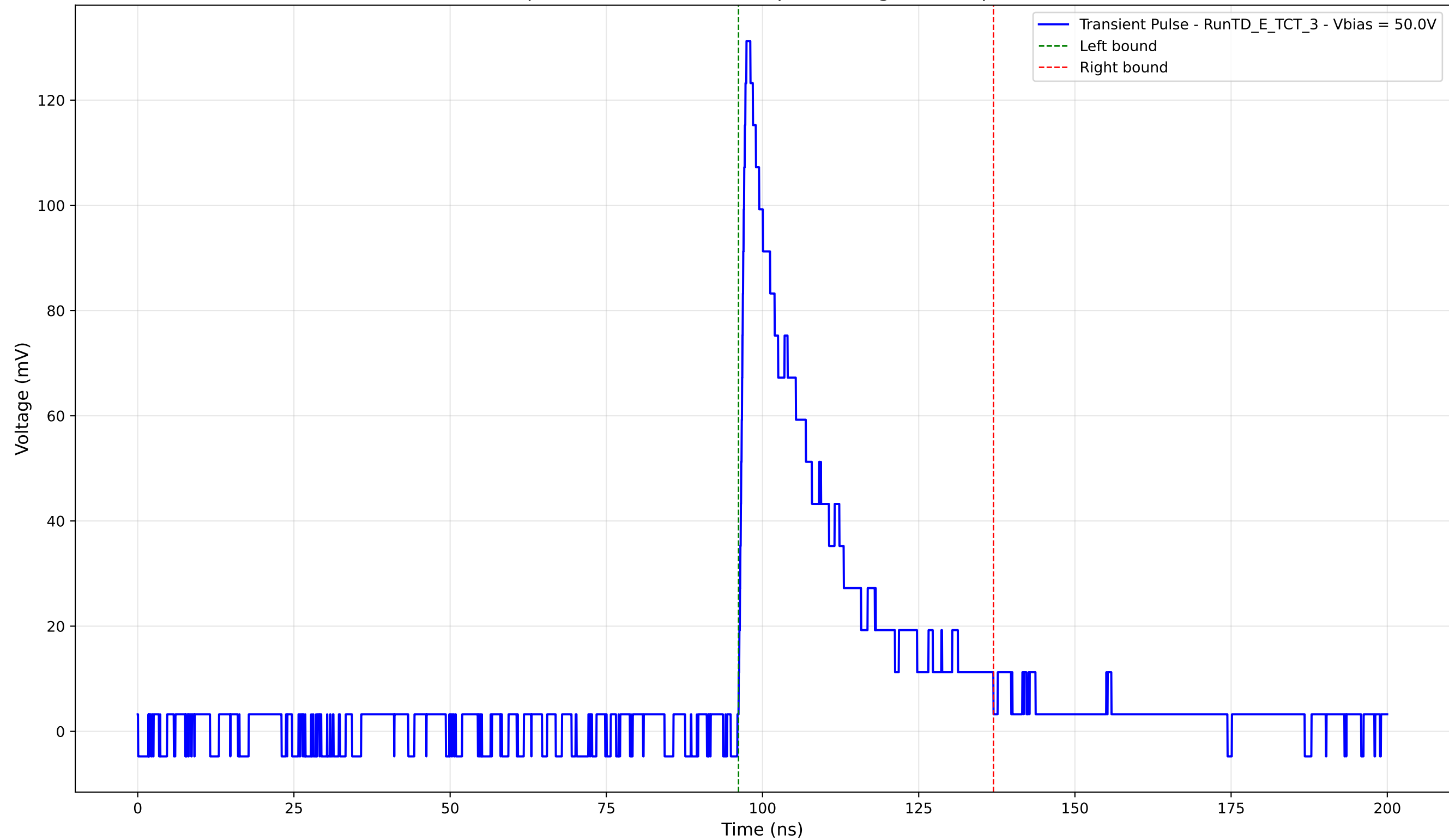
Transient Pulse - Sample: TD - Position: 515.0 \mu\text{m} - Charge: 31.04 pC - Rise Time: 1.00 ns
