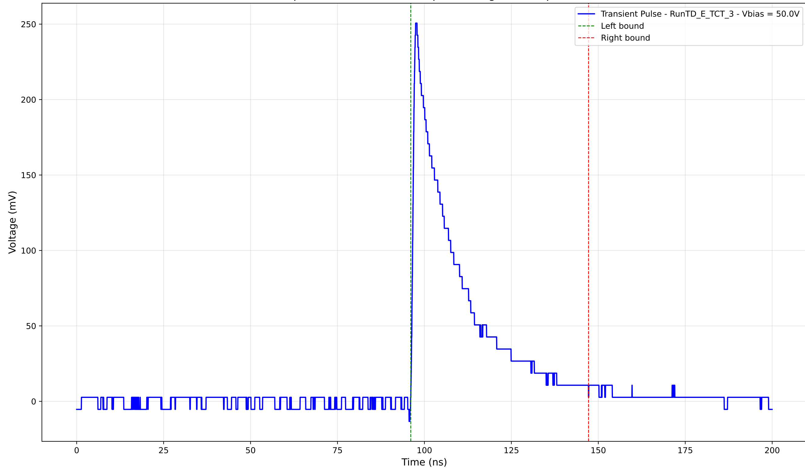
Transient Pulse - Sample: TD - Position: 460.0 \mu\text{m} - Charge: 63.87 pC - Rise Time: 0.98 ns
