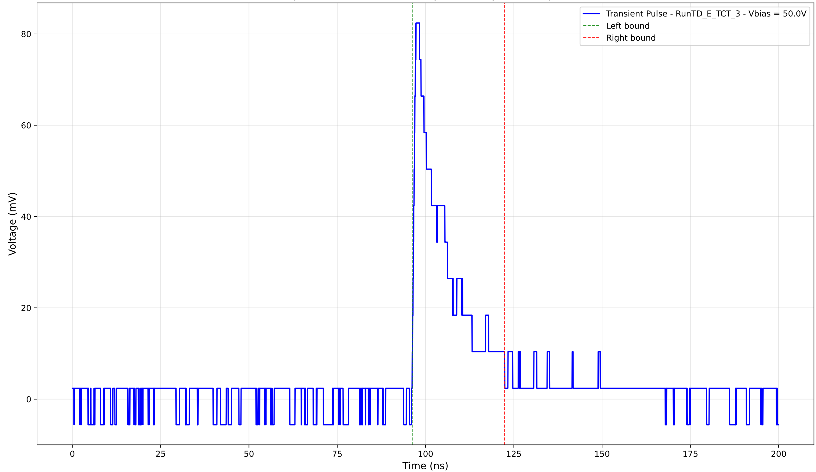
Transient Pulse - Sample: TD - Position: 590.0 \mu\text{m} - Charge: 15.42 pC - Rise Time: 0.89 ns
