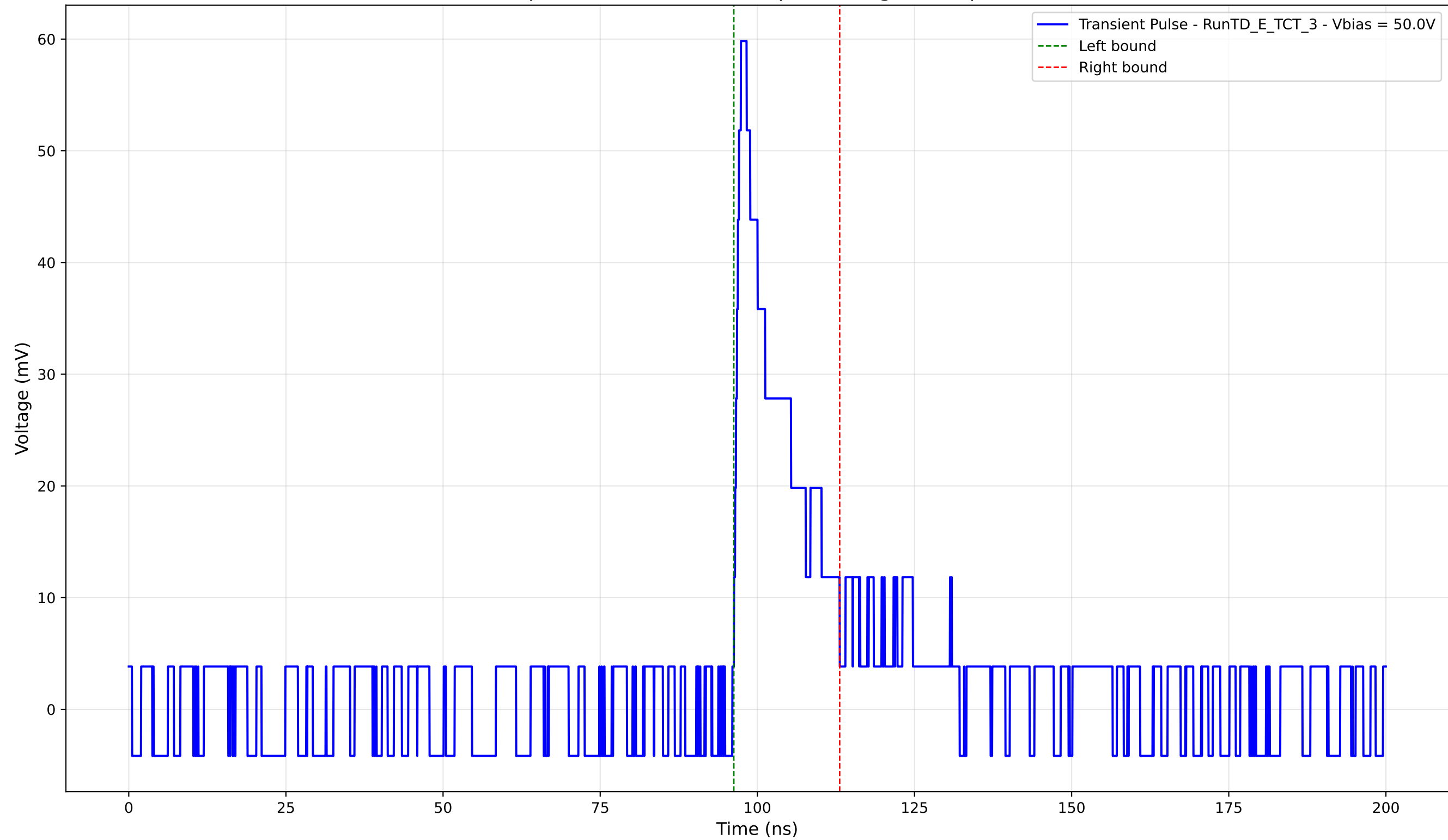
Transient Pulse - Sample: TD - Position: 620.0 \mu\text{m} - Charge: 9.12 pC - Rise Time: 1.11 ns
