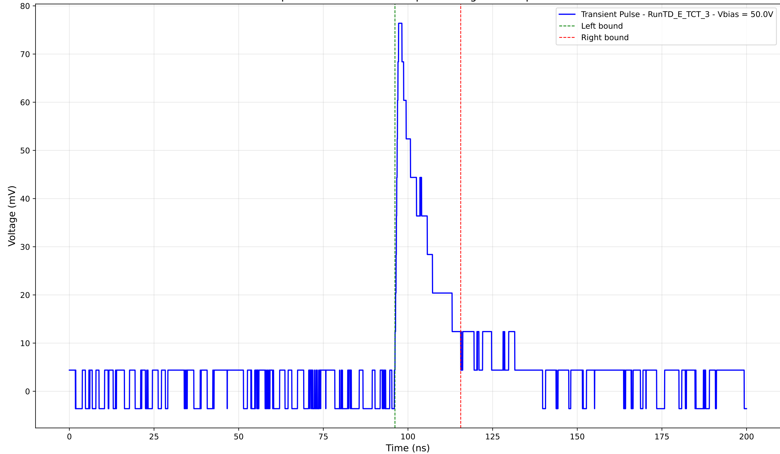
Transient Pulse - Sample: TD - Position: 610.0 \mu\text{m} - Charge: 13.12 pC - Rise Time: 1.05 ns
