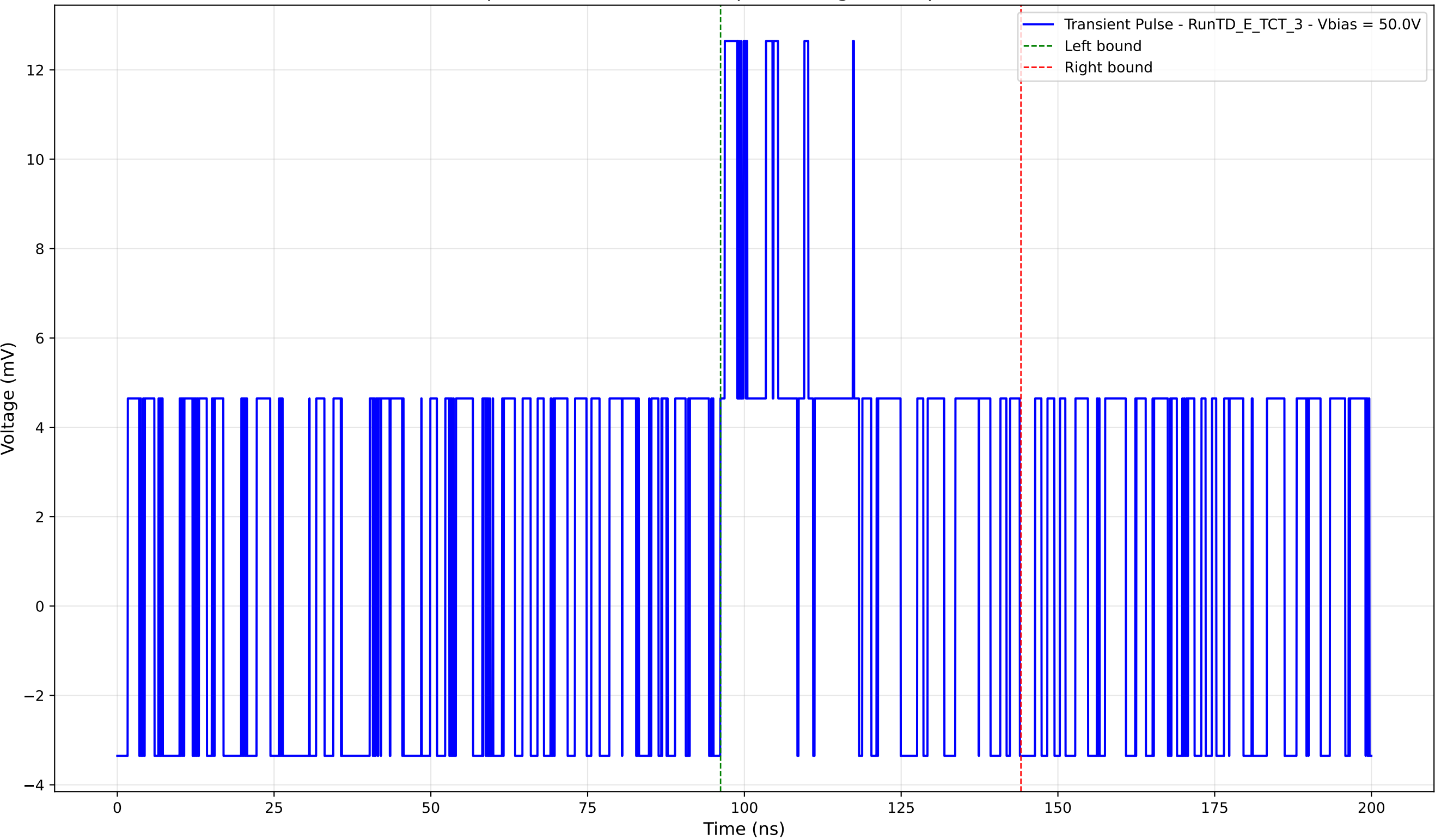
Transient Pulse - - Sample: TD - Position: 300.0 \mu\text{m} - Charge: 3.81 pC - Rise Time: 0.00 ns (N/A)
