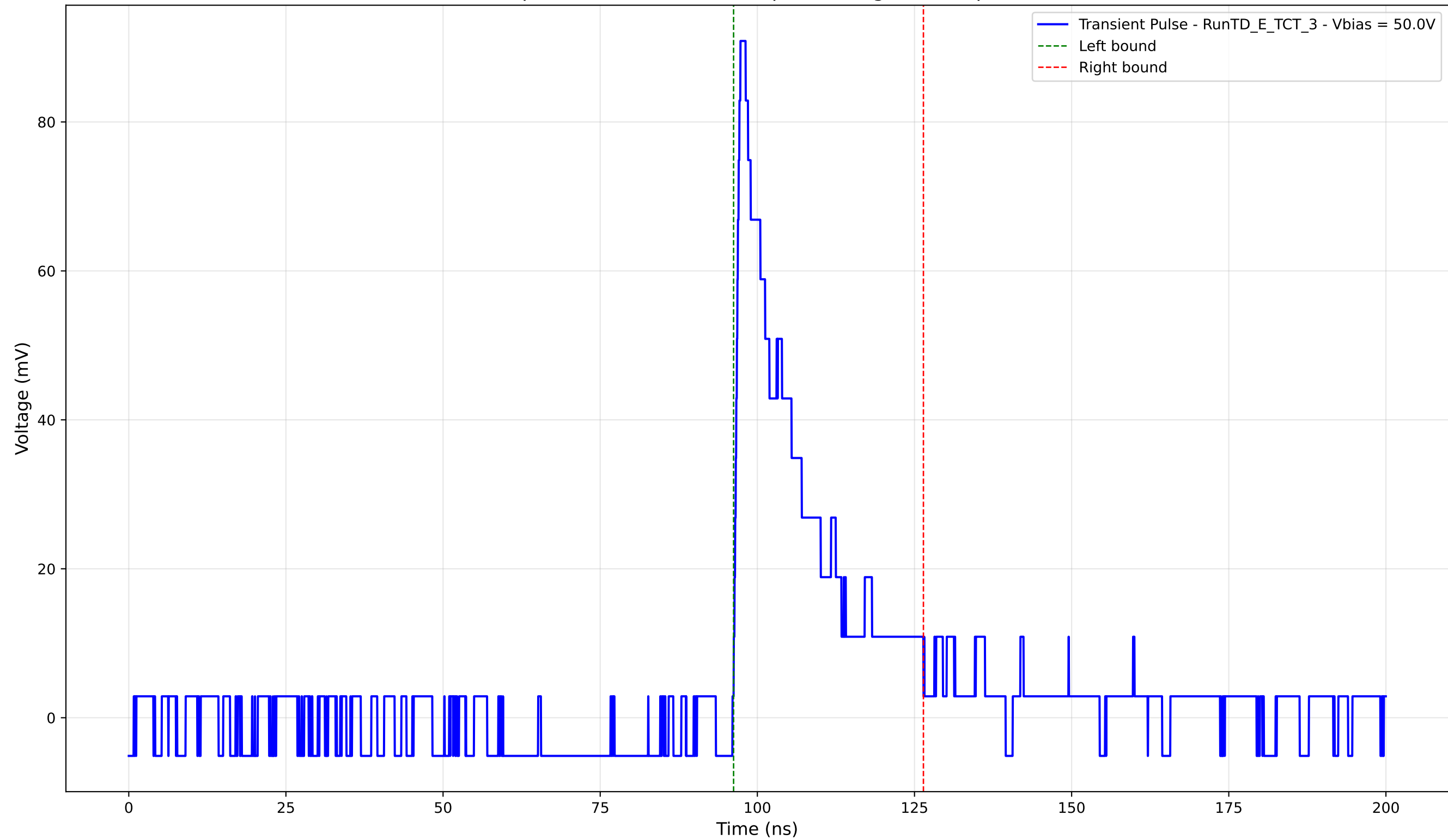
Transient Pulse - Sample: TD - Position: 570.0 \mu\text{m} - Charge: 17.80 pC - Rise Time: 0.90 ns
