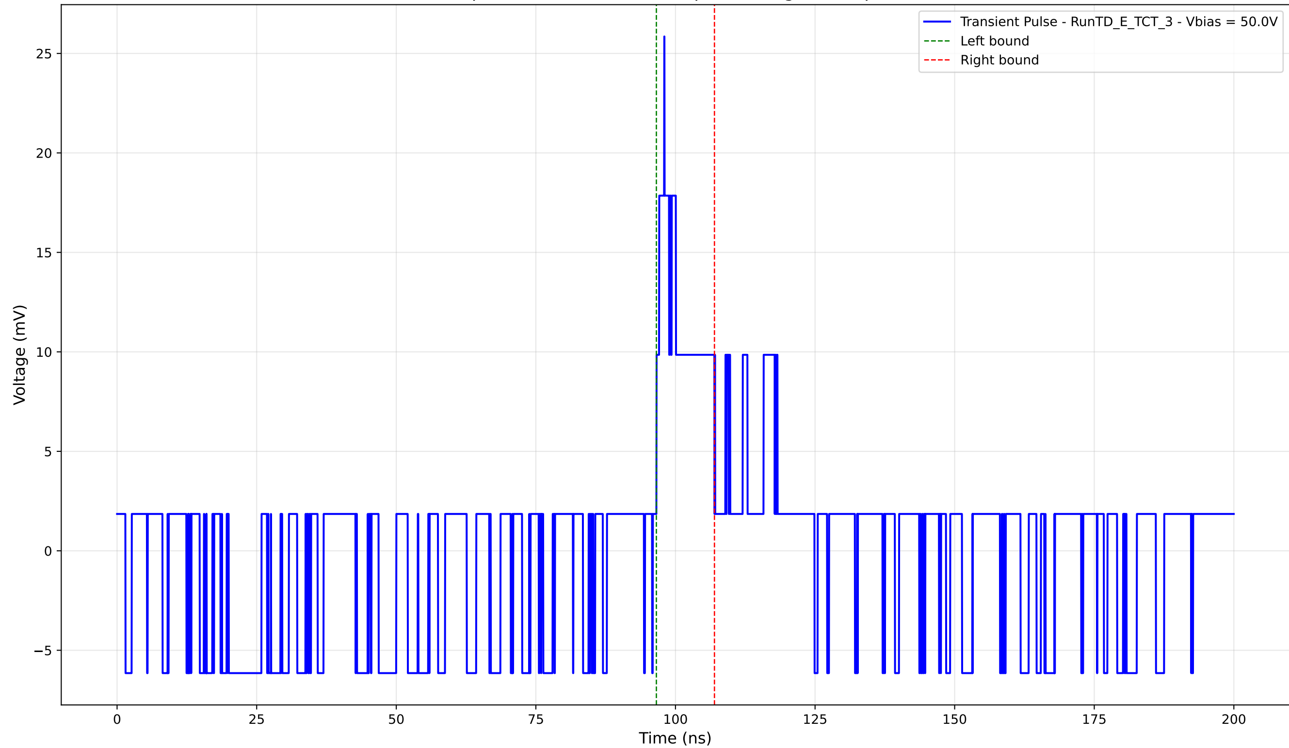
Transient Pulse - Sample: TD - Position: 315.0 \mu\text{m} - Charge: 2.50 pC - Rise Time: 1.40 ns
