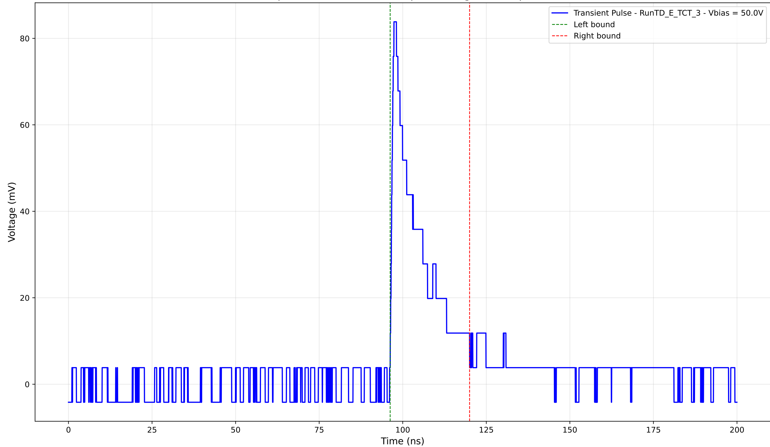
Transient Pulse - Sample: TD - Position: 600.0 \mu\text{m} - Charge: 14.62 pC - Rise Time: 0.89 ns
