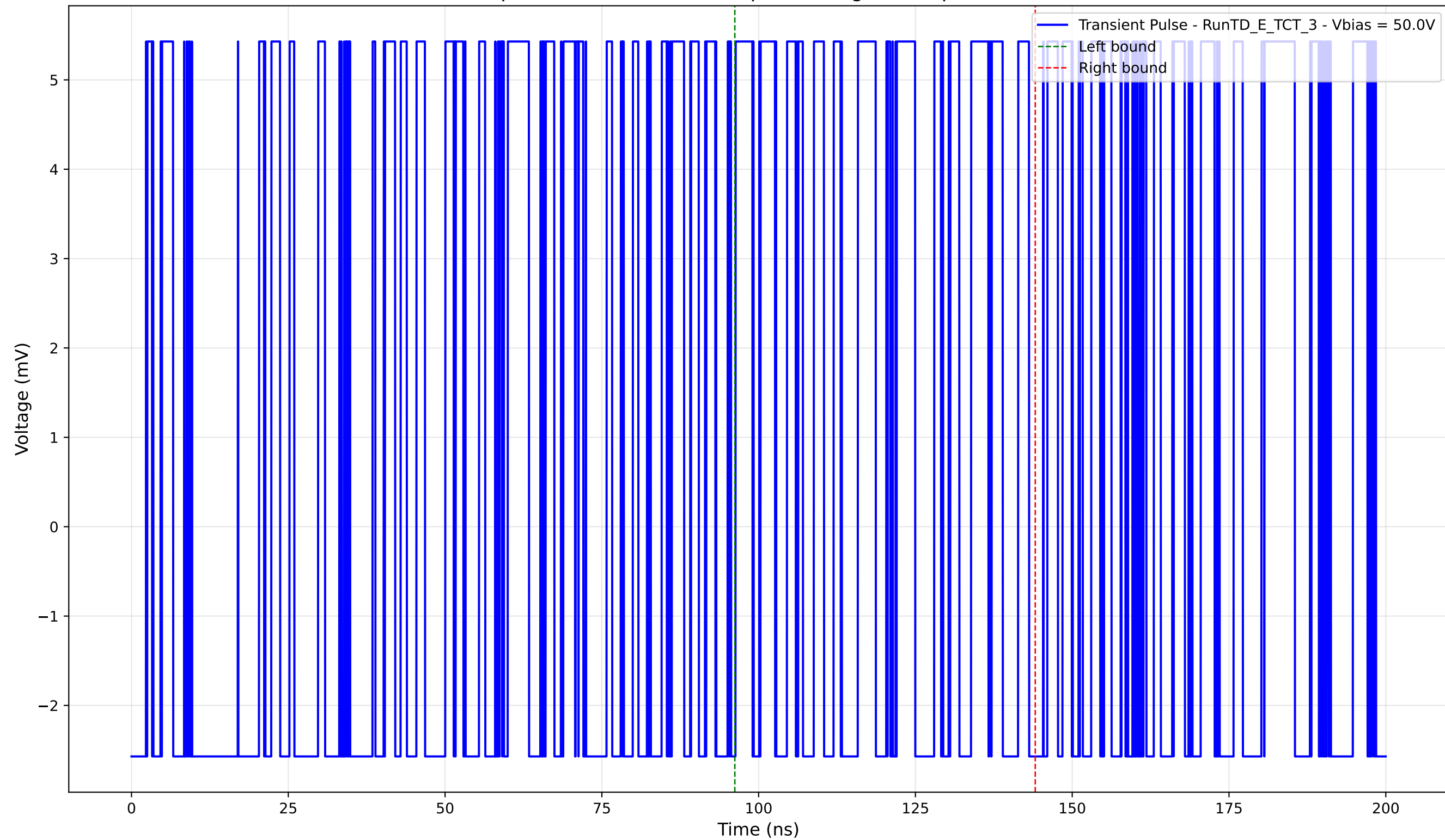
Transient Pulse - Sample: TD - Position: 150.0 \mu\text{m} - Charge: 1.71 pC - Rise Time: 0.00 ns (N/A)
