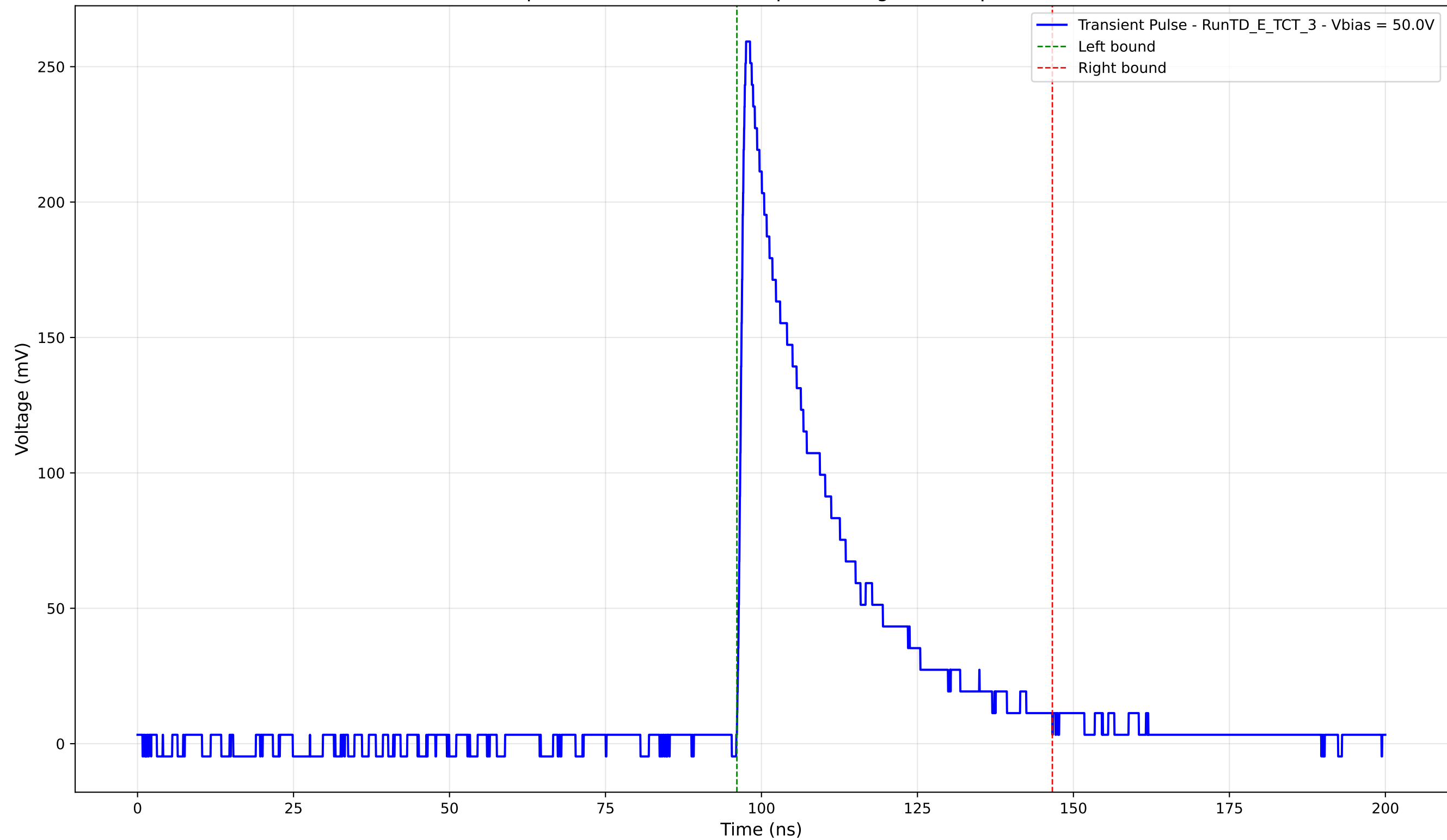
Transient Pulse - Sample: TD - Position: 425.0 \mu\text{m} - Charge: 70.11 pC - Rise Time: 1.06 ns
