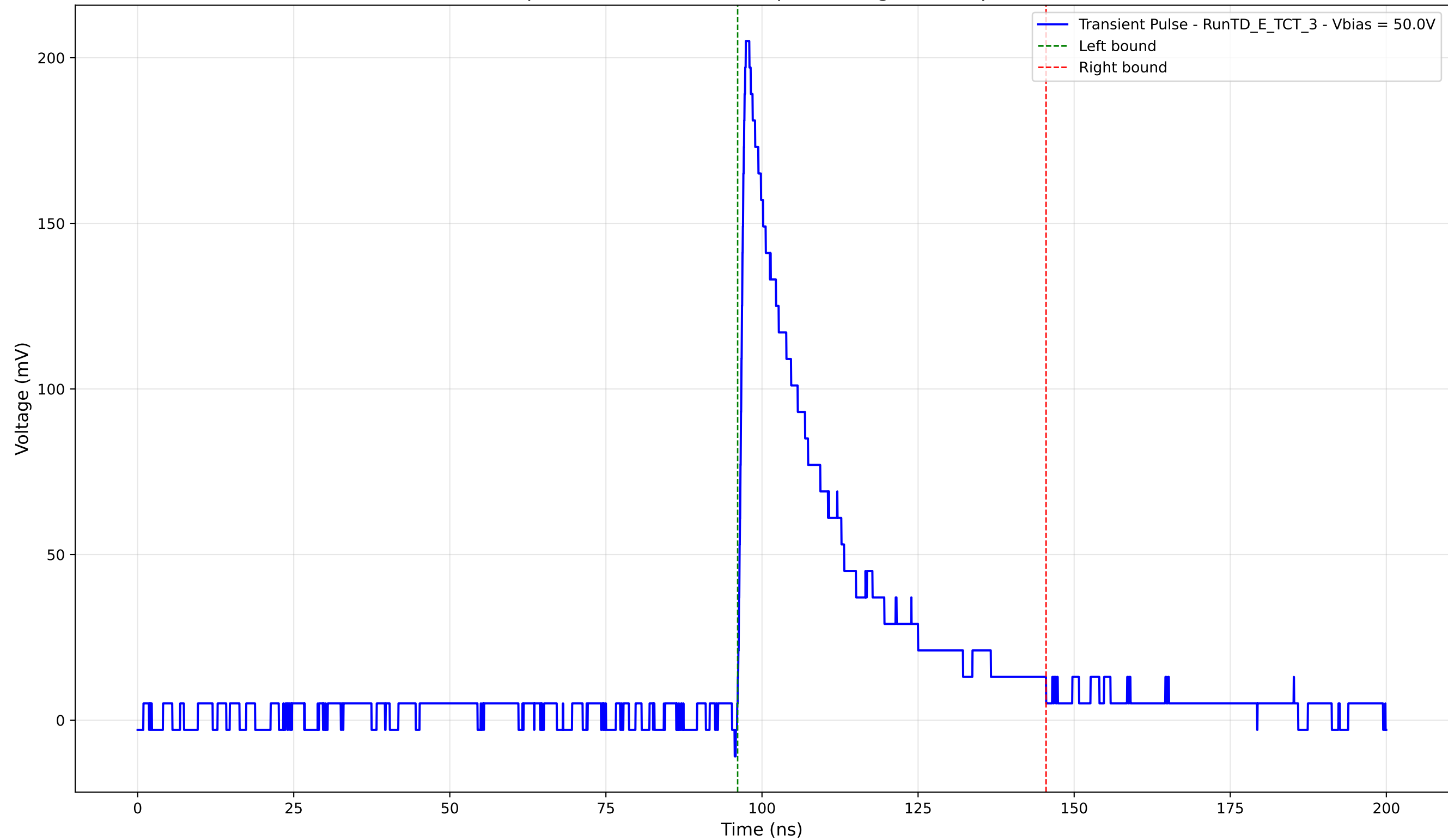
Transient Pulse - Sample: TD - Position: 480.0 \mu\text{m} - Charge: 52.61 pC - Rise Time: 1.00 ns
