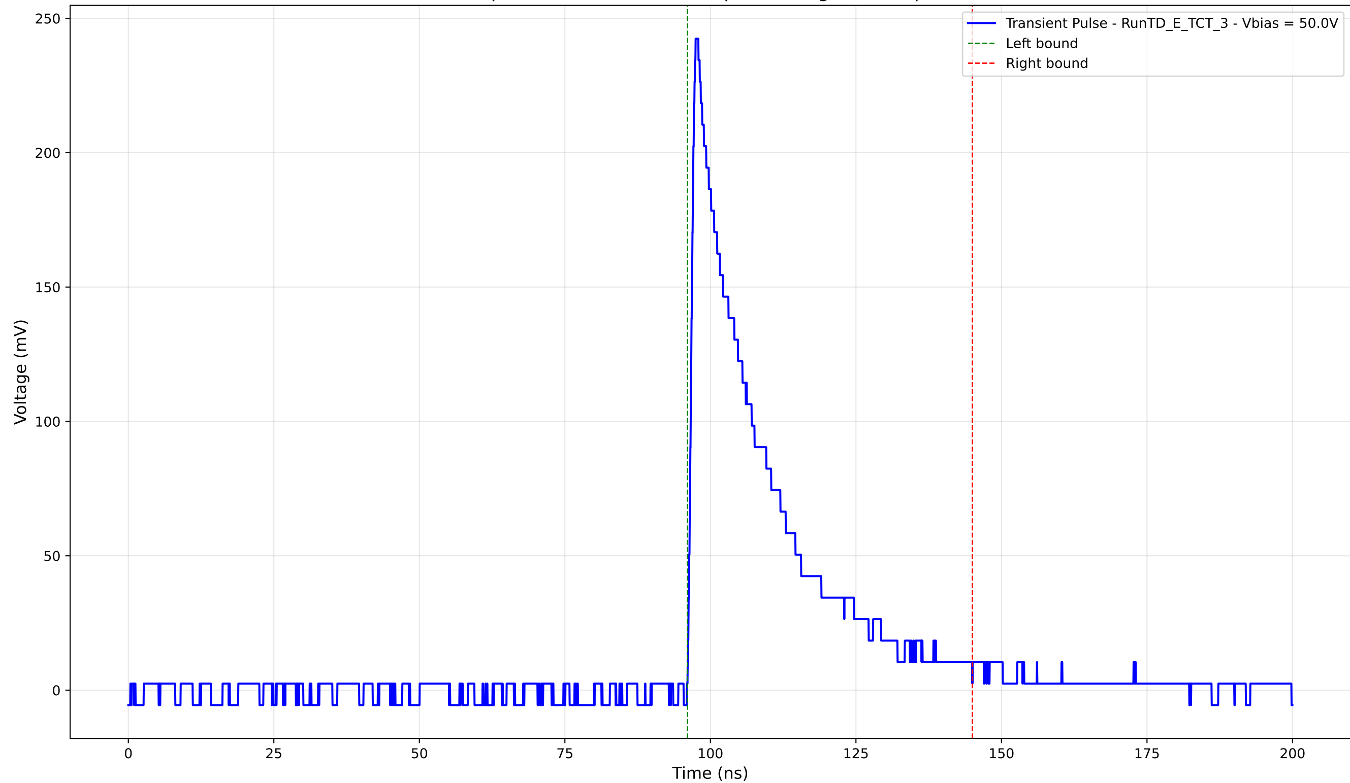
Transient Pulse - Sample: TD - Position: 465.0 \mu\text{m} - Charge: 60.02 pC - Rise Time: 0.97 ns
