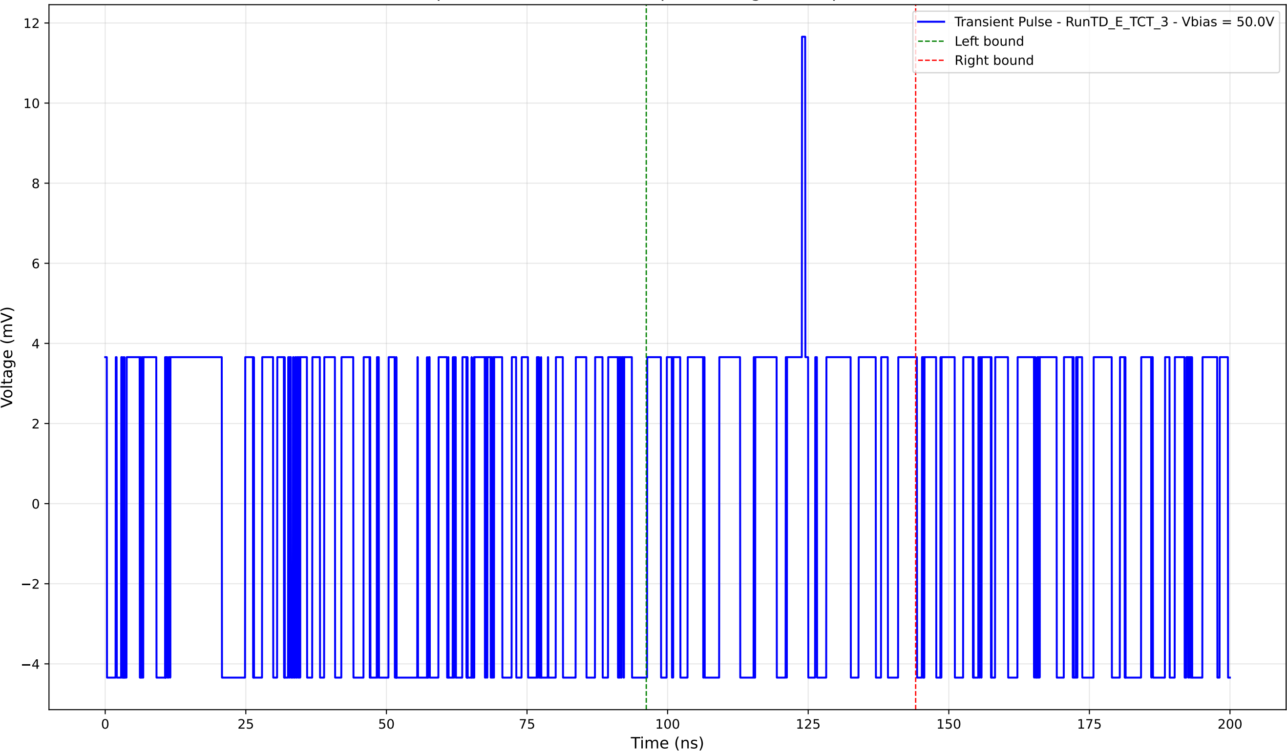
Transient Pulse - Sample: TD - Position: 225.0 \mu\text{m} - Charge: 0.94 pC - Rise Time: 0.00 ns (N/A)
