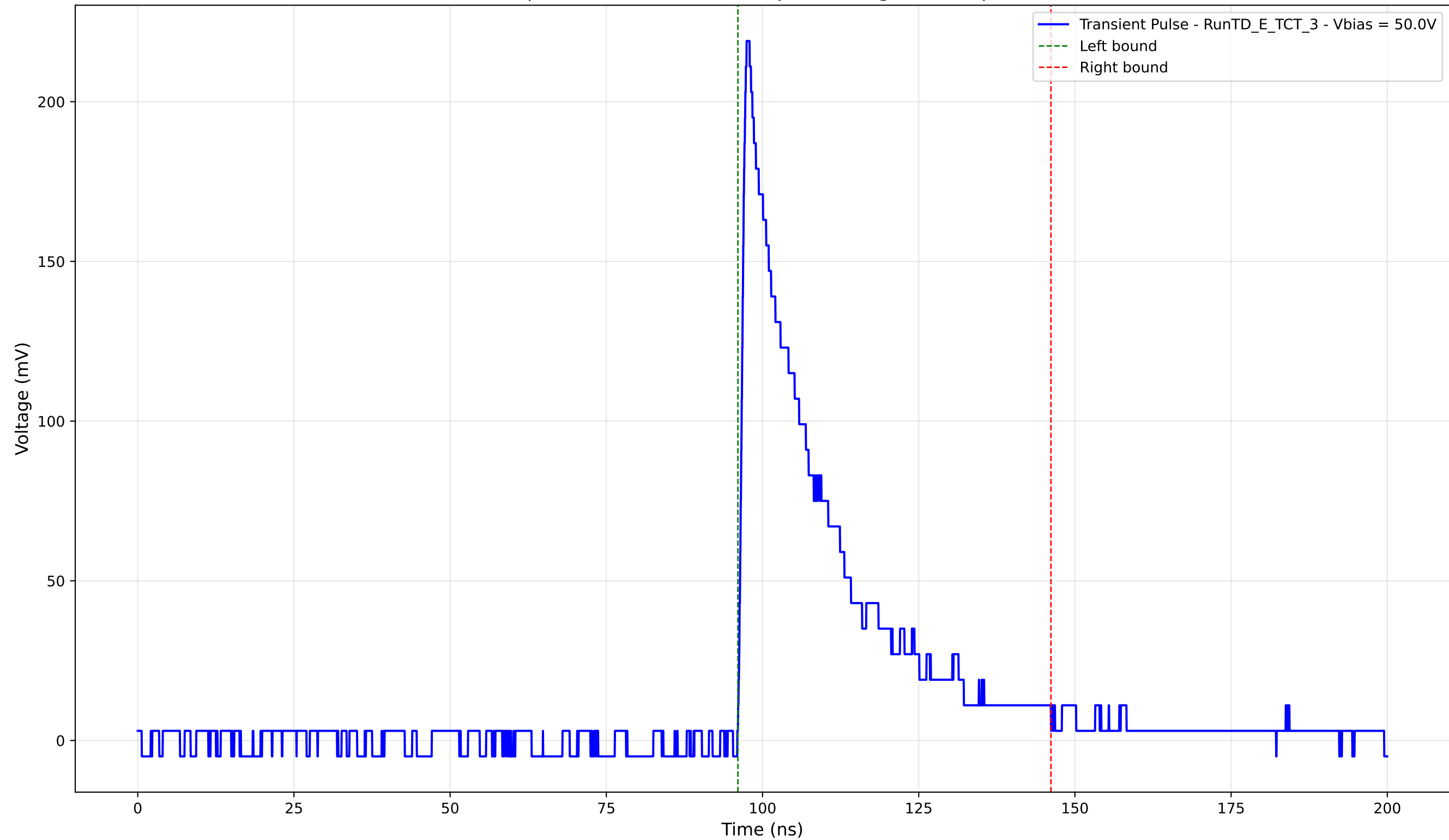
Transient Pulse - Sample: TD - Position: 475.0 \mu\text{m} - Charge: 54.39 pC - Rise Time: 1.01 ns
