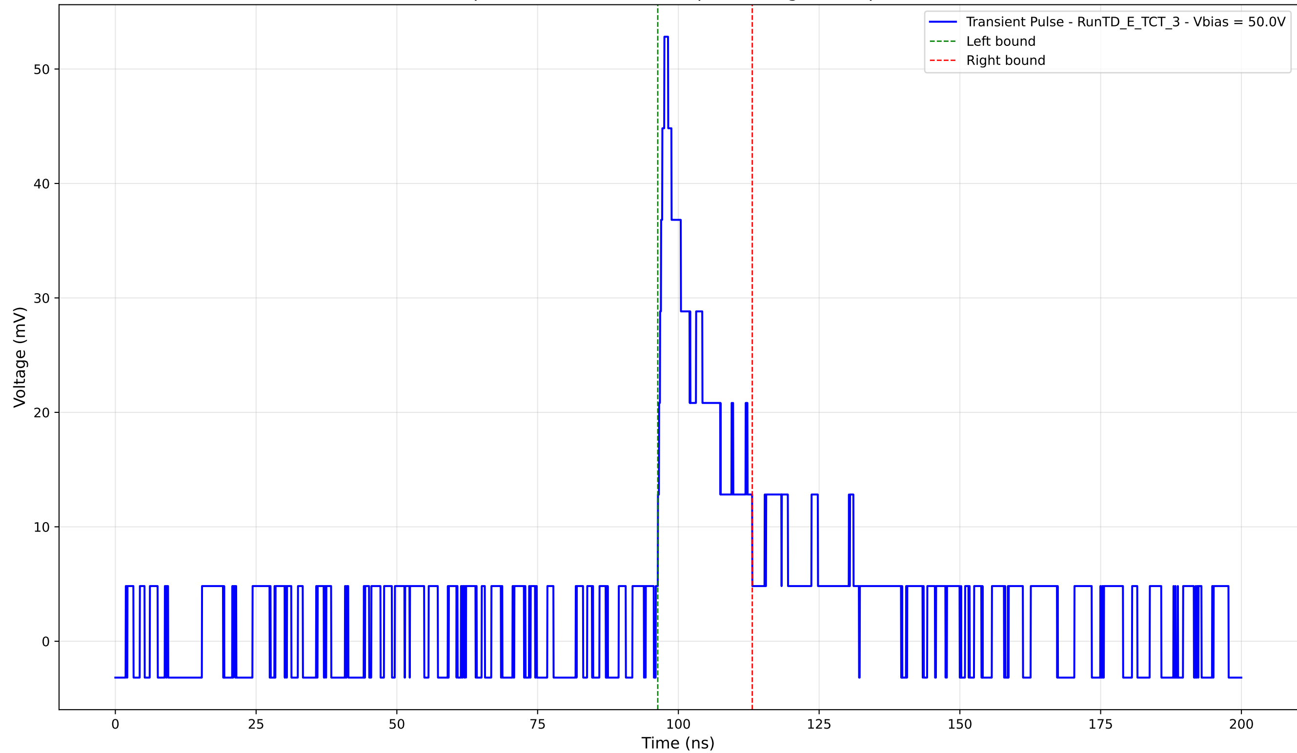
Transient Pulse - Sample: TD - Position: 640.0 \mu\text{m} - Charge: 8.09 pC - Rise Time: 1.16 ns
