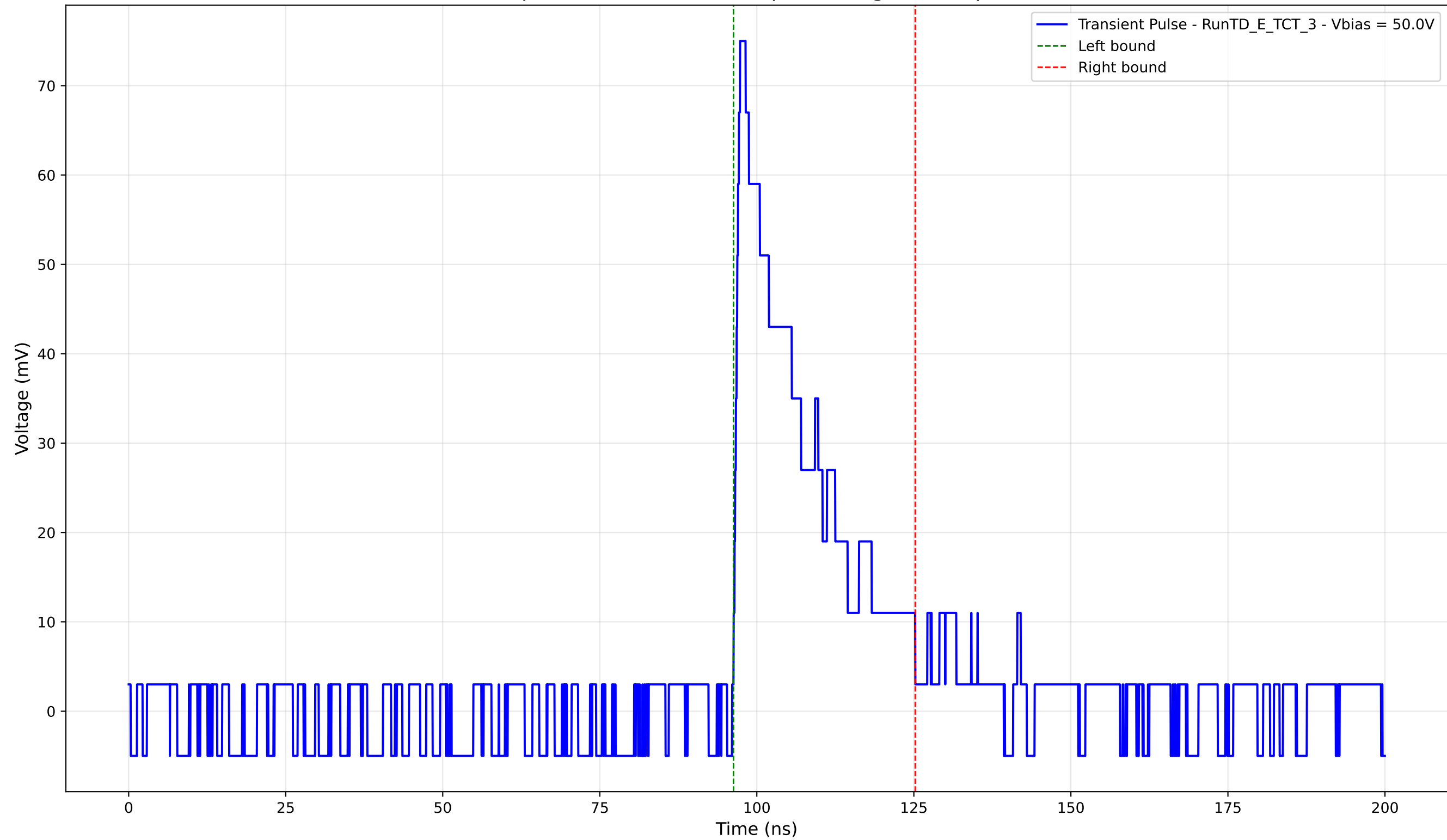
Transient Pulse - Sample: TD - Position: 335.0 \mu\text{m} - Charge: 16.92 pC - Rise Time: 1.03 ns
