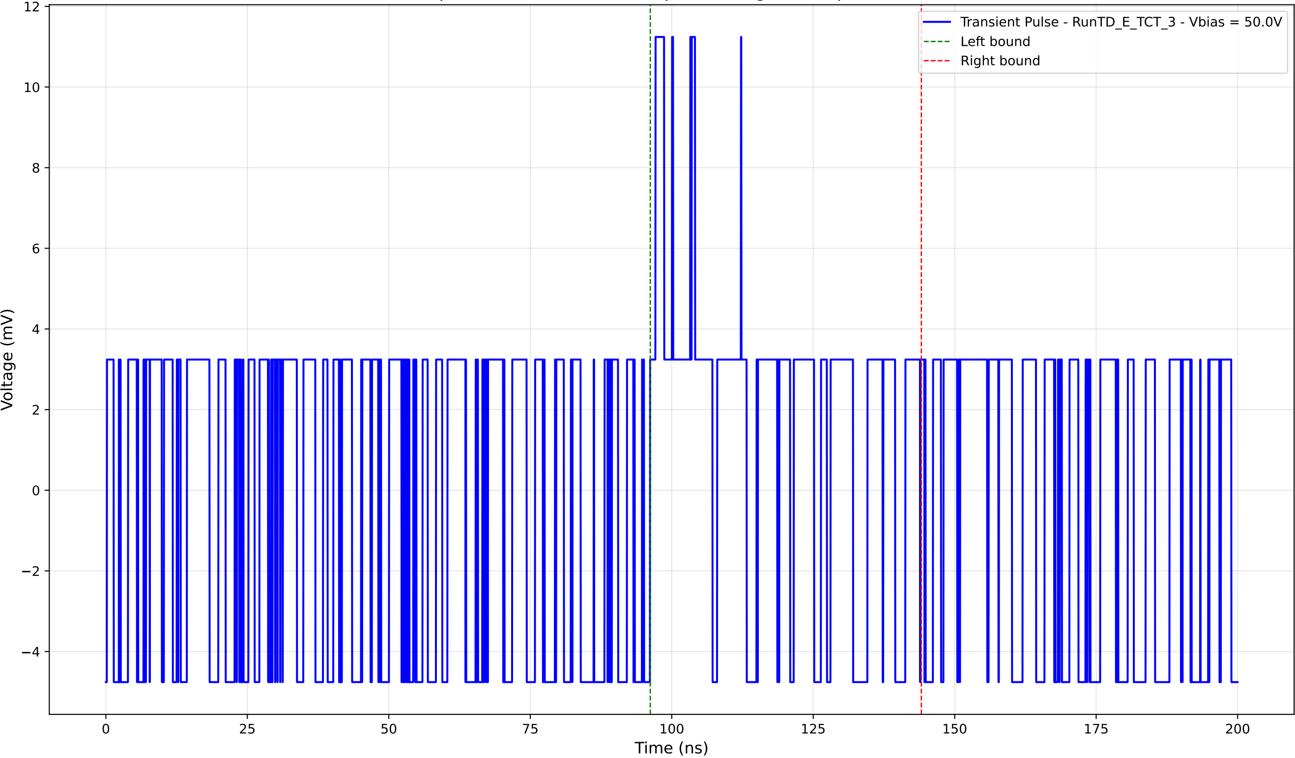
Transient Pulse - Sample: TD - Position: 290.0 \mu\text{m} - Charge: 1.94 pC - Rise Time: 0.00 ns (N/A)
