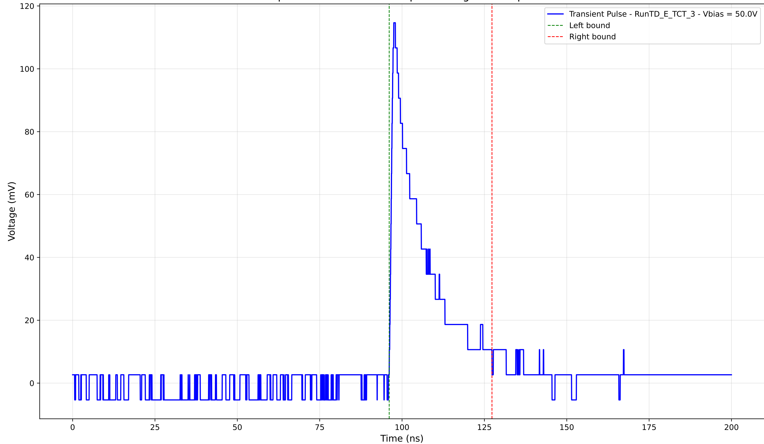
Transient Pulse - Sample: TD - Position: 555.0 \mu\text{m} - Charge: 22.98 pC - Rise Time: 1.02 ns
