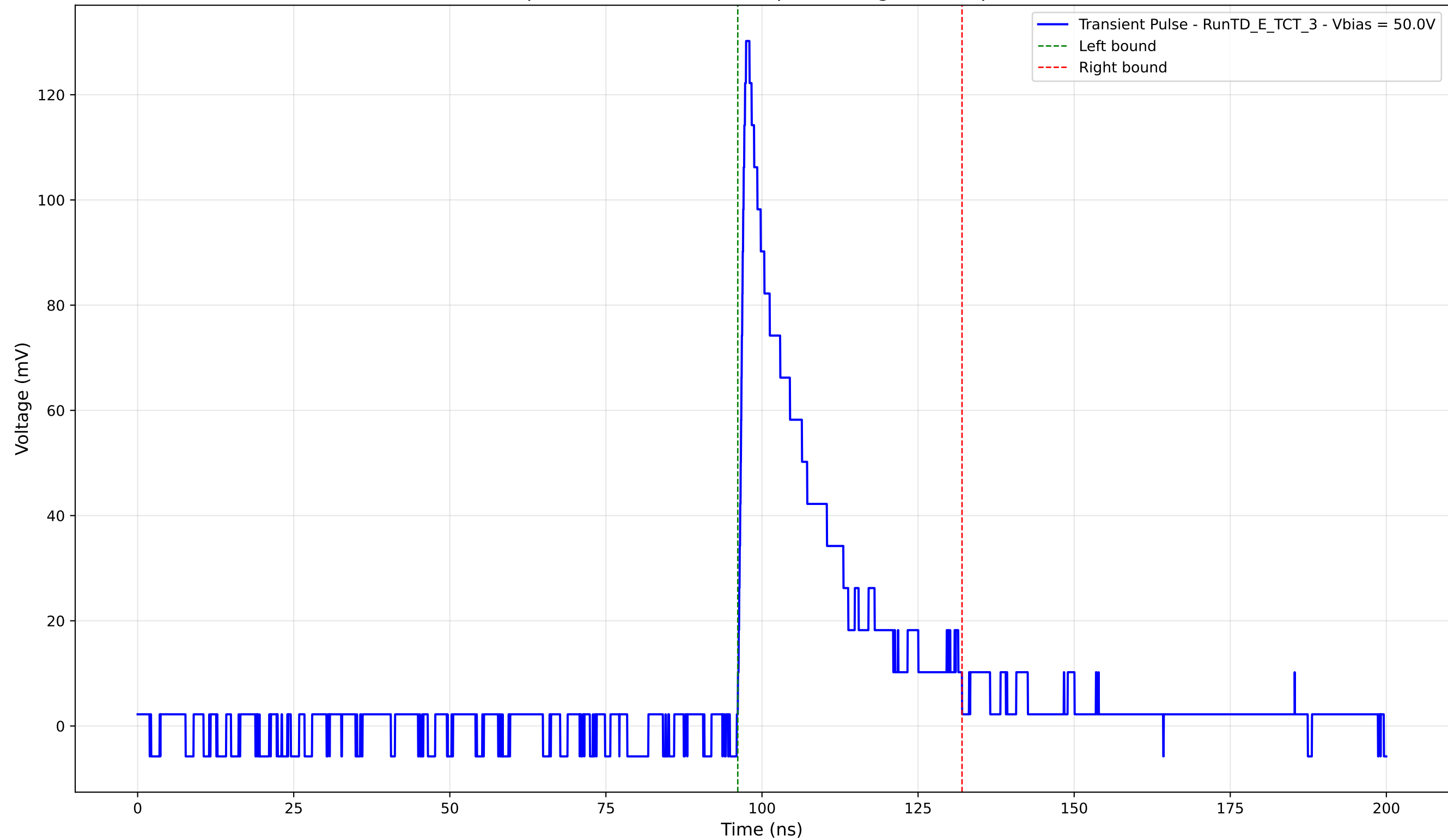
Transient Pulse - Sample: TD - Position: 520.0 \mu\text{m} - Charge: 27.77 pC - Rise Time: 1.03 ns
