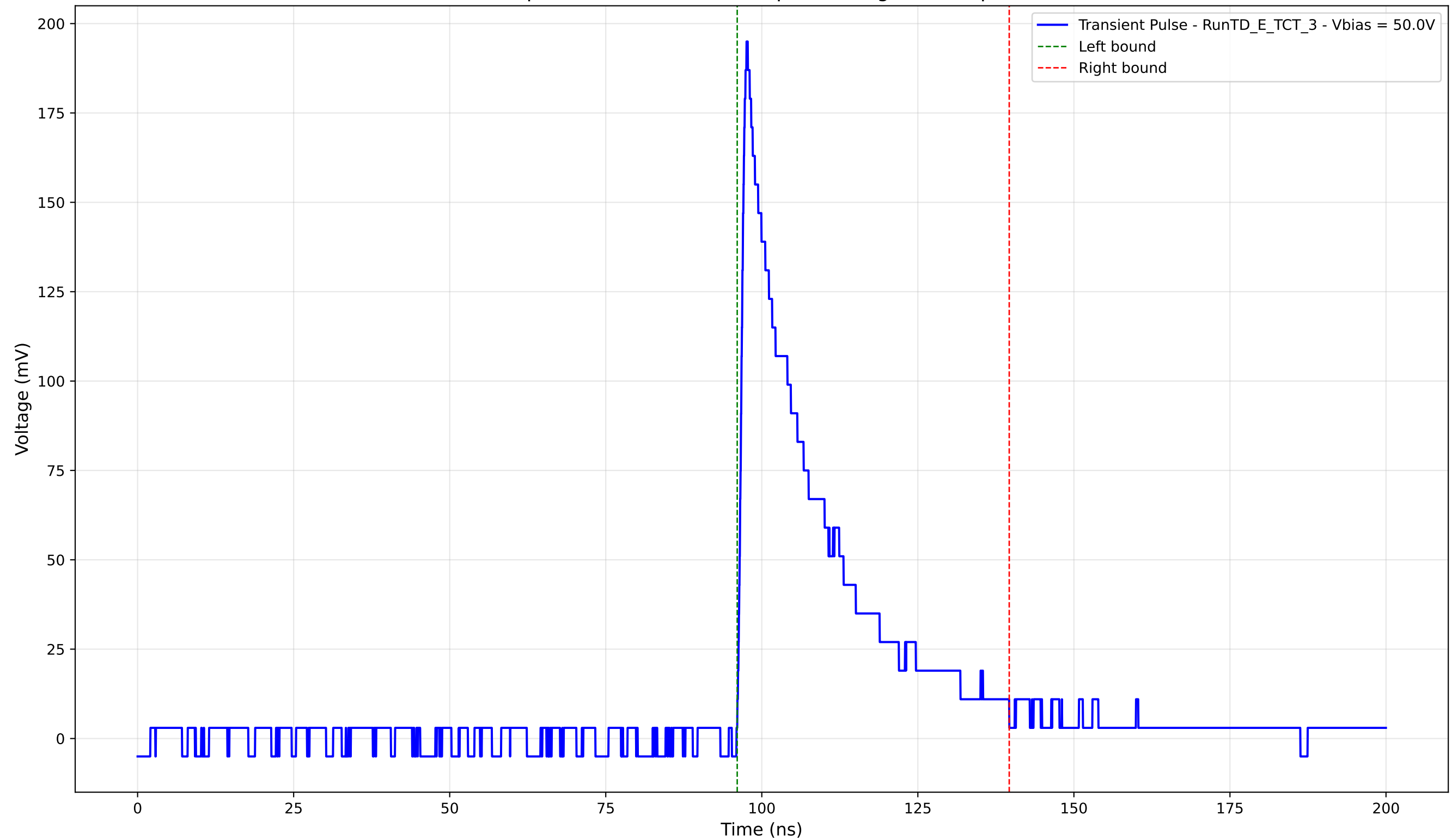
Transient Pulse - Sample: TD - Position: 485.0 \mu\text{m} - Charge: 45.34 pC - Rise Time: 1.02 ns
