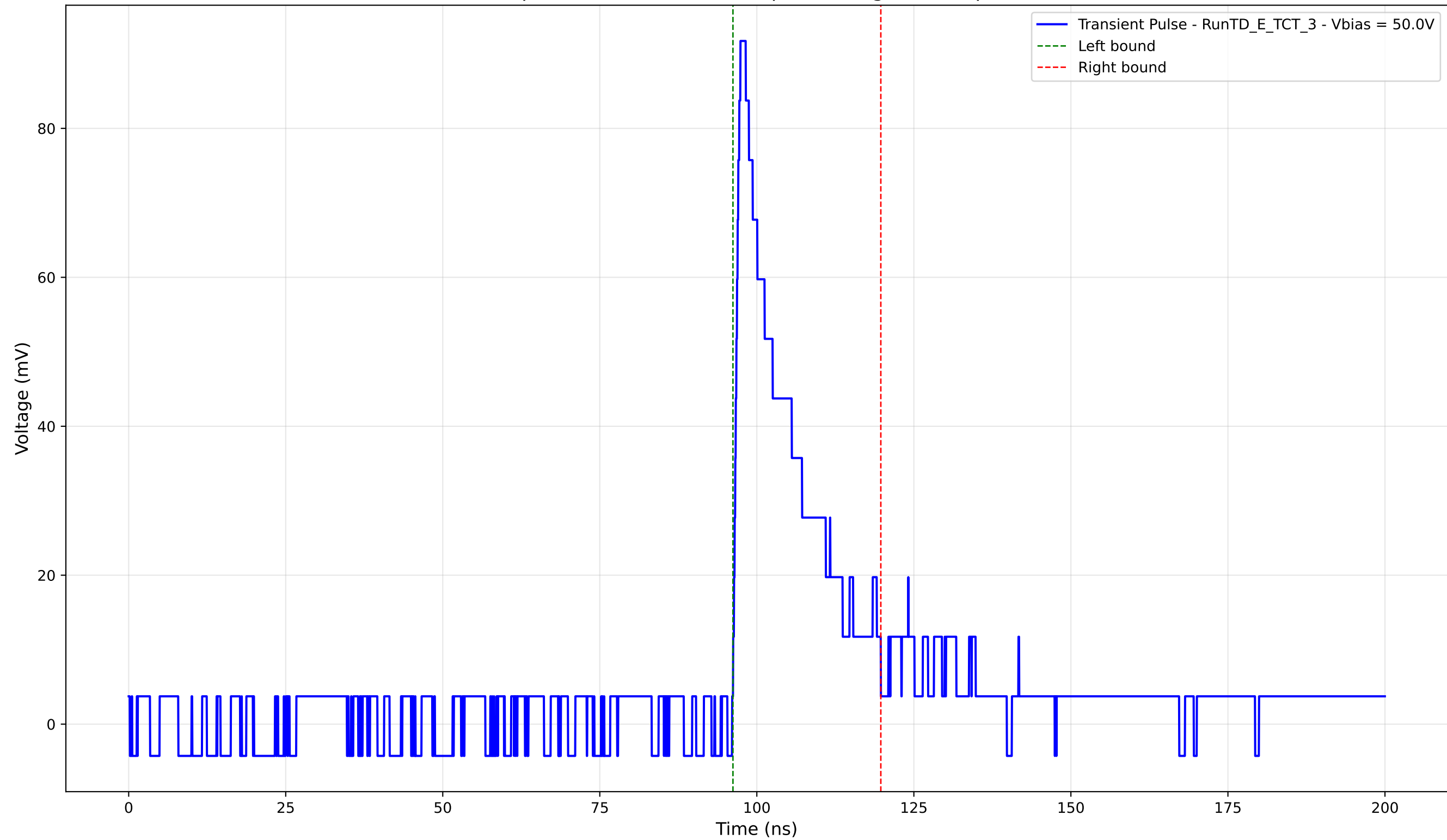
Transient Pulse - Sample: TD - Position: 575.0 \mu\text{m} - Charge: 16.83 pC - Rise Time: 0.99 ns
