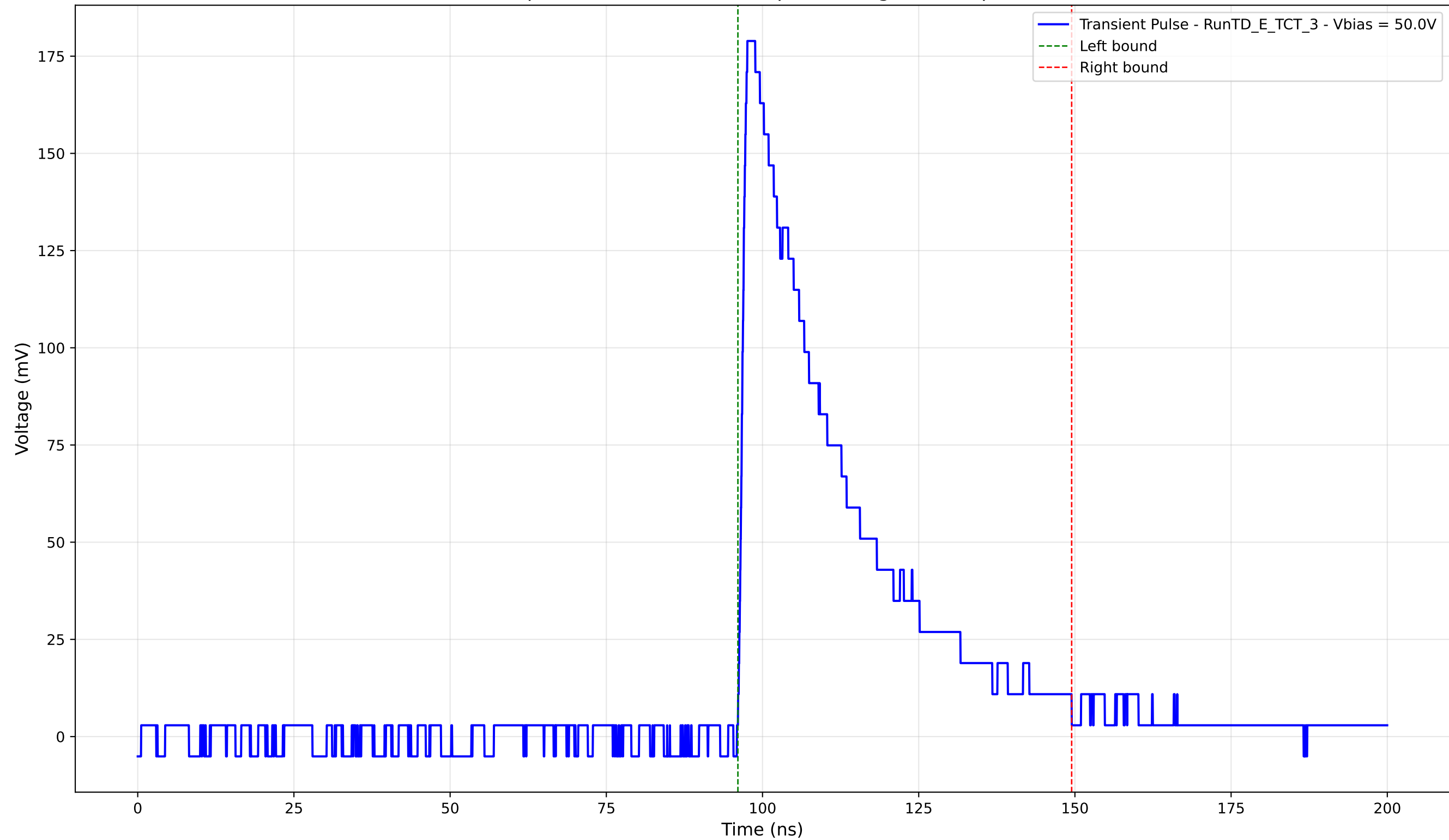
Transient Pulse - Sample: TD - Position: 380.0 \mu\text{m} - Charge: 59.08 pC - Rise Time: 1.12 ns
