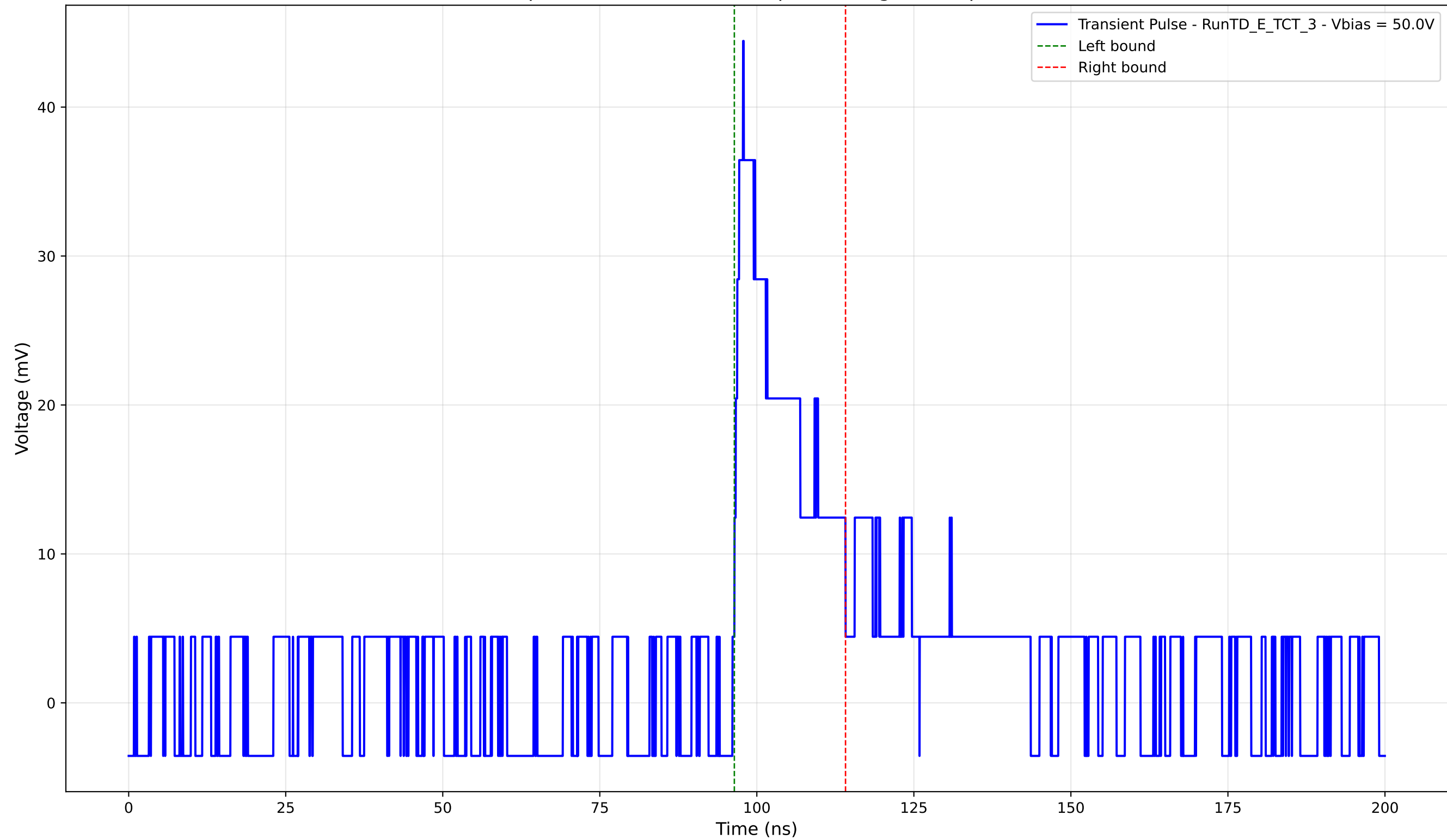
Transient Pulse - Sample: TD - Position: 325.0 \mu\text{m} - Charge: 7.28 pC - Rise Time: 1.38 ns
