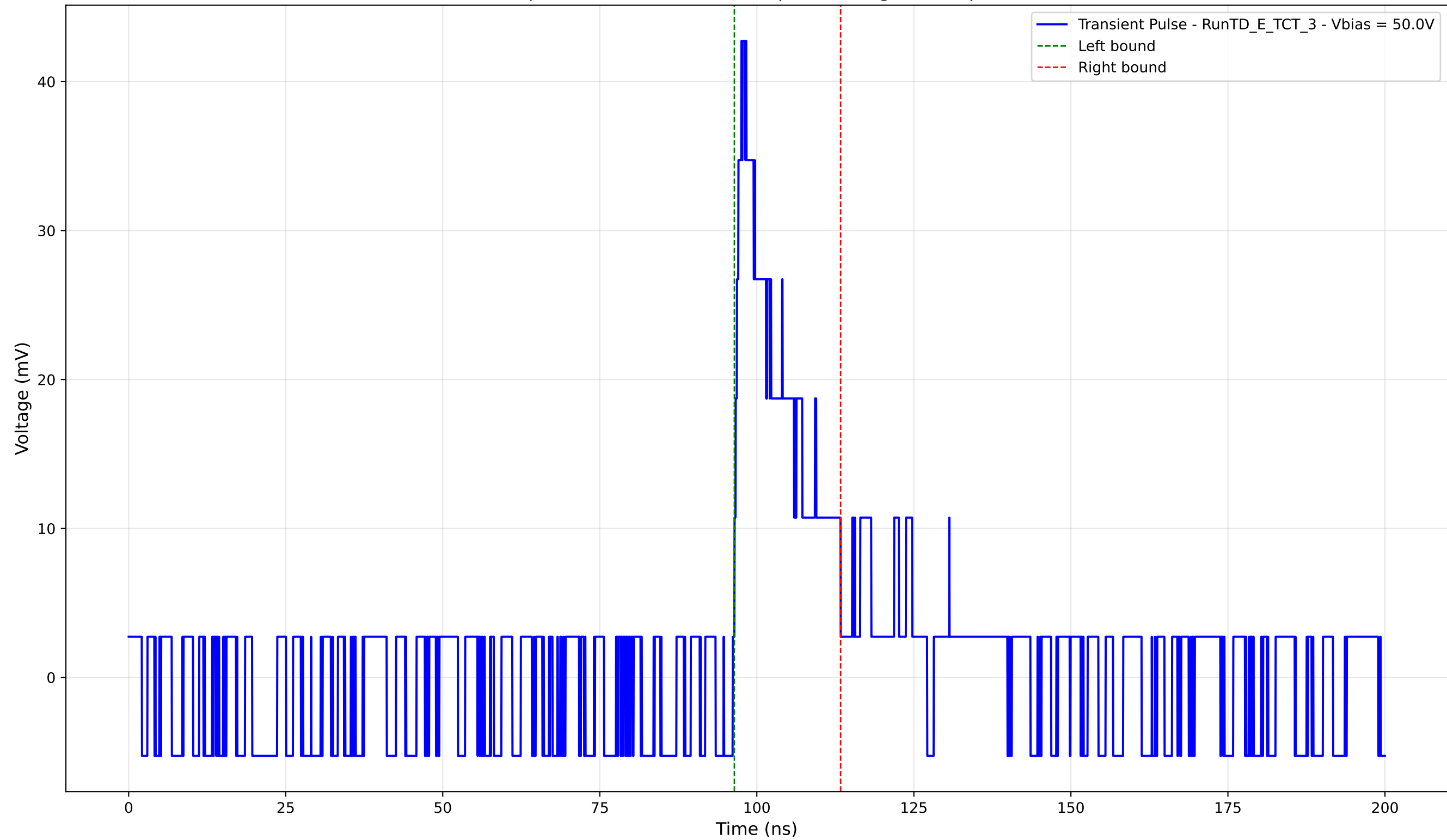
Transient Pulse - Sample: TD - Position: 650.0 \mu\text{m} - Charge: 6.68 pC - Rise Time: 1.12 ns
