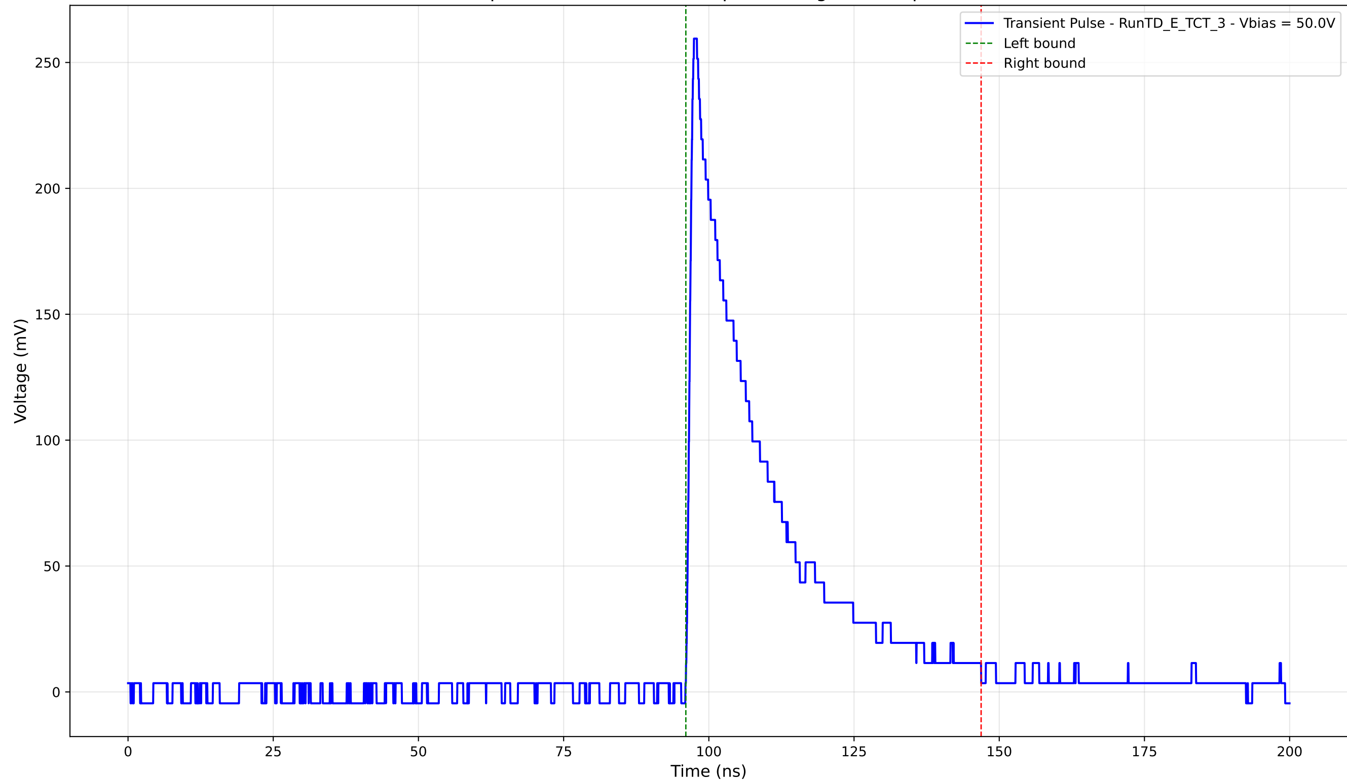
Transient Pulse - Sample: TD - Position: 455.0 \mu\text{m} - Charge: 65.74 pC - Rise Time: 0.98 ns
