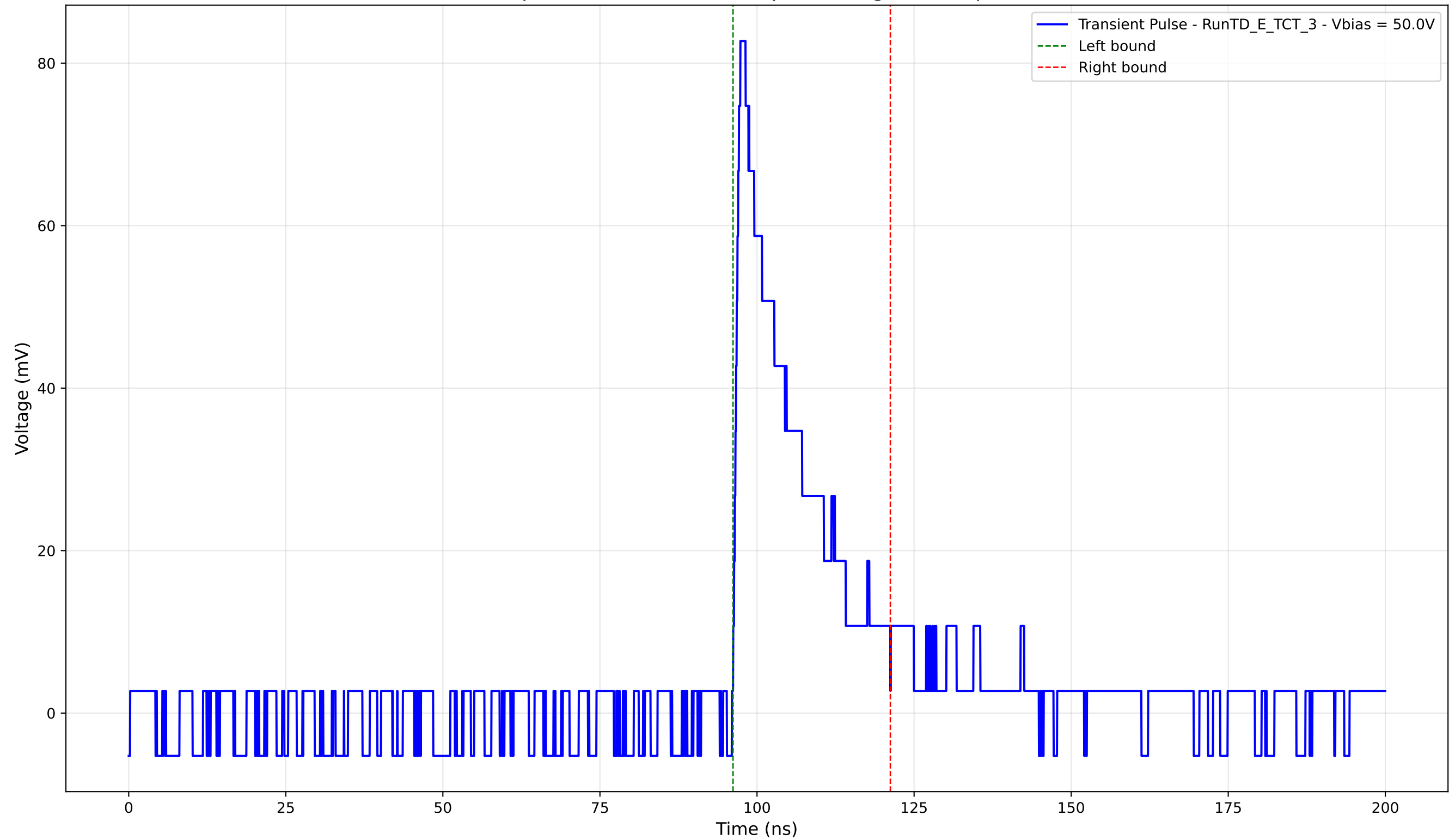
Transient Pulse - Sample: TD - Position: 580.0 \mu\text{m} - Charge: 15.97 pC - Rise Time: 0.93 ns
