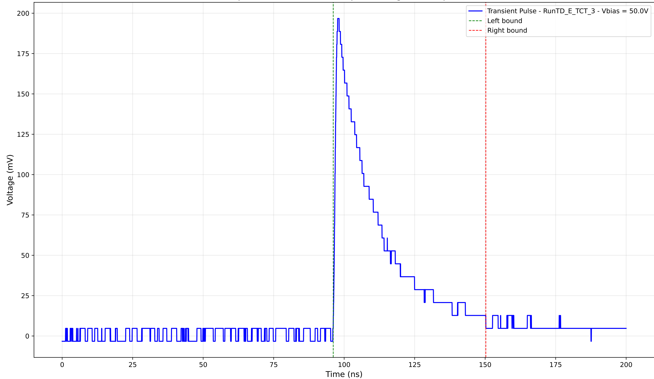
Transient Pulse - Sample: TD - Position: 400.0 \mu\text{m} - Charge: 60.94 pC - Rise Time: 1.14 ns
