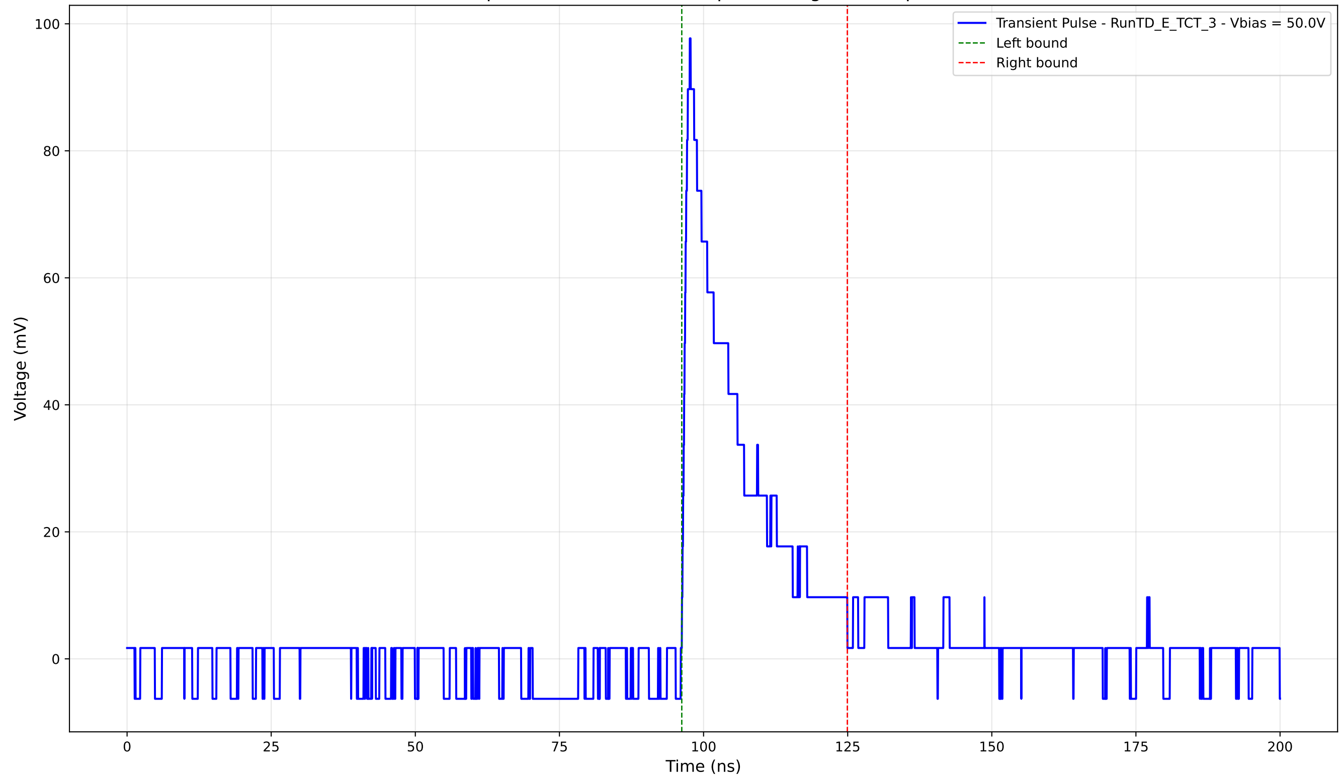
Transient Pulse - Sample: TD - Position: 565.0 \mu\text{m} - Charge: 18.07 pC - Rise Time: 0.94 ns
