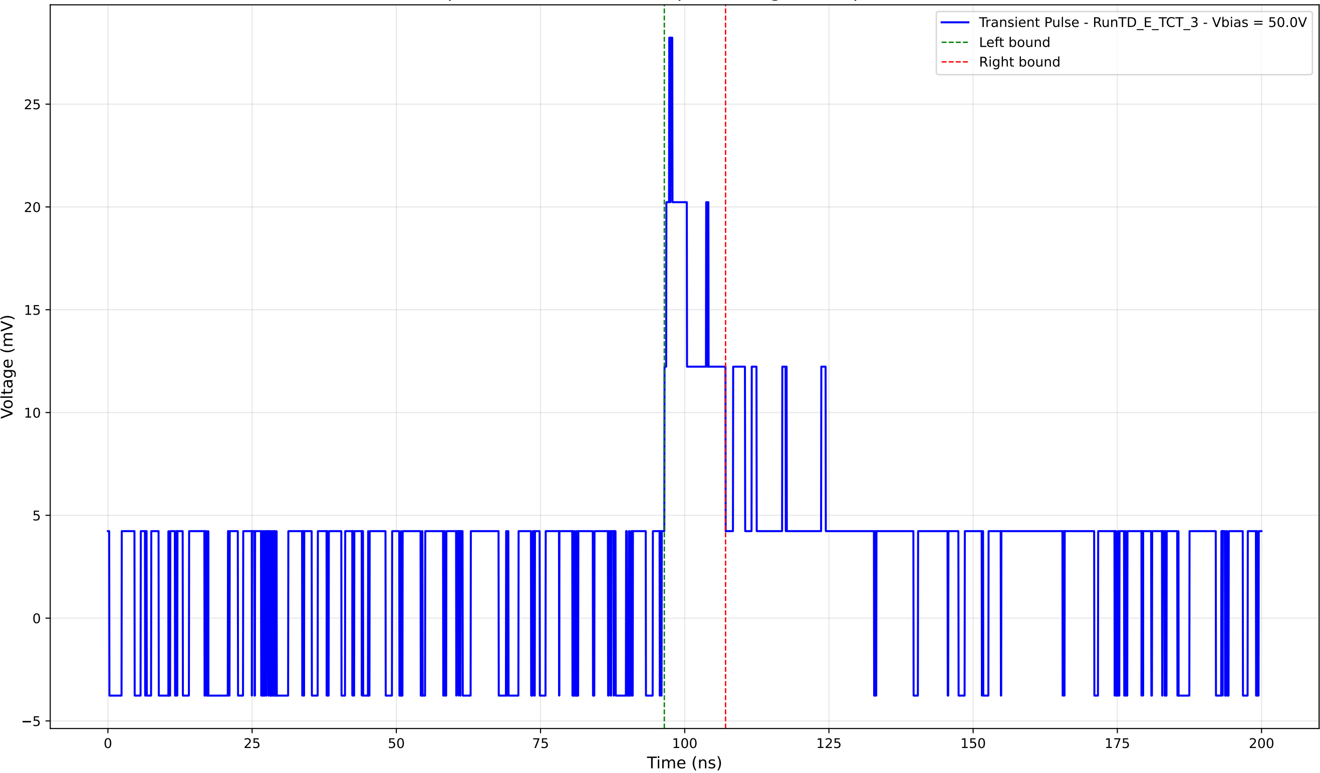
Transient Pulse - Sample: TD - Position: 680.0 \mu\text{m} - Charge: 3.28 pC - Rise Time: 0.00 ns (N/A)
