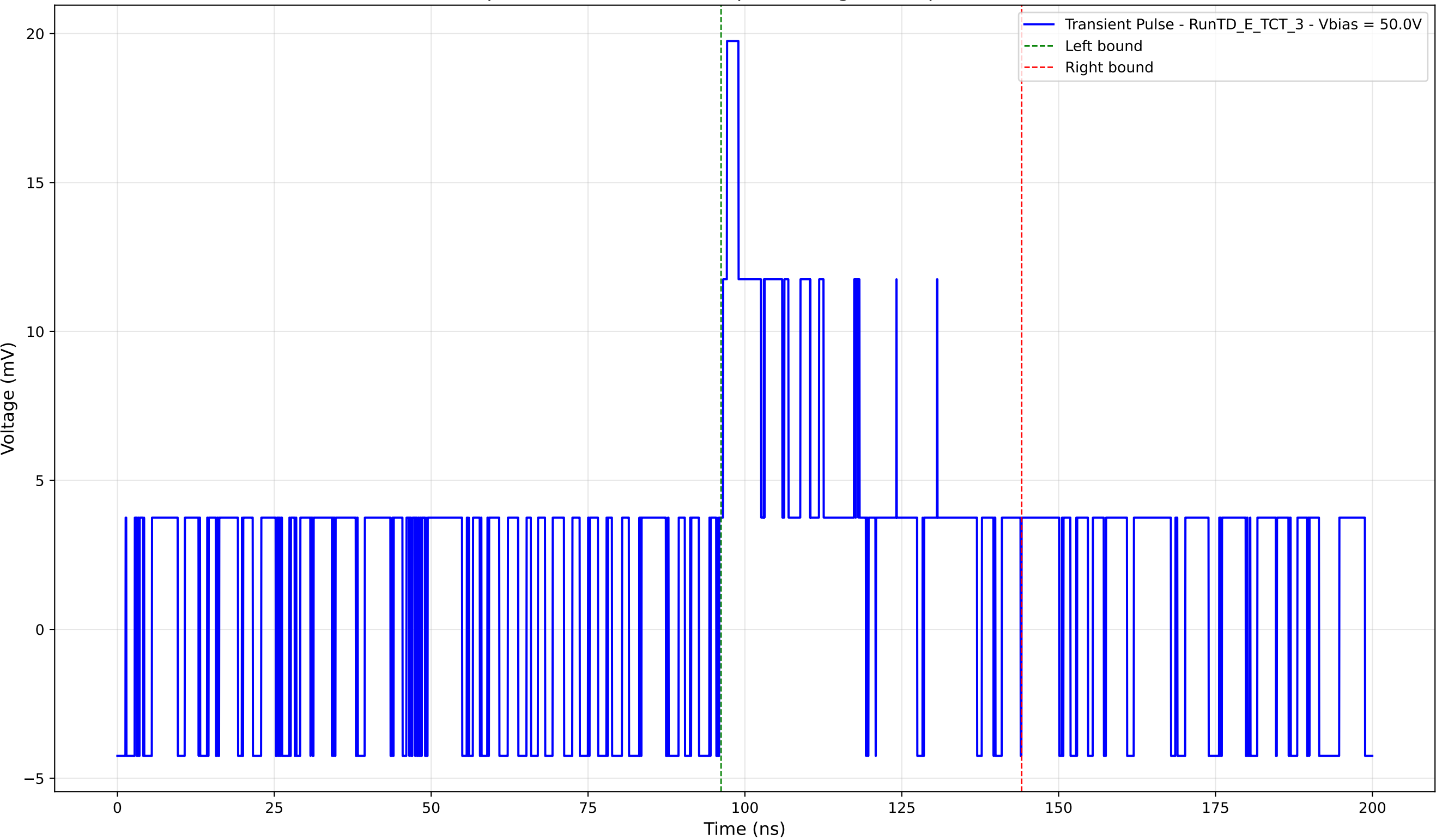
Transient Pulse - Sample: TD - Position: 675.0 \mu\text{m} - Charge: 5.40 pC - Rise Time: 0.00 ns (N/A)
