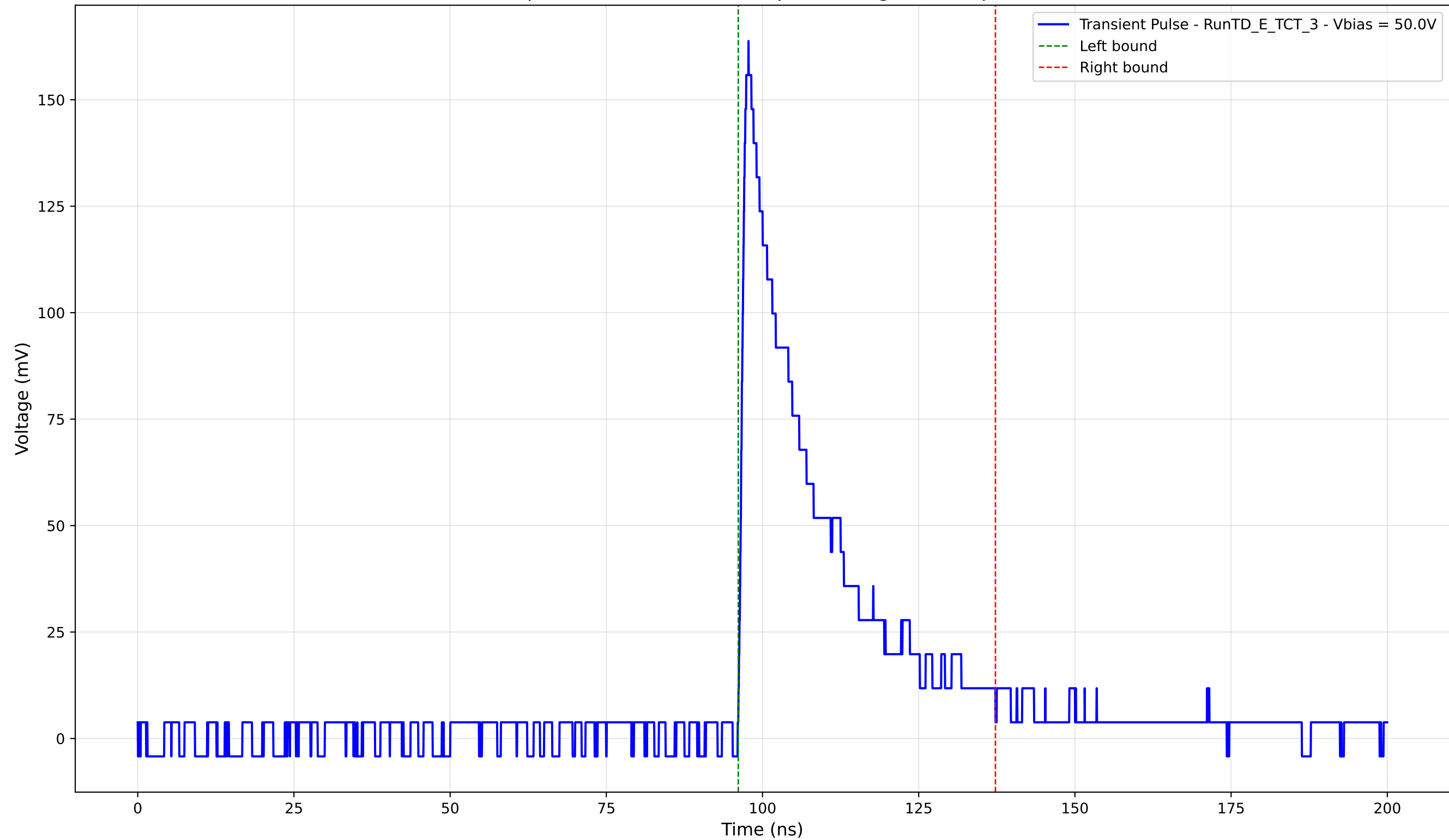
Transient Pulse - Sample: TD - Position: 495.0 \mu\text{m} - Charge: 38.23 pC - Rise Time: 1.03 ns
