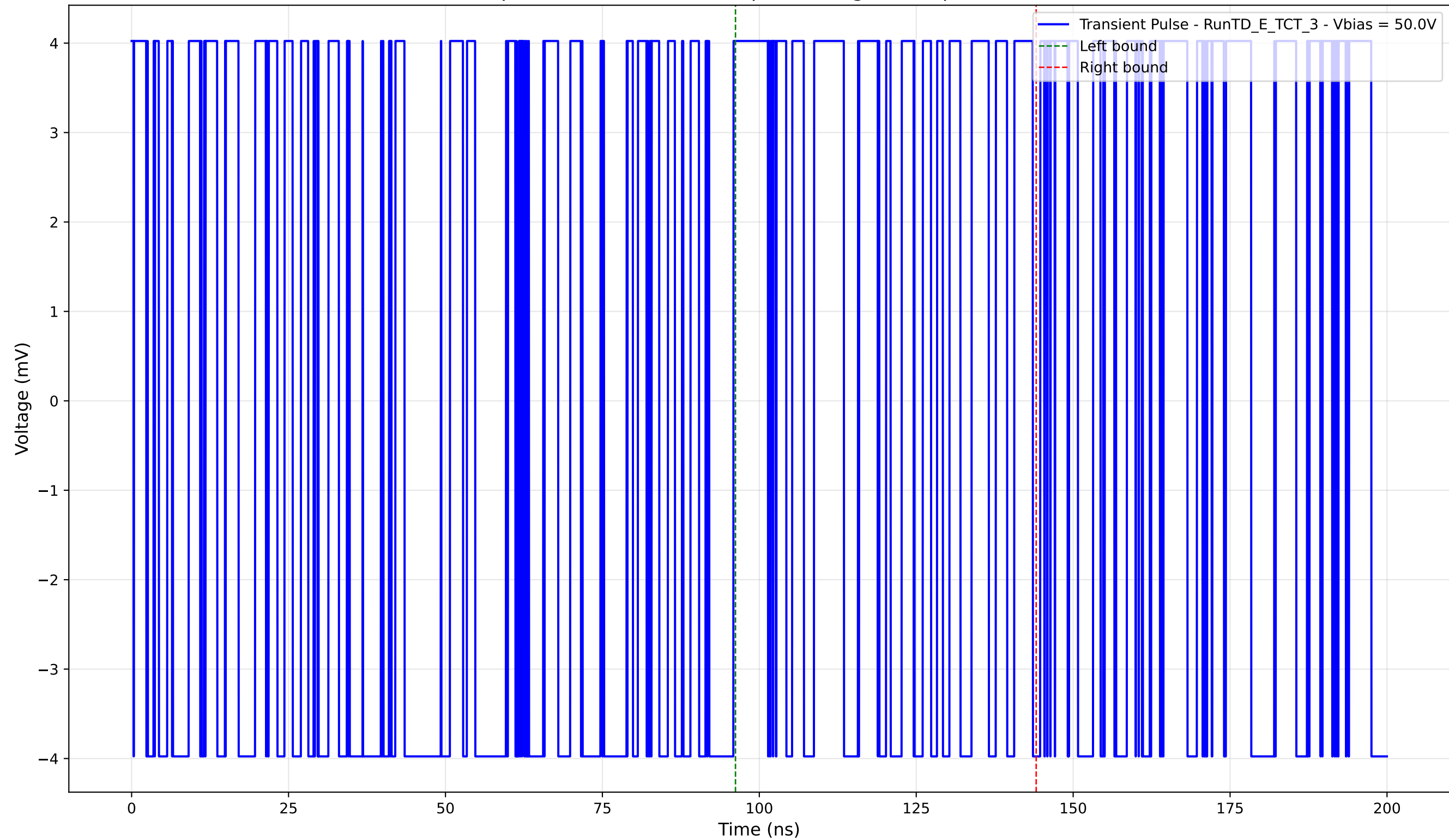
Transient Pulse - Sample: TD - Position: 120.0 \mu\text{m} - Charge: 1.27 pC - Rise Time: 0.00 ns (N/A)
