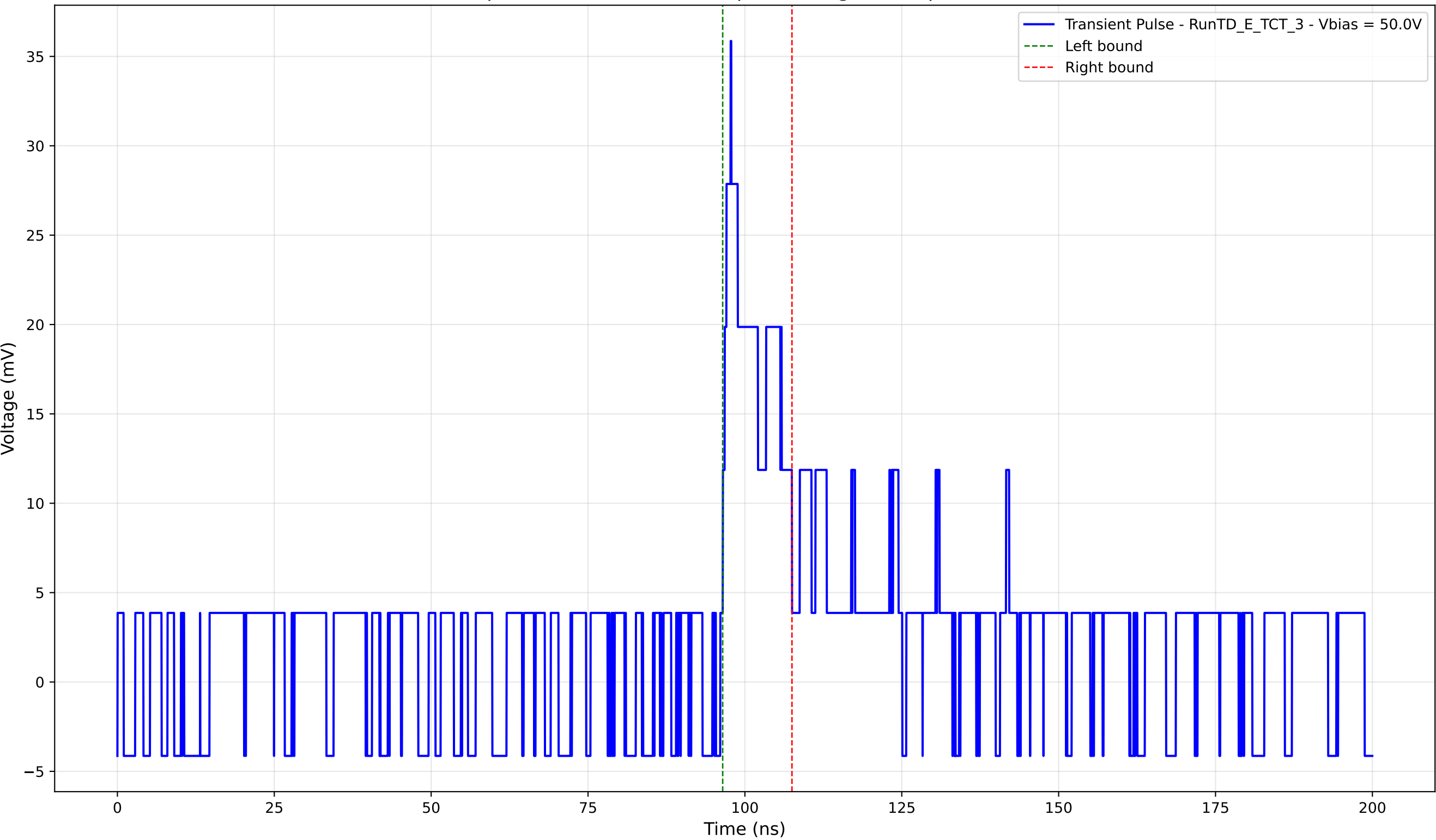
Transient Pulse - Sample: TD - Position: 685.0 \mu\text{m} - Charge: 4.16 pC - Rise Time: 0.00 ns (N/A)
