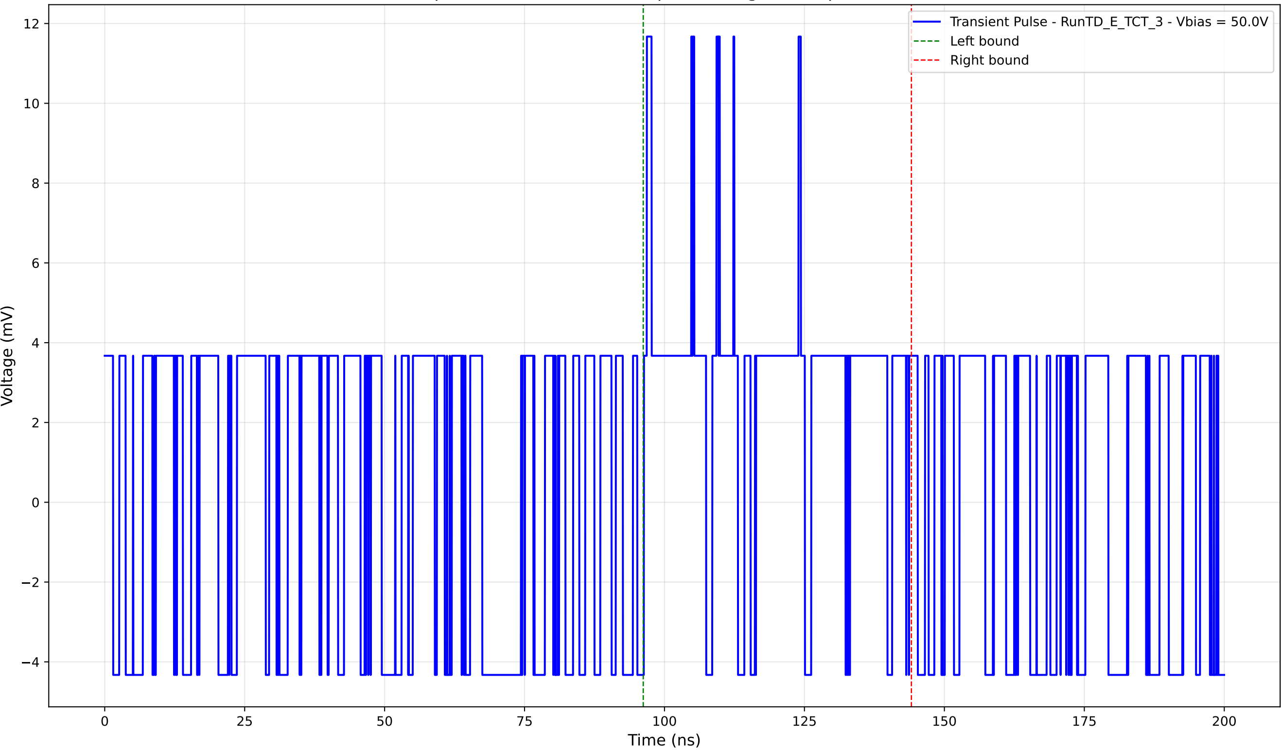
Transient Pulse - Sample: TD - Position: 275.0 \mu\text{m} - Charge: 3.01 pC - Rise Time: 0.00 ns (N/A)
