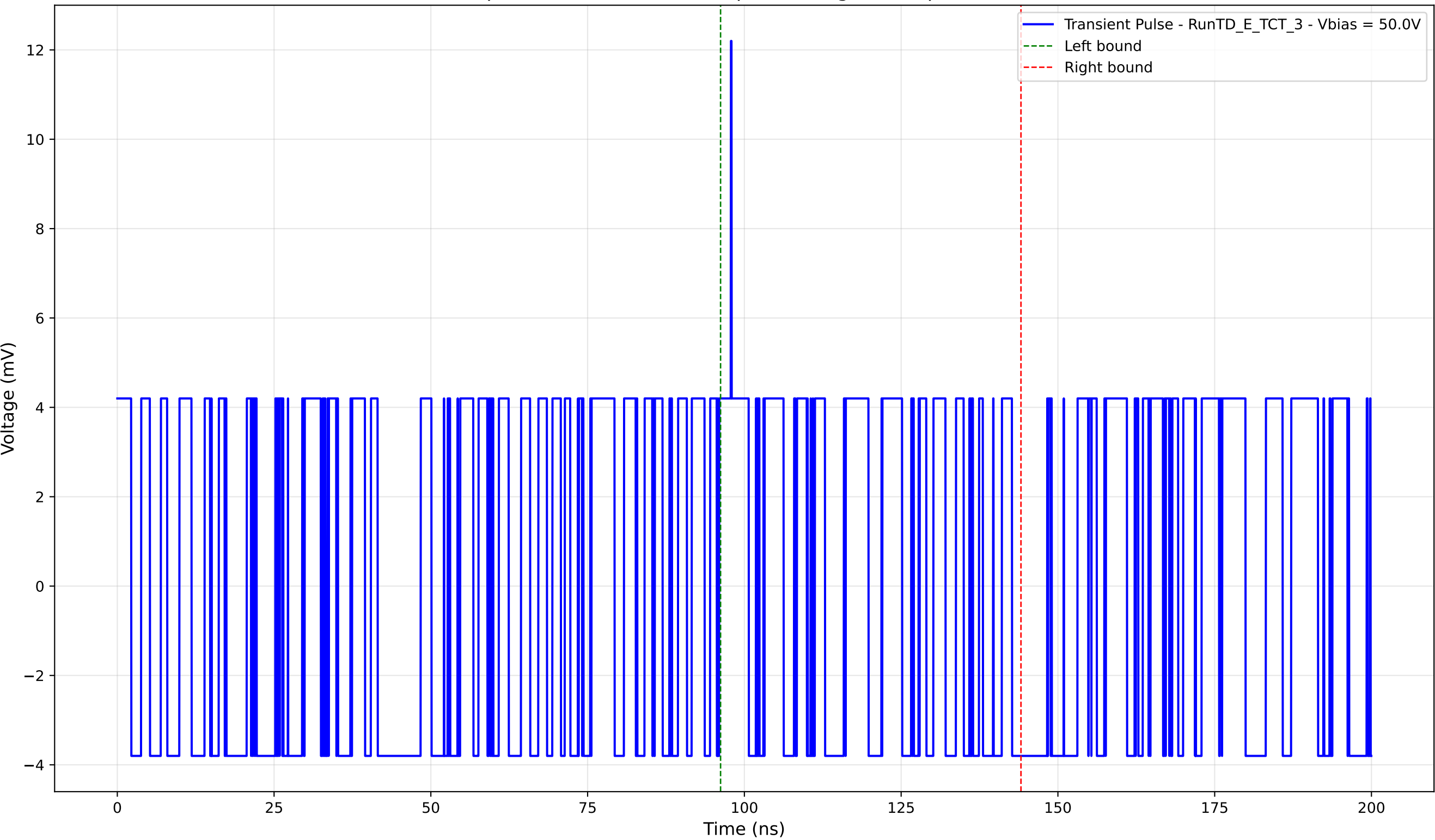
Transient Pulse - Sample: TD - Position: 195.0 \mu\text{m} - Charge: 0.54 pC - Rise Time: 0.00 ns (N/A)
