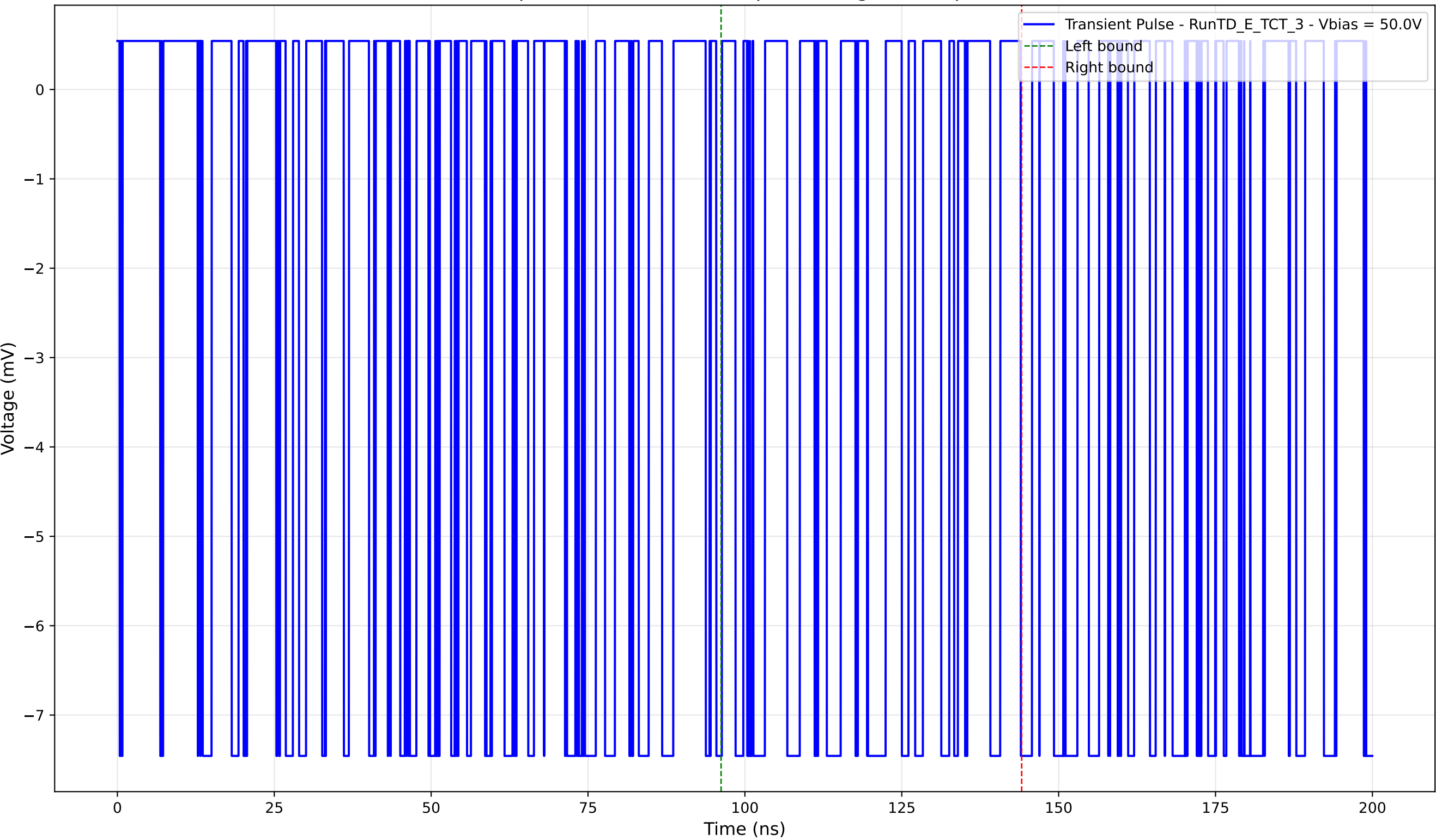
Transient Pulse - Sample: TD - Position: 75.0 \mu\text{m} - Charge: -2.37 pC - Rise Time: 0.02 ns
