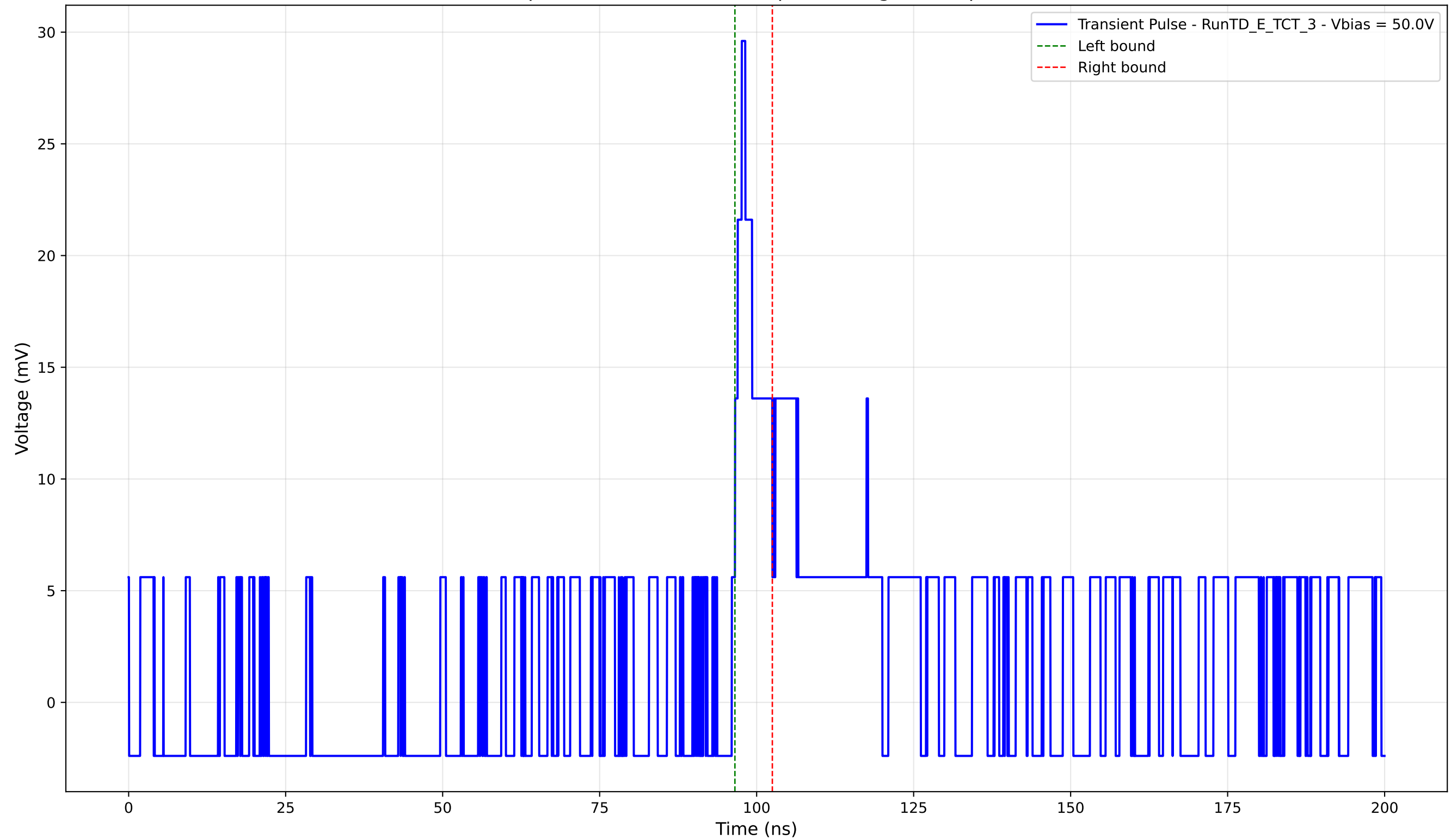
Transient Pulse - Sample: TD - Position: 665.0 \mu\text{m} - Charge: 2.08 pC - Rise Time: 1.60 ns
