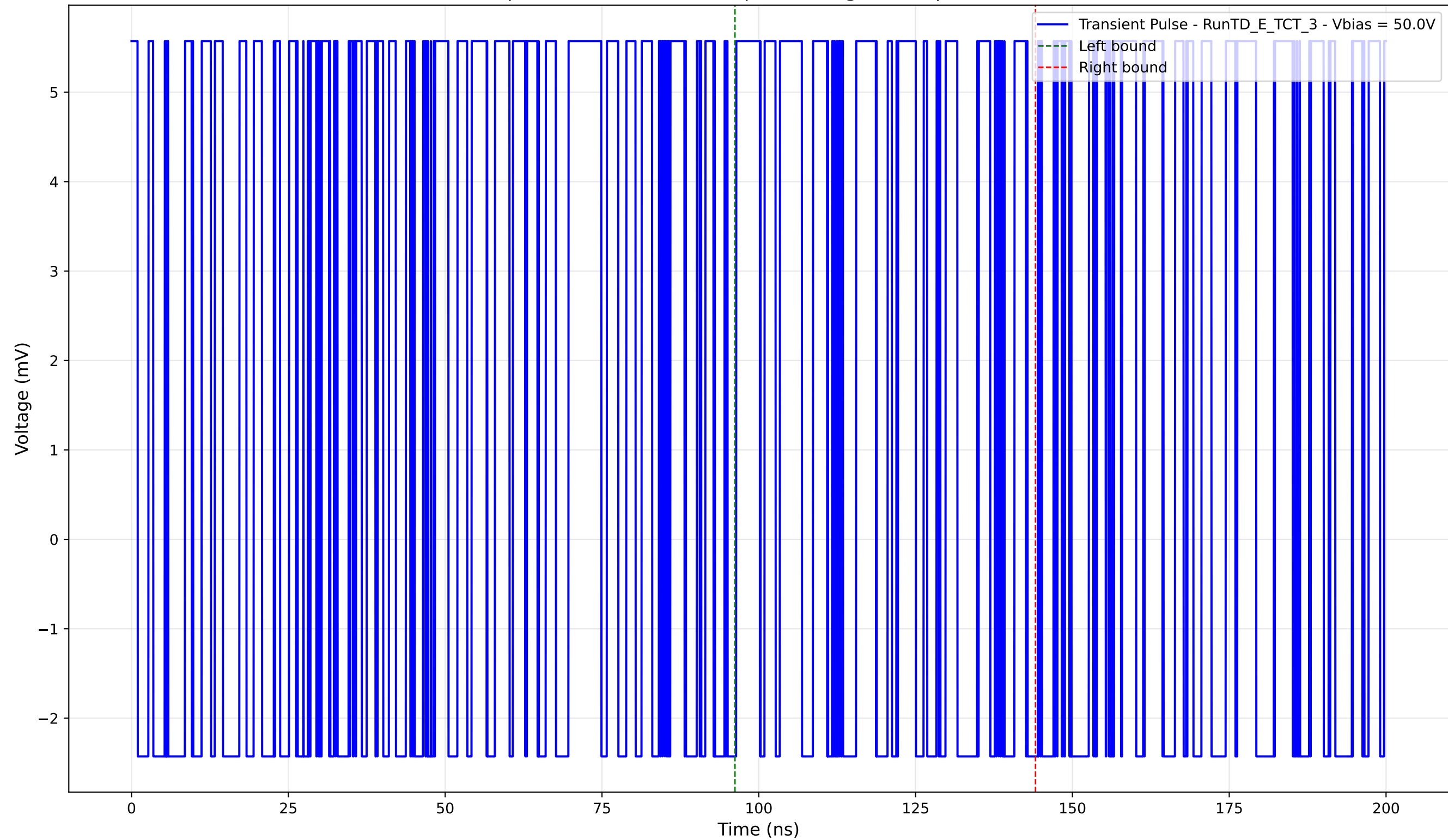
Transient Pulse - Sample: TD - Position: 95.0 \mu\text{m} - Charge: 1.97 pC - Rise Time: 0.00 ns (N/A)
