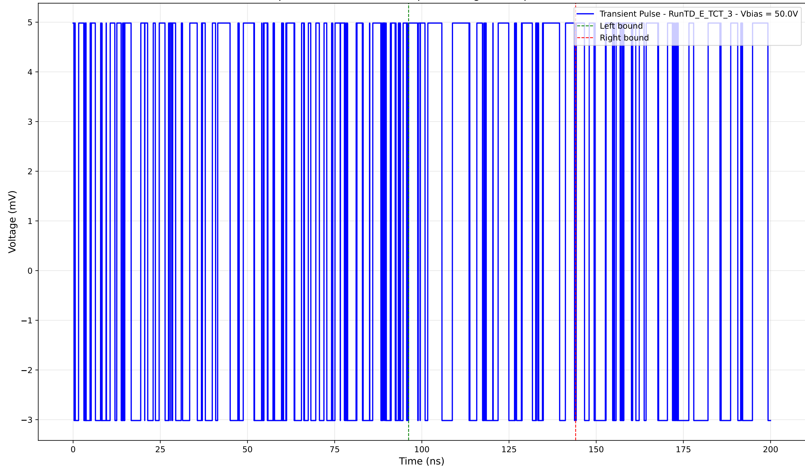
Transient Pulse - Sample: TD - Position: 215.0 \mu\text{m} - Charge: 1.96 pC - Rise Time: 0.00 ns (N/A)
