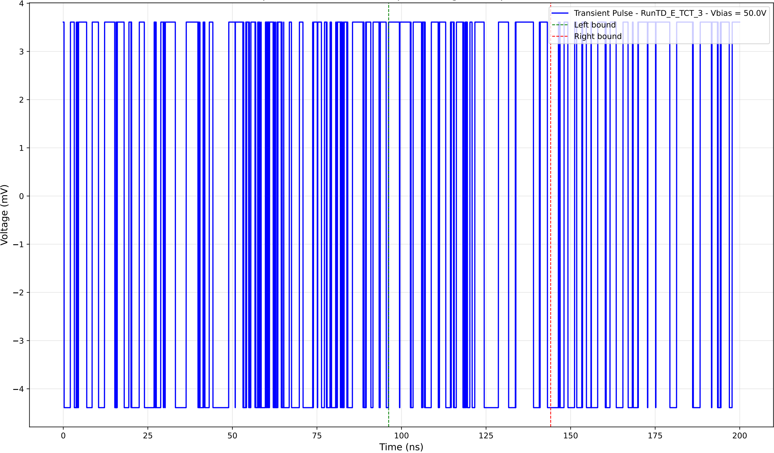
Transient Pulse - Sample: TD - Position: 170.0 \mu\text{m} - Charge: 0.76 pC - Rise Time: 0.00 ns (N/A)
