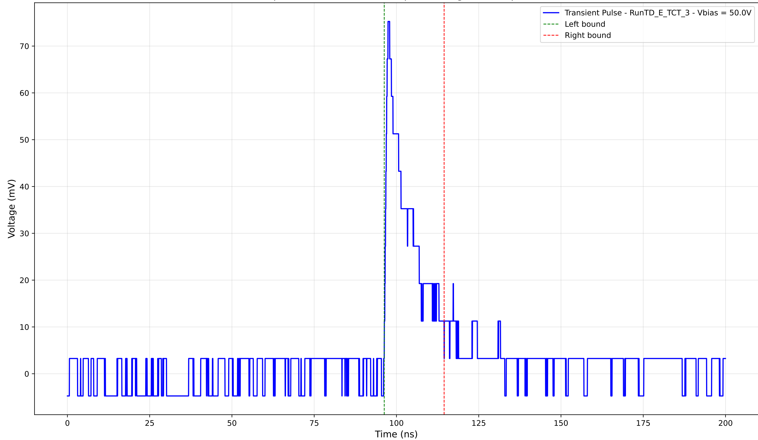
Transient Pulse - Sample: TD - Position: 615.0 \mu\text{m} - Charge: 11.46 pC - Rise Time: 1.13 ns
