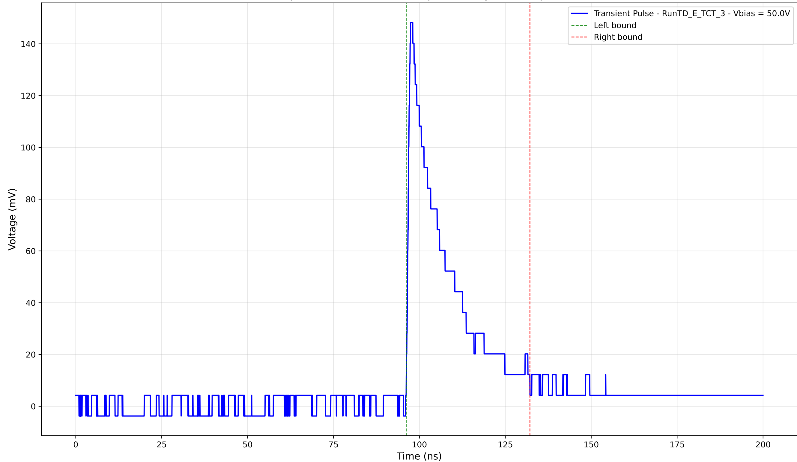
Transient Pulse - Sample: TD - Position: 505.0 \mu\text{m} - Charge: 33.72 pC - Rise Time: 1.03 ns
