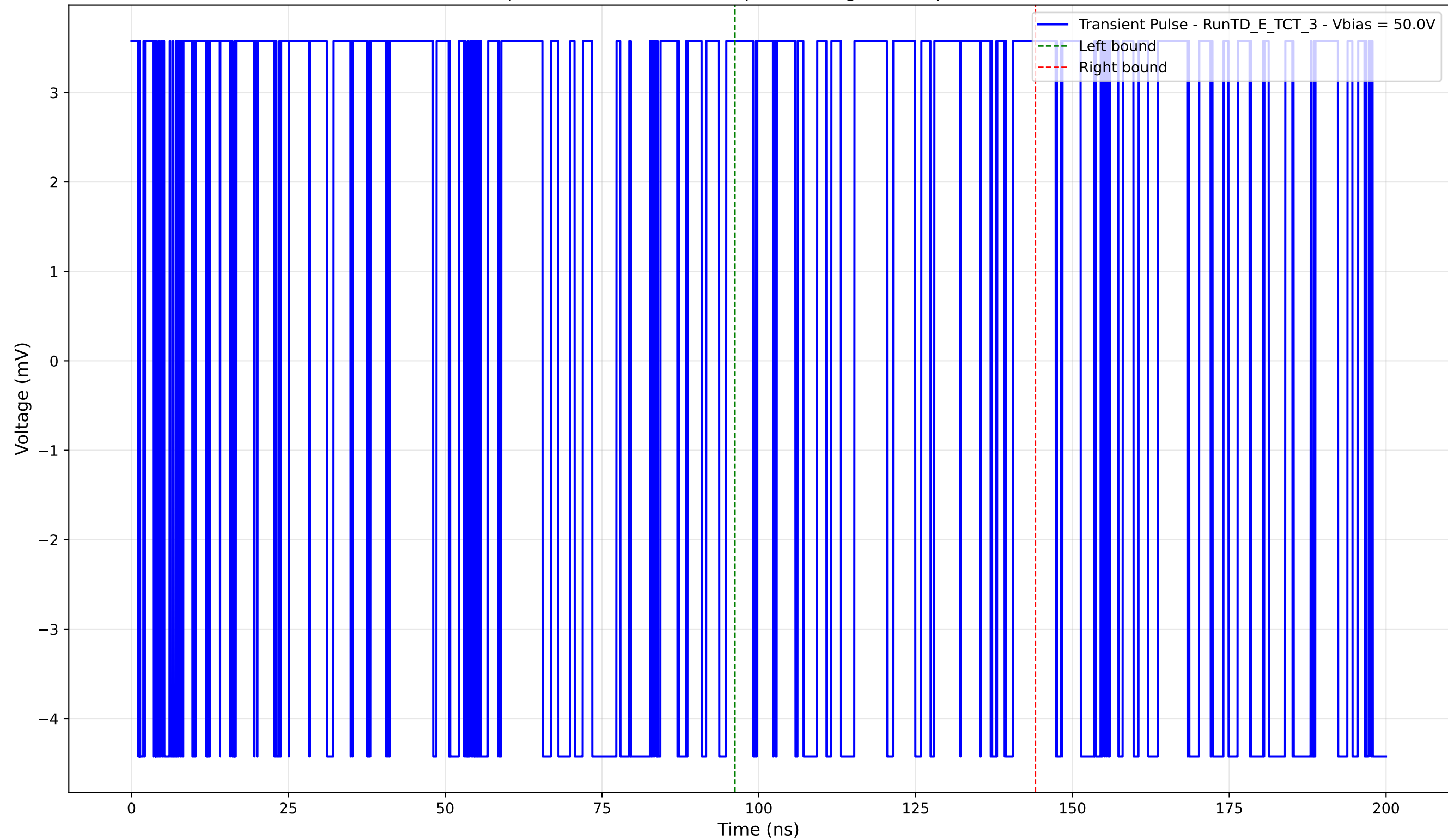
Transient Pulse - Sample: TD - Position: 25.0 \mu\text{m} - Charge: 1.68 pC - Rise Time: 0.00 ns (N/A)
