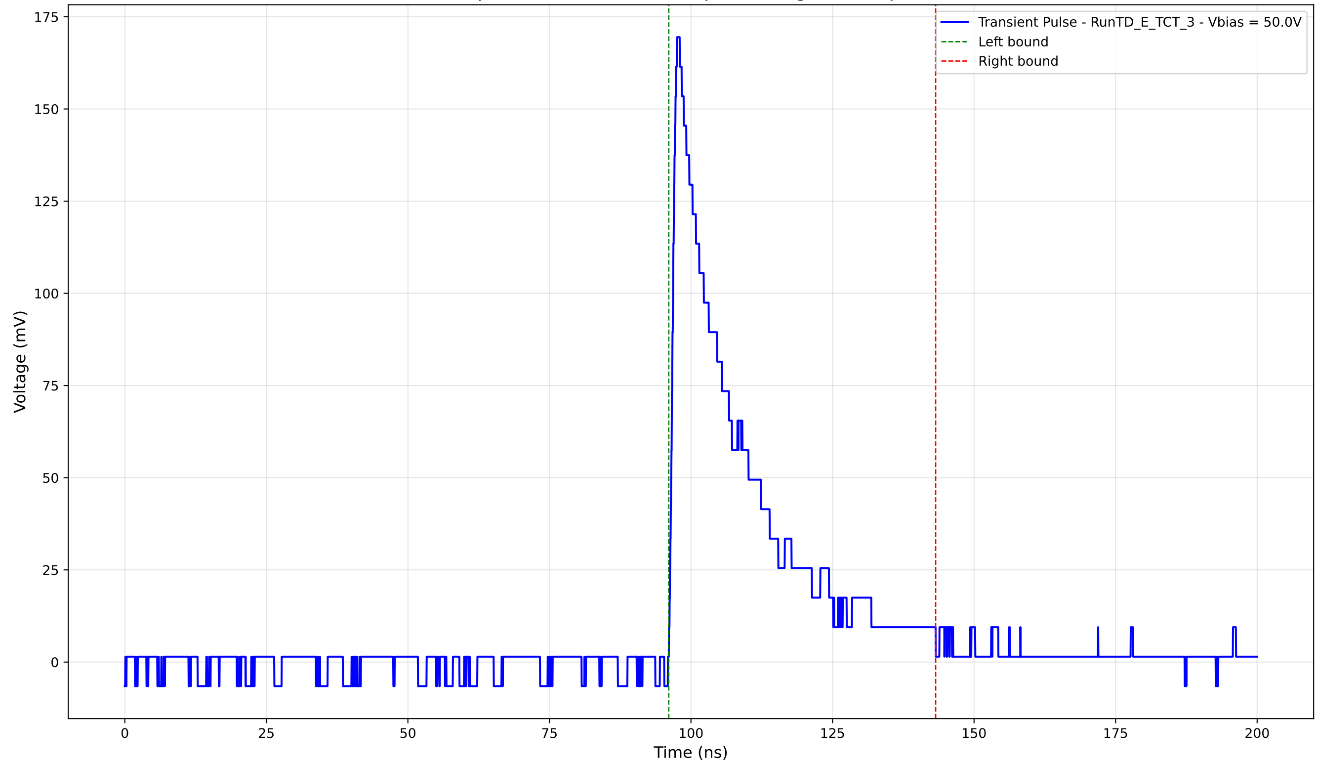
Transient Pulse - Sample: TD - Position: 490.0 \mu\text{m} - Charge: 40.38 pC - Rise Time: 1.04 ns
