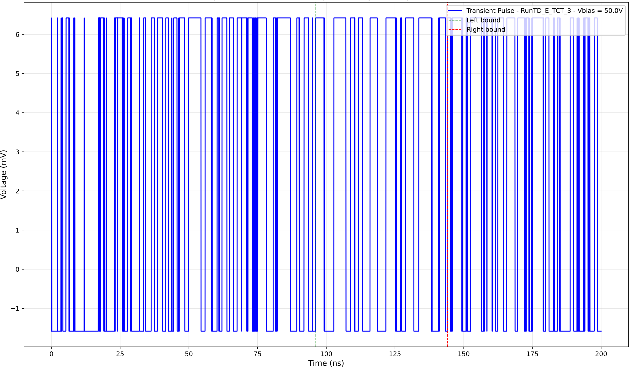
Transient Pulse - Sample: TD - Position: 110.0 \mu\text{m} - Charge: 2.86 pC - Rise Time: 0.00 ns (N/A)
