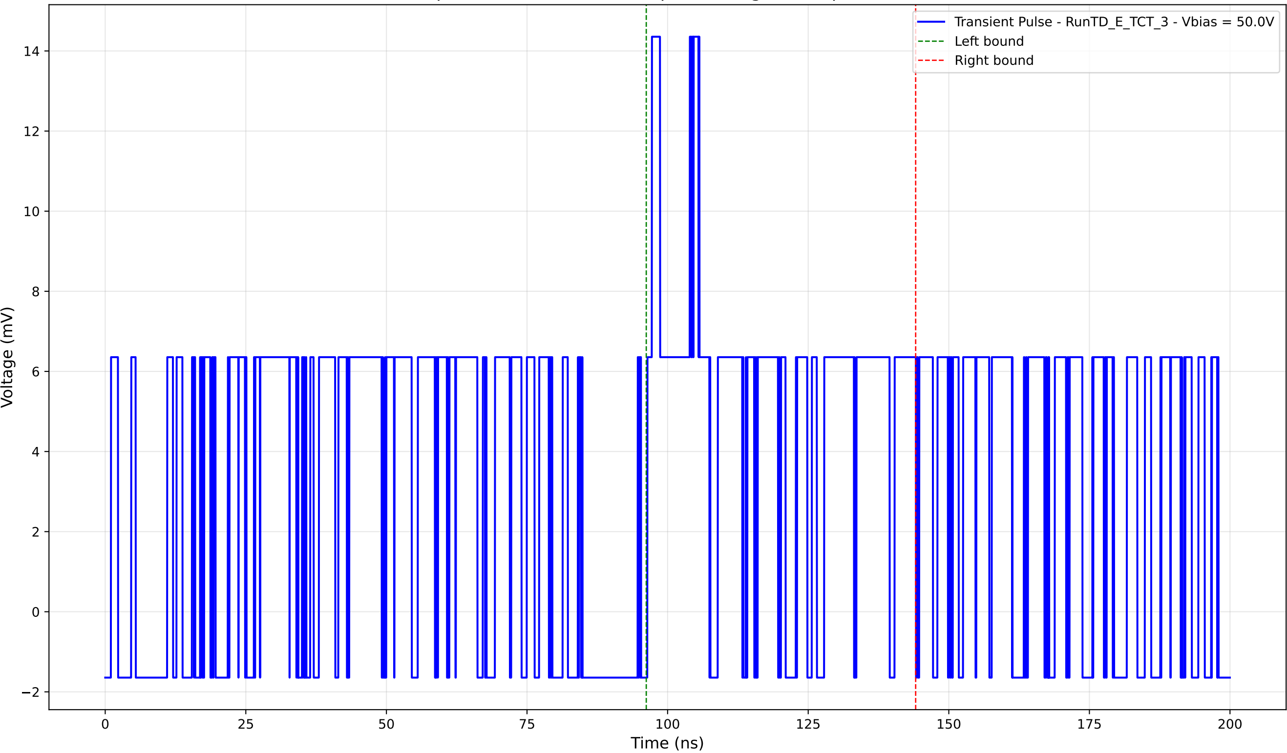
Transient Pulse - Sample: TD - Position: 295.0 \mu\text{m} - Charge: 5.18 pC - Rise Time: 0.00 ns (N/A)
