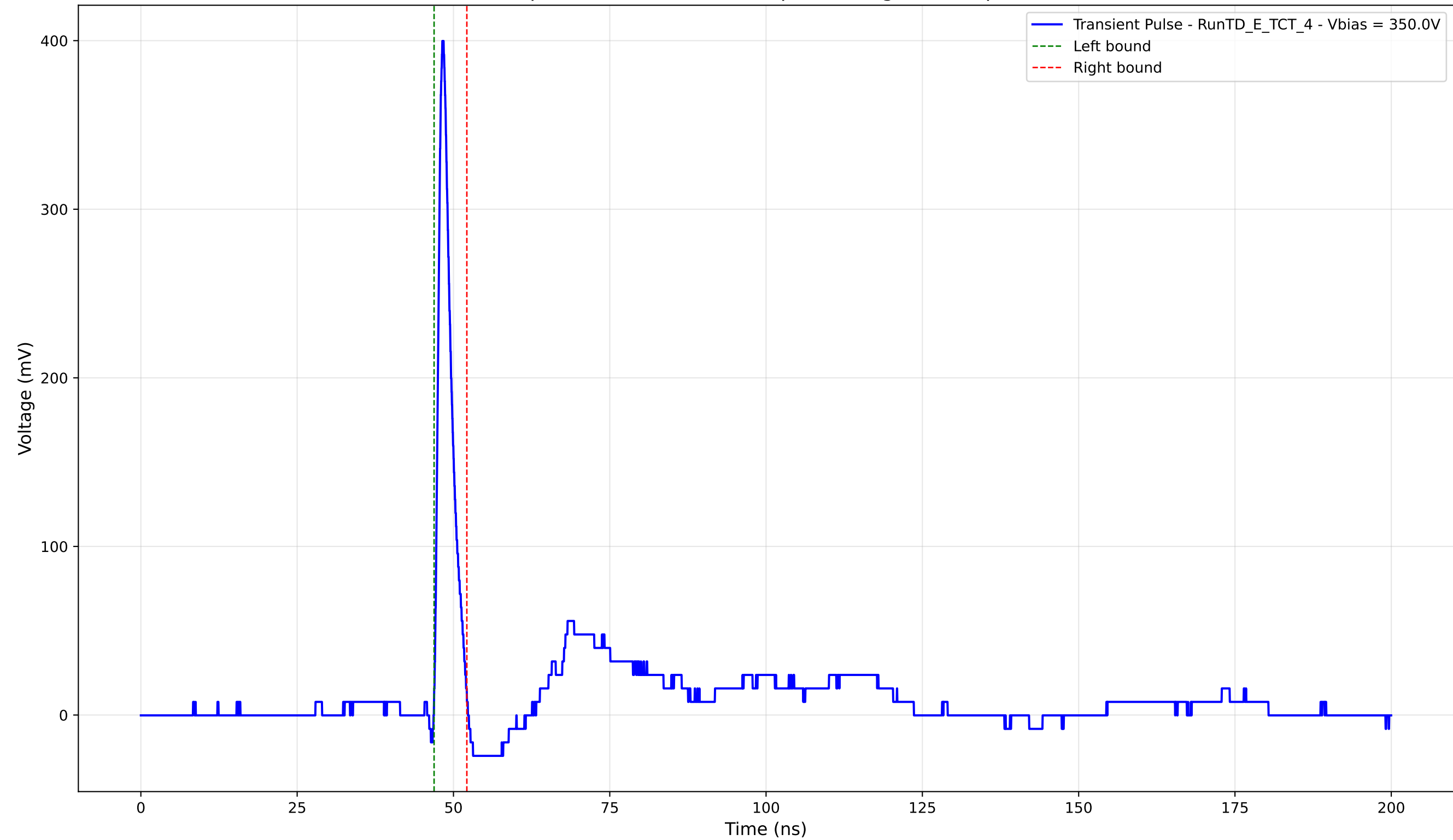
Transient Pulse - Sample: TD - Position: 175.0 \mu\text{m} - Charge: 19.07 pC - Rise Time: 0.92 ns
