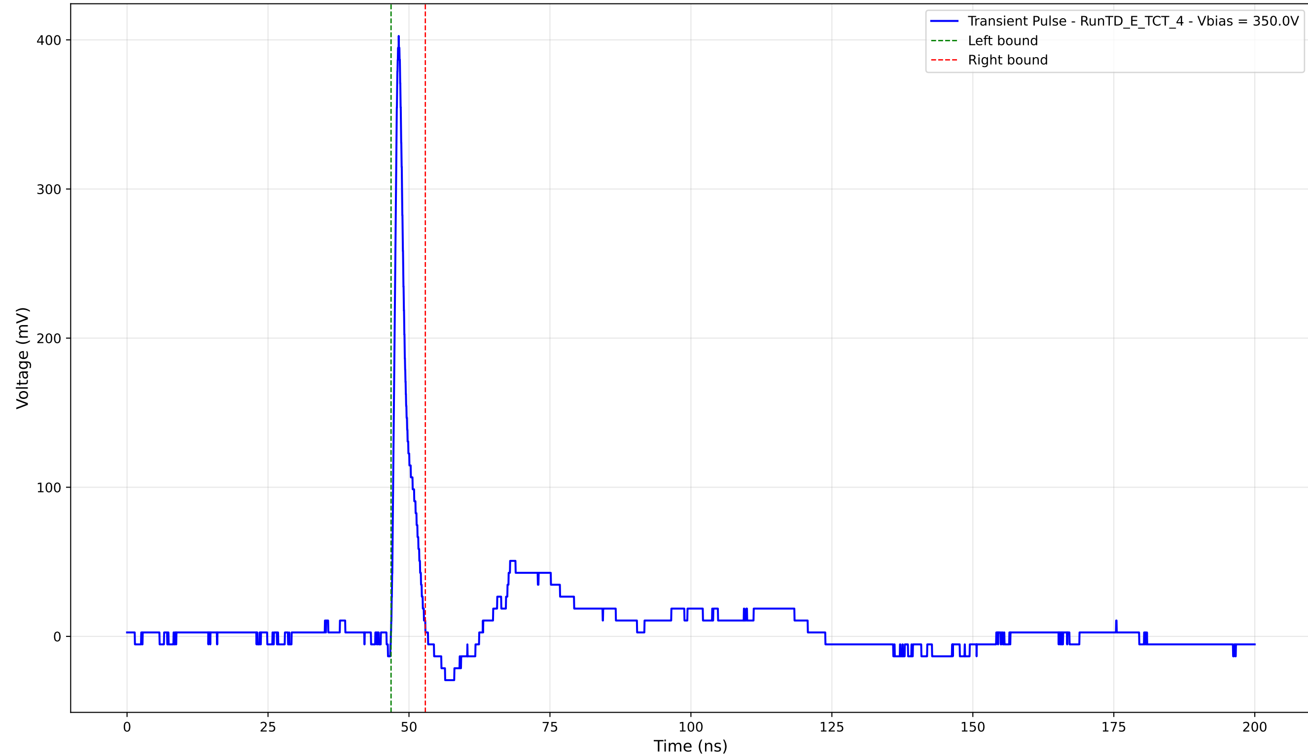
Transient Pulse - Sample: TD - Position: 100.0 \mu\text{m} - Charge: 18.58 pC - Rise Time: 0.87 ns
