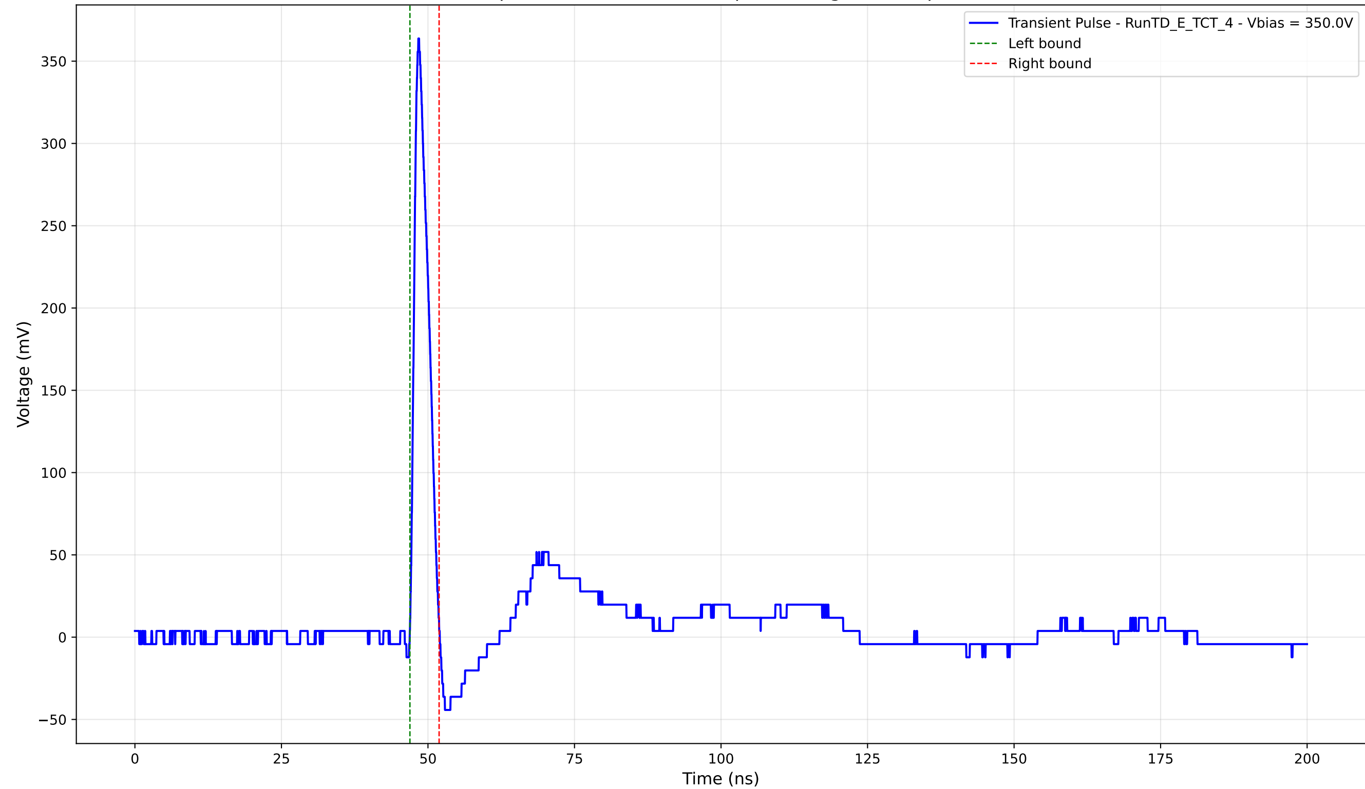
Transient Pulse - Sample: TD - Position: 260.0 \mu\text{m} - Charge: 19.45 pC - Rise Time: 0.94 ns
