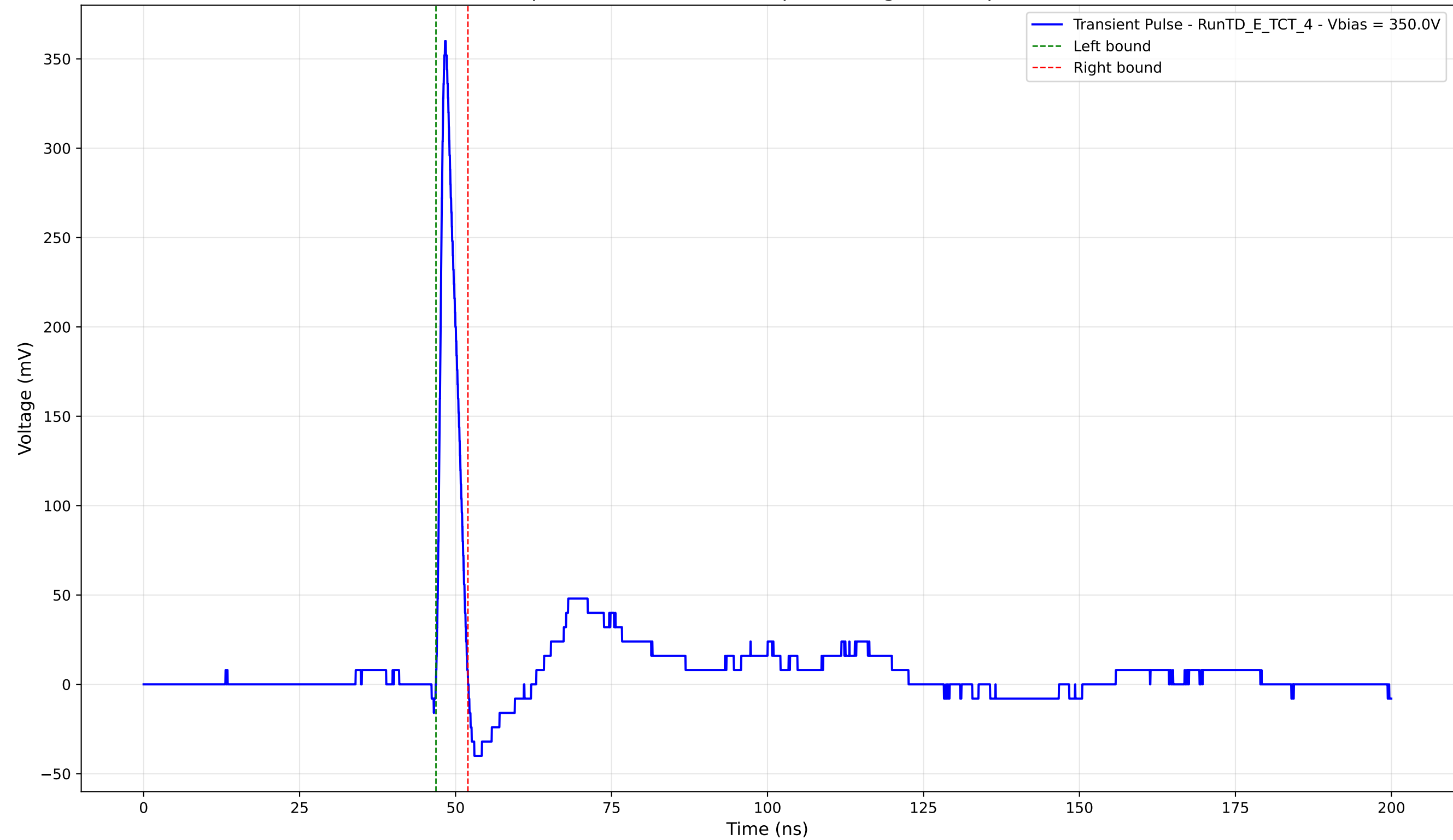
Transient Pulse - Sample: TD - Position: 270.0 \mu\text{m} - Charge: 19.03 pC - Rise Time: 0.95 ns
