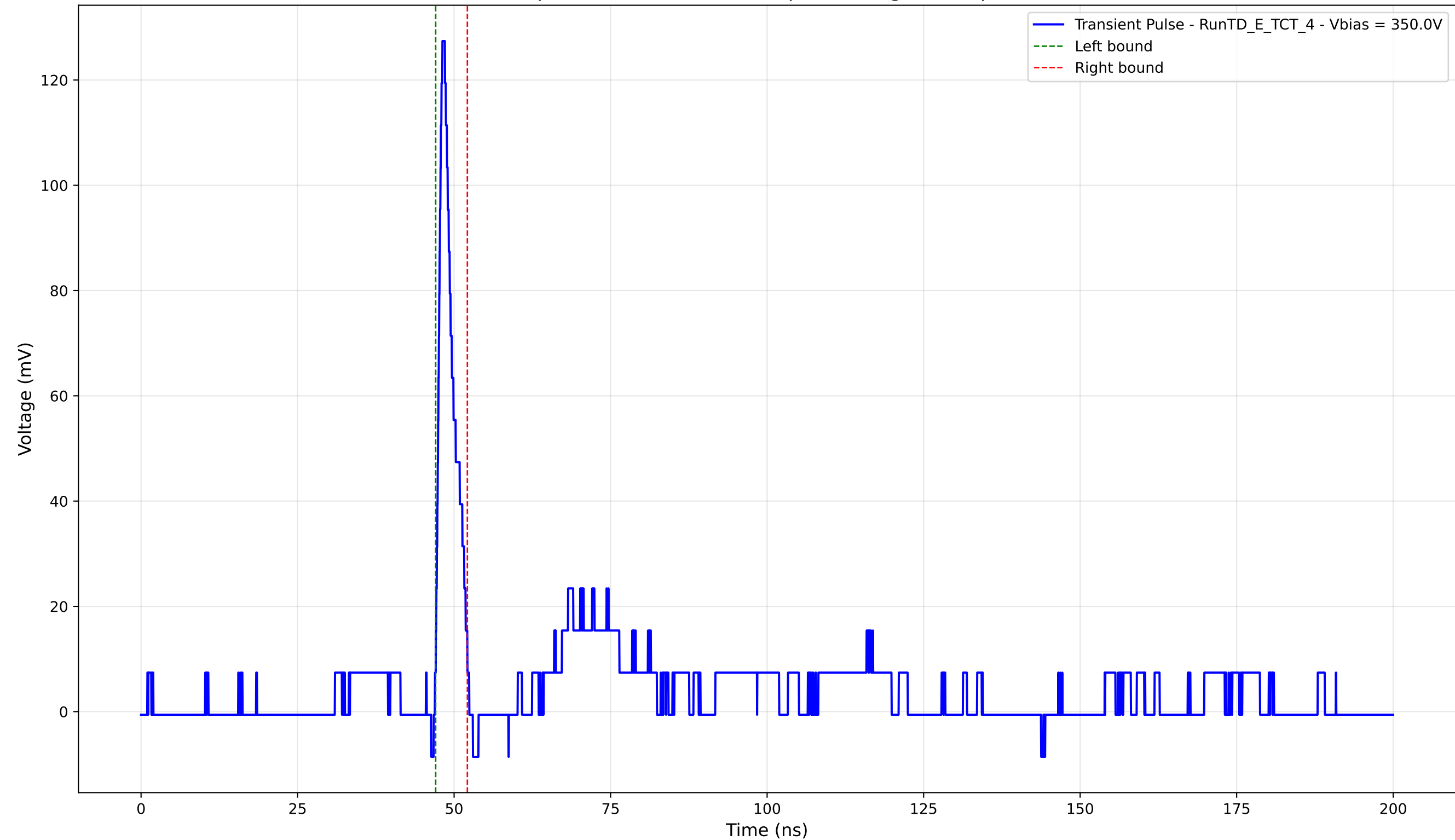
Transient Pulse - Sample: TD - Position: 340.0 \mu\text{m} - Charge: 6.67 pC - Rise Time: 0.91 ns
