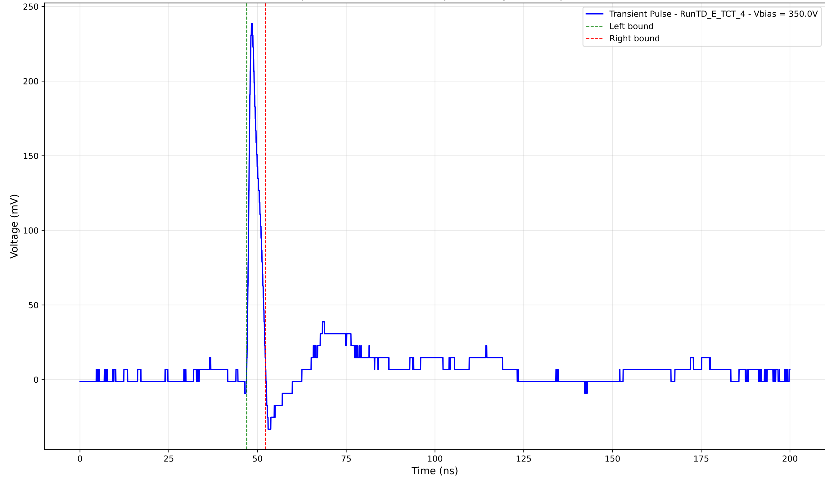
Transient Pulse - Sample: TD - Position: 330.0 \mu\text{m} - Charge: 13.95 pC - Rise Time: 0.98 ns
