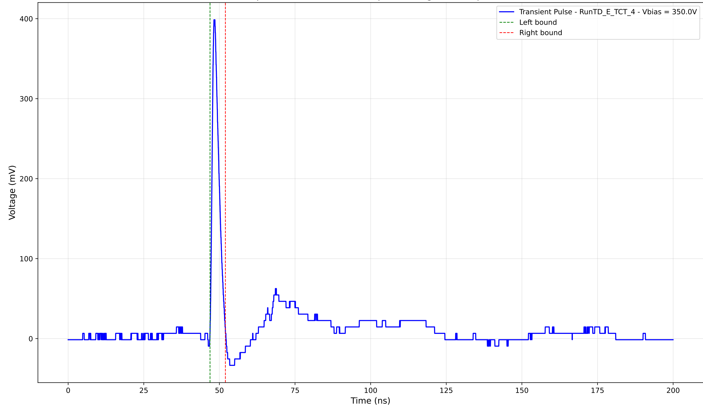
Transient Pulse - Sample: TD - Position: 205.0 \mu\text{m} - Charge: 20.10 pC - Rise Time: 0.94 ns
