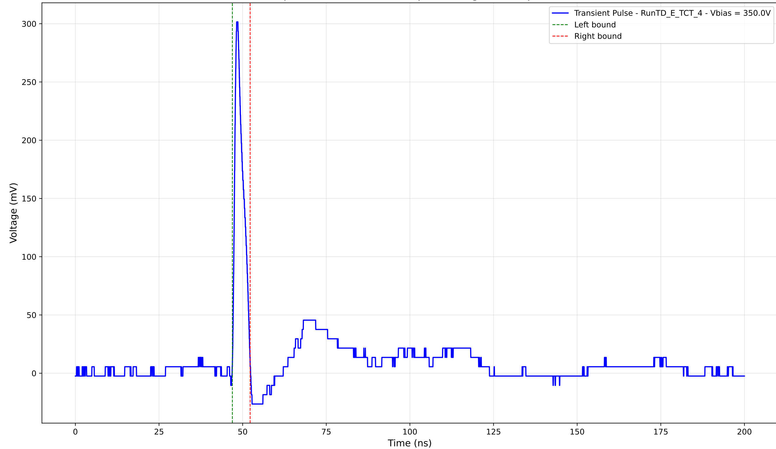
Transient Pulse - Sample: TD - Position: 235.0 \mu\text{m} - Charge: 17.33 pC - Rise Time: 0.94 ns
