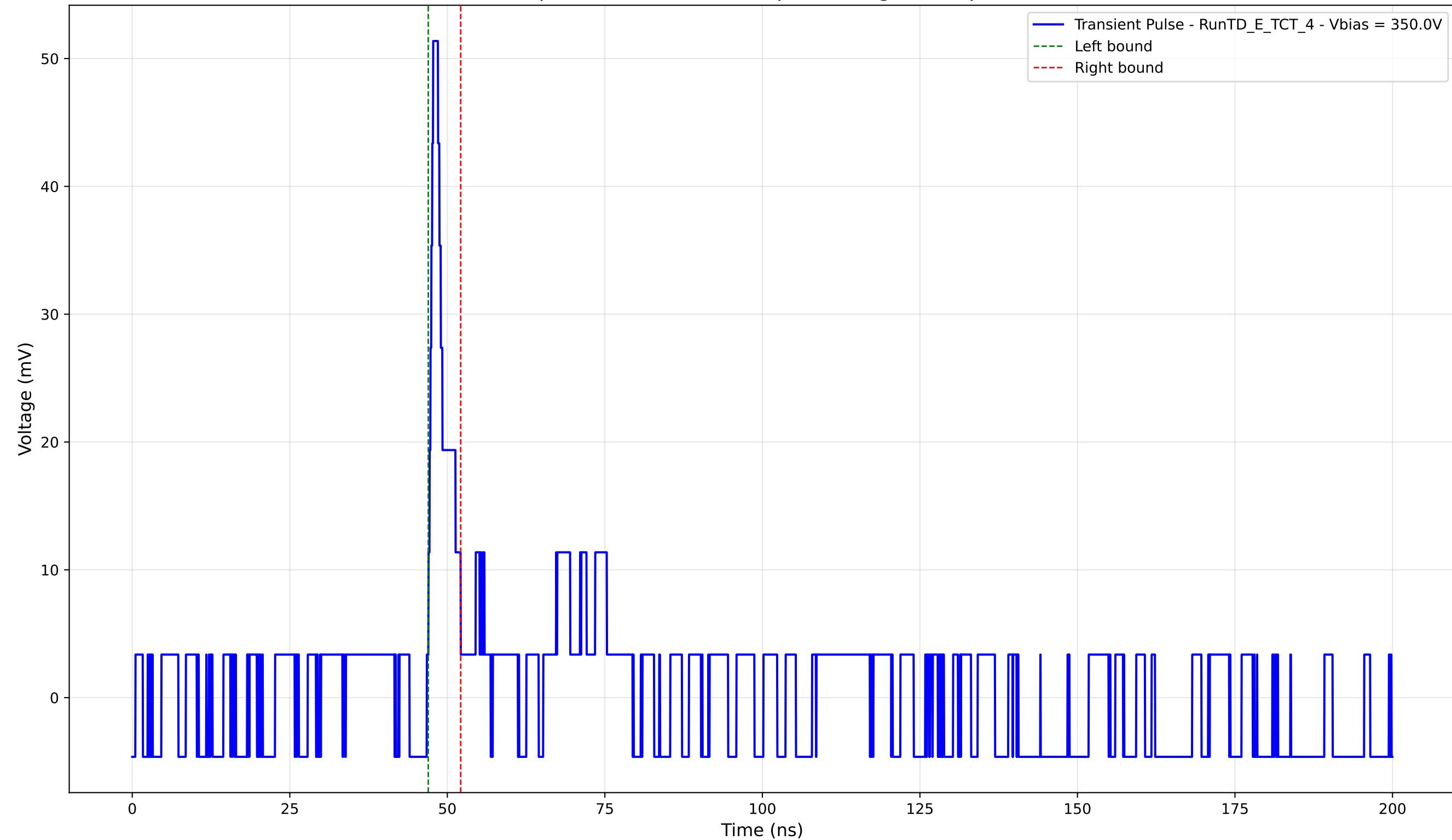
Transient Pulse - Sample: TD - Position: 25.0 \mu\text{m} - Charge: 2.68 pC - Rise Time: 0.76 ns
