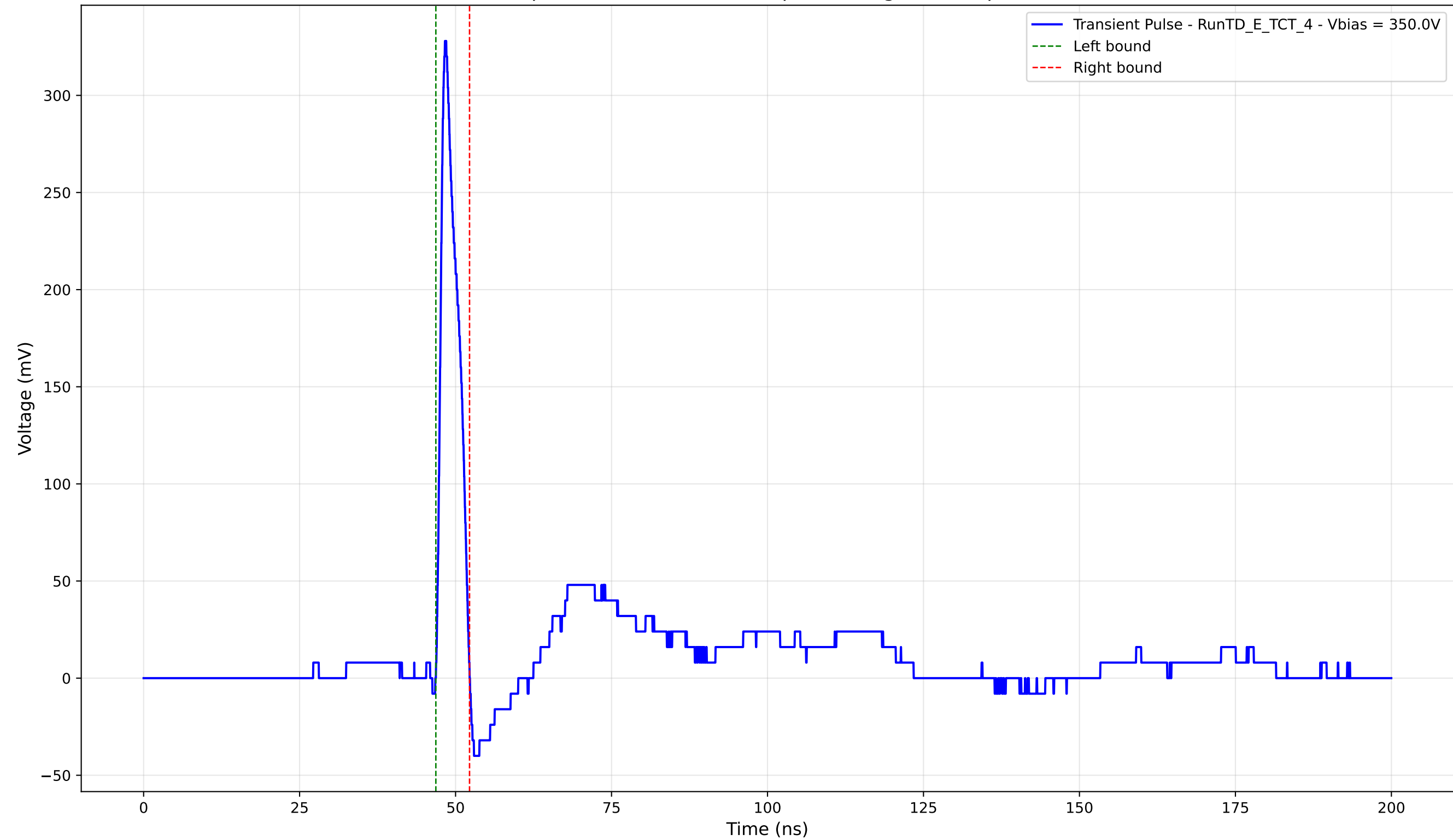
Transient Pulse - Sample: TD - Position: 240.0 \mu\text{m} - Charge: 19.68 pC - Rise Time: 0.96 ns
