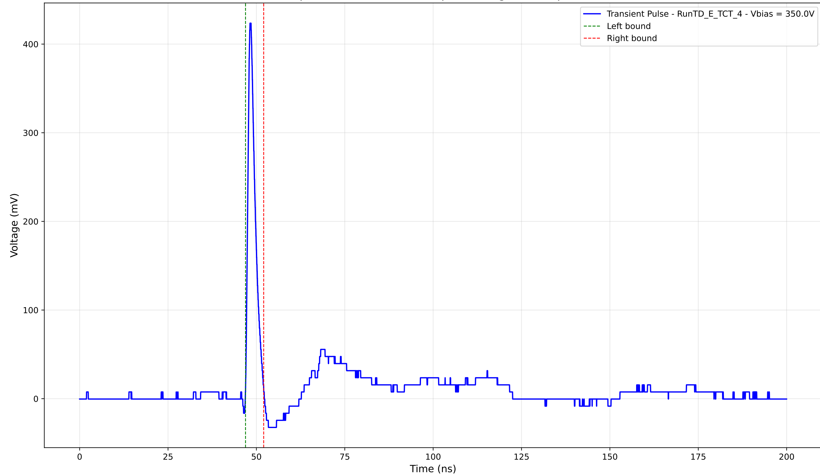
Transient Pulse - Sample: TD - Position: 180.0 \mu\text{m} - Charge: 20.13 pC - Rise Time: 0.89 ns
