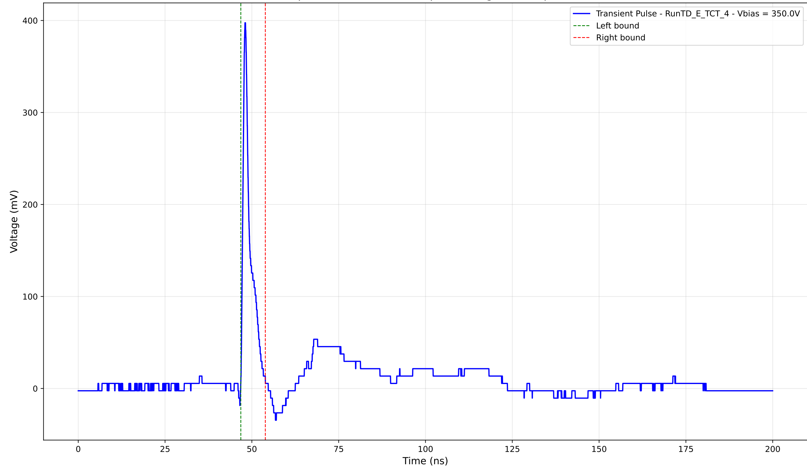
Transient Pulse - Sample: TD - Position: 40.0 \mu\text{m} - Charge: 19.38 pC - Rise Time: 0.83 ns
