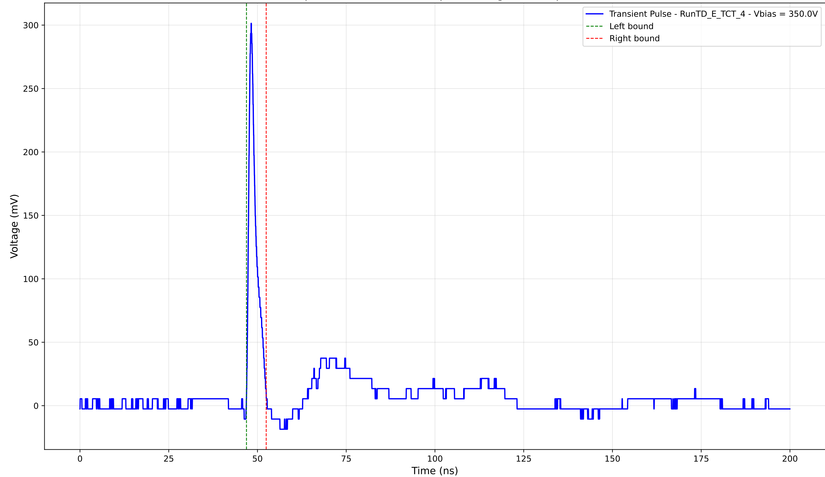
Transient Pulse - Sample: TD - Position: 90.0 \mu\text{m} - Charge: 14.30 pC - Rise Time: 0.88 ns
