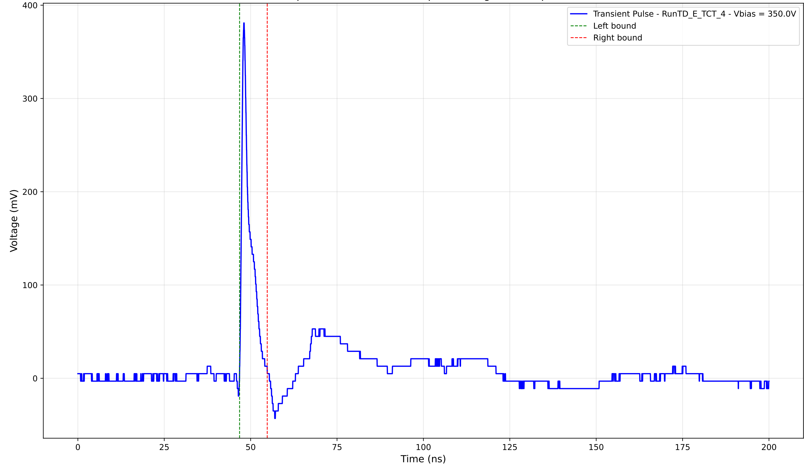
Transient Pulse - Sample: TD - Position: 65.0 \mu\text{m} - Charge: 20.94 pC - Rise Time: 0.82 ns
