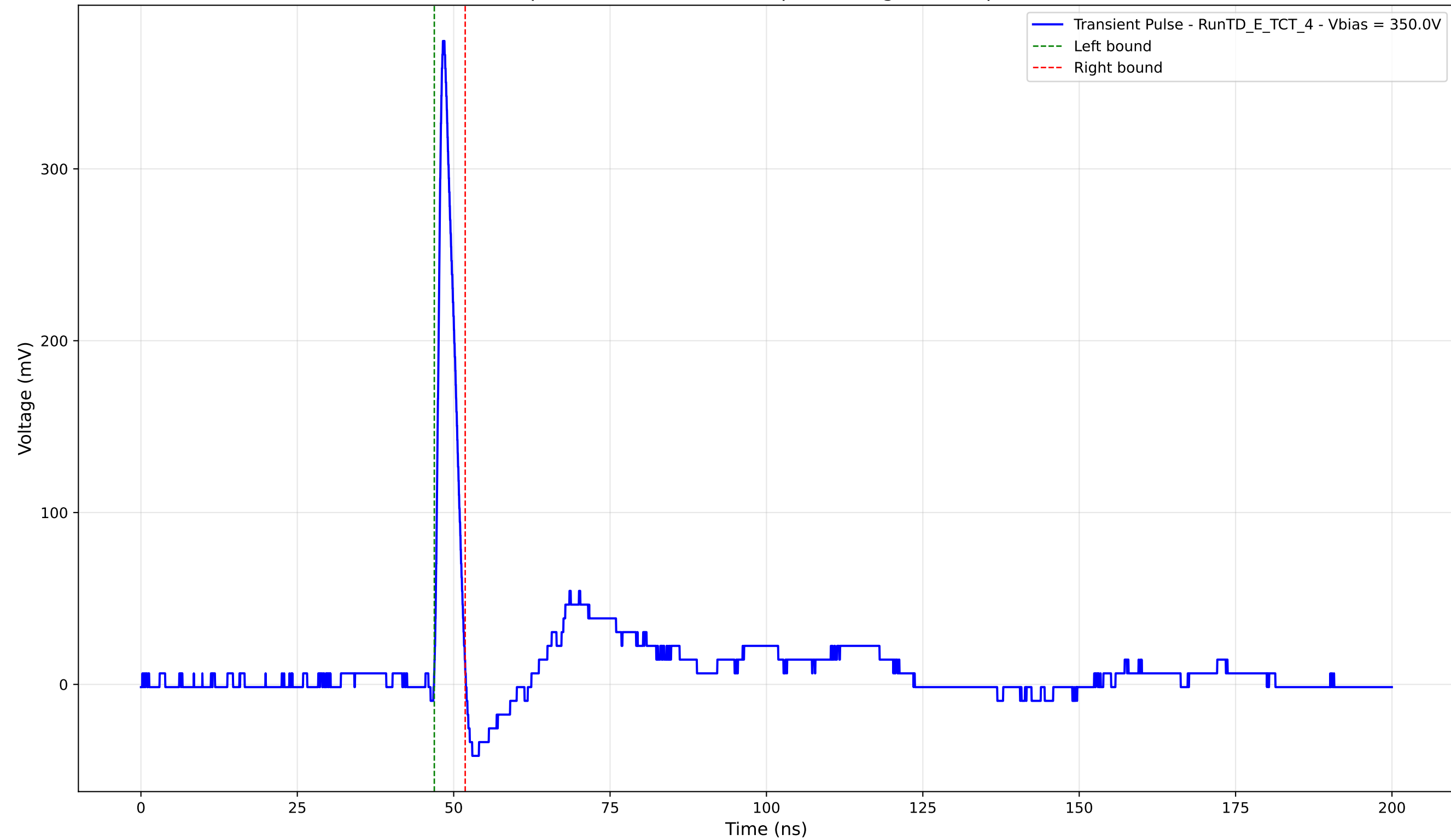
Transient Pulse - Sample: TD - Position: 265.0 \mu\text{m} - Charge: 19.77 pC - Rise Time: 0.96 ns
