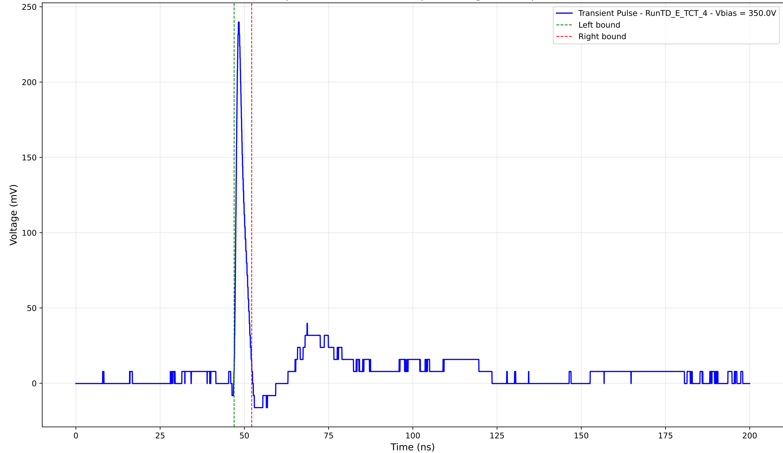
Transient Pulse - Sample: TD - Position: 310.0 \mu\text{m} - Charge: 12.30 pC - Rise Time: 0.96 ns
