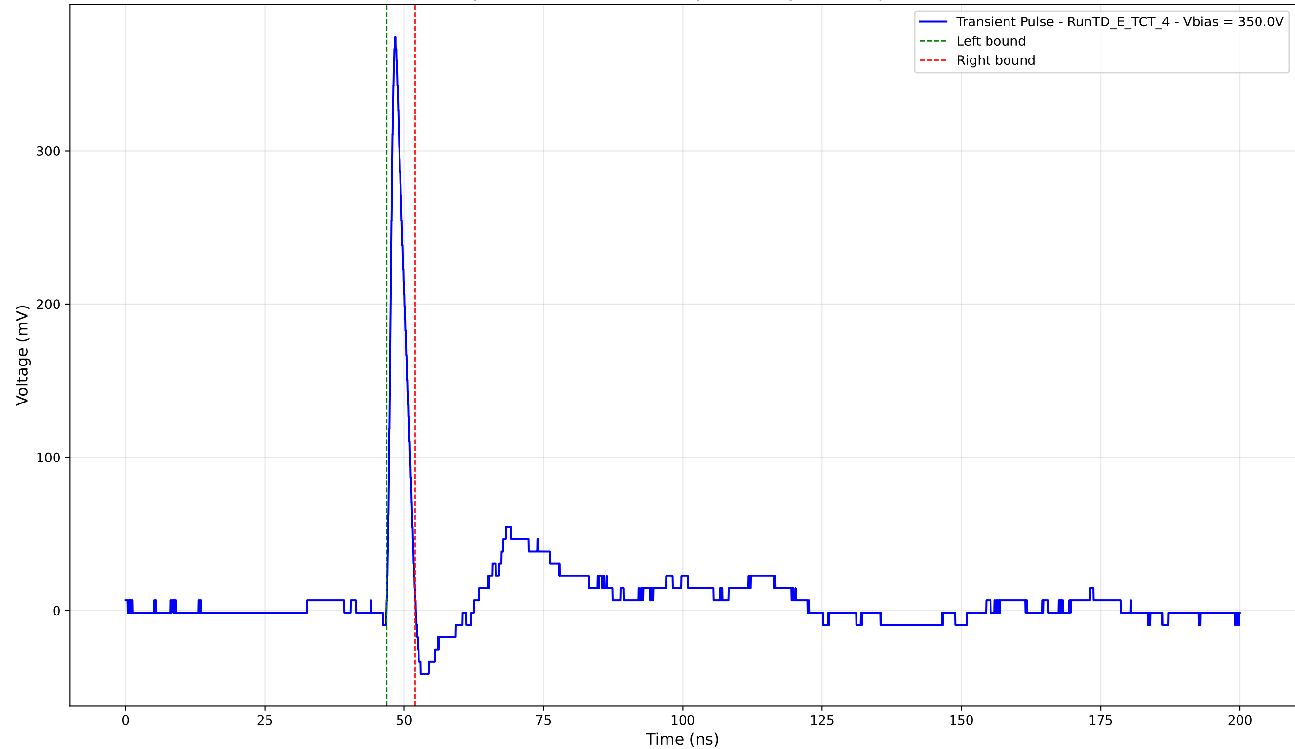
Transient Pulse - Sample: TD - Position: 155.0 \mu\text{m} - Charge: 19.96 pC - Rise Time: 1.00 ns
