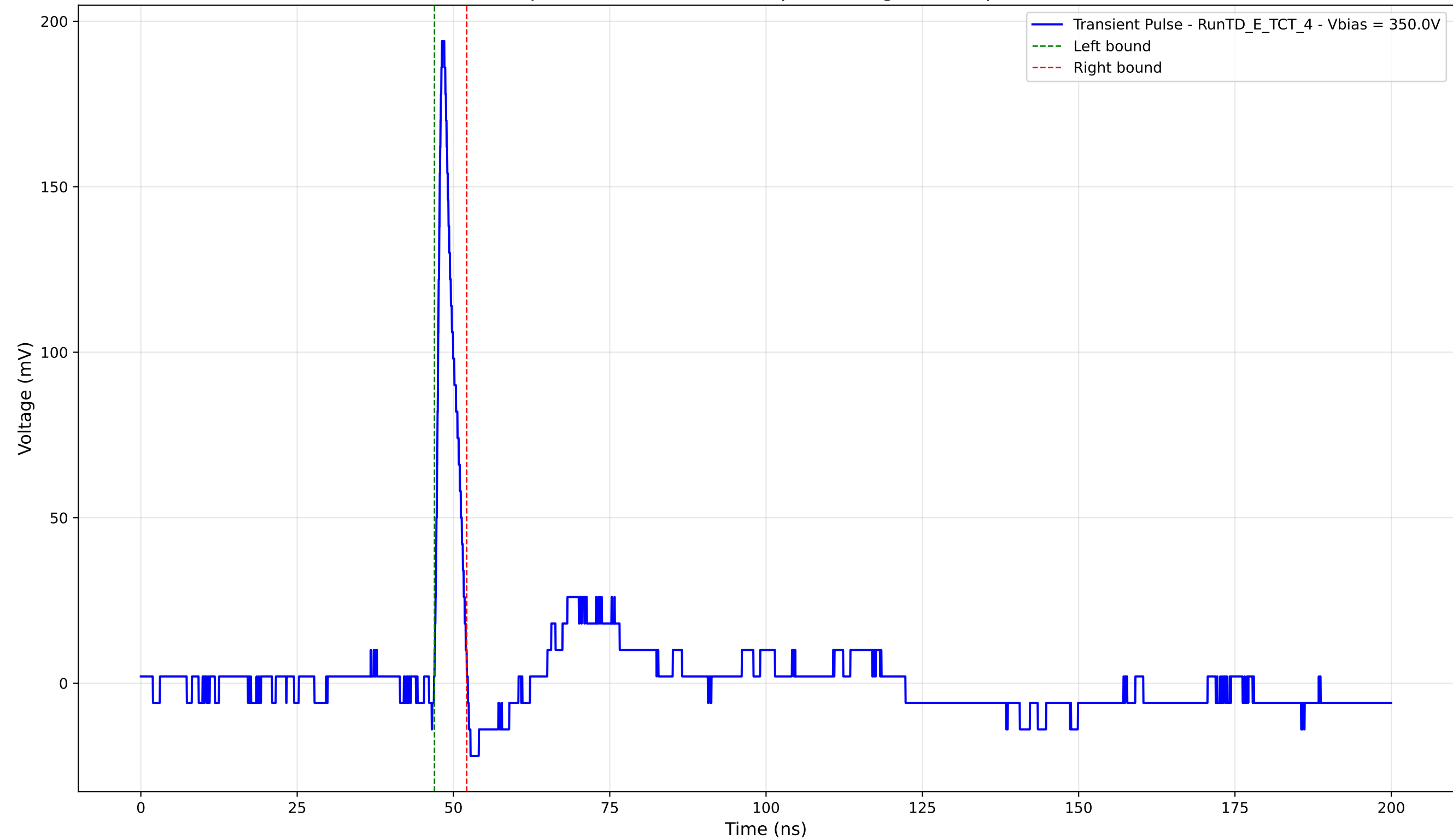
Transient Pulse - Sample: TD - Position: 335.0 \mu\text{m} - Charge: 10.38 pC - Rise Time: 0.88 ns
