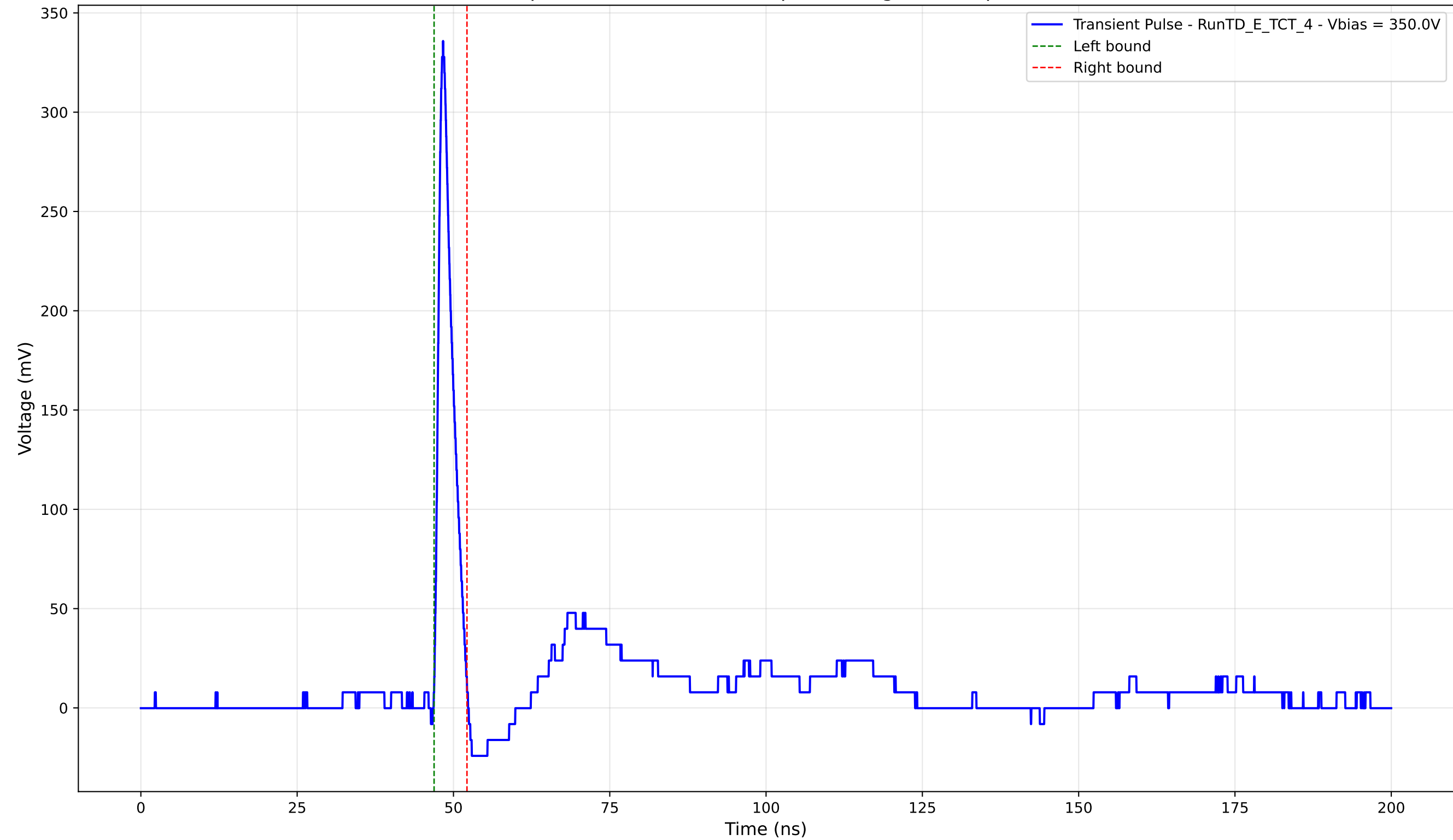
Transient Pulse - Sample: TD - Position: 230.0 \mu\text{m} - Charge: 17.16 pC - Rise Time: 0.96 ns
