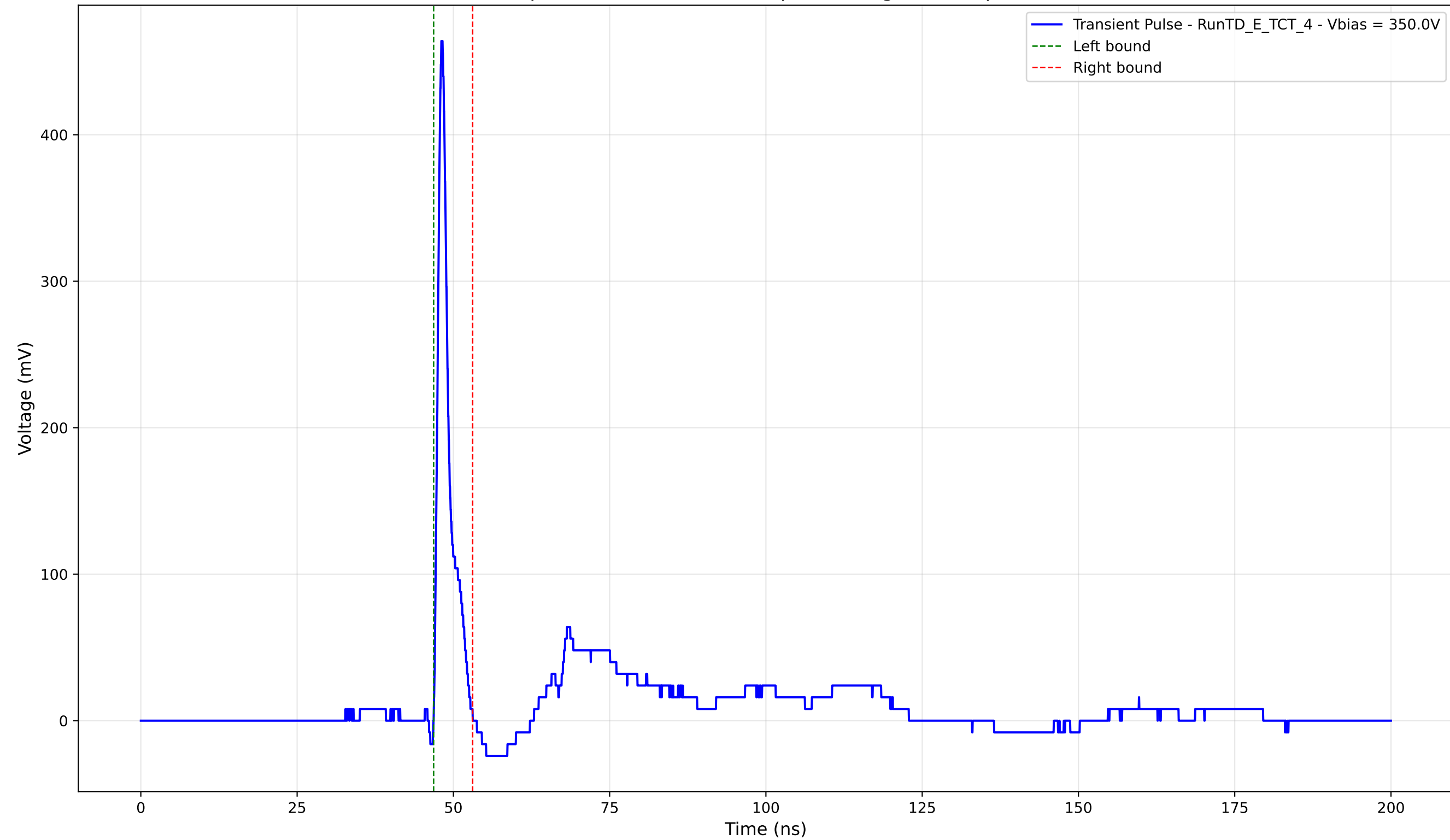
Transient Pulse - Sample: TD - Position: 110.0 \mu\text{m} - Charge: 20.16 pC - Rise Time: 0.85 ns
