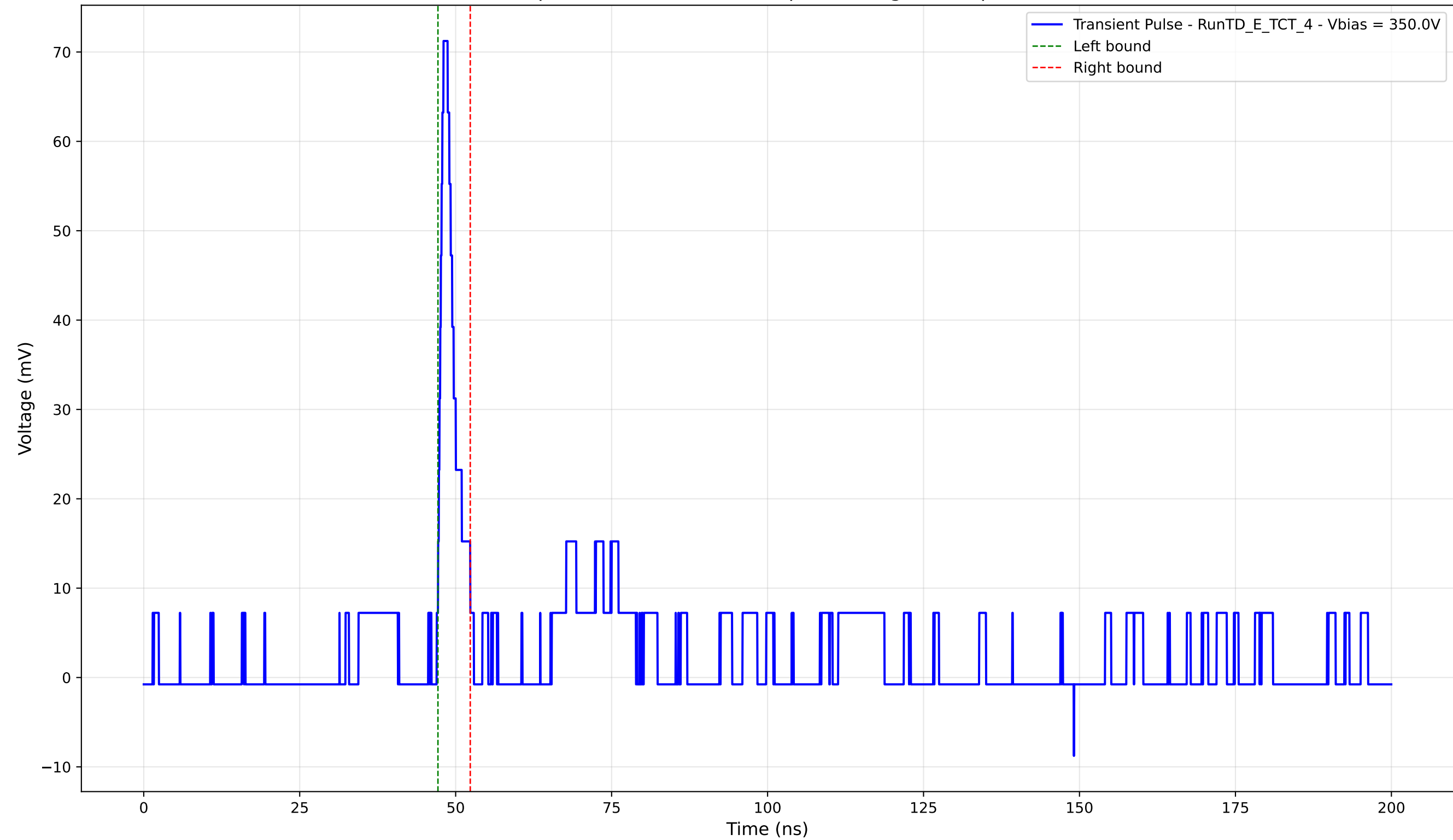
Transient Pulse - Sample: TD - Position: 370.0 \mu\text{m} - Charge: 3.74 pC - Rise Time: 1.08 ns
