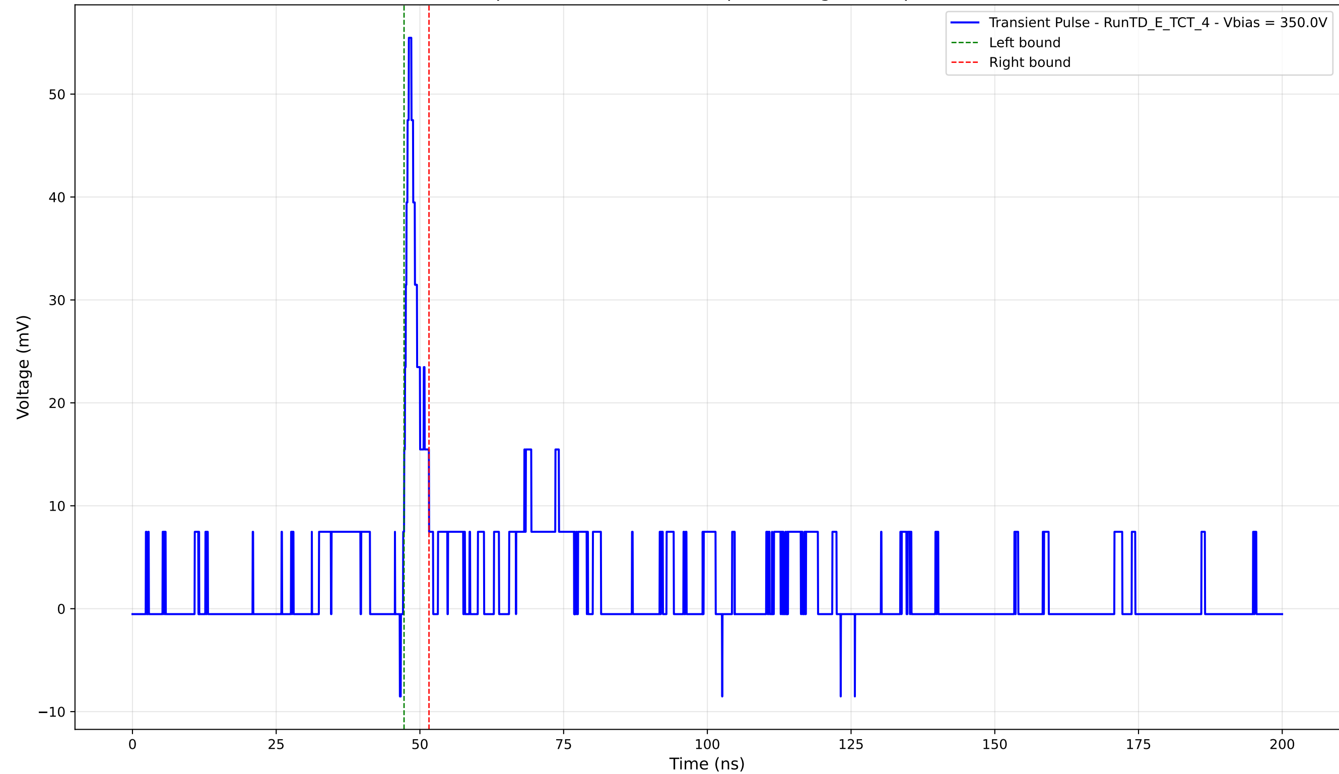
Transient Pulse - Sample: TD - Position: 365.0 \mu\text{m} - Charge: 2.56 pC - Rise Time: 0.99 ns
