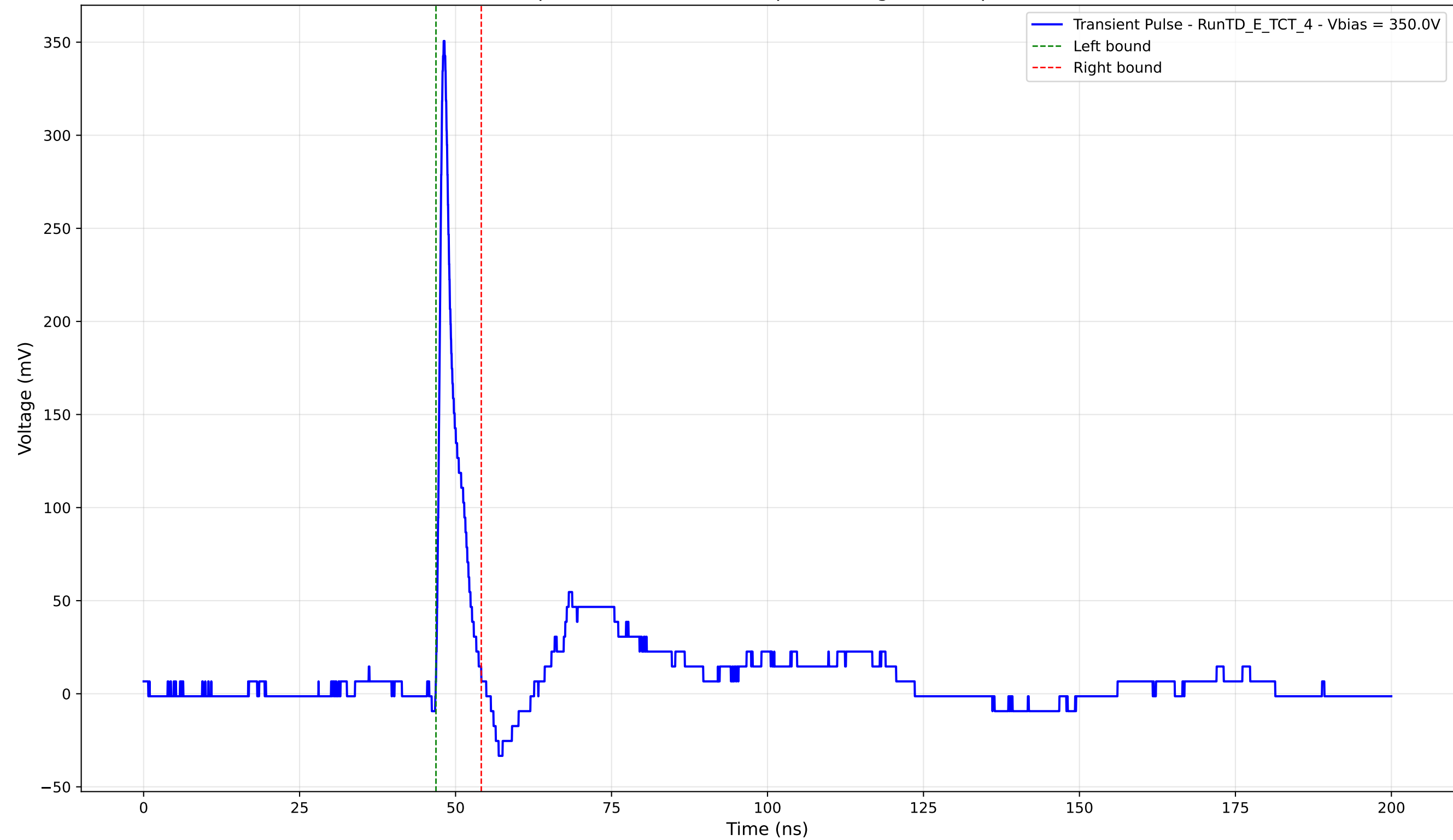
Transient Pulse - Sample: TD - Position: 75.0 \mu\text{m} - Charge: 19.41 pC - Rise Time: 0.85 ns
