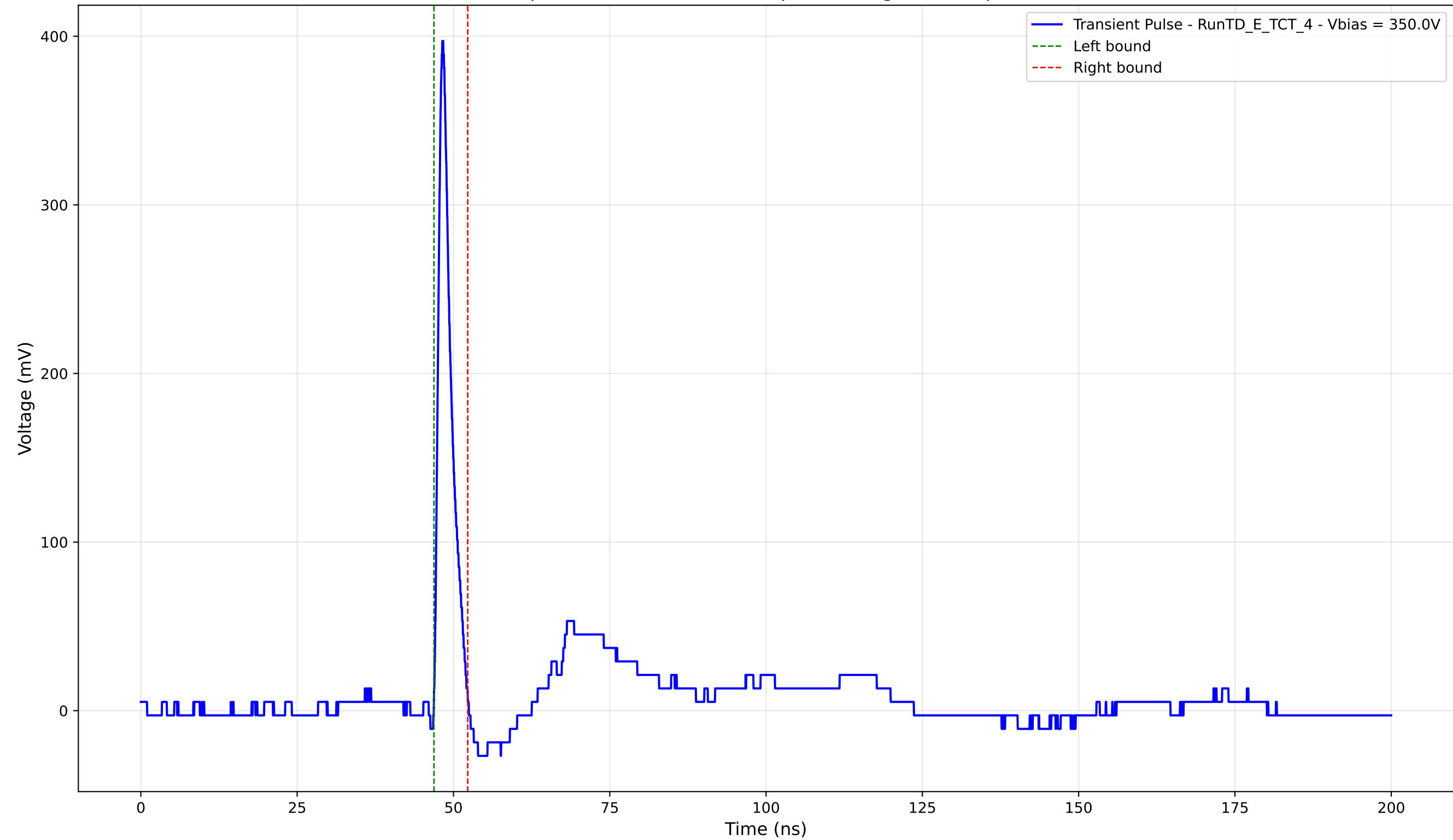
Transient Pulse - Sample: TD - Position: 170.0 \mu\text{m} - Charge: 18.78 pC - Rise Time: 0.91 ns
