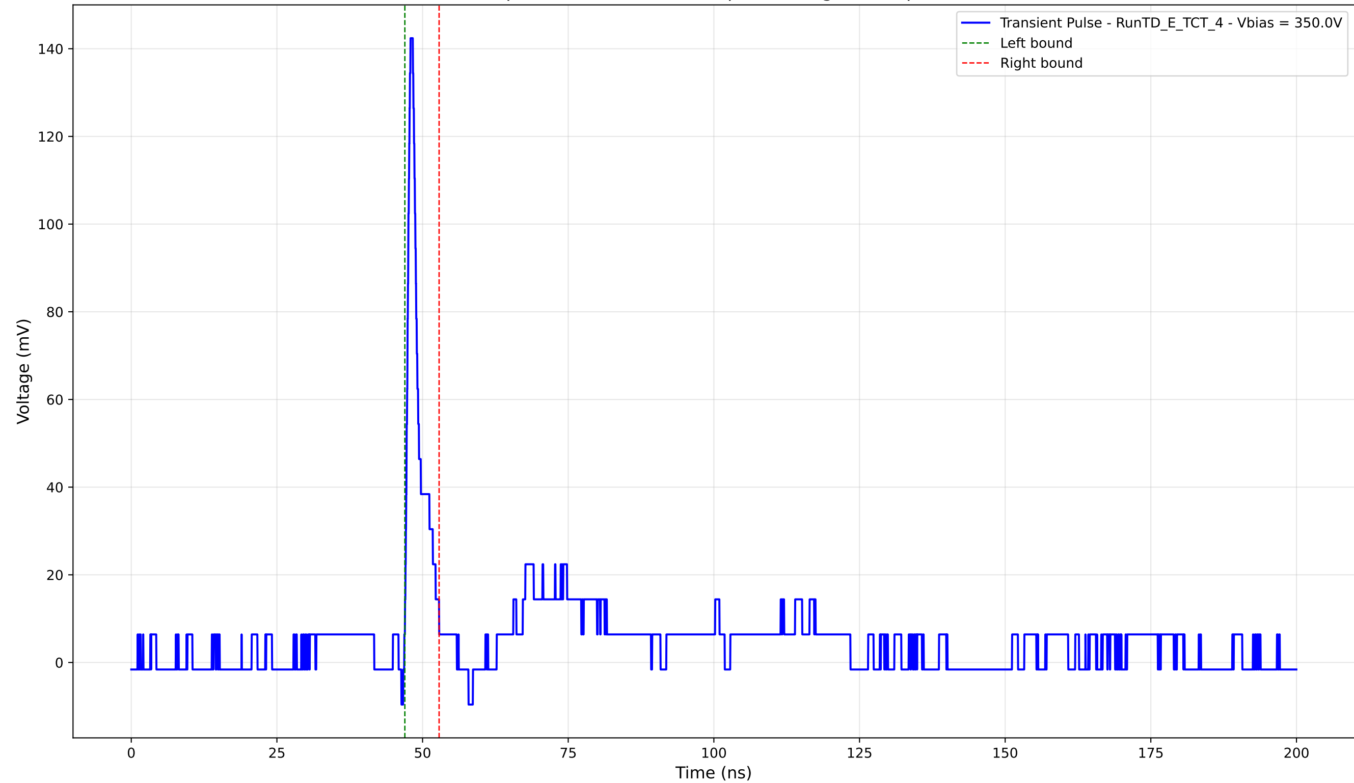
Transient Pulse - Sample: TD - Position: 30.0 \mu\text{m} - Charge: 6.68 pC - Rise Time: 0.84 ns
