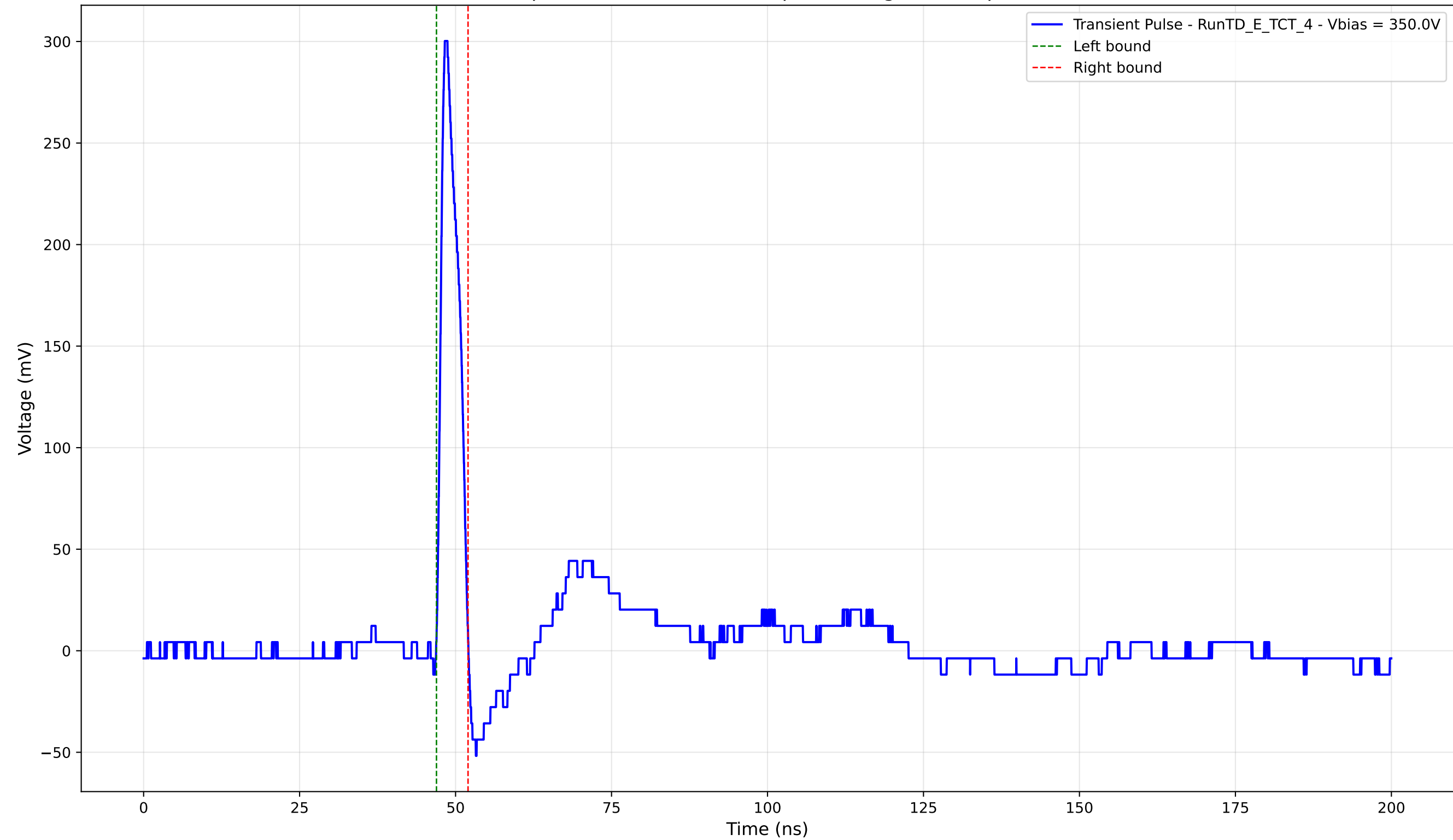
Transient Pulse - Sample: TD - Position: 285.0 \mu\text{m} - Charge: 18.31 pC - Rise Time: 0.96 ns
