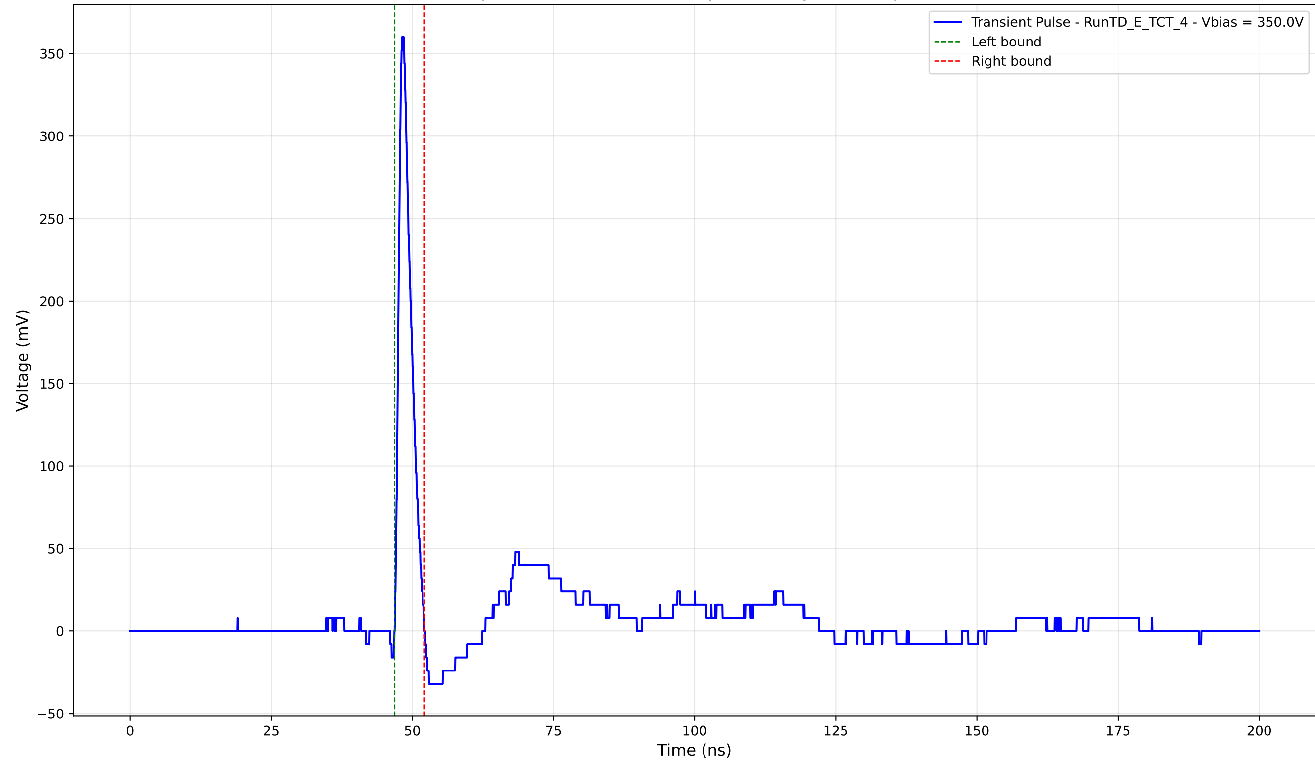
Transient Pulse - Sample: TD - Position: 225.0 \mu\text{m} - Charge: 17.96 pC - Rise Time: 0.89 ns
