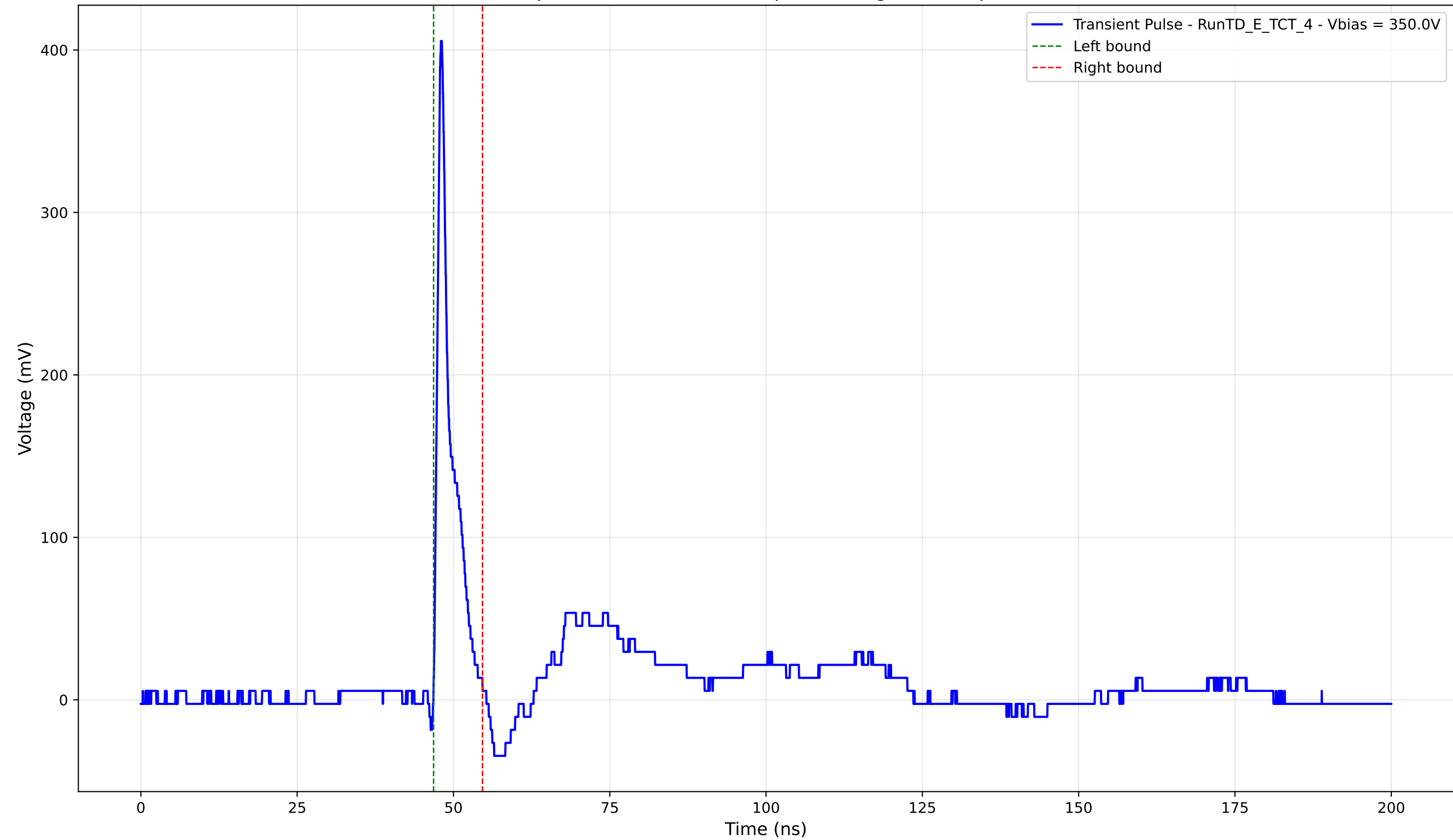
Transient Pulse - Sample: TD - Position: 50.0 \mu\text{m} - Charge: 20.98 pC - Rise Time: 0.79 ns
