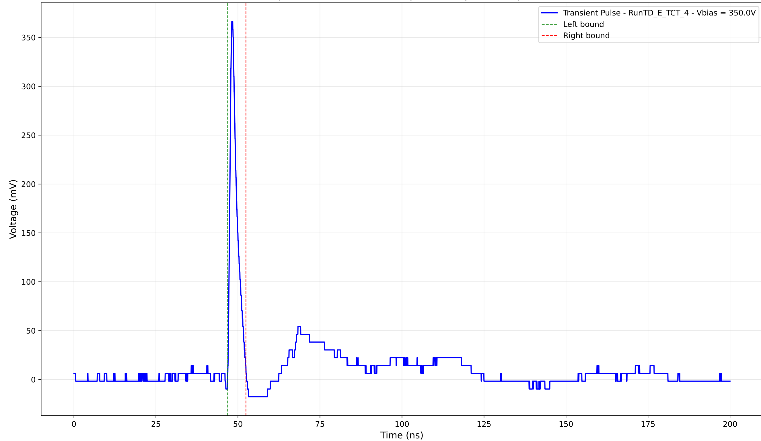
Transient Pulse - Sample: TD - Position: 195.0 \mu\text{m} - Charge: 18.00 pC - Rise Time: 0.88 ns
