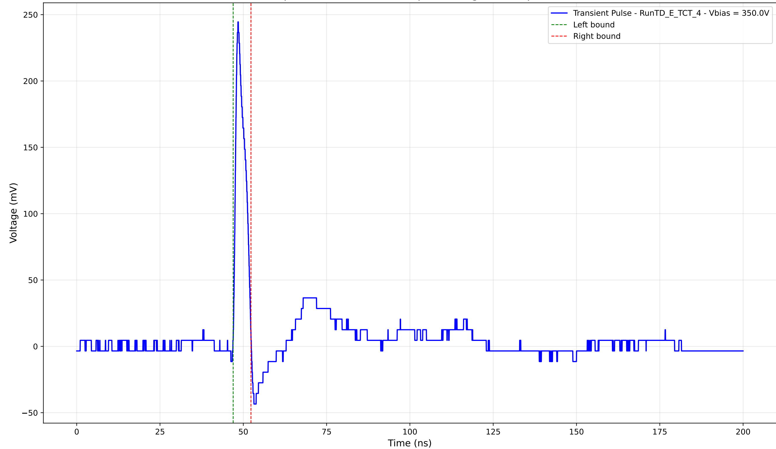
Transient Pulse - Sample: TD - Position: 325.0 \mu\text{m} - Charge: 15.14 pC - Rise Time: 0.95 ns
