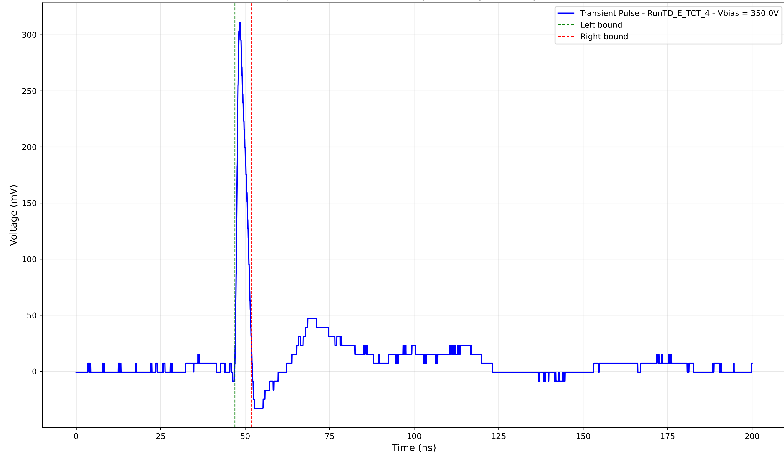
Transient Pulse - Sample: TD - Position: 280.0 \mu\text{m} - Charge: 17.66 pC - Rise Time: 0.98 ns
