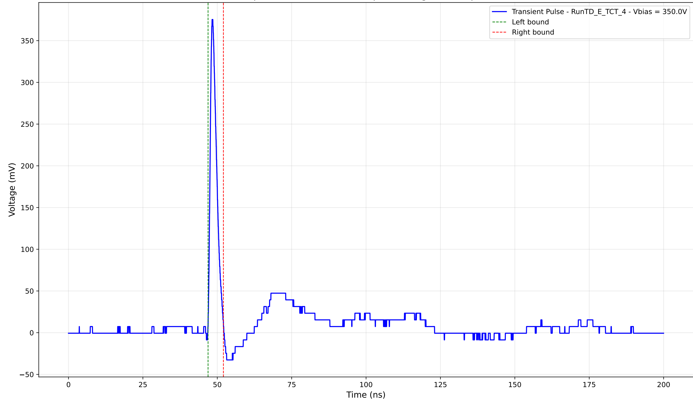
Transient Pulse - Sample: TD - Position: 215.0 \mu\text{m} - Charge: 18.66 pC - Rise Time: 0.96 ns
