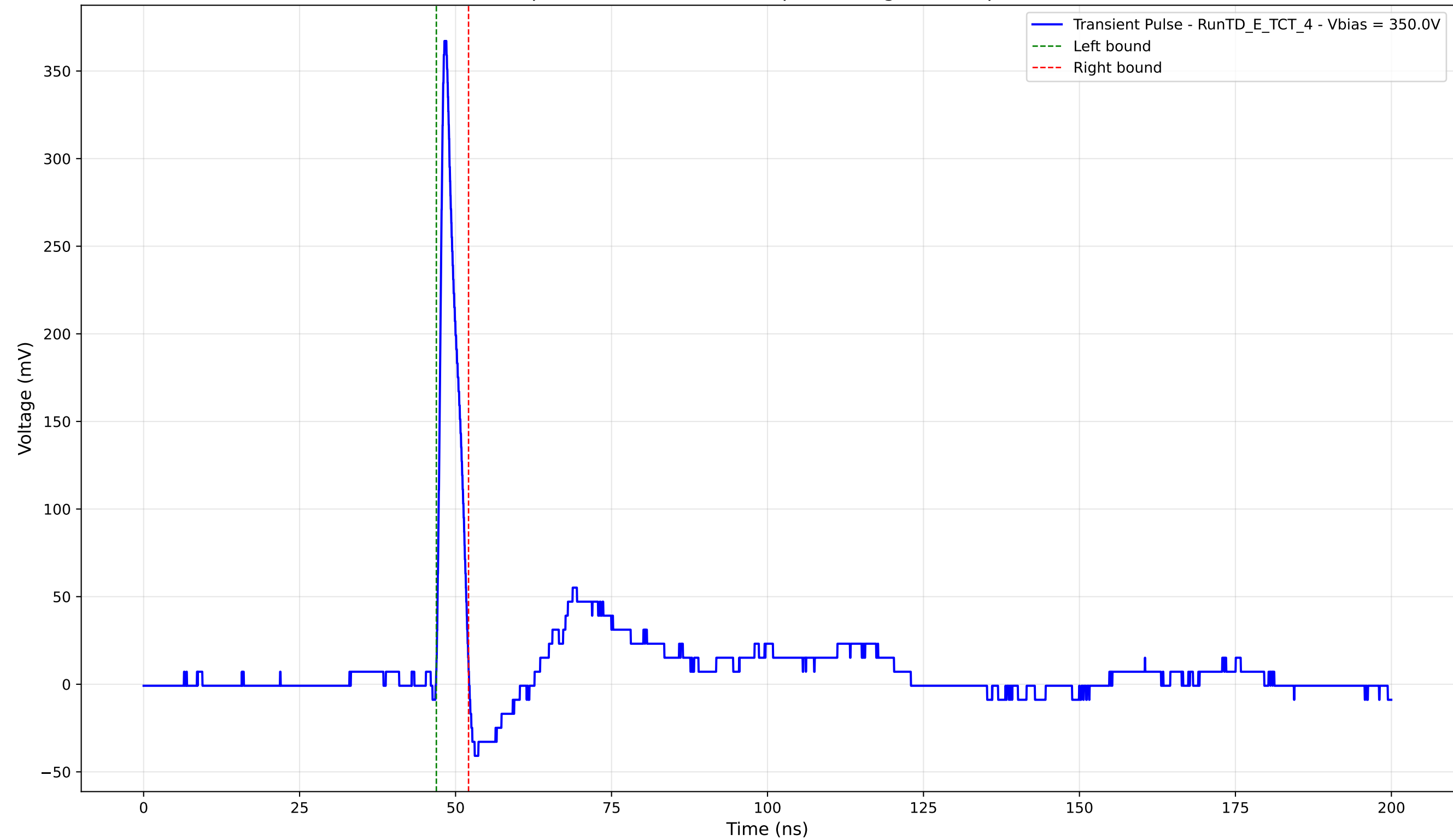
Transient Pulse - Sample: TD - Position: 245.0 \mu\text{m} - Charge: 20.27 pC - Rise Time: 0.91 ns
