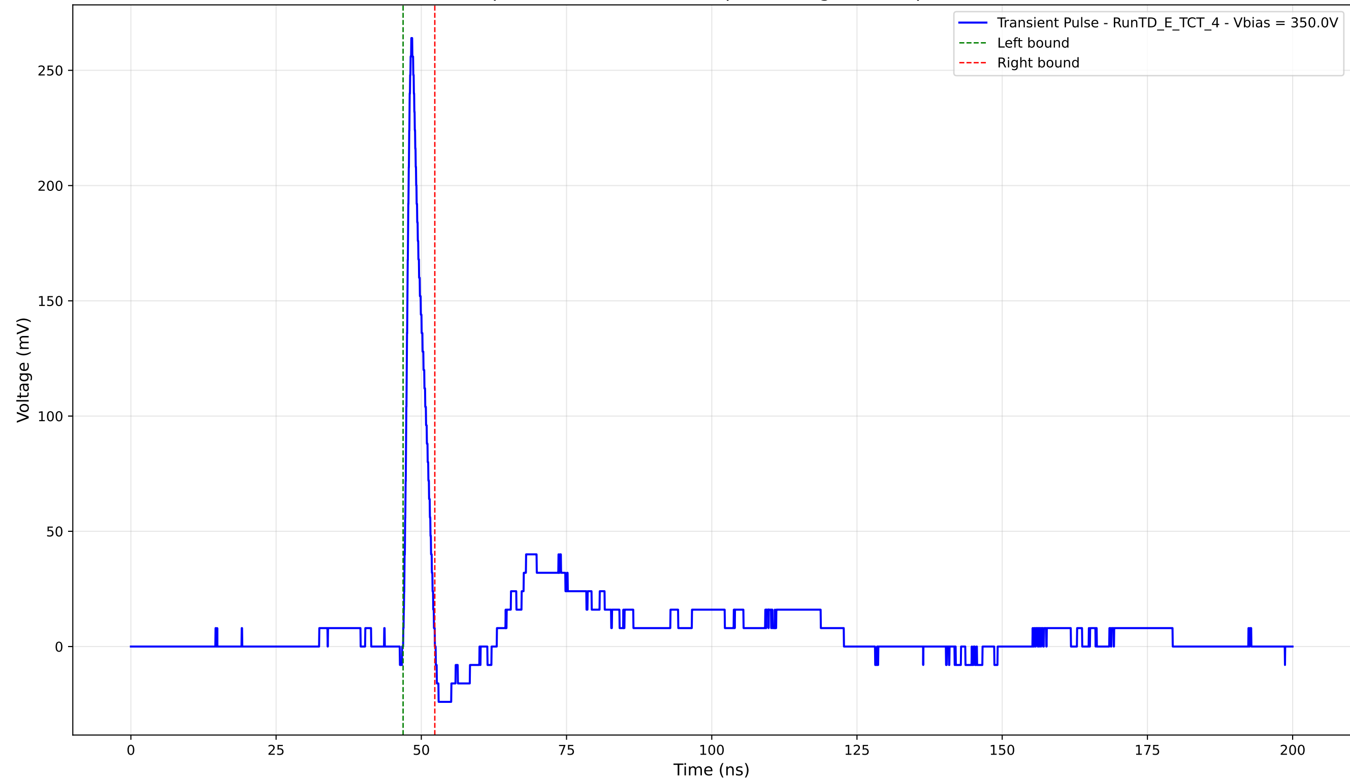
Transient Pulse - Sample: TD - Position: 315.0 \mu\text{m} - Charge: 14.39 pC - Rise Time: 0.93 ns
