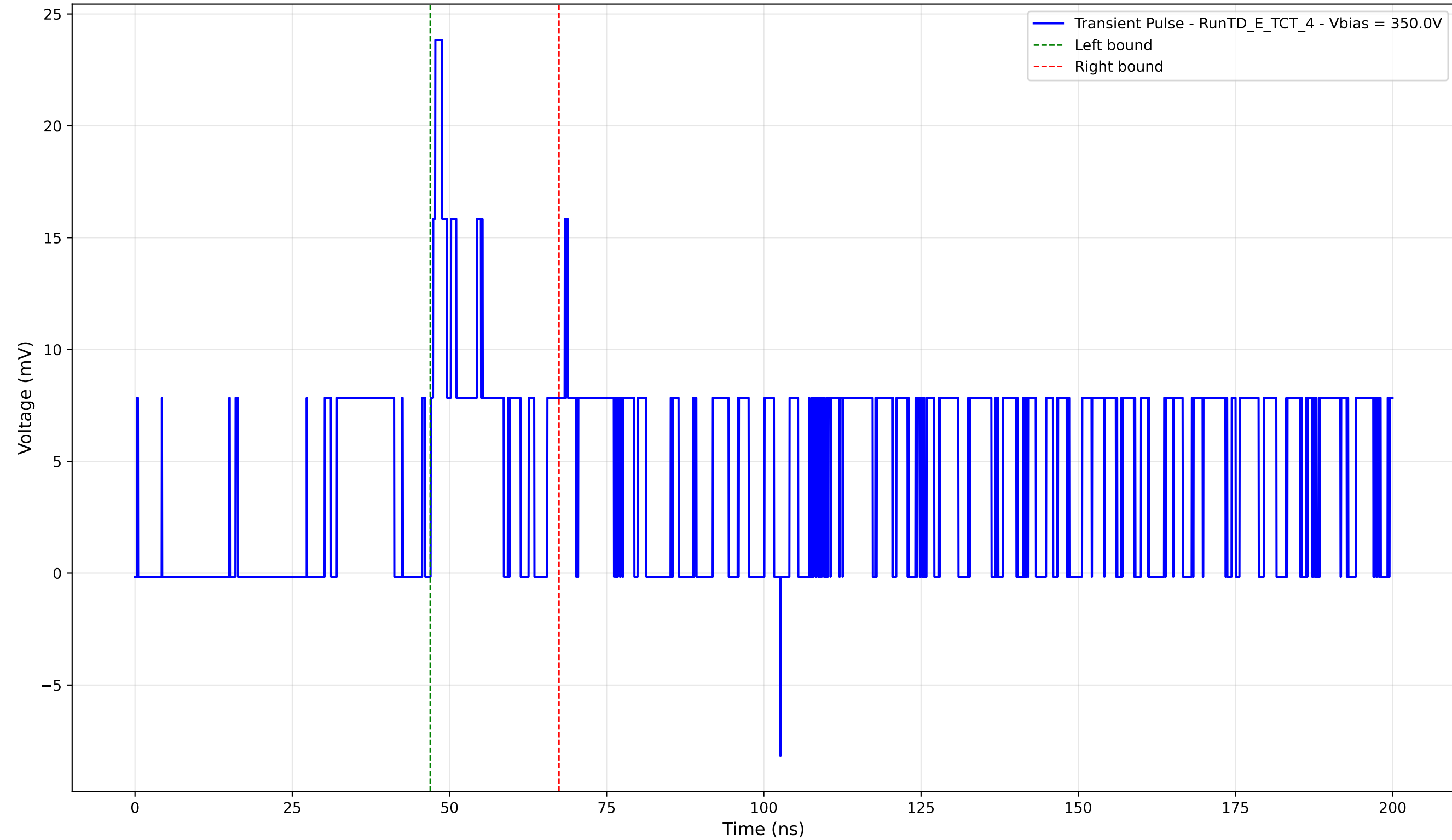
Transient Pulse - Sample: TD - Position: 10.0 \mu\text{m} - Charge: 3.31 pC - Rise Time: 0.73 ns
