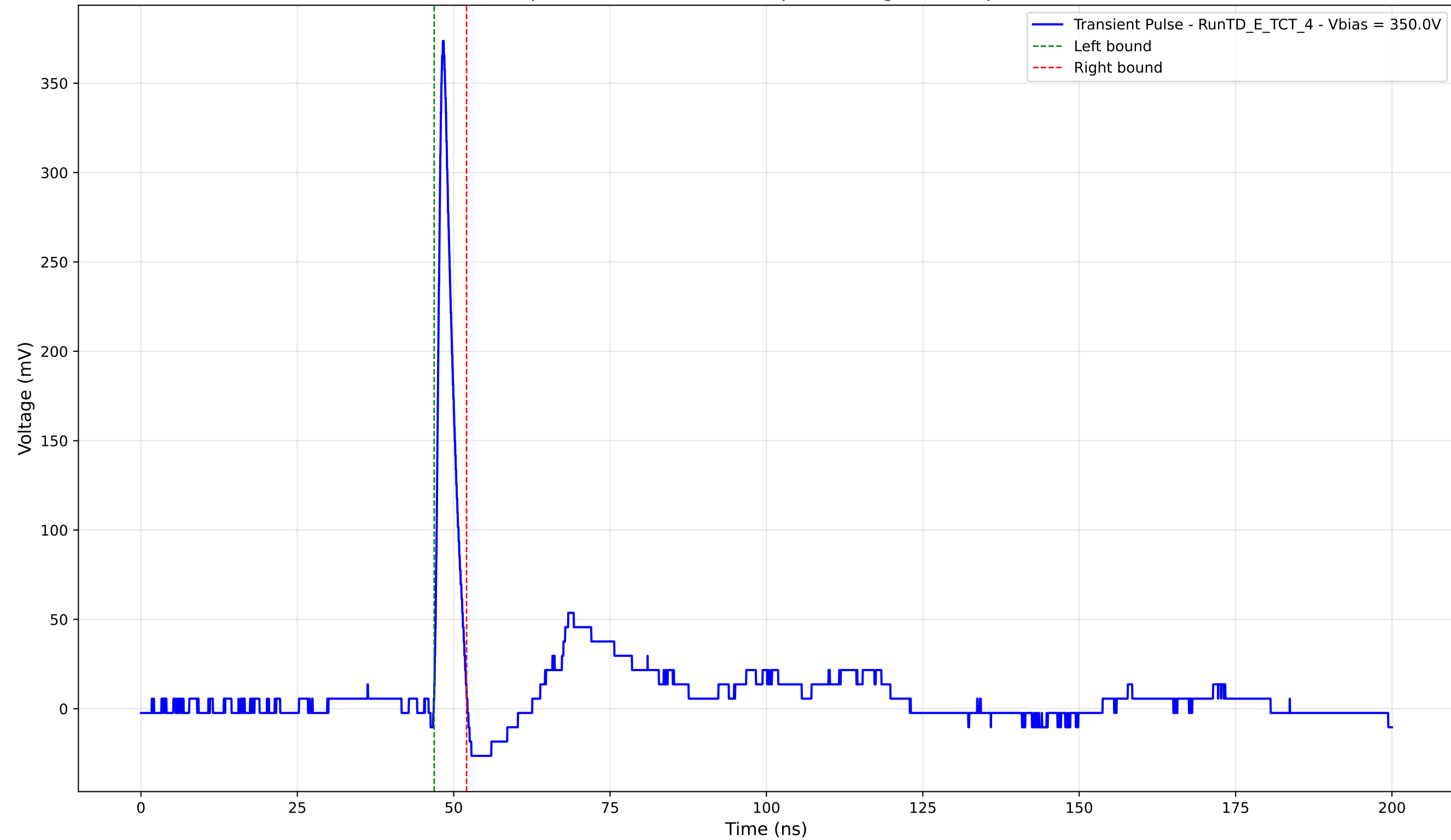
Transient Pulse - Sample: TD - Position: 190.0 \mu\text{m} - Charge: 18.62 pC - Rise Time: 0.96 ns
