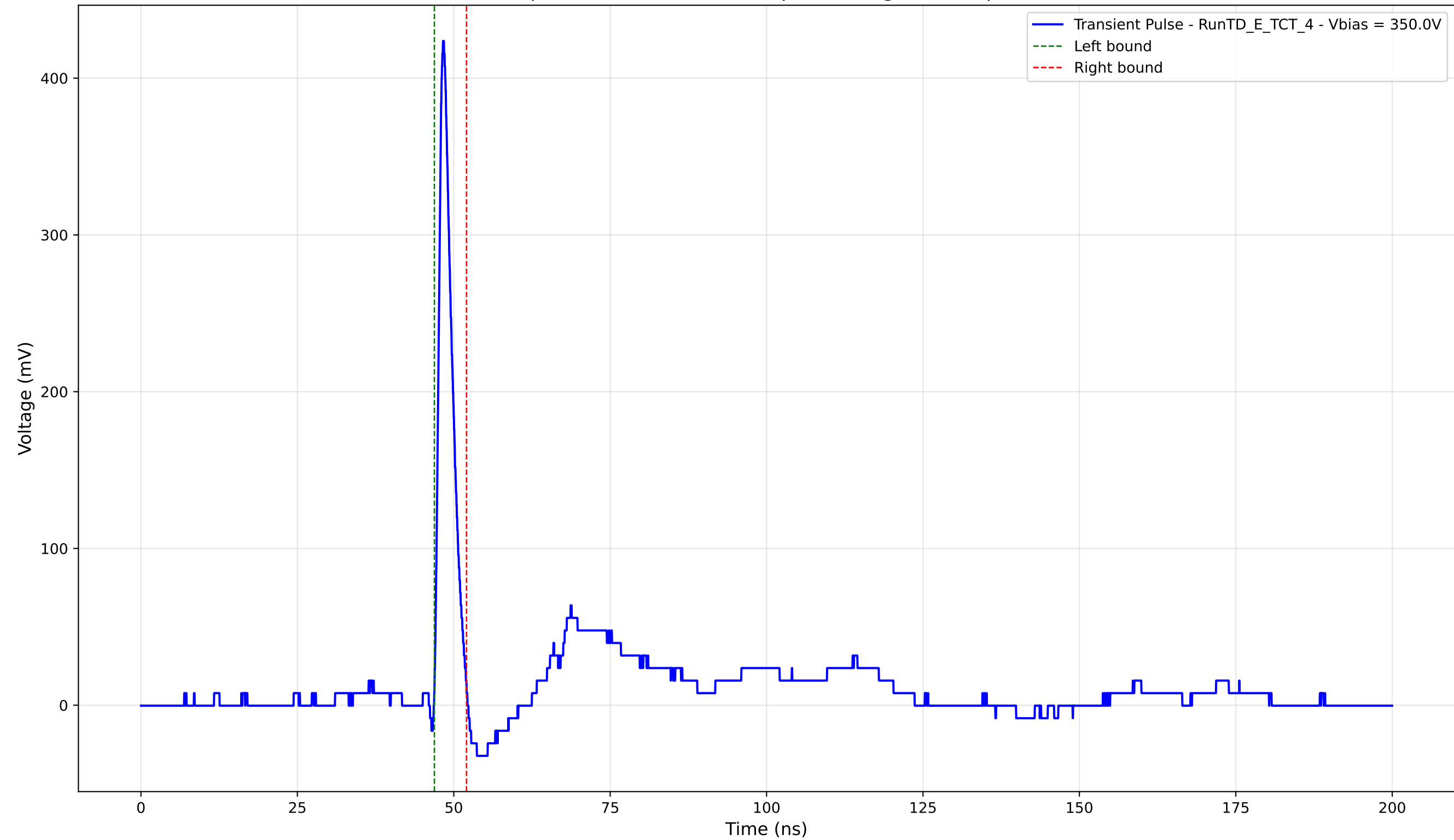
Transient Pulse - Sample: TD - Position: 185.0 \mu\text{m} - Charge: 20.56 pC - Rise Time: 0.91 ns
