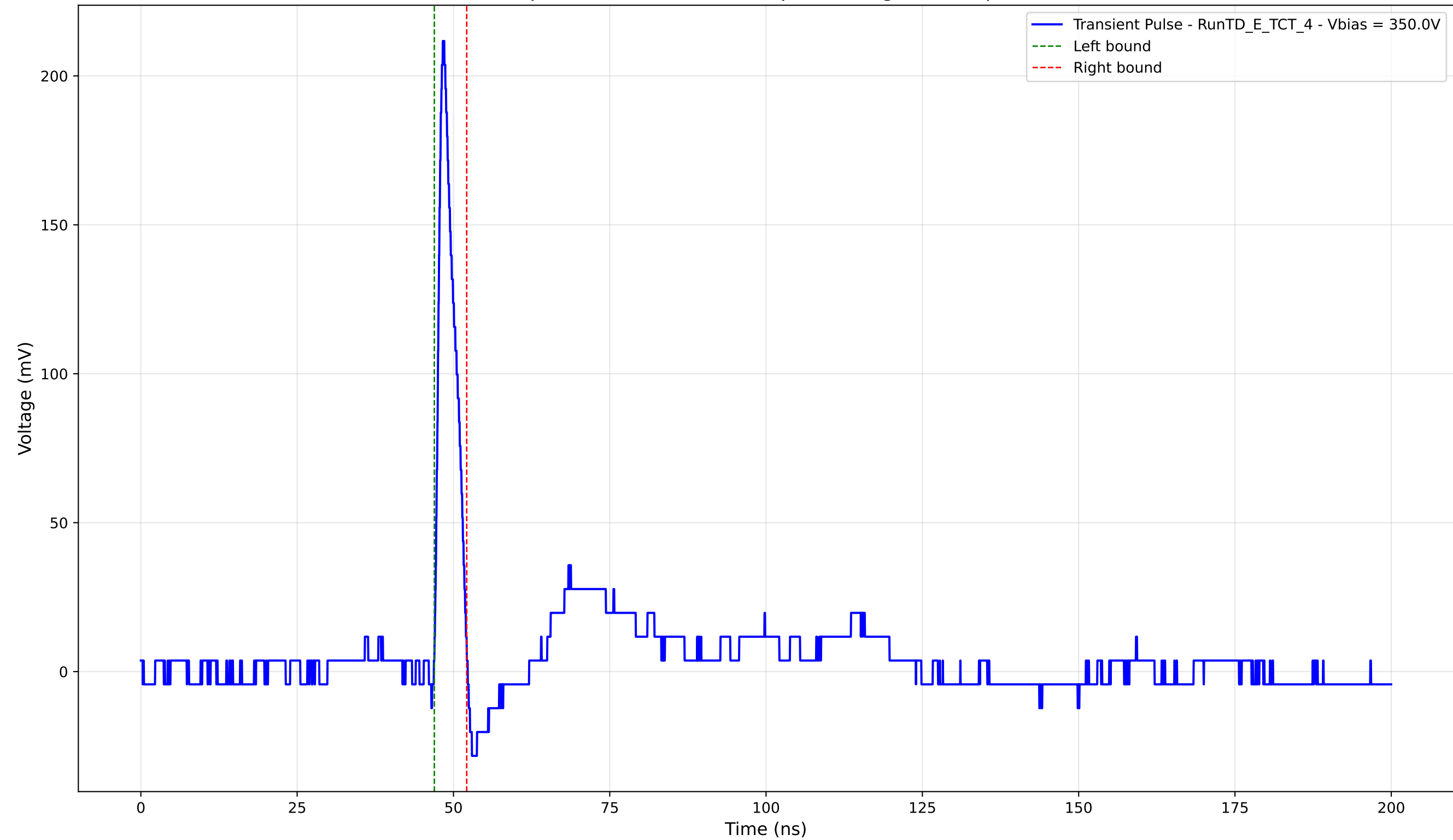
Transient Pulse - Sample: TD - Position: 300.0 \mu\text{m} - Charge: 11.96 pC - Rise Time: 0.98 ns
