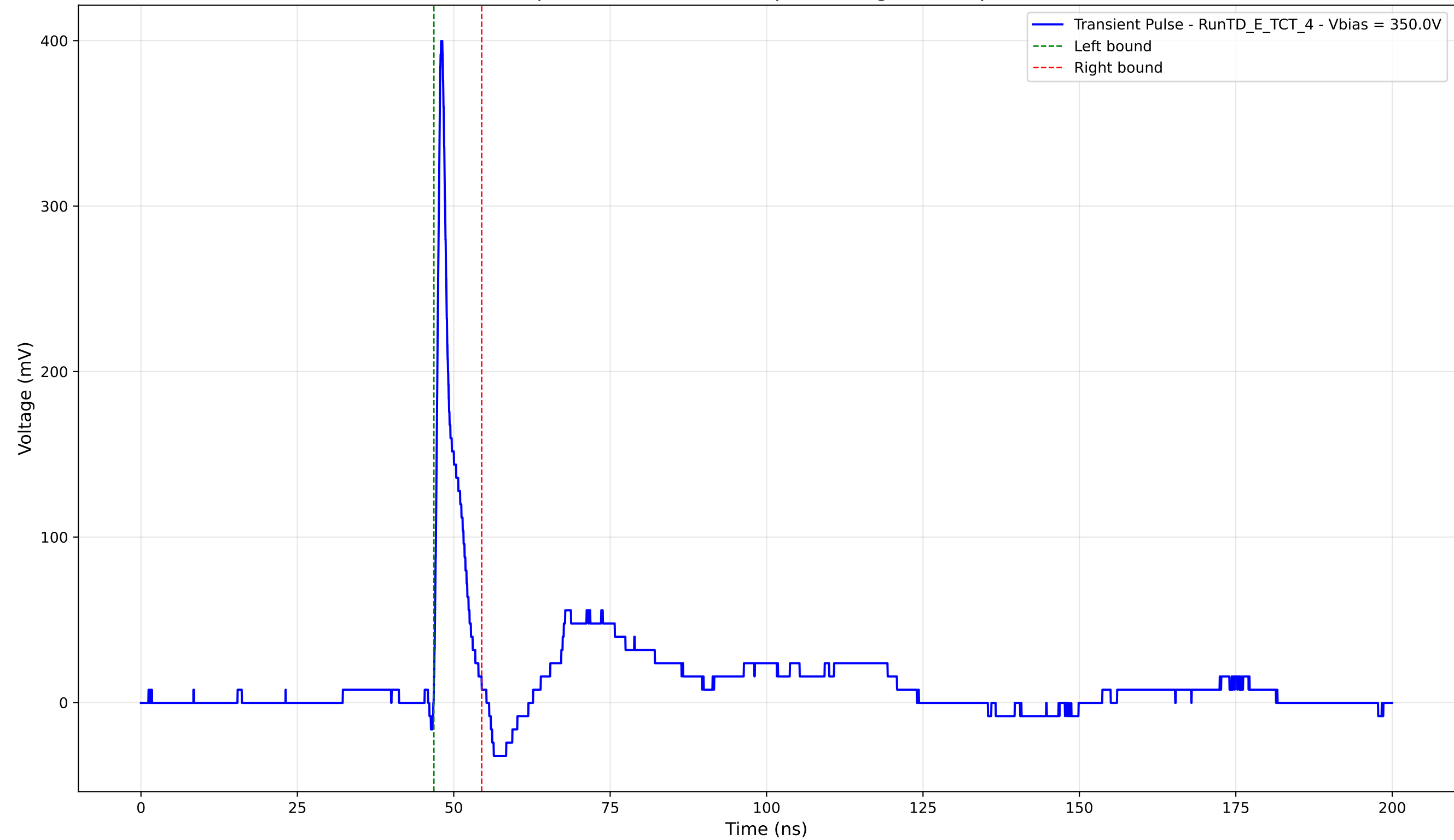
Transient Pulse - Sample: TD - Position: 60.0 \mu\text{m} - Charge: 21.38 pC - Rise Time: 0.82 ns
