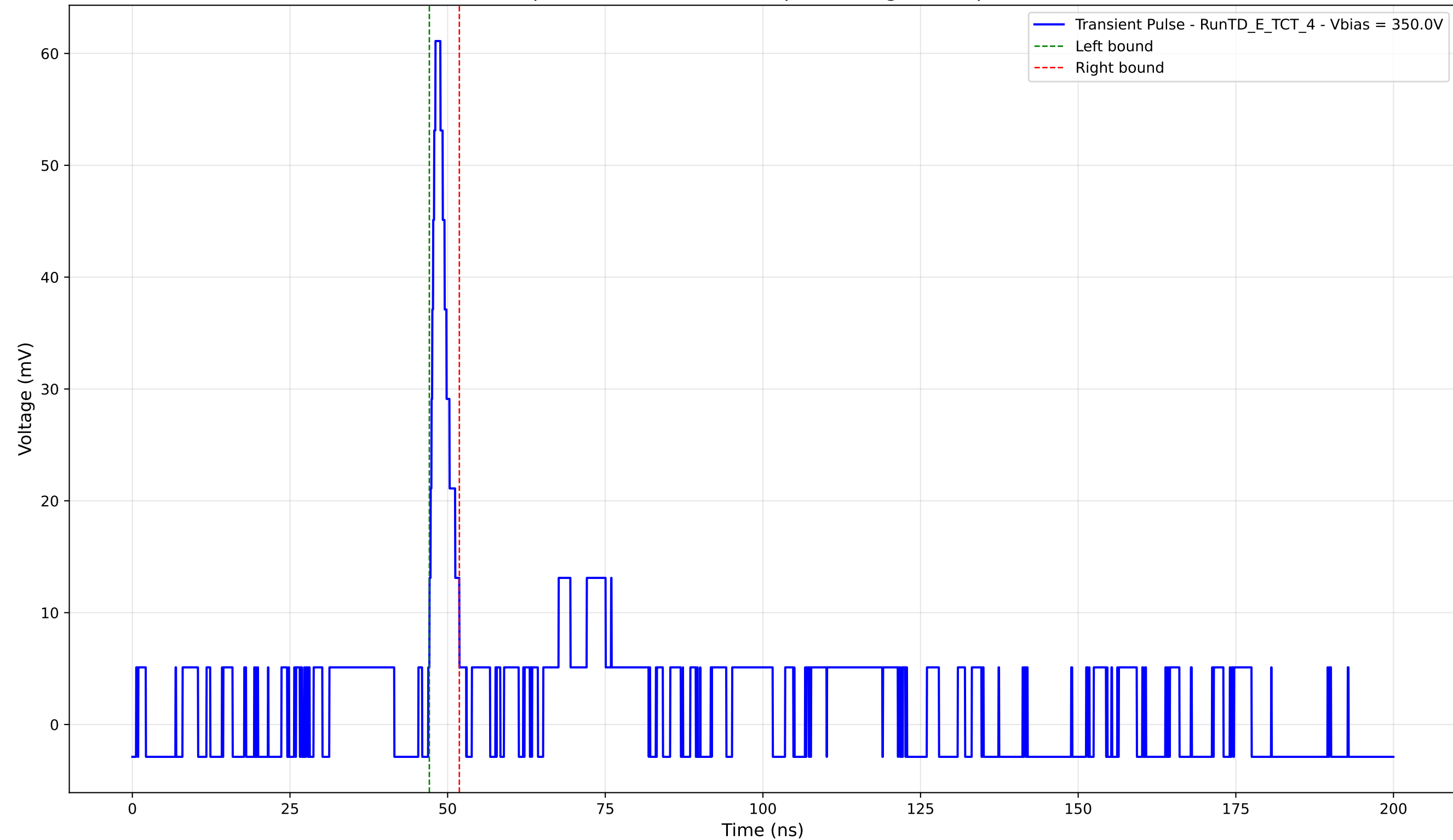
Transient Pulse - Sample: TD - Position: 345.0 \mu\text{m} - Charge: 3.32 pC - Rise Time: 0.96 ns
