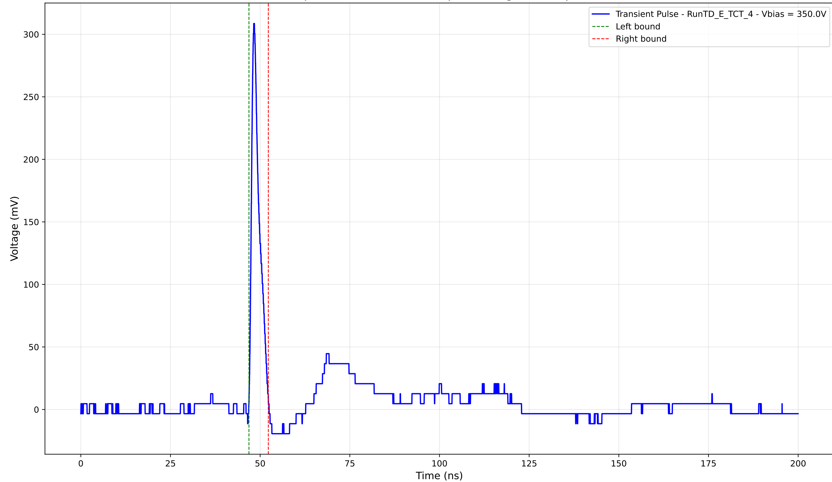
Transient Pulse - Sample: TD - Position: 145.0 \mu\text{m} - Charge: 15.50 pC - Rise Time: 0.93 ns
