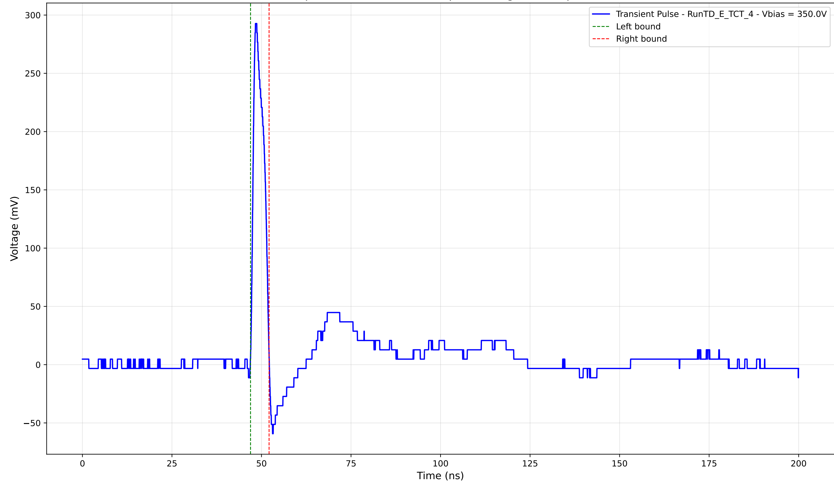
Transient Pulse - Sample: TD - Position: 290.0 \mu\text{m} - Charge: 19.05 pC - Rise Time: 0.96 ns
