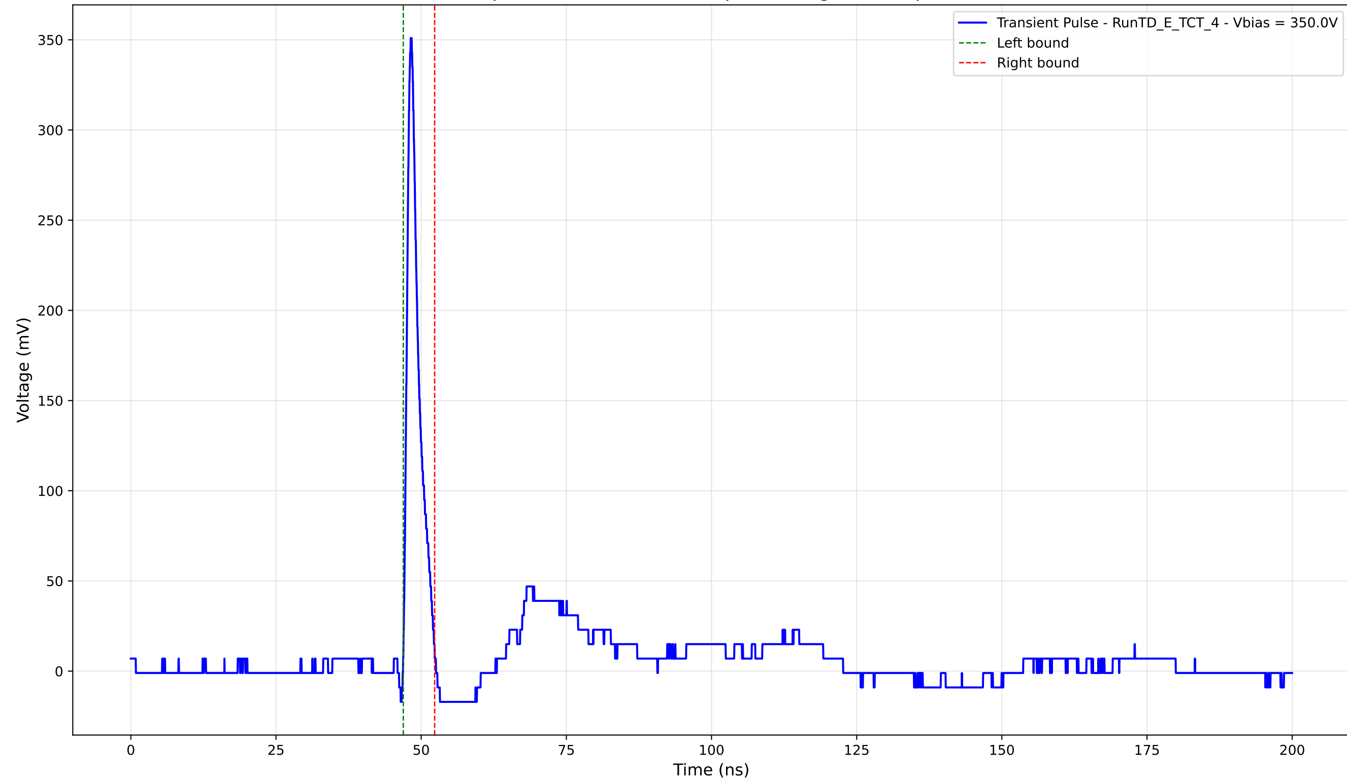
Transient Pulse - Sample: TD - Position: 140.0 \mu\text{m} - Charge: 16.68 pC - Rise Time: 0.89 ns
