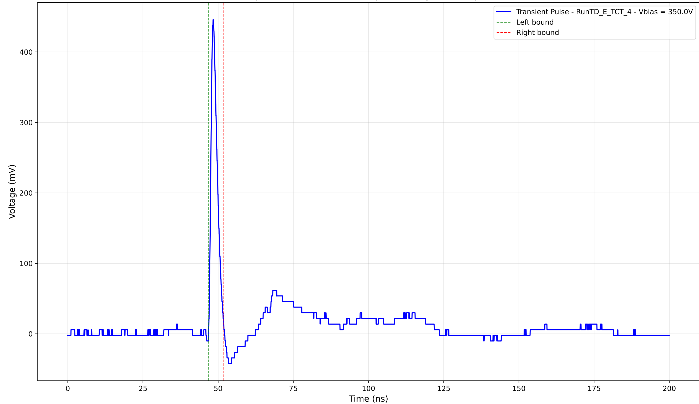
Transient Pulse - Sample: TD - Position: 160.0 \mu\text{m} - Charge: 21.34 pC - Rise Time: 0.95 ns
