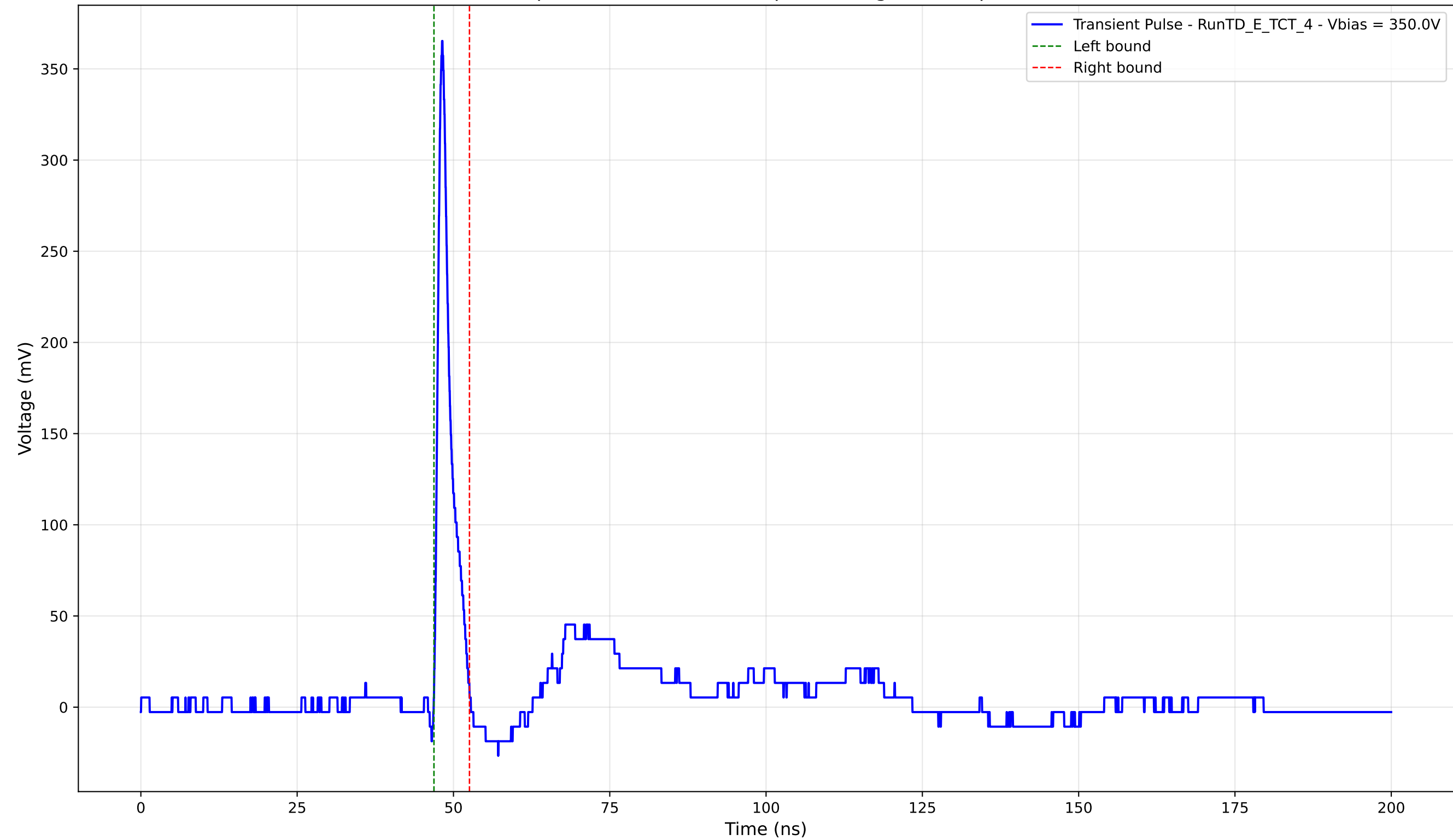
Transient Pulse - Sample: TD - Position: 95.0 \mu\text{m} - Charge: 17.02 pC - Rise Time: 0.88 ns
