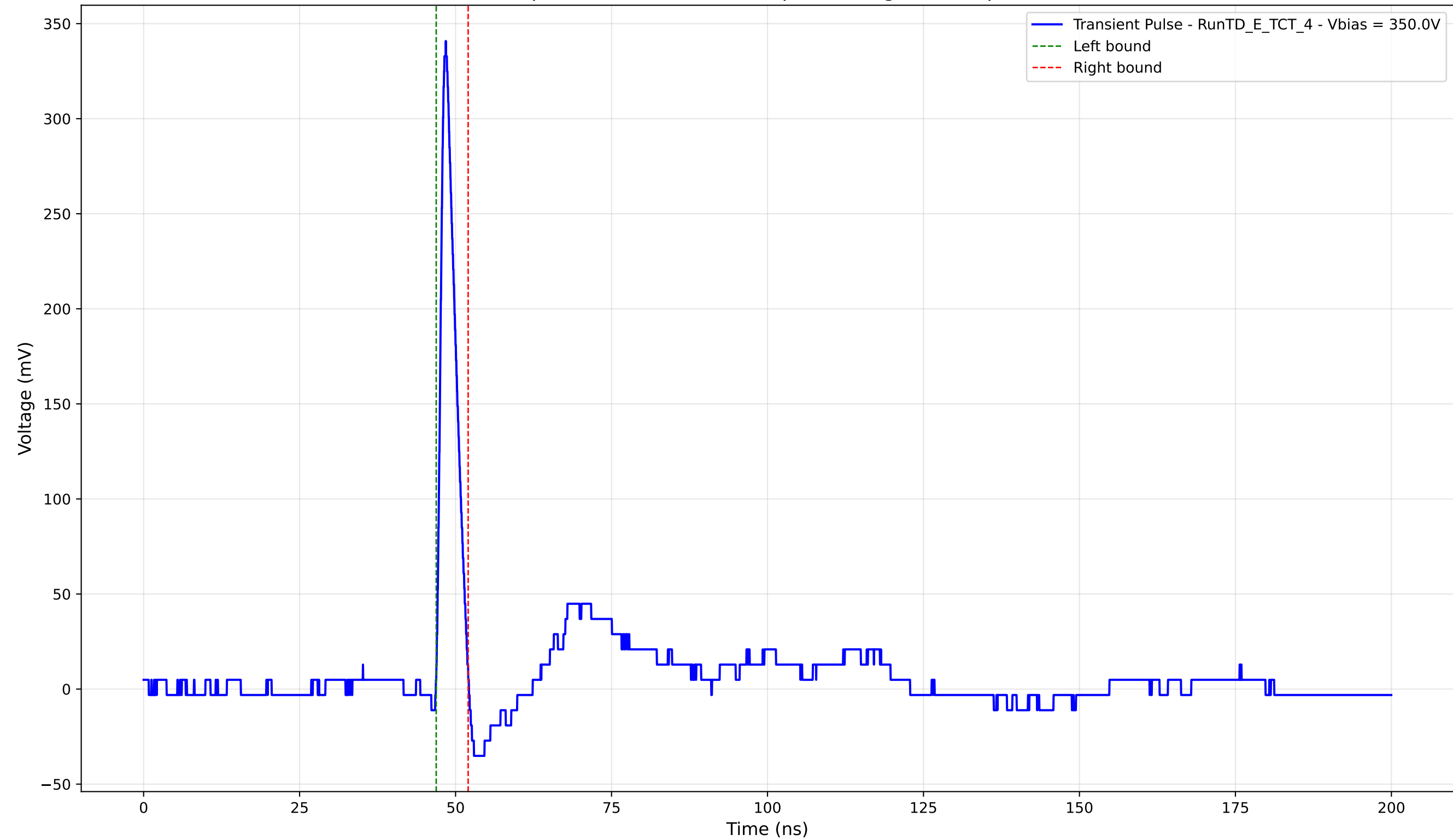
Transient Pulse - Sample: TD - Position: 210.0 \mu\text{m} - Charge: 17.86 pC - Rise Time: 0.97 ns
