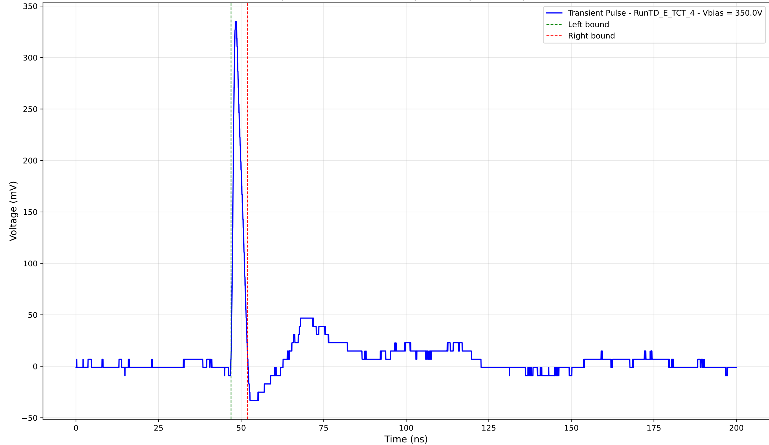
Transient Pulse - Sample: TD - Position: 275.0 \mu\text{m} - Charge: 18.22 pC - Rise Time: 0.91 ns
