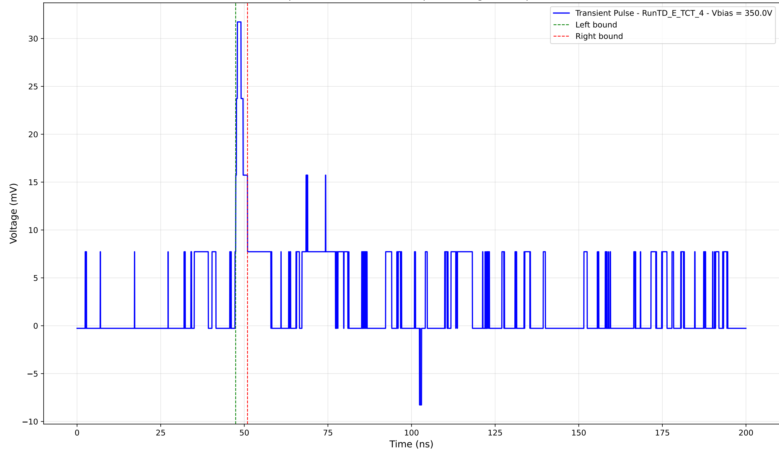
Transient Pulse - Sample: TD - Position: 360.0 \mu\text{m} - Charge: 1.61 pC - Rise Time: 0.71 ns
