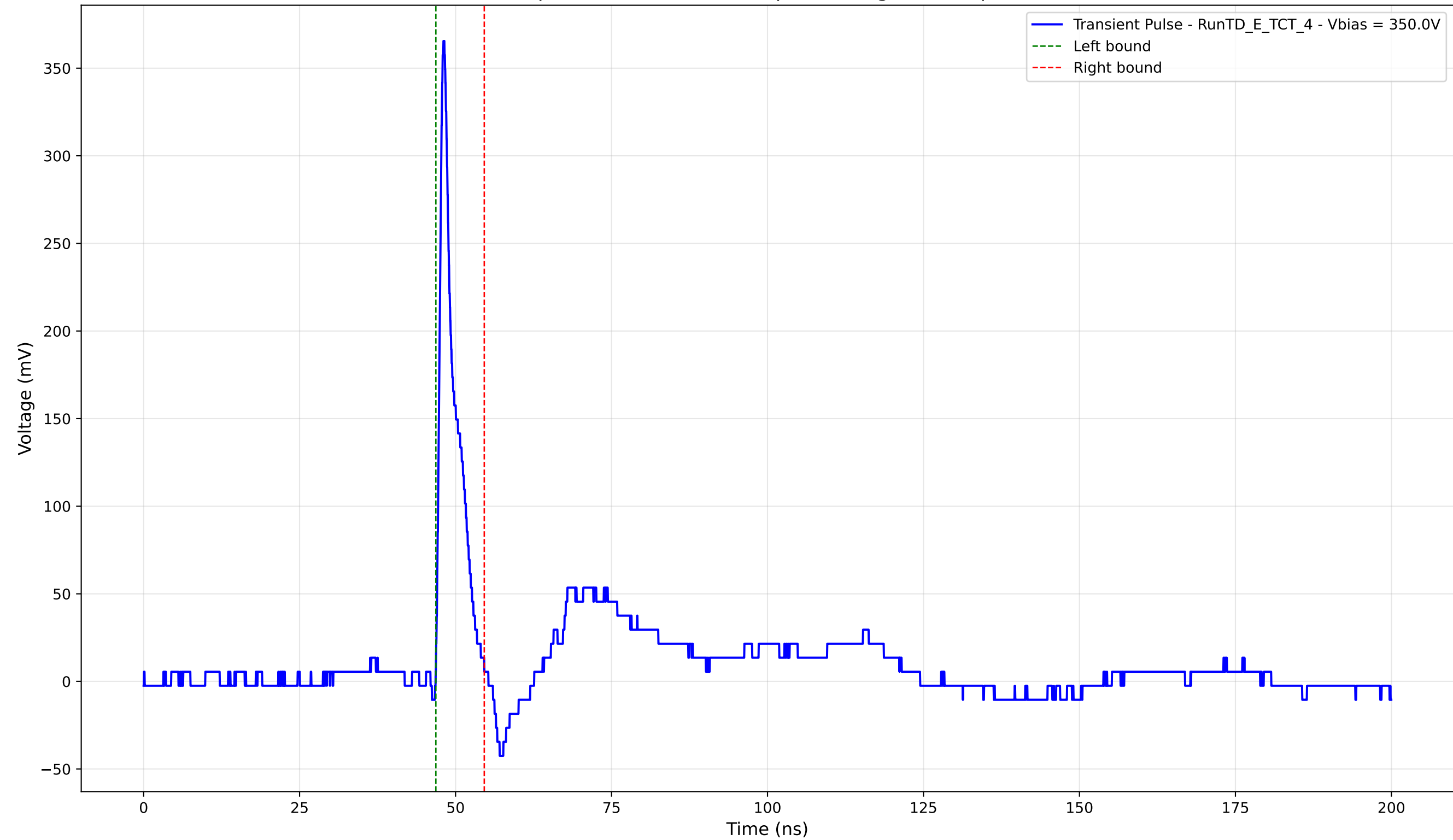
Transient Pulse - Sample: TD - Position: 70.0 \mu\text{m} - Charge: 20.97 pC - Rise Time: 0.84 ns
