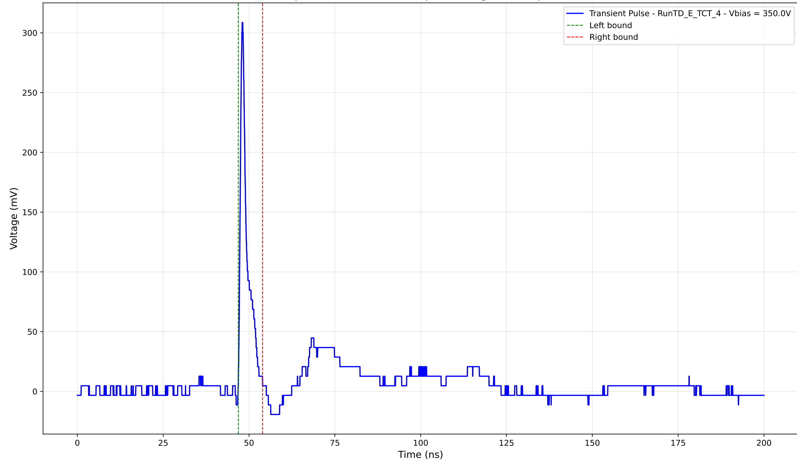
Transient Pulse - Sample: TD - Position: 35.0 \mu\text{m} - Charge: 14.44 pC - Rise Time: 0.81 ns
