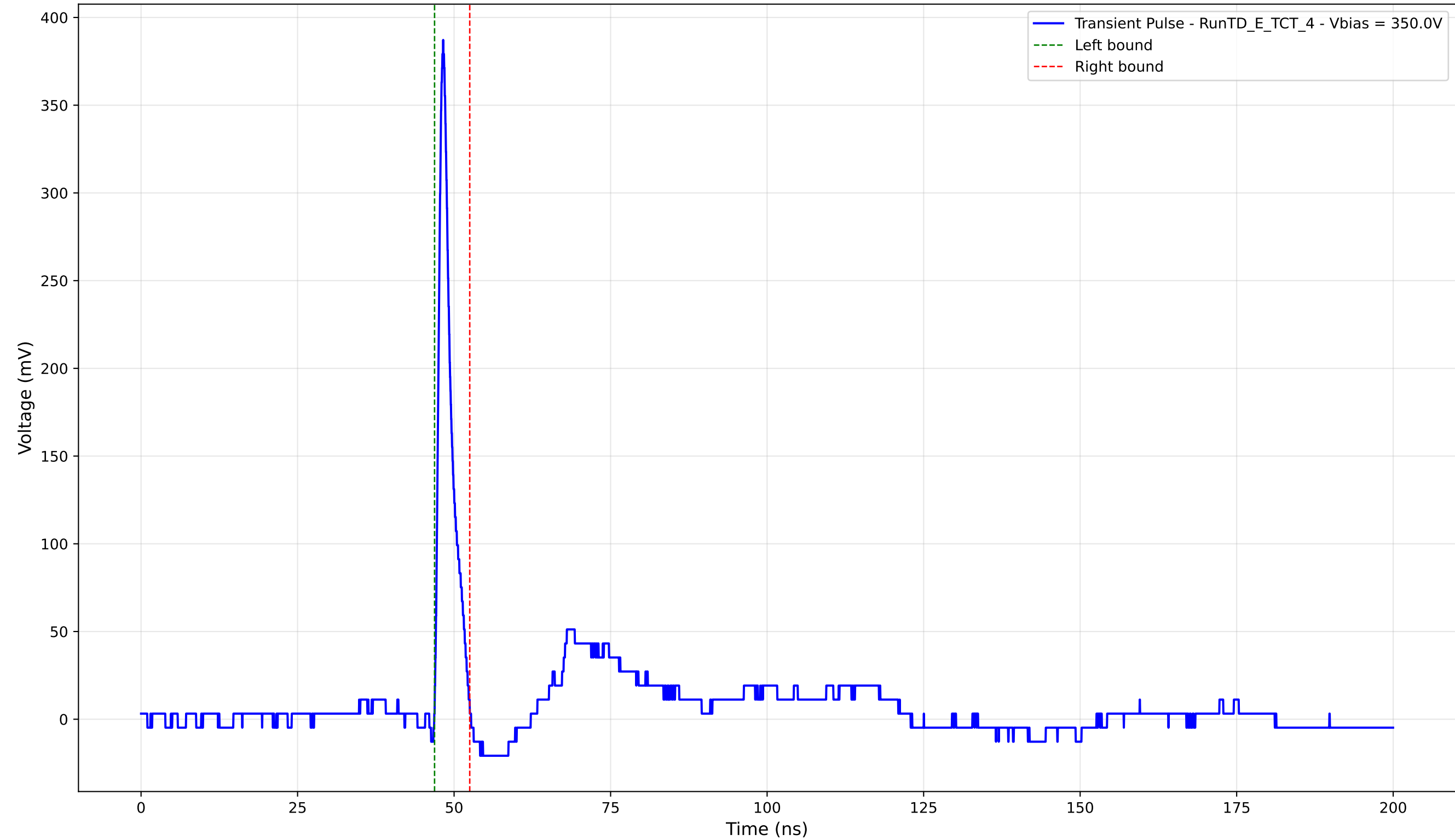
Transient Pulse - Sample: TD - Position: 135.0 \mu\text{m} - Charge: 17.85 pC - Rise Time: 0.91 ns
