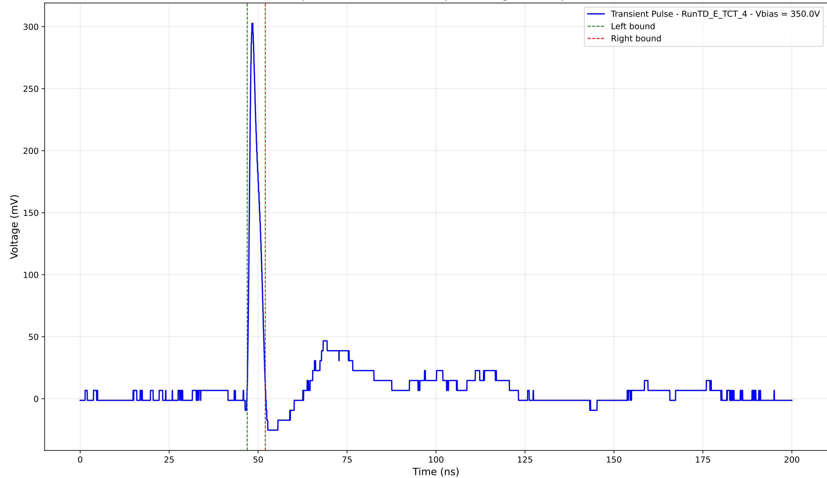
Transient Pulse - Sample: TD - Position: 150.0 \mu\text{m} - Charge: 16.88 pC - Rise Time: 0.98 ns
