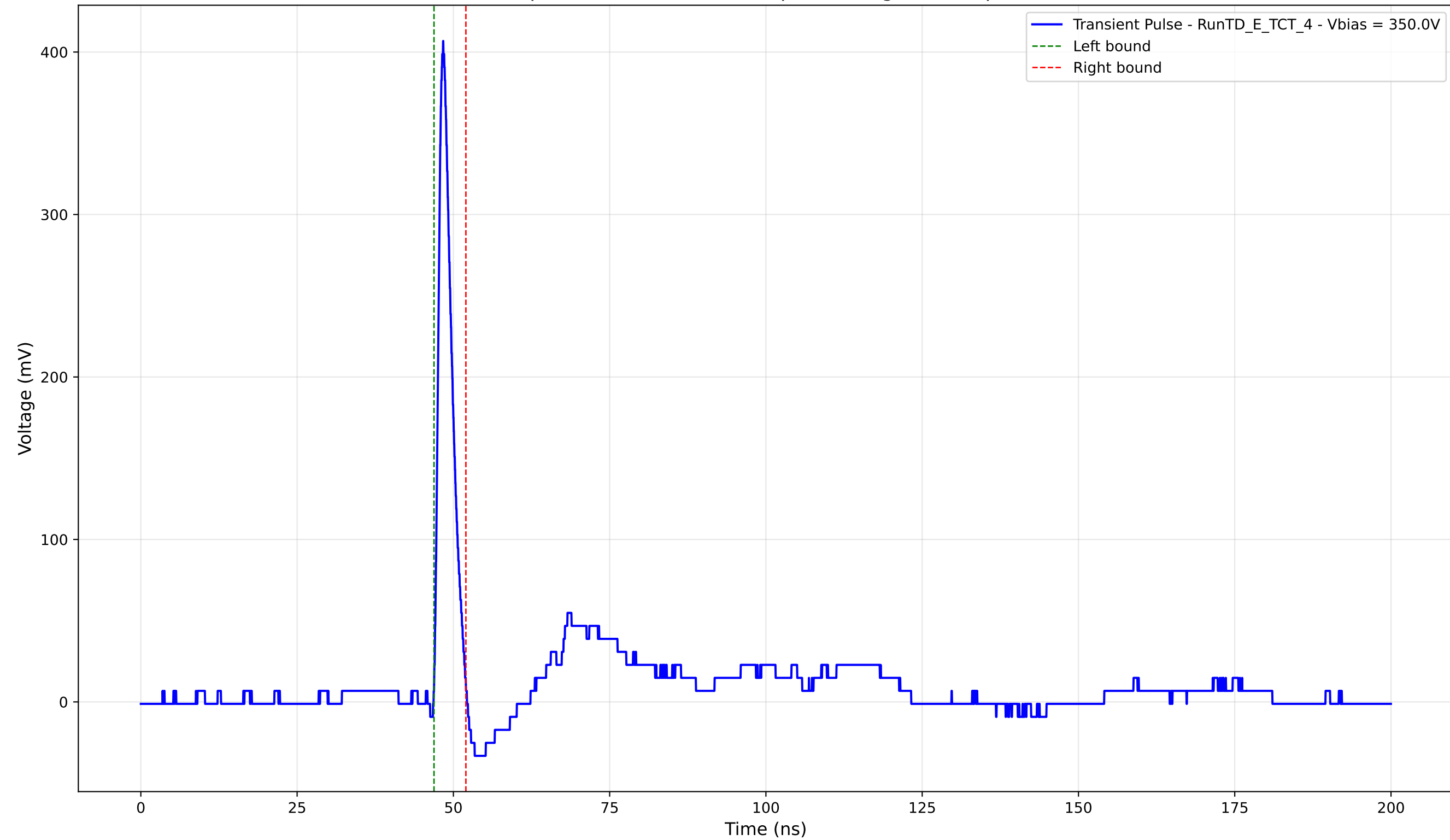
Transient Pulse - Sample: TD - Position: 220.0 \mu\text{m} - Charge: 19.68 pC - Rise Time: 0.94 ns
