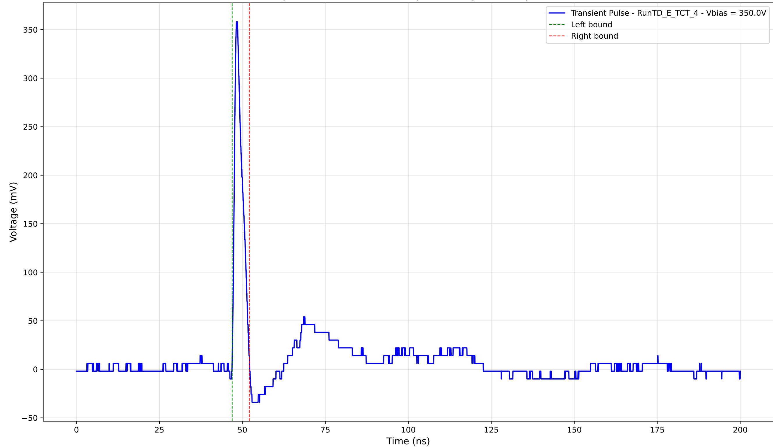
Transient Pulse - Sample: TD - Position: 250.0 \mu\text{m} - Charge: 19.37 pC - Rise Time: 0.93 ns
