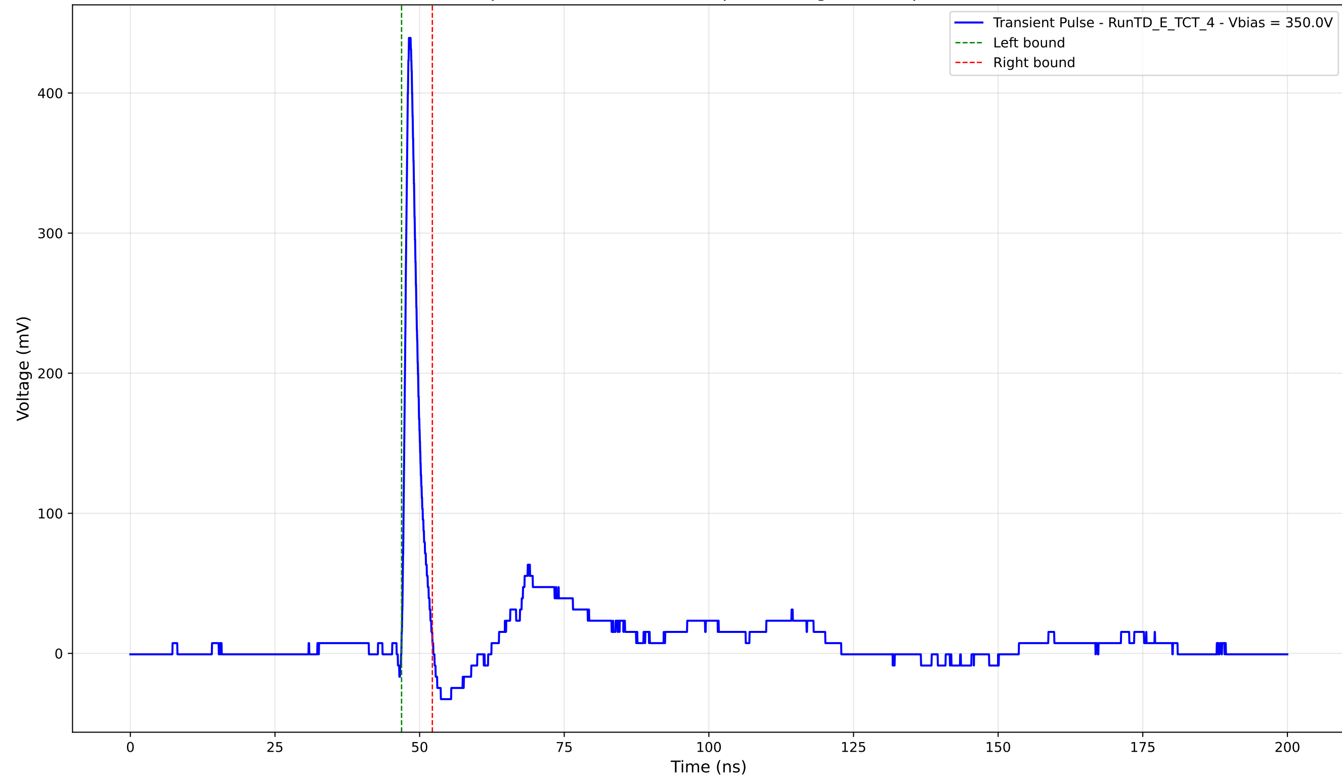
Transient Pulse - Sample: TD - Position: 165.0 \mu\text{m} - Charge: 20.52 pC - Rise Time: 0.91 ns
