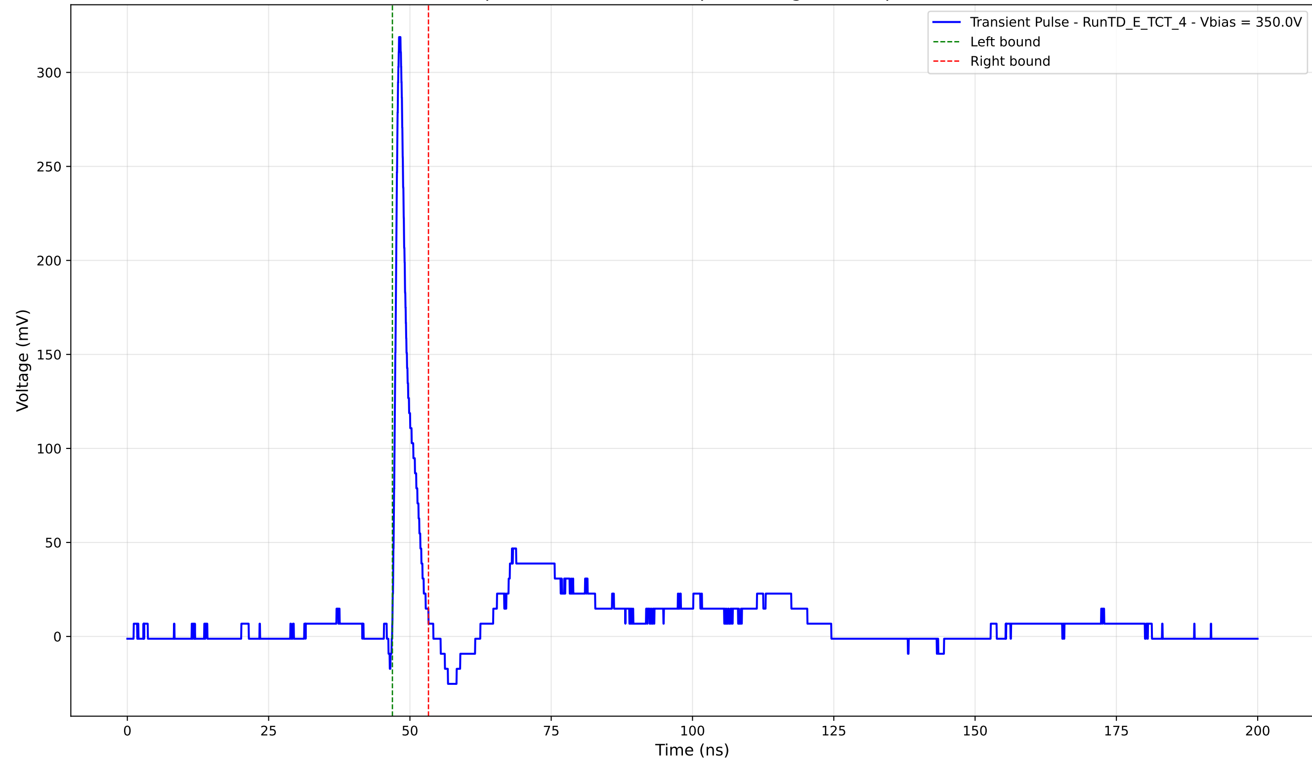
Transient Pulse - Sample: TD - Position: 80.0 \mu\text{m} - Charge: 16.10 pC - Rise Time: 0.88 ns
