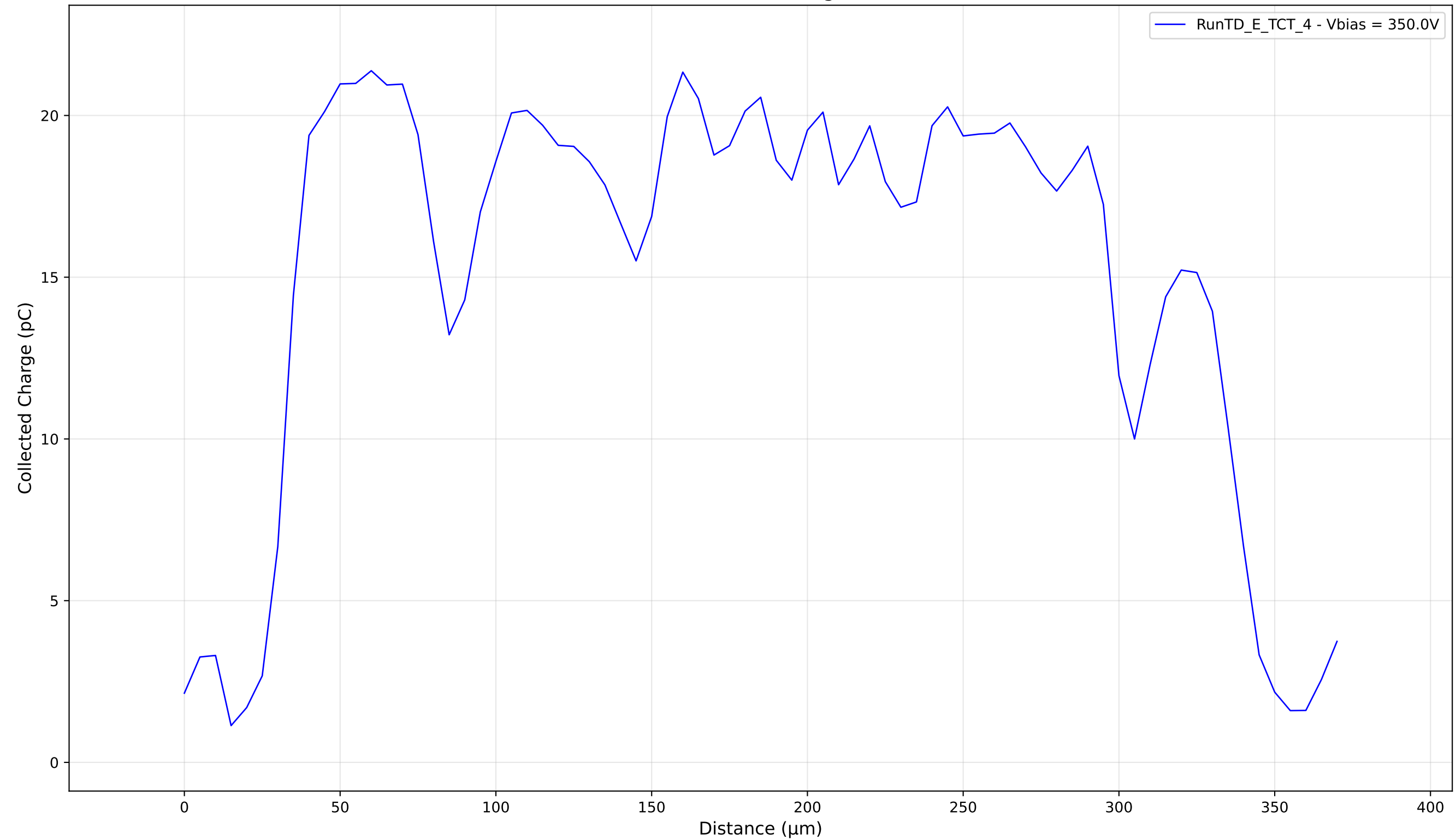
Collected Charge
