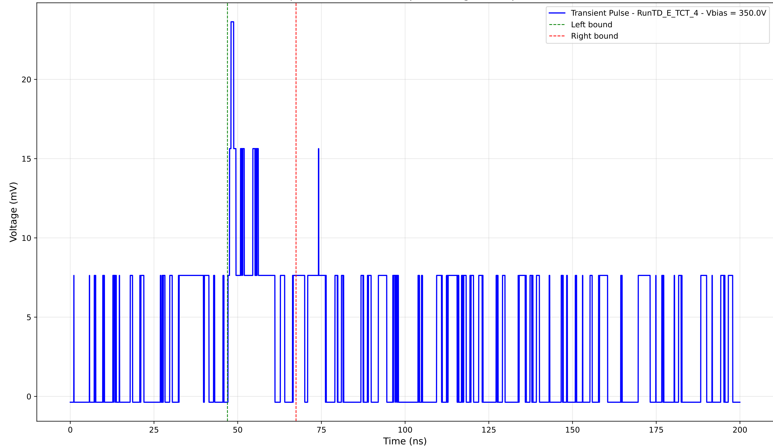
Transient Pulse - Sample: TD - Position: 5.0 \mu\text{m} - Charge: 3.26 pC - Rise Time: 0.91 ns
