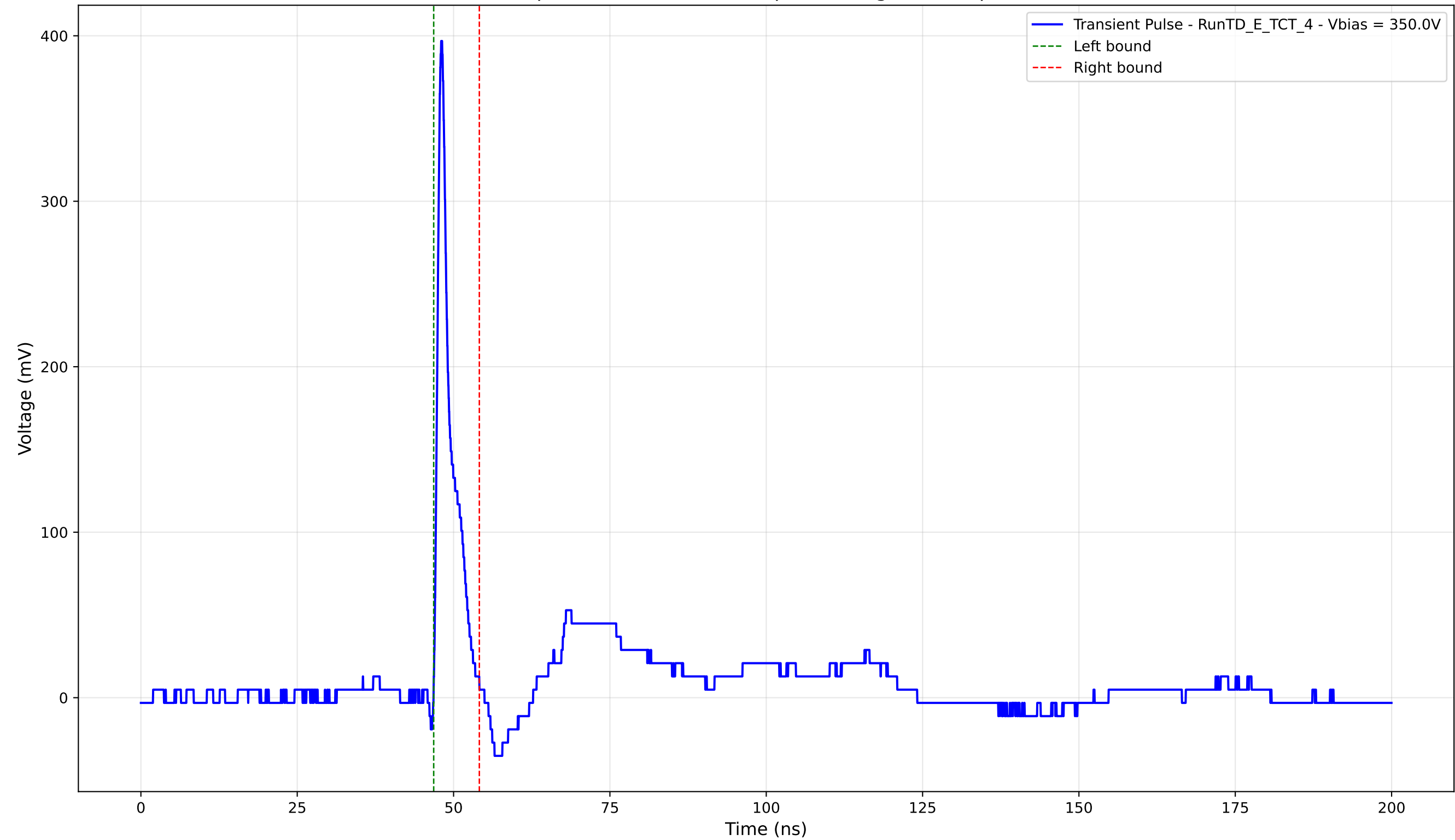
Transient Pulse - Sample: TD - Position: 45.0 \mu\text{m} - Charge: 20.12 pC - Rise Time: 0.81 ns
