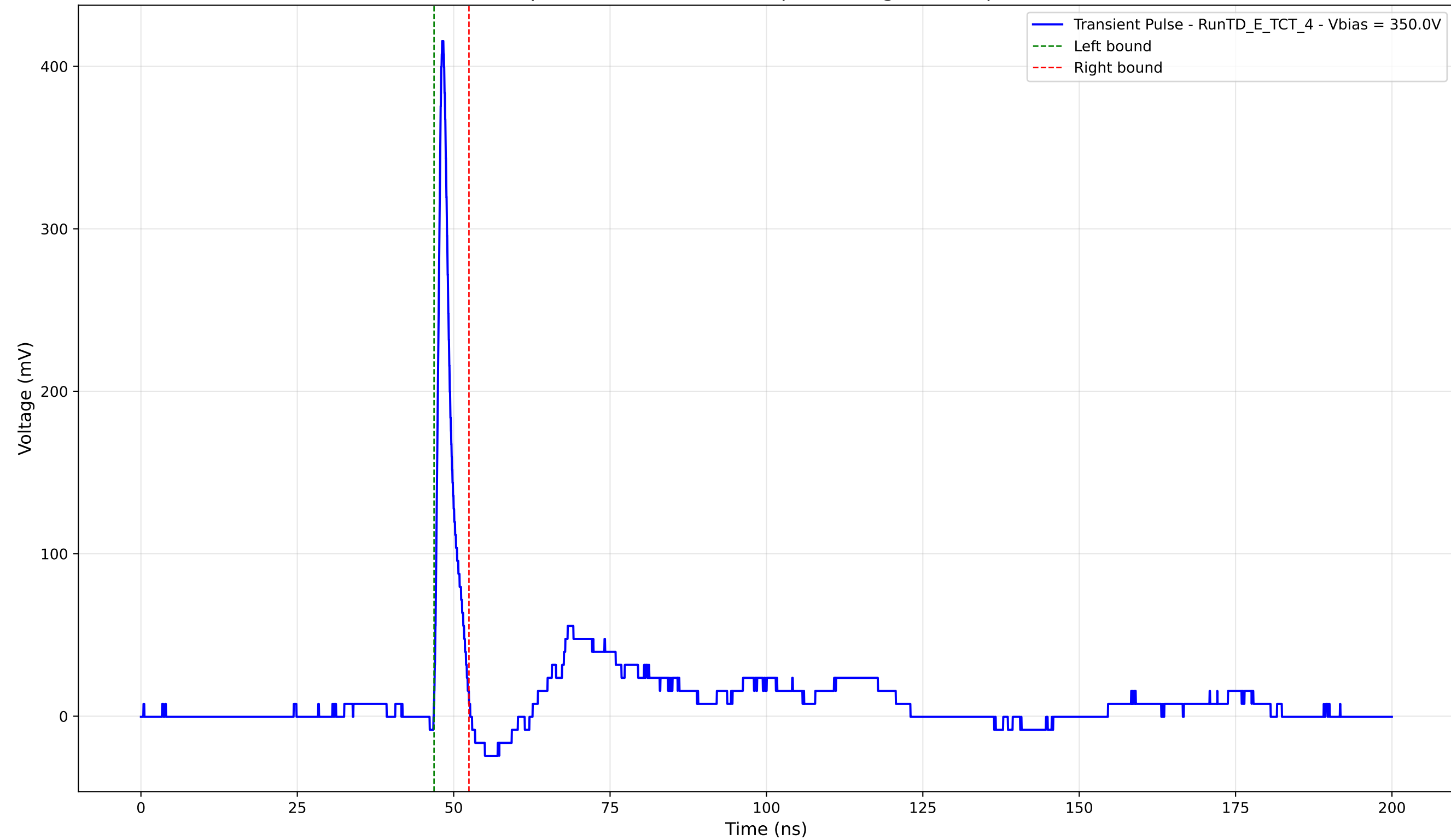
Transient Pulse - Sample: TD - Position: 125.0 \mu\text{m} - Charge: 19.04 pC - Rise Time: 0.88 ns
