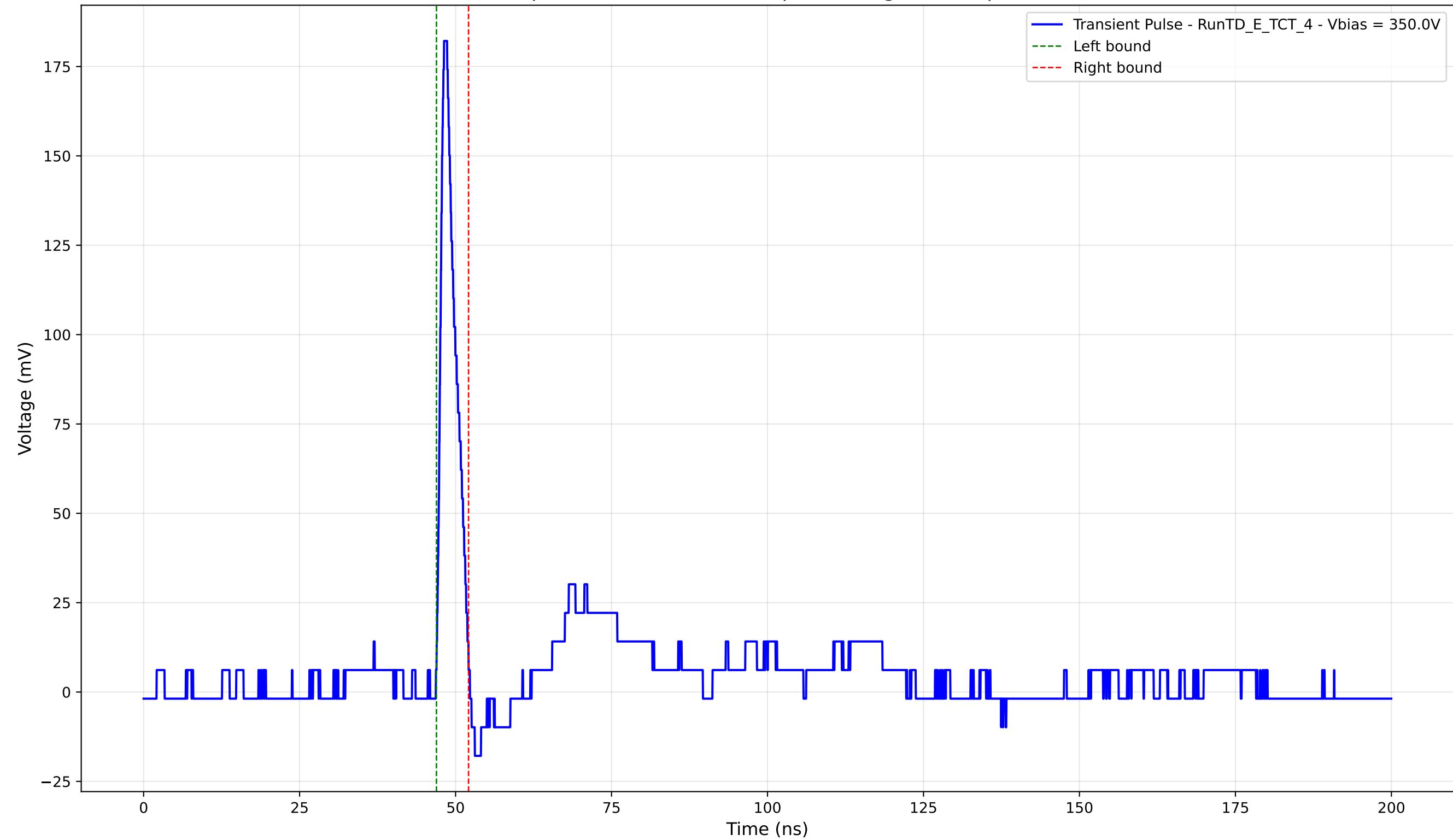
Transient Pulse - Sample: TD - Position: 305.0 \mu\text{m} - Charge: 10.00 pC - Rise Time: 0.93 ns
