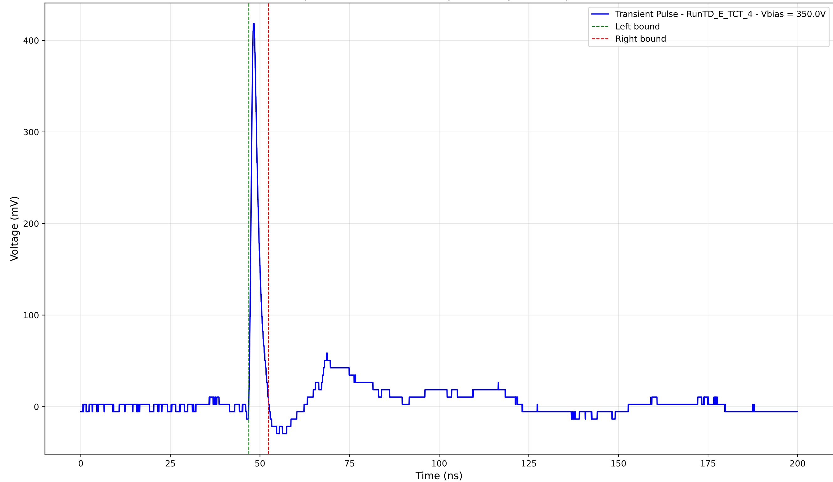
Transient Pulse - Sample: TD - Position: 200.0 \mu\text{m} - Charge: 19.54 pC - Rise Time: 0.88 ns
