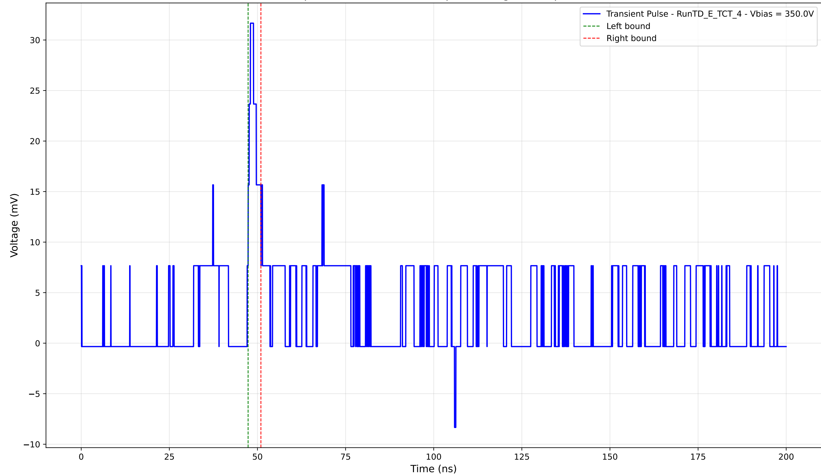
Transient Pulse - Sample: TD - Position: 355.0 \mu\text{m} - Charge: 1.60 pC - Rise Time: 0.93 ns
