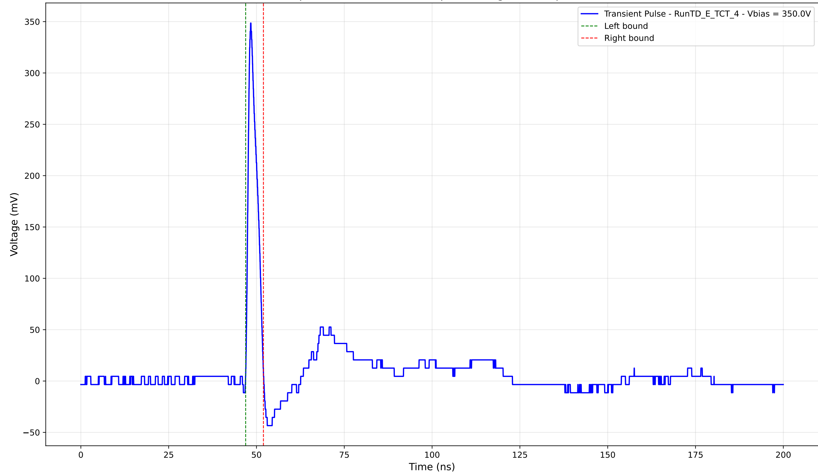
Transient Pulse - Sample: TD - Position: 255.0 \mu\text{m} - Charge: 19.42 pC - Rise Time: 0.94 ns
