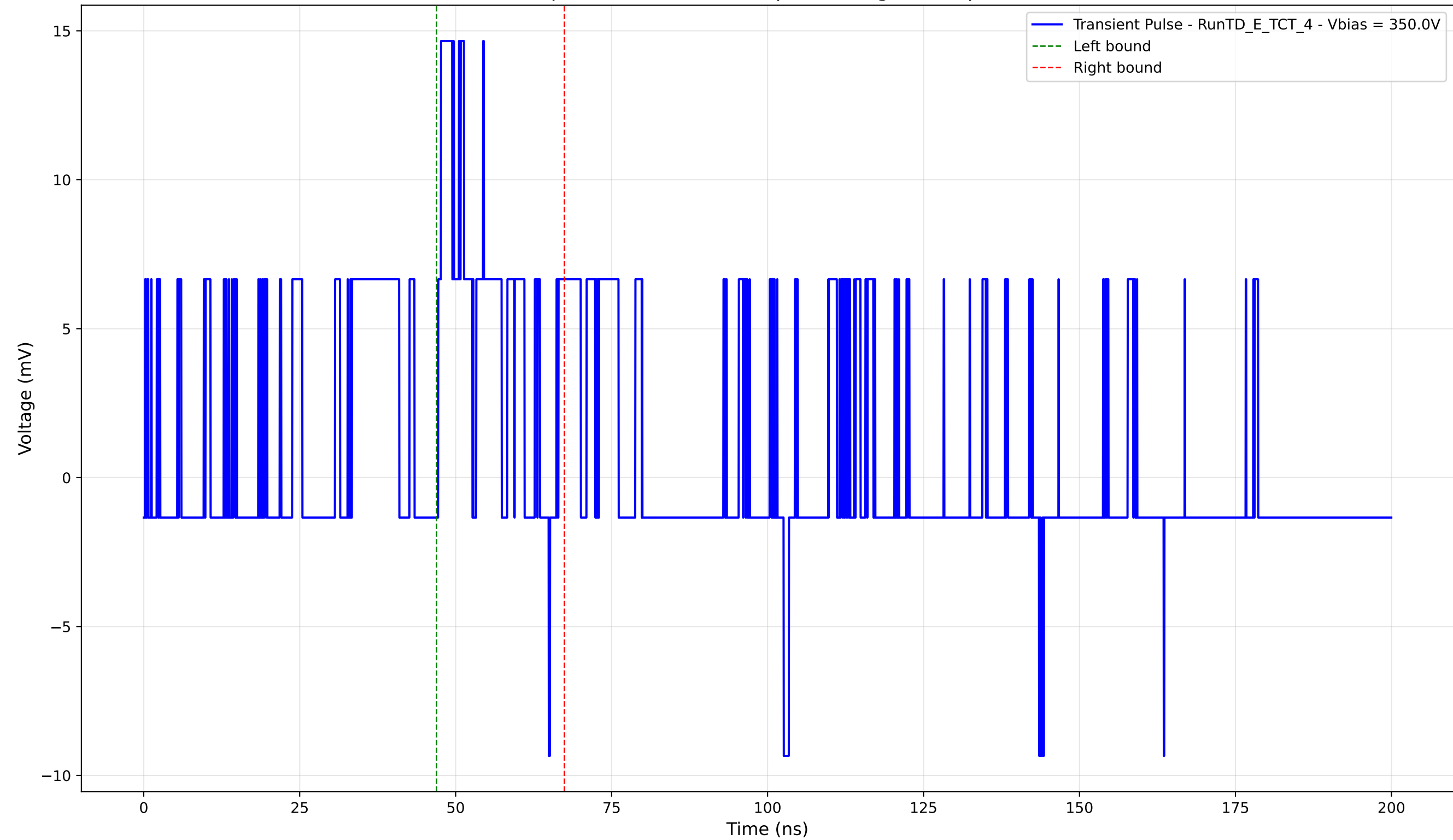
Transient Pulse - Sample: TD - Position: 0.0 \mu\text{m} - Charge: 2.14 pC - Rise Time: 0.46 ns
