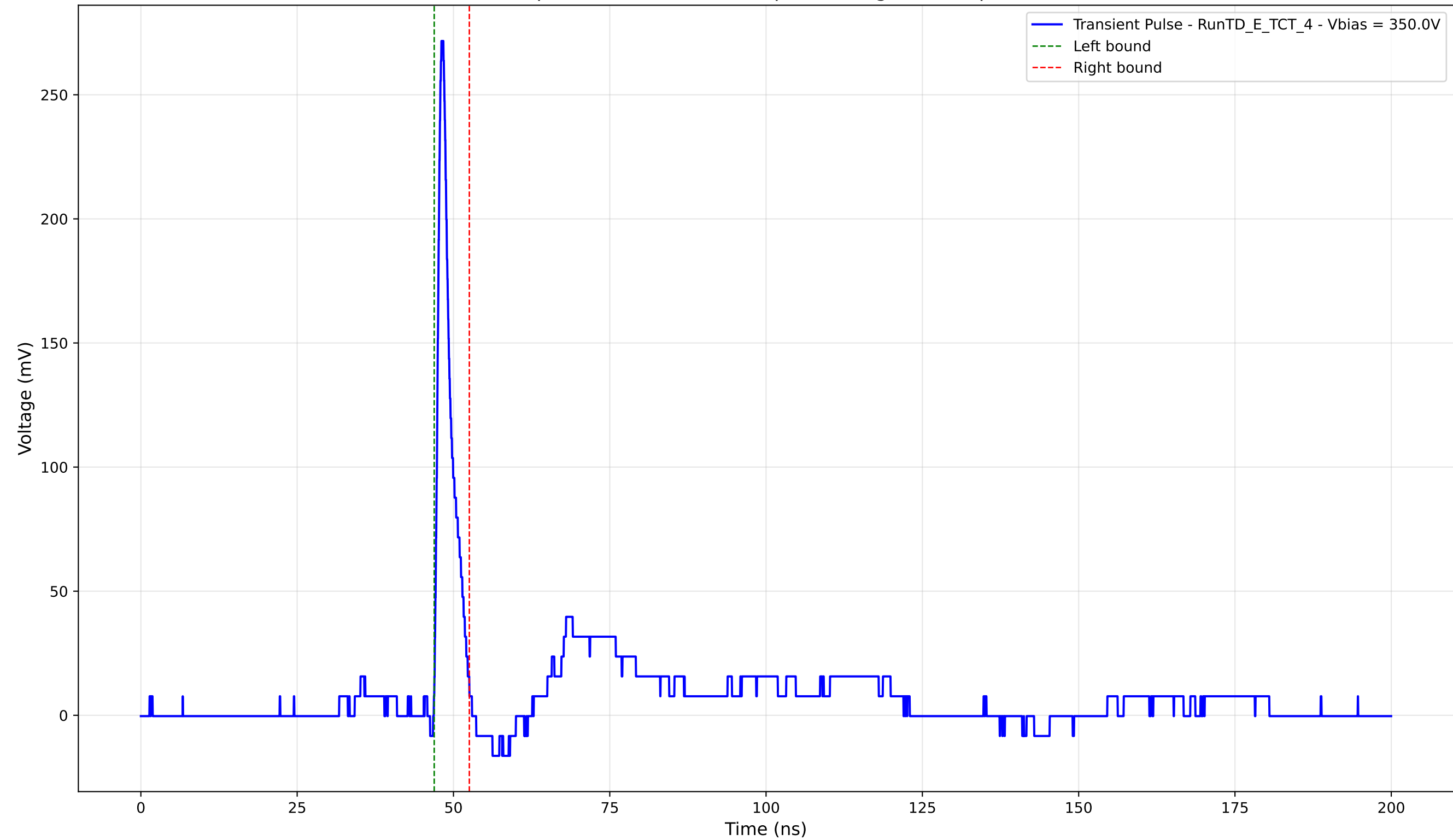
Transient Pulse - Sample: TD - Position: 85.0 \mu\text{m} - Charge: 13.22 pC - Rise Time: 0.85 ns
