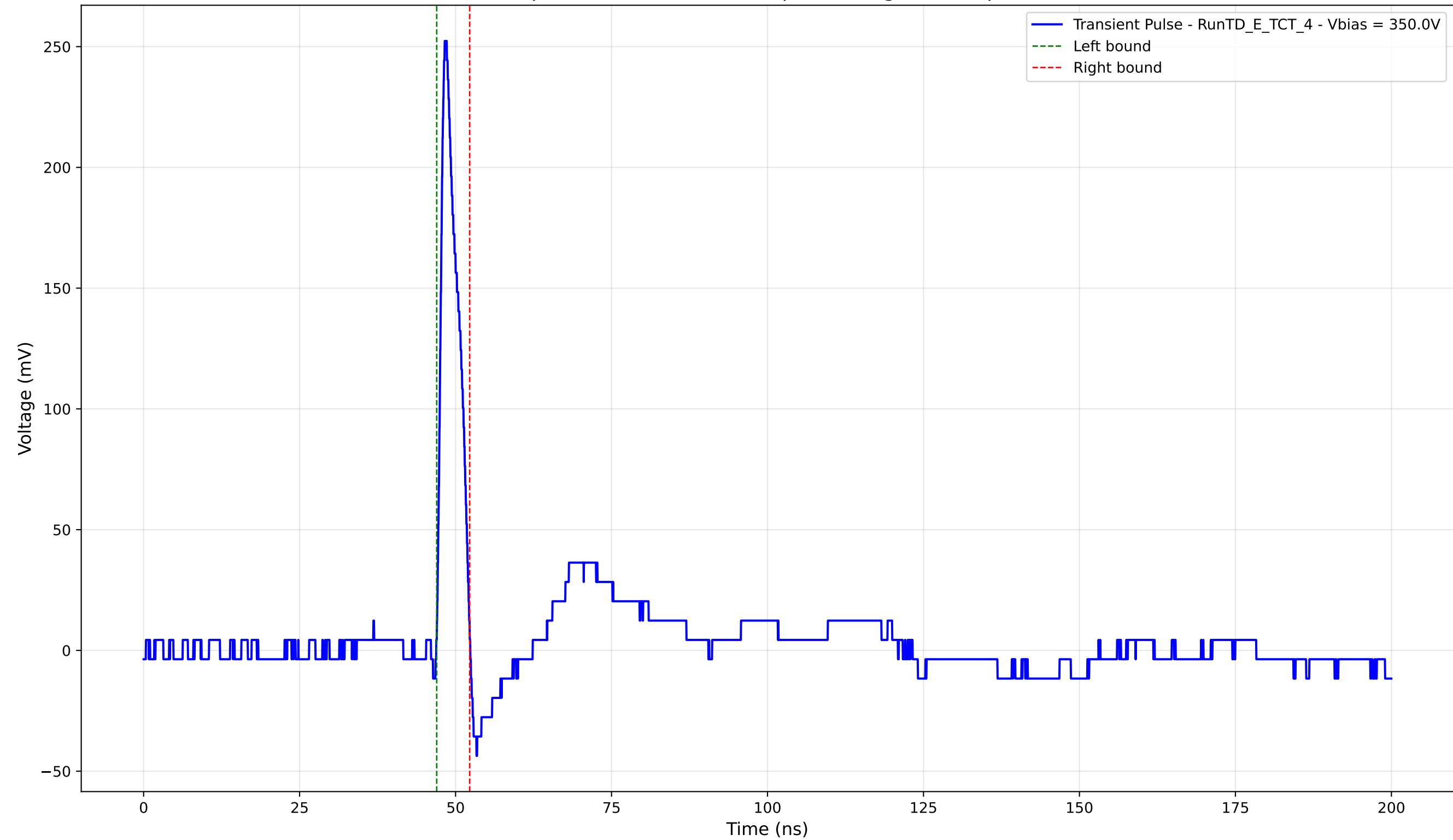
Transient Pulse - Sample: TD - Position: 320.0 \mu\text{m} - Charge: 15.22 pC - Rise Time: 0.91 ns
