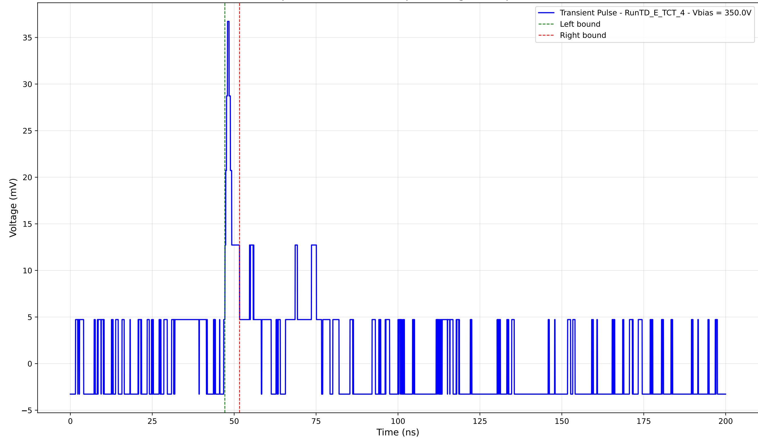
Transient Pulse - Sample: TD - Position: 20.0 \mu\text{m} - Charge: 1.69 pC - Rise Time: 1.17 ns
