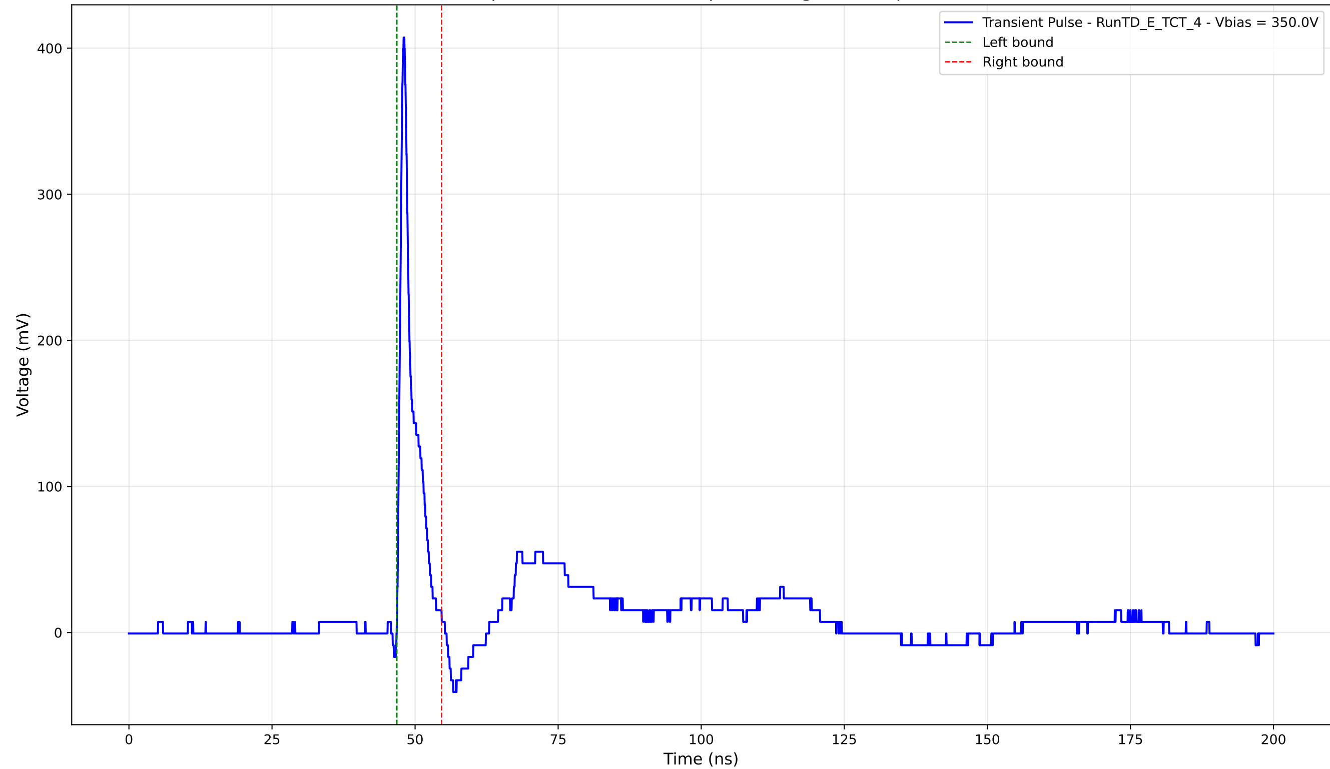
Transient Pulse - Sample: TD - Position: 55.0 \mu\text{m} - Charge: 20.99 pC - Rise Time: 0.79 ns
