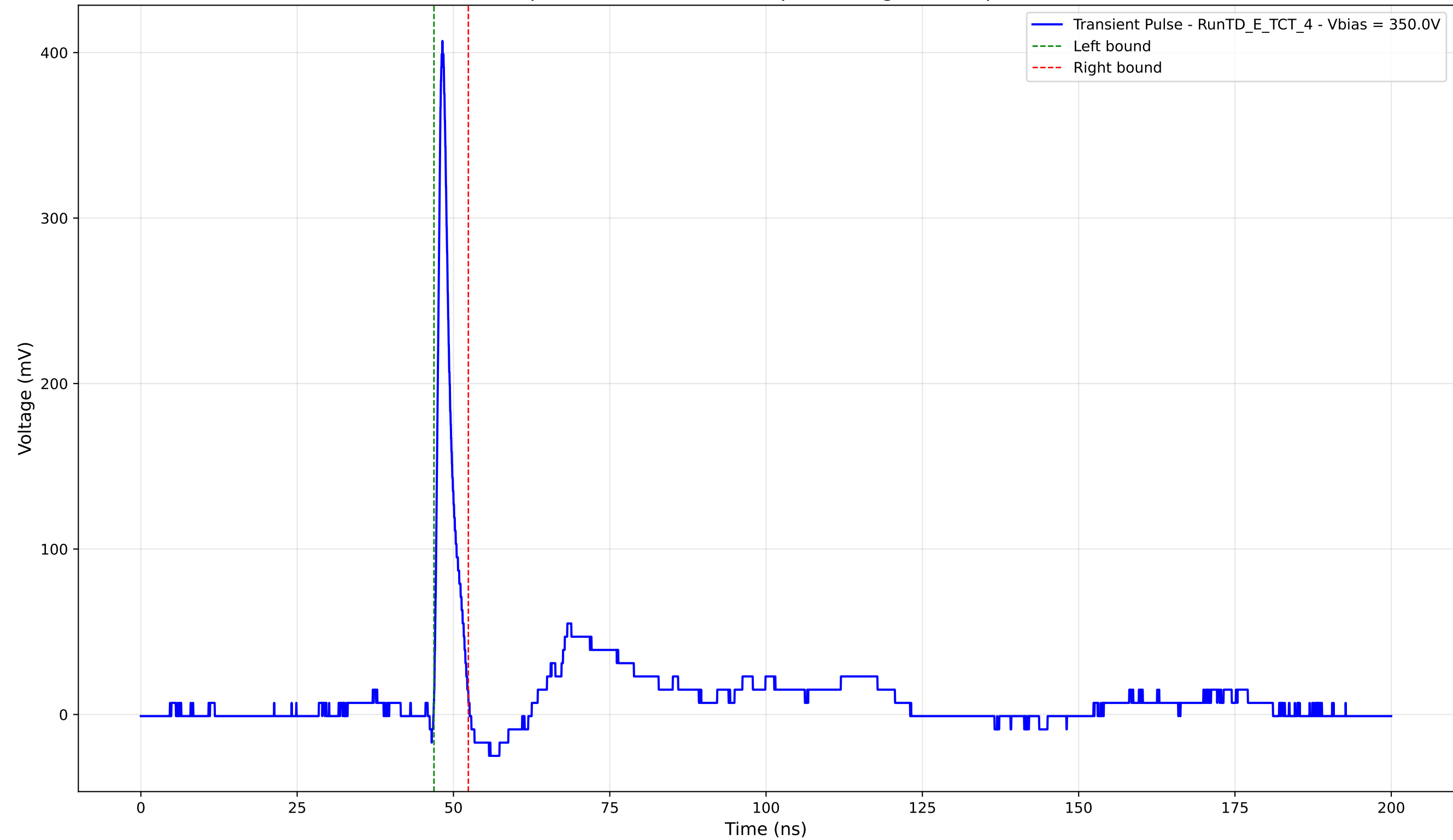
Transient Pulse - Sample: TD - Position: 130.0 \mu\text{m} - Charge: 18.57 pC - Rise Time: 0.88 ns
