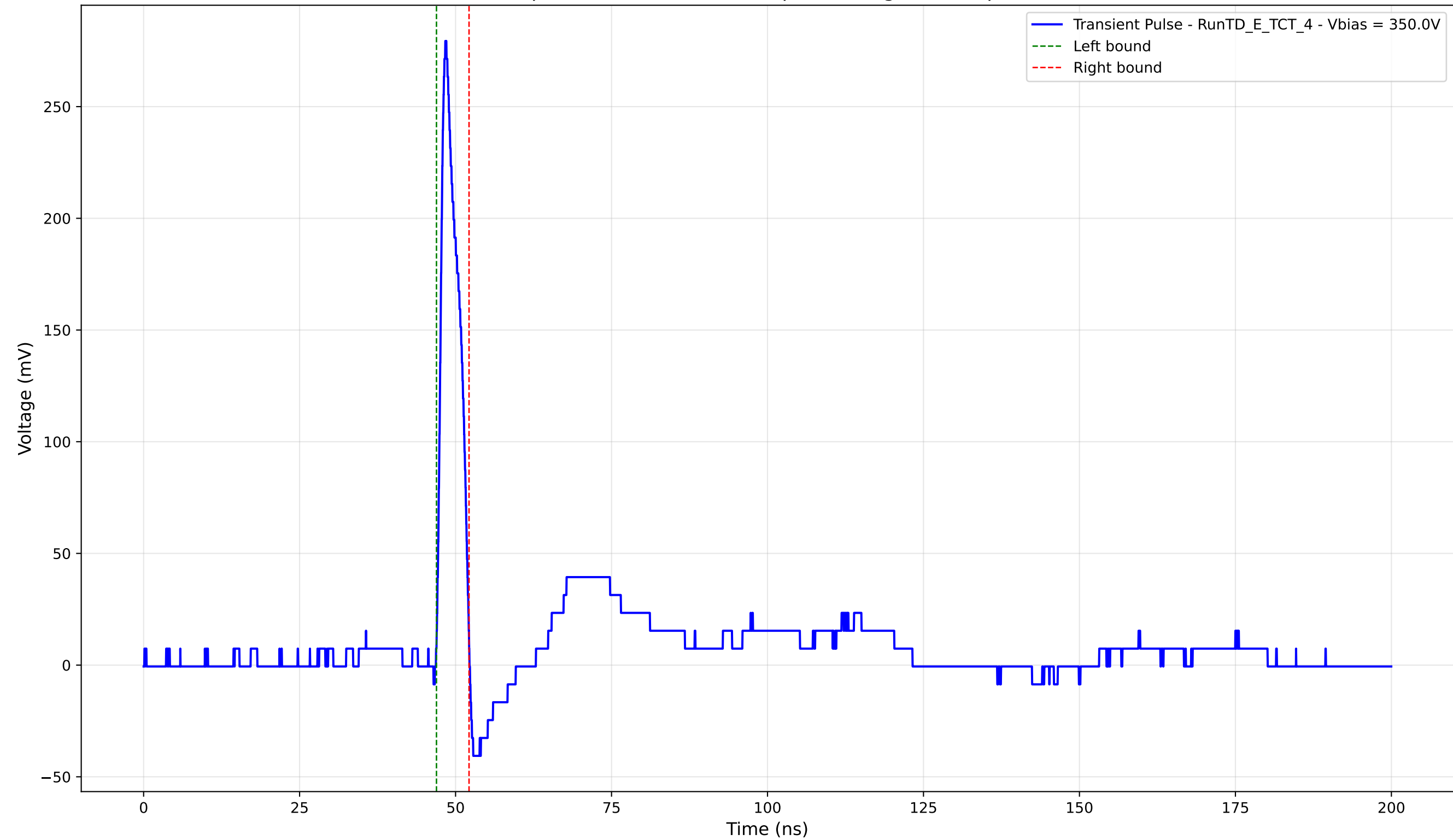
Transient Pulse - Sample: TD - Position: 295.0 \mu\text{m} - Charge: 17.25 pC - Rise Time: 0.99 ns
