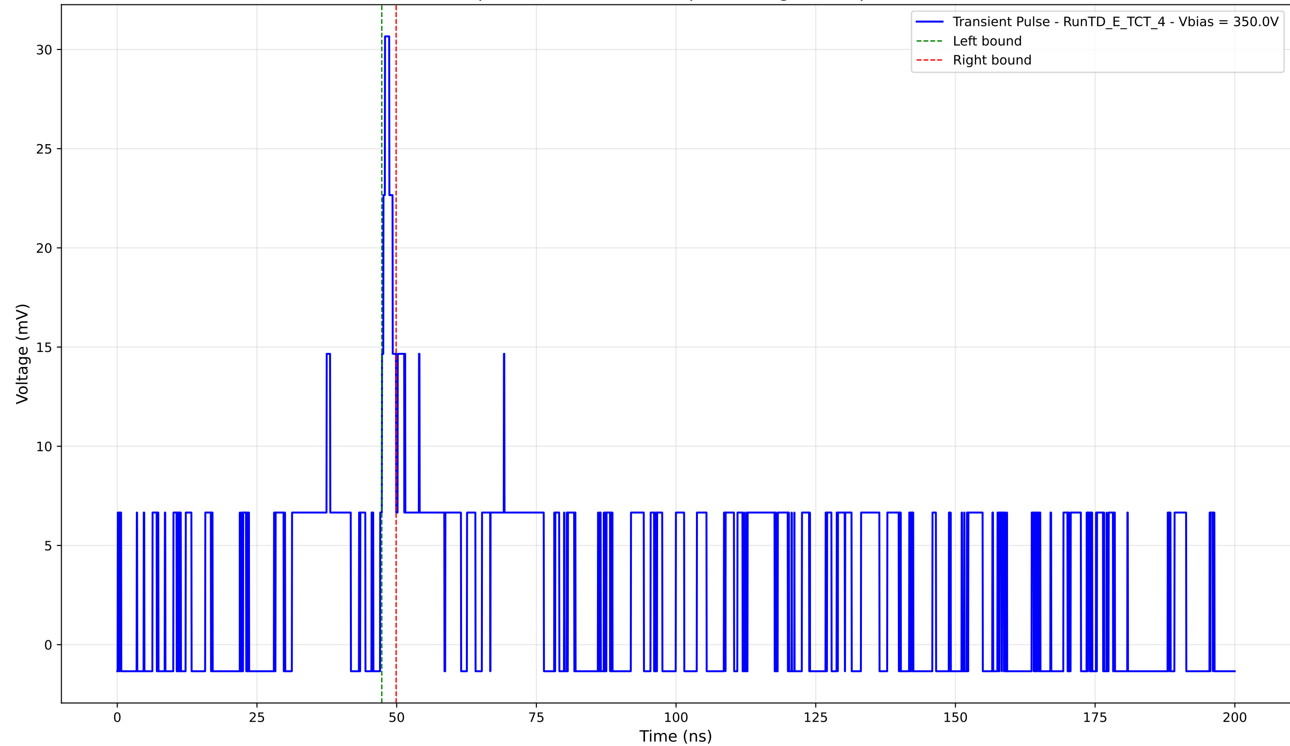
Transient Pulse - Sample: TD - Position: 15.0 \mu\text{m} - Charge: 1.14 pC - Rise Time: 0.87 ns
