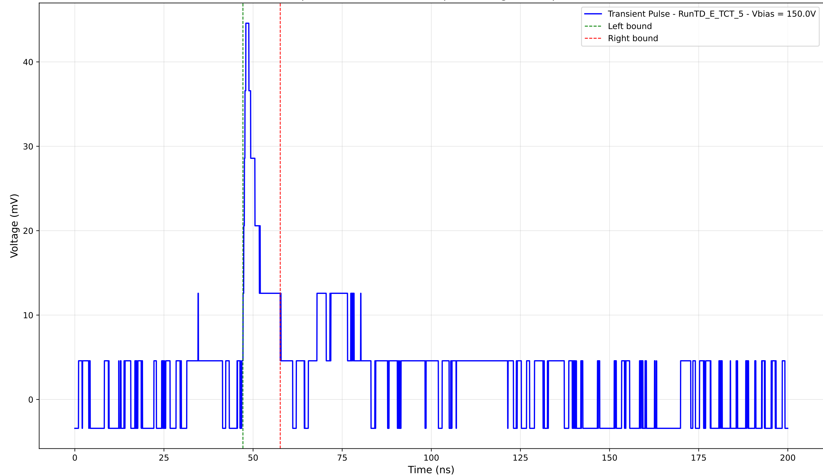
Transient Pulse - Sample: TD - Position: 370.0 \mu\text{m} - Charge: 4.22 pC - Rise Time: 1.14 ns
