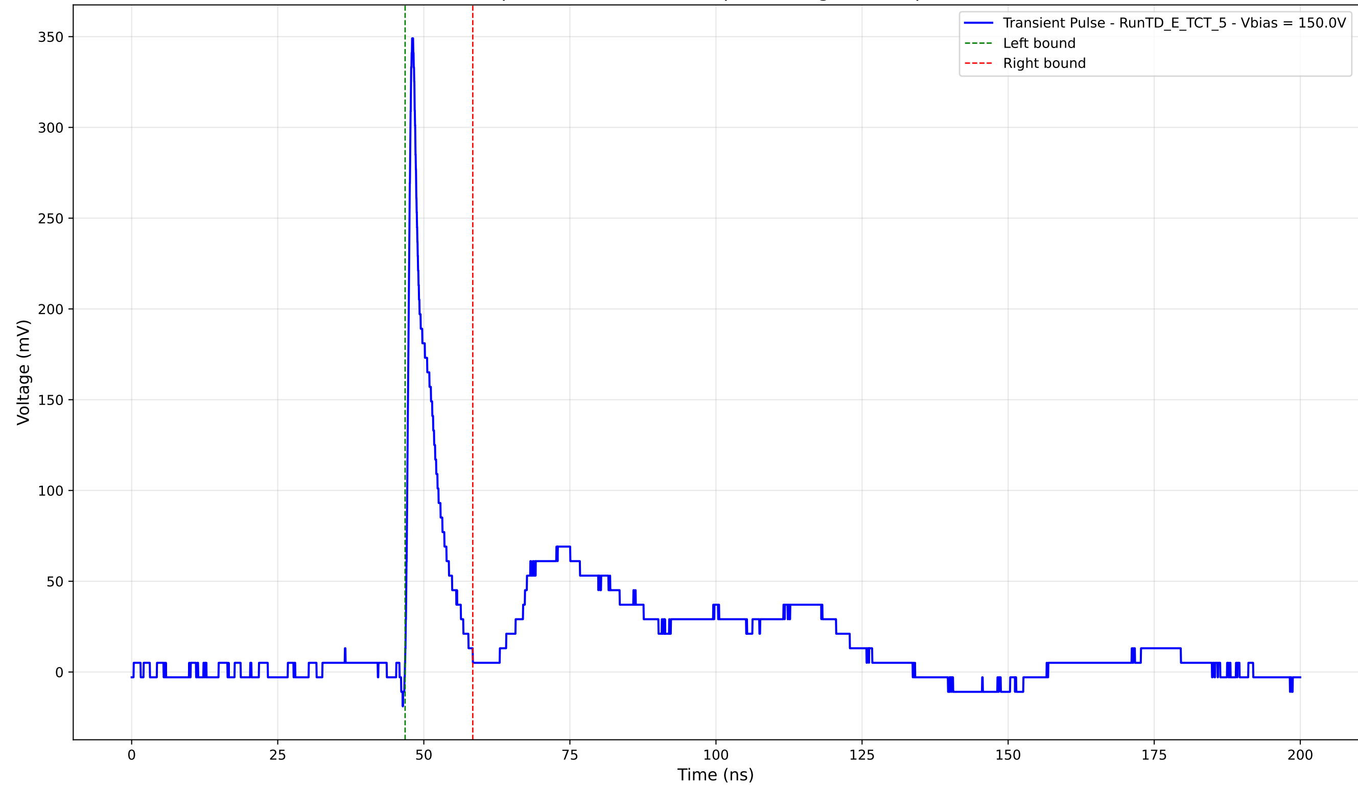
Transient Pulse - Sample: TD - Position: 70.0 \mu\text{m} - Charge: 26.94 pC - Rise Time: 0.82 ns
