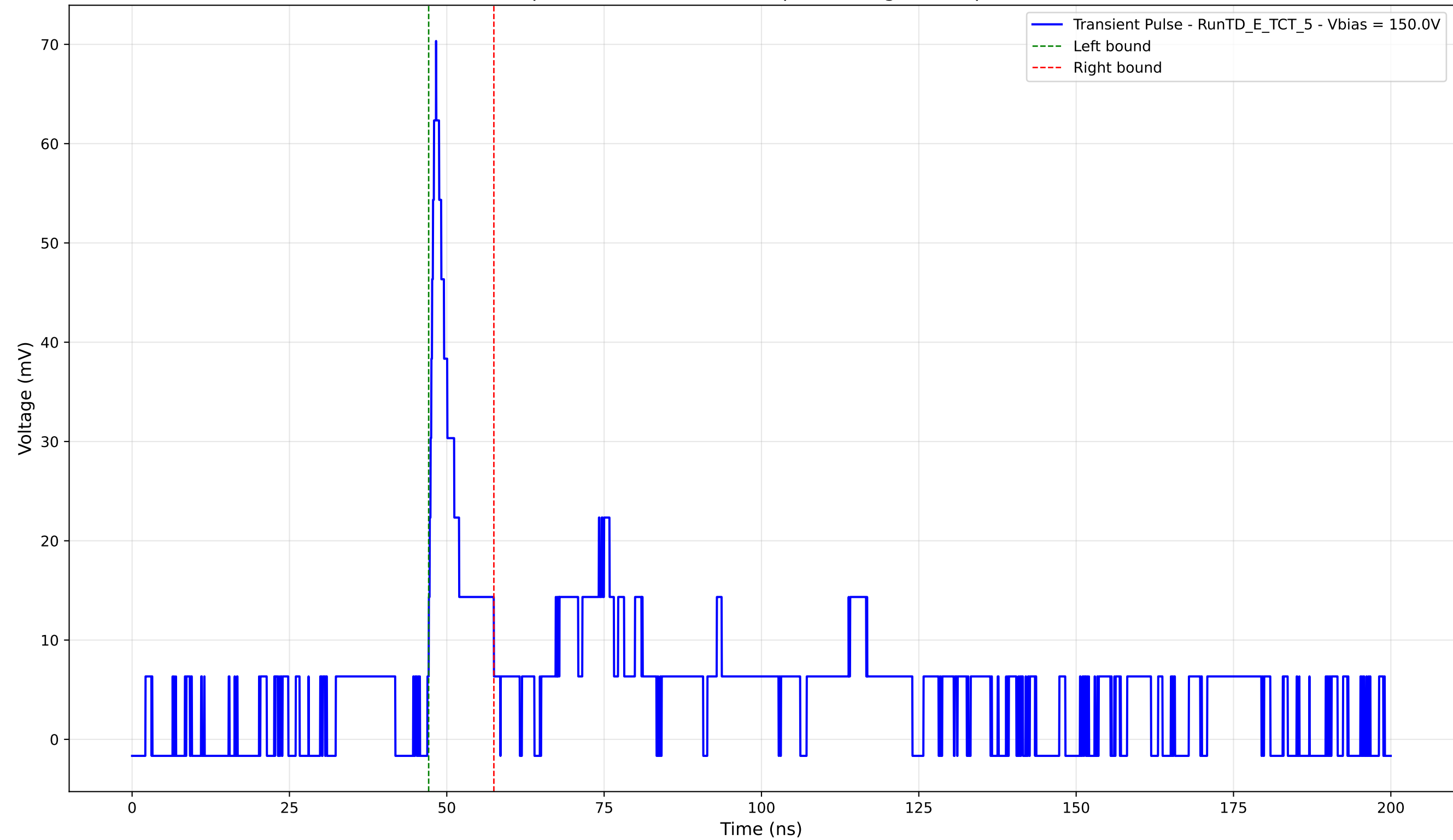
Transient Pulse - Sample: TD - Position: 390.0 \mu\text{m} - Charge: 5.37 pC - Rise Time: 1.18 ns
