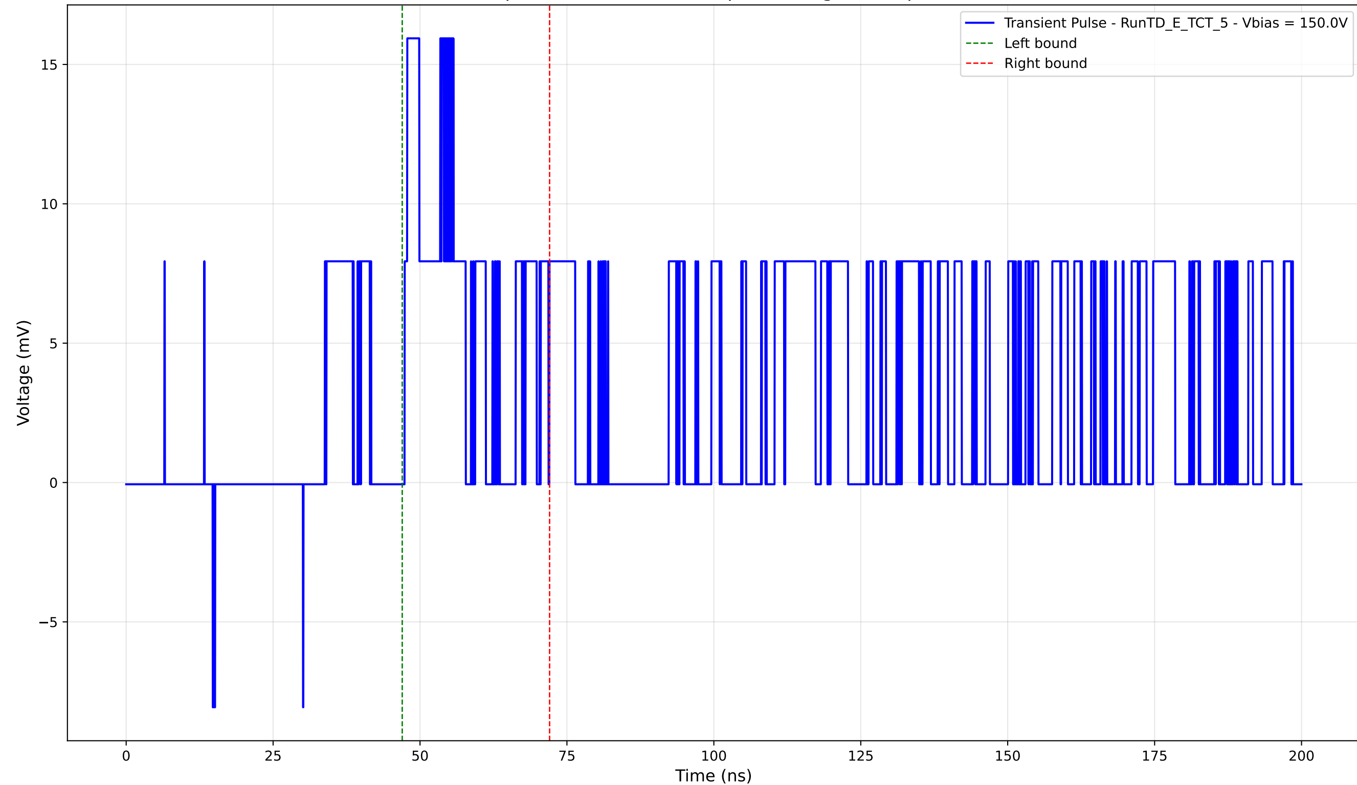
Transient Pulse - Sample: TD - Position: 10.0 \mu\text{m} - Charge: 3.31 pC - Rise Time: 0.46 ns
