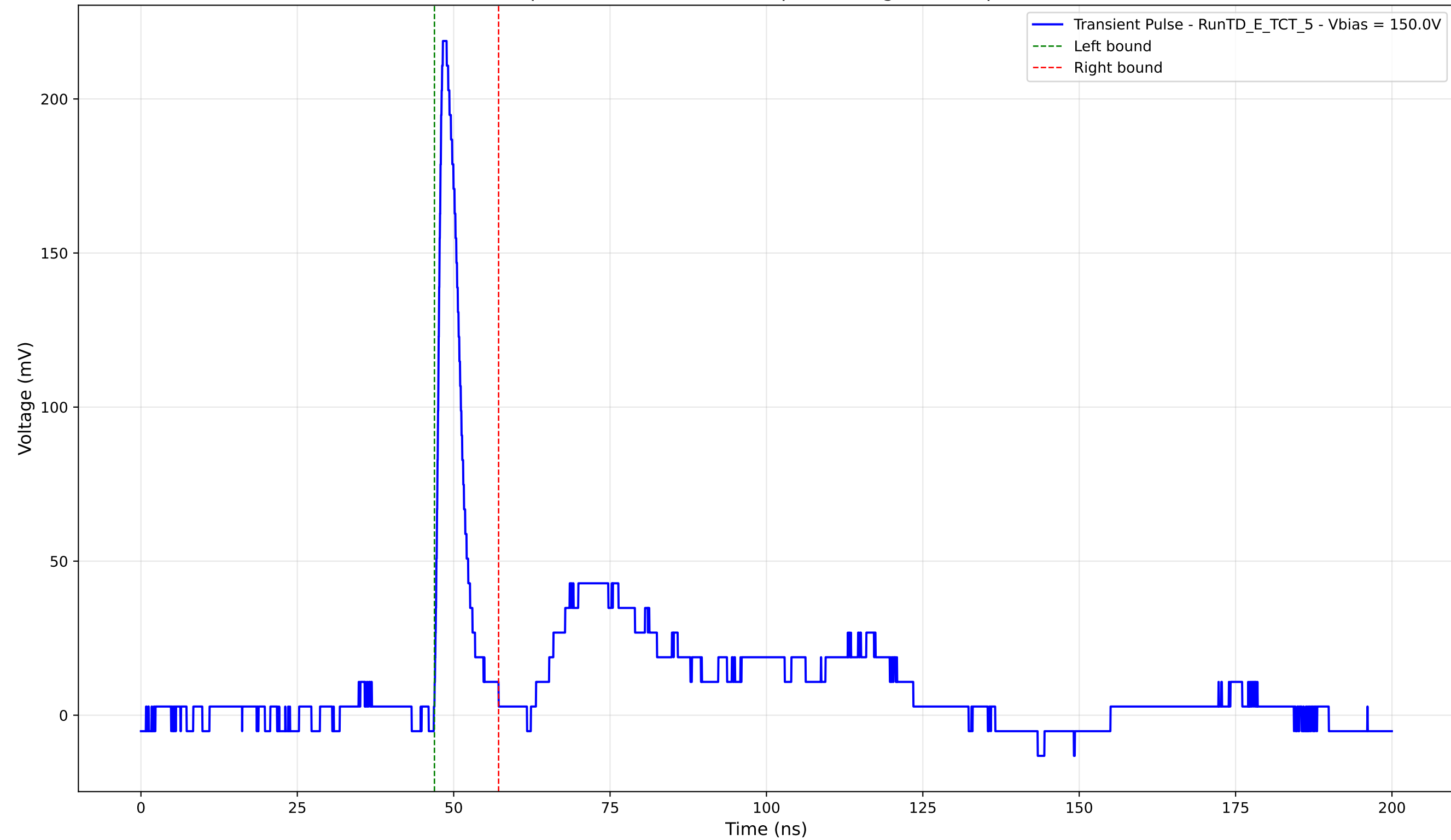
Transient Pulse - Sample: TD - Position: 210.0 \mu\text{m} - Charge: 16.73 pC - Rise Time: 0.99 ns
