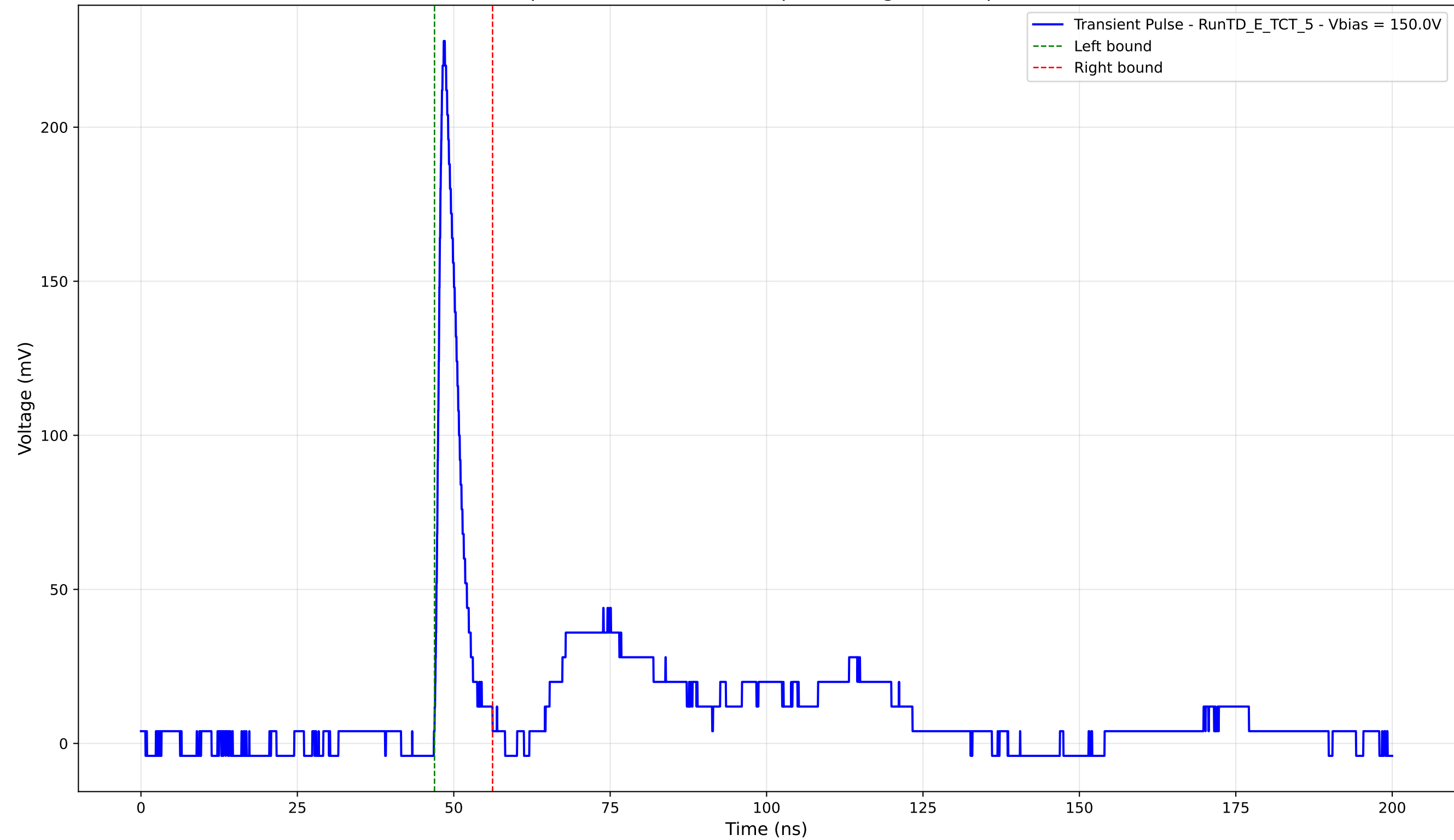
Transient Pulse - Sample: TD - Position: 220.0 \mu\text{m} - Charge: 15.48 pC - Rise Time: 1.03 ns
