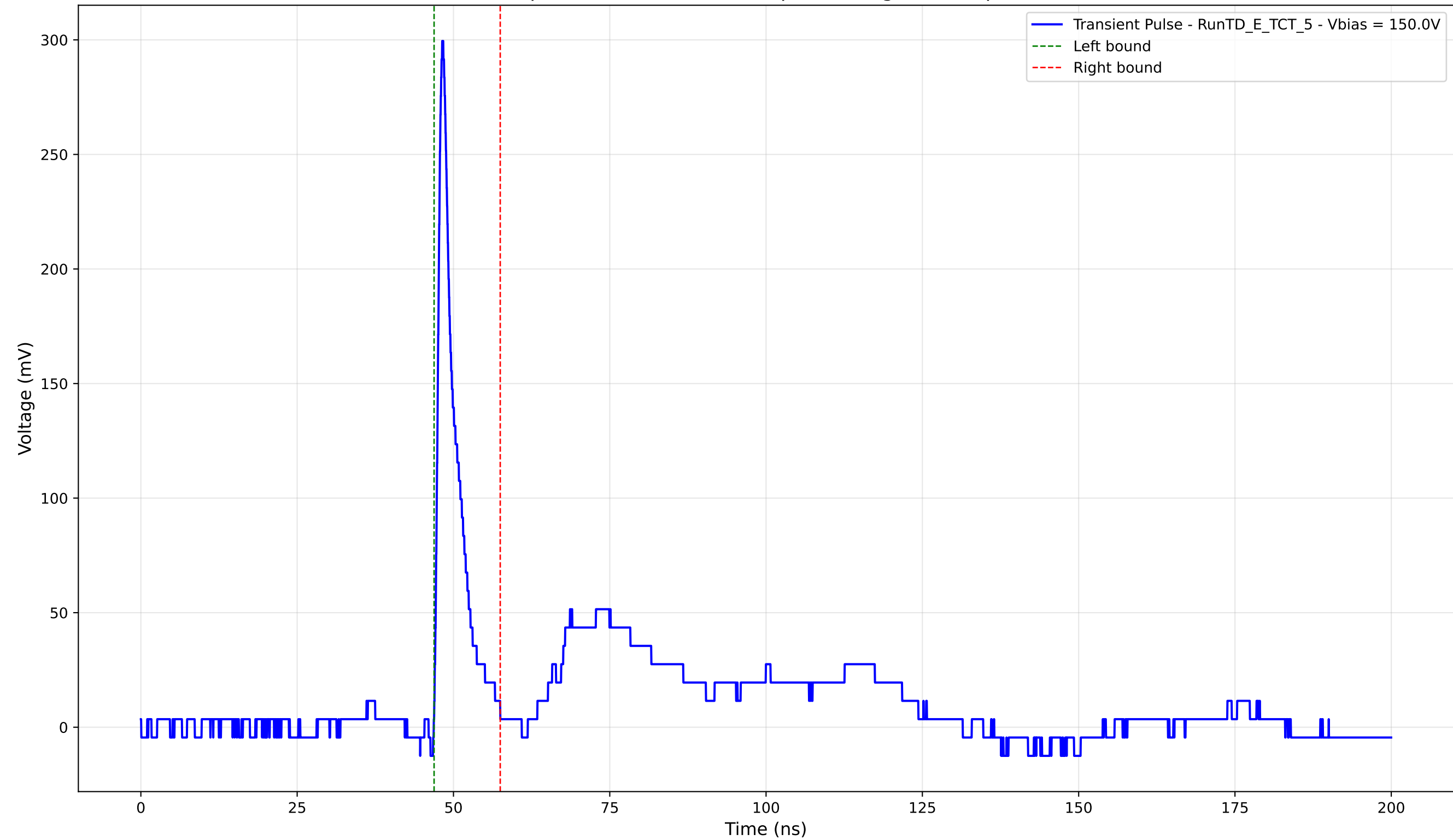
Transient Pulse - Sample: TD - Position: 140.0 \mu\text{m} - Charge: 19.34 pC - Rise Time: 0.89 ns
