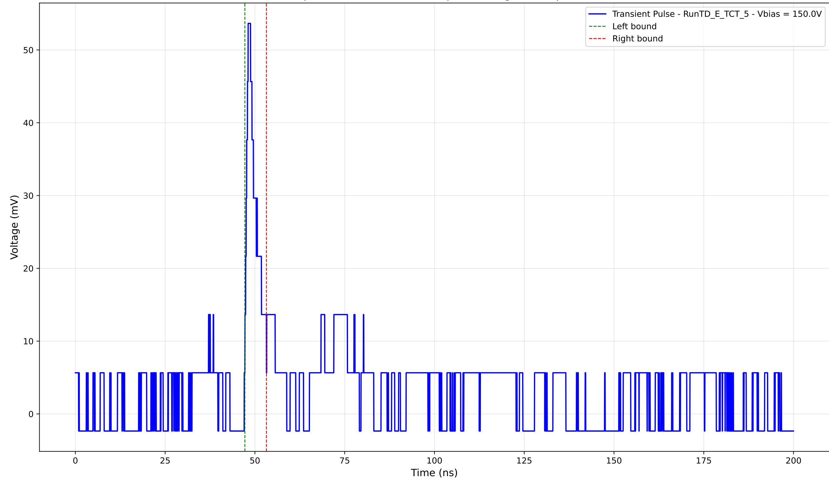
Transient Pulse - Sample: TD - Position: 400.0 \mu\text{m} - Charge: 3.43 pC - Rise Time: 1.08 ns
