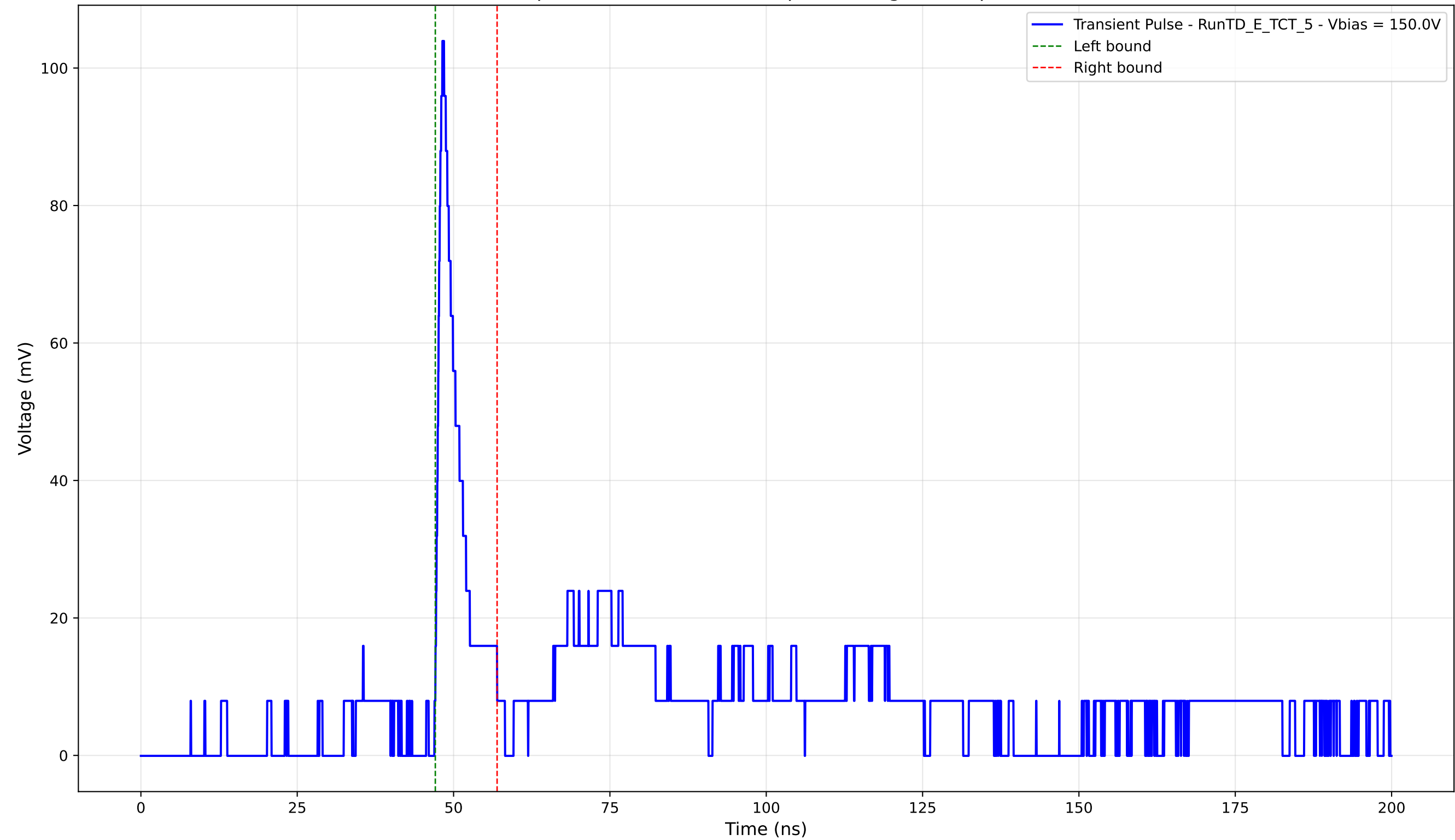
Transient Pulse - Sample: TD - Position: 340.0 \mu\text{m} - Charge: 7.66 pC - Rise Time: 0.93 ns
