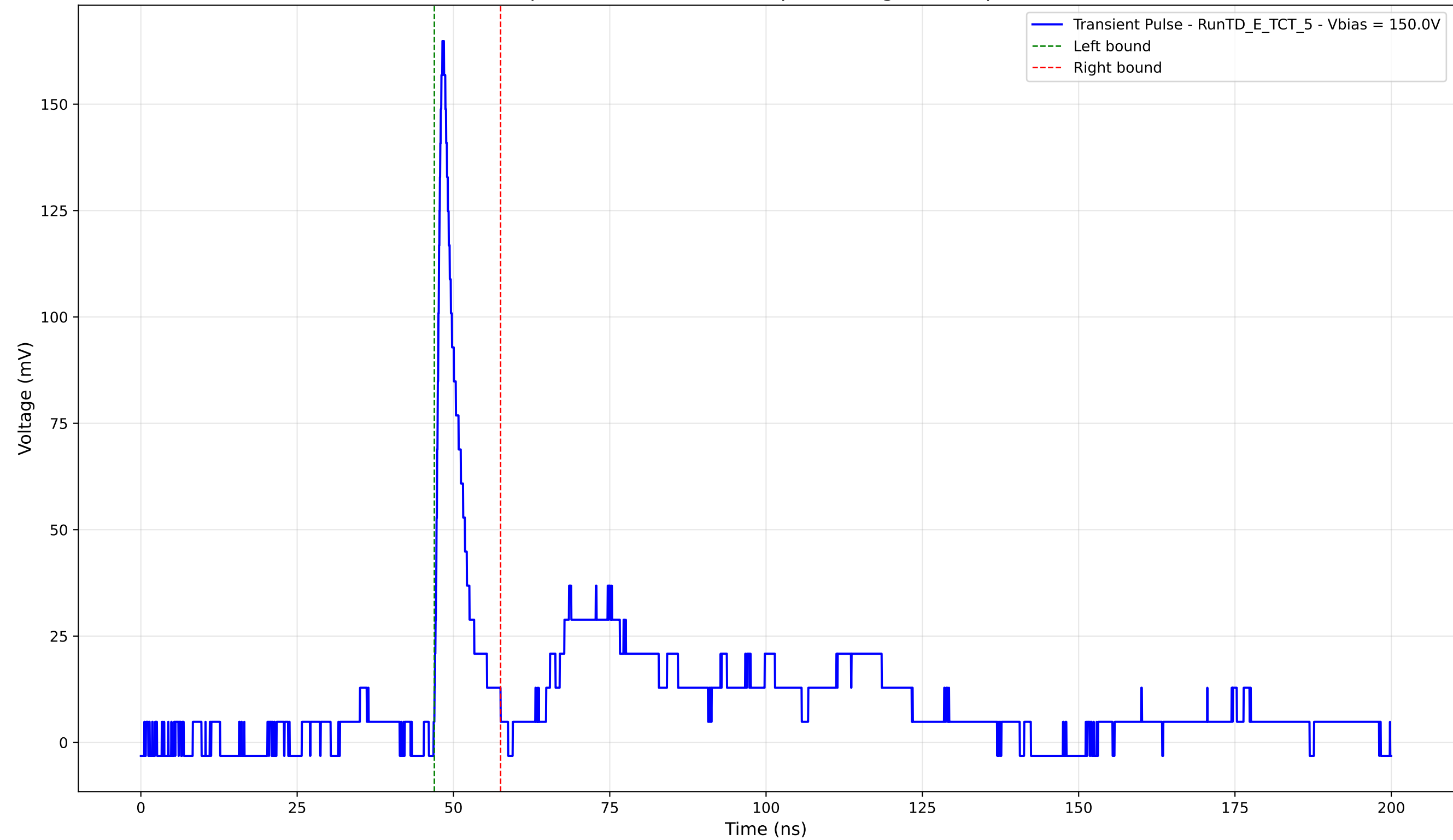
Transient Pulse - Sample: TD - Position: 235.0 \mu\text{m} - Charge: 11.90 pC - Rise Time: 0.93 ns
