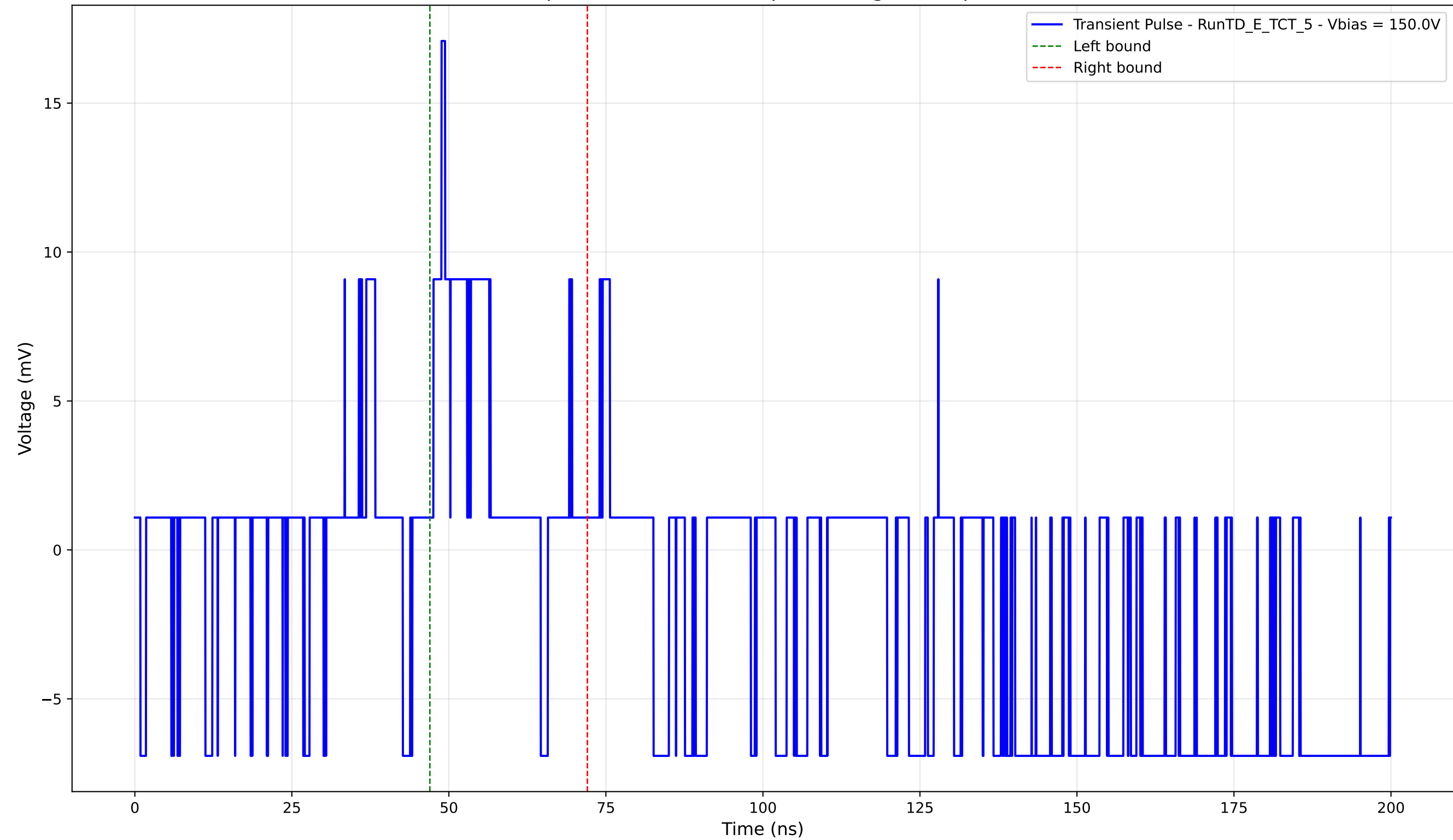
Transient Pulse - Sample: TD - Position: 0.0 \mu\text{m} - Charge: 1.89 pC - Rise Time: 1.30 ns
