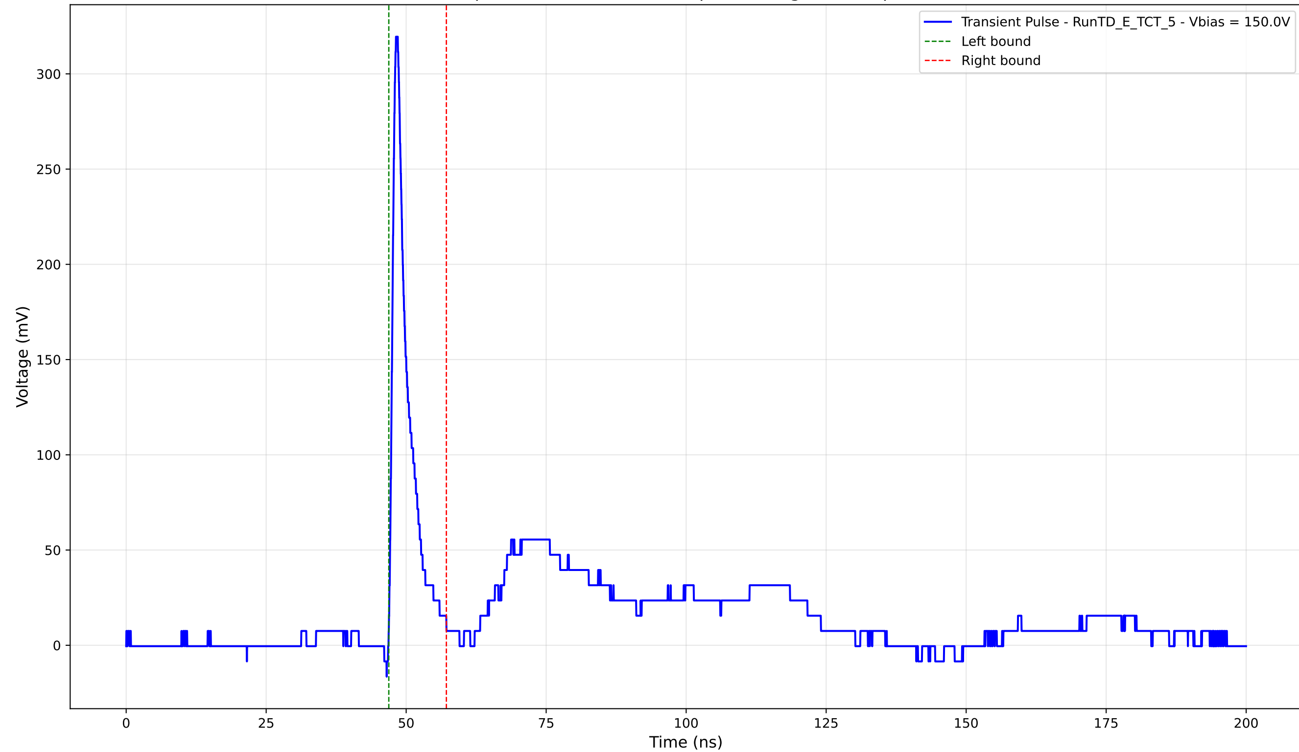
Transient Pulse - Sample: TD - Position: 130.0 \mu\text{m} - Charge: 20.71 pC - Rise Time: 0.92 ns
