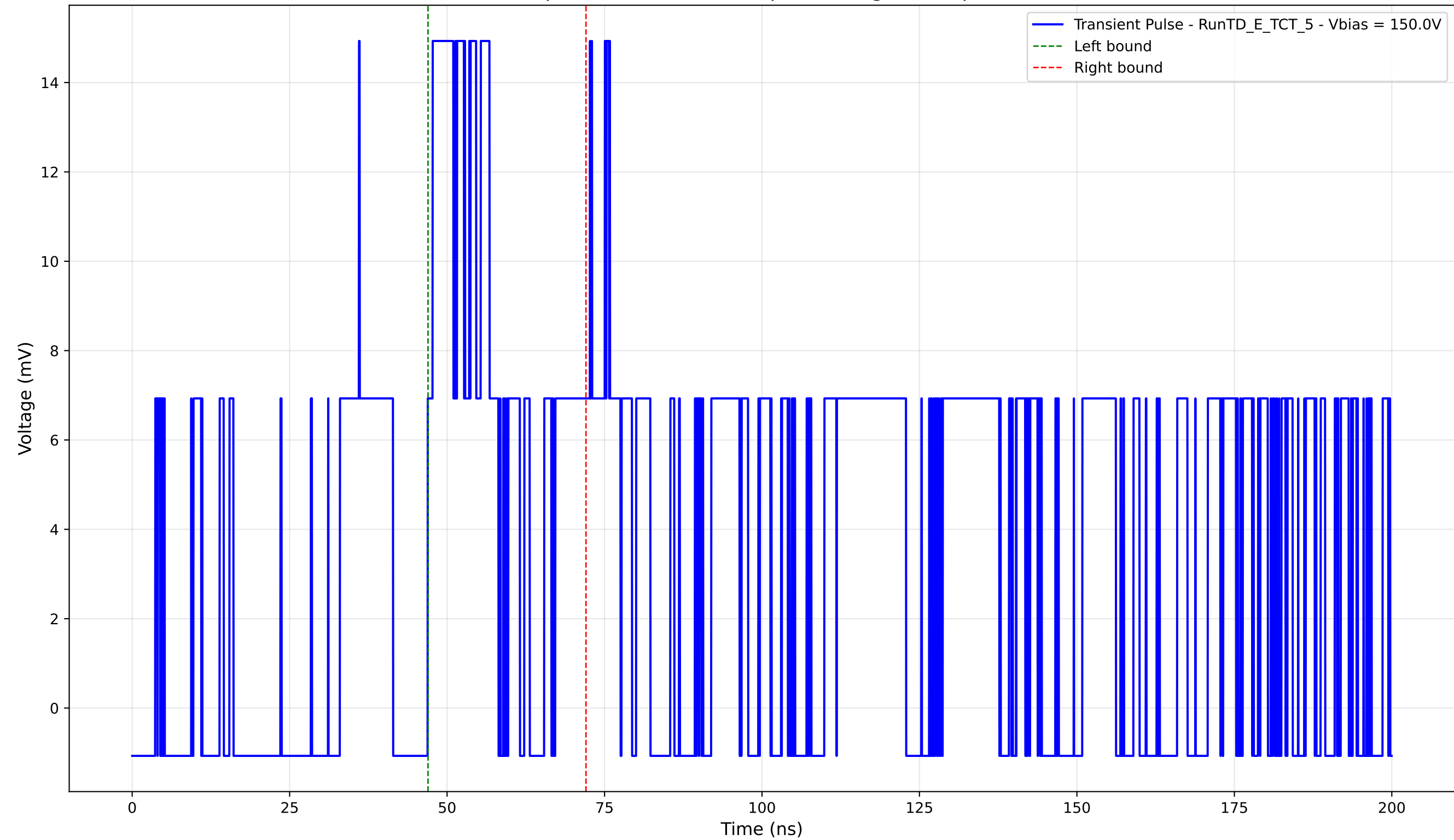
Transient Pulse - Sample: TD - Position: 5.0 \mu\text{m} - Charge: 3.83 pC - Rise Time: 3.04 ns
