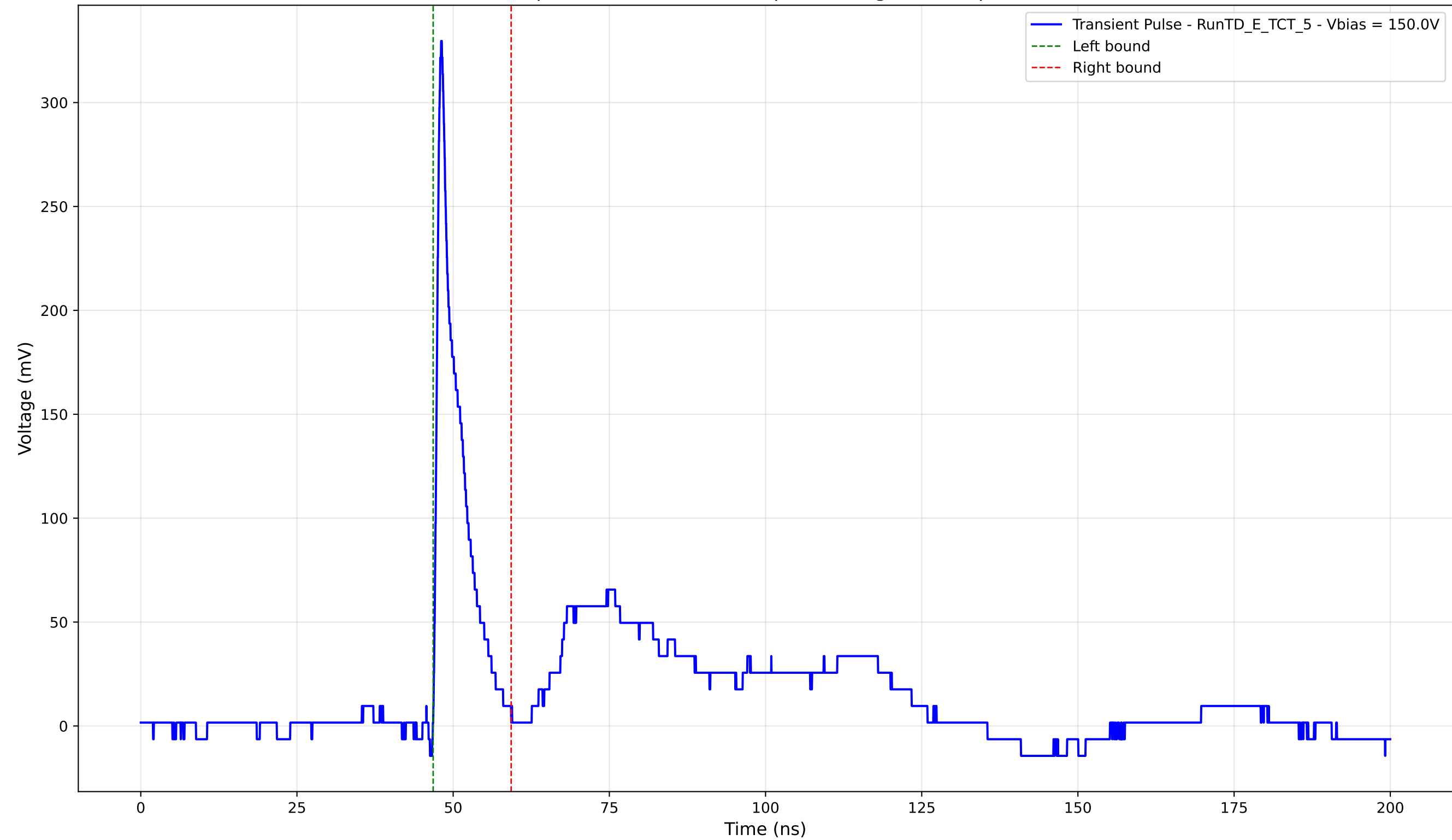
Transient Pulse - Sample: TD - Position: 75.0 \mu\text{m} - Charge: 25.82 pC - Rise Time: 0.84 ns
