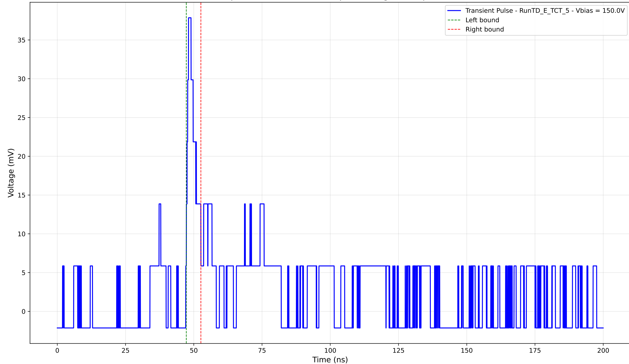
Transient Pulse - Sample: TD - Position: 415.0 \mu\text{m} - Charge: 2.48 pC - Rise Time: 1.01 ns
