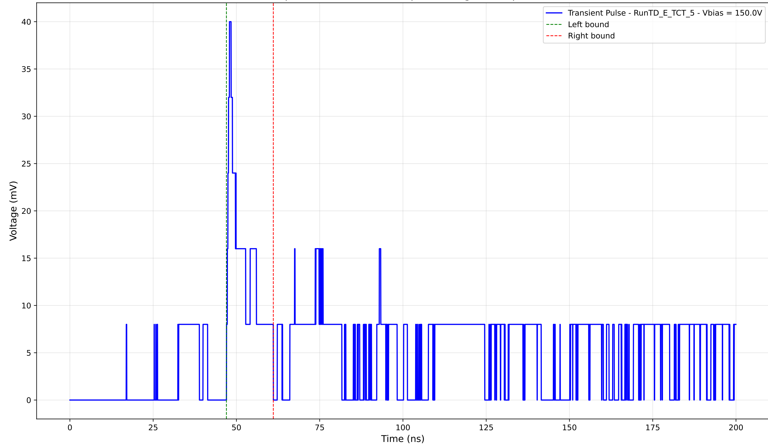
Transient Pulse - Sample: TD - Position: 25.0 \mu\text{m} - Charge: 4.07 pC - Rise Time: 0.89 ns
