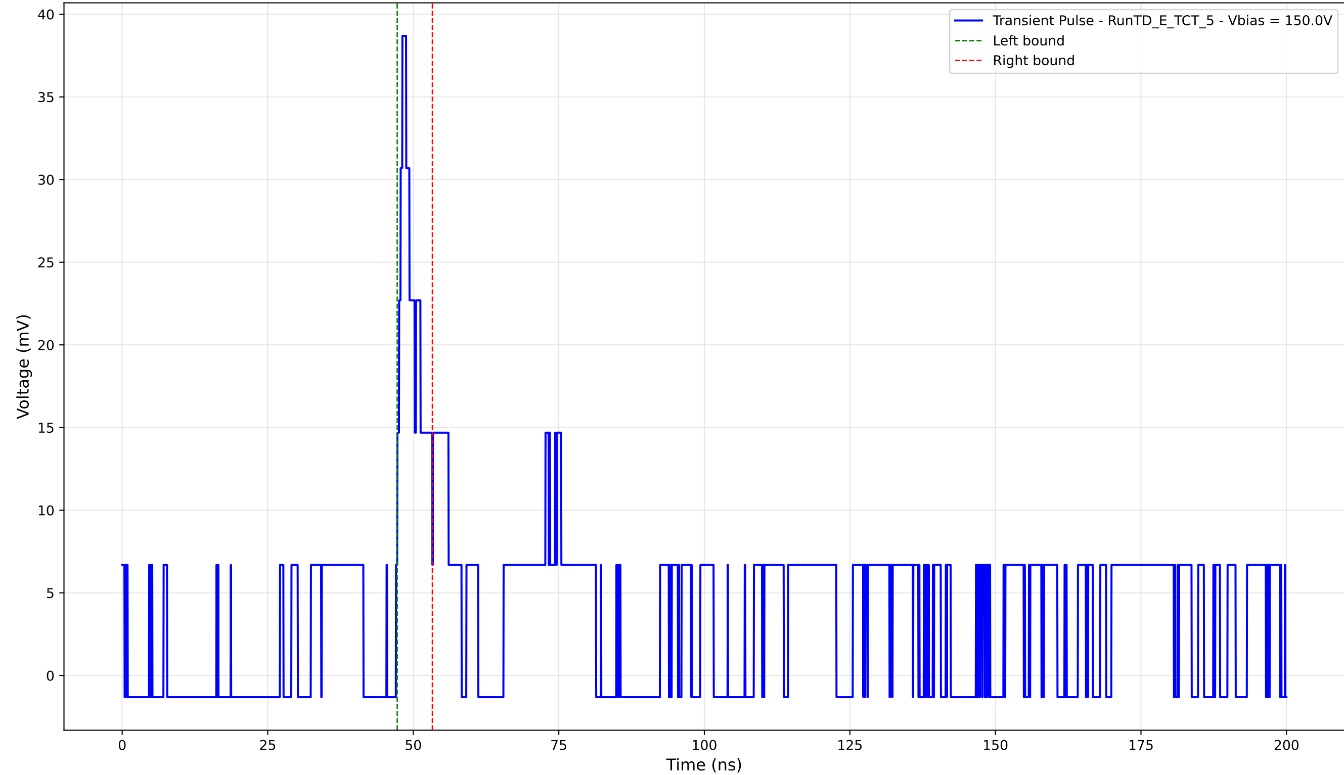
Transient Pulse - Sample: TD - Position: 350.0 \mu\text{m} - Charge: 2.67 pC - Rise Time: 1.11 ns
