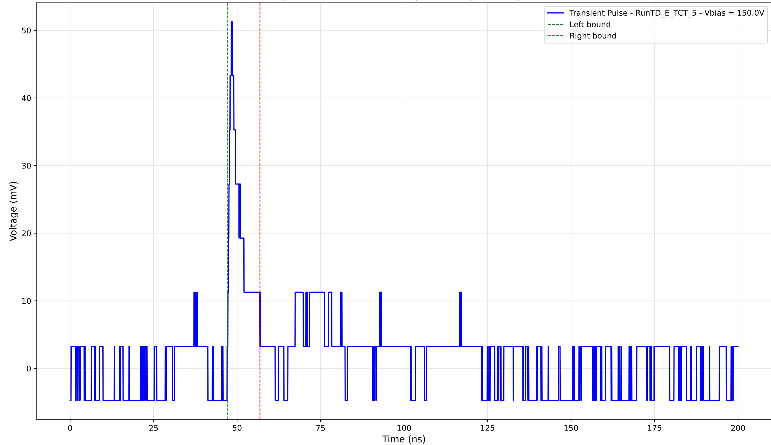
Transient Pulse - Sample: TD - Position: 405.0 \mu\text{m} - Charge: 3.97 pC - Rise Time: 1.02 ns
