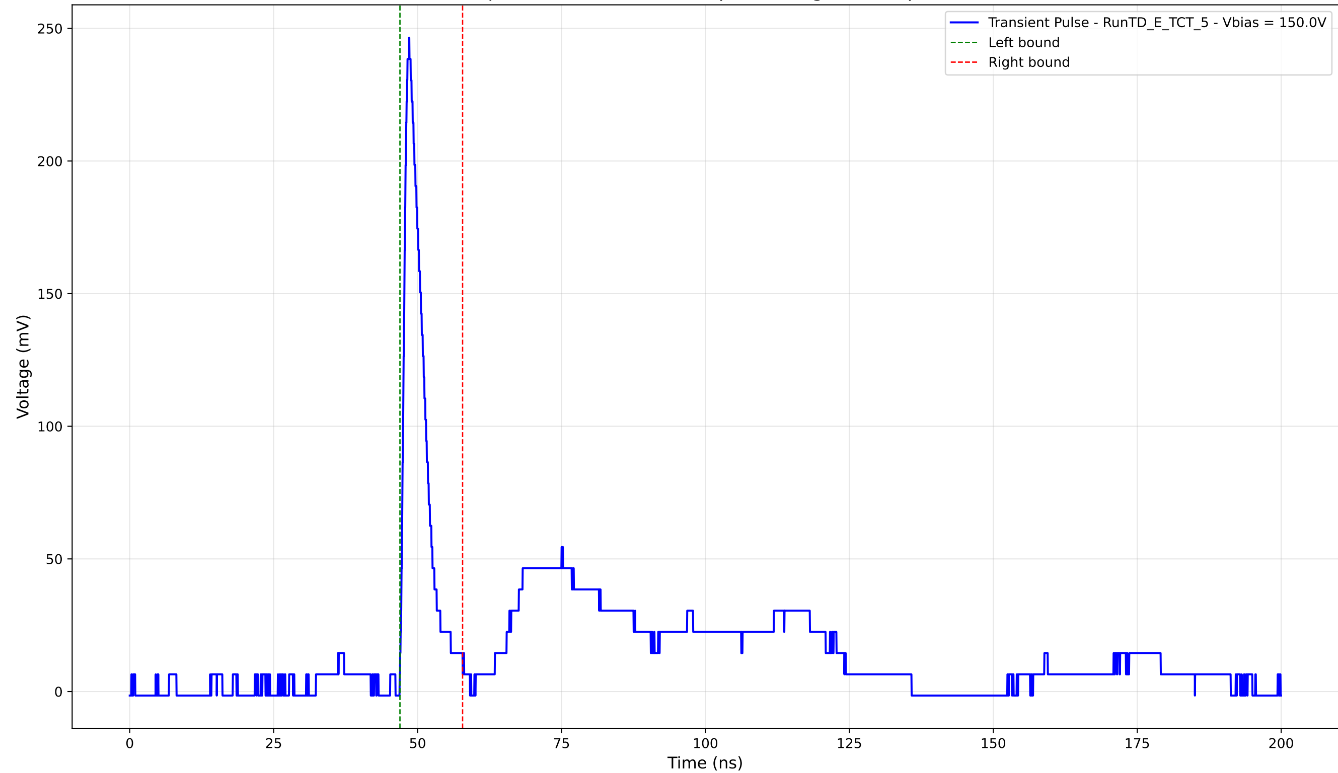
Transient Pulse - Sample: TD - Position: 190.0 \mu\text{m} - Charge: 18.89 pC - Rise Time: 0.97 ns
