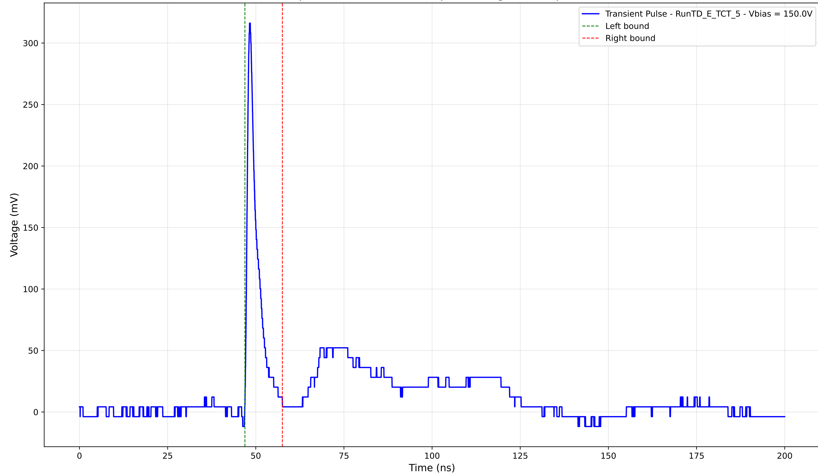
Transient Pulse - Sample: TD - Position: 170.0 \mu\text{m} - Charge: 20.58 pC - Rise Time: 0.93 ns
