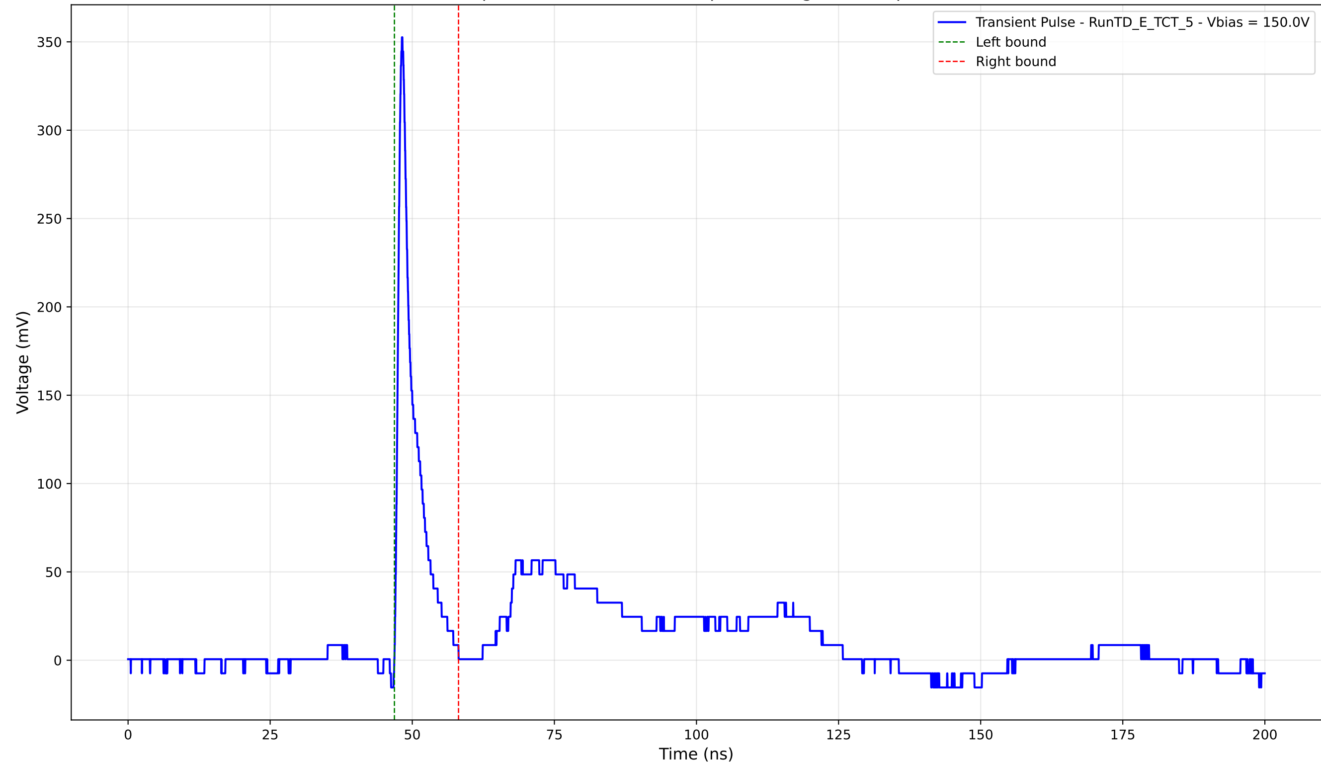
Transient Pulse - Sample: TD - Position: 105.0 \mu\text{m} - Charge: 22.67 pC - Rise Time: 0.87 ns
