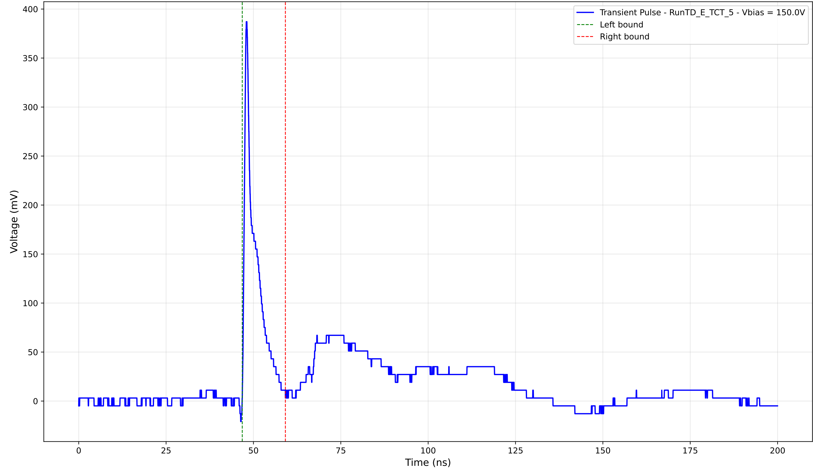
Transient Pulse - Sample: TD - Position: 60.0 \mu\text{m} - Charge: 27.33 pC - Rise Time: 0.81 ns
