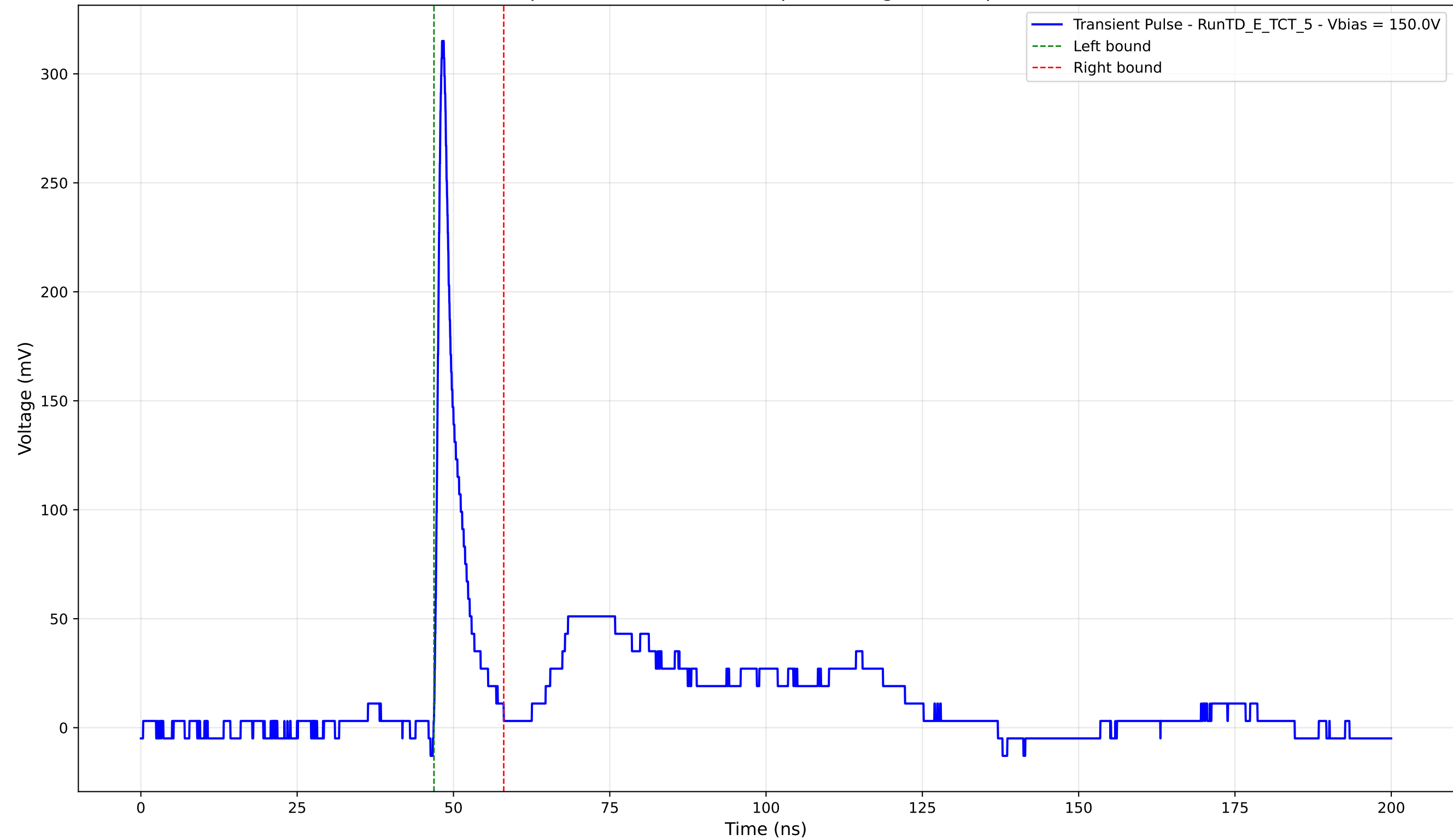
Transient Pulse - Sample: TD - Position: 125.0 \mu\text{m} - Charge: 20.62 pC - Rise Time: 0.93 ns
