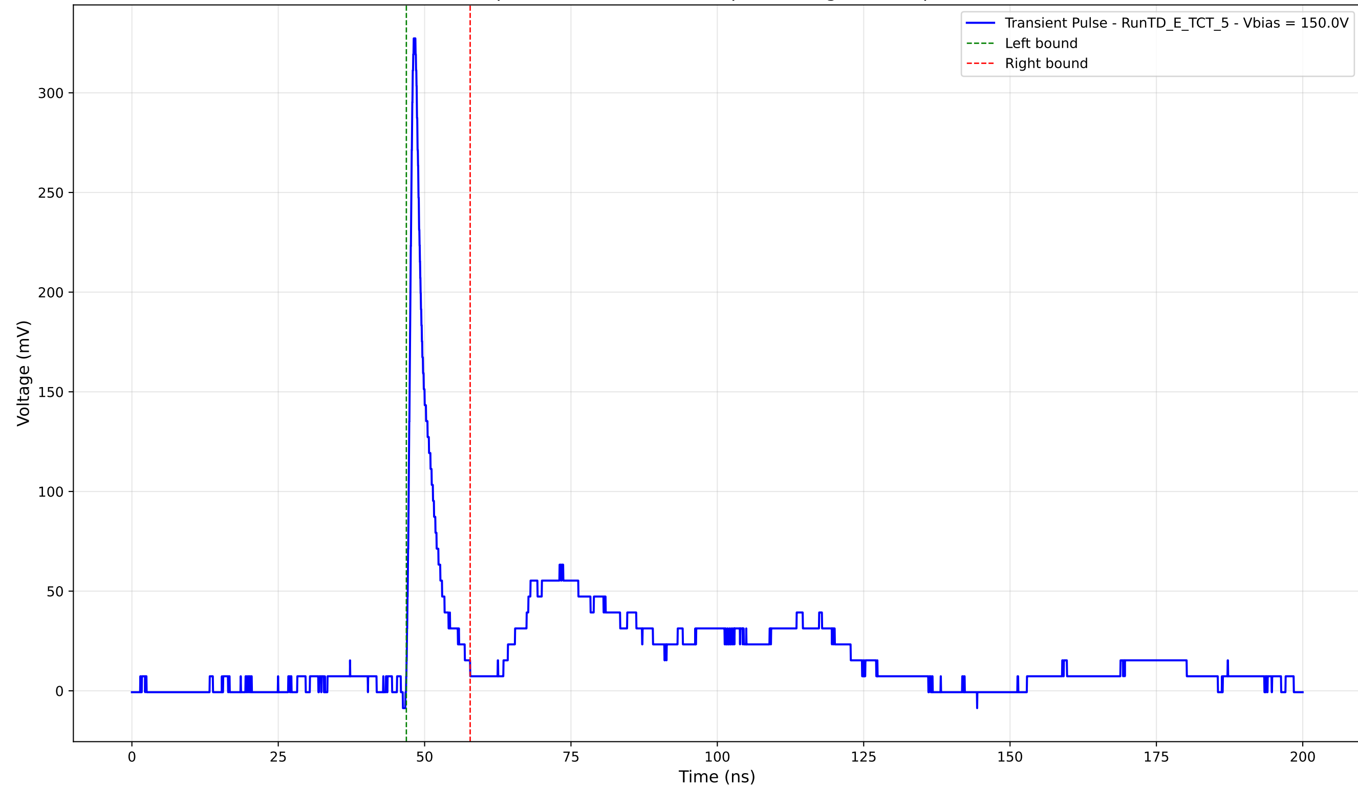
Transient Pulse - Sample: TD - Position: 120.0 \mu\text{m} - Charge: 21.81 pC - Rise Time: 0.88 ns
