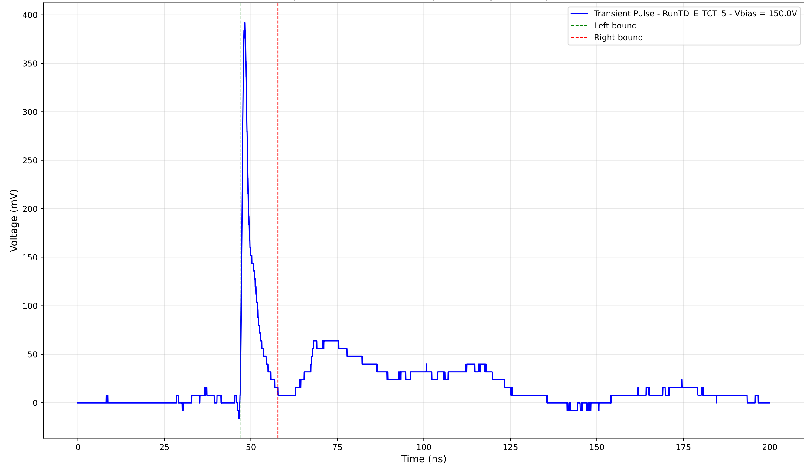
Transient Pulse - Sample: TD - Position: 110.0 \mu\text{m} - Charge: 24.76 pC - Rise Time: 0.88 ns
