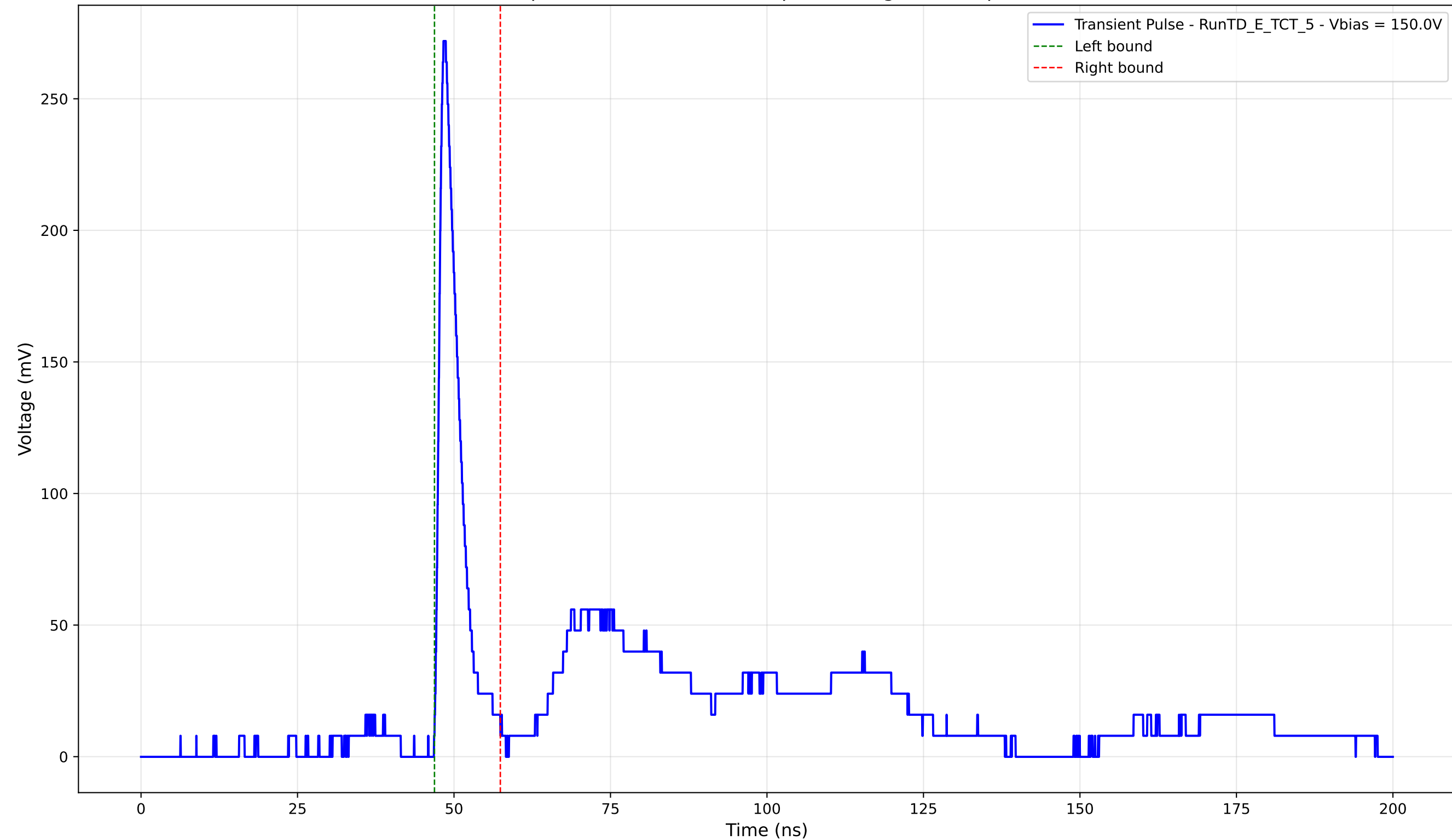
Transient Pulse - Sample: TD - Position: 185.0 \mu\text{m} - Charge: 20.20 pC - Rise Time: 1.01 ns
