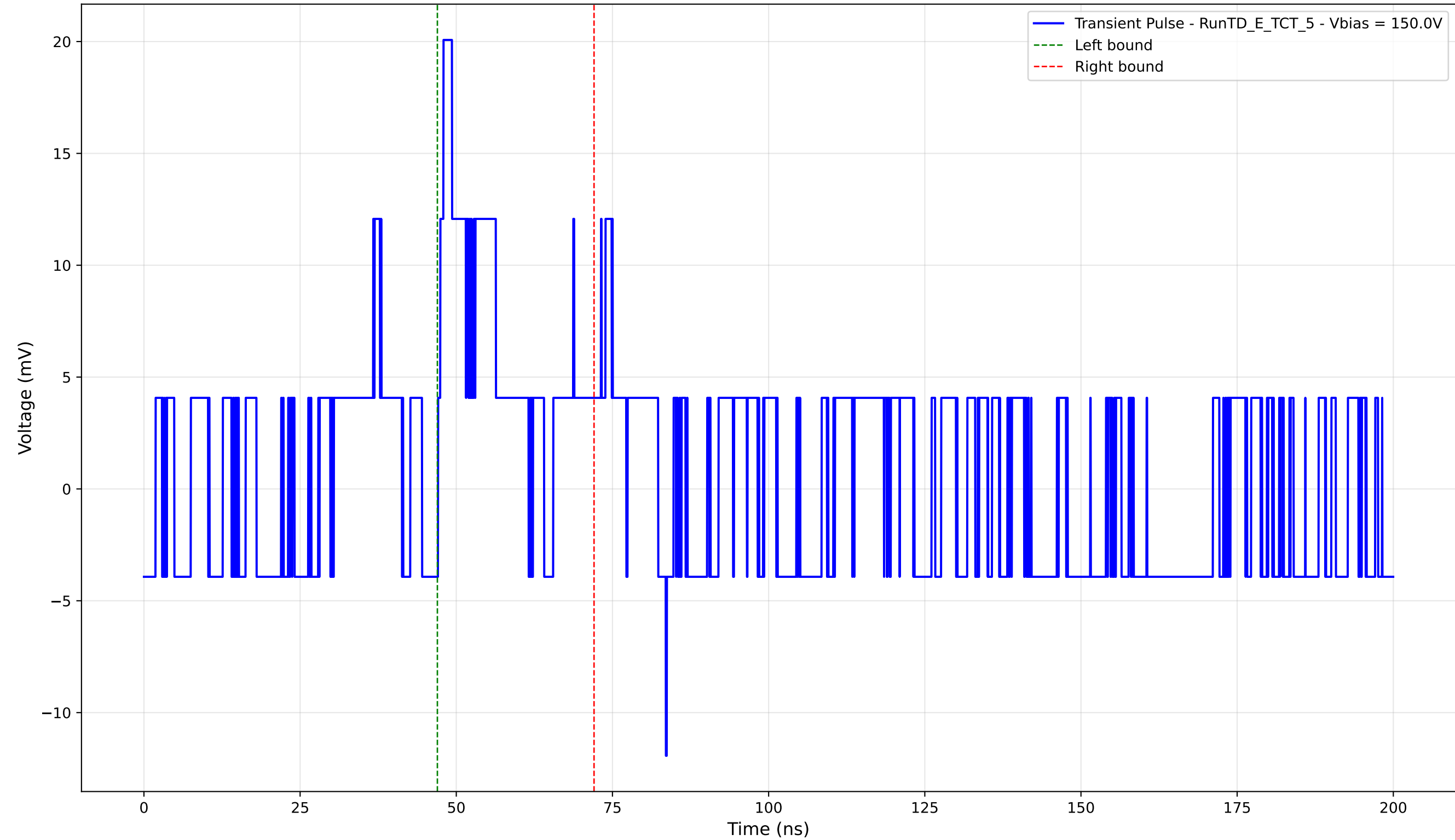
Transient Pulse - Sample: TD - Position: 360.0 \mu\text{m} - Charge: 3.26 pC - Rise Time: 0.00 ns (N/A)
