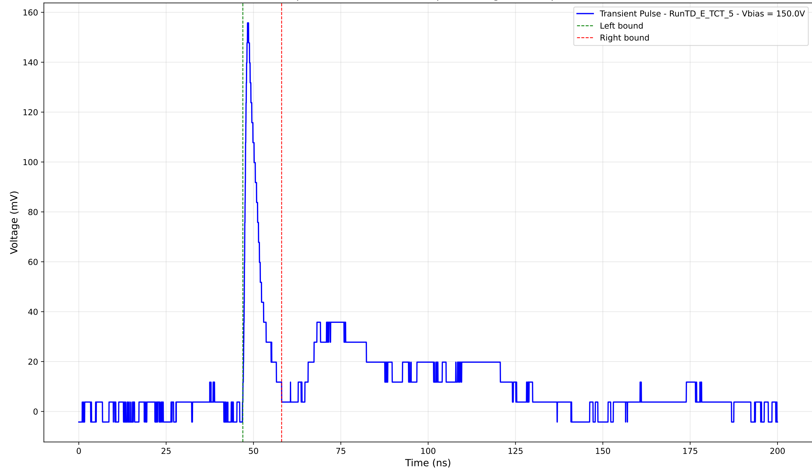
Transient Pulse - Sample: TD - Position: 155.0 \mu\text{m} - Charge: 13.18 pC - Rise Time: 1.05 ns
