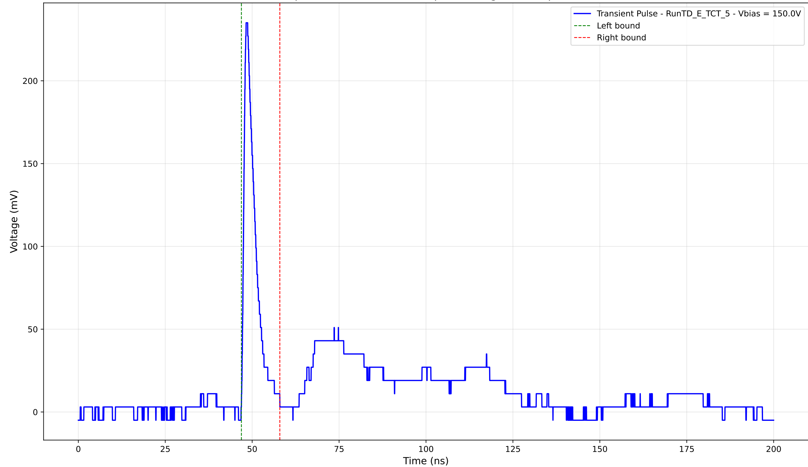
Transient Pulse - Sample: TD - Position: 180.0 \mu\text{m} - Charge: 17.66 pC - Rise Time: 0.99 ns
