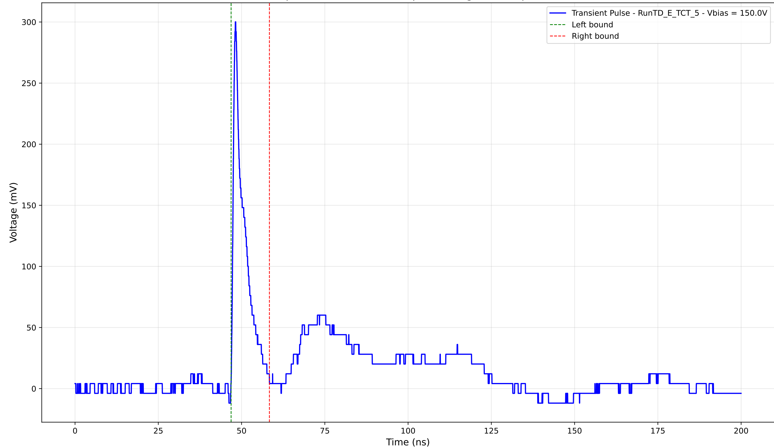
Transient Pulse - Sample: TD - Position: 80.0 \mu\text{m} - Charge: 22.79 pC - Rise Time: 0.90 ns
