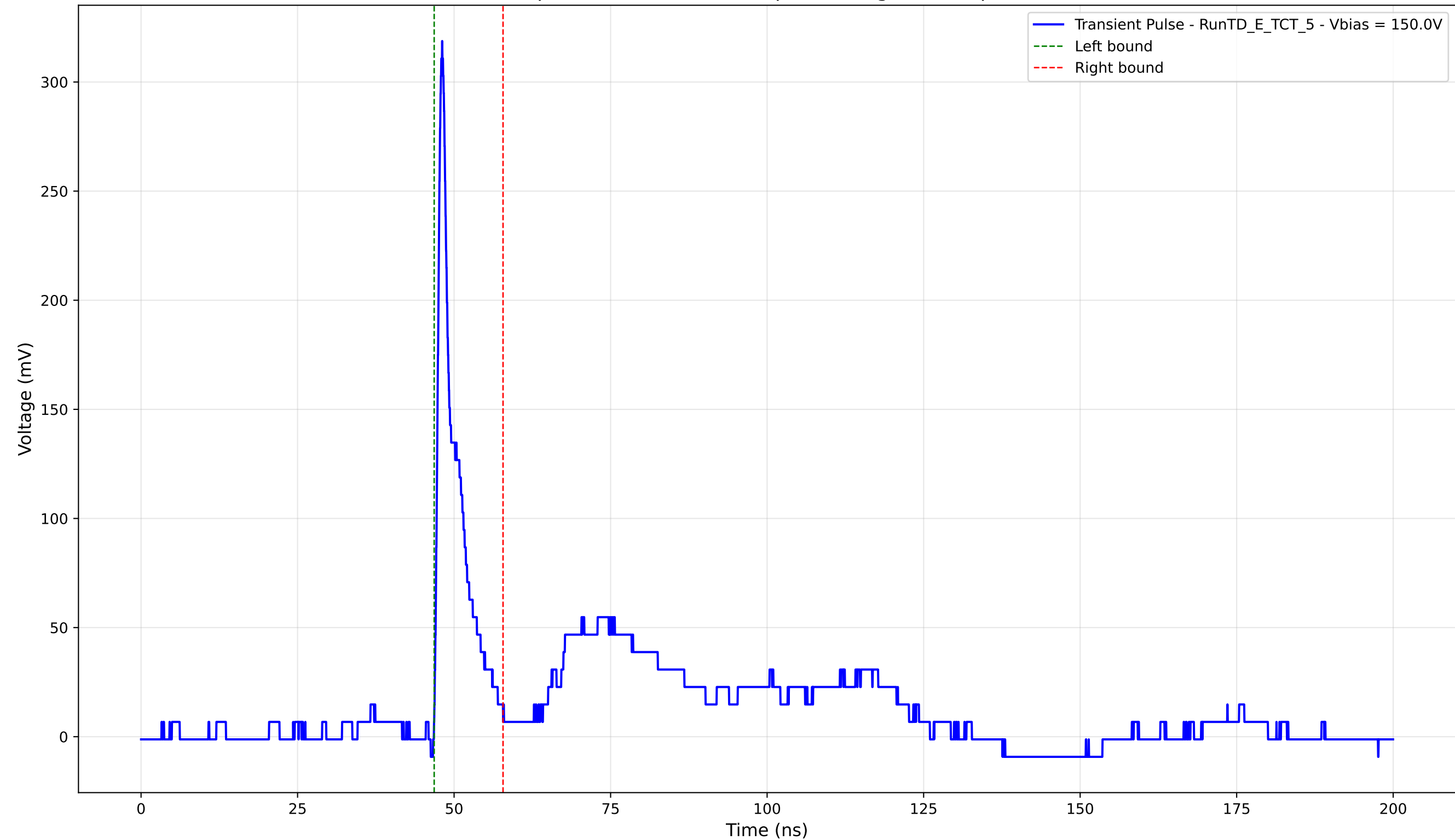
Transient Pulse - Sample: TD - Position: 40.0 \mu\text{m} - Charge: 21.03 pC - Rise Time: 0.88 ns
