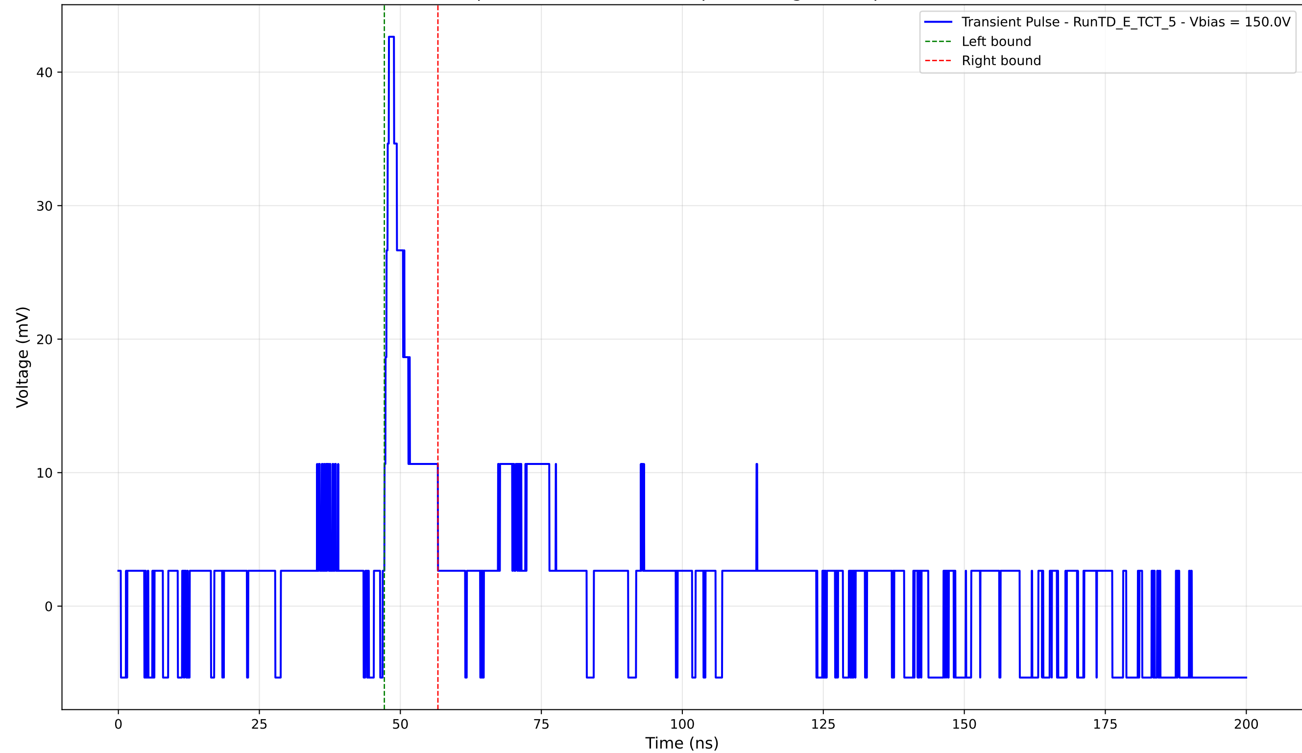
Transient Pulse - Sample: TD - Position: 410.0 \mu\text{m} - Charge: 3.57 pC - Rise Time: 0.80 ns
