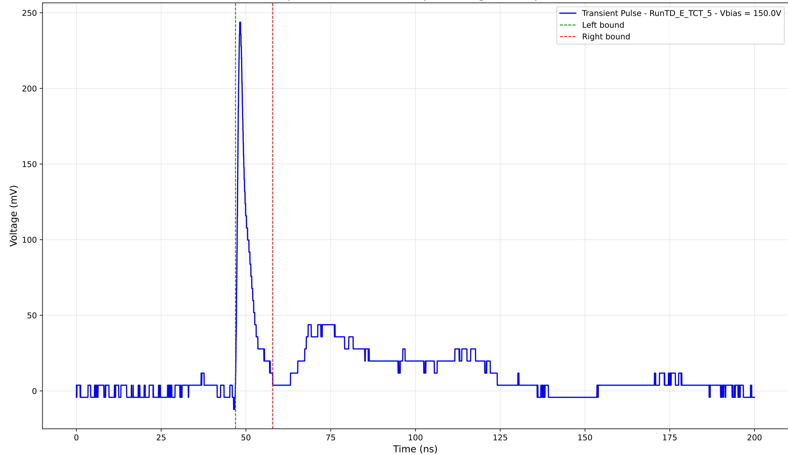
Transient Pulse - Sample: TD - Position: 145.0 \mu\text{m} - Charge: 16.78 pC - Rise Time: 0.89 ns
