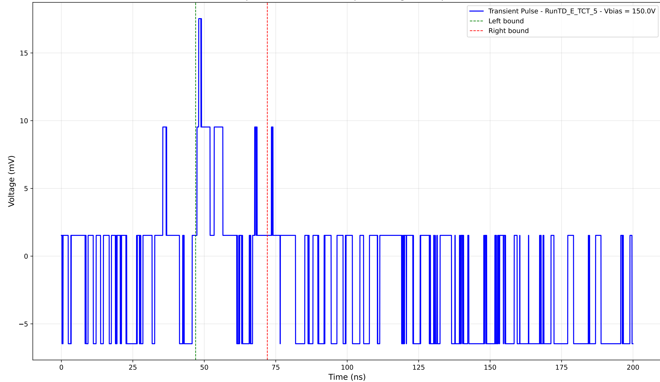
Transient Pulse - Sample: TD - Position: 15.0 \mu\text{m} - Charge: 1.59 pC - Rise Time: 0.62 ns
