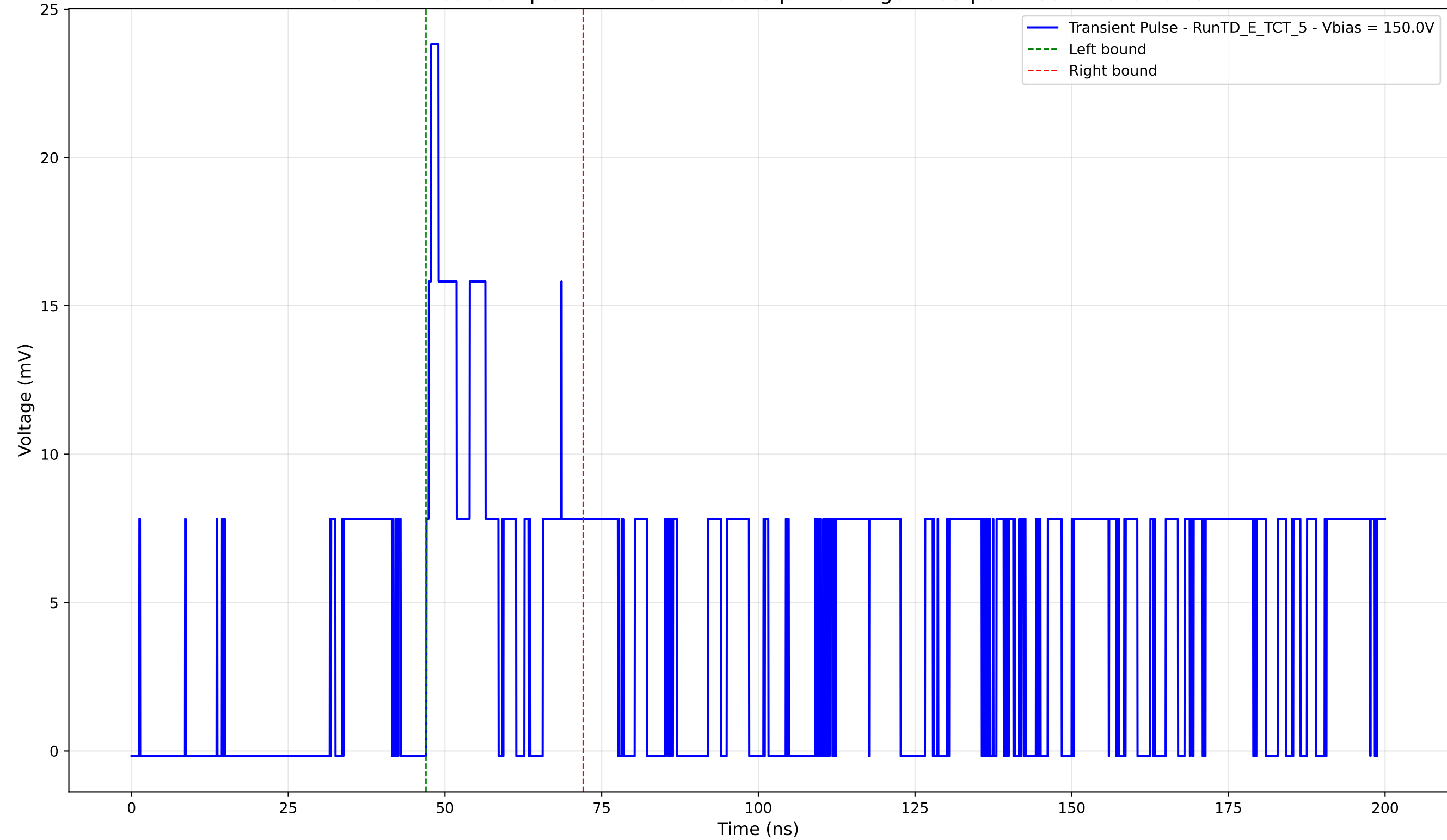
Transient Pulse - Sample: TD - Position: 355.0 \mu\text{m} - Charge: 4.55 pC - Rise Time: 0.73 ns
