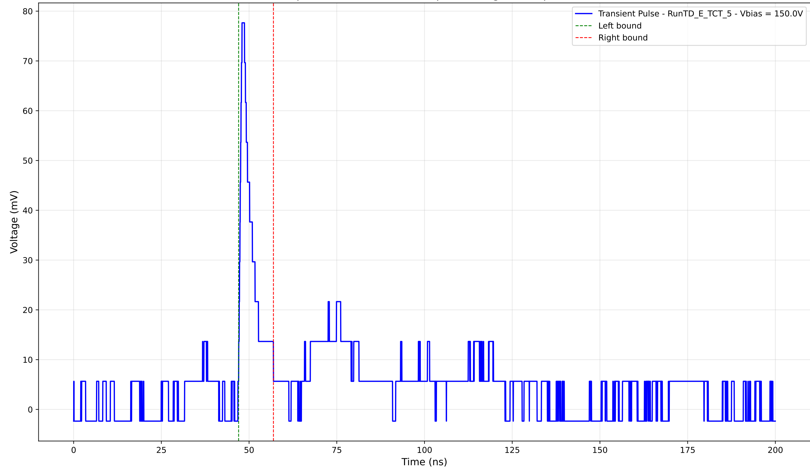
Transient Pulse - Sample: TD - Position: 380.0 \mu\text{m} - Charge: 6.14 pC - Rise Time: 0.95 ns
