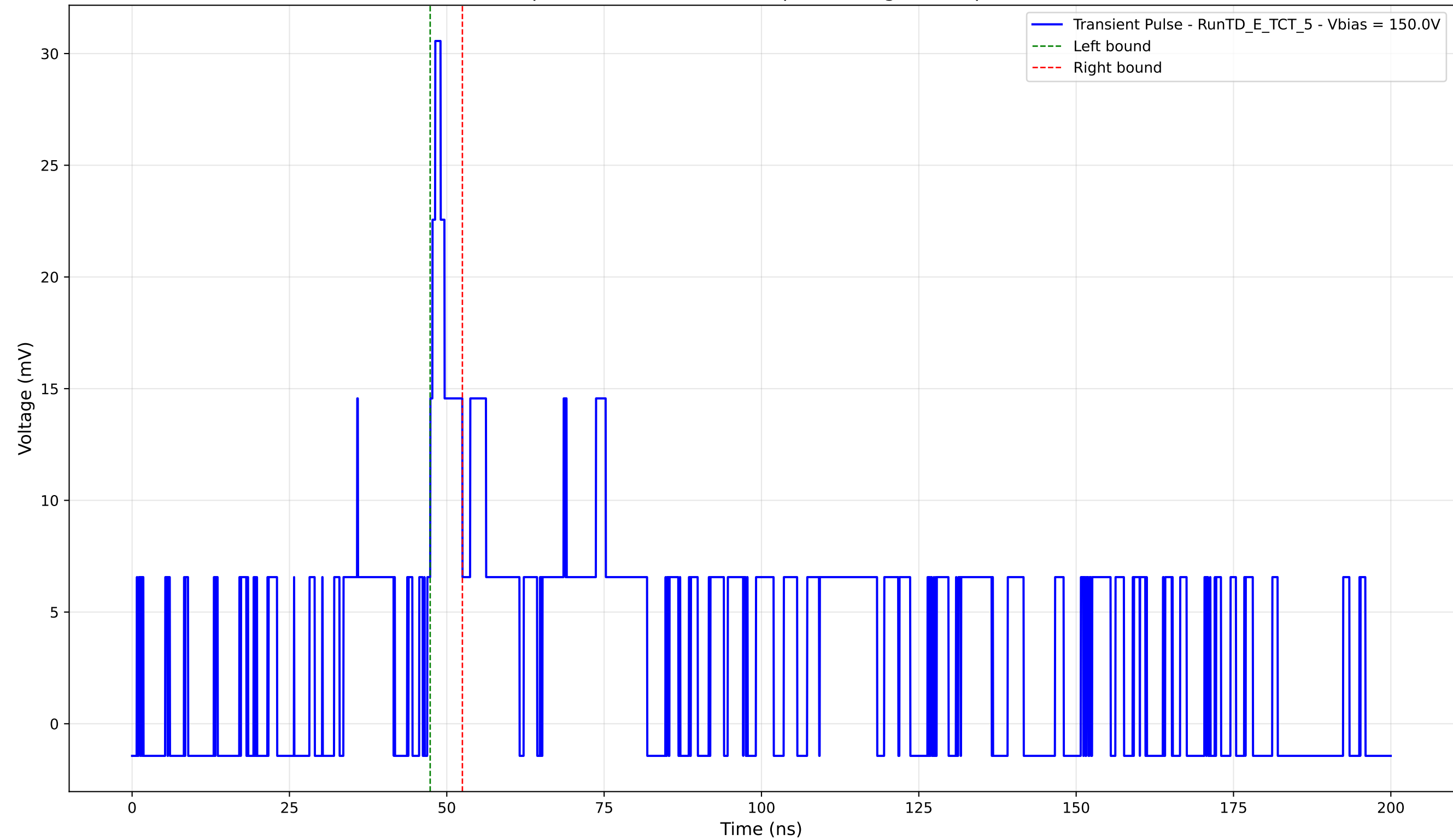
Transient Pulse - Sample: TD - Position: 365.0 \mu\text{m} - Charge: 1.93 pC - Rise Time: 1.27 ns
