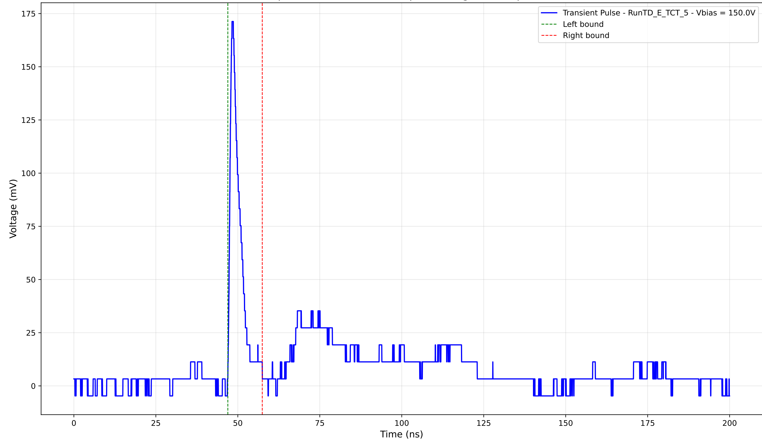
Transient Pulse - Sample: TD - Position: 275.0 \mu\text{m} - Charge: 11.79 pC - Rise Time: 0.95 ns
