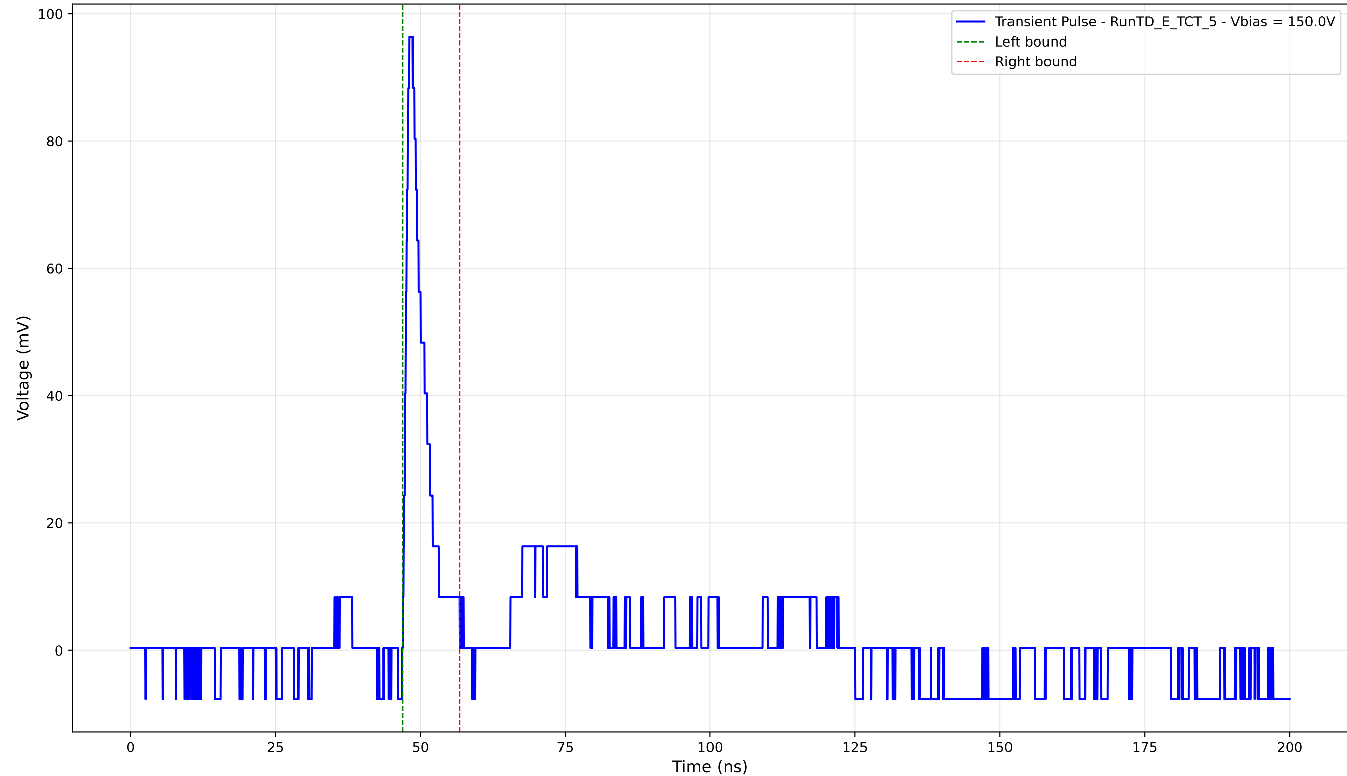
Transient Pulse - Sample: TD - Position: 335.0 \mu\text{m} - Charge: 6.64 pC - Rise Time: 0.84 ns
