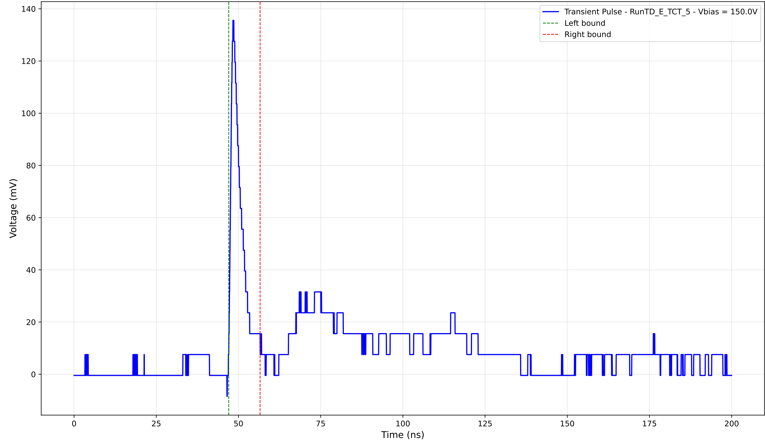
Transient Pulse - Sample: TD - Position: 245.0 \mu\text{m} - Charge: 9.94 pC - Rise Time: 1.06 ns
