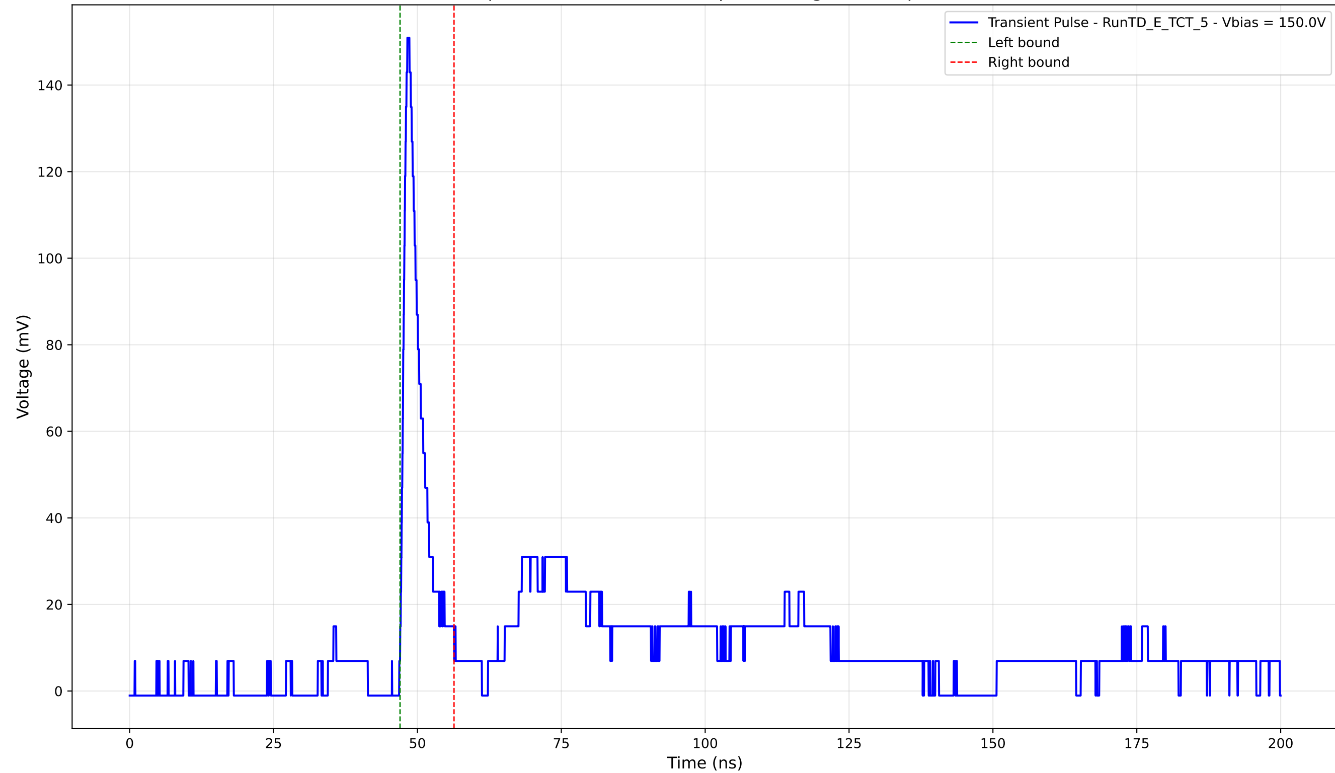
Transient Pulse - Sample: TD - Position: 255.0 \mu\text{m} - Charge: 10.56 pC - Rise Time: 1.02 ns
