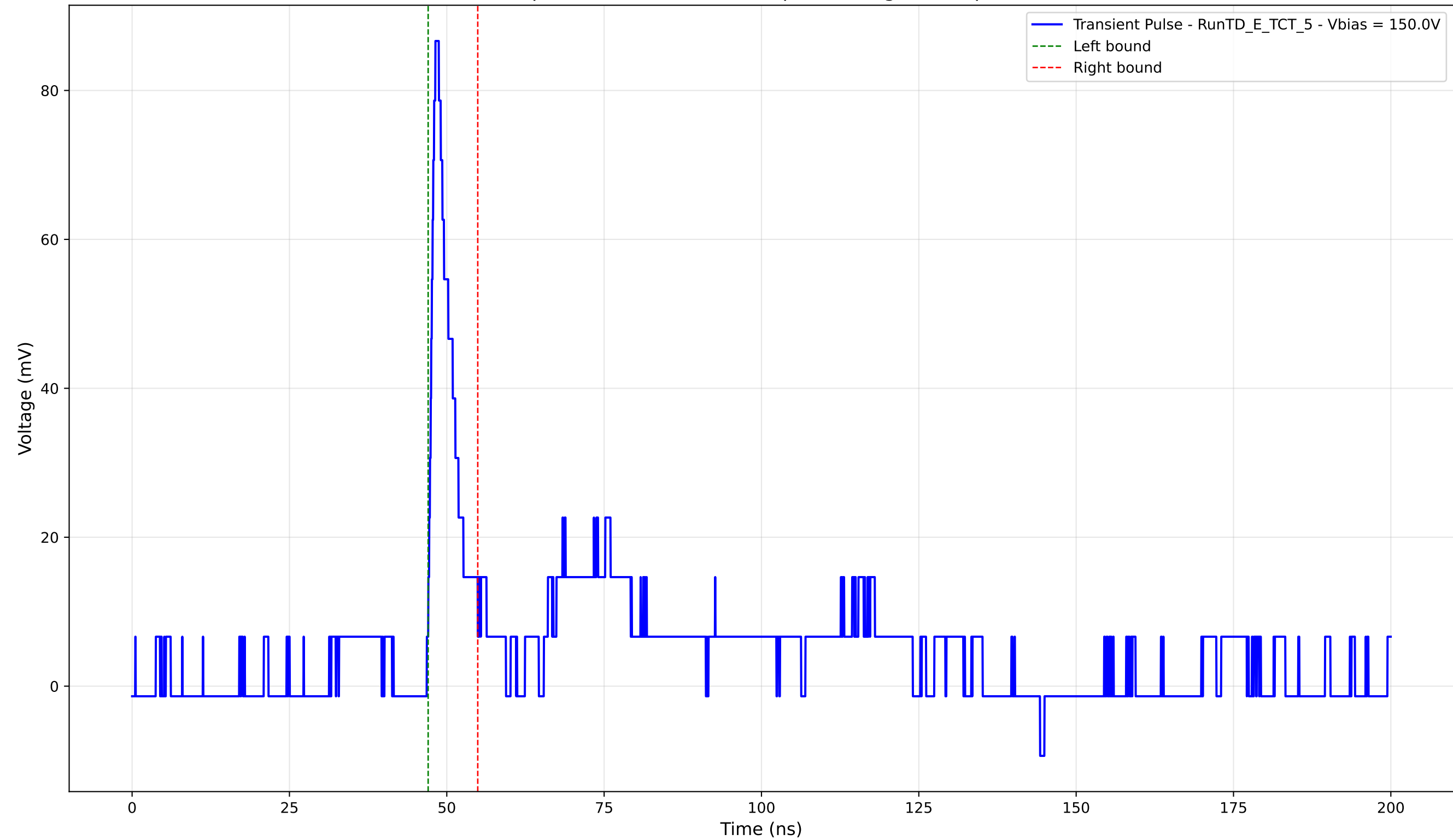
Transient Pulse - Sample: TD - Position: 305.0 \mu\text{m} - Charge: 6.28 pC - Rise Time: 0.93 ns
