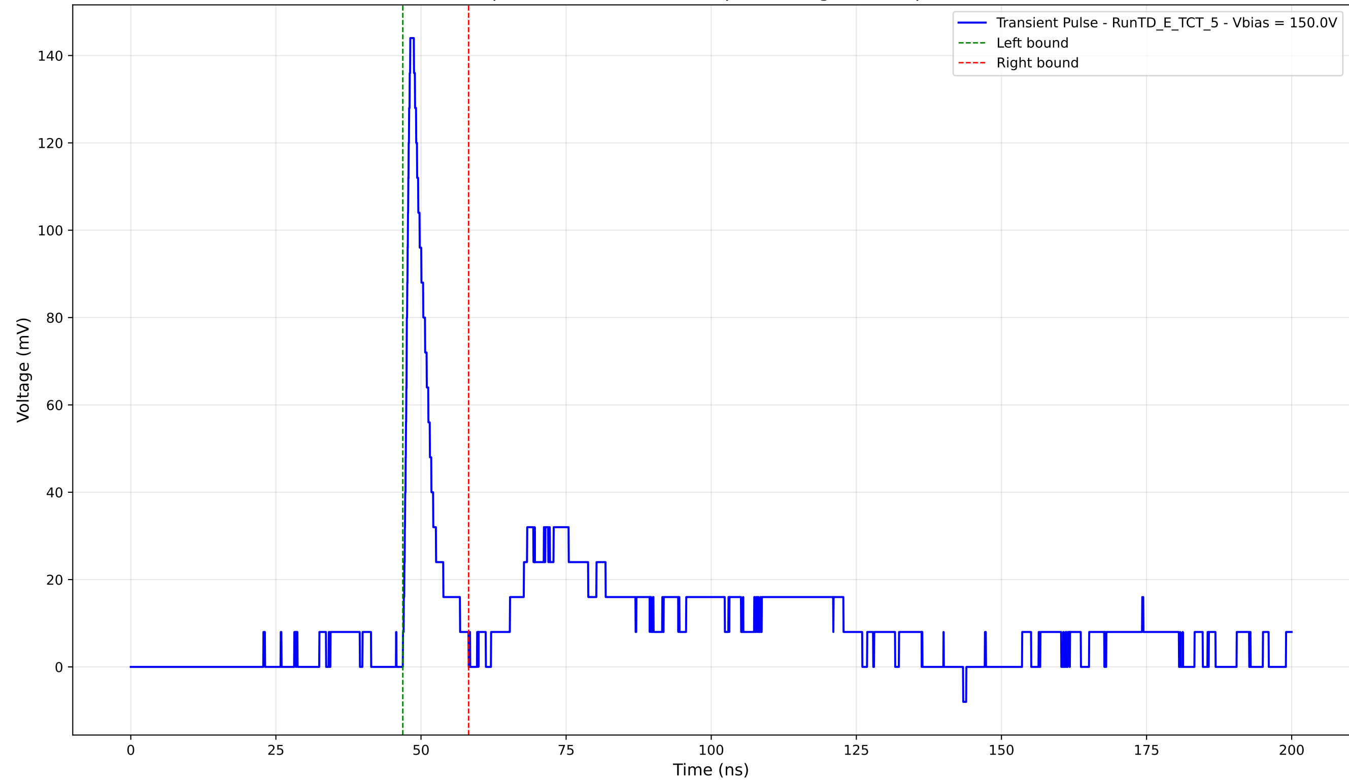
Transient Pulse - Sample: TD - Position: 280.0 \mu\text{m} - Charge: 11.21 pC - Rise Time: 1.02 ns
