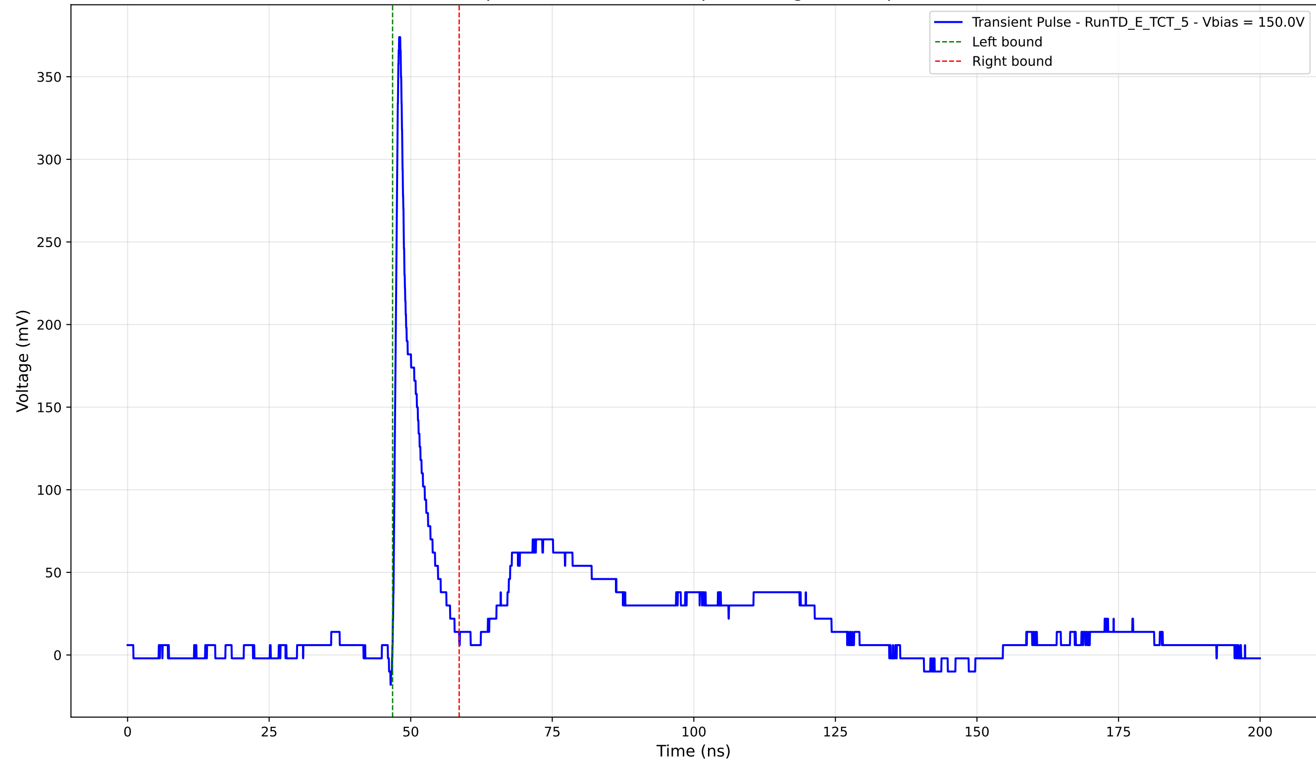
Transient Pulse - Sample: TD - Position: 65.0 \mu\text{m} - Charge: 27.39 pC - Rise Time: 0.81 ns
