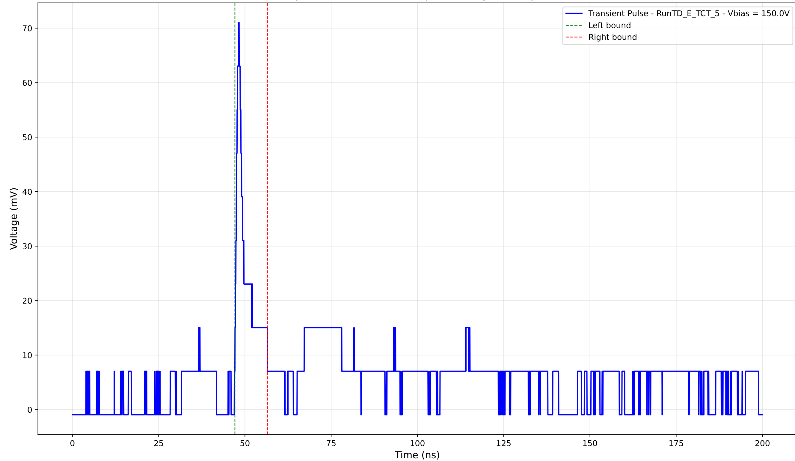
Transient Pulse - Sample: TD - Position: 30.0 \mu\text{m} - Charge: 4.82 pC - Rise Time: 1.10 ns
