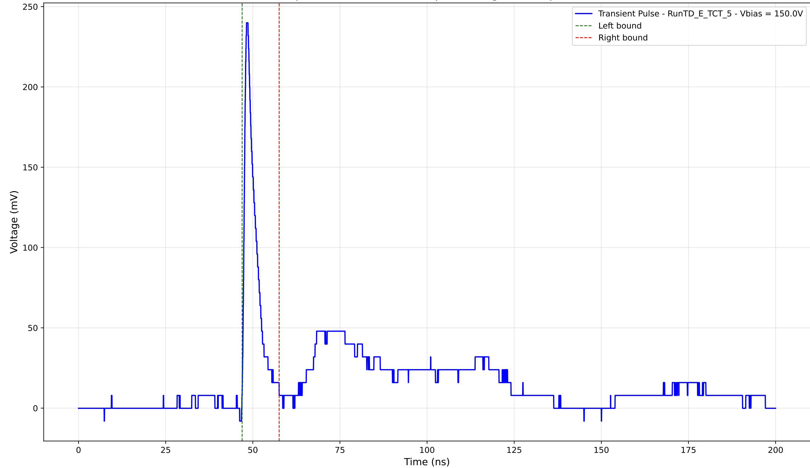
Transient Pulse - Sample: TD - Position: 175.0 \mu\text{m} - Charge: 17.86 pC - Rise Time: 0.96 ns
