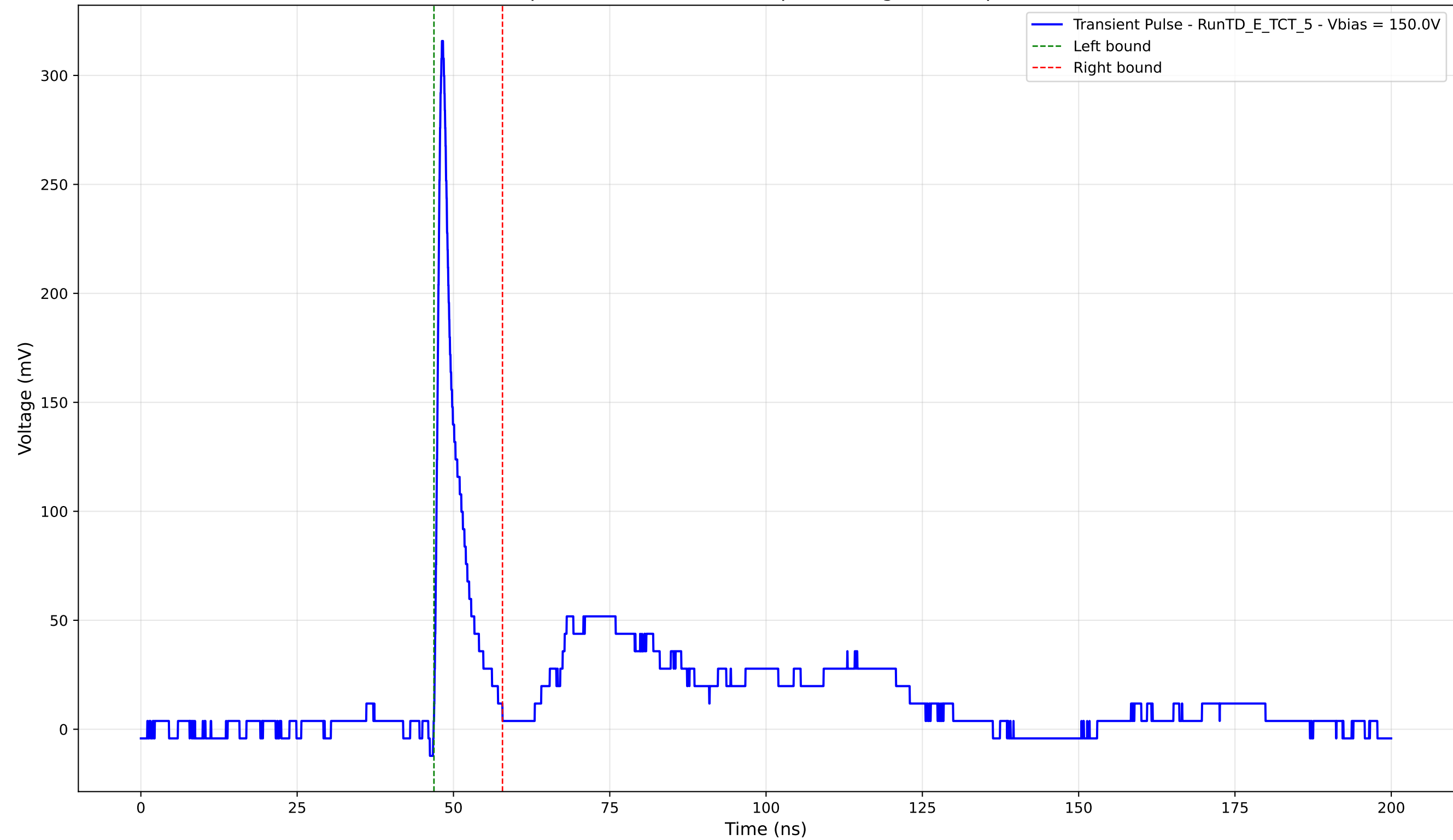
Transient Pulse - Sample: TD - Position: 100.0 \mu\text{m} - Charge: 21.07 pC - Rise Time: 0.91 ns
