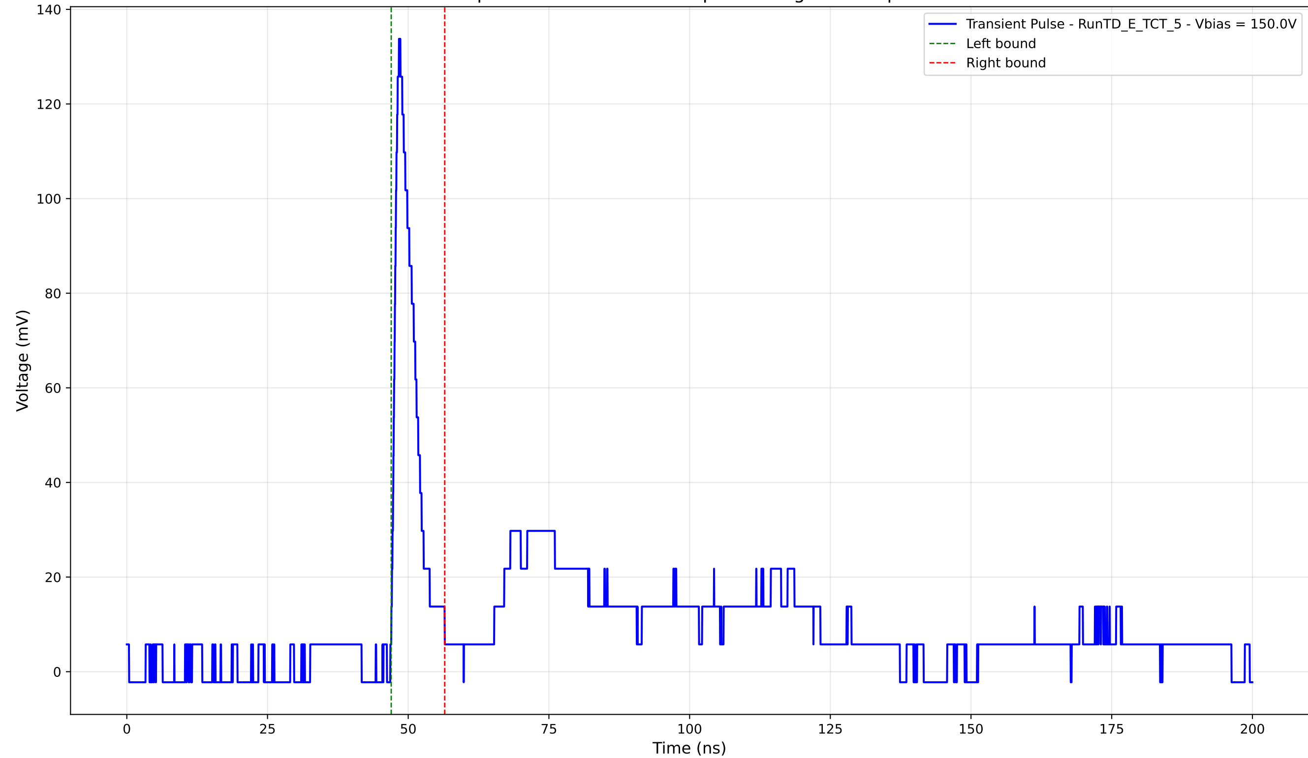
Transient Pulse - Sample: TD - Position: 265.0 \mu\text{m} - Charge: 10.41 pC - Rise Time: 1.12 ns
