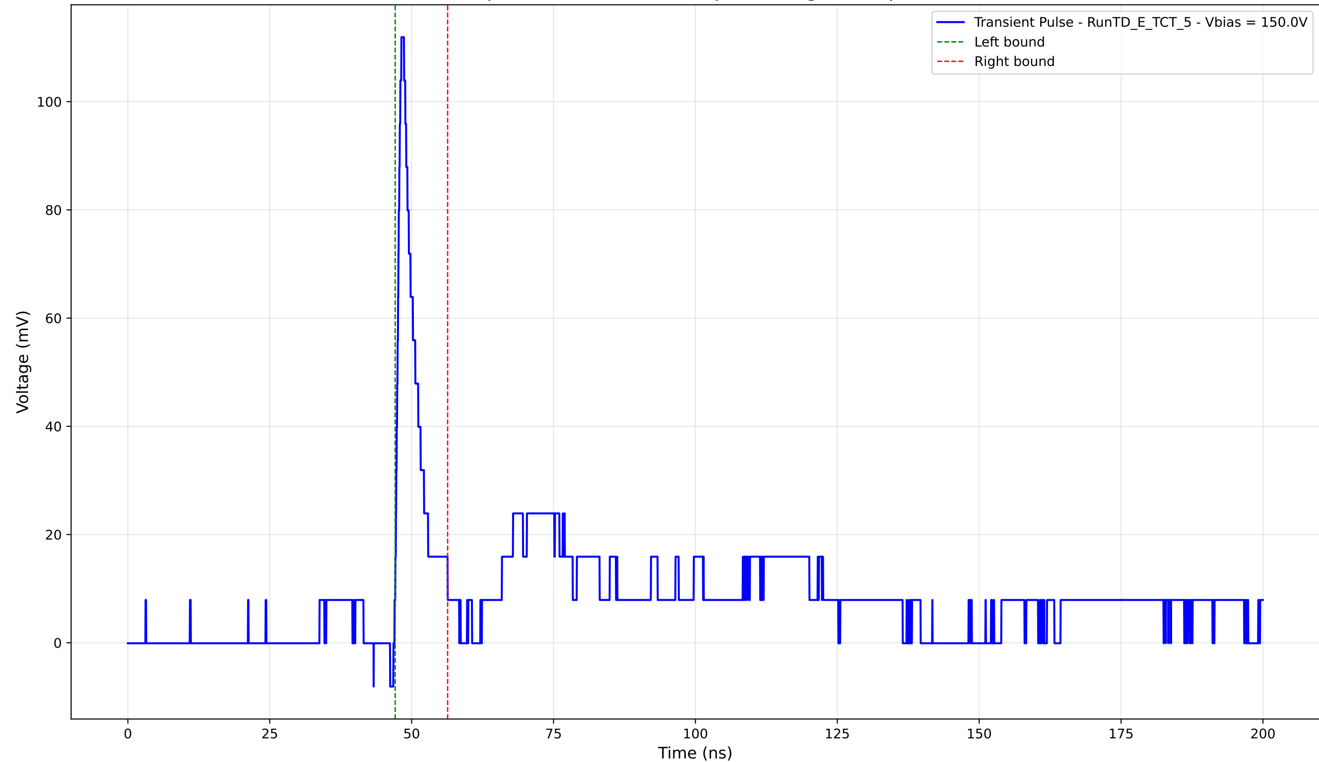
Transient Pulse - Sample: TD - Position: 310.0 \mu\text{m} - Charge: 8.08 pC - Rise Time: 0.89 ns
