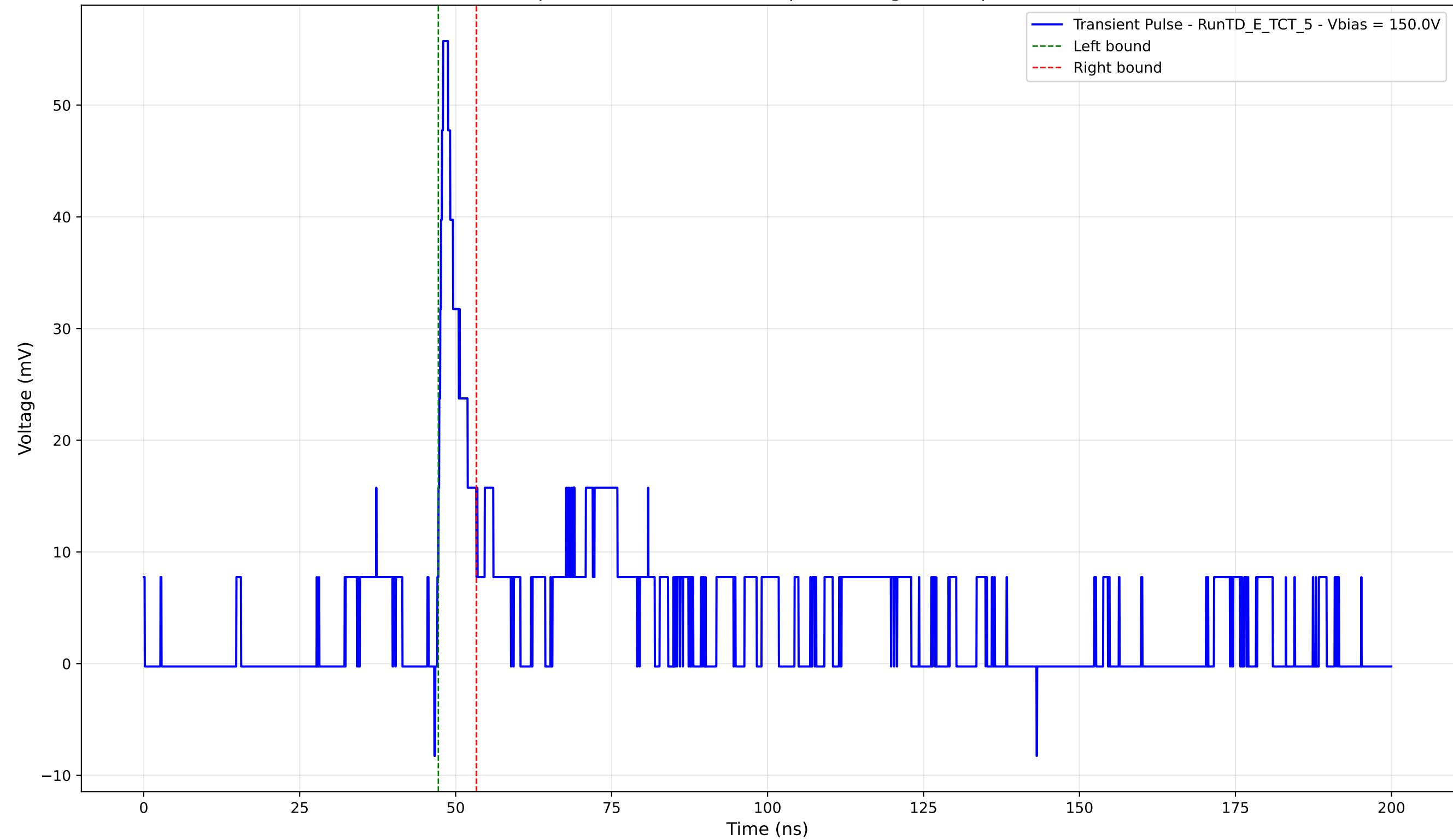
Transient Pulse - Sample: TD - Position: 395.0 \mu\text{m} - Charge: 3.78 pC - Rise Time: 0.93 ns
