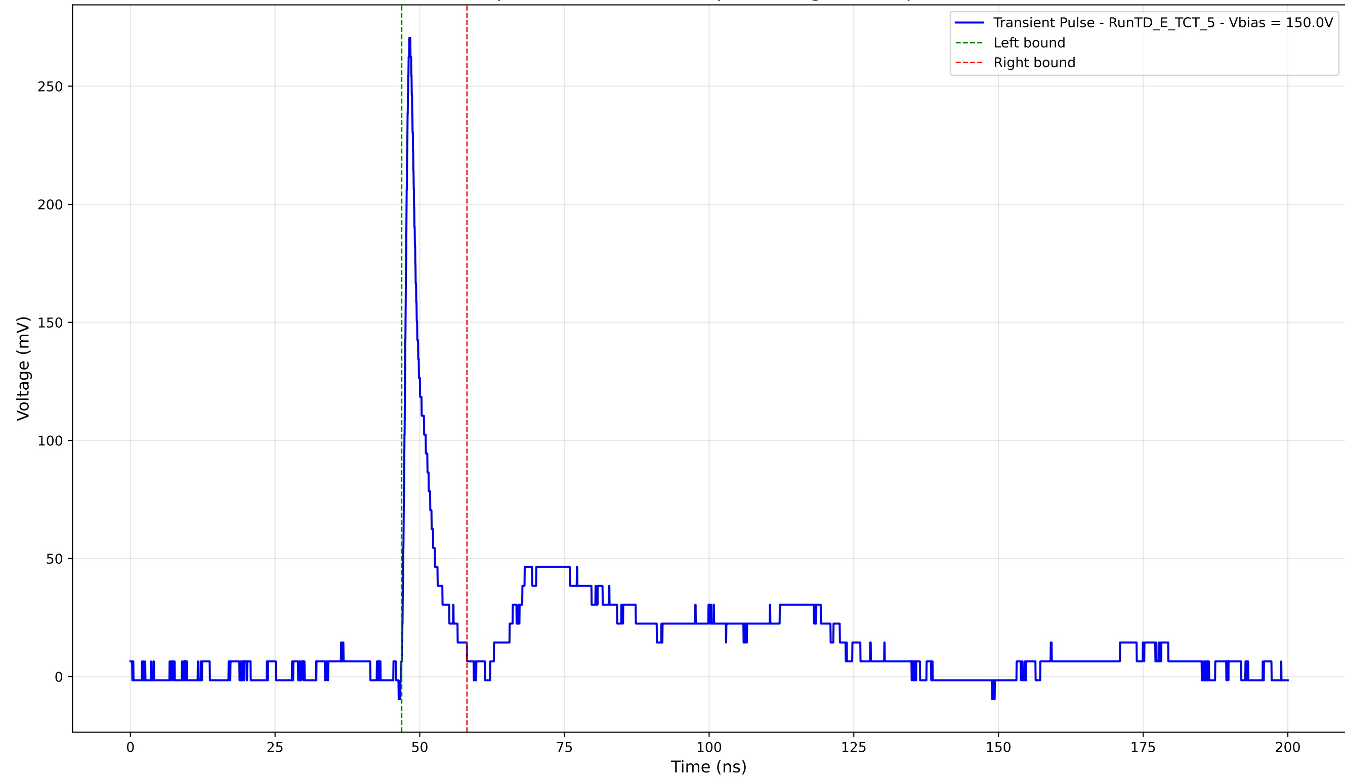
Transient Pulse - Sample: TD - Position: 95.0 \mu\text{m} - Charge: 18.41 pC - Rise Time: 0.91 ns
