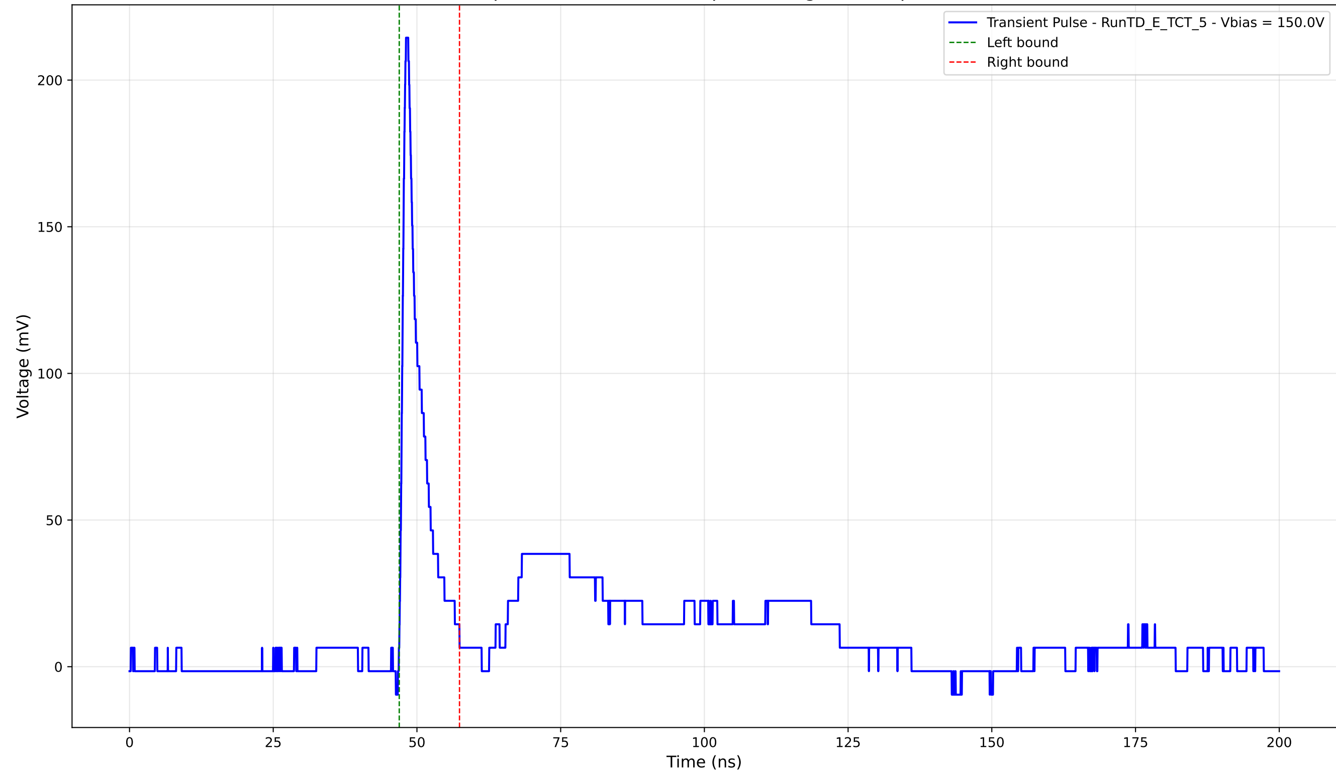
Transient Pulse - Sample: TD - Position: 90.0 \mu\text{m} - Charge: 15.55 pC - Rise Time: 0.92 ns
