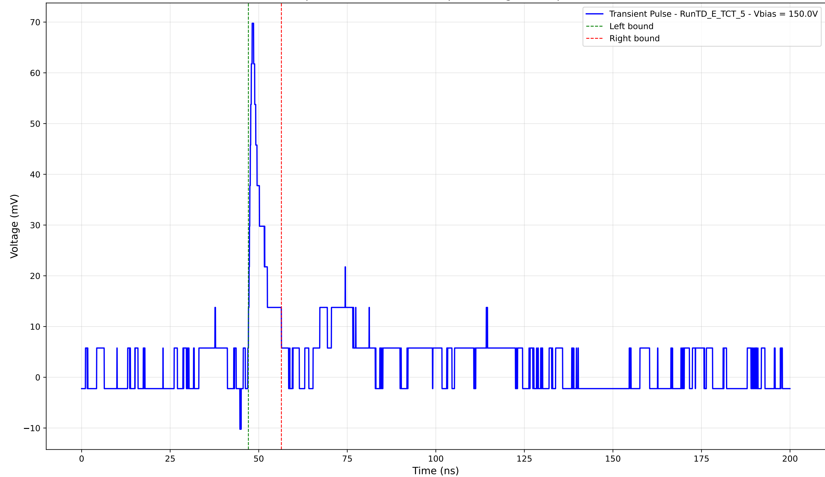
Transient Pulse - Sample: TD - Position: 345.0 \mu\text{m} - Charge: 5.26 pC - Rise Time: 1.06 ns
