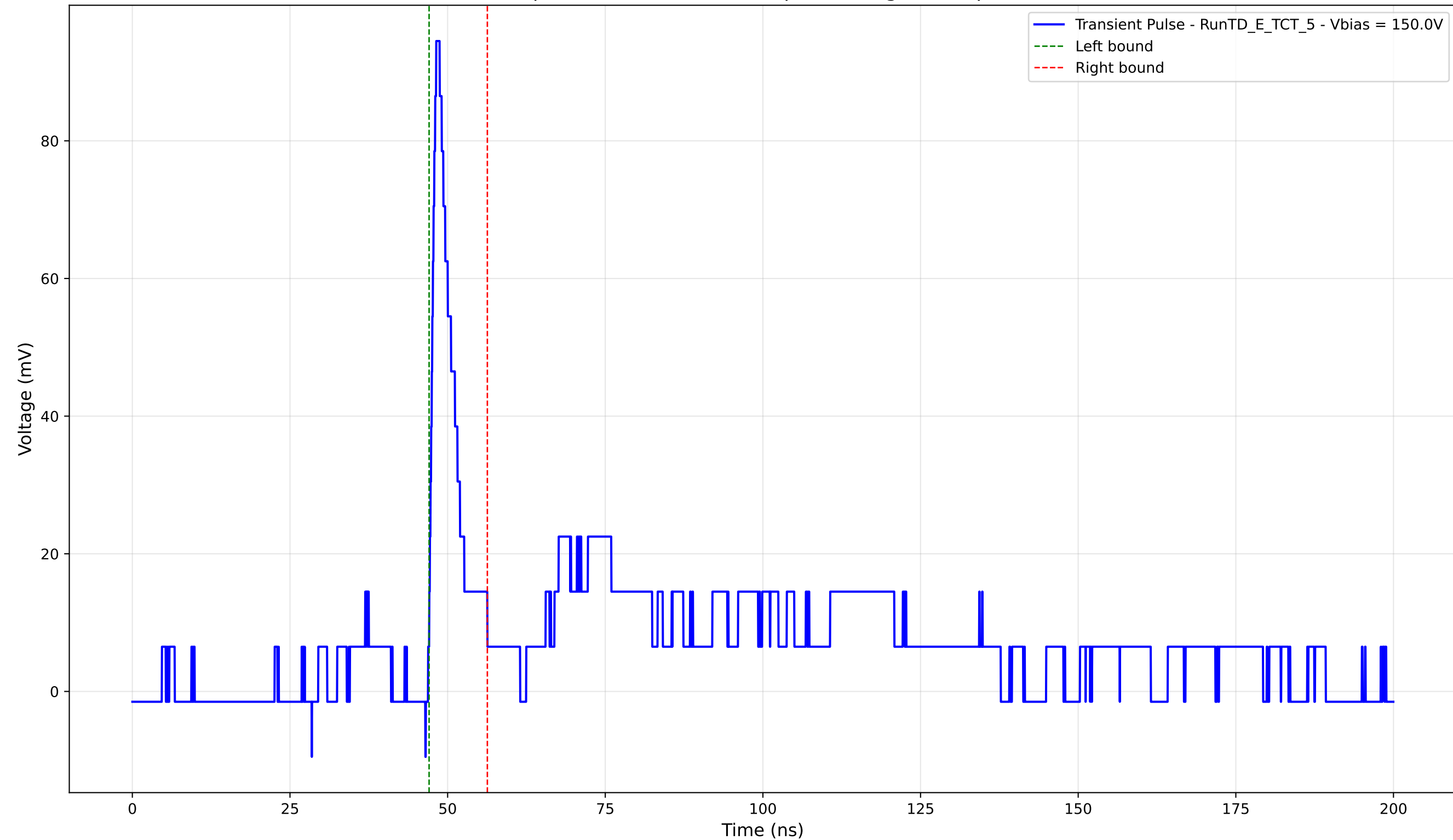
Transient Pulse - Sample: TD - Position: 300.0 \mu\text{m} - Charge: 7.19 pC - Rise Time: 0.95 ns
