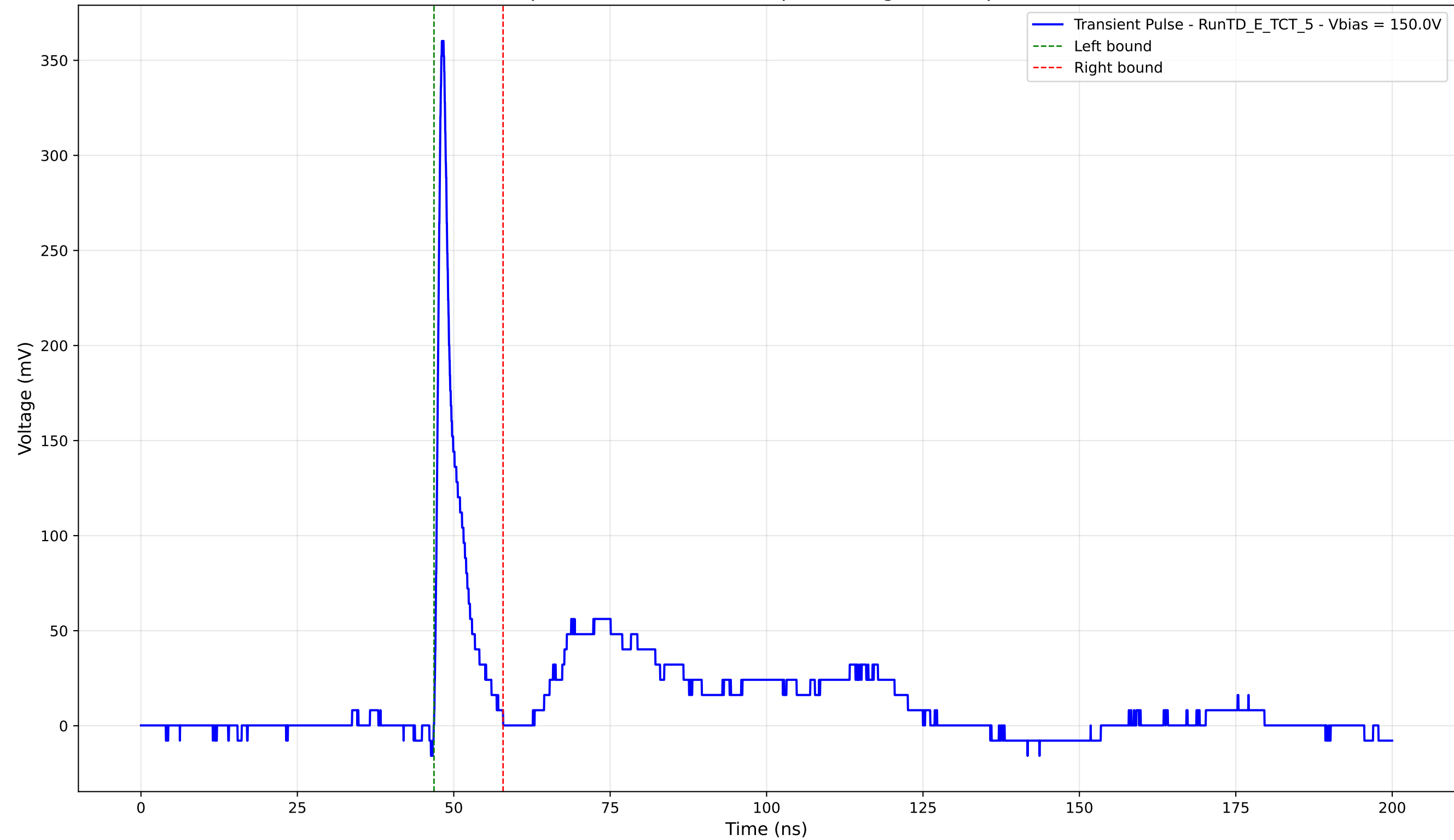
Transient Pulse - Sample: TD - Position: 115.0 \mu\text{m} - Charge: 22.33 pC - Rise Time: 0.87 ns
