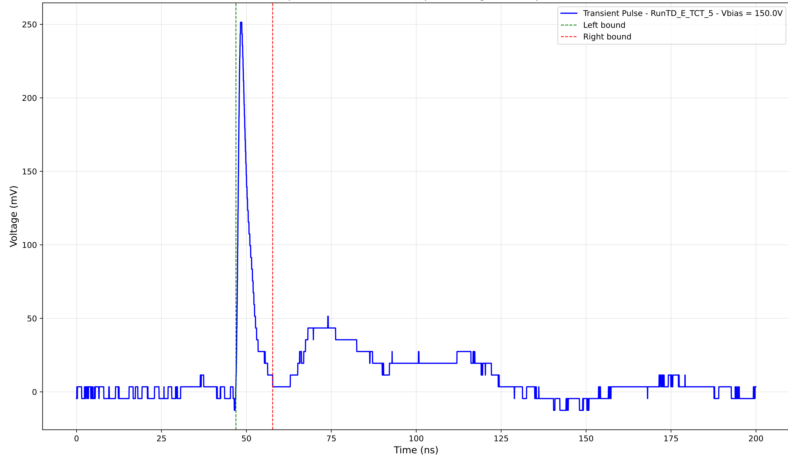
Transient Pulse - Sample: TD - Position: 160.0 \mu\text{m} - Charge: 18.12 pC - Rise Time: 0.95 ns
