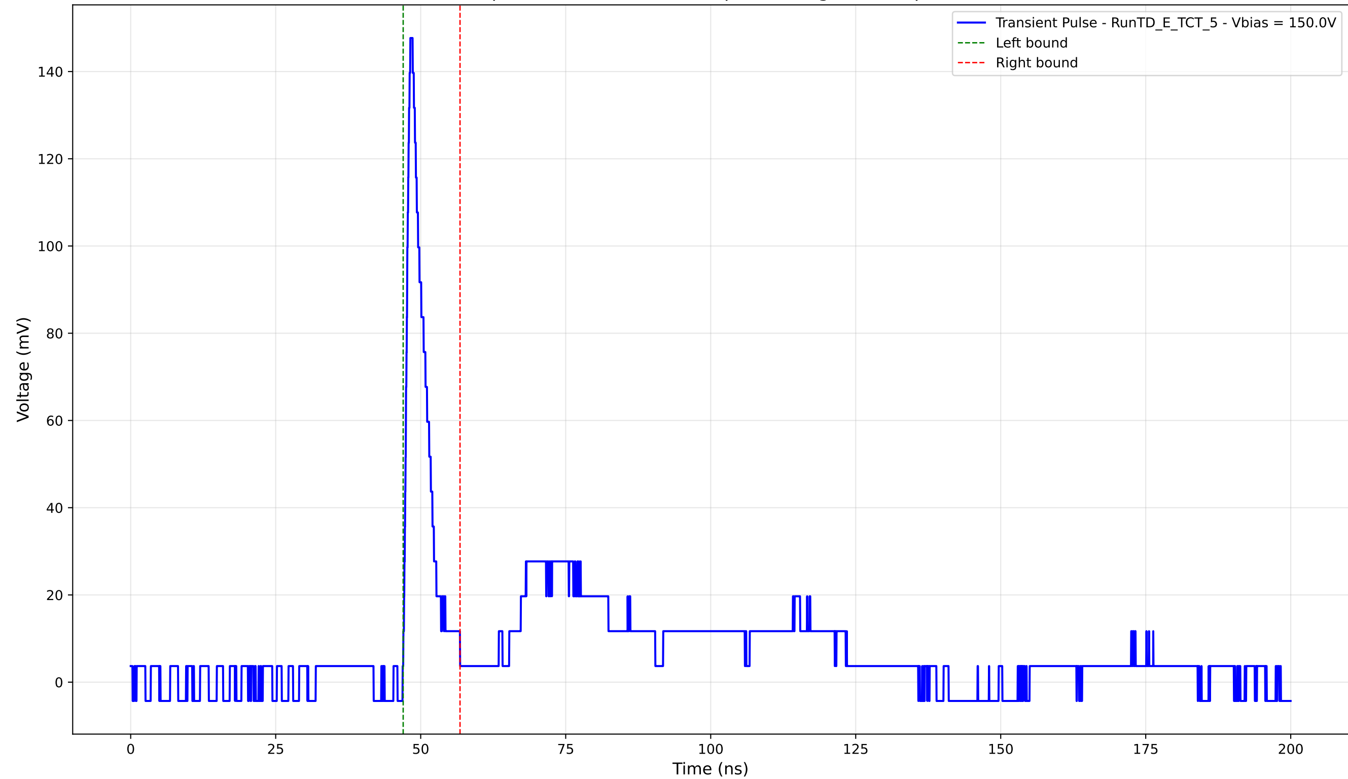
Transient Pulse - Sample: TD - Position: 270.0 \mu\text{m} - Charge: 10.53 pC - Rise Time: 0.97 ns
