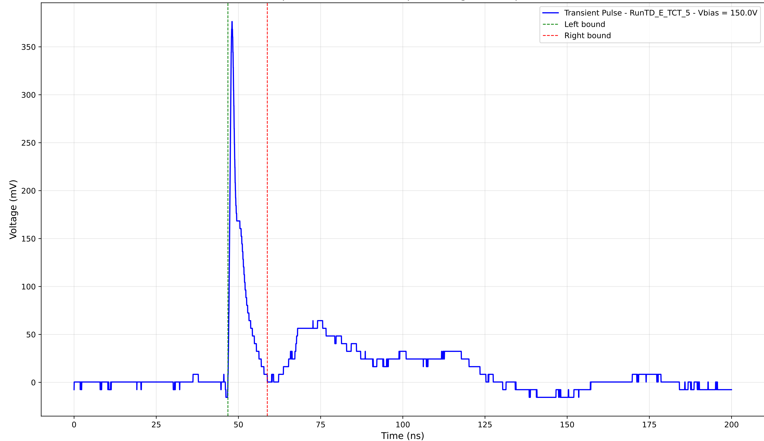
Transient Pulse - Sample: TD - Position: 50.0 \mu\text{m} - Charge: 25.66 pC - Rise Time: 0.83 ns
