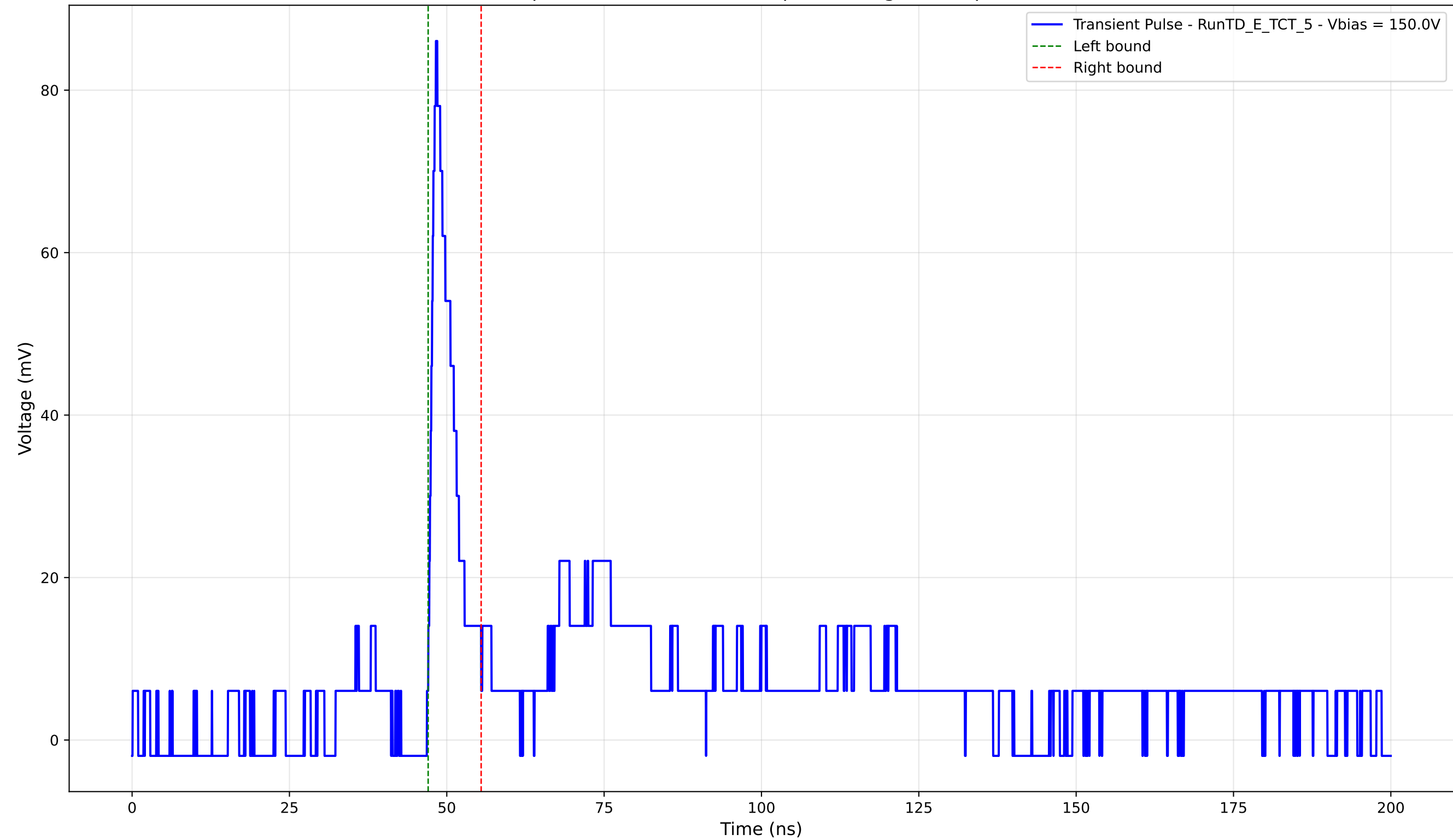
Transient Pulse - Sample: TD - Position: 295.0 \mu\text{m} - Charge: 6.43 pC - Rise Time: 1.01 ns
