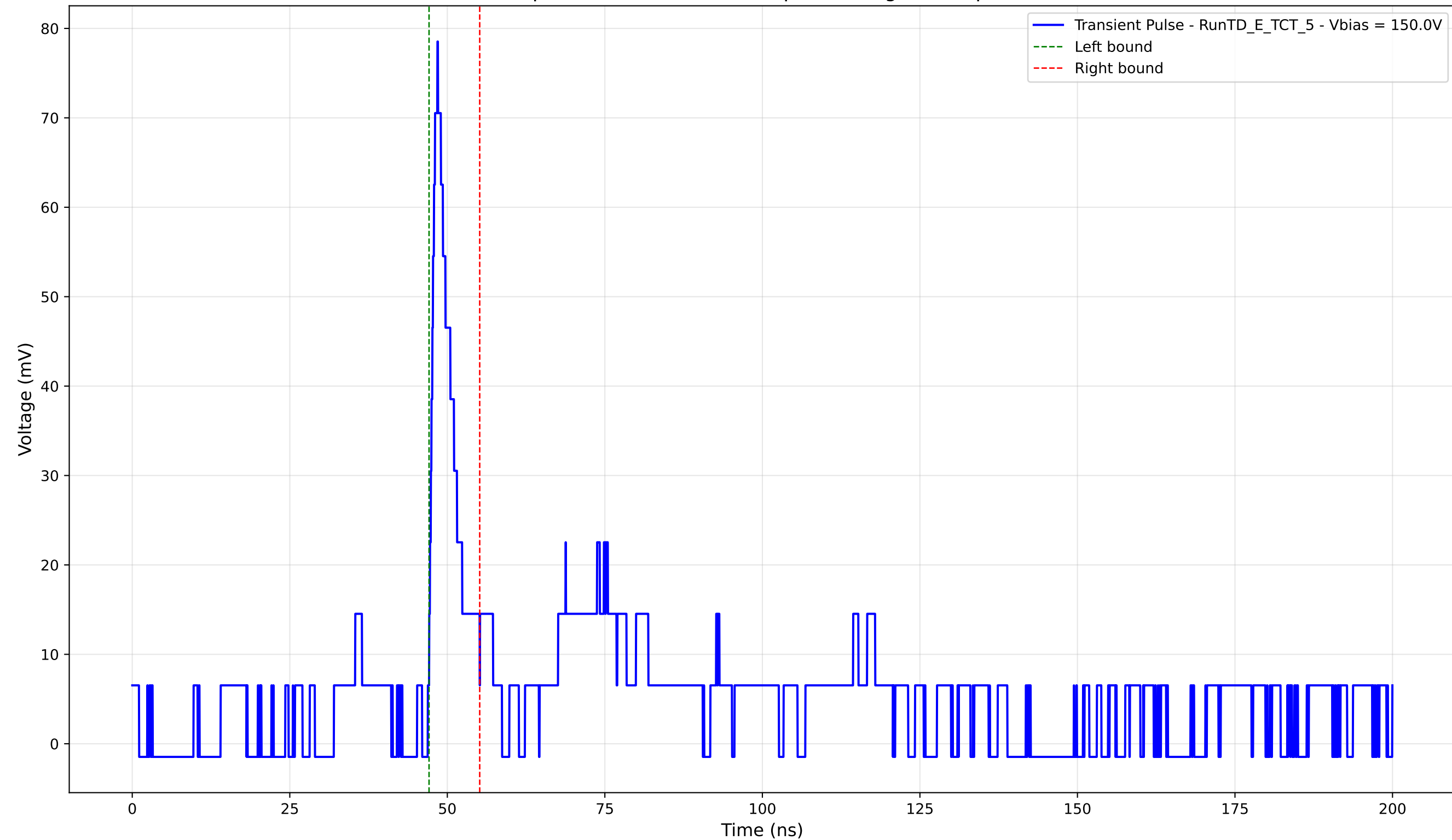
Transient Pulse - Sample: TD - Position: 325.0 \mu\text{m} - Charge: 5.56 pC - Rise Time: 1.32 ns
