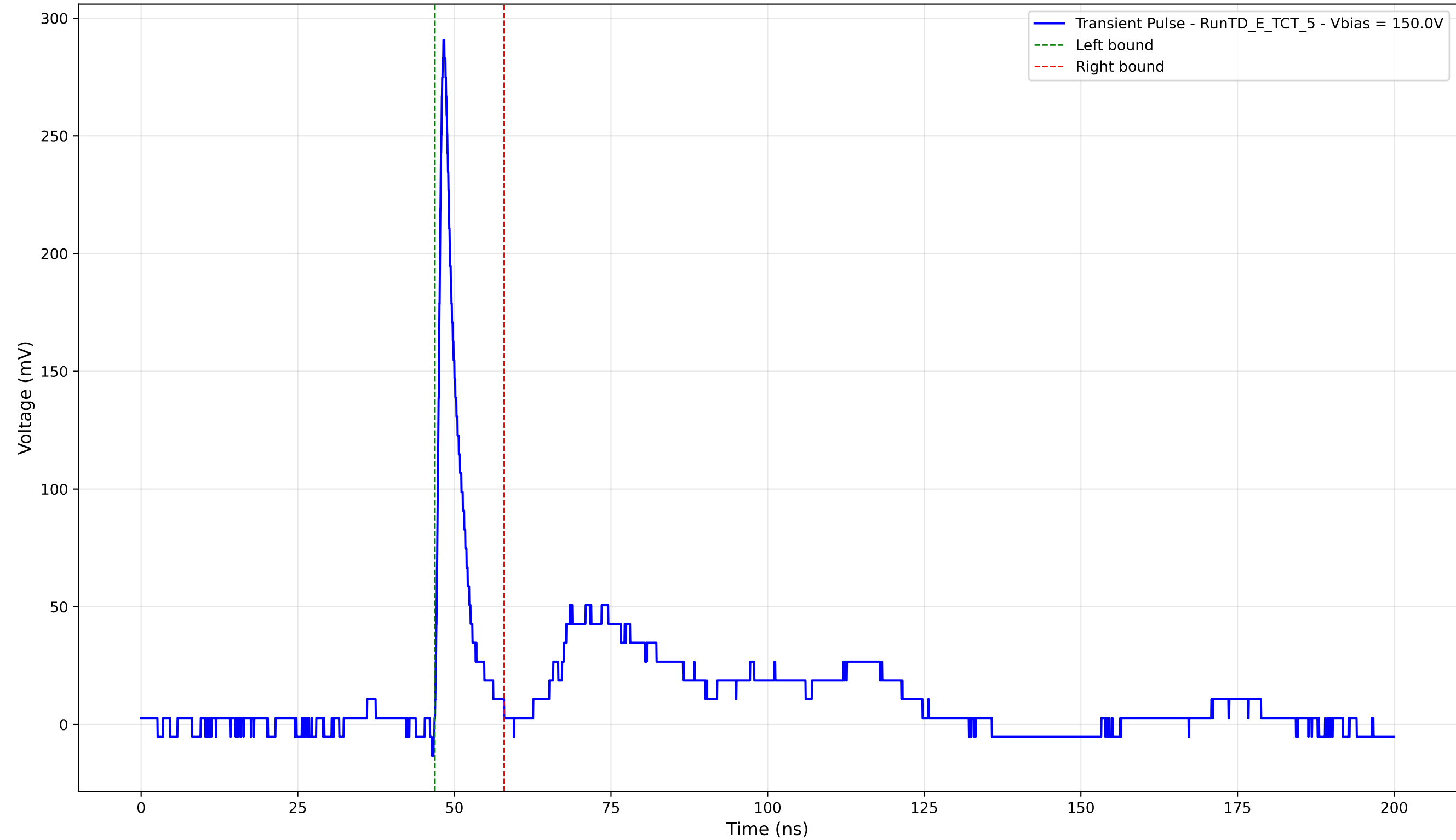
Transient Pulse - Sample: TD - Position: 200.0 \mu\text{m} - Charge: 19.23 pC - Rise Time: 0.93 ns
