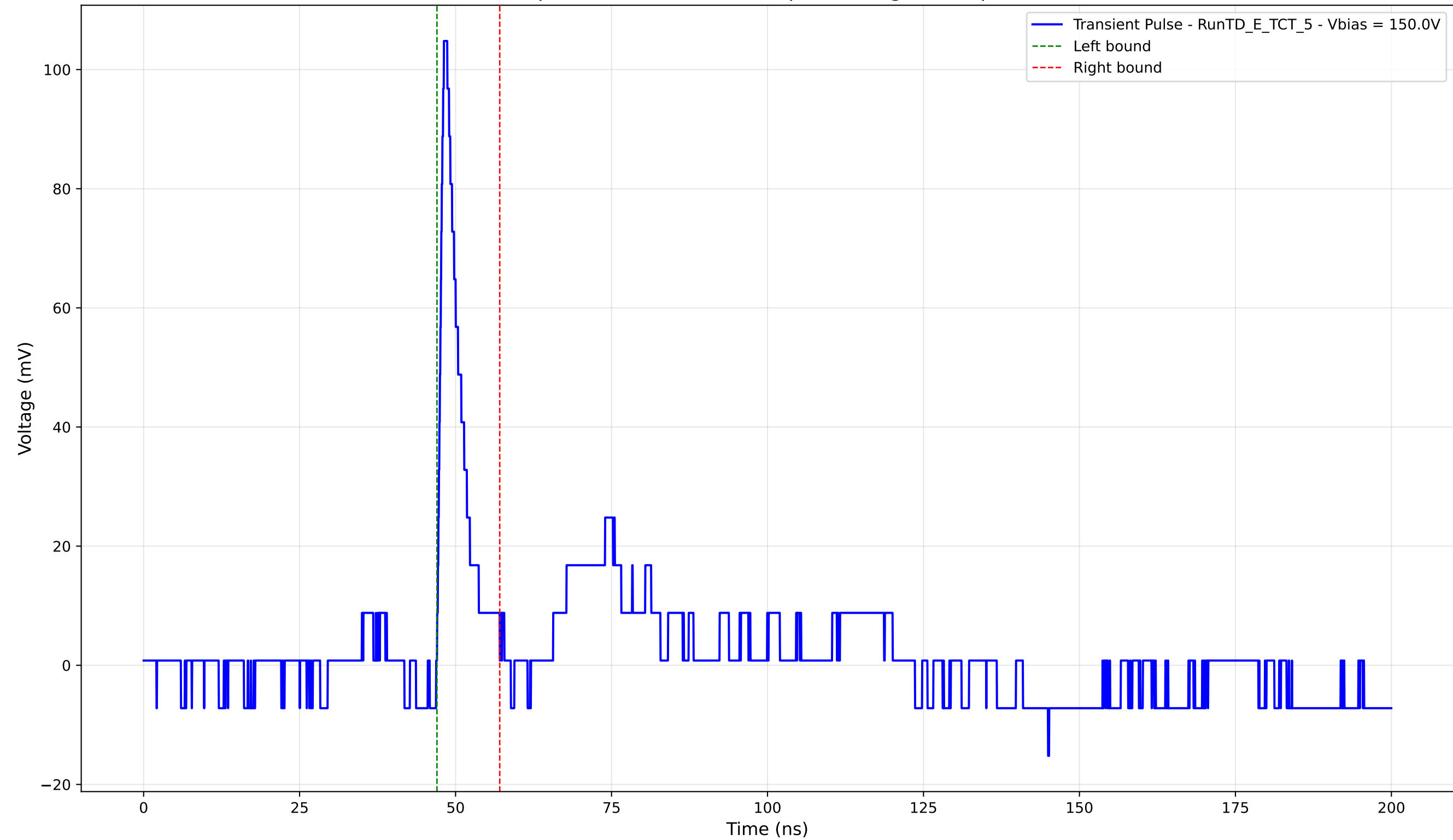
Transient Pulse - Sample: TD - Position: 320.0 \mu\text{m} - Charge: 7.41 pC - Rise Time: 0.86 ns
