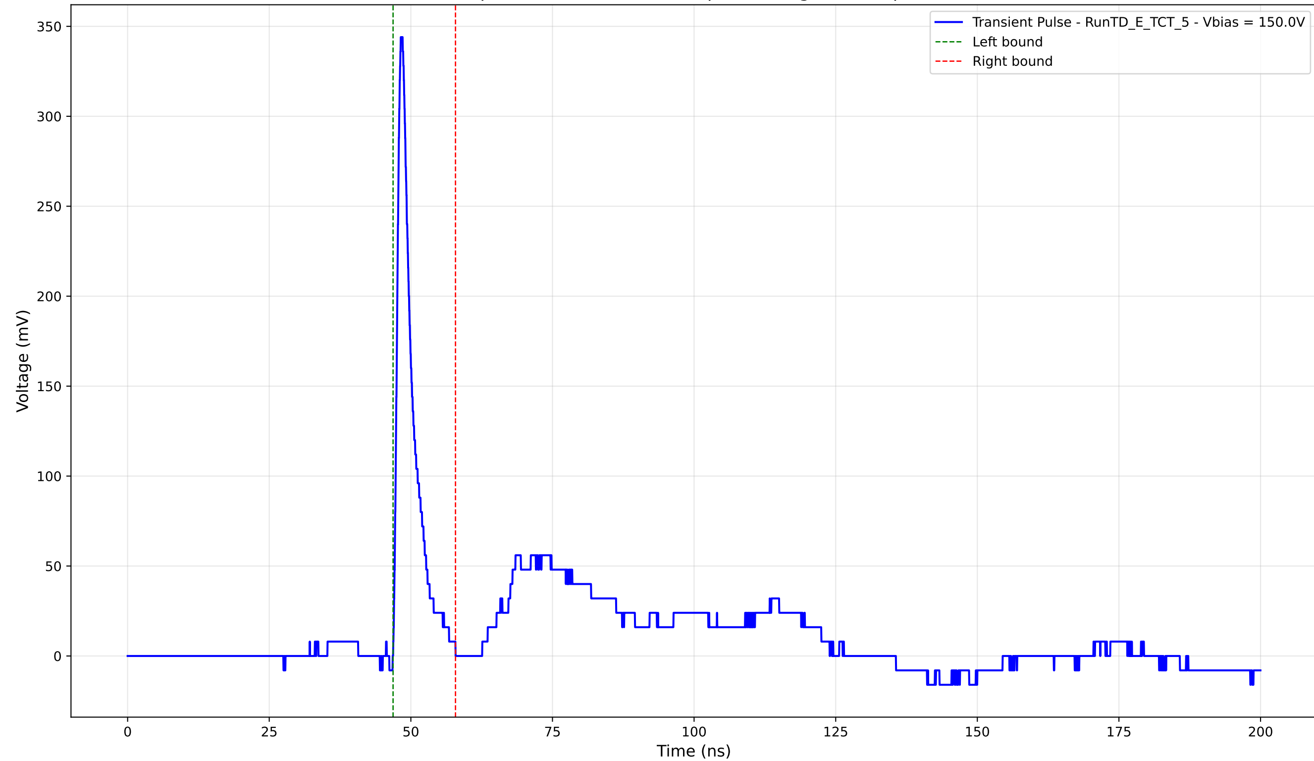
Transient Pulse - Sample: TD - Position: 165.0 \mu\text{m} - Charge: 21.88 pC - Rise Time: 0.93 ns
