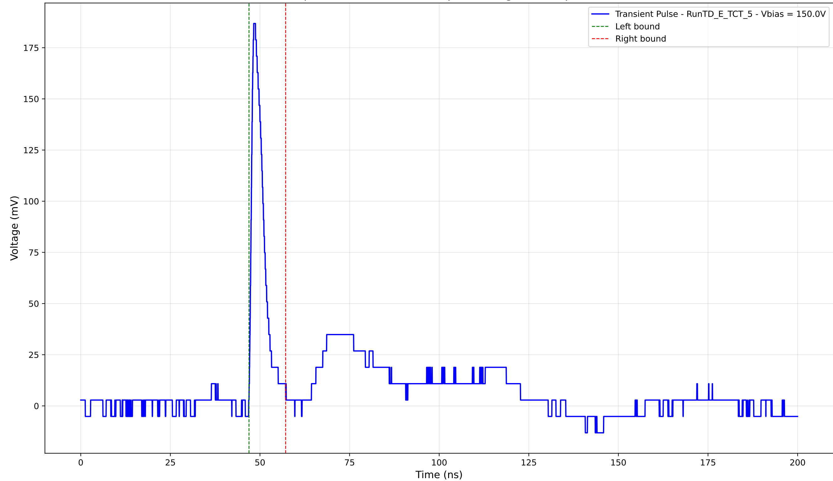
Transient Pulse - Sample: TD - Position: 215.0 \mu\text{m} - Charge: 14.26 pC - Rise Time: 0.98 ns
