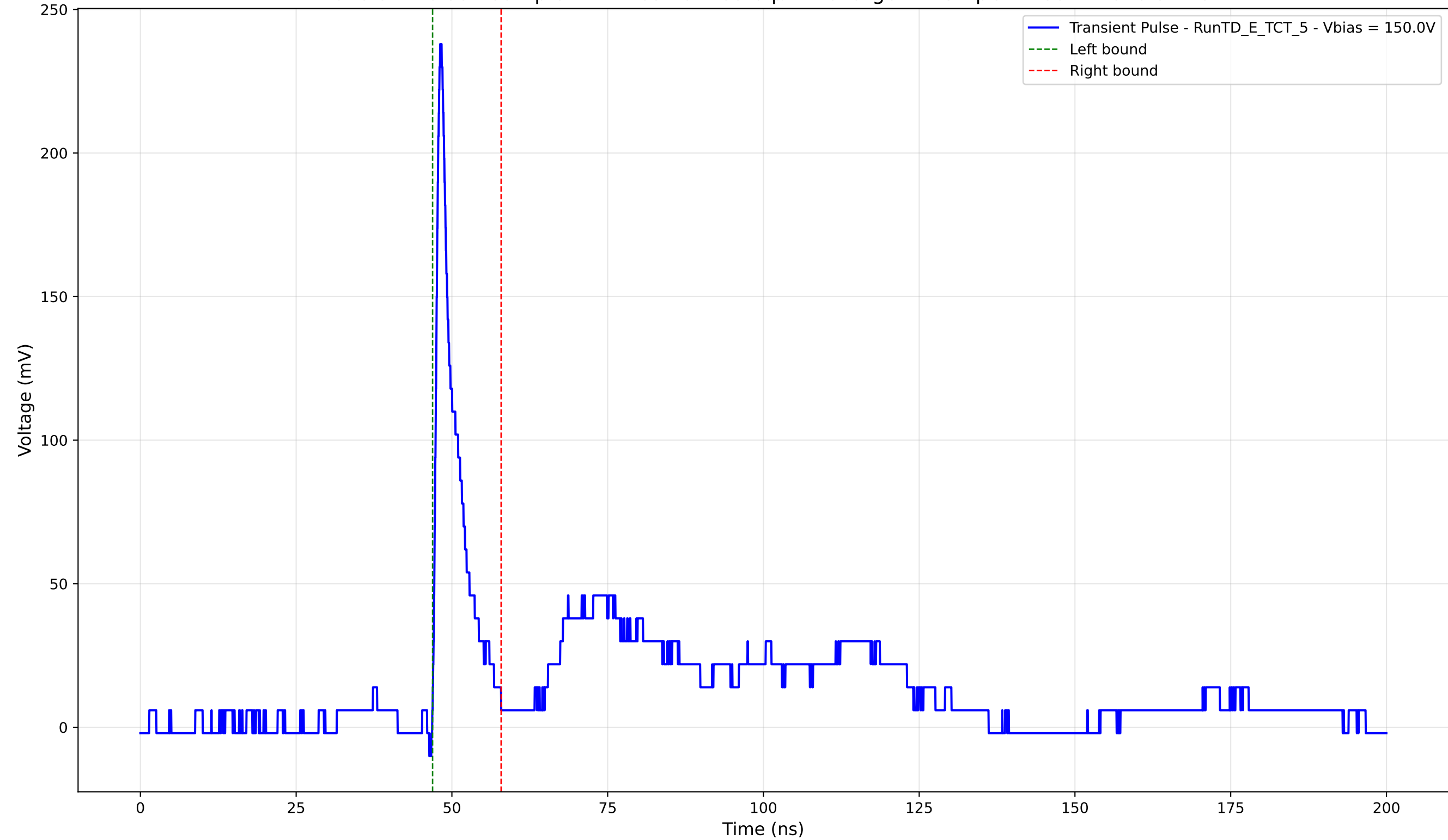
Transient Pulse - Sample: TD - Position: 85.0 \mu\text{m} - Charge: 17.32 pC - Rise Time: 0.92 ns
