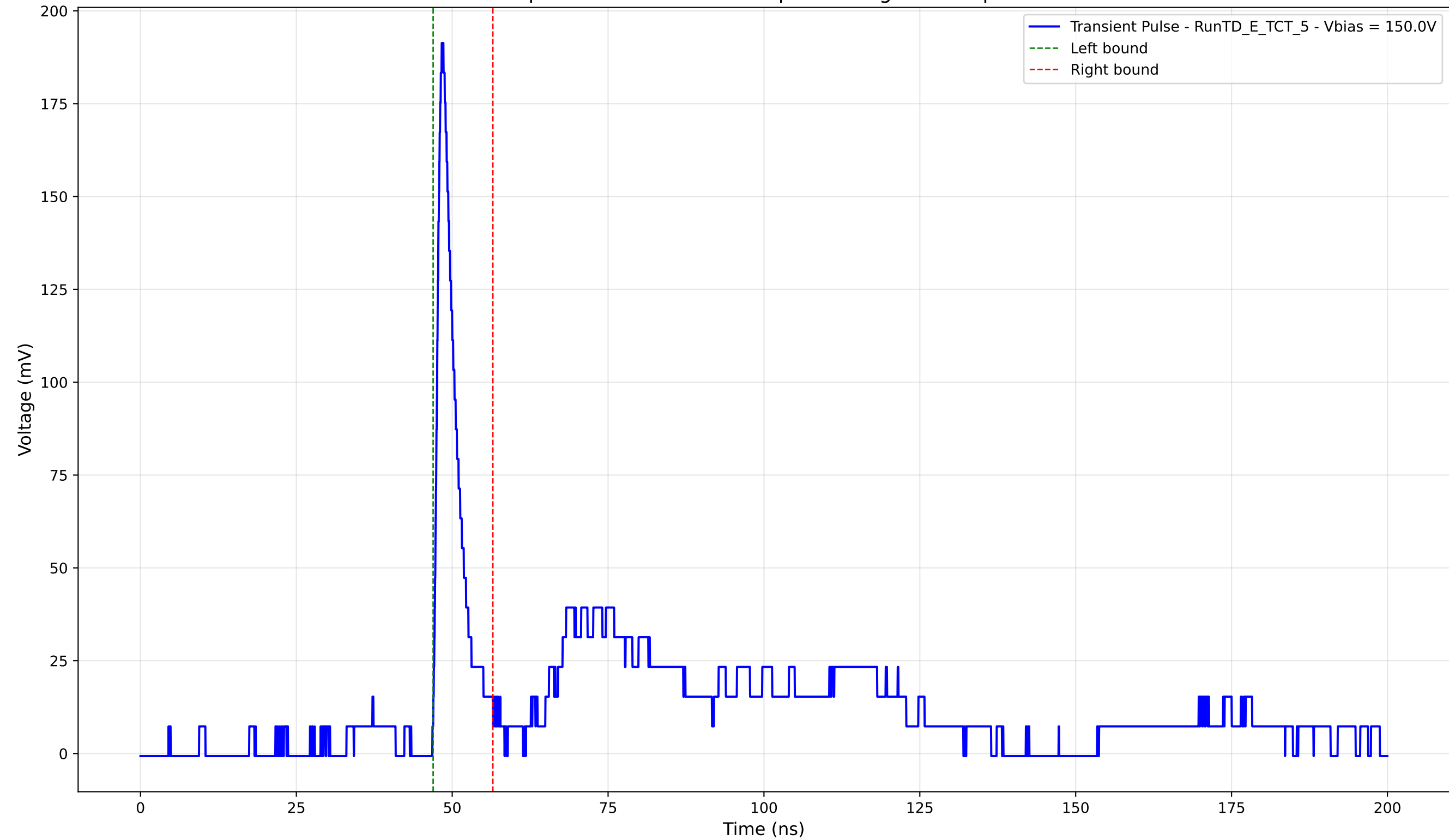
Transient Pulse - Sample: TD - Position: 250.0 \mu\text{m} - Charge: 13.50 pC - Rise Time: 1.03 ns
