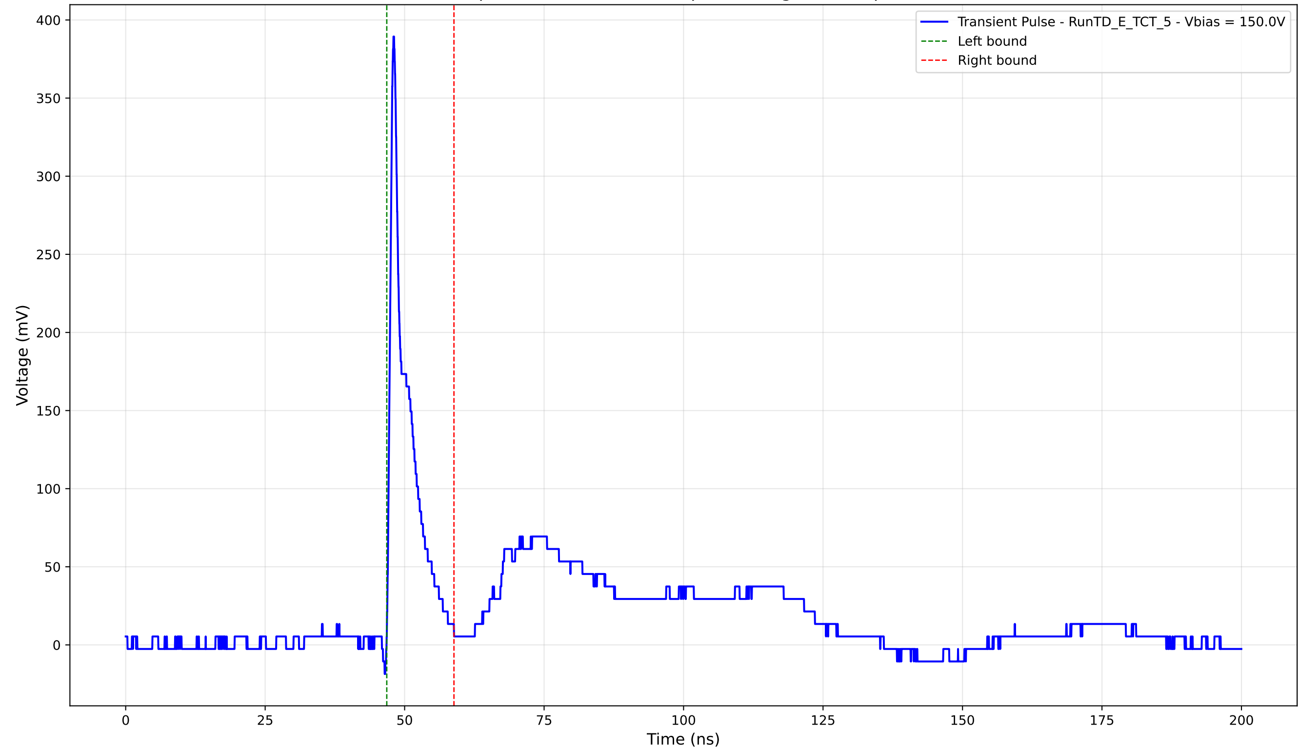
Transient Pulse - Sample: TD - Position: 55.0 \mu\text{m} - Charge: 27.19 pC - Rise Time: 0.84 ns
