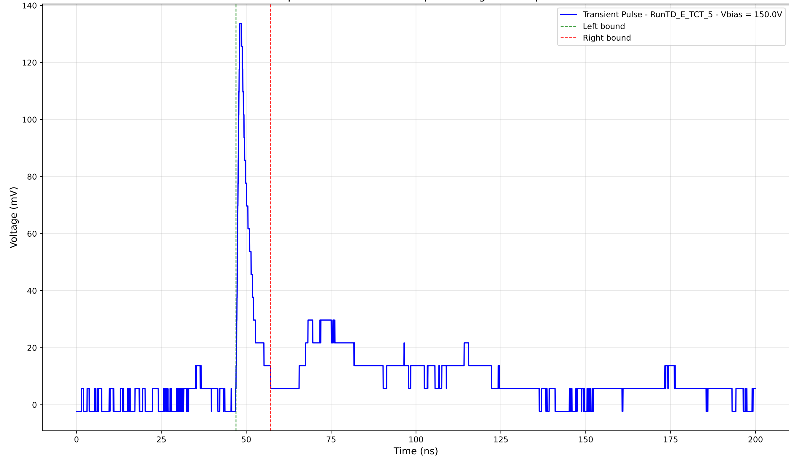
Transient Pulse - Sample: TD - Position: 315.0 \mu\text{m} - Charge: 10.08 pC - Rise Time: 0.98 ns
