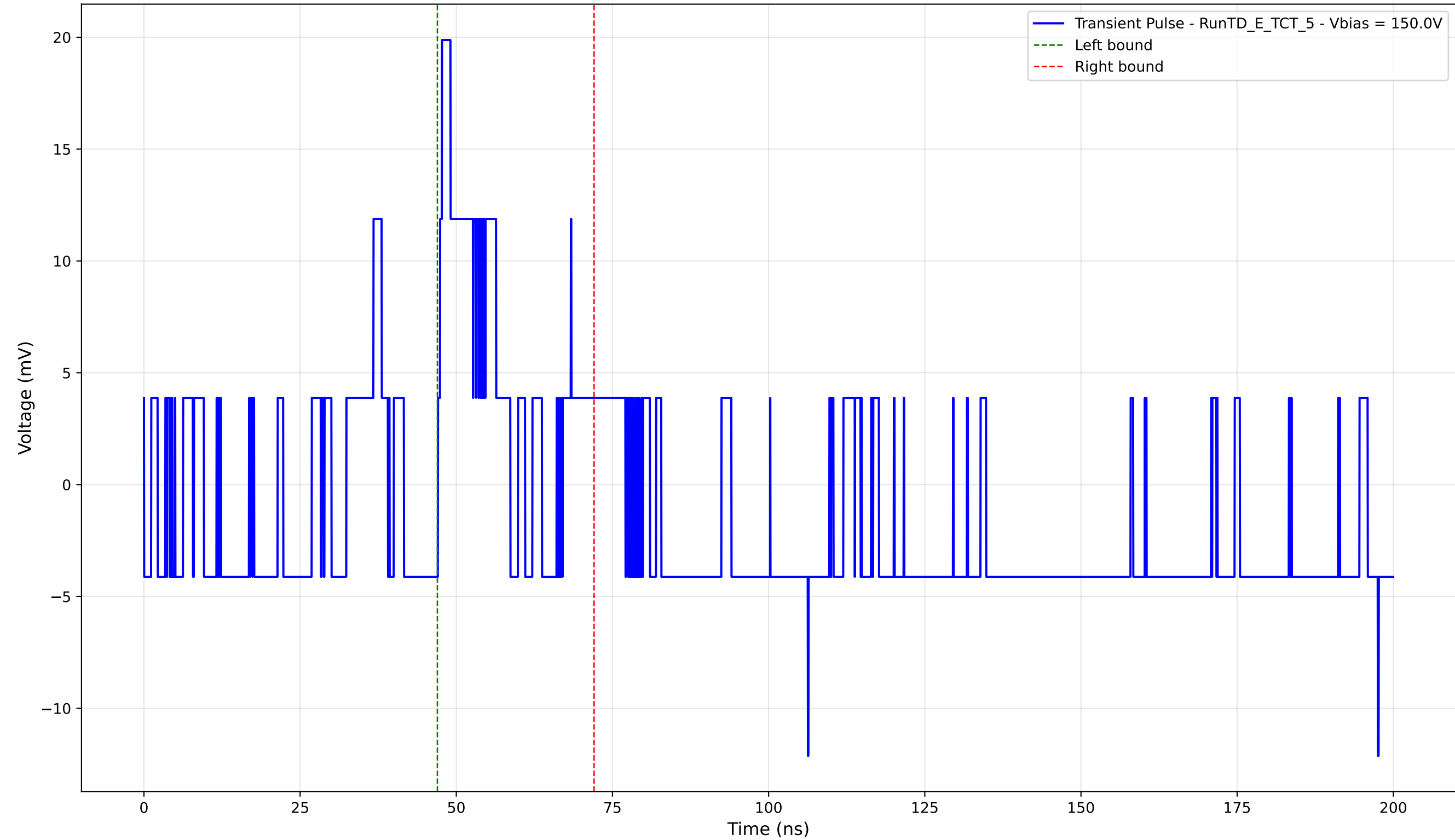
Transient Pulse - Sample: TD - Position: 20.0 \mu\text{m} - Charge: 2.69 pC - Rise Time: 0.00 ns (N/A)
