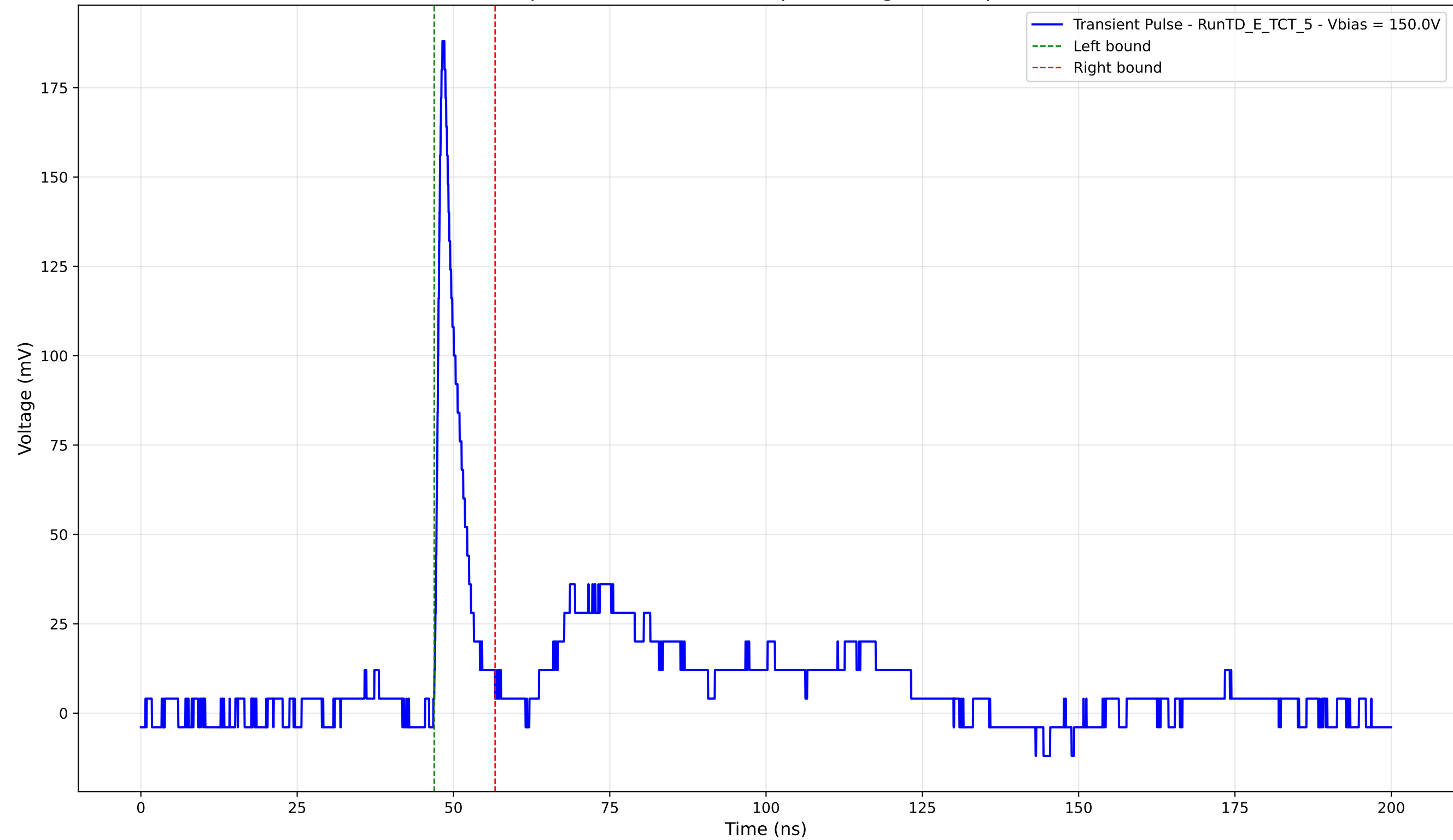
Transient Pulse - Sample: TD - Position: 230.0 \mu\text{m} - Charge: 13.05 pC - Rise Time: 0.98 ns
