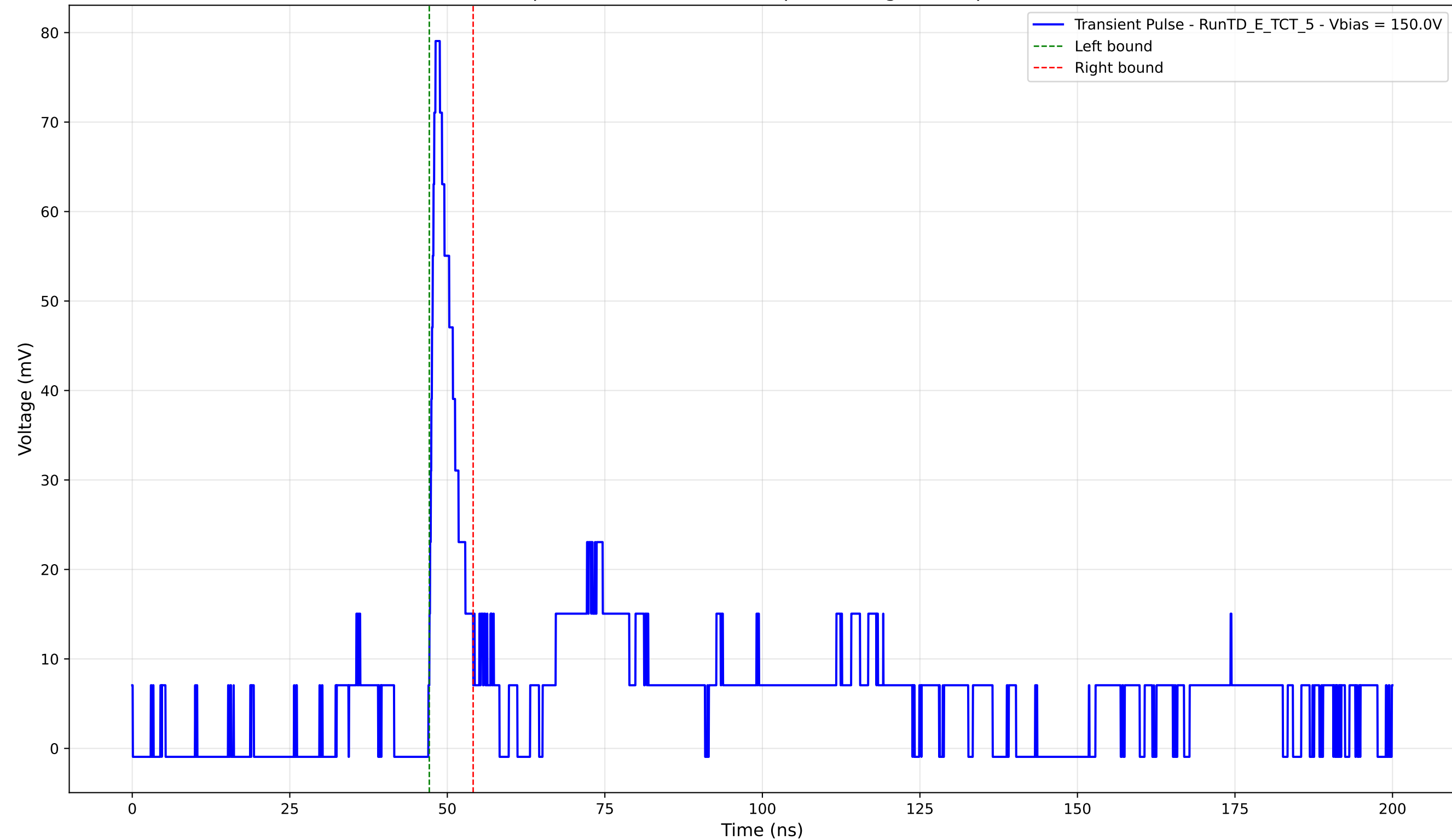
Transient Pulse - Sample: TD - Position: 290.0 \mu\text{m} - Charge: 5.84 pC - Rise Time: 0.98 ns
