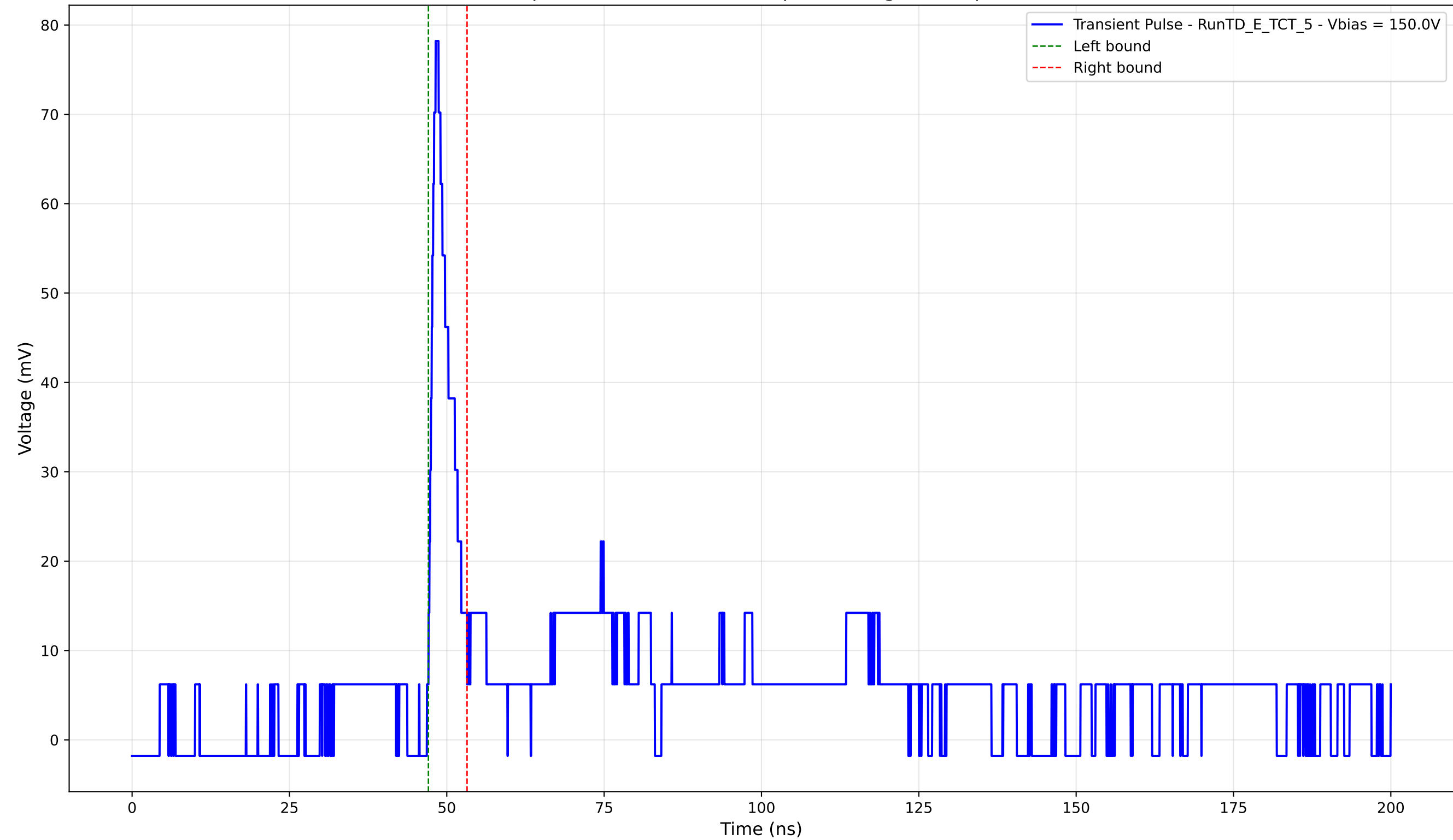
Transient Pulse - Sample: TD - Position: 330.0 \mu\text{m} - Charge: 5.08 pC - Rise Time: 1.14 ns
