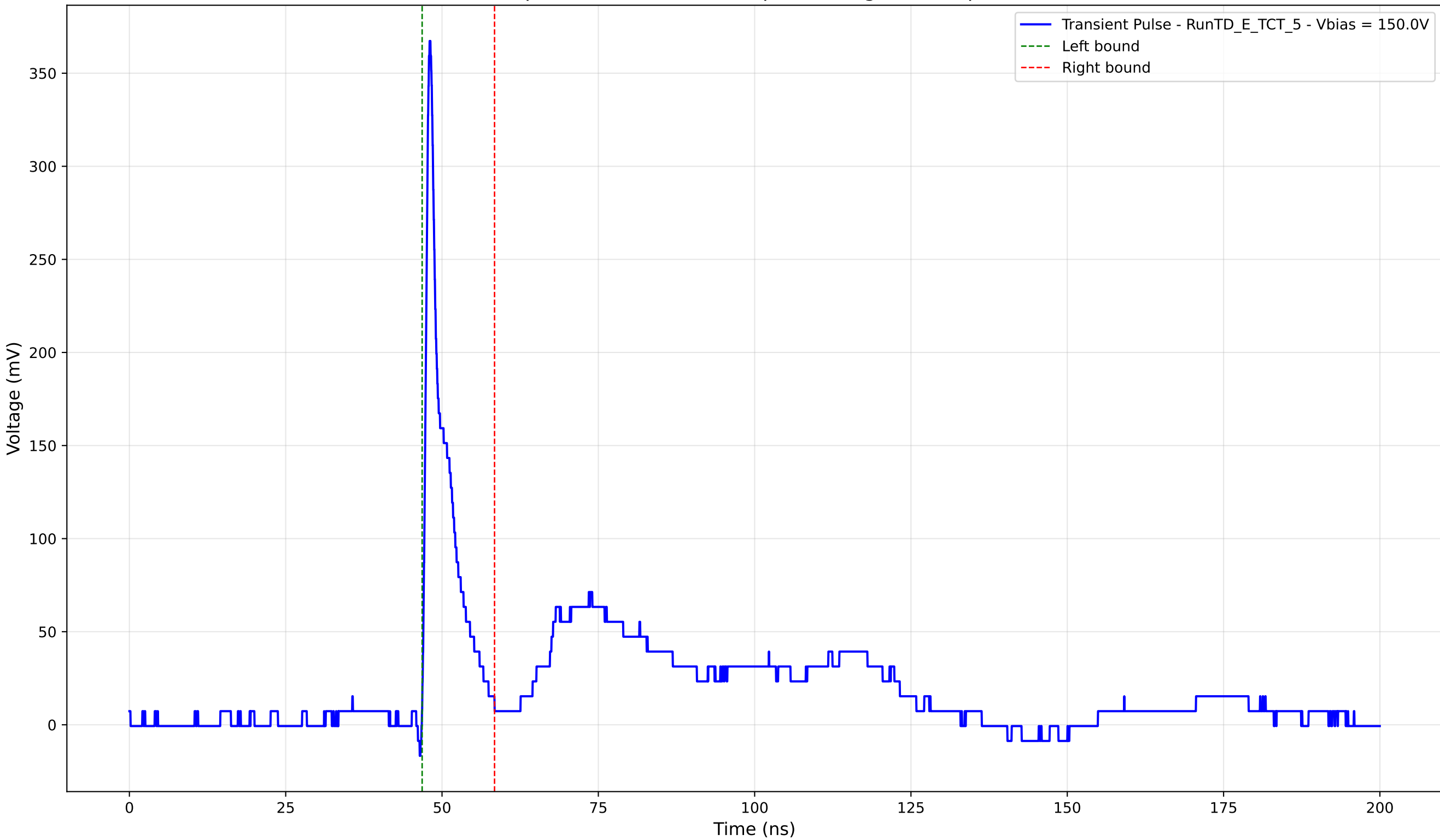
Transient Pulse - Sample: TD - Position: 45.0 \mu\text{m} - Charge: 25.66 pC - Rise Time: 0.85 ns
