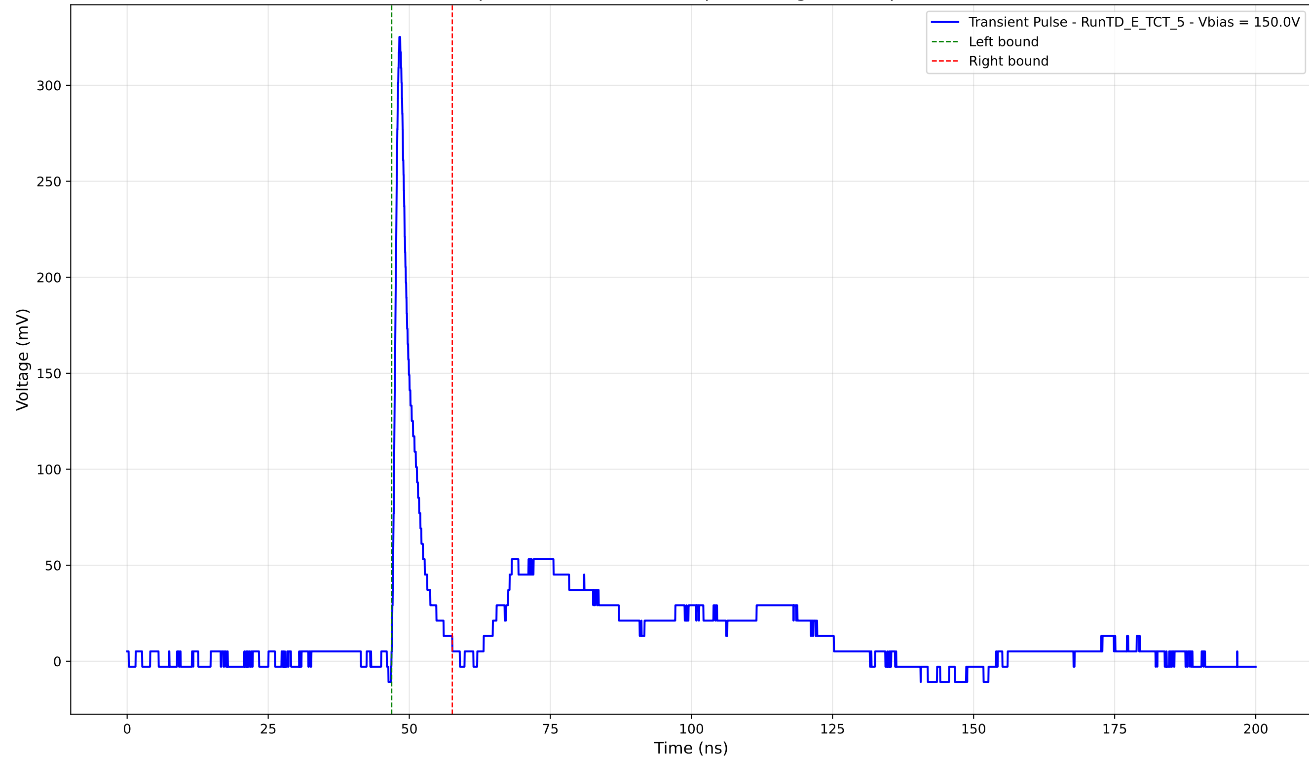
Transient Pulse - Sample: TD - Position: 135.0 \mu\text{m} - Charge: 20.73 pC - Rise Time: 0.91 ns
