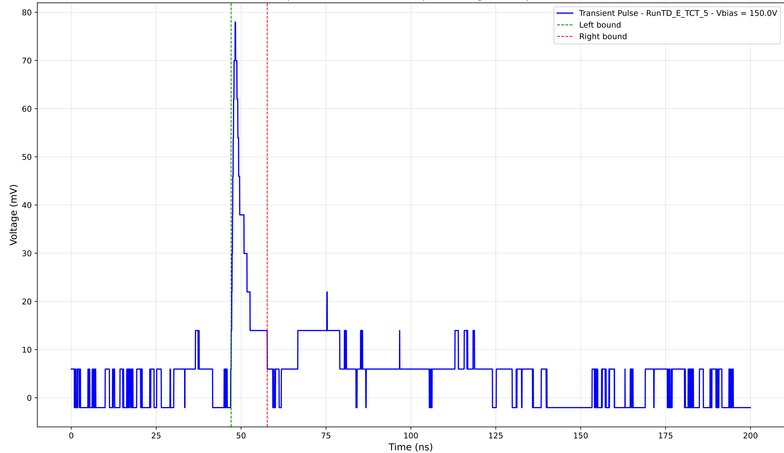
Transient Pulse - Sample: TD - Position: 375.0 \mu\text{m} - Charge: 6.03 pC - Rise Time: 1.18 ns
