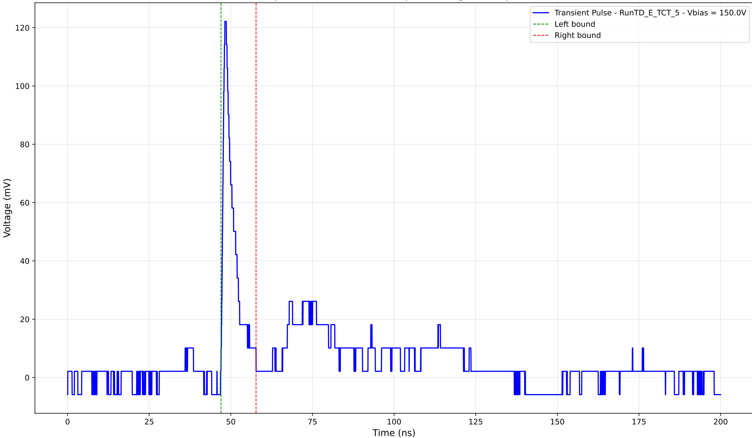
Transient Pulse - Sample: TD - Position: 240.0 \mu\text{m} - Charge: 9.09 pC - Rise Time: 0.91 ns
