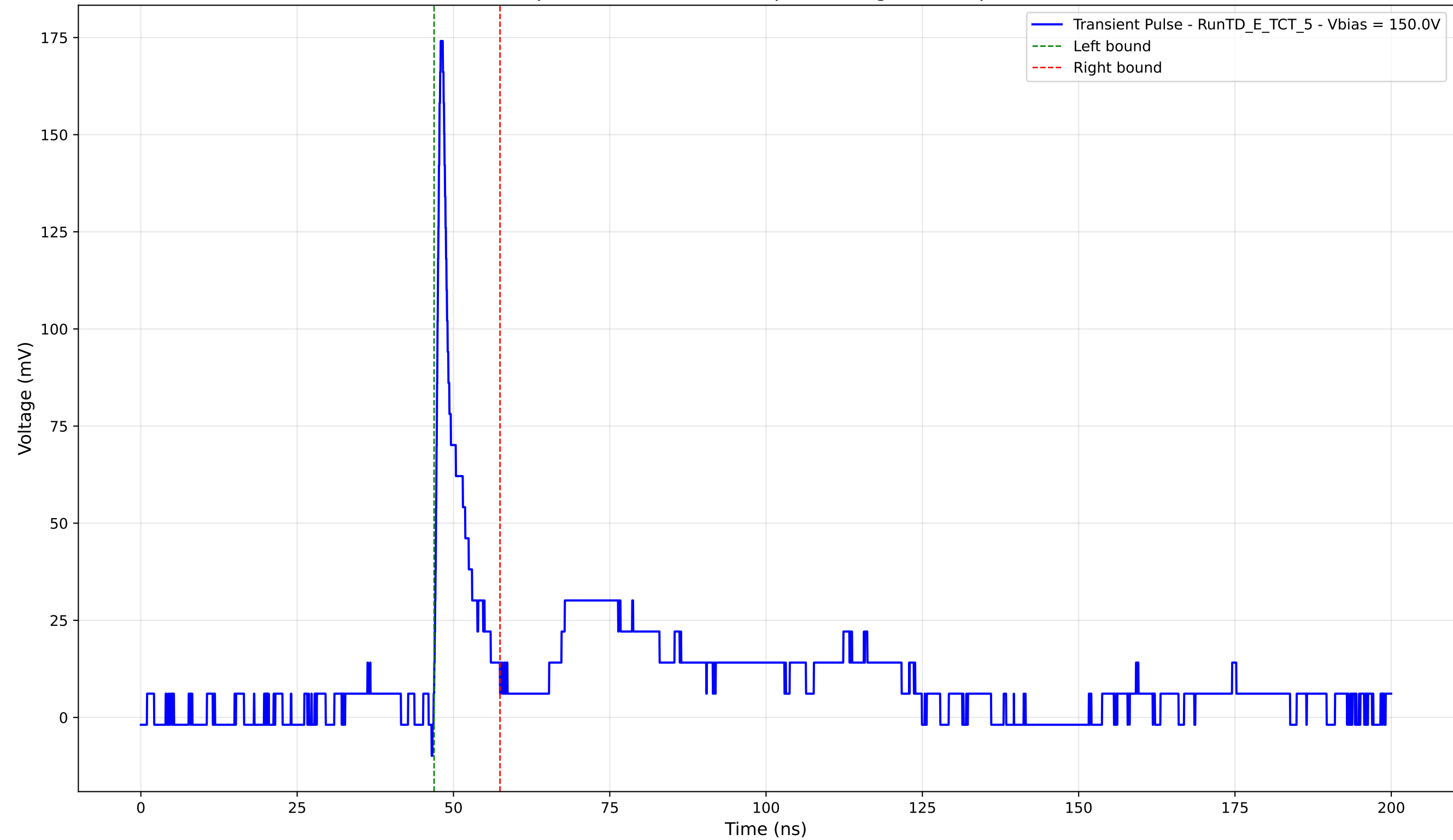
Transient Pulse - Sample: TD - Position: 35.0 \mu\text{m} - Charge: 11.89 pC - Rise Time: 0.79 ns
