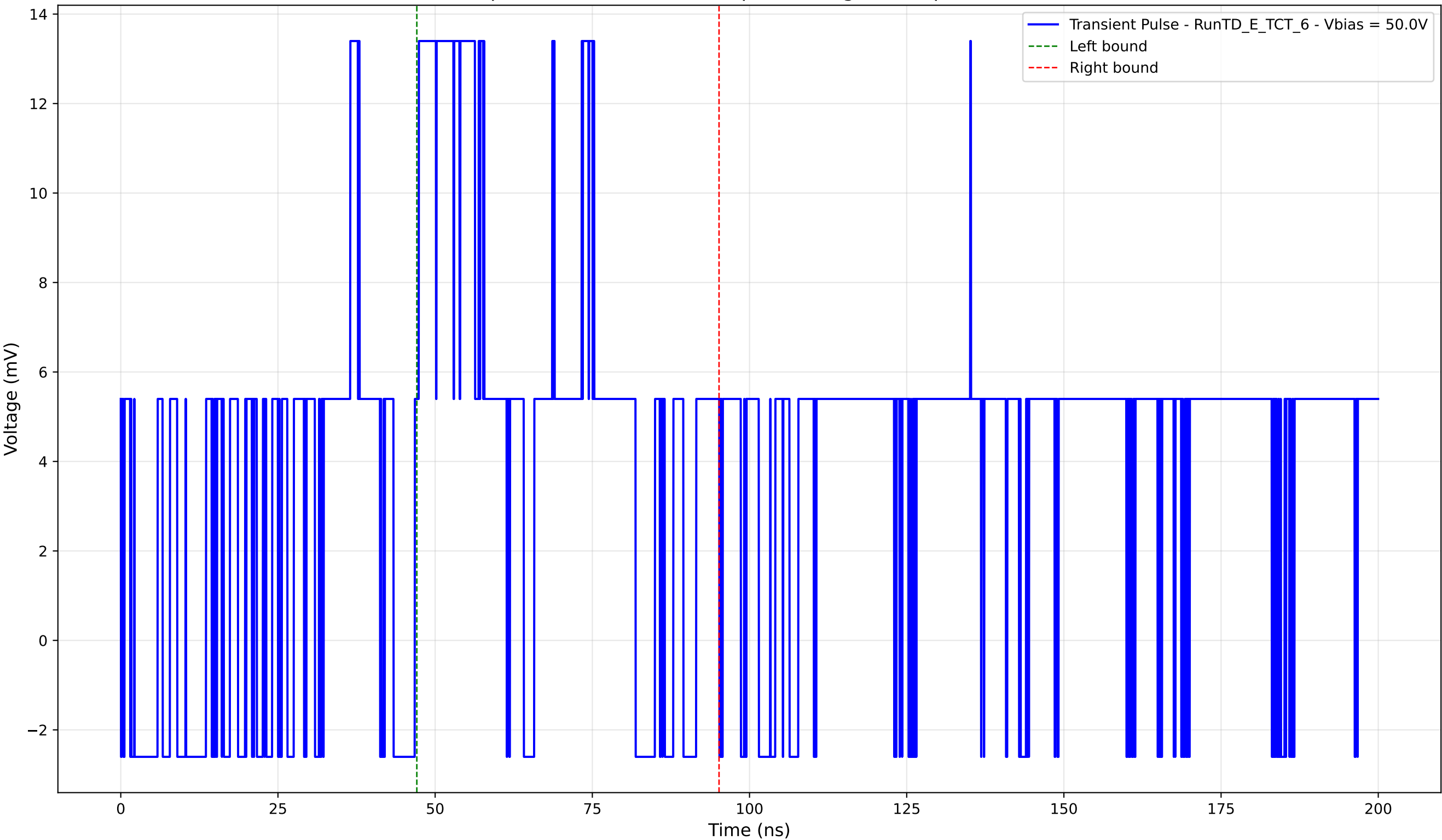
Transient Pulse - Sample: TD - Position: 355.0 \mu\text{m} - Charge: 5.64 pC - Rise Time: 0.00 ns (N/A)
