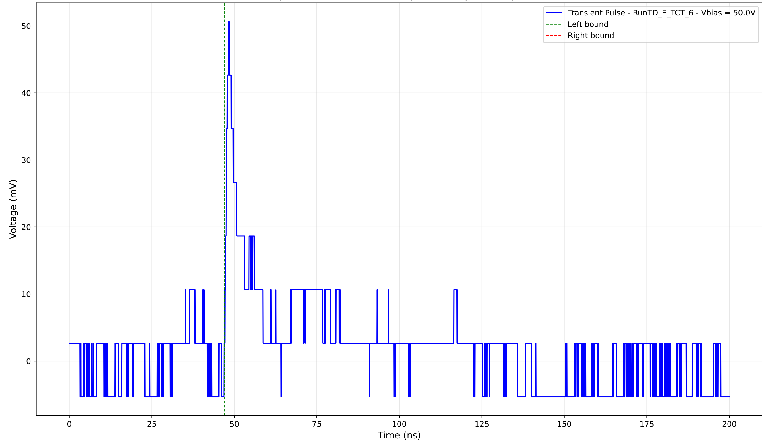
Transient Pulse - Sample: TD - Position: 270.0 \mu\text{m} - Charge: 4.67 pC - Rise Time: 1.11 ns
