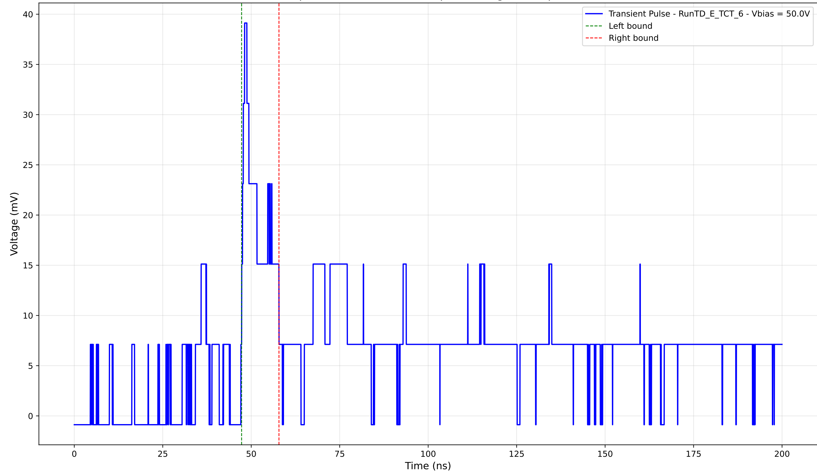
Transient Pulse - Sample: TD - Position: 265.0 \mu\text{m} - Charge: 4.31 pC - Rise Time: 1.05 ns
