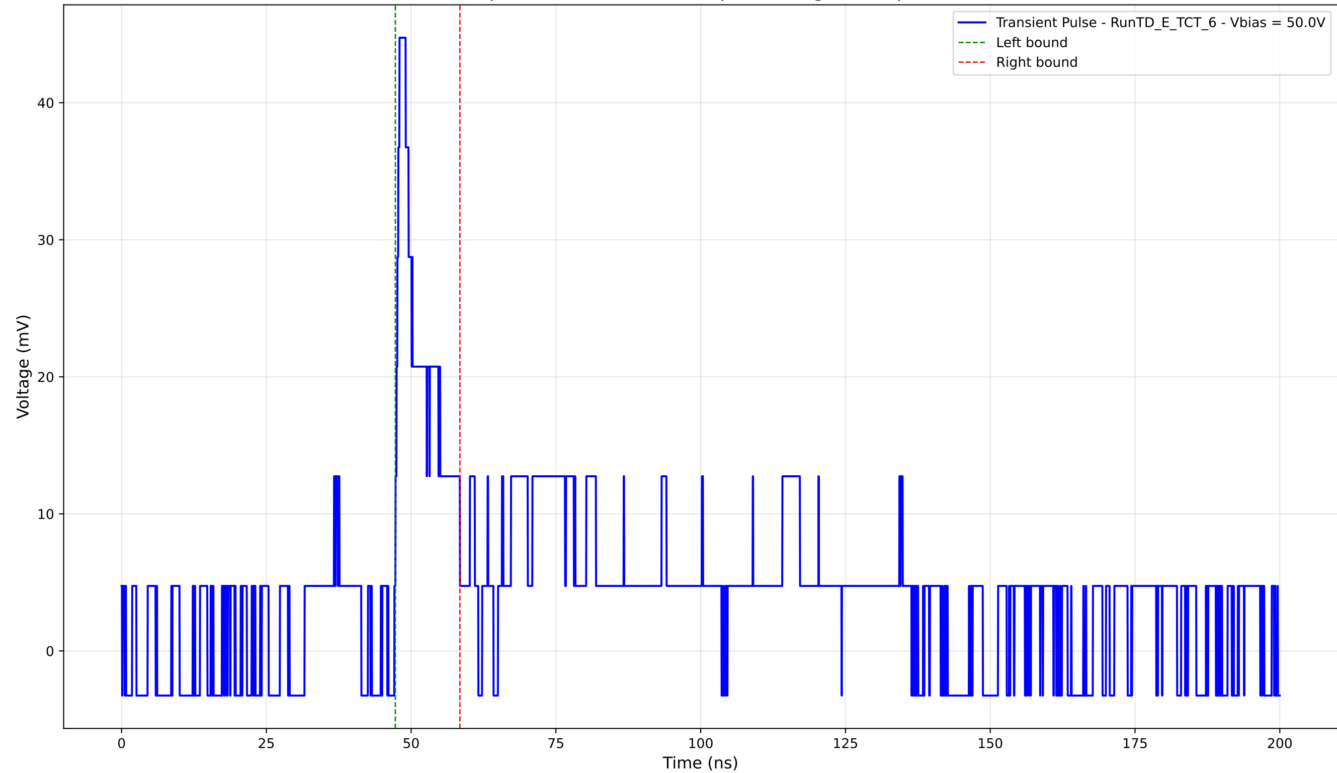
Transient Pulse - Sample: TD - Position: 320.0 \mu\text{m} - Charge: 4.88 pC - Rise Time: 0.88 ns
