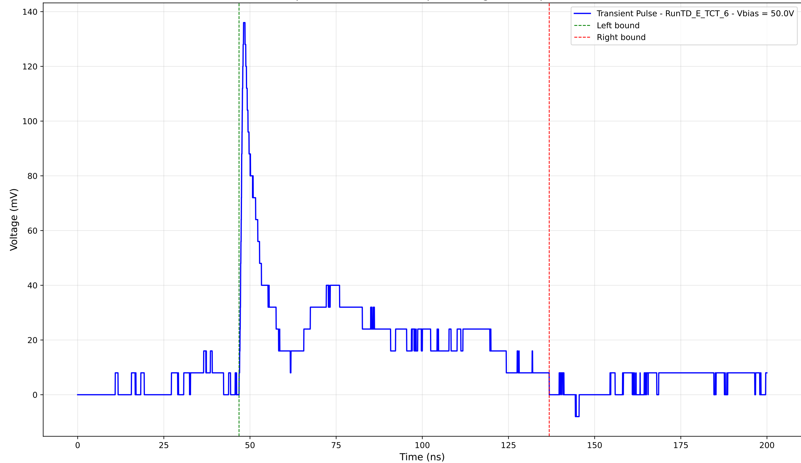
Transient Pulse - Sample: TD - Position: 90.0 \mu\text{m} - Charge: 46.82 pC - Rise Time: 1.01 ns
