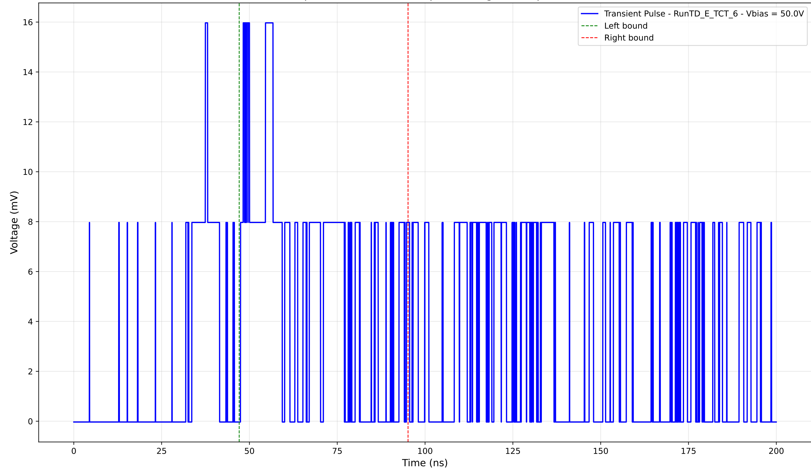
Transient Pulse - Sample: TD - Position: 0.0 \mu\text{m} - Charge: 5.36 pC - Rise Time: 3.86 ns
