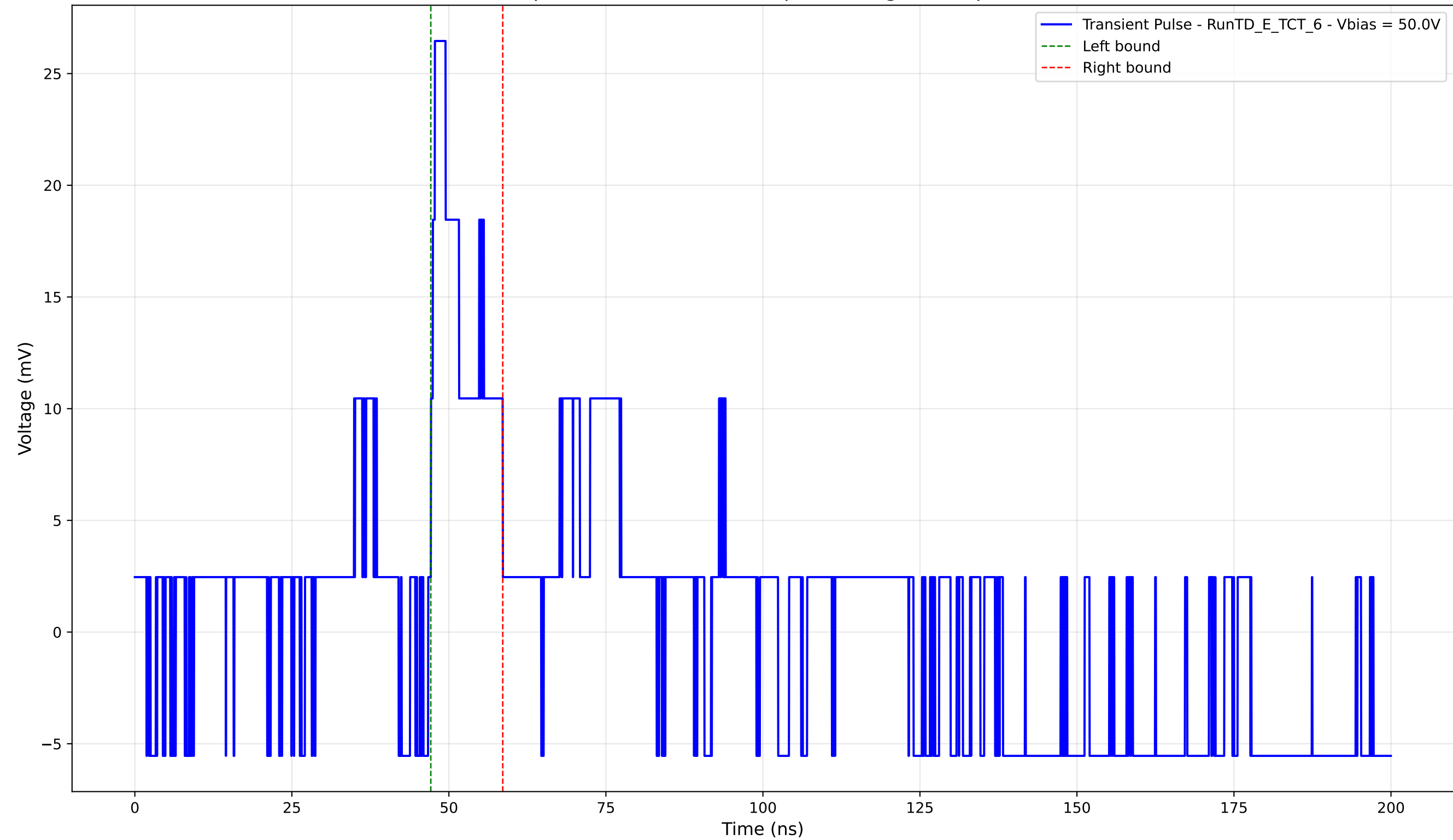
Transient Pulse - Sample: TD - Position: 305.0 \mu\text{m} - Charge: 3.41 pC - Rise Time: 0.64 ns
