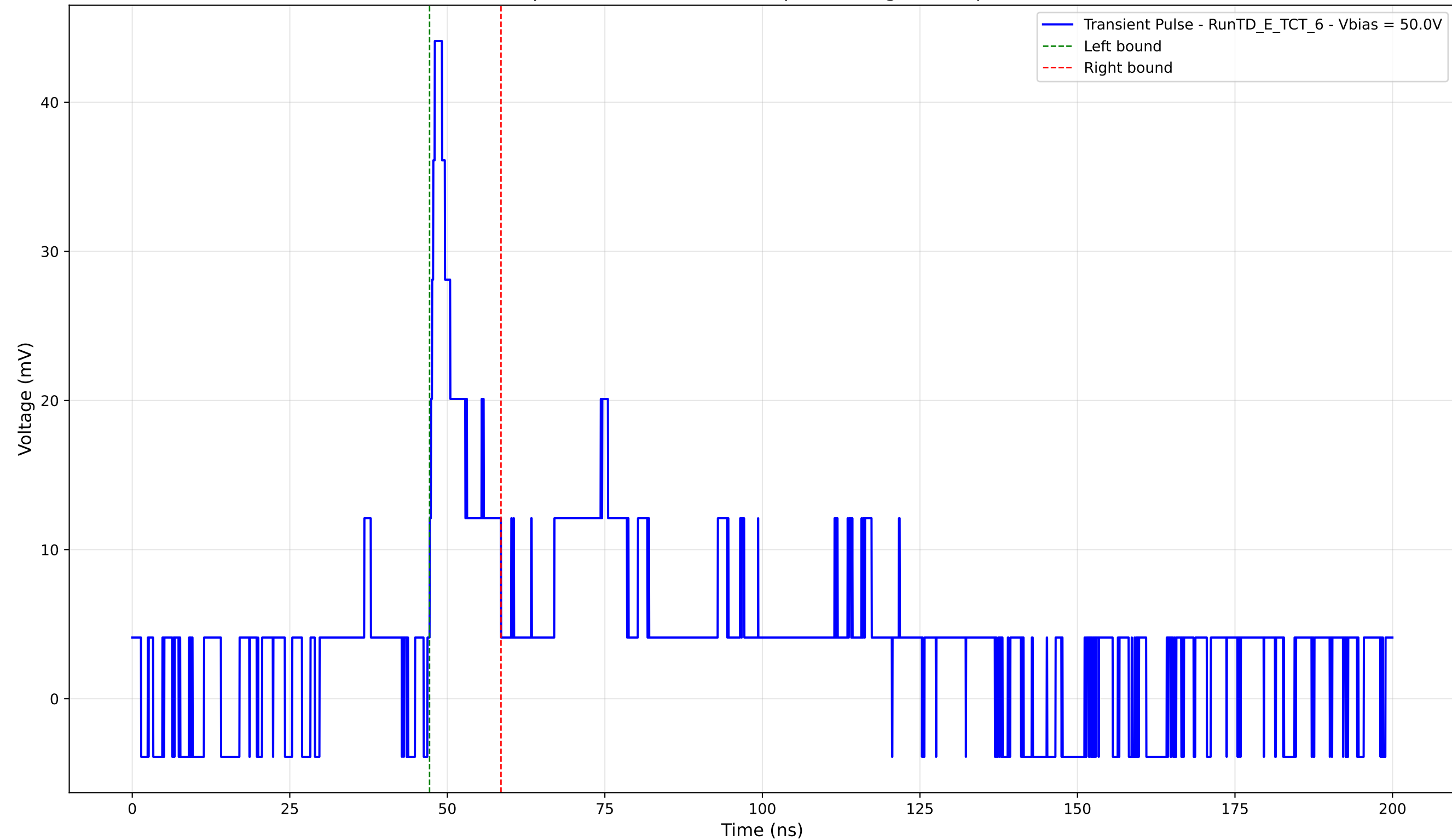
Transient Pulse - Sample: TD - Position: 280.0 \mu\text{m} - Charge: 4.61 pC - Rise Time: 0.82 ns
