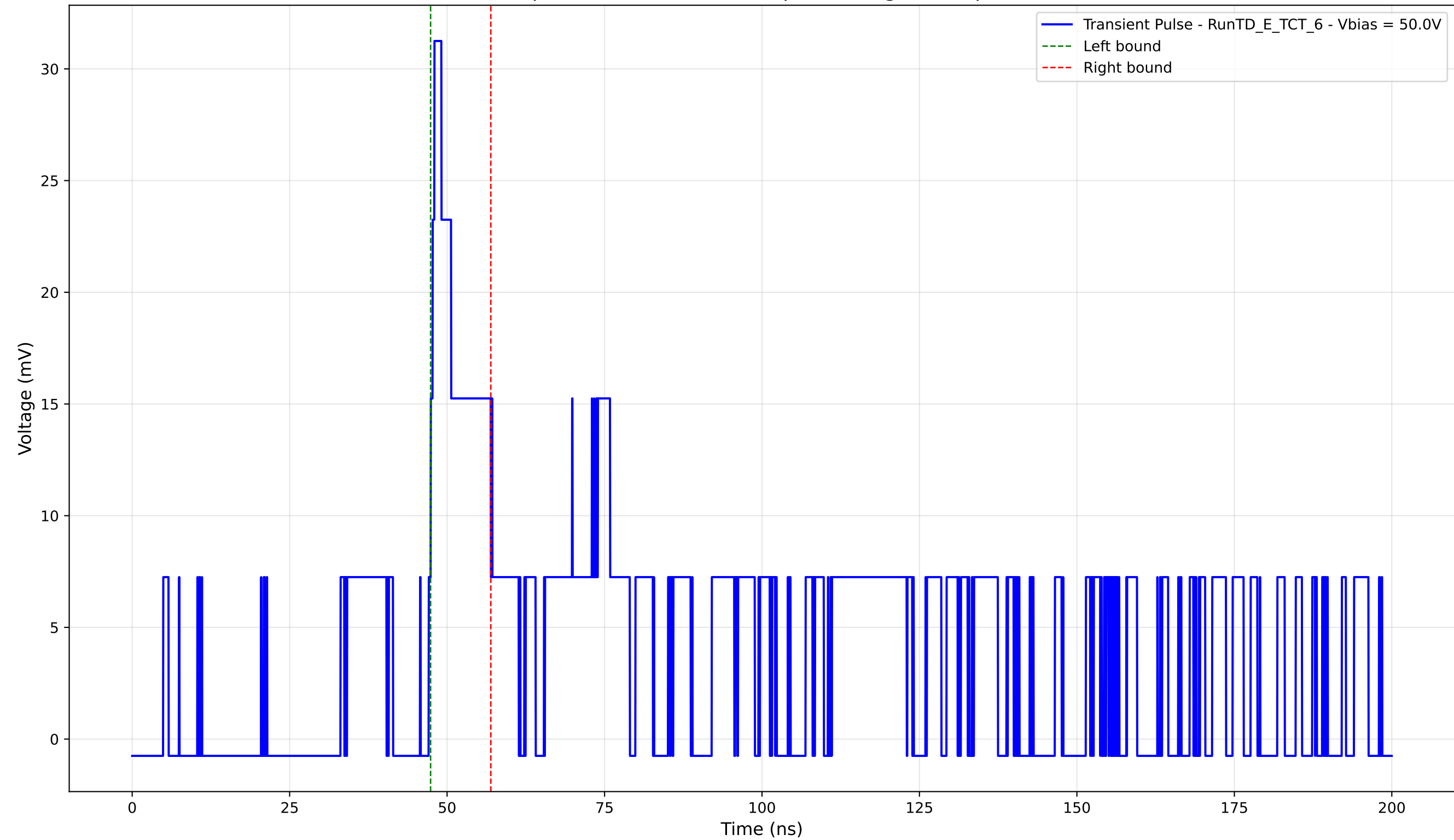
Transient Pulse - Sample: TD - Position: 300.0 \mu\text{m} - Charge: 3.56 pC - Rise Time: 0.91 ns
