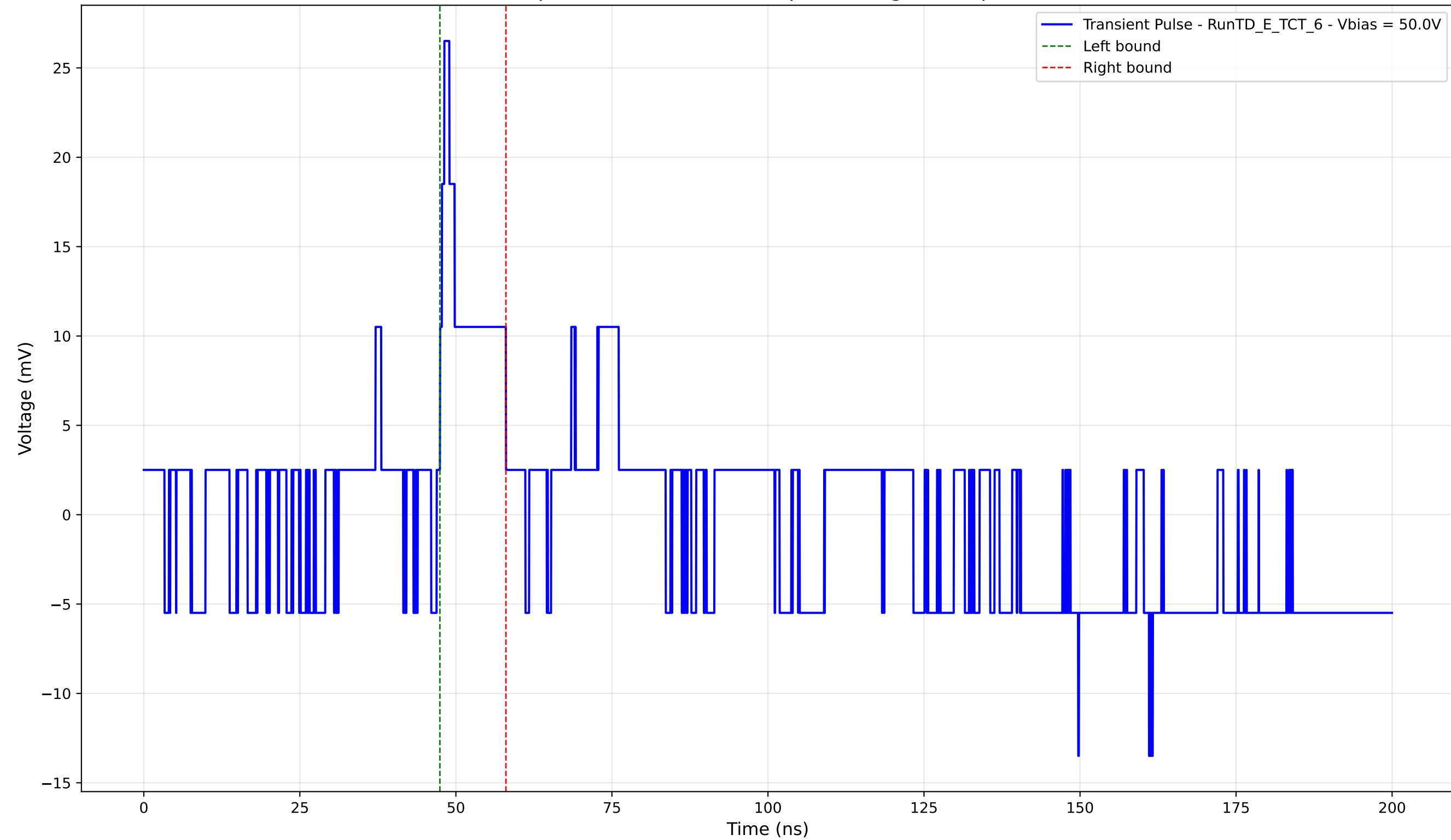
Transient Pulse - Sample: TD - Position: 325.0 \mu\text{m} - Charge: 2.68 pC - Rise Time: 0.70 ns
