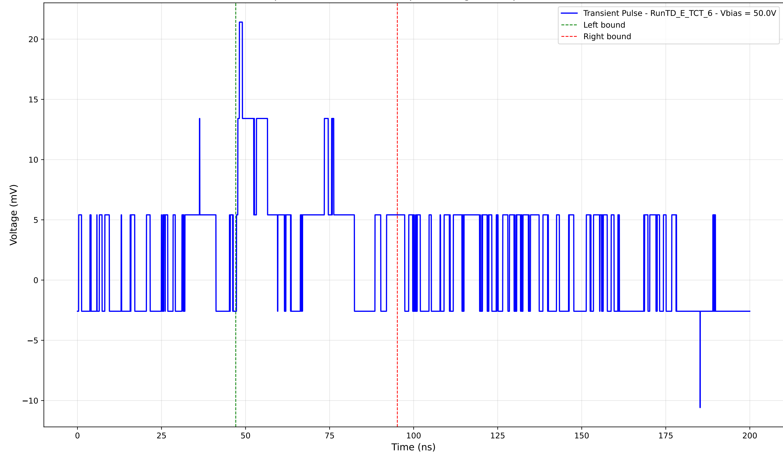
Transient Pulse - Sample: TD - Position: 350.0 \mu\text{m} - Charge: 5.11 pC - Rise Time: 0.00 ns (N/A)
