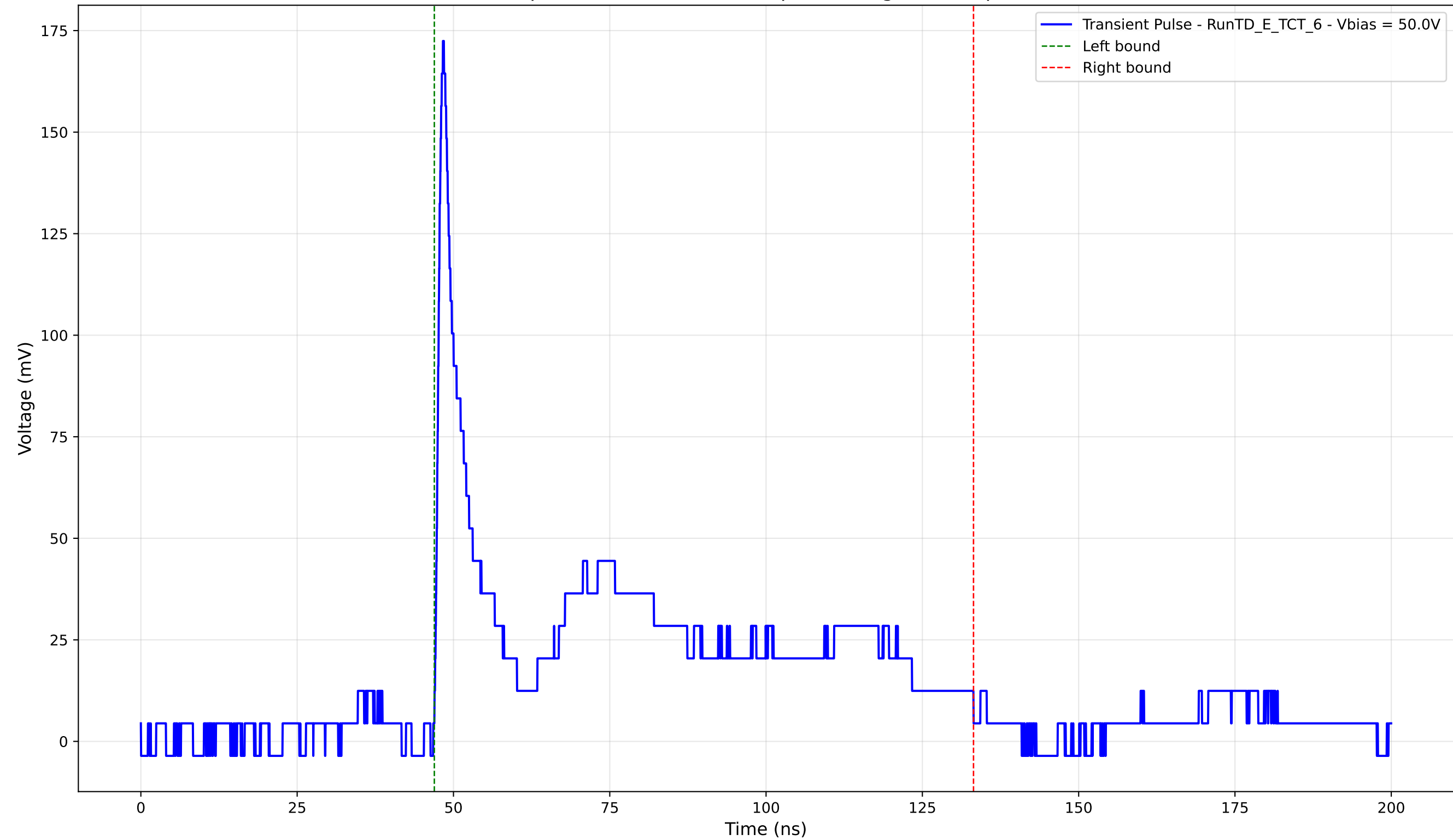
Transient Pulse - Sample: TD - Position: 140.0 \mu\text{m} - Charge: 51.92 pC - Rise Time: 0.97 ns
