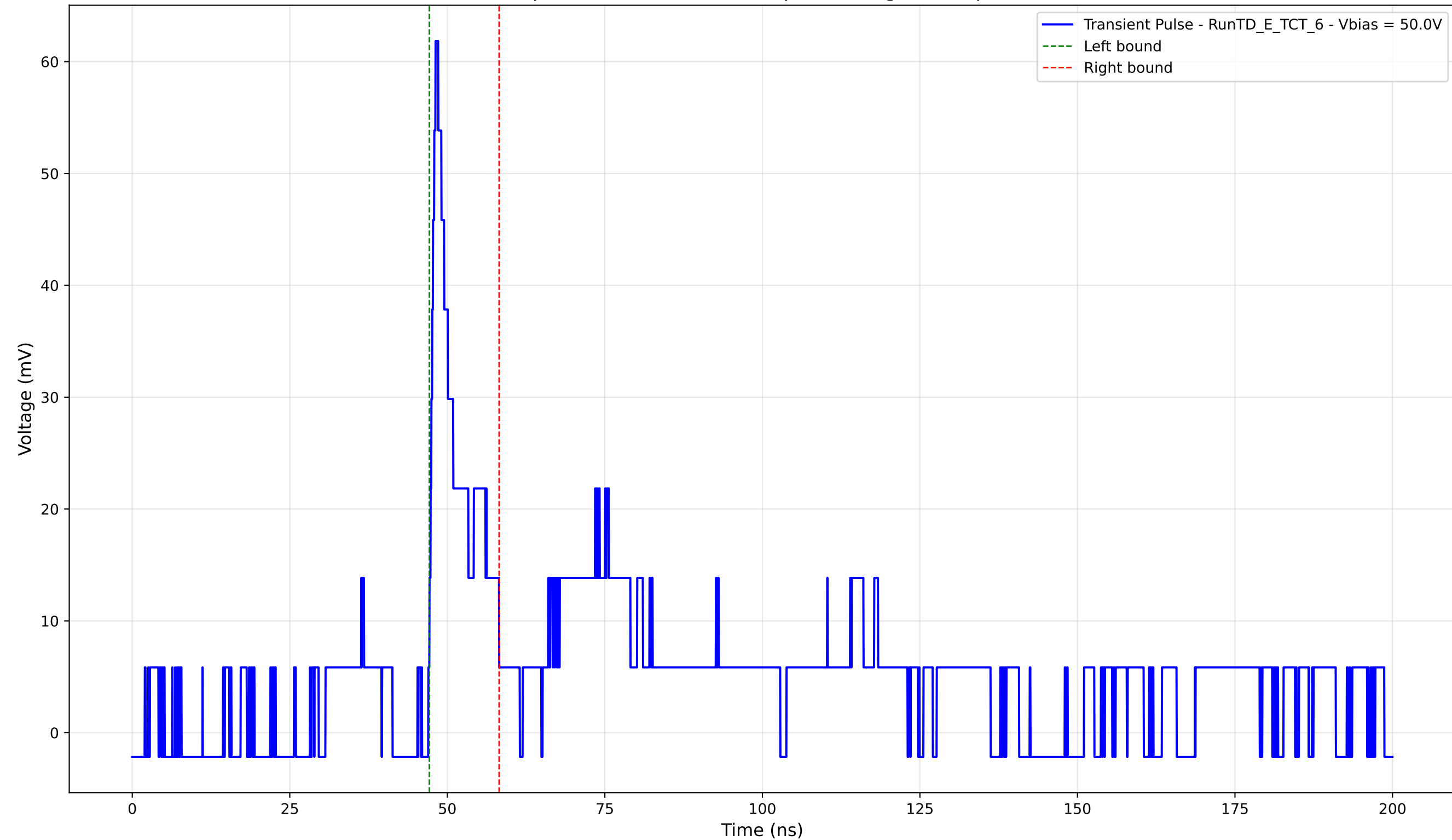
Transient Pulse - Sample: TD - Position: 275.0 \mu\text{m} - Charge: 5.82 pC - Rise Time: 0.98 ns
