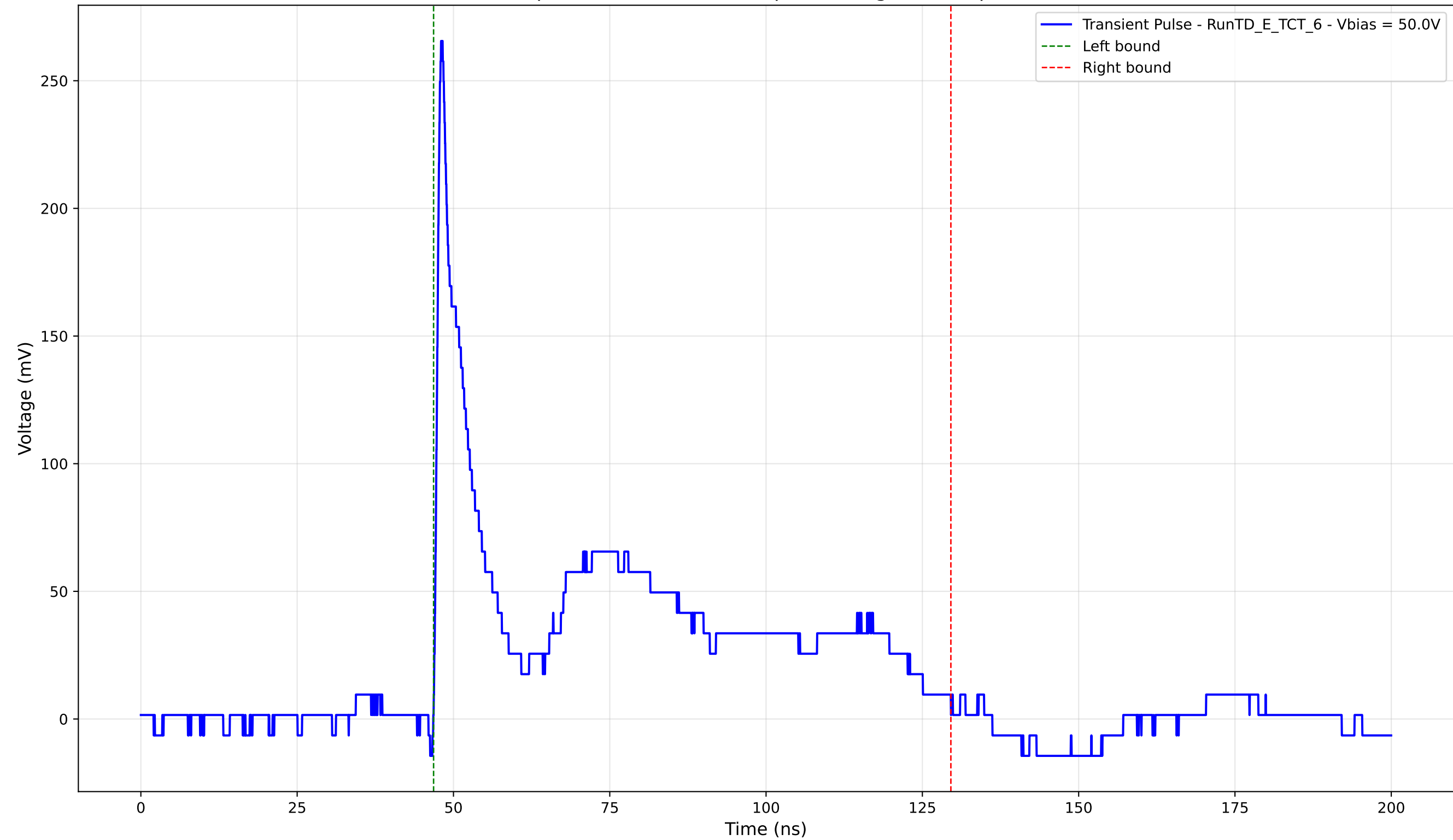
Transient Pulse - Sample: TD - Position: 75.0 \mu\text{m} - Charge: 77.88 pC - Rise Time: 0.82 ns
