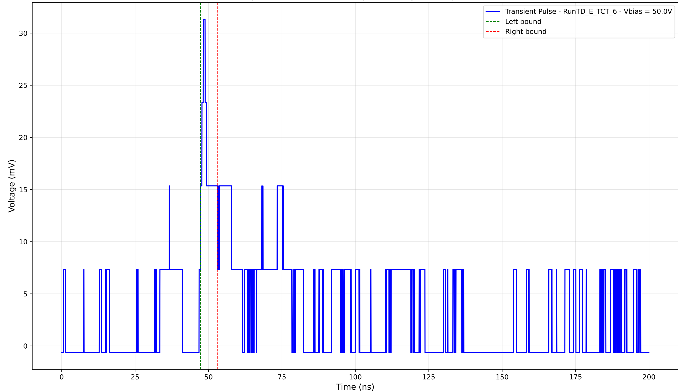
Transient Pulse - Sample: TD - Position: 25.0 \mu\text{m} - Charge: 2.15 pC - Rise Time: 1.43 ns
