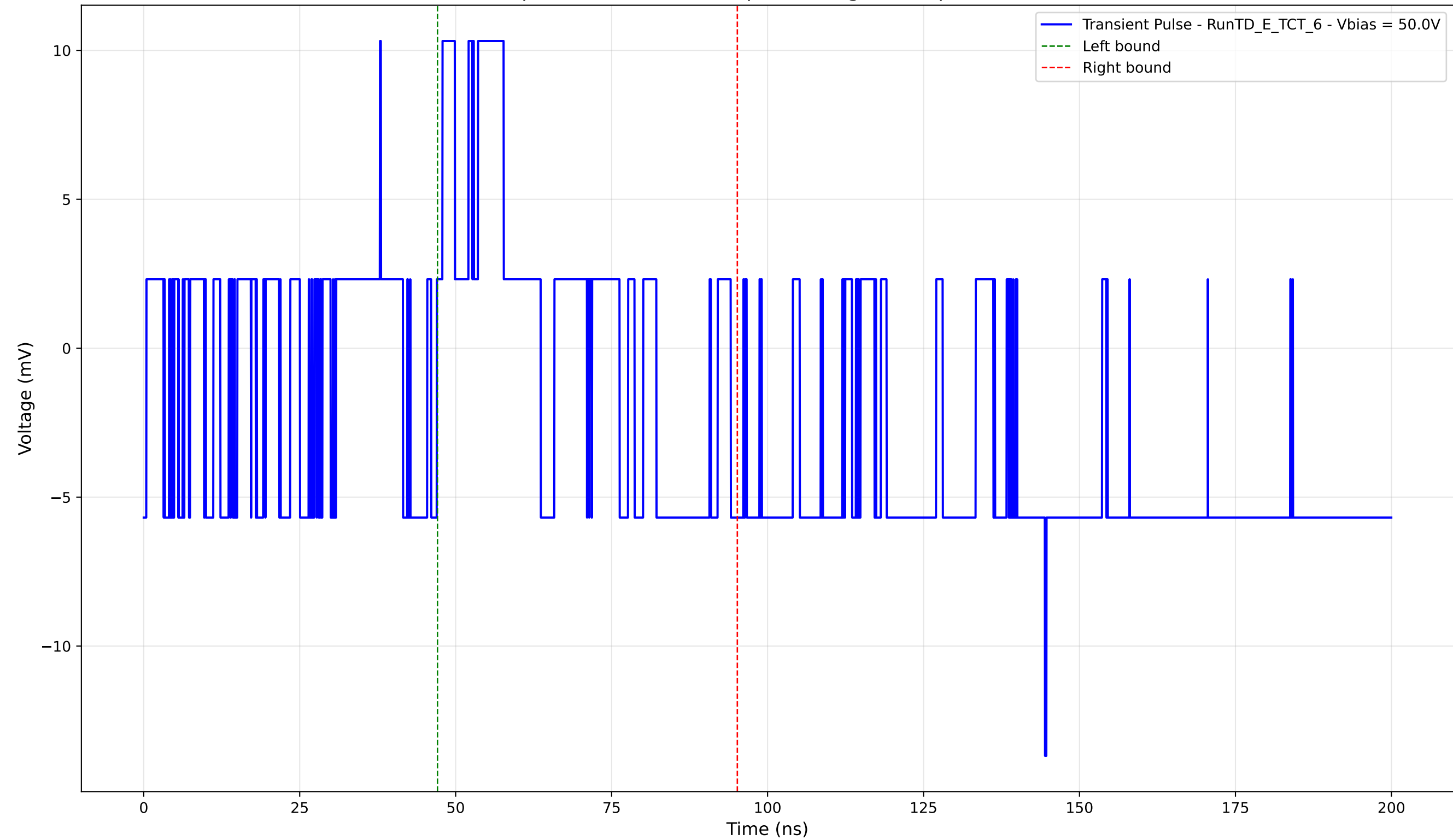
Transient Pulse - Sample: TD - Position: 5.0 \mu\text{m} - Charge: 0.82 pC - Rise Time: 0.00 ns (N/A)
