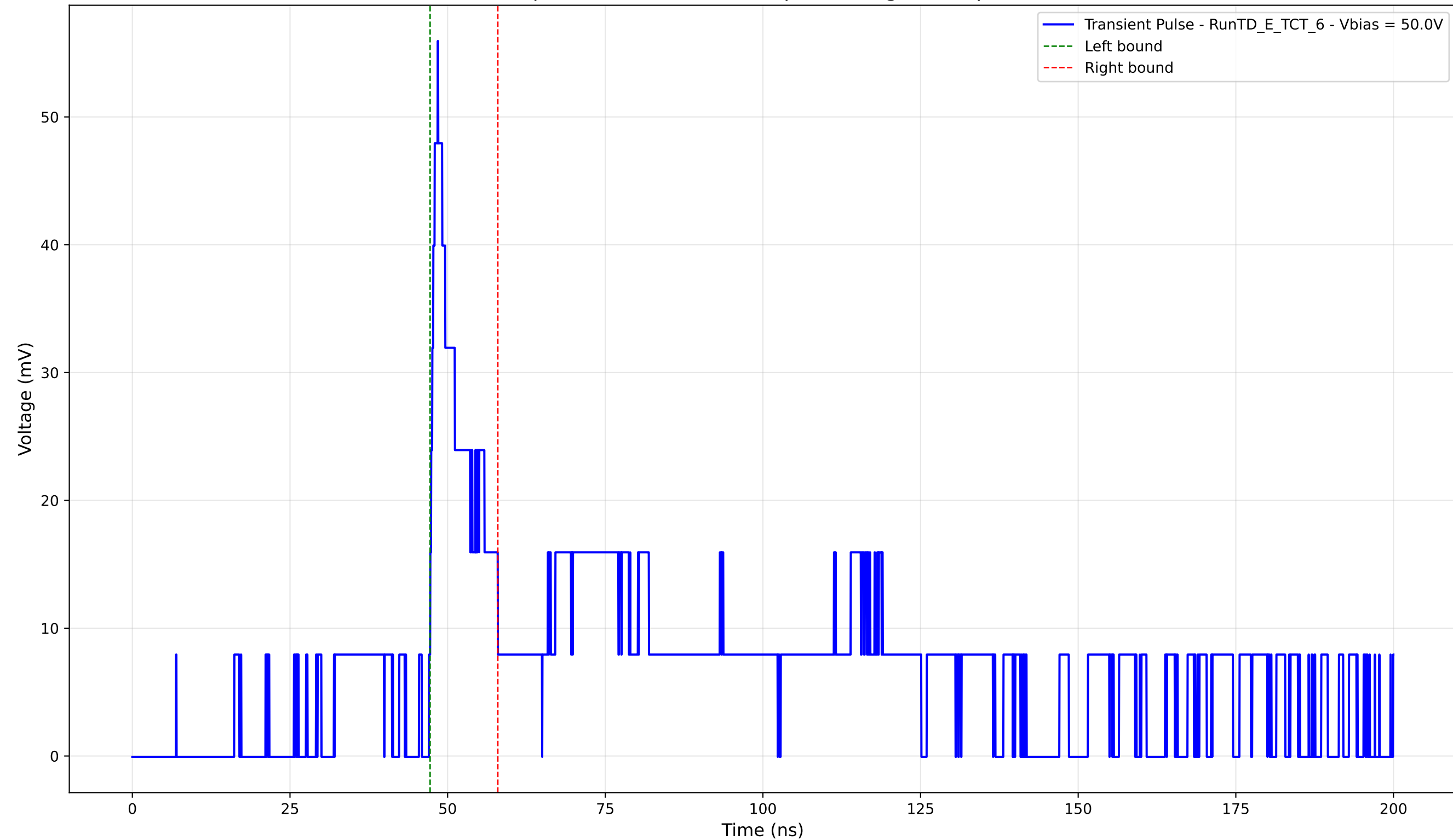
Transient Pulse - Sample: TD - Position: 240.0 \mu\text{m} - Charge: 5.70 pC - Rise Time: 1.39 ns
