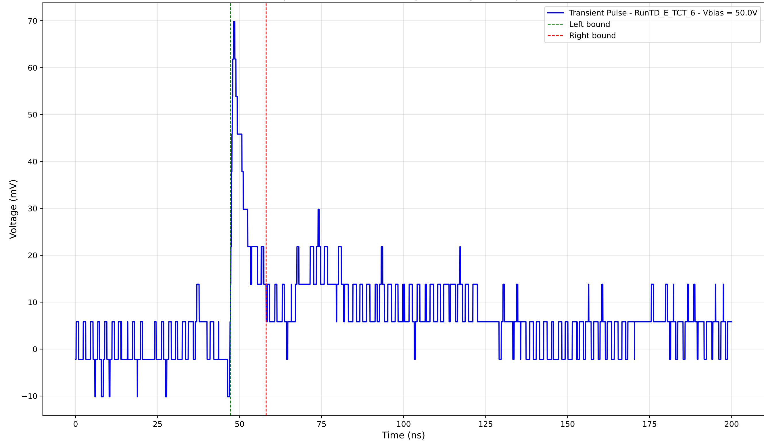
Transient Pulse - Sample: TD - Position: 190.0 \mu\text{m} - Charge: 6.69 pC - Rise Time: 0.96 ns
