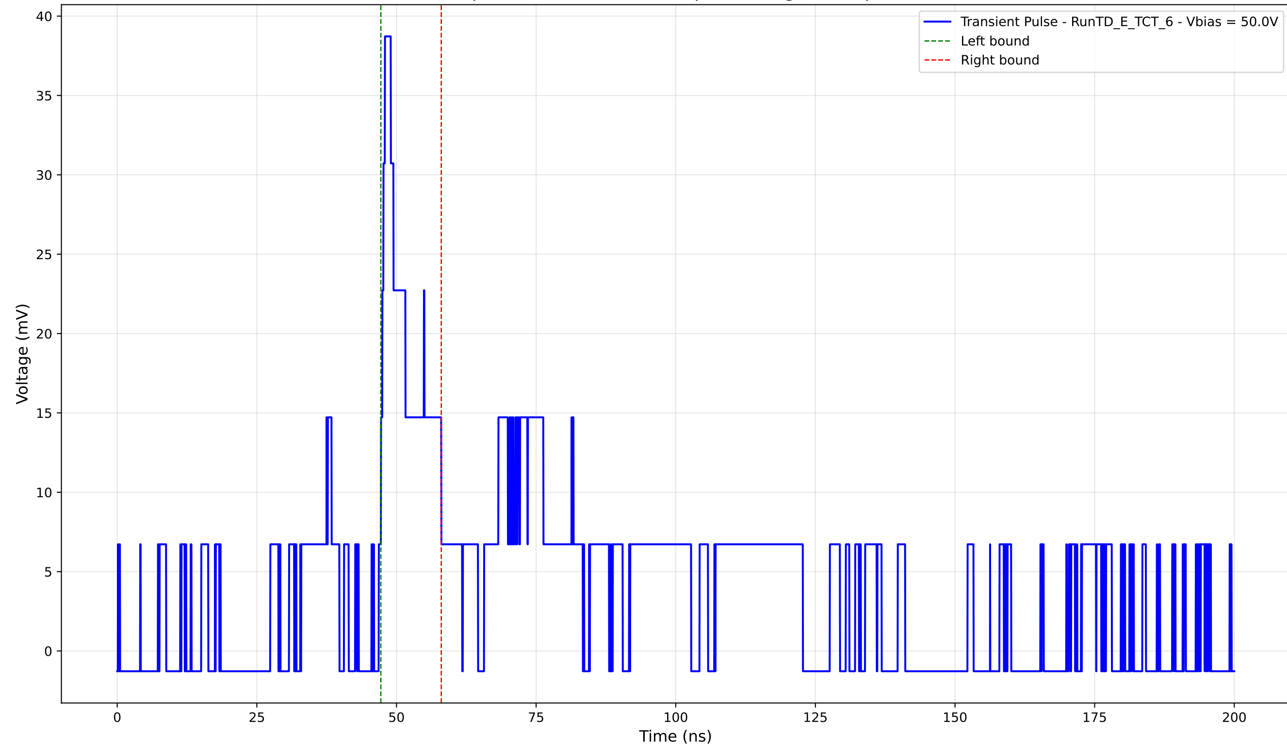
Transient Pulse - Sample: TD - Position: 335.0 \mu\text{m} - Charge: 4.32 pC - Rise Time: 1.11 ns
