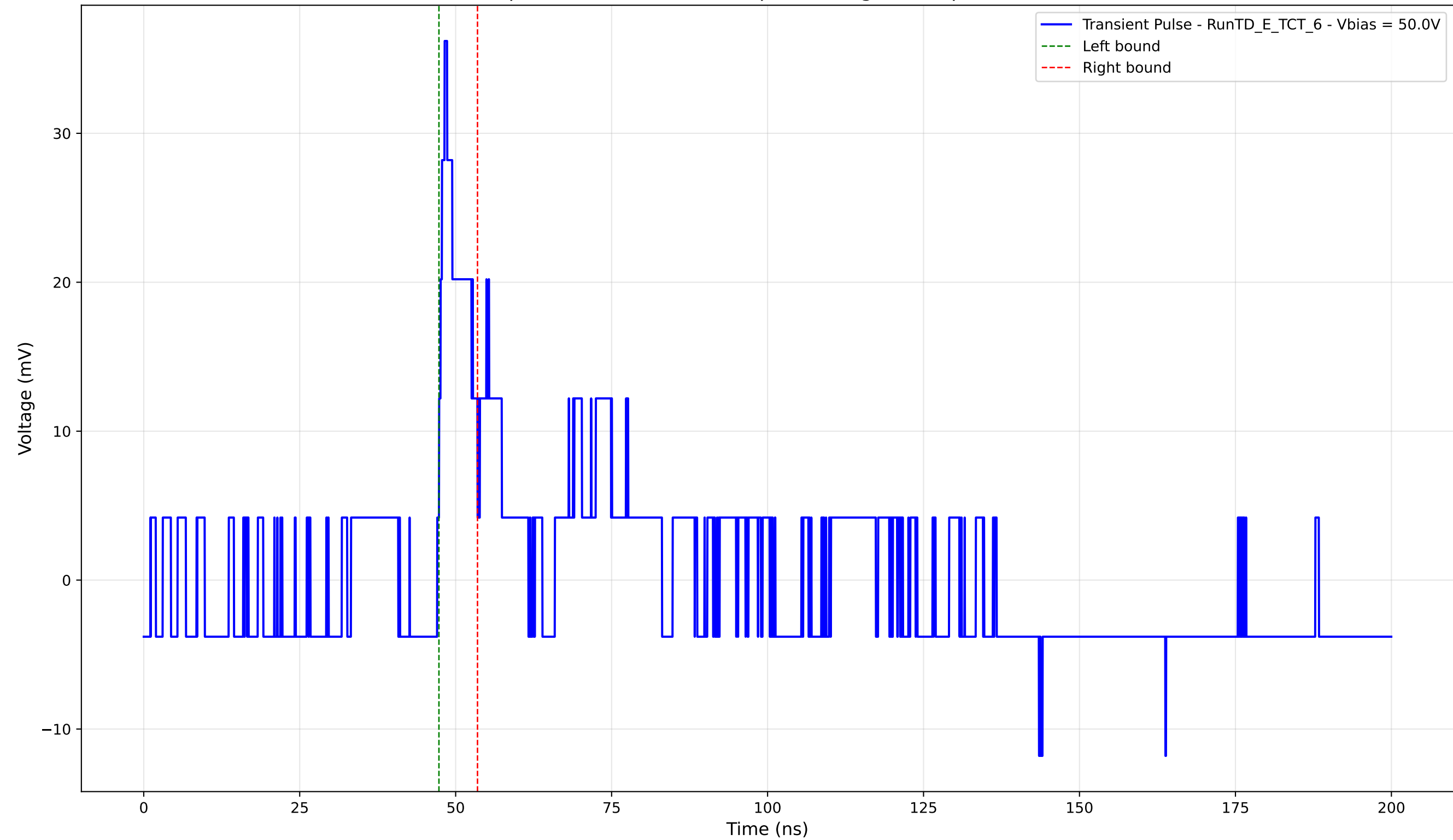
Transient Pulse - Sample: TD - Position: 385.0 \mu\text{m} - Charge: 2.64 pC - Rise Time: 0.00 ns (N/A)
