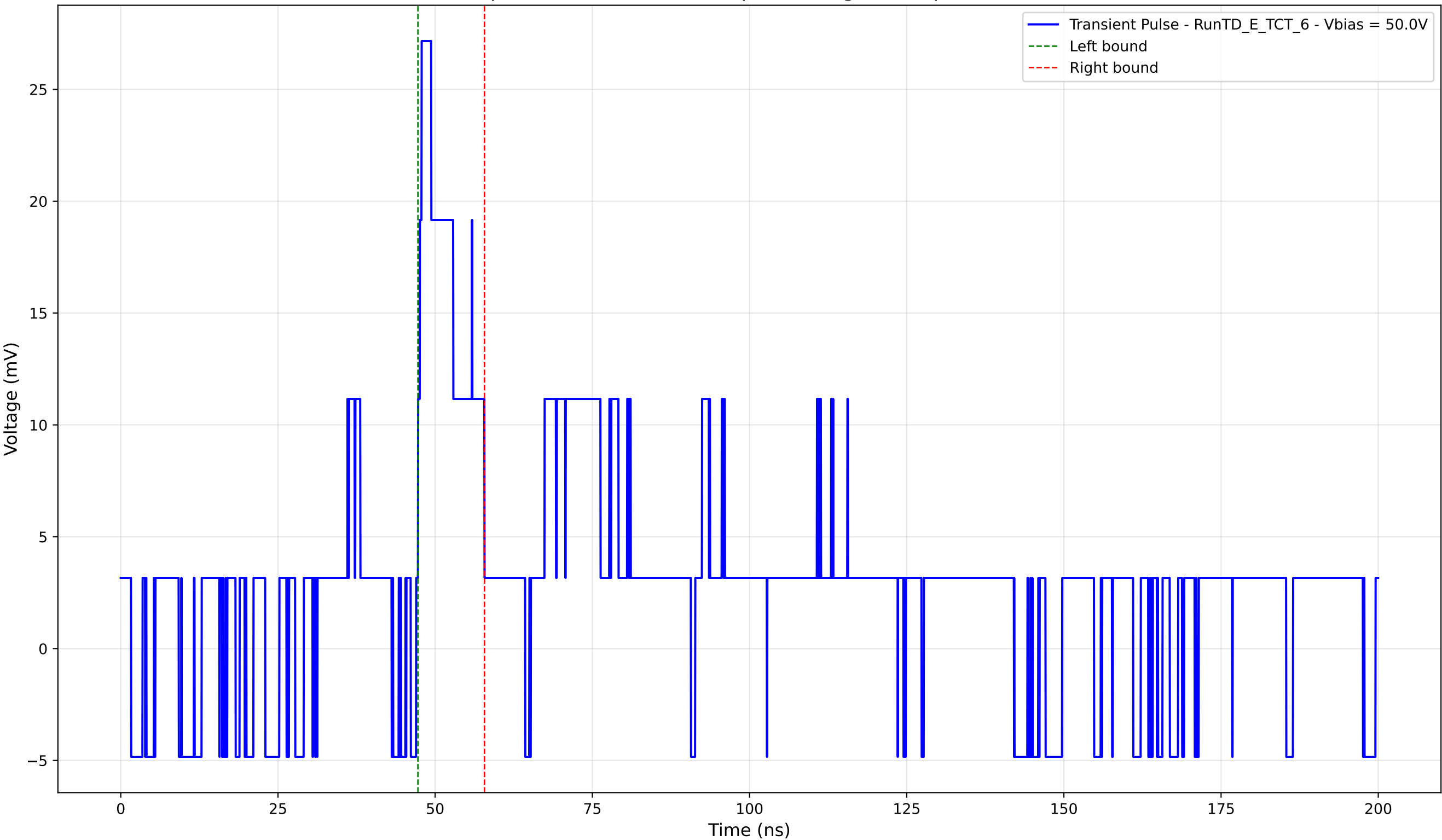
Transient Pulse - Sample: TD - Position: 390.0 \mu\text{m} - Charge: 3.47 pC - Rise Time: 0.00 ns (N/A)
