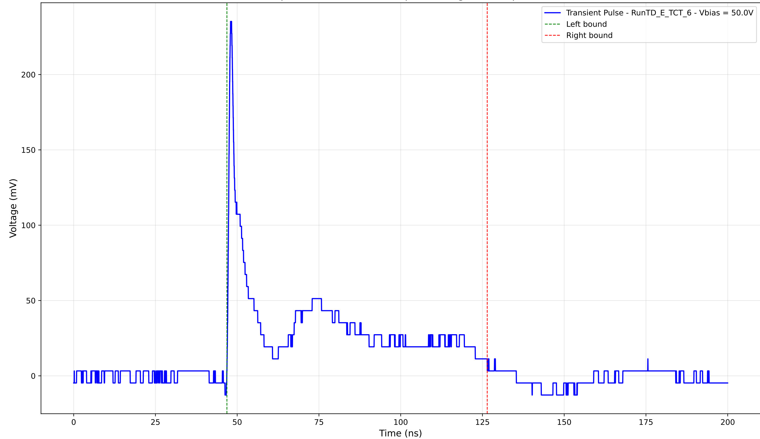
Transient Pulse - Sample: TD - Position: 40.0 \mu\text{m} - Charge: 55.37 pC - Rise Time: 0.83 ns
