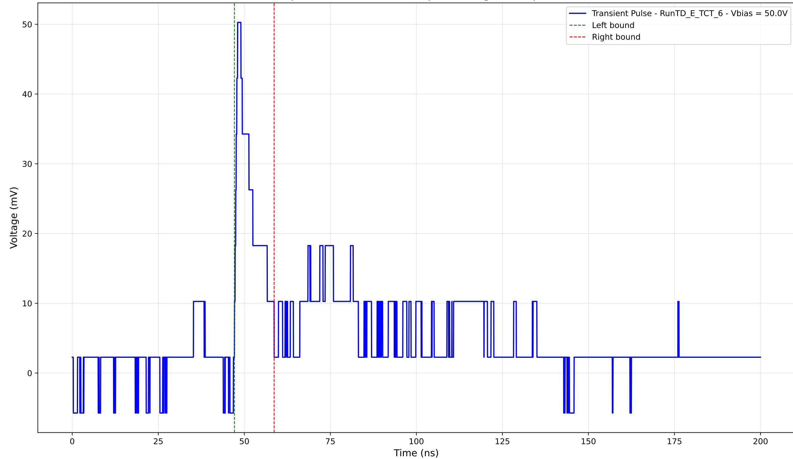
Transient Pulse - Sample: TD - Position: 155.0 \mu\text{m} - Charge: 5.66 pC - Rise Time: 0.91 ns
