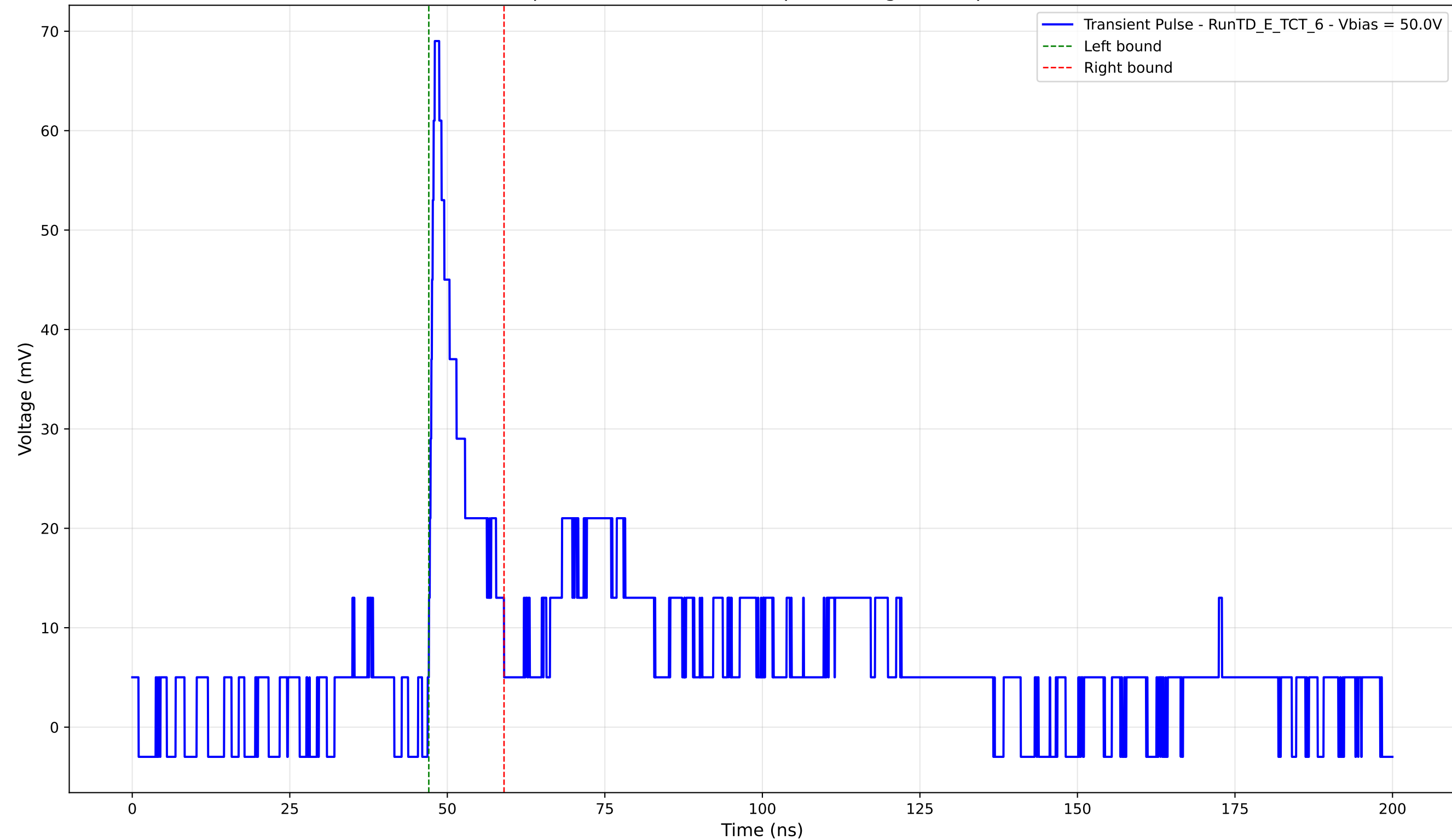
Transient Pulse - Sample: TD - Position: 225.0 \mu\text{m} - Charge: 7.28 pC - Rise Time: 0.94 ns
