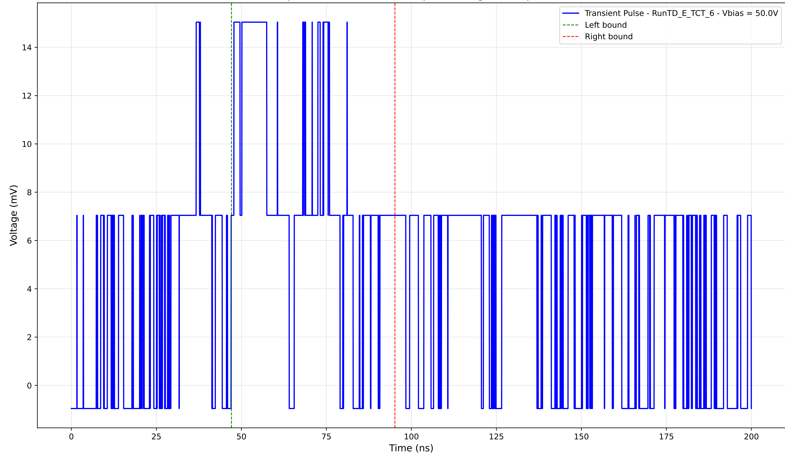
Transient Pulse - Sample: TD - Position: 360.0 \mu\text{m} - Charge: 7.84 pC - Rise Time: 5.00 ns
