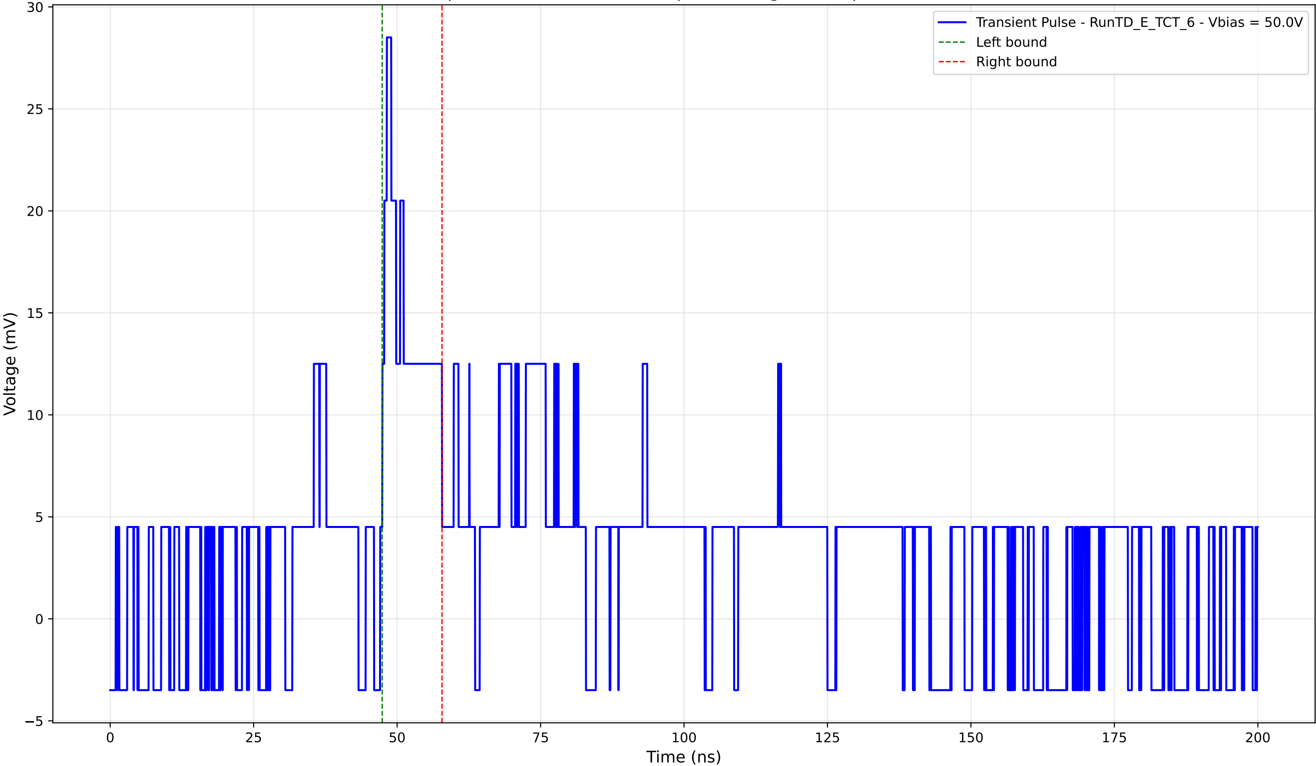
Transient Pulse - Sample: TD - Position: 400.0 \mu\text{m} - Charge: 3.16 pC - Rise Time: 0.00 ns (N/A)
