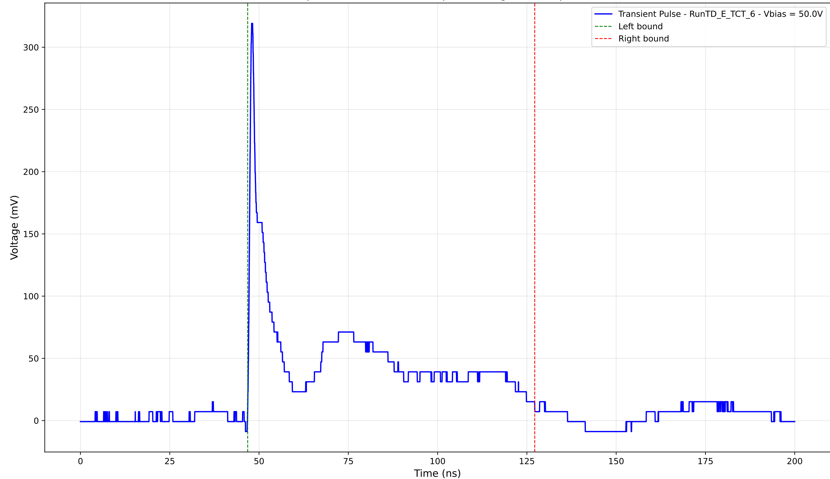
Transient Pulse - Sample: TD - Position: 65.0 \mu\text{m} - Charge: 84.59 pC - Rise Time: 0.80 ns
