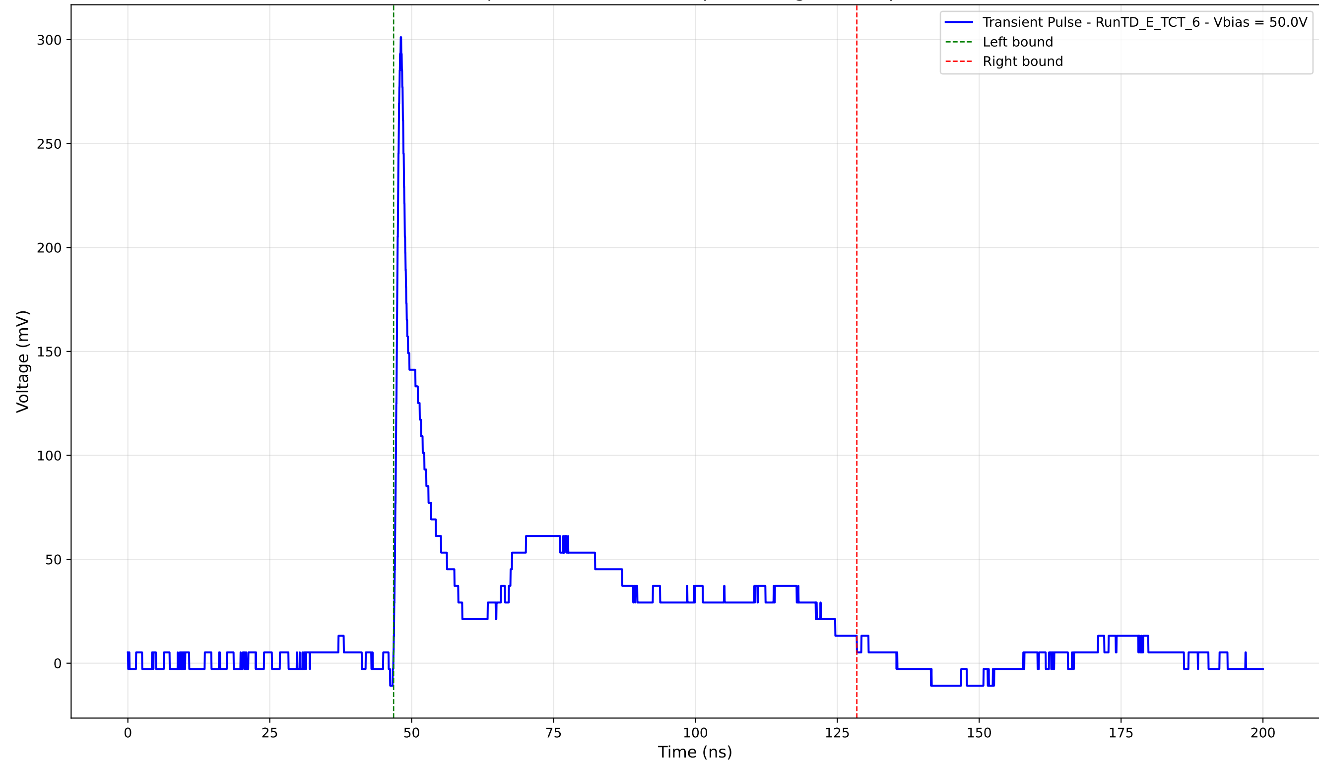
Transient Pulse - Sample: TD - Position: 45.0 \mu\text{m} - Charge: 74.60 pC - Rise Time: 0.86 ns
