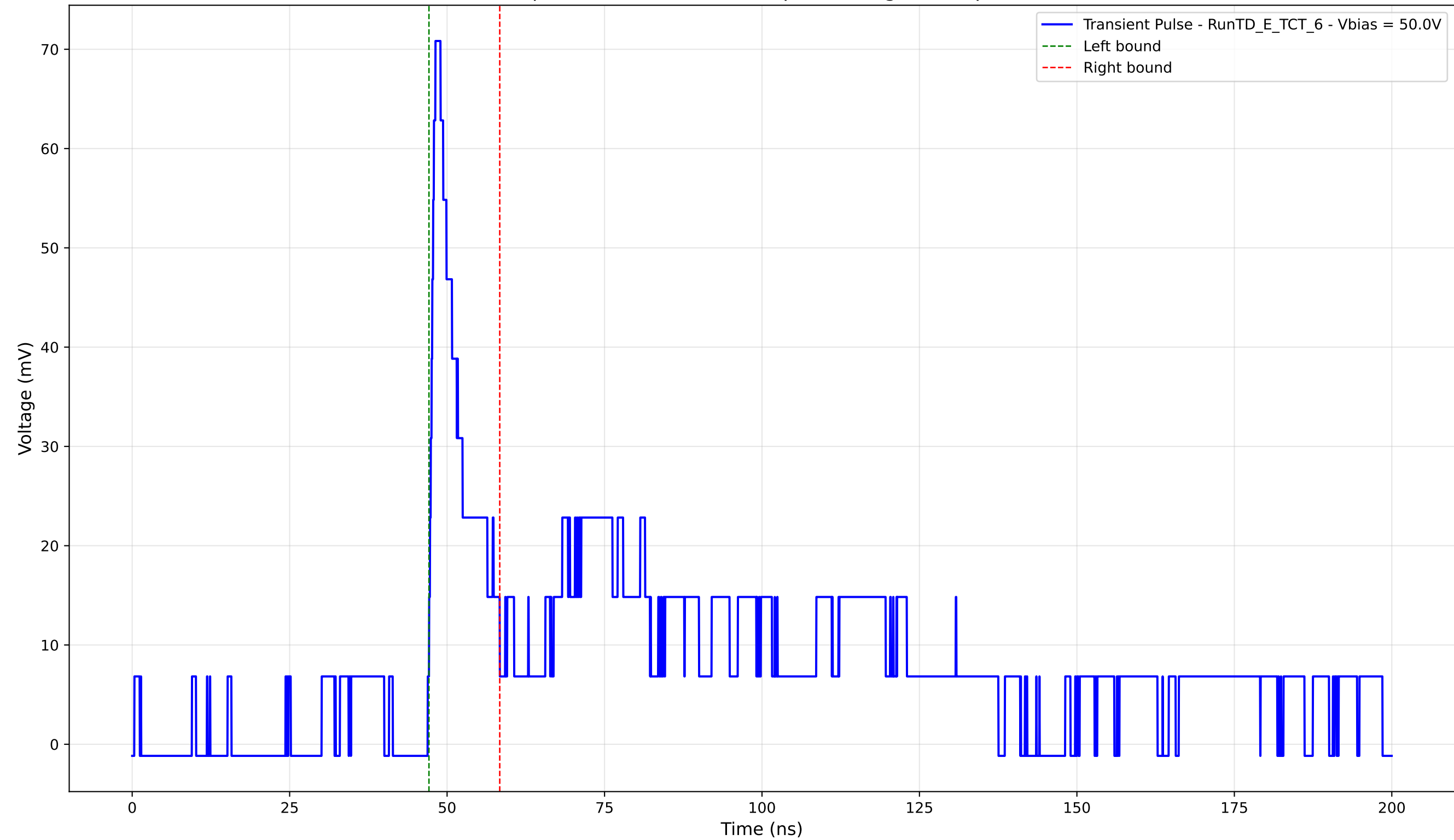
Transient Pulse - Sample: TD - Position: 180.0 \mu\text{m} - Charge: 7.49 pC - Rise Time: 1.02 ns
