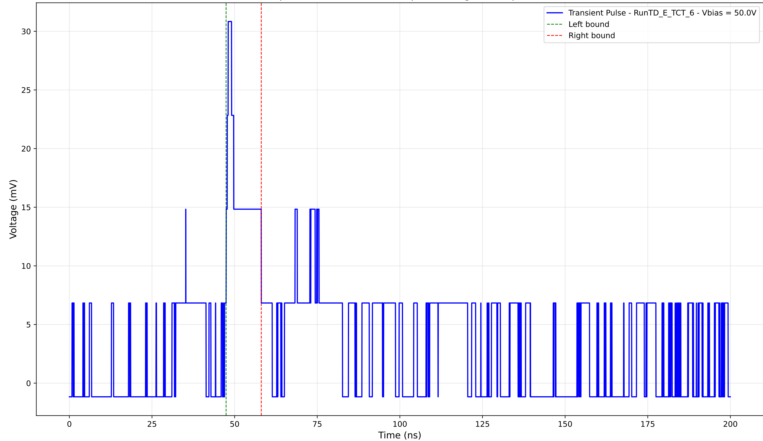
Transient Pulse - Sample: TD - Position: 330.0 \mu\text{m} - Charge: 3.63 pC - Rise Time: 1.09 ns
