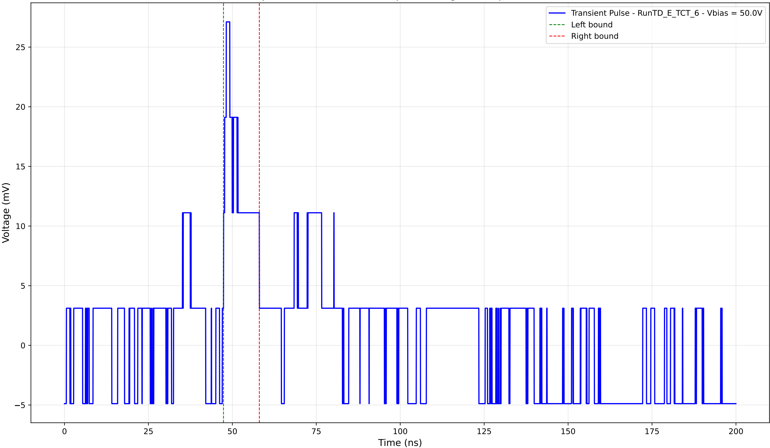
Transient Pulse - Sample: TD - Position: 395.0 \mu\text{m} - Charge: 3.13 pC - Rise Time: 0.00 ns (N/A)
