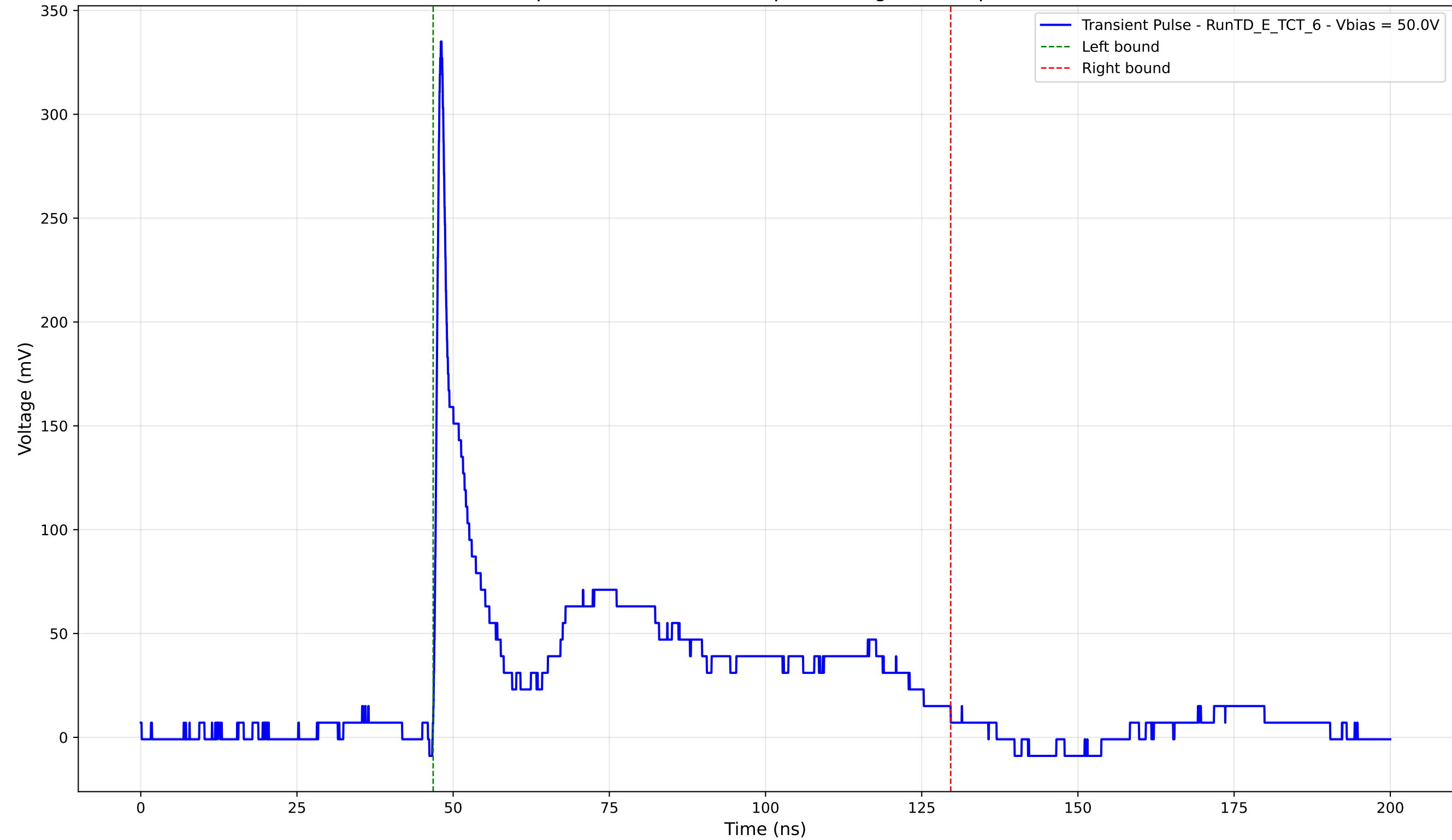
Transient Pulse - Sample: TD - Position: 60.0 \mu\text{m} - Charge: 86.50 pC - Rise Time: 0.83 ns
