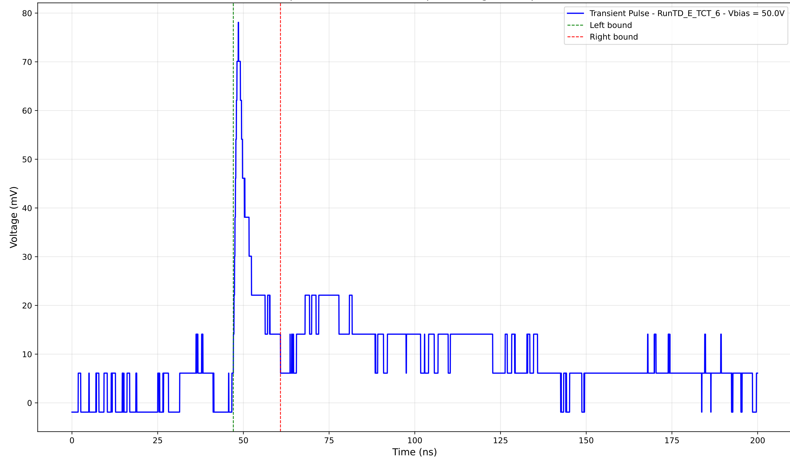
Transient Pulse - Sample: TD - Position: 185.0 \mu\text{m} - Charge: 8.04 pC - Rise Time: 1.44 ns
