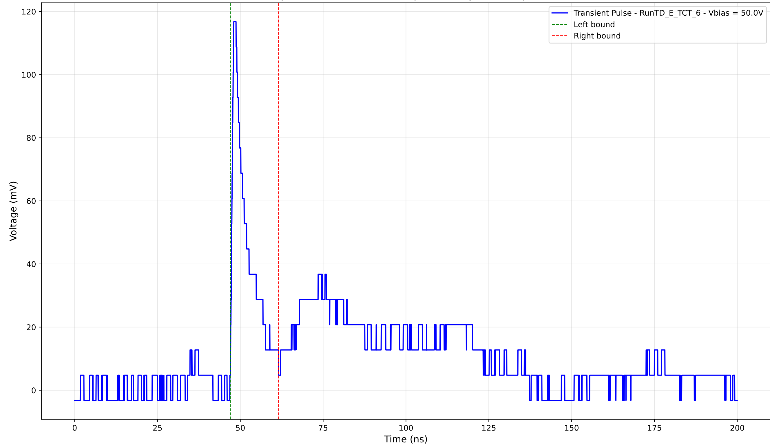
Transient Pulse - Sample: TD - Position: 200.0 \mu\text{m} - Charge: 12.33 pC - Rise Time: 0.92 ns
