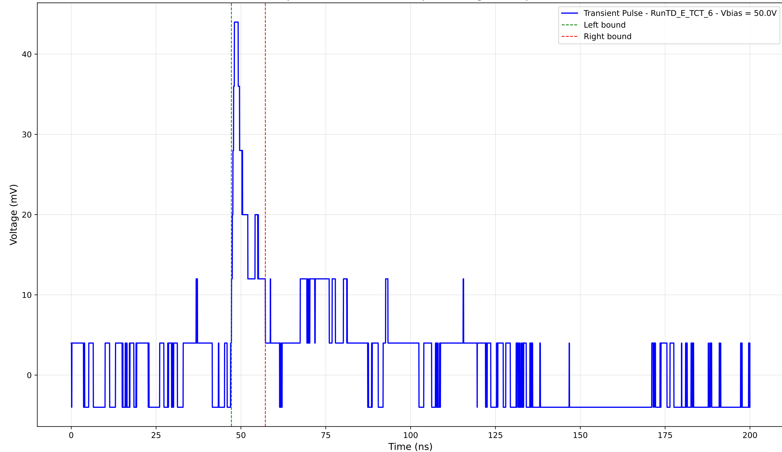
Transient Pulse - Sample: TD - Position: 255.0 \mu\text{m} - Charge: 4.17 pC - Rise Time: 0.86 ns
