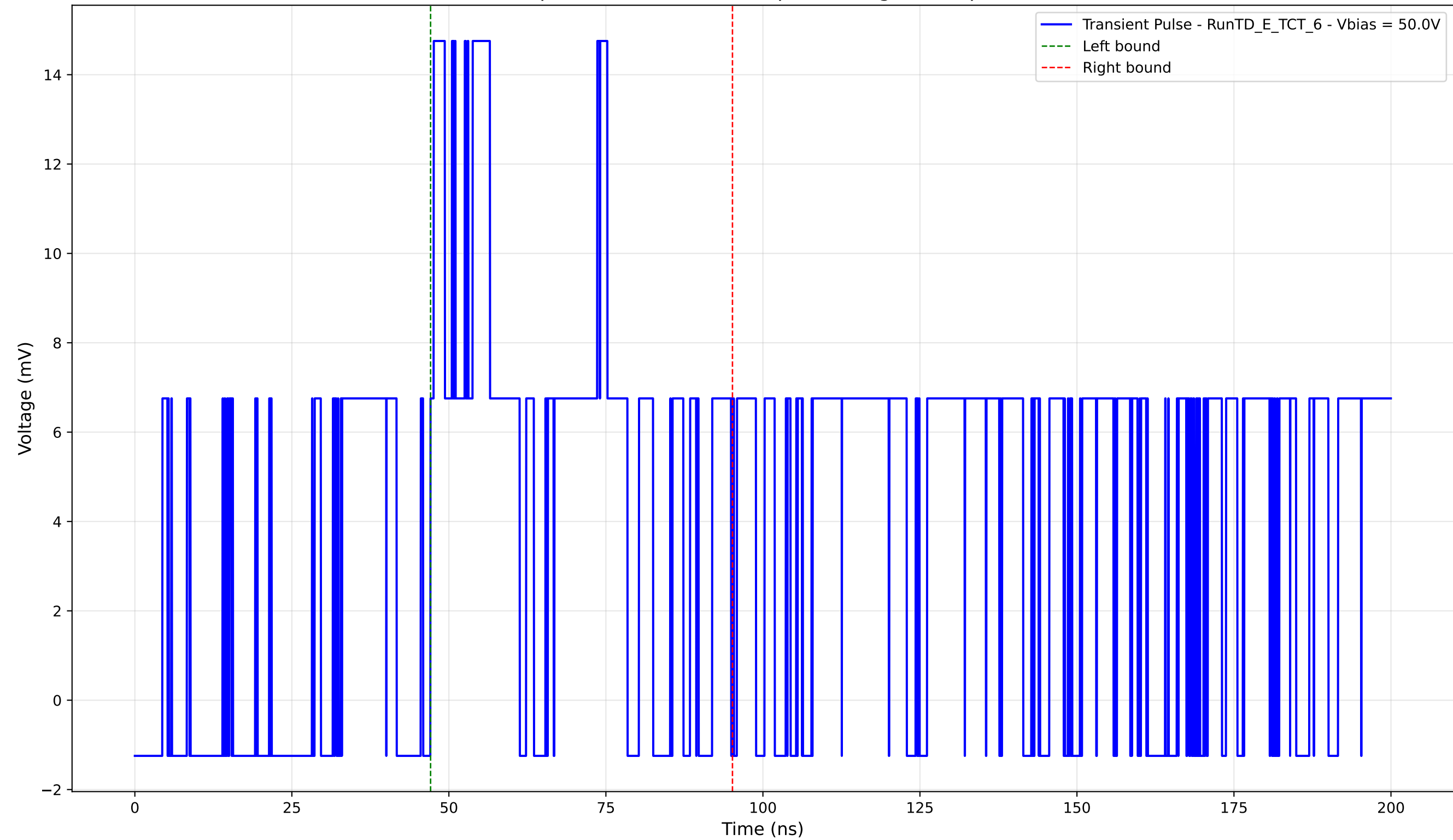
Transient Pulse - Sample: TD - Position: 10.0 \mu\text{m} - Charge: 5.74 pC - Rise Time: 0.54 ns
