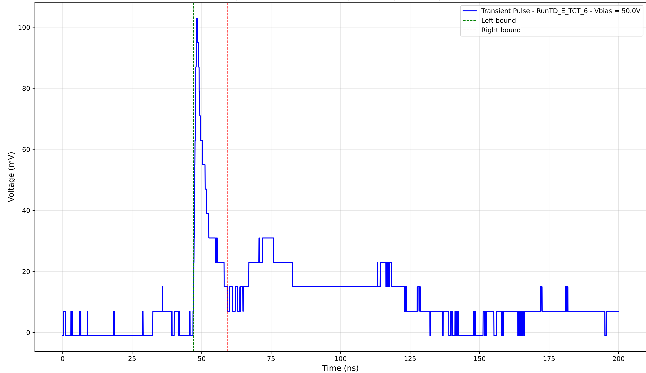
Transient Pulse - Sample: TD - Position: 175.0 \mu\text{m} - Charge: 10.16 pC - Rise Time: 0.97 ns
