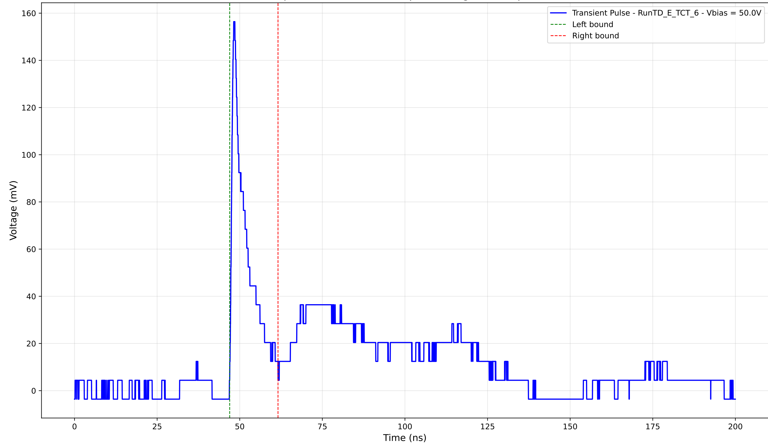
Transient Pulse - Sample: TD - Position: 95.0 \mu\text{m} - Charge: 15.78 pC - Rise Time: 0.95 ns
