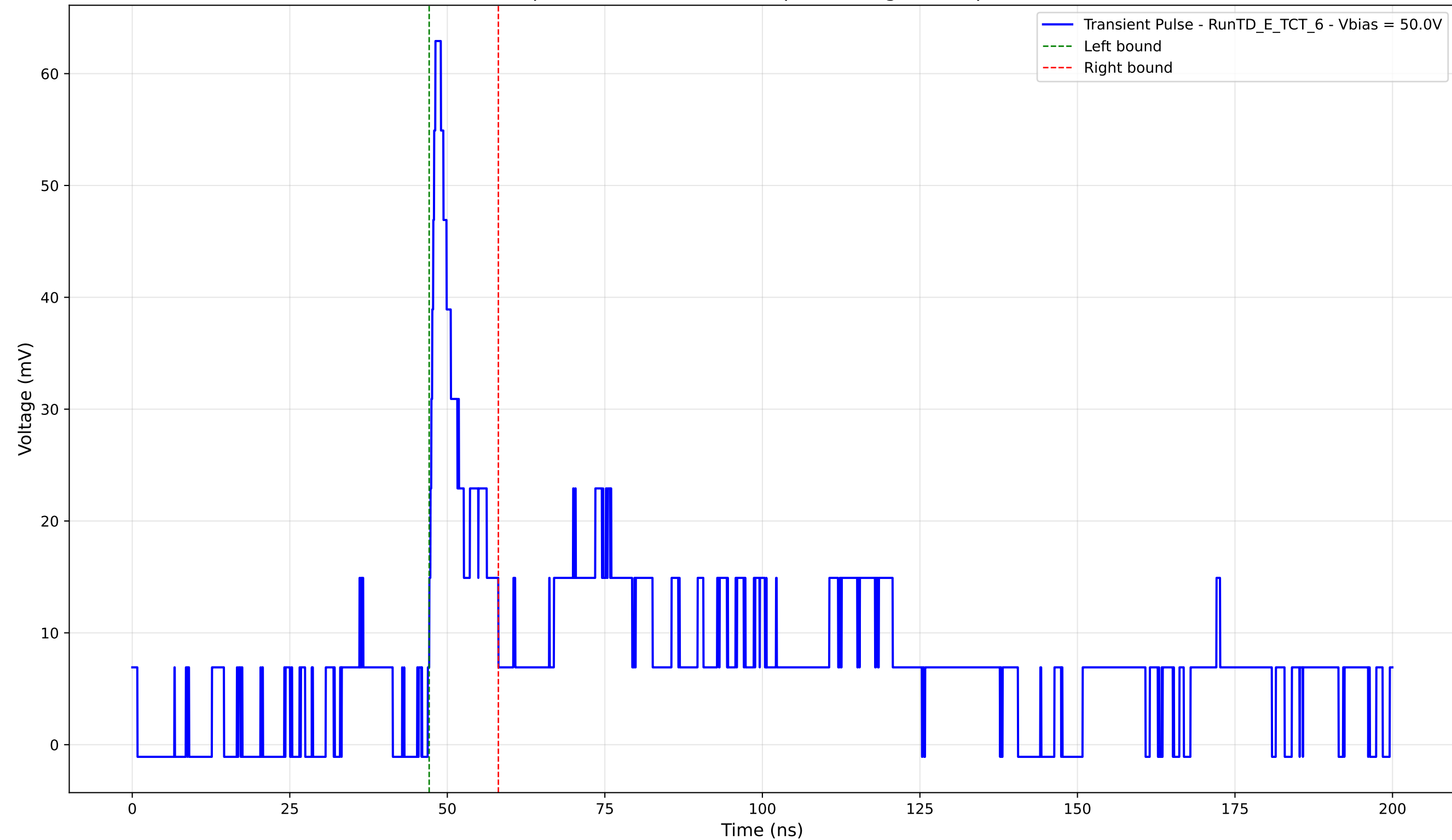
Transient Pulse - Sample: TD - Position: 315.0 \mu\text{m} - Charge: 6.41 pC - Rise Time: 1.20 ns
