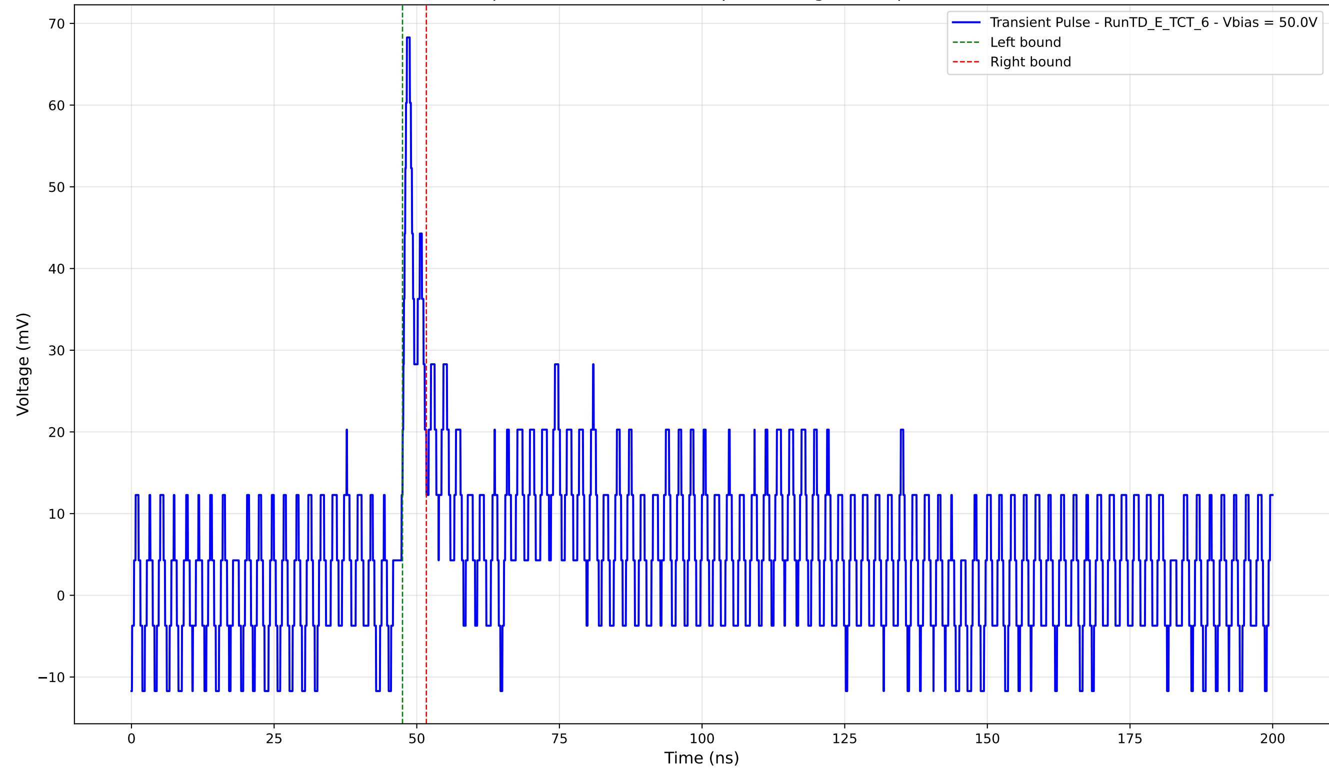
Transient Pulse - Sample: TD - Position: 220.0 \mu\text{m} - Charge: 3.46 pC - Rise Time: 0.93 ns
