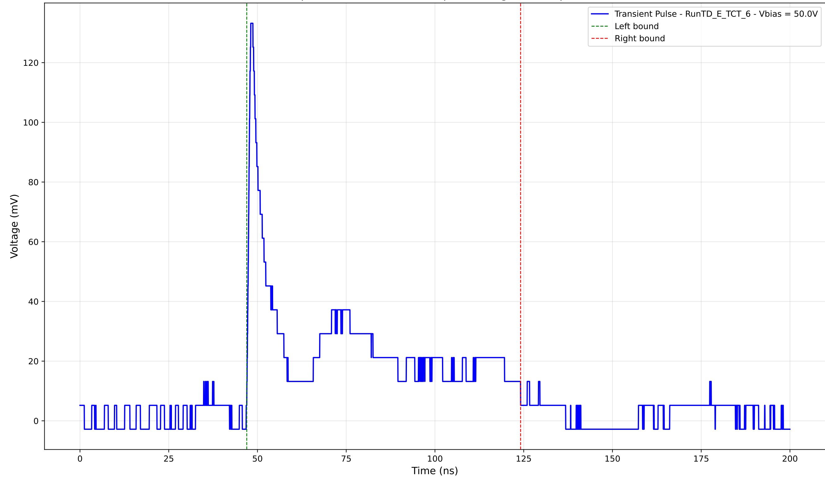
Transient Pulse - Sample: TD - Position: 145.0 \mu\text{m} - Charge: 40.41 pC - Rise Time: 0.94 ns
