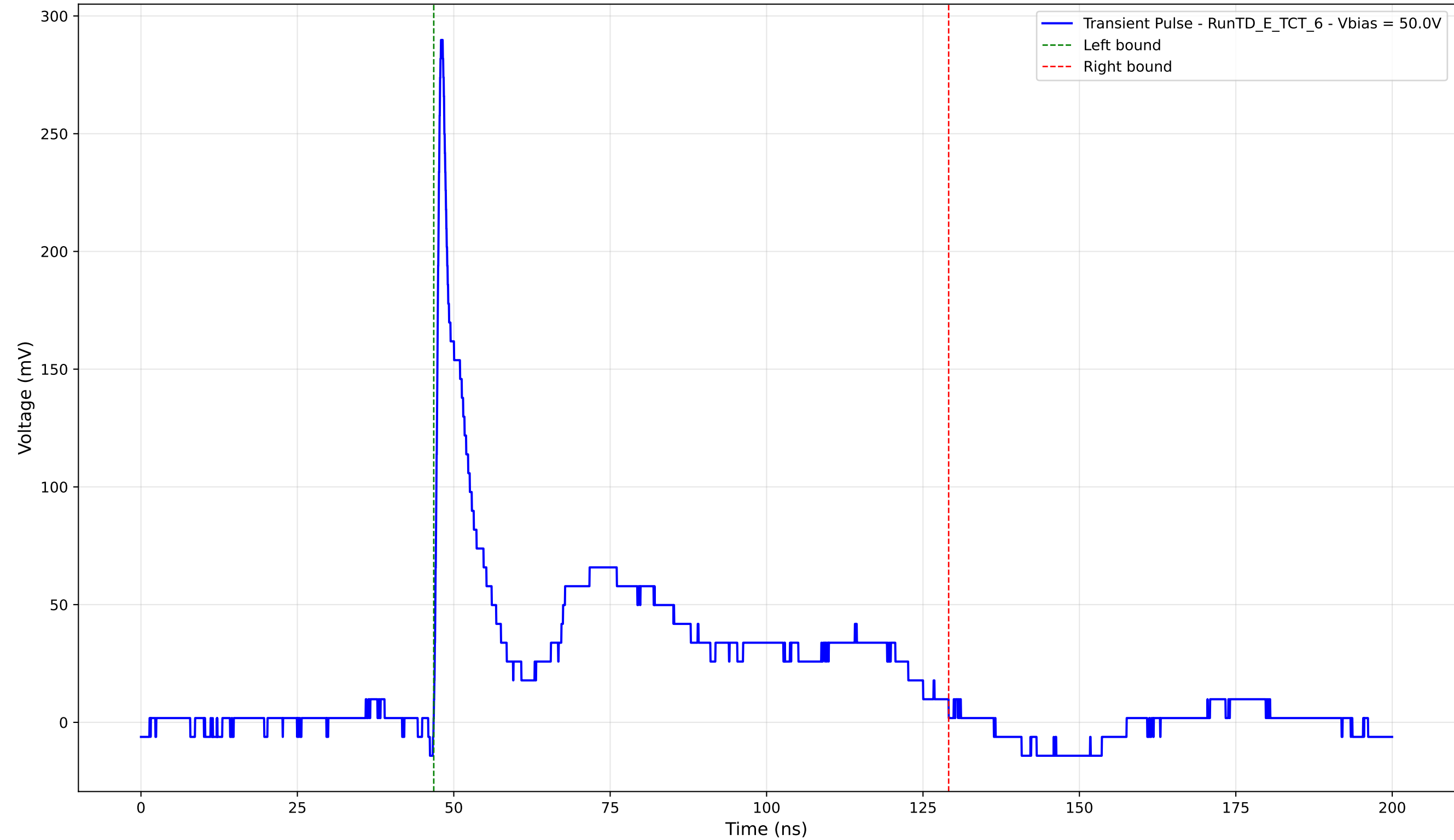
Transient Pulse - Sample: TD - Position: 70.0 \mu\text{m} - Charge: 77.36 pC - Rise Time: 0.81 ns
