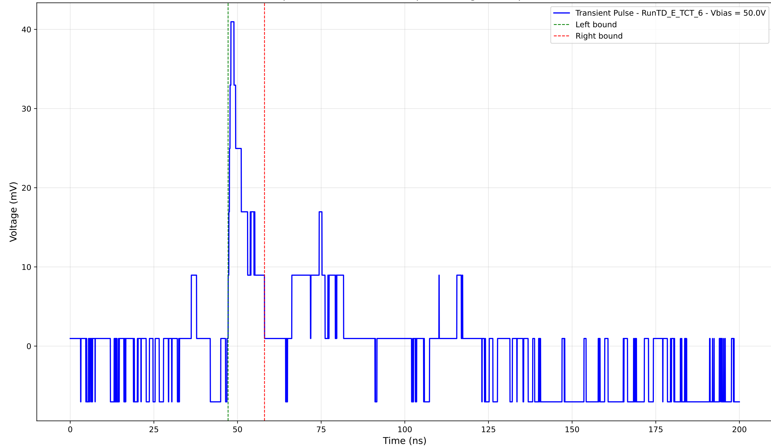
Transient Pulse - Sample: TD - Position: 340.0 \mu\text{m} - Charge: 4.02 pC - Rise Time: 0.83 ns
