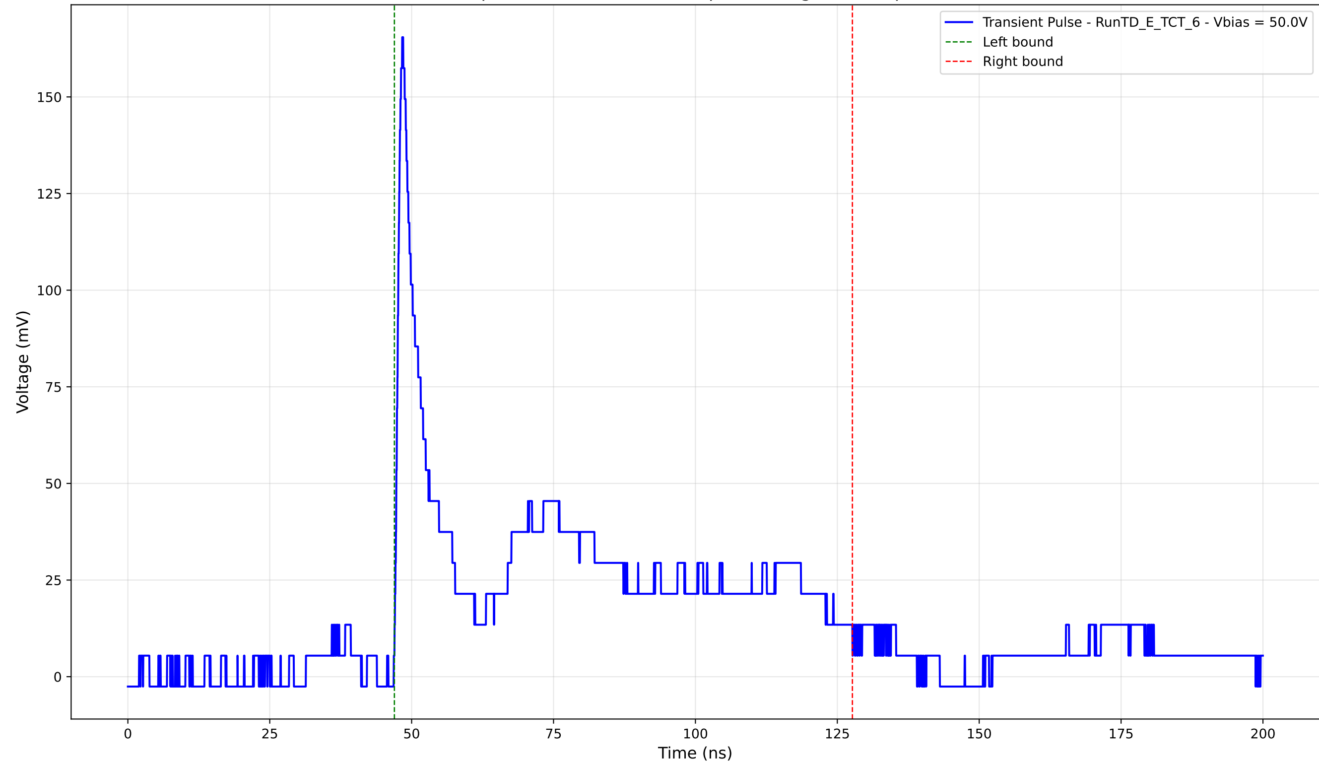
Transient Pulse - Sample: TD - Position: 135.0 \mu\text{m} - Charge: 51.91 pC - Rise Time: 0.97 ns
