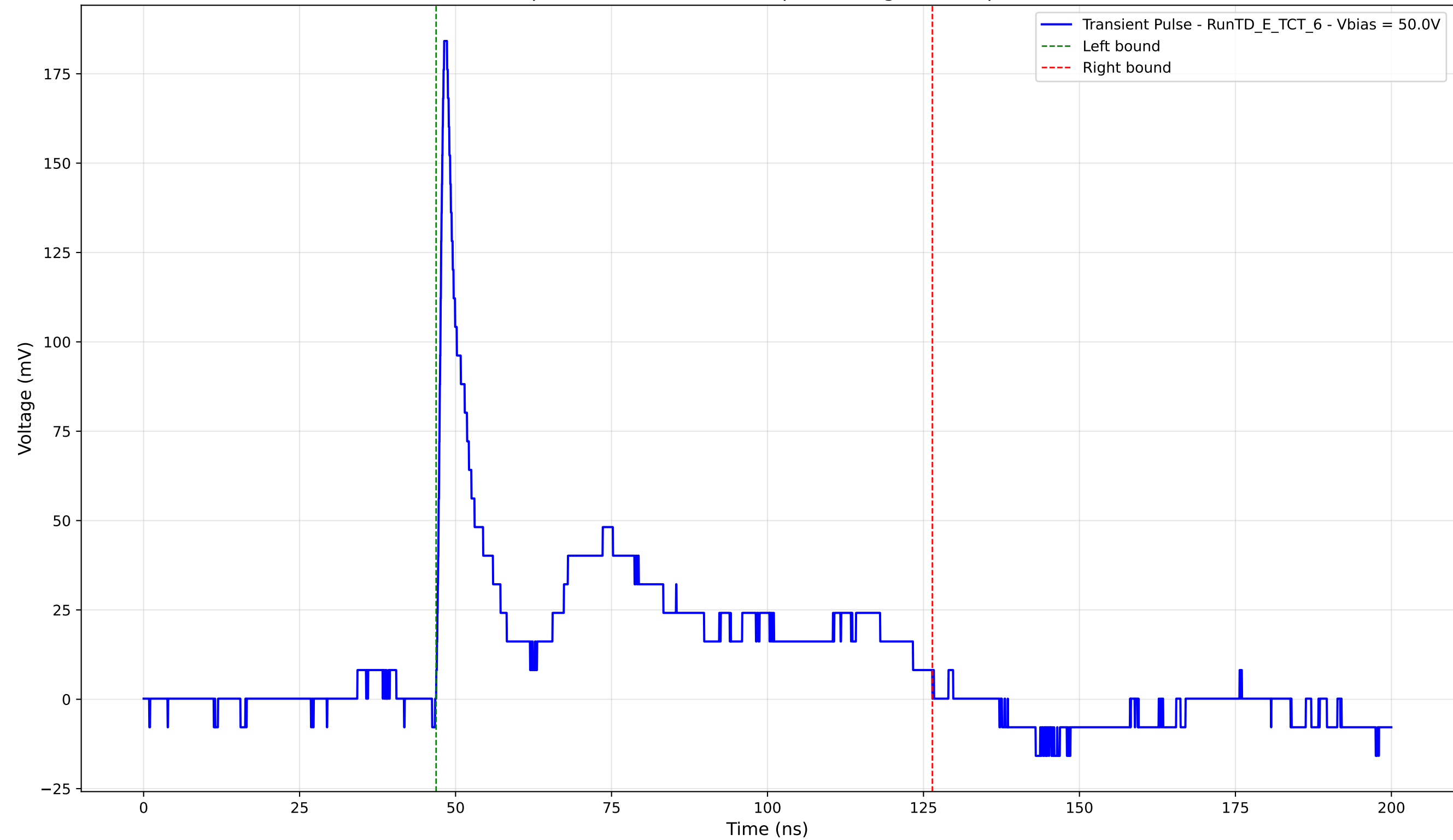
Transient Pulse - Sample: TD - Position: 120.0 \mu\text{m} - Charge: 48.54 pC - Rise Time: 0.91 ns
