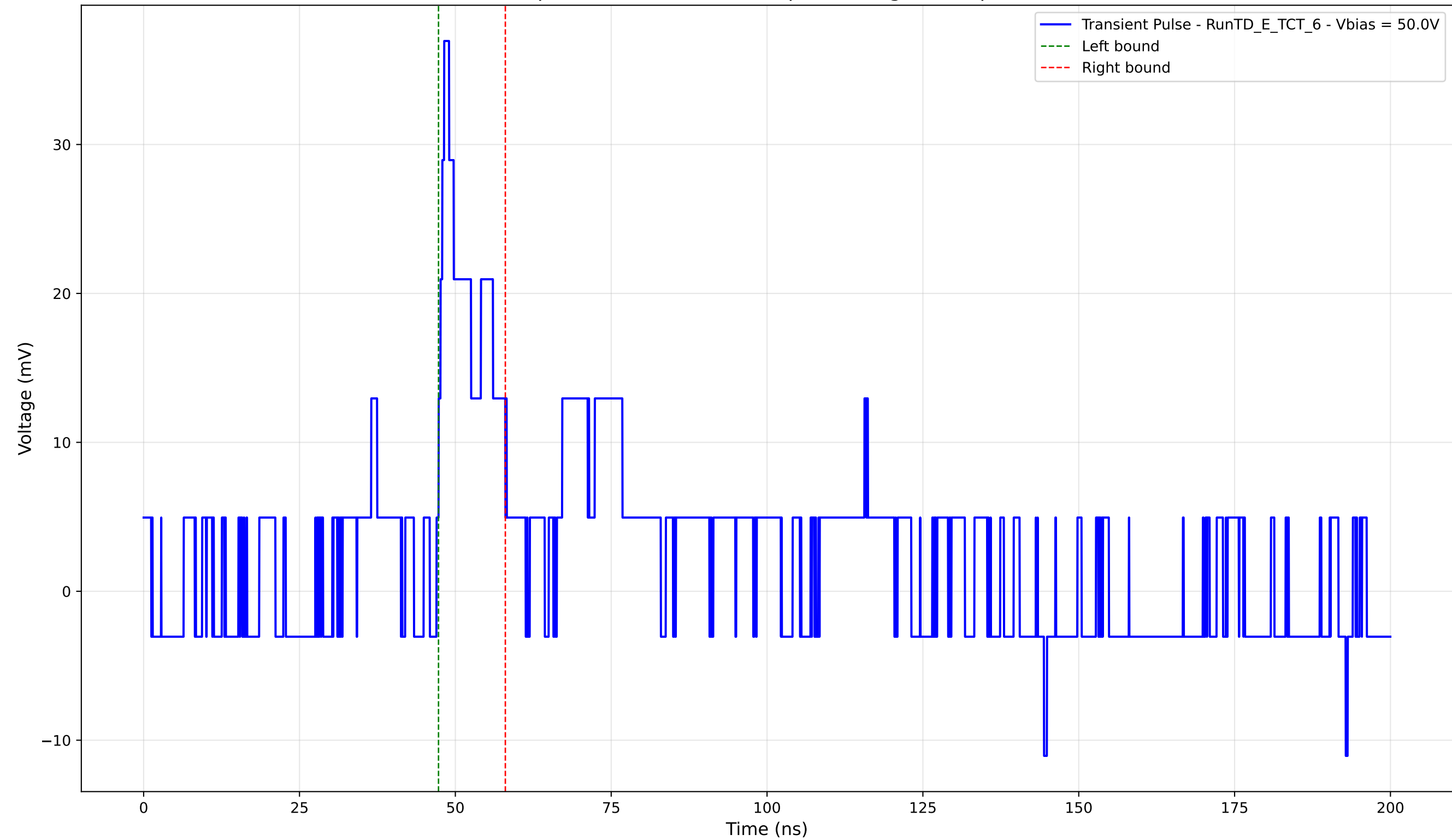
Transient Pulse - Sample: TD - Position: 345.0 \mu\text{m} - Charge: 4.29 pC - Rise Time: 1.23 ns
