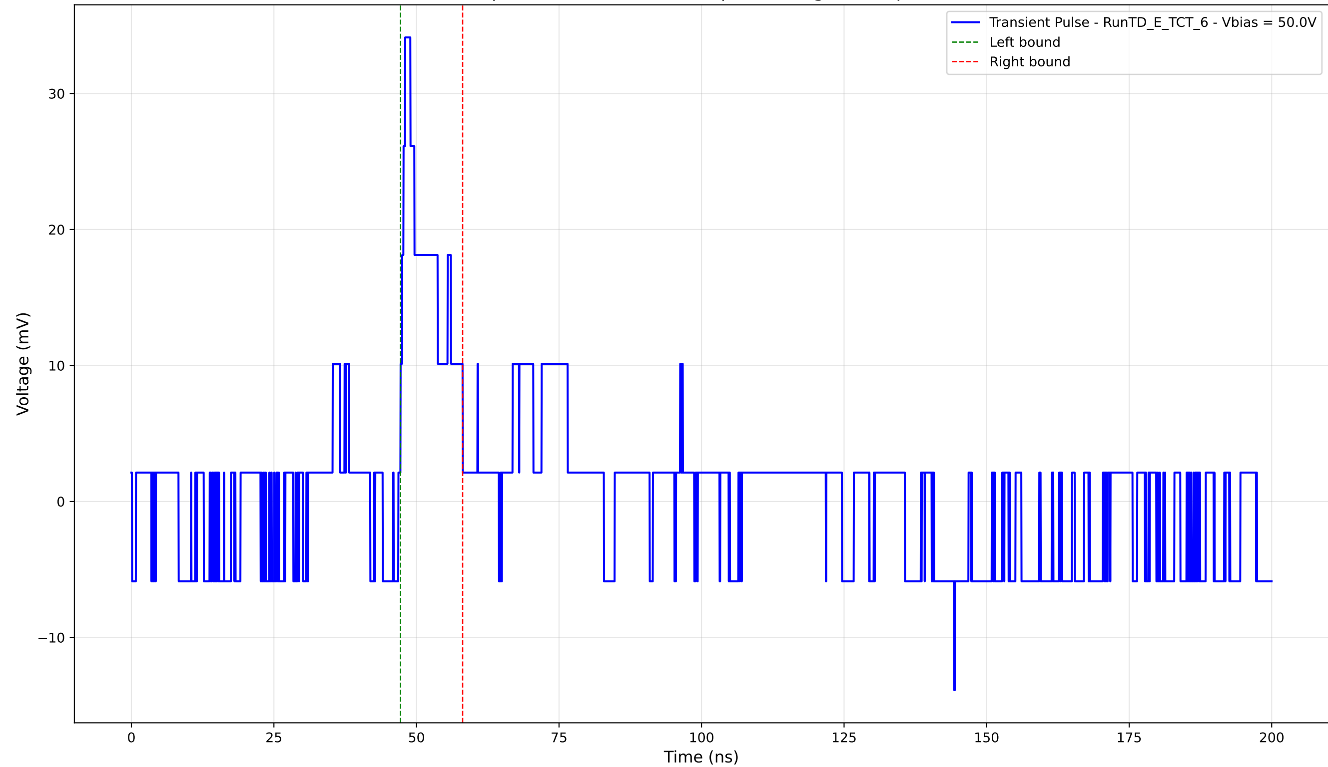
Transient Pulse - Sample: TD - Position: 375.0 \mu\text{m} - Charge: 3.76 pC - Rise Time: 0.82 ns
