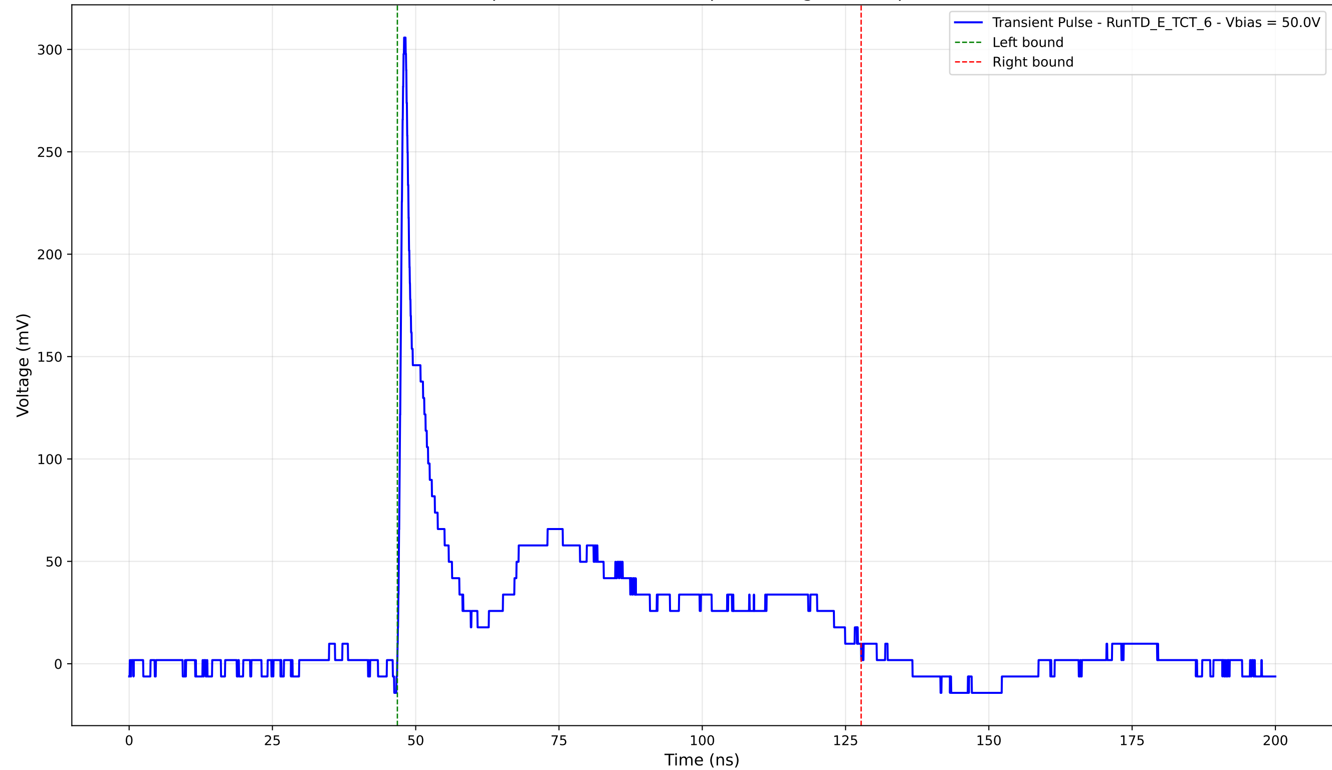
Transient Pulse - Sample: TD - Position: 50.0 \mu\text{m} - Charge: 74.54 pC - Rise Time: 0.83 ns
