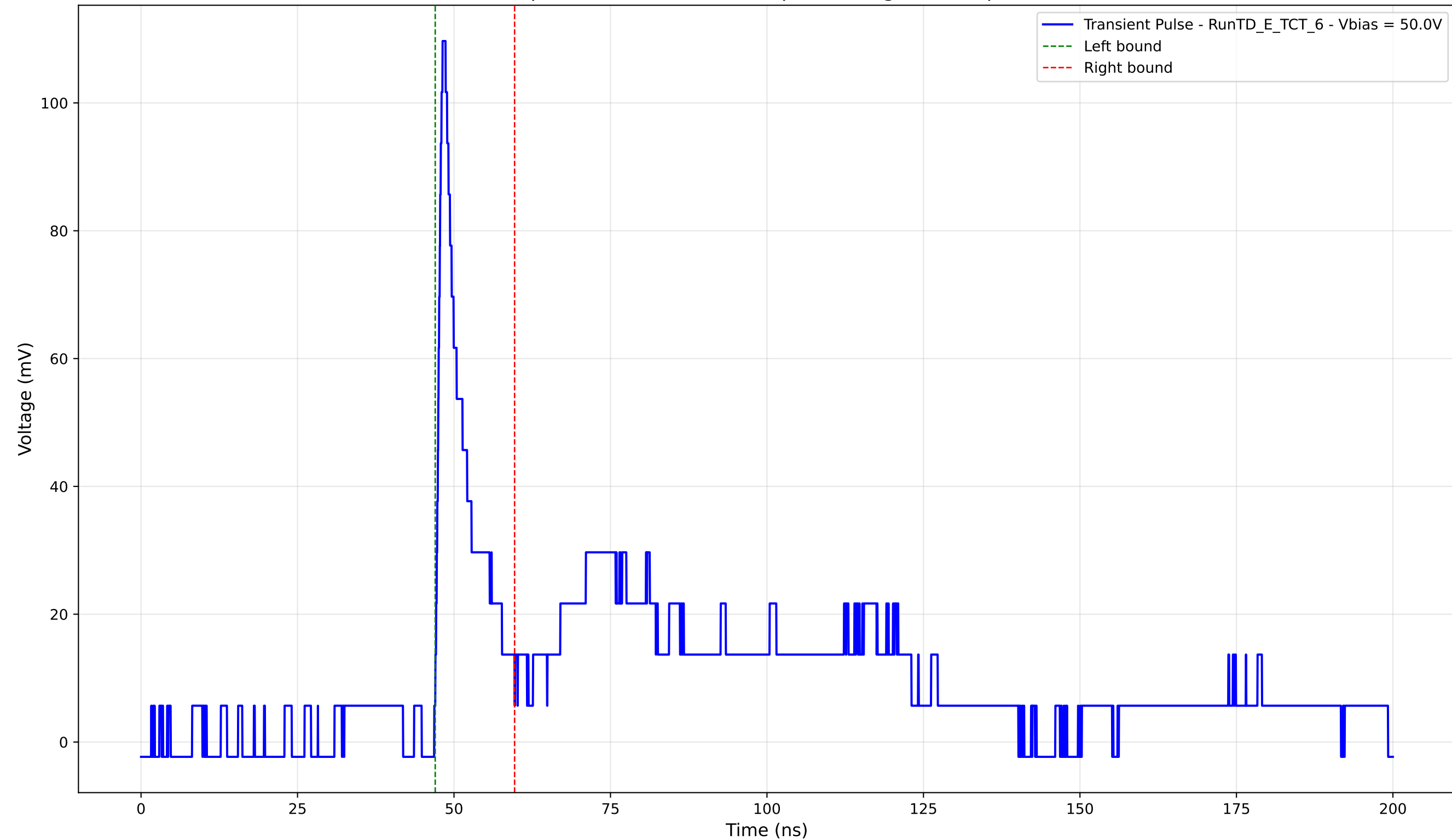
Transient Pulse - Sample: TD - Position: 205.0 \mu\text{m} - Charge: 10.56 pC - Rise Time: 0.99 ns
