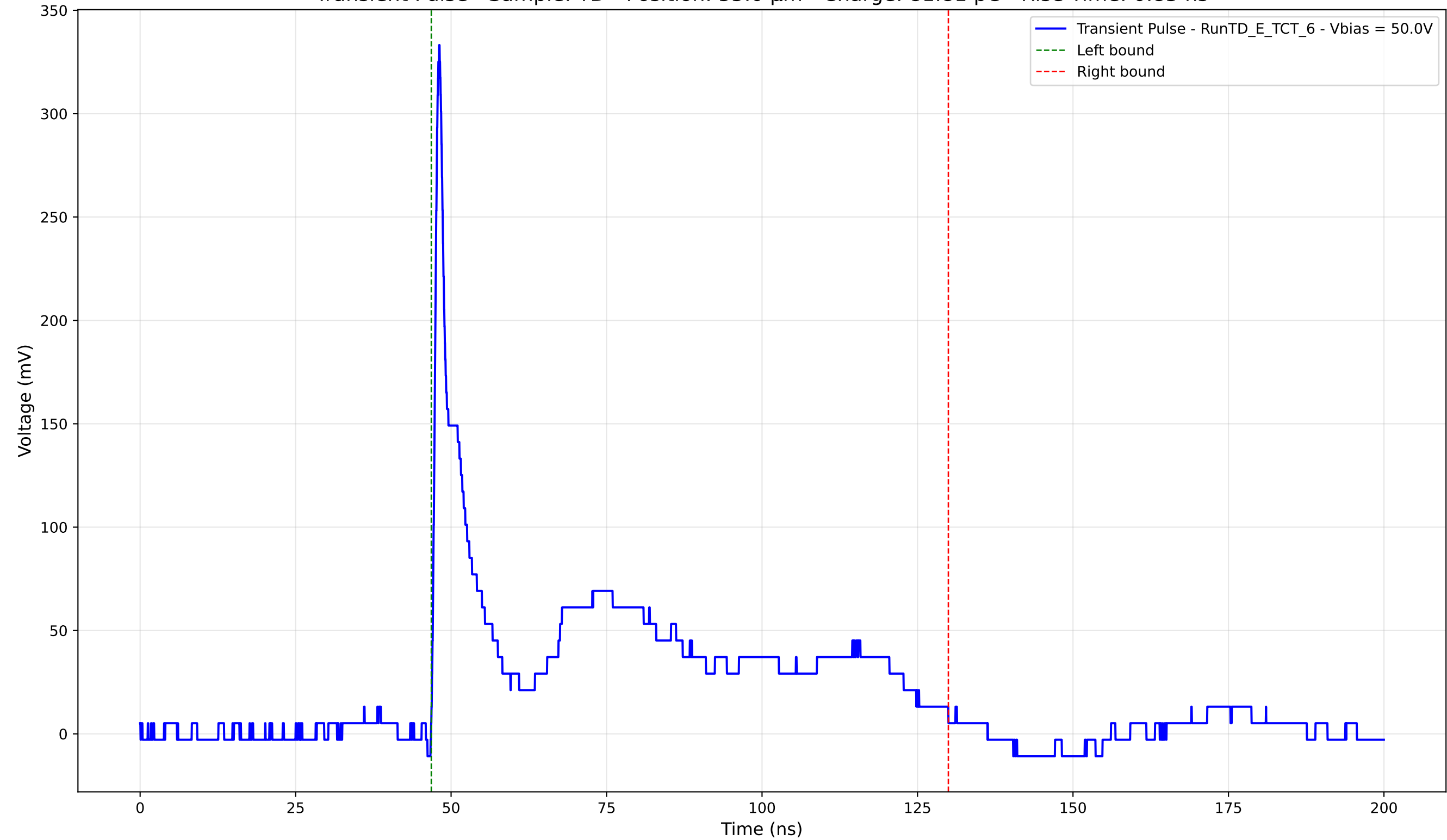
Transient Pulse - Sample: TD - Position: 55.0 \mu\text{m} - Charge: 81.81 pC - Rise Time: 0.83 ns
