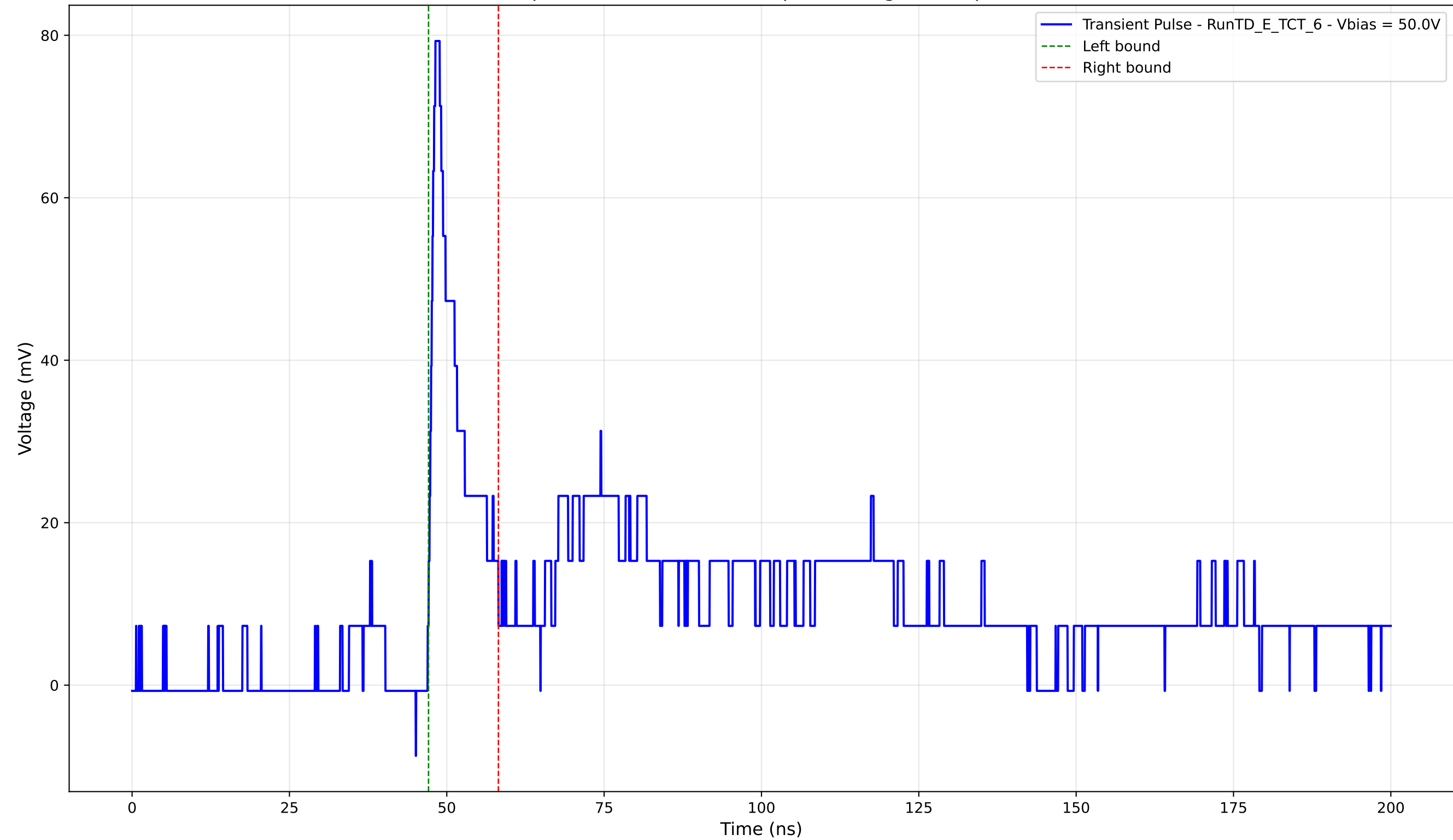
Transient Pulse - Sample: TD - Position: 195.0 \mu\text{m} - Charge: 7.88 pC - Rise Time: 1.08 ns
