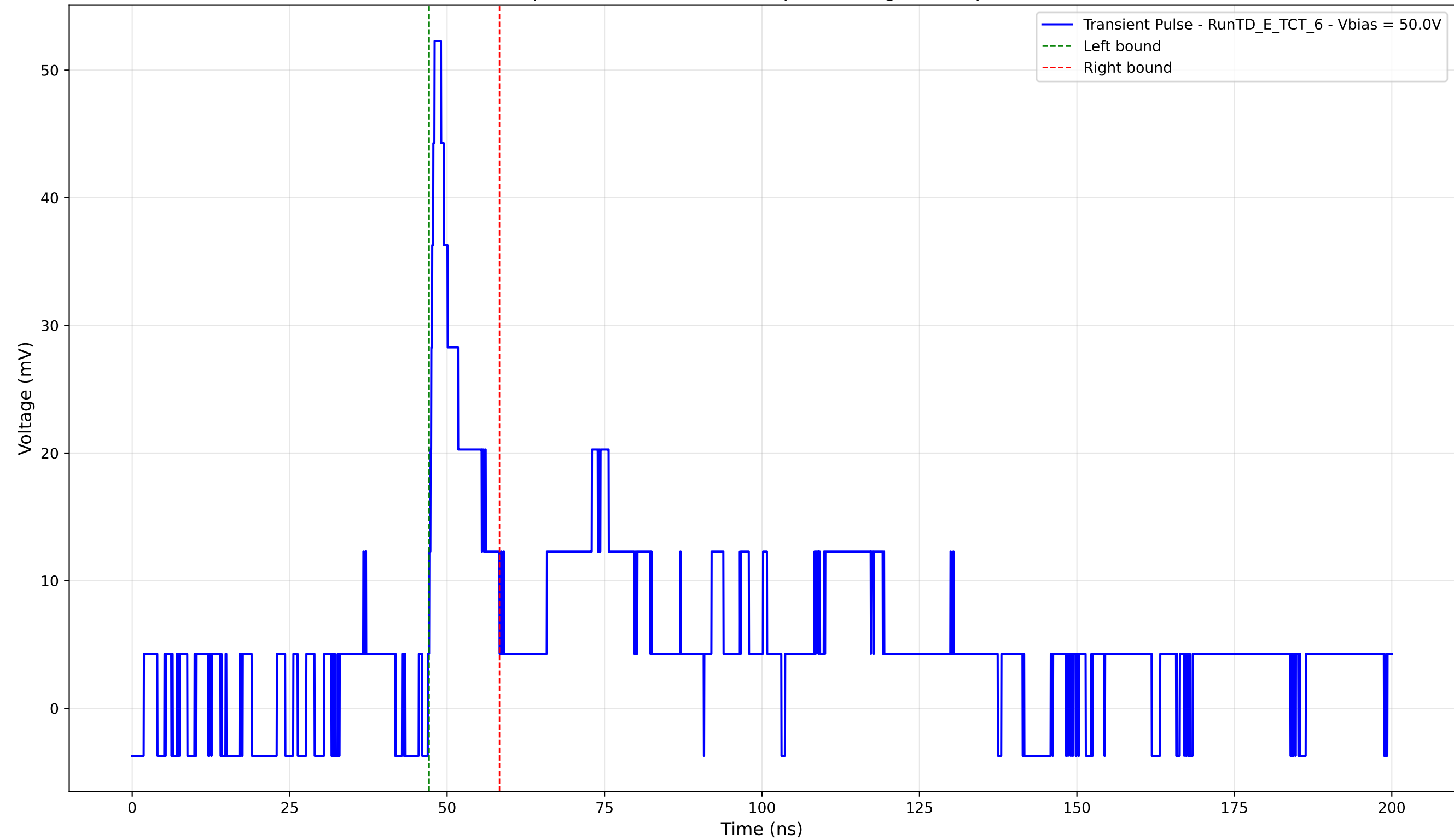
Transient Pulse - Sample: TD - Position: 210.0 \mu\text{m} - Charge: 5.62 pC - Rise Time: 0.86 ns
