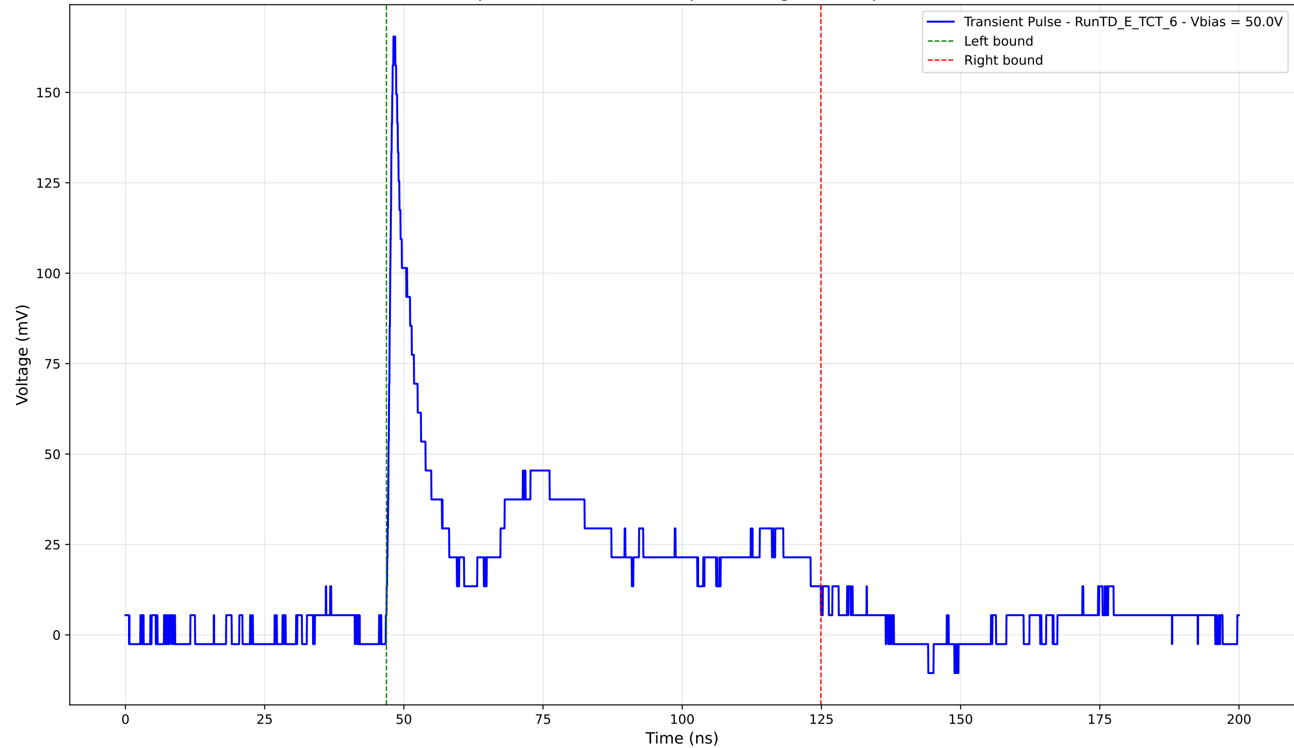
Transient Pulse - Sample: TD - Position: 85.0 \mu\text{m} - Charge: 50.46 pC - Rise Time: 0.91 ns
