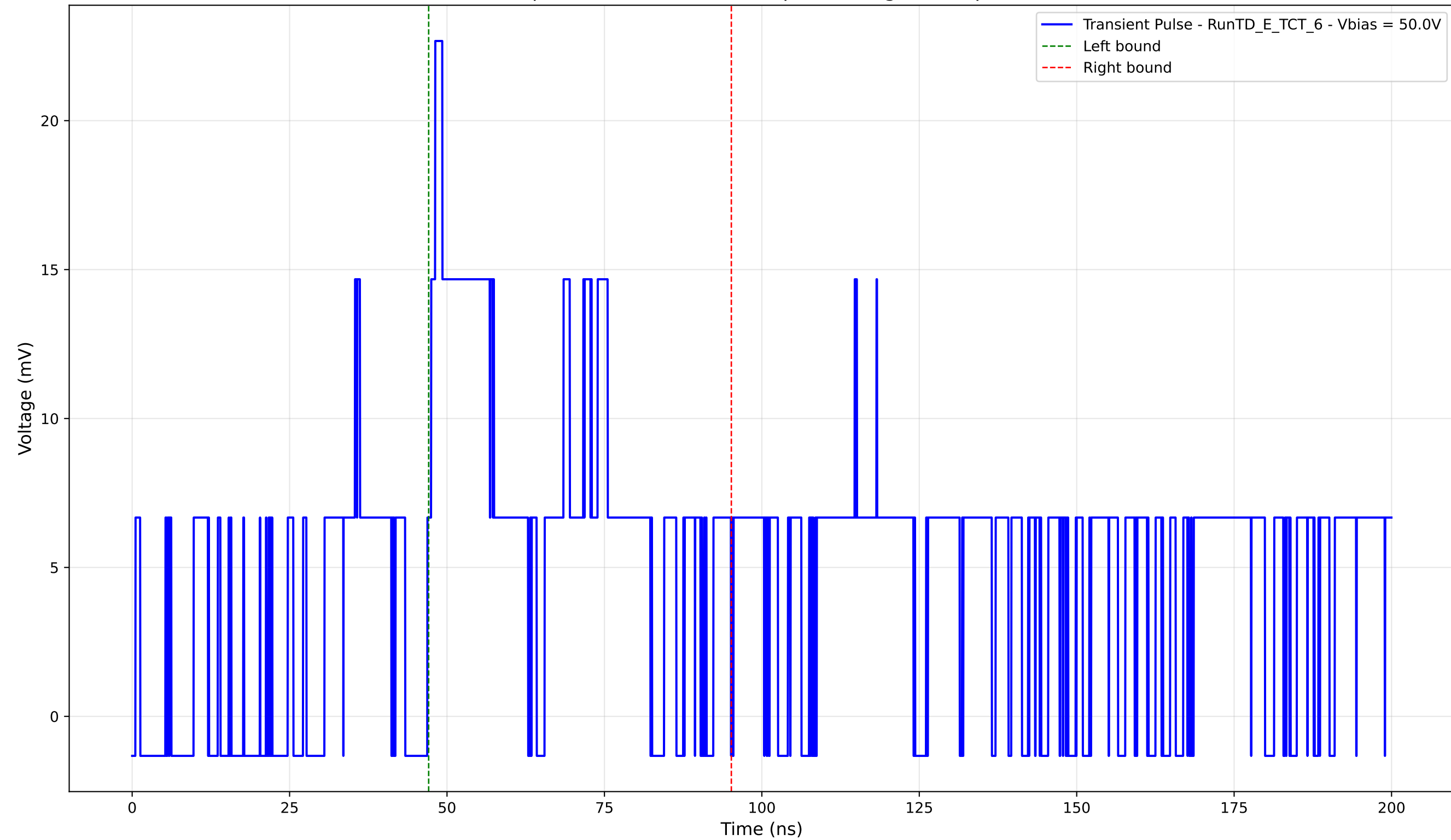
Transient Pulse - Sample: TD - Position: 410.0 \mu\text{m} - Charge: 7.72 pC - Rise Time: 1.26 ns
