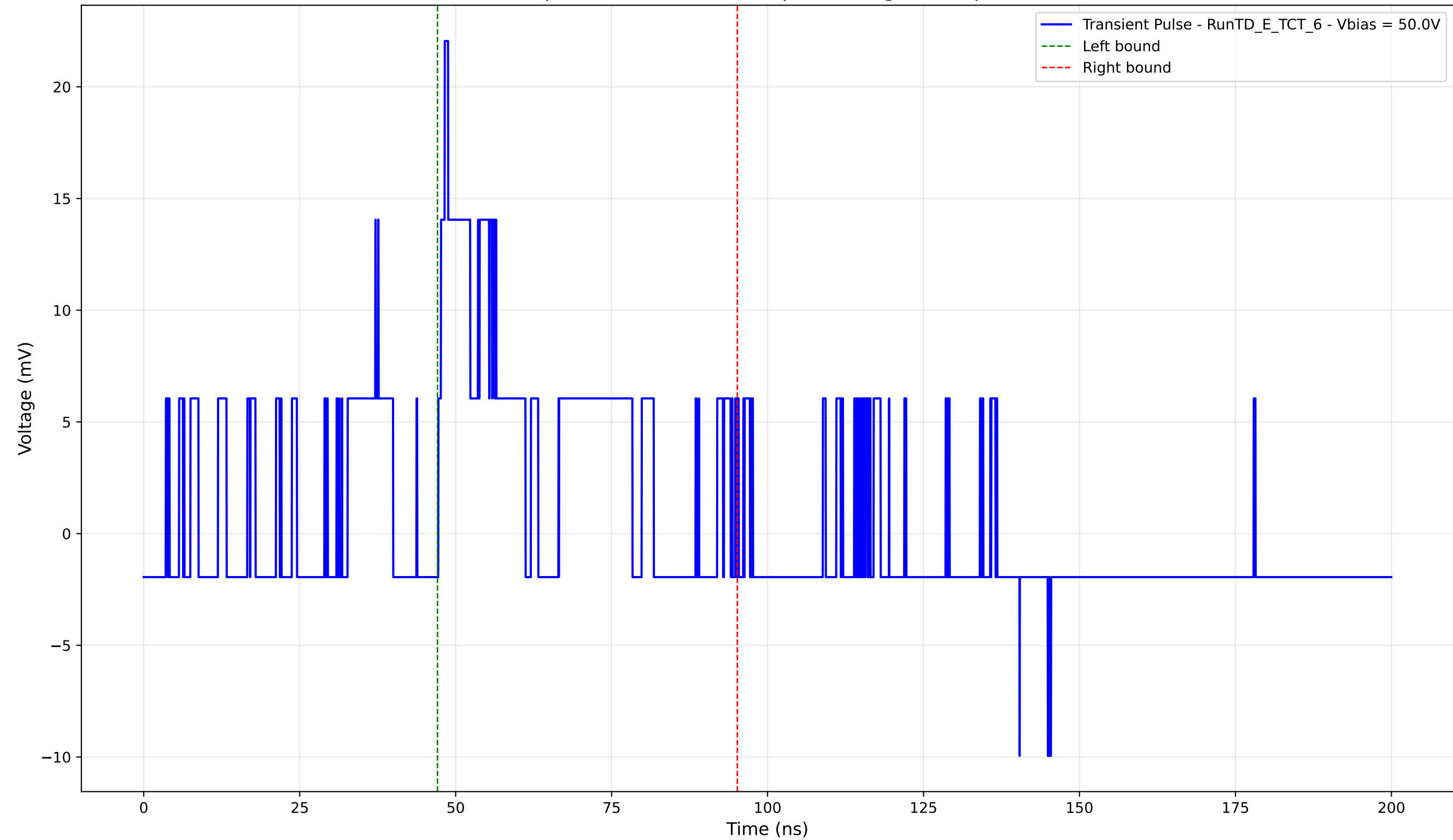
Transient Pulse - Sample: TD - Position: 20.0 \mu\text{m} - Charge: 4.40 pC - Rise Time: 1.04 ns
