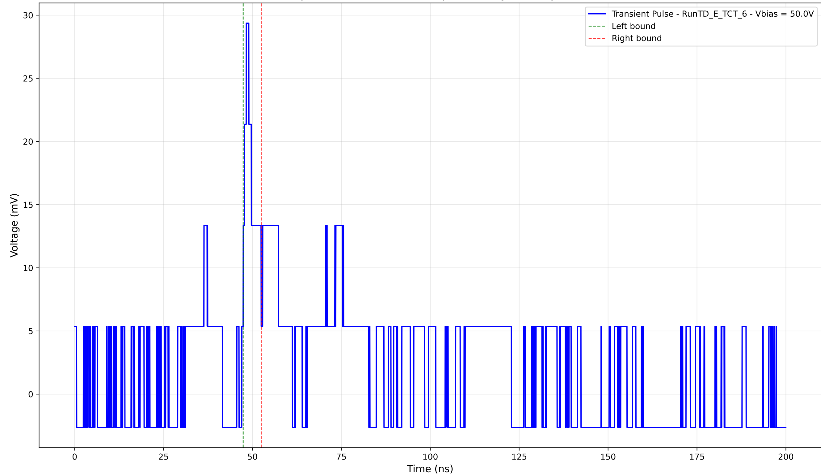
Transient Pulse - Sample: TD - Position: 295.0 \mu\text{m} - Charge: 1.77 pC - Rise Time: 1.28 ns
