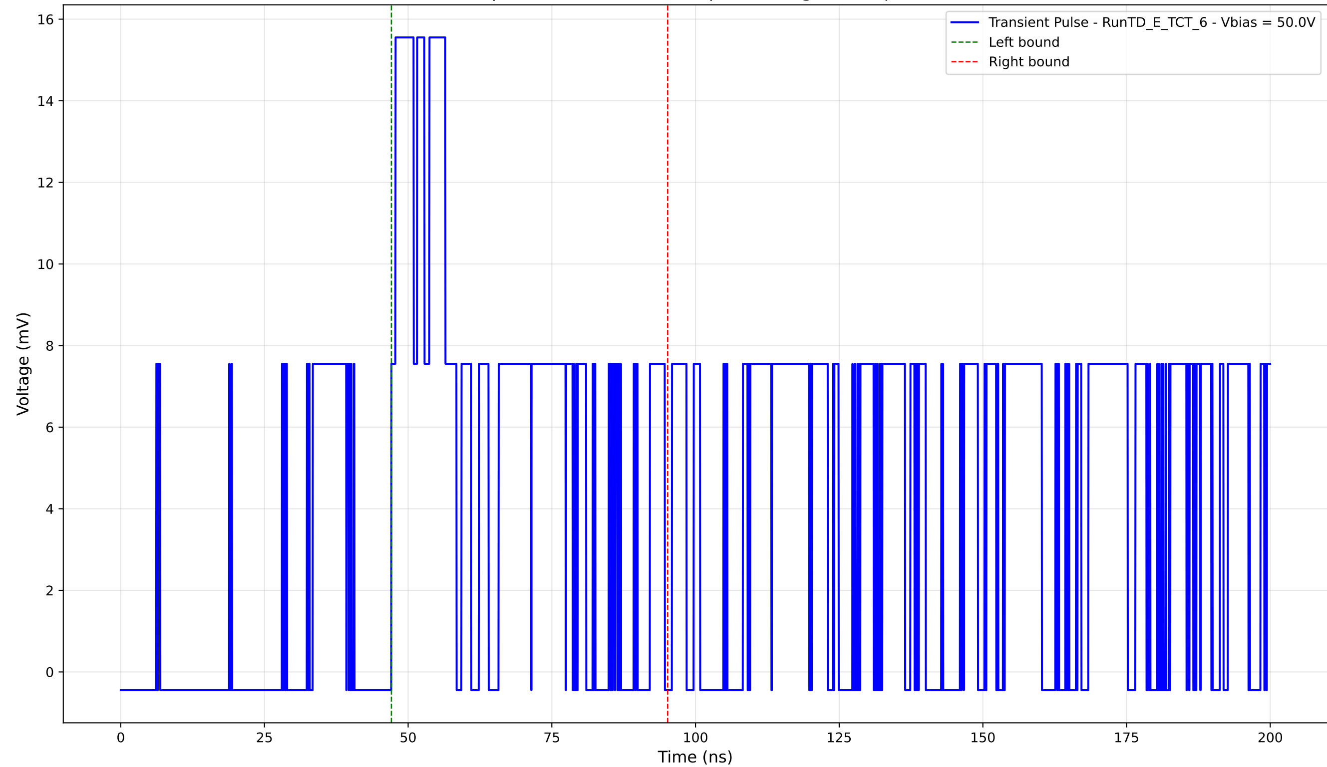
Transient Pulse - Sample: TD - Position: 15.0 \mu\text{m} - Charge: 6.16 pC - Rise Time: 0.74 ns
