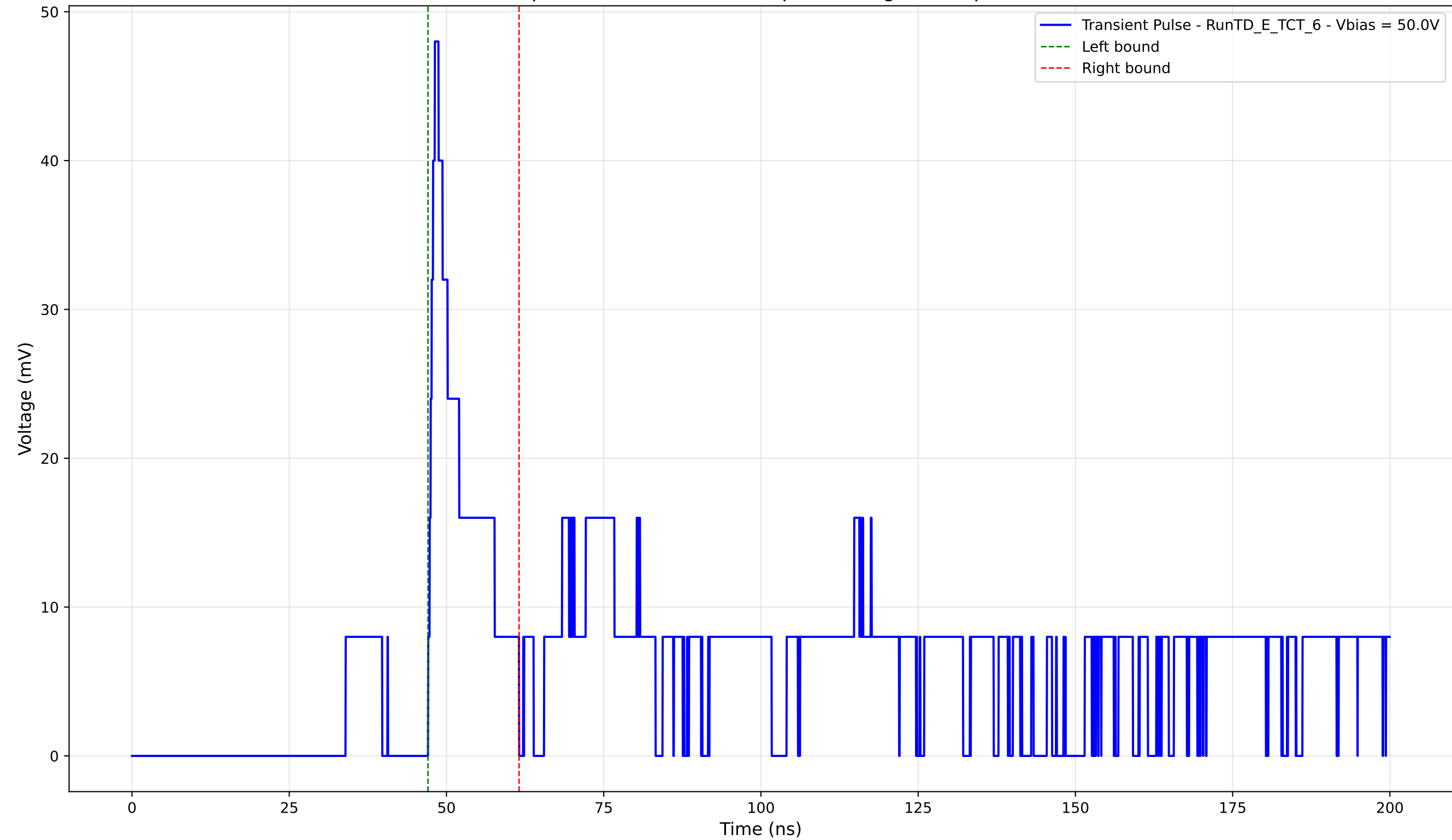
Transient Pulse - Sample: TD - Position: 310.0 \mu\text{m} - Charge: 5.44 pC - Rise Time: 1.07 ns
