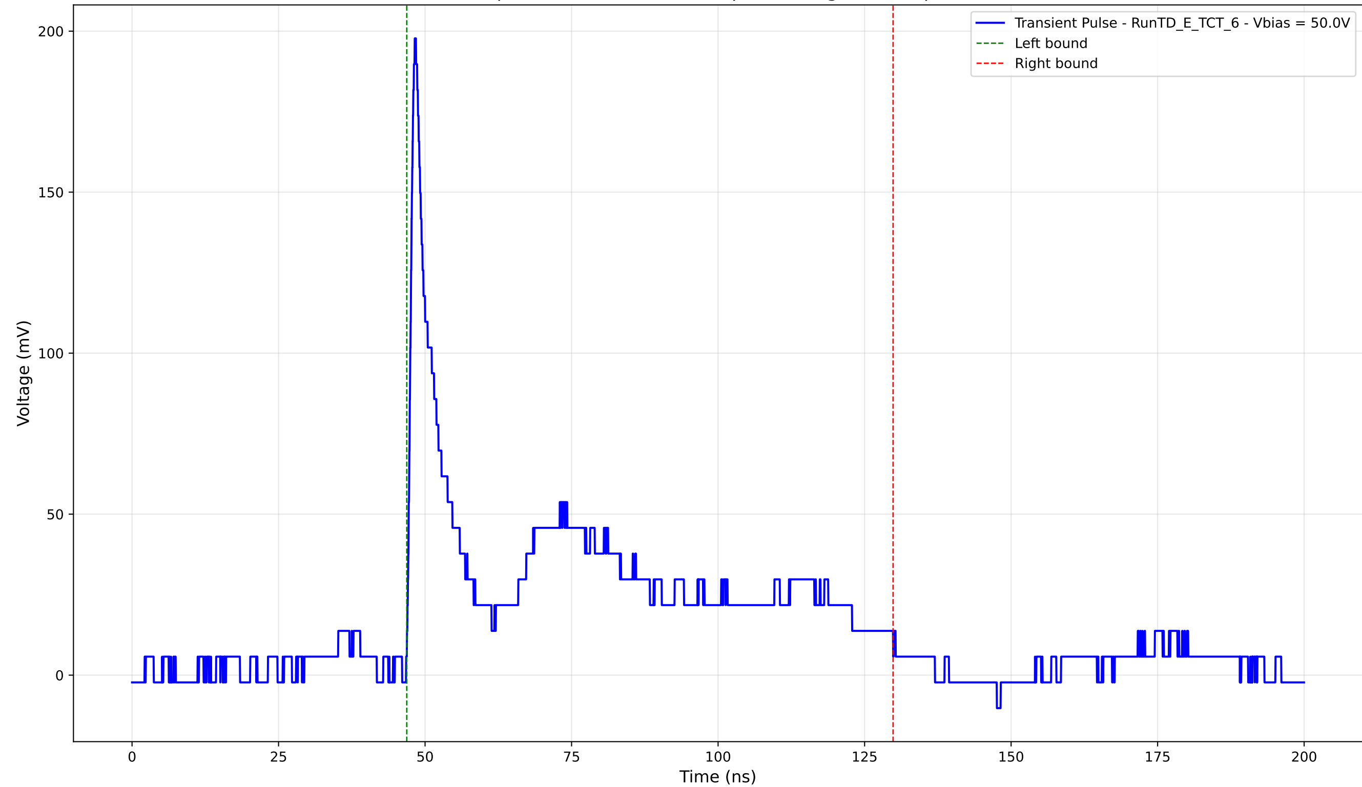
Transient Pulse - Sample: TD - Position: 100.0 \mu\text{m} - Charge: 58.08 pC - Rise Time: 1.00 ns
