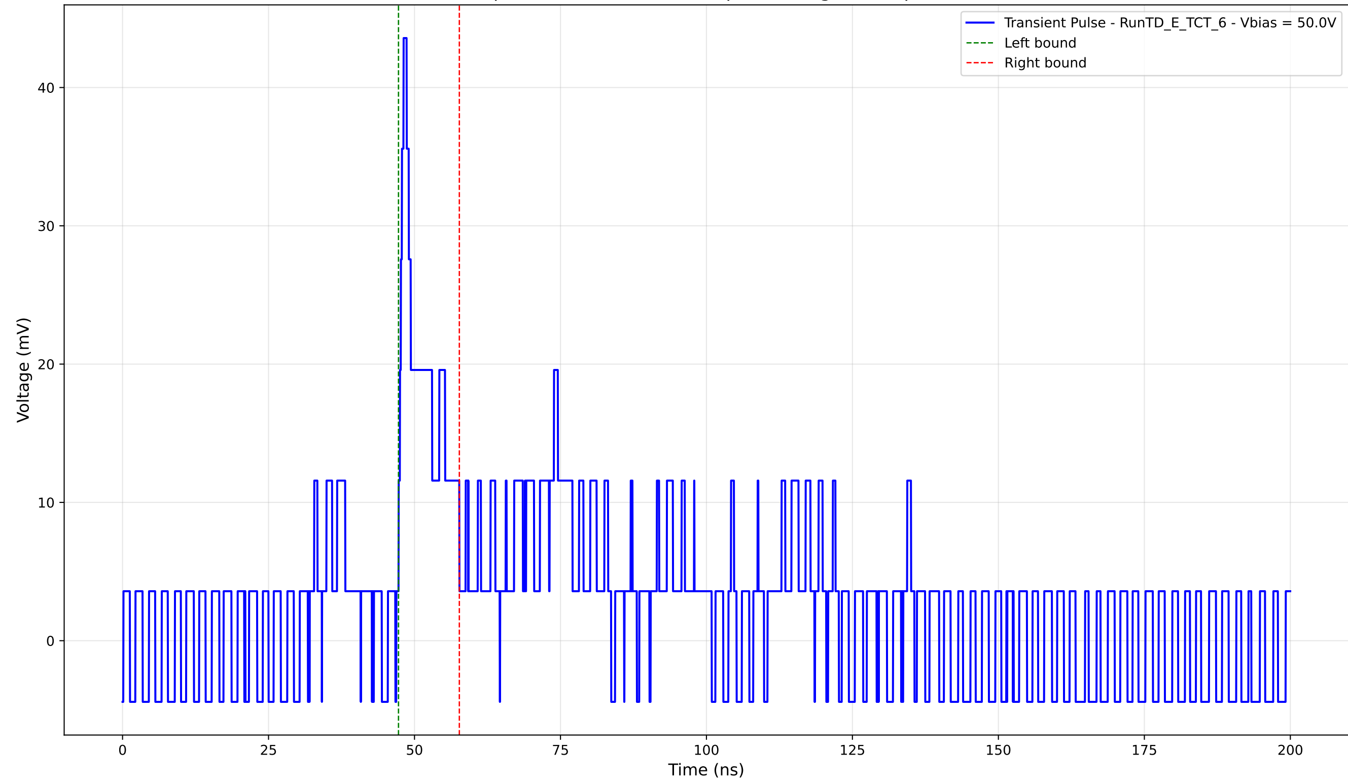
Transient Pulse - Sample: TD - Position: 245.0 \mu\text{m} - Charge: 4.00 pC - Rise Time: 0.86 ns
