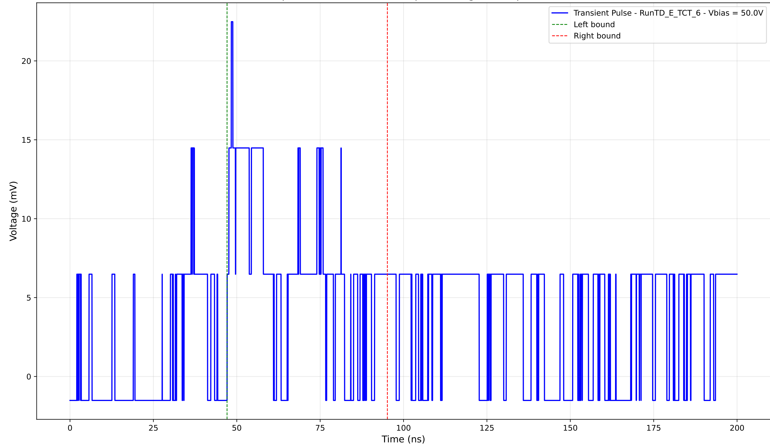
Transient Pulse - Sample: TD - Position: 415.0 \mu\text{m} - Charge: 6.85 pC - Rise Time: 1.28 ns
