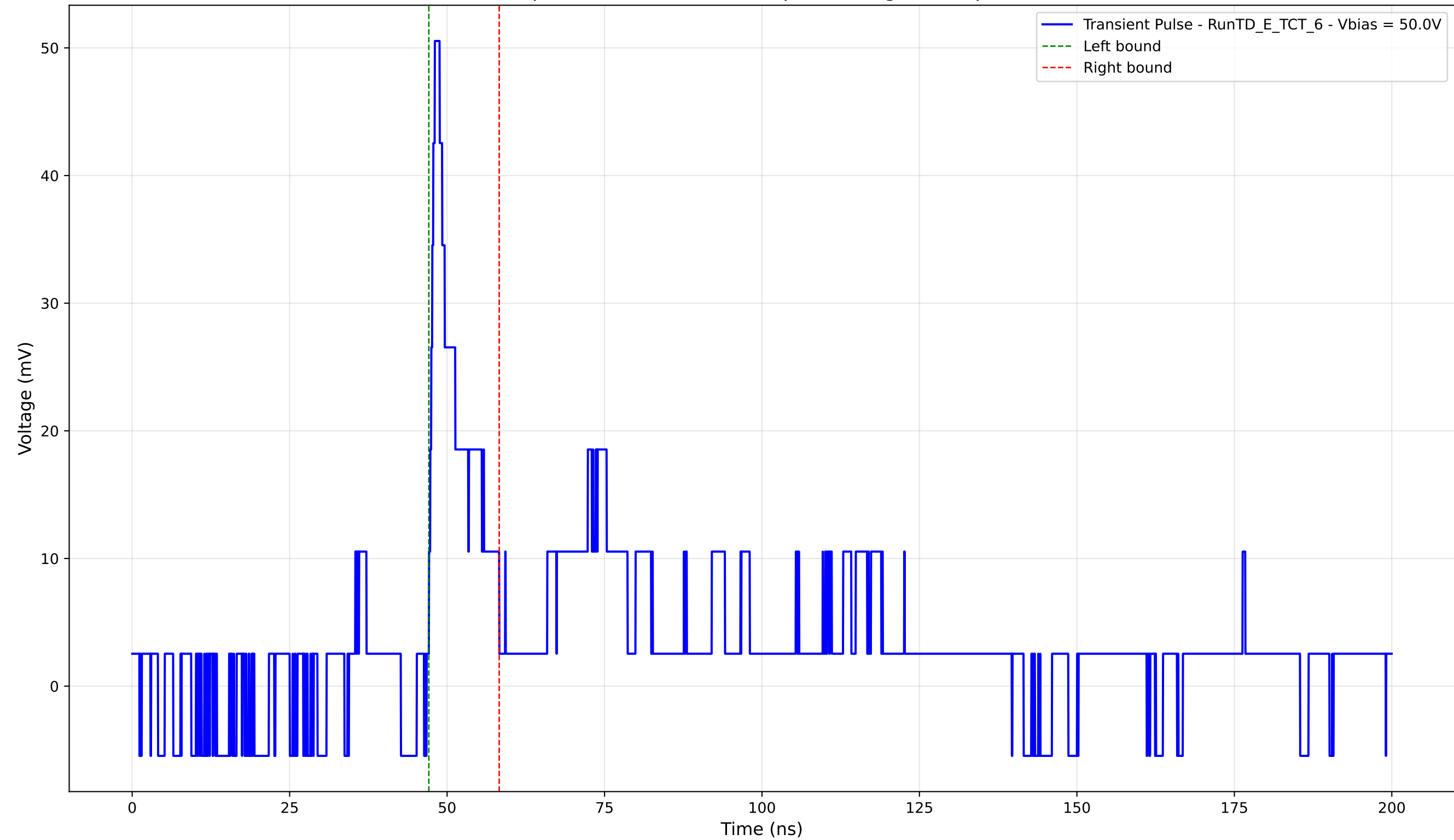
Transient Pulse - Sample: TD - Position: 250.0 \mu\text{m} - Charge: 4.94 pC - Rise Time: 0.93 ns
