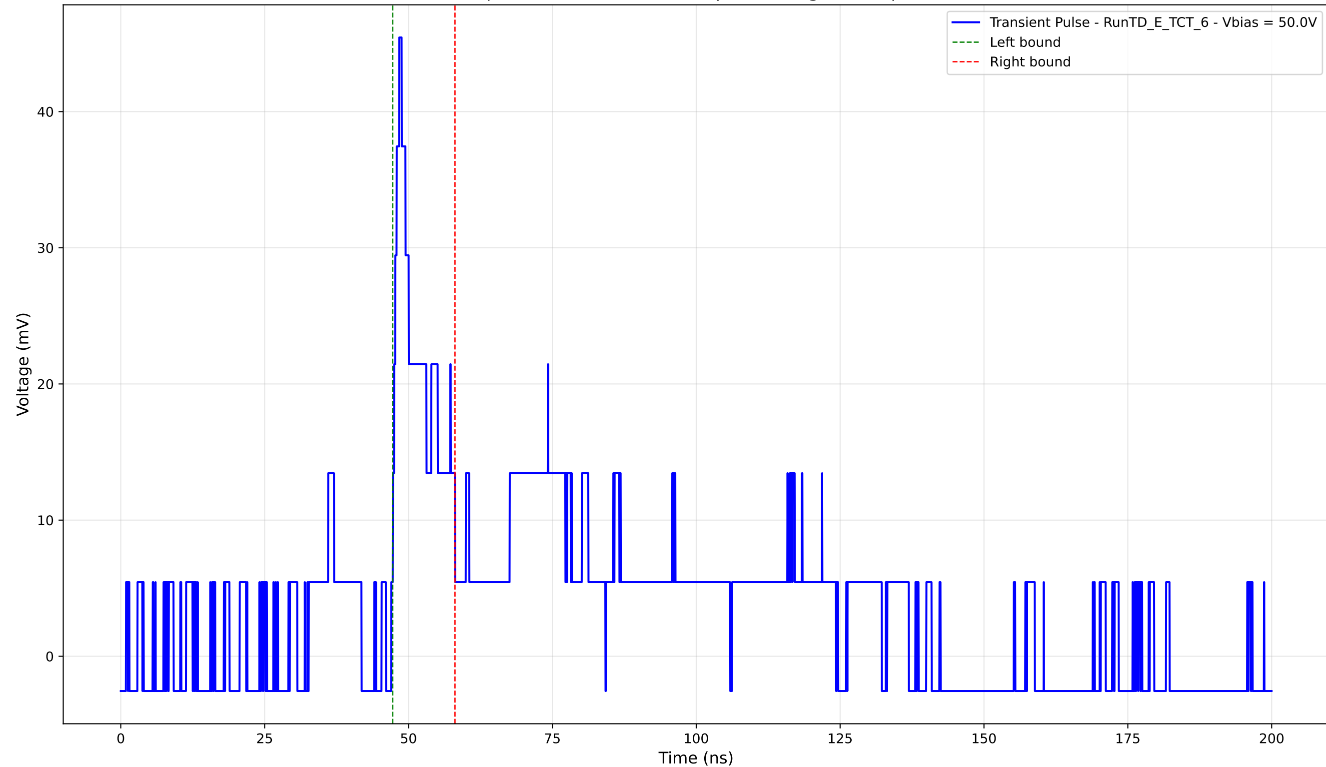
Transient Pulse - Sample: TD - Position: 380.0 \mu\text{m} - Charge: 4.69 pC - Rise Time: 1.39 ns
