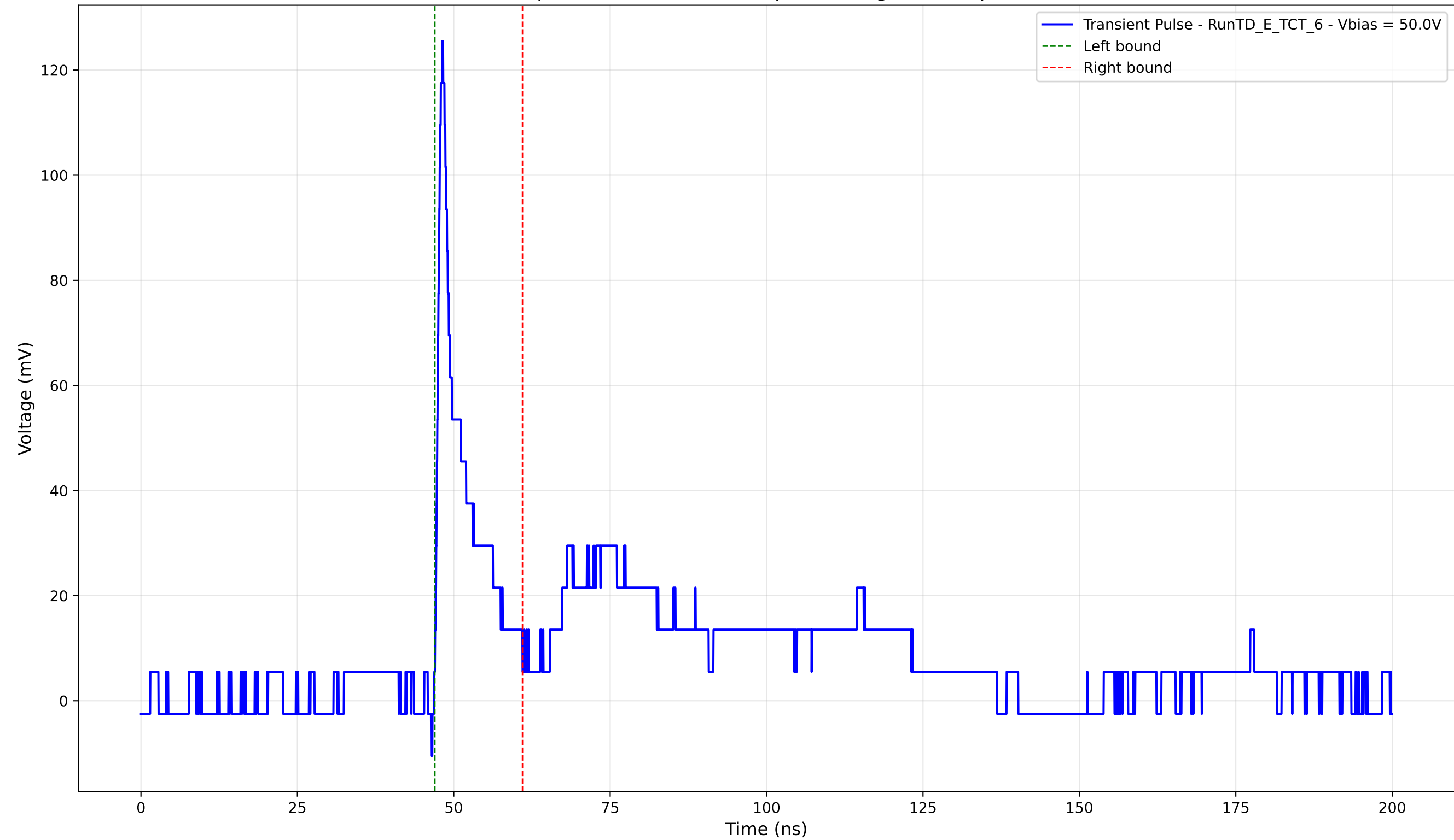
Transient Pulse - Sample: TD - Position: 35.0 \mu\text{m} - Charge: 10.99 pC - Rise Time: 0.92 ns
