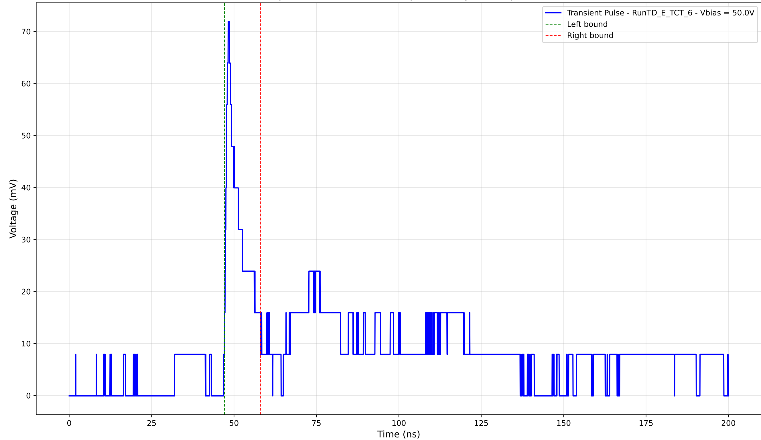
Transient Pulse - Sample: TD - Position: 235.0 \mu\text{m} - Charge: 7.13 pC - Rise Time: 1.38 ns
