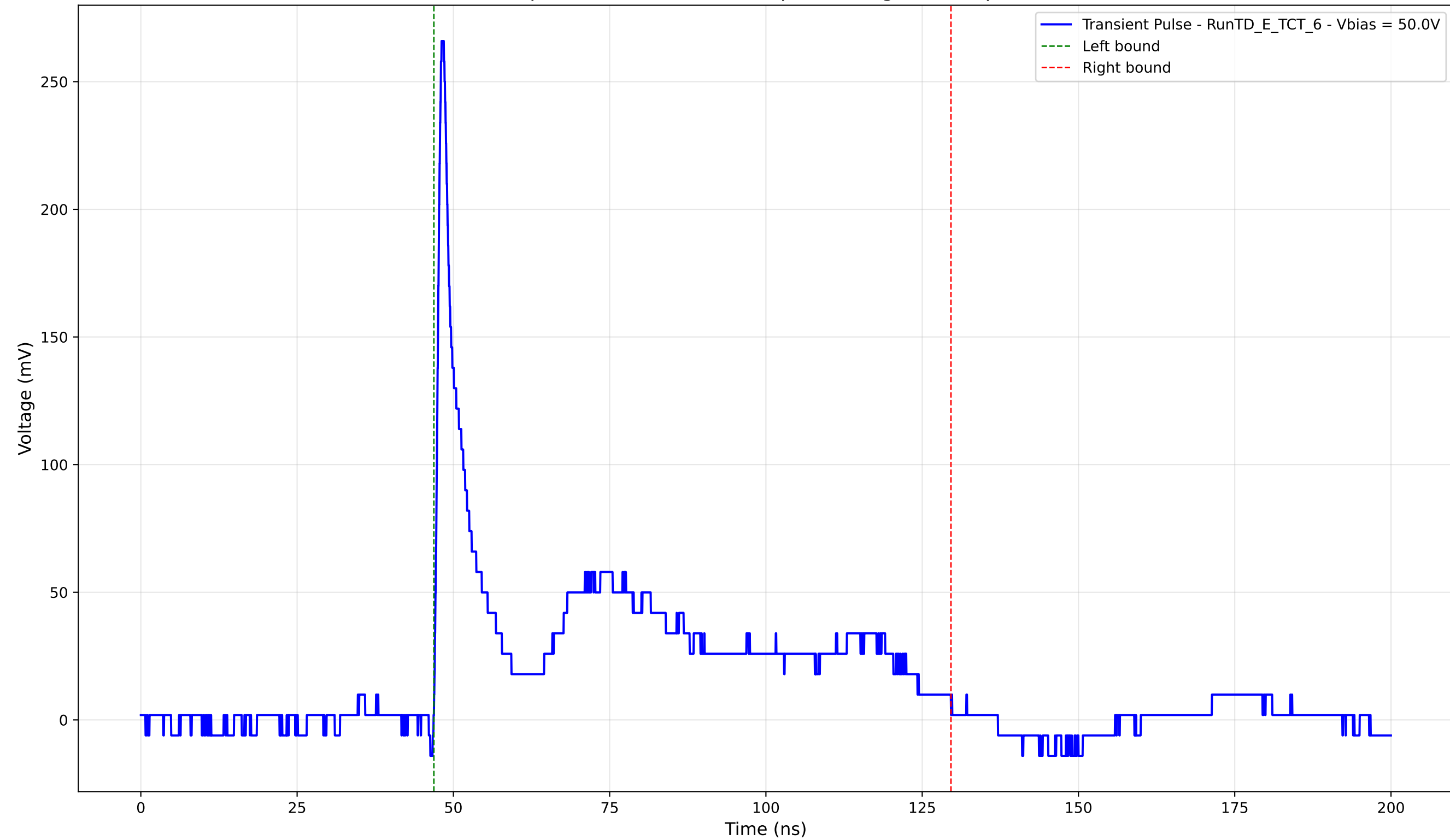
Transient Pulse - Sample: TD - Position: 110.0 \mu\text{m} - Charge: 65.70 pC - Rise Time: 0.88 ns
