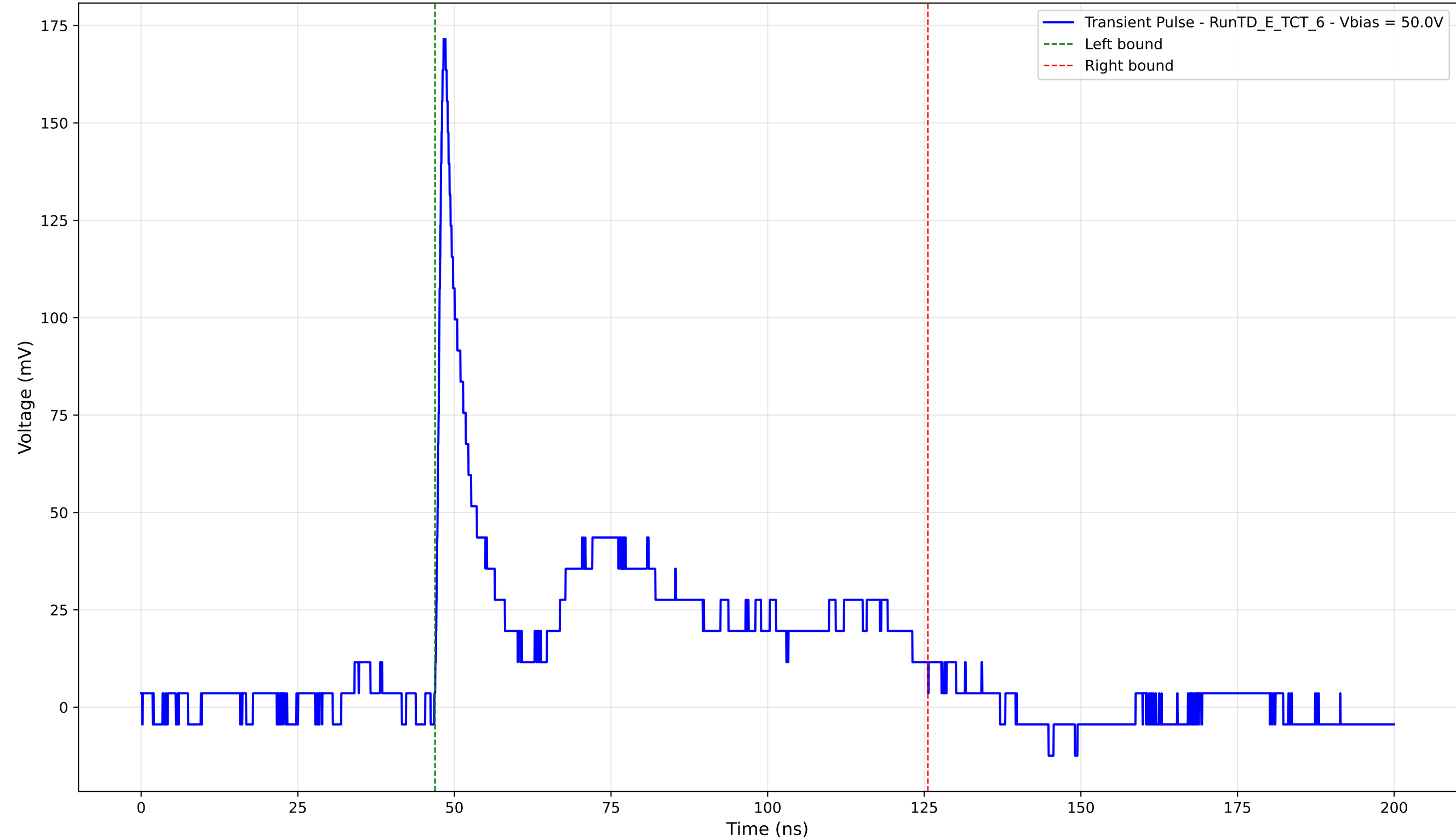
Transient Pulse - Sample: TD - Position: 125.0 \mu\text{m} - Charge: 49.73 pC - Rise Time: 0.97 ns
