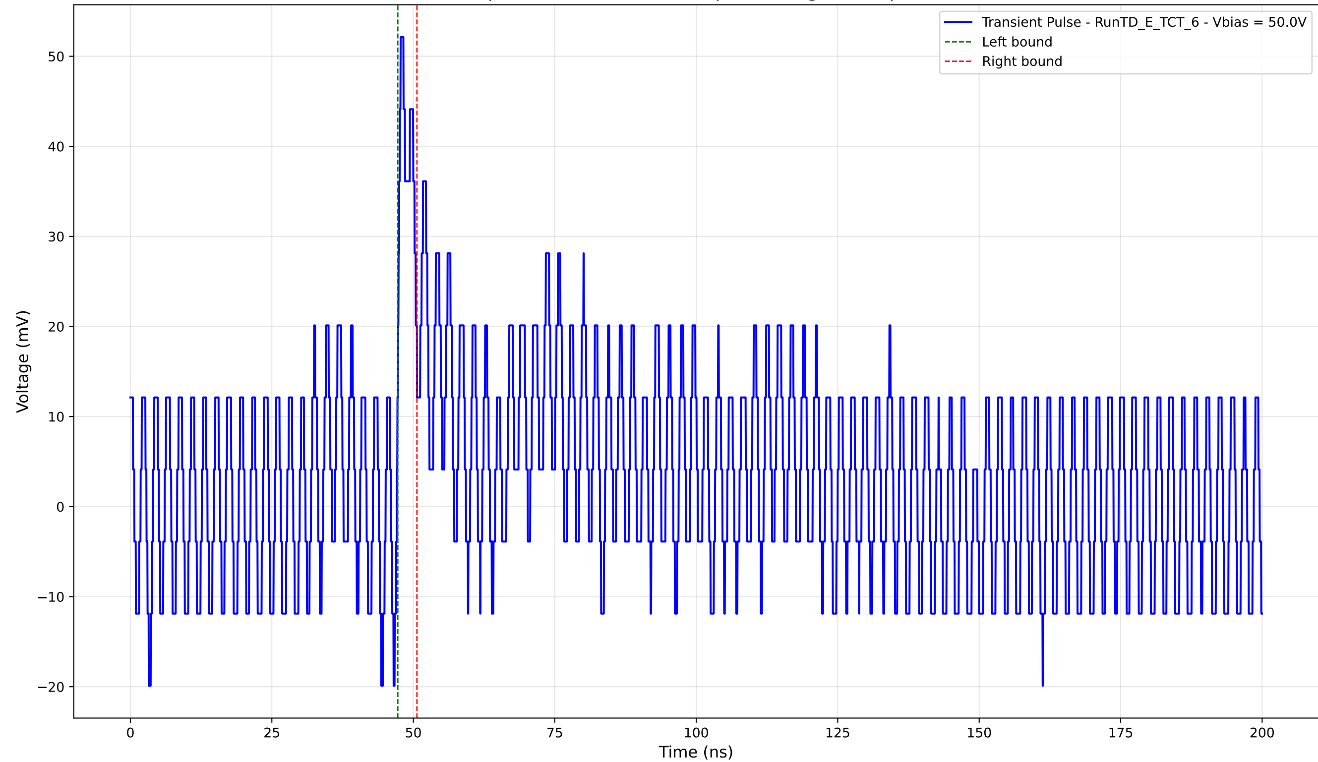
Transient Pulse - Sample: TD - Position: 215.0 \mu\text{m} - Charge: 2.61 pC - Rise Time: 0.58 ns
