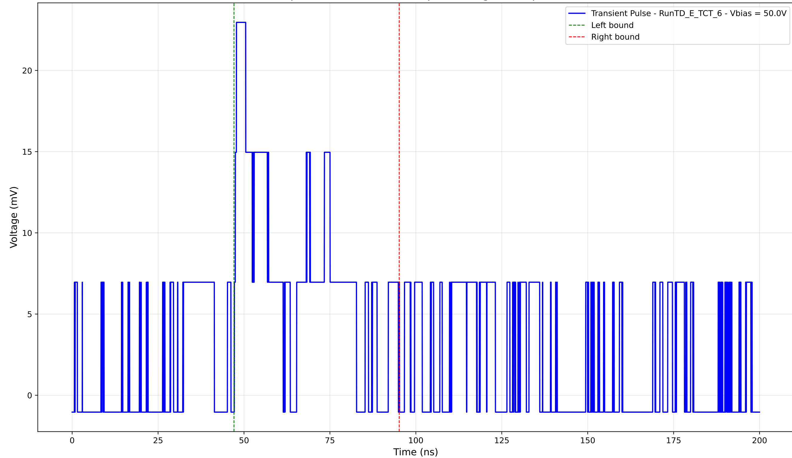
Transient Pulse - Sample: TD - Position: 290.0 \mu\text{m} - Charge: 7.50 pC - Rise Time: 0.64 ns
