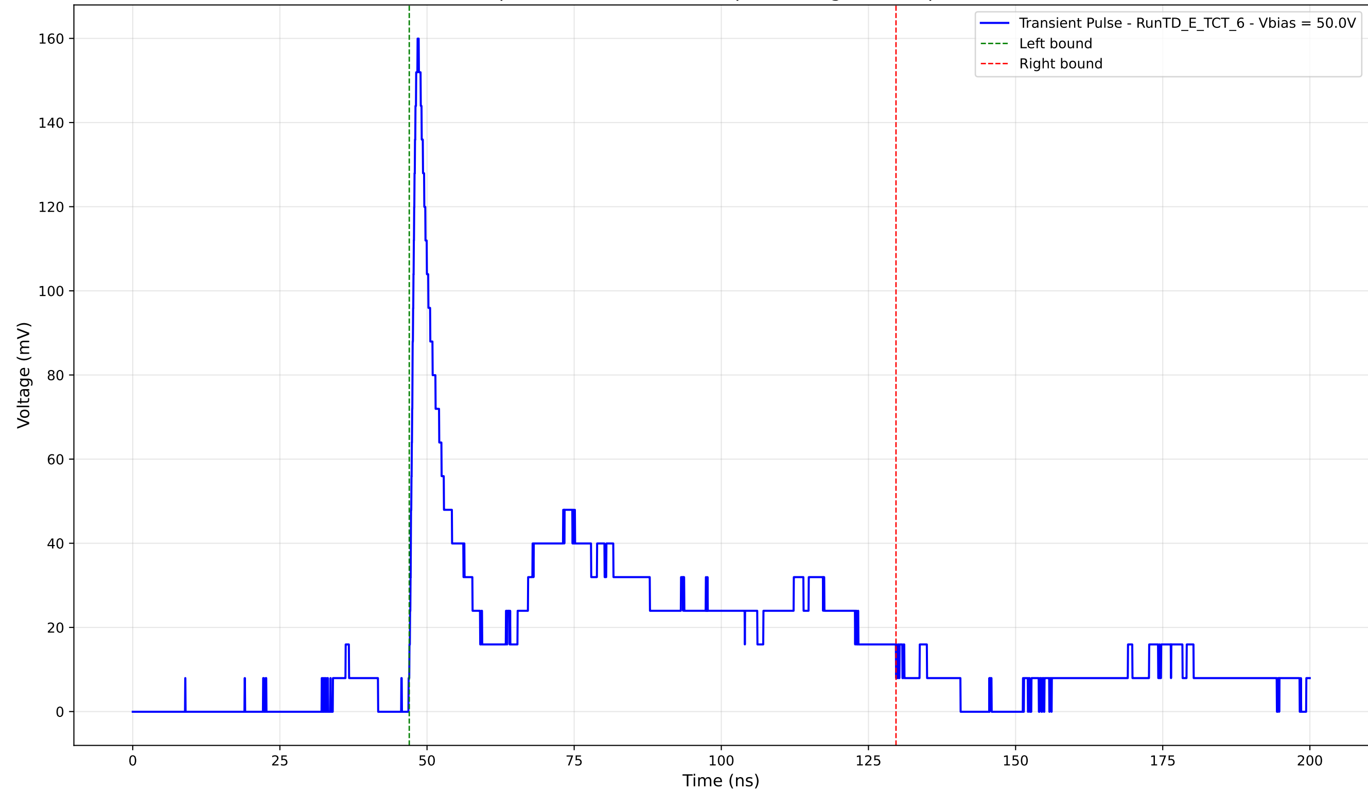
Transient Pulse - Sample: TD - Position: 130.0 \mu\text{m} - Charge: 54.00 pC - Rise Time: 1.06 ns
