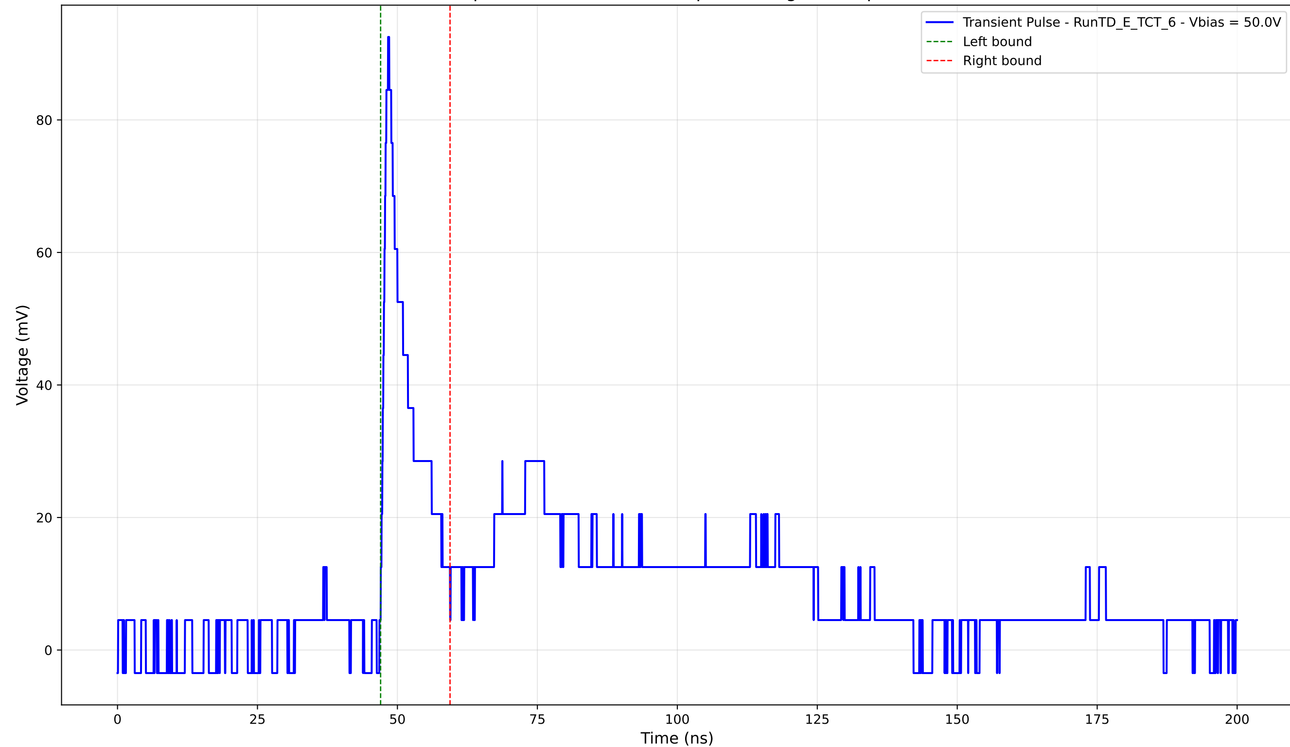
Transient Pulse - Sample: TD - Position: 150.0 \mu\text{m} - Charge: 9.41 pC - Rise Time: 1.01 ns
