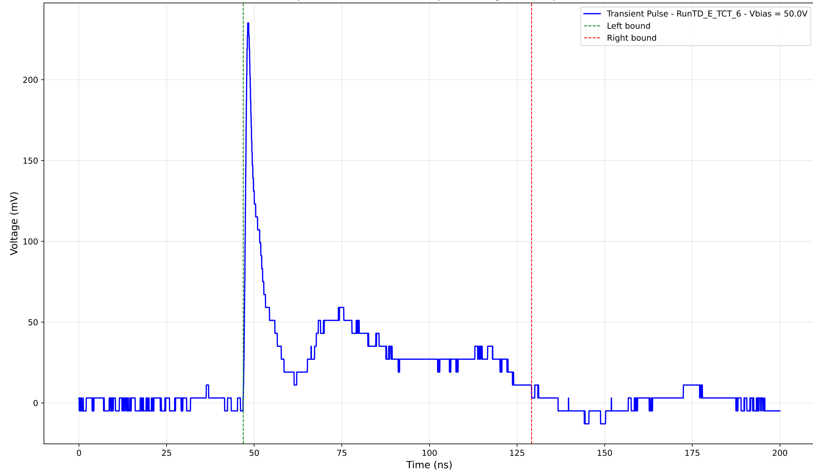
Transient Pulse - Sample: TD - Position: 105.0 \mu\text{m} - Charge: 63.79 pC - Rise Time: 0.93 ns
