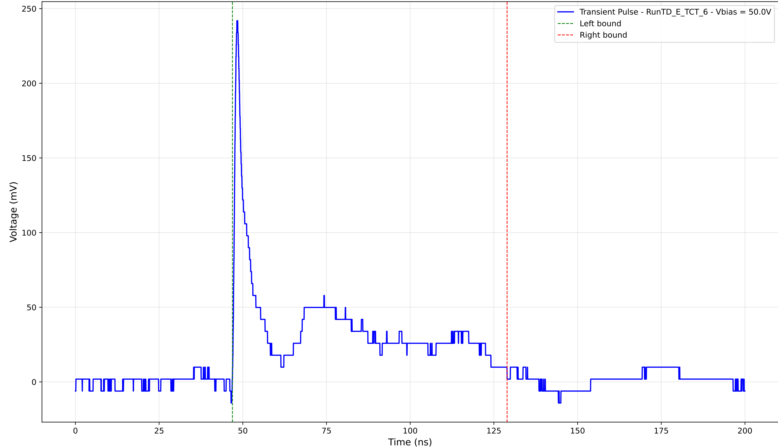
Transient Pulse - Sample: TD - Position: 115.0 \mu\text{m} - Charge: 61.23 pC - Rise Time: 0.90 ns
