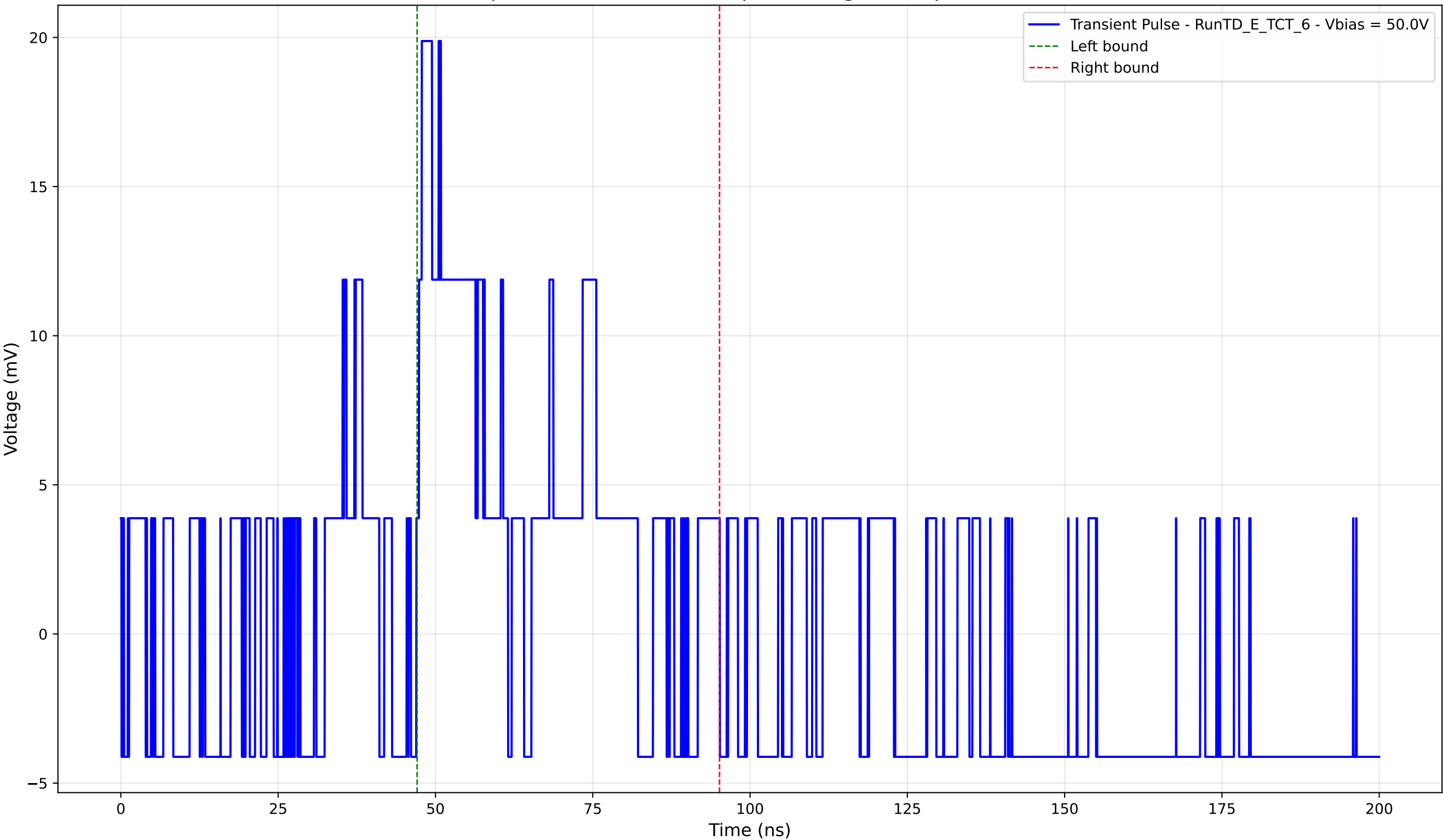
Transient Pulse - Sample: TD - Position: 370.0 \mu\text{m} - Charge: 4.97 pC - Rise Time: 0.00 ns (N/A)
