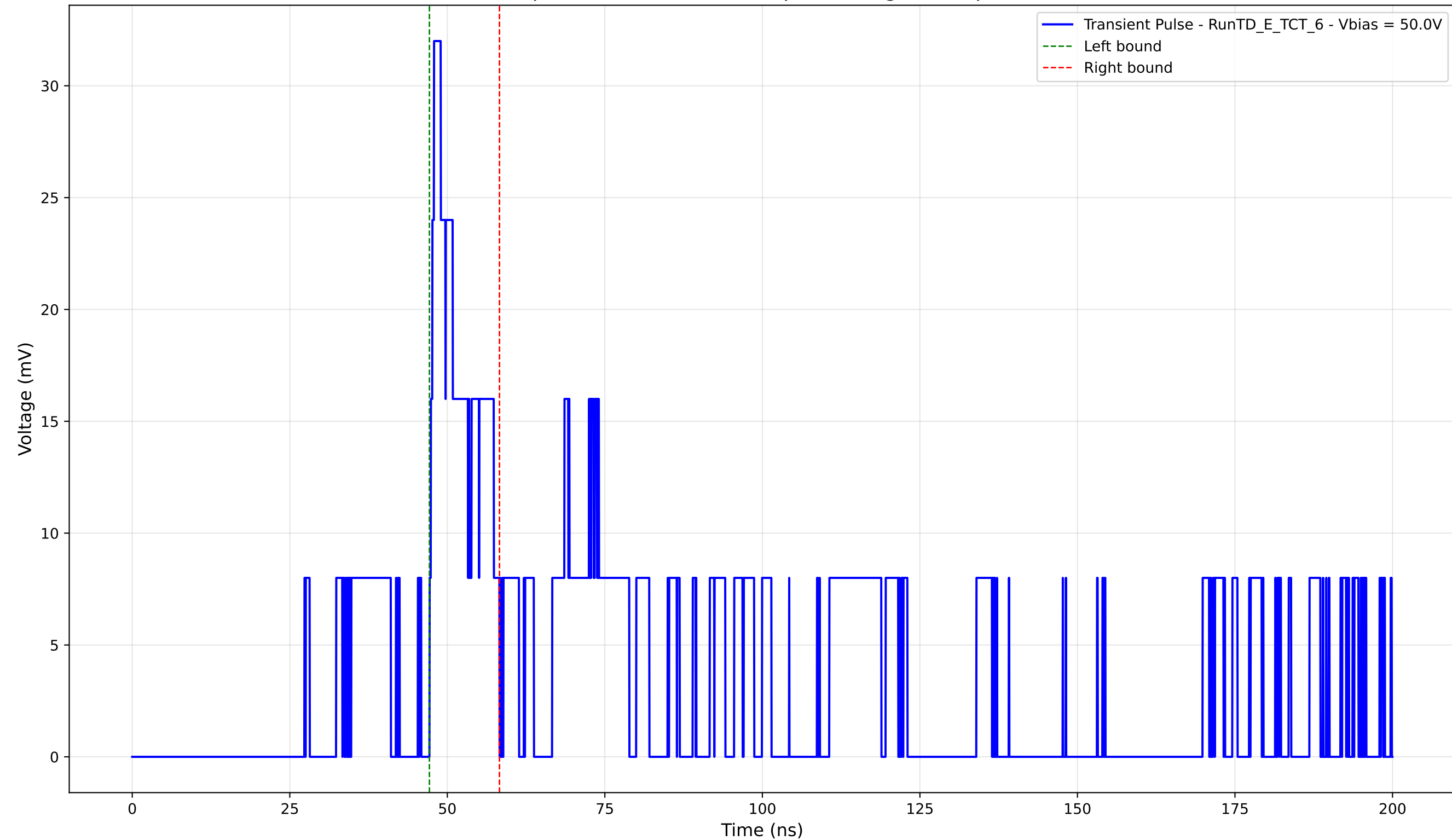
Transient Pulse - Sample: TD - Position: 260.0 \mu\text{m} - Charge: 3.99 pC - Rise Time: 0.71 ns
