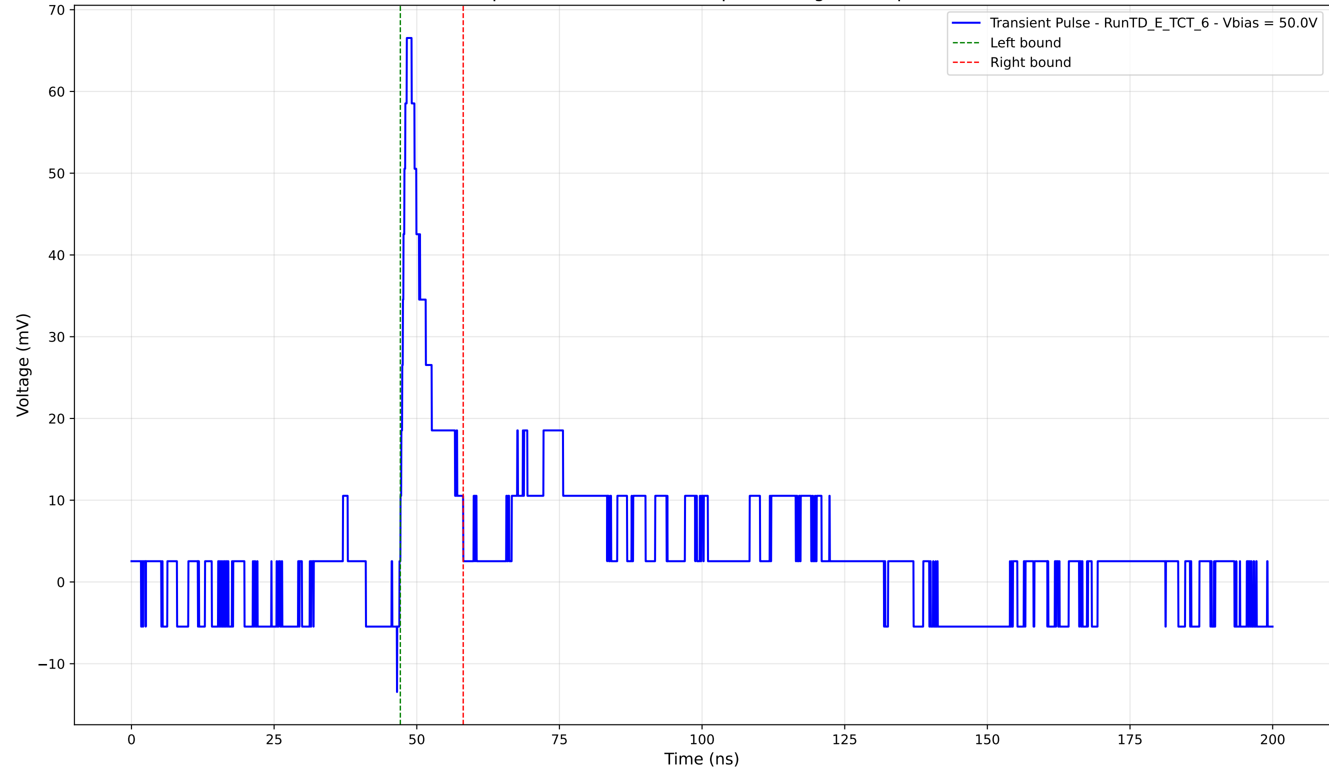
Transient Pulse - Sample: TD - Position: 160.0 \mu\text{m} - Charge: 6.50 pC - Rise Time: 1.11 ns
