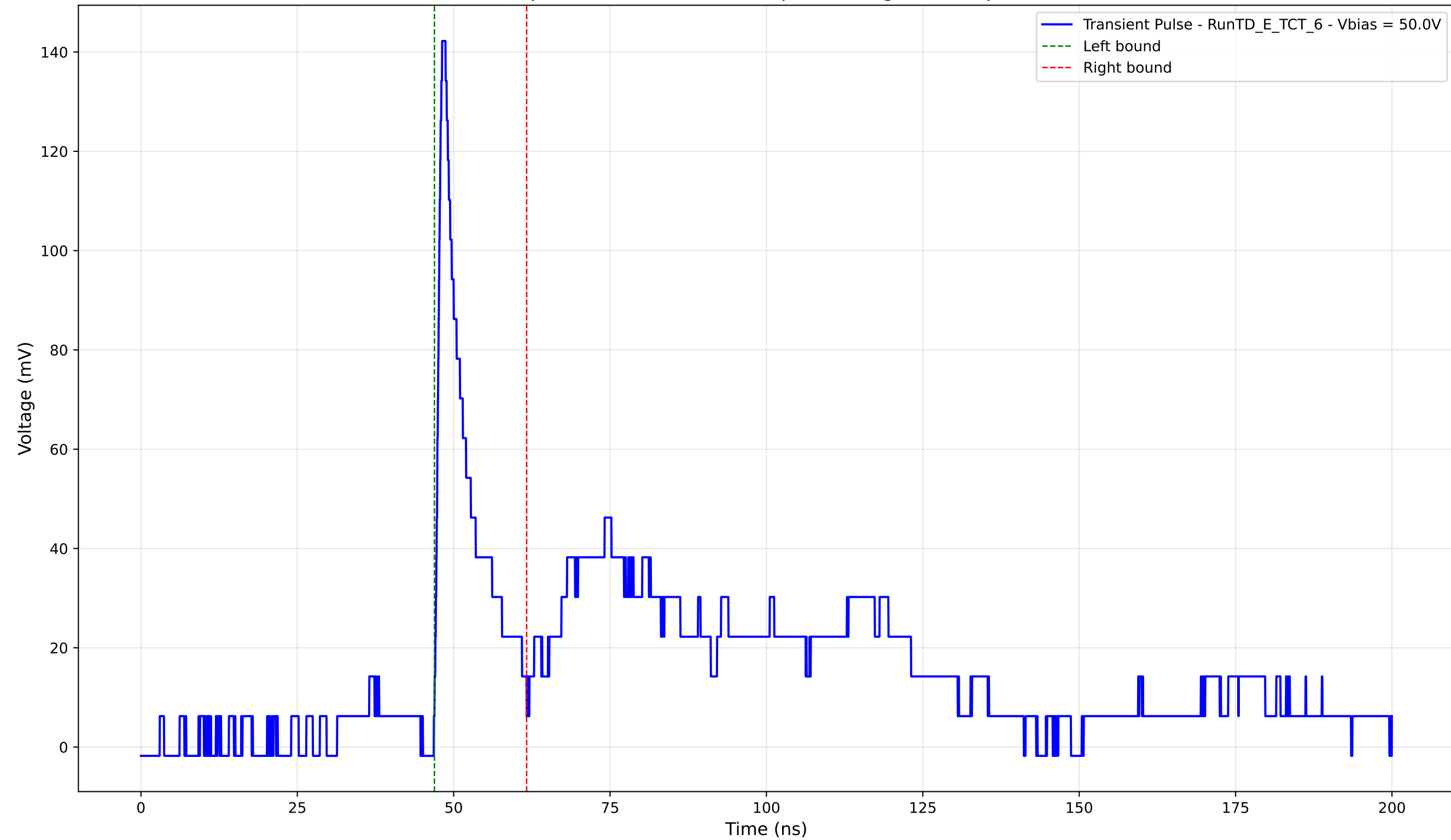
Transient Pulse - Sample: TD - Position: 170.0 \mu\text{m} - Charge: 15.38 pC - Rise Time: 1.08 ns
