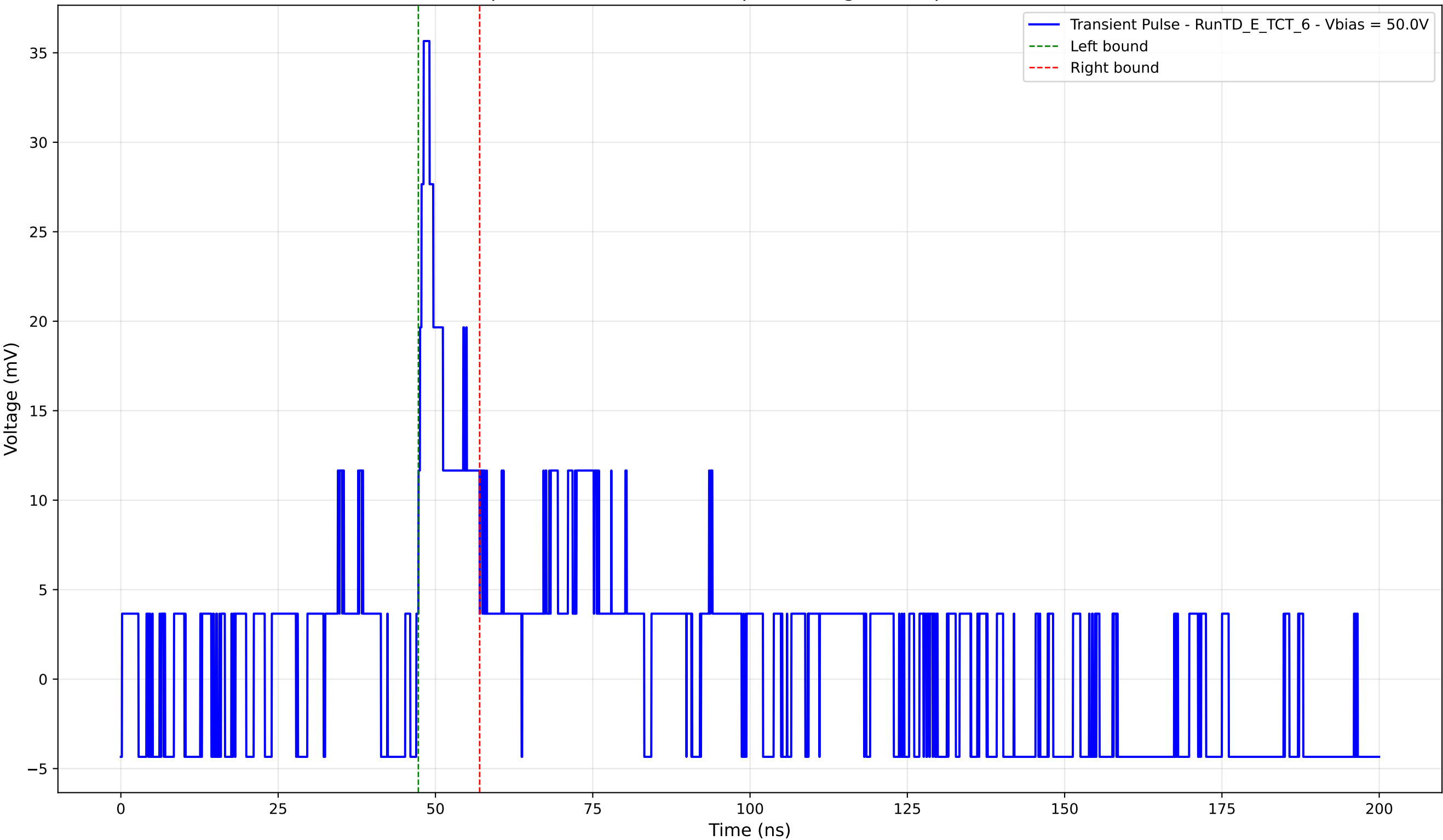
Transient Pulse - Sample: TD - Position: 285.0 \mu\text{m} - Charge: 3.34 pC - Rise Time: 0.00 ns (N/A)
