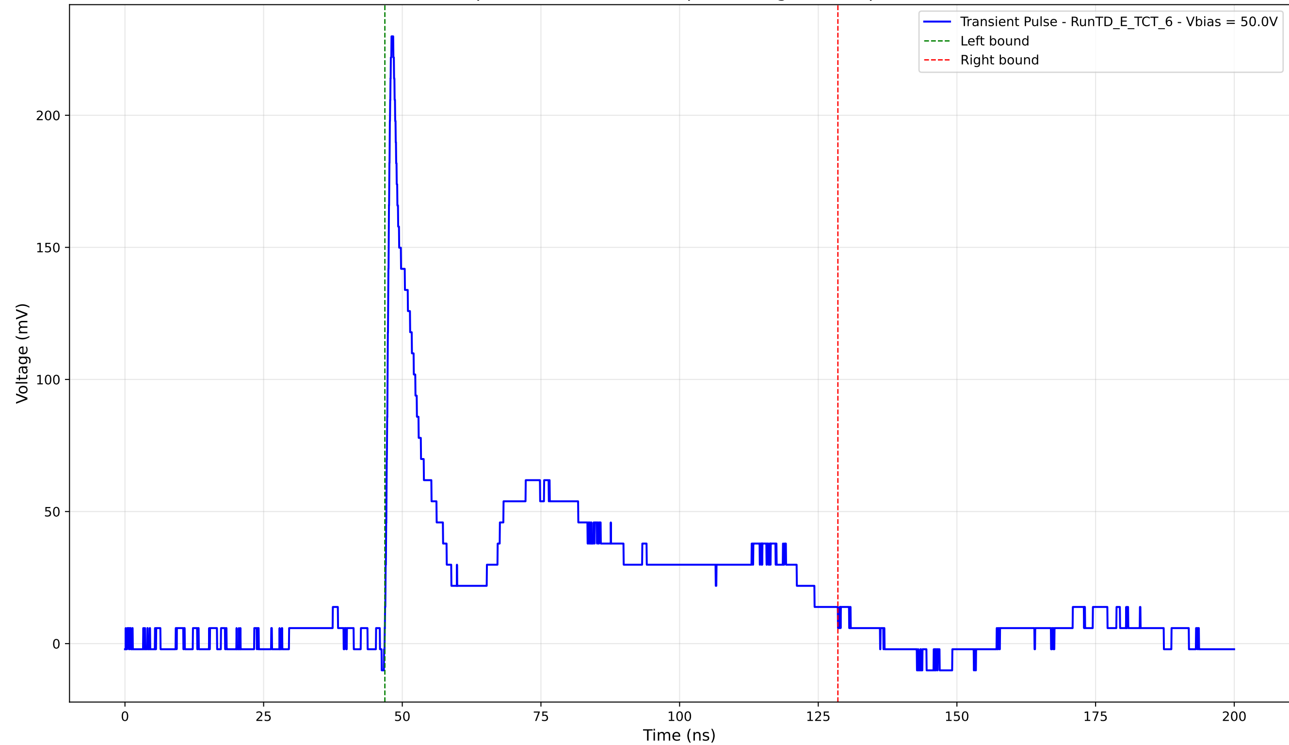
Transient Pulse - Sample: TD - Position: 80.0 \mu\text{m} - Charge: 71.72 pC - Rise Time: 0.88 ns
