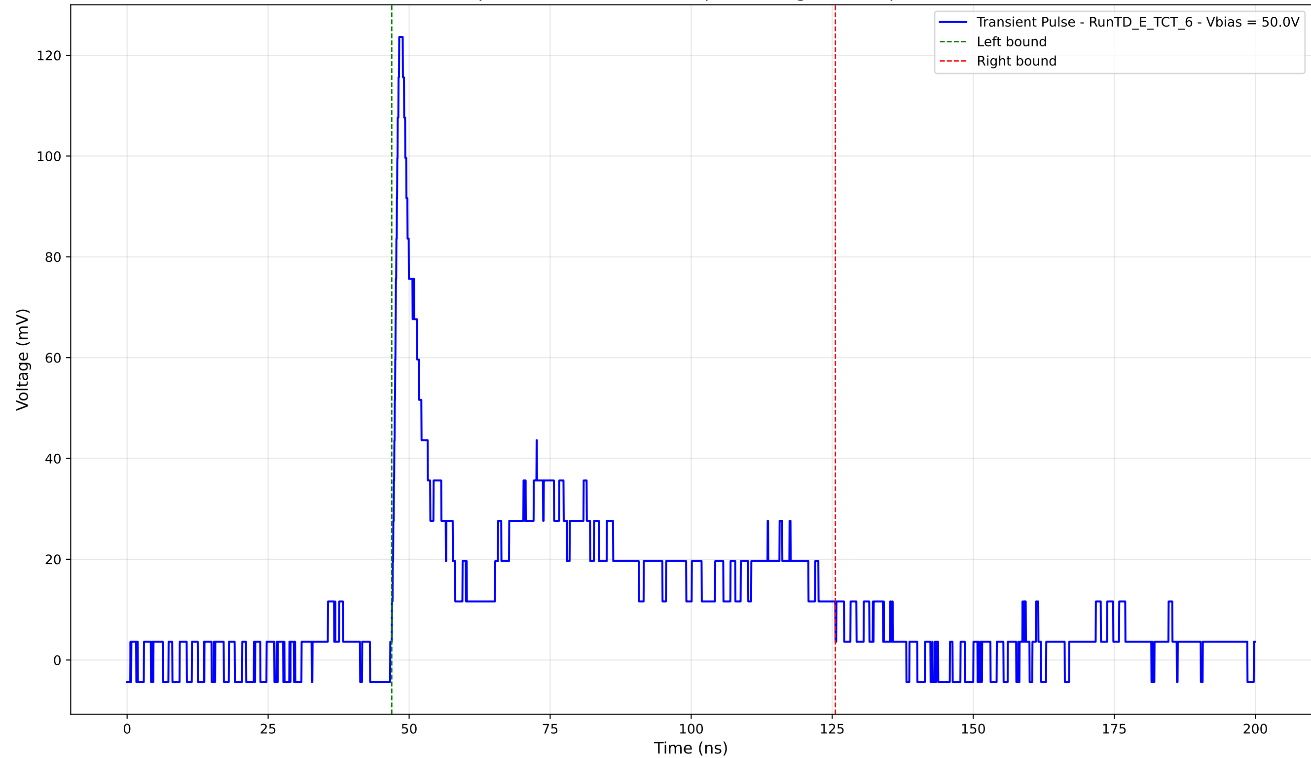
Transient Pulse - Sample: TD - Position: 165.0 \mu\text{m} - Charge: 39.34 pC - Rise Time: 1.04 ns
