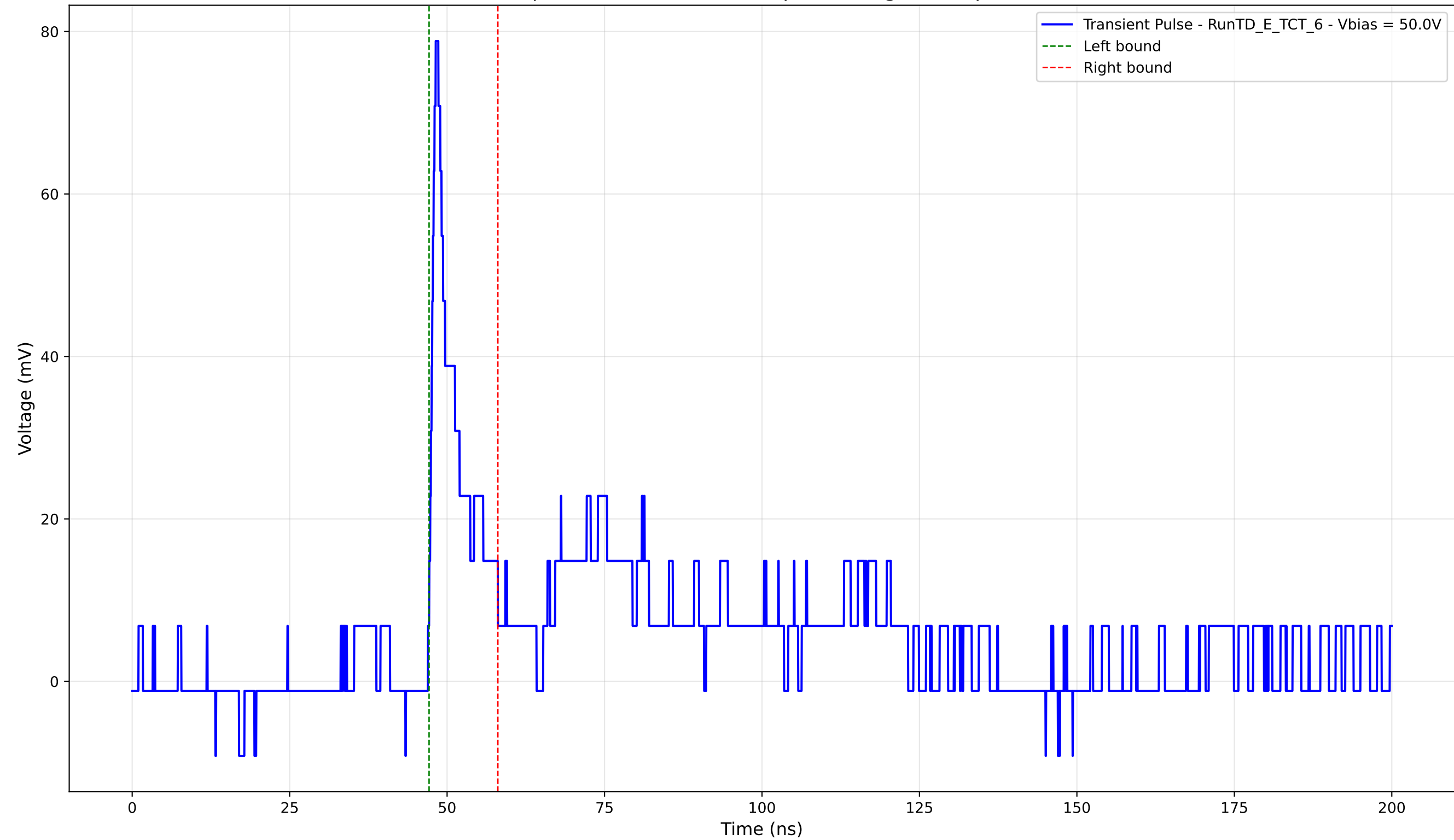
Transient Pulse - Sample: TD - Position: 230.0 \mu\text{m} - Charge: 6.82 pC - Rise Time: 1.04 ns
