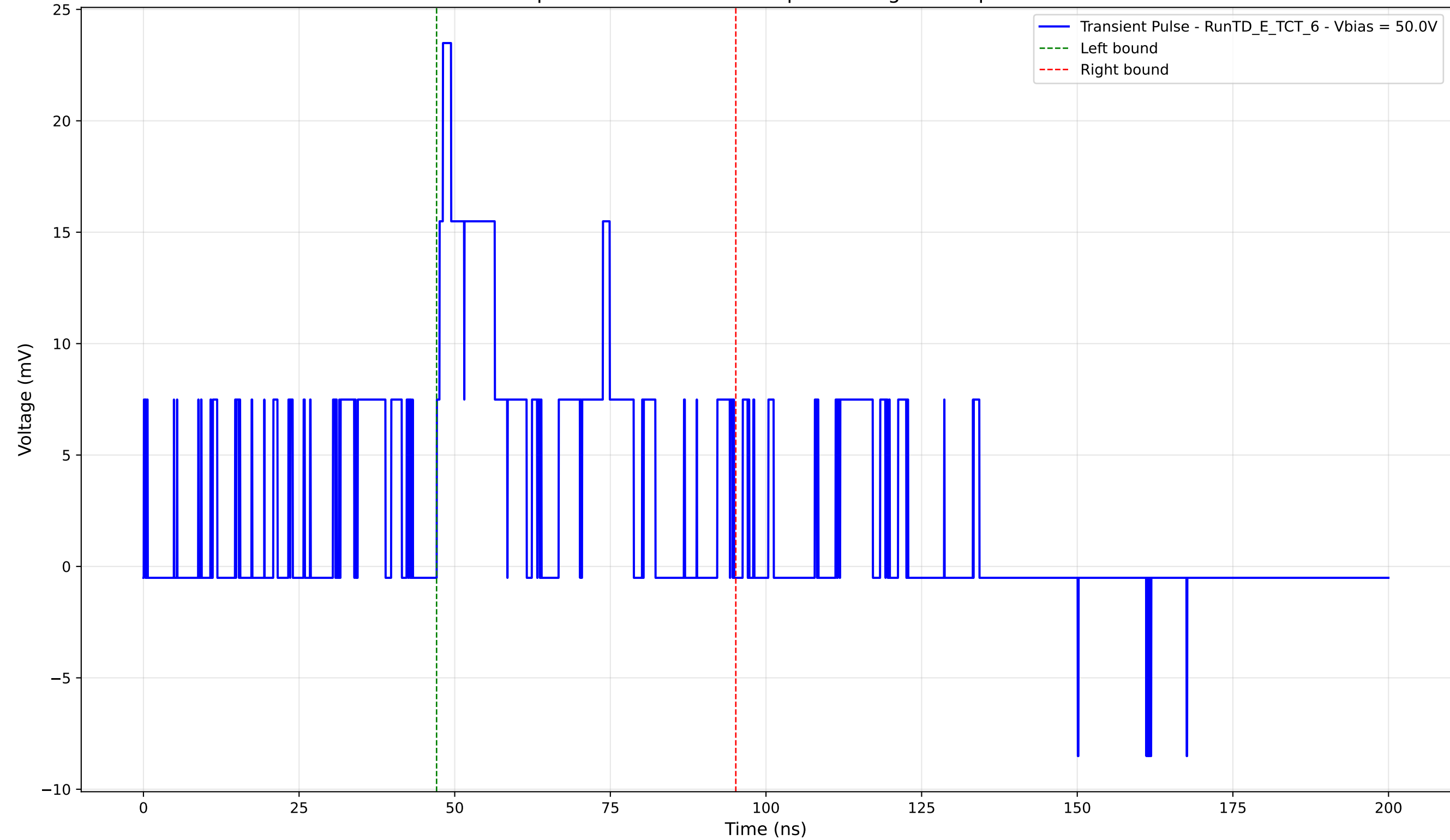
Transient Pulse - Sample: TD - Position: 405.0 \mu\text{m} - Charge: 6.48 pC - Rise Time: 0.99 ns
