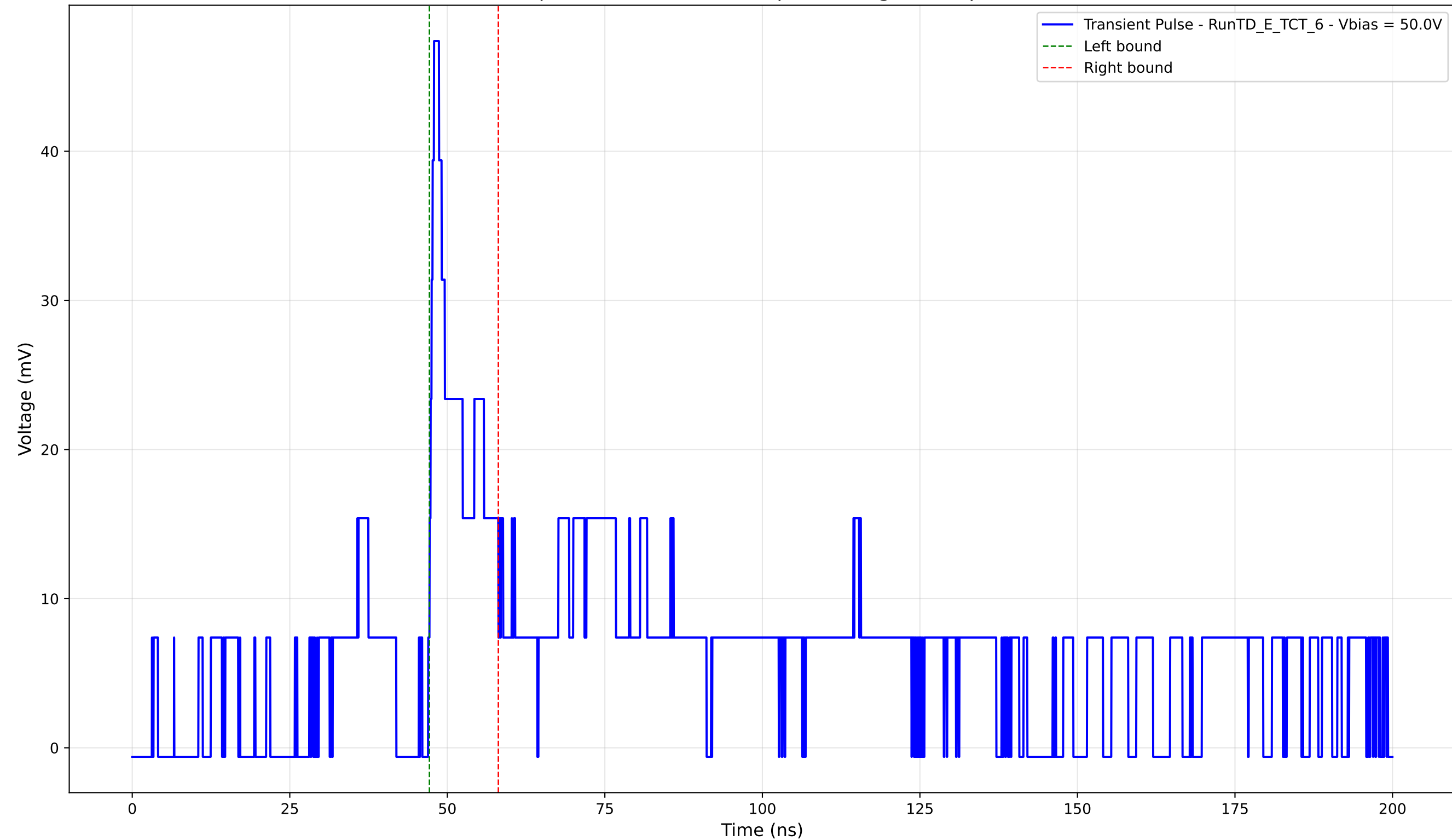
Transient Pulse - Sample: TD - Position: 30.0 \mu\text{m} - Charge: 5.12 pC - Rise Time: 0.93 ns
