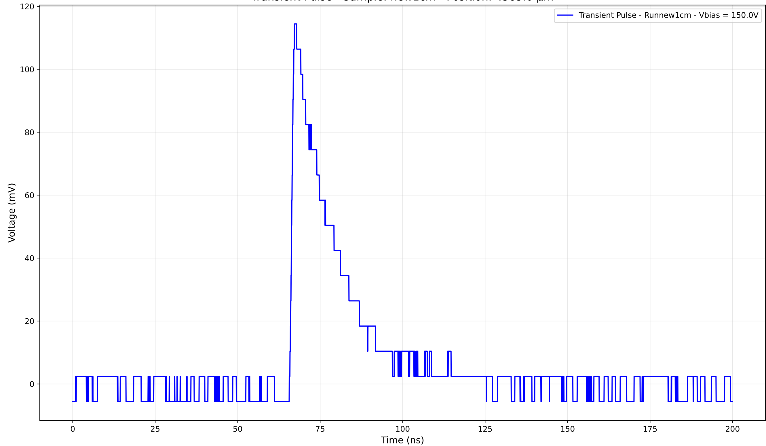
Transient Pulse - Sample: new1cm - Position: 4585.0 \mu\text{m}
