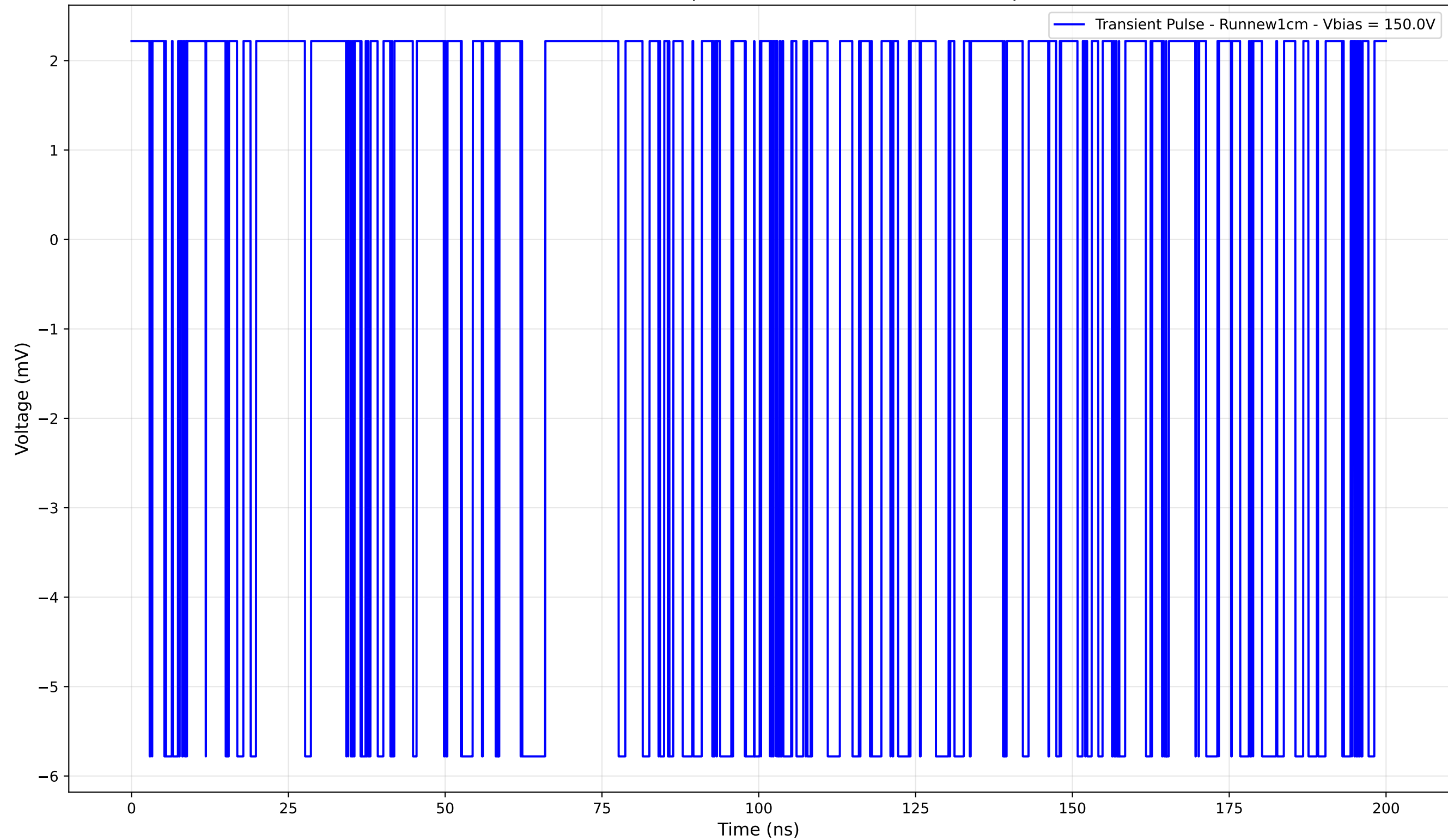
Transient Pulse - Sample: new1cm - Position: 4980.0 \mu\text{m}
