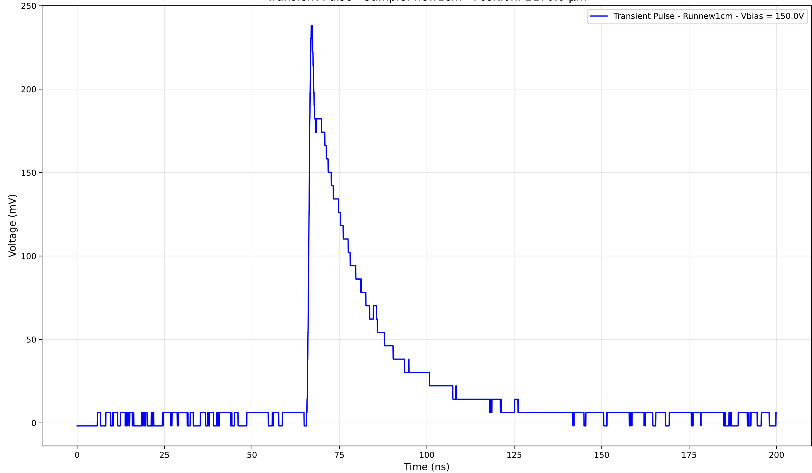
Transient Pulse - Sample: new1cm - Position: 2170.0 \mu\text{m}
