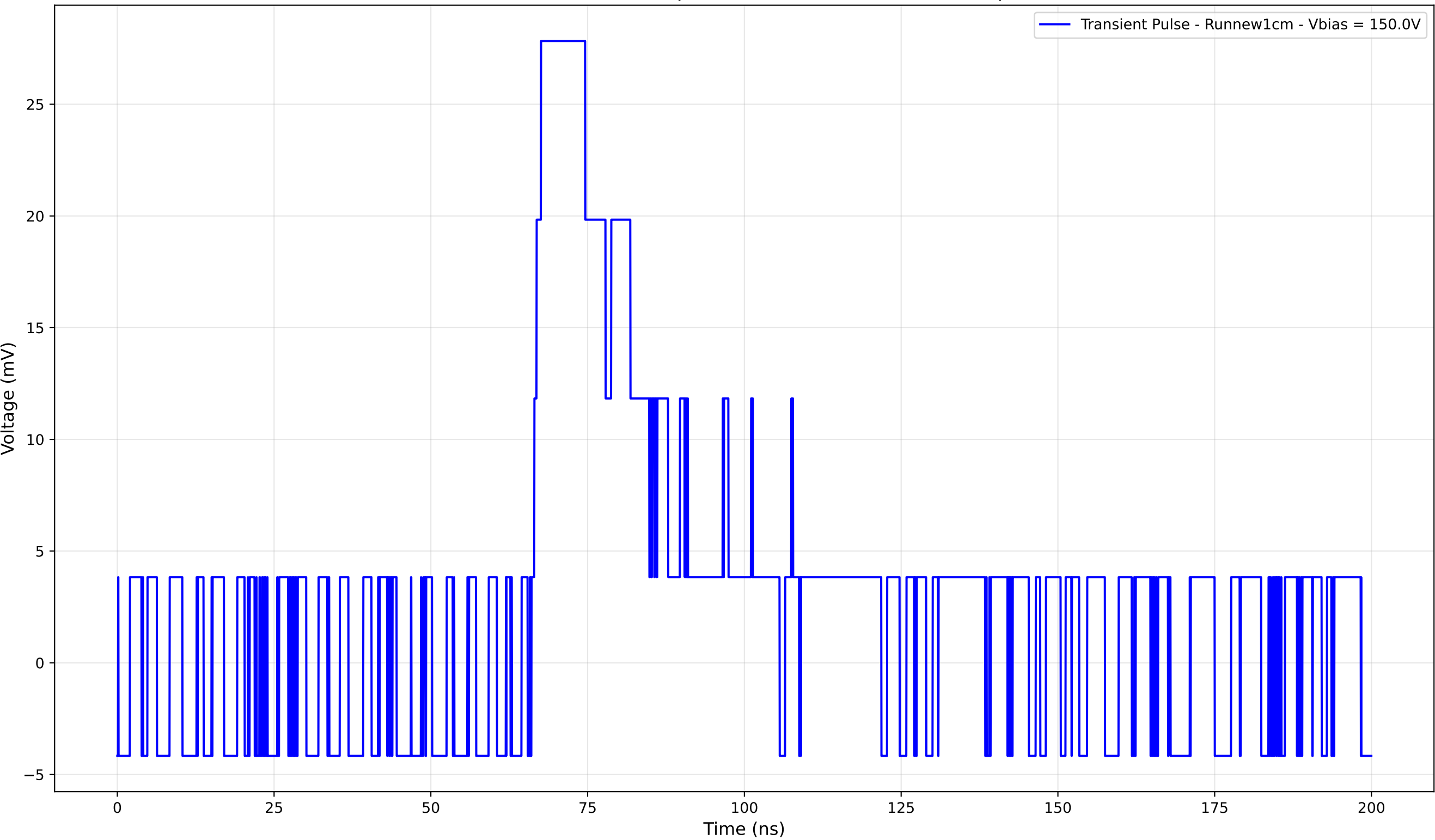
Transient Pulse - Sample: new1cm - Position: 1590.0 \mu\text{m}
