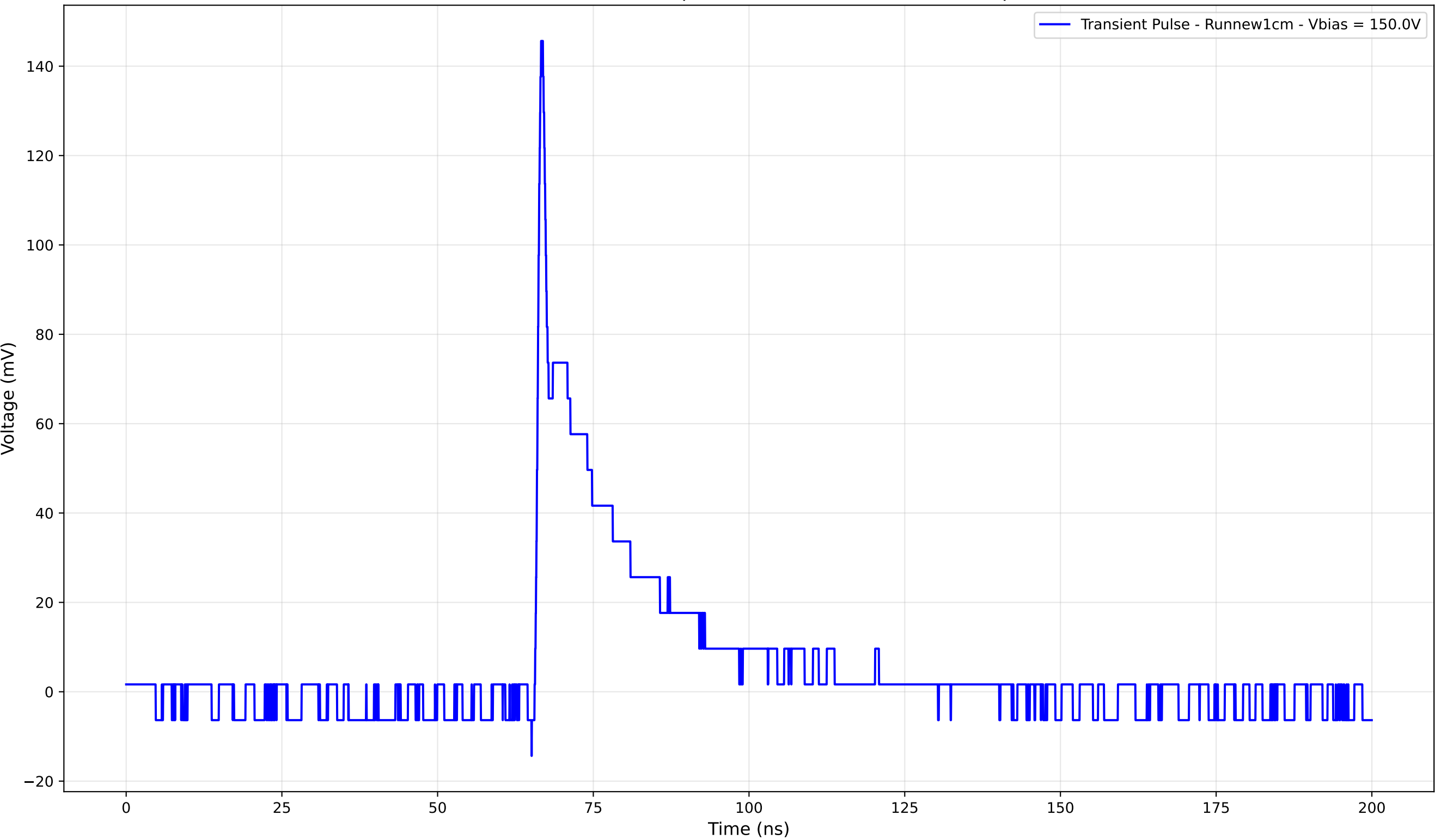
Transient Pulse - Sample: new1cm - Position: 2635.0 \mu\text{m}
