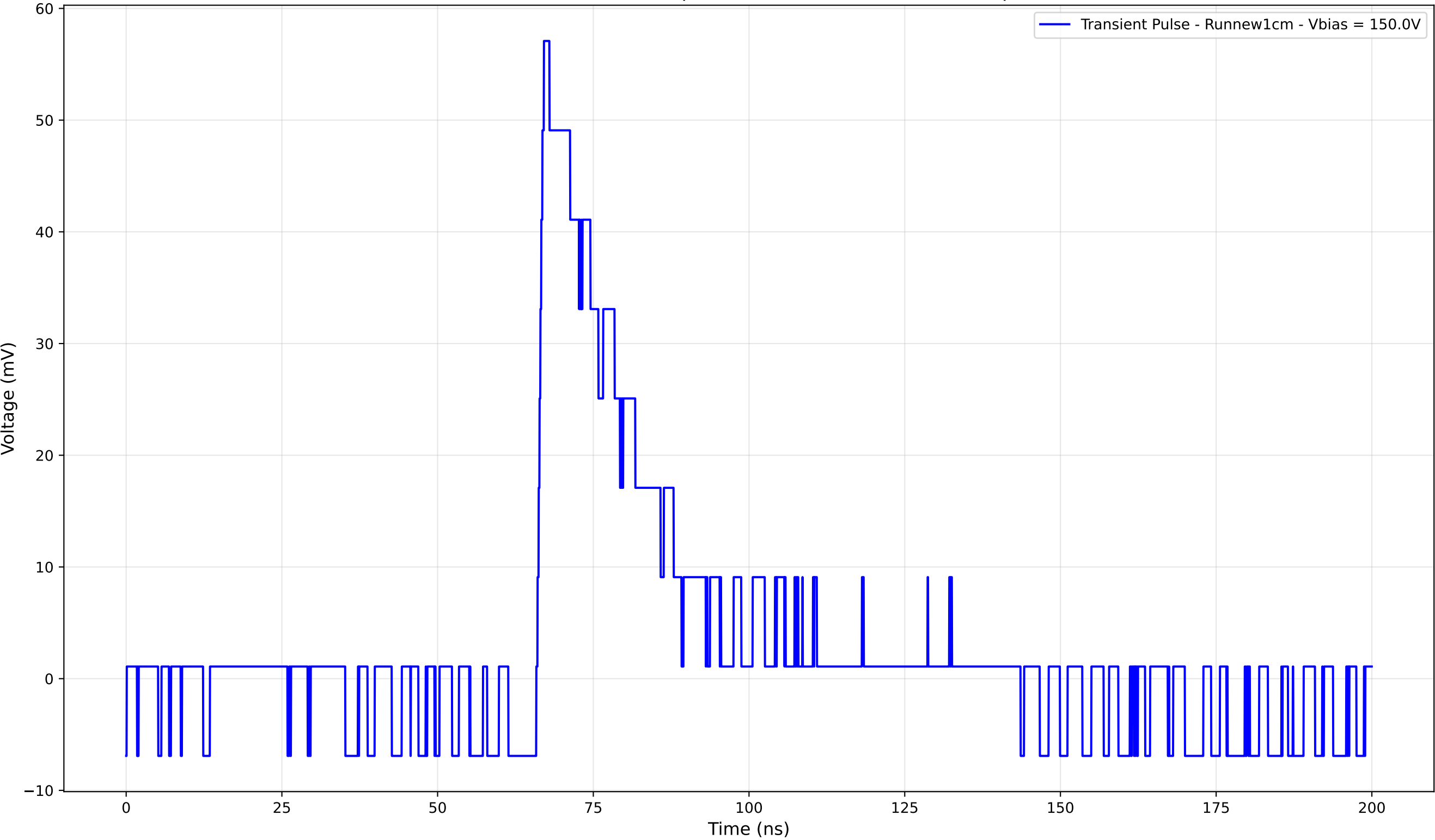
Transient Pulse - Sample: new1cm - Position: 3130.0 \mu\text{m}
