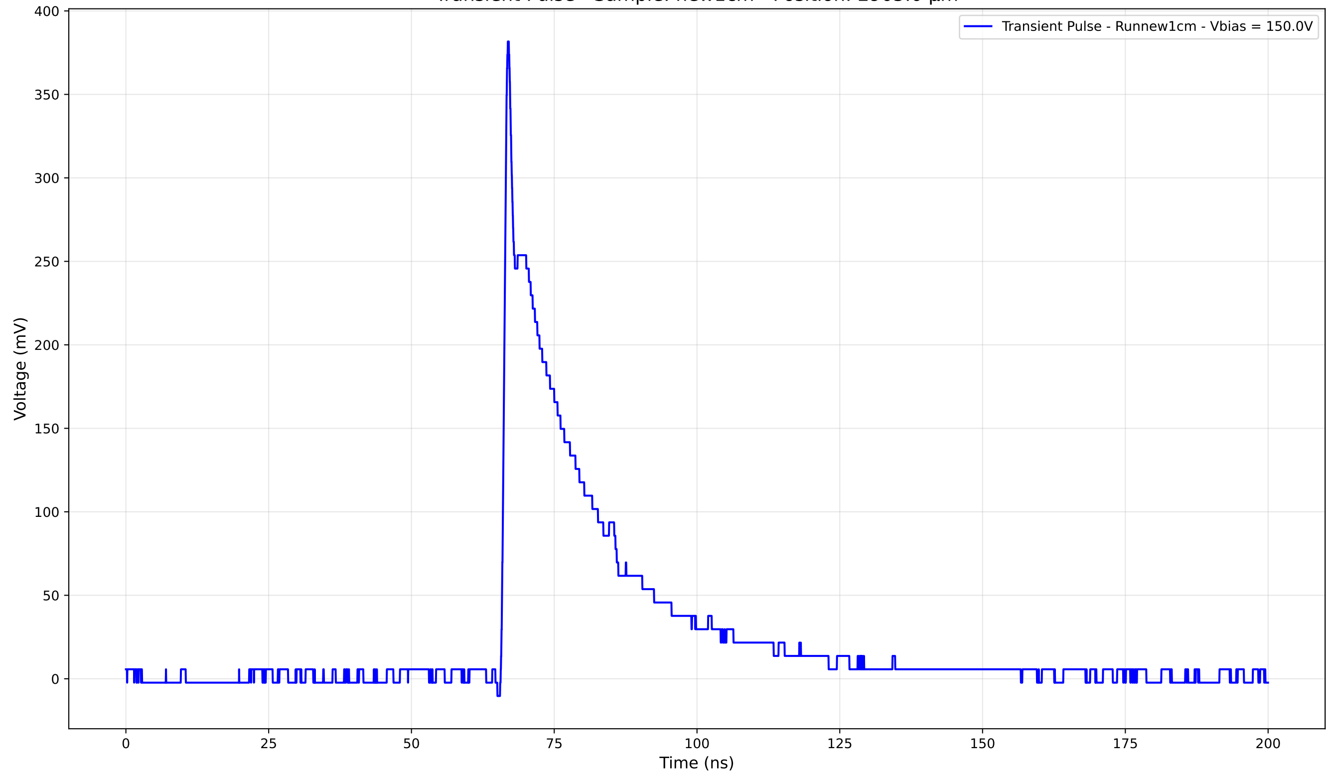
Transient Pulse - Sample: new1cm - Position: 2905.0 \mu\text{m}
