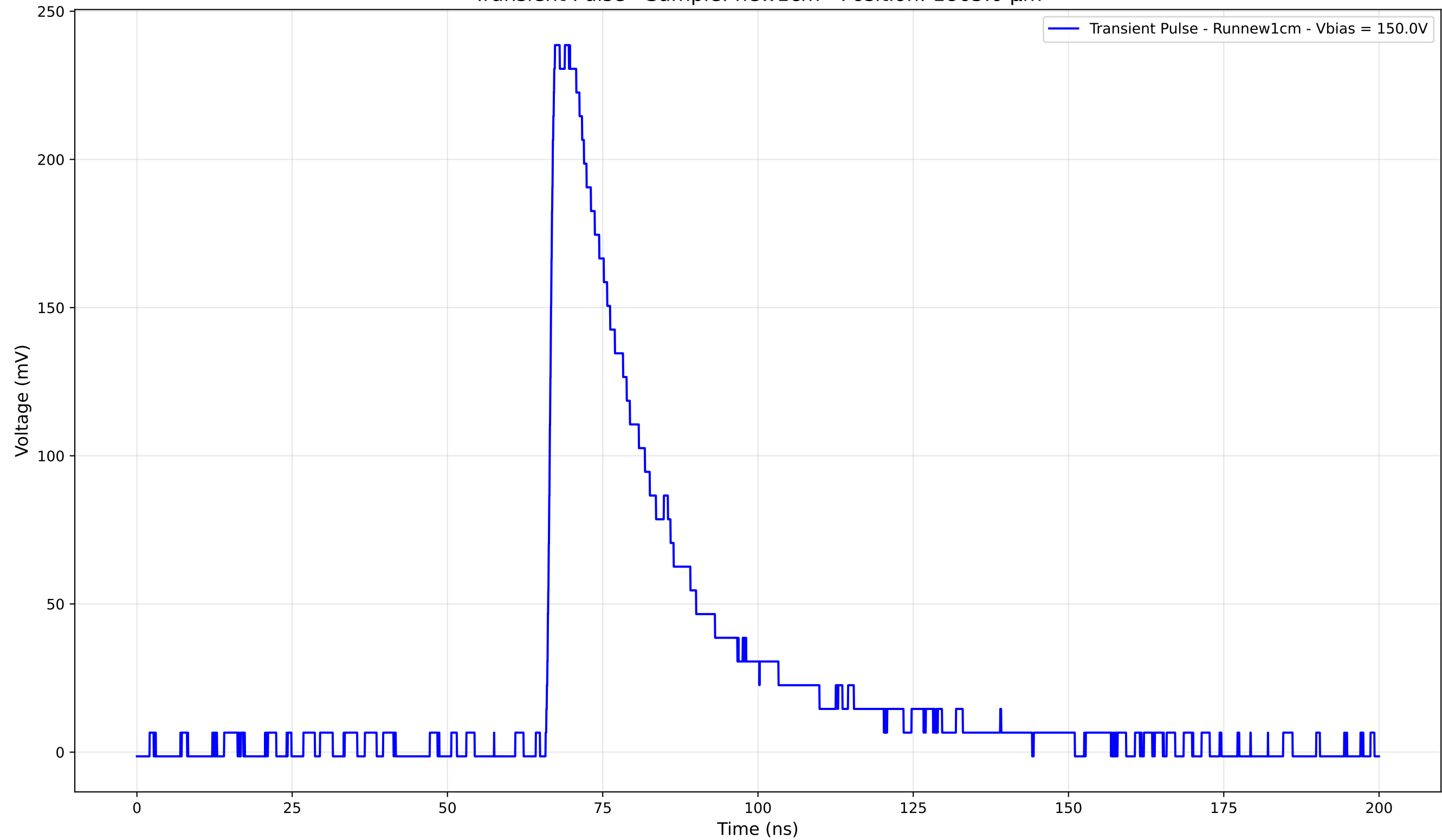
Transient Pulse - Sample: new1cm - Position: 1865.0 \mu\text{m}
