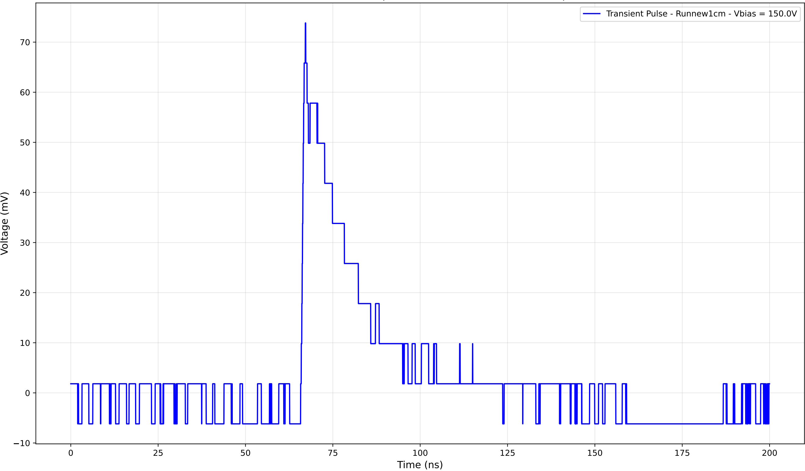
Transient Pulse - Sample: new1cm - Position: 3085.0 \mu\text{m}
