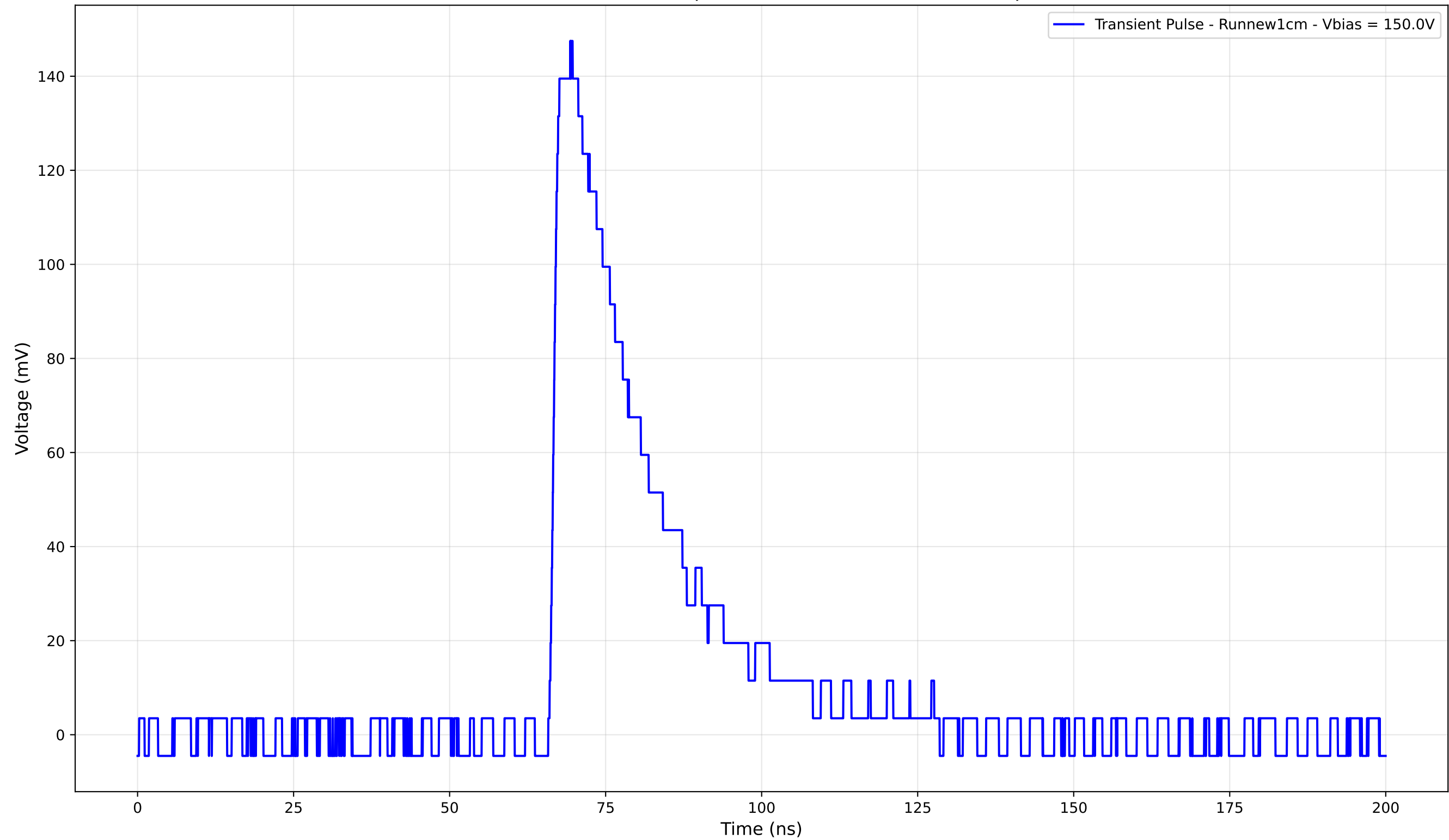
Transient Pulse - Sample: new1cm - Position: 1655.0 \mu\text{m}
