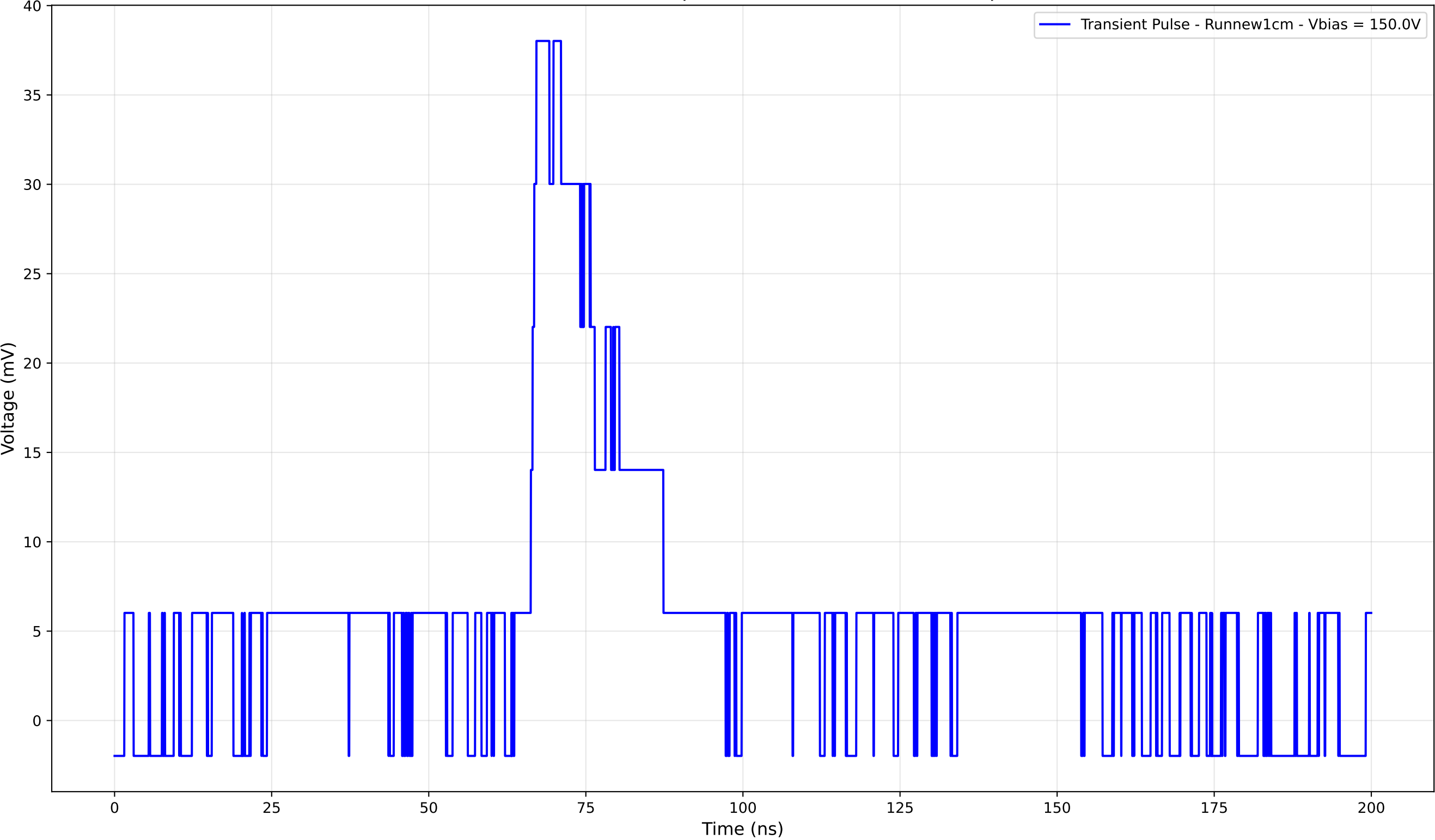
Transient Pulse - Sample: new1cm - Position: 570.0 \mu\text{m}
