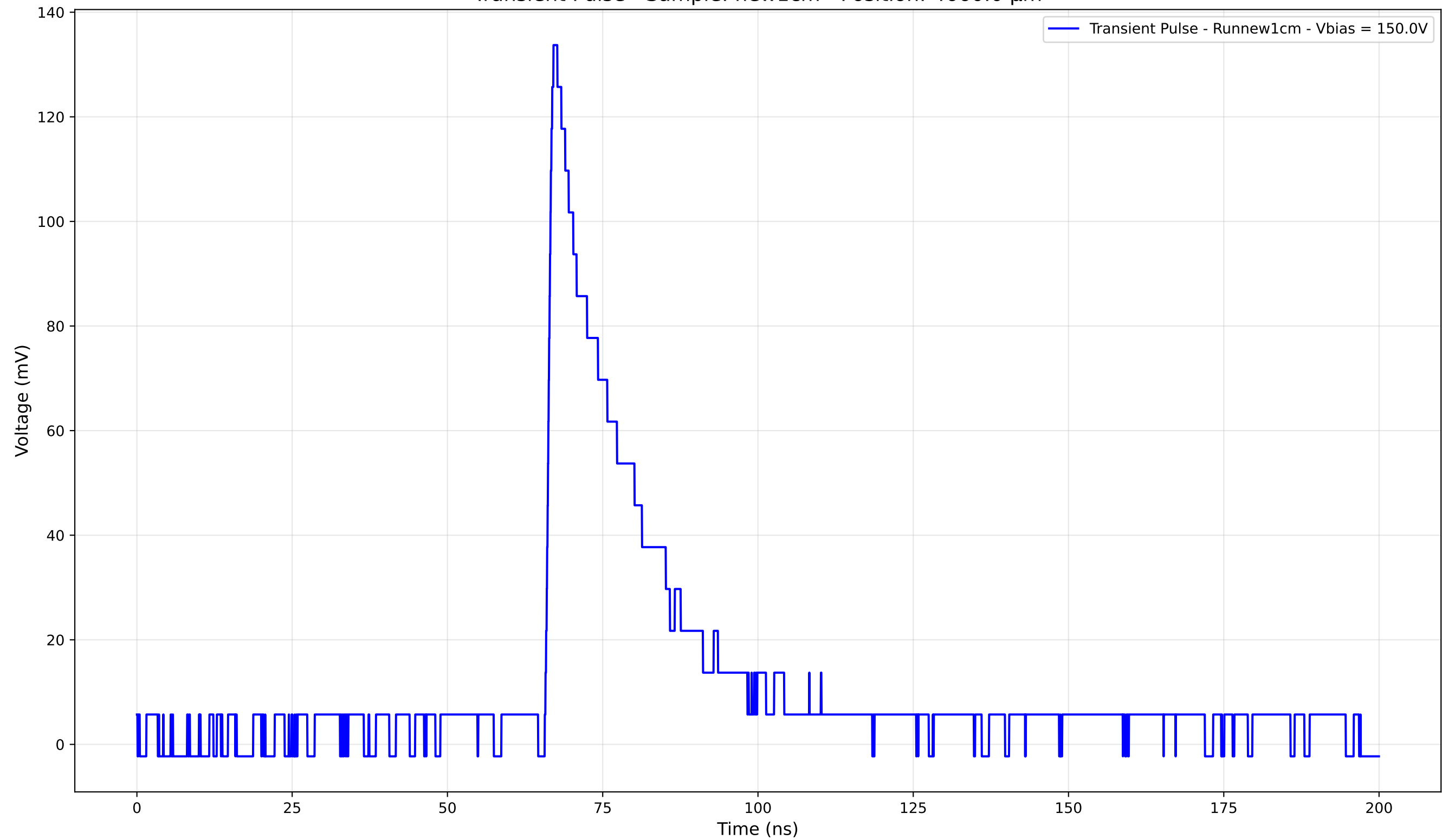
Transient Pulse - Sample: new1cm - Position: 4660.0 \mu\text{m}
