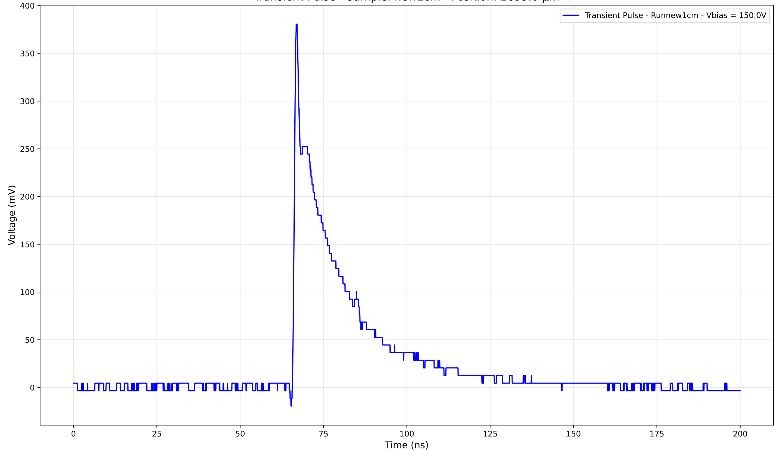
Transient Pulse - Sample: new1cm - Position: 2895.0 \mu\text{m}
