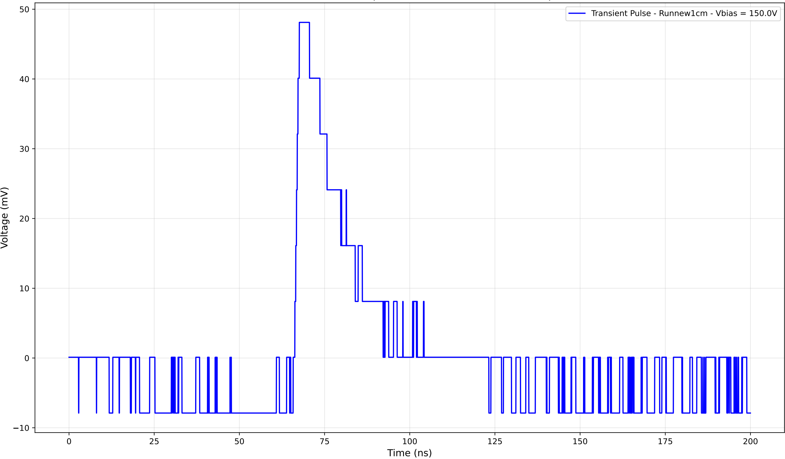
Transient Pulse - Sample: new1cm - Position: 4105.0 \mu\text{m}
