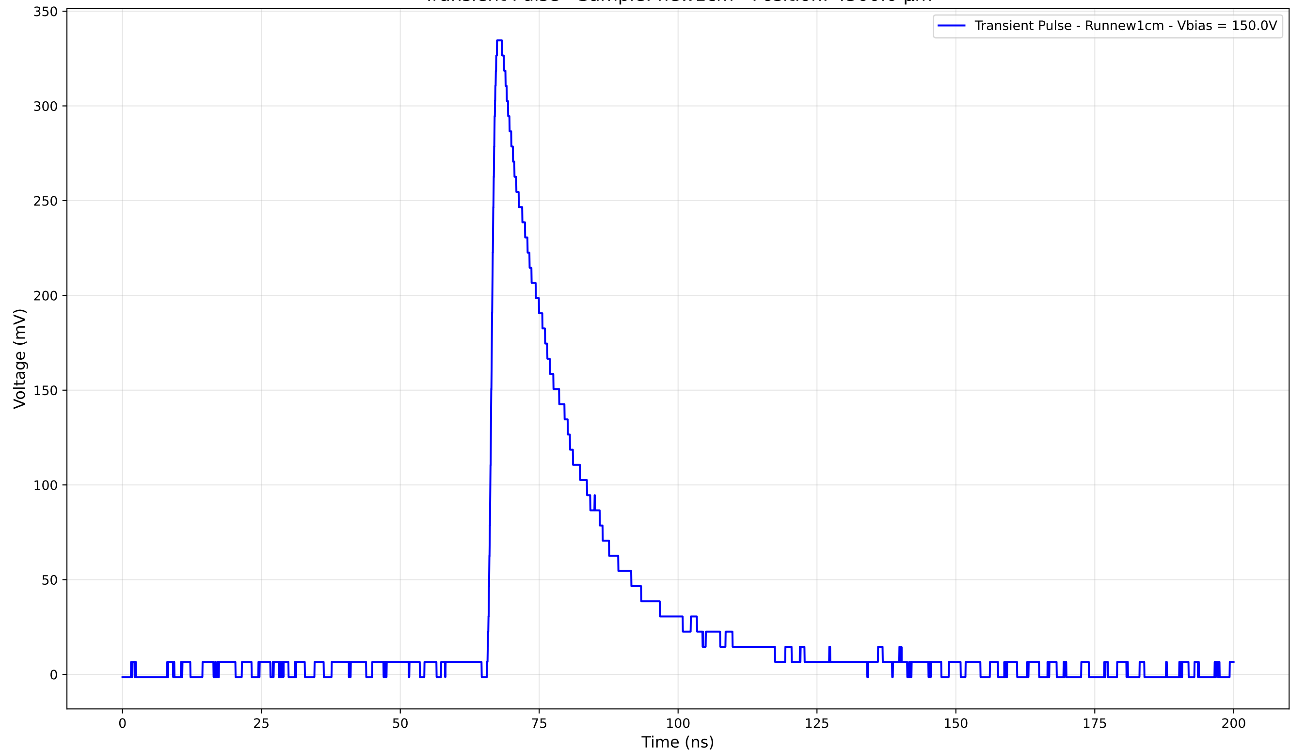
Transient Pulse - Sample: new1cm - Position: 4500.0 \mu\text{m}
