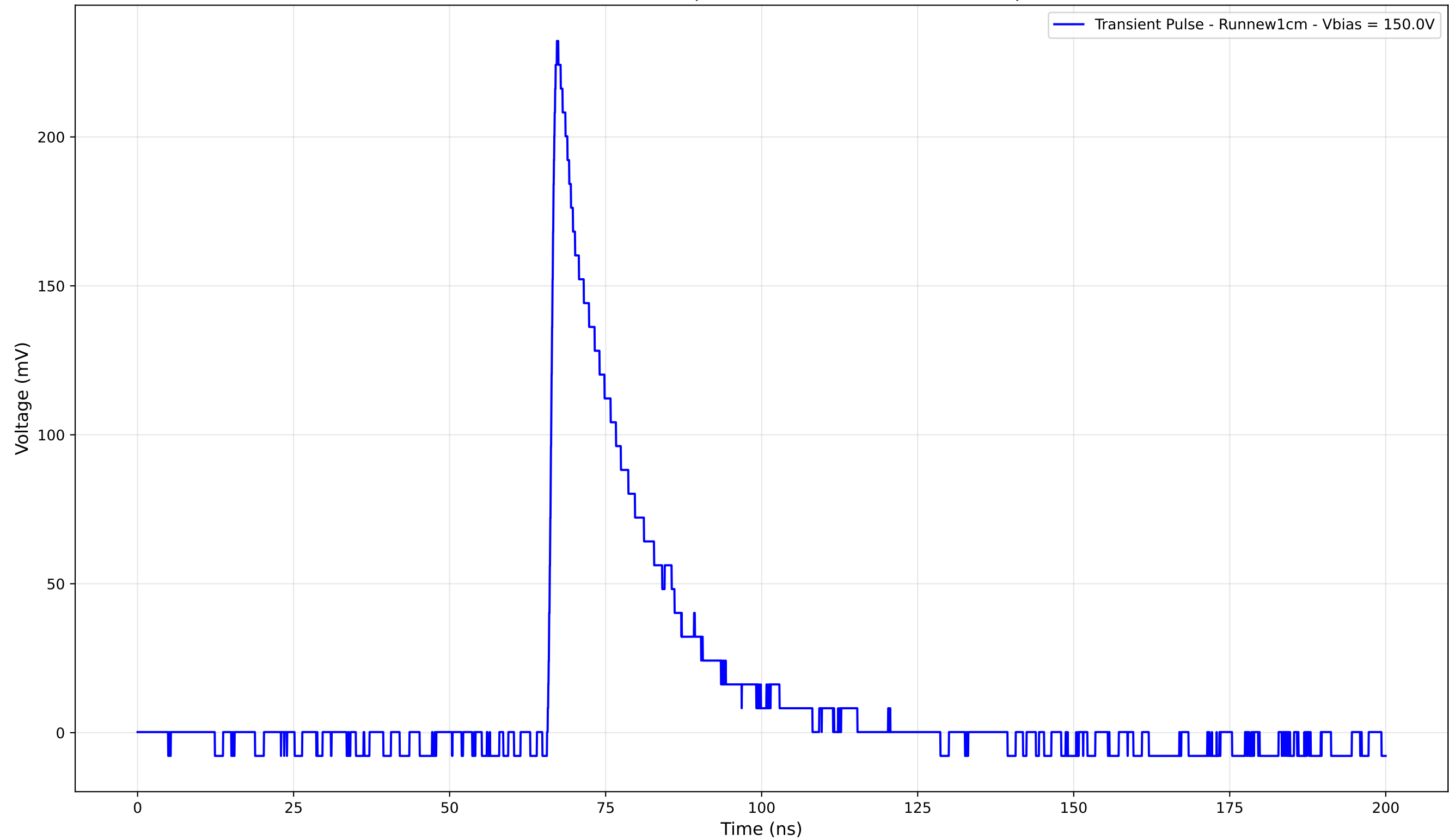
Transient Pulse - Sample: new1cm - Position: 4690.0 \mu\text{m}
