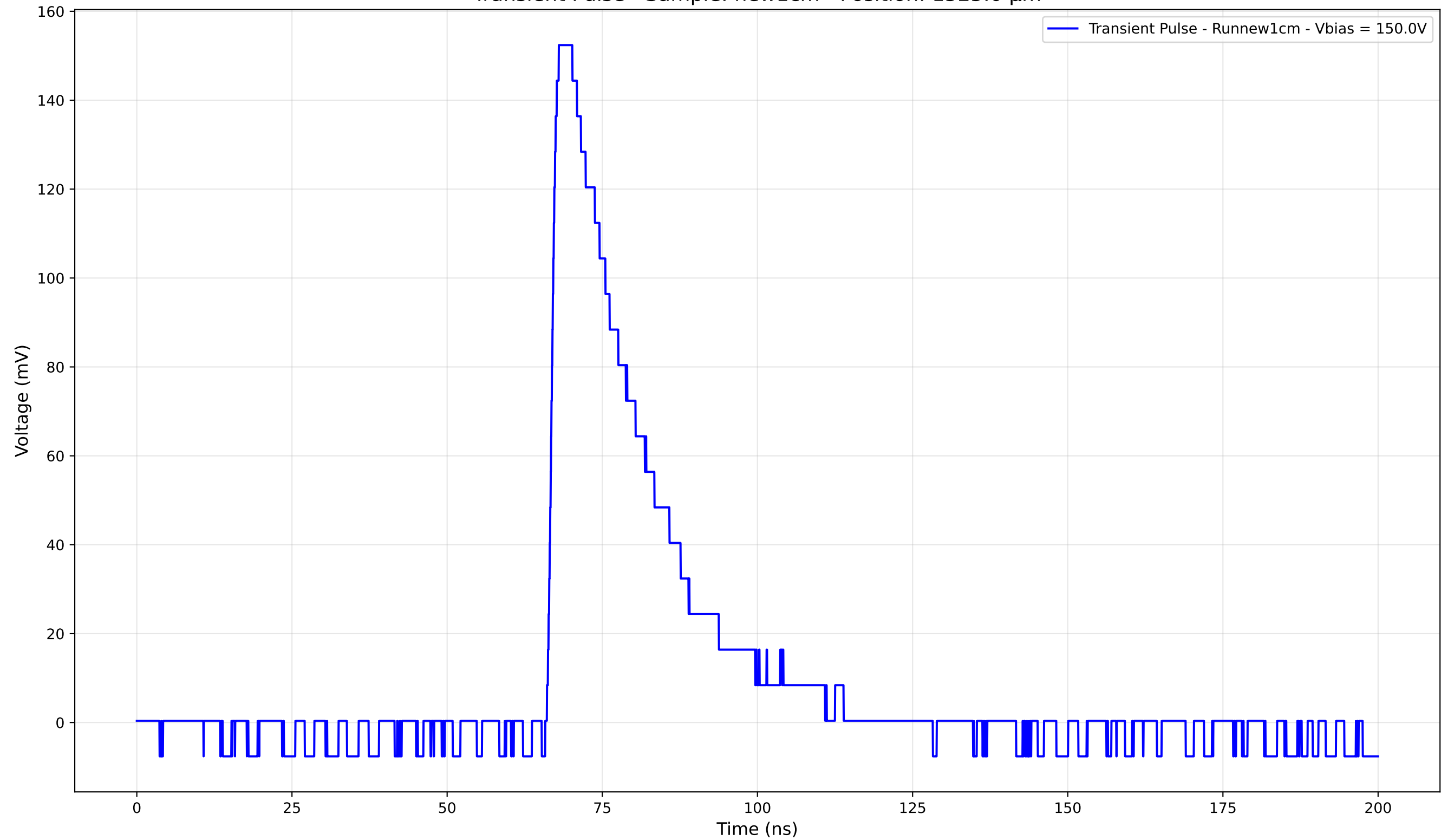
Transient Pulse - Sample: new1cm - Position: 1525.0 \mu\text{m}
