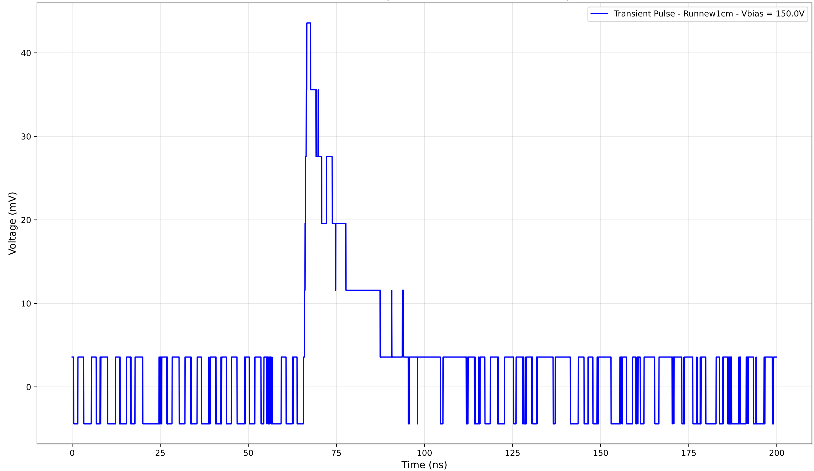
Transient Pulse - Sample: new1cm - Position: 4940.0 \mu\text{m}
