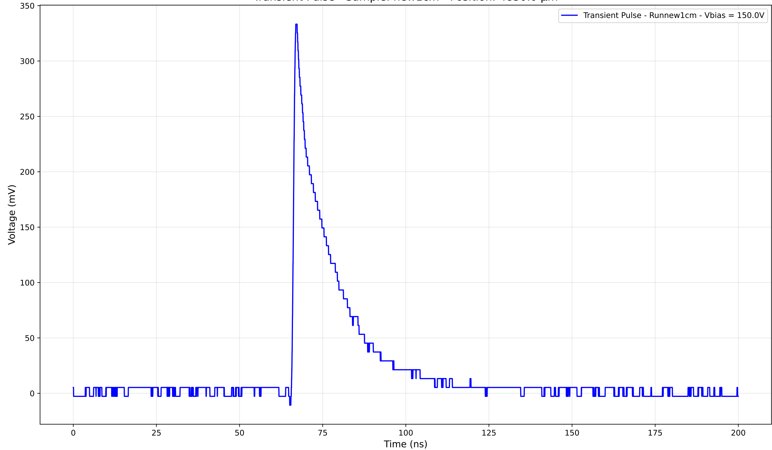
Transient Pulse - Sample: new1cm - Position: 4830.0 \mu\text{m}
