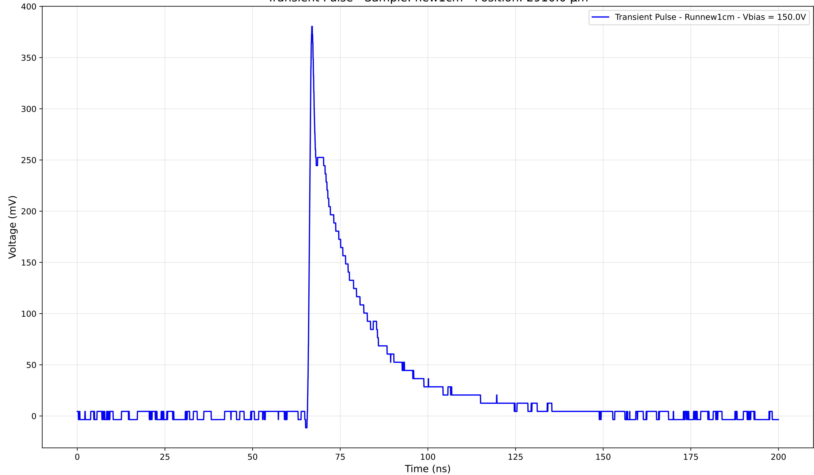
Transient Pulse - Sample: new1cm - Position: 2910.0 \mu\text{m}
