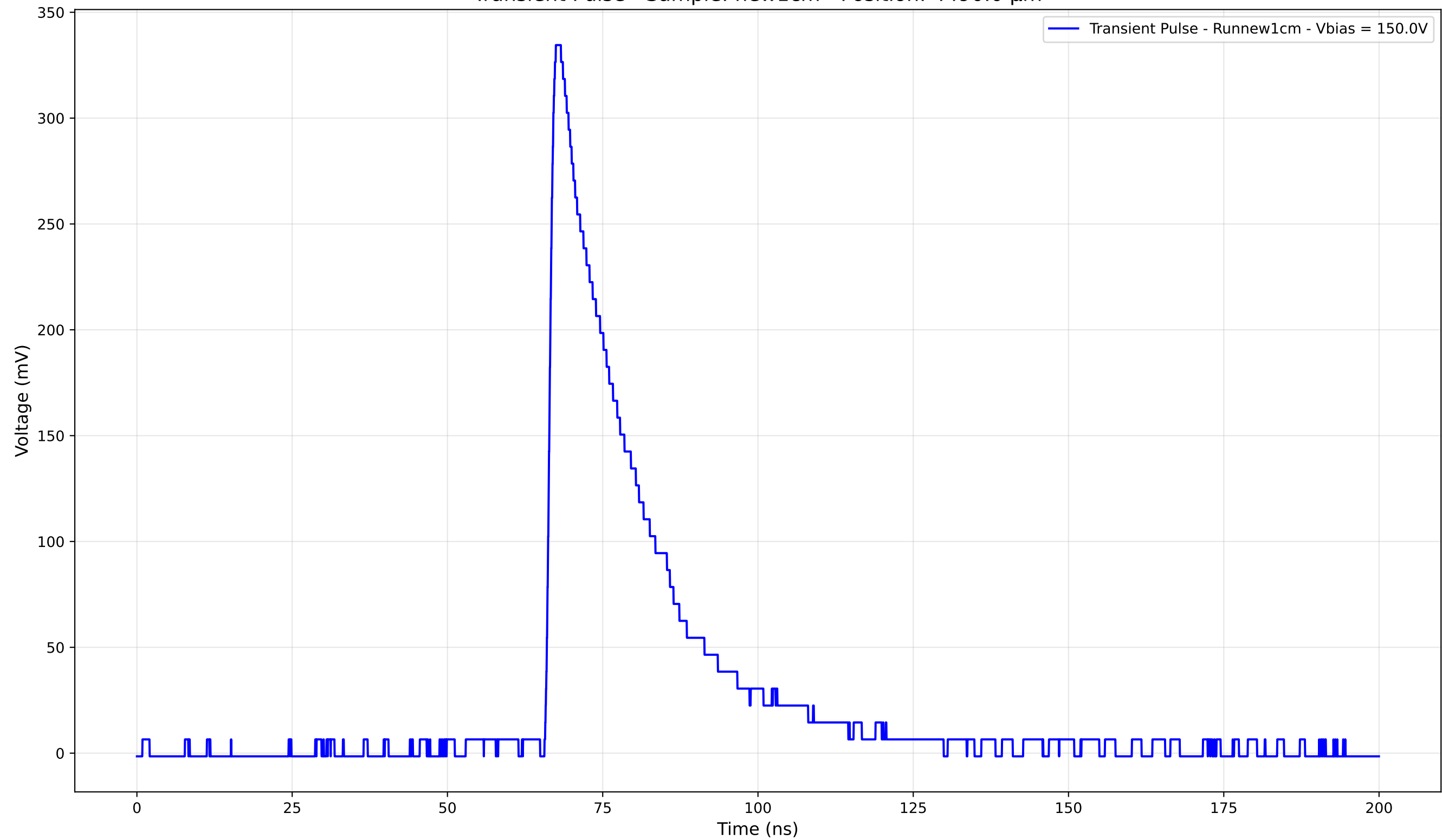
Transient Pulse - Sample: new1cm - Position: 4490.0 \mu\text{m}
