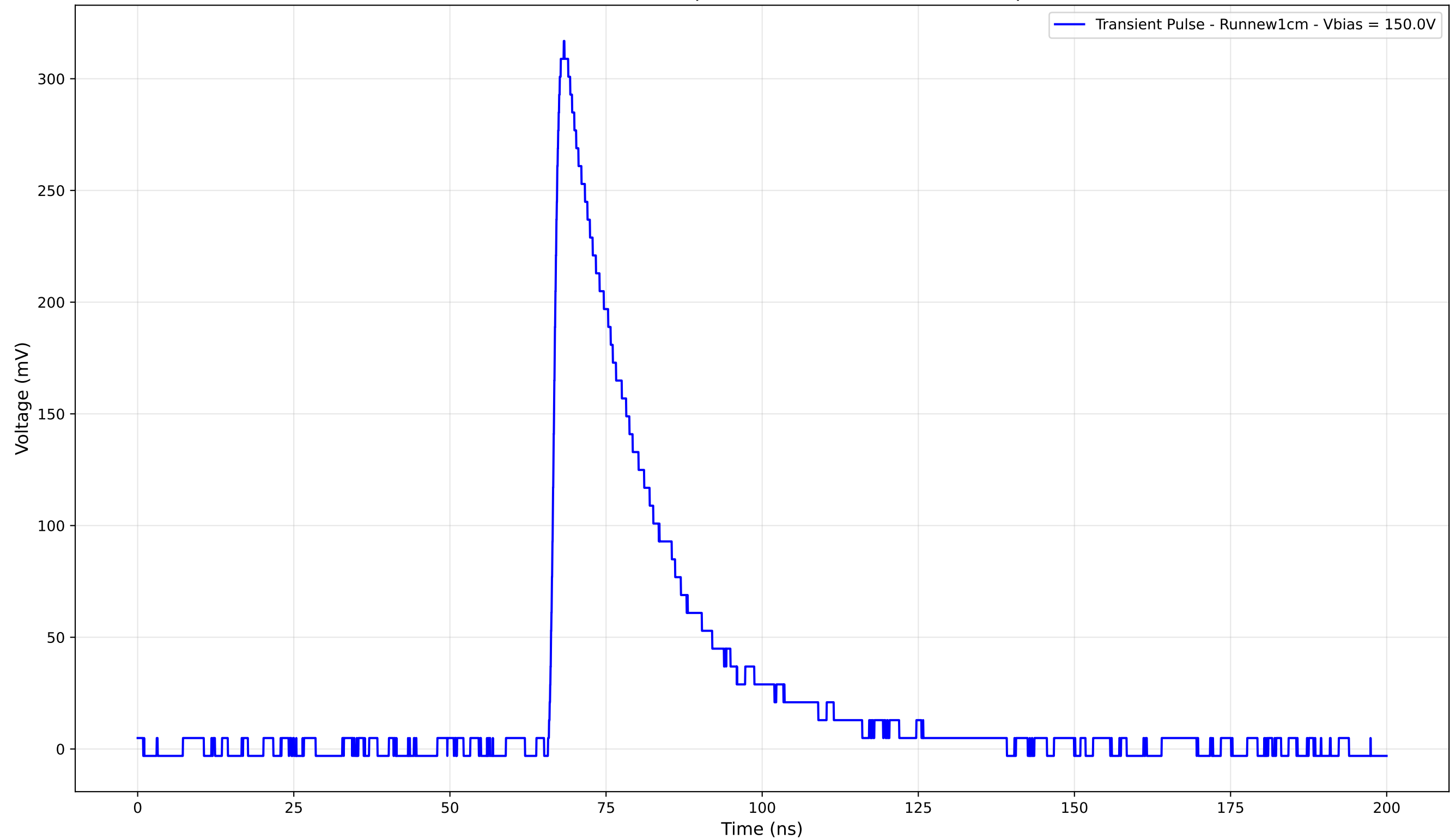
Transient Pulse - Sample: new1cm - Position: 4225.0 \mu\text{m}
