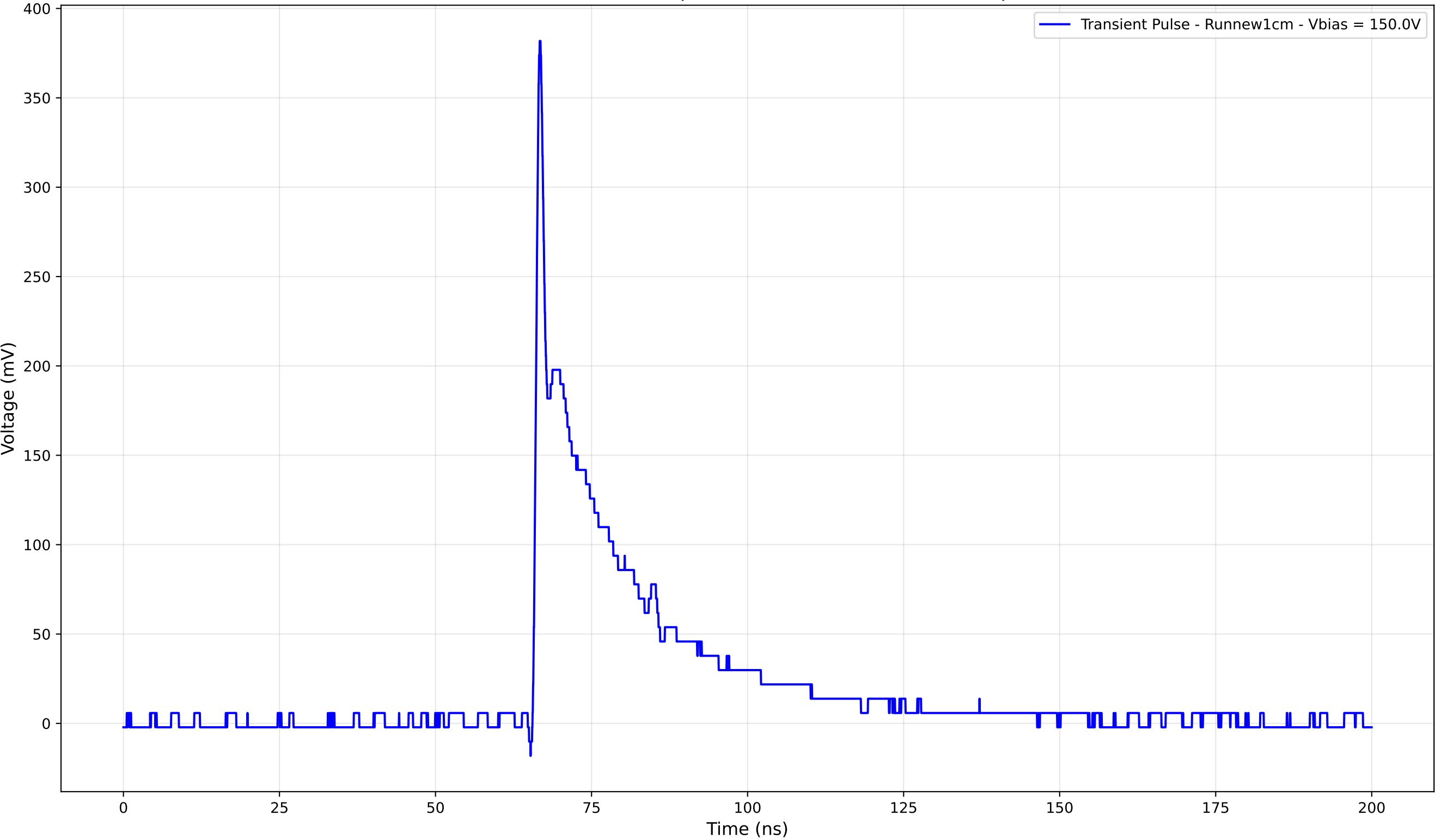
Transient Pulse - Sample: new1cm - Position: 2520.0 \mu\text{m}
