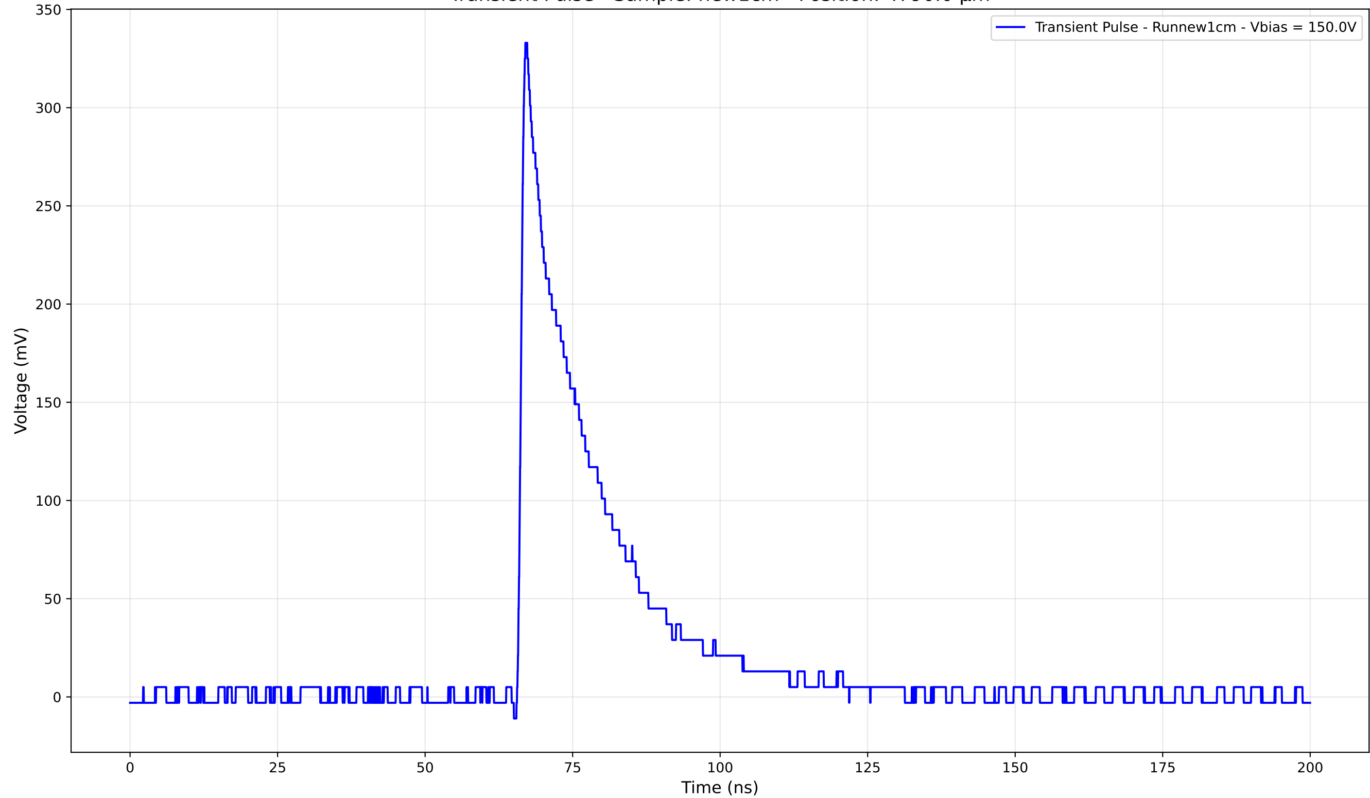
Transient Pulse - Sample: new1cm - Position: 4790.0 \mu\text{m}
