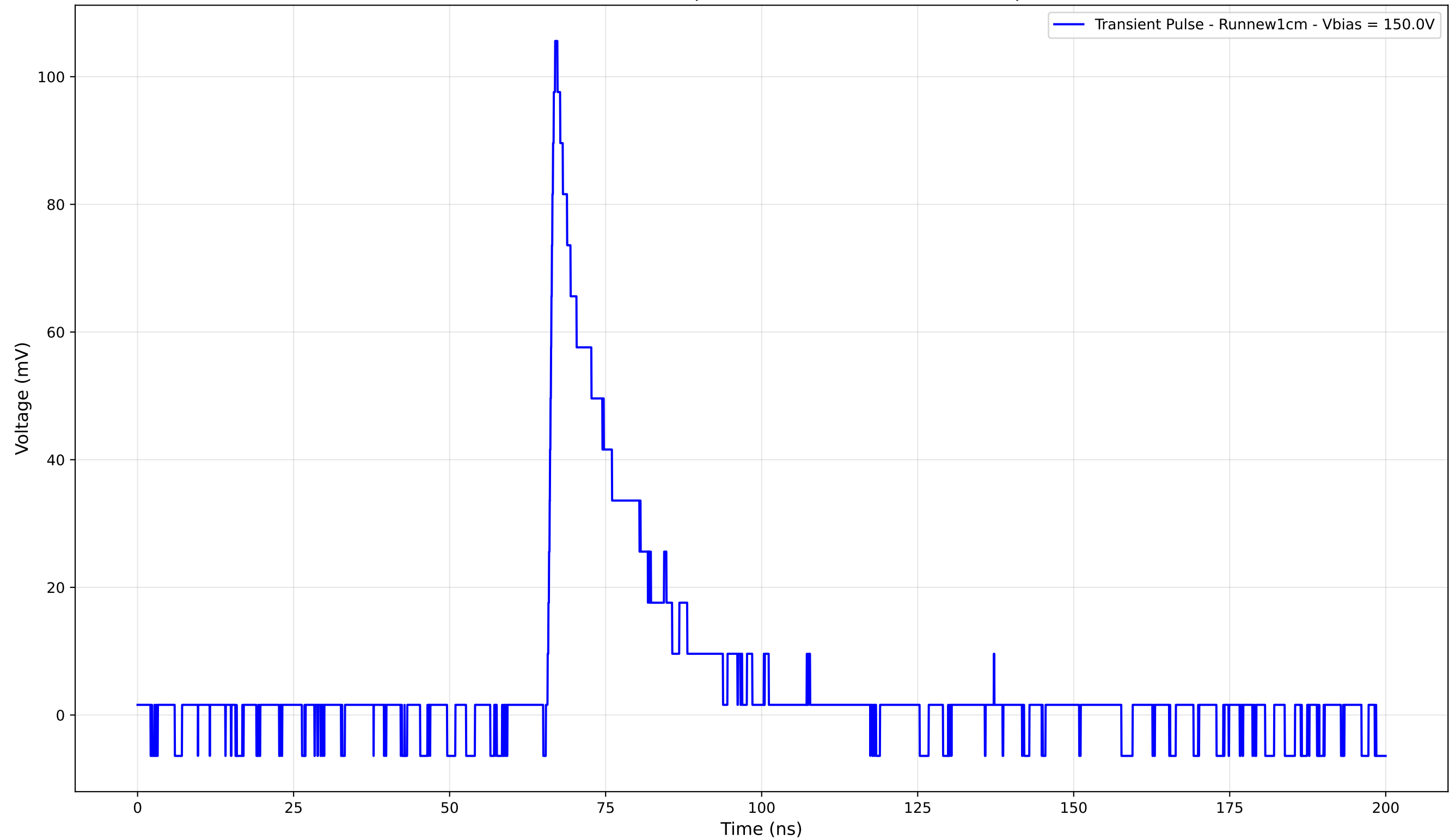
Transient Pulse - Sample: new1cm - Position: 4920.0 \mu\text{m}
