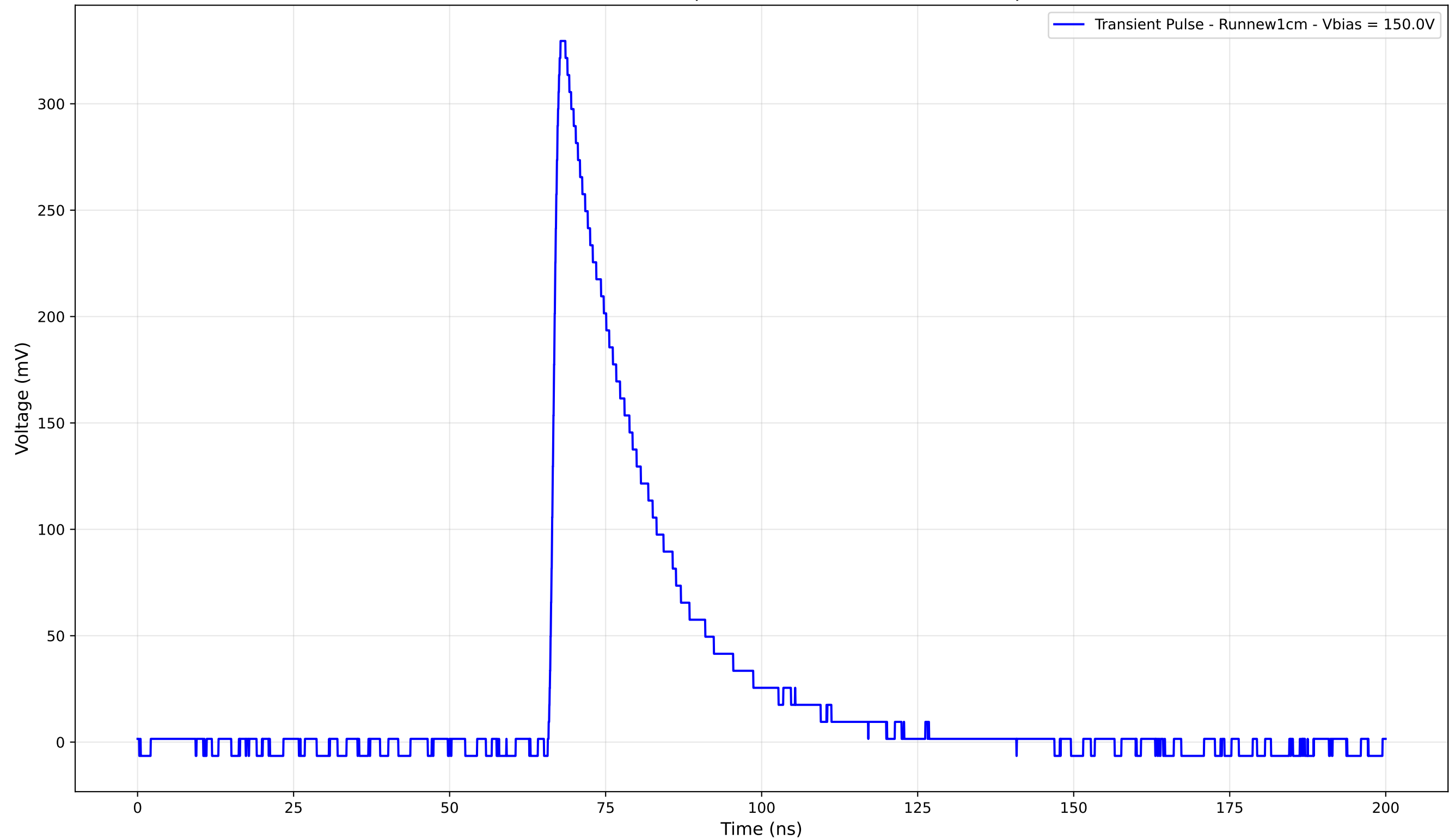
Transient Pulse - Sample: new1cm - Position: 4245.0 \mu\text{m}
