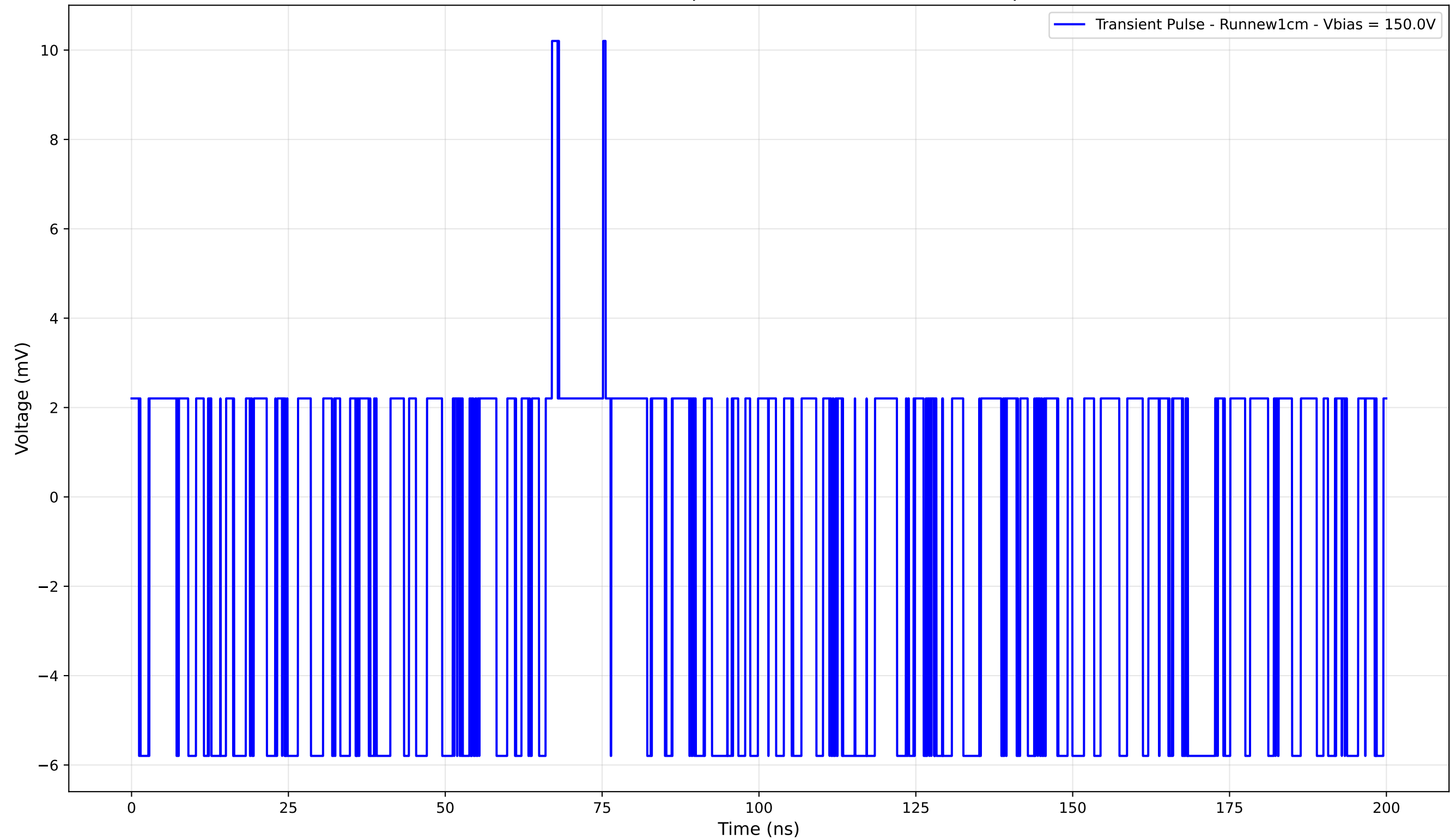
Transient Pulse - Sample: new1cm - Position: 4990.0 \mu\text{m}
