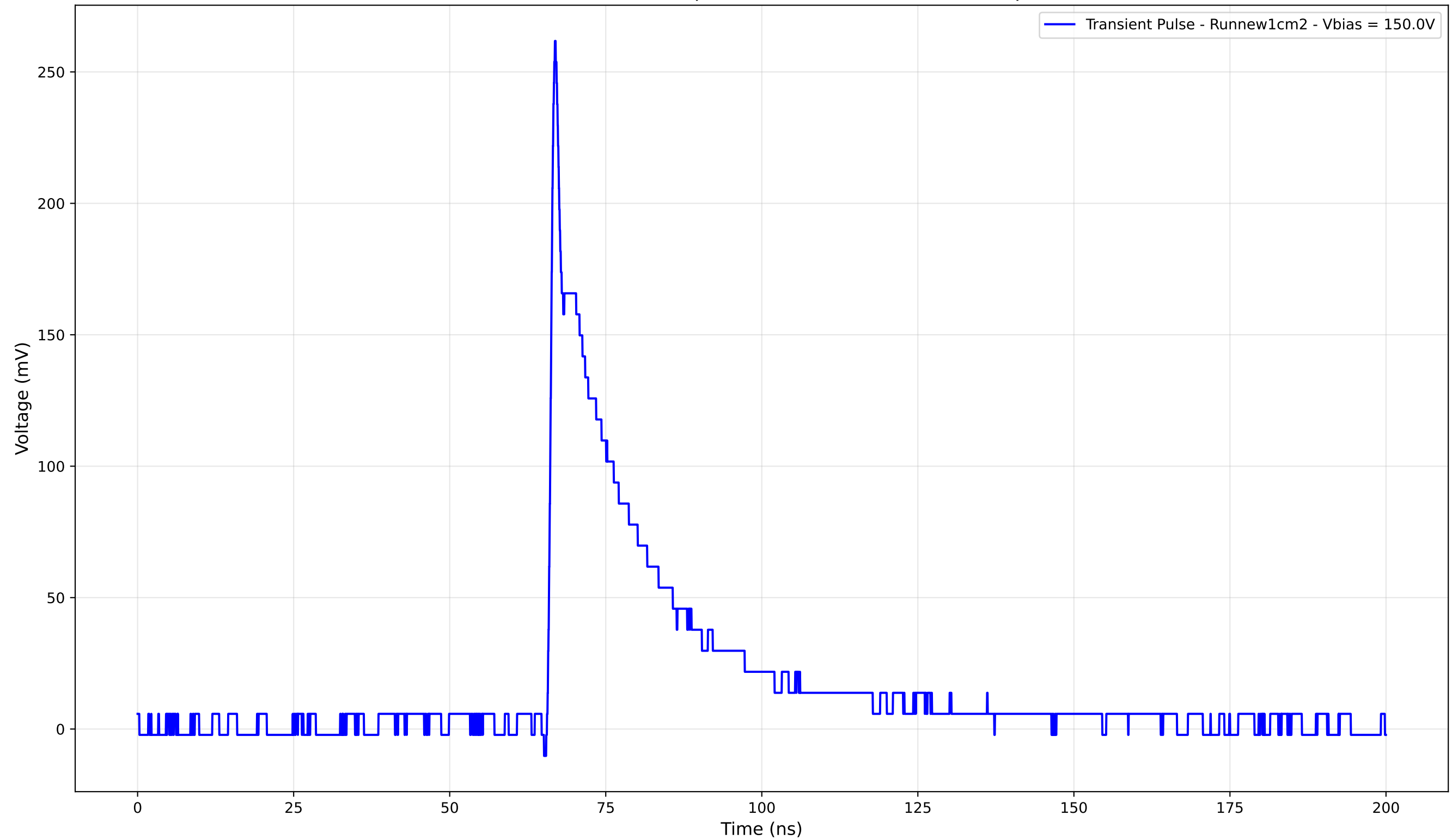
Transient Pulse - Sample: new1cm - Position: 2850.0 \mu\text{m}
