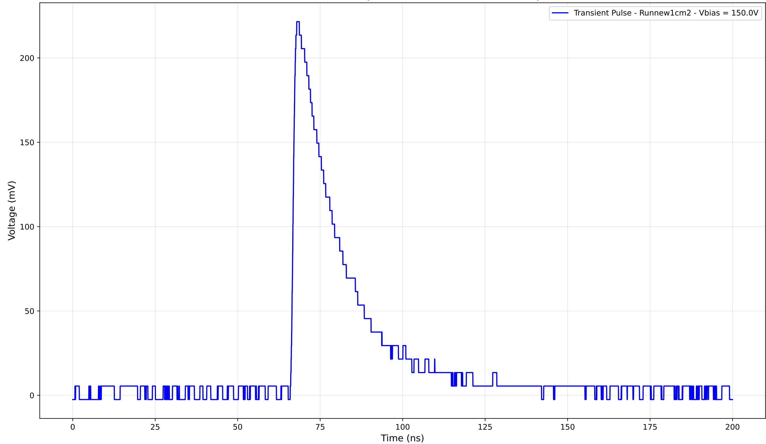
Transient Pulse - Sample: new1cm - Position: 3705.0 \mu\text{m}
