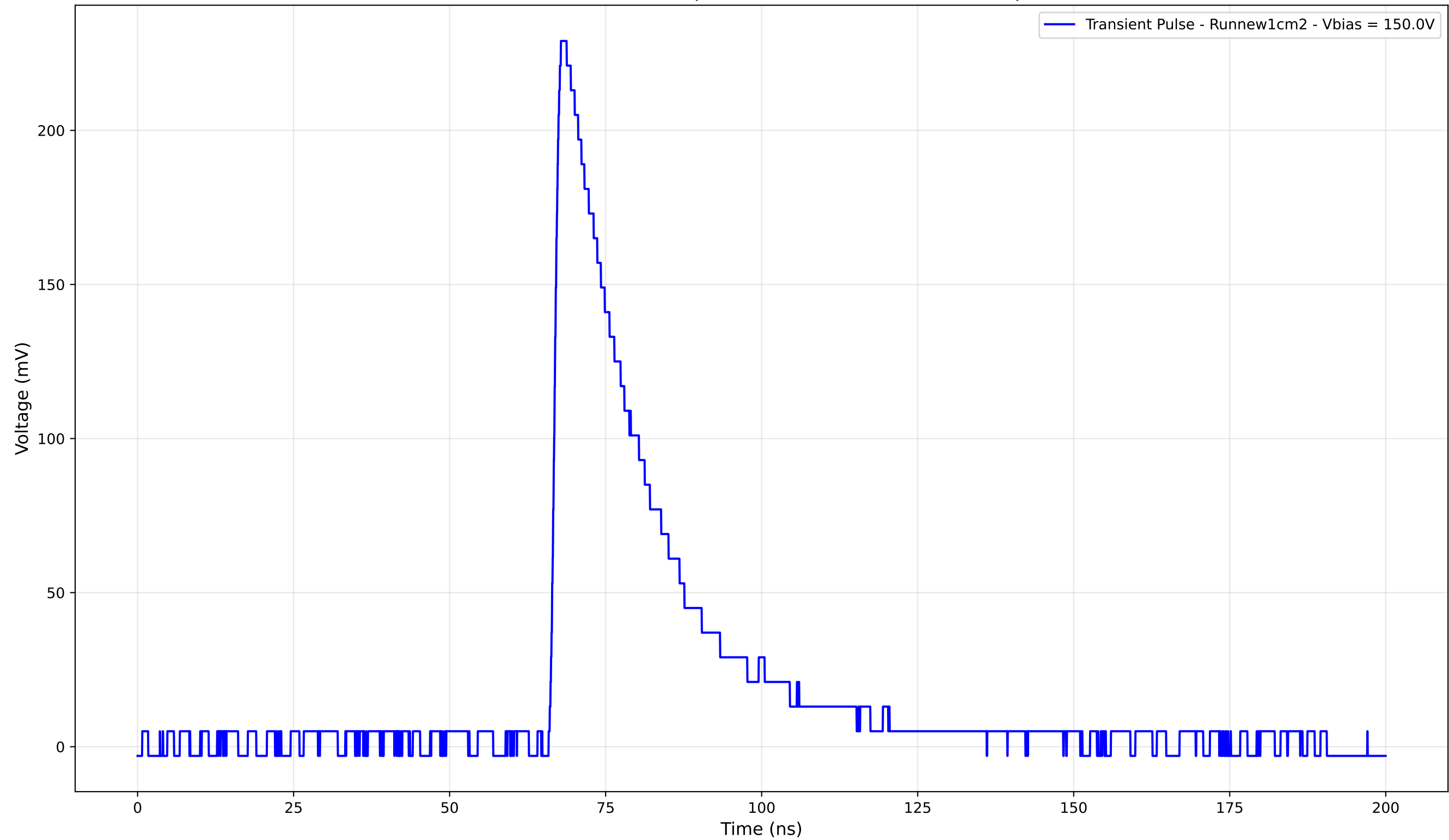
Transient Pulse - Sample: new1cm - Position: 3860.0 \mu\text{m}
