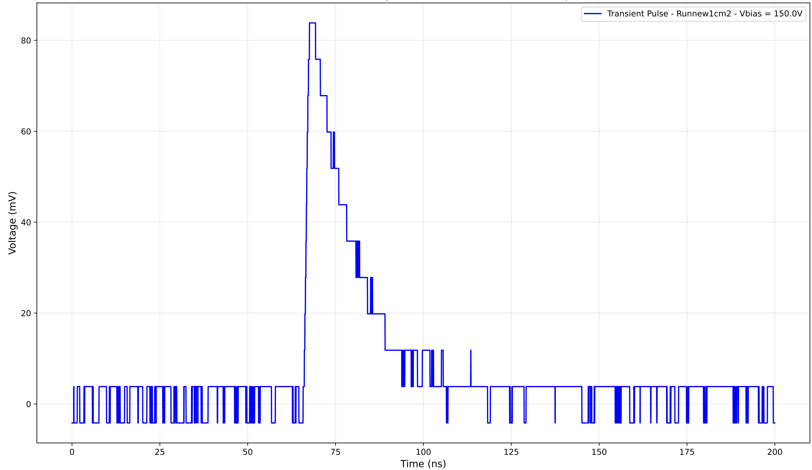
Transient Pulse - Sample: new1cm - Position: 4130.0 \mu\text{m}
