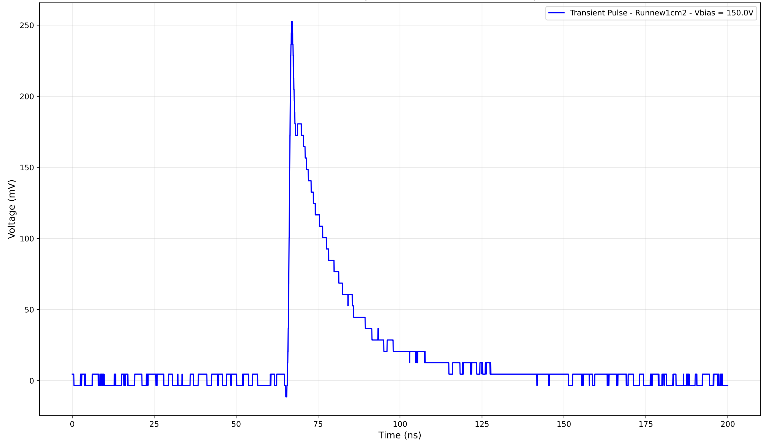
Transient Pulse - Sample: new1cm - Position: 2930.0 \mu\text{m}
