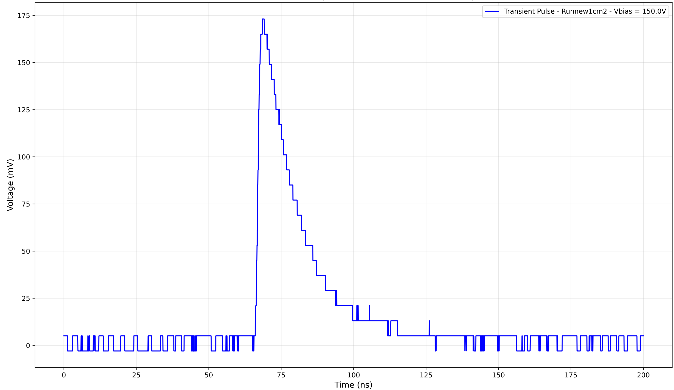
Transient Pulse - Sample: new1cm - Position: 1345.0 \mu\text{m}
