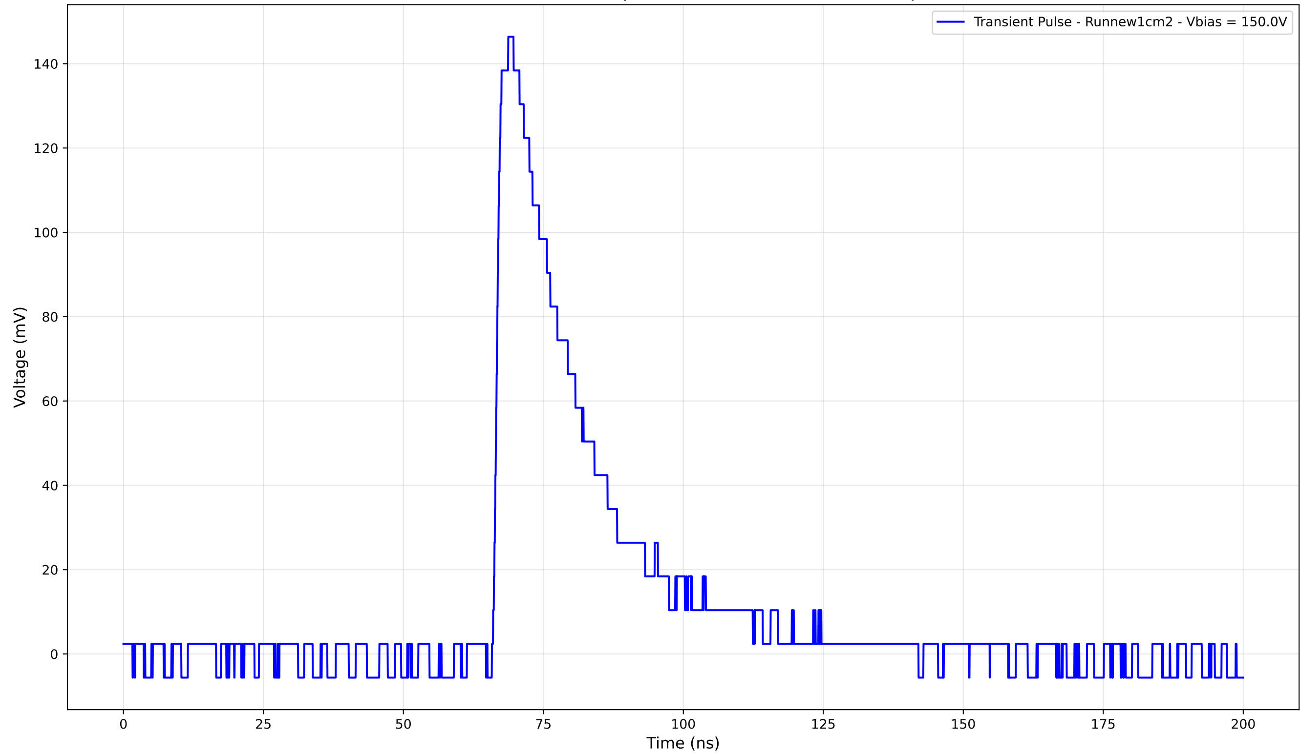
Transient Pulse - Sample: new1cm - Position: 1675.0 \mu\text{m}
