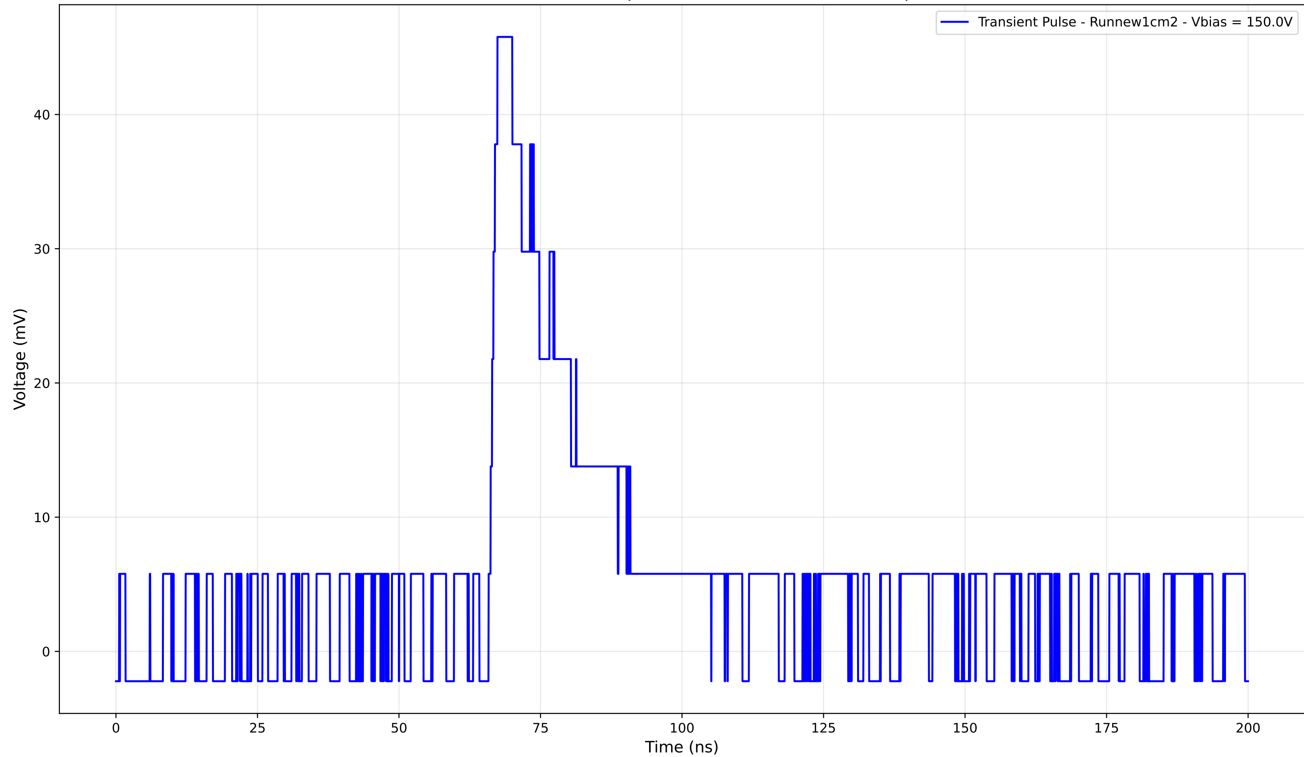
Transient Pulse - Sample: new1cm - Position: 580.0 \mu\text{m}
