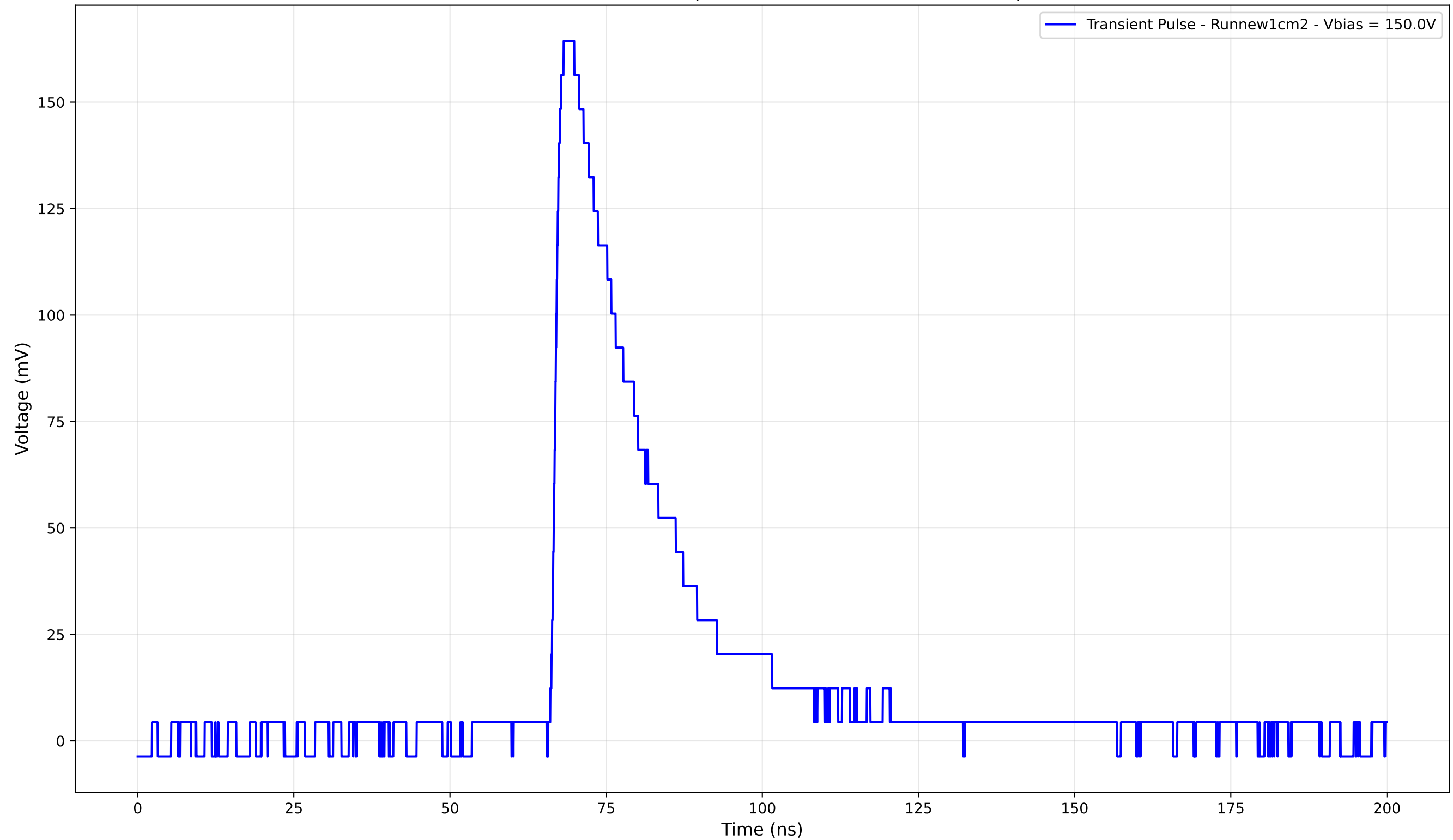
Transient Pulse - Sample: new1cm - Position: 1400.0 \mu\text{m}
