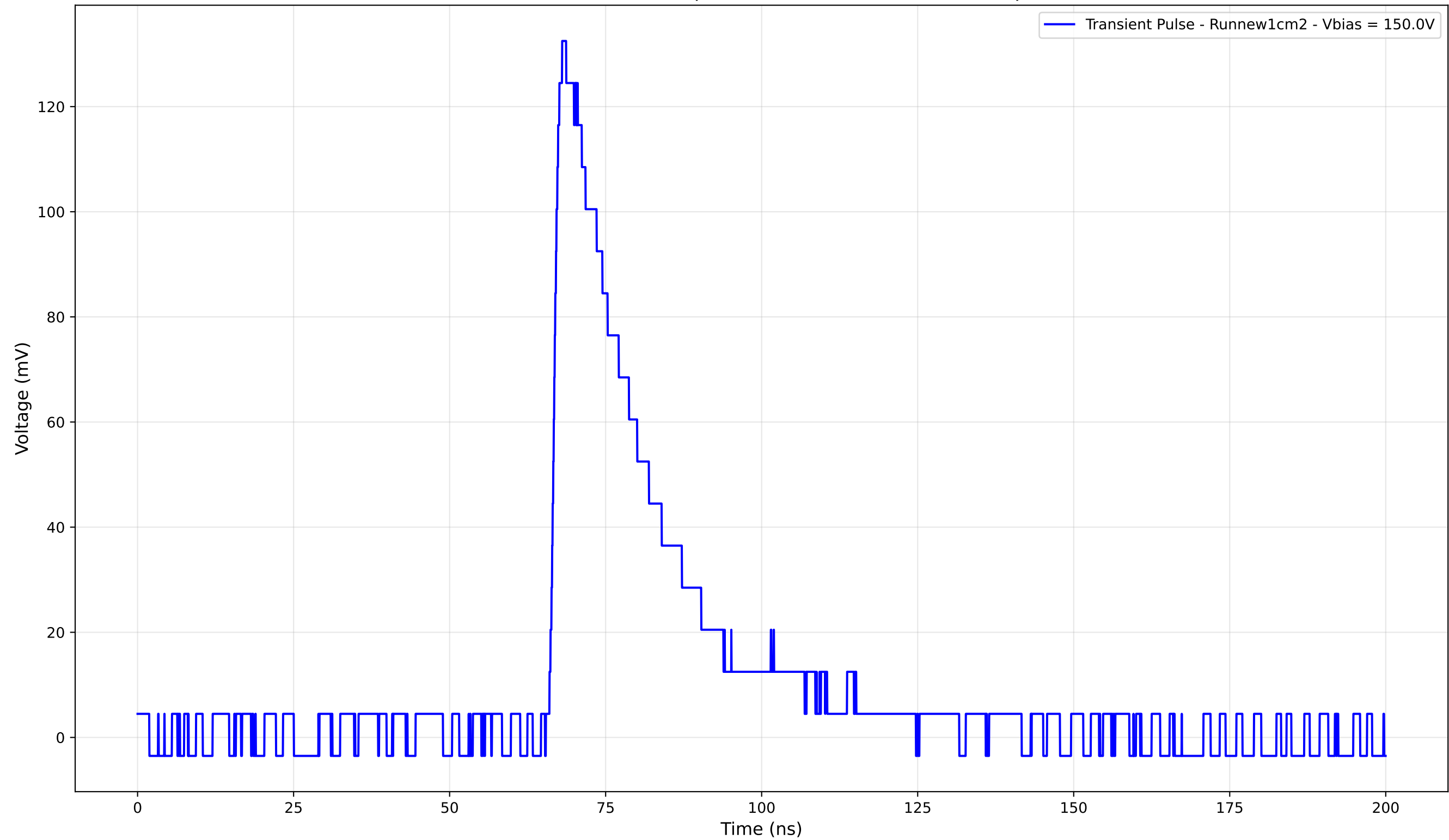
Transient Pulse - Sample: new1cm - Position: 3645.0 \mu\text{m}
