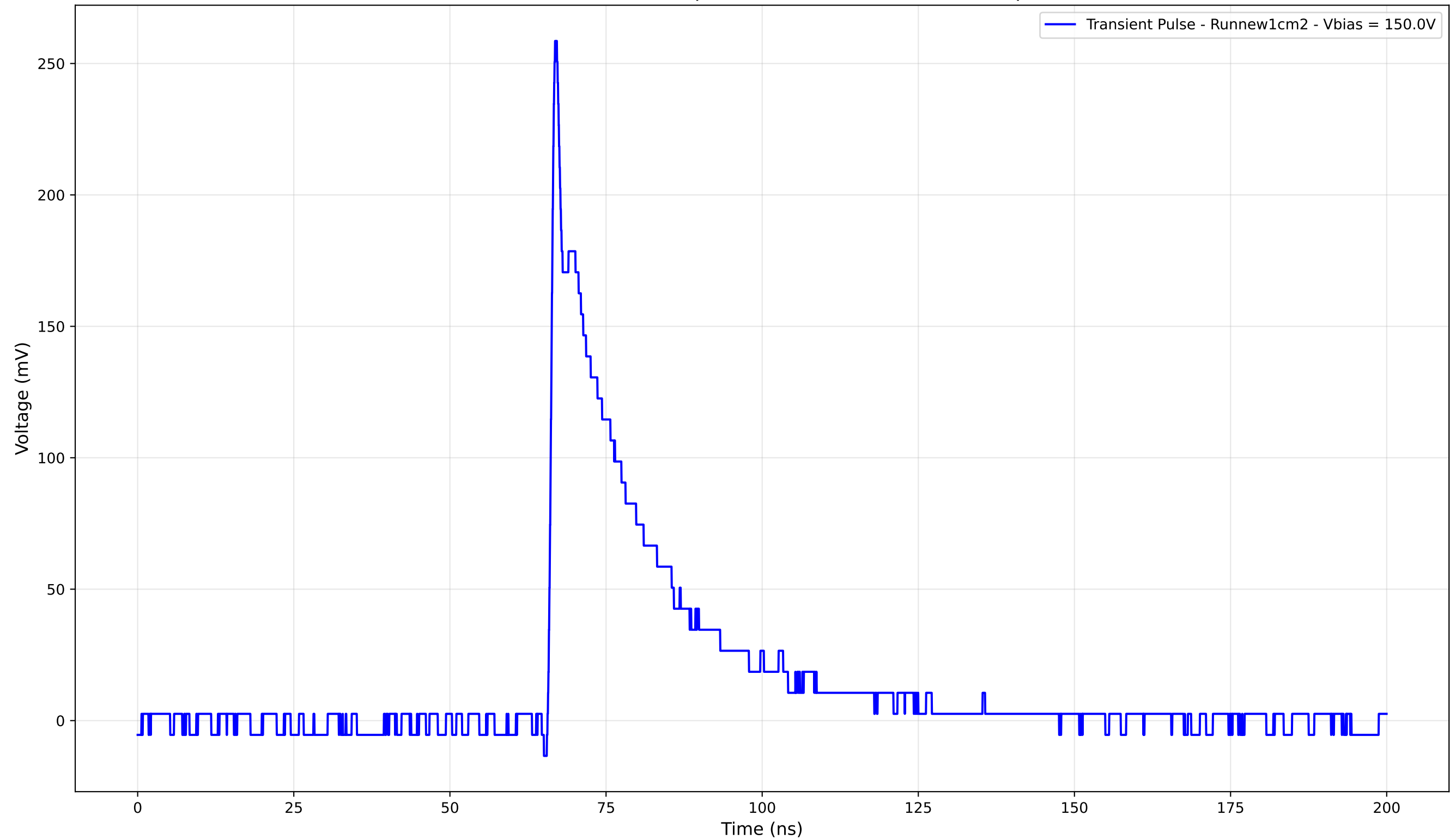
Transient Pulse - Sample: new1cm - Position: 2895.0 \mu\text{m}
