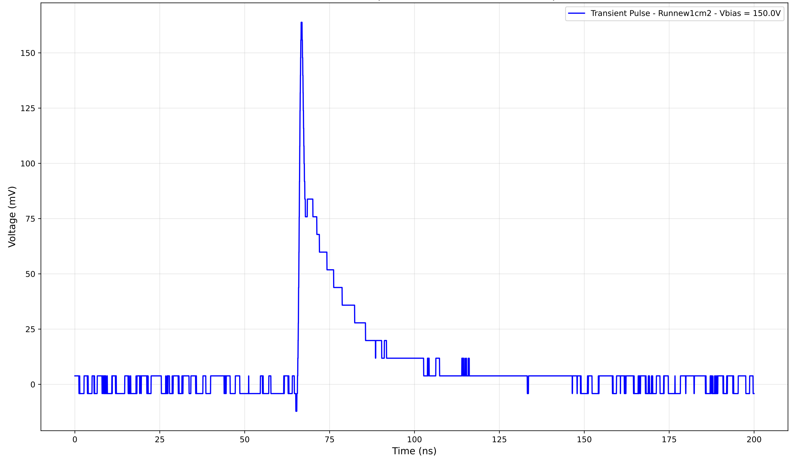
Transient Pulse - Sample: new1cm - Position: 2630.0 \mu\text{m}
