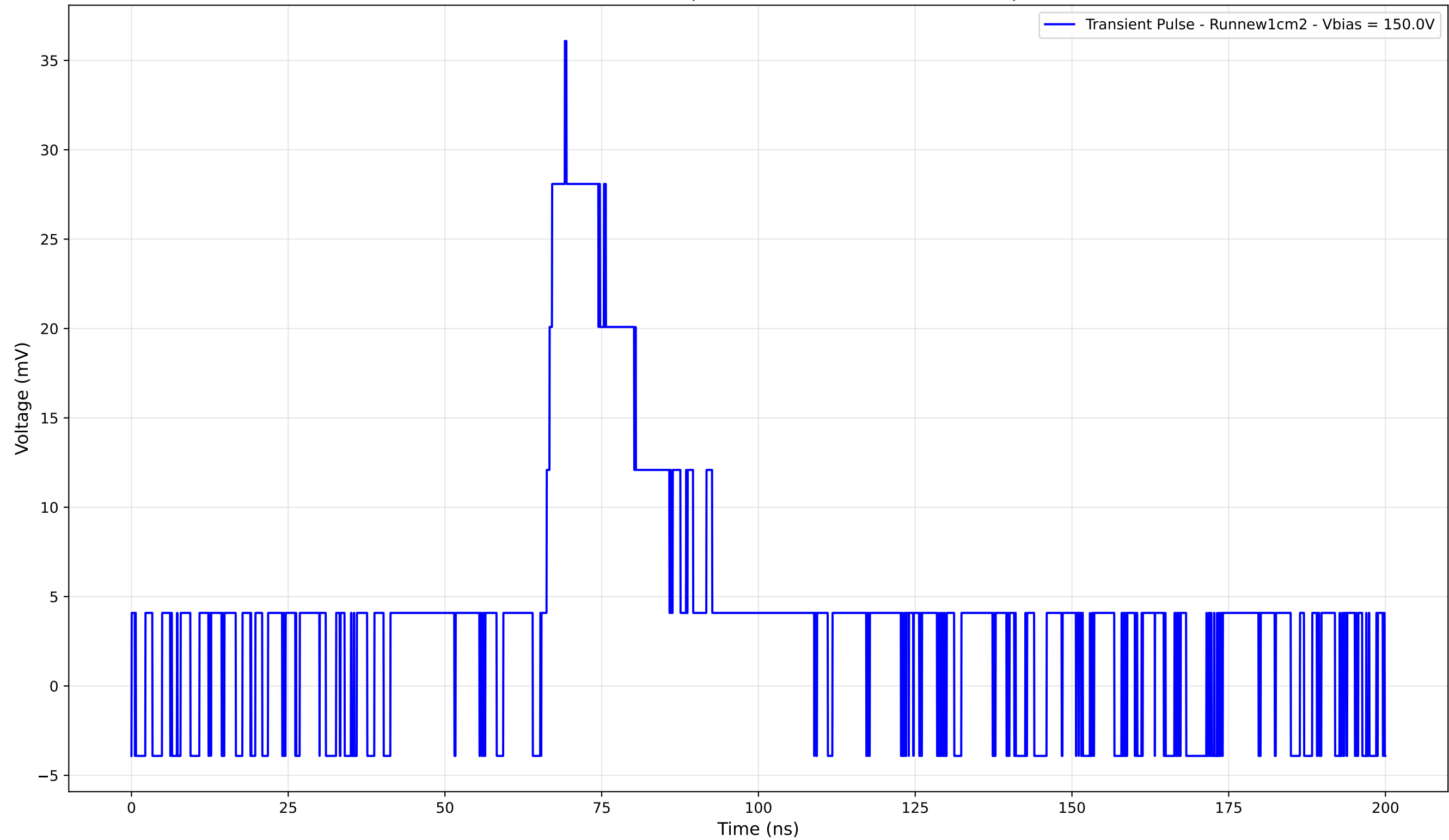
Transient Pulse - Sample: new1cm - Position: 3595.0 \mu\text{m}
