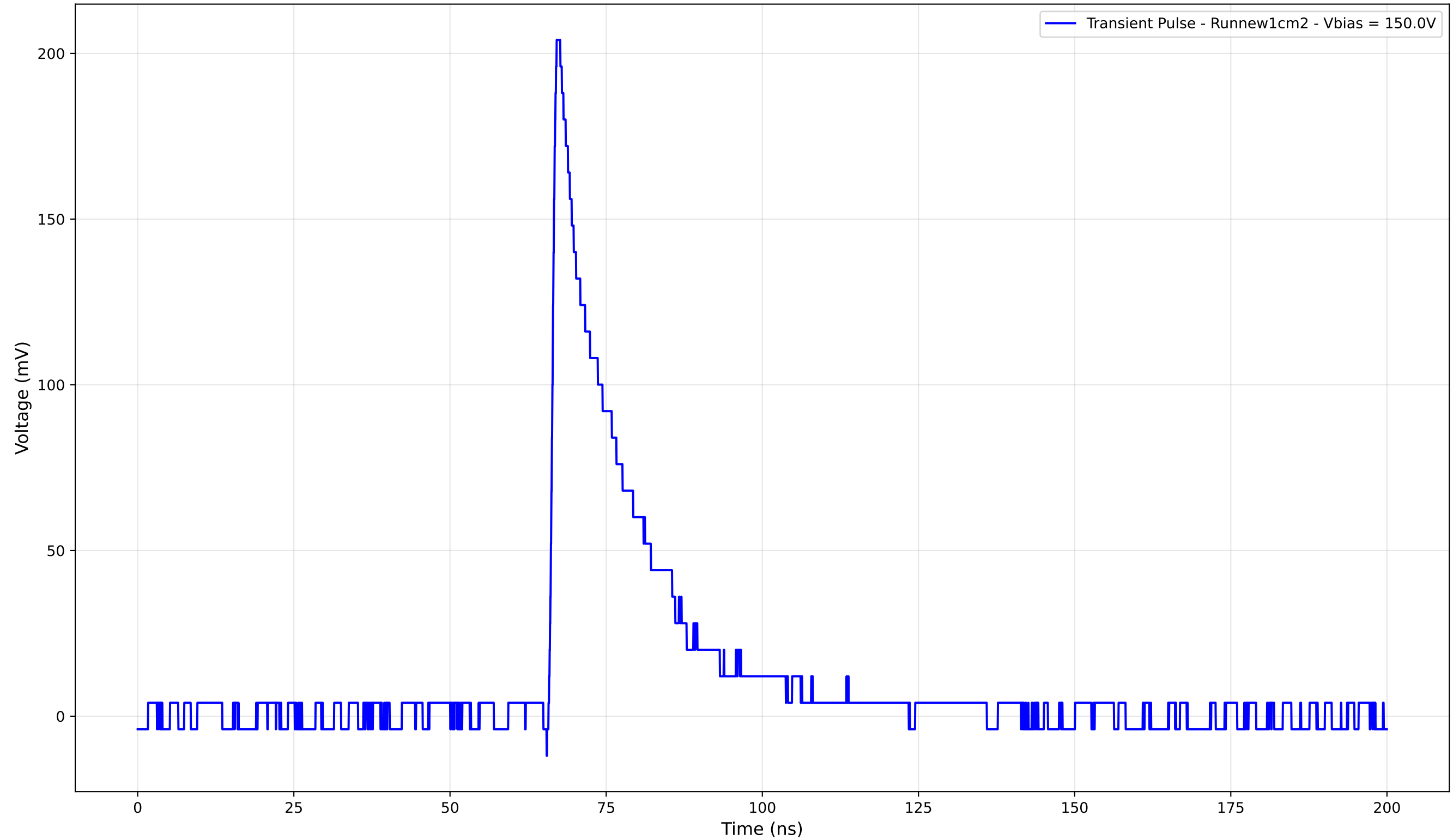
Transient Pulse - Sample: new1cm - Position: 260.0 \mu\text{m}
