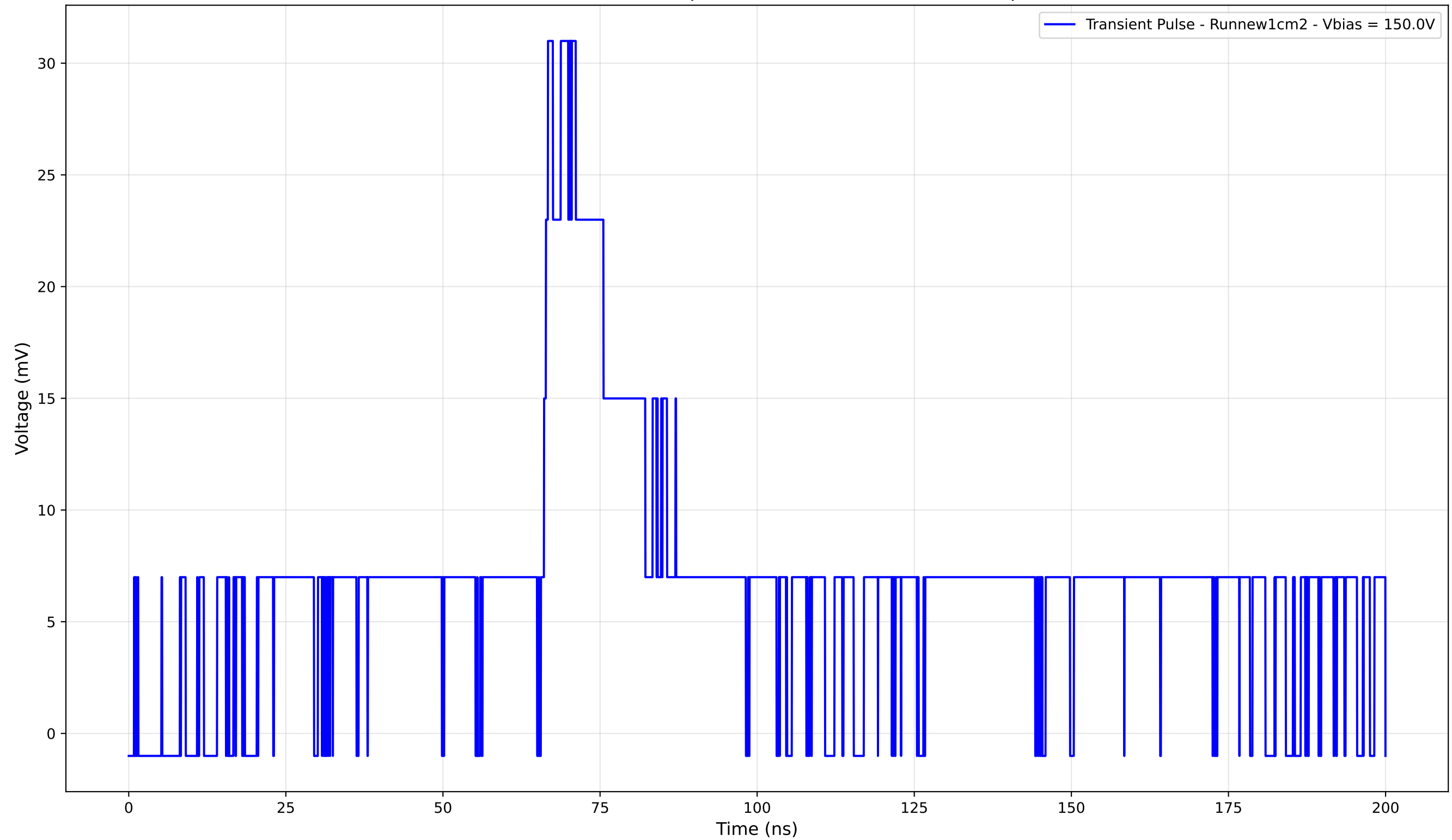
Transient Pulse - Sample: new1cm - Position: 2065.0 \mu\text{m}
