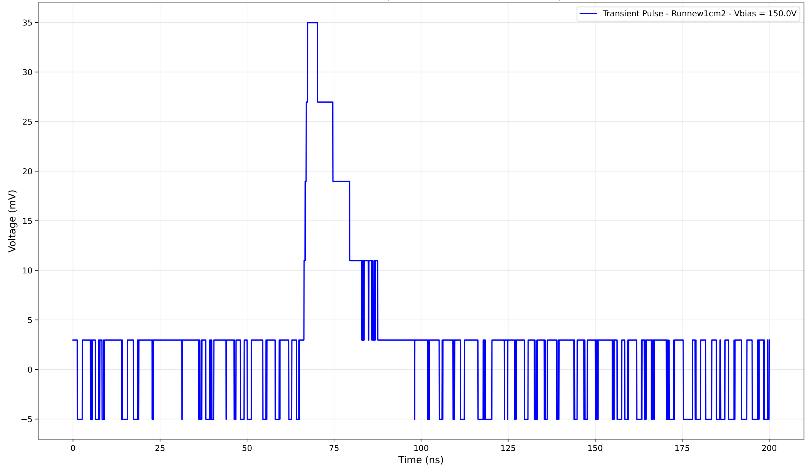
Transient Pulse - Sample: new1cm - Position: 575.0 \mu\text{m}
