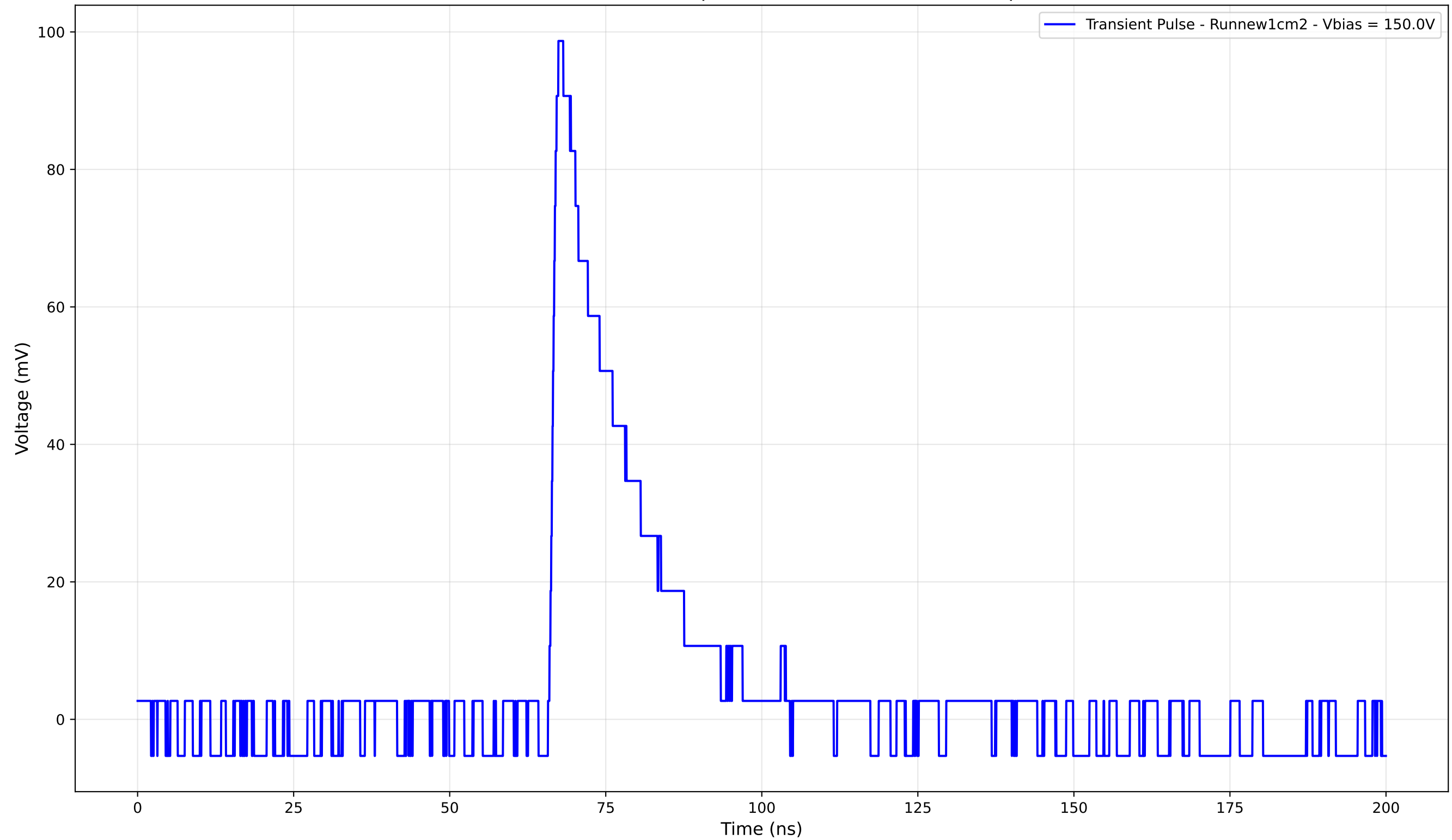
Transient Pulse - Sample: new1cm - Position: 505.0 \mu\text{m}
