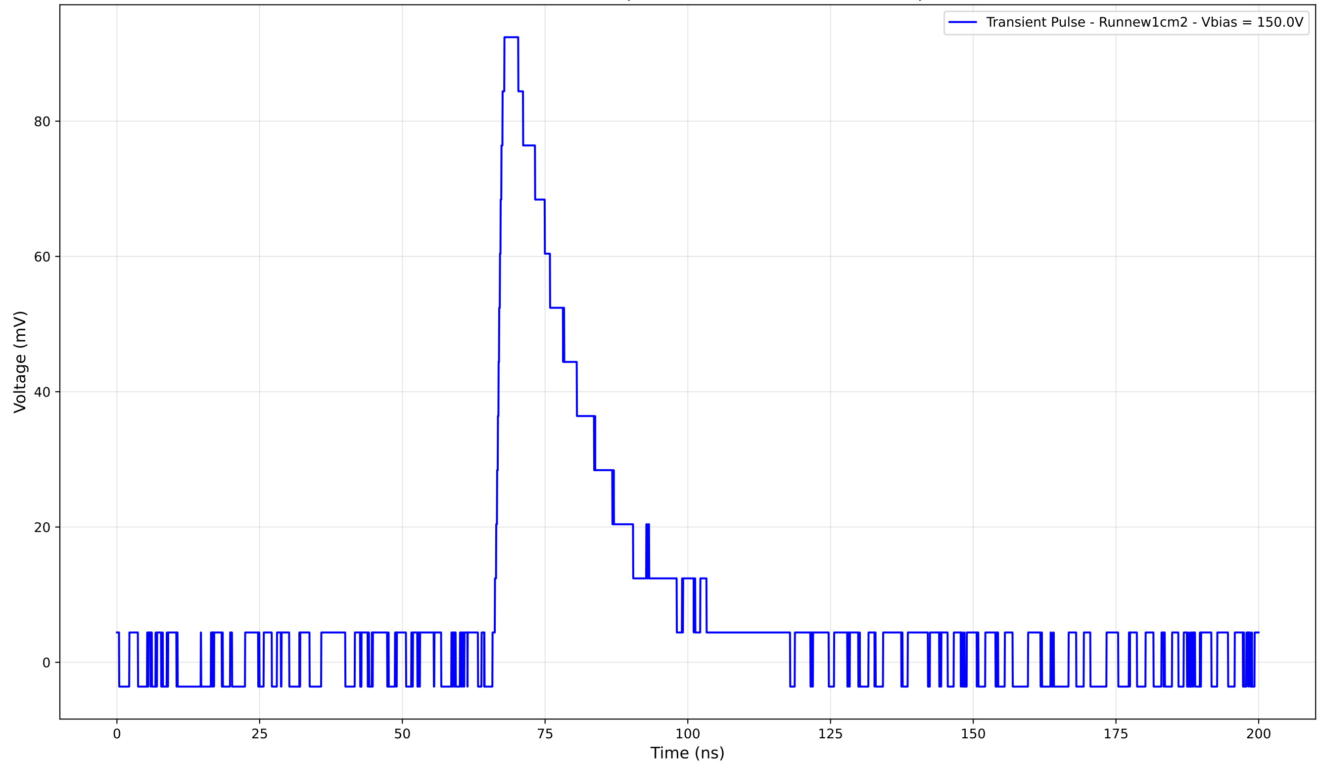
Transient Pulse - Sample: new1cm - Position: 1120.0 \mu\text{m}
