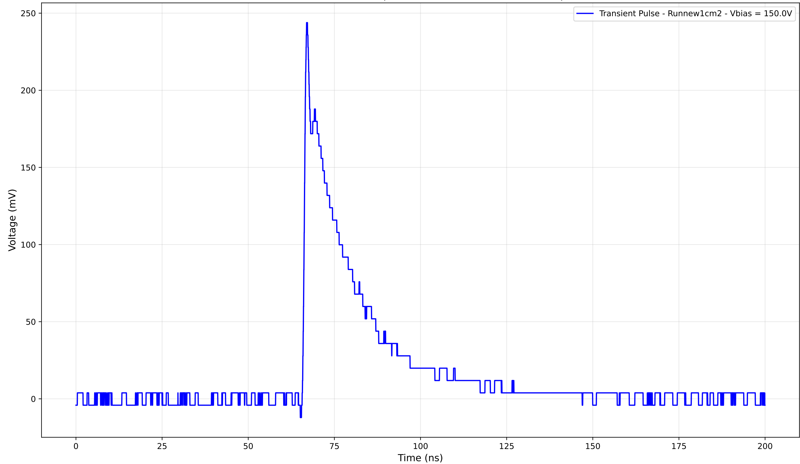
Transient Pulse - Sample: new1cm - Position: 2975.0 \mu\text{m}
