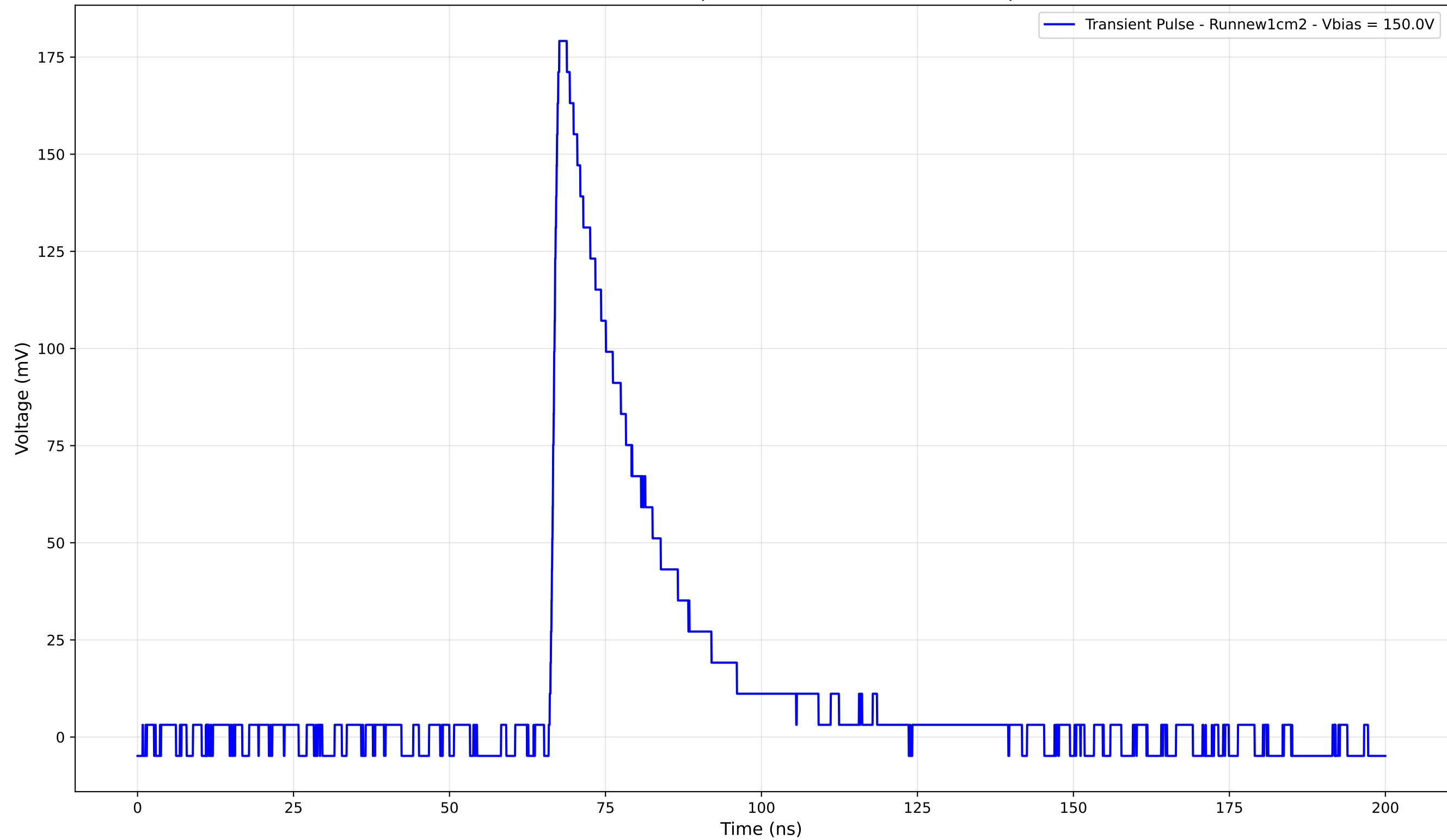
Transient Pulse - Sample: new1cm - Position: 685.0 \mu\text{m}
