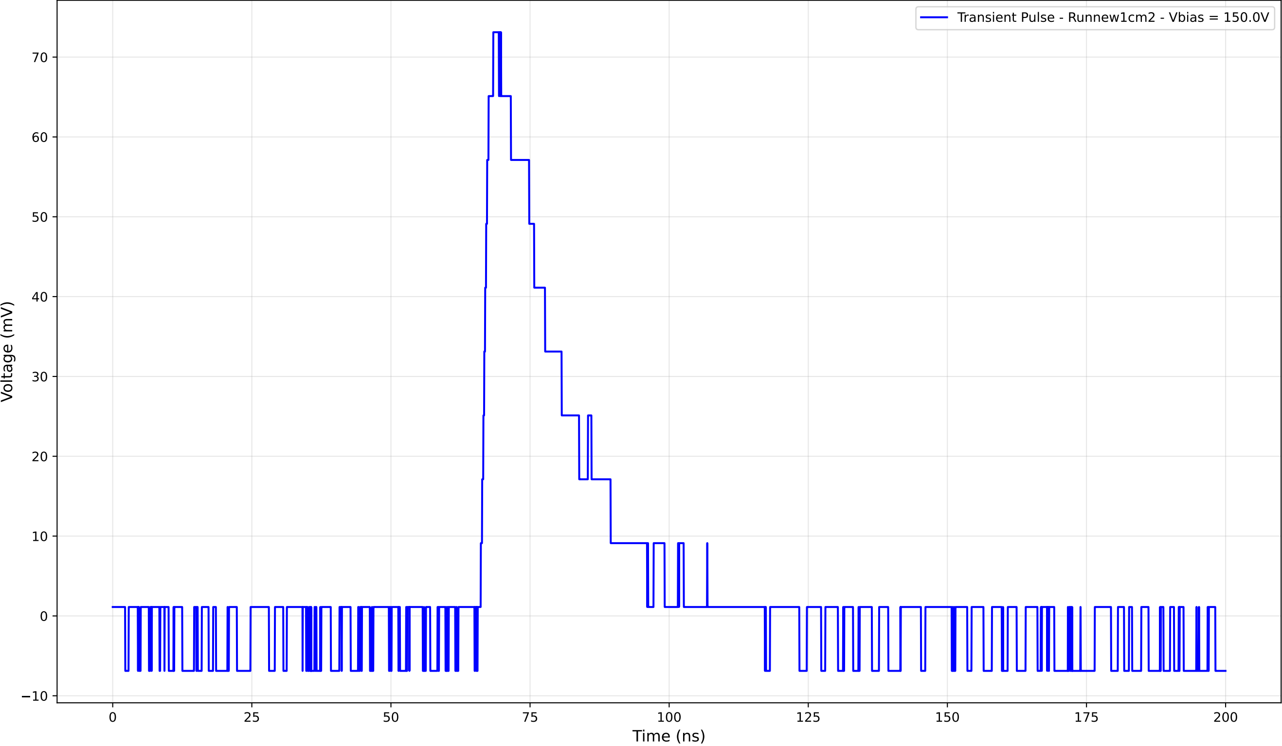
Transient Pulse - Sample: new1cm - Position: 1520.0 \mu\text{m}
