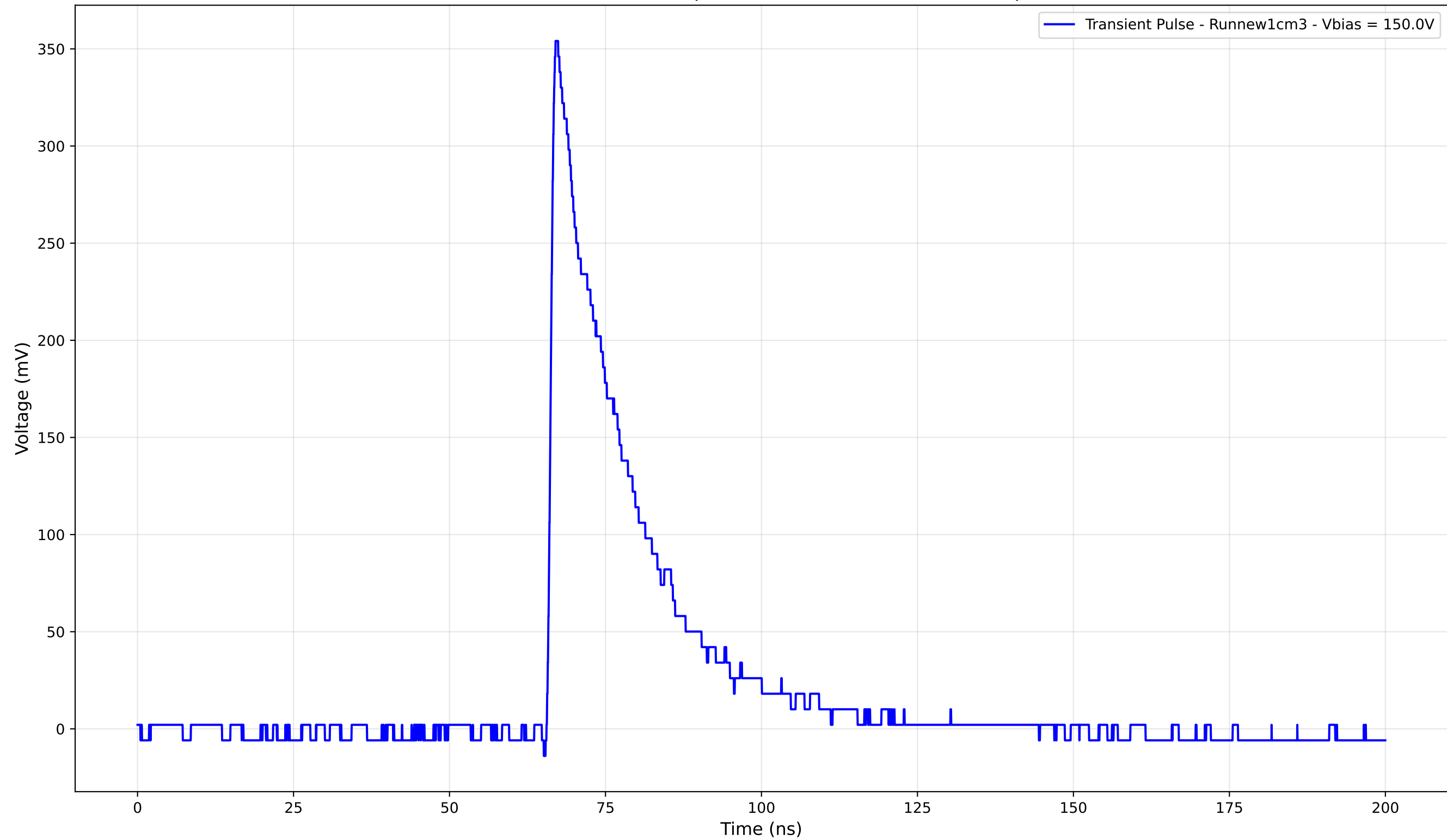
Transient Pulse - Sample: new1cm - Position: 4730.0 \mu\text{m}
