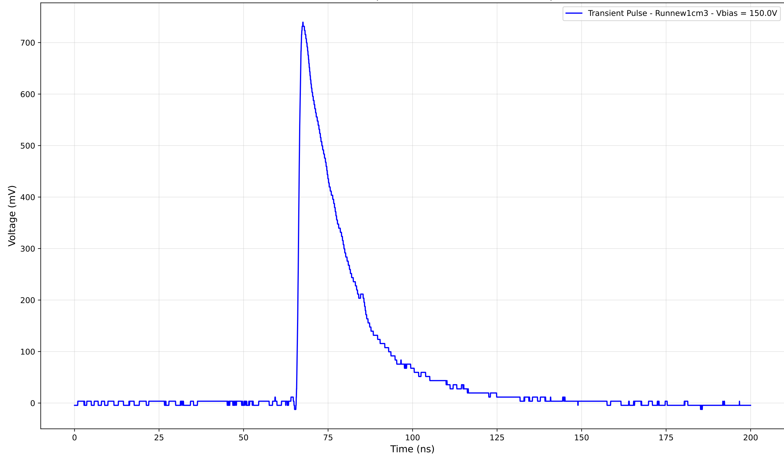
Transient Pulse - Sample: new1cm - Position: 4545.0 \mu\text{m}
