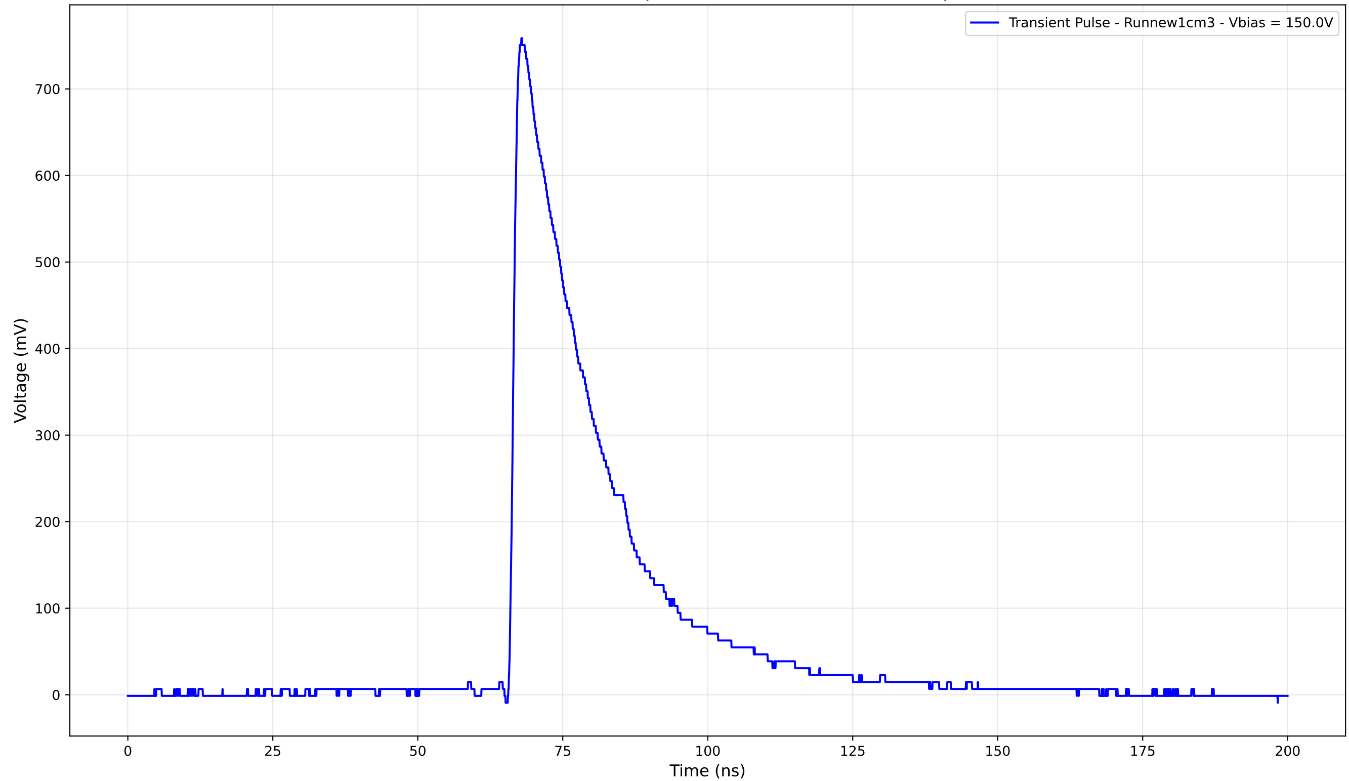
Transient Pulse - Sample: new1cm - Position: 4360.0 \mu\text{m}
