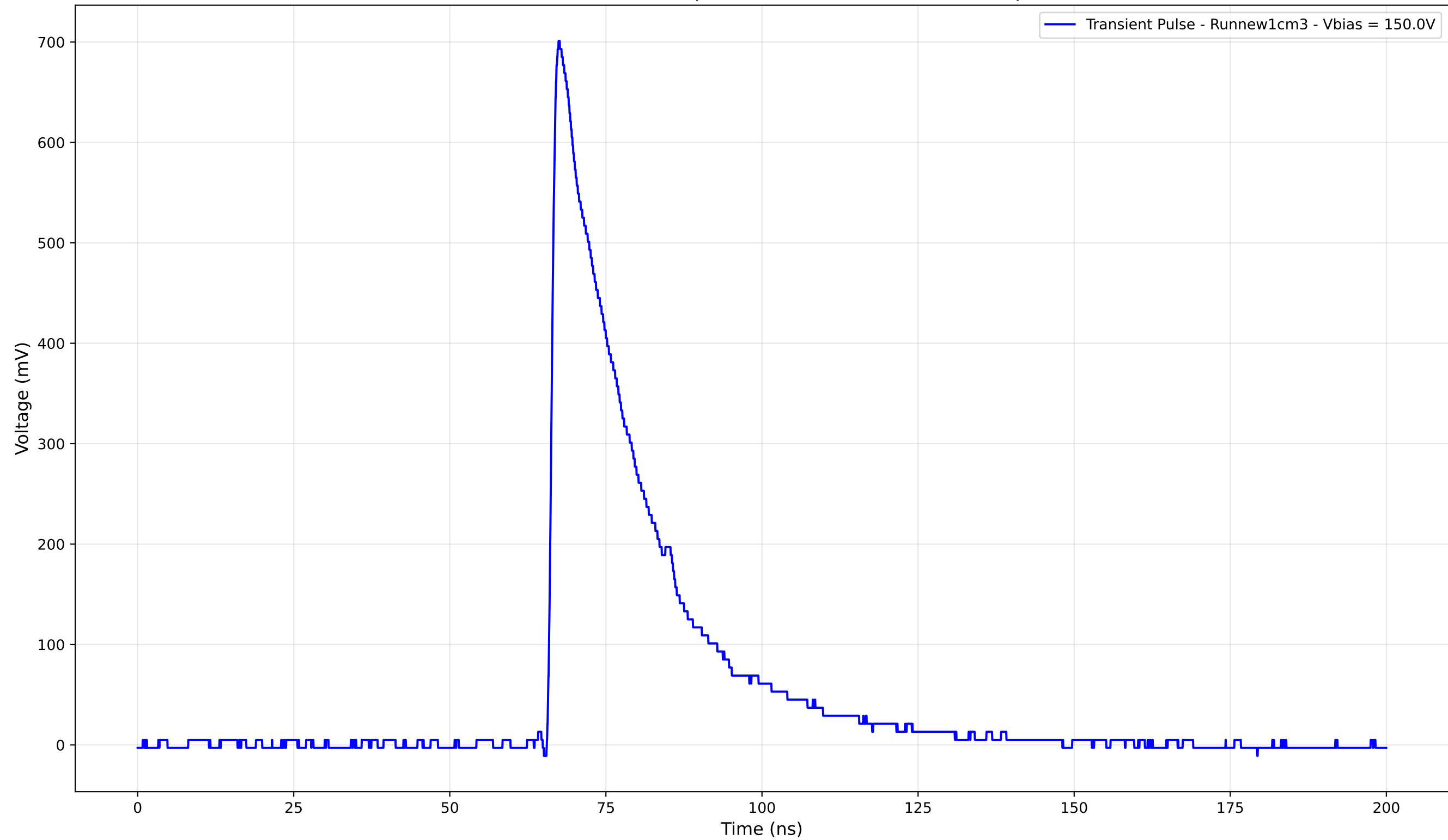
Transient Pulse - Sample: new1cm - Position: 4575.0 \mu\text{m}
