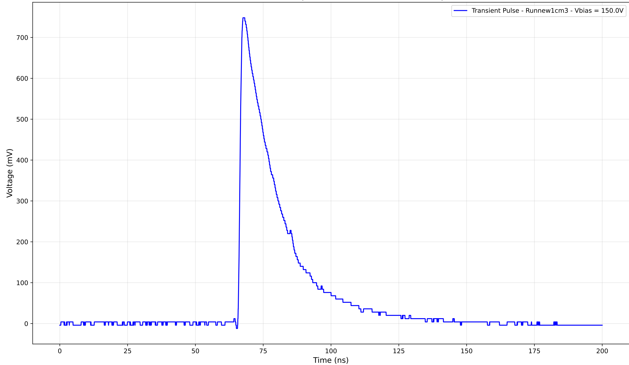
Transient Pulse - Sample: new1cm - Position: 4435.0 \mu\text{m}
