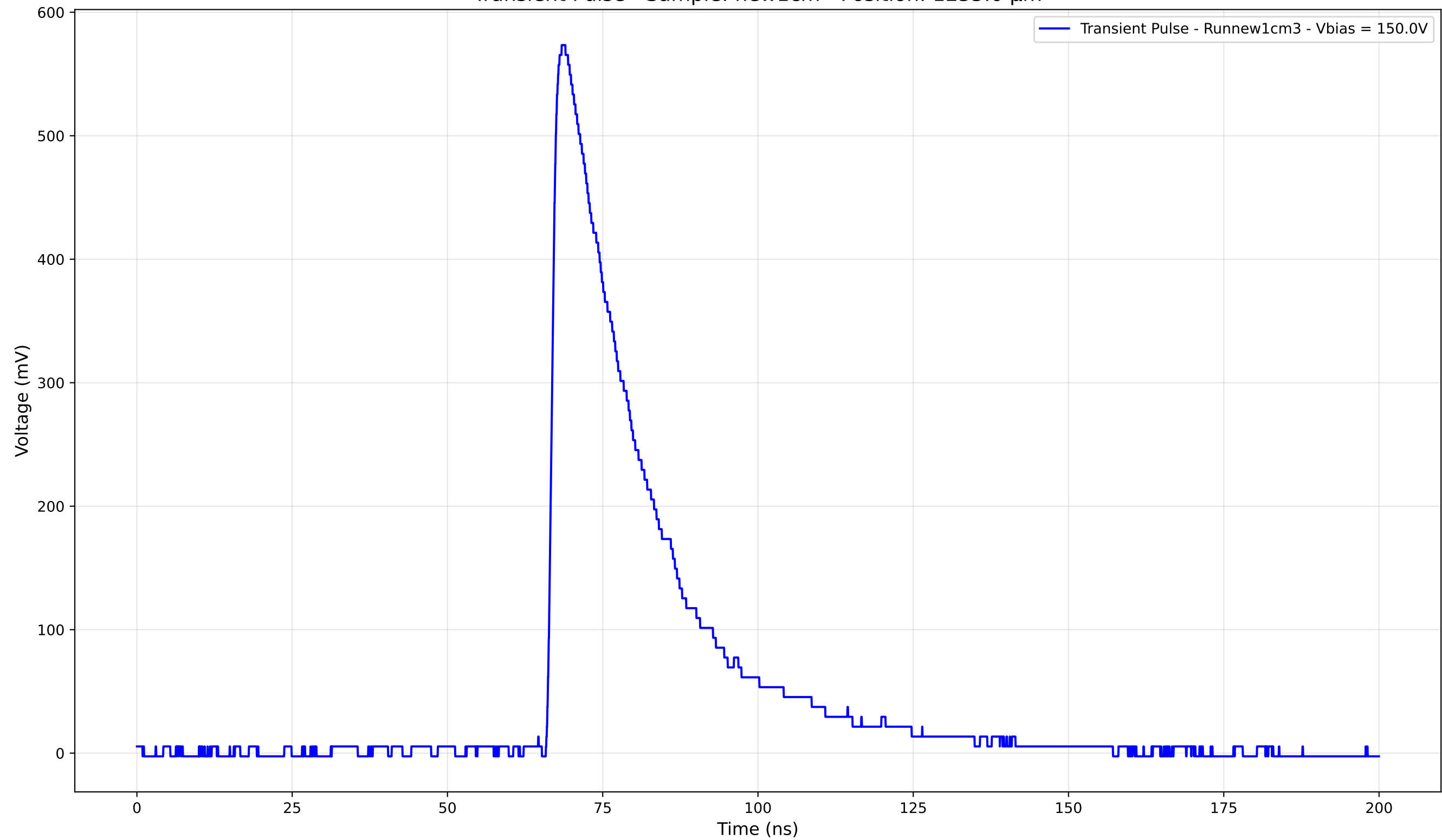
Transient Pulse - Sample: new1cm - Position: 1255.0 \mu\text{m}
