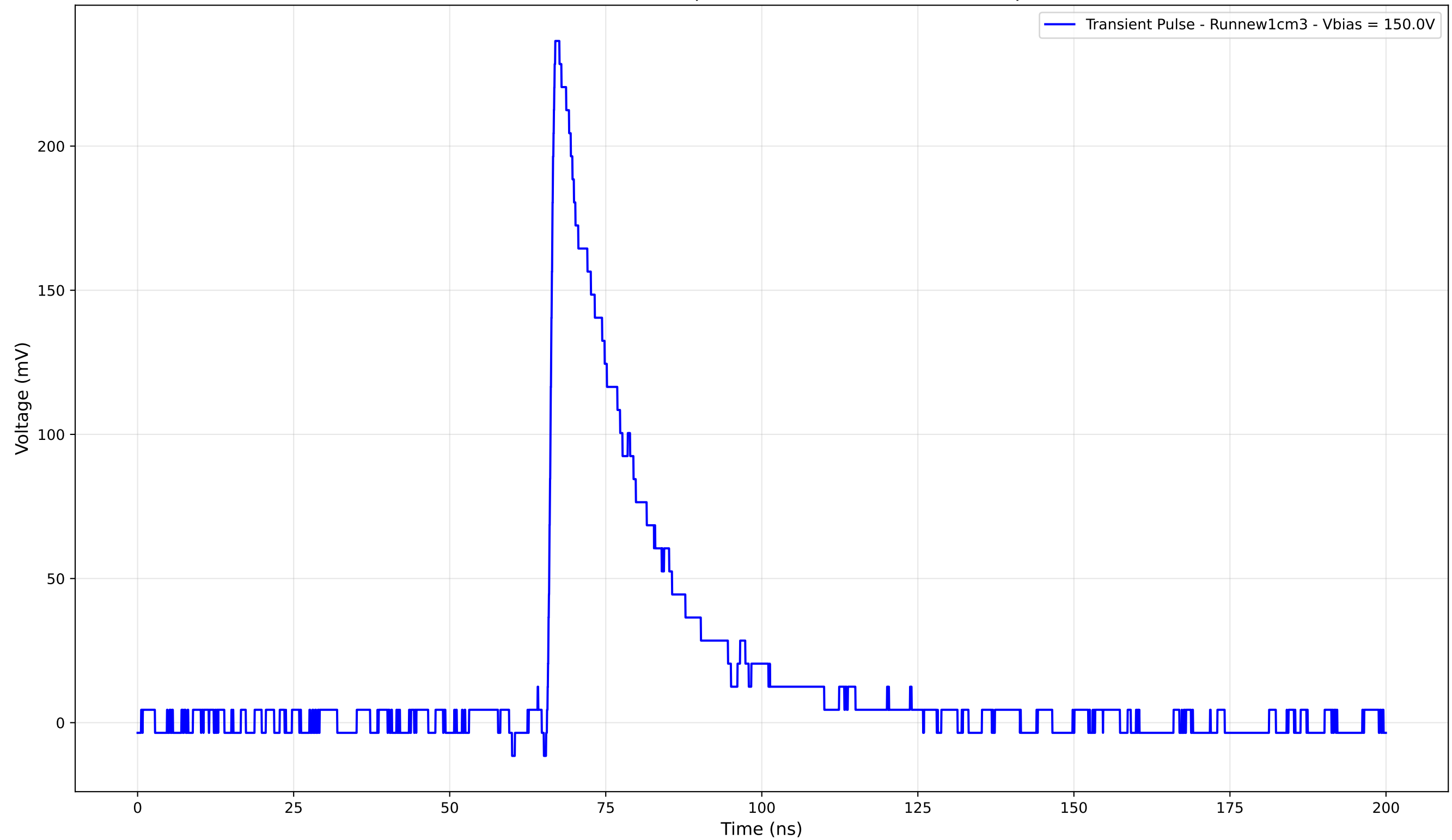
Transient Pulse - Sample: new1cm - Position: 4710.0 \mu\text{m}
