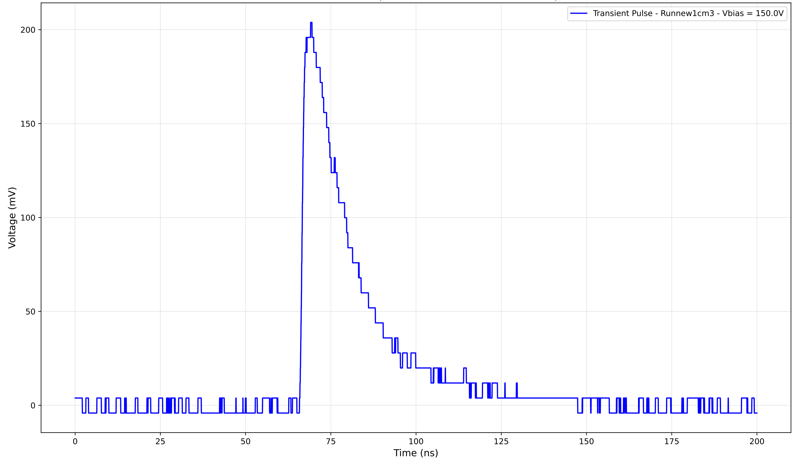
Transient Pulse - Sample: new1cm - Position: 1680.0 \mu\text{m}
