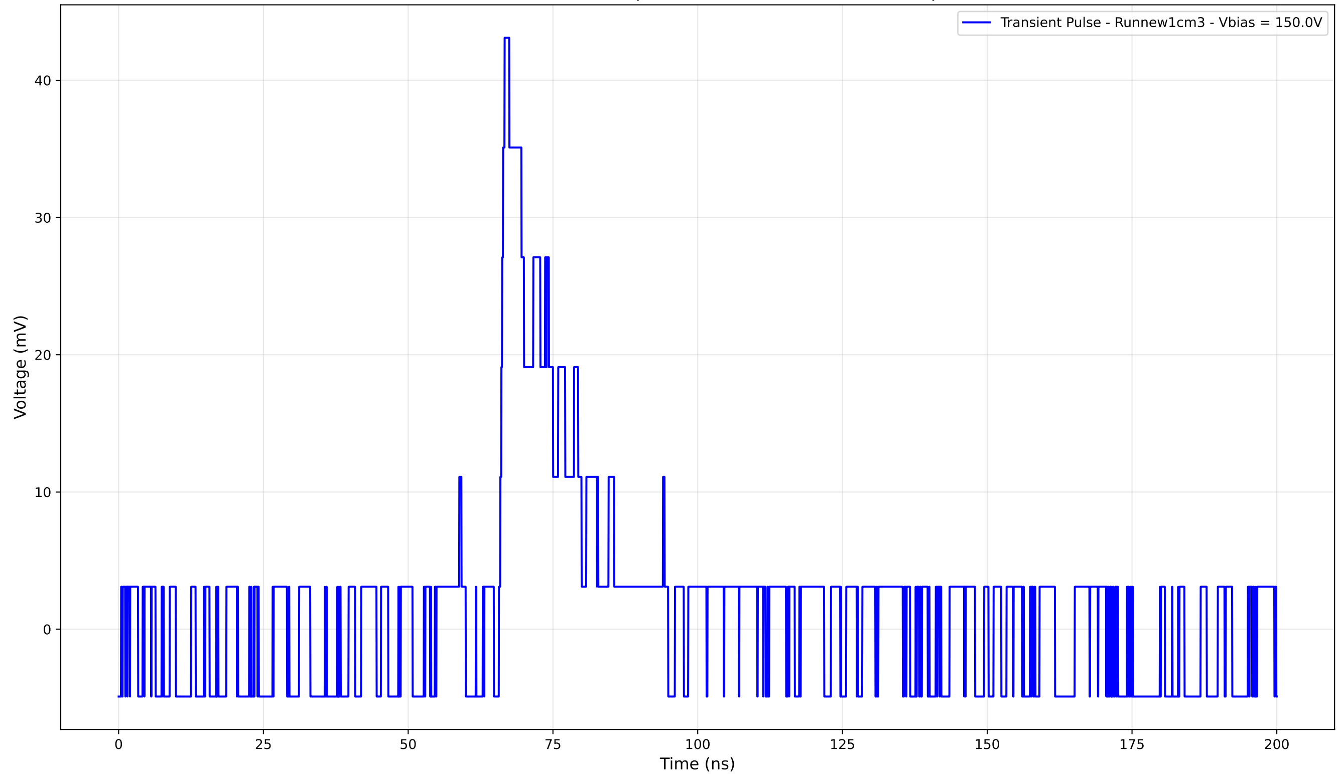
Transient Pulse - Sample: new1cm - Position: 5015.0 \mu\text{m}
