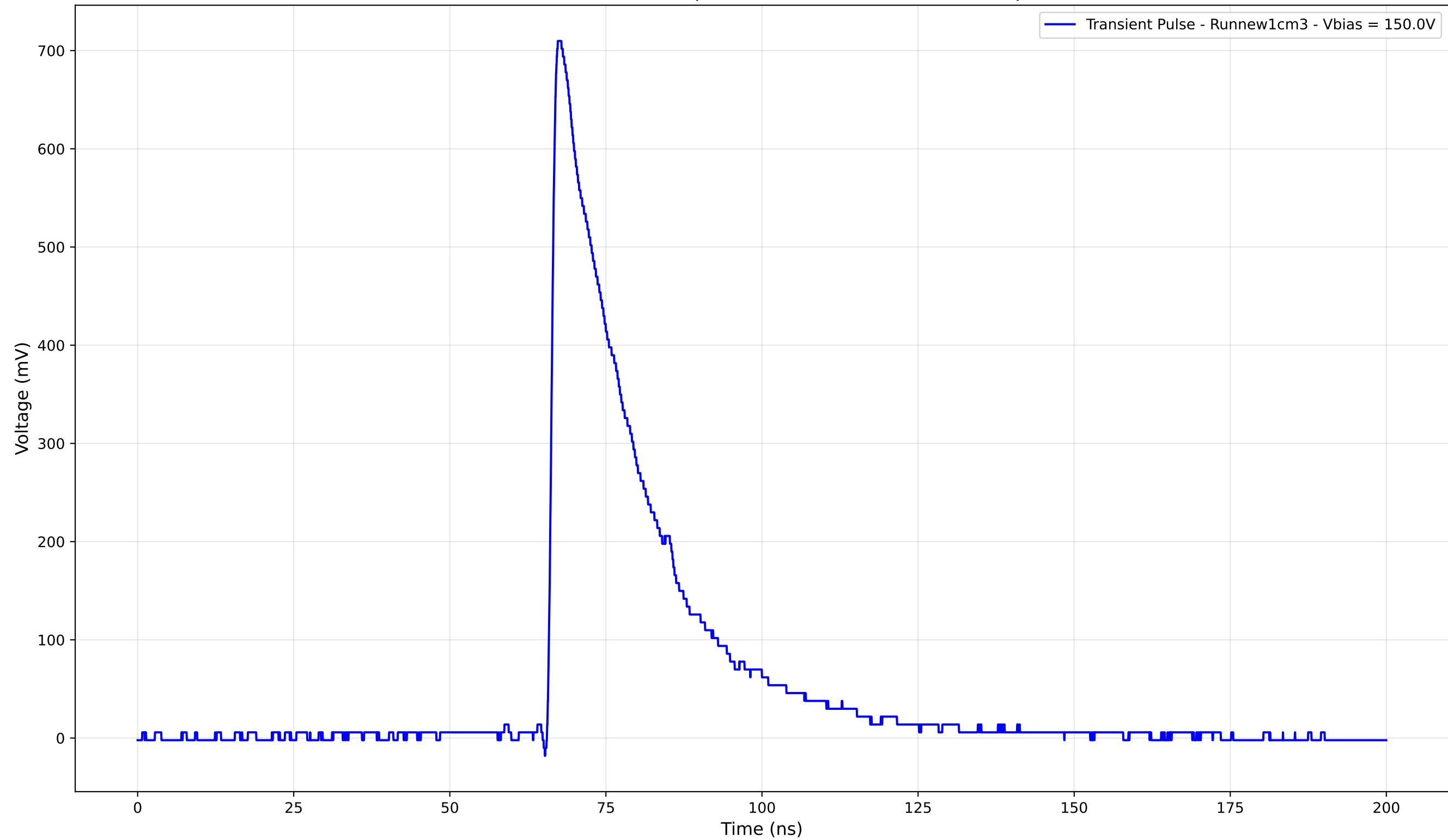
Transient Pulse - Sample: new1cm - Position: 4570.0 \mu\text{m}
