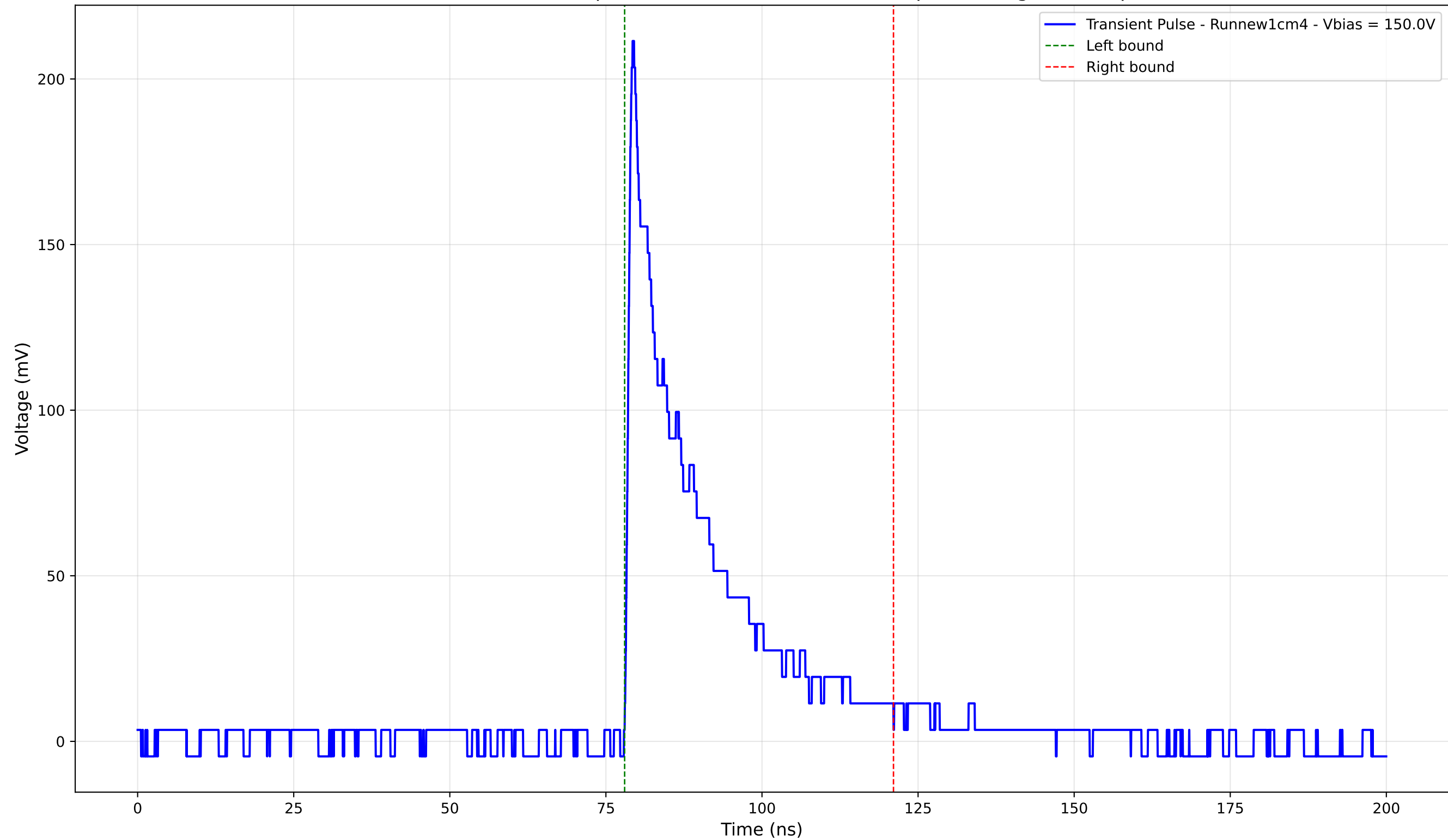
Transient Pulse - Sample: new1cm - Position: 4715.0 \mu\text{m} - Charge: 44.86 pC
