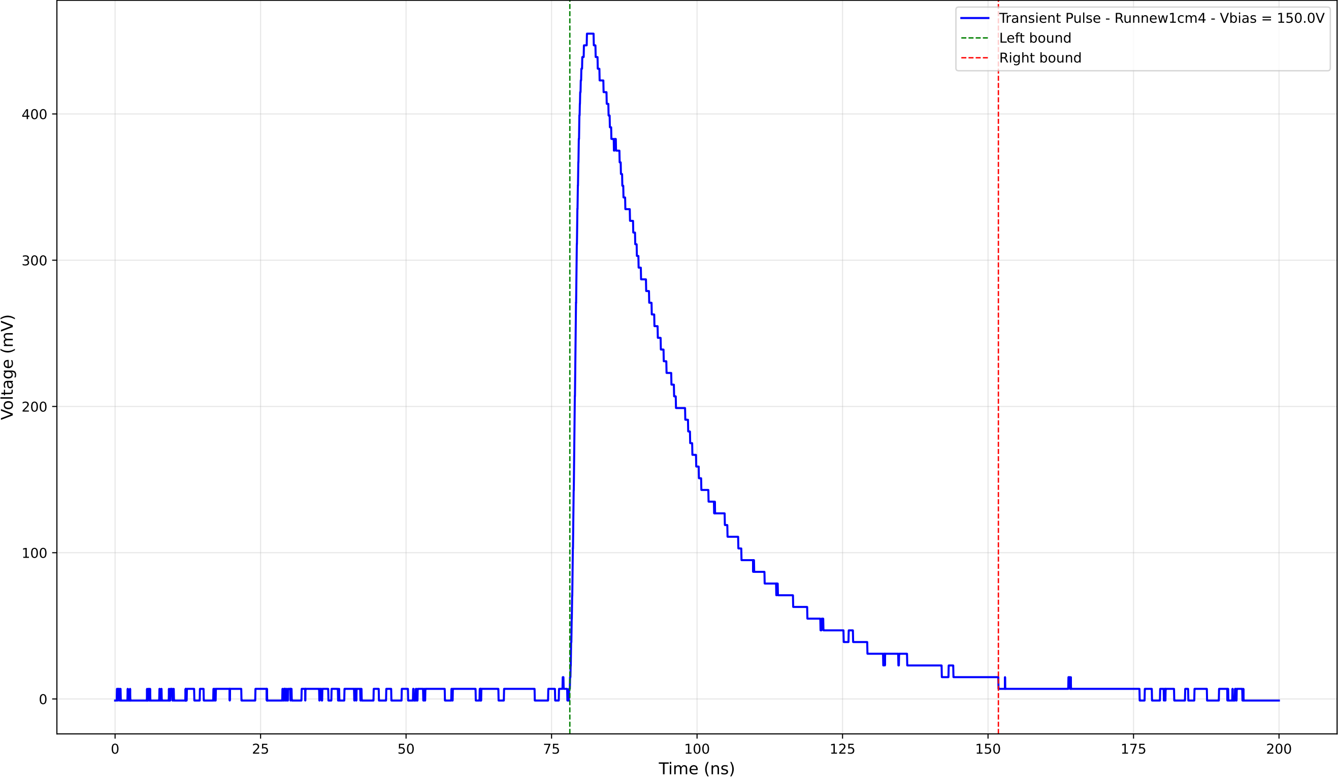
Transient Pulse - Sample: new1cm - Position: 3660.0 \mu\text{m} - Charge: 188.49 pC
