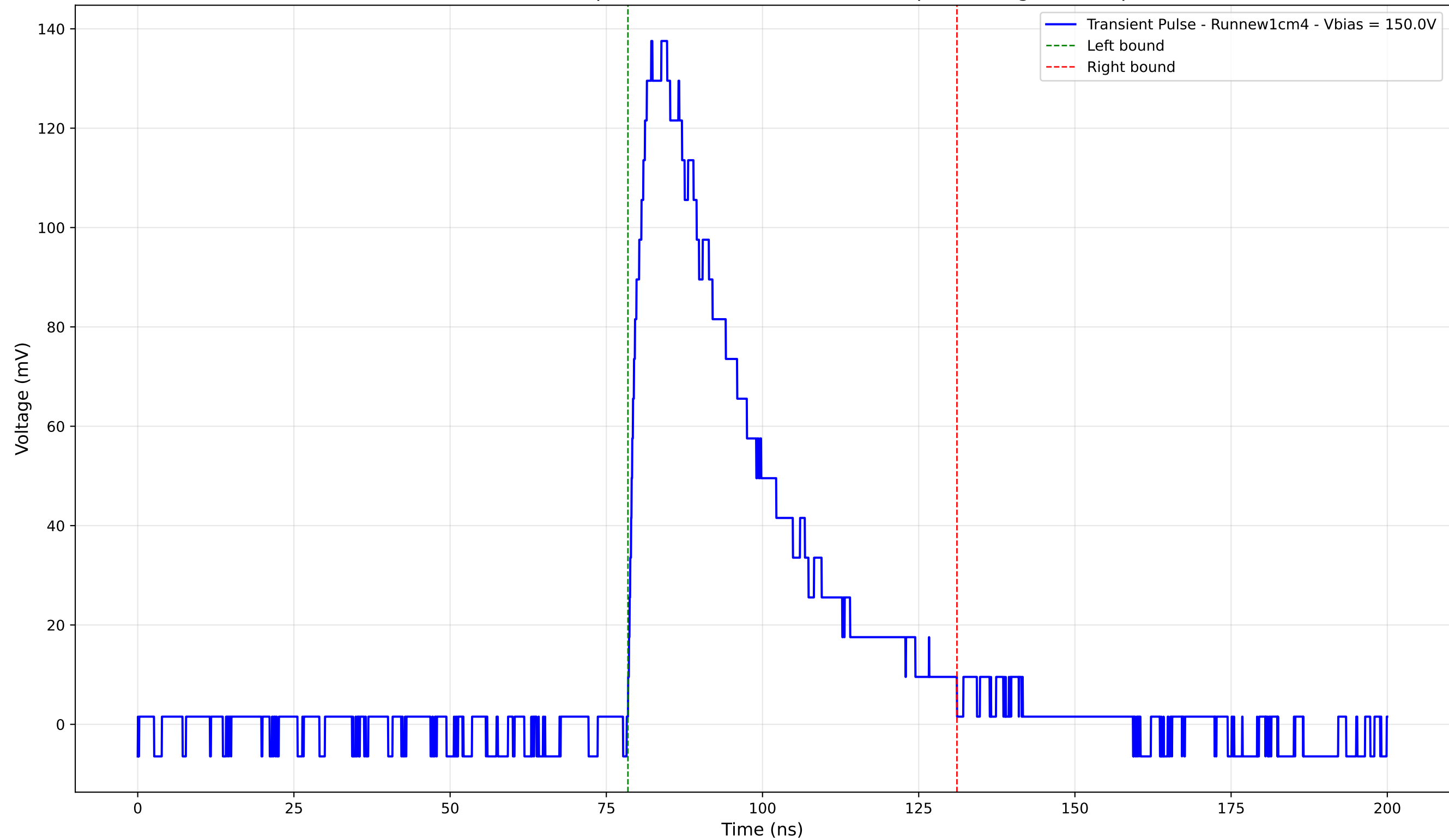
Transient Pulse - Sample: new1cm - Position: 2740.0 \mu\text{m} - Charge: 54.87 pC
