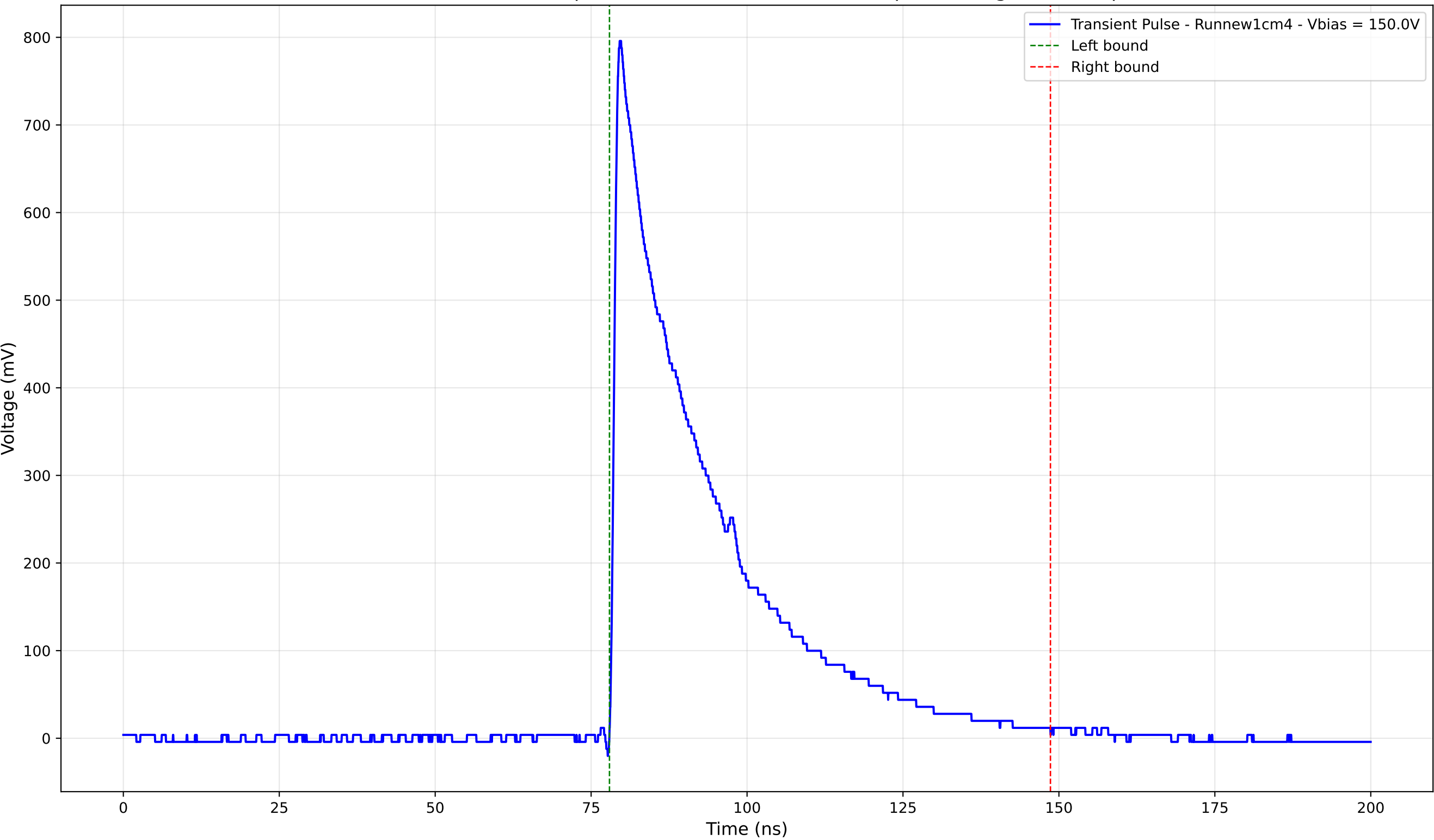
Transient Pulse - Sample: new1cm - Position: 4395.0 \mu\text{m} - Charge: 243.76 pC
