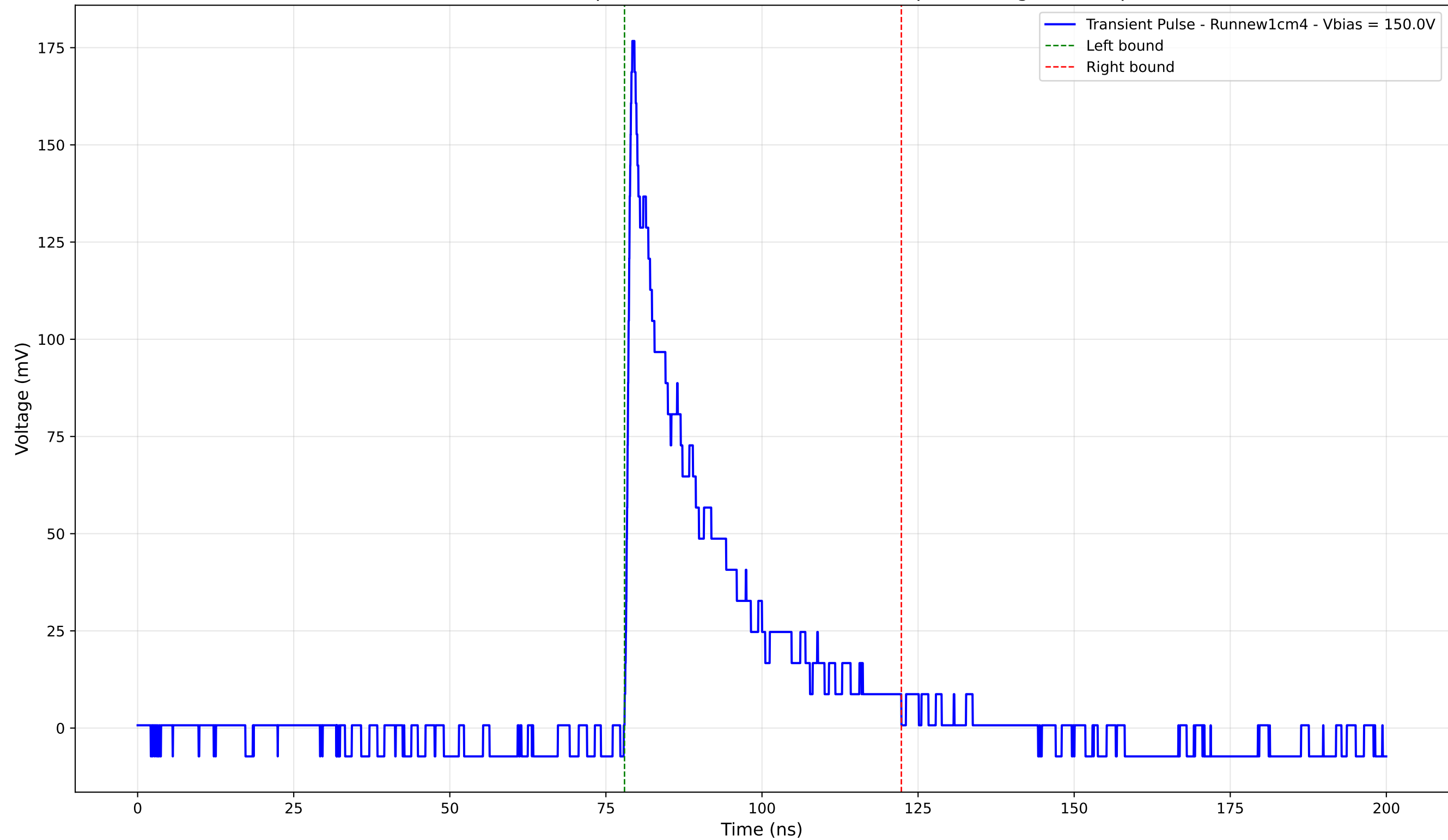
Transient Pulse - Sample: new1cm - Position: 4720.0 \mu\text{m} - Charge: 38.08 pC
