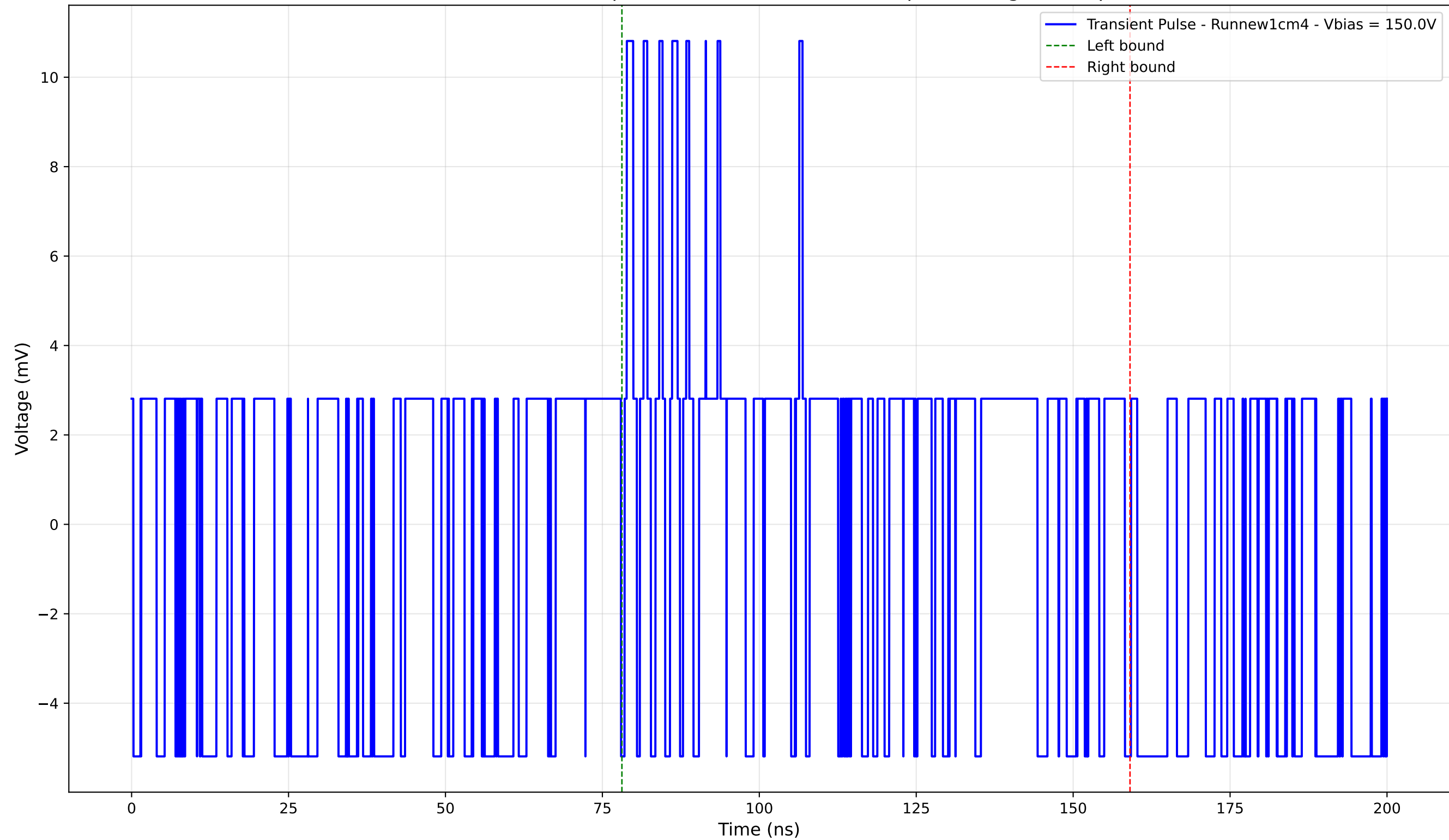
Transient Pulse - Sample: new1cm - Position: 15.0 \mu\text{m} - Charge: 2.29 pC
