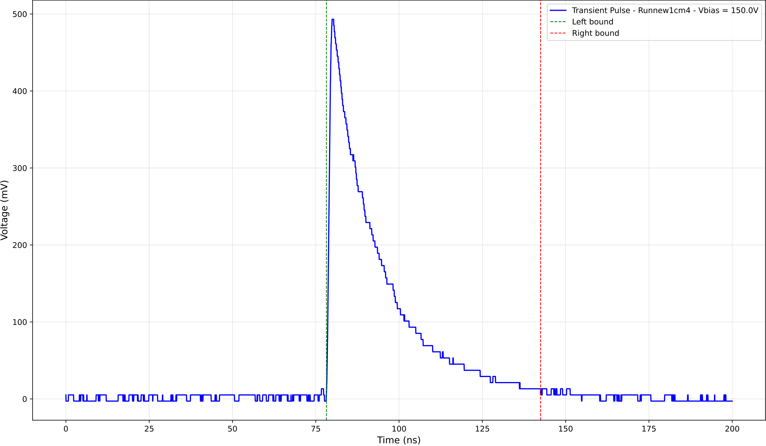
Transient Pulse - Sample: new1cm - Position: 1130.0 \mu\text{m} - Charge: 153.35 pC
