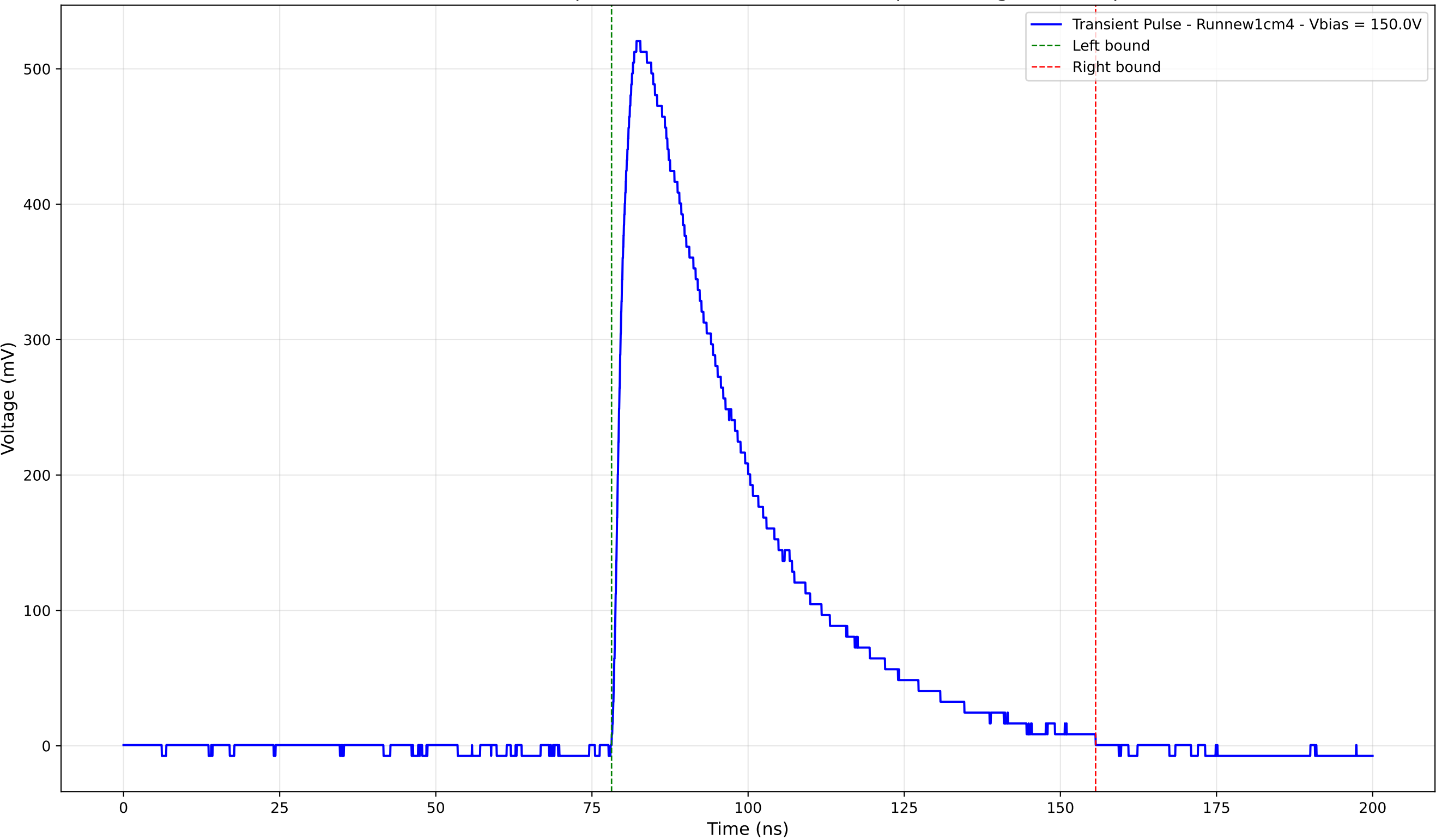
Transient Pulse - Sample: new1cm - Position: 2400.0 \mu\text{m} - Charge: 222.99 pC
