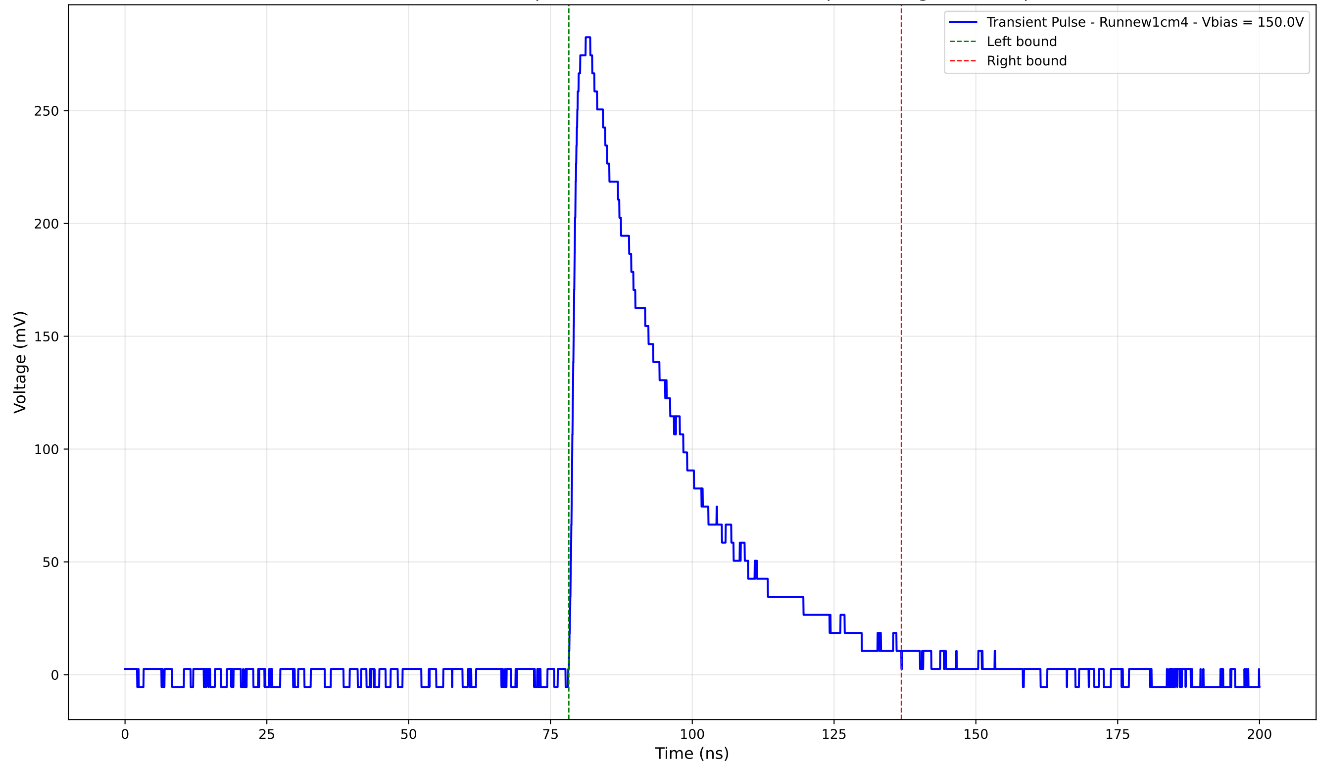
Transient Pulse - Sample: new1cm - Position: 3770.0 \mu\text{m} - Charge: 104.09 pC
