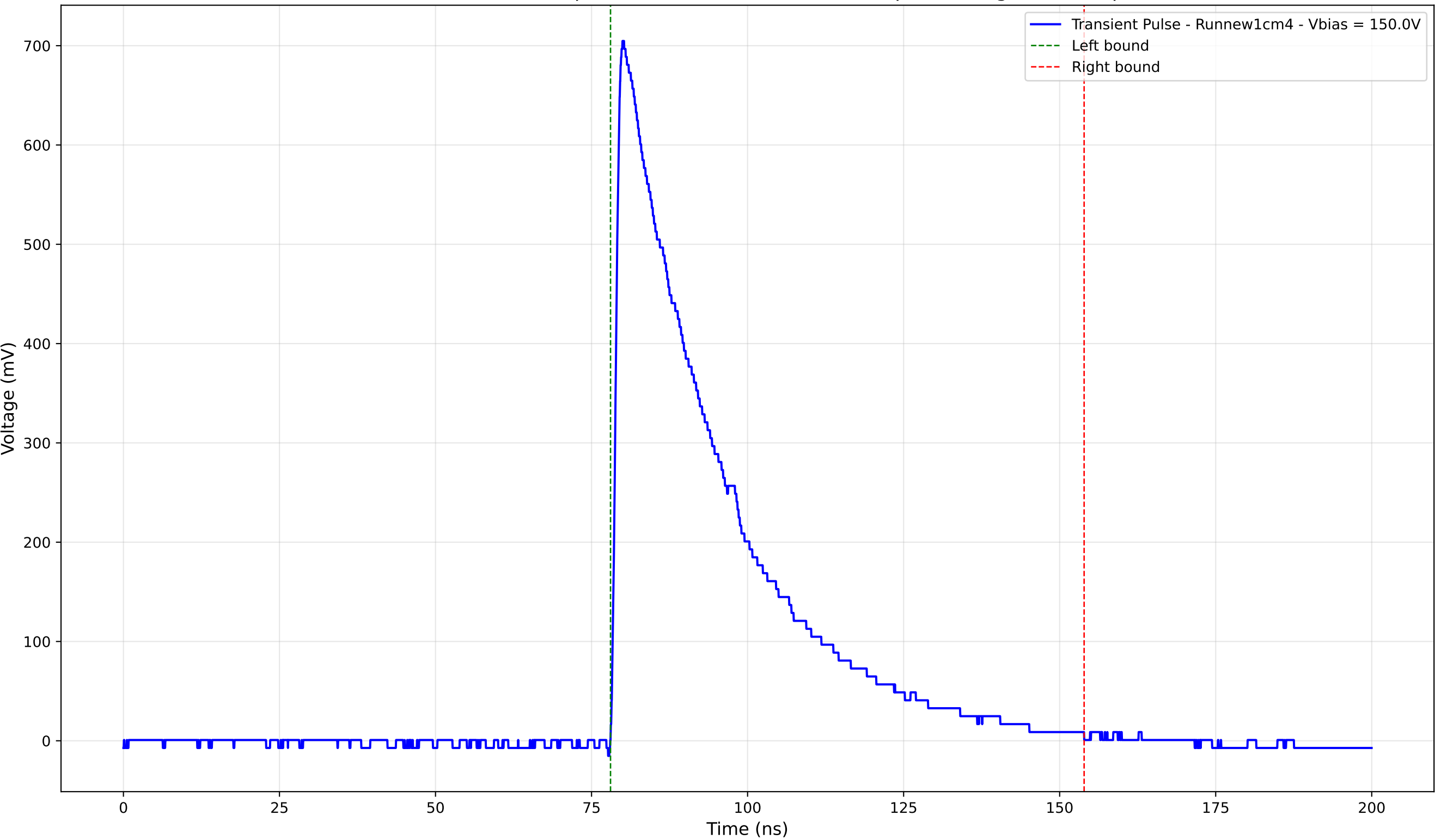
Transient Pulse - Sample: new1cm - Position: 4090.0 \mu\text{m} - Charge: 247.99 pC
