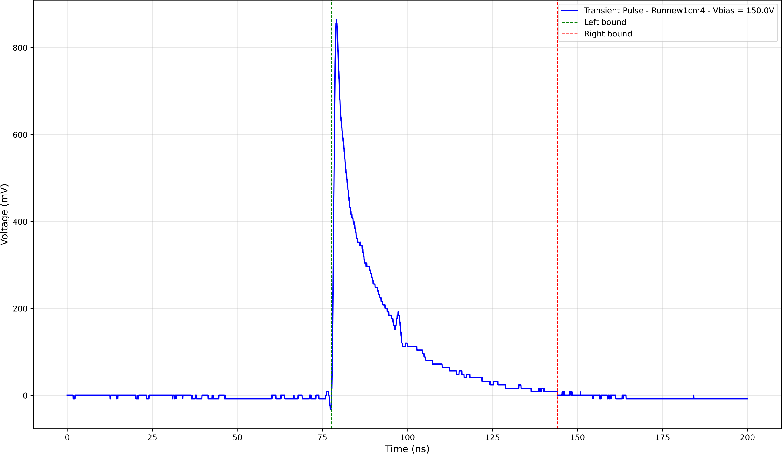
Transient Pulse - Sample: new1cm - Position: 4915.0 \mu\text{m} - Charge: 183.79 pC
