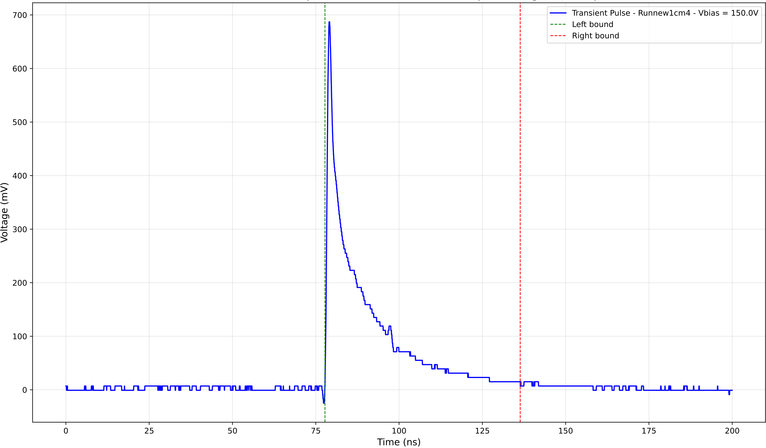
Transient Pulse - Sample: new1cm - Position: 5010.0 \mu\text{m} - Charge: 122.01 pC
