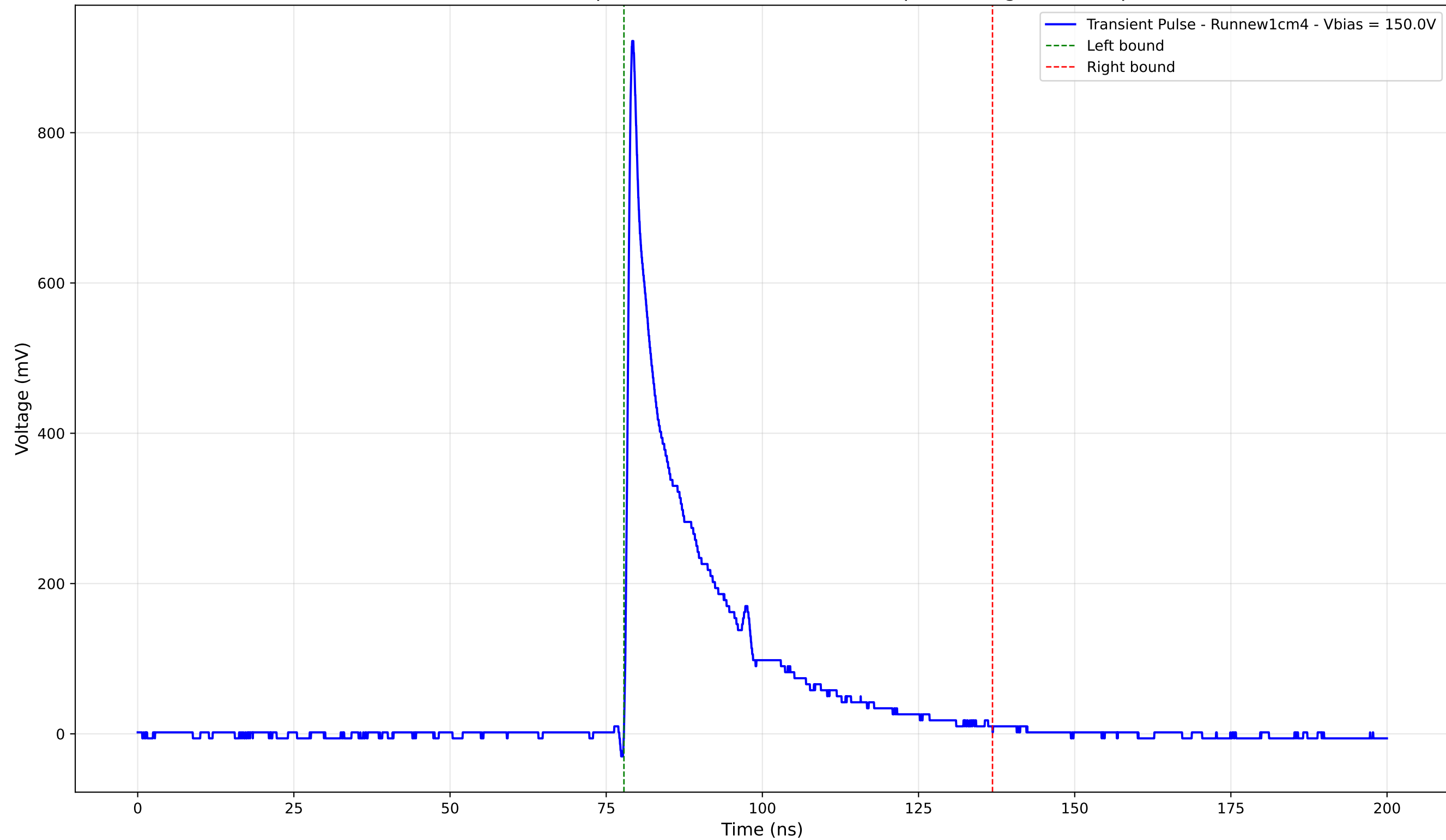
Transient Pulse - Sample: new1cm - Position: 295.0 \mu\text{m} - Charge: 171.23 pC
