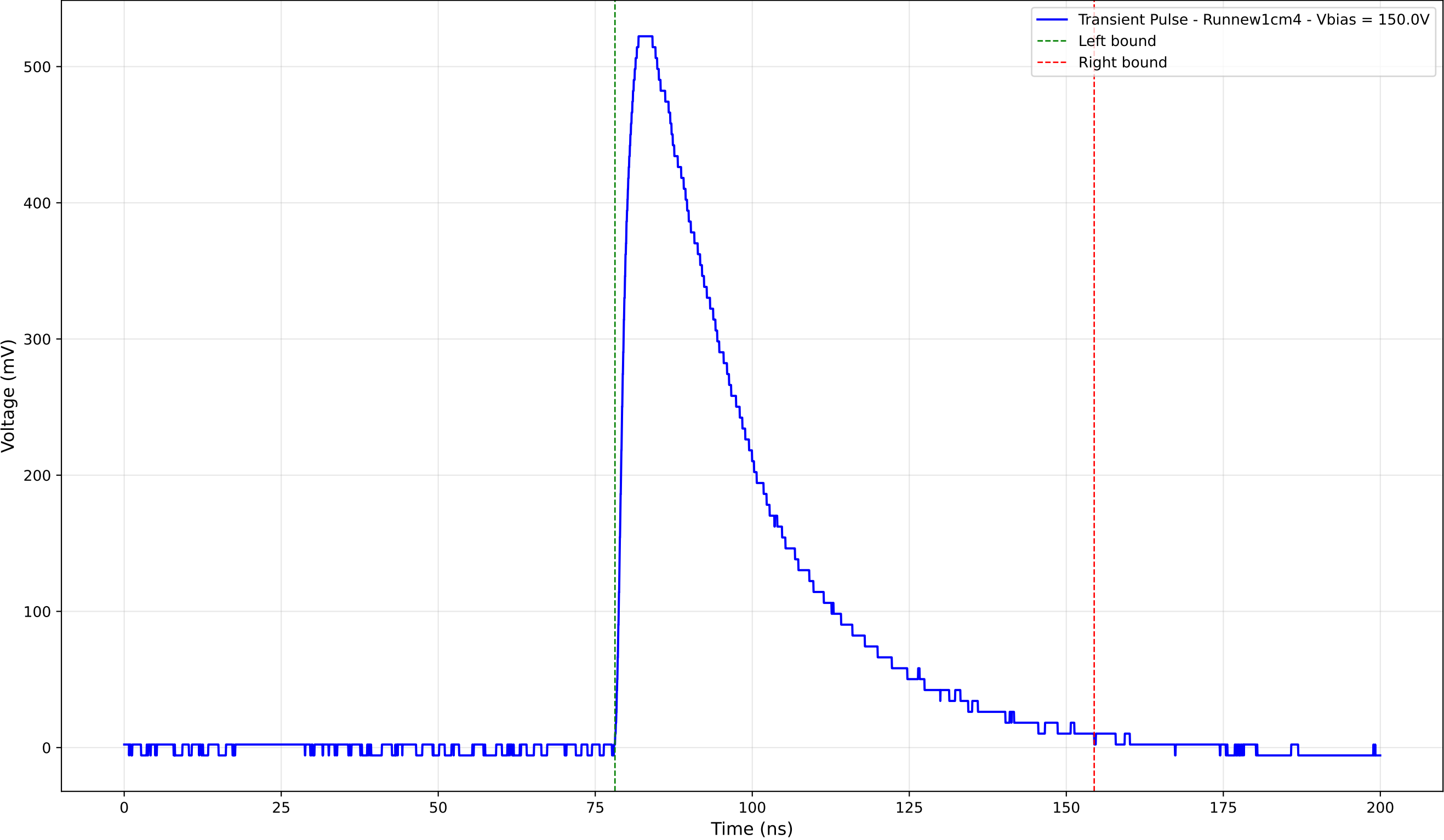
Transient Pulse - Sample: new1cm - Position: 2860.0 \mu\text{m} - Charge: 232.43 pC
