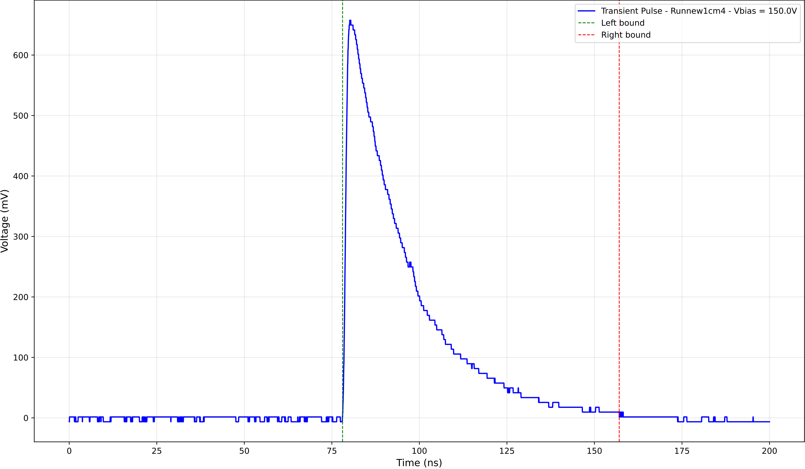
Transient Pulse - Sample: new1cm - Position: 3975.0 \mu\text{m} - Charge: 245.22 pC
