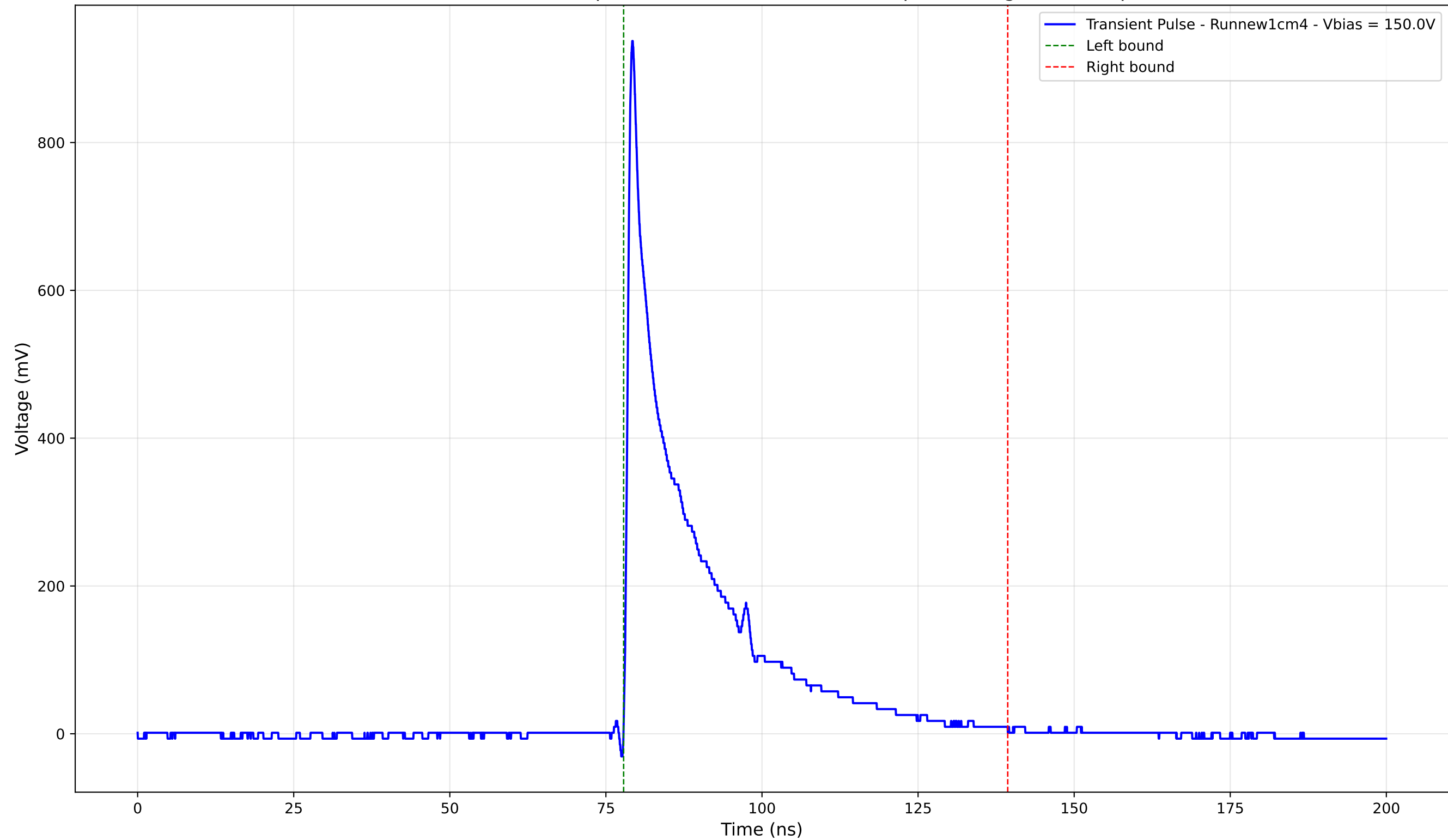
Transient Pulse - Sample: new1cm - Position: 305.0 \mu\text{m} - Charge: 175.26 pC
