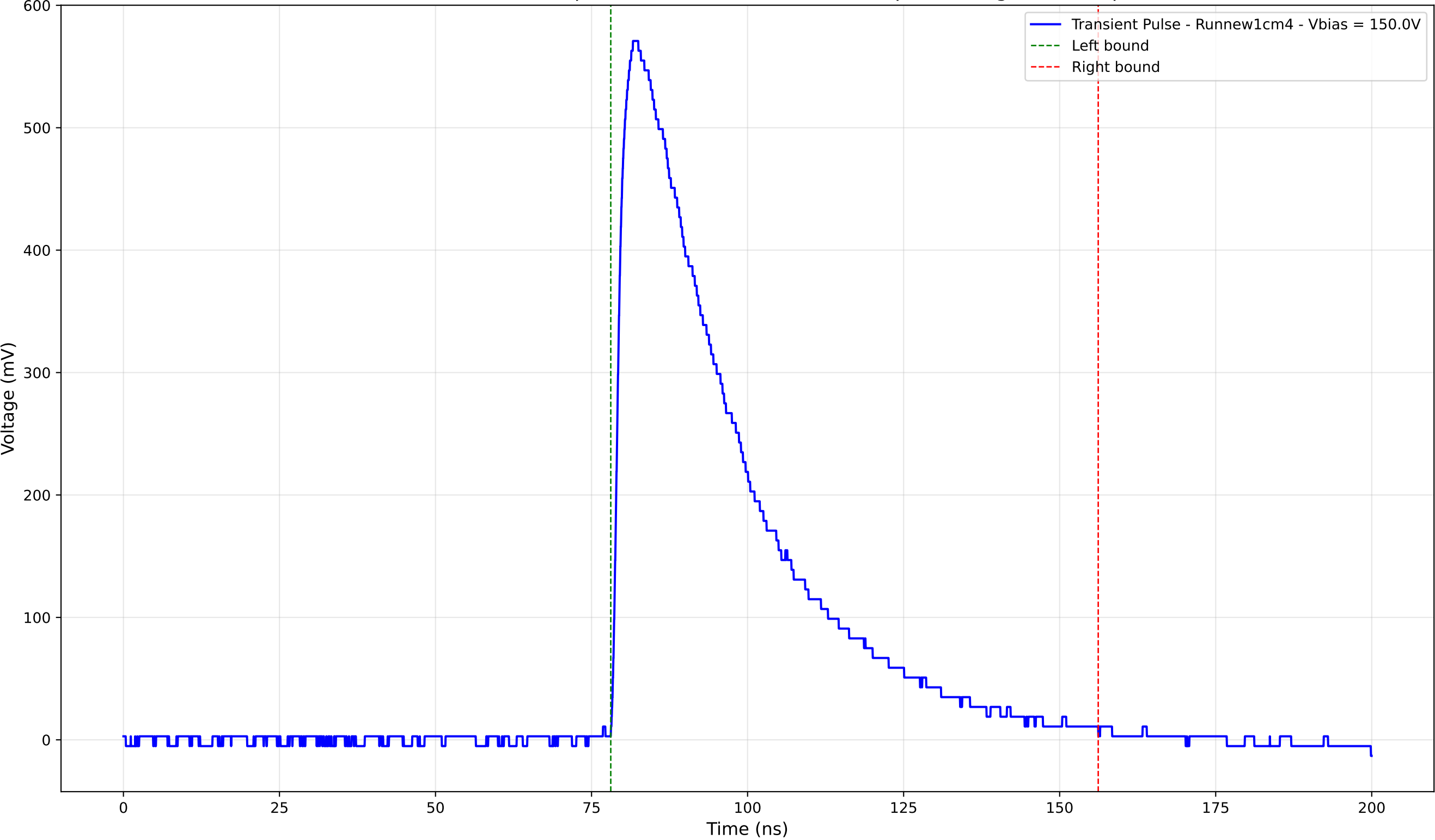
Transient Pulse - Sample: new1cm - Position: 3350.0 \mu\text{m} - Charge: 244.39 pC
