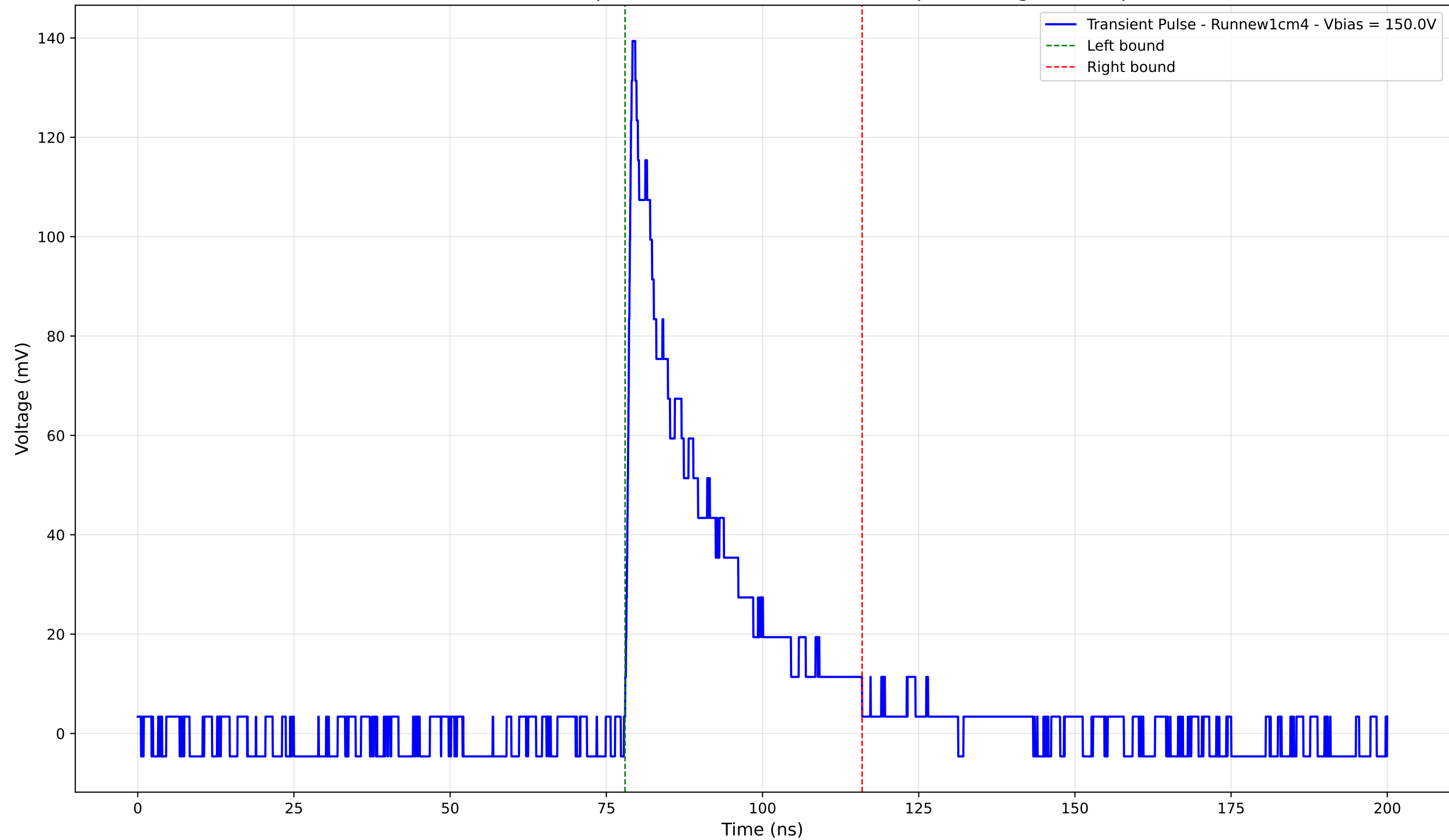
Transient Pulse - Sample: new1cm - Position: 4730.0 \mu\text{m} - Charge: 30.42 pC
