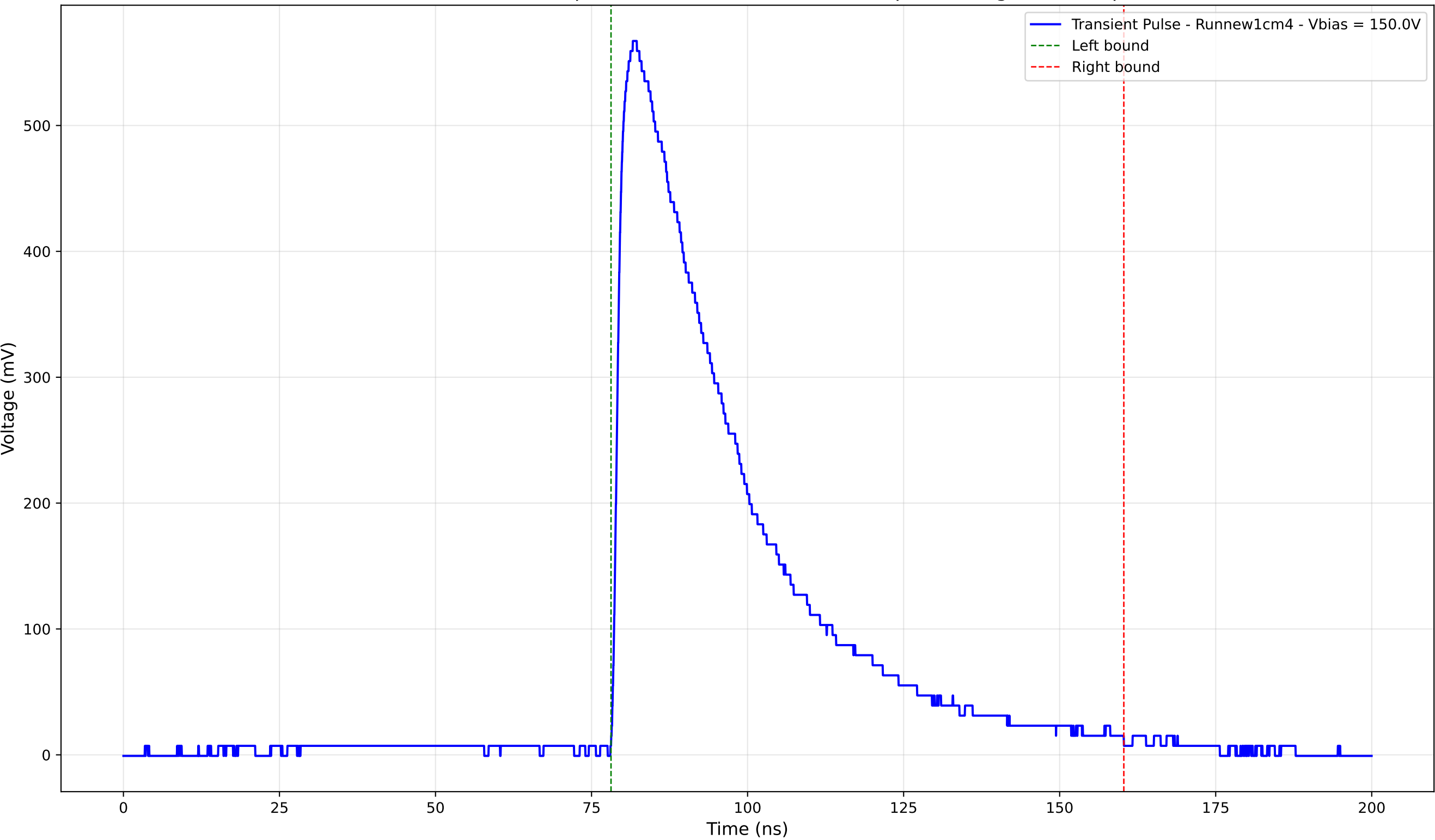
Transient Pulse - Sample: new1cm - Position: 3465.0 \mu\text{m} - Charge: 245.24 pC
