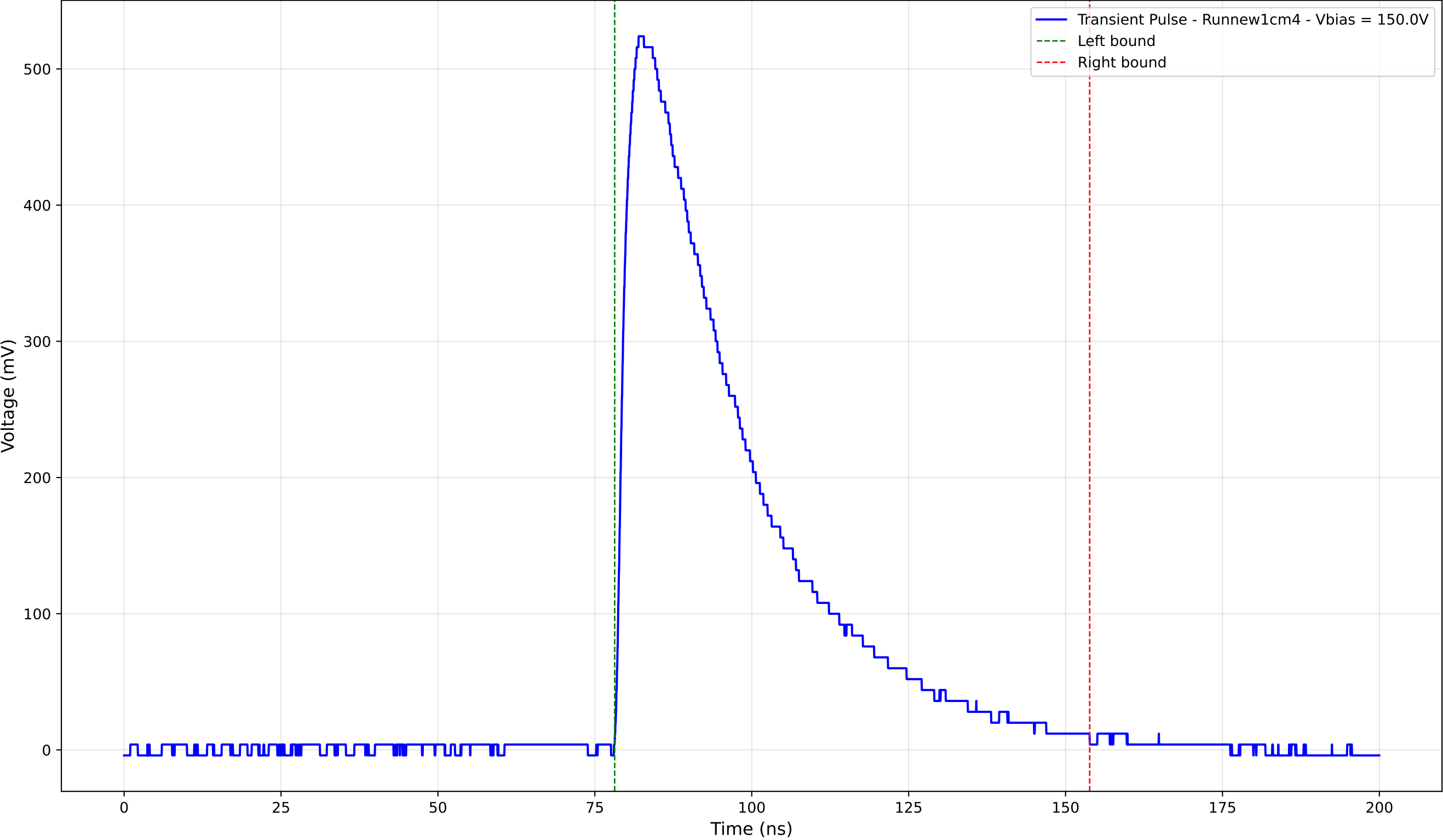
Transient Pulse - Sample: new1cm - Position: 2965.0 \mu\text{m} - Charge: 230.44 pC
