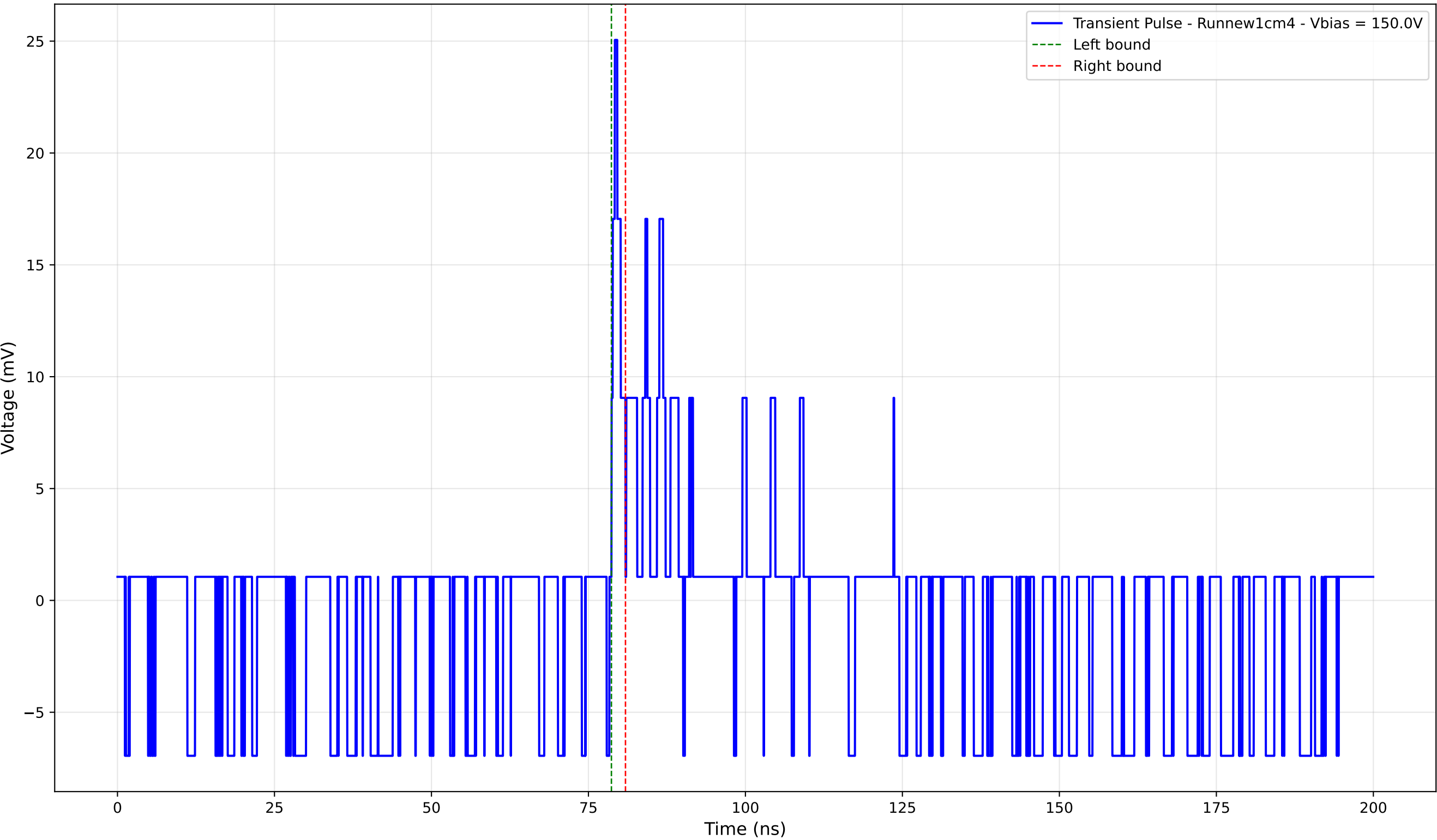
Transient Pulse - Sample: new1cm - Position: 115.0 \mu\text{m} - Charge: 0.67 pC
