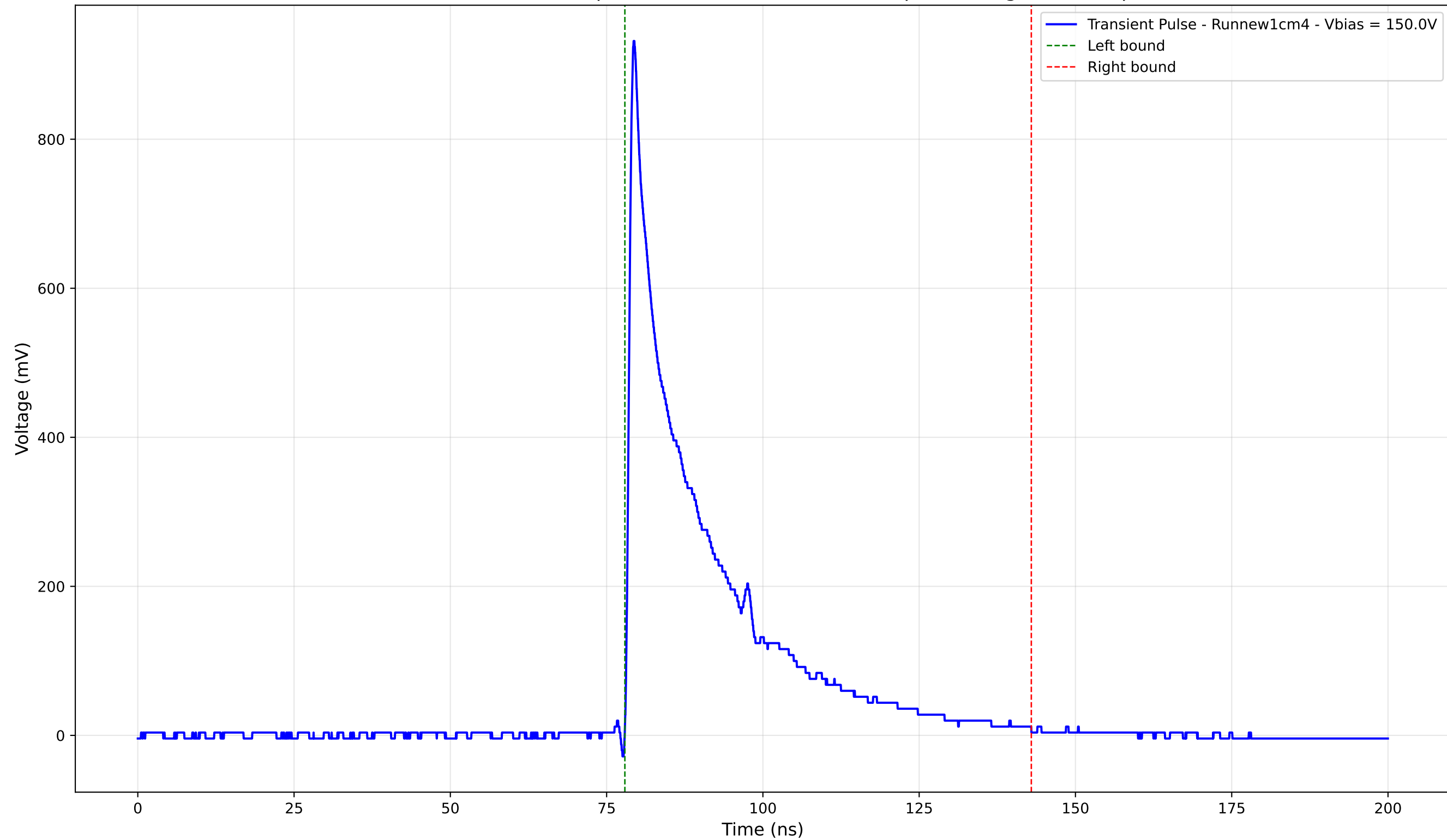
Transient Pulse - Sample: new1cm - Position: 455.0 \mu\text{m} - Charge: 201.59 pC
