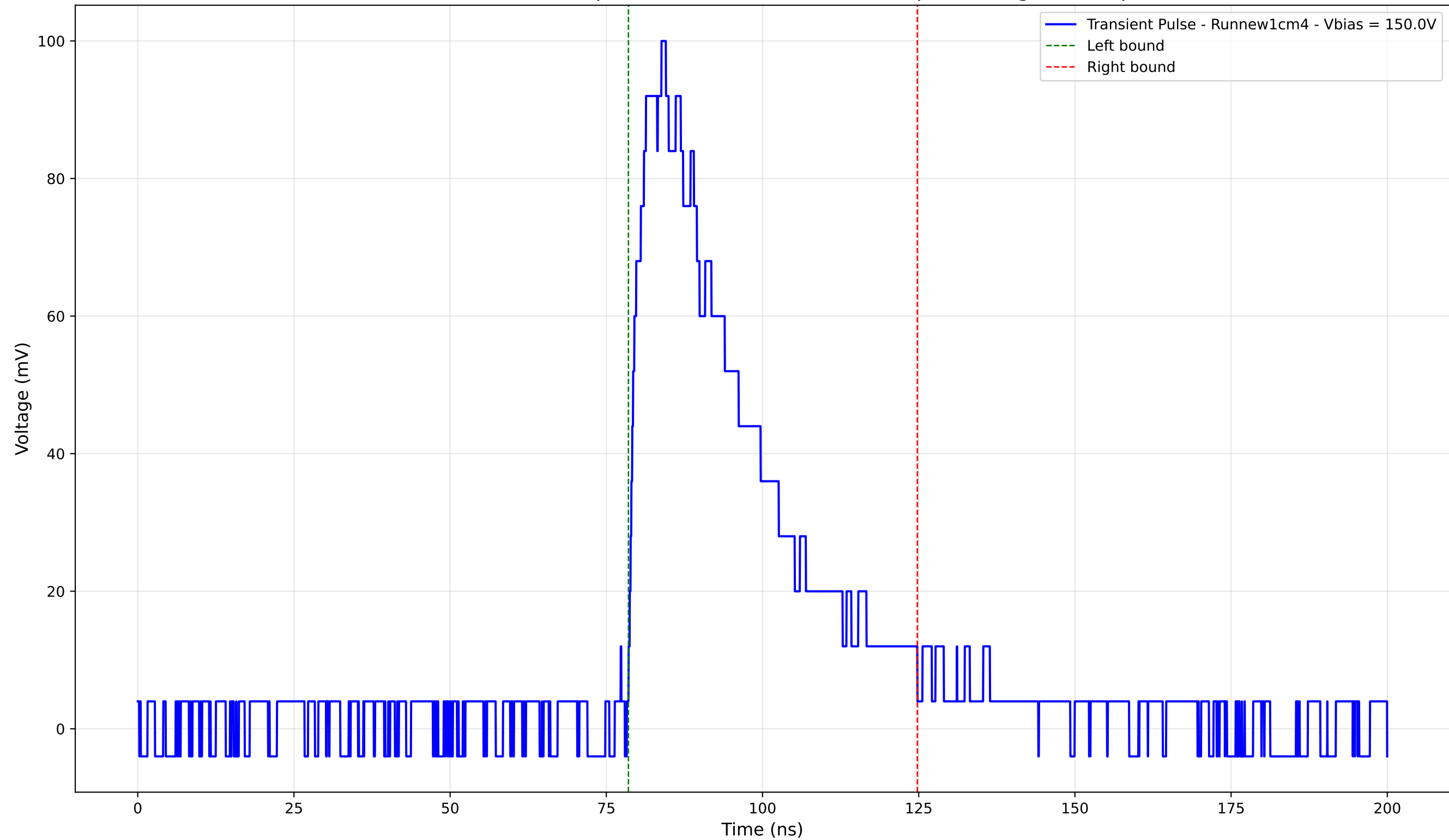
Transient Pulse - Sample: new1cm - Position: 3235.0 \mu\text{m} - Charge: 38.44 pC
