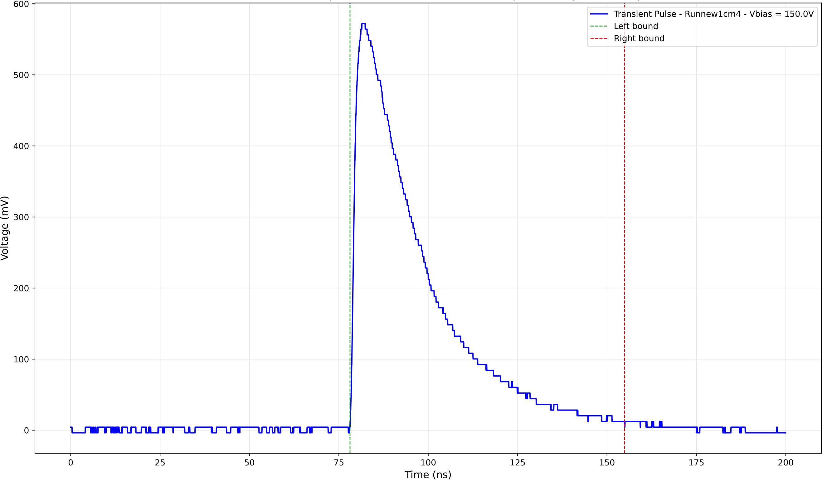
Transient Pulse - Sample: new1cm - Position: 3405.0 \mu\text{m} - Charge: 245.38 pC
