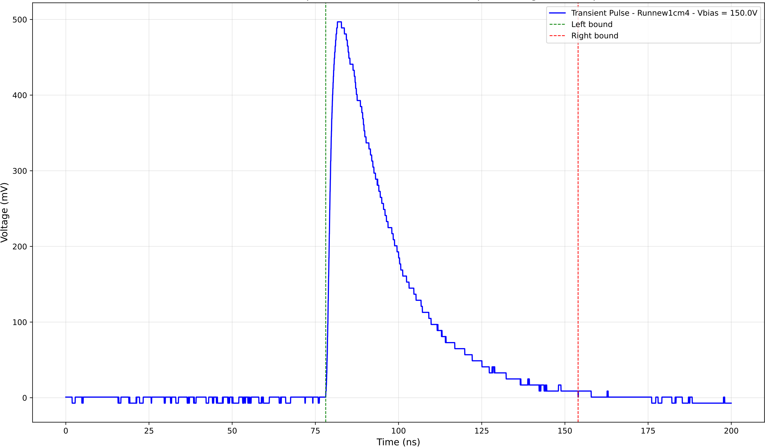
Transient Pulse - Sample: new1cm - Position: 2110.0 \mu\text{m} - Charge: 207.47 pC
