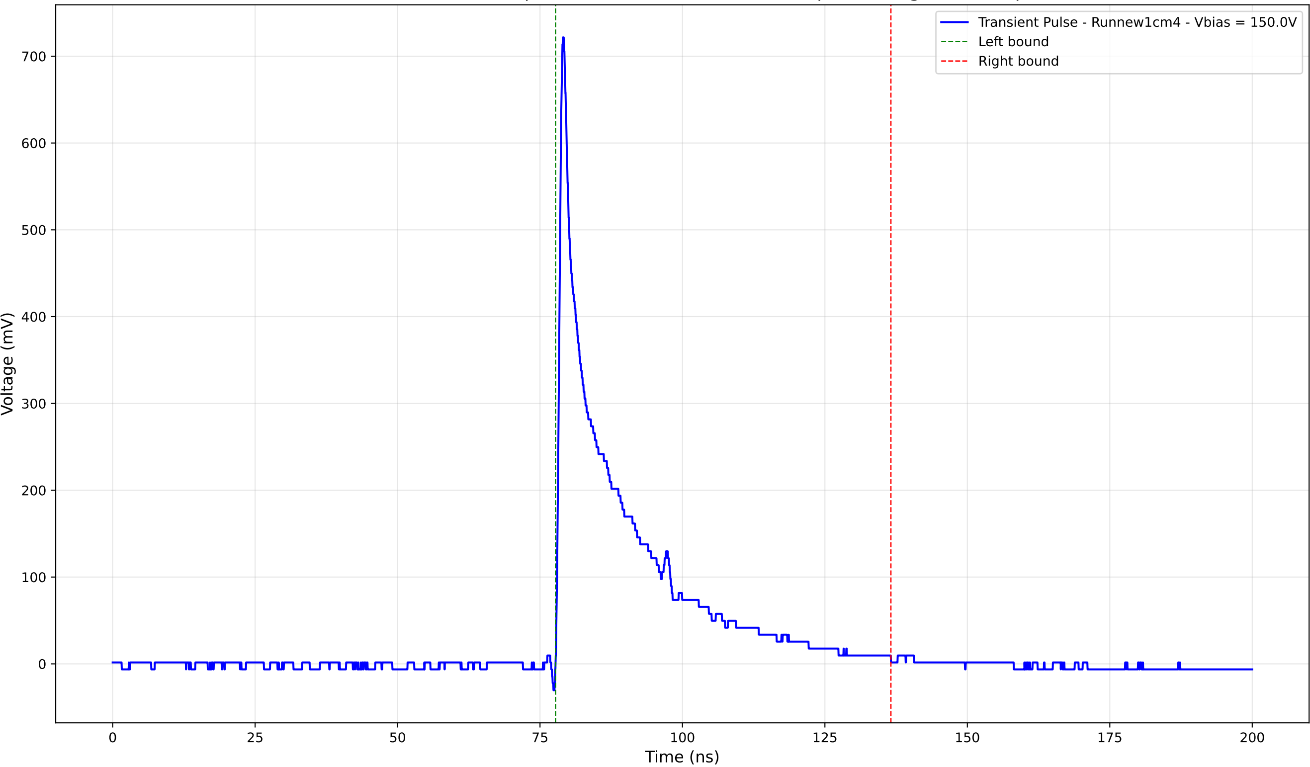
Transient Pulse - Sample: new1cm - Position: 5005.0 \mu\text{m} - Charge: 126.10 pC
