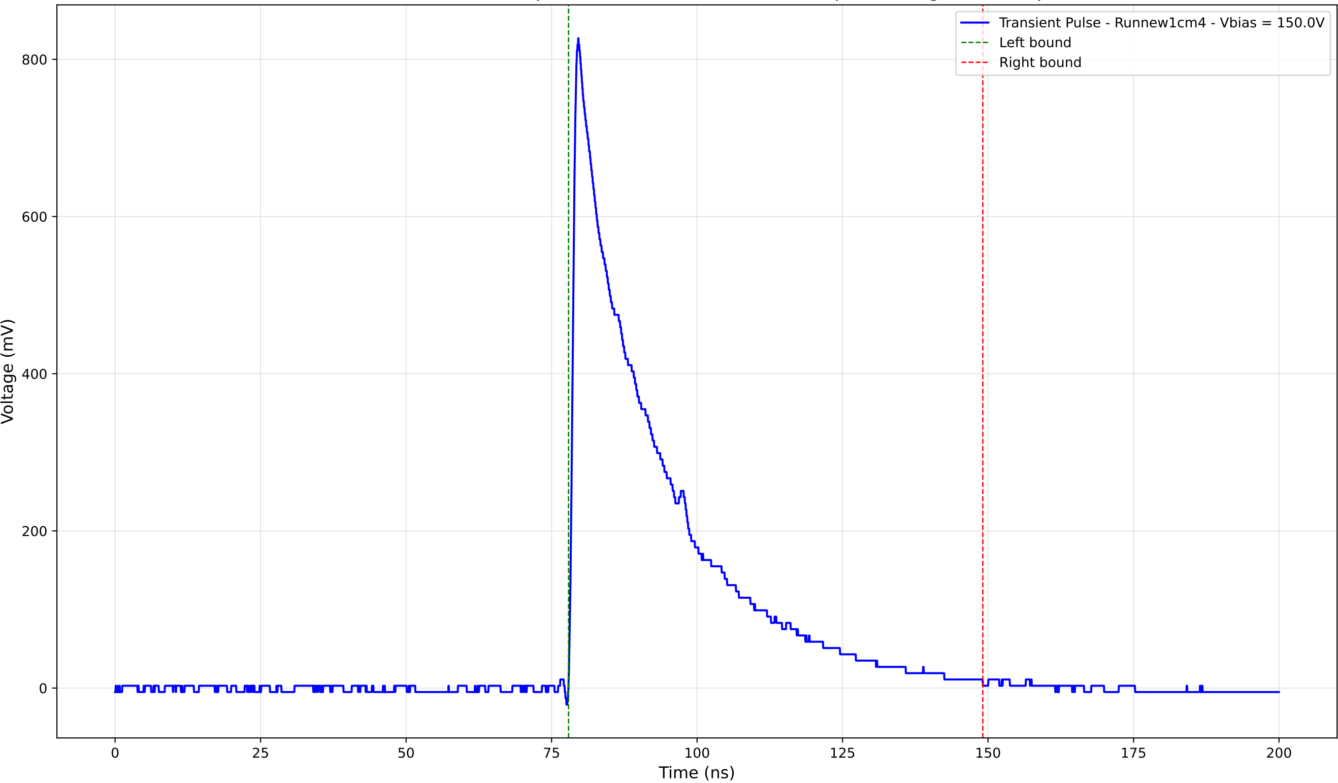
Transient Pulse - Sample: new1cm - Position: 4465.0 \mu\text{m} - Charge: 243.65 pC
