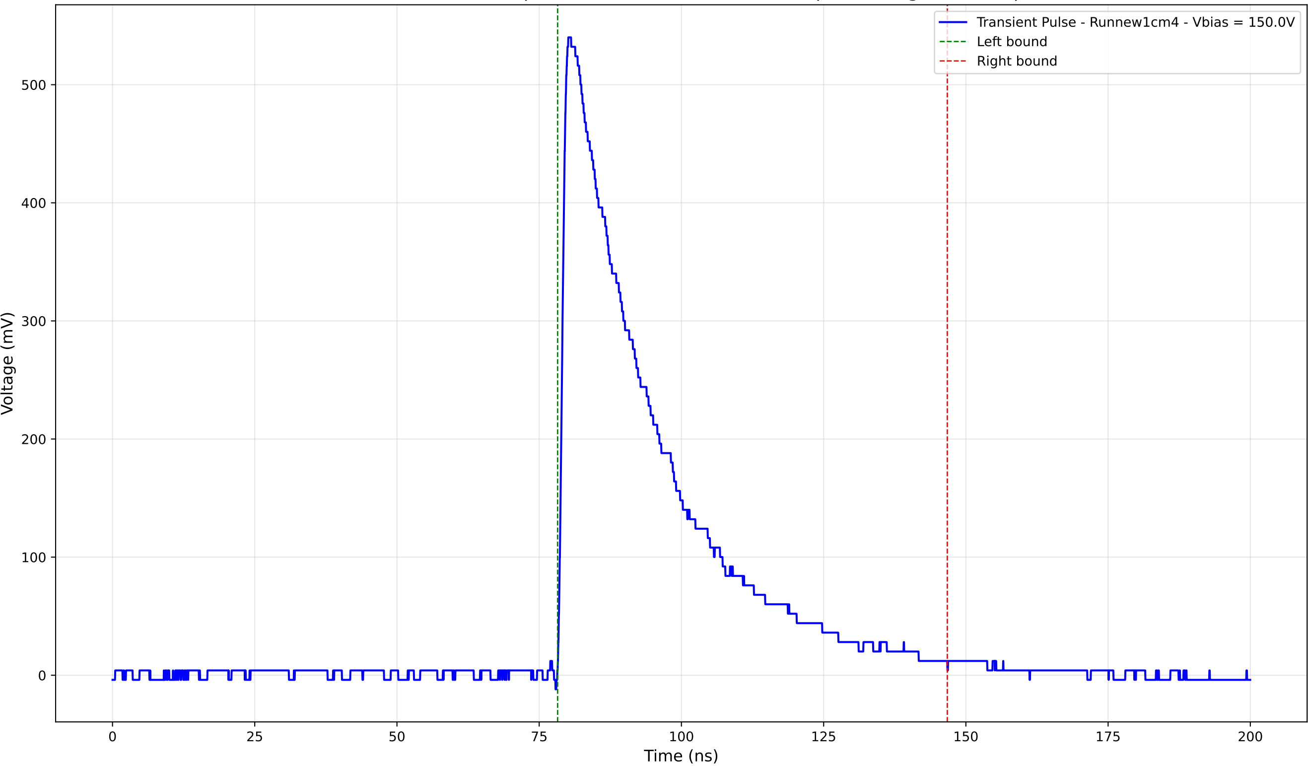
Transient Pulse - Sample: new1cm - Position: 1295.0 \mu\text{m} - Charge: 188.83 pC
