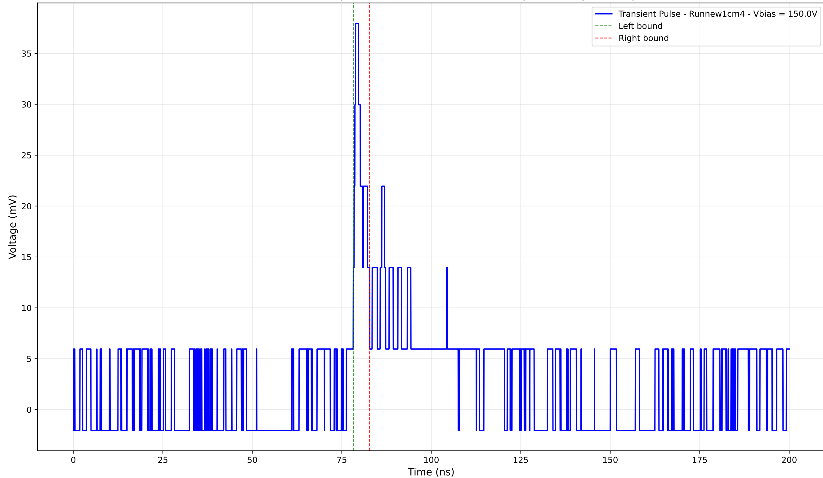
Transient Pulse - Sample: new1cm -Position: 5090.0 \mu\text{m} - Charge: 2.23 pC
