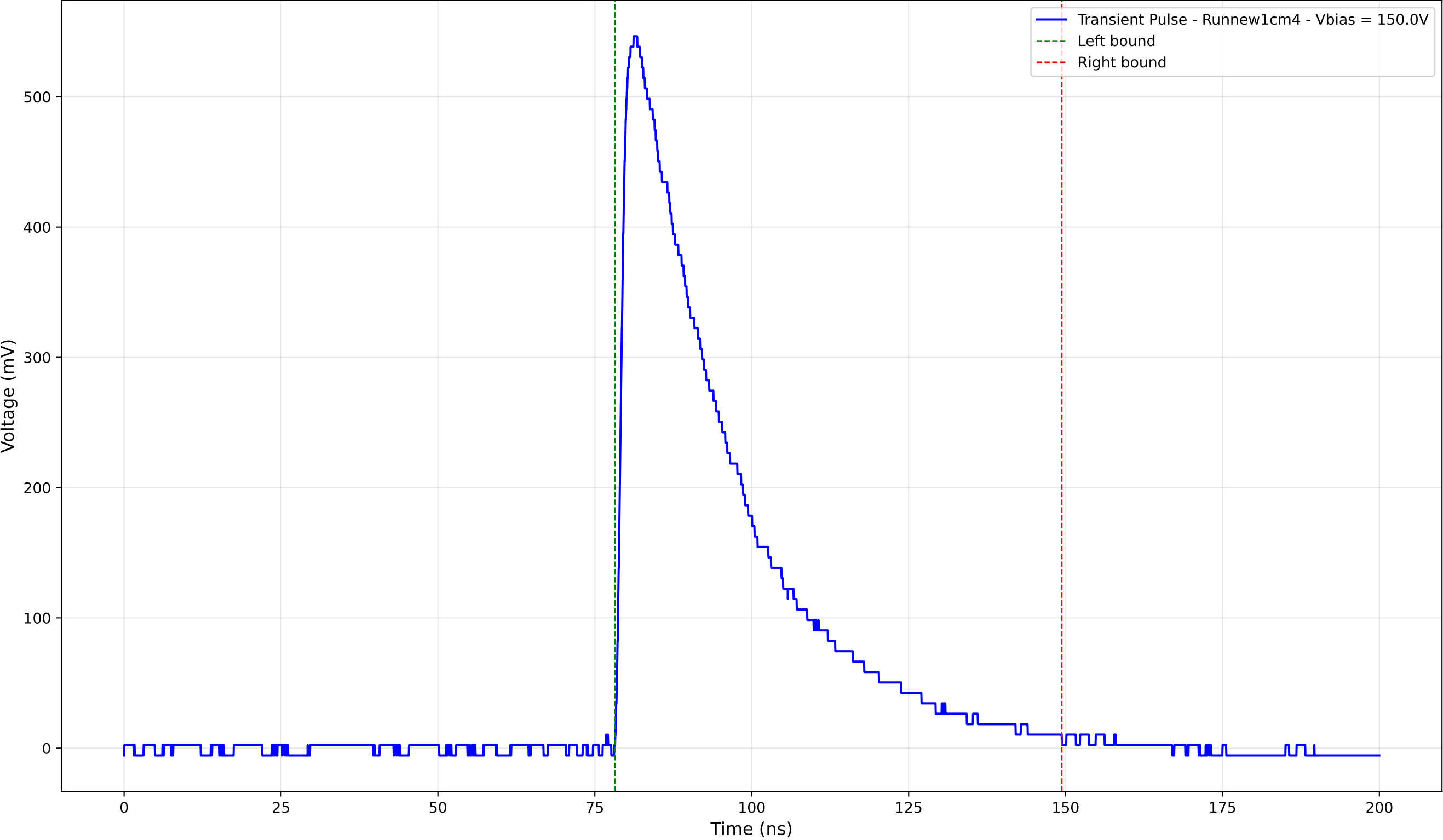
Transient Pulse - Sample: new1cm - Position: 1595.0 \mu\text{m} - Charge: 207.38 pC
