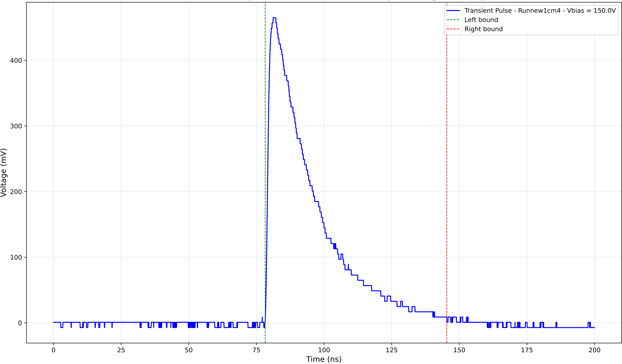
Transient Pulse - Sample: new1cm - Position: 1625.0 \mu\text{m} - Charge: 174.07 pC
