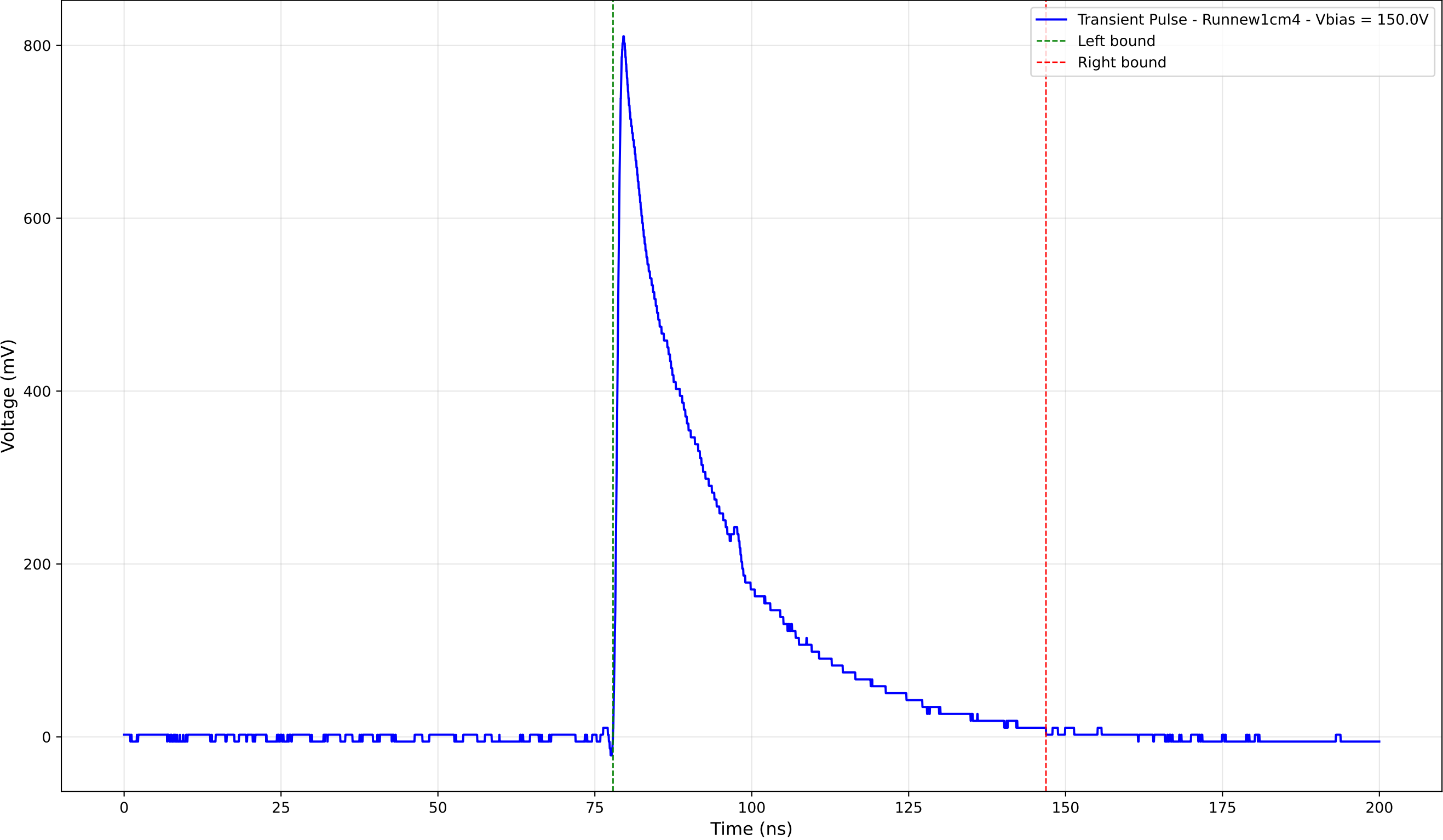
Transient Pulse - Sample: new1cm - Position: 4485.0 \mu\text{m} - Charge: 236.15 pC
