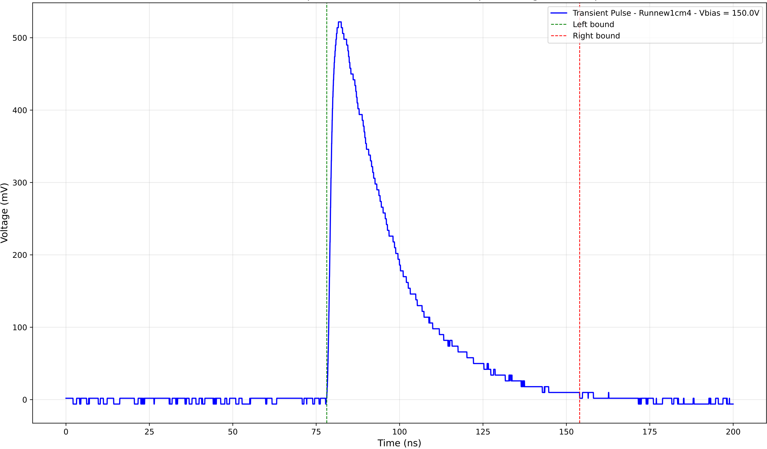
Transient Pulse - Sample: new1cm - Position: 1910.0 \mu\text{m} - Charge: 213.16 pC
