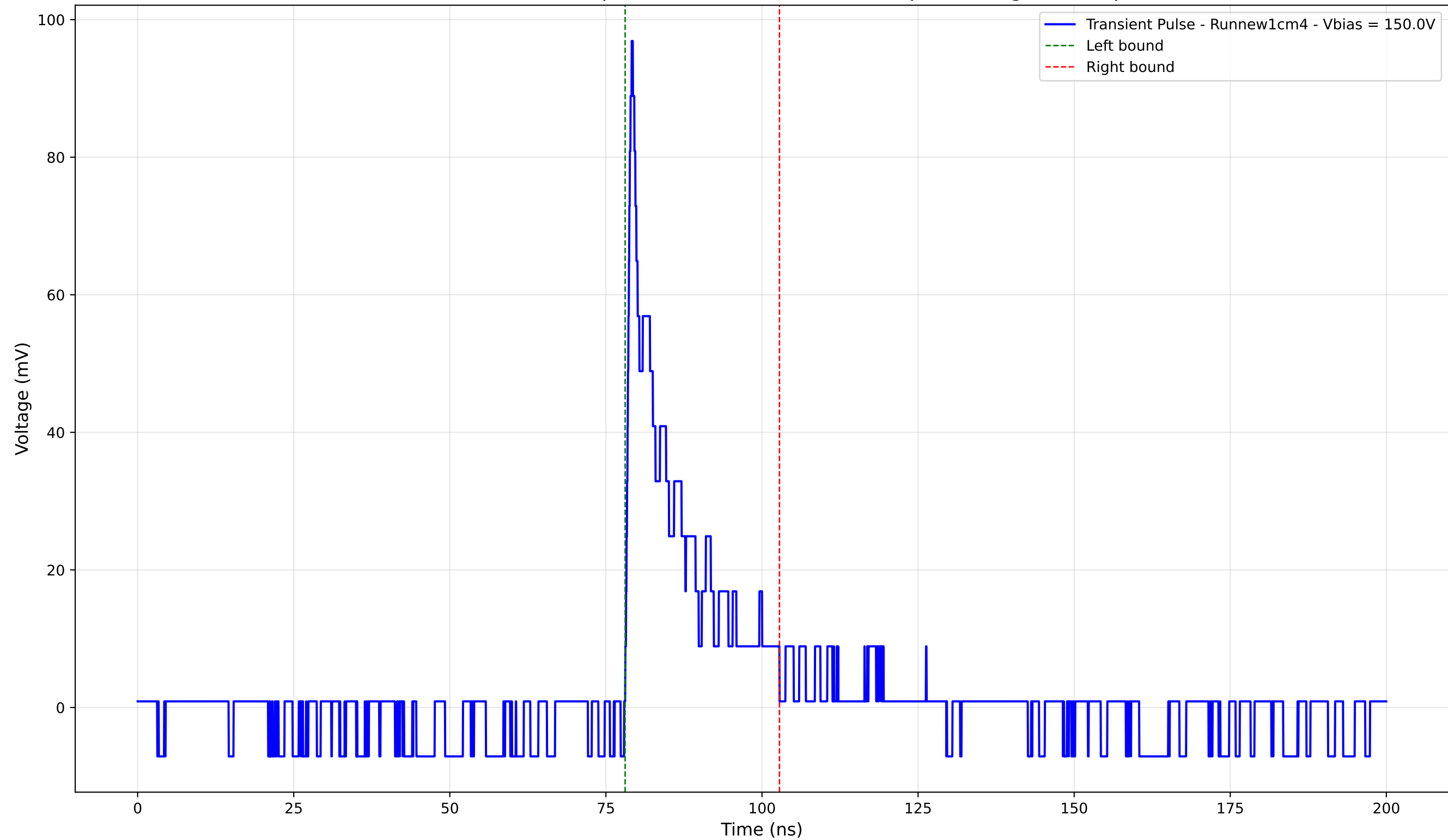
Transient Pulse - Sample: new1cm - Position: 190.0 \mu\text{m} - Charge: 12.79 pC
