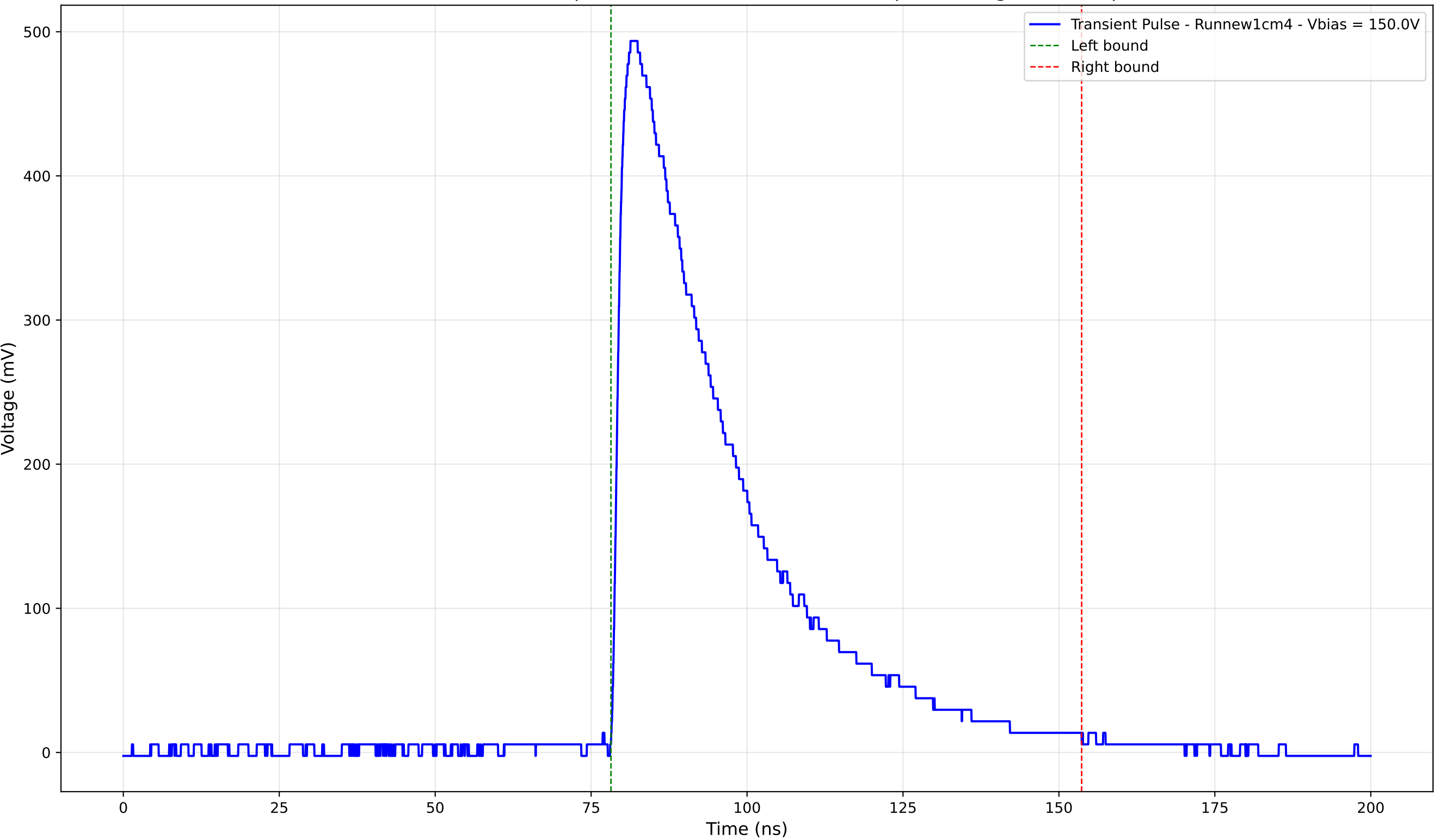
Transient Pulse - Sample: new1cm - Position: 1800.0 \mu\text{m} - Charge: 201.97 pC
