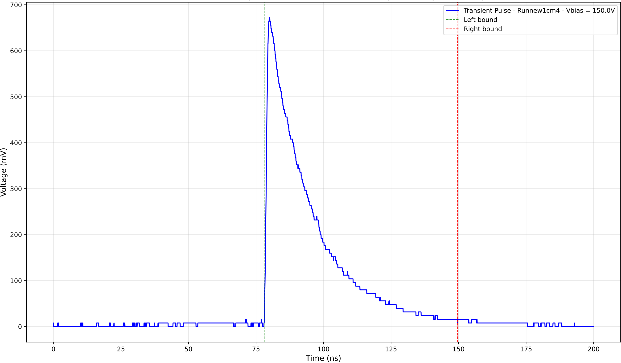
Transient Pulse - Sample: new1cm - Position: 4145.0 \mu\text{m} - Charge: 232.05 pC
