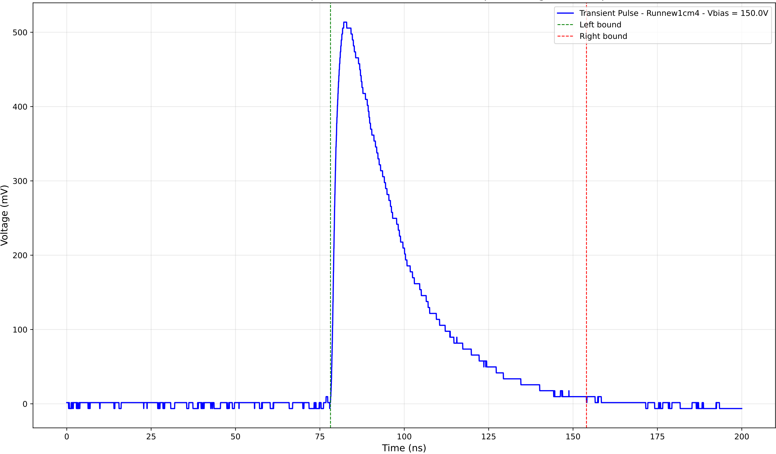
Transient Pulse - Sample: new1cm - Position: 2960.0 \mu\text{m} - Charge: 224.06 pC
