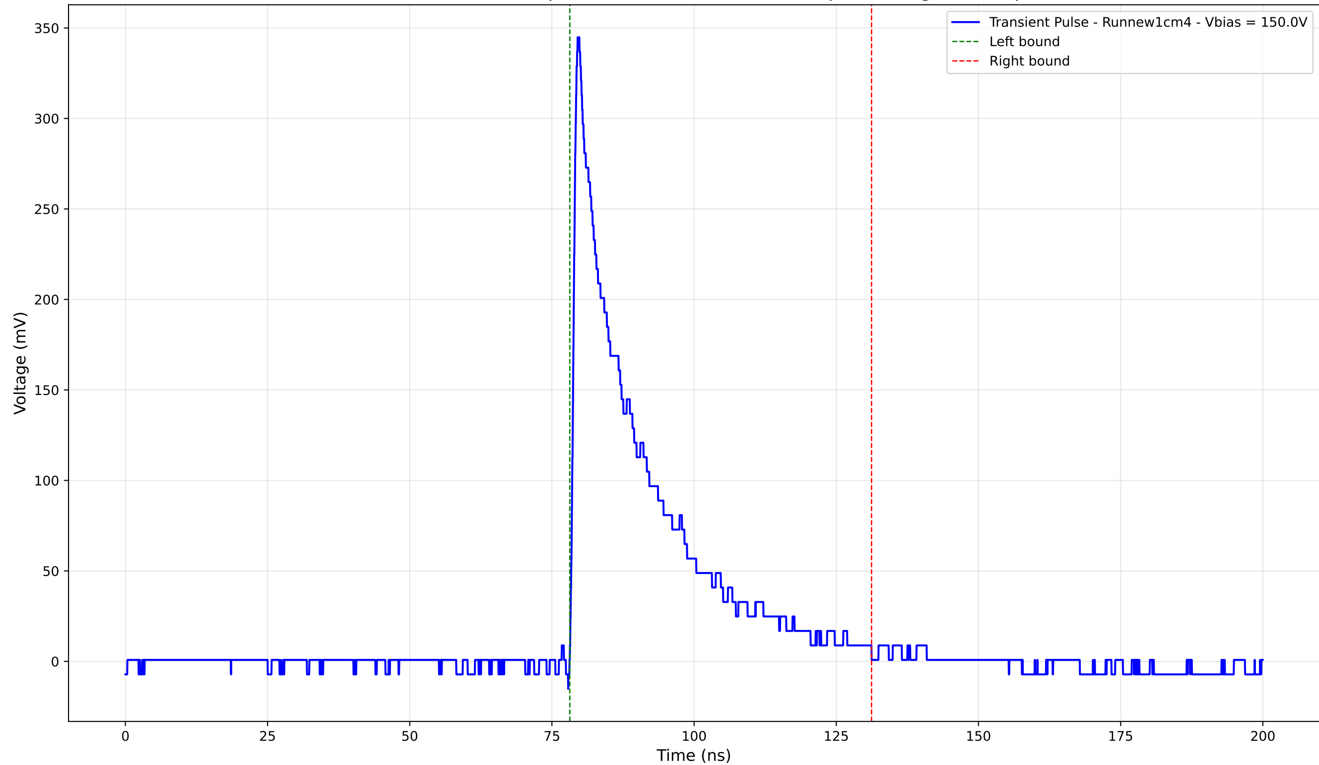
Transient Pulse - Sample: new1cm - Position: 735.0 \mu\text{m} - Charge: 79.39 pC
