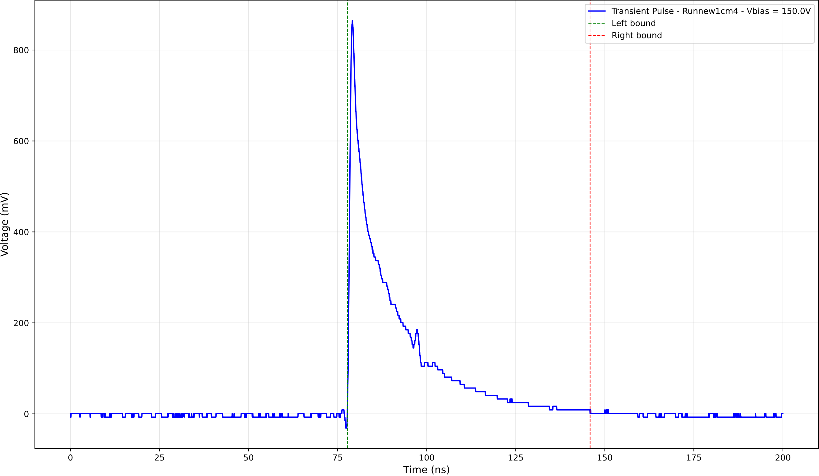
Transient Pulse - Sample: new1cm - Position: 4945.0 \mu\text{m} - Charge: 177.23 pC
