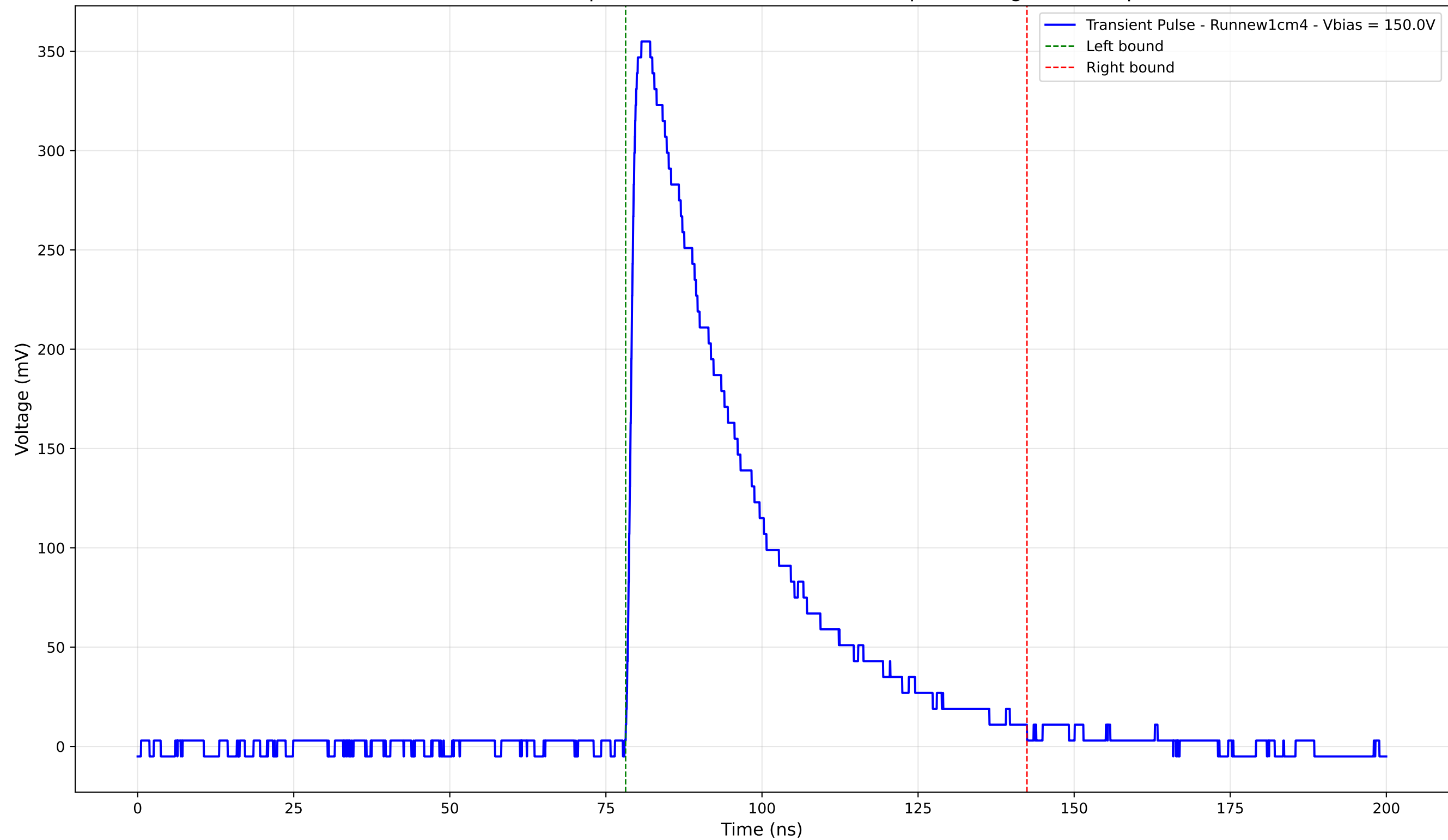
Transient Pulse - Sample: new1cm - Position: 3780.0 \mu\text{m} - Charge: 135.35 pC
