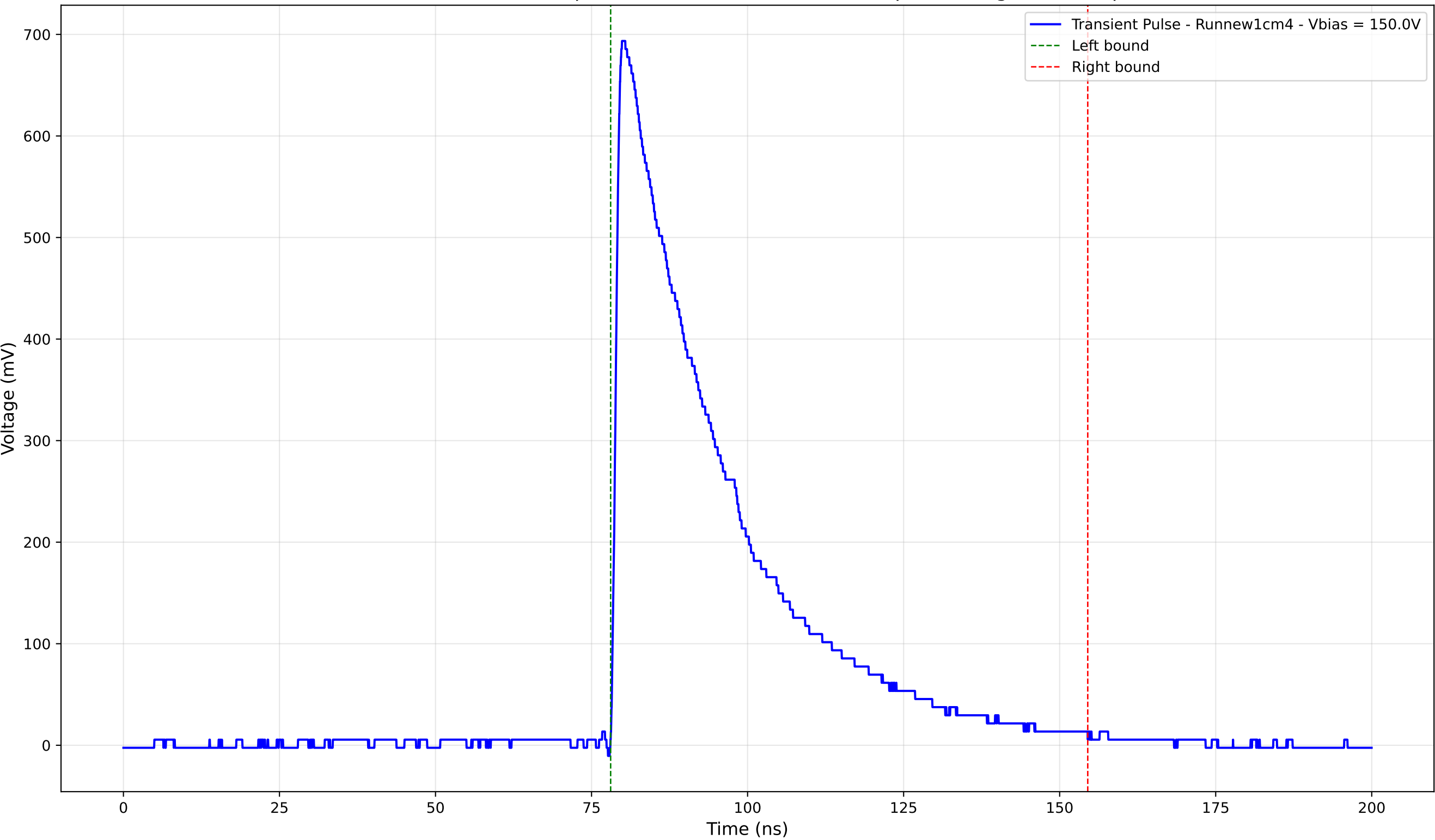
Transient Pulse - Sample: new1cm - Position: 4065.0 \mu\text{m} - Charge: 254.23 pC
