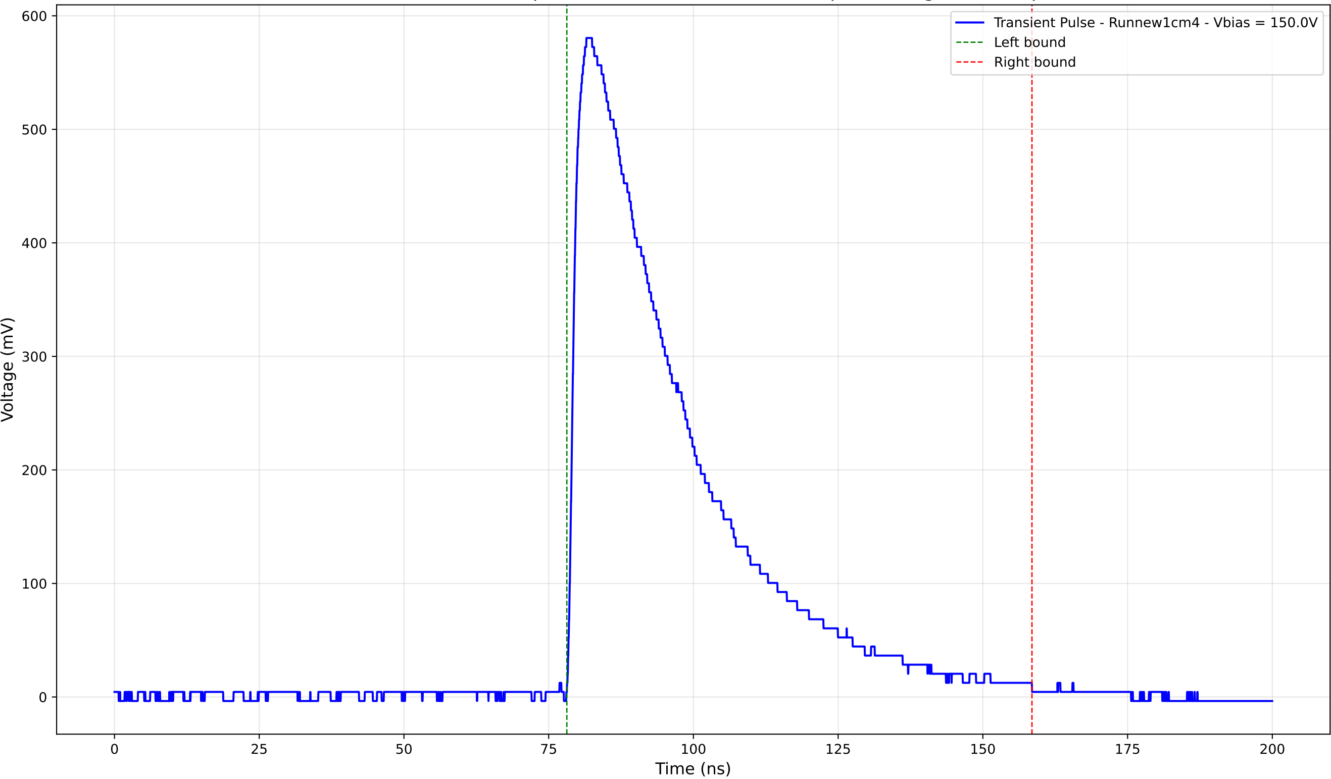
Transient Pulse - Sample: new1cm - Position: 3370.0 \mu\text{m} - Charge: 249.72 pC
