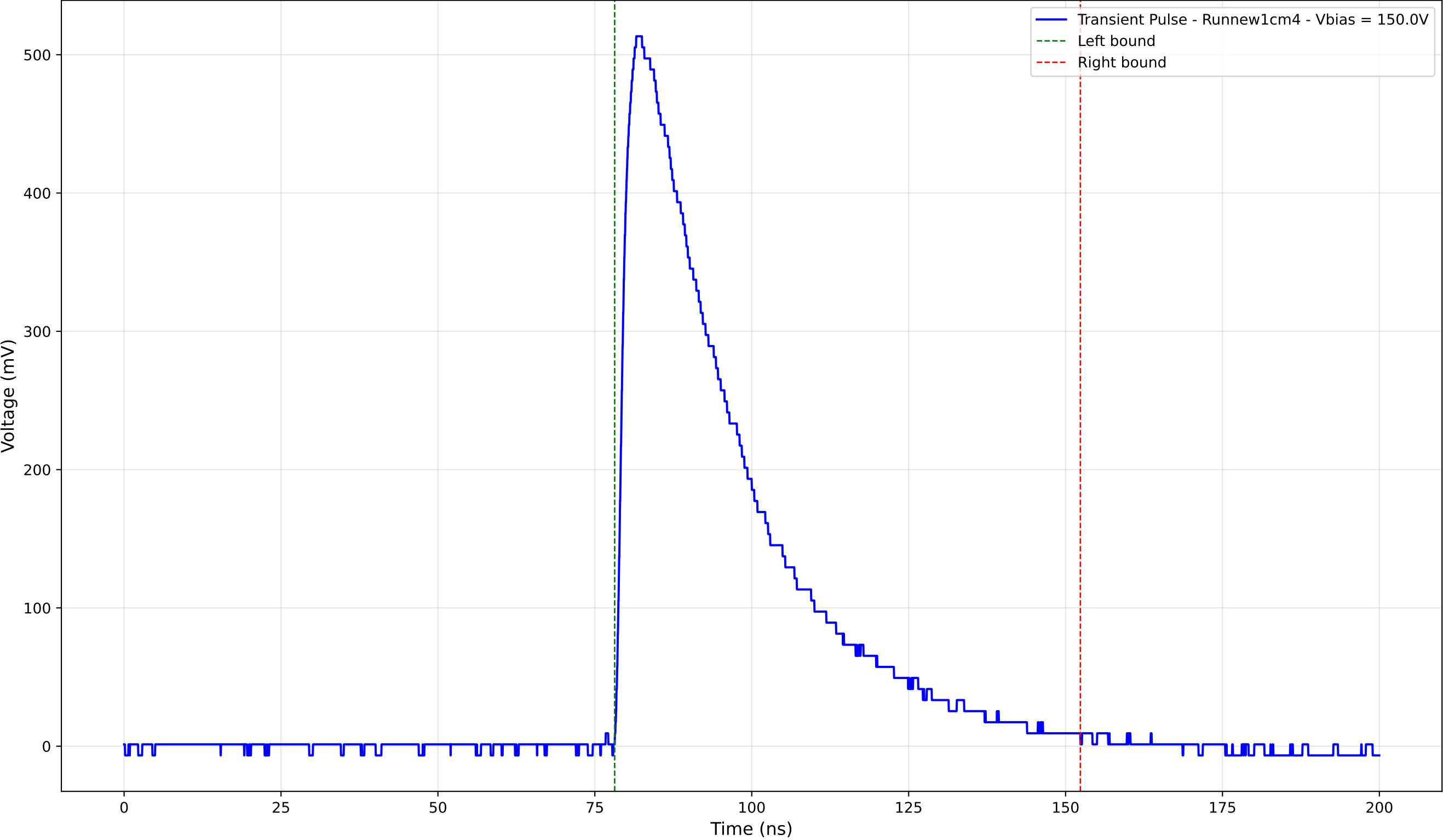
Transient Pulse - Sample: new1cm - Position: 1970.0 \mu\text{m} - Charge: 211.55 pC
