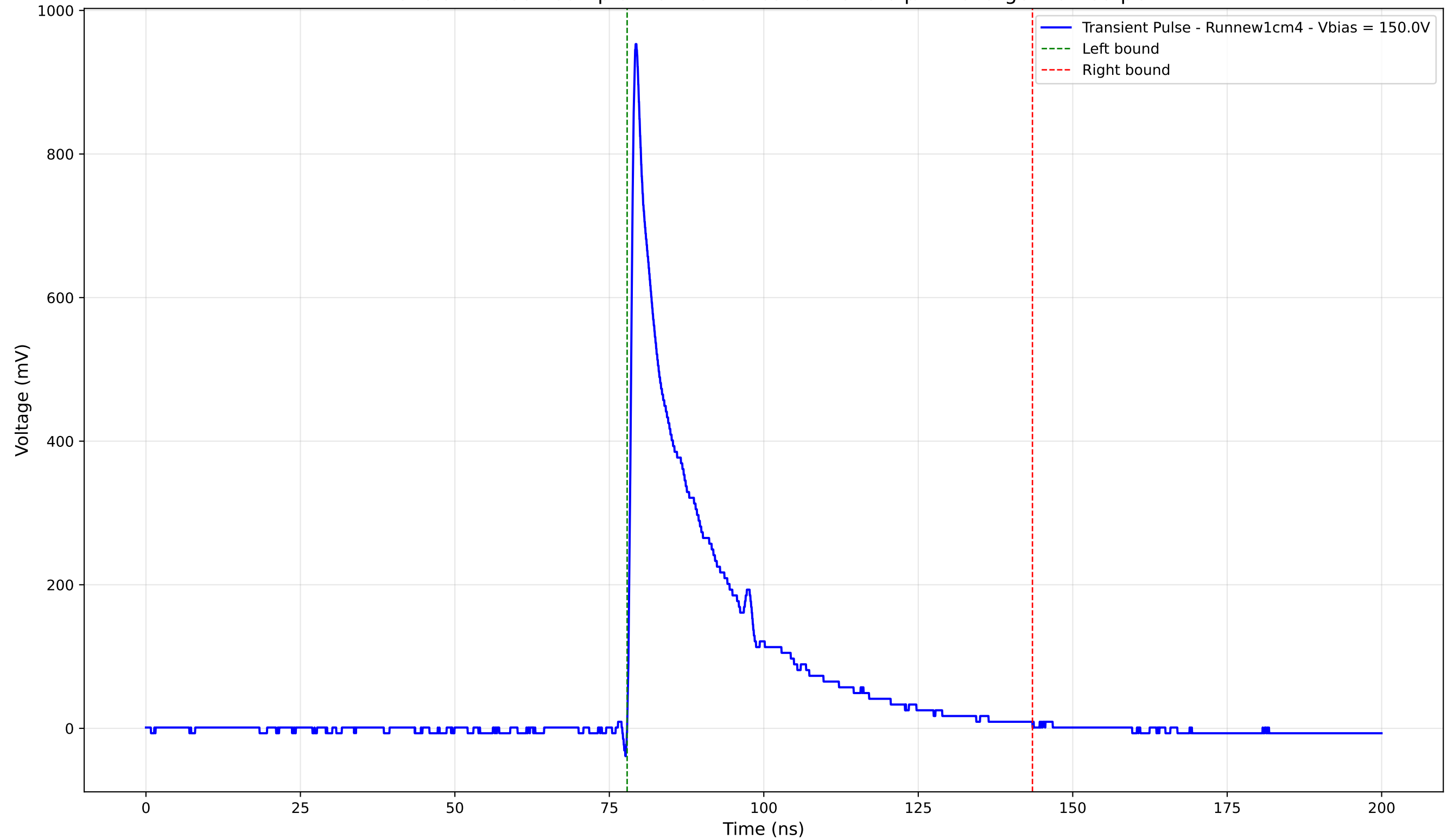
Transient Pulse - Sample: new1cm - Position: 375.0 \mu\text{m} - Charge: 194.89 pC
