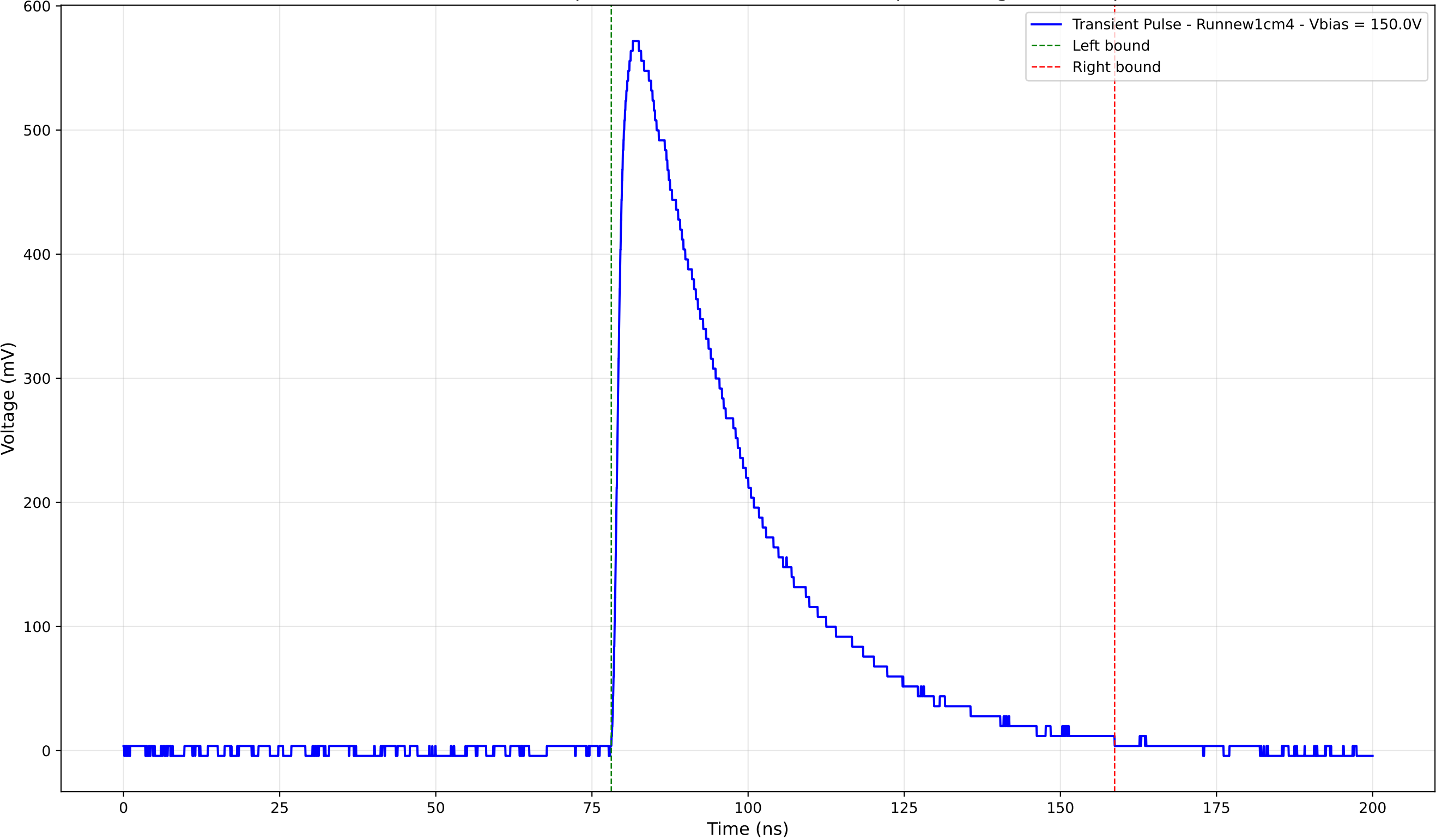
Transient Pulse - Sample: new1cm - Position: 3410.0 \mu\text{m} - Charge: 245.18 pC
