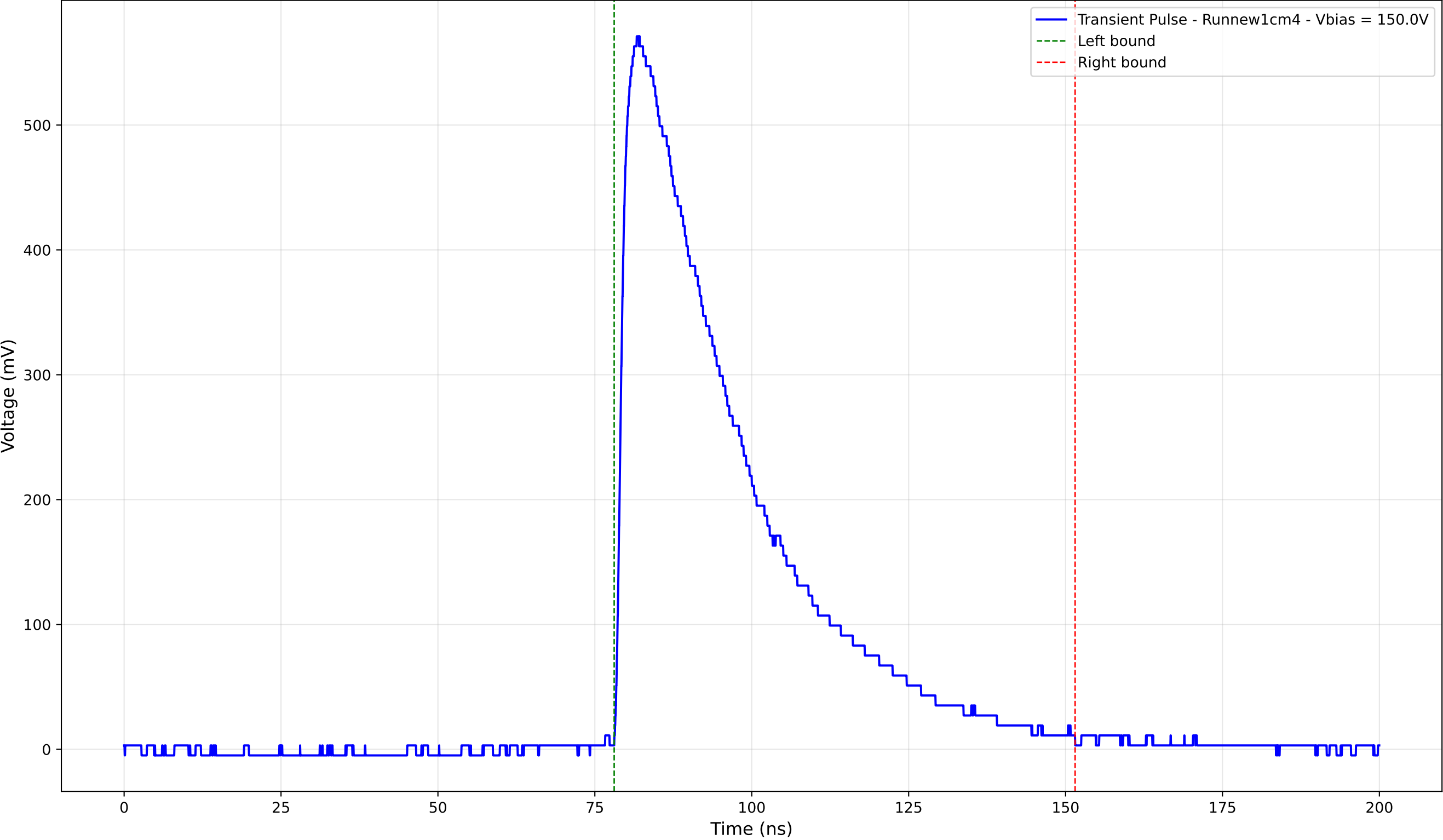
Transient Pulse - Sample: new1cm - Position: 3430.0 \mu\text{m} - Charge: 240.64 pC
