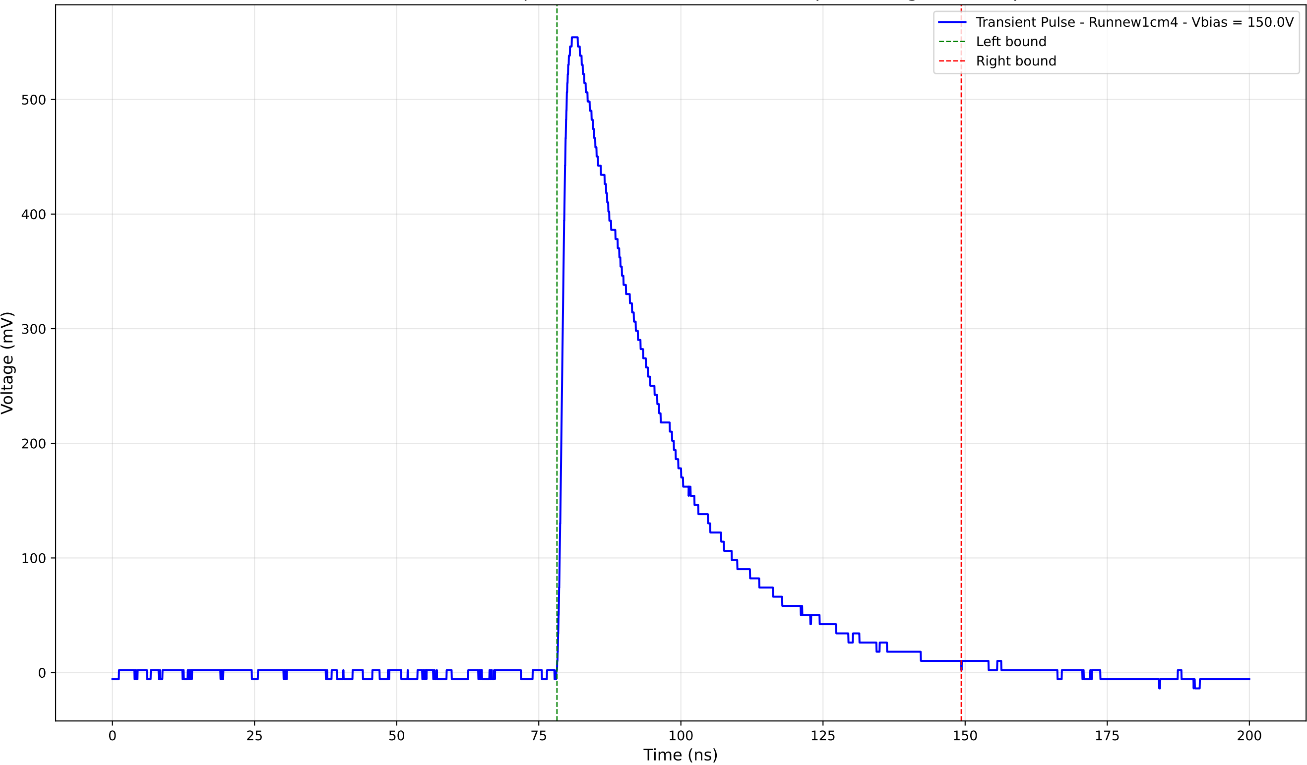
Transient Pulse - Sample: new1cm - Position: 1530.0 \mu\text{m} - Charge: 209.23 pC
