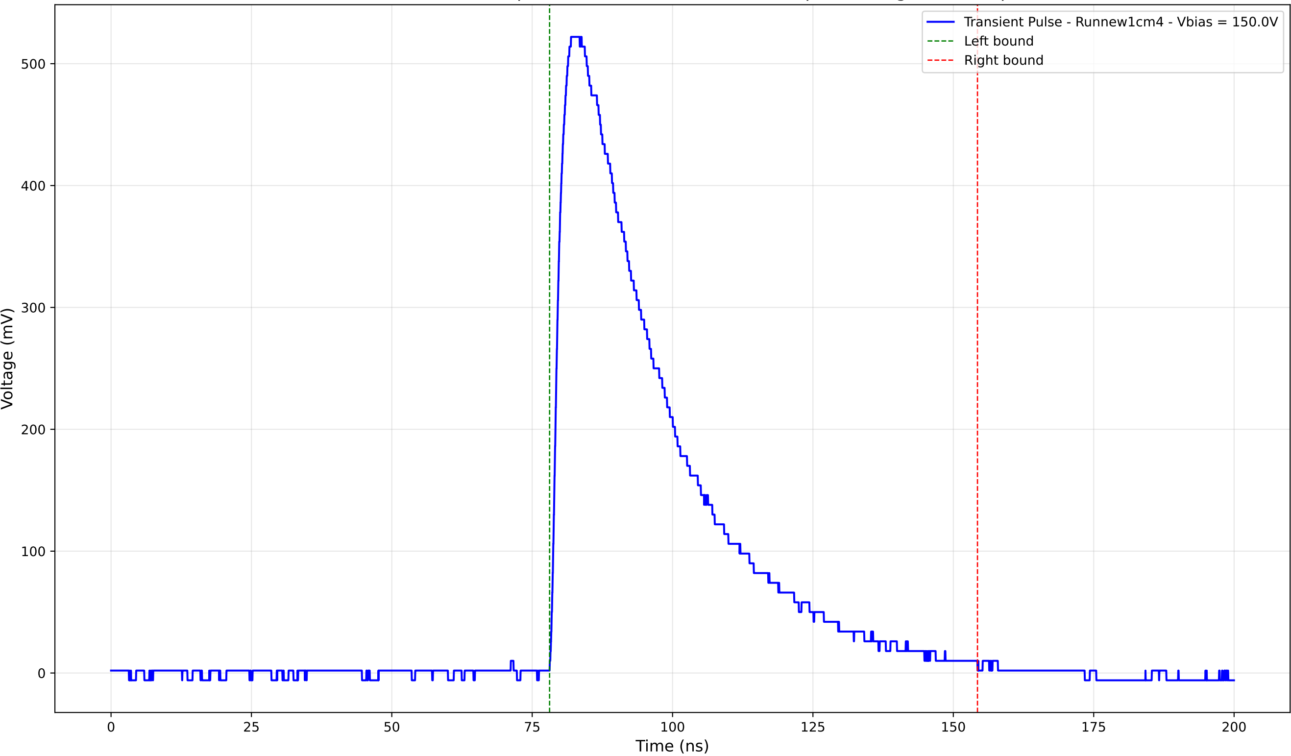
Transient Pulse - Sample: new1cm - Position: 2360.0 \mu\text{m} - Charge: 226.05 pC
