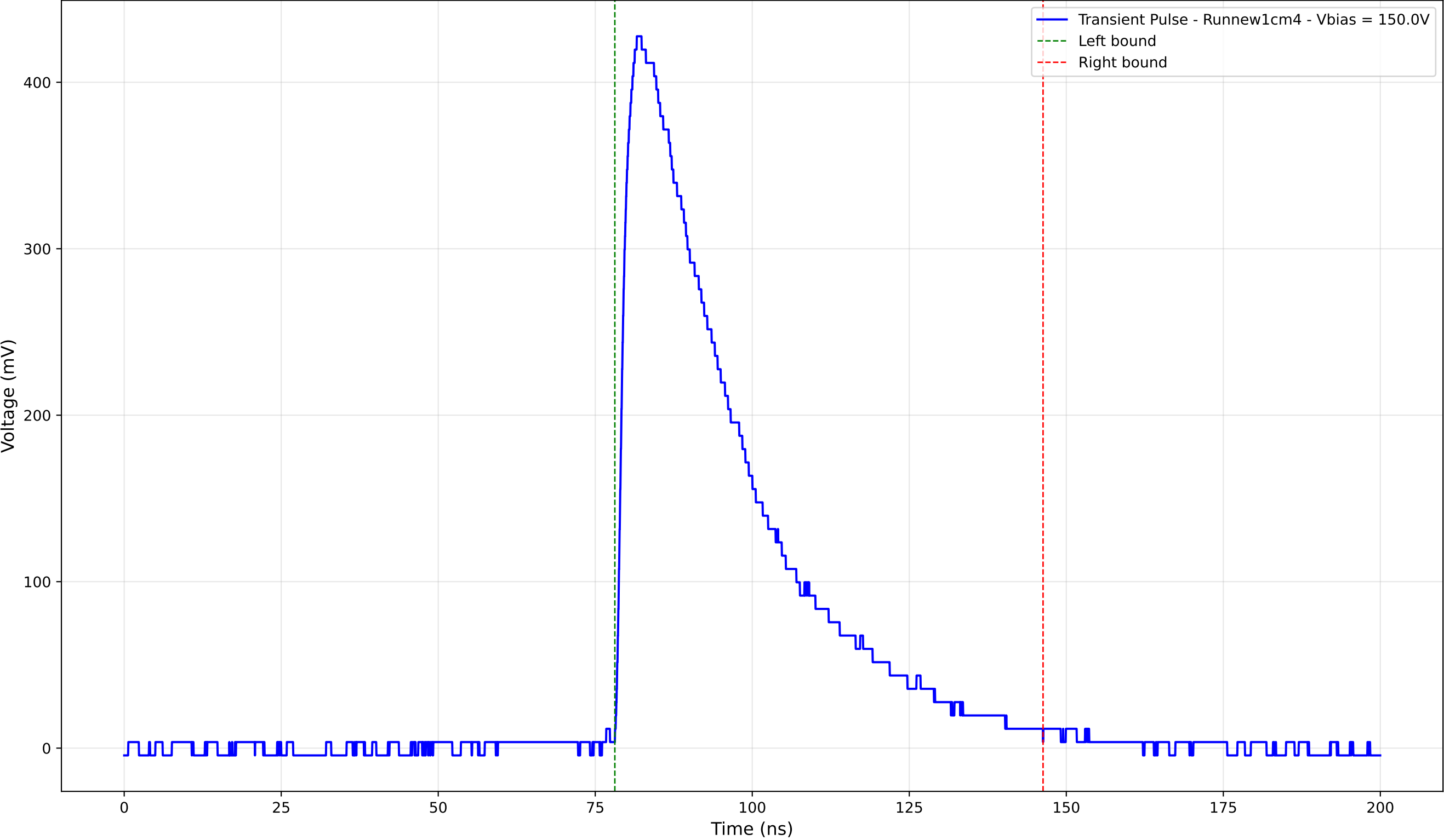
Transient Pulse - Sample: new1cm - Position: 3295.0 \mu\text{m} - Charge: 178.80 pC
