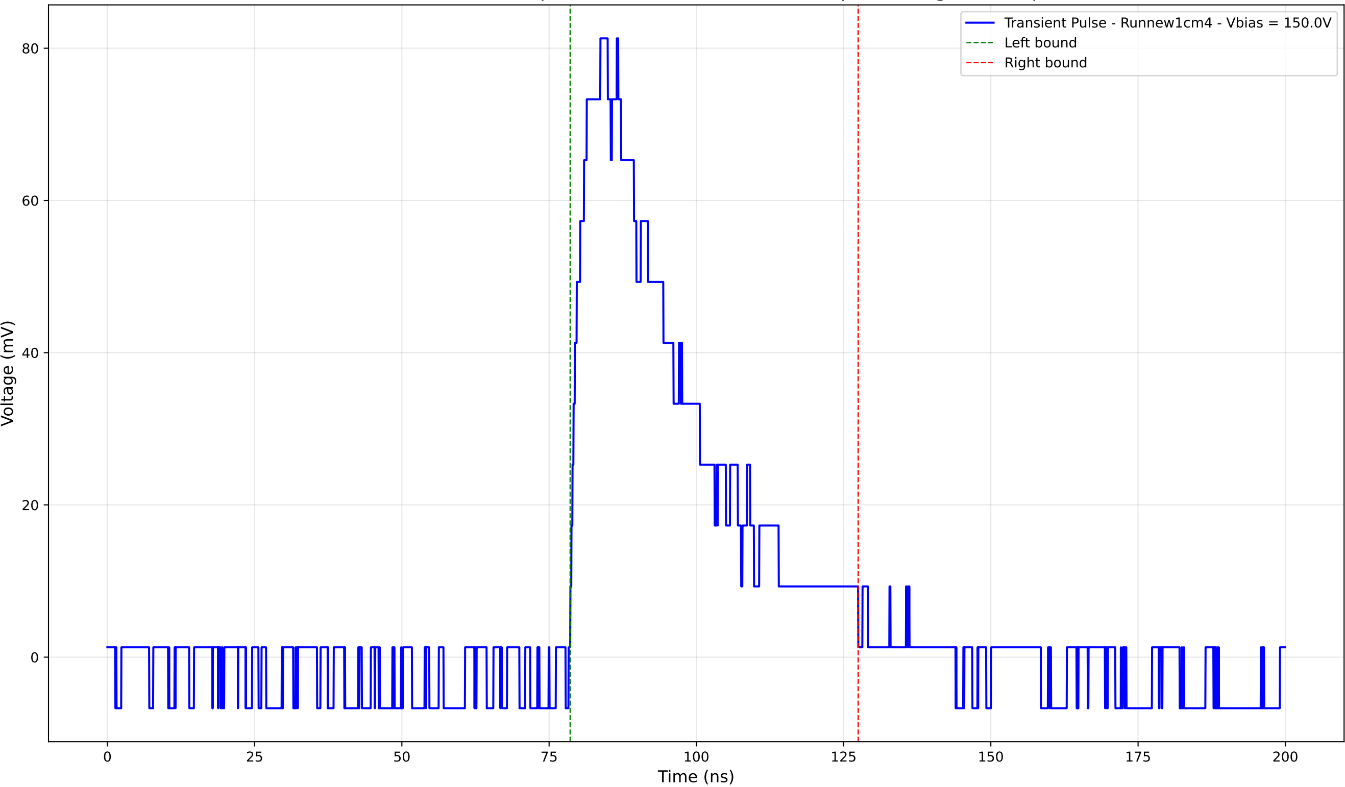
Transient Pulse - Sample: new1cm - Position: 2710.0 \mu\text{m} - Charge: 31.71 pC
