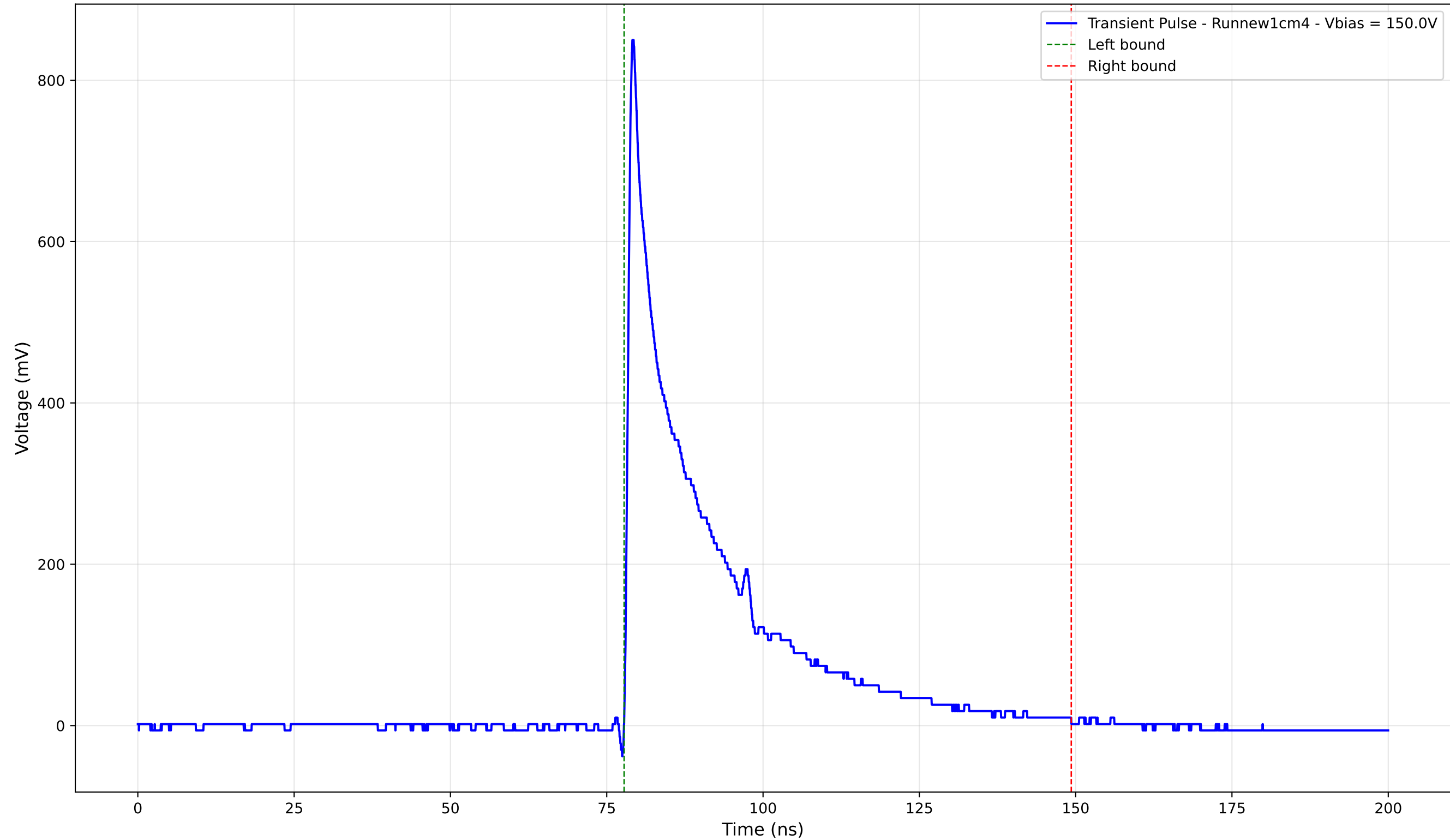
Transient Pulse - Sample: new1cm - Position: 4865.0 \mu\text{m} - Charge: 189.39 pC
