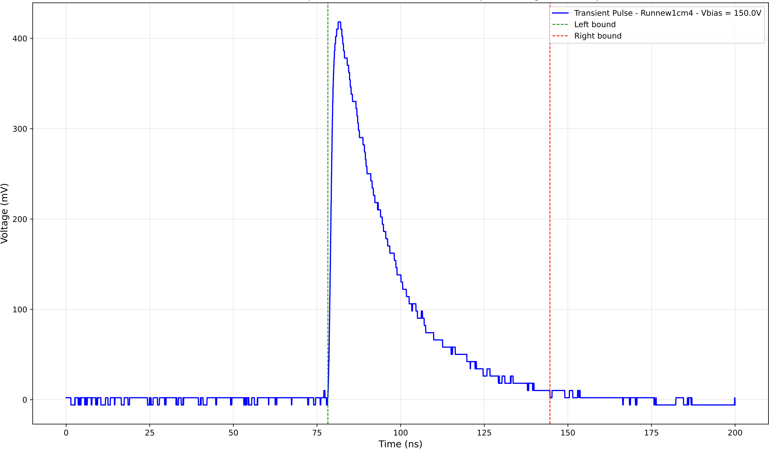
Transient Pulse - Sample: new1cm - Position: 1635.0 \mu\text{m} - Charge: 156.44 pC
