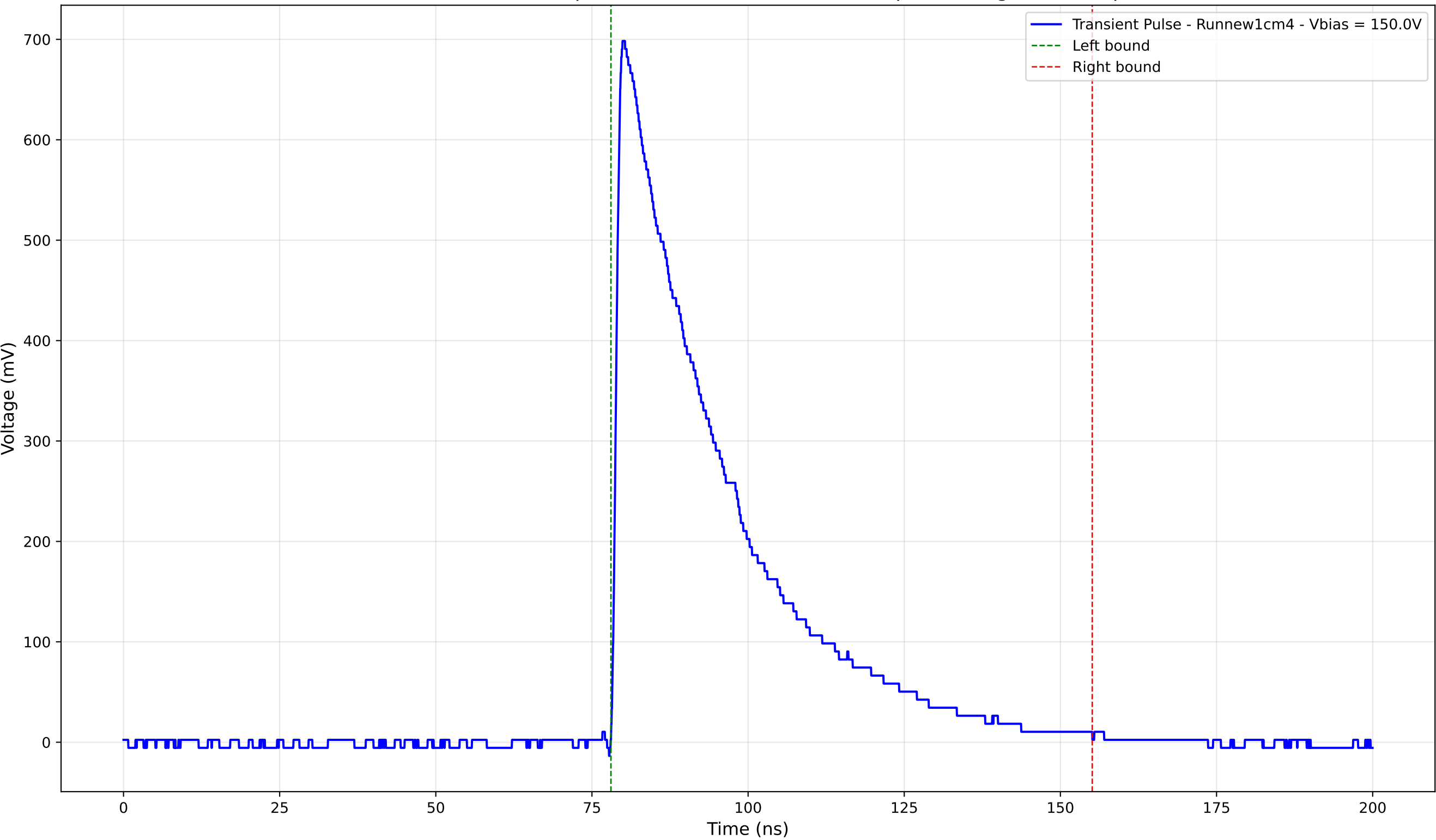
Transient Pulse - Sample: new1cm - Position: 4075.0 \mu\text{m} - Charge: 251.06 pC
