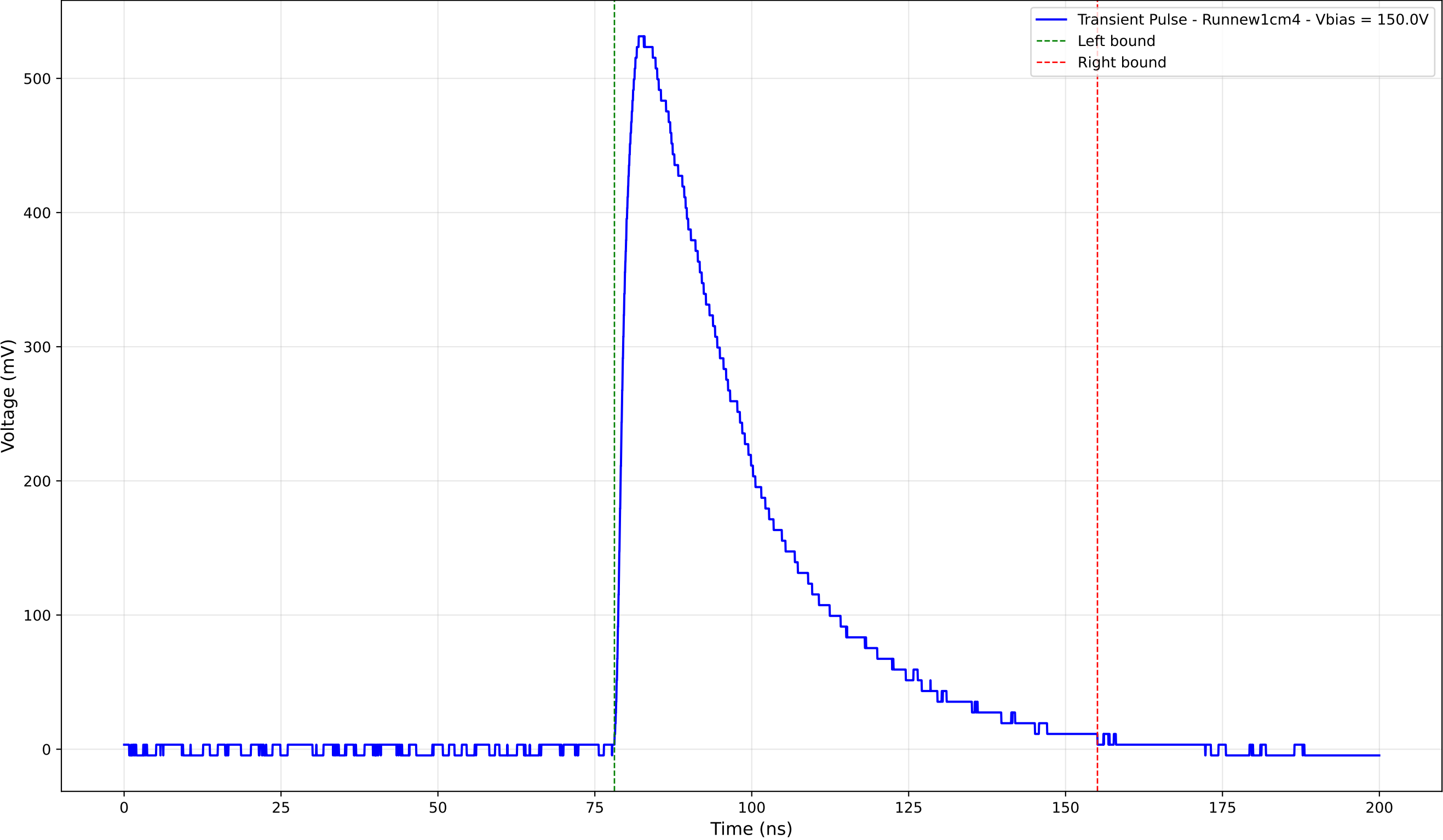
Transient Pulse - Sample: new1cm - Position: 2855.0 \mu\text{m} - Charge: 233.87 pC
