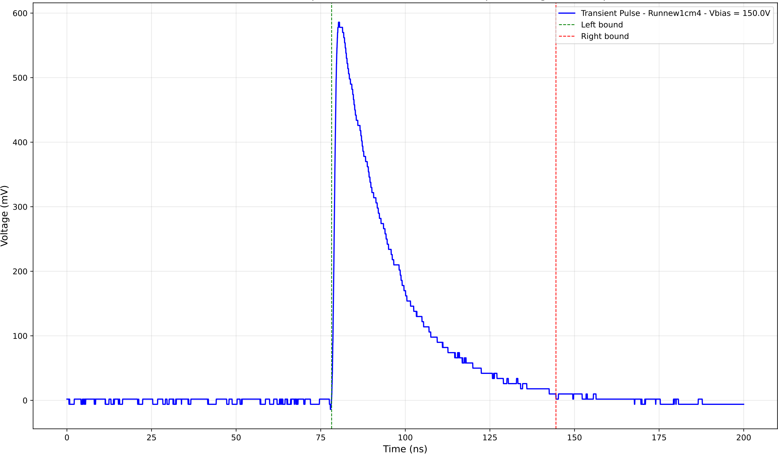
Transient Pulse - Sample: new1cm - Position: 1340.0 \mu\text{m} - Charge: 205.33 pC
