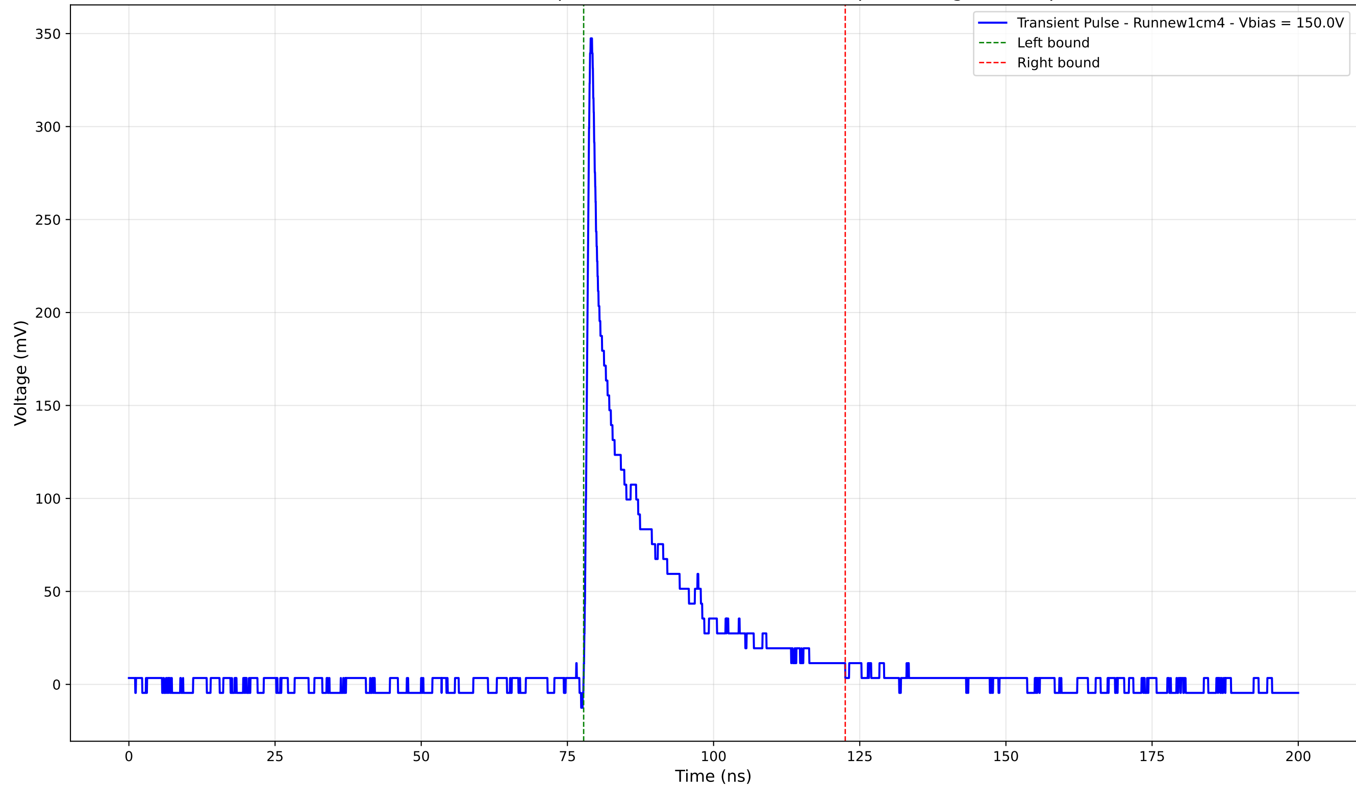
Transient Pulse - Sample: new1cm - Position: 5040.0 \mu\text{m} - Charge: 54.08 pC
