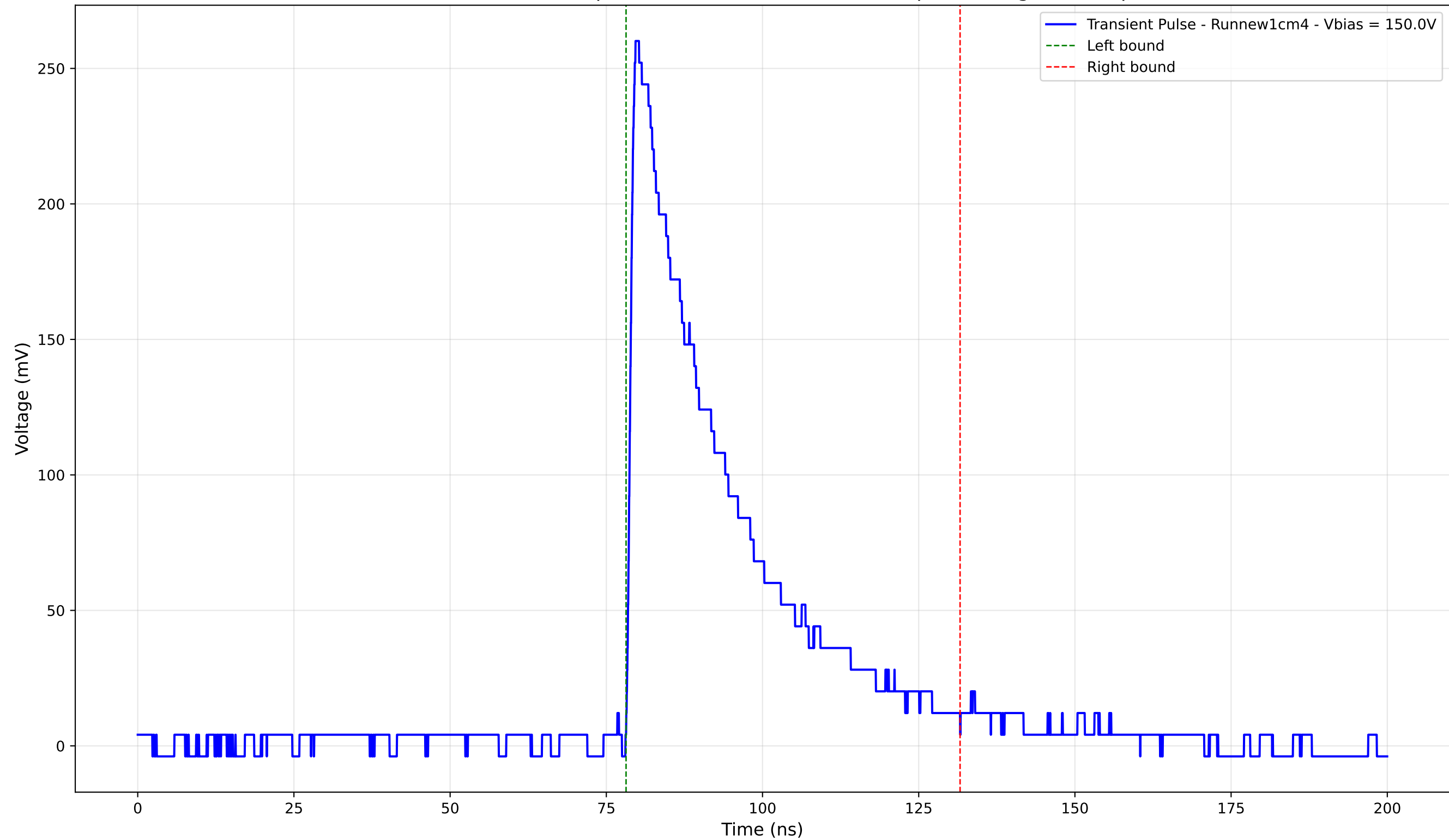
Transient Pulse - Sample: new1cm - Position: 4200.0 \mu\text{m} - Charge: 82.86 pC
