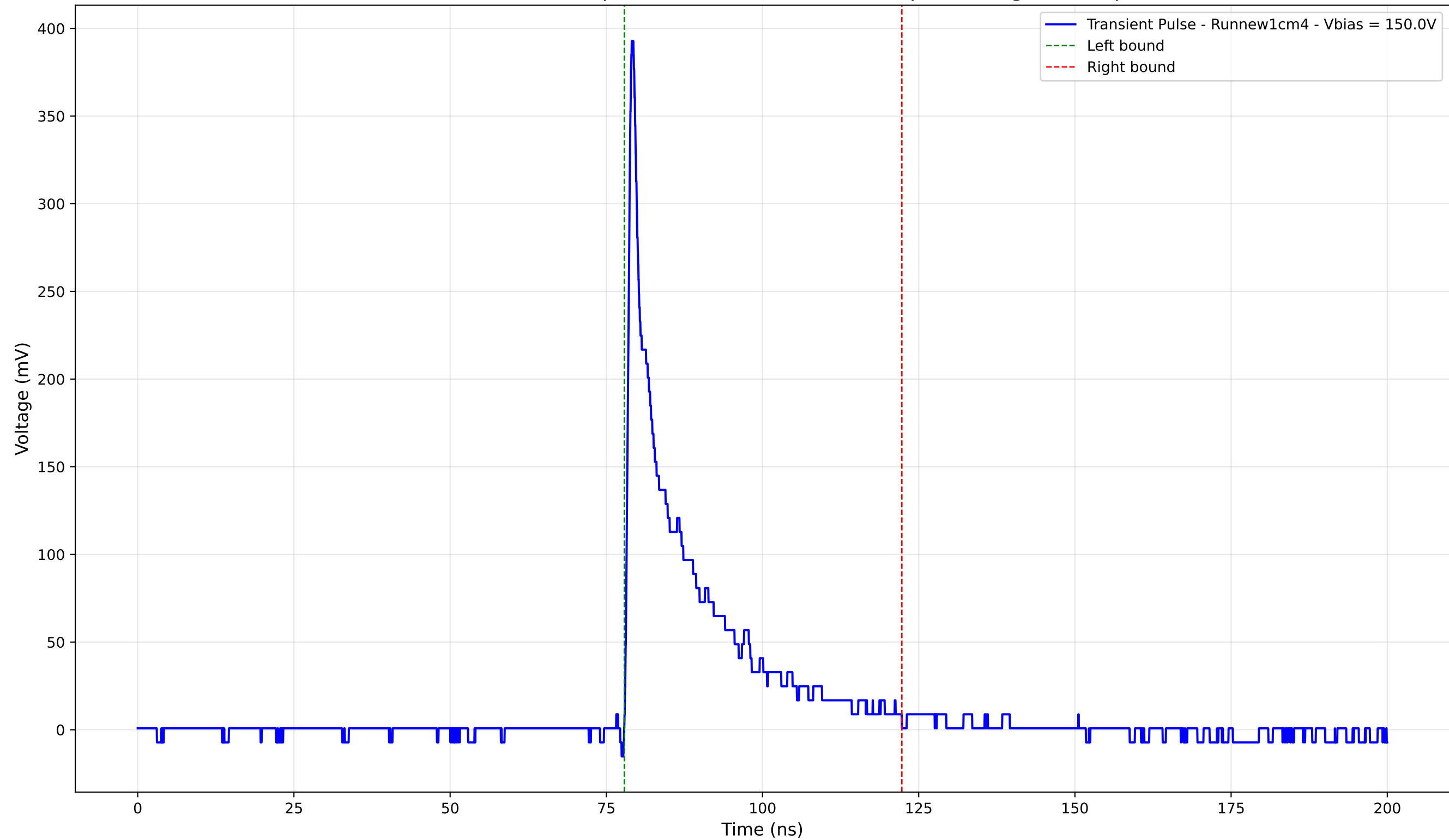
Transient Pulse - Sample: new1cm - Position: 225.0 \mu\text{m} - Charge: 58.71 pC
