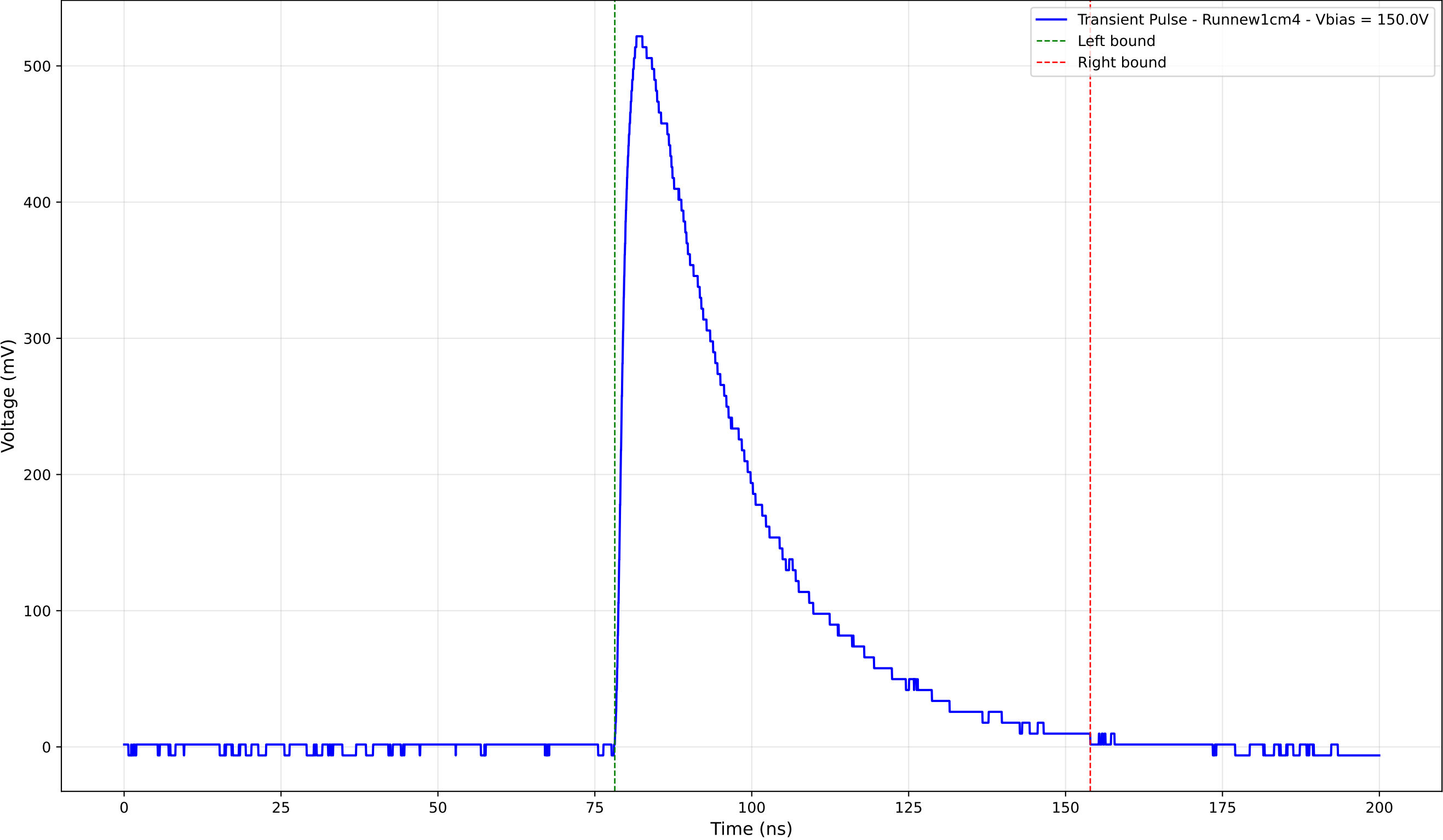
Transient Pulse - Sample: new1cm - Position: 2055.0 \mu\text{m} - Charge: 216.85 pC
