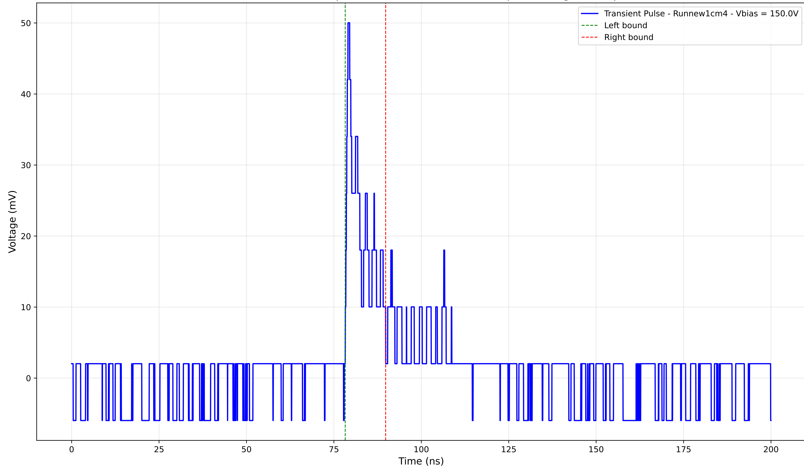
Transient Pulse - Sample: new1cm - Position: 165.0 \mu\text{m} - Charge: 4.90 pC
