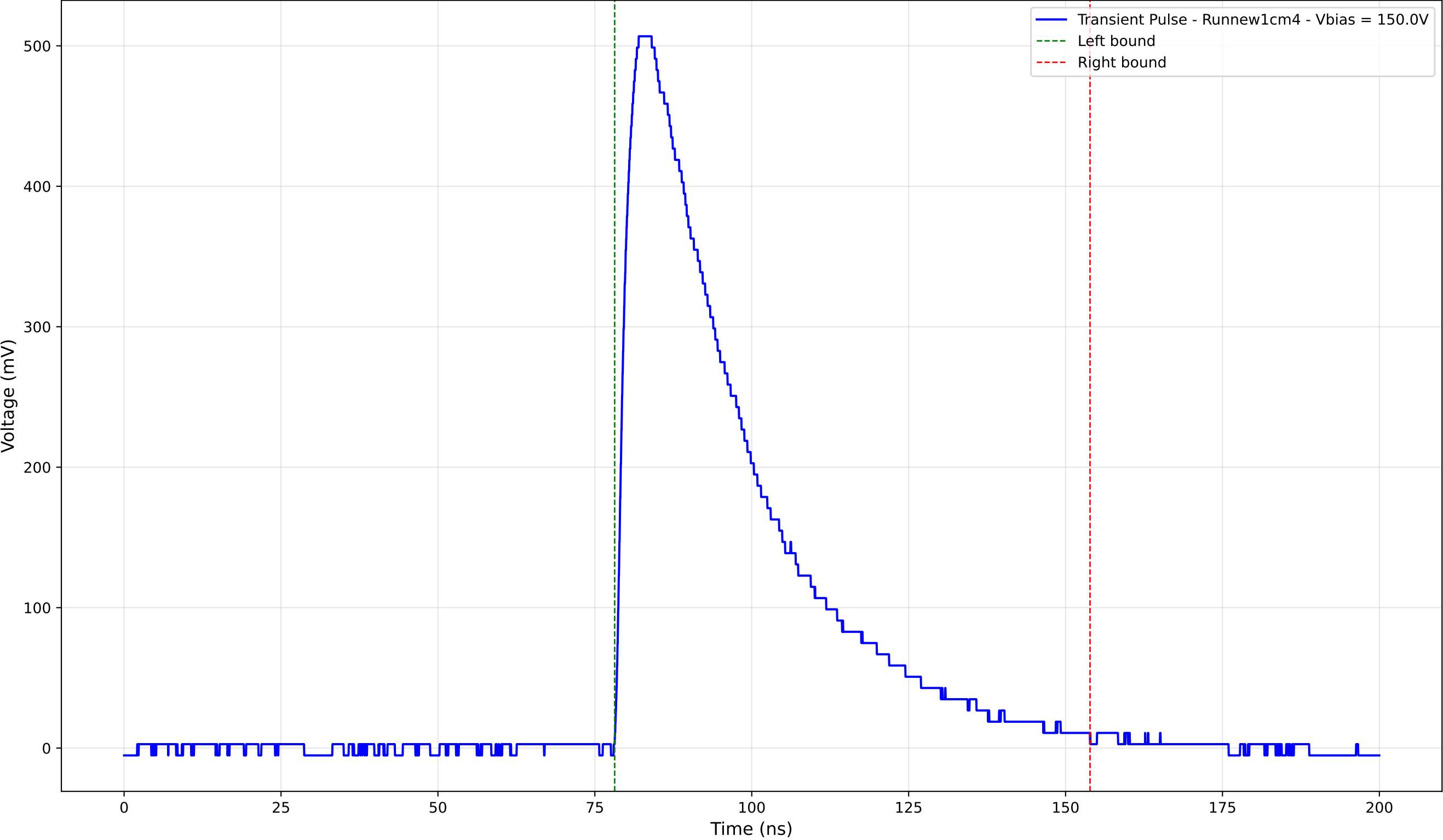
Transient Pulse - Sample: new1cm - Position: 2600.0 \mu\text{m} - Charge: 223.97 pC
