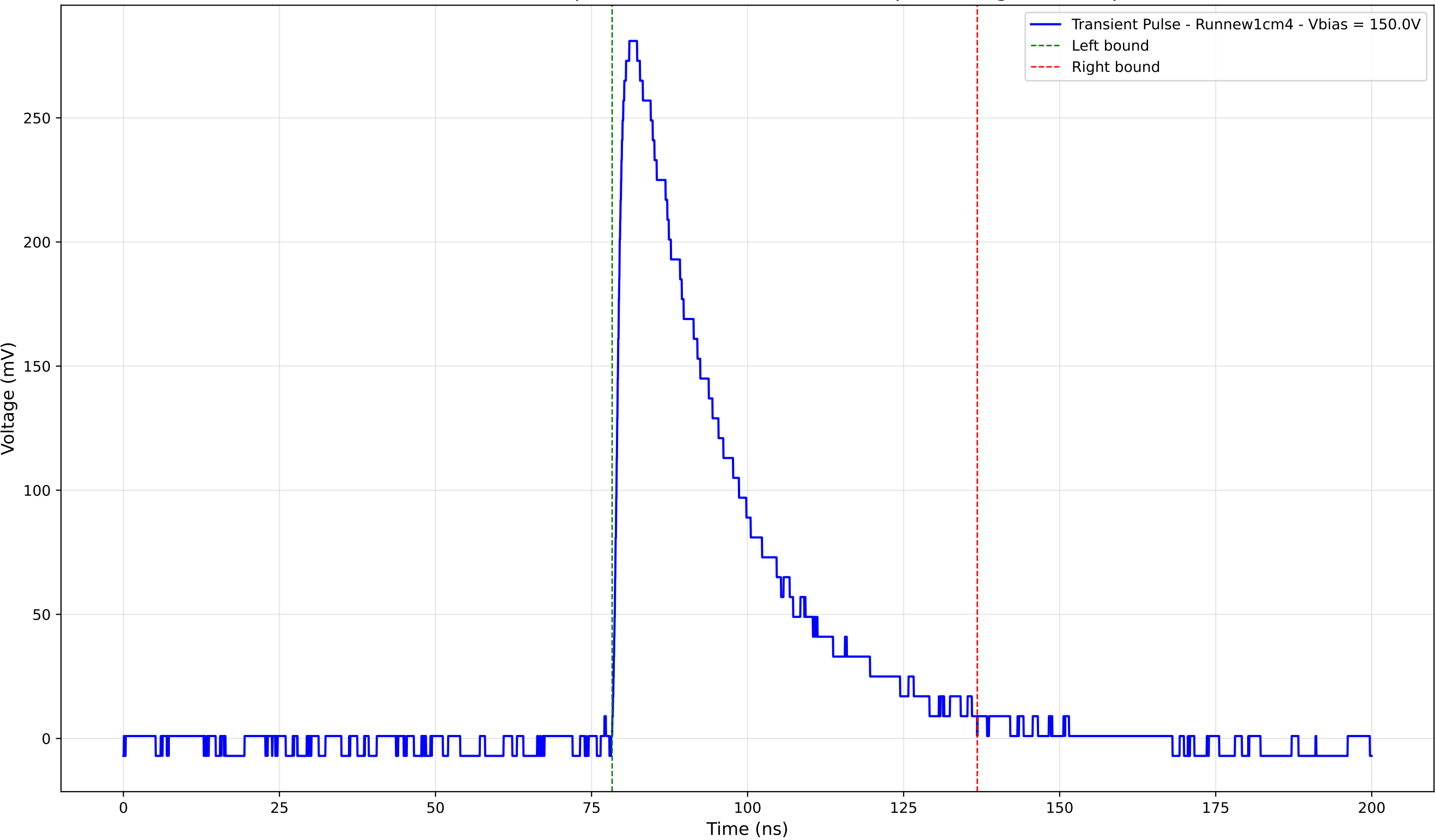
Transient Pulse - Sample: new1cm - Position: 1655.0 \mu\text{m} - Charge: 103.95 pC
