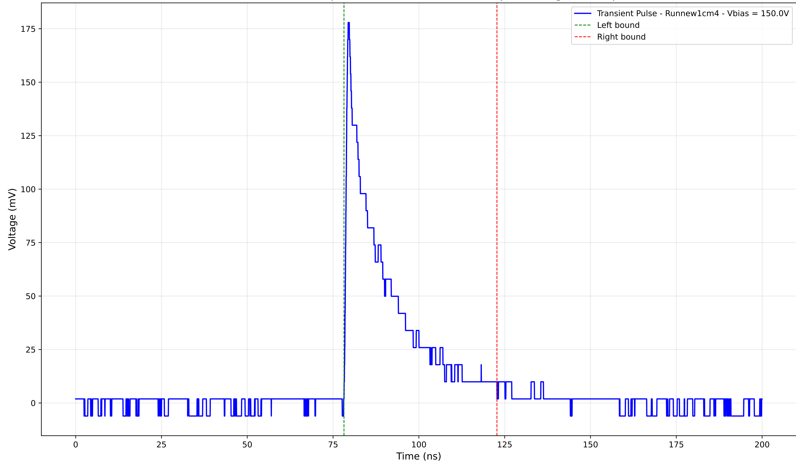
Transient Pulse - Sample: new1cm - Position: 675.0 \mu\text{m} - Charge: 38.77 pC
