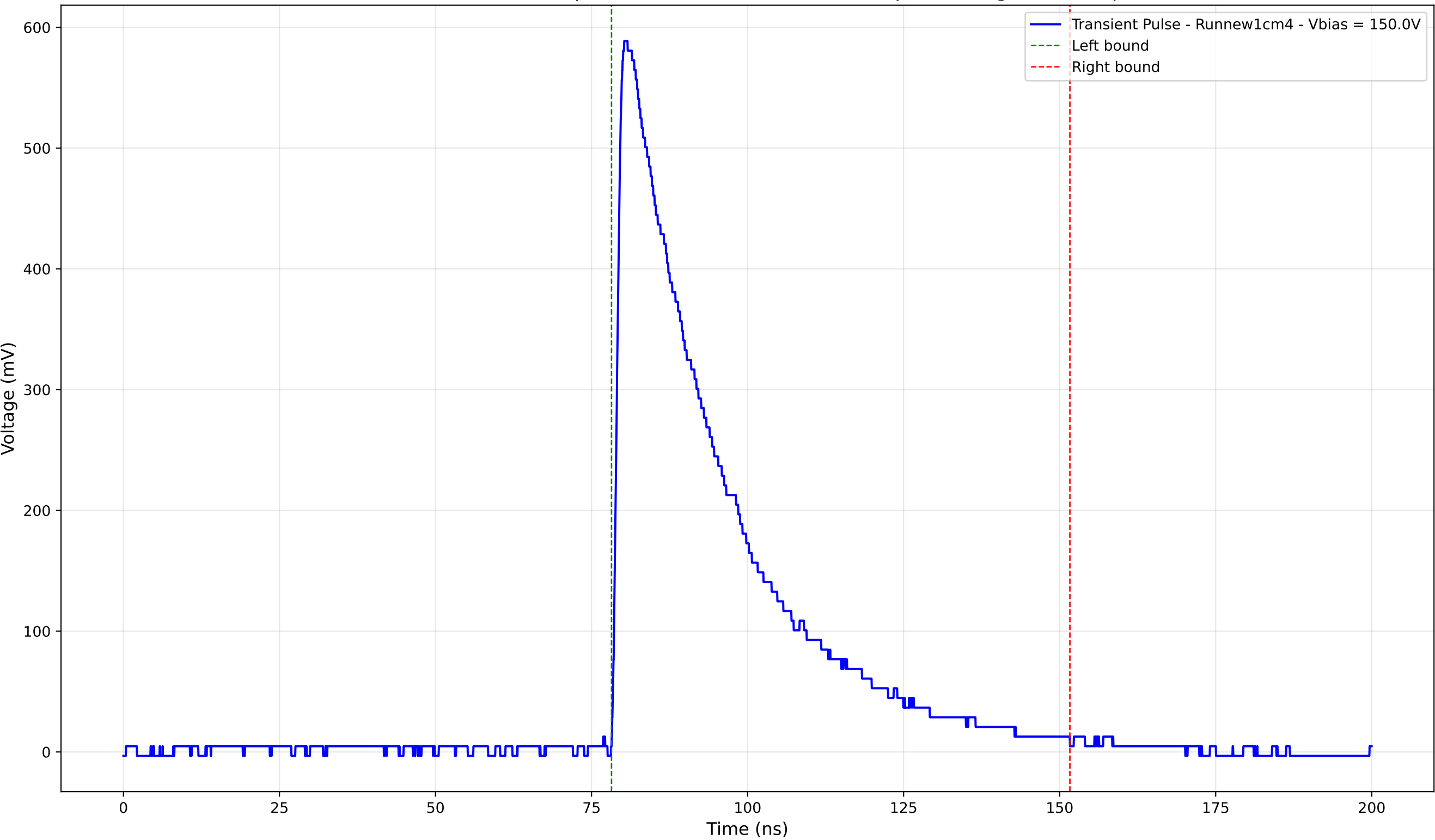
Transient Pulse - Sample: new1cm - Position: 1350.0 \mu\text{m} - Charge: 212.33 pC
