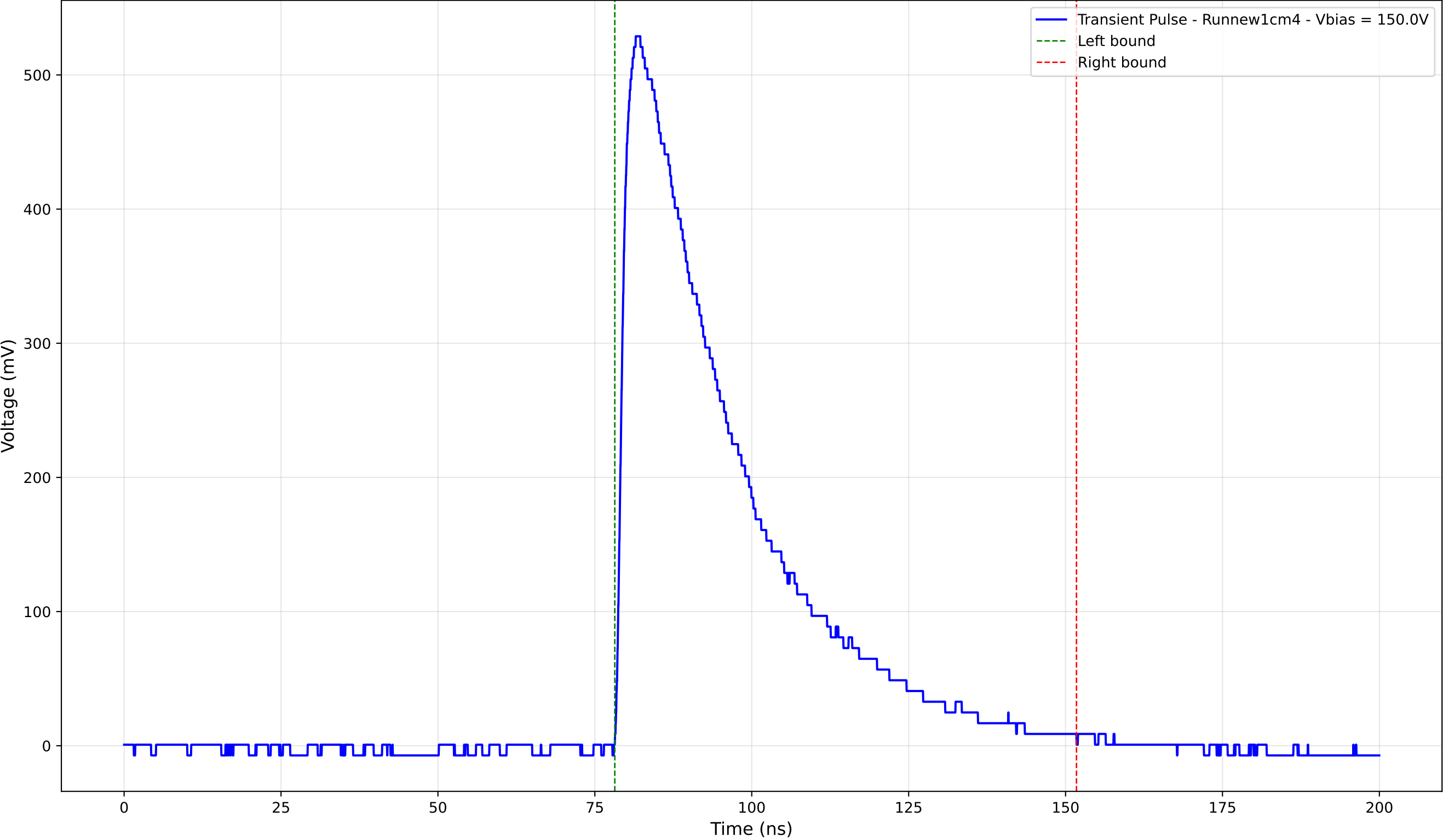
Transient Pulse - Sample: new1cm - Position: 1850.0 \mu\text{m} - Charge: 210.92 pC
