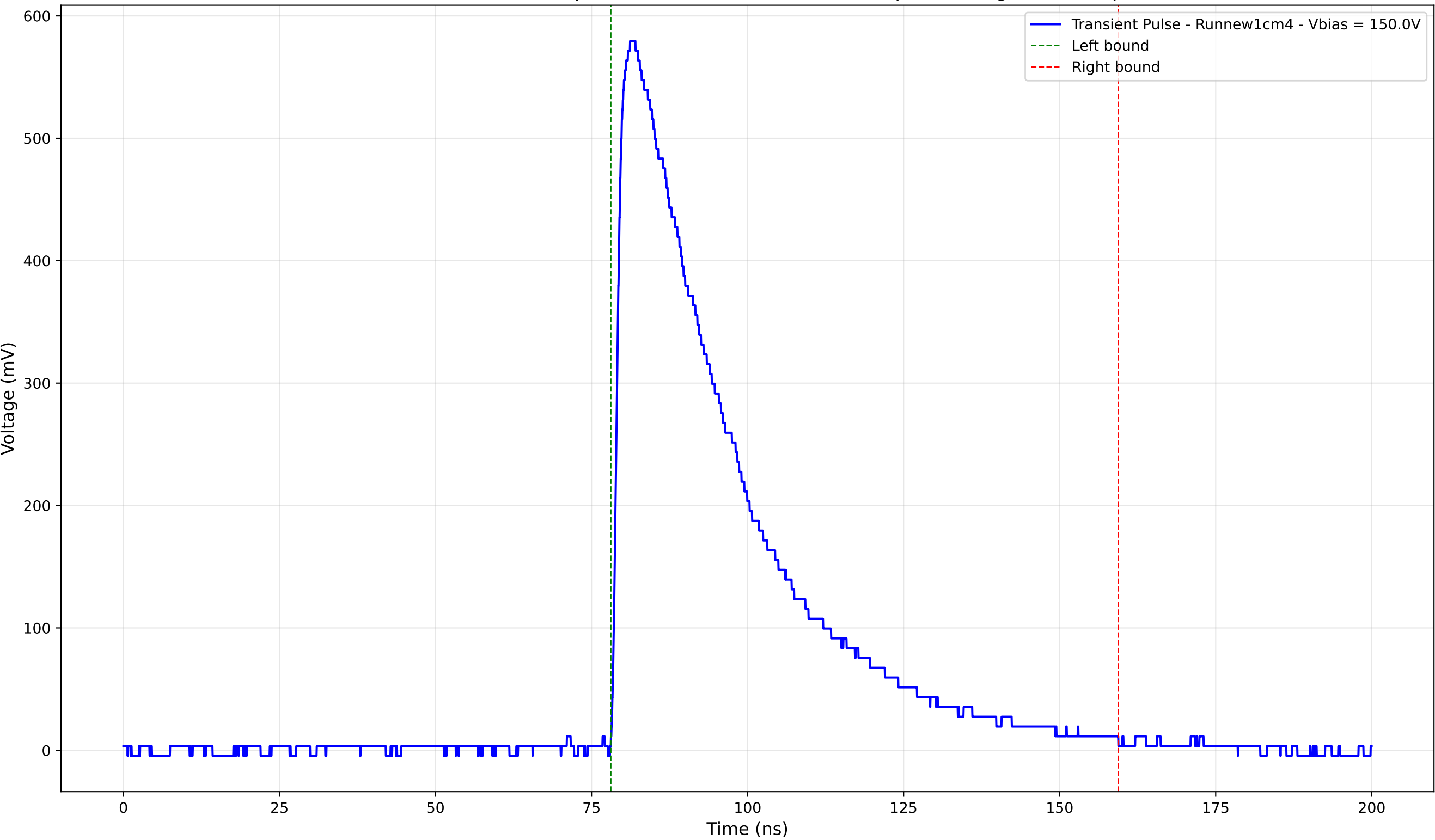
Transient Pulse - Sample: new1cm - Position: 3625.0 \mu\text{m} - Charge: 241.67 pC
