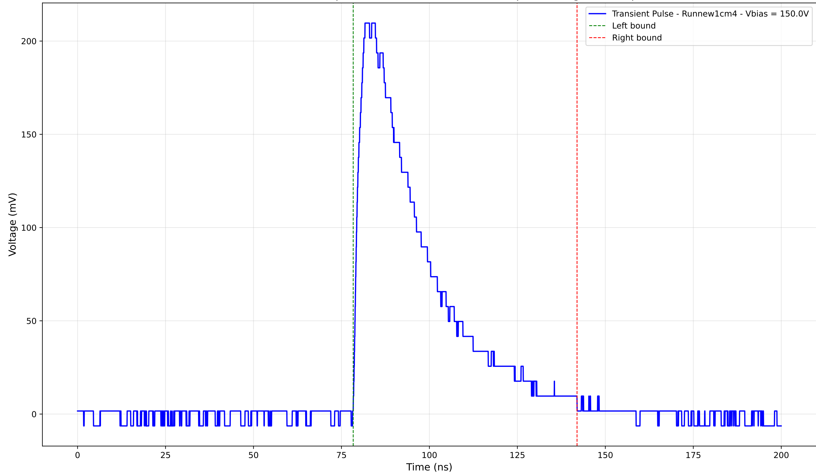
Transient Pulse - Sample: new1cm - Position: 2755.0 \mu\text{m} - Charge: 88.22 pC
