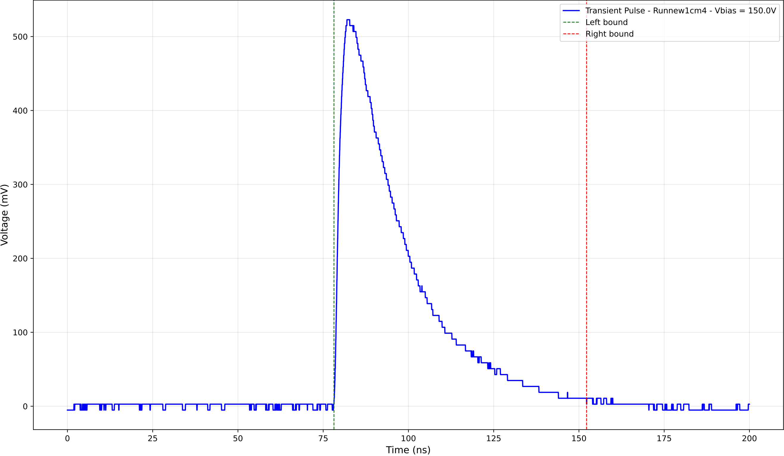
Transient Pulse - Sample: new1cm - Position: 2395.0 \mu\text{m} - Charge: 223.34 pC
