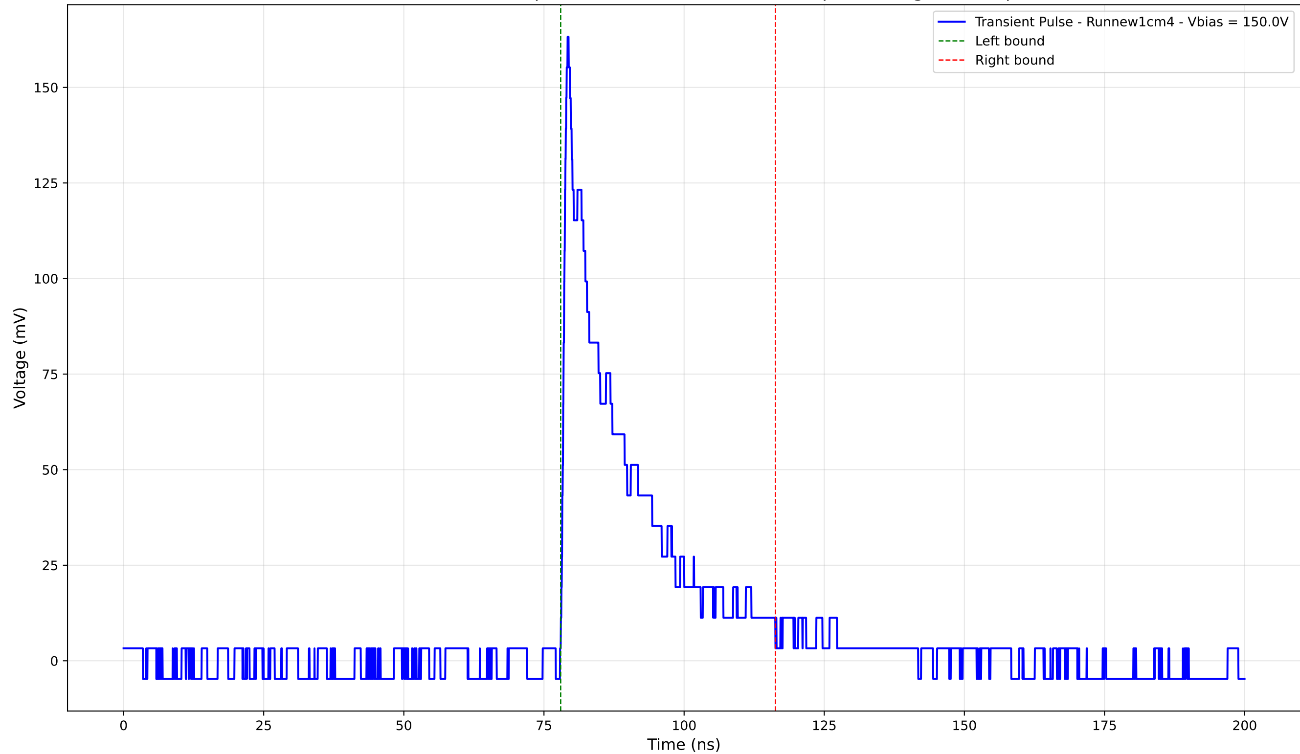
Transient Pulse - Sample: new1cm - Position: 4745.0 \mu\text{m} - Charge: 33.16 pC
