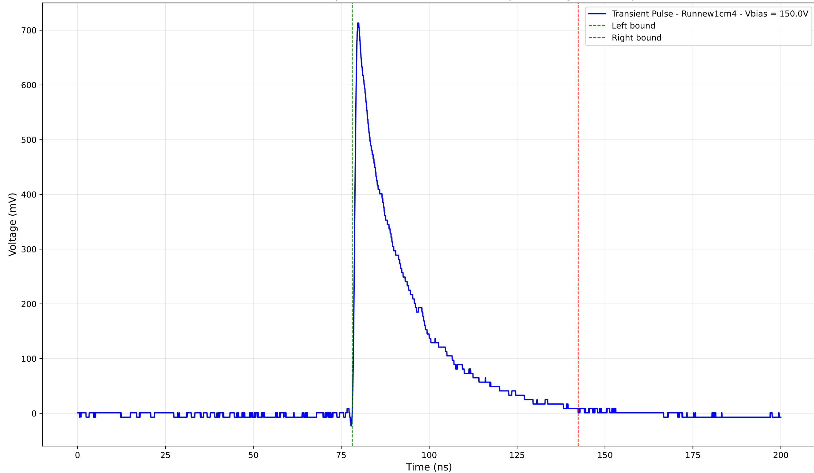
Transient Pulse - Sample: new1cm - Position: 905.0 \mu\text{m} - Charge: 196.23 pC
