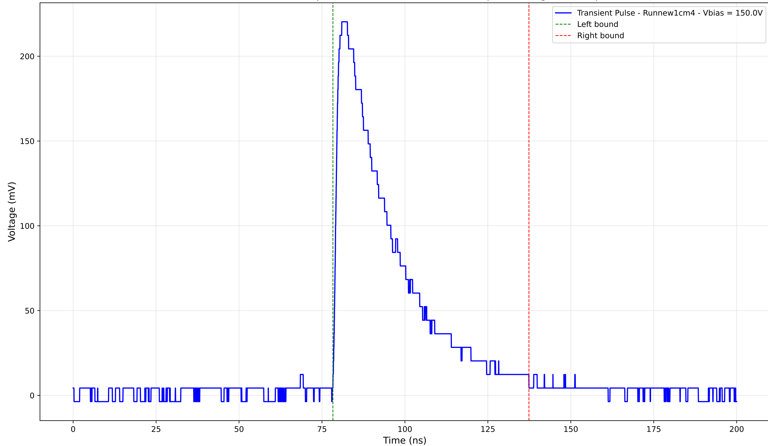
Transient Pulse - Sample: new1cm - Position: 1665.0 \mu\text{m} - Charge: 83.70 pC
