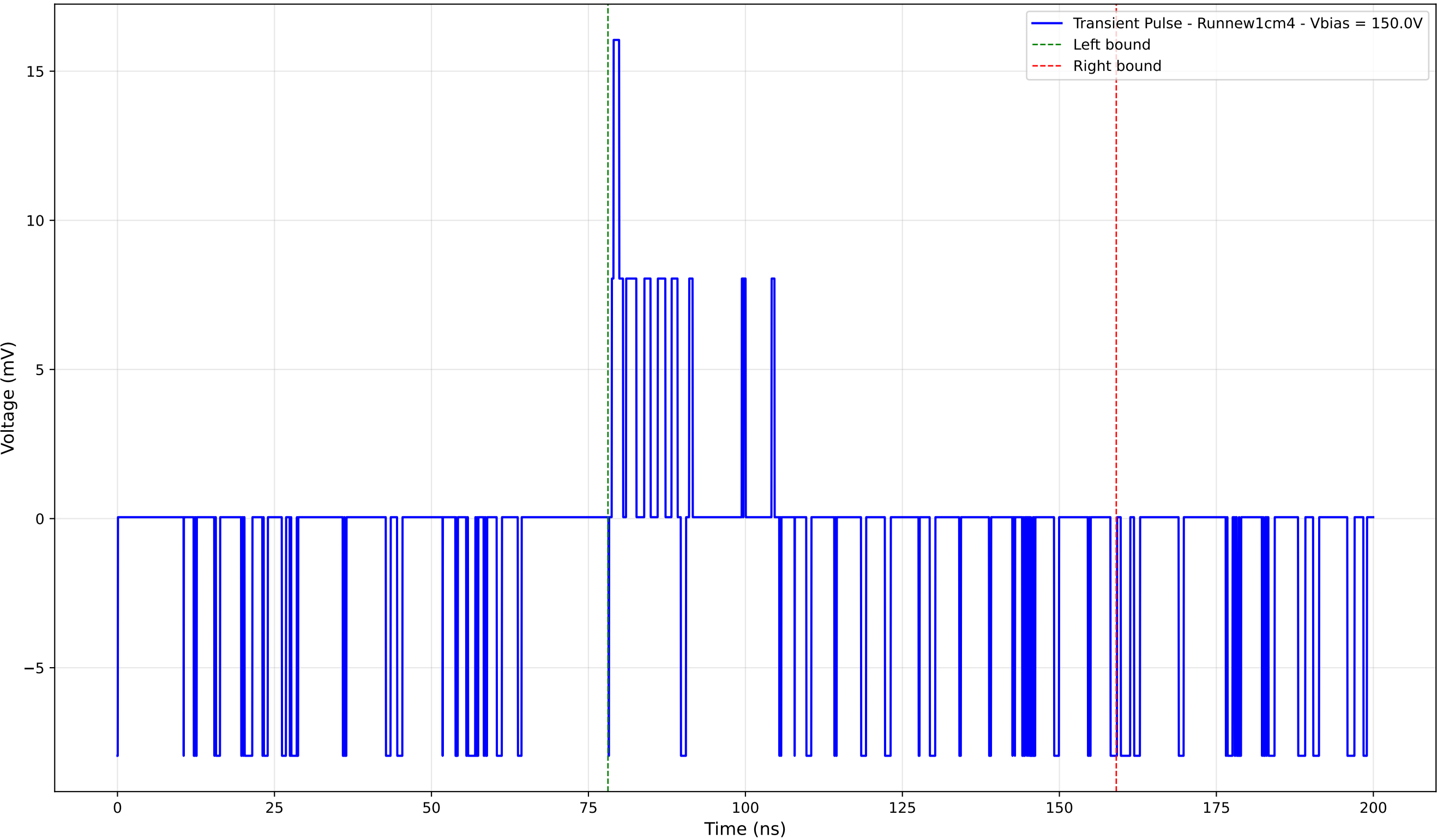
Transient Pulse - Sample: new1cm - Position: 110.0 \mu\text{m} - Charge: 0.15 pC
