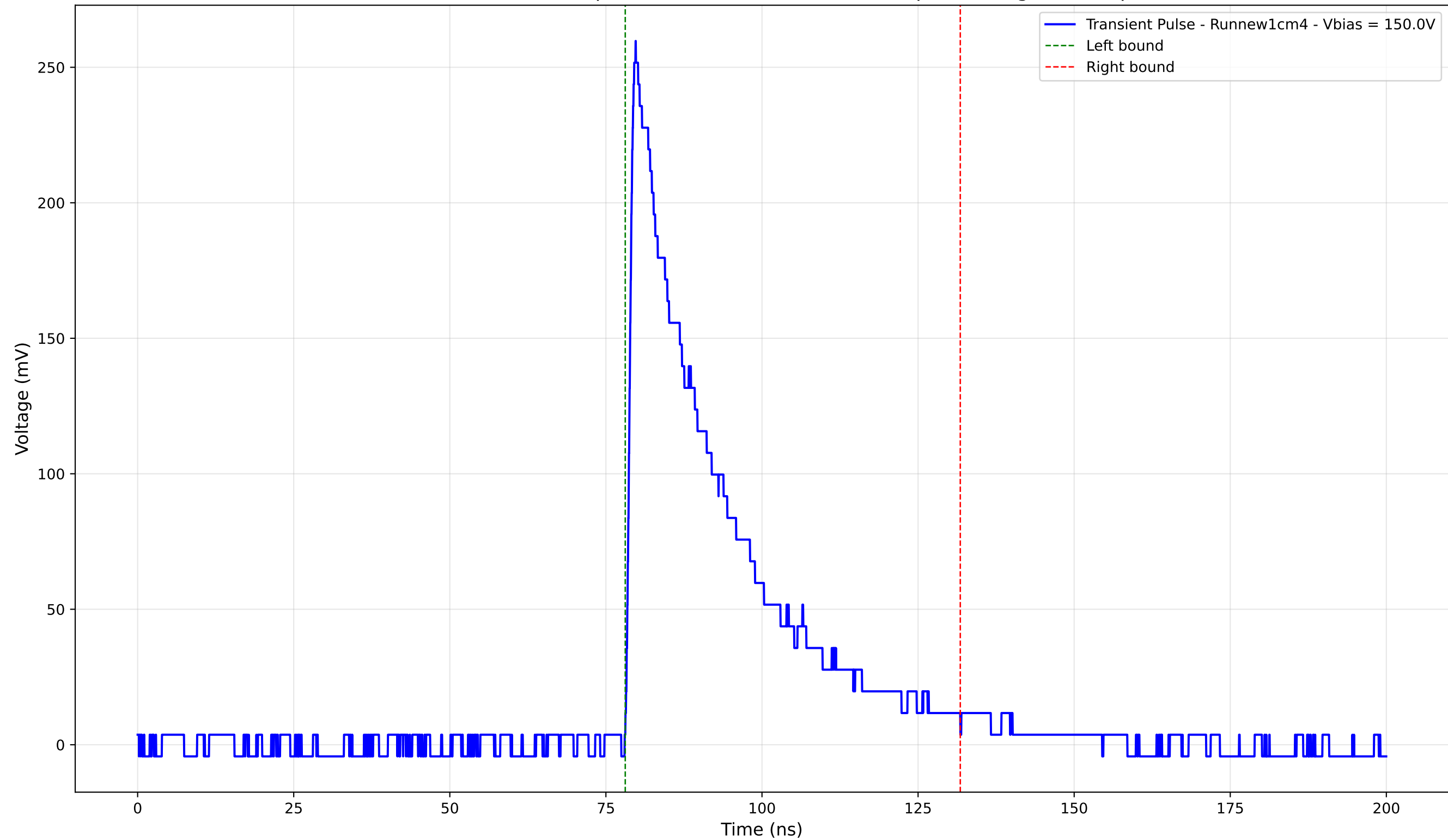
Transient Pulse - Sample: new1cm - Position: 4265.0 \mu\text{m} - Charge: 75.25 pC
