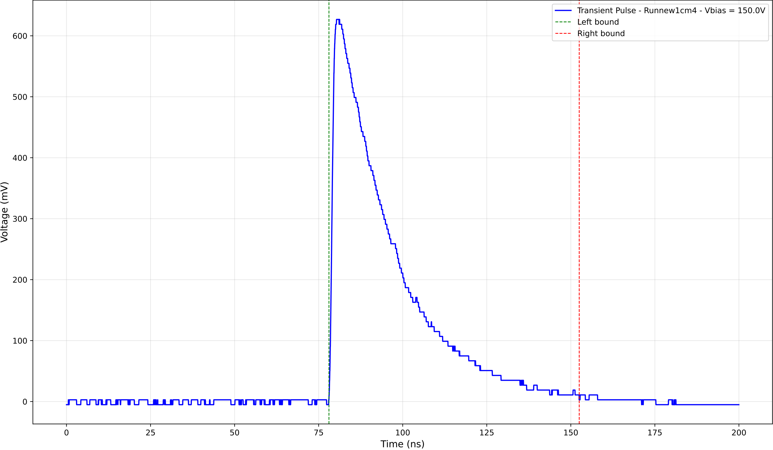
Transient Pulse - Sample: new1cm - Position: 3840.0 \mu\text{m} - Charge: 244.89 pC
