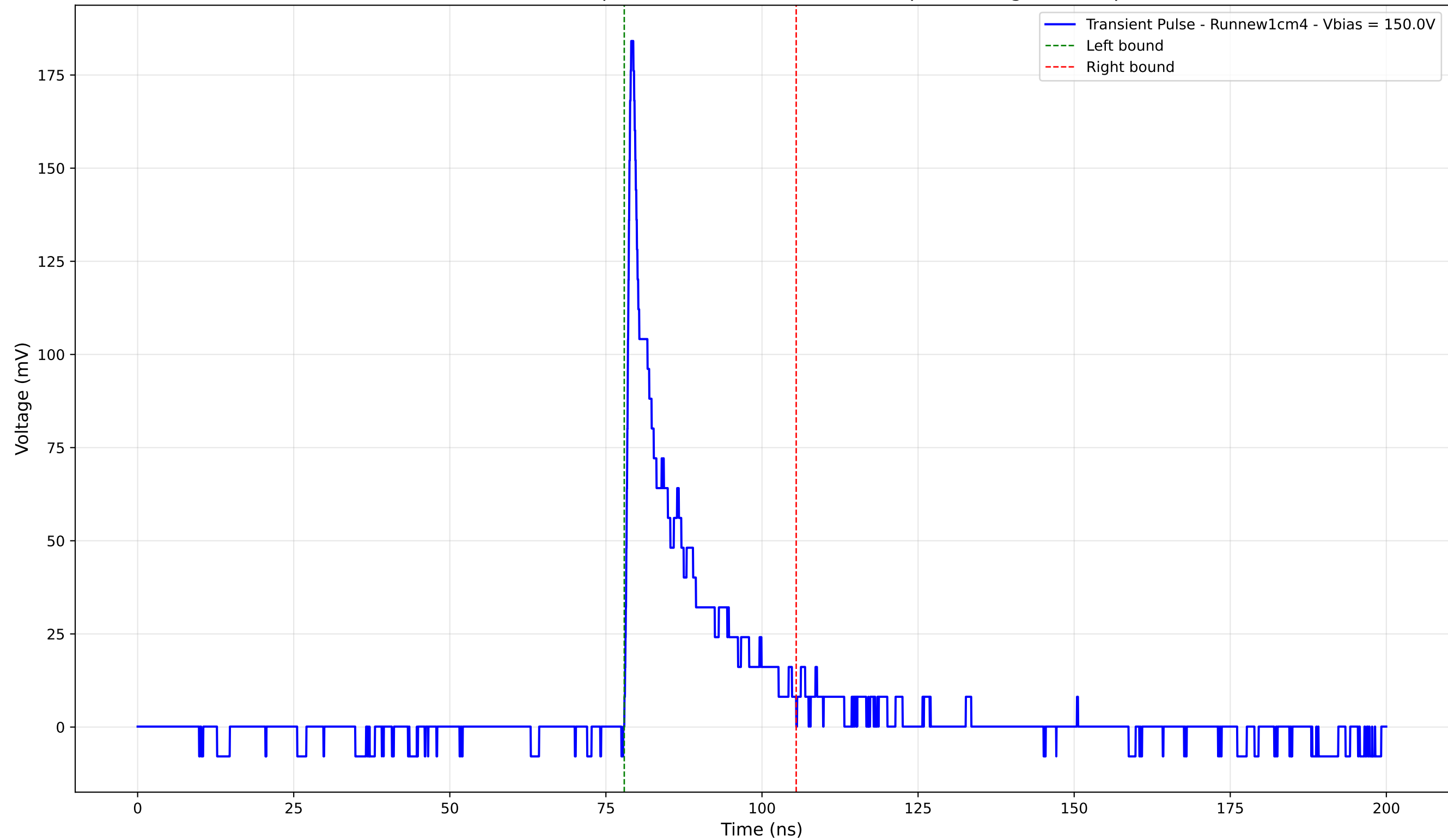
Transient Pulse - Sample: new1cm - Position: 205.0 \mu\text{m} - Charge: 24.82 pC
