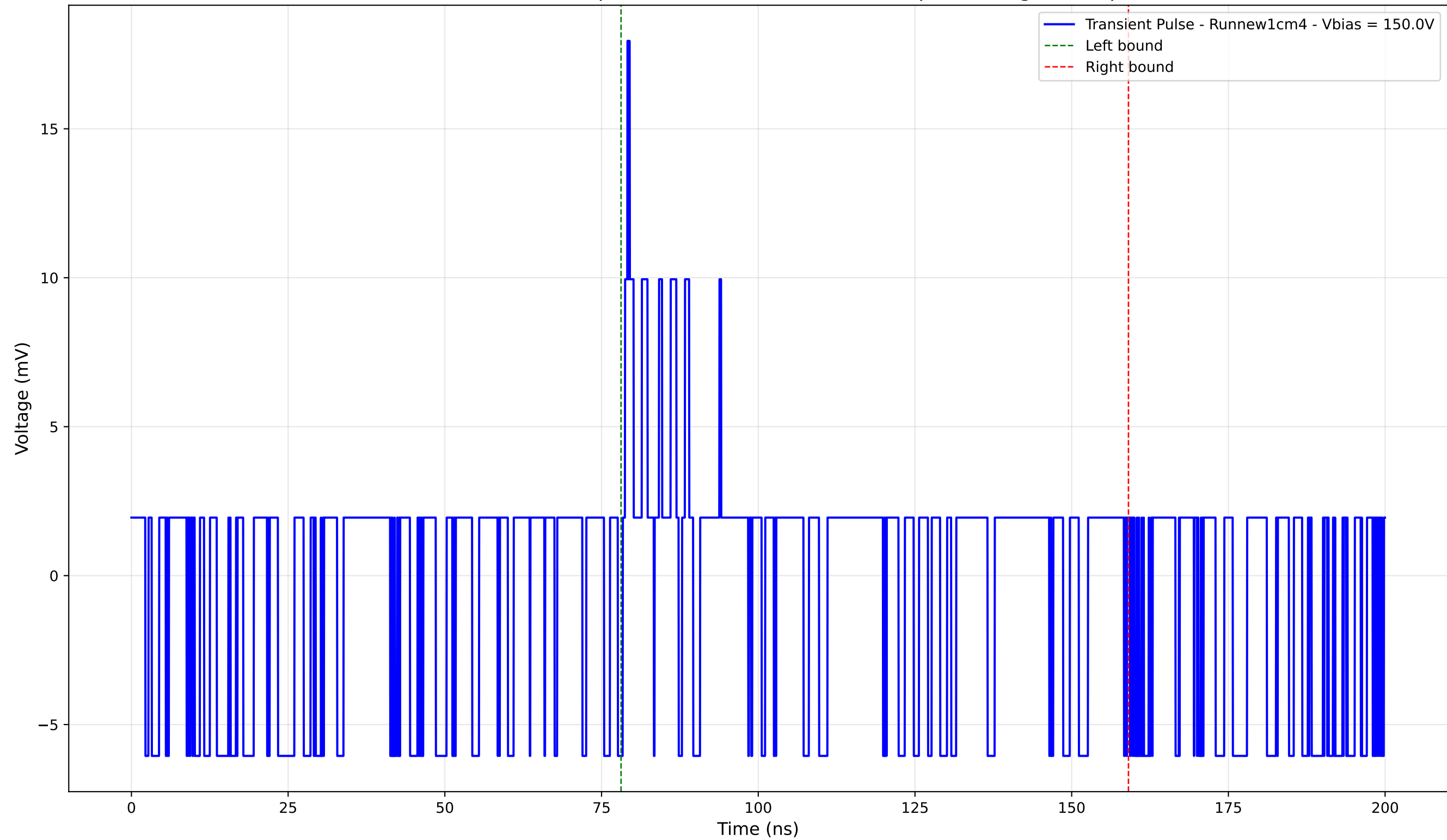
Transient Pulse - Sample: new1cm - Position: 5135.0 \mu\text{m} - Charge: 1.65 pC
