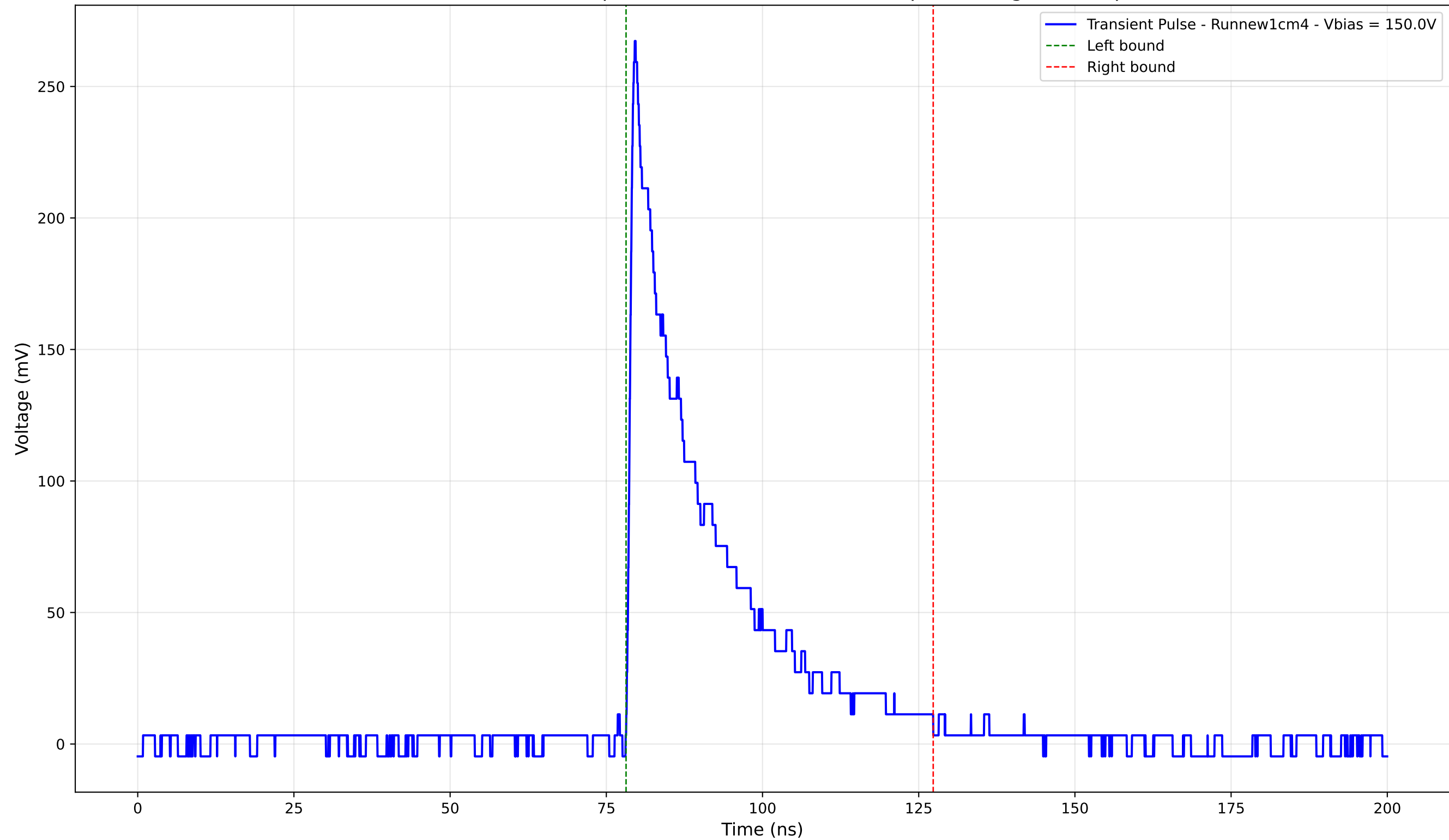
Transient Pulse - Sample: new1cm - Position: 725.0 \mu\text{m} - Charge: 62.62 pC
