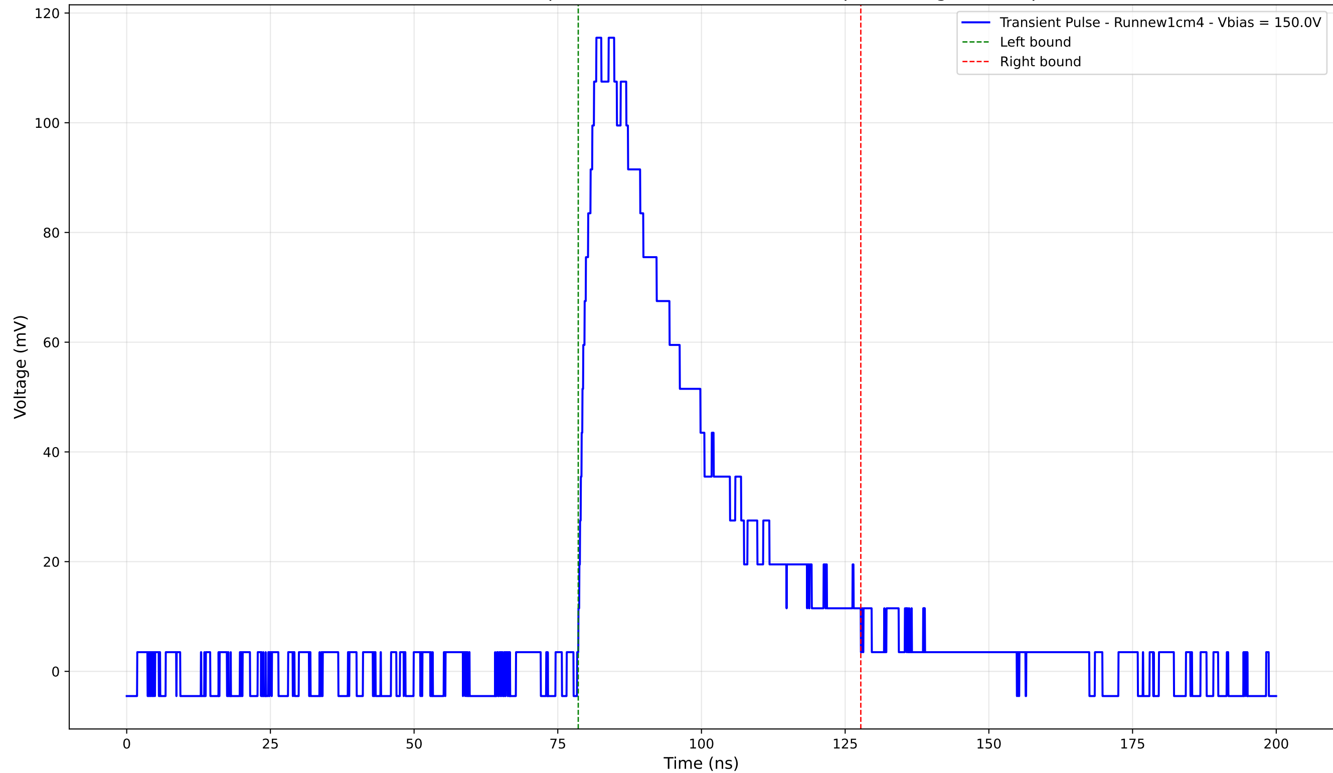
Transient Pulse - Sample: new1cm - Position: 2735.0 \mu\text{m} - Charge: 45.96 pC
