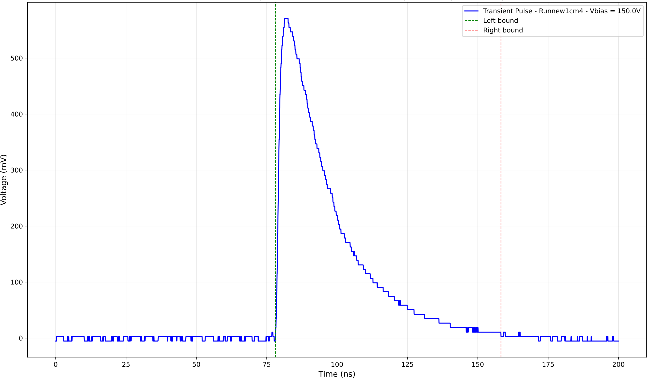
Transient Pulse - Sample: new1cm - Position: 3385.0 \mu\text{m} - Charge: 244.93 pC
