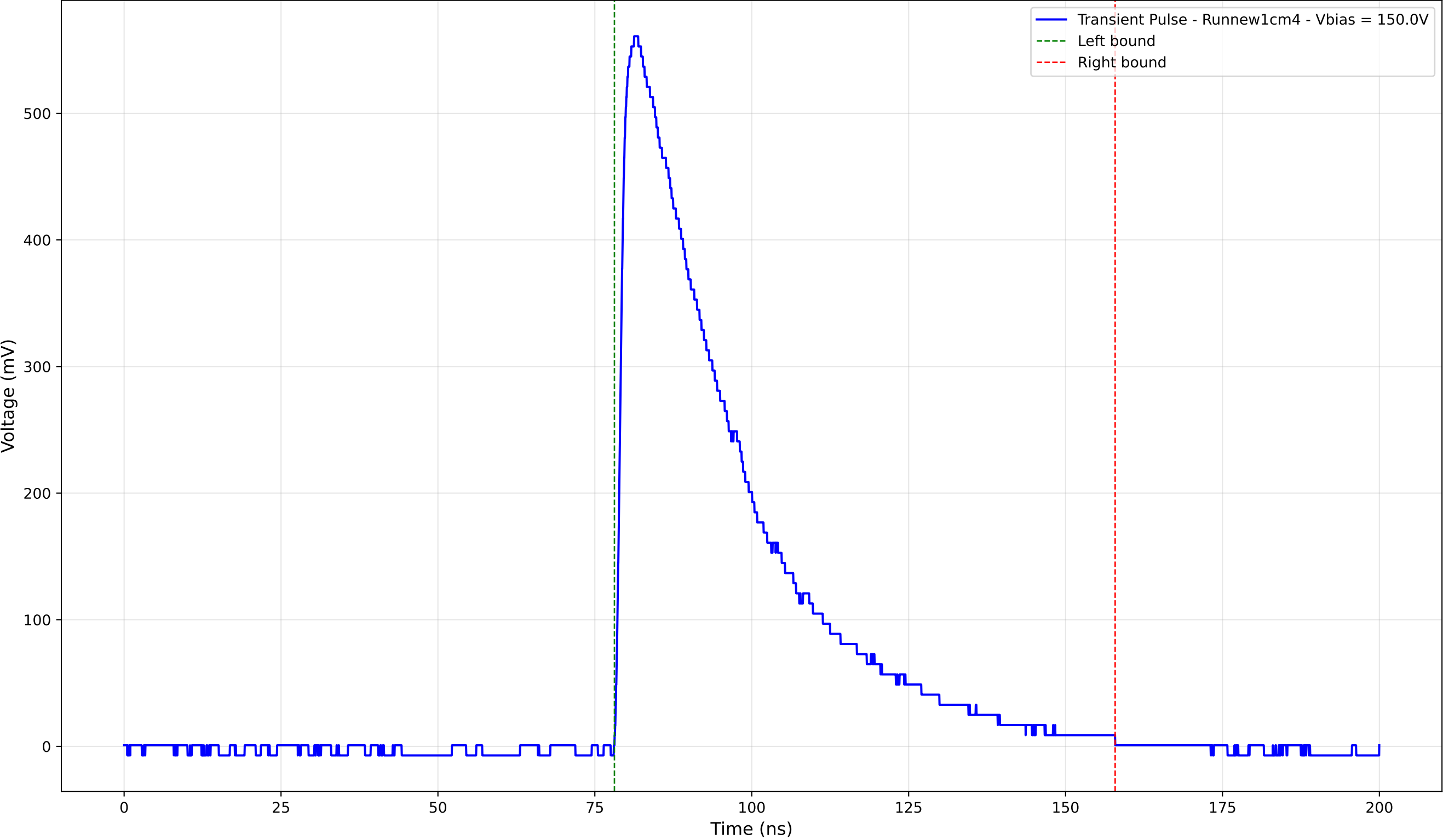
Transient Pulse - Sample: new1cm - Position: 3635.0 \mu\text{m} - Charge: 228.27 pC
