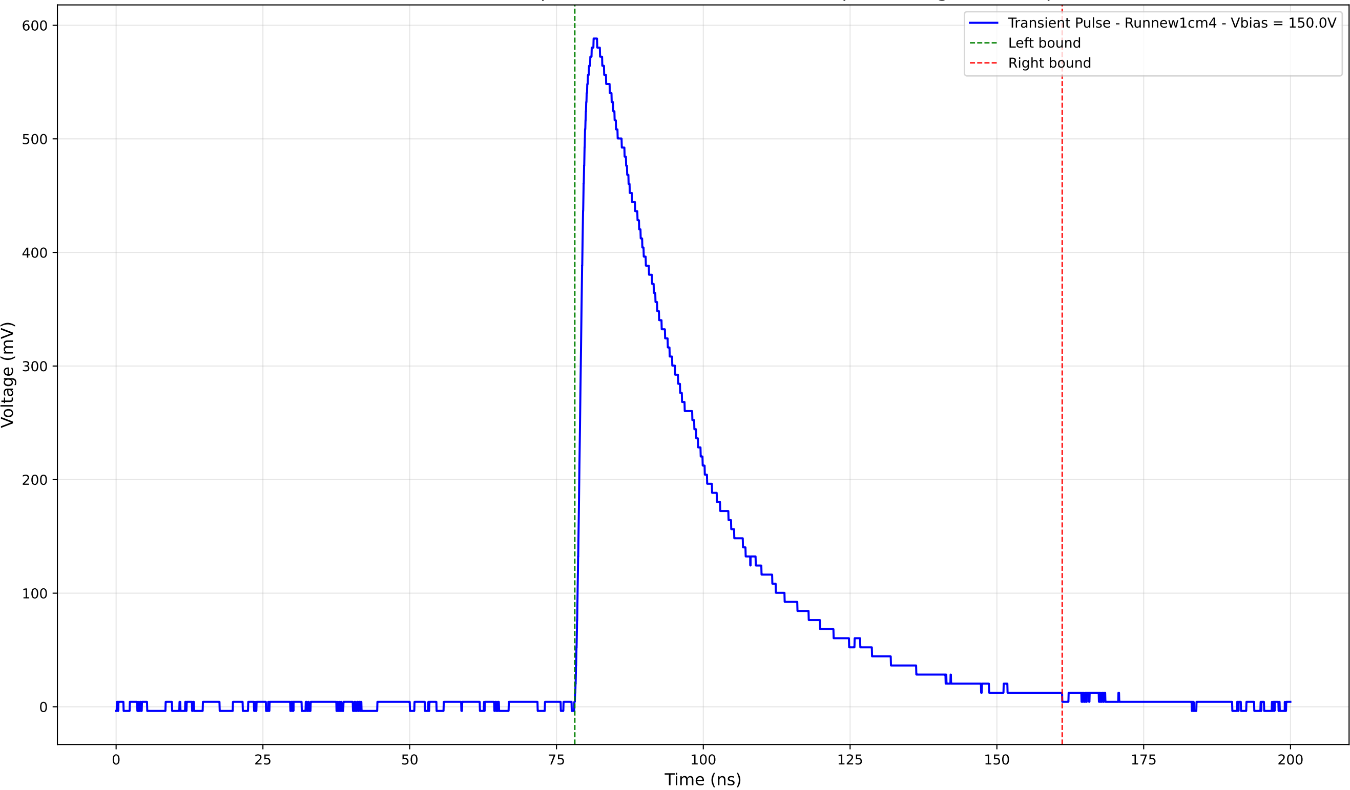
Transient Pulse - Sample: new1cm - Position: 3570.0 \mu\text{m} - Charge: 248.77 pC
