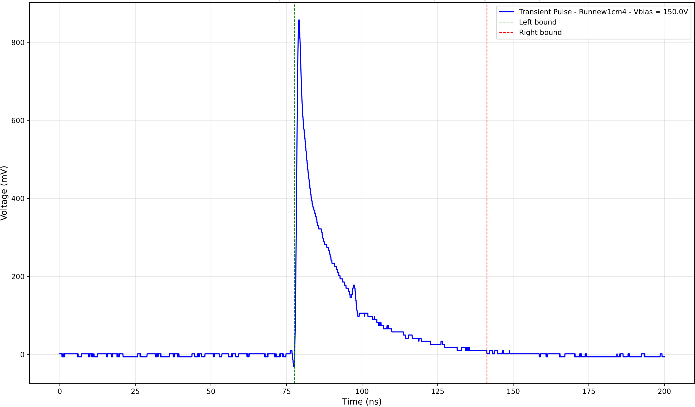
Transient Pulse - Sample: new1cm - Position: 4965.0 \mu\text{m} - Charge: 171.34 pC
