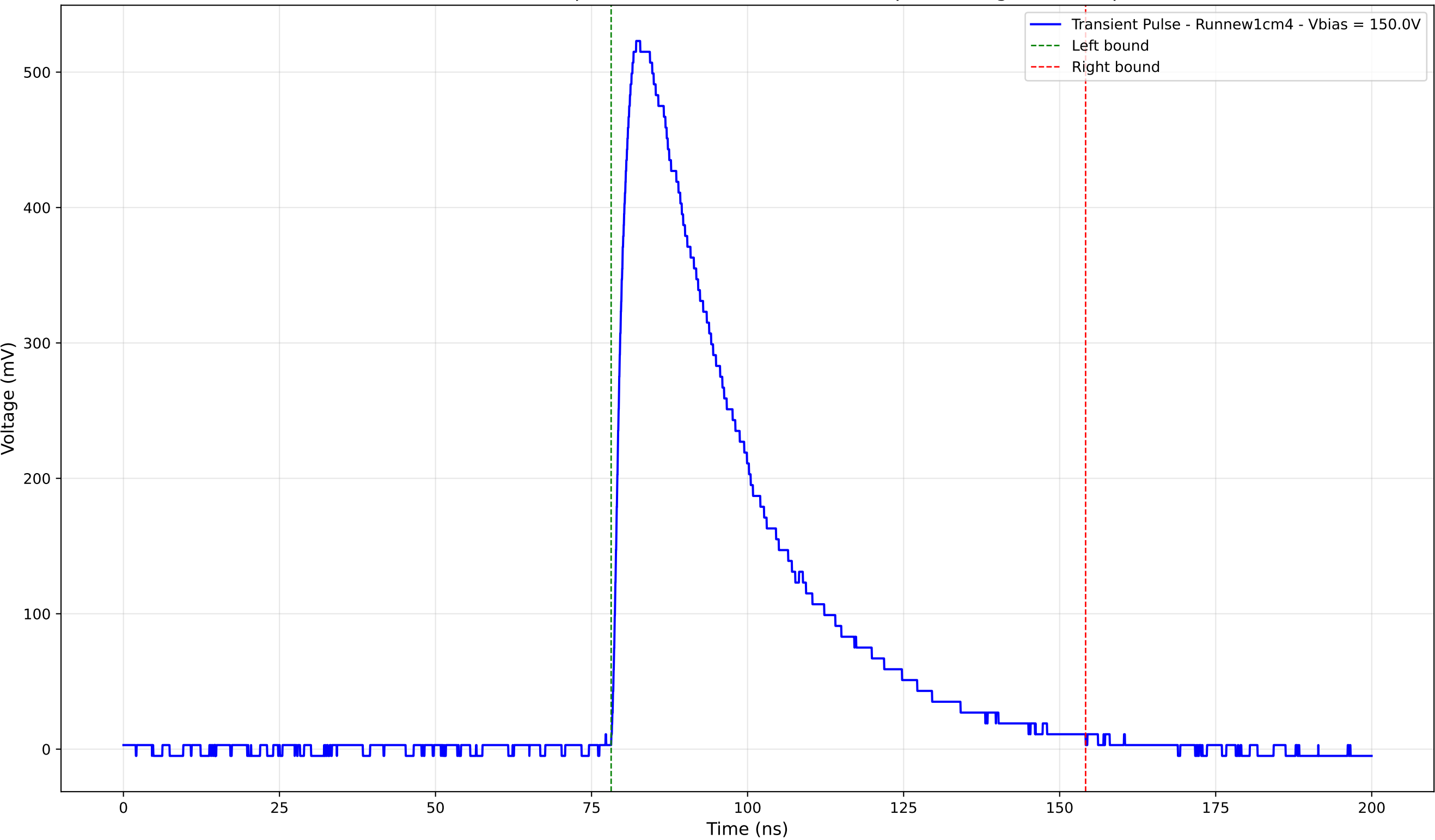
Transient Pulse - Sample: new1cm - Position: 2540.0 \mu\text{m} - Charge: 228.59 pC
