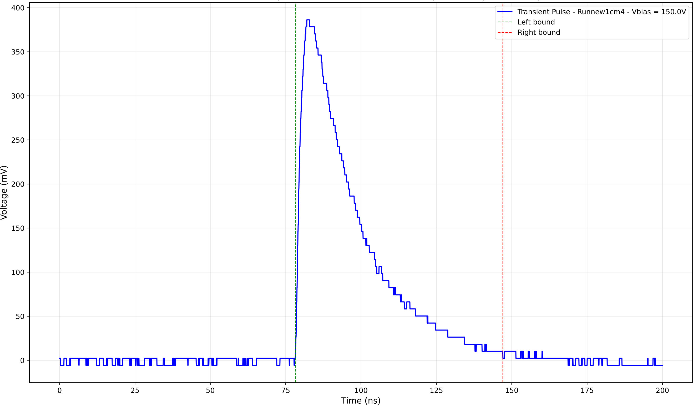
Transient Pulse - Sample: new1cm - Position: 2785.0 \mu\text{m} - Charge: 165.17 pC
