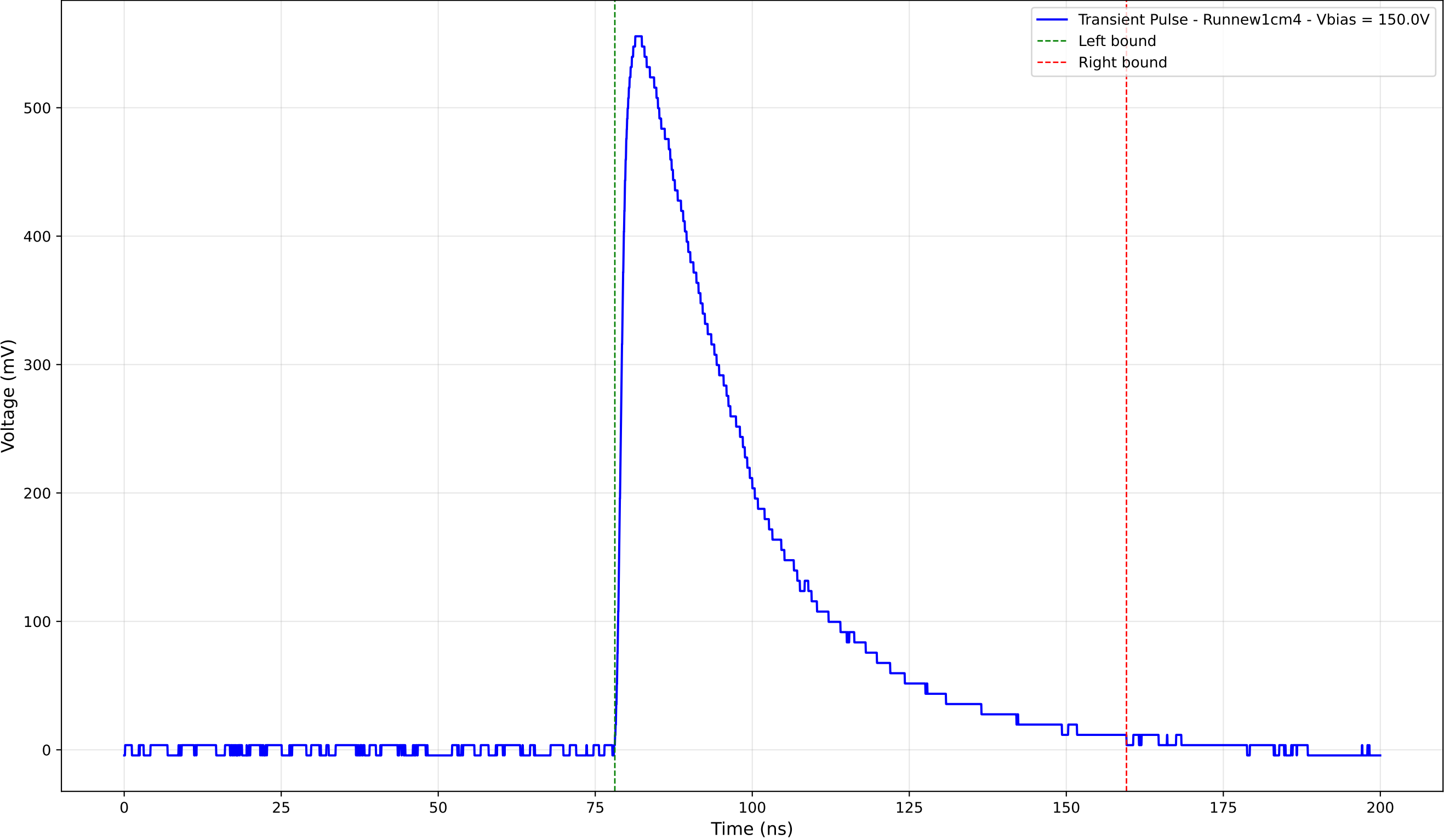
Transient Pulse - Sample: new1cm - Position: 3455.0 \mu\text{m} - Charge: 239.89 pC
