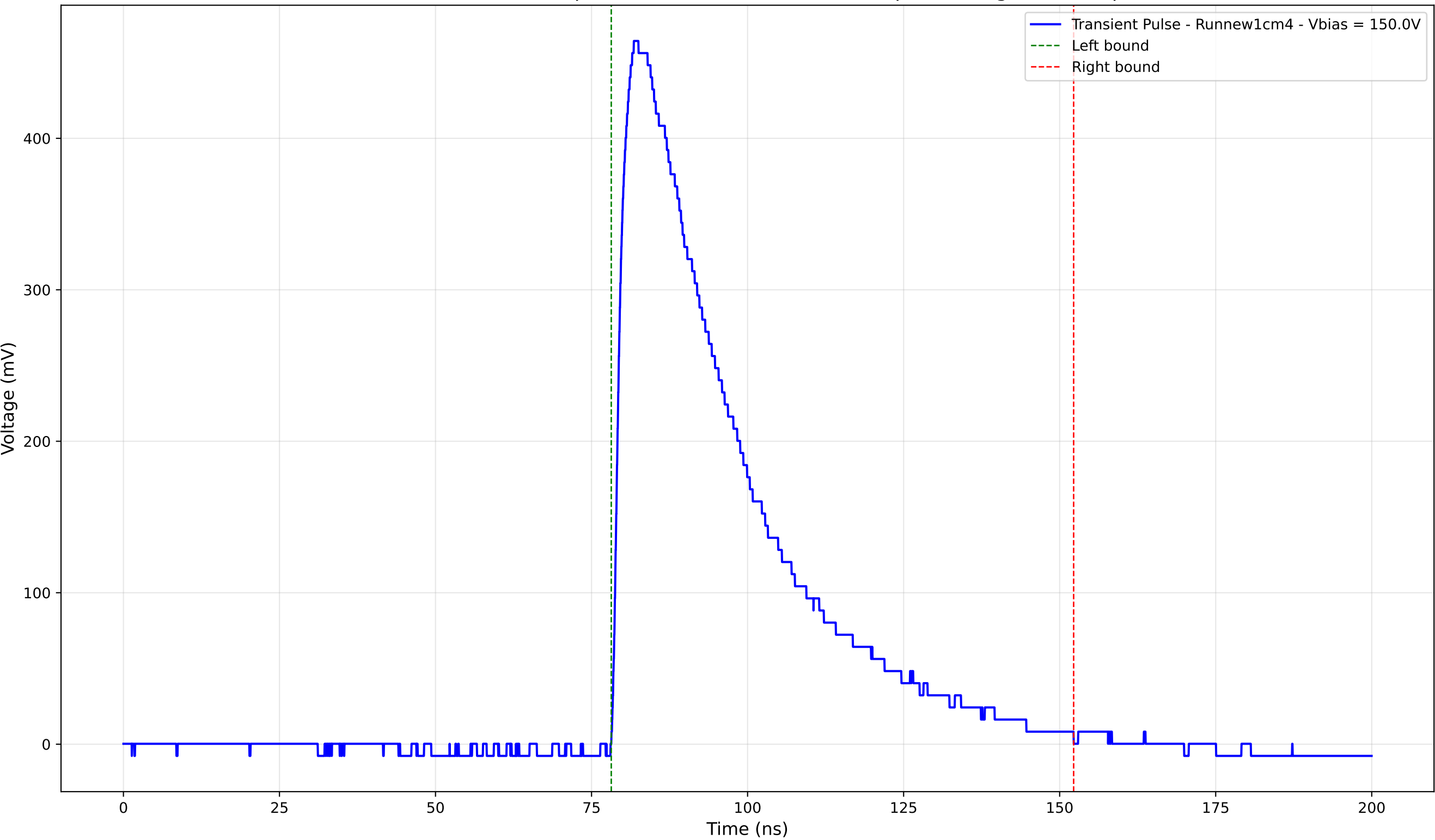
Transient Pulse - Sample: new1cm - Position: 3145.0 \mu\text{m} - Charge: 197.80 pC
