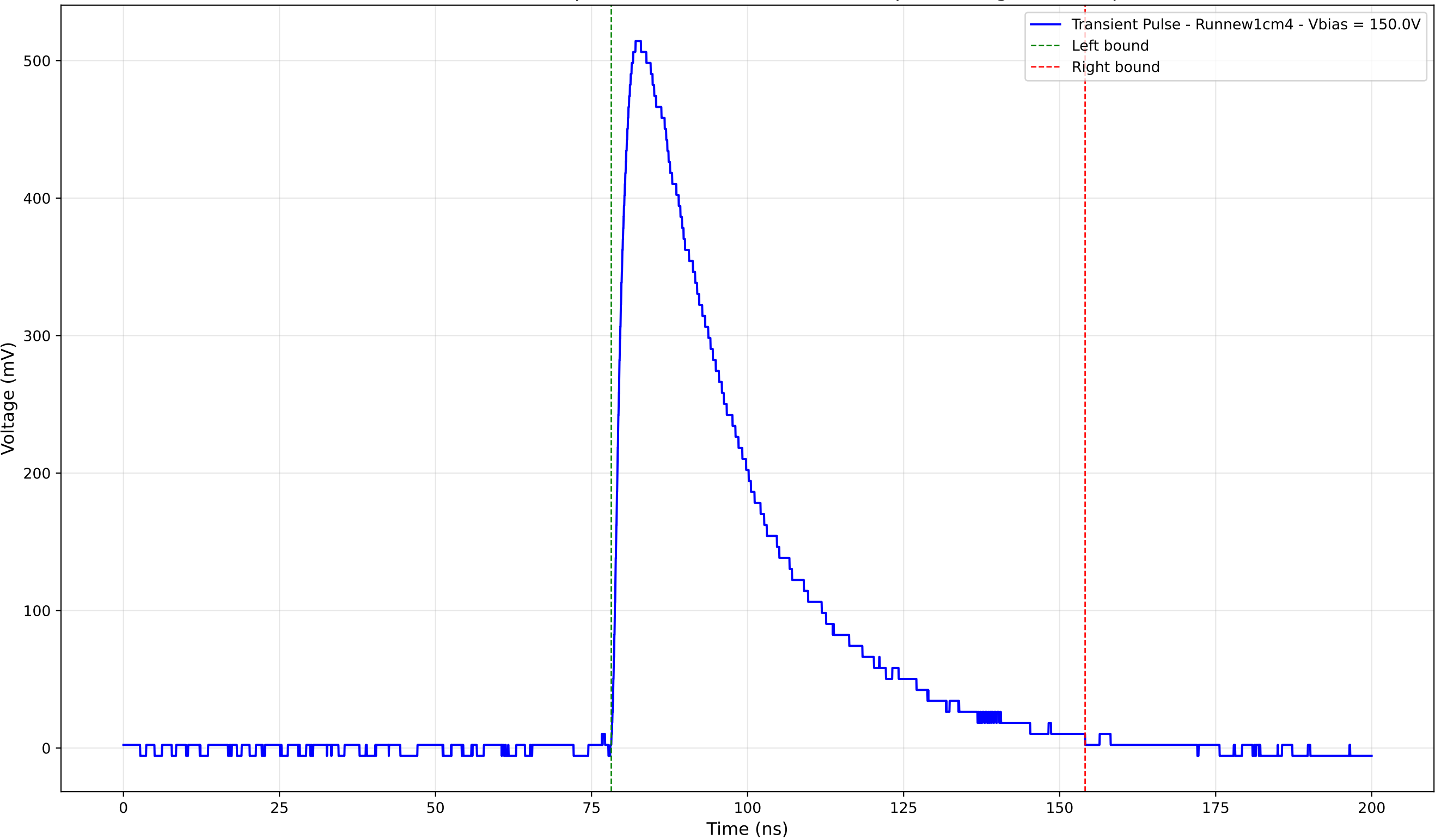
Transient Pulse - Sample: new1cm - Position: 2320.0 \mu\text{m} - Charge: 220.10 pC
