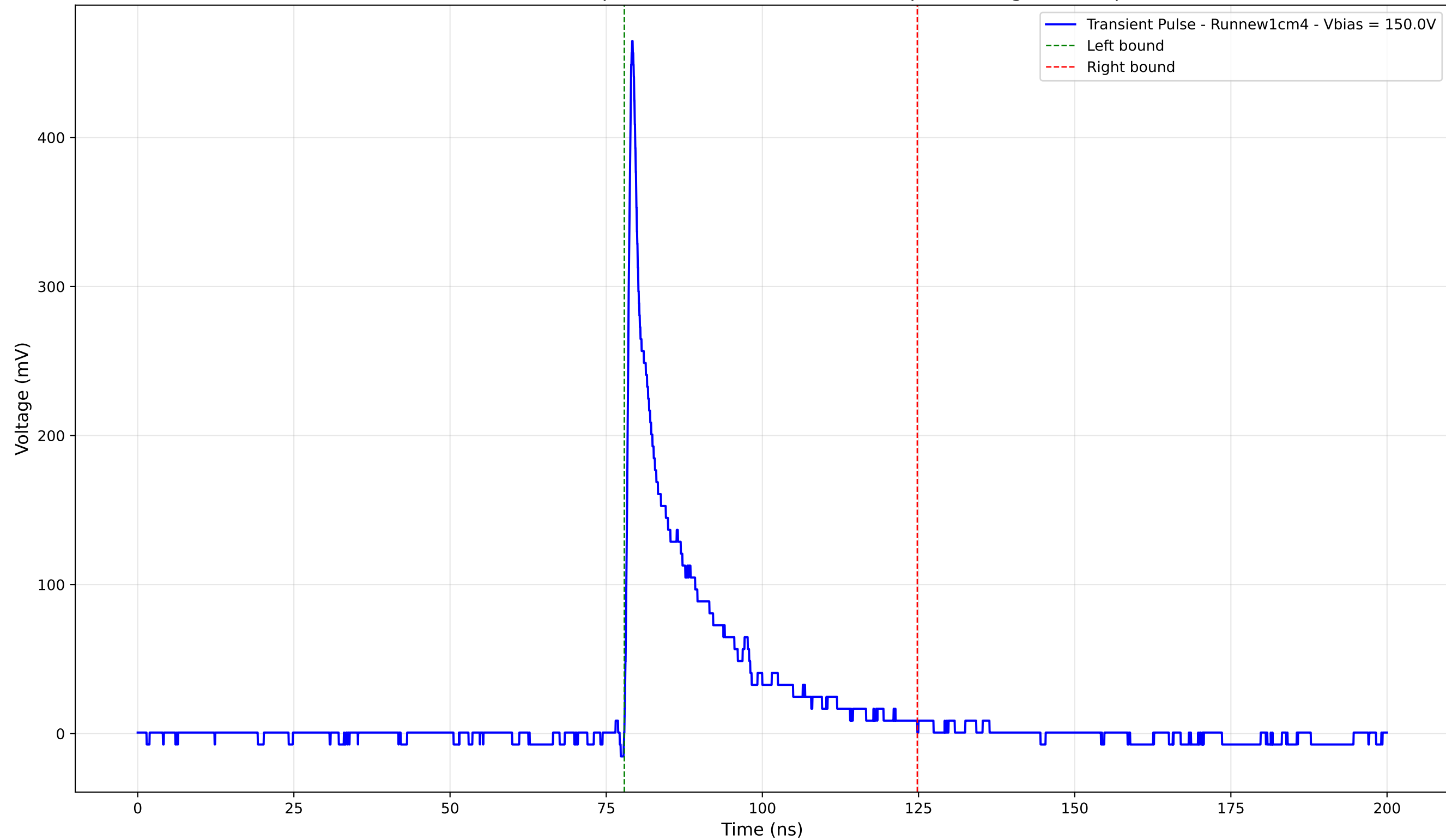
Transient Pulse - Sample: new1cm - Position: 230.0 \mu\text{m} - Charge: 67.26 pC
