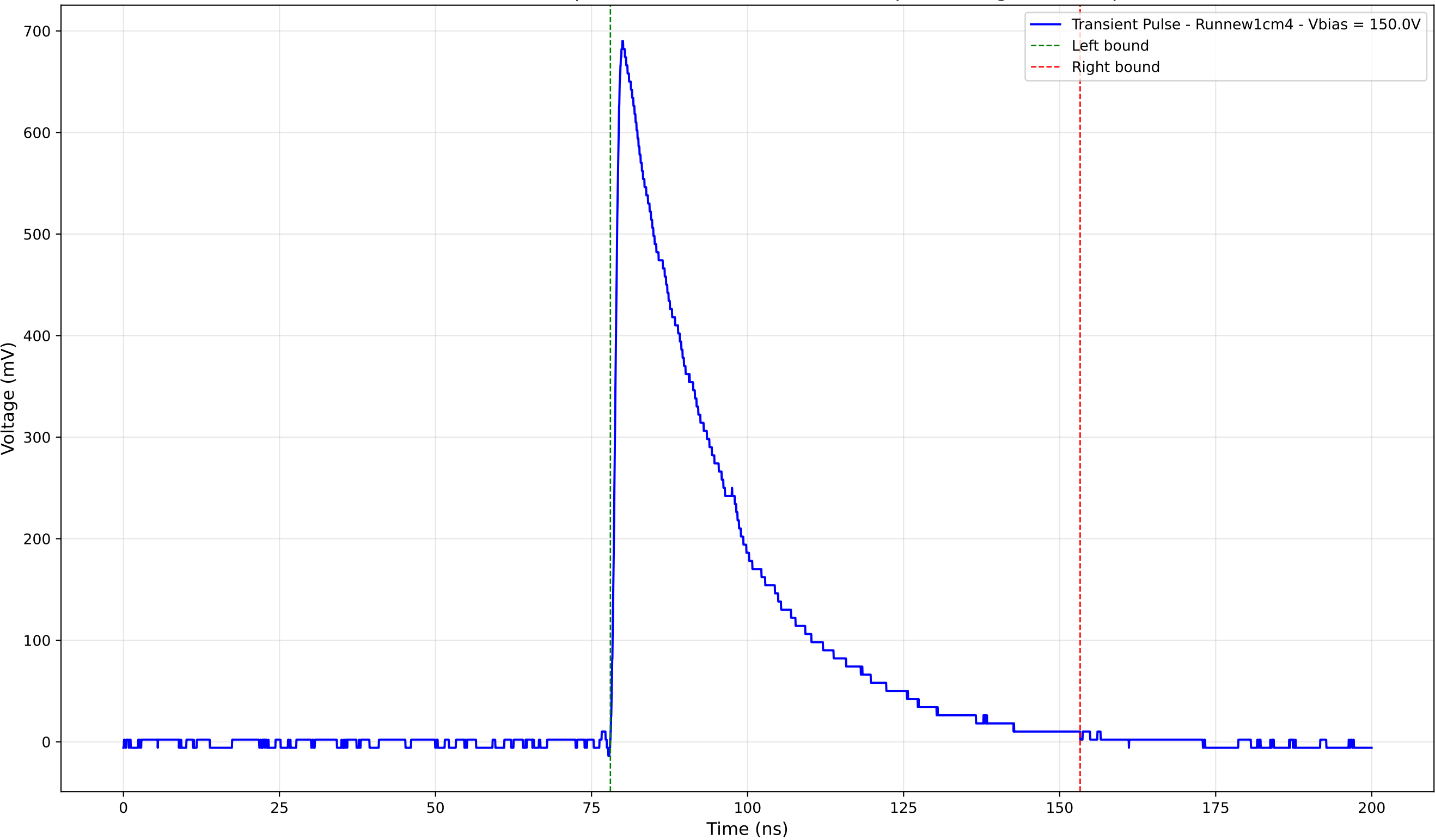
Transient Pulse - Sample: new1cm - Position: 4135.0 \mu\text{m} - Charge: 236.26 pC
