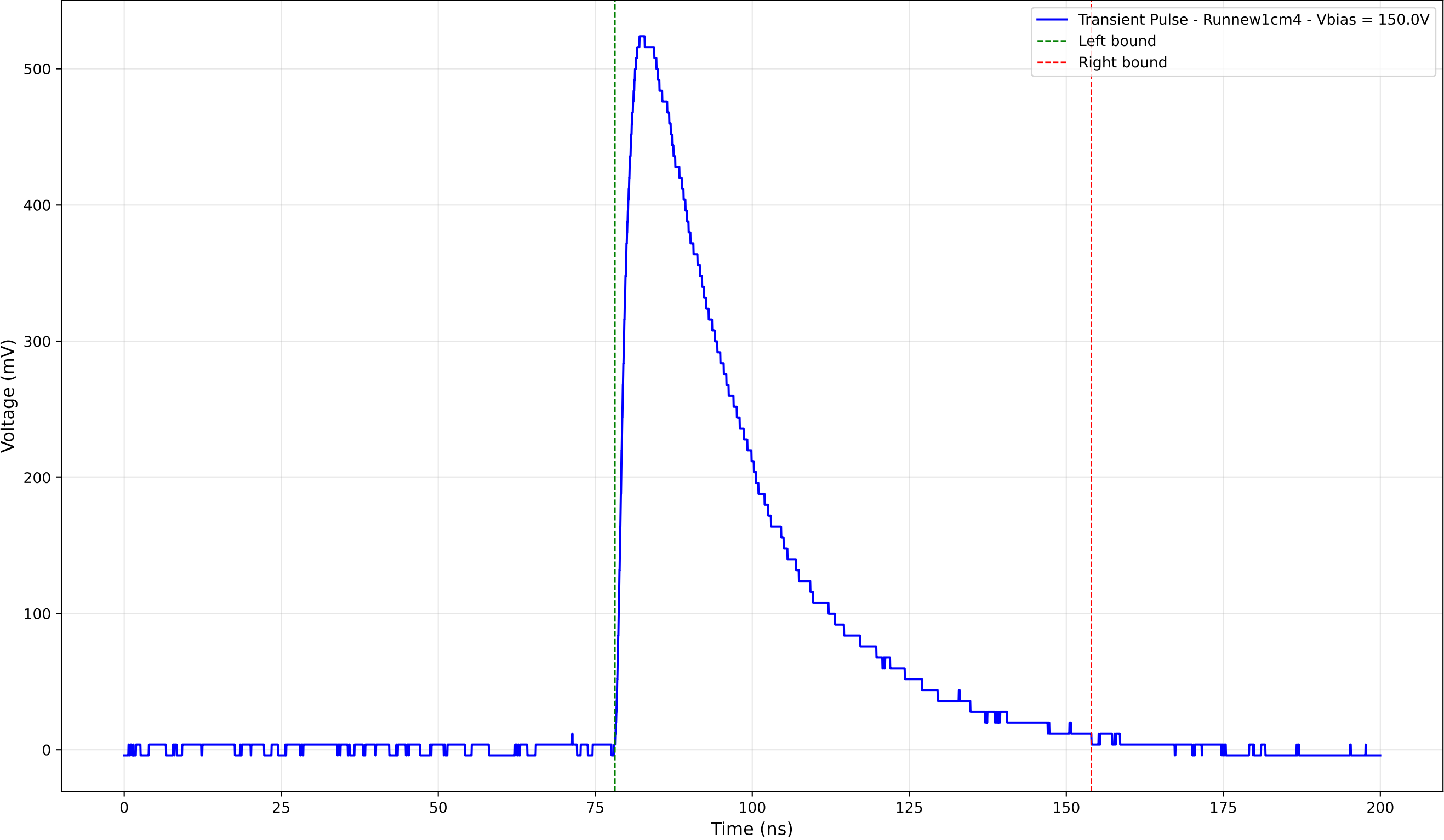
Transient Pulse - Sample: new1cm - Position: 2435.0 \mu\text{m} - Charge: 228.80 pC
