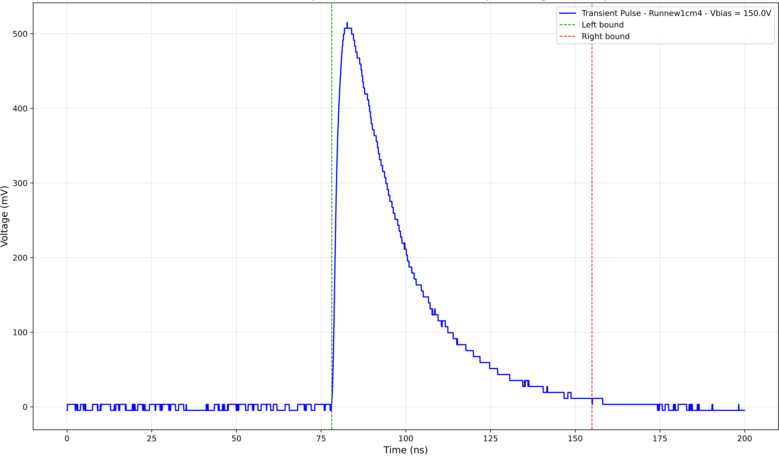
Transient Pulse - Sample: new1cm - Position: 2875.0 \mu\text{m} - Charge: 228.27 pC
