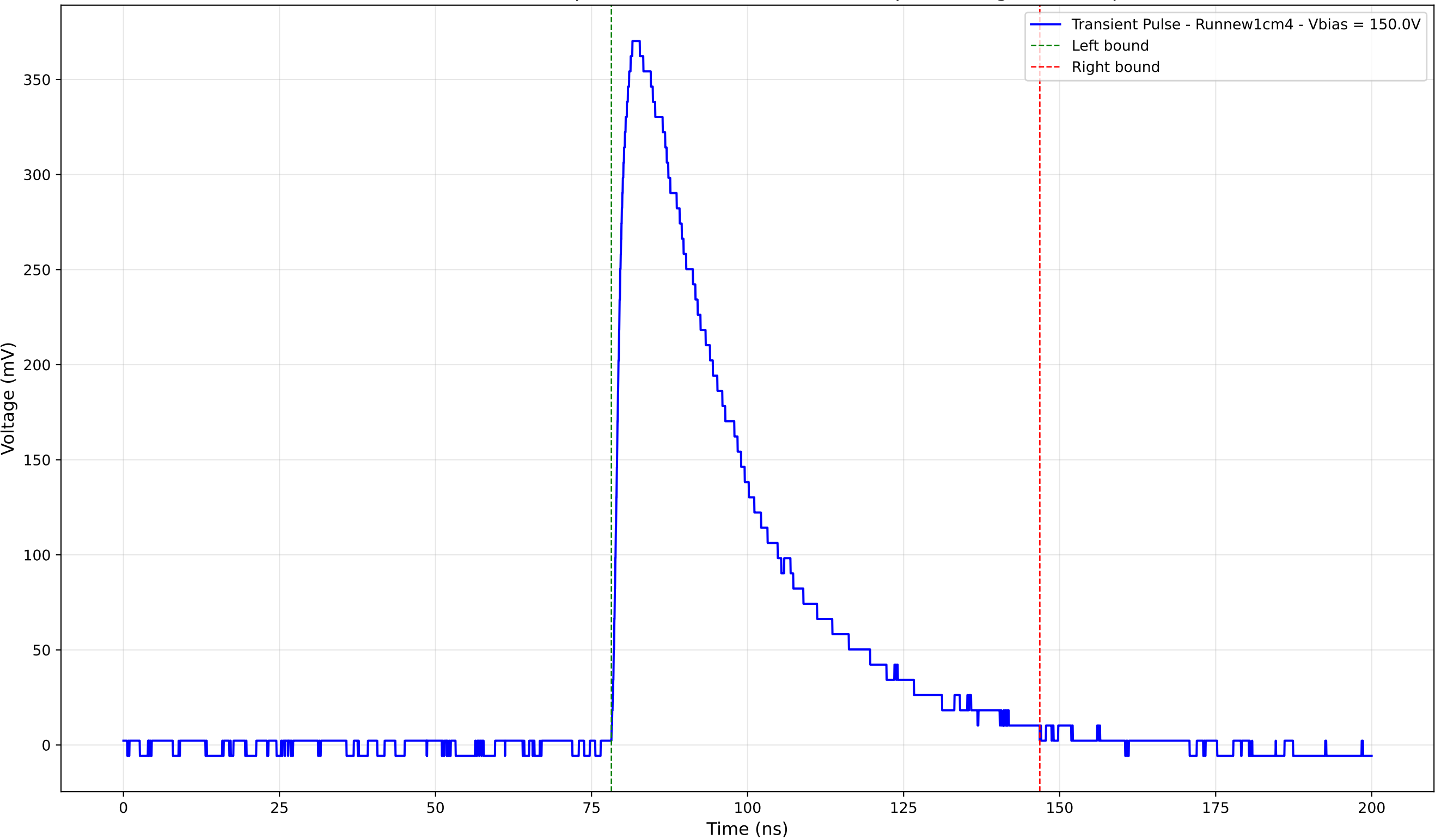
Transient Pulse - Sample: new1cm - Position: 3285.0 \mu\text{m} - Charge: 154.32 pC
