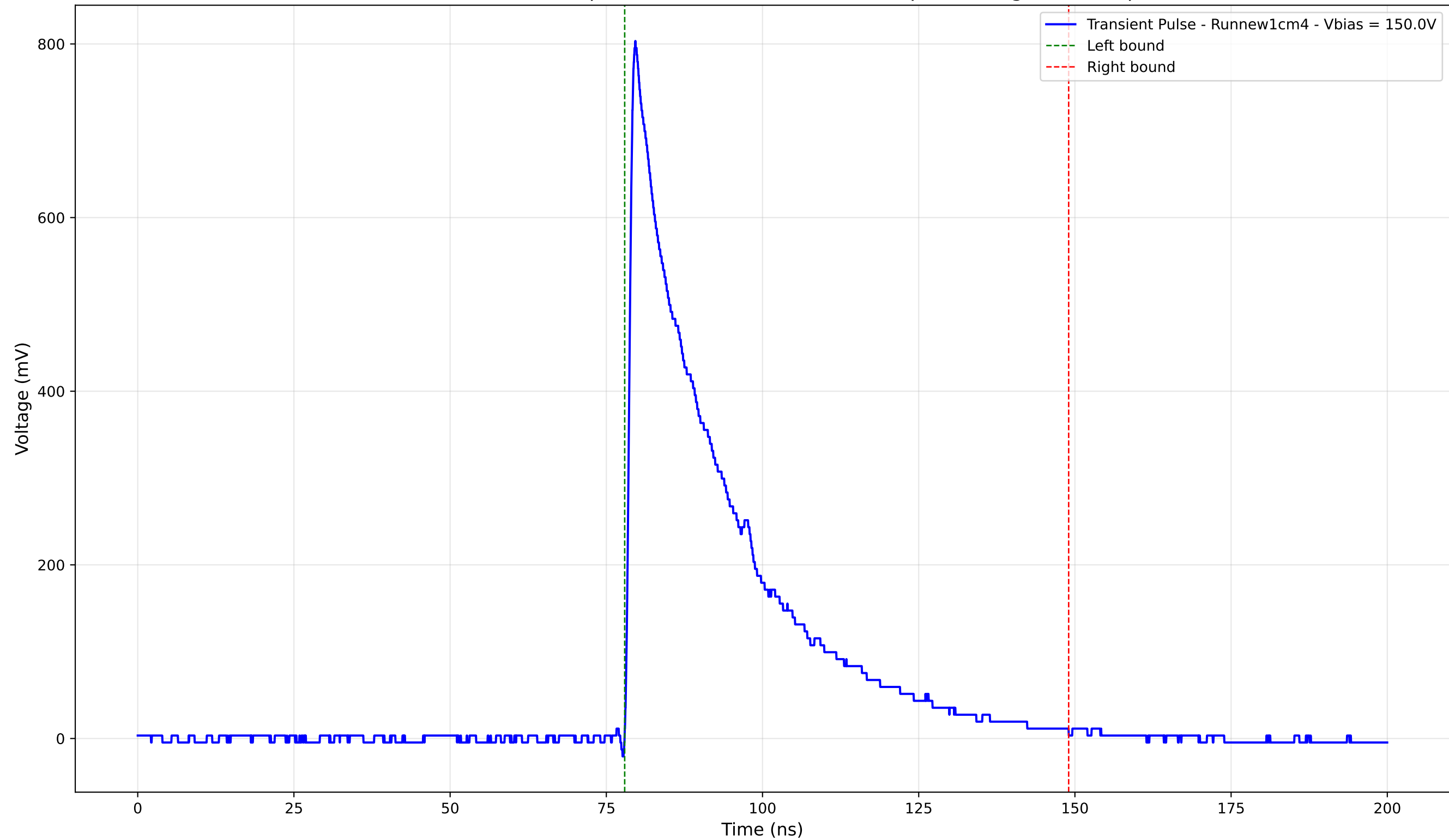
Transient Pulse - Sample: new1cm - Position: 4400.0 \mu\text{m} - Charge: 242.97 pC
