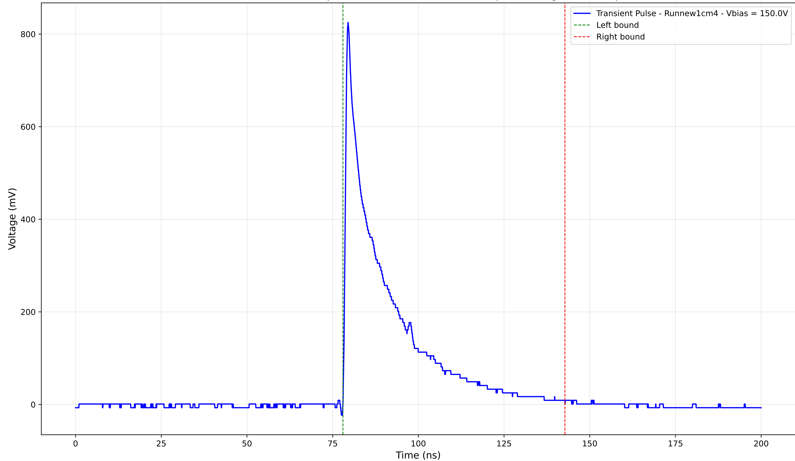
Transient Pulse - Sample: new1cm - Position: 595.0 \mu\text{m} - Charge: 182.59 pC
