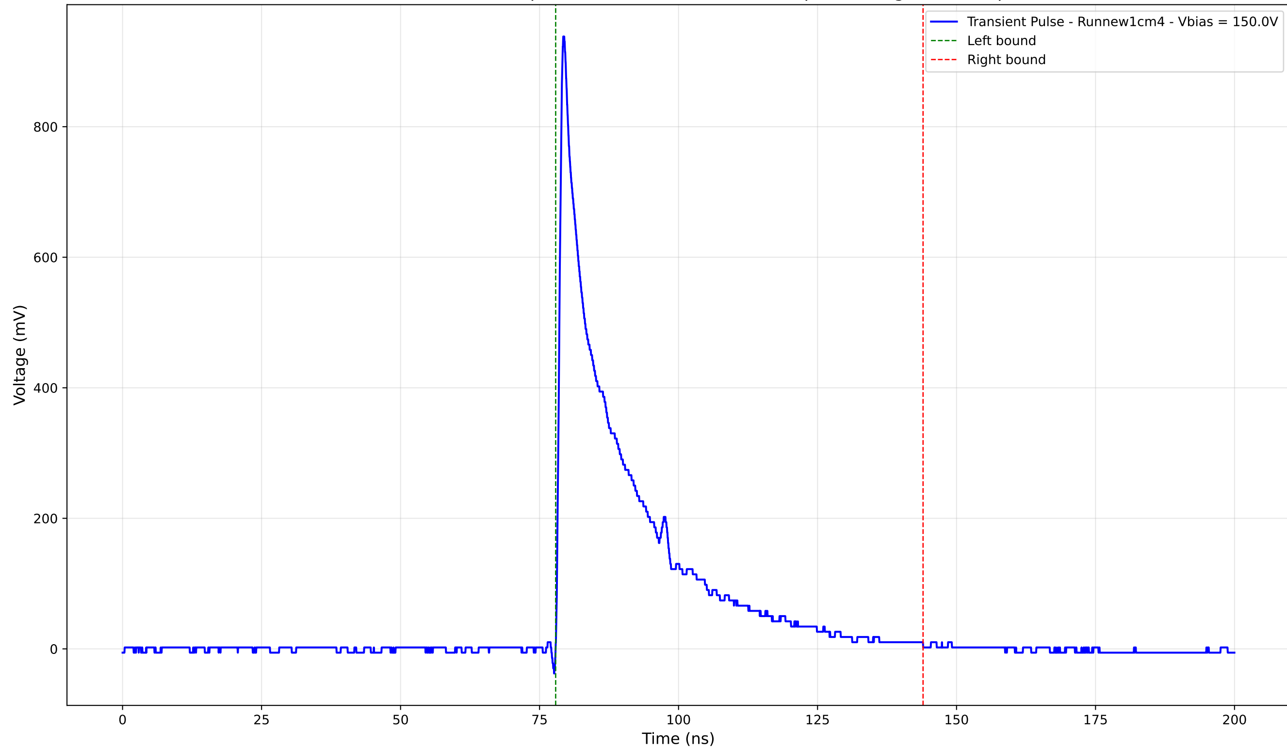
Transient Pulse - Sample: new1cm - Position: 435.0 \mu\text{m} - Charge: 199.79 pC
