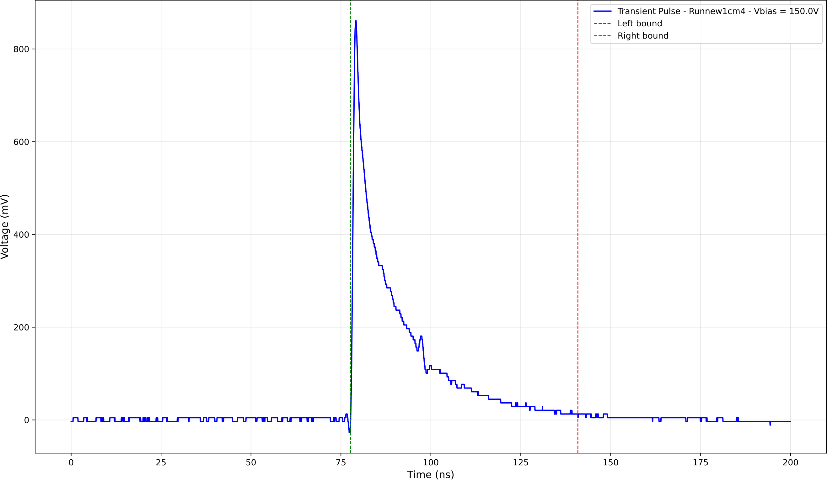
Transient Pulse - Sample: new1cm - Position: 4955.0 \mu\text{m} - Charge: 178.53 pC
