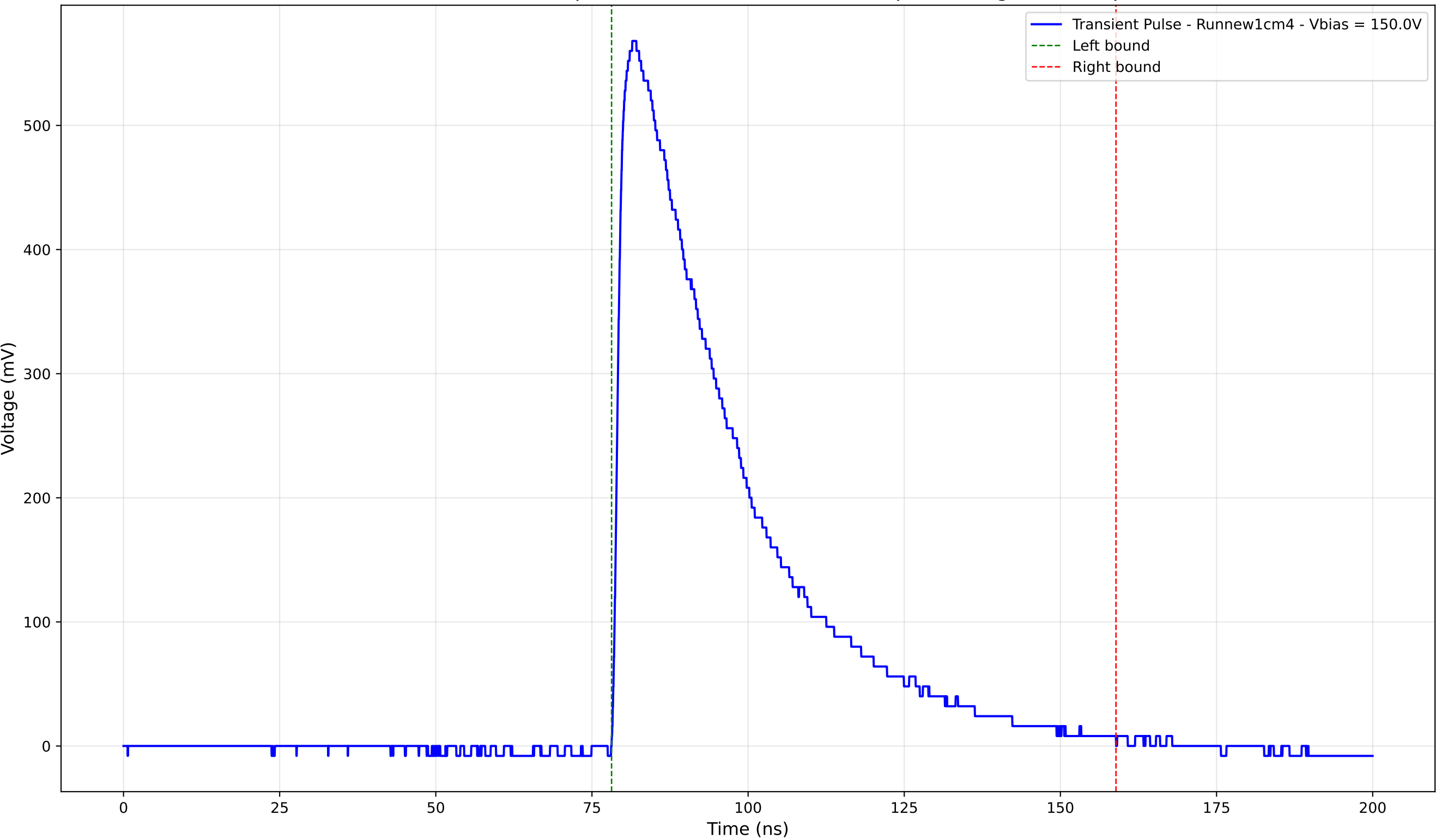
Transient Pulse - Sample: new1cm - Position: 3530.0 \mu\text{m} - Charge: 237.82 pC
