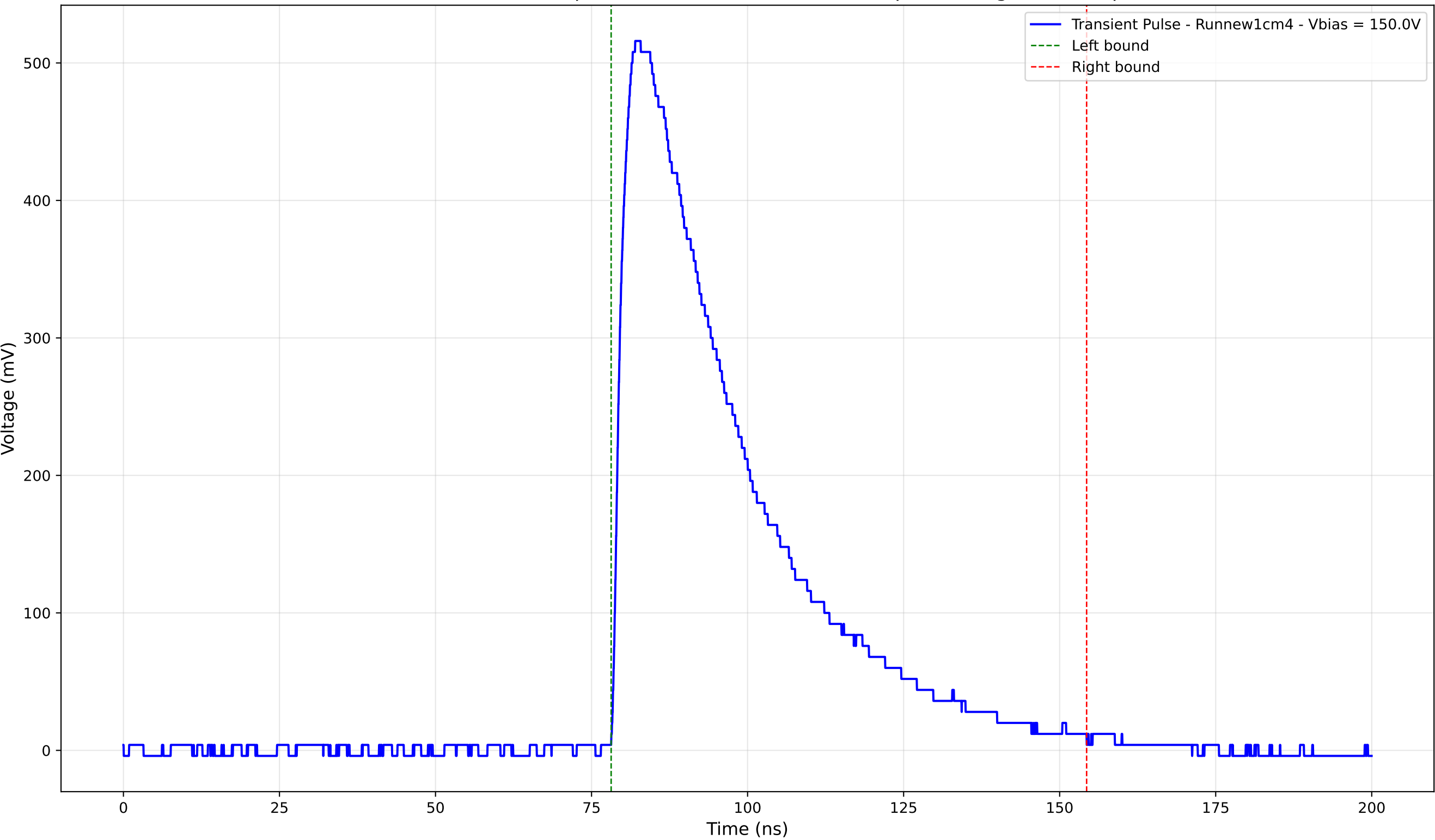
Transient Pulse - Sample: new1cm - Position: 2915.0 \mu\text{m} - Charge: 228.75 pC
