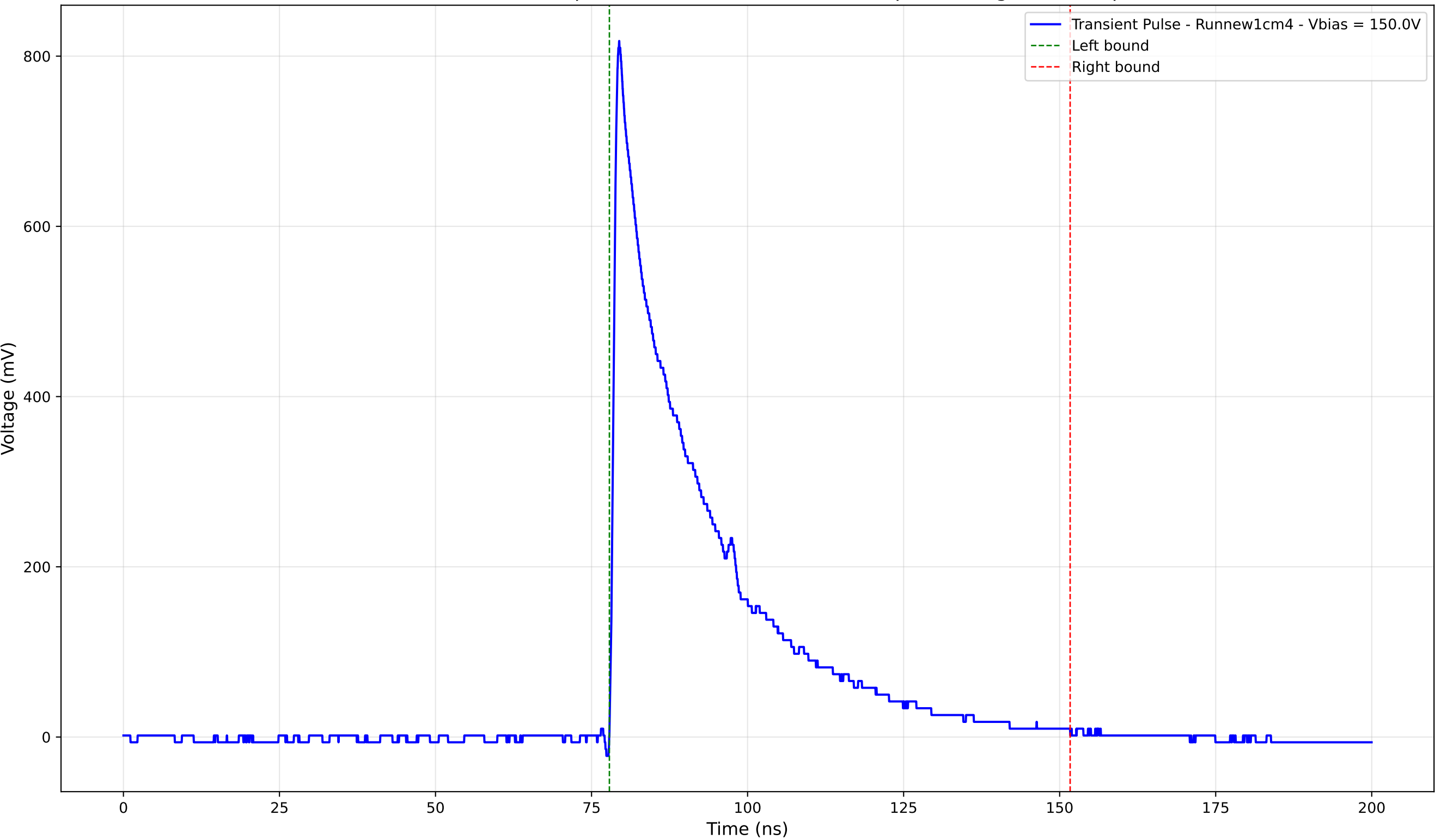
Transient Pulse - Sample: new1cm - Position: 4595.0 \mu\text{m} - Charge: 226.37 pC
