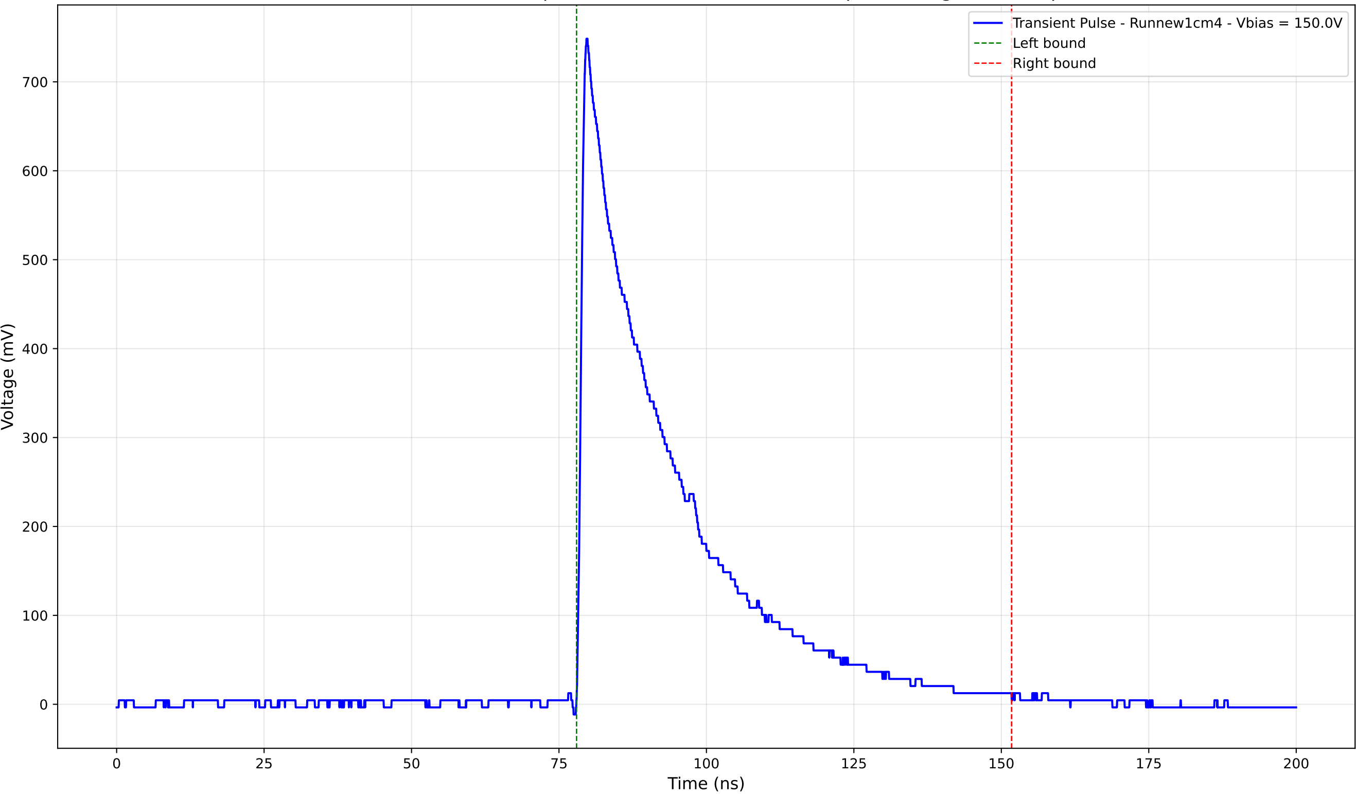
Transient Pulse - Sample: new1cm - Position: 4340.0 \mu\text{m} - Charge: 233.16 pC
