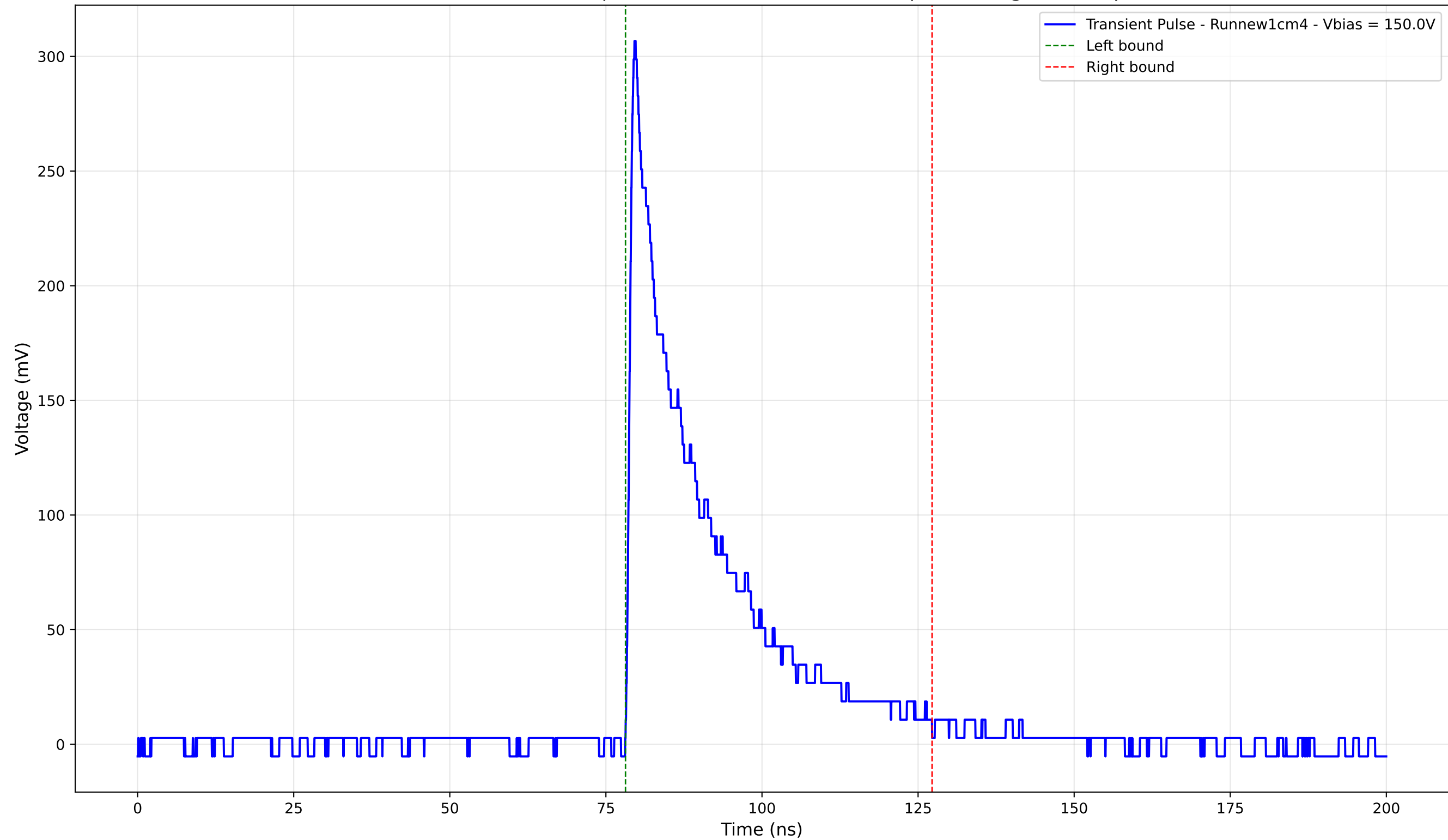
Transient Pulse - Sample: new1cm - Position: 730.0 \mu\text{m} - Charge: 71.00 pC
