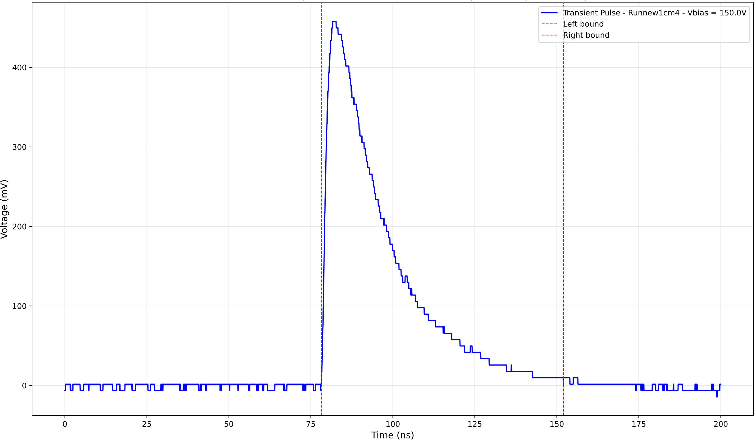
Transient Pulse - Sample: new1cm - Position: 2125.0 \mu\text{m} - Charge: 189.30 pC
