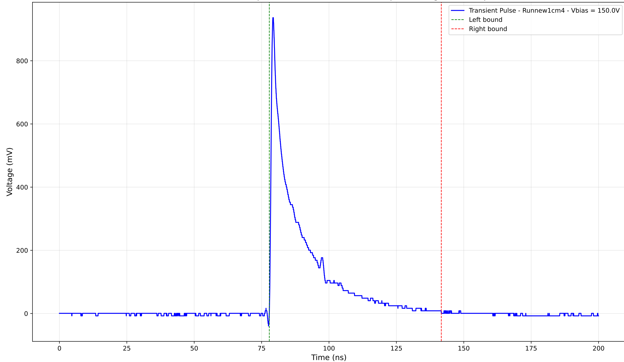
Transient Pulse - Sample: new1cm - Position: 310.0 \mu\text{m} - Charge: 177.52 pC
