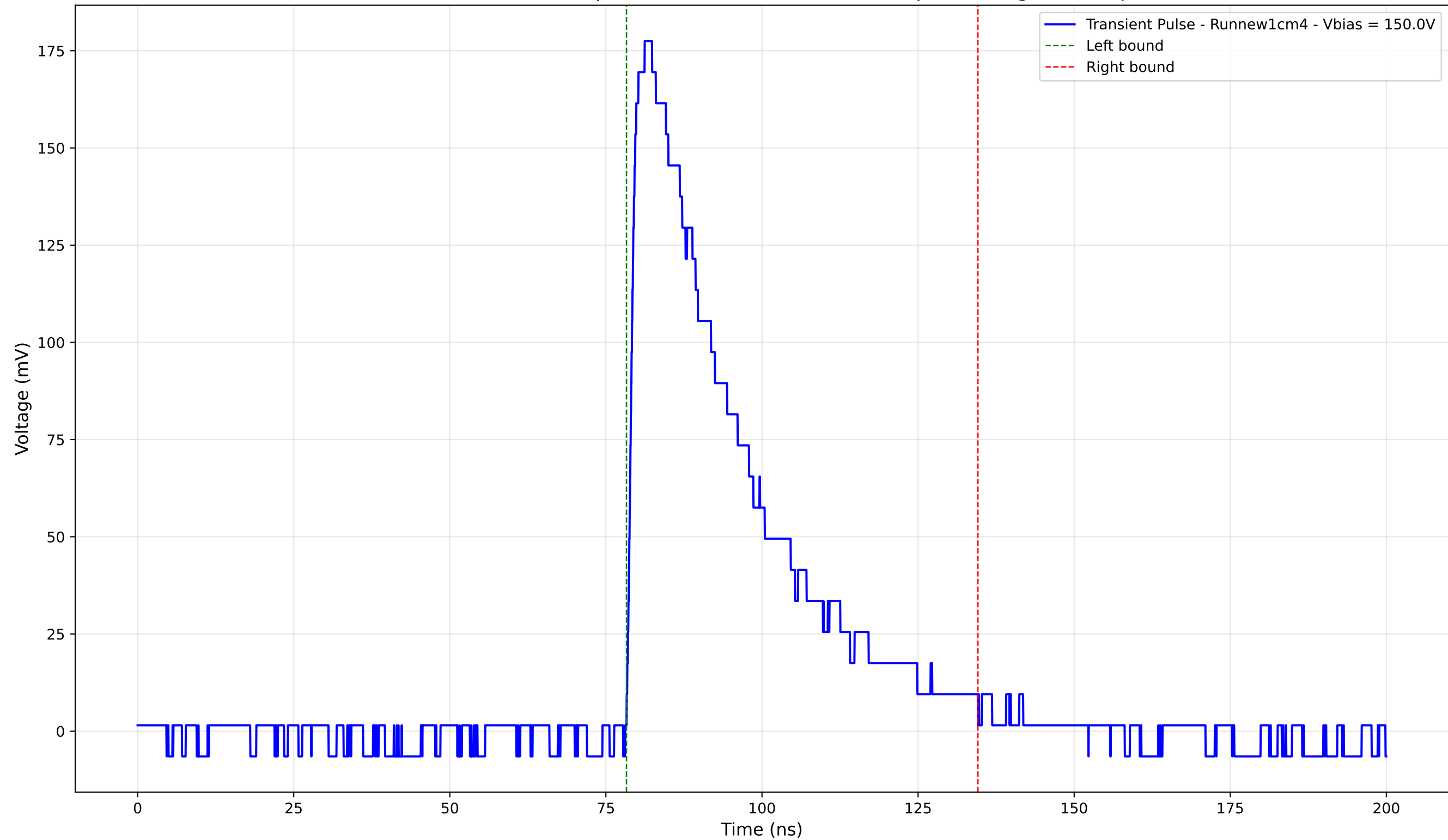
Transient Pulse - Sample: new1cm - Position: 3755.0 \mu\text{m} - Charge: 66.60 pC
