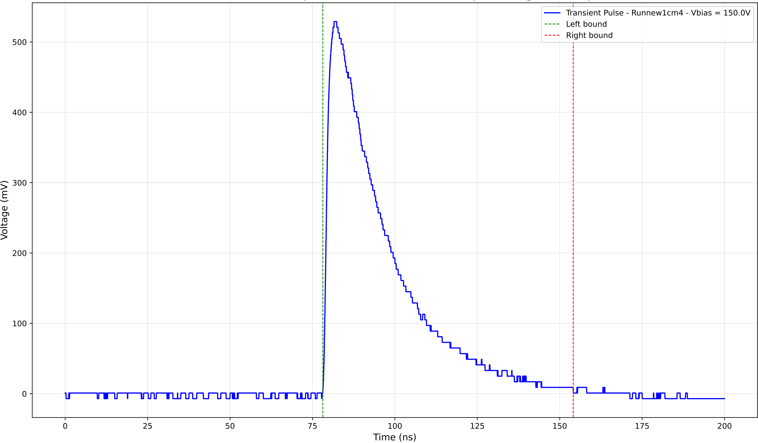
Transient Pulse - Sample: new1cm - Position: 1855.0 \mu\text{m} - Charge: 212.90 pC
