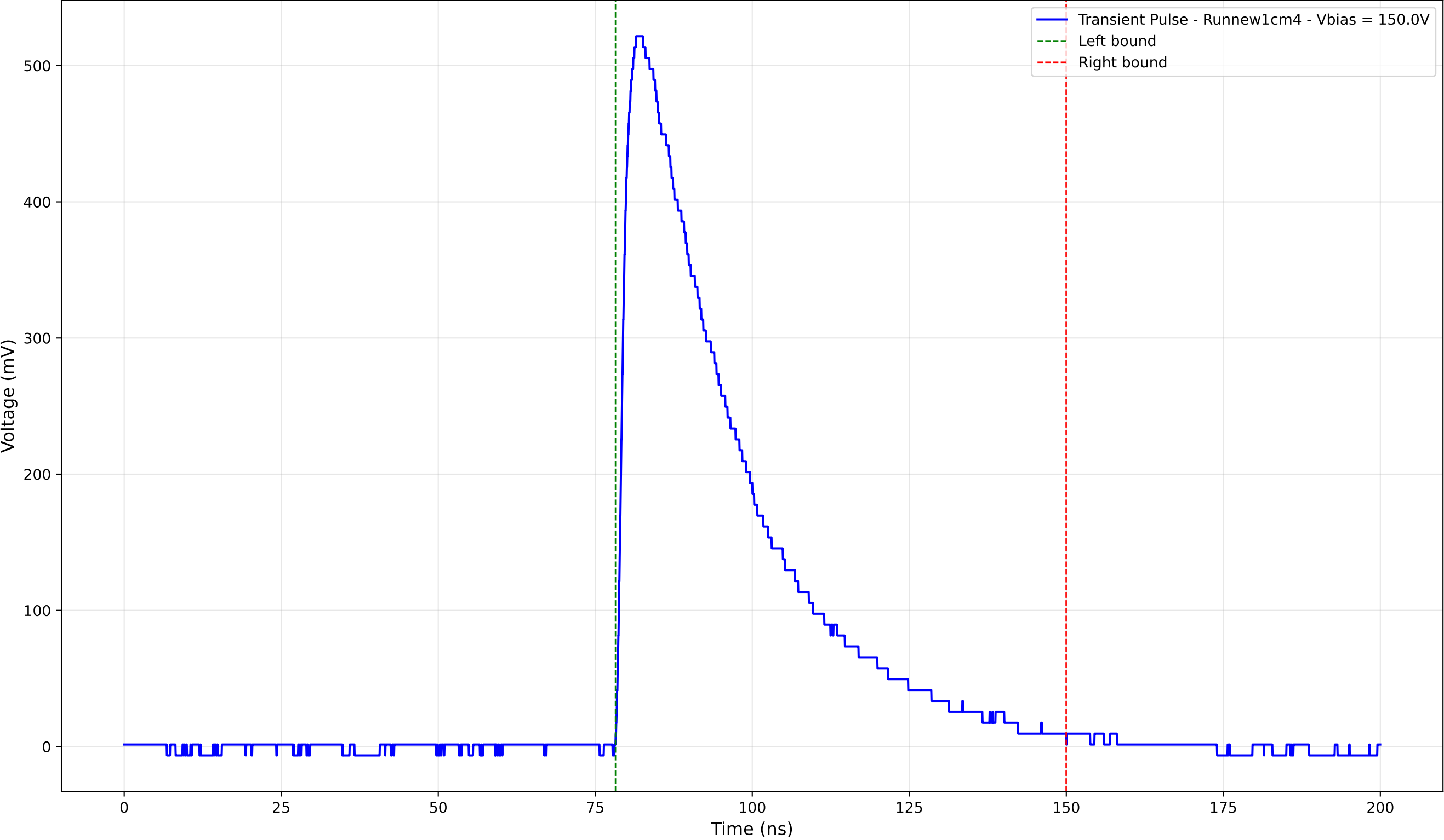
Transient Pulse - Sample: new1cm - Position: 1900.0 \mu\text{m} - Charge: 211.83 pC
