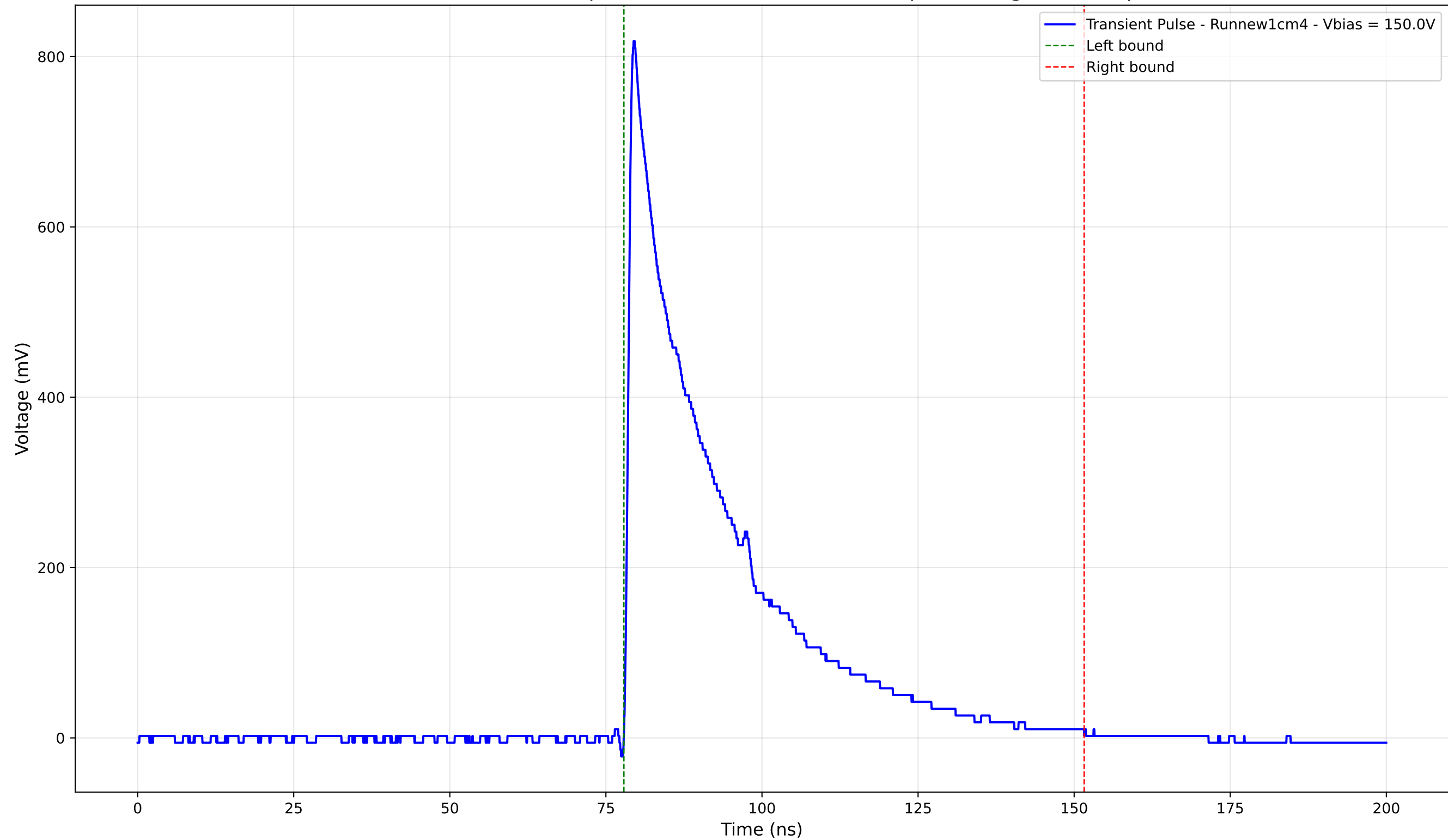
Transient Pulse - Sample: new1cm - Position: 4530.0 \mu\text{m} - Charge: 234.85 pC
