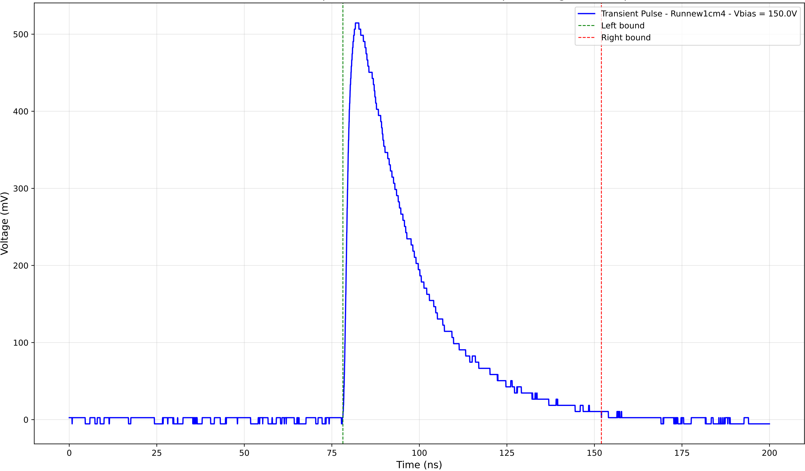
Transient Pulse - Sample: new1cm - Position: 2025.0 \mu\text{m} - Charge: 214.22 pC
