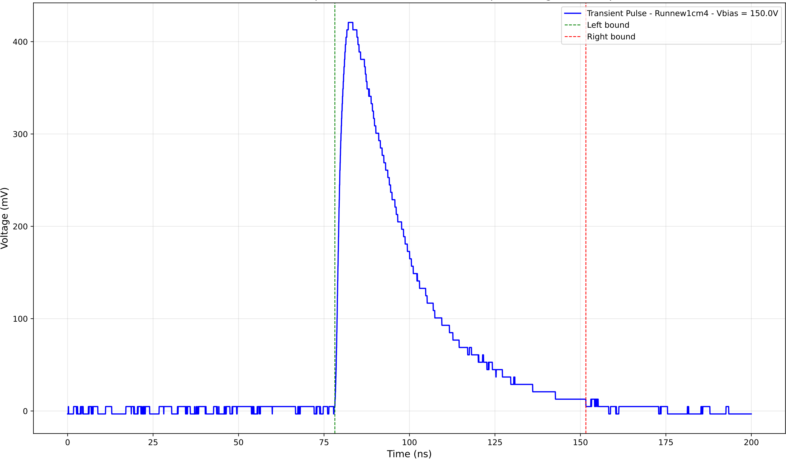
Transient Pulse - Sample: new1cm - Position: 2795.0 \mu\text{m} - Charge: 185.87 pC
