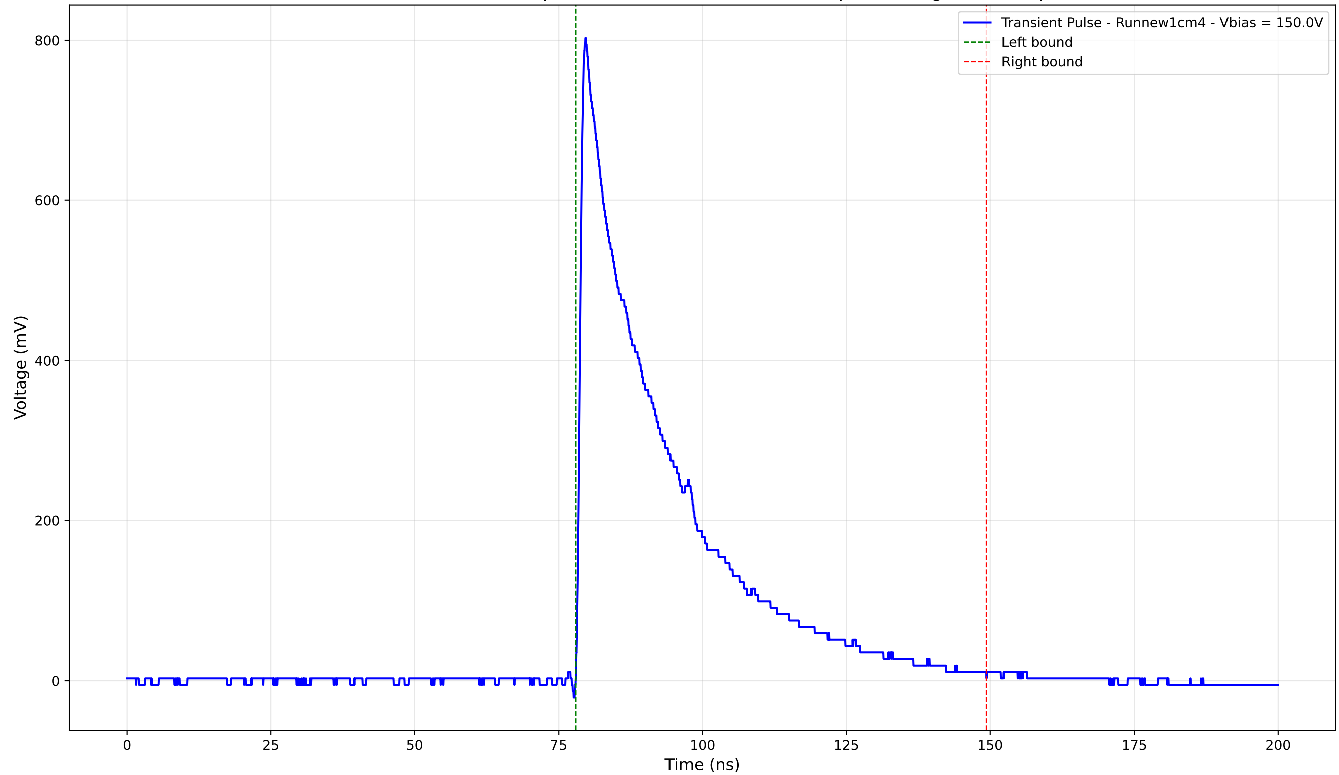
Transient Pulse - Sample: new1cm - Position: 4405.0 \mu\text{m} - Charge: 242.27 pC
