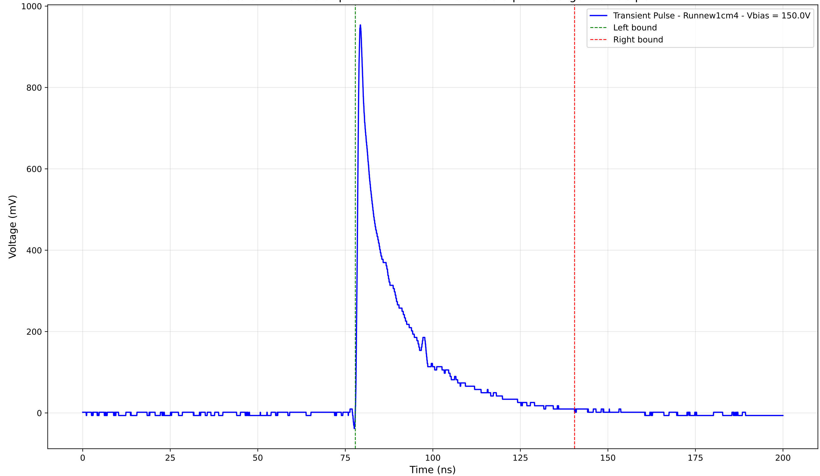
Transient Pulse - Sample: new1cm - Position: 350.0 \mu\text{m} - Charge: 191.30 pC
