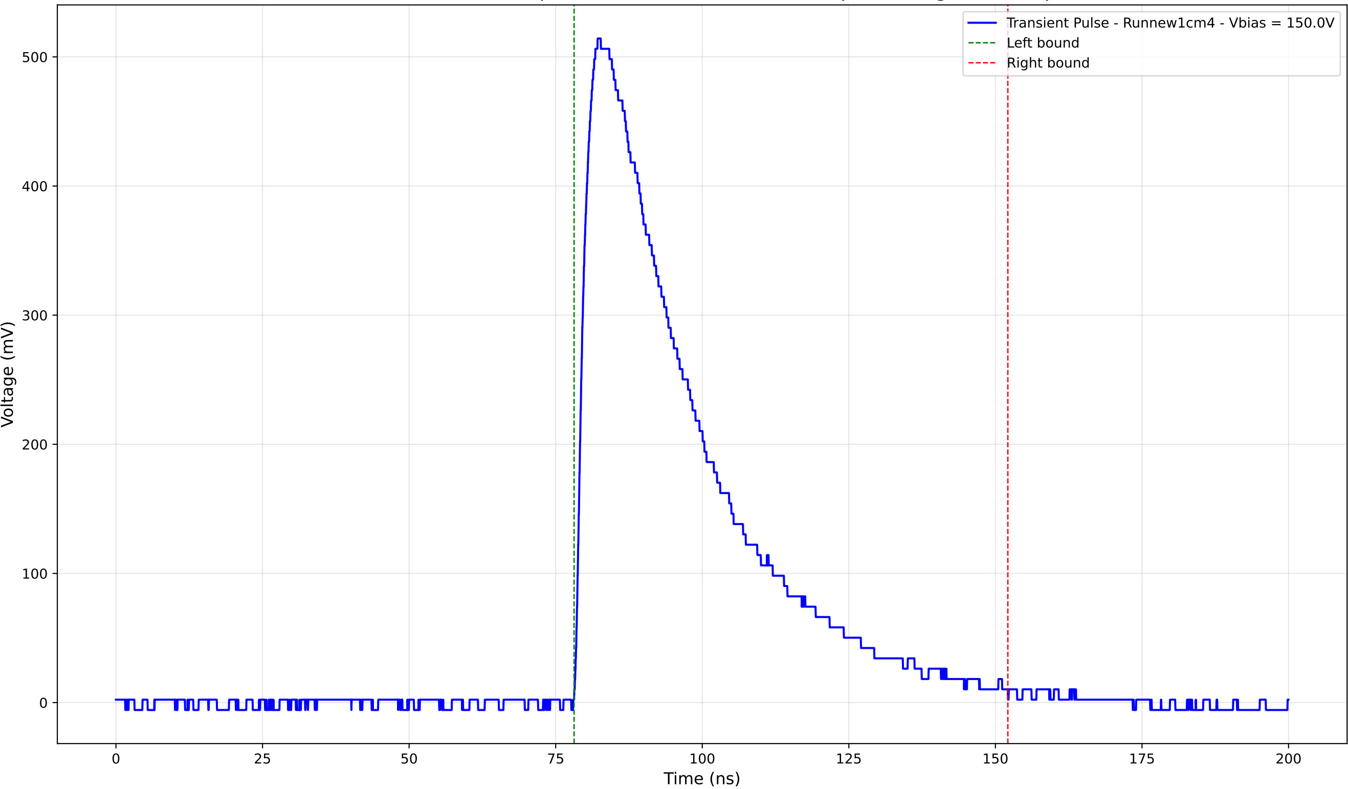
Transient Pulse - Sample: new1cm - Position: 2515.0 \mu\text{m} - Charge: 223.59 pC
