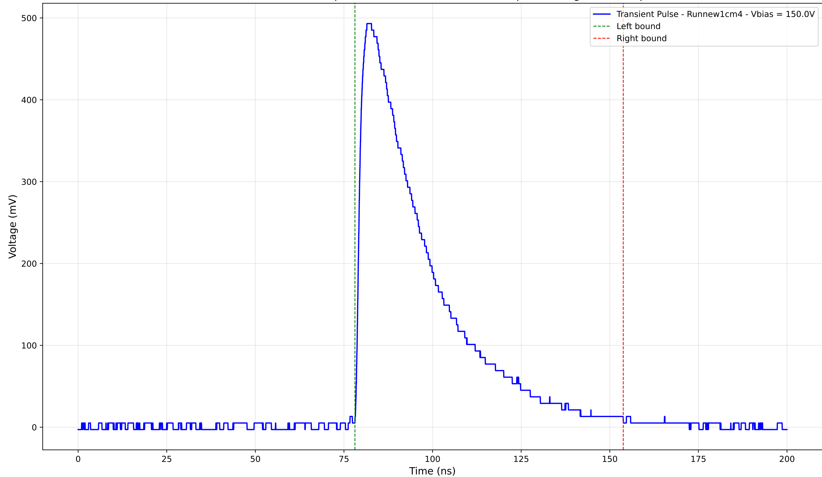
Transient Pulse - Sample: new1cm - Position: 3310.0 \mu\text{m} - Charge: 213.28 pC
