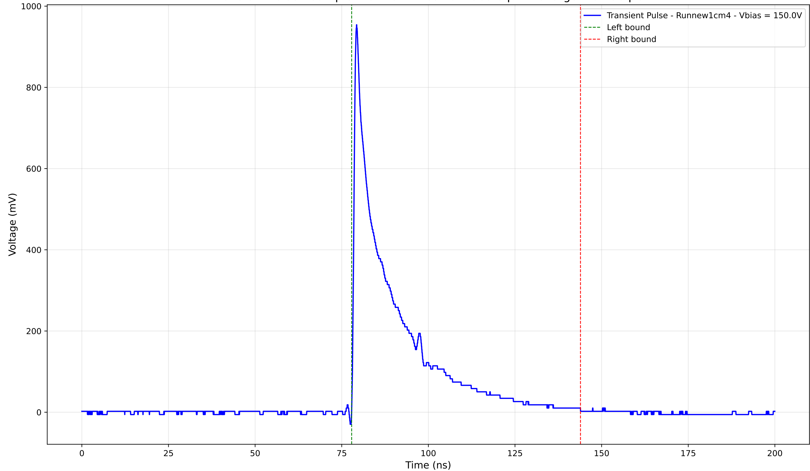
Transient Pulse - Sample: new1cm - Position: 365.0 \mu\text{m} - Charge: 194.38 pC
