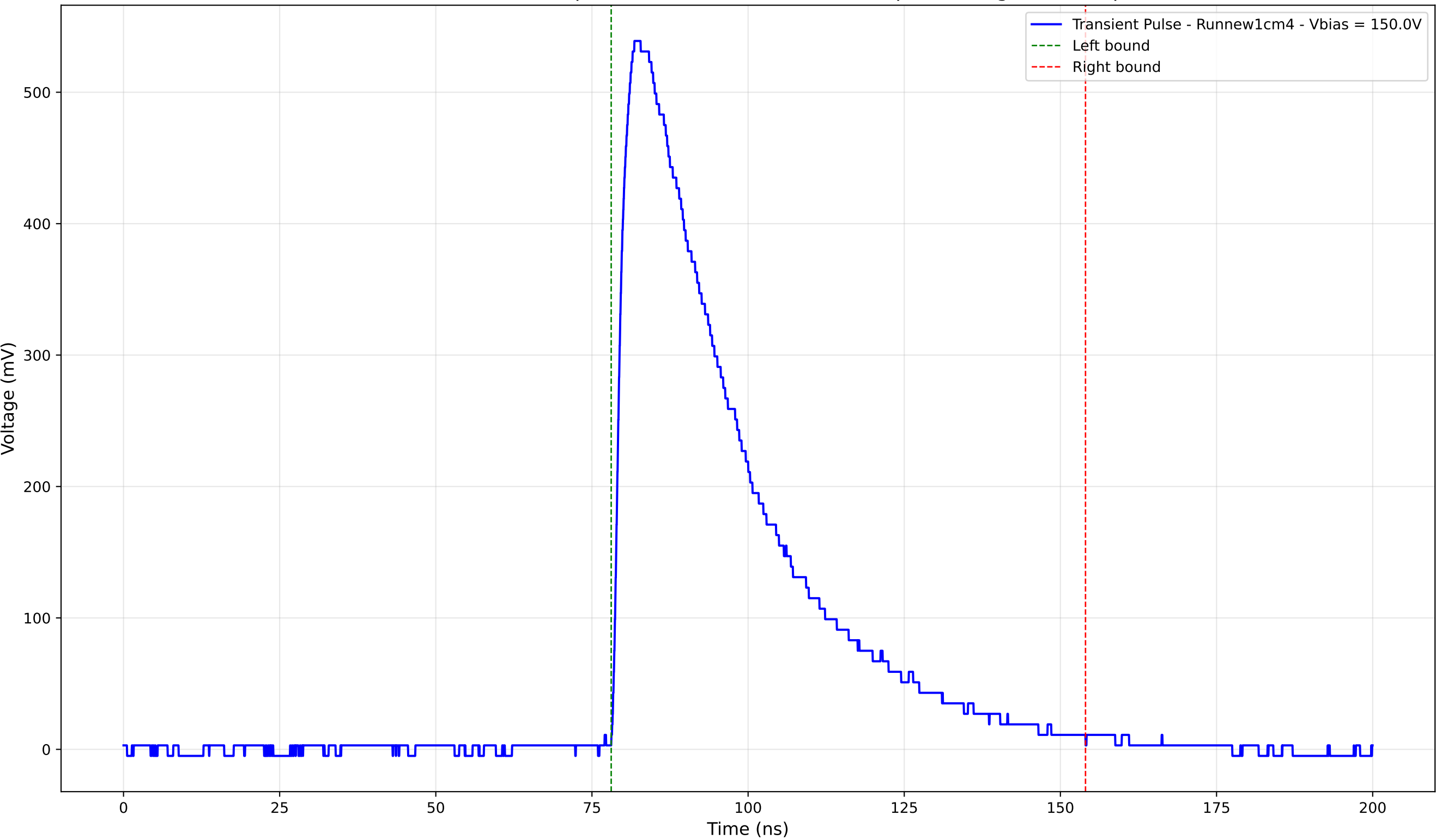
Transient Pulse - Sample: new1cm - Position: 3075.0 \mu\text{m} - Charge: 236.52 pC
