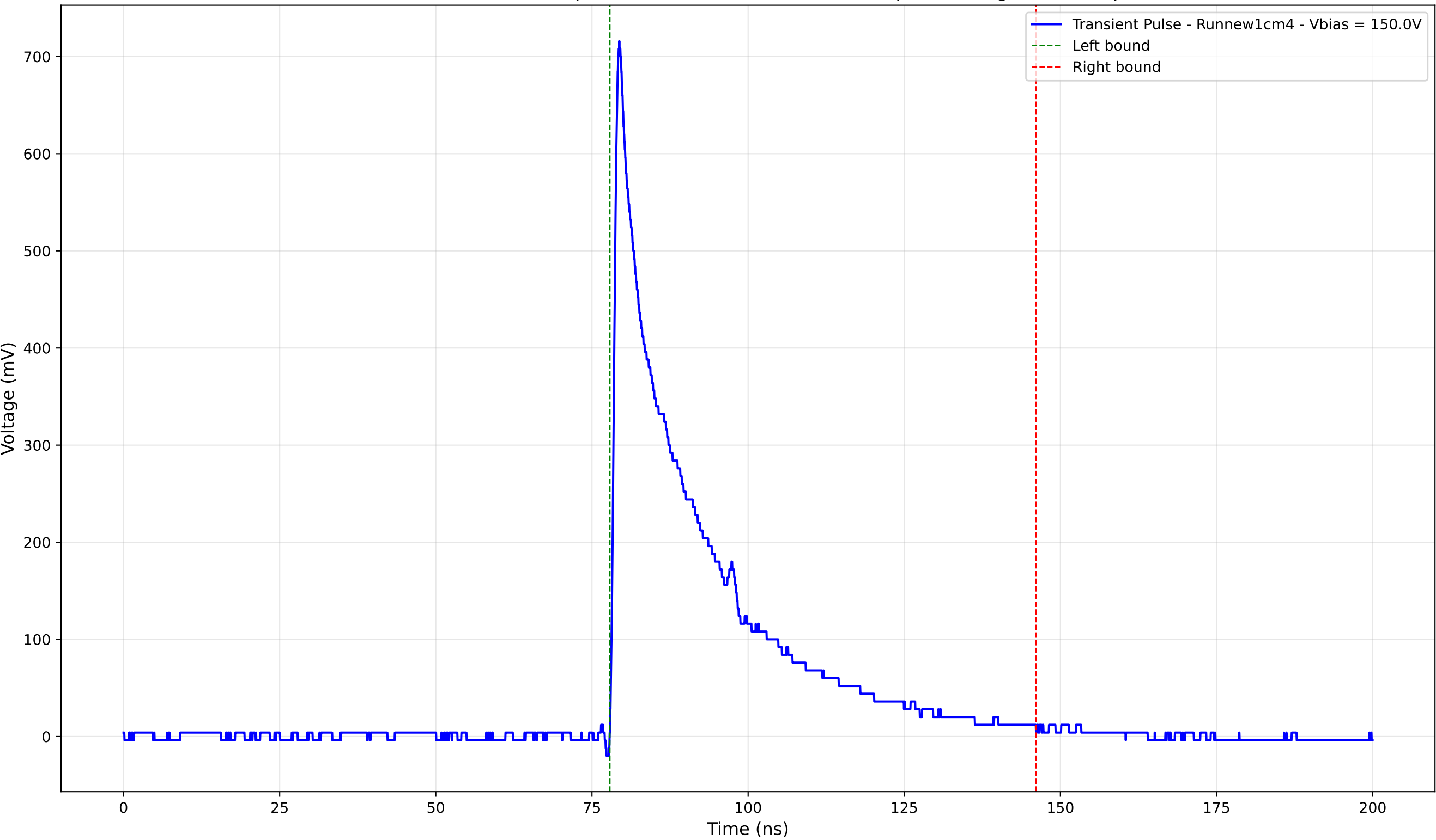
Transient Pulse - Sample: new1cm - Position: 4660.0 \mu\text{m} - Charge: 174.61 pC
