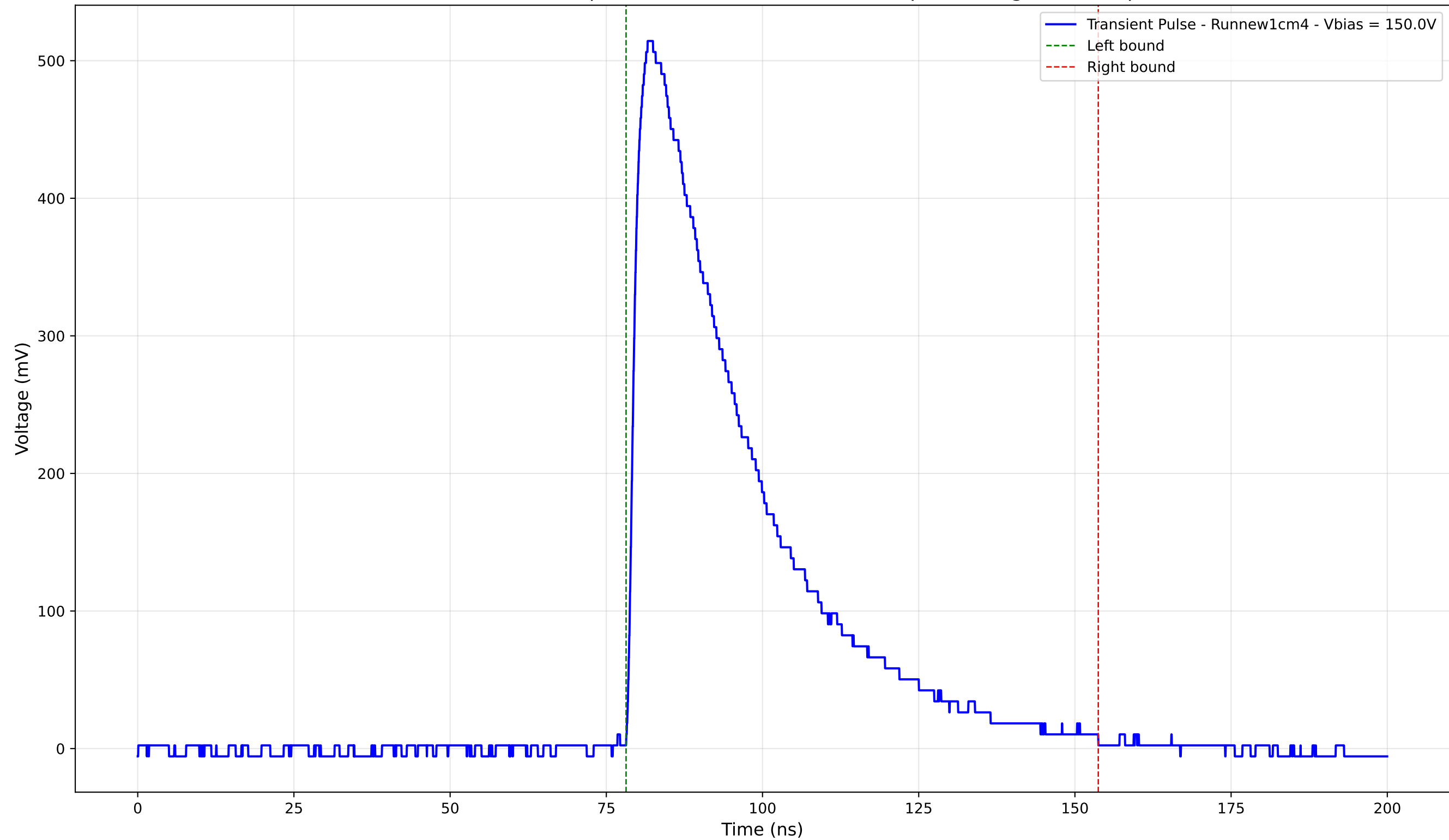
Transient Pulse - Sample: new1cm - Position: 1955.0 \mu\text{m} - Charge: 211.39 pC
