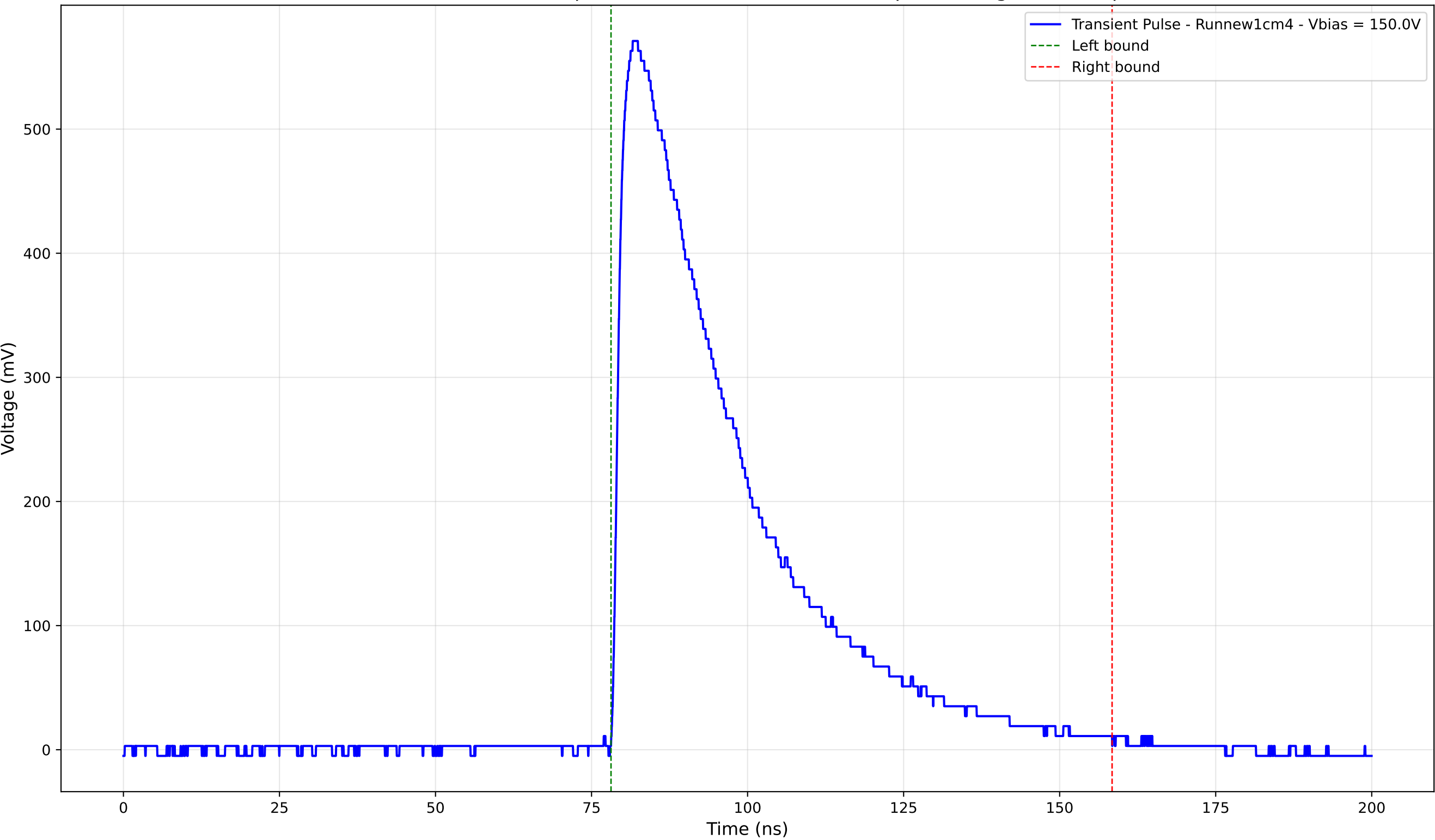
Transient Pulse - Sample: new1cm - Position: 3390.0 \mu\text{m} - Charge: 245.80 pC
