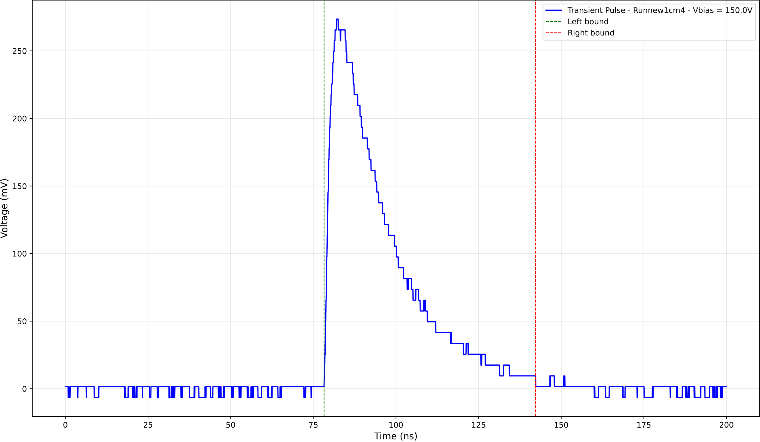
Transient Pulse - Sample: new1cm - Position: 2250.0 \mu\text{m} - Charge: 110.50 pC
