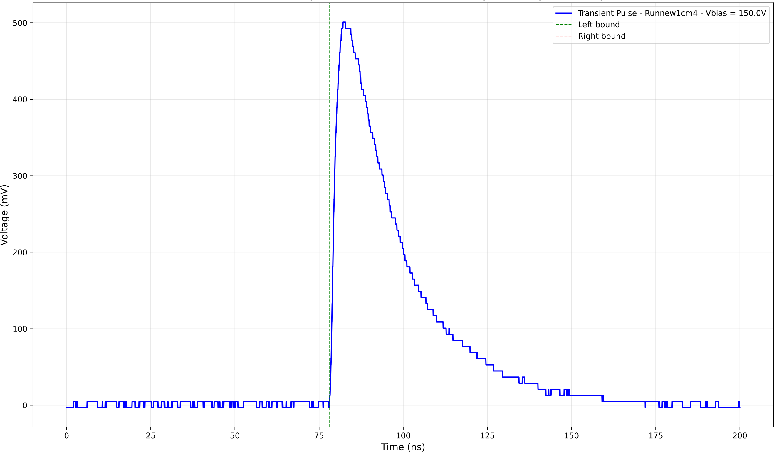
Transient Pulse - Sample: new1cm - Position: 2545.0 \mu\text{m} - Charge: 224.02 pC
