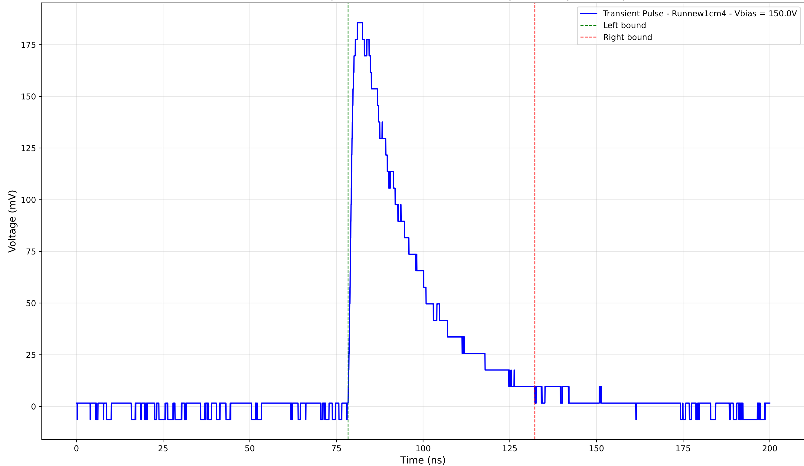
Transient Pulse - Sample: new1cm - Position: 1670.0 \mu\text{m} - Charge: 68.25 pC
