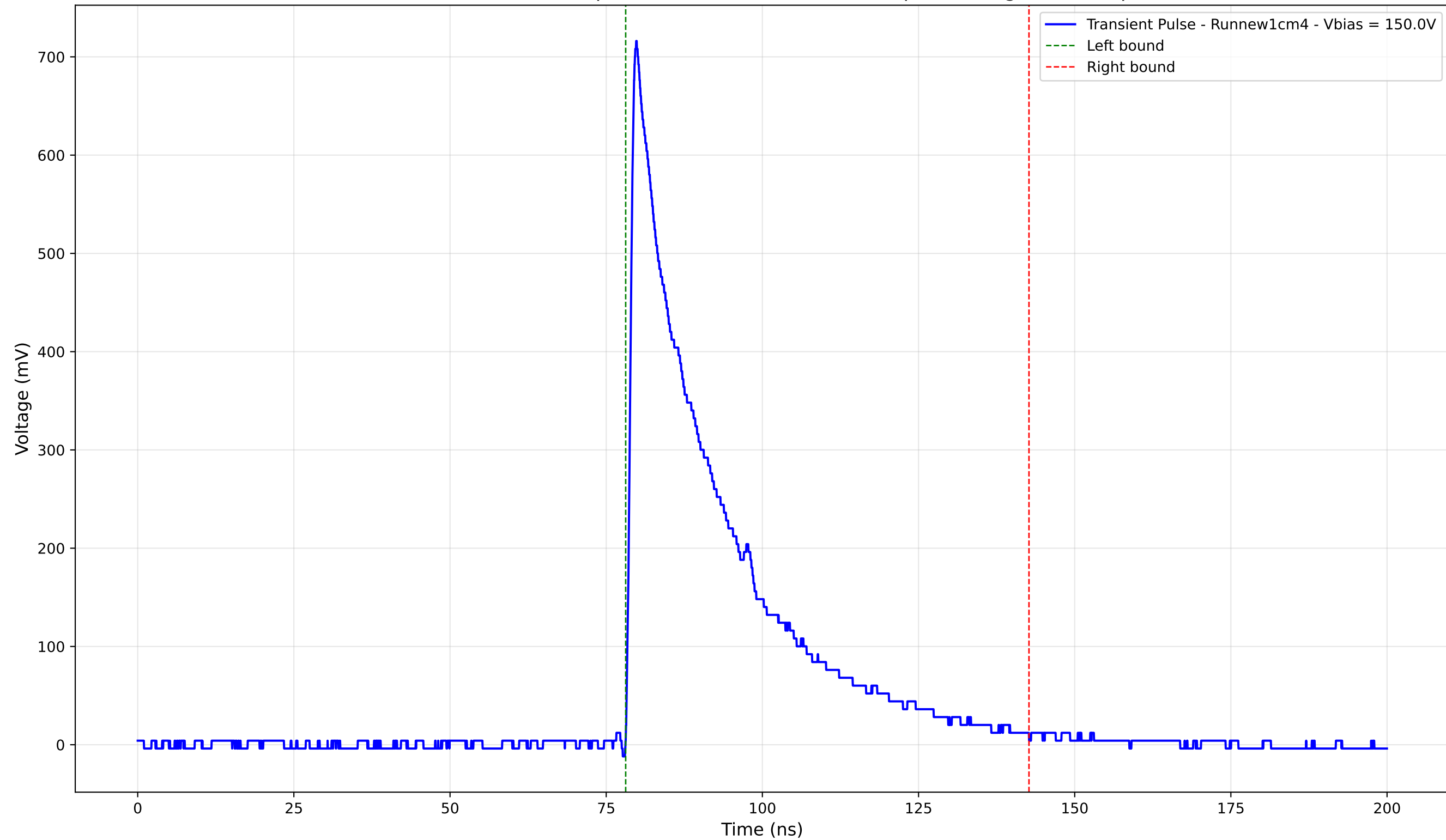
Transient Pulse - Sample: new1cm - Position: 910.0 \mu\text{m} - Charge: 200.10 pC
