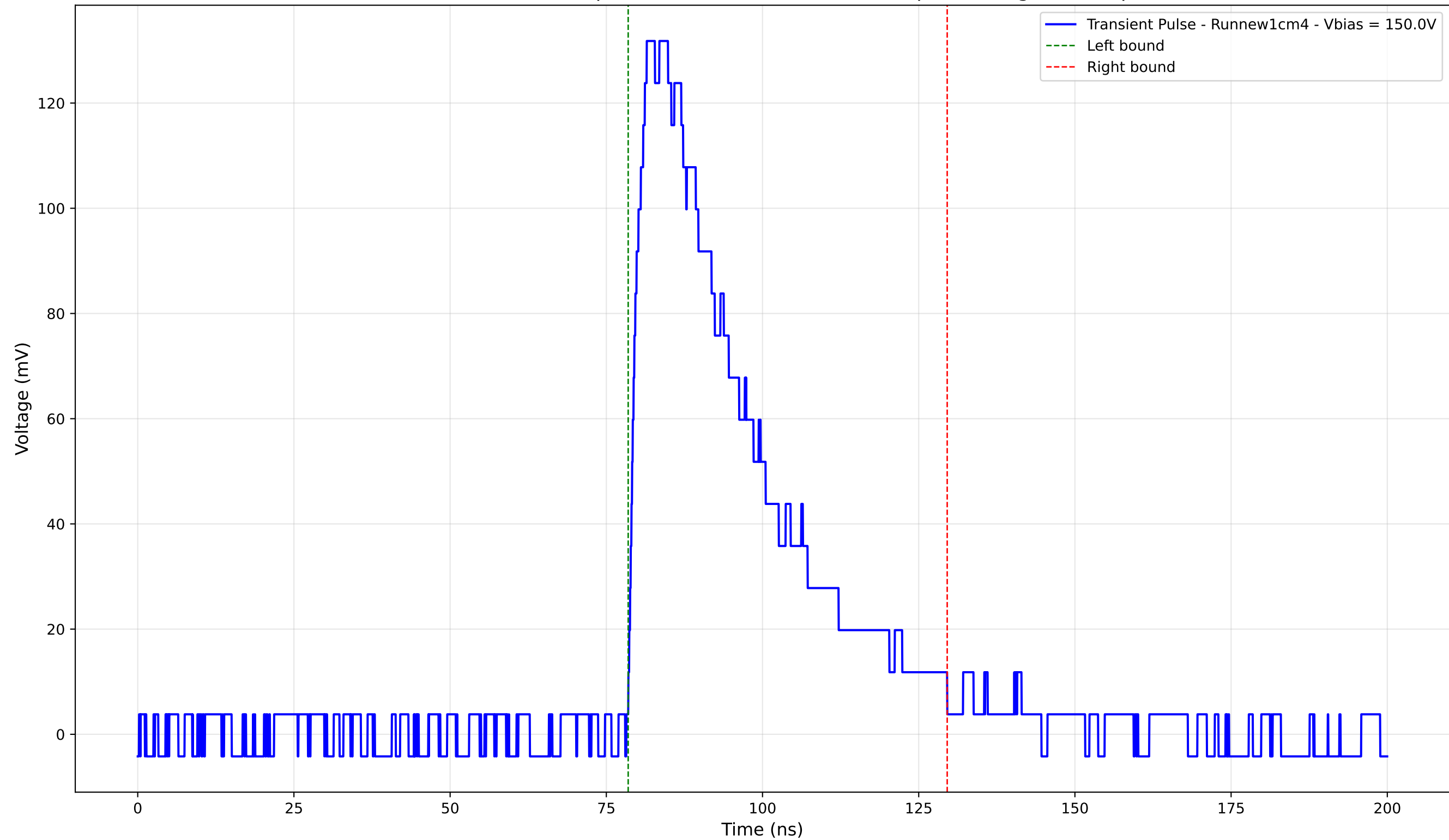
Transient Pulse - Sample: new1cm - Position: 2225.0 \mu\text{m} - Charge: 53.70 pC
