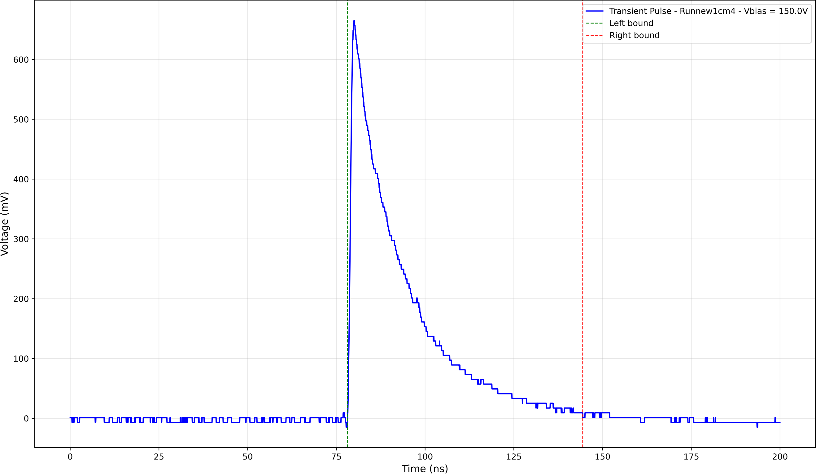
Transient Pulse - Sample: new1cm - Position: 1065.0 \mu\text{m} - Charge: 199.59 pC
