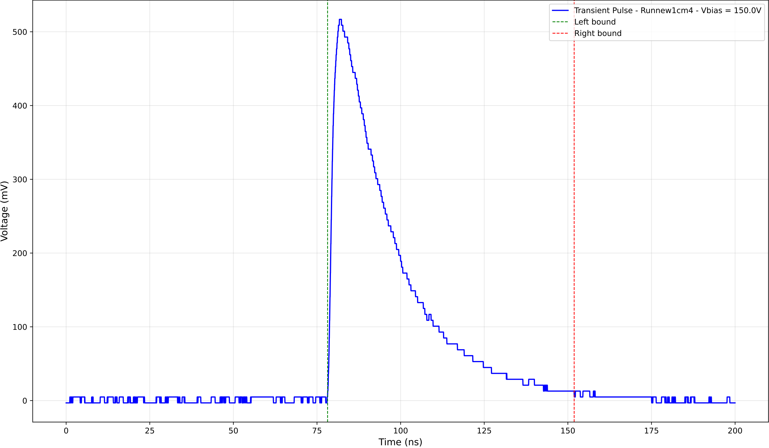
Transient Pulse - Sample: new1cm - Position: 2000.0 \mu\text{m} - Charge: 213.87 pC
