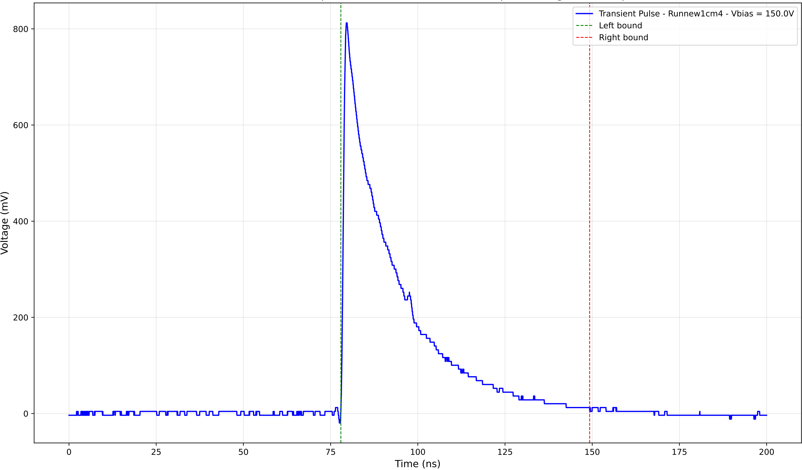
Transient Pulse - Sample: new1cm - Position: 4445.0 \mu\text{m} - Charge: 243.10 pC
