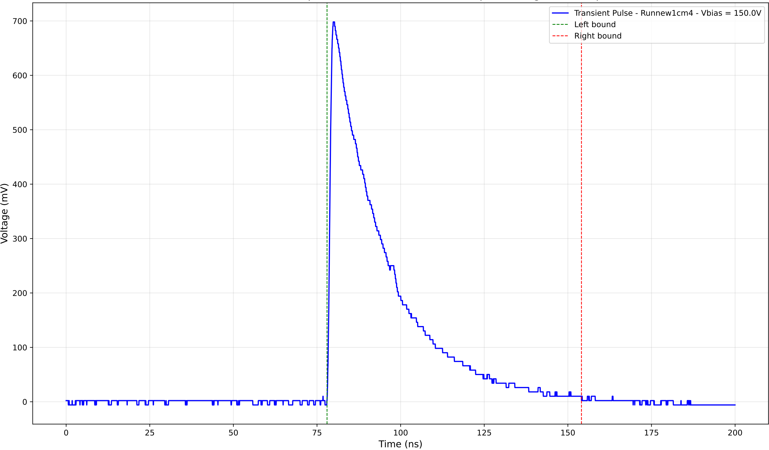
Transient Pulse - Sample: new1cm - Position: 4130.0 \mu\text{m} - Charge: 243.06 pC
