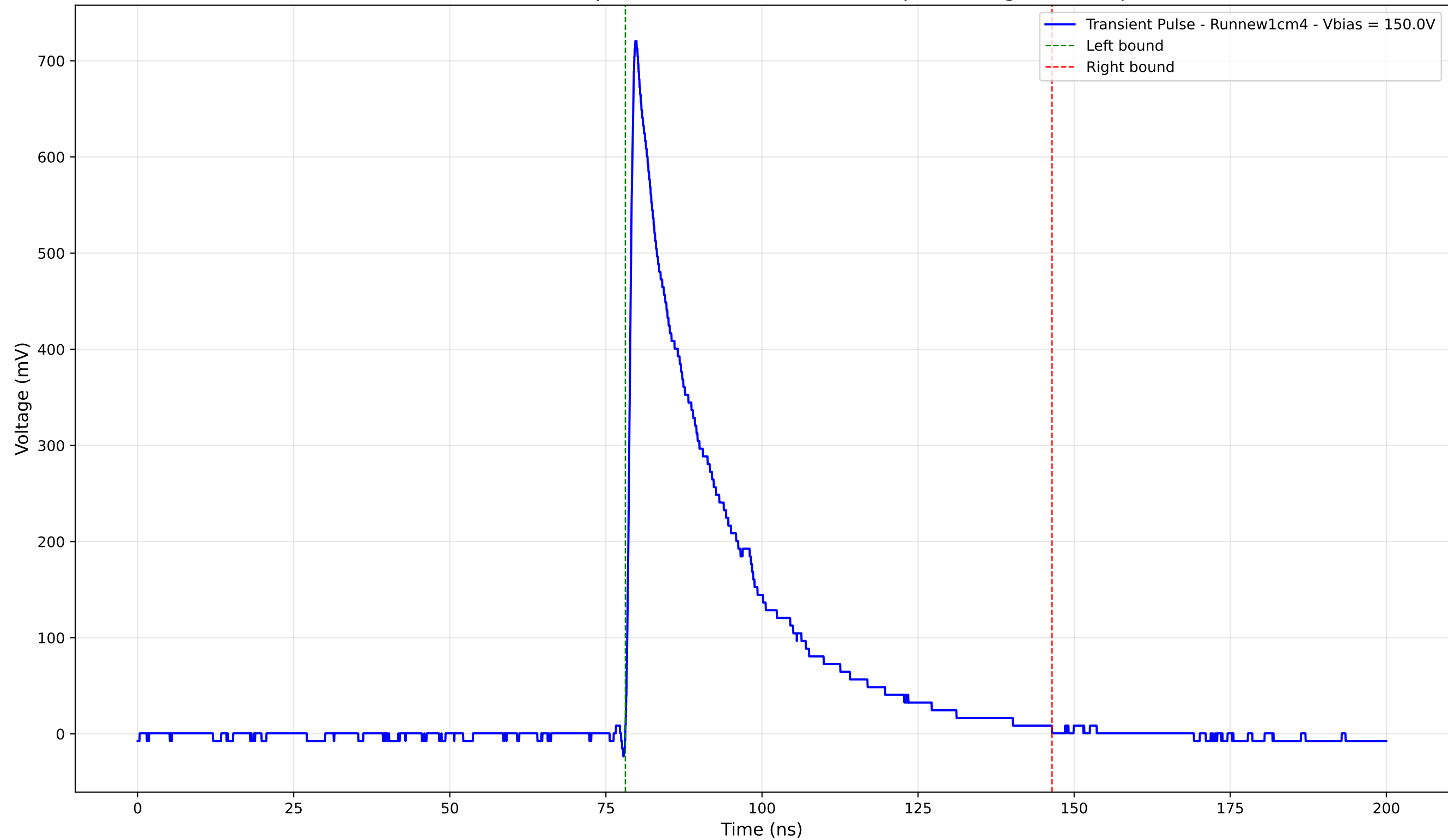
Transient Pulse - Sample: new1cm - Position: 895.0 \mu\text{m} - Charge: 196.85 pC
