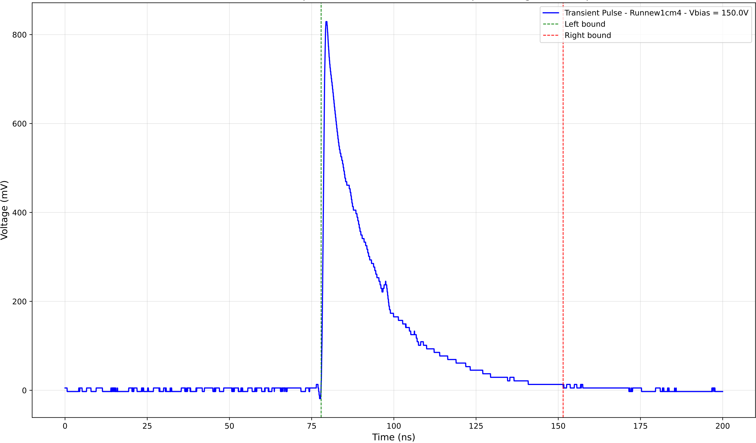
Transient Pulse - Sample: new1cm - Position: 4550.0 \mu\text{m} - Charge: 238.96 pC
