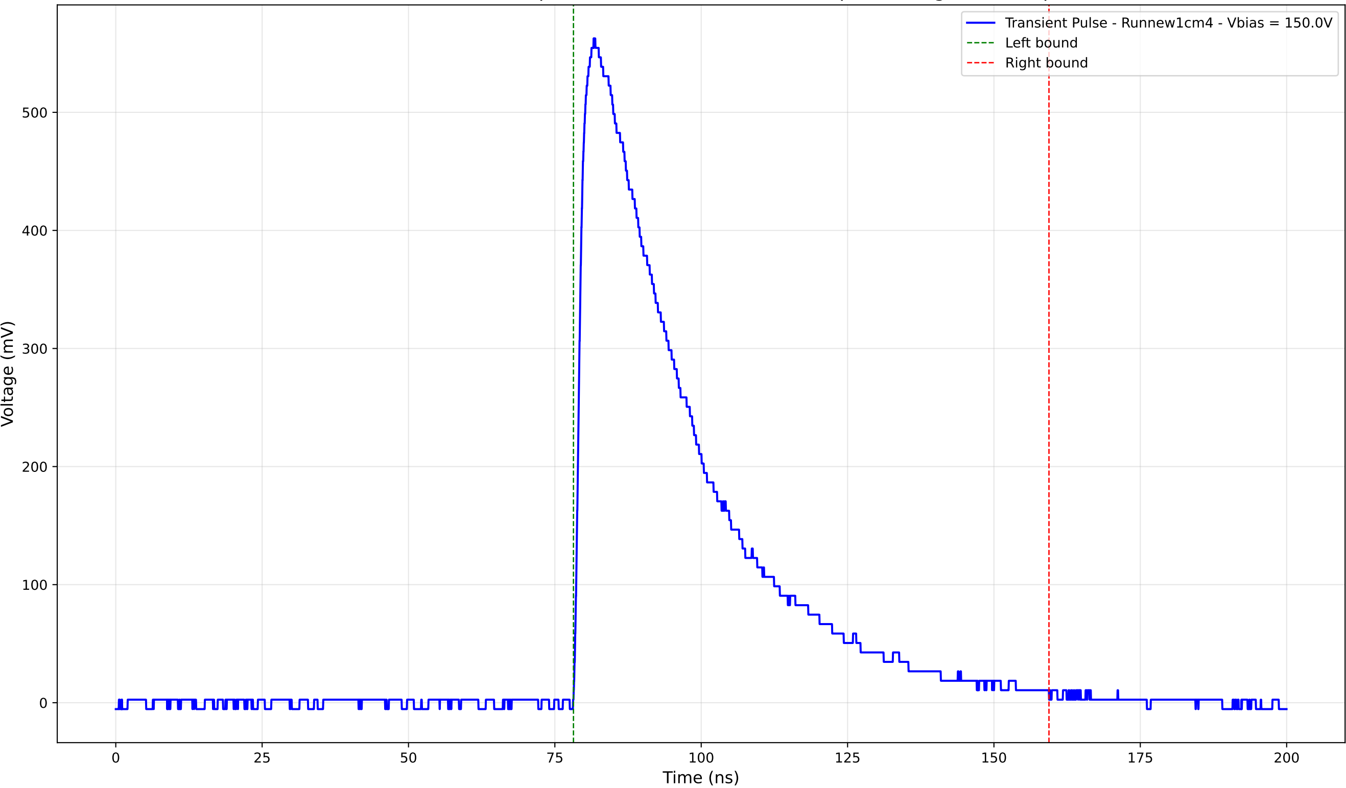
Transient Pulse - Sample: new1cm - Position: 3470.0 \mu\text{m} - Charge: 238.93 pC
