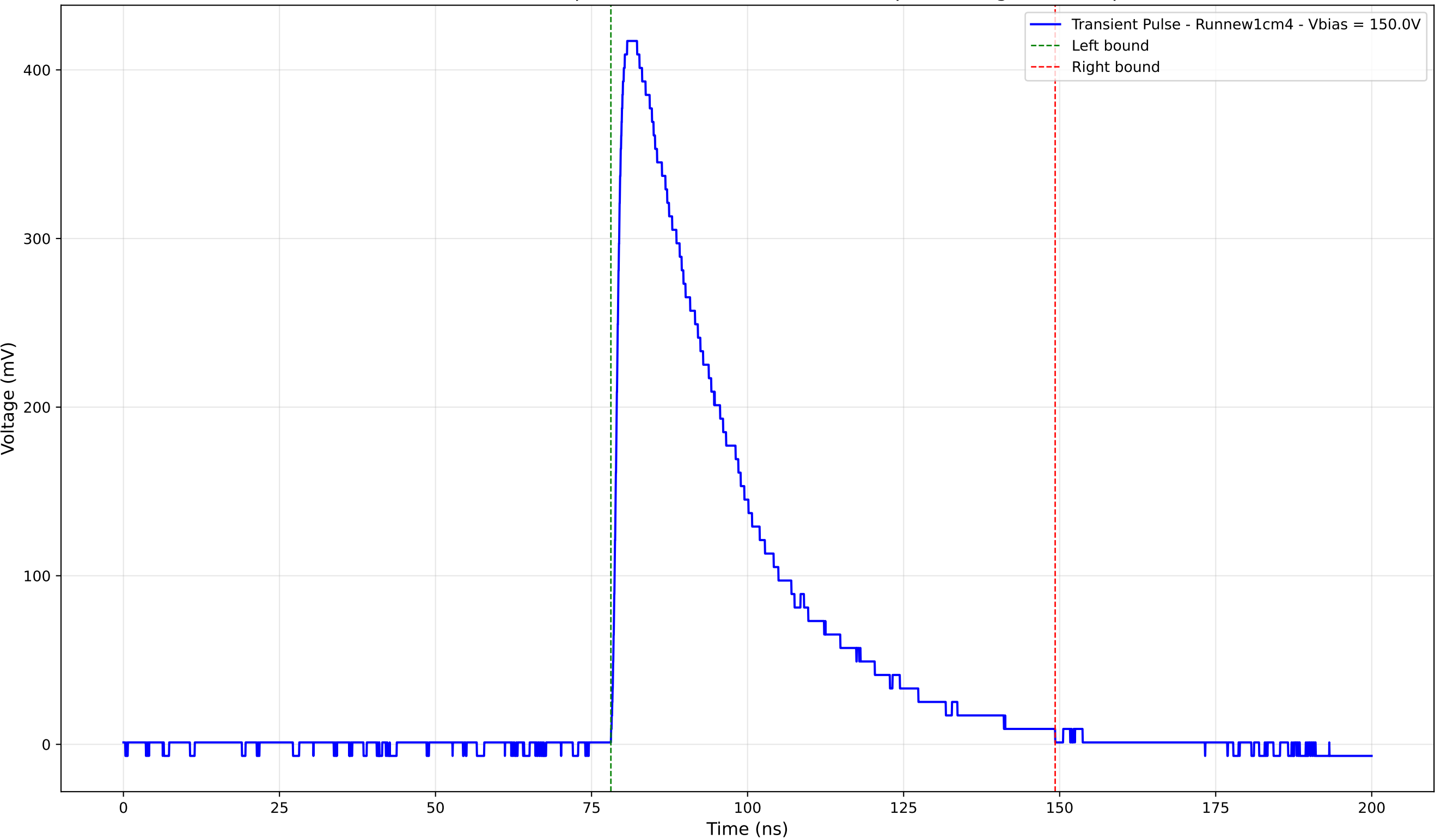
Transient Pulse - Sample: new1cm - Position: 3665.0 \mu\text{m} - Charge: 166.25 pC
