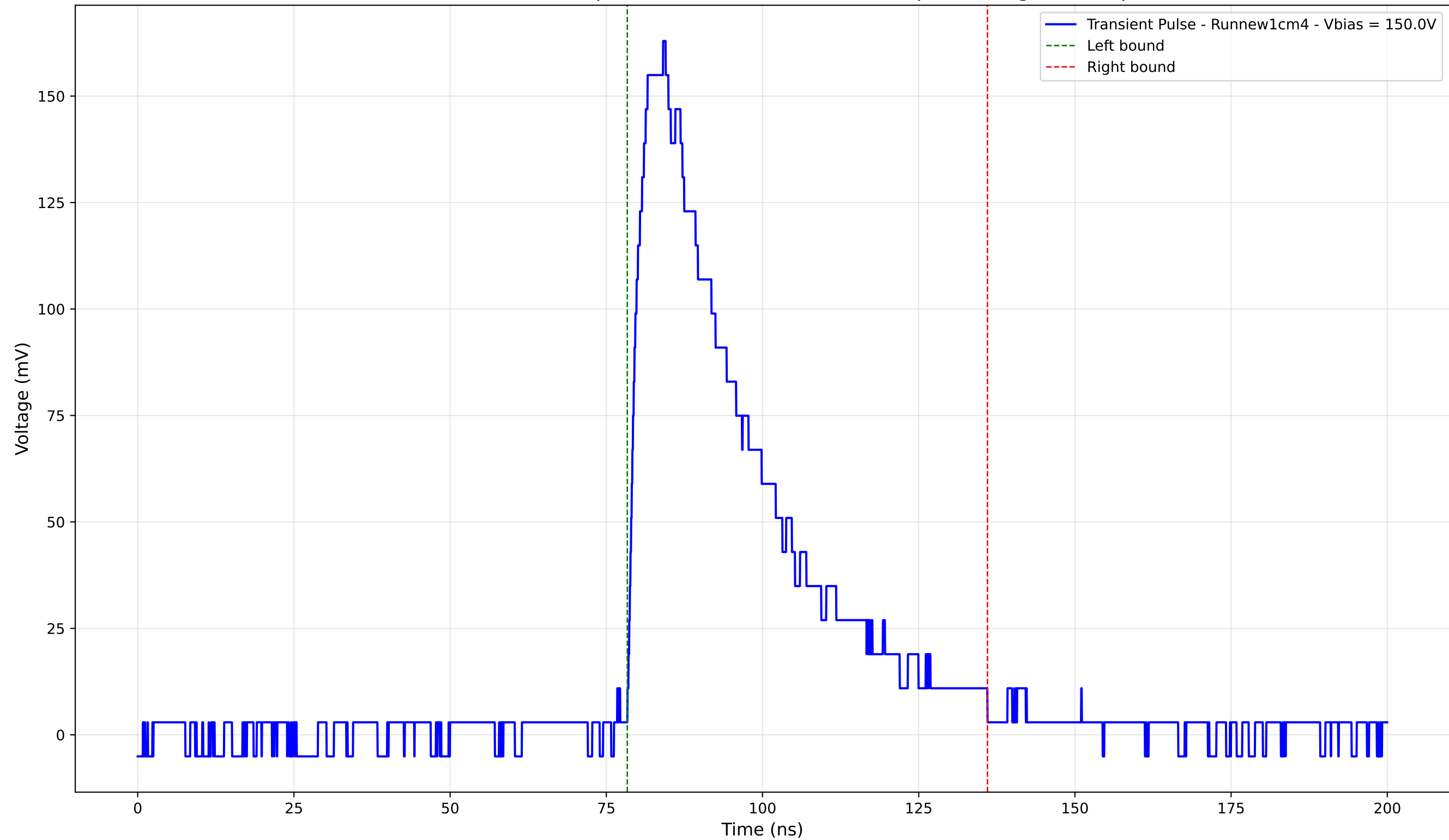
Transient Pulse - Sample: new1cm - Position: 2230.0 \mu\text{m} - Charge: 65.01 pC
