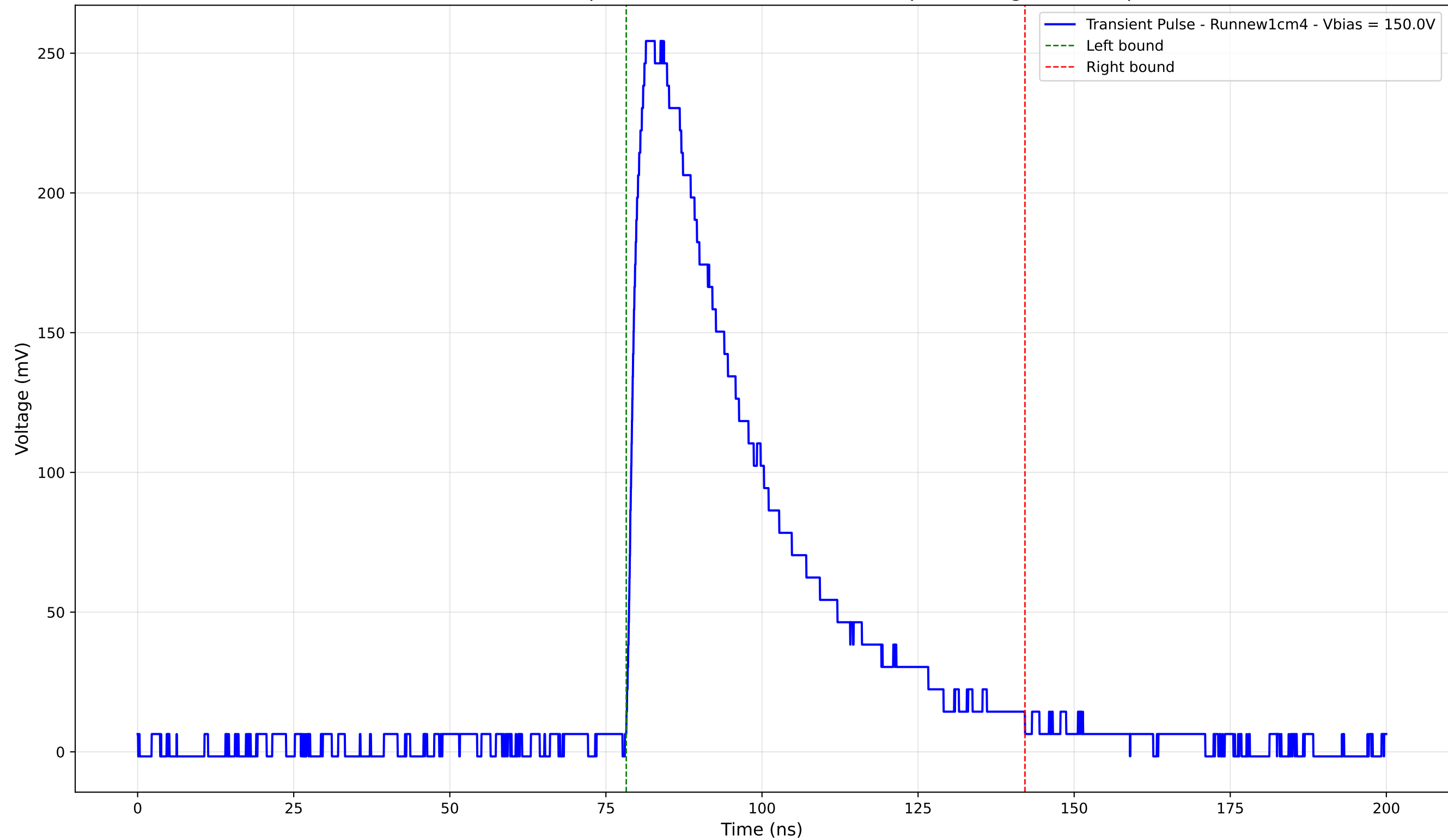
Transient Pulse - Sample: new1cm - Position: 3180.0 \mu\text{m} - Charge: 109.71 pC
