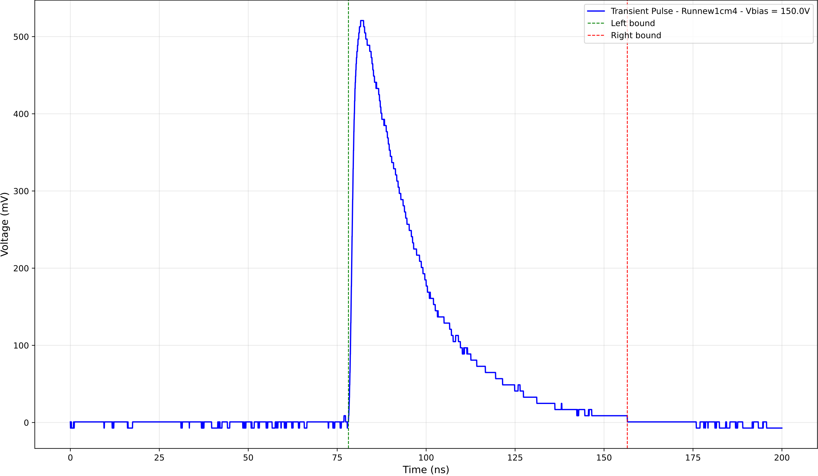
Transient Pulse - Sample: new1cm - Position: 1820.0 \mu\text{m} - Charge: 208.47 pC
