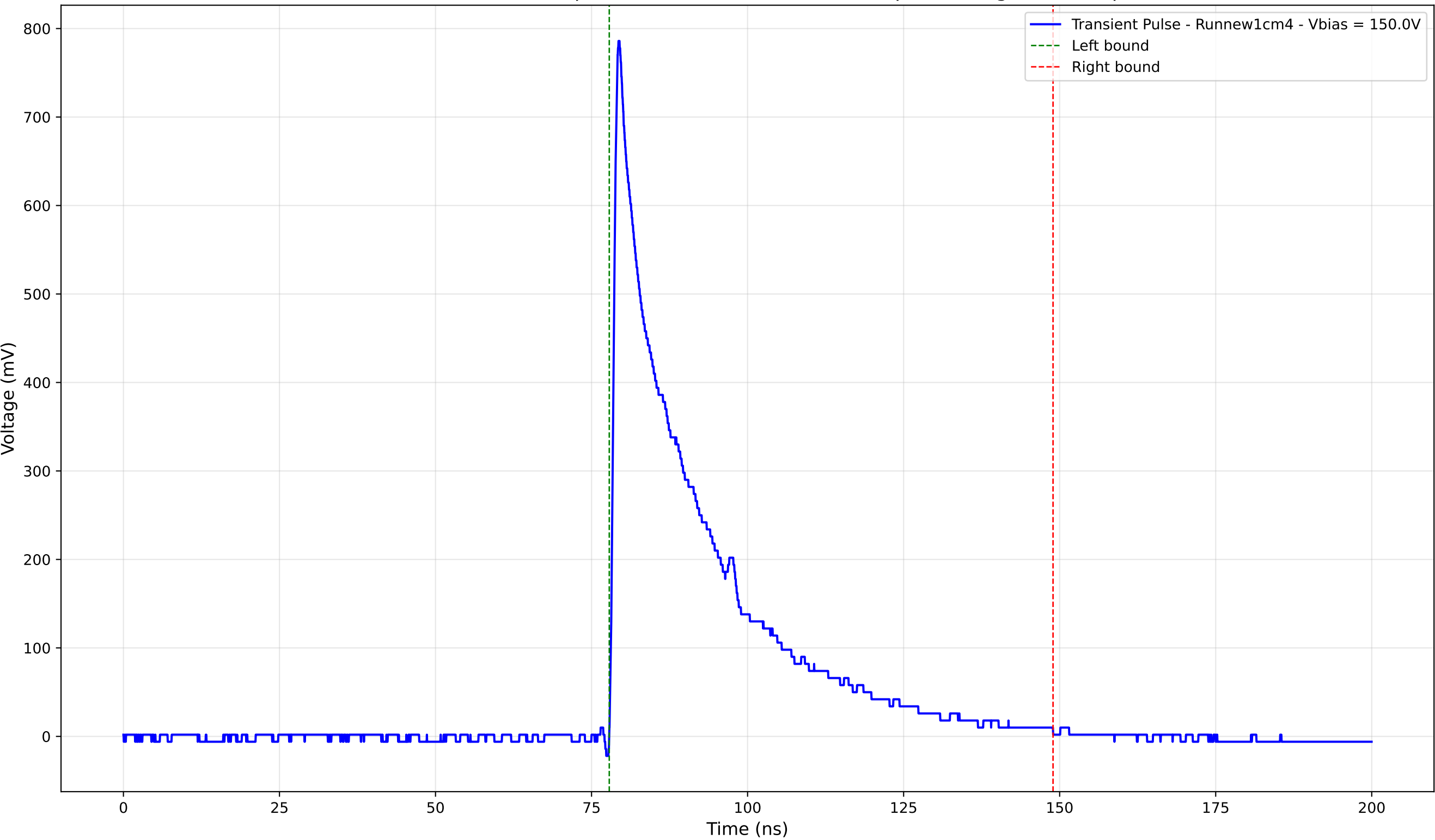
Transient Pulse - Sample: new1cm - Position: 4645.0 \mu\text{m} - Charge: 200.90 pC
