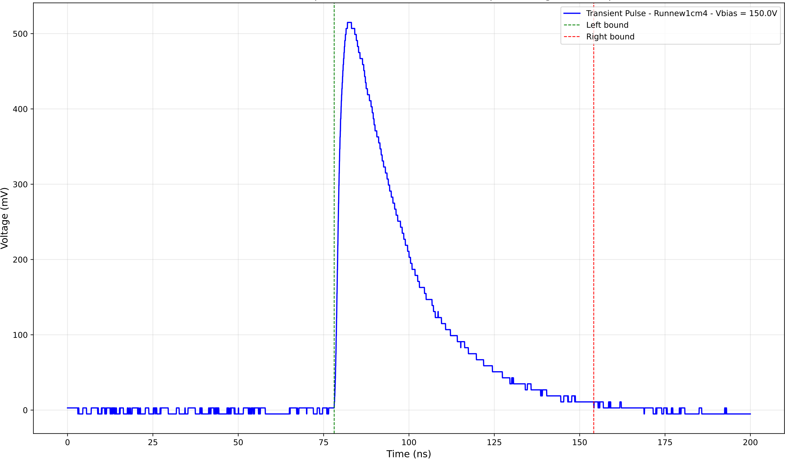
Transient Pulse - Sample: new1cm - Position: 3025.0 \mu\text{m} - Charge: 227.34 pC
