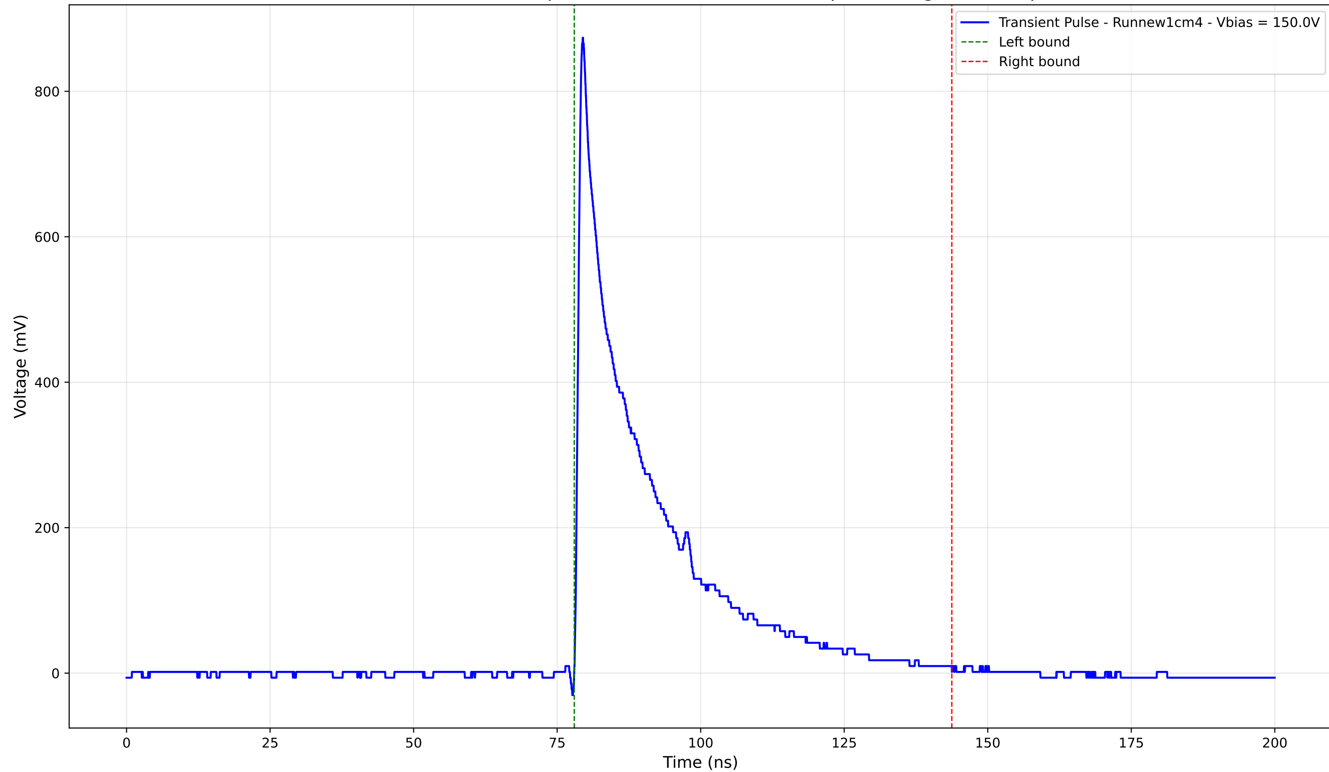
Transient Pulse - Sample: new1cm - Position: 570.0 \mu\text{m} - Charge: 195.37 pC
