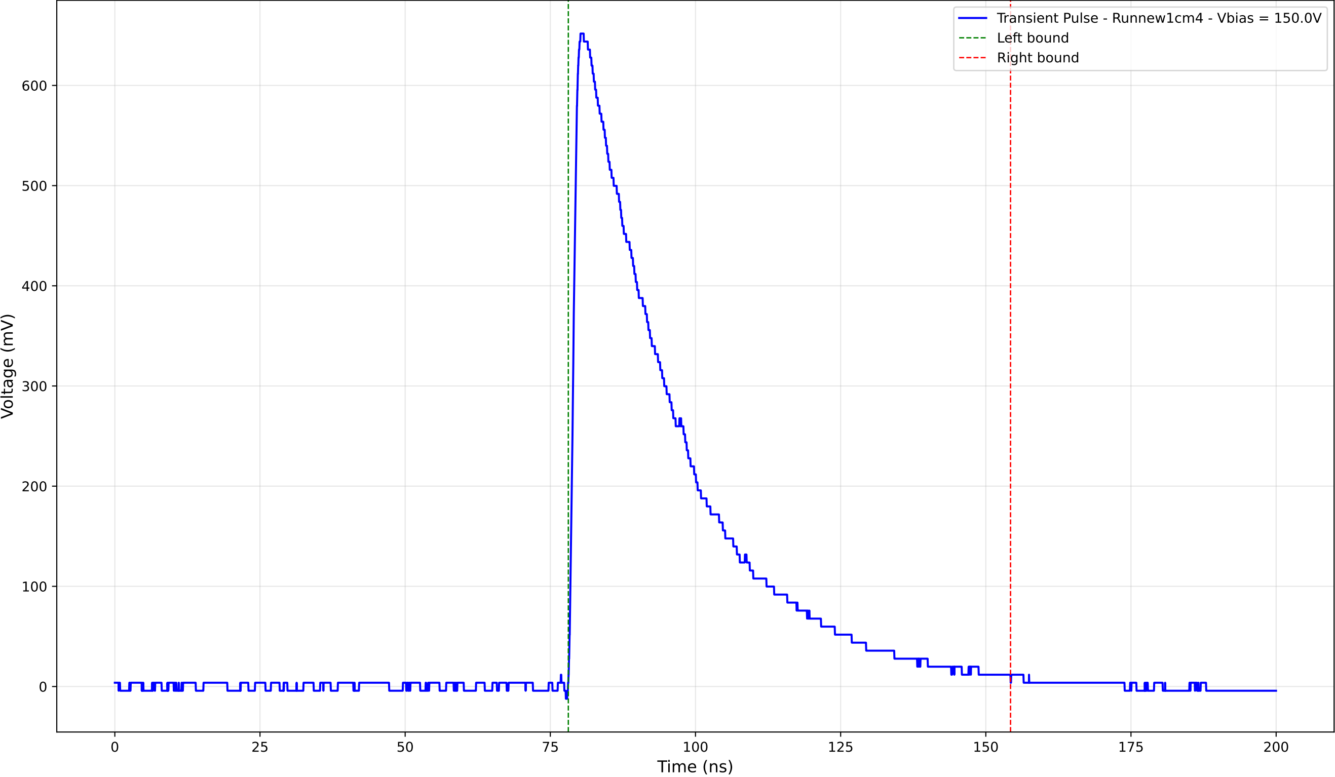
Transient Pulse - Sample: new1cm - Position: 3900.0 \mu\text{m} - Charge: 250.93 pC
