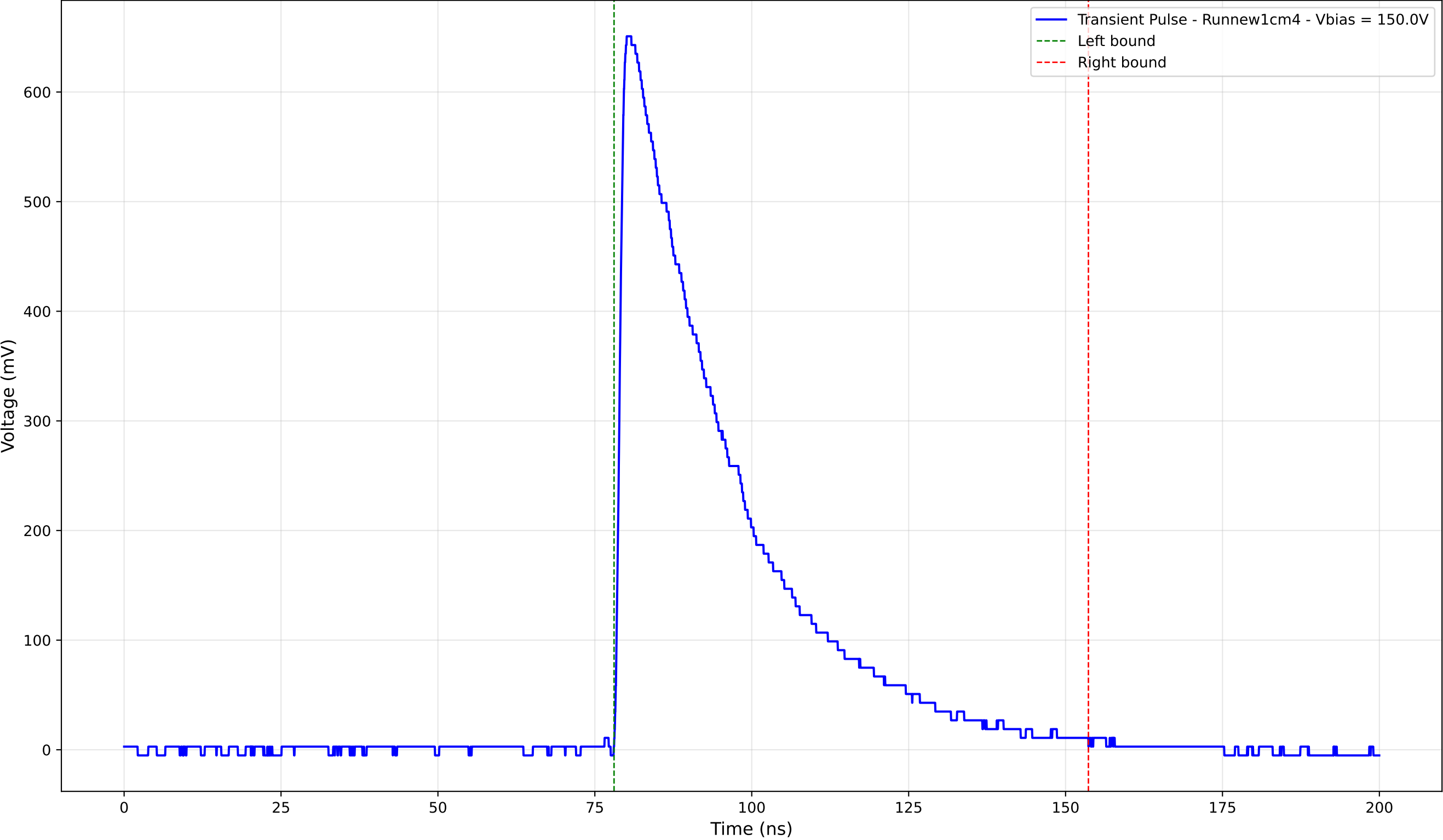
Transient Pulse - Sample: new1cm - Position: 3935.0 \mu\text{m} - Charge: 247.21 pC
