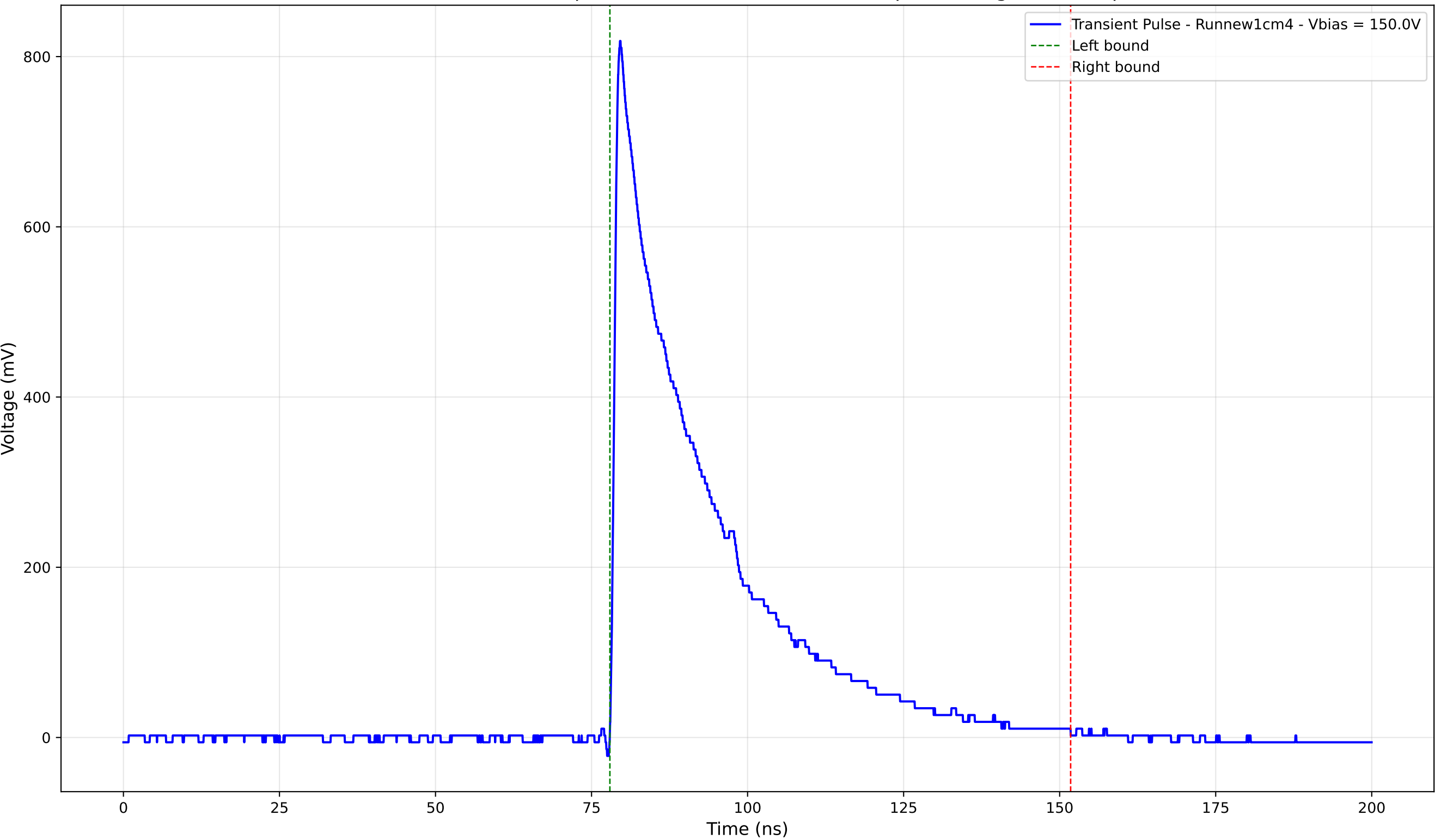
Transient Pulse - Sample: new1cm - Position: 4460.0 \mu\text{m} - Charge: 240.51 pC
