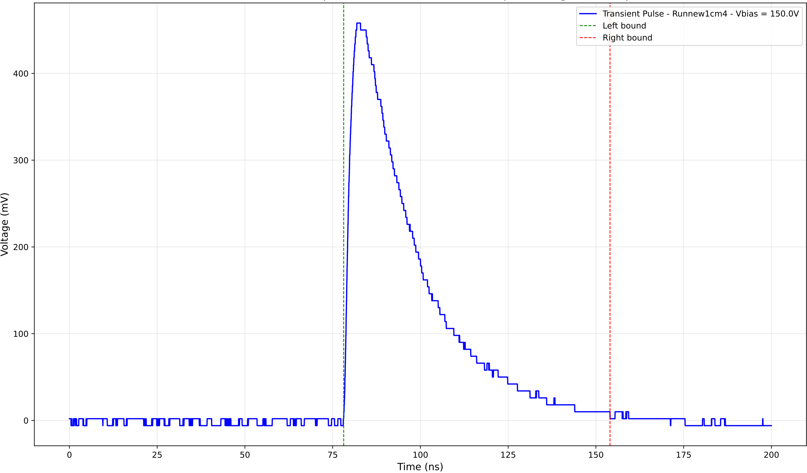
Transient Pulse - Sample: new1cm - Position: 2630.0 \mu\text{m} - Charge: 197.50 pC
