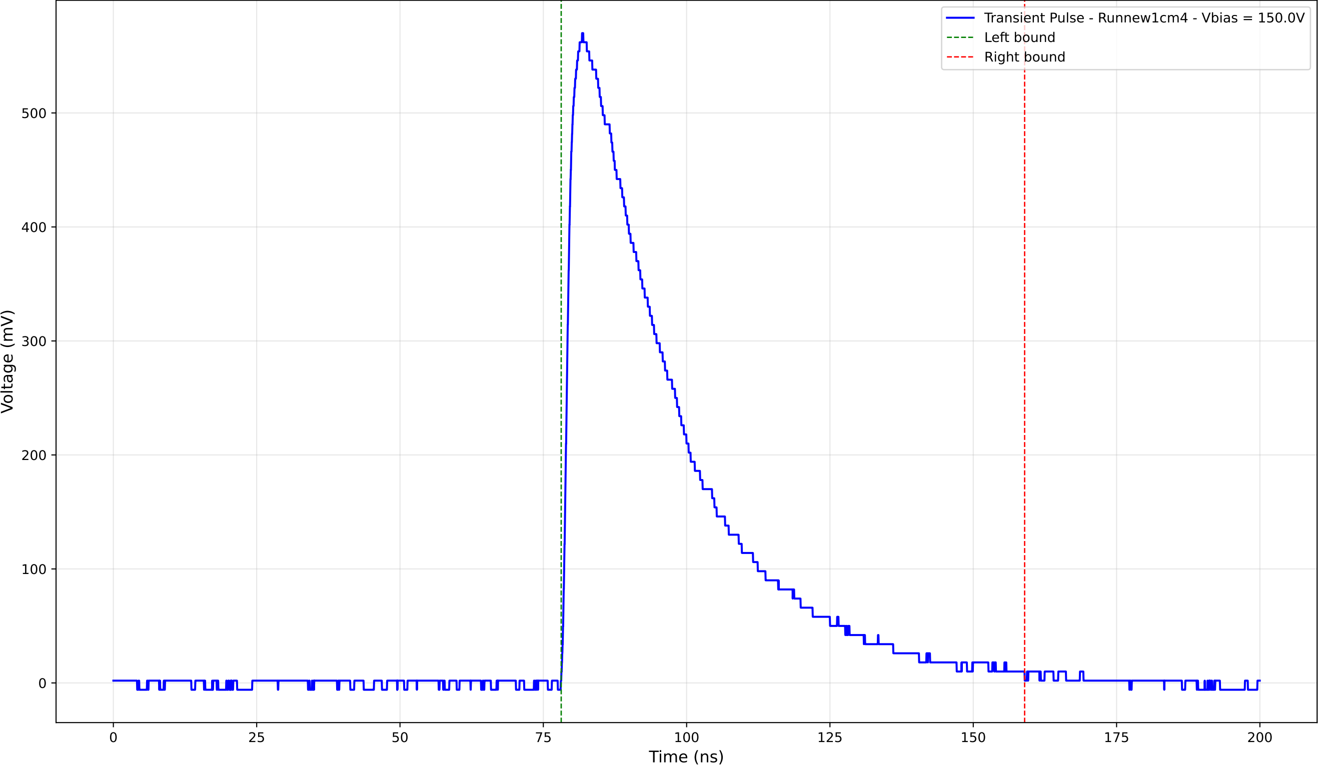
Transient Pulse - Sample: new1cm - Position: 3415.0 \mu\text{m} - Charge: 242.26 pC
