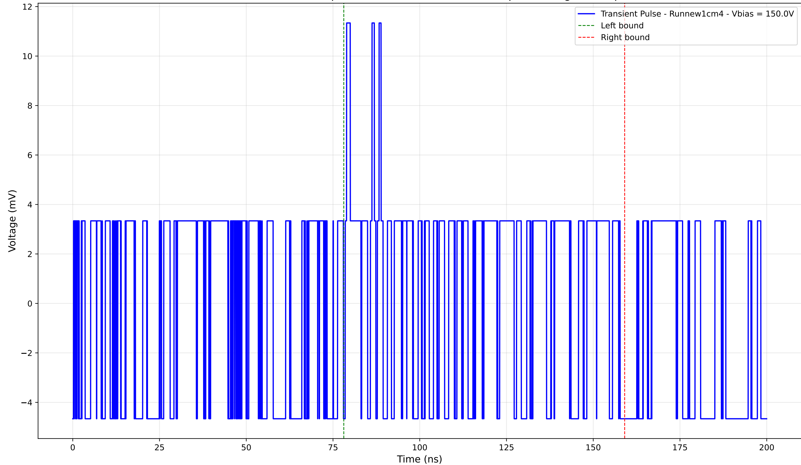
Transient Pulse - Sample: new1cm - Position: 5150.0 \mu\text{m} - Charge: 2.11 pC
