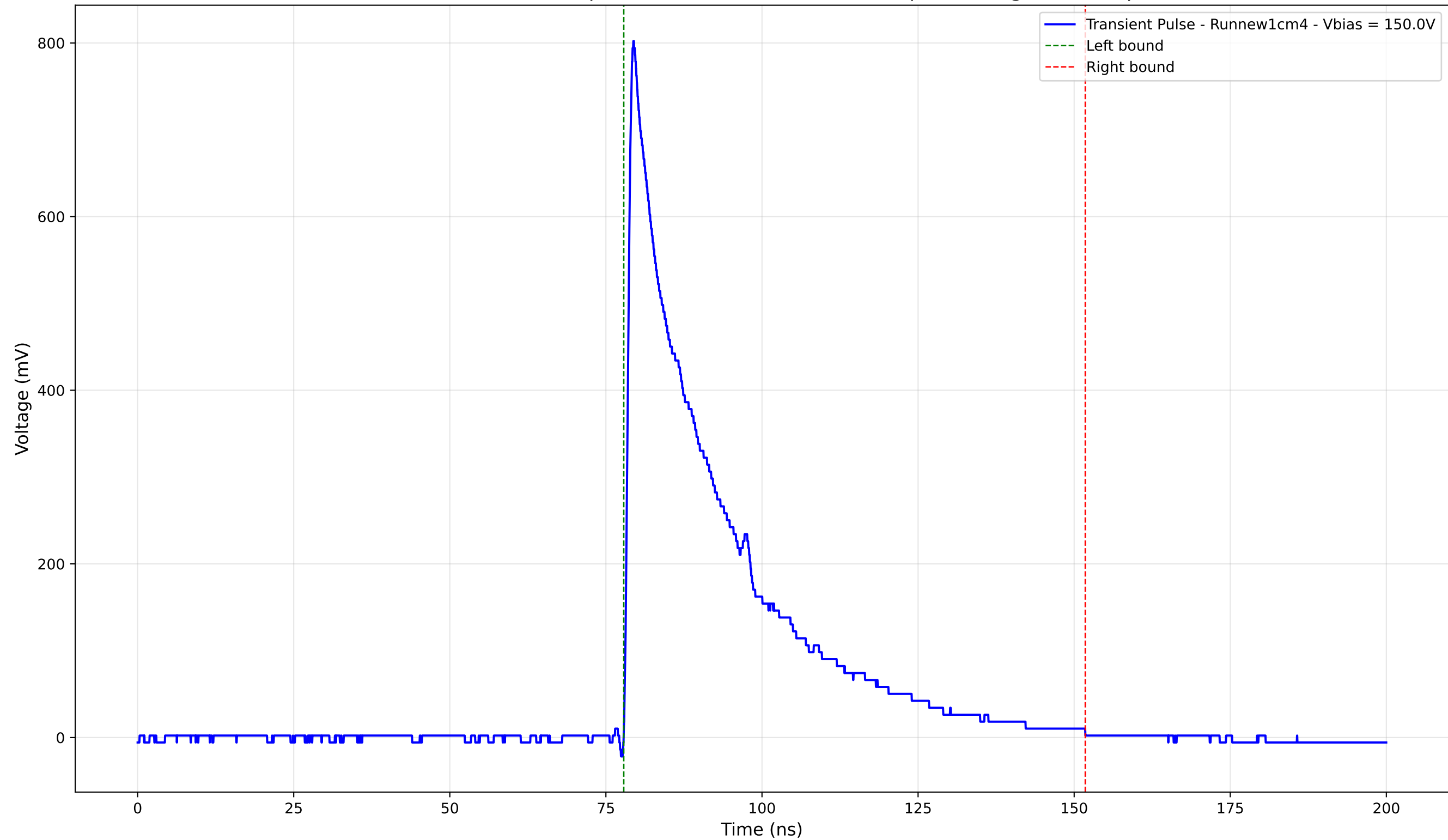
Transient Pulse - Sample: new1cm - Position: 4585.0 \mu\text{m} - Charge: 226.82 pC
