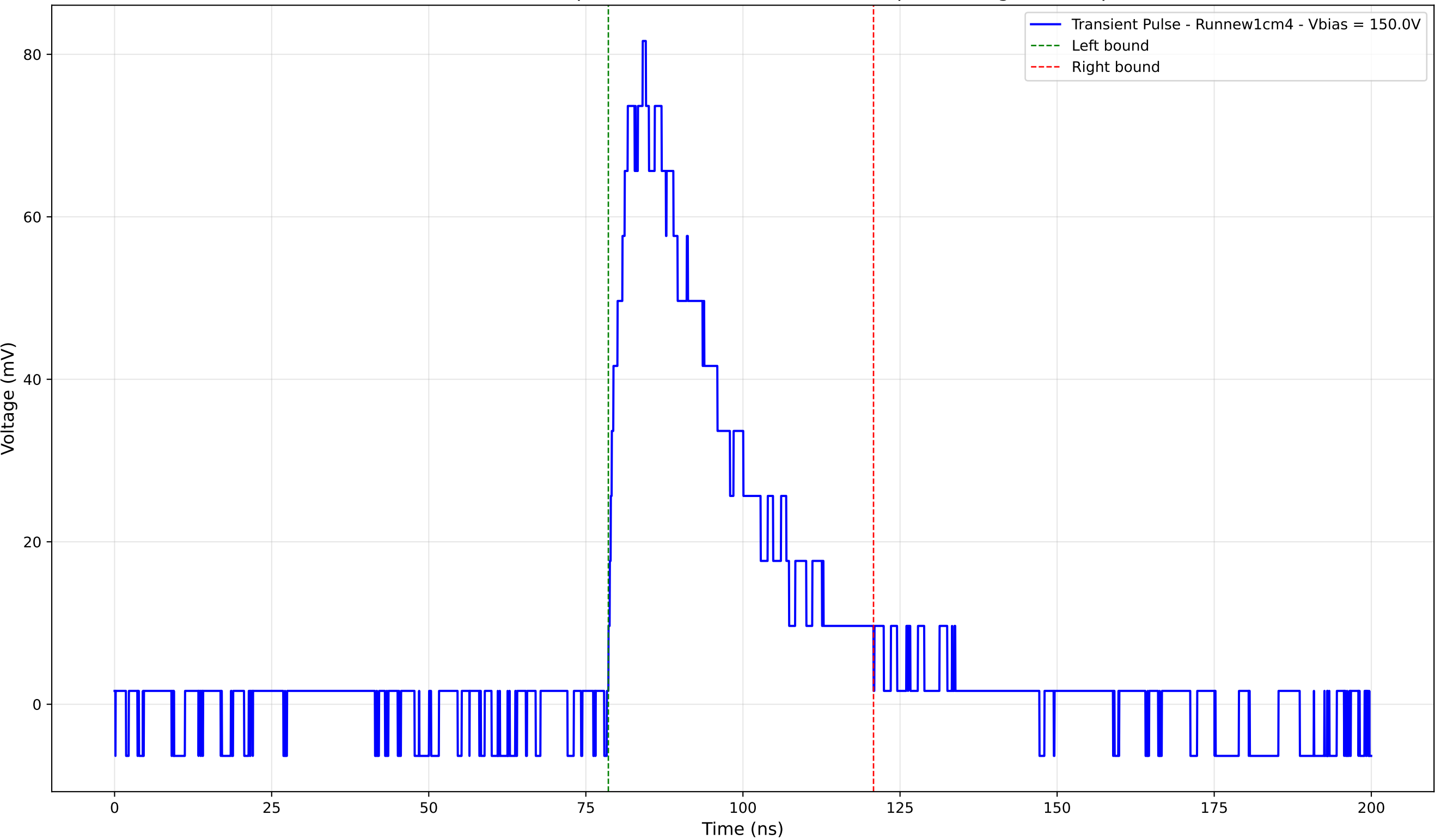
Transient Pulse - Sample: new1cm - Position: 2715.0 \mu\text{m} - Charge: 28.82 pC
