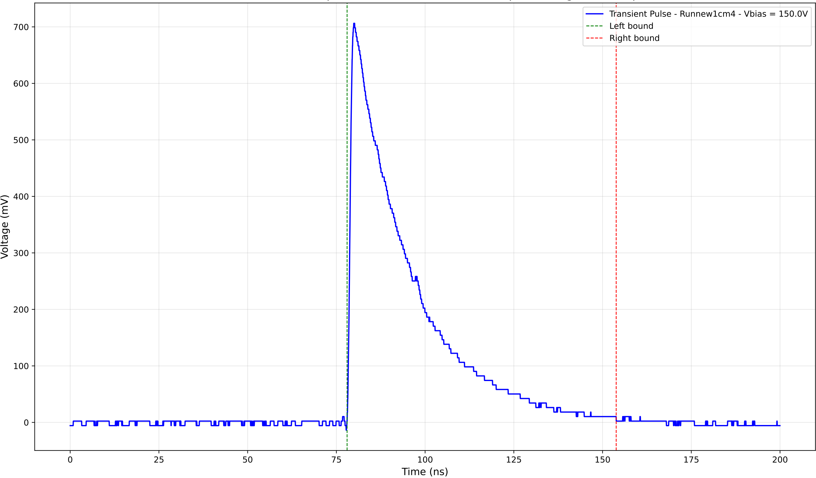
Transient Pulse - Sample: new1cm - Position: 4120.0 \mu\text{m} - Charge: 246.90 pC
