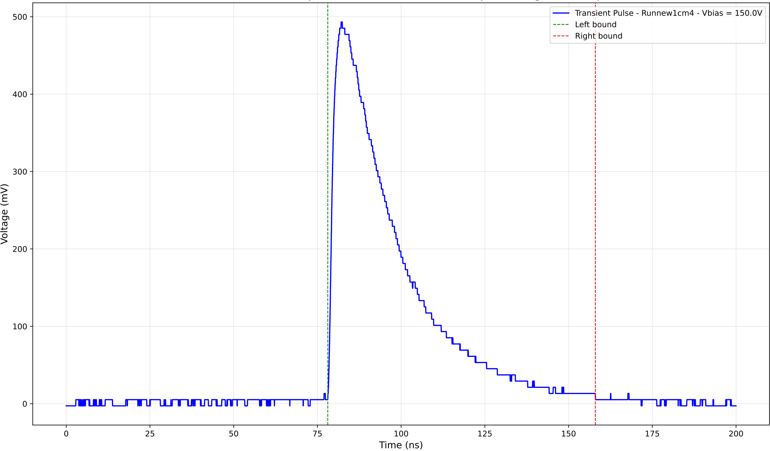
Transient Pulse - Sample: new1cm - Position: 3140.0 \mu\text{m} - Charge: 215.90 pC
