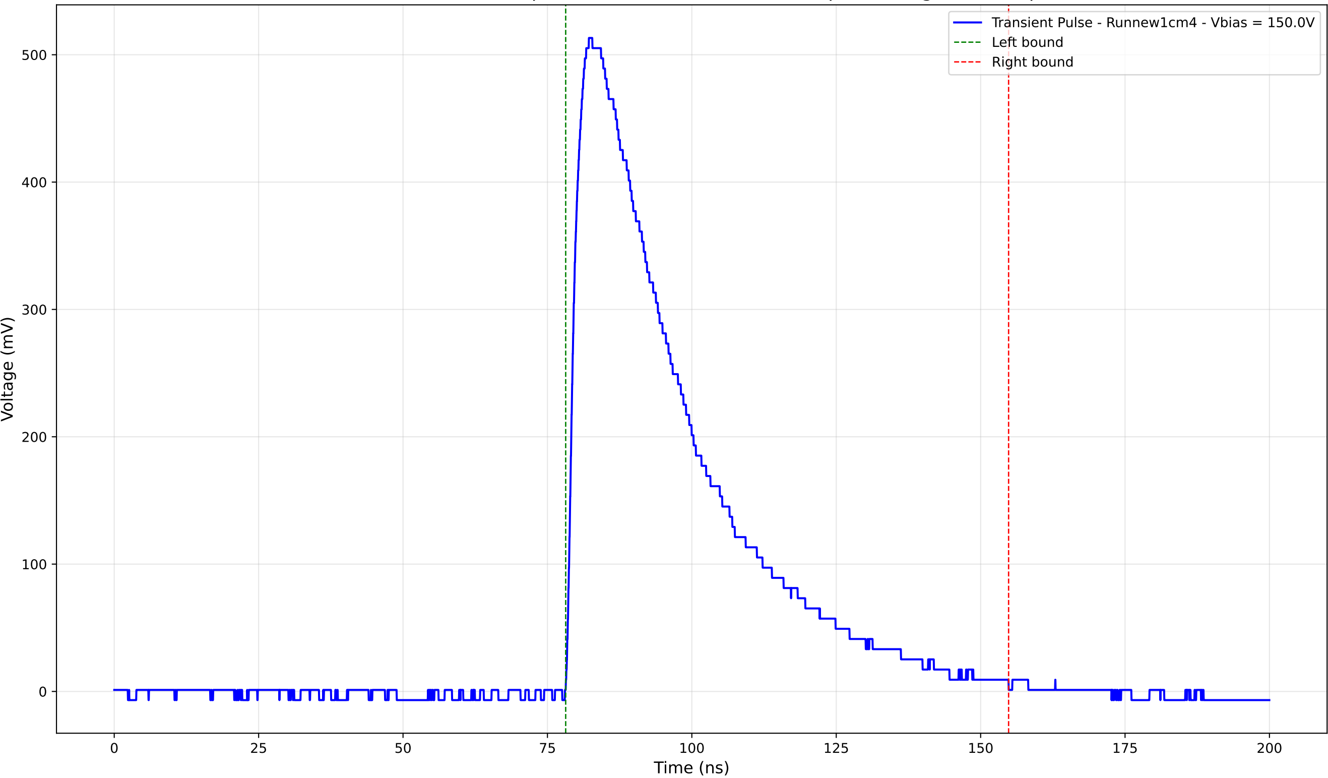
Transient Pulse - Sample: new1cm - Position: 2850.0 \mu\text{m} - Charge: 225.33 pC
