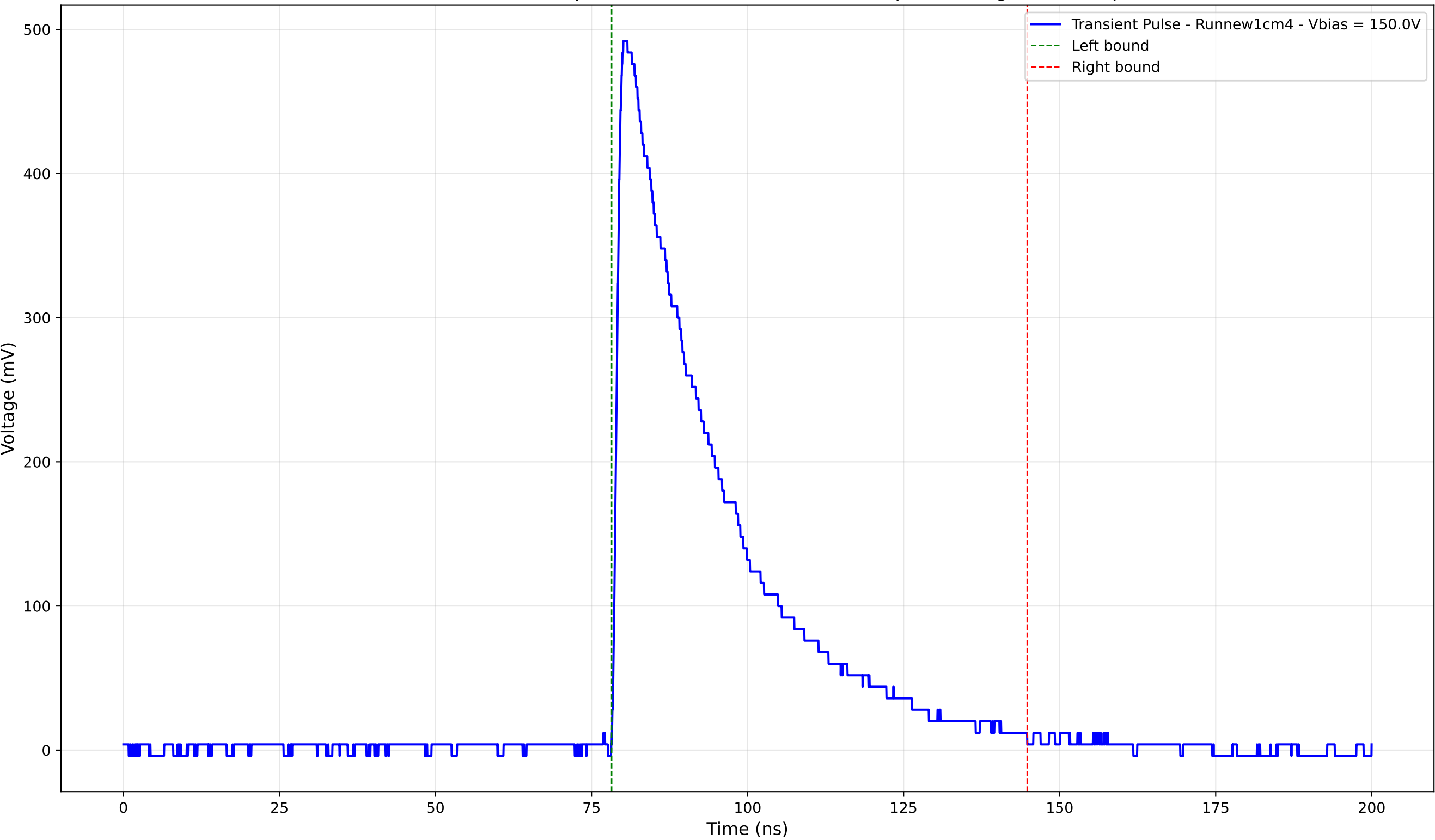
Transient Pulse - Sample: new1cm - Position: 1280.0 \mu\text{m} - Charge: 170.40 pC
