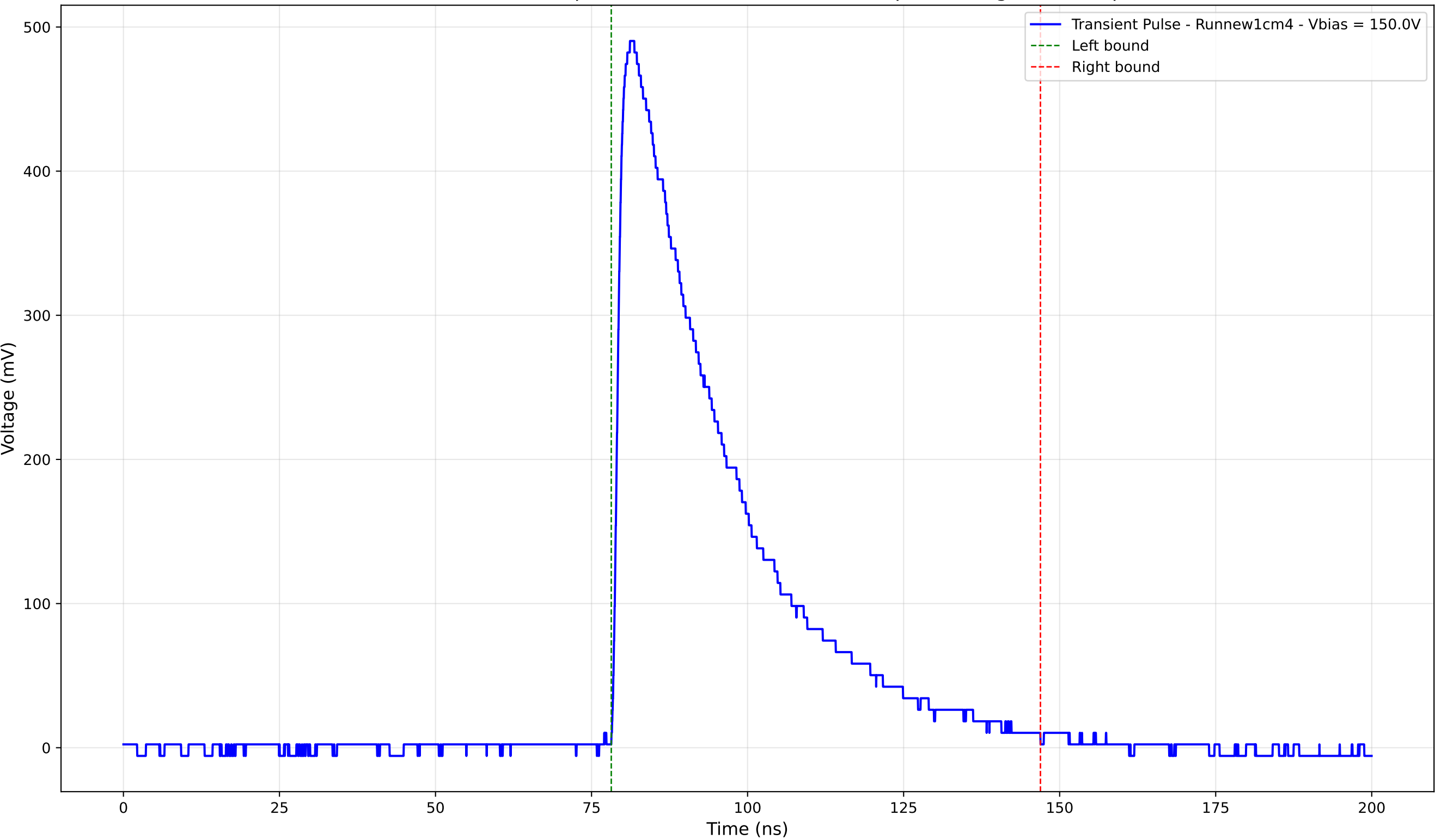
Transient Pulse - Sample: new1cm - Position: 1620.0 \mu\text{m} - Charge: 187.10 pC
