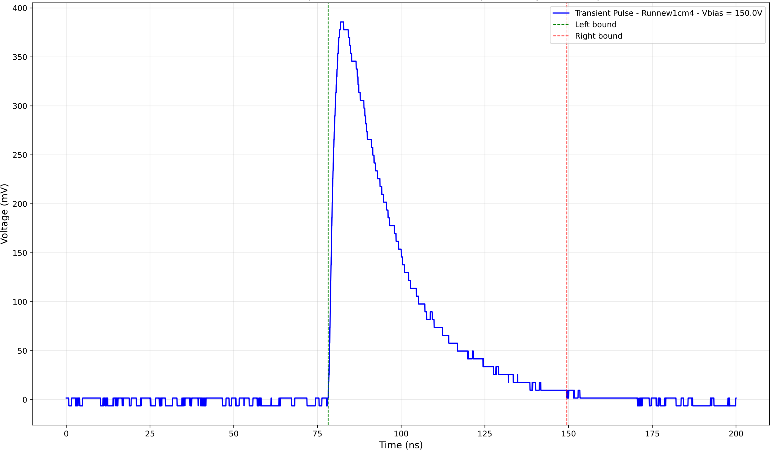
Transient Pulse - Sample: new1cm - Position: 2270.0 \mu\text{m} - Charge: 160.80 pC
