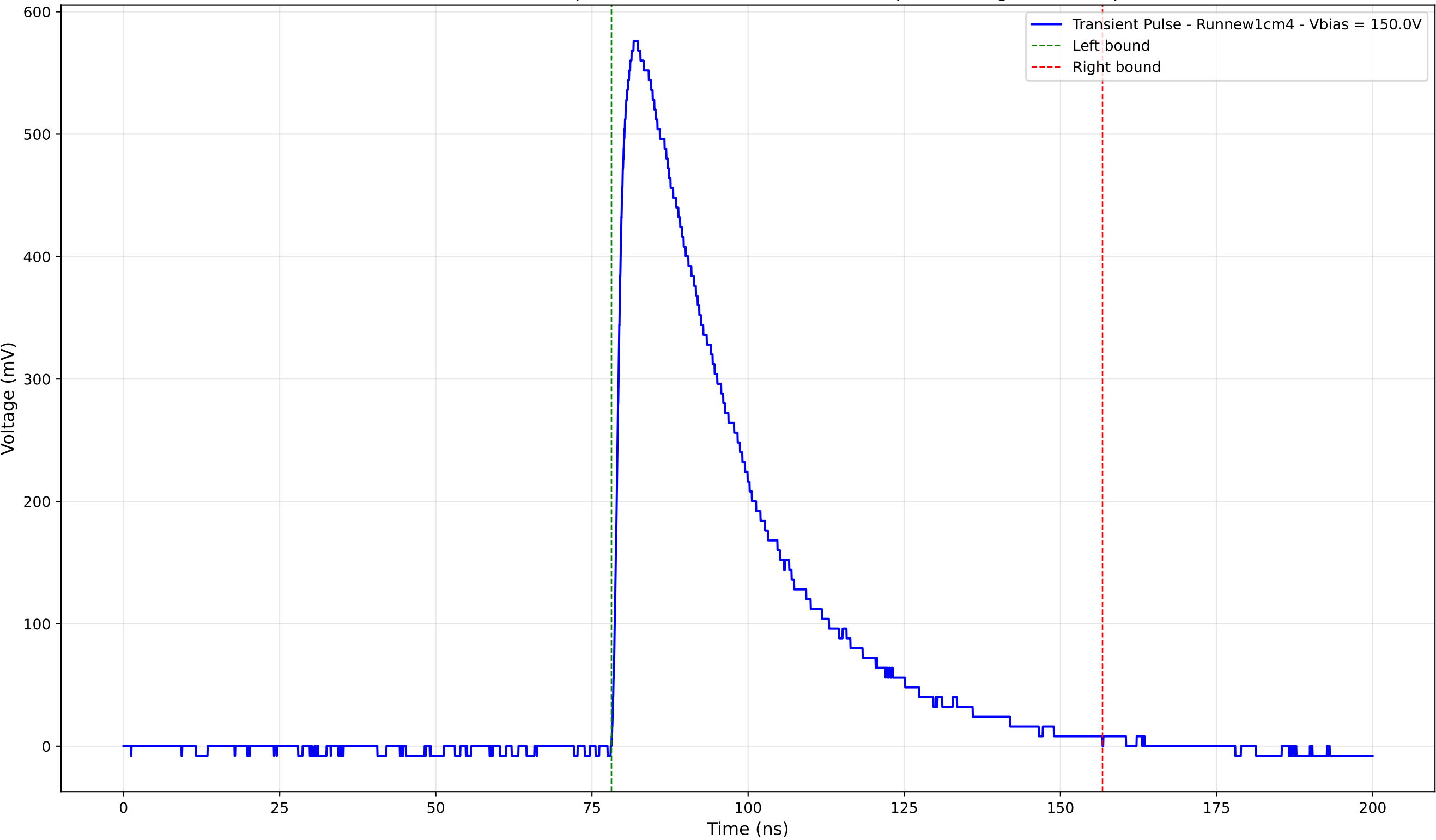
Transient Pulse - Sample: new1cm - Position: 3375.0 \mu\text{m} - Charge: 242.90 pC
