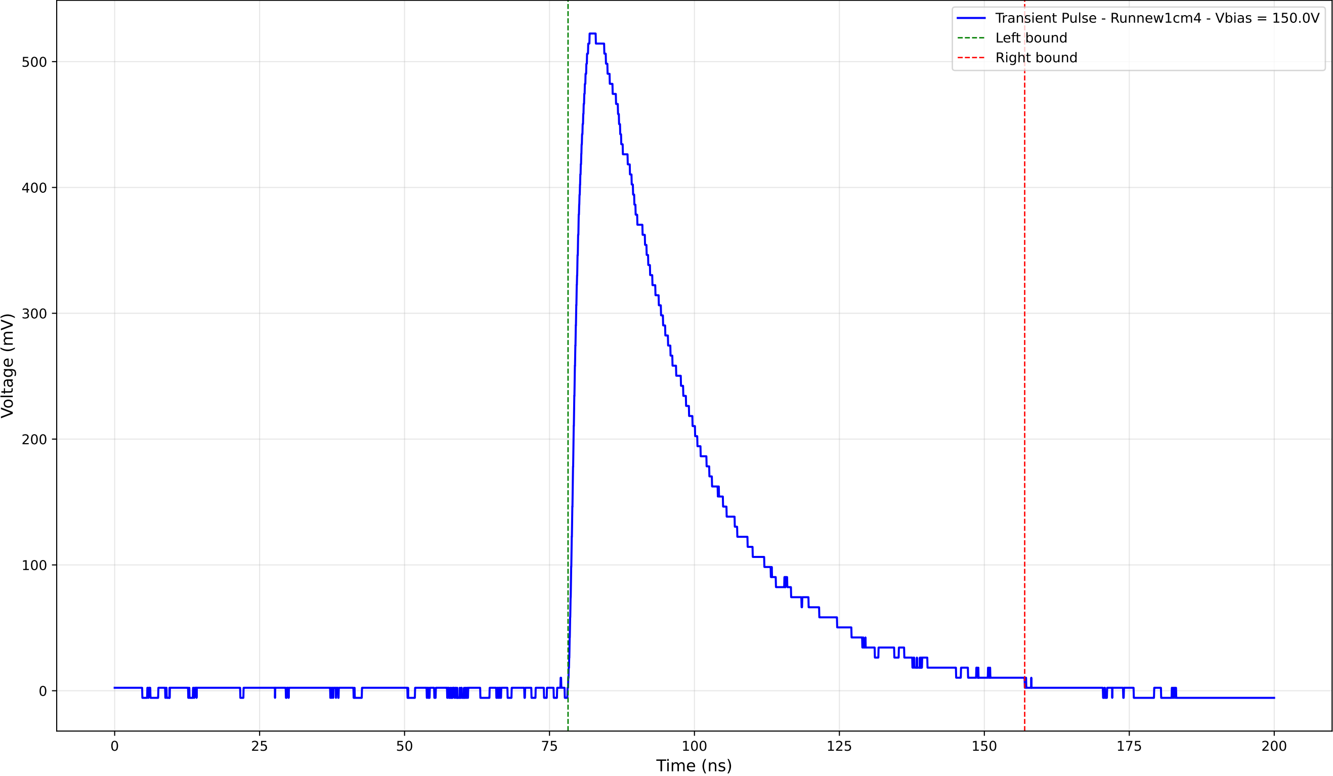
Transient Pulse - Sample: new1cm - Position: 2455.0 \mu\text{m} - Charge: 226.80 pC
