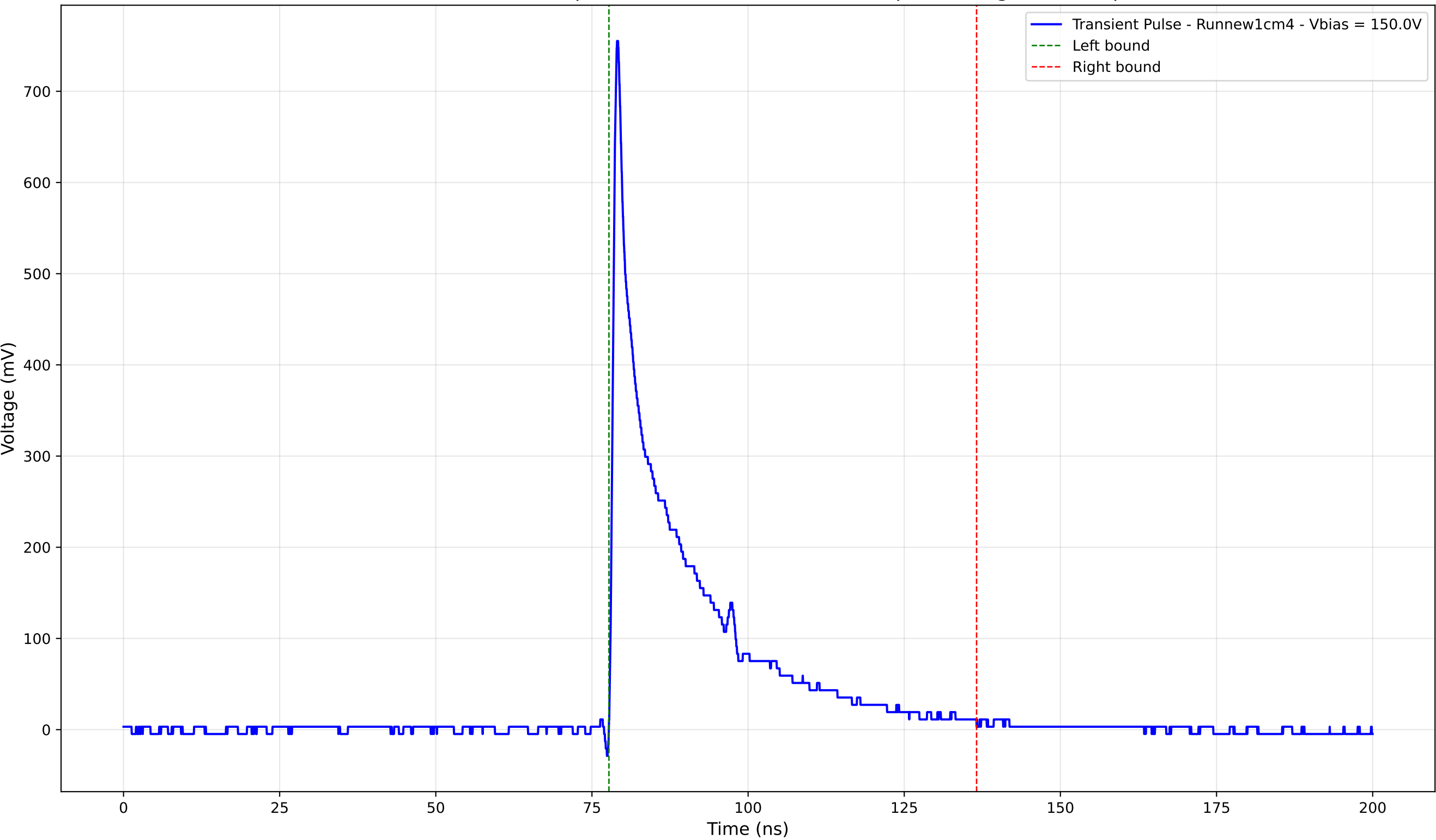
Transient Pulse - Sample: new1cm - Position: 5000.0 \mu\text{m} - Charge: 135.33 pC
