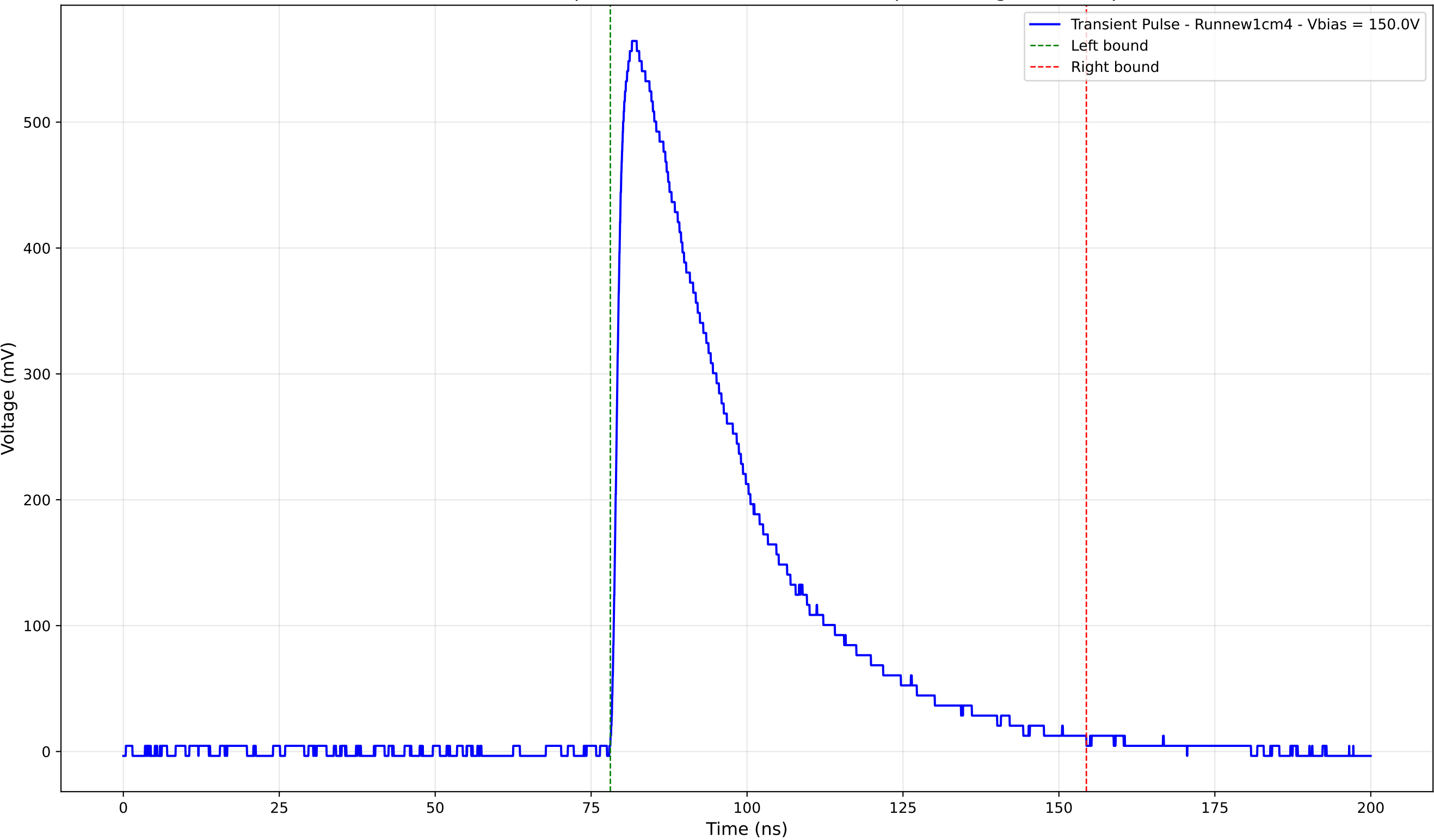
Transient Pulse - Sample: new1cm - Position: 3440.0 \mu\text{m} - Charge: 240.99 pC
