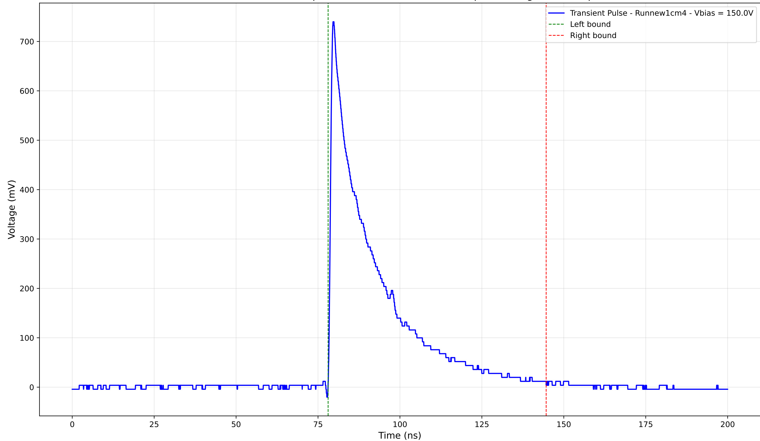
Transient Pulse - Sample: new1cm - Position: 810.0 \mu\text{m} - Charge: 195.92 pC
