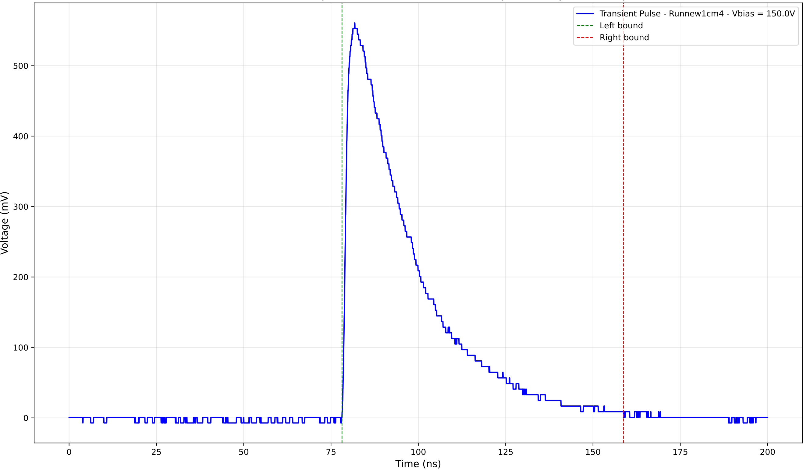
Transient Pulse - Sample: new1cm - Position: 3450.0 \mu\text{m} - Charge: 236.86 pC
