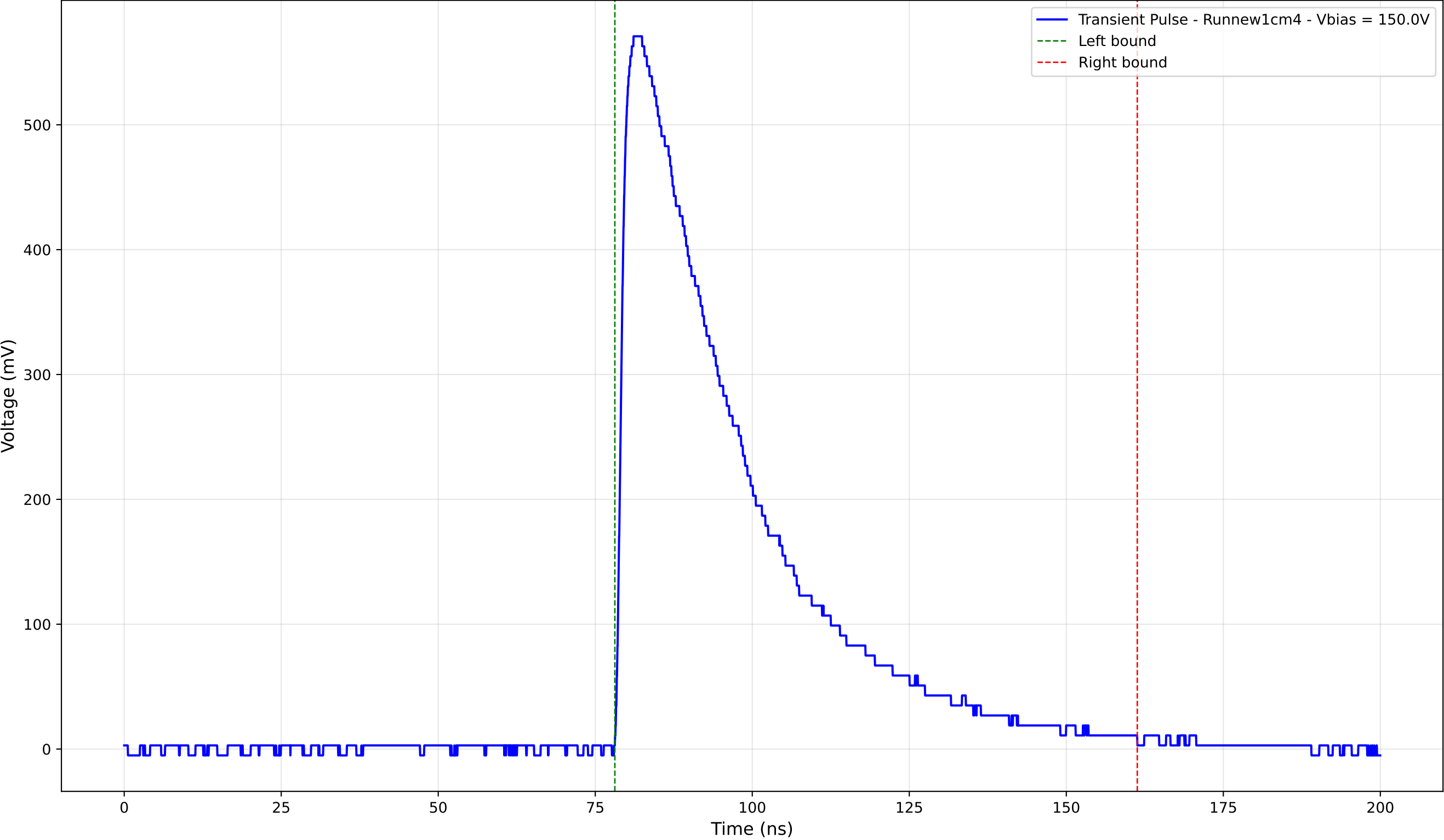
Transient Pulse - Sample: new1cm - Position: 3545.0 \mu\text{m} - Charge: 243.40 pC
