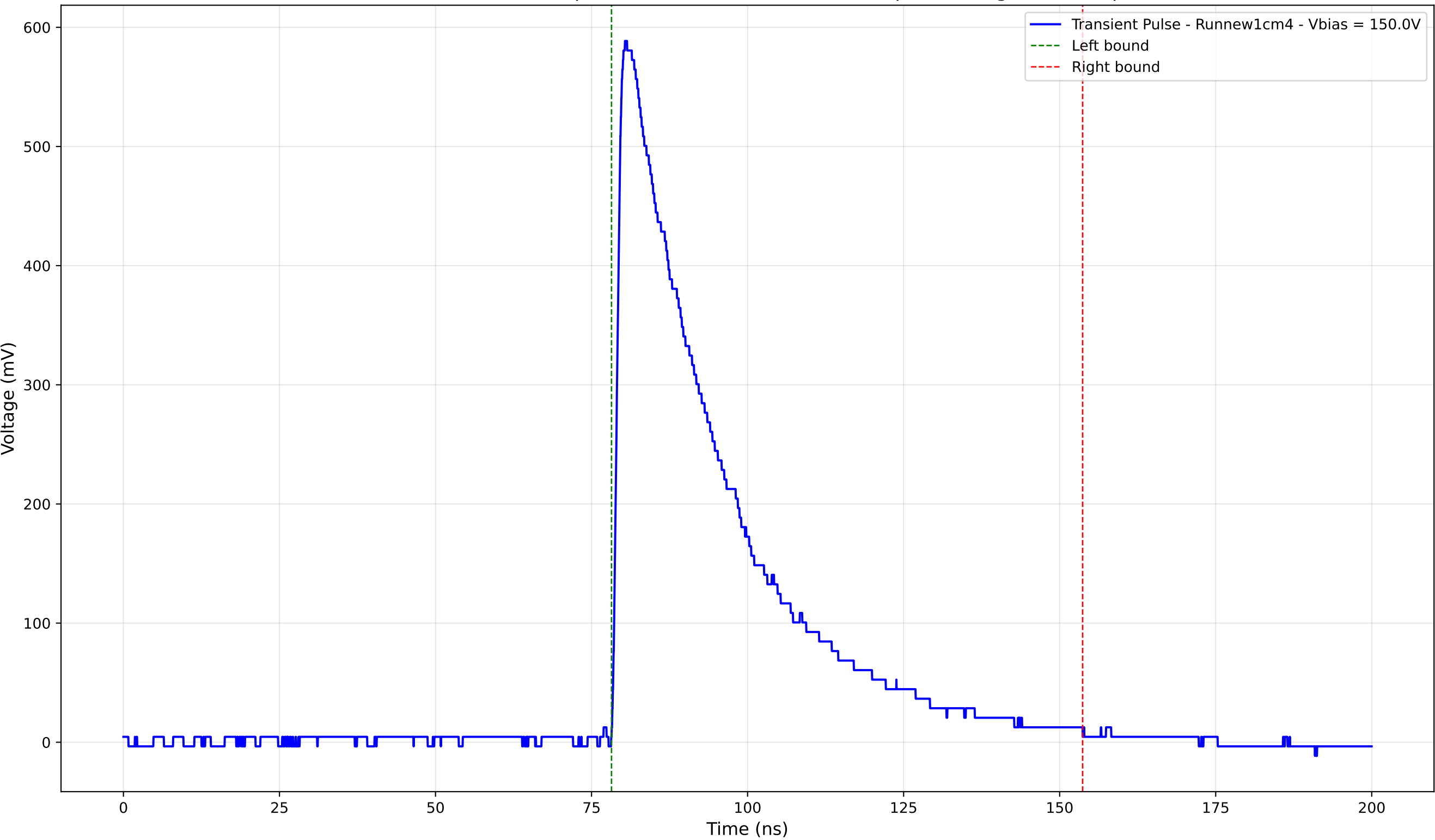
Transient Pulse - Sample: new1cm - Position: 1355.0 \mu\text{m} - Charge: 212.00 pC
