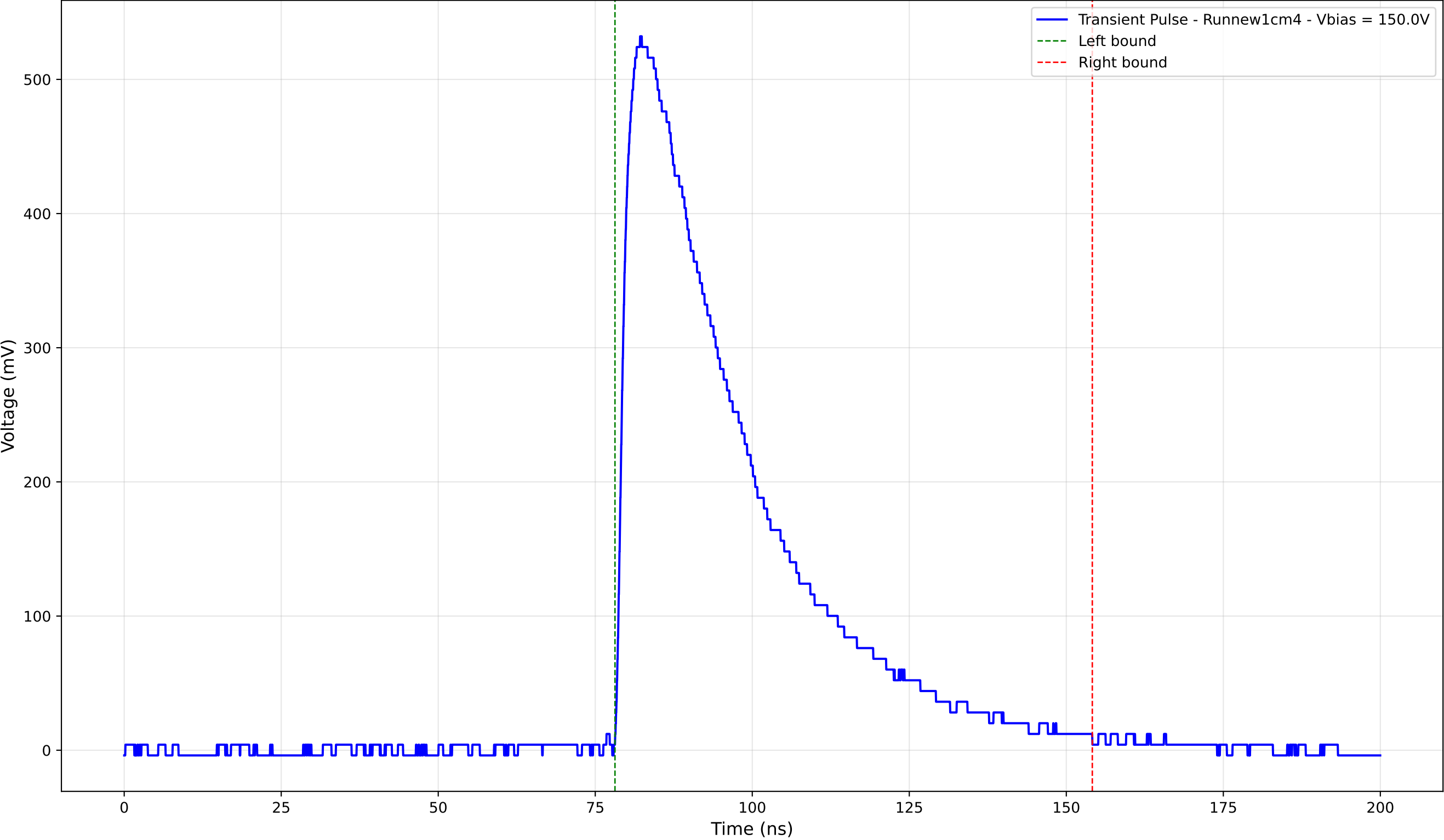
Transient Pulse - Sample: new1cm - Position: 3125.0 \mu\text{m} - Charge: 230.17 pC
