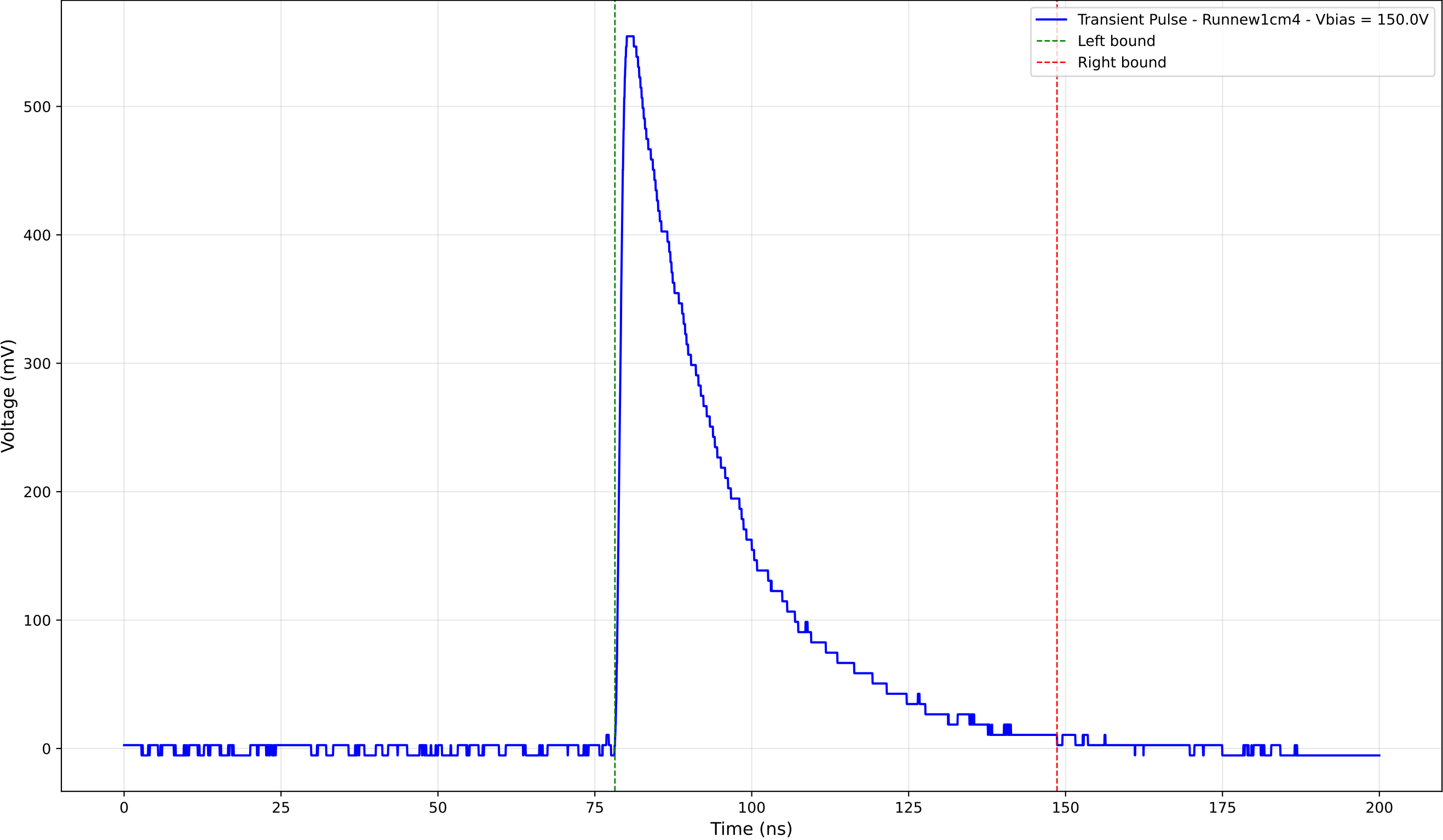
Transient Pulse - Sample: new1cm - Position: 1305.0 \mu\text{m} - Charge: 193.82 pC
