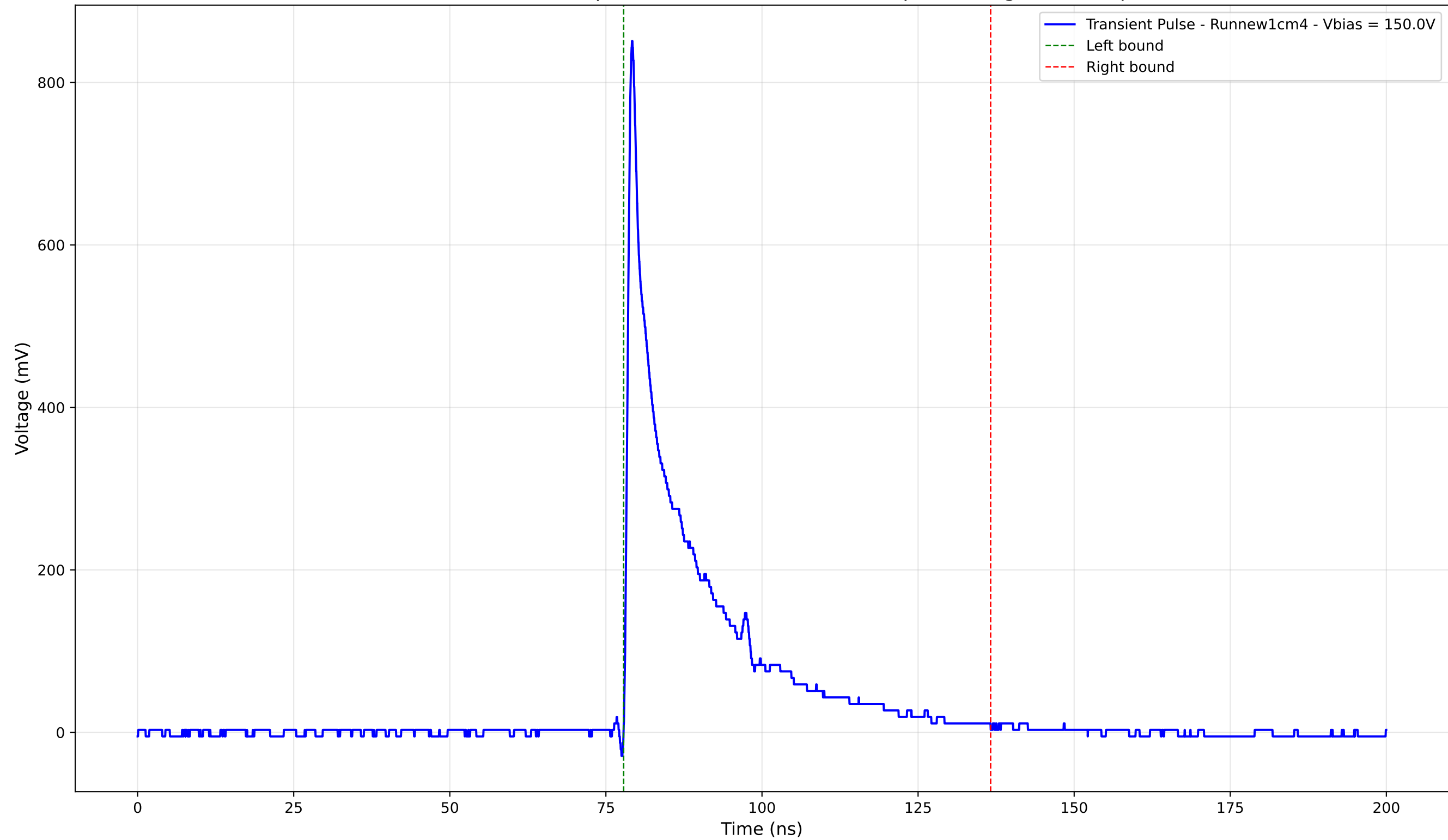
Transient Pulse - Sample: new1cm - Position: 270.0 \mu\text{m} - Charge: 145.54 pC
