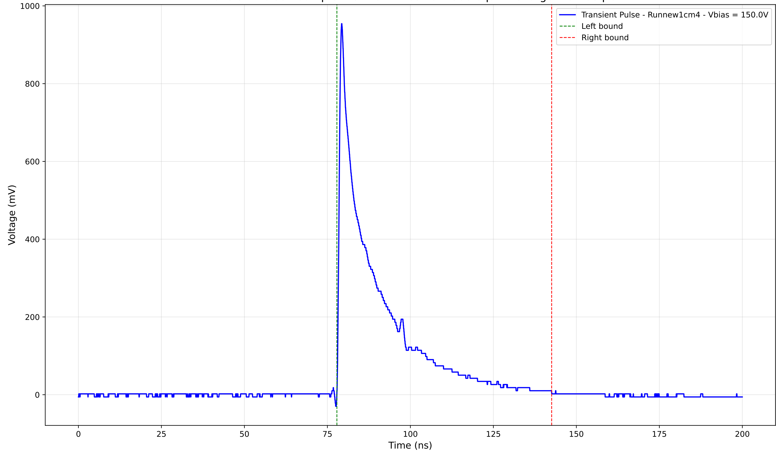
Transient Pulse - Sample: new1cm - Position: 380.0 \mu\text{m} - Charge: 197.08 pC
