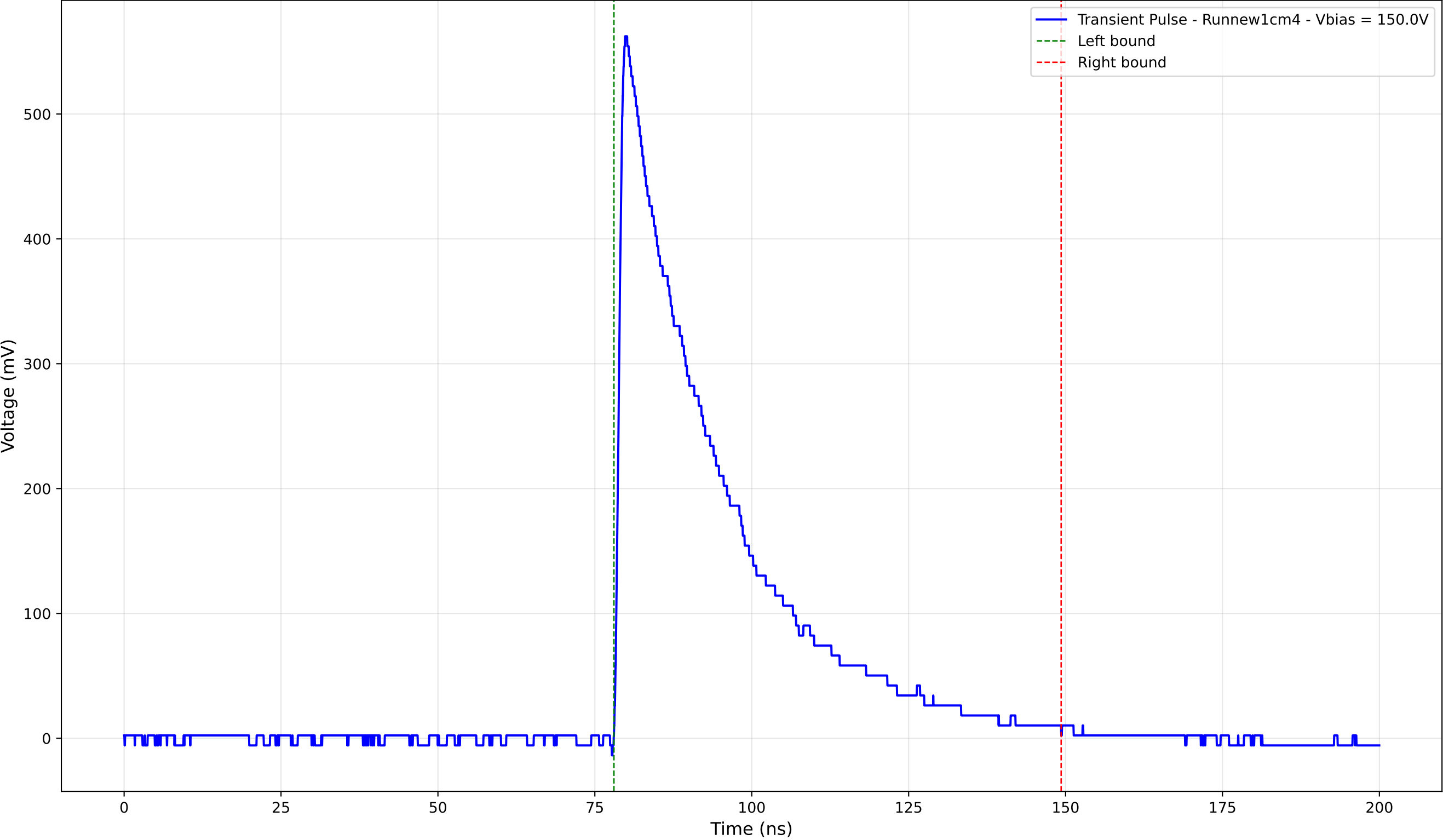
Transient Pulse - Sample: new1cm - Position: 4165.0 \mu\text{m} - Charge: 185.56 pC
