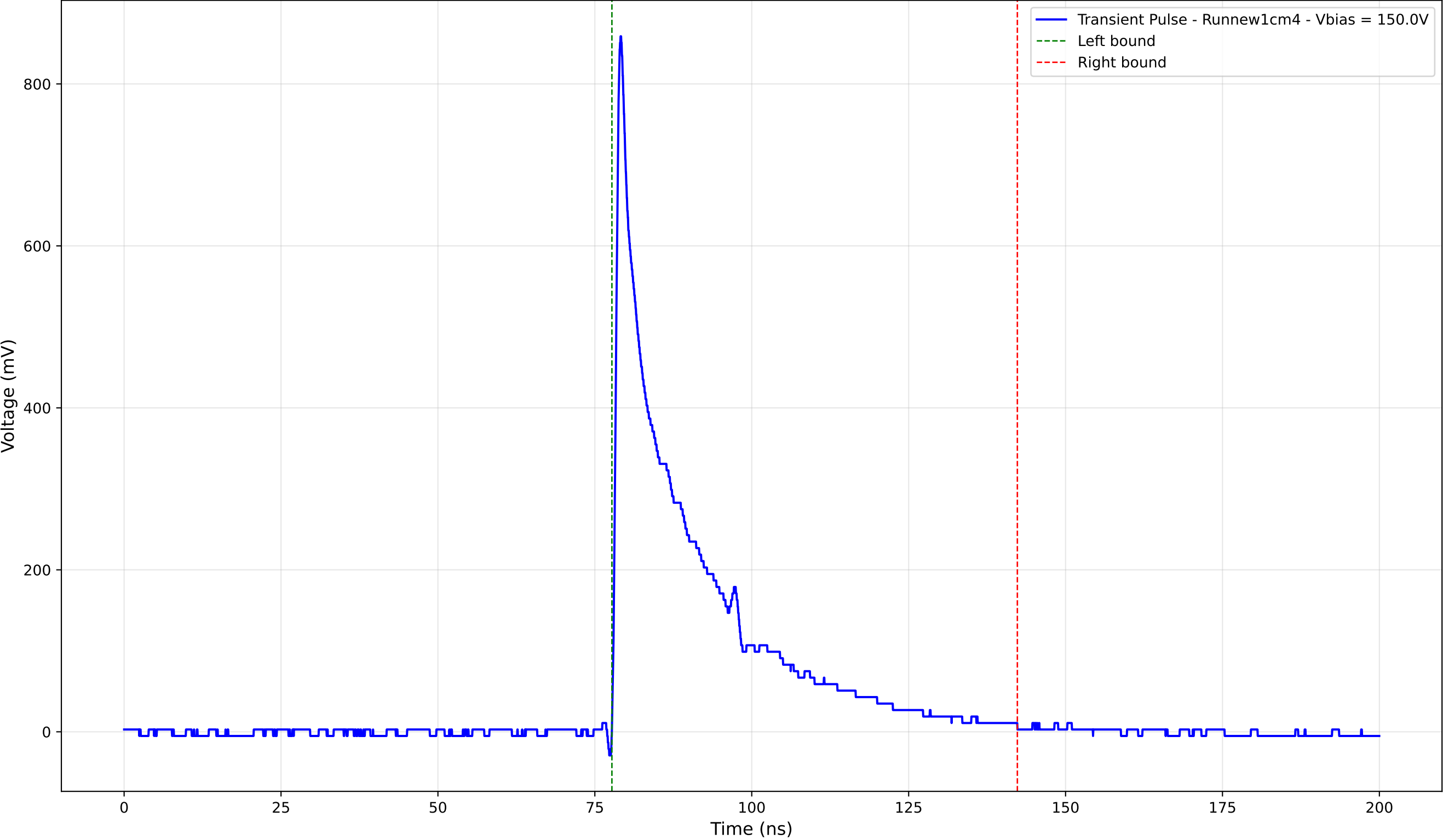
Transient Pulse - Sample: new1cm - Position: 4960.0 \mu\text{m} - Charge: 174.64 pC
