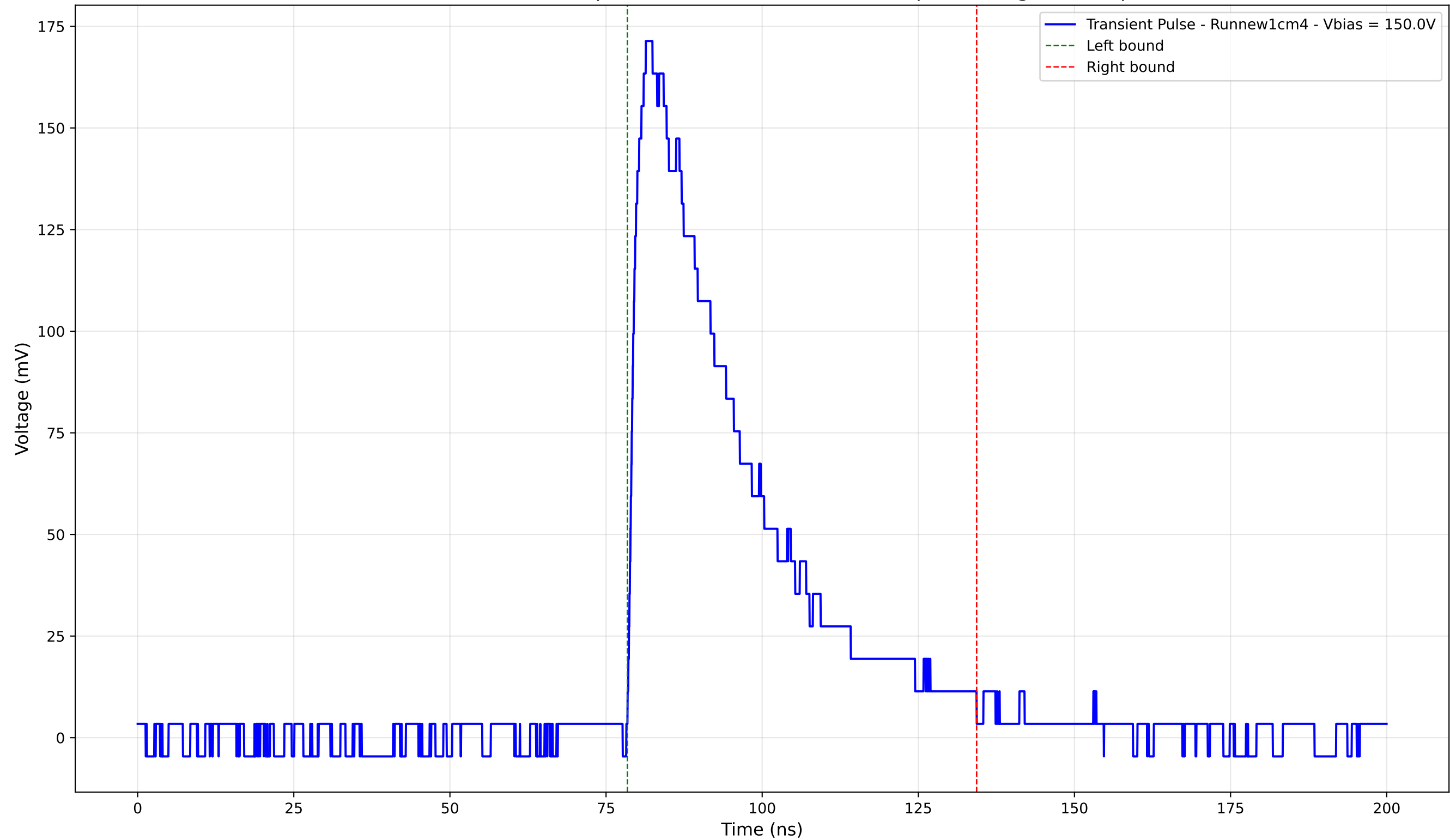
Transient Pulse - Sample: new1cm - Position: 1735.0 \mu\text{m} - Charge: 64.95 pC
