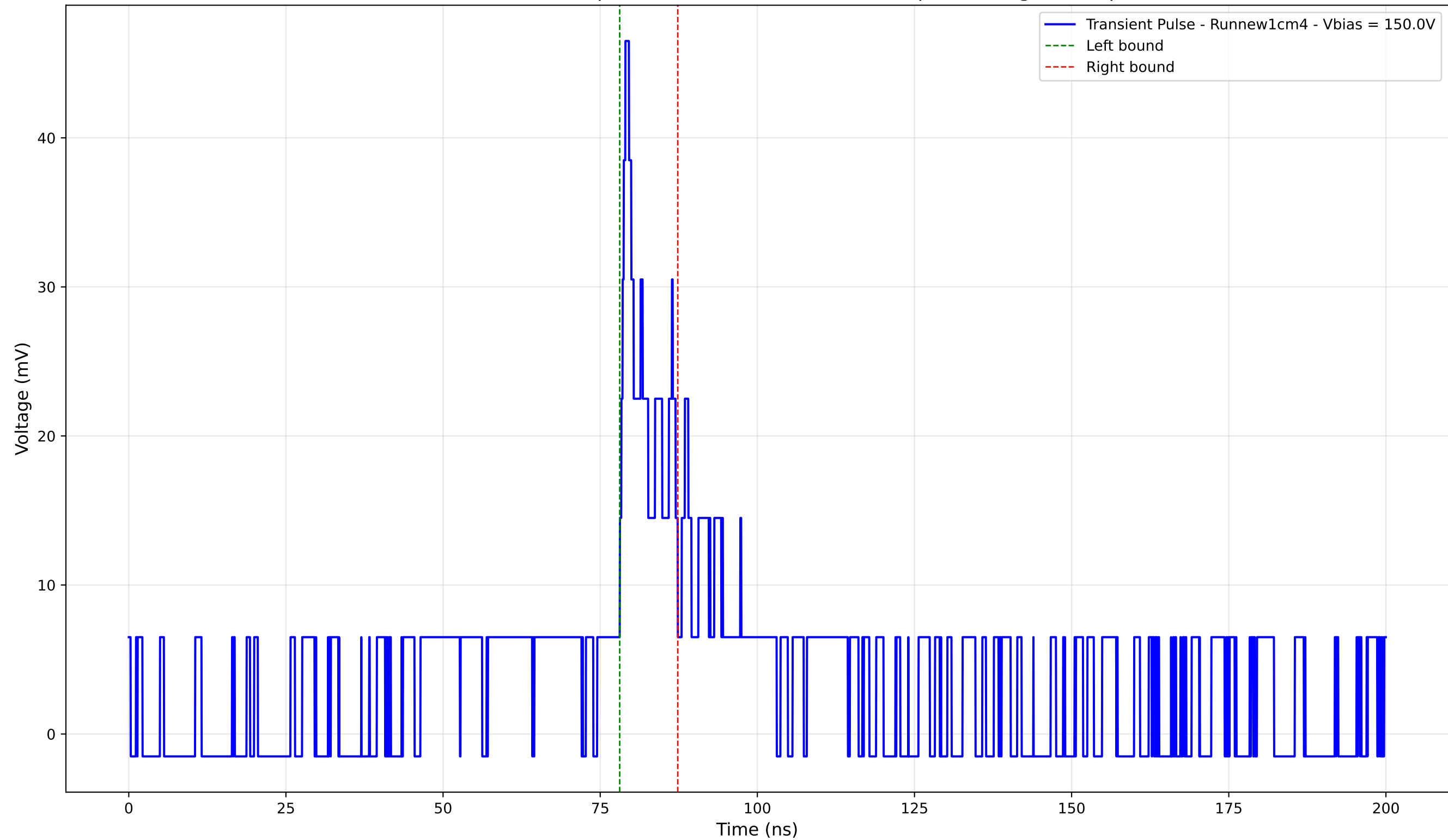
Transient Pulse - Sample: new1cm -Position: 5085.0 \mu\text{m} - Charge: 4.36 pC
