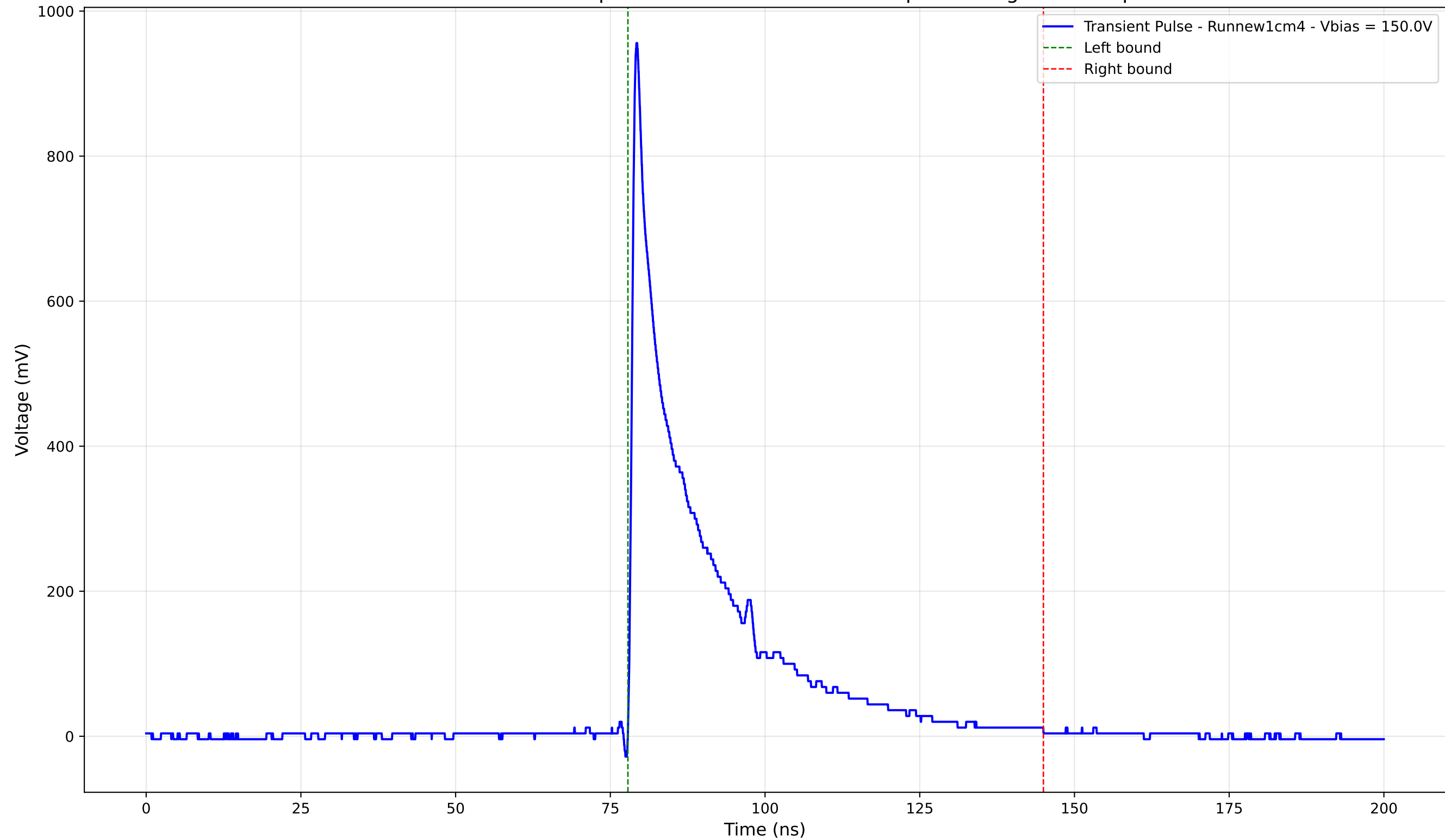
Transient Pulse - Sample: new1cm - Position: 330.0 \mu\text{m} - Charge: 191.80 pC
