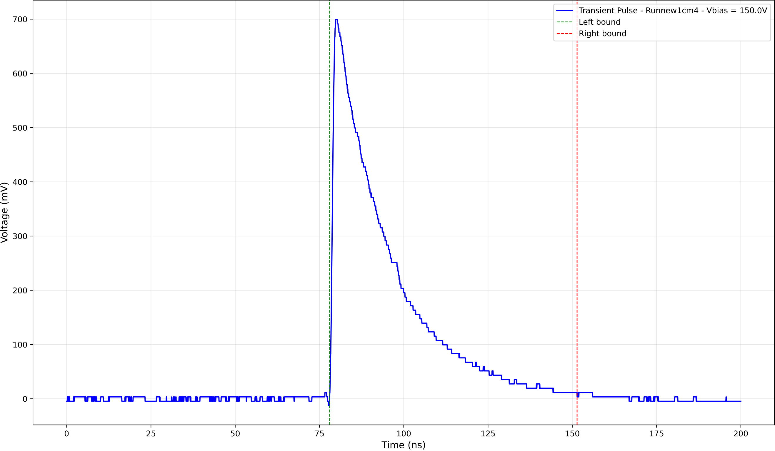
Transient Pulse - Sample: new1cm - Position: 4125.0 \mu\text{m} - Charge: 245.66 pC
