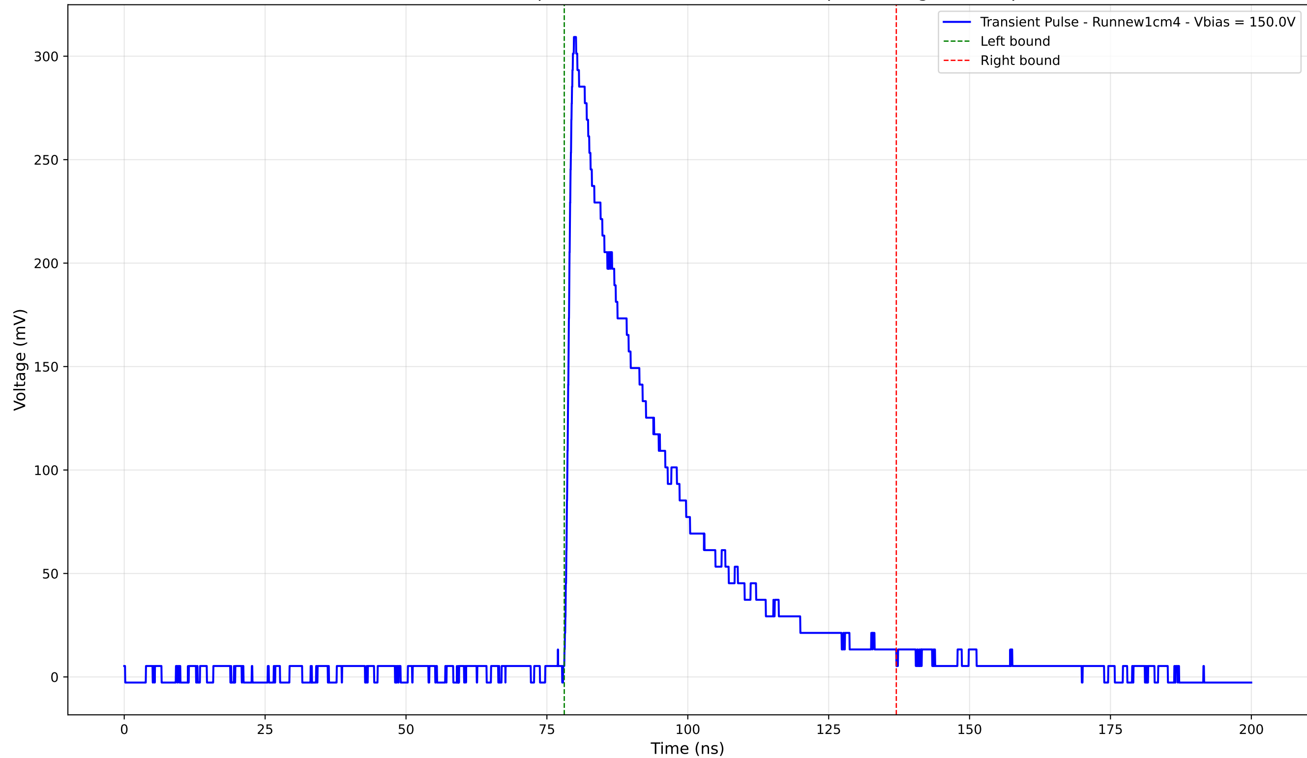
Transient Pulse - Sample: new1cm - Position: 4195.0 \mu\text{m} - Charge: 98.64 pC
