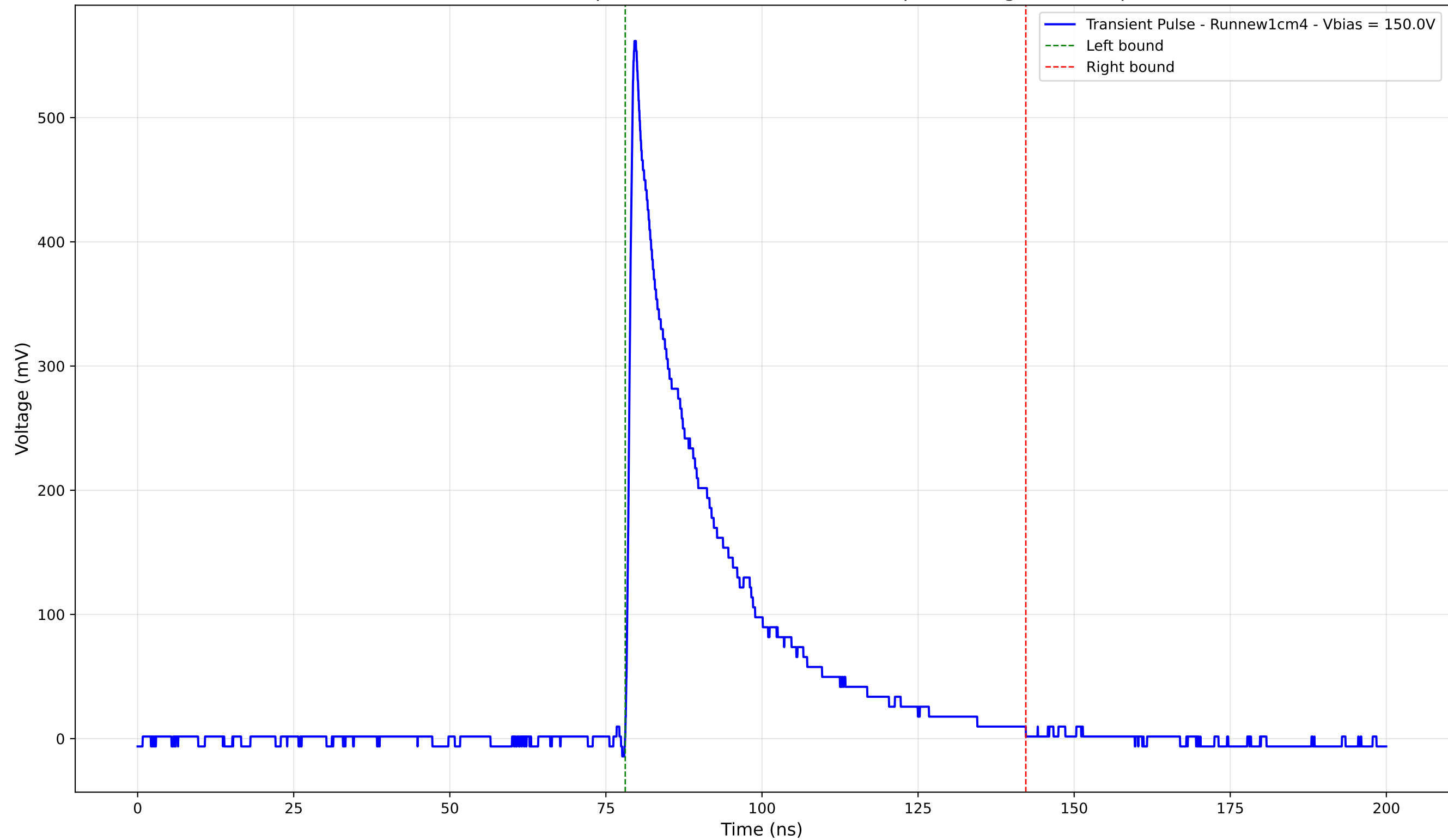
Transient Pulse - Sample: new1cm - Position: 760.0 \mu\text{m} - Charge: 138.87 pC
