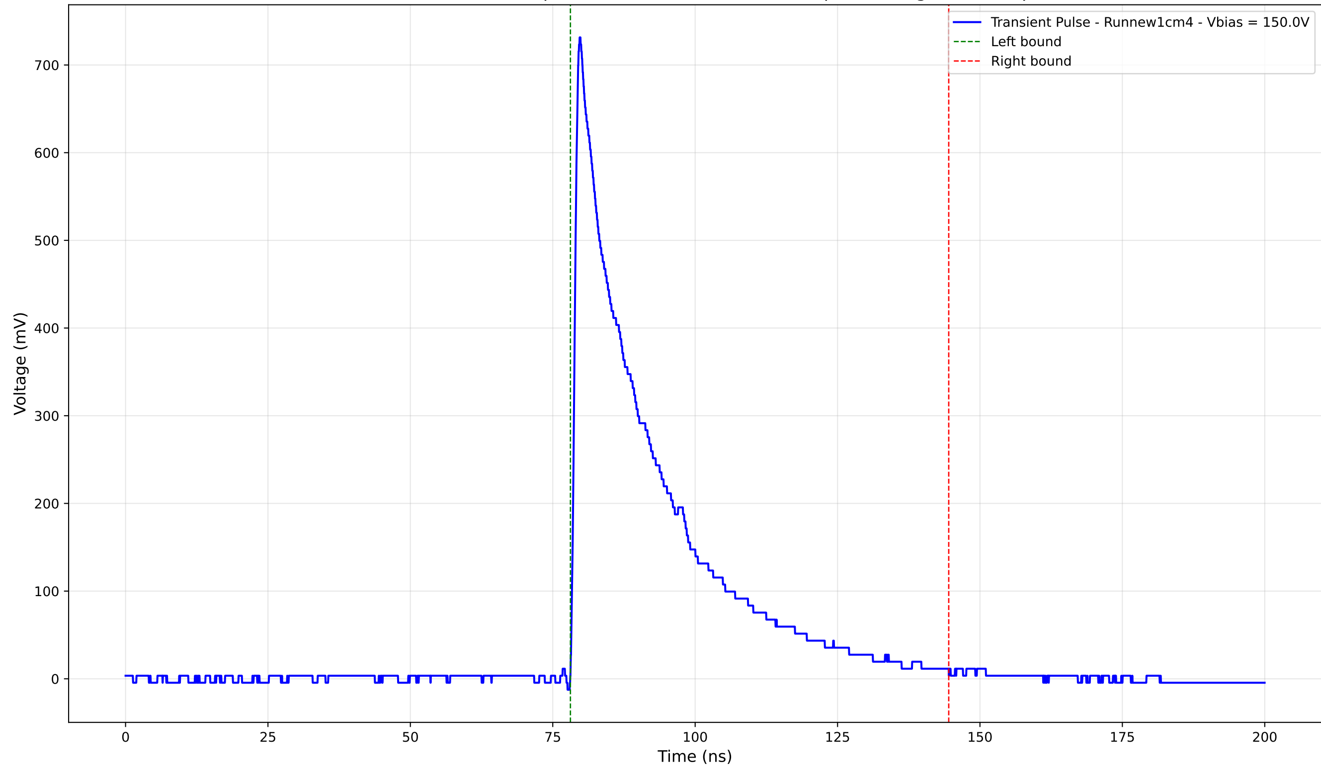
Transient Pulse - Sample: new1cm - Position: 880.0 \mu\text{m} - Charge: 200.05 pC
