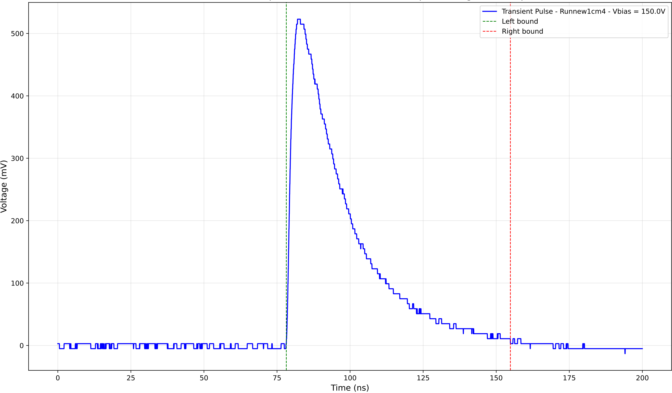
Transient Pulse - Sample: new1cm - Position: 2385.0 \mu\text{m} - Charge: 226.85 pC
