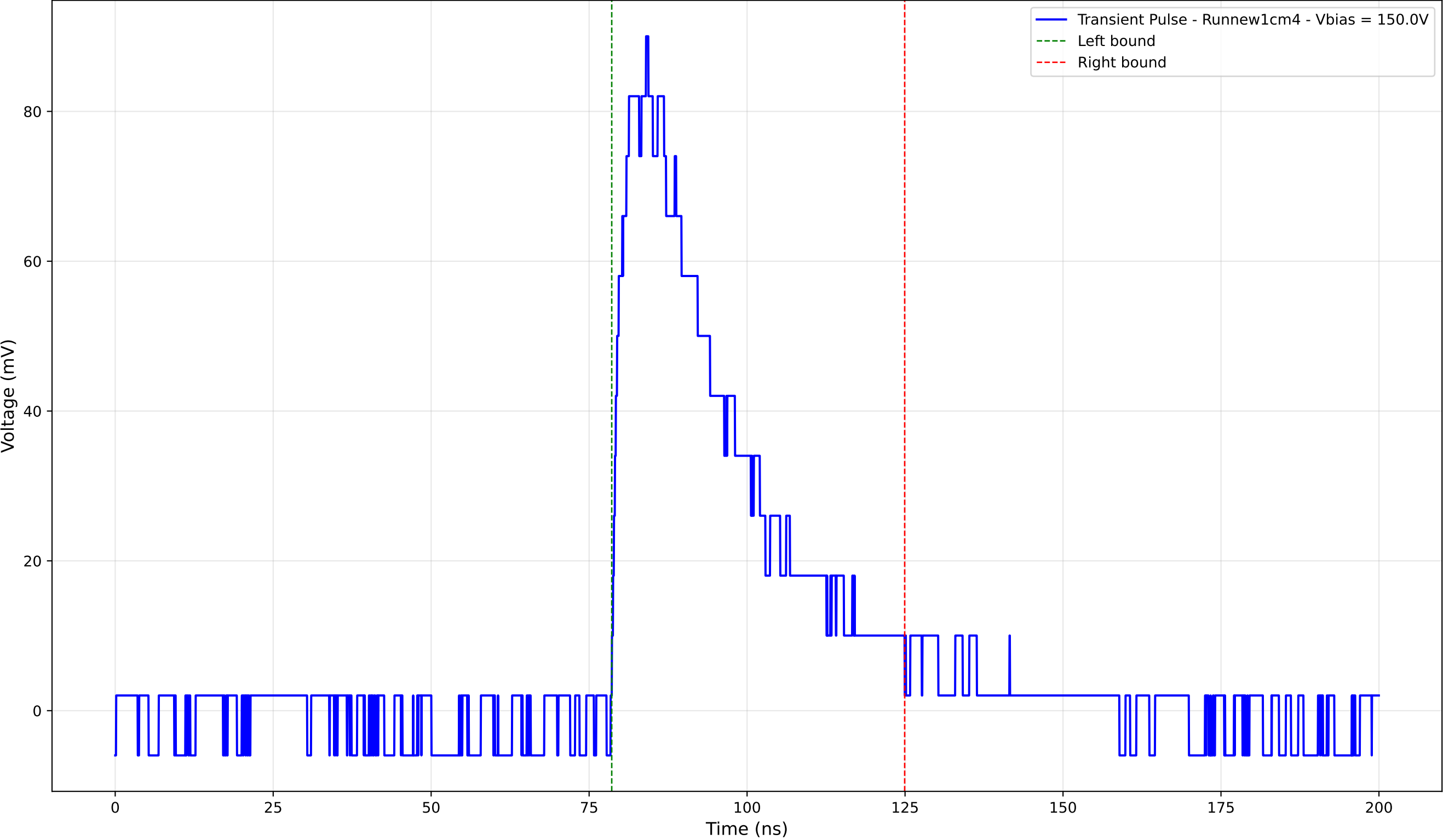
Transient Pulse - Sample: new1cm - Position: 3220.0 \mu\text{m} - Charge: 33.46 pC
