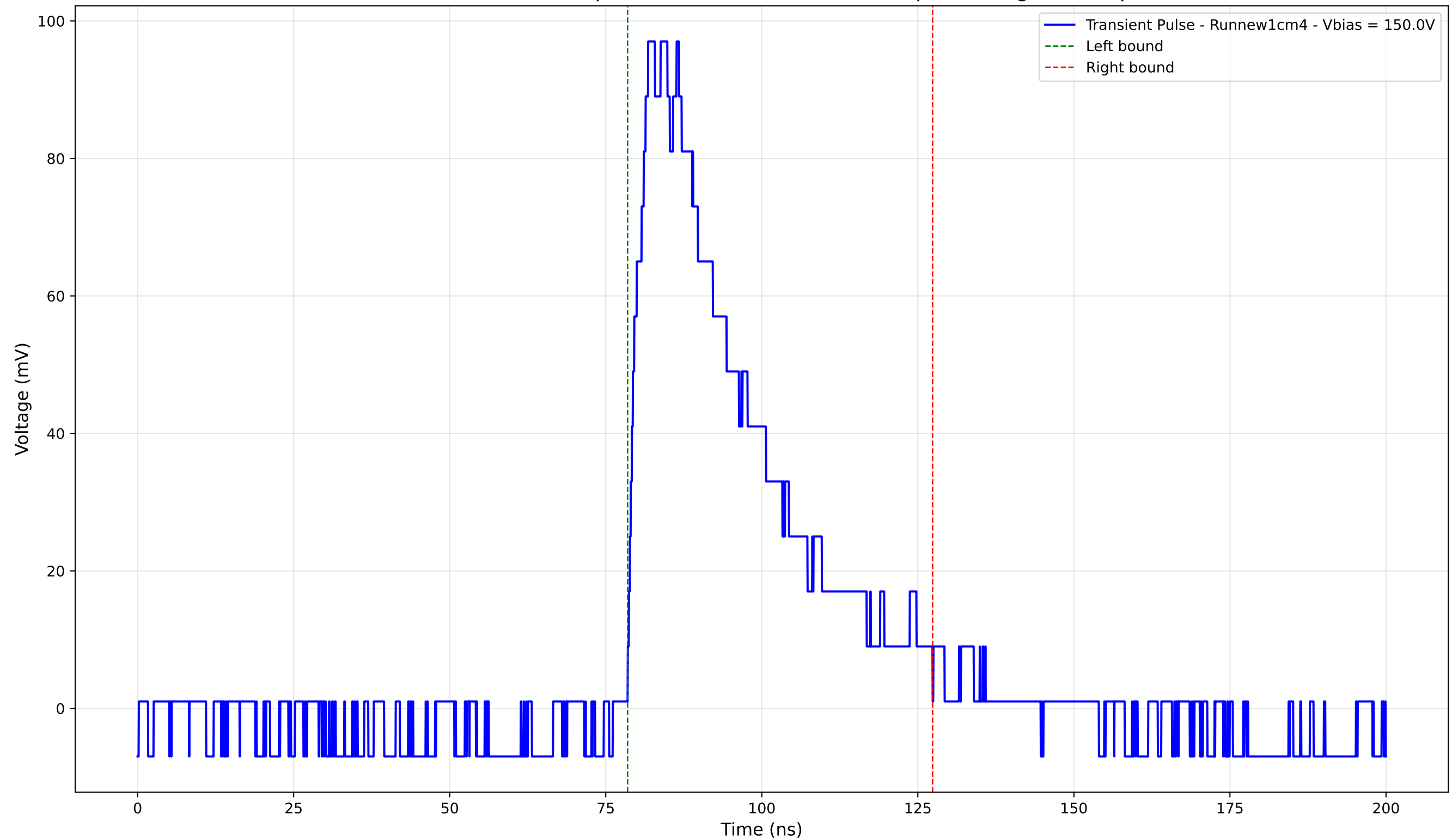
Transient Pulse - Sample: new1cm - Position: 2730.0 \mu\text{m} - Charge: 38.54 pC
