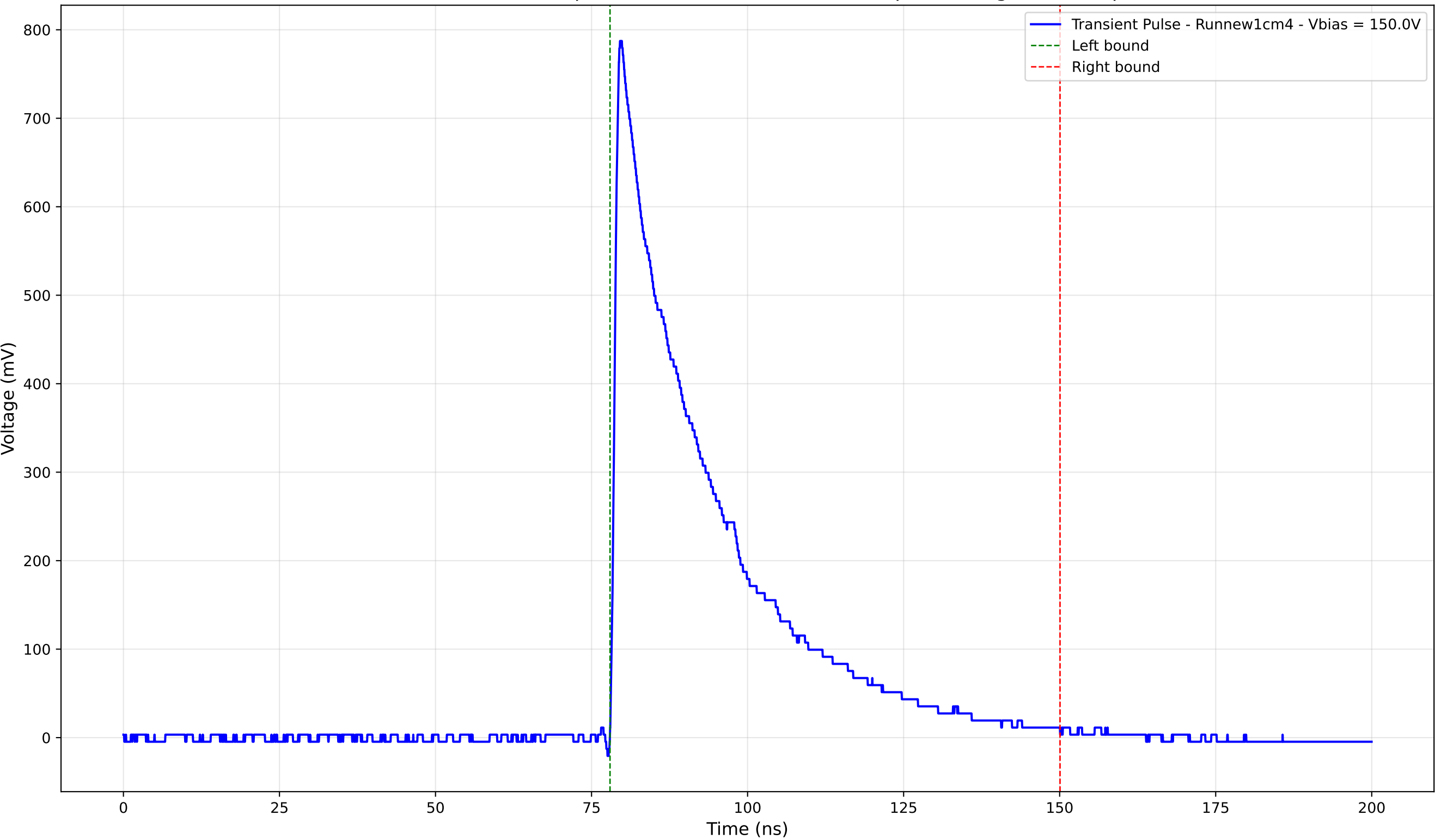
Transient Pulse - Sample: new1cm - Position: 4380.0 \mu\text{m} - Charge: 243.50 pC
