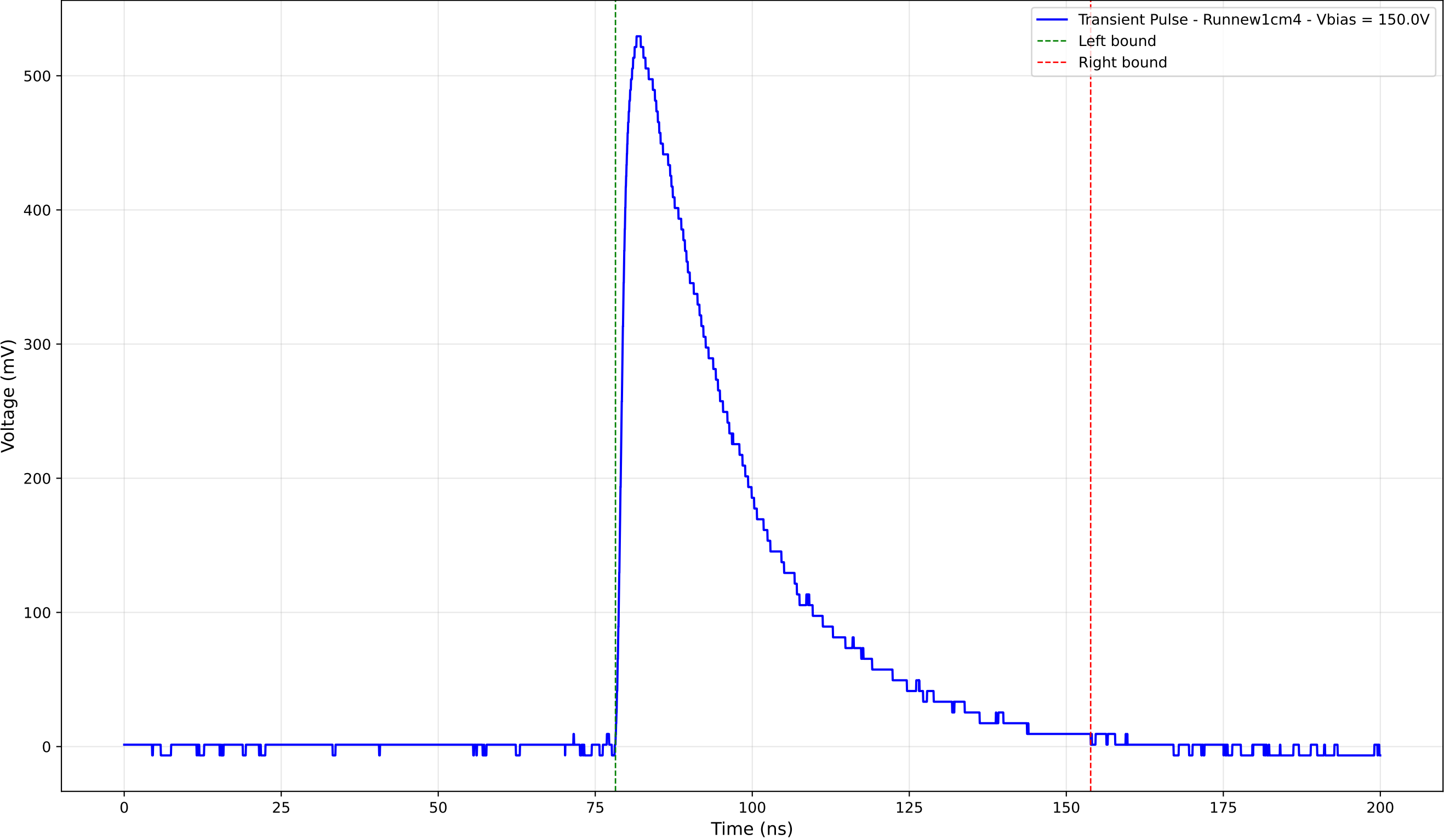
Transient Pulse - Sample: new1cm - Position: 1830.0 \mu\text{m} - Charge: 212.62 pC
