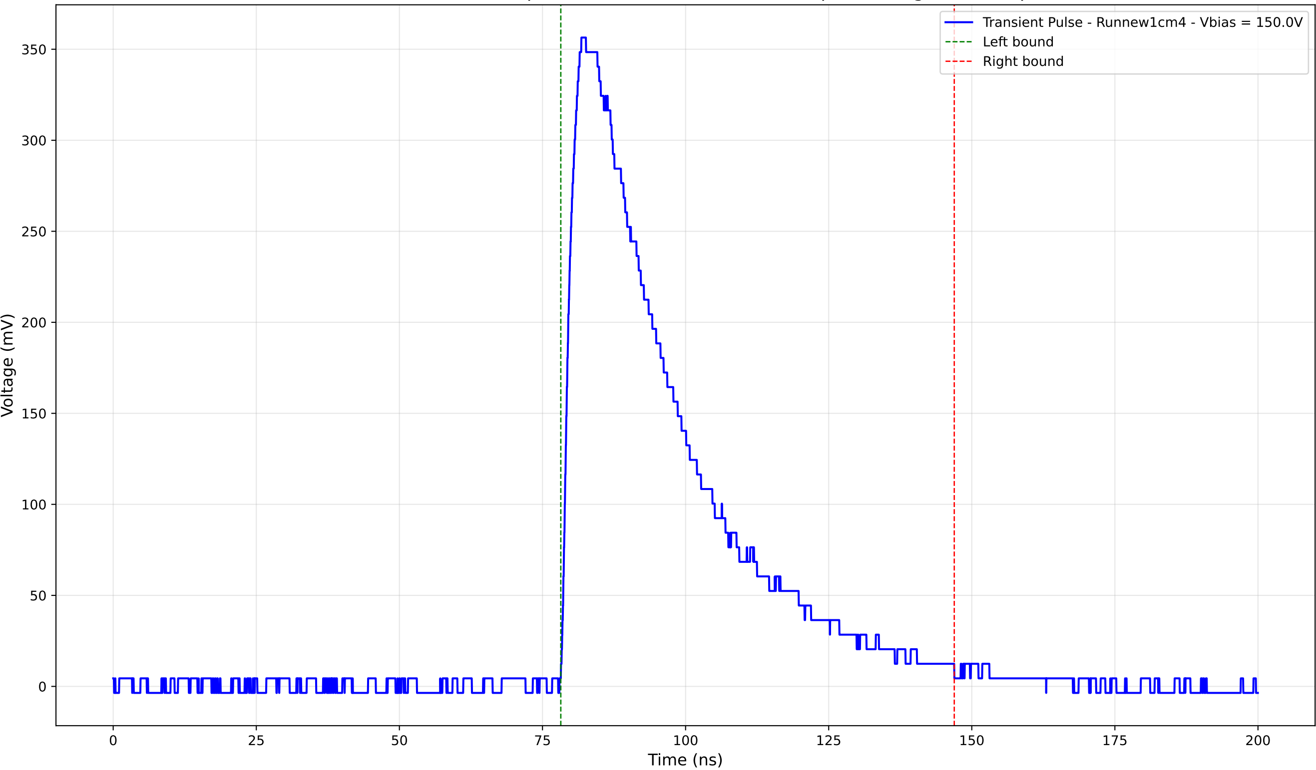
Transient Pulse - Sample: new1cm - Position: 2265.0 \mu\text{m} - Charge: 151.21 pC
