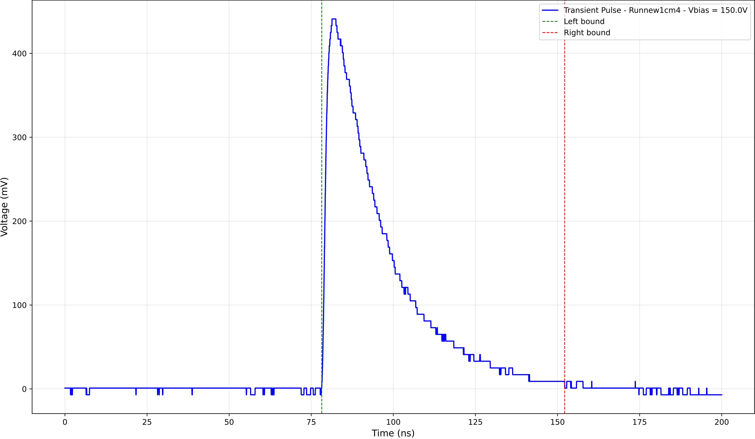
Transient Pulse - Sample: new1cm - Position: 1785.0 \mu\text{m} - Charge: 175.06 pC
