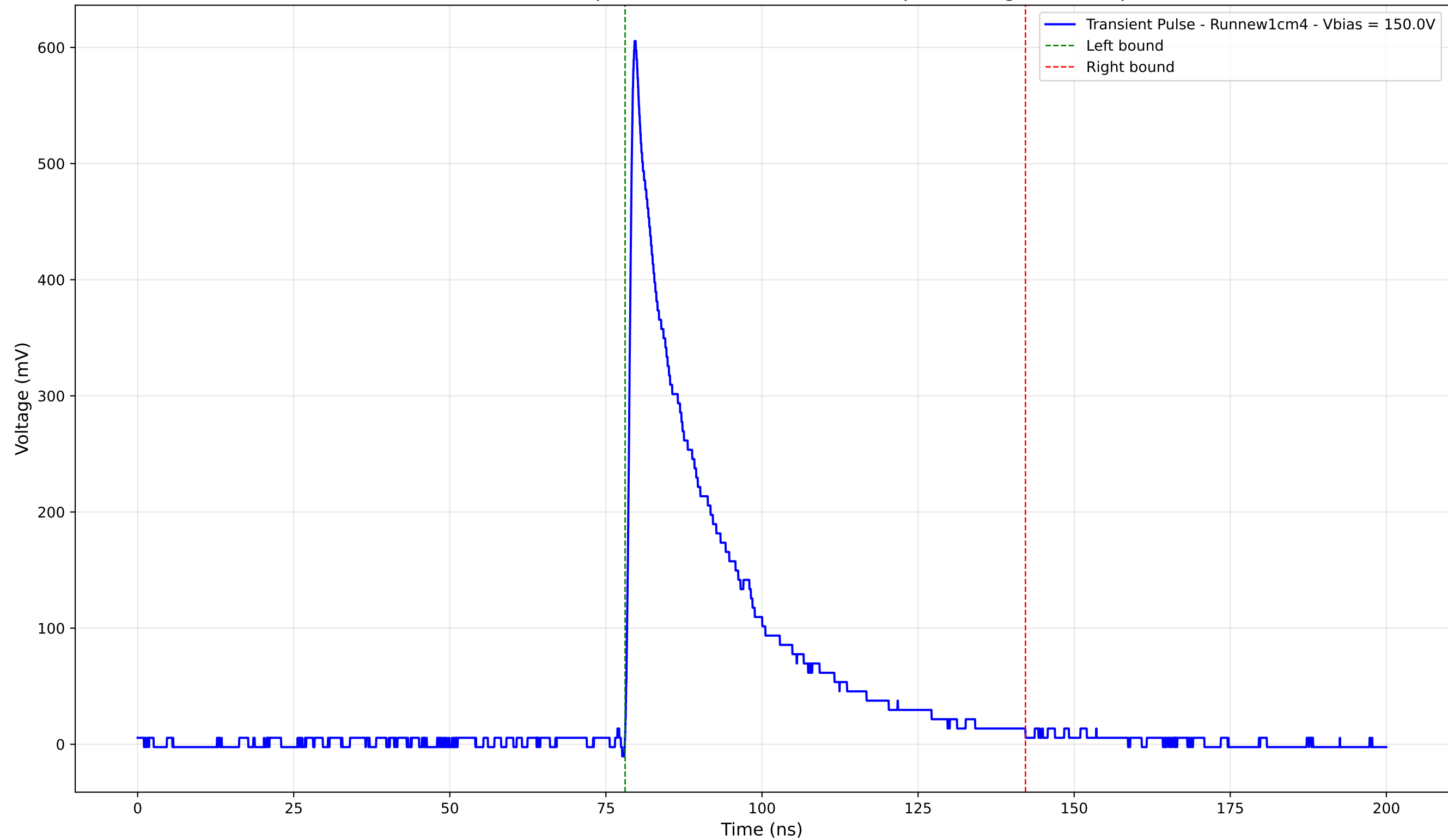
Transient Pulse - Sample: new1cm - Position: 765.0 \mu\text{m} - Charge: 151.69 pC
