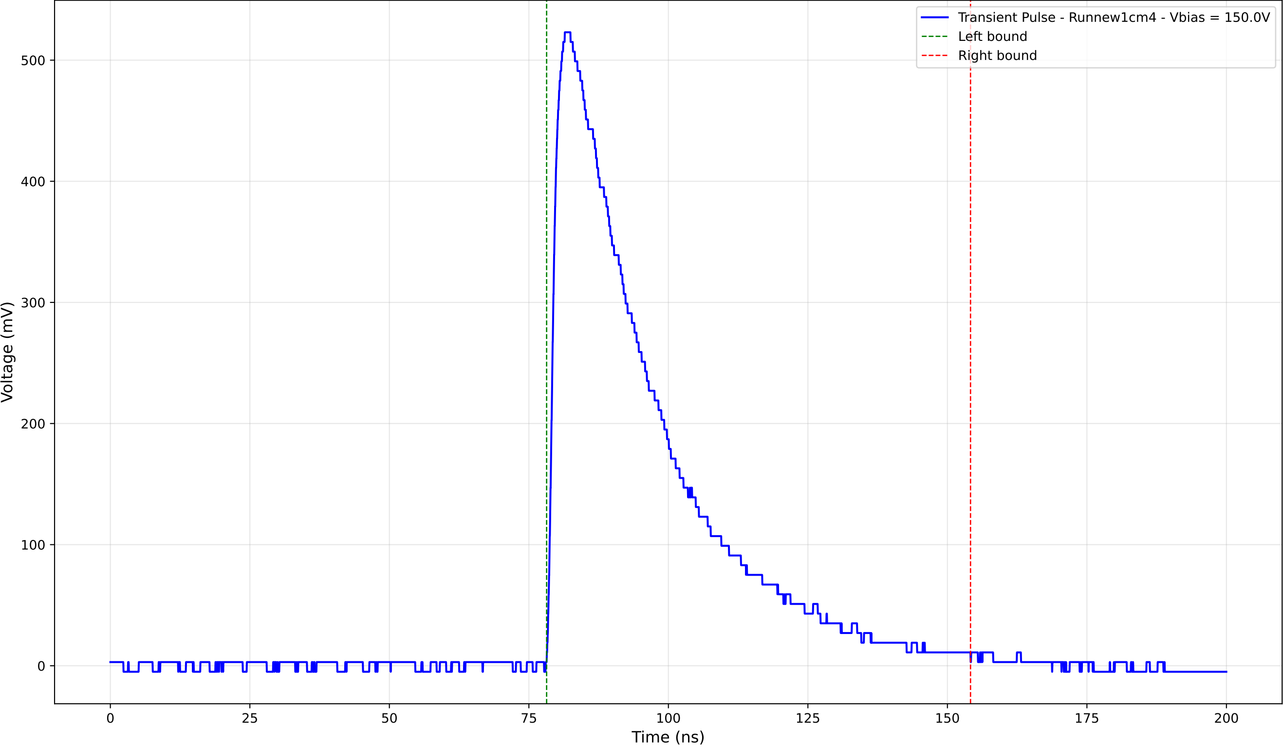
Transient Pulse - Sample: new1cm - Position: 1825.0 \mu\text{m} - Charge: 211.61 pC
