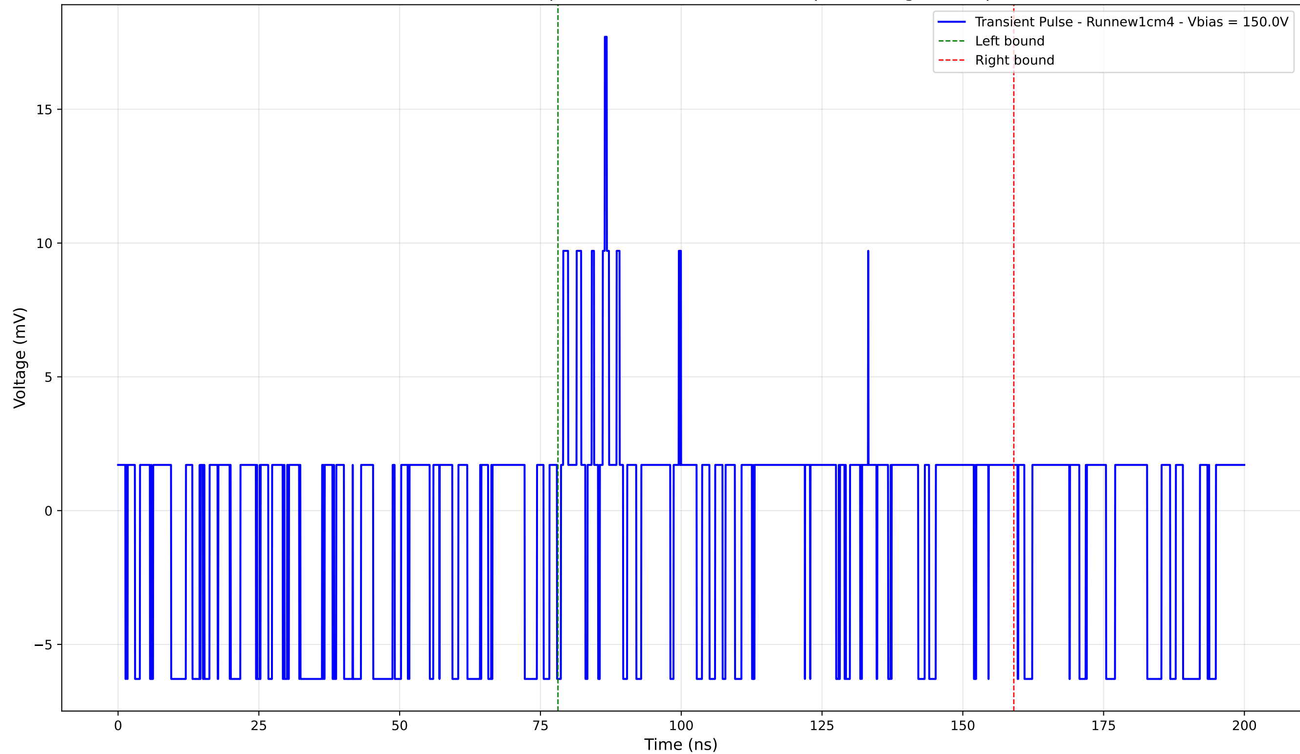
Transient Pulse - Sample: new1cm - Position: 55.0 \mu\text{m} - Charge: 1.48 pC
