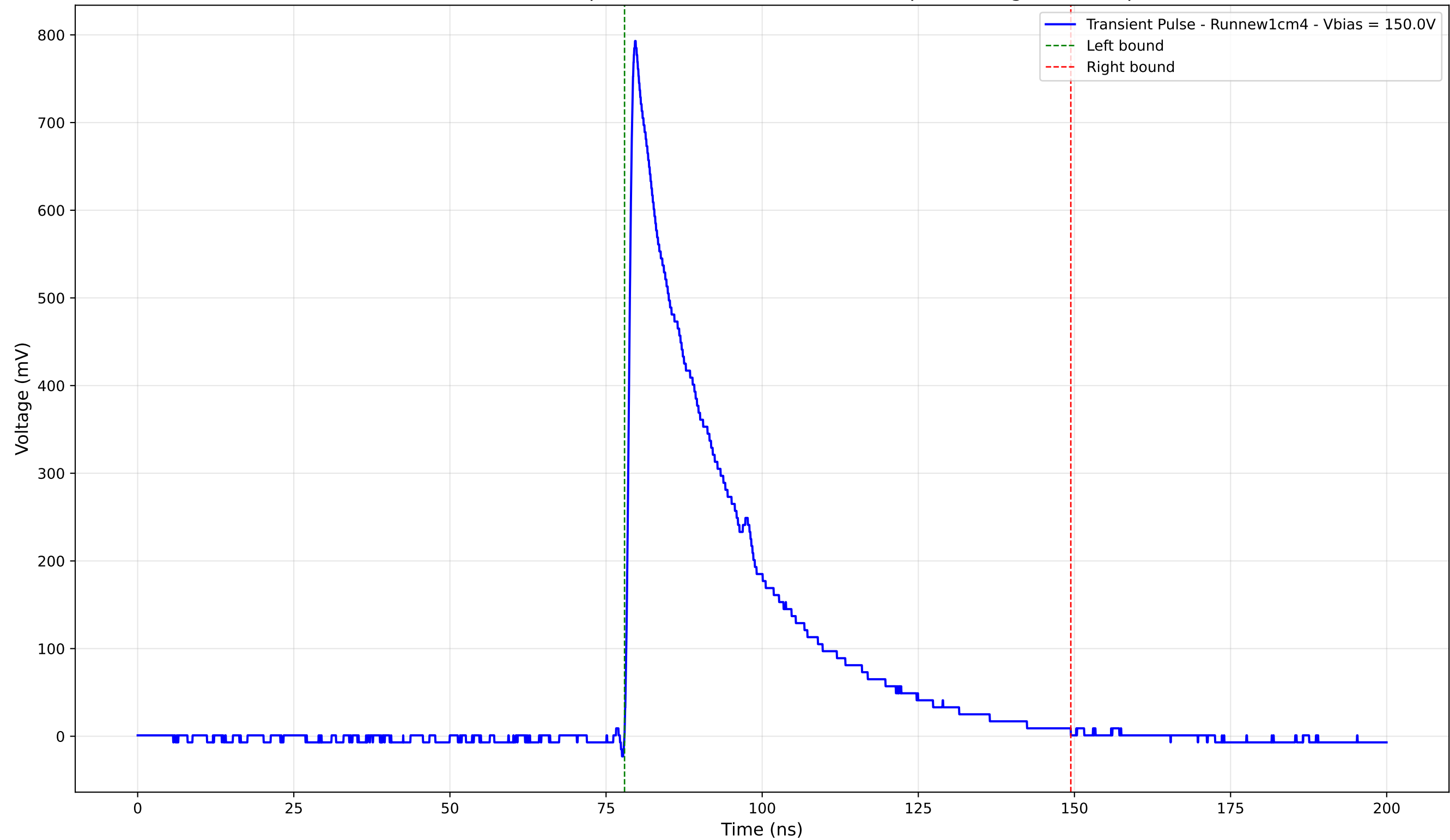
Transient Pulse - Sample: new1cm - Position: 4390.0 \mu\text{m} - Charge: 239.91 pC
