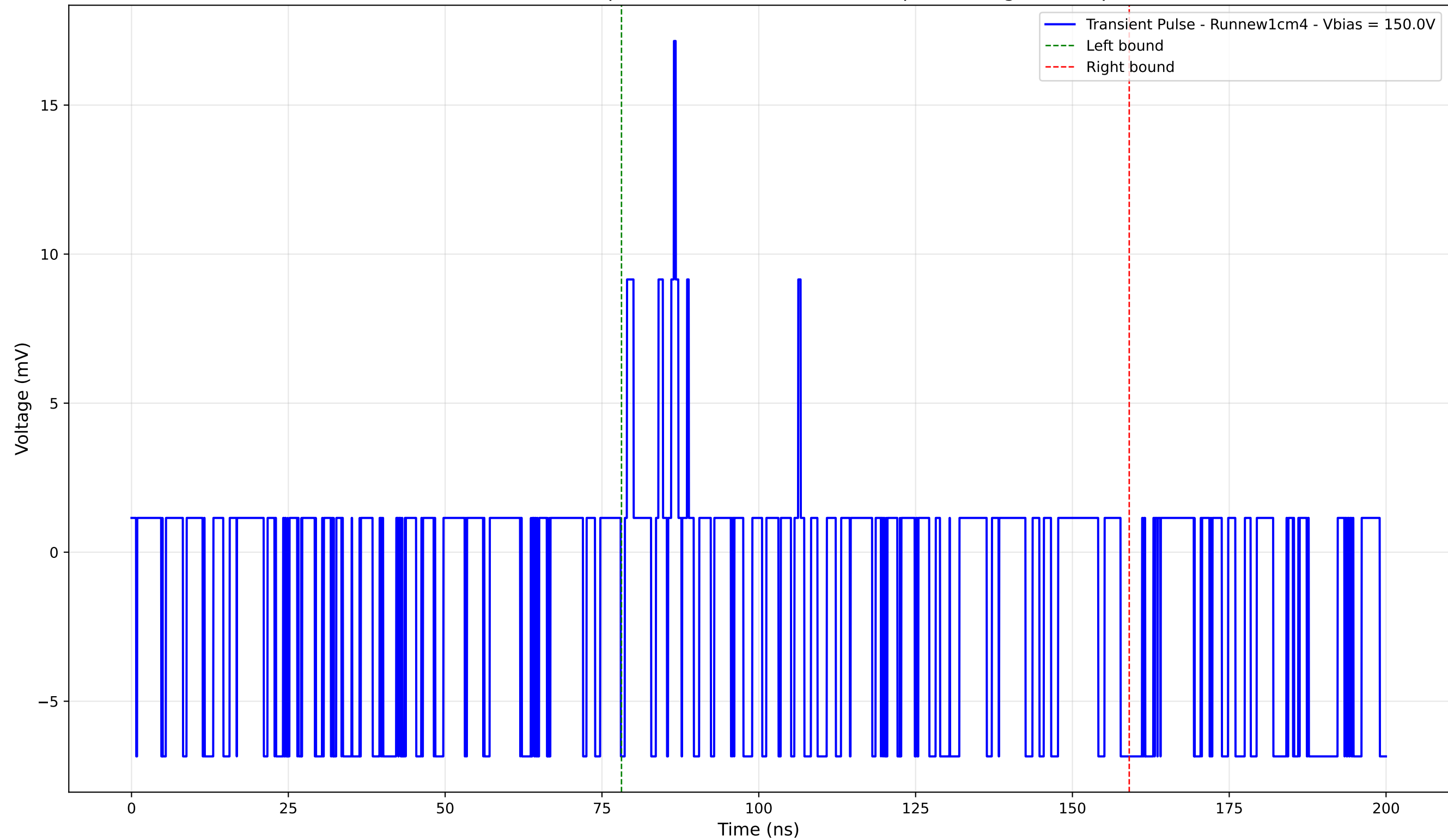
Transient Pulse - Sample: new1cm - Position: 70.0 \mu\text{m} - Charge: -1.01 pC
