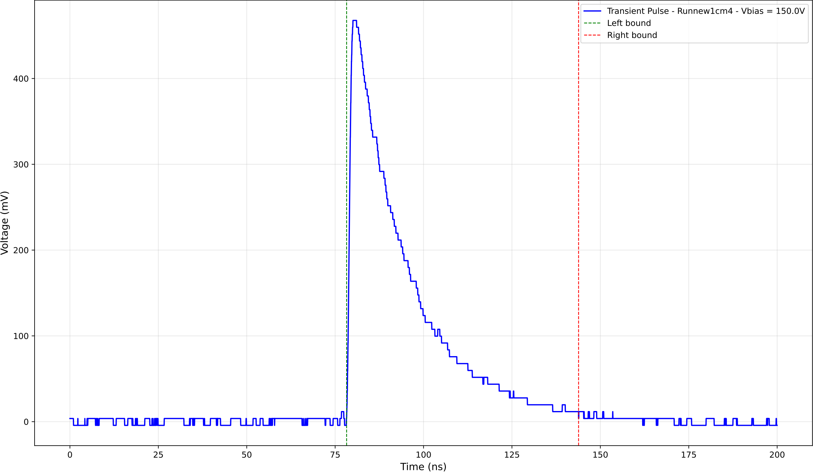
Transient Pulse - Sample: new1cm - Position: 1275.0 \mu\text{m} - Charge: 160.67 pC
