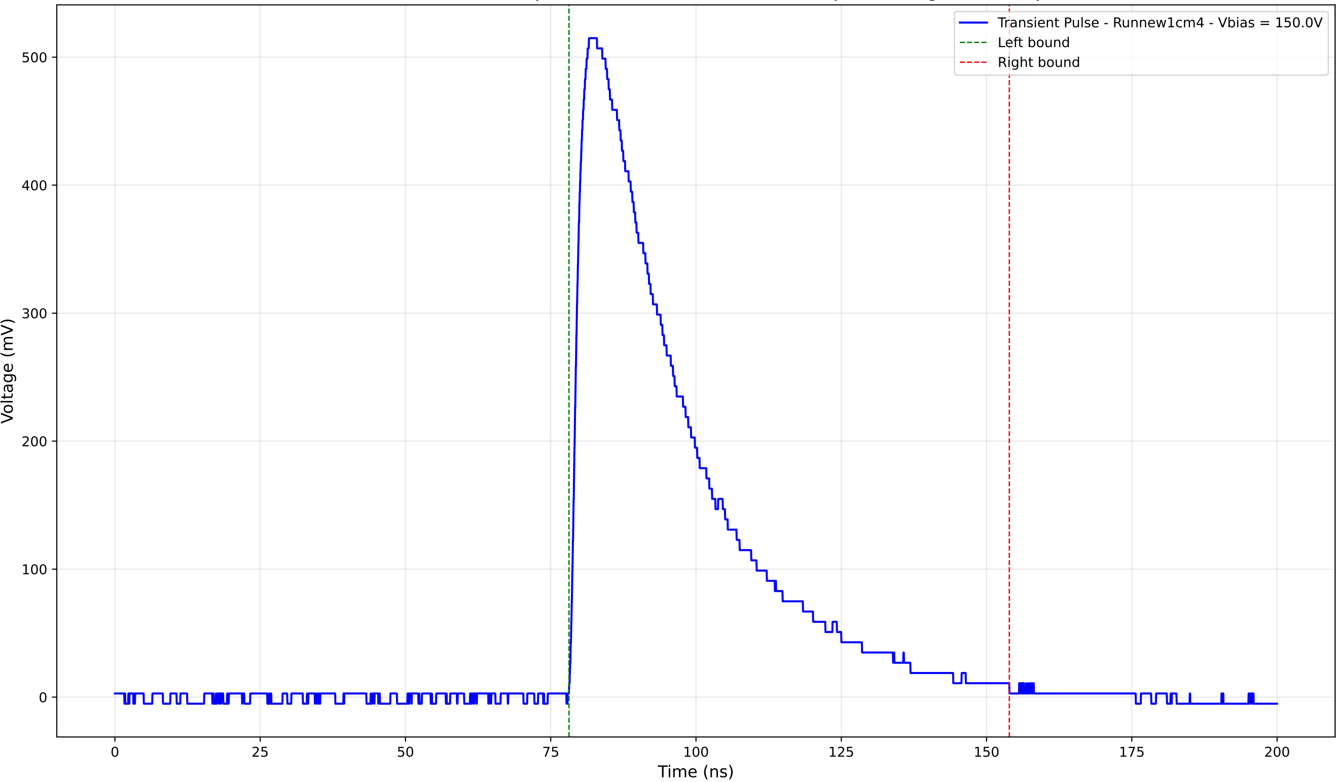
Transient Pulse - Sample: new1cm - Position: 2095.0 \mu\text{m} - Charge: 217.88 pC
