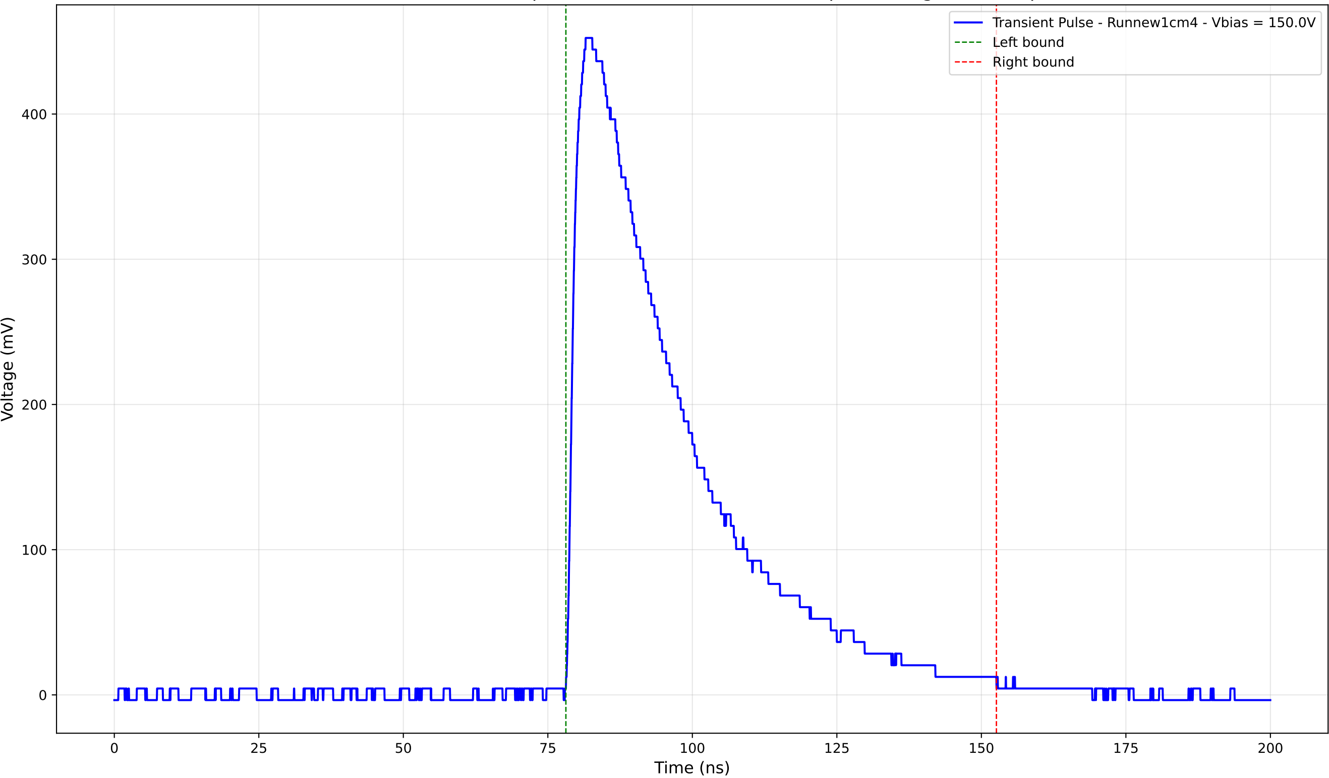
Transient Pulse - Sample: new1cm - Position: 3300.0 \mu\text{m} - Charge: 193.91 pC
