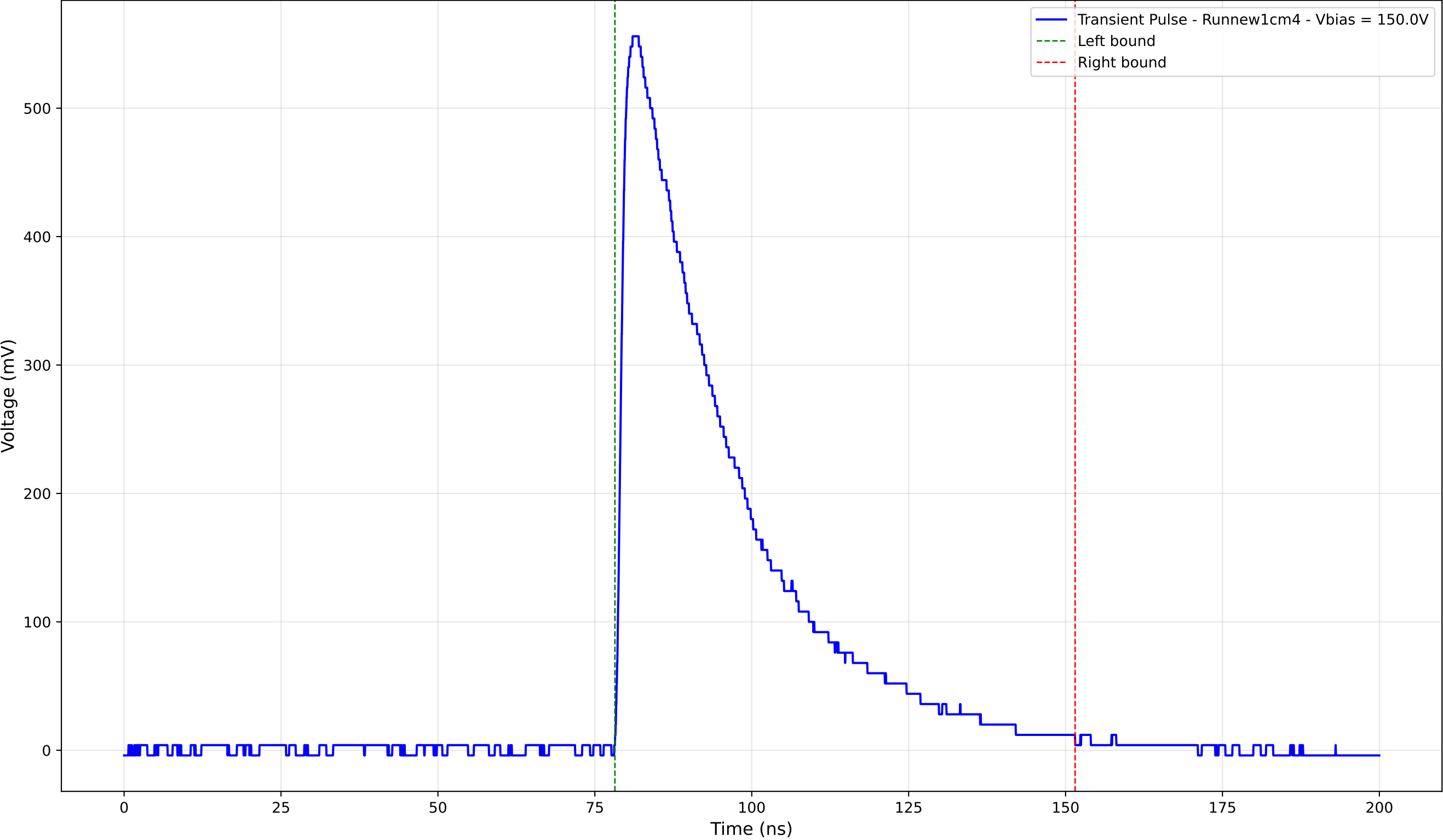
Transient Pulse - Sample: new1cm - Position: 1575.0 \mu\text{m} - Charge: 213.75 pC
