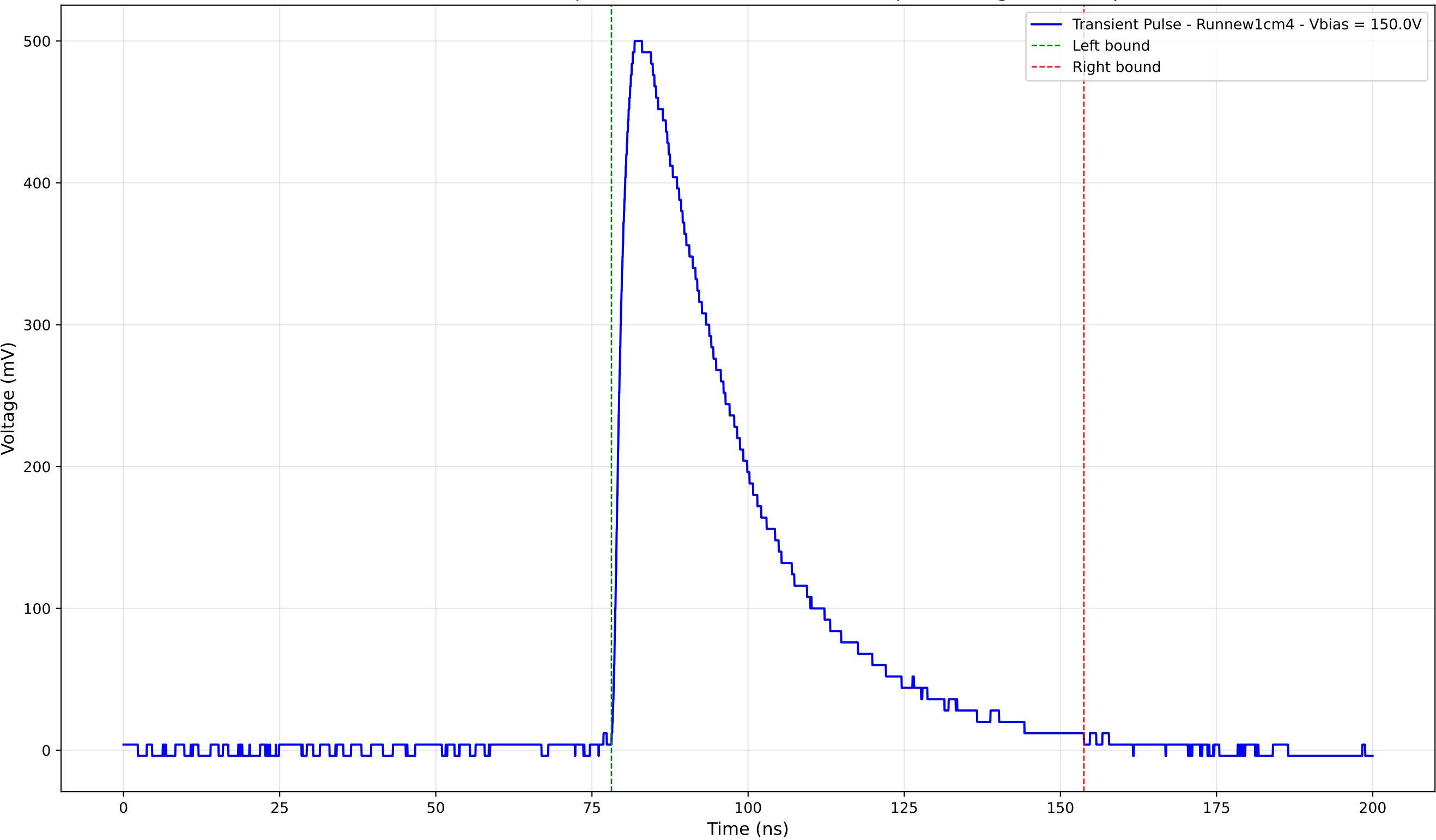
Transient Pulse - Sample: new1cm - Position: 2310.0 \mu\text{m} - Charge: 216.04 pC
