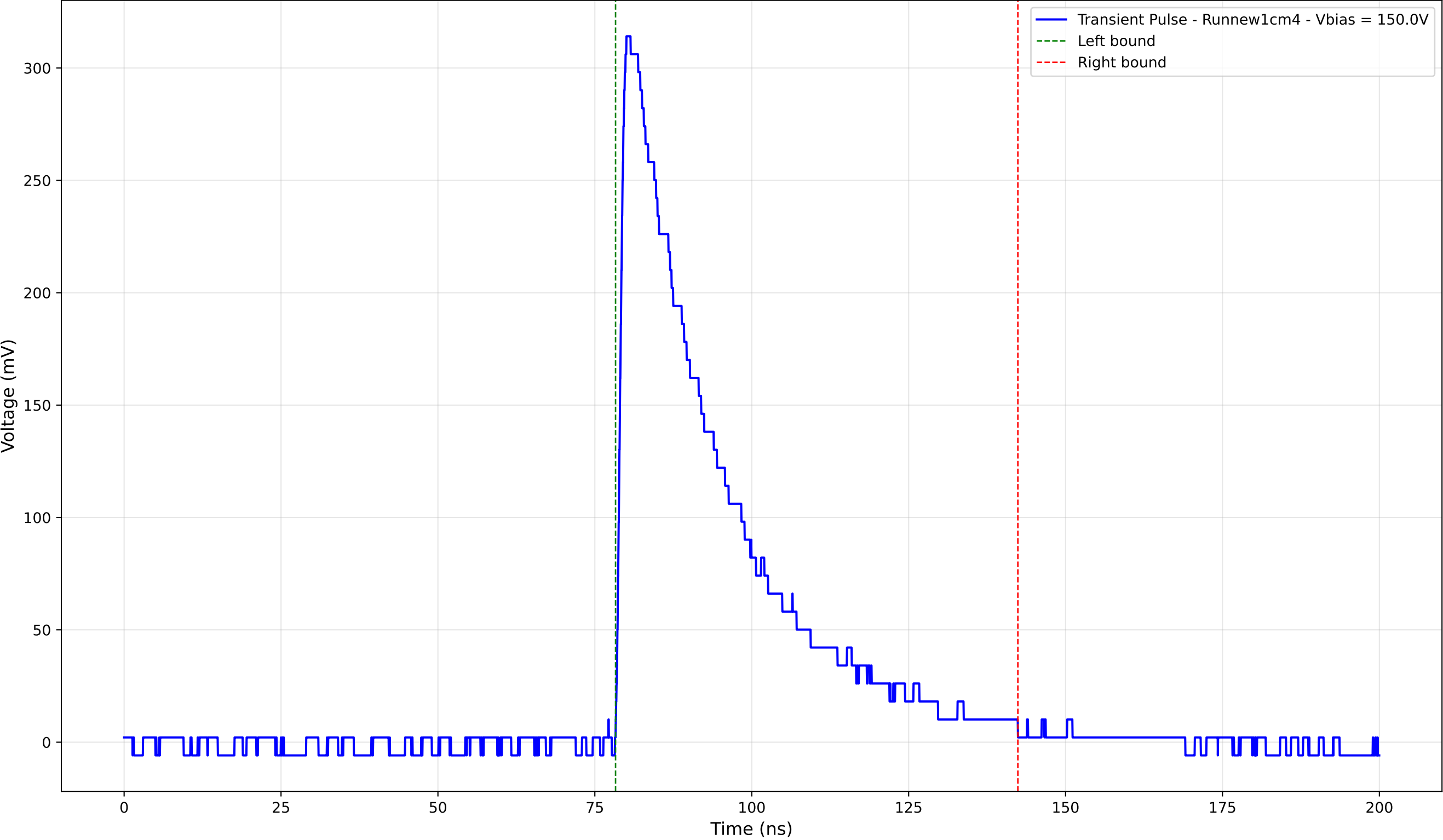
Transient Pulse - Sample: new1cm - Position: 1250.0 \mu\text{m} - Charge: 106.37 pC
