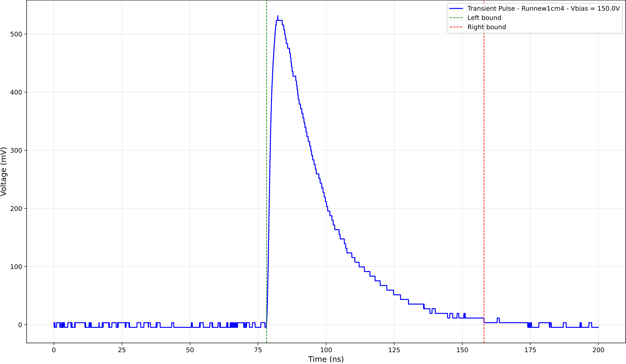
Transient Pulse - Sample: new1cm - Position: 3040.0 \mu\text{m} - Charge: 232.96 pC
