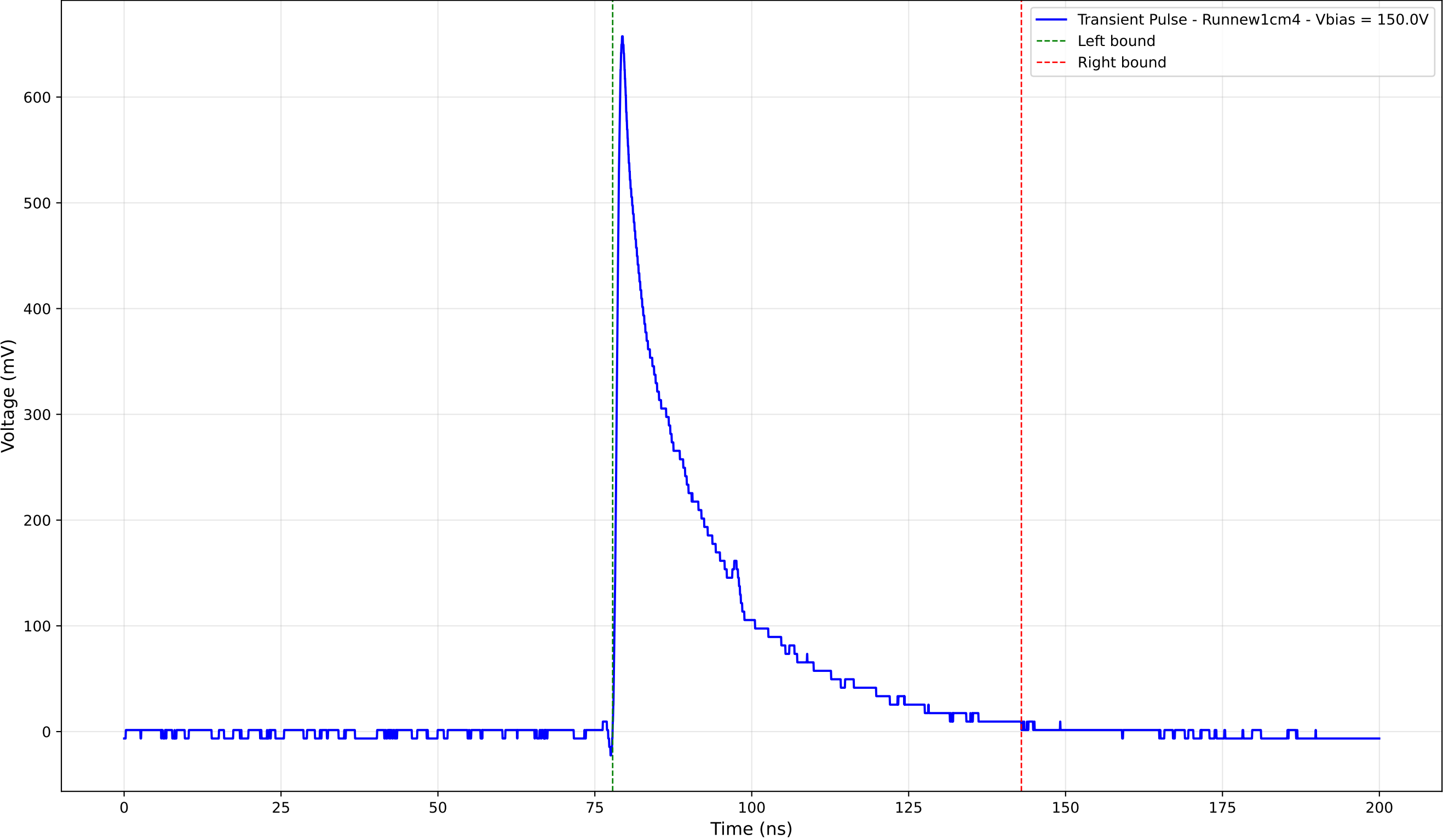
Transient Pulse - Sample: new1cm - Position: 4665.0 \mu\text{m} - Charge: 156.83 pC
