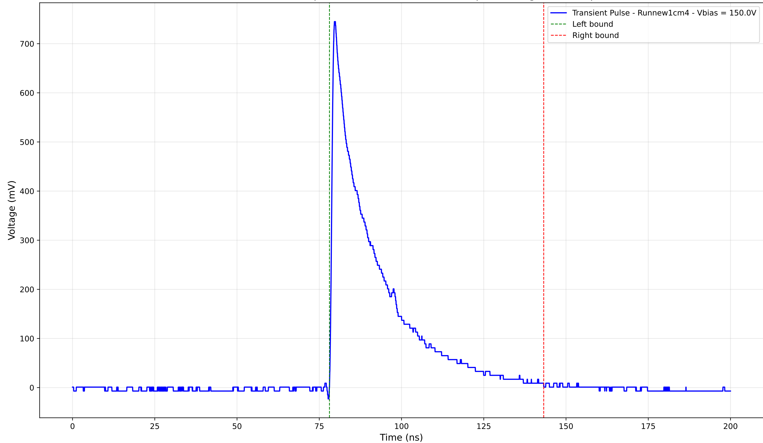
Transient Pulse - Sample: new1cm - Position: 835.0 \mu\text{m} - Charge: 197.69 pC
