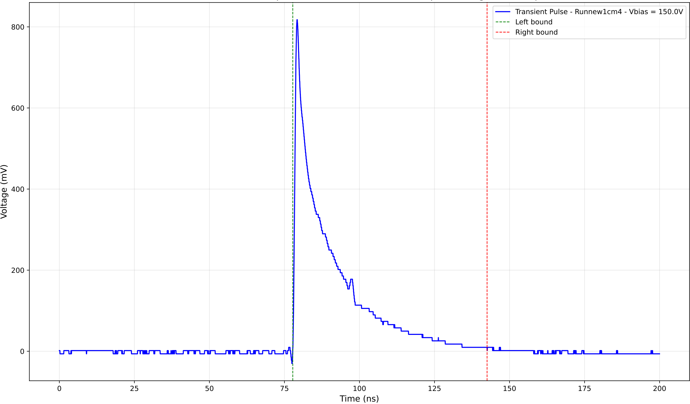
Transient Pulse - Sample: new1cm - Position: 4830.0 \mu\text{m} - Charge: 176.33 pC
