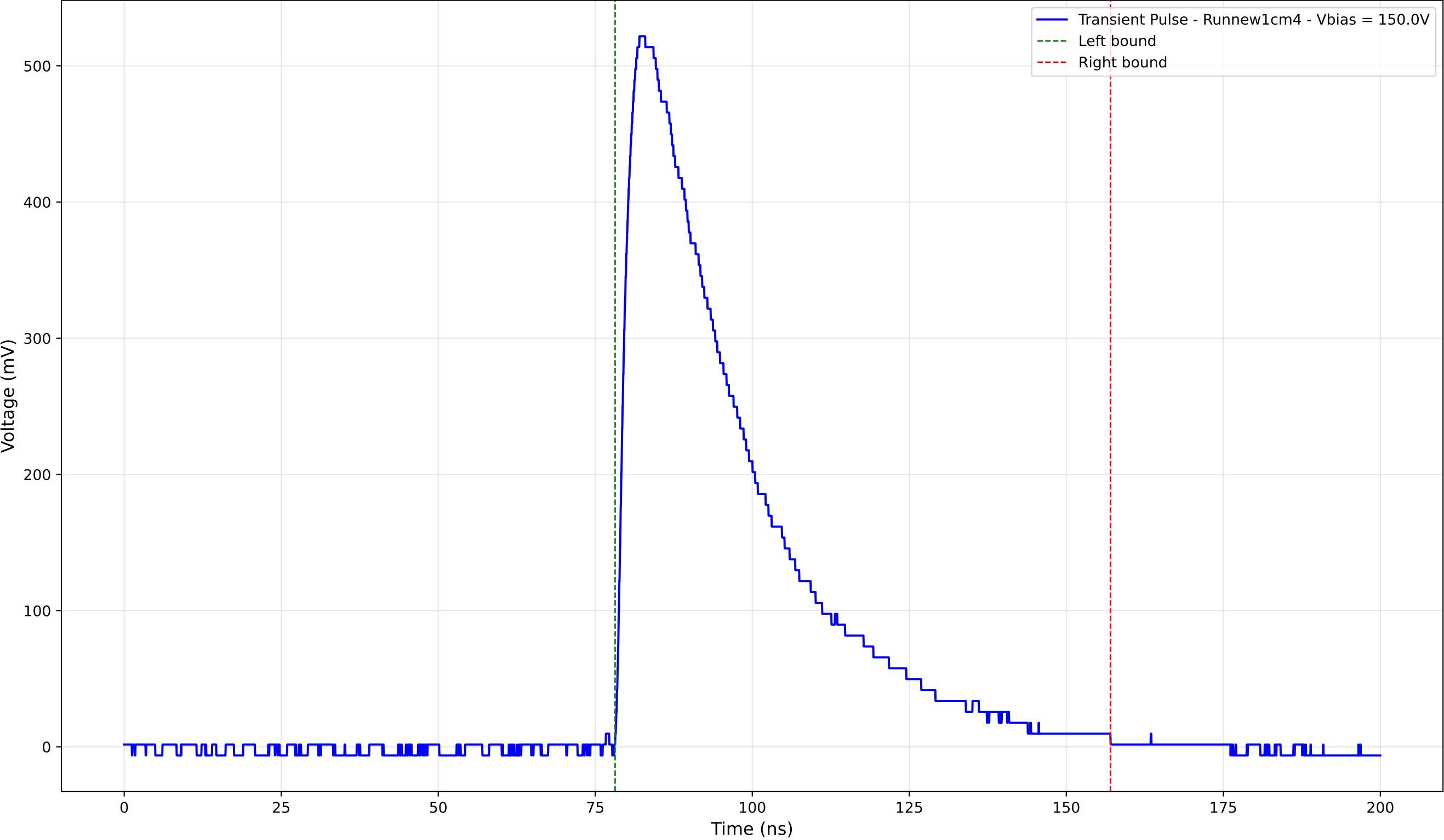
Transient Pulse - Sample: new1cm - Position: 2465.0 \mu\text{m} - Charge: 225.60 pC
