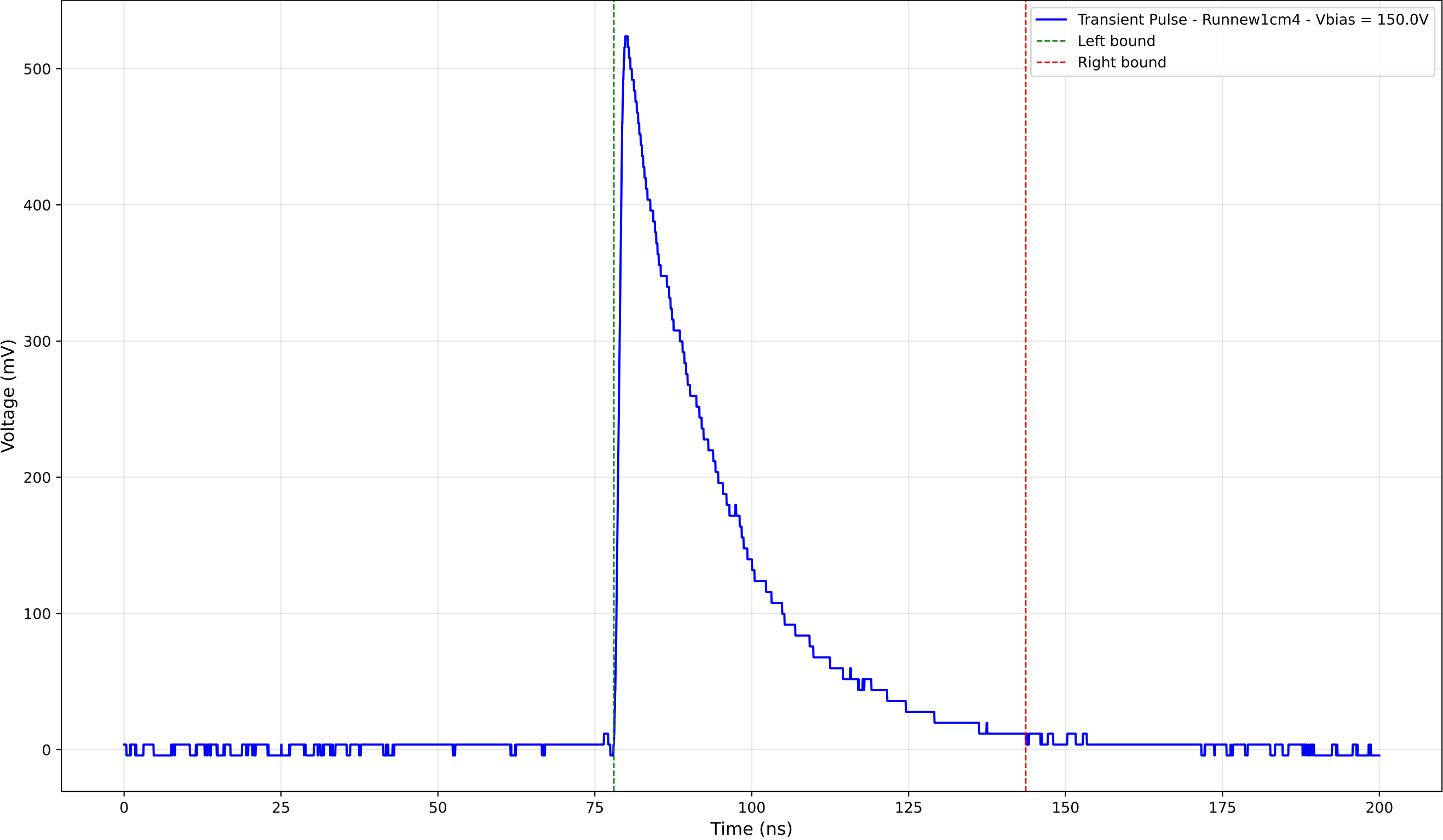
Transient Pulse - Sample: new1cm - Position: 4170.0 \mu\text{m} - Charge: 170.41 pC
