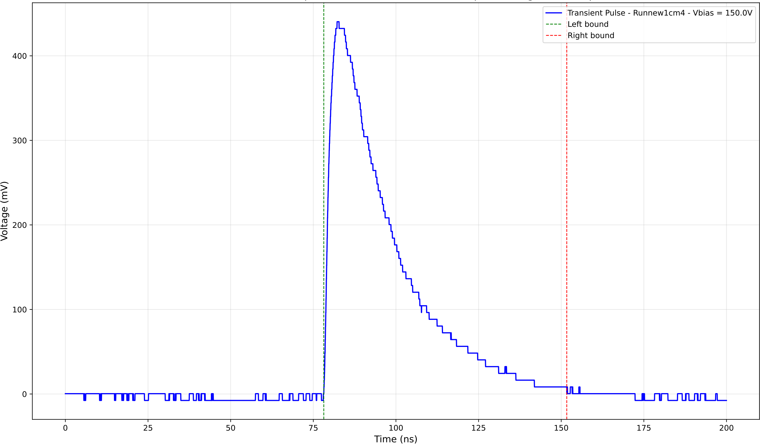
Transient Pulse - Sample: new1cm - Position: 2635.0 \mu\text{m} - Charge: 188.35 pC
