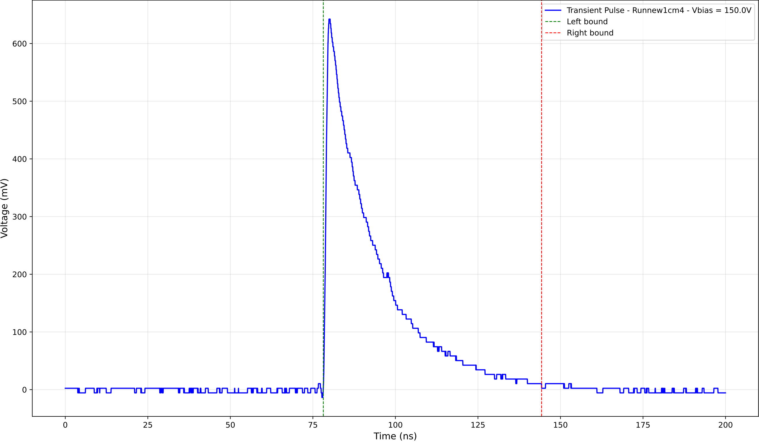
Transient Pulse - Sample: new1cm - Position: 1090.0 \mu\text{m} - Charge: 198.07 pC
