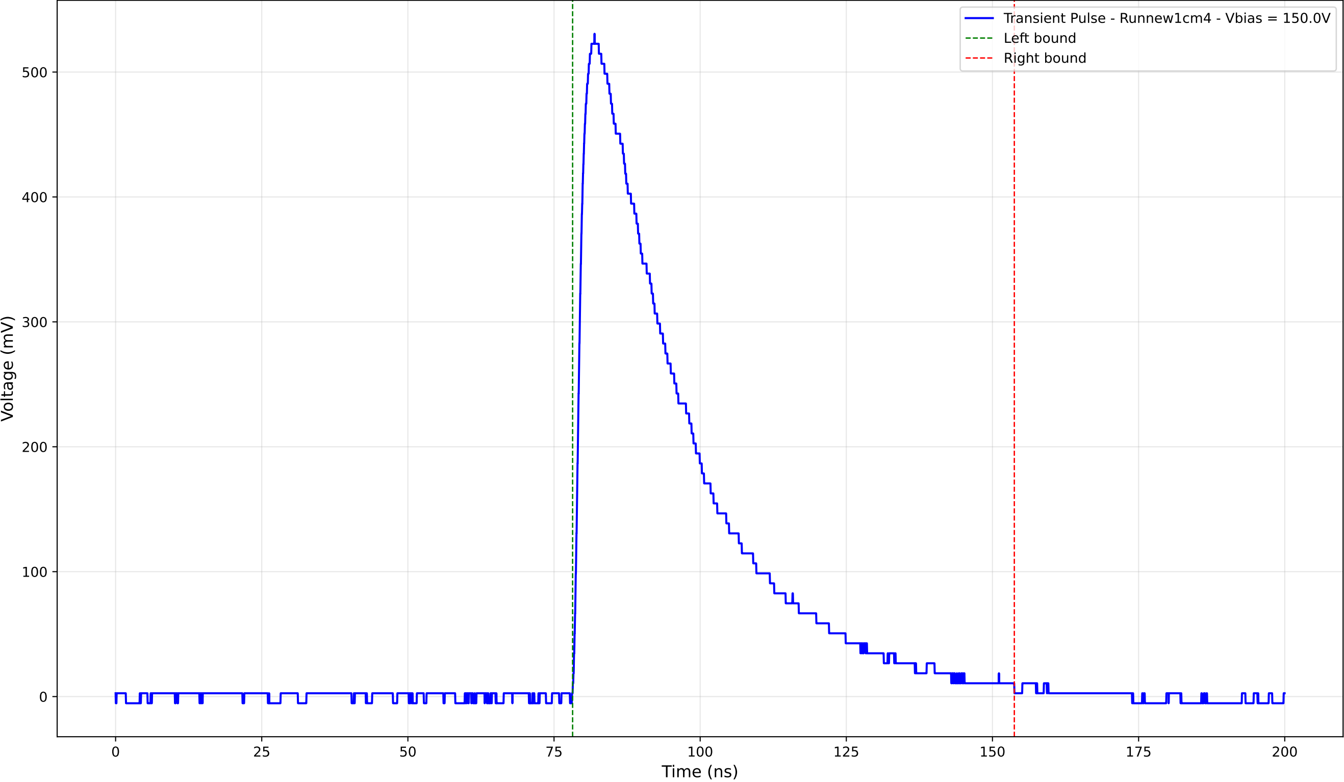
Transient Pulse - Sample: new1cm - Position: 1885.0 \mu\text{m} - Charge: 214.31 pC
