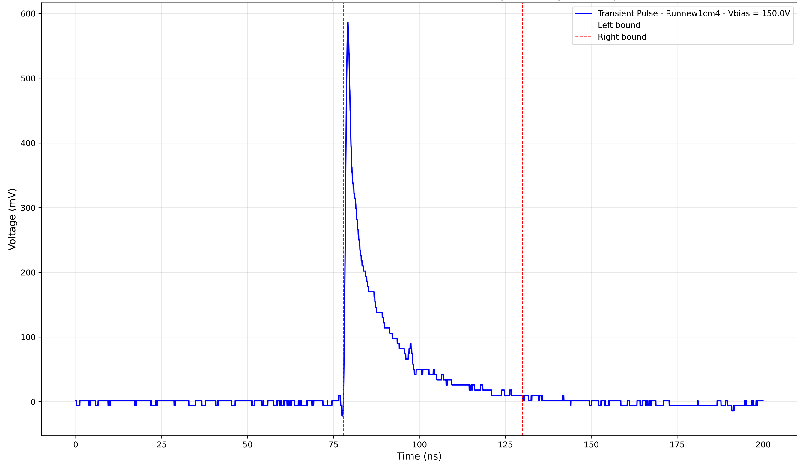
Transient Pulse - Sample: new1cm - Position: 240.0 \mu\text{m} - Charge: 89.18 pC
