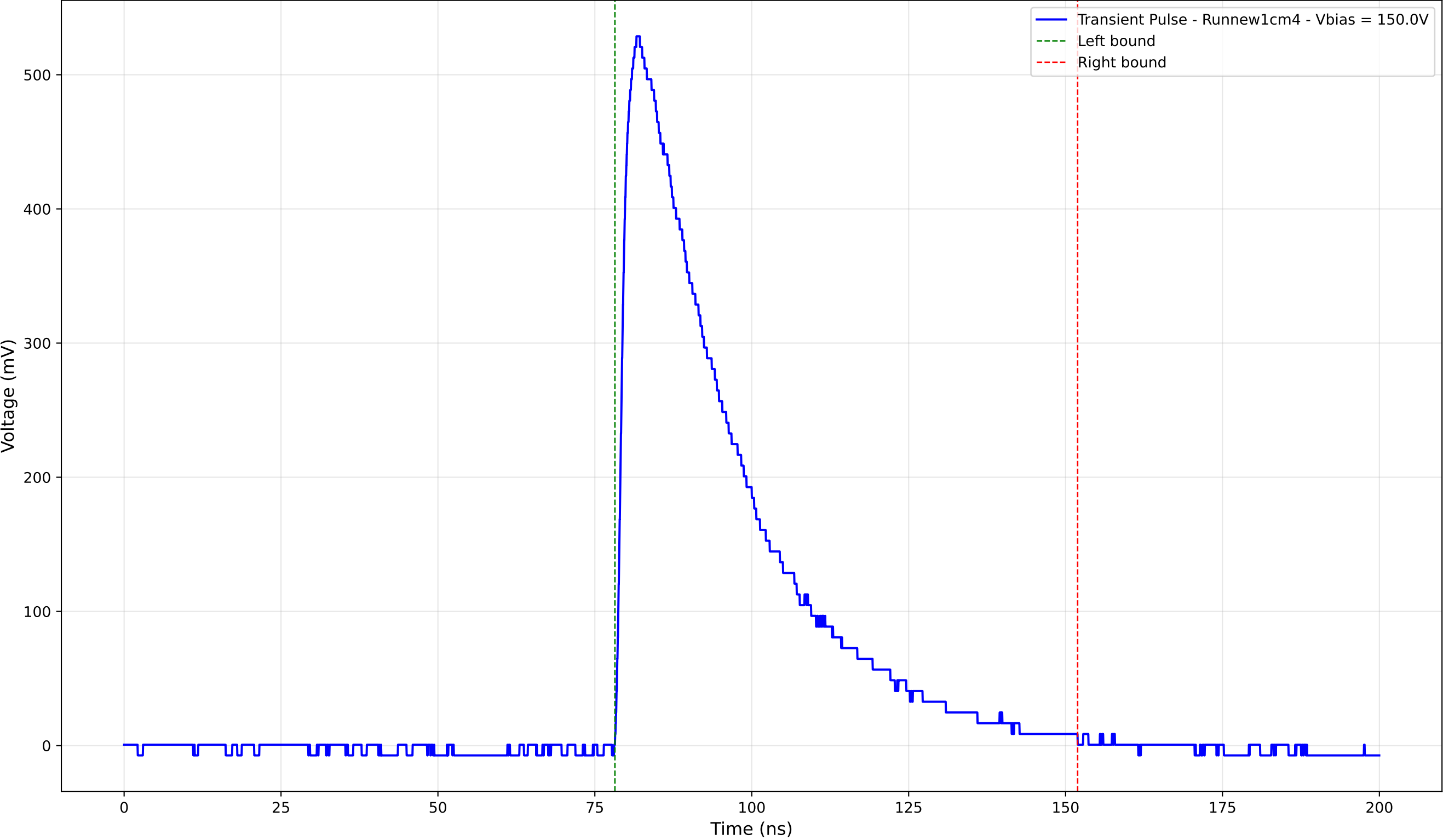
Transient Pulse - Sample: new1cm - Position: 1835.0 \mu\text{m} - Charge: 208.73 pC
