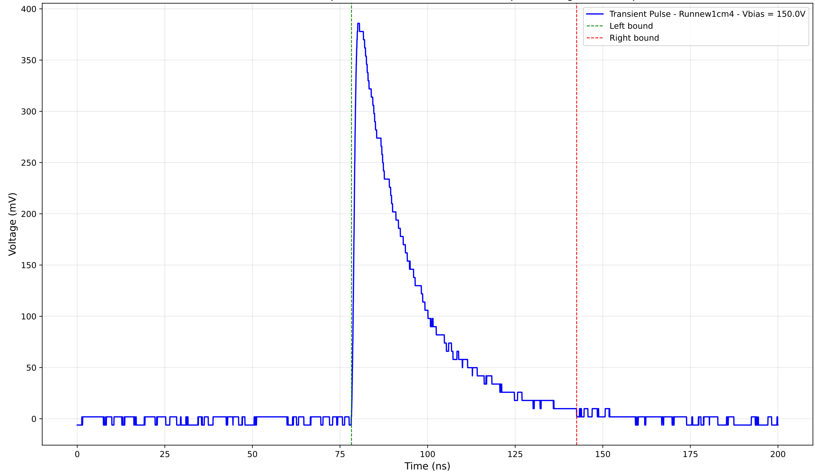
Transient Pulse - Sample: new1cm - Position: 1260.0 \mu\text{m} - Charge: 129.59 pC
