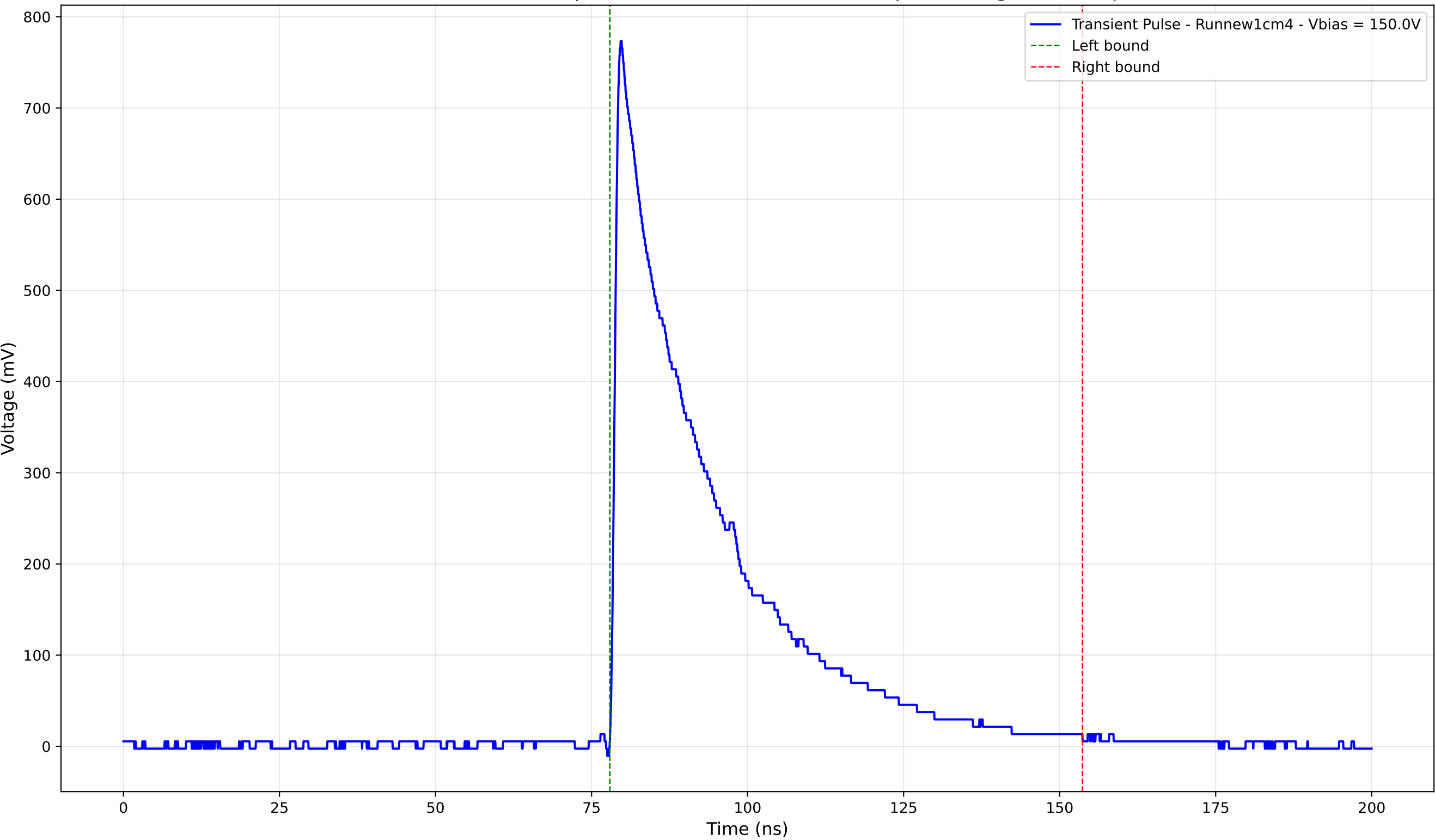
Transient Pulse - Sample: new1cm - Position: 4355.0 \mu\text{m} - Charge: 242.40 pC
