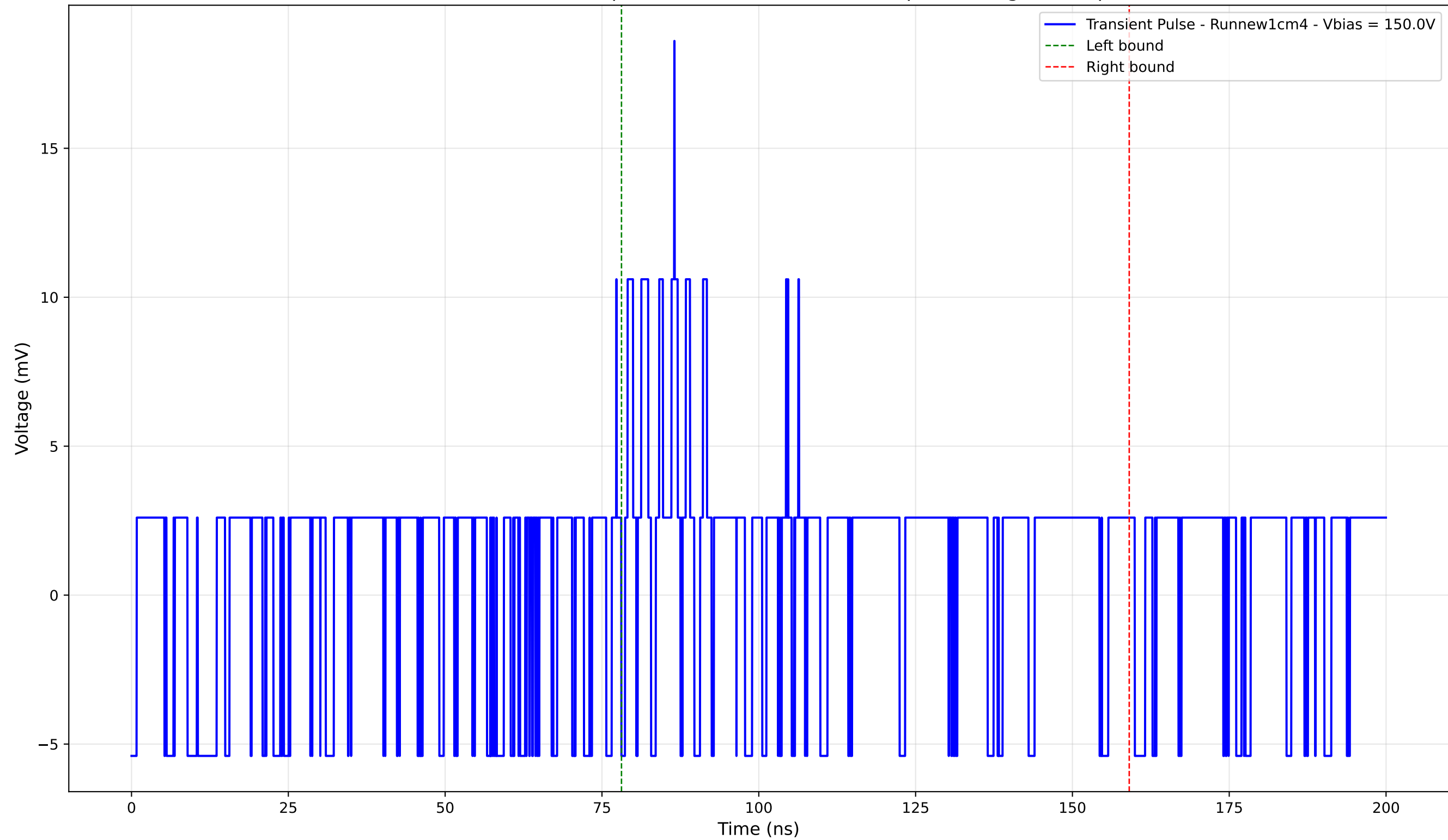
Transient Pulse - Sample: new1cm - Position: 40.0 \mu\text{m} - Charge: 2.98 pC
