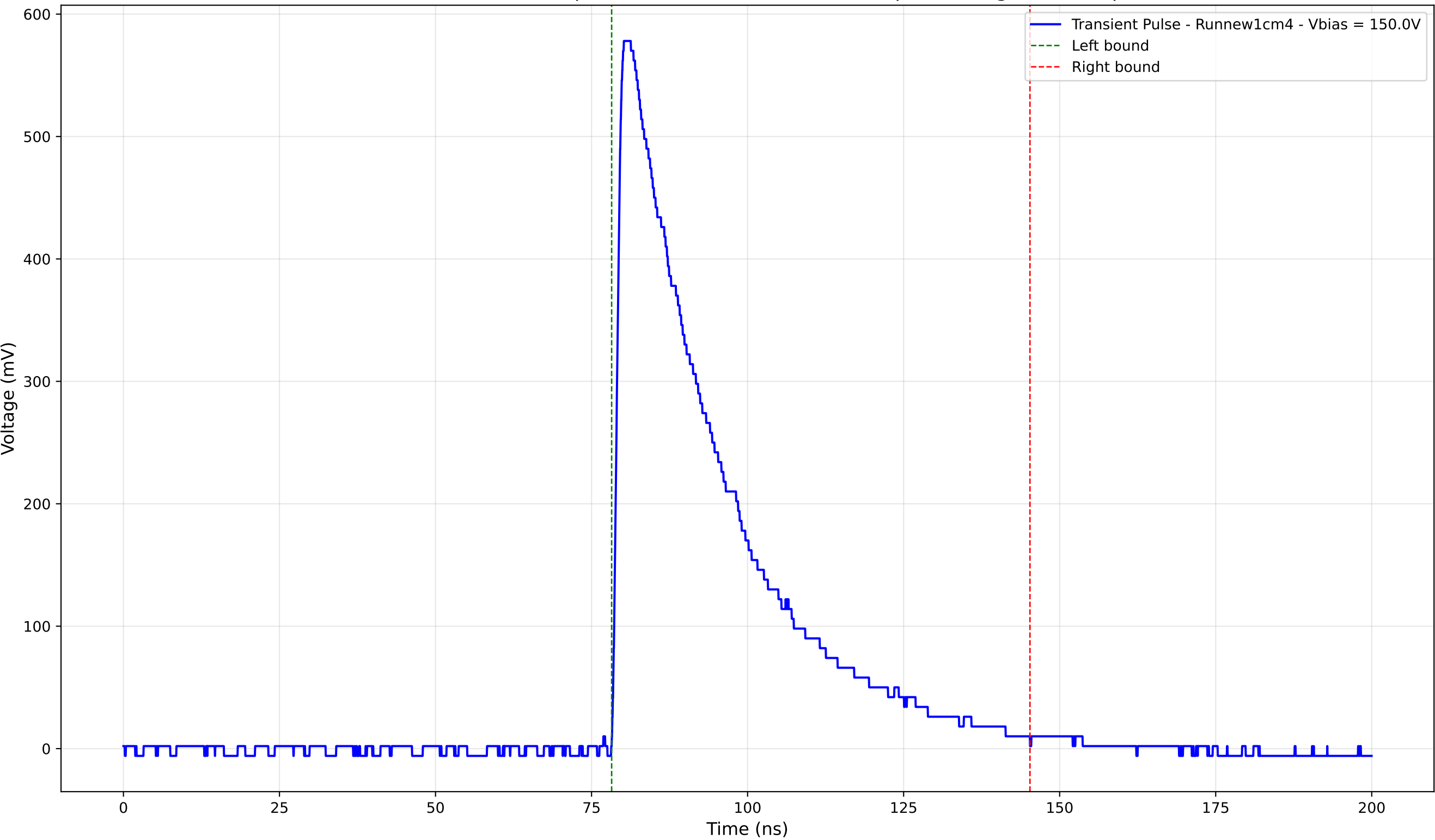
Transient Pulse - Sample: new1cm - Position: 1360.0 \mu\text{m} - Charge: 205.10 pC
