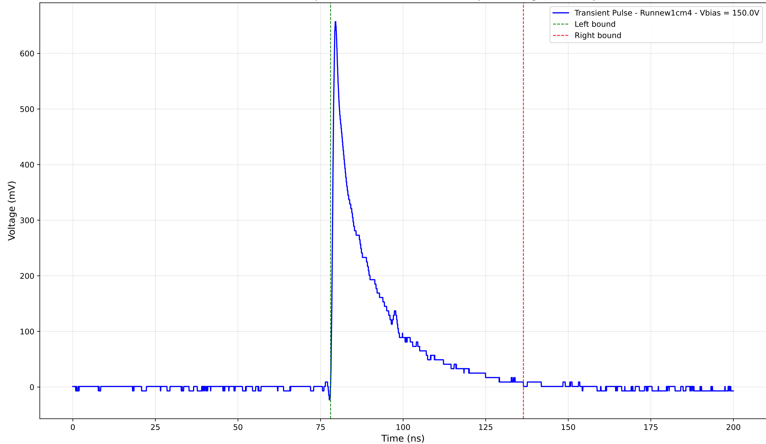
Transient Pulse - Sample: new1cm - Position: 625.0 \mu\text{m} - Charge: 137.79 pC
