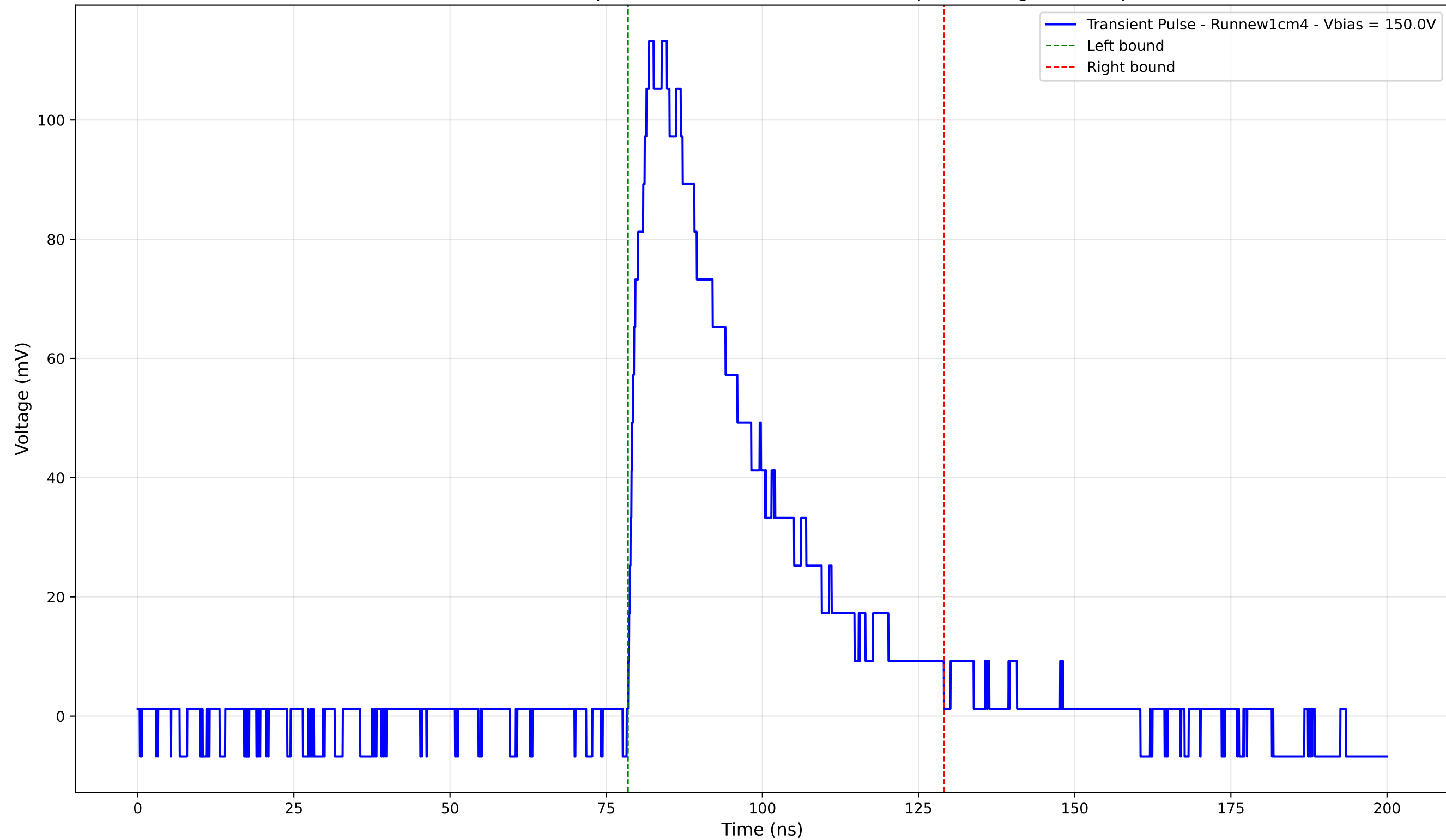
Transient Pulse - Sample: new1cm - Position: 2220.0 \mu\text{m} - Charge: 43.35 pC
