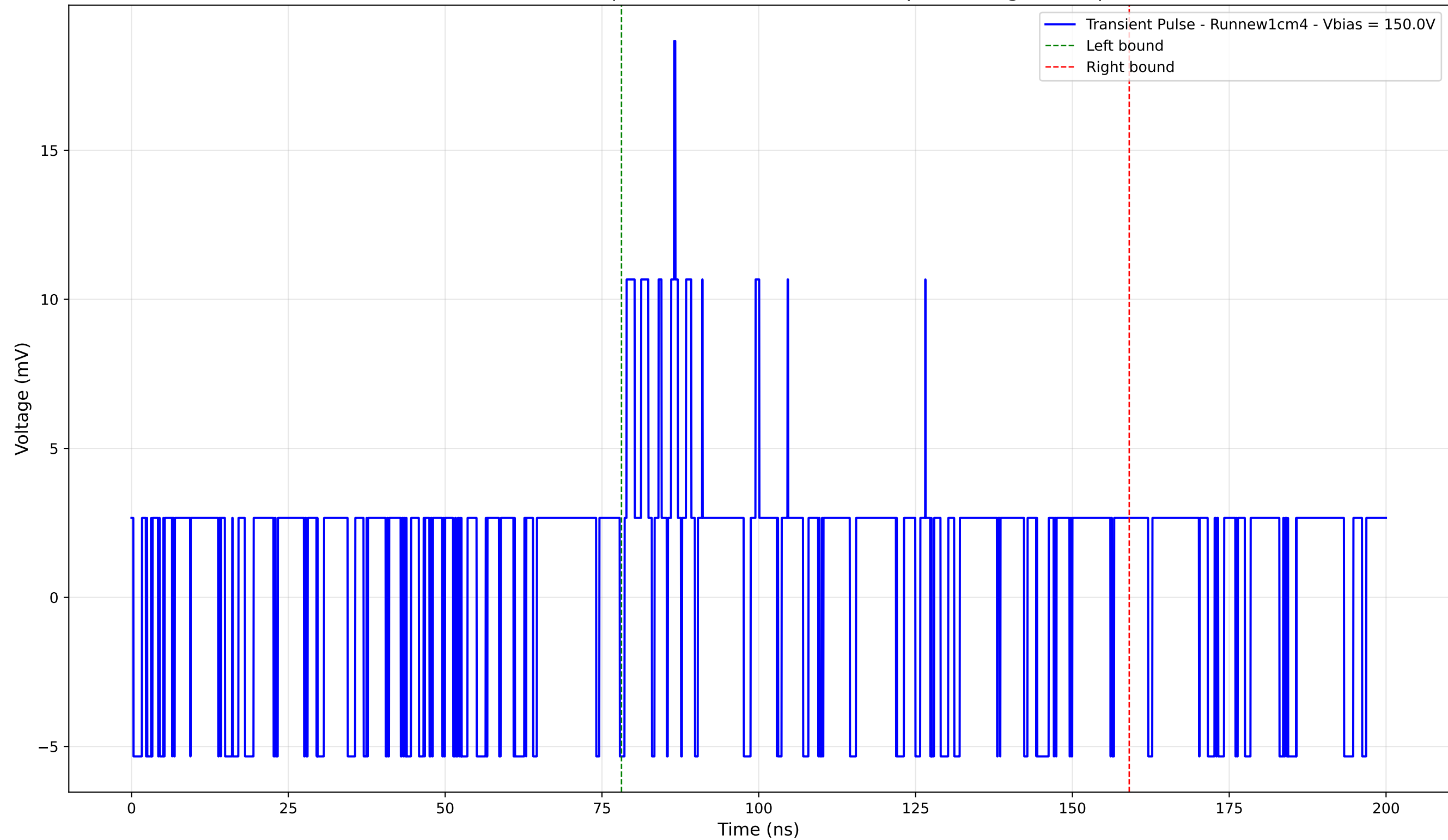
Transient Pulse - Sample: new1cm - Position: 50.0 \mu\text{m} - Charge: 3.04 pC
