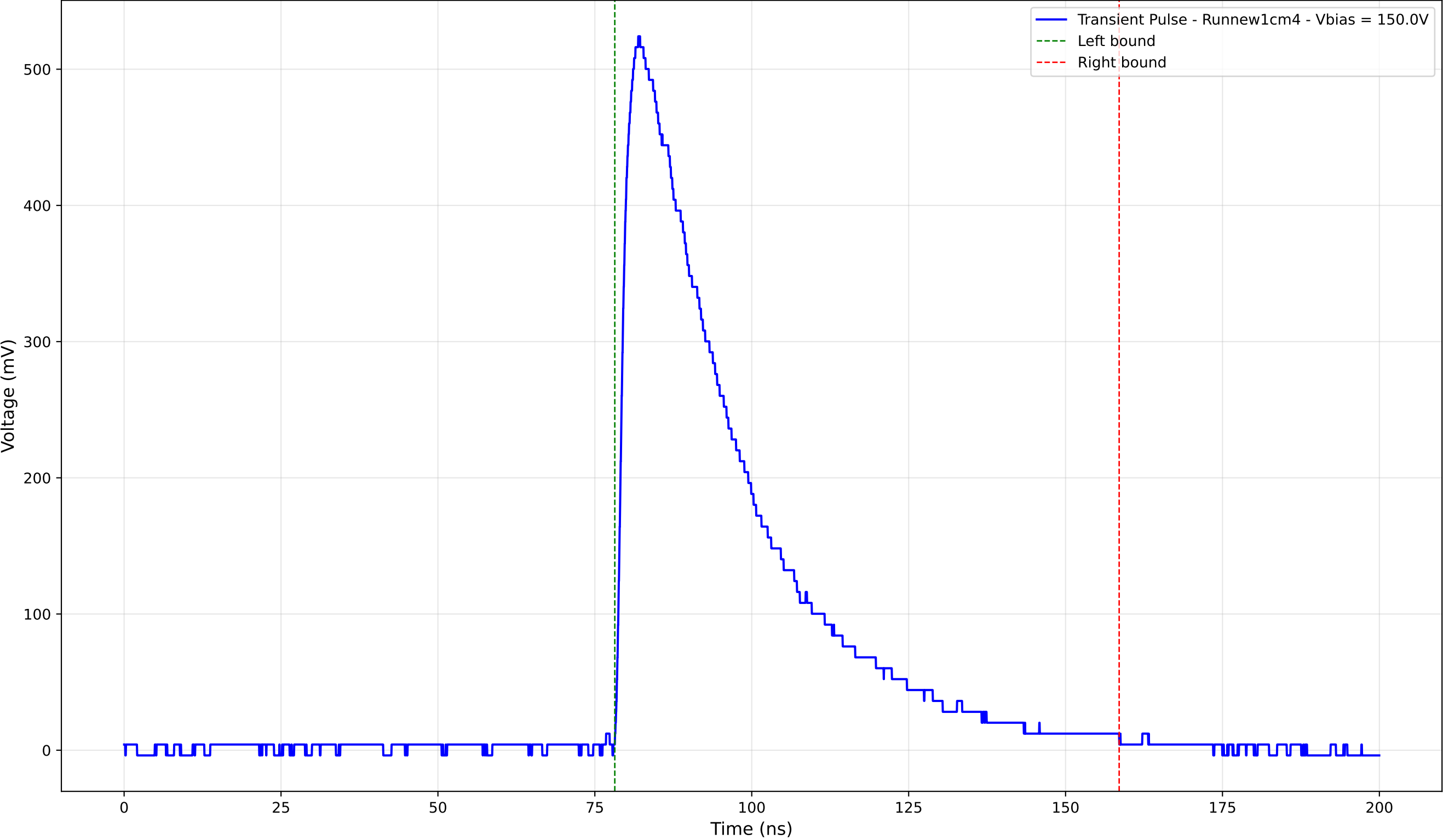
Transient Pulse - Sample: new1cm - Position: 1935.0 \mu\text{m} - Charge: 215.58 pC
