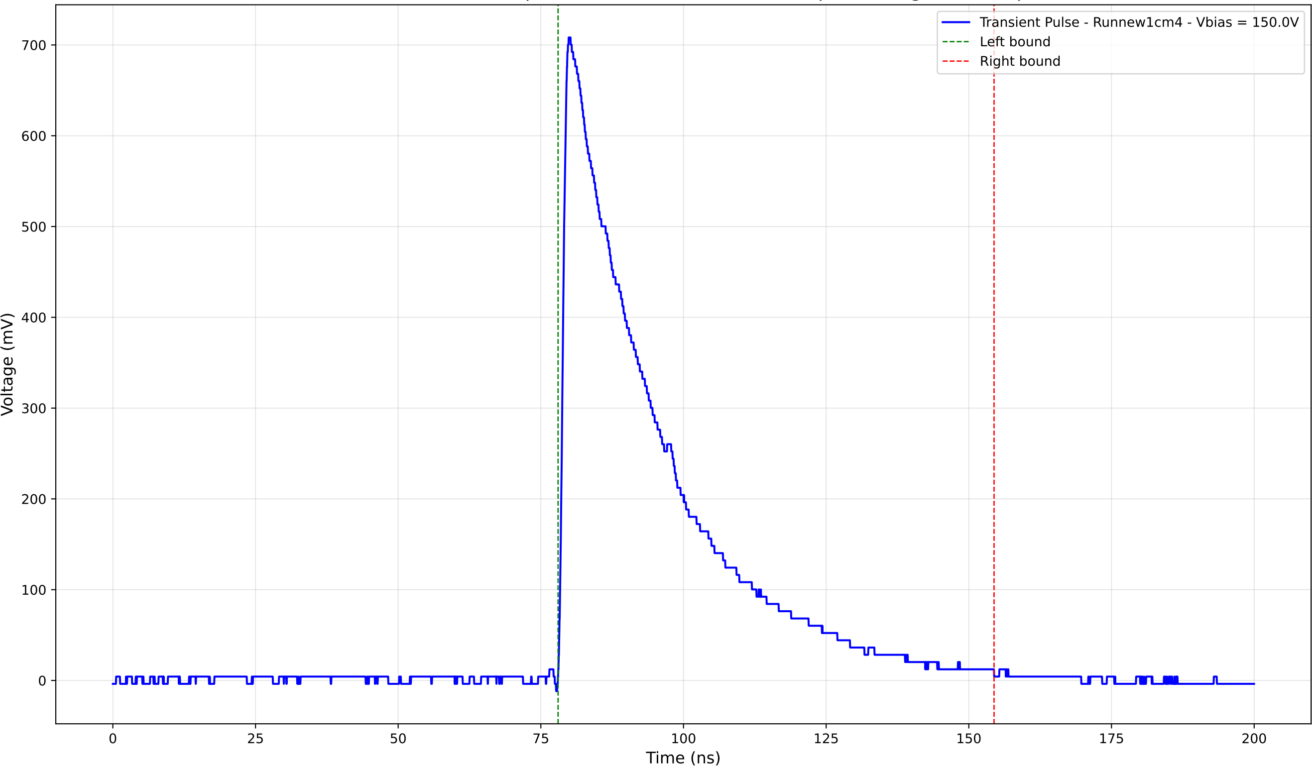
Transient Pulse - Sample: new1cm - Position: 4110.0 \mu\text{m} - Charge: 252.11 pC
