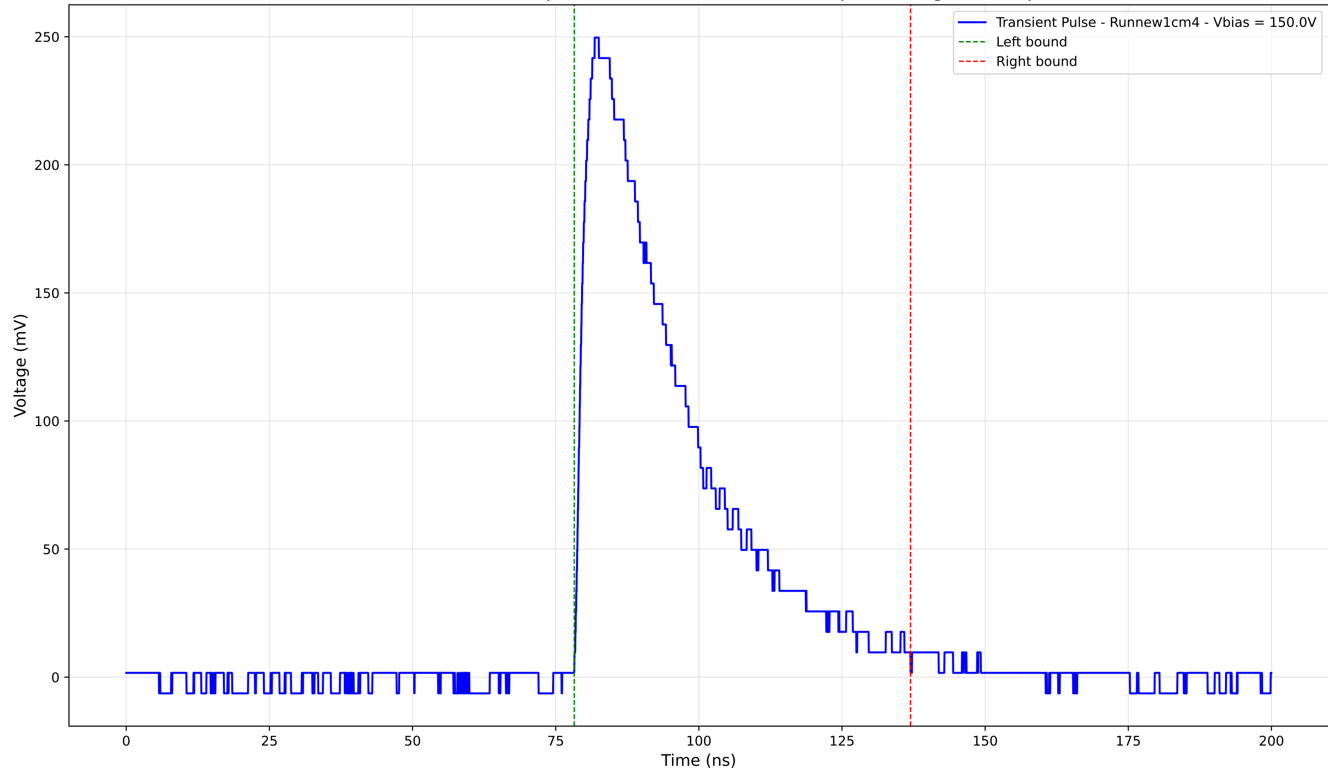
Transient Pulse - Sample: new1cm - Position: 2160.0 \mu\text{m} - Charge: 99.04 pC
