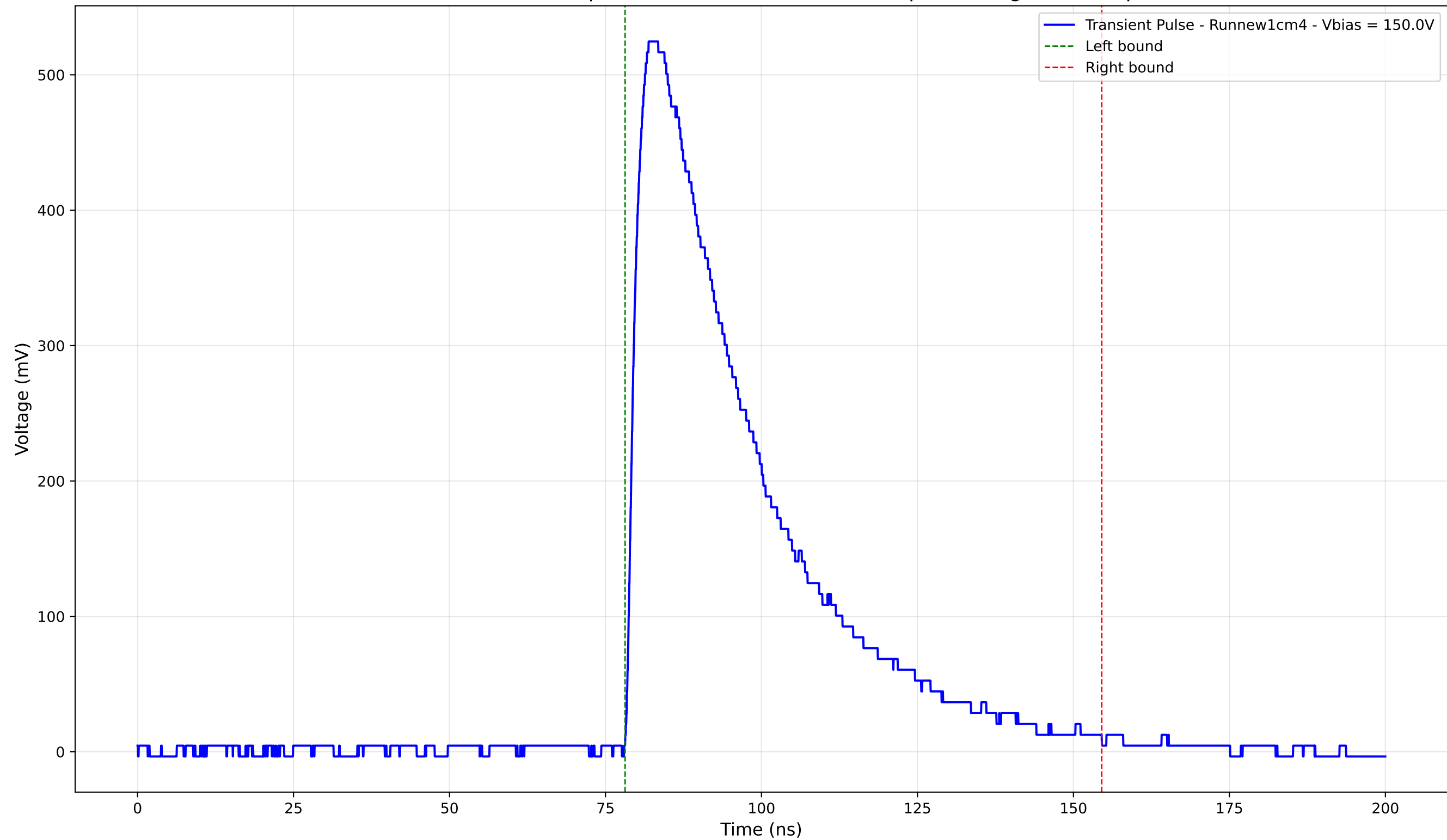
Transient Pulse - Sample: new1cm - Position: 2380.0 \mu\text{m} - Charge: 229.54 pC
