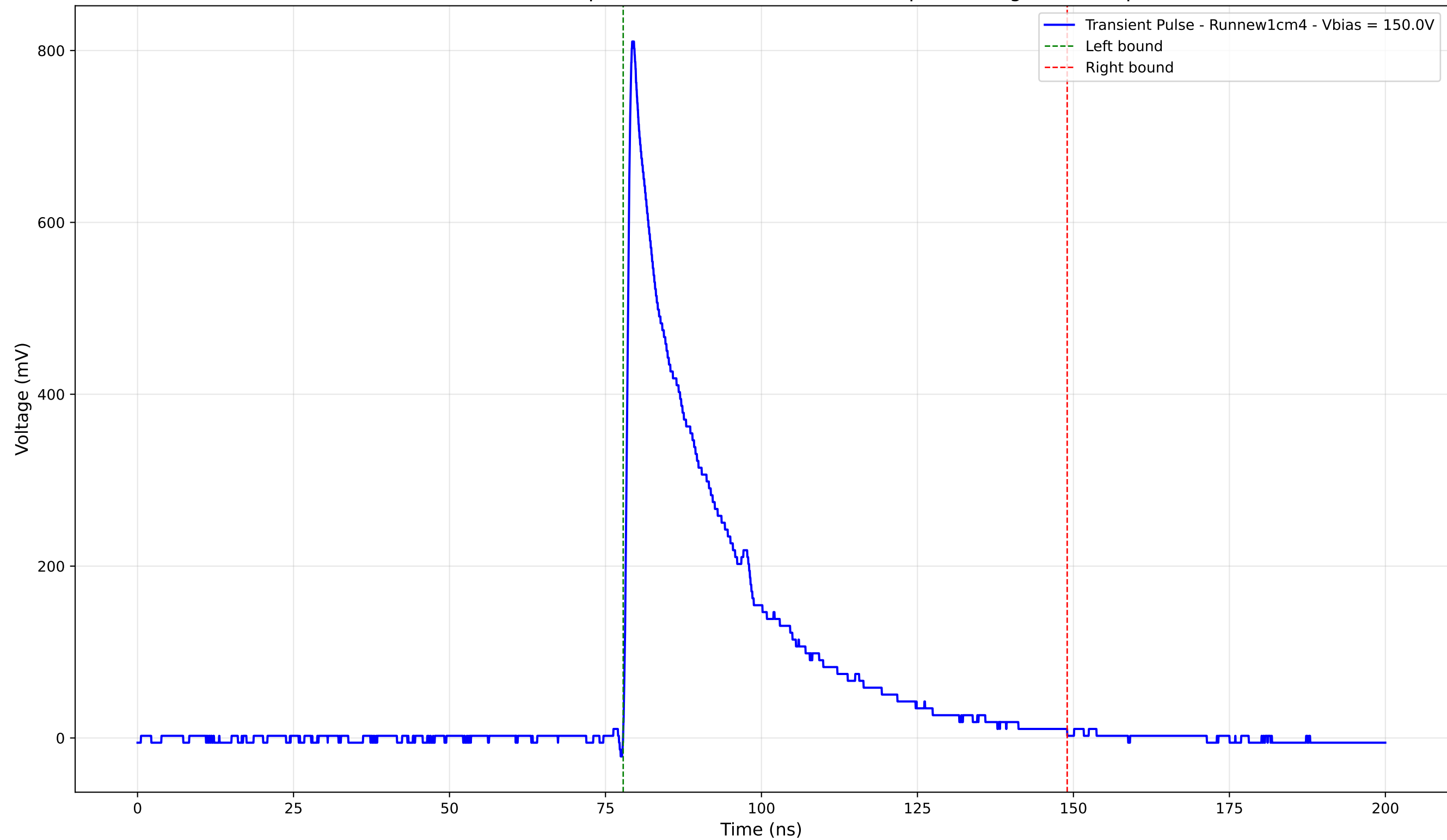
Transient Pulse - Sample: new1cm - Position: 4630.0 \mu\text{m} - Charge: 217.03 pC
