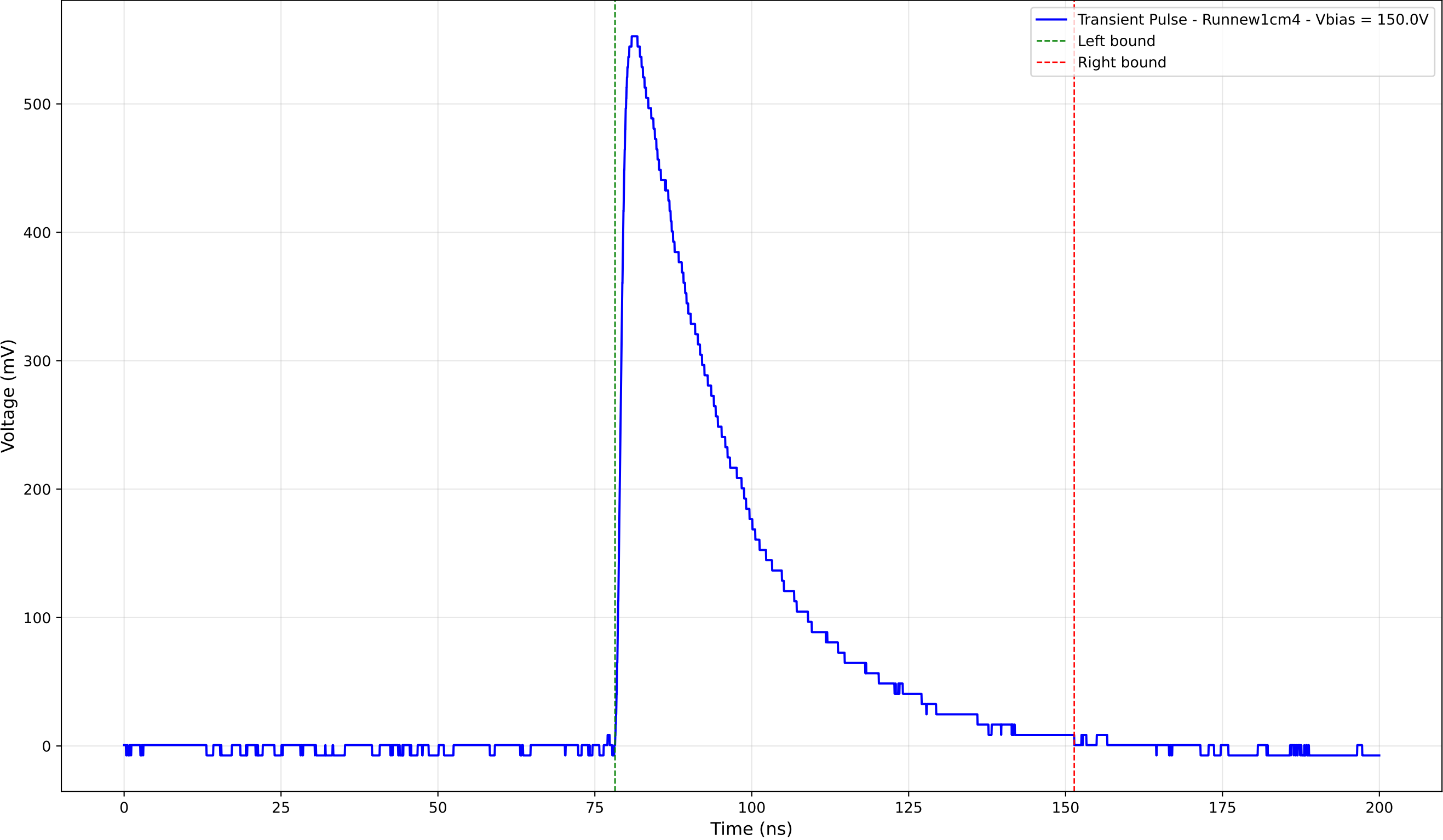
Transient Pulse - Sample: new1cm - Position: 1540.0 \mu\text{m} - Charge: 206.15 pC
