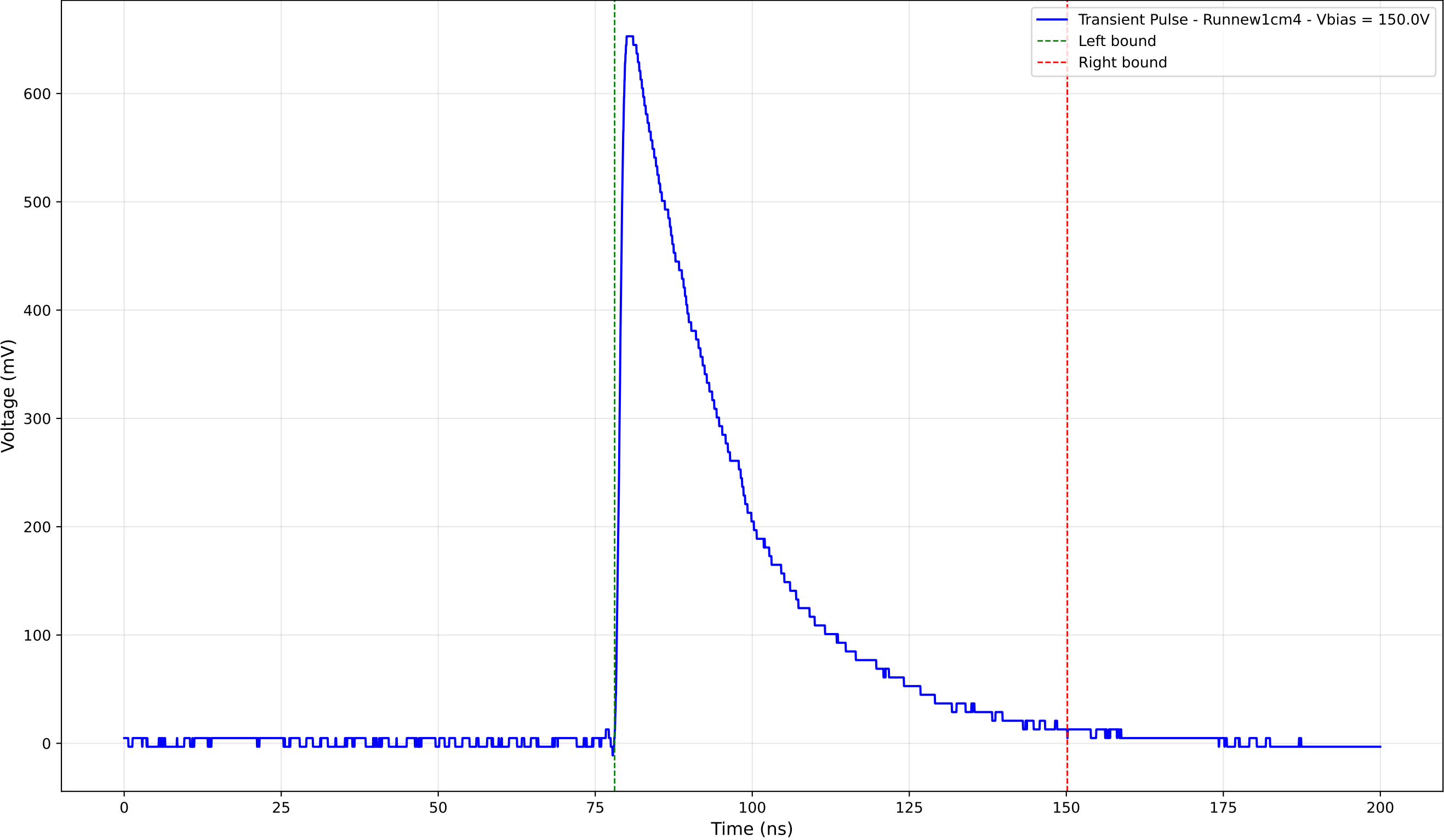
Transient Pulse - Sample: new1cm - Position: 3955.0 \mu\text{m} - Charge: 249.01 pC
