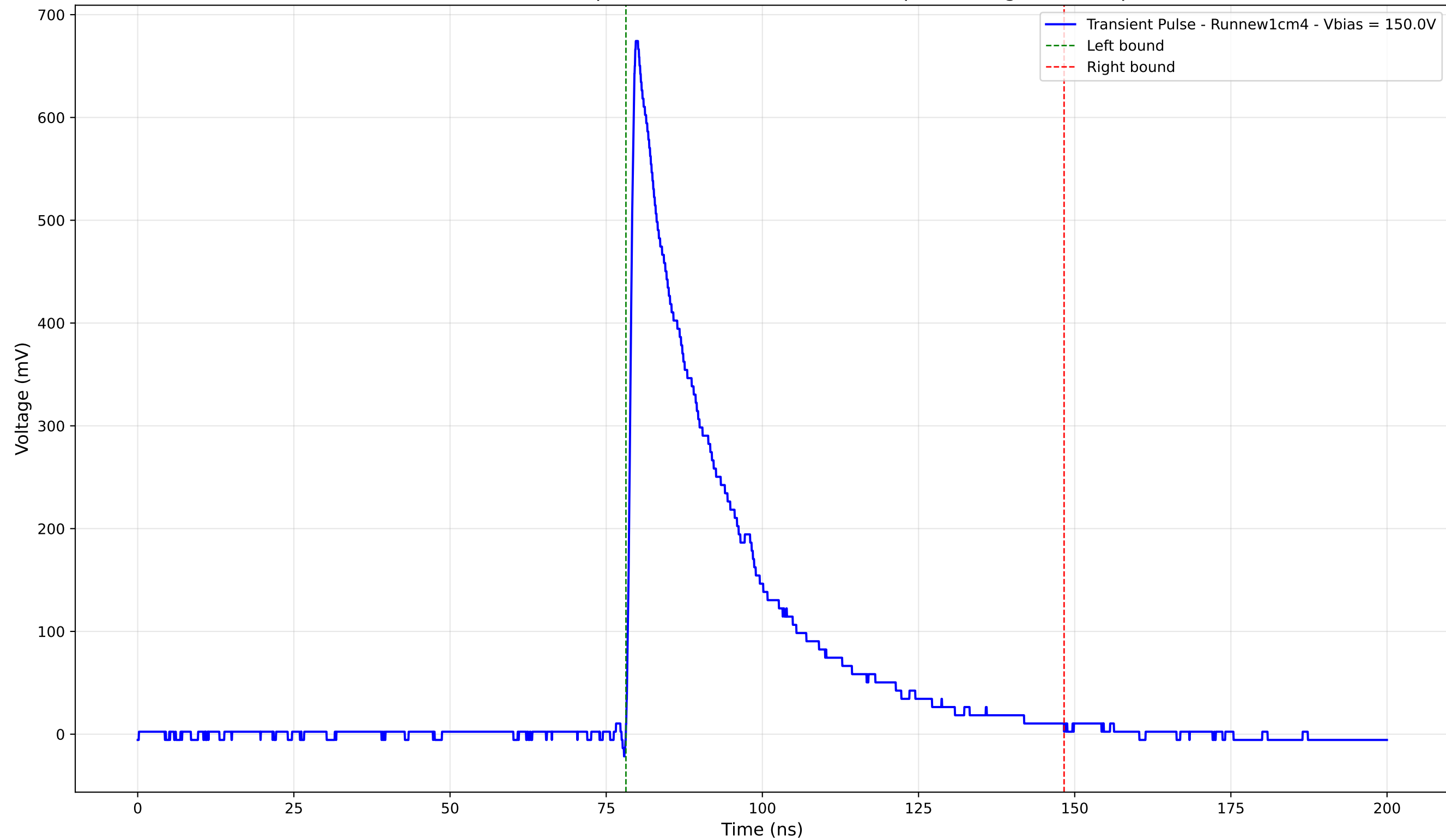
Transient Pulse - Sample: new1cm - Position: 985.0 \mu\text{m} - Charge: 197.83 pC
