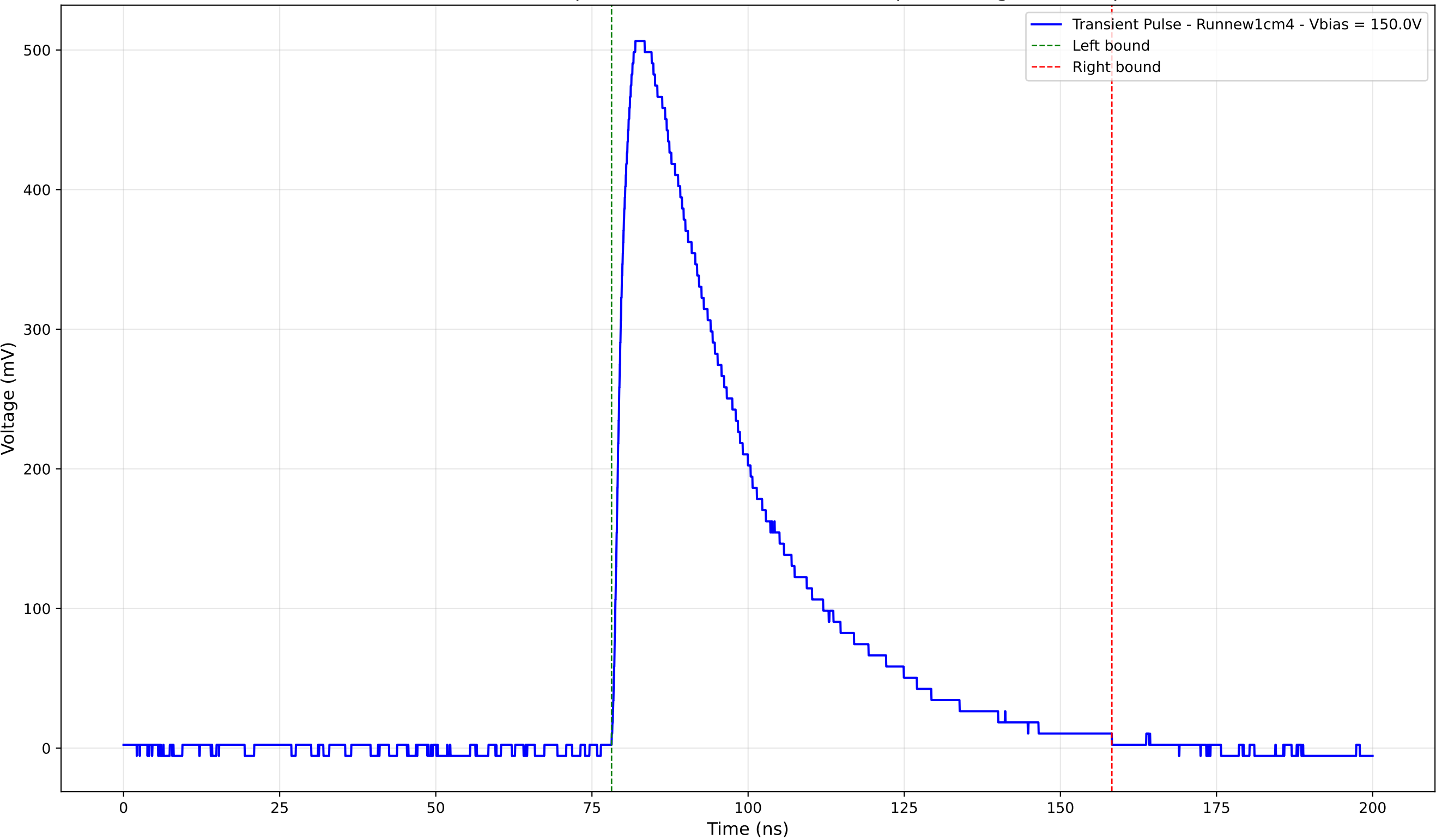
Transient Pulse - Sample: new1cm - Position: 2595.0 \mu\text{m} - Charge: 224.16 pC
