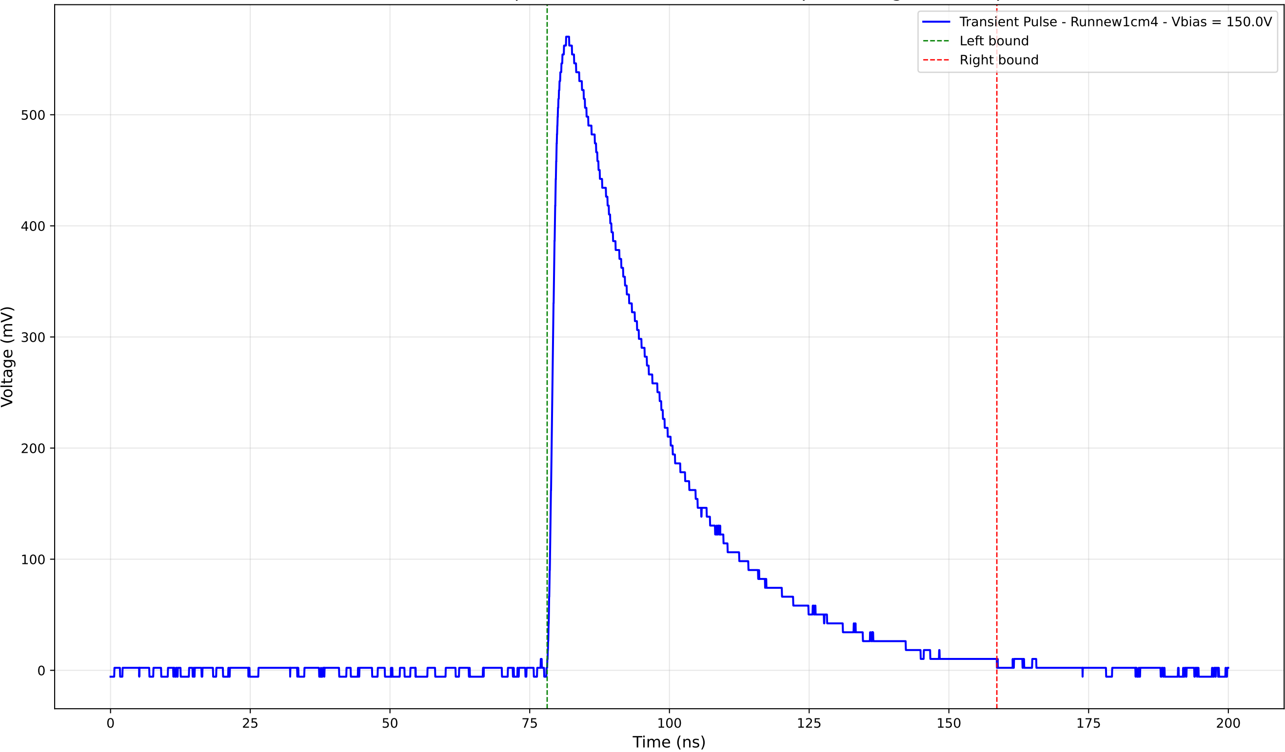
Transient Pulse - Sample: new1cm - Position: 3500.0 \mu\text{m} - Charge: 239.98 pC
