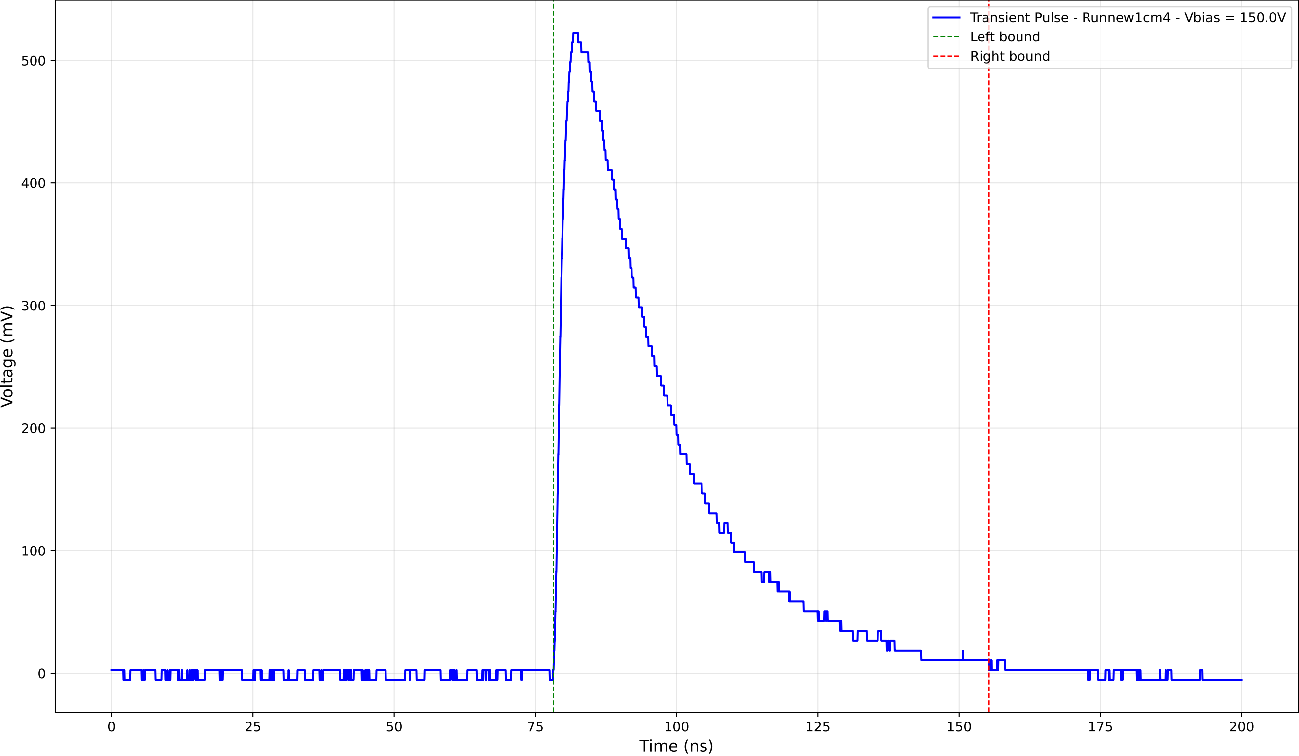
Transient Pulse - Sample: new1cm - Position: 2090.0 \mu\text{m} - Charge: 218.99 pC
