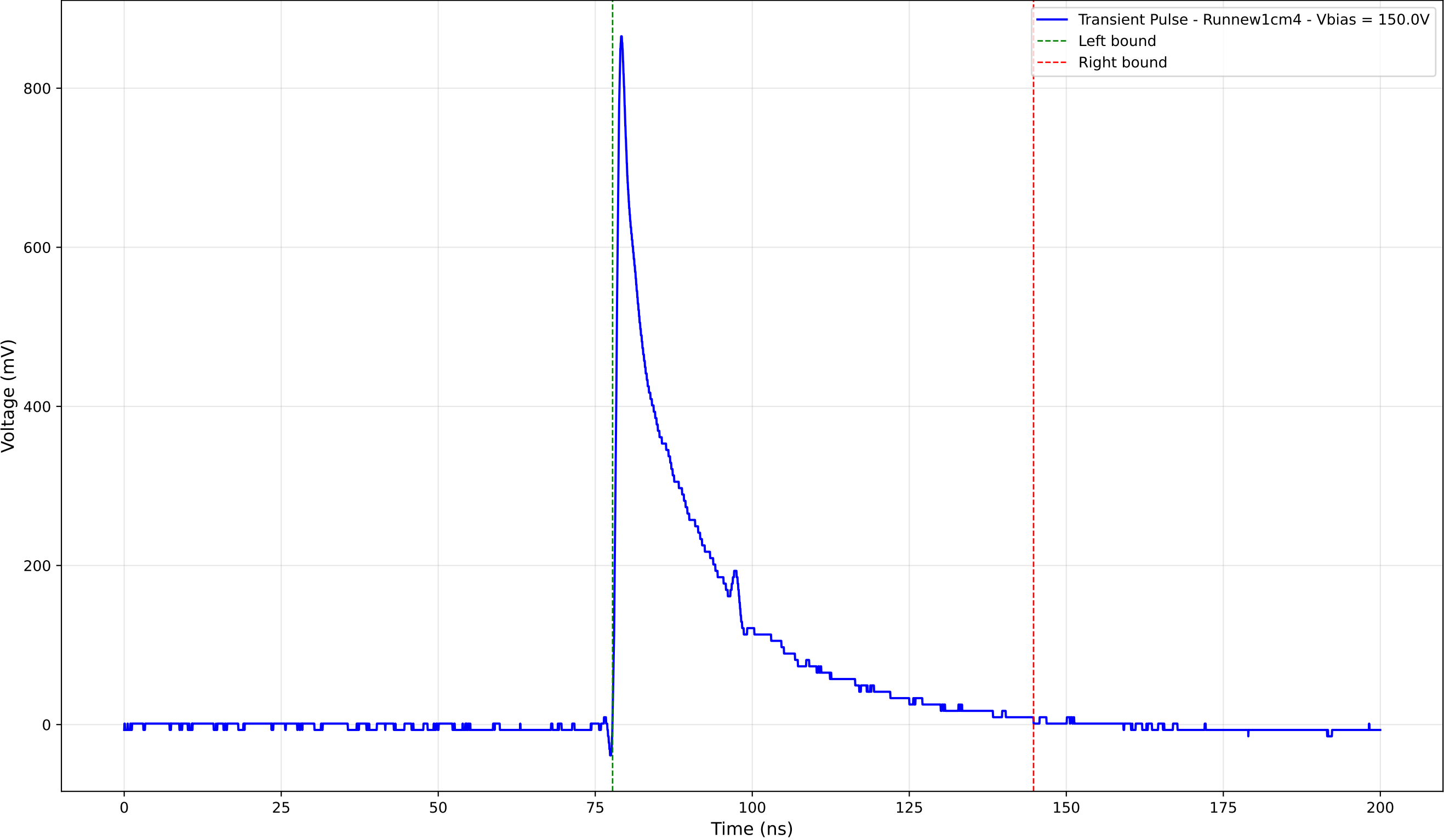
Transient Pulse - Sample: new1cm - Position: 4905.0 \mu\text{m} - Charge: 187.17 pC
