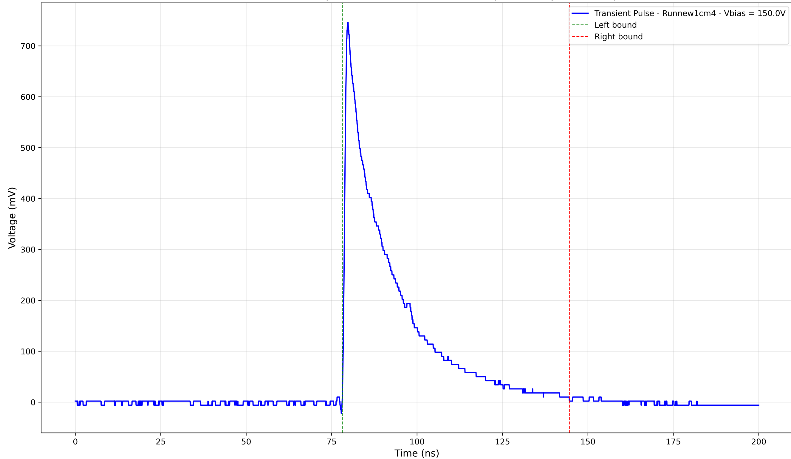
Transient Pulse - Sample: new1cm - Position: 855.0 \mu\text{m} - Charge: 199.75 pC
