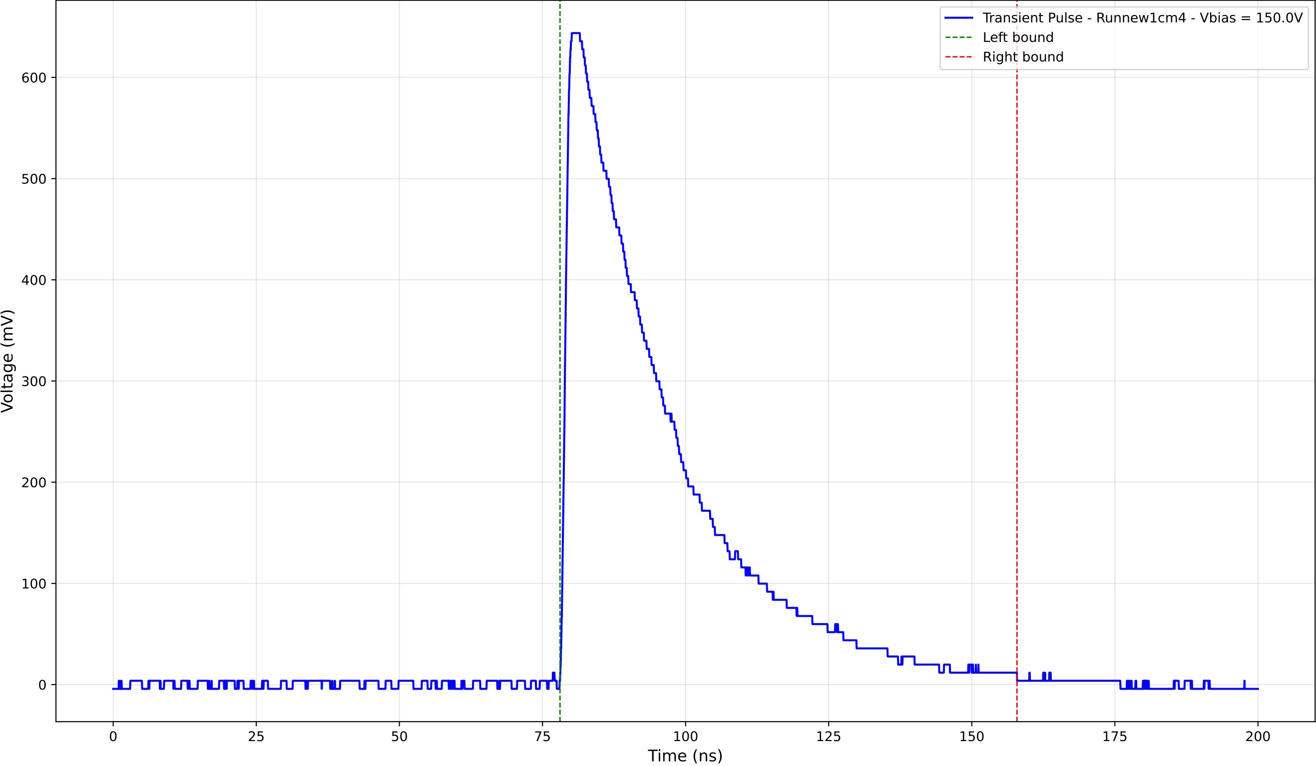
Transient Pulse - Sample: new1cm - Position: 3875.0 \mu\text{m} - Charge: 253.93 pC
