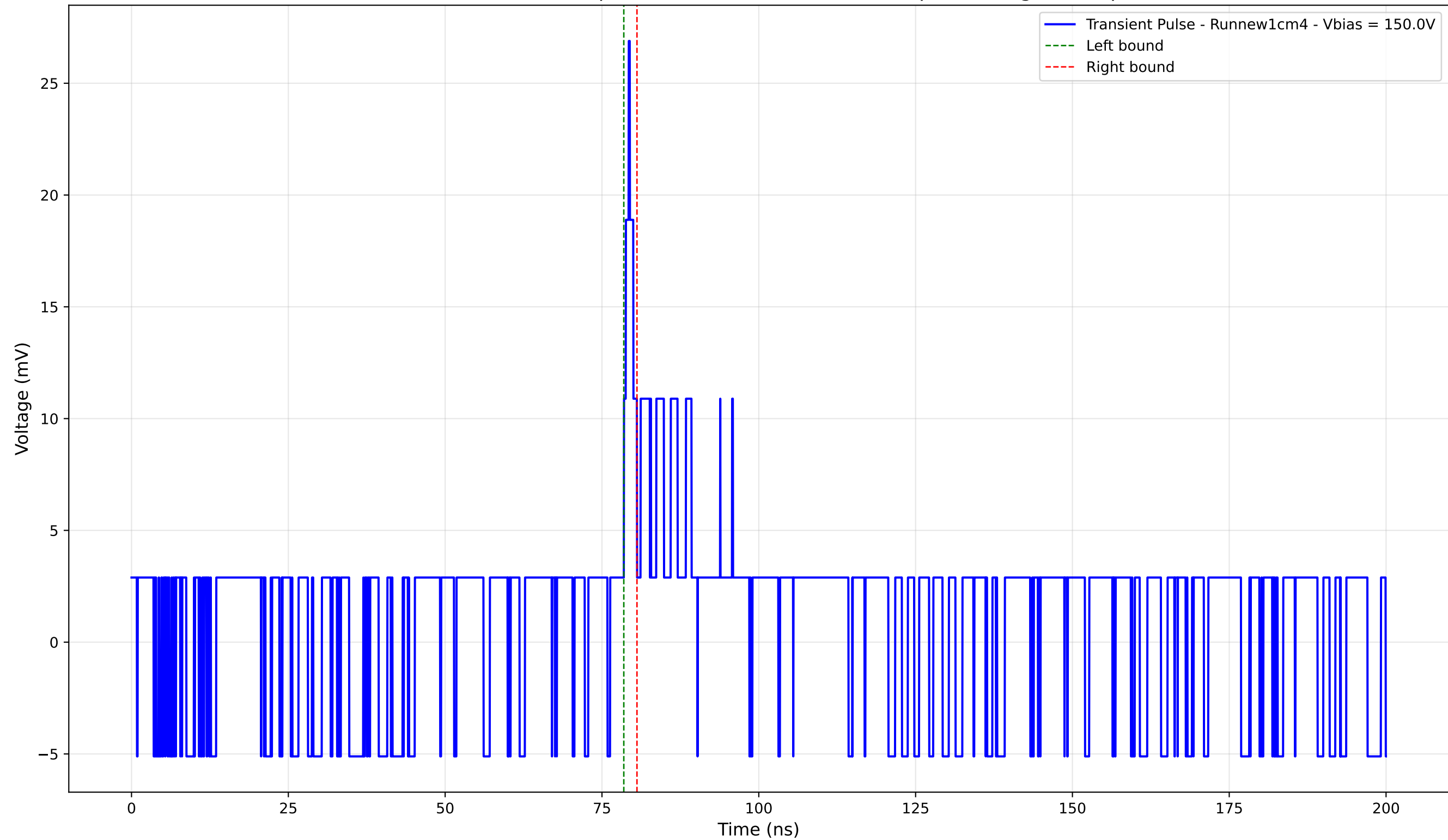
Transient Pulse - Sample: new1cm - Position: 5105.0 \mu\text{m} - Charge: 0.67 pC
