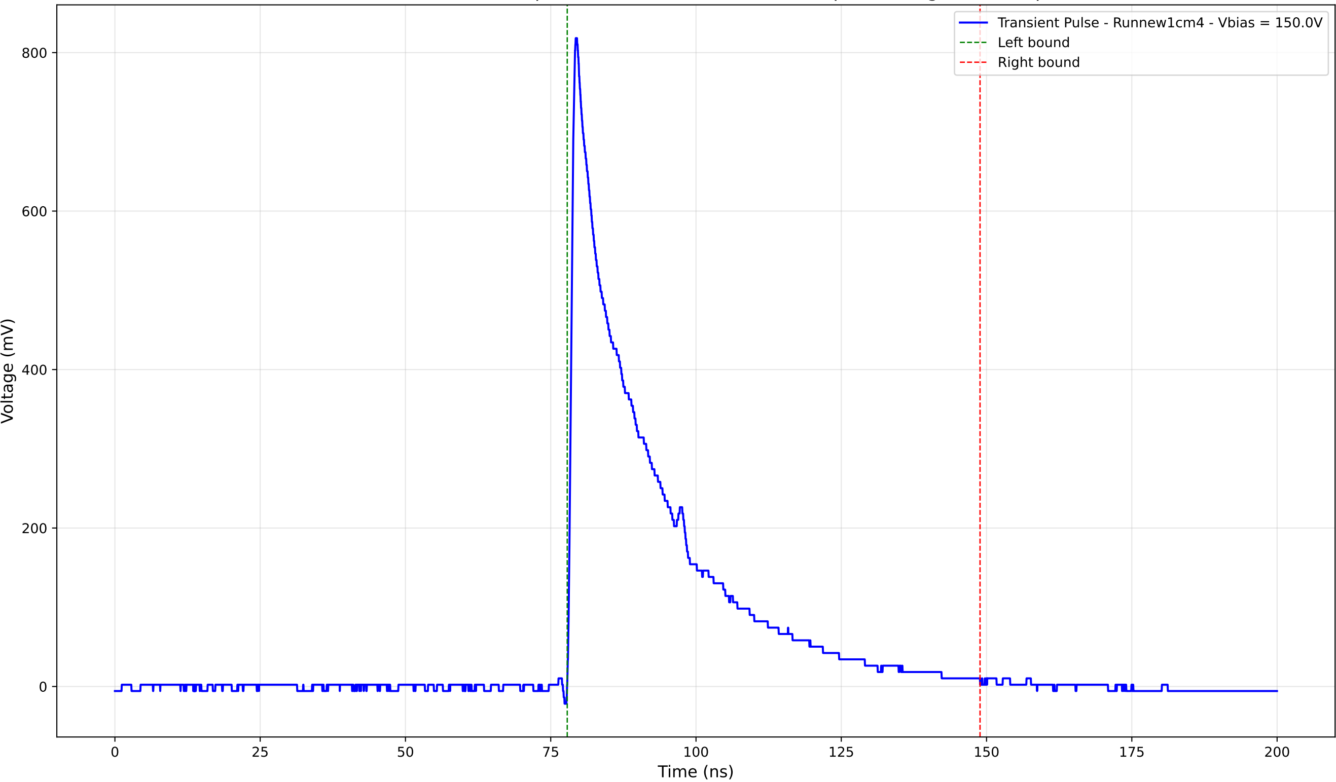
Transient Pulse - Sample: new1cm - Position: 4625.0 \mu\text{m} - Charge: 219.74 pC
