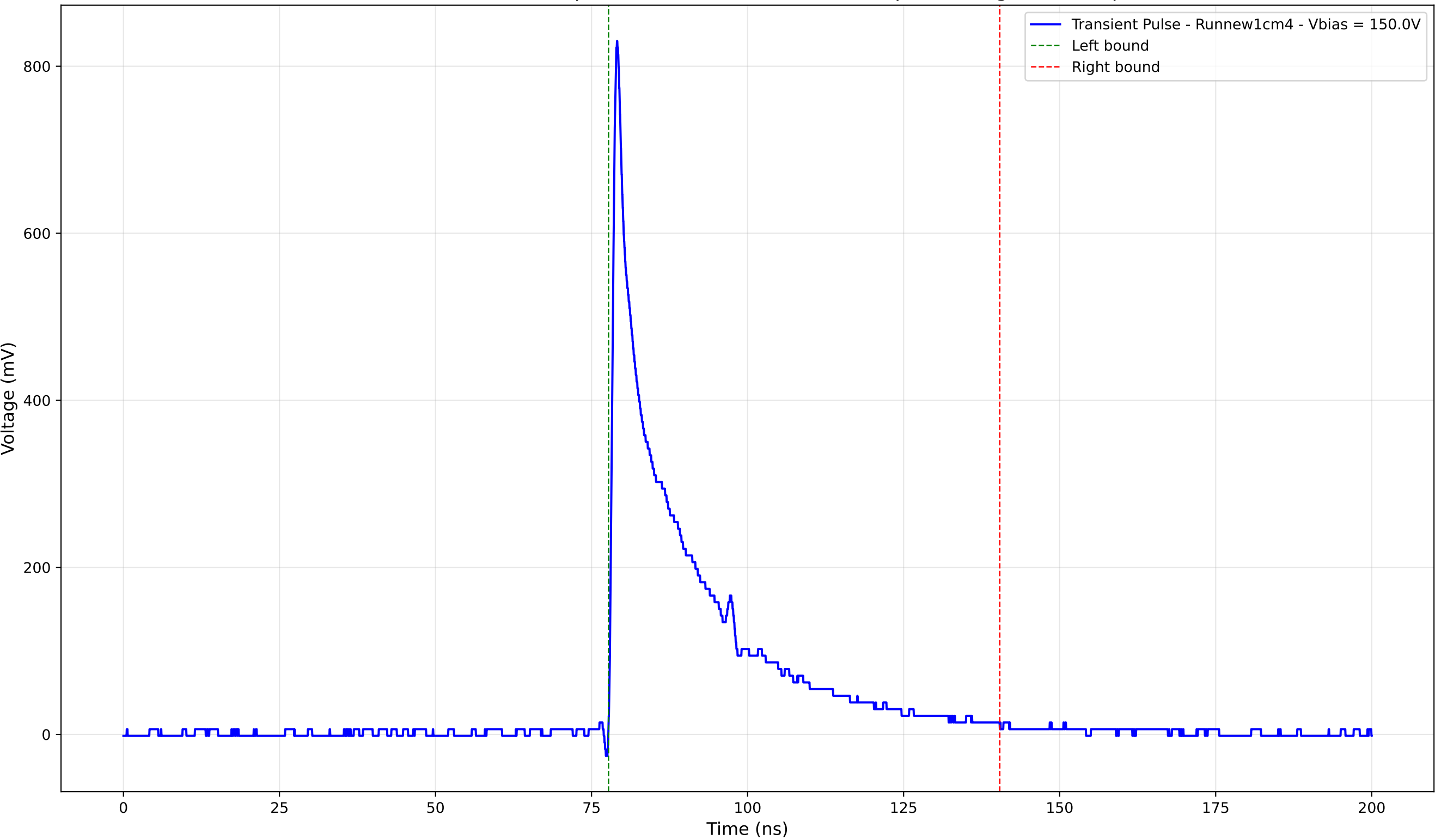
Transient Pulse - Sample: new1cm - Position: 4985.0 \mu\text{m} - Charge: 162.07 pC
