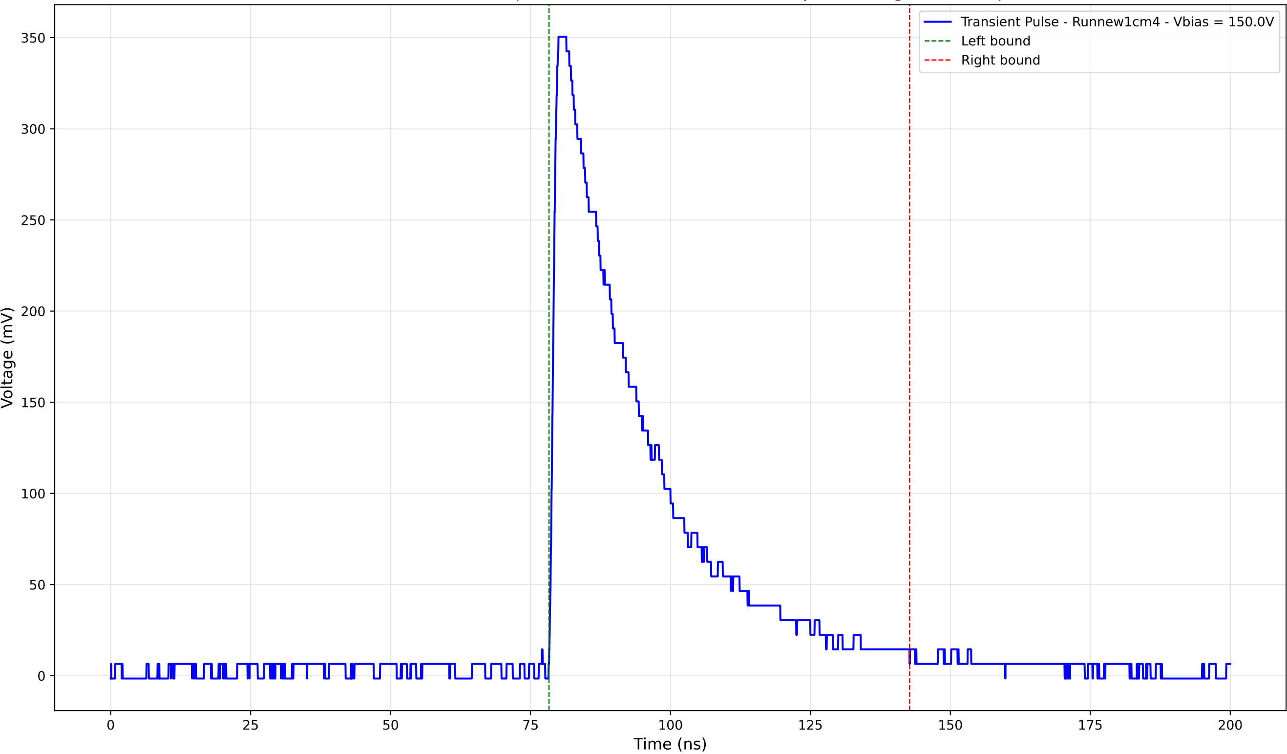
Transient Pulse - Sample: new1cm - Position: 1255.0 \mu\text{m} - Charge: 122.33 pC
