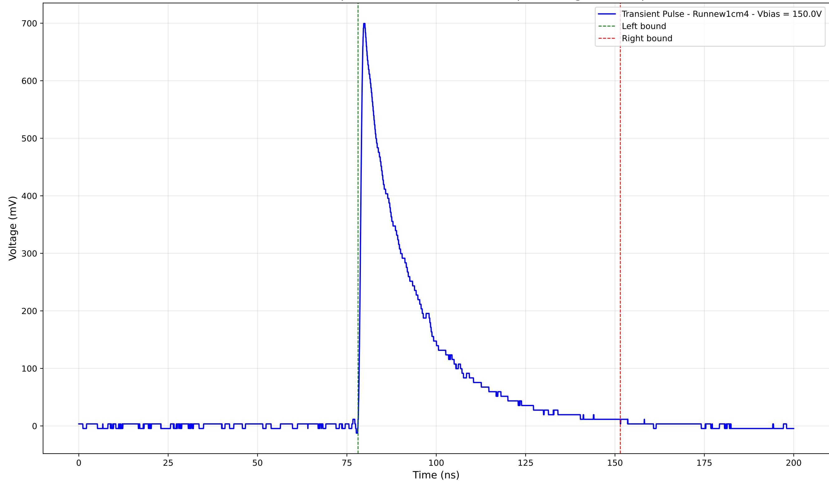
Transient Pulse - Sample: new1cm - Position: 940.0 \mu\text{m} - Charge: 201.24 pC
