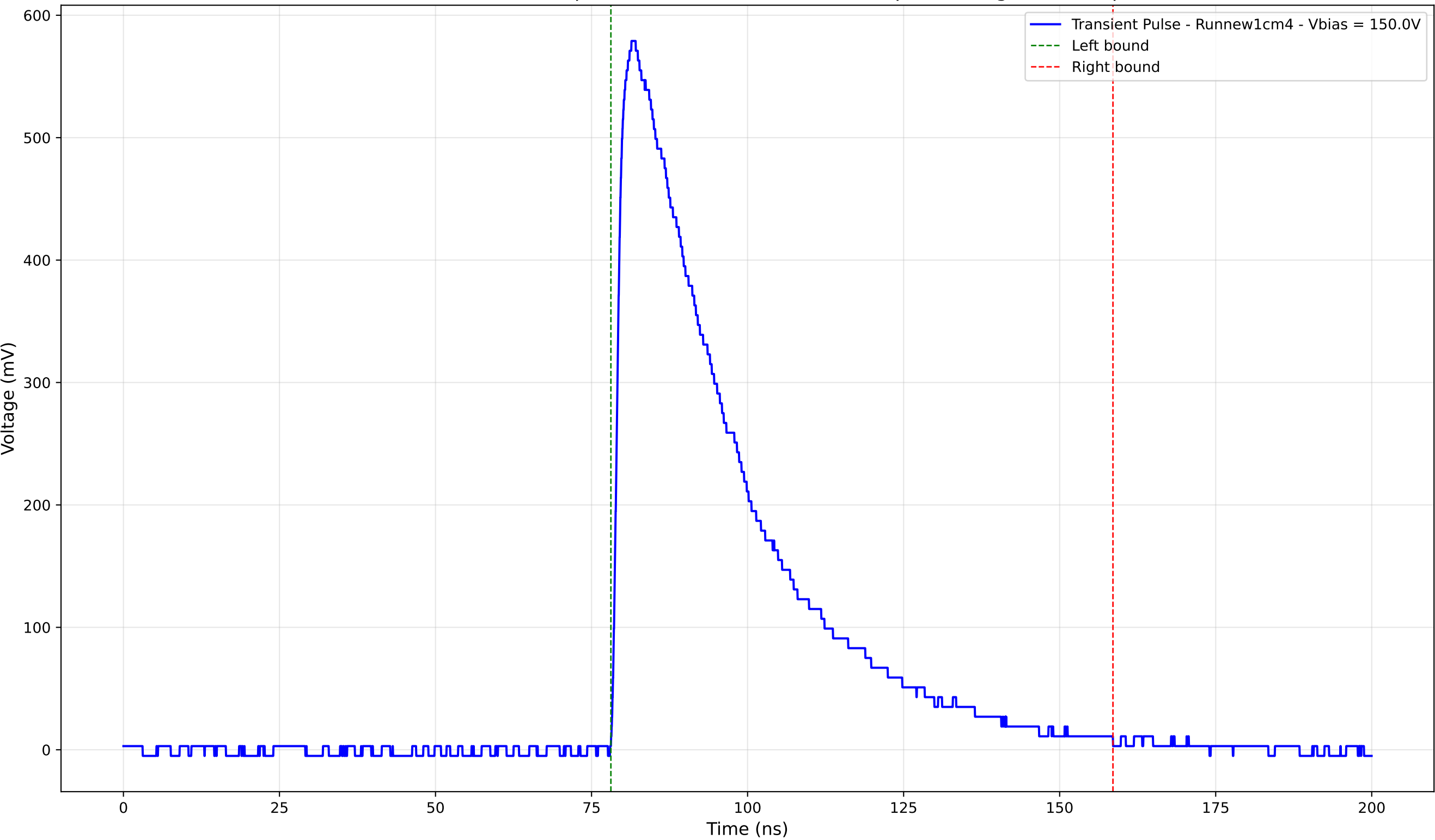
Transient Pulse - Sample: new1cm - Position: 3555.0 \mu\text{m} - Charge: 243.56 pC
