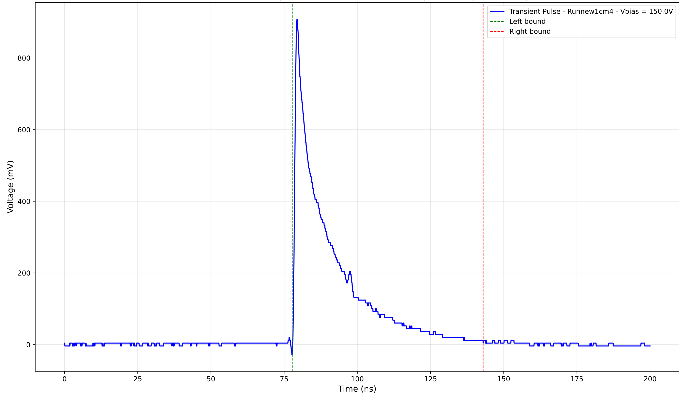
Transient Pulse - Sample: new1cm - Position: 525.0 \mu\text{m} - Charge: 204.00 pC
