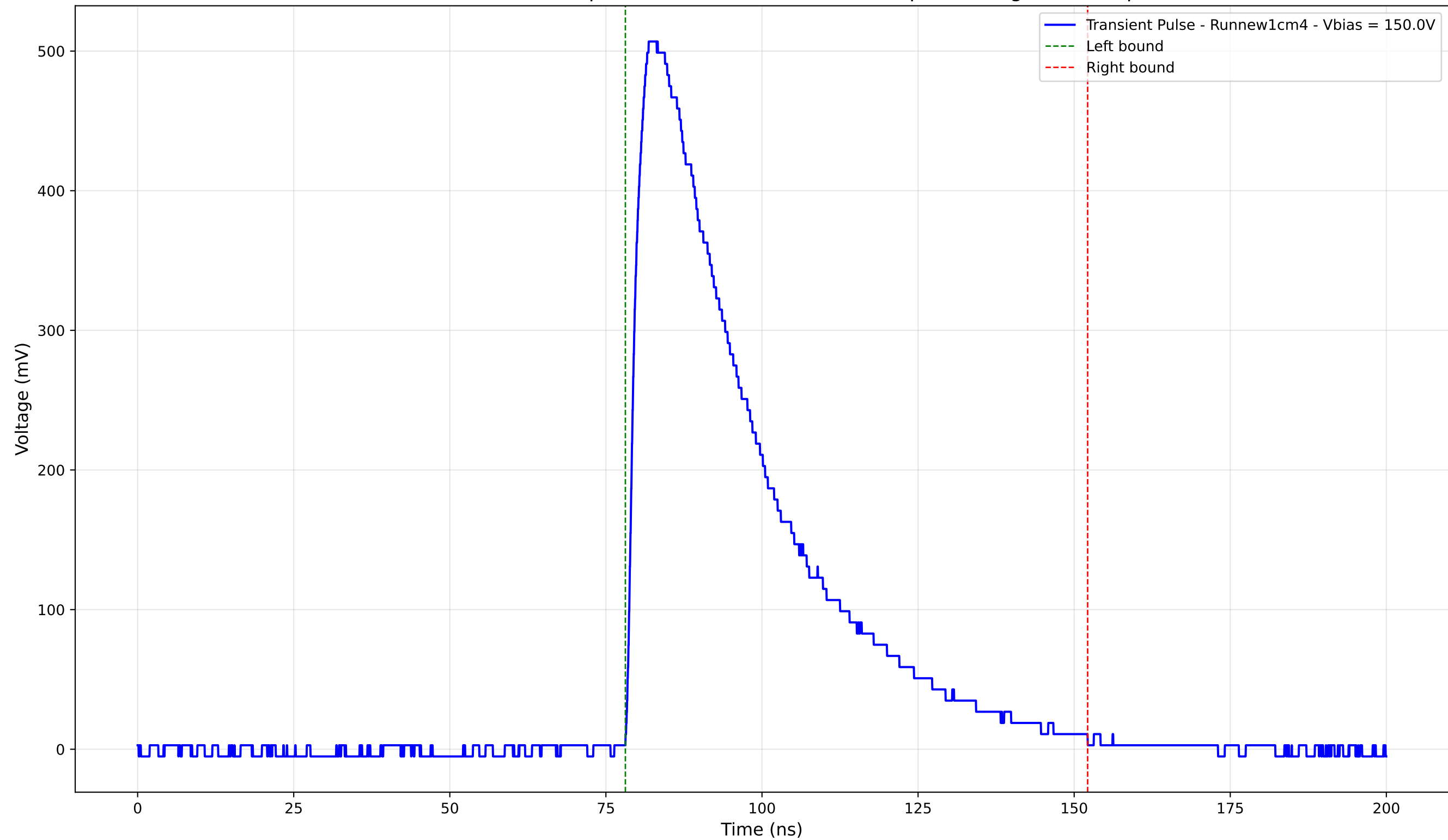
Transient Pulse - Sample: new1cm - Position: 2845.0 \mu\text{m} - Charge: 225.45 pC
