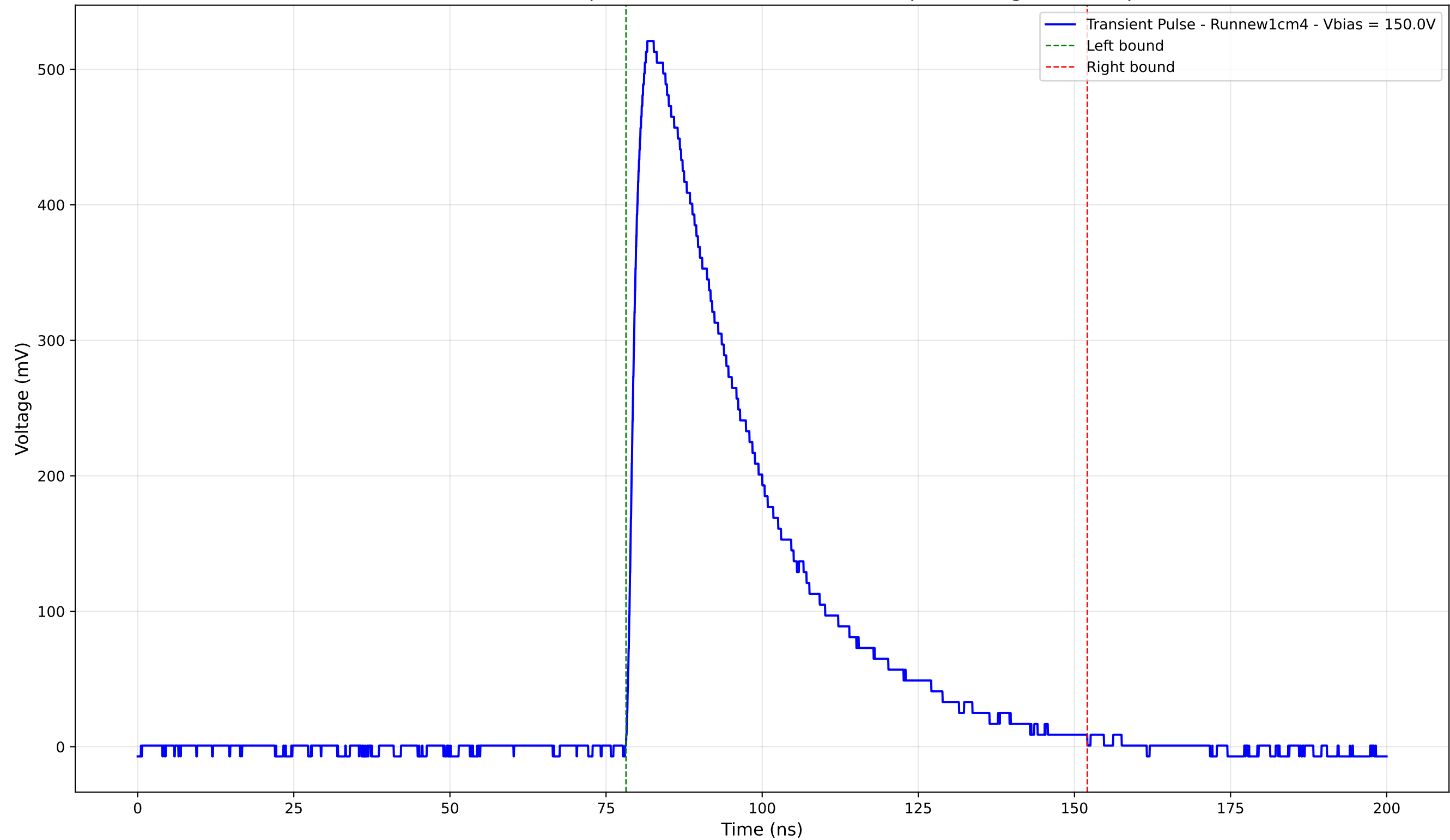
Transient Pulse - Sample: new1cm - Position: 2065.0 \mu\text{m} - Charge: 216.72 pC
