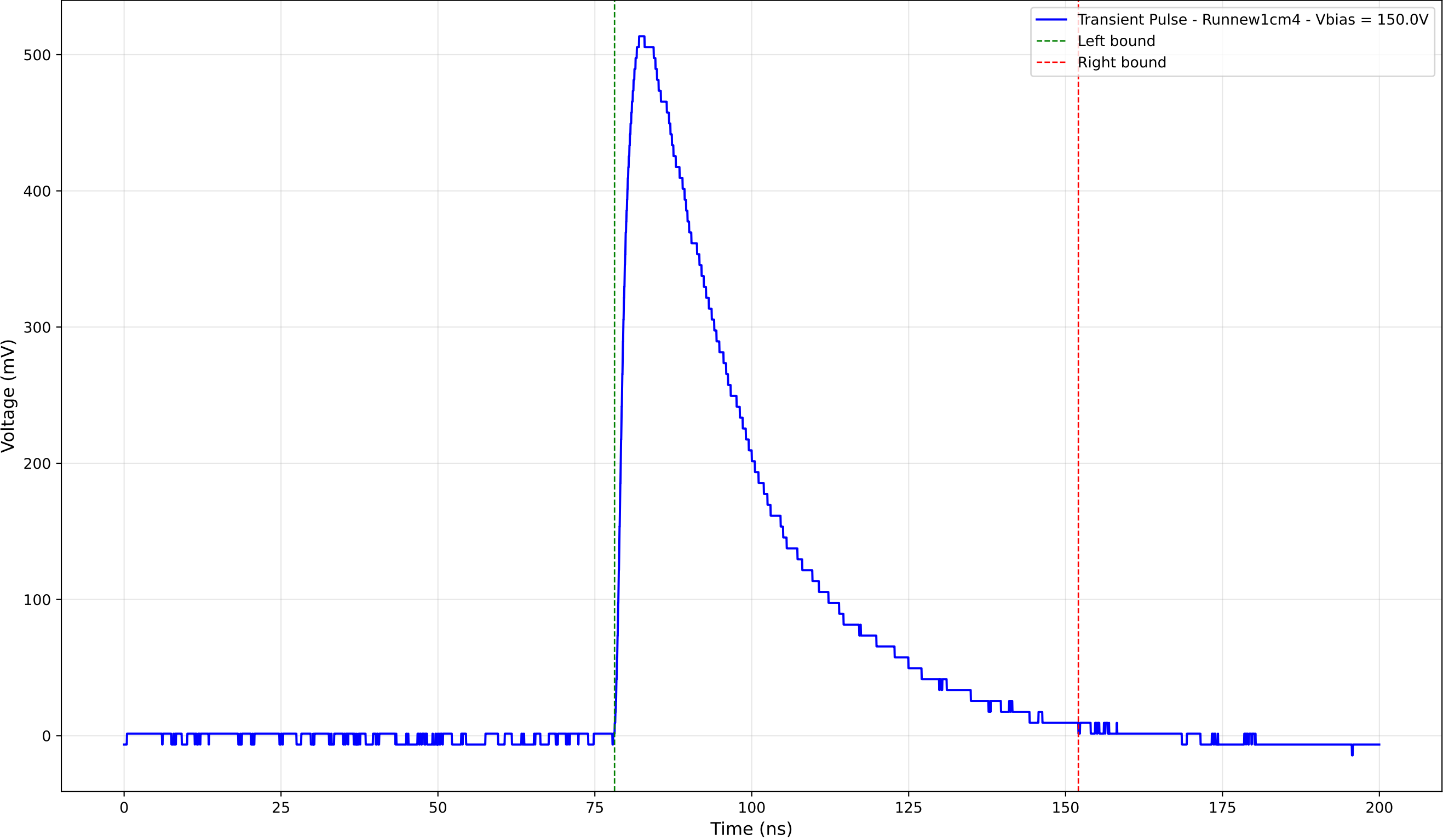
Transient Pulse - Sample: new1cm - Position: 2955.0 \mu\text{m} - Charge: 224.27 pC
