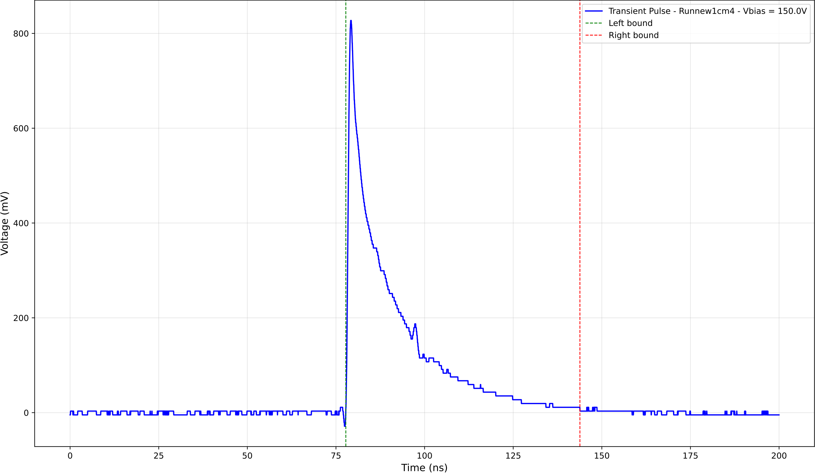
Transient Pulse - Sample: new1cm - Position: 4835.0 \mu\text{m} - Charge: 181.60 pC
