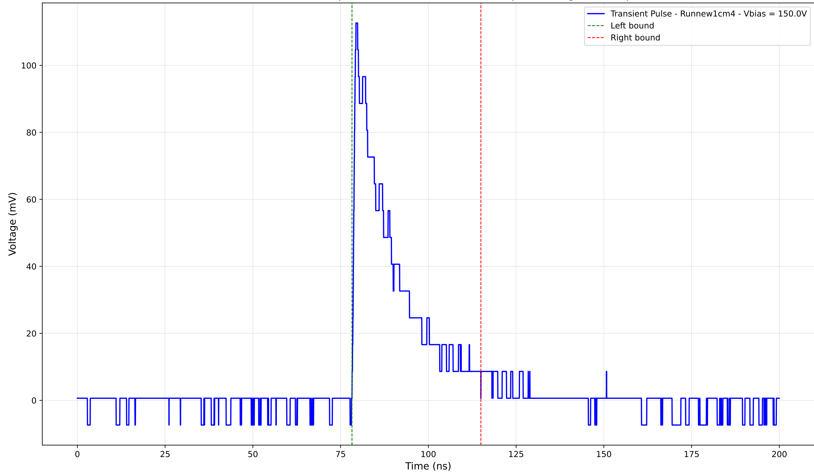
Transient Pulse - Sample: new1cm - Position: 695.0 \mu\text{m} - Charge: 25.67 pC
