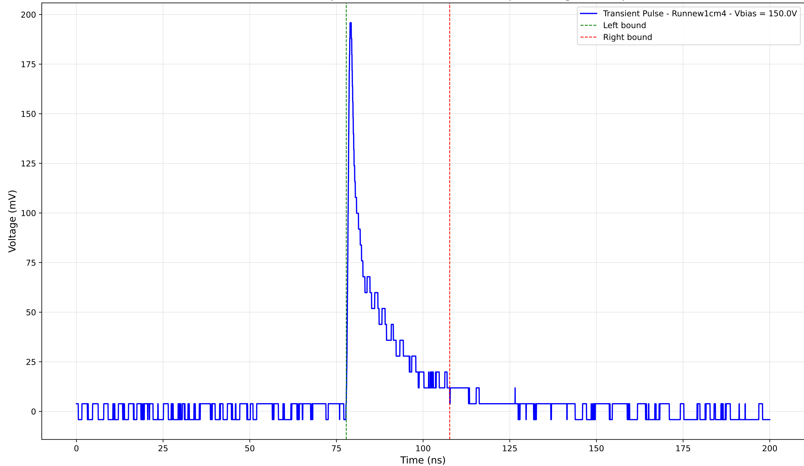
Transient Pulse - Sample: new1cm - Position: 5055.0 \mu\text{m} - Charge: 26.98 pC
