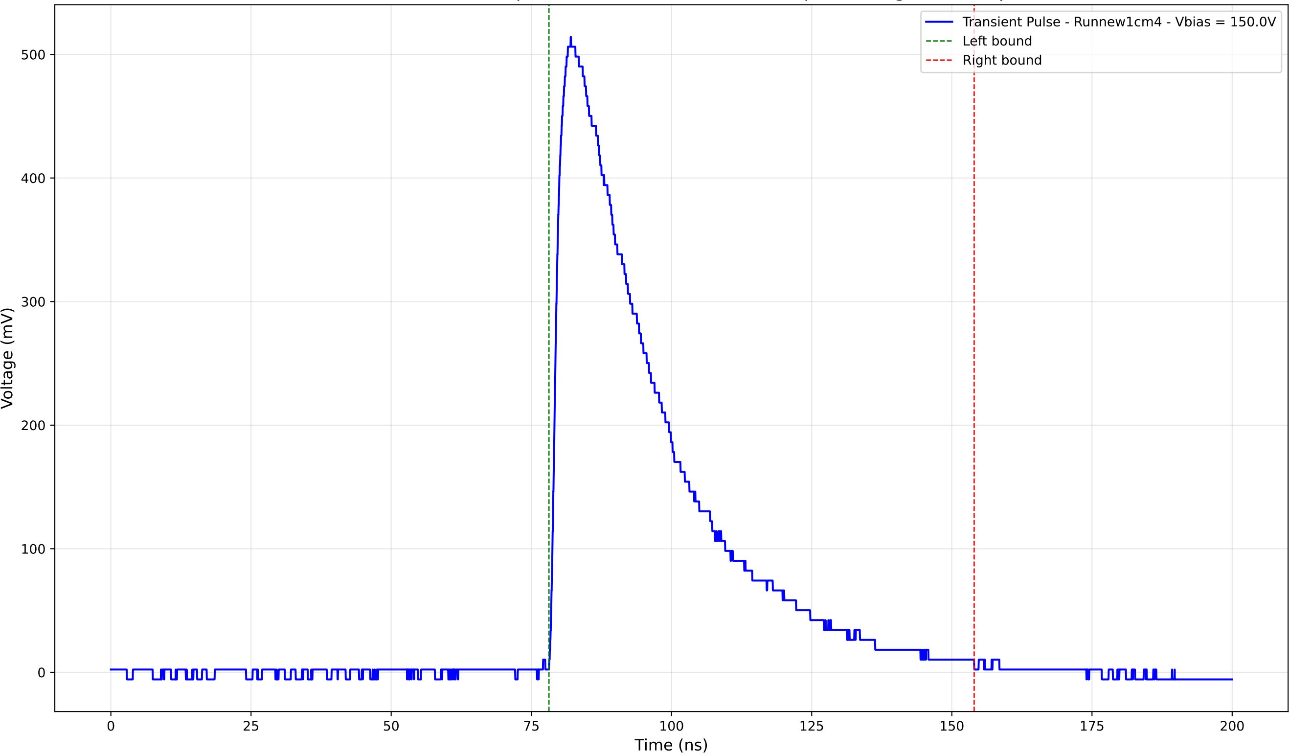
Transient Pulse - Sample: new1cm - Position: 1980.0 \mu\text{m} - Charge: 210.89 pC
