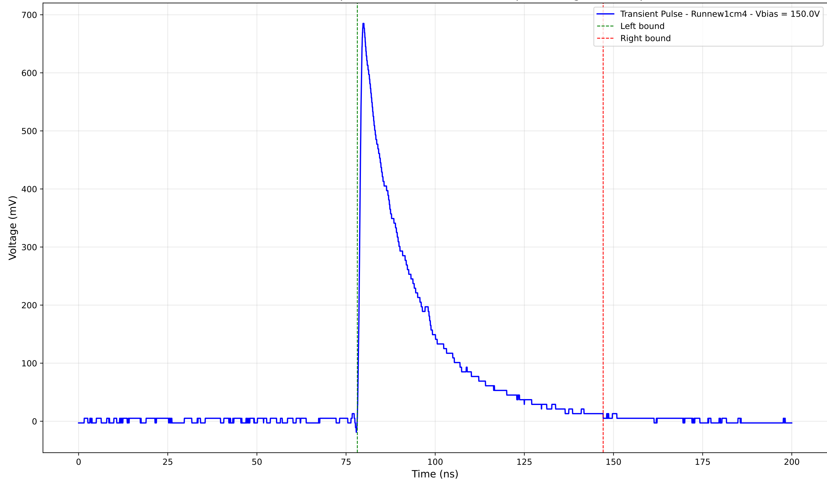
Transient Pulse - Sample: new1cm - Position: 960.0 \mu\text{m} - Charge: 199.07 pC
