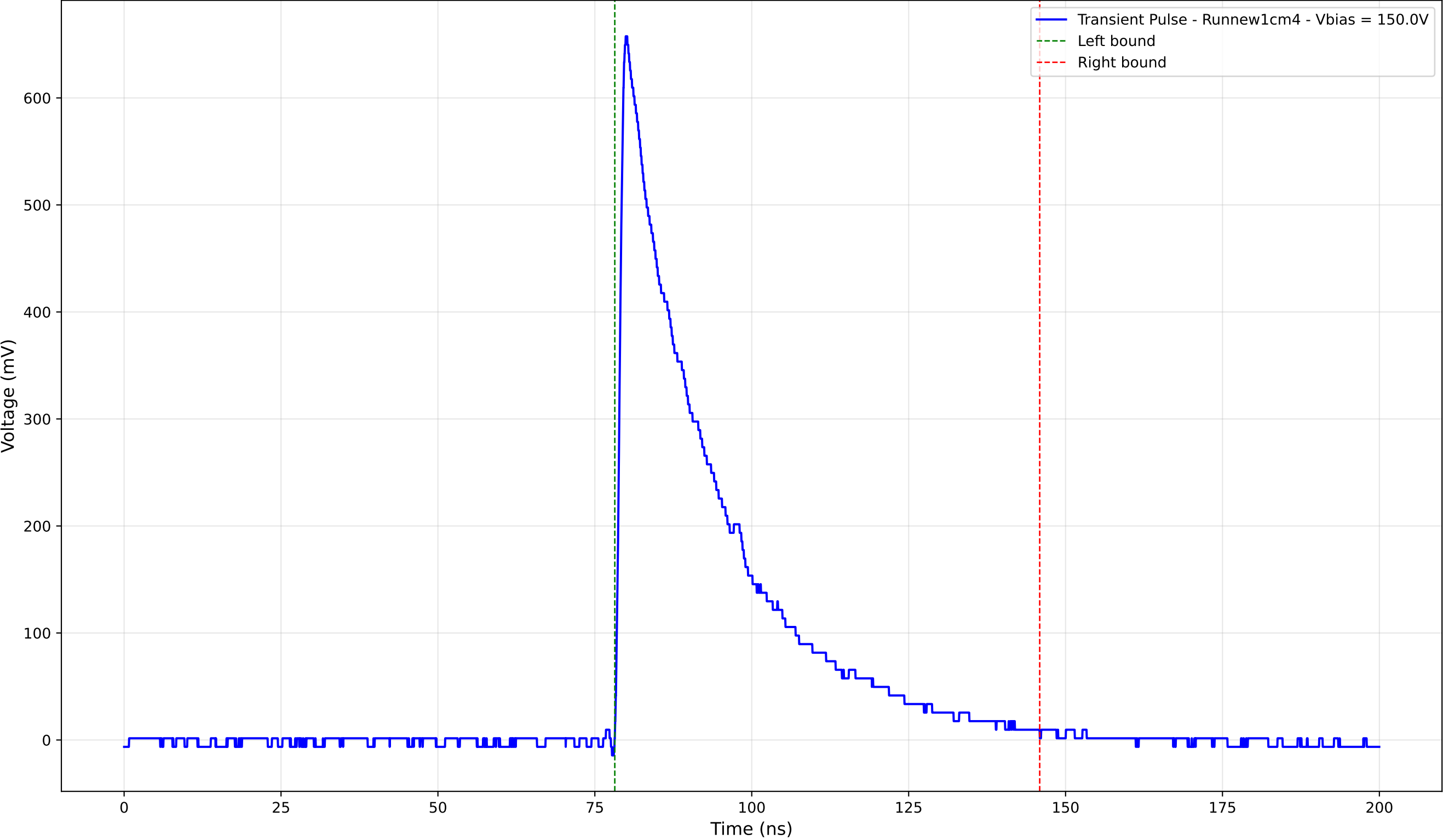
Transient Pulse - Sample: new1cm - Position: 1080.0 \mu\text{m} - Charge: 200.74 pC
