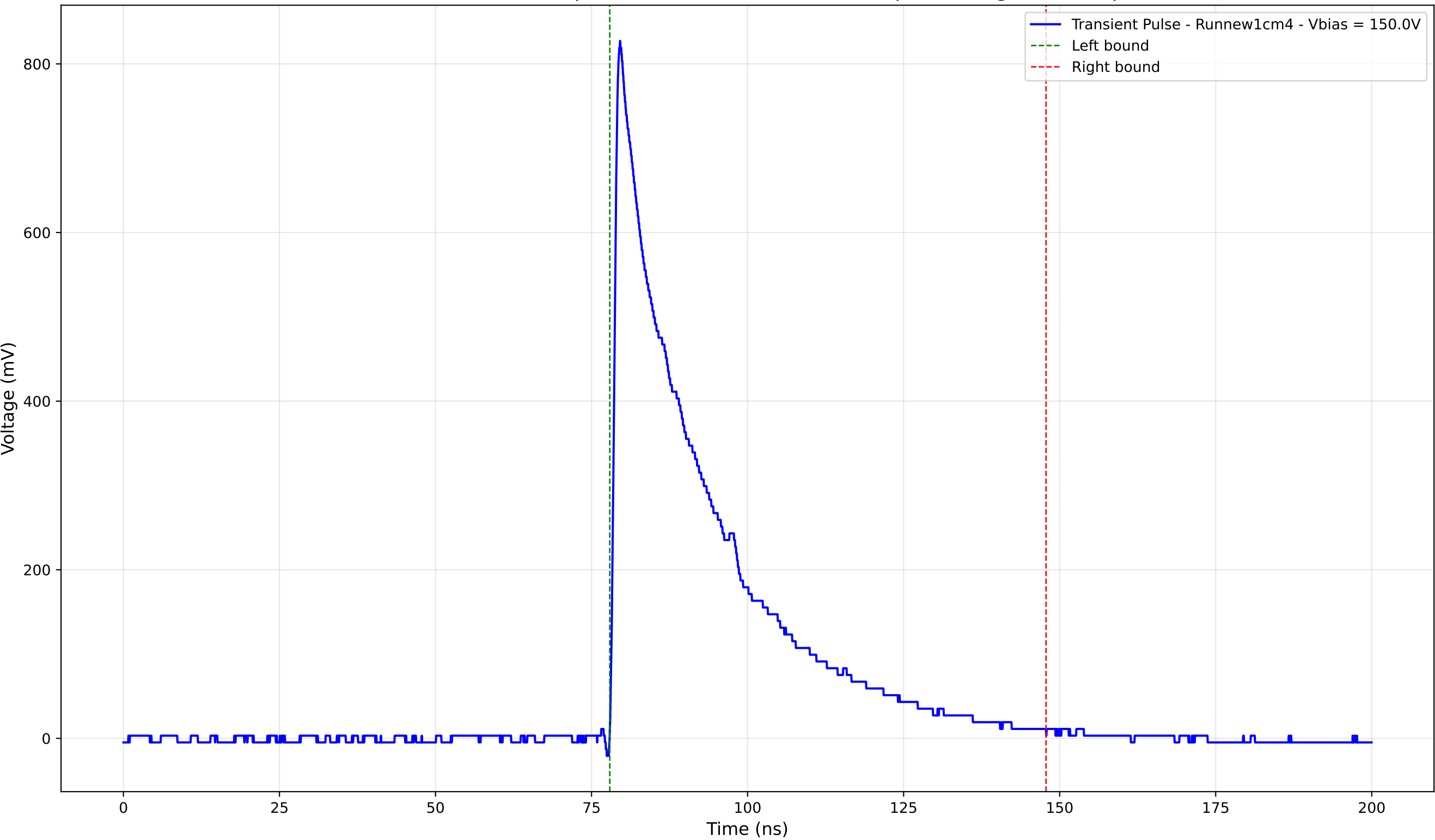
Transient Pulse - Sample: new1cm - Position: 4475.0 \mu\text{m} - Charge: 241.51 pC
