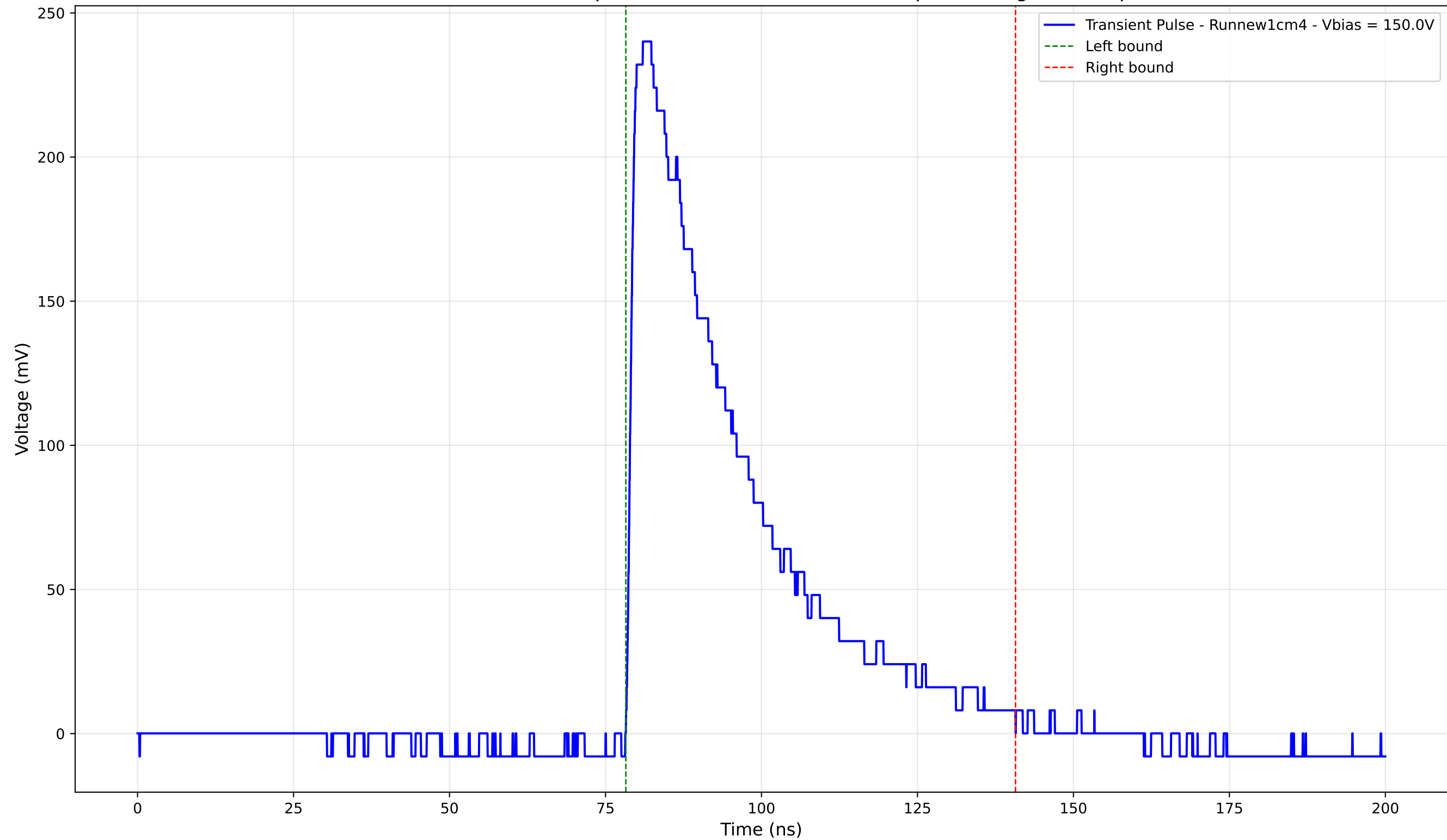
Transient Pulse - Sample: new1cm - Position: 3765.0 \mu\text{m} - Charge: 91.09 pC
