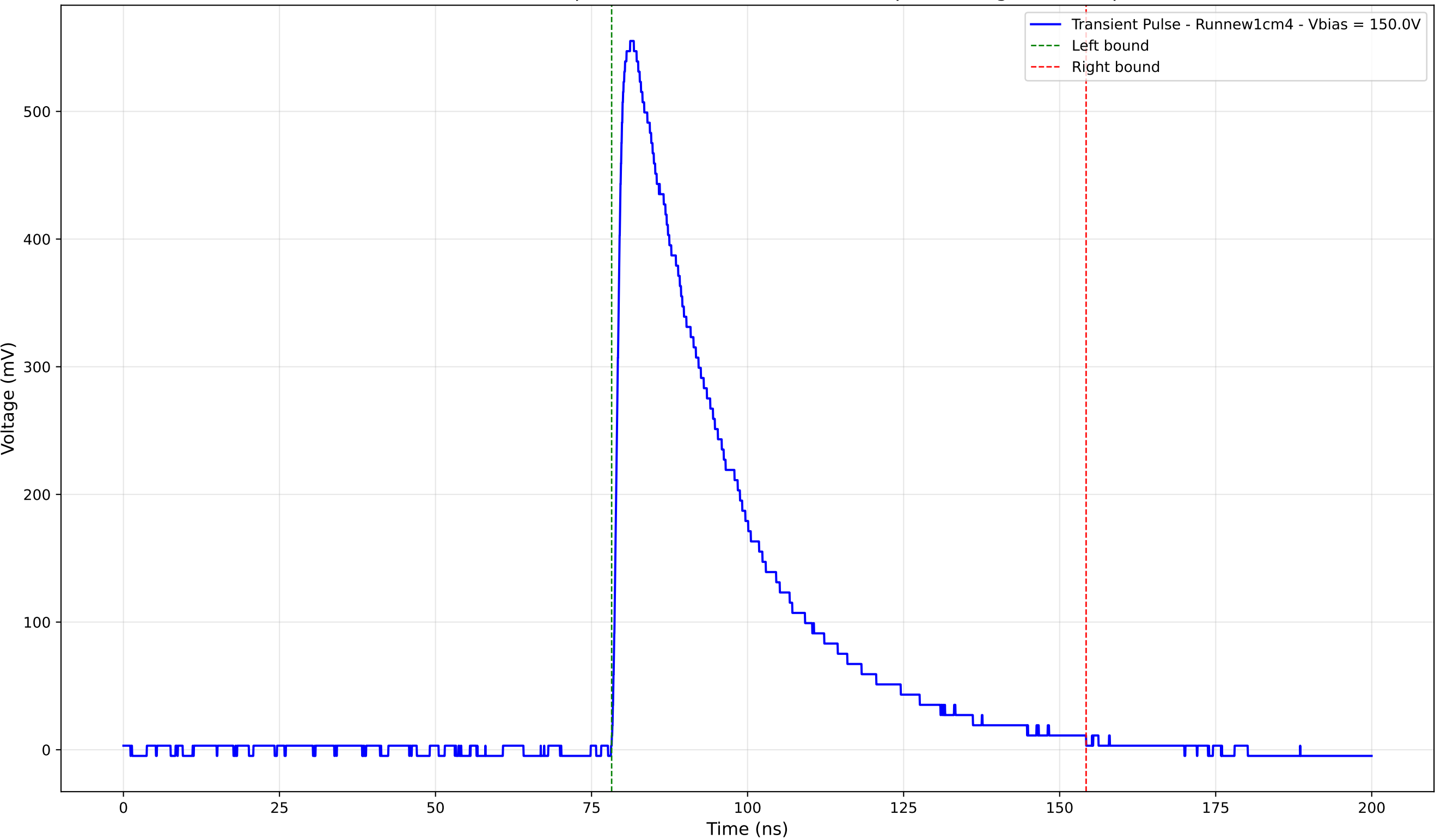
Transient Pulse - Sample: new1cm - Position: 1545.0 \mu\text{m} - Charge: 212.42 pC
