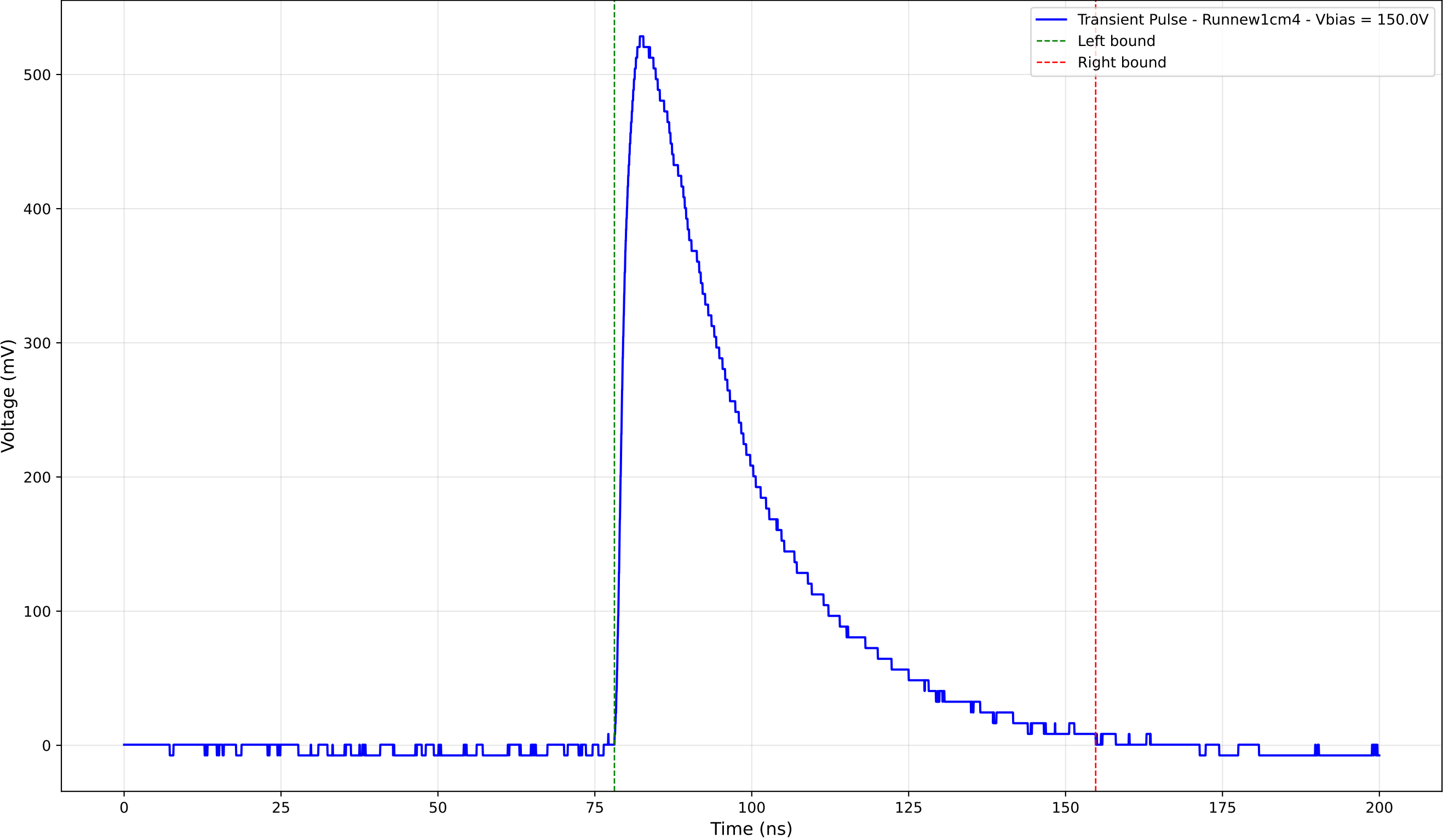
Transient Pulse - Sample: new1cm - Position: 2985.0 \mu\text{m} - Charge: 228.77 pC
