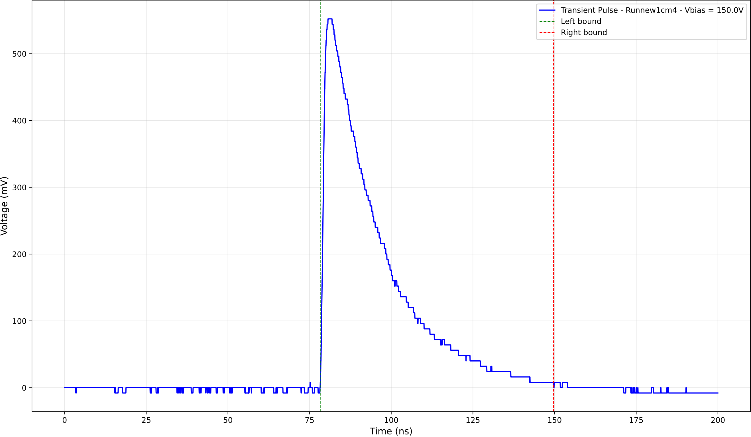
Transient Pulse - Sample: new1cm - Position: 1515.0 \mu\text{m} - Charge: 205.98 pC
