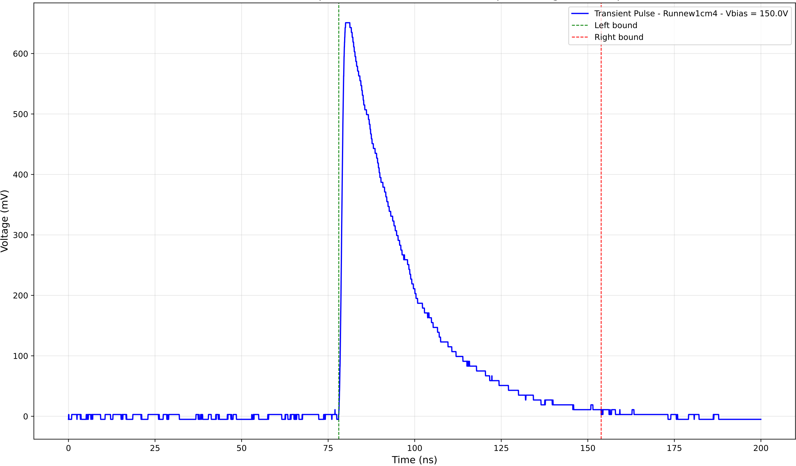
Transient Pulse - Sample: new1cm - Position: 3930.0 \mu\text{m} - Charge: 250.86 pC
