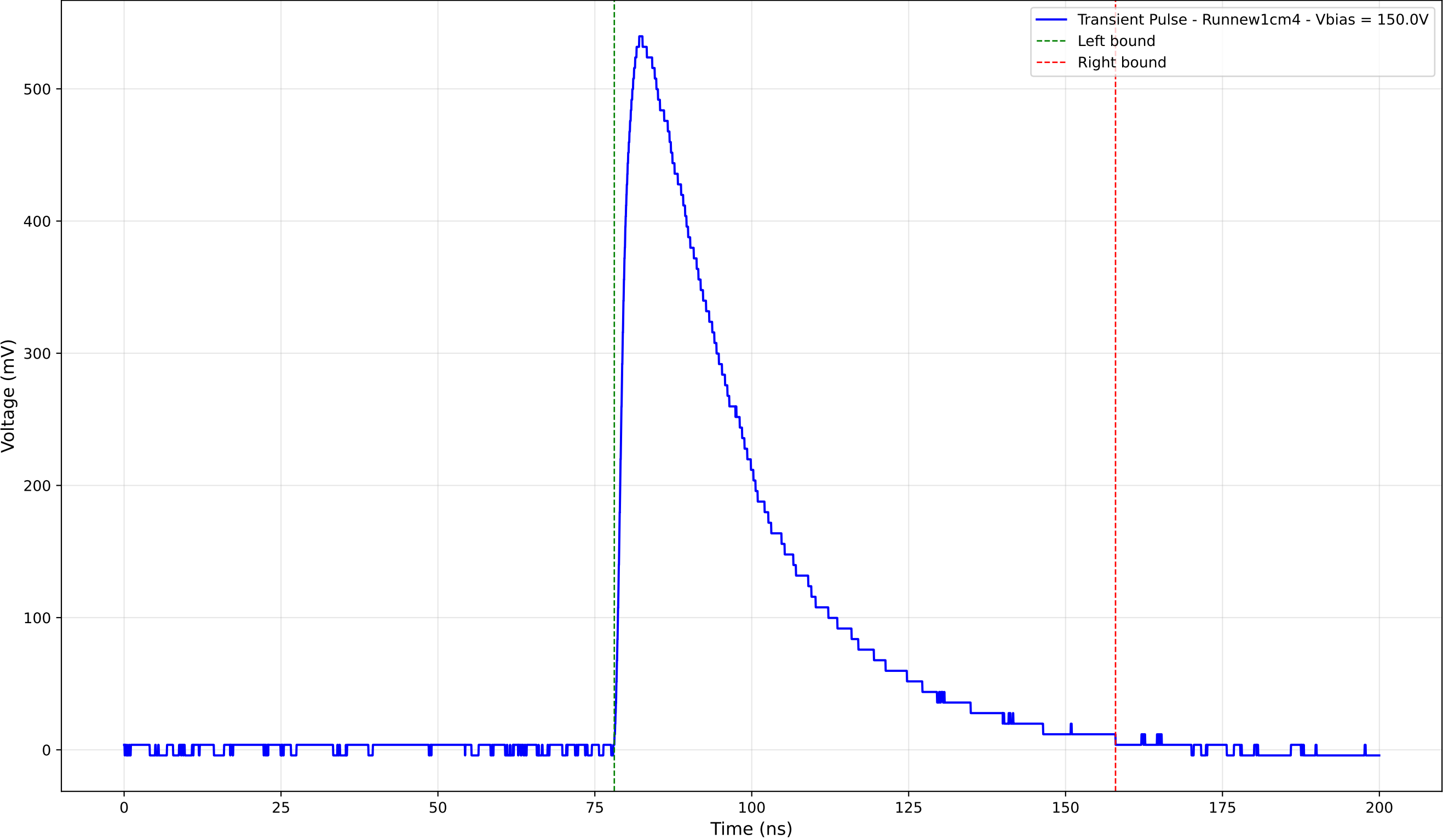
Transient Pulse - Sample: new1cm - Position: 3120.0 \mu\text{m} - Charge: 234.93 pC
