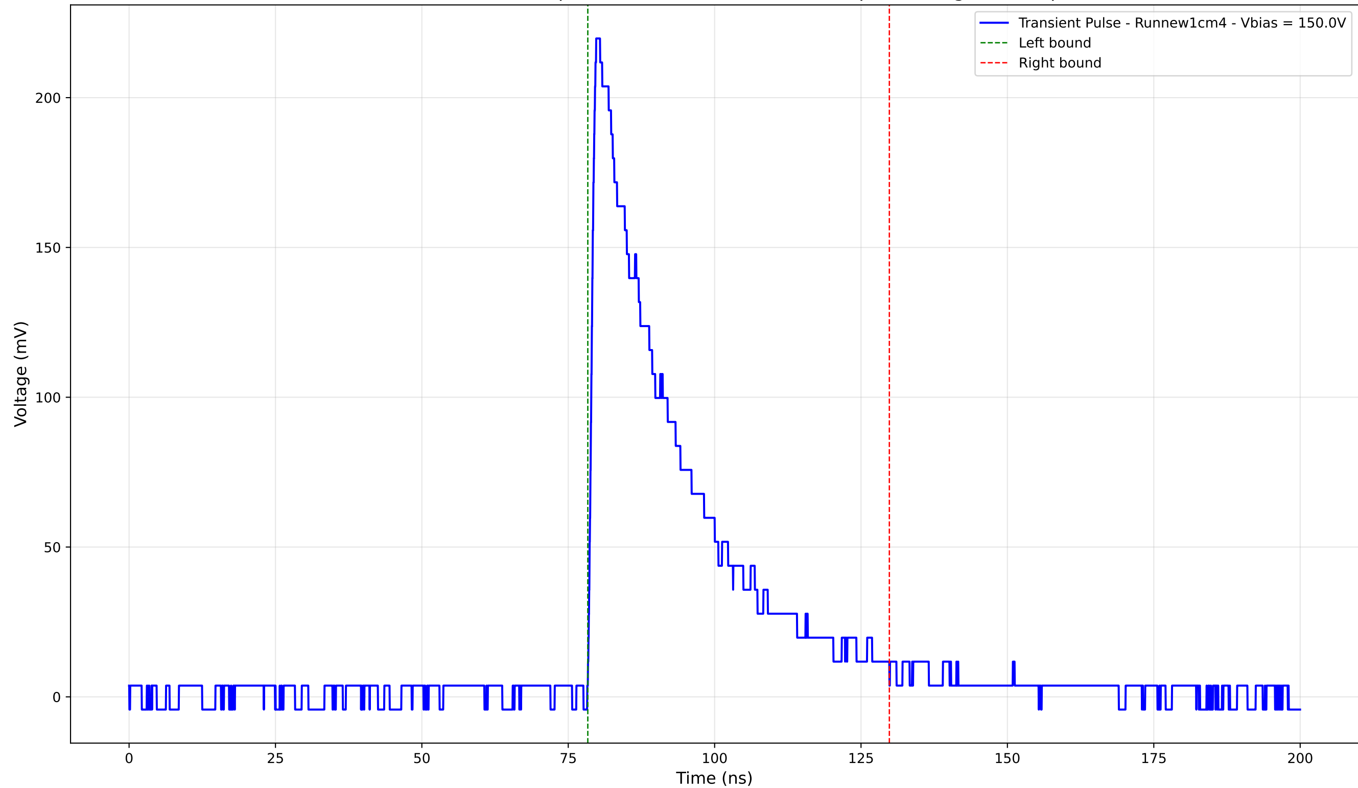
Transient Pulse - Sample: new1cm - Position: 1165.0 \mu\text{m} - Charge: 67.16 pC
