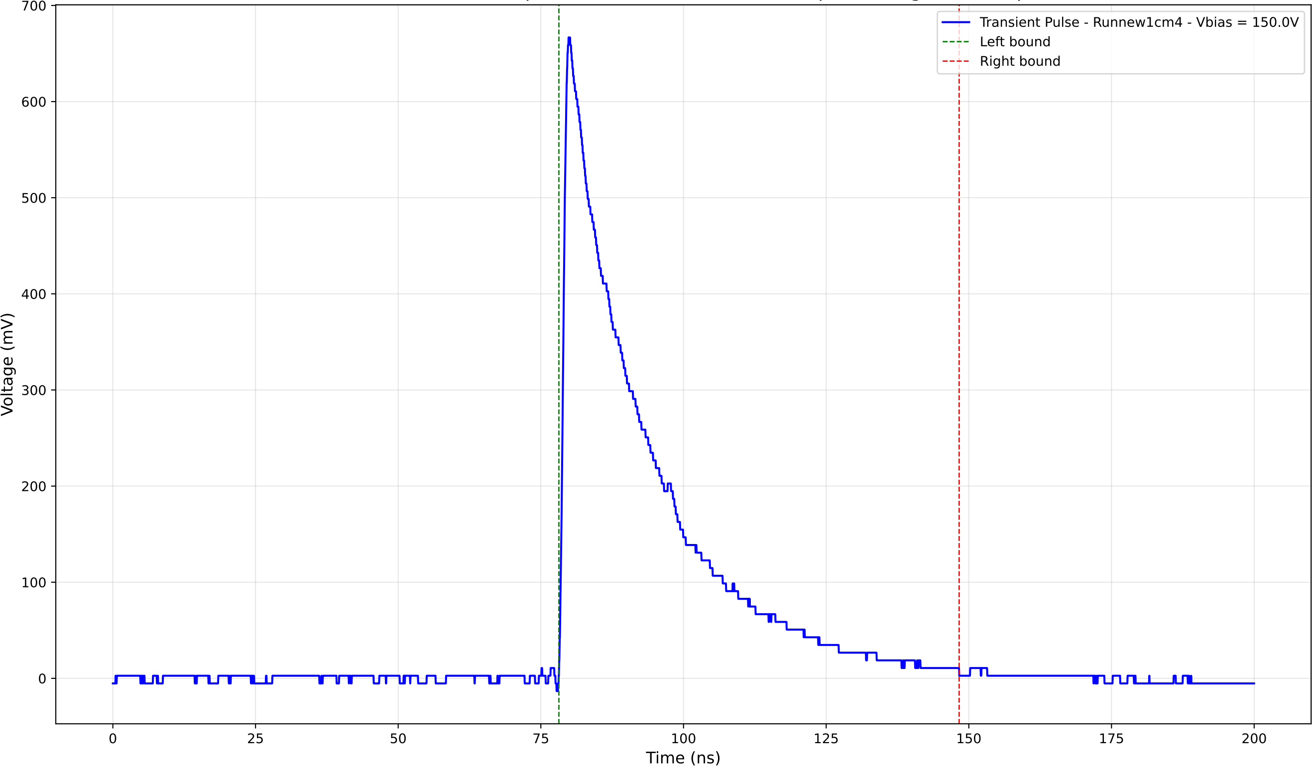
Transient Pulse - Sample: new1cm - Position: 1045.0 \mu\text{m} - Charge: 201.74 pC
