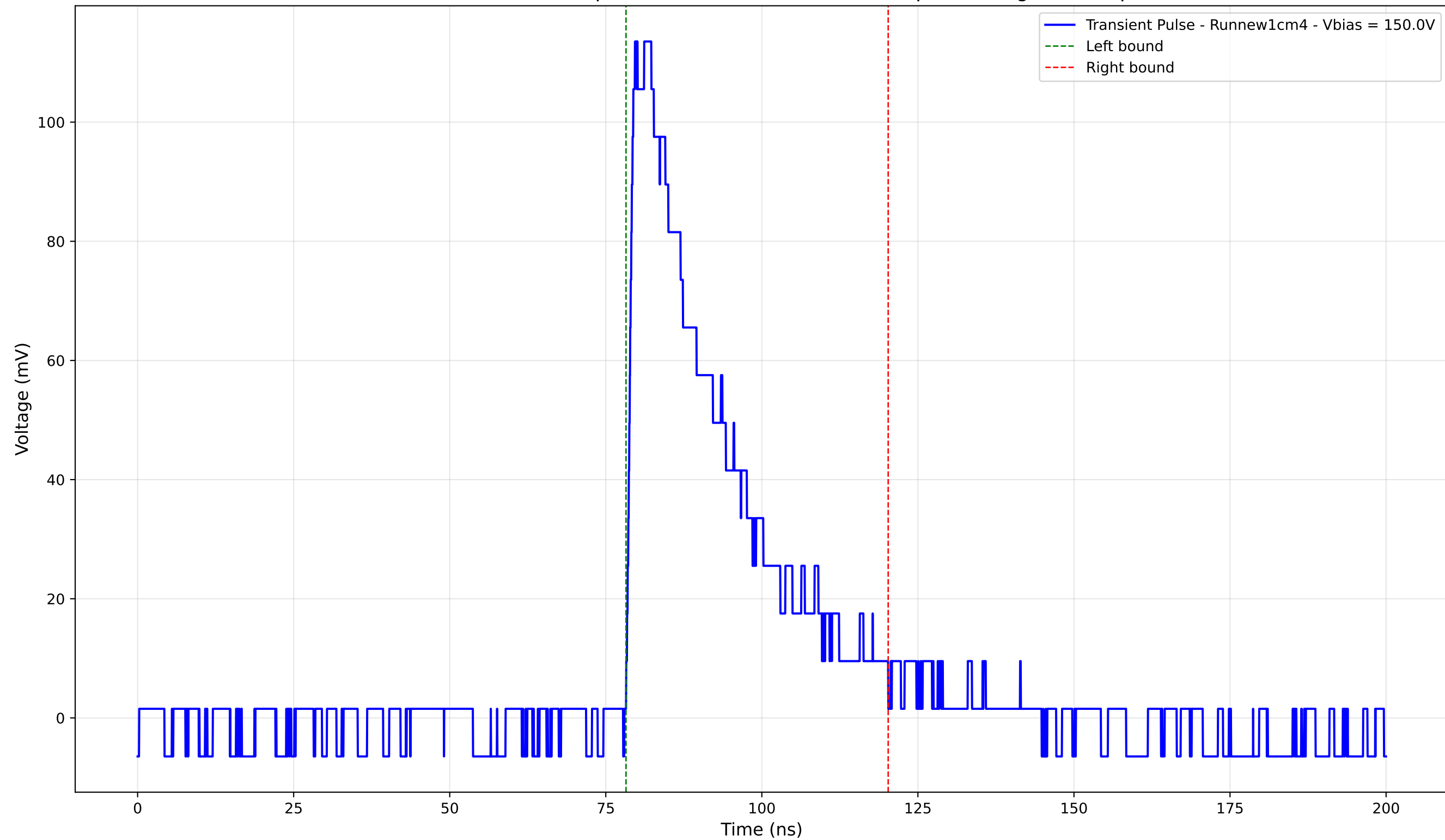
Transient Pulse - Sample: new1cm - Position: 4225.0 \mu\text{m} - Charge: 35.67 pC
