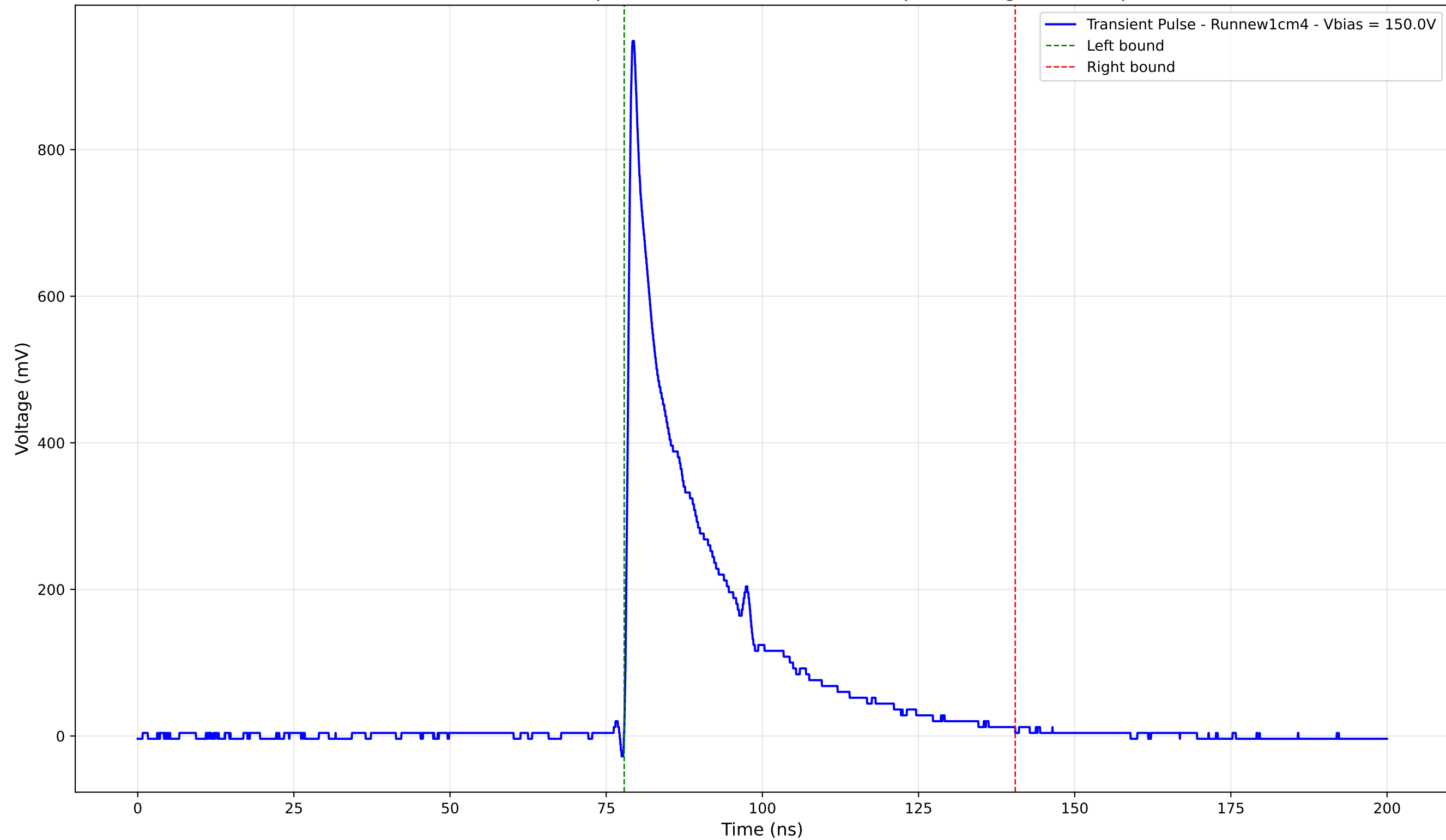
Transient Pulse - Sample: new1cm - Position: 390.0 \mu\text{m} - Charge: 199.43 pC
