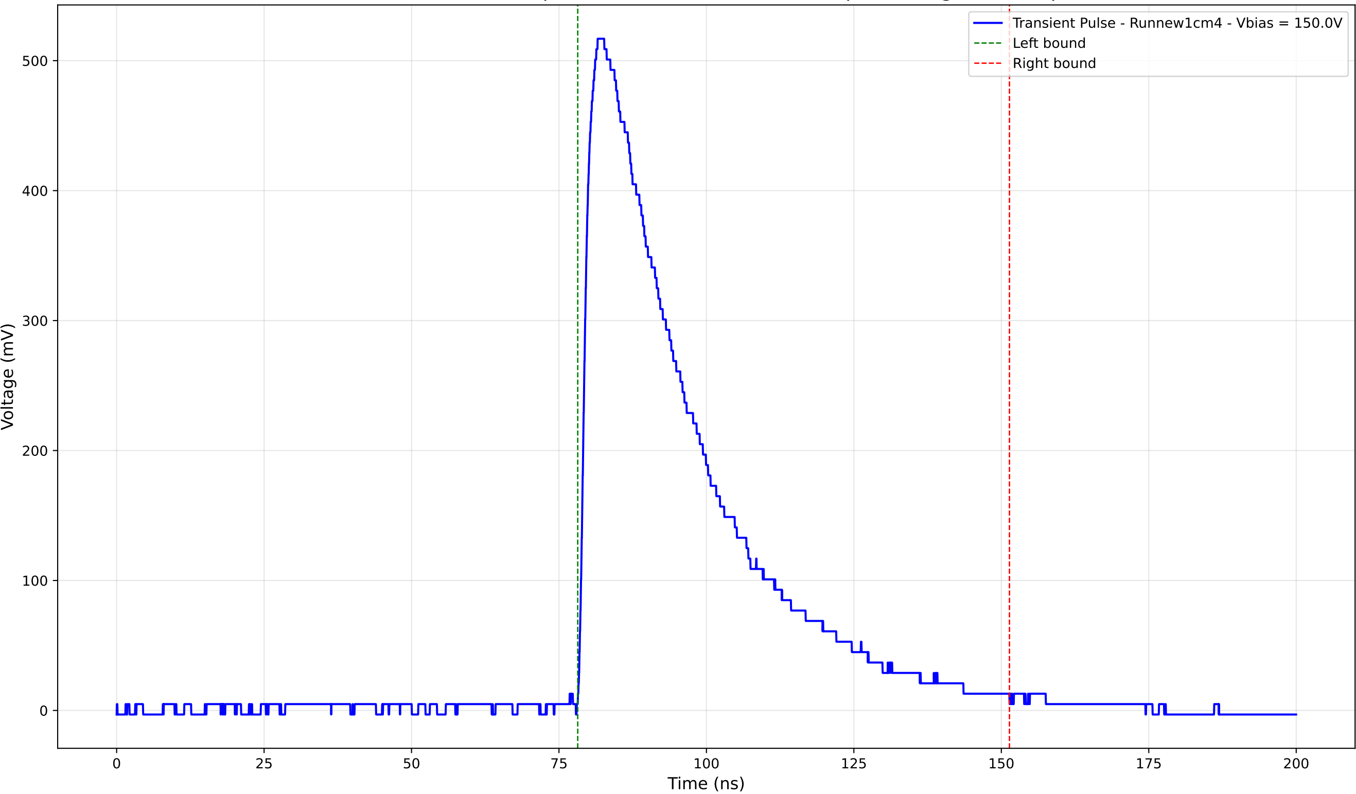
Transient Pulse - Sample: new1cm - Position: 1940.0 \mu\text{m} - Charge: 214.25 pC
