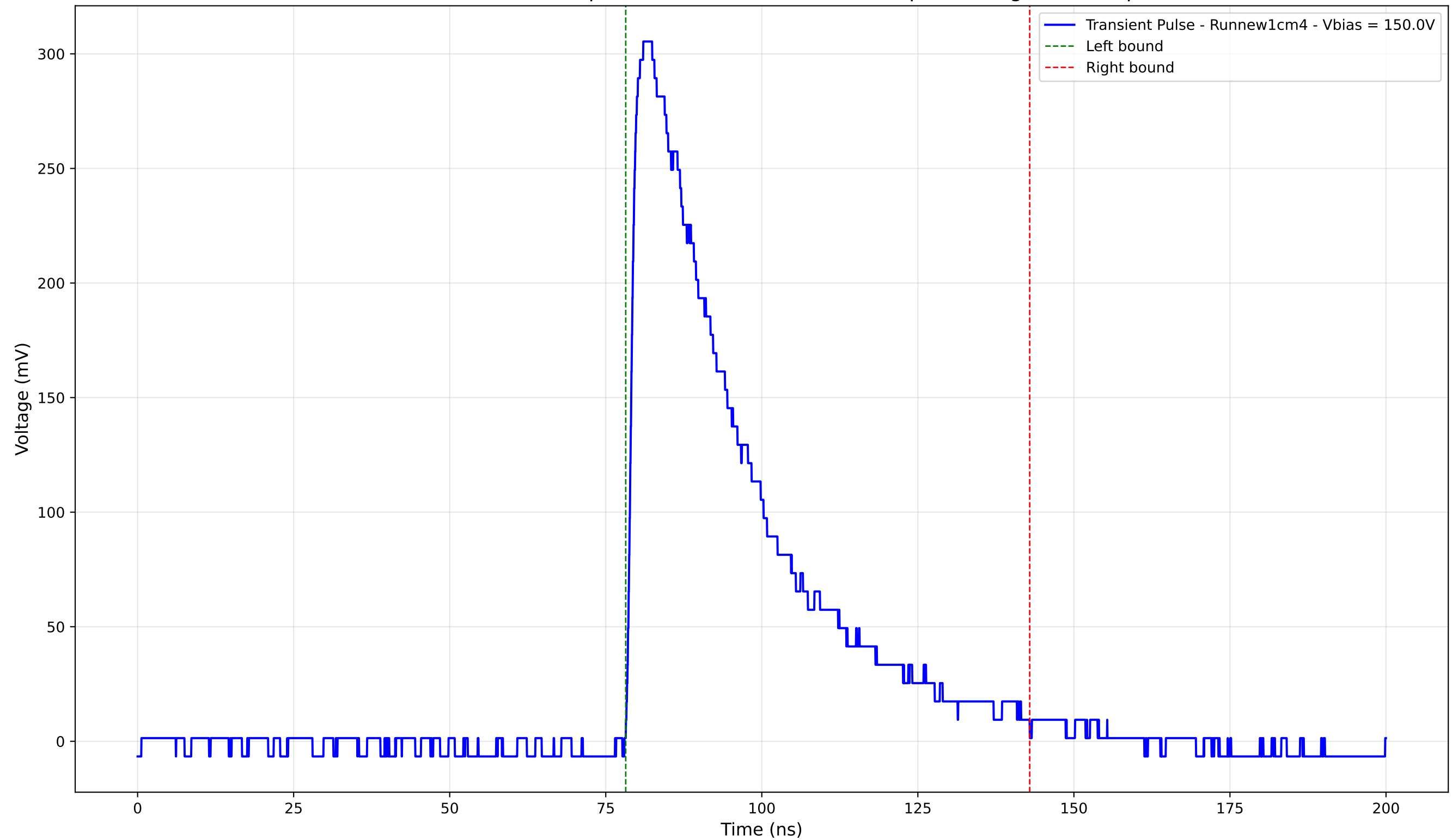
Transient Pulse - Sample: new1cm - Position: 3680.0 \mu\text{m} - Charge: 120.68 pC
