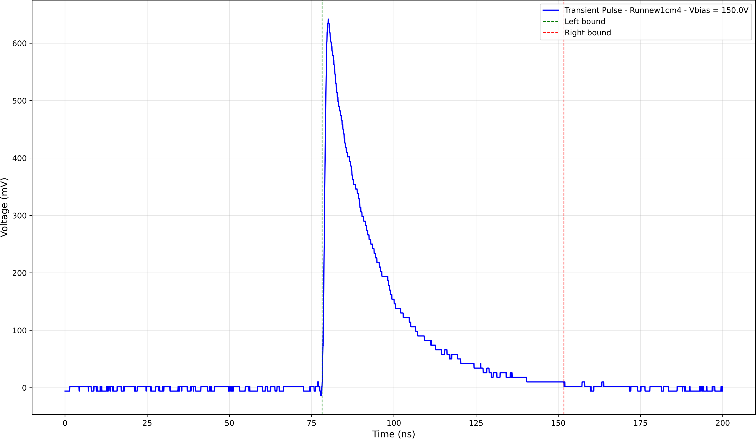
Transient Pulse - Sample: new1cm - Position: 1095.0 \mu\text{m} - Charge: 197.90 pC
