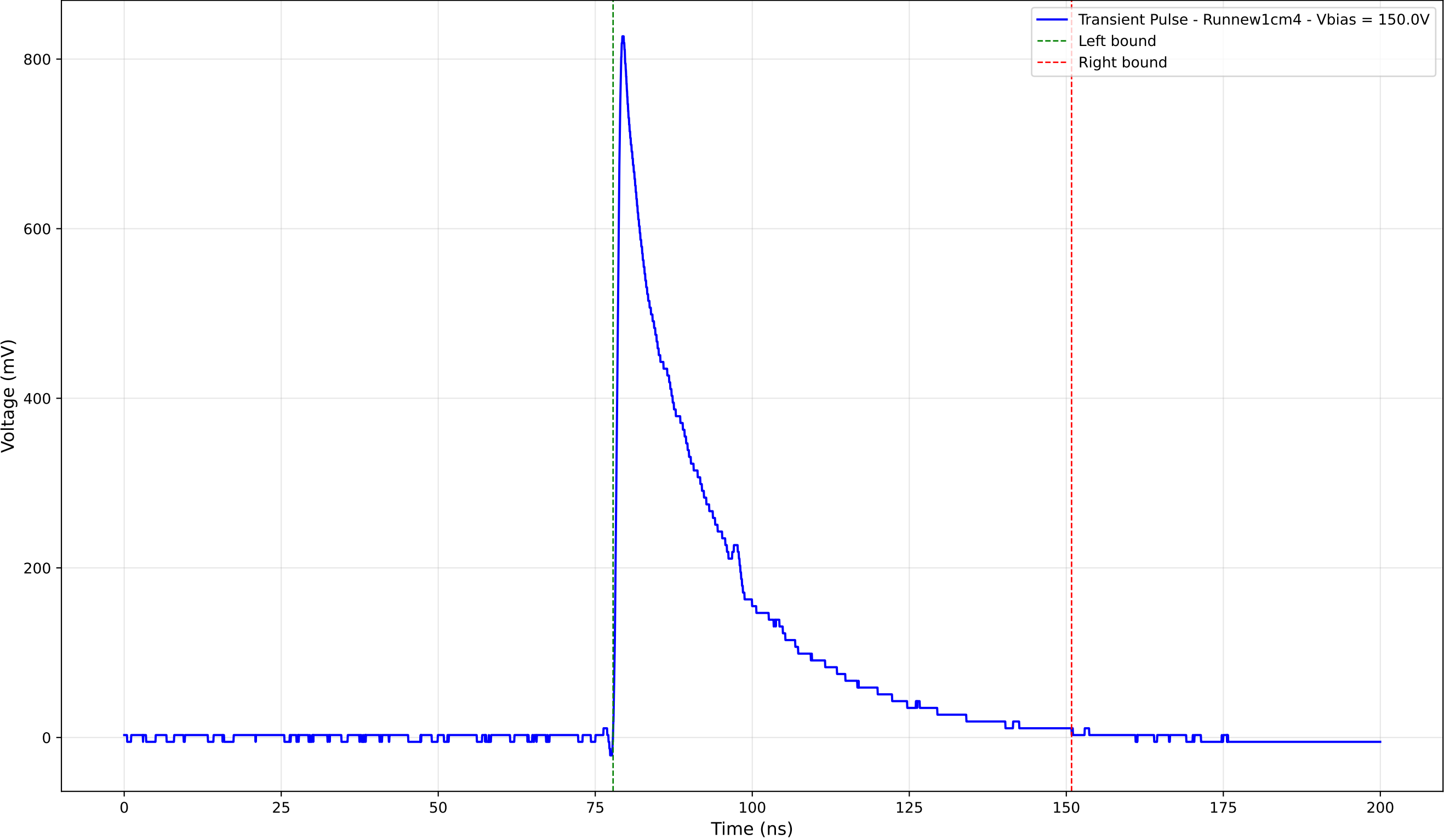
Transient Pulse - Sample: new1cm - Position: 4620.0 \mu\text{m} - Charge: 225.59 pC
