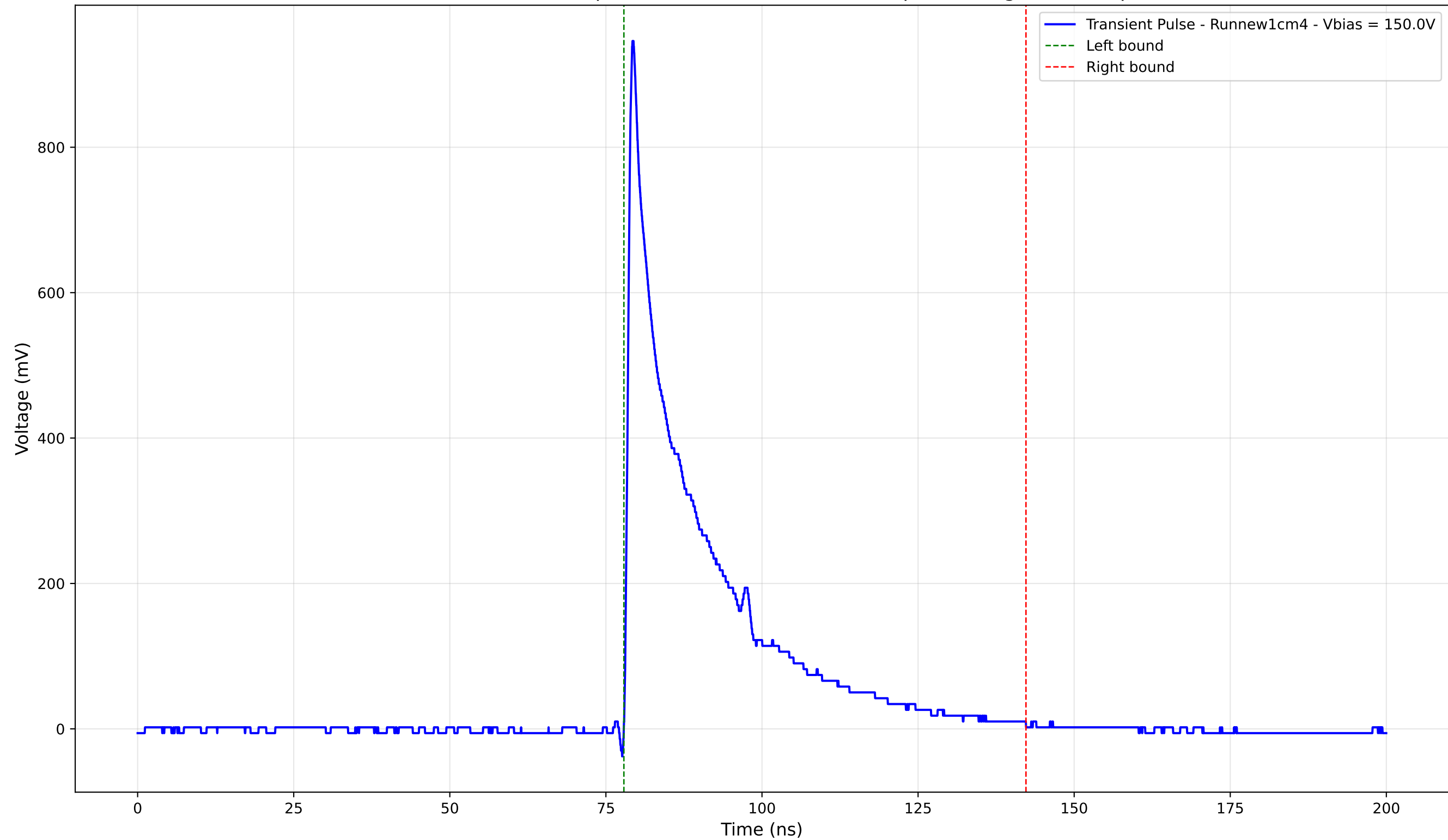
Transient Pulse - Sample: new1cm - Position: 400.0 \mu\text{m} - Charge: 196.36 pC
