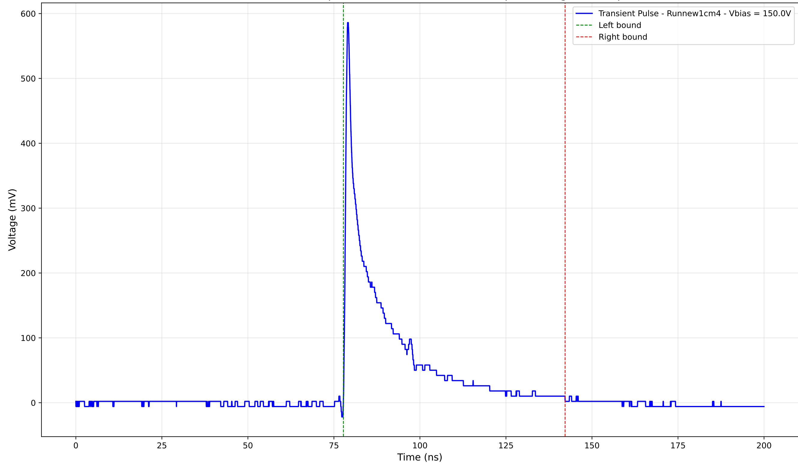
Transient Pulse - Sample: new1cm - Position: 5020.0 \mu\text{m} - Charge: 99.76 pC
