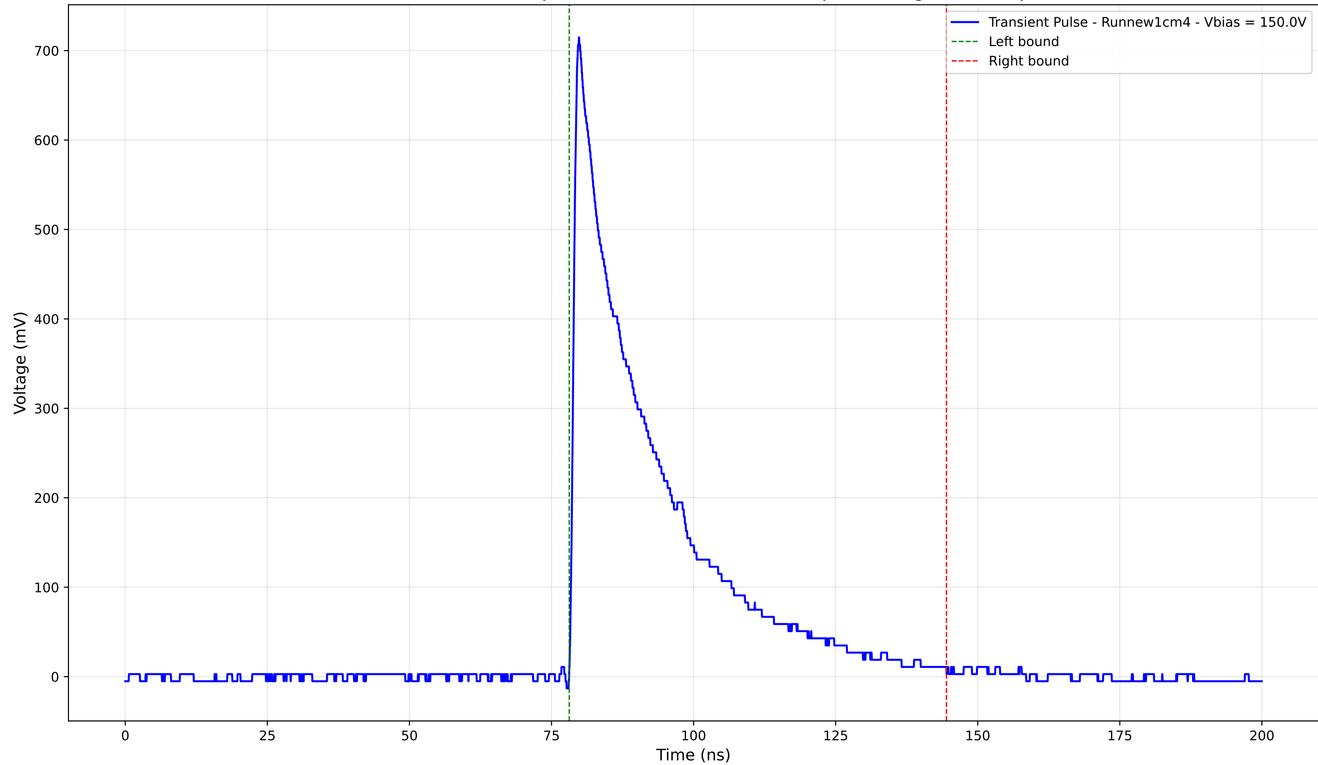
Transient Pulse - Sample: new1cm - Position: 920.0 \mu\text{m} - Charge: 199.27 pC
