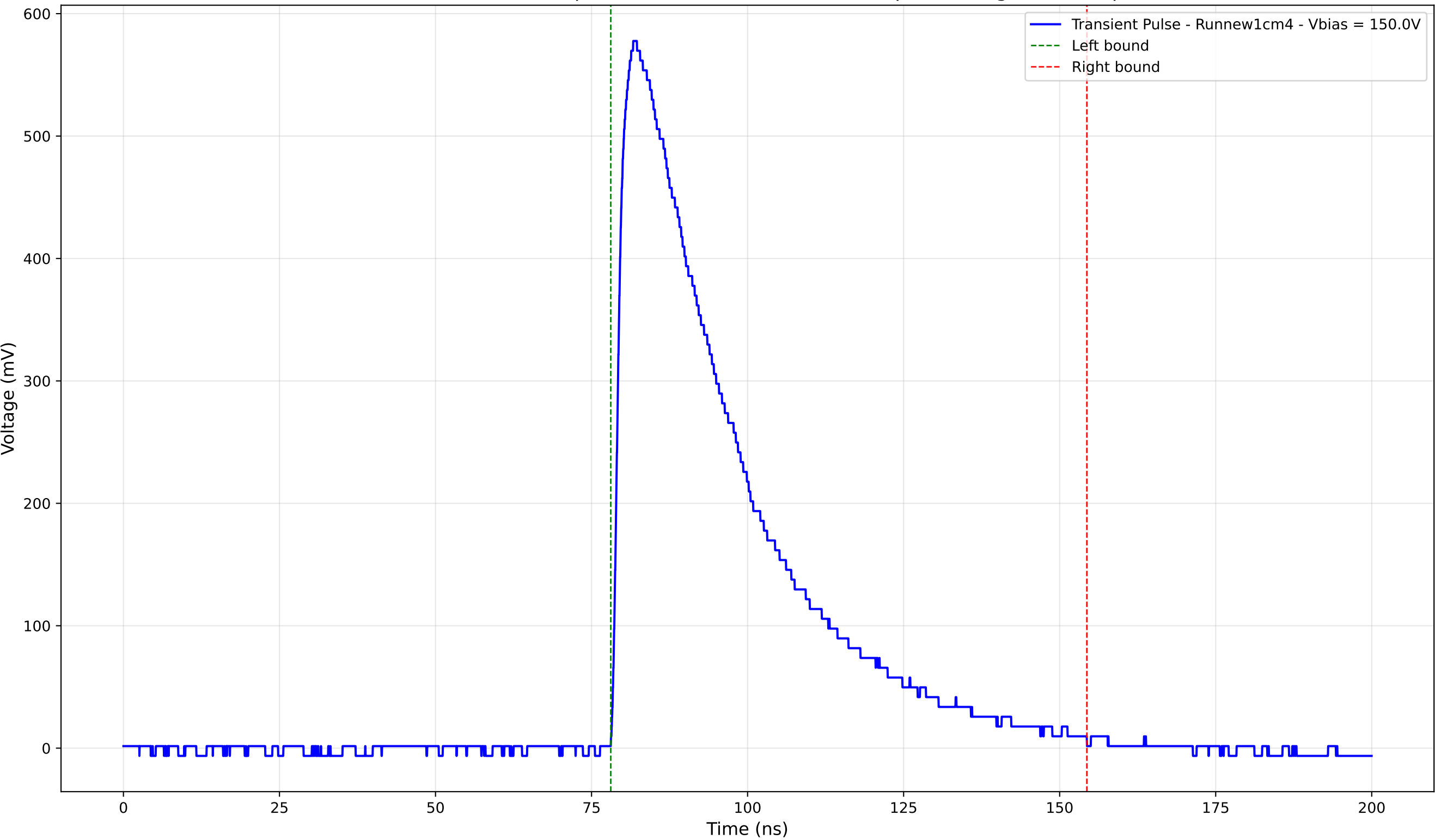
Transient Pulse - Sample: new1cm - Position: 3380.0 \mu\text{m} - Charge: 244.00 pC
