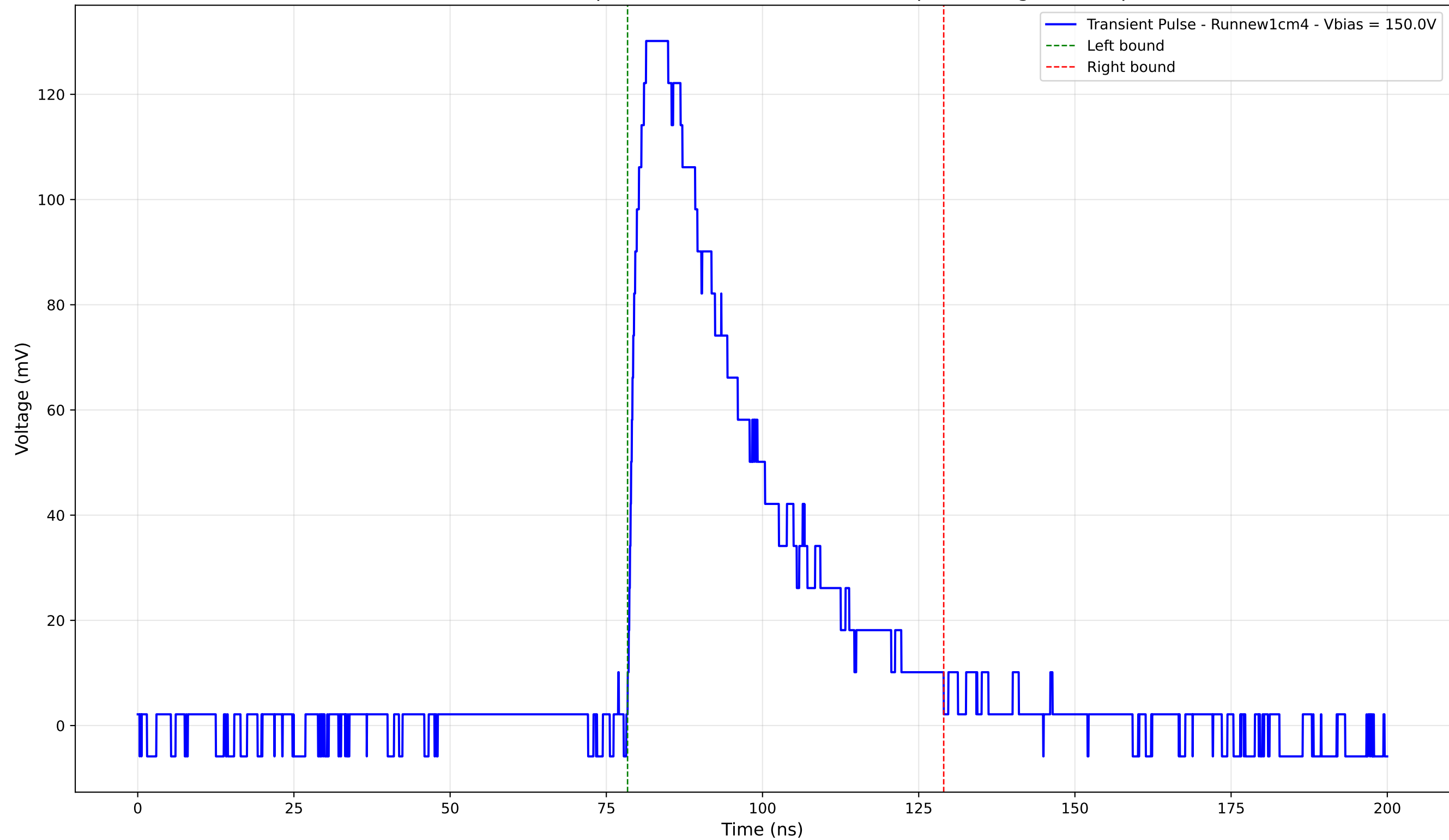
Transient Pulse - Sample: new1cm - Position: 2180.0 \mu\text{m} - Charge: 52.40 pC
