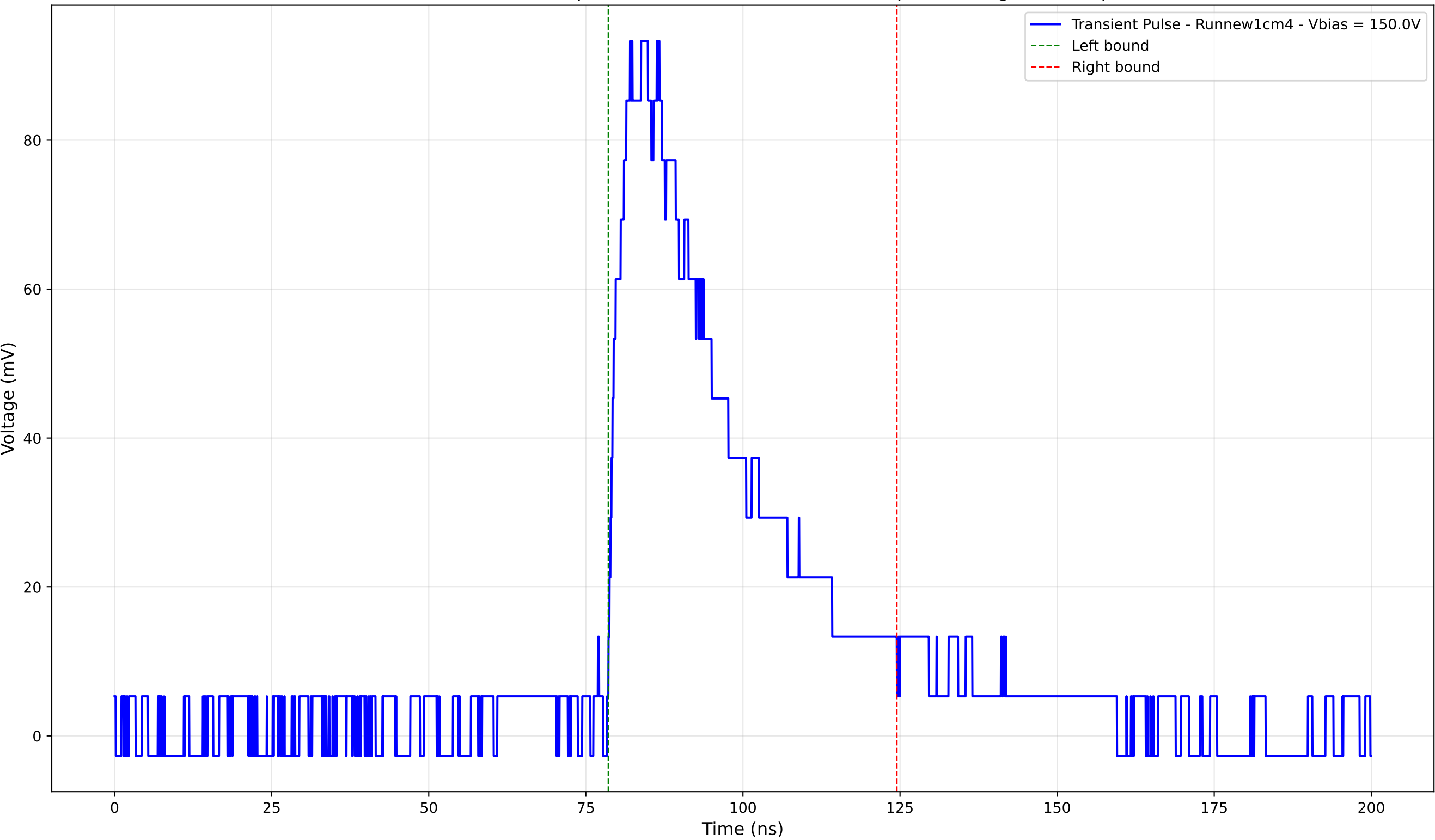
Transient Pulse - Sample: new1cm - Position: 2705.0 \mu\text{m} - Charge: 37.69 pC
