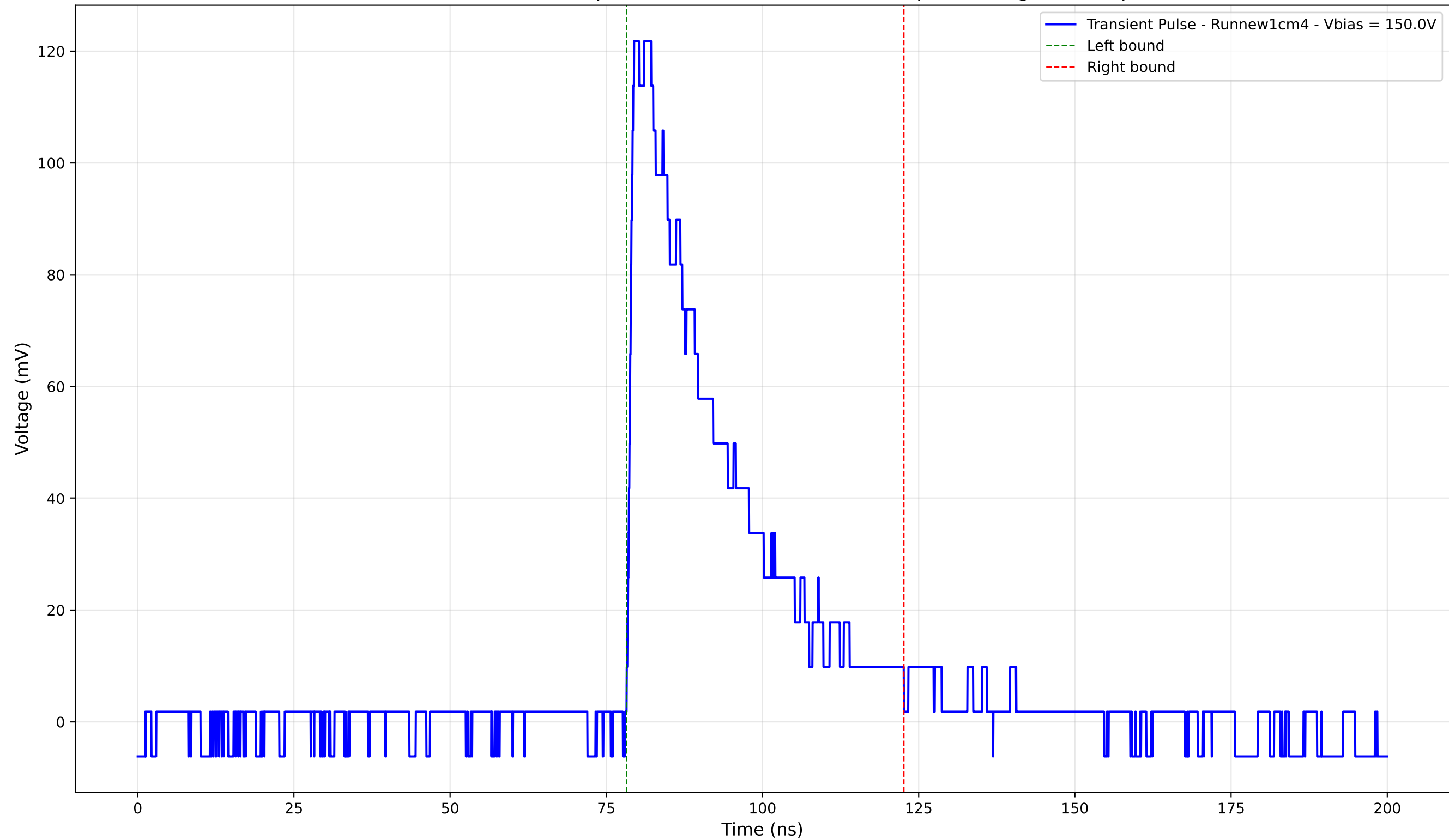
Transient Pulse - Sample: new1cm - Position: 4245.0 \mu\text{m} - Charge: 37.87 pC
