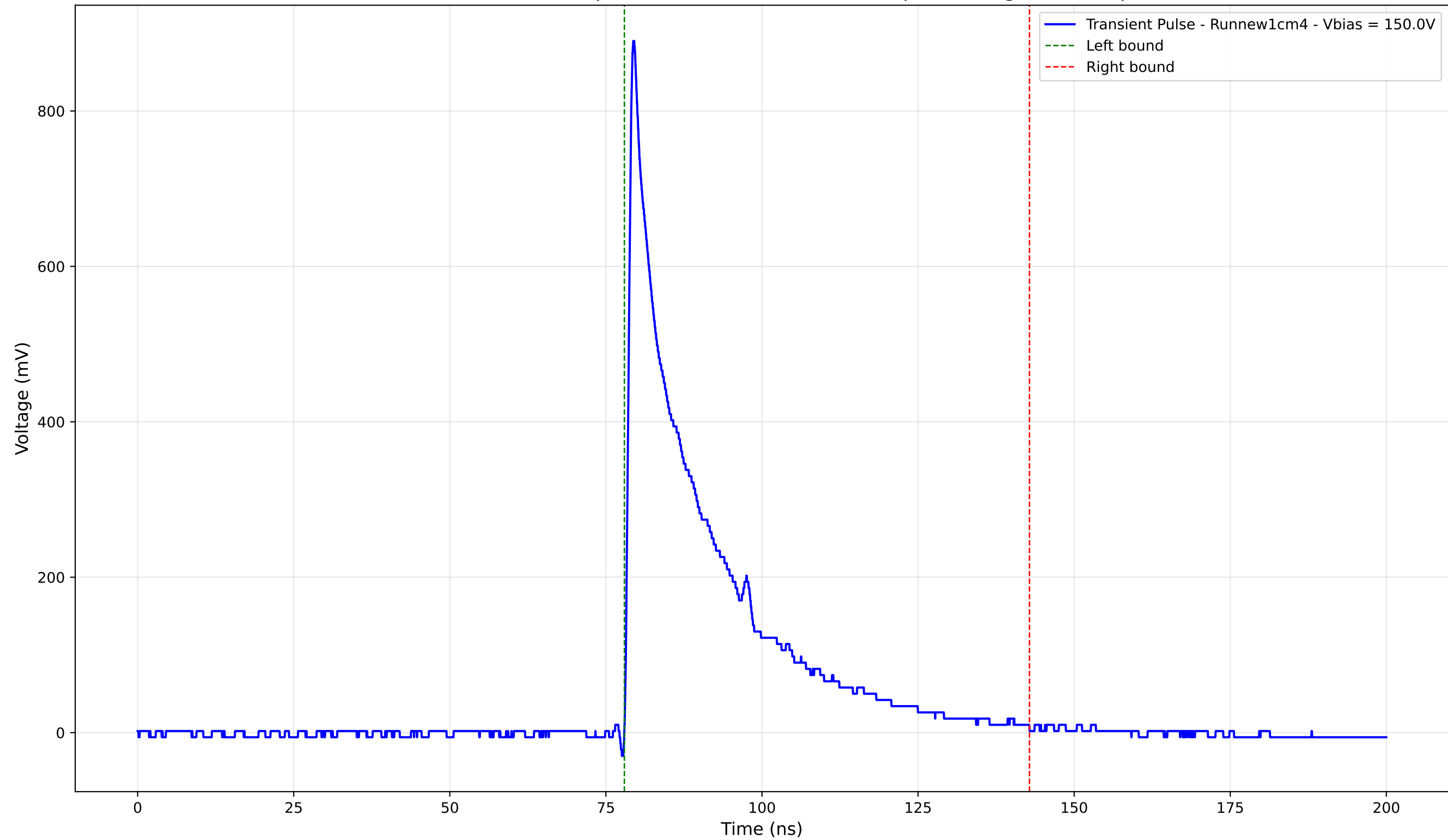
Transient Pulse - Sample: new1cm - Position: 545.0 \mu\text{m} - Charge: 198.40 pC
