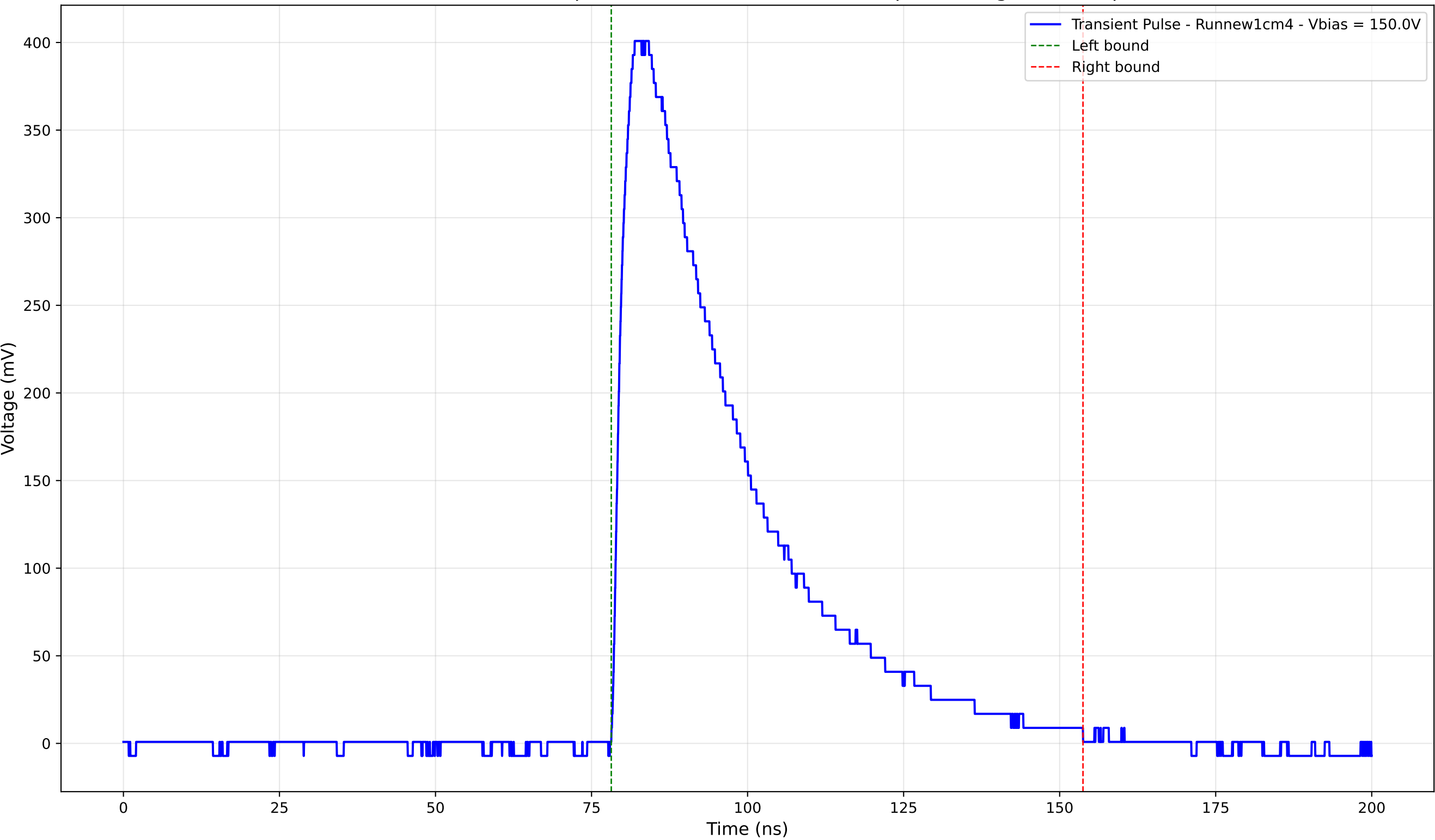
Transient Pulse - Sample: new1cm - Position: 2790.0 \mu\text{m} - Charge: 173.48 pC
