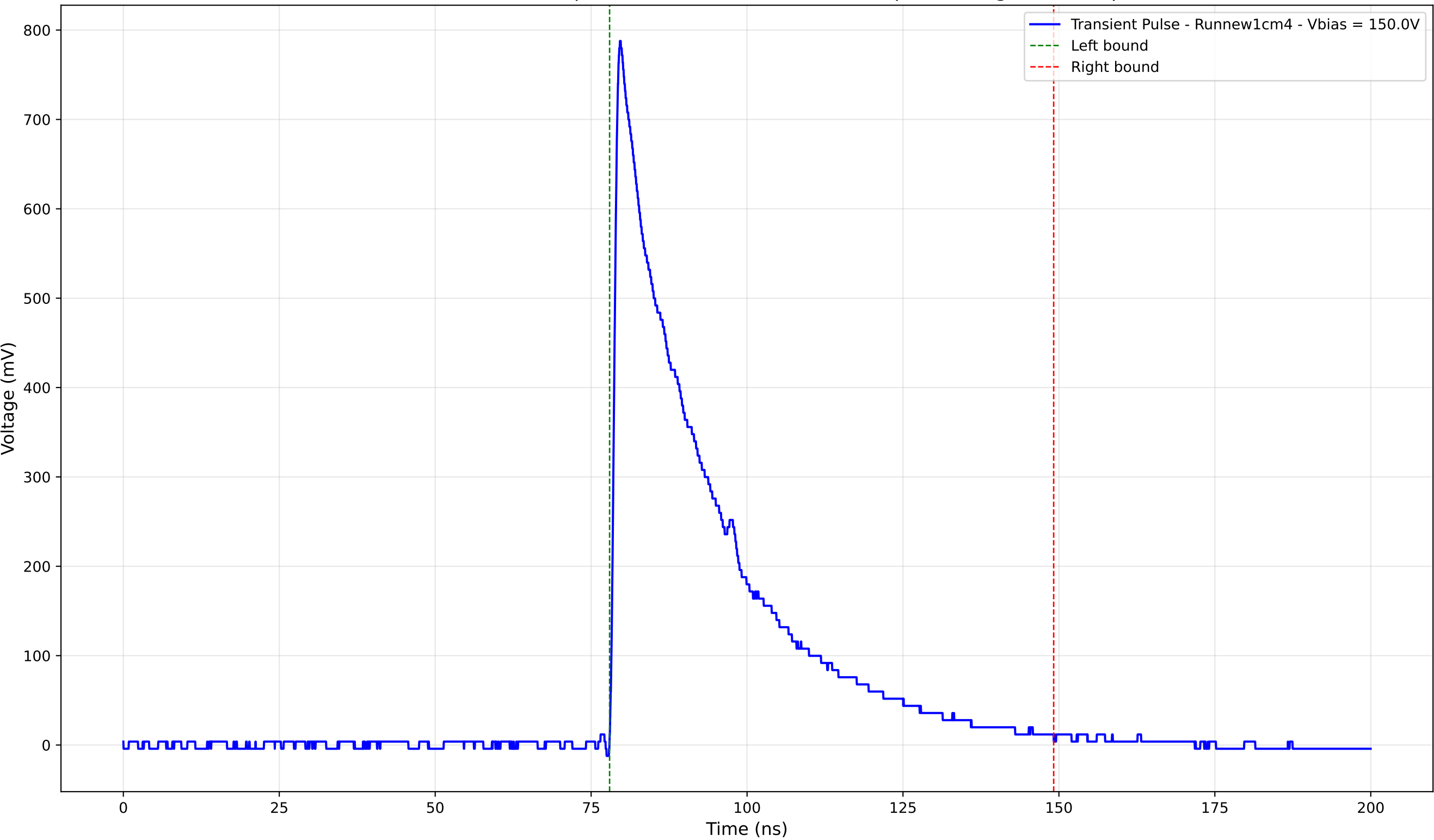
Transient Pulse - Sample: new1cm - Position: 4375.0 \mu\text{m} - Charge: 242.98 pC
