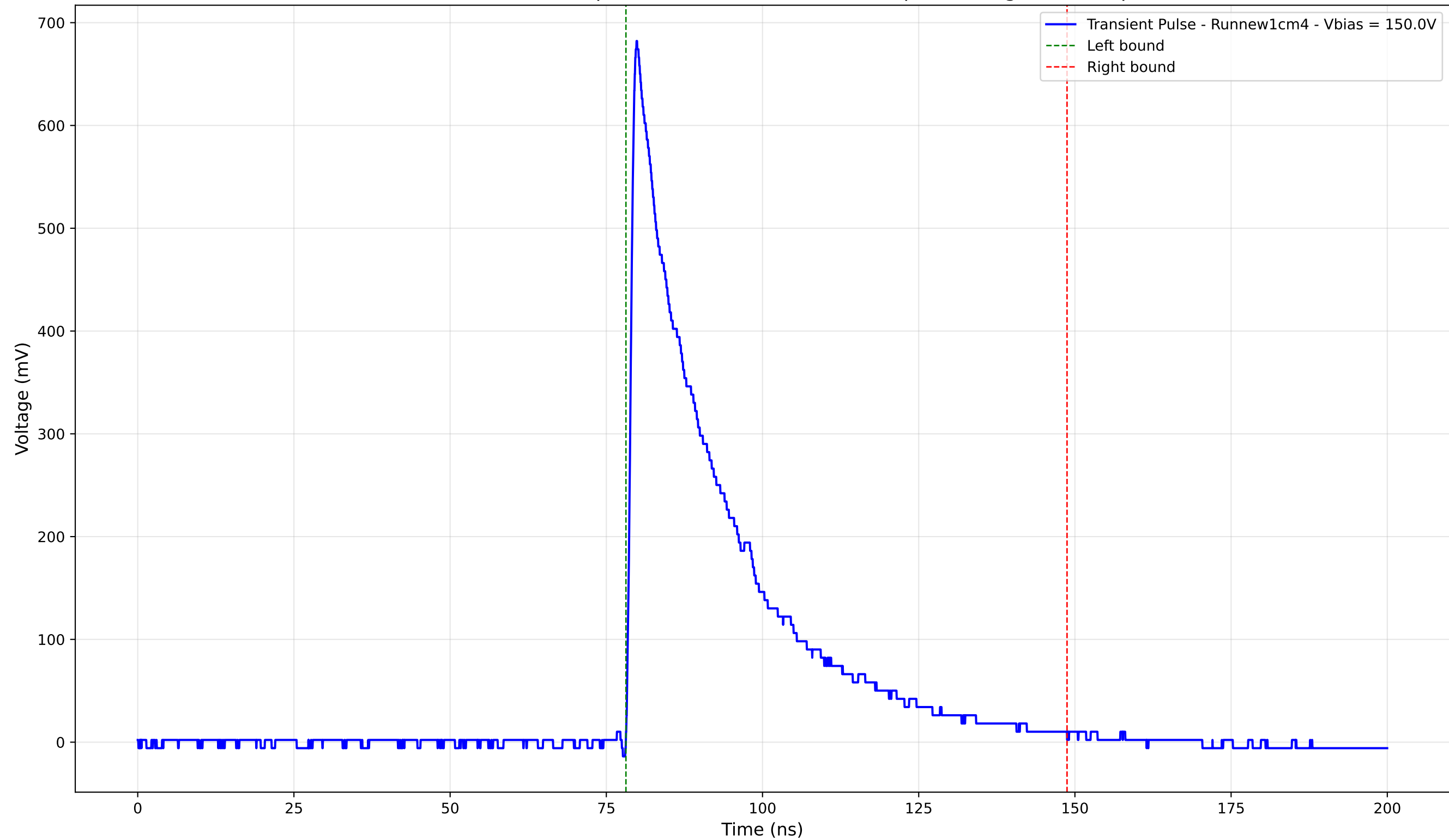
Transient Pulse - Sample: new1cm - Position: 975.0 \mu\text{m} - Charge: 198.00 pC
