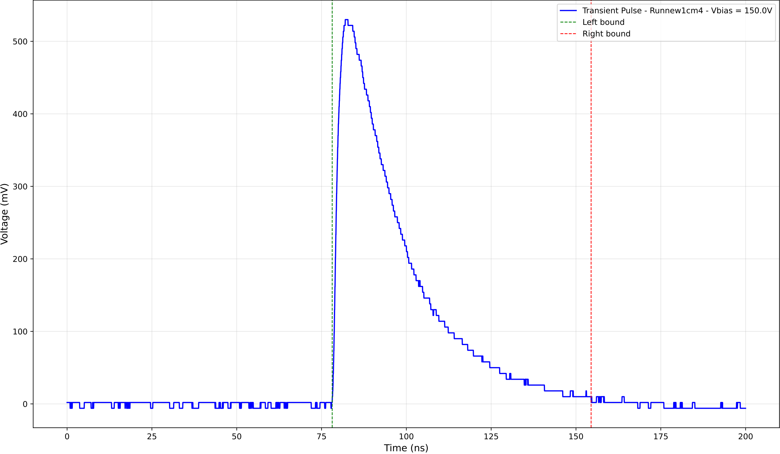
Transient Pulse - Sample: new1cm - Position: 2970.0 \mu\text{m} - Charge: 231.52 pC
