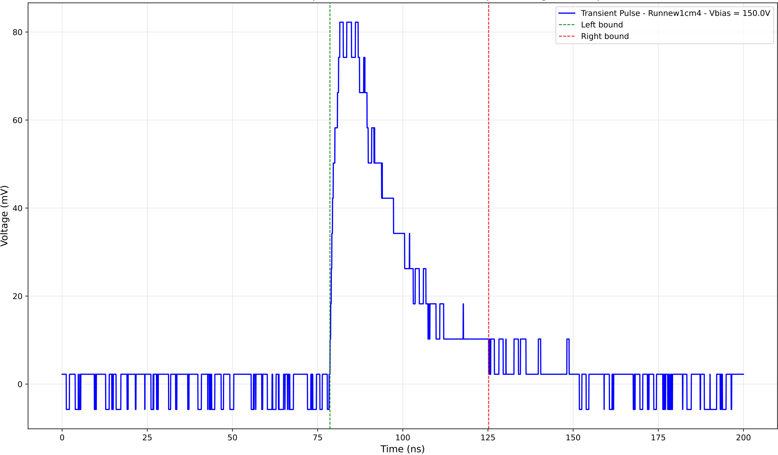
Transient Pulse - Sample: new1cm - Position: 2195.0 \mu\text{m} - Charge: 31.96 pC
