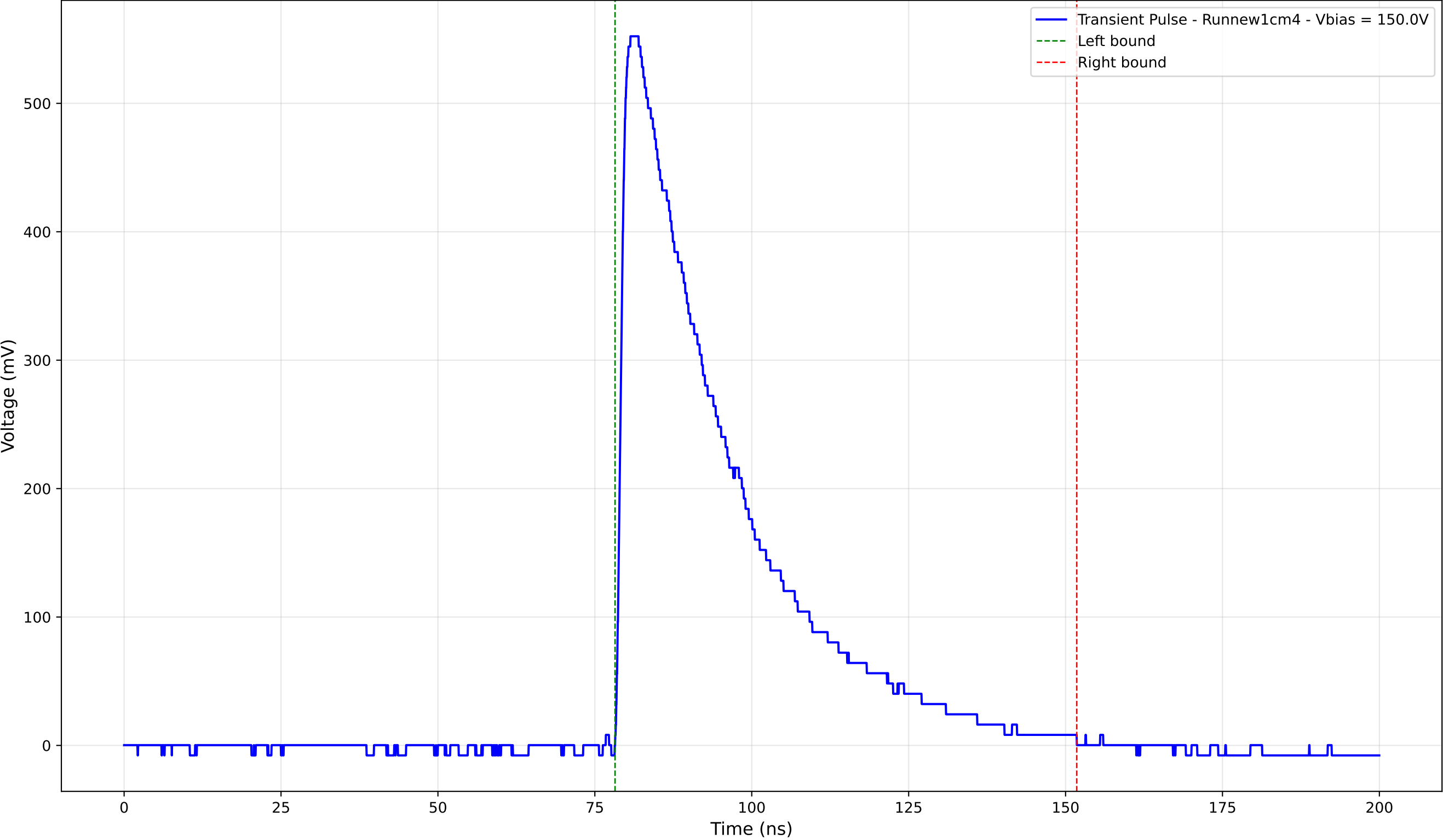
Transient Pulse - Sample: new1cm - Position: 1505.0 \mu\text{m} - Charge: 206.15 pC
