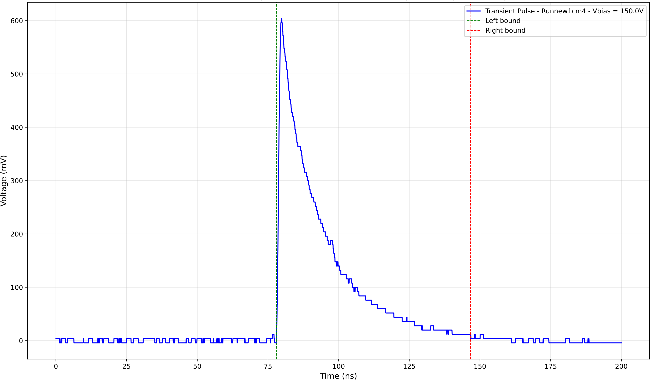
Transient Pulse - Sample: new1cm - Position: 4305.0 \mu\text{m} - Charge: 182.98 pC
