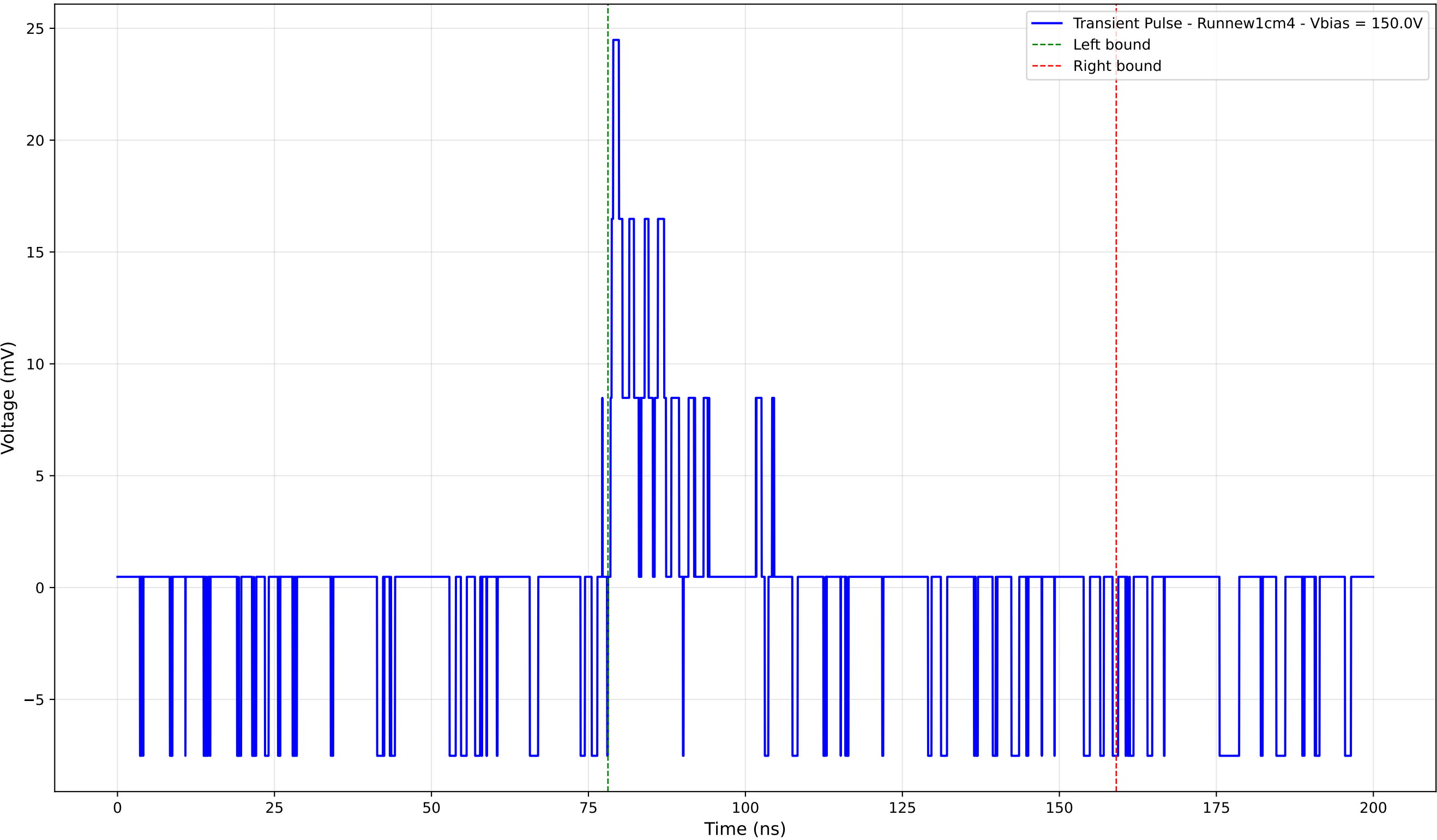
Transient Pulse - Sample: new1cm - Position: 135.0 \mu\text{m} - Charge: 2.12 pC
