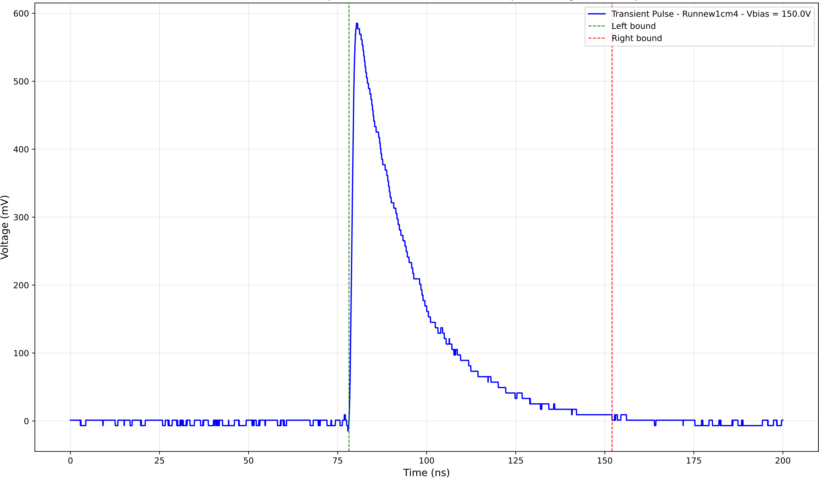
Transient Pulse - Sample: new1cm - Position: 1345.0 \mu\text{m} - Charge: 204.79 pC
