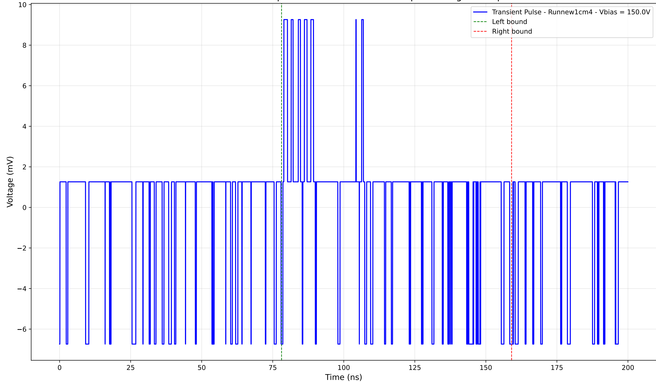
Transient Pulse - Sample: new1cm - Position: 30.0 \mu\text{m} - Charge: 1.14 pC
