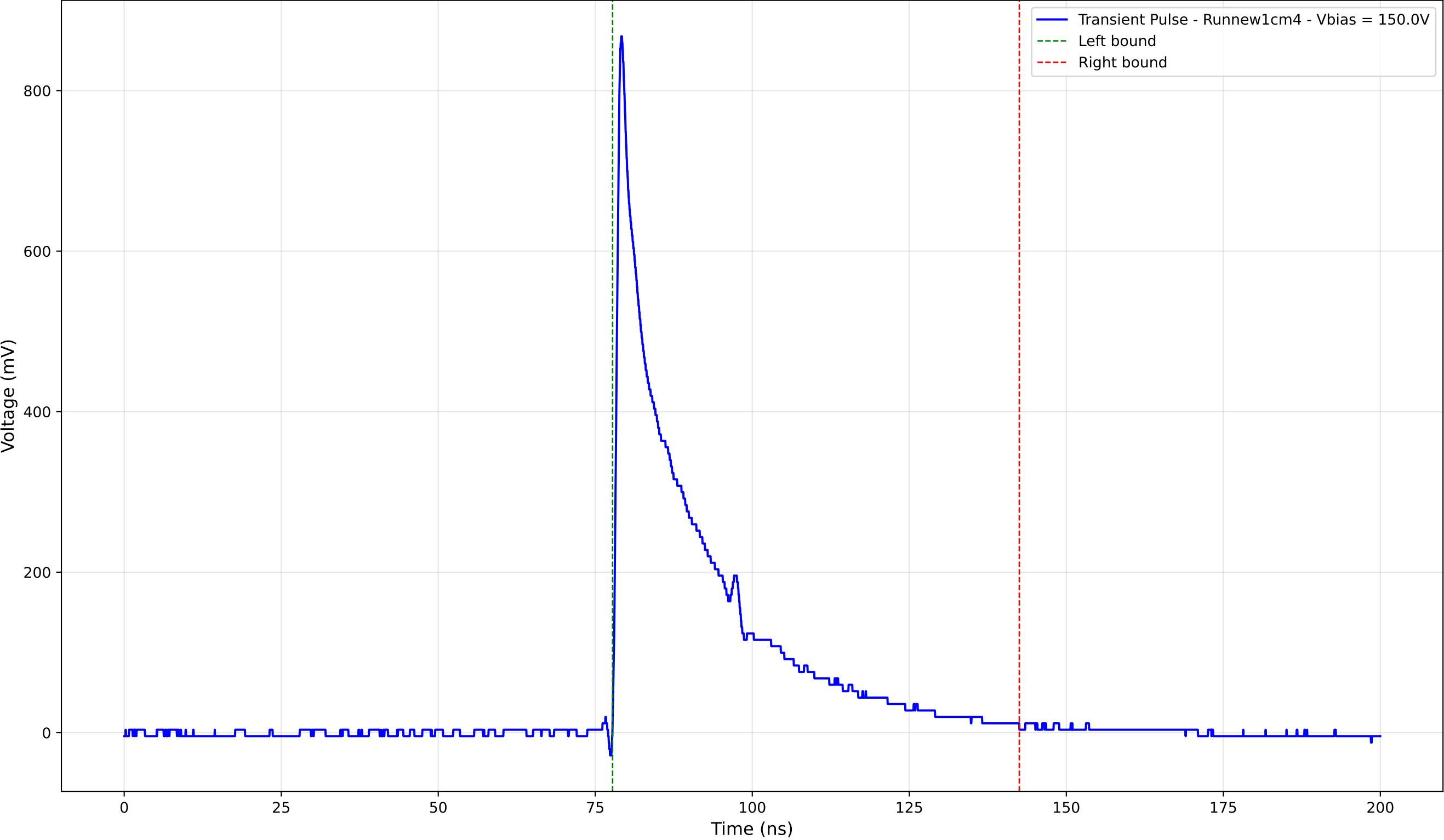
Transient Pulse - Sample: new1cm - Position: 4885.0 \mu\text{m} - Charge: 190.62 pC
