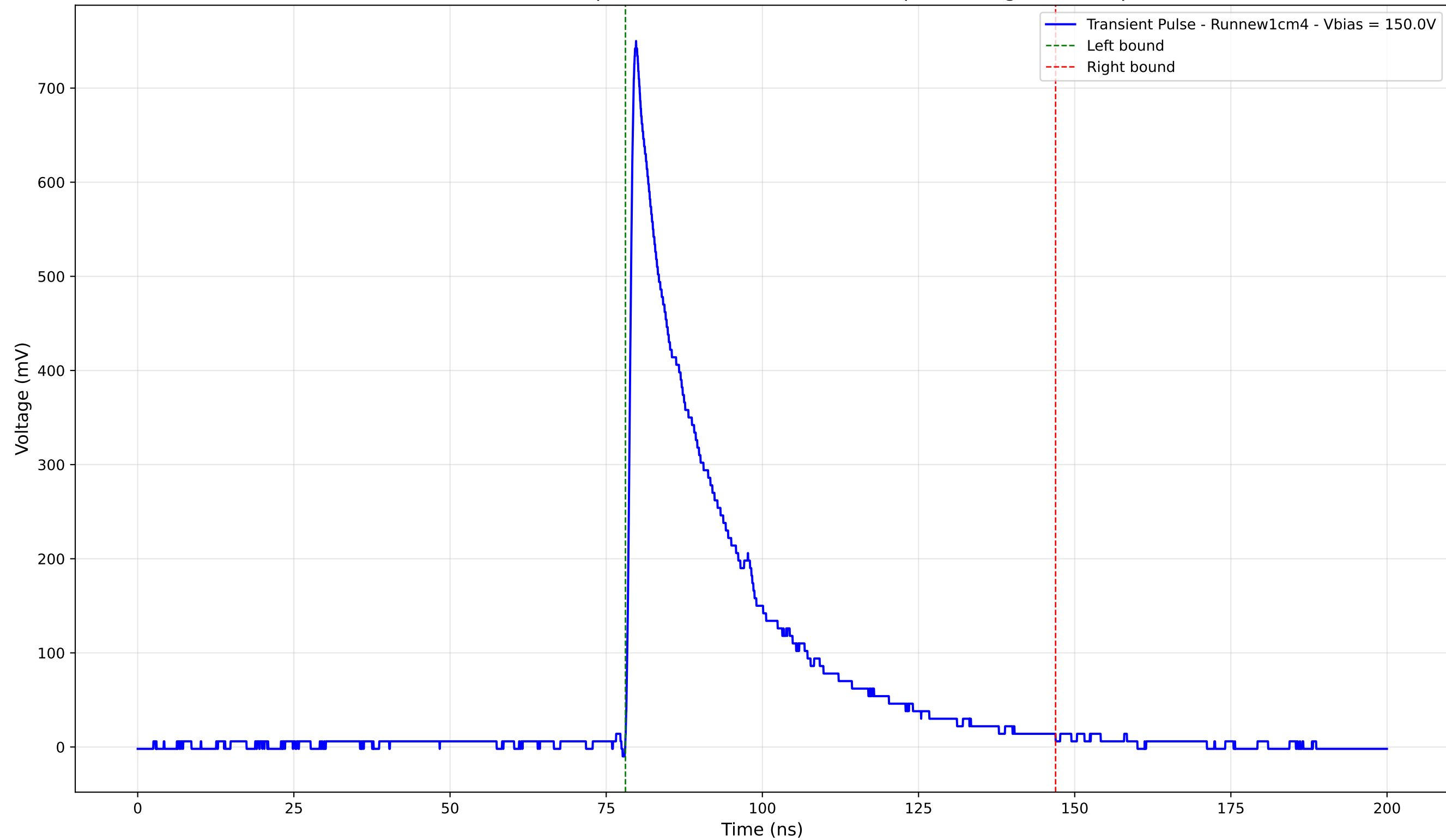
Transient Pulse - Sample: new1cm - Position: 860.0 \mu\text{m} - Charge: 206.19 pC
