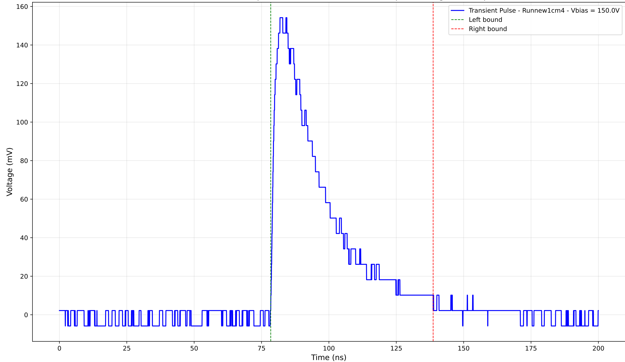
Transient Pulse - Sample: new1cm - Position: 3250.0 \mu\text{m} - Charge: 62.65 pC
