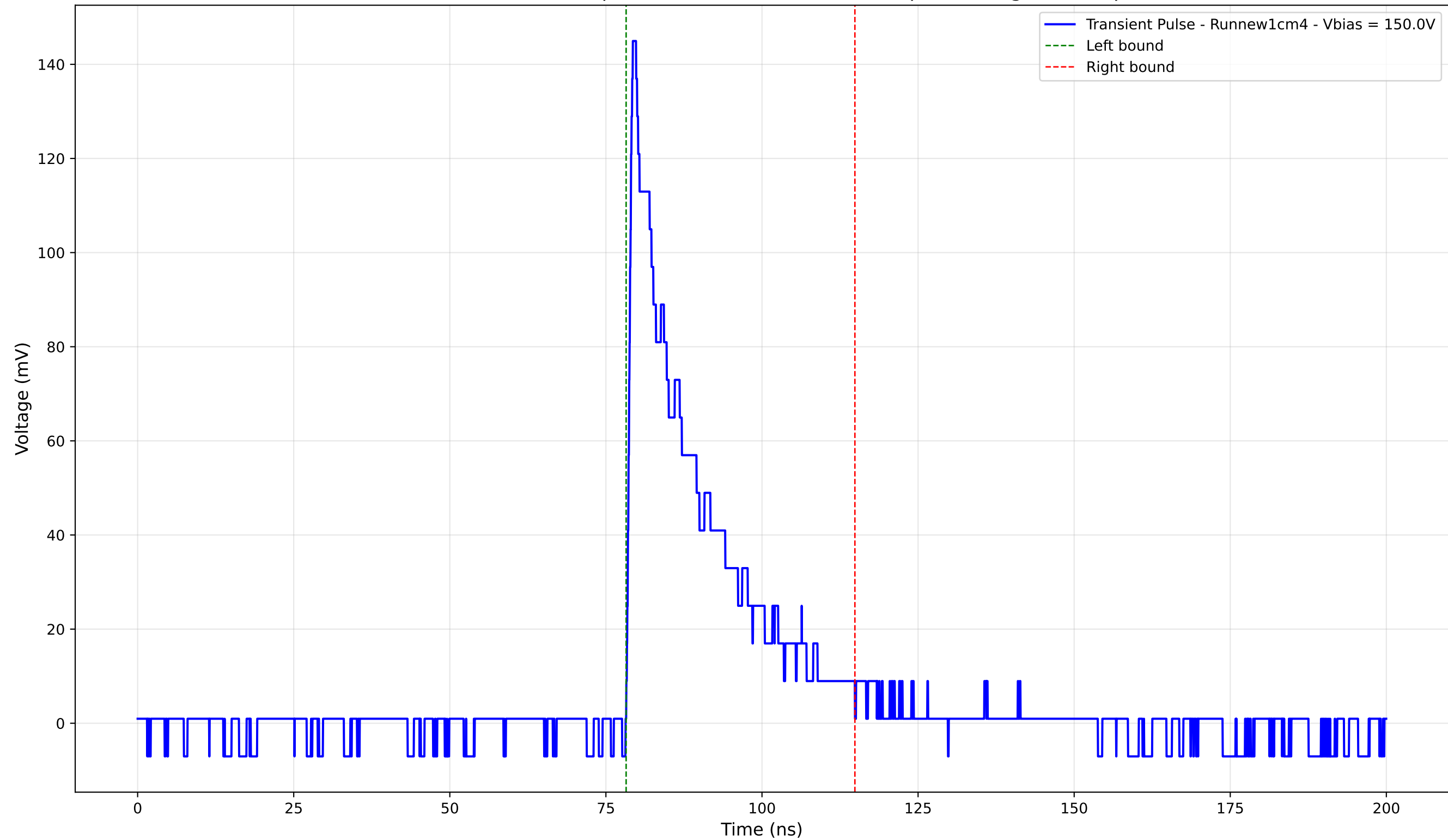
Transient Pulse - Sample: new1cm - Position: 680.0 \mu\text{m} - Charge: 30.46 pC
