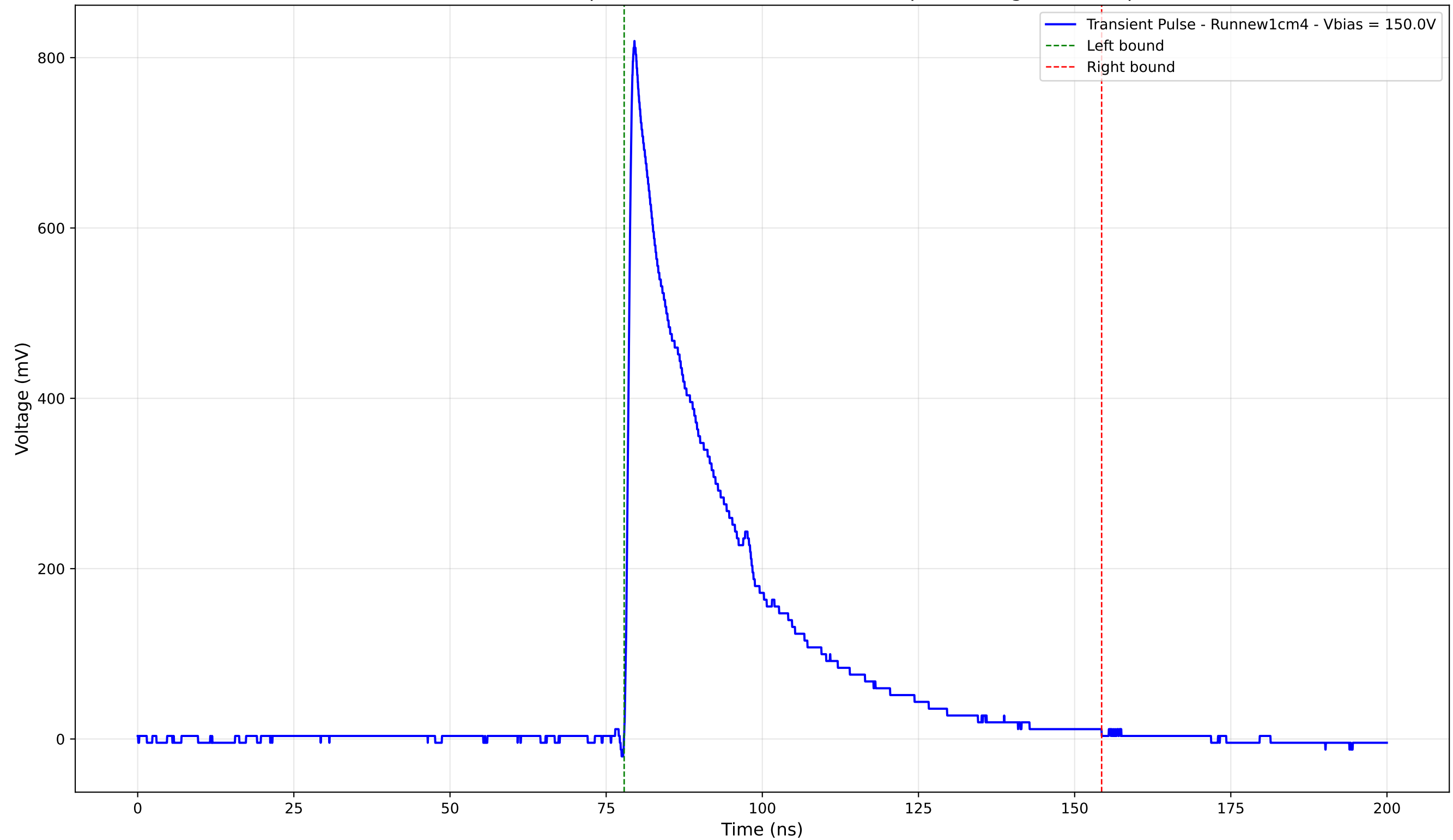
Transient Pulse - Sample: new1cm - Position: 4510.0 \mu\text{m} - Charge: 237.64 pC
