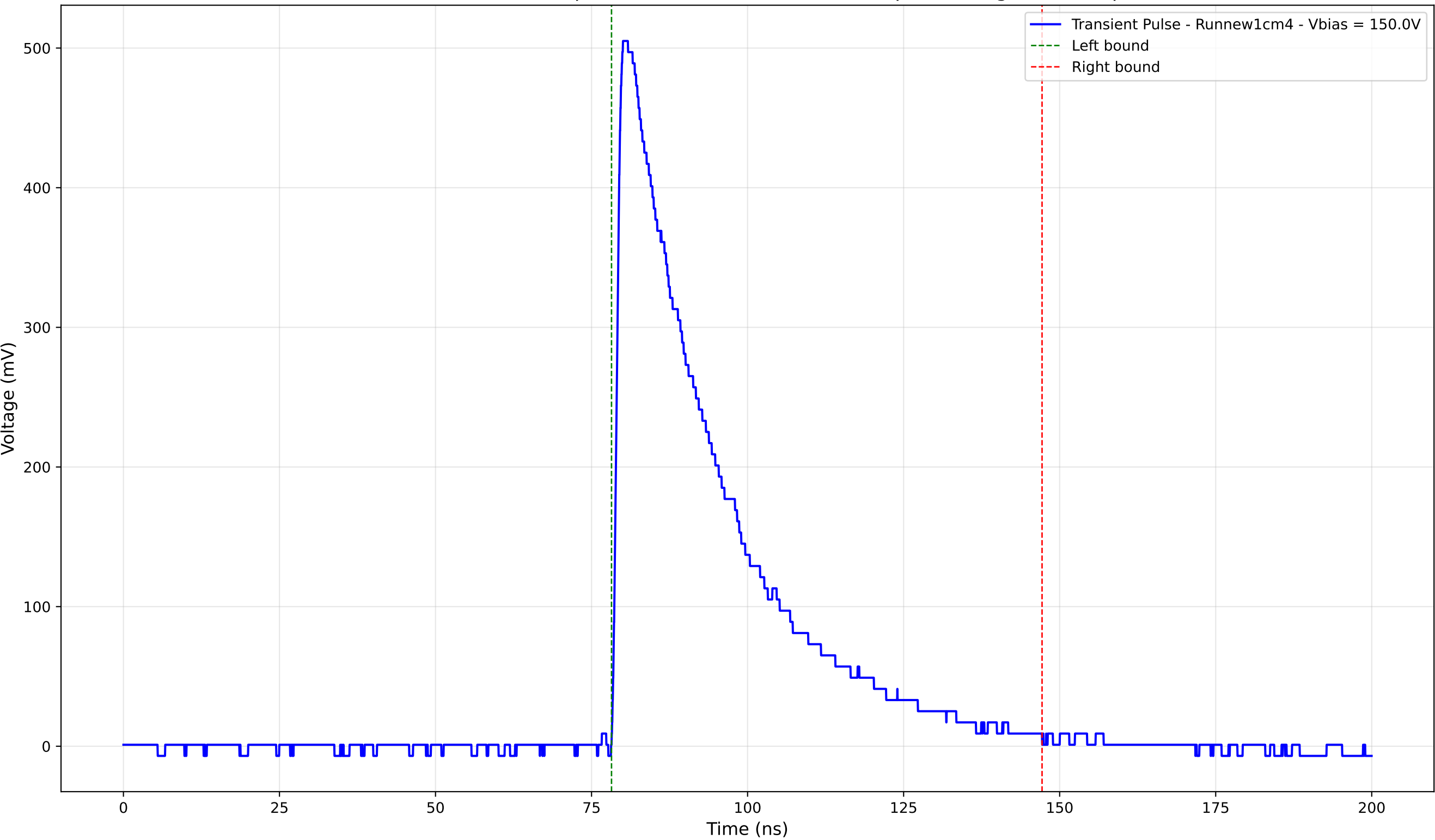
Transient Pulse - Sample: new1cm - Position: 1285.0 \mu\text{m} - Charge: 174.19 pC
