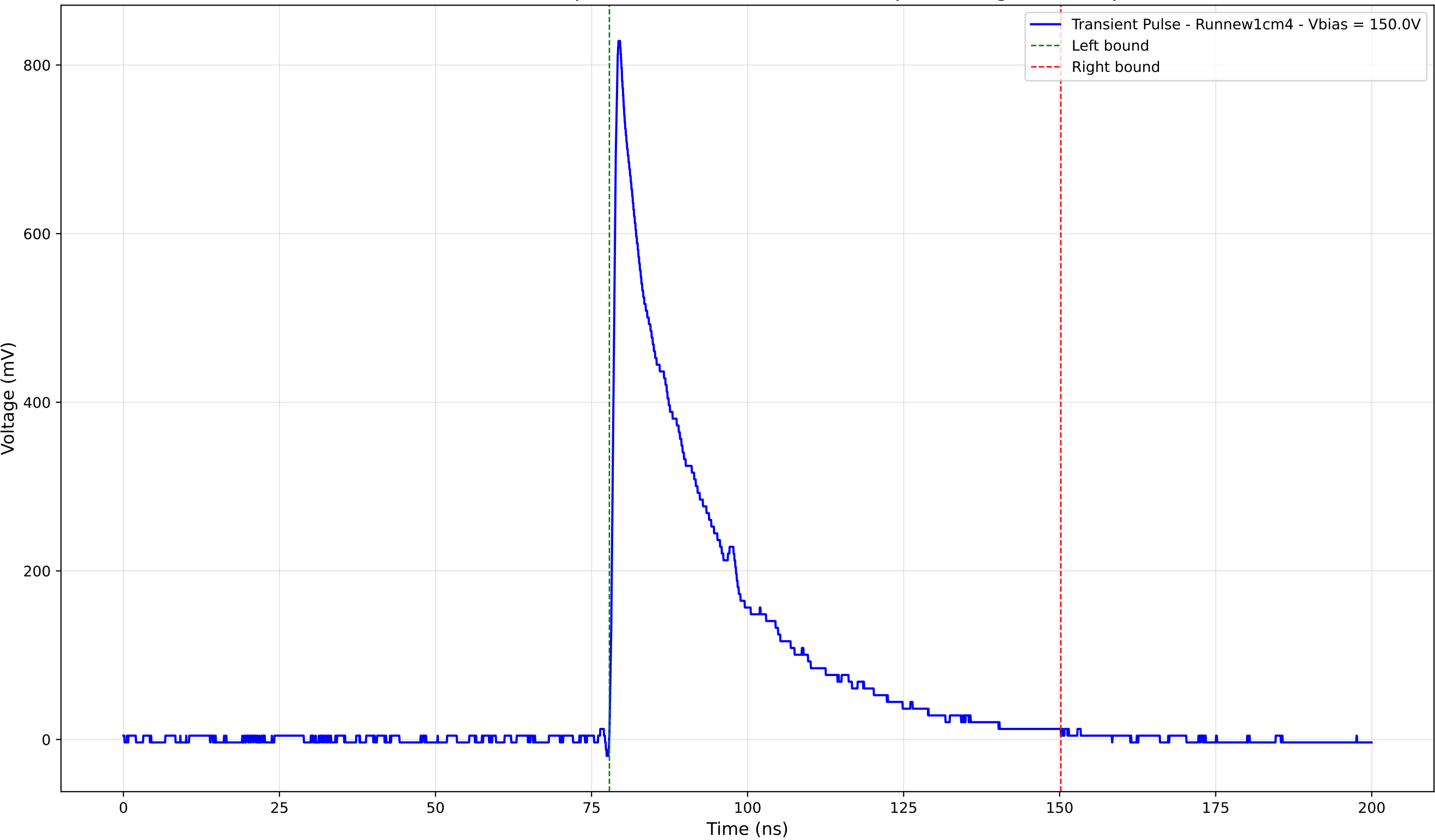
Transient Pulse - Sample: new1cm - Position: 4610.0 \mu\text{m} - Charge: 228.06 pC
