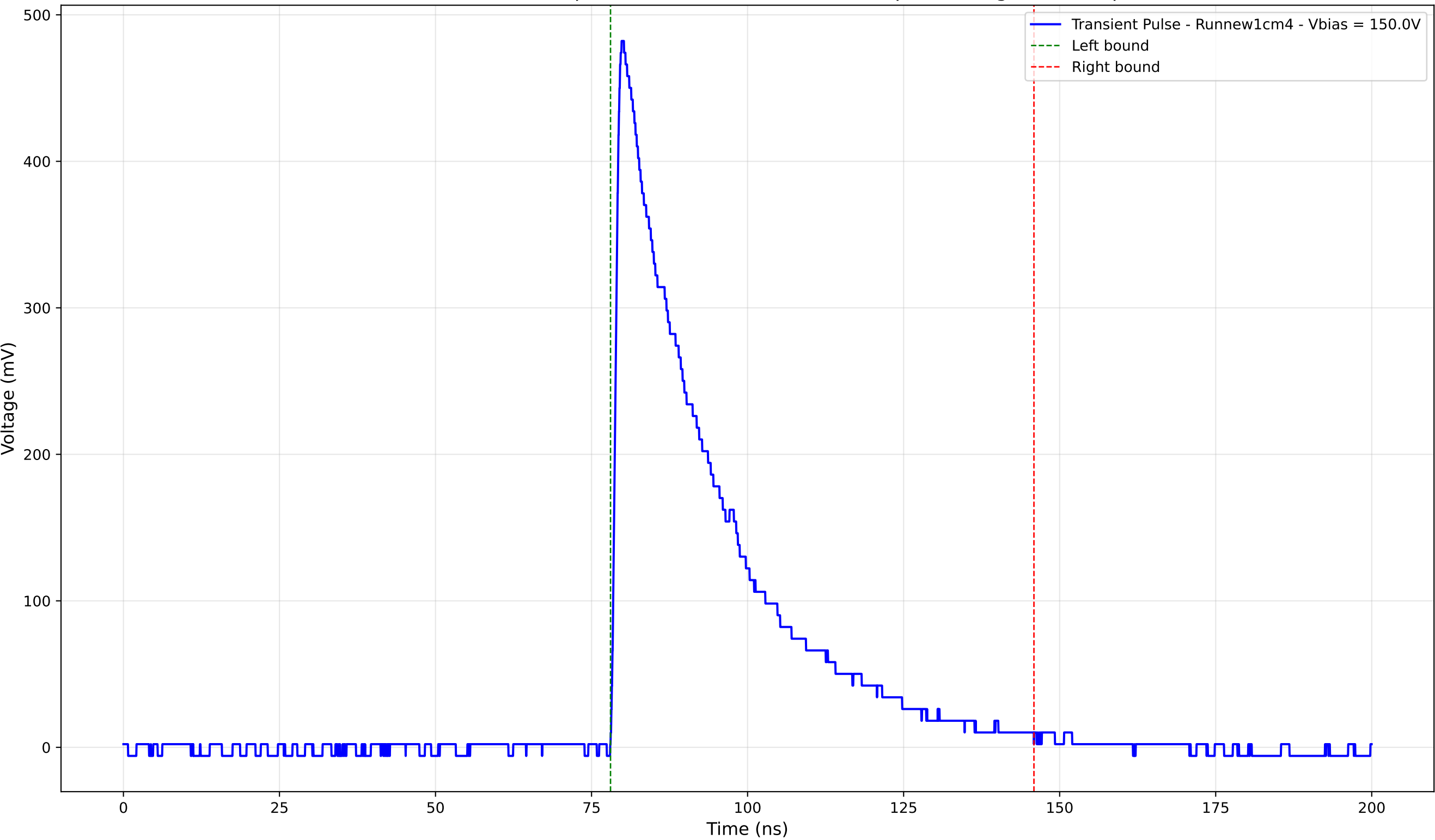
Transient Pulse - Sample: new1cm - Position: 4175.0 \mu\text{m} - Charge: 156.52 pC
