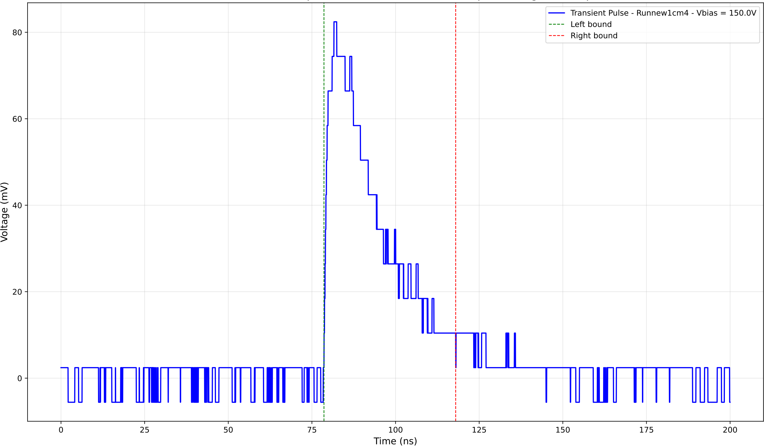
Transient Pulse - Sample: new1cm - Position: 1700.0 \mu\text{m} - Charge: 28.16 pC
