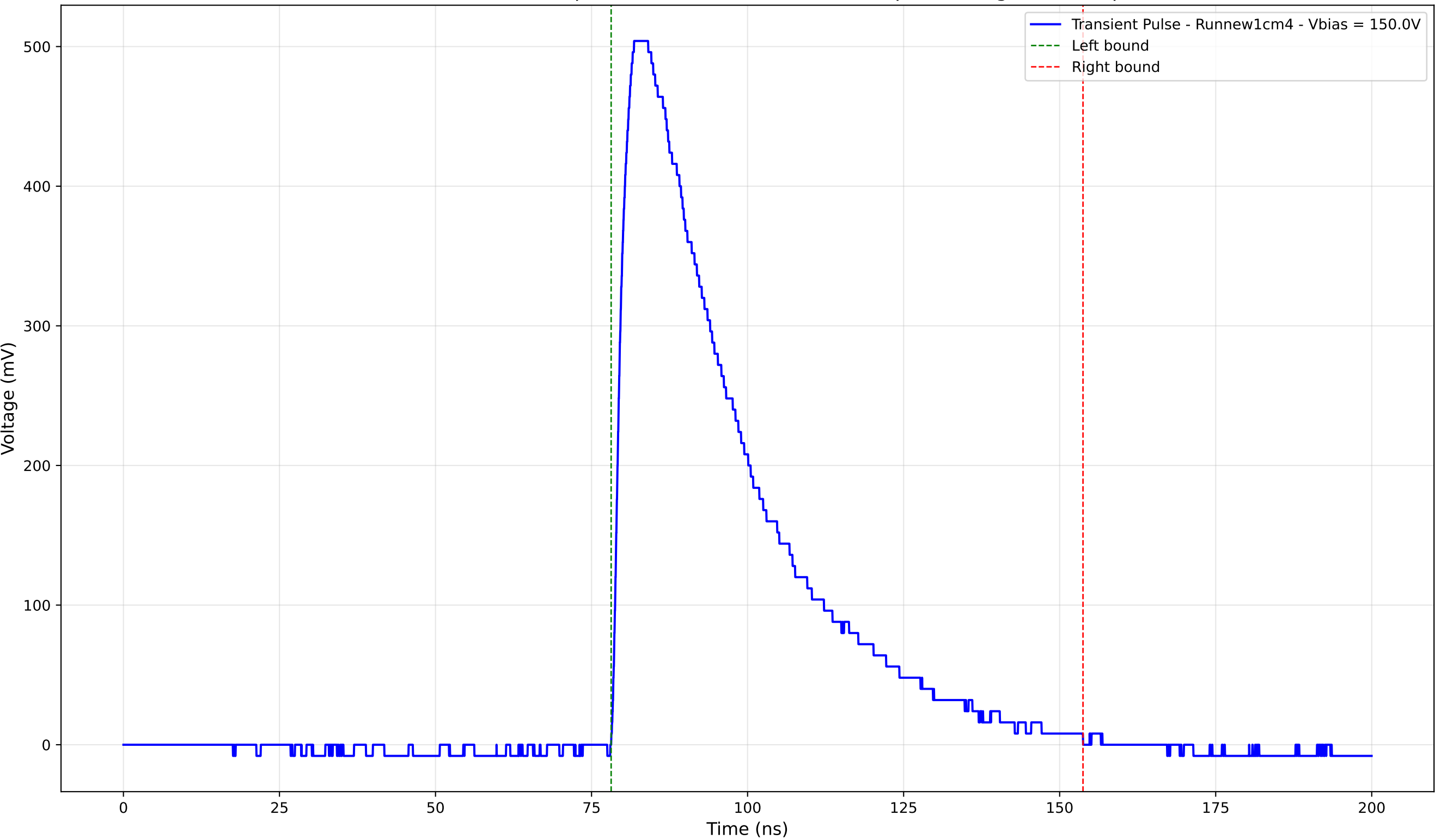
Transient Pulse - Sample: new1cm - Position: 2550.0 \mu\text{m} - Charge: 221.40 pC
