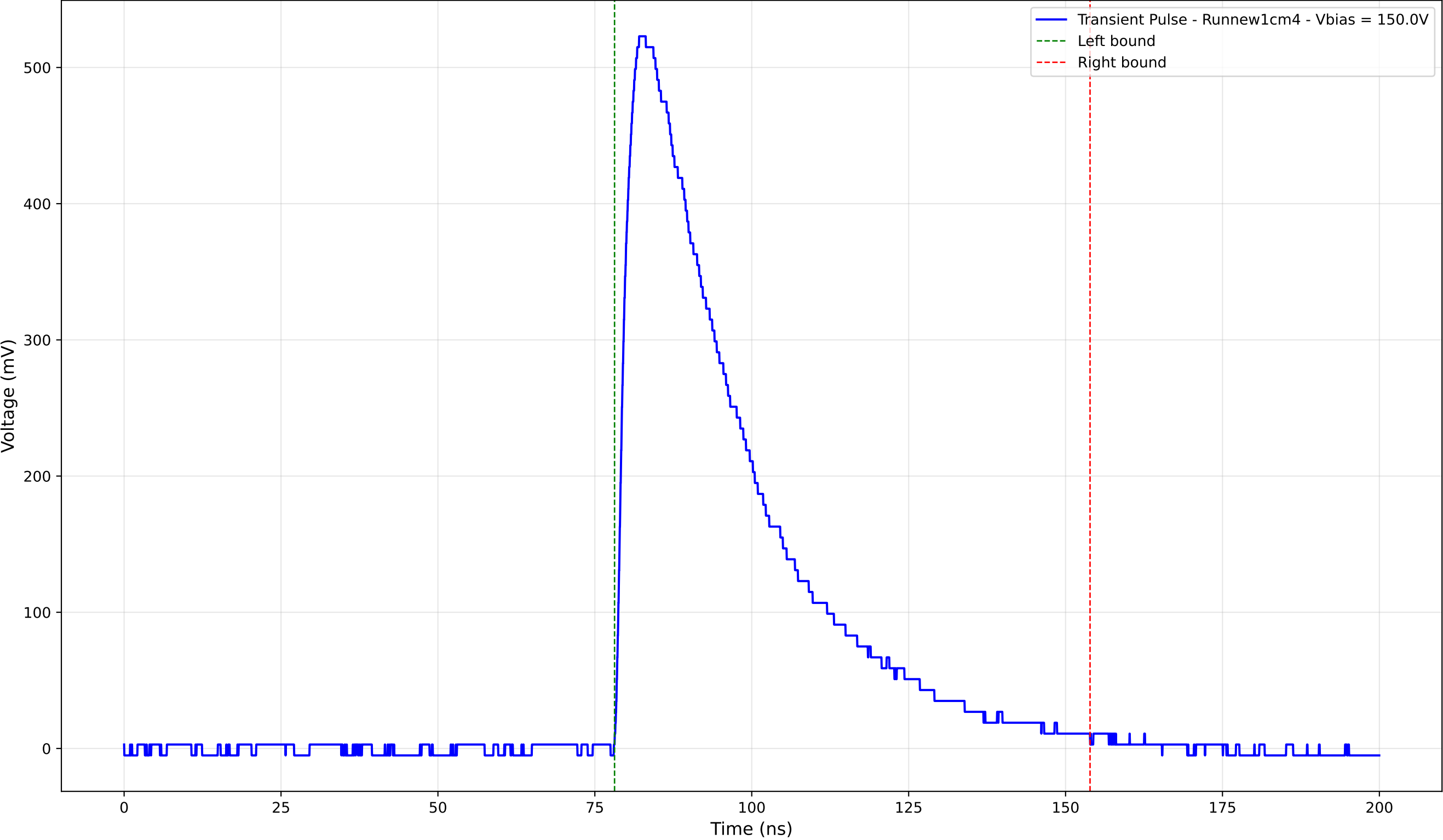
Transient Pulse - Sample: new1cm - Position: 2430.0 \mu\text{m} - Charge: 226.13 pC
