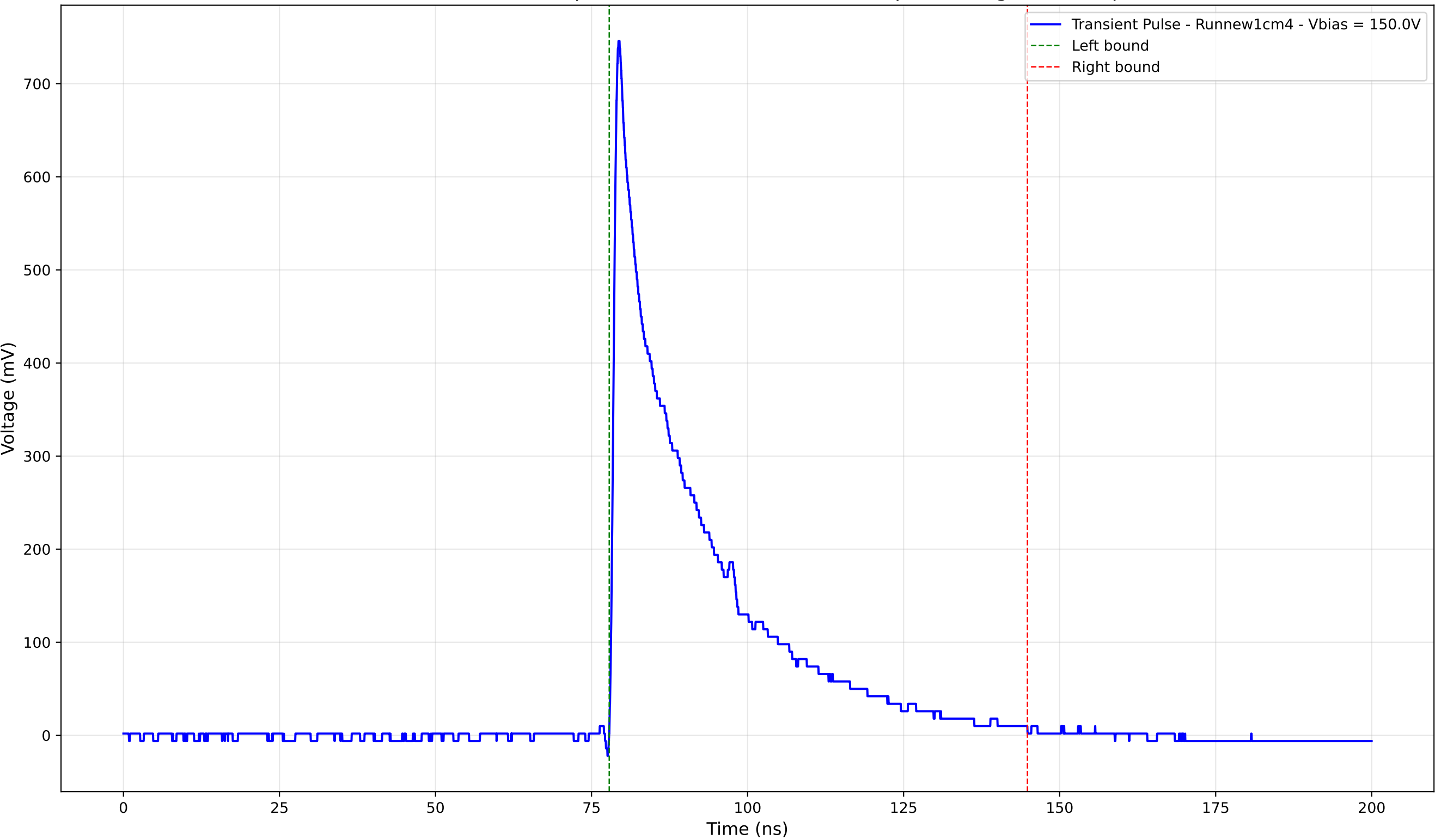
Transient Pulse - Sample: new1cm - Position: 4655.0 \mu\text{m} - Charge: 185.58 pC
