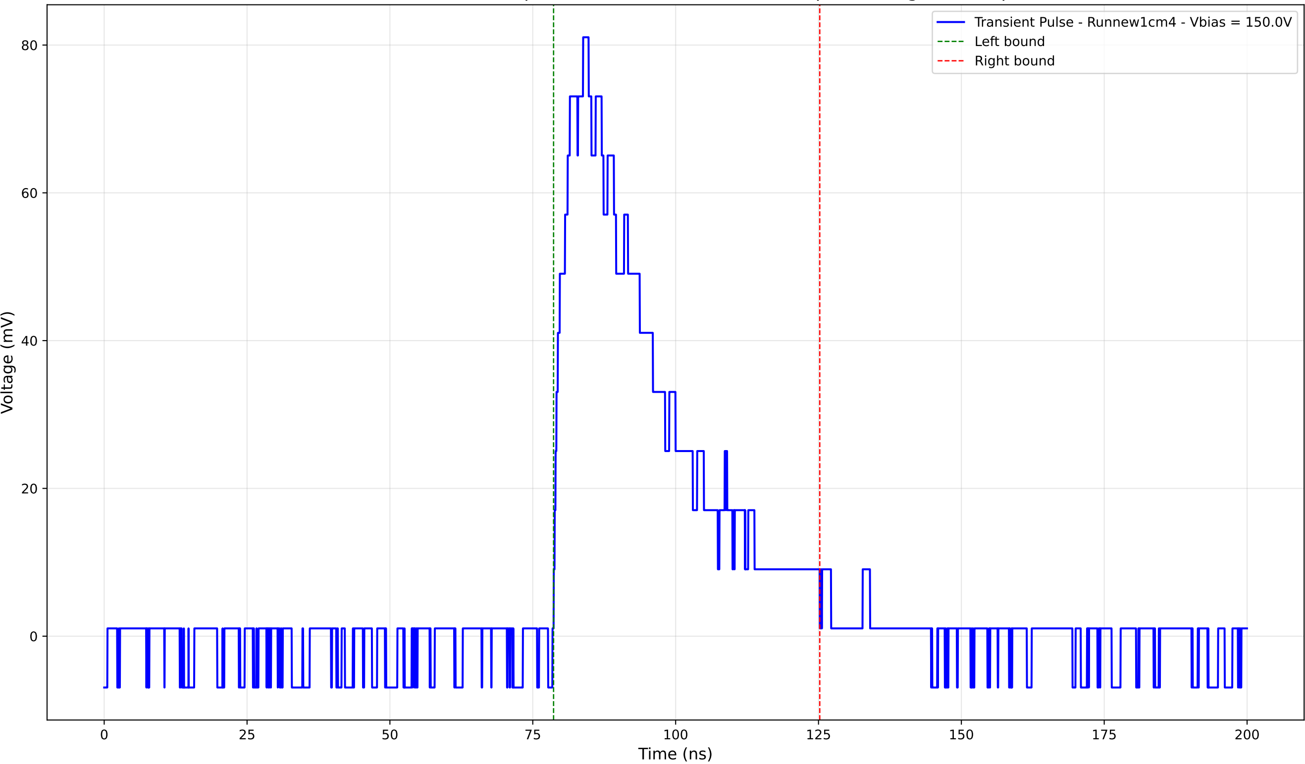
Transient Pulse - Sample: new1cm - Position: 2205.0 \mu\text{m} - Charge: 29.72 pC
