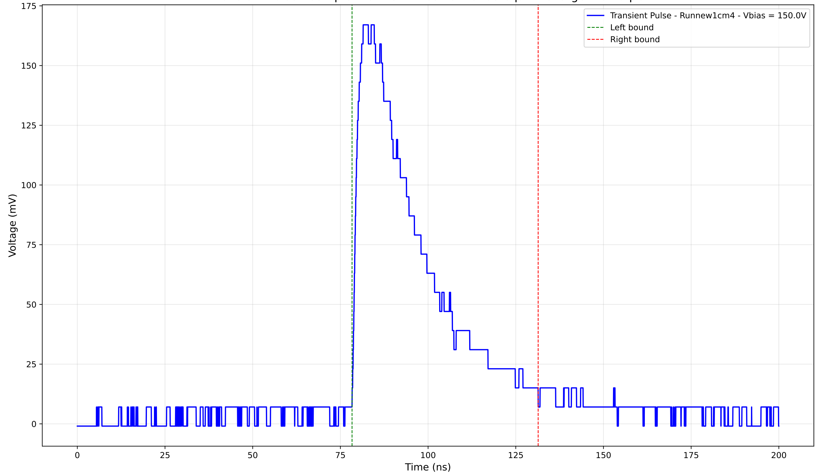
Transient Pulse - Sample: new1cm - Position: 3195.0 \mu\text{m} - Charge: 70.79 pC
