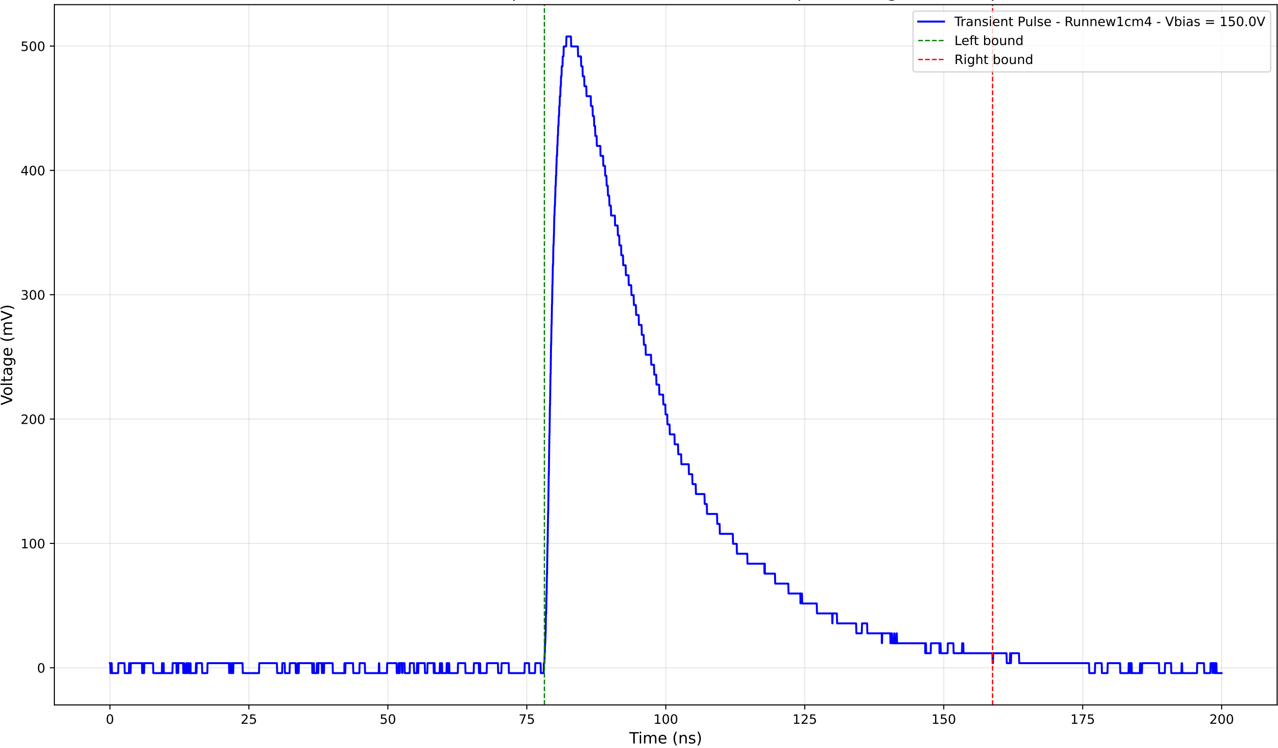
Transient Pulse - Sample: new1cm - Position: 2885.0 \mu\text{m} - Charge: 226.63 pC
