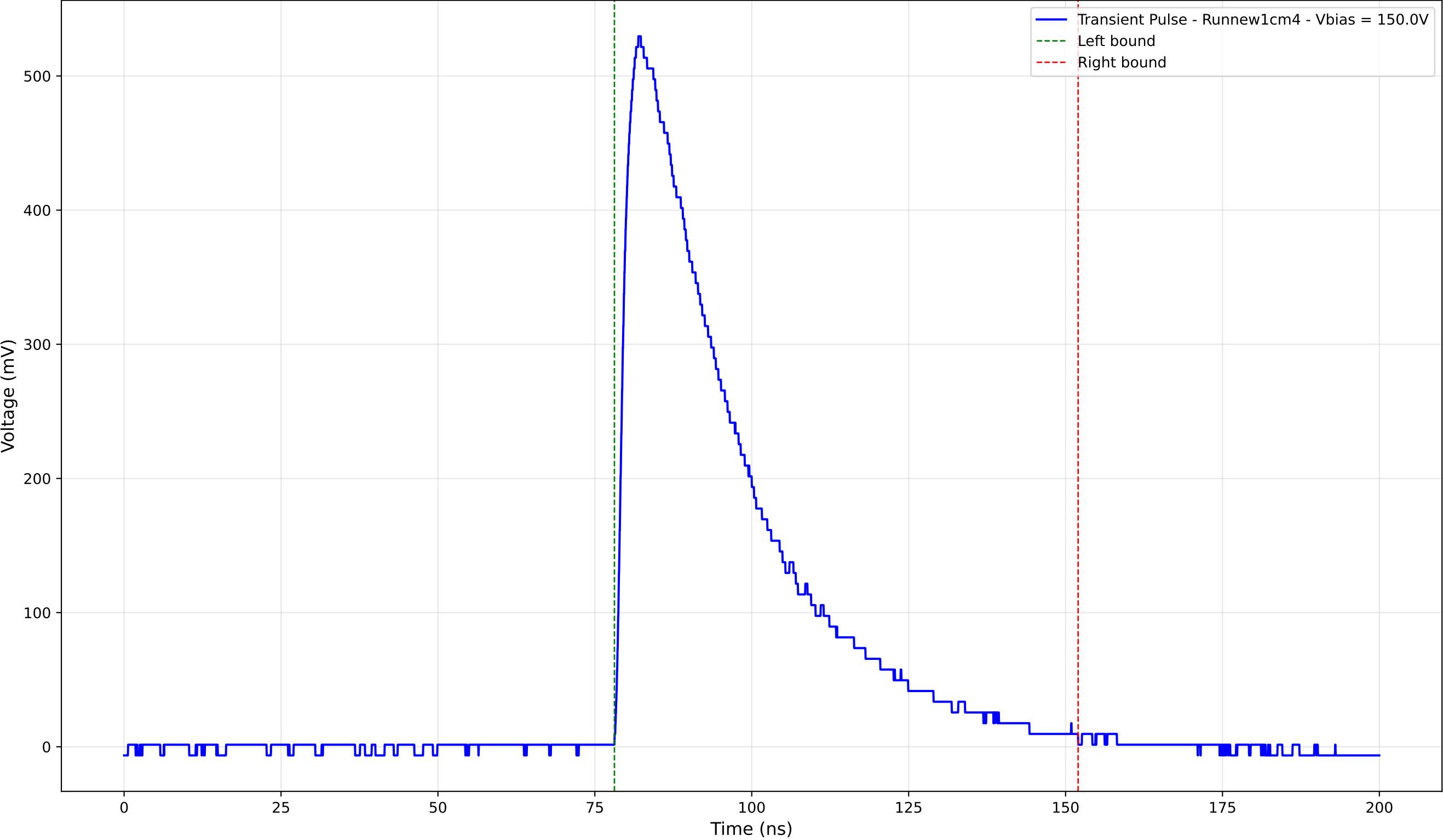
Transient Pulse - Sample: new1cm - Position: 2075.0 \mu\text{m} - Charge: 218.09 pC
