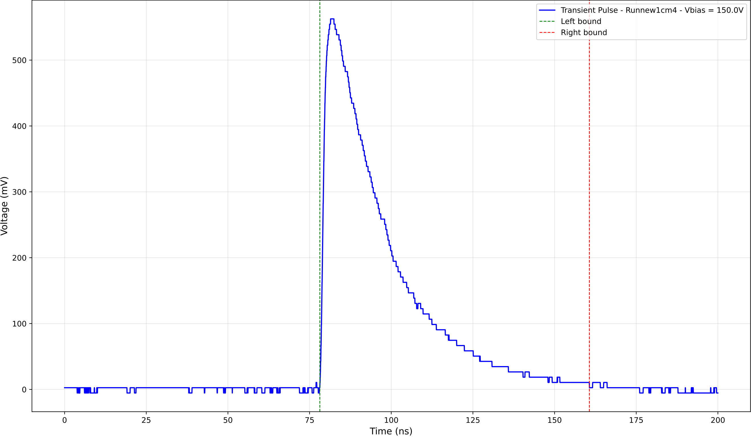
Transient Pulse - Sample: new1cm - Position: 3435.0 \mu\text{m} - Charge: 241.30 pC
