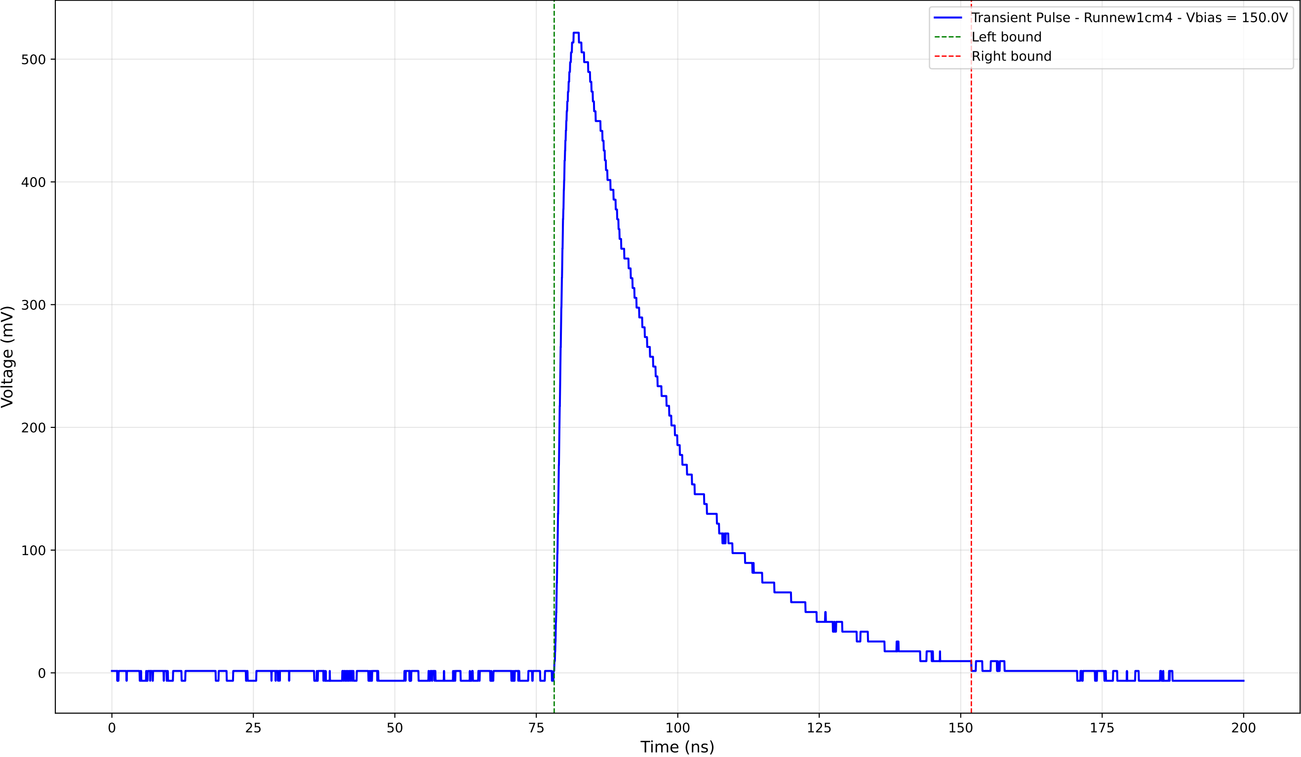
Transient Pulse - Sample: new1cm - Position: 1915.0 \mu\text{m} - Charge: 212.02 pC
