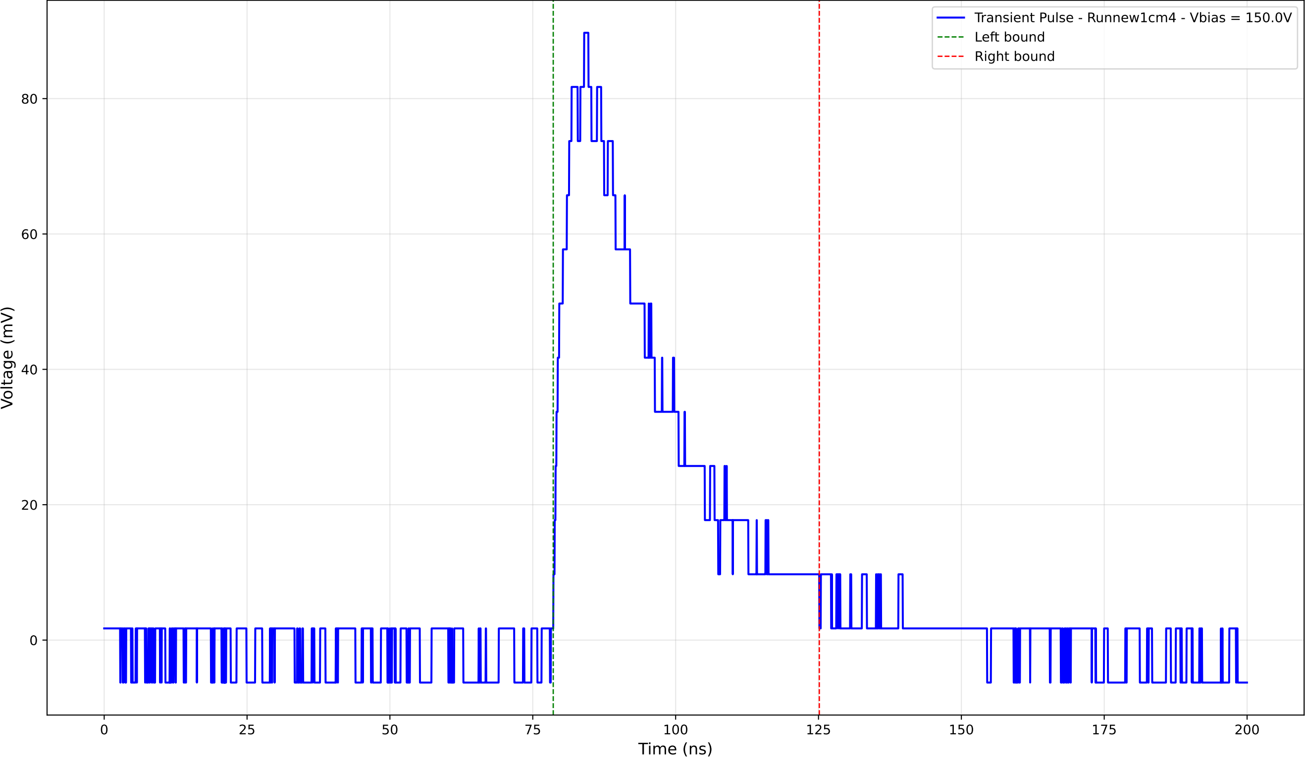
Transient Pulse - Sample: new1cm - Position: 2725.0 \mu\text{m} - Charge: 32.55 pC
