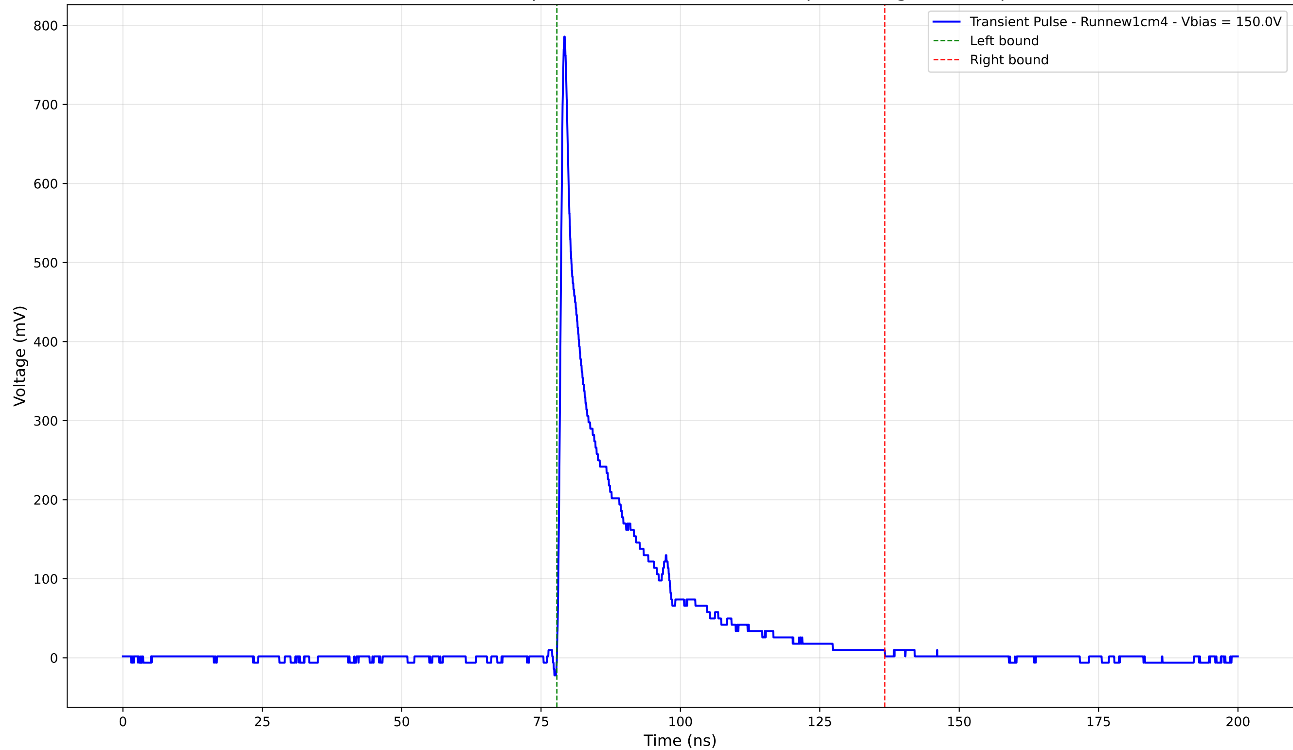
Transient Pulse - Sample: new1cm - Position: 260.0 \mu\text{m} - Charge: 128.38 pC
