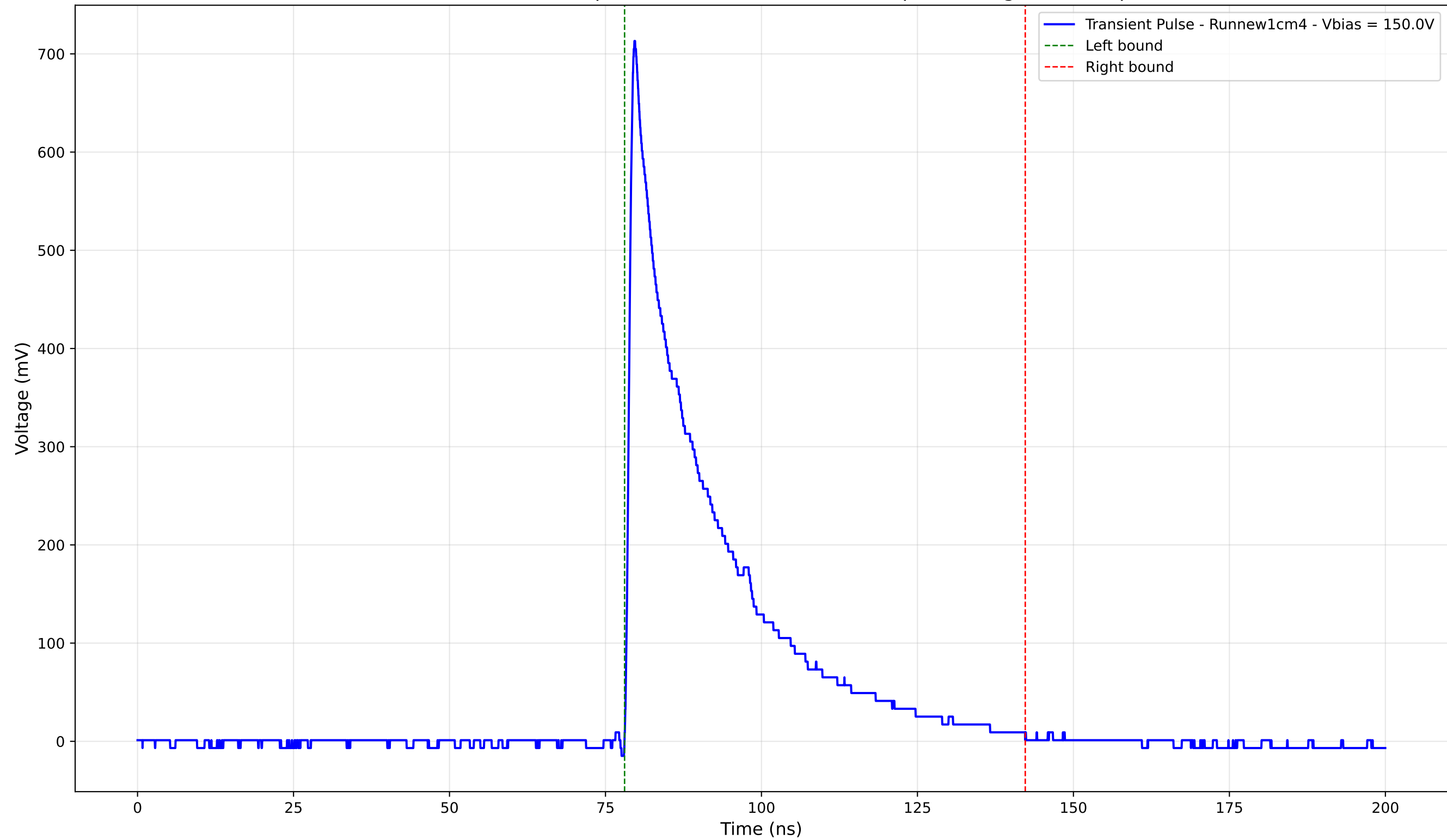
Transient Pulse - Sample: new1cm - Position: 790.0 \mu\text{m} - Charge: 180.31 pC
