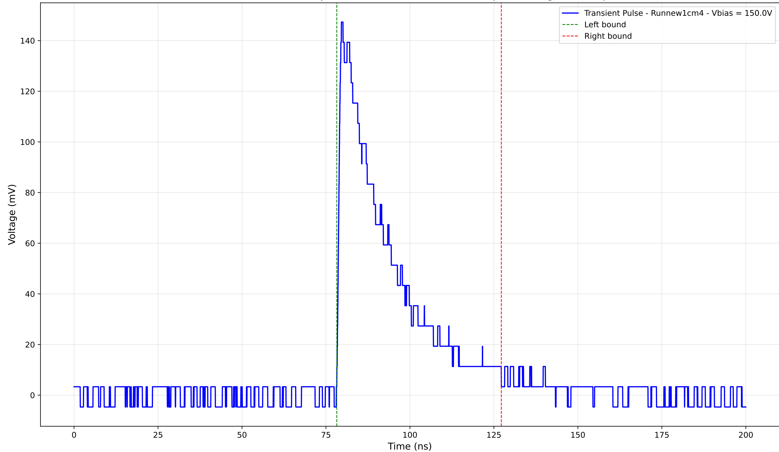
Transient Pulse - Sample: new1cm - Position: 4250.0 \mu\text{m} - Charge: 45.56 pC
