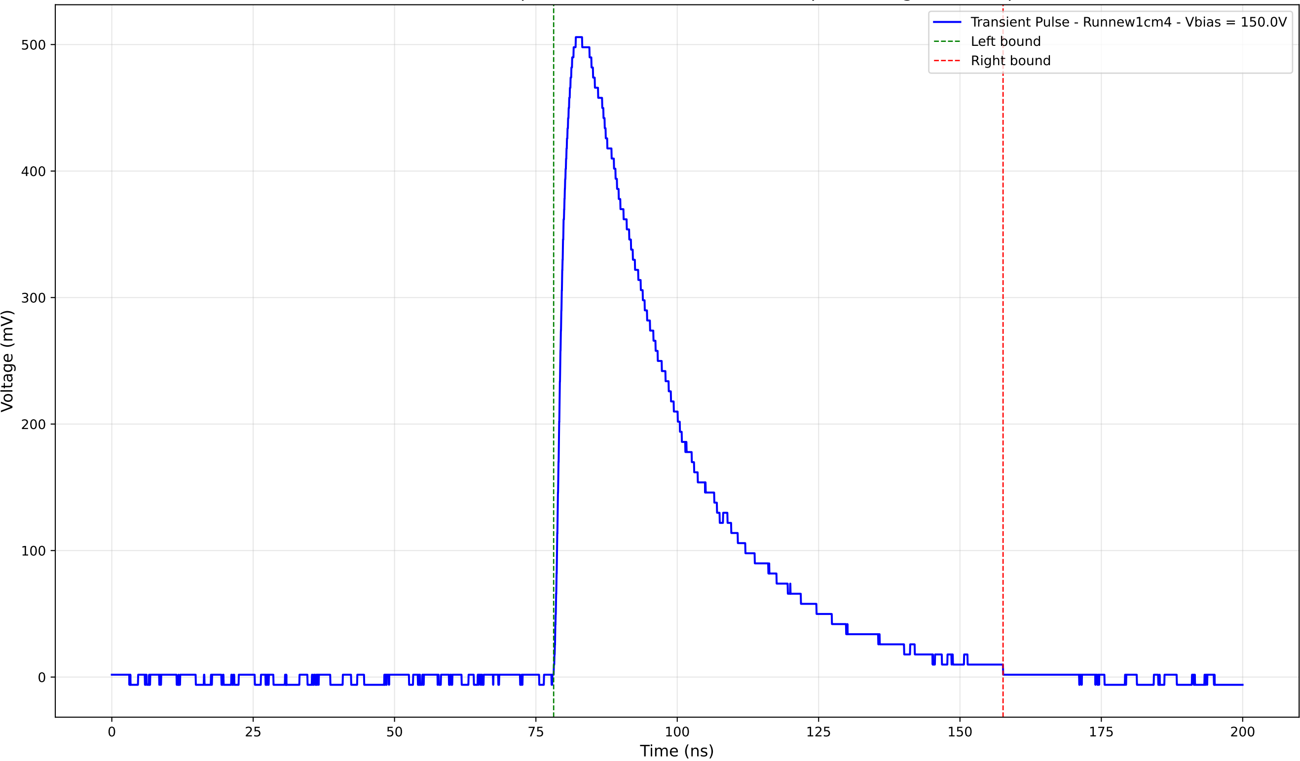
Transient Pulse - Sample: new1cm - Position: 2900.0 \mu\text{m} - Charge: 224.94 pC
