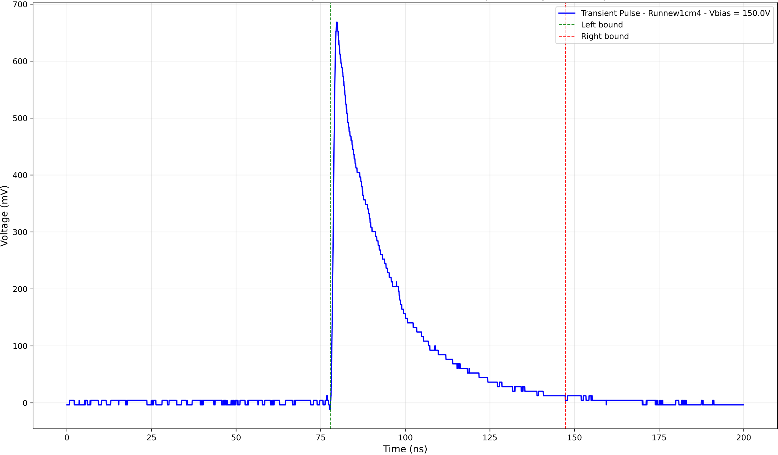
Transient Pulse - Sample: new1cm - Position: 4315.0 \mu\text{m} - Charge: 204.73 pC
