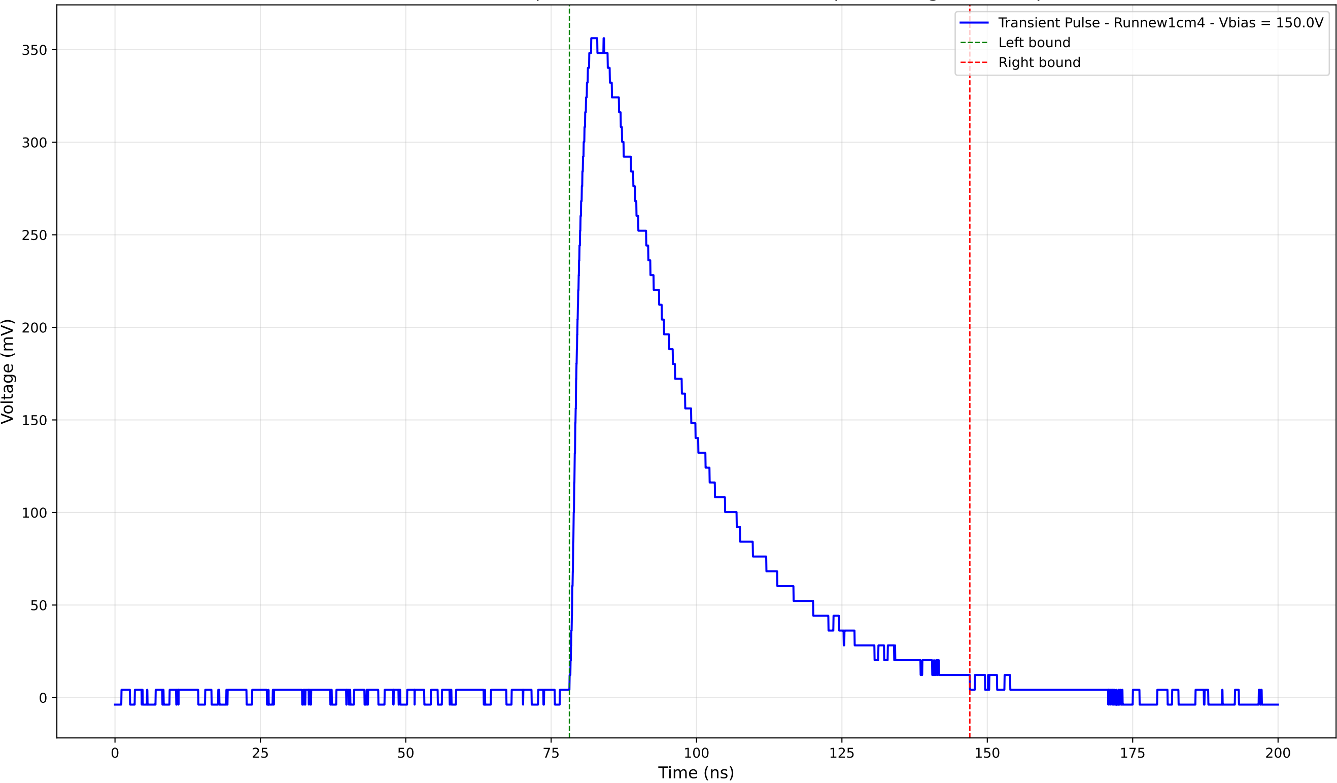
Transient Pulse - Sample: new1cm - Position: 2780.0 \mu\text{m} - Charge: 155.14 pC
