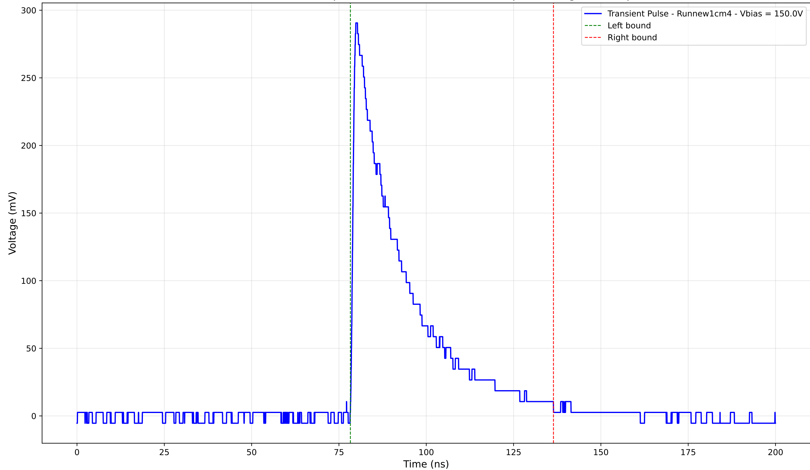
Transient Pulse - Sample: new1cm - Position: 1155.0 \mu\text{m} - Charge: 86.87 pC
