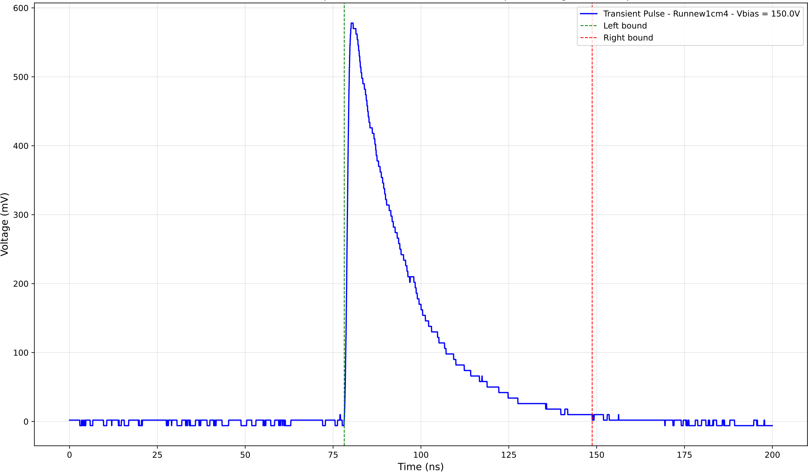
Transient Pulse - Sample: new1cm - Position: 1325.0 \mu\text{m} - Charge: 202.23 pC
