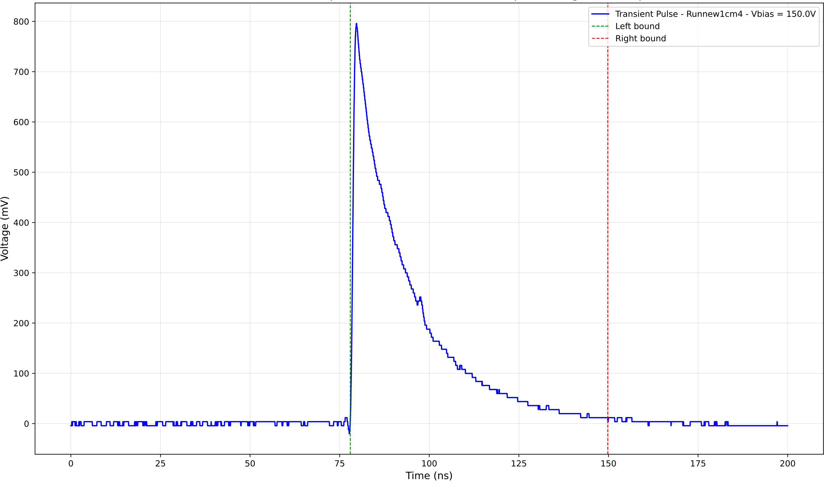
Transient Pulse - Sample: new1cm - Position: 4385.0 \mu\text{m} - Charge: 243.69 pC
