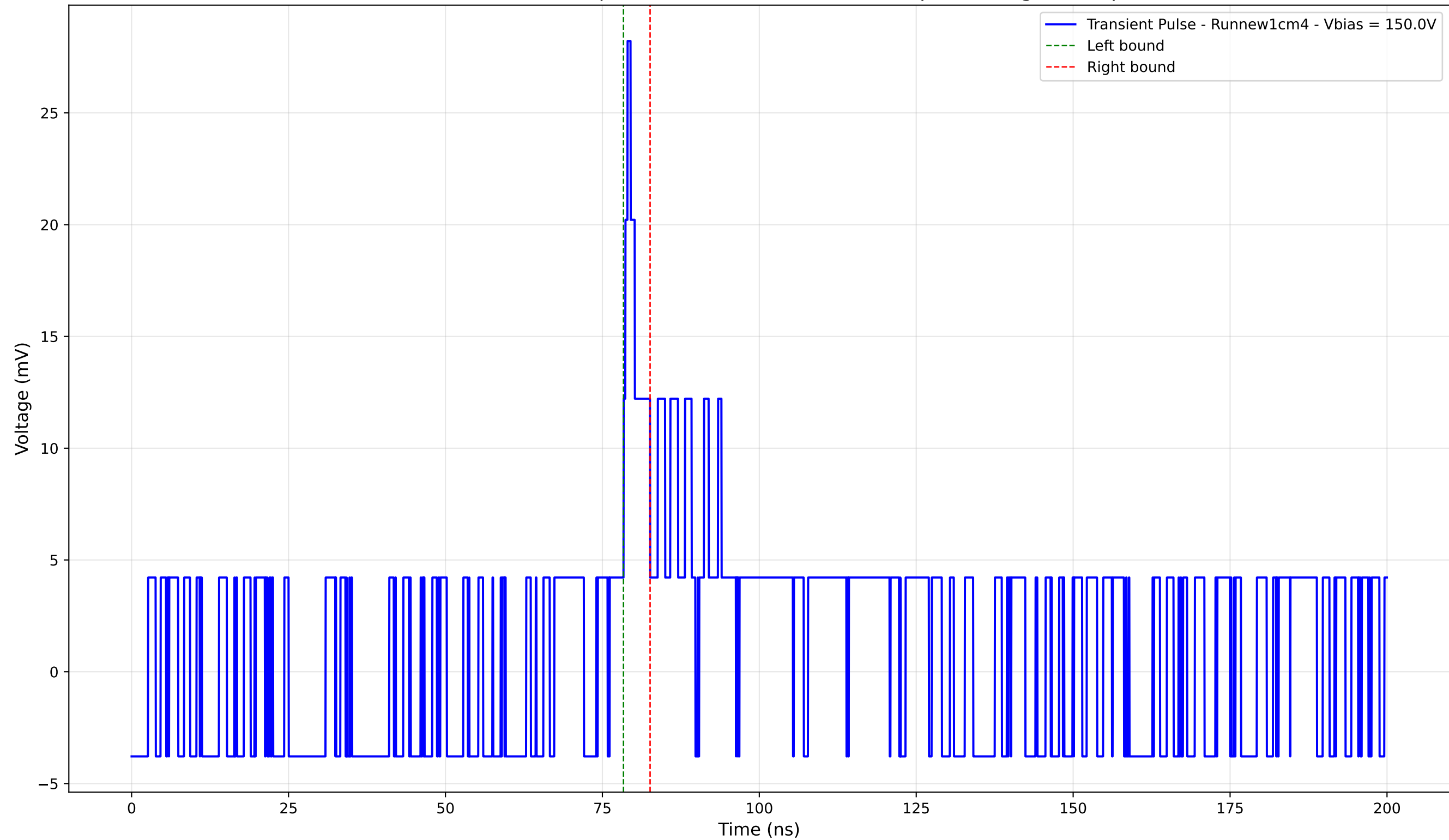
Transient Pulse - Sample: new1cm - Position: 5100.0 \mu\text{m} - Charge: 1.35 pC
