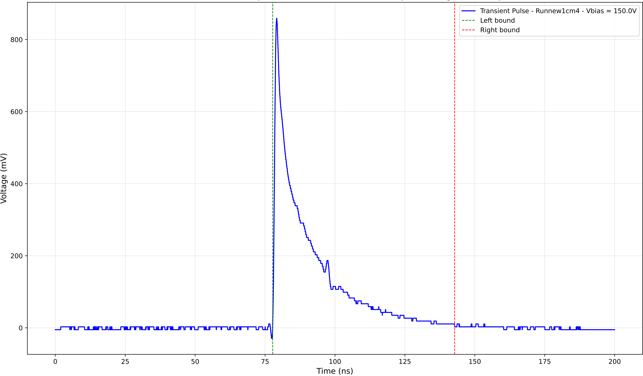
Transient Pulse - Sample: new1cm - Position: 4935.0 \mu\text{m} - Charge: 180.12 pC
