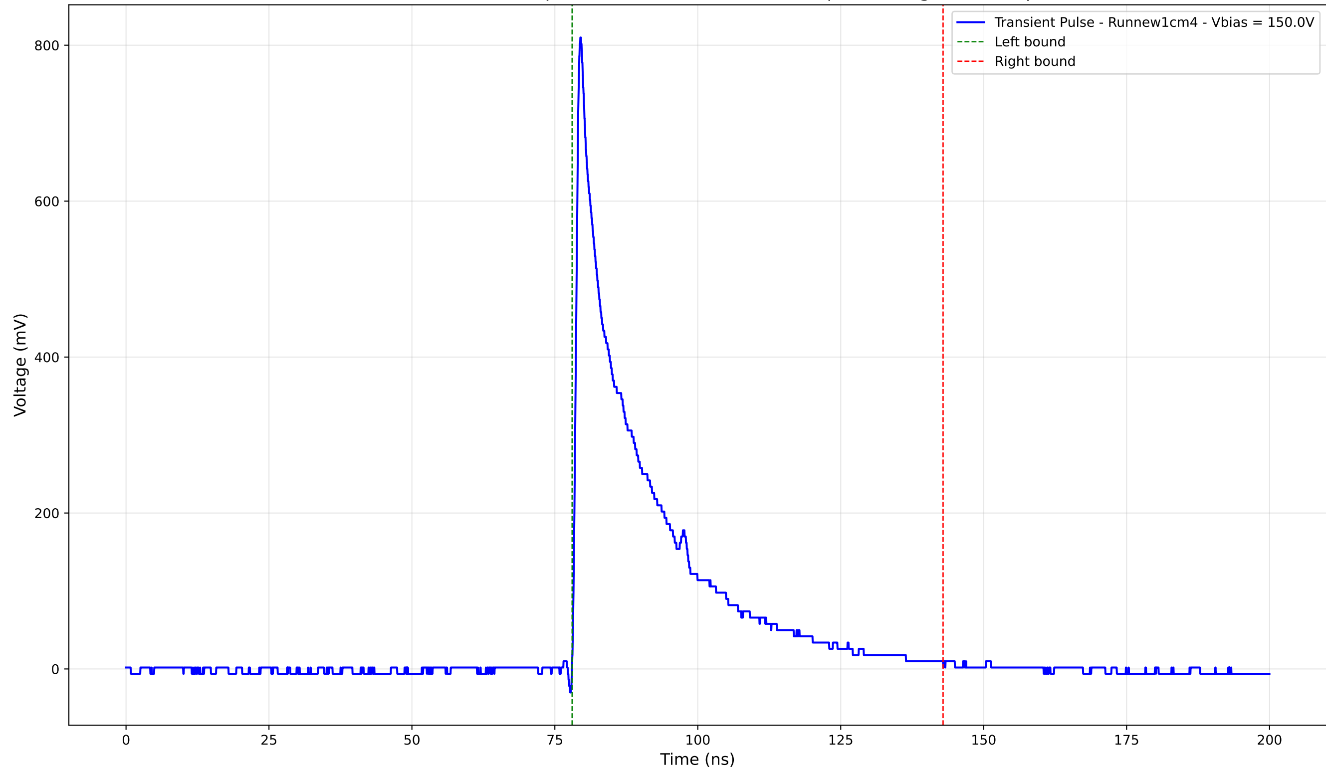
Transient Pulse - Sample: new1cm - Position: 600.0 \mu\text{m} - Charge: 179.81 pC
