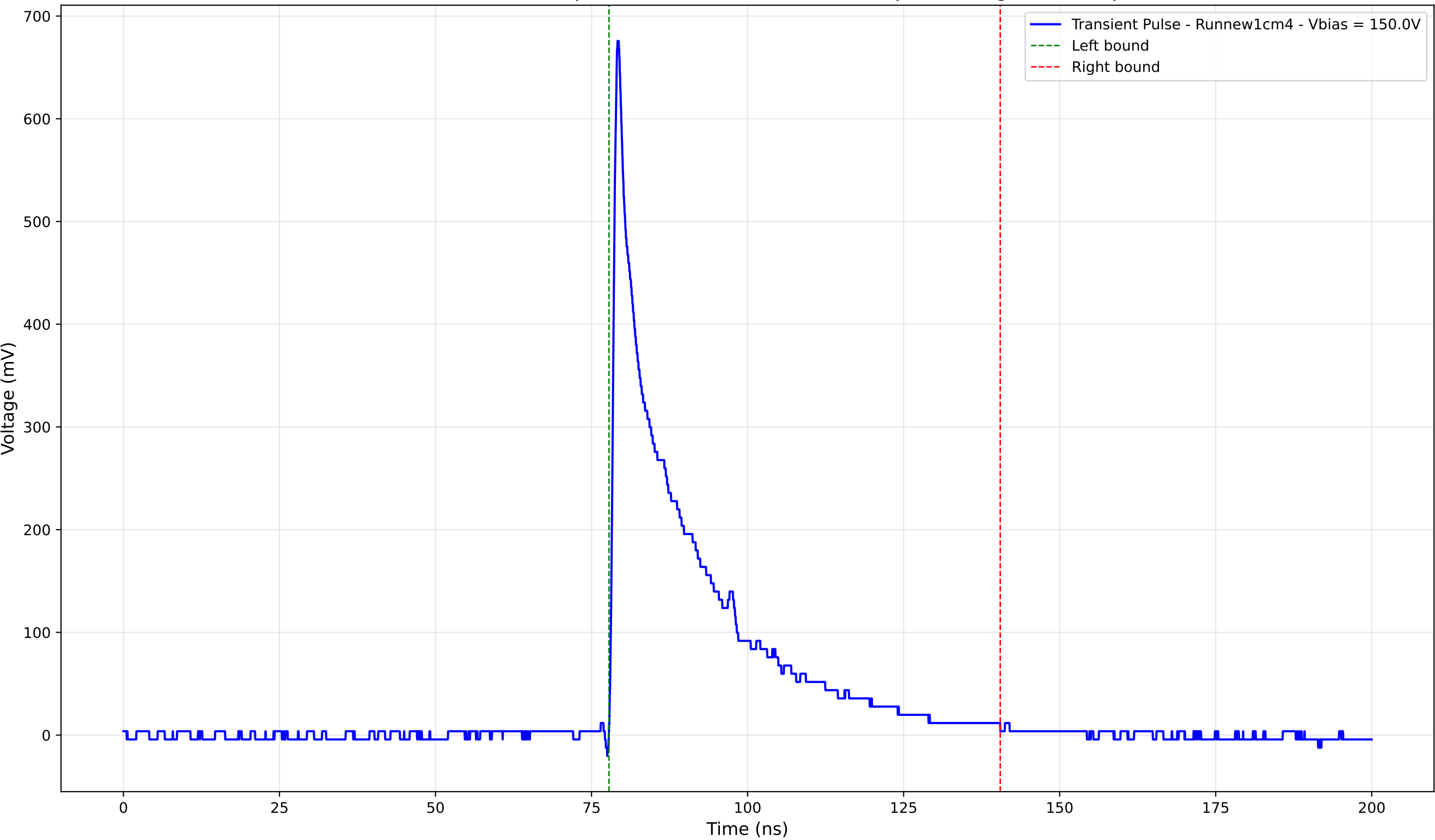
Transient Pulse - Sample: new1cm - Position: 4800.0 \mu\text{m} - Charge: 140.54 pC
