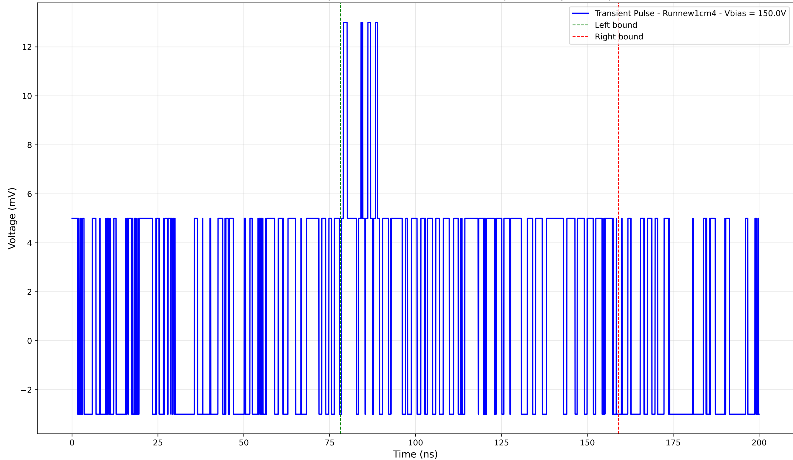
Transient Pulse - Sample: new1cm - Position: 5180.0 \mu\text{m} - Charge: 4.98 pC
