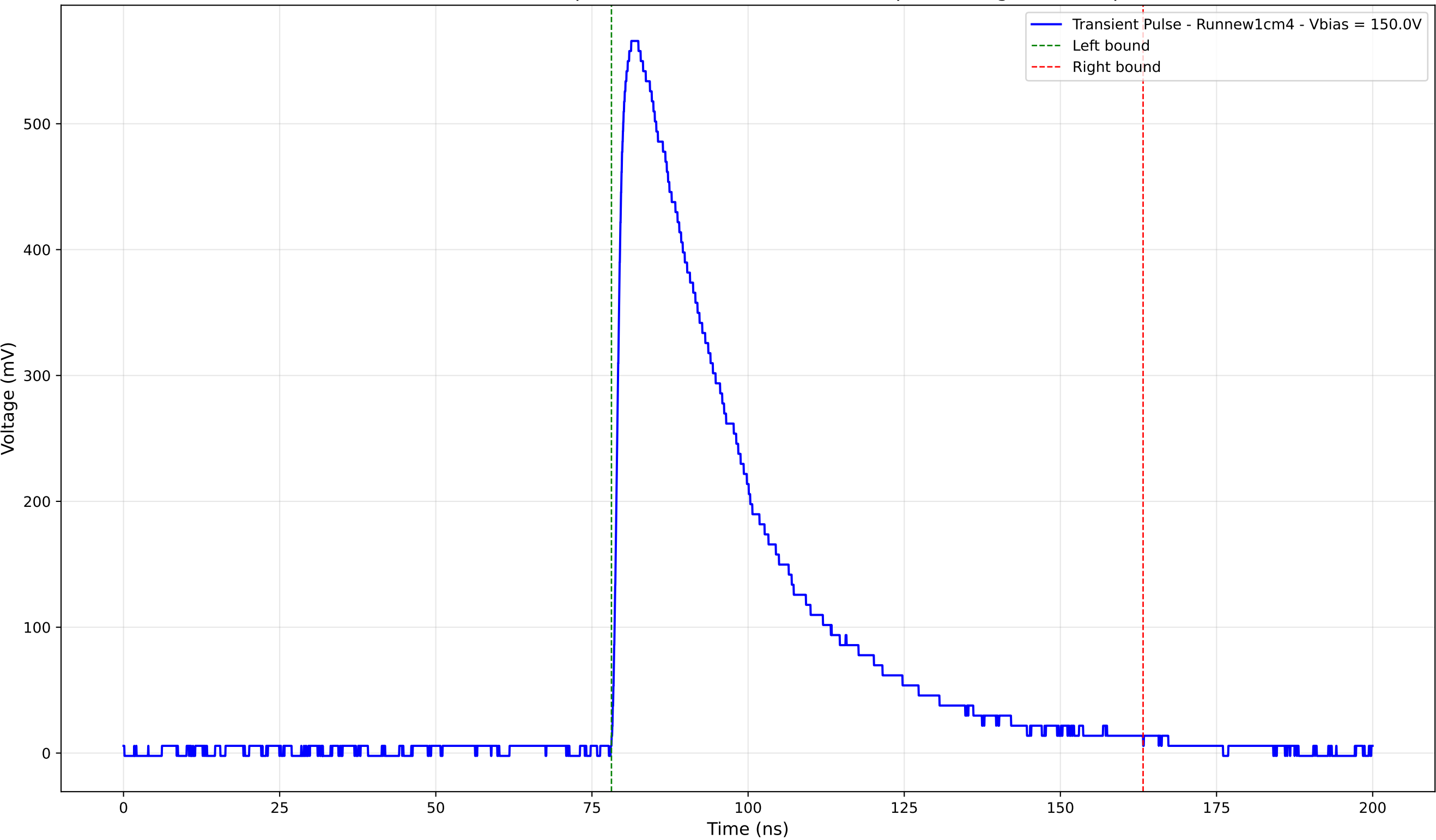
Transient Pulse - Sample: new1cm - Position: 3505.0 \mu\text{m} - Charge: 245.09 pC
