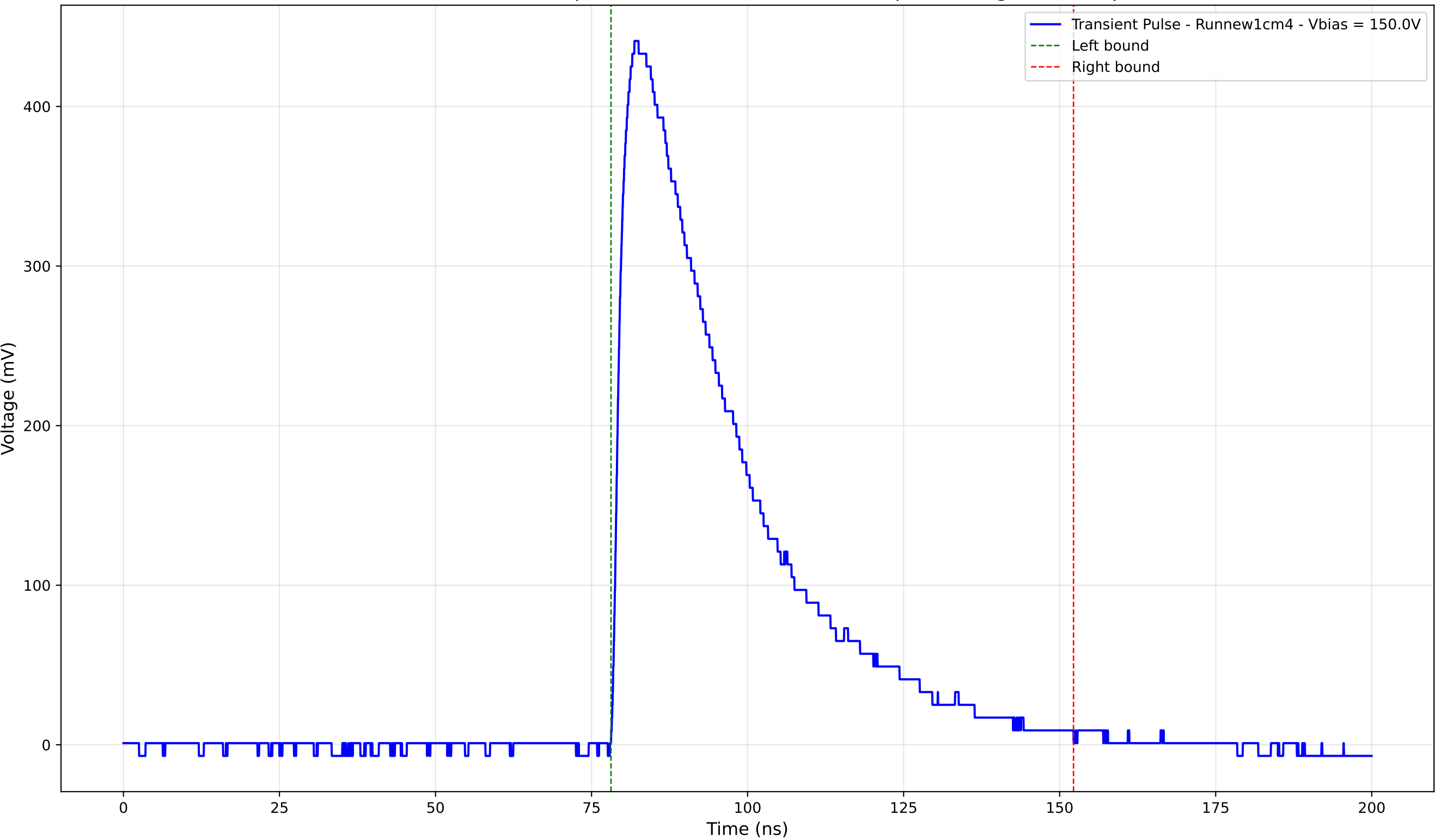
Transient Pulse - Sample: new1cm - Position: 3150.0 \mu\text{m} - Charge: 187.24 pC
