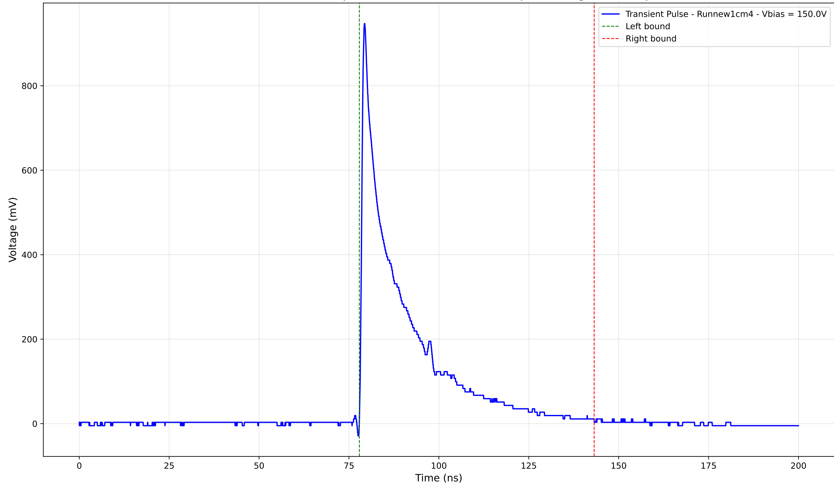
Transient Pulse - Sample: new1cm - Position: 405.0 \mu\text{m} - Charge: 199.73 pC
