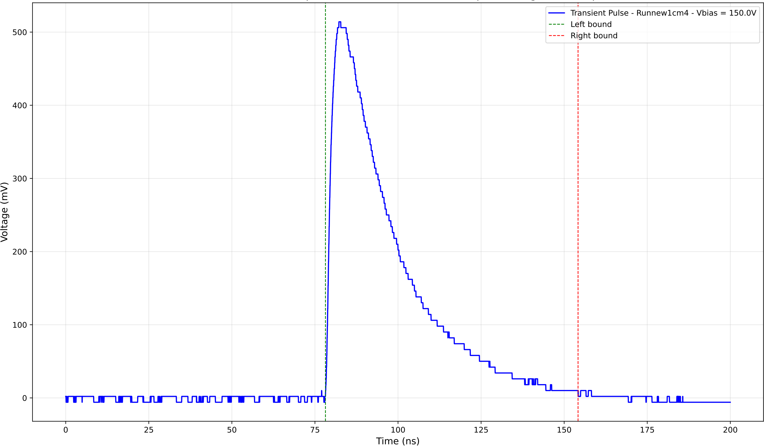
Transient Pulse - Sample: new1cm - Position: 2510.0 \mu\text{m} - Charge: 223.63 pC
