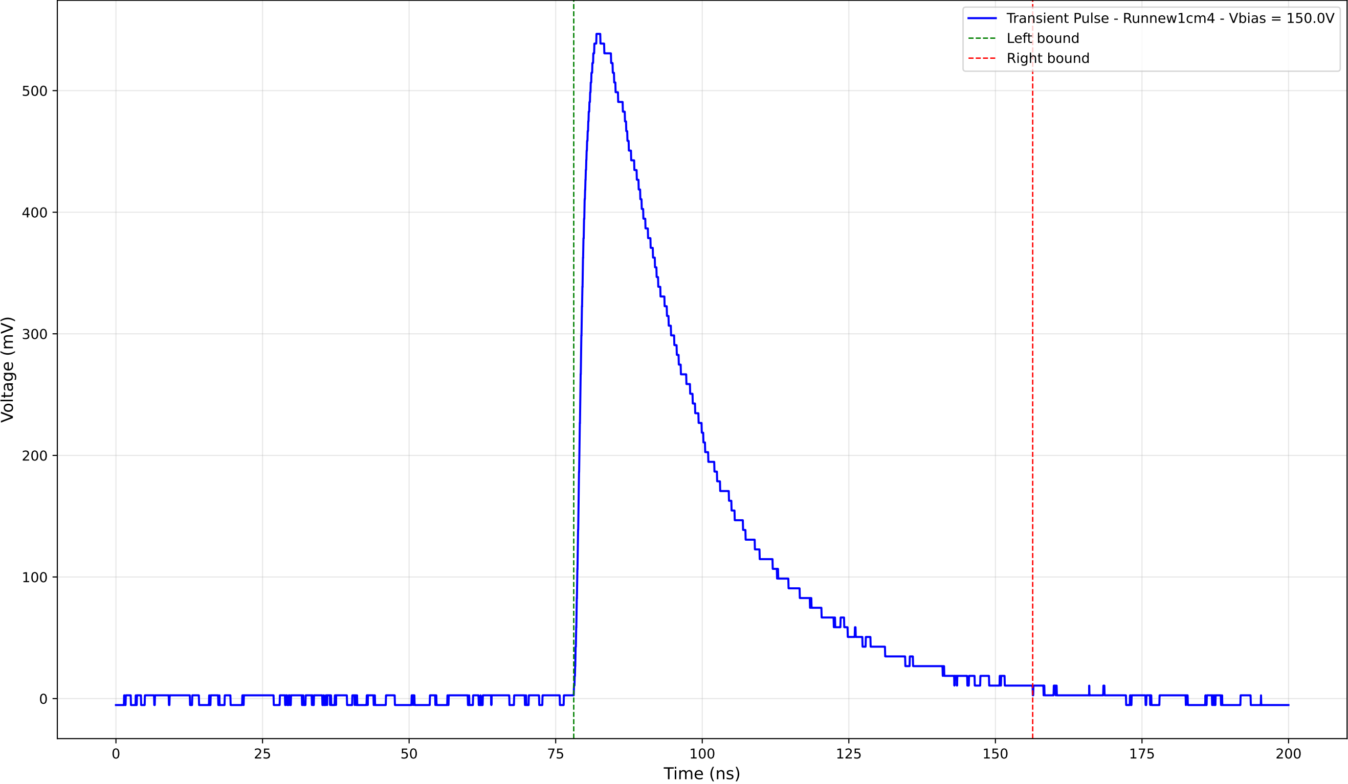
Transient Pulse - Sample: new1cm - Position: 3095.0 \mu\text{m} - Charge: 239.29 pC
