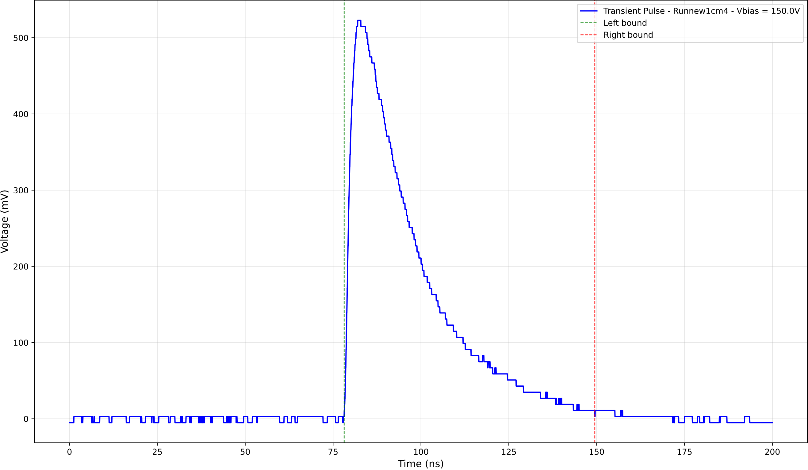
Transient Pulse - Sample: new1cm - Position: 2405.0 \mu\text{m} - Charge: 224.54 pC
