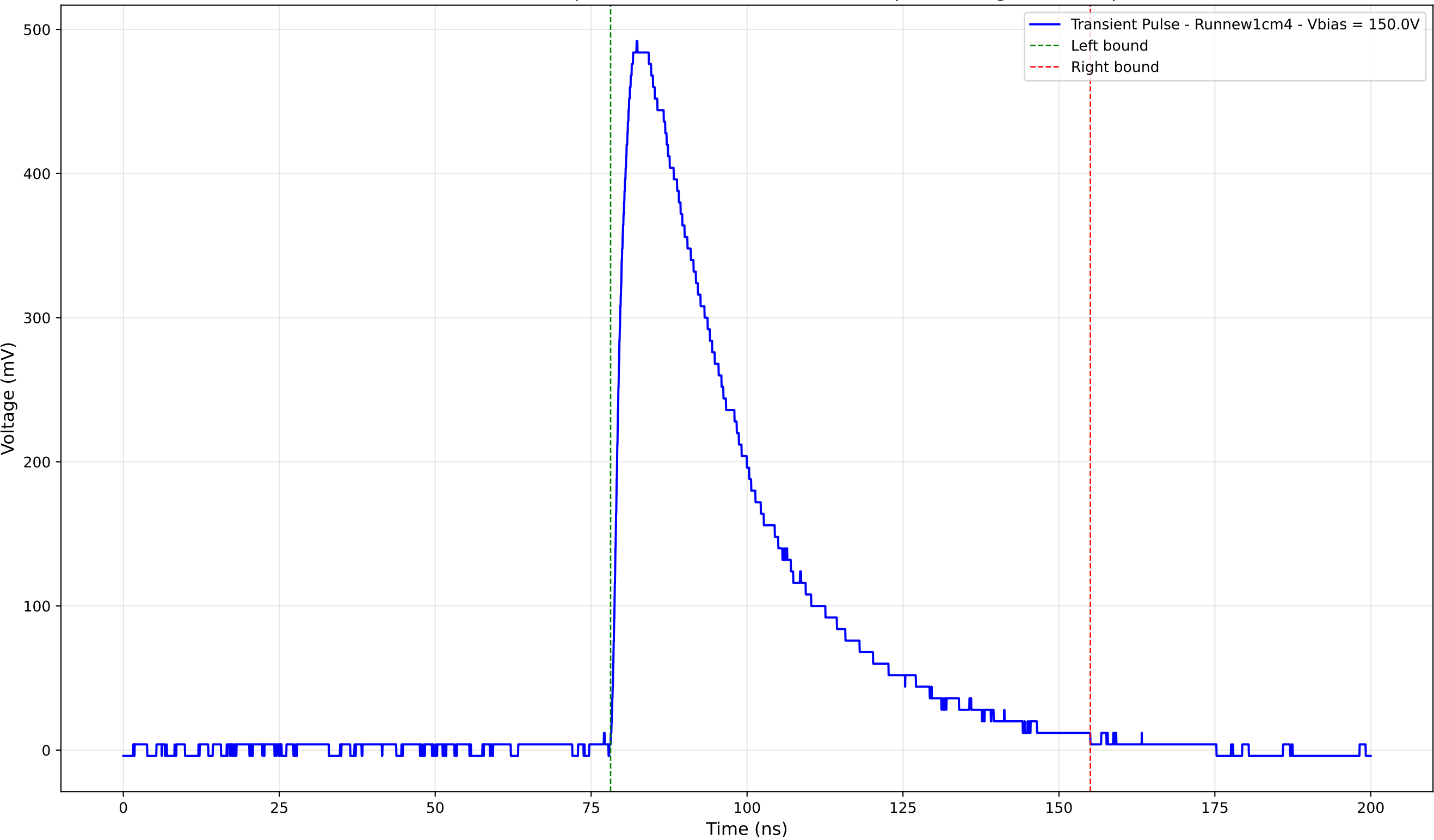
Transient Pulse - Sample: new1cm - Position: 2620.0 \mu\text{m} - Charge: 215.80 pC
