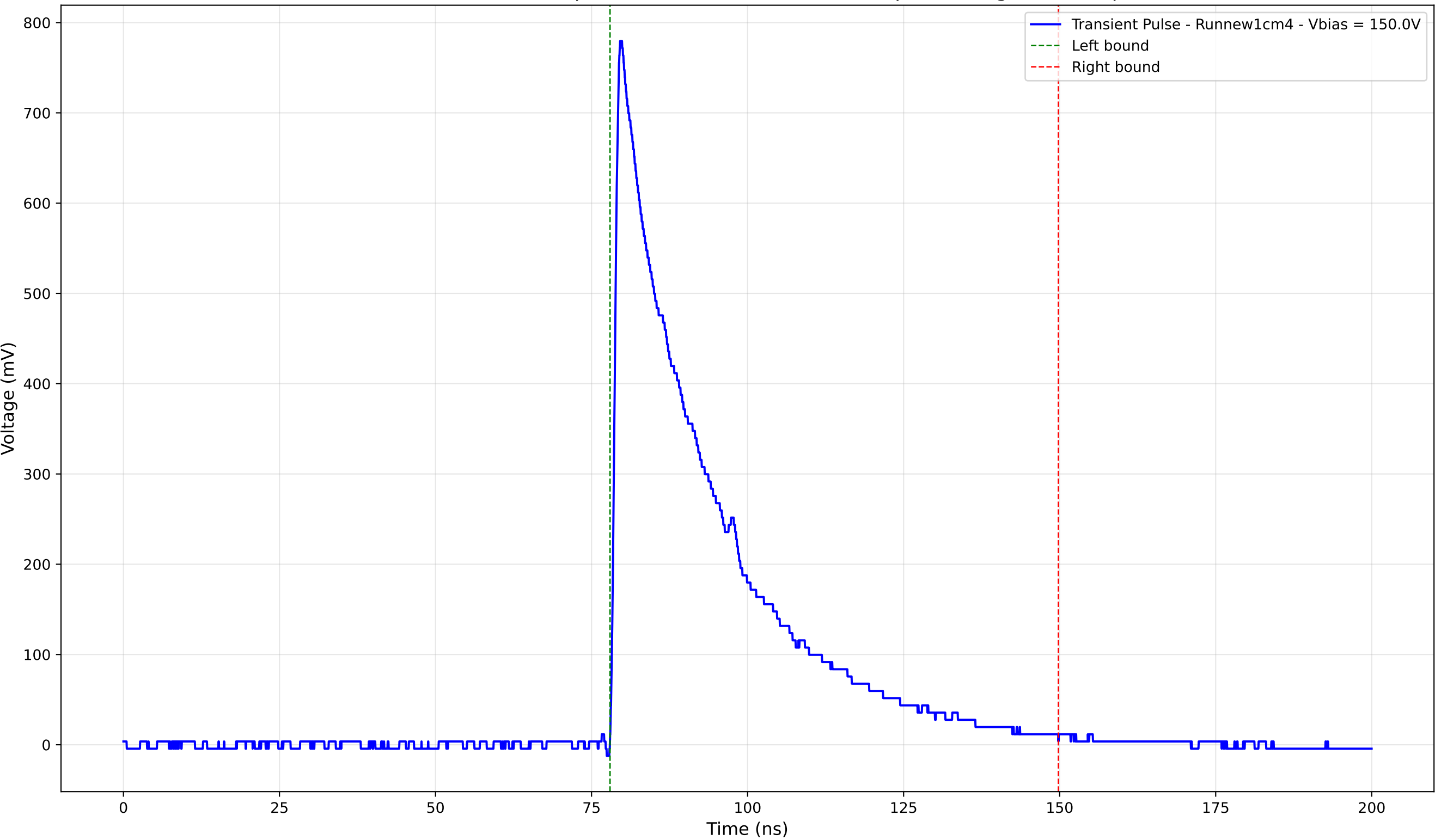
Transient Pulse - Sample: new1cm - Position: 4365.0 \mu\text{m} - Charge: 242.57 pC
