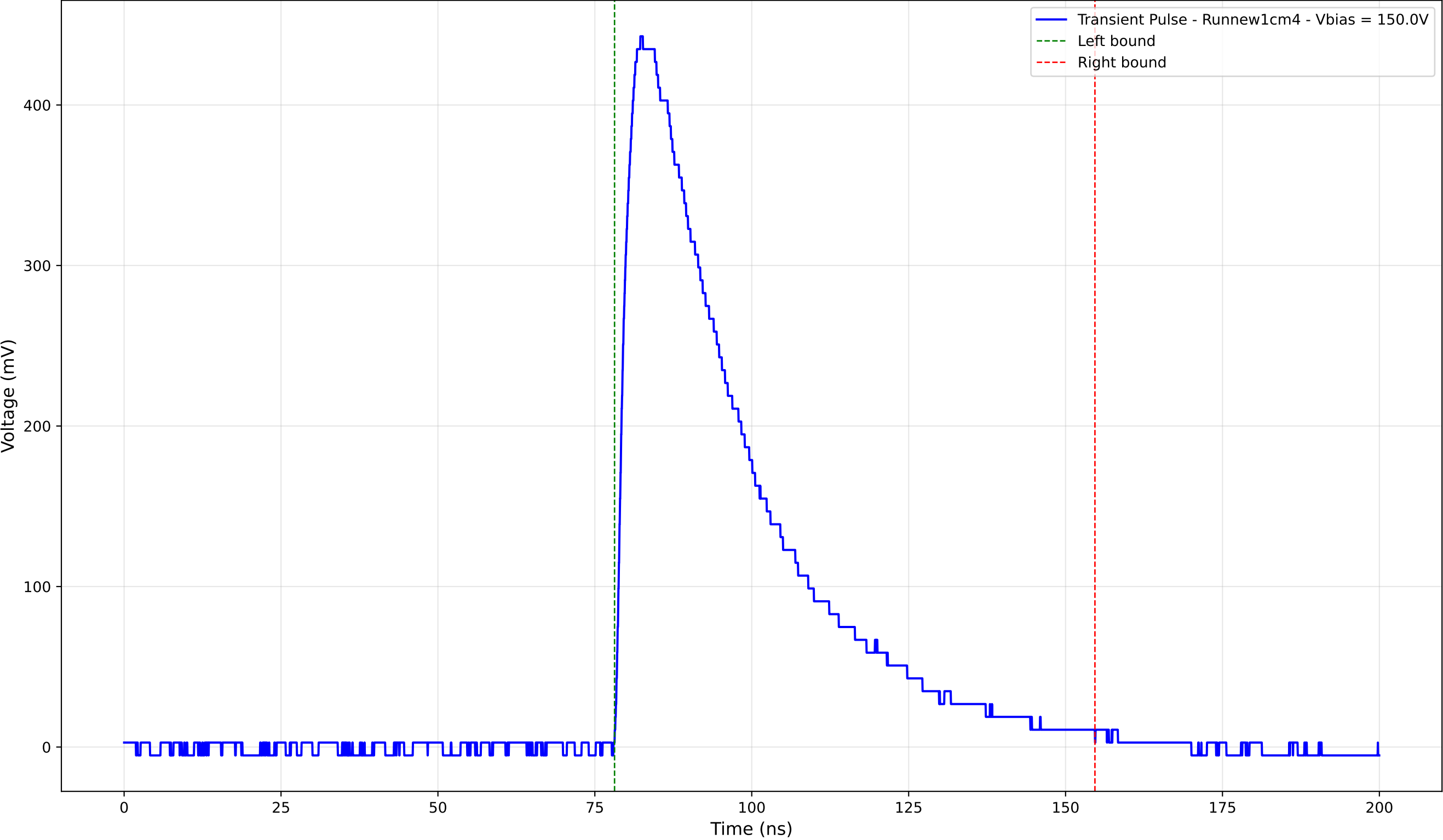
Transient Pulse - Sample: new1cm - Position: 2800.0 \mu\text{m} - Charge: 193.63 pC
