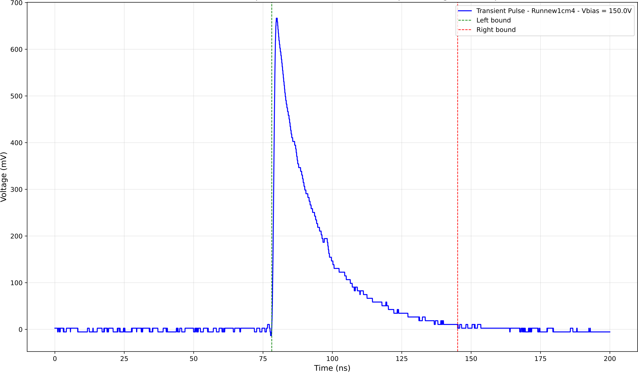
Transient Pulse - Sample: new1cm - Position: 1005.0 \mu\text{m} - Charge: 196.13 pC
