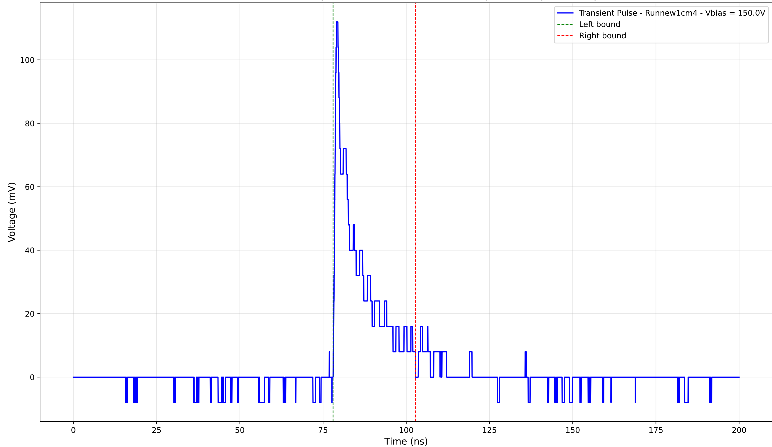
Transient Pulse - Sample: new1cm - Position: 195.0 \mu\text{m} - Charge: 15.36 pC
