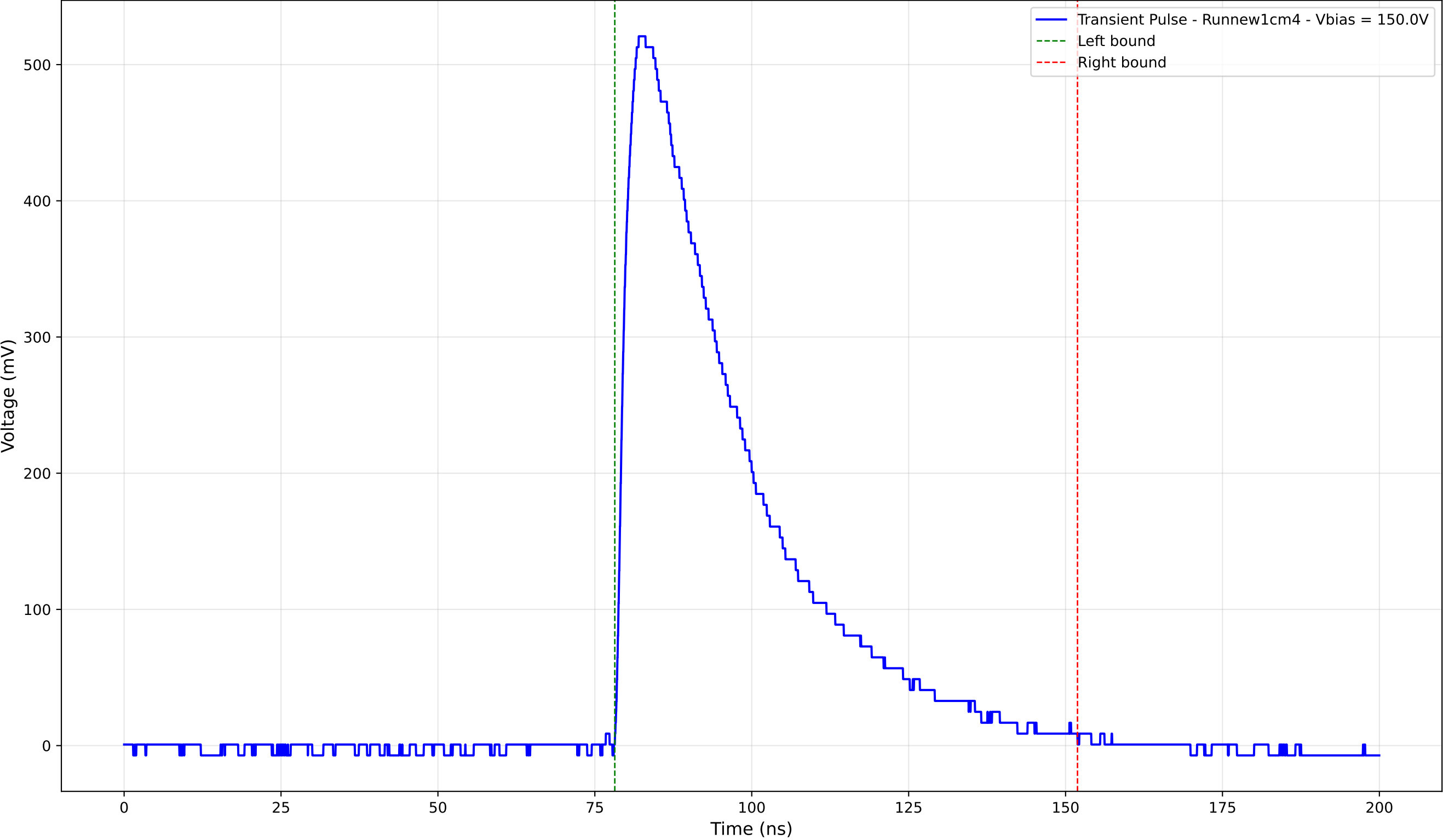
Transient Pulse - Sample: new1cm - Position: 2440.0 \mu\text{m} - Charge: 222.29 pC
