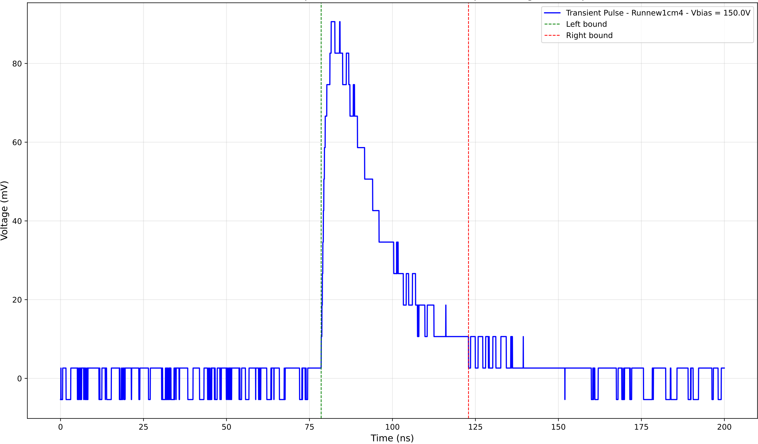
Transient Pulse - Sample: new1cm - Position: 1715.0 \mu\text{m} - Charge: 32.93 pC
