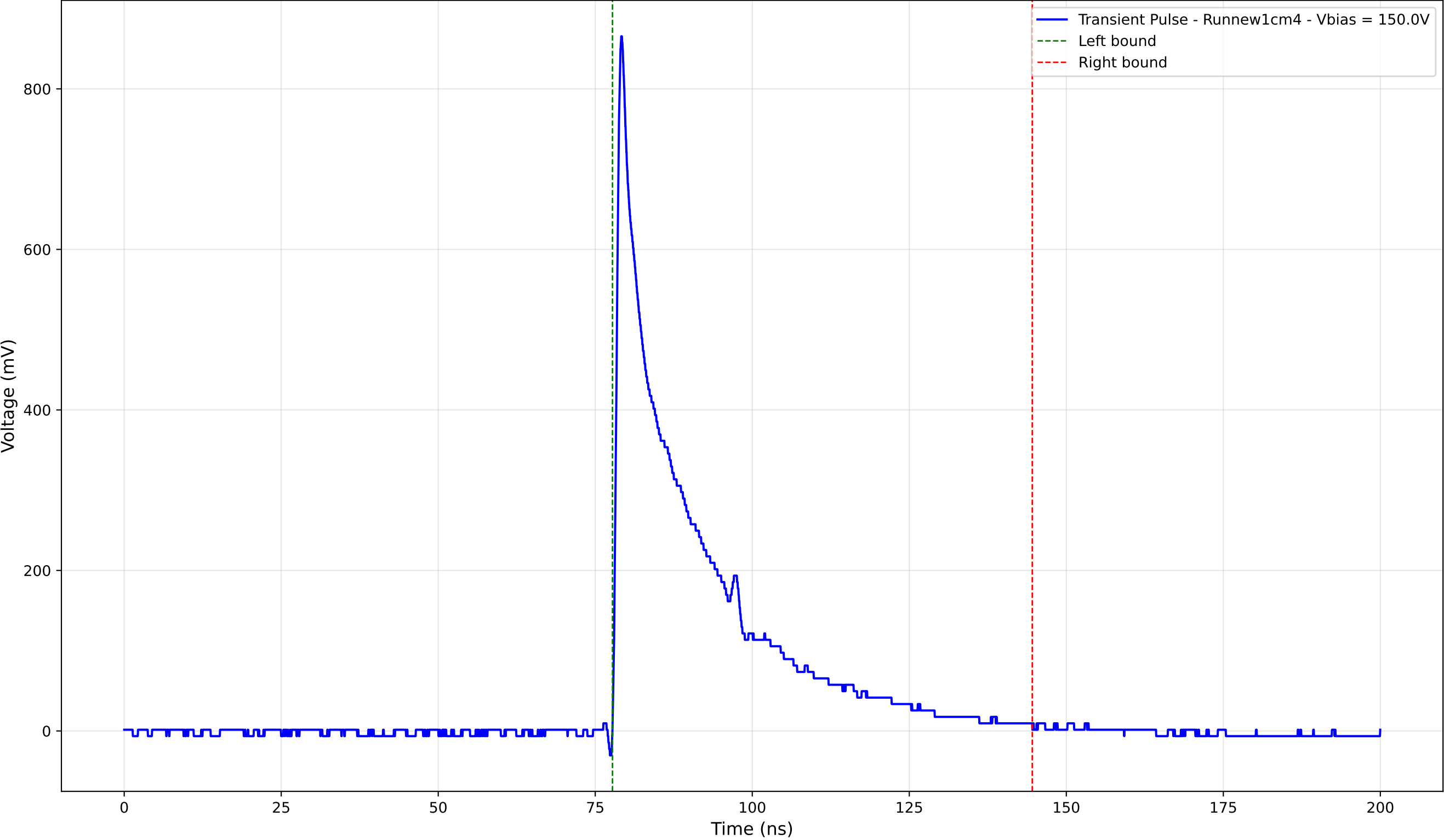
Transient Pulse - Sample: new1cm - Position: 4890.0 \mu\text{m} - Charge: 187.76 pC
