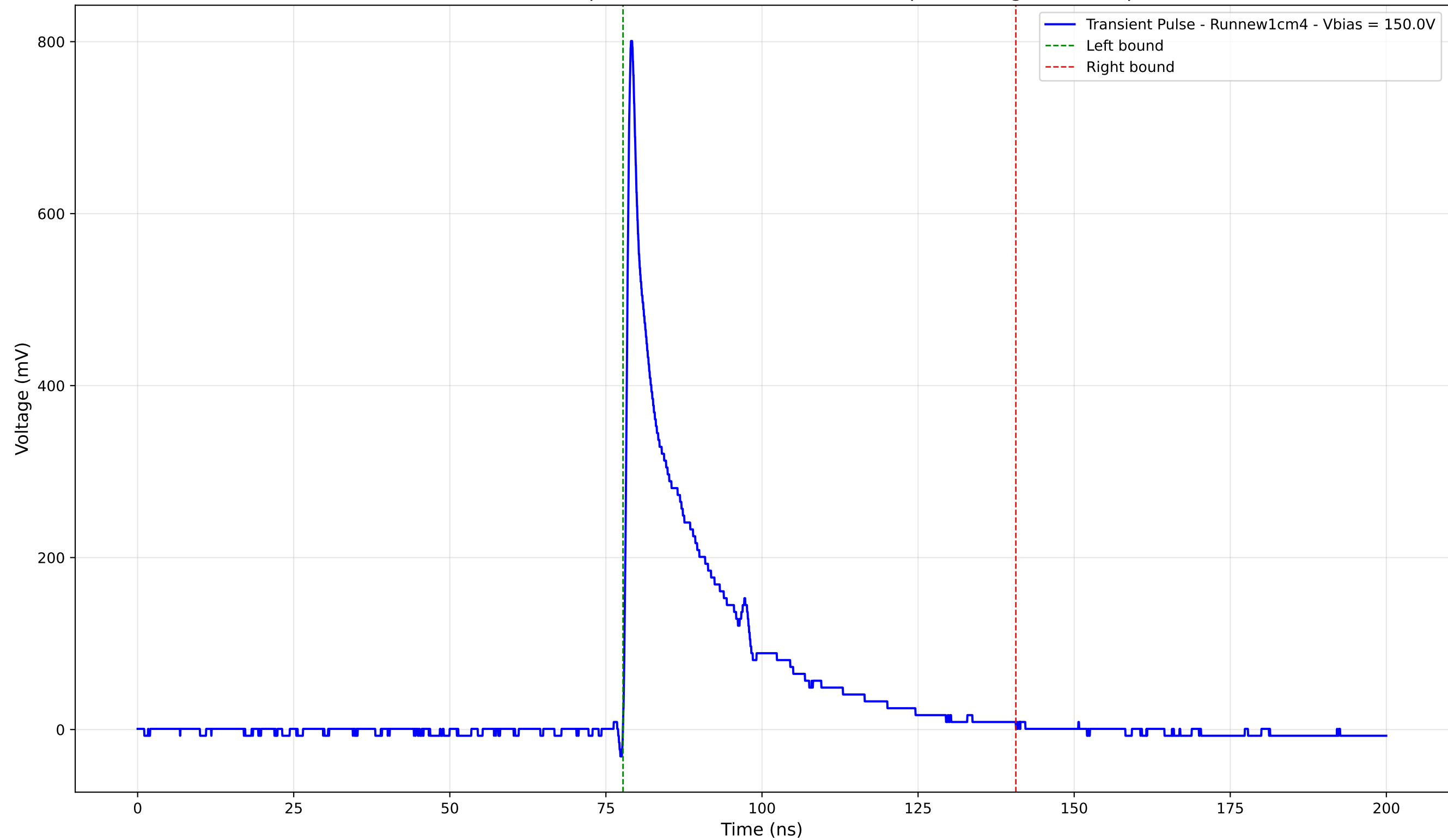
Transient Pulse - Sample: new1cm - Position: 4990.0 \mu\text{m} - Charge: 147.99 pC
