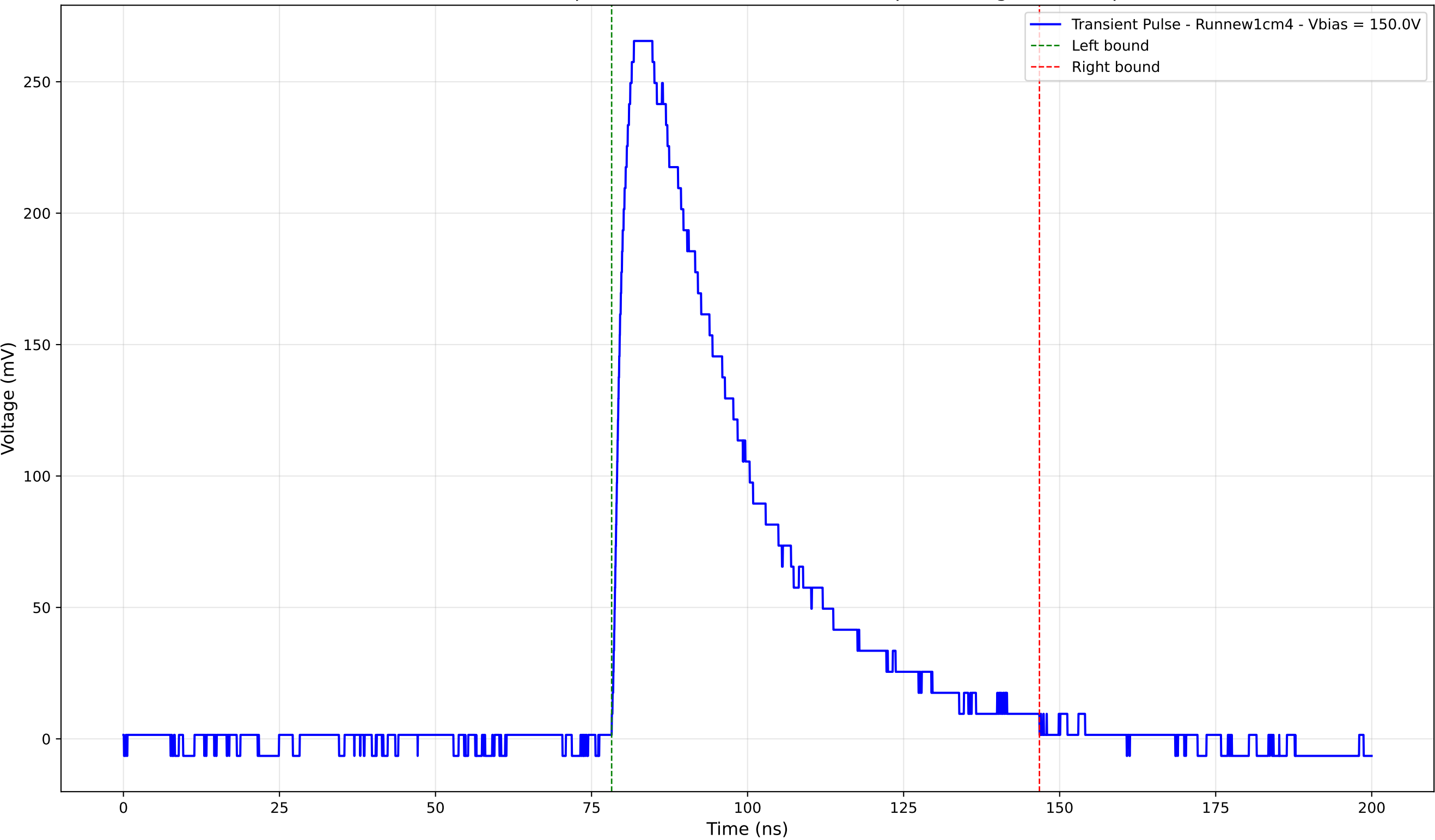
Transient Pulse - Sample: new1cm - Position: 2765.0 \mu\text{m} - Charge: 114.79 pC
