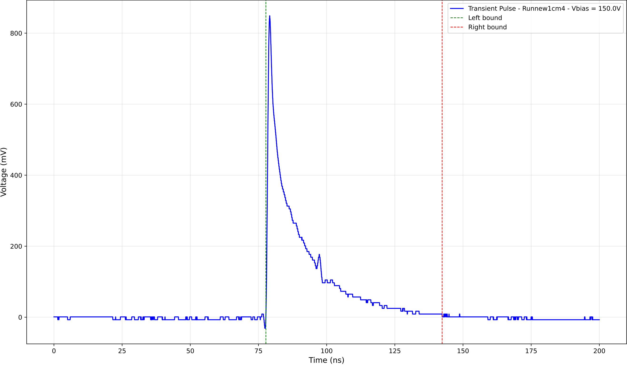
Transient Pulse - Sample: new1cm - Position: 4975.0 \mu\text{m} - Charge: 165.32 pC
