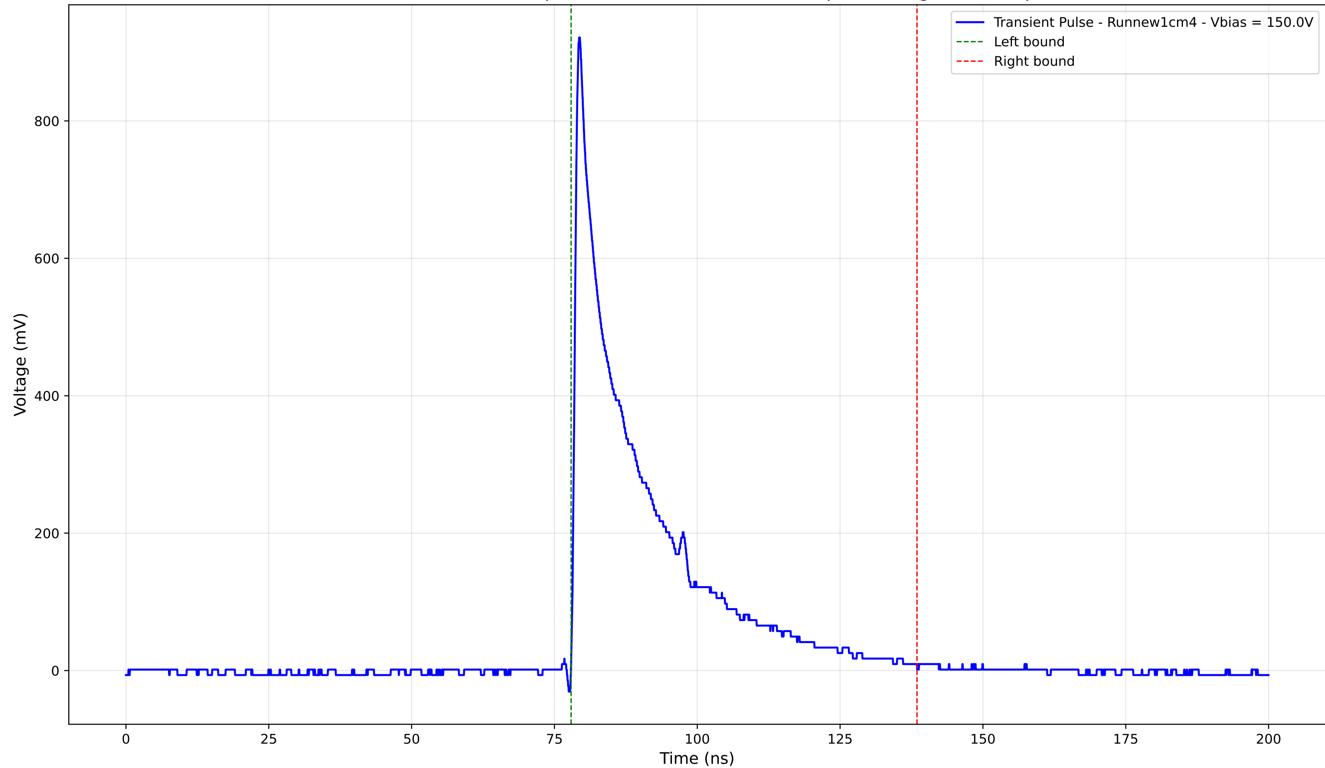
Transient Pulse - Sample: new1cm - Position: 450.0 \mu\text{m} - Charge: 197.66 pC
