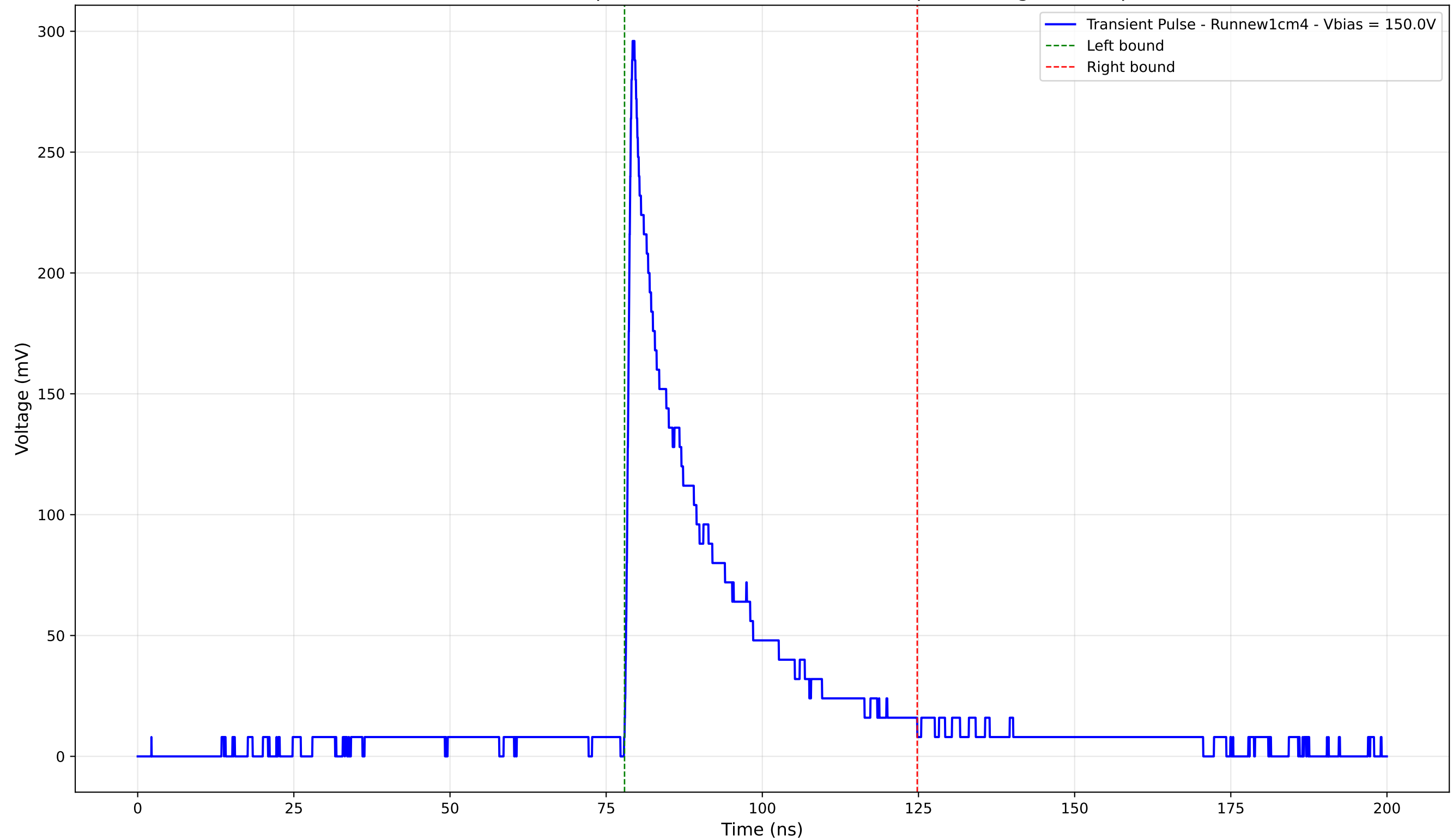
Transient Pulse - Sample: new1cm - Position: 4705.0 \mu\text{m} - Charge: 66.72 pC
