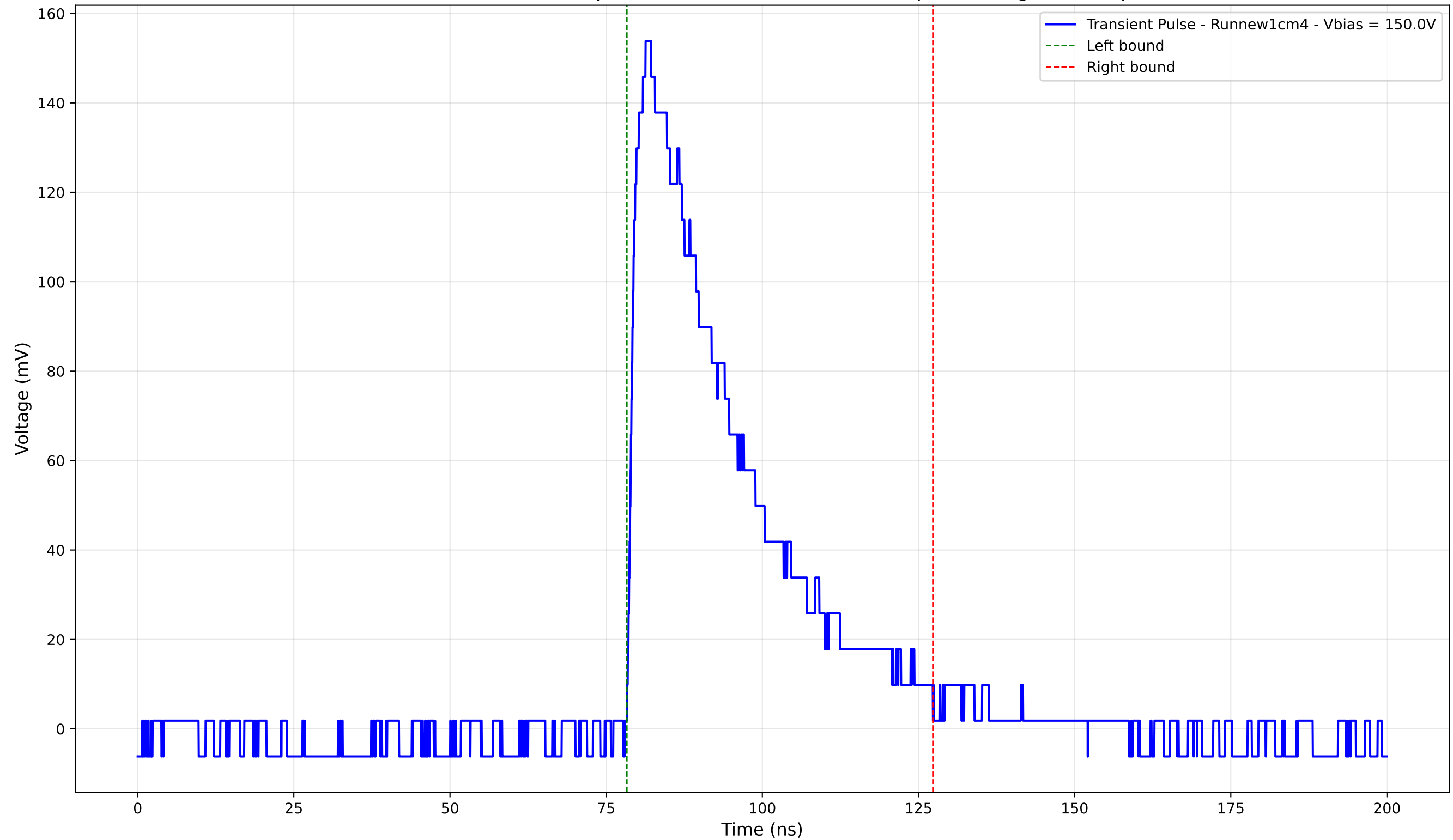
Transient Pulse - Sample: new1cm - Position: 3705.0 \mu\text{m} - Charge: 54.93 pC
