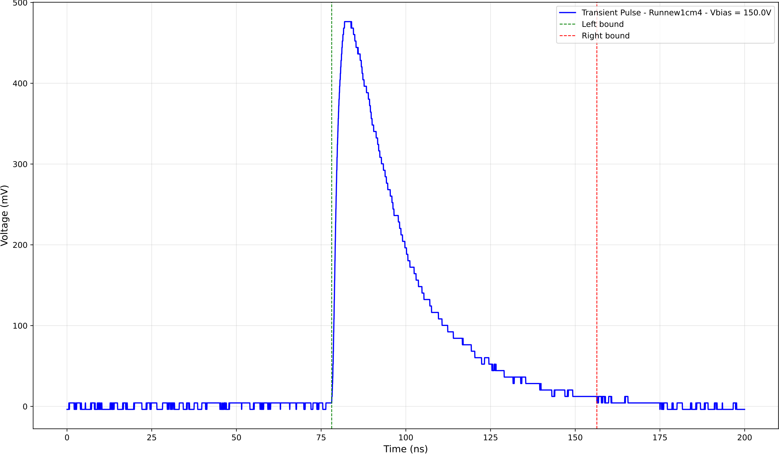
Transient Pulse - Sample: new1cm - Position: 2820.0 \mu\text{m} - Charge: 215.13 pC
