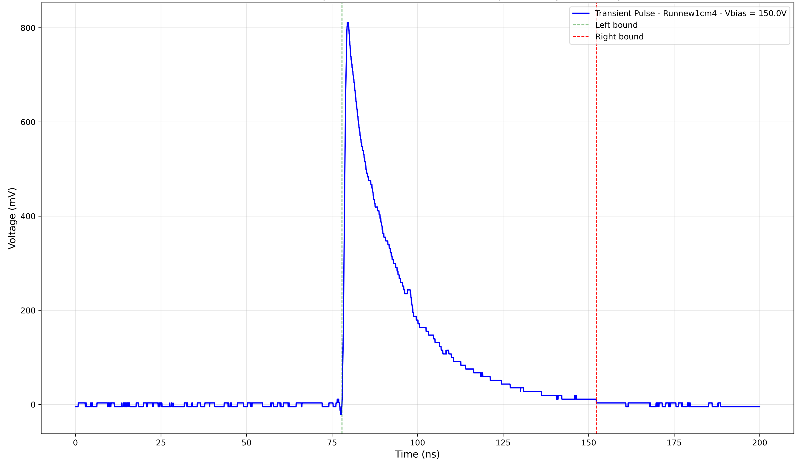
Transient Pulse - Sample: new1cm - Position: 4455.0 \mu\text{m} - Charge: 241.88 pC
