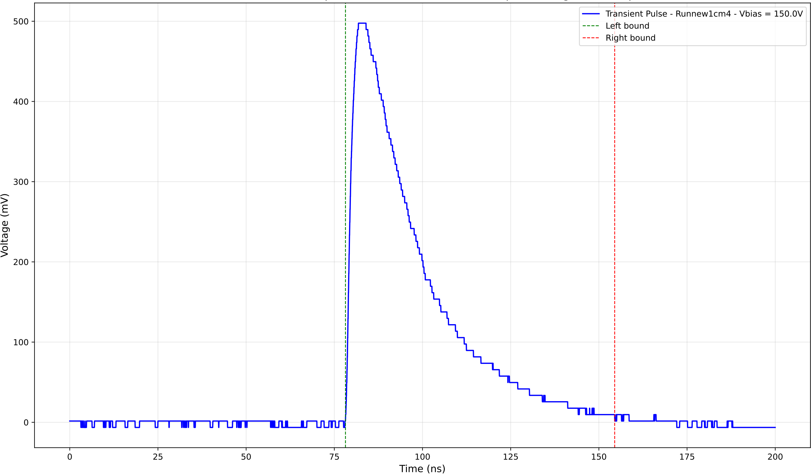
Transient Pulse - Sample: new1cm - Position: 2495.0 \mu\text{m} - Charge: 218.90 pC
