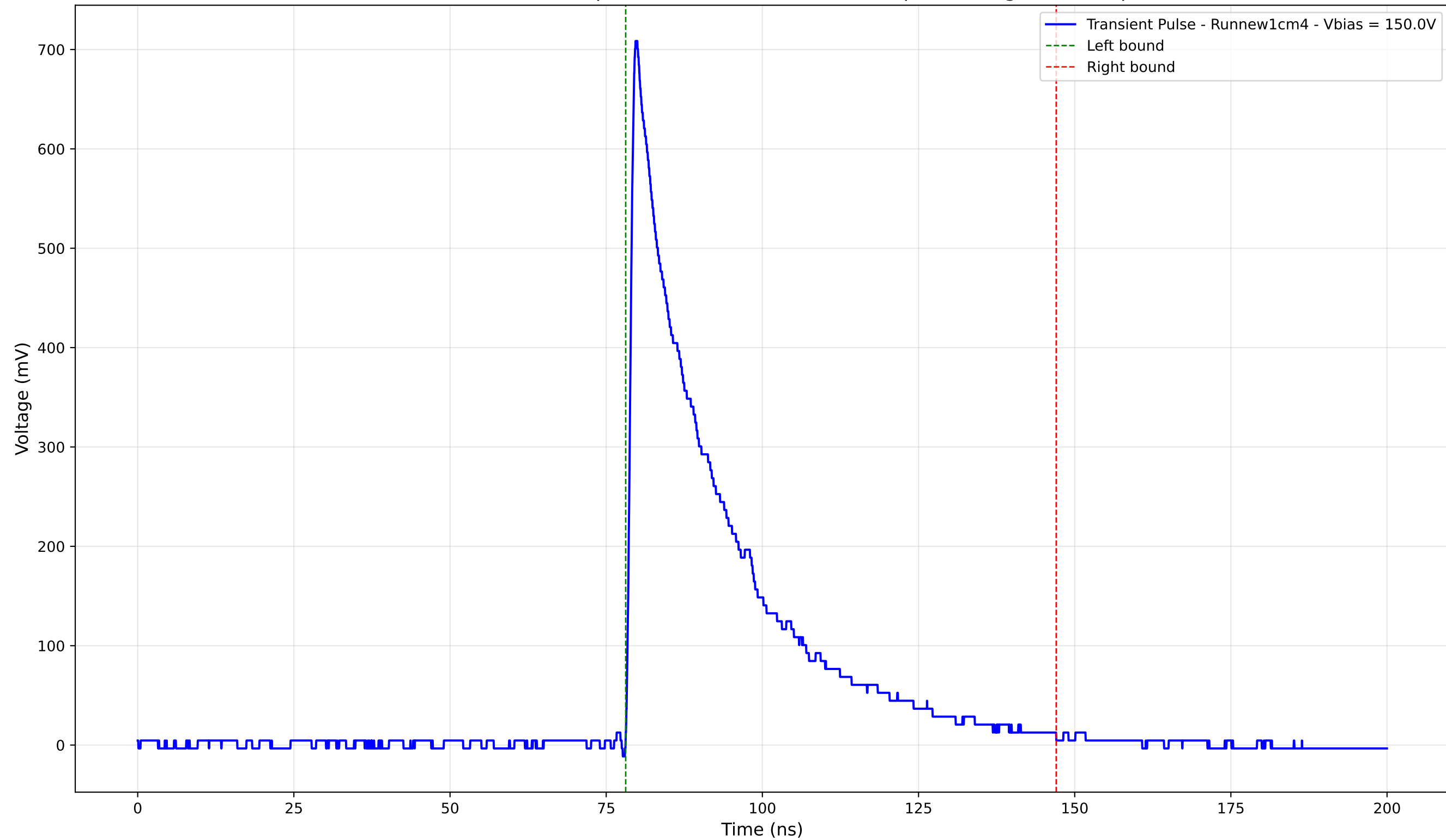
Transient Pulse - Sample: new1cm - Position: 915.0 \mu\text{m} - Charge: 201.61 pC
