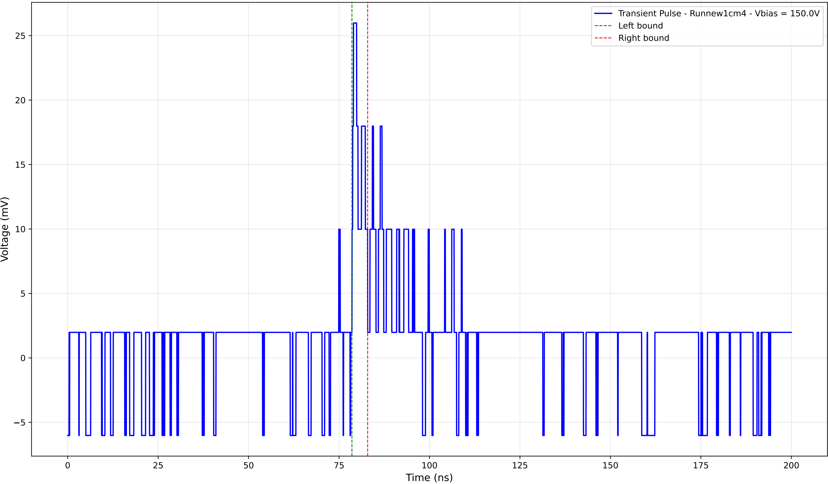
Transient Pulse - Sample: new1cm - Position: 130.0 \mu\text{m} - Charge: 1.41 pC
