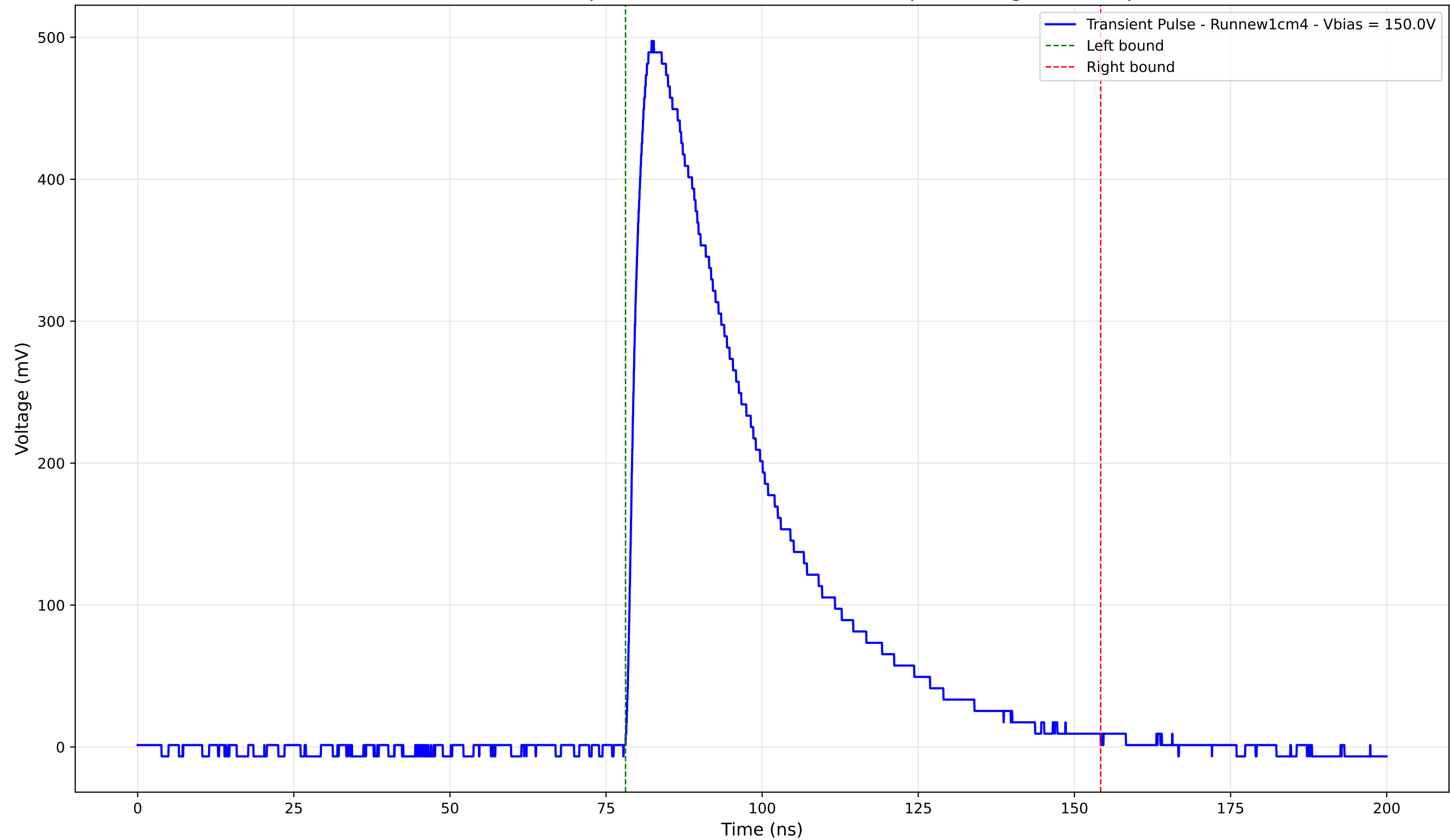
Transient Pulse - Sample: new1cm - Position: 2560.0 \mu\text{m} - Charge: 216.06 pC
