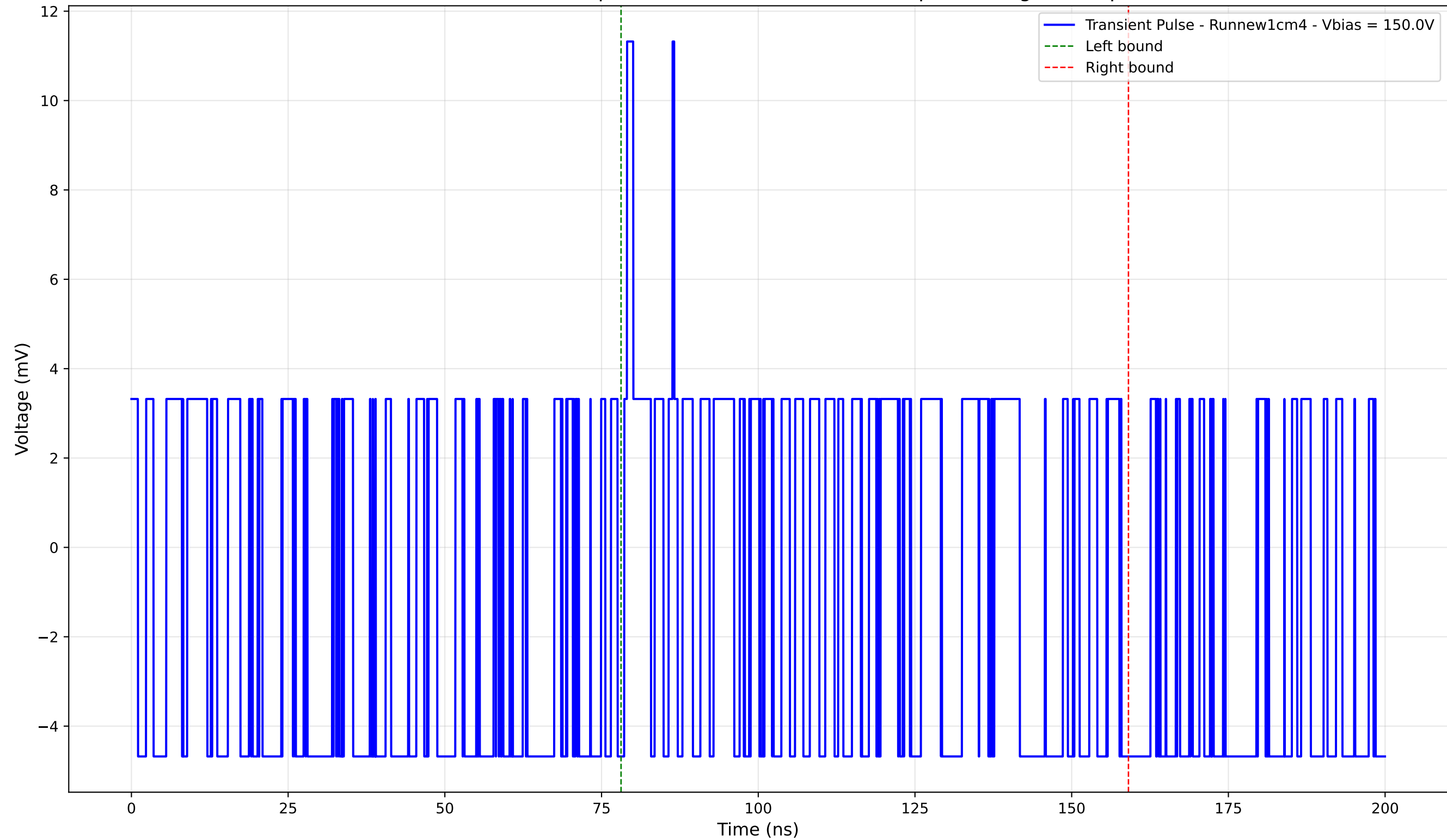
Transient Pulse - Sample: new1cm - Position: 5165.0 \mu\text{m} - Charge: 0.23 pC
