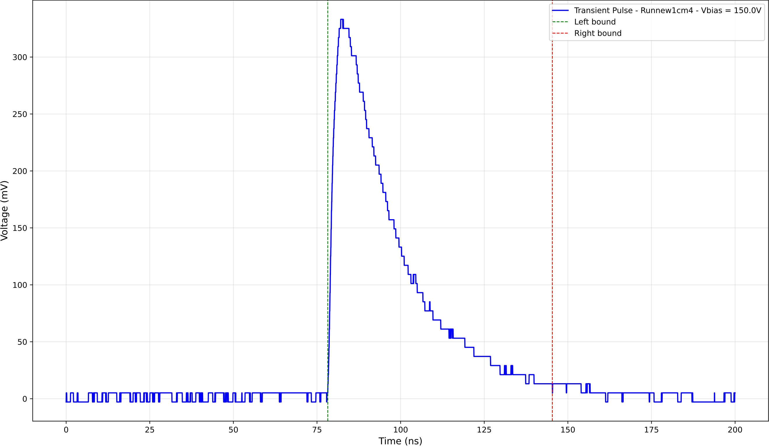
Transient Pulse - Sample: new1cm - Position: 2775.0 \mu\text{m} - Charge: 144.23 pC
