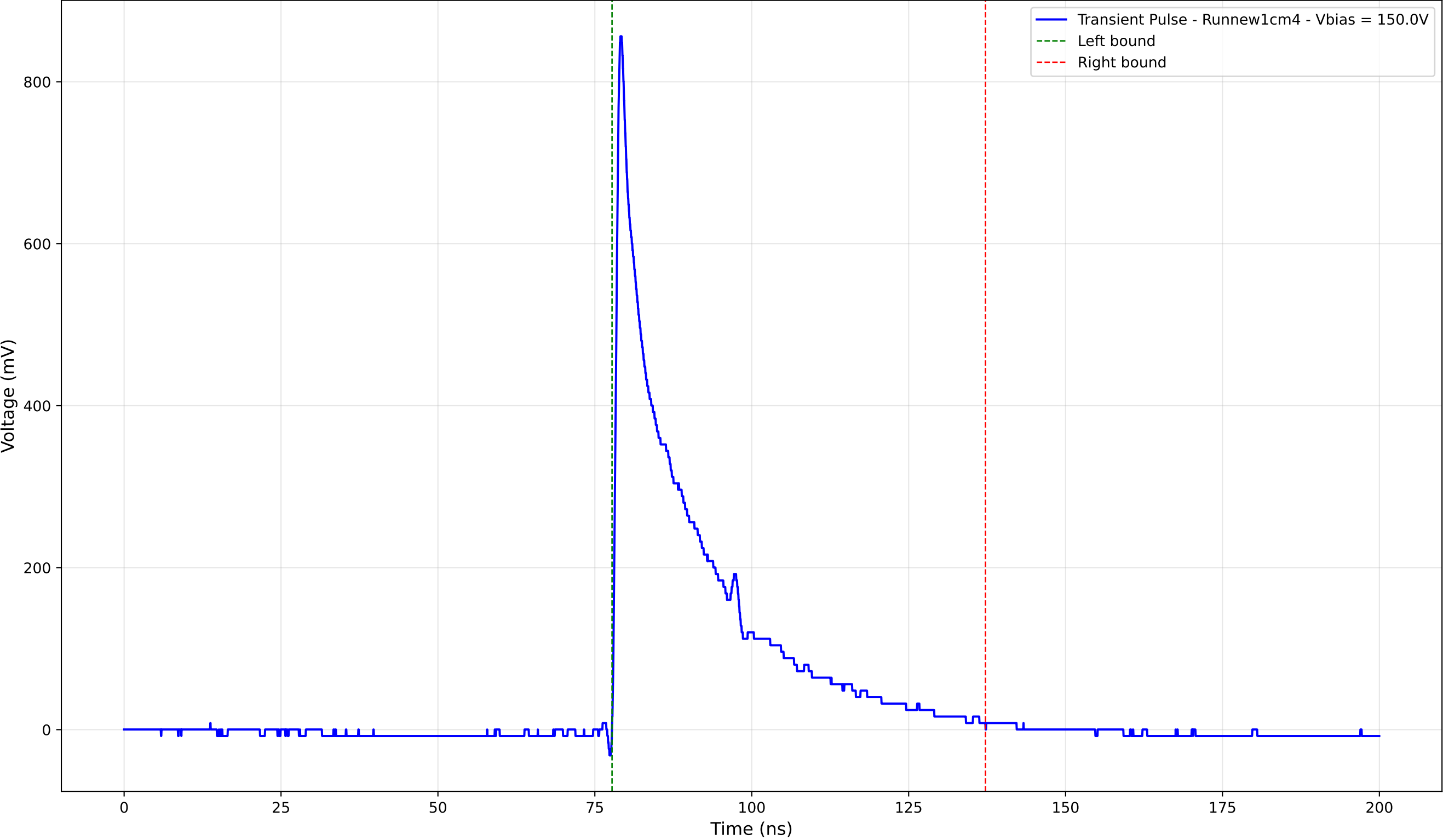
Transient Pulse - Sample: new1cm - Position: 4910.0 \mu\text{m} - Charge: 182.65 pC
