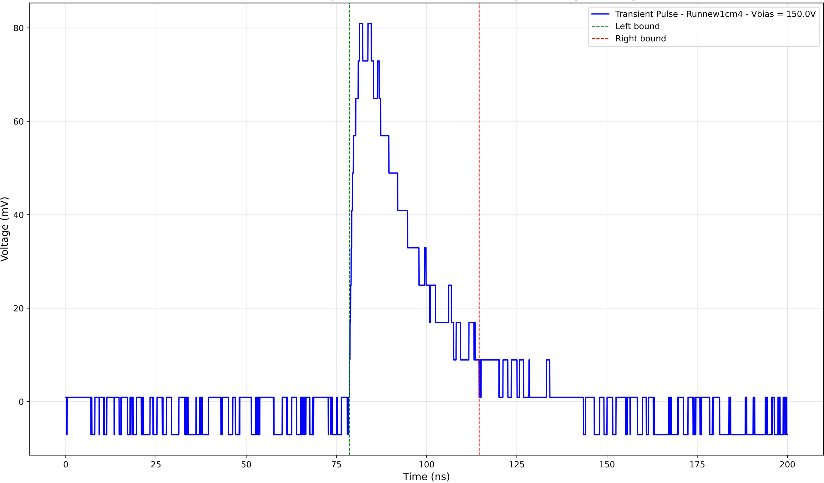
Transient Pulse - Sample: new1cm - Position: 1710.0 \mu\text{m} - Charge: 26.57 pC
