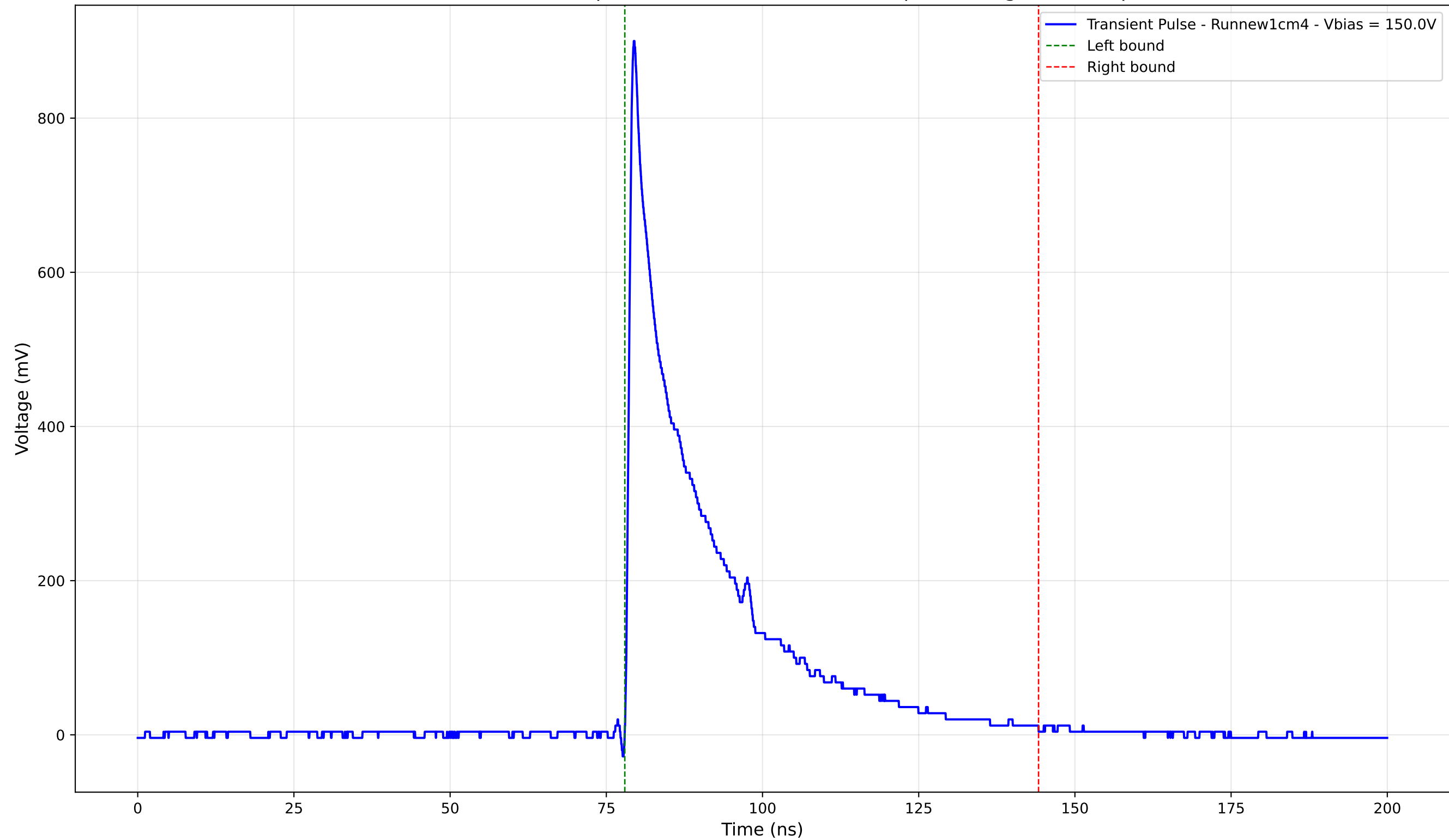
Transient Pulse - Sample: new1cm - Position: 535.0 \mu\text{m} - Charge: 202.81 pC
