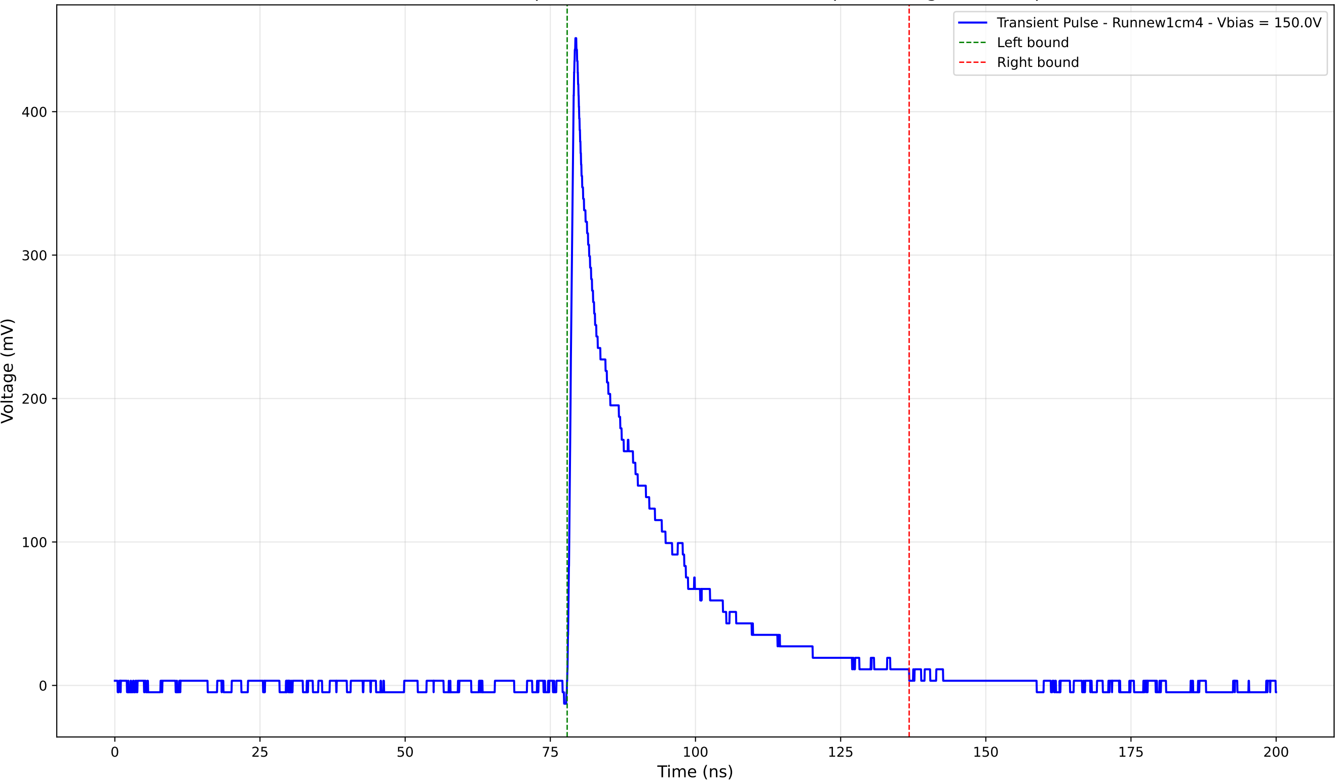
Transient Pulse - Sample: new1cm - Position: 4690.0 \mu\text{m} - Charge: 101.30 pC
