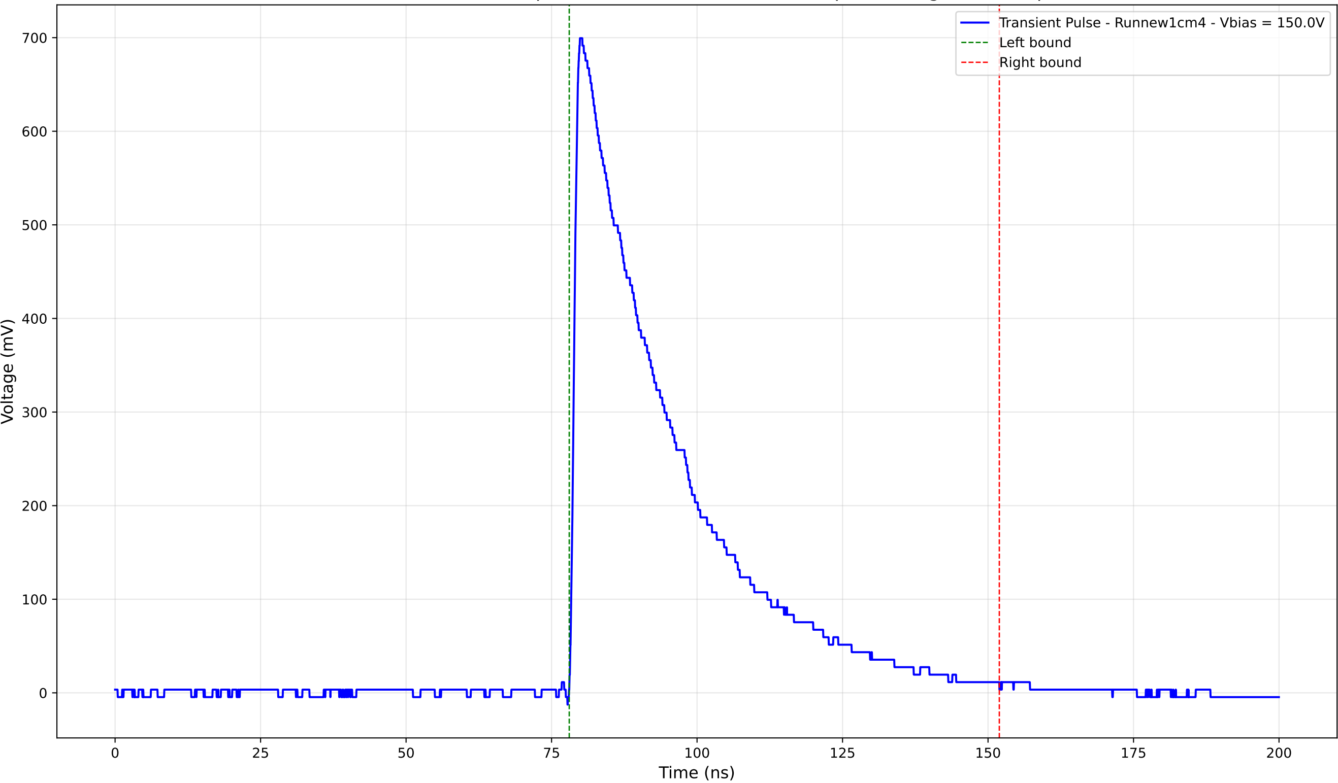
Transient Pulse - Sample: new1cm - Position: 4085.0 \mu\text{m} - Charge: 251.13 pC
