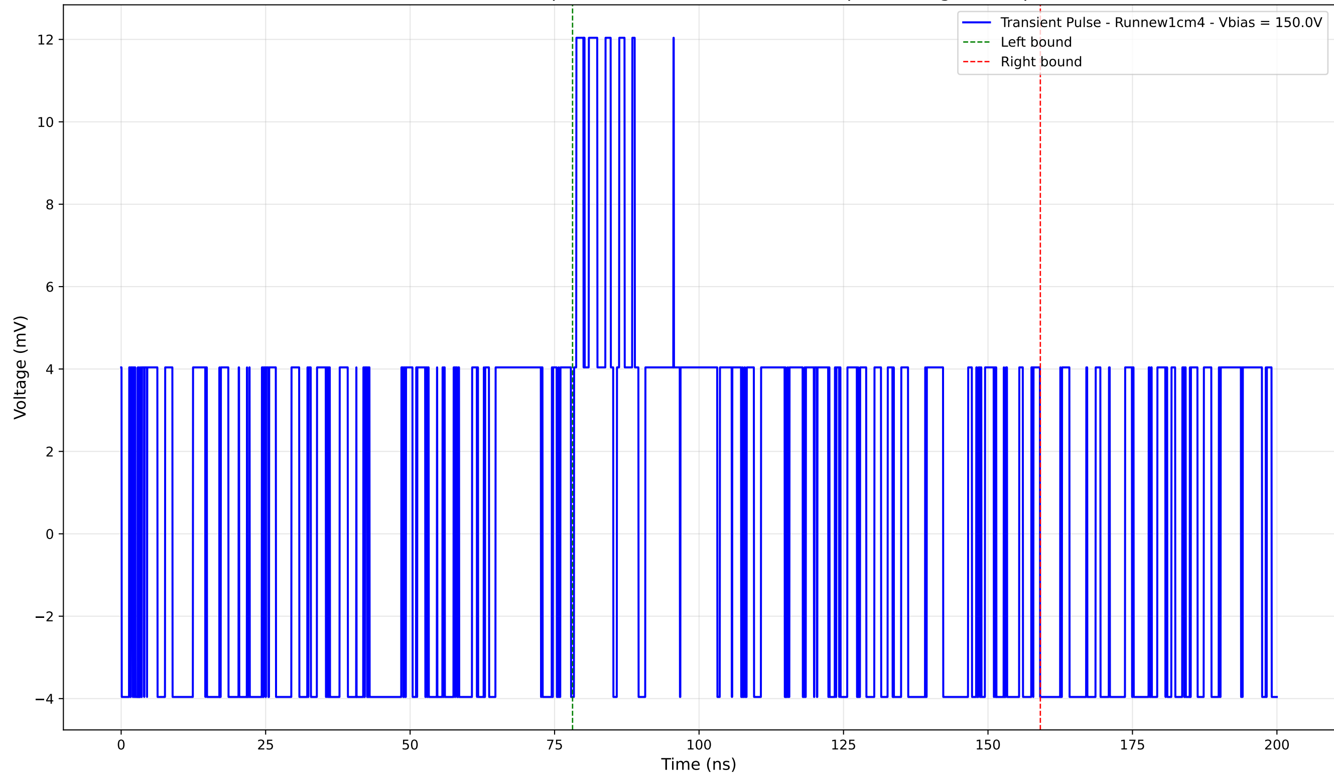
Transient Pulse - Sample: new1cm - Position: 5155.0 \mu\text{m} - Charge: 3.02 pC
