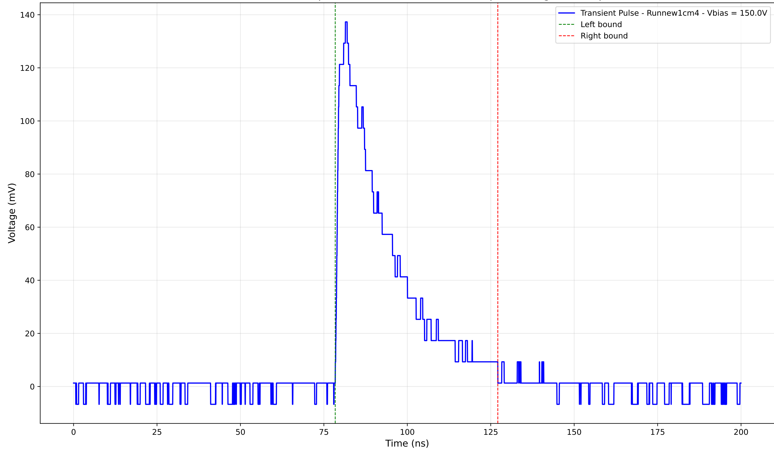
Transient Pulse - Sample: new1cm - Position: 1220.0 \mu\text{m} - Charge: 43.38 pC
