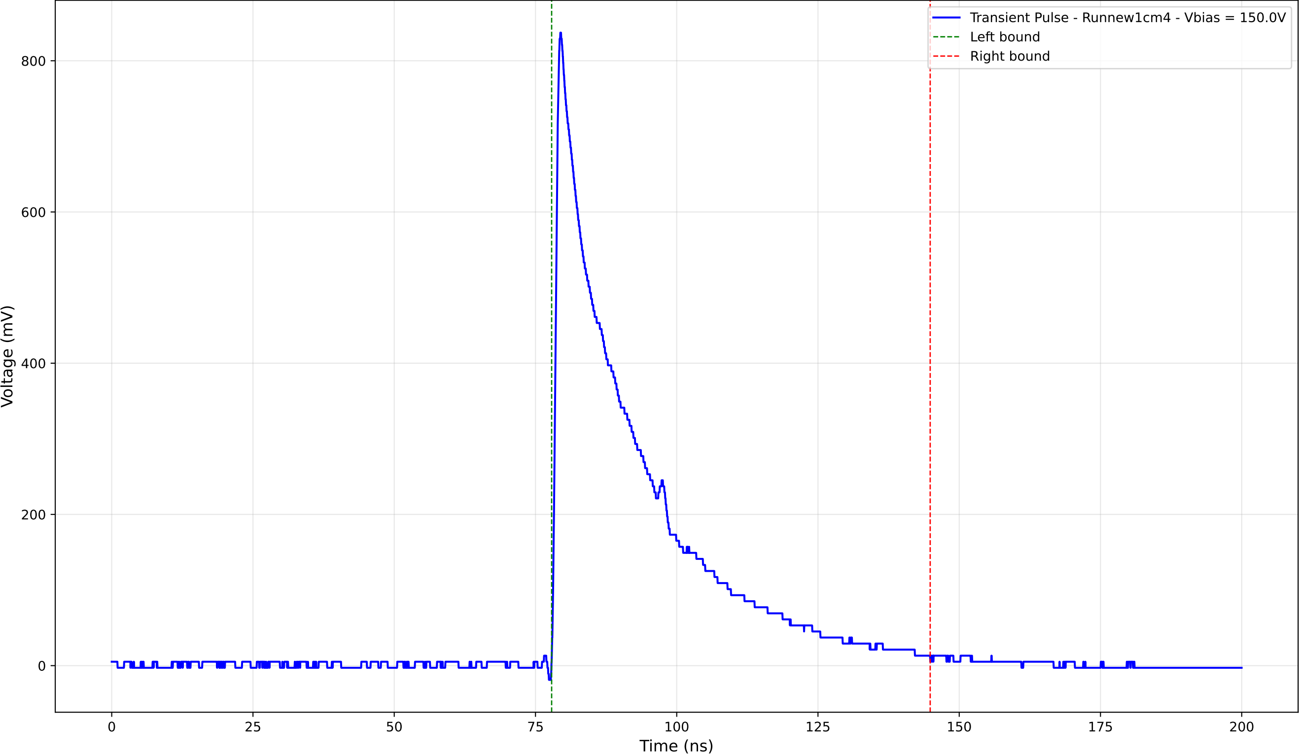
Transient Pulse - Sample: new1cm - Position: 4580.0 \mu\text{m} - Charge: 235.37 pC
