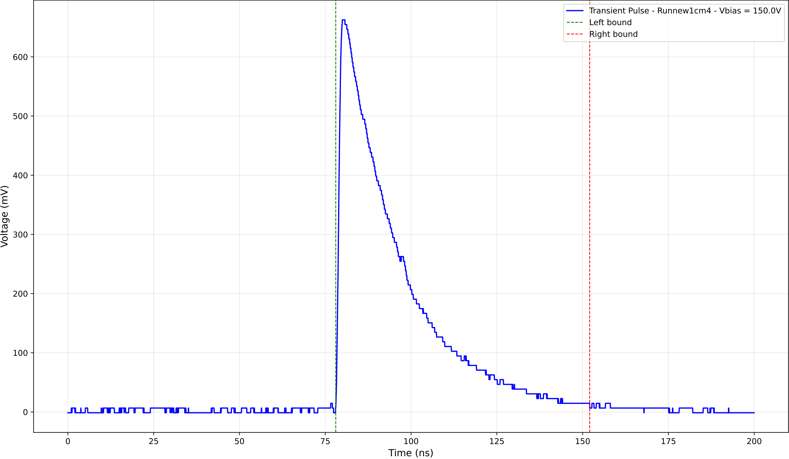
Transient Pulse - Sample: new1cm - Position: 3990.0 \mu\text{m} - Charge: 251.68 pC
