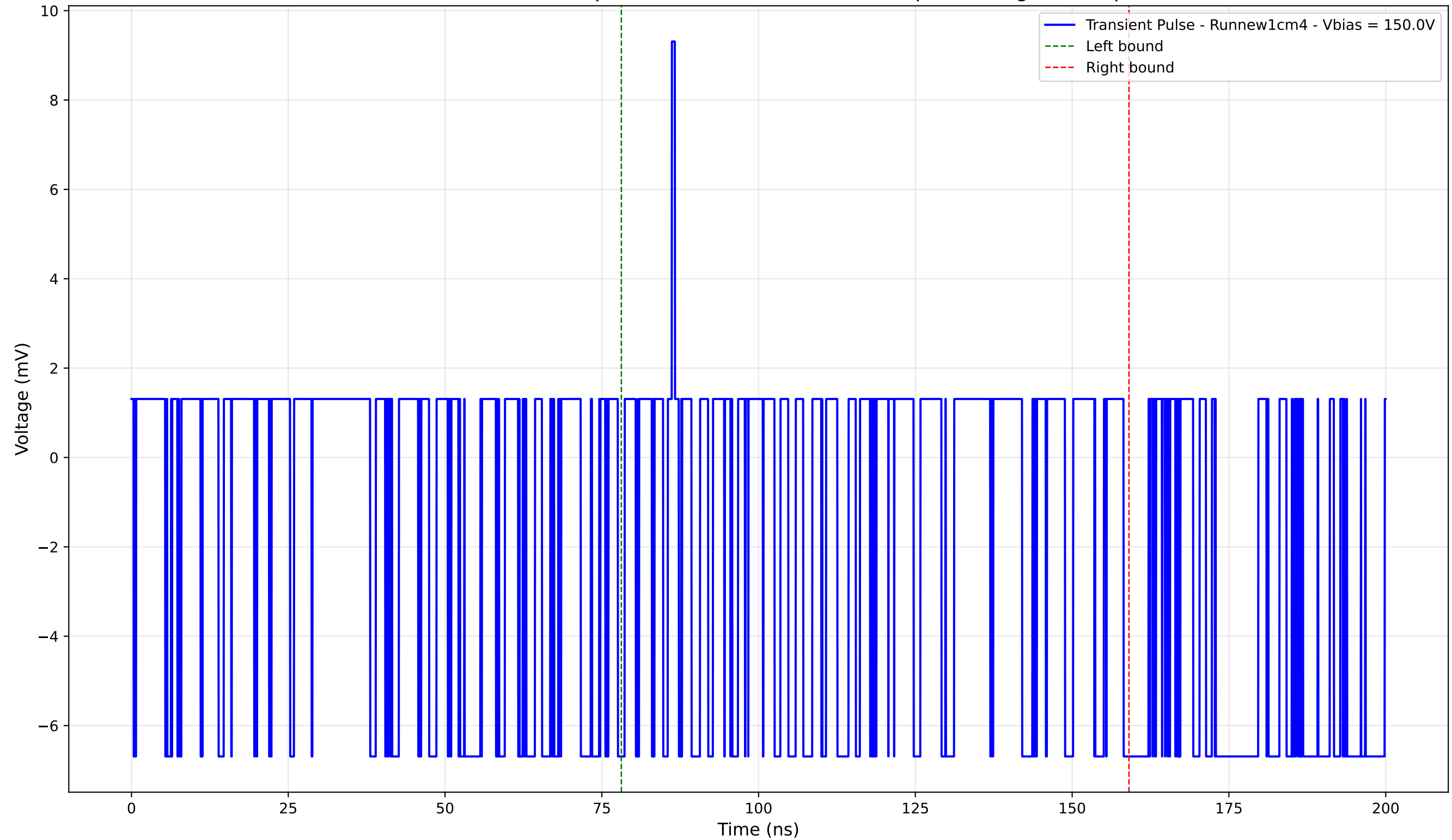
Transient Pulse - Sample: new1cm - Position: 5195.0 \mu\text{m} - Charge: -1.38 pC
