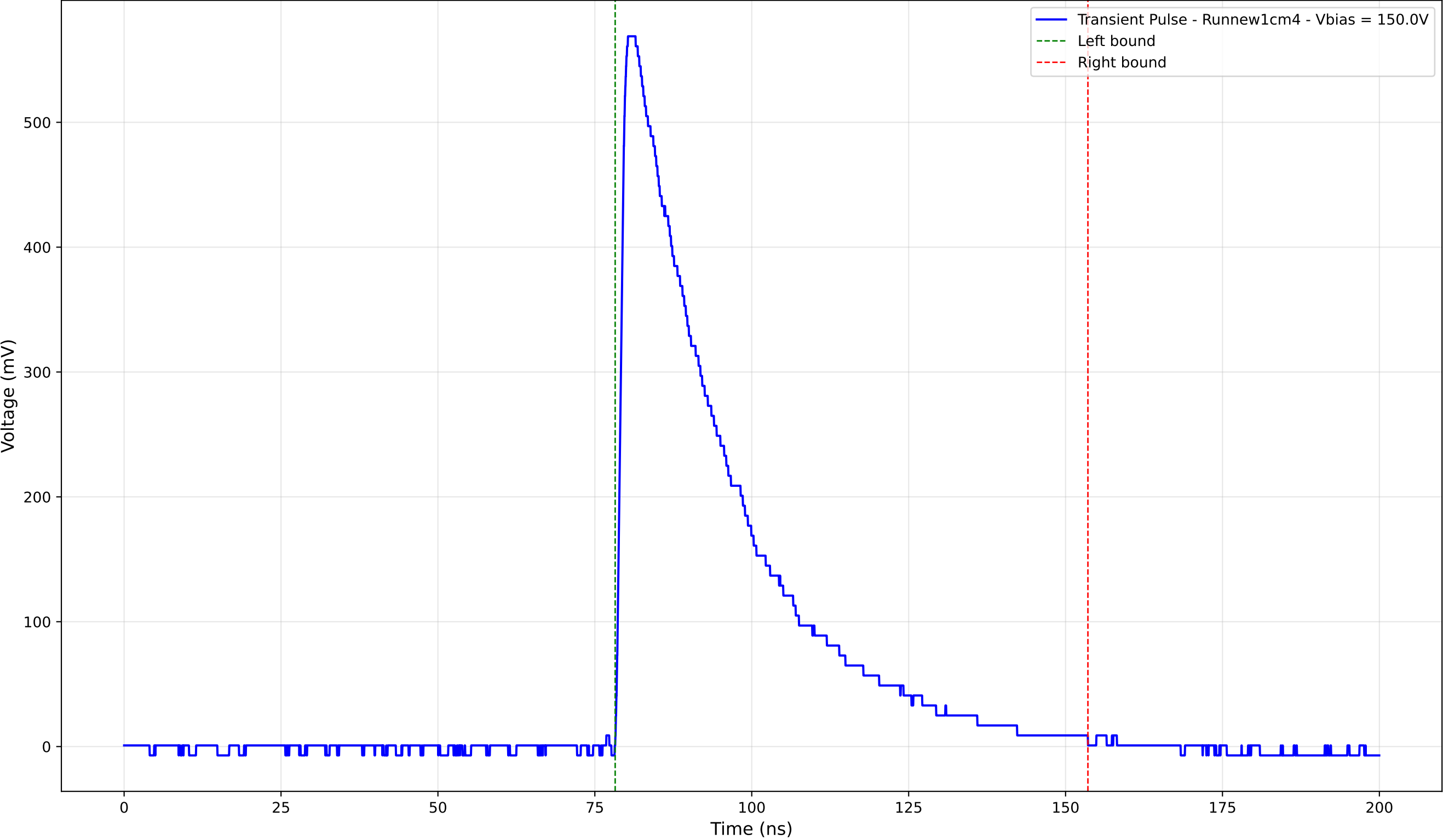
Transient Pulse - Sample: new1cm - Position: 1415.0 \mu\text{m} - Charge: 207.03 pC
