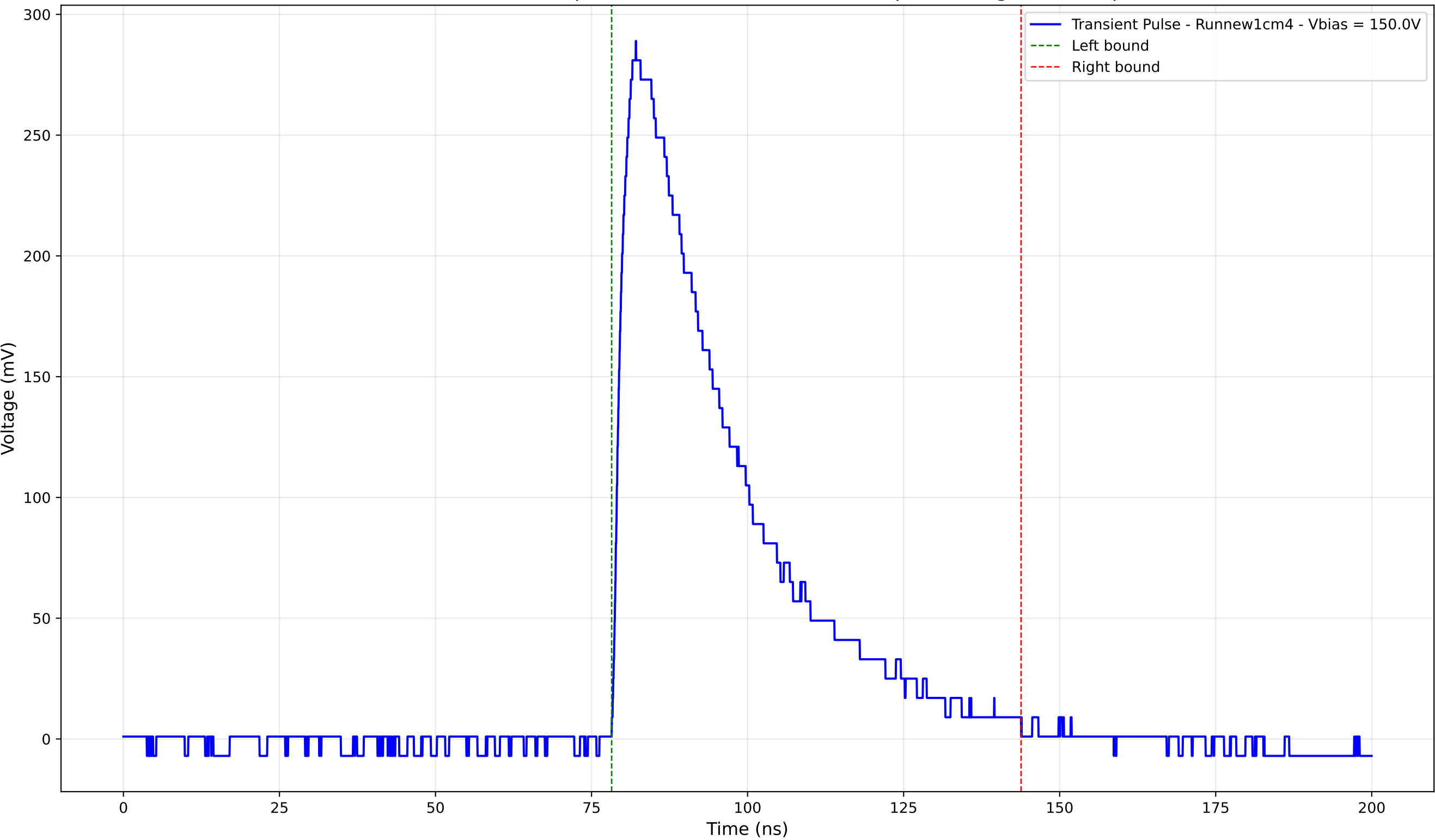
Transient Pulse - Sample: new1cm - Position: 2155.0 \mu\text{m} - Charge: 114.34 pC
