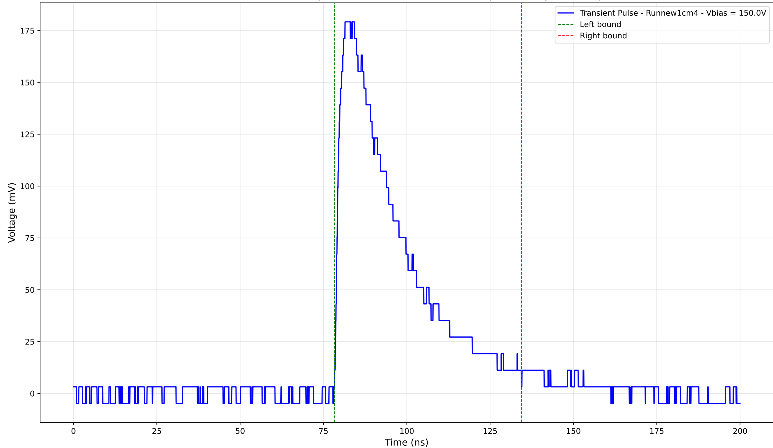
Transient Pulse - Sample: new1cm - Position: 3255.0 \mu\text{m} - Charge: 73.64 pC
