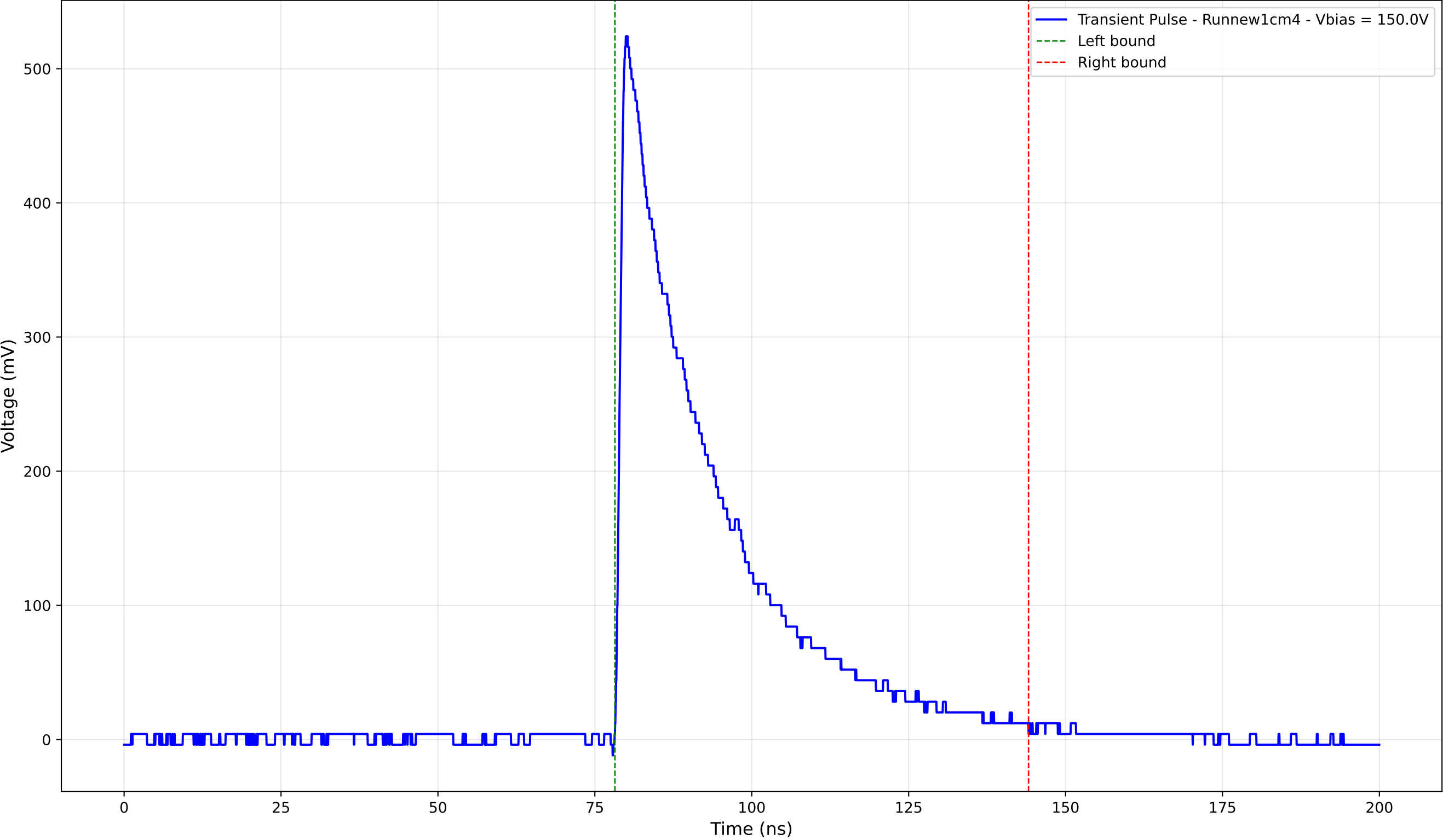
Transient Pulse - Sample: new1cm - Position: 1125.0 \mu\text{m} - Charge: 162.64 pC
