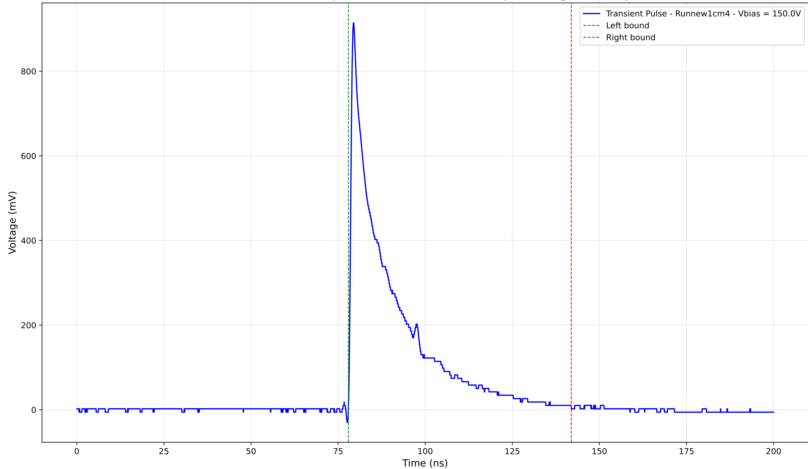
Transient Pulse - Sample: new1cm - Position: 510.0 \mu\text{m} - Charge: 200.25 pC
