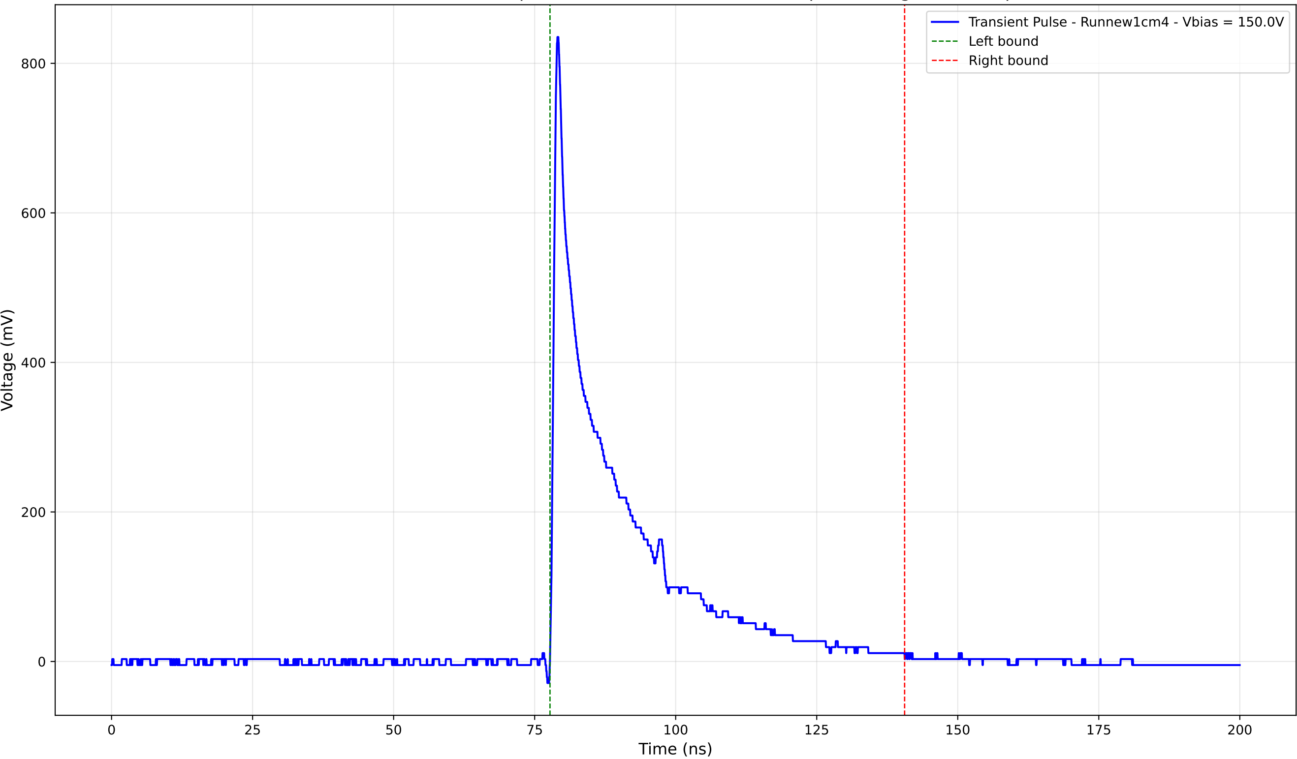
Transient Pulse - Sample: new1cm - Position: 4980.0 \mu\text{m} - Charge: 162.59 pC
