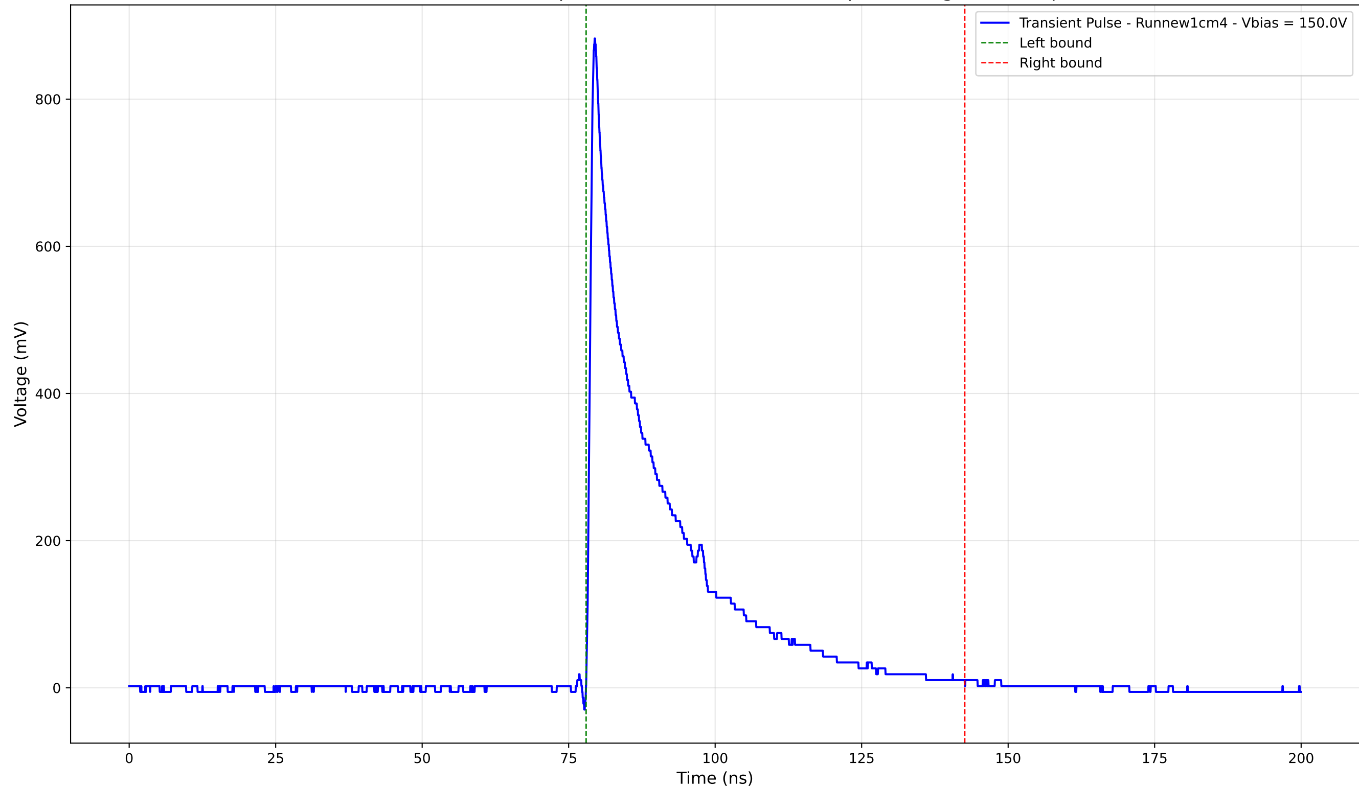
Transient Pulse - Sample: new1cm - Position: 565.0 \mu\text{m} - Charge: 197.93 pC
