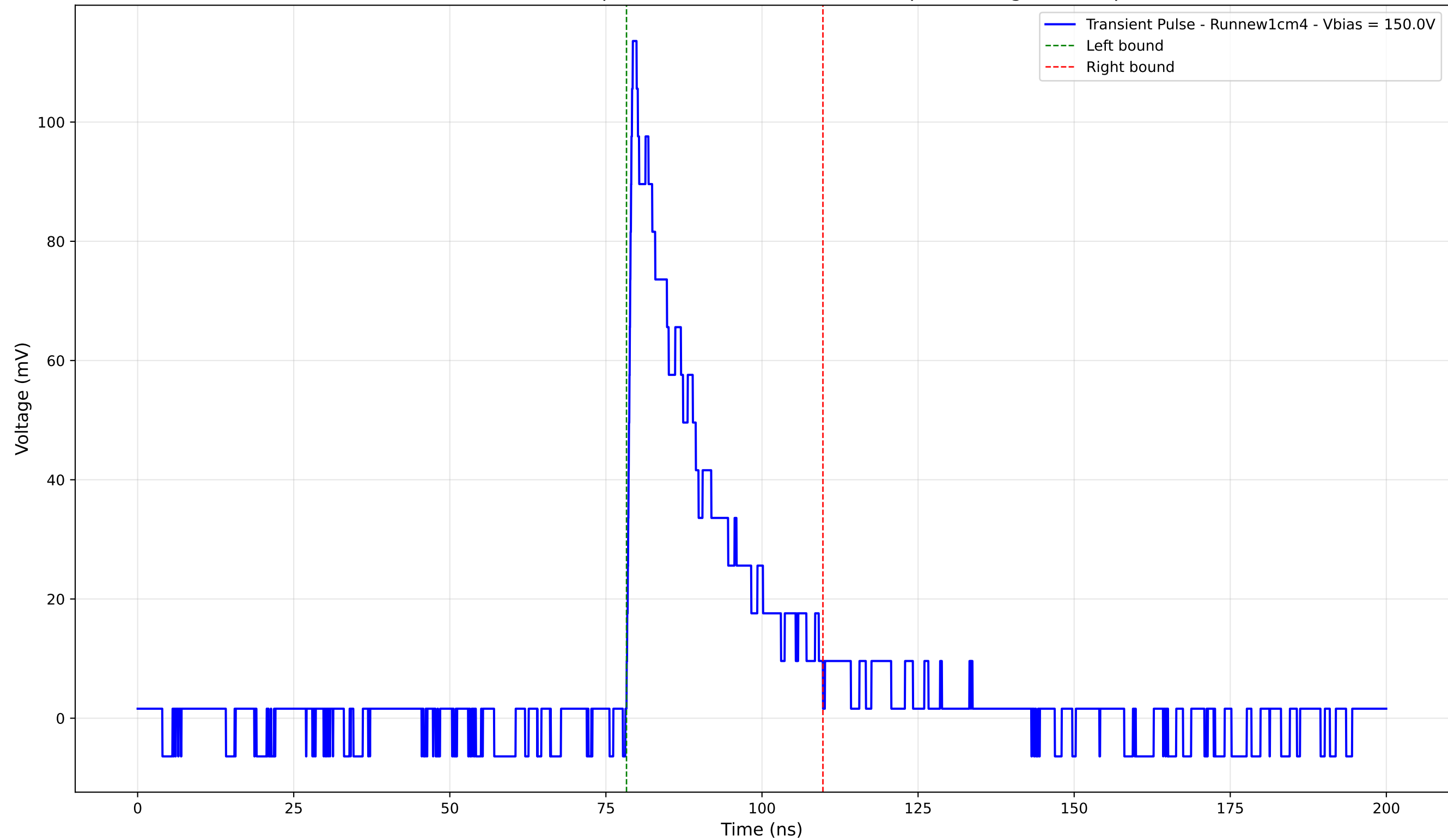
Transient Pulse - Sample: new1cm - Position: 690.0 \mu\text{m} - Charge: 25.53 pC
