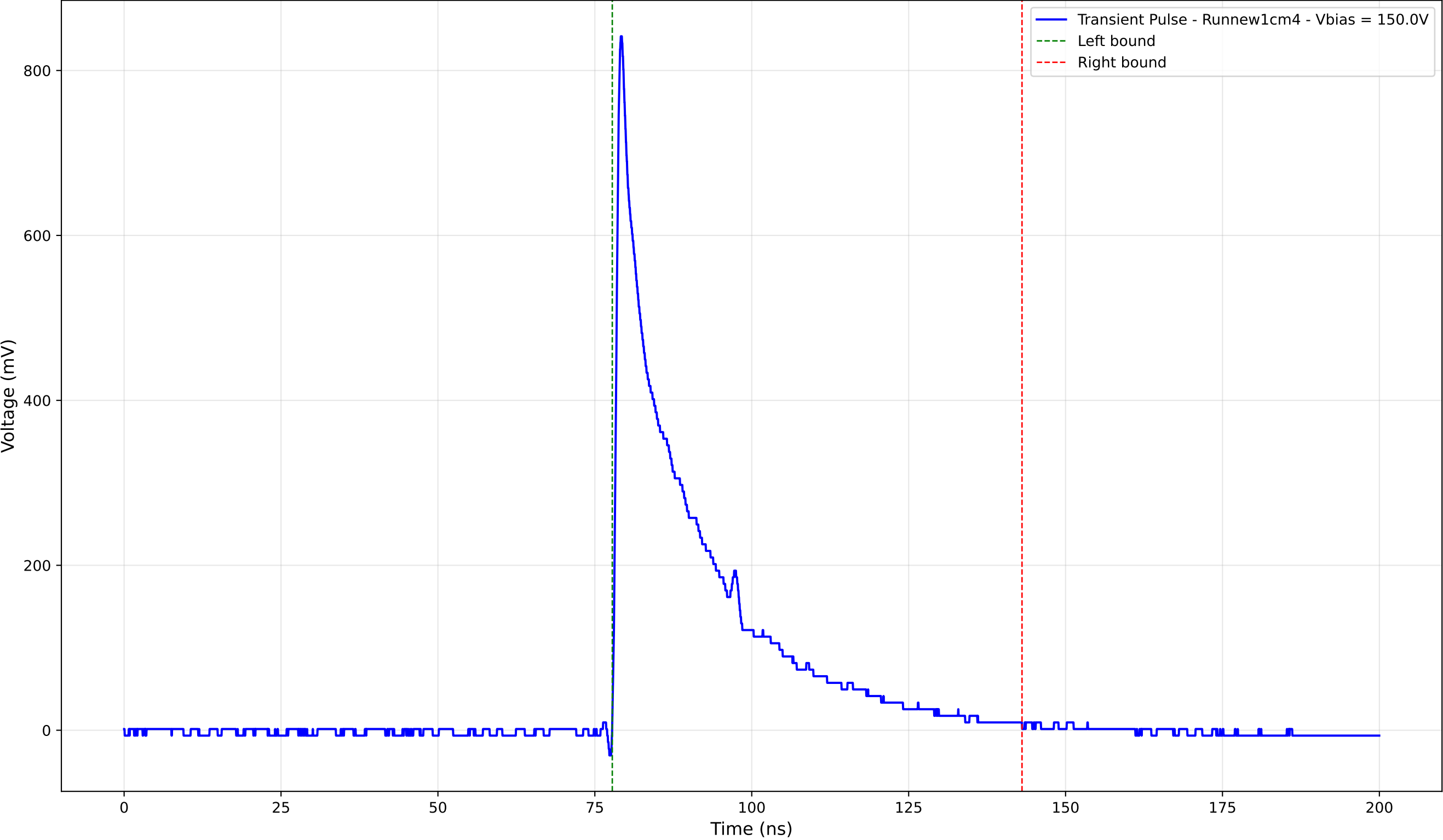
Transient Pulse - Sample: new1cm - Position: 4855.0 \mu\text{m} - Charge: 185.29 pC
