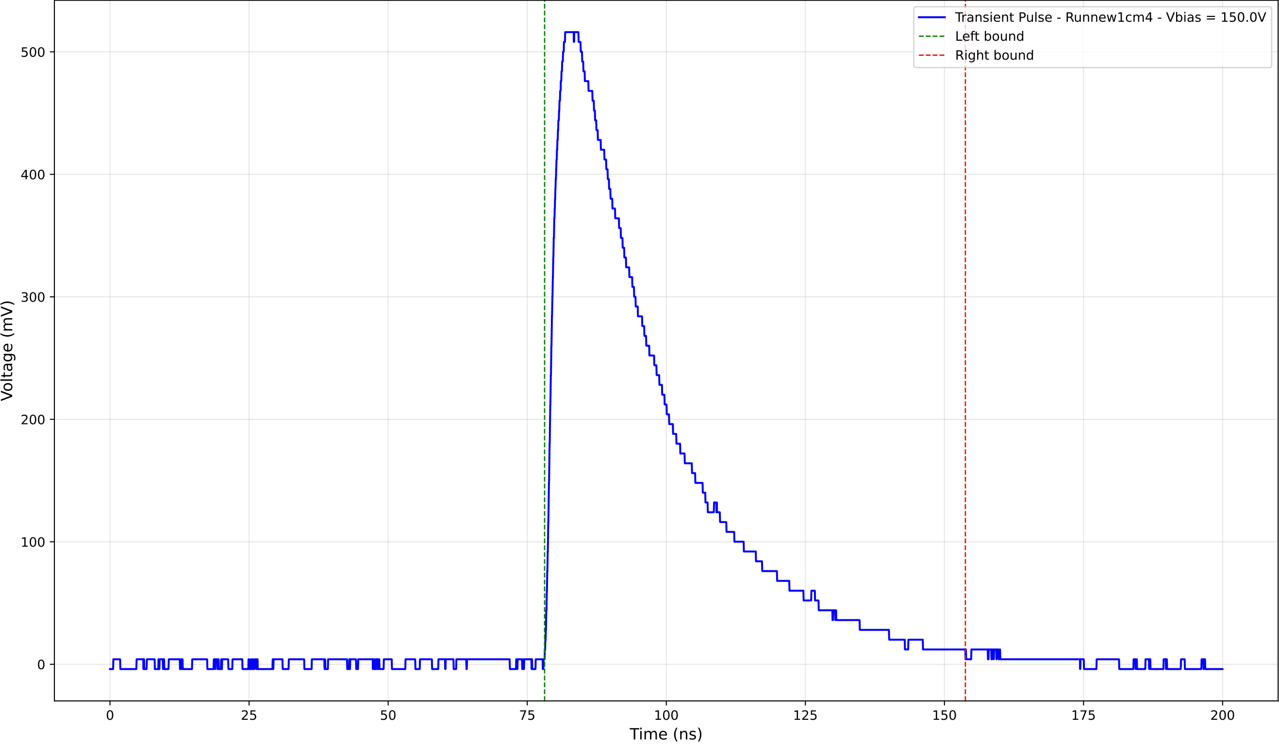
Transient Pulse - Sample: new1cm - Position: 2910.0 \mu\text{m} - Charge: 230.55 pC
