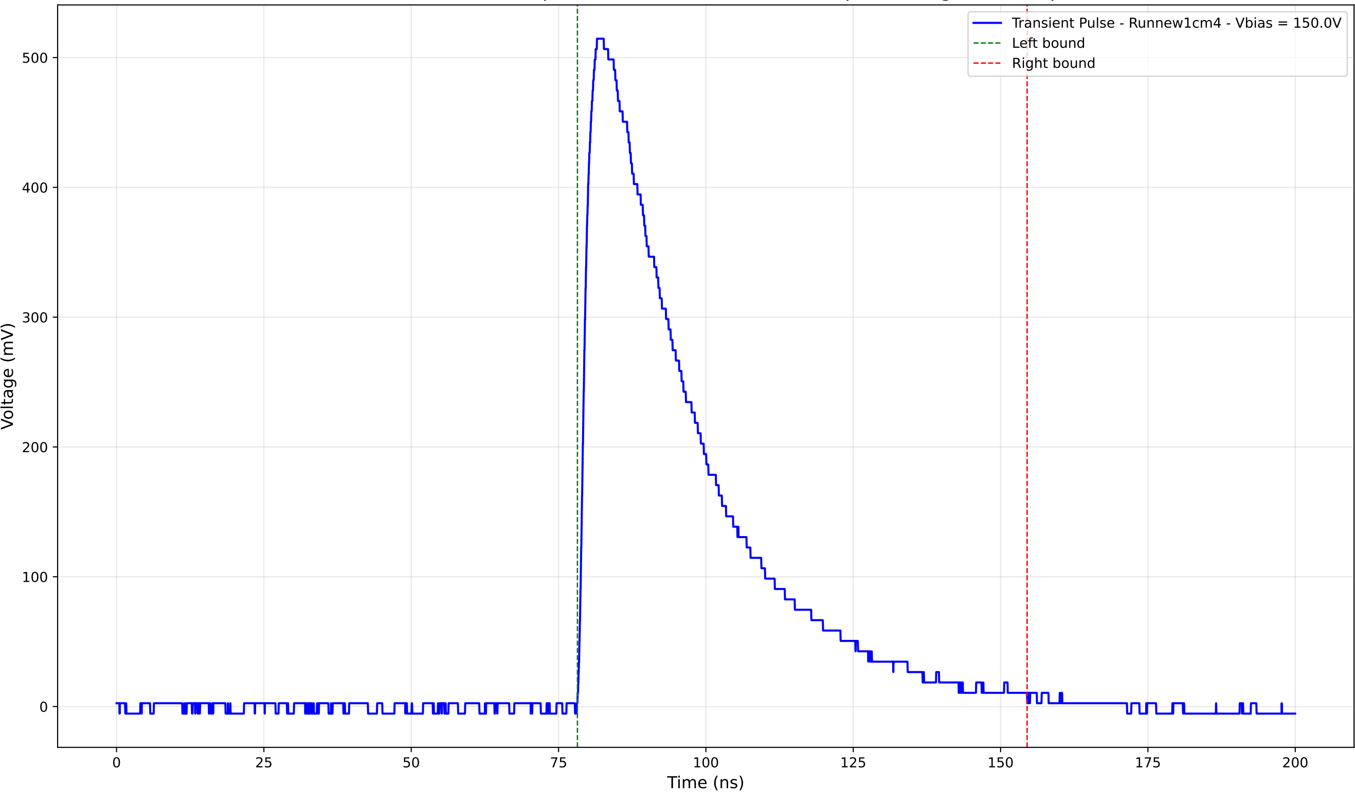
Transient Pulse - Sample: new1cm - Position: 2035.0 \mu\text{m} - Charge: 215.94 pC
