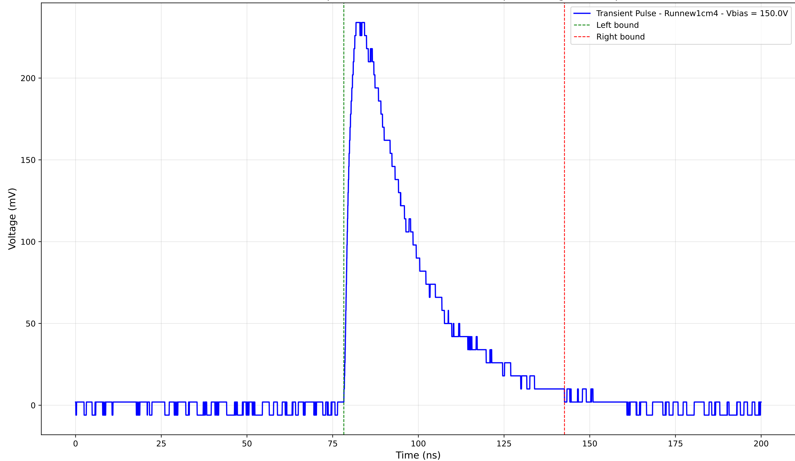
Transient Pulse - Sample: new1cm - Position: 2760.0 \mu\text{m} - Charge: 98.97 pC
