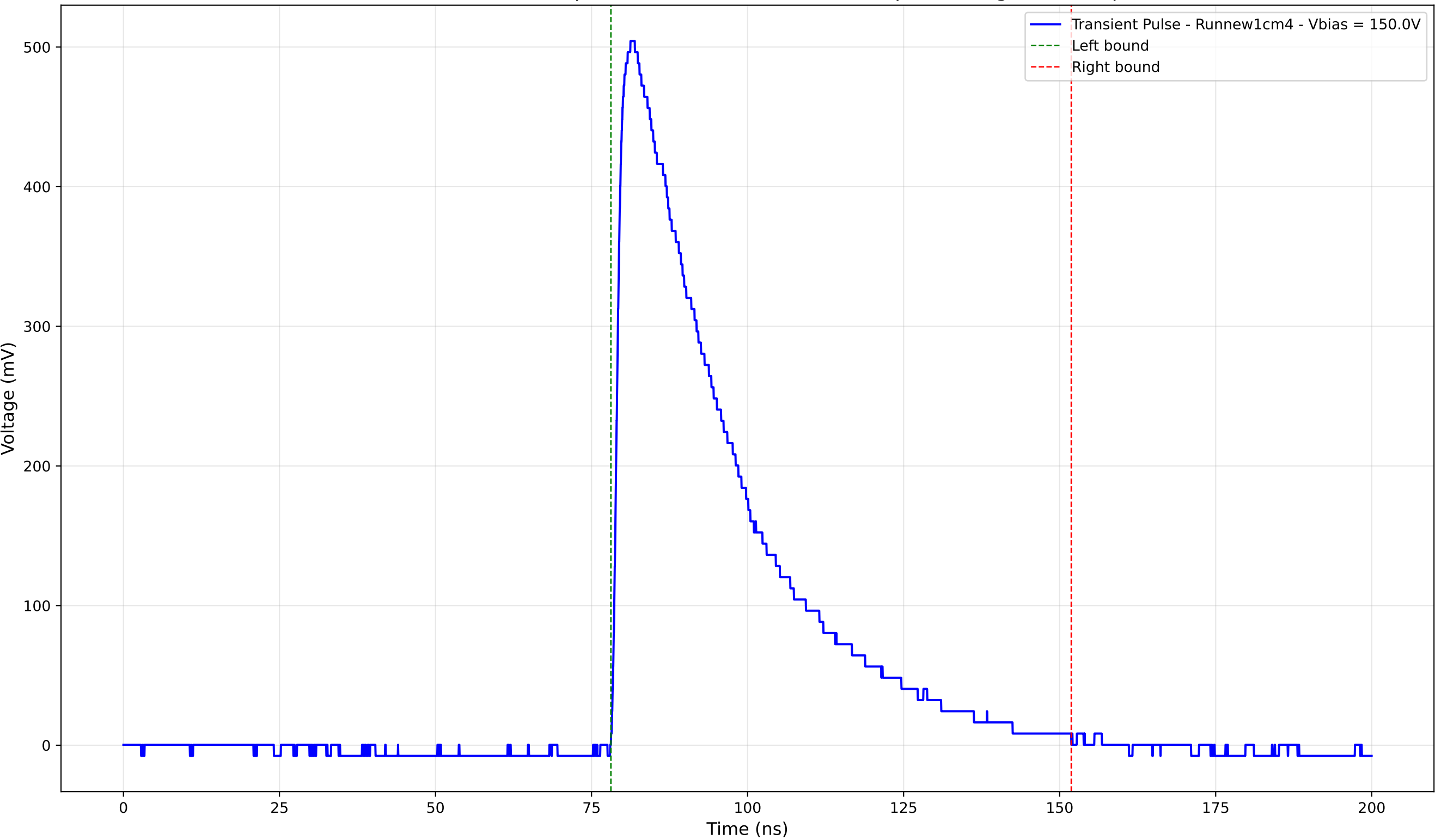
Transient Pulse - Sample: new1cm - Position: 3650.0 \mu\text{m} - Charge: 201.12 pC
