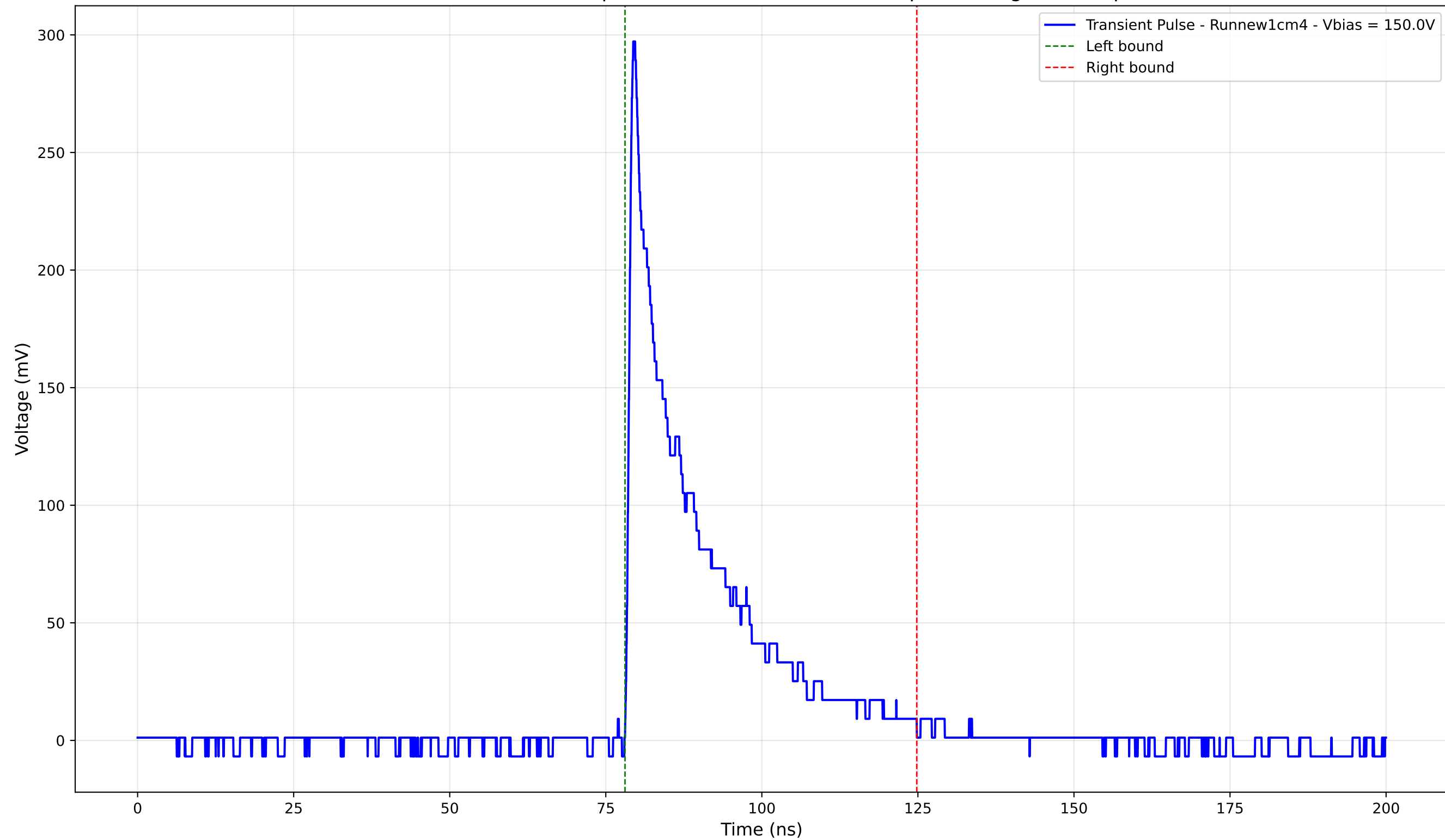
Transient Pulse - Sample: new1cm - Position: 660.0 \mu\text{m} - Charge: 59.63 pC
