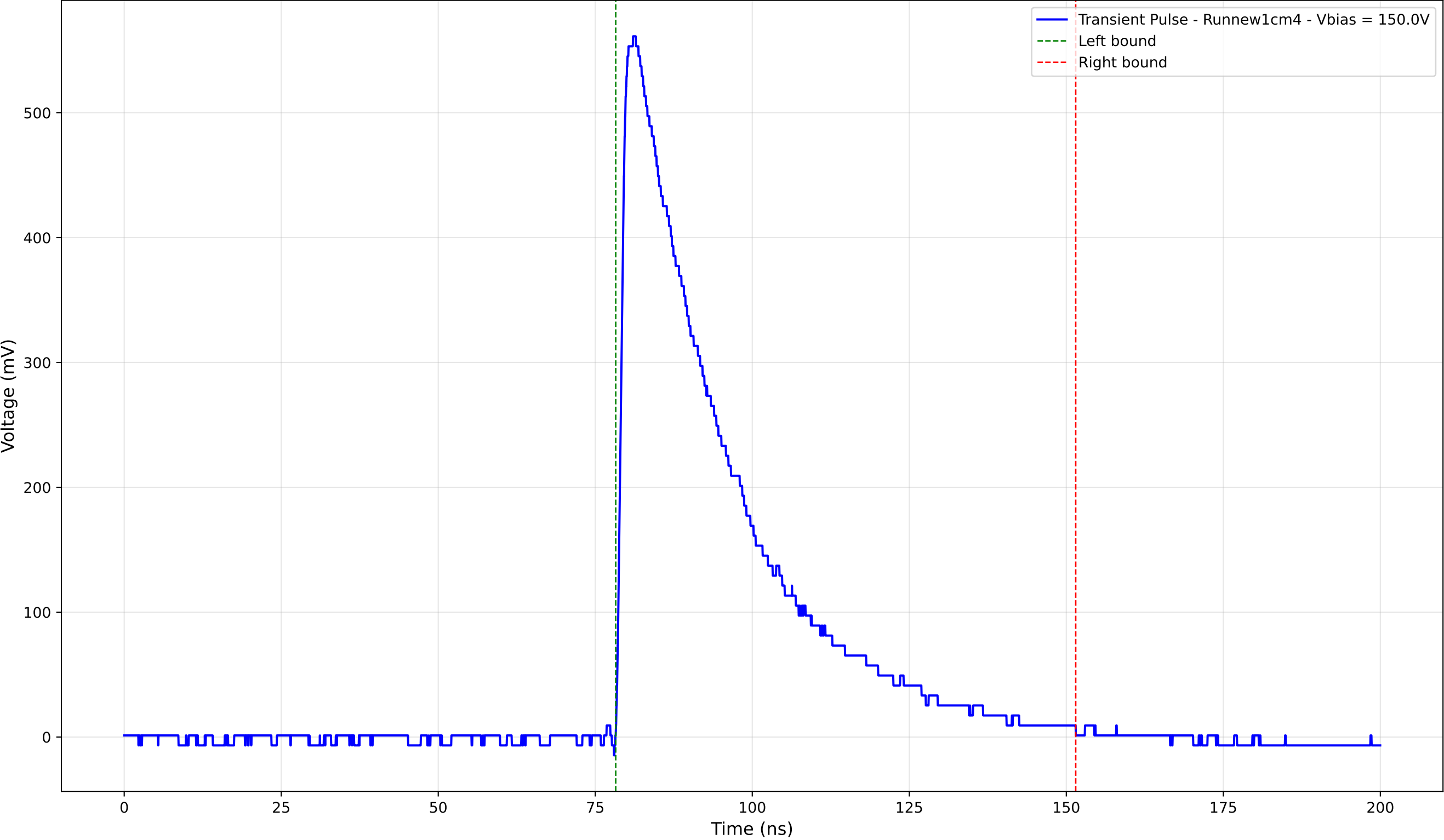
Transient Pulse - Sample: new1cm - Position: 1435.0 \mu\text{m} - Charge: 203.62 pC
