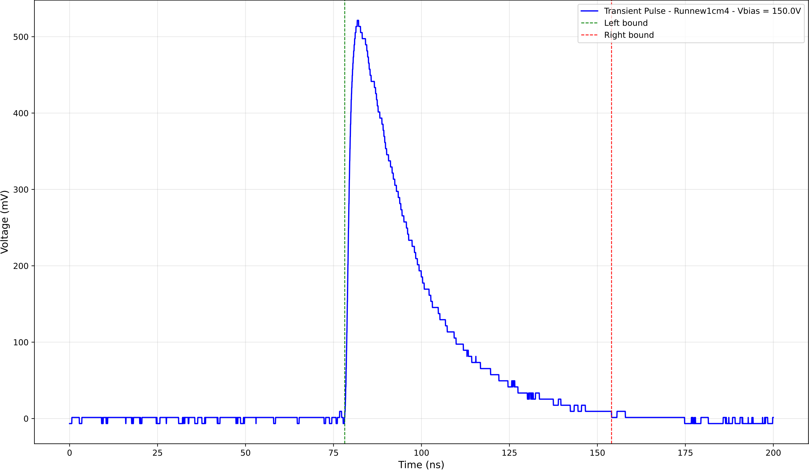
Transient Pulse - Sample: new1cm - Position: 1930.0 \mu\text{m} - Charge: 211.94 pC
