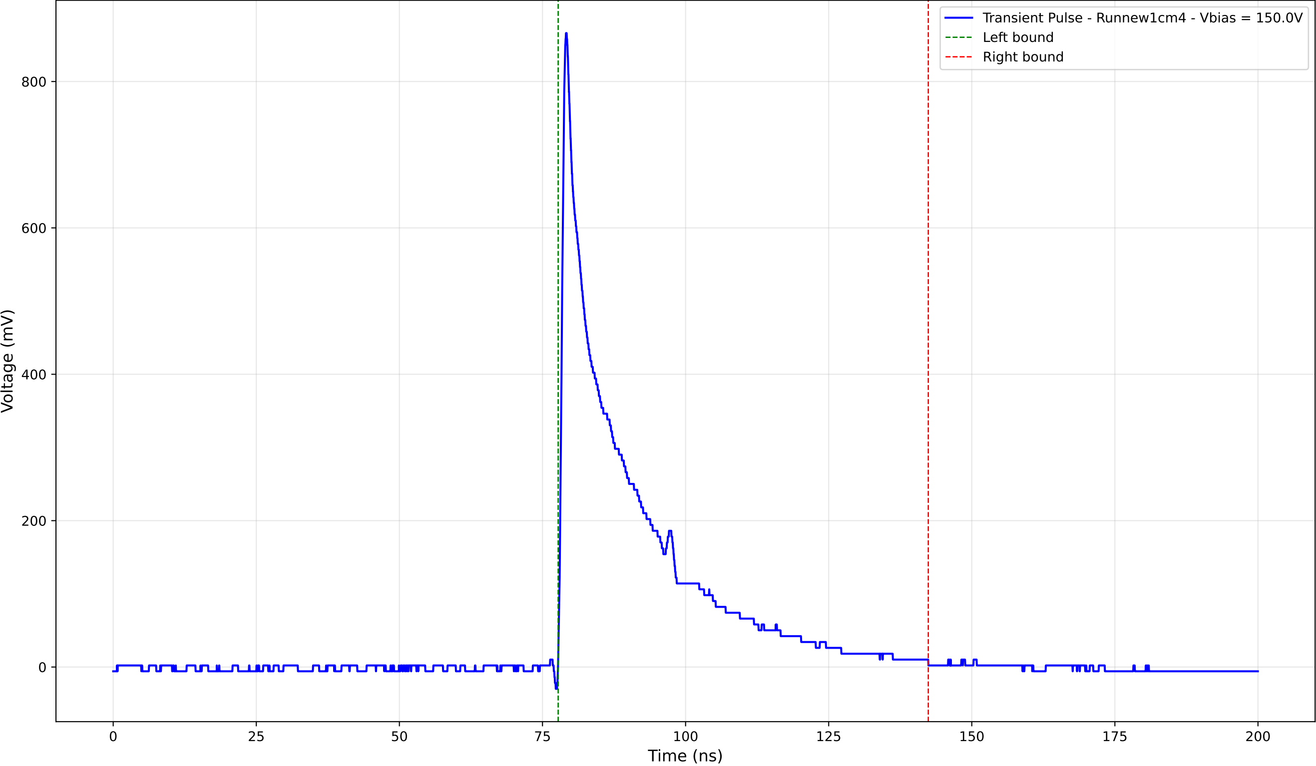
Transient Pulse - Sample: new1cm - Position: 4925.0 \mu\text{m} - Charge: 182.11 pC
