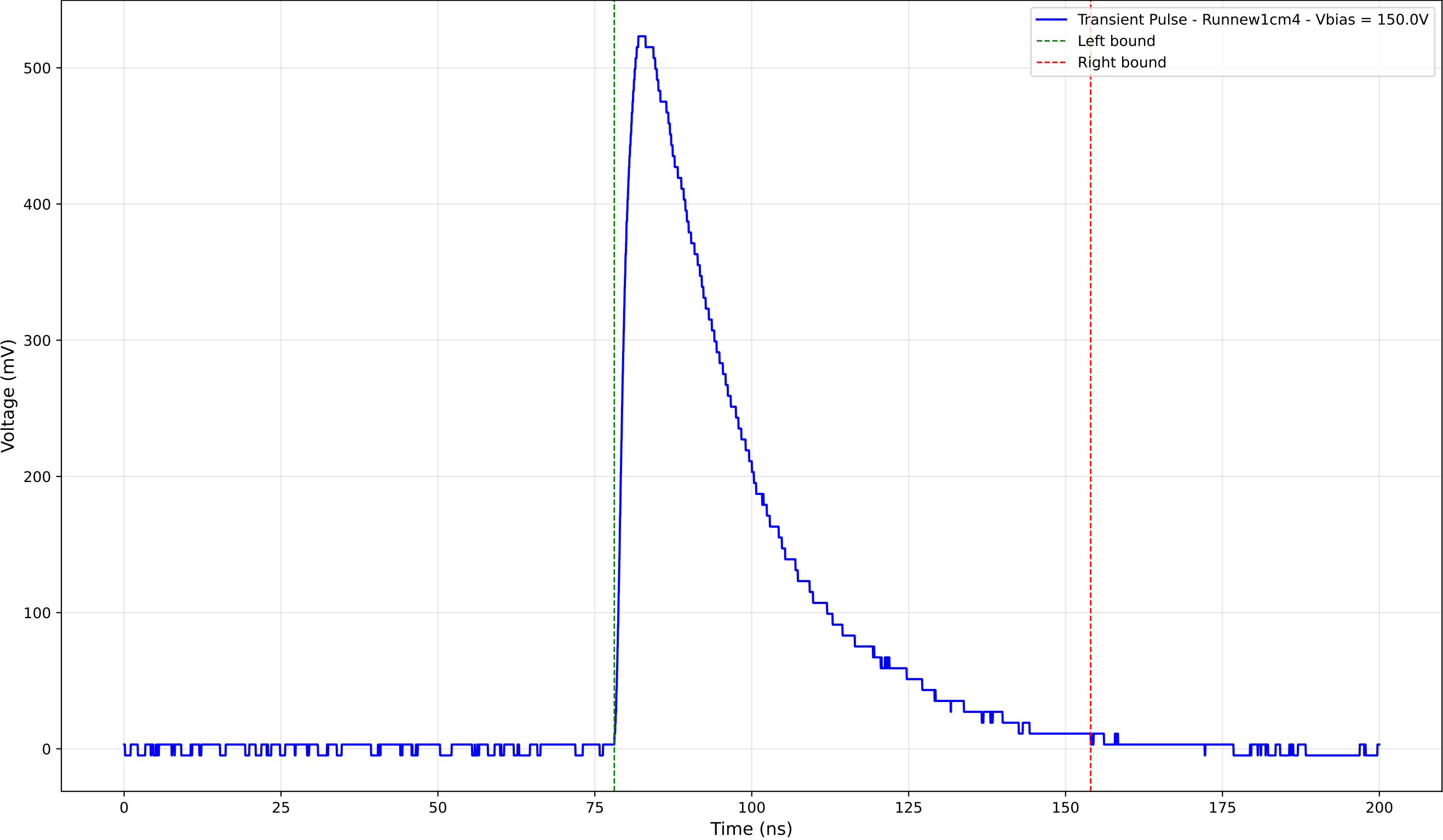
Transient Pulse - Sample: new1cm - Position: 2375.0 \mu\text{m} - Charge: 226.15 pC
