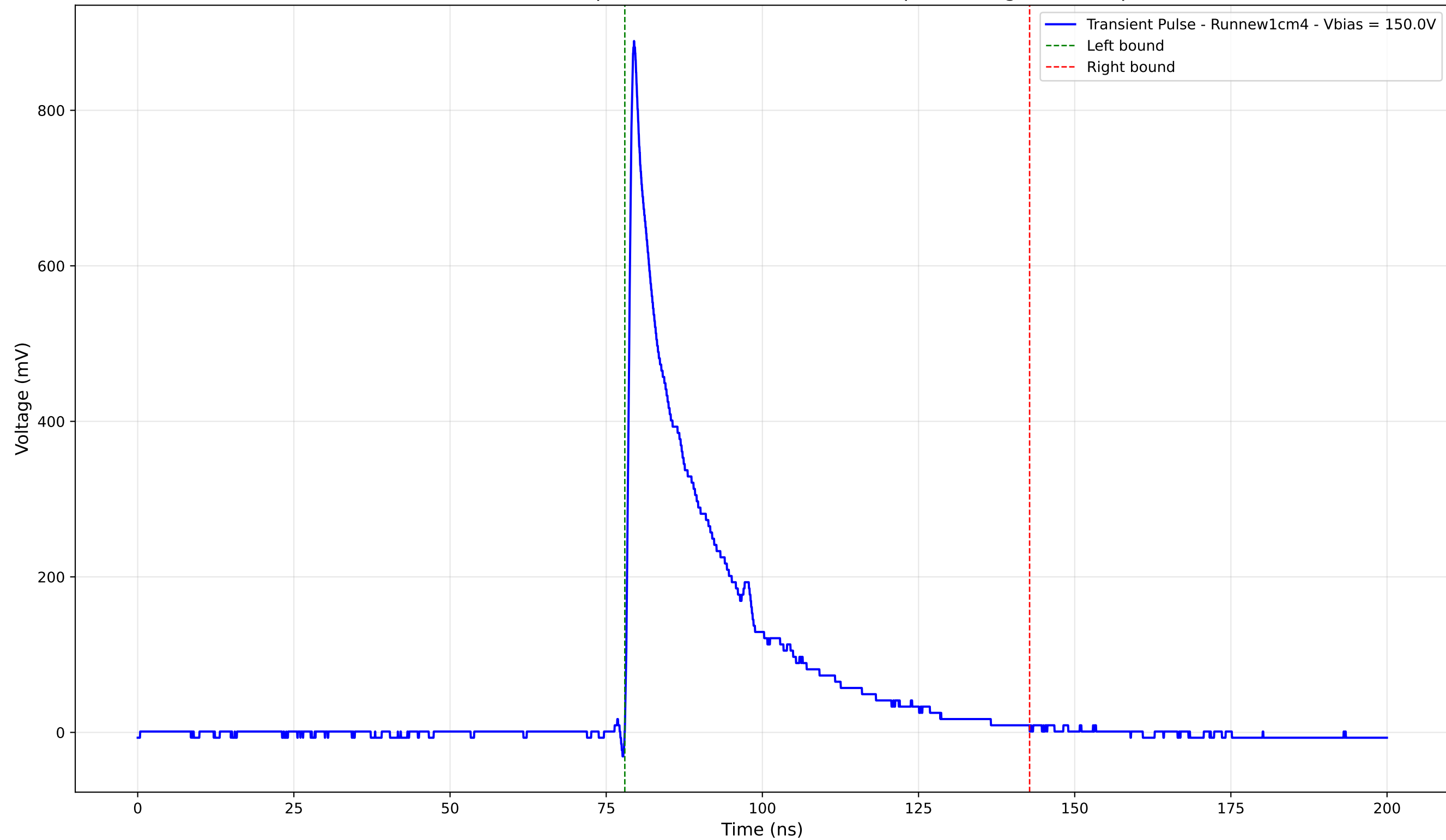
Transient Pulse - Sample: new1cm - Position: 555.0 \mu\text{m} - Charge: 197.66 pC
