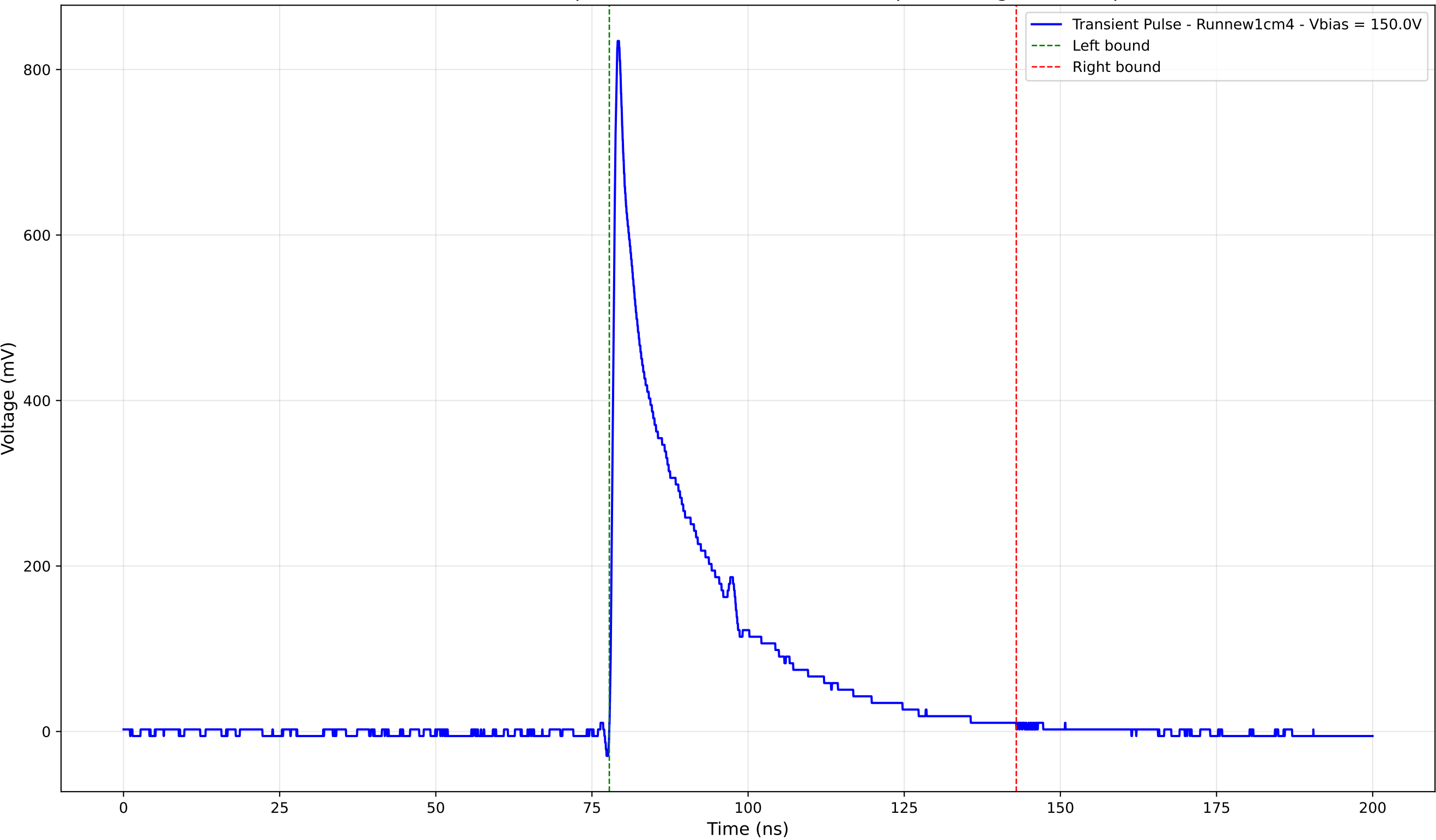
Transient Pulse - Sample: new1cm - Position: 4845.0 \mu\text{m} - Charge: 183.92 pC
