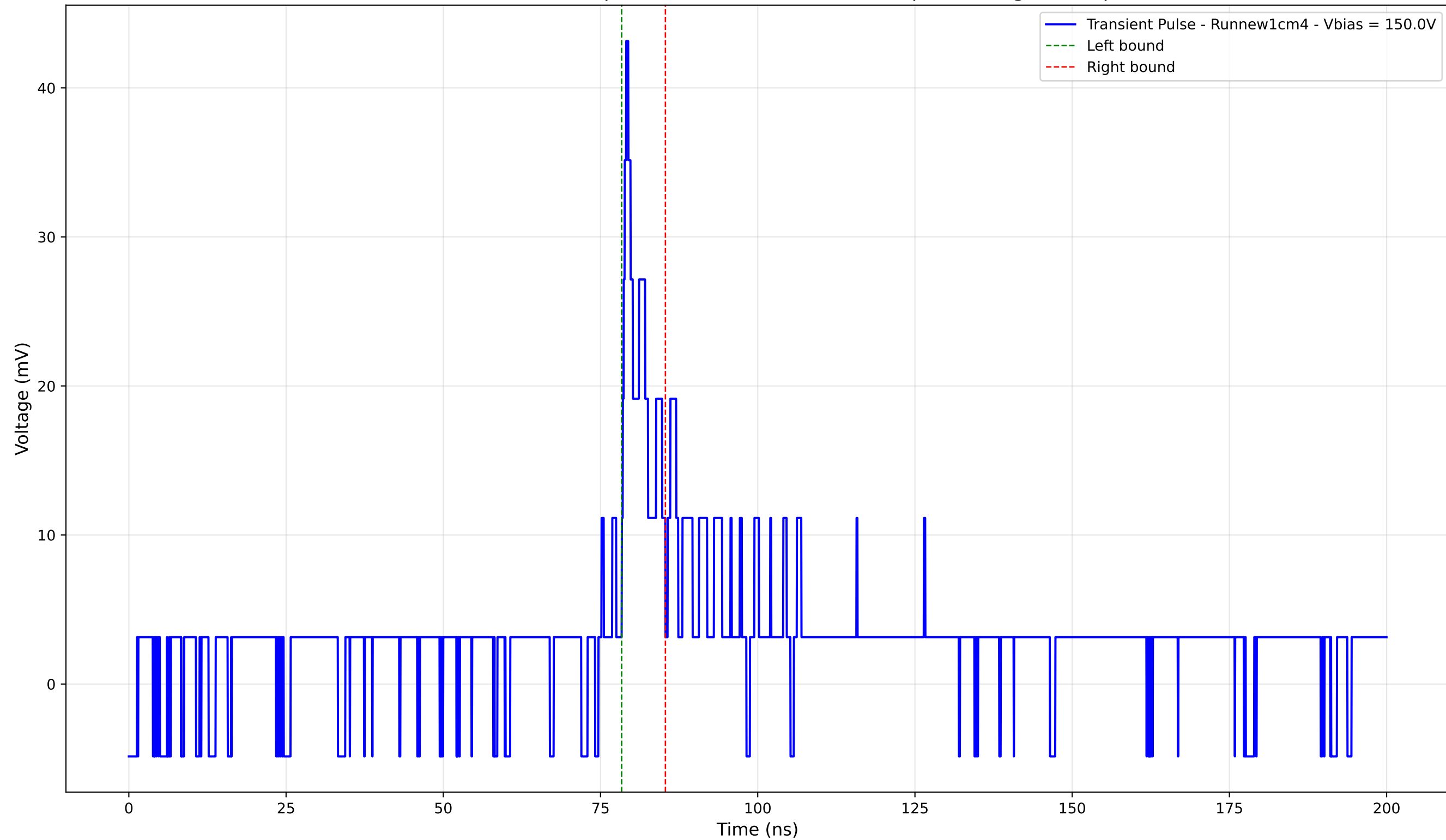
Transient Pulse - Sample: new1cm - Position: 155.0 \mu\text{m} - Charge: 2.94 pC
