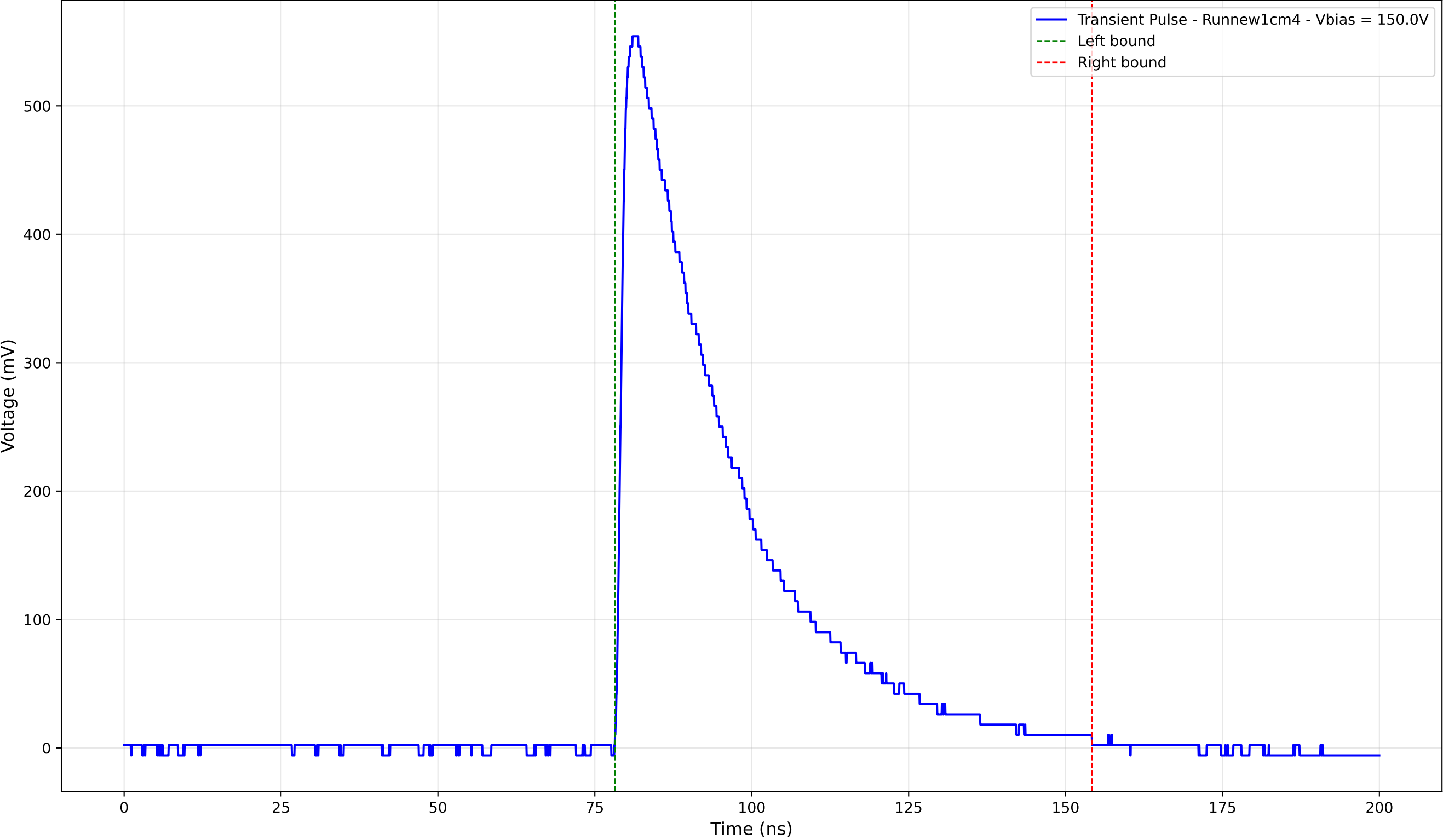
Transient Pulse - Sample: new1cm - Position: 1560.0 \mu\text{m} - Charge: 210.94 pC
