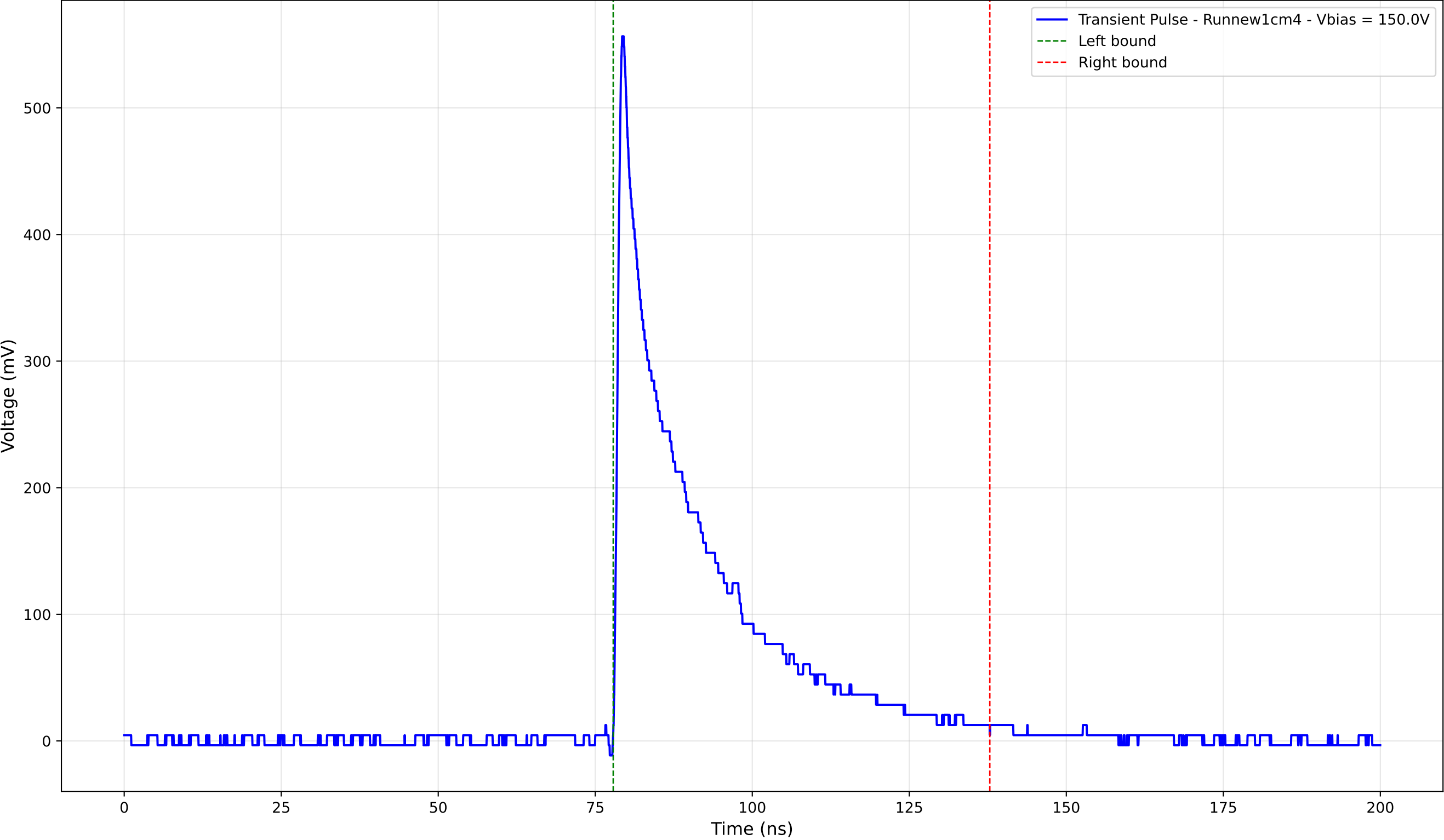
Transient Pulse - Sample: new1cm - Position: 4680.0 \mu\text{m} - Charge: 129.47 pC
