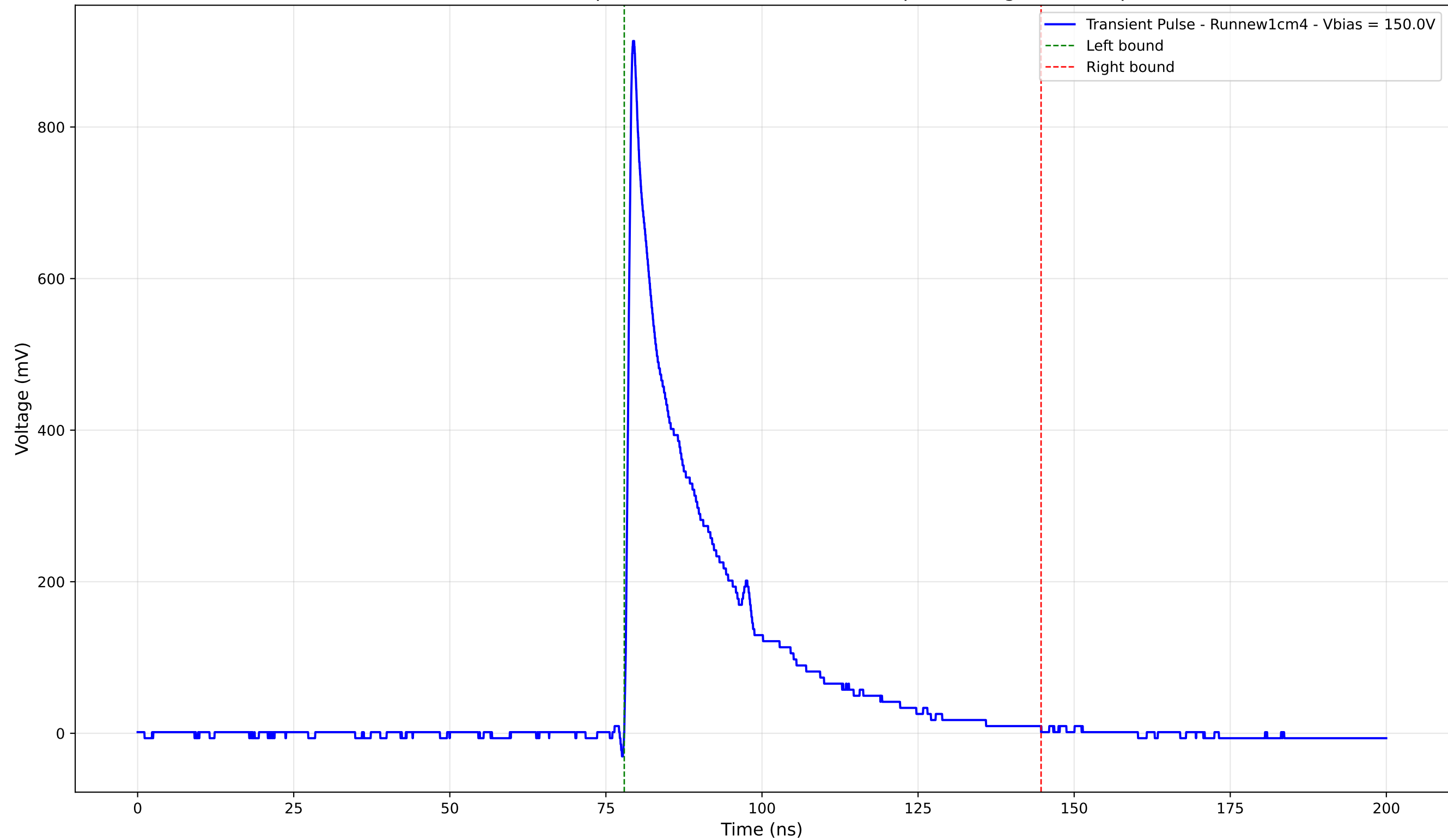
Transient Pulse - Sample: new1cm - Position: 495.0 \mu\text{m} - Charge: 200.40 pC
