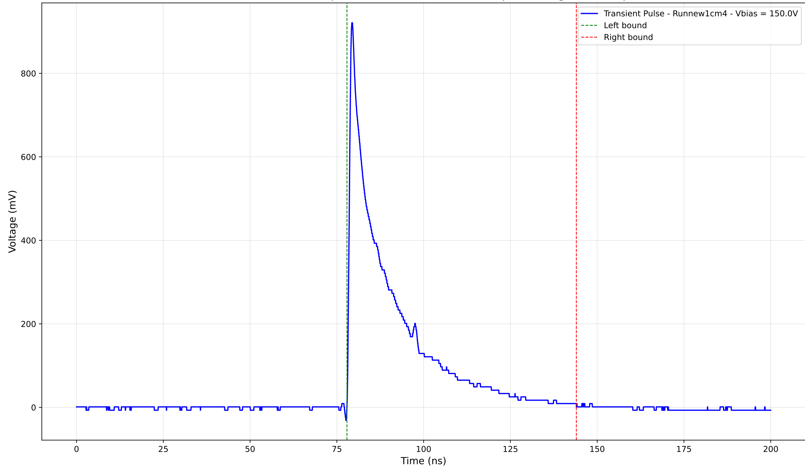
Transient Pulse - Sample: new1cm - Position: 475.0 \mu\text{m} - Charge: 199.68 pC
