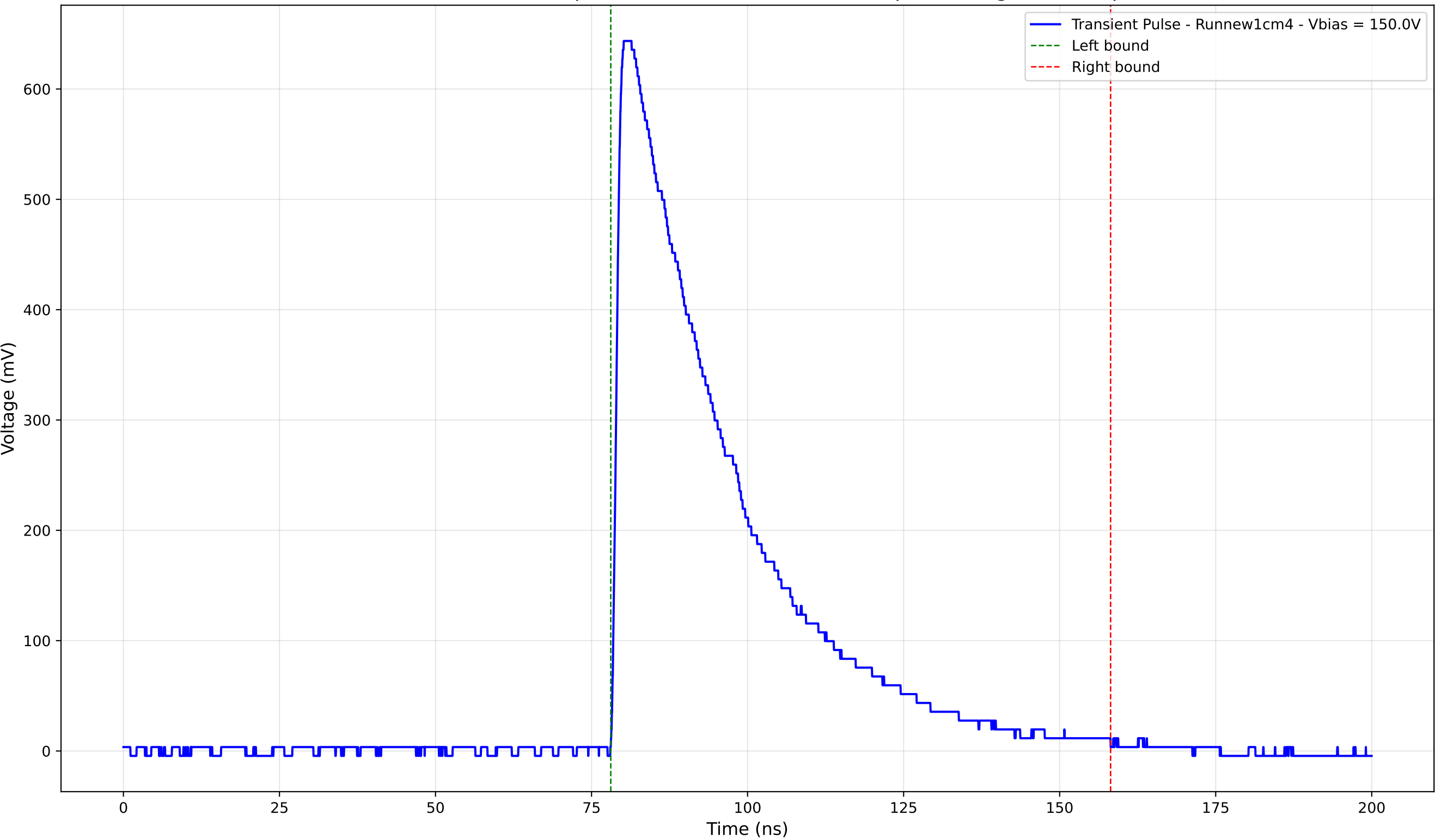
Transient Pulse - Sample: new1cm - Position: 3865.0 \mu\text{m} - Charge: 252.82 pC
