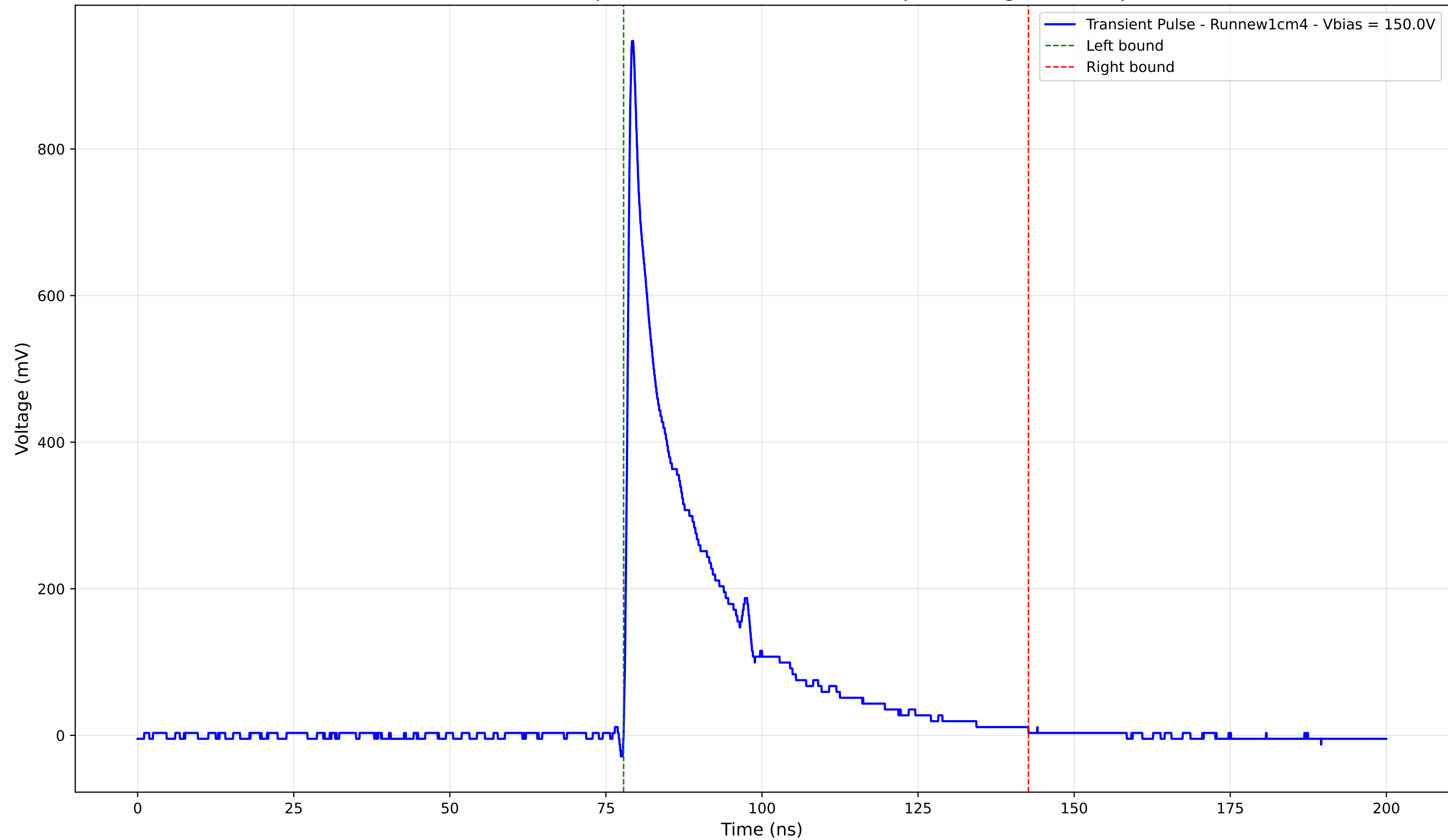
Transient Pulse - Sample: new1cm - Position: 325.0 \mu\text{m} - Charge: 187.78 pC
