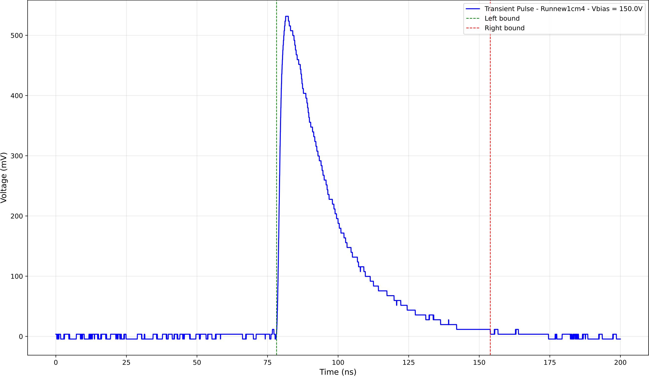
Transient Pulse - Sample: new1cm - Position: 1875.0 \mu\text{m} - Charge: 216.41 pC
