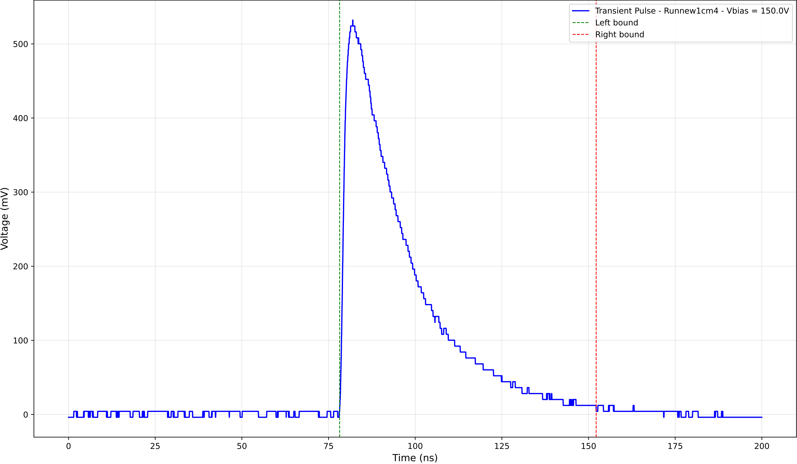
Transient Pulse - Sample: new1cm - Position: 1890.0 \mu\text{m} - Charge: 216.21 pC
