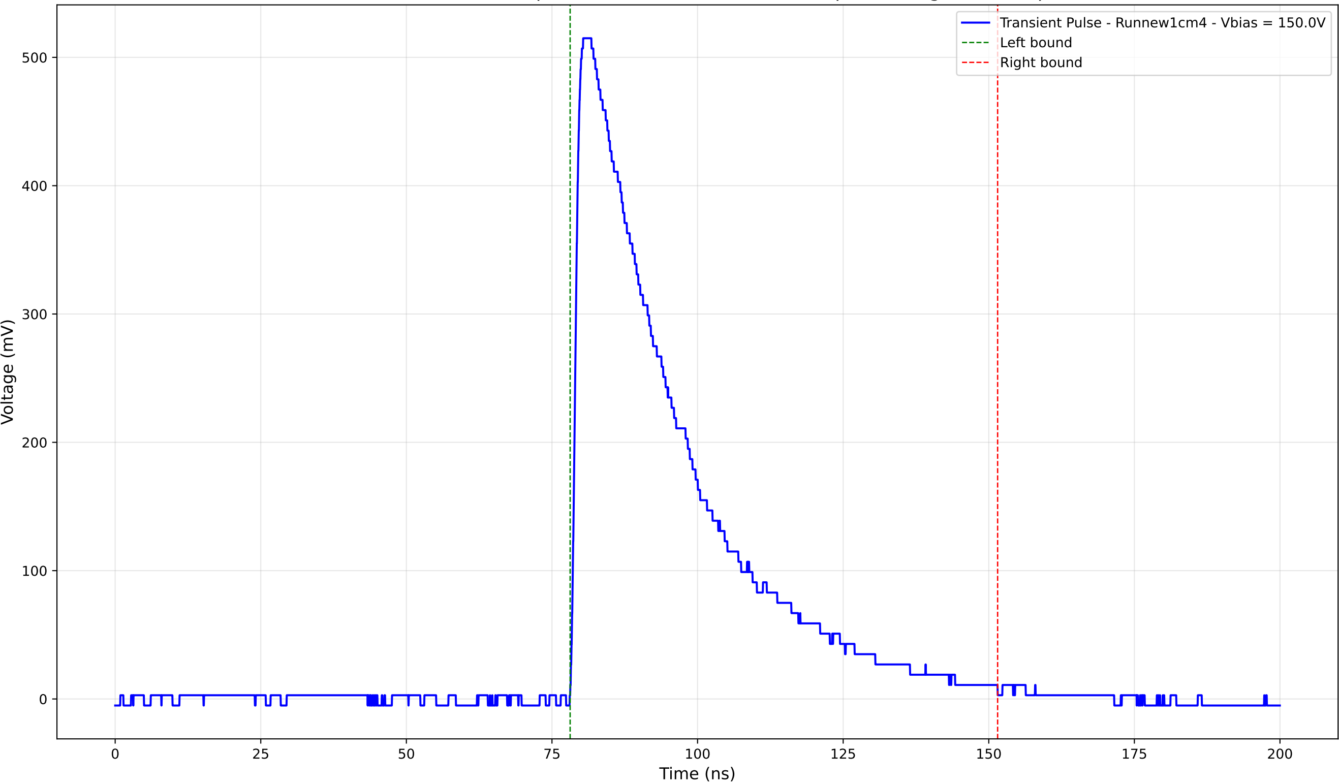
Transient Pulse - Sample: new1cm - Position: 3805.0 \mu\text{m} - Charge: 201.38 pC
