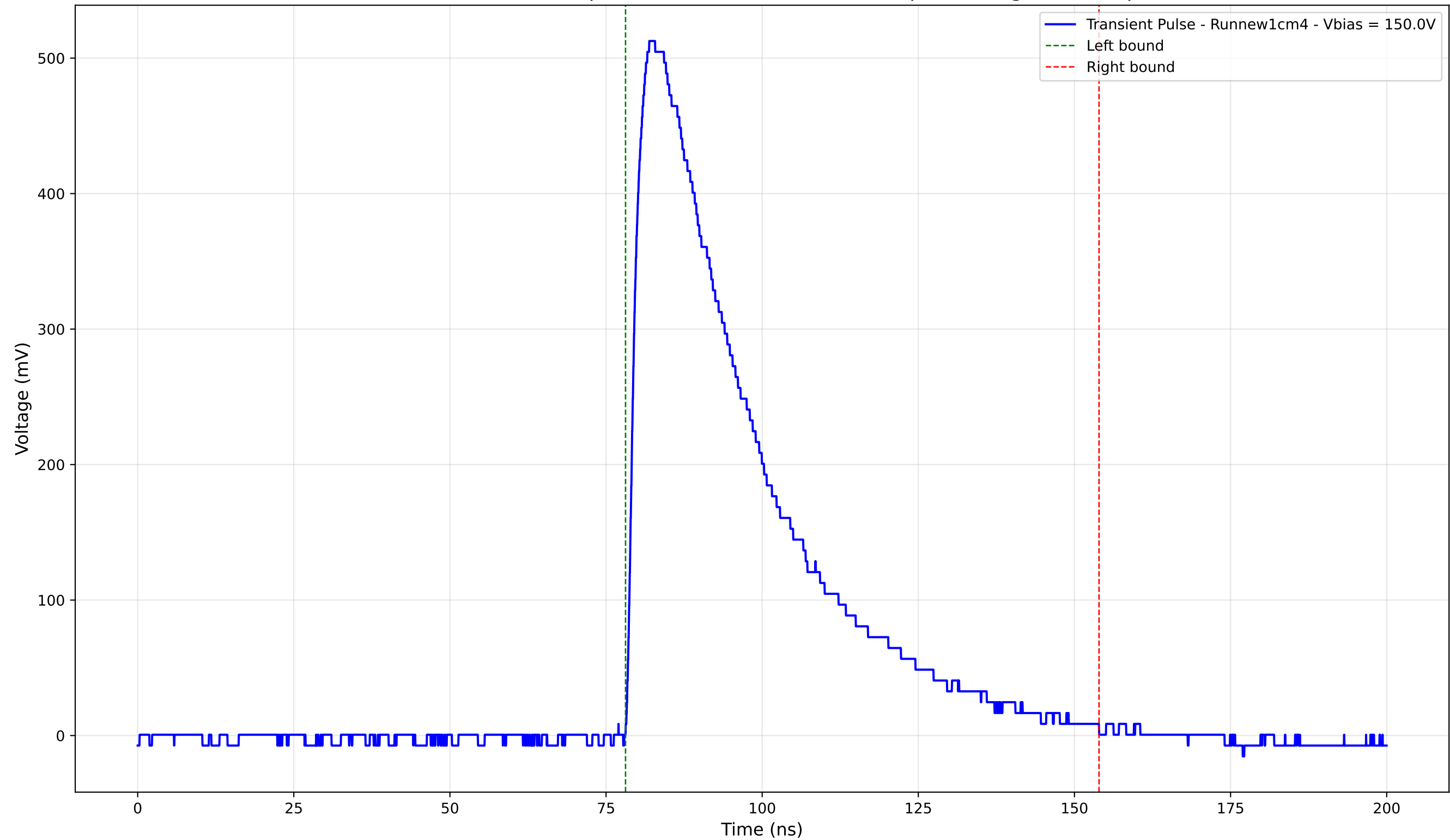
Transient Pulse - Sample: new1cm - Position: 3030.0 \mu\text{m} - Charge: 223.16 pC
