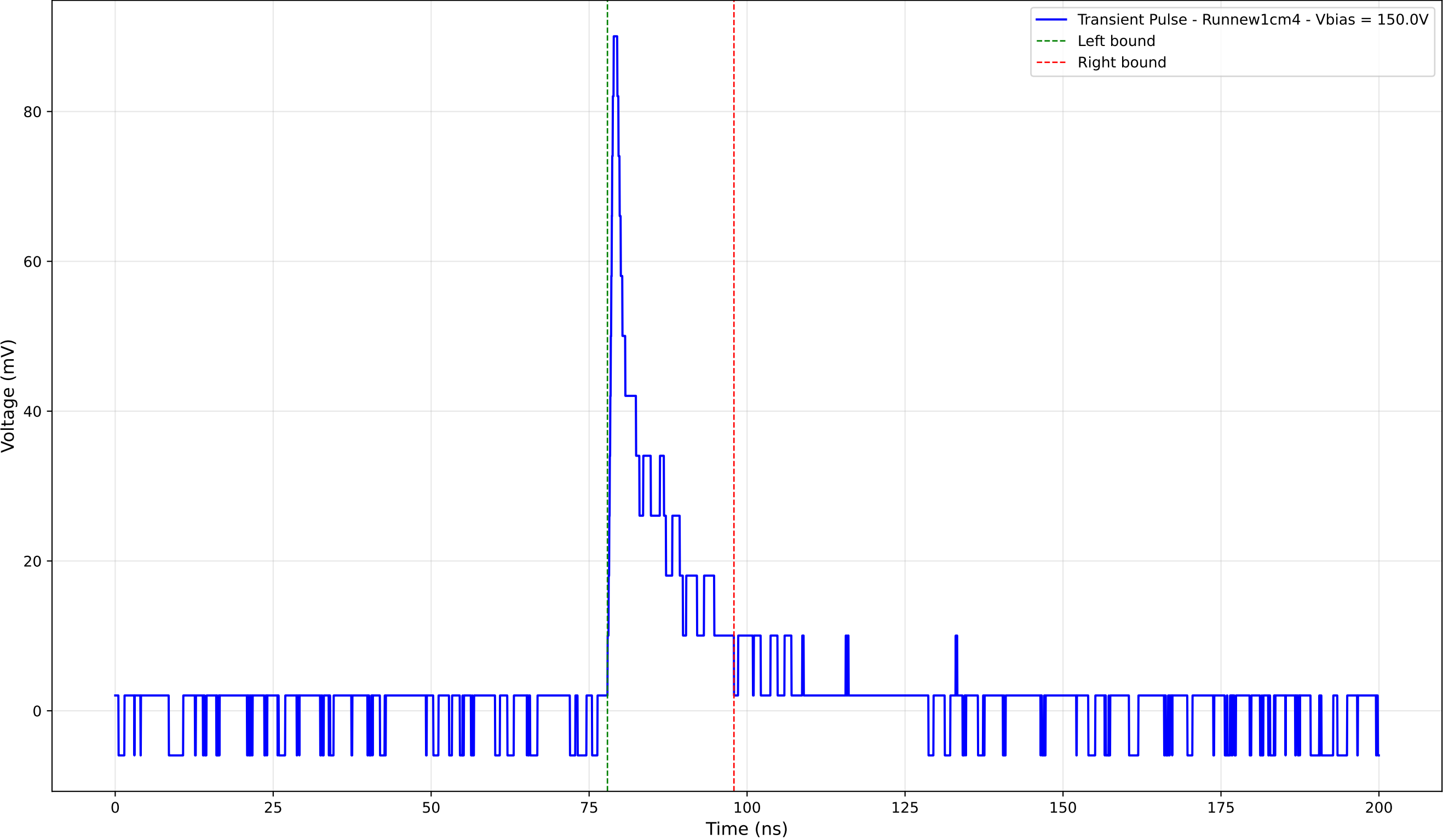
Transient Pulse - Sample: new1cm - Position: 5070.0 \mu\text{m} - Charge: 11.06 pC
