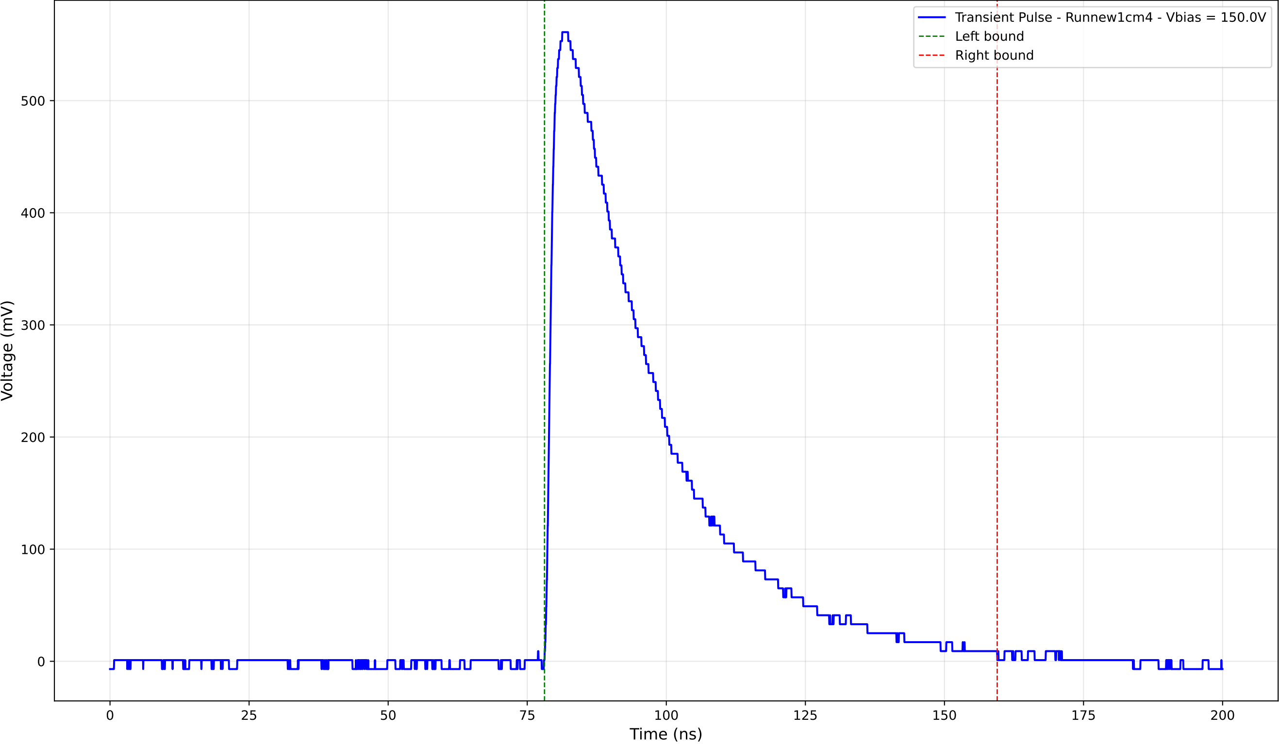
Transient Pulse - Sample: new1cm - Position: 3495.0 \mu\text{m} - Charge: 237.95 pC
