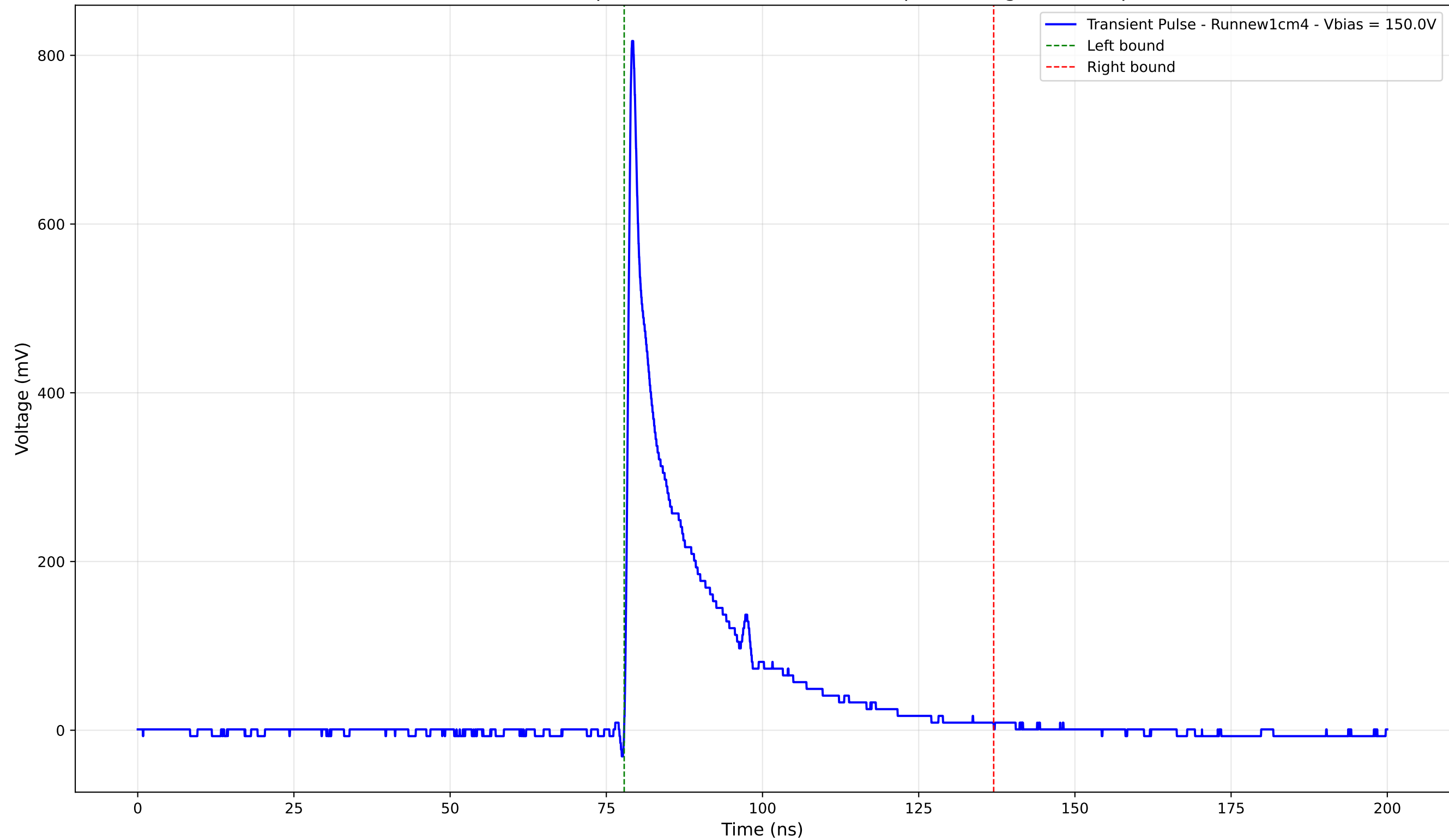
Transient Pulse - Sample: new1cm - Position: 265.0 \mu\text{m} - Charge: 135.02 pC
