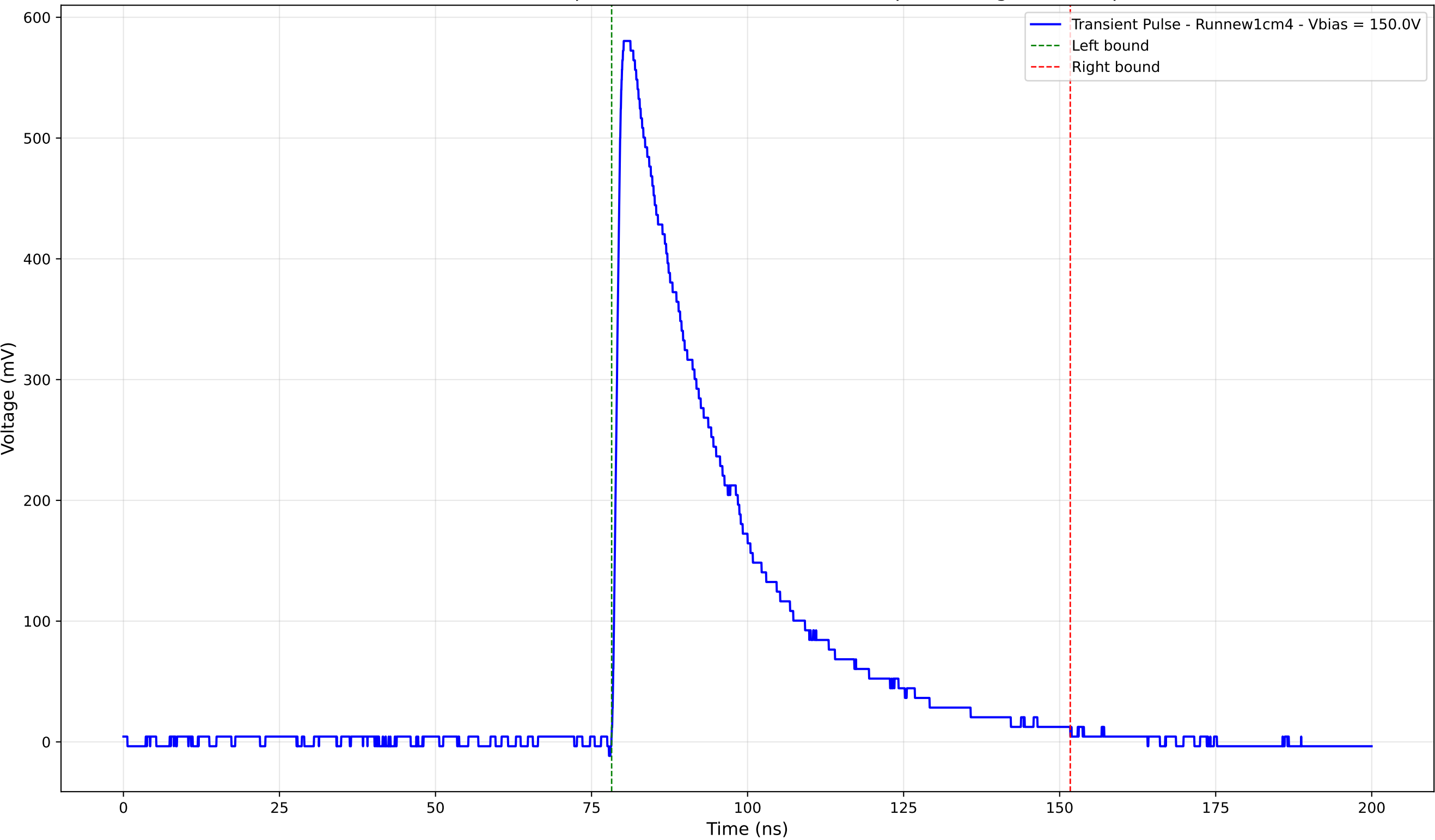
Transient Pulse - Sample: new1cm - Position: 1335.0 \mu\text{m} - Charge: 208.40 pC
