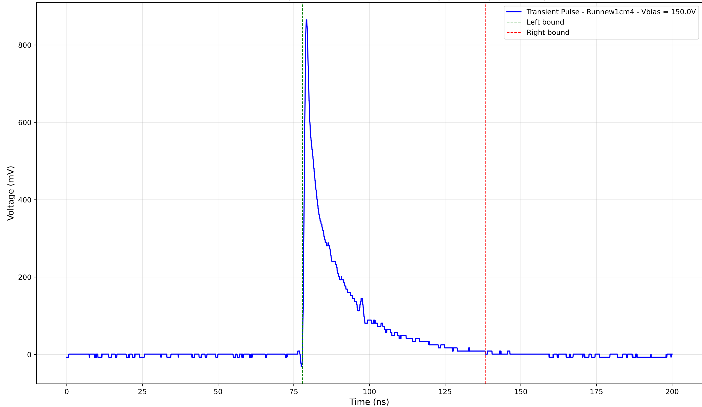
Transient Pulse - Sample: new1cm - Position: 275.0 \mu\text{m} - Charge: 149.43 pC
