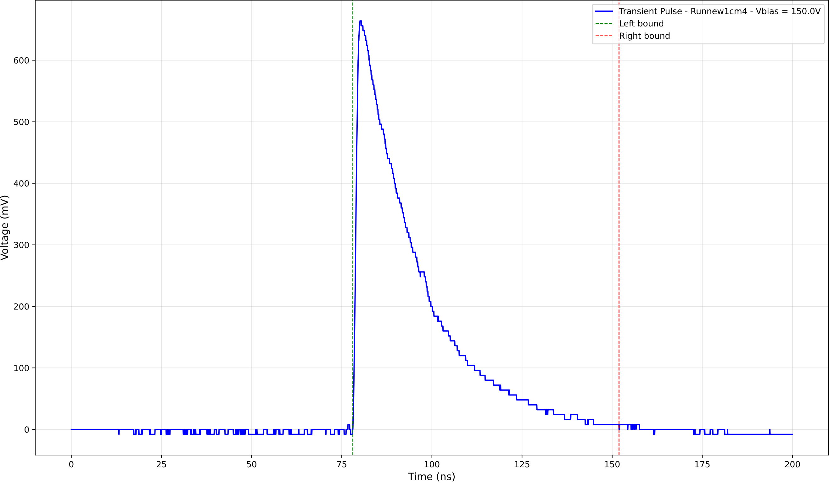
Transient Pulse - Sample: new1cm - Position: 3995.0 \mu\text{m} - Charge: 242.78 pC
