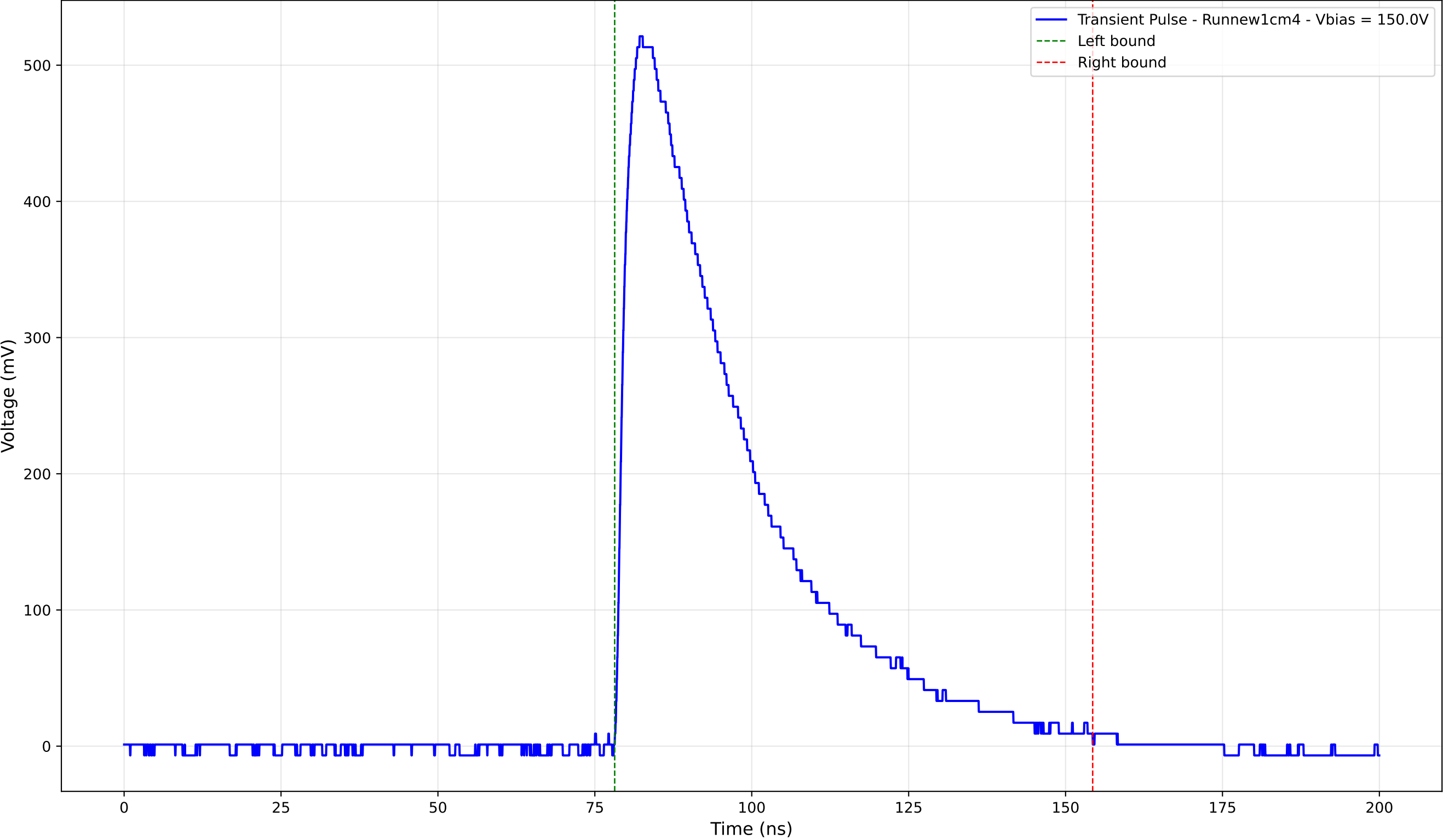
Transient Pulse - Sample: new1cm - Position: 2945.0 \mu\text{m} - Charge: 227.47 pC
