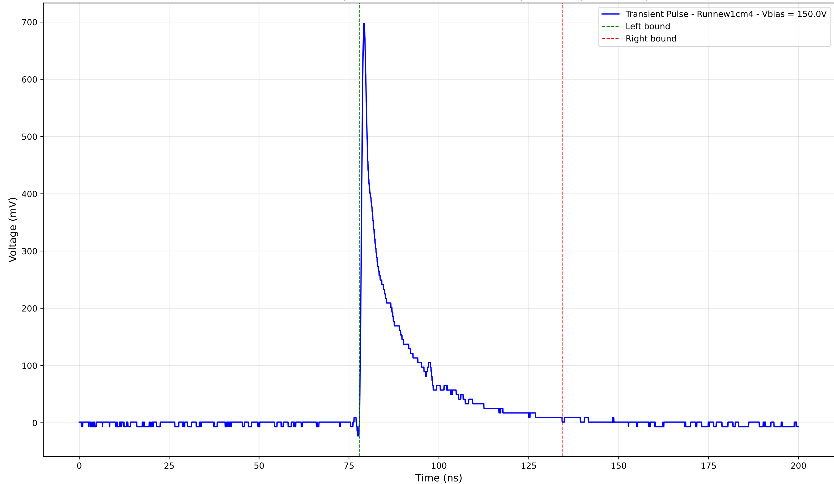
Transient Pulse - Sample: new1cm - Position: 250.0 \mu\text{m} - Charge: 109.63 pC
