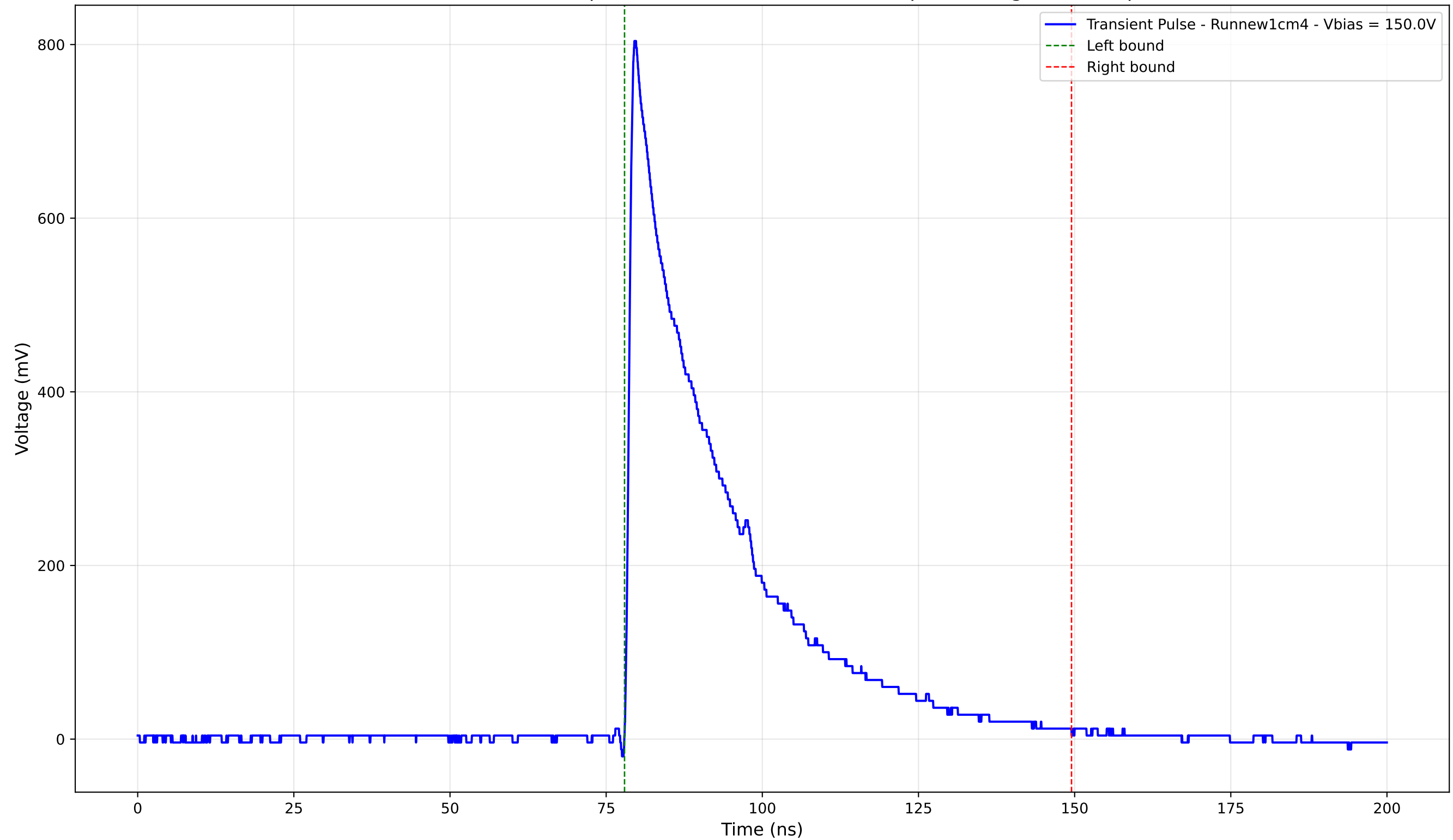
Transient Pulse - Sample: new1cm - Position: 4420.0 \mu\text{m} - Charge: 243.07 pC
