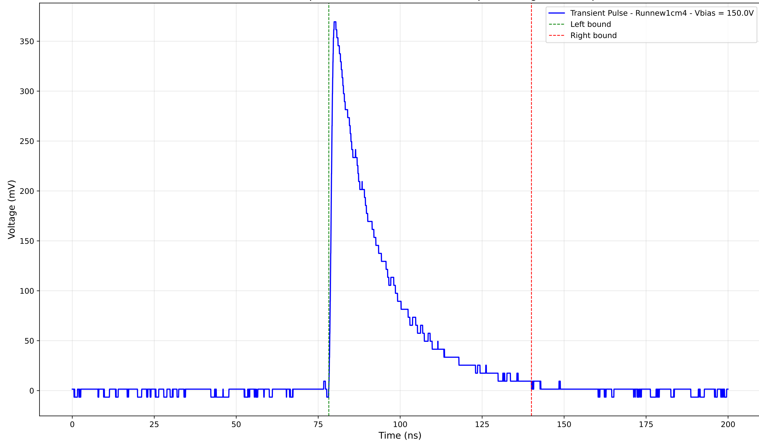
Transient Pulse - Sample: new1cm - Position: 1145.0 \mu\text{m} - Charge: 112.47 pC
