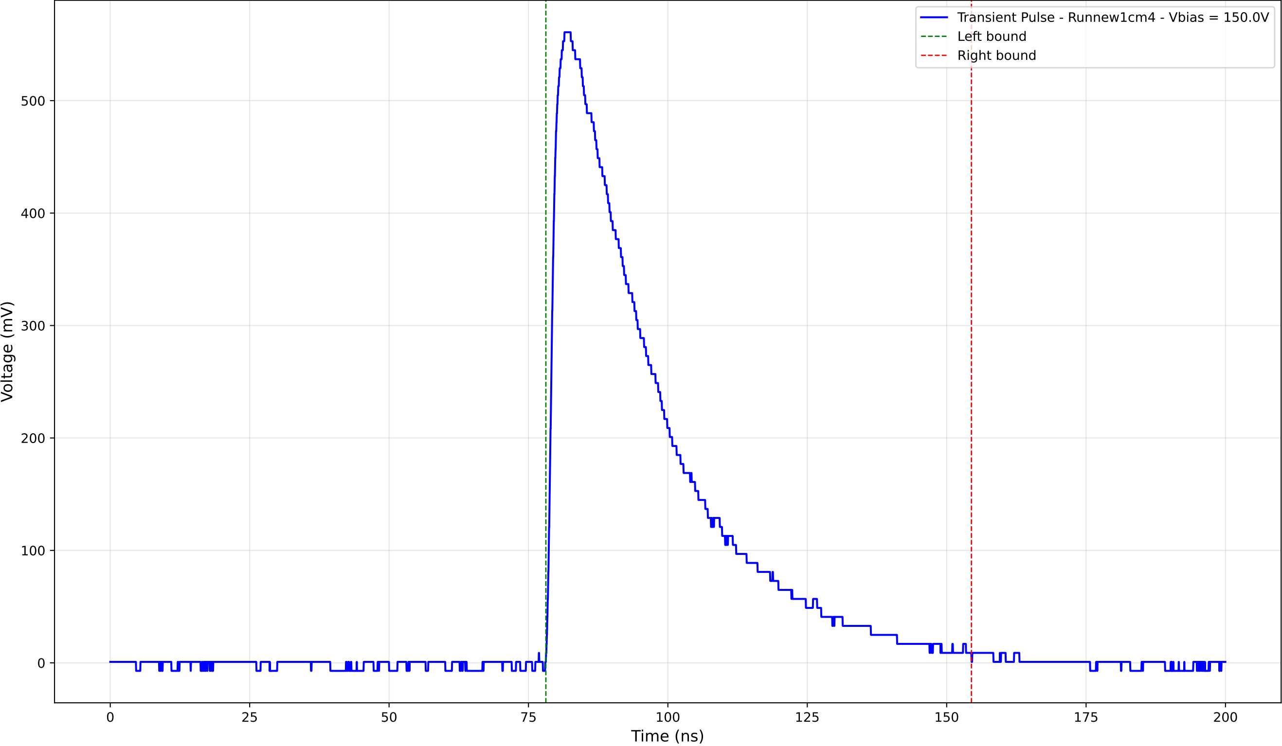
Transient Pulse - Sample: new1cm - Position: 3425.0 \mu\text{m} - Charge: 238.24 pC
