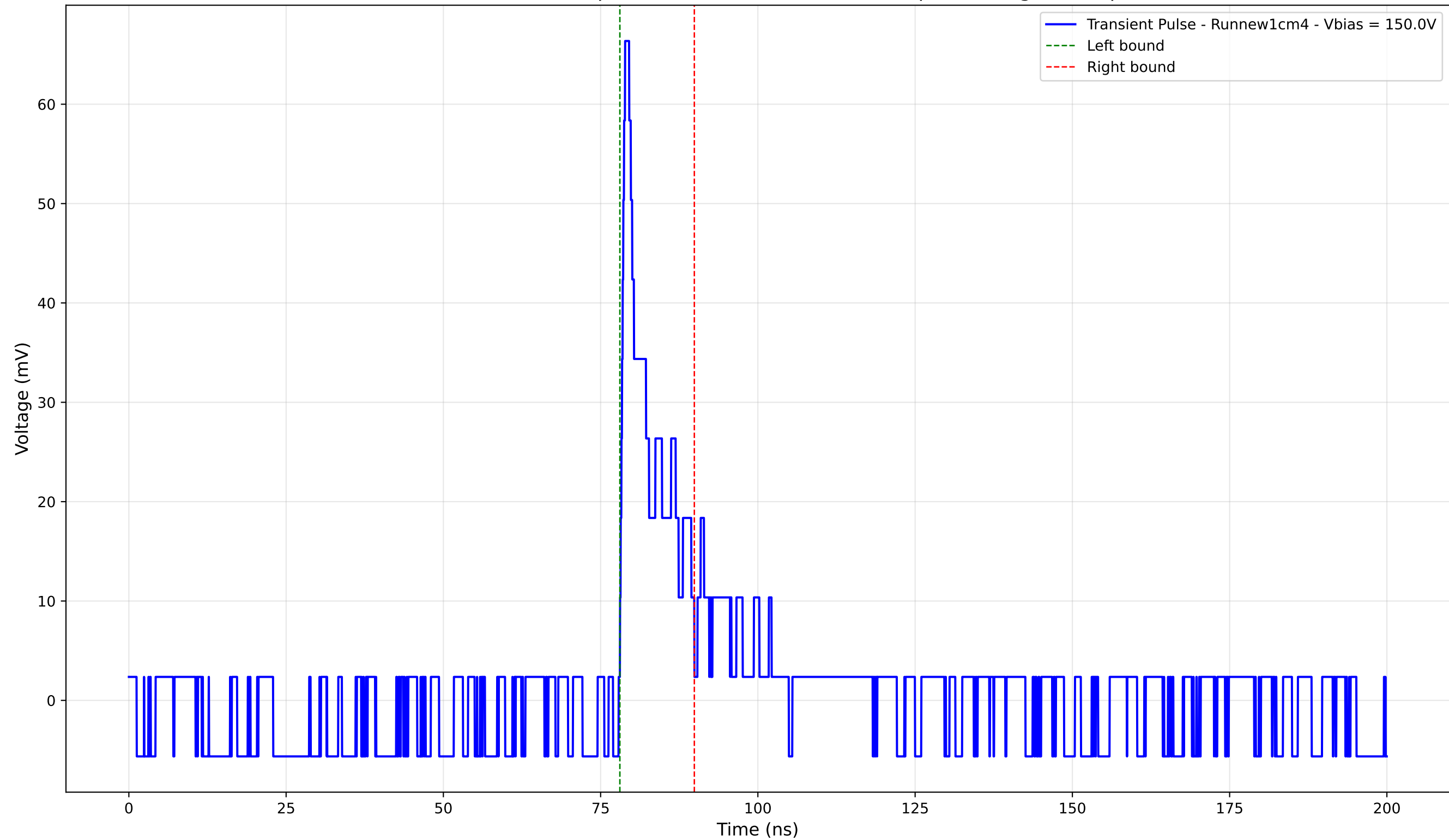
Transient Pulse - Sample: new1cm -Position: 5075.0 \mu\text{m} - Charge: 6.54 pC
