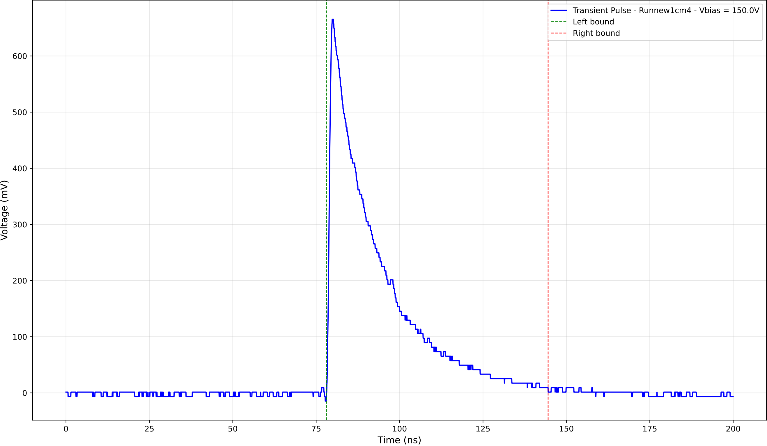
Transient Pulse - Sample: new1cm - Position: 1035.0 \mu\text{m} - Charge: 199.45 pC
