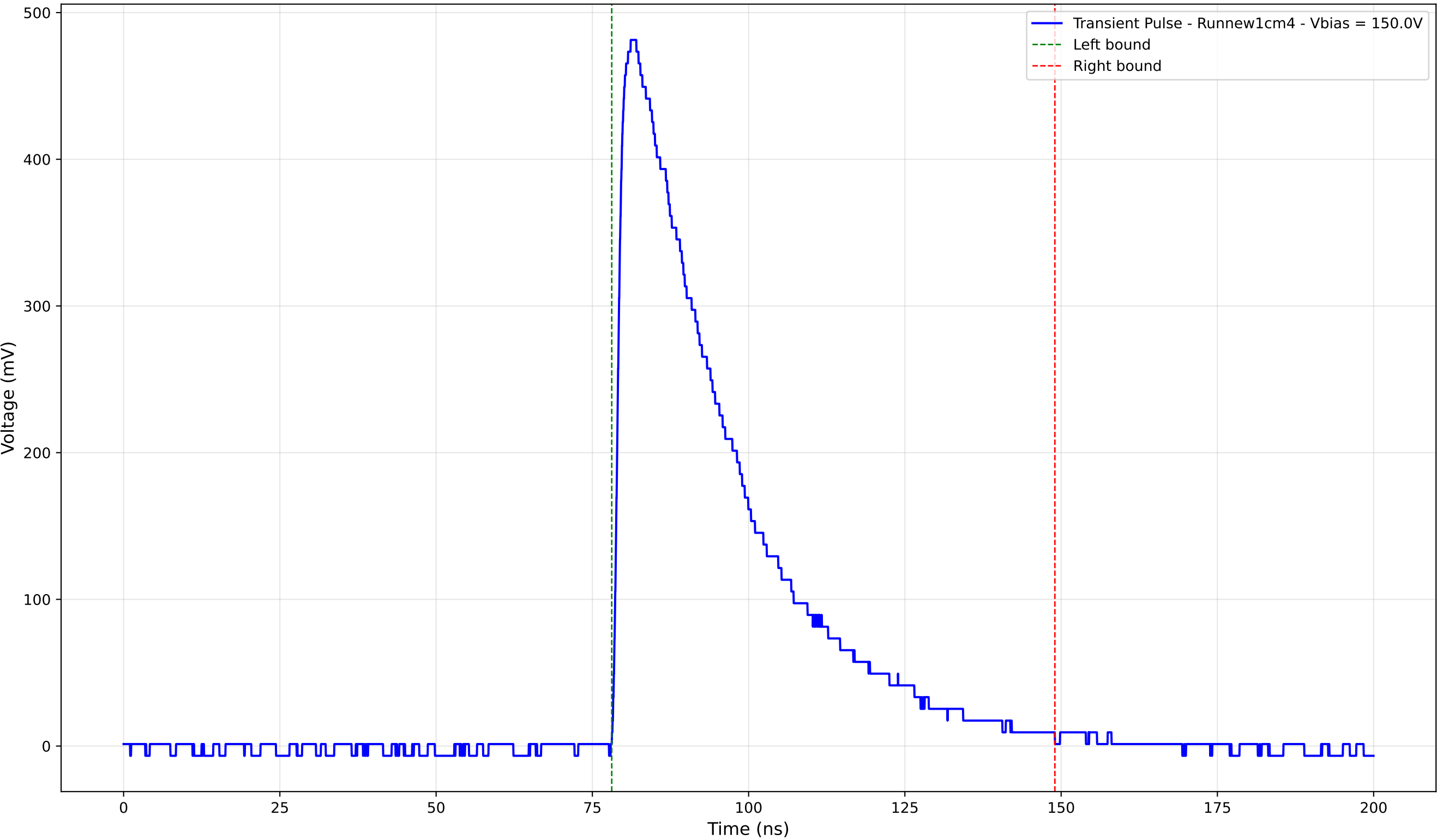
Transient Pulse - Sample: new1cm - Position: 3655.0 \mu\text{m} - Charge: 190.28 pC
