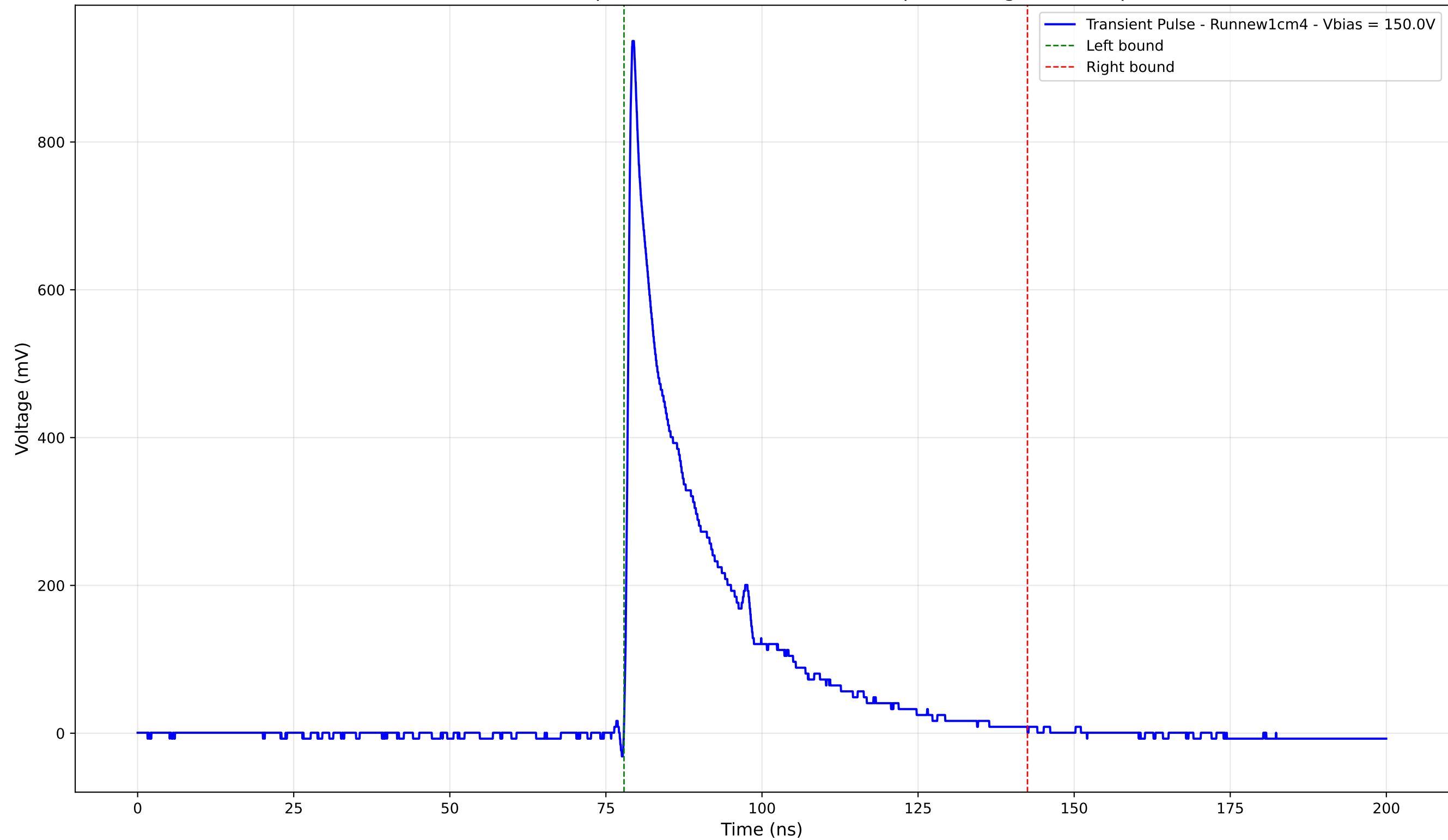
Transient Pulse - Sample: new1cm - Position: 425.0 \mu\text{m} - Charge: 198.33 pC
