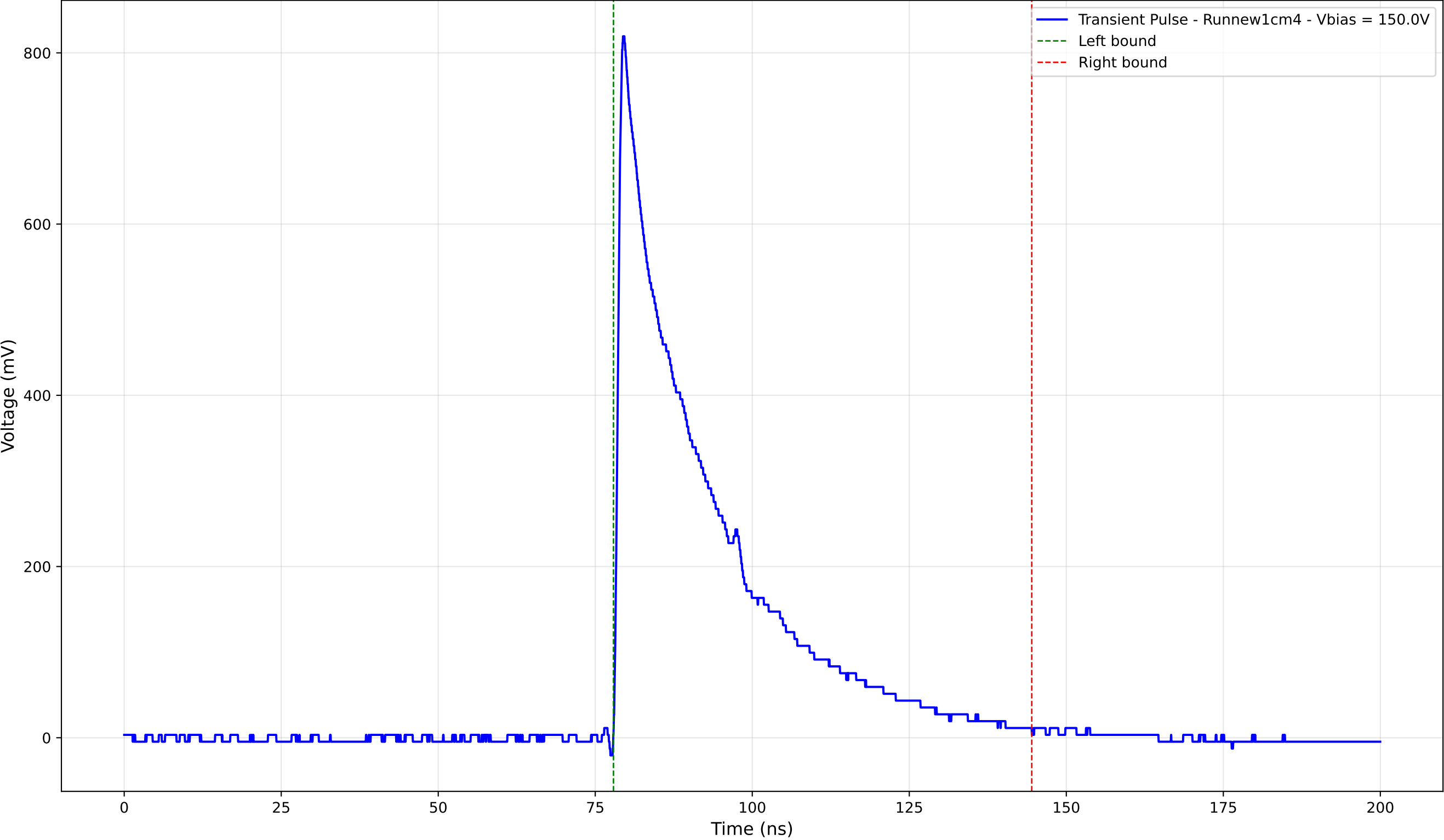
Transient Pulse - Sample: new1cm - Position: 4520.0 \mu\text{m} - Charge: 234.15 pC
