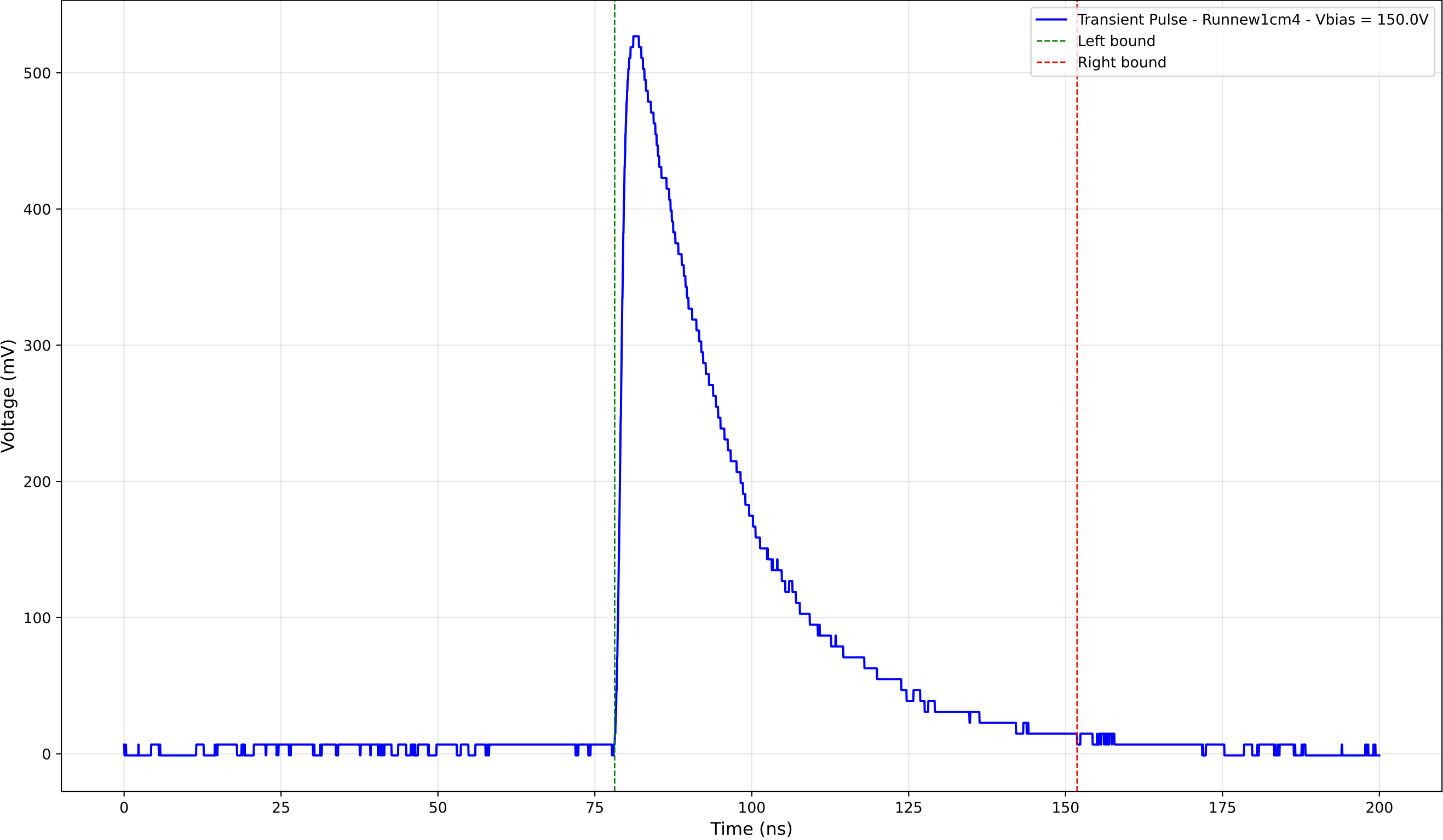
Transient Pulse - Sample: new1cm - Position: 1610.0 \mu\text{m} - Charge: 206.29 pC
