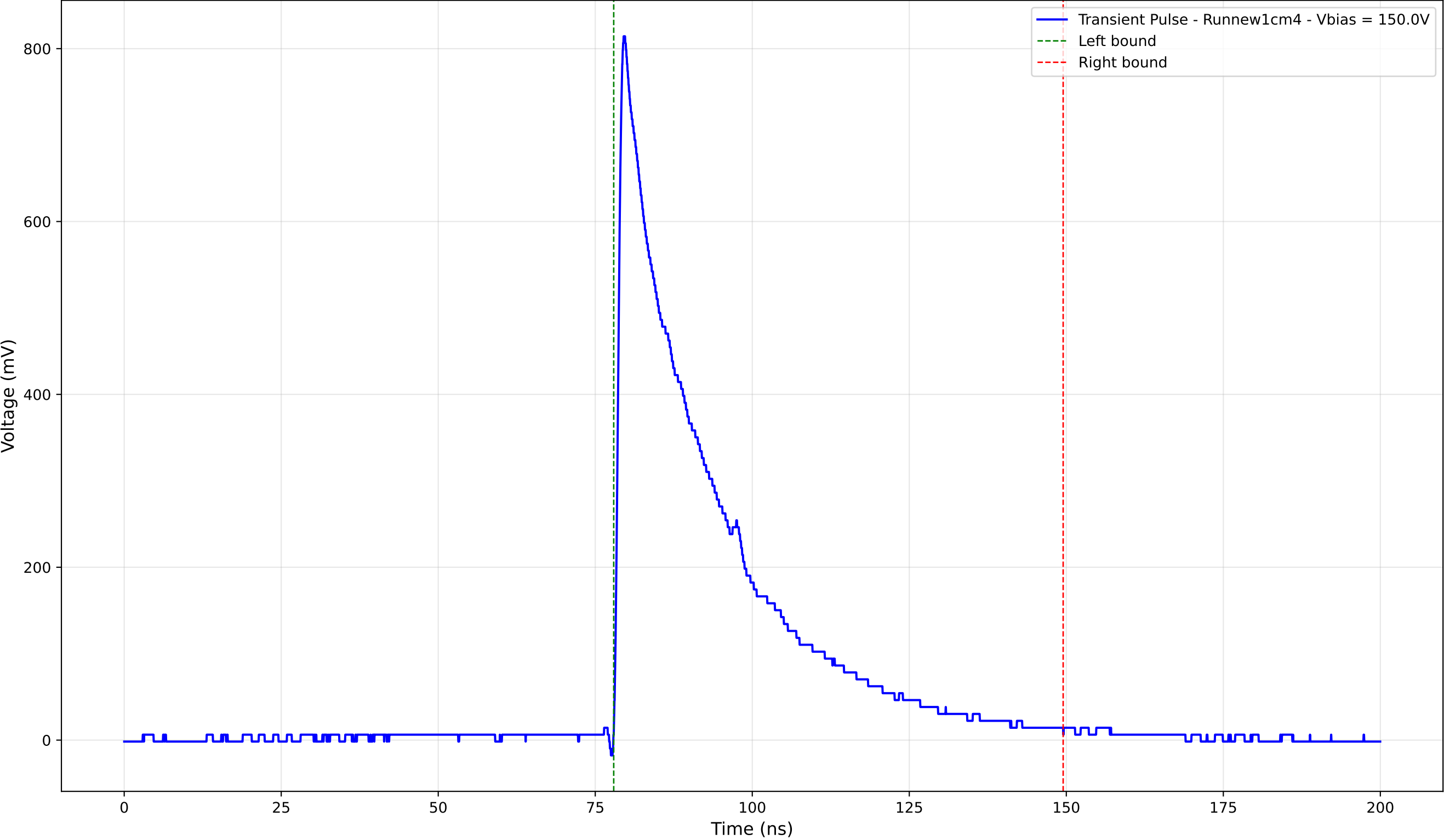
Transient Pulse - Sample: new1cm - Position: 4440.0 \mu\text{m} - Charge: 245.16 pC
