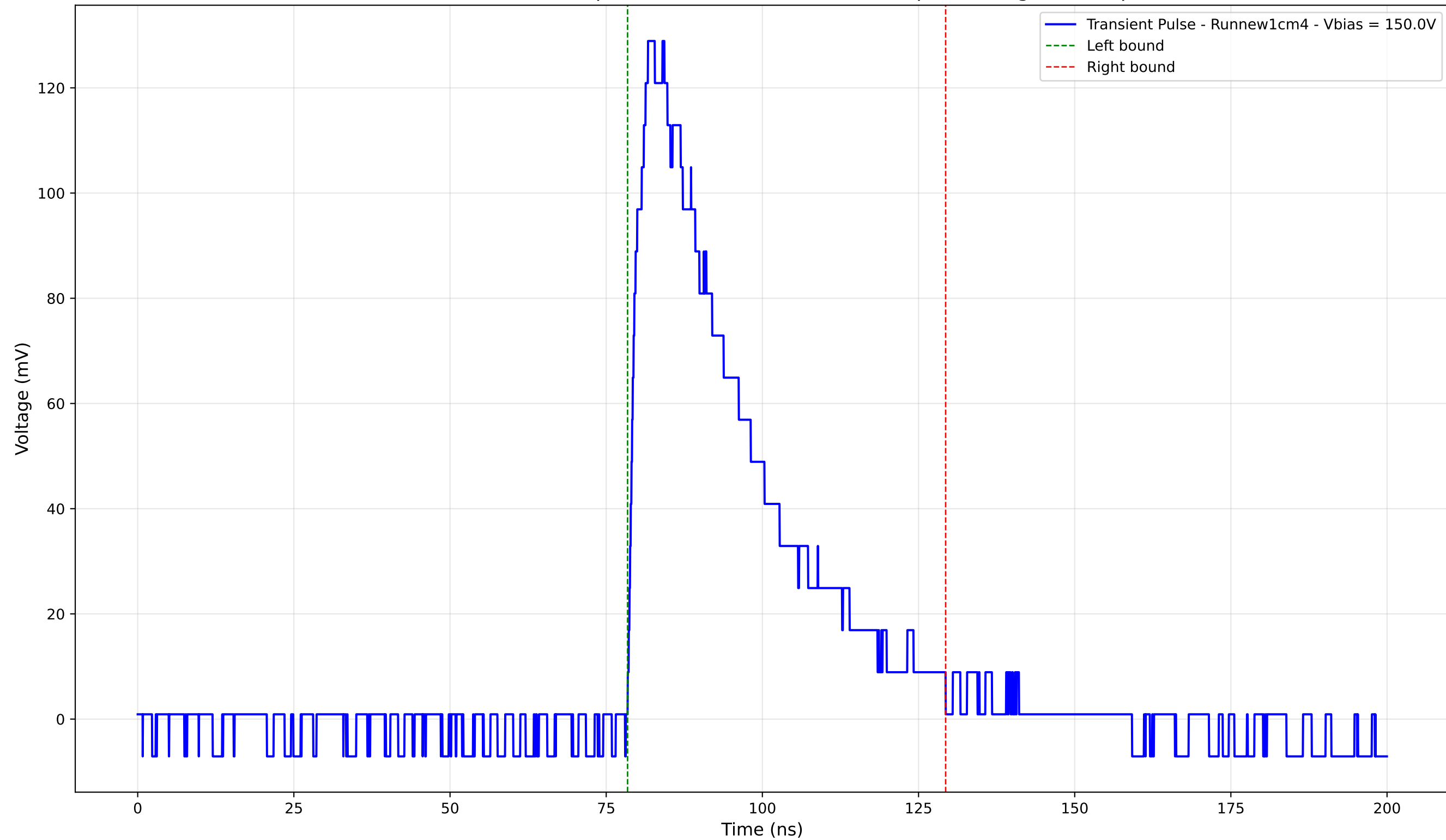
Transient Pulse - Sample: new1cm - Position: 3245.0 \mu\text{m} - Charge: 49.07 pC
