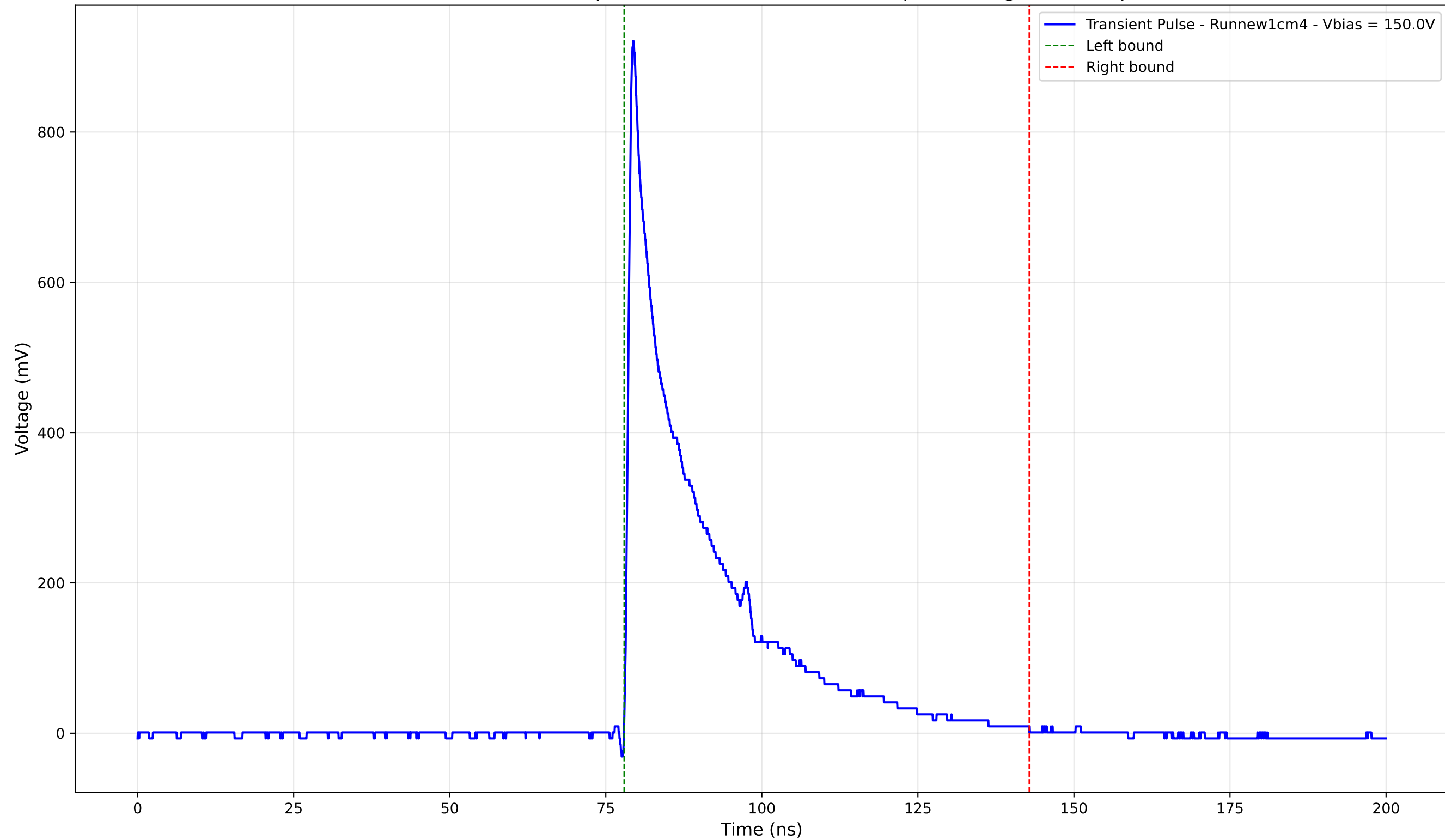
Transient Pulse - Sample: new1cm - Position: 485.0 \mu\text{m} - Charge: 199.20 pC
