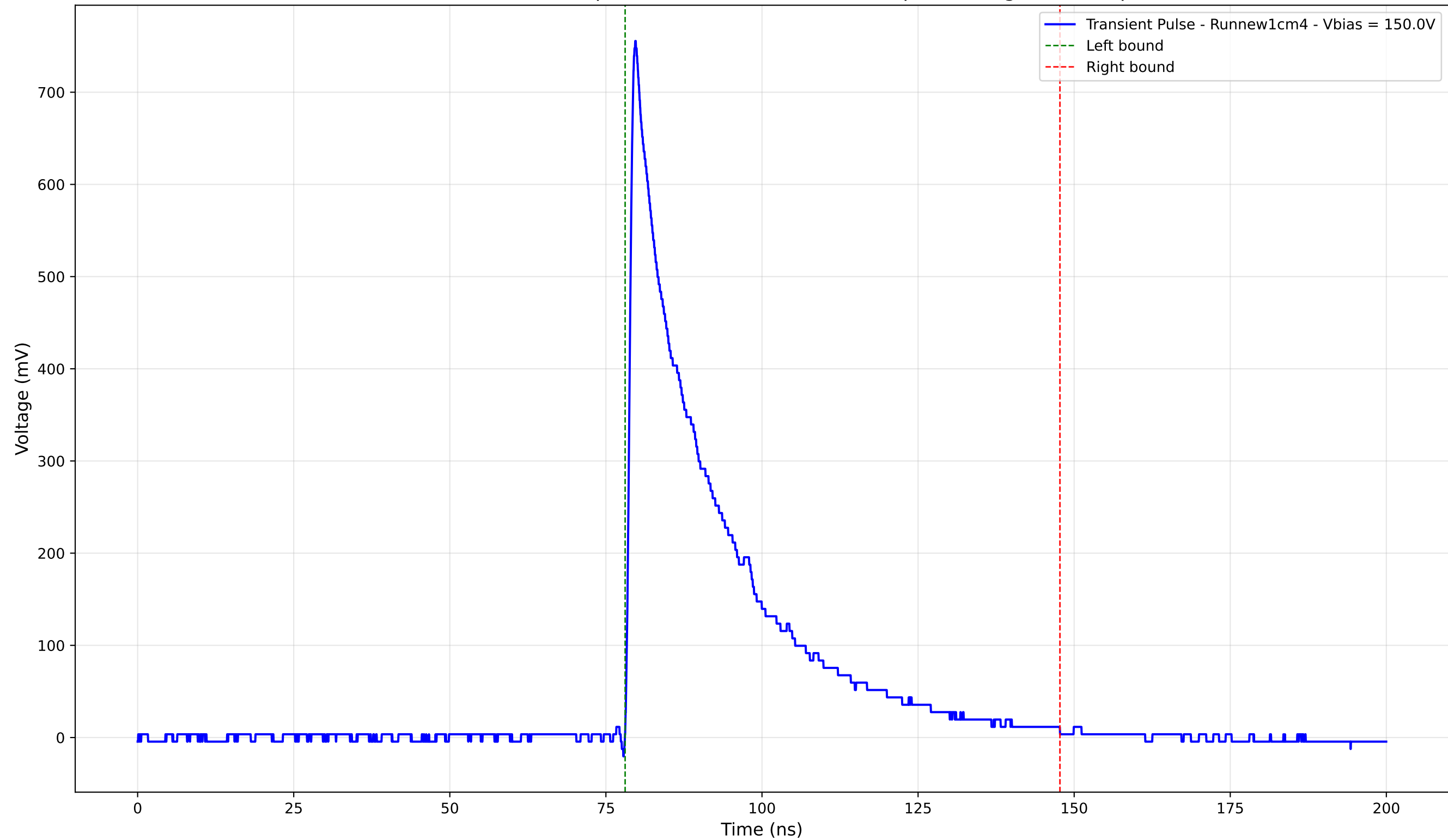
Transient Pulse - Sample: new1cm - Position: 830.0 \mu\text{m} - Charge: 201.68 pC
