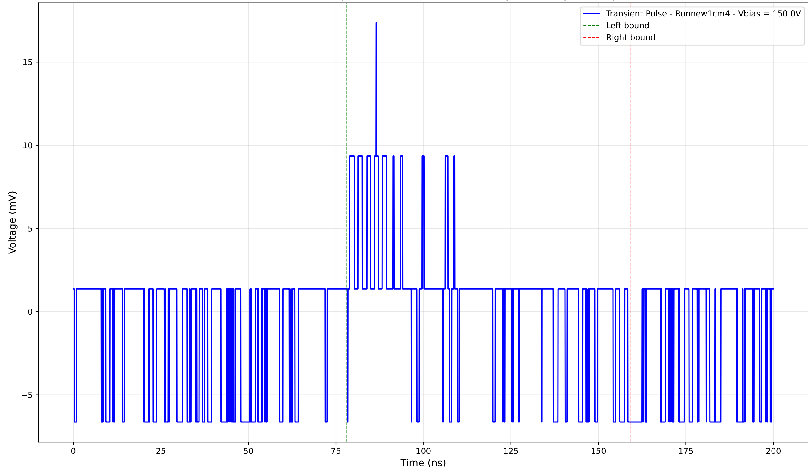
Transient Pulse - Sample: new1cm - Position: 90.0 \mu\text{m} - Charge: 1.82 pC
