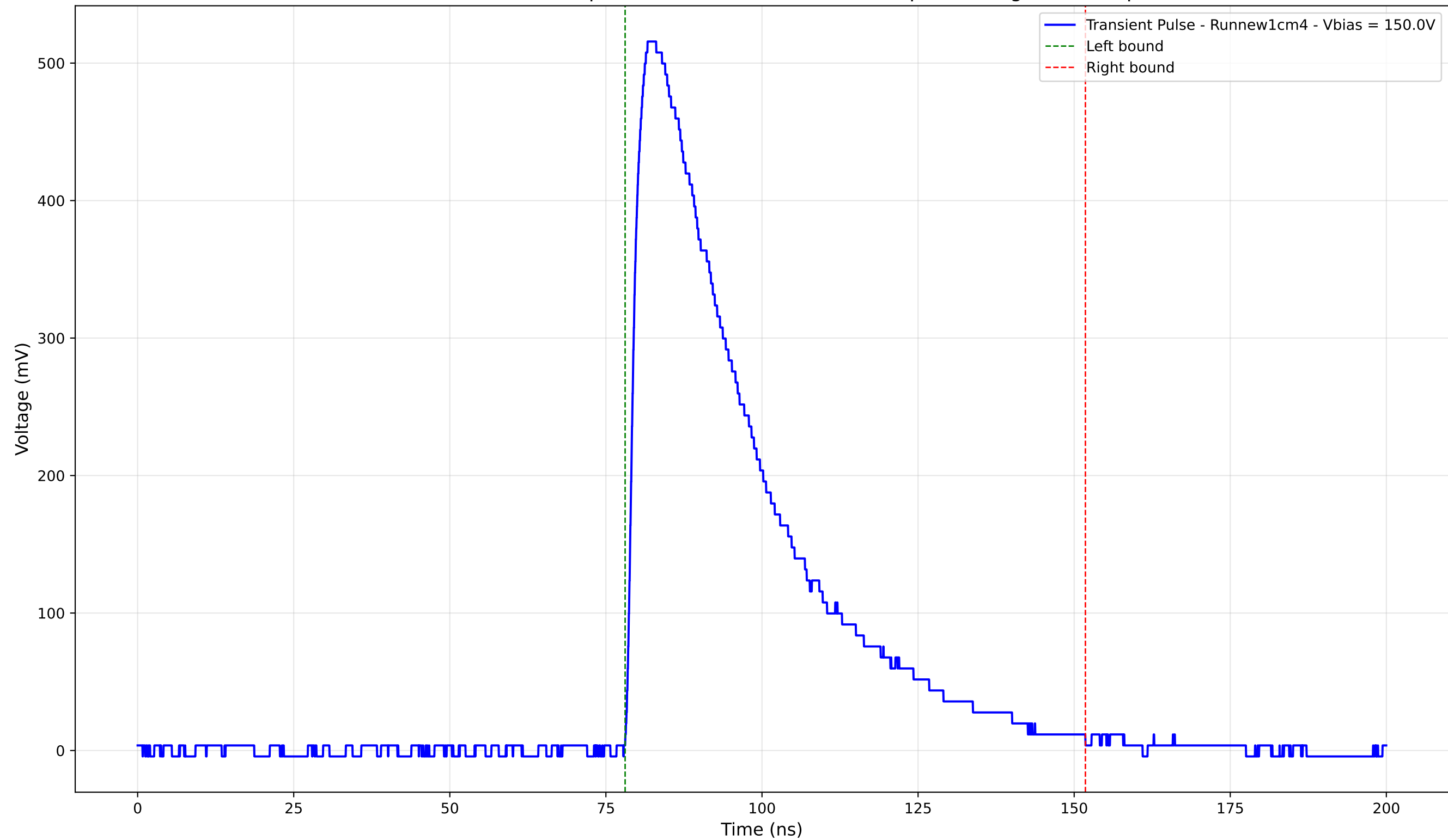
Transient Pulse - Sample: new1cm - Position: 3130.0 \mu\text{m} - Charge: 224.56 pC
