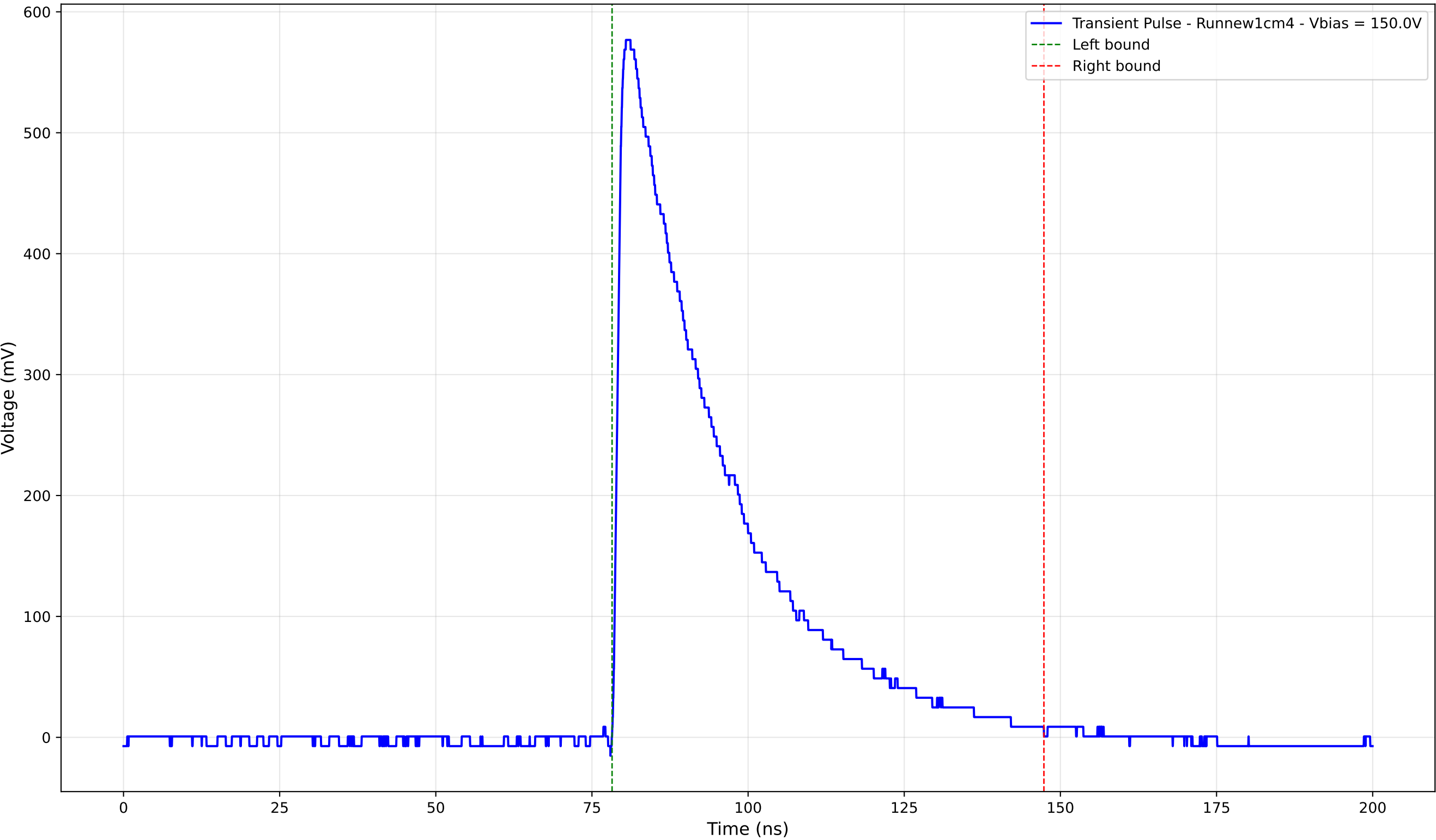
Transient Pulse - Sample: new1cm - Position: 1400.0 \mu\text{m} - Charge: 207.08 pC
