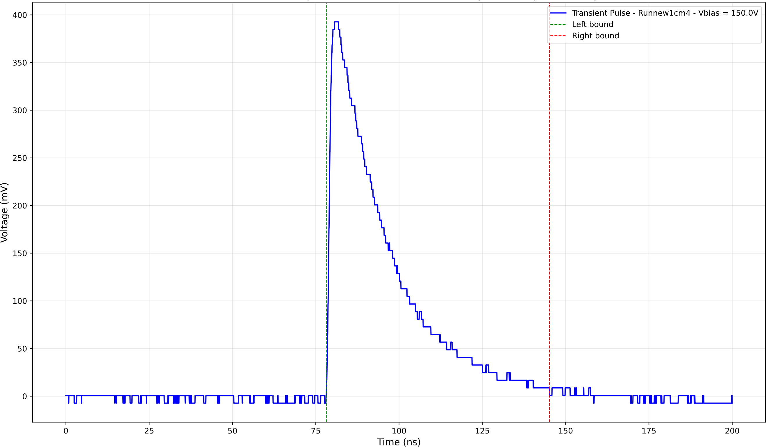
Transient Pulse - Sample: new1cm - Position: 3785.0 \mu\text{m} - Charge: 147.77 pC
