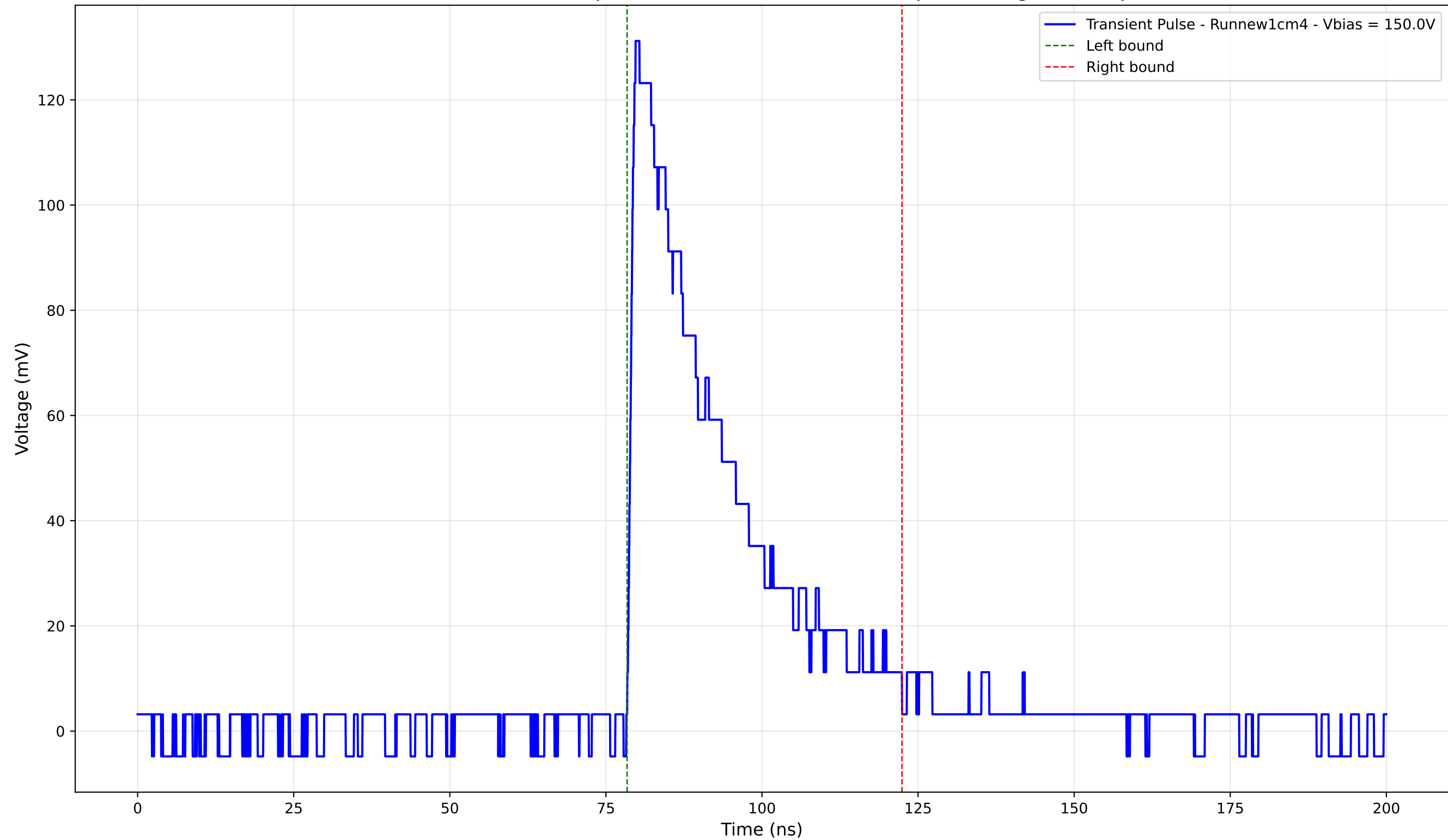
Transient Pulse - Sample: new1cm - Position: 1180.0 \mu\text{m} - Charge: 40.48 pC
