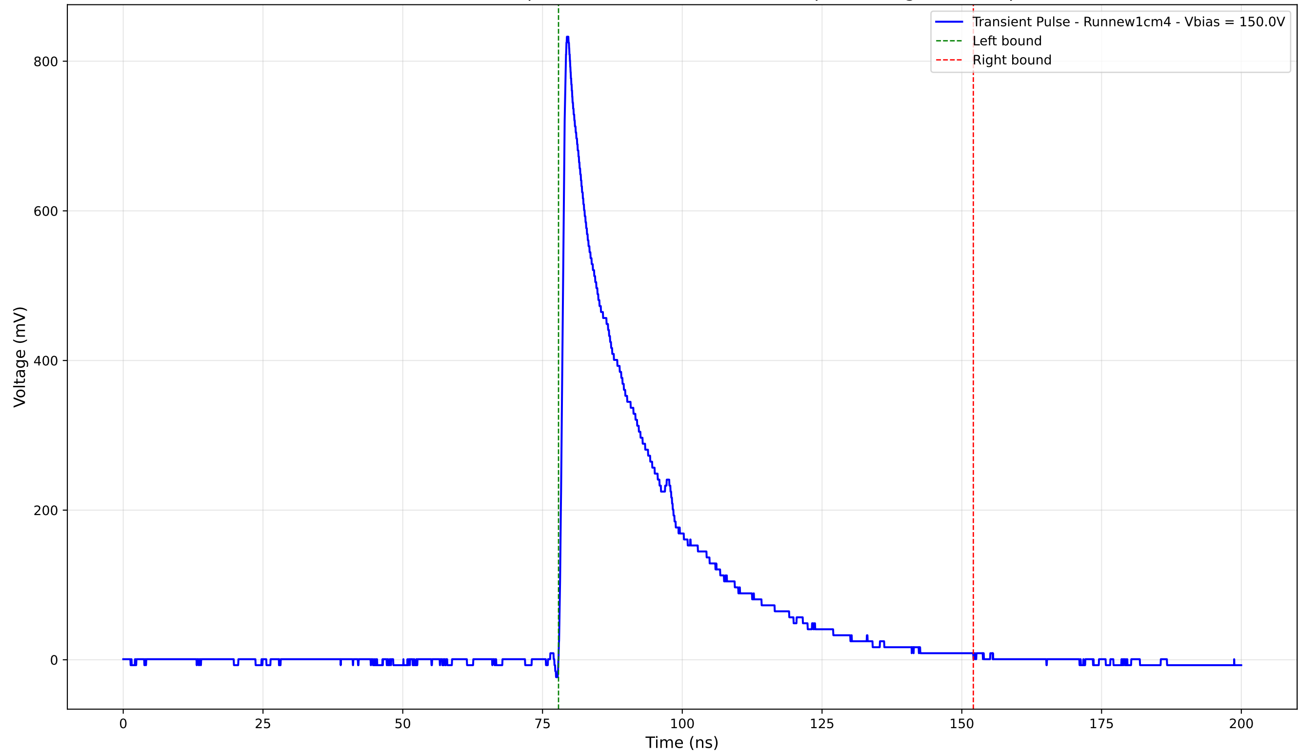
Transient Pulse - Sample: new1cm - Position: 4560.0 \mu\text{m} - Charge: 234.84 pC
