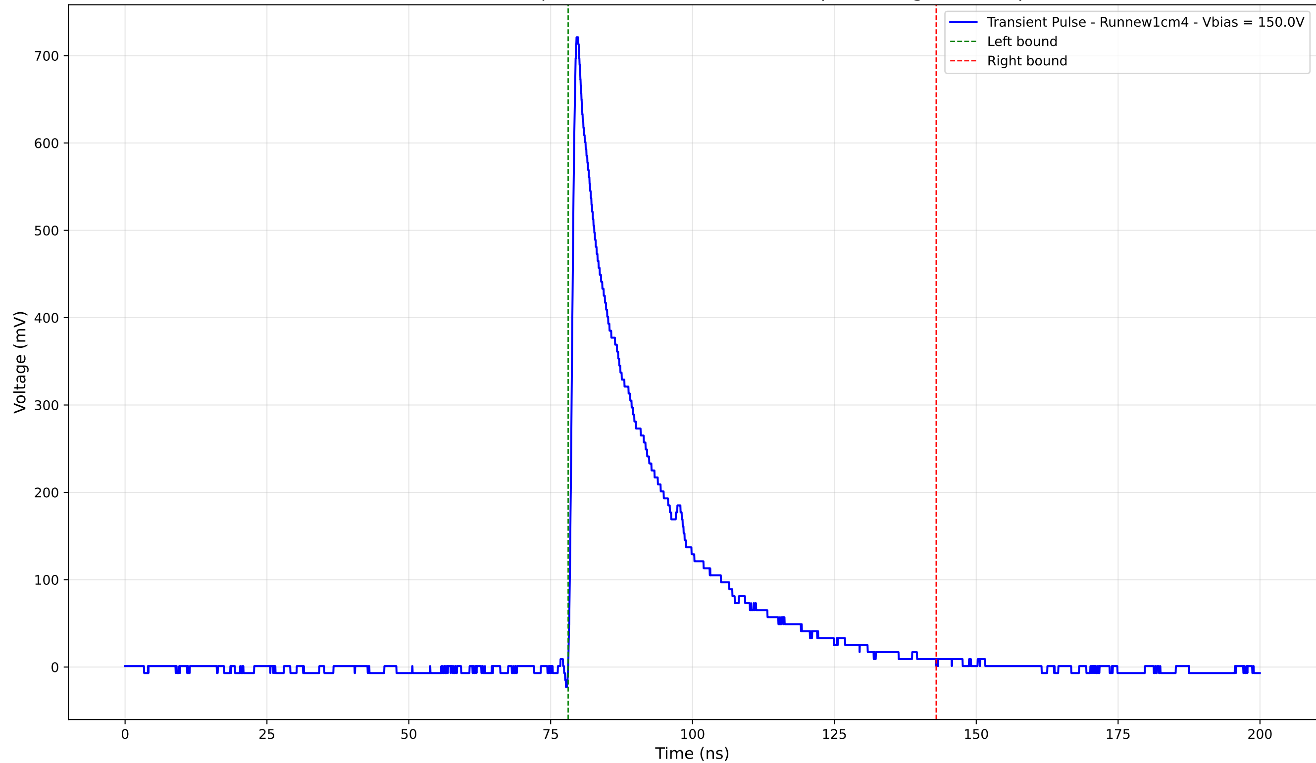
Transient Pulse - Sample: new1cm - Position: 795.0 \mu\text{m} - Charge: 185.18 pC
