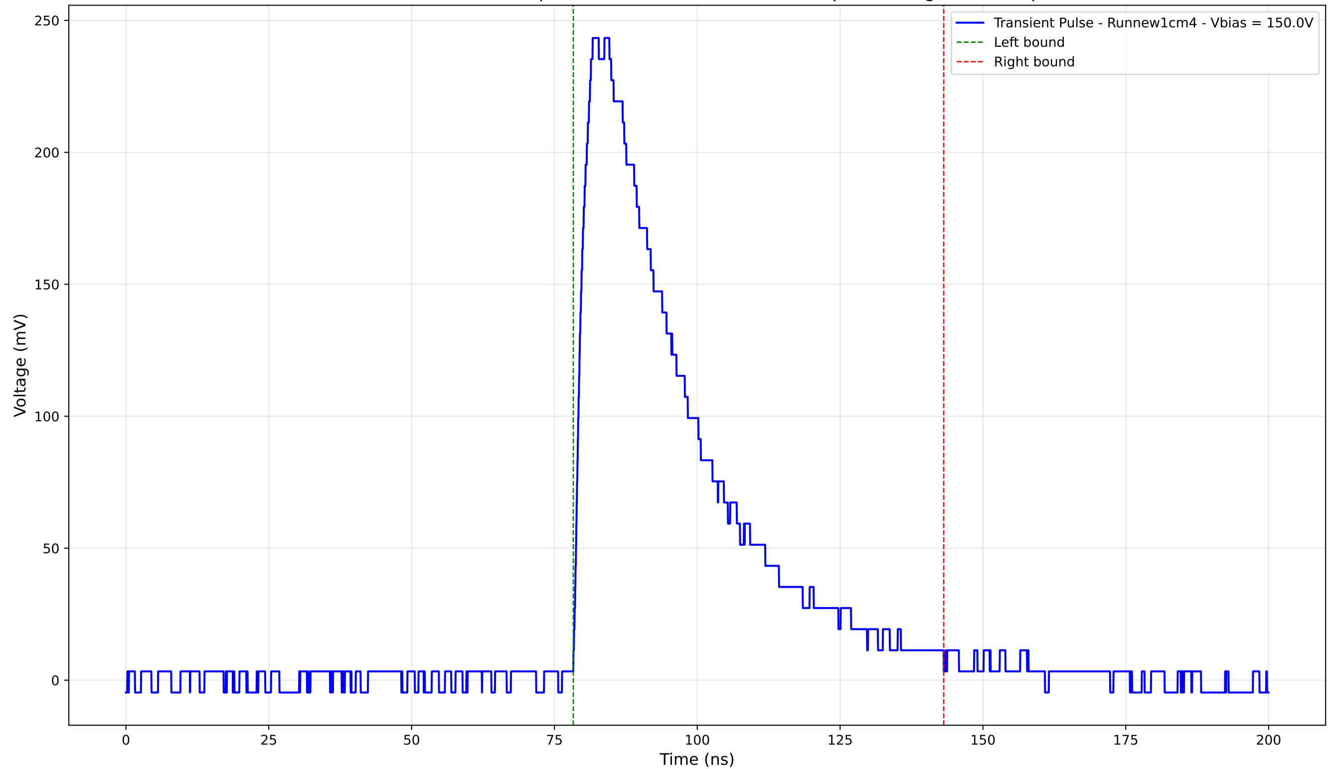
Transient Pulse - Sample: new1cm - Position: 2670.0 \mu\text{m} - Charge: 103.24 pC
