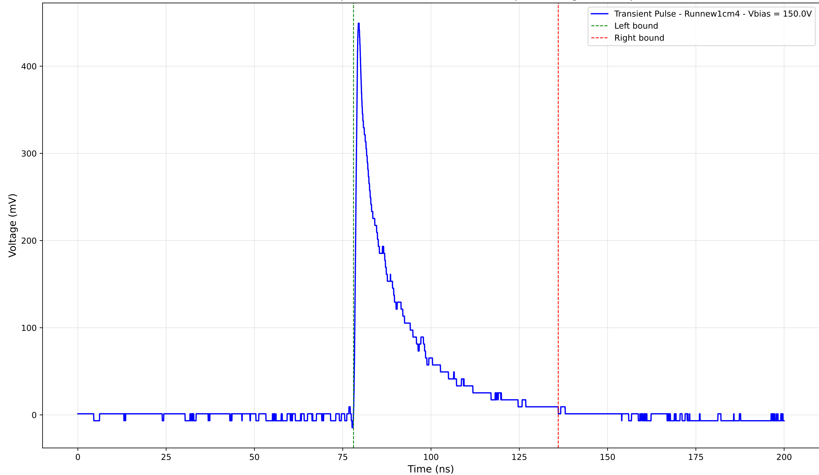
Transient Pulse - Sample: new1cm - Position: 645.0 \mu\text{m} - Charge: 92.84 pC
