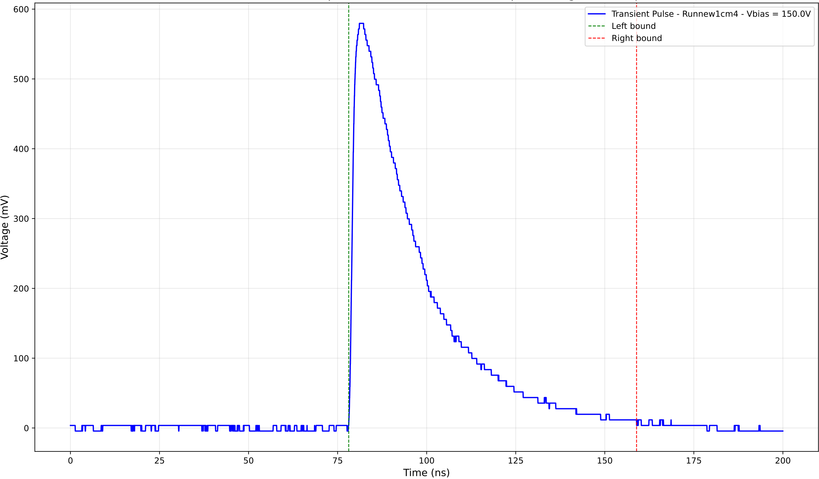
Transient Pulse - Sample: new1cm - Position: 3560.0 \mu\text{m} - Charge: 245.89 pC
