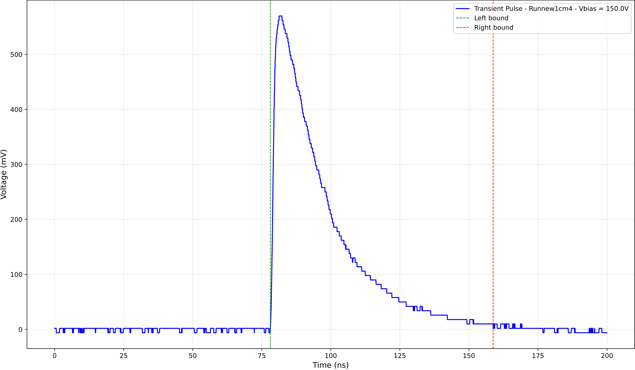
Transient Pulse - Sample: new1cm - Position: 3525.0 \mu\text{m} - Charge: 241.73 pC
