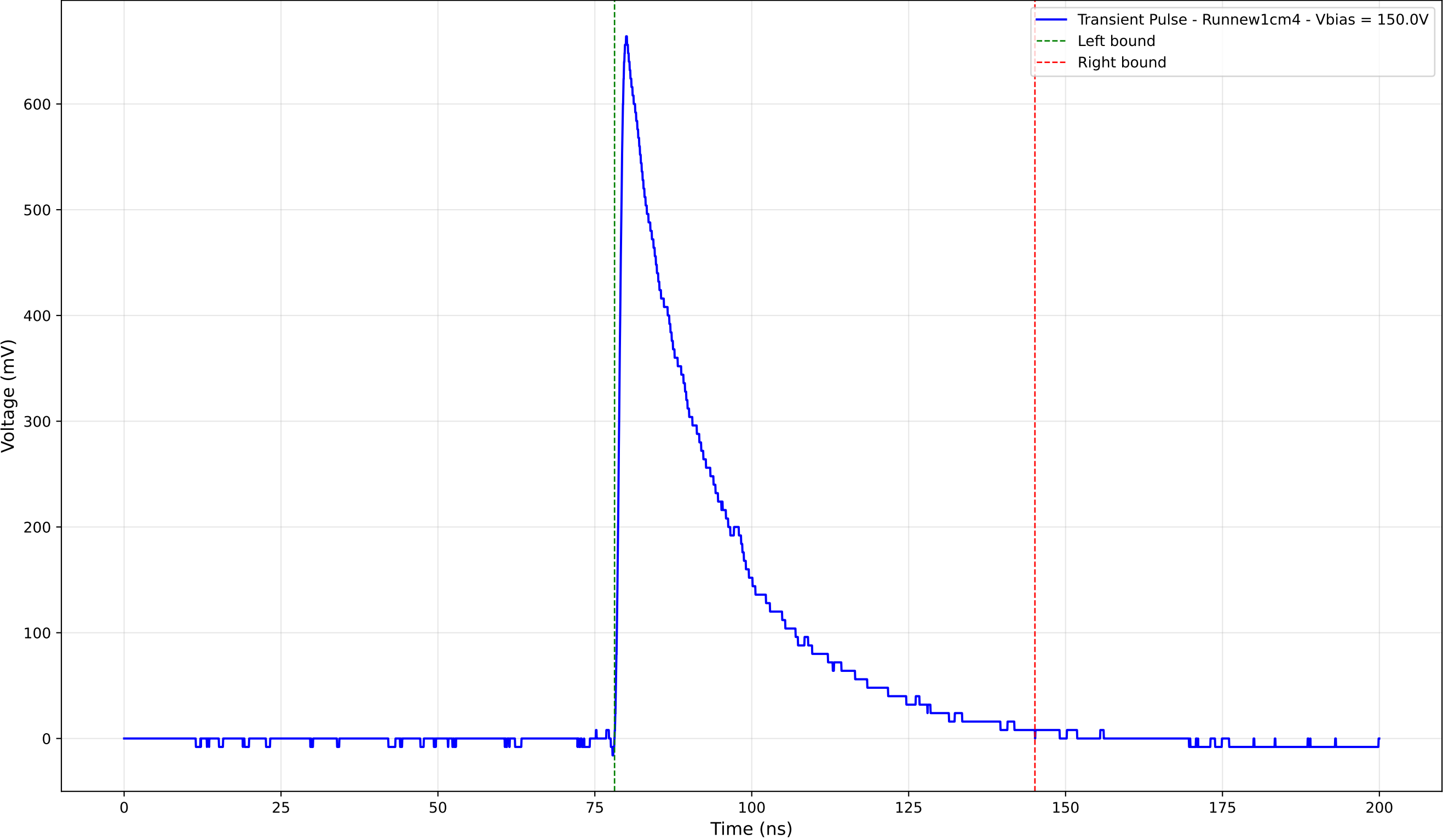
Transient Pulse - Sample: new1cm - Position: 1060.0 \mu\text{m} - Charge: 198.85 pC
