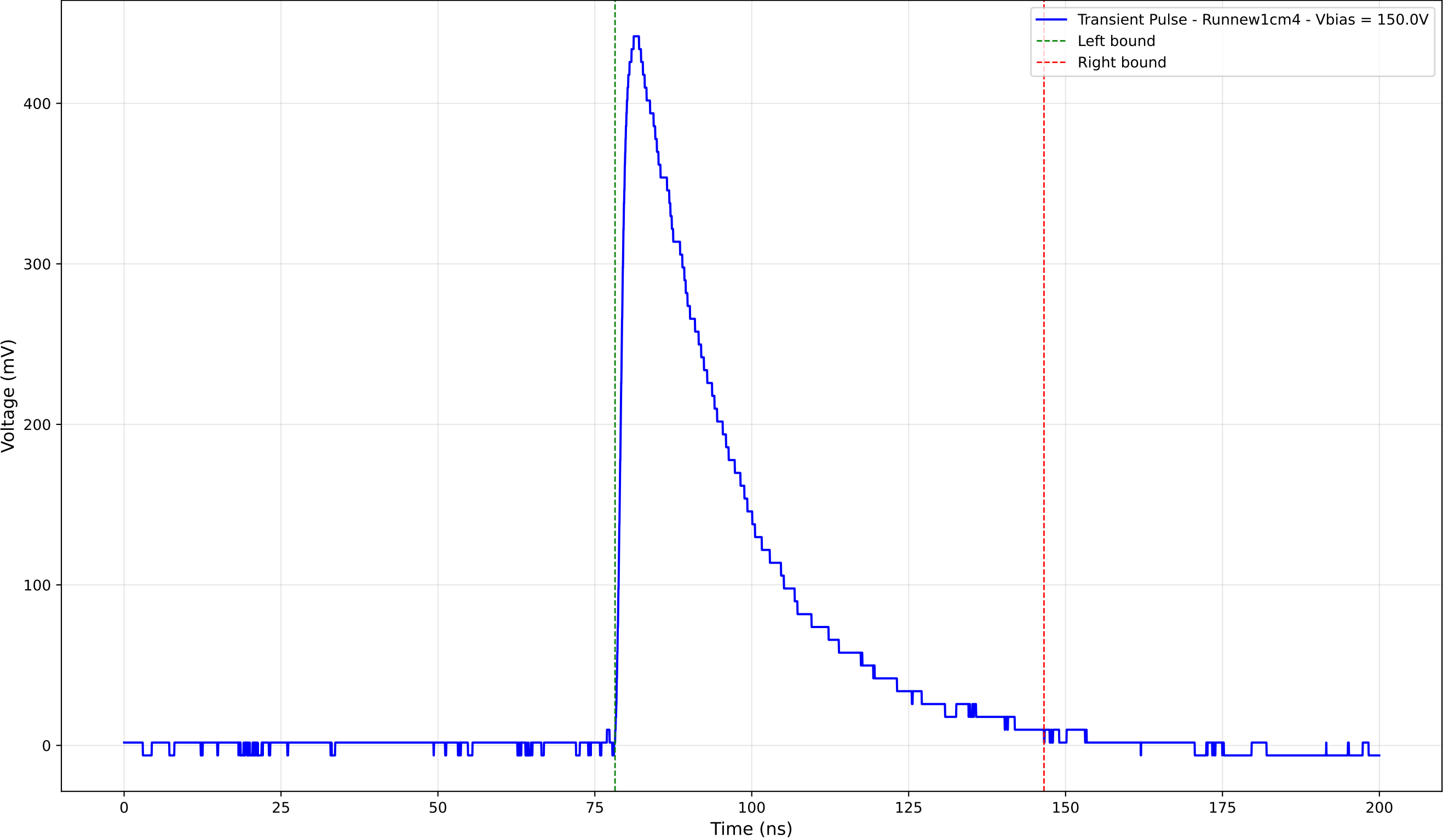
Transient Pulse - Sample: new1cm - Position: 1630.0 \mu\text{m} - Charge: 167.04 pC
