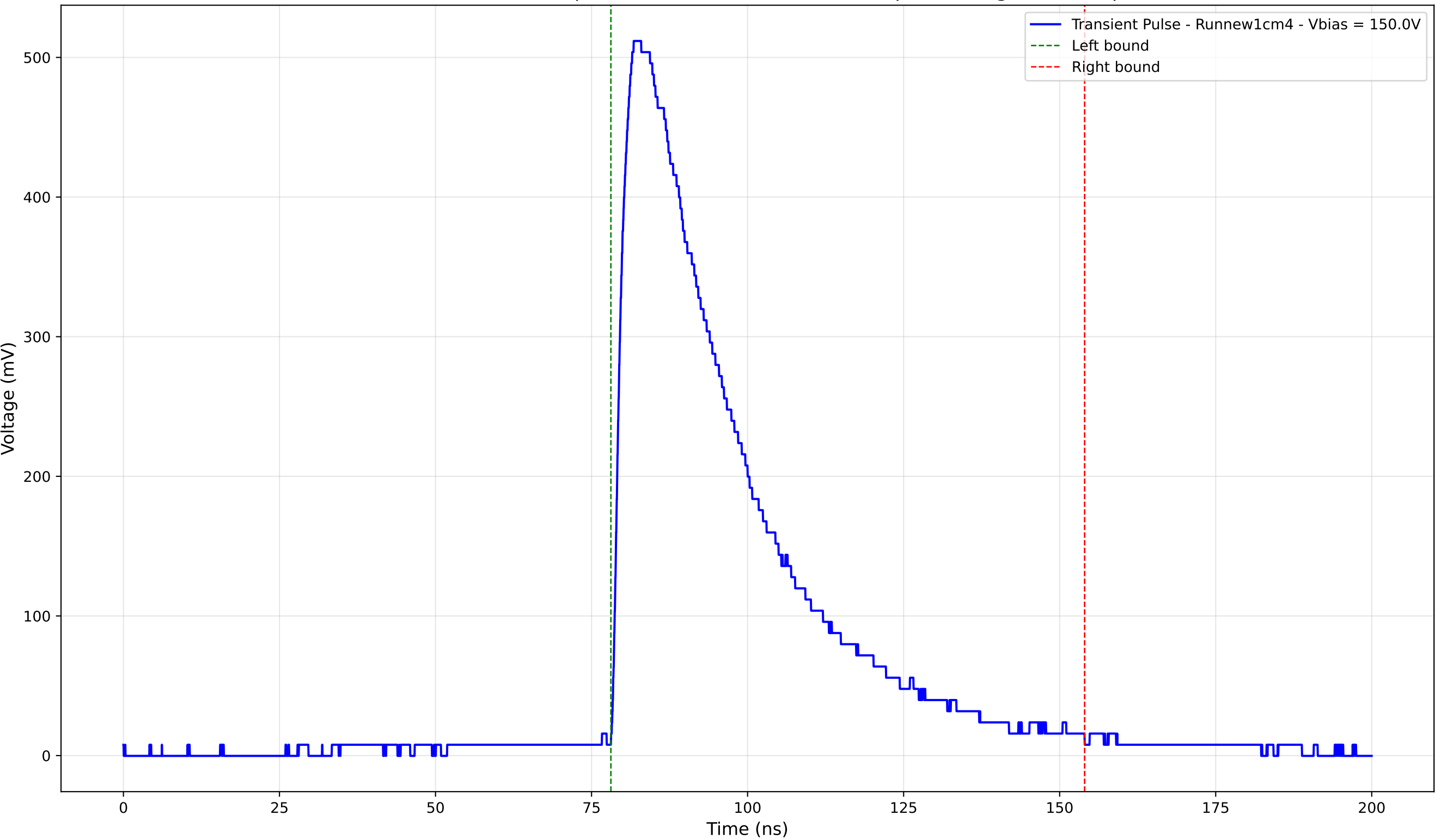
Transient Pulse - Sample: new1cm - Position: 2315.0 \mu\text{m} - Charge: 224.80 pC
