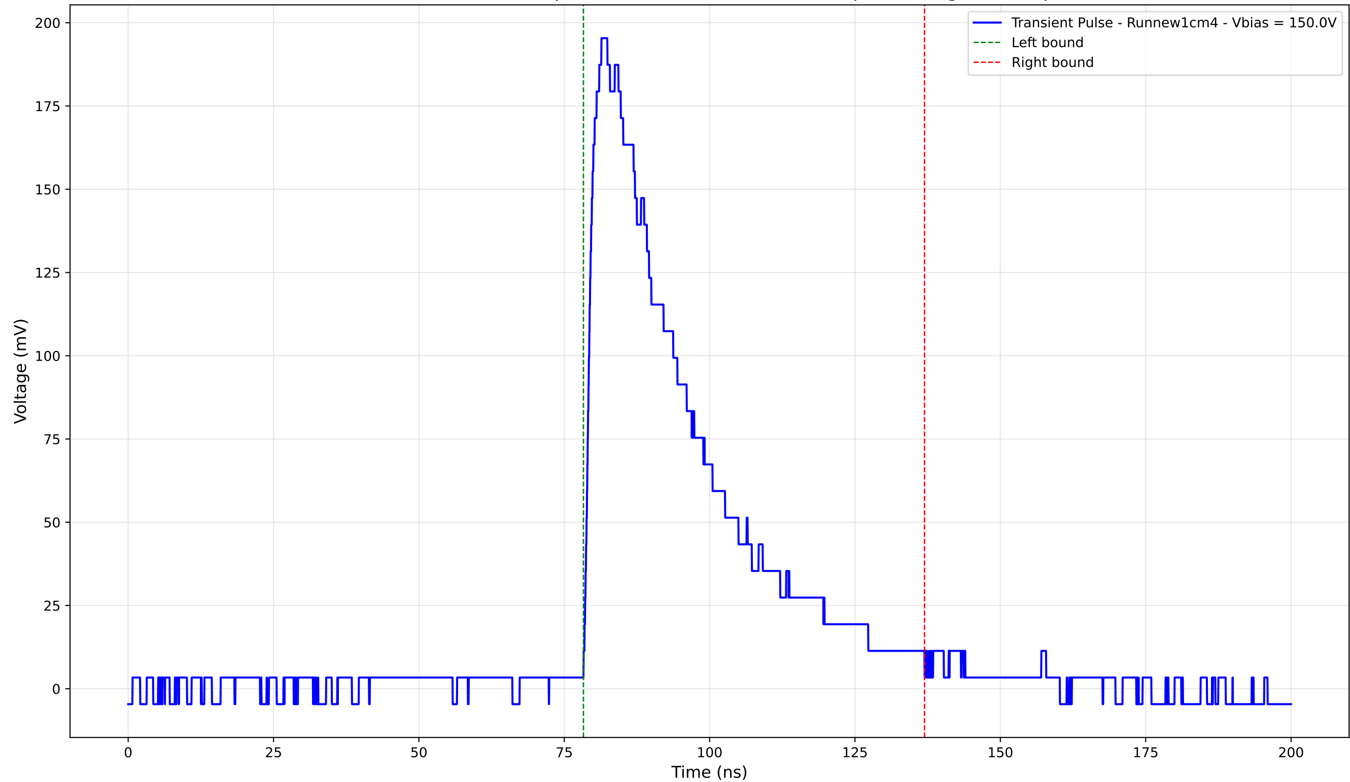
Transient Pulse - Sample: new1cm - Position: 1740.0 \mu\text{m} - Charge: 75.34 pC
