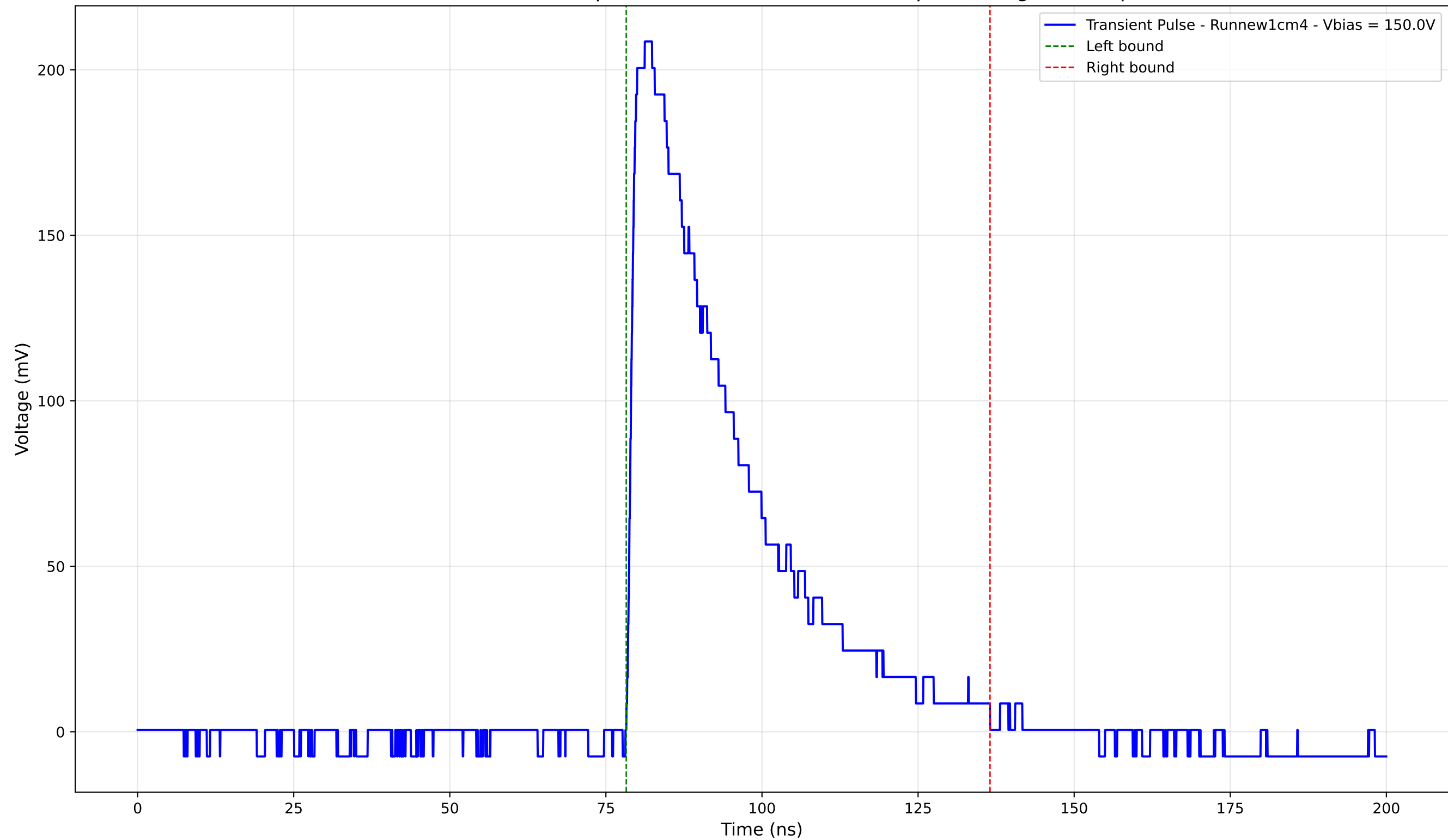
Transient Pulse - Sample: new1cm - Position: 3760.0 \mu\text{m} - Charge: 76.75 pC
