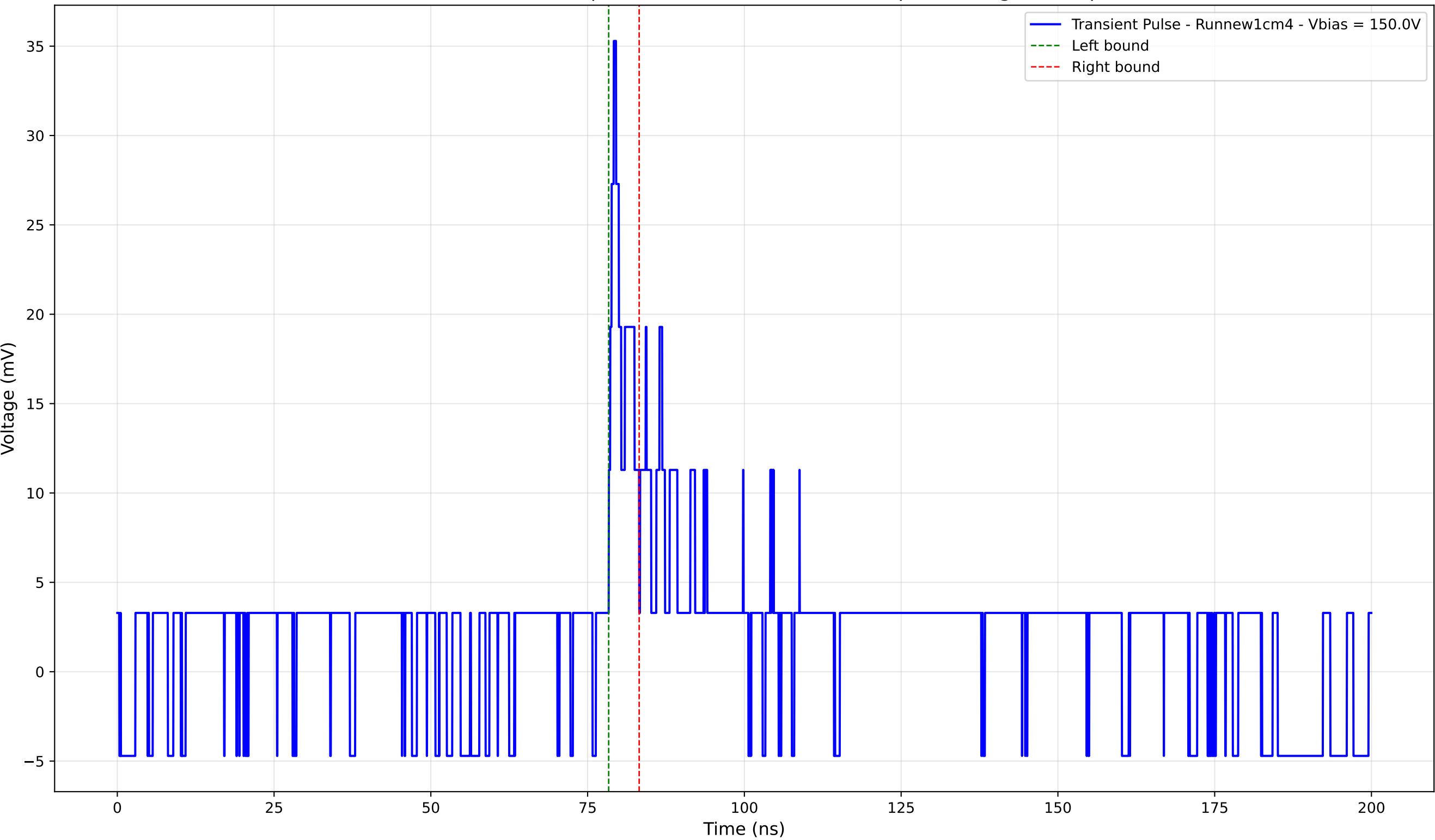
Transient Pulse - Sample: new1cm - Position: 145.0 \mu\text{m} - Charge: 1.87 pC
