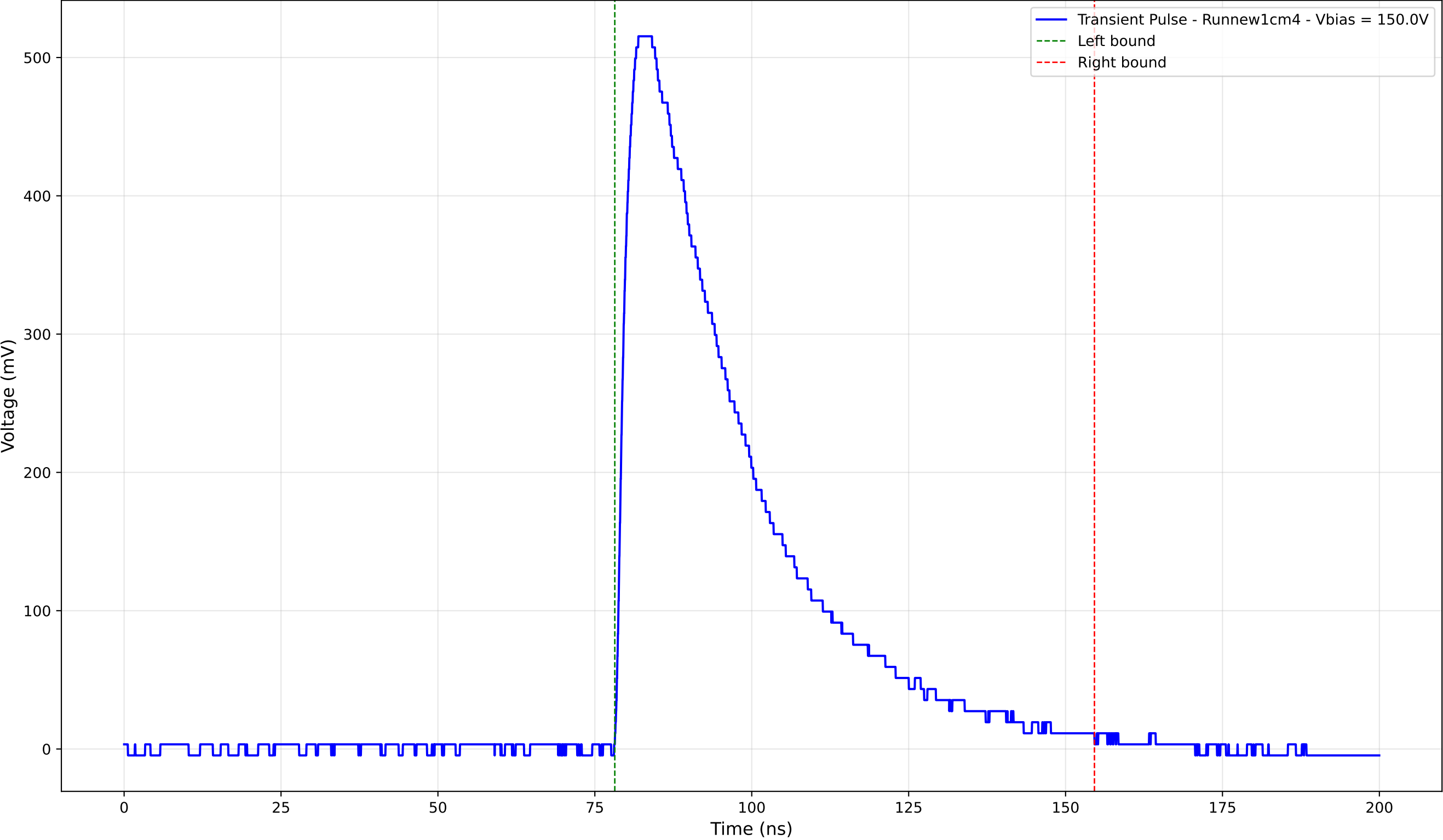
Transient Pulse - Sample: new1cm - Position: 2410.0 \mu\text{m} - Charge: 224.57 pC
