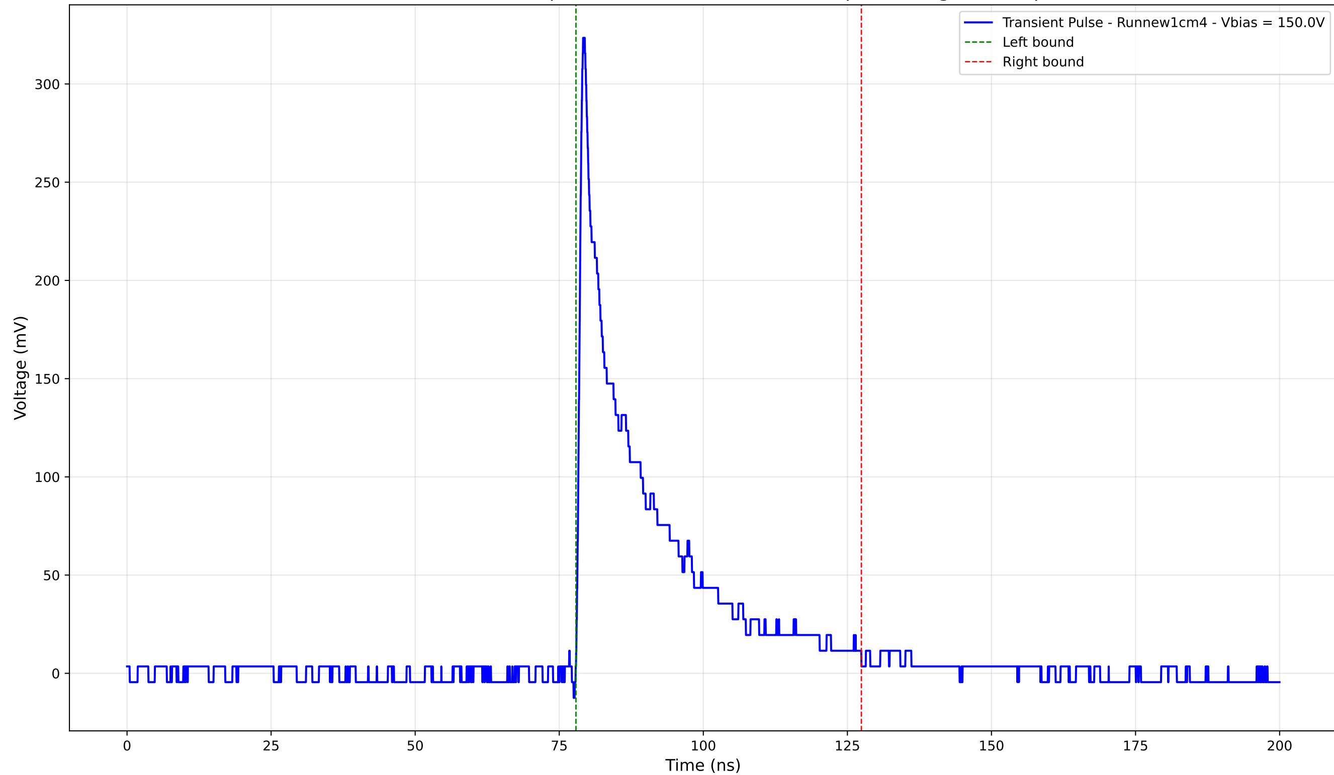
Transient Pulse - Sample: new1cm - Position: 4765.0 \mu\text{m} - Charge: 64.64 pC
