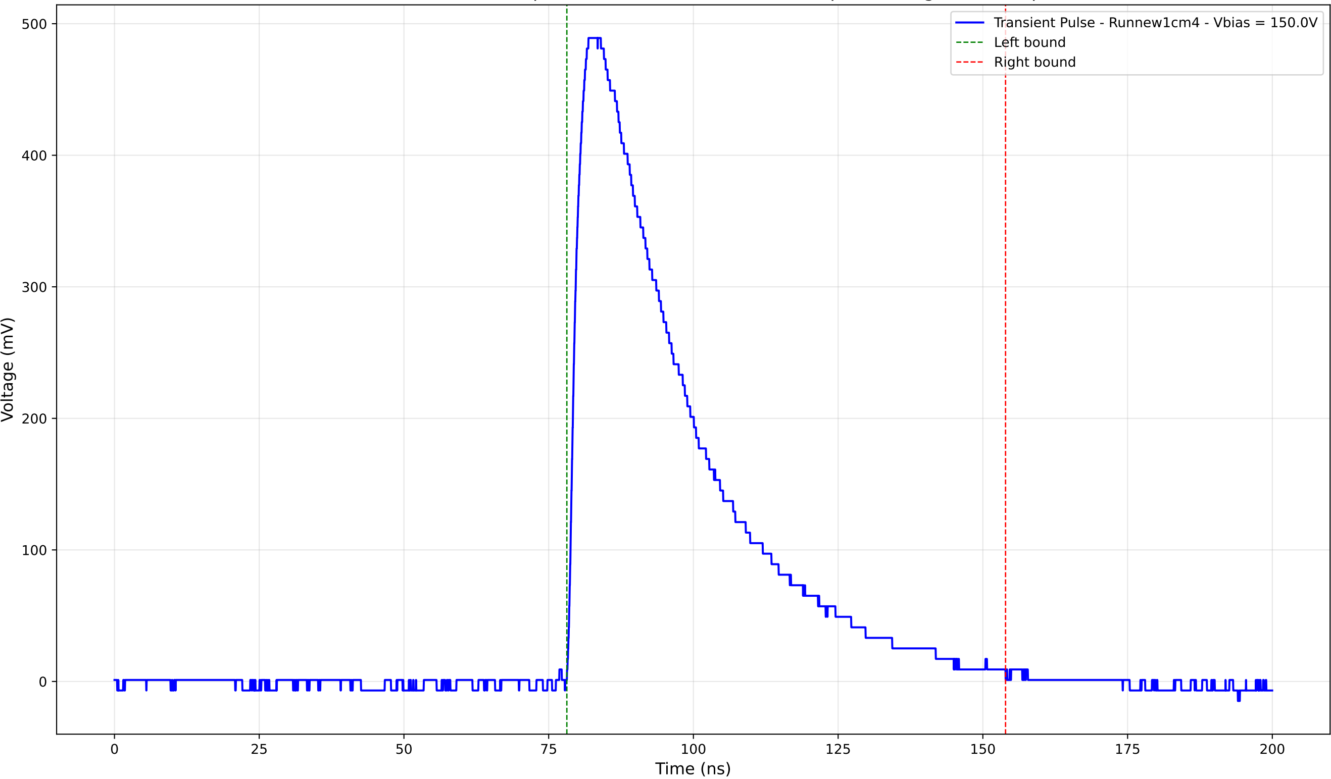
Transient Pulse - Sample: new1cm - Position: 2555.0 \mu\text{m} - Charge: 216.50 pC
