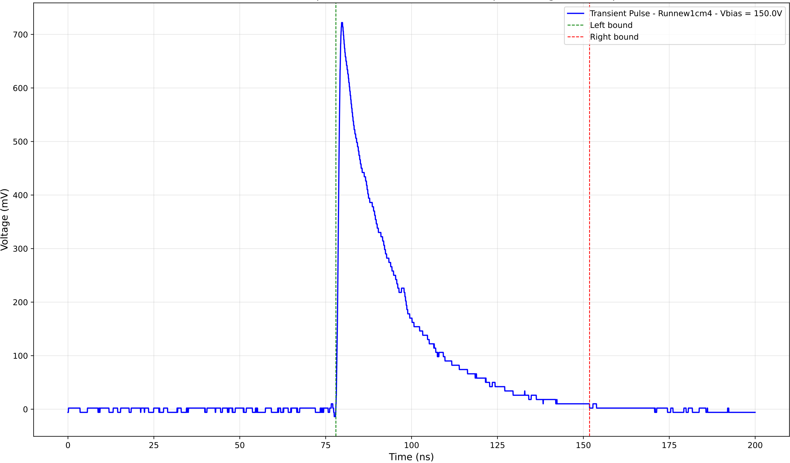
Transient Pulse - Sample: new1cm - Position: 4330.0 \mu\text{m} - Charge: 223.40 pC
