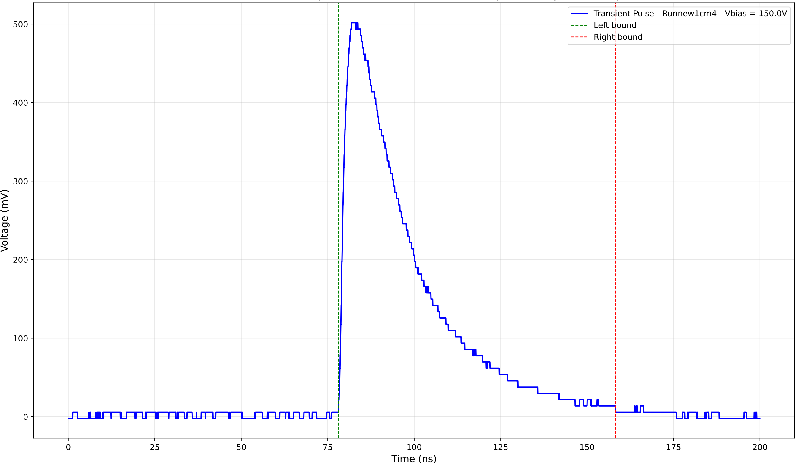
Transient Pulse - Sample: new1cm - Position: 2830.0 \mu\text{m} - Charge: 227.99 pC
