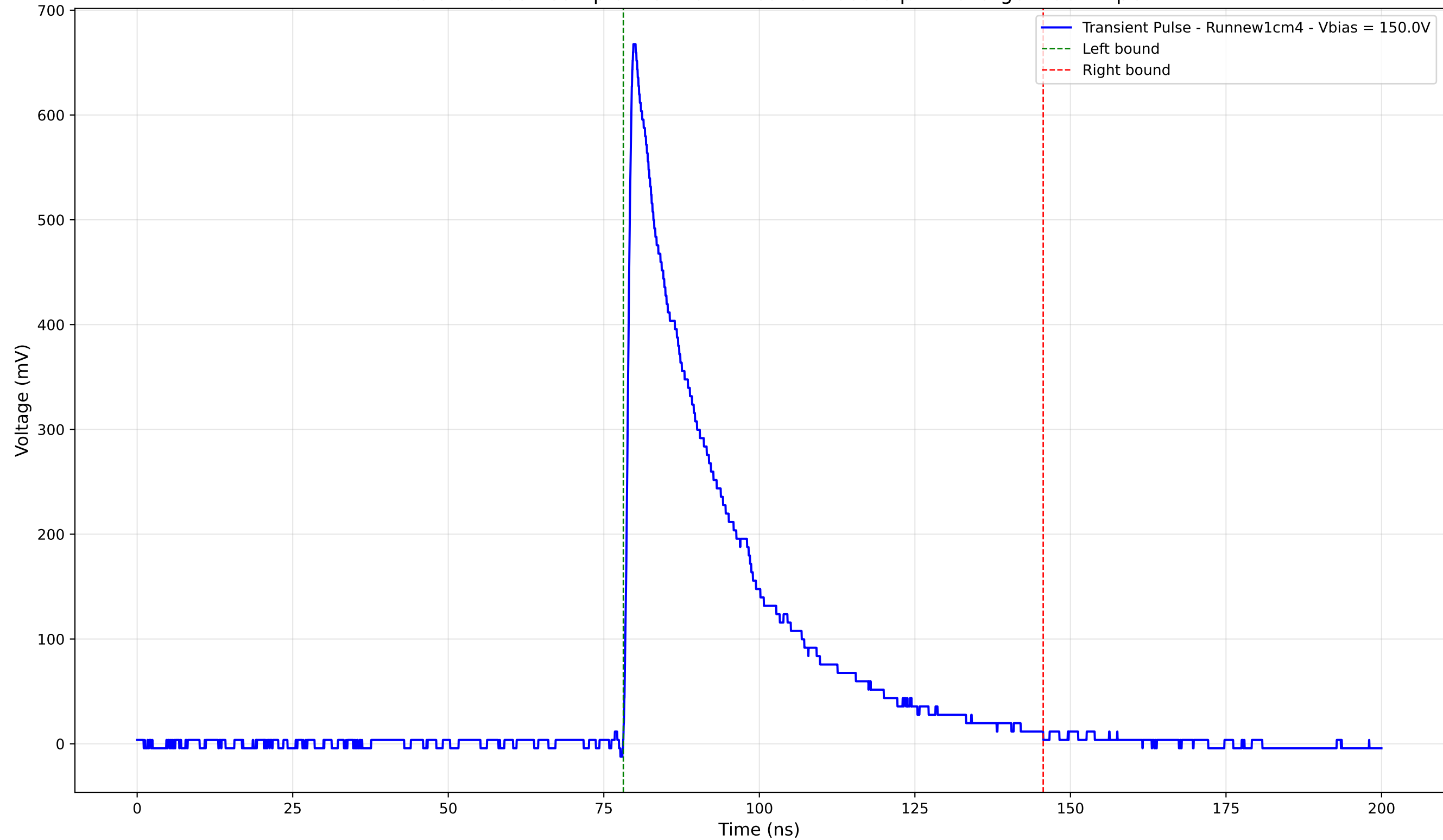
Transient Pulse - Sample: new1cm - Position: 995.0 \mu\text{m} - Charge: 198.12 pC
