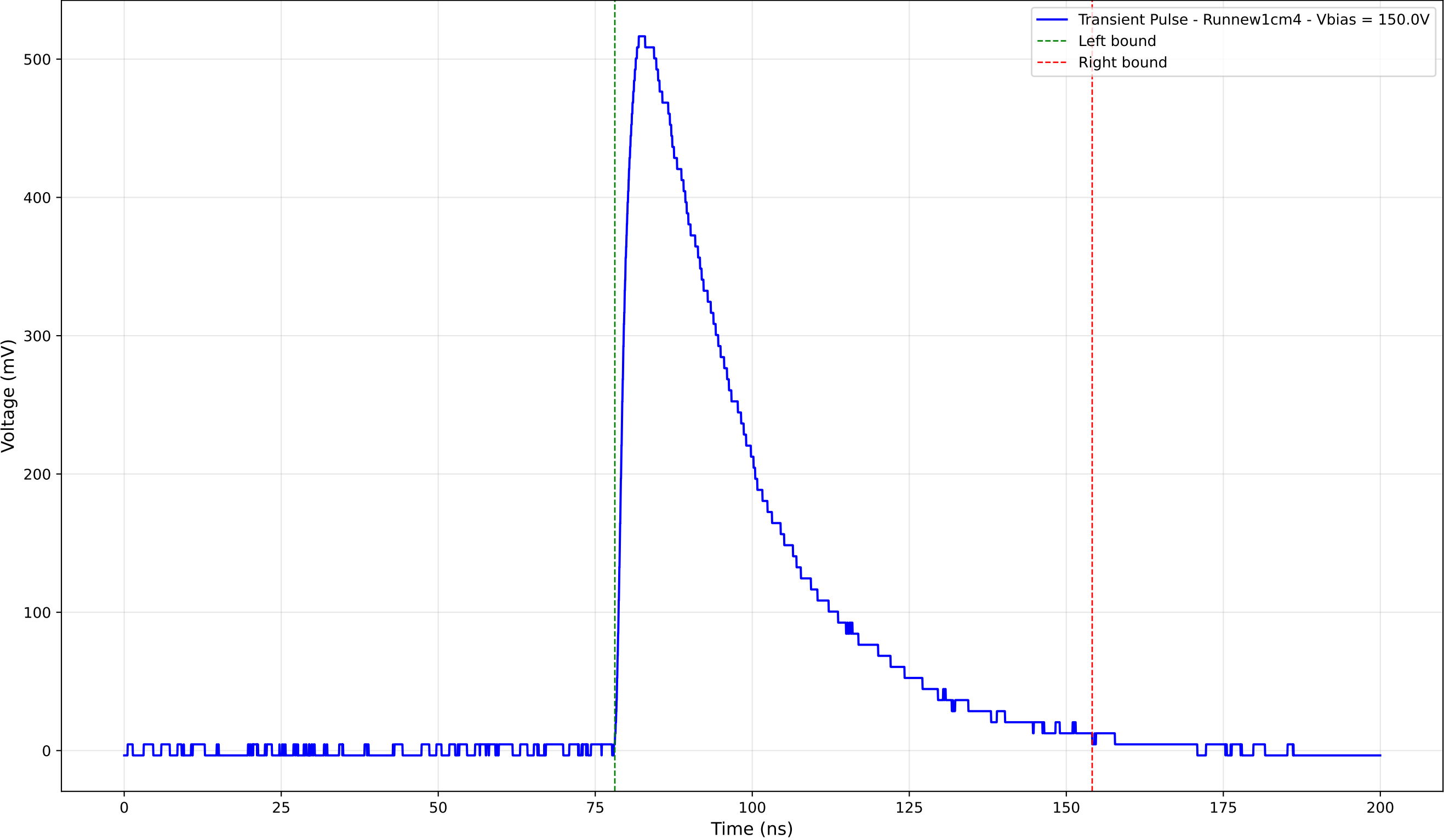
Transient Pulse - Sample: new1cm - Position: 2880.0 \mu\text{m} - Charge: 229.54 pC
