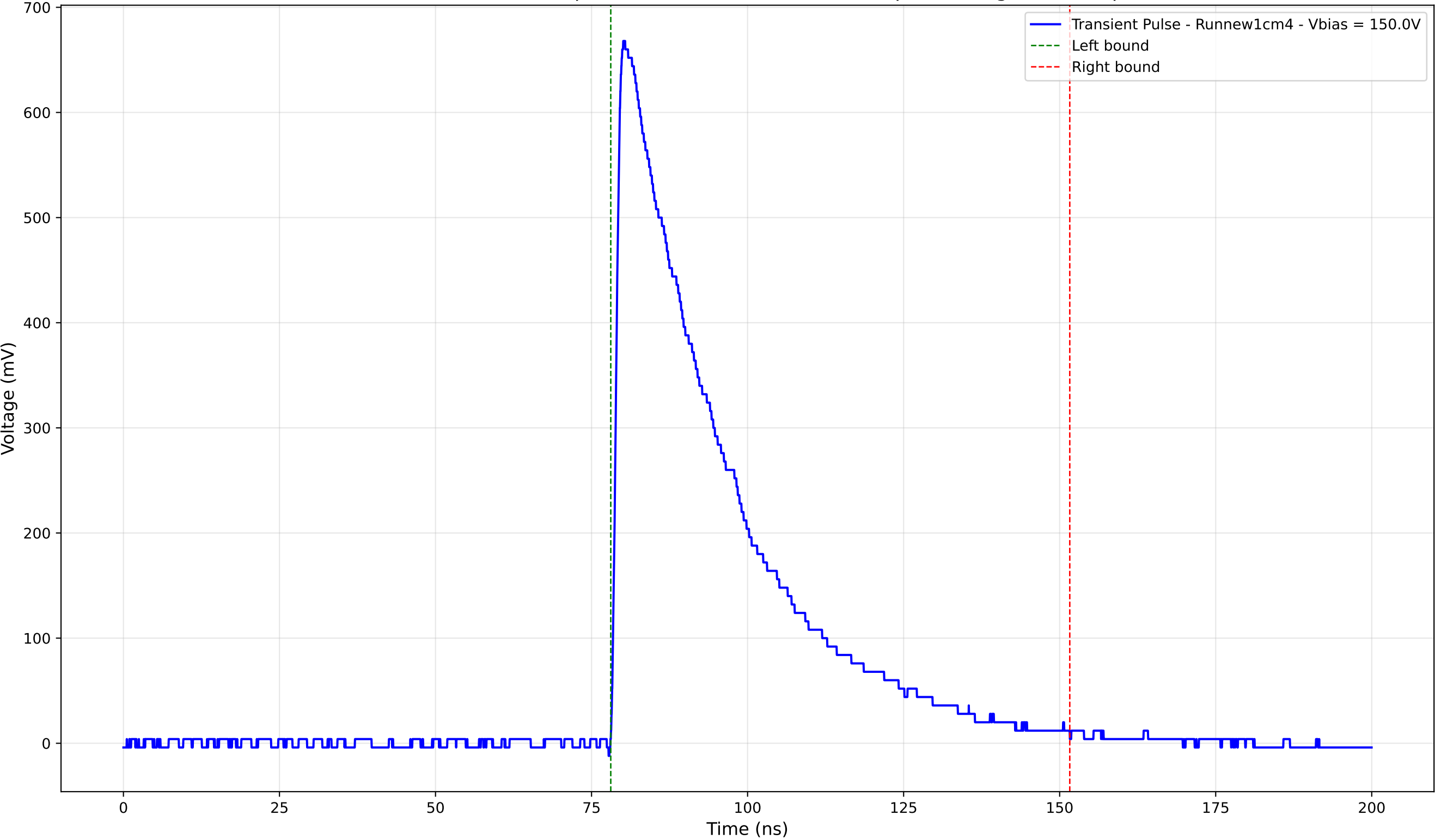
Transient Pulse - Sample: new1cm - Position: 3985.0 \mu\text{m} - Charge: 248.63 pC
