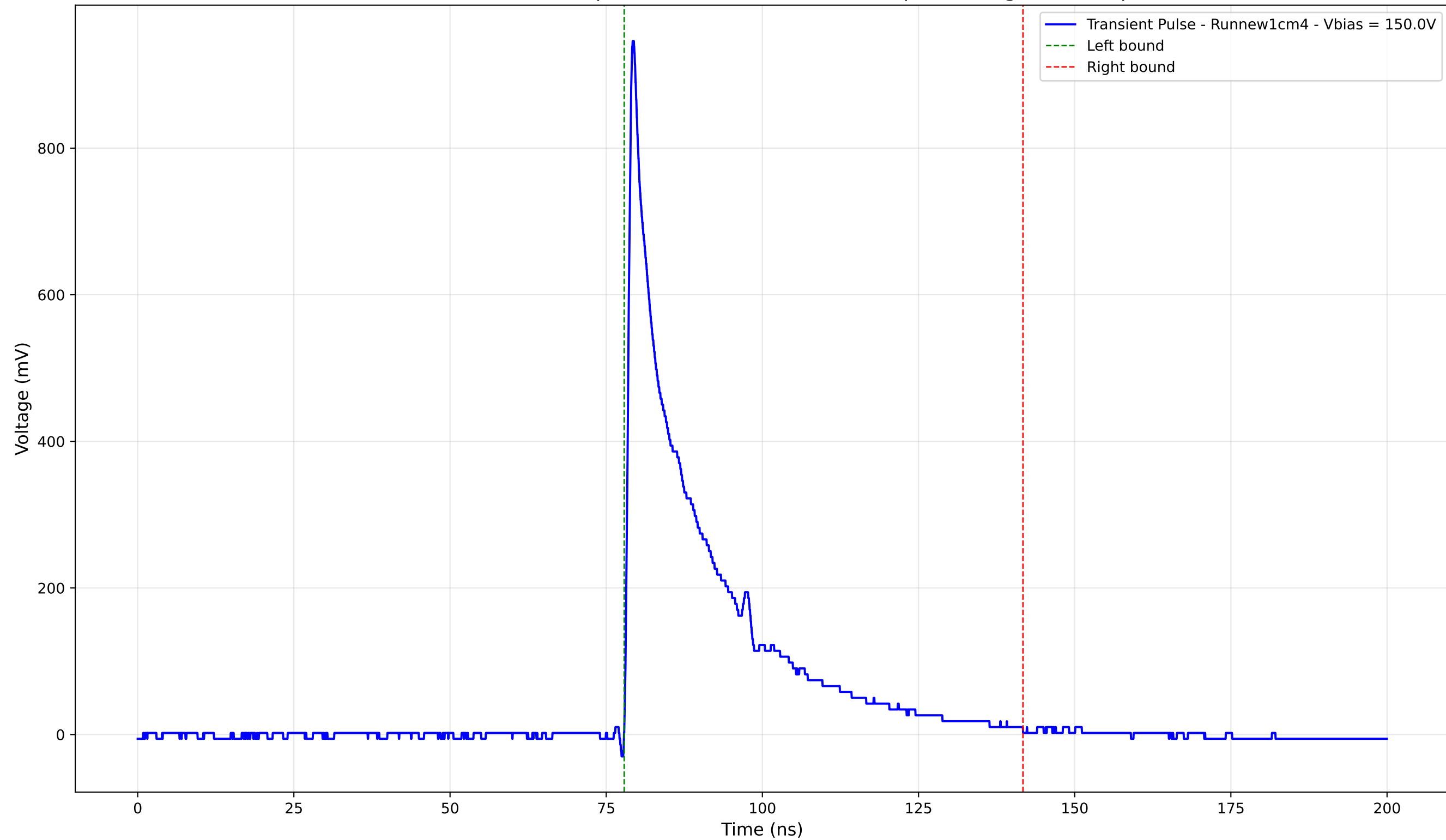
Transient Pulse - Sample: new1cm - Position: 385.0 \mu\text{m} - Charge: 195.79 pC
