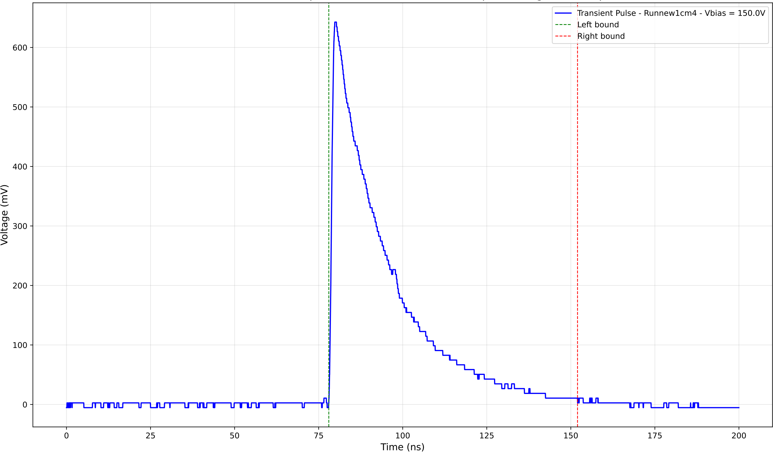
Transient Pulse - Sample: new1cm - Position: 4150.0 \mu\text{m} - Charge: 219.14 pC
