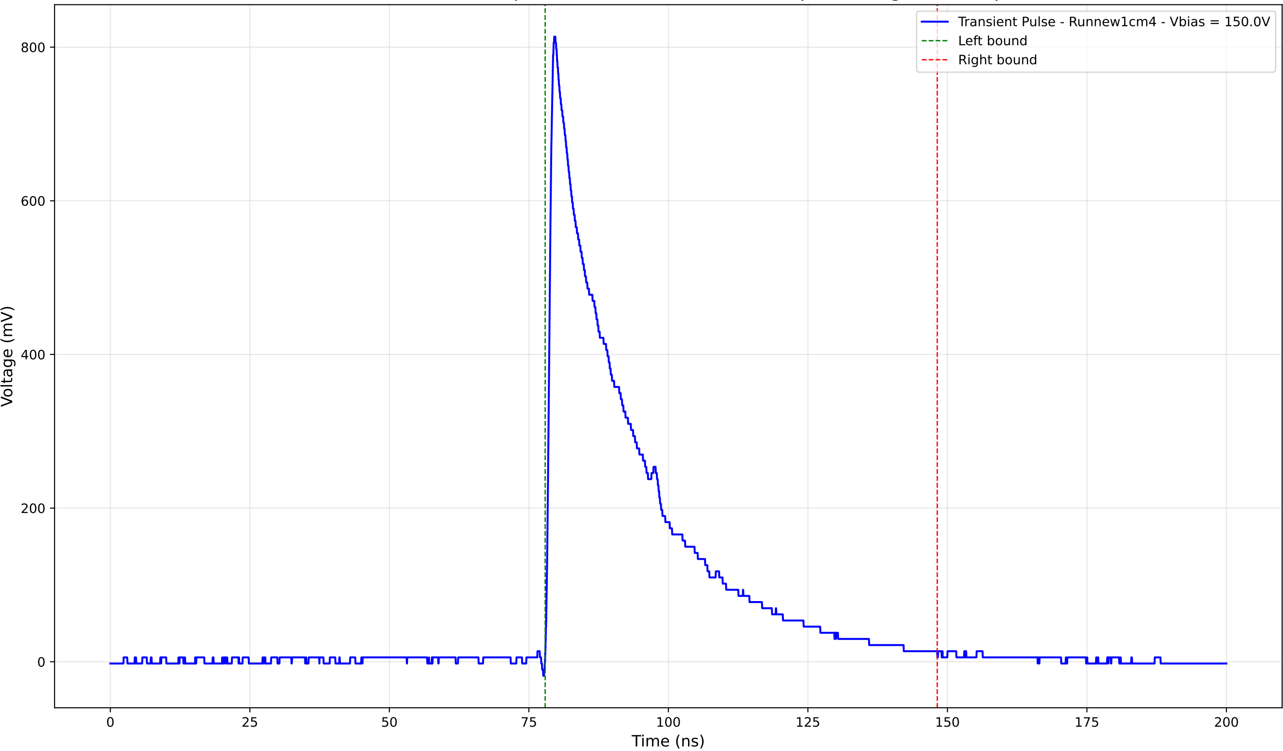
Transient Pulse - Sample: new1cm - Position: 4430.0 \mu\text{m} - Charge: 244.70 pC
