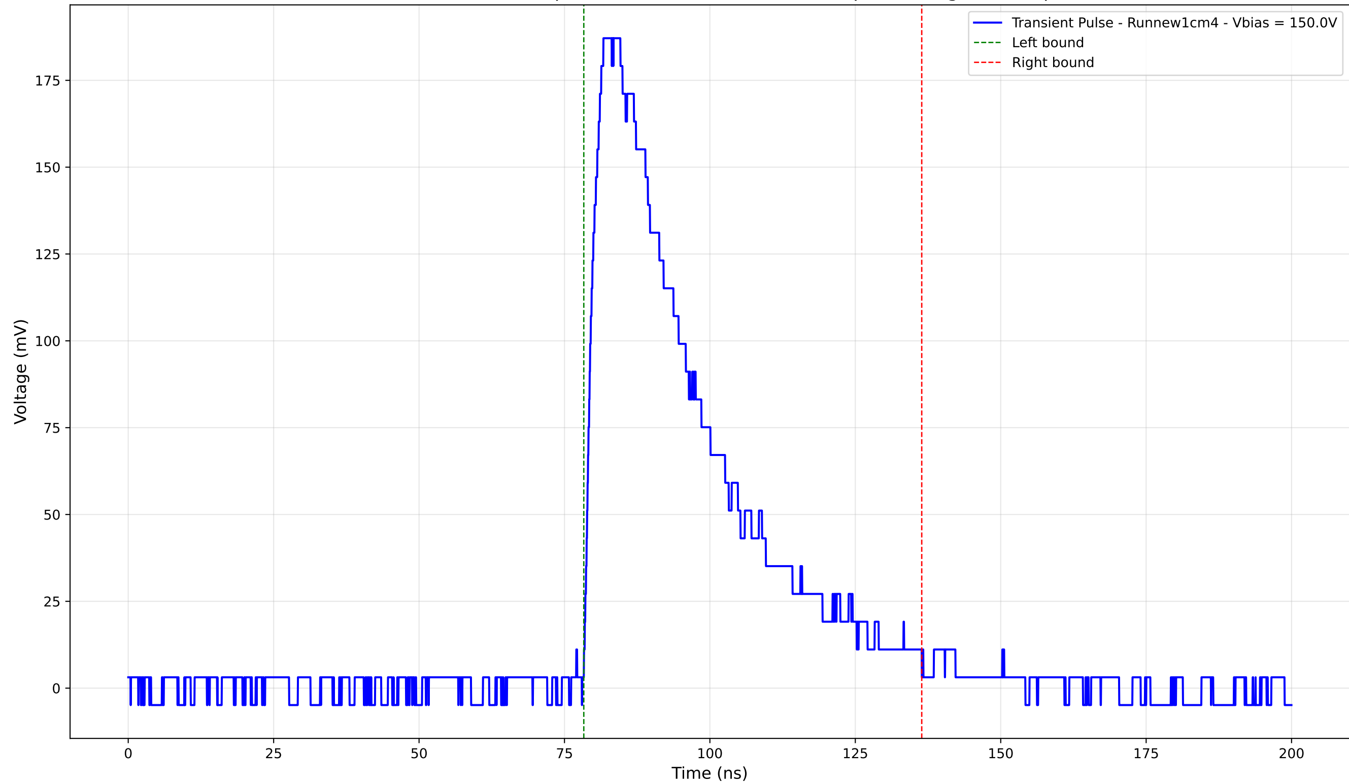
Transient Pulse - Sample: new1cm - Position: 2680.0 \mu\text{m} - Charge: 78.13 pC
