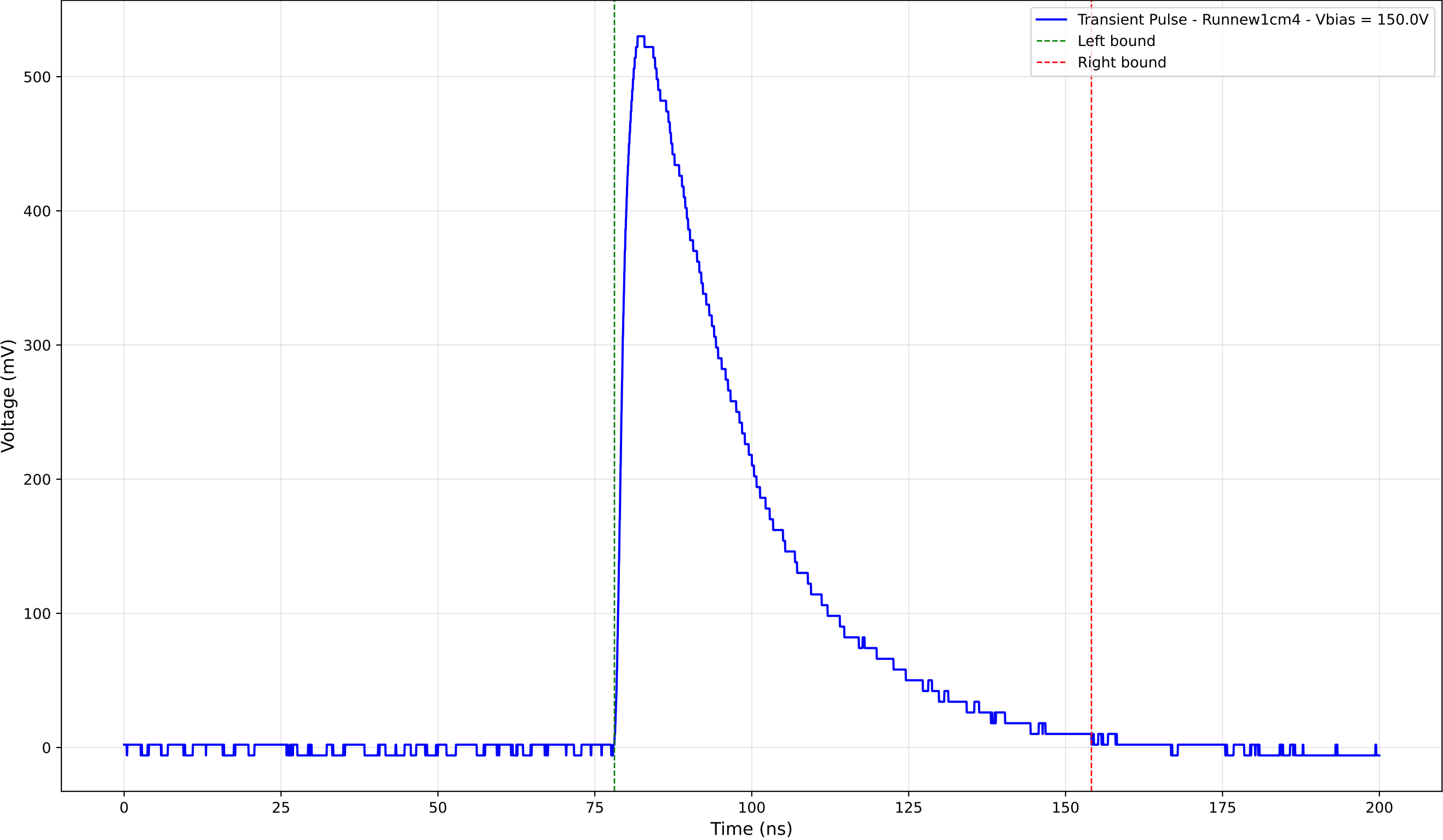
Transient Pulse - Sample: new1cm - Position: 3060.0 \mu\text{m} - Charge: 231.62 pC
