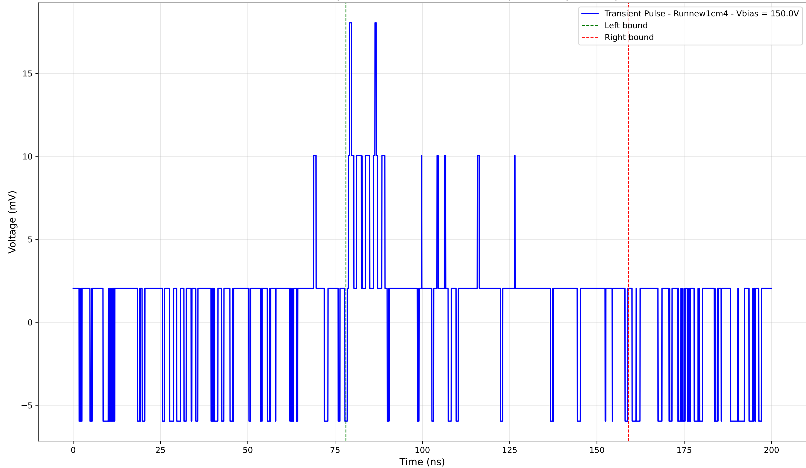
Transient Pulse - Sample: new1cm - Position: 100.0 \mu\text{m} - Charge: 3.60 pC
