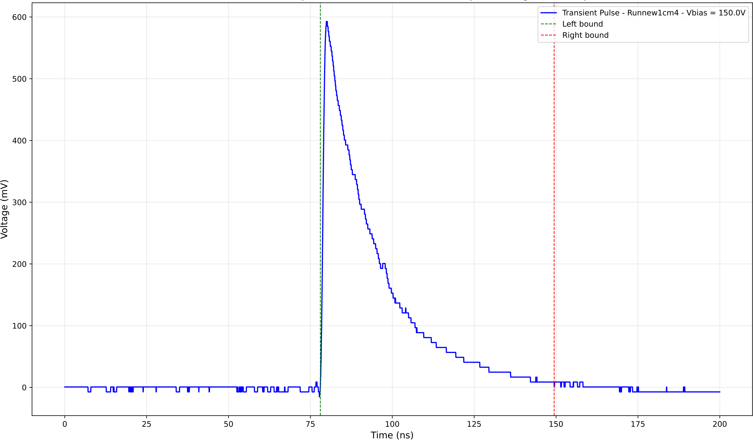
Transient Pulse - Sample: new1cm - Position: 4160.0 \mu\text{m} - Charge: 195.27 pC
