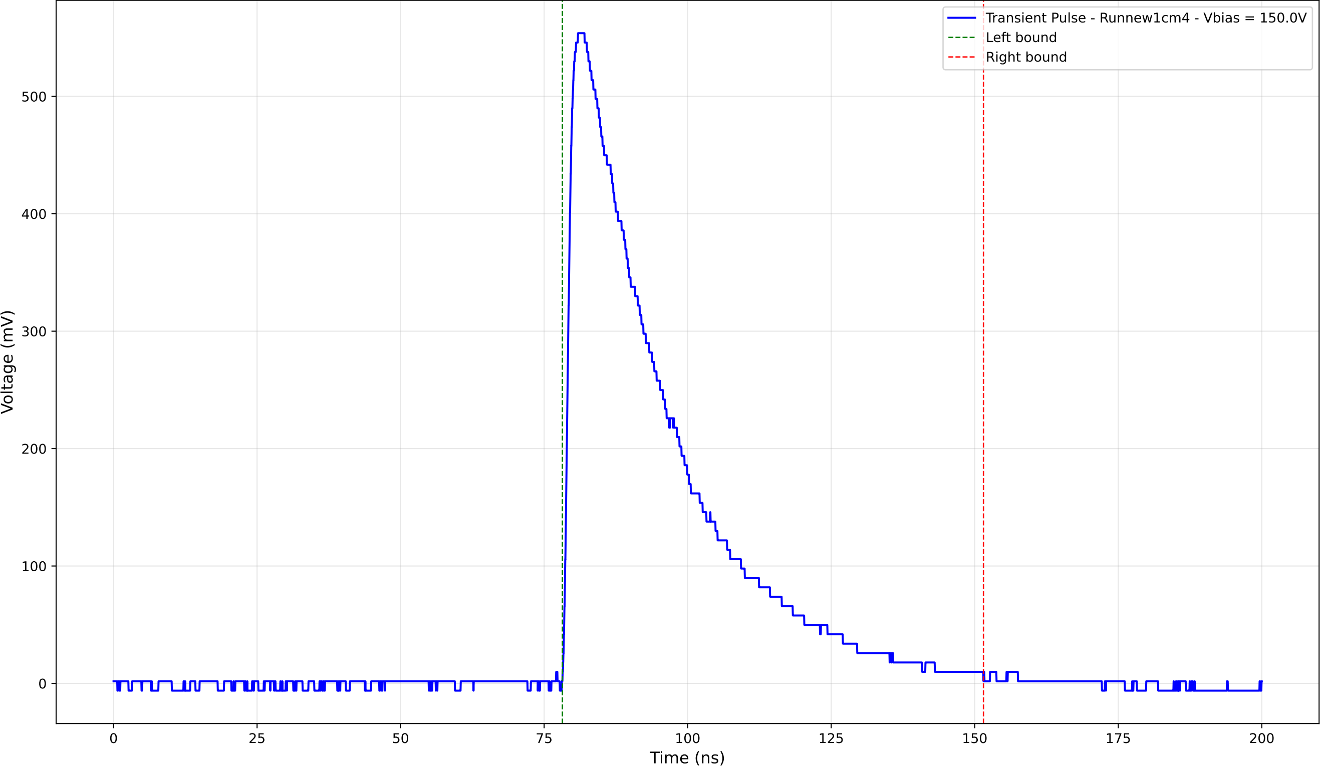
Transient Pulse - Sample: new1cm - Position: 1570.0 \mu\text{m} - Charge: 211.45 pC
