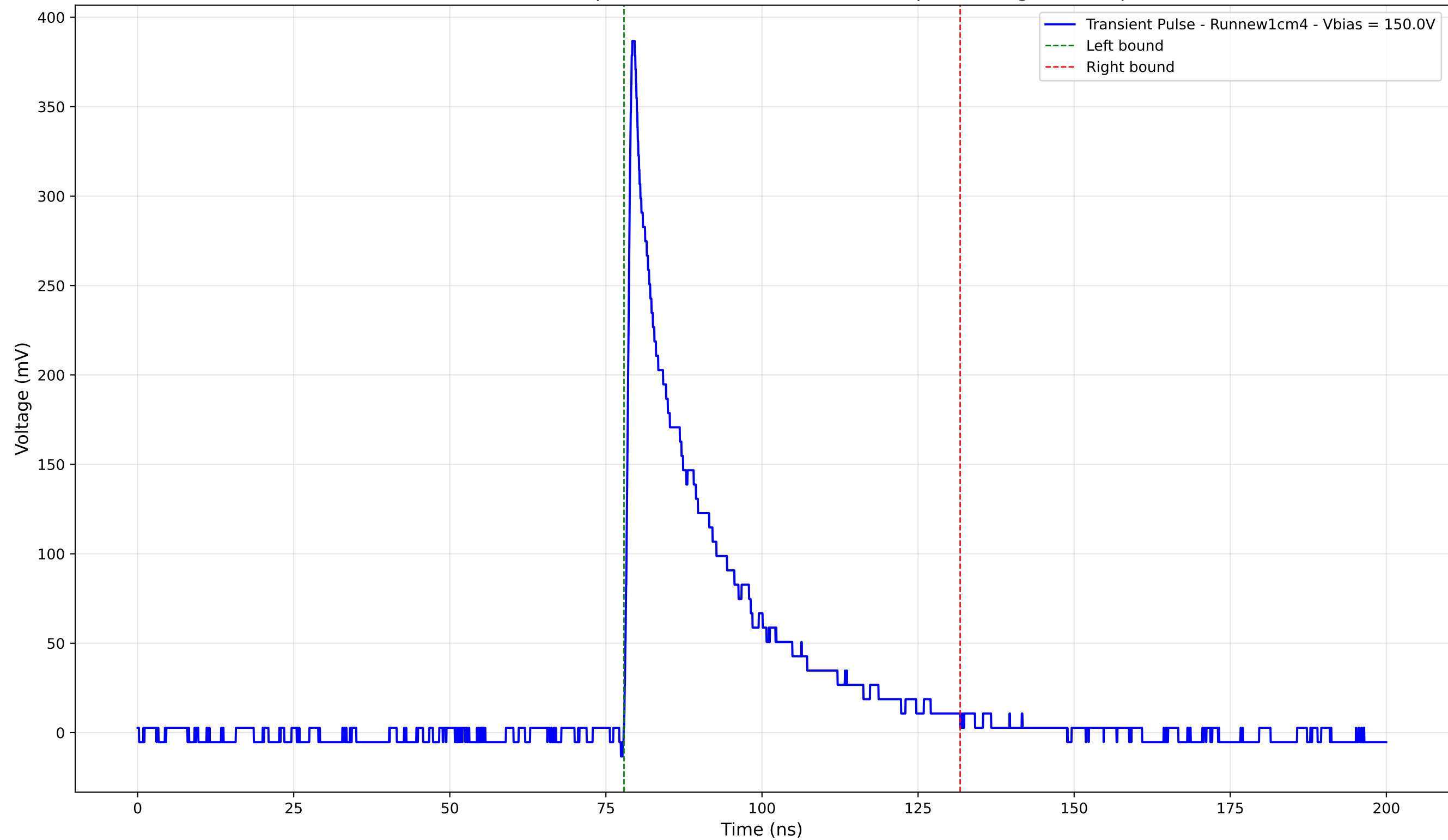
Transient Pulse - Sample: new1cm - Position: 4695.0 \mu\text{m} - Charge: 86.77 pC
