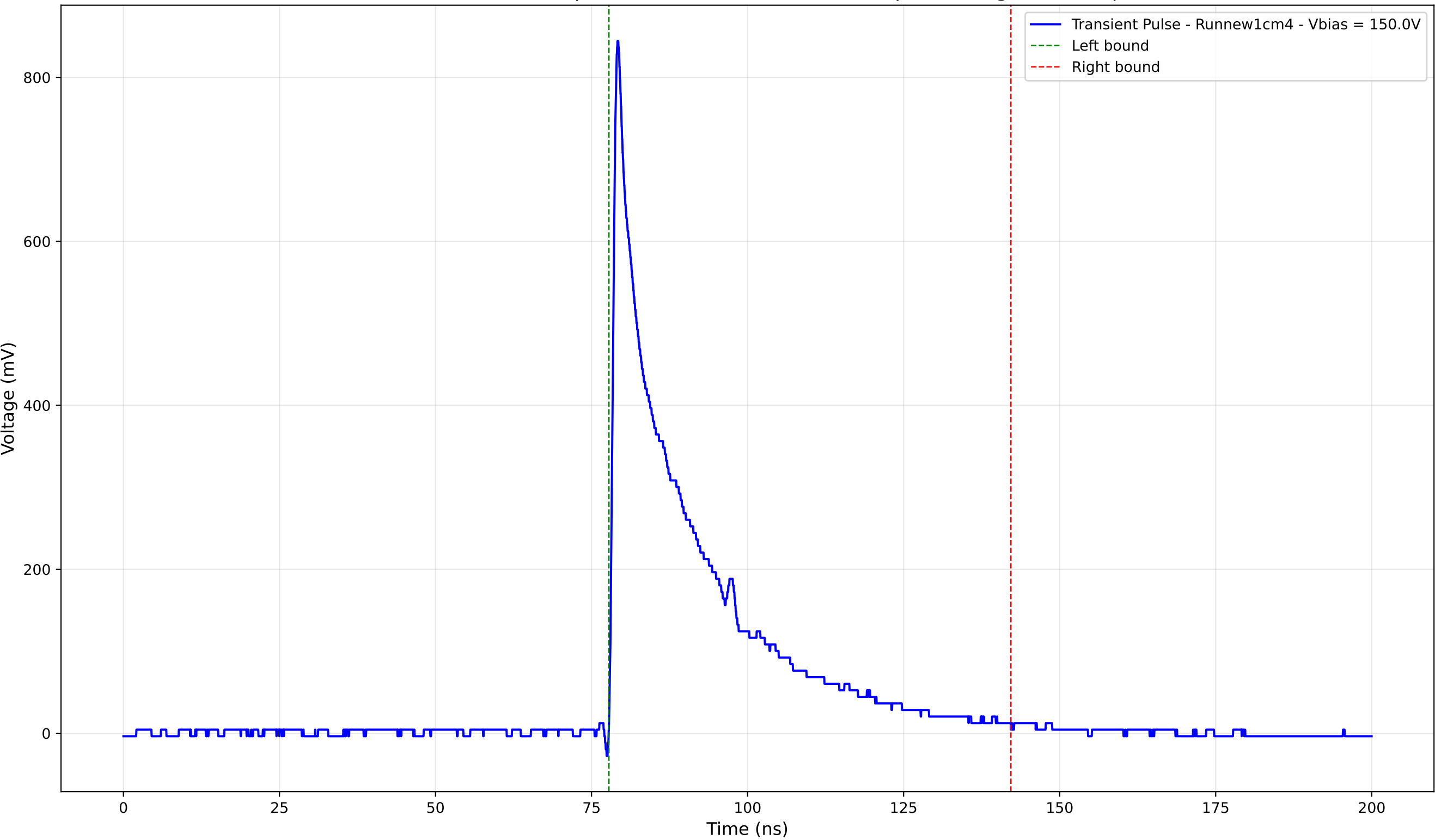
Transient Pulse - Sample: new1cm - Position: 4850.0 \mu\text{m} - Charge: 188.33 pC
