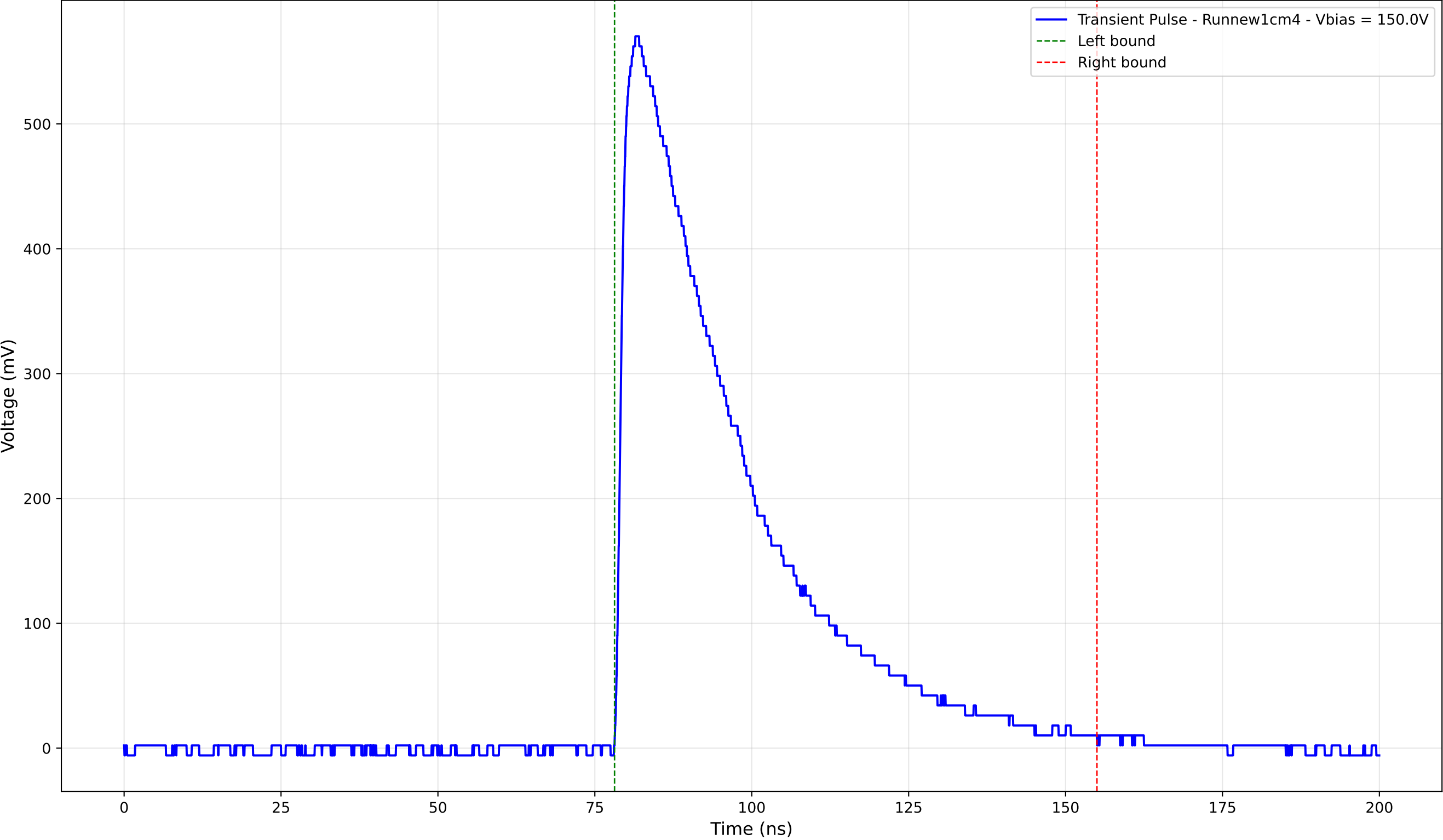
Transient Pulse - Sample: new1cm - Position: 3510.0 \mu\text{m} - Charge: 237.41 pC
