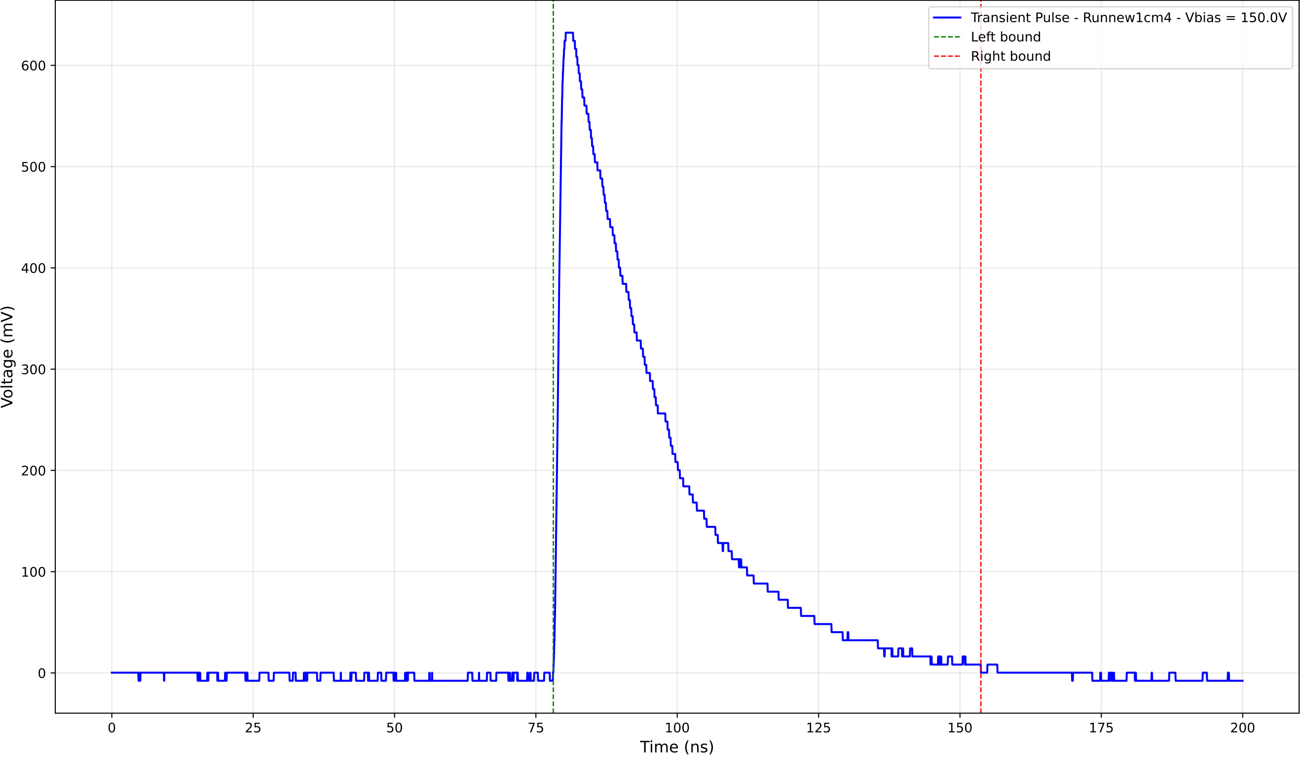
Transient Pulse - Sample: new1cm - Position: 3850.0 \mu\text{m} - Charge: 244.85 pC
