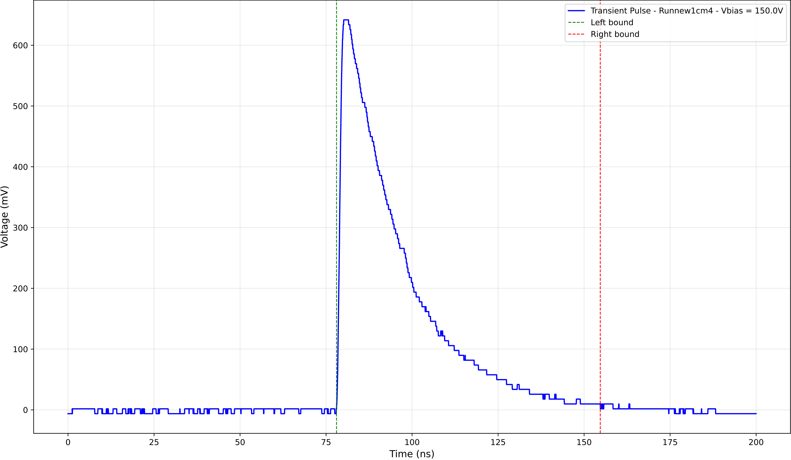
Transient Pulse - Sample: new1cm - Position: 3870.0 \mu\text{m} - Charge: 249.16 pC
