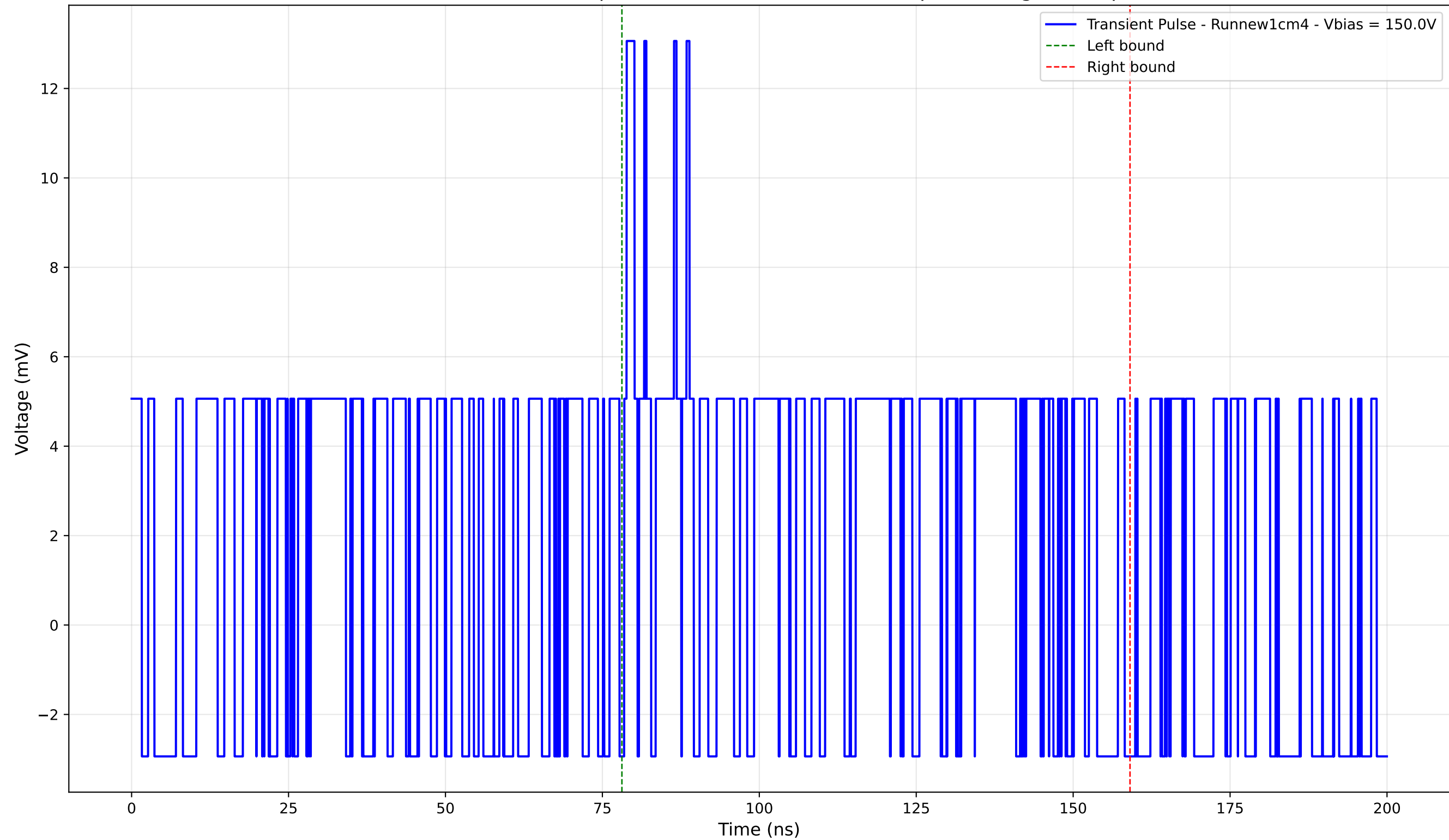
Transient Pulse - Sample: new1cm - Position: 5175.0 \mu\text{m} - Charge: 5.03 pC
