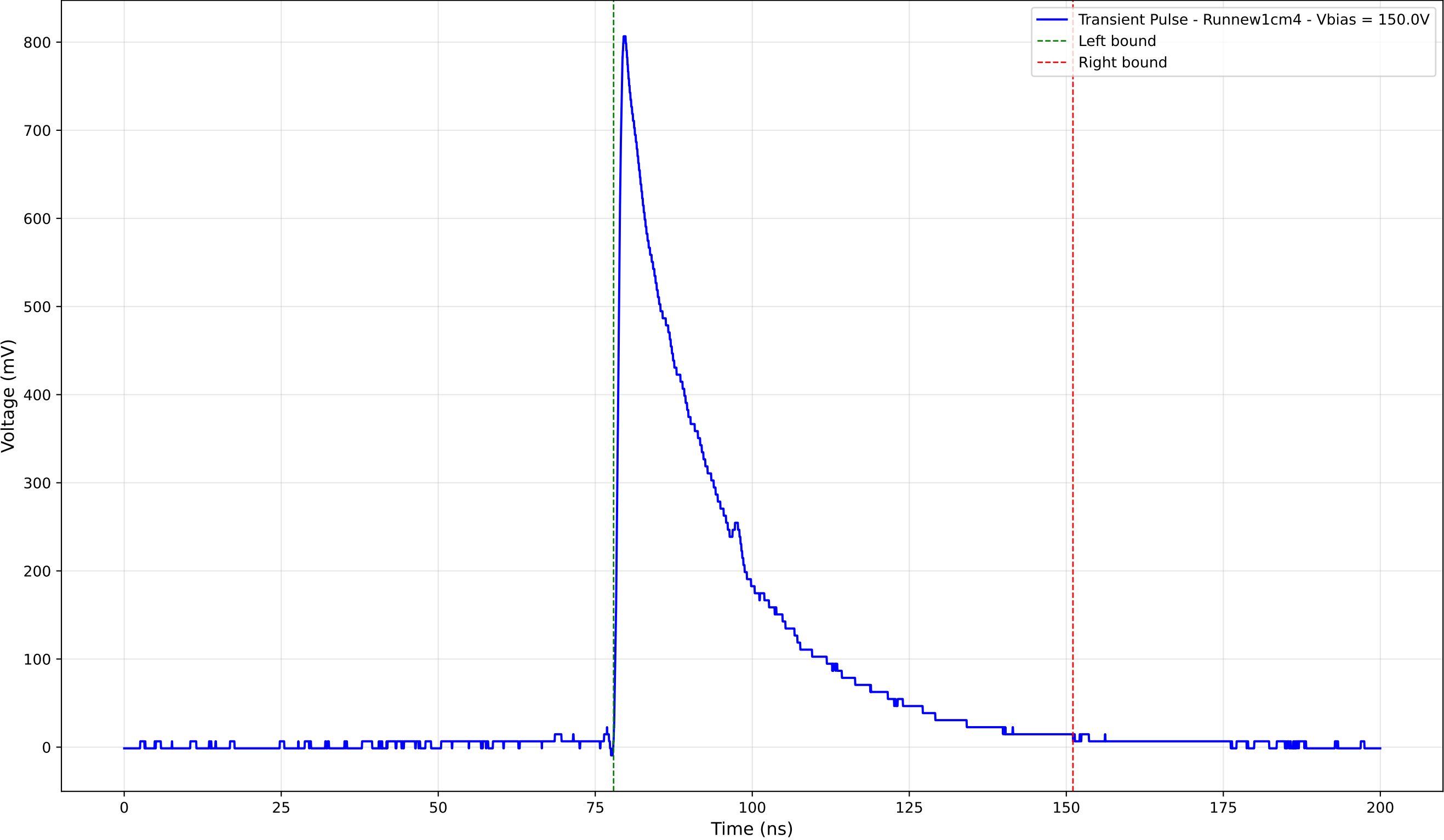
Transient Pulse - Sample: new1cm - Position: 4410.0 \mu\text{m} - Charge: 248.02 pC
