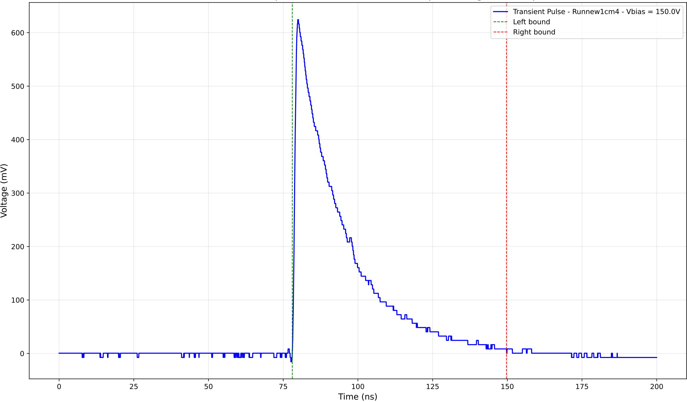
Transient Pulse - Sample: new1cm - Position: 4155.0 \mu\text{m} - Charge: 207.89 pC
