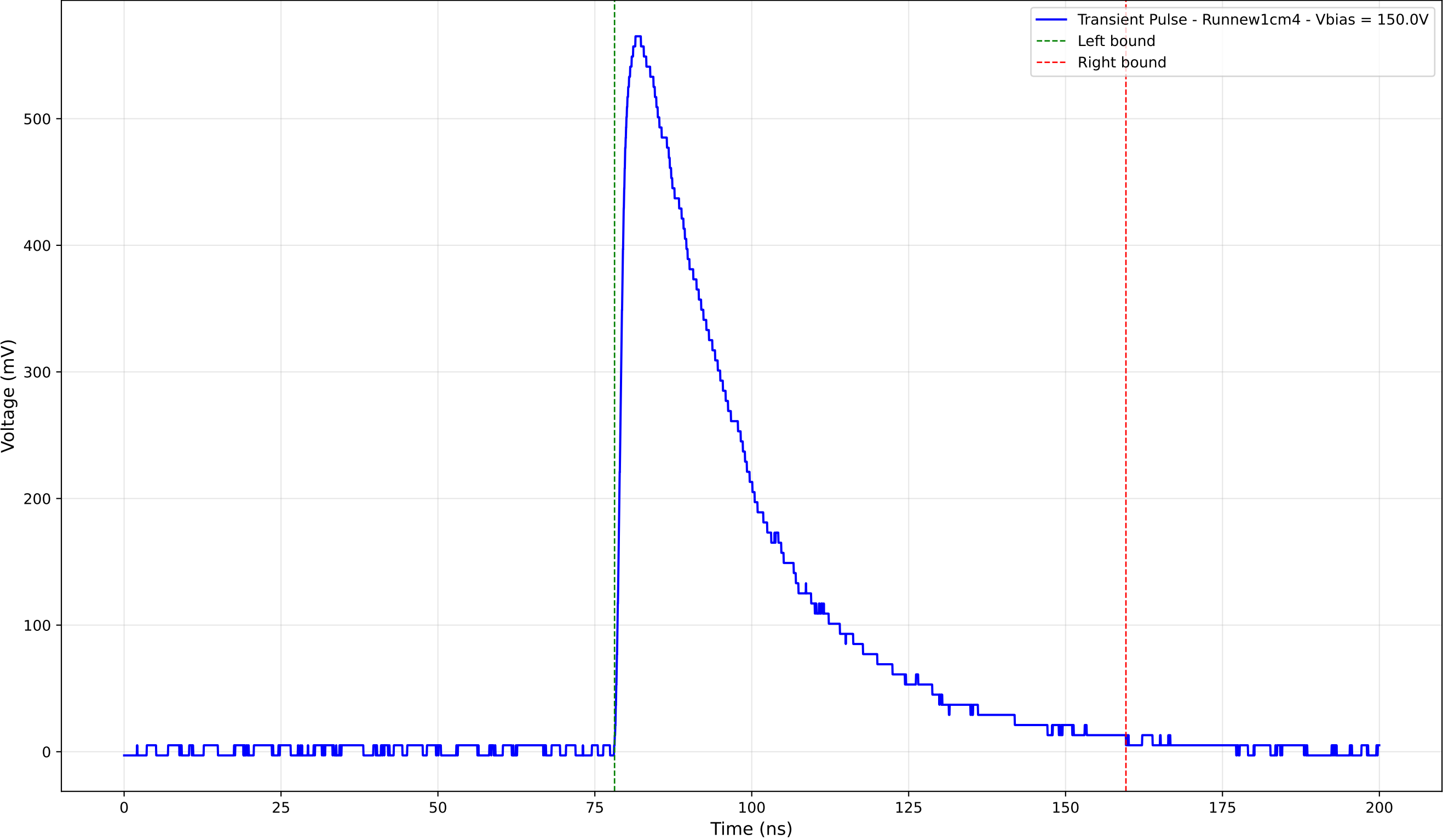
Transient Pulse - Sample: new1cm - Position: 3490.0 \mu\text{m} - Charge: 244.05 pC
