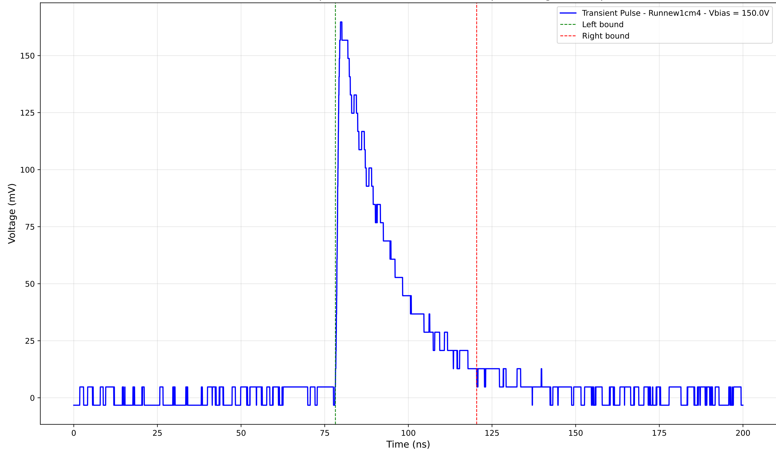
Transient Pulse - Sample: new1cm - Position: 4215.0 \mu\text{m} - Charge: 51.15 pC
