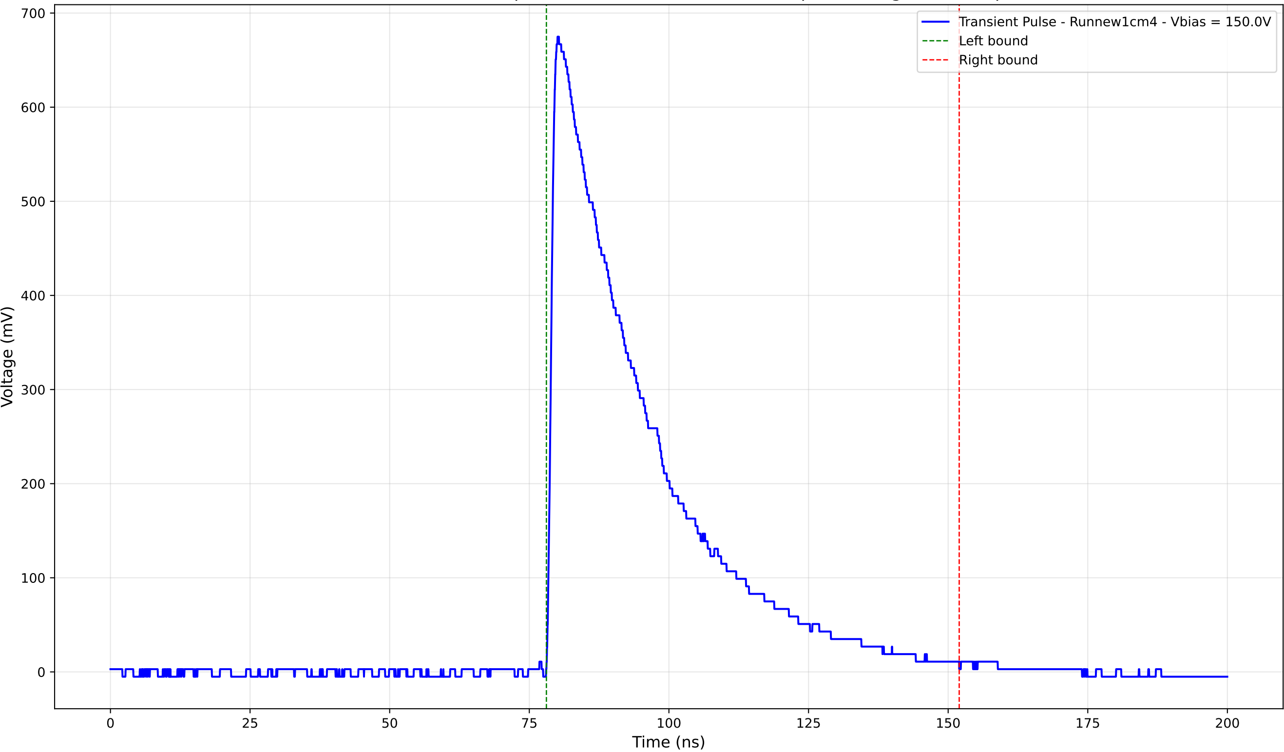
Transient Pulse - Sample: new1cm - Position: 4015.0 \mu\text{m} - Charge: 248.22 pC
