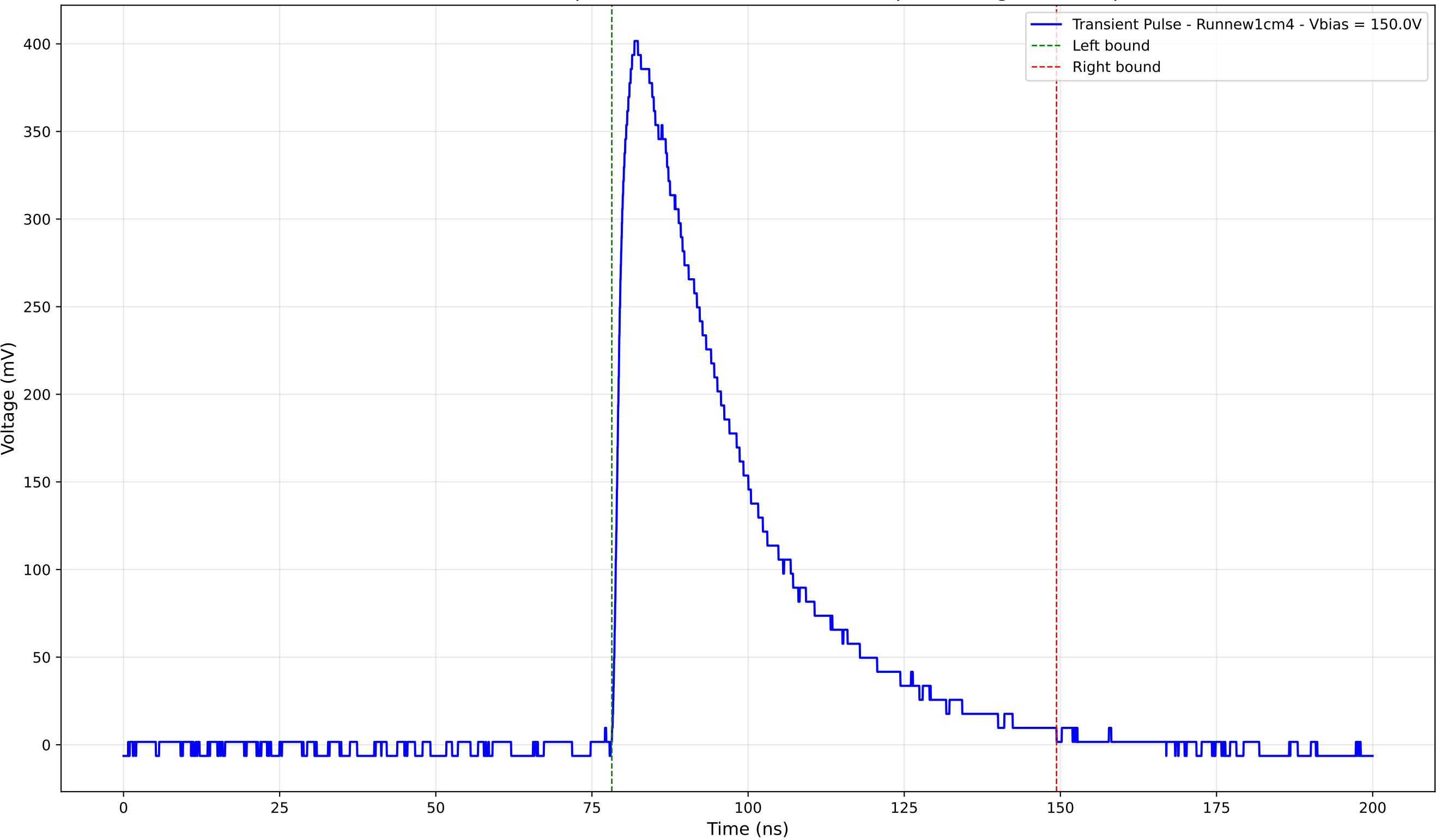
Transient Pulse - Sample: new1cm - Position: 3290.0 \mu\text{m} - Charge: 166.21 pC
