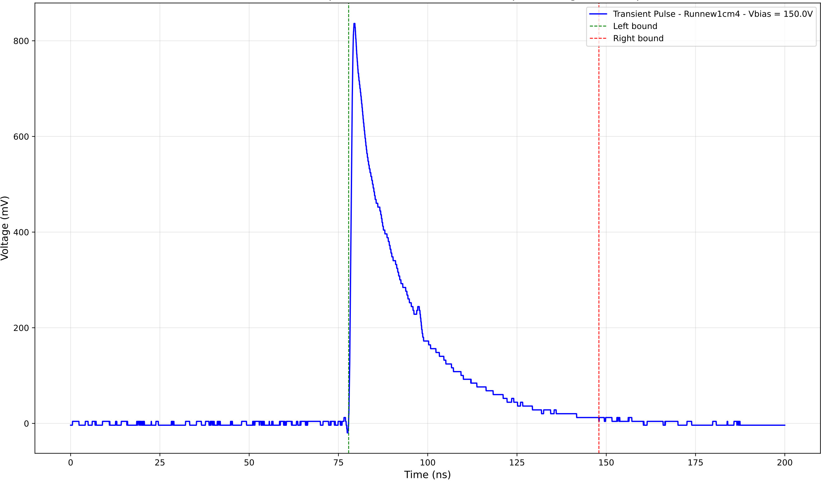
Transient Pulse - Sample: new1cm - Position: 4575.0 \mu\text{m} - Charge: 236.02 pC
