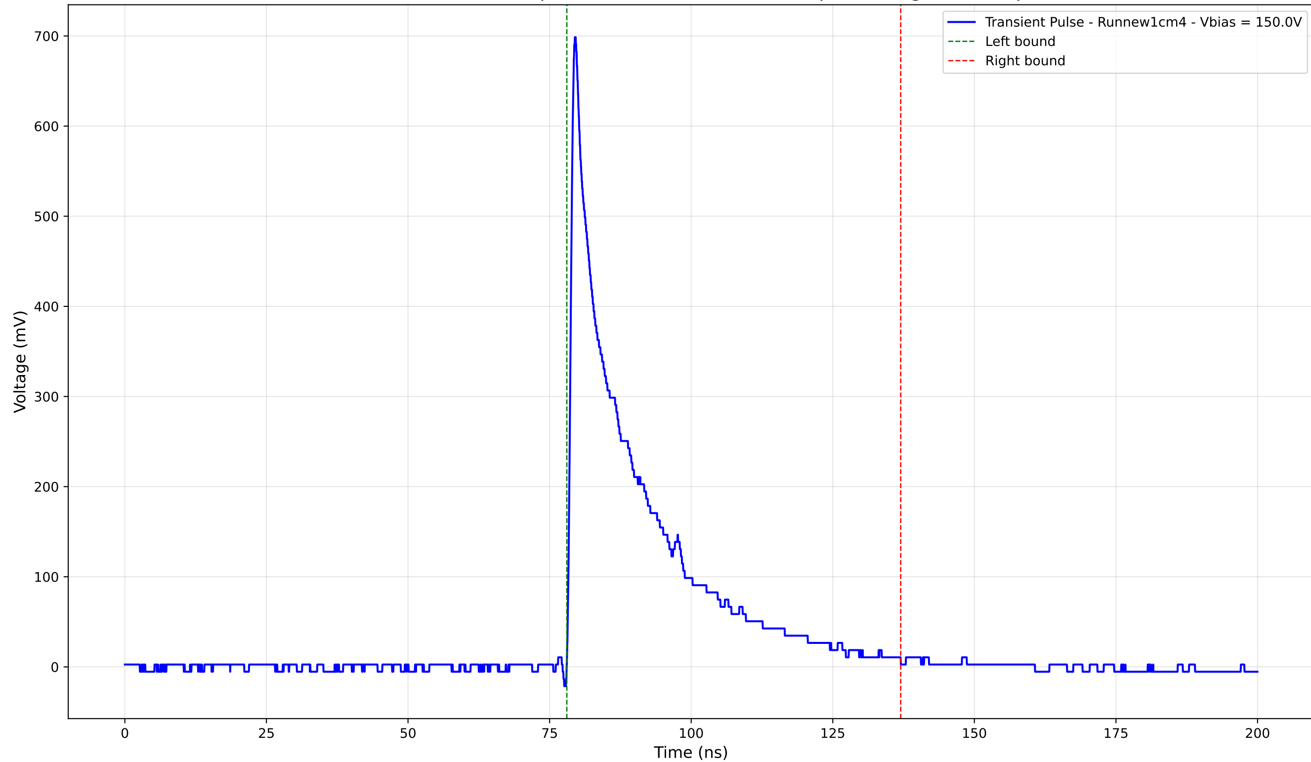
Transient Pulse - Sample: new1cm - Position: 620.0 \mu\text{m} - Charge: 148.40 pC
