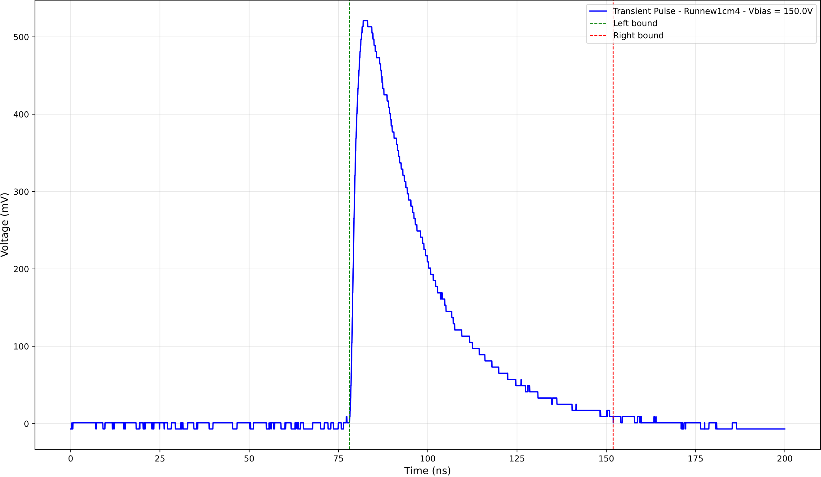
Transient Pulse - Sample: new1cm - Position: 2930.0 \mu\text{m} - Charge: 228.57 pC
