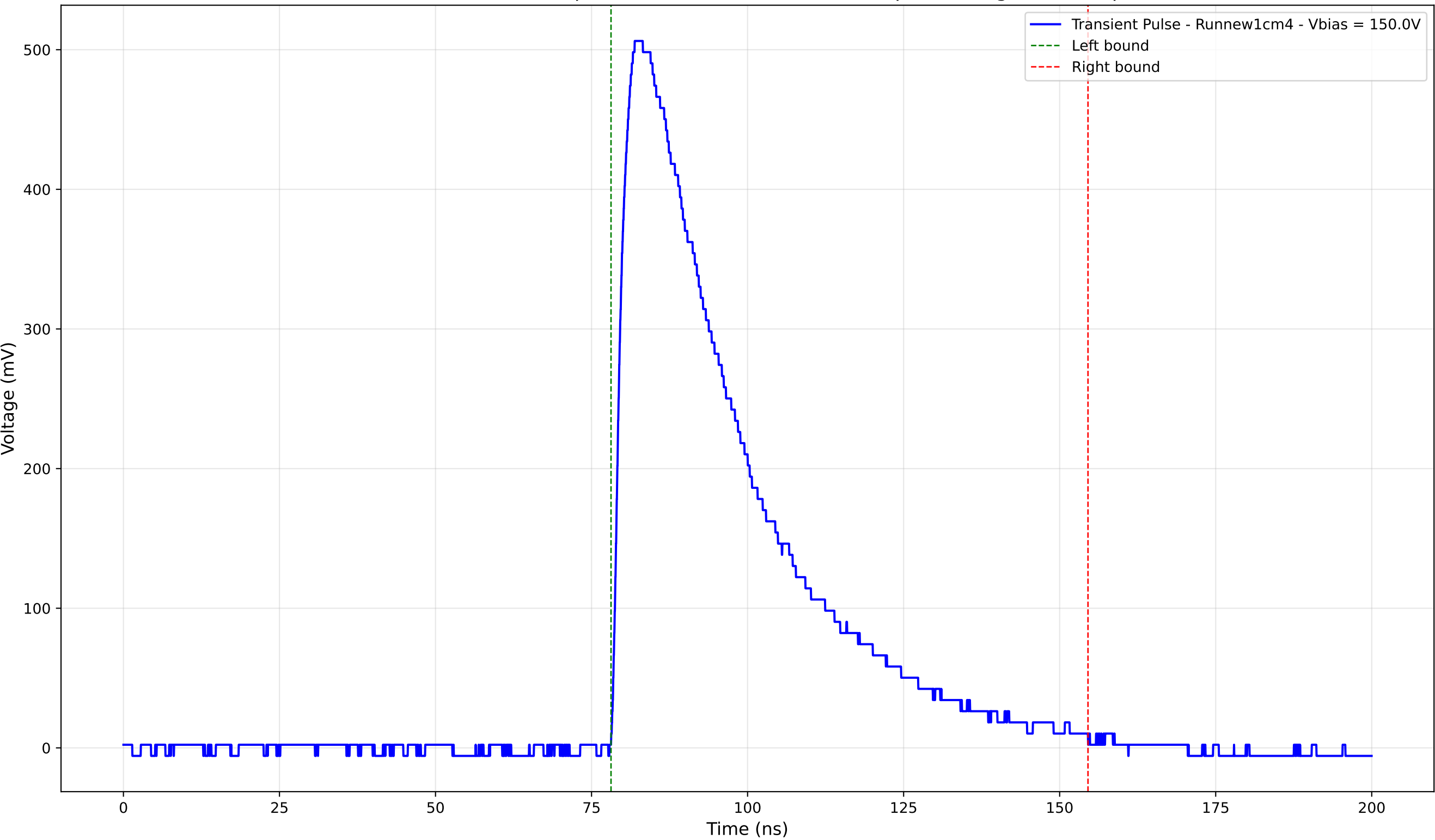
Transient Pulse - Sample: new1cm - Position: 2840.0 \mu\text{m} - Charge: 224.80 pC
