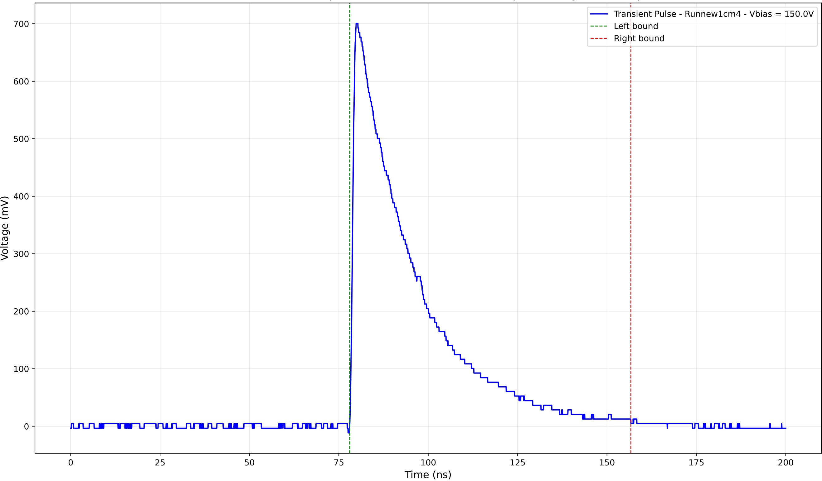
Transient Pulse - Sample: new1cm - Position: 4095.0 \mu\text{m} - Charge: 253.26 pC
