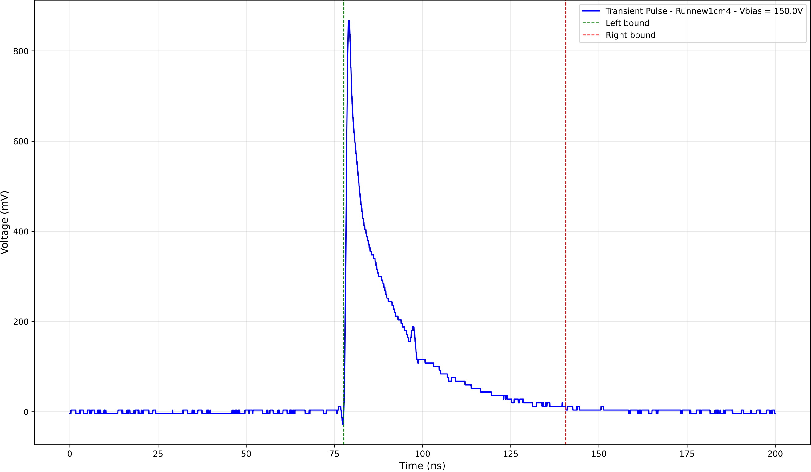
Transient Pulse - Sample: new1cm - Position: 4940.0 \mu\text{m} - Charge: 181.91 pC
