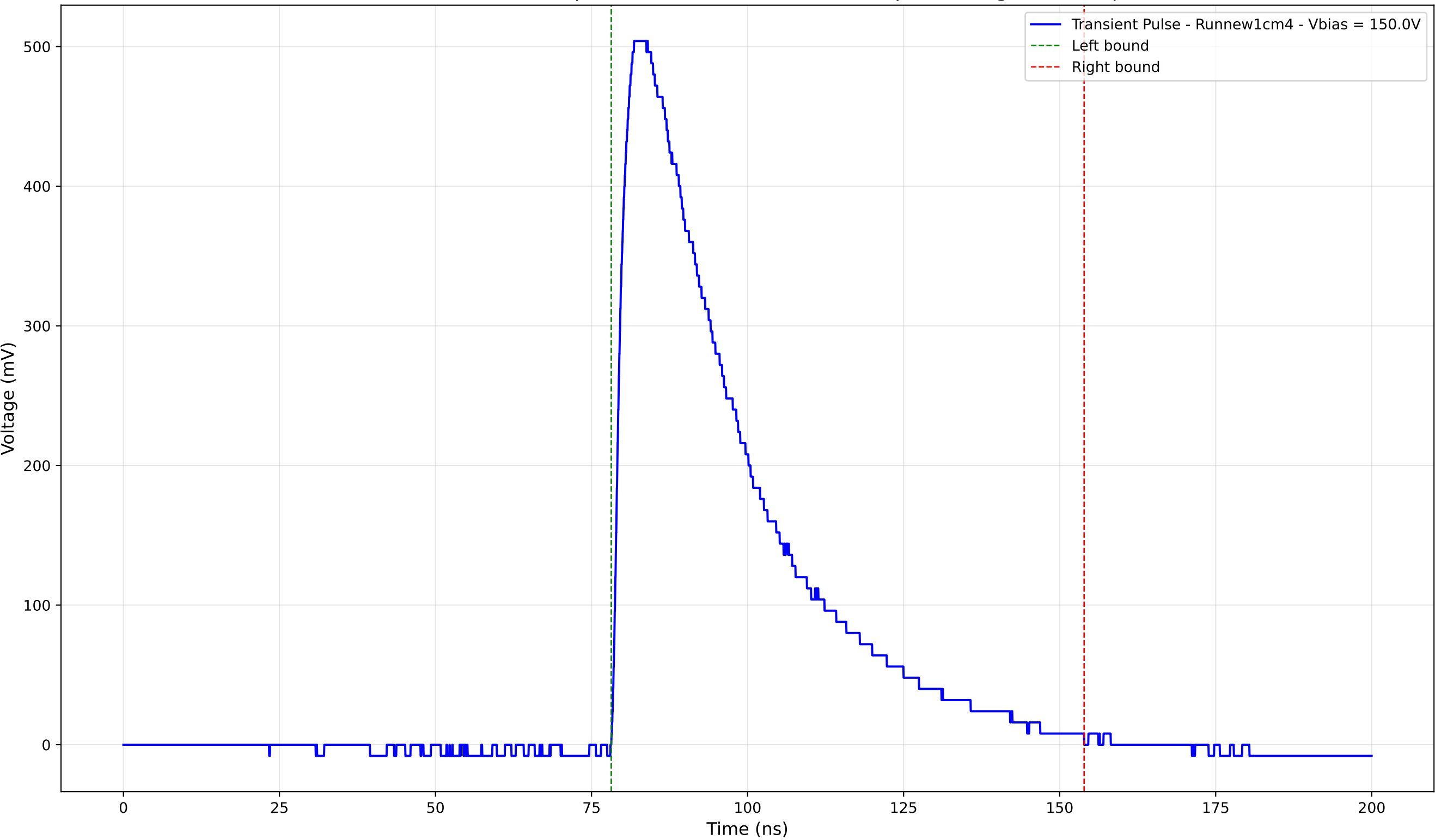
Transient Pulse - Sample: new1cm - Position: 2865.0 \mu\text{m} - Charge: 223.06 pC
