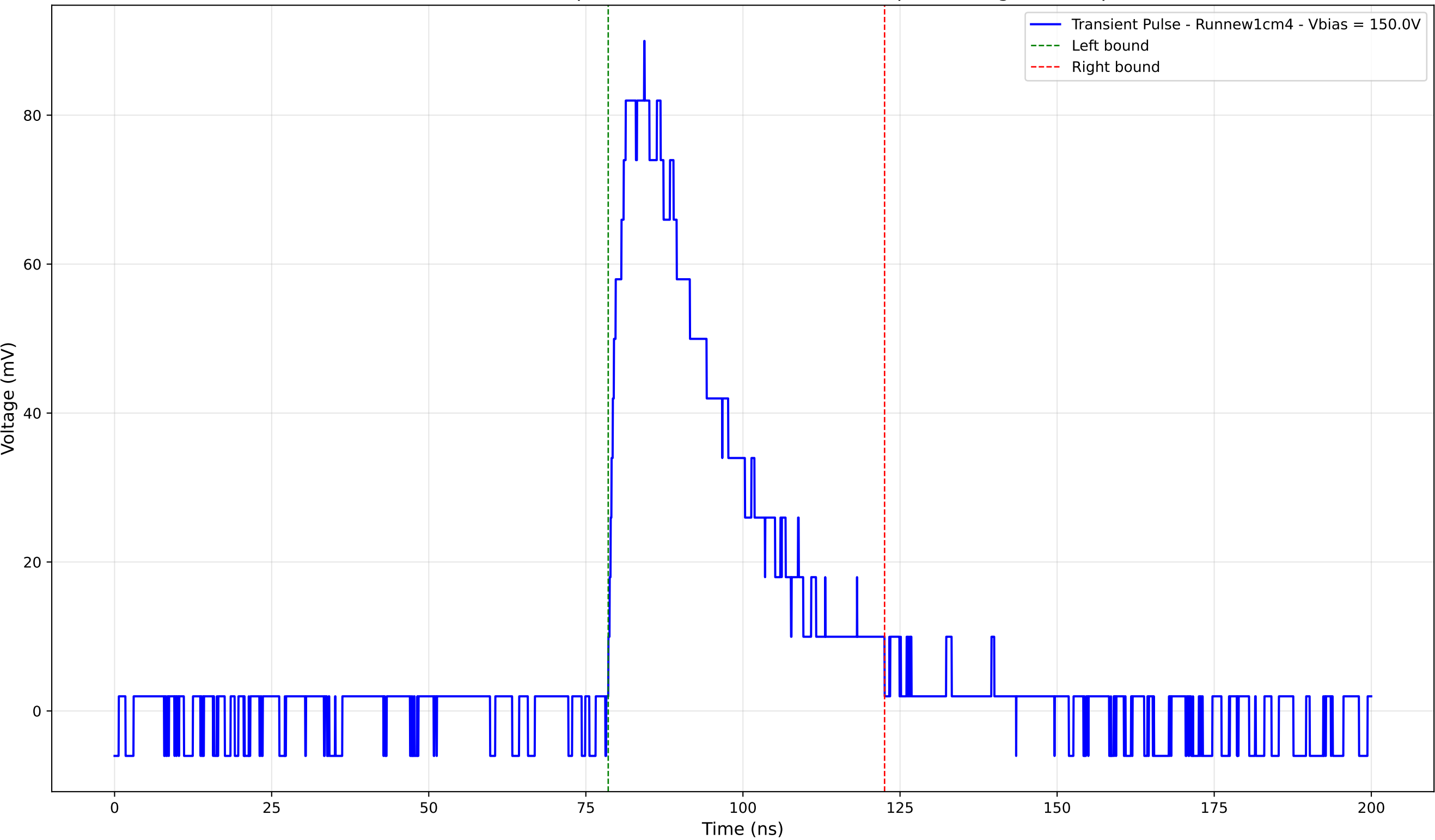
Transient Pulse - Sample: new1cm - Position: 3225.0 \mu\text{m} - Charge: 32.00 pC
