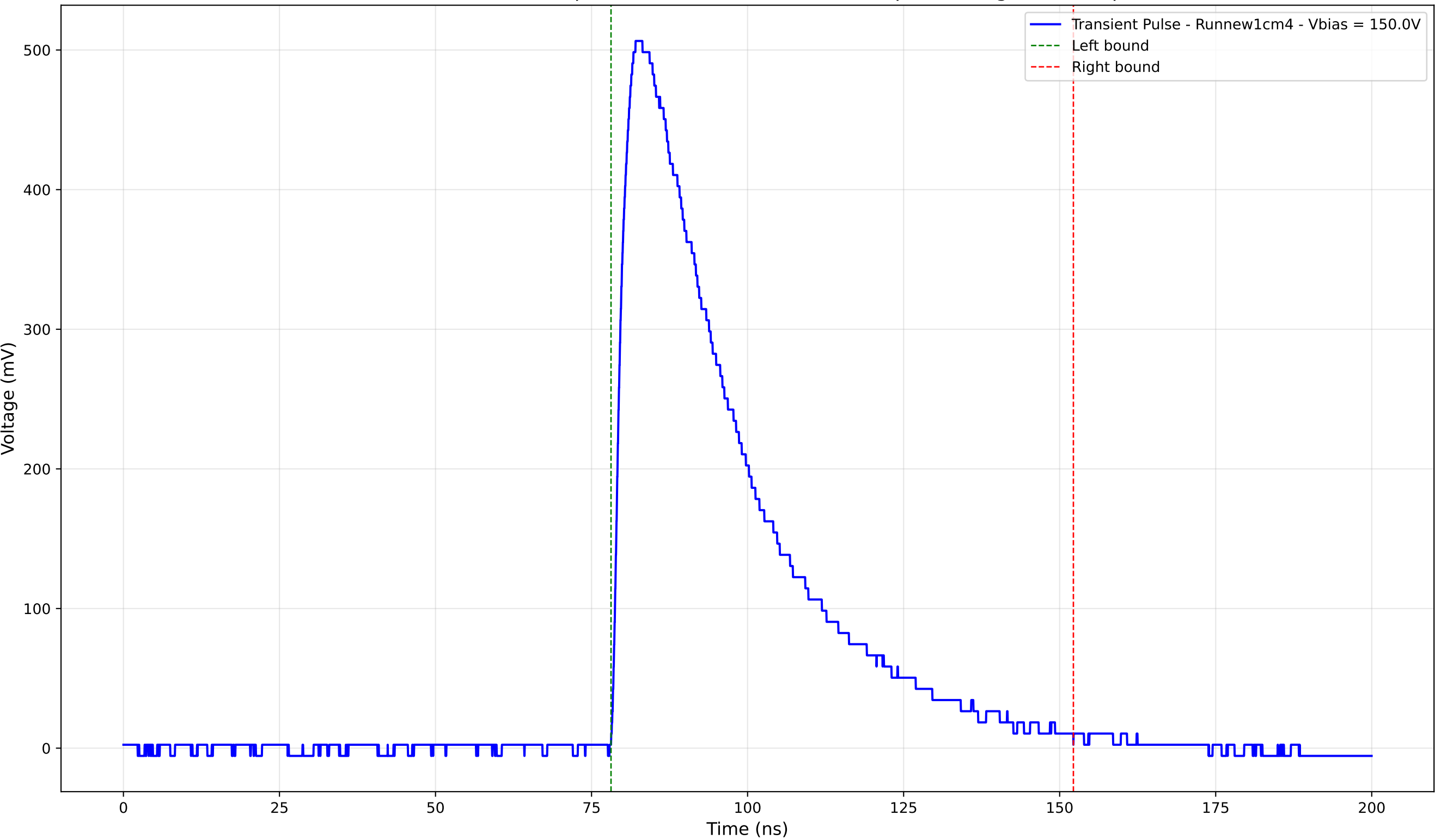
Transient Pulse - Sample: new1cm - Position: 2505.0 \mu\text{m} - Charge: 220.48 pC
