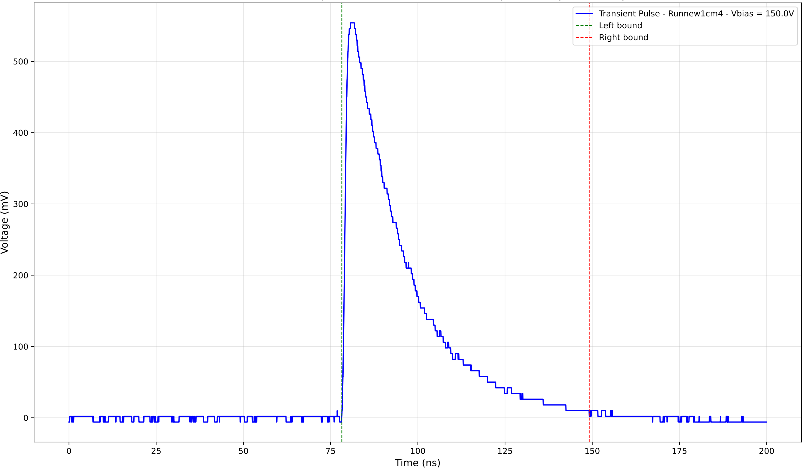
Transient Pulse - Sample: new1cm - Position: 1480.0 \mu\text{m} - Charge: 204.93 pC
