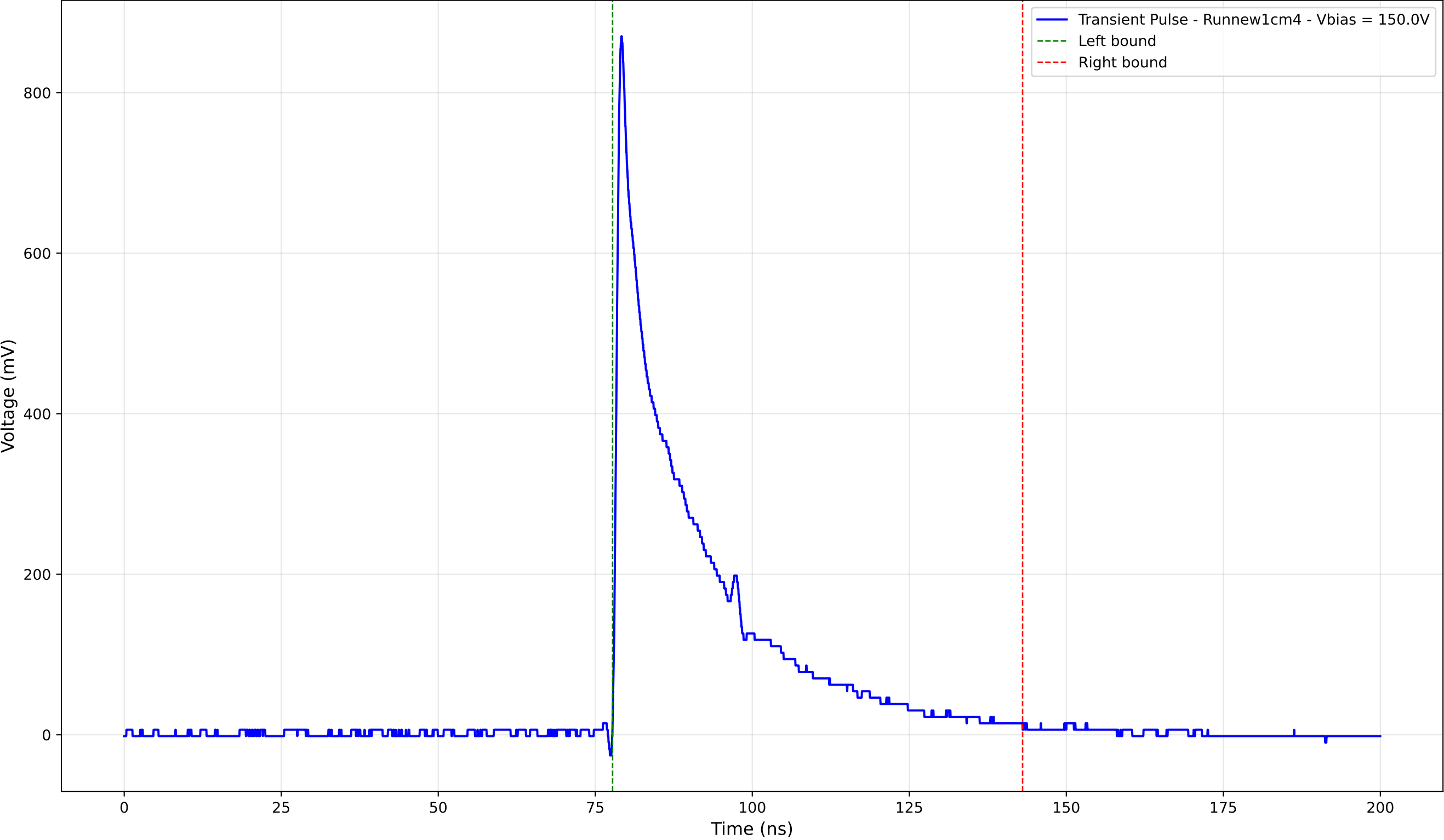
Transient Pulse - Sample: new1cm - Position: 4880.0 \mu\text{m} - Charge: 193.93 pC
