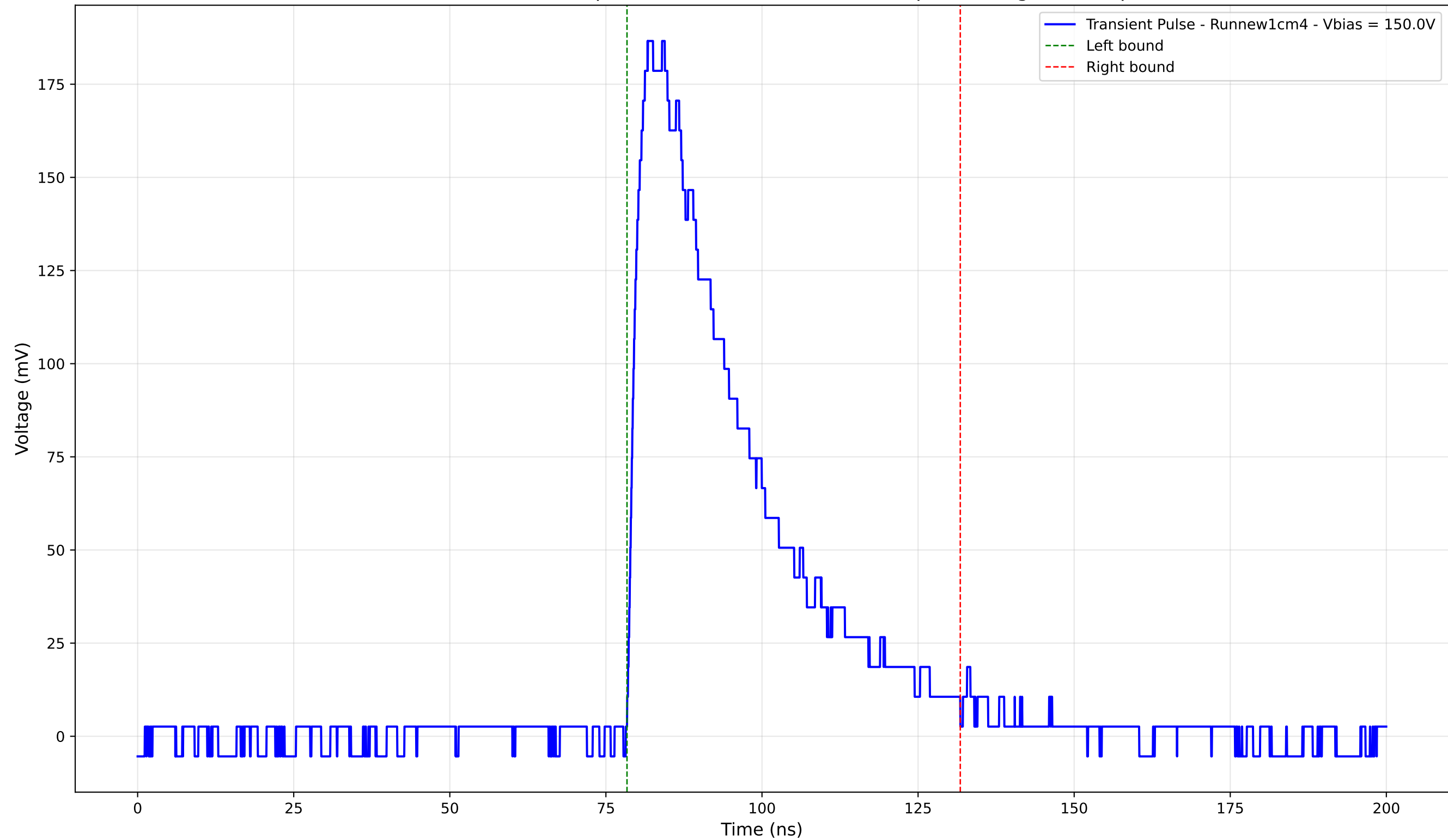
Transient Pulse - Sample: new1cm - Position: 2170.0 \mu\text{m} - Charge: 72.65 pC
