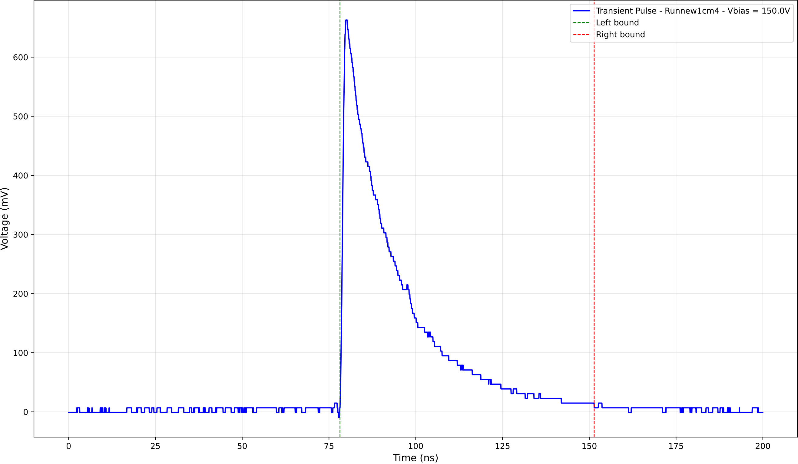
Transient Pulse - Sample: new1cm - Position: 1070.0 \mu\text{m} - Charge: 210.72 pC
