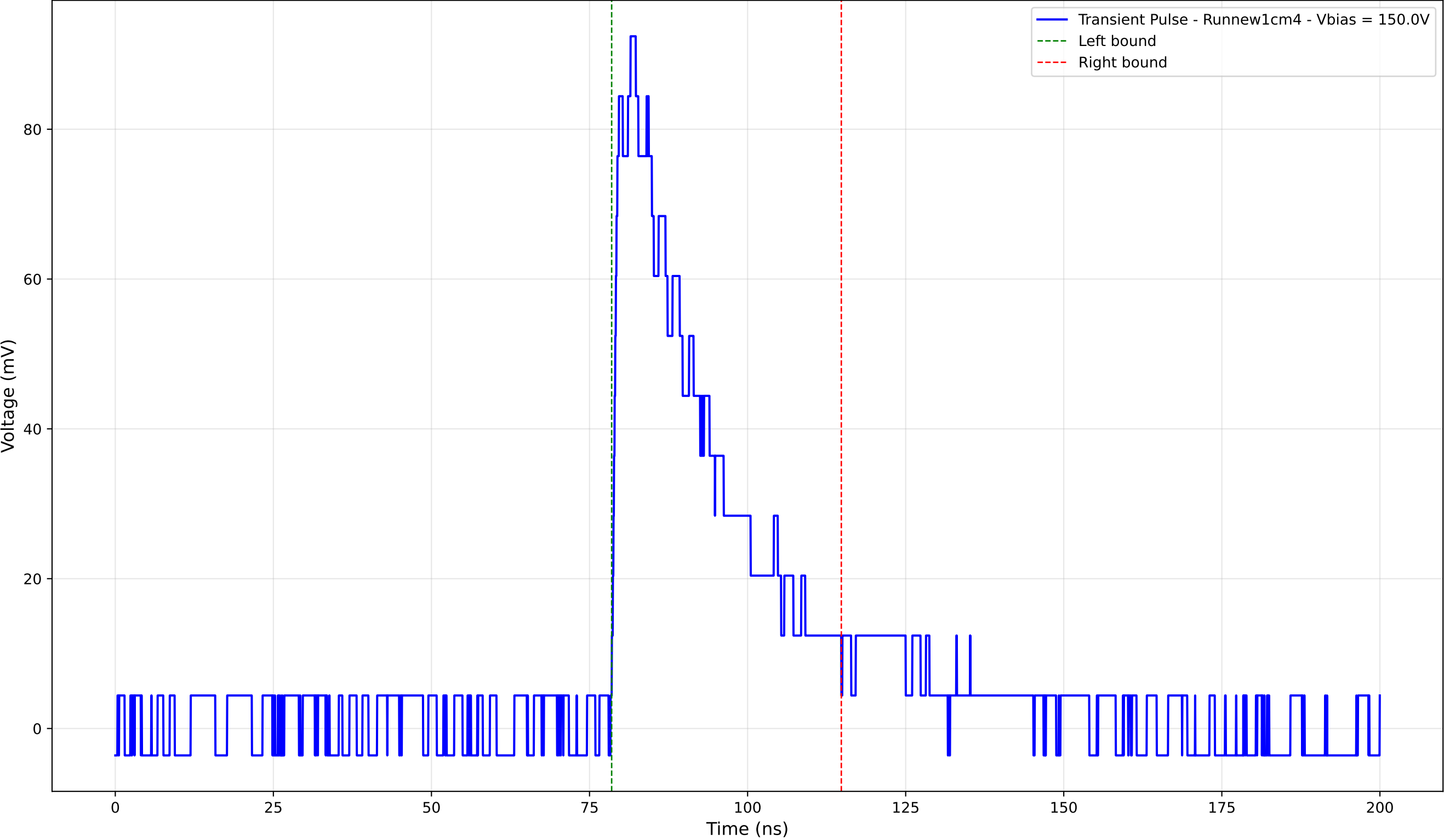
Transient Pulse - Sample: new1cm - Position: 1195.0 \mu\text{m} - Charge: 28.12 pC
