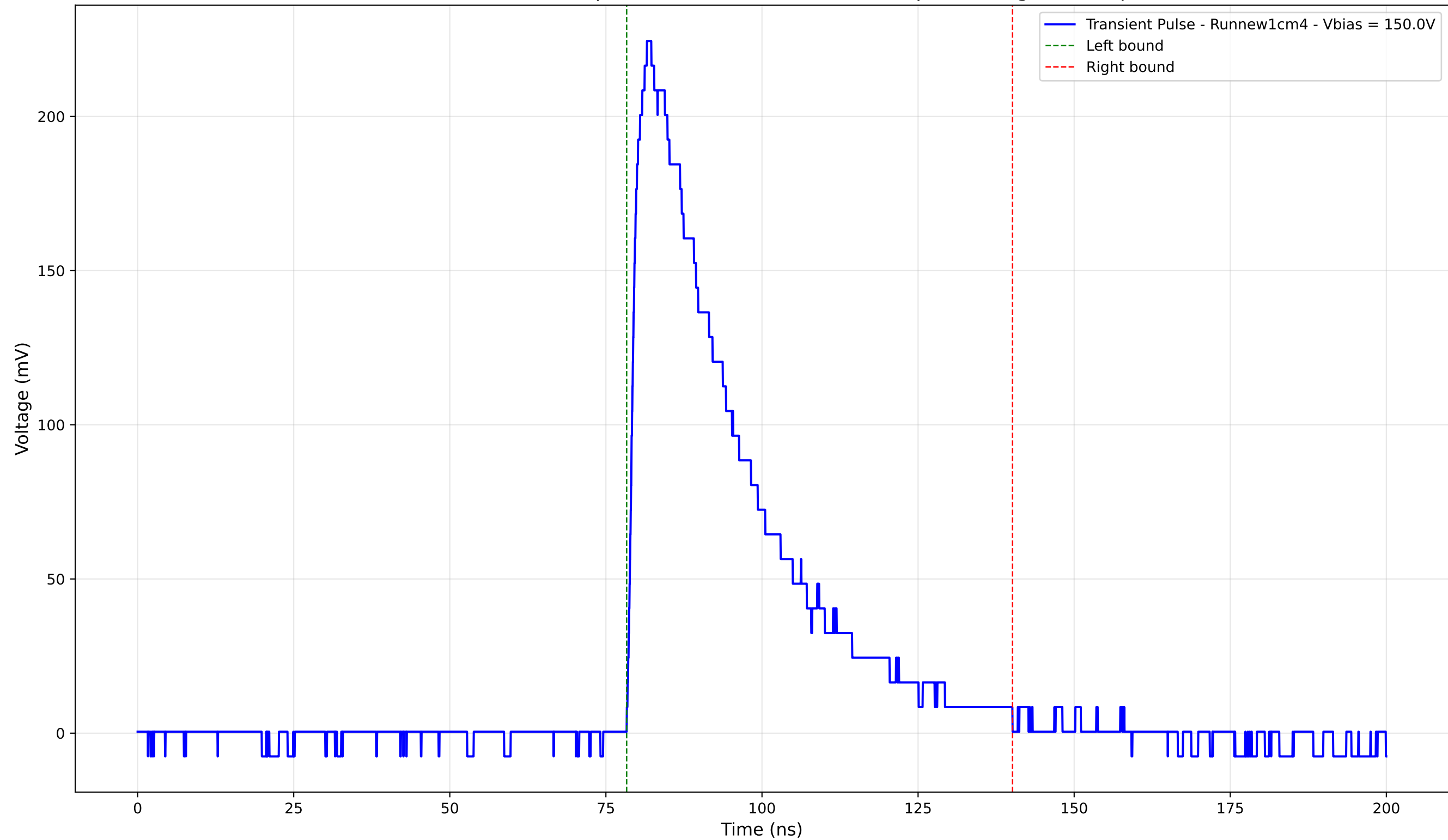
Transient Pulse - Sample: new1cm - Position: 1745.0 \mu\text{m} - Charge: 83.08 pC
