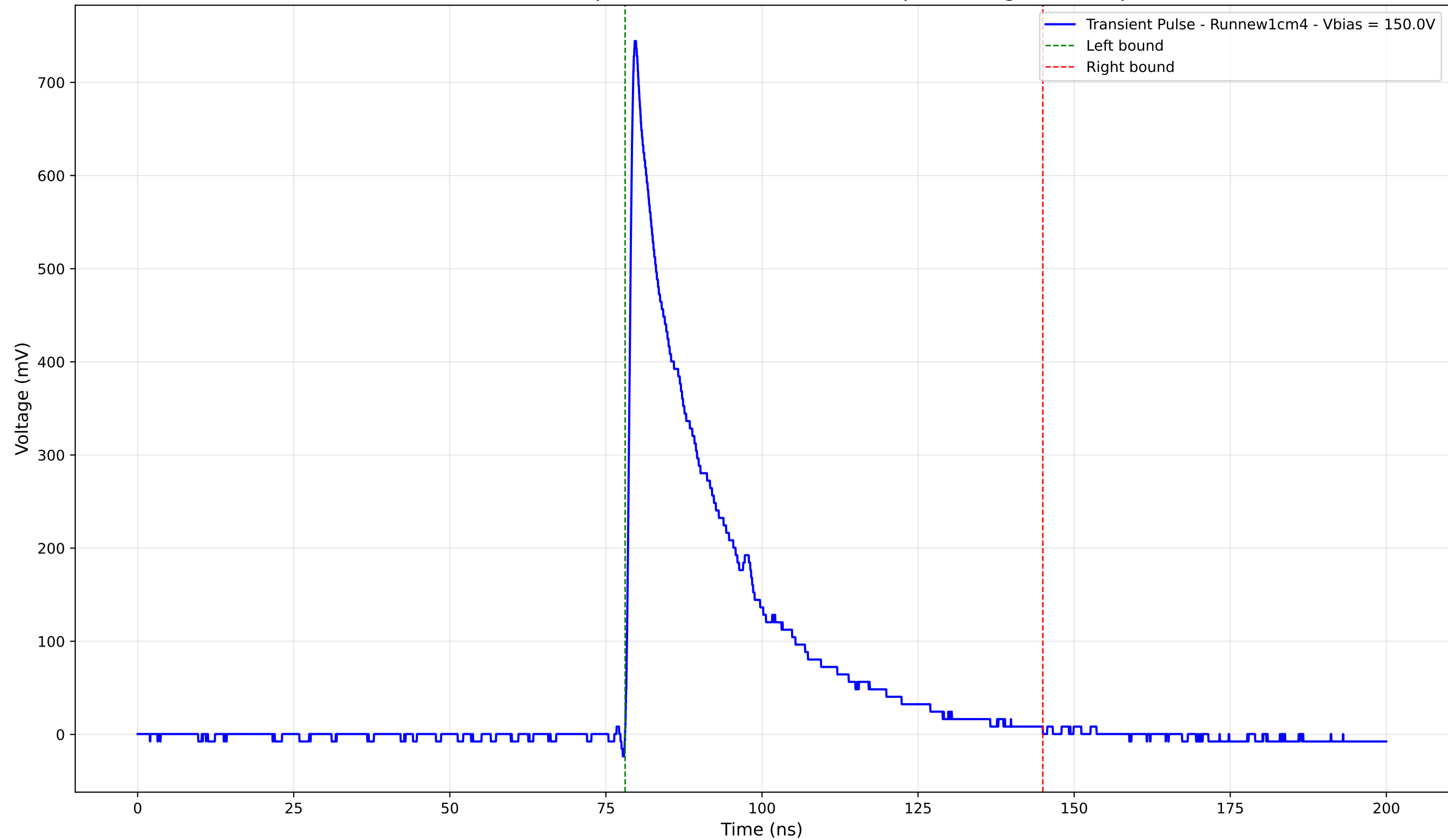
Transient Pulse - Sample: new1cm - Position: 815.0 \mu\text{m} - Charge: 192.75 pC
