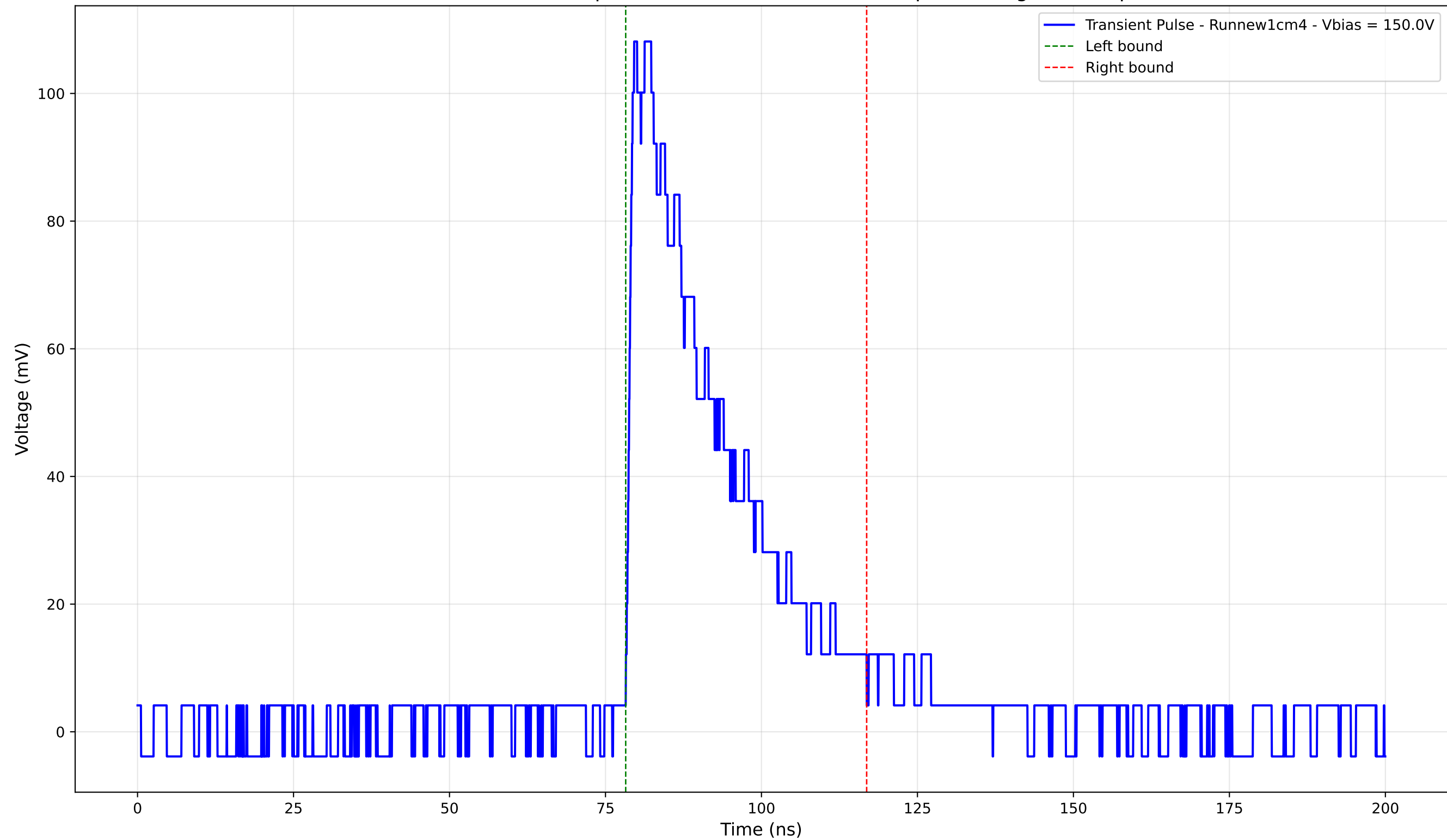
Transient Pulse - Sample: new1cm - Position: 4235.0 \mu\text{m} - Charge: 34.30 pC
