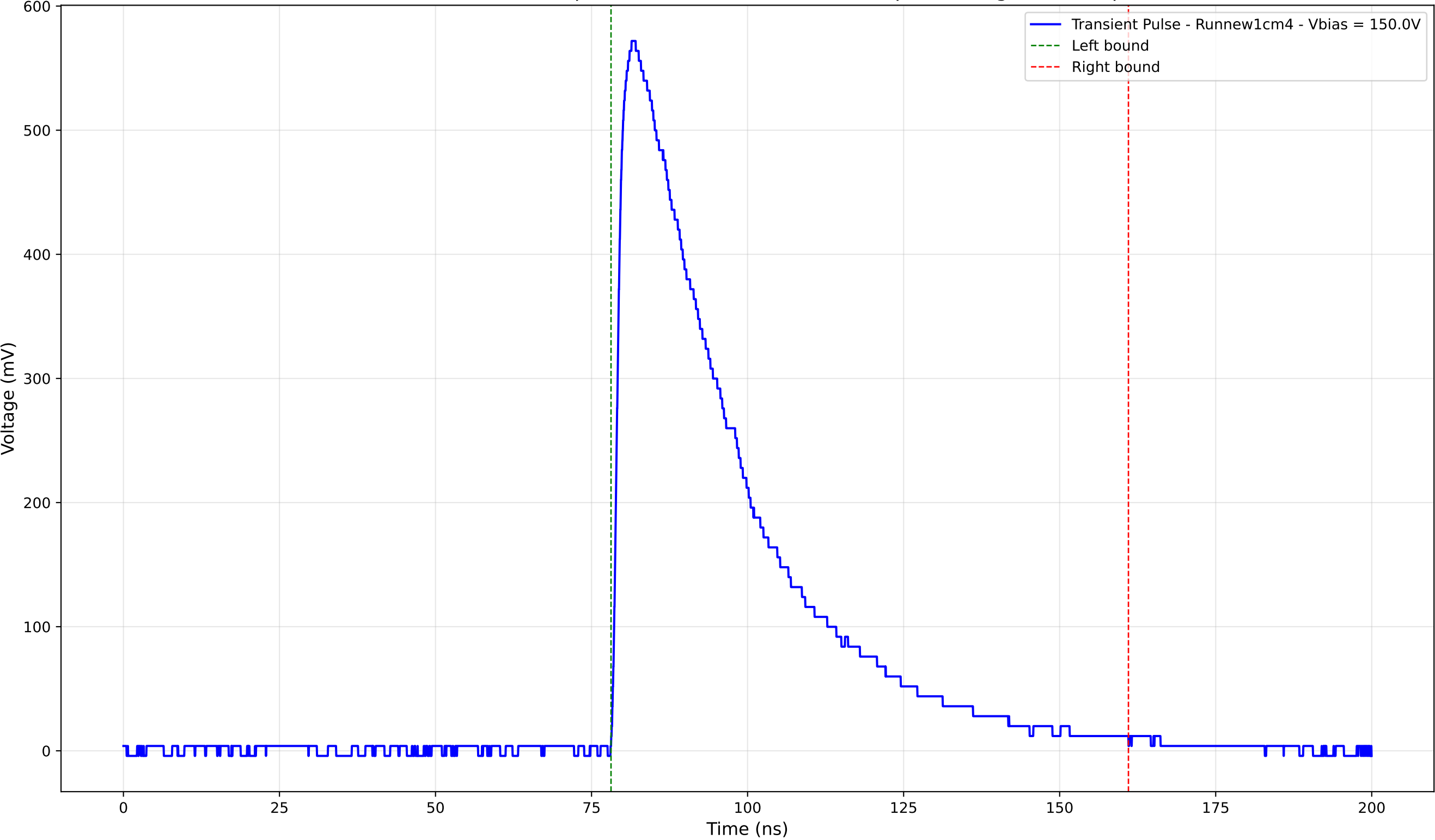
Transient Pulse - Sample: new1cm - Position: 3515.0 \mu\text{m} - Charge: 243.55 pC
