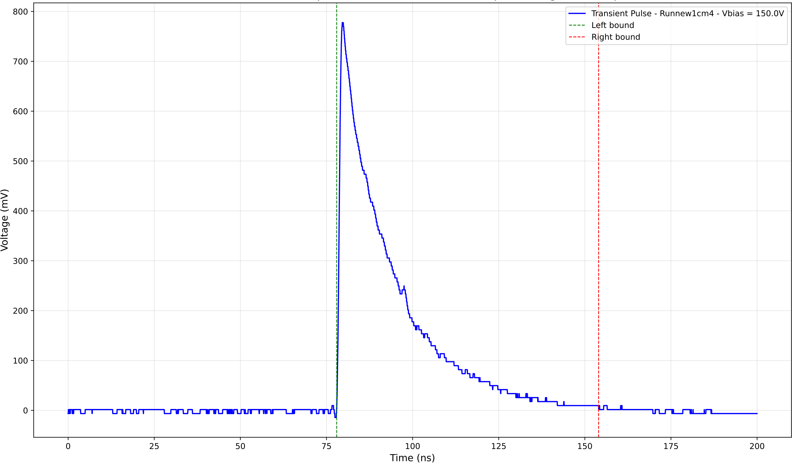
Transient Pulse - Sample: new1cm - Position: 4370.0 \mu\text{m} - Charge: 239.71 pC
