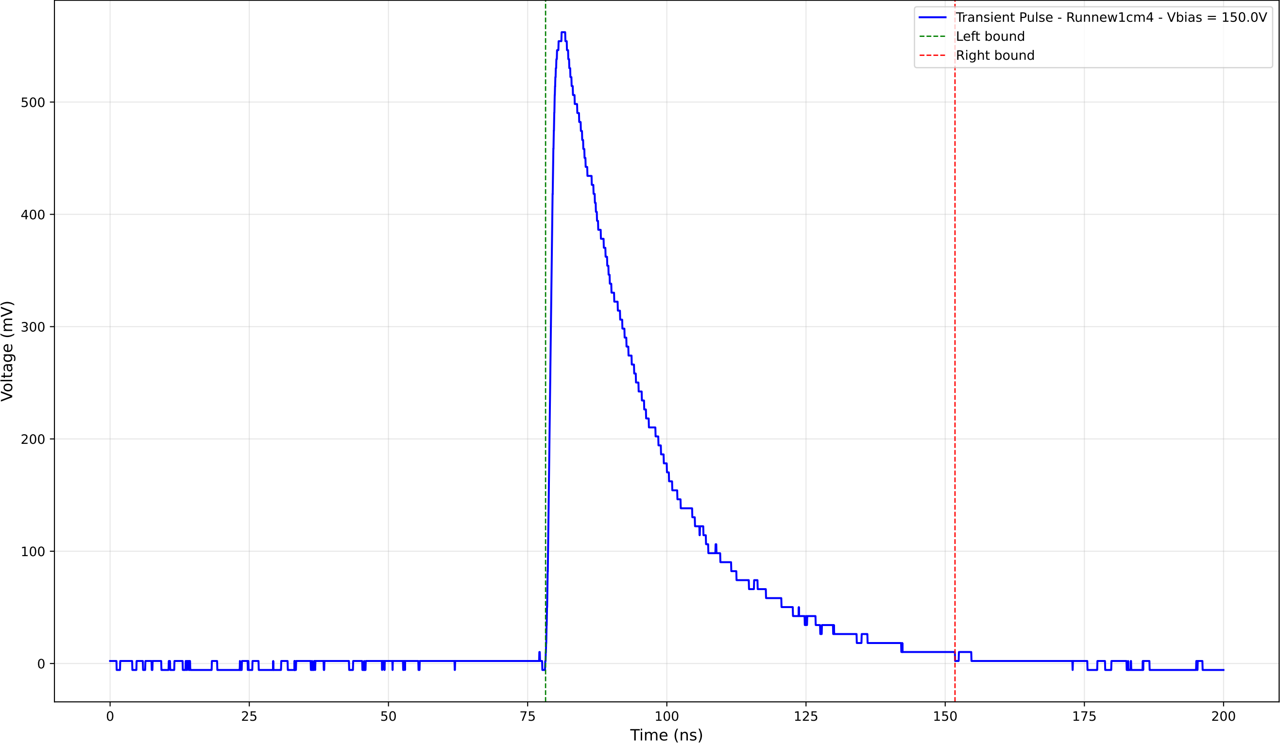
Transient Pulse - Sample: new1cm - Position: 1475.0 \mu\text{m} - Charge: 207.23 pC
