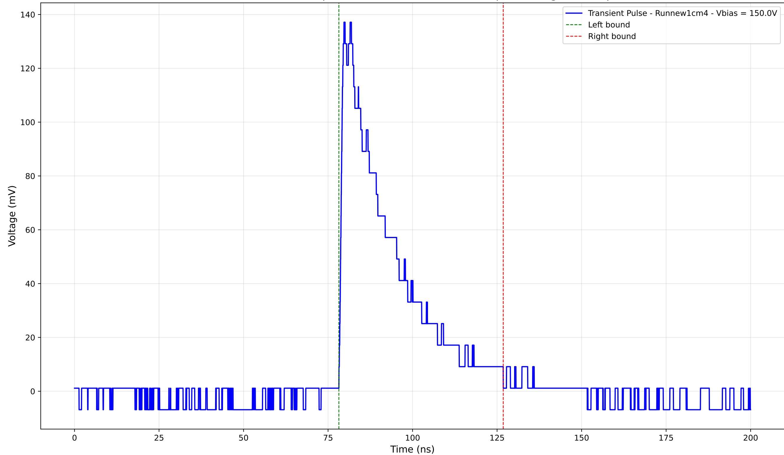
Transient Pulse - Sample: new1cm - Position: 4220.0 \mu\text{m} - Charge: 42.42 pC
