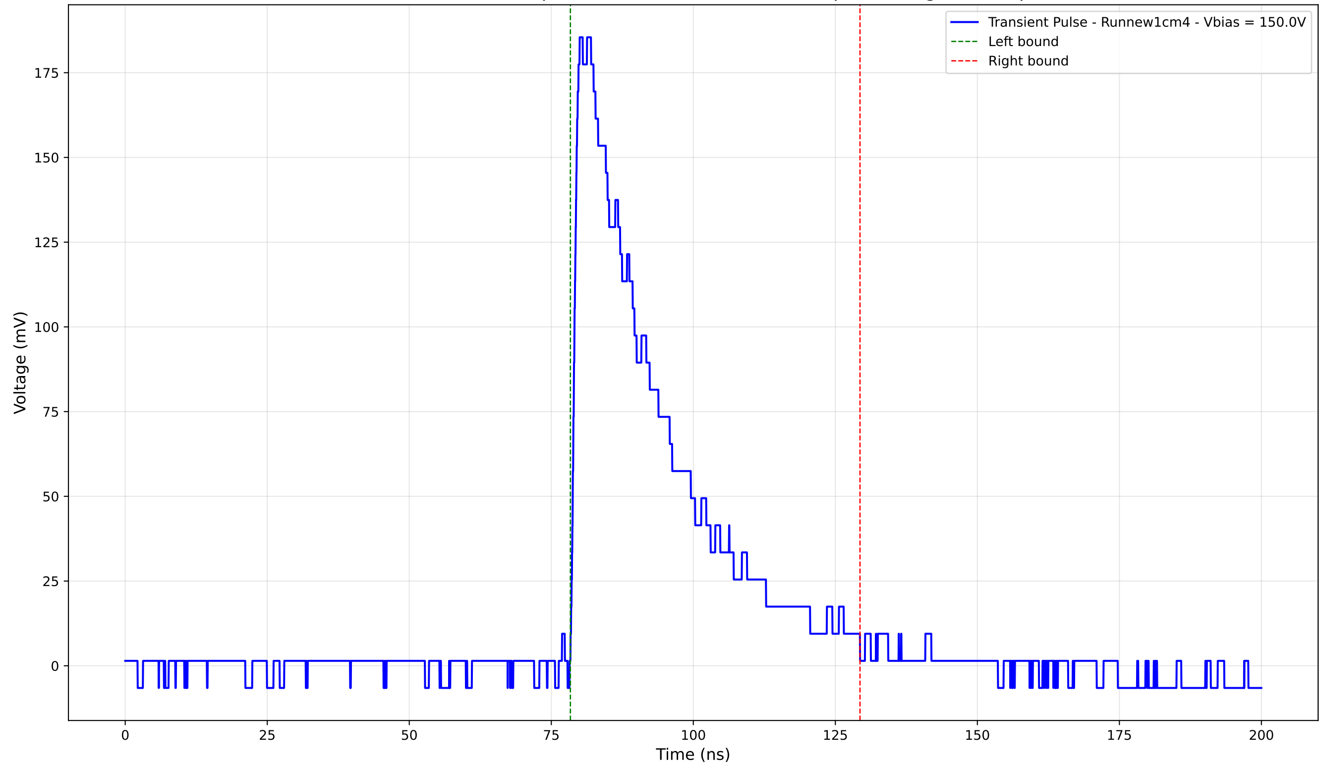
Transient Pulse - Sample: new1cm - Position: 1230.0 \mu\text{m} - Charge: 60.10 pC
