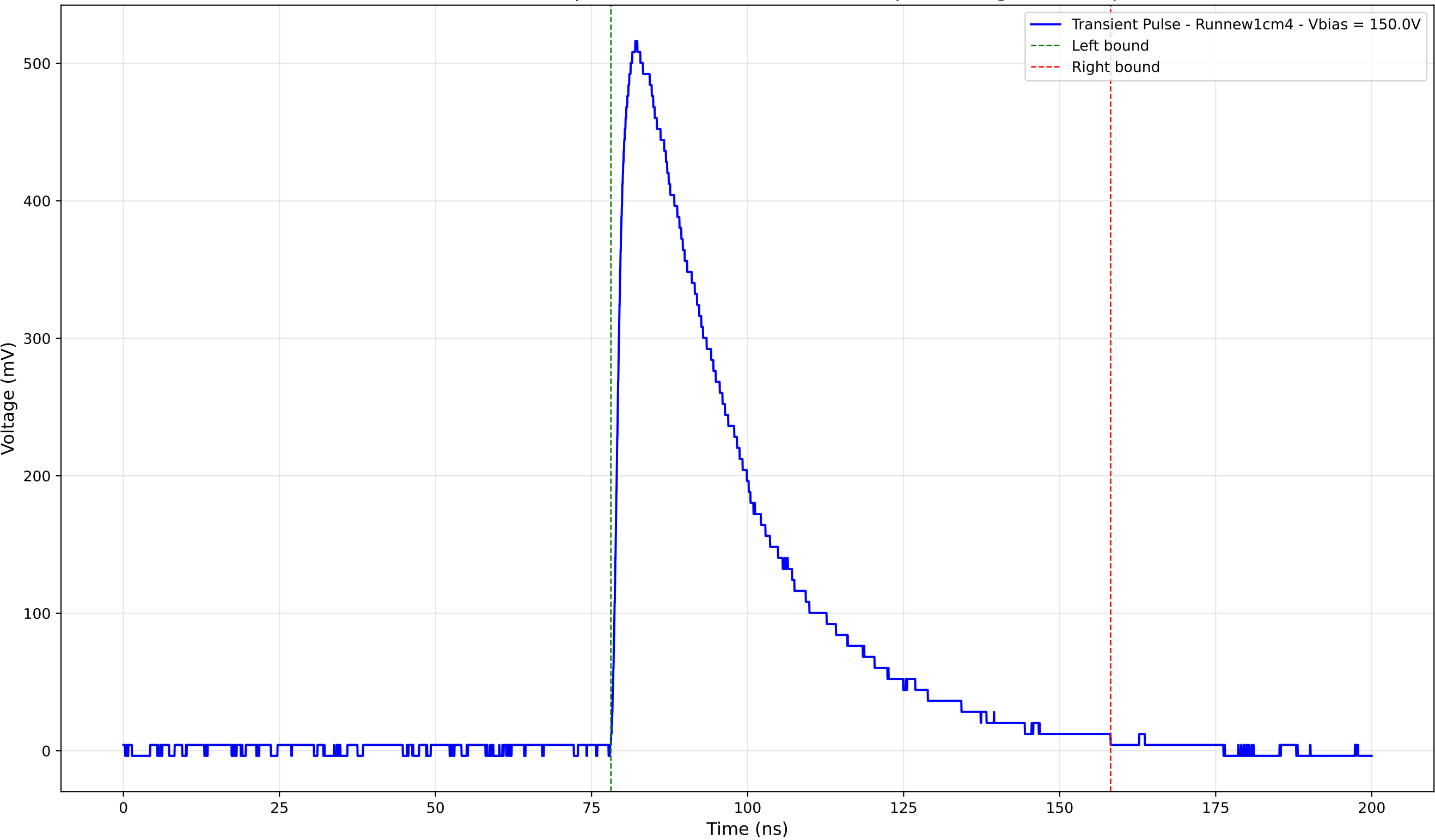
Transient Pulse - Sample: new1cm - Position: 3315.0 \mu\text{m} - Charge: 220.72 pC
