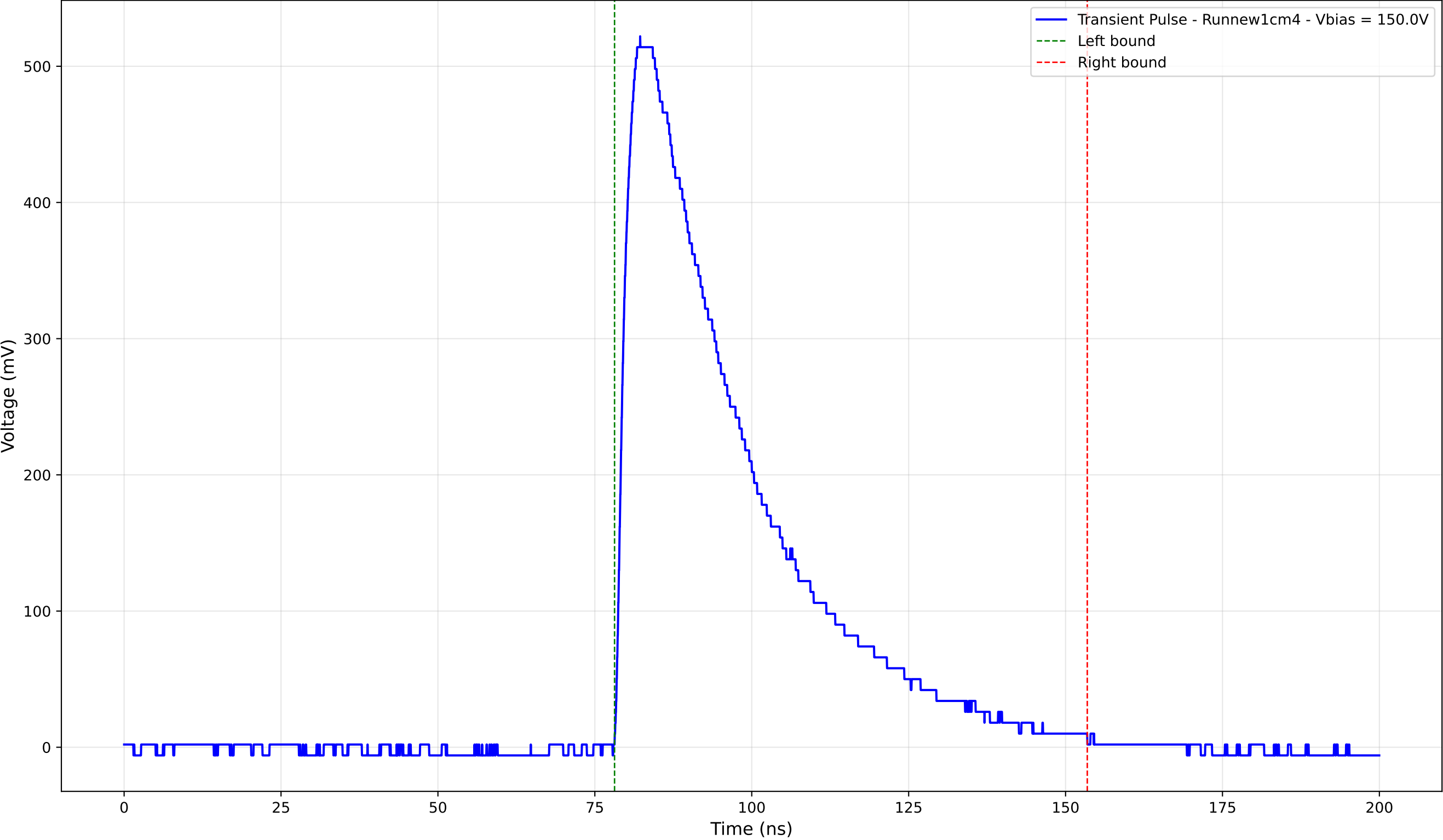
Transient Pulse - Sample: new1cm - Position: 2335.0 \mu\text{m} - Charge: 223.84 pC
