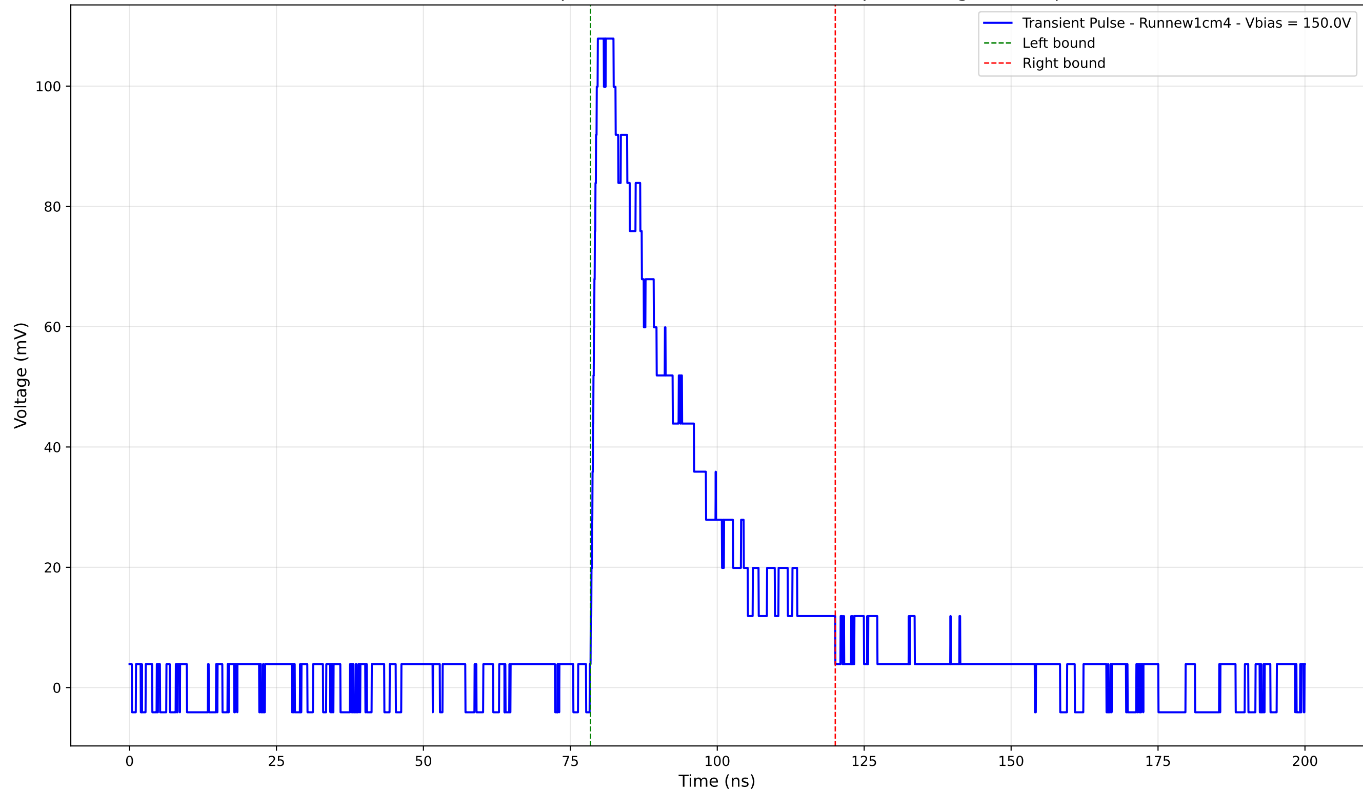
Transient Pulse - Sample: new1cm - Position: 1185.0 \mu\text{m} - Charge: 34.22 pC
