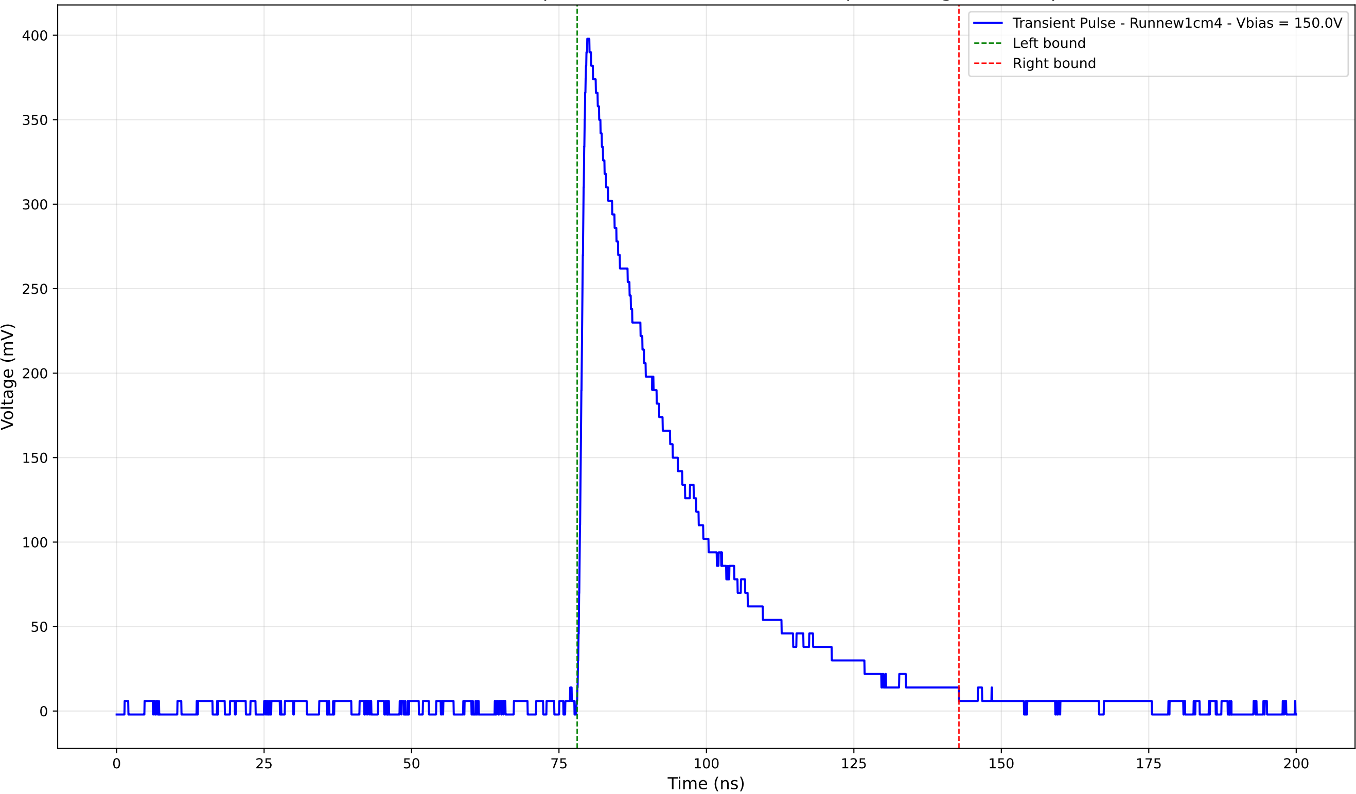
Transient Pulse - Sample: new1cm - Position: 4185.0 \mu\text{m} - Charge: 130.31 pC
