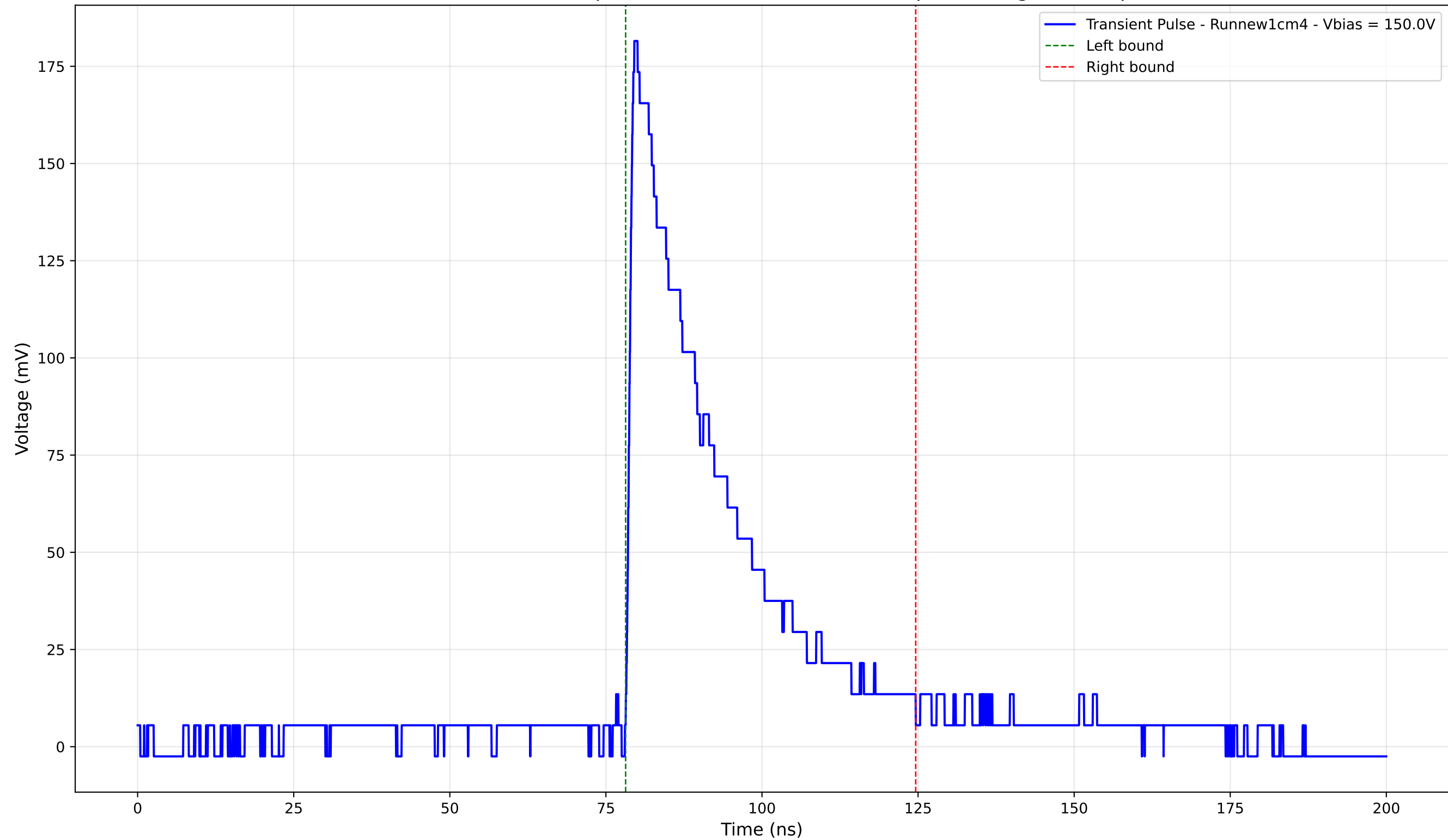
Transient Pulse - Sample: new1cm - Position: 4255.0 \mu\text{m} - Charge: 53.82 pC
