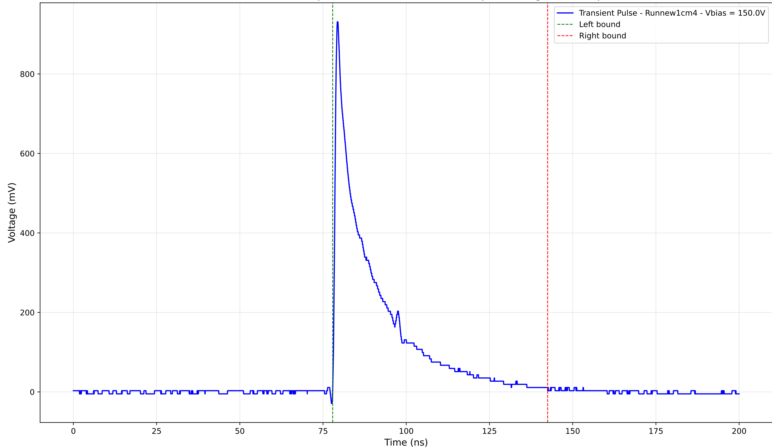
Transient Pulse - Sample: new1cm - Position: 445.0 \mu\text{m} - Charge: 200.69 pC
