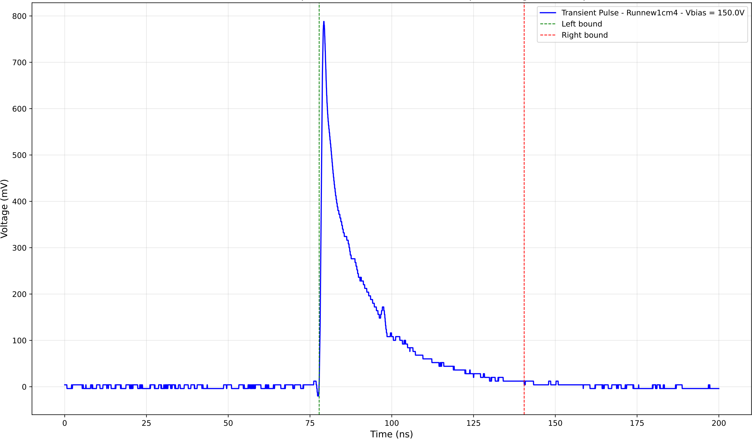
Transient Pulse - Sample: new1cm - Position: 4820.0 \mu\text{m} - Charge: 168.79 pC
