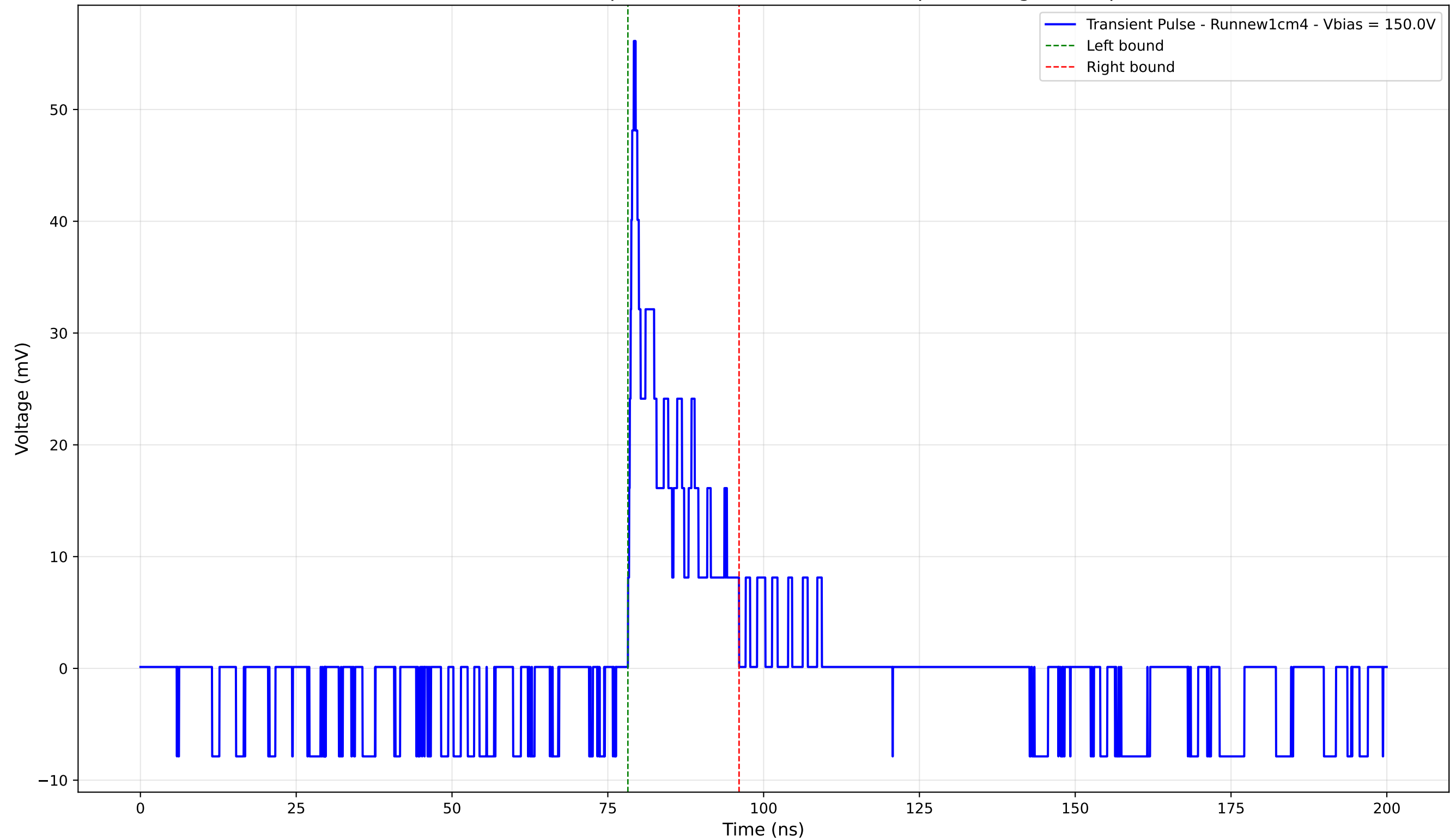
Transient Pulse - Sample: new1cm - Position: 175.0 \mu\text{m} - Charge: 6.52 pC
