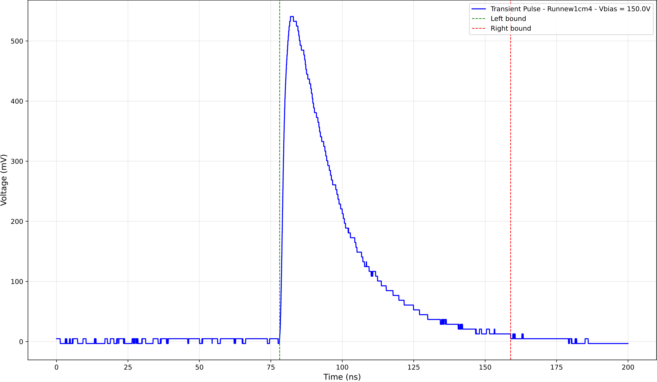
Transient Pulse - Sample: new1cm - Position: 3070.0 \mu\text{m} - Charge: 238.88 pC
