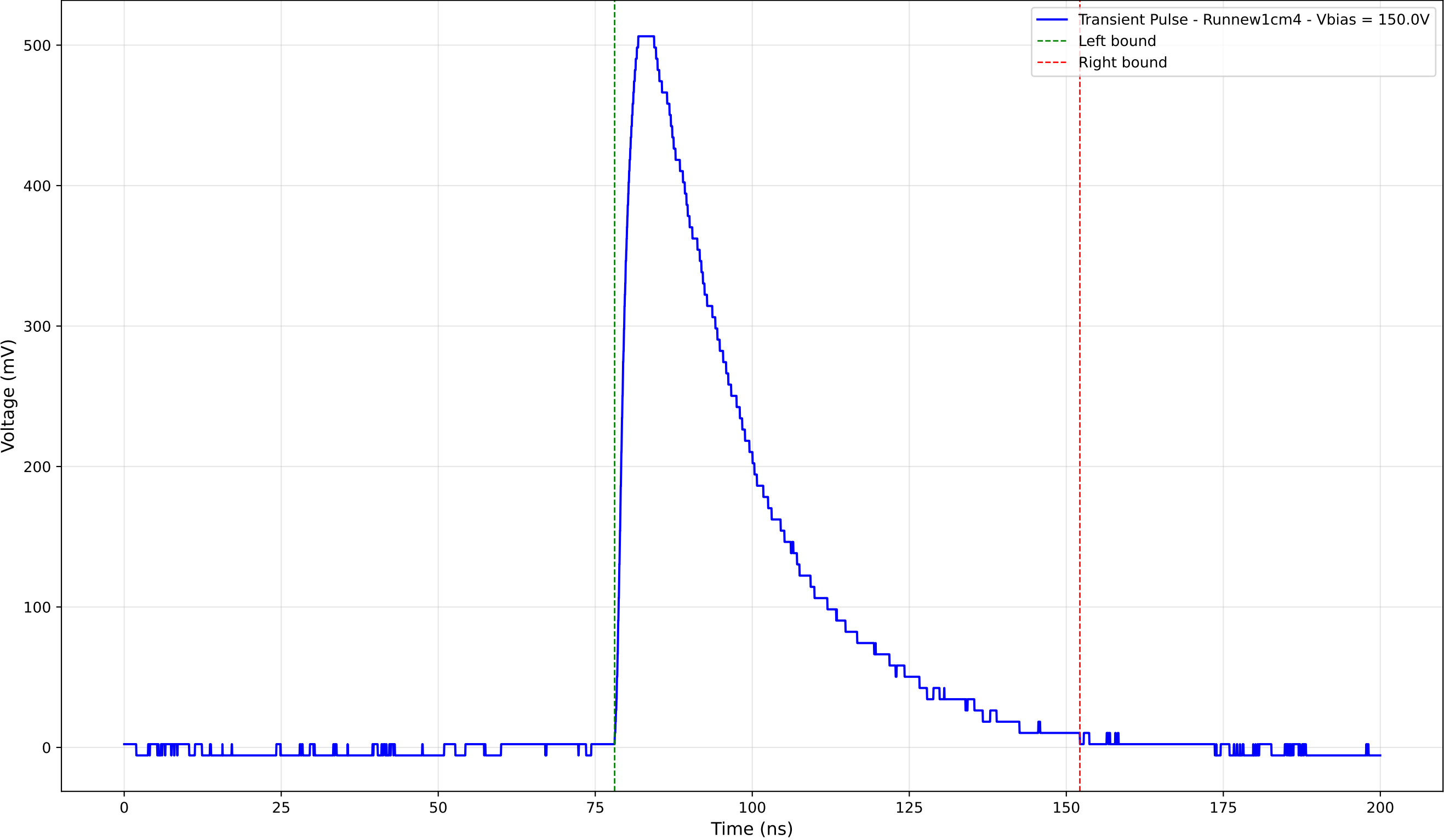
Transient Pulse - Sample: new1cm - Position: 2590.0 \mu\text{m} - Charge: 222.83 pC
