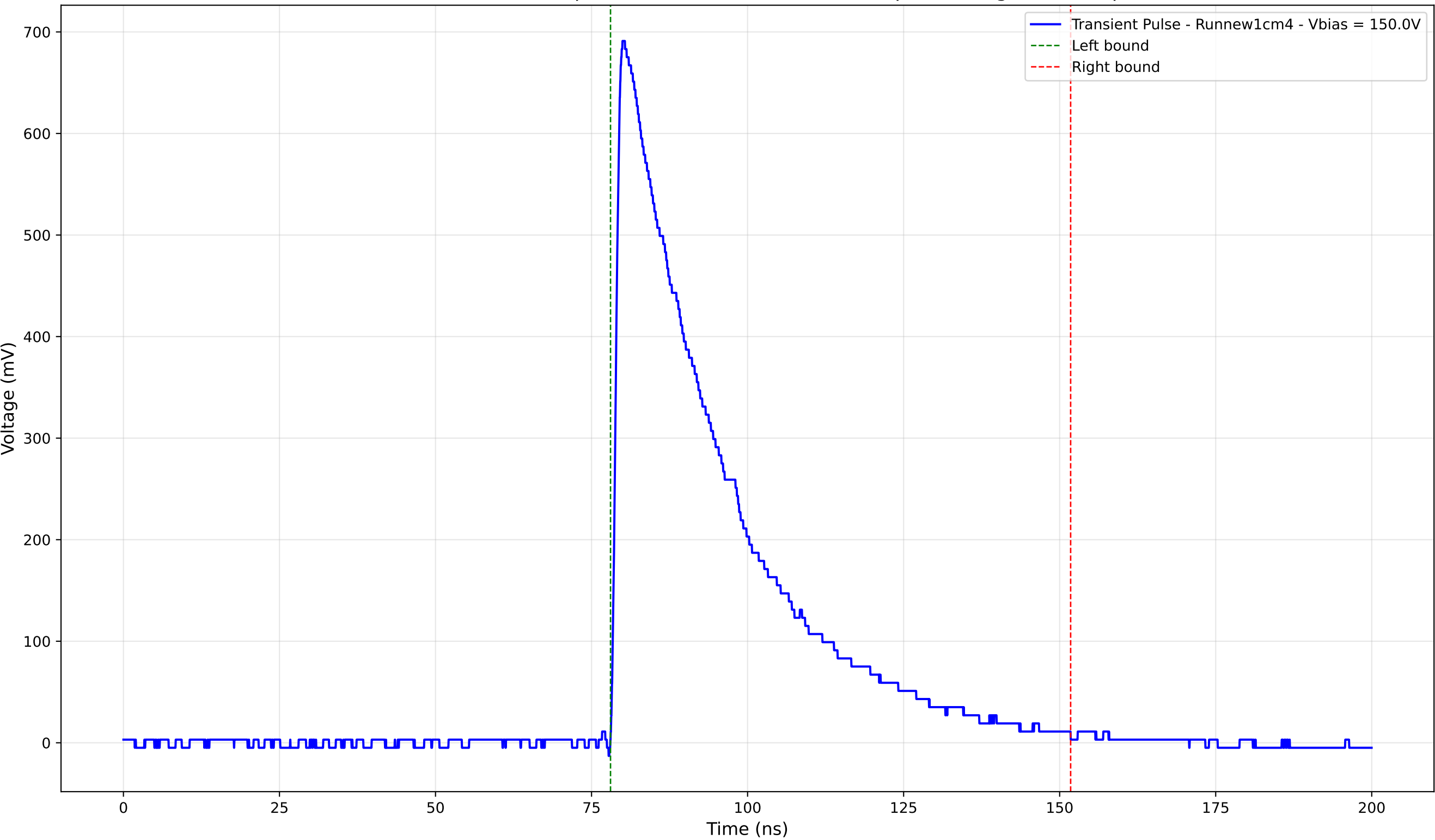
Transient Pulse - Sample: new1cm - Position: 4050.0 \mu\text{m} - Charge: 250.78 pC
