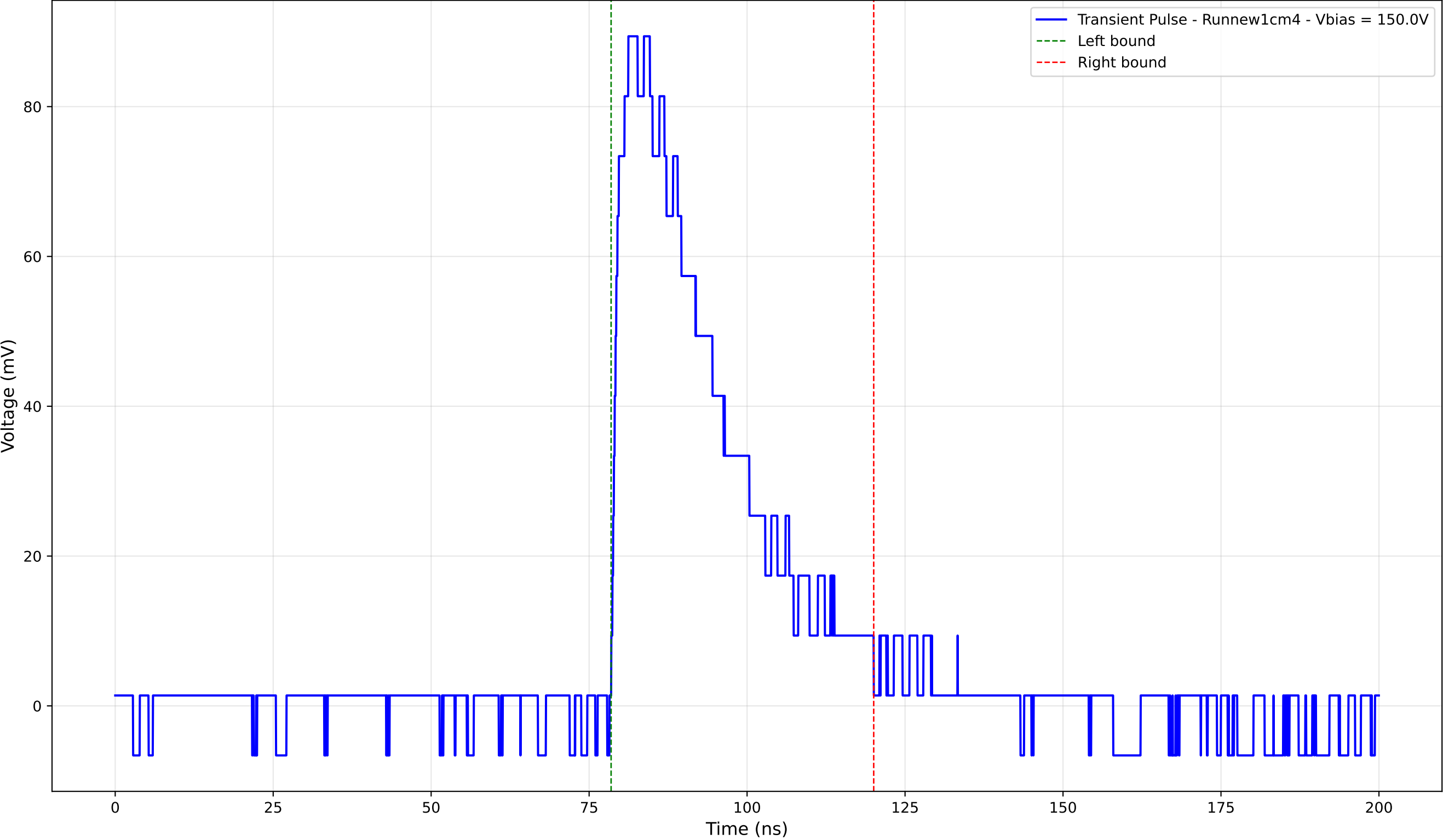
Transient Pulse - Sample: new1cm - Position: 3730.0 \mu\text{m} - Charge: 31.88 pC
