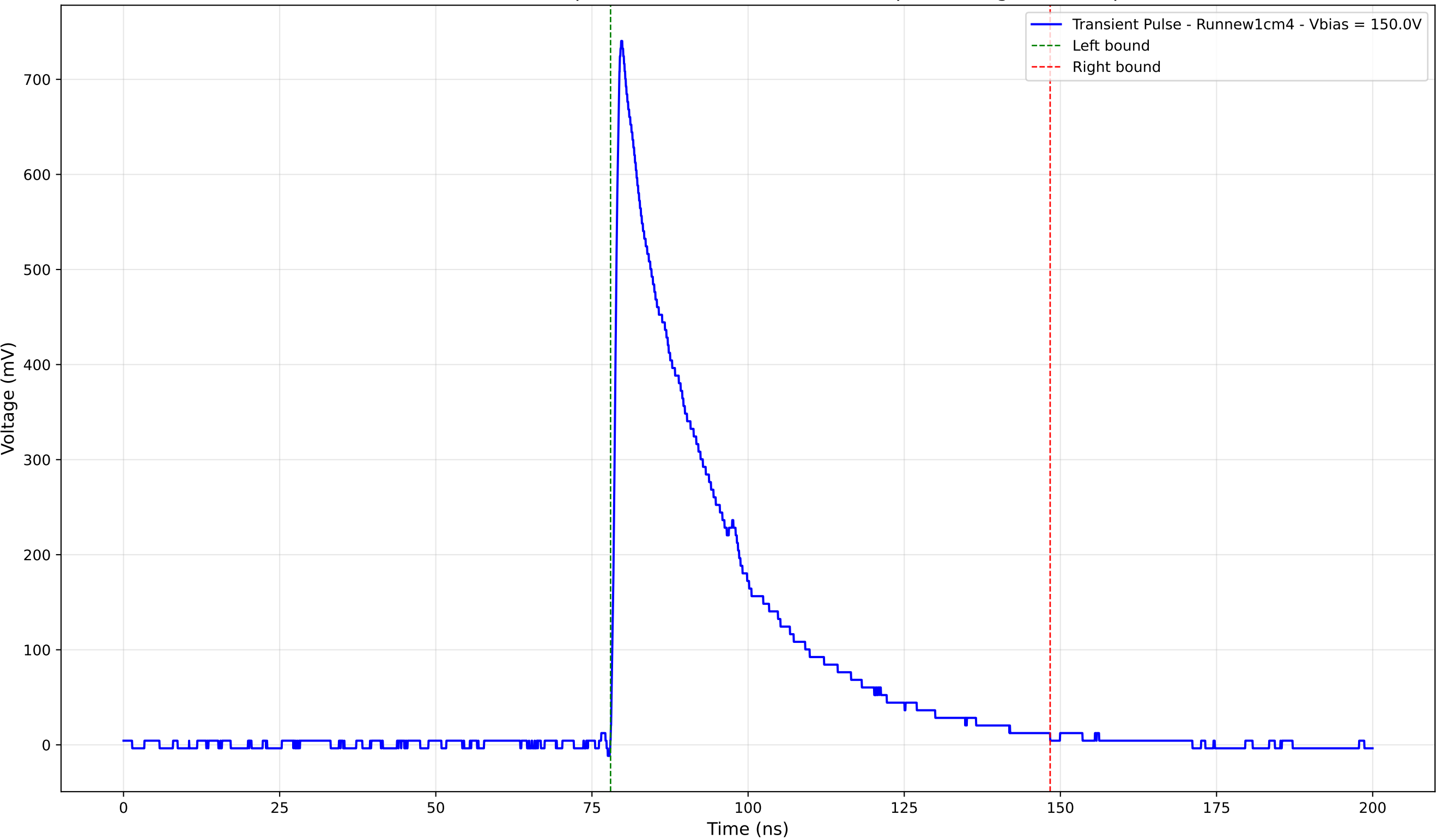
Transient Pulse - Sample: new1cm - Position: 4335.0 \mu\text{m} - Charge: 229.04 pC
