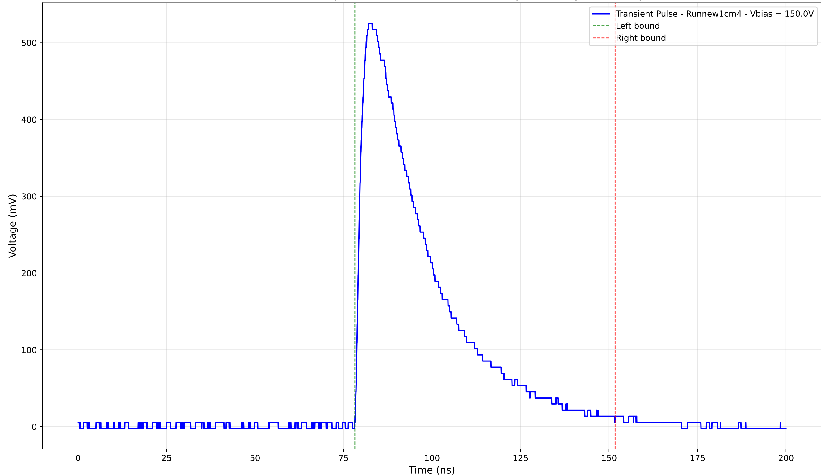
Transient Pulse - Sample: new1cm - Position: 2460.0 \mu\text{m} - Charge: 228.28 pC
