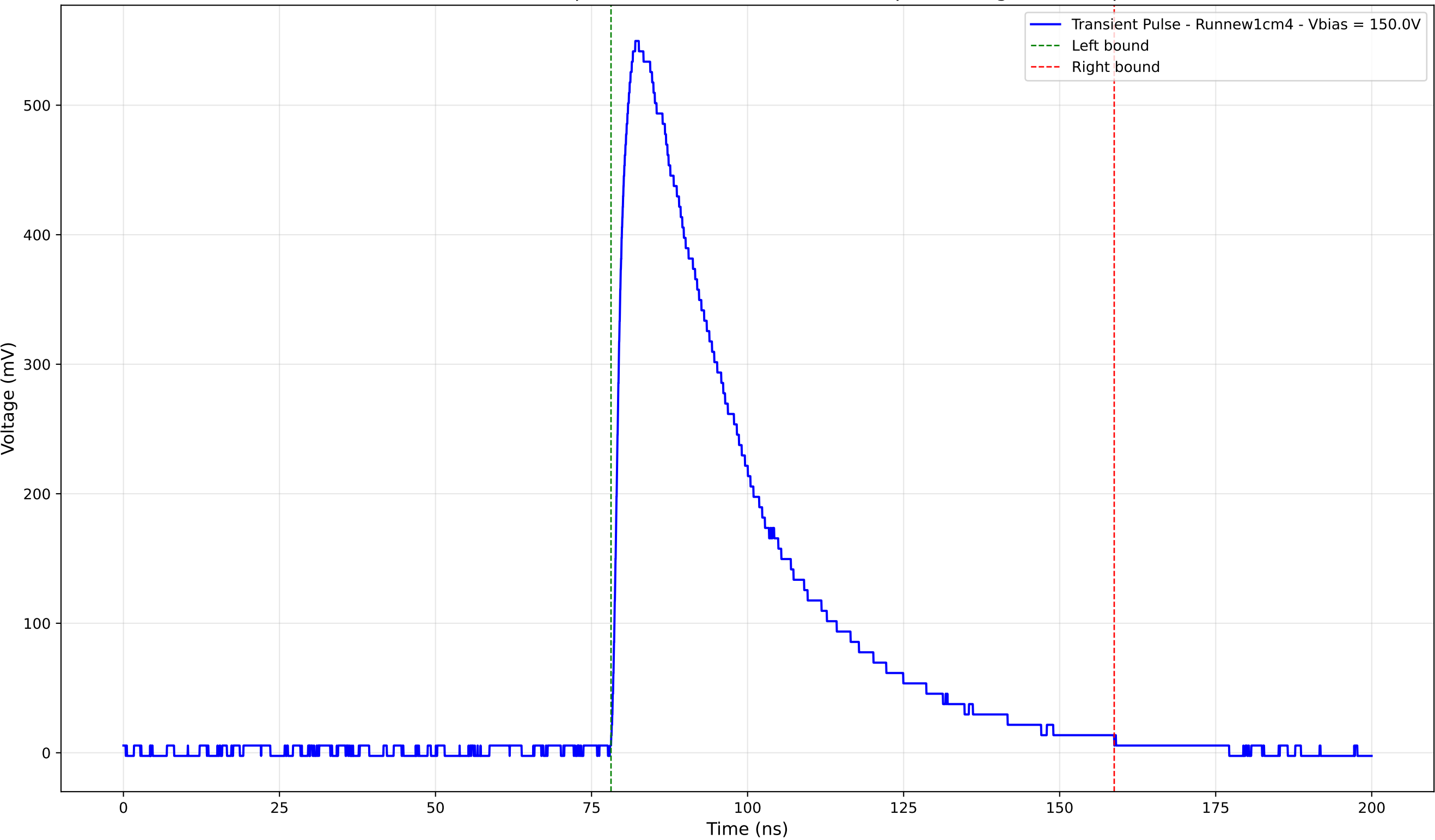
Transient Pulse - Sample: new1cm - Position: 3105.0 \mu\text{m} - Charge: 243.55 pC
