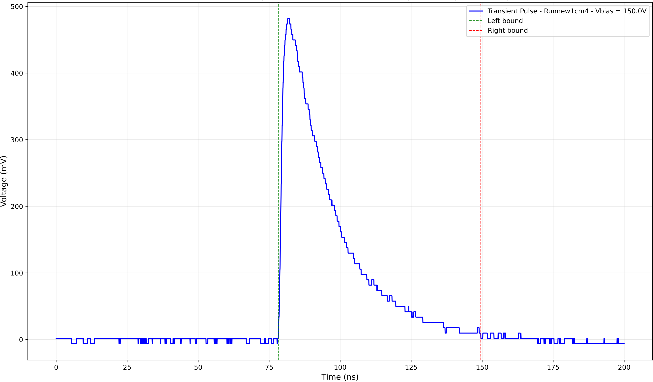
Transient Pulse - Sample: new1cm - Position: 1795.0 \mu\text{m} - Charge: 190.42 pC
