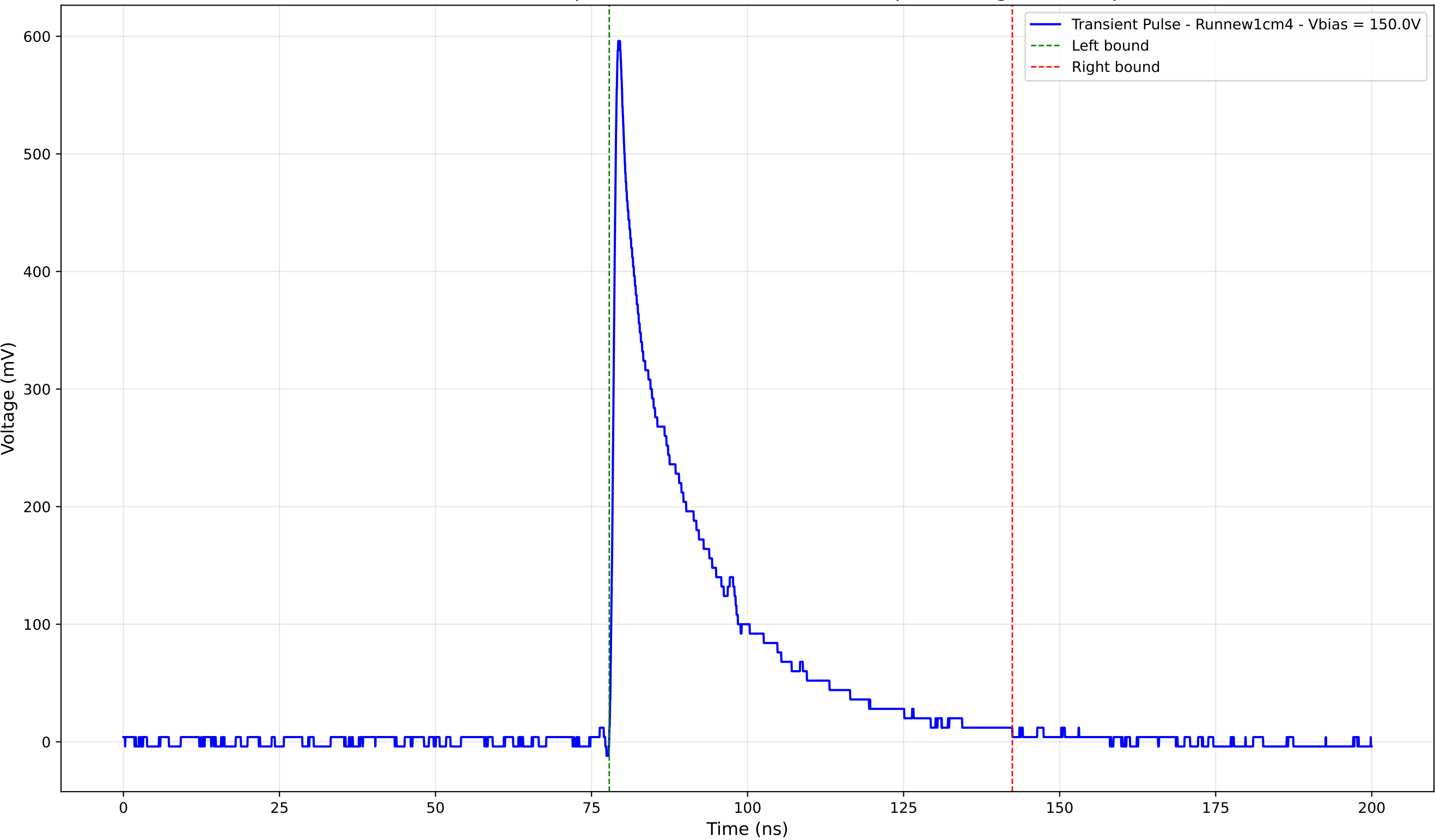
Transient Pulse - Sample: new1cm - Position: 4675.0 \mu\text{m} - Charge: 141.13 pC
