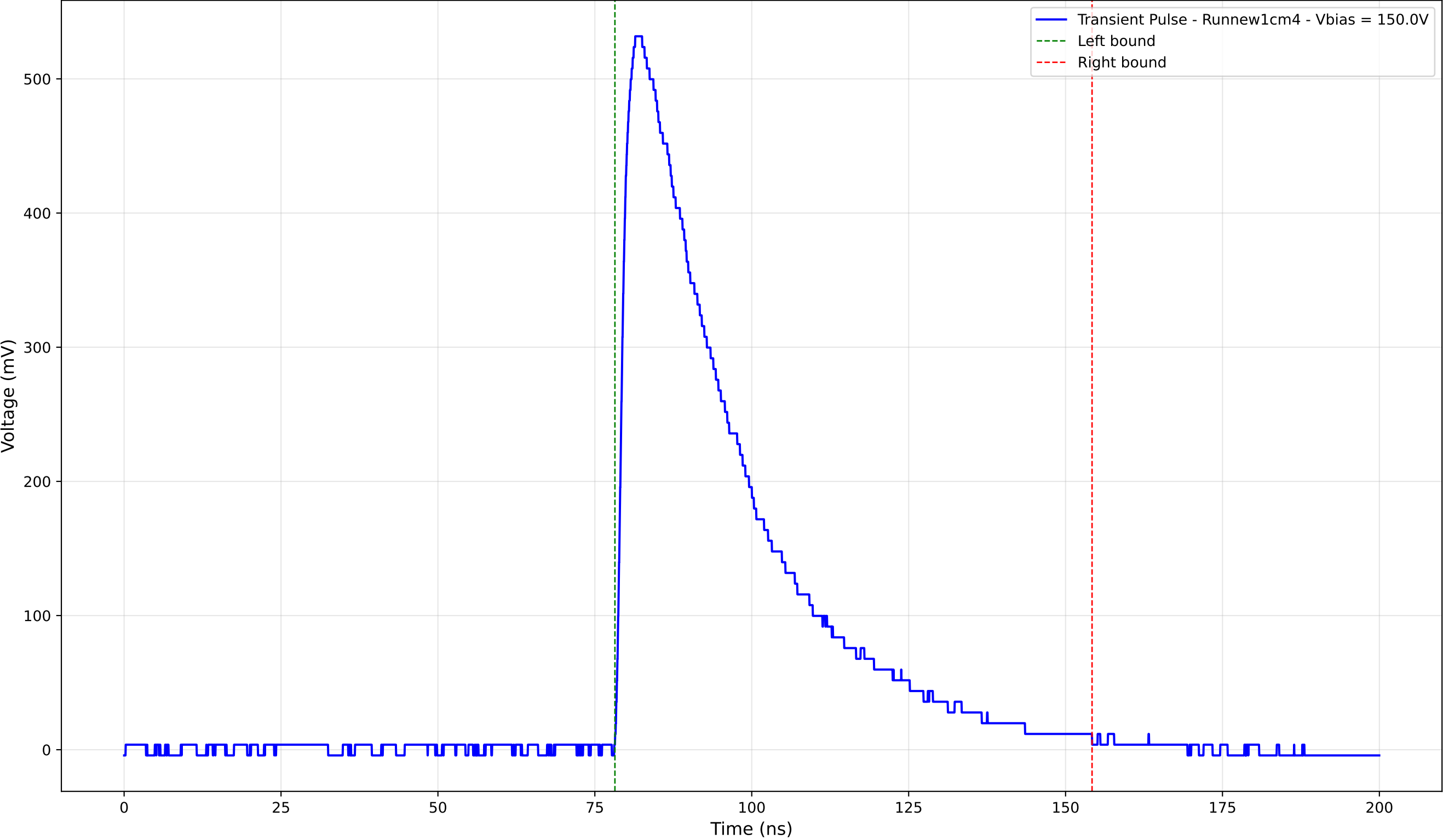
Transient Pulse - Sample: new1cm - Position: 1865.0 \mu\text{m} - Charge: 217.80 pC
