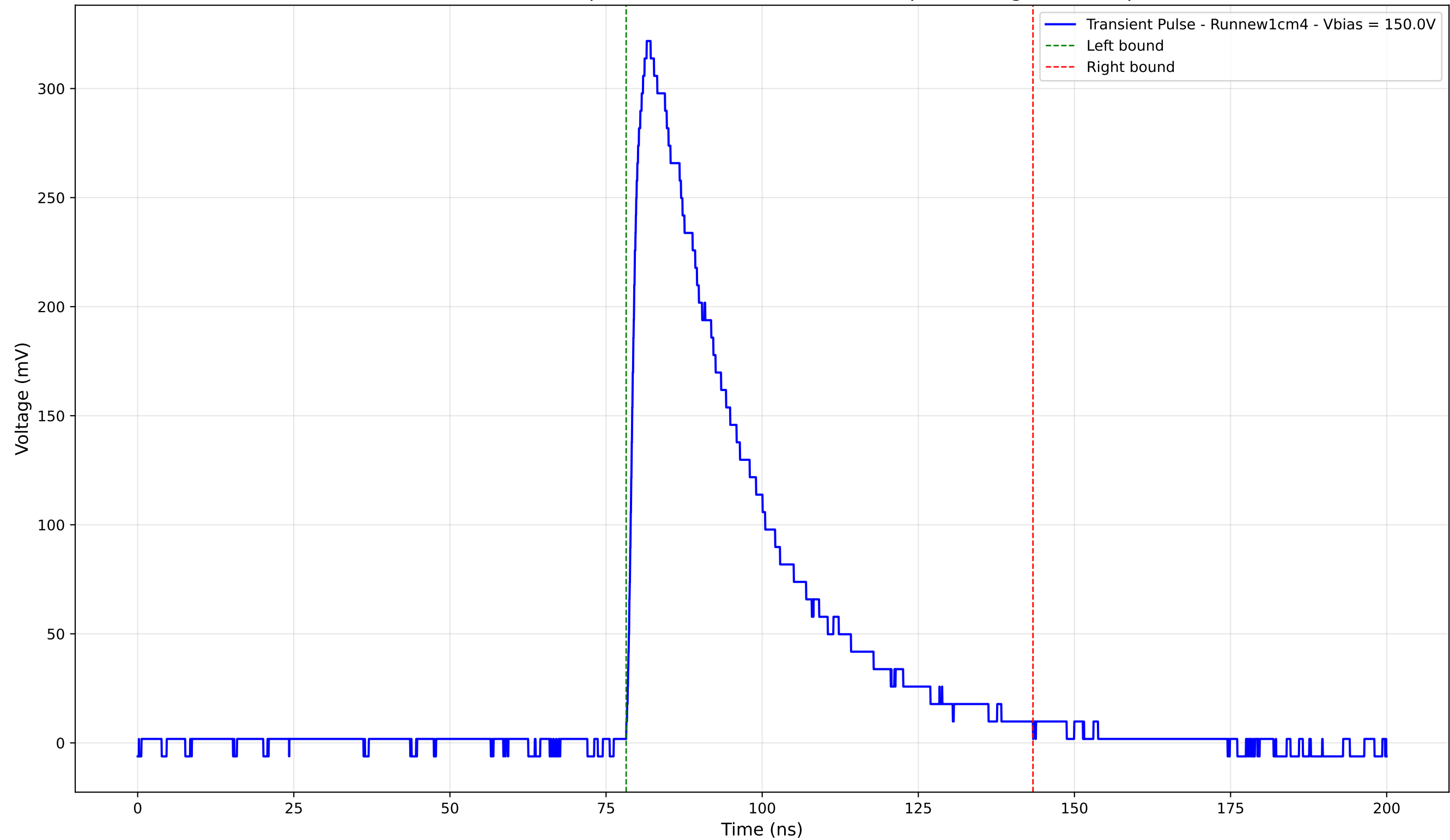
Transient Pulse - Sample: new1cm - Position: 1760.0 \mu\text{m} - Charge: 123.20 pC
