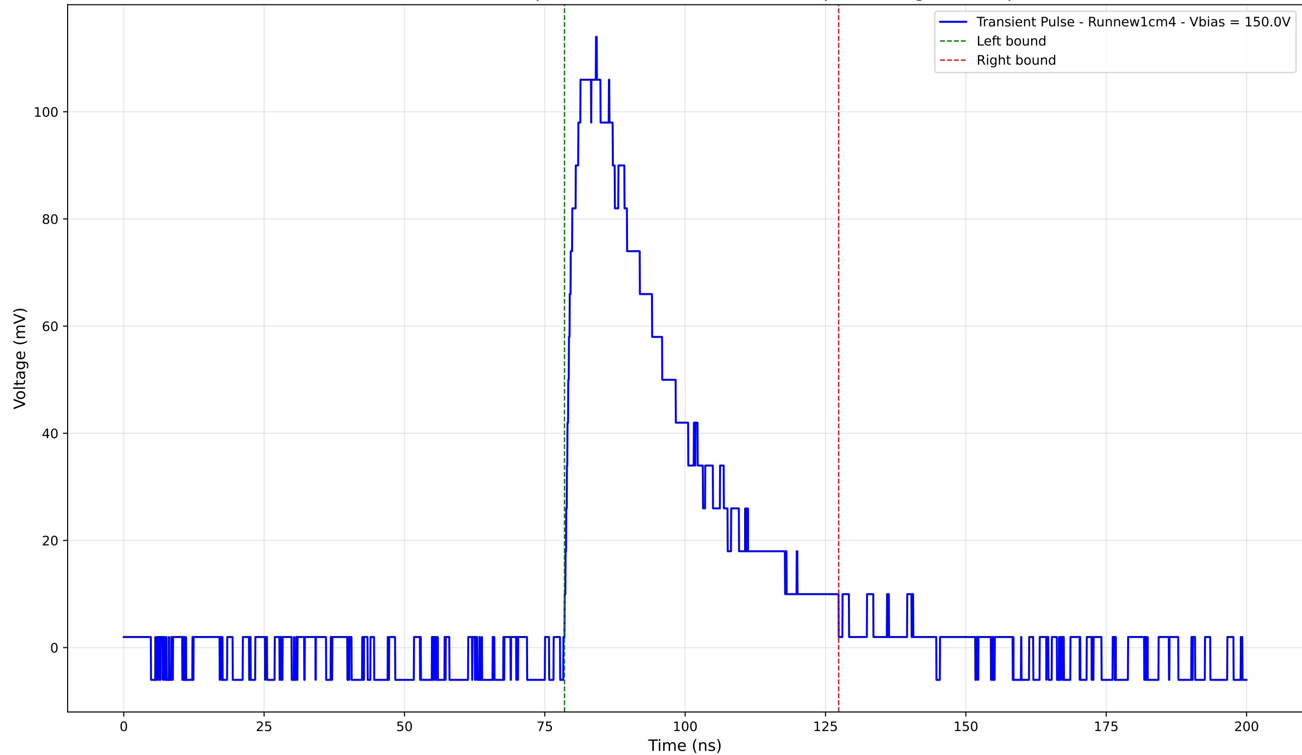
Transient Pulse - Sample: new1cm - Position: 3240.0 \mu\text{m} - Charge: 43.11 pC
