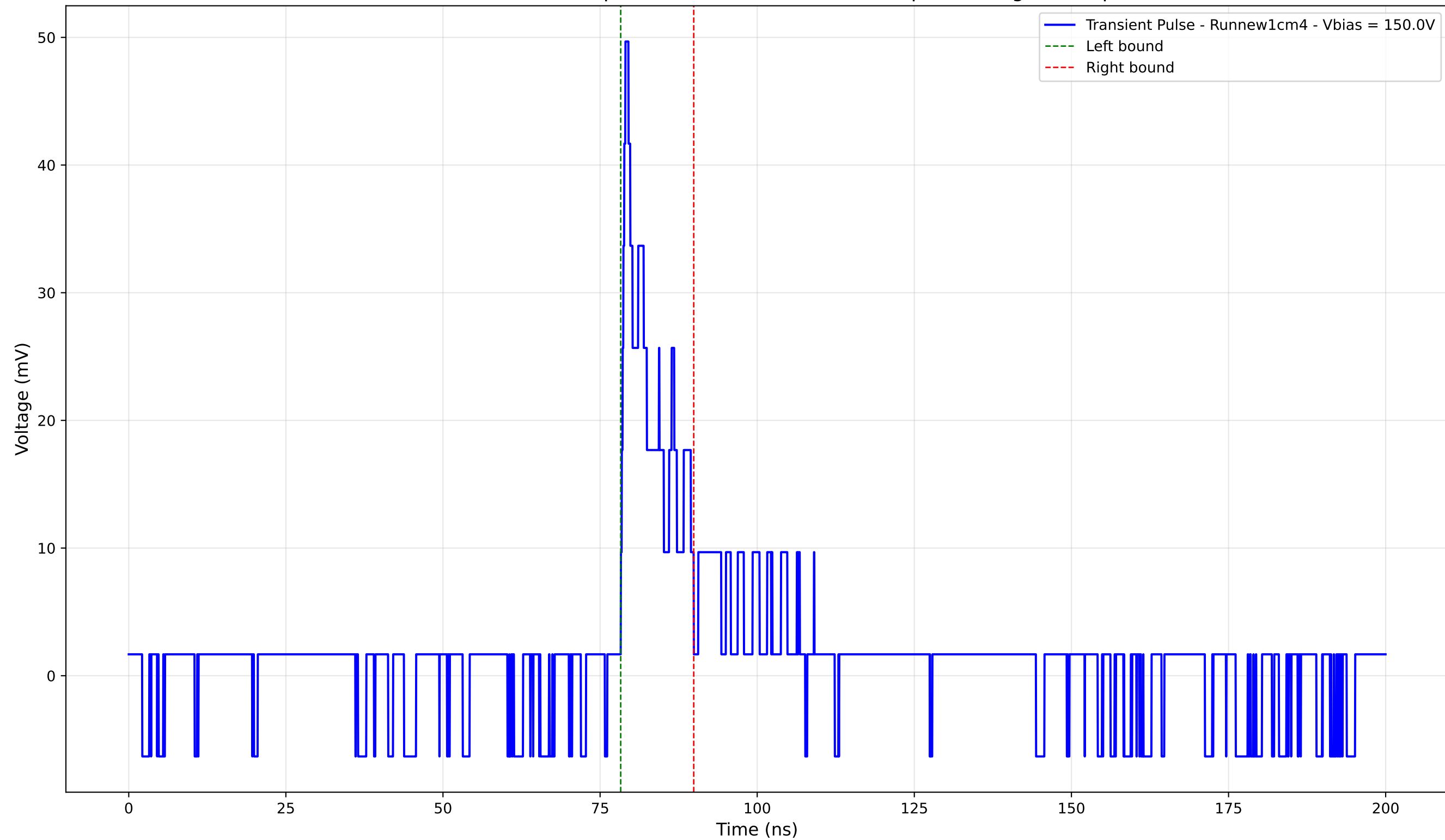
Transient Pulse - Sample: new1cm - Position: 170.0 \mu\text{m} - Charge: 5.00 pC
