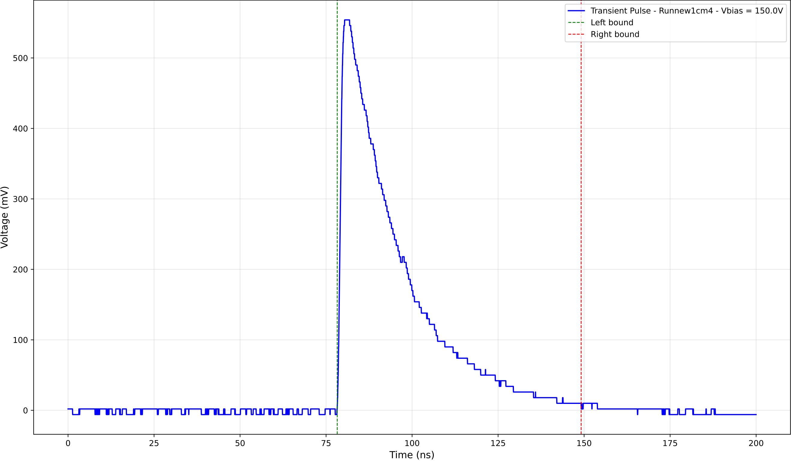
Transient Pulse - Sample: new1cm - Position: 1465.0 \mu\text{m} - Charge: 206.22 pC
