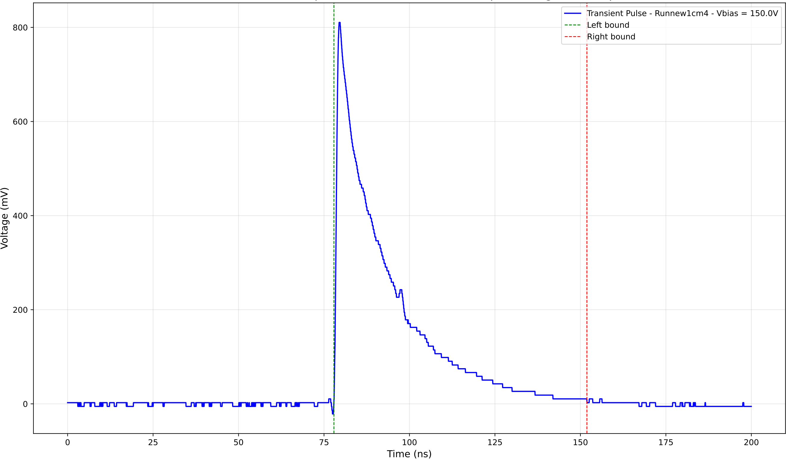
Transient Pulse - Sample: new1cm - Position: 4505.0 \mu\text{m} - Charge: 237.07 pC
