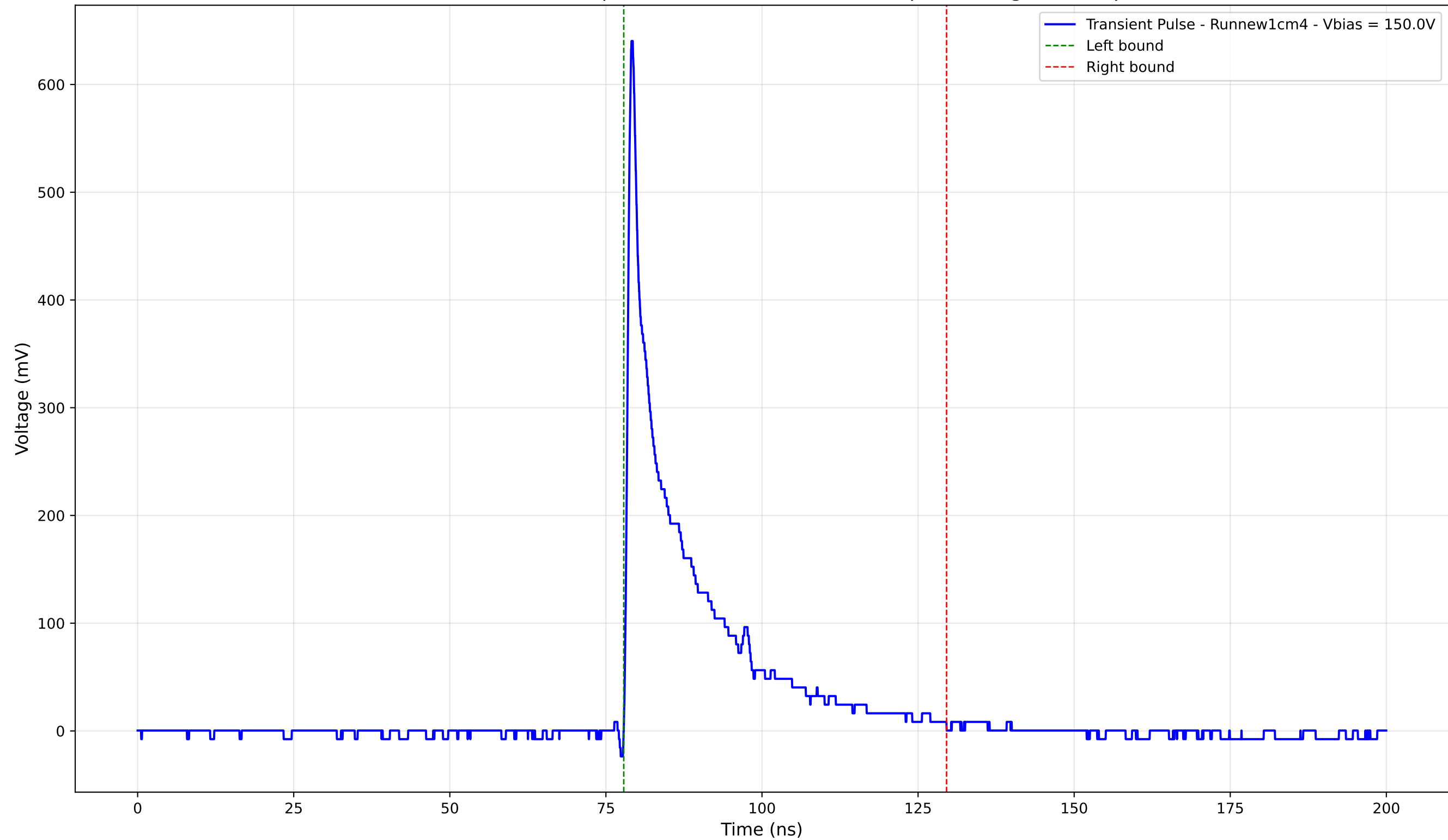
Transient Pulse - Sample: new1cm - Position: 245.0 \mu\text{m} - Charge: 98.58 pC
