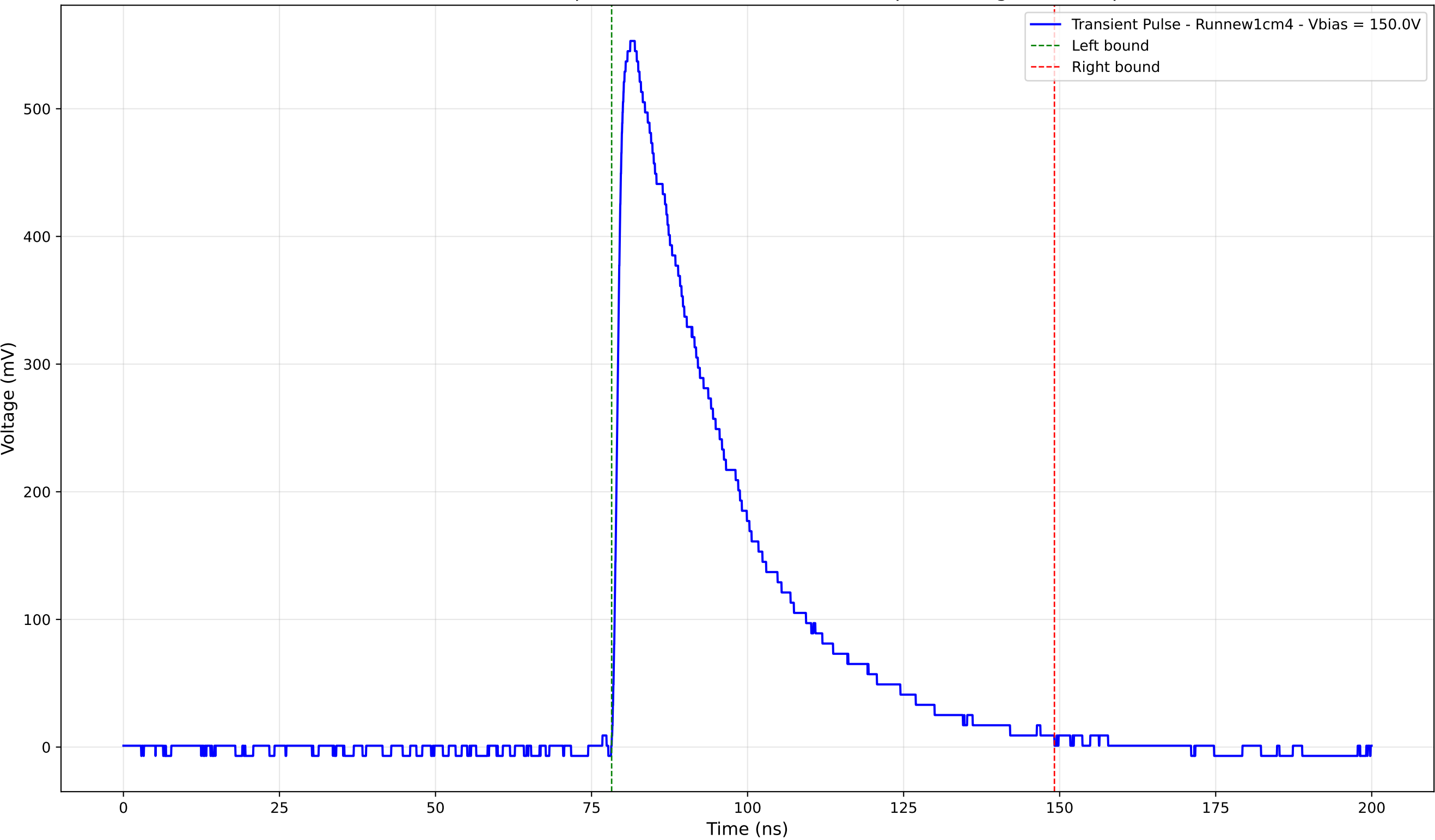
Transient Pulse - Sample: new1cm - Position: 1565.0 \mu\text{m} - Charge: 207.99 pC
