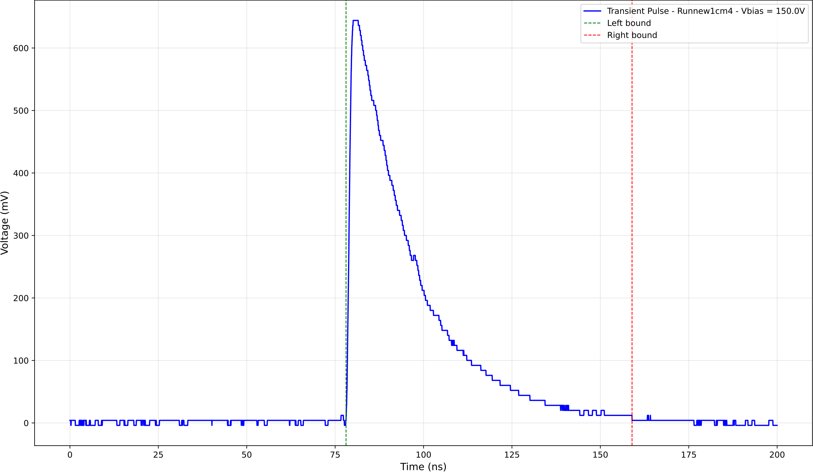
Transient Pulse - Sample: new1cm - Position: 3880.0 \mu\text{m} - Charge: 254.40 pC
