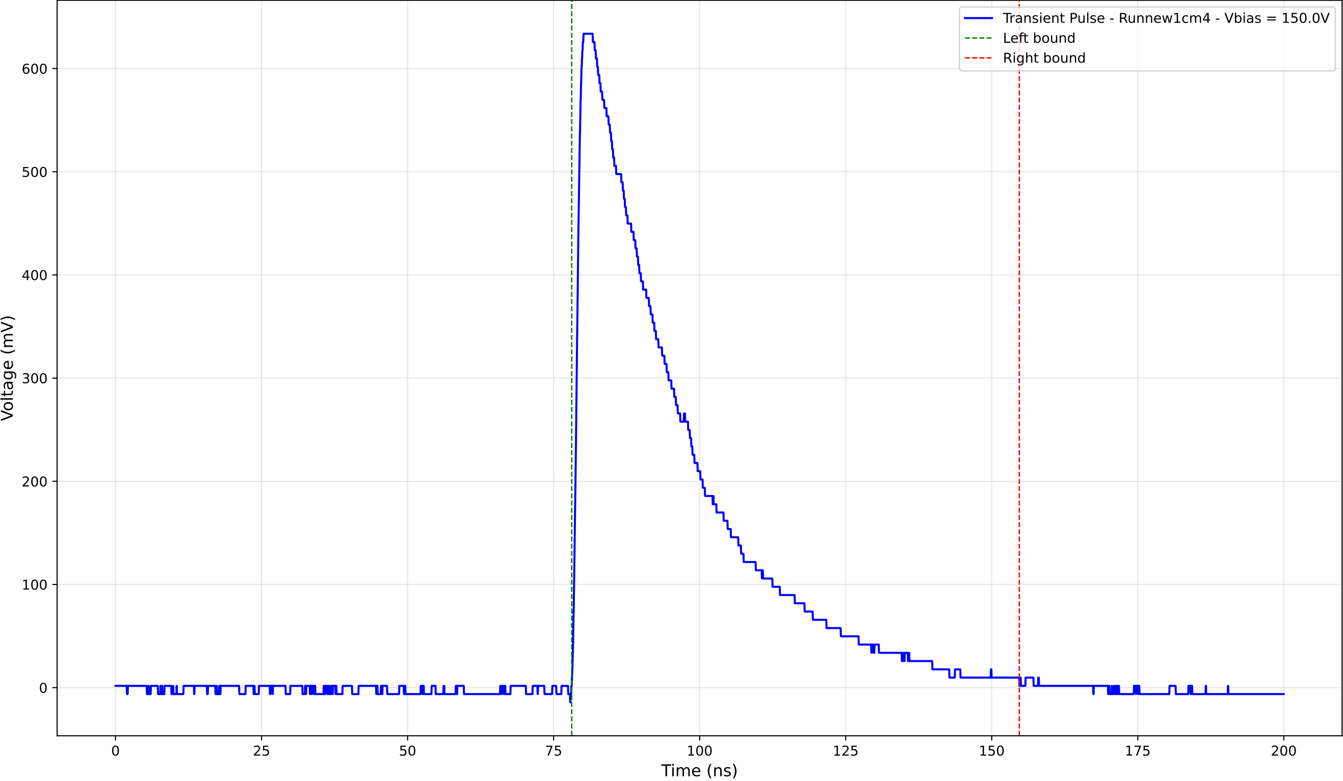
Transient Pulse - Sample: new1cm - Position: 3860.0 \mu\text{m} - Charge: 247.50 pC
