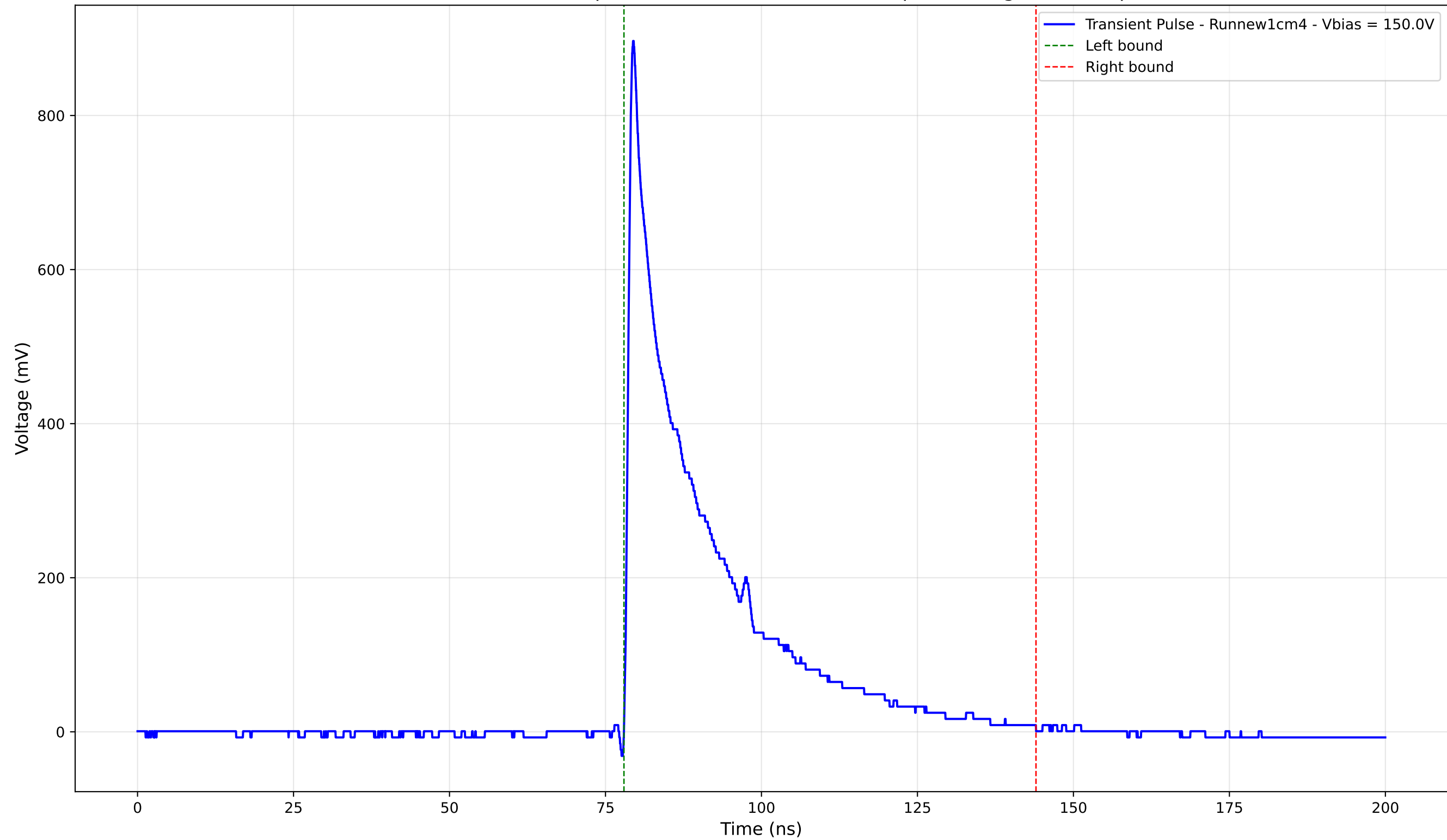
Transient Pulse - Sample: new1cm - Position: 540.0 \mu\text{m} - Charge: 199.03 pC
