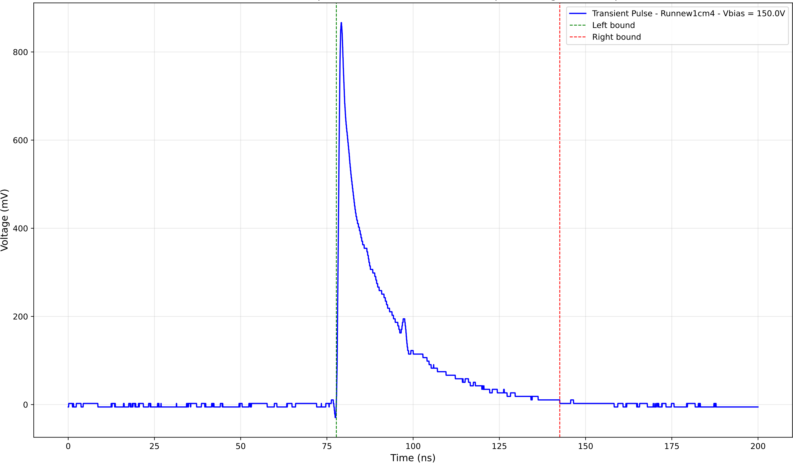
Transient Pulse - Sample: new1cm - Position: 4895.0 \mu\text{m} - Charge: 186.87 pC
