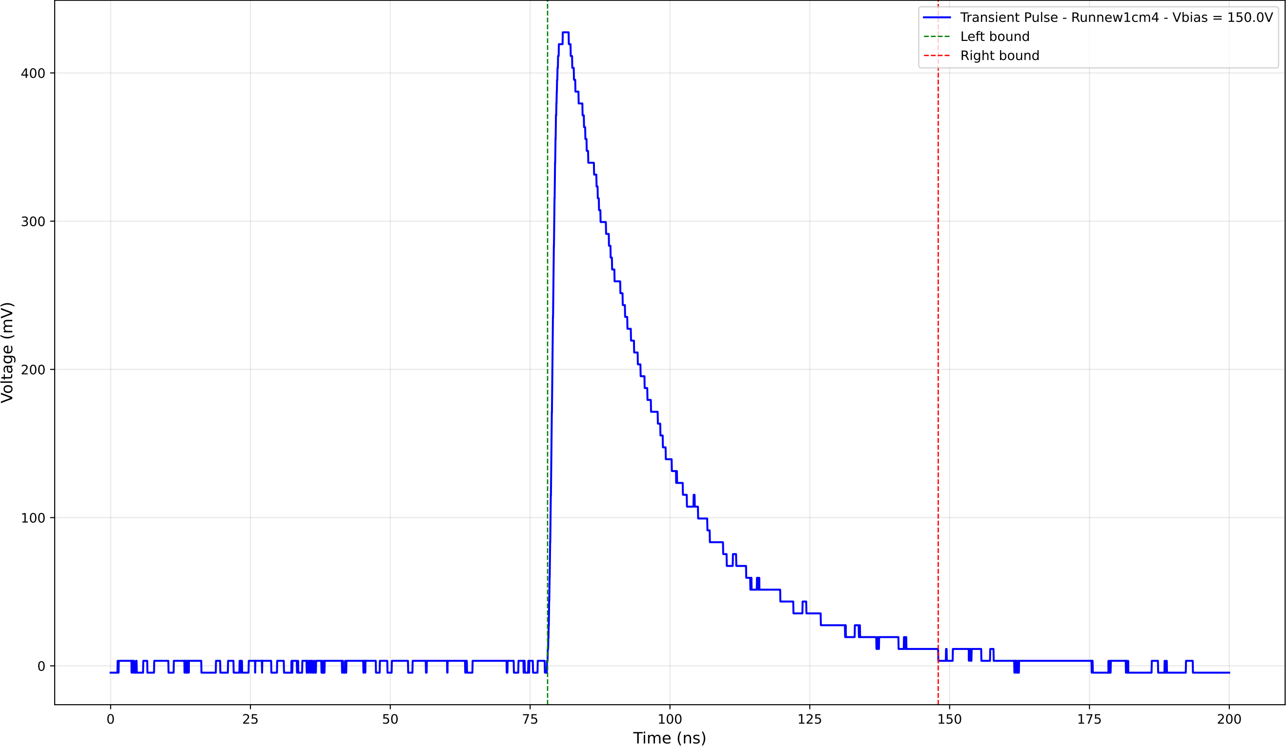
Transient Pulse - Sample: new1cm - Position: 3790.0 \mu\text{m} - Charge: 164.87 pC
