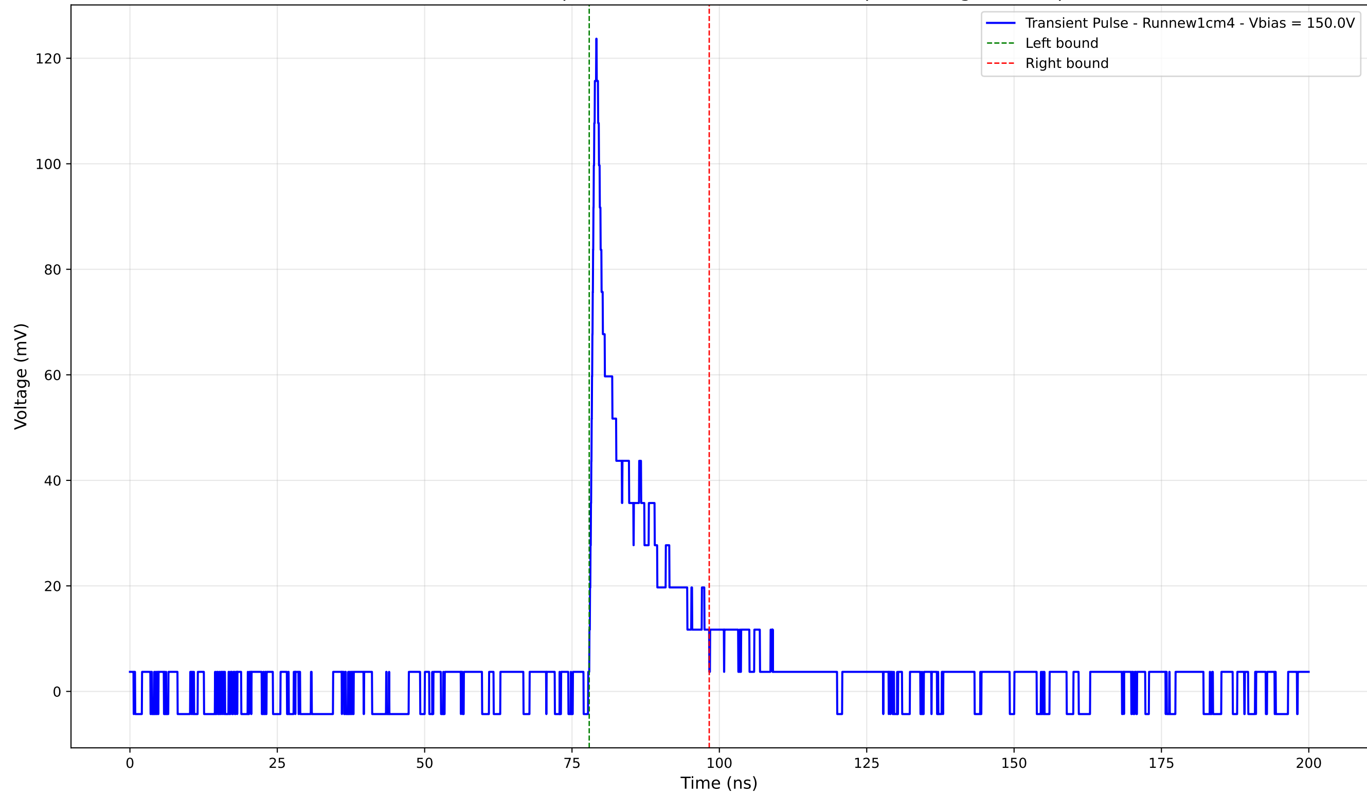
Transient Pulse - Sample: new1cm - Position: 5065.0 \mu\text{m} - Charge: 14.74 pC
