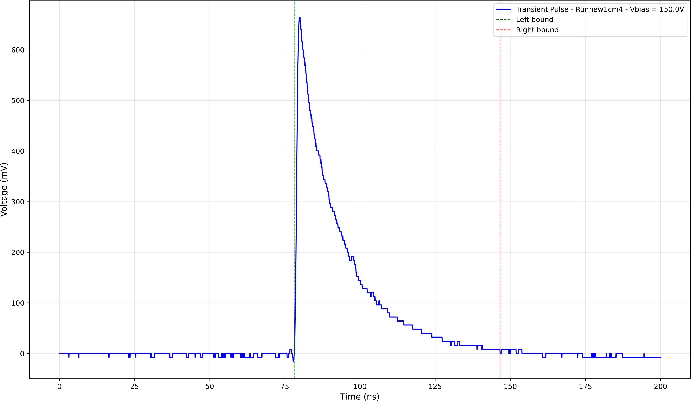
Transient Pulse - Sample: new1cm - Position: 1000.0 \mu\text{m} - Charge: 192.35 pC
