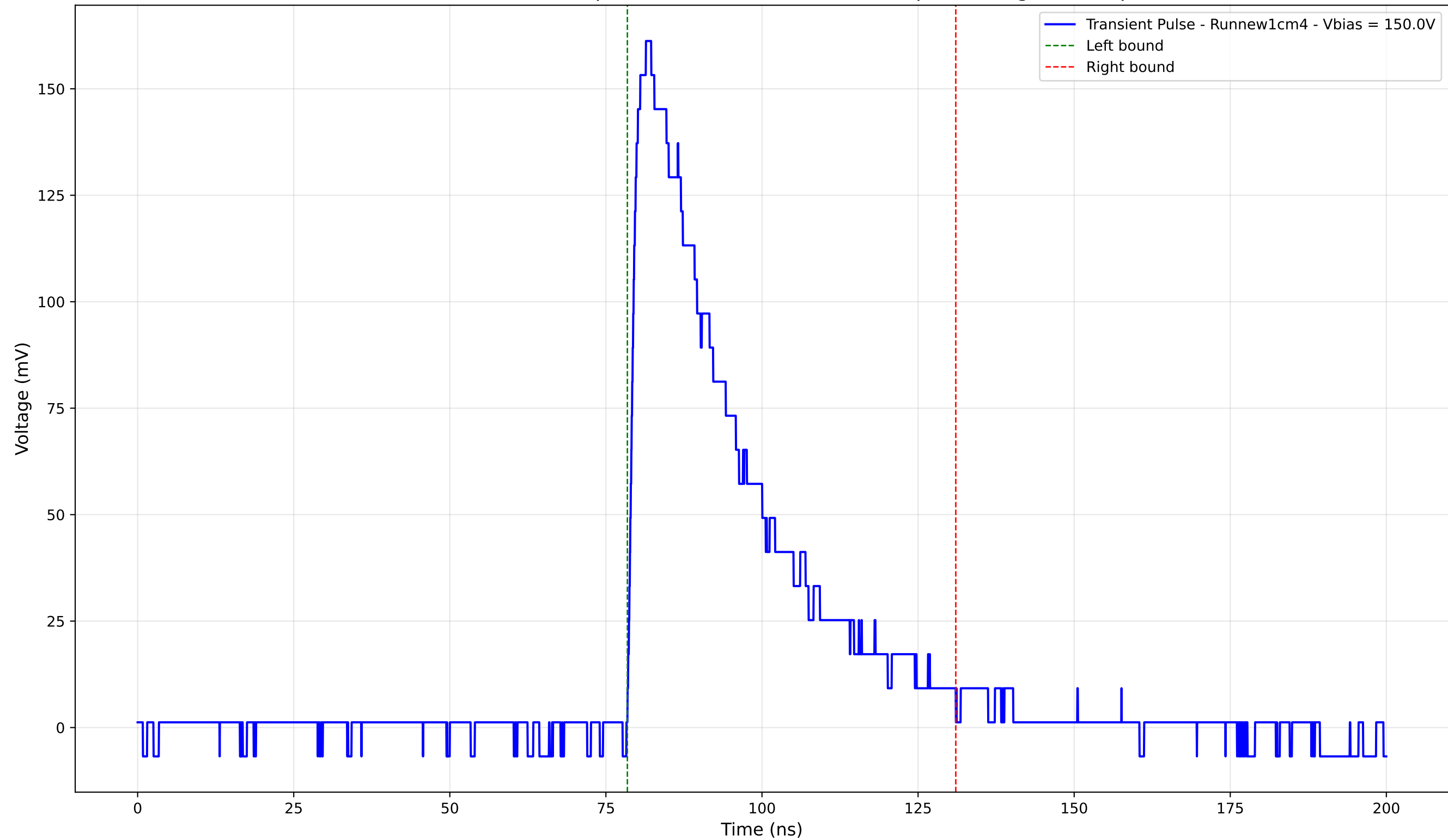
Transient Pulse - Sample: new1cm - Position: 1675.0 \mu\text{m} - Charge: 58.44 pC
