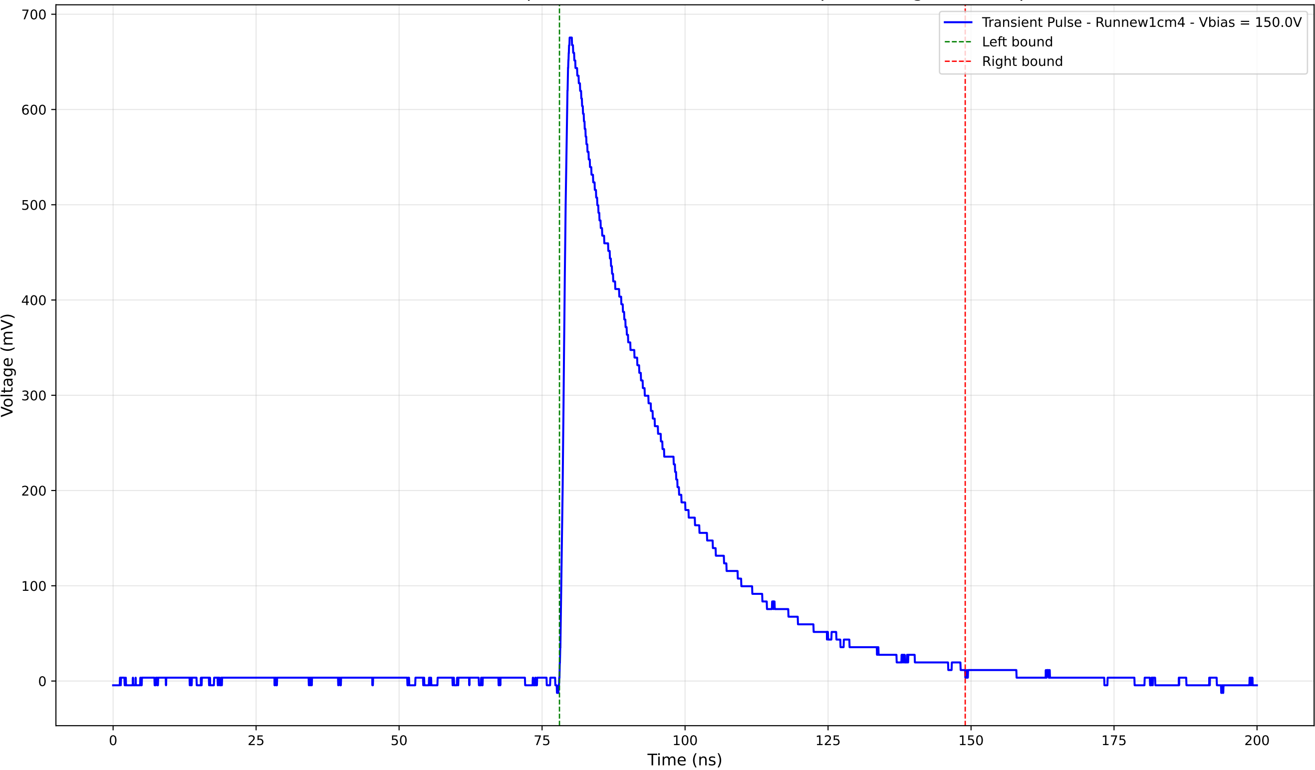
Transient Pulse - Sample: new1cm - Position: 4140.0 \mu\text{m} - Charge: 234.29 pC
