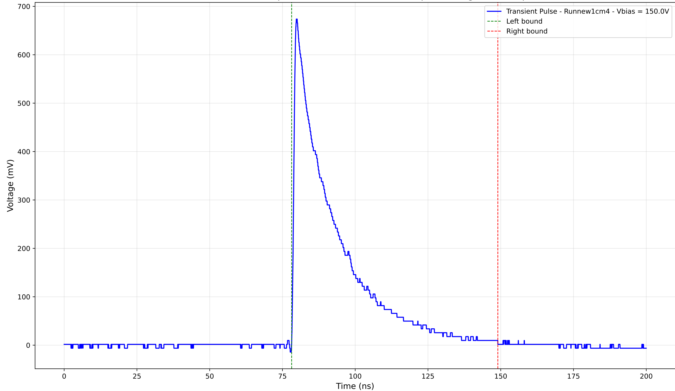
Transient Pulse - Sample: new1cm - Position: 980.0 \mu\text{m} - Charge: 195.04 pC
