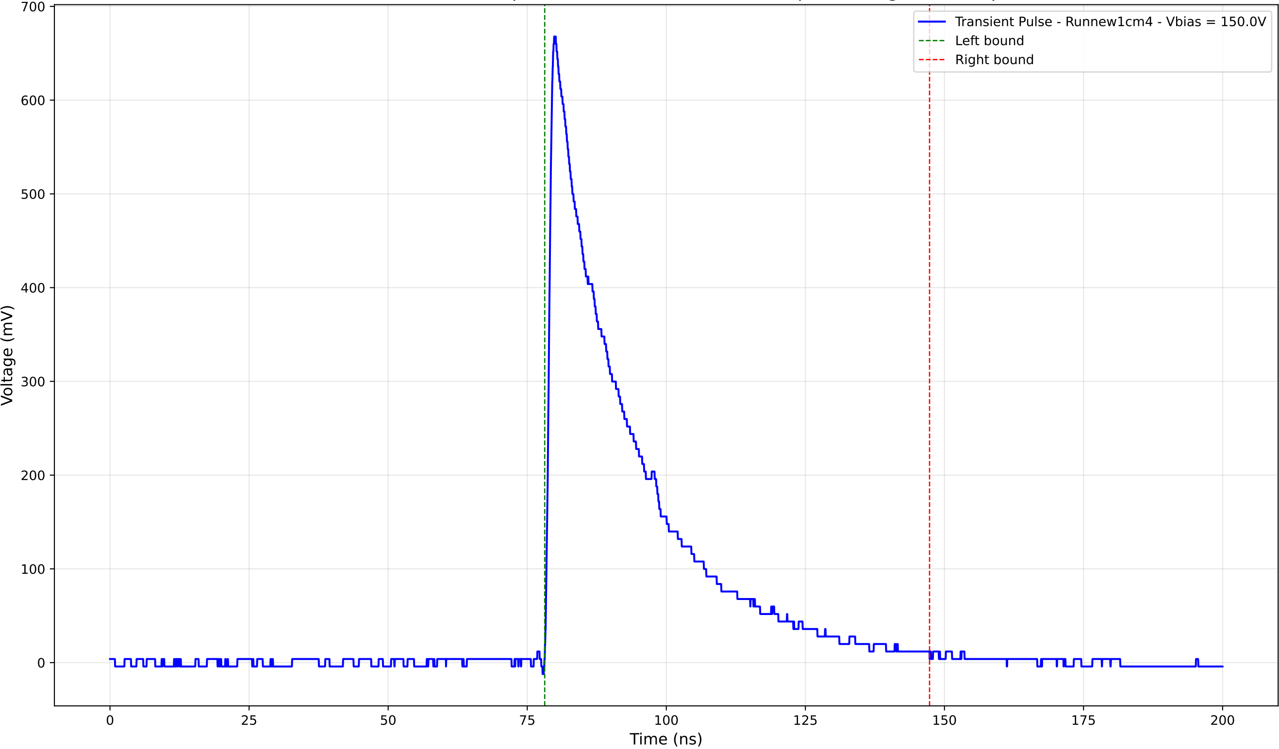
Transient Pulse - Sample: new1cm - Position: 1025.0 \mu\text{m} - Charge: 200.52 pC
