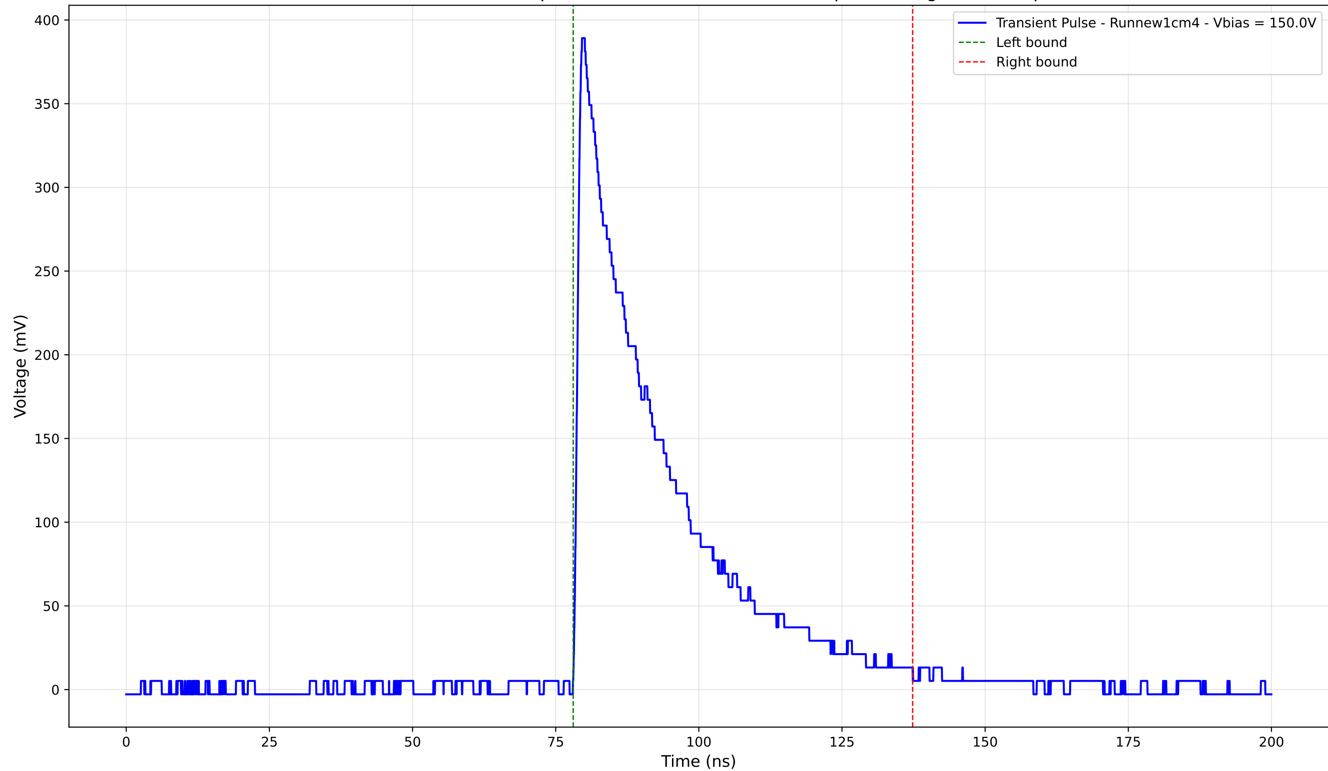
Transient Pulse - Sample: new1cm - Position: 4280.0 \mu\text{m} - Charge: 117.51 pC
