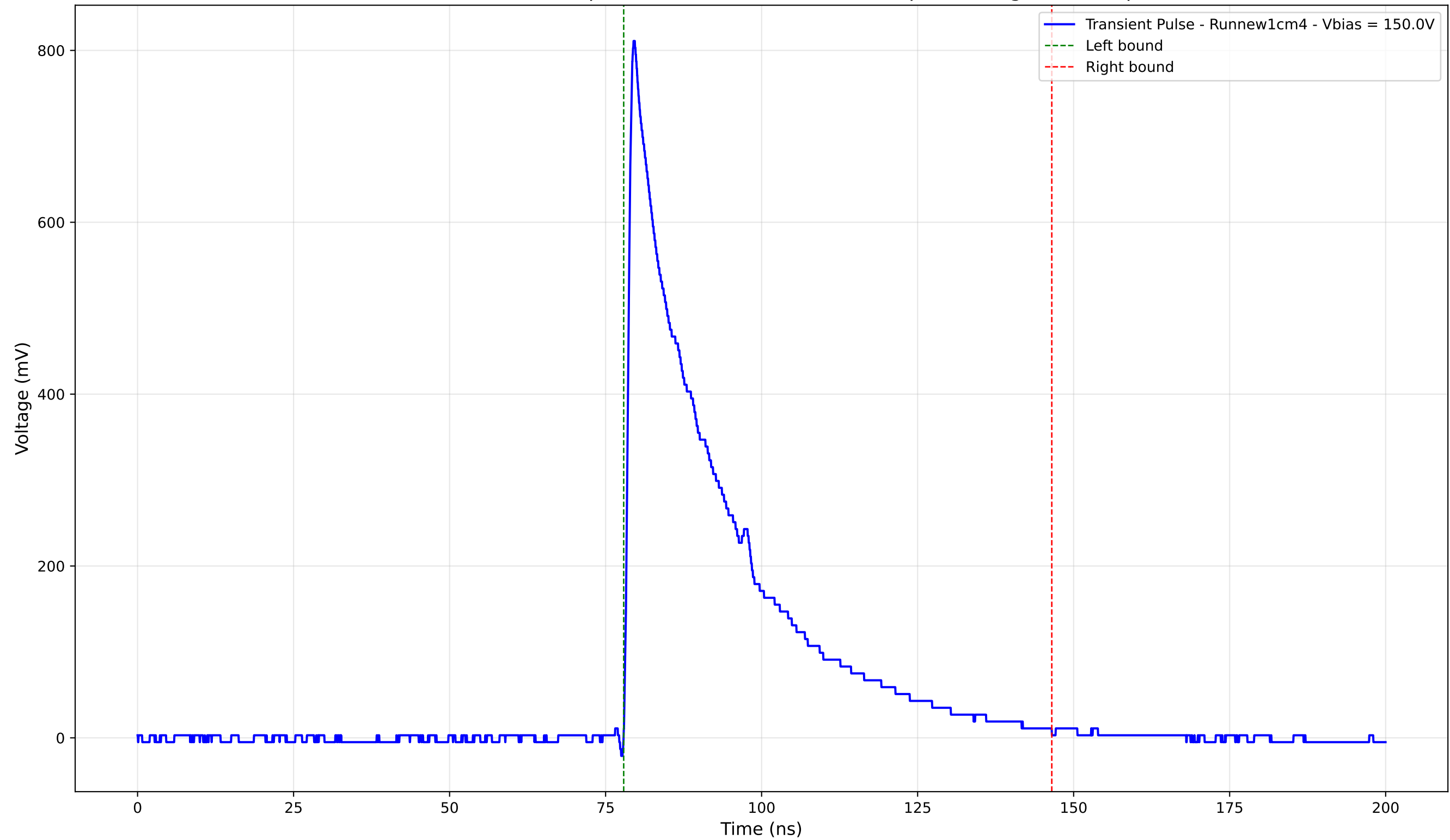
Transient Pulse - Sample: new1cm - Position: 4495.0 \mu\text{m} - Charge: 236.39 pC
