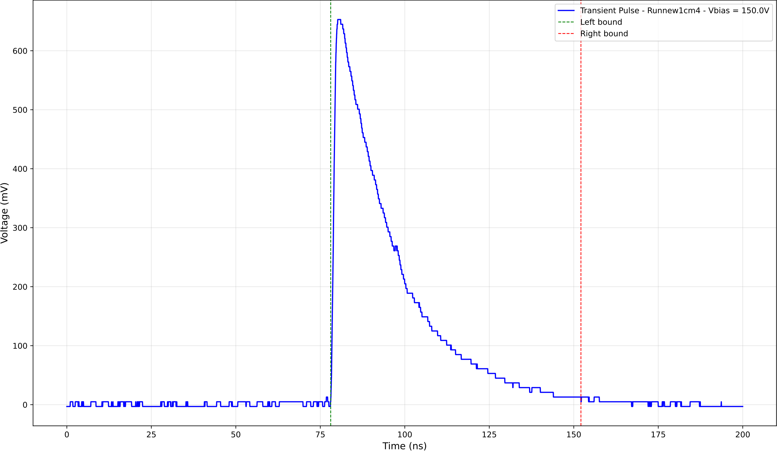
Transient Pulse - Sample: new1cm - Position: 3915.0 \mu\text{m} - Charge: 252.29 pC
