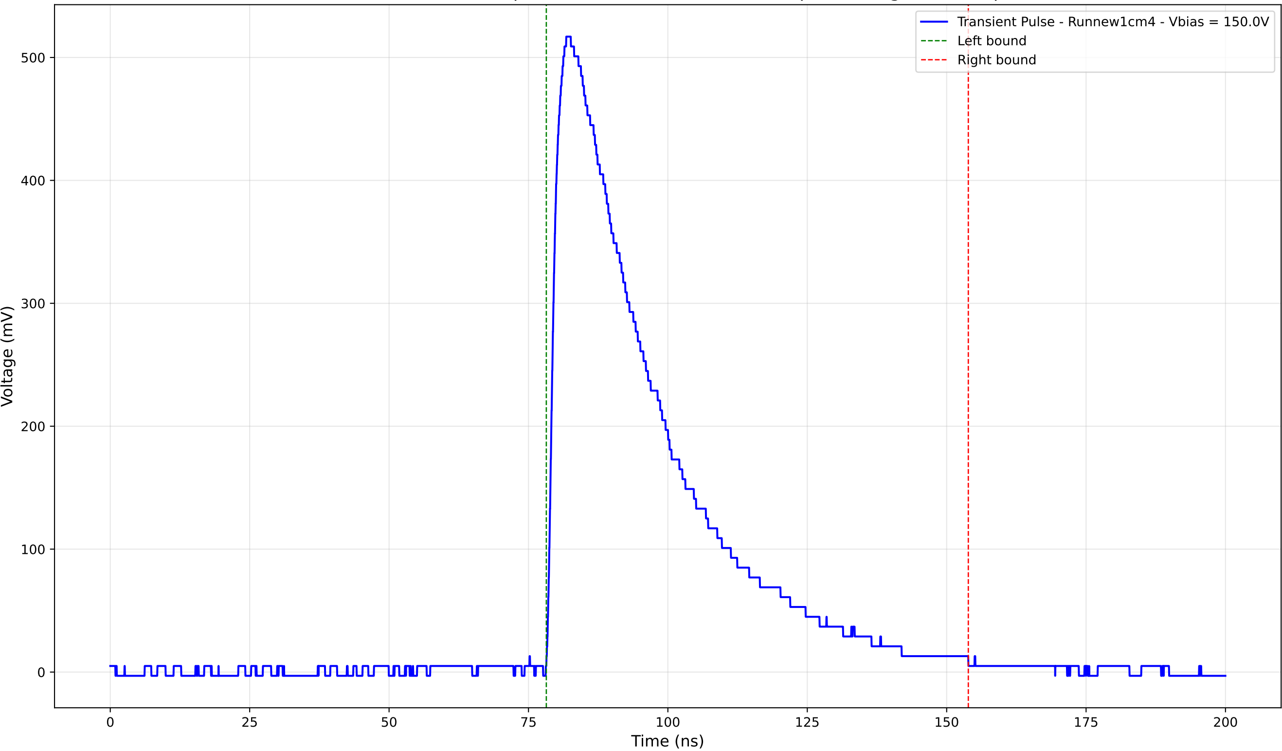
Transient Pulse - Sample: new1cm - Position: 2010.0 \mu\text{m} - Charge: 215.66 pC
