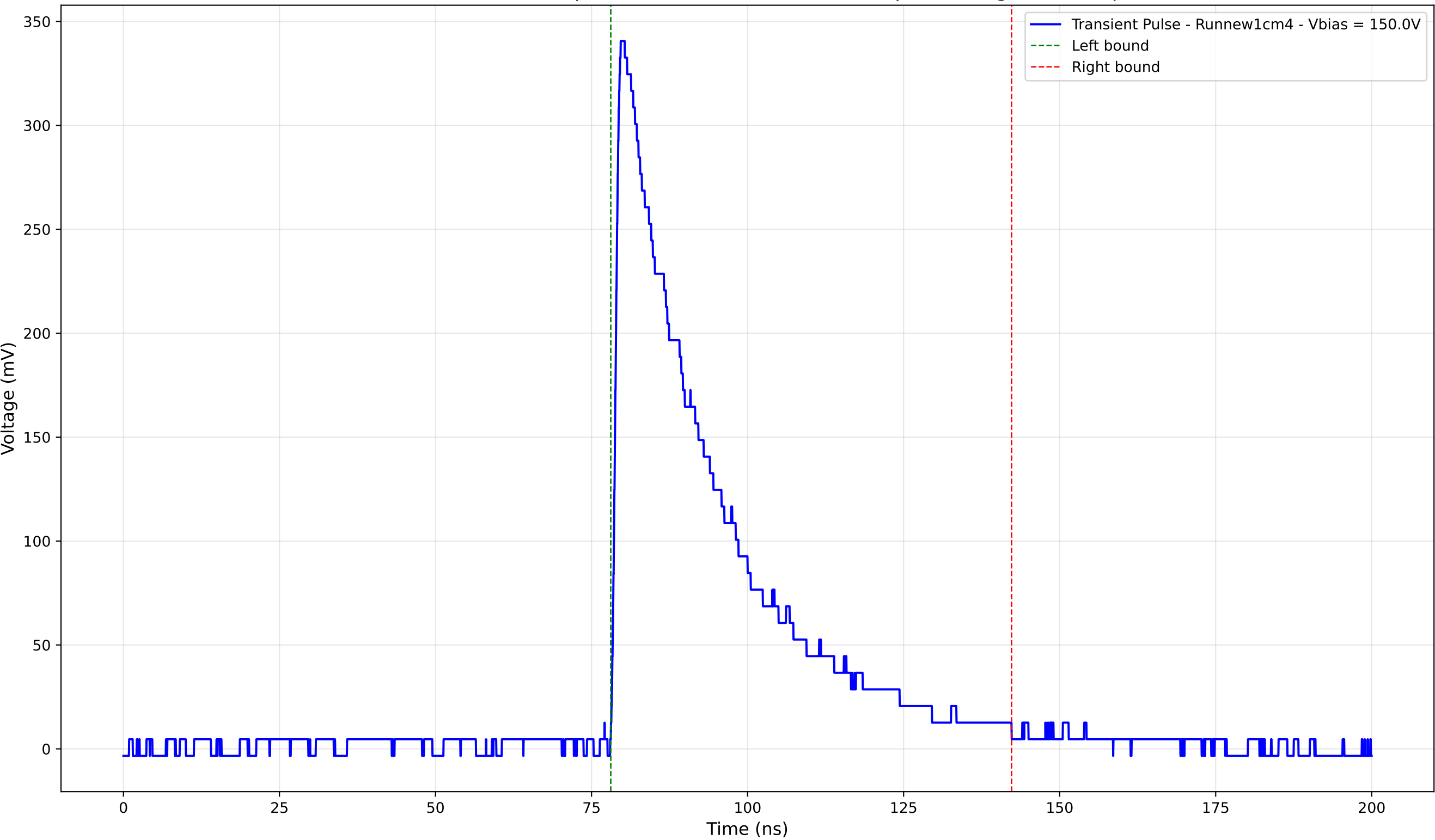
Transient Pulse - Sample: new1cm - Position: 4190.0 \mu\text{m} - Charge: 111.89 pC
