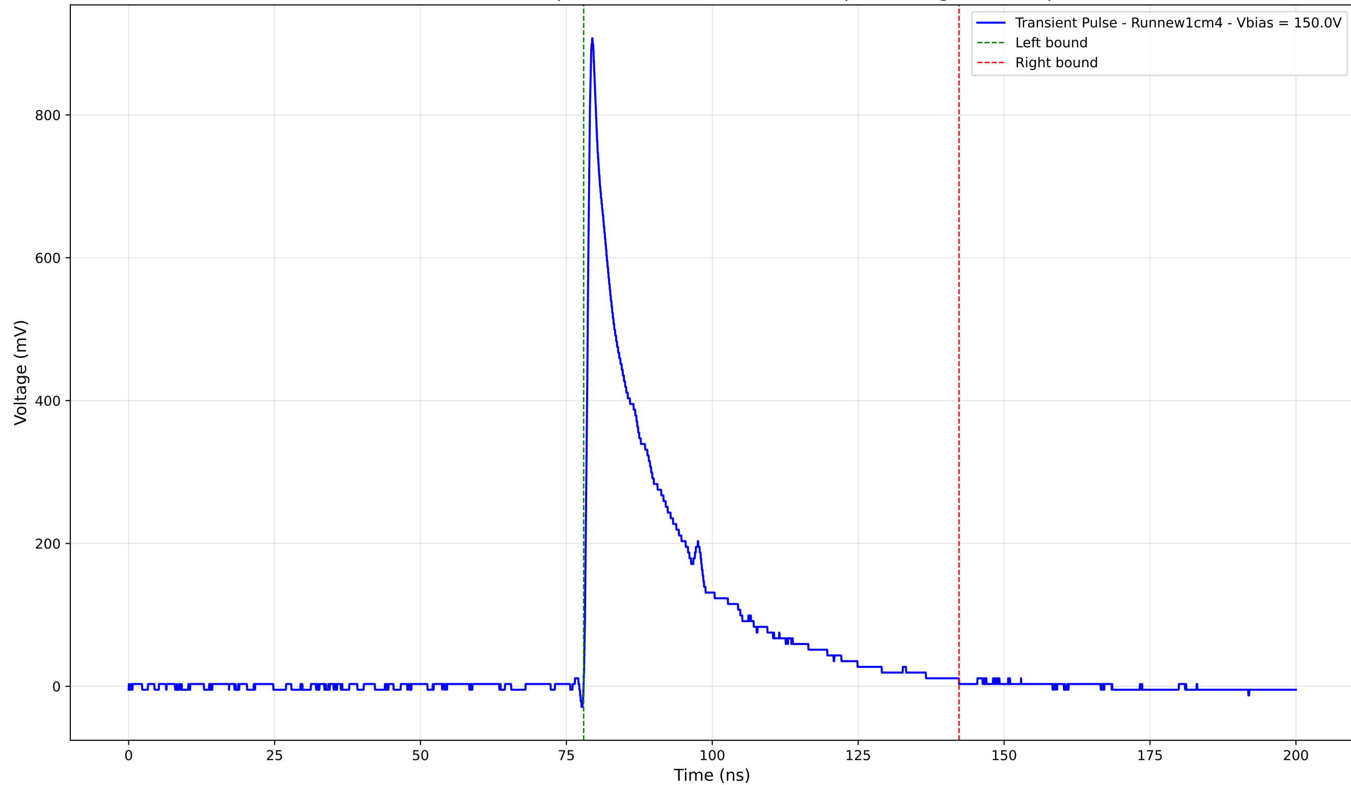
Transient Pulse - Sample: new1cm - Position: 520.0 \mu\text{m} - Charge: 202.00 pC
