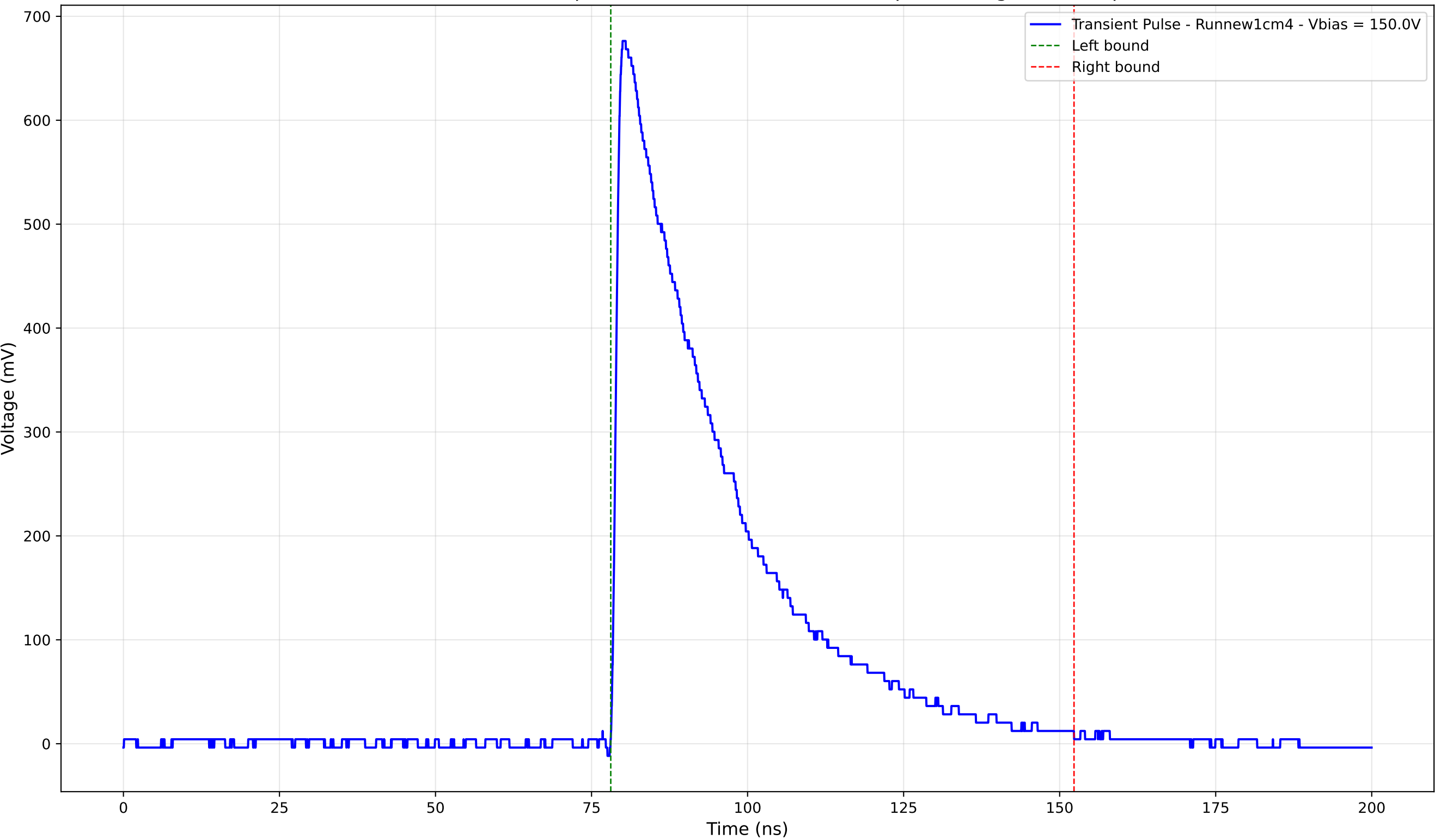
Transient Pulse - Sample: new1cm - Position: 4020.0 \mu\text{m} - Charge: 249.37 pC
