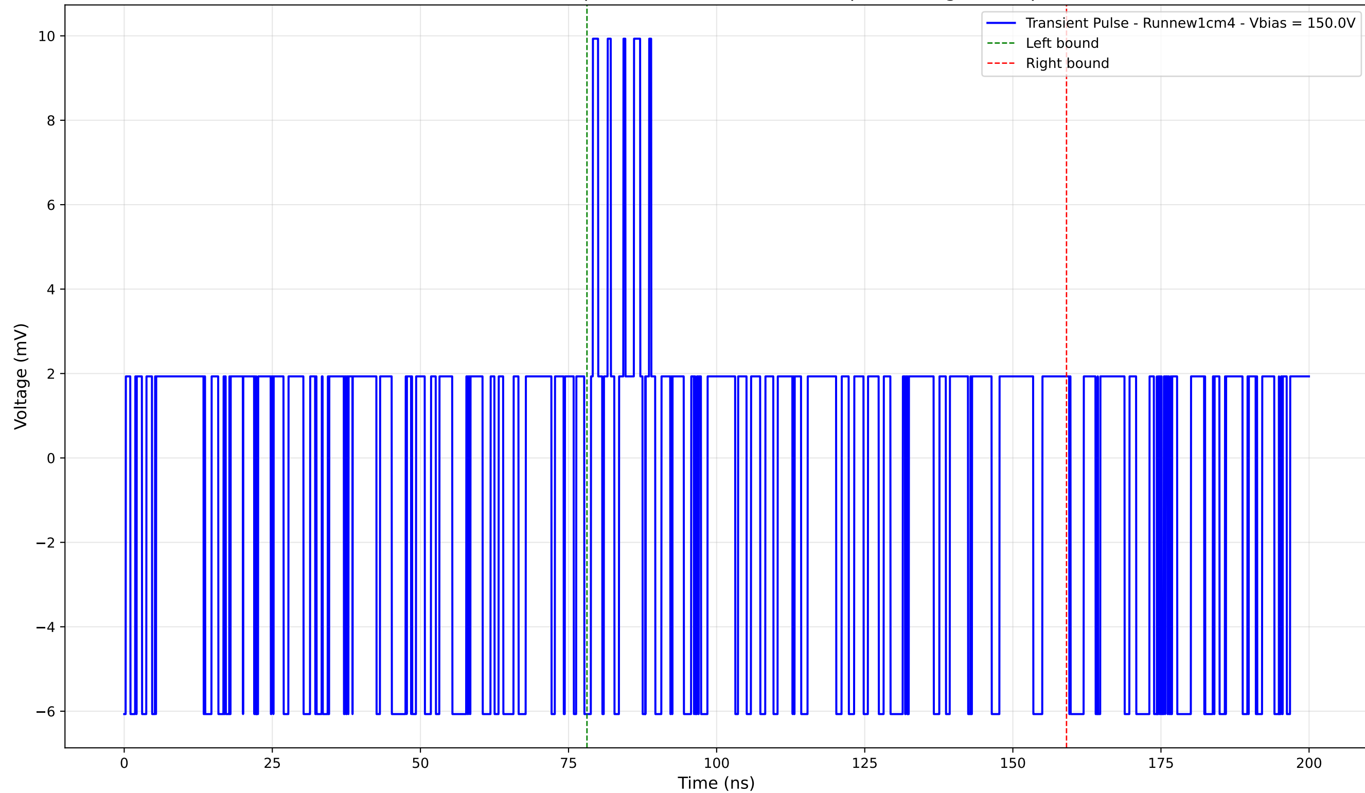
Transient Pulse - Sample: new1cm - Position: 0.0 \mu\text{m} - Charge: 0.26 pC
