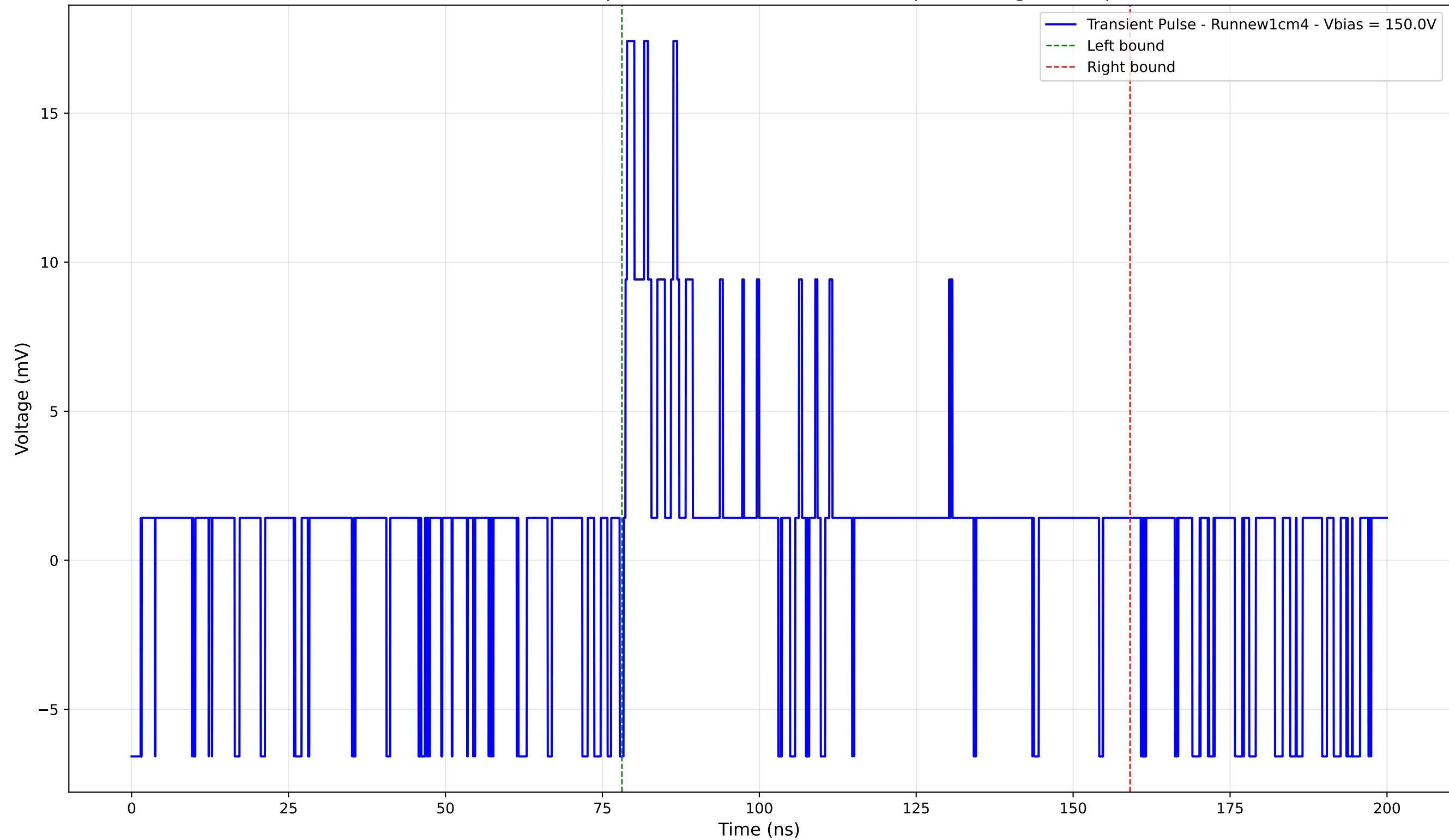
Transient Pulse - Sample: new1cm - Position: 120.0 \mu\text{m} - Charge: 3.60 pC
