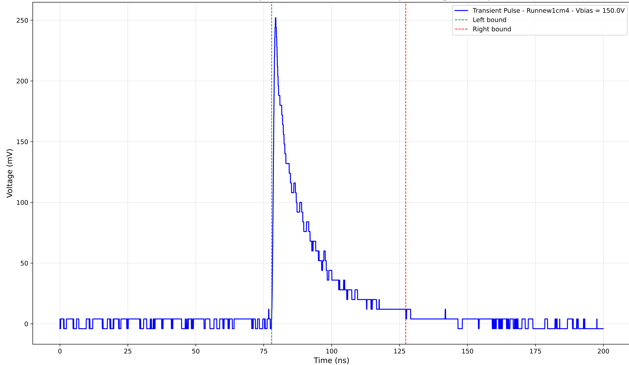
Transient Pulse - Sample: new1cm - Position: 4710.0 \mu\text{m} - Charge: 55.51 pC
