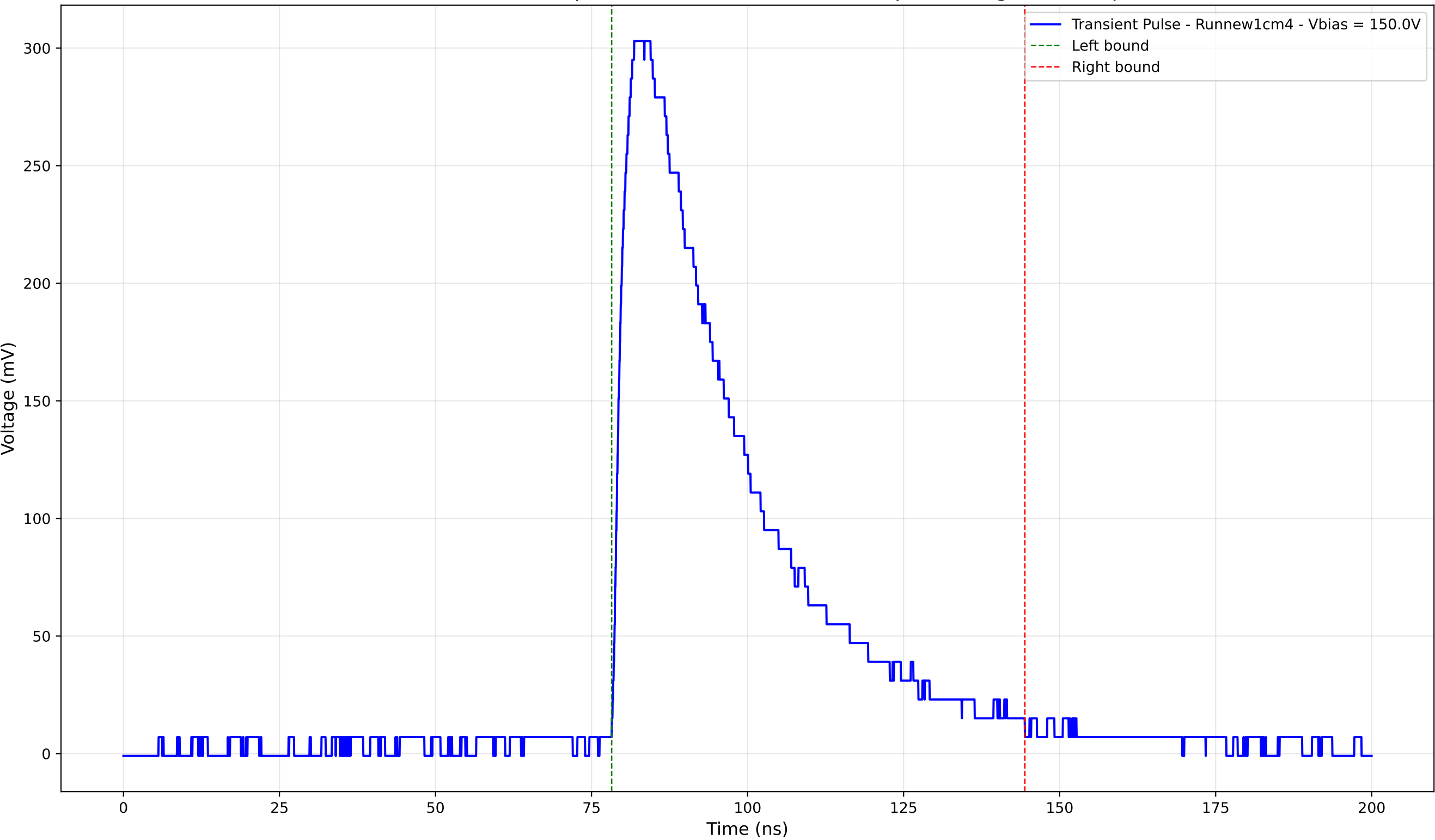
Transient Pulse - Sample: new1cm - Position: 2770.0 \mu\text{m} - Charge: 133.54 pC
