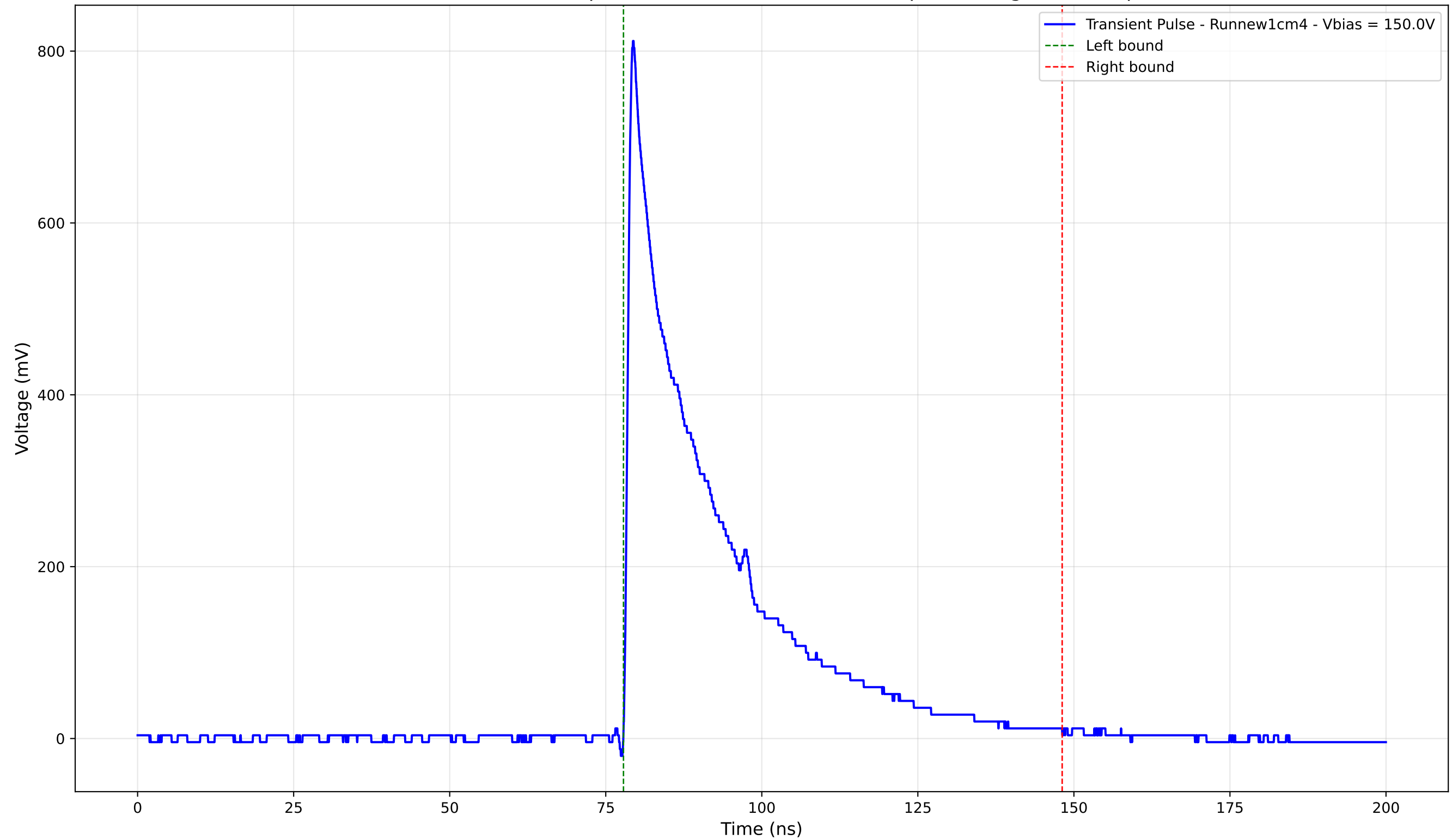
Transient Pulse - Sample: new1cm - Position: 4635.0 \mu\text{m} - Charge: 214.70 pC
