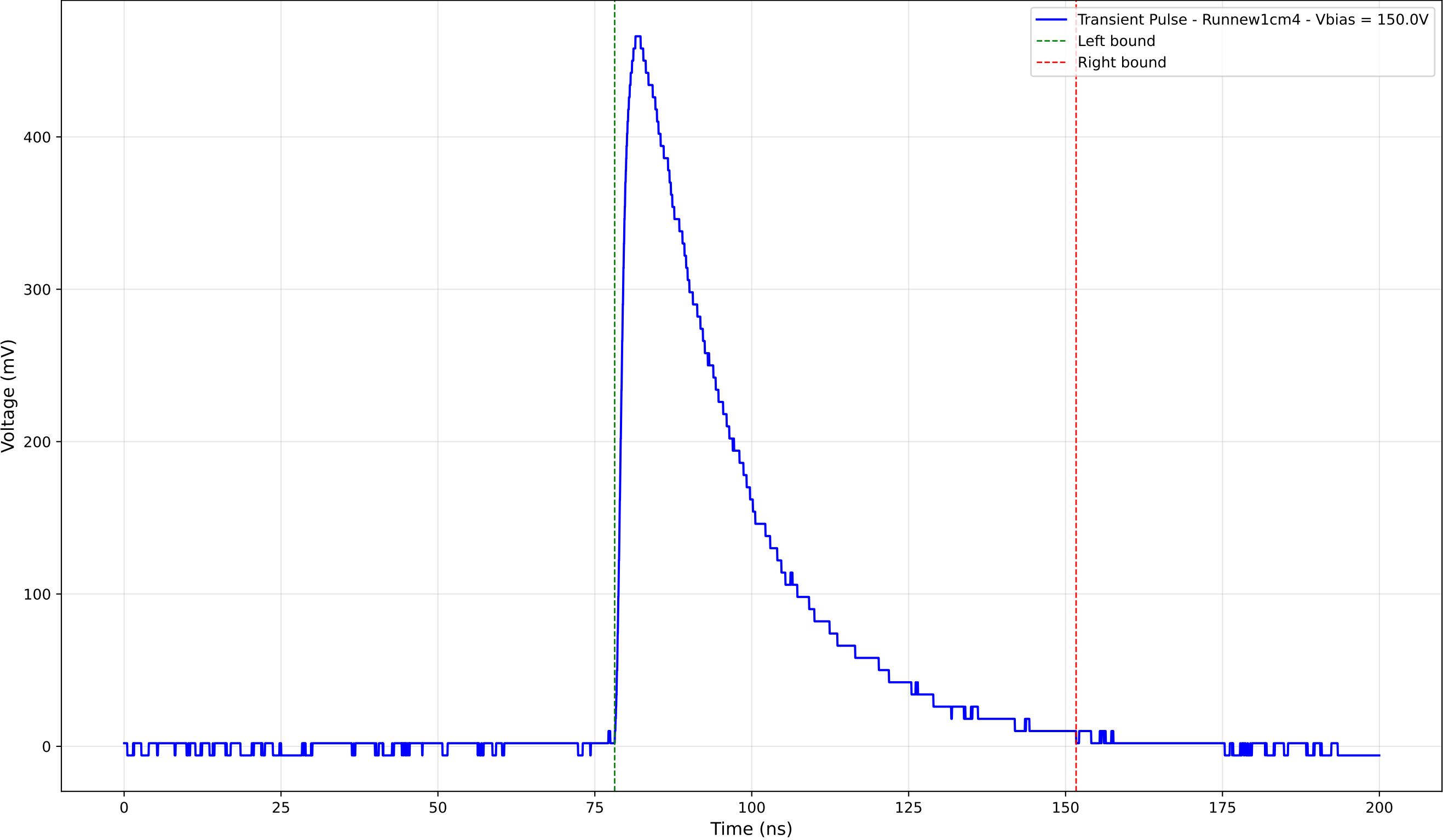
Transient Pulse - Sample: new1cm - Position: 1790.0 \mu\text{m} - Charge: 185.45 pC
