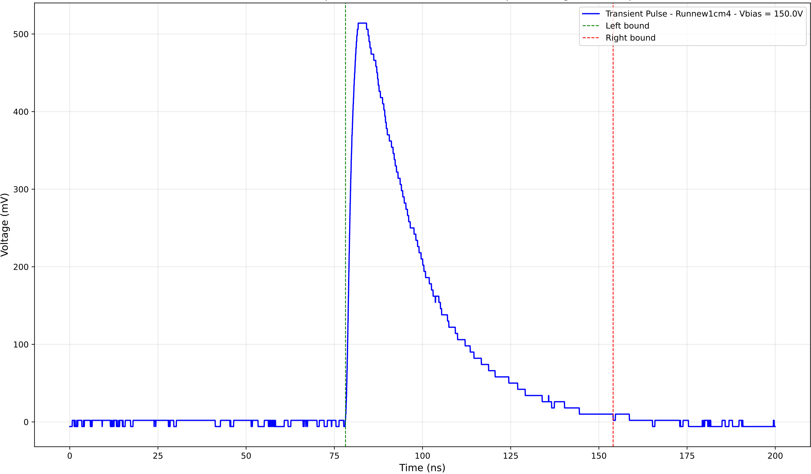
Transient Pulse - Sample: new1cm - Position: 2475.0 \mu\text{m} - Charge: 224.00 pC
