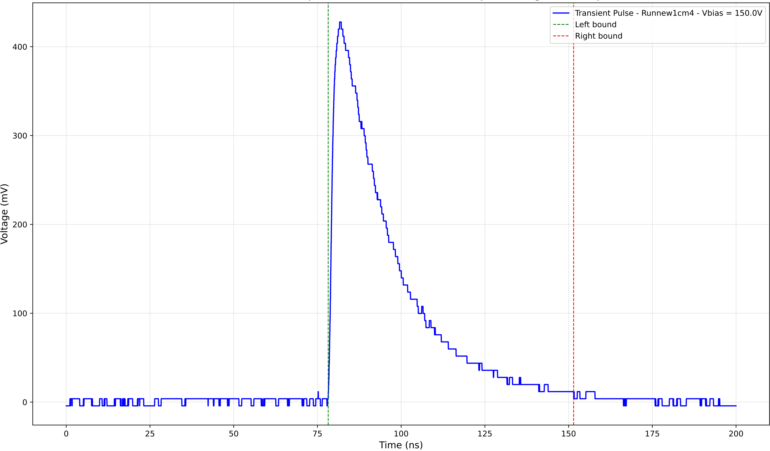
Transient Pulse - Sample: new1cm - Position: 1780.0 \mu\text{m} - Charge: 169.62 pC
