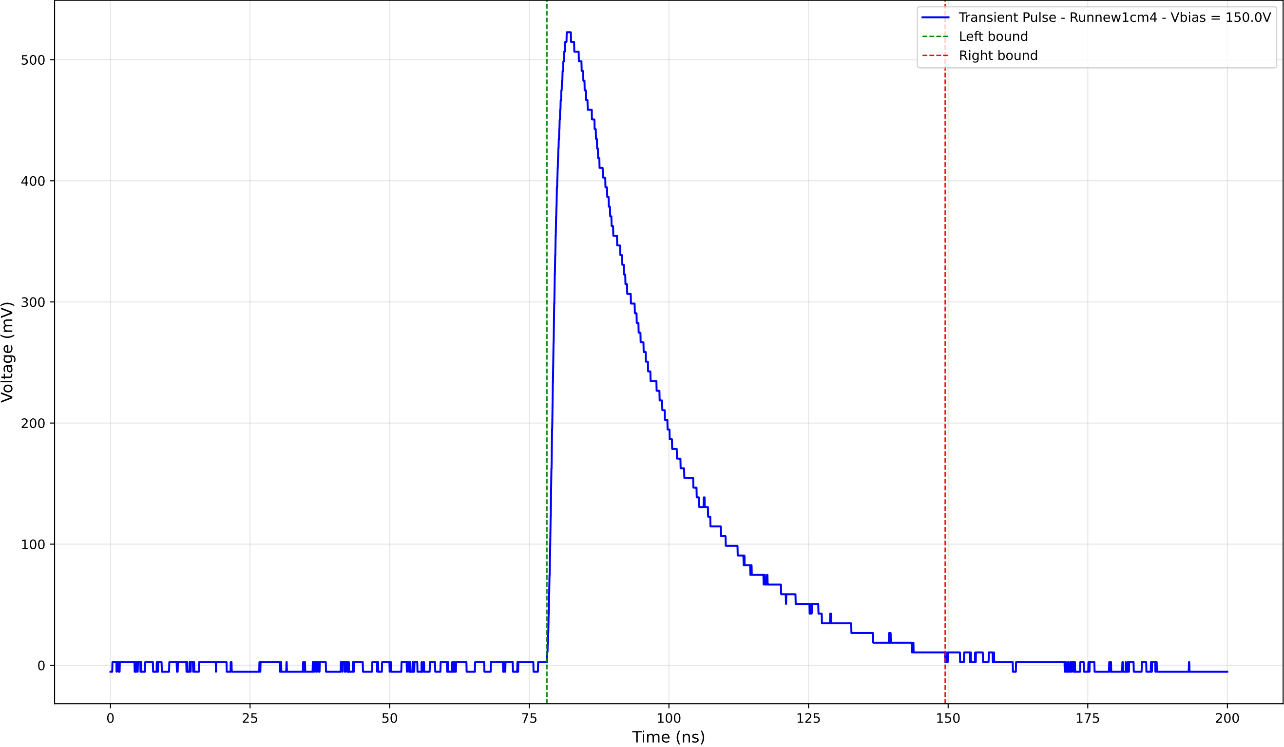
Transient Pulse - Sample: new1cm - Position: 2045.0 \mu\text{m} - Charge: 215.76 pC
