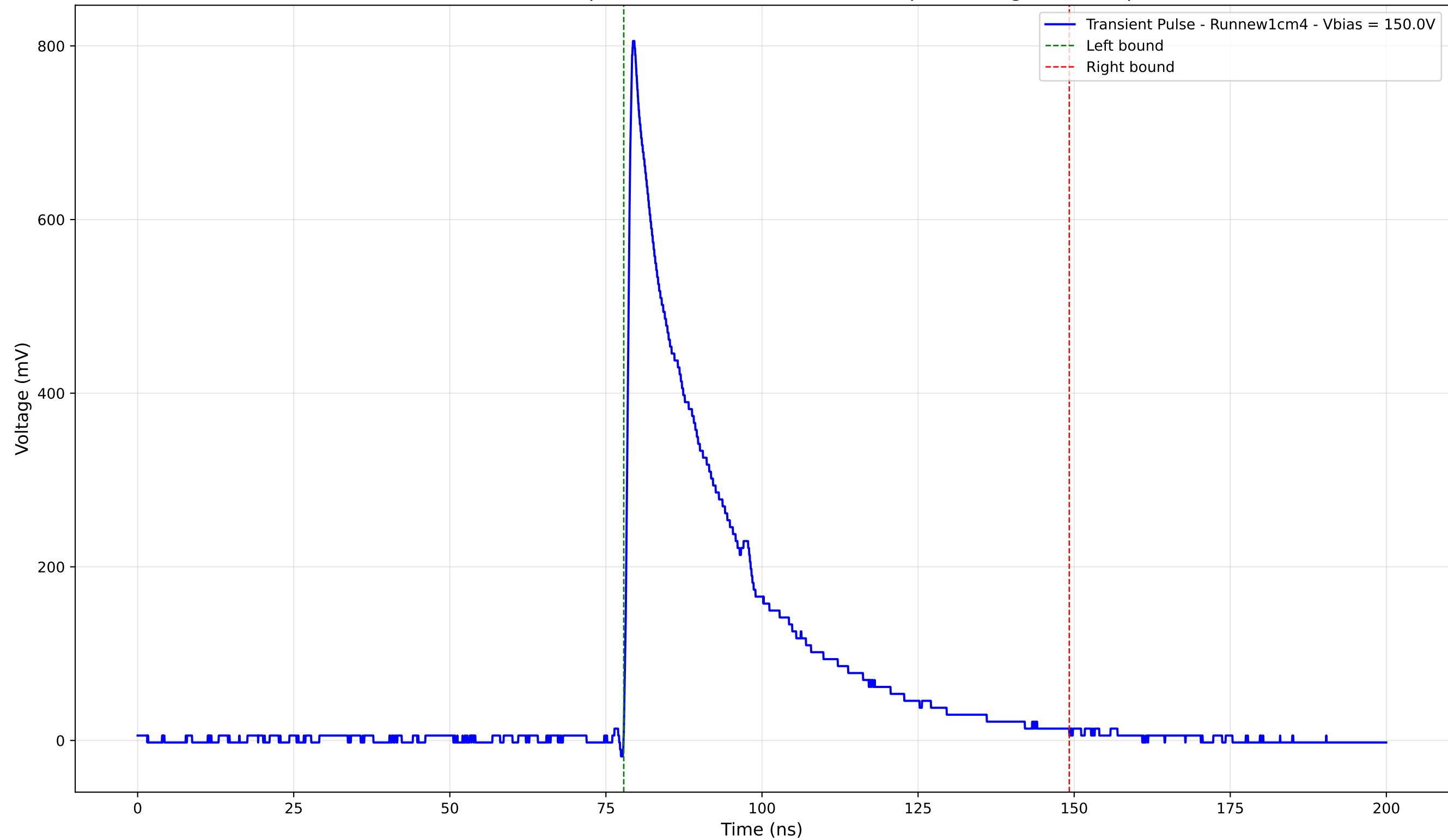
Transient Pulse - Sample: new1cm - Position: 4590.0 \mu\text{m} - Charge: 231.27 pC
