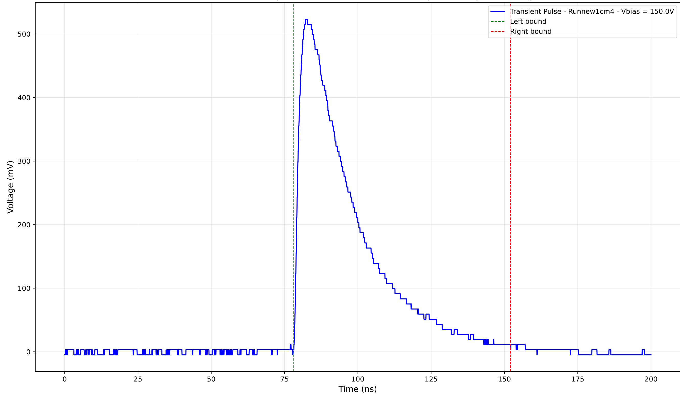
Transient Pulse - Sample: new1cm - Position: 2420.0 \mu\text{m} - Charge: 224.50 pC
