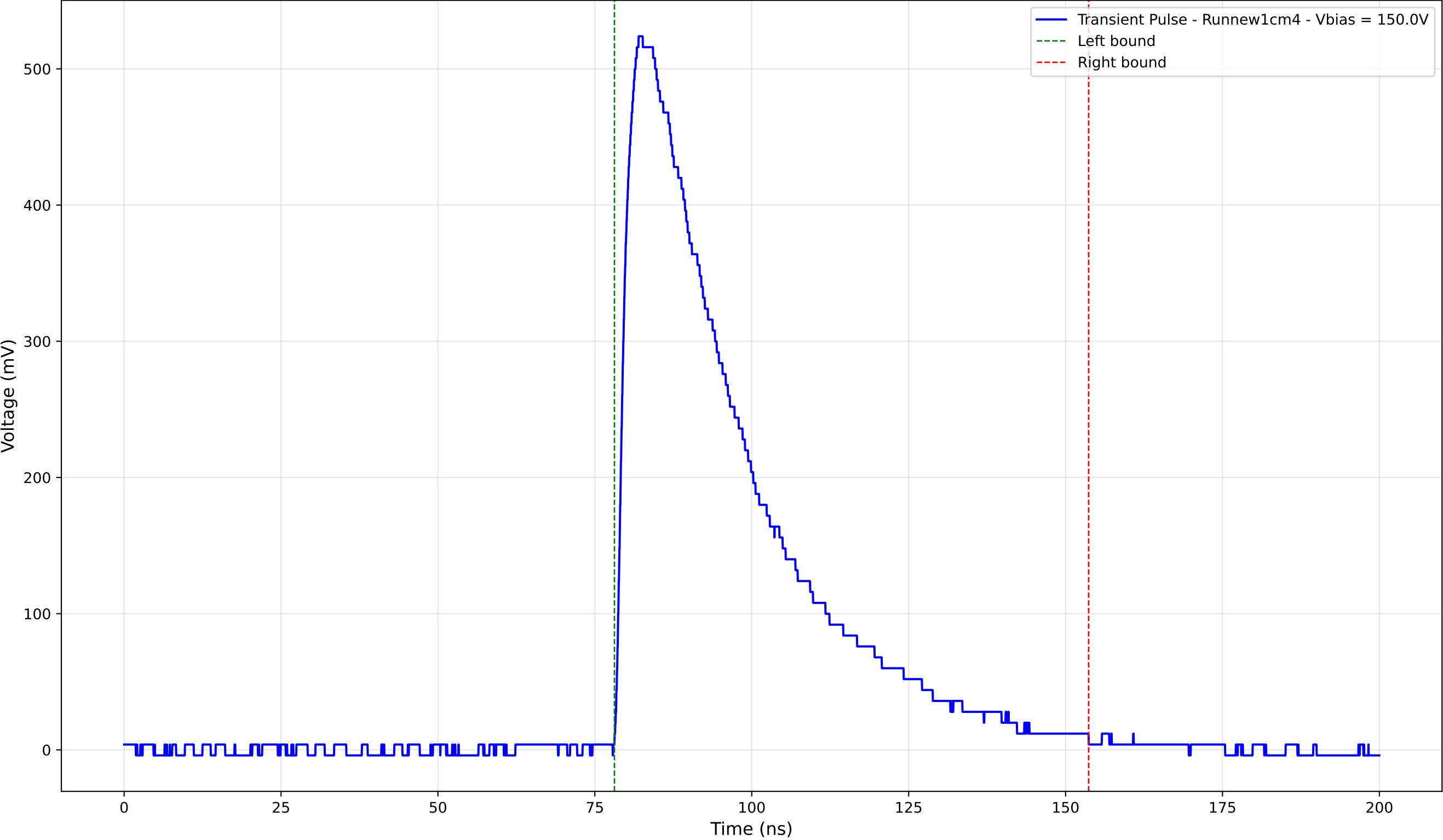
Transient Pulse - Sample: new1cm - Position: 2340.0 \mu\text{m} - Charge: 226.43 pC
