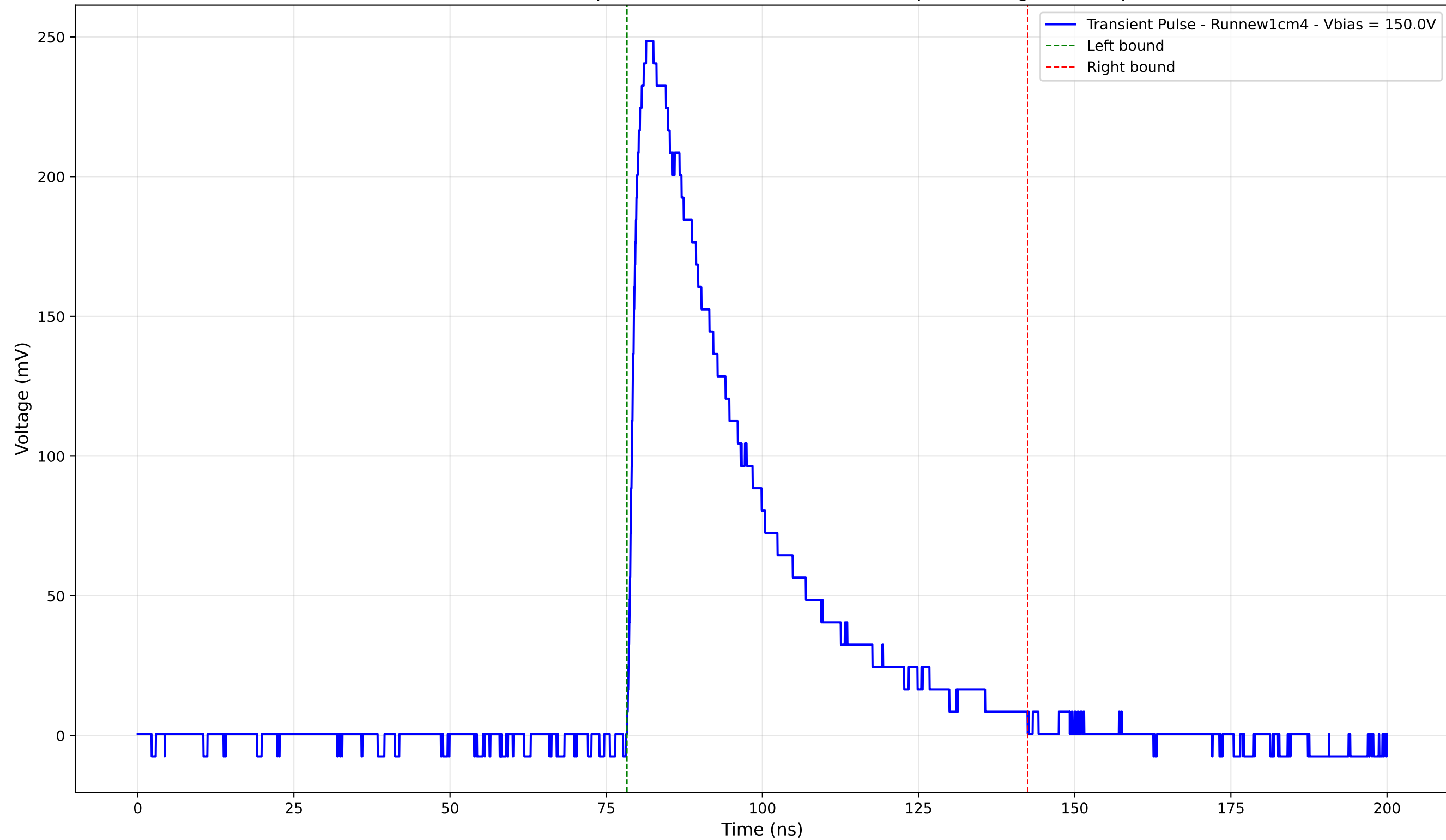
Transient Pulse - Sample: new1cm - Position: 1750.0 \mu\text{m} - Charge: 95.28 pC
