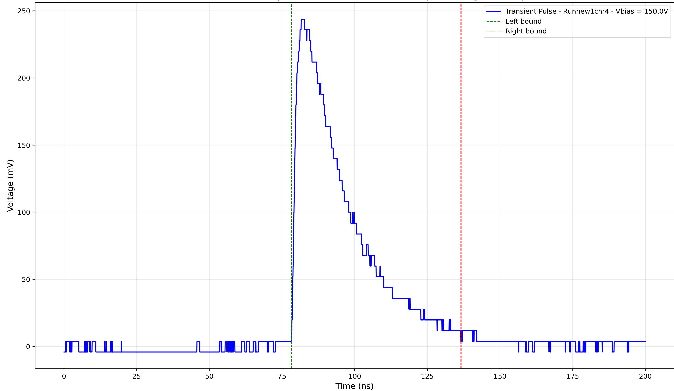
Transient Pulse - Sample: new1cm - Position: 3265.0 \mu\text{m} - Charge: 99.03 pC
