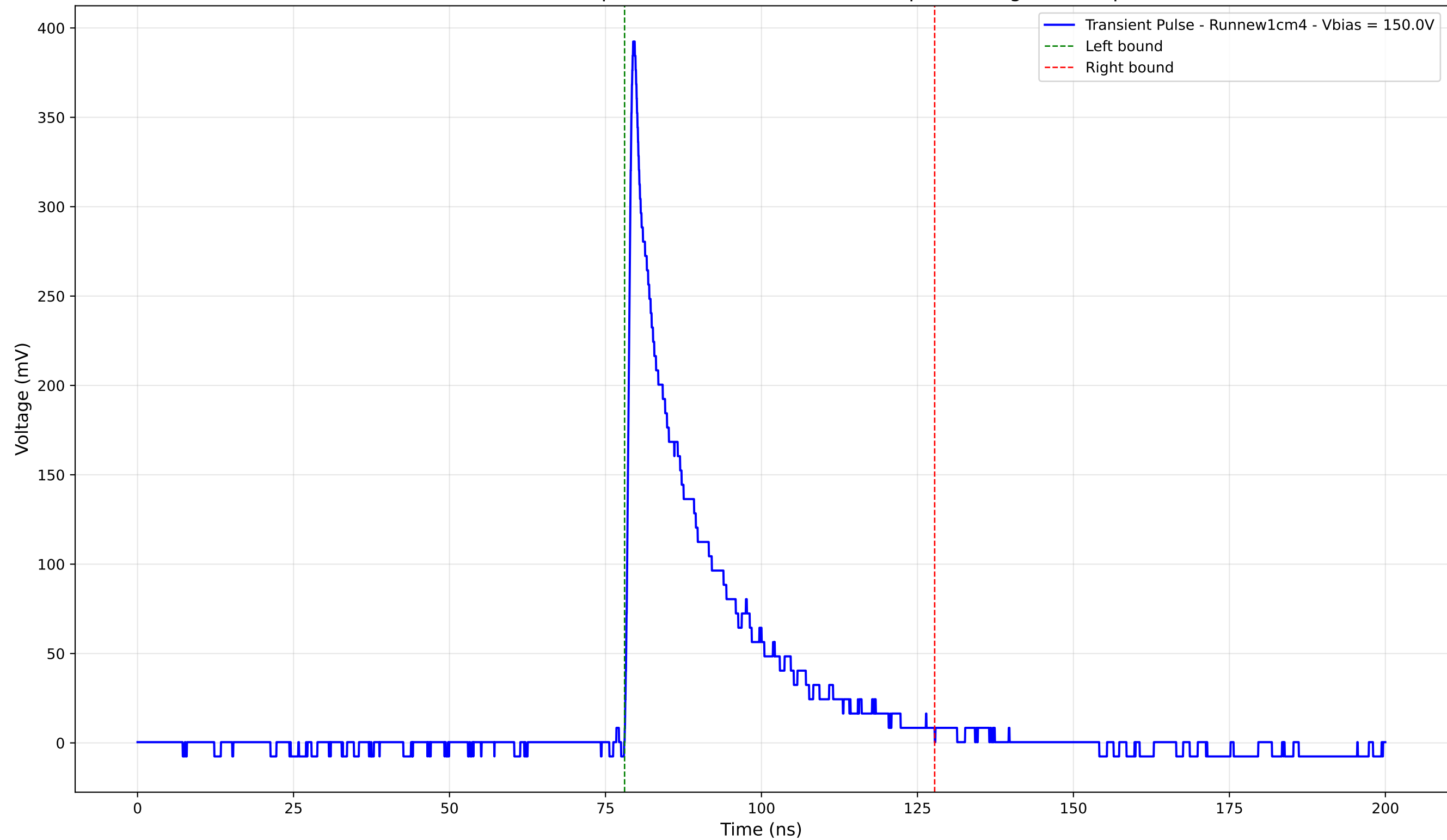
Transient Pulse - Sample: new1cm - Position: 650.0 \mu\text{m} - Charge: 79.47 pC
