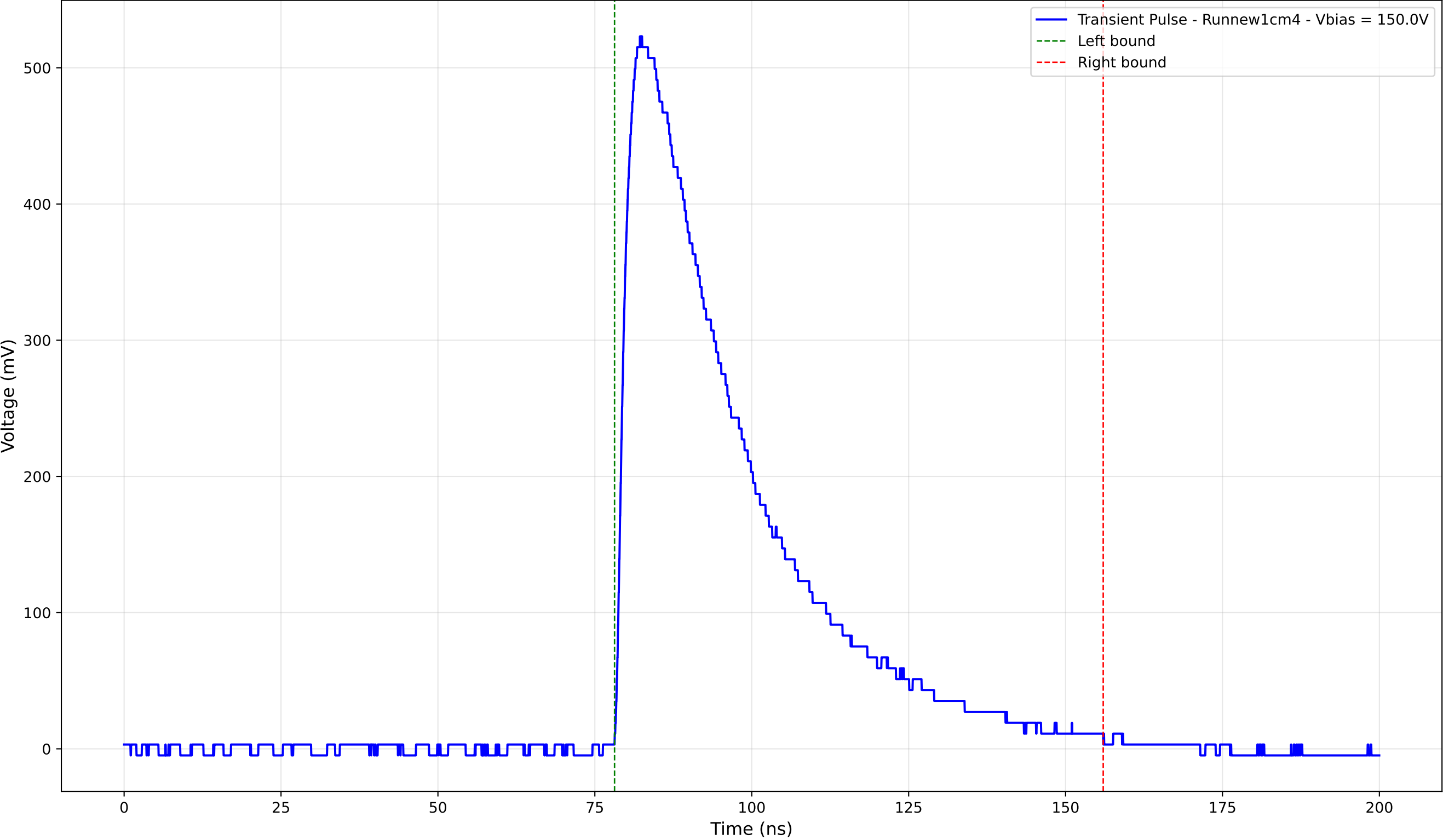
Transient Pulse - Sample: new1cm - Position: 2355.0 \mu\text{m} - Charge: 224.65 pC
