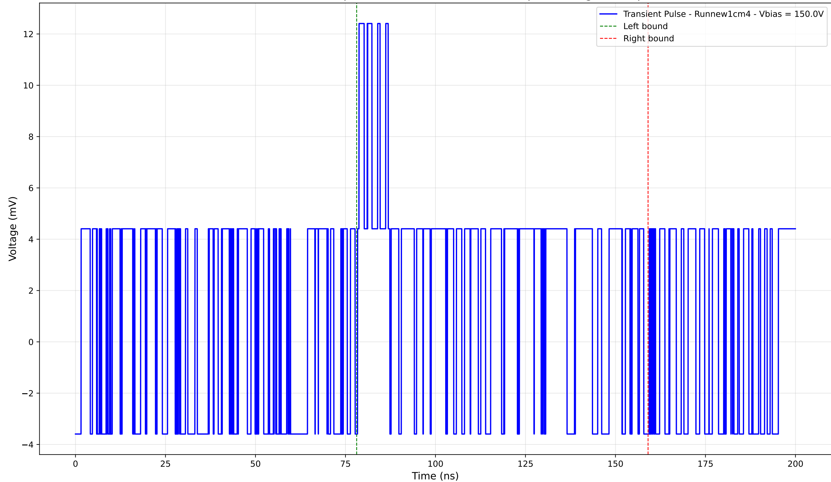
Transient Pulse - Sample: new1cm - Position: 5120.0 \mu\text{m} - Charge: 5.11 pC
