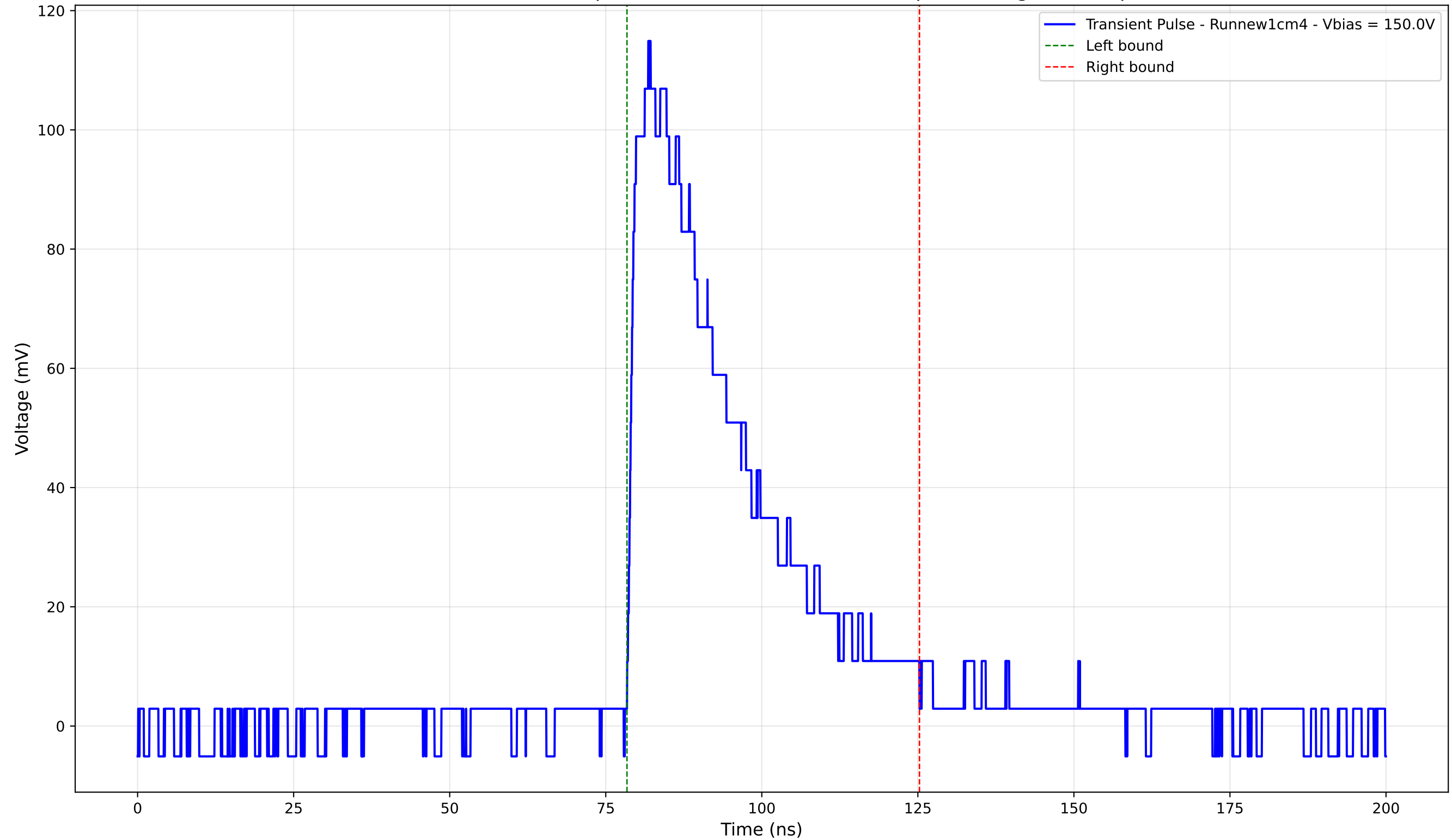
Transient Pulse - Sample: new1cm - Position: 3740.0 \mu\text{m} - Charge: 41.10 pC
