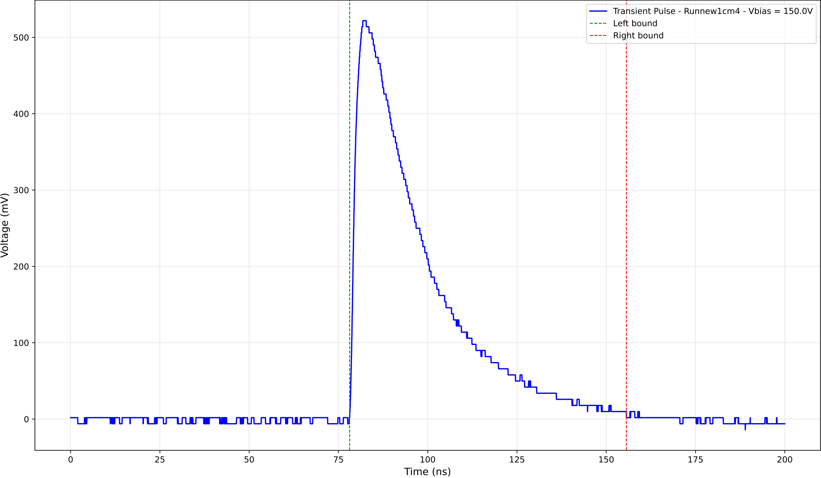
Transient Pulse - Sample: new1cm - Position: 3045.0 \mu\text{m} - Charge: 229.21 pC
