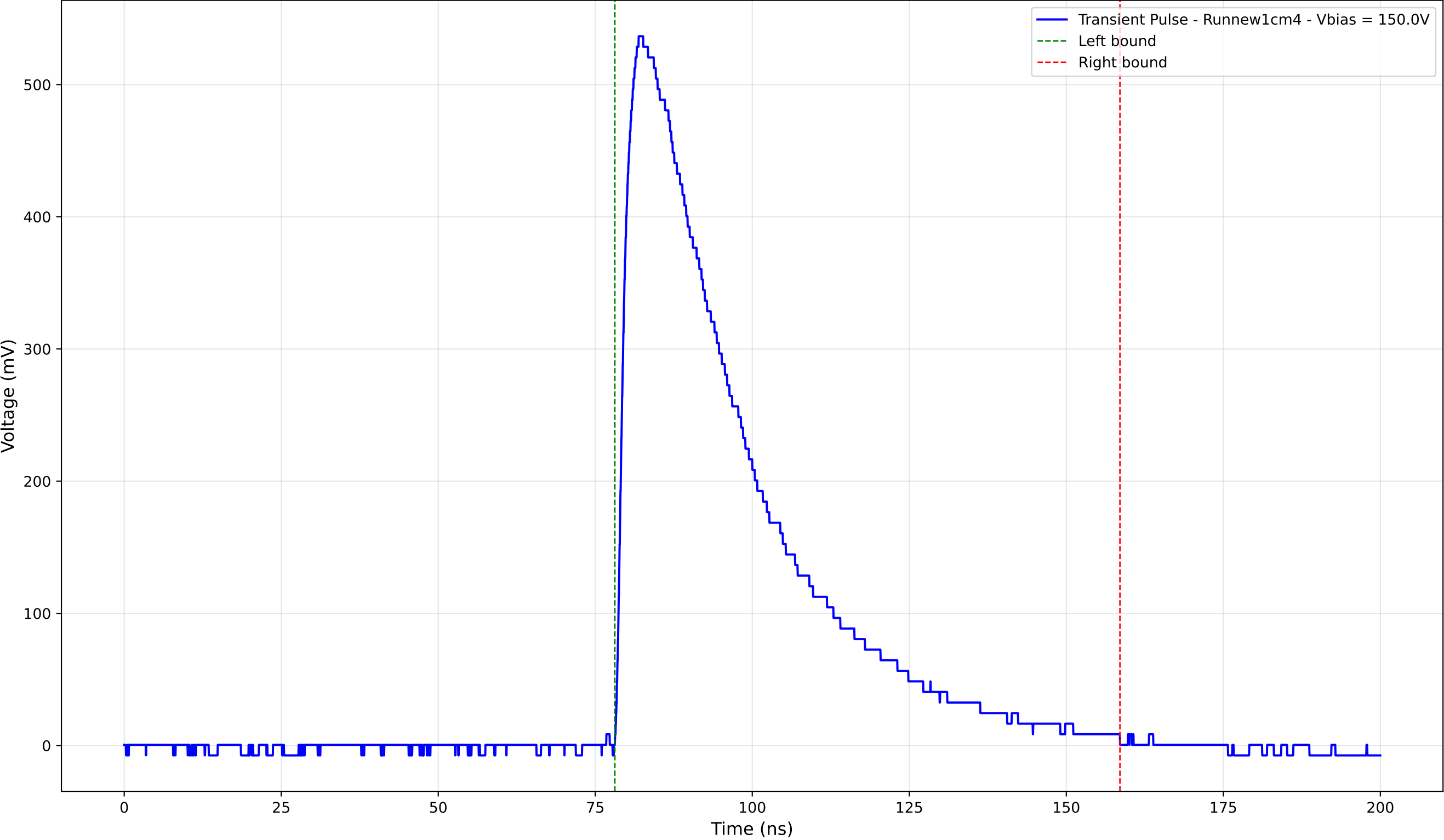
Transient Pulse - Sample: new1cm - Position: 3065.0 \mu\text{m} - Charge: 234.15 pC
