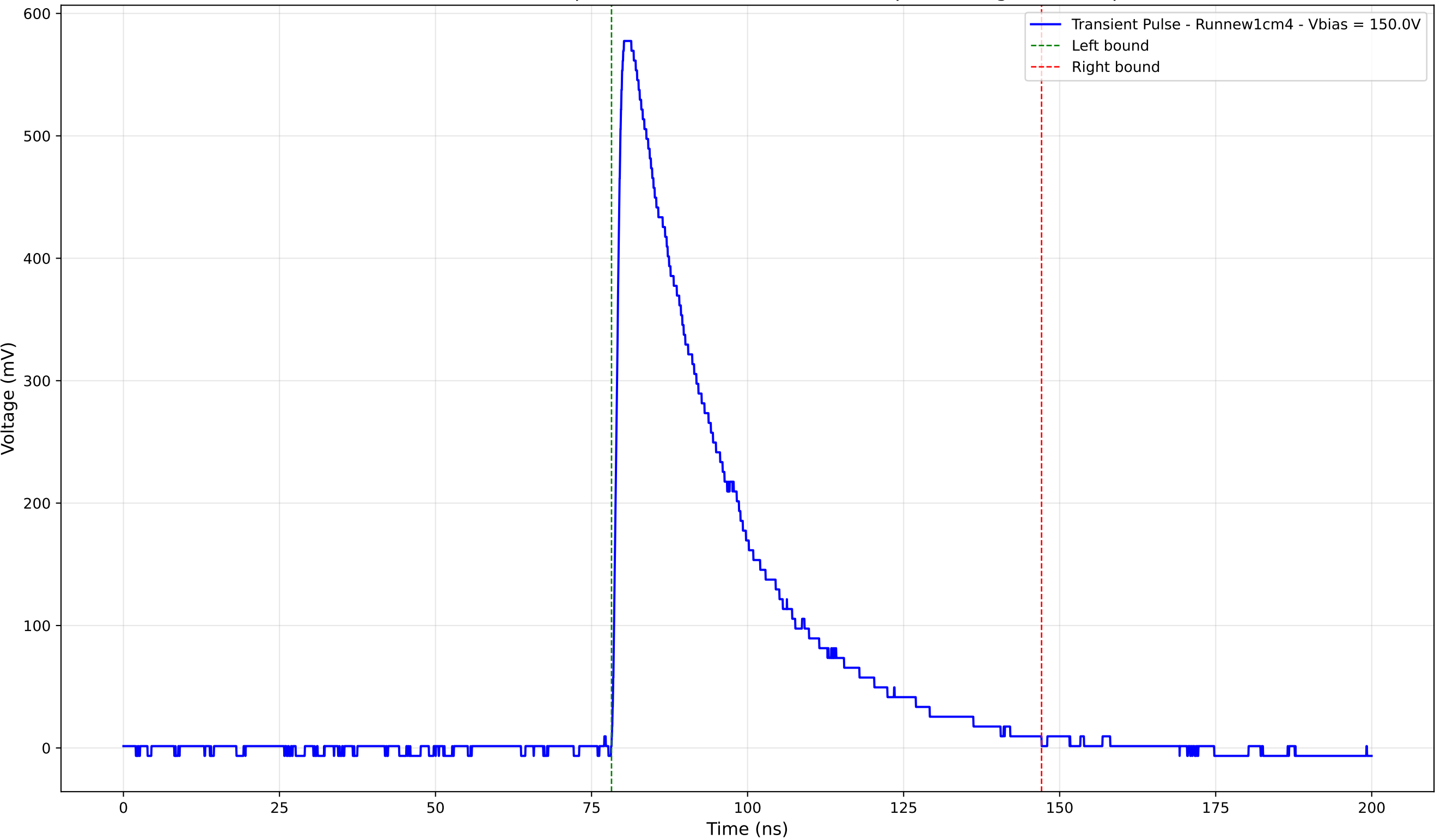
Transient Pulse - Sample: new1cm - Position: 1380.0 \mu\text{m} - Charge: 207.64 pC
