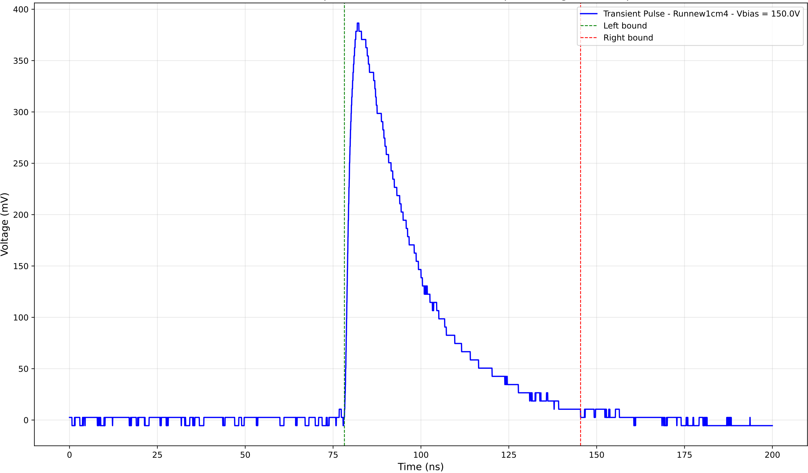
Transient Pulse - Sample: new1cm - Position: 2140.0 \mu\text{m} - Charge: 157.97 pC
