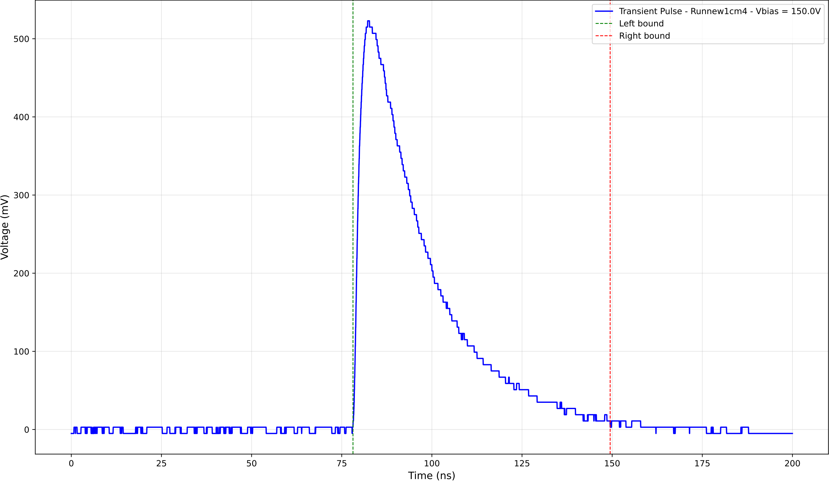
Transient Pulse - Sample: new1cm - Position: 2390.0 \mu\text{m} - Charge: 223.00 pC
