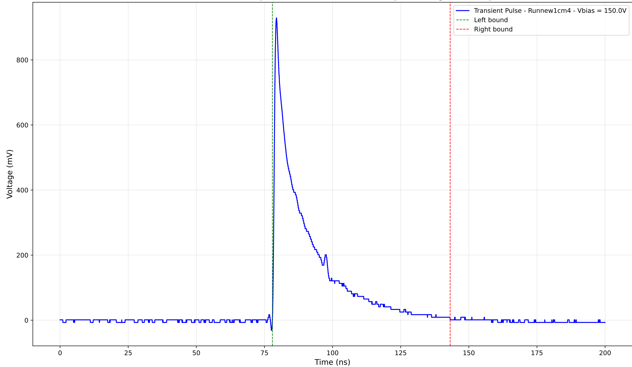
Transient Pulse - Sample: new1cm - Position: 460.0 \mu\text{m} - Charge: 198.74 pC
