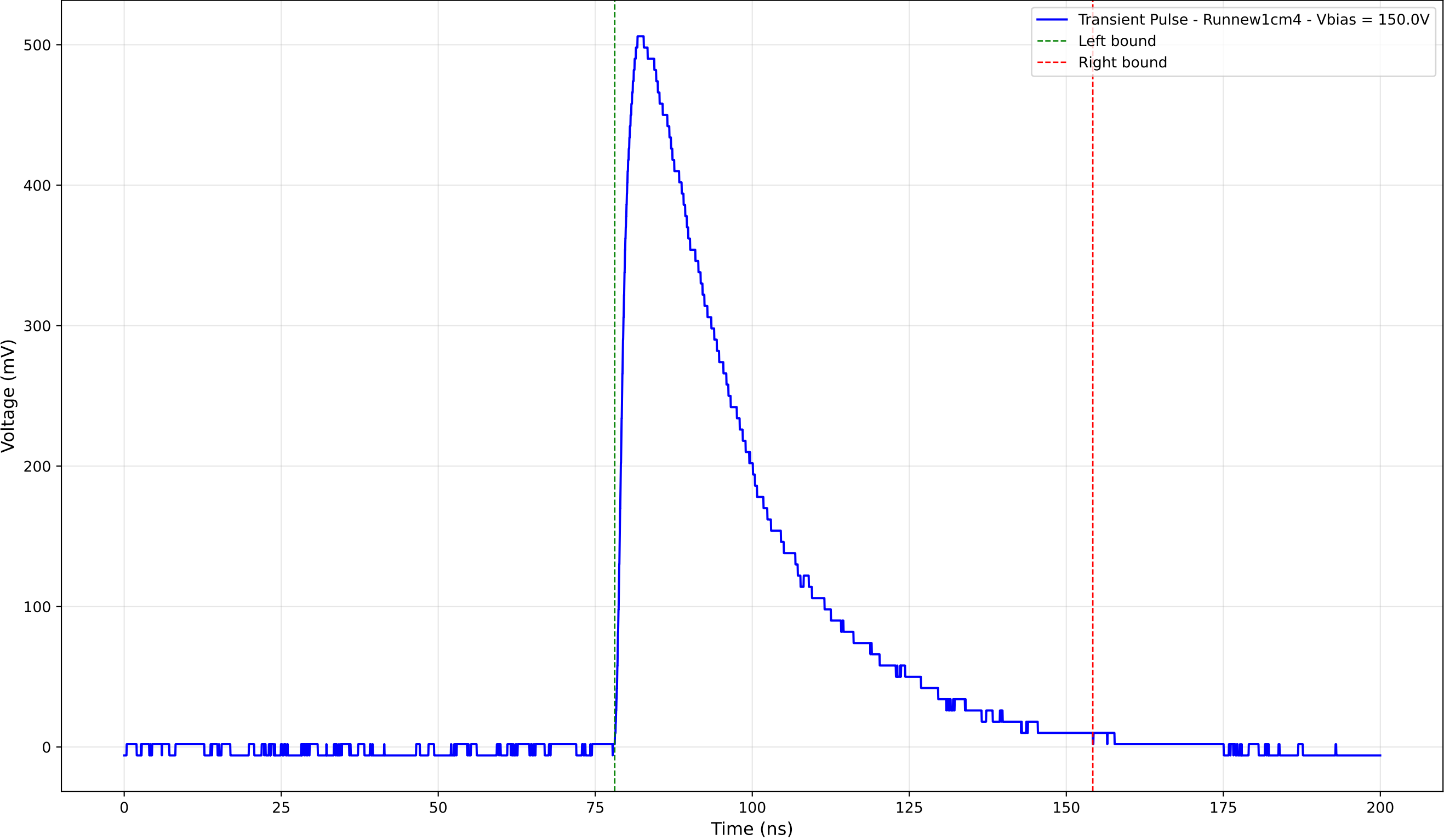
Transient Pulse - Sample: new1cm - Position: 3135.0 \mu\text{m} - Charge: 218.07 pC
