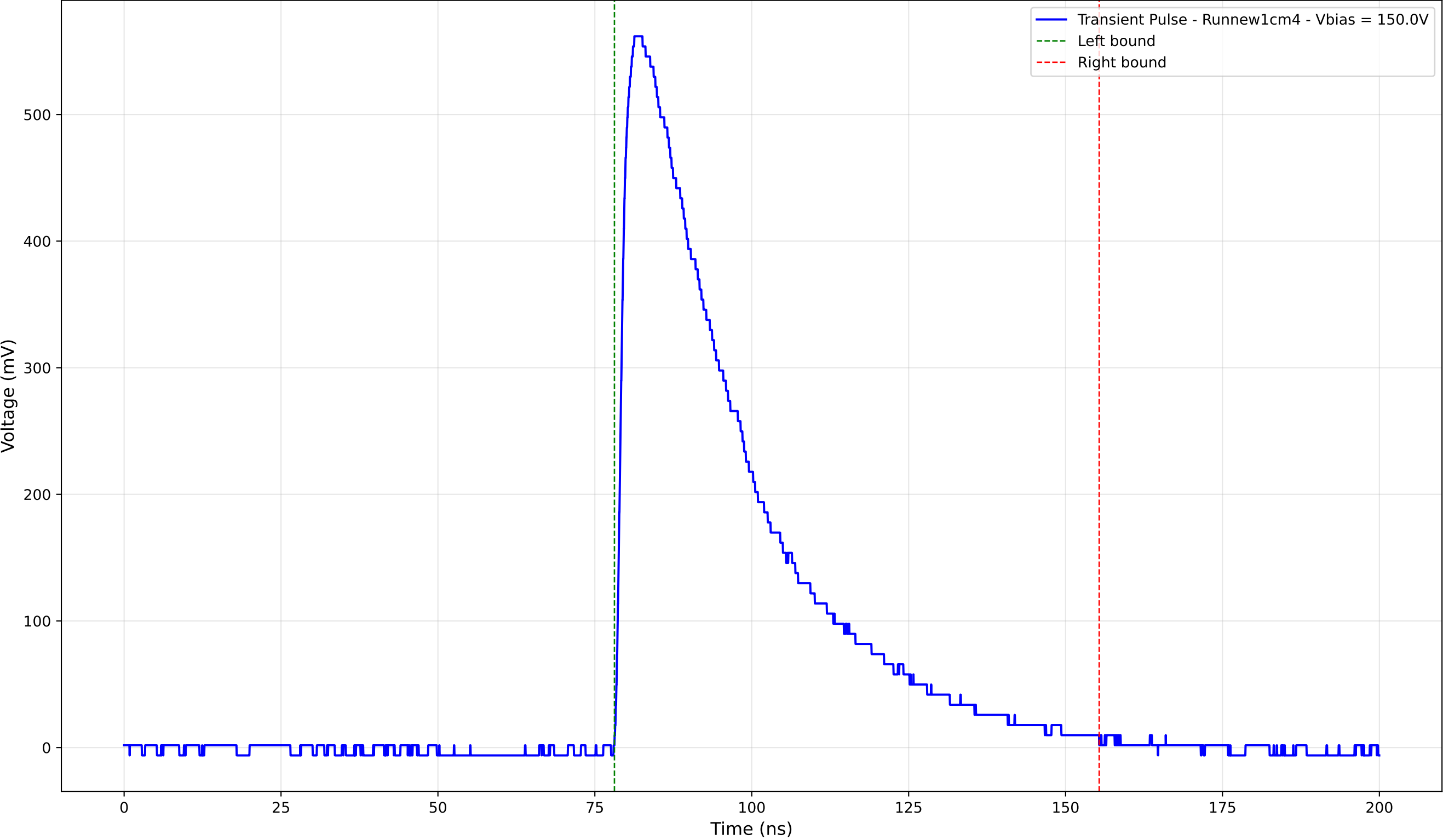
Transient Pulse - Sample: new1cm - Position: 3400.0 \mu\text{m} - Charge: 242.60 pC
