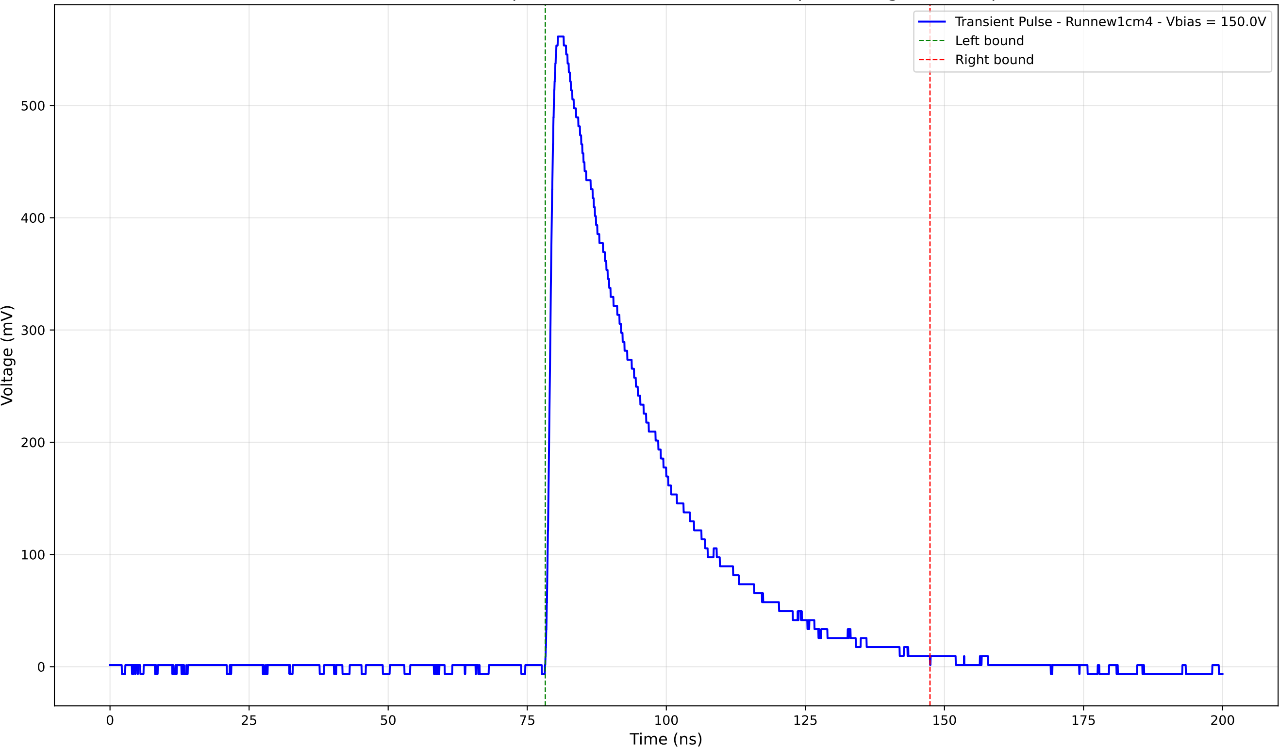
Transient Pulse - Sample: new1cm - Position: 1450.0 \mu\text{m} - Charge: 205.46 pC
