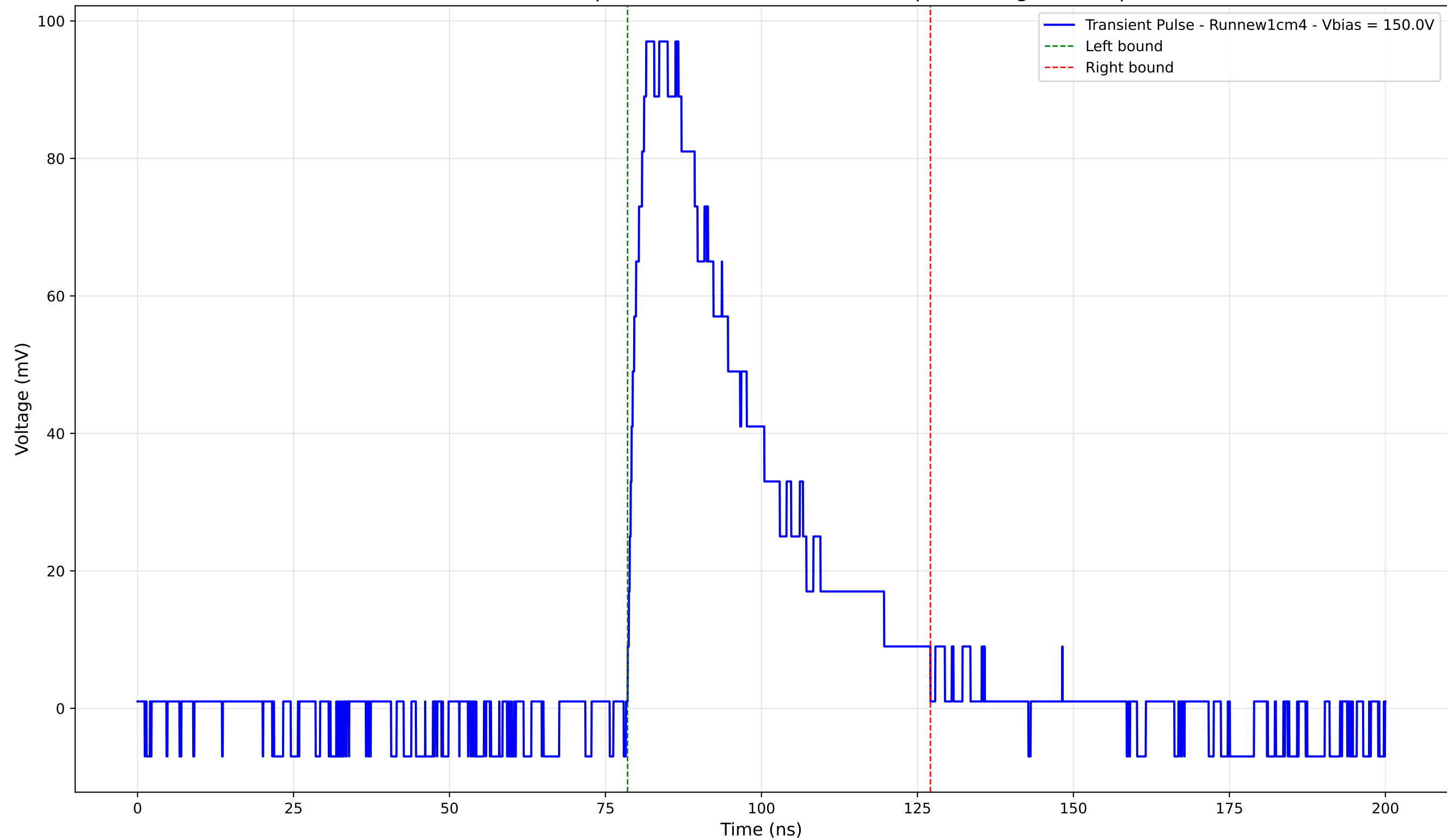
Transient Pulse - Sample: new1cm - Position: 2700.0 \mu\text{m} - Charge: 39.10 pC
