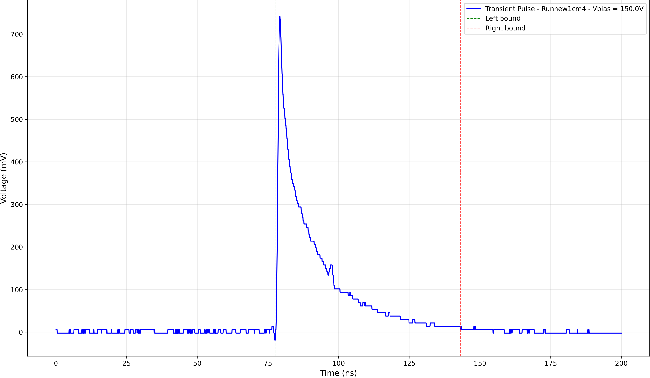
Transient Pulse - Sample: new1cm - Position: 4810.0 \mu\text{m} - Charge: 158.91 pC
