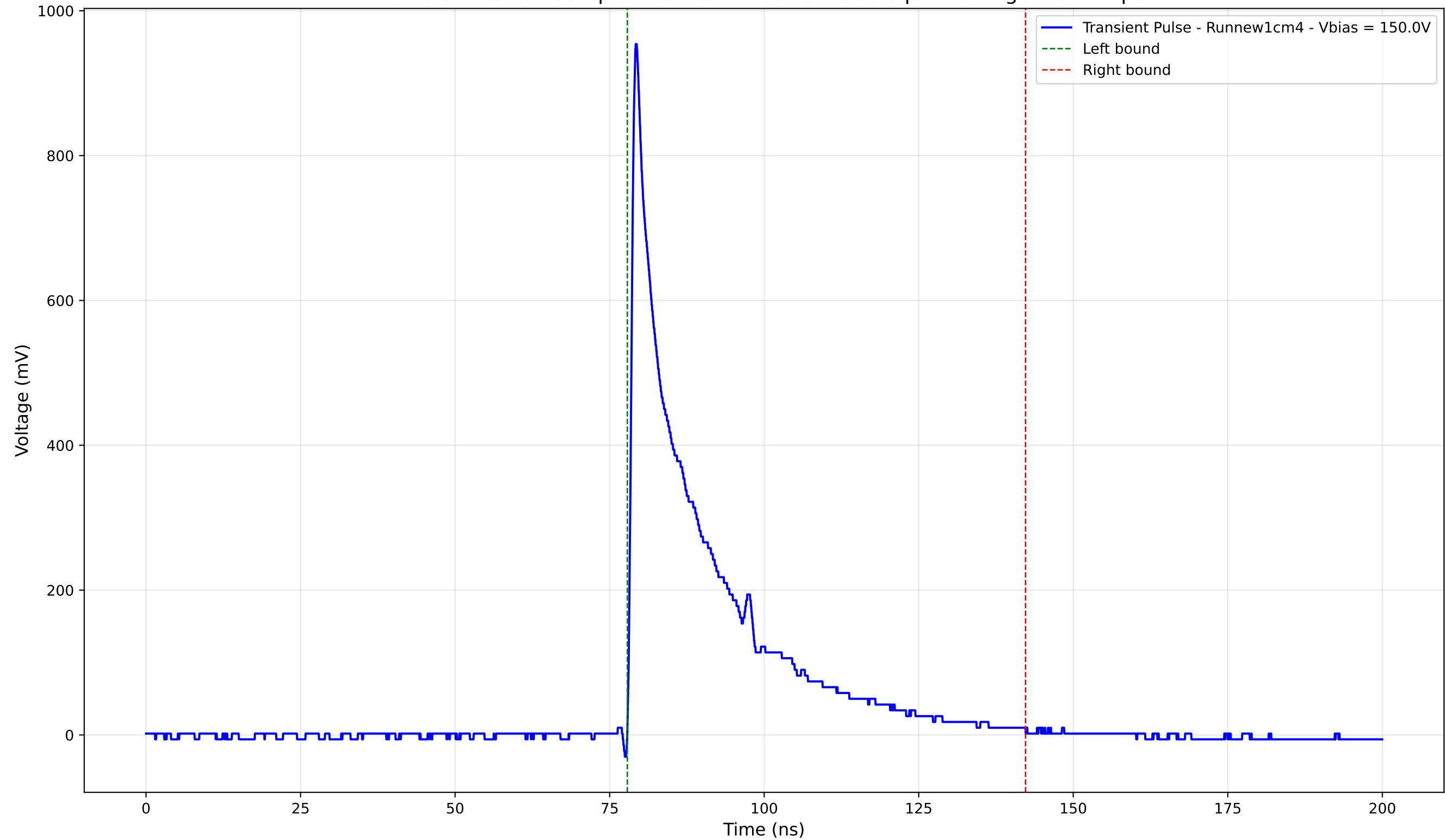
Transient Pulse - Sample: new1cm - Position: 360.0 \mu\text{m} - Charge: 194.71 pC
