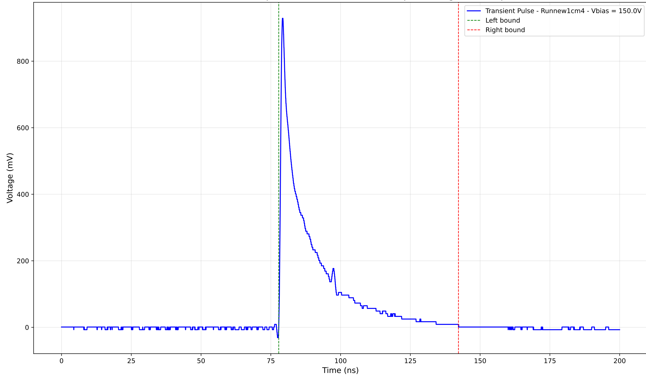
Transient Pulse - Sample: new1cm - Position: 300.0 \mu\text{m} - Charge: 174.47 pC
