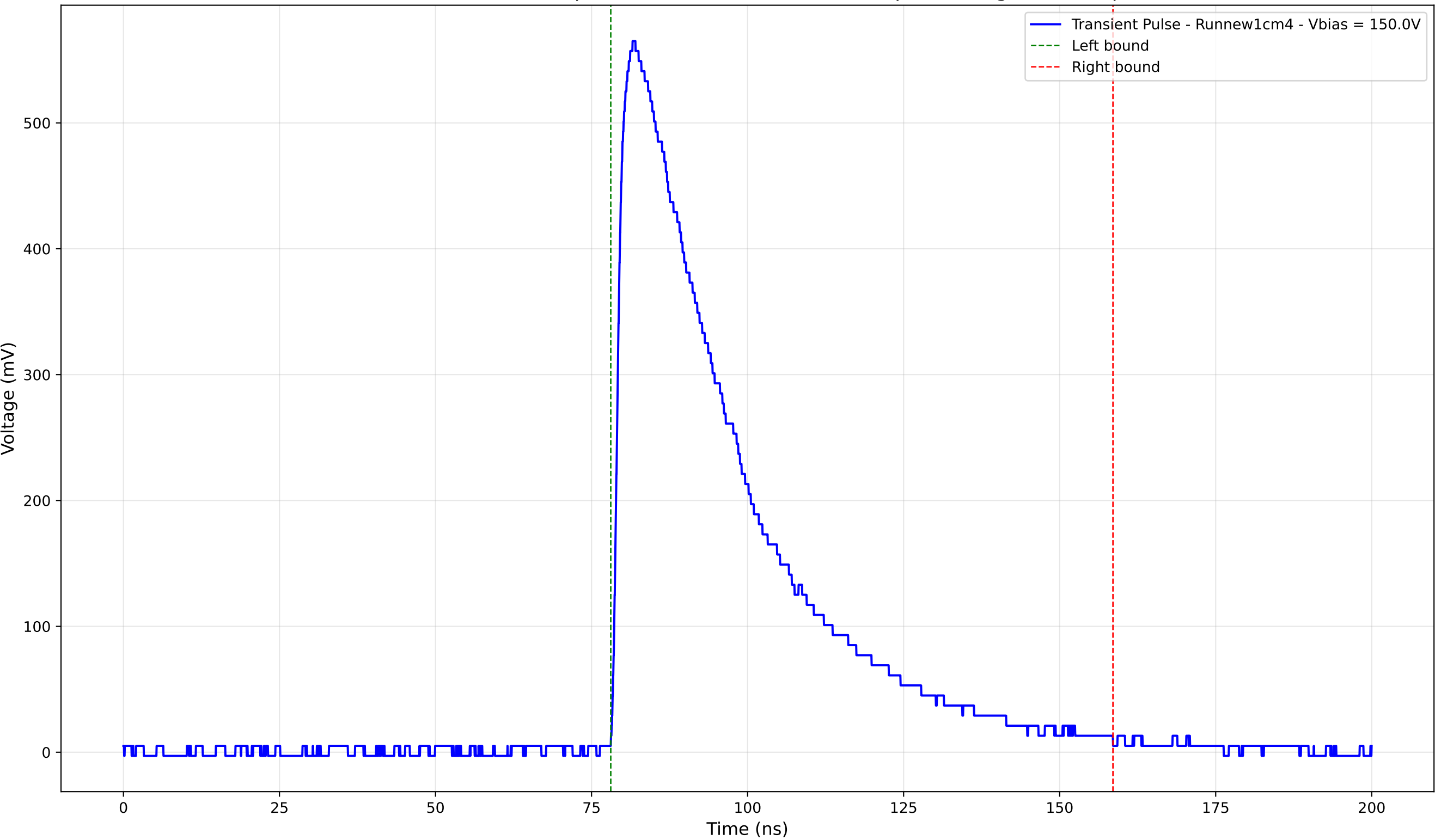
Transient Pulse - Sample: new1cm - Position: 3460.0 \mu\text{m} - Charge: 242.62 pC
