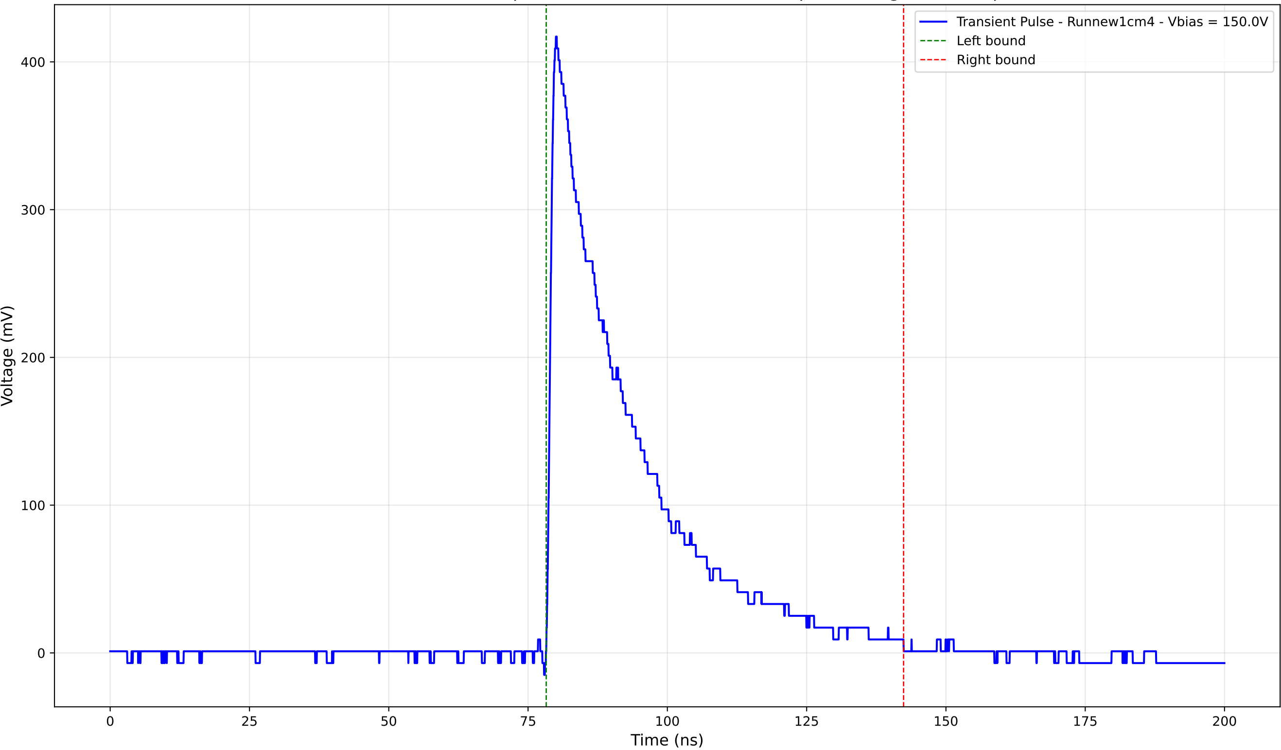
Transient Pulse - Sample: new1cm - Position: 1140.0 \mu\text{m} - Charge: 124.90 pC
