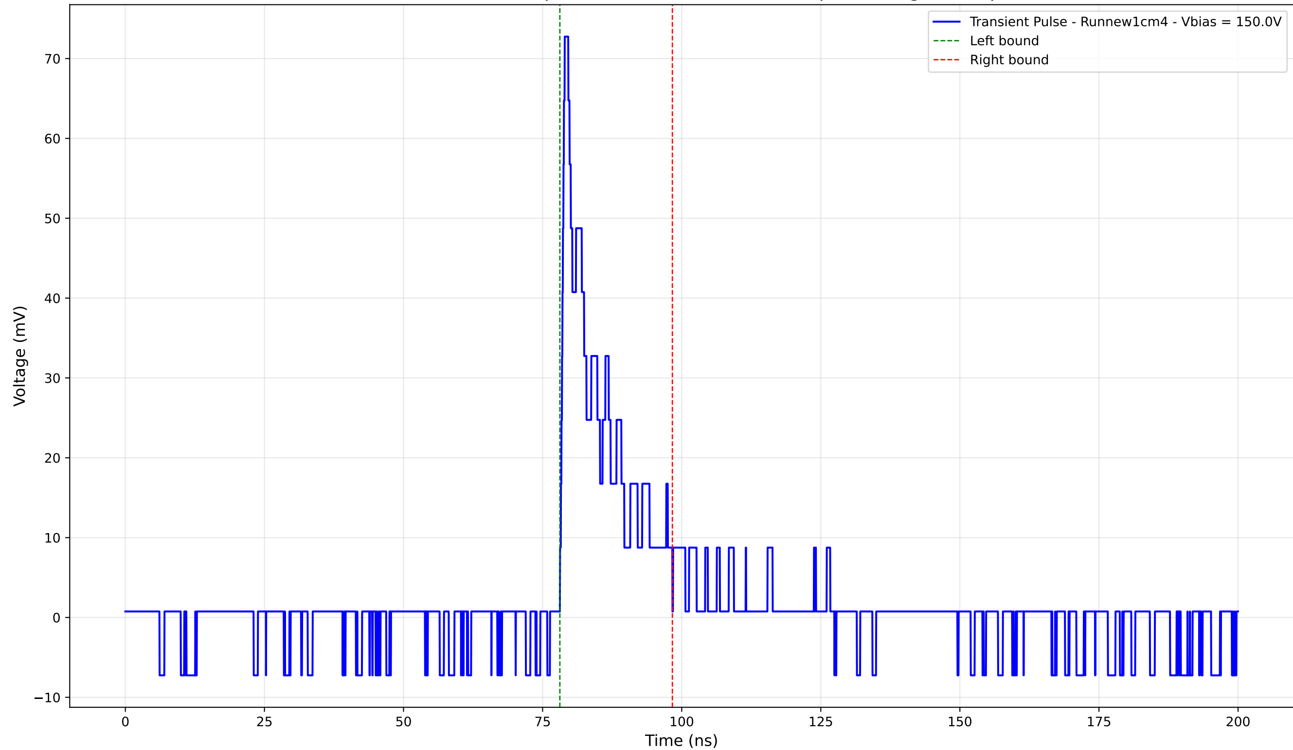
Transient Pulse - Sample: new1cm - Position: 185.0 \mu\text{m} - Charge: 9.83 pC
