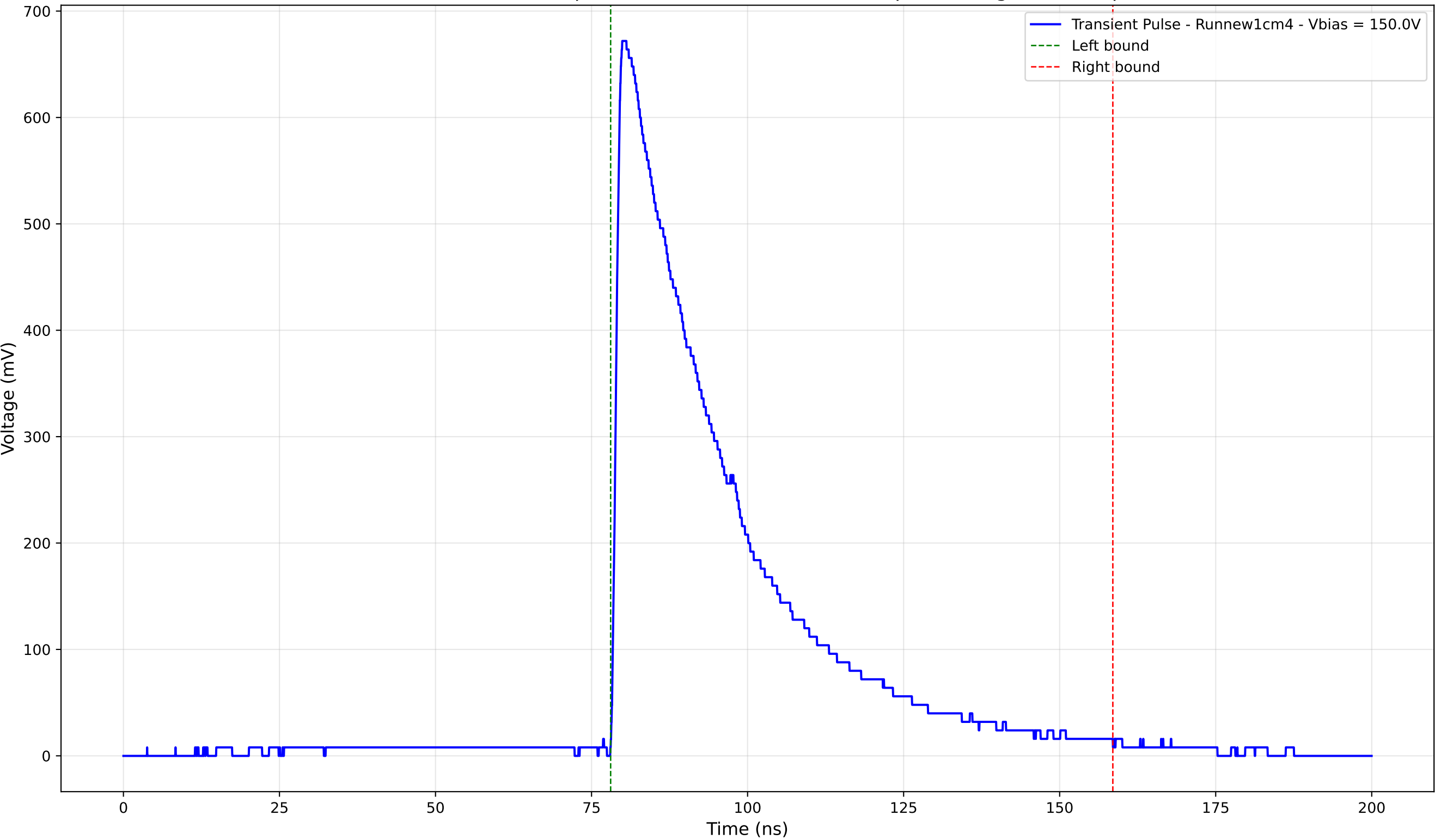
Transient Pulse - Sample: new1cm - Position: 4010.0 \mu\text{m} - Charge: 255.86 pC
