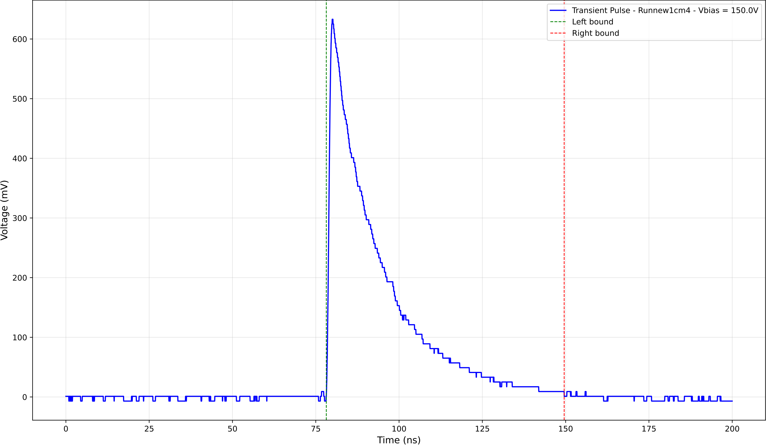
Transient Pulse - Sample: new1cm - Position: 1100.0 \mu\text{m} - Charge: 195.71 pC
