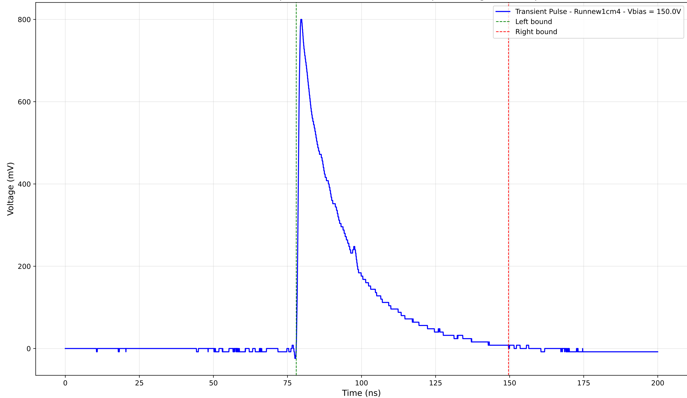
Transient Pulse - Sample: new1cm - Position: 4425.0 \mu\text{m} - Charge: 238.99 pC
