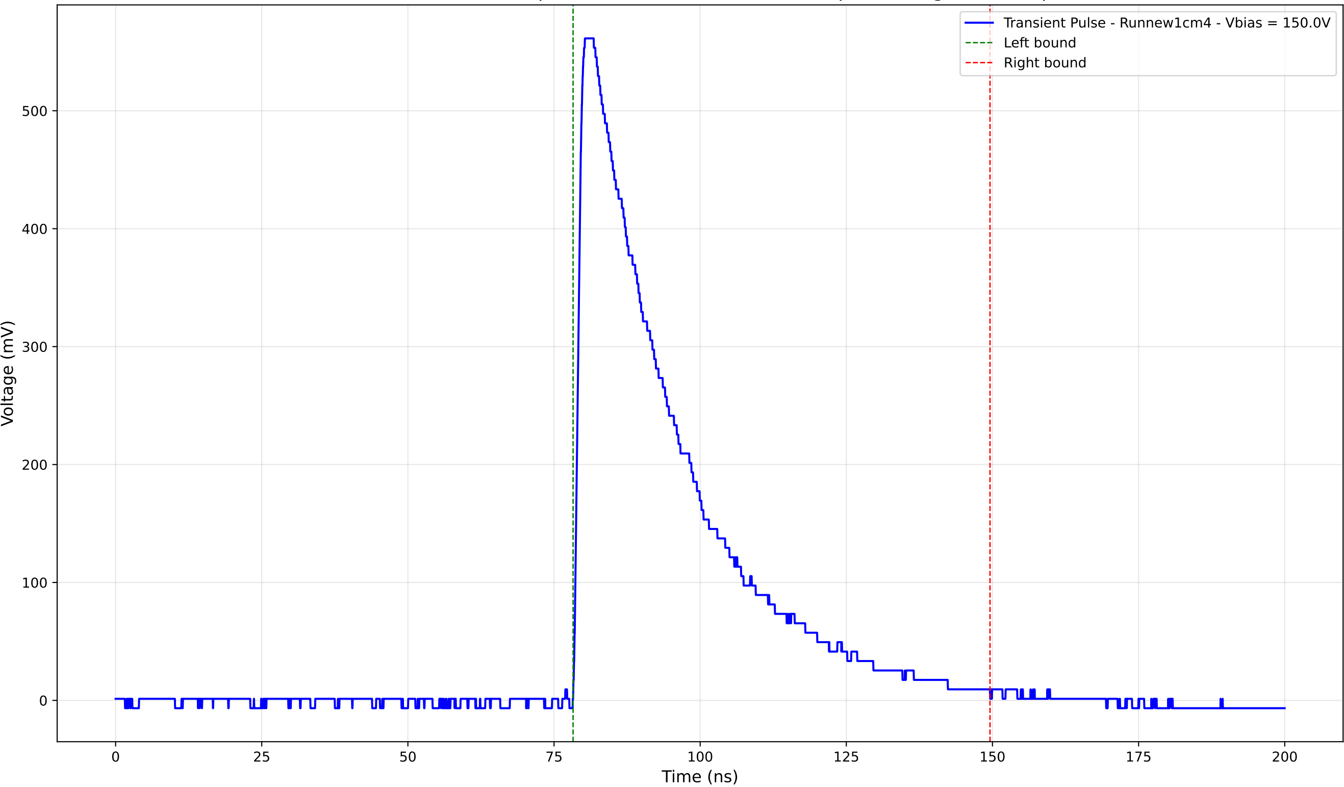
Transient Pulse - Sample: new1cm - Position: 1420.0 \mu\text{m} - Charge: 205.28 pC
