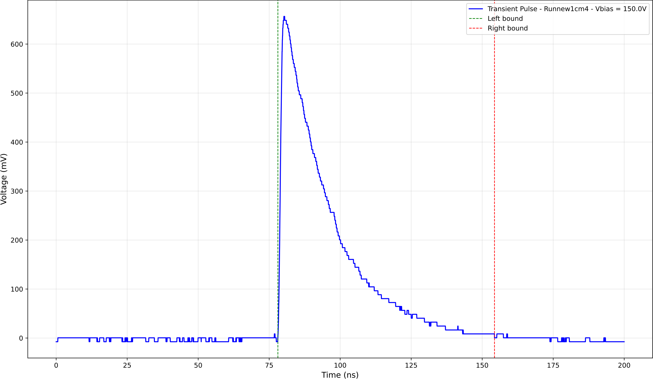
Transient Pulse - Sample: new1cm - Position: 3960.0 \mu\text{m} - Charge: 242.83 pC
