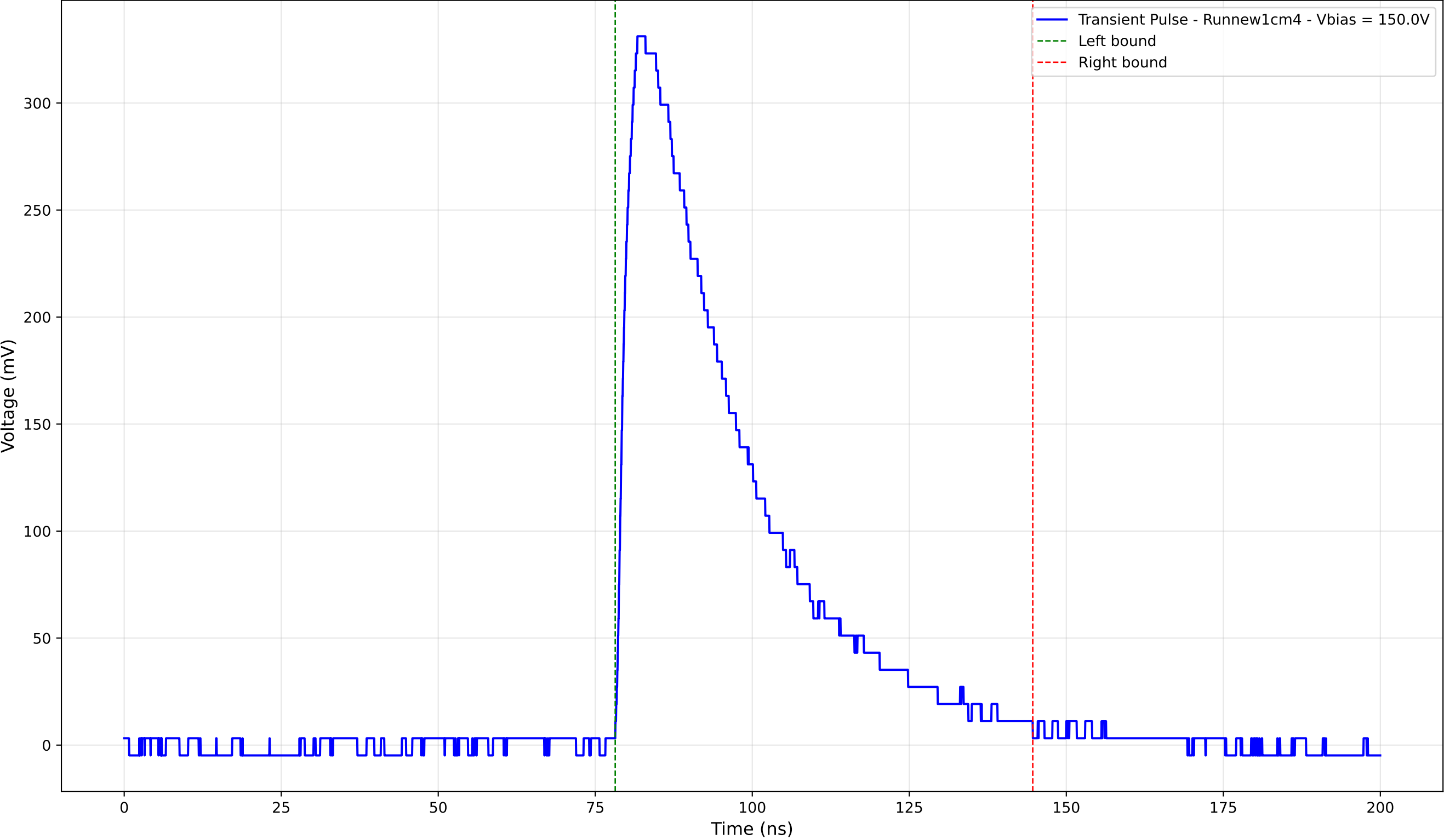
Transient Pulse - Sample: new1cm - Position: 2260.0 \mu\text{m} - Charge: 138.79 pC
