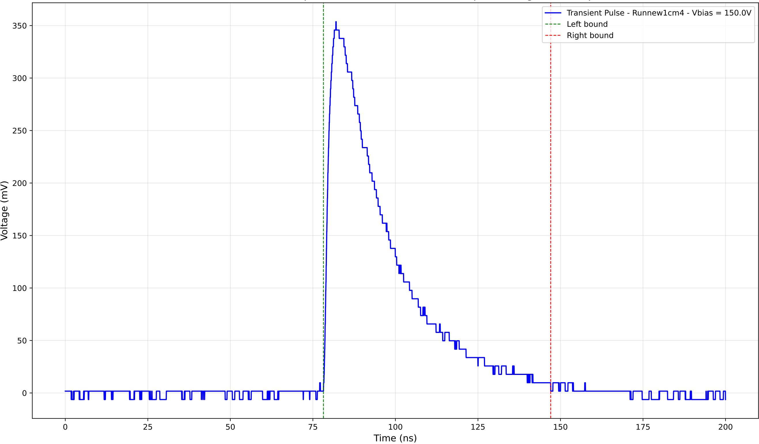
Transient Pulse - Sample: new1cm - Position: 2145.0 \mu\text{m} - Charge: 144.87 pC
