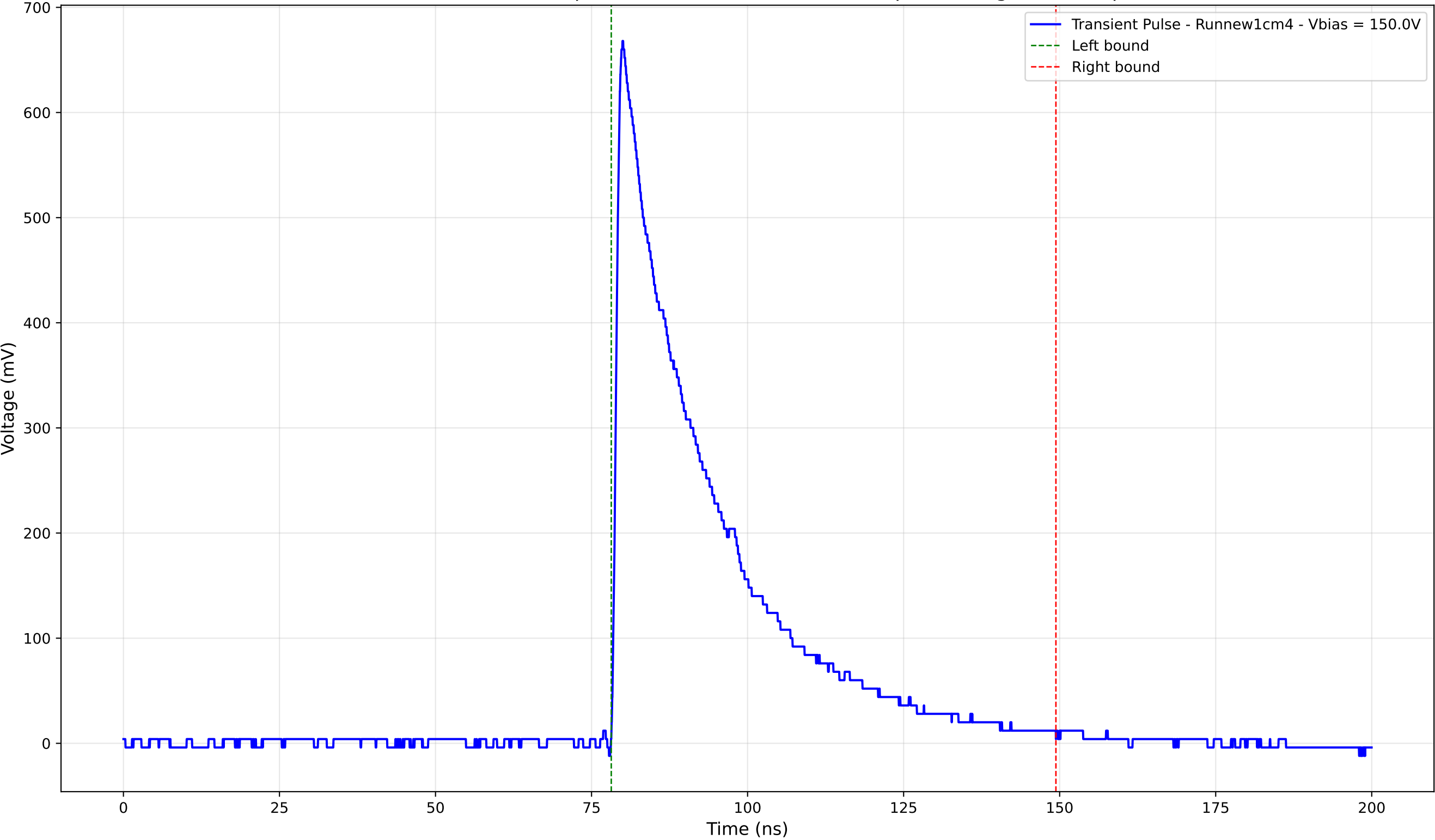
Transient Pulse - Sample: new1cm - Position: 1055.0 \mu\text{m} - Charge: 204.41 pC
