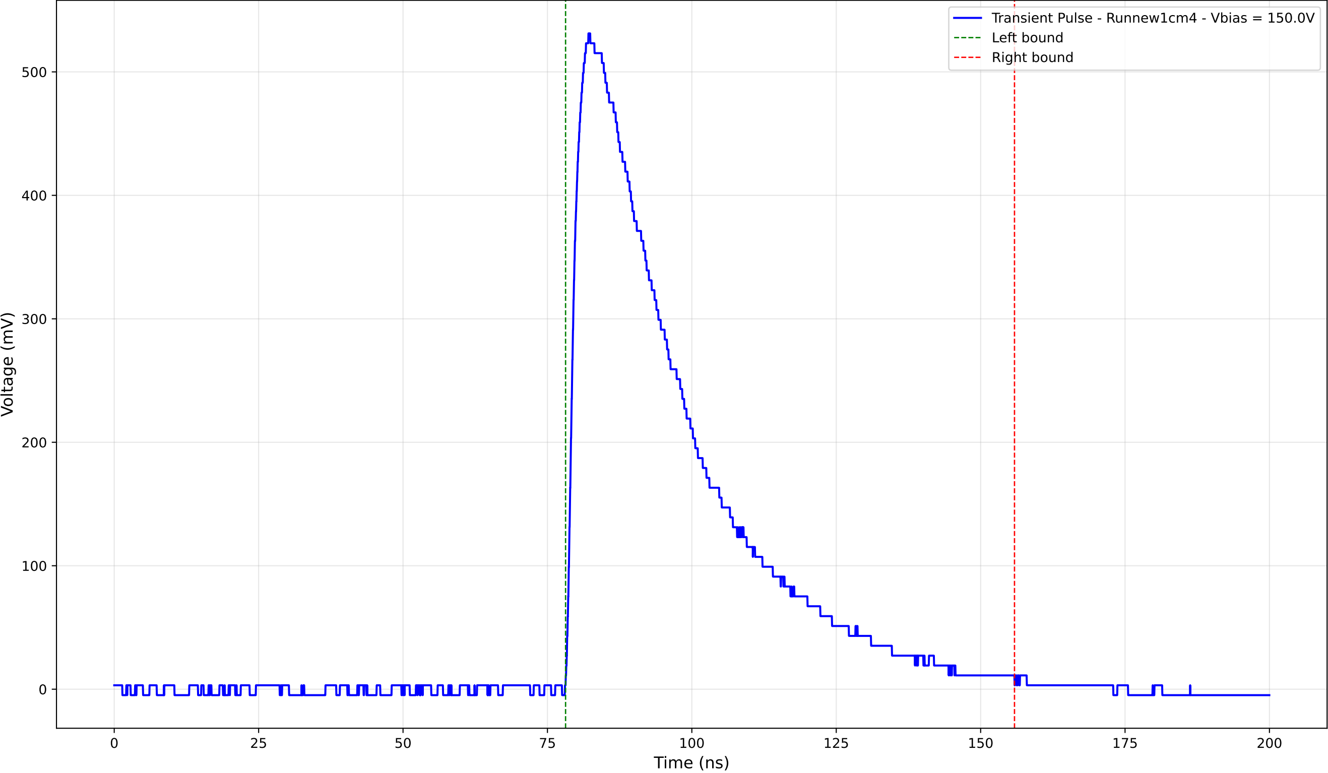
Transient Pulse - Sample: new1cm - Position: 3050.0 \mu\text{m} - Charge: 231.70 pC
