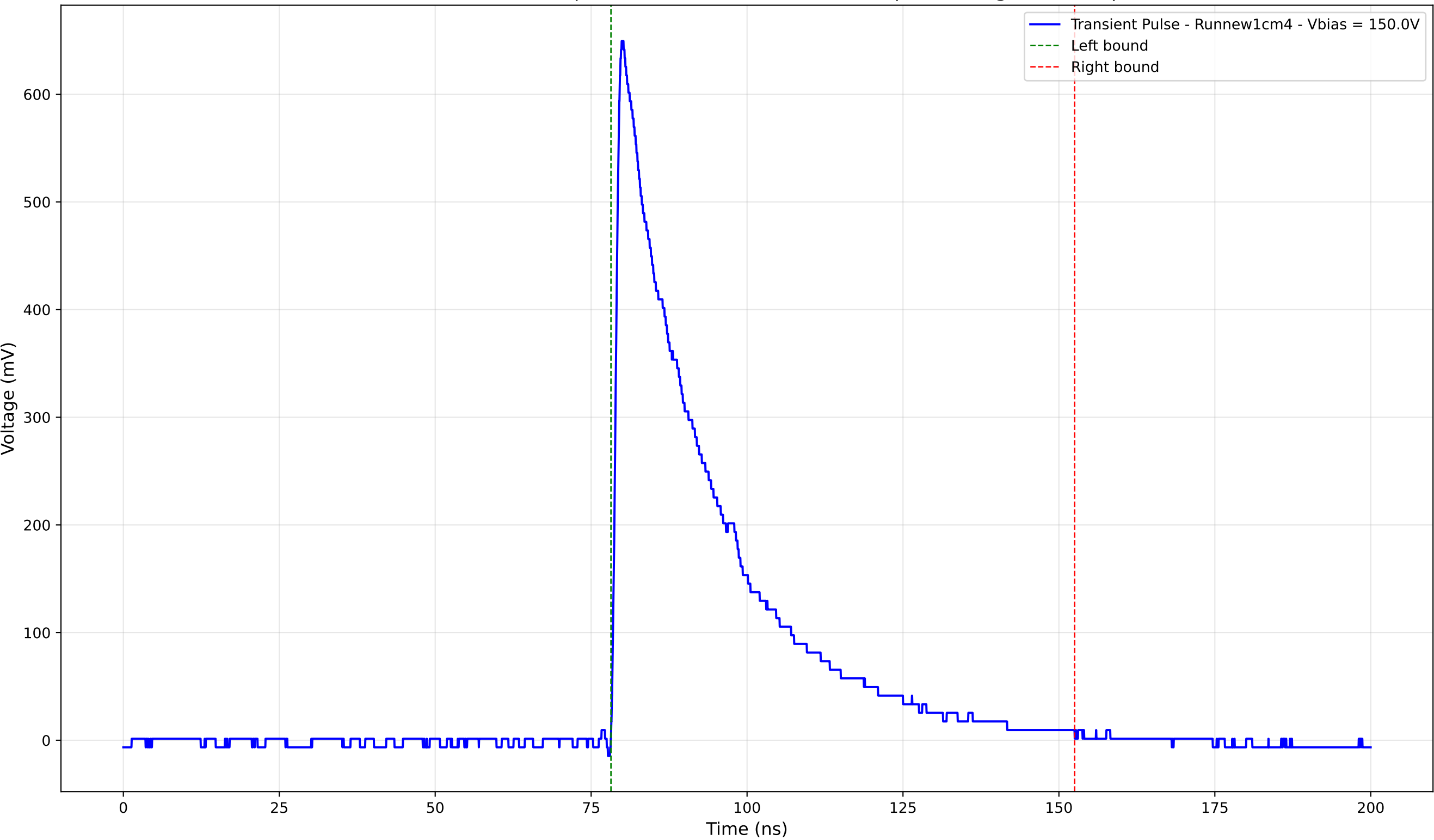
Transient Pulse - Sample: new1cm - Position: 1085.0 \mu\text{m} - Charge: 200.43 pC
