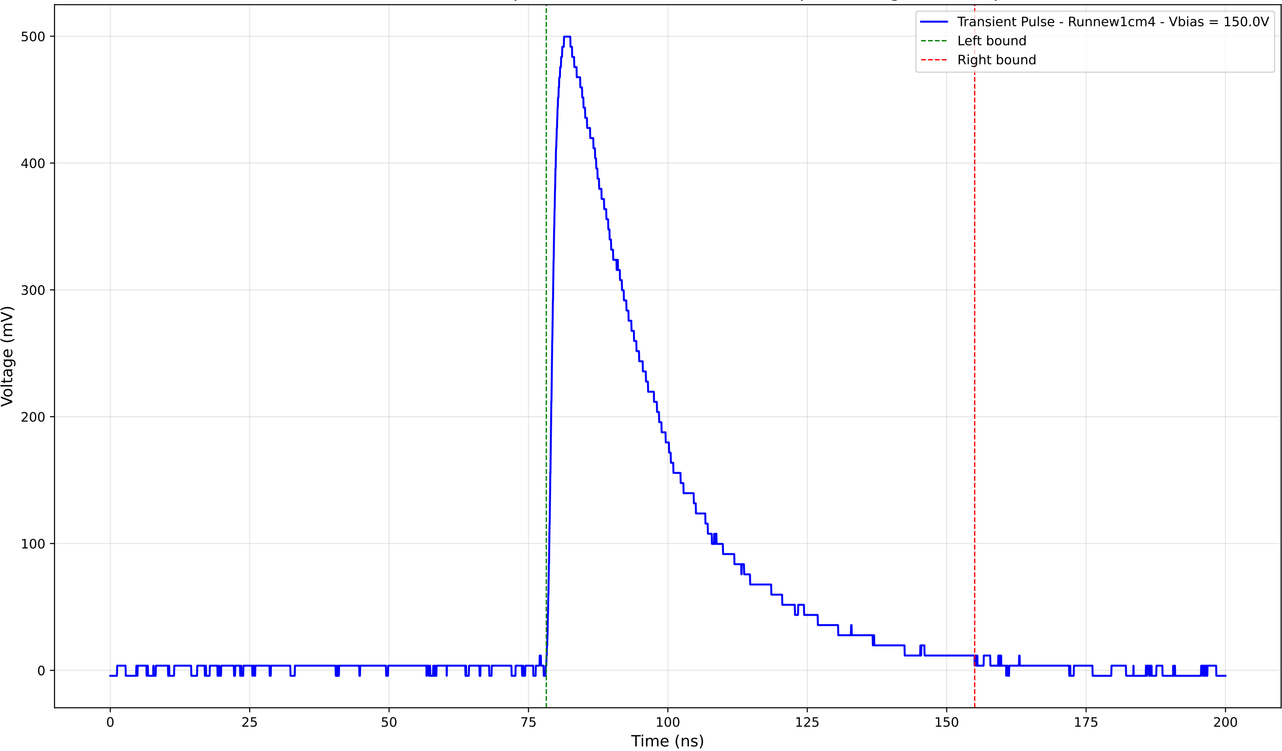
Transient Pulse - Sample: new1cm - Position: 1805.0 \mu\text{m} - Charge: 203.31 pC
