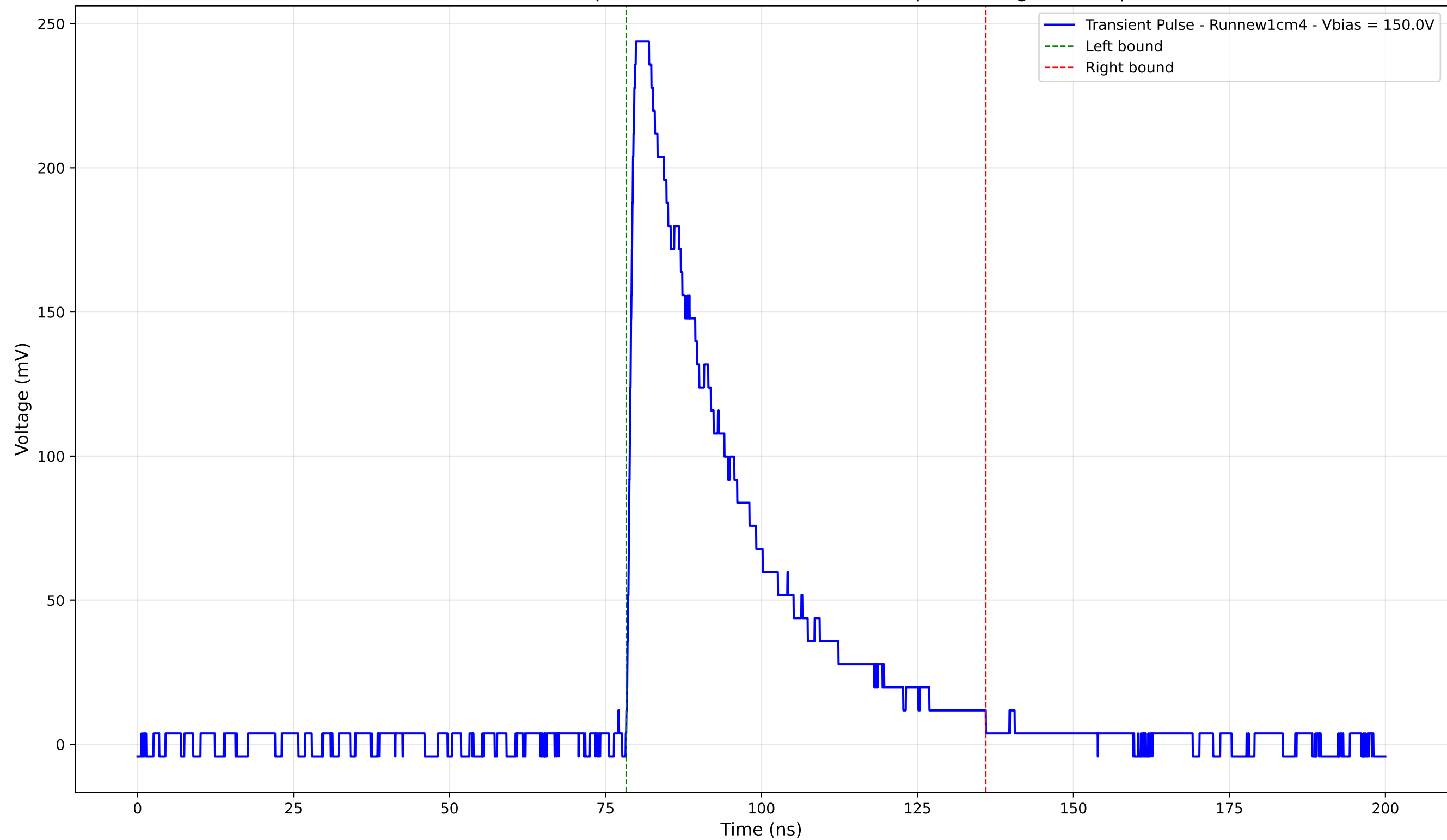
Transient Pulse - Sample: new1cm - Position: 1240.0 \mu\text{m} - Charge: 83.15 pC
