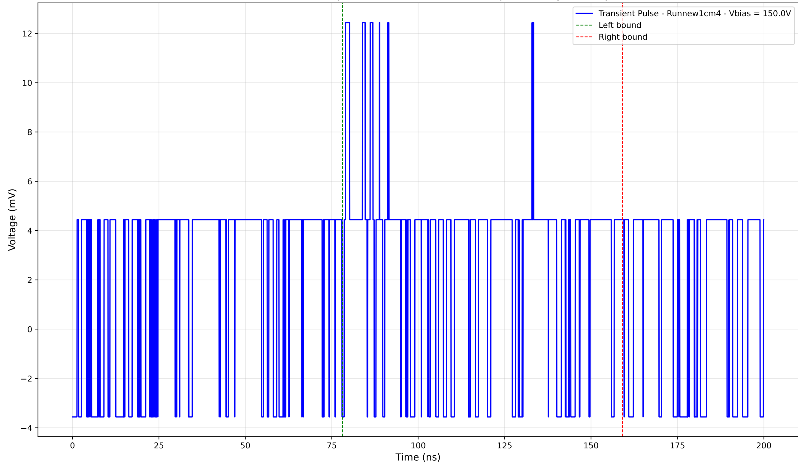
Transient Pulse - Sample: new1cm - Position: 75.0 \mu\text{m} - Charge: 5.08 pC
