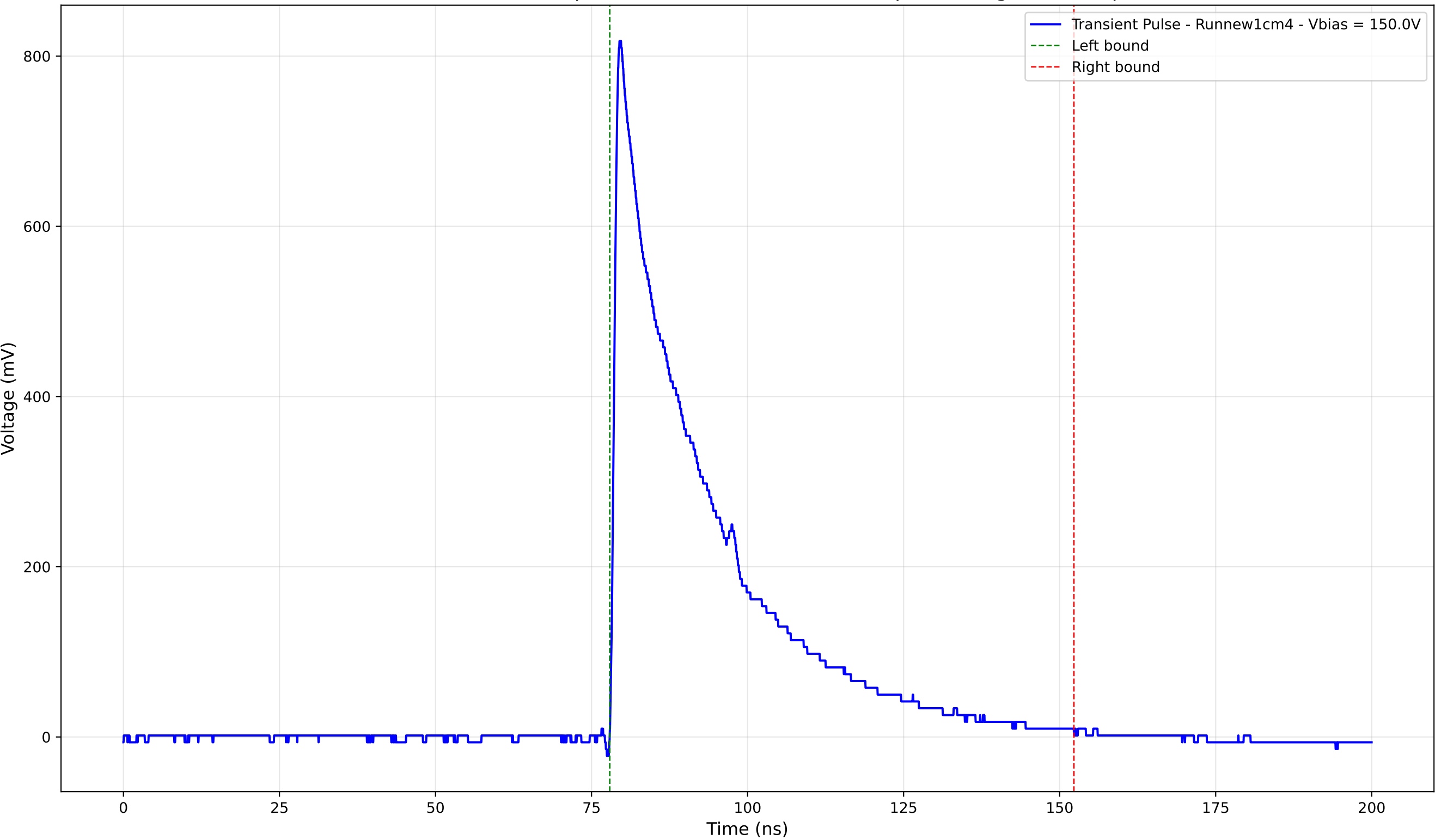
Transient Pulse - Sample: new1cm - Position: 4470.0 \mu\text{m} - Charge: 240.25 pC
