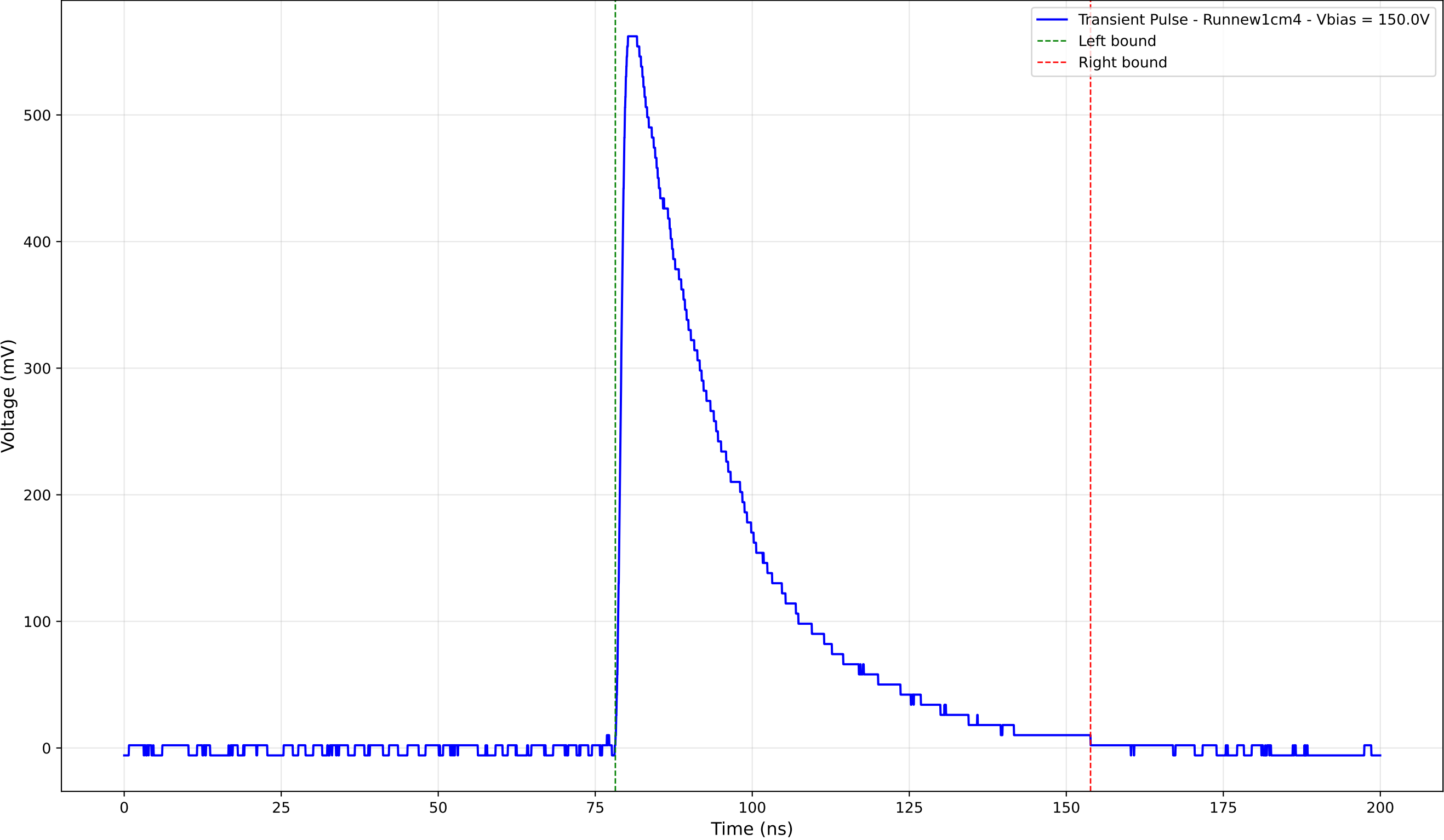
Transient Pulse - Sample: new1cm - Position: 1410.0 \mu\text{m} - Charge: 205.47 pC
