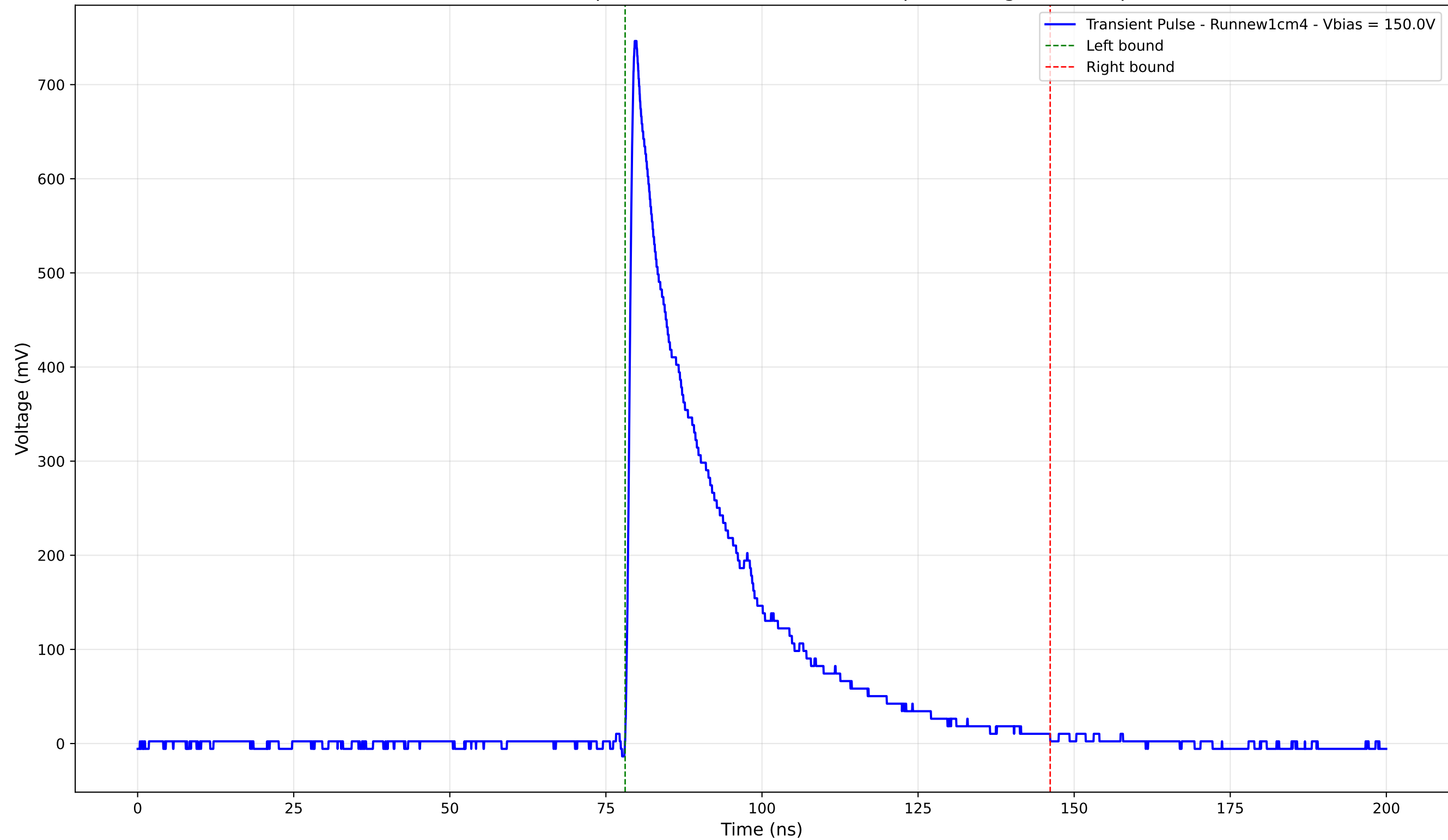
Transient Pulse - Sample: new1cm - Position: 850.0 \mu\text{m} - Charge: 201.51 pC
