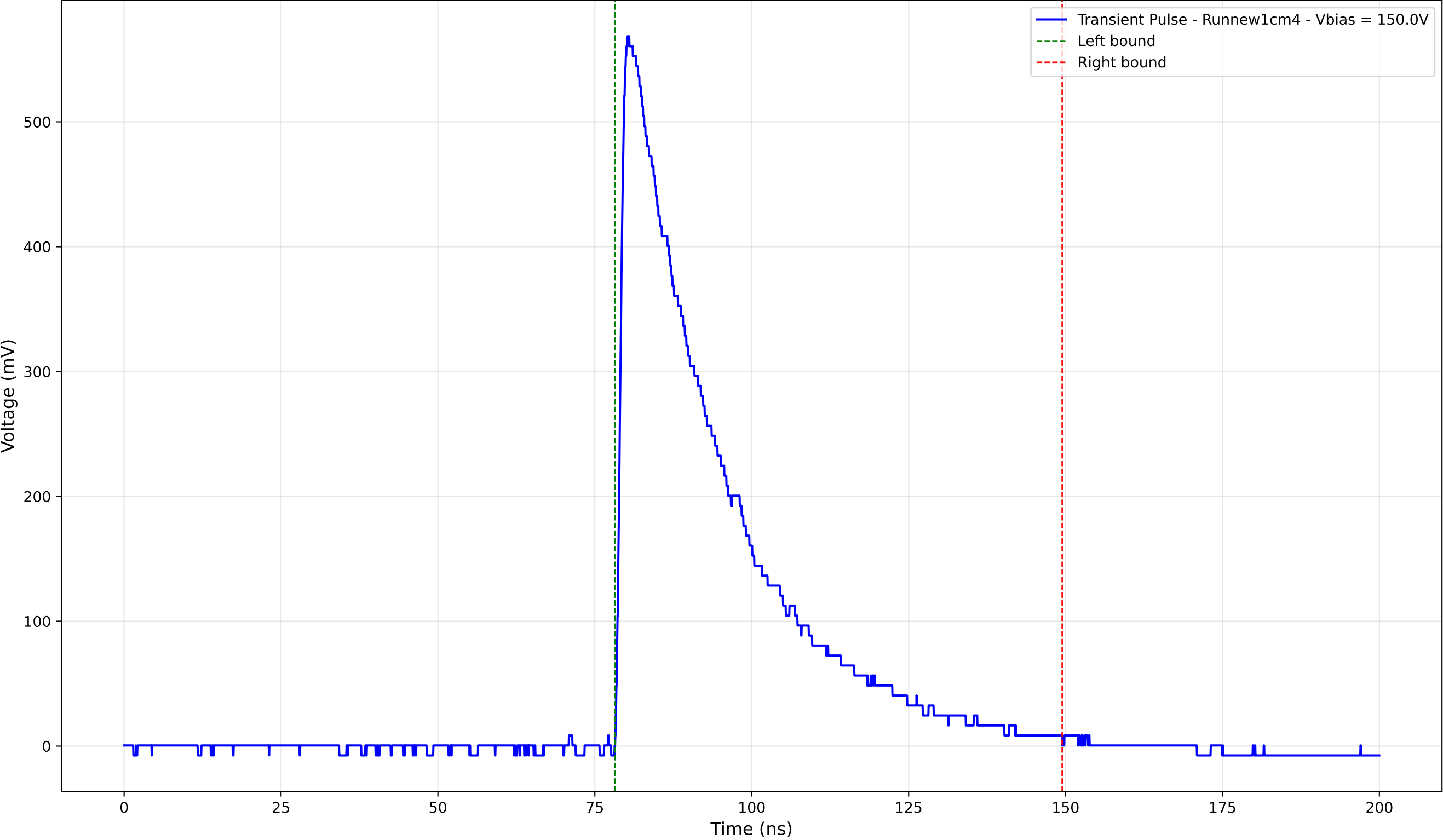
Transient Pulse - Sample: new1cm - Position: 1310.0 \mu\text{m} - Charge: 195.69 pC
