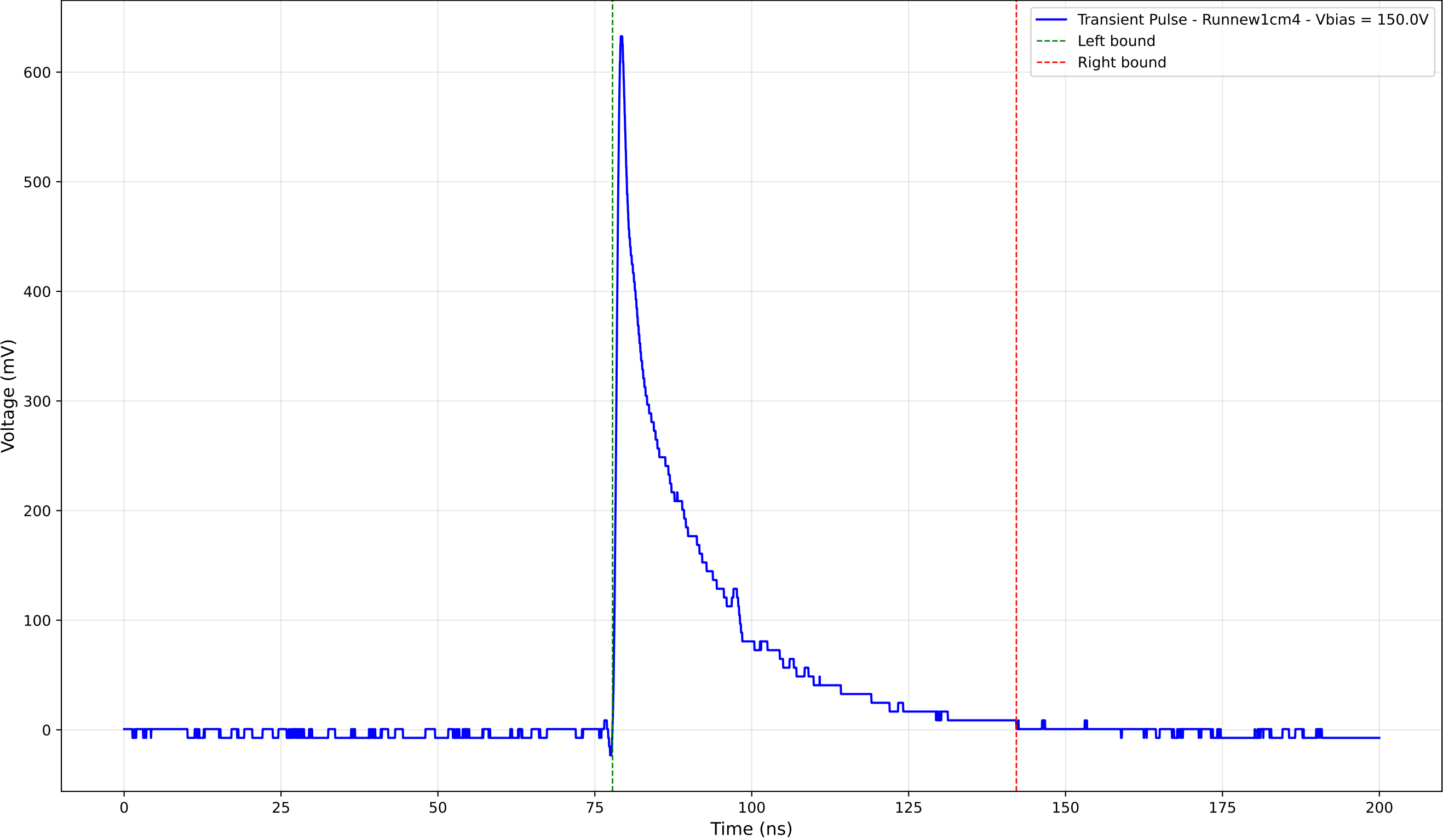
Transient Pulse - Sample: new1cm - Position: 4795.0 \mu\text{m} - Charge: 127.90 pC
