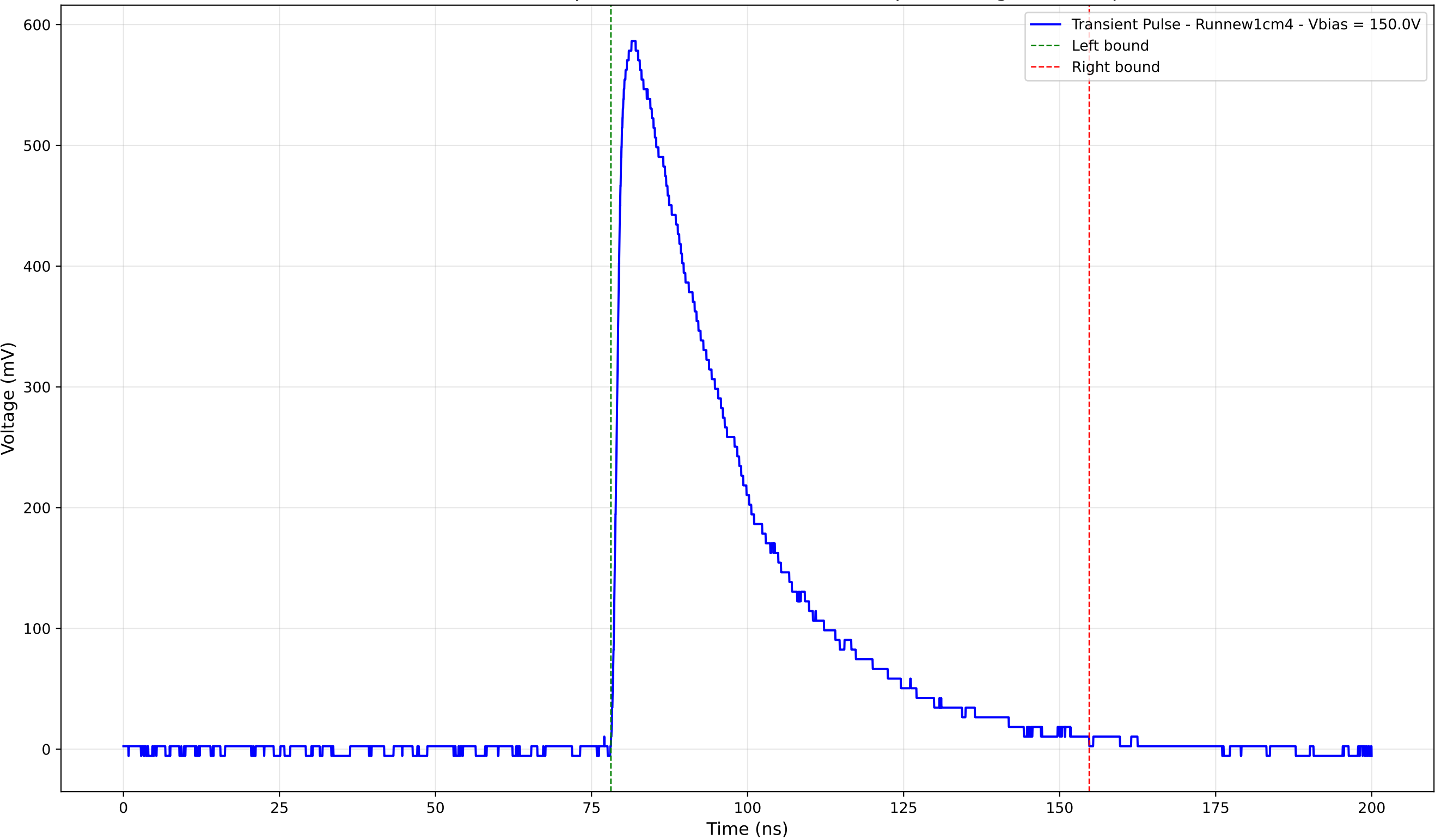
Transient Pulse - Sample: new1cm - Position: 3585.0 \mu\text{m} - Charge: 242.77 pC
