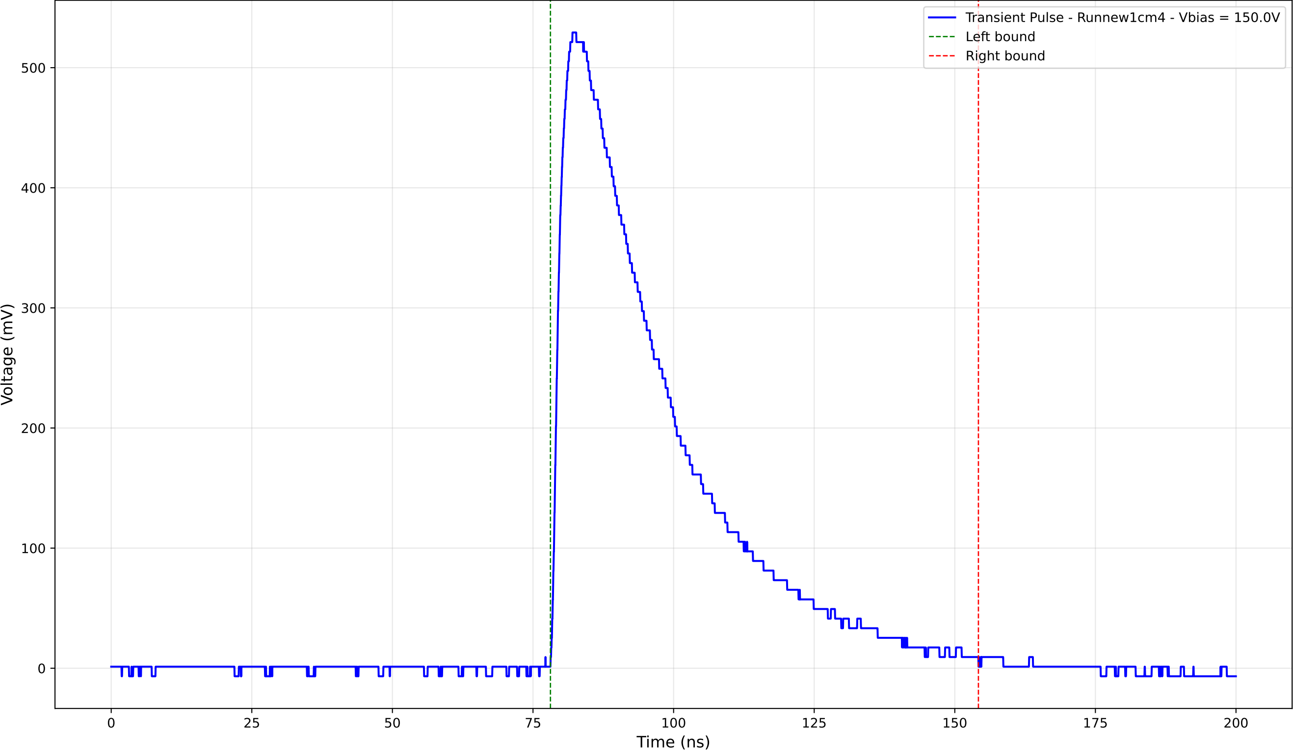
Transient Pulse - Sample: new1cm - Position: 3055.0 \mu\text{m} - Charge: 231.31 pC
