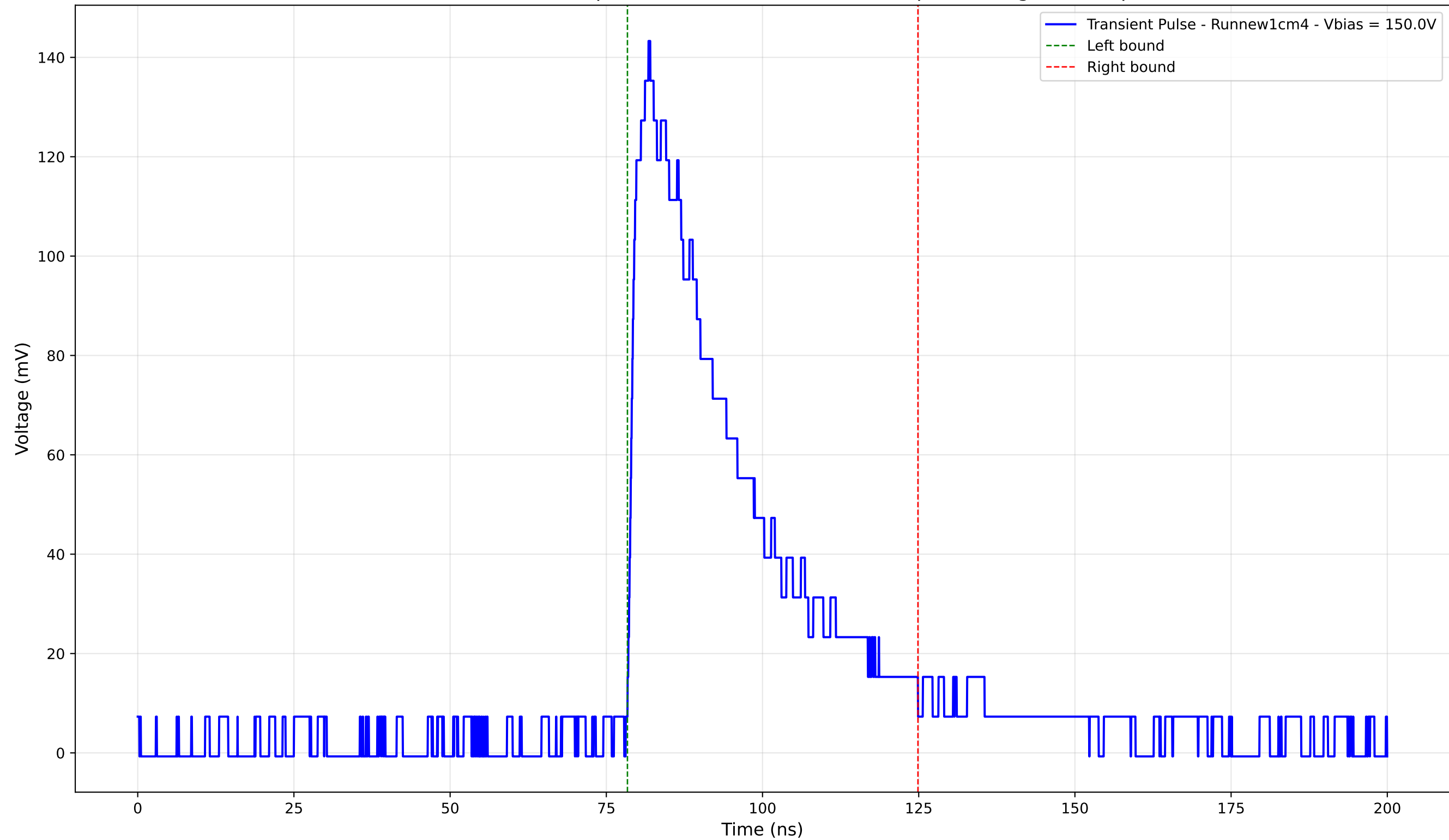
Transient Pulse - Sample: new1cm - Position: 3745.0 \mu\text{m} - Charge: 51.08 pC
