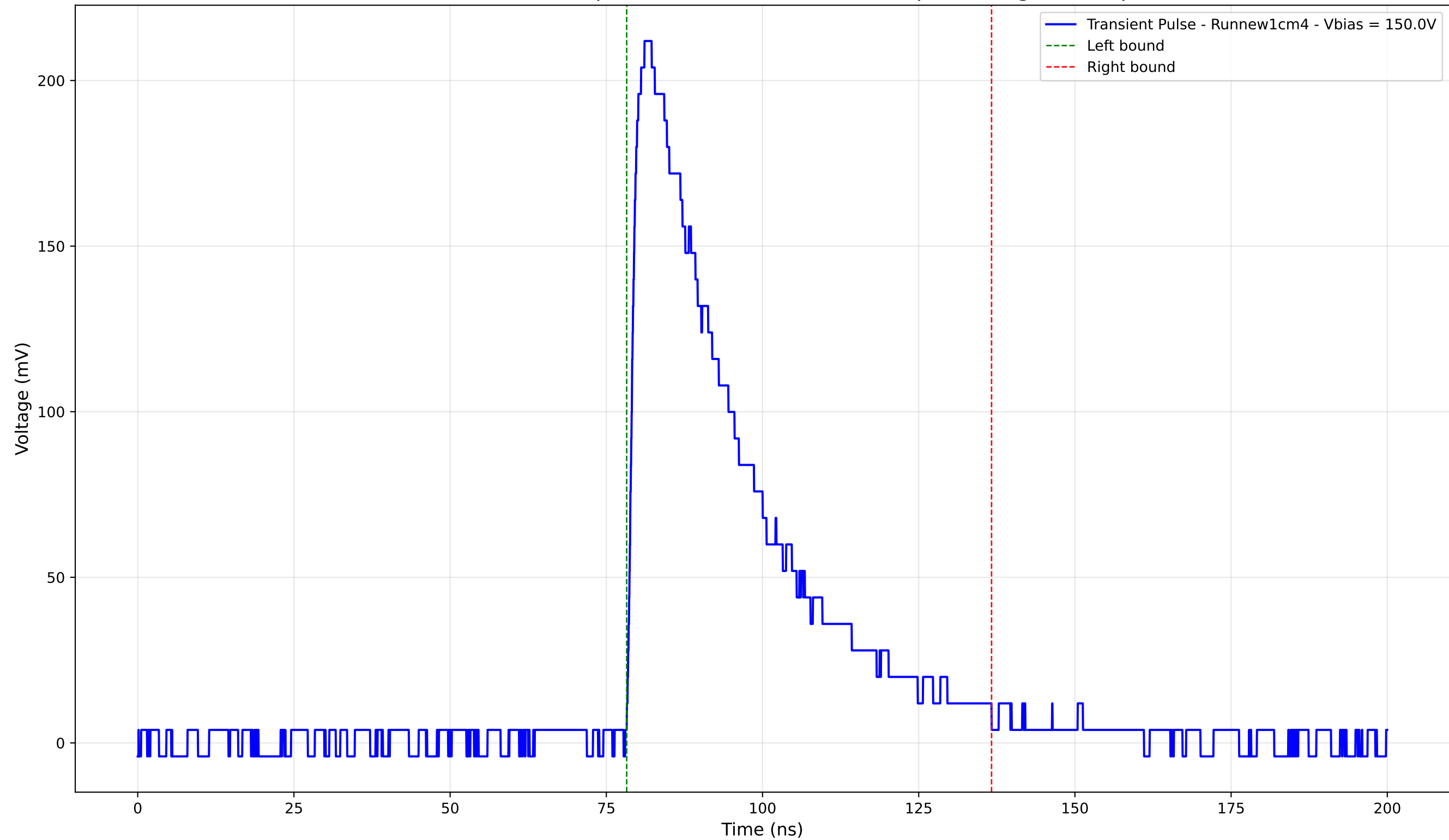
Transient Pulse - Sample: new1cm - Position: 3695.0 \mu\text{m} - Charge: 81.28 pC
