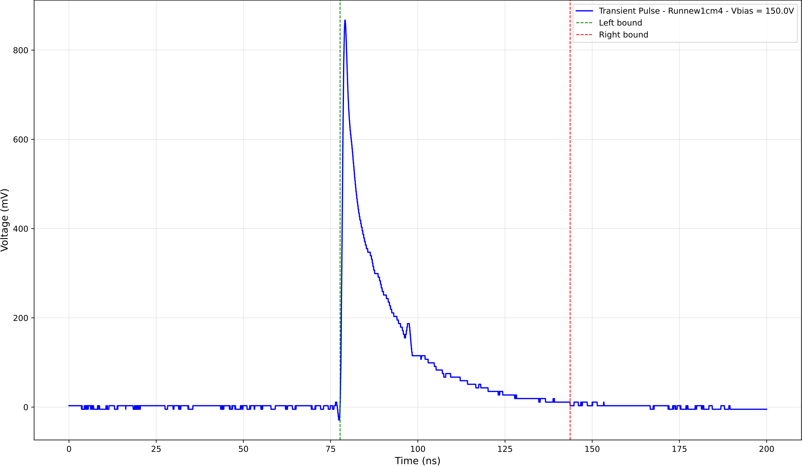
Transient Pulse - Sample: new1cm - Position: 4930.0 \mu\text{m} - Charge: 183.88 pC
