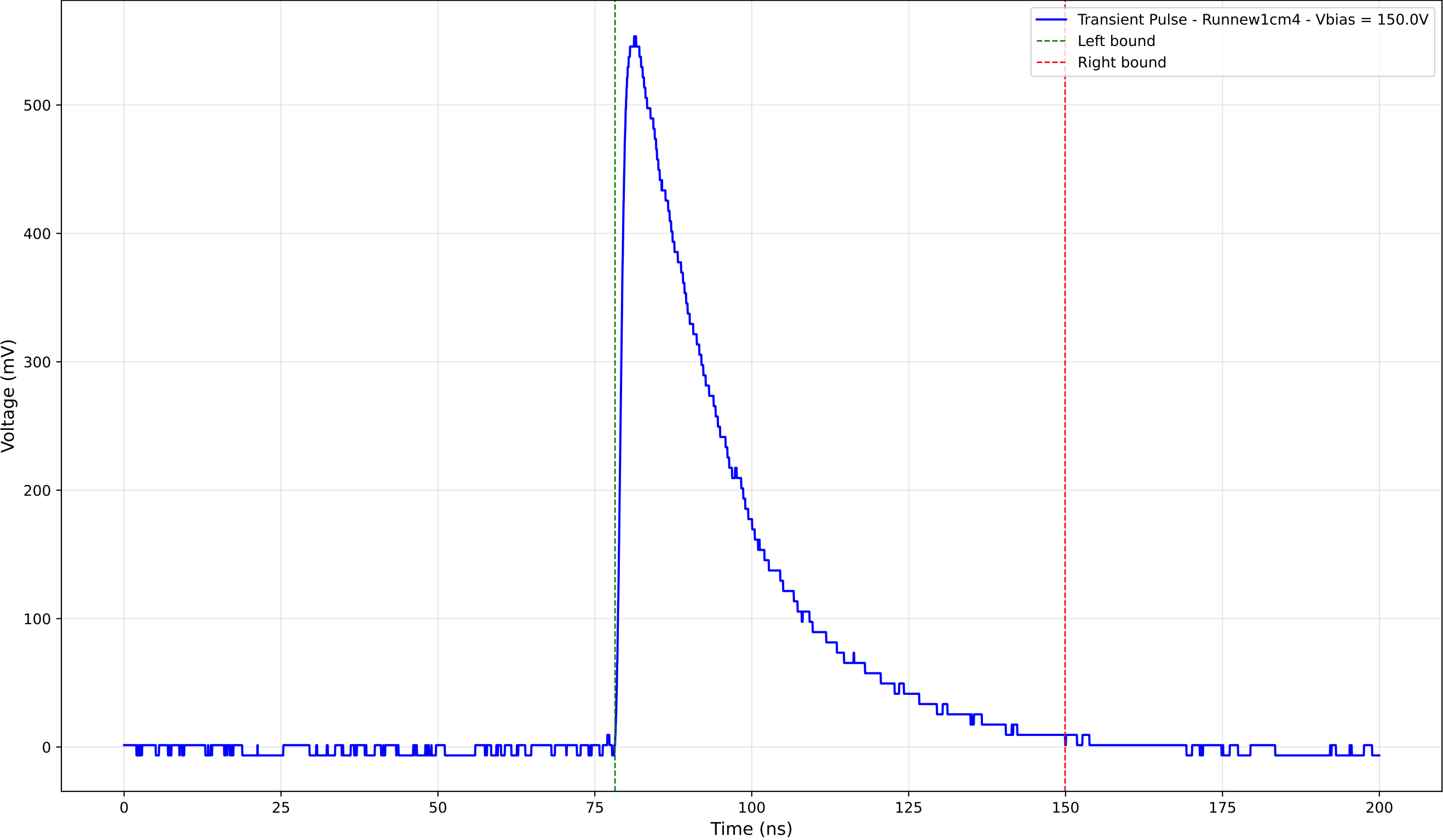
Transient Pulse - Sample: new1cm - Position: 1525.0 \mu\text{m} - Charge: 205.96 pC
