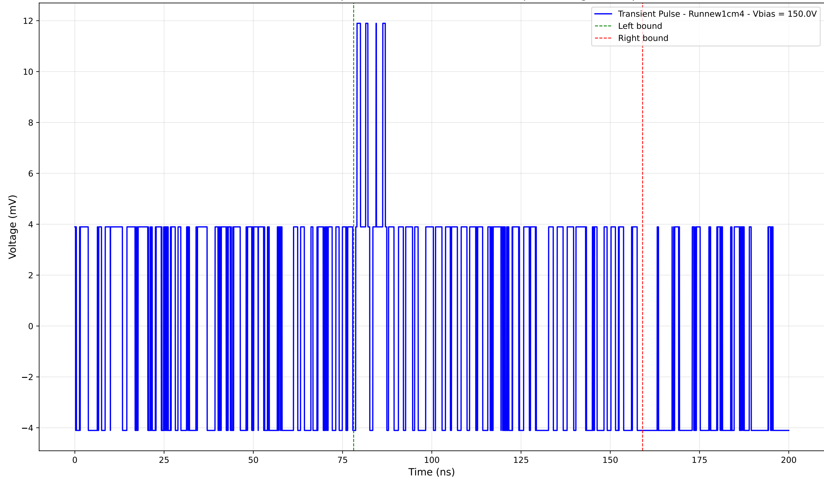
Transient Pulse - Sample: new1cm - Position: 5140.0 \mu\text{m} - Charge: 1.55 pC
