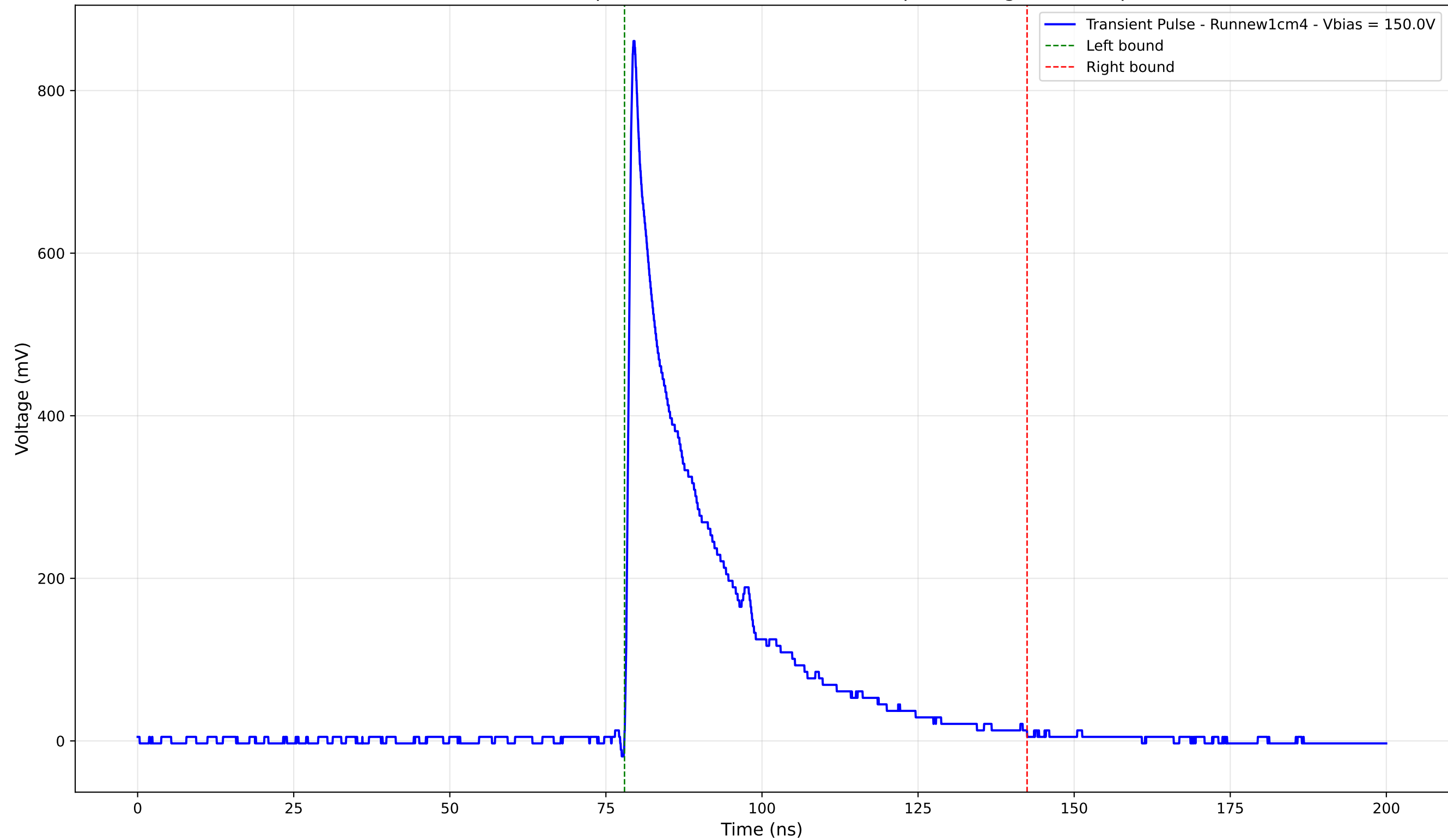
Transient Pulse - Sample: new1cm - Position: 580.0 \mu\text{m} - Charge: 195.45 pC
