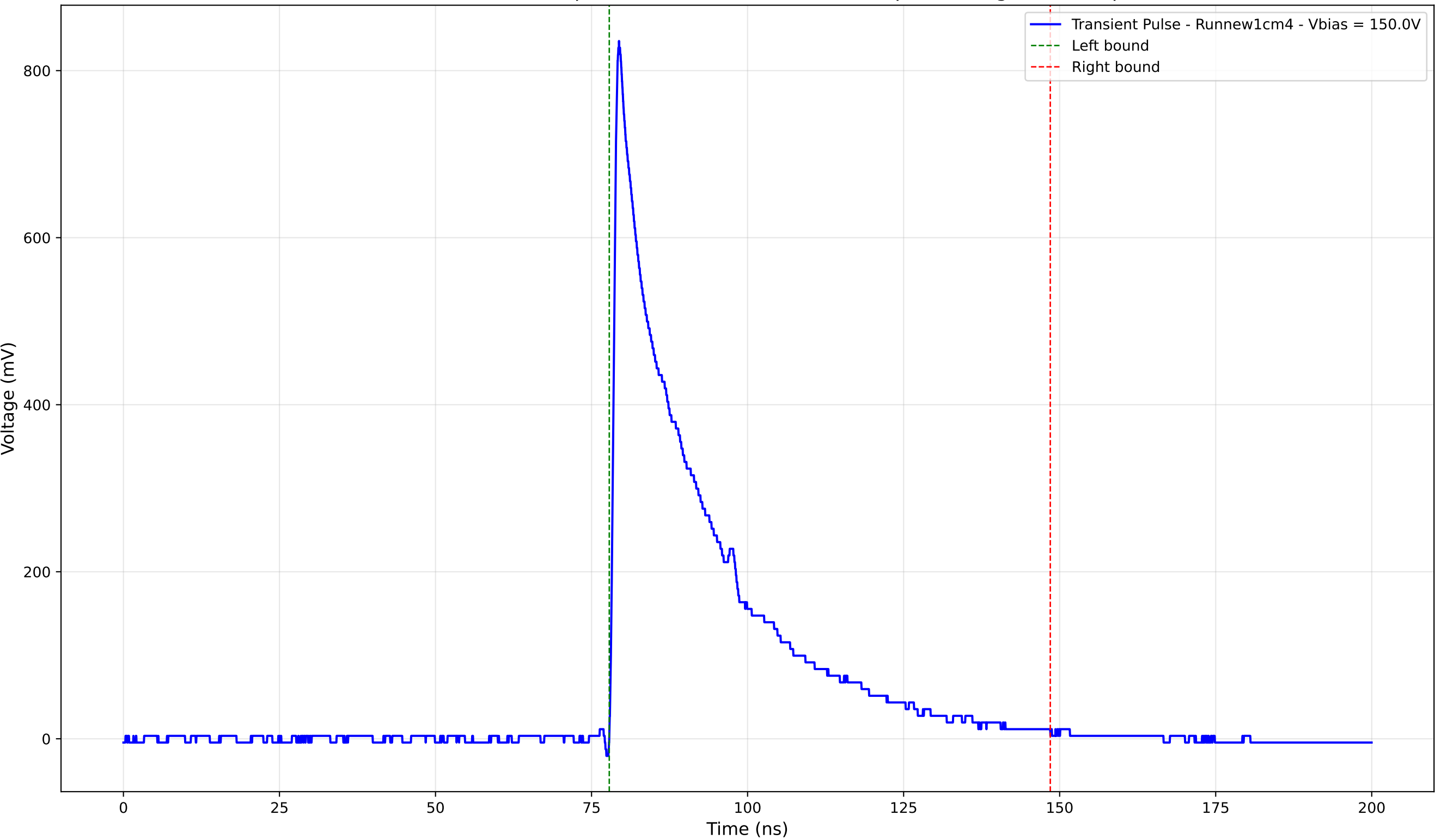
Transient Pulse - Sample: new1cm - Position: 4615.0 \mu\text{m} - Charge: 225.91 pC
