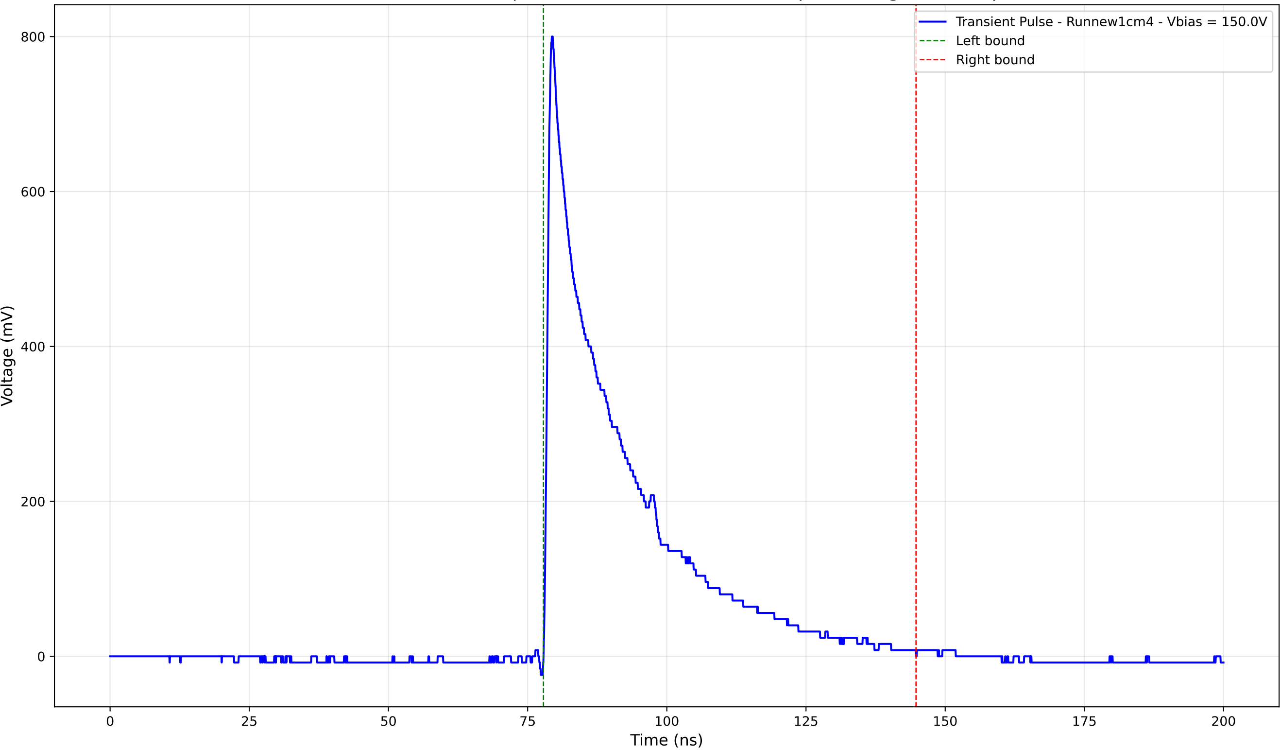
Transient Pulse - Sample: new1cm - Position: 4640.0 \mu\text{m} - Charge: 205.84 pC
