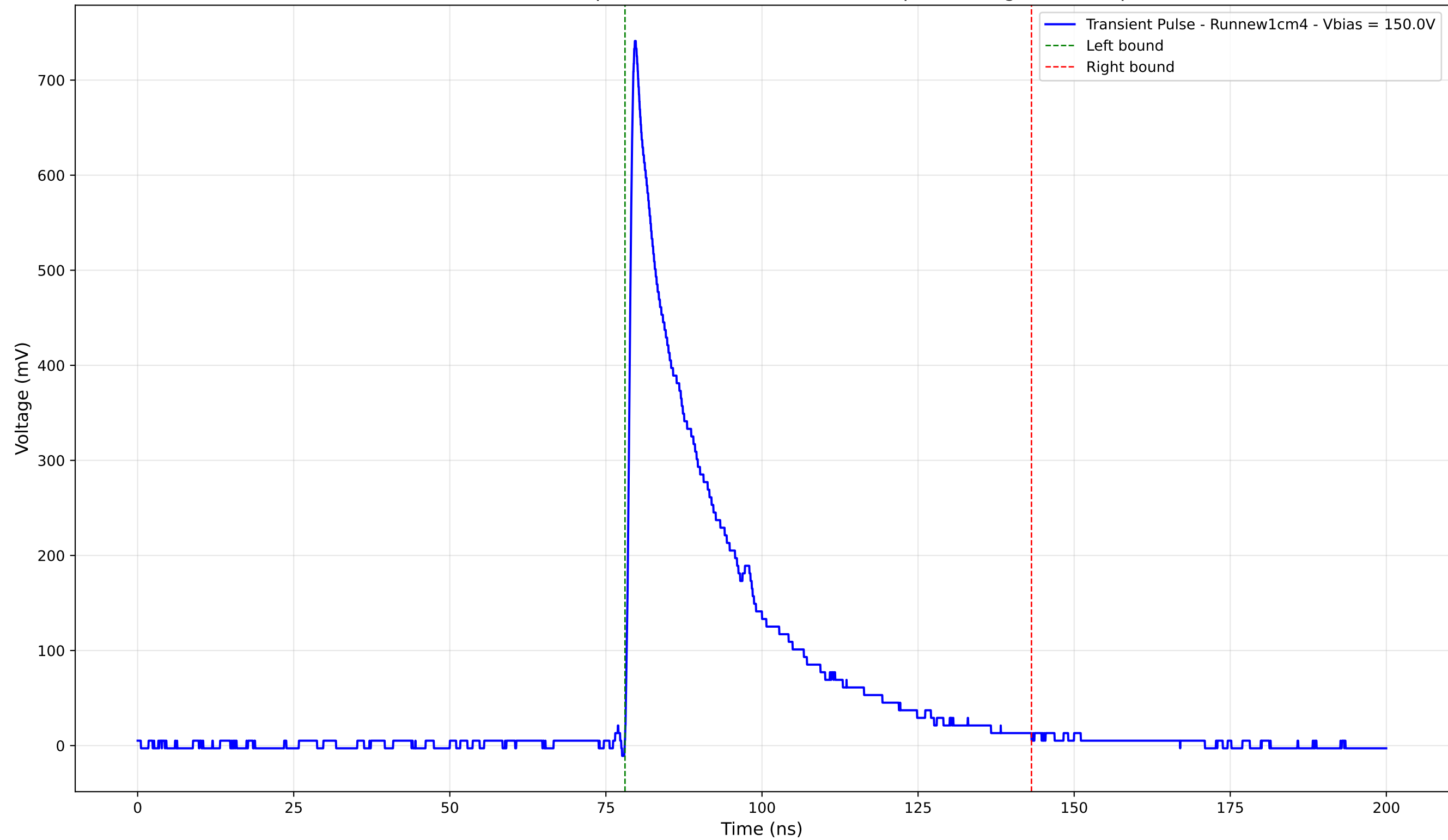
Transient Pulse - Sample: new1cm - Position: 805.0 \mu\text{m} - Charge: 194.21 pC
