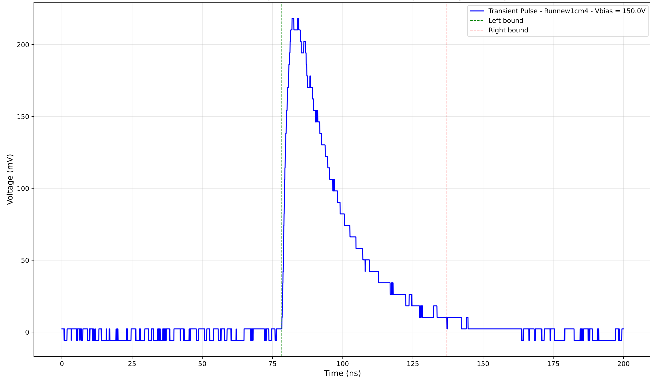
Transient Pulse - Sample: new1cm - Position: 2675.0 \mu\text{m} - Charge: 88.97 pC
