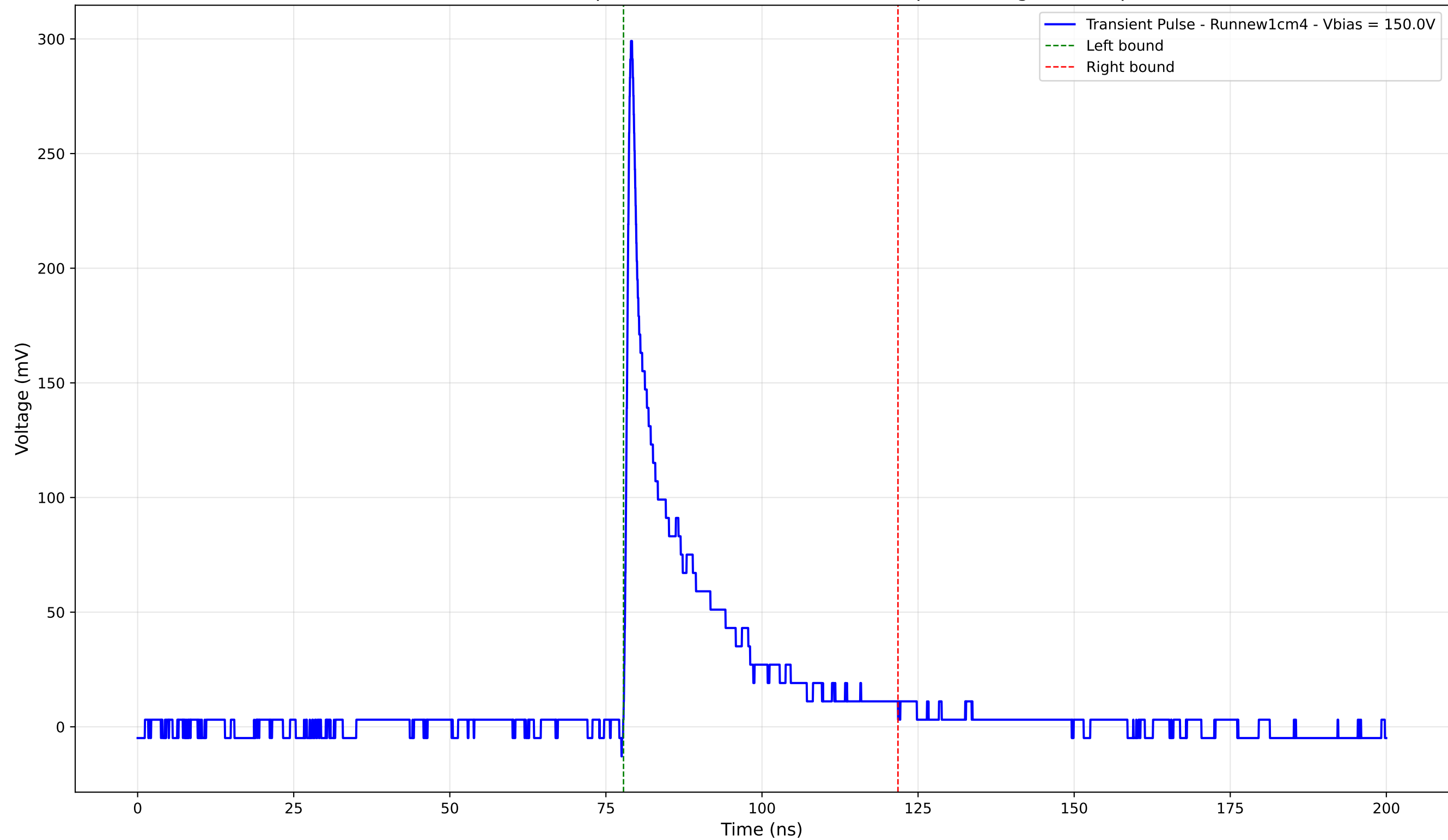
Transient Pulse - Sample: new1cm - Position: 5045.0 \mu\text{m} - Charge: 44.62 pC
