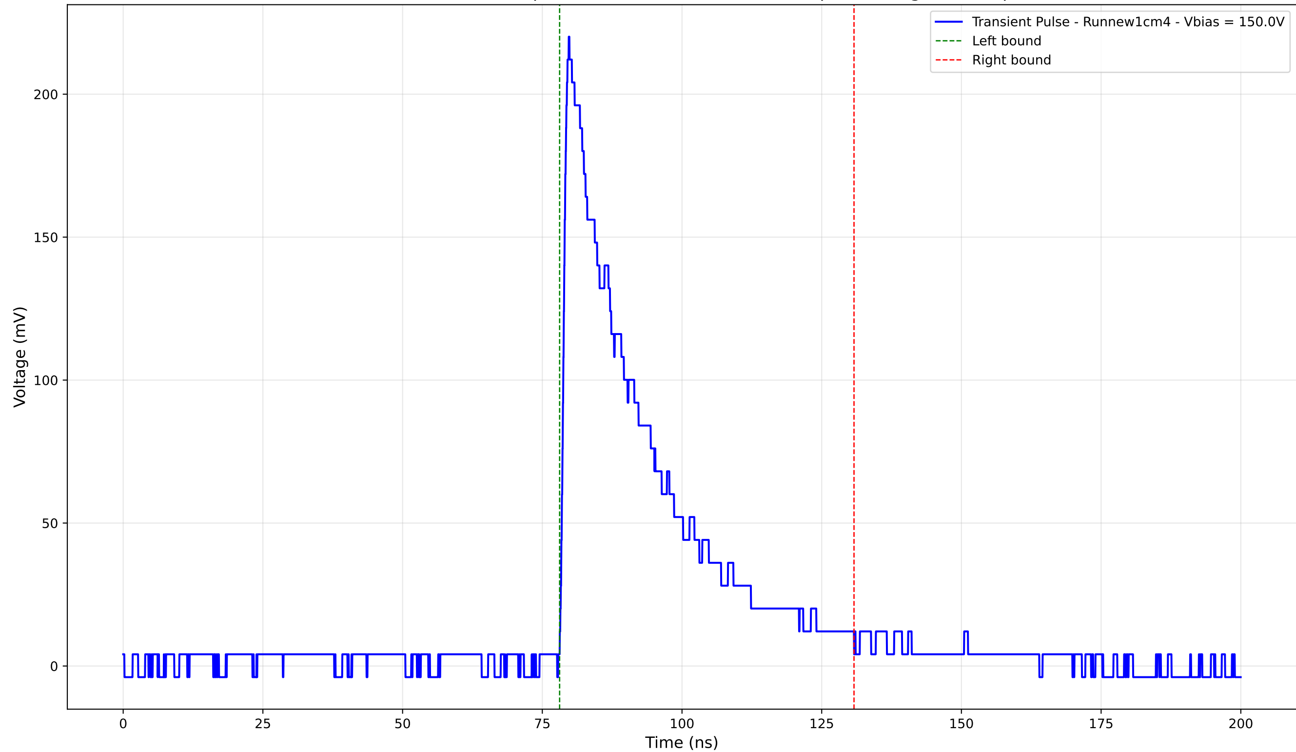
Transient Pulse - Sample: new1cm - Position: 4260.0 \mu\text{m} - Charge: 65.16 pC
