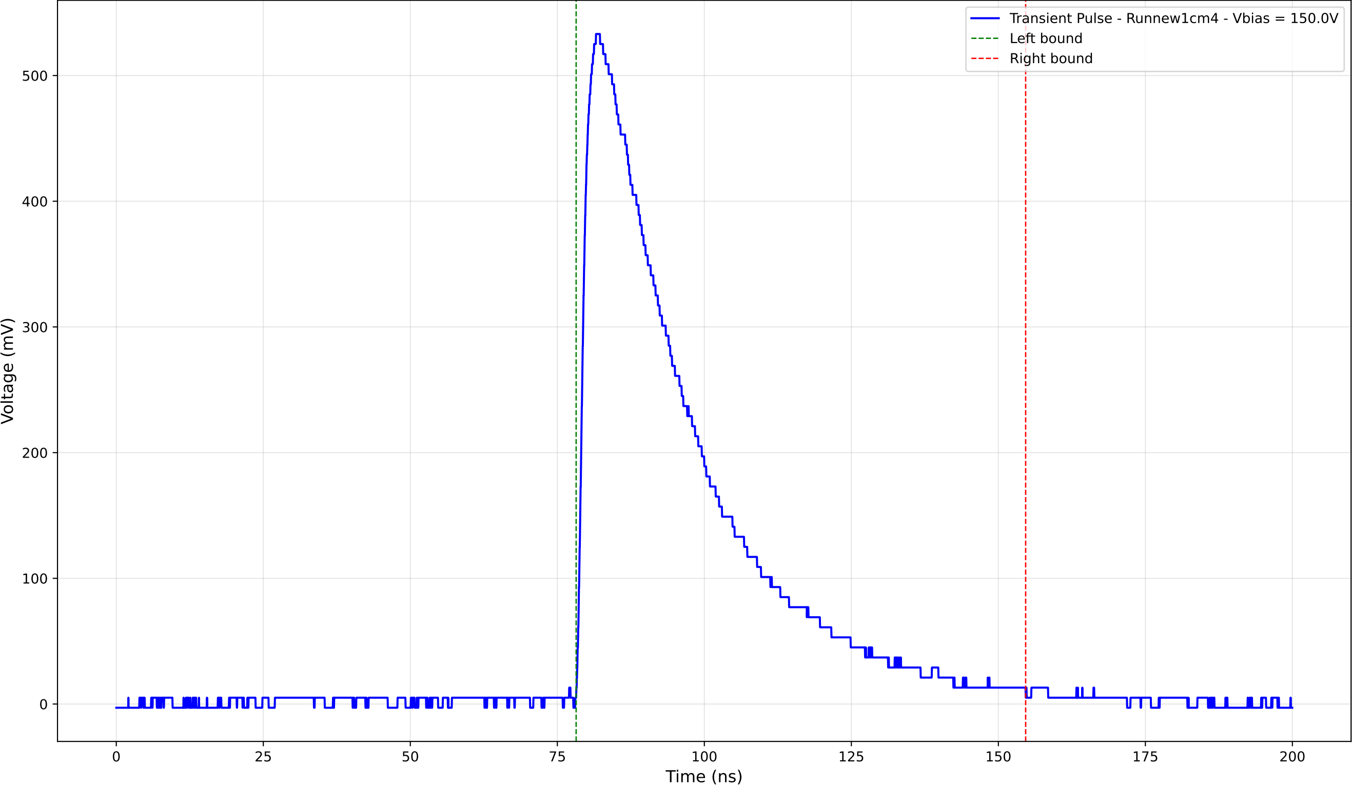
Transient Pulse - Sample: new1cm - Position: 1870.0 \mu\text{m} - Charge: 219.05 pC
