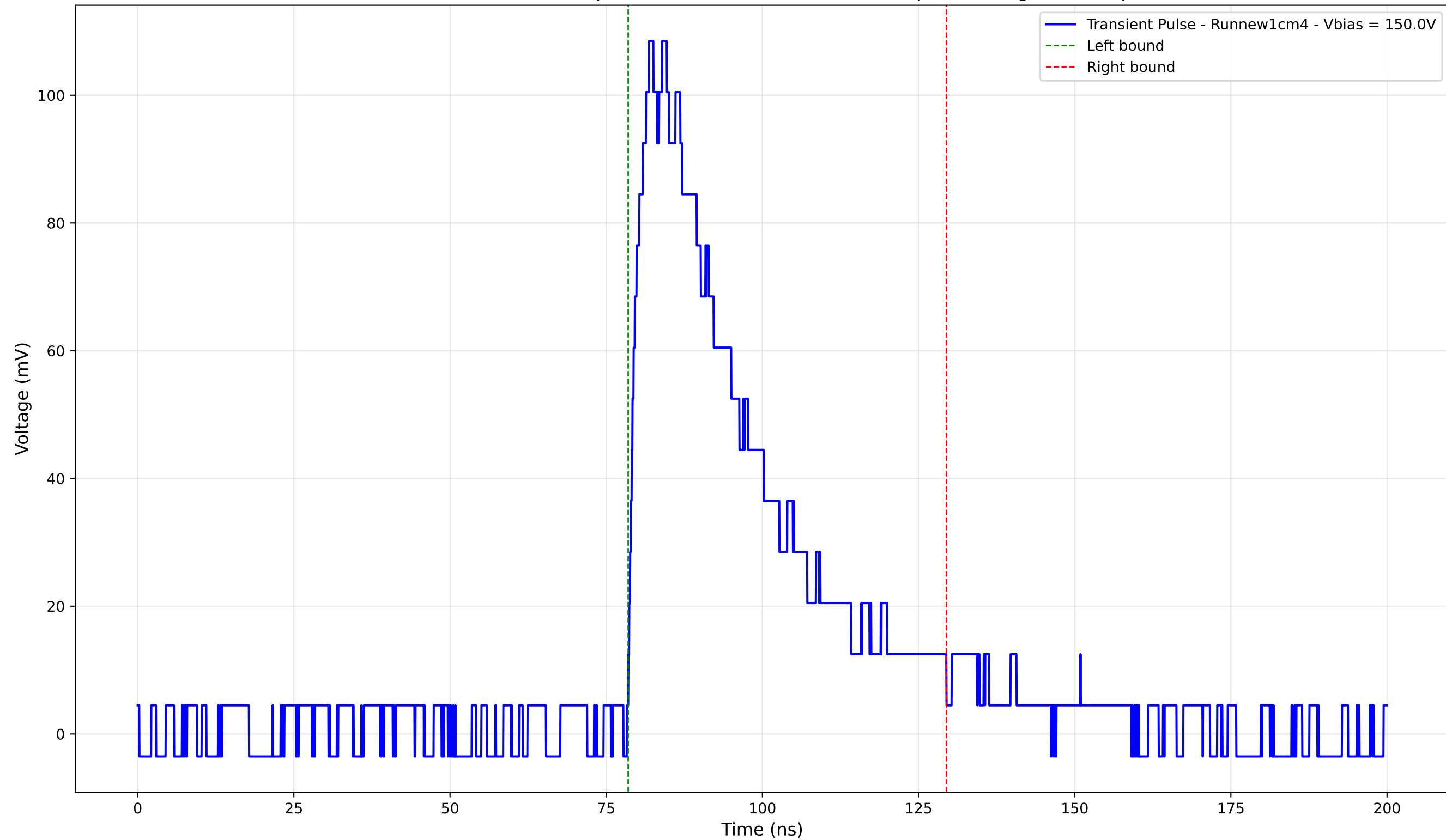
Transient Pulse - Sample: new1cm - Position: 3210.0 \mu\text{m} - Charge: 43.26 pC
