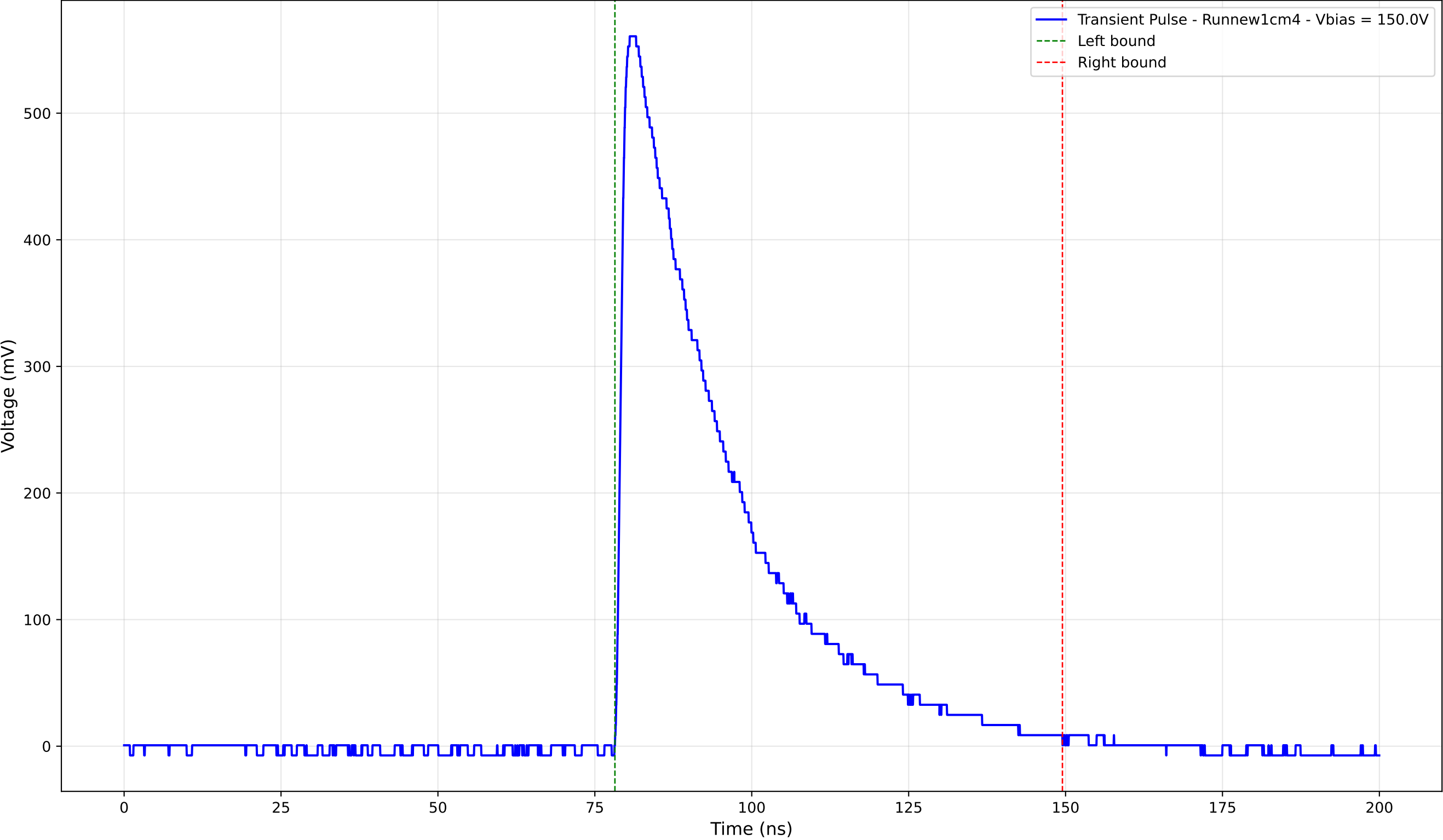
Transient Pulse - Sample: new1cm - Position: 1460.0 \mu\text{m} - Charge: 205.35 pC
