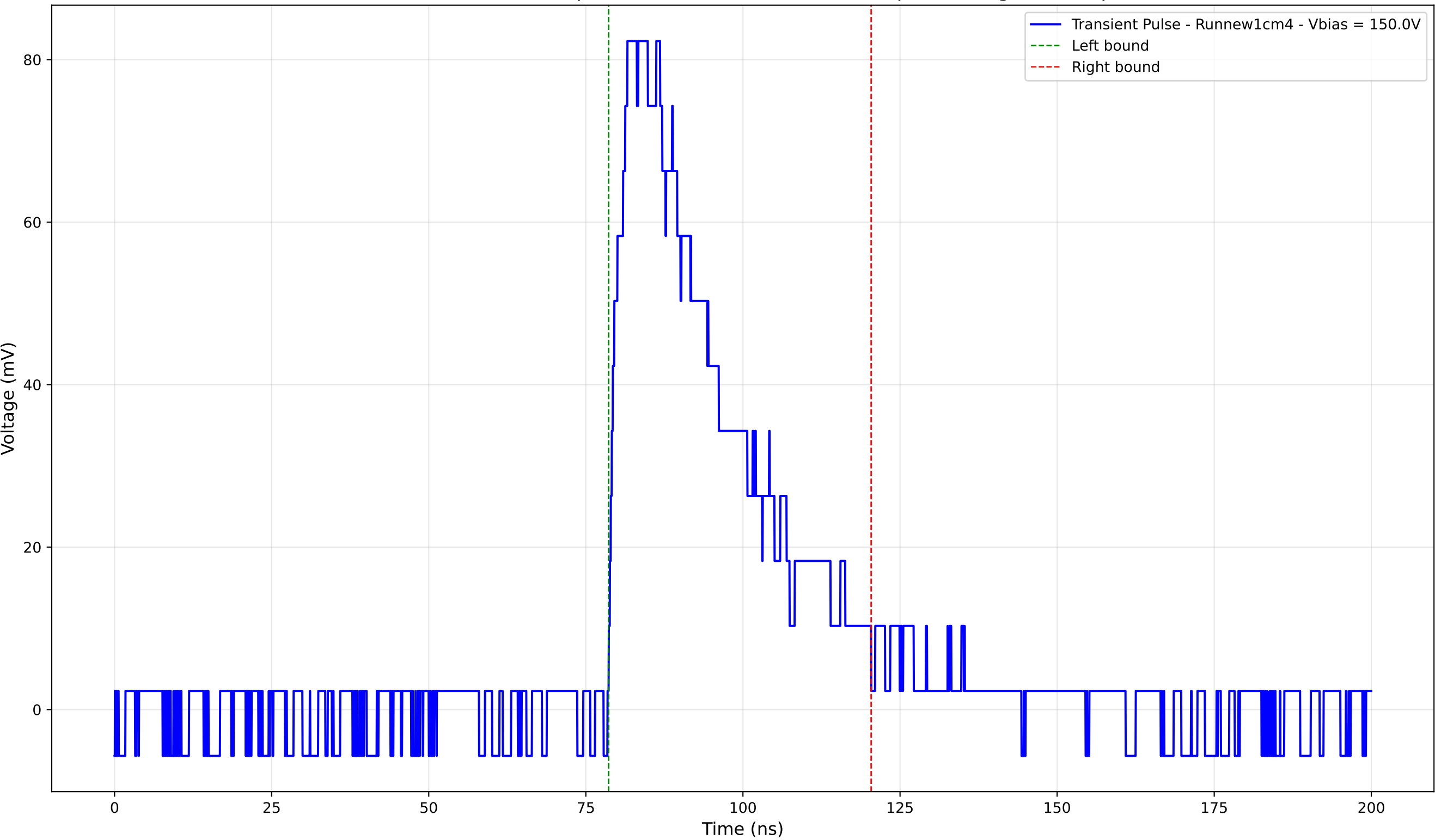
Transient Pulse - Sample: new1cm - Position: 2210.0 \mu\text{m} - Charge: 31.90 pC
