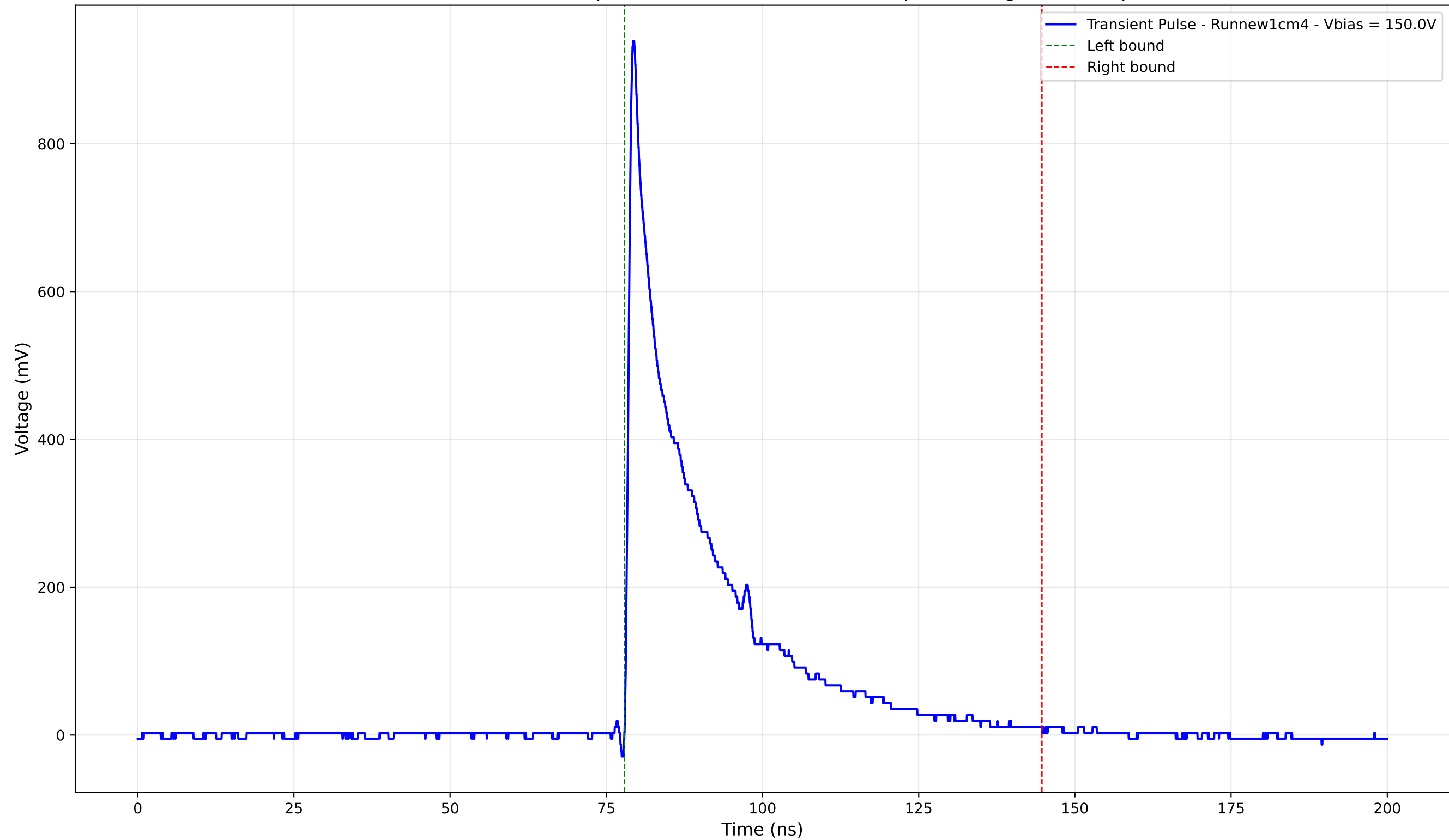
Transient Pulse - Sample: new1cm - Position: 430.0 \mu\text{m} - Charge: 202.51 pC
