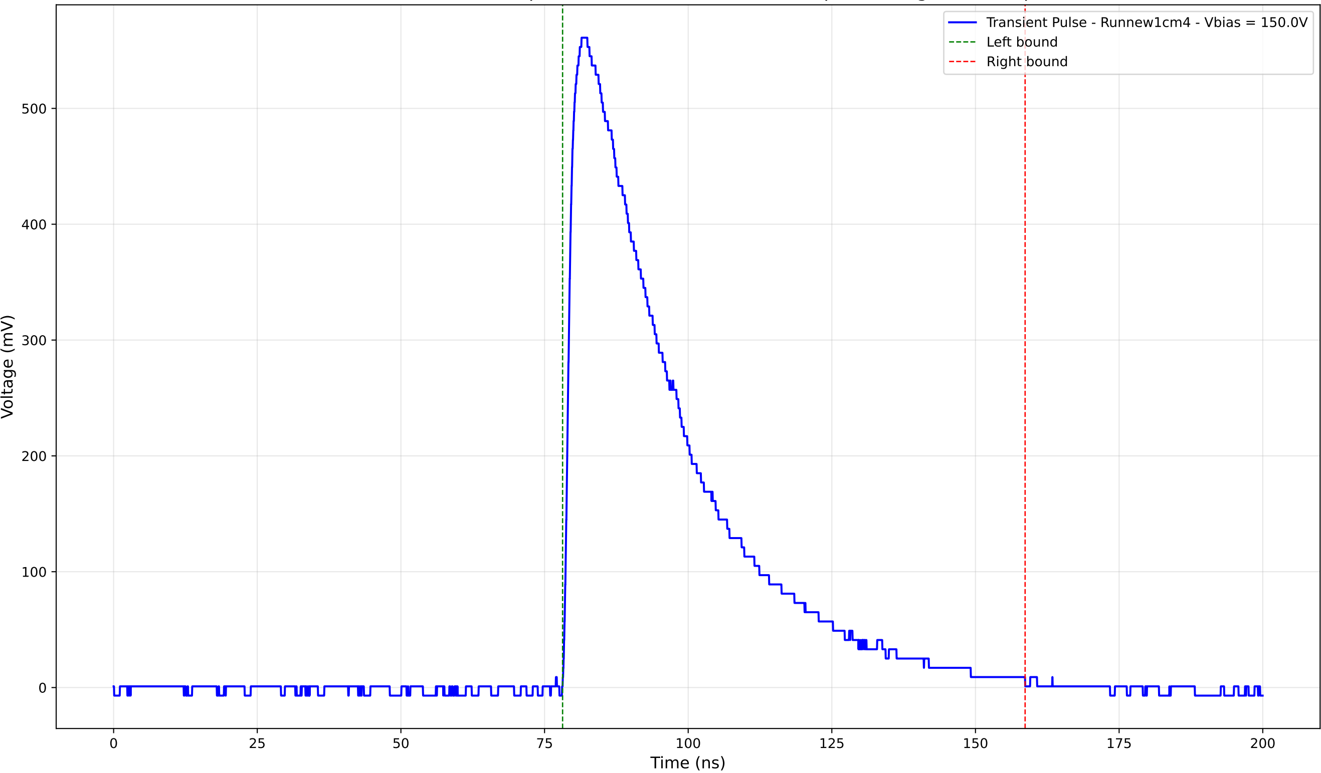
Transient Pulse - Sample: new1cm - Position: 3445.0 \mu\text{m} - Charge: 238.87 pC
