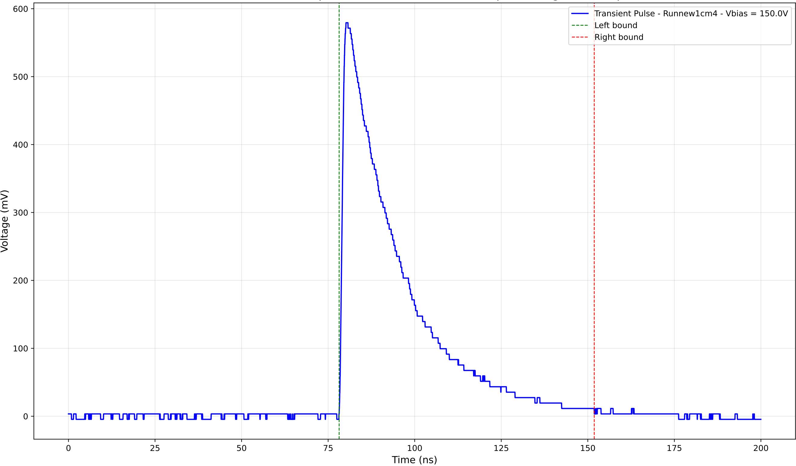
Transient Pulse - Sample: new1cm - Position: 1320.0 \mu\text{m} - Charge: 205.16 pC
