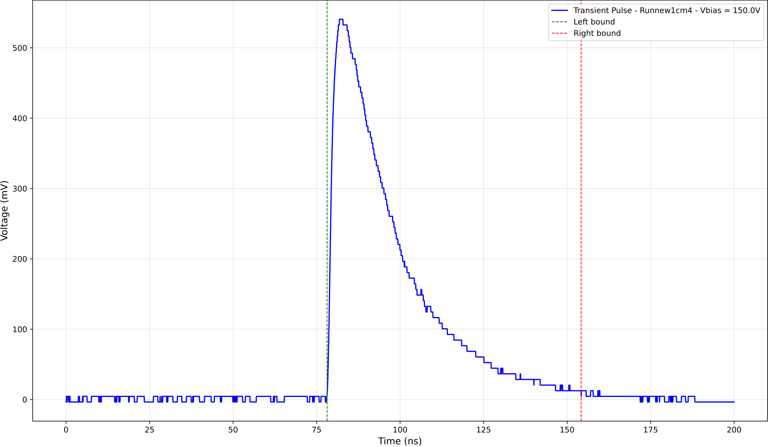
Transient Pulse - Sample: new1cm - Position: 3110.0 \mu\text{m} - Charge: 238.50 pC
