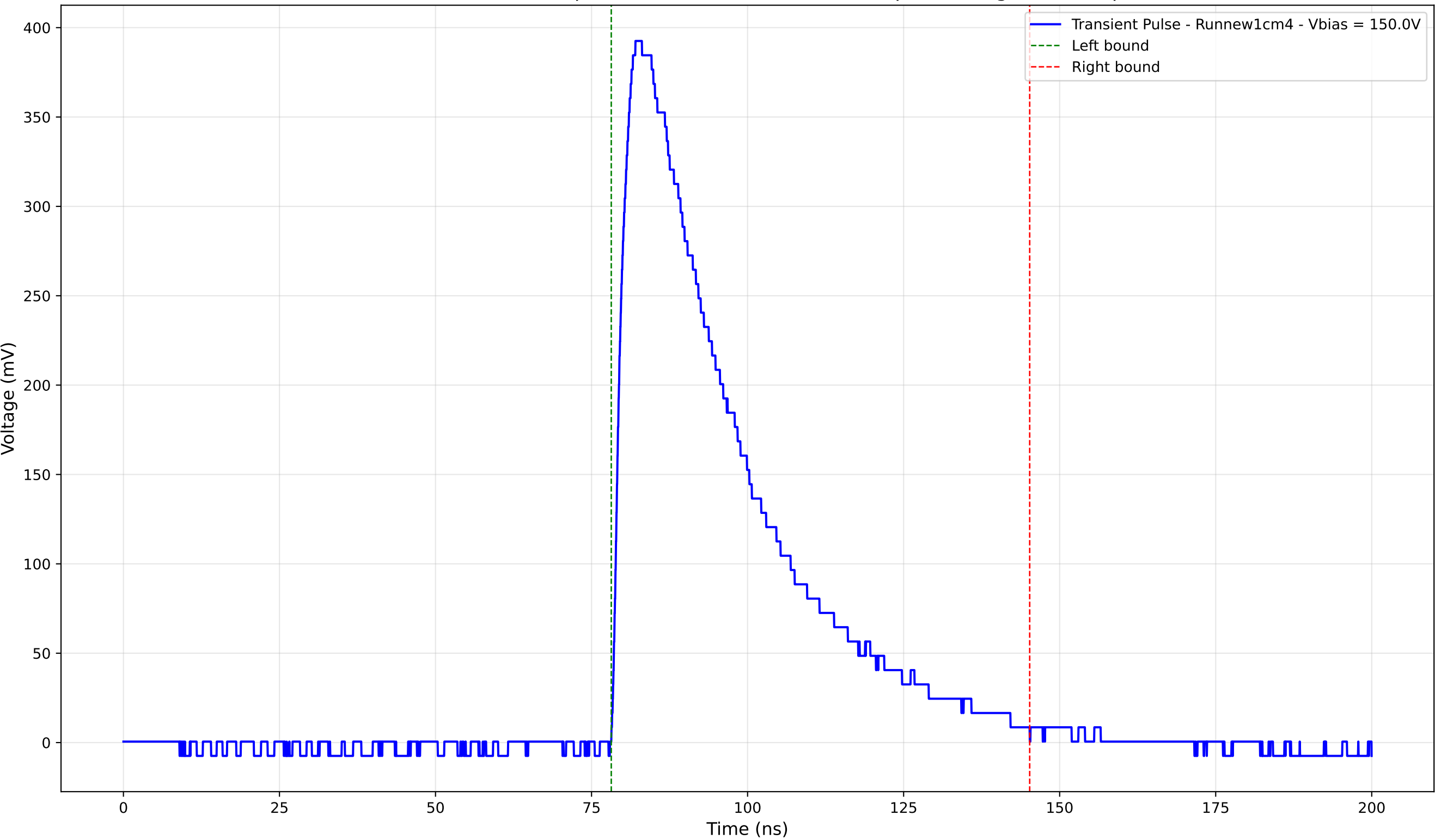
Transient Pulse - Sample: new1cm - Position: 2645.0 \mu\text{m} - Charge: 166.13 pC
