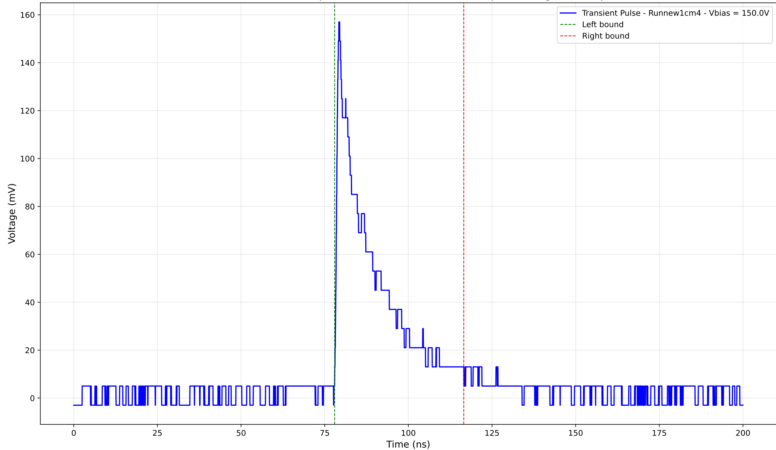
Transient Pulse - Sample: new1cm - Position: 4725.0 \mu\text{m} - Charge: 34.44 pC
