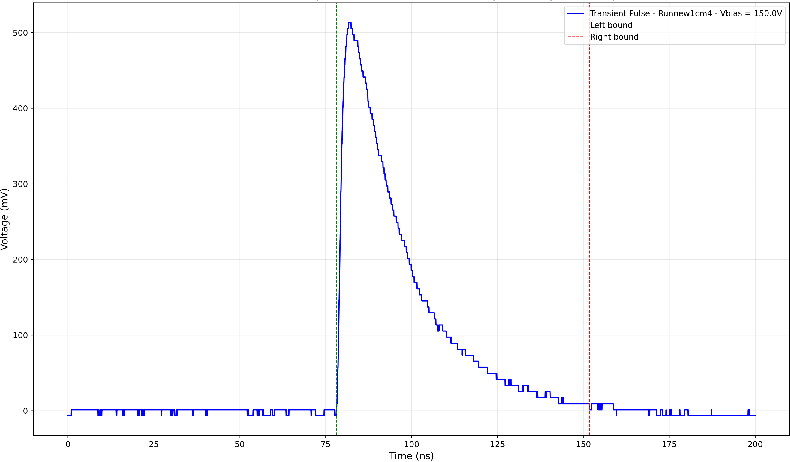
Transient Pulse - Sample: new1cm - Position: 1990.0 \mu\text{m} - Charge: 209.78 pC
