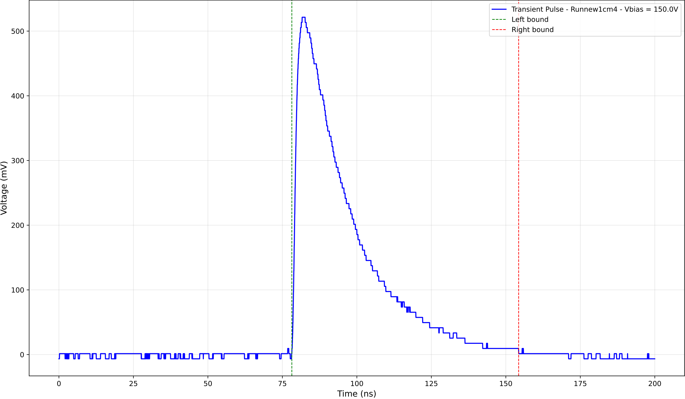
Transient Pulse - Sample: new1cm - Position: 1925.0 \mu\text{m} - Charge: 212.73 pC
