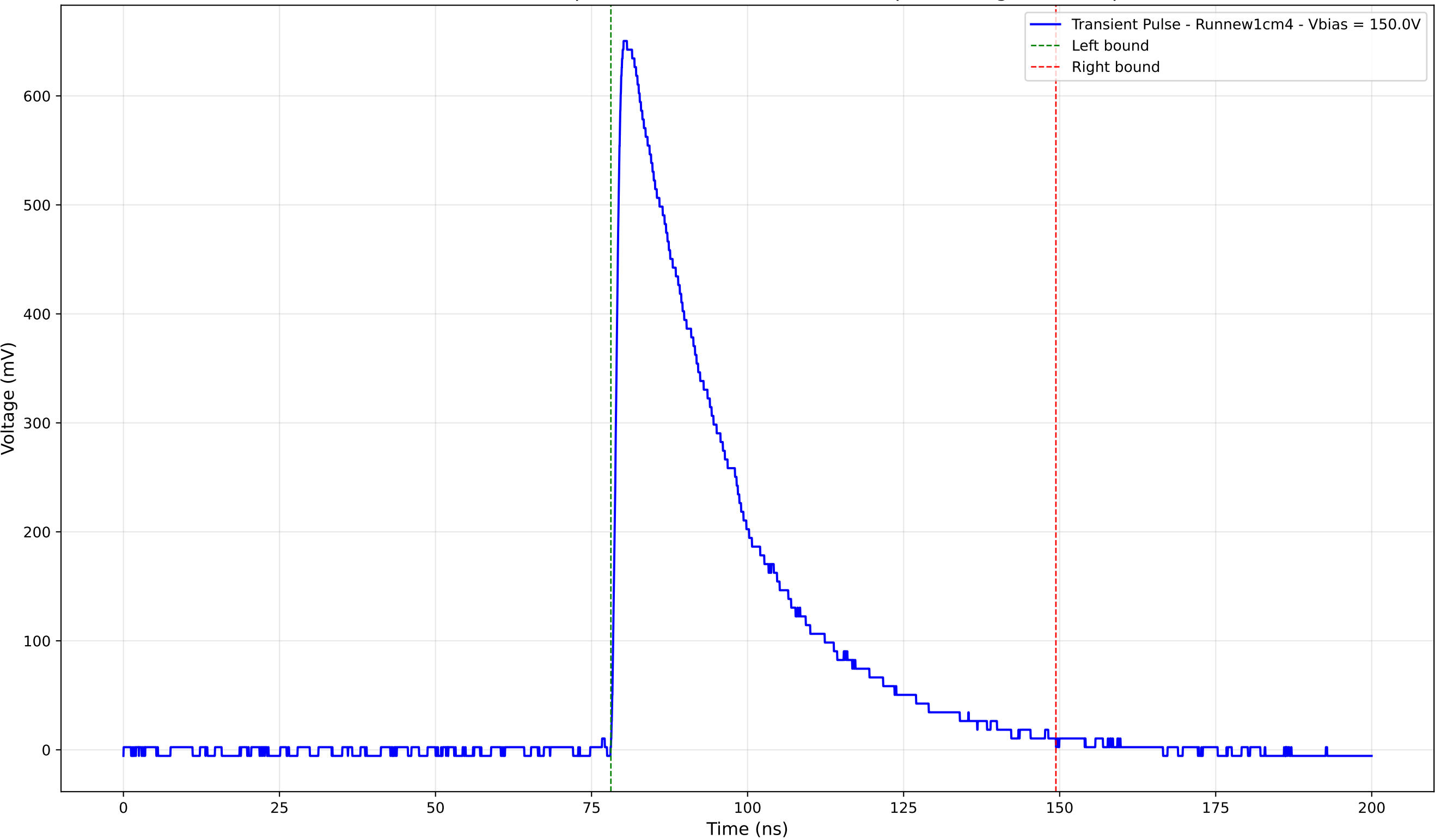
Transient Pulse - Sample: new1cm - Position: 3920.0 \mu\text{m} - Charge: 246.76 pC
