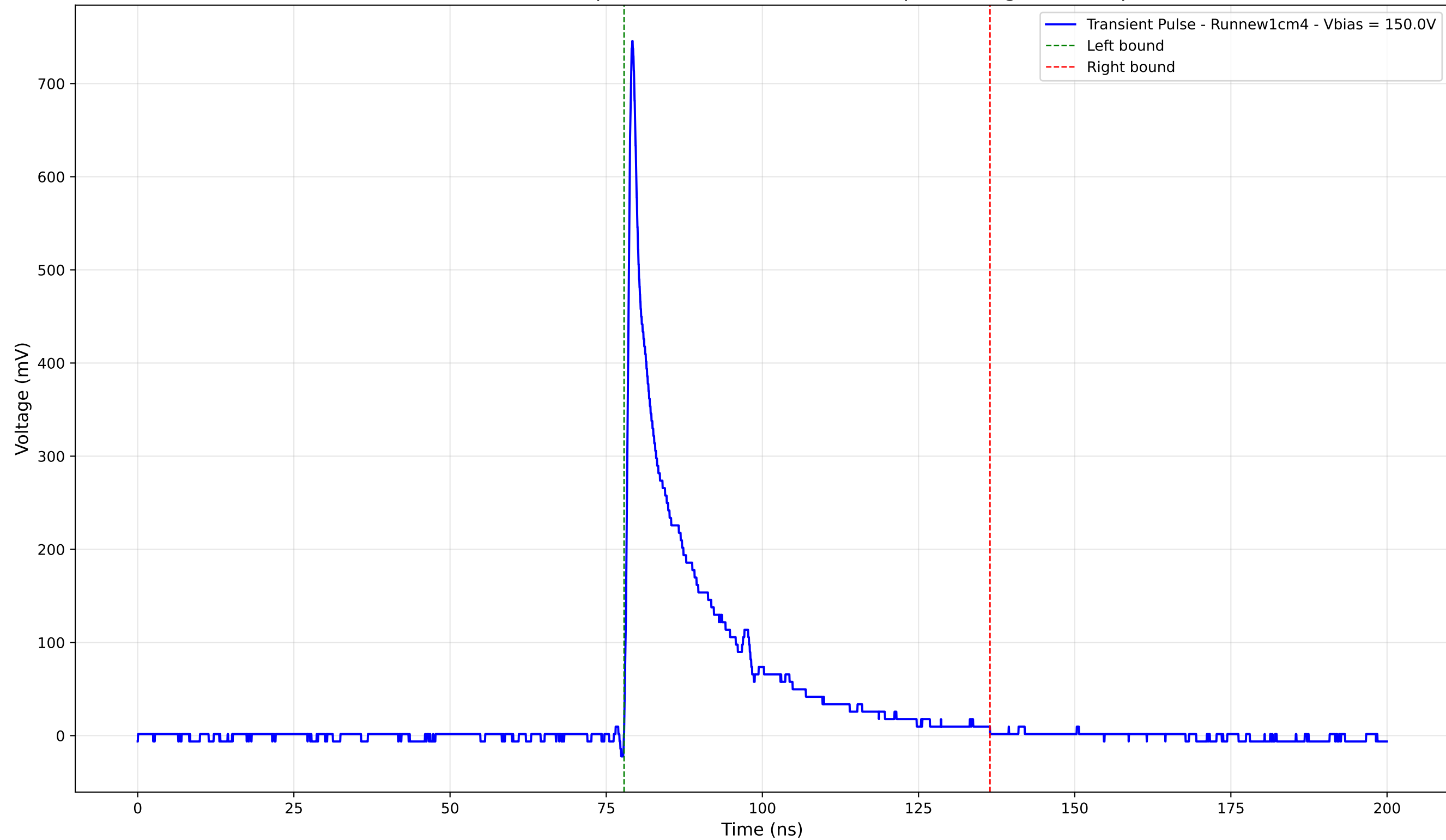
Transient Pulse - Sample: new1cm - Position: 255.0 \mu\text{m} - Charge: 119.10 pC
