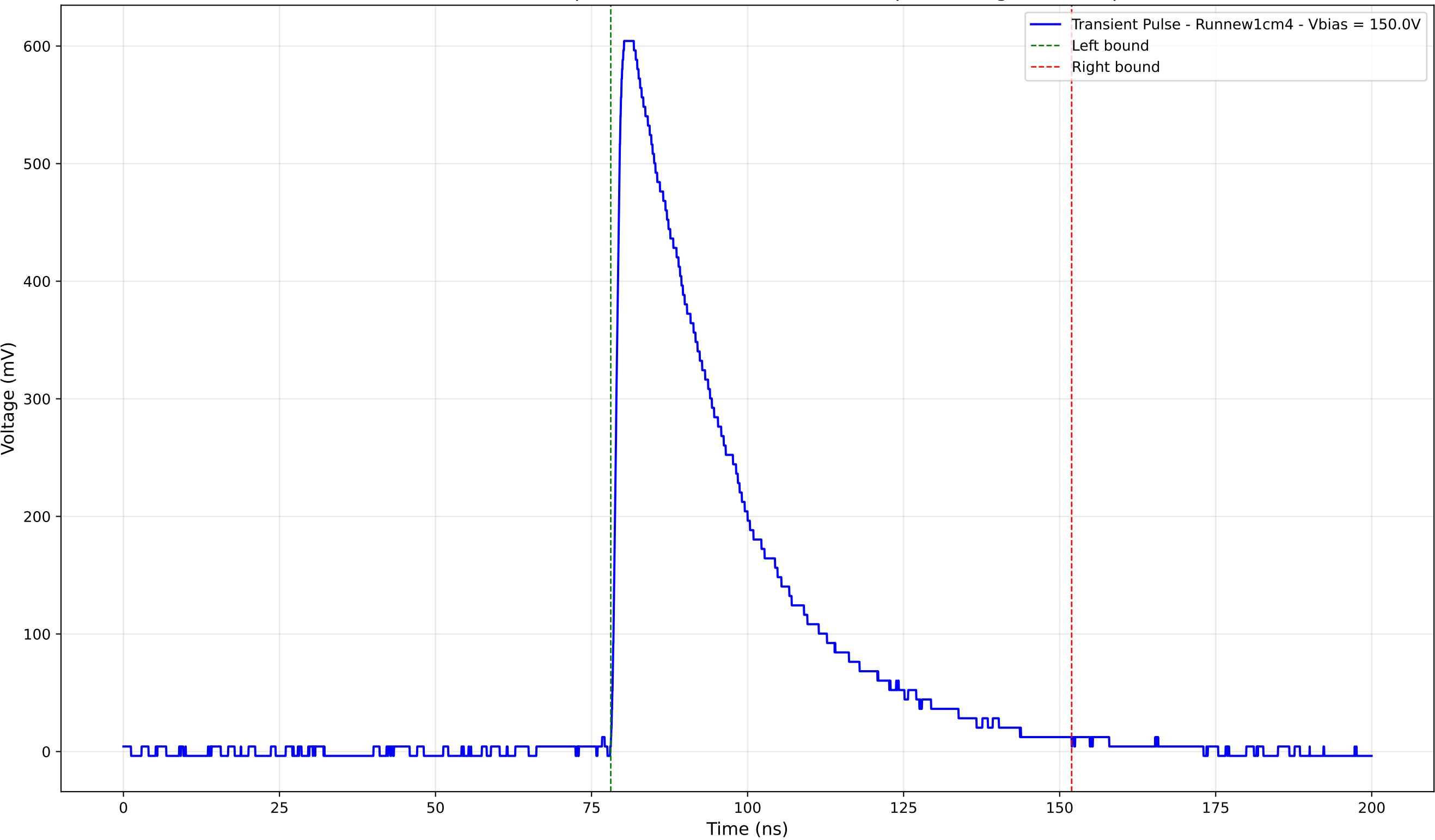
Transient Pulse - Sample: new1cm - Position: 3830.0 \mu\text{m} - Charge: 238.73 pC
