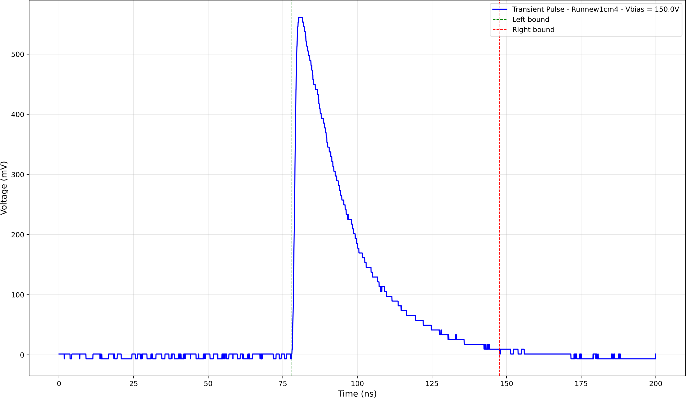
Transient Pulse - Sample: new1cm - Position: 3815.0 \mu\text{m} - Charge: 215.98 pC
