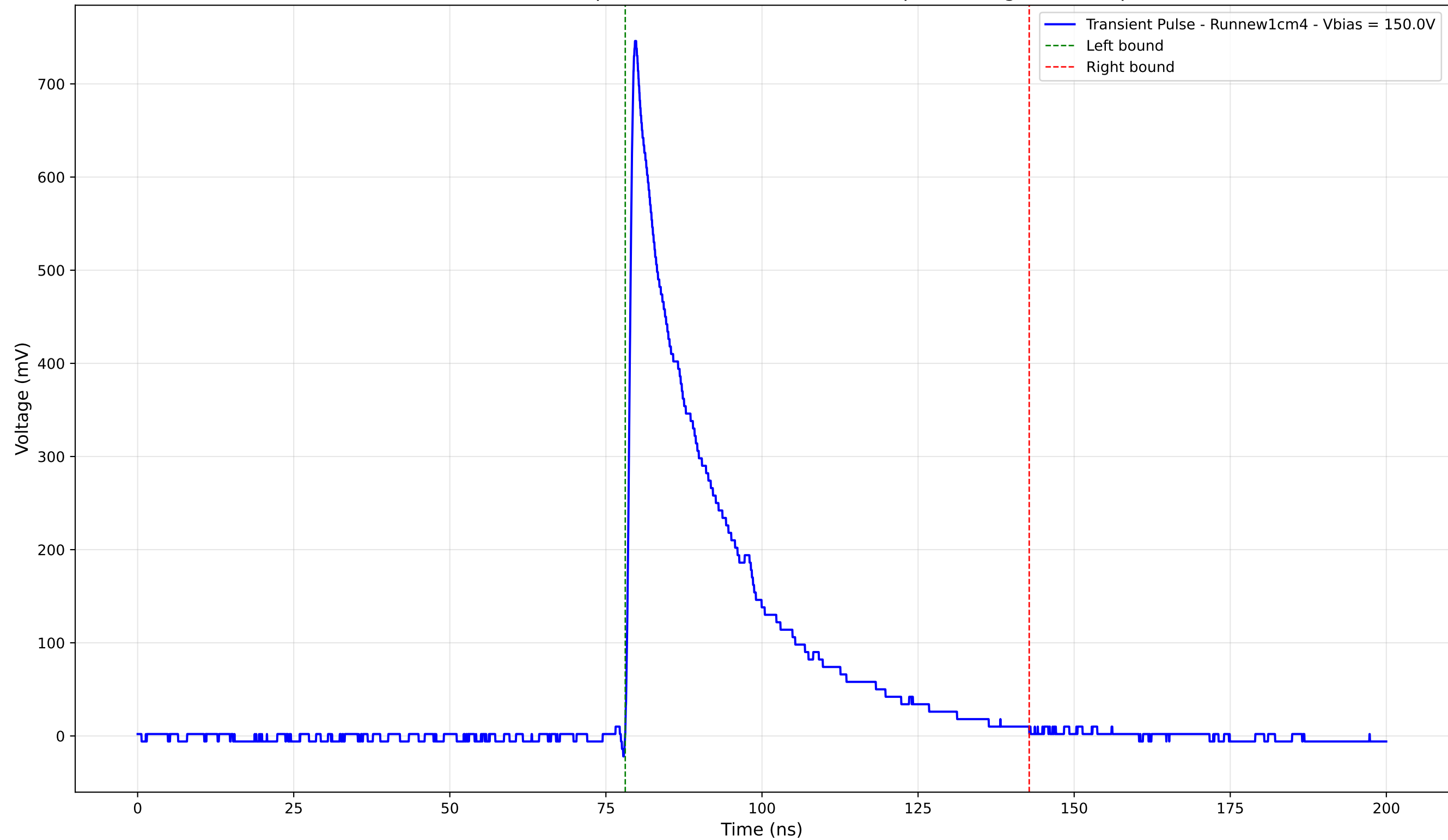
Transient Pulse - Sample: new1cm - Position: 840.0 \mu\text{m} - Charge: 197.81 pC
