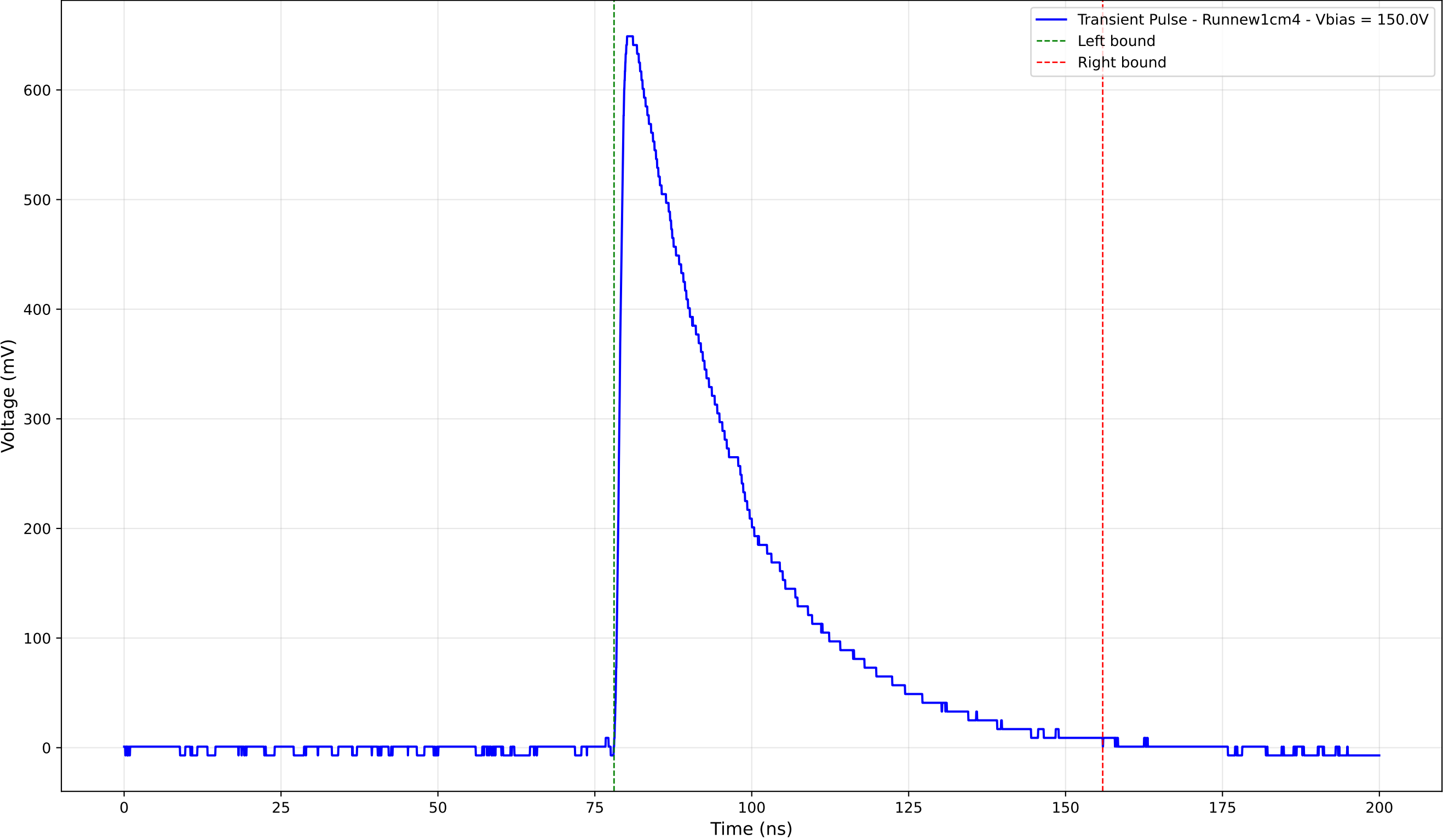
Transient Pulse - Sample: new1cm - Position: 3895.0 \mu\text{m} - Charge: 250.14 pC
