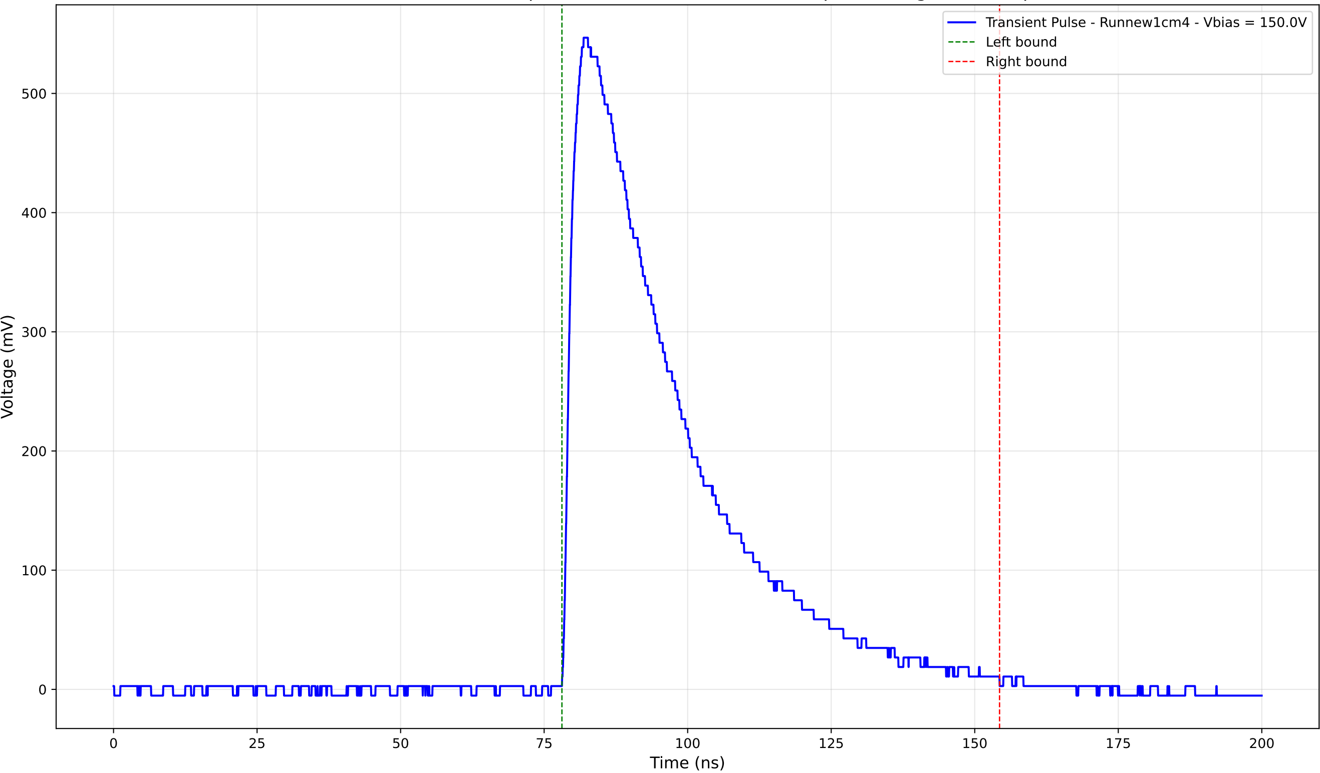
Transient Pulse - Sample: new1cm - Position: 3100.0 \mu\text{m} - Charge: 237.12 pC
