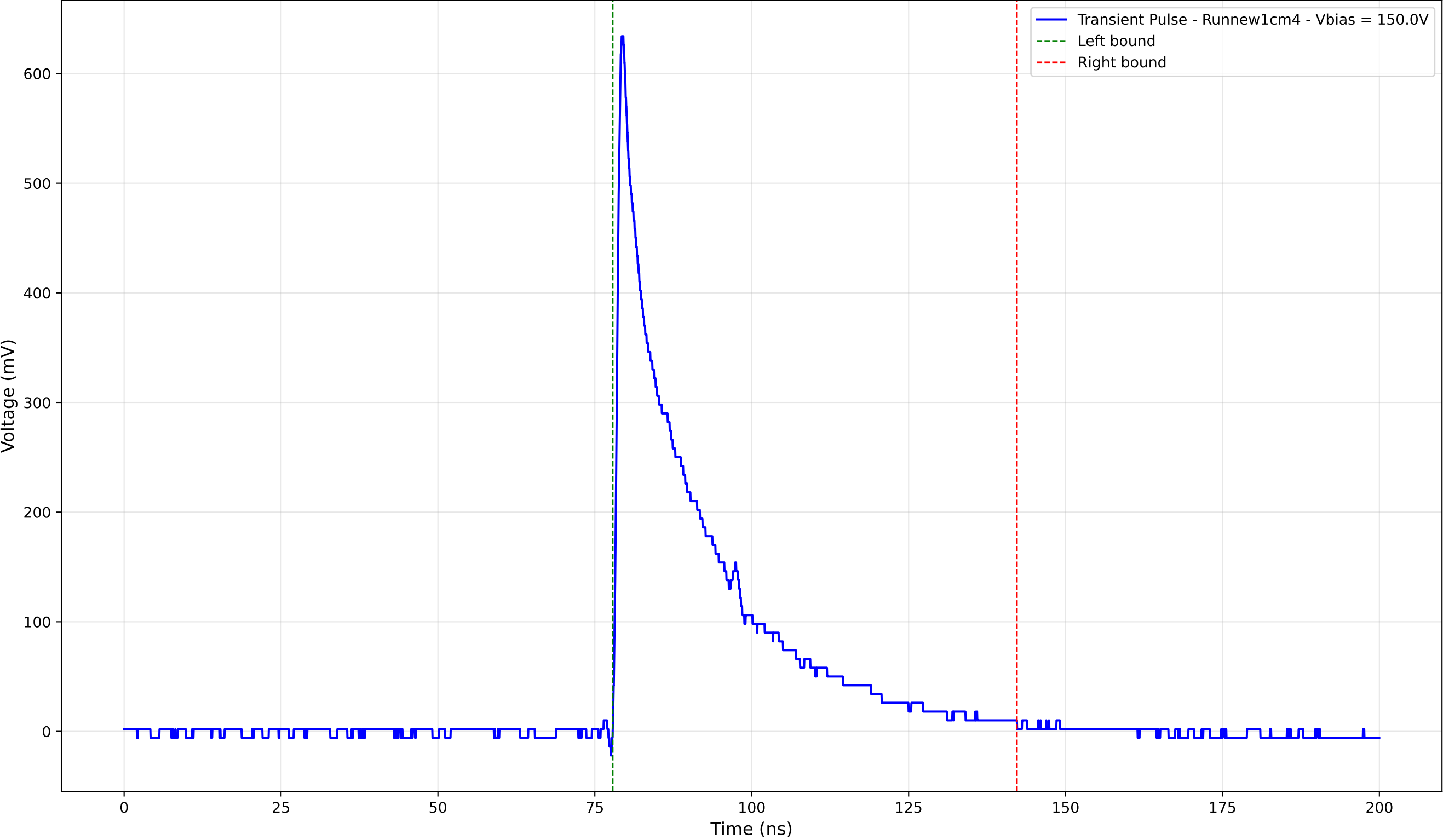
Transient Pulse - Sample: new1cm - Position: 4670.0 \mu\text{m} - Charge: 150.07 pC
