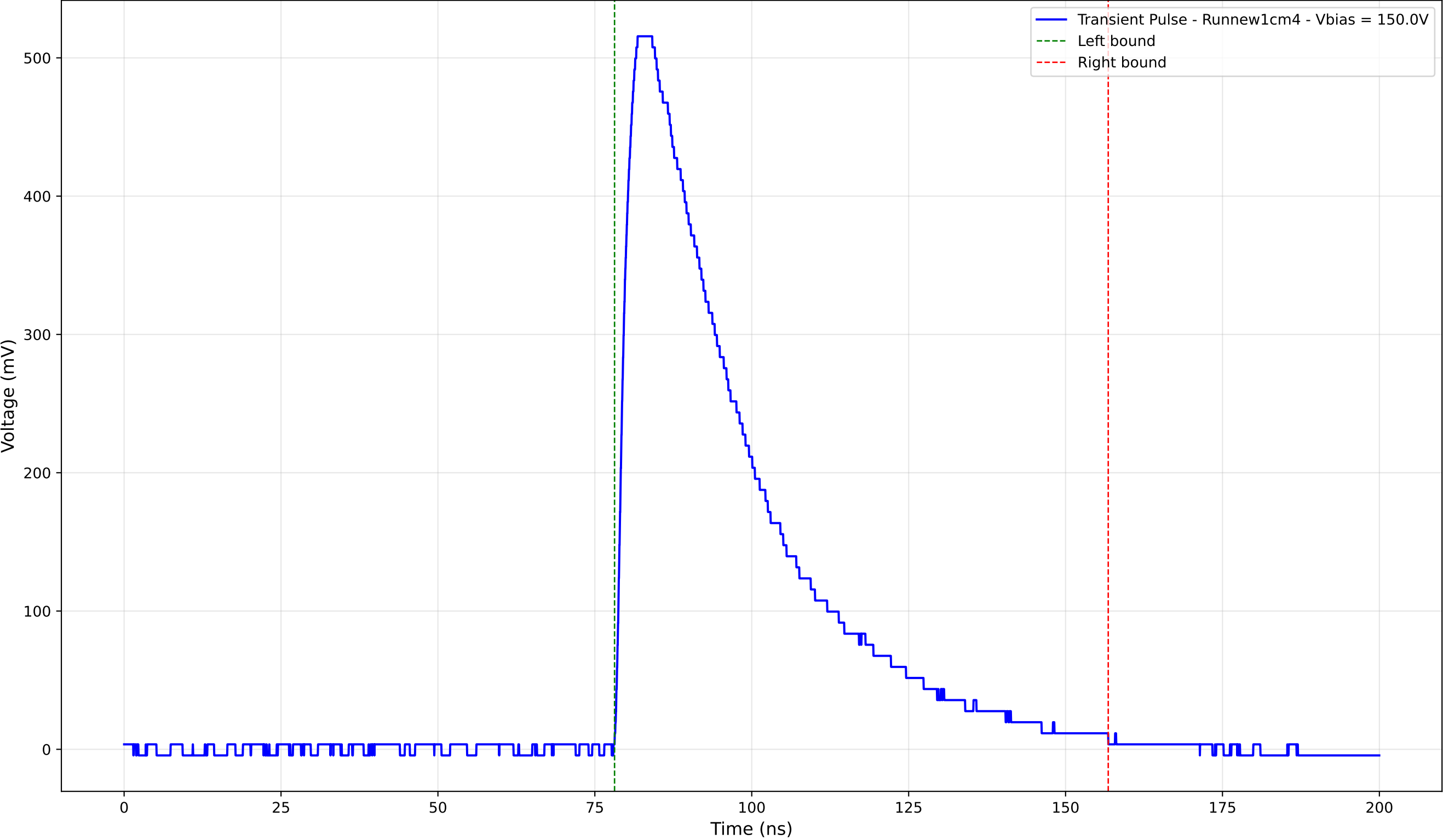
Transient Pulse - Sample: new1cm - Position: 2525.0 \mu\text{m} - Charge: 228.86 pC
