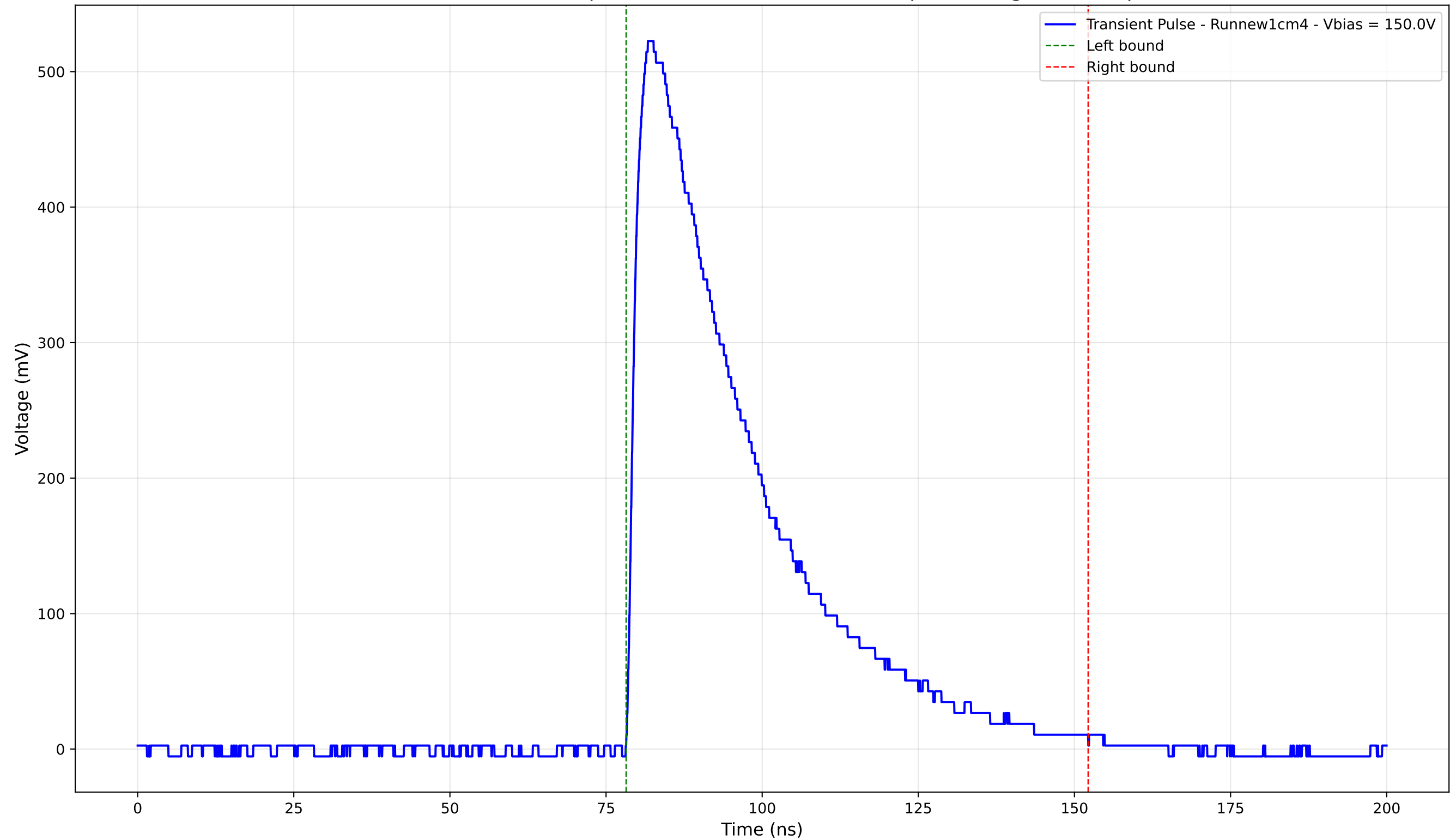
Transient Pulse - Sample: new1cm - Position: 2060.0 \mu\text{m} - Charge: 217.24 pC
