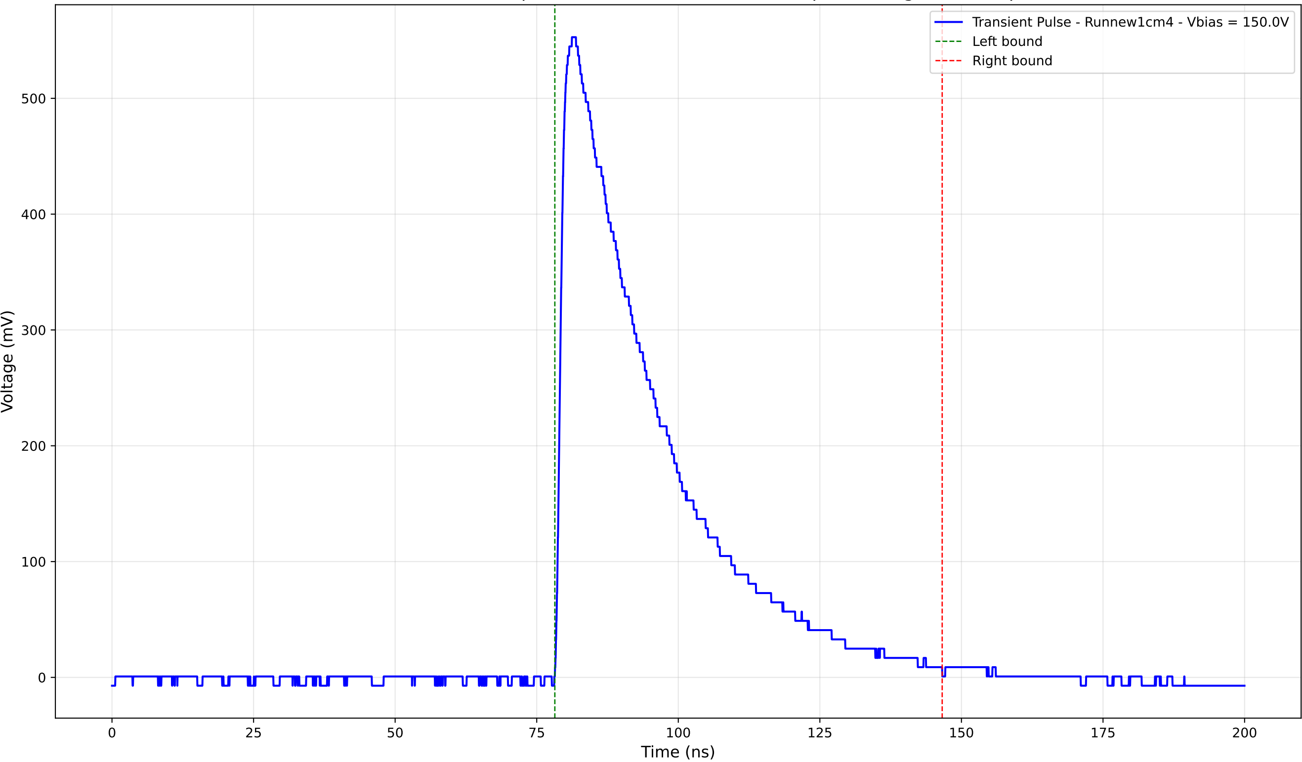
Transient Pulse - Sample: new1cm - Position: 1580.0 \mu\text{m} - Charge: 207.41 pC
