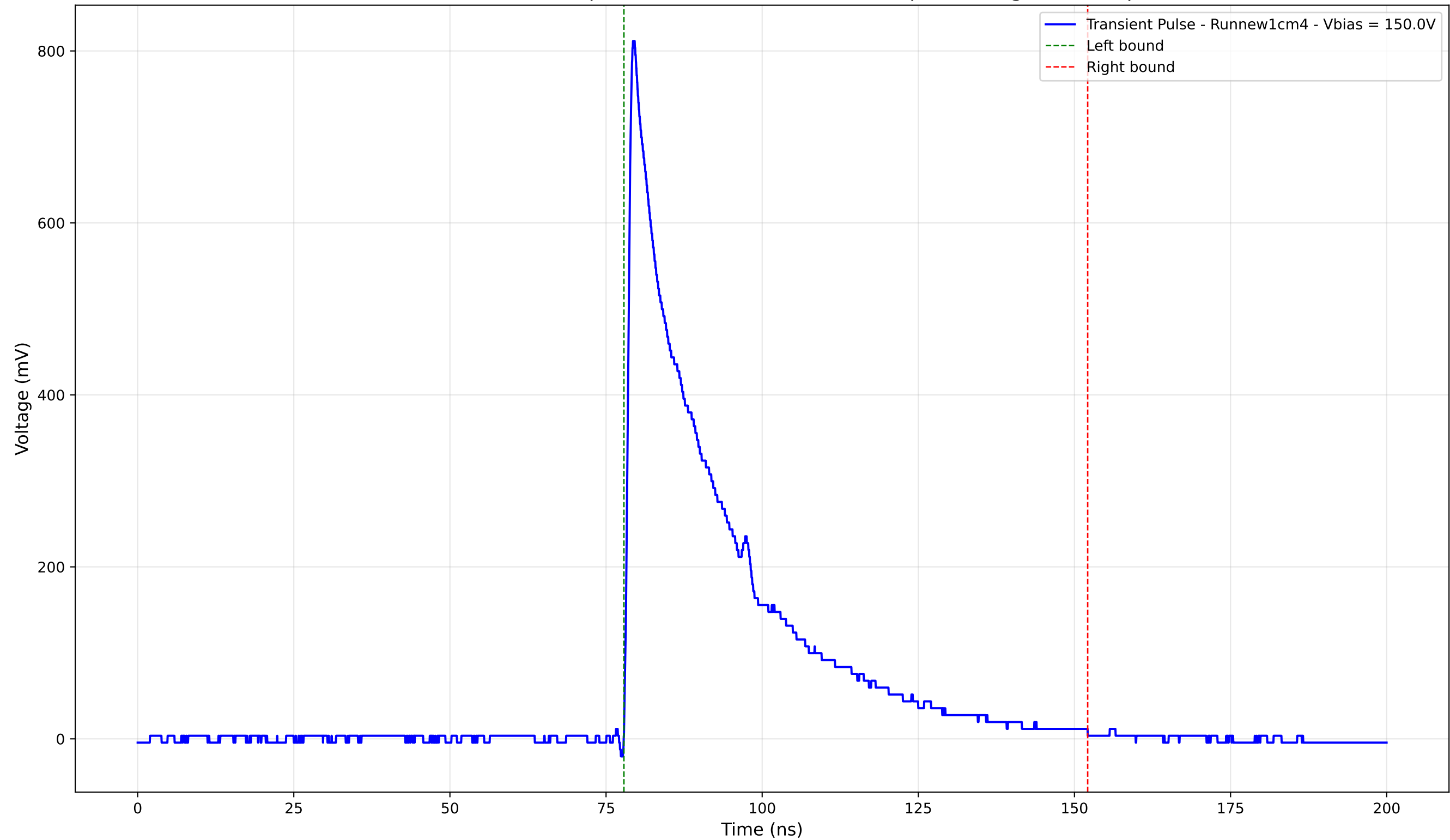
Transient Pulse - Sample: new1cm - Position: 4600.0 \mu\text{m} - Charge: 228.28 pC
