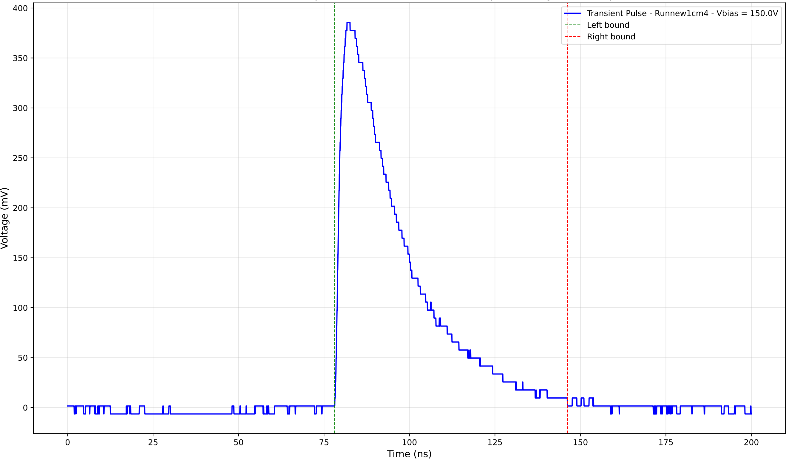
Transient Pulse - Sample: new1cm - Position: 3160.0 \mu\text{m} - Charge: 161.07 pC
