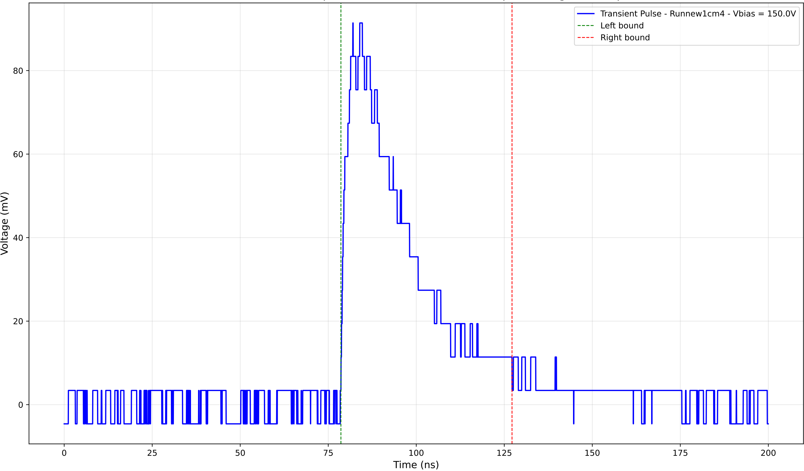
Transient Pulse - Sample: new1cm - Position: 3230.0 \mu\text{m} - Charge: 35.28 pC
