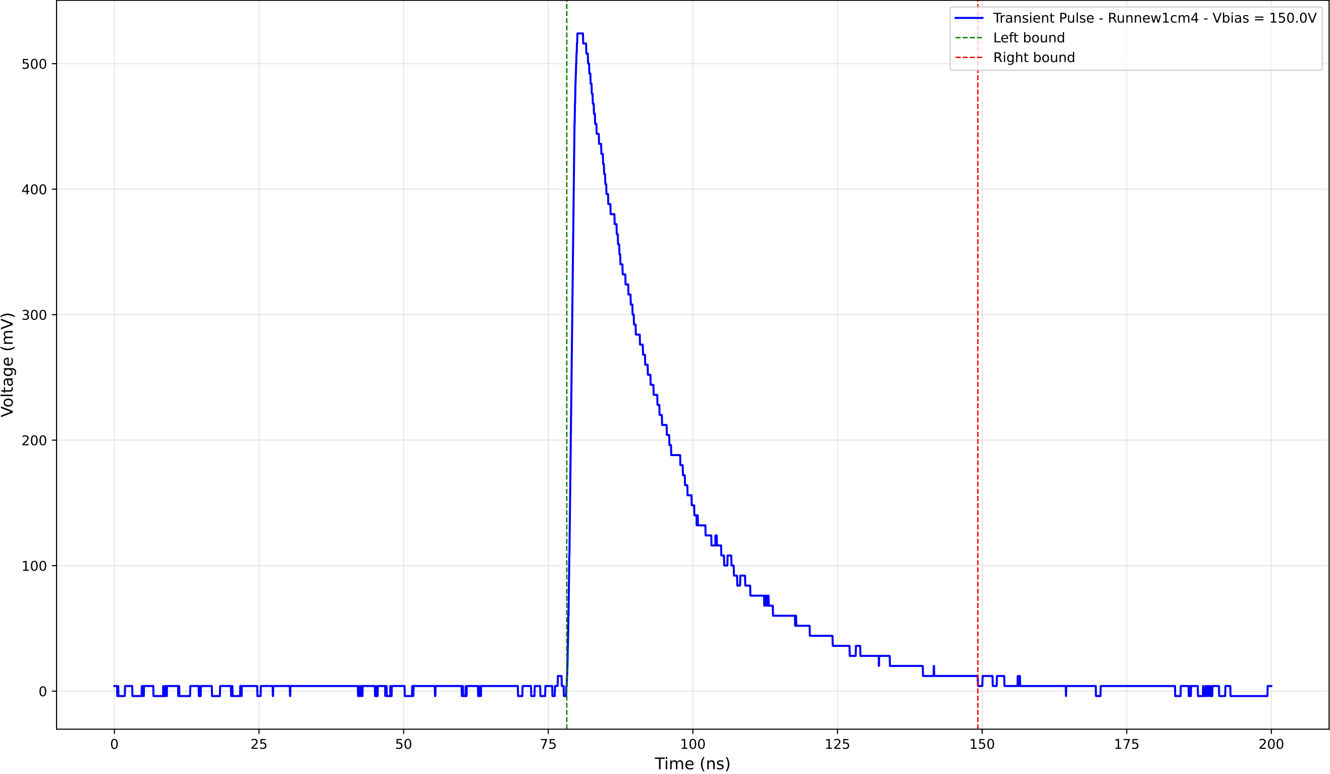
Transient Pulse - Sample: new1cm - Position: 1290.0 \mu\text{m} - Charge: 185.01 pC
