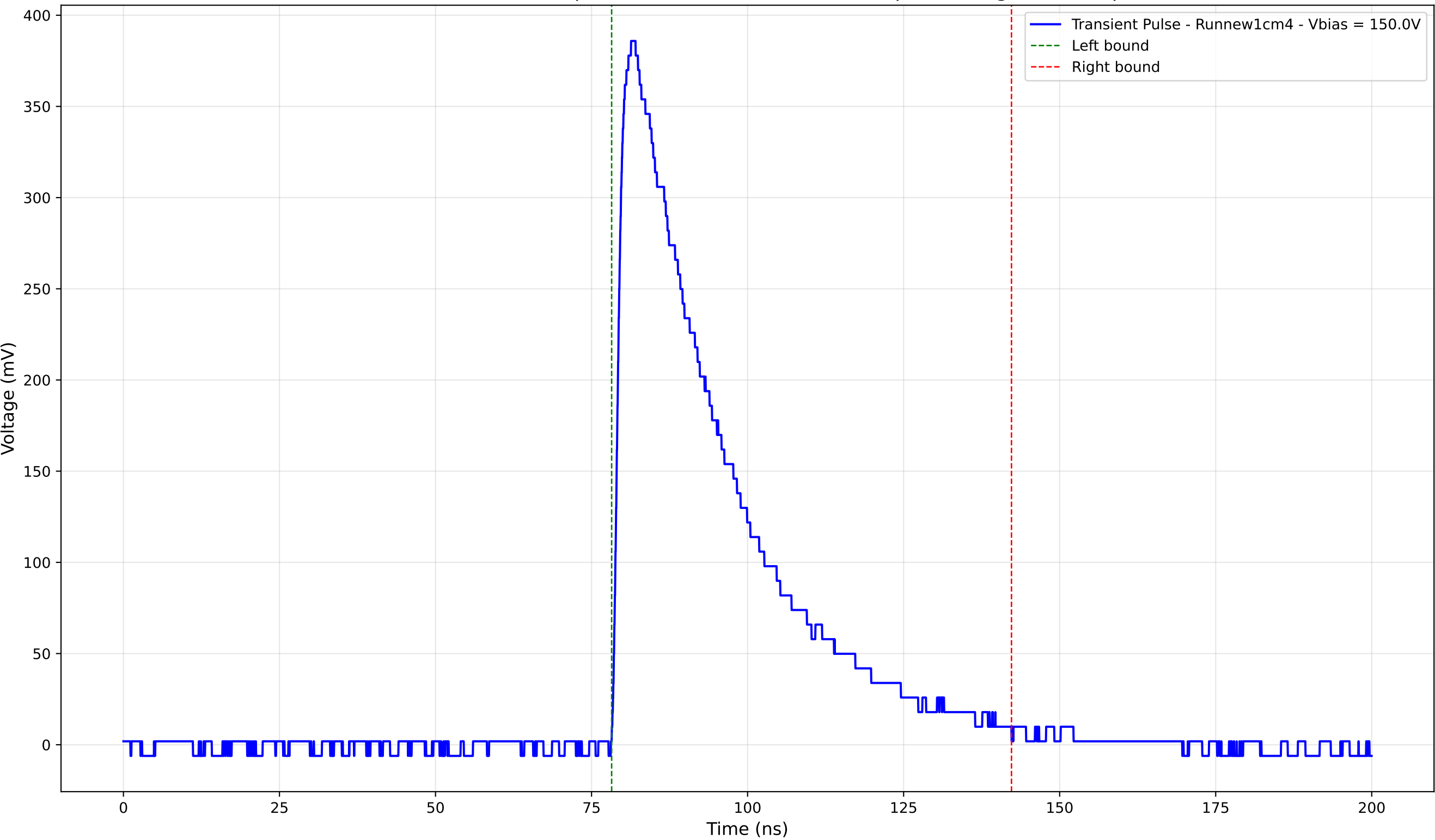
Transient Pulse - Sample: new1cm - Position: 1640.0 \mu\text{m} - Charge: 143.65 pC
