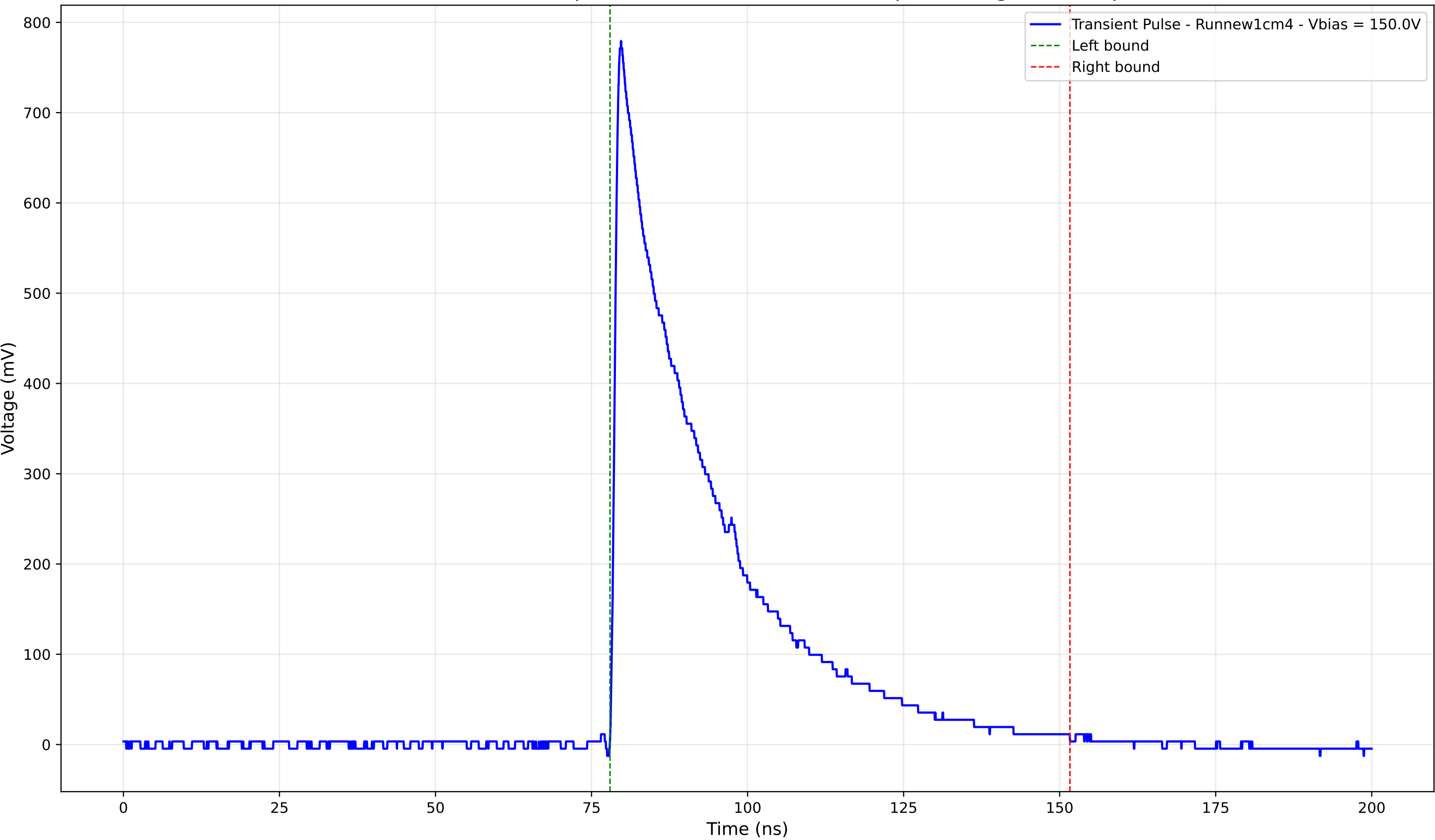
Transient Pulse - Sample: new1cm - Position: 4360.0 \mu\text{m} - Charge: 241.20 pC
