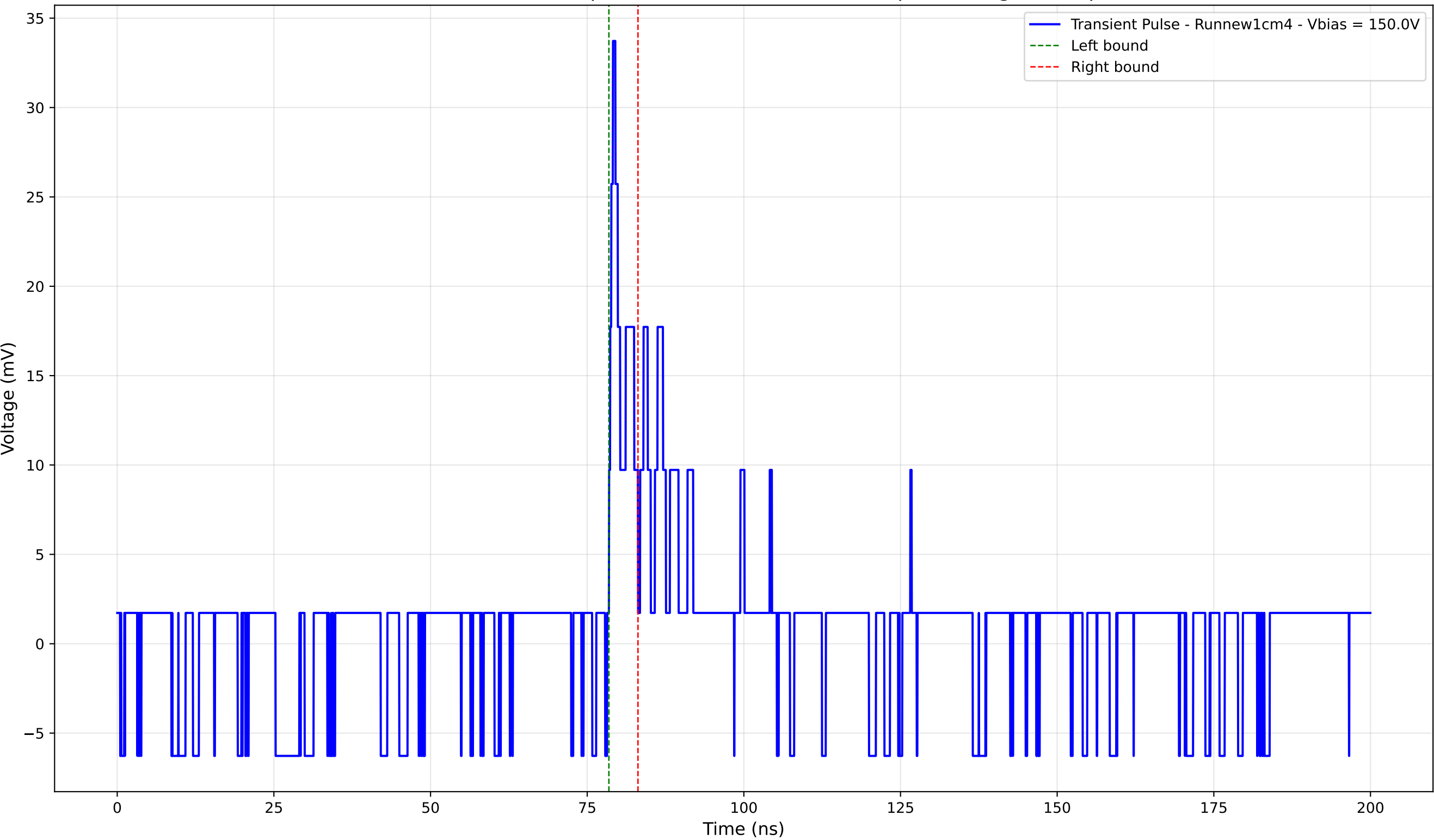
Transient Pulse - Sample: new1cm - Position: 140.0 \mu\text{m} - Charge: 1.60 pC
