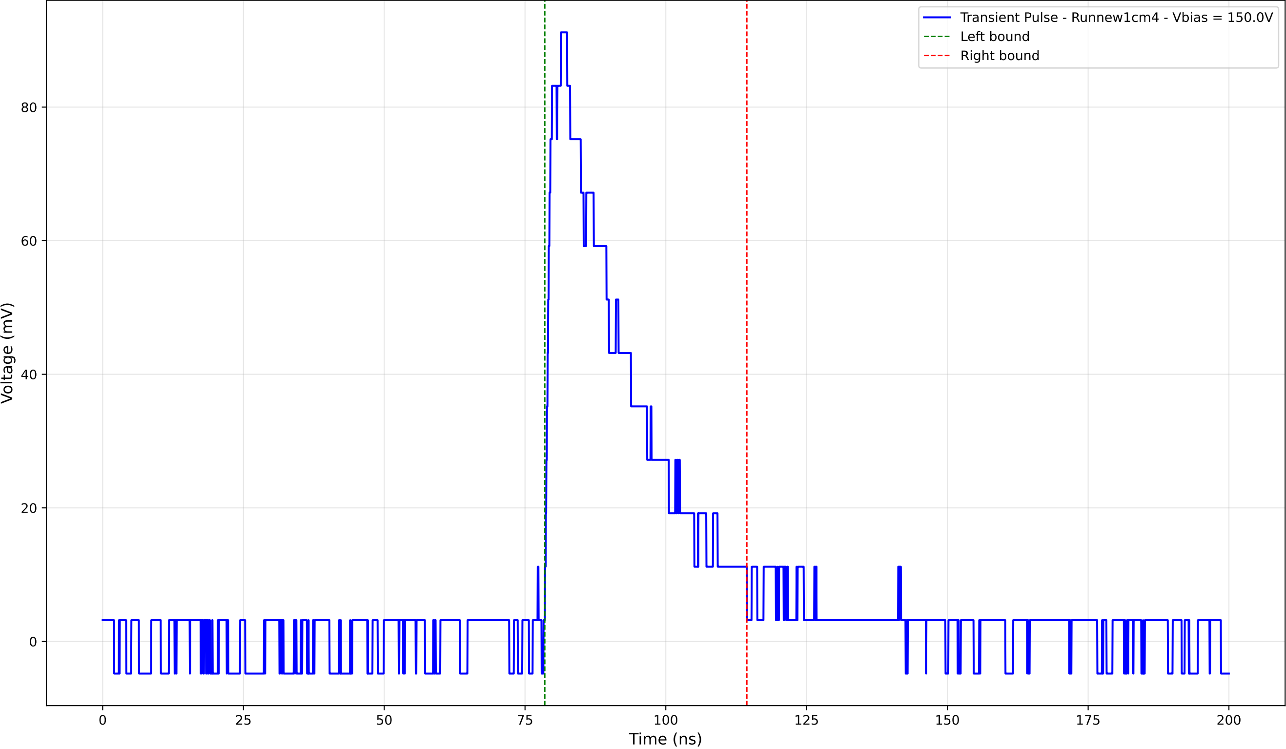
Transient Pulse - Sample: new1cm - Position: 1205.0 \mu\text{m} - Charge: 27.59 pC
