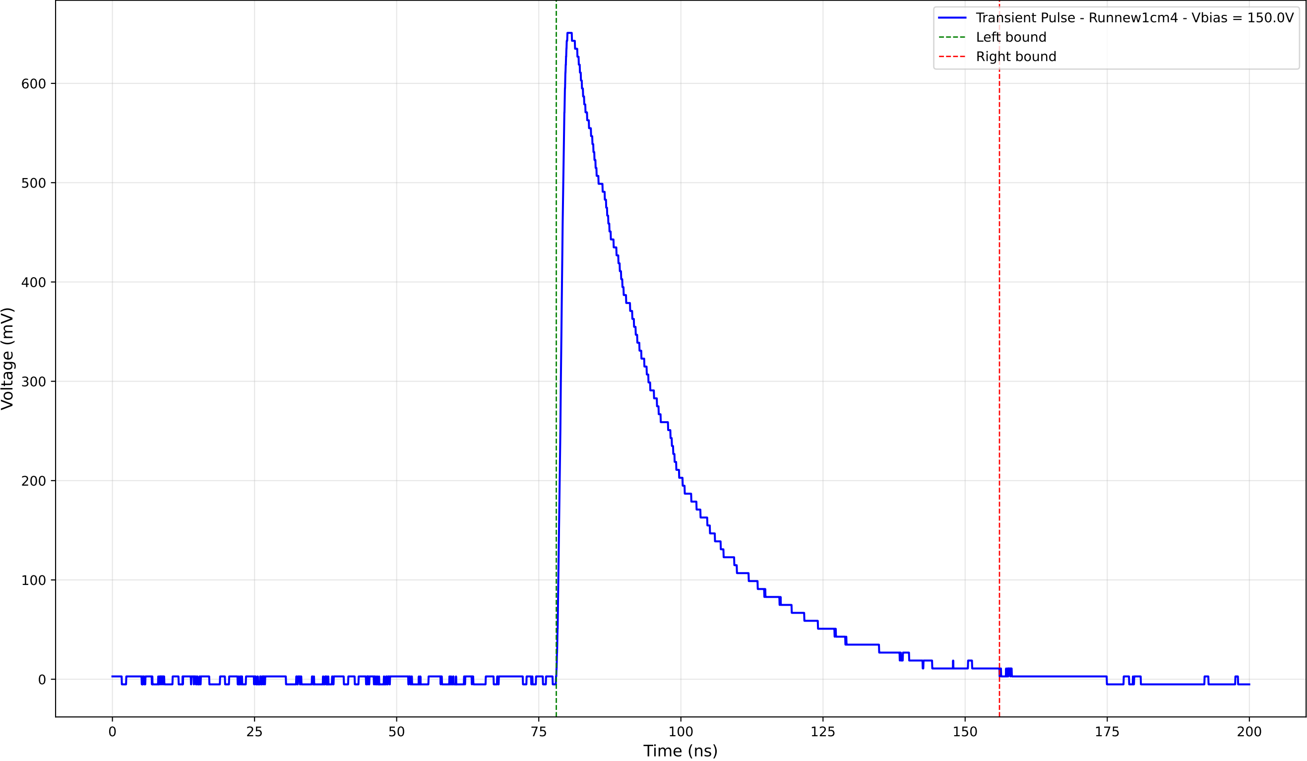
Transient Pulse - Sample: new1cm - Position: 3950.0 \mu\text{m} - Charge: 247.33 pC
