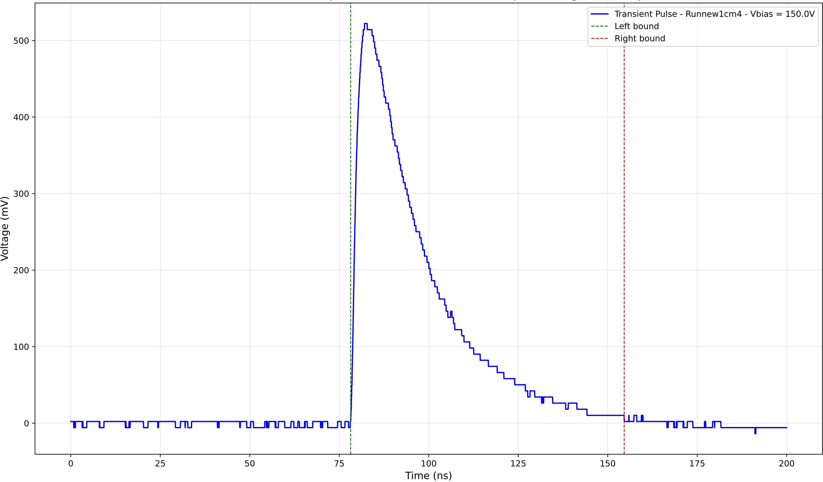
Transient Pulse - Sample: new1cm - Position: 2365.0 \mu\text{m} - Charge: 224.05 pC
