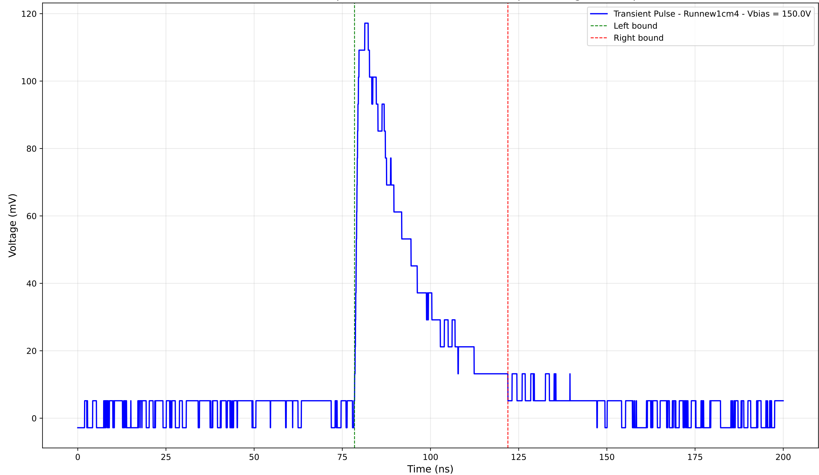
Transient Pulse - Sample: new1cm - Position: 1215.0 \mu\text{m} - Charge: 38.41 pC
