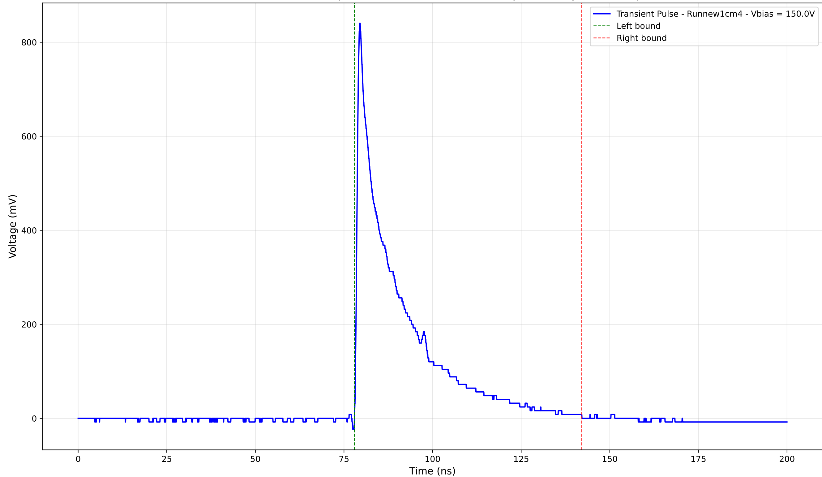
Transient Pulse - Sample: new1cm - Position: 590.0 \mu\text{m} - Charge: 185.34 pC
