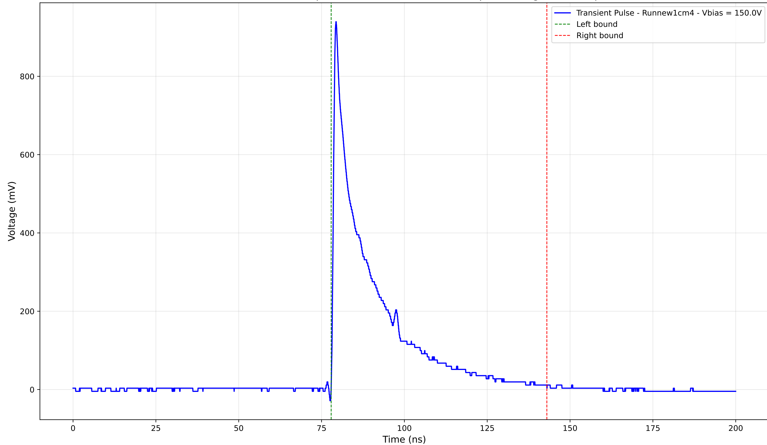
Transient Pulse - Sample: new1cm - Position: 440.0 \mu\text{m} - Charge: 201.37 pC
