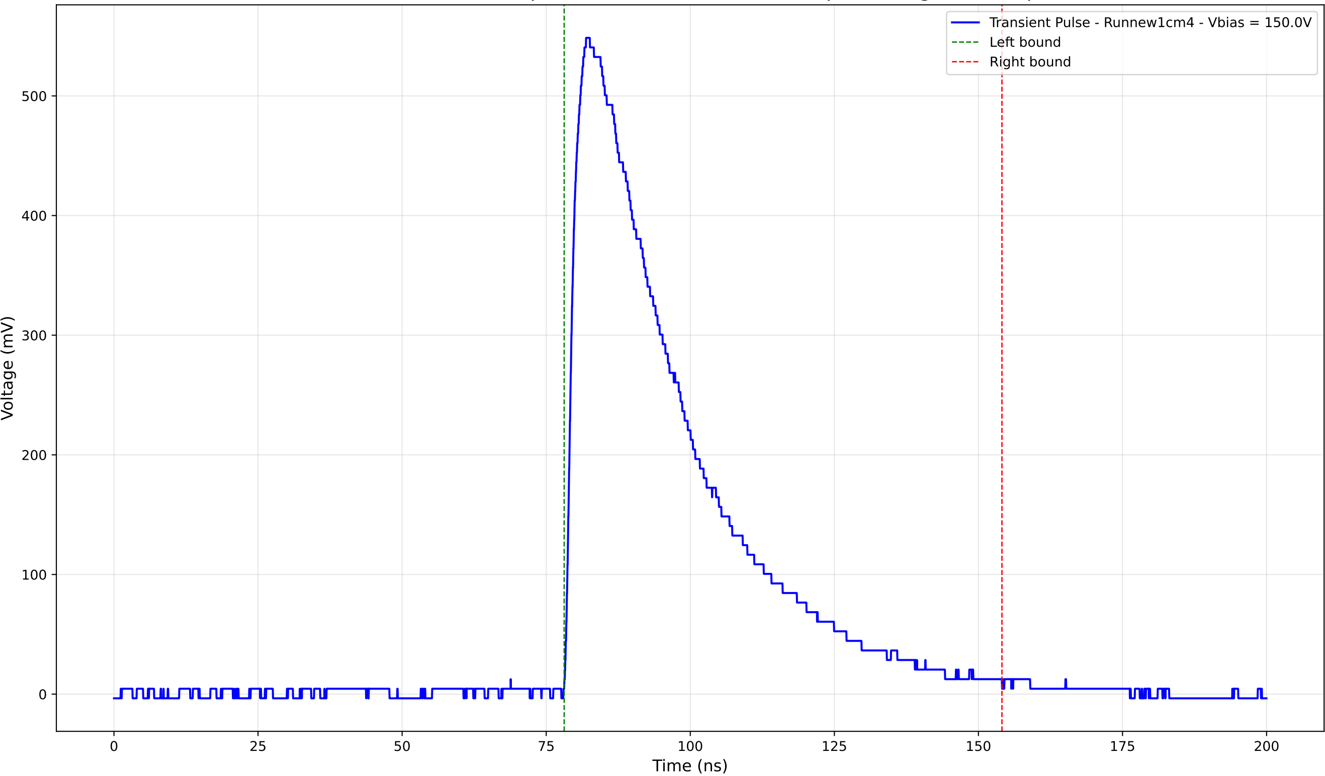
Transient Pulse - Sample: new1cm - Position: 3085.0 \mu\text{m} - Charge: 239.36 pC
