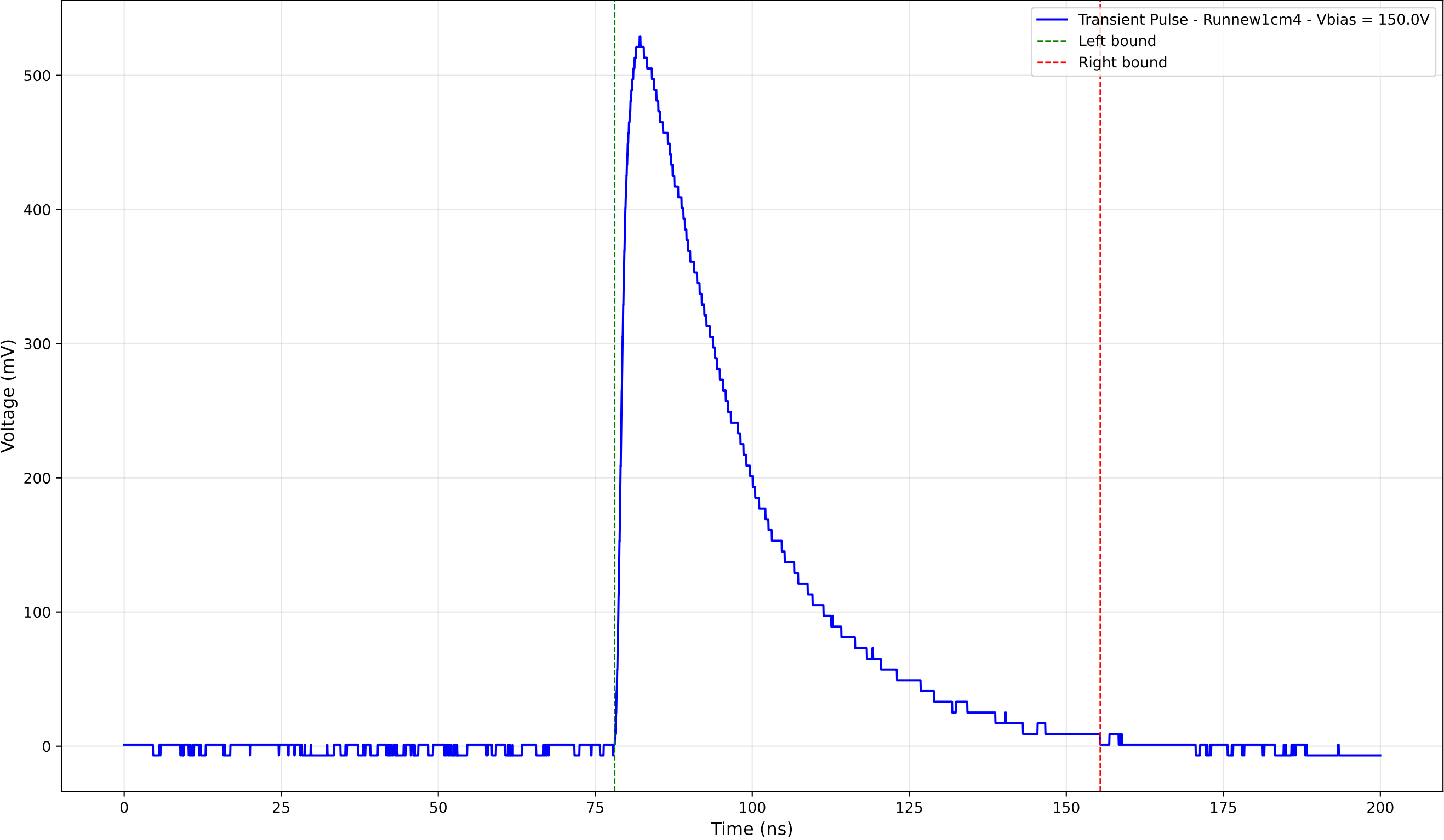
Transient Pulse - Sample: new1cm - Position: 3320.0 \mu\text{m} - Charge: 221.11 pC
