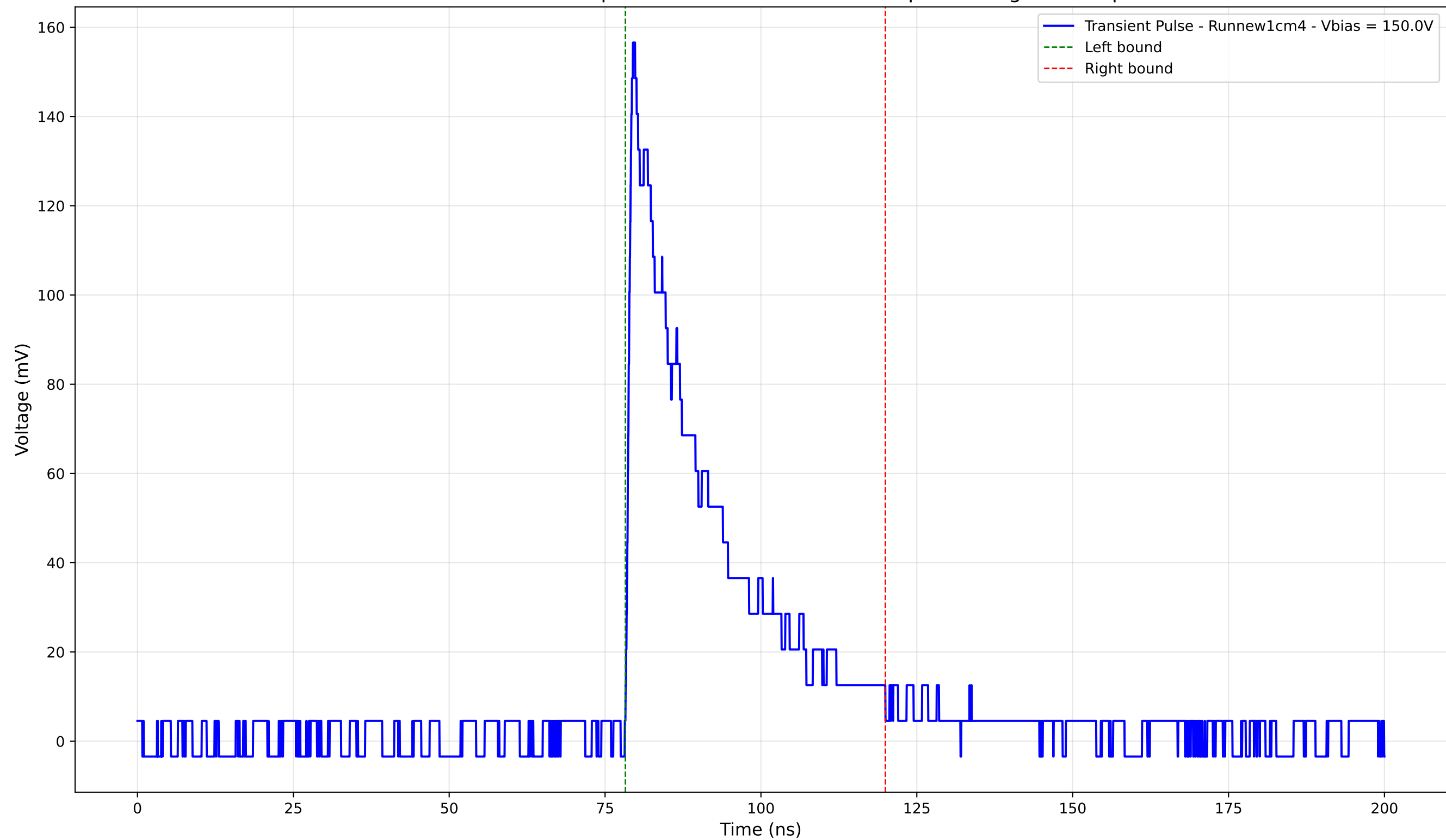
Transient Pulse - Sample: new1cm - Position: 710.0 \mu\text{m} - Charge: 38.84 pC
