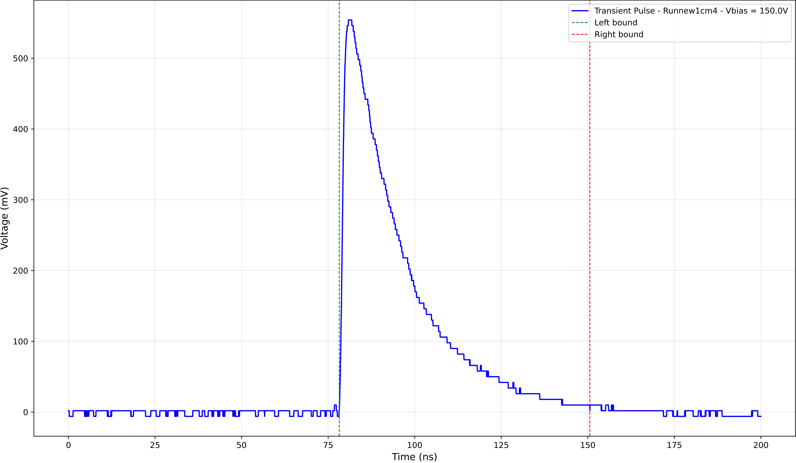
Transient Pulse - Sample: new1cm - Position: 1550.0 \mu\text{m} - Charge: 210.22 pC
