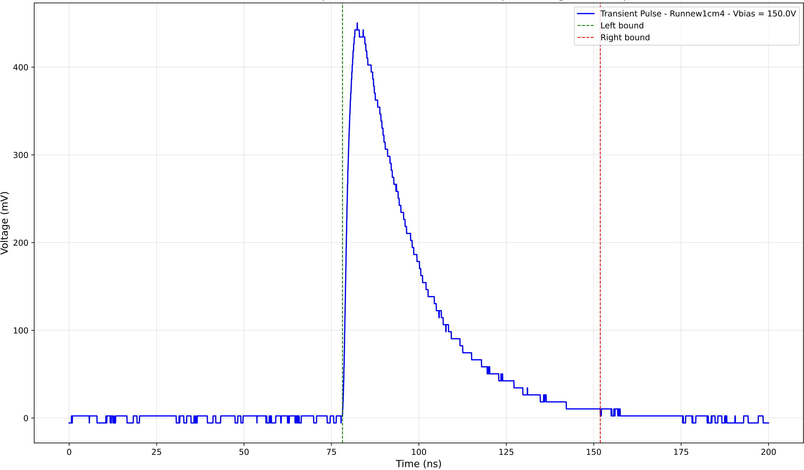
Transient Pulse - Sample: new1cm - Position: 2285.0 \mu\text{m} - Charge: 189.17 pC
