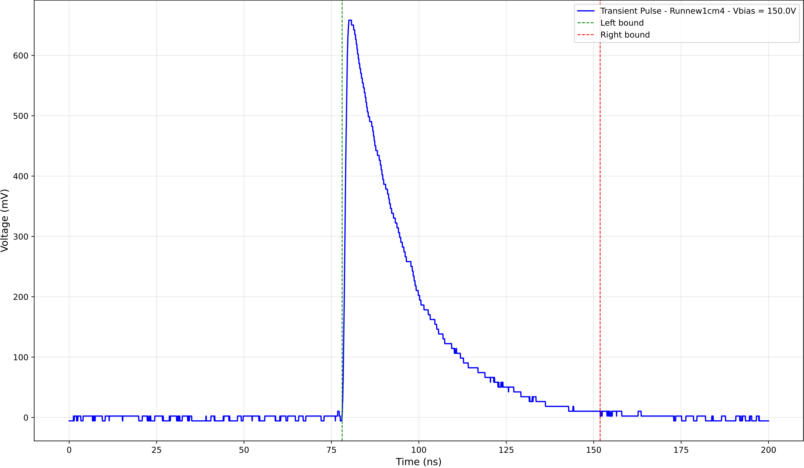
Transient Pulse - Sample: new1cm - Position: 3980.0 \mu\text{m} - Charge: 244.71 pC
