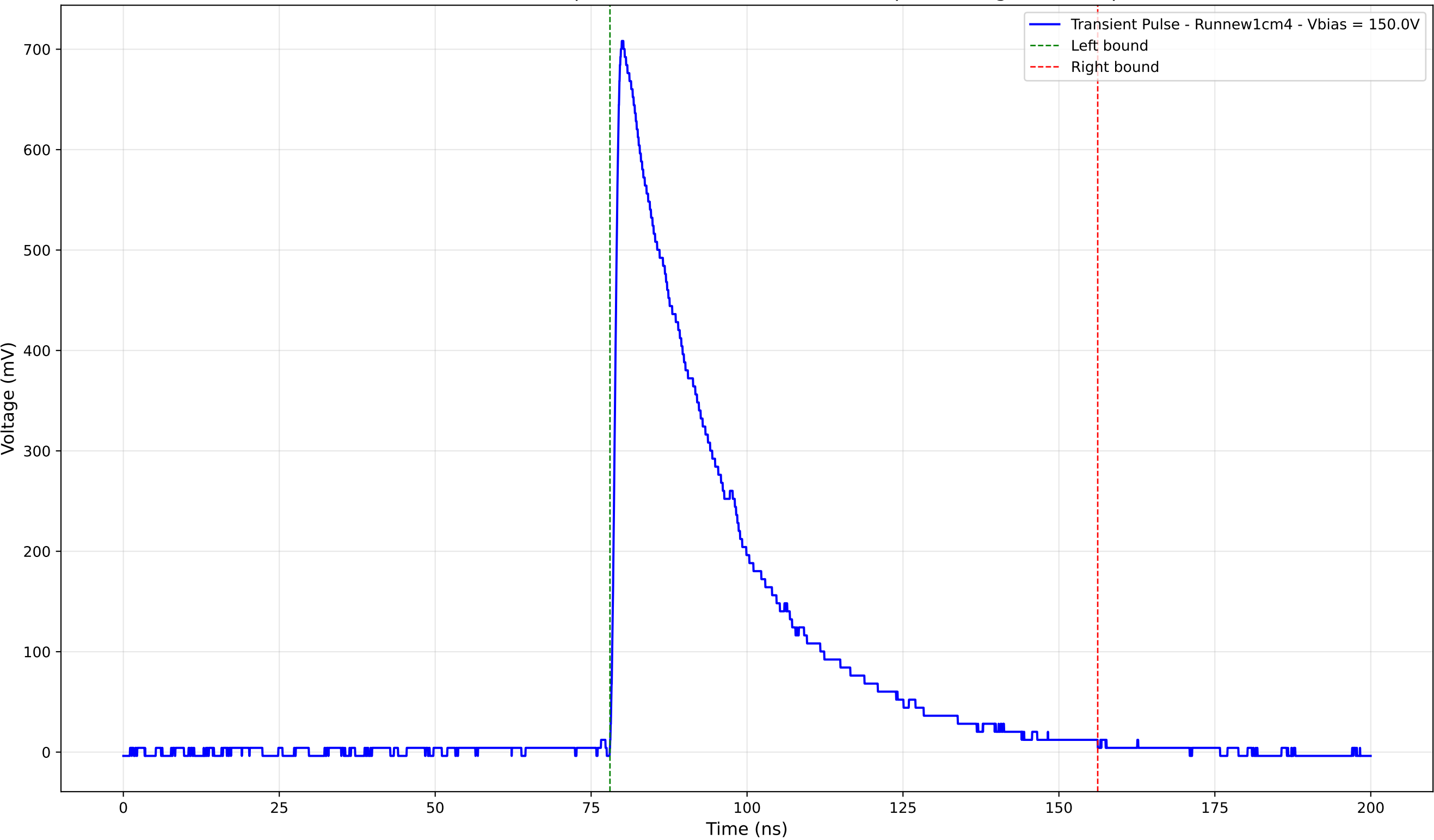
Transient Pulse - Sample: new1cm - Position: 4115.0 \mu\text{m} - Charge: 250.77 pC
