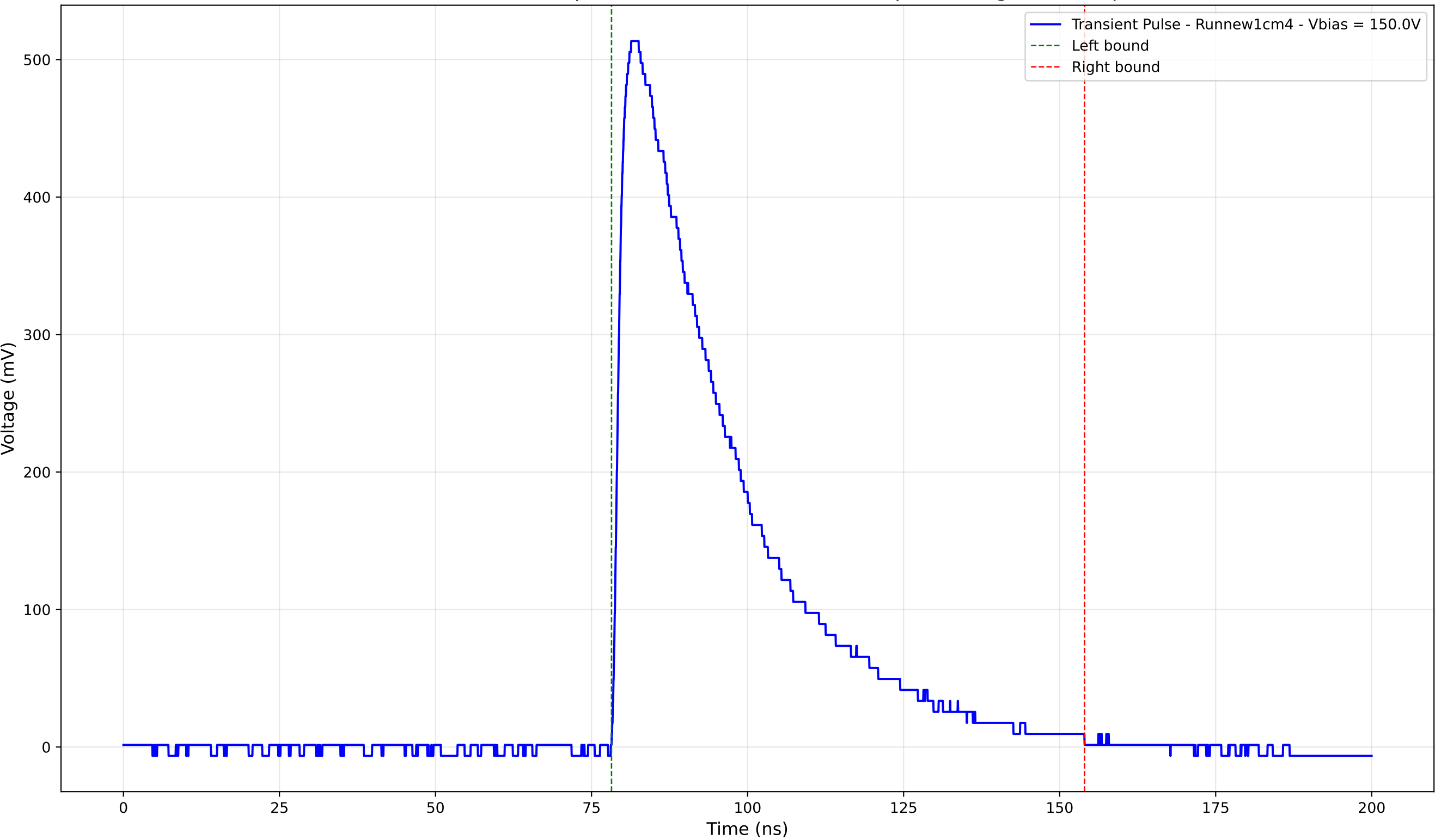
Transient Pulse - Sample: new1cm - Position: 1815.0 \mu\text{m} - Charge: 206.65 pC
