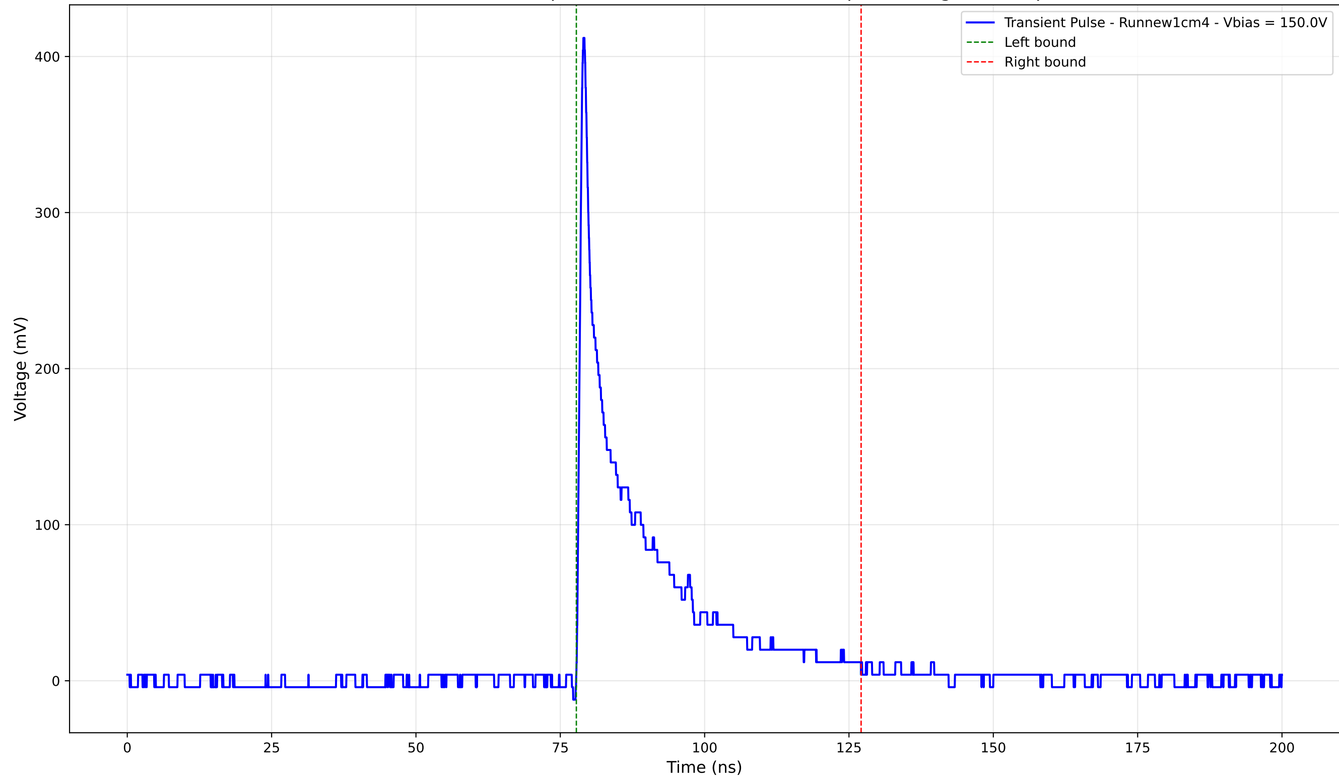
Transient Pulse - Sample: new1cm - Position: 5035.0 \mu\text{m} - Charge: 66.03 pC
