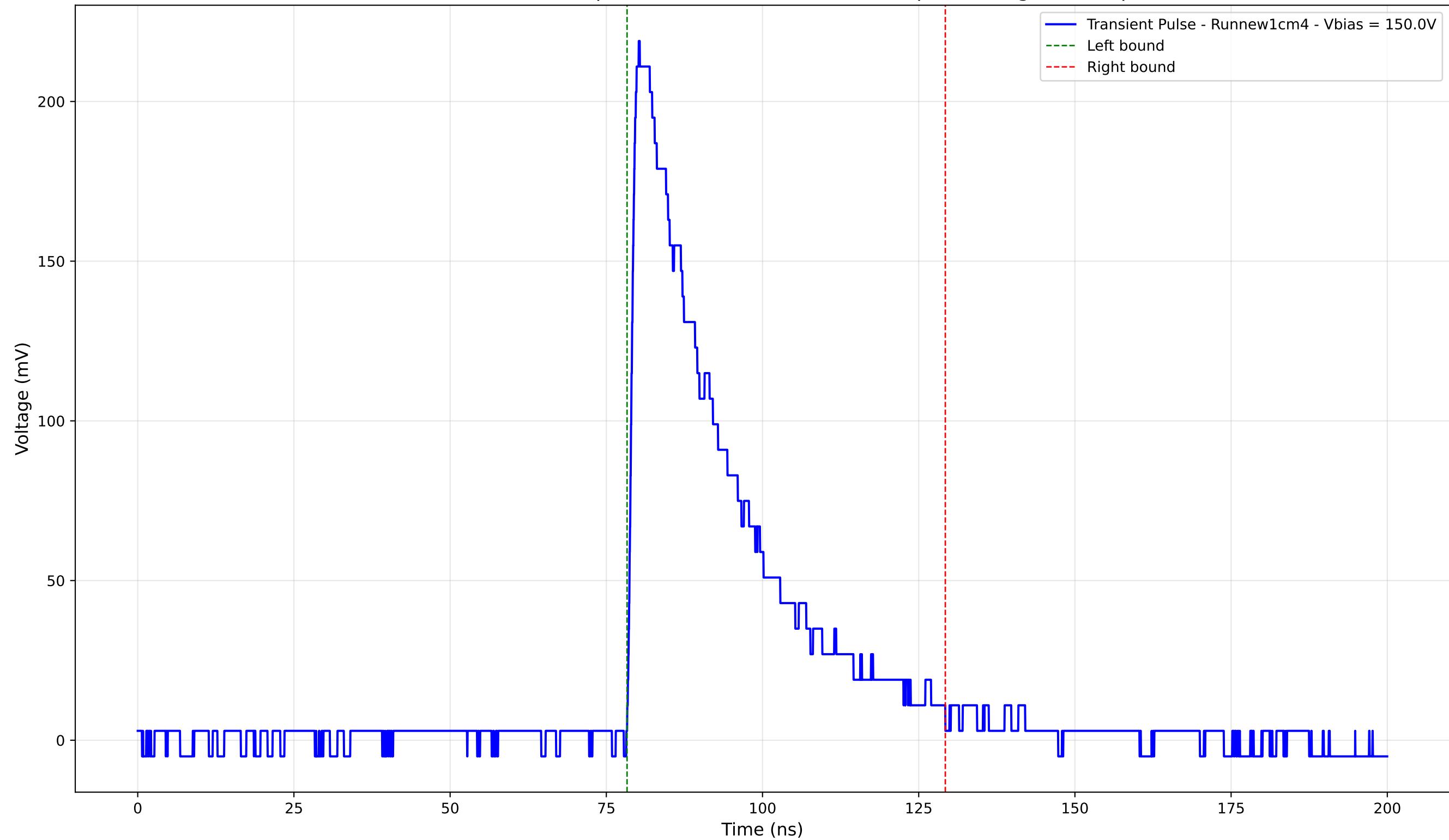
Transient Pulse - Sample: new1cm - Position: 1235.0 \mu\text{m} - Charge: 70.19 pC
