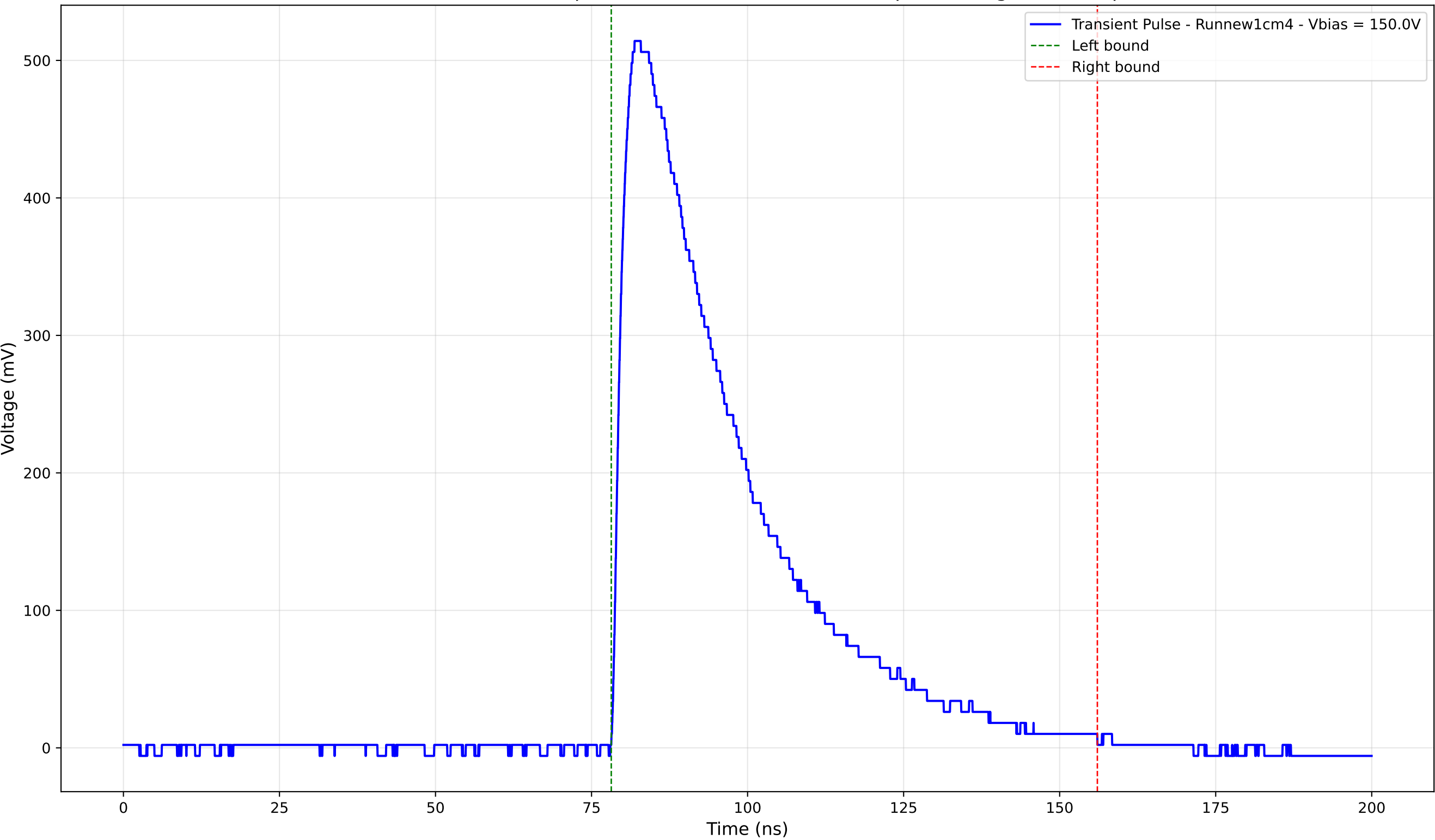
Transient Pulse - Sample: new1cm - Position: 2325.0 \mu\text{m} - Charge: 220.03 pC
