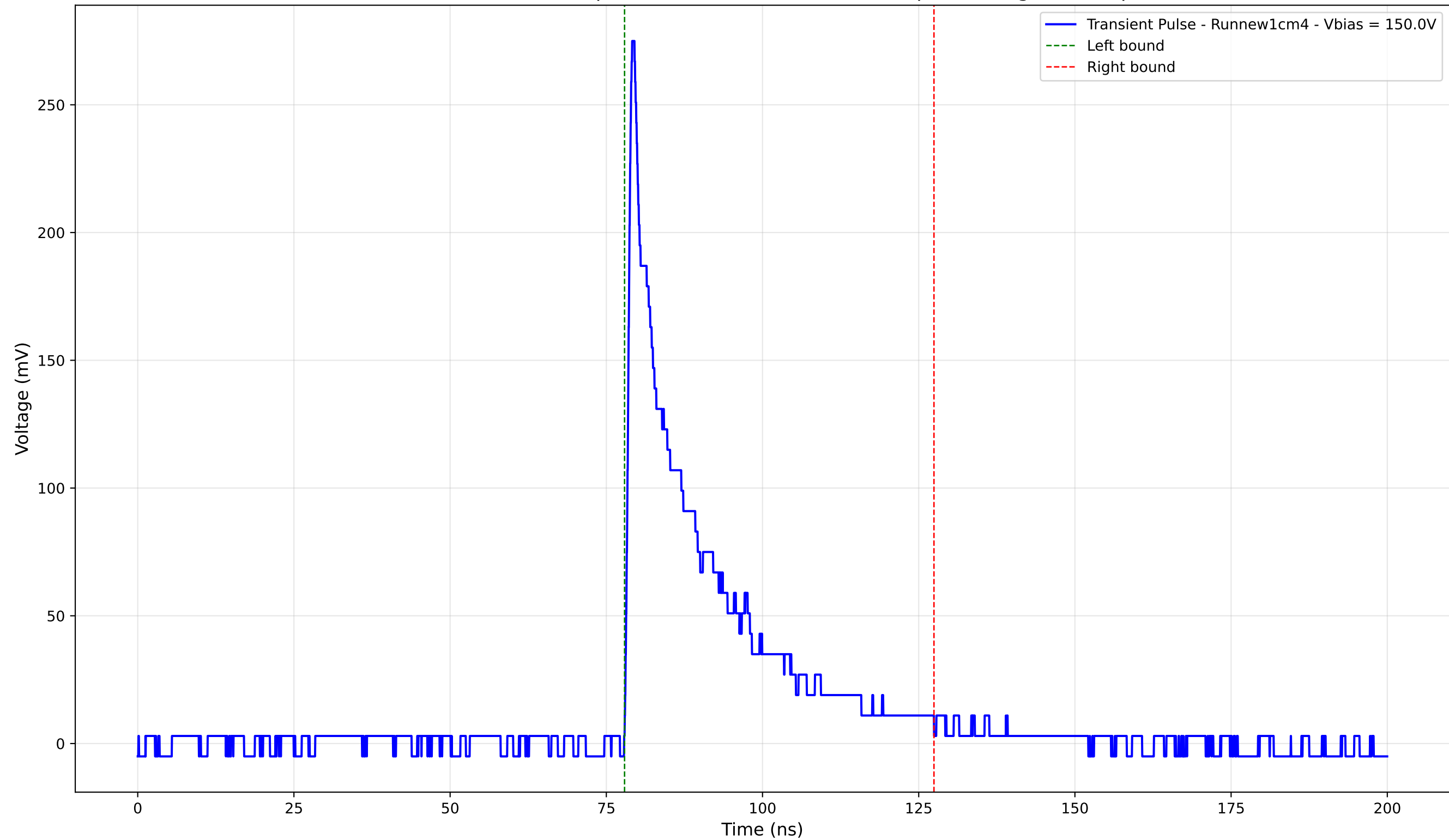
Transient Pulse - Sample: new1cm - Position: 4760.0 \mu\text{m} - Charge: 54.90 pC
