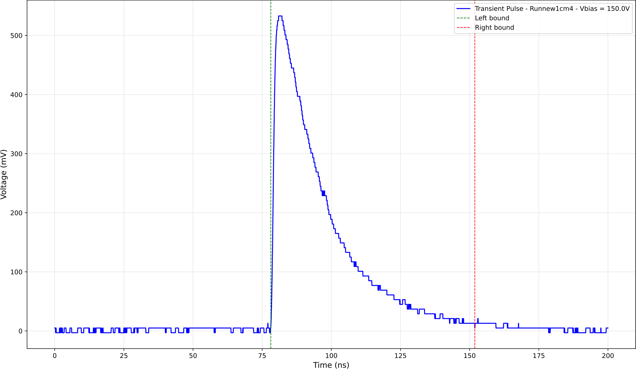
Transient Pulse - Sample: new1cm - Position: 3645.0 \mu\text{m} - Charge: 220.07 pC
