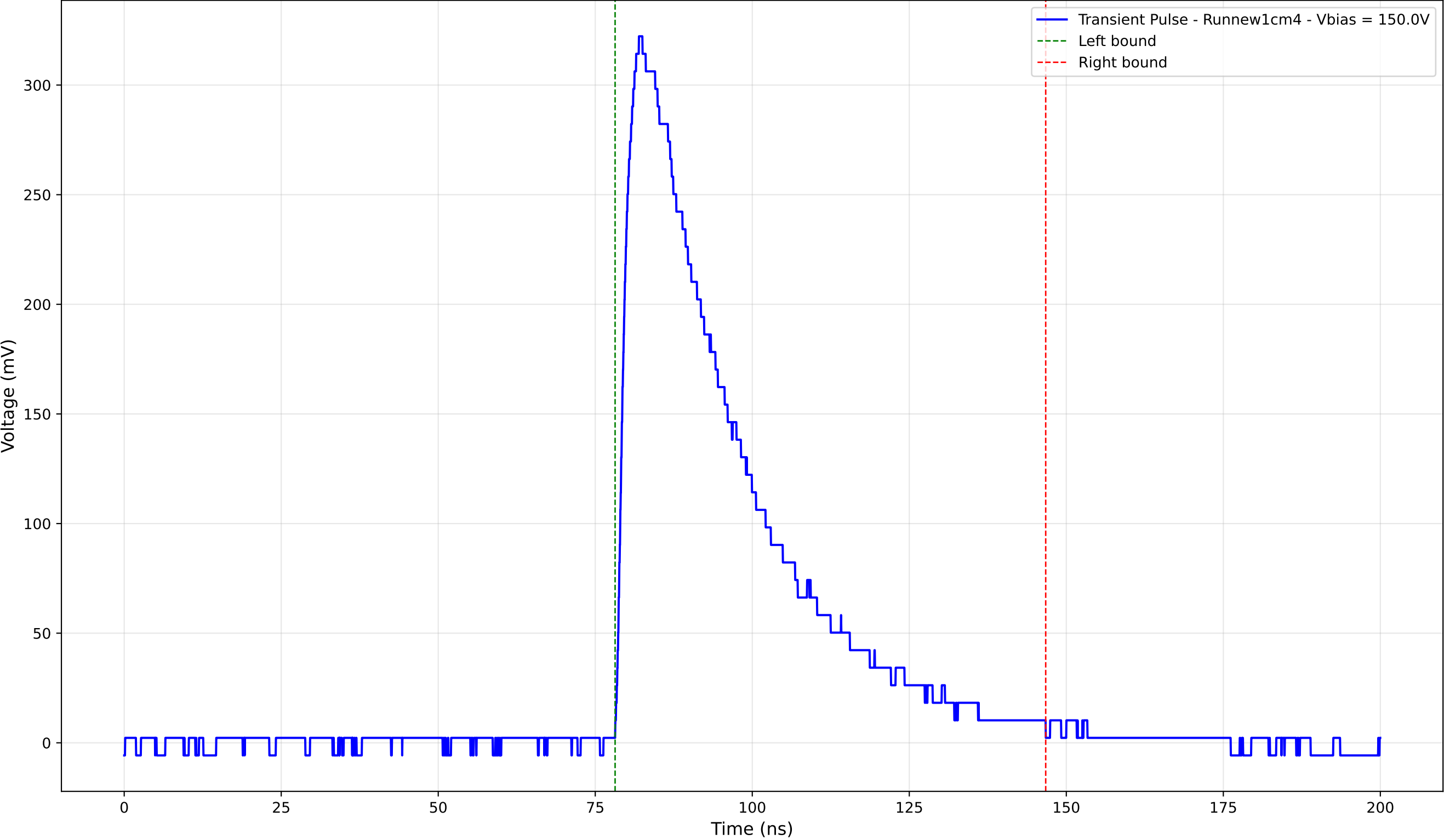
Transient Pulse - Sample: new1cm - Position: 2150.0 \mu\text{m} - Charge: 129.91 pC
