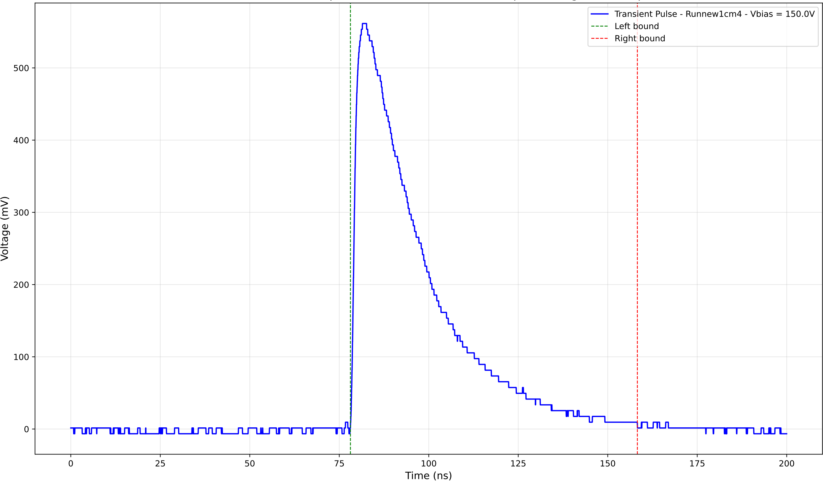
Transient Pulse - Sample: new1cm - Position: 3420.0 \mu\text{m} - Charge: 238.95 pC
