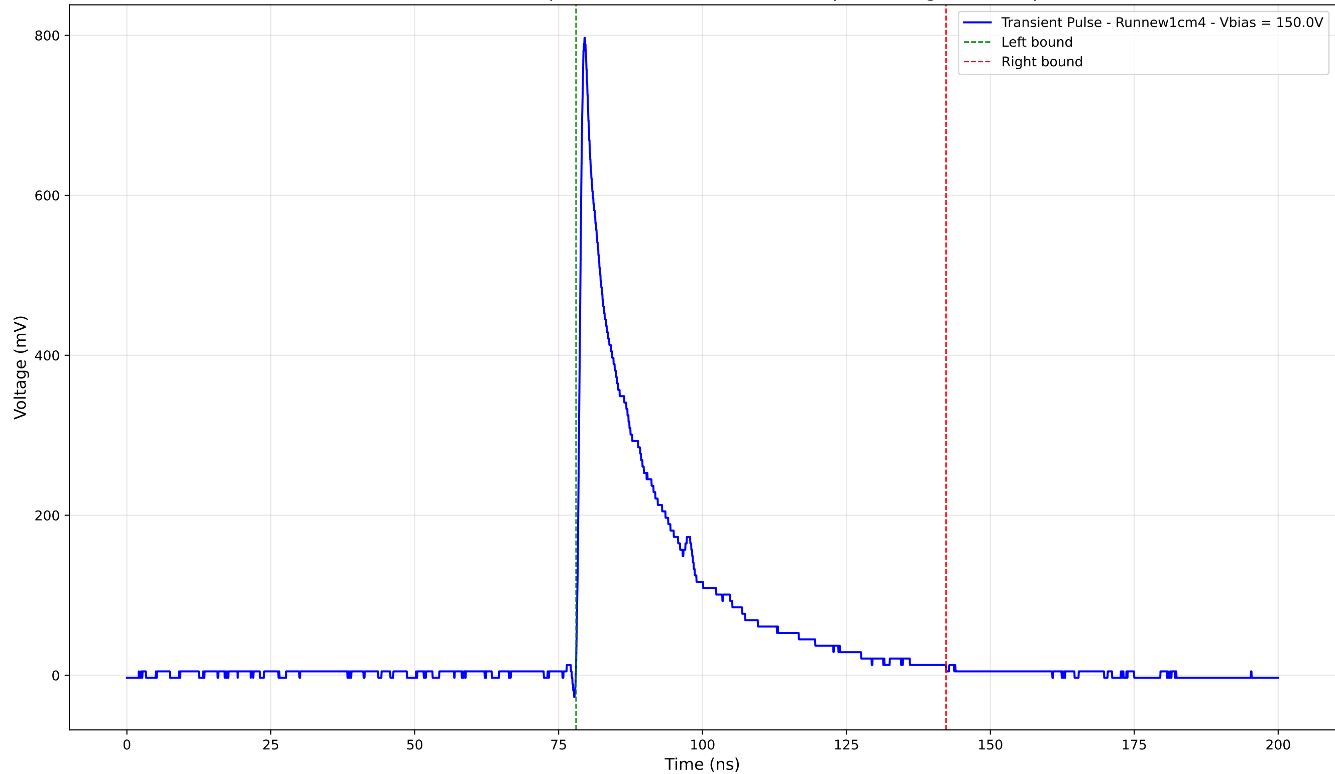
Transient Pulse - Sample: new1cm - Position: 605.0 \mu\text{m} - Charge: 177.27 pC
