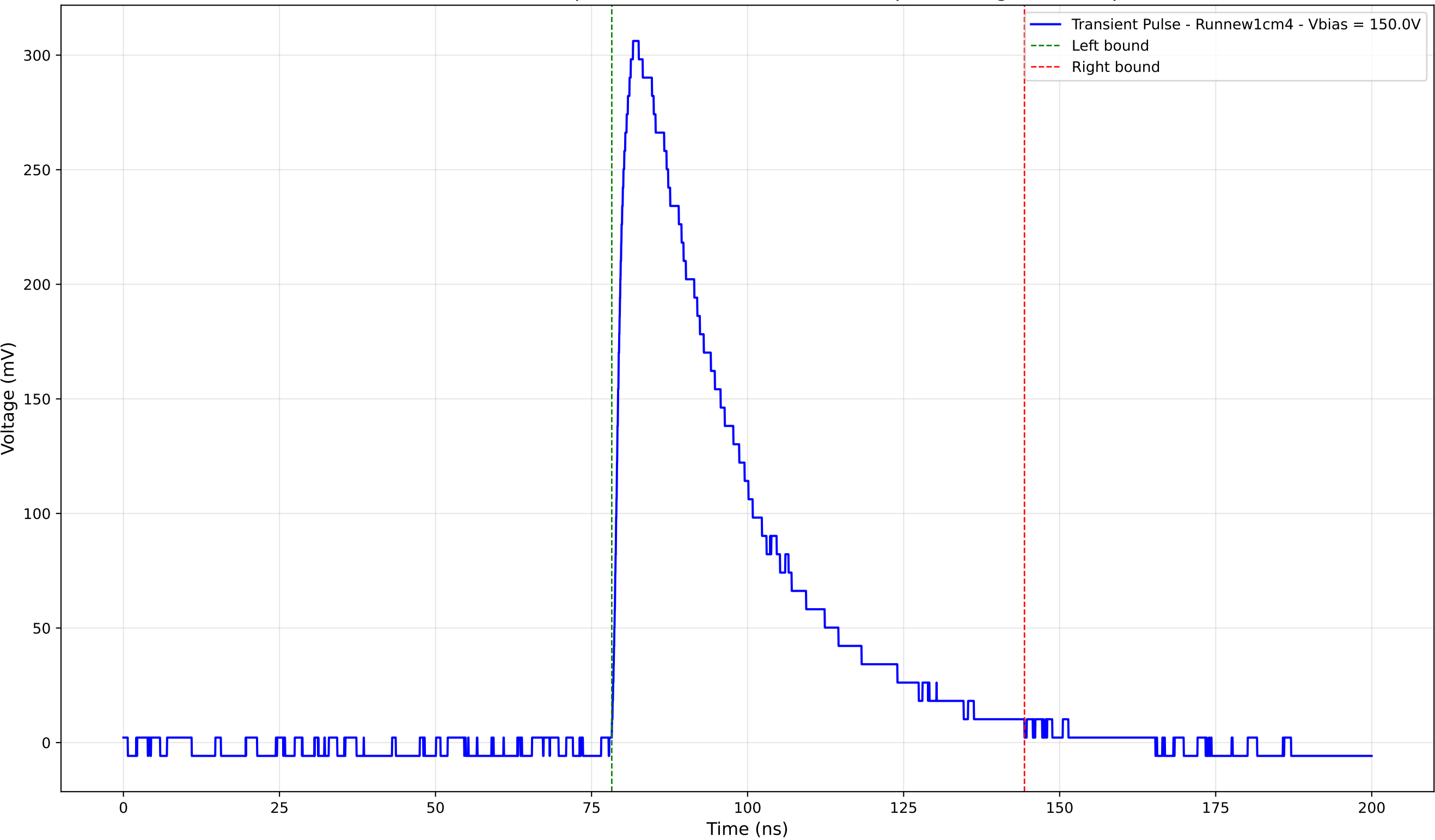
Transient Pulse - Sample: new1cm - Position: 3275.0 \mu\text{m} - Charge: 124.56 pC
