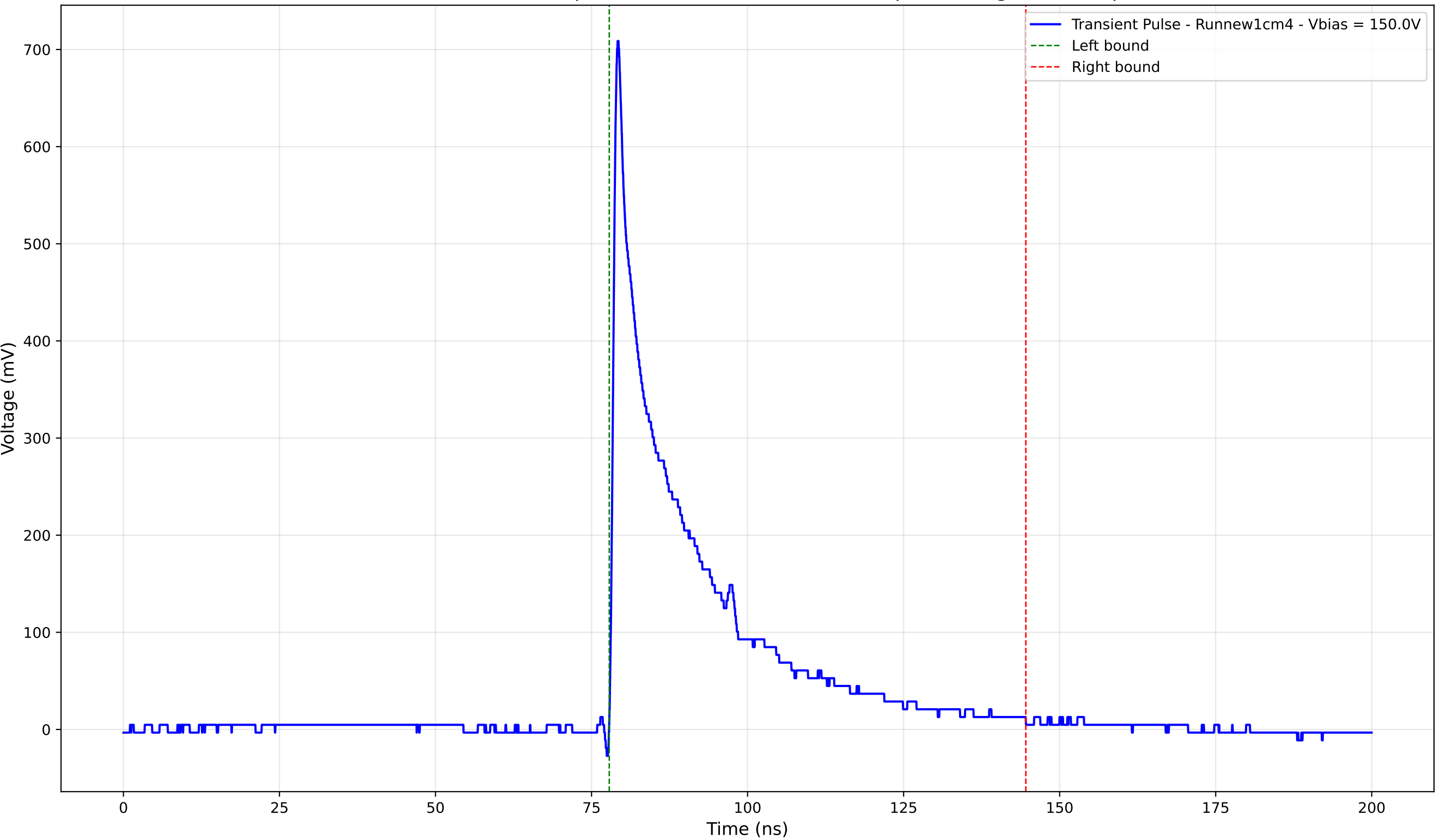
Transient Pulse - Sample: new1cm - Position: 4805.0 \mu\text{m} - Charge: 150.09 pC
