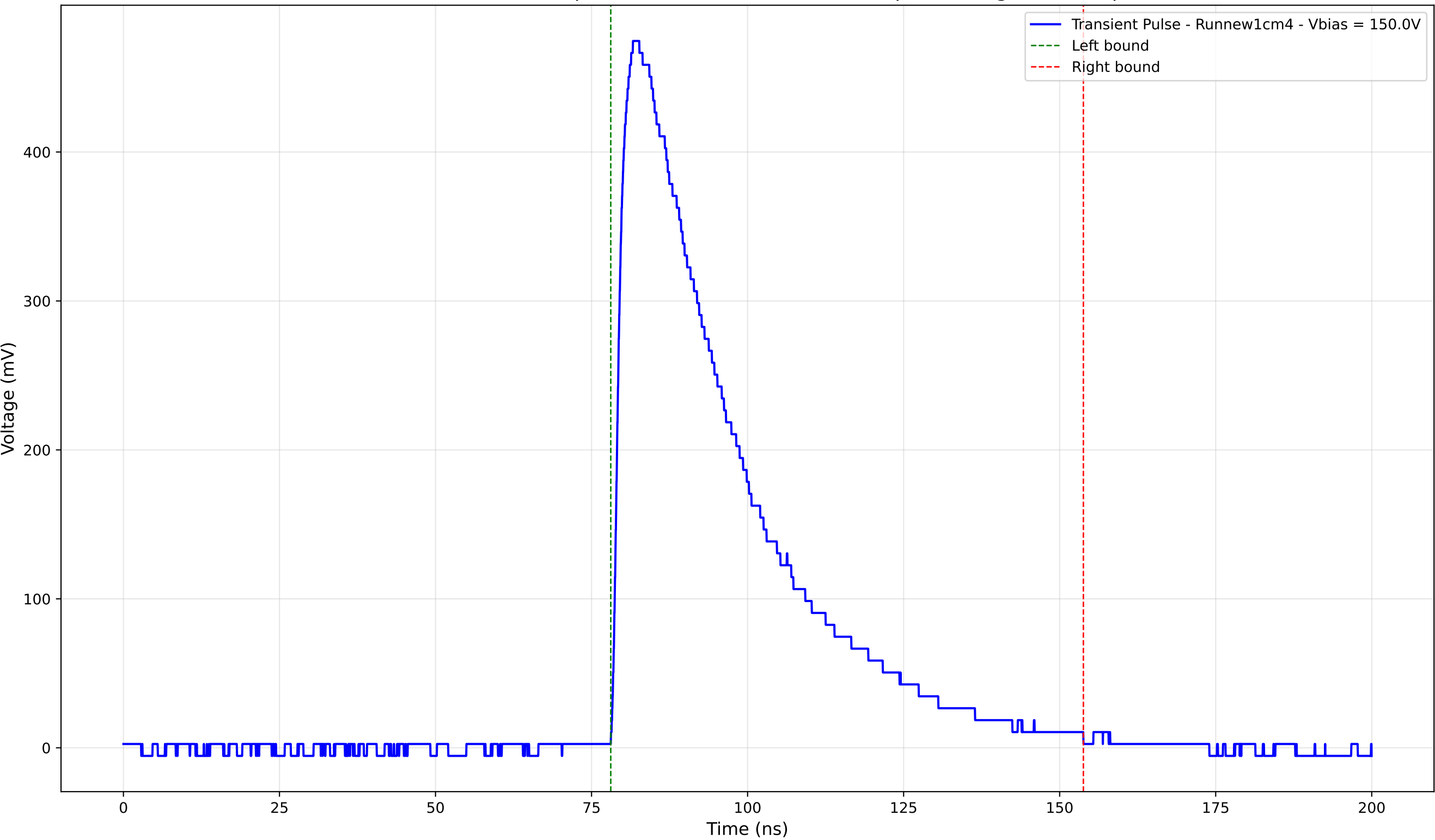
Transient Pulse - Sample: new1cm - Position: 3305.0 \mu\text{m} - Charge: 200.61 pC
