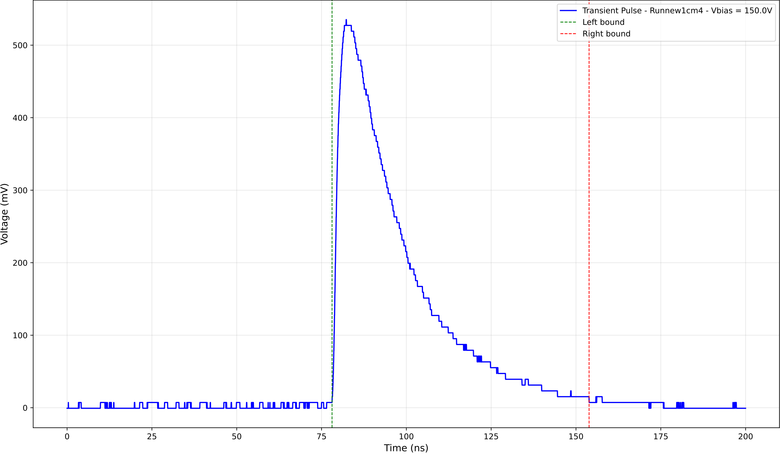
Transient Pulse - Sample: new1cm - Position: 2980.0 \mu\text{m} - Charge: 236.40 pC
