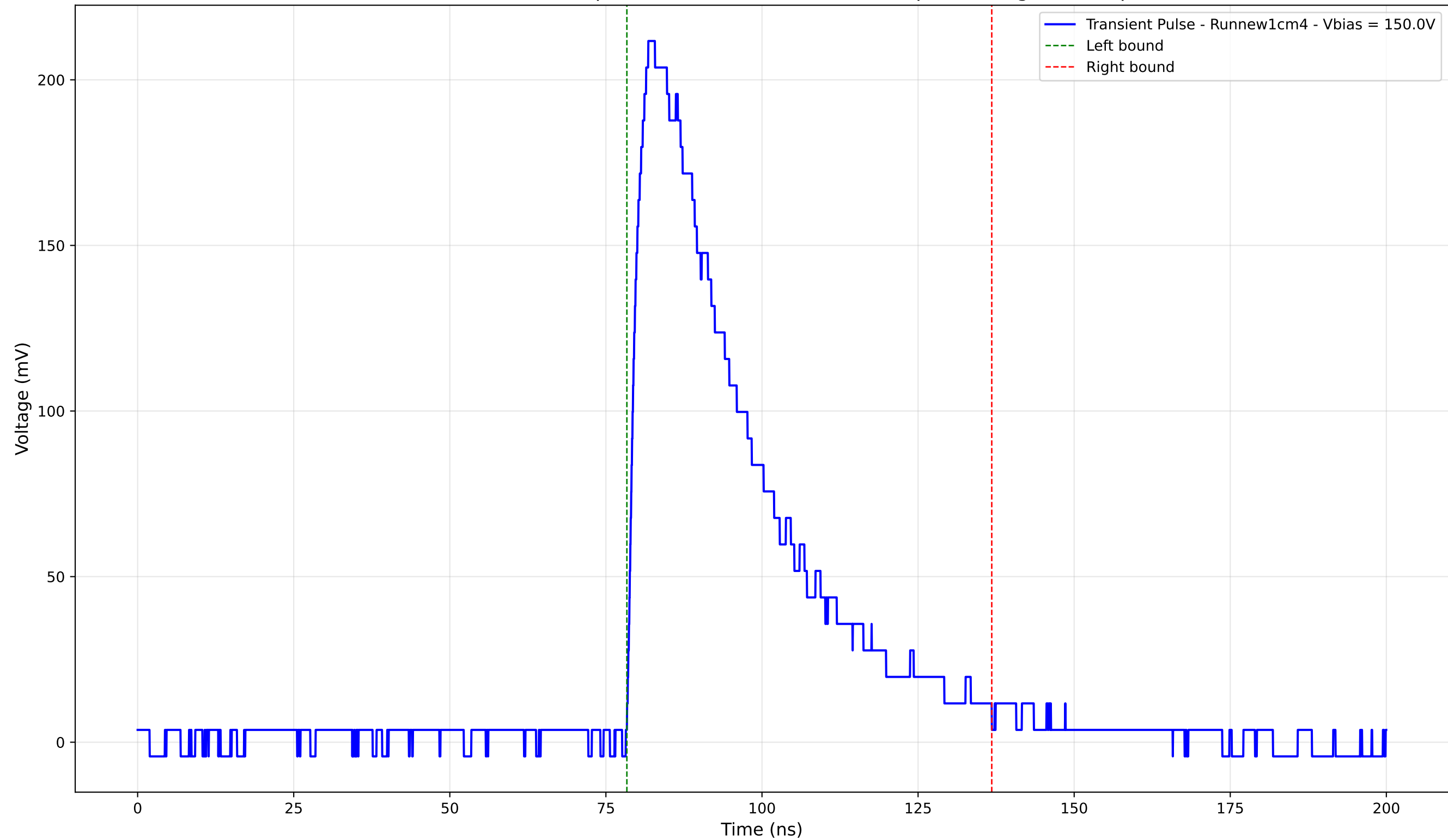
Transient Pulse - Sample: new1cm - Position: 2240.0 \mu\text{m} - Charge: 86.92 pC
