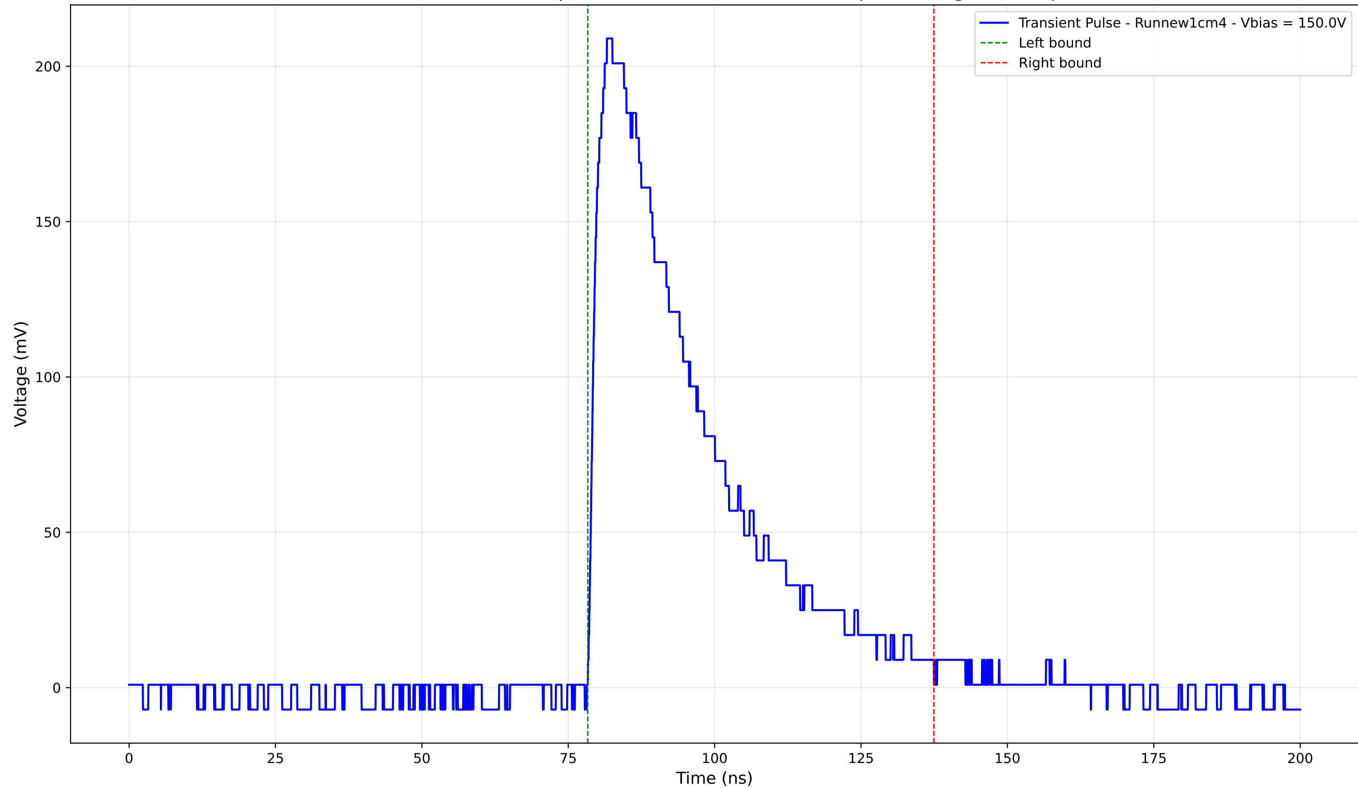
Transient Pulse - Sample: new1cm - Position: 3260.0 \mu\text{m} - Charge: 83.61 pC
