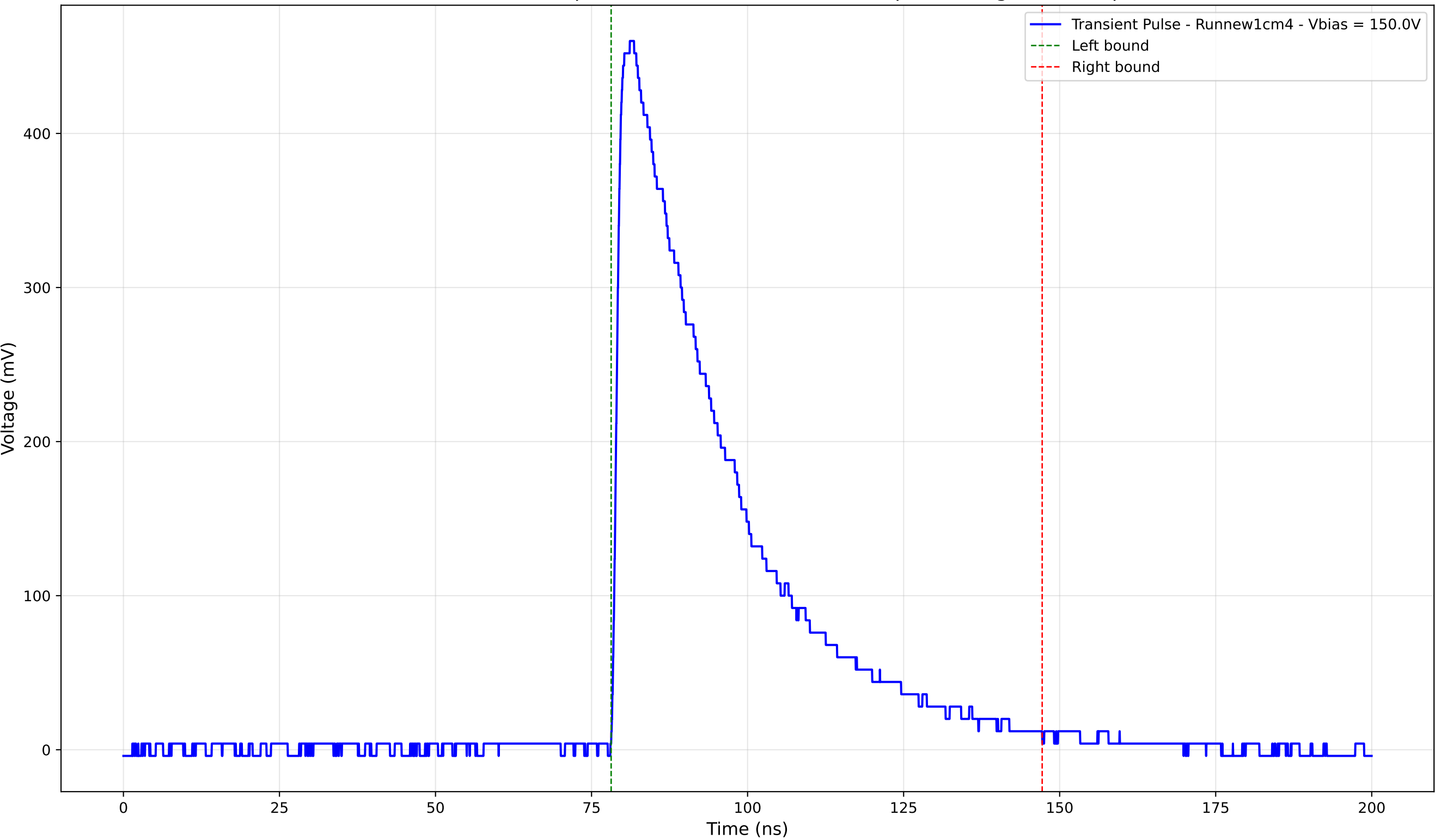
Transient Pulse - Sample: new1cm - Position: 3795.0 \mu\text{m} - Charge: 177.19 pC
