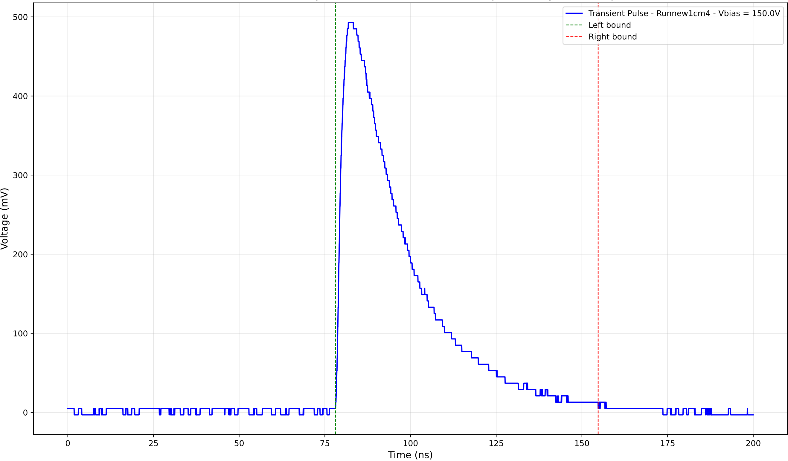
Transient Pulse - Sample: new1cm - Position: 2305.0 \mu\text{m} - Charge: 214.46 pC
