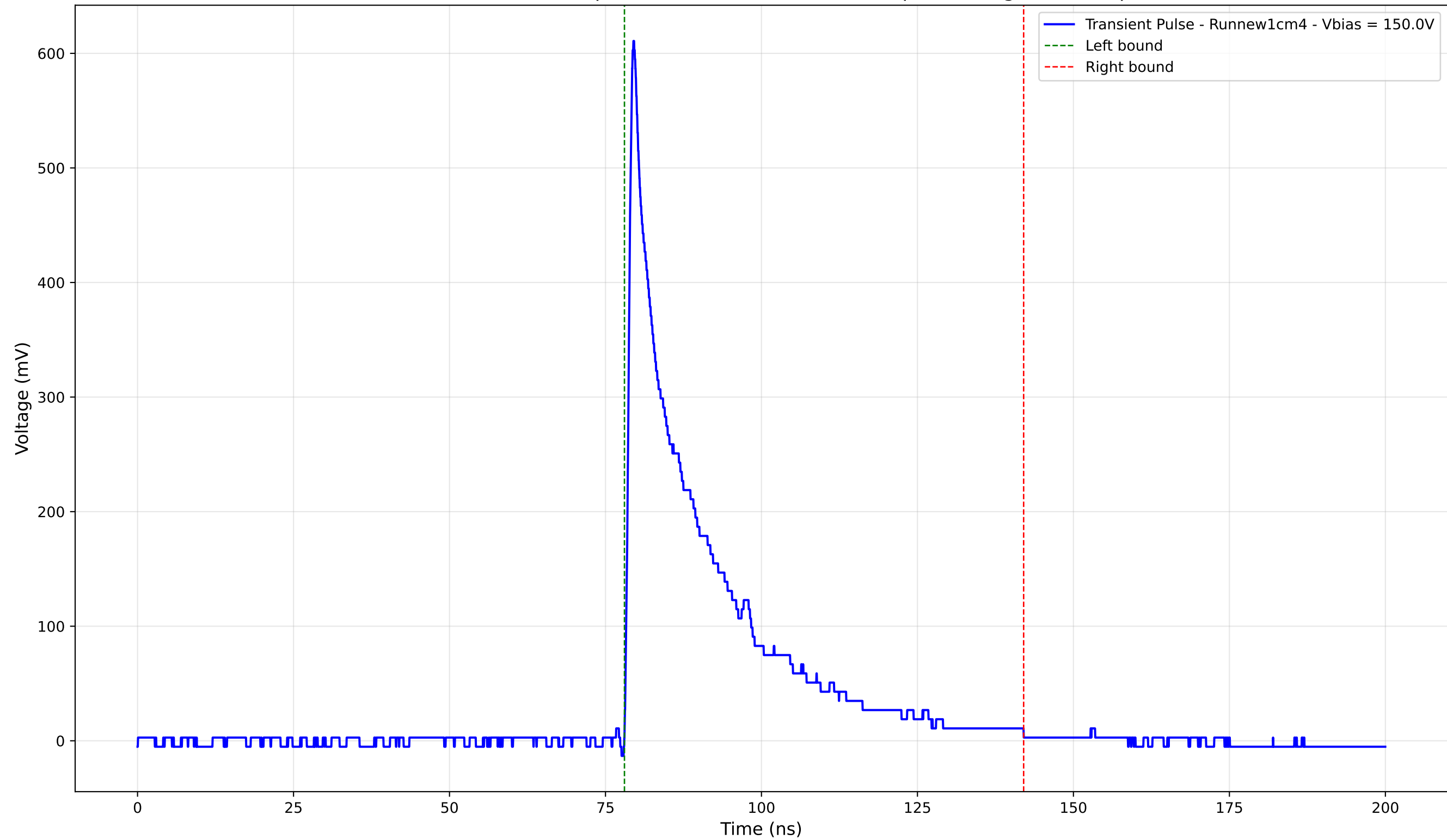
Transient Pulse - Sample: new1cm - Position: 630.0 \mu\text{m} - Charge: 129.14 pC
