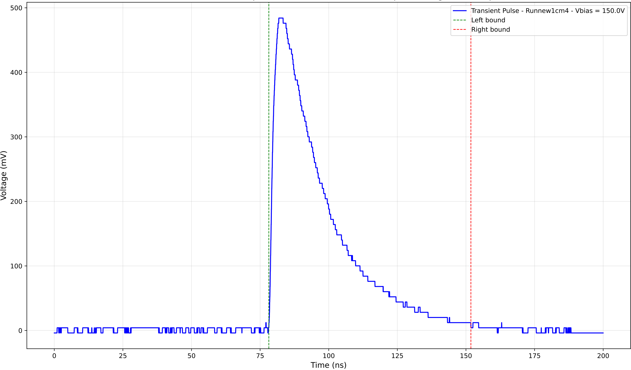
Transient Pulse - Sample: new1cm - Position: 2300.0 \mu\text{m} - Charge: 207.97 pC
