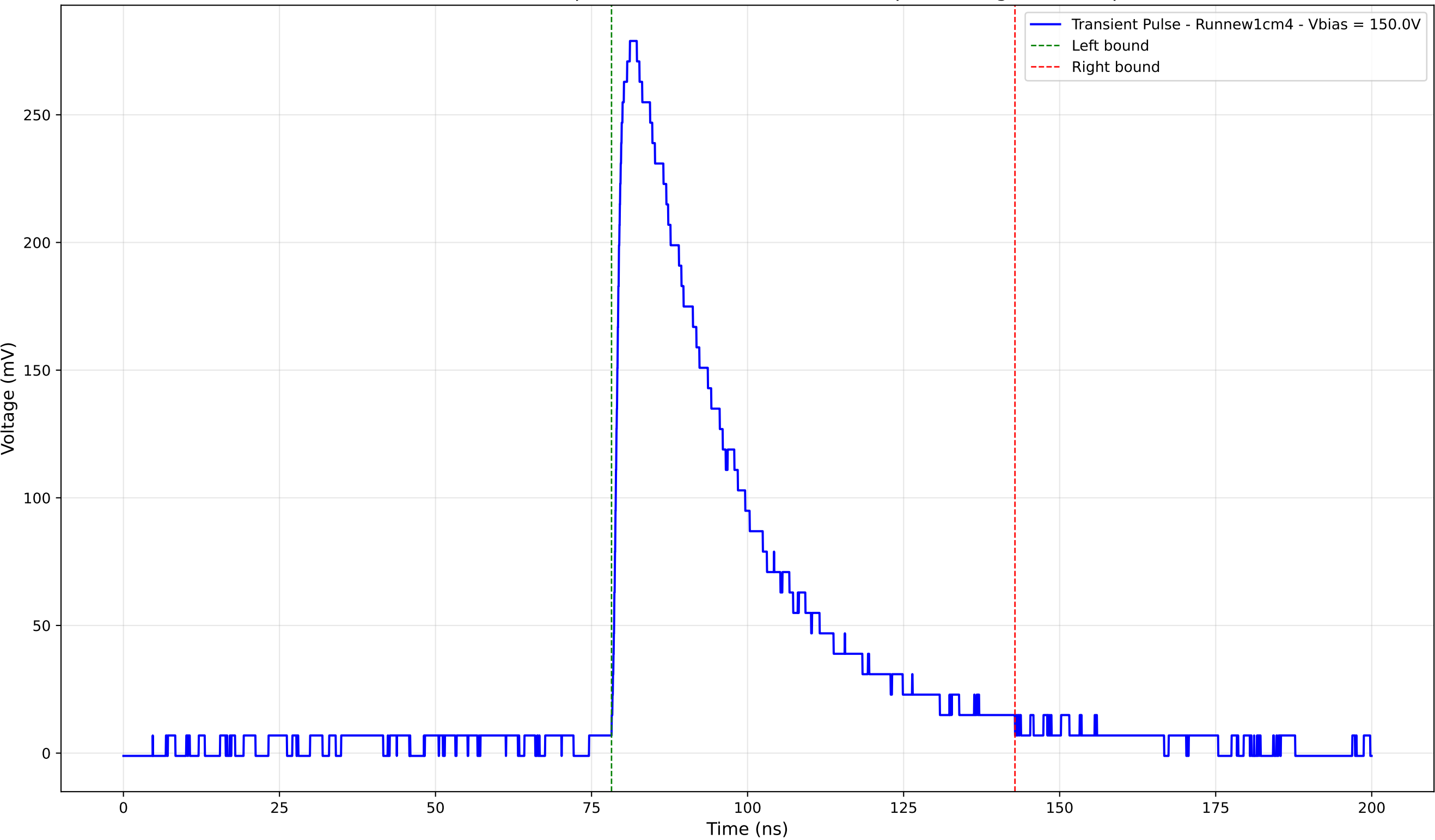
Transient Pulse - Sample: new1cm - Position: 3685.0 \mu\text{m} - Charge: 111.49 pC
