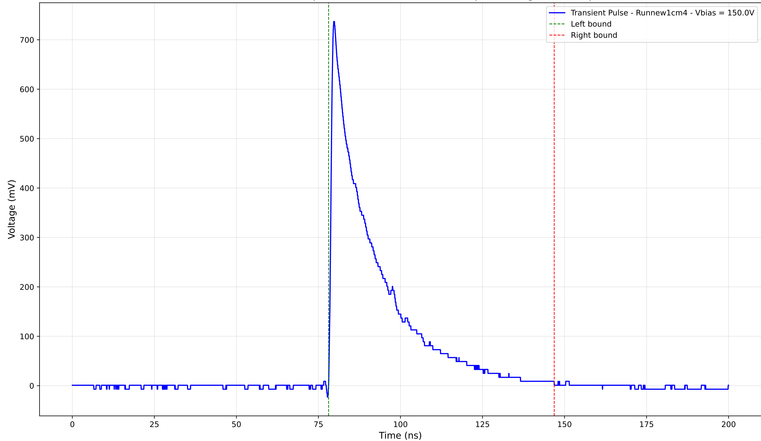
Transient Pulse - Sample: new1cm - Position: 865.0 \mu\text{m} - Charge: 198.23 pC
