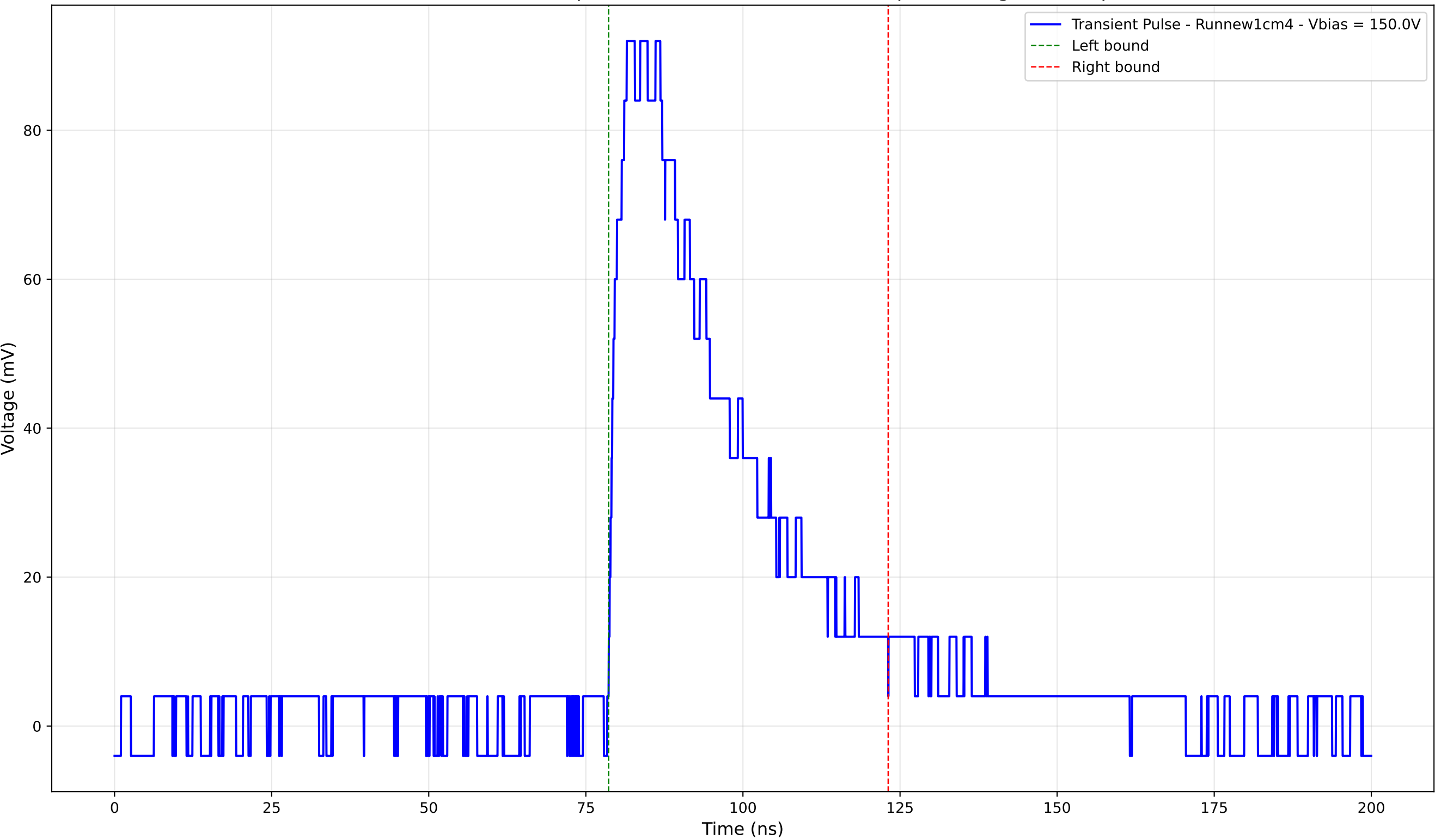
Transient Pulse - Sample: new1cm - Position: 3215.0 \mu\text{m} - Charge: 37.15 pC
