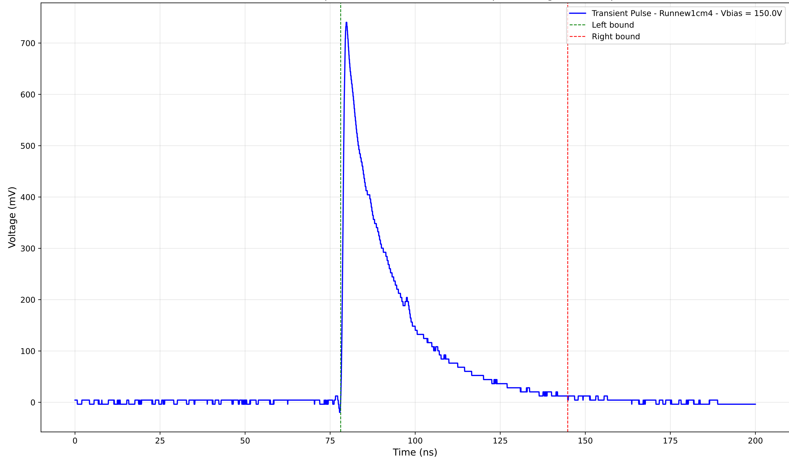
Transient Pulse - Sample: new1cm - Position: 870.0 \mu\text{m} - Charge: 202.37 pC
