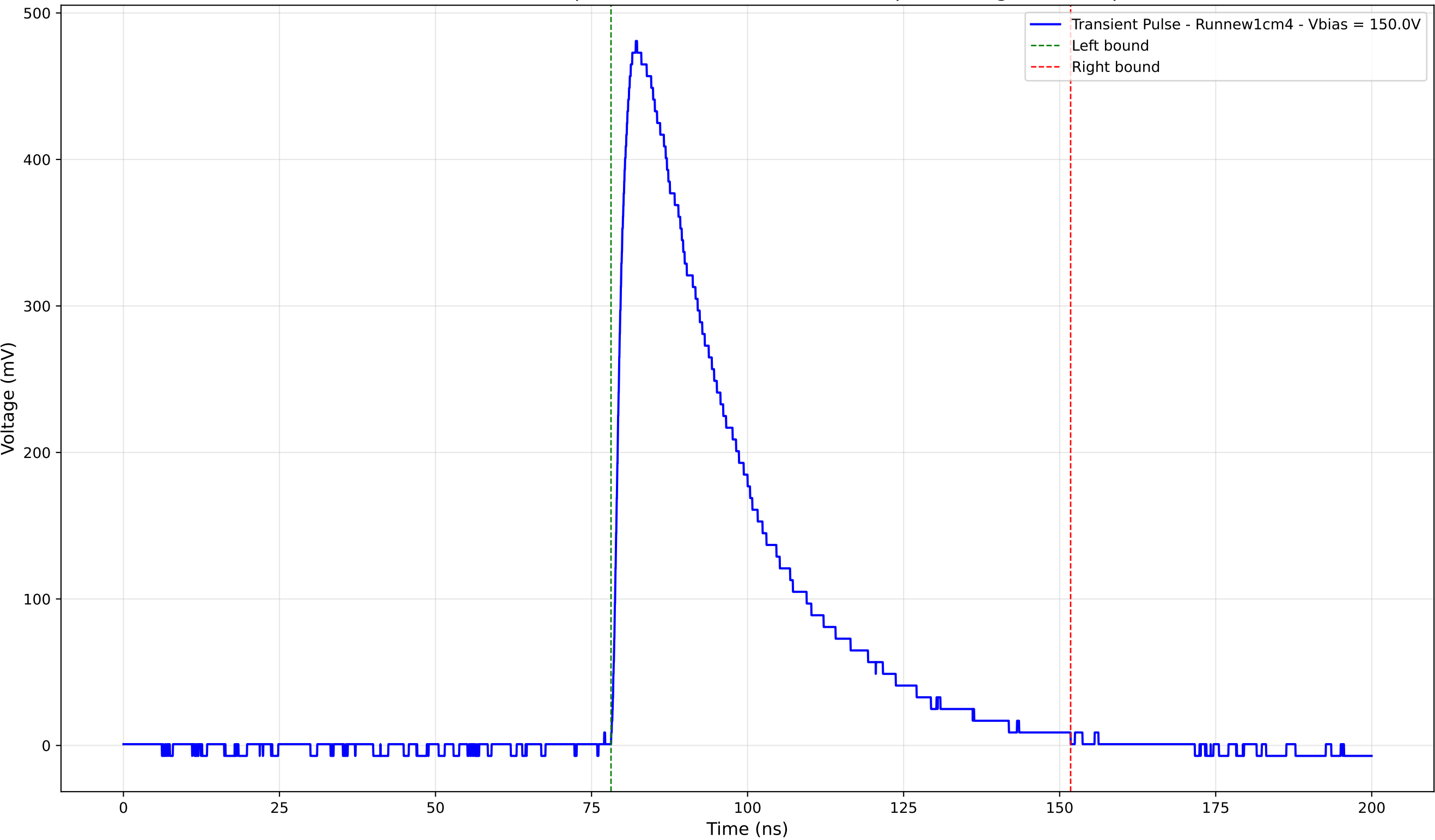
Transient Pulse - Sample: new1cm - Position: 2120.0 \mu\text{m} - Charge: 197.21 pC
