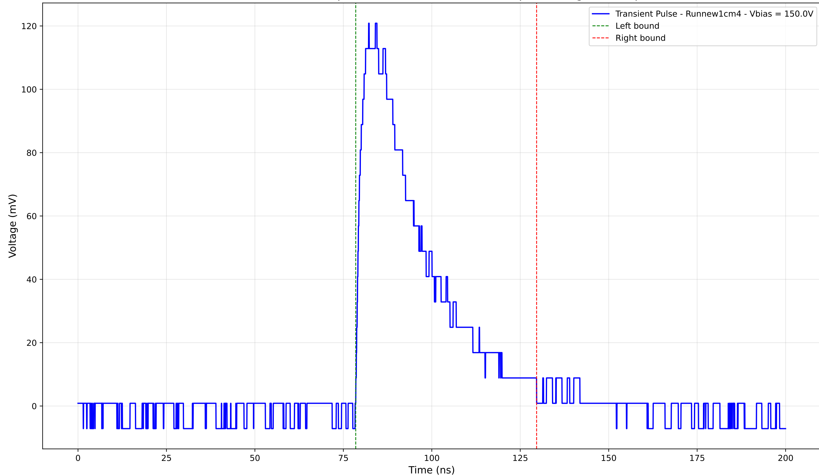
Transient Pulse - Sample: new1cm - Position: 3205.0 \mu\text{m} - Charge: 46.20 pC
