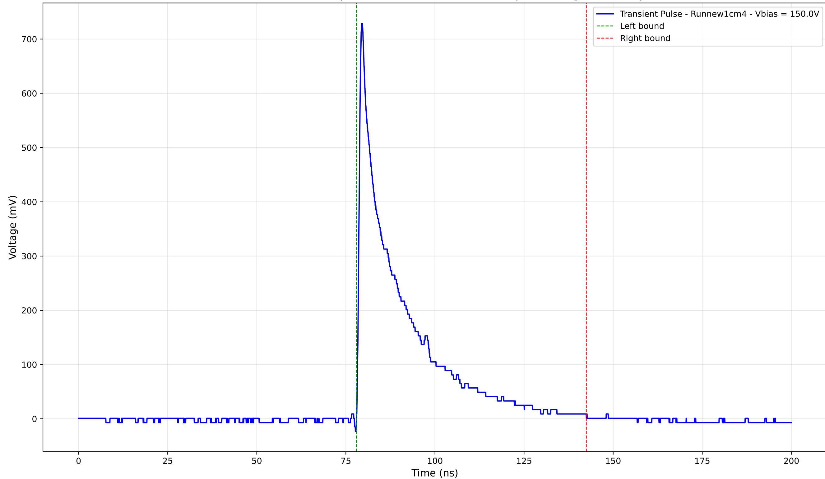
Transient Pulse - Sample: new1cm - Position: 615.0 \mu\text{m} - Charge: 158.09 pC
