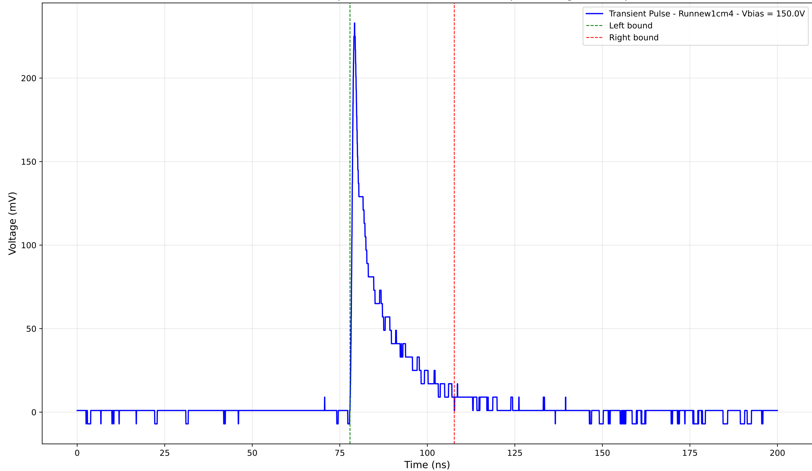
Transient Pulse - Sample: new1cm - Position: 210.0 \mu\text{m} - Charge: 31.45 pC
