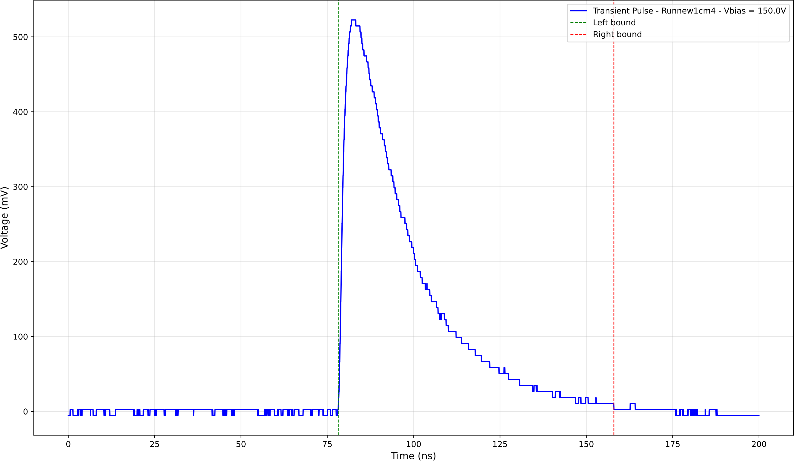
Transient Pulse - Sample: new1cm - Position: 2940.0 \mu\text{m} - Charge: 231.26 pC
