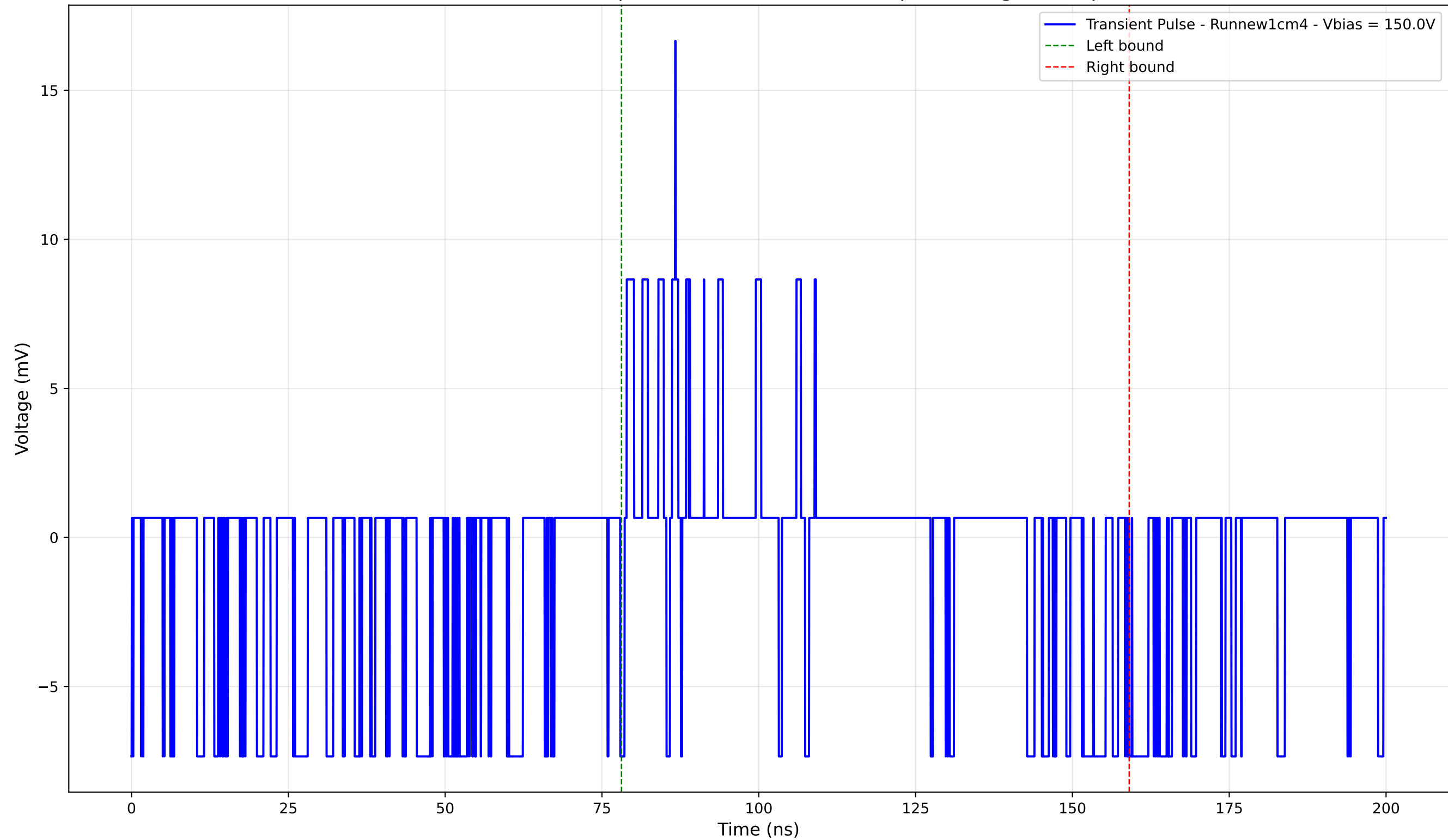
Transient Pulse - Sample: new1cm - Position: 5.0 \mu\text{m} - Charge: 0.34 pC
