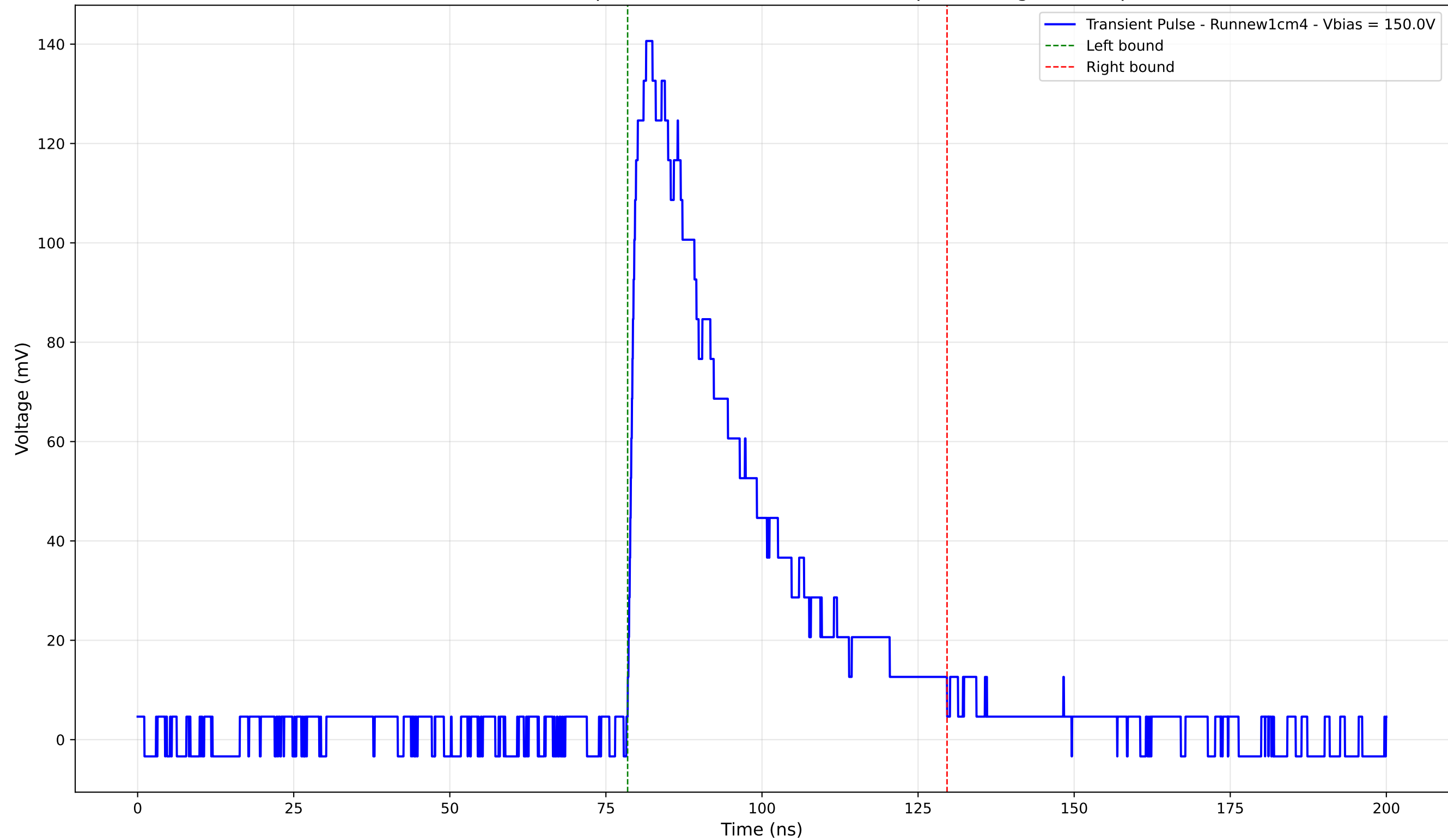
Transient Pulse - Sample: new1cm - Position: 1680.0 \mu\text{m} - Charge: 51.80 pC
