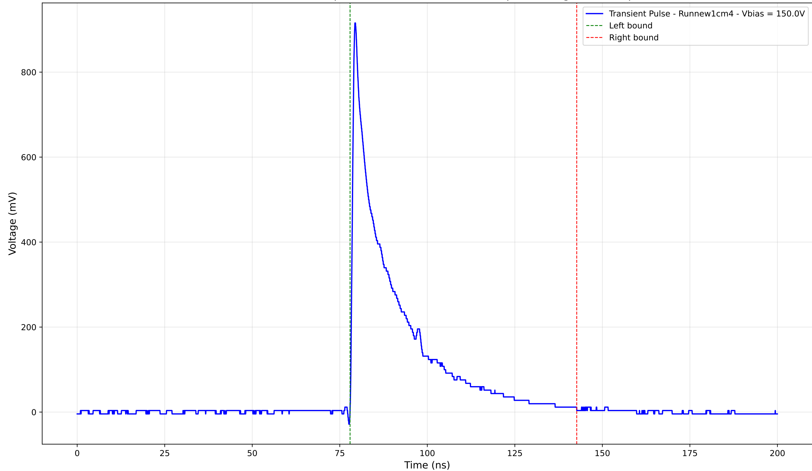
Transient Pulse - Sample: new1cm - Position: 500.0 \mu\text{m} - Charge: 202.42 pC
