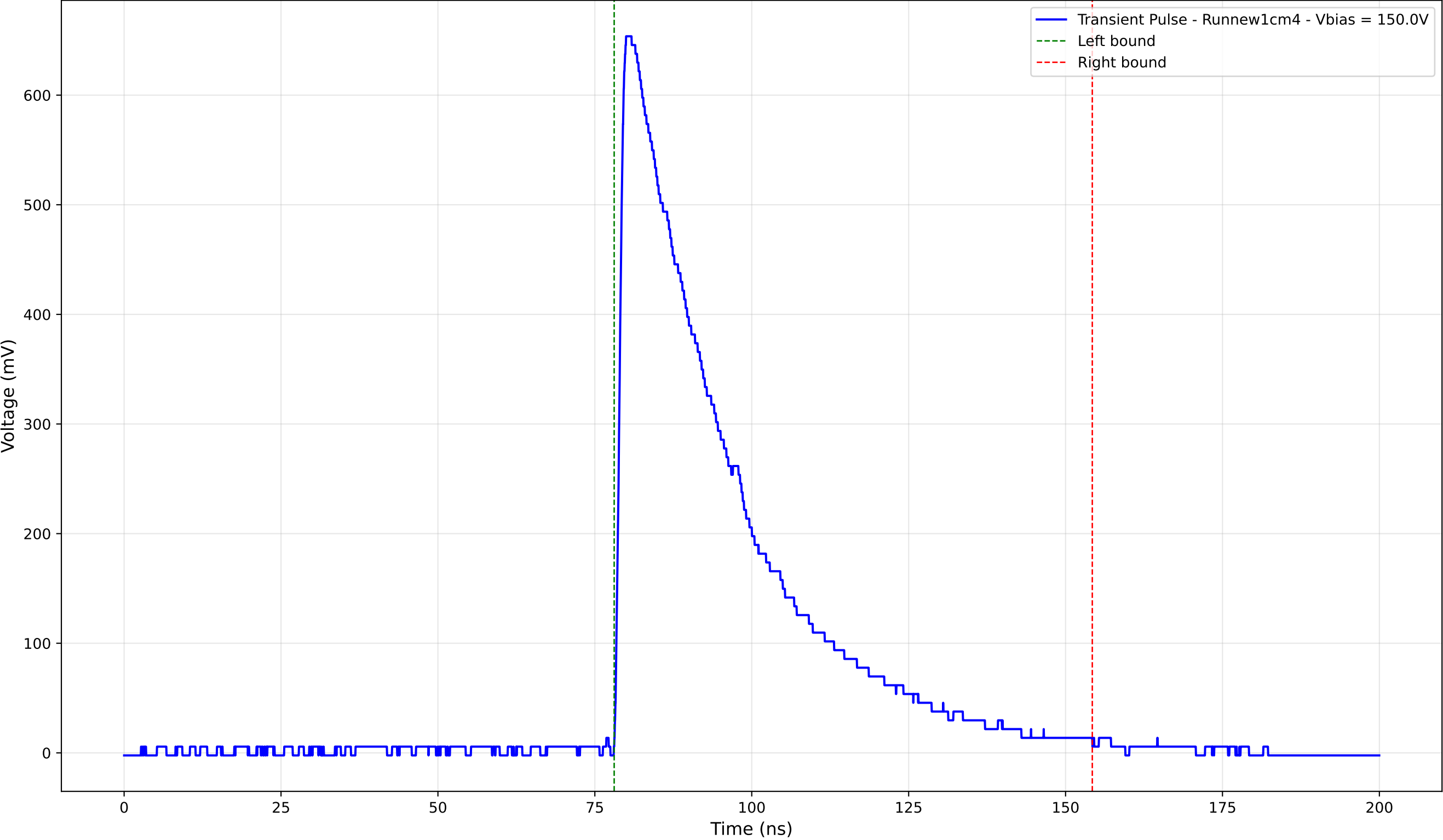
Transient Pulse - Sample: new1cm - Position: 3965.0 \mu\text{m} - Charge: 248.78 pC
