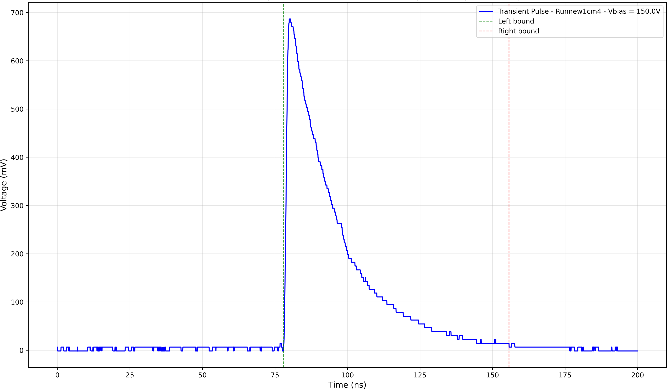
Transient Pulse - Sample: new1cm - Position: 4040.0 \mu\text{m} - Charge: 256.56 pC
