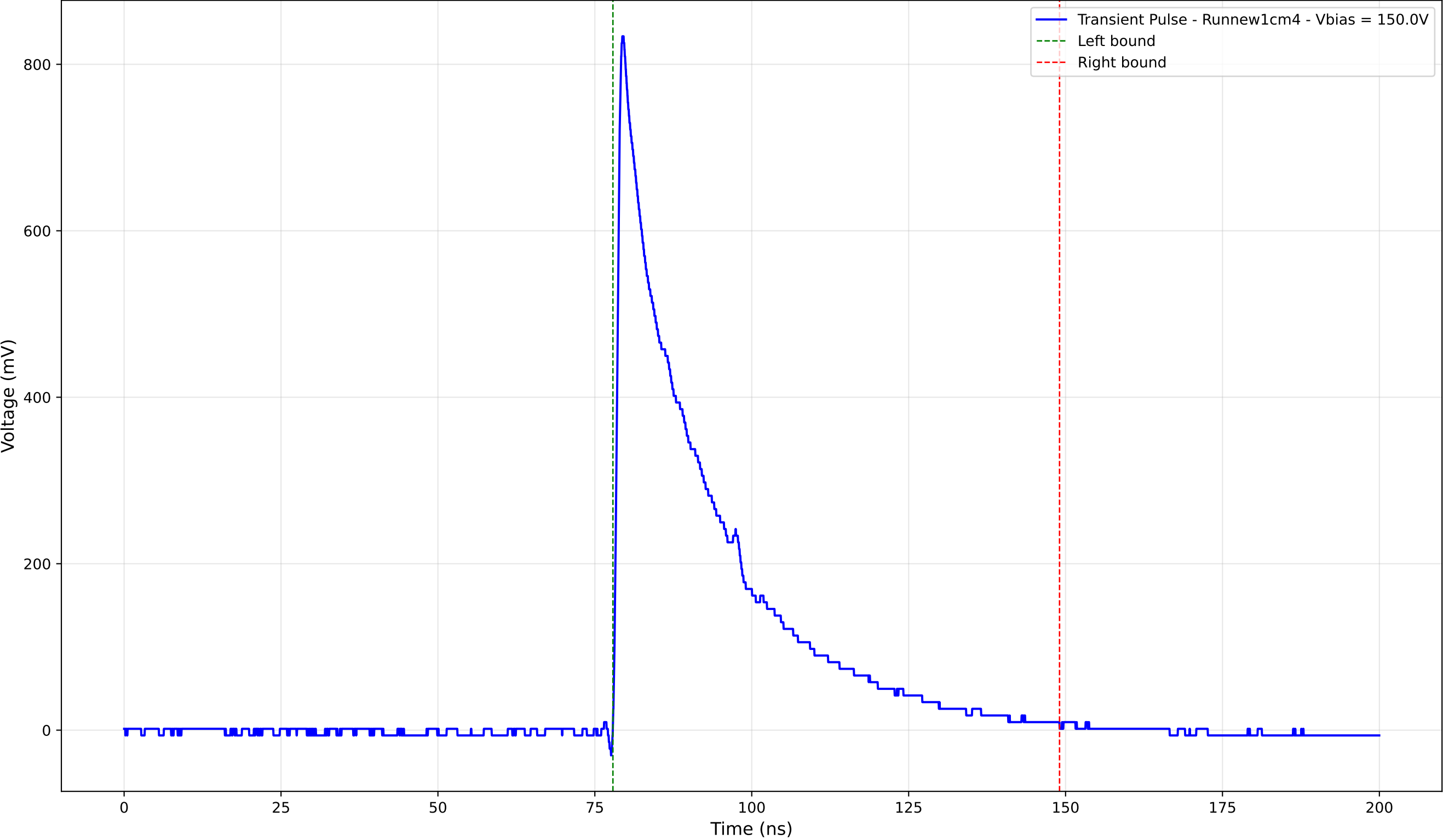
Transient Pulse - Sample: new1cm - Position: 4570.0 \mu\text{m} - Charge: 233.12 pC
