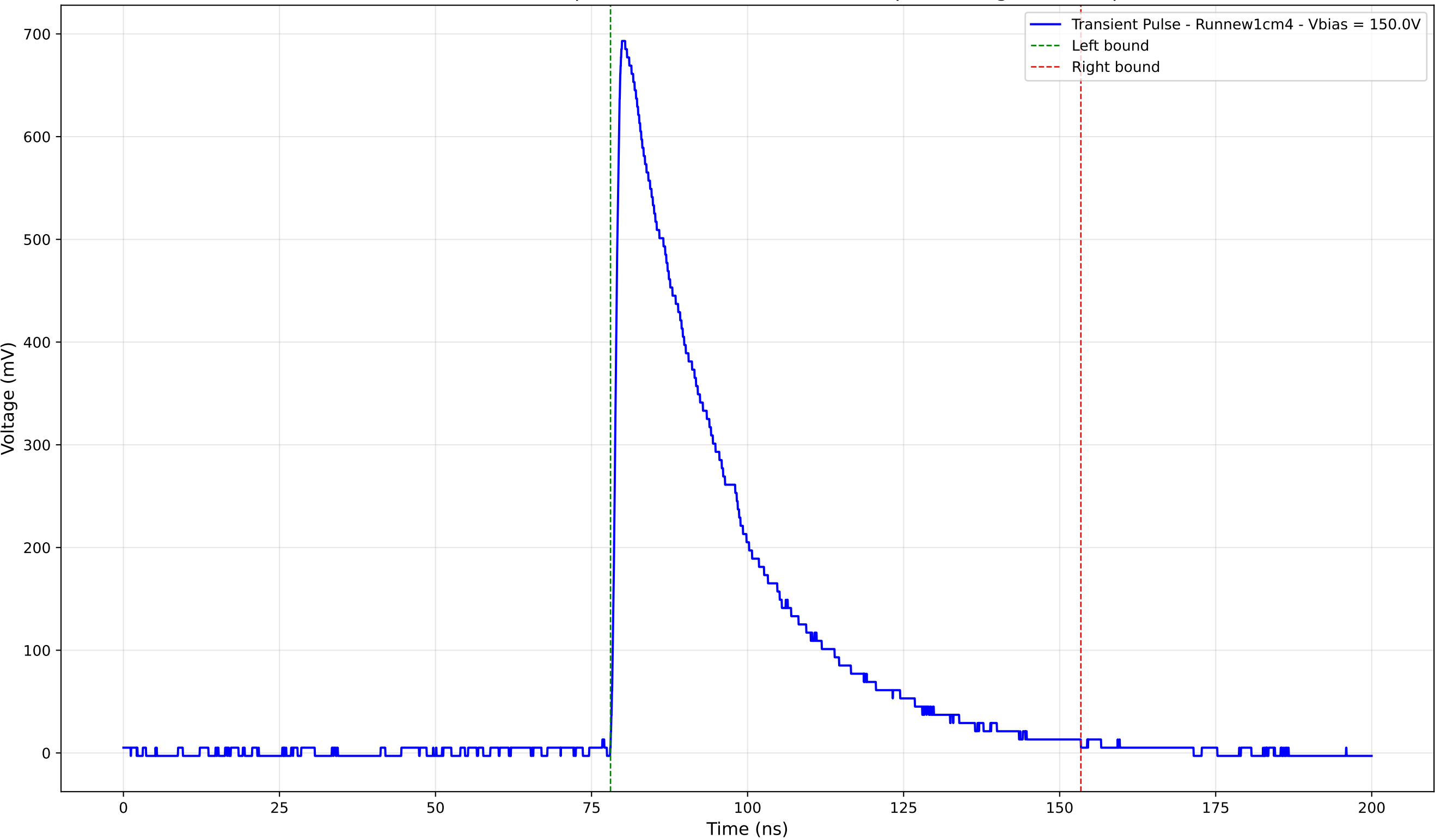
Transient Pulse - Sample: new1cm - Position: 4060.0 \mu\text{m} - Charge: 254.29 pC
