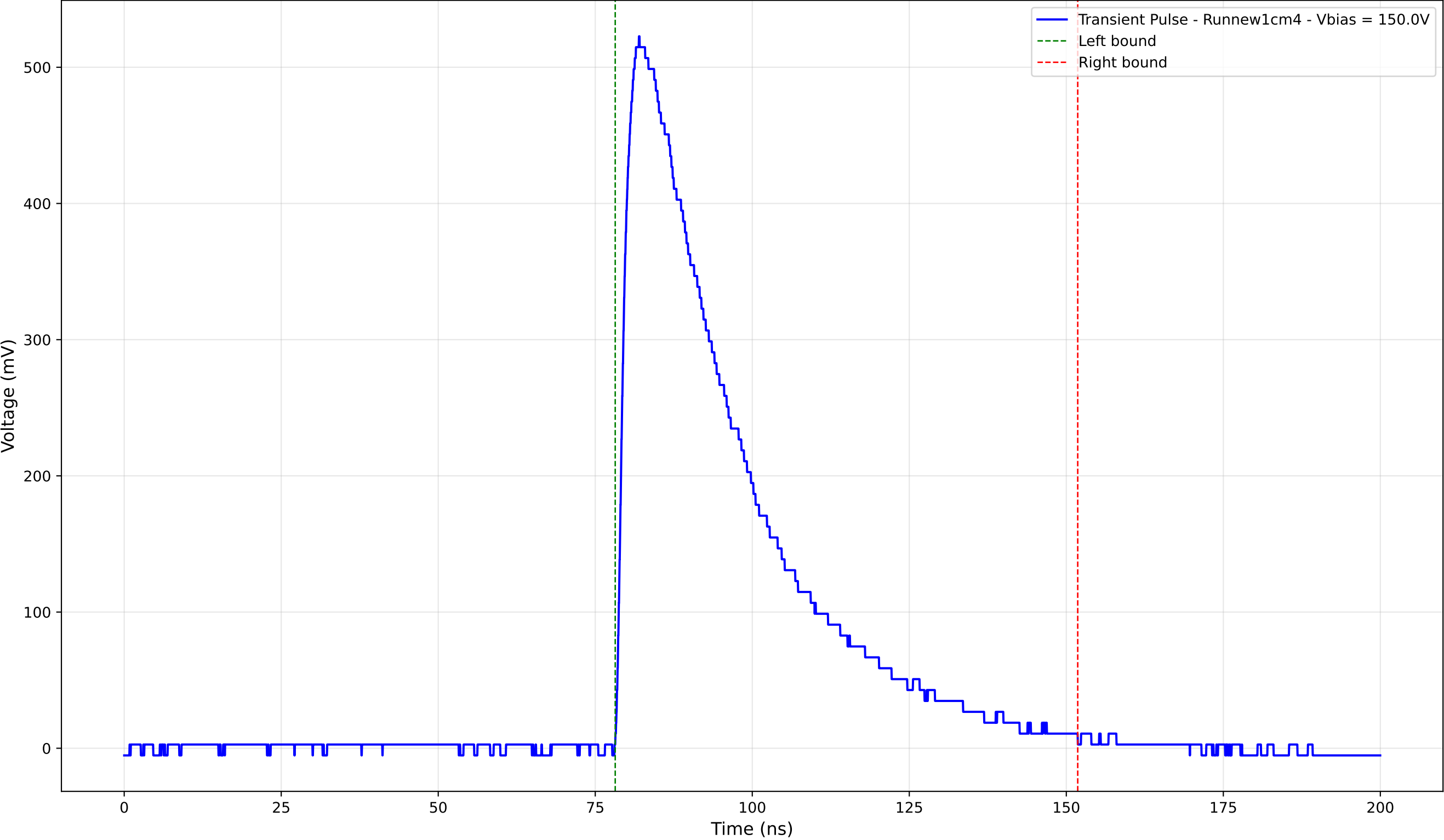
Transient Pulse - Sample: new1cm - Position: 2040.0 \mu\text{m} - Charge: 216.29 pC
