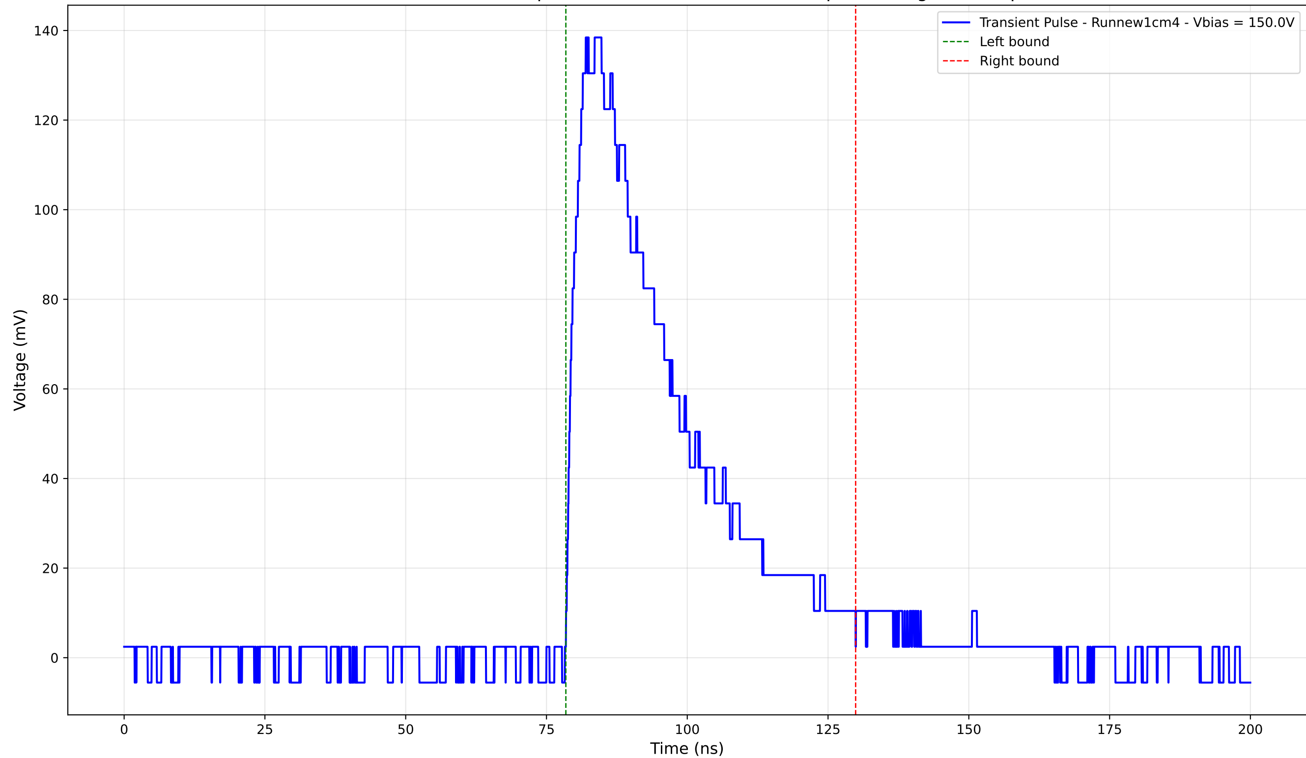
Transient Pulse - Sample: new1cm - Position: 2690.0 \mu\text{m} - Charge: 55.07 pC
