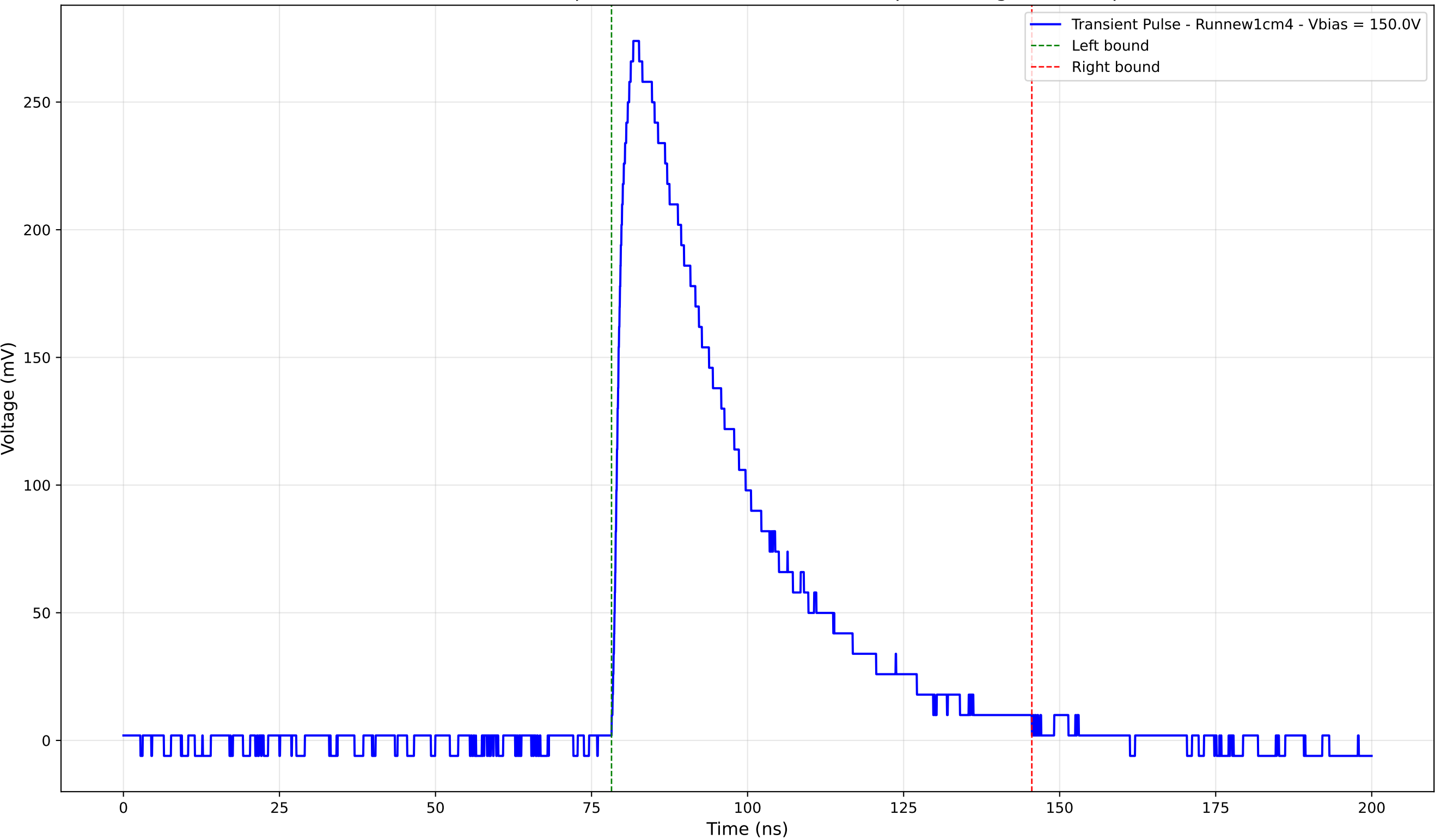
Transient Pulse - Sample: new1cm - Position: 3270.0 \mu\text{m} - Charge: 111.51 pC
