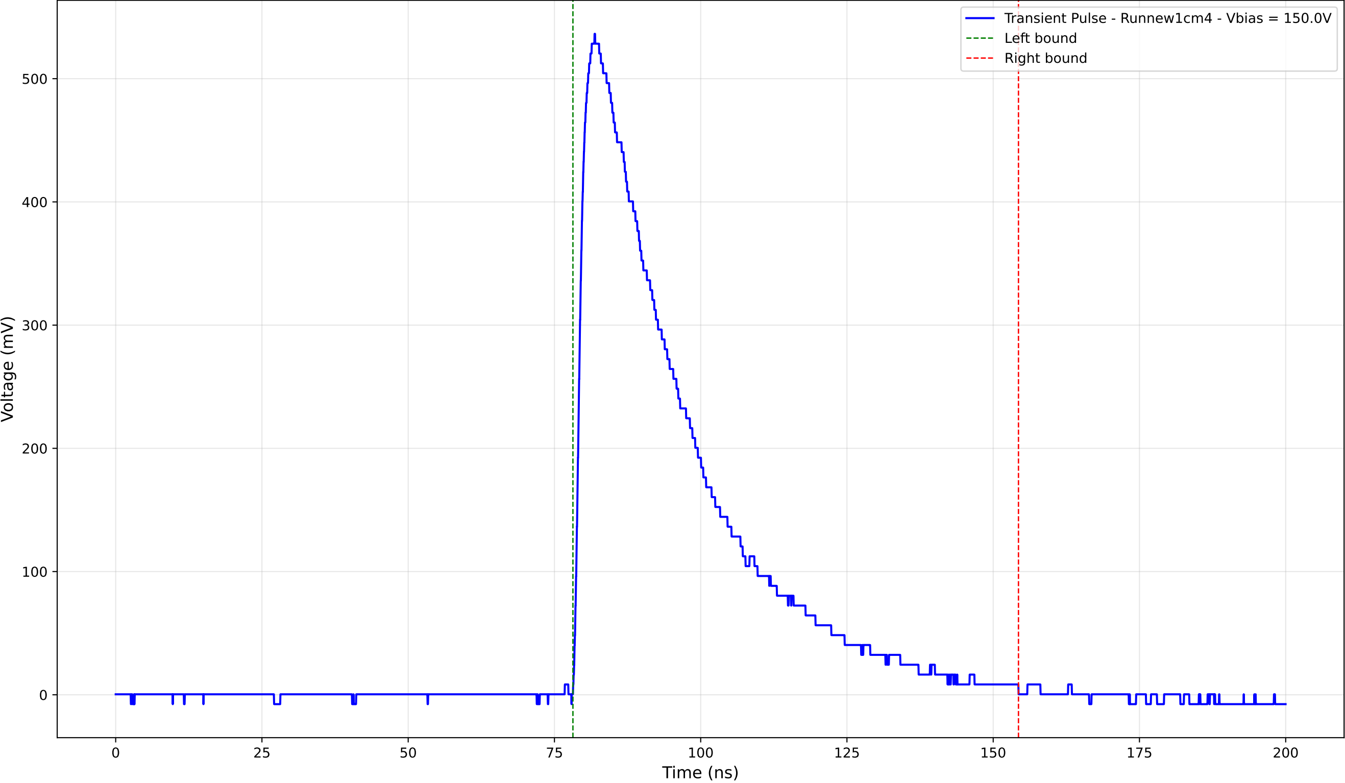
Transient Pulse - Sample: new1cm - Position: 1845.0 \mu\text{m} - Charge: 213.61 pC
