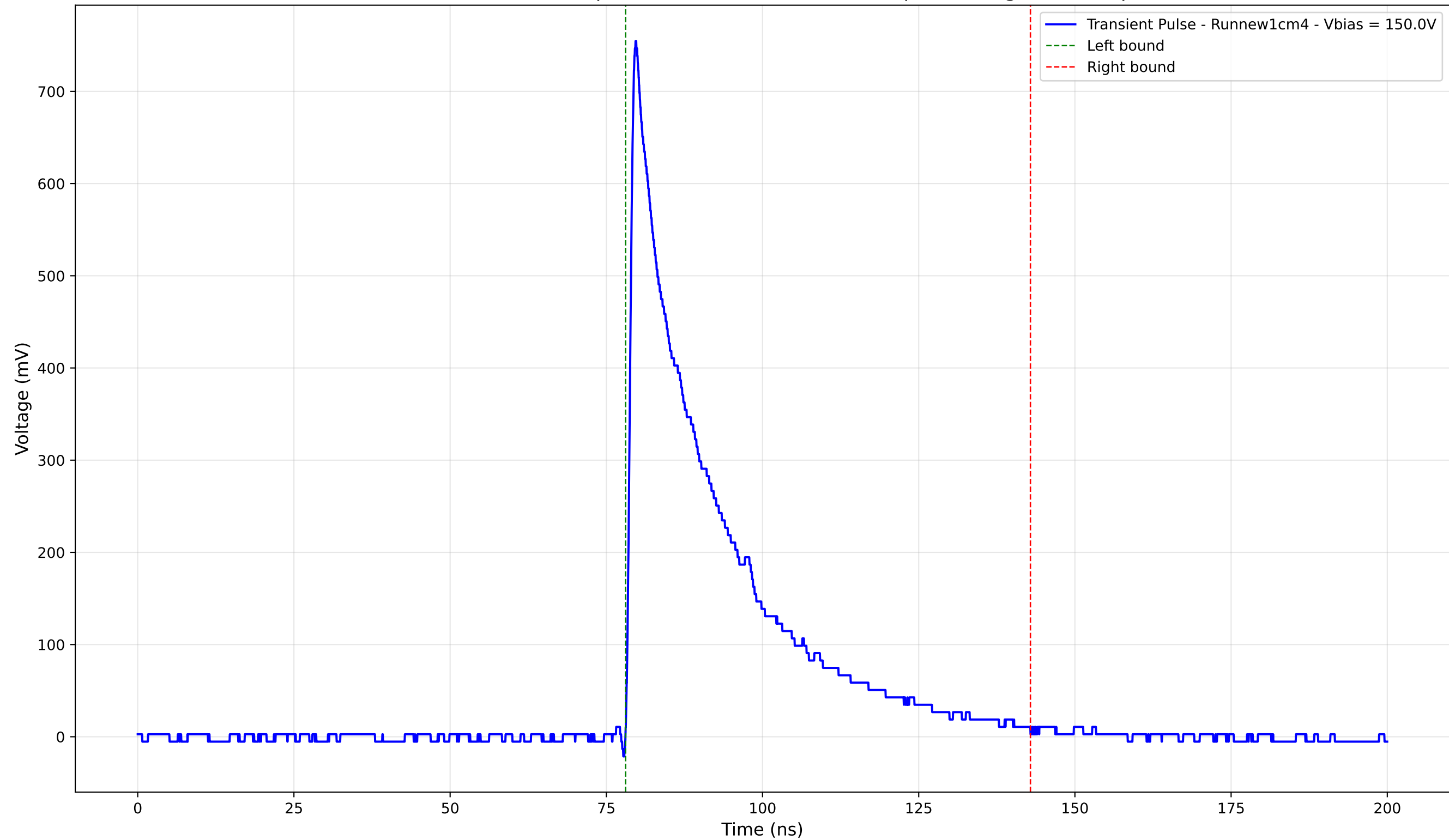
Transient Pulse - Sample: new1cm - Position: 825.0 \mu\text{m} - Charge: 199.23 pC
