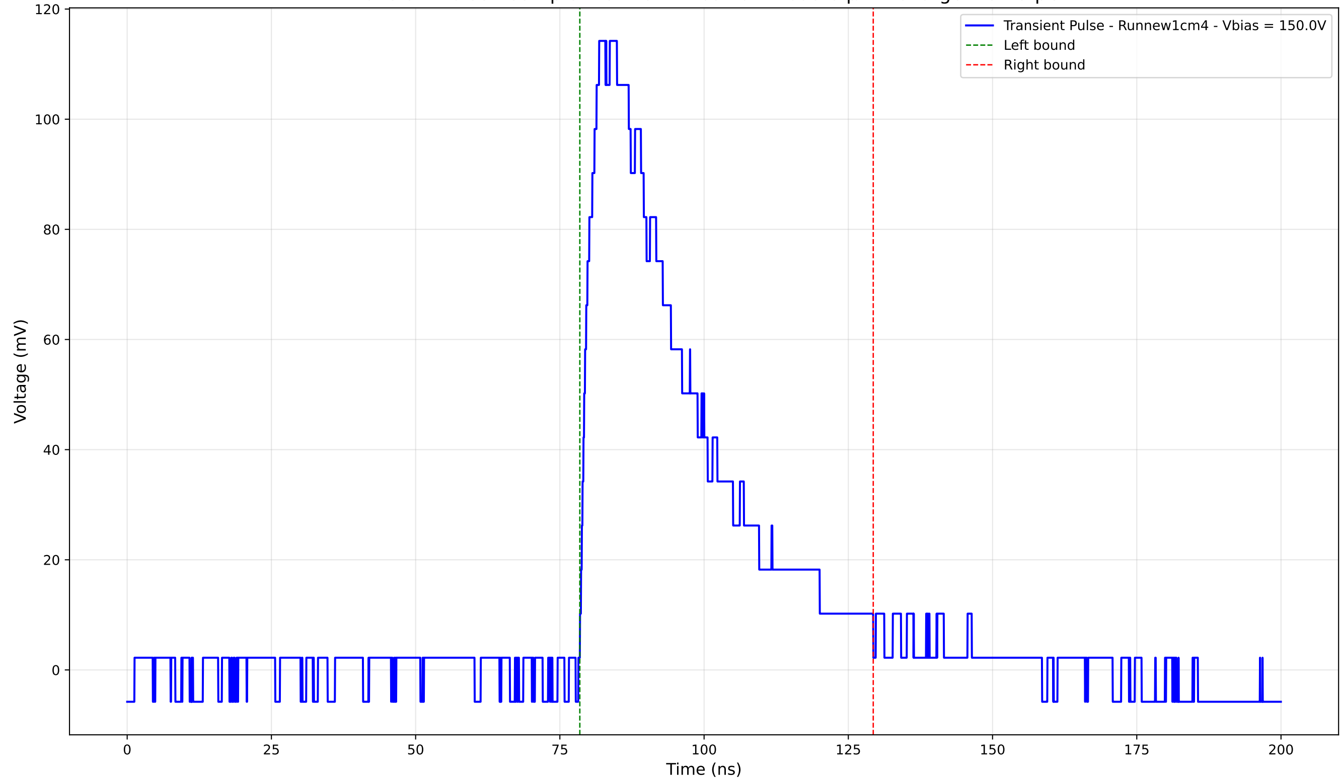
Transient Pulse - Sample: new1cm - Position: 2695.0 \mu\text{m} - Charge: 45.79 pC
