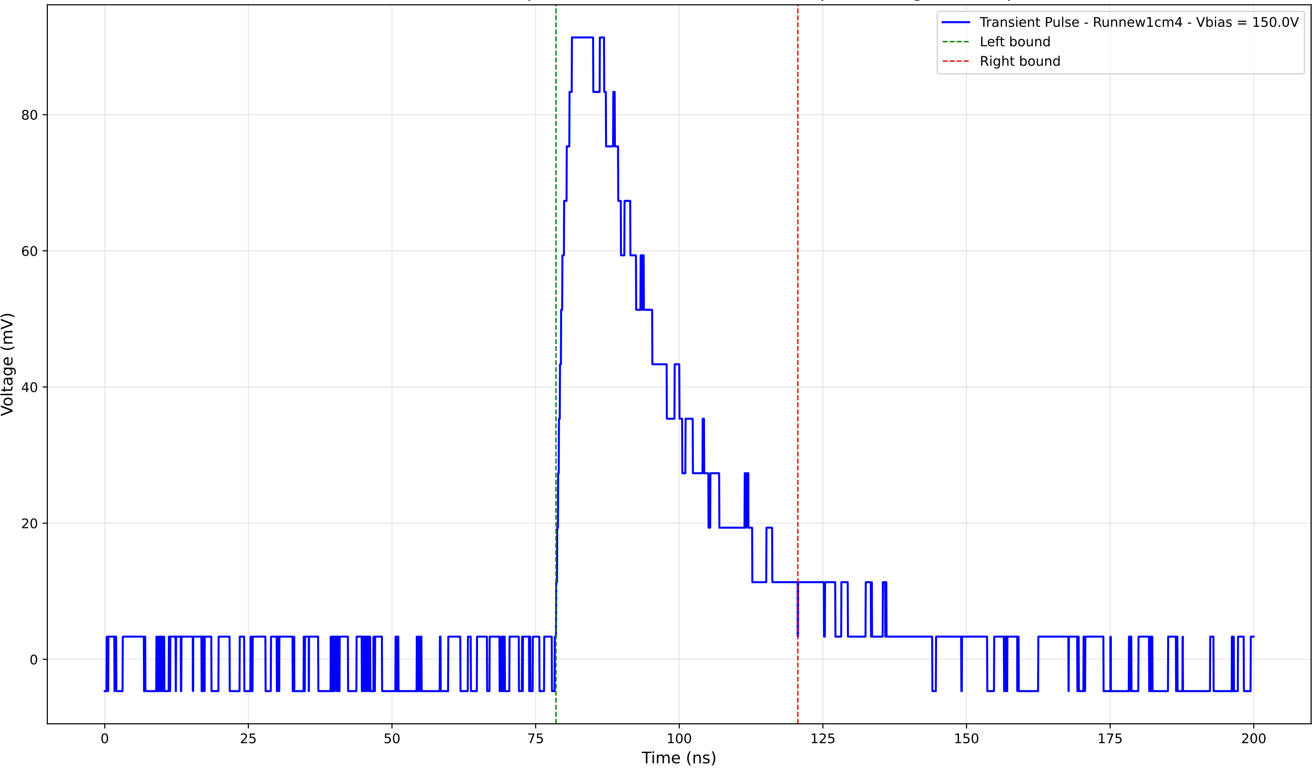
Transient Pulse - Sample: new1cm - Position: 2190.0 \mu\text{m} - Charge: 36.07 pC
