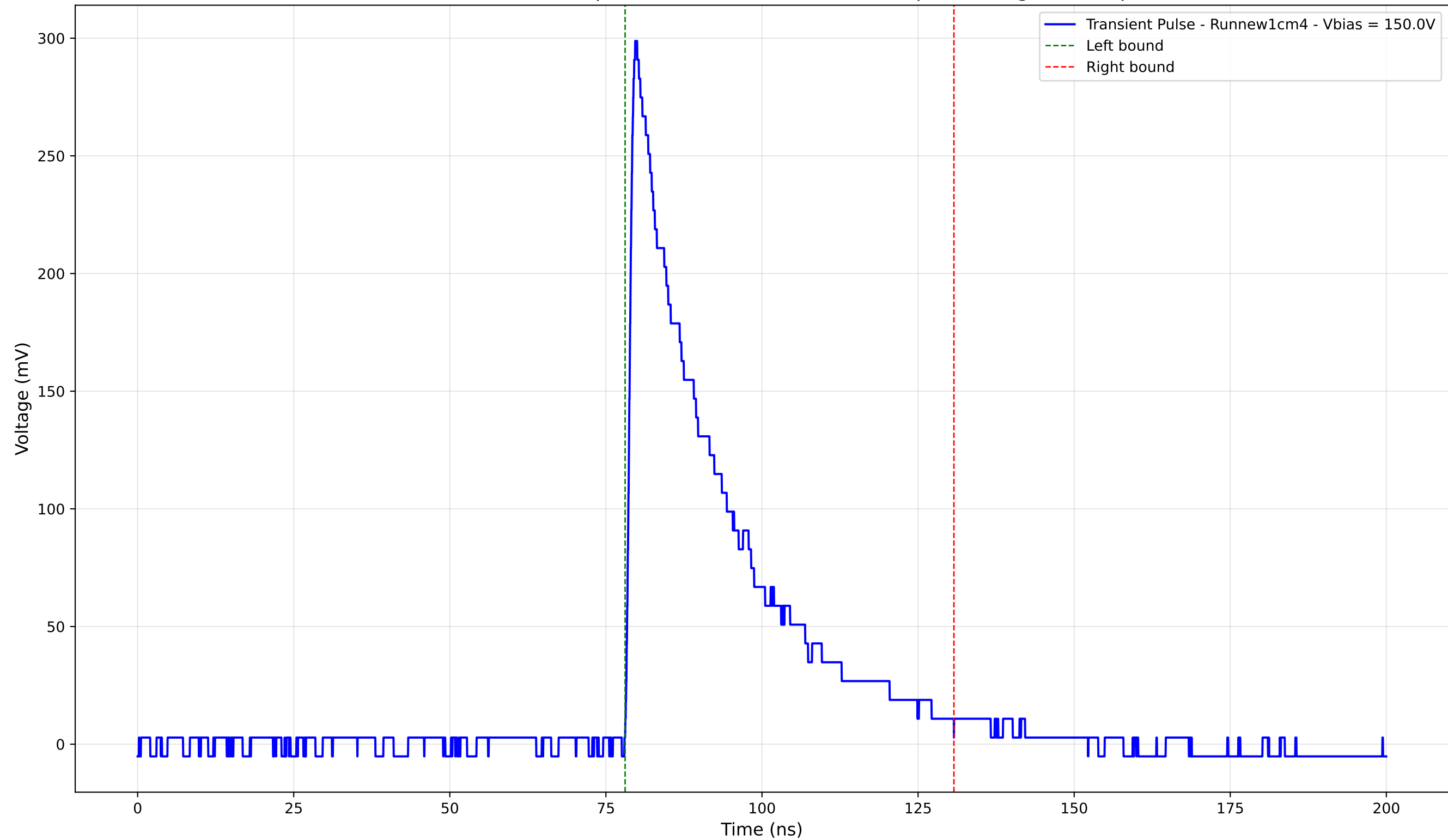
Transient Pulse - Sample: new1cm - Position: 4270.0 \mu\text{m} - Charge: 86.82 pC
