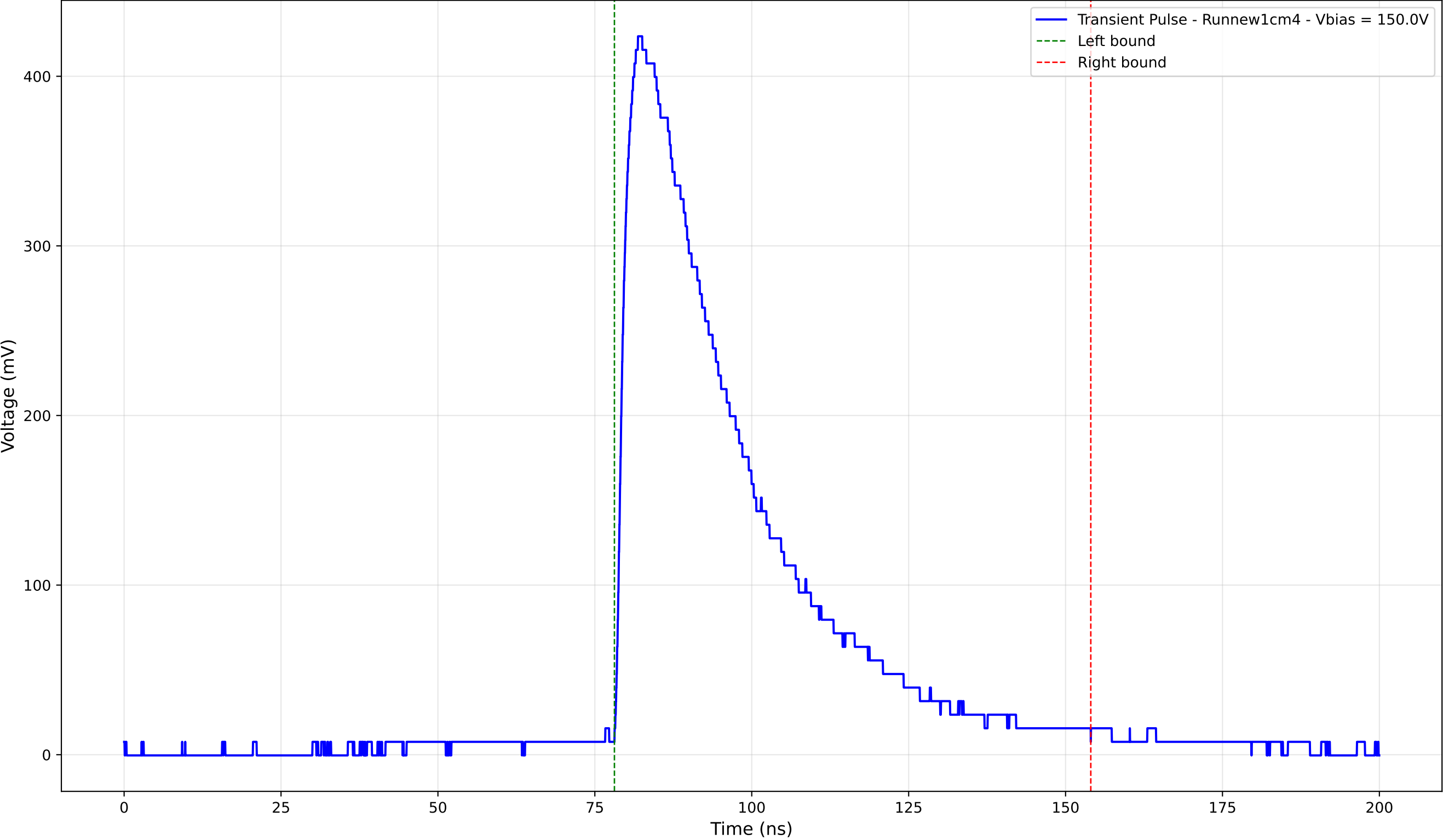
Transient Pulse - Sample: new1cm - Position: 3155.0 \mu\text{m} - Charge: 182.48 pC
