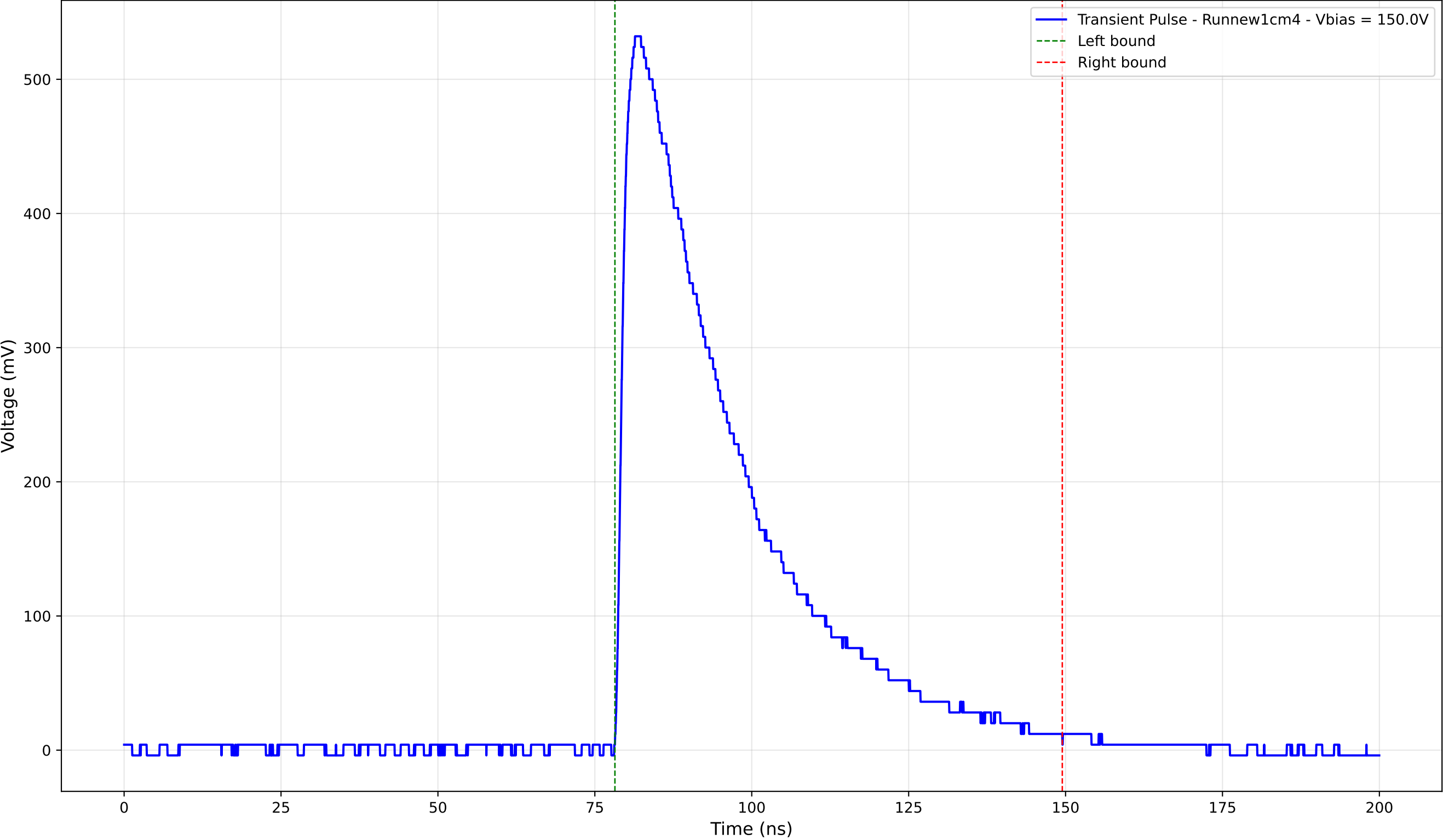
Transient Pulse - Sample: new1cm - Position: 1840.0 \mu\text{m} - Charge: 216.14 pC
