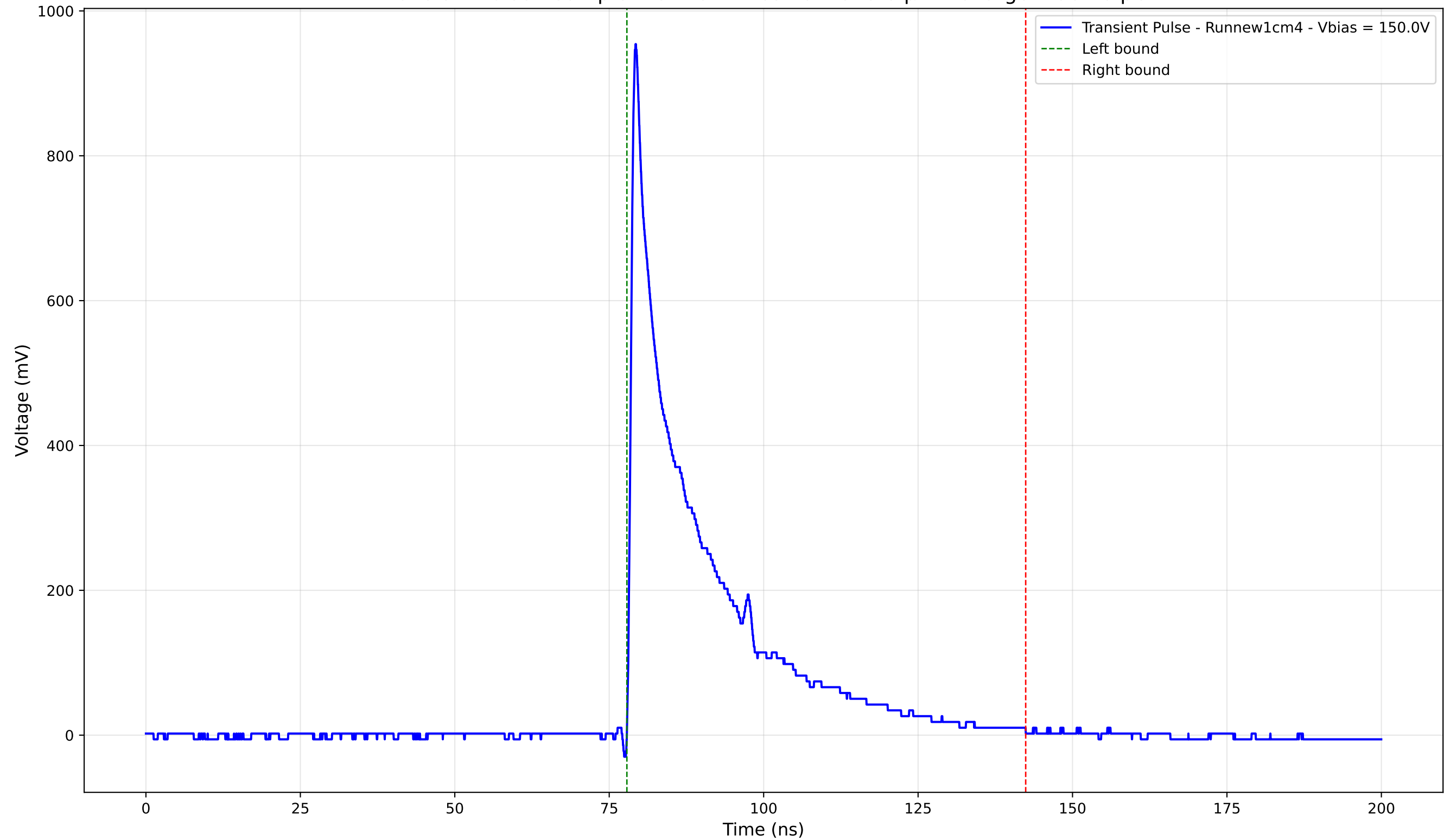
Transient Pulse - Sample: new1cm - Position: 345.0 \mu\text{m} - Charge: 190.20 pC
