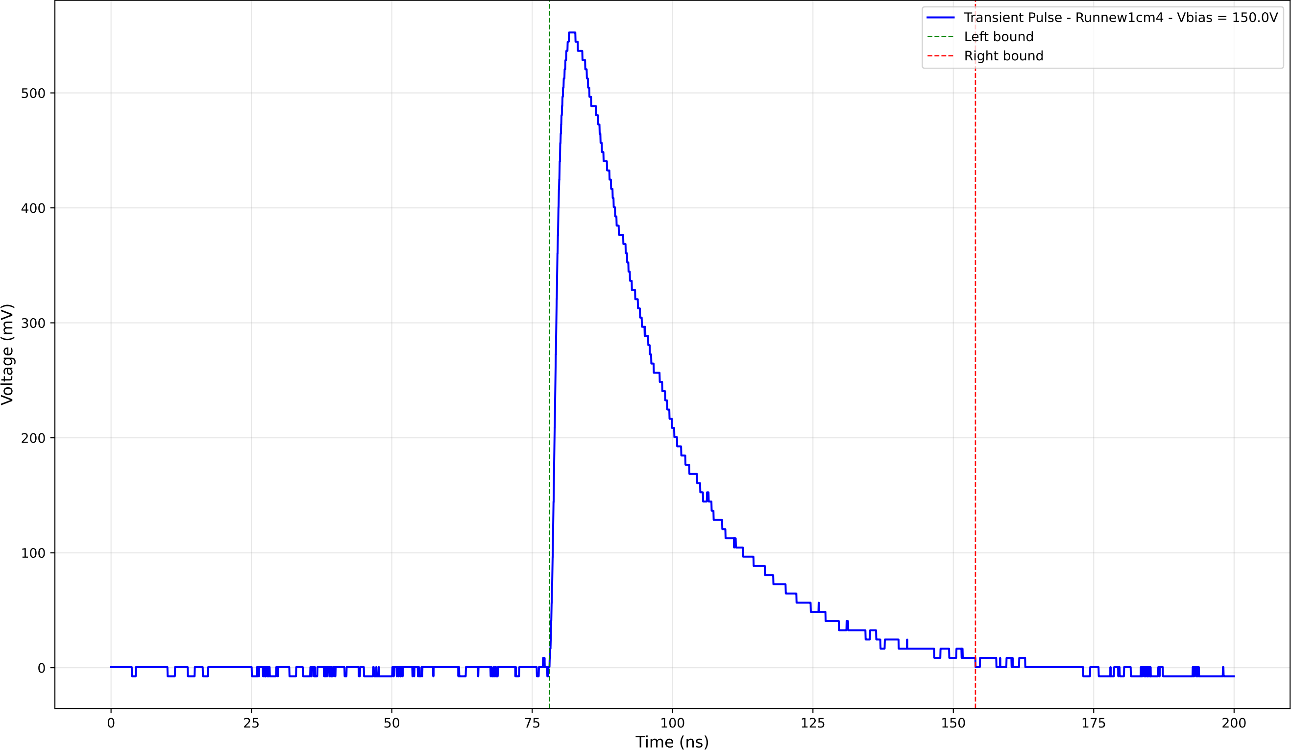
Transient Pulse - Sample: new1cm - Position: 3335.0 \mu\text{m} - Charge: 235.57 pC
