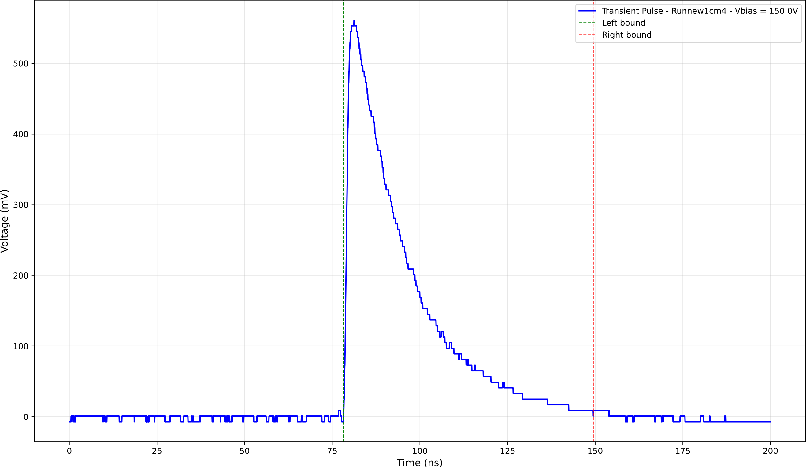
Transient Pulse - Sample: new1cm - Position: 1470.0 \mu\text{m} - Charge: 204.89 pC
