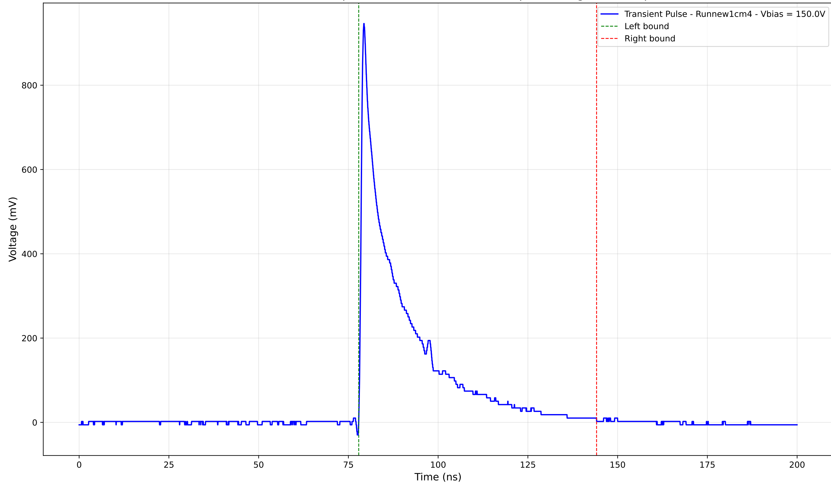
Transient Pulse - Sample: new1cm - Position: 410.0 \mu\text{m} - Charge: 198.36 pC
