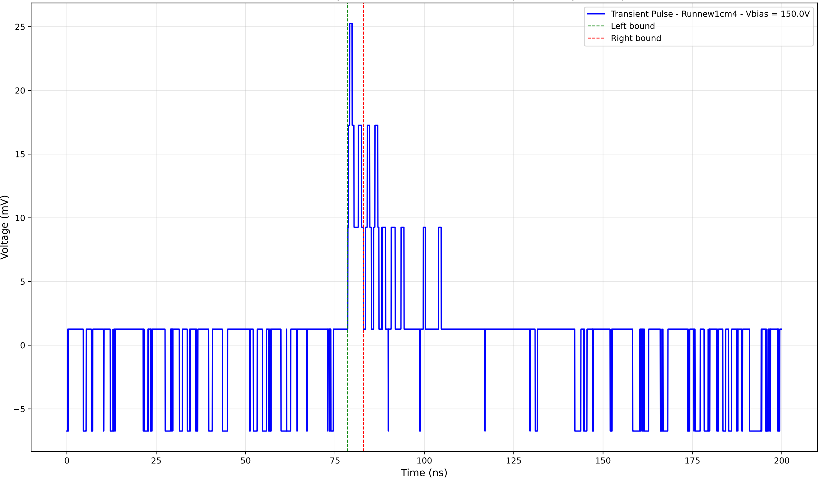
Transient Pulse - Sample: new1cm - Position: 125.0 \mu\text{m} - Charge: 1.32 pC
