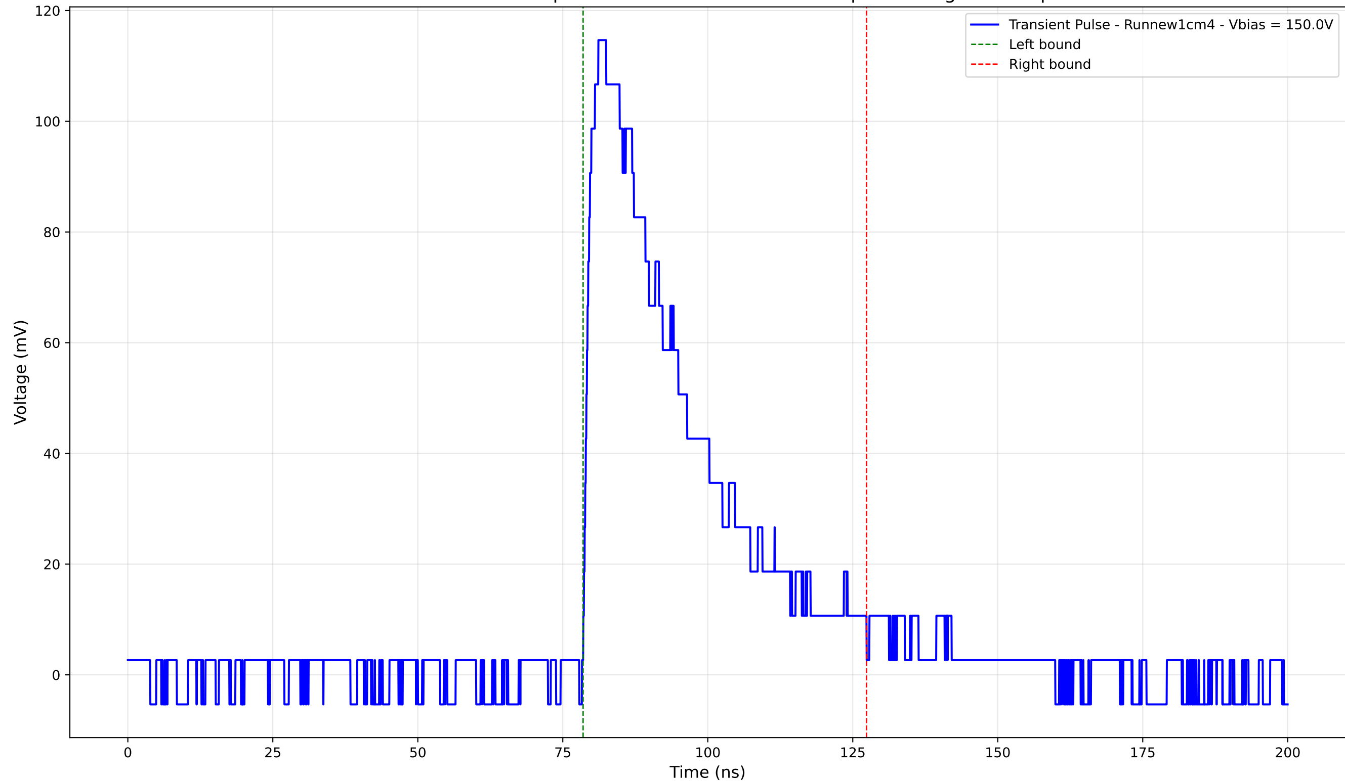
Transient Pulse - Sample: new1cm - Position: 1685.0 \mu\text{m} - Charge: 42.56 pC
