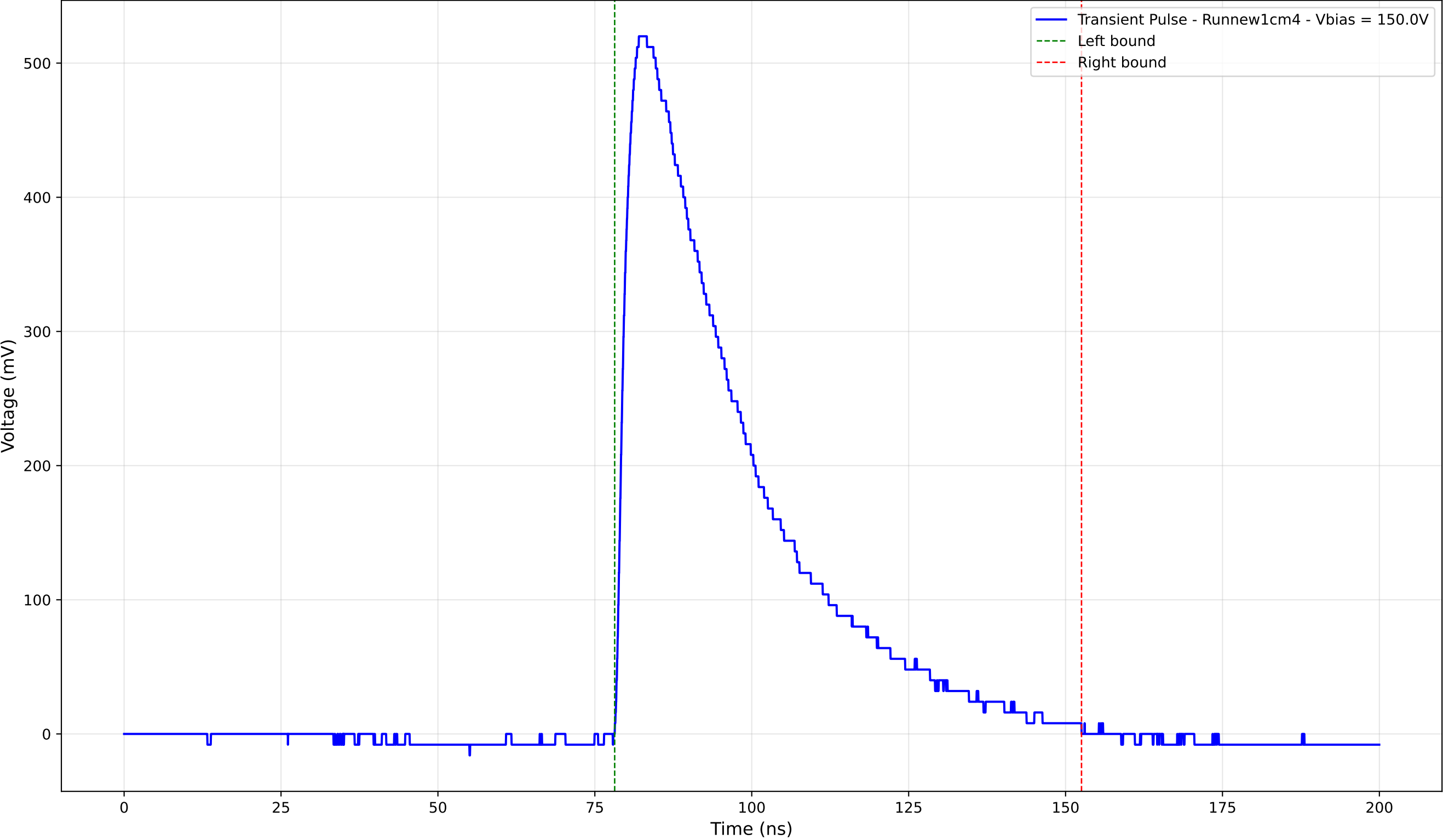
Transient Pulse - Sample: new1cm - Position: 2425.0 \mu\text{m} - Charge: 224.45 pC
