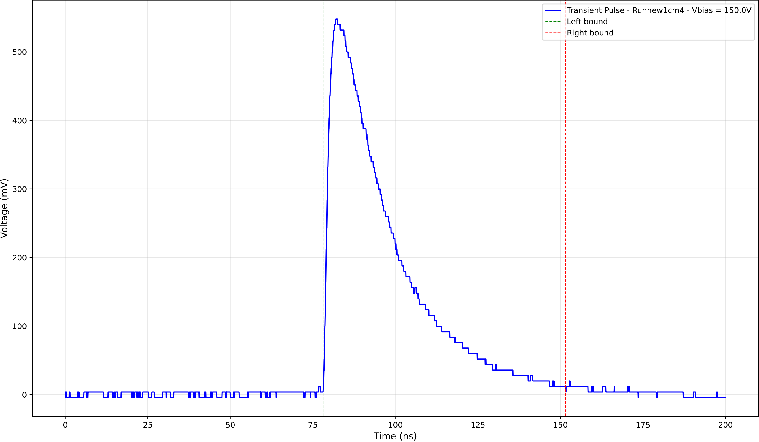
Transient Pulse - Sample: new1cm - Position: 3080.0 \mu\text{m} - Charge: 239.14 pC
