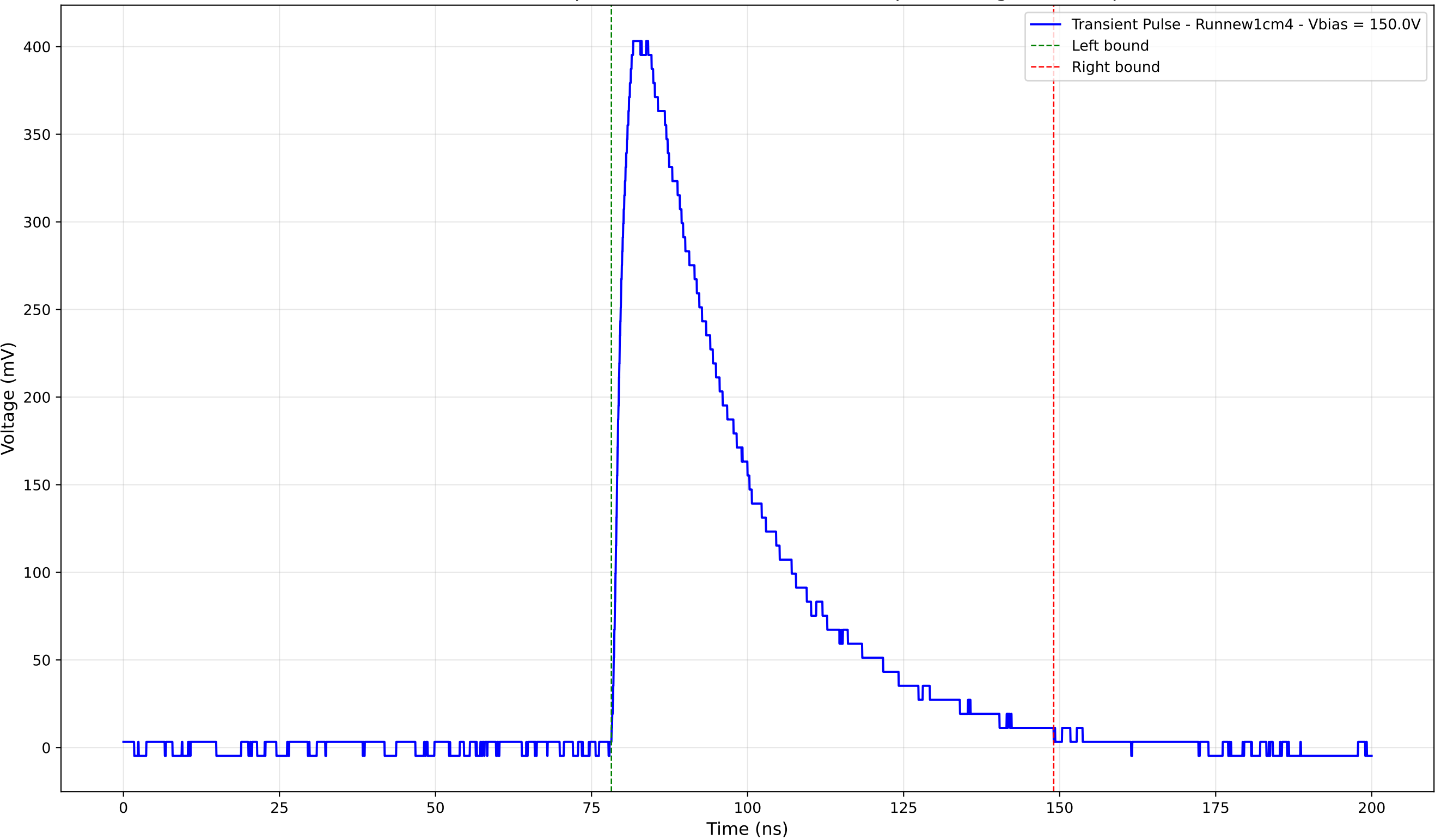
Transient Pulse - Sample: new1cm - Position: 2275.0 \mu\text{m} - Charge: 171.75 pC
