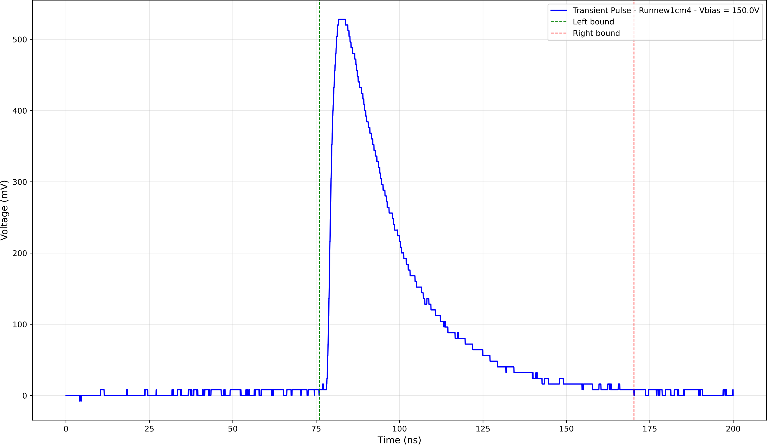
Transient Pulse - Sample: new1cm - Position: 2975.0 \mu\text{m} - Charge: 242.00 pC
