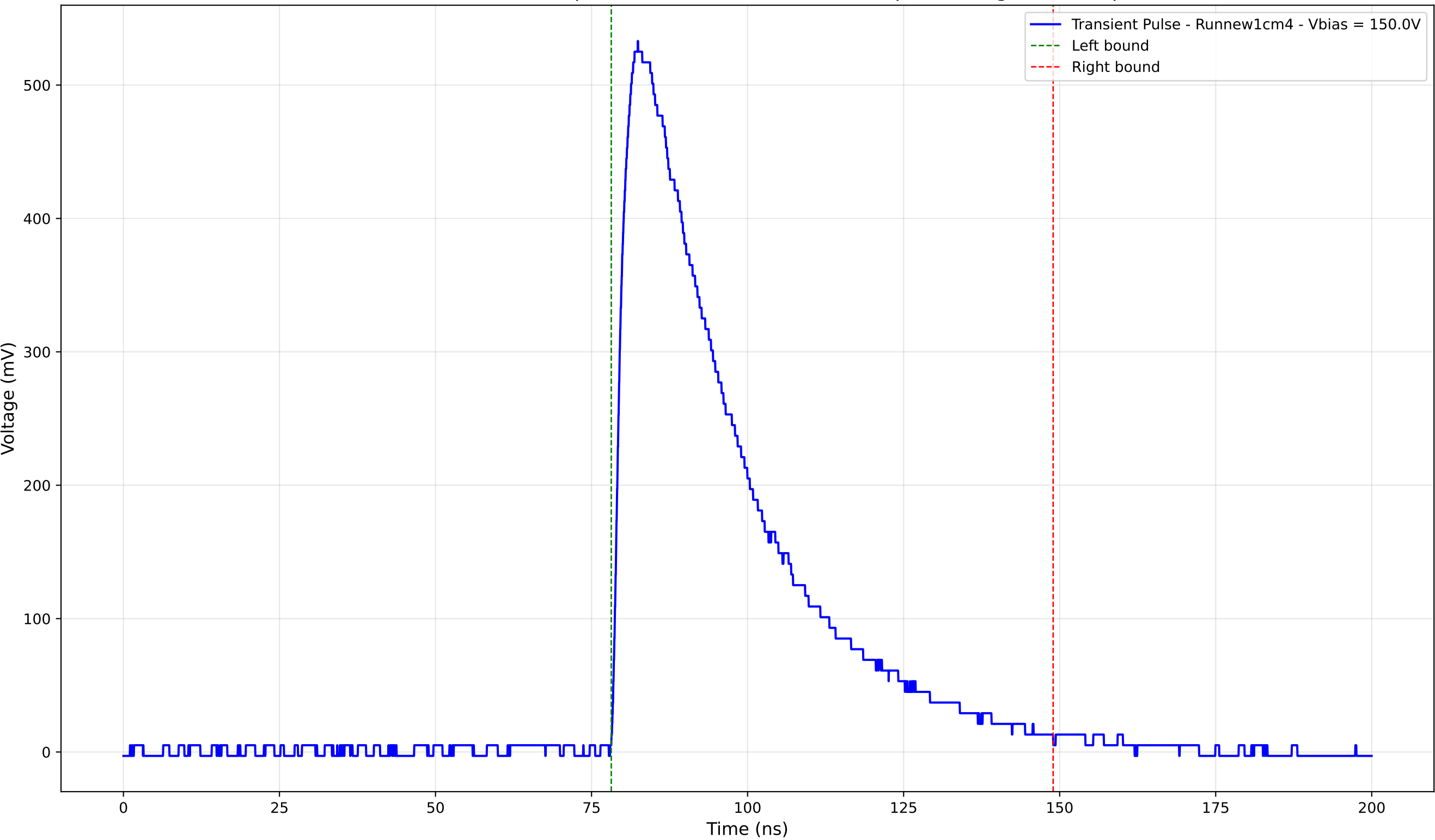
Transient Pulse - Sample: new1cm - Position: 2345.0 \mu\text{m} - Charge: 227.52 pC
