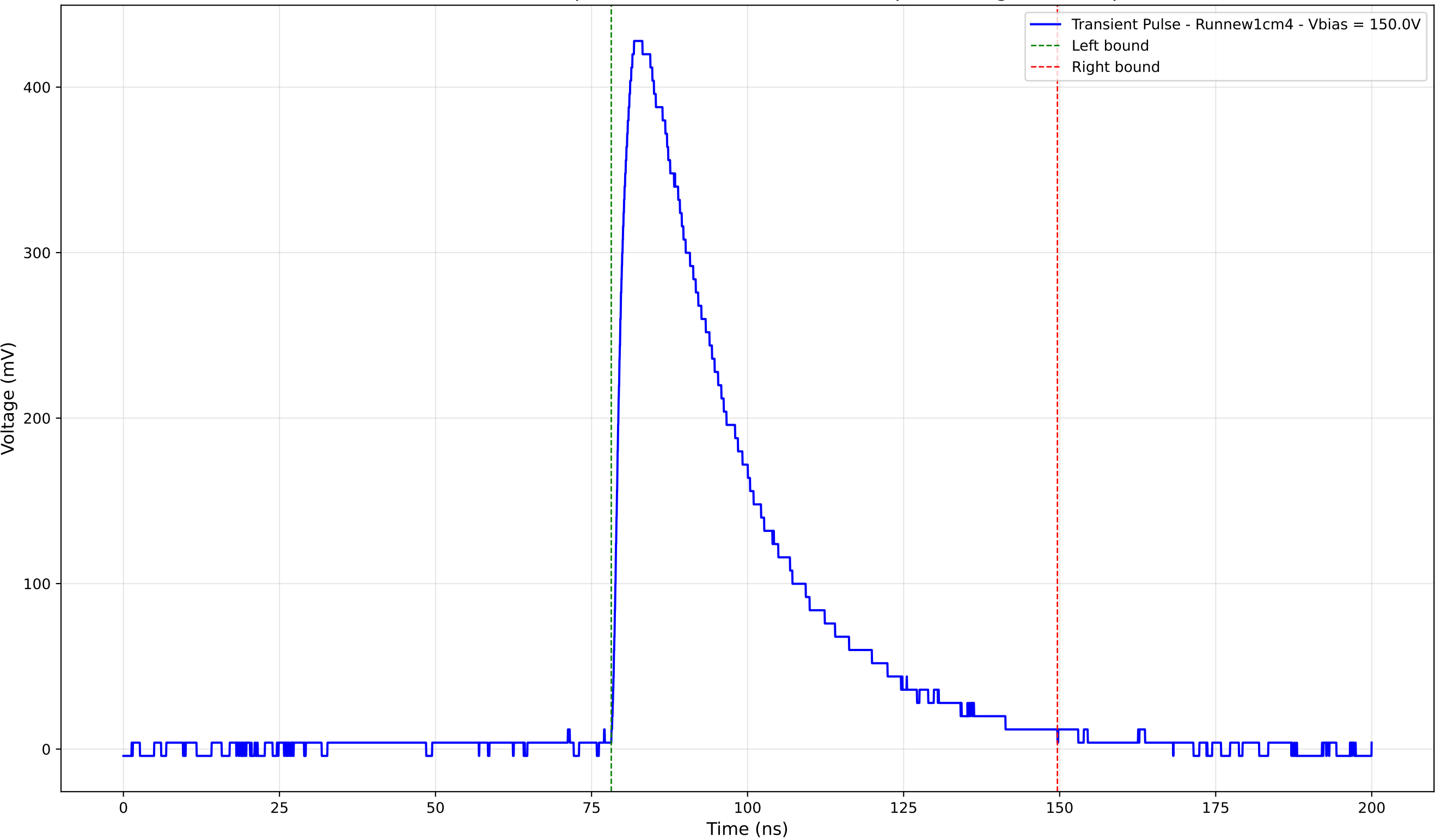
Transient Pulse - Sample: new1cm - Position: 2280.0 \mu\text{m} - Charge: 182.12 pC
