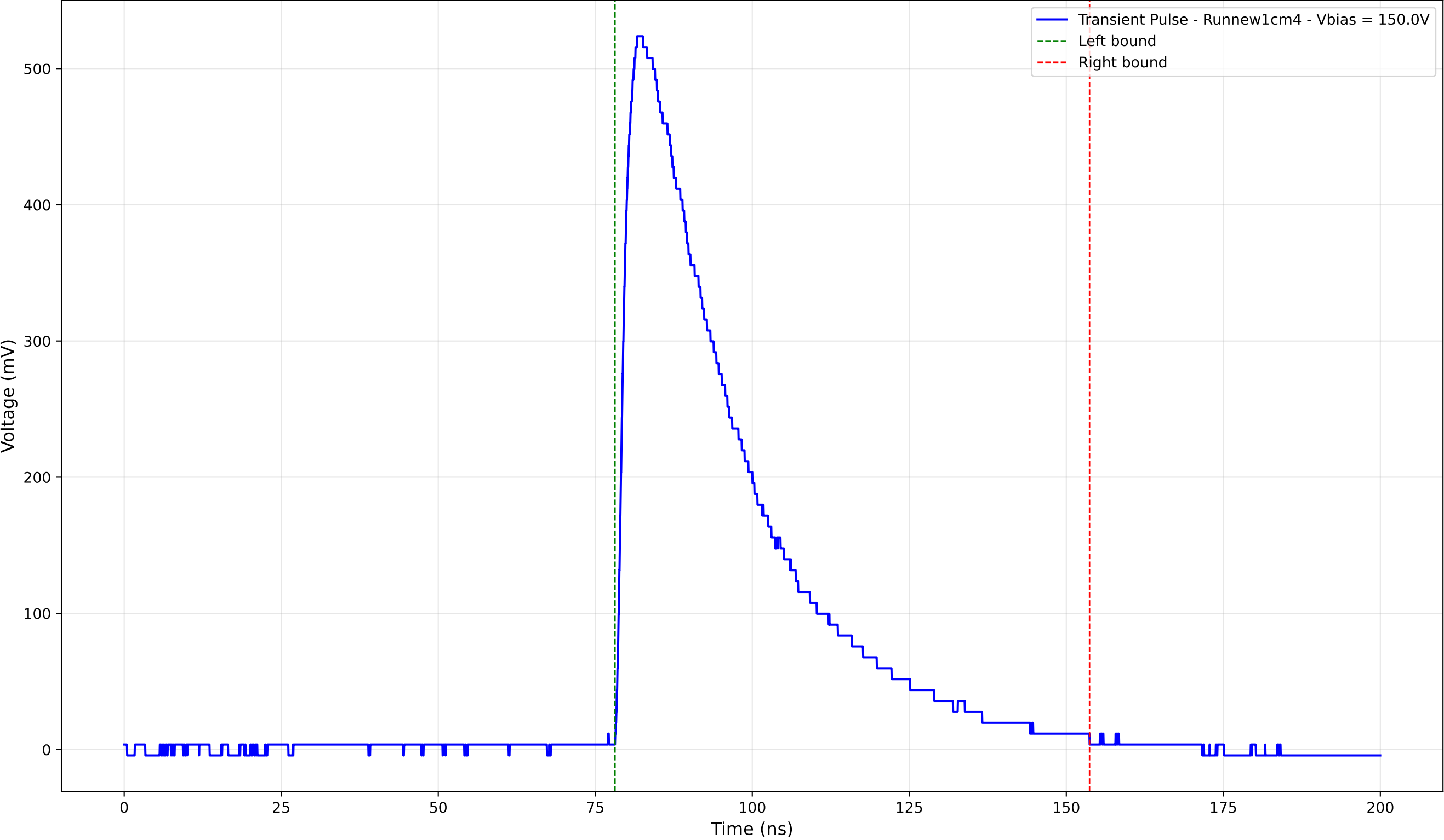
Transient Pulse - Sample: new1cm - Position: 2080.0 \mu\text{m} - Charge: 220.06 pC
