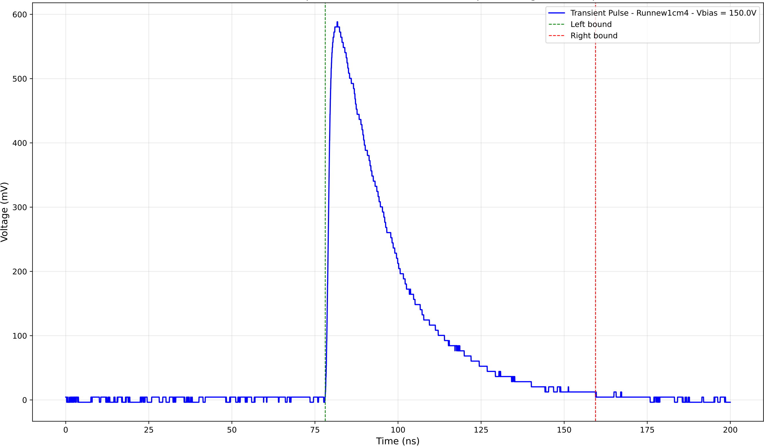
Transient Pulse - Sample: new1cm - Position: 3580.0 \mu\text{m} - Charge: 246.05 pC
