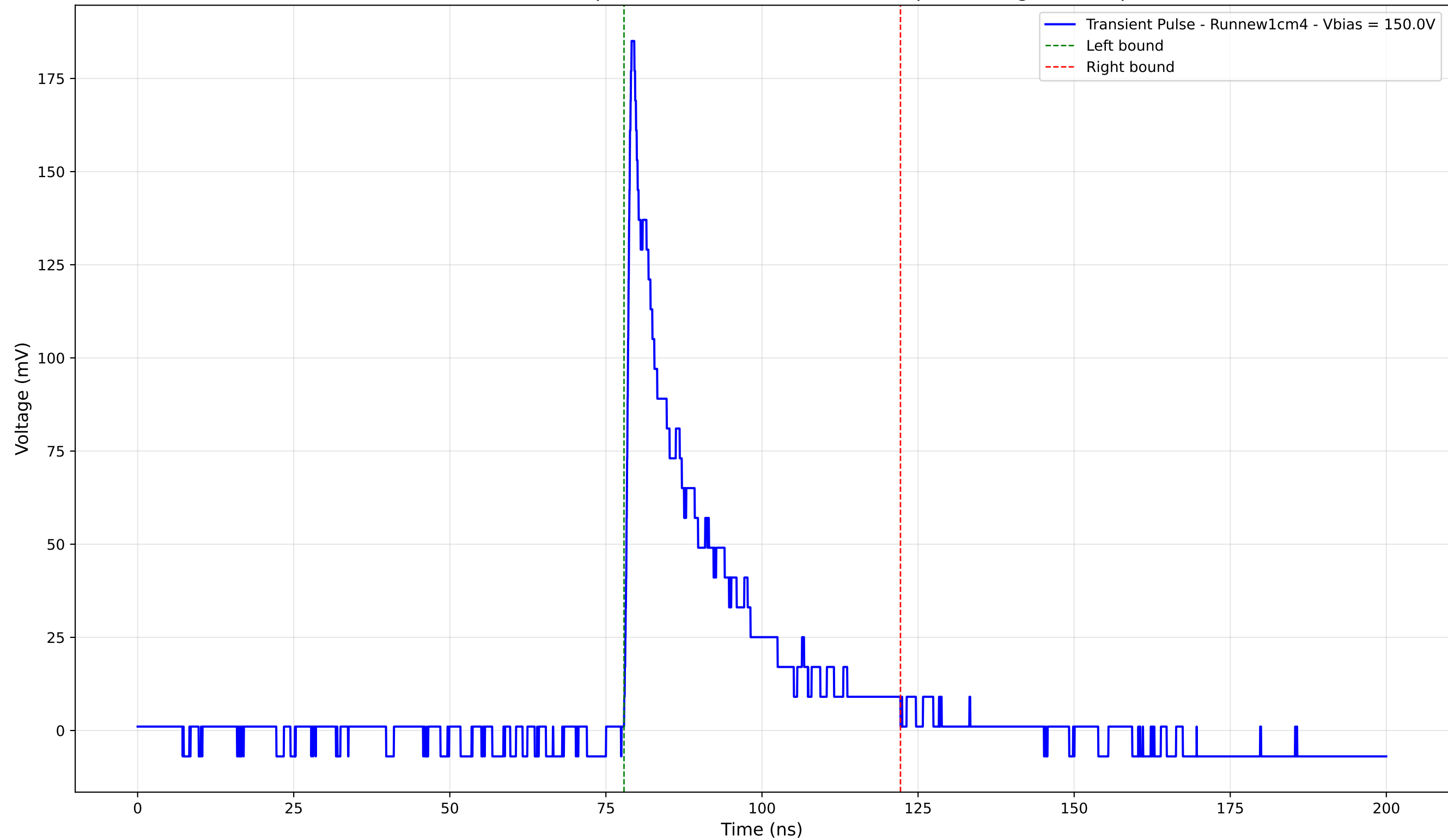
Transient Pulse - Sample: new1cm - Position: 4750.0 \mu\text{m} - Charge: 37.29 pC
