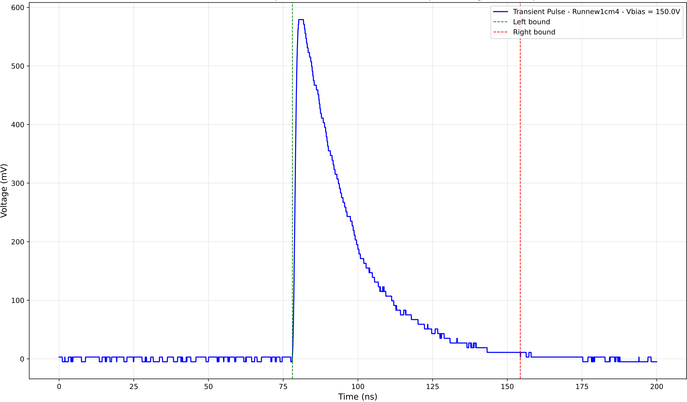
Transient Pulse - Sample: new1cm - Position: 3820.0 \mu\text{m} - Charge: 227.50 pC
