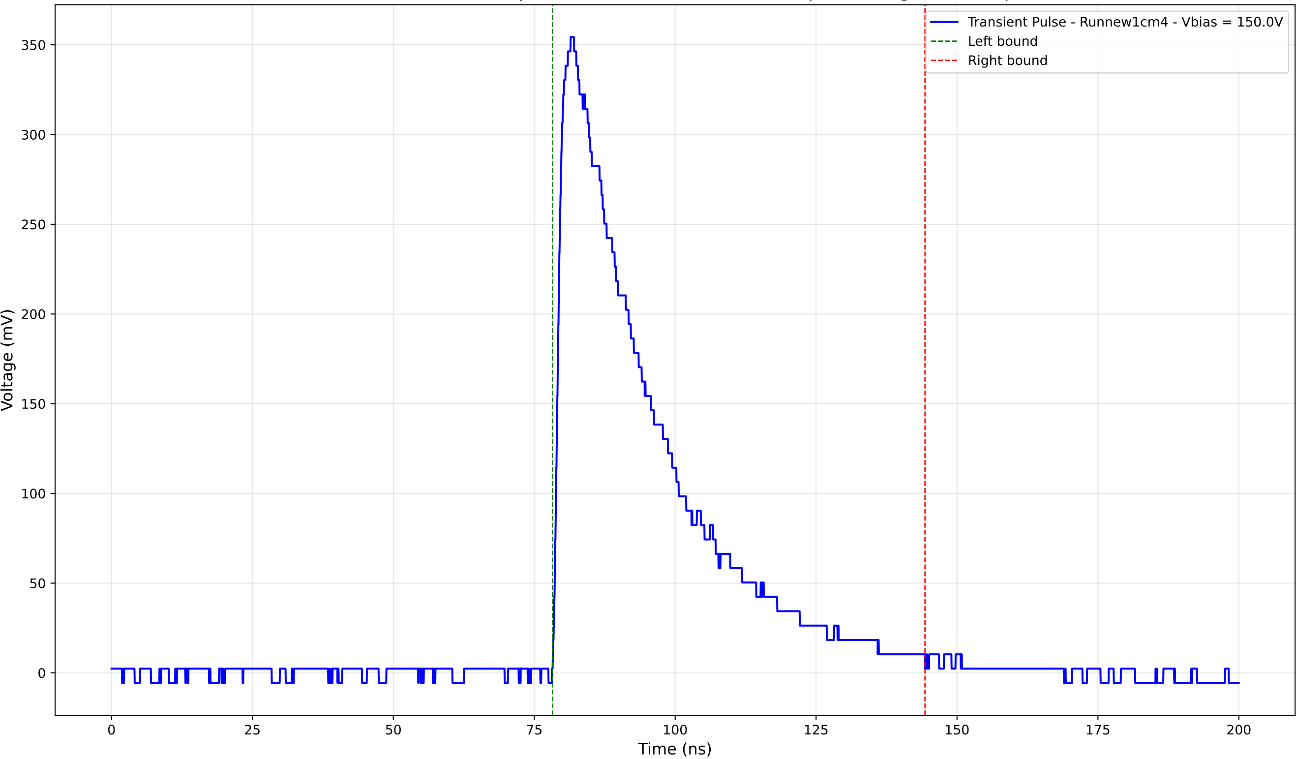
Transient Pulse - Sample: new1cm - Position: 1645.0 \mu\text{m} - Charge: 130.88 pC
