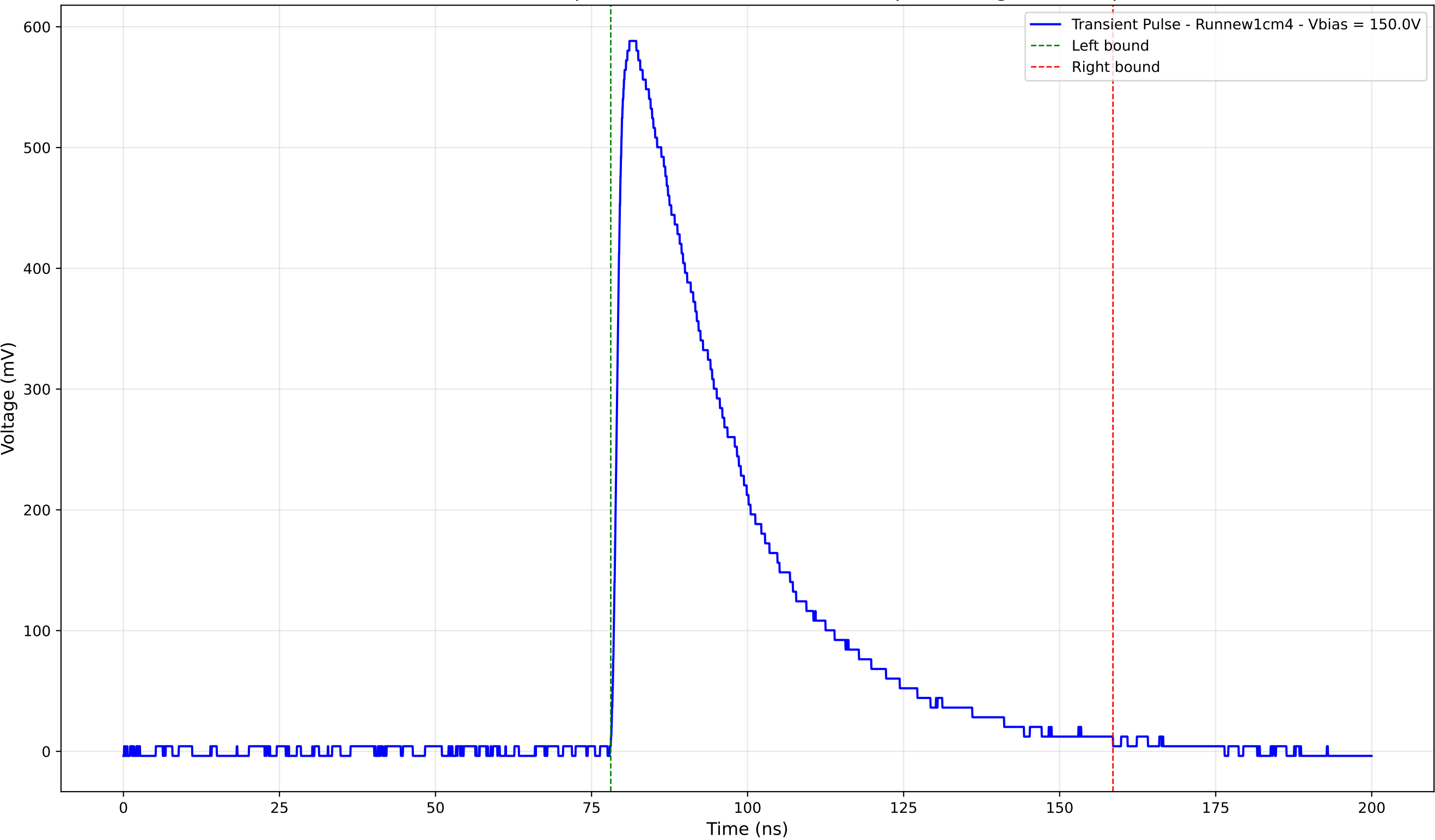
Transient Pulse - Sample: new1cm - Position: 3605.0 \mu\text{m} - Charge: 246.77 pC
