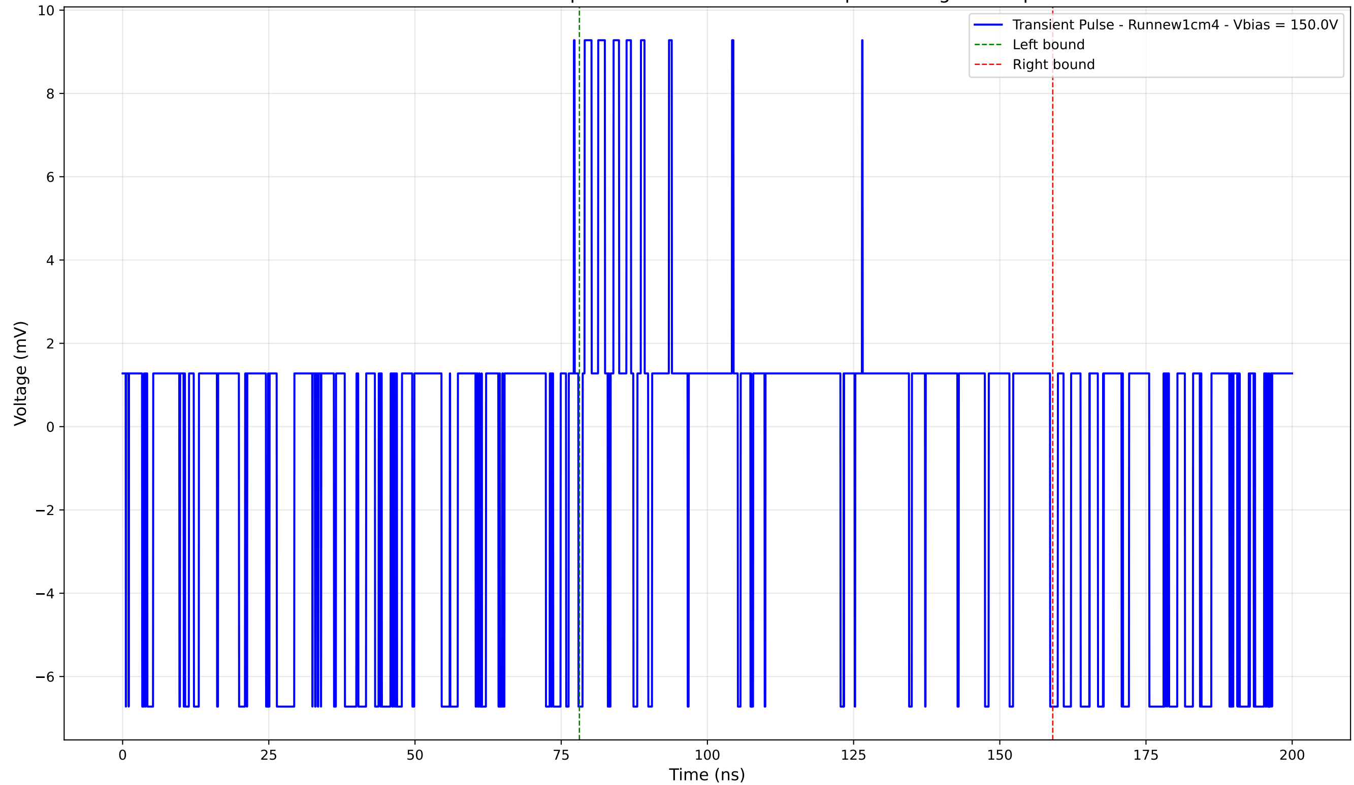
Transient Pulse - Sample: new1cm - Position: 35.0 \mu\text{m} - Charge: 1.90 pC
