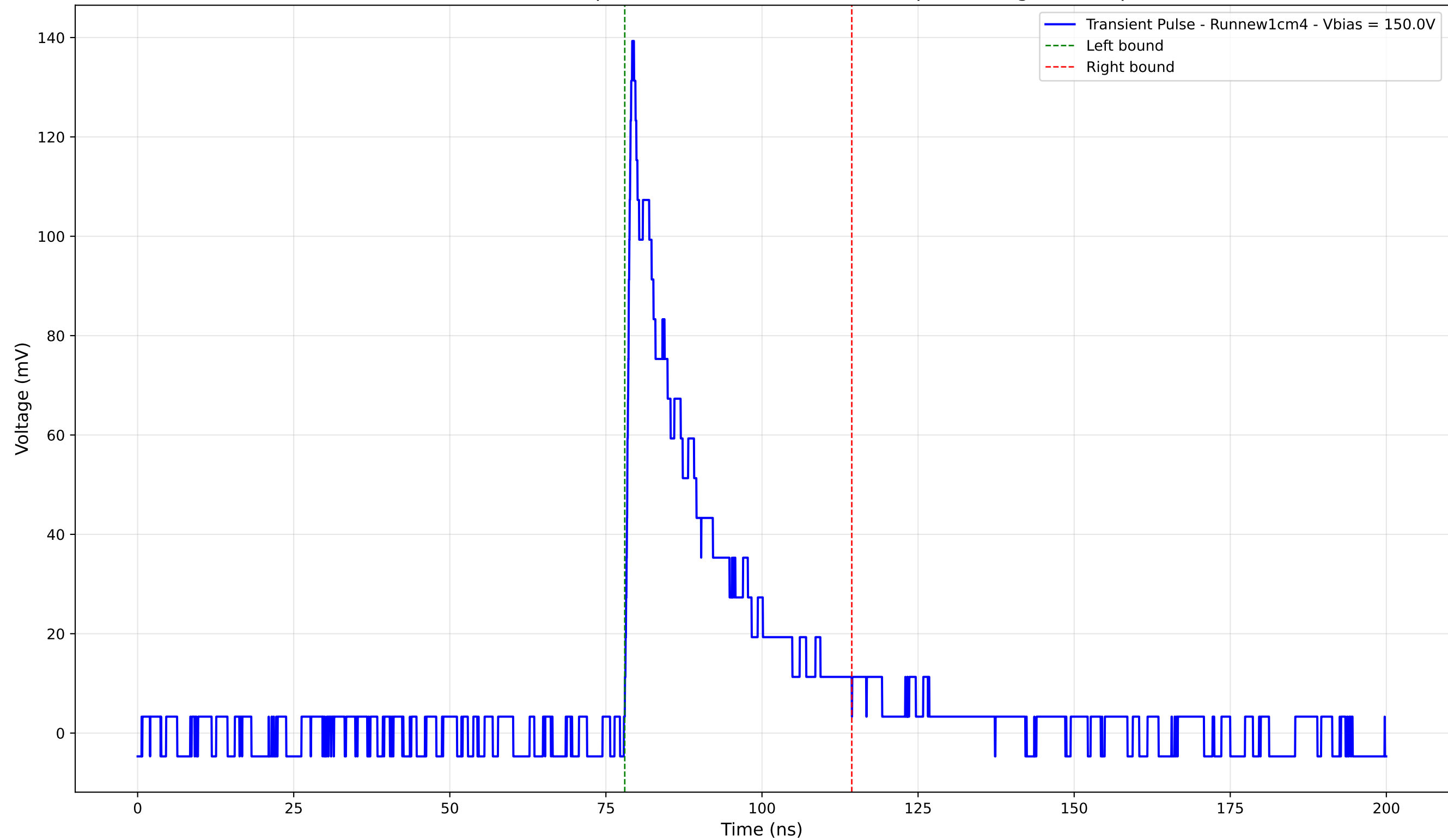
Transient Pulse - Sample: new1cm - Position: 4735.0 \mu\text{m} - Charge: 29.58 pC
