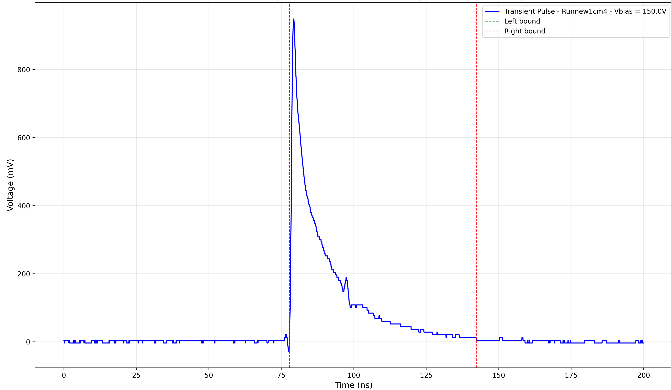
Transient Pulse - Sample: new1cm - Position: 320.0 \mu\text{m} - Charge: 188.45 pC
