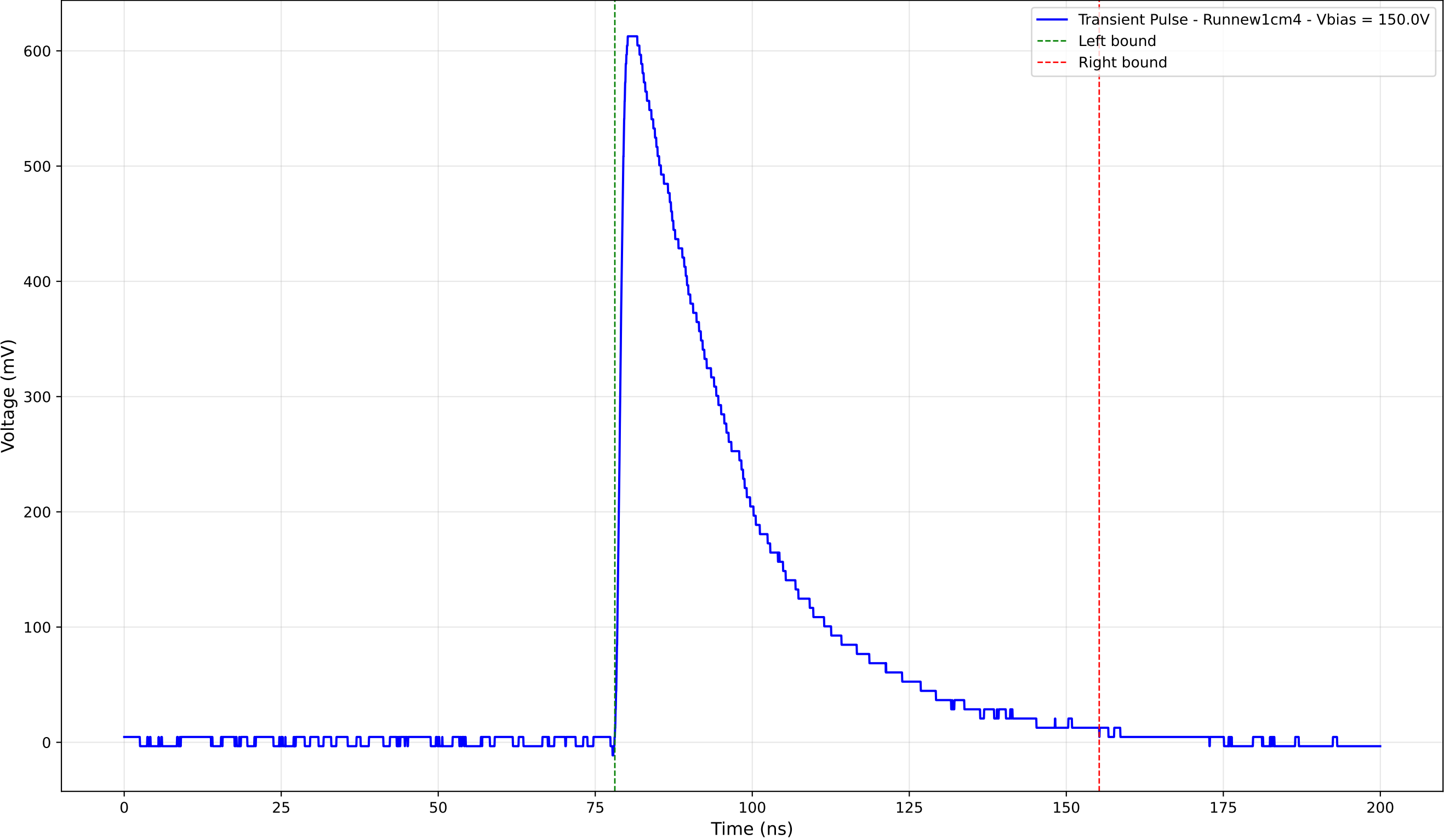
Transient Pulse - Sample: new1cm - Position: 3835.0 \mu\text{m} - Charge: 243.28 pC
