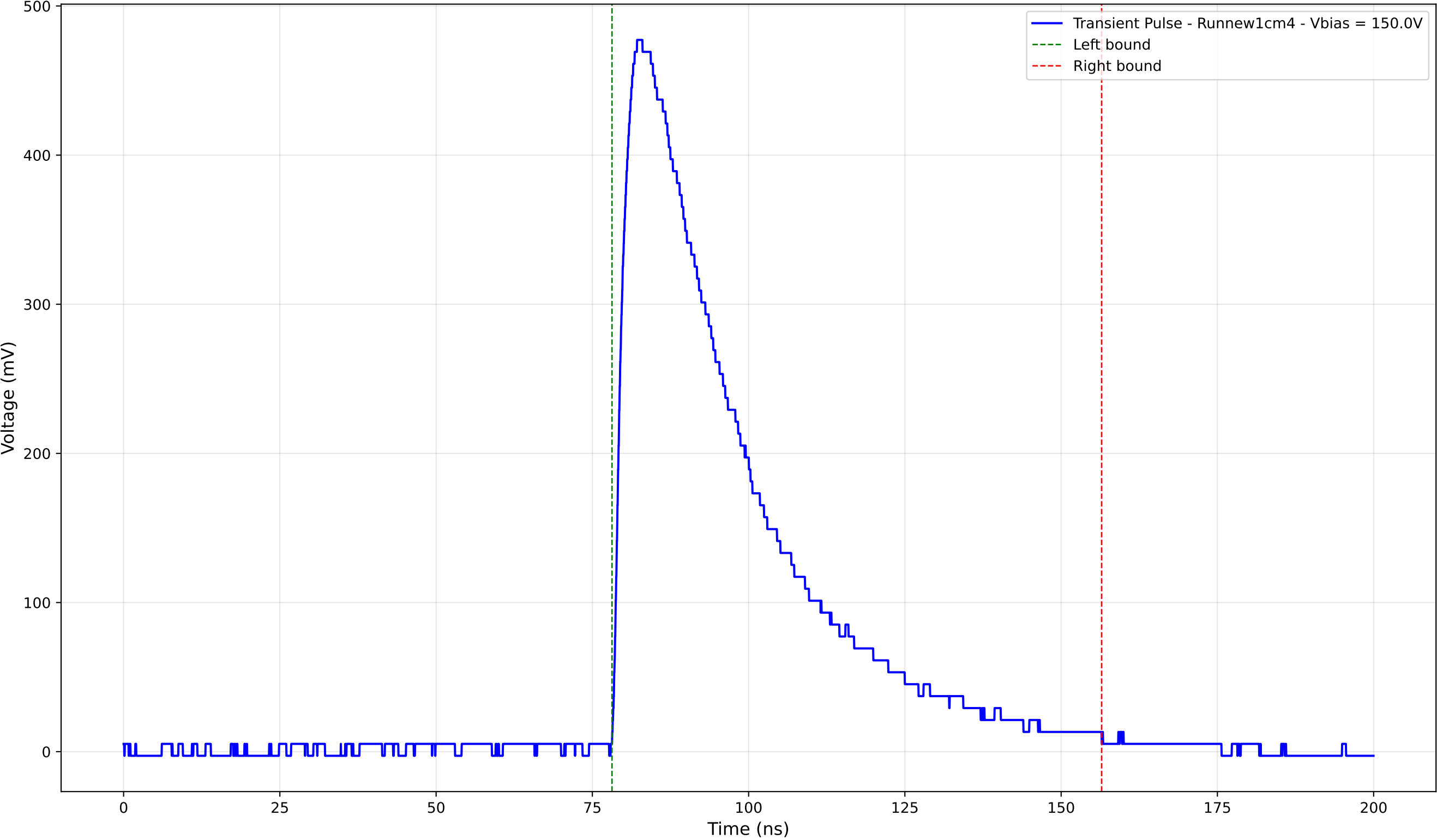
Transient Pulse - Sample: new1cm - Position: 2625.0 \mu\text{m} - Charge: 211.27 pC
