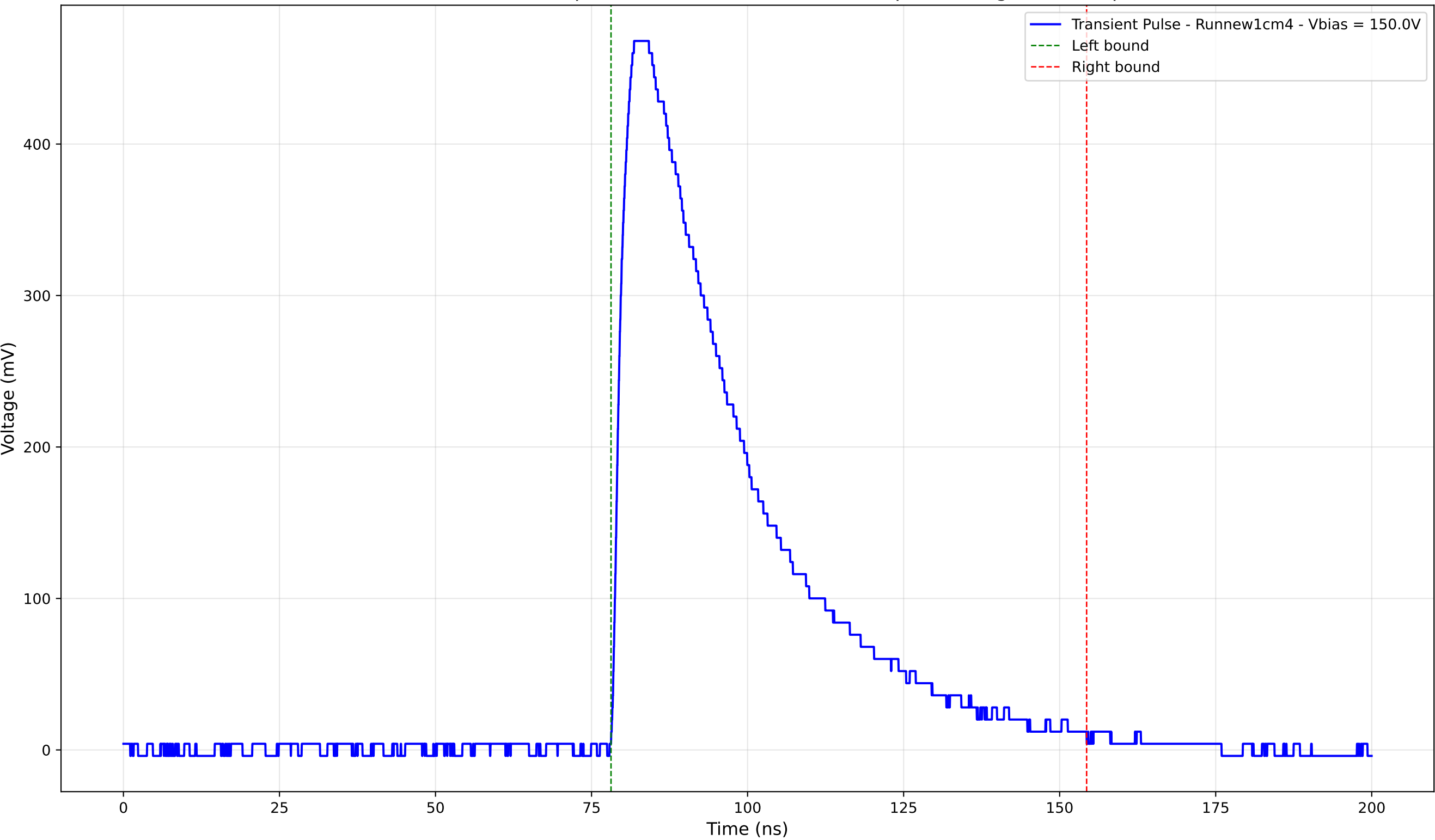
Transient Pulse - Sample: new1cm - Position: 2815.0 \mu\text{m} - Charge: 210.47 pC
