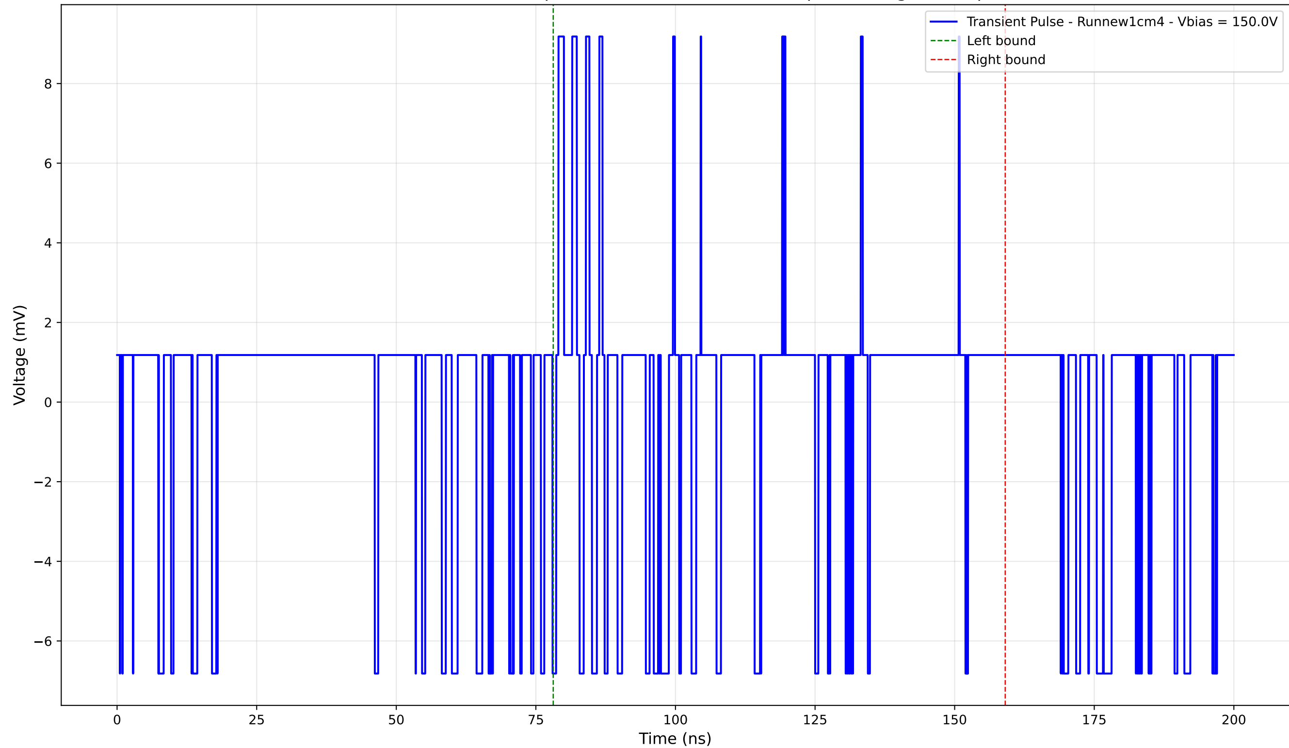
Transient Pulse - Sample: new1cm - Position: 20.0 \mu\text{m} - Charge: 0.69 pC
