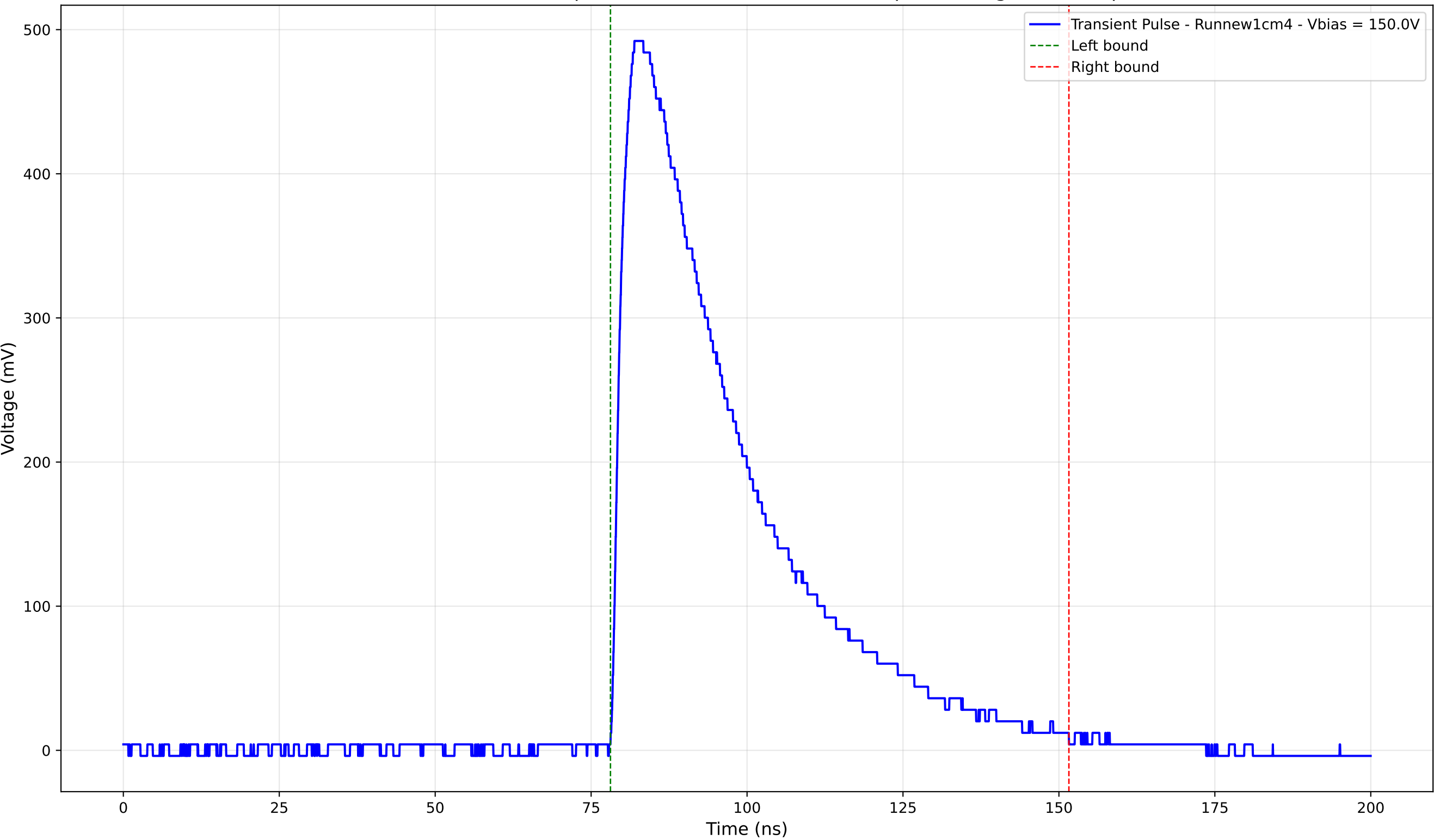
Transient Pulse - Sample: new1cm - Position: 2615.0 \mu\text{m} - Charge: 217.15 pC
