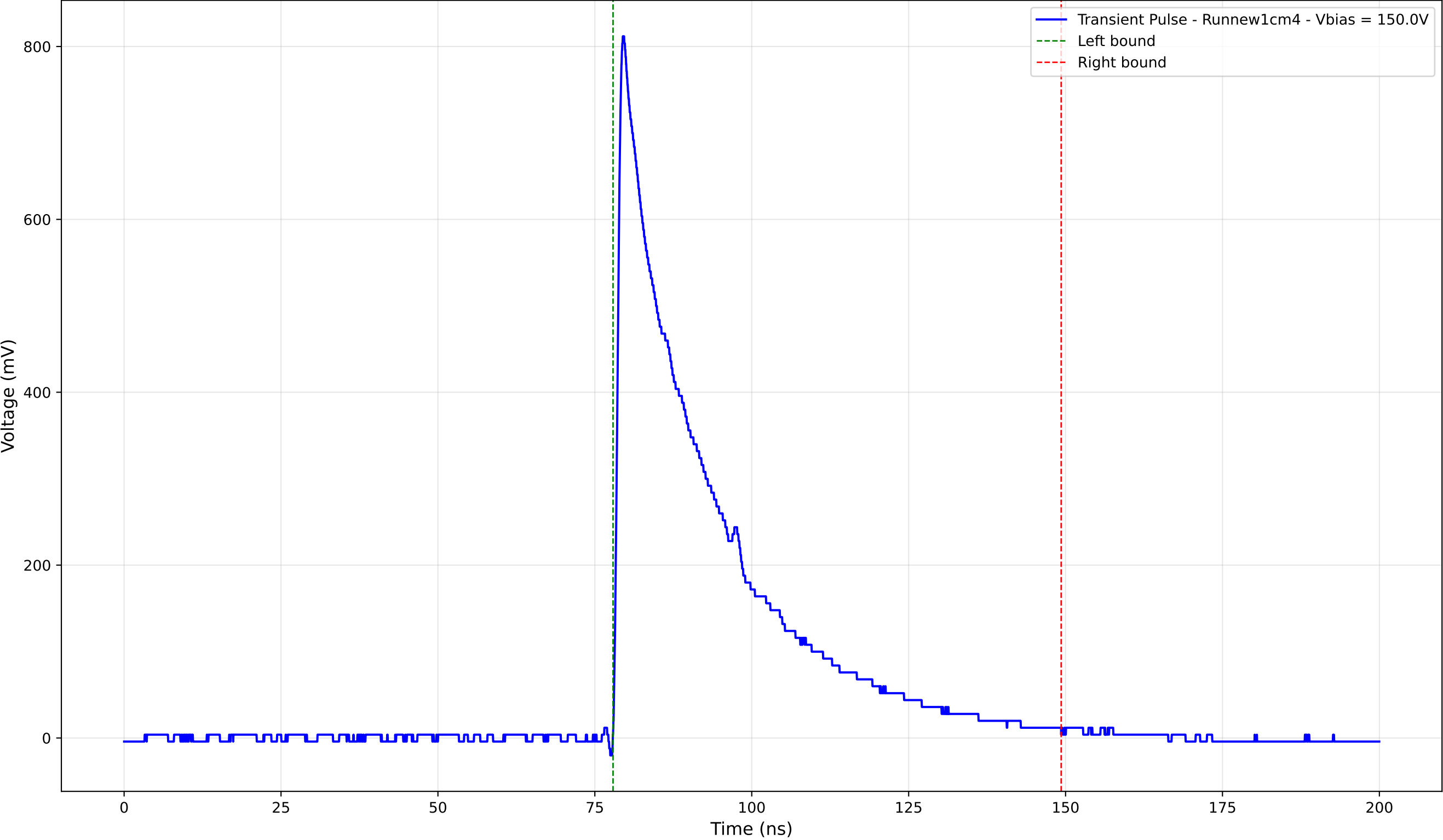
Transient Pulse - Sample: new1cm - Position: 4490.0 \mu\text{m} - Charge: 238.90 pC
