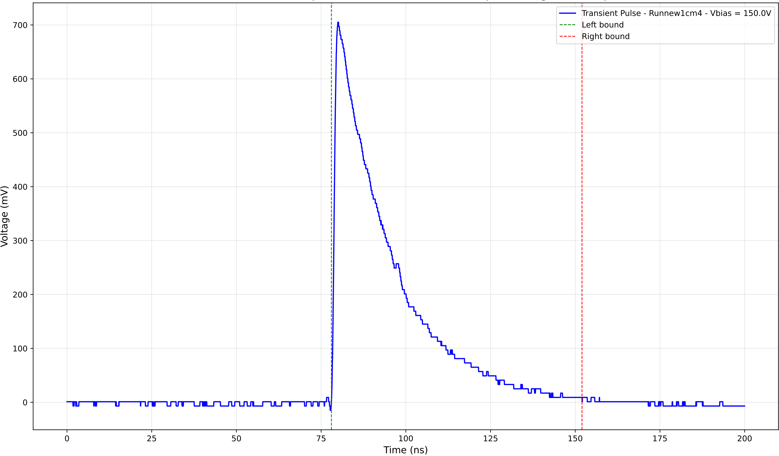
Transient Pulse - Sample: new1cm - Position: 4100.0 \mu\text{m} - Charge: 246.47 pC
