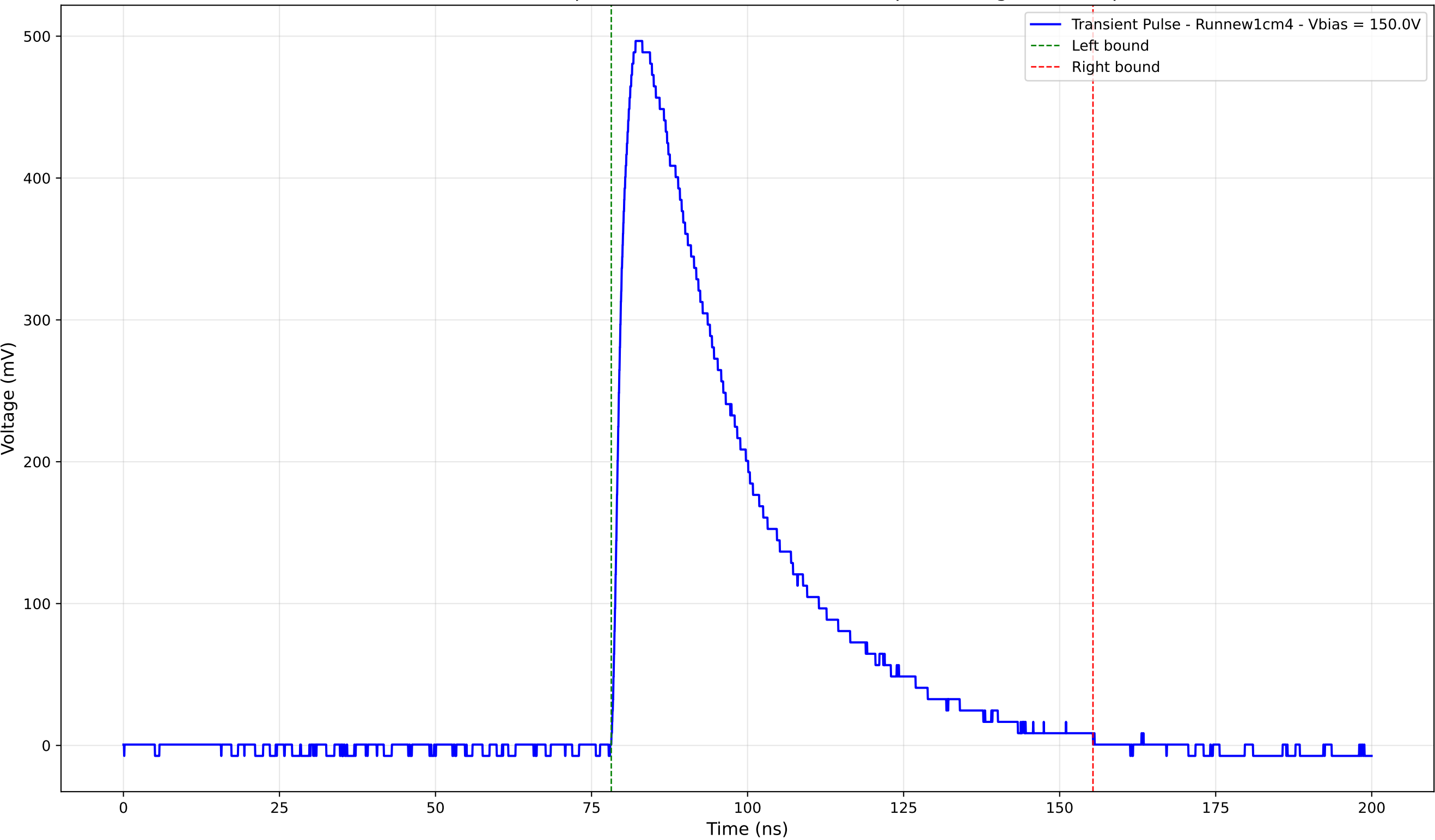
Transient Pulse - Sample: new1cm - Position: 2490.0 \mu\text{m} - Charge: 214.75 pC
