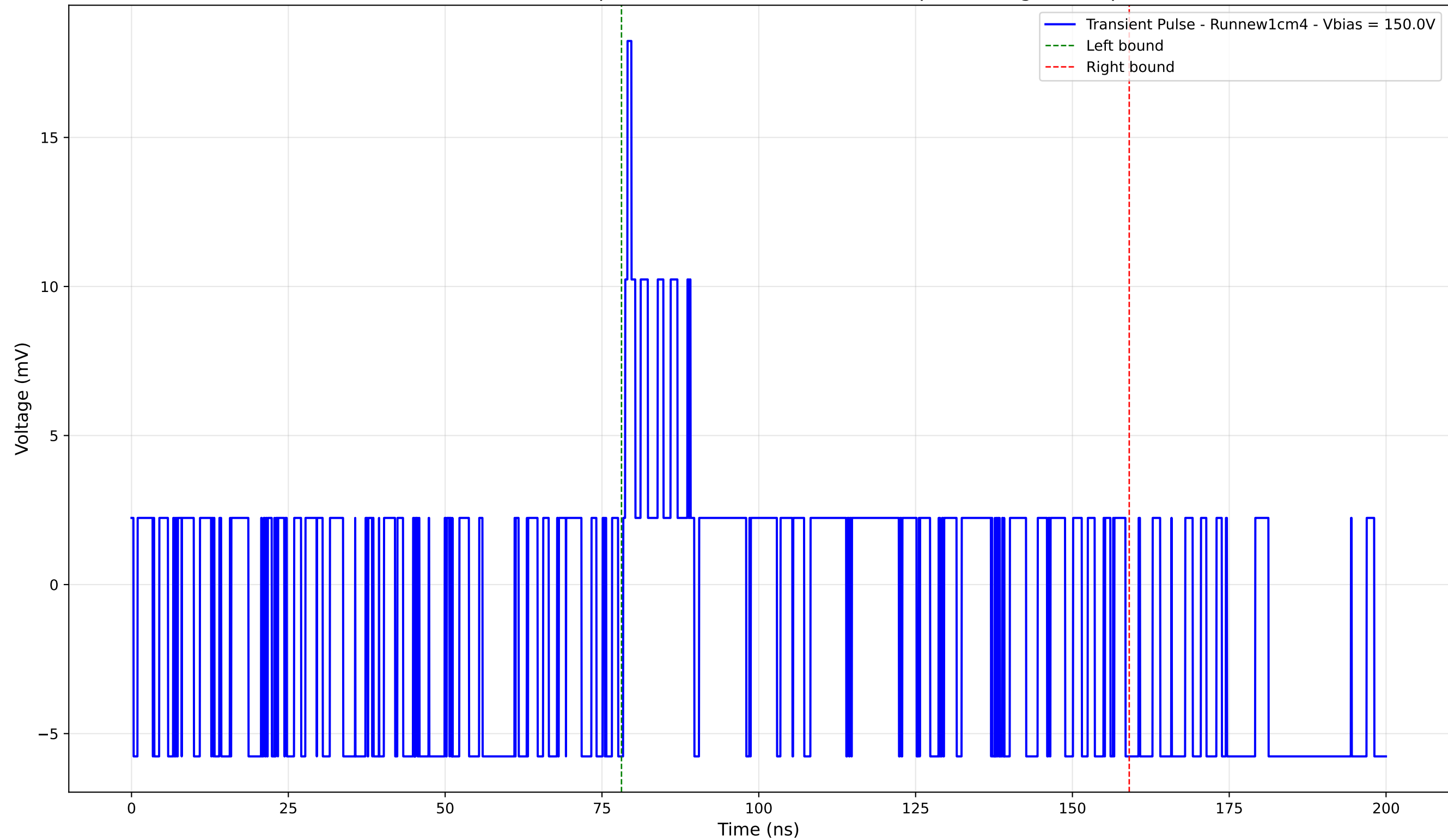
Transient Pulse - Sample: new1cm - Position: 5110.0 \mu\text{m} - Charge: 1.93 pC
