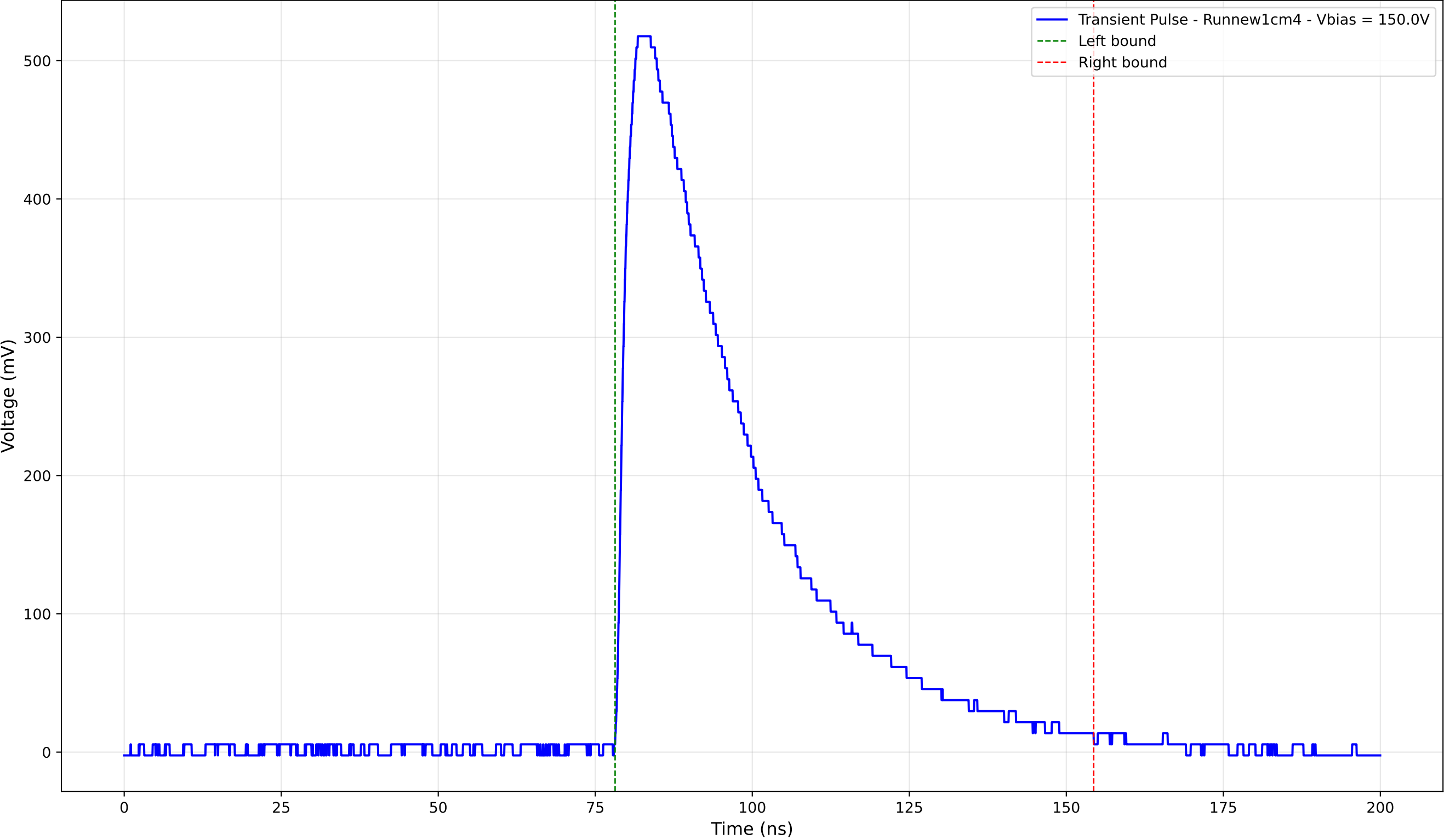
Transient Pulse - Sample: new1cm - Position: 2950.0 \mu\text{m} - Charge: 232.34 pC
