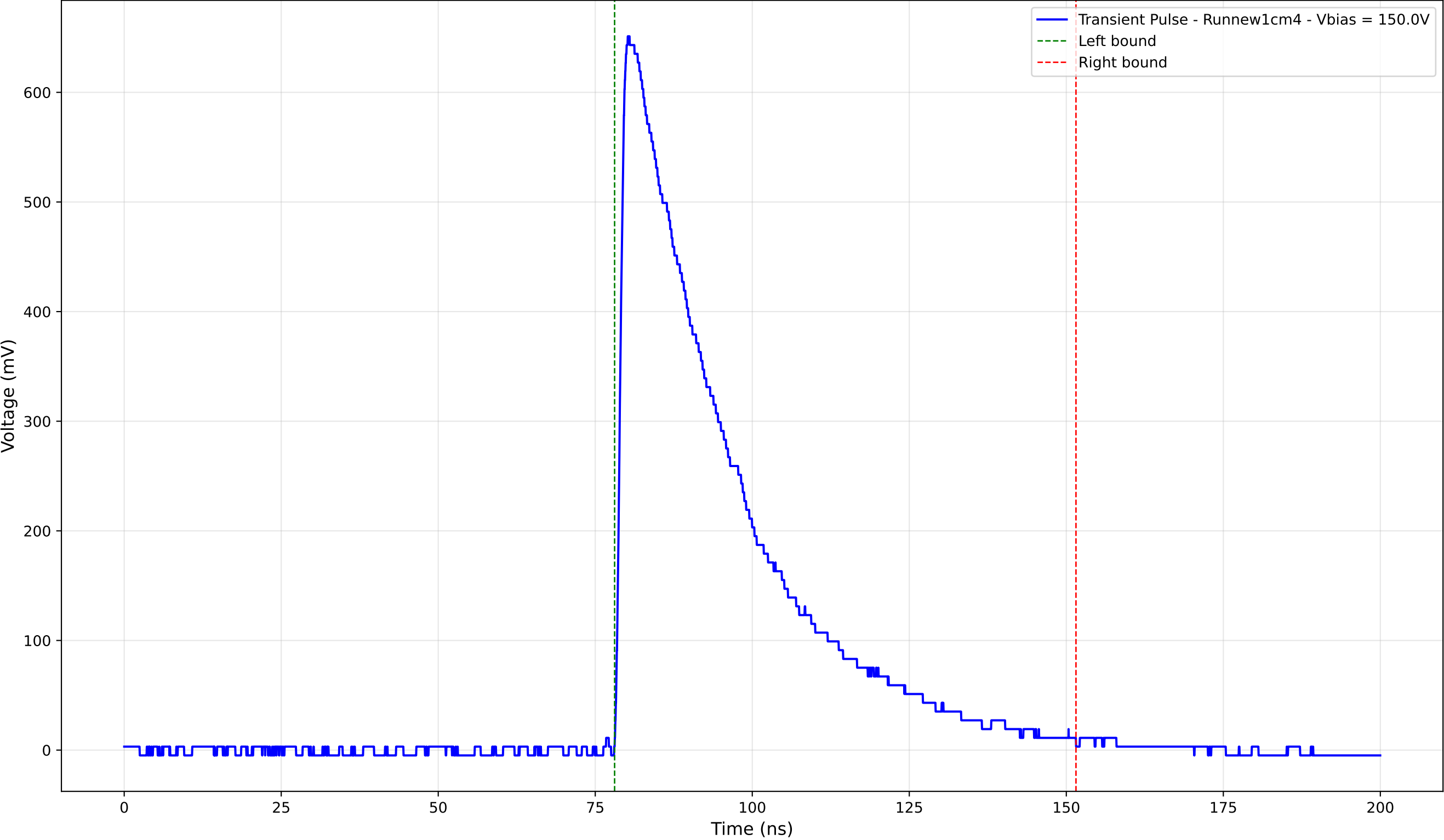
Transient Pulse - Sample: new1cm - Position: 3925.0 \mu\text{m} - Charge: 246.98 pC
