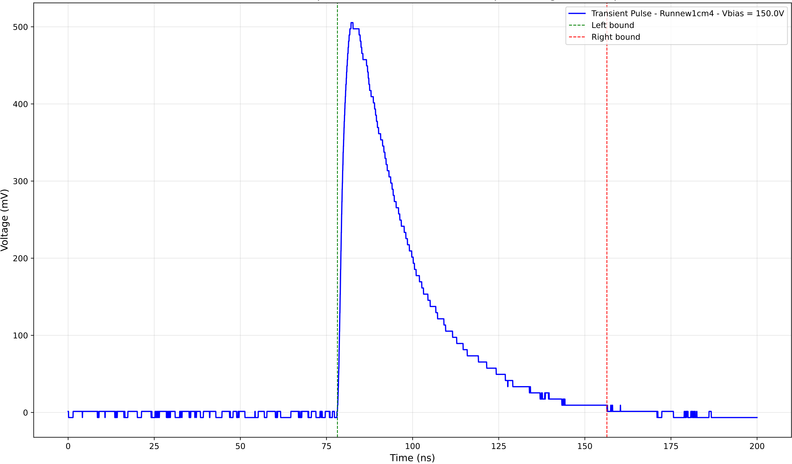
Transient Pulse - Sample: new1cm - Position: 2500.0 \mu\text{m} - Charge: 217.98 pC
