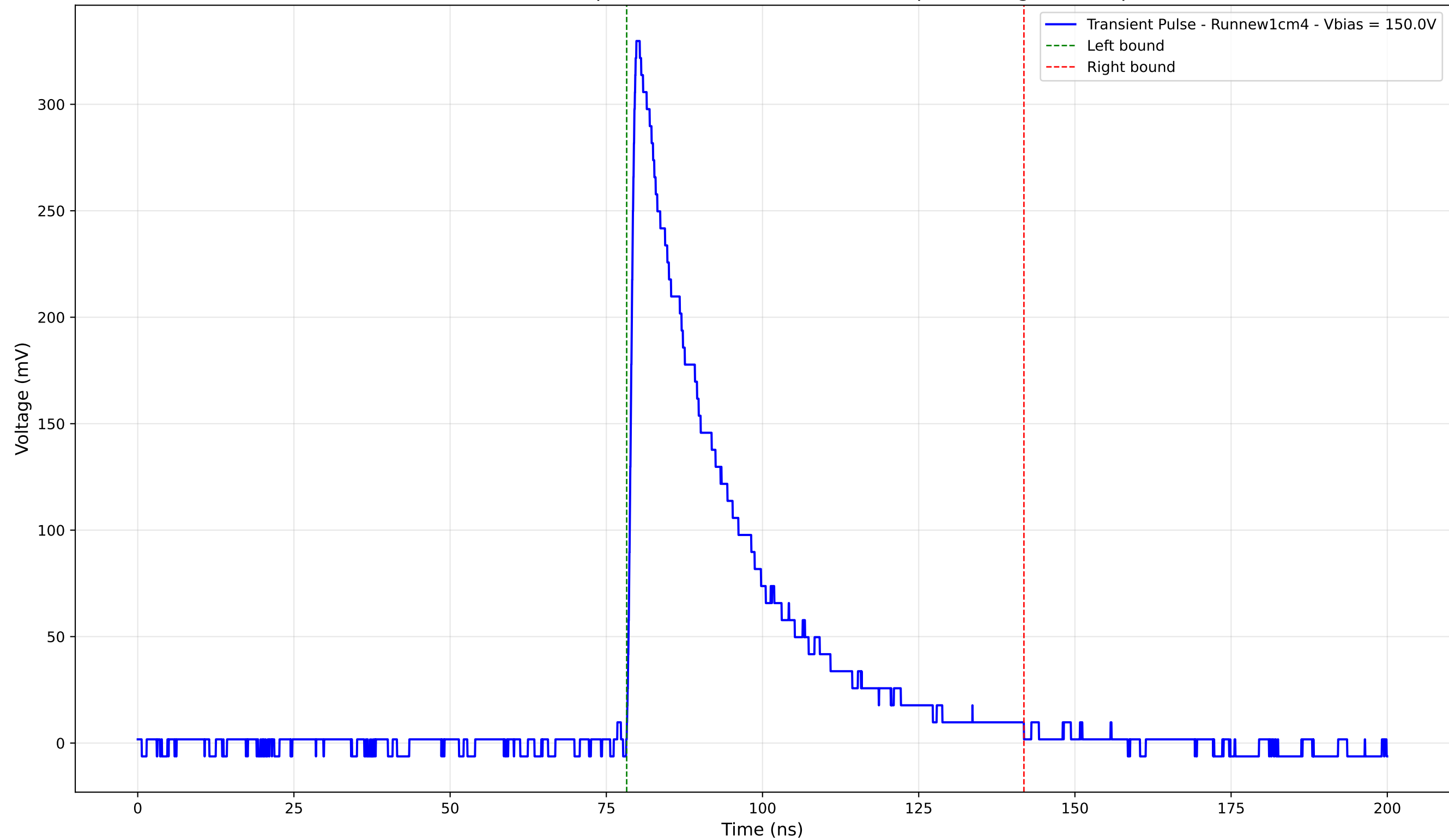
Transient Pulse - Sample: new1cm - Position: 1150.0 \mu\text{m} - Charge: 99.12 pC
