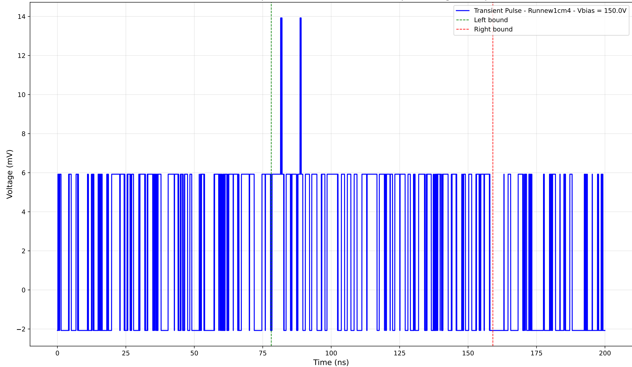
Transient Pulse - Sample: new1cm - Position: 5185.0 \mu\text{m} - Charge: 5.17 pC
