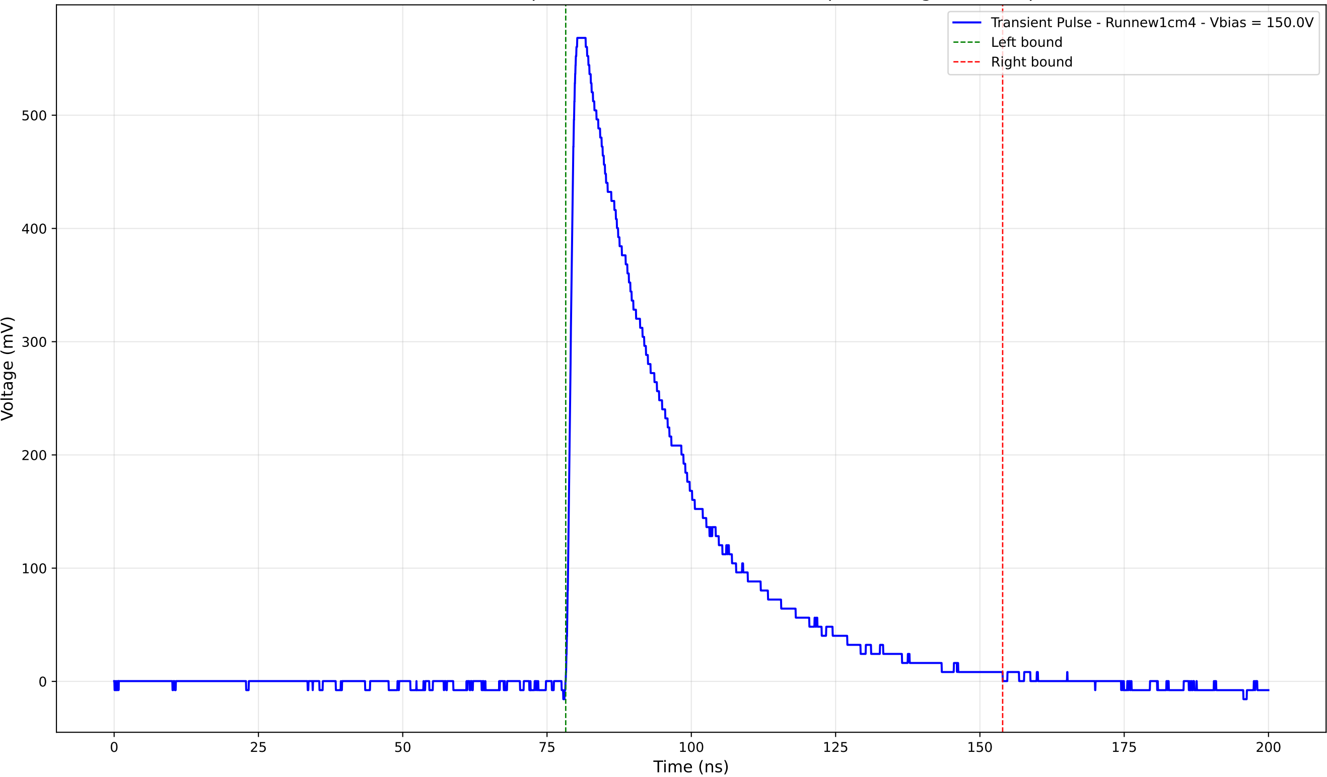
Transient Pulse - Sample: new1cm - Position: 1395.0 \mu\text{m} - Charge: 206.50 pC
