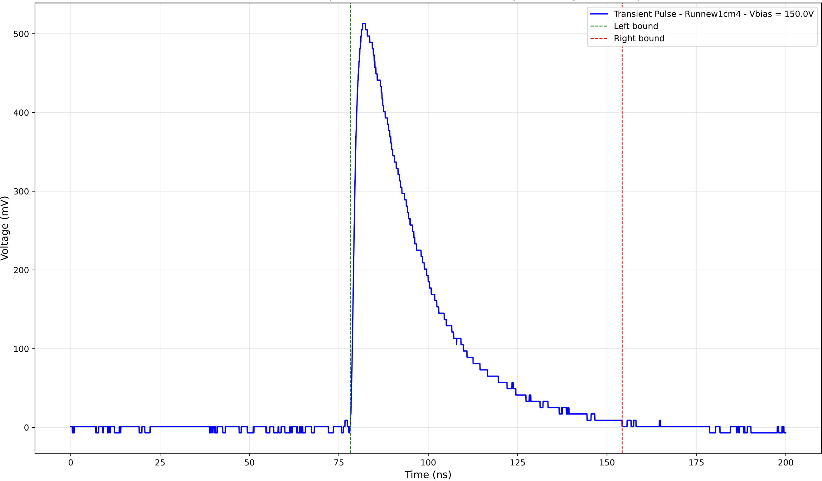
Transient Pulse - Sample: new1cm - Position: 1960.0 \mu\text{m} - Charge: 210.10 pC
