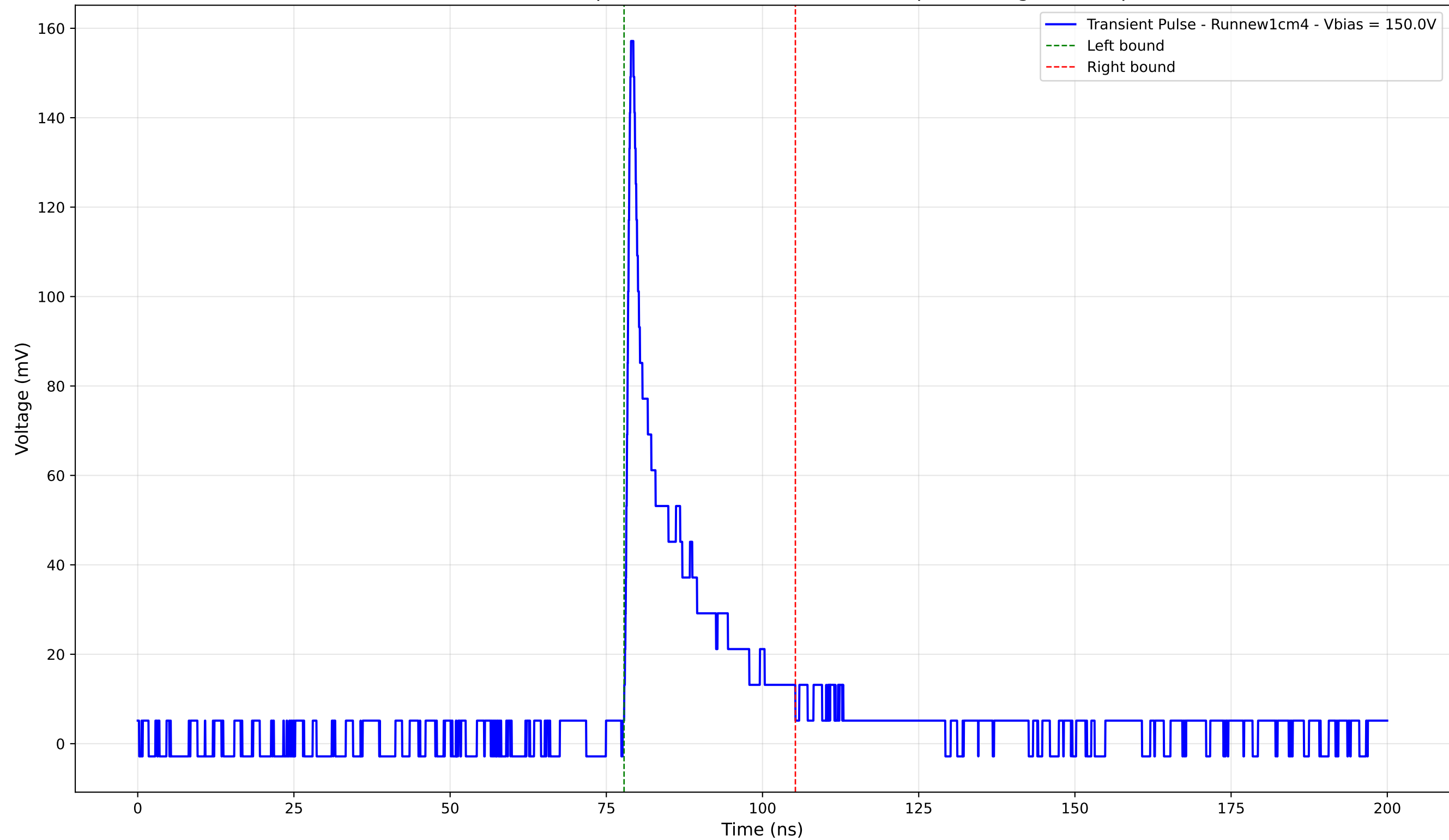
Transient Pulse - Sample: new1cm - Position: 5060.0 \mu\text{m} - Charge: 21.54 pC
