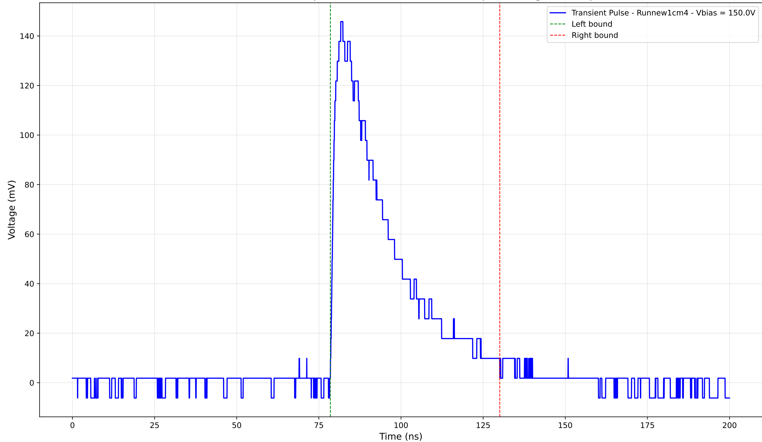
Transient Pulse - Sample: new1cm - Position: 1730.0 \mu\text{m} - Charge: 53.34 pC
