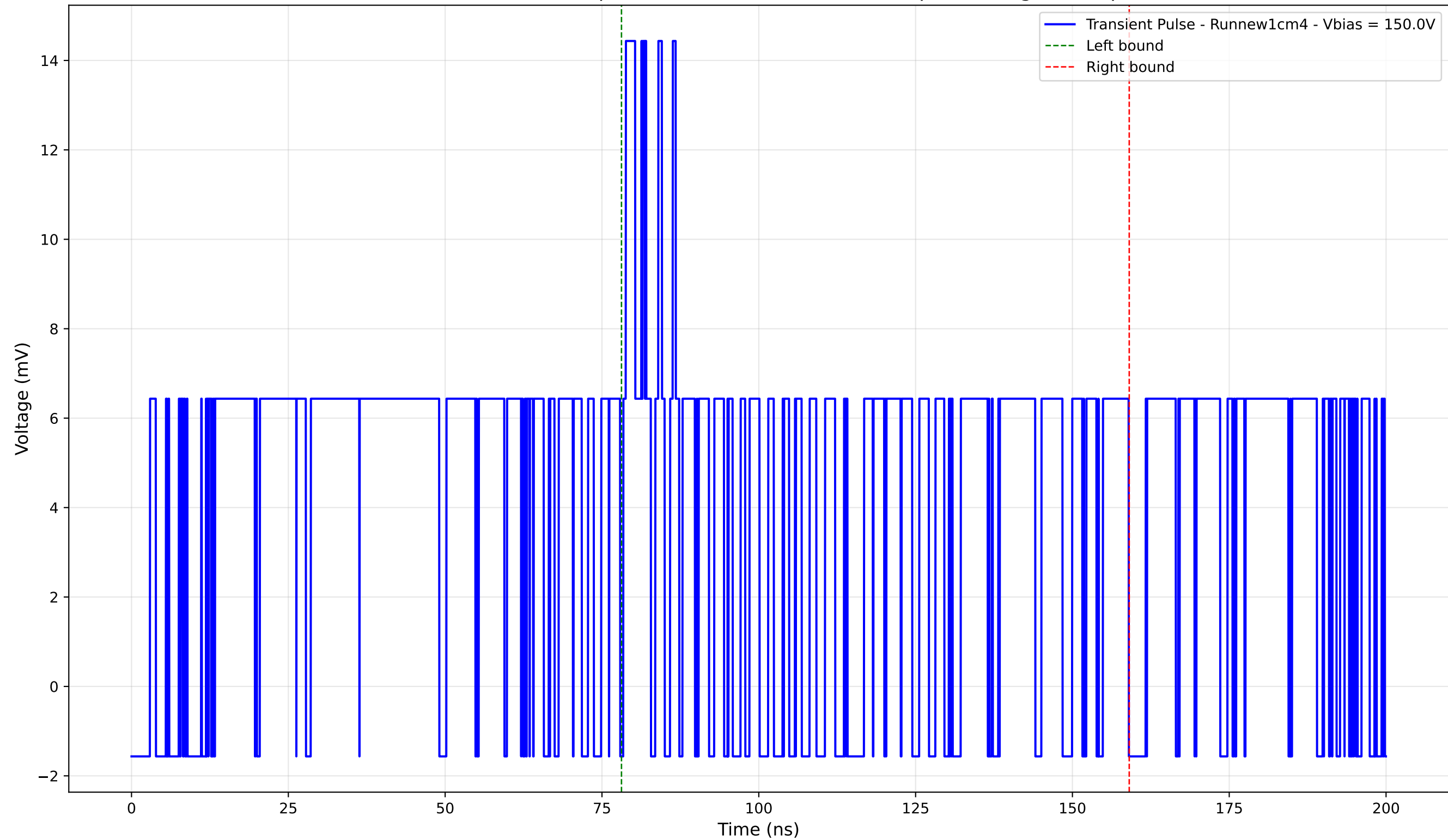
Transient Pulse - Sample: new1cm - Position: 5130.0 \mu\text{m} - Charge: 6.49 pC
