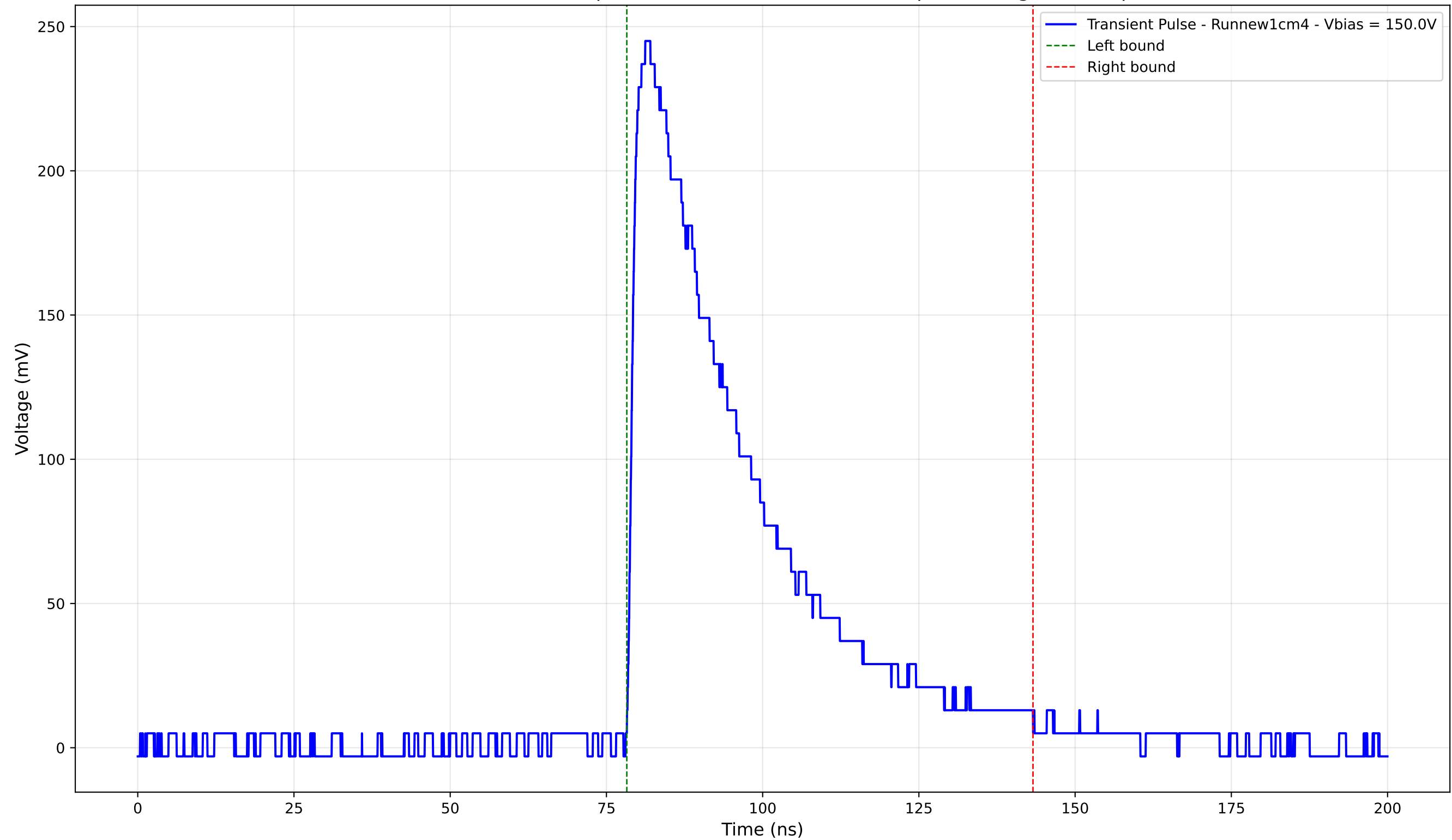
Transient Pulse - Sample: new1cm - Position: 3690.0 \mu\text{m} - Charge: 96.98 pC
