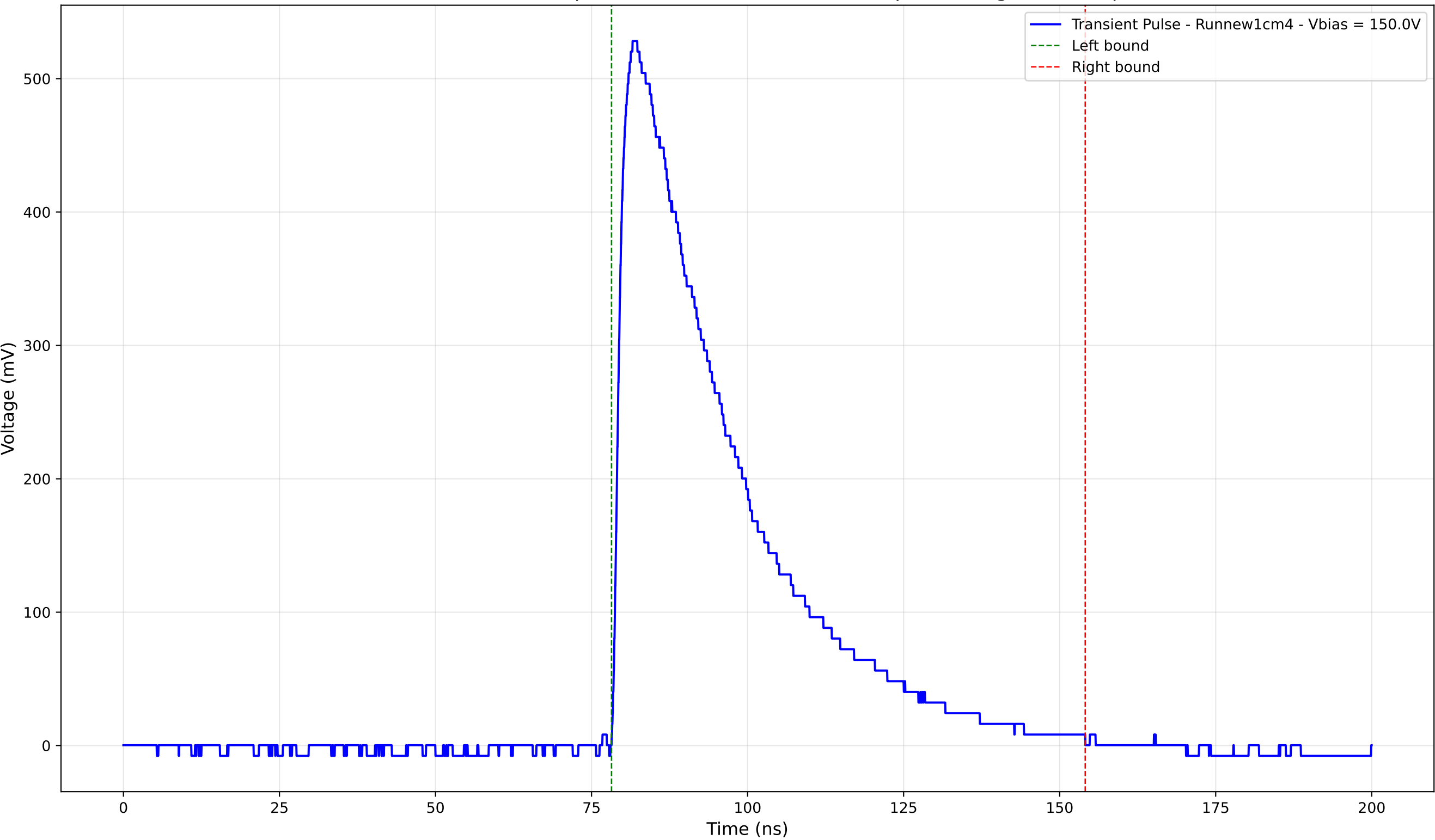
Transient Pulse - Sample: new1cm - Position: 1895.0 \mu\text{m} - Charge: 212.47 pC
