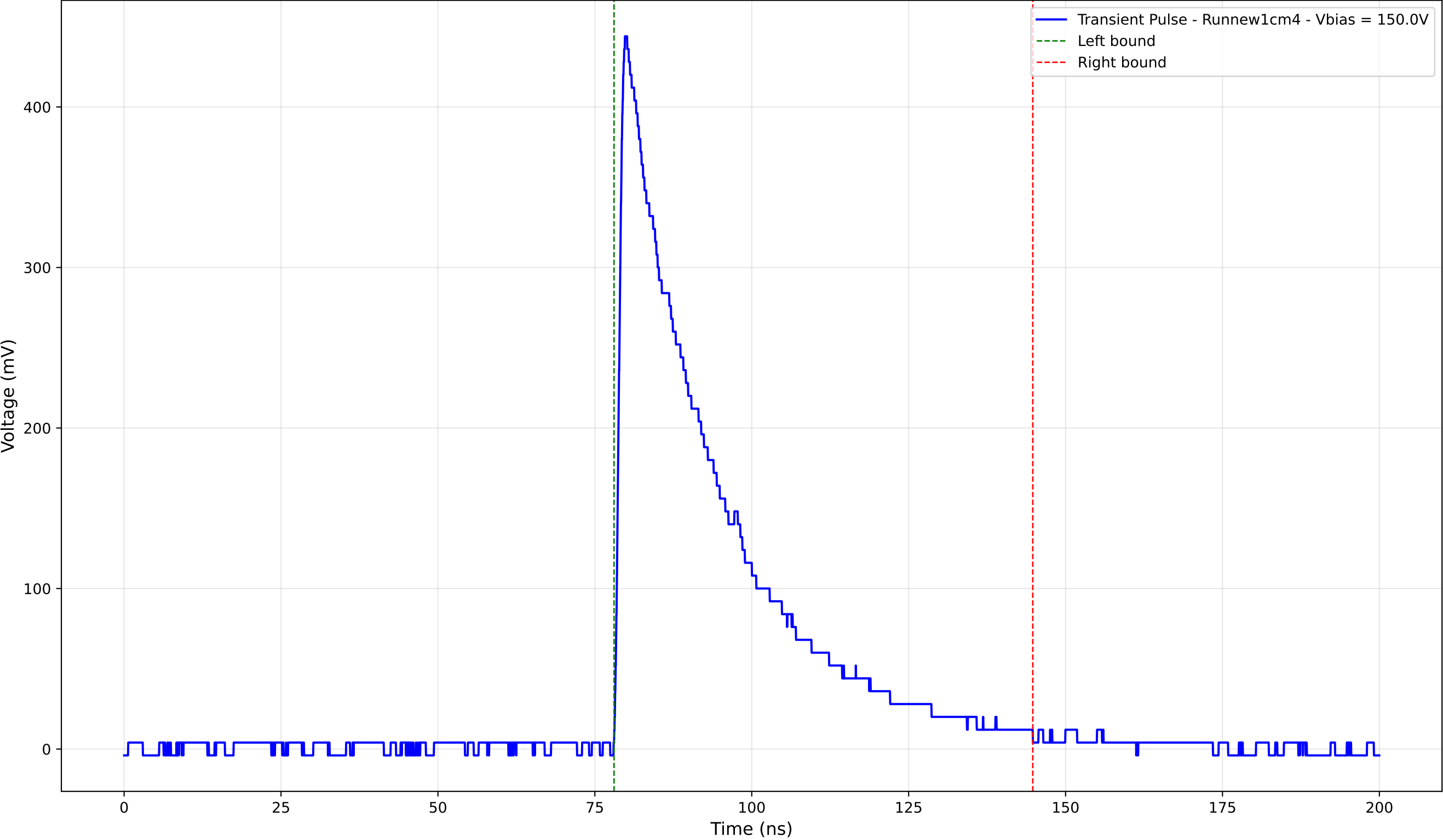
Transient Pulse - Sample: new1cm - Position: 4180.0 \mu\text{m} - Charge: 143.56 pC
