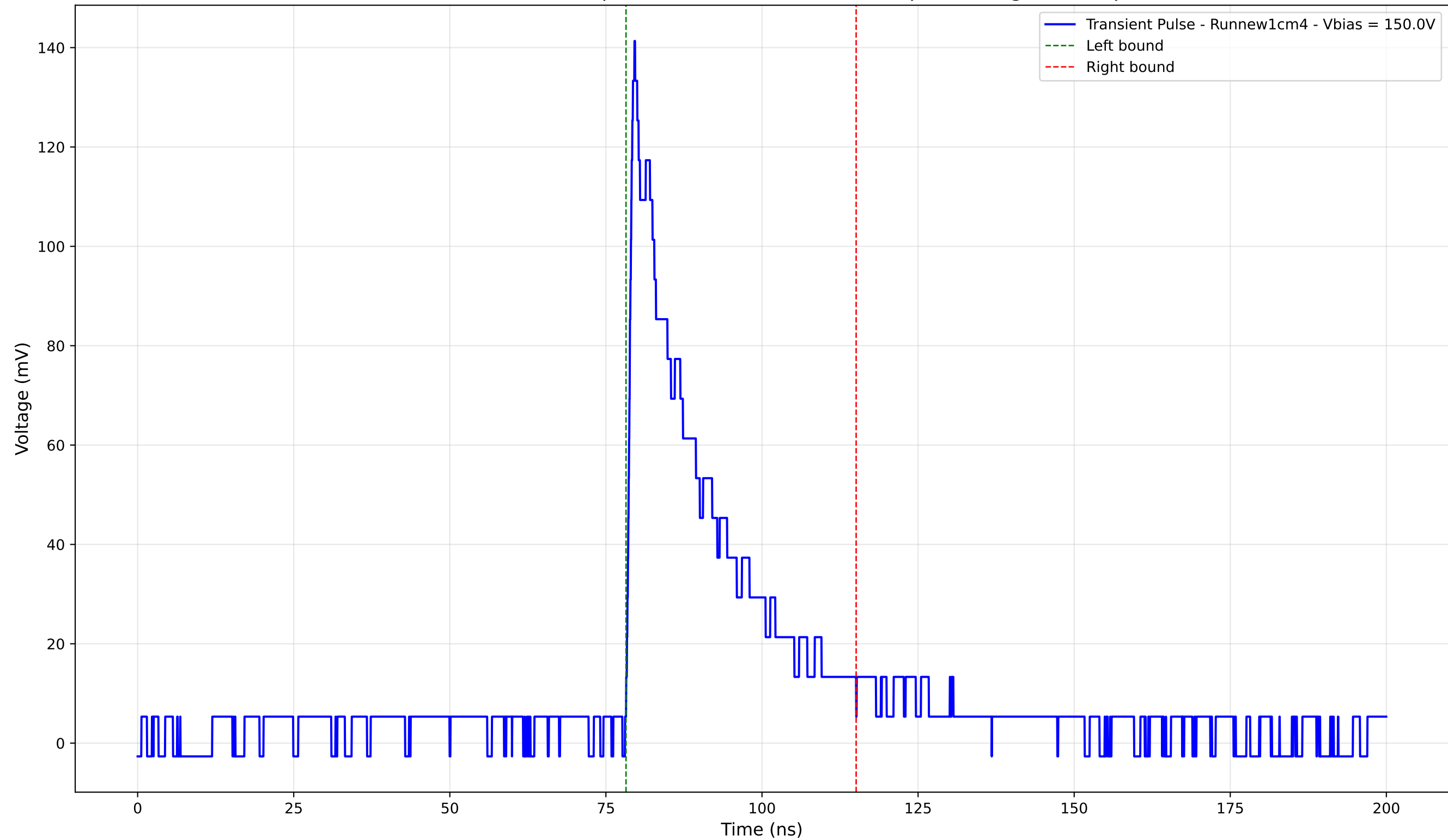
Transient Pulse - Sample: new1cm - Position: 705.0 \mu\text{m} - Charge: 33.36 pC
