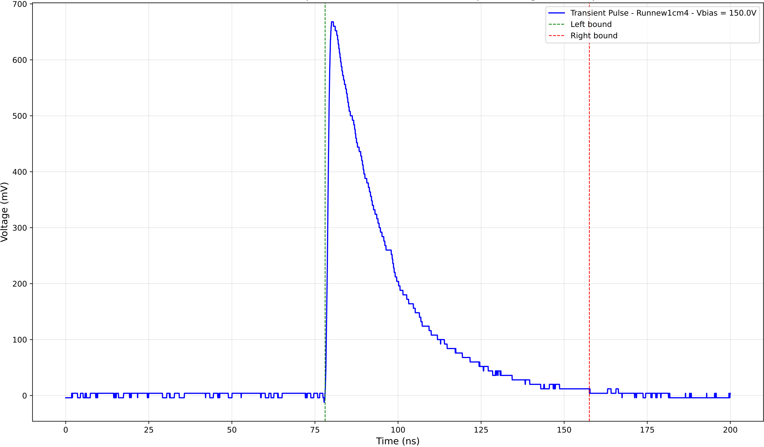
Transient Pulse - Sample: new1cm - Position: 4005.0 \mu\text{m} - Charge: 251.36 pC
