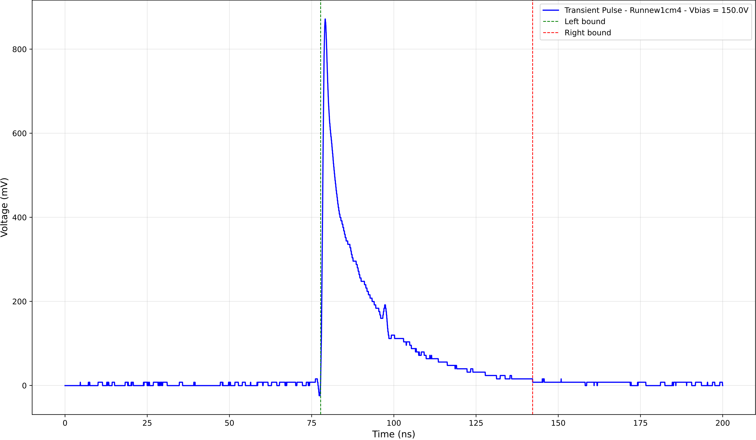
Transient Pulse - Sample: new1cm - Position: 4950.0 \mu\text{m} - Charge: 184.14 pC
