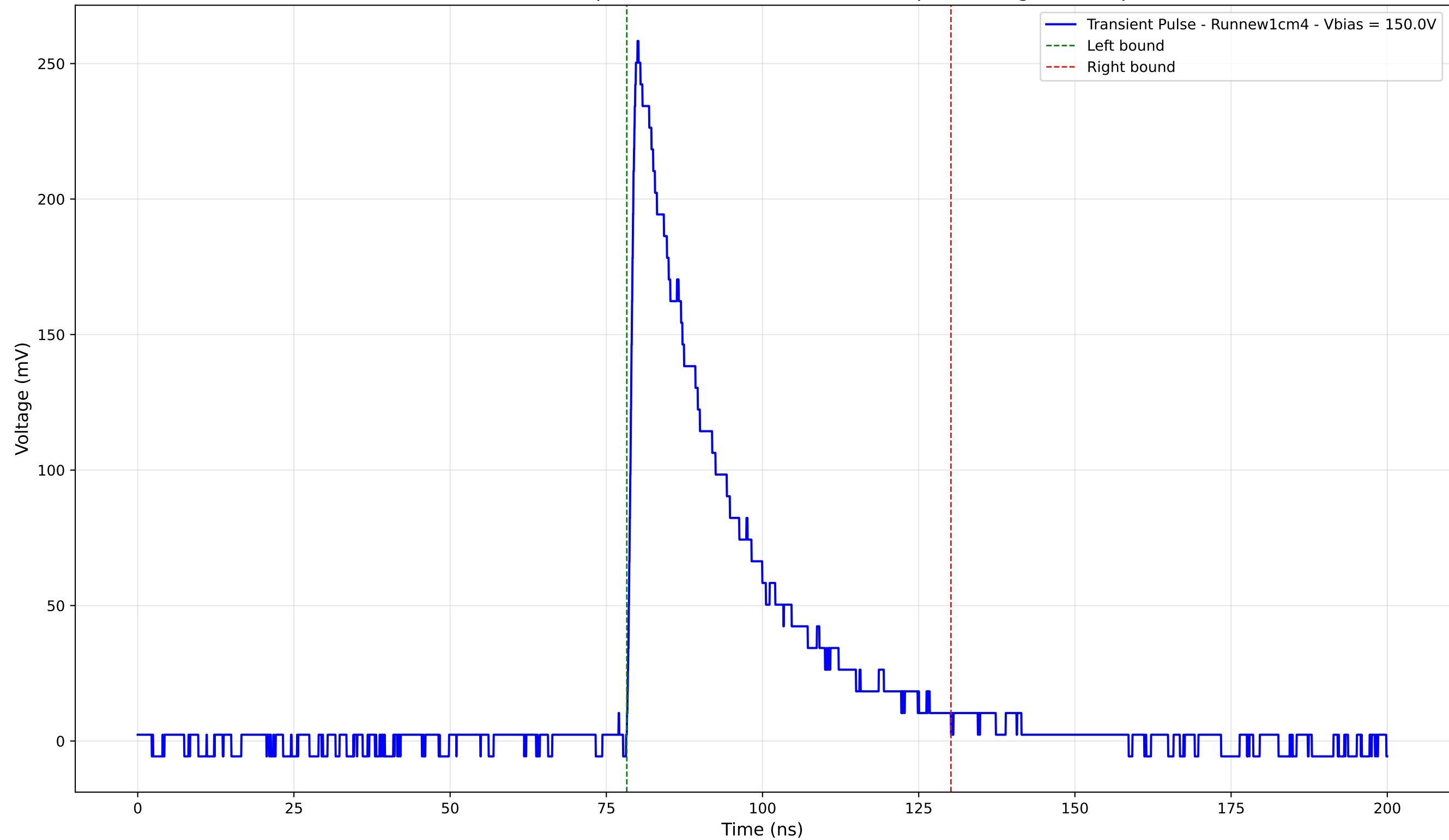
Transient Pulse - Sample: new1cm - Position: 1160.0 \mu\text{m} - Charge: 75.97 pC
