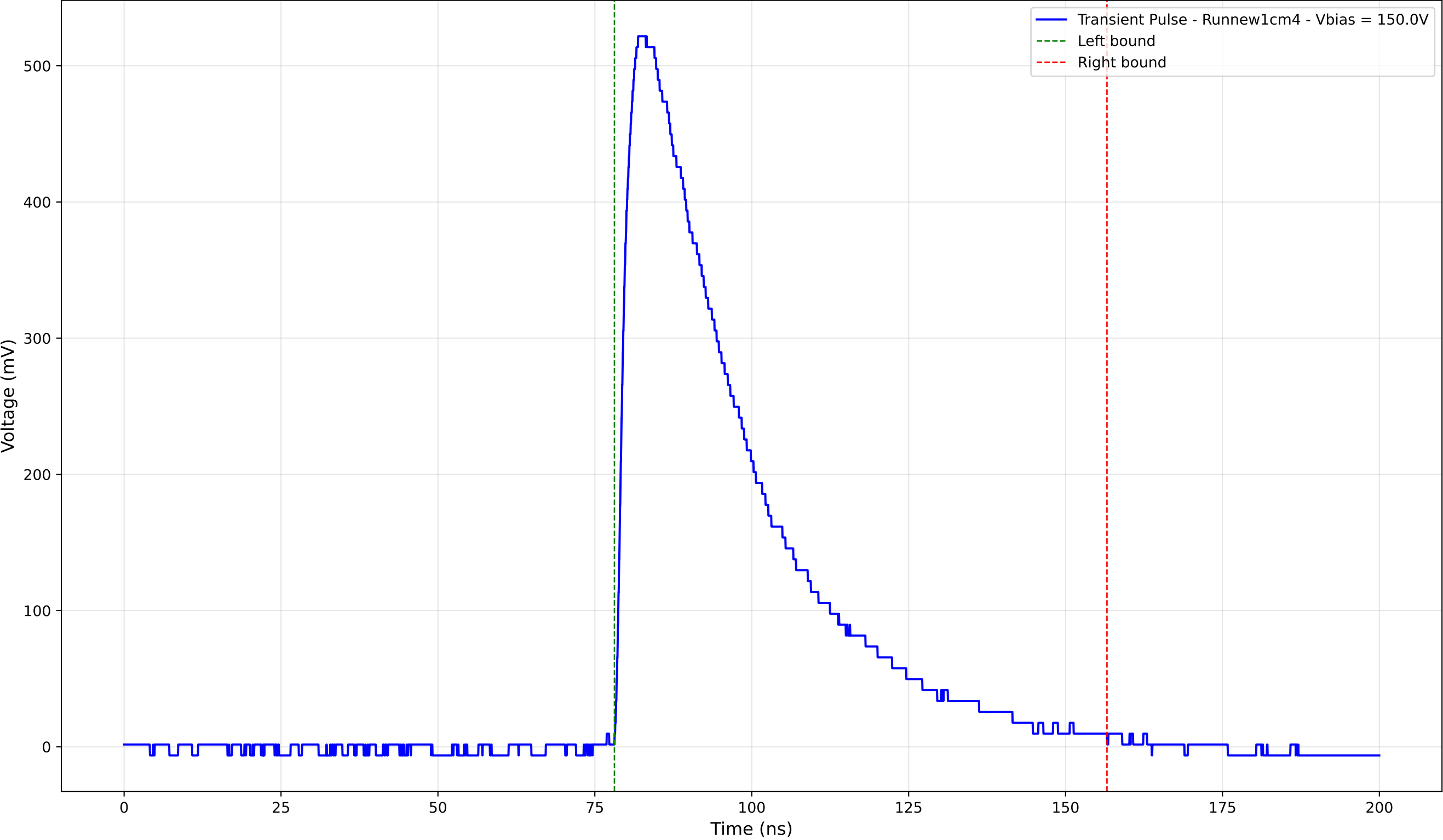
Transient Pulse - Sample: new1cm - Position: 2935.0 \mu\text{m} - Charge: 230.17 pC
