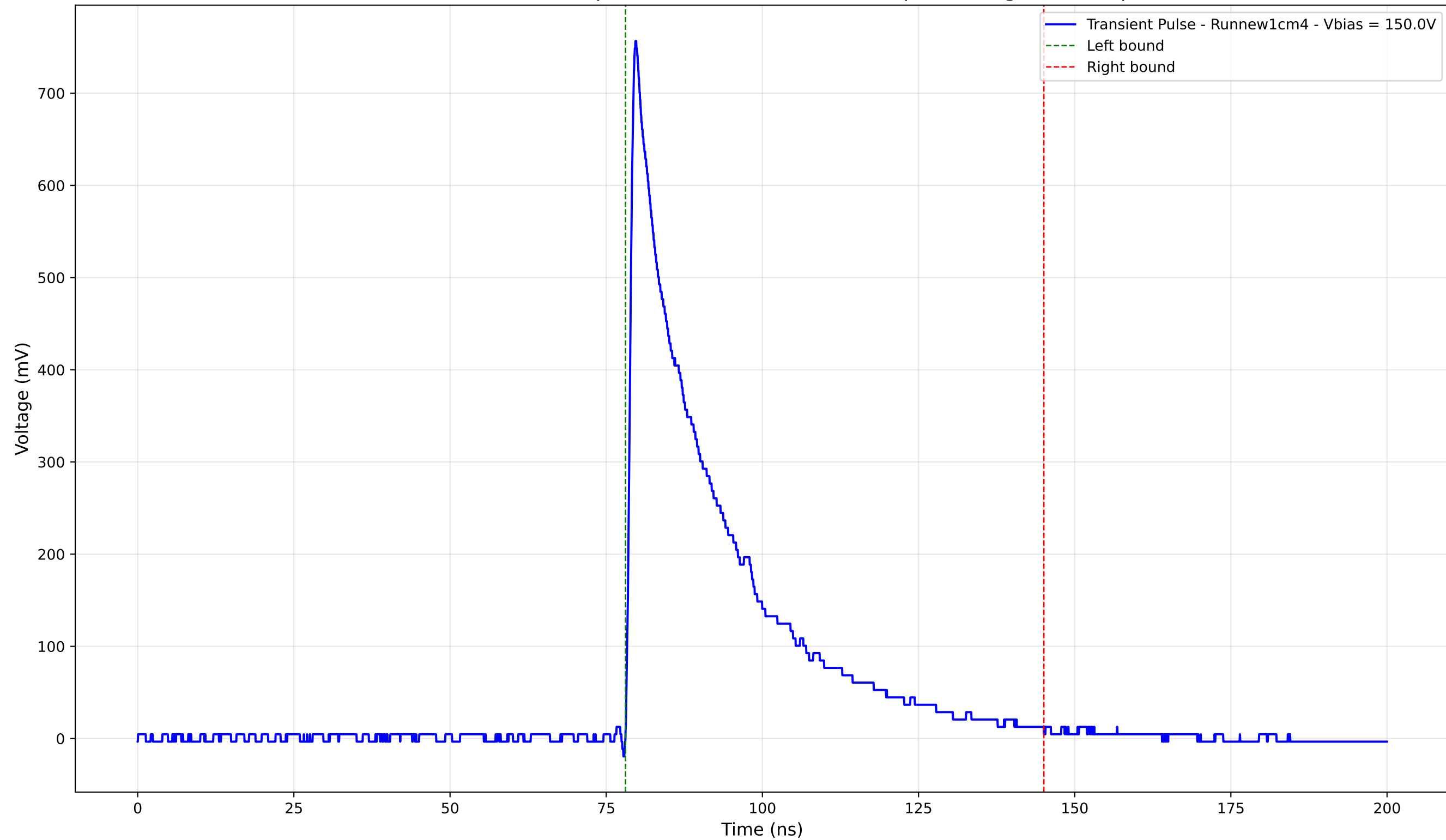
Transient Pulse - Sample: new1cm - Position: 845.0 \mu\text{m} - Charge: 204.09 pC
