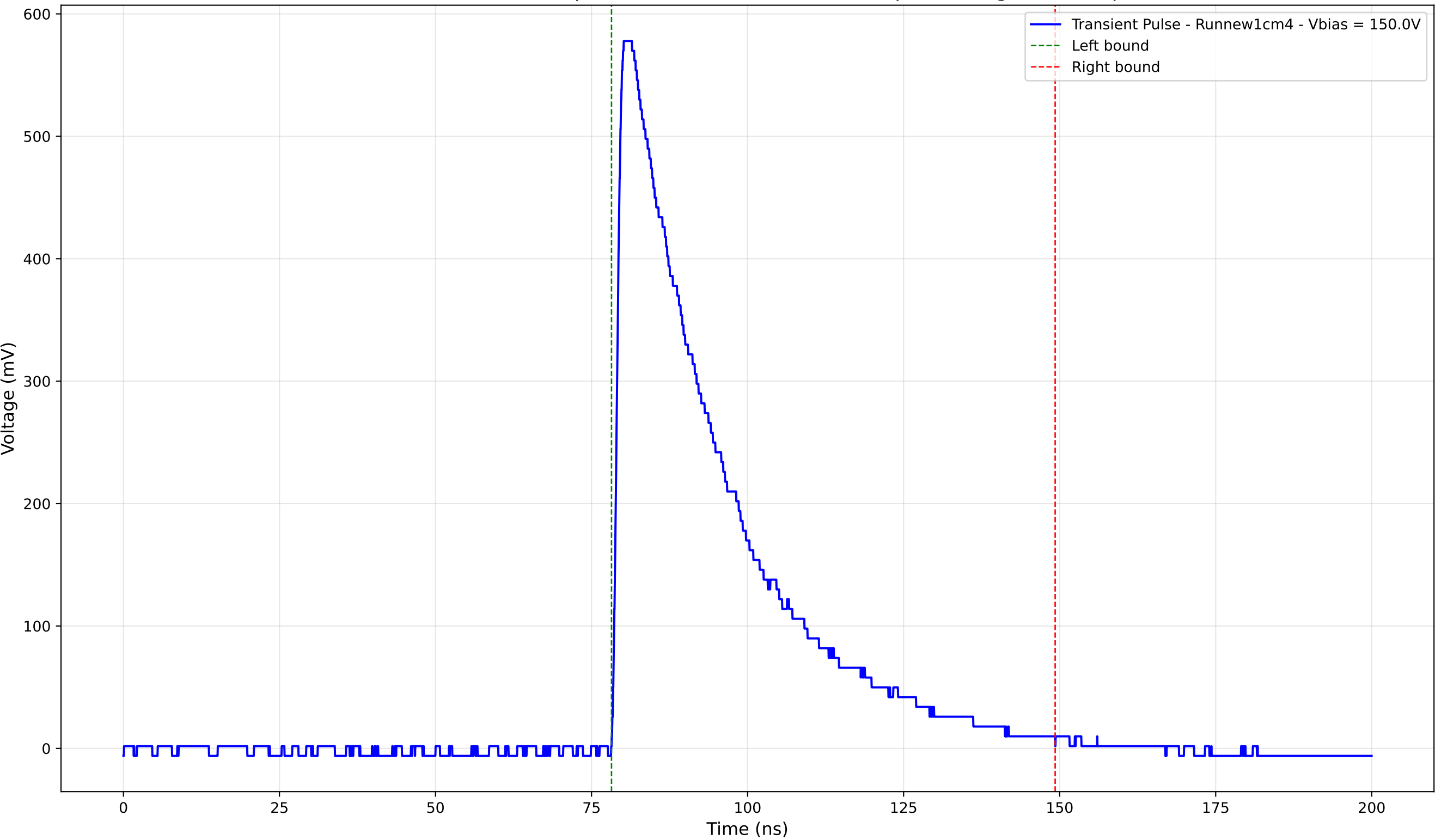
Transient Pulse - Sample: new1cm - Position: 1375.0 \mu\text{m} - Charge: 208.46 pC
