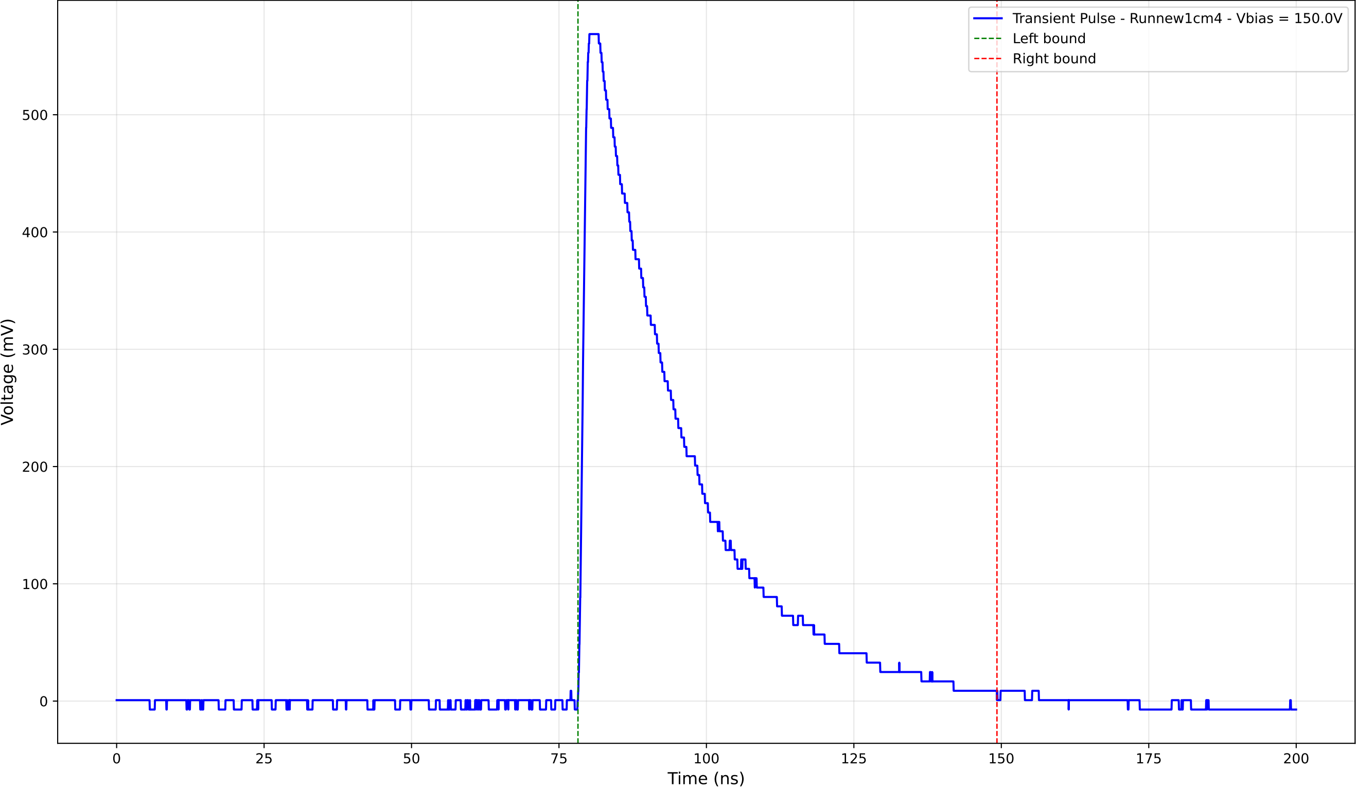
Transient Pulse - Sample: new1cm - Position: 1390.0 \mu\text{m} - Charge: 205.77 pC
