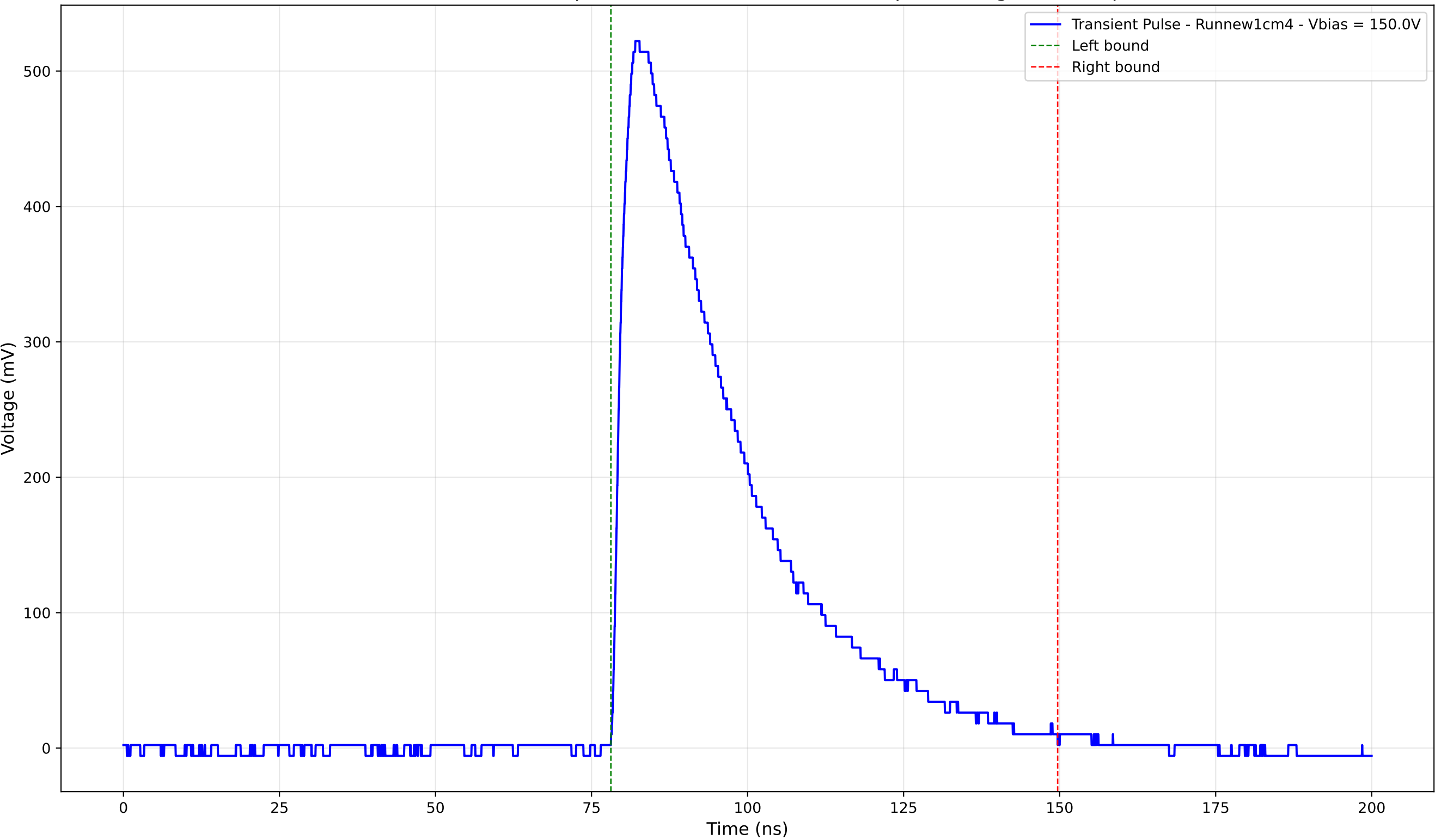
Transient Pulse - Sample: new1cm - Position: 2415.0 \mu\text{m} - Charge: 221.66 pC
