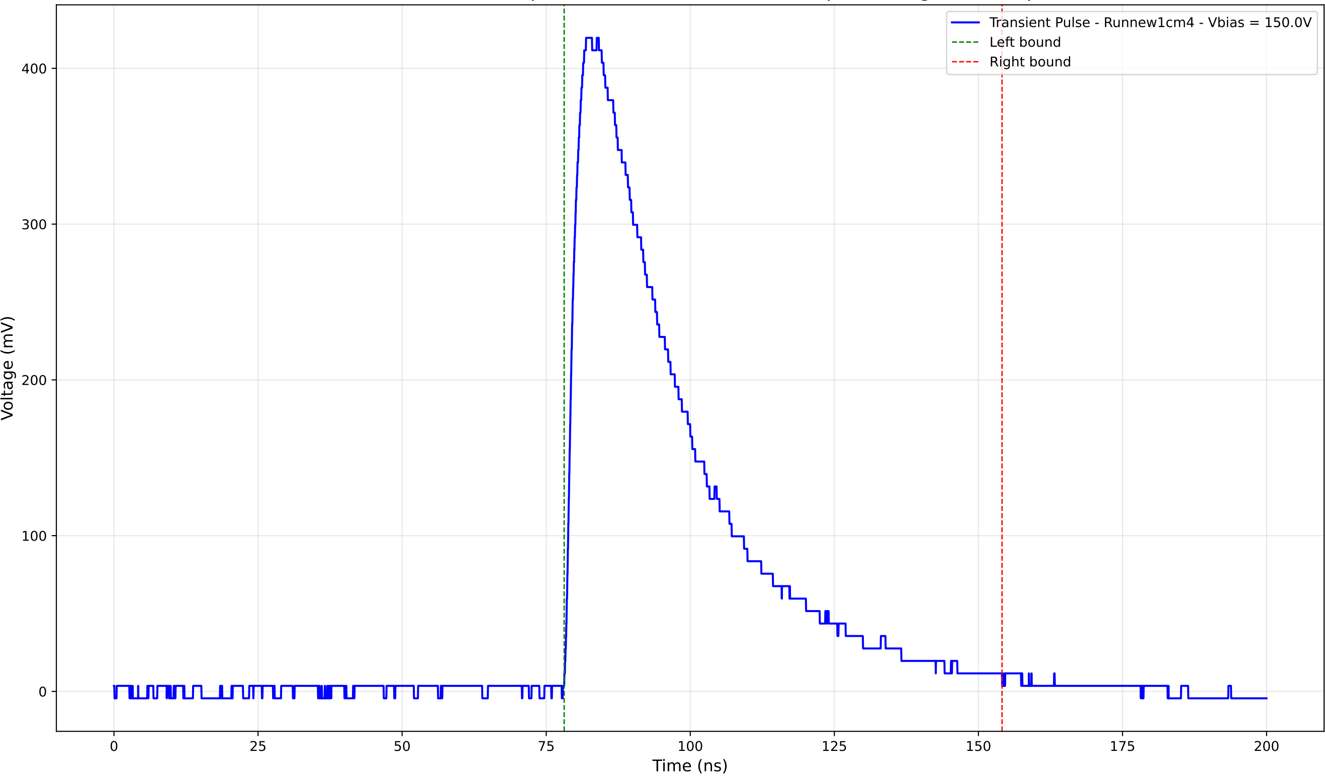
Transient Pulse - Sample: new1cm - Position: 2640.0 \mu\text{m} - Charge: 183.73 pC
