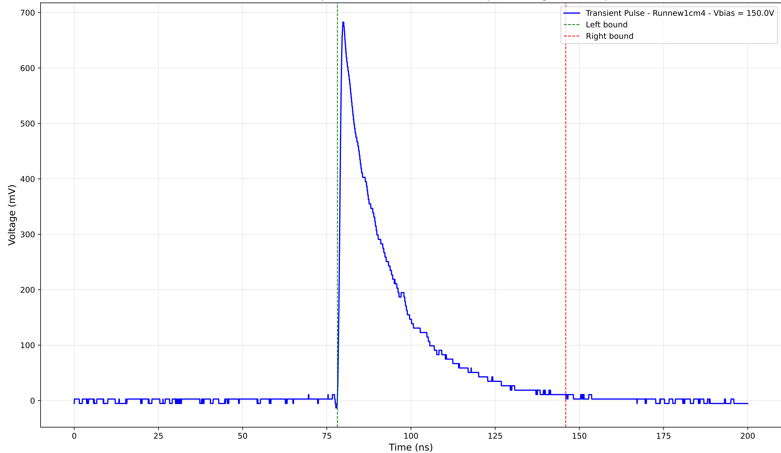
Transient Pulse - Sample: new1cm - Position: 970.0 \mu\text{m} - Charge: 196.50 pC
