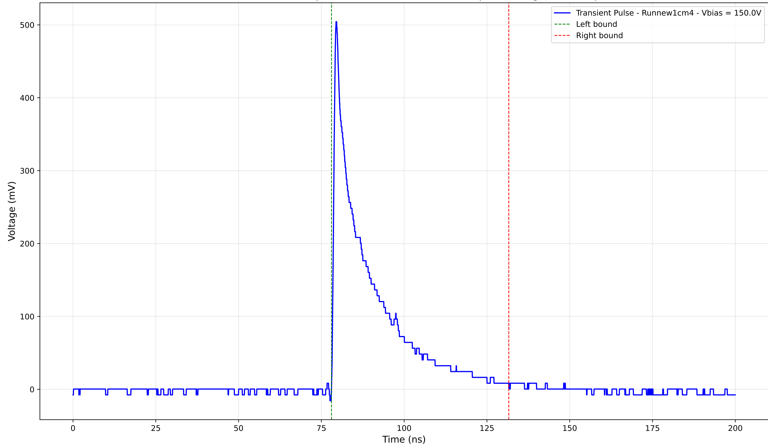
Transient Pulse - Sample: new1cm - Position: 640.0 \mu\text{m} - Charge: 102.08 pC
