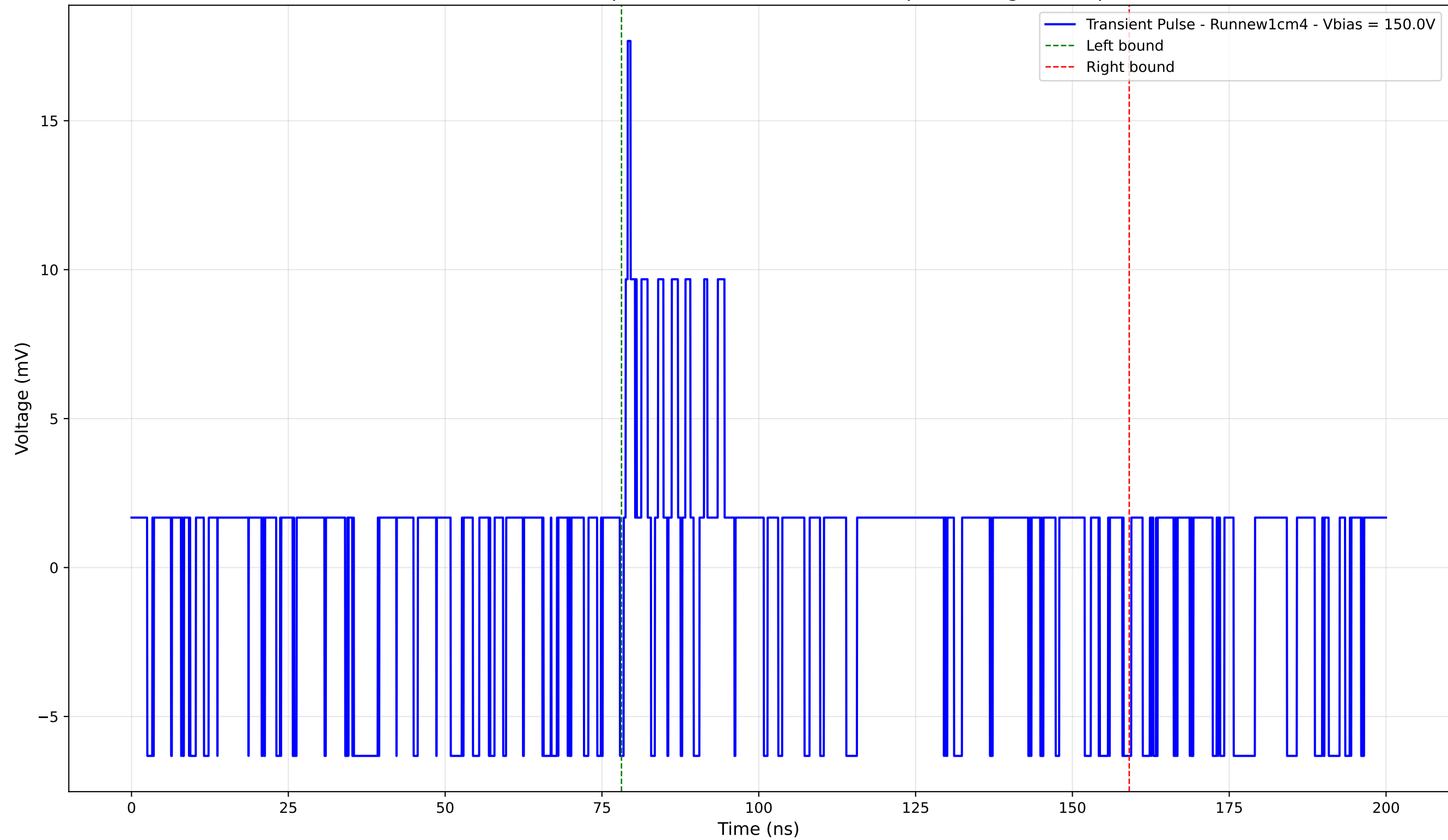
Transient Pulse - Sample: new1cm - Position: 95.0 \mu\text{m} - Charge: 1.70 pC
