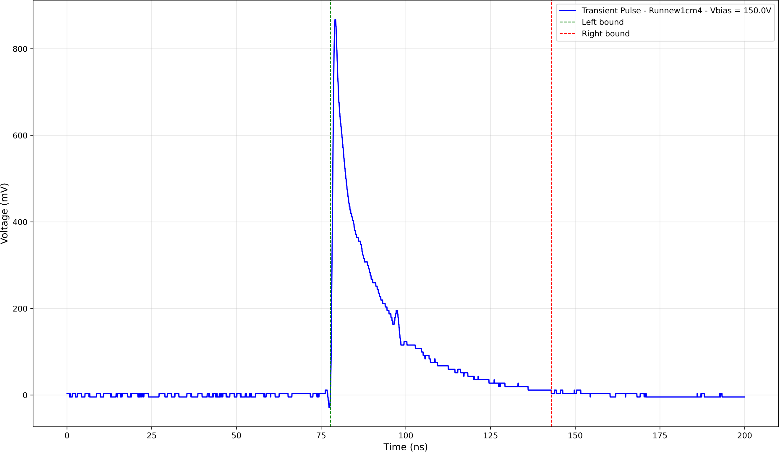
Transient Pulse - Sample: new1cm - Position: 4900.0 \mu\text{m} - Charge: 189.87 pC
