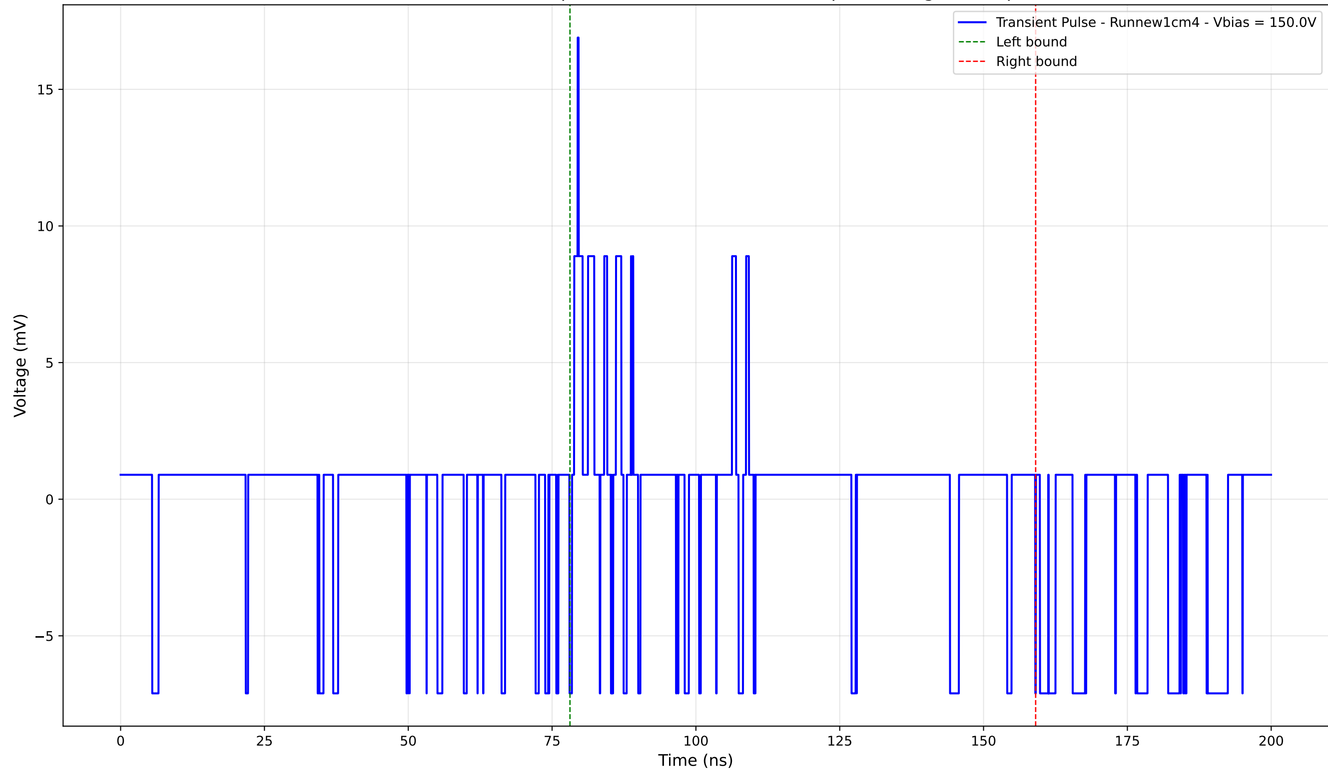
Transient Pulse - Sample: new1cm - Position: 45.0 \mu\text{m} - Charge: 1.18 pC
