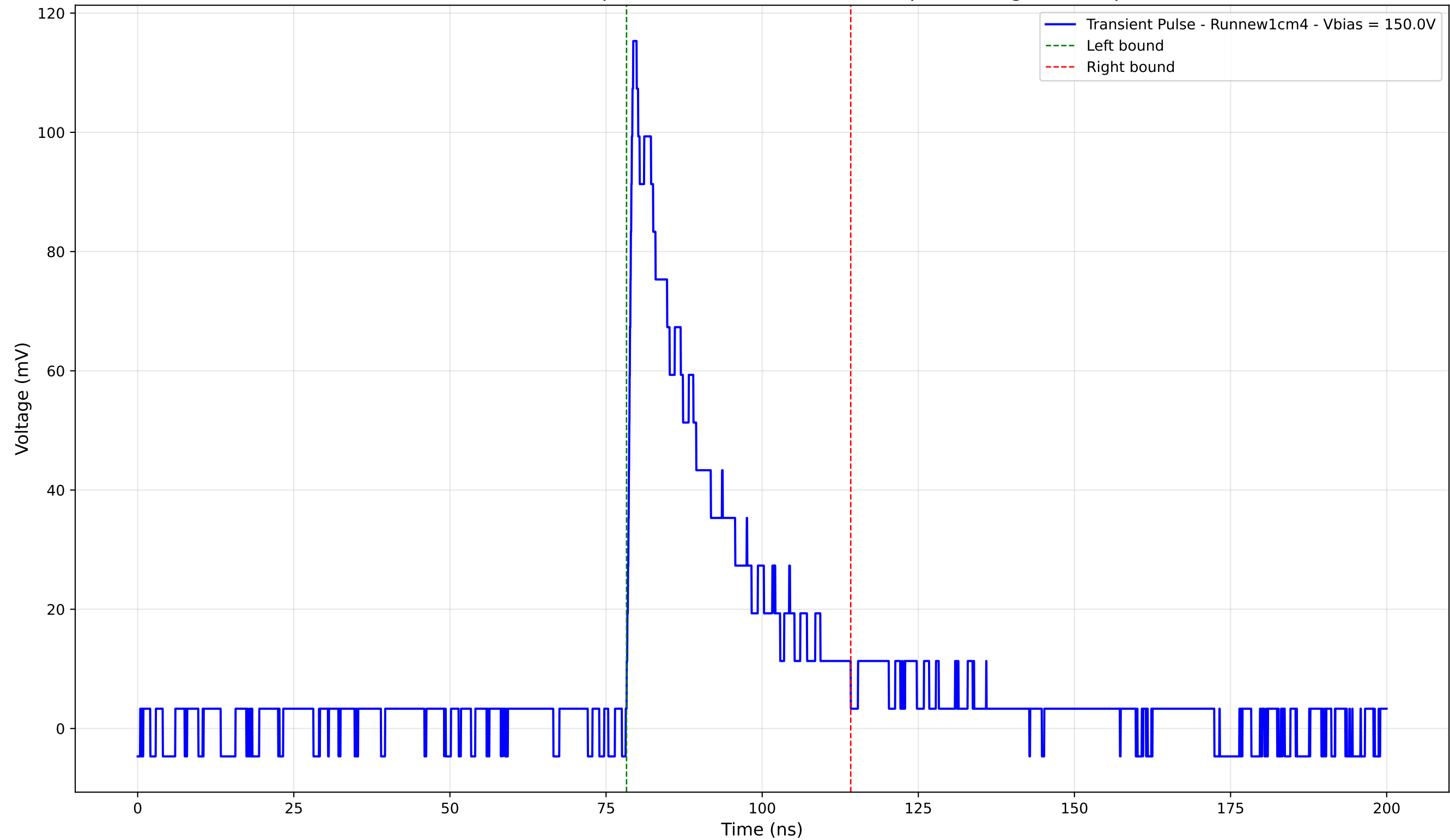
Transient Pulse - Sample: new1cm - Position: 700.0 \mu\text{m} - Charge: 28.03 pC
