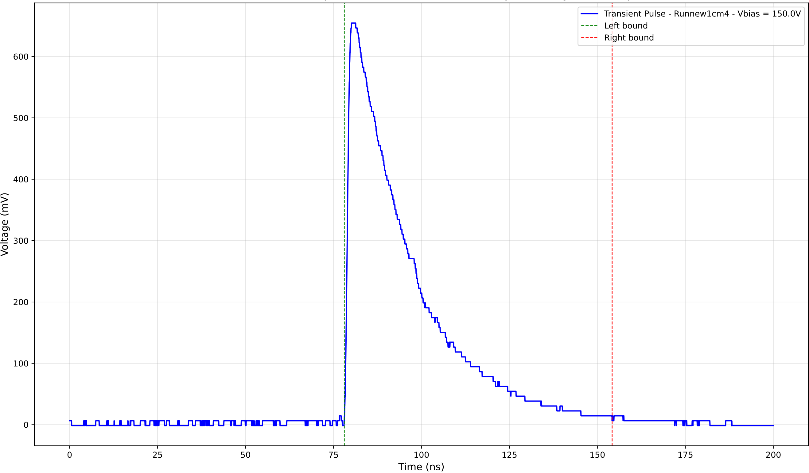
Transient Pulse - Sample: new1cm - Position: 3890.0 \mu\text{m} - Charge: 257.61 pC
