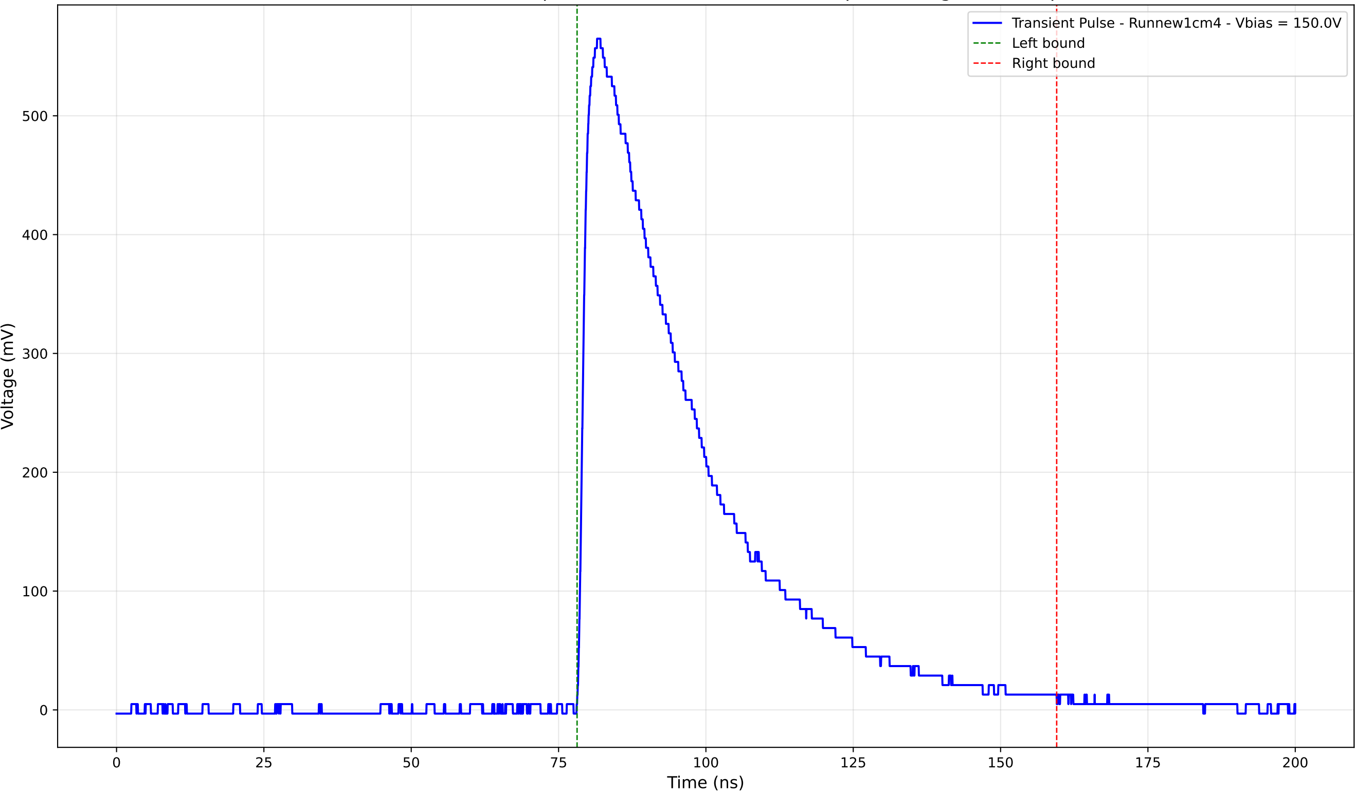
Transient Pulse - Sample: new1cm - Position: 3475.0 \mu\text{m} - Charge: 241.91 pC
