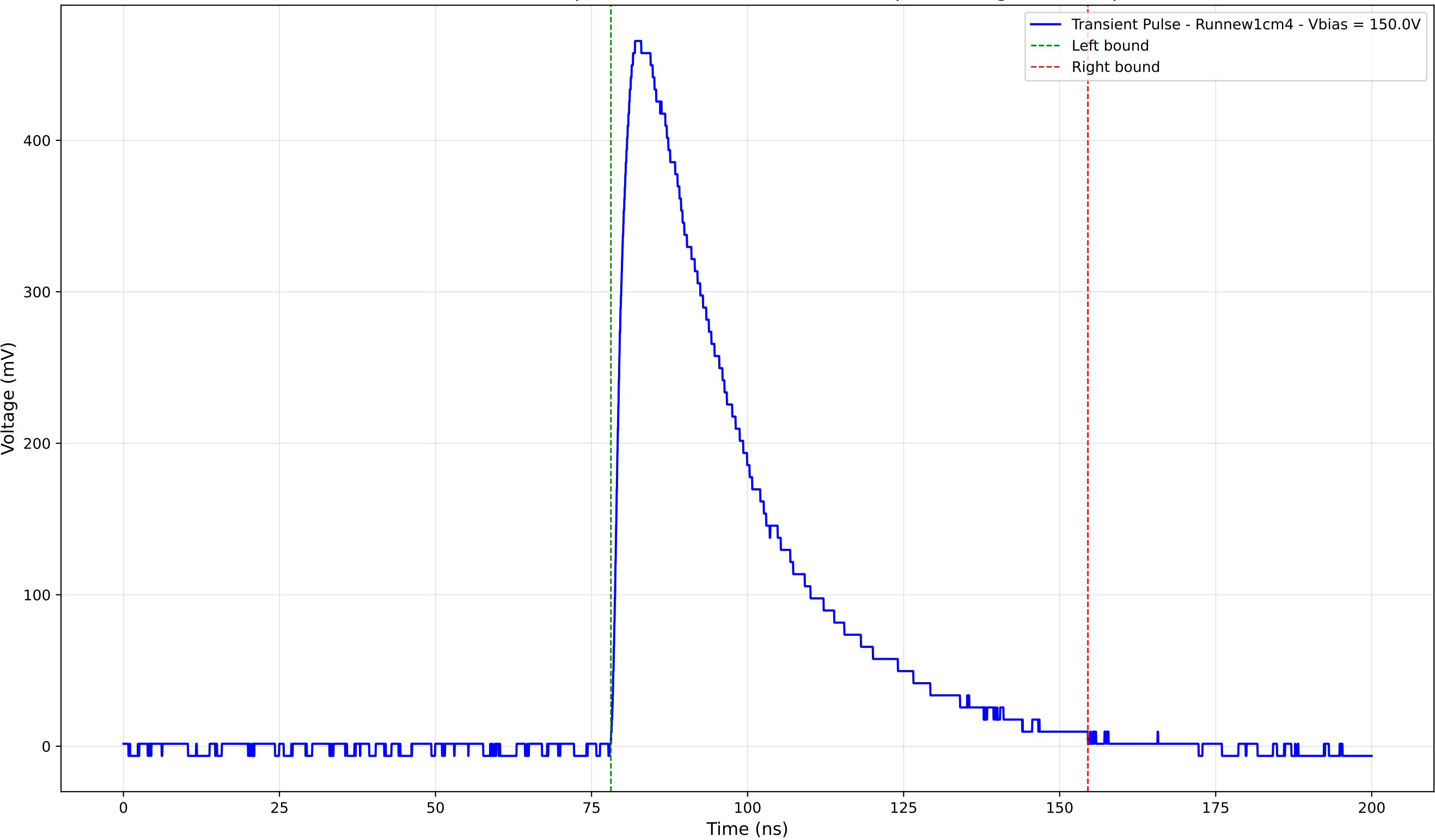
Transient Pulse - Sample: new1cm - Position: 2810.0 \mu\text{m} - Charge: 205.32 pC
