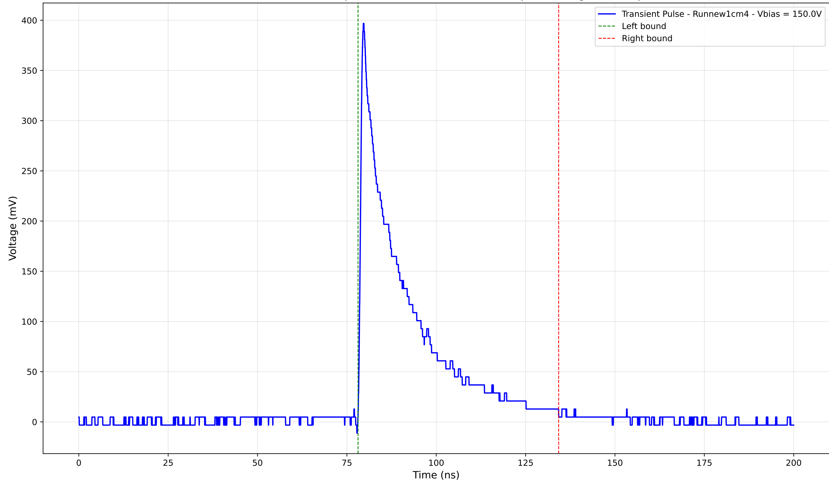
Transient Pulse - Sample: new1cm - Position: 740.0 \mu\text{m} - Charge: 95.68 pC
