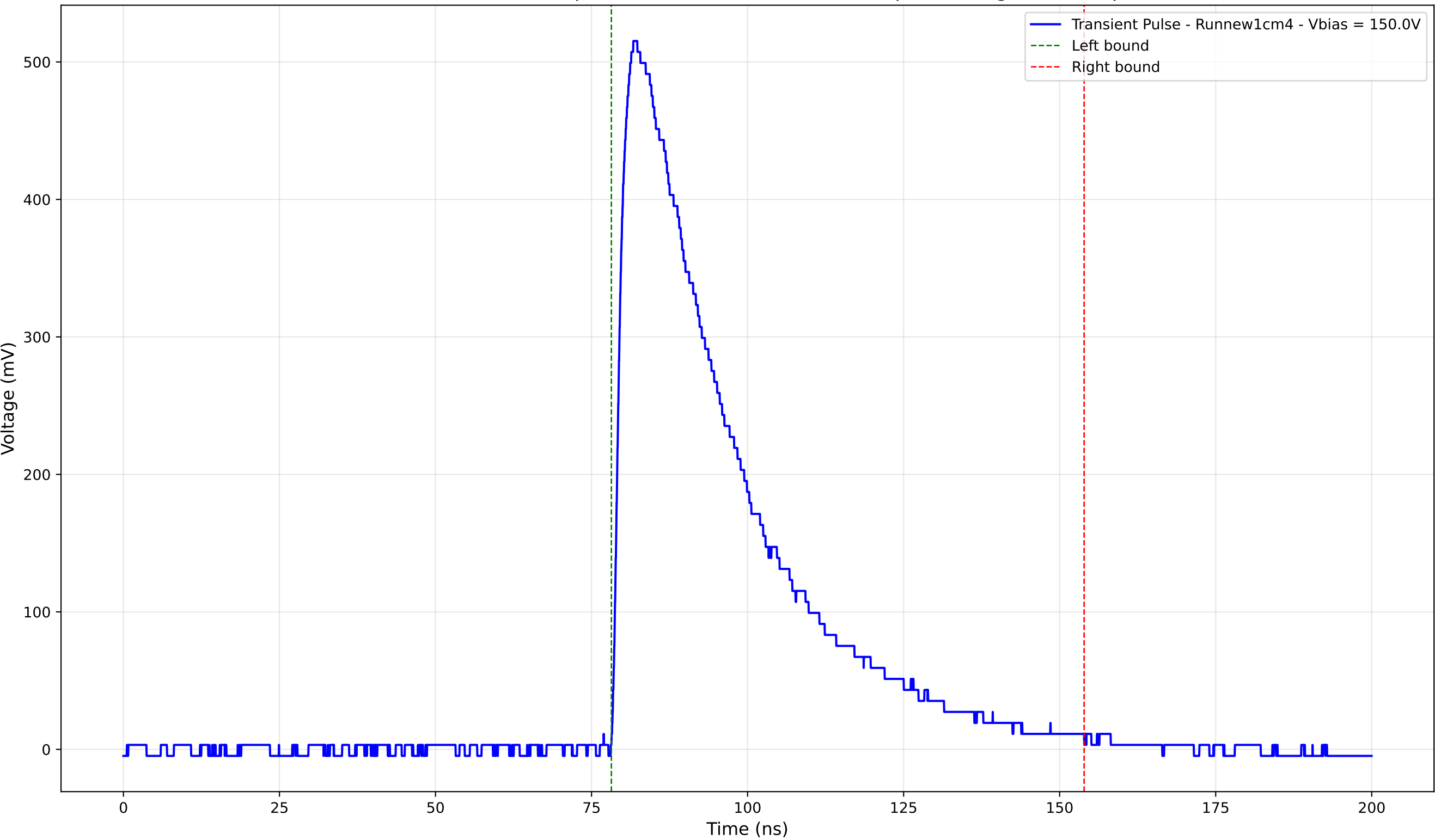
Transient Pulse - Sample: new1cm - Position: 1985.0 \mu\text{m} - Charge: 213.06 pC
