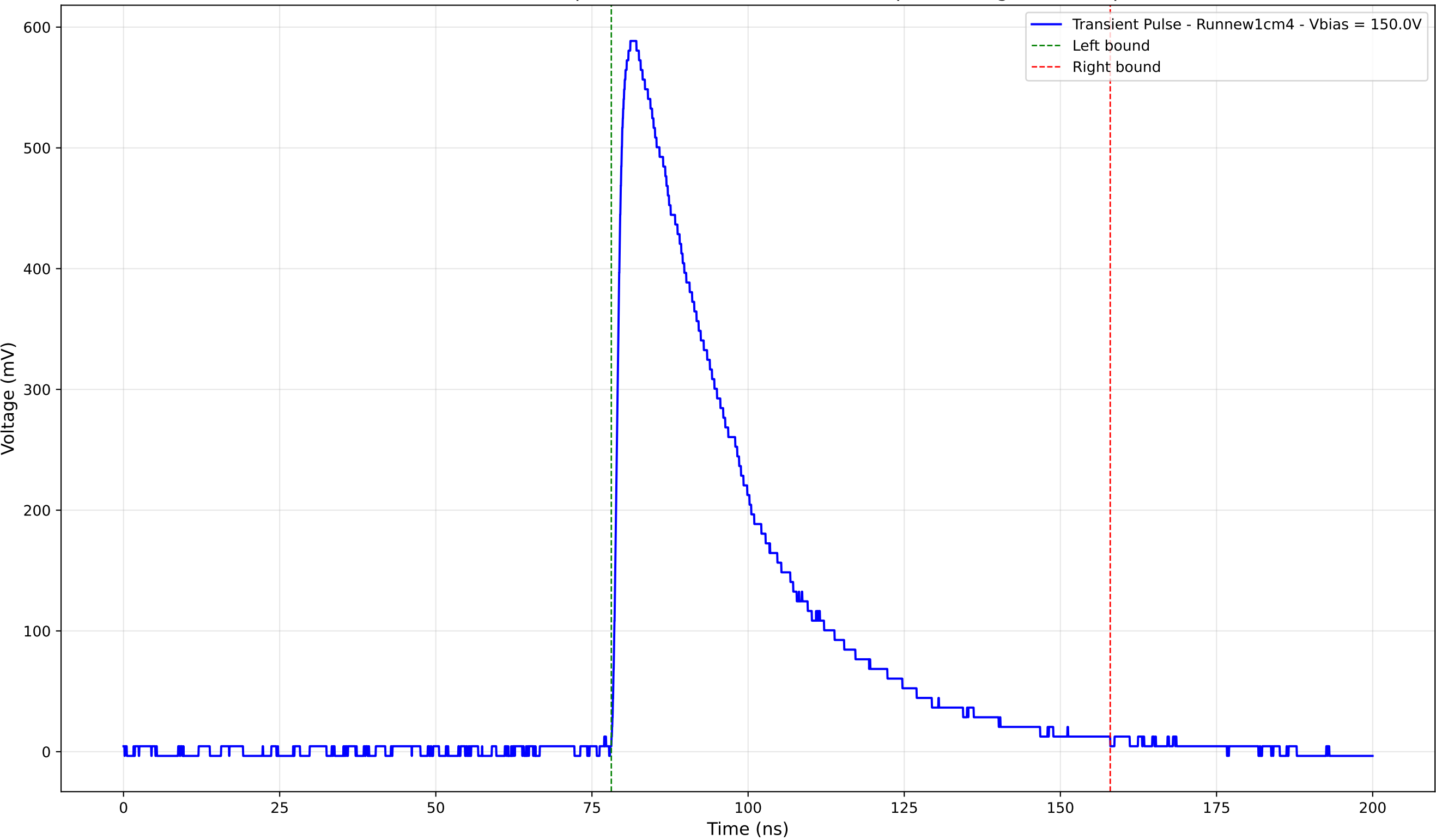
Transient Pulse - Sample: new1cm - Position: 3595.0 \mu\text{m} - Charge: 245.65 pC
