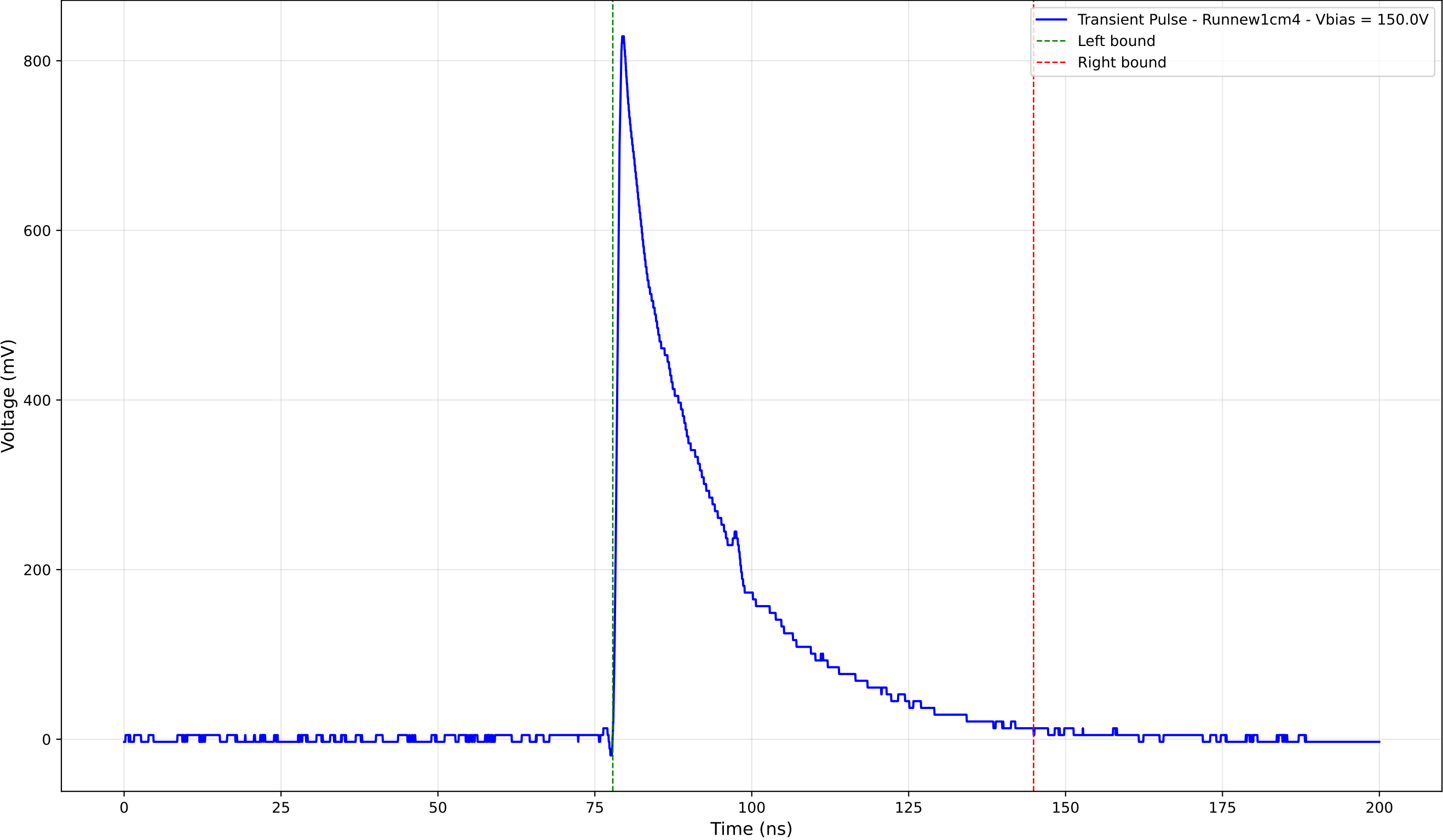
Transient Pulse - Sample: new1cm - Position: 4555.0 \mu\text{m} - Charge: 236.05 pC
