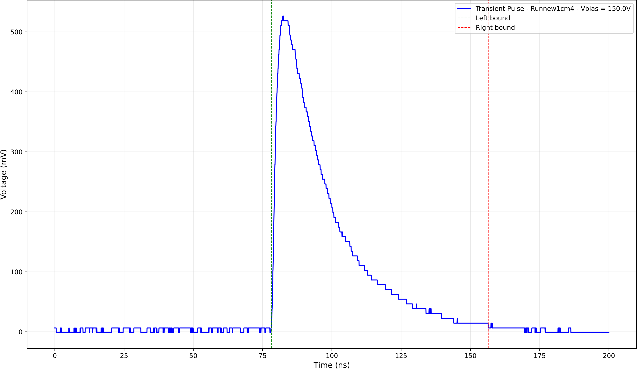
Transient Pulse - Sample: new1cm - Position: 2445.0 \mu\text{m} - Charge: 230.97 pC
