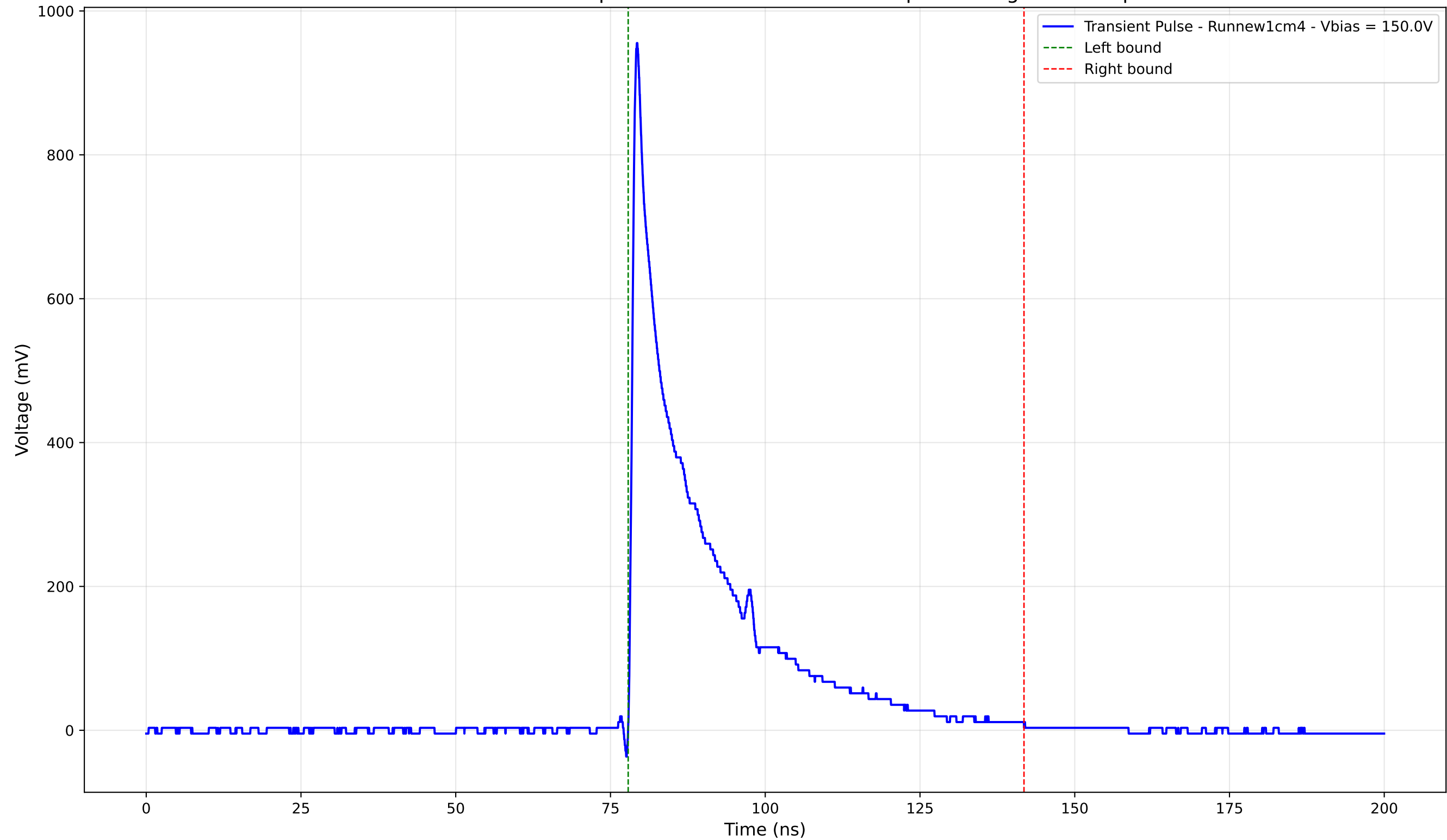
Transient Pulse - Sample: new1cm - Position: 355.0 \mu\text{m} - Charge: 193.39 pC
