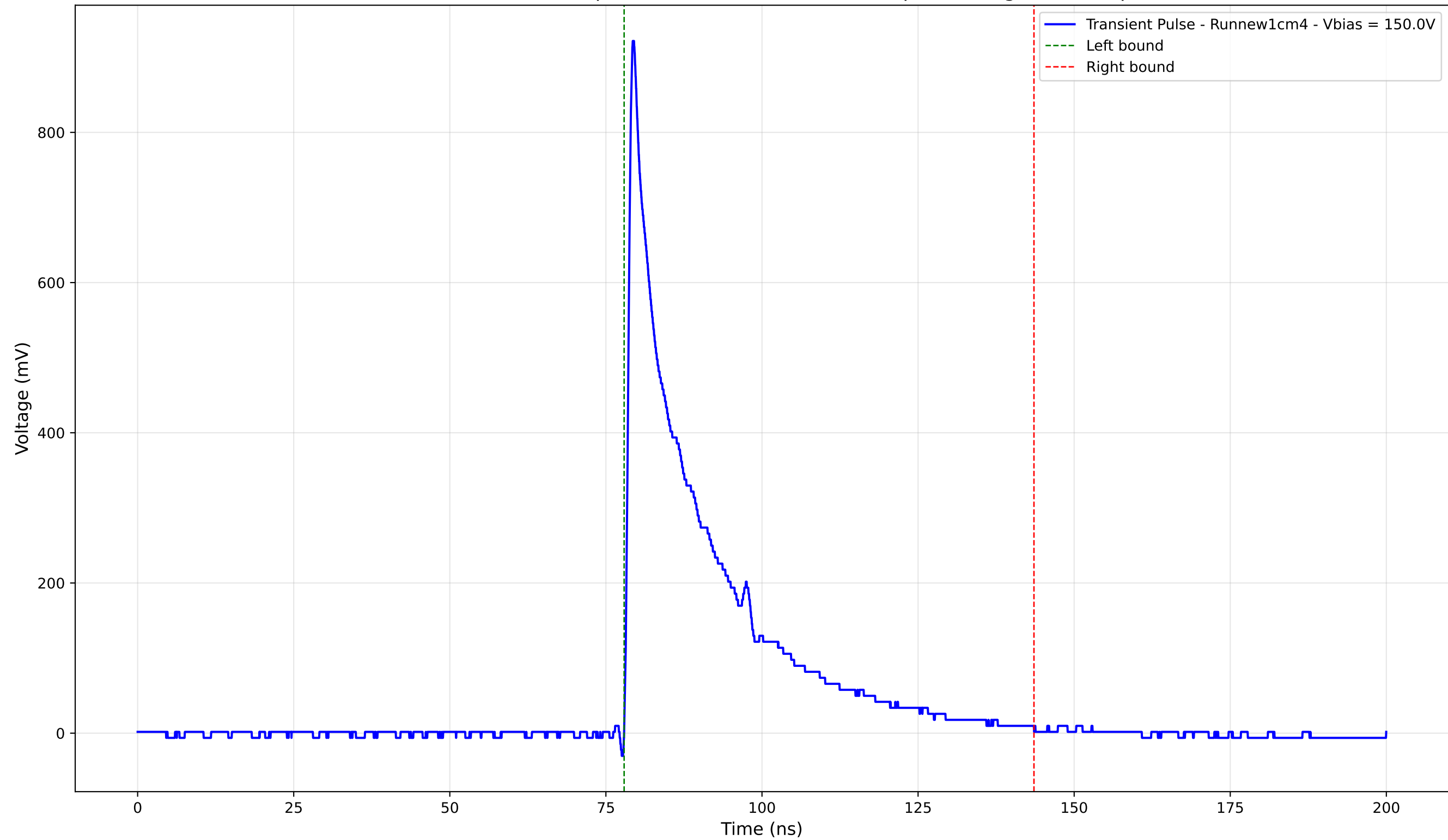
Transient Pulse - Sample: new1cm - Position: 470.0 \mu\text{m} - Charge: 199.44 pC
