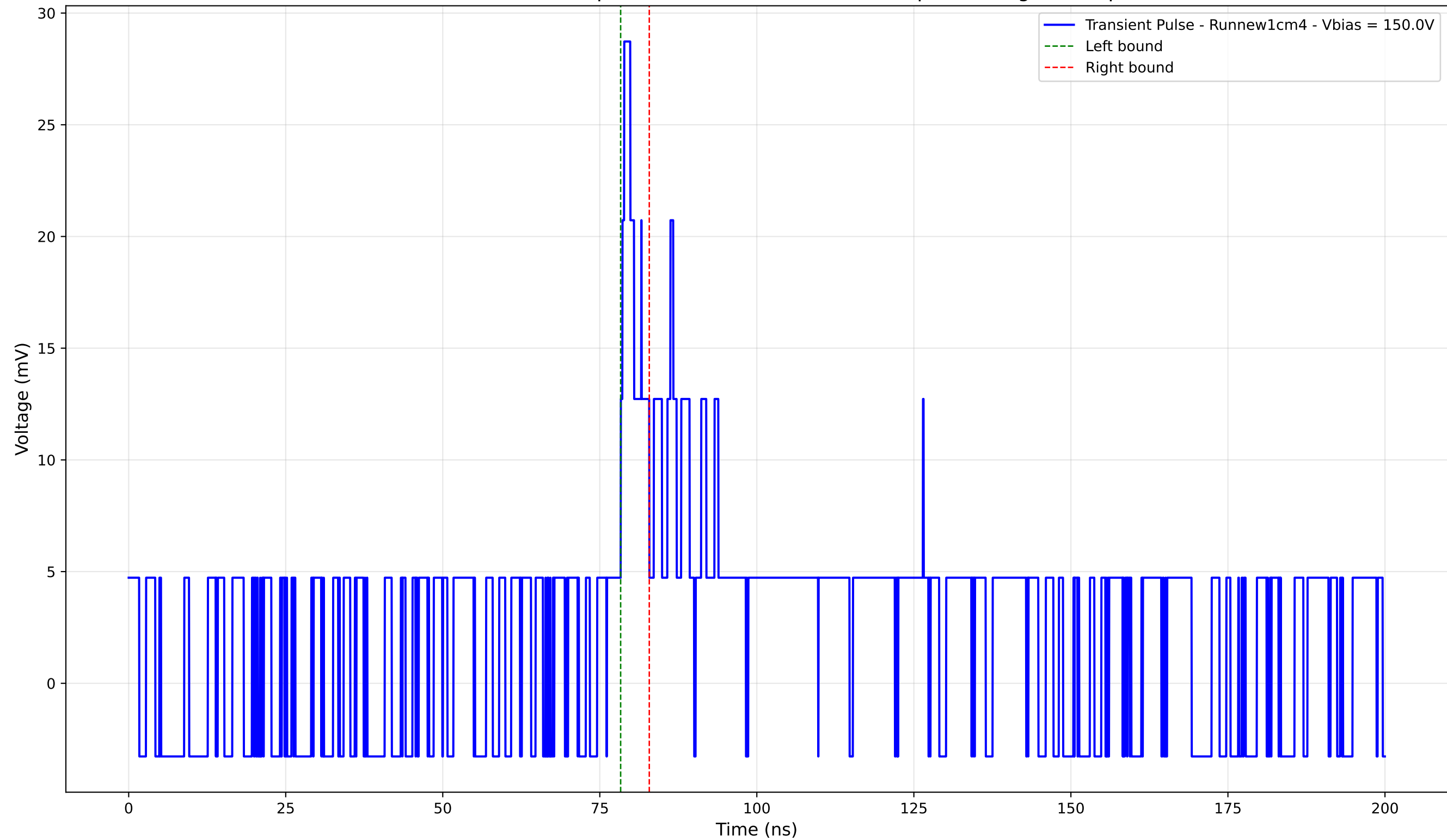
Transient Pulse - Sample: new1cm -Position: 5095.0 \mu\text{m} - Charge: 1.62 pC
