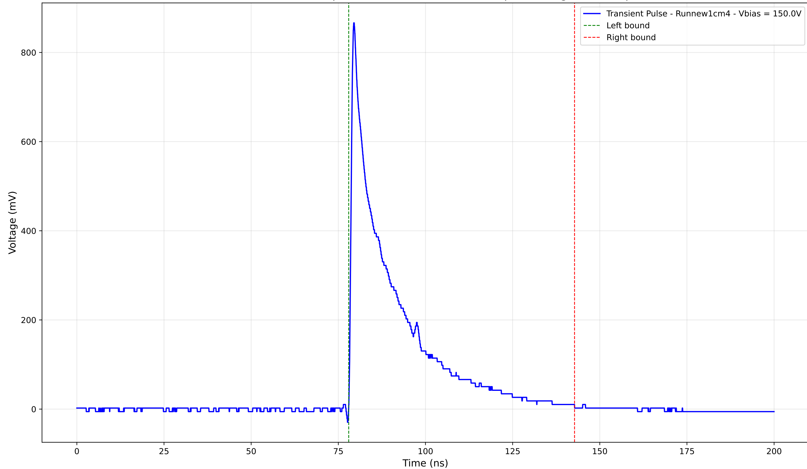
Transient Pulse - Sample: new1cm - Position: 575.0 \mu\text{m} - Charge: 194.18 pC
