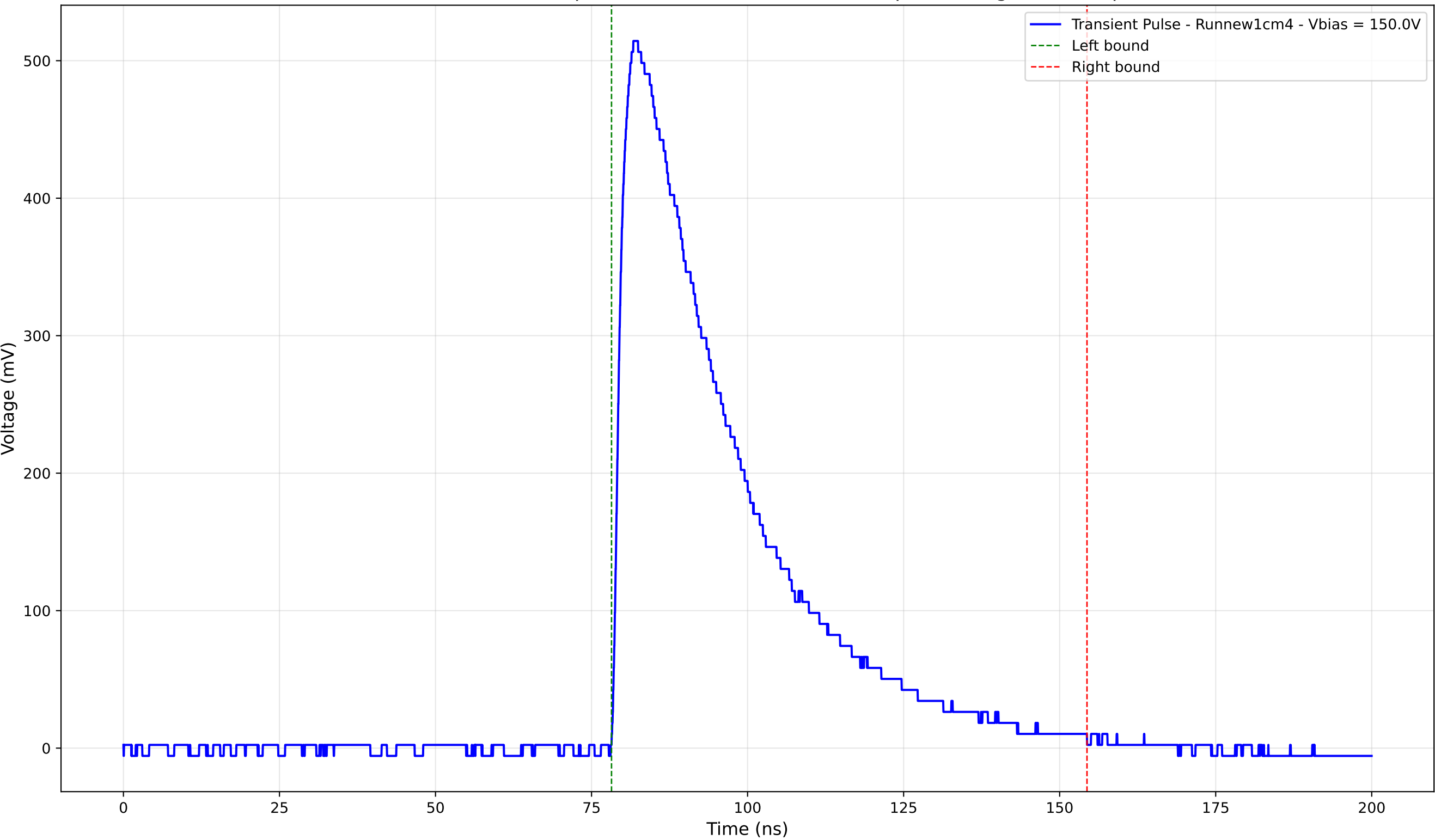
Transient Pulse - Sample: new1cm - Position: 2005.0 \mu\text{m} - Charge: 211.58 pC
