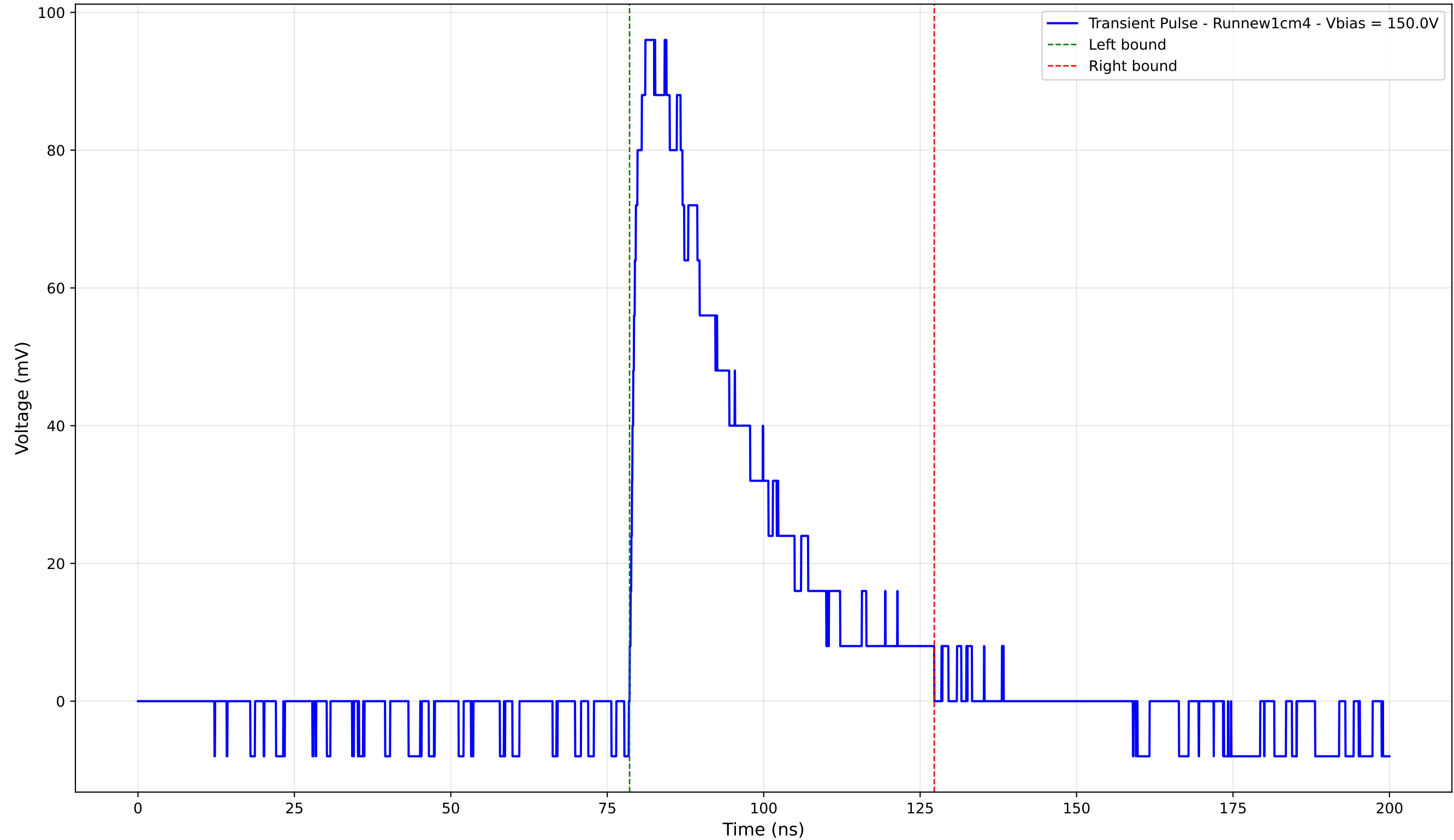
Transient Pulse - Sample: new1cm - Position: 1690.0 \mu\text{m} - Charge: 34.19 pC
