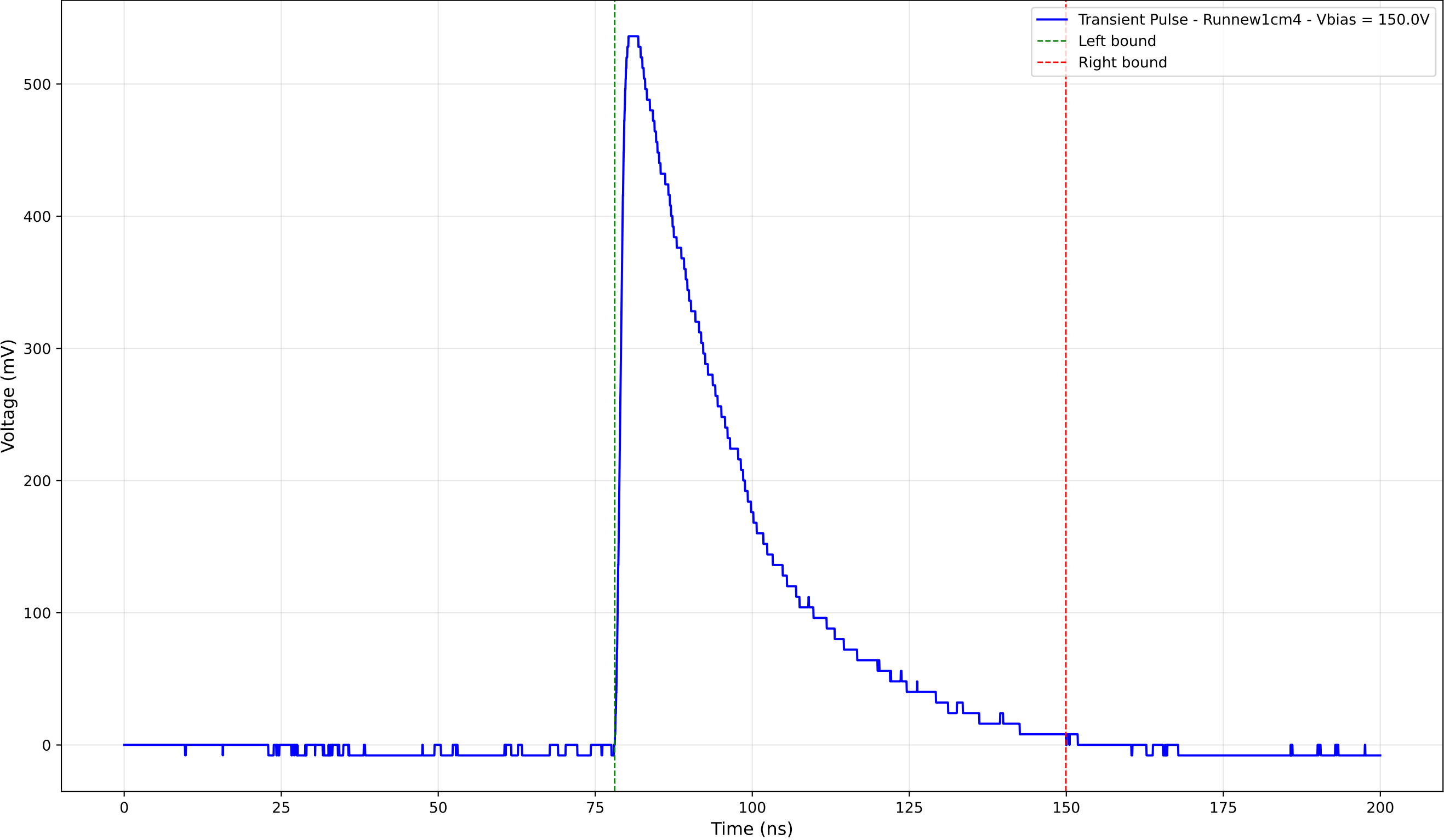
Transient Pulse - Sample: new1cm - Position: 3810.0 \mu\text{m} - Charge: 208.99 pC
