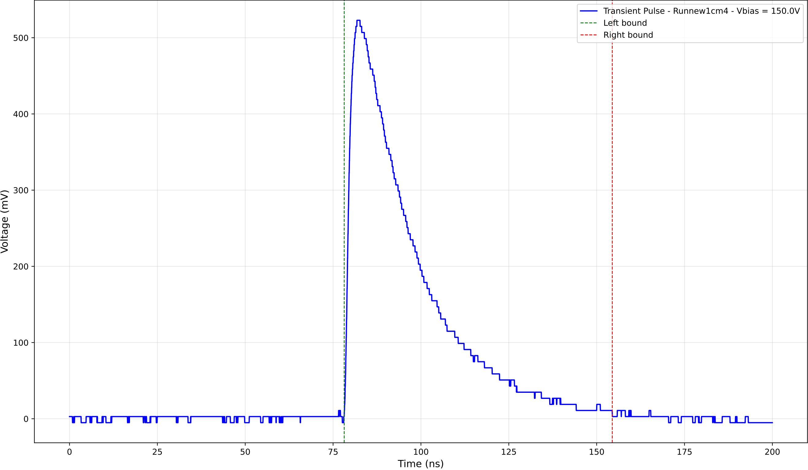
Transient Pulse - Sample: new1cm - Position: 2050.0 \mu\text{m} - Charge: 219.50 pC
