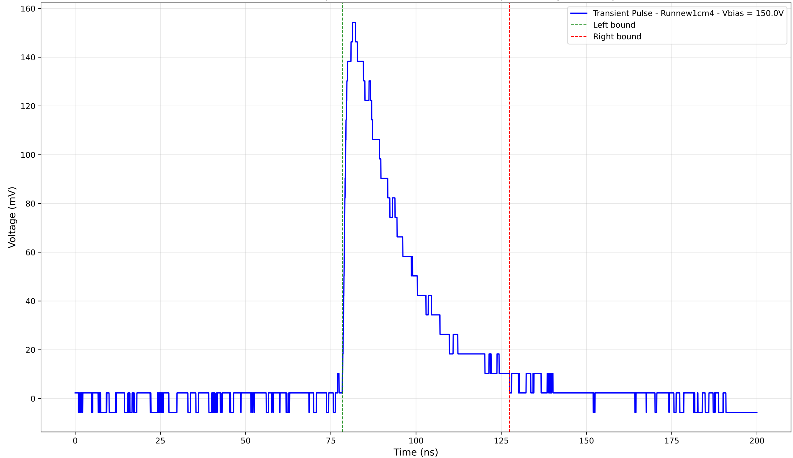
Transient Pulse - Sample: new1cm - Position: 3750.0 \mu\text{m} - Charge: 54.62 pC
