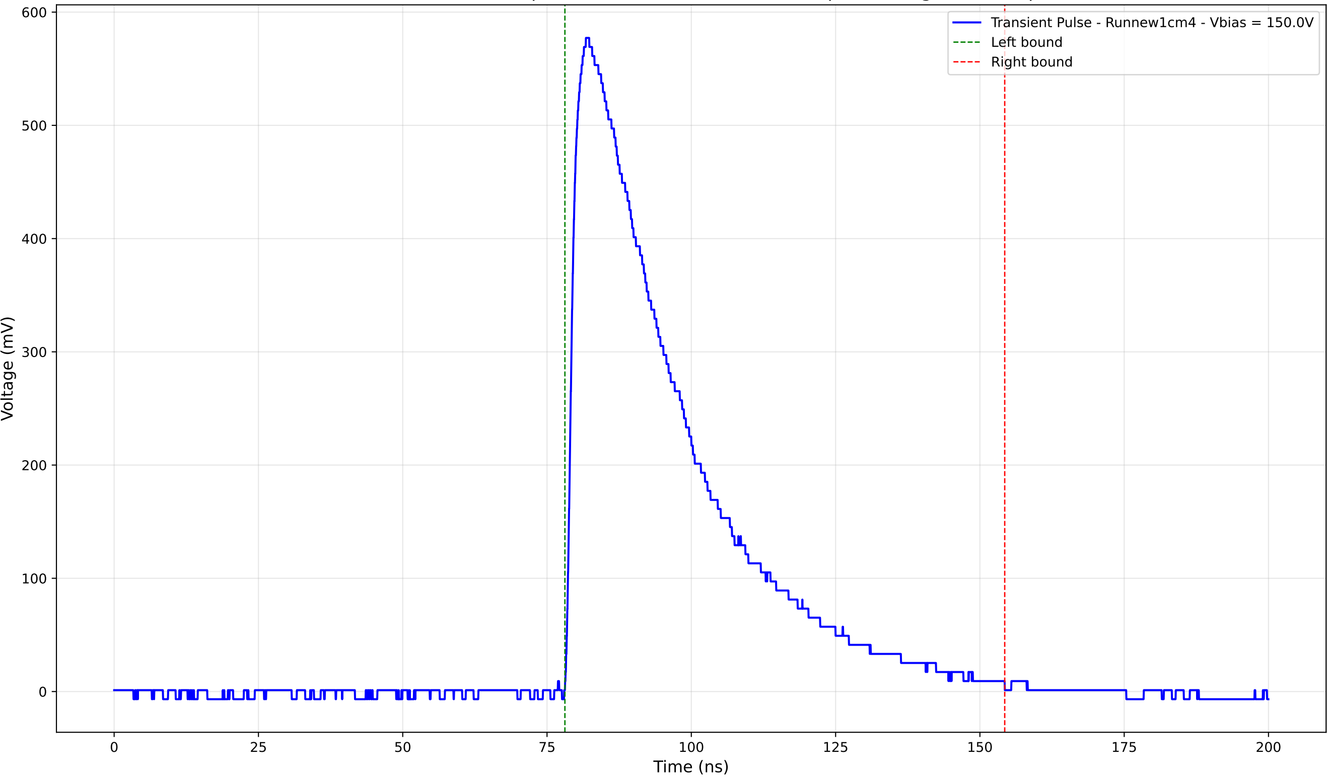
Transient Pulse - Sample: new1cm - Position: 3365.0 \mu\text{m} - Charge: 244.79 pC
