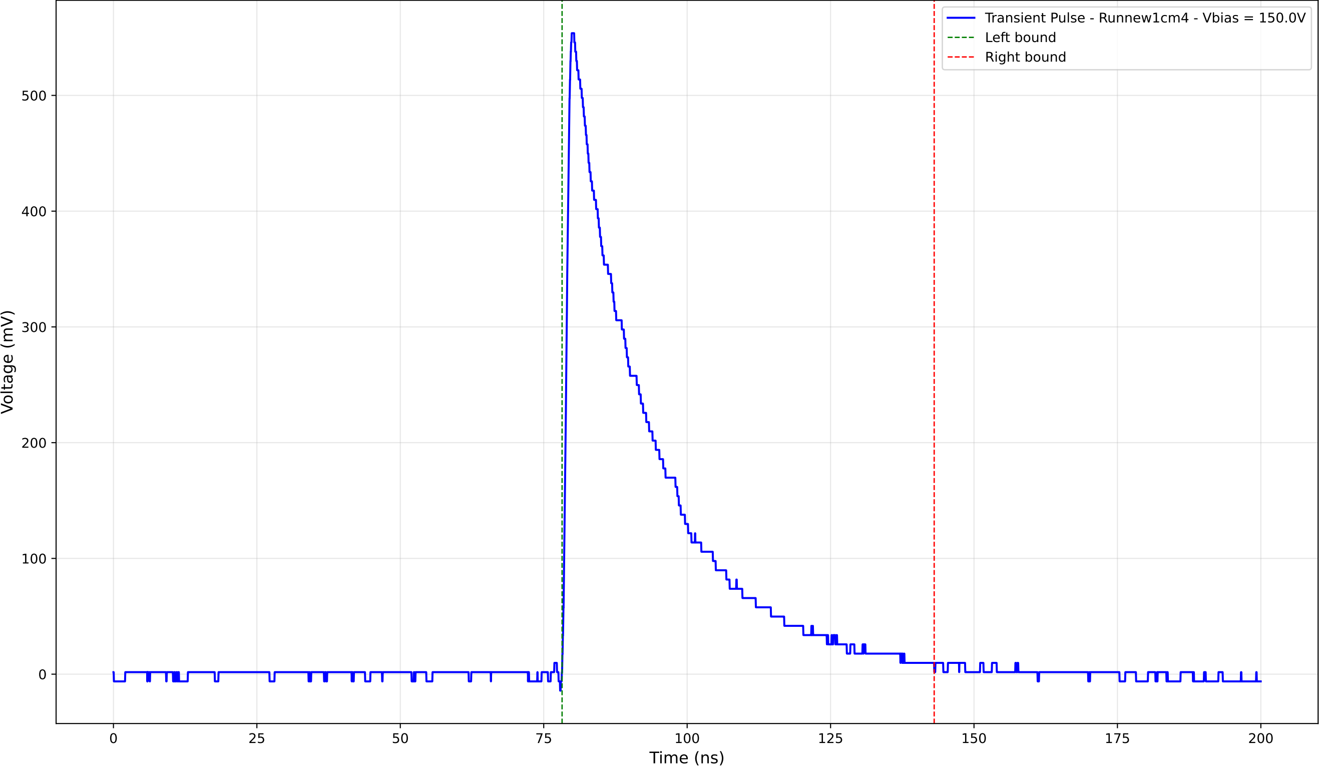
Transient Pulse - Sample: new1cm - Position: 1120.0 \mu\text{m} - Charge: 167.96 pC
