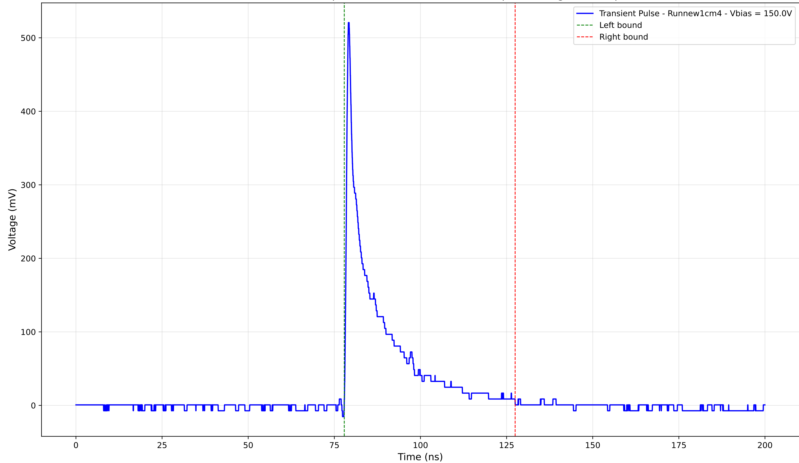
Transient Pulse - Sample: new1cm - Position: 235.0 \mu\text{m} - Charge: 76.56 pC
