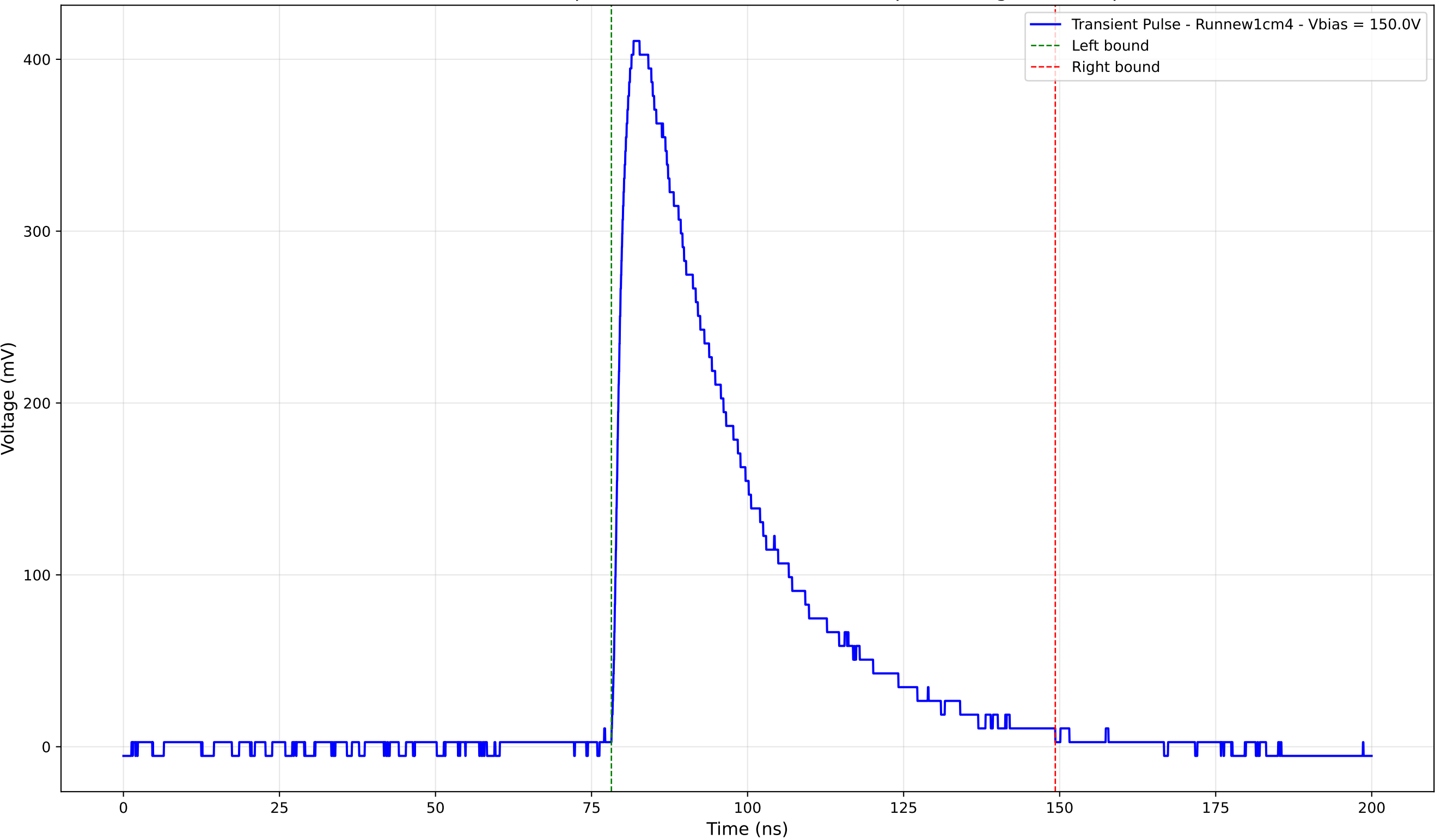
Transient Pulse - Sample: new1cm - Position: 2135.0 \mu\text{m} - Charge: 169.26 pC
