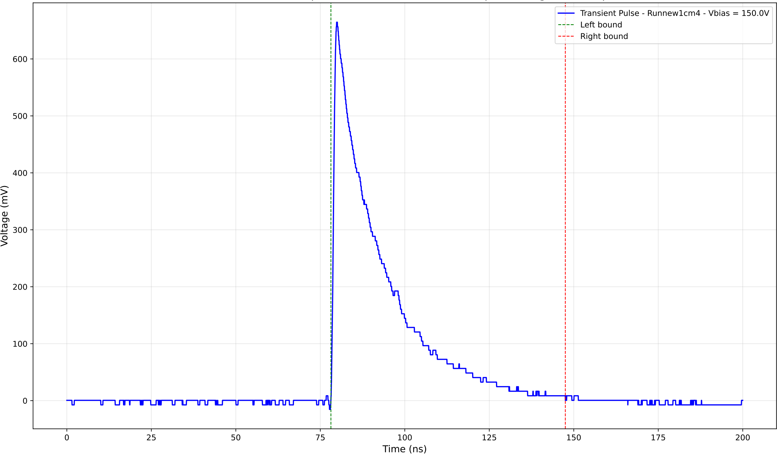
Transient Pulse - Sample: new1cm - Position: 1010.0 \mu\text{m} - Charge: 193.03 pC
