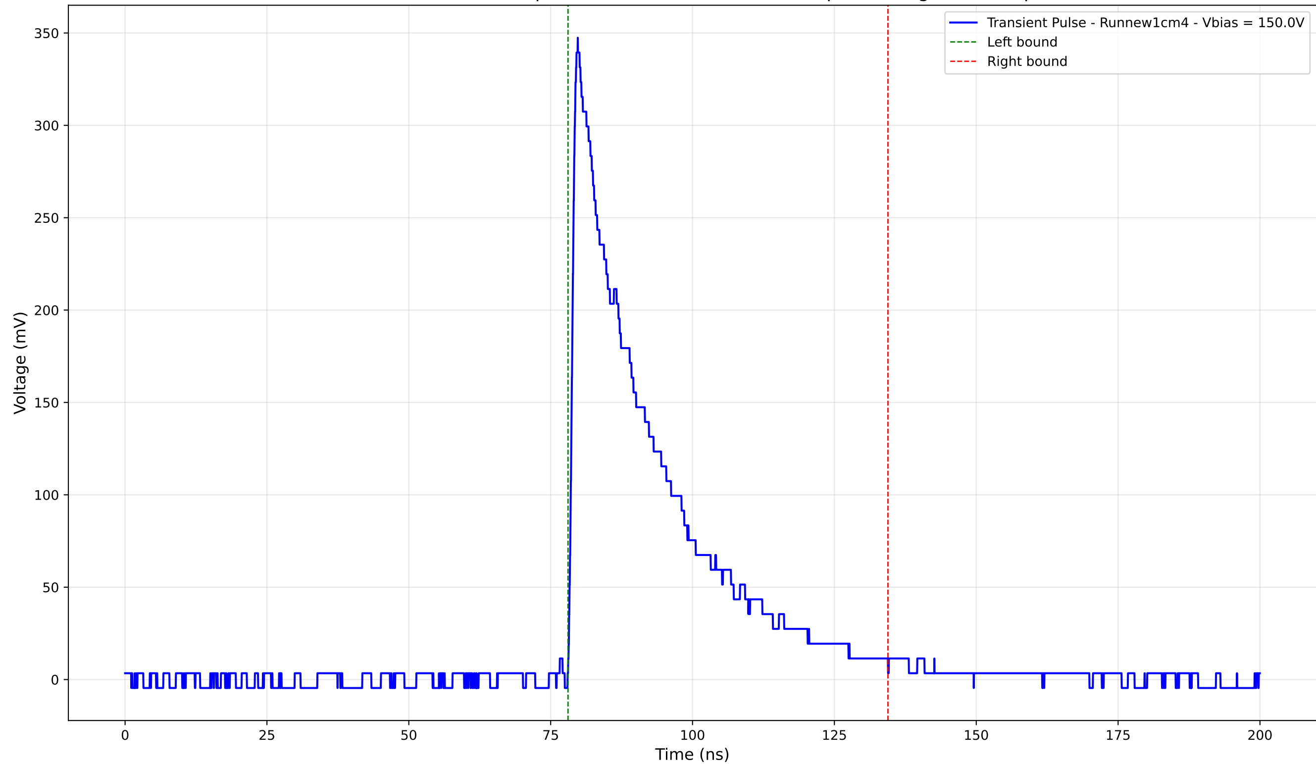
Transient Pulse - Sample: new1cm - Position: 4275.0 \mu\text{m} - Charge: 100.02 pC
