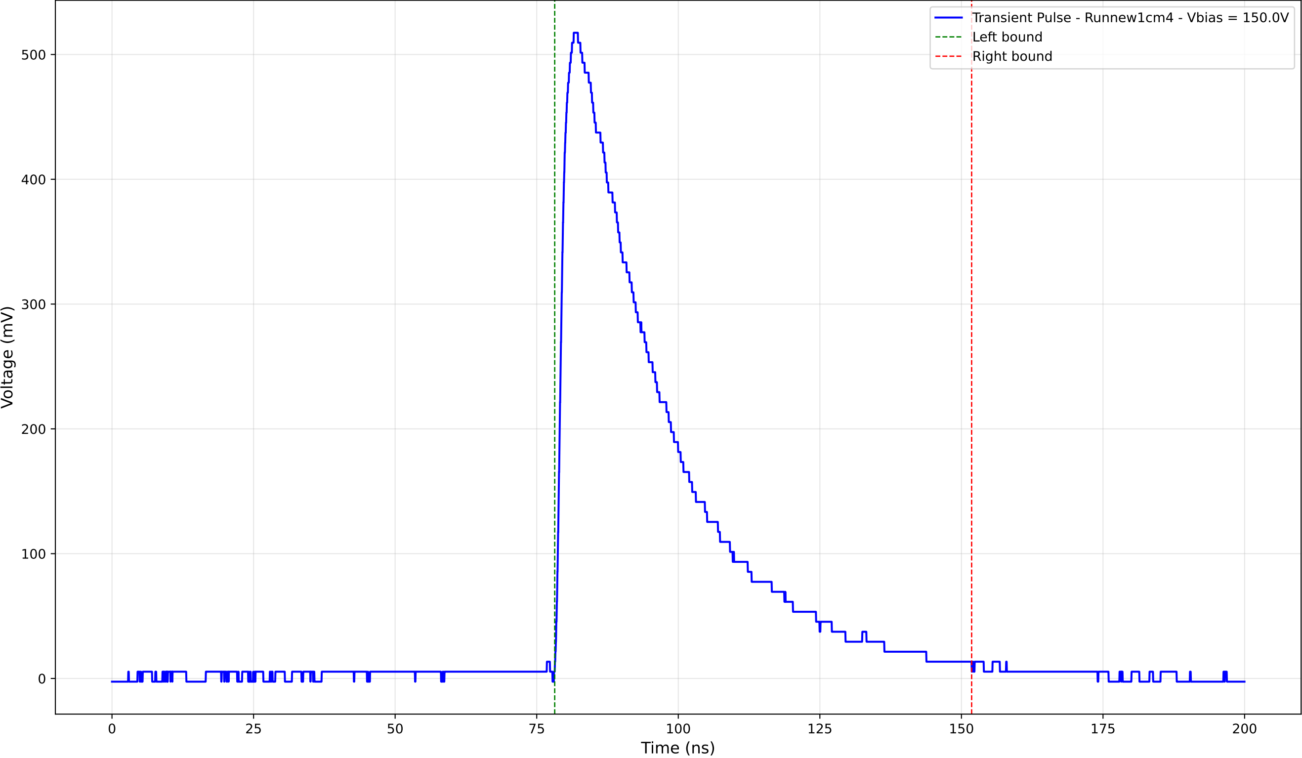
Transient Pulse - Sample: new1cm - Position: 1810.0 \mu\text{m} - Charge: 209.51 pC
