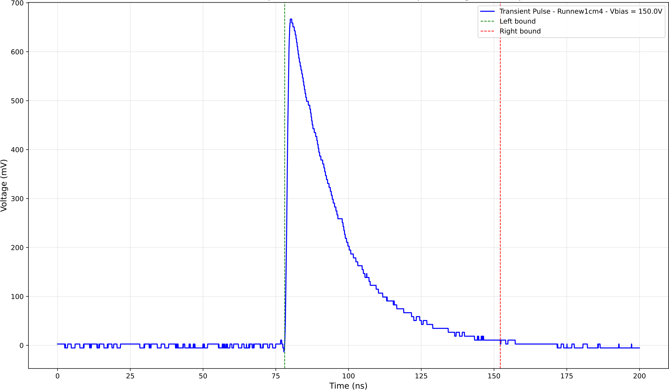
Transient Pulse - Sample: new1cm - Position: 4000.0 \mu\text{m} - Charge: 247.05 pC
