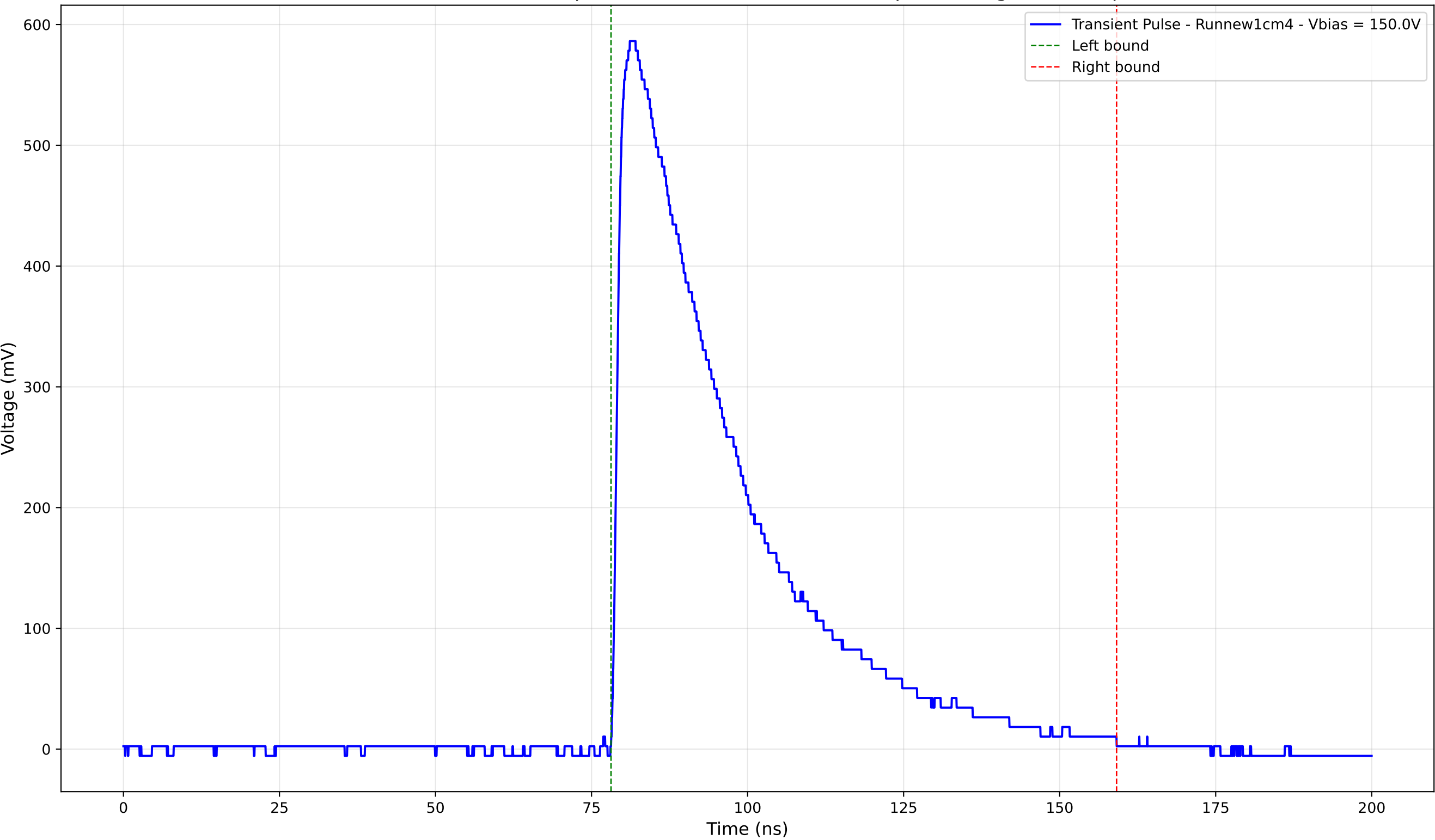
Transient Pulse - Sample: new1cm - Position: 3610.0 \mu\text{m} - Charge: 243.12 pC
