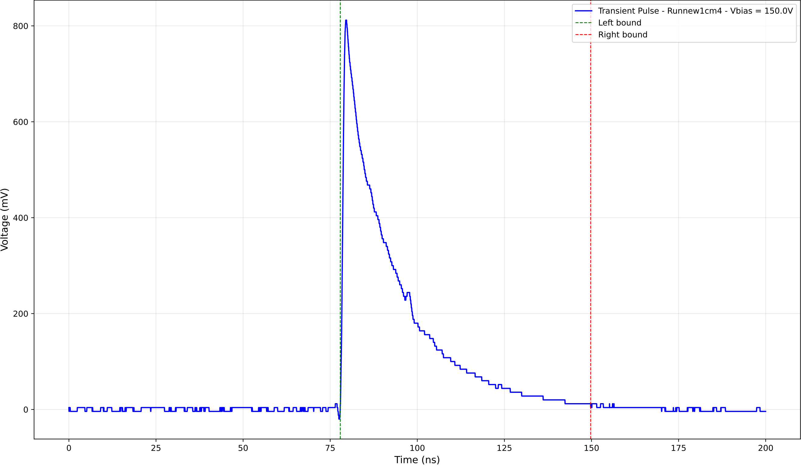
Transient Pulse - Sample: new1cm - Position: 4480.0 \mu\text{m} - Charge: 239.61 pC
