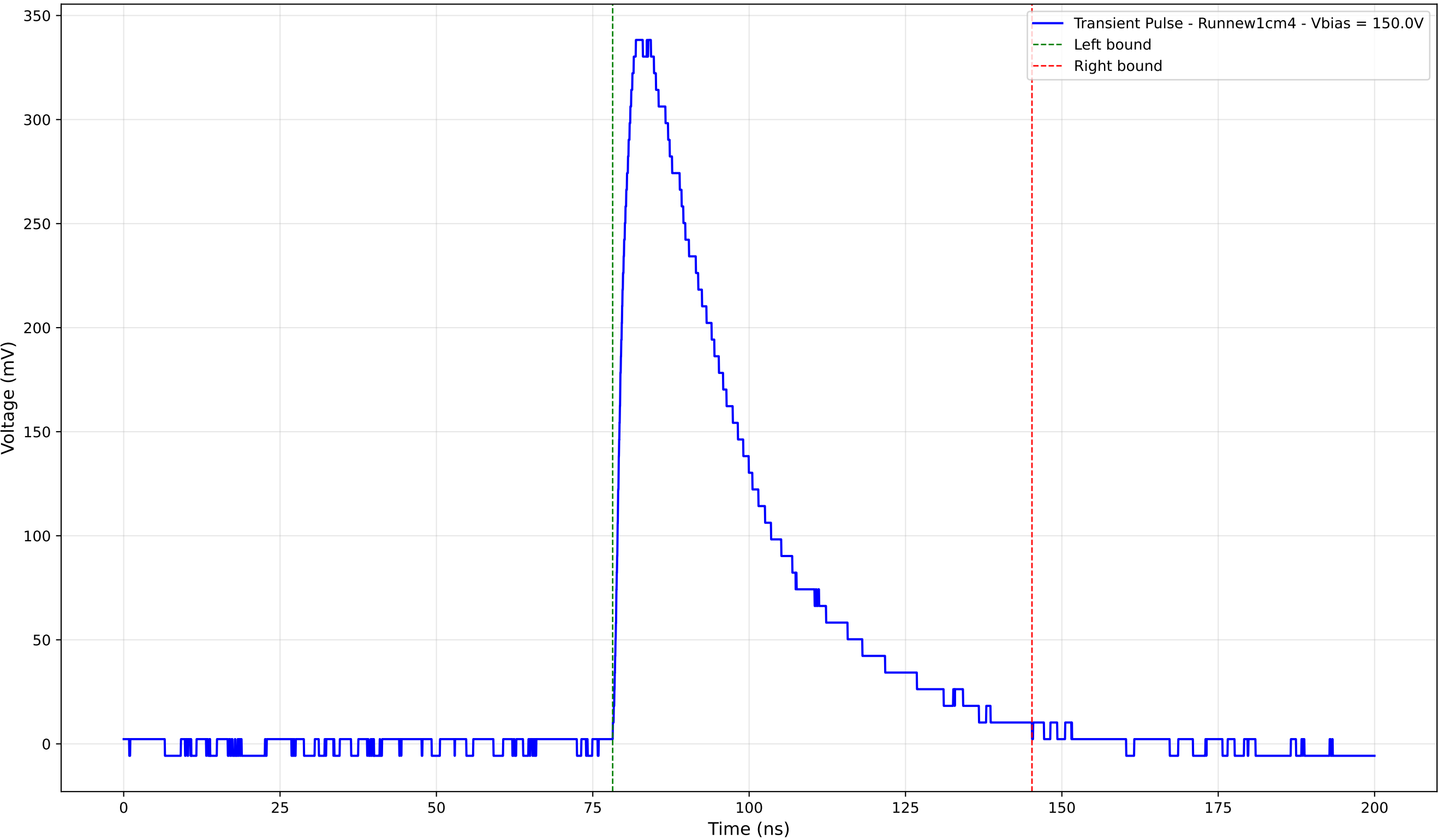
Transient Pulse - Sample: new1cm - Position: 2655.0 \mu\text{m} - Charge: 143.78 pC
