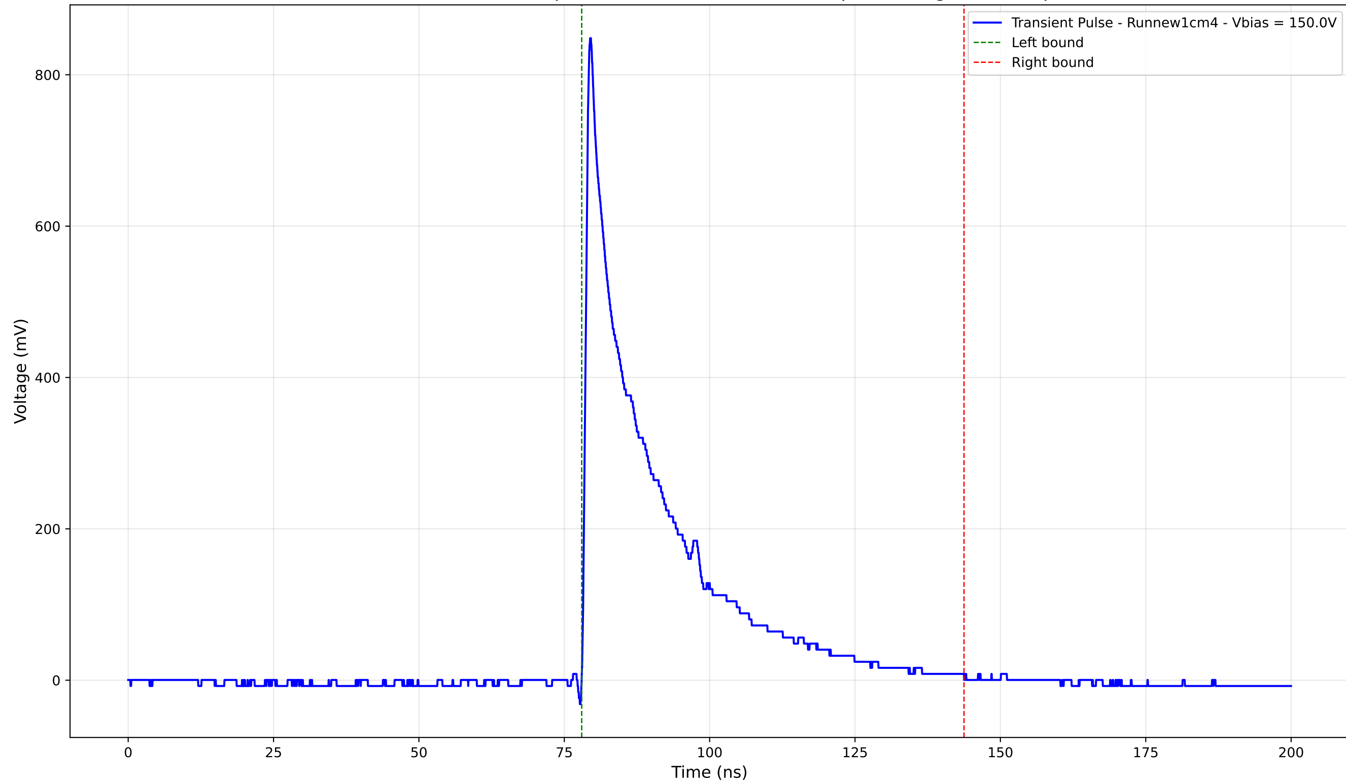
Transient Pulse - Sample: new1cm - Position: 585.0 \mu\text{m} - Charge: 188.04 pC
