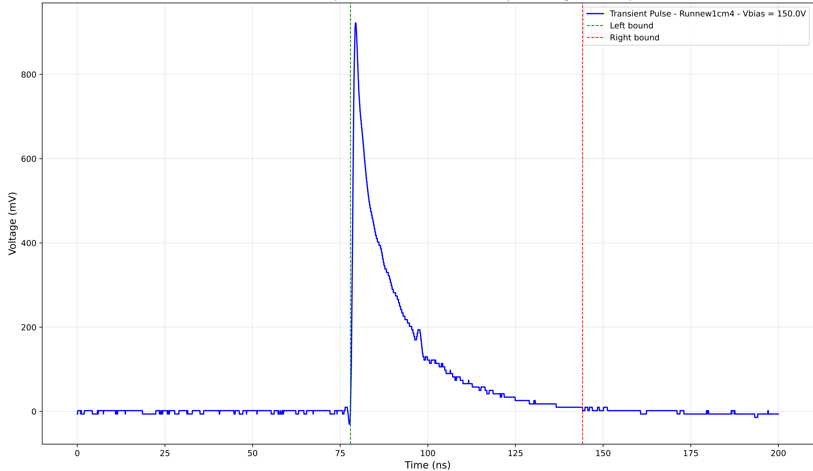
Transient Pulse - Sample: new1cm - Position: 480.0 \mu\text{m} - Charge: 200.49 pC
