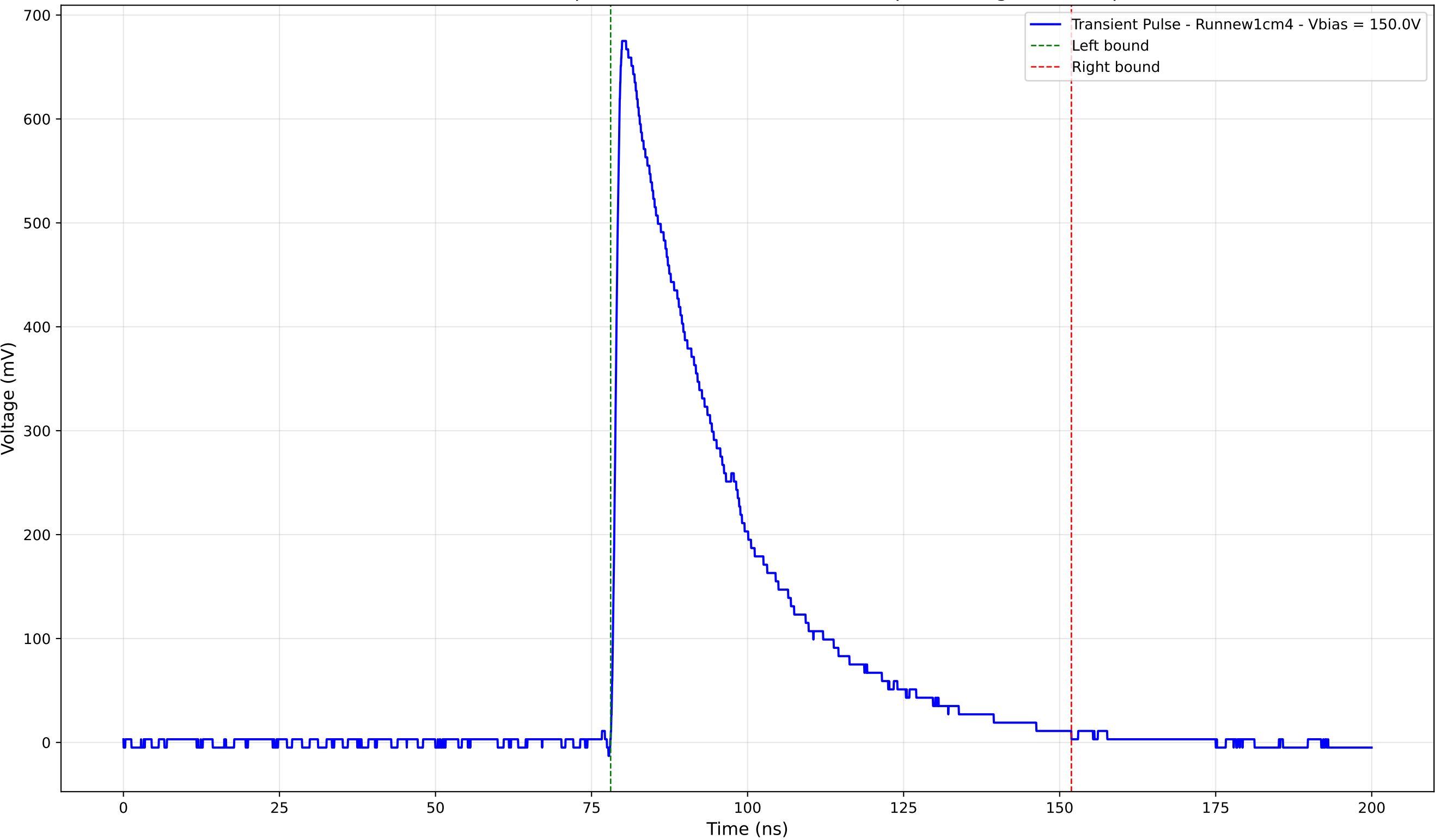
Transient Pulse - Sample: new1cm - Position: 4035.0 \mu\text{m} - Charge: 248.12 pC
