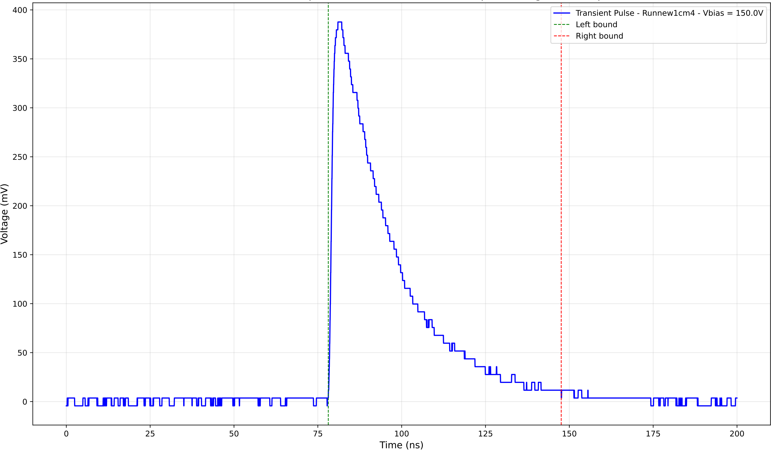
Transient Pulse - Sample: new1cm - Position: 3670.0 \mu\text{m} - Charge: 153.20 pC
