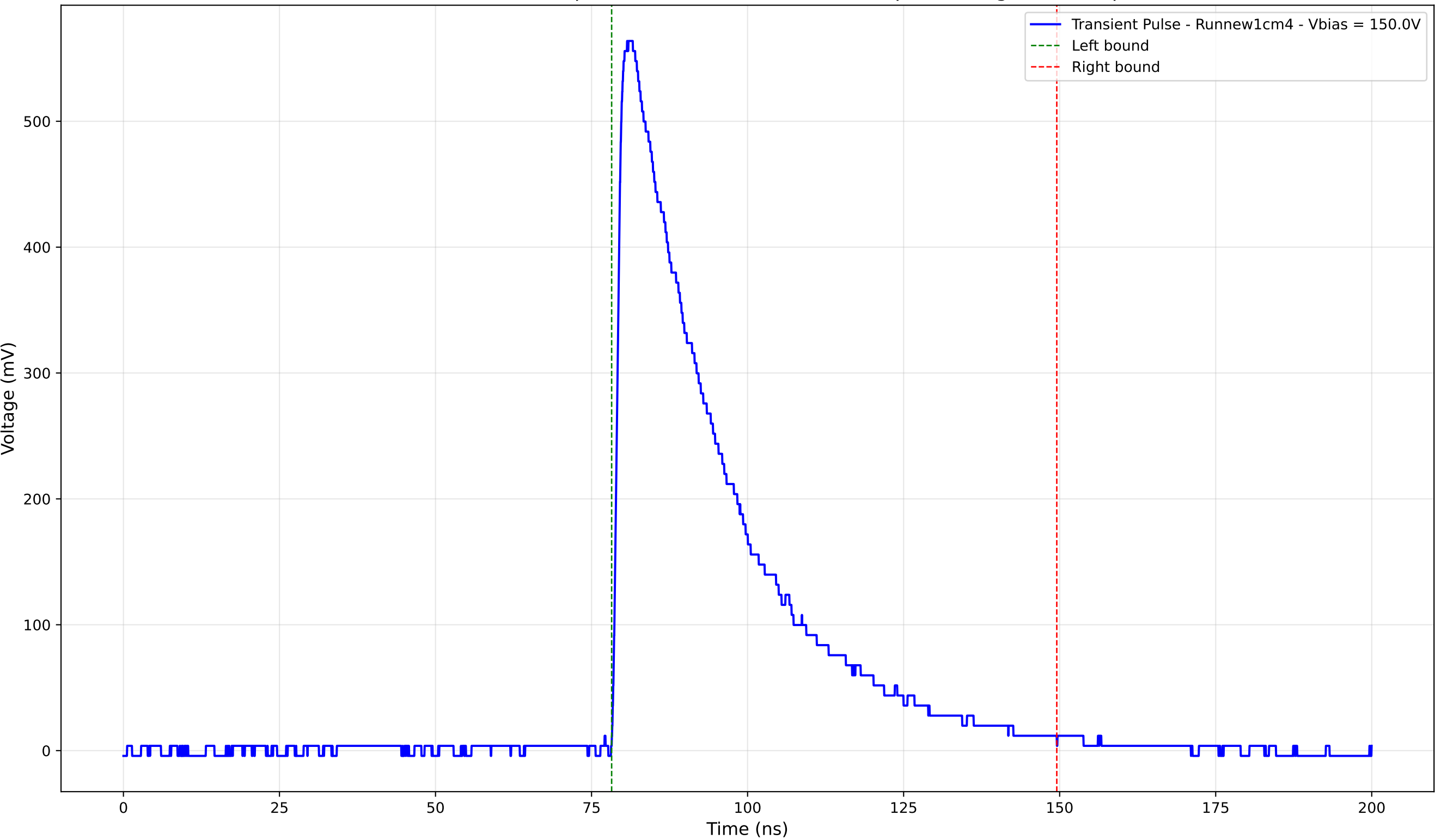
Transient Pulse - Sample: new1cm - Position: 1440.0 \mu\text{m} - Charge: 207.94 pC
