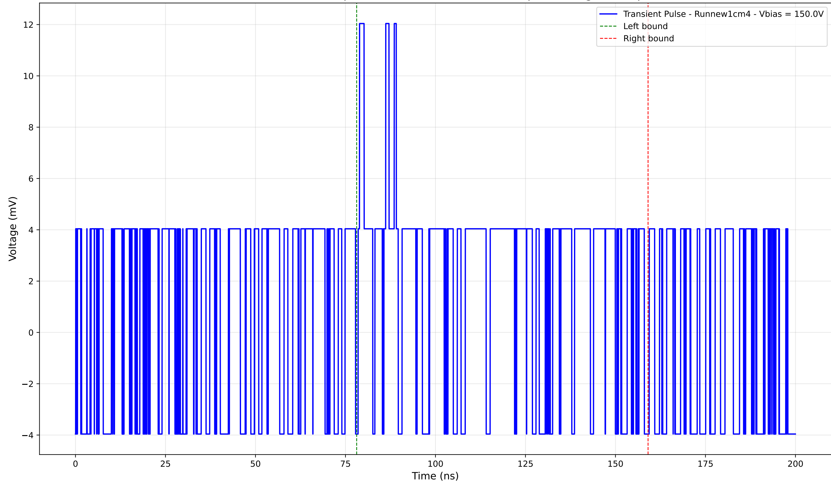
Transient Pulse - Sample: new1cm - Position: 5145.0 \mu\text{m} - Charge: 3.87 pC
