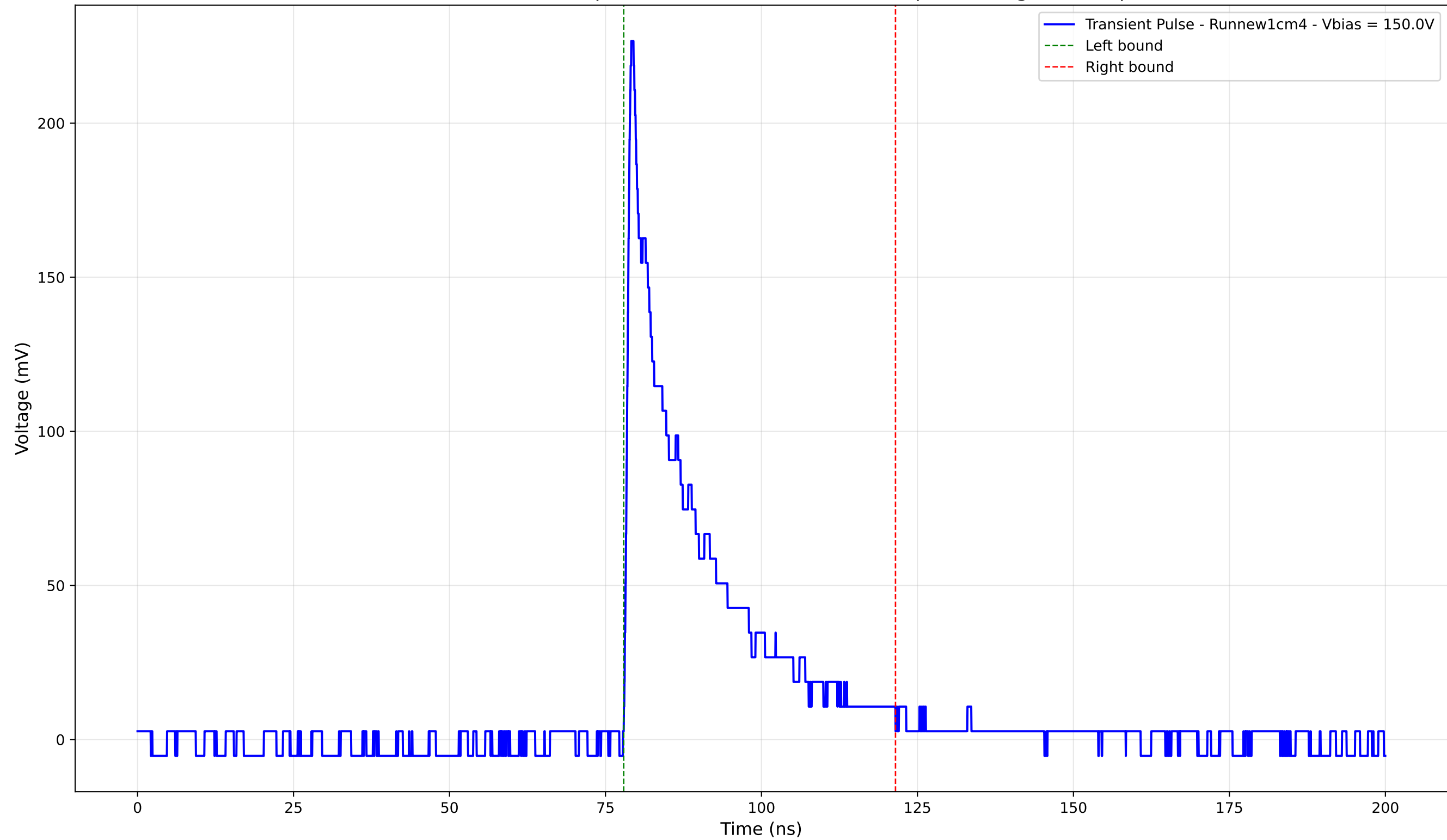
Transient Pulse - Sample: new1cm - Position: 4755.0 \mu\text{m} - Charge: 45.13 pC
