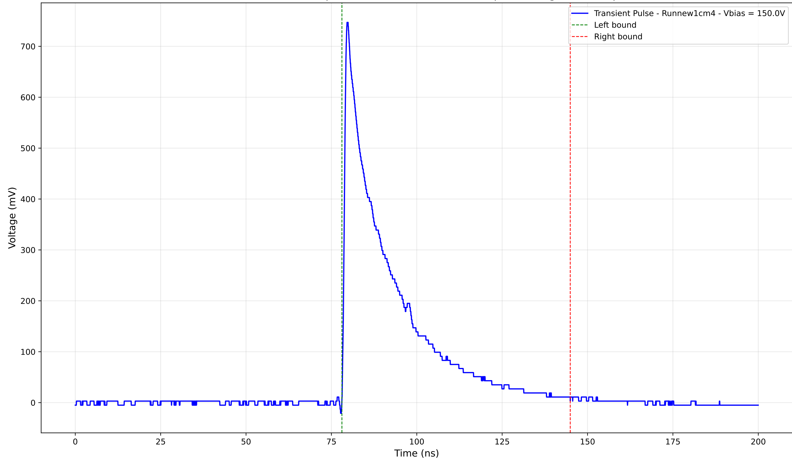
Transient Pulse - Sample: new1cm - Position: 820.0 \mu\text{m} - Charge: 198.31 pC
