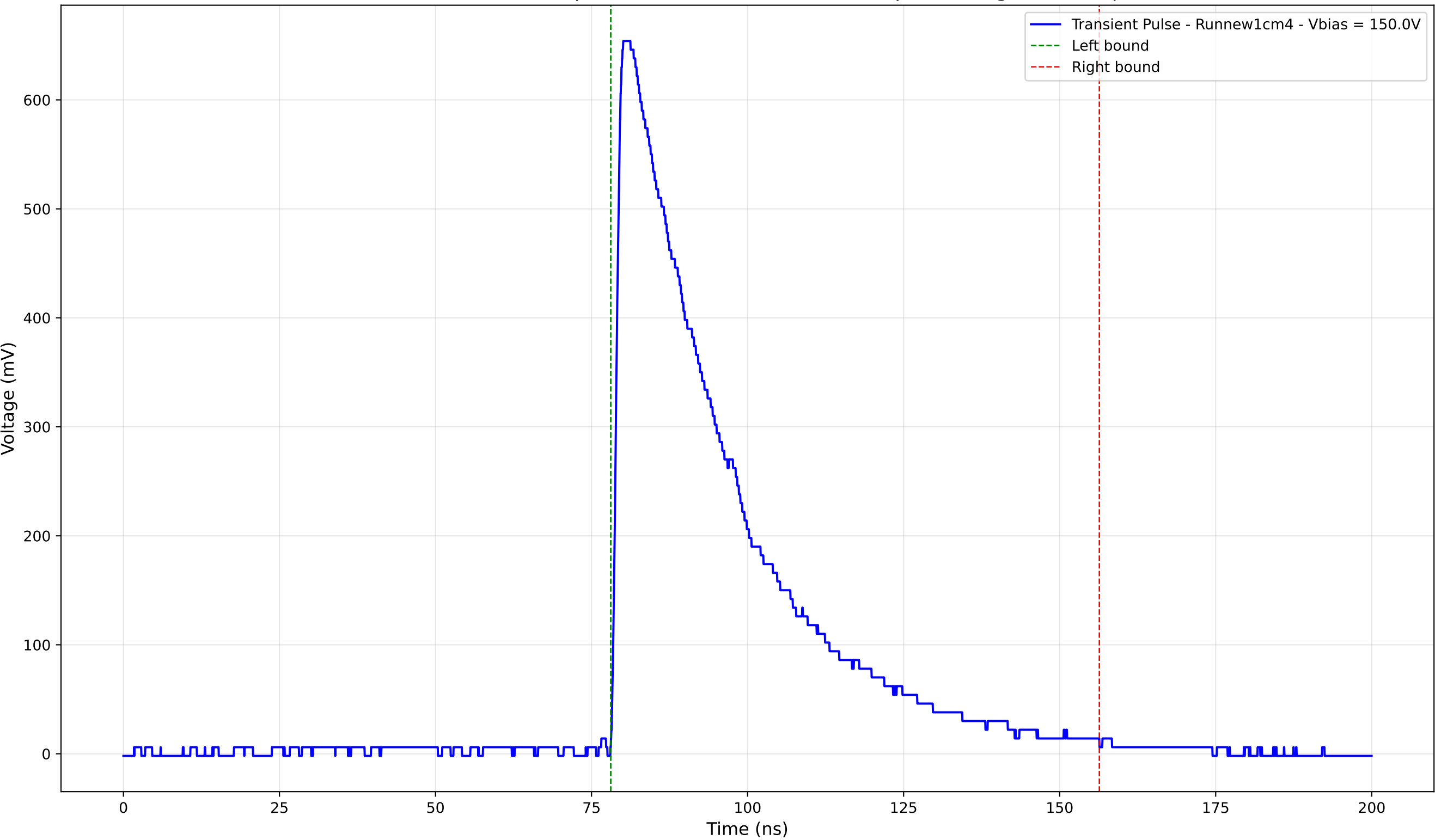
Transient Pulse - Sample: new1cm - Position: 3905.0 \mu\text{m} - Charge: 256.66 pC
