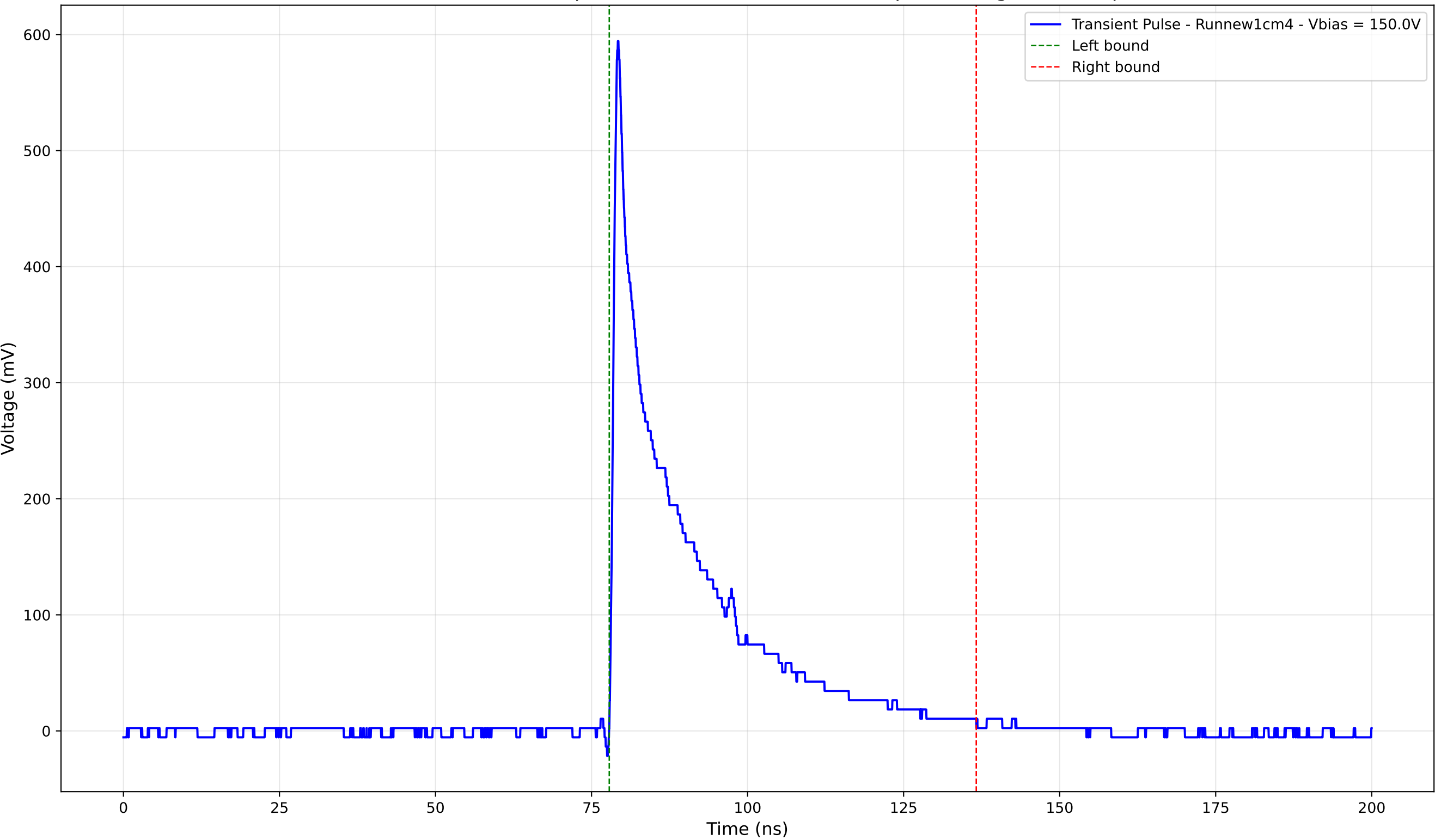
Transient Pulse - Sample: new1cm - Position: 4790.0 \mu\text{m} - Charge: 118.98 pC
