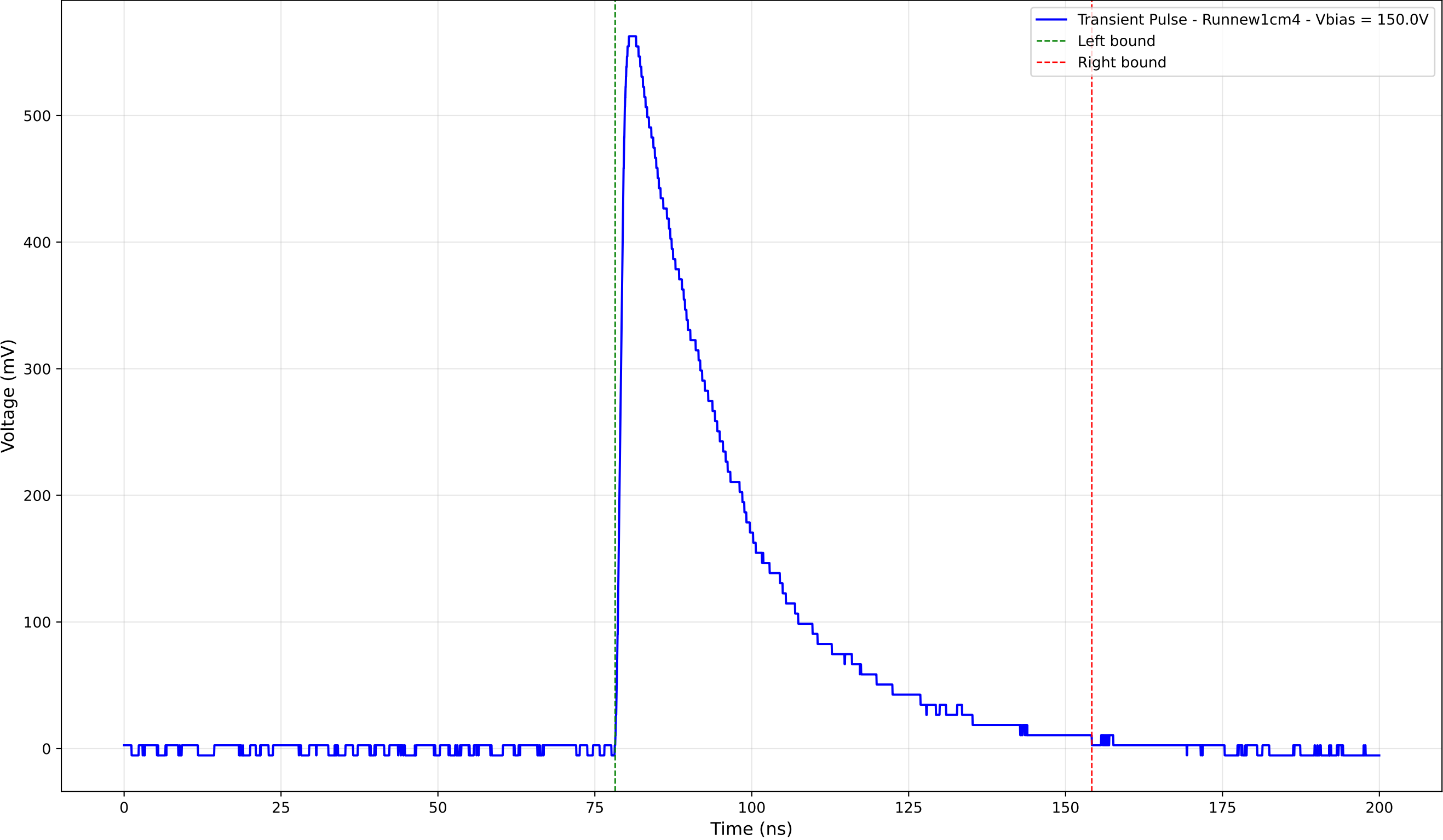
Transient Pulse - Sample: new1cm - Position: 1430.0 \mu\text{m} - Charge: 207.50 pC
