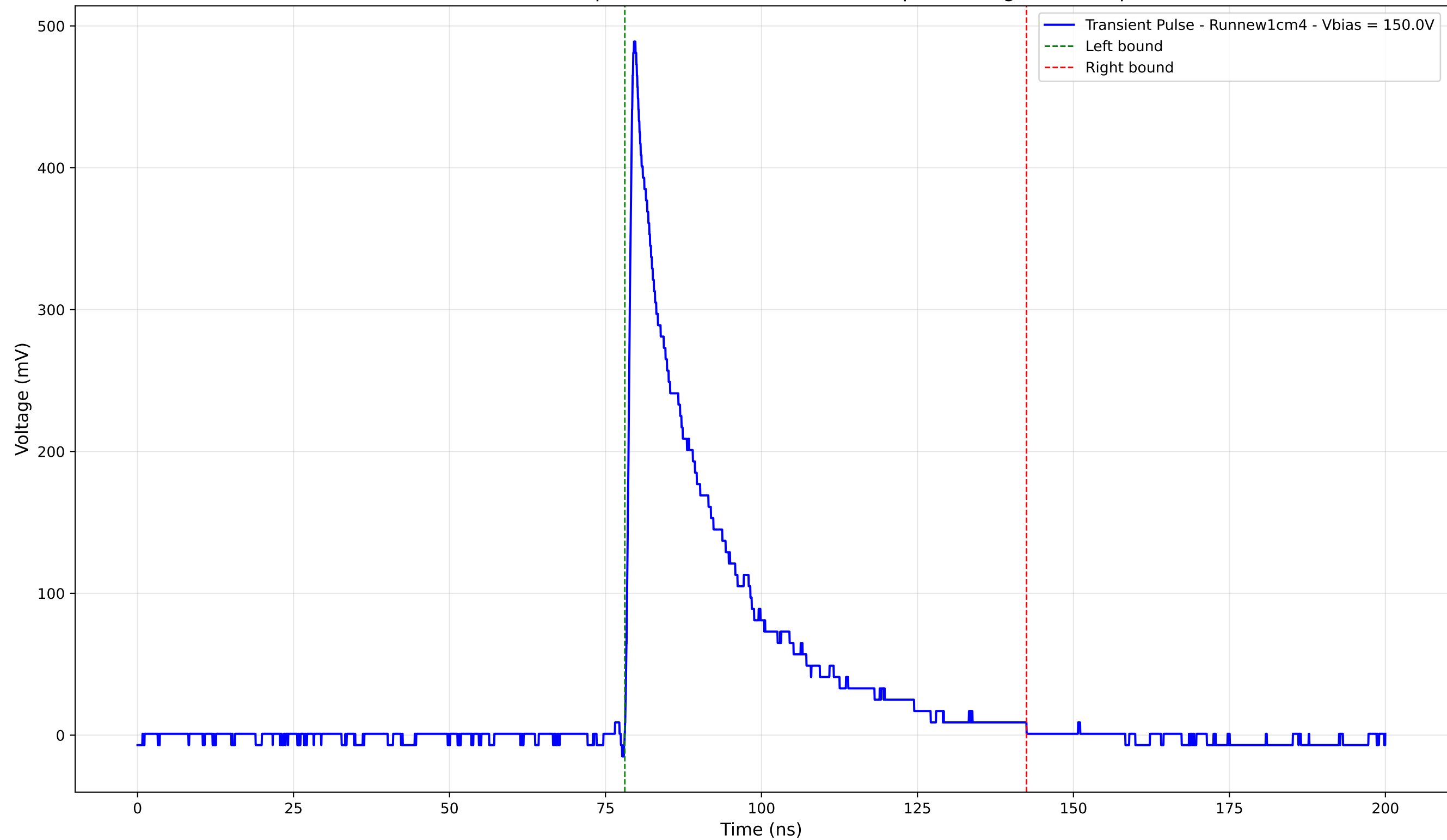
Transient Pulse - Sample: new1cm - Position: 750.0 \mu\text{m} - Charge: 118.30 pC
