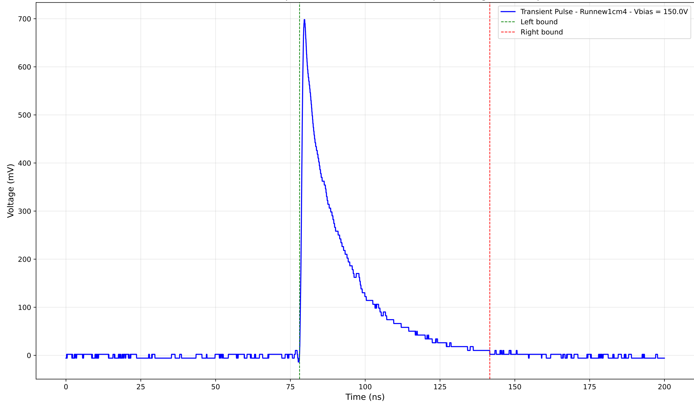
Transient Pulse - Sample: new1cm - Position: 785.0 \mu\text{m} - Charge: 175.98 pC
