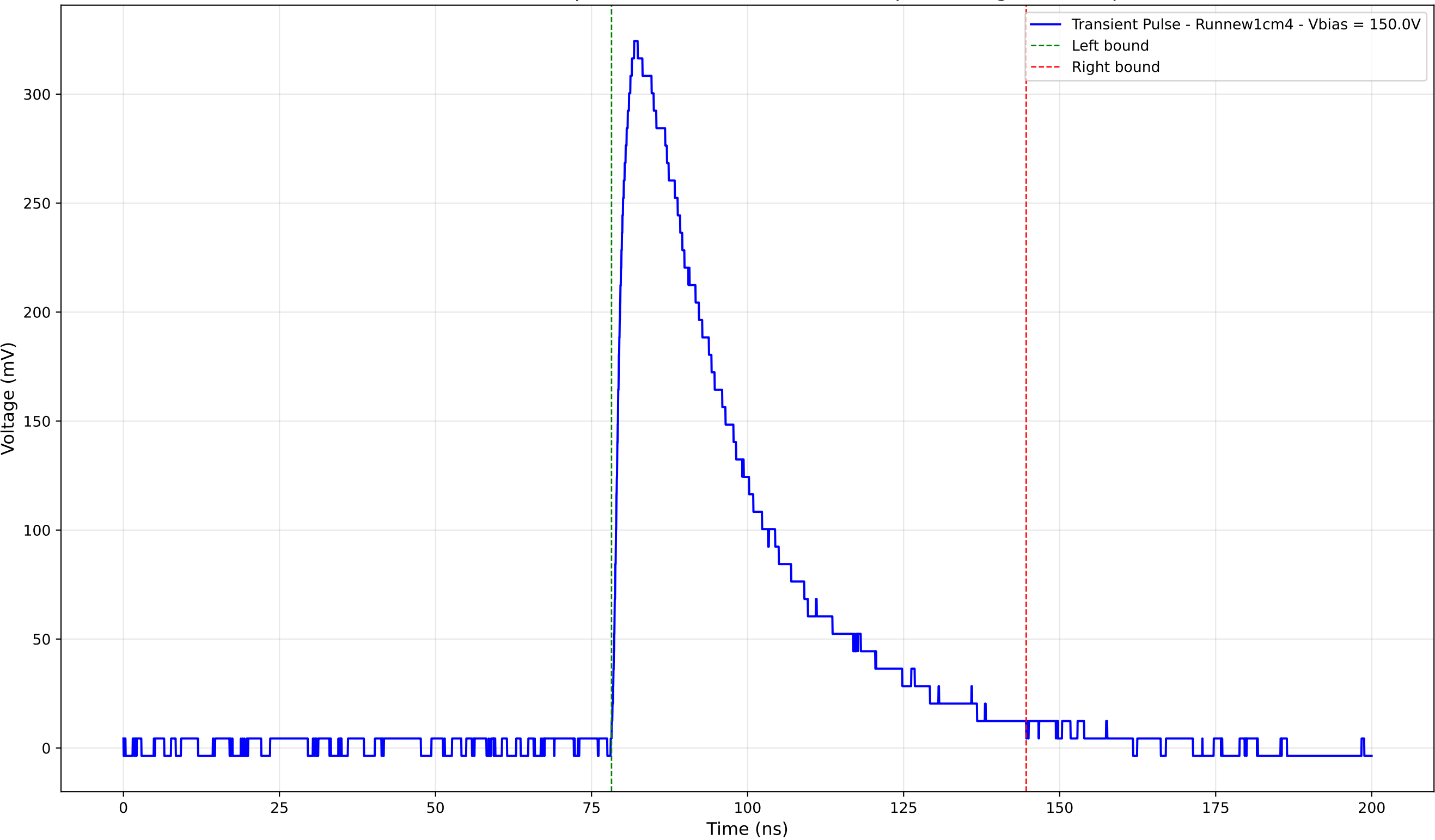
Transient Pulse - Sample: new1cm - Position: 3170.0 \mu\text{m} - Charge: 135.68 pC
