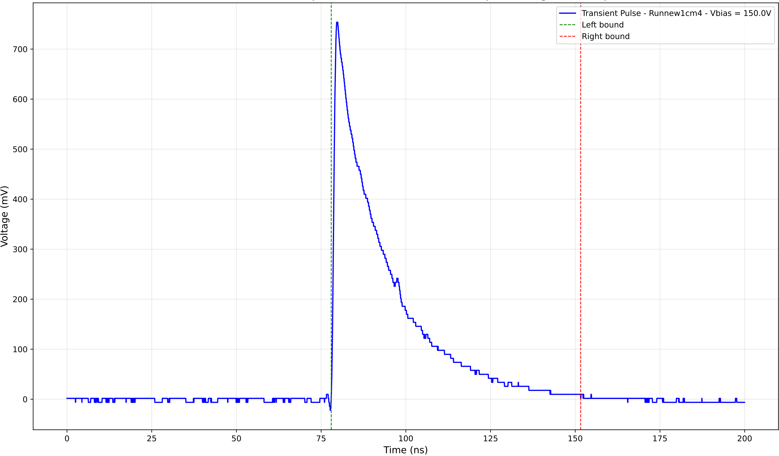
Transient Pulse - Sample: new1cm - Position: 4345.0 \mu\text{m} - Charge: 233.20 pC
