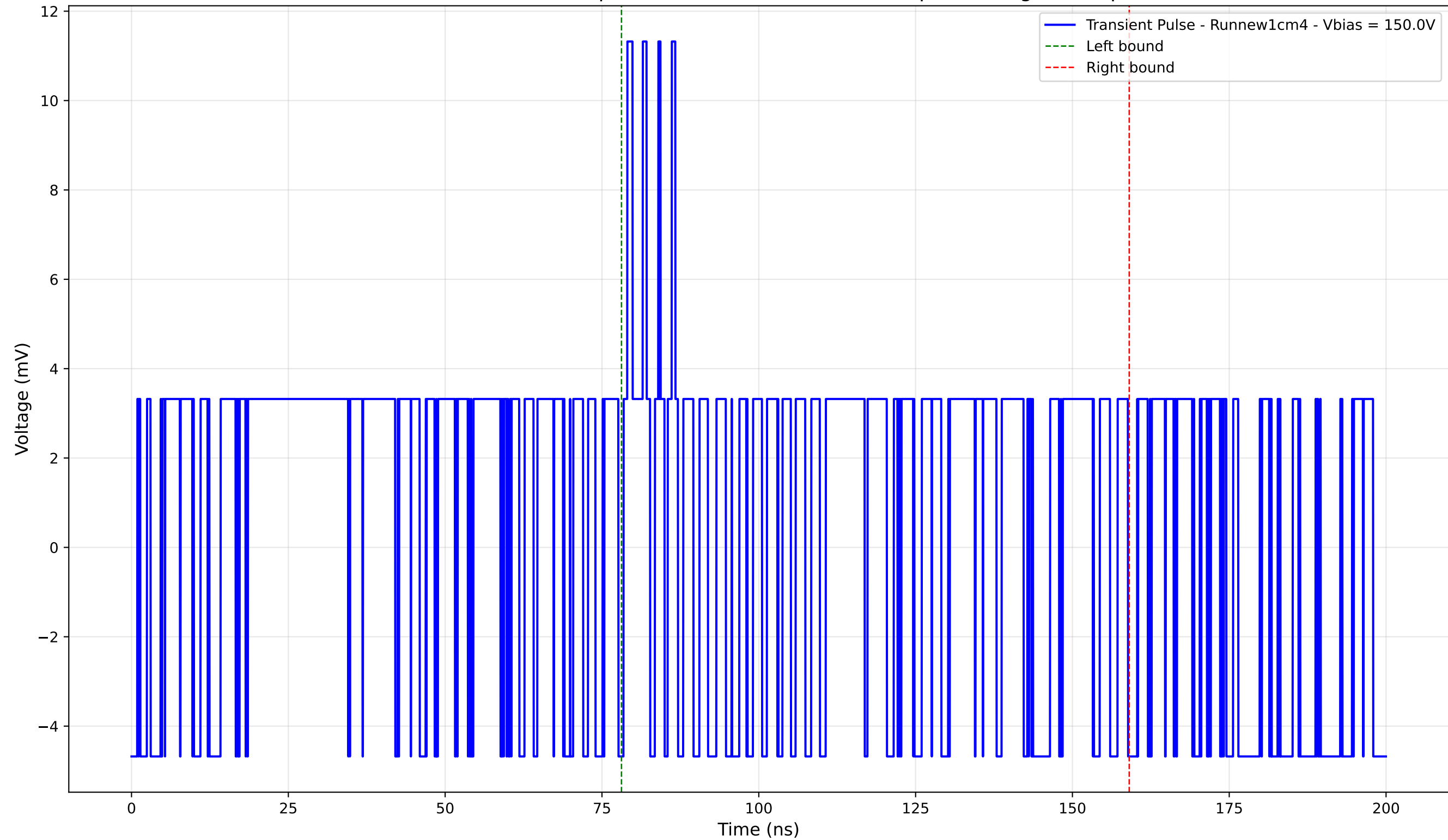
Transient Pulse - Sample: new1cm - Position: 5160.0 \mu\text{m} - Charge: 1.94 pC
