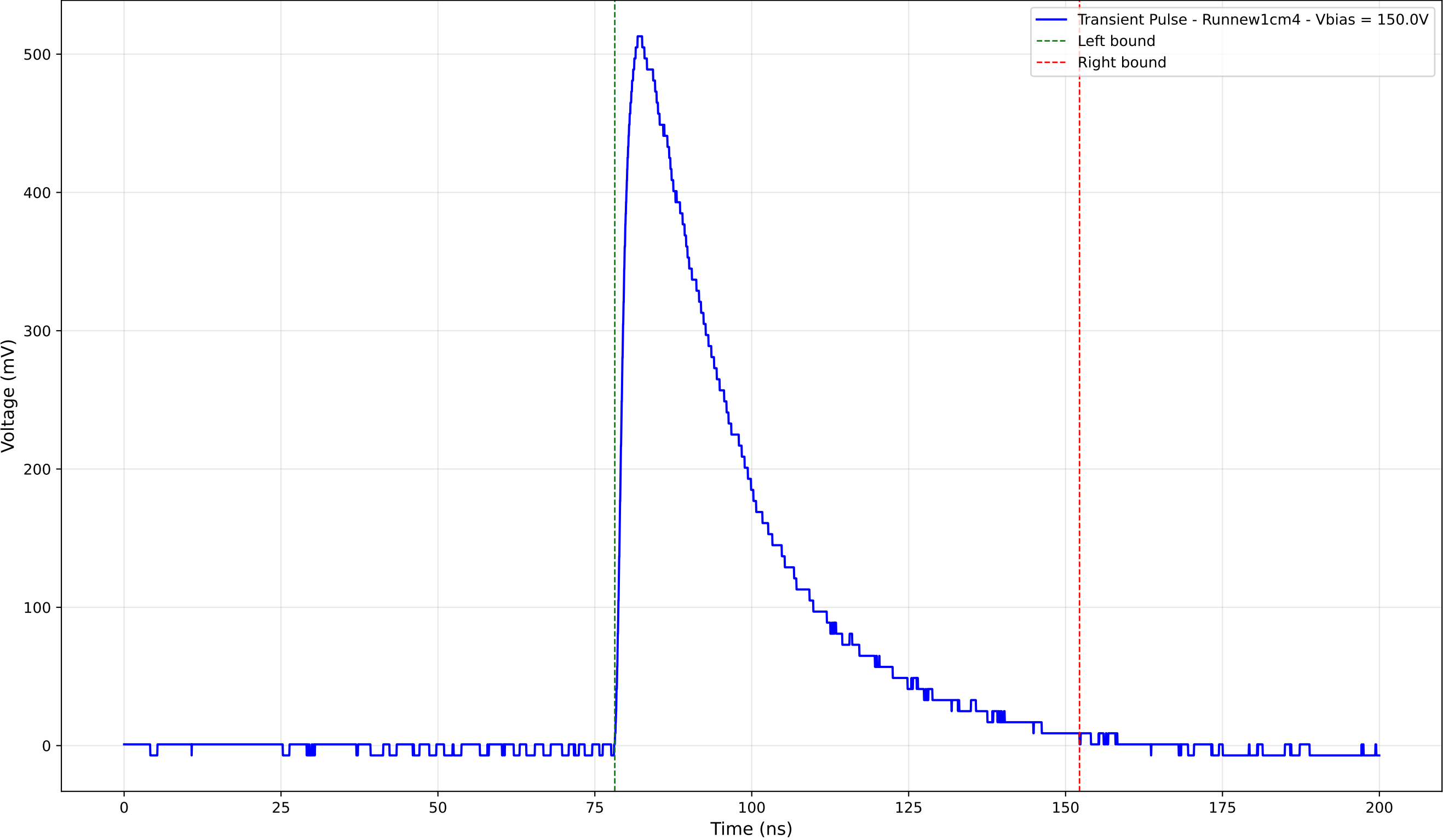
Transient Pulse - Sample: new1cm - Position: 1995.0 \mu\text{m} - Charge: 210.29 pC
