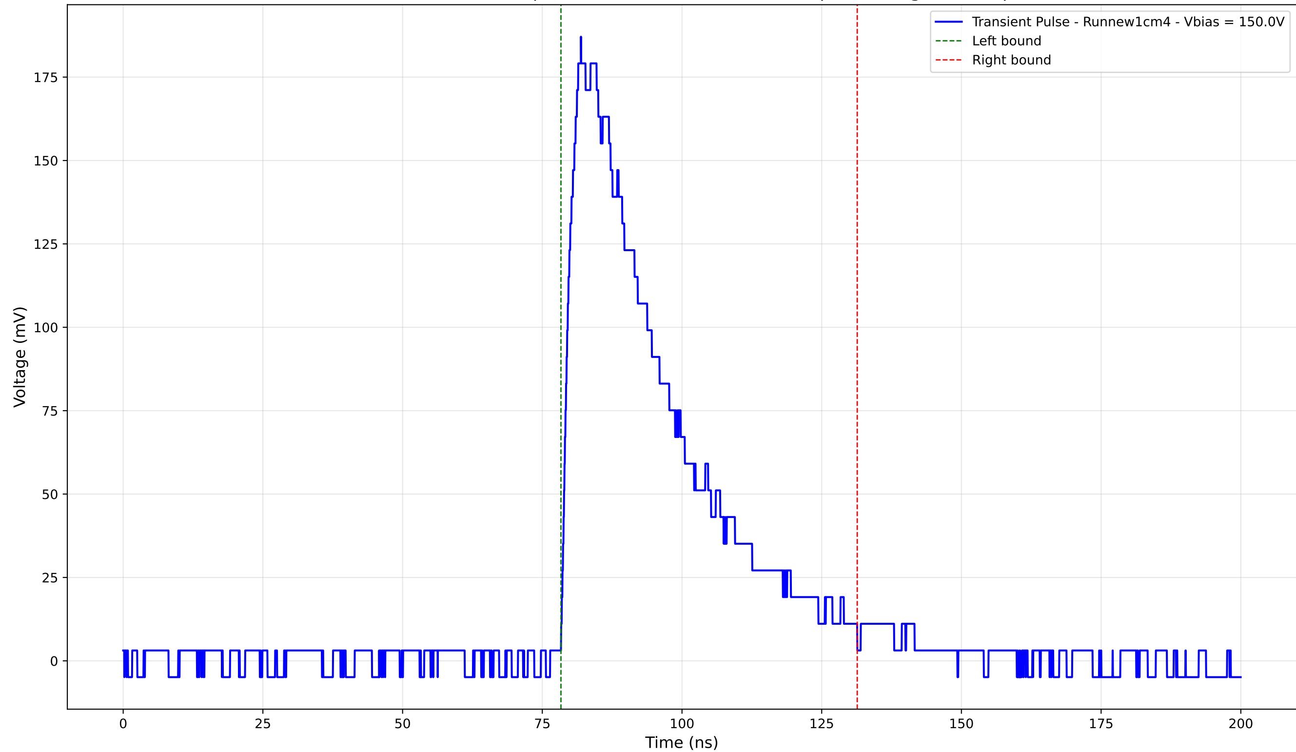
Transient Pulse - Sample: new1cm - Position: 2235.0 \mu\text{m} - Charge: 72.25 pC
