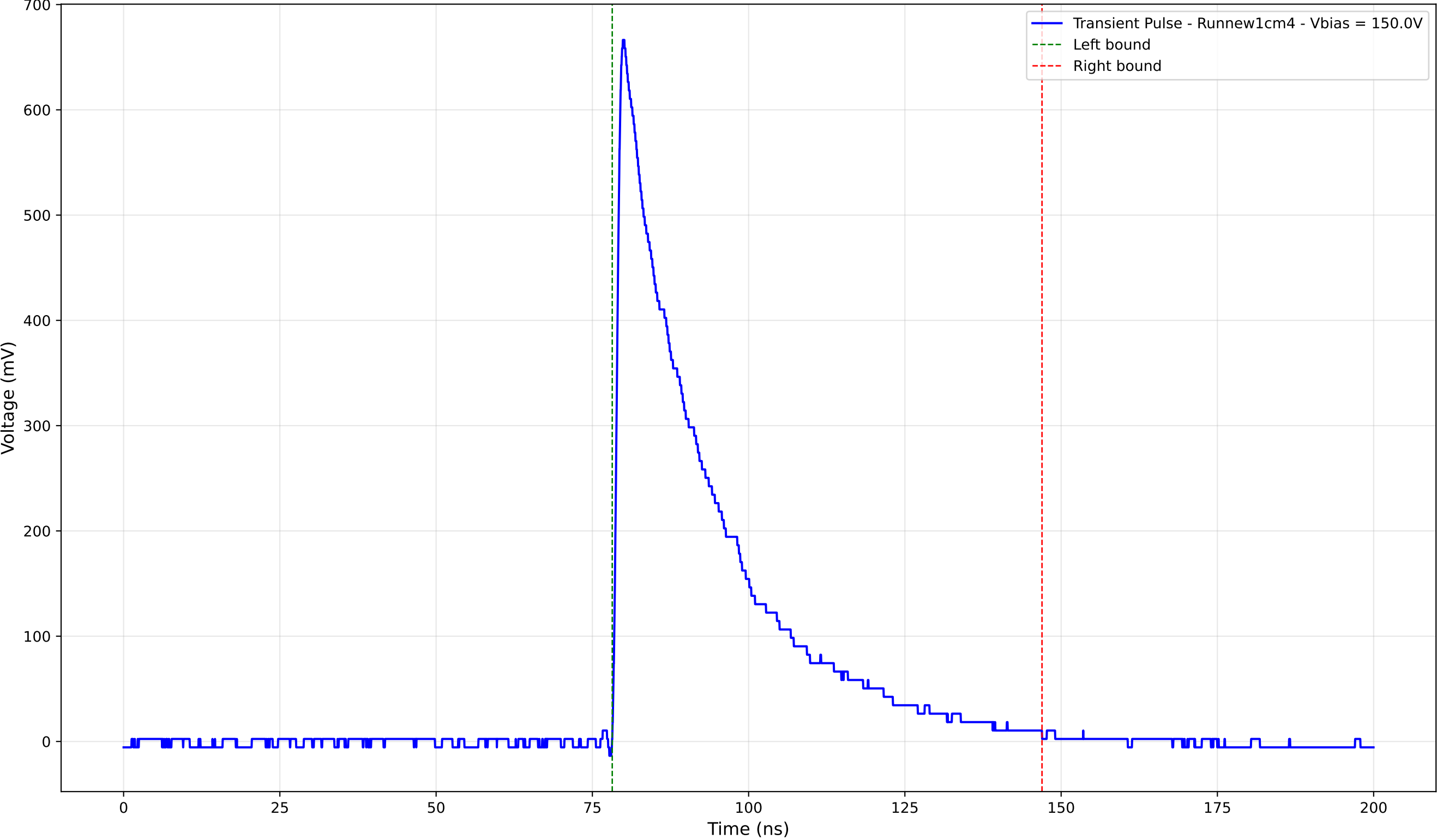
Transient Pulse - Sample: new1cm - Position: 1040.0 \mu\text{m} - Charge: 199.82 pC
