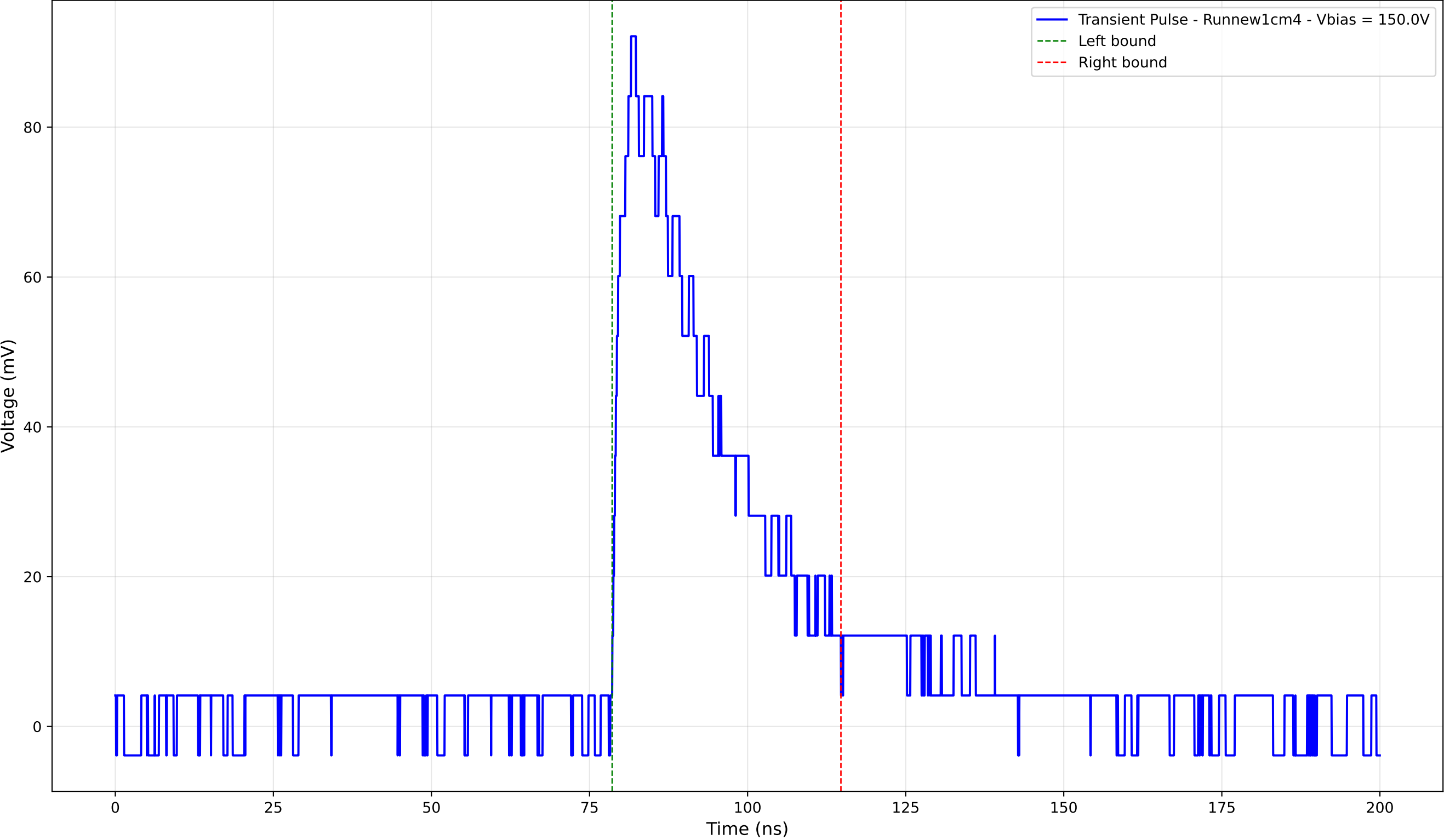
Transient Pulse - Sample: new1cm - Position: 1695.0 \mu\text{m} - Charge: 30.74 pC
