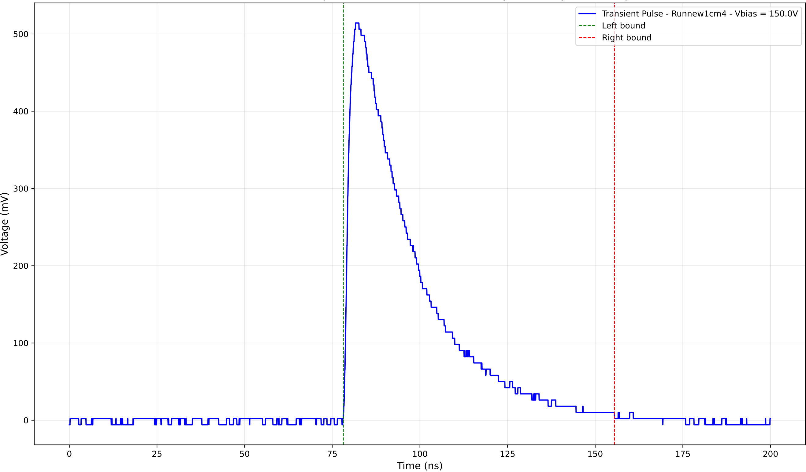
Transient Pulse - Sample: new1cm - Position: 2020.0 \mu\text{m} - Charge: 213.52 pC
