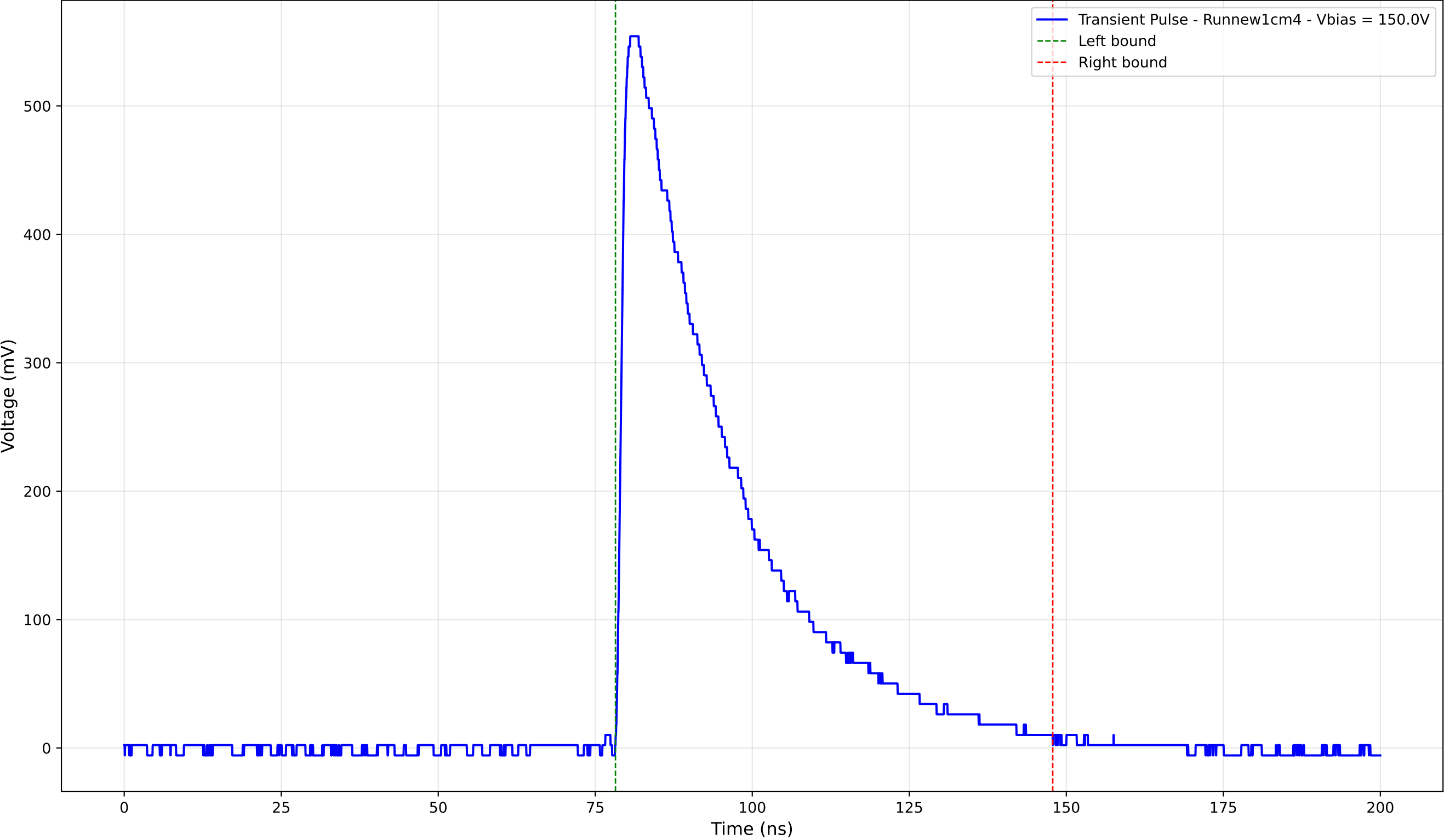
Transient Pulse - Sample: new1cm - Position: 1490.0 \mu\text{m} - Charge: 207.73 pC
