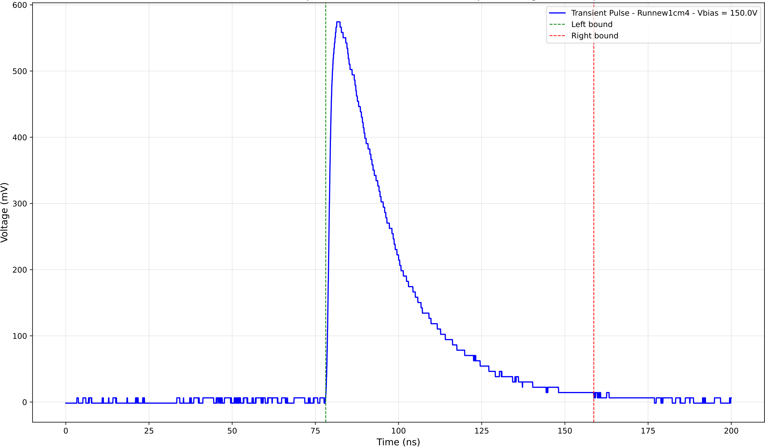
Transient Pulse - Sample: new1cm - Position: 3395.0 \mu\text{m} - Charge: 248.66 pC
