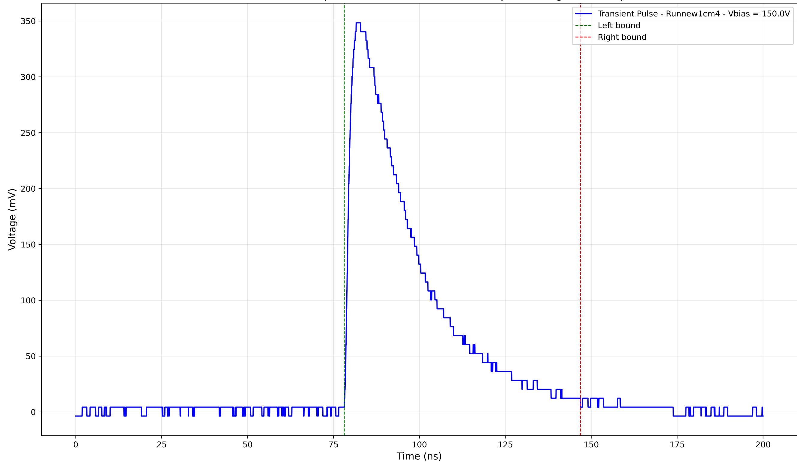
Transient Pulse - Sample: new1cm - Position: 3165.0 \mu\text{m} - Charge: 149.78 pC
