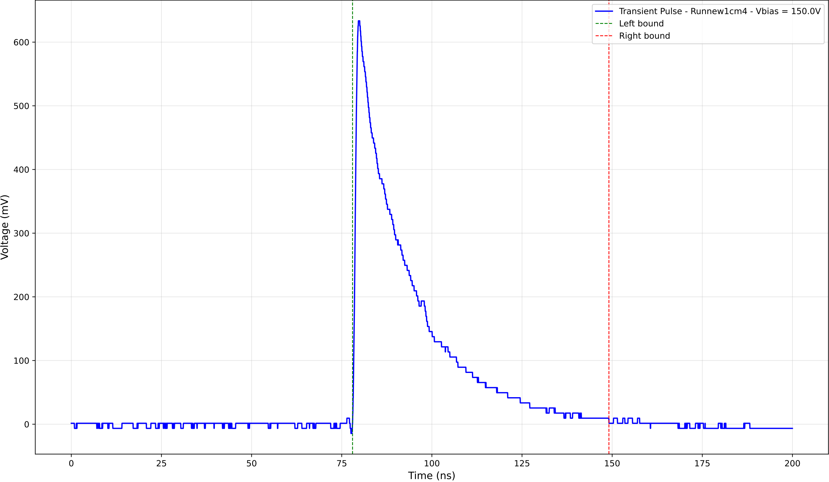
Transient Pulse - Sample: new1cm - Position: 4310.0 \mu\text{m} - Charge: 192.28 pC
