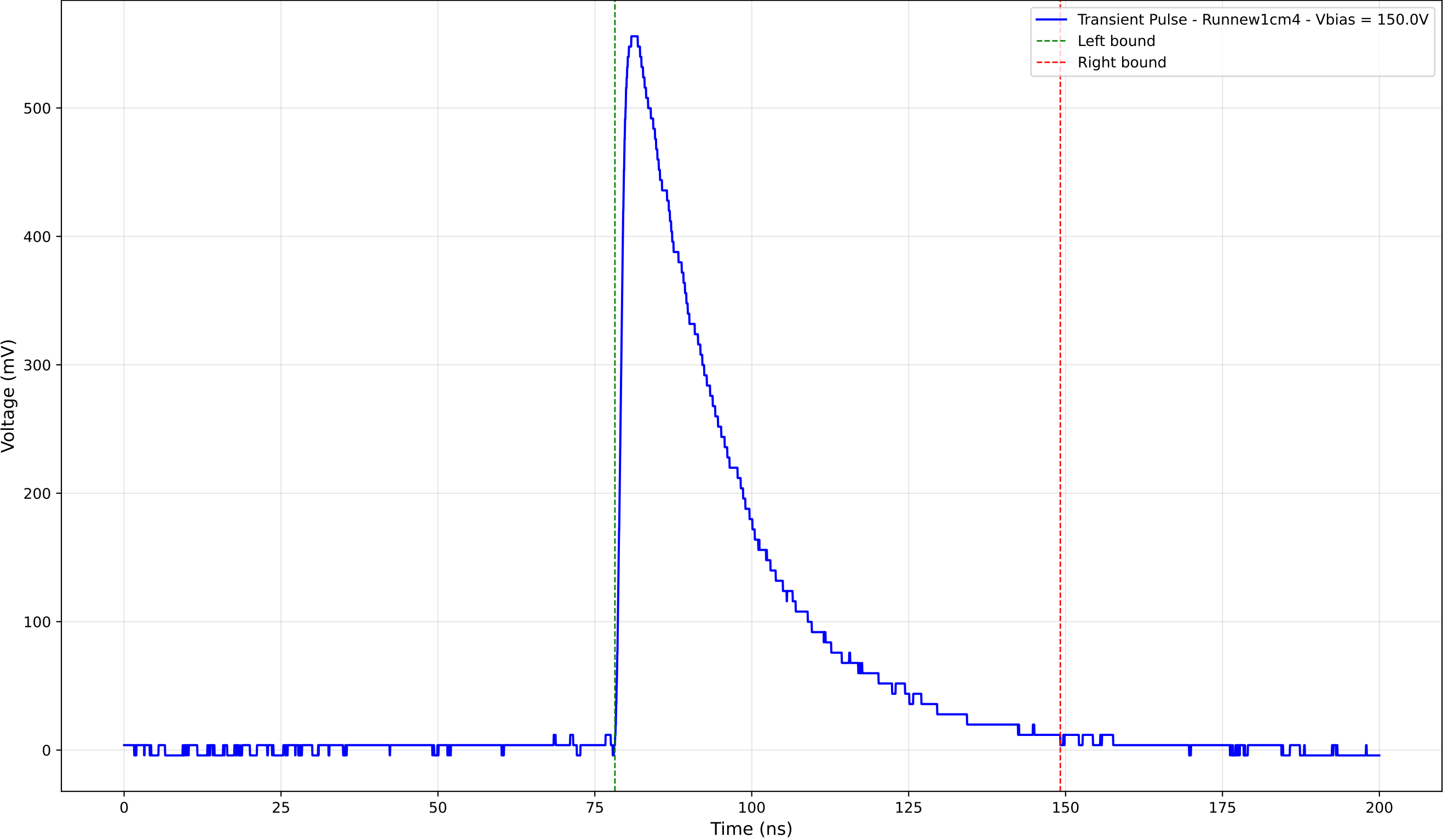
Transient Pulse - Sample: new1cm - Position: 1520.0 \mu\text{m} - Charge: 209.38 pC
