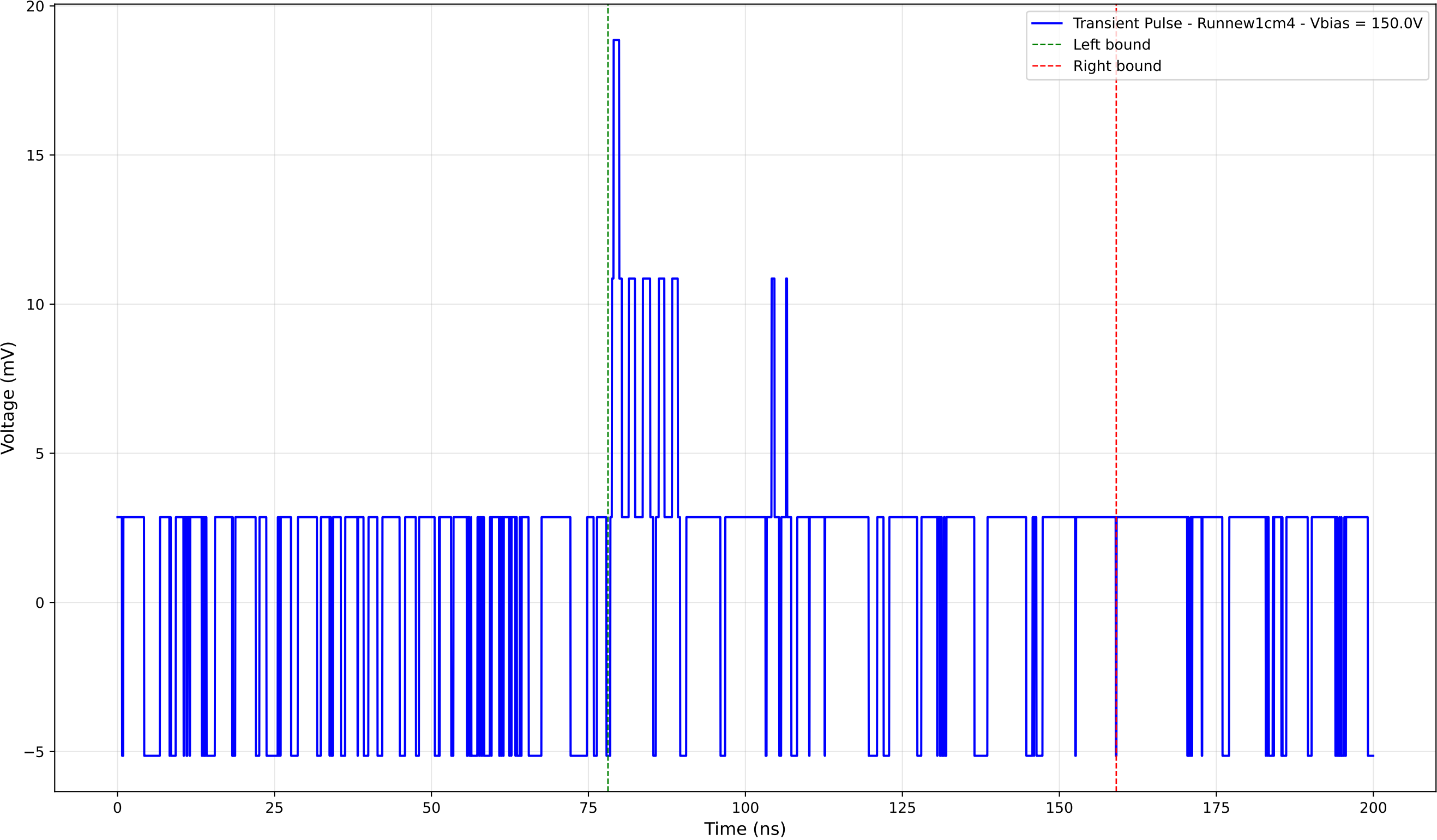
Transient Pulse - Sample: new1cm - Position: 105.0 \mu\text{m} - Charge: 3.84 pC
