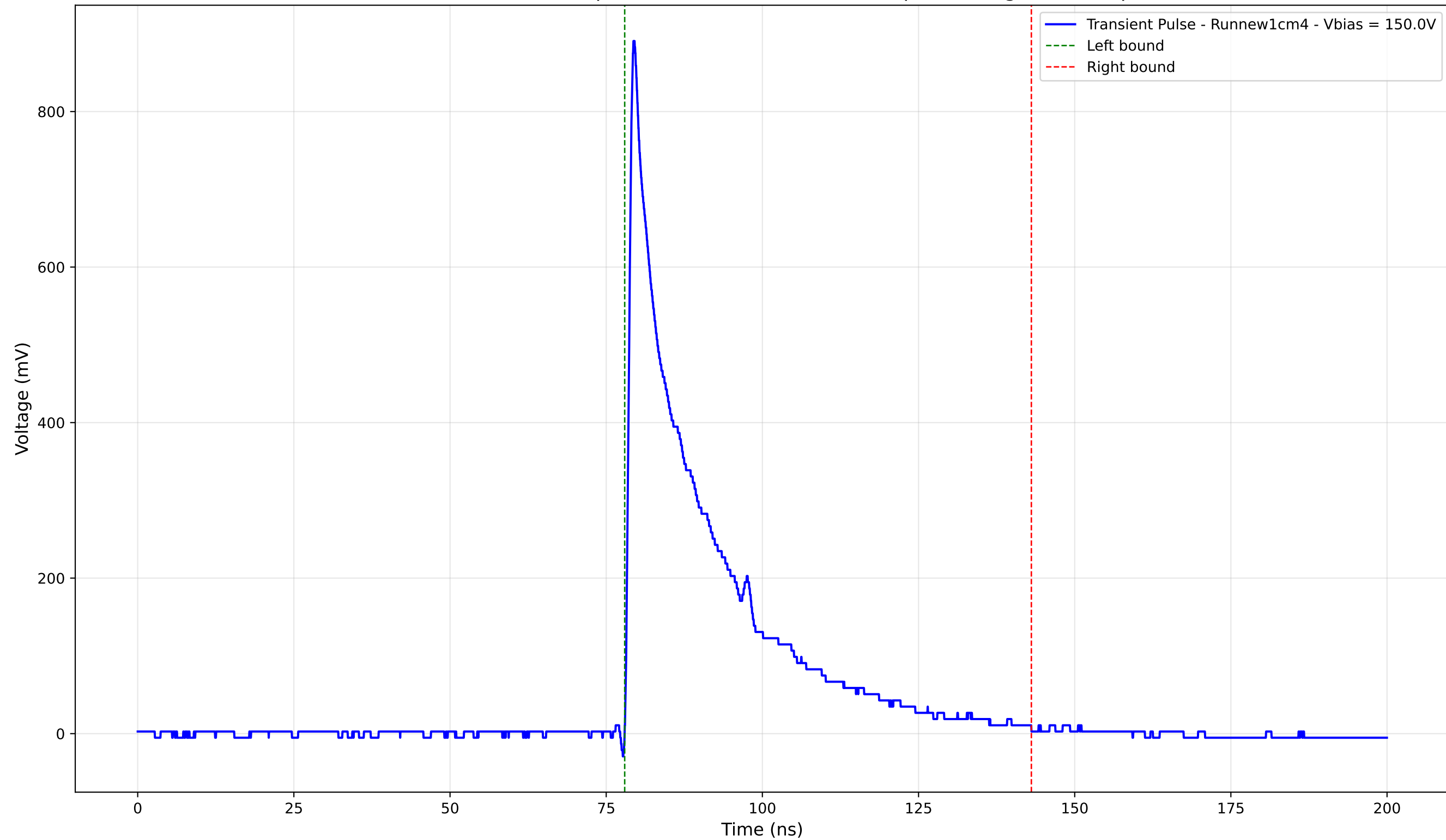
Transient Pulse - Sample: new1cm - Position: 550.0 \mu\text{m} - Charge: 200.92 pC
