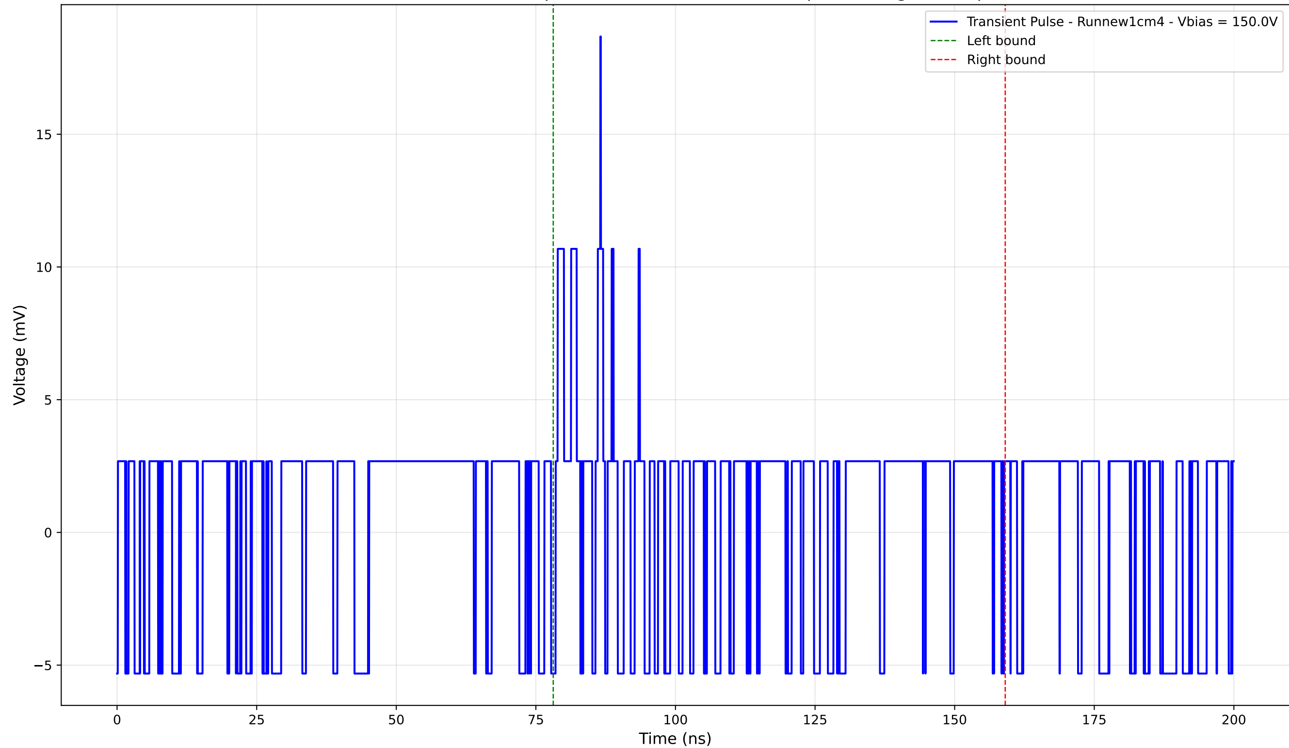
Transient Pulse - Sample: new1cm - Position: 85.0 \mu\text{m} - Charge: 2.22 pC
