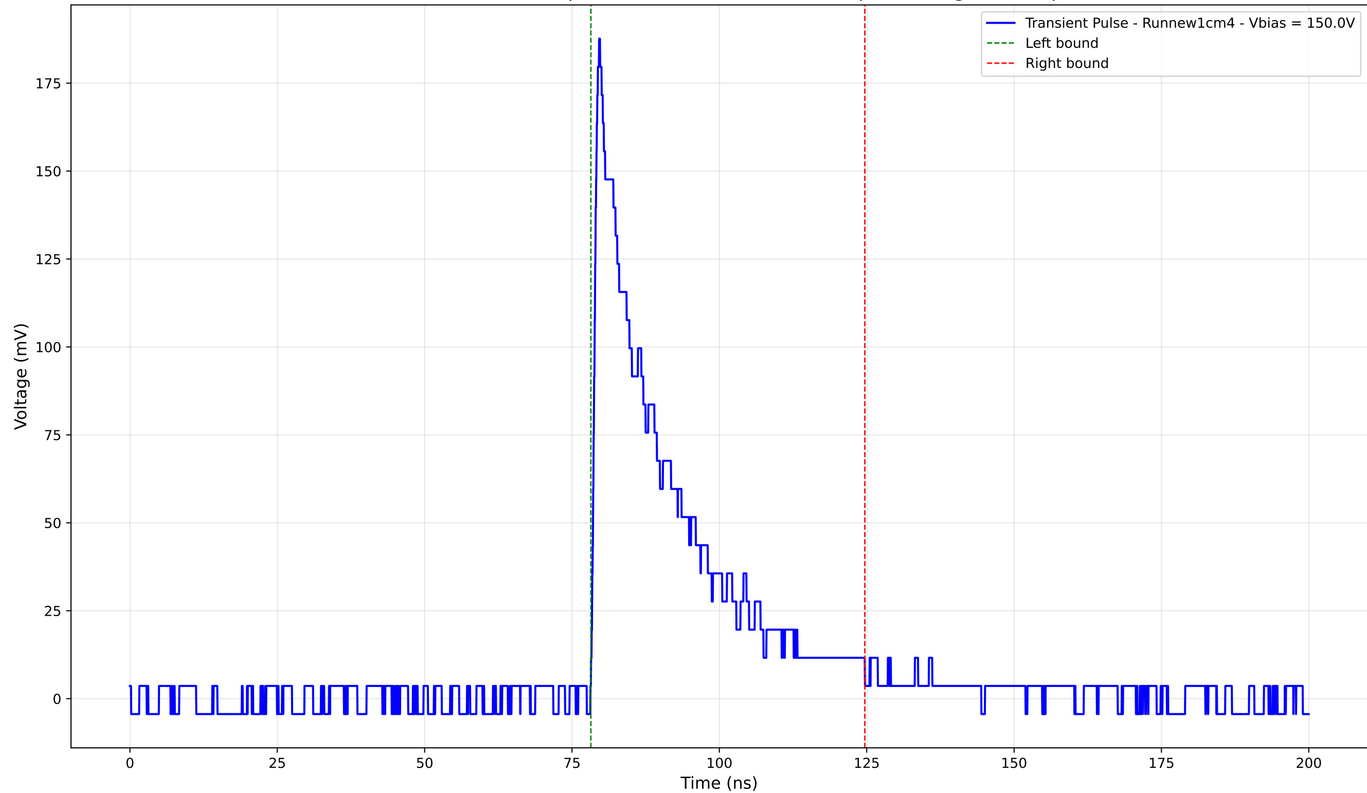
Transient Pulse - Sample: new1cm - Position: 715.0 \mu\text{m} - Charge: 45.00 pC
