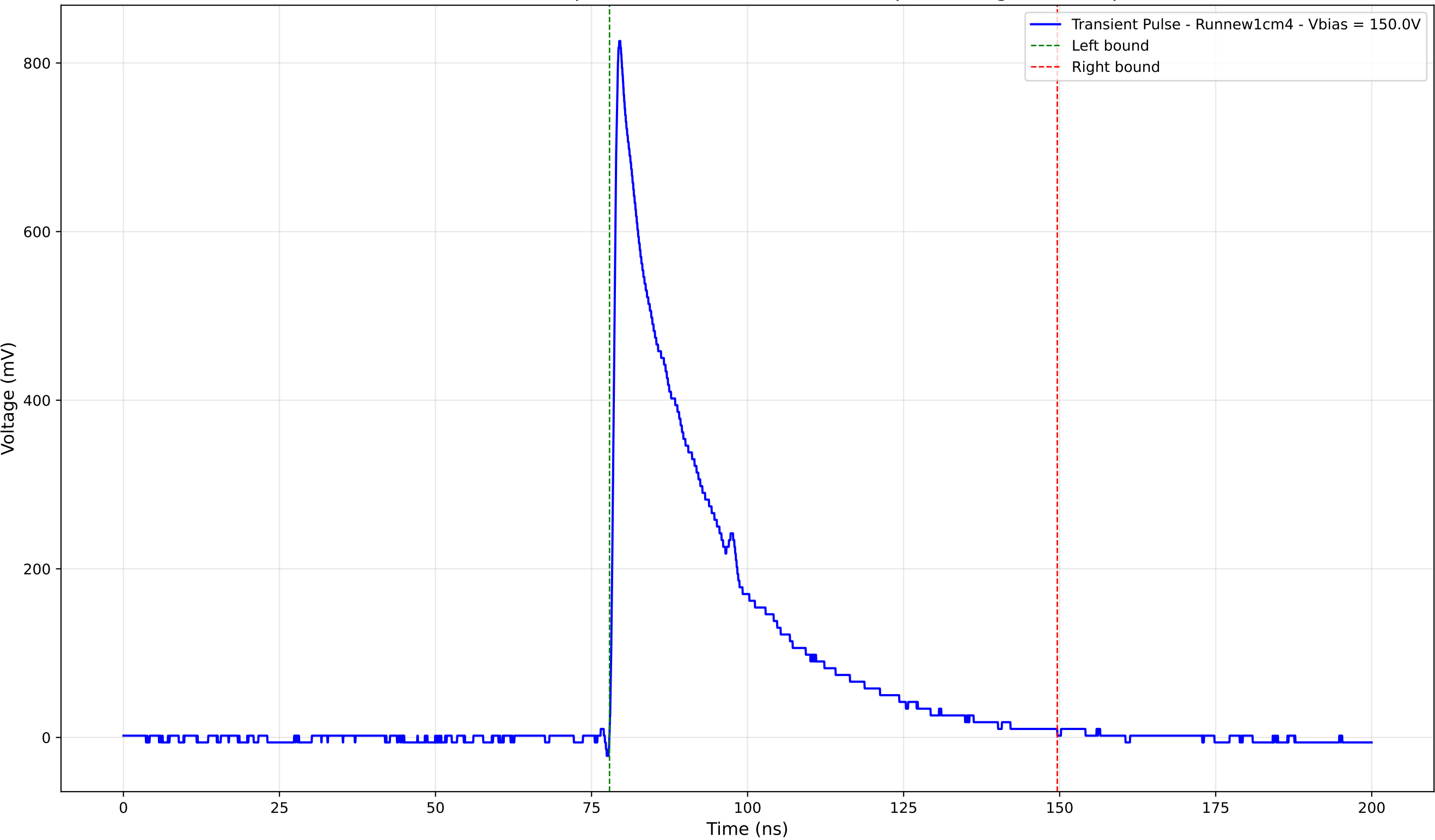
Transient Pulse - Sample: new1cm - Position: 4545.0 \mu\text{m} - Charge: 234.61 pC
