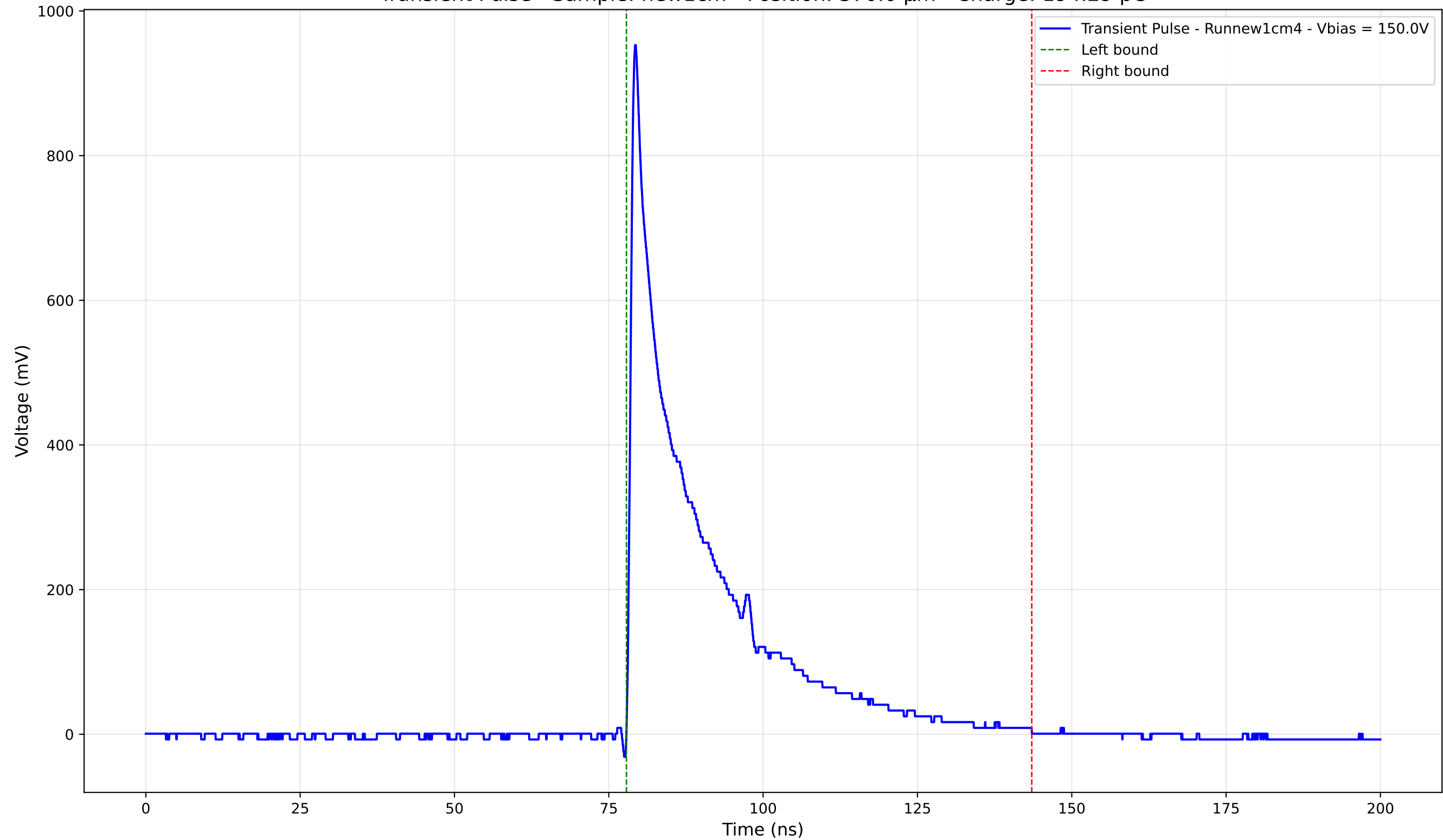
Transient Pulse - Sample: new1cm - Position: 370.0 \mu\text{m} - Charge: 194.29 pC
