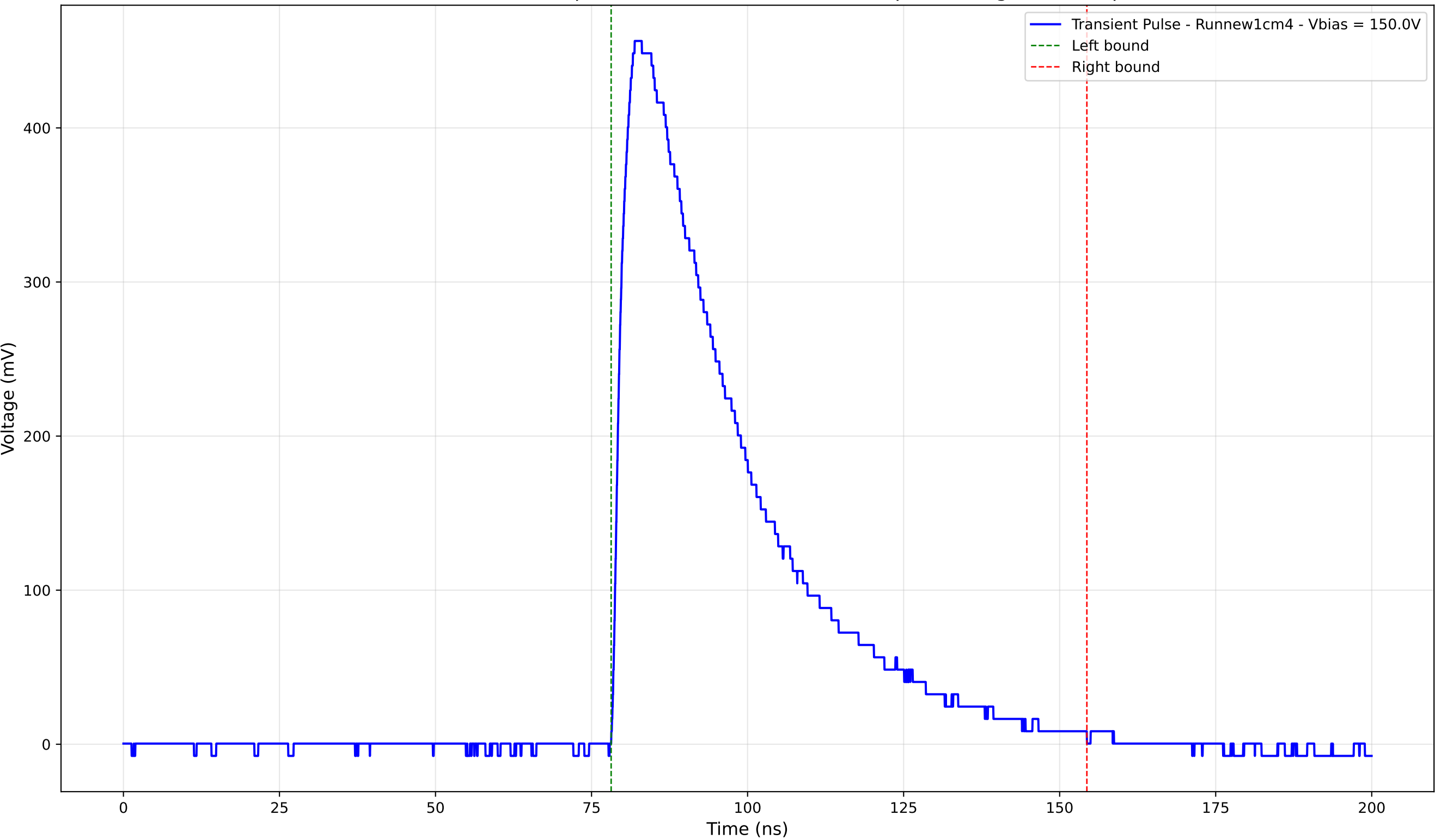
Transient Pulse - Sample: new1cm - Position: 2805.0 \mu\text{m} - Charge: 199.22 pC
