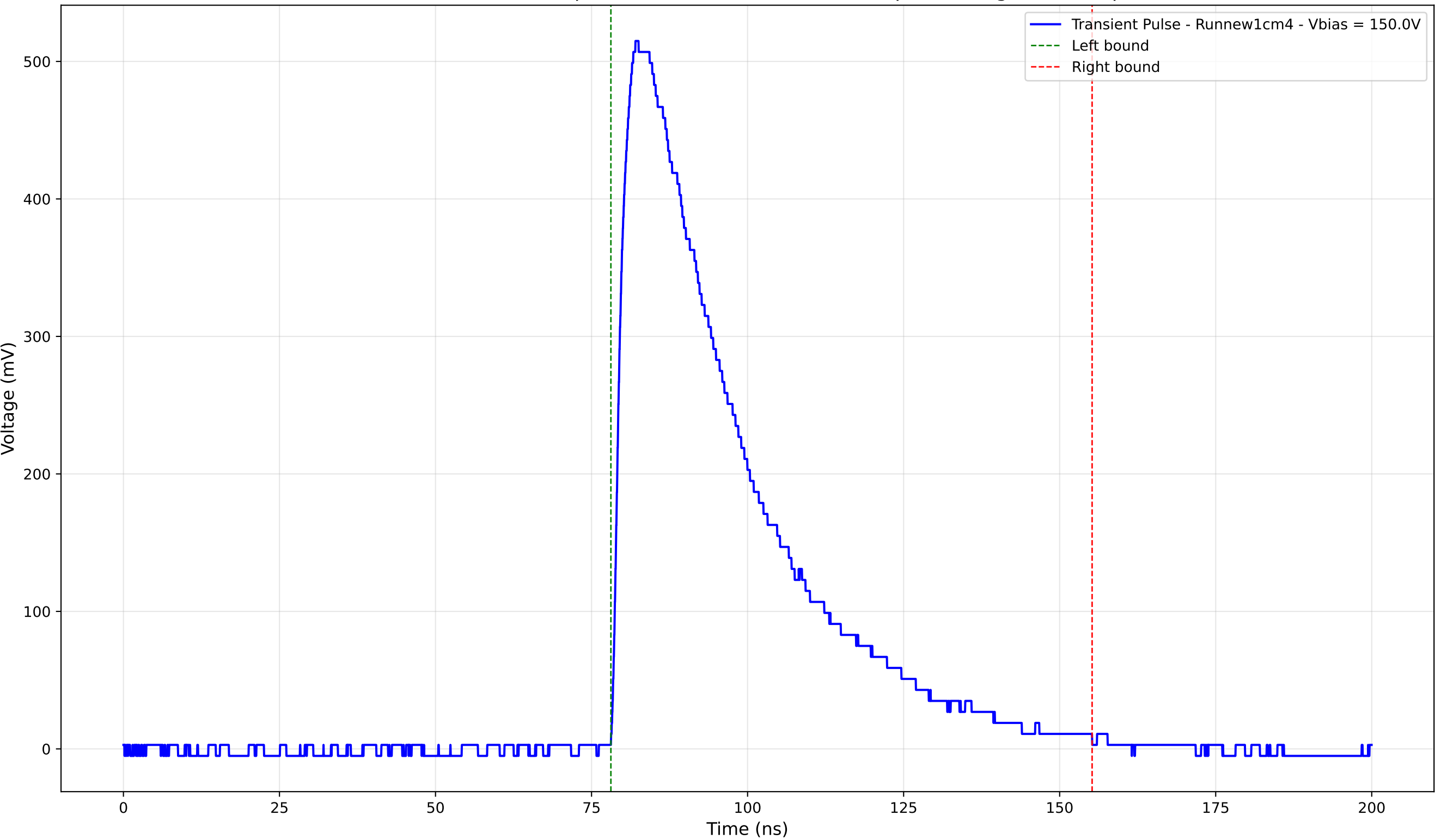
Transient Pulse - Sample: new1cm - Position: 2870.0 \mu\text{m} - Charge: 226.63 pC
