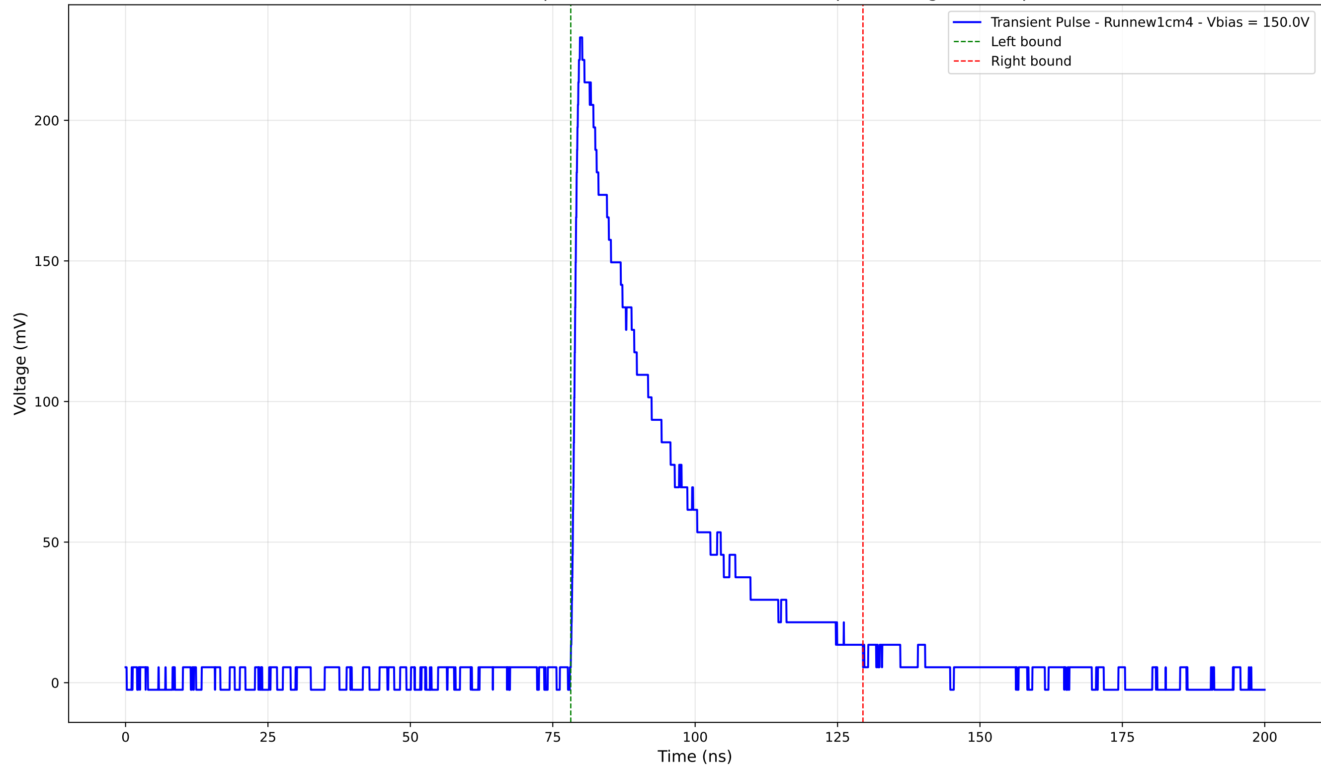
Transient Pulse - Sample: new1cm - Position: 4205.0 \mu\text{m} - Charge: 72.69 pC
