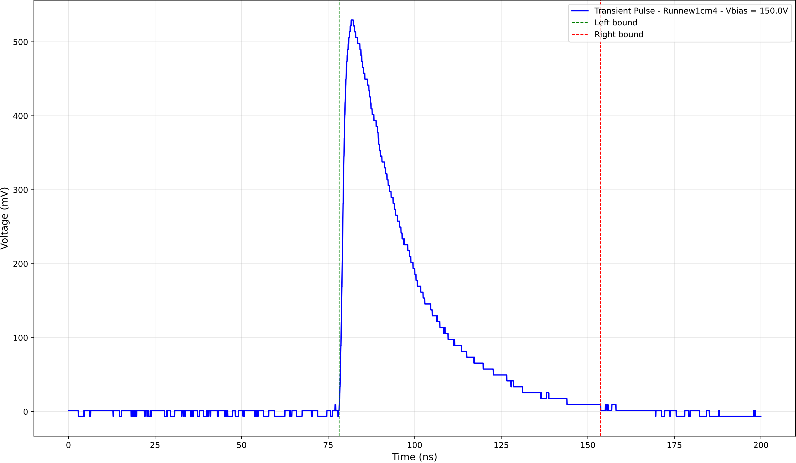
Transient Pulse - Sample: new1cm - Position: 1860.0 \mu\text{m} - Charge: 213.33 pC
