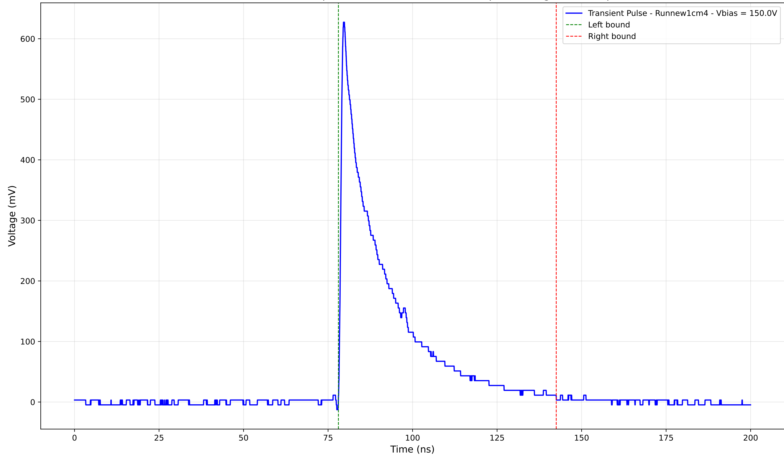
Transient Pulse - Sample: new1cm - Position: 770.0 \mu\text{m} - Charge: 158.35 pC
