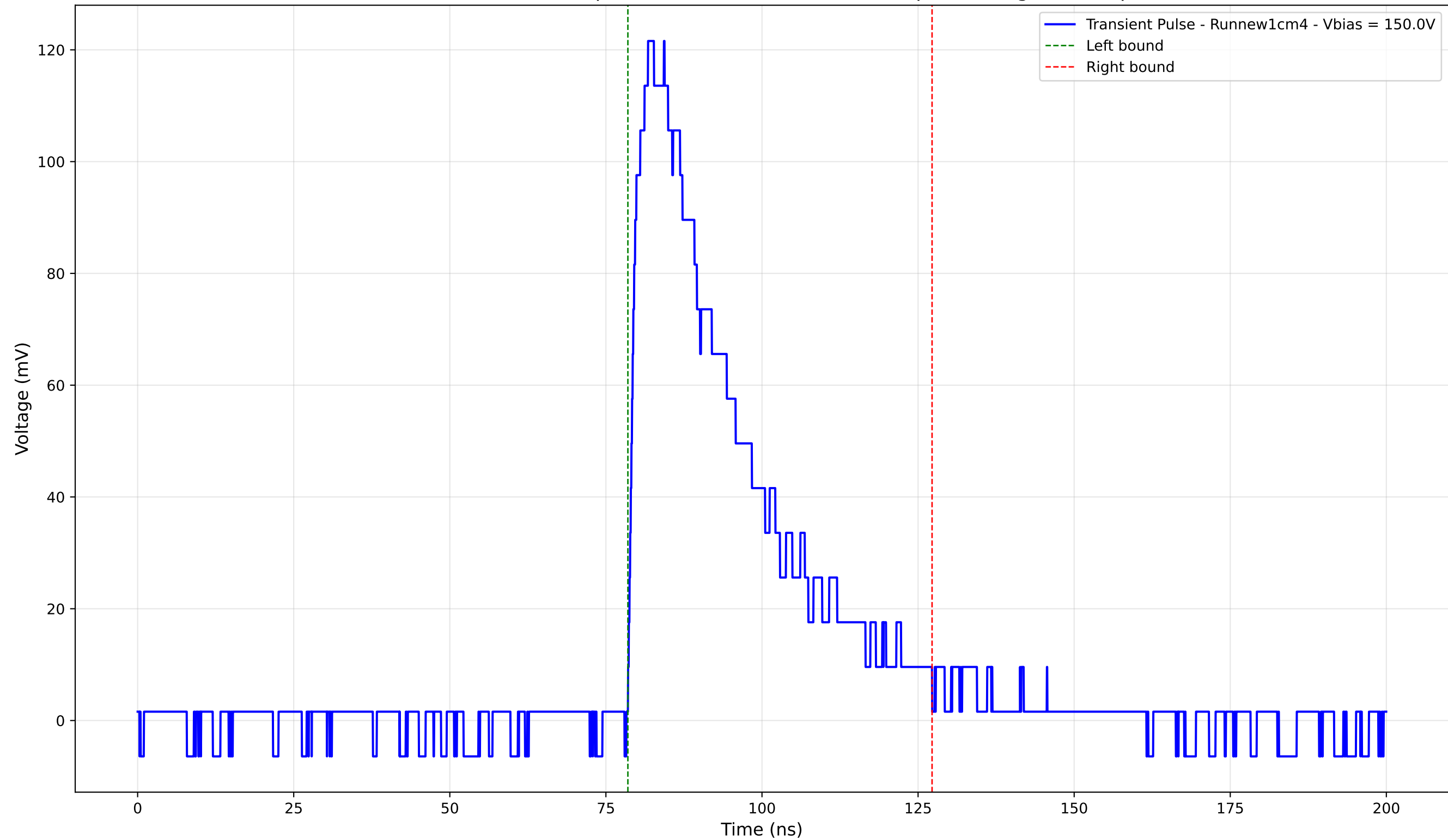
Transient Pulse - Sample: new1cm - Position: 1725.0 \mu\text{m} - Charge: 44.71 pC
