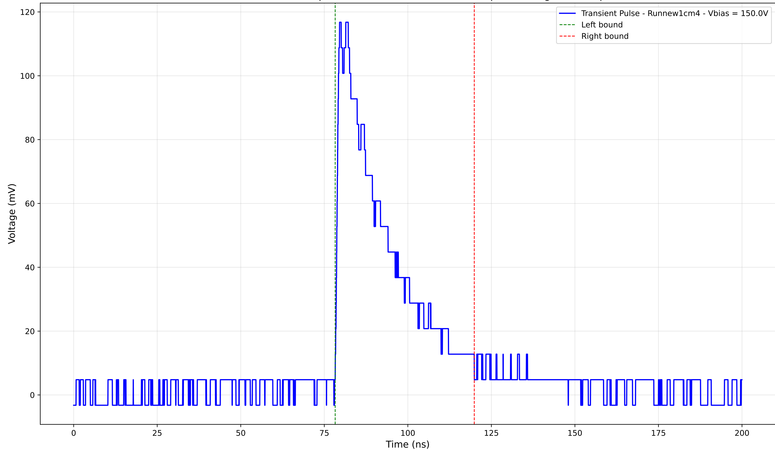
Transient Pulse - Sample: new1cm - Position: 4240.0 \mu\text{m} - Charge: 37.40 pC
