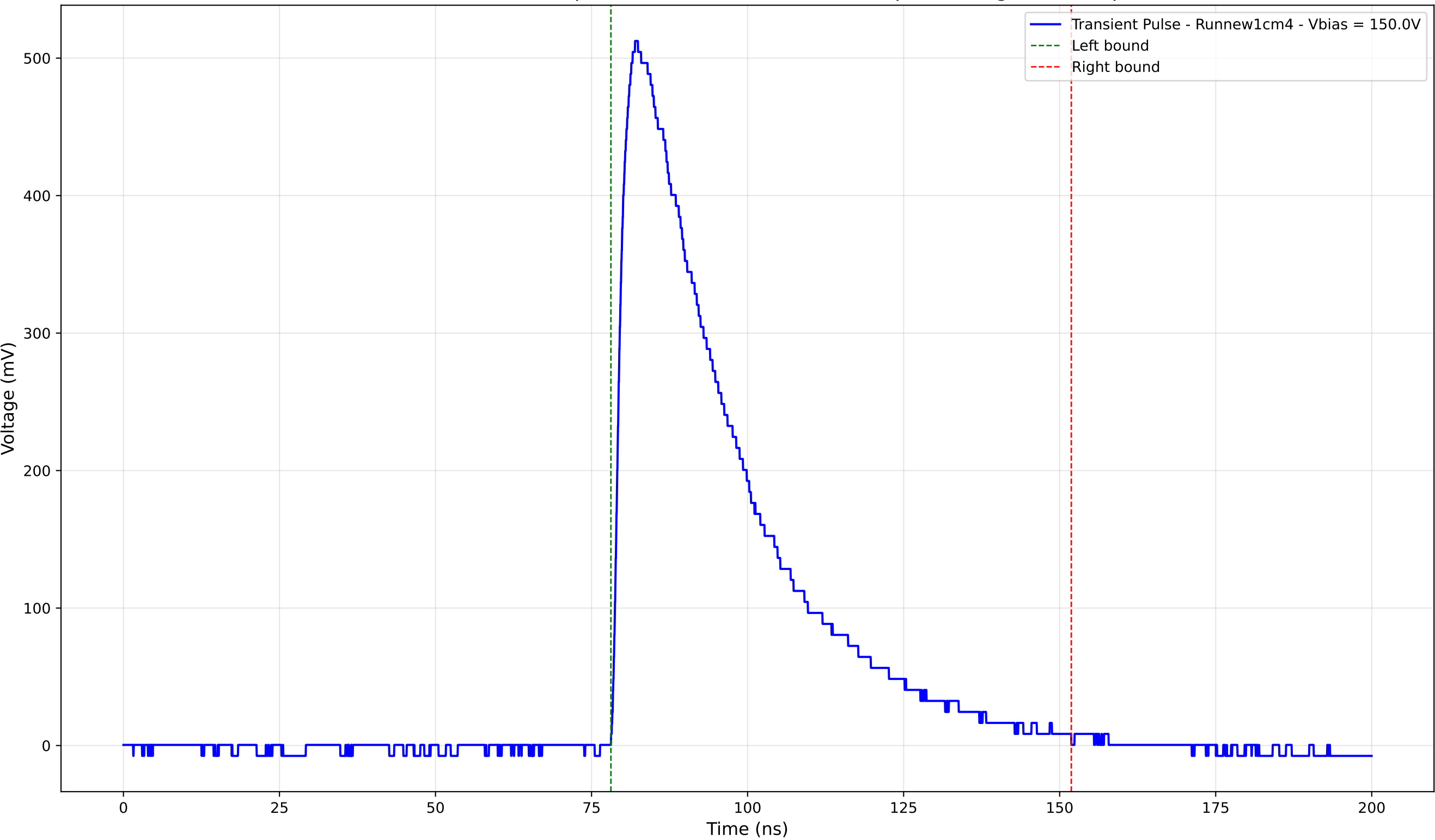
Transient Pulse - Sample: new1cm - Position: 2105.0 \mu\text{m} - Charge: 211.51 pC
