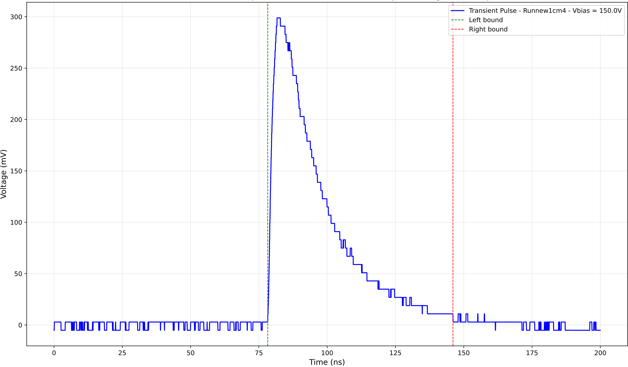
Transient Pulse - Sample: new1cm - Position: 2255.0 \mu\text{m} - Charge: 126.06 pC
