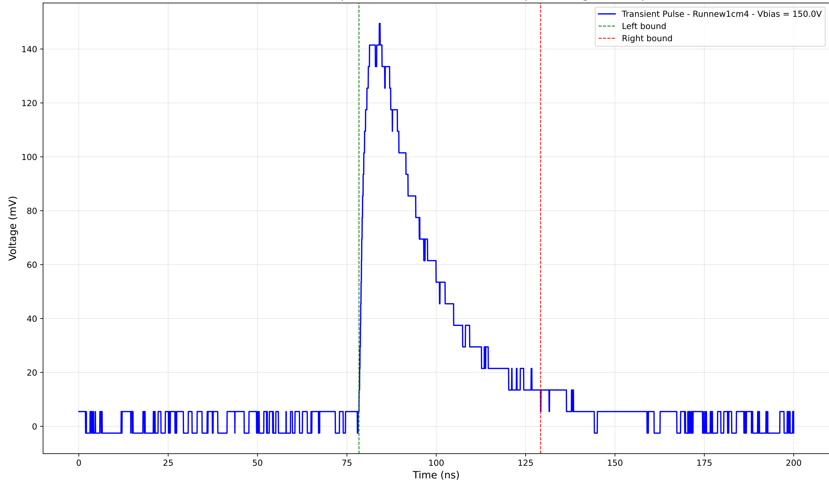
Transient Pulse - Sample: new1cm - Position: 3200.0 \mu\text{m} - Charge: 59.40 pC
