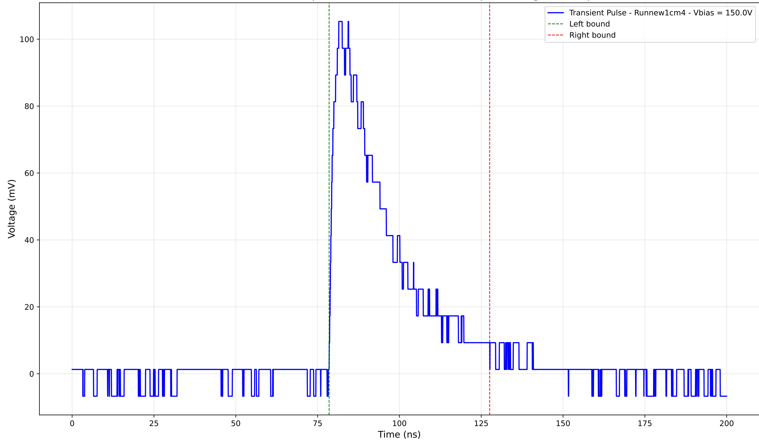
Transient Pulse - Sample: new1cm - Position: 1720.0 \mu\text{m} - Charge: 38.41 pC
