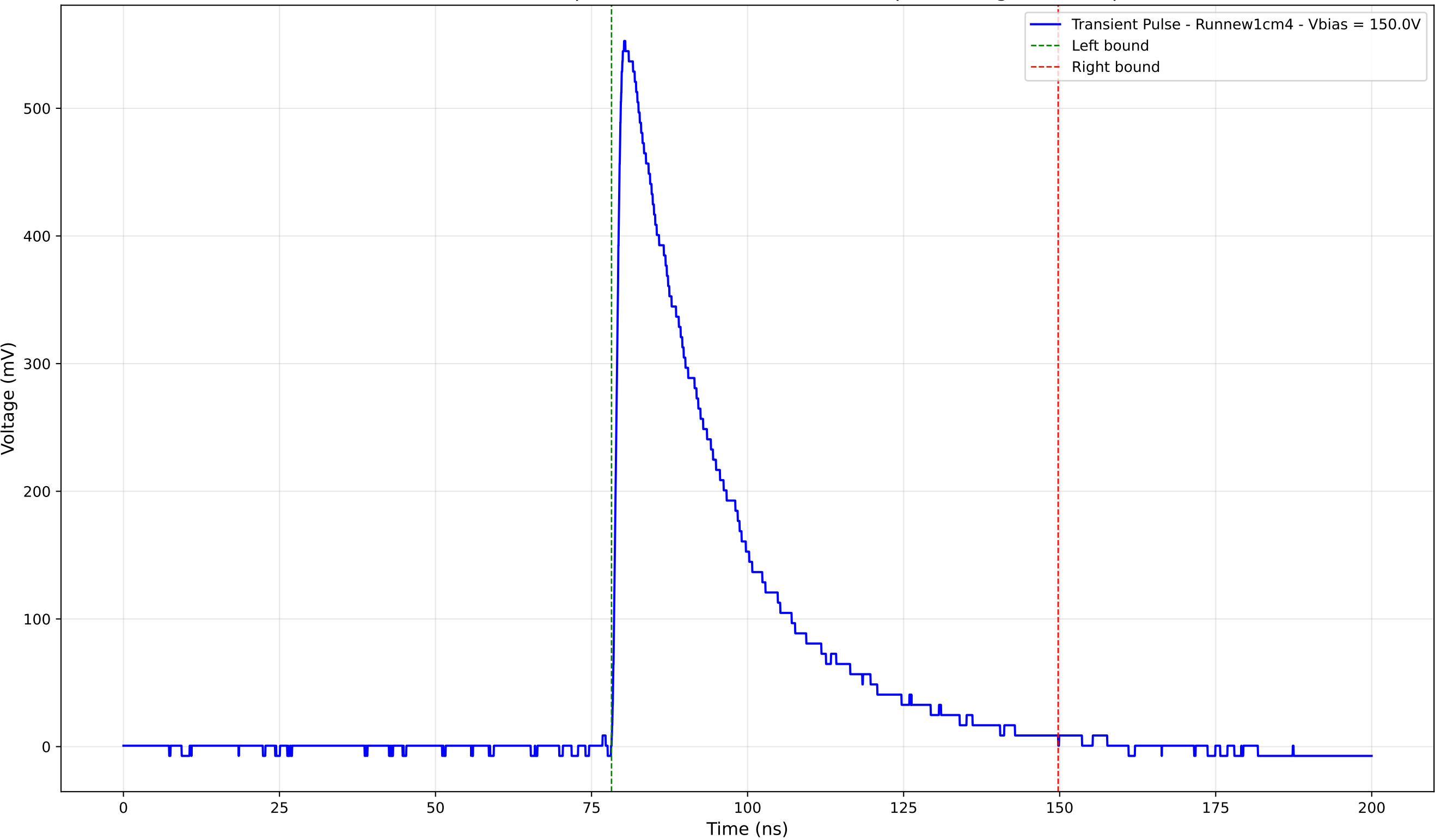
Transient Pulse - Sample: new1cm - Position: 1300.0 \mu\text{m} - Charge: 190.65 pC
