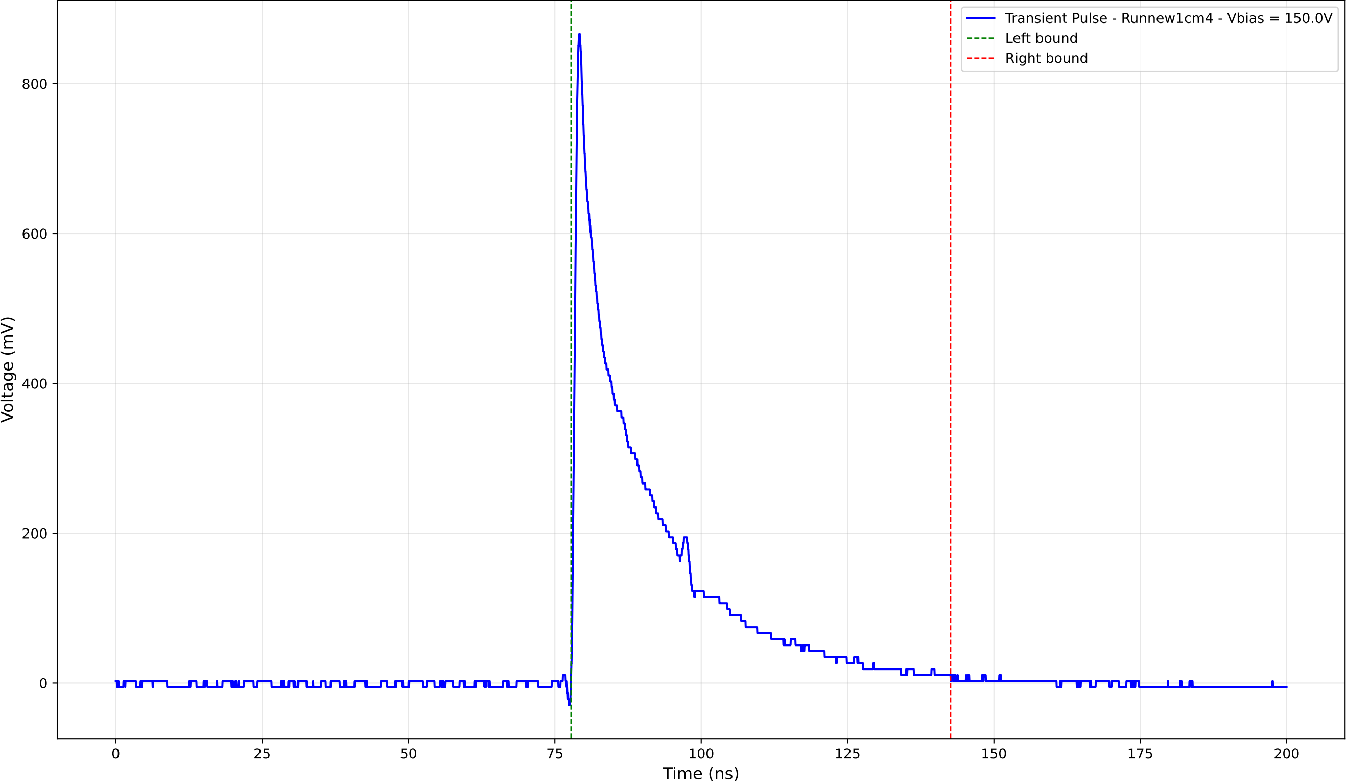
Transient Pulse - Sample: new1cm - Position: 4875.0 \mu\text{m} - Charge: 189.19 pC
