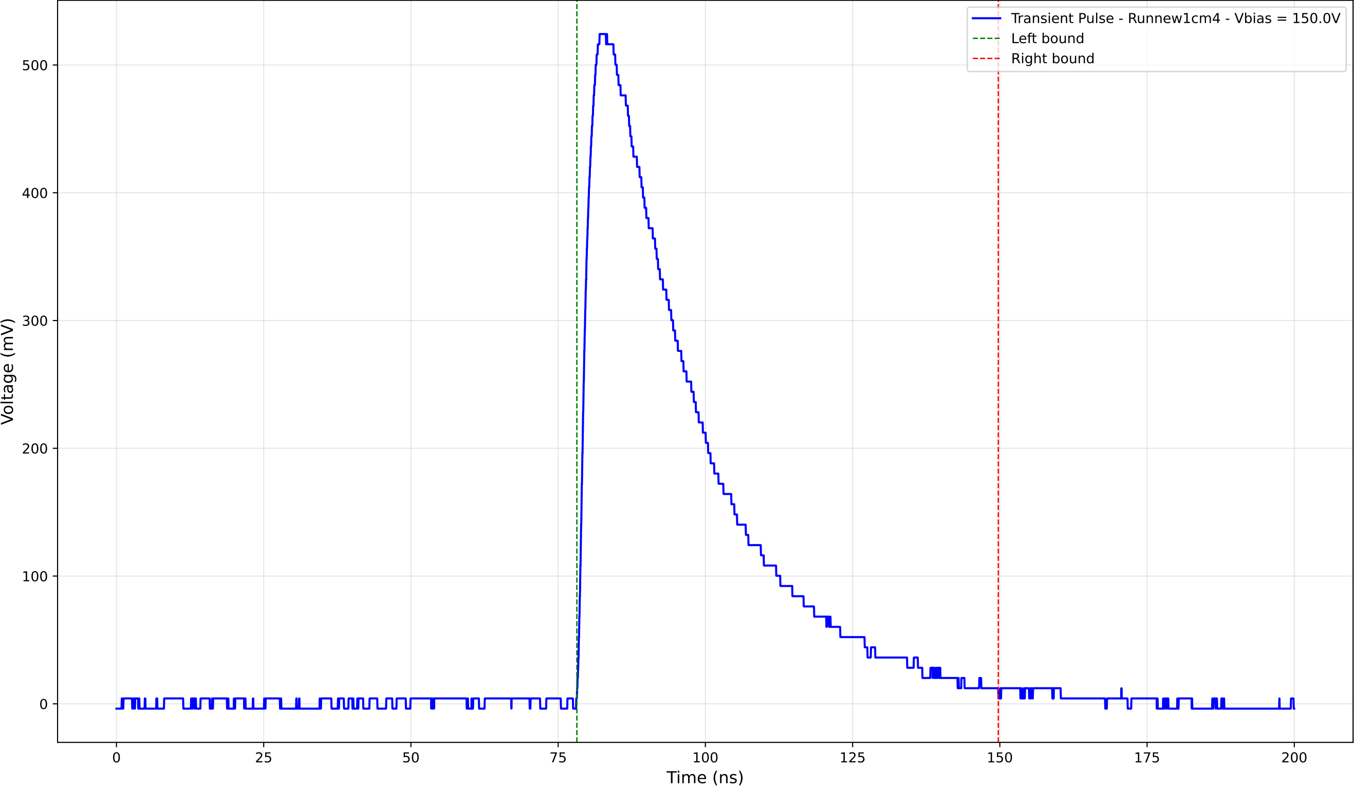
Transient Pulse - Sample: new1cm - Position: 2470.0 \mu\text{m} - Charge: 226.49 pC
