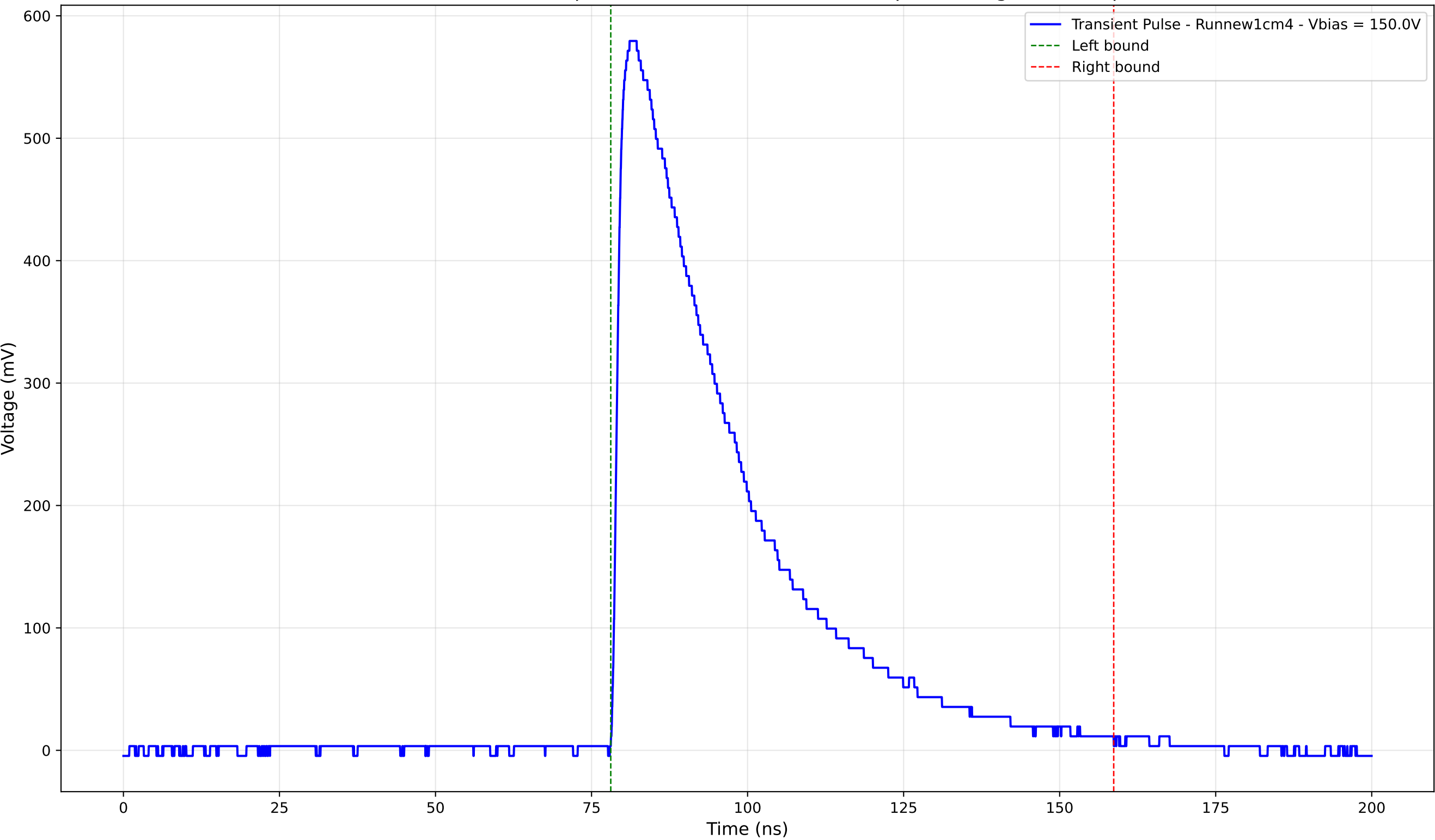
Transient Pulse - Sample: new1cm - Position: 3575.0 \mu\text{m} - Charge: 246.25 pC
