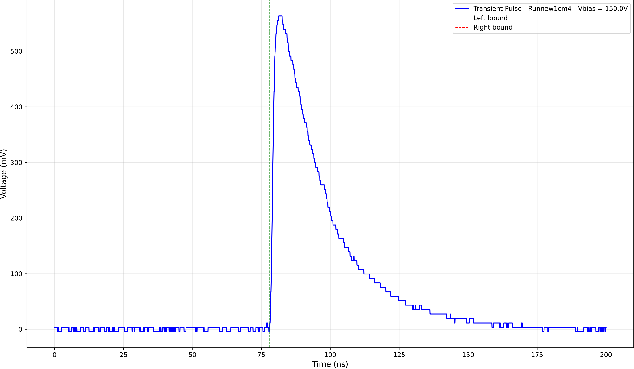
Transient Pulse - Sample: new1cm - Position: 3520.0 \mu\text{m} - Charge: 241.10 pC
