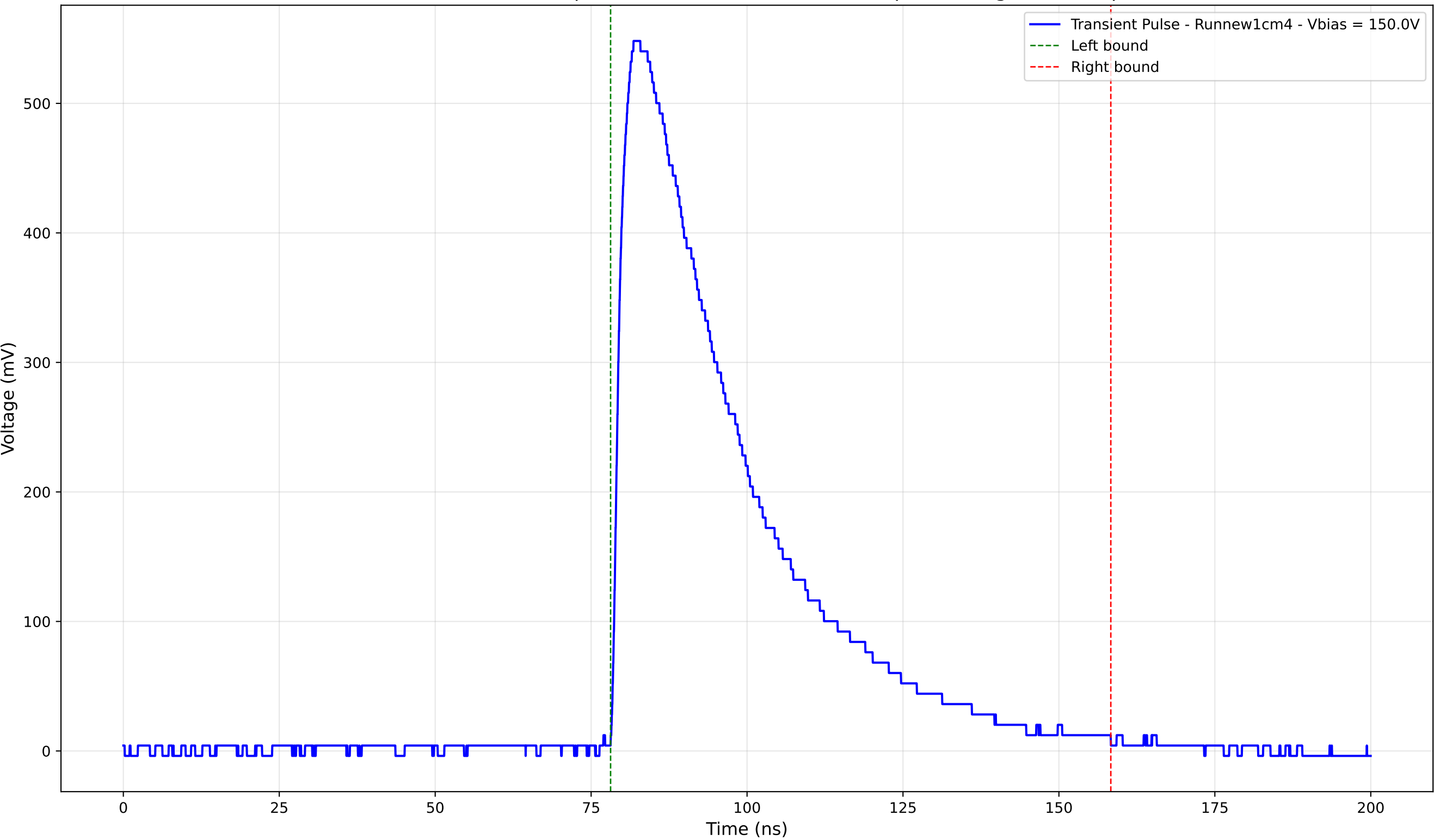
Transient Pulse - Sample: new1cm - Position: 3090.0 \mu\text{m} - Charge: 242.24 pC
