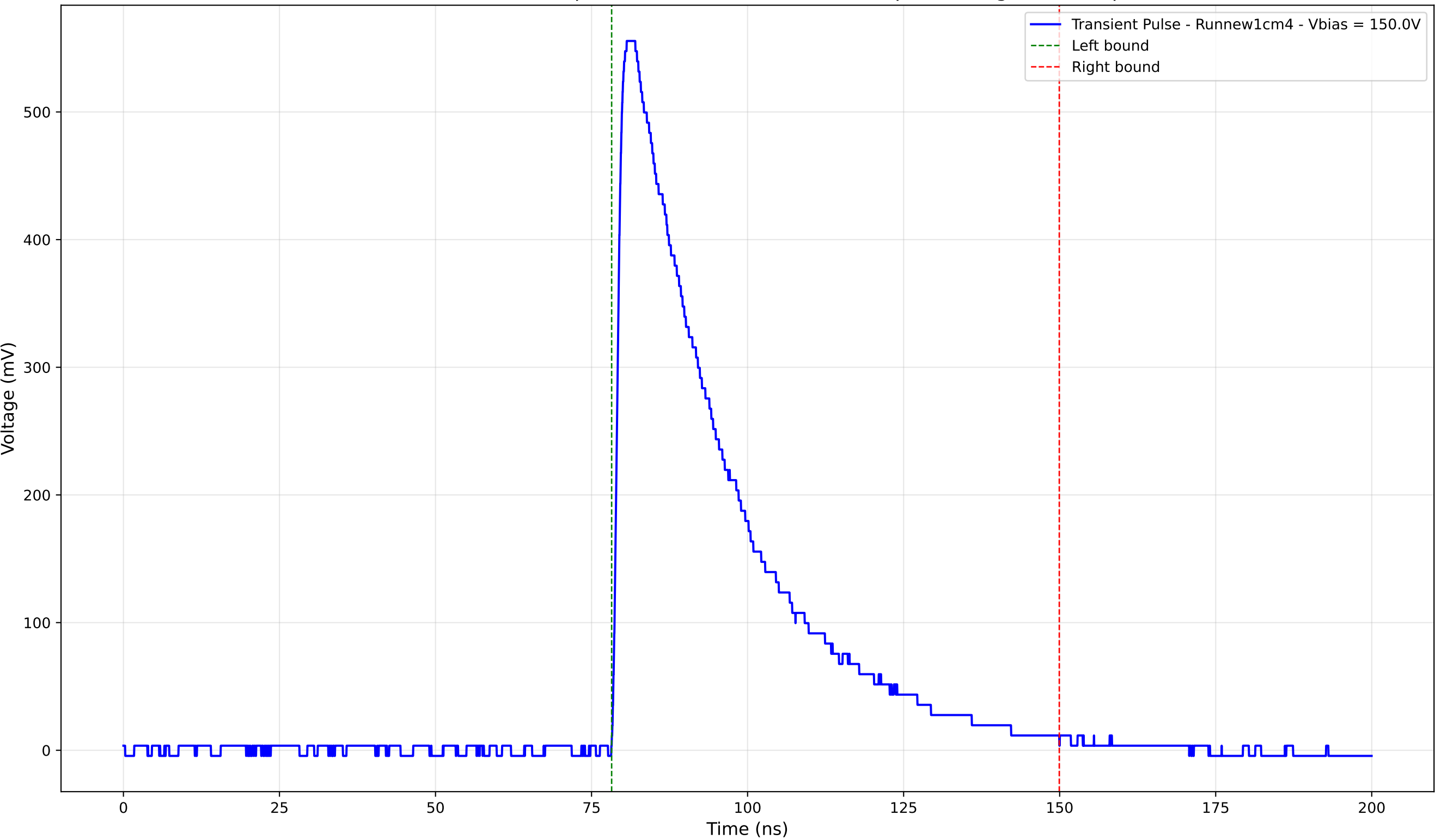
Transient Pulse - Sample: new1cm - Position: 1500.0 \mu\text{m} - Charge: 209.73 pC
