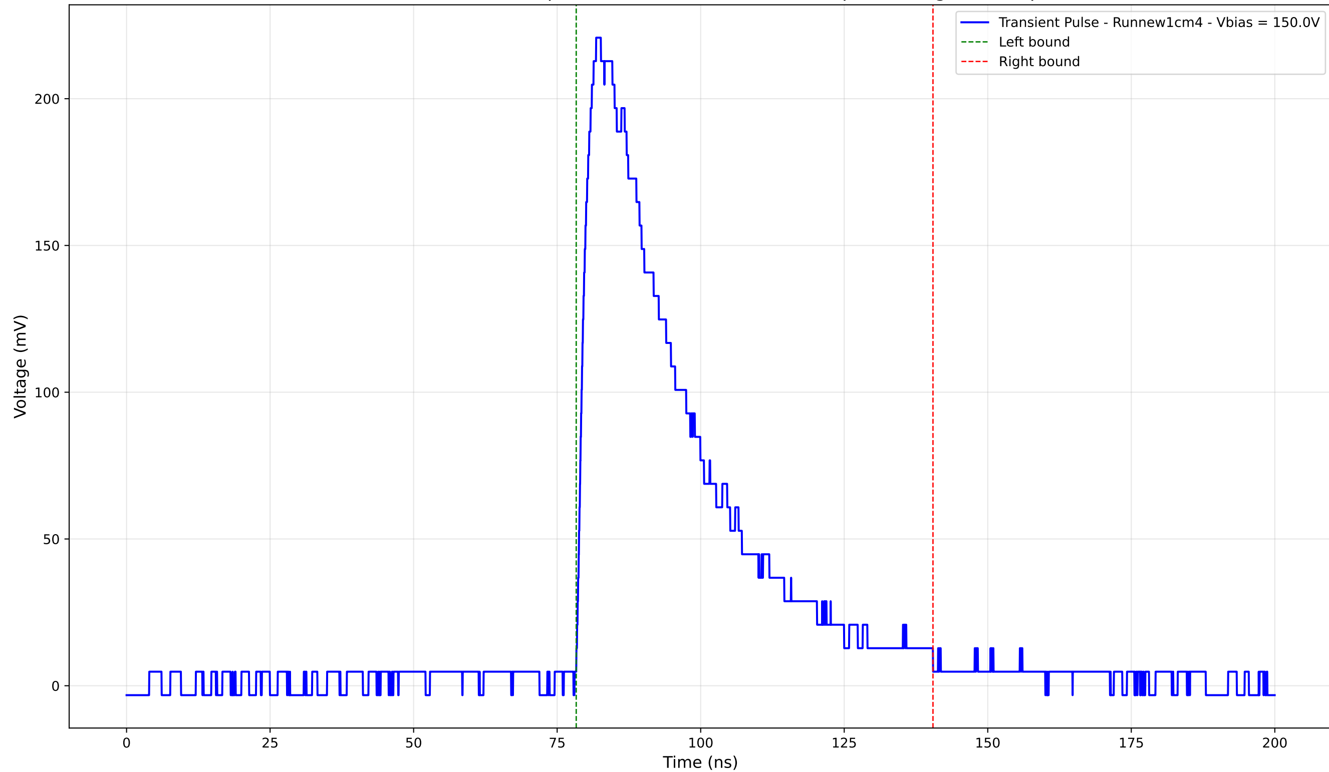
Transient Pulse - Sample: new1cm - Position: 2165.0 \mu\text{m} - Charge: 88.89 pC
