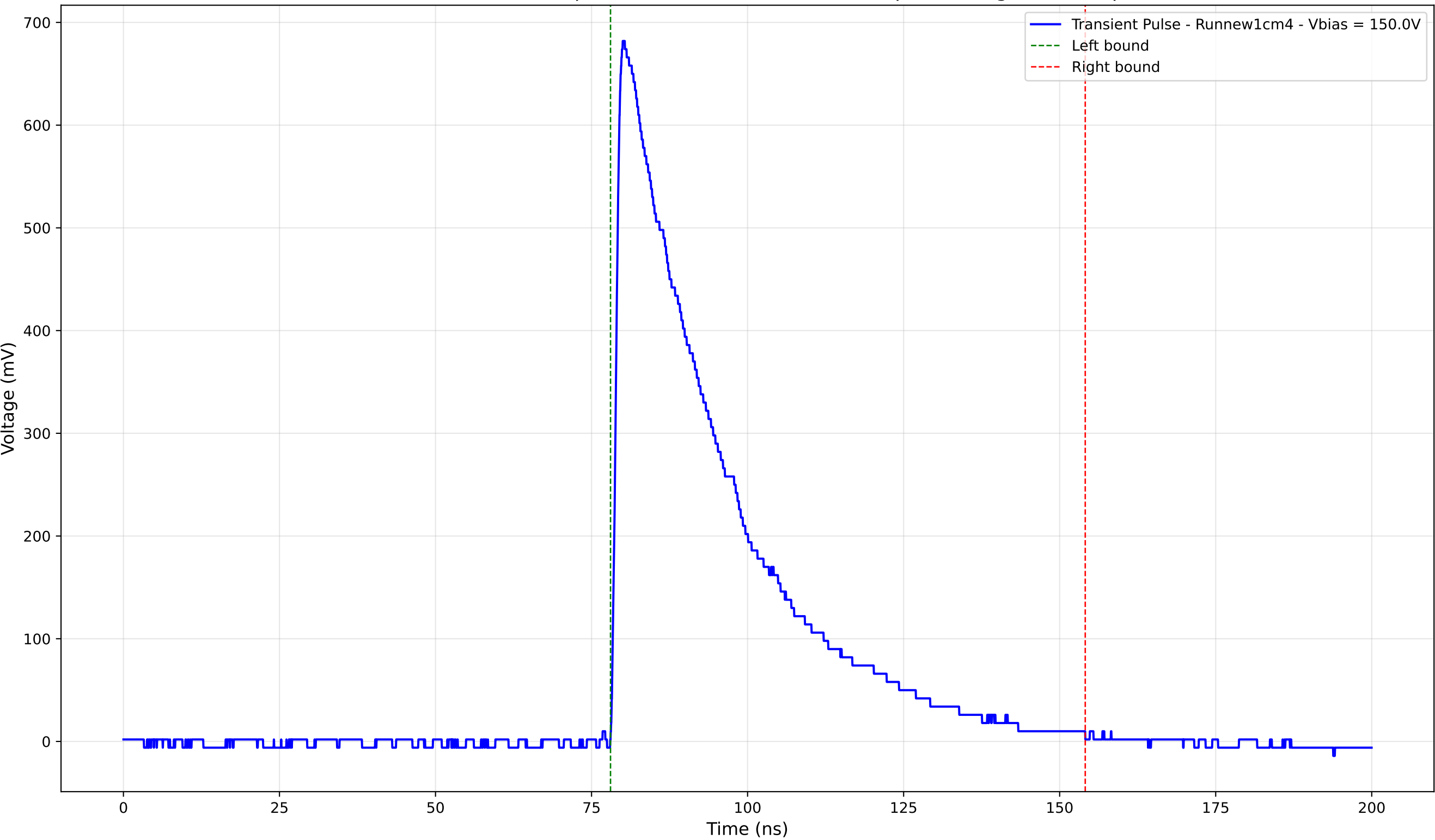
Transient Pulse - Sample: new1cm - Position: 4025.0 \mu\text{m} - Charge: 248.50 pC
