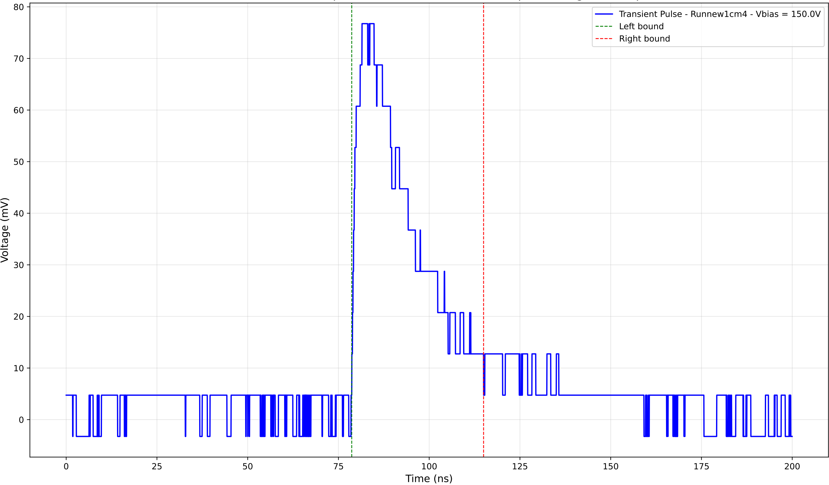
Transient Pulse - Sample: new1cm - Position: 1705.0 \mu\text{m} - Charge: 27.50 pC
