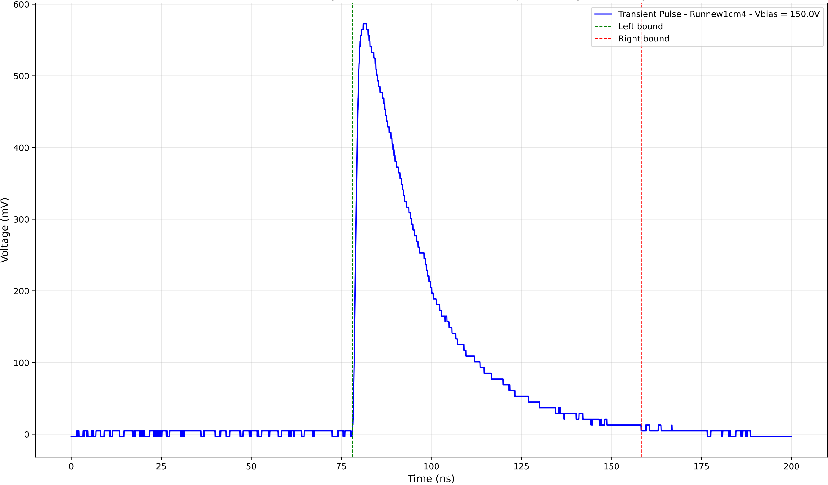
Transient Pulse - Sample: new1cm - Position: 3630.0 \mu\text{m} - Charge: 239.72 pC
