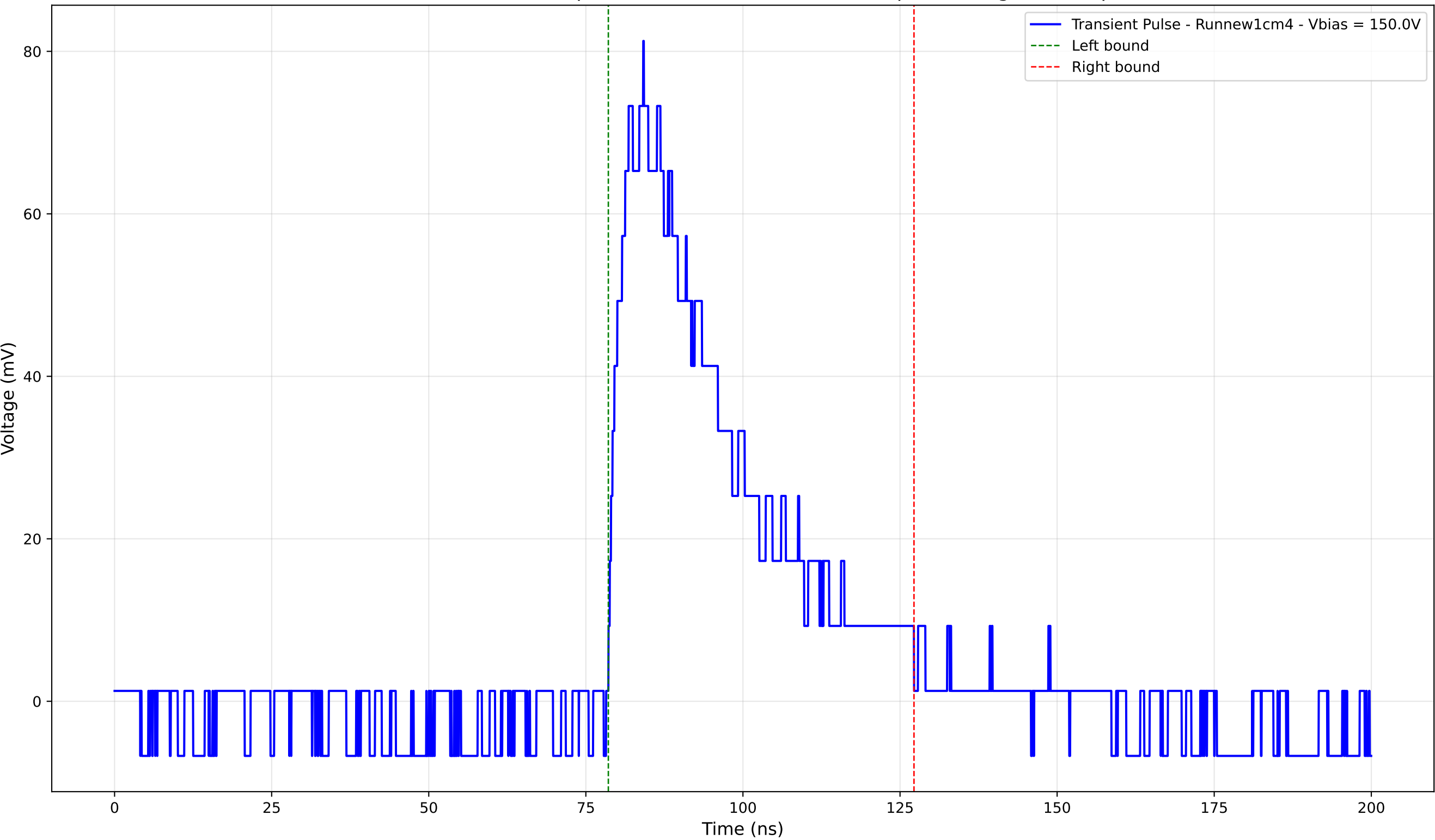
Transient Pulse - Sample: new1cm - Position: 2720.0 \mu\text{m} - Charge: 29.54 pC
