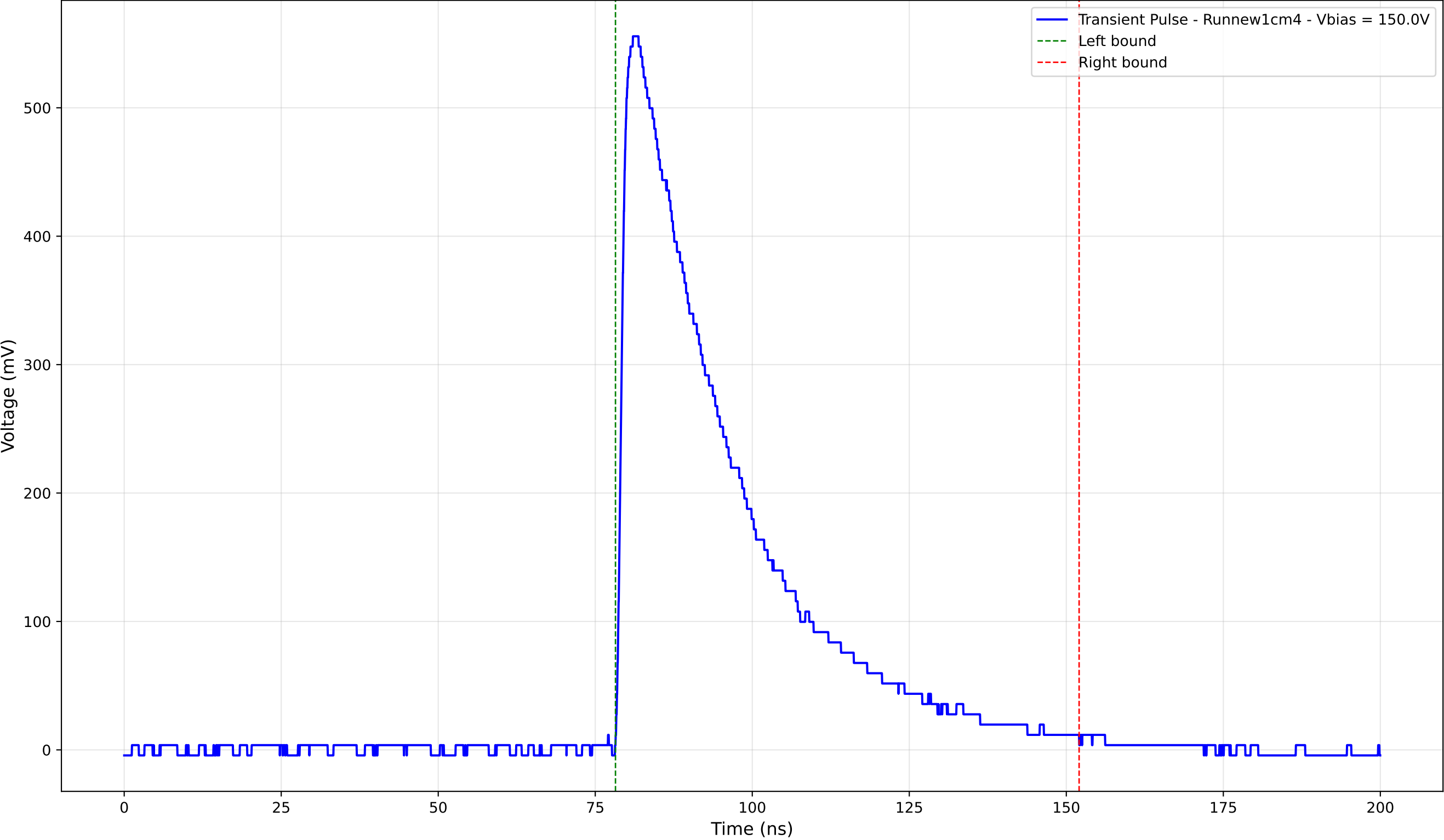
Transient Pulse - Sample: new1cm - Position: 1555.0 \mu\text{m} - Charge: 213.18 pC
