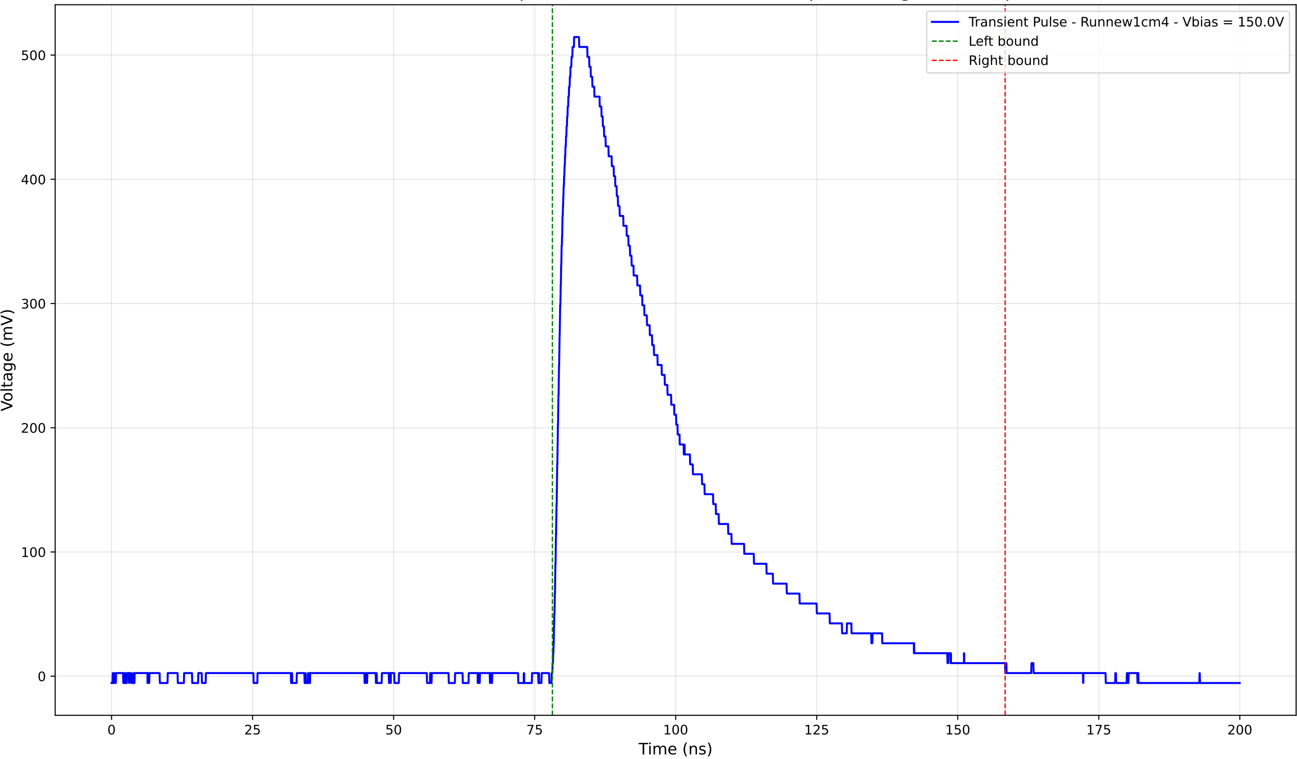
Transient Pulse - Sample: new1cm - Position: 2920.0 \mu\text{m} - Charge: 228.20 pC
