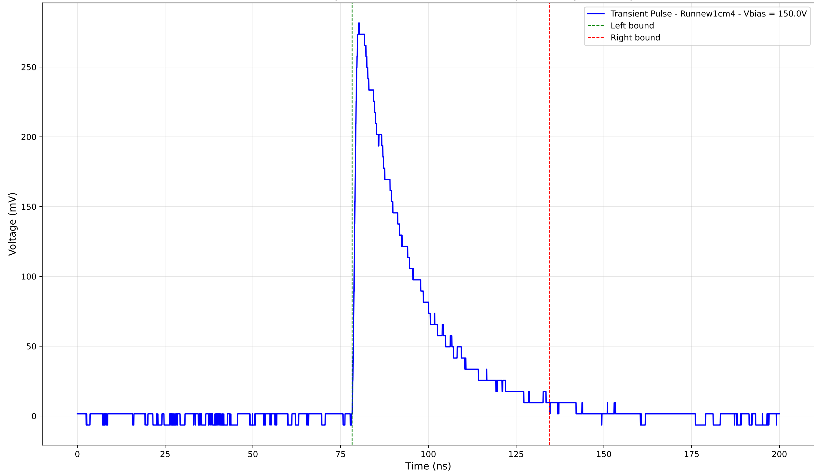
Transient Pulse - Sample: new1cm - Position: 1245.0 \mu\text{m} - Charge: 92.03 pC
