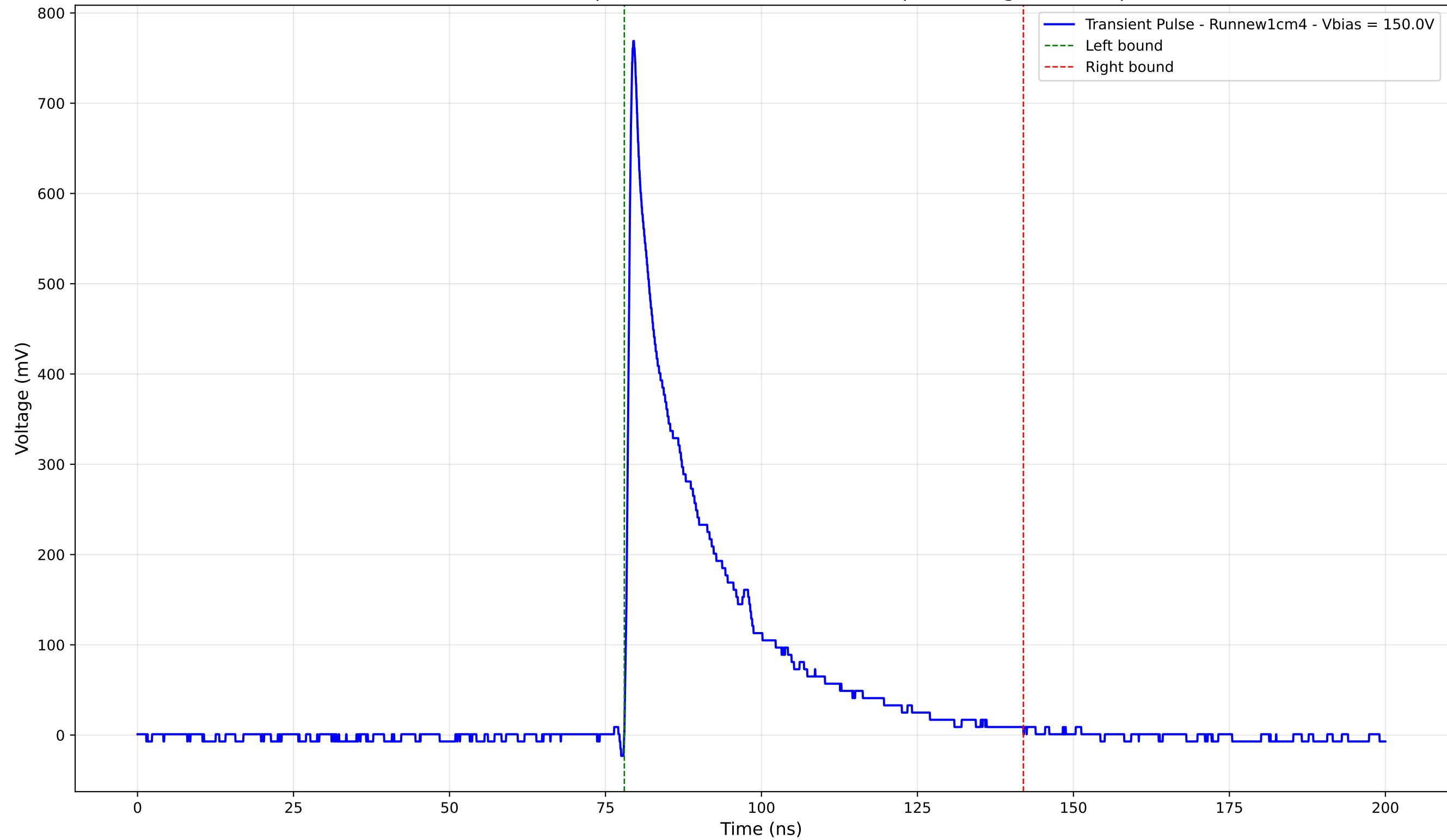
Transient Pulse - Sample: new1cm - Position: 610.0 \mu\text{m} - Charge: 166.91 pC
