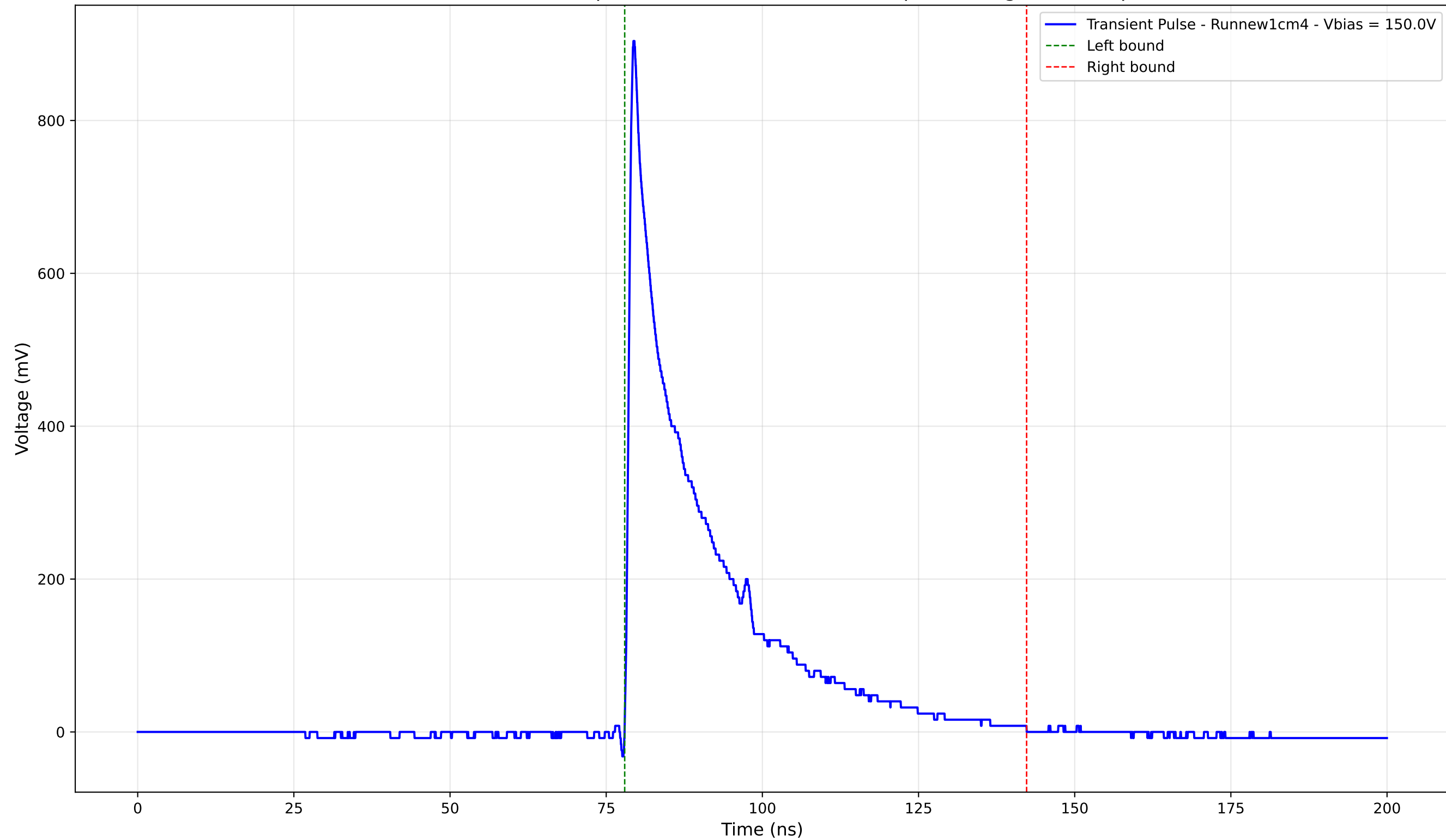
Transient Pulse - Sample: new1cm - Position: 515.0 \mu\text{m} - Charge: 197.24 pC
