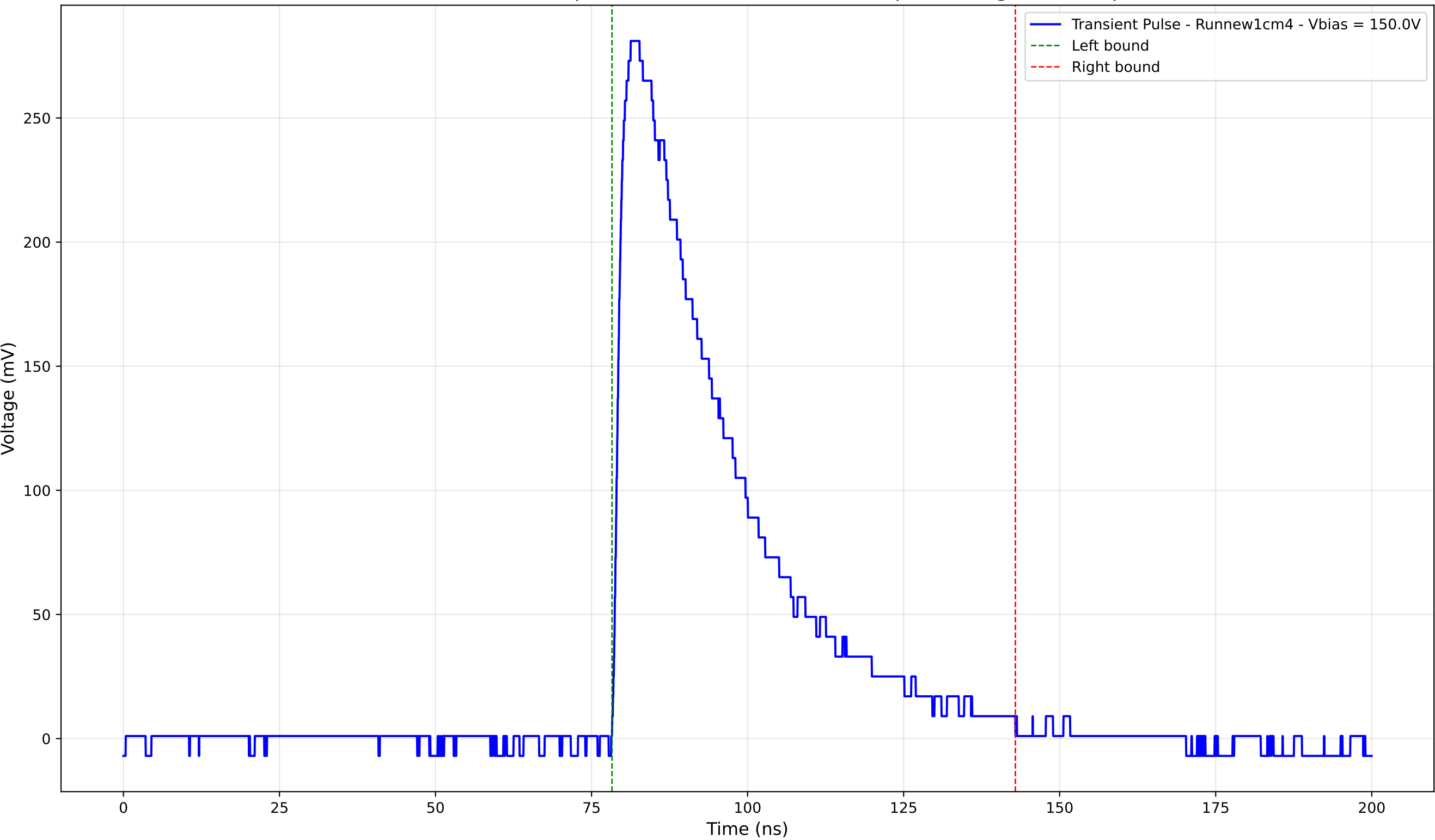
Transient Pulse - Sample: new1cm - Position: 1755.0 \mu\text{m} - Charge: 109.11 pC
