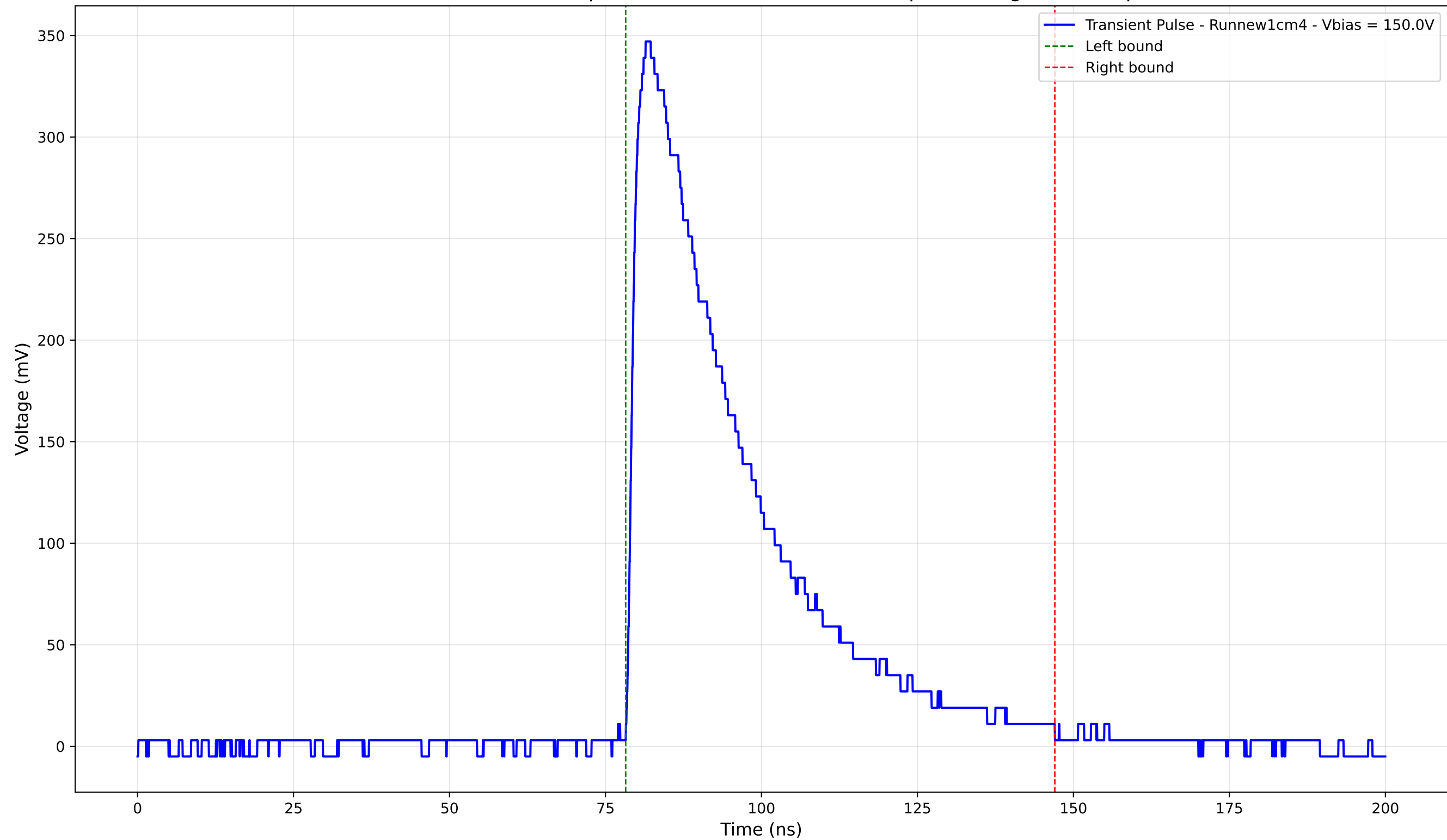
Transient Pulse - Sample: new1cm - Position: 1765.0 \mu\text{m} - Charge: 135.69 pC
