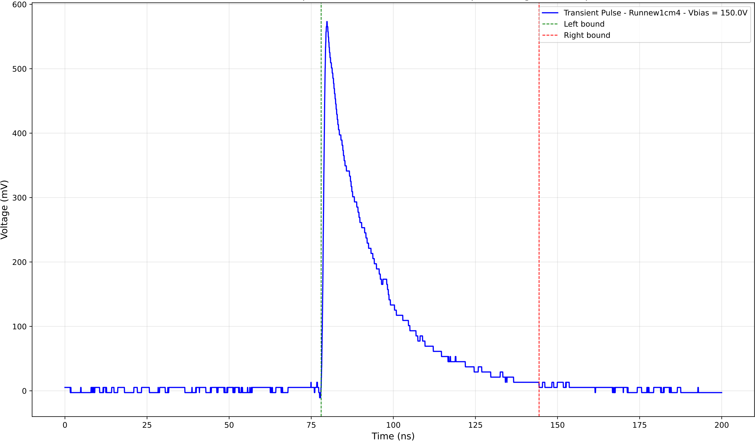
Transient Pulse - Sample: new1cm - Position: 4300.0 \mu\text{m} - Charge: 172.69 pC
