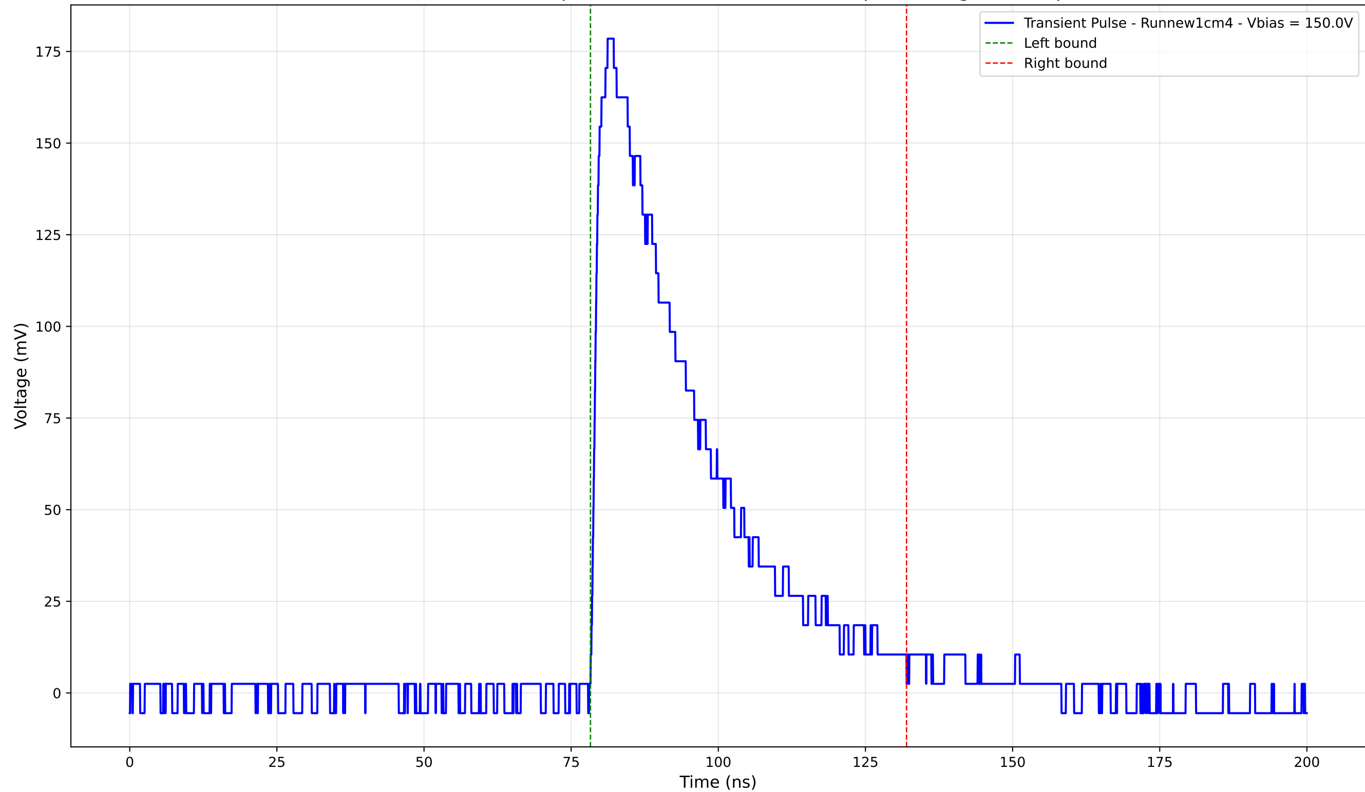
Transient Pulse - Sample: new1cm - Position: 3700.0 \mu\text{m} - Charge: 66.35 pC
