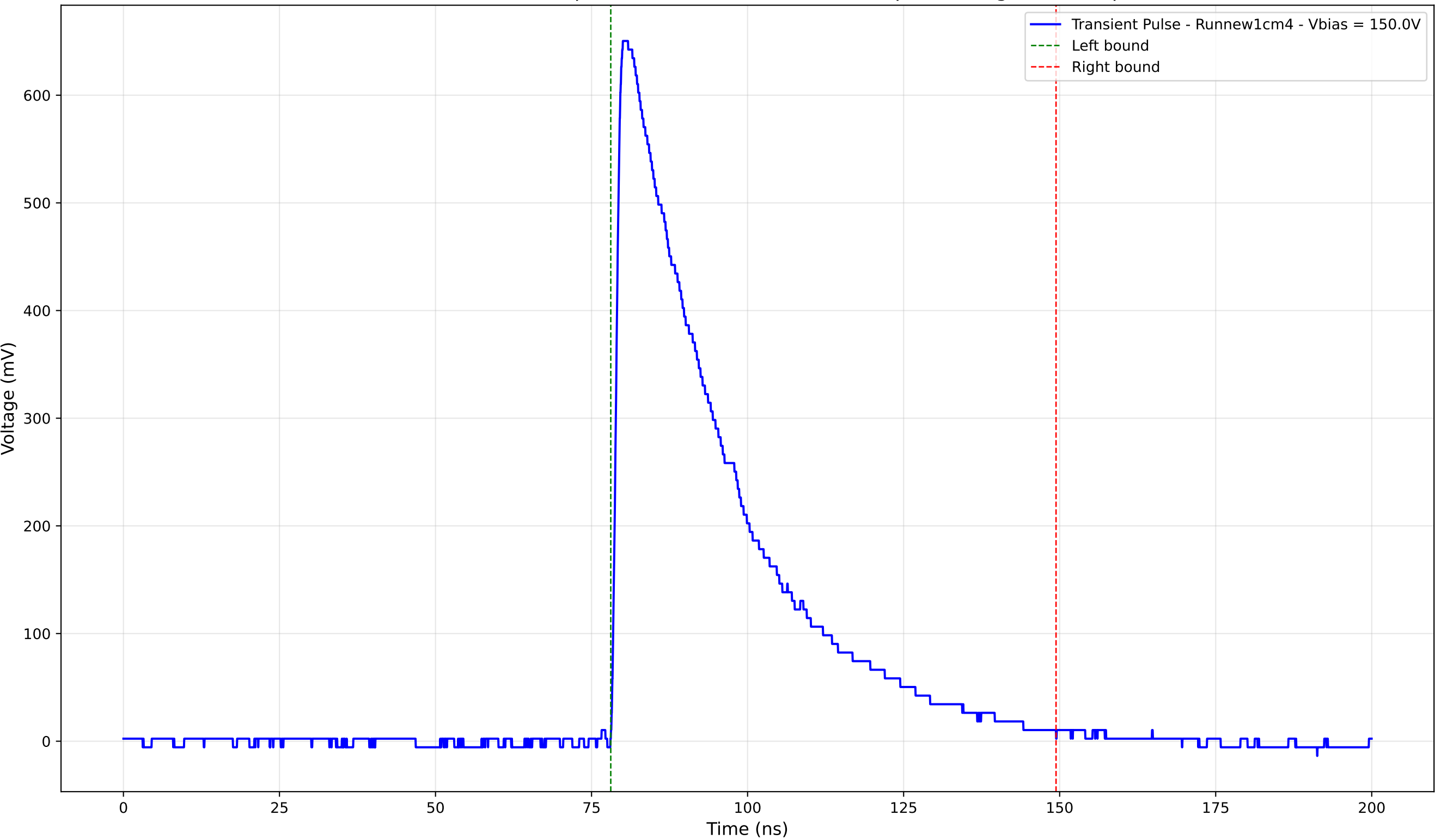
Transient Pulse - Sample: new1cm - Position: 3945.0 \mu\text{m} - Charge: 245.94 pC
