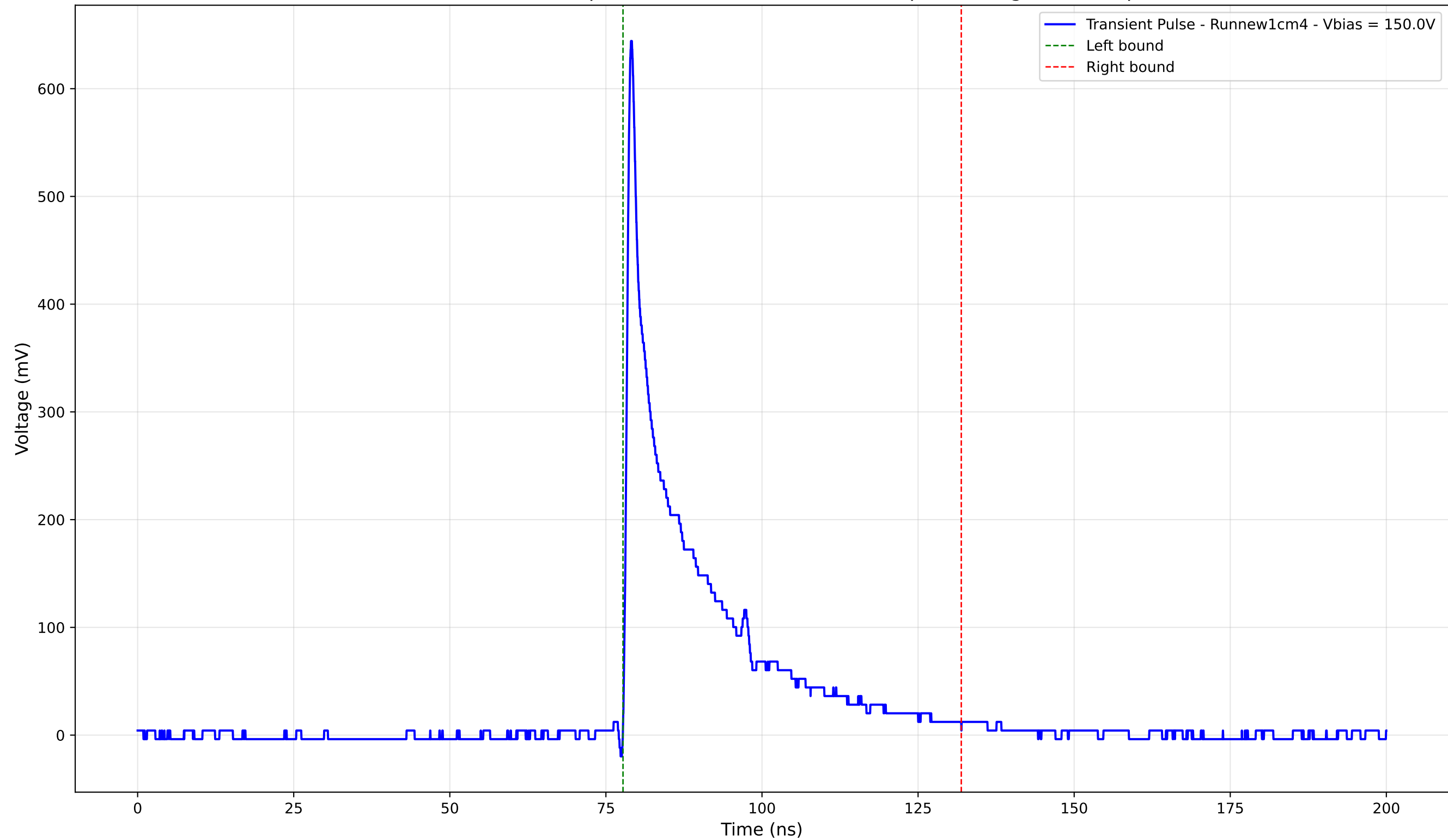
Transient Pulse - Sample: new1cm - Position: 5015.0 \mu\text{m} - Charge: 110.72 pC
