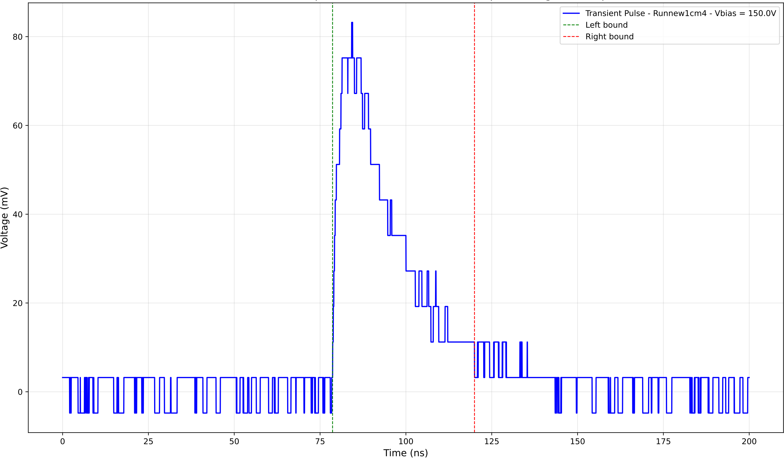
Transient Pulse - Sample: new1cm - Position: 2200.0 \mu\text{m} - Charge: 29.51 pC
