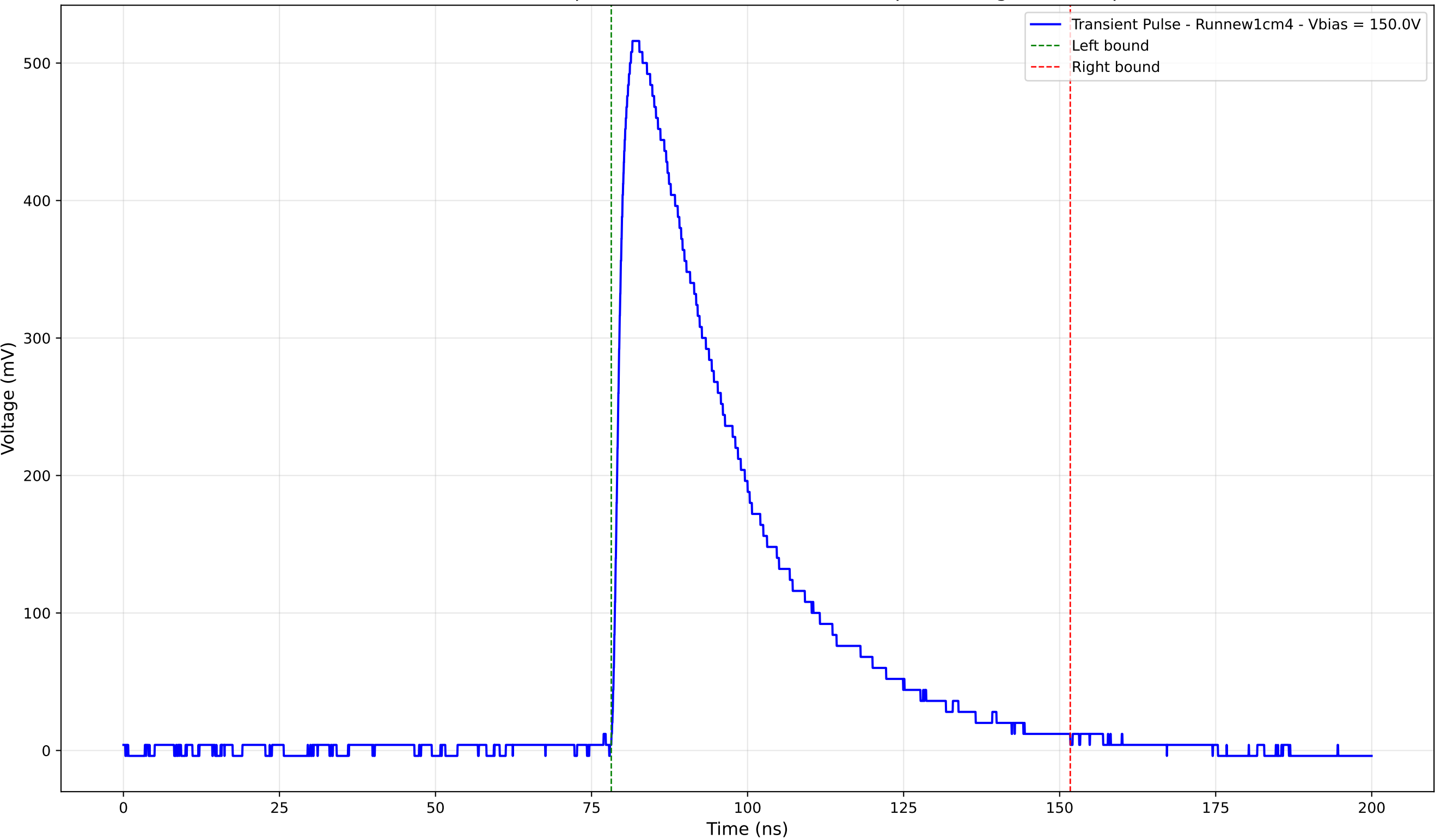
Transient Pulse - Sample: new1cm - Position: 1975.0 \mu\text{m} - Charge: 215.65 pC
