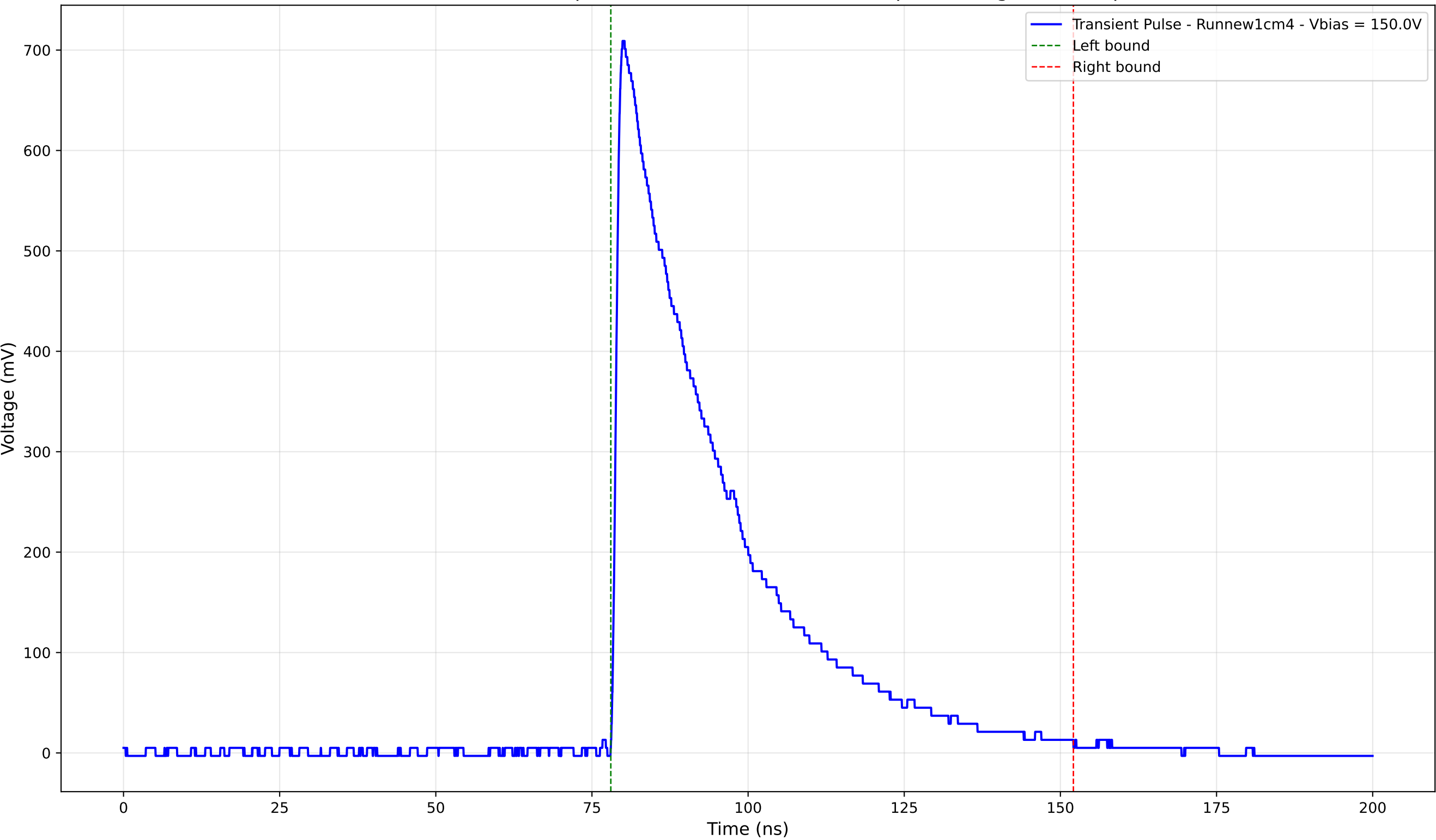
Transient Pulse - Sample: new1cm - Position: 4105.0 \mu\text{m} - Charge: 251.35 pC
