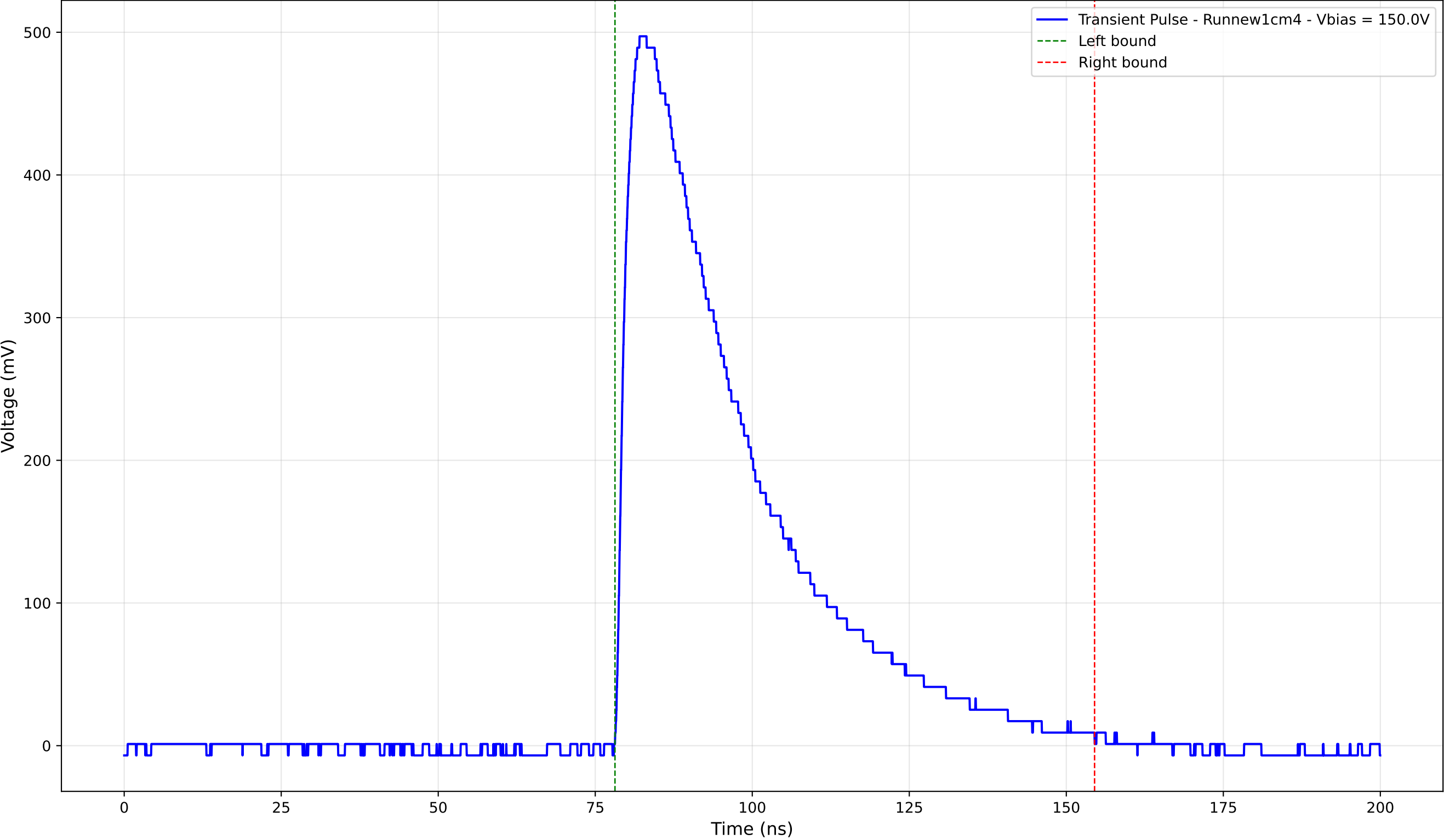
Transient Pulse - Sample: new1cm - Position: 2835.0 \mu\text{m} - Charge: 219.72 pC
