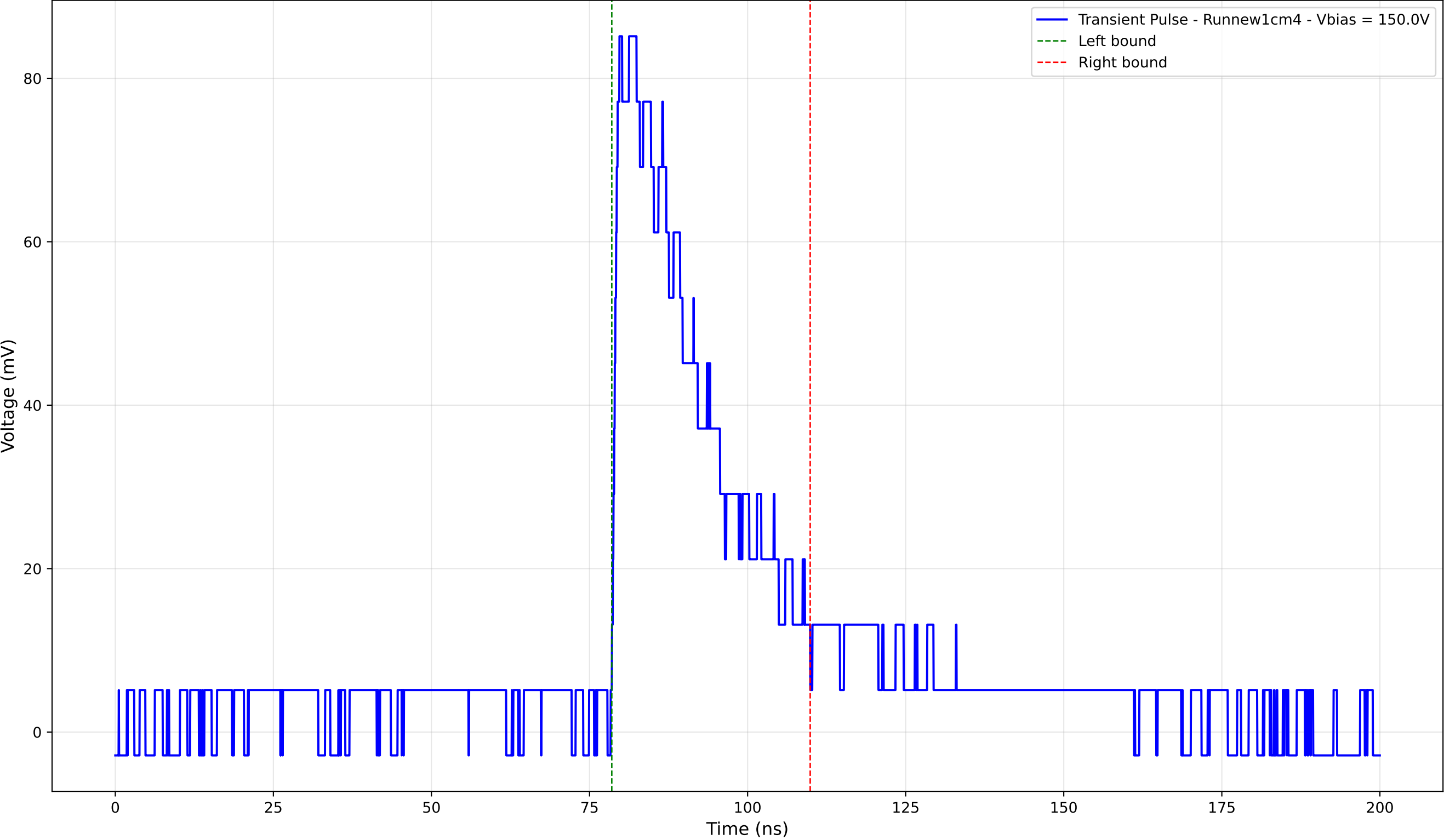
Transient Pulse - Sample: new1cm - Position: 1200.0 \mu\text{m} - Charge: 26.35 pC
