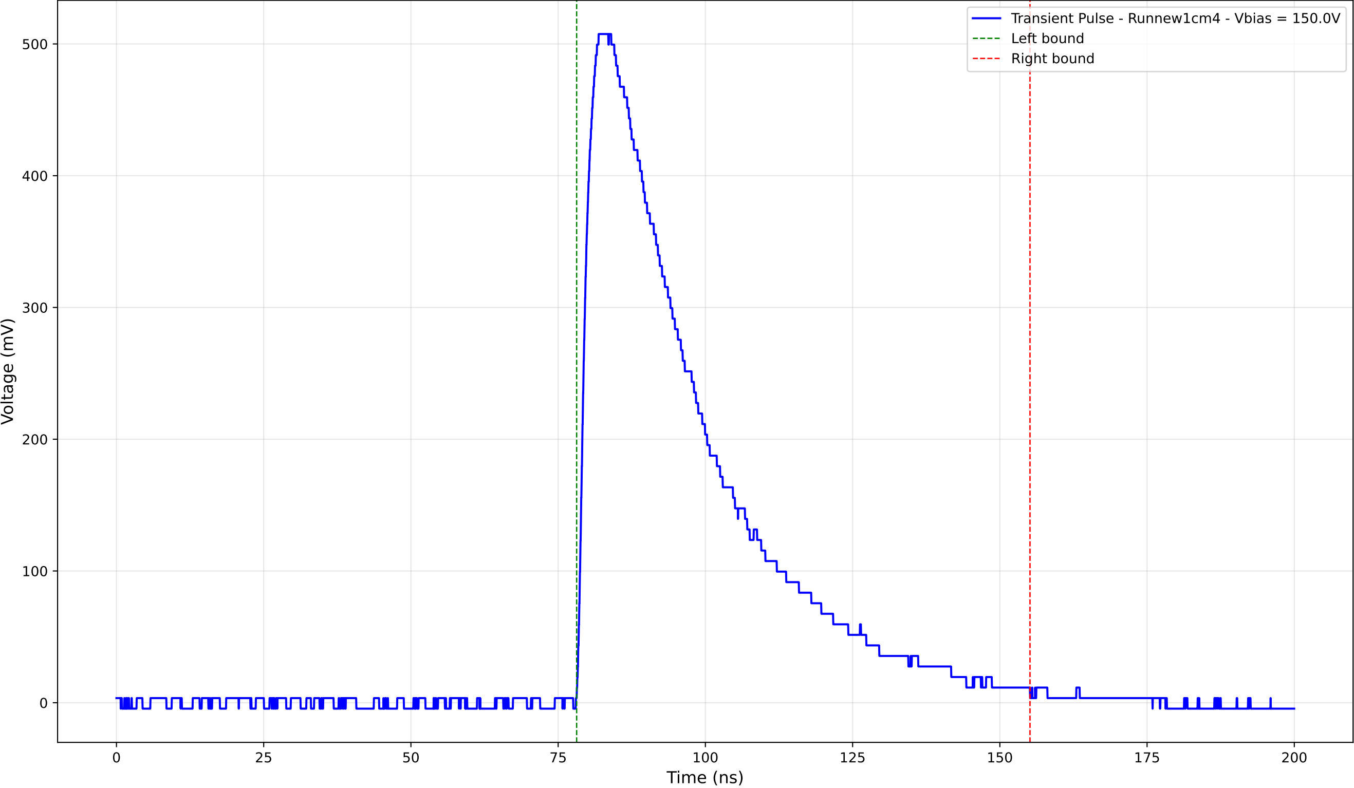
Transient Pulse - Sample: new1cm - Position: 2895.0 \mu\text{m} - Charge: 227.73 pC
