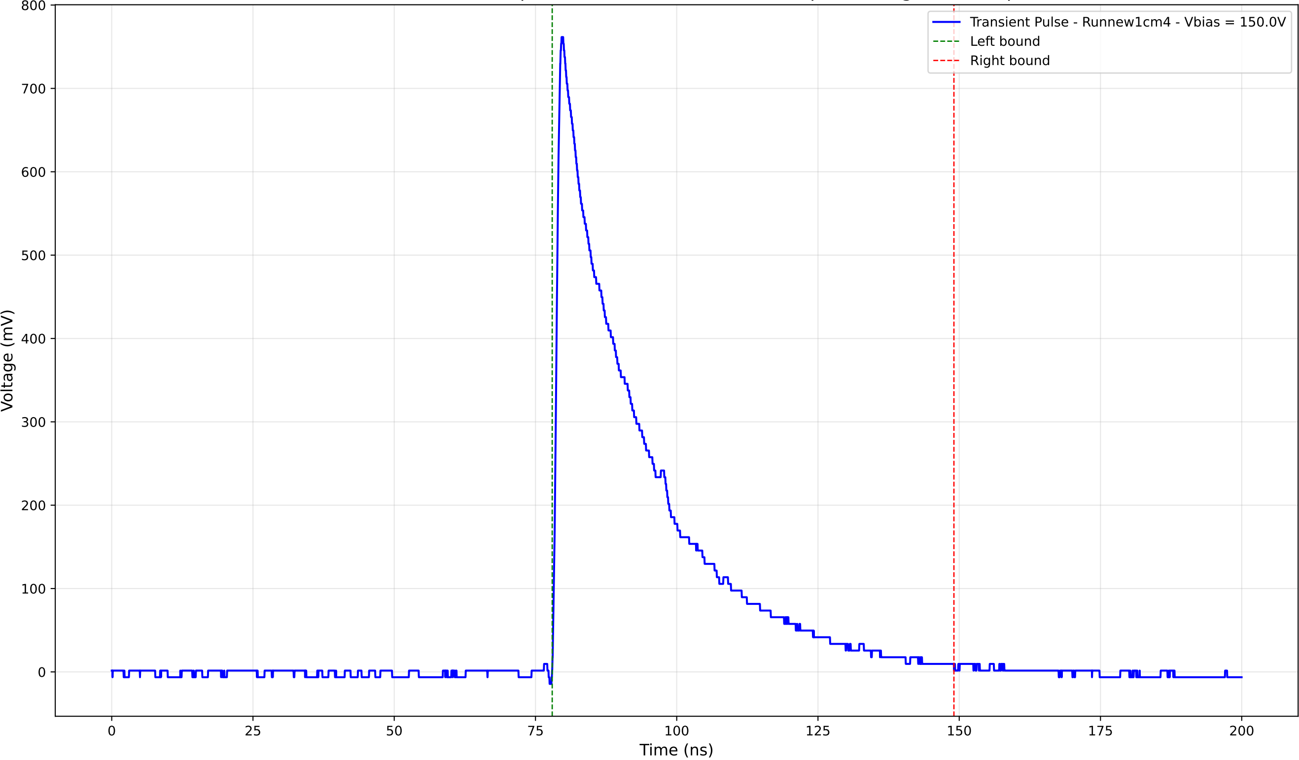
Transient Pulse - Sample: new1cm - Position: 4350.0 \mu\text{m} - Charge: 234.27 pC
