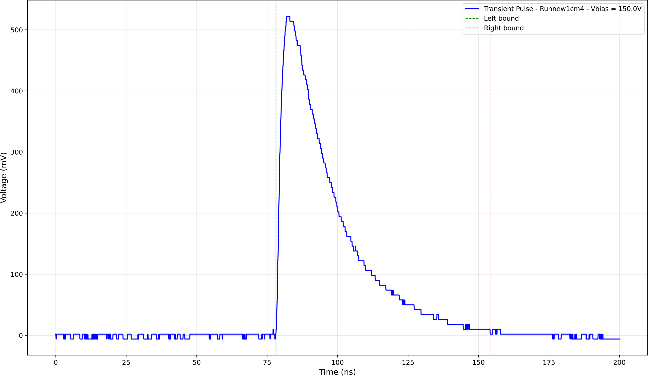
Transient Pulse - Sample: new1cm - Position: 2535.0 \mu\text{m} - Charge: 226.89 pC
