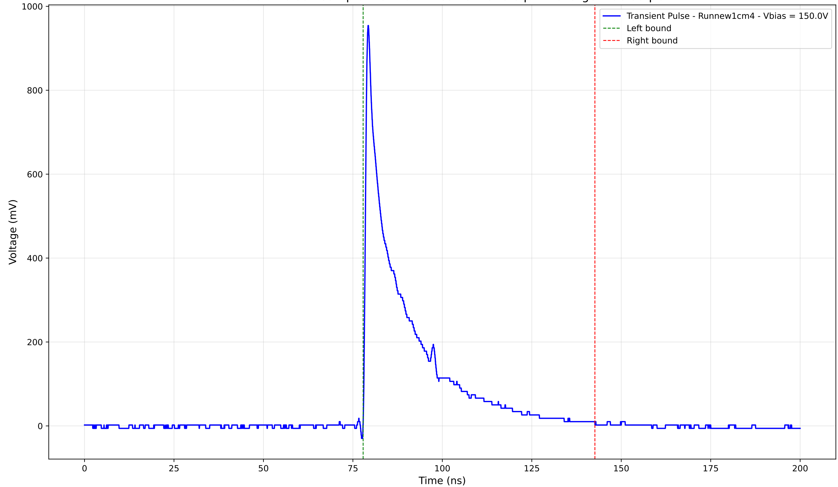
Transient Pulse - Sample: new1cm - Position: 340.0 \mu\text{m} - Charge: 190.35 pC
