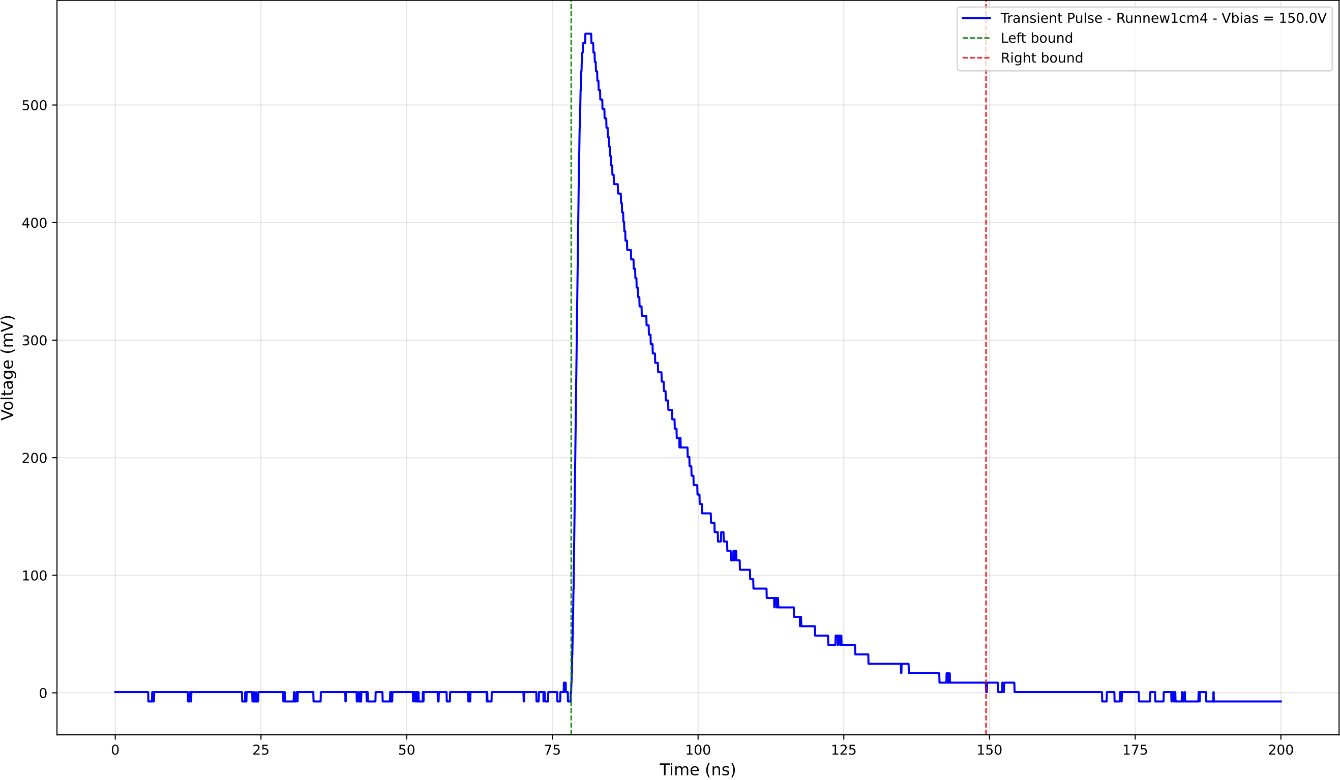
Transient Pulse - Sample: new1cm - Position: 1445.0 \mu\text{m} - Charge: 205.00 pC
