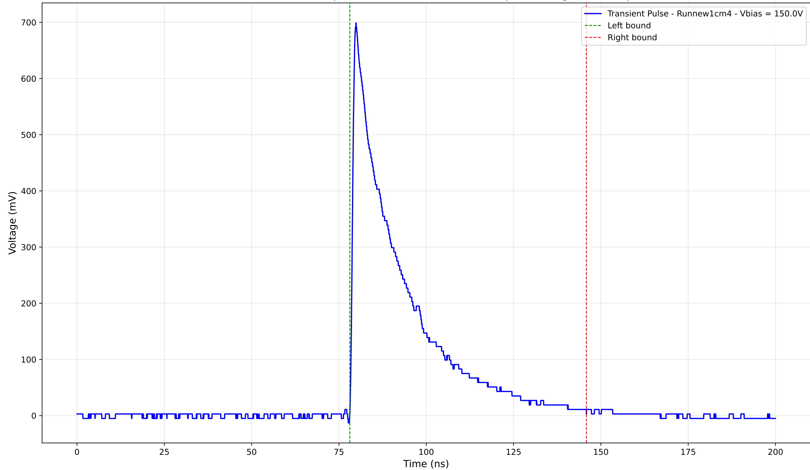
Transient Pulse - Sample: new1cm - Position: 950.0 \mu\text{m} - Charge: 199.18 pC
