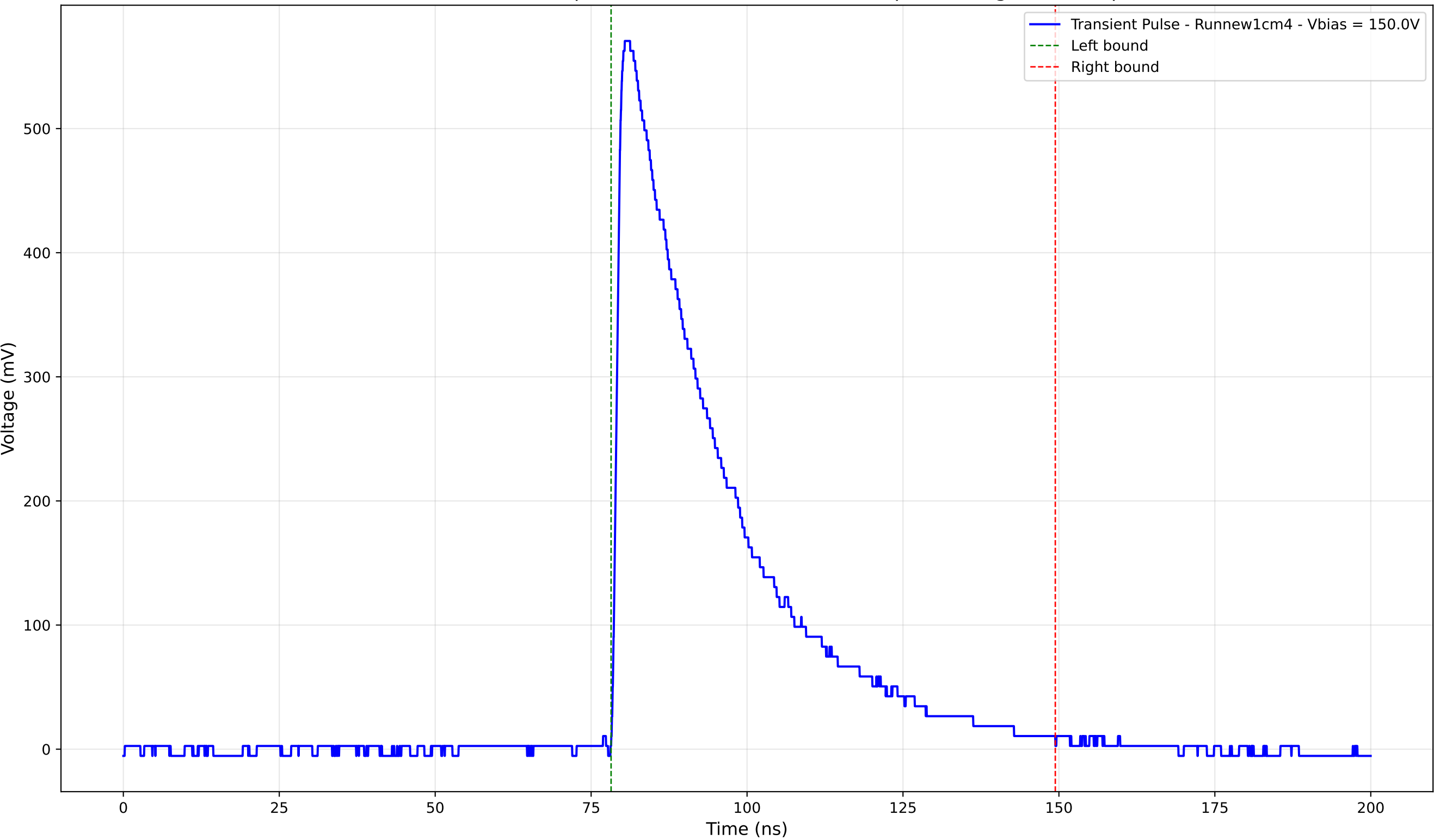
Transient Pulse - Sample: new1cm - Position: 1405.0 \mu\text{m} - Charge: 207.52 pC
