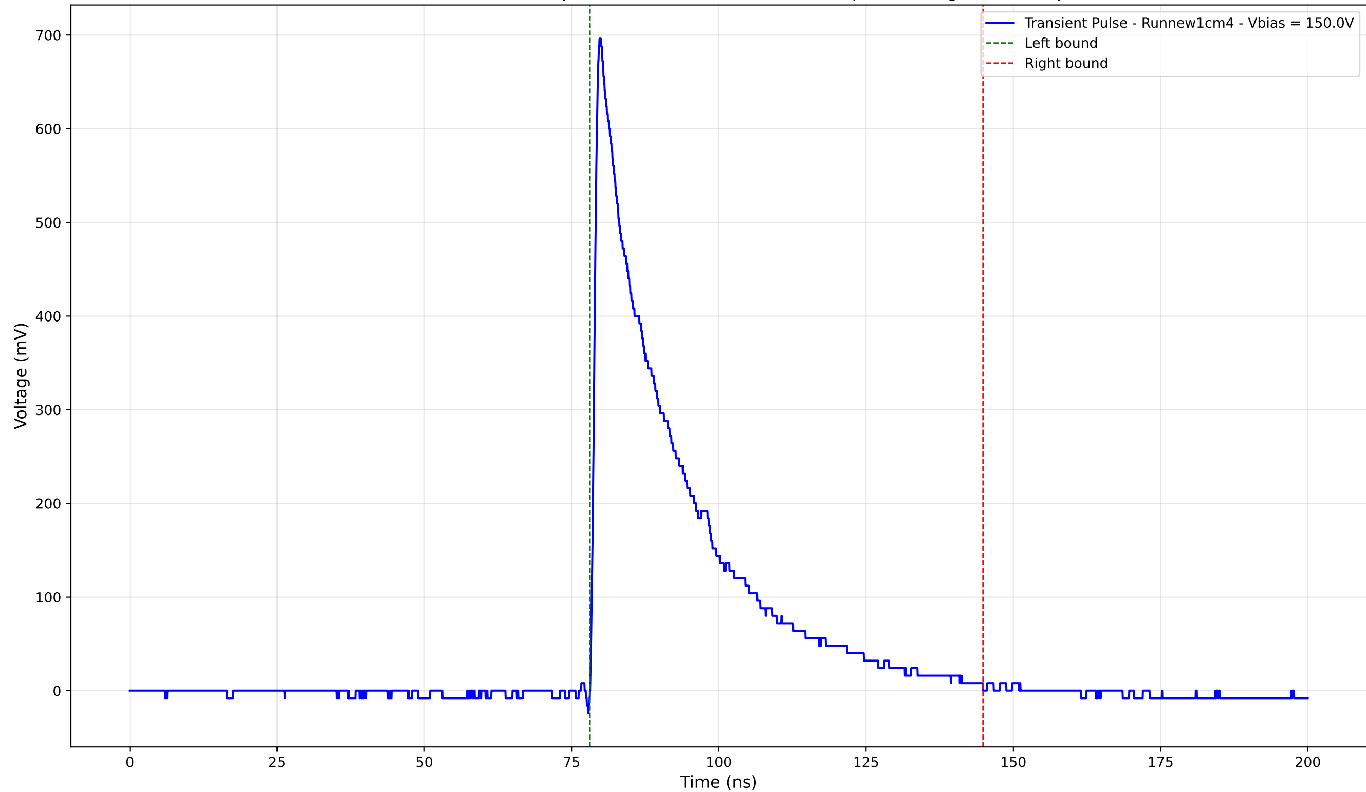
Transient Pulse - Sample: new1cm - Position: 935.0 \mu\text{m} - Charge: 196.08 pC
