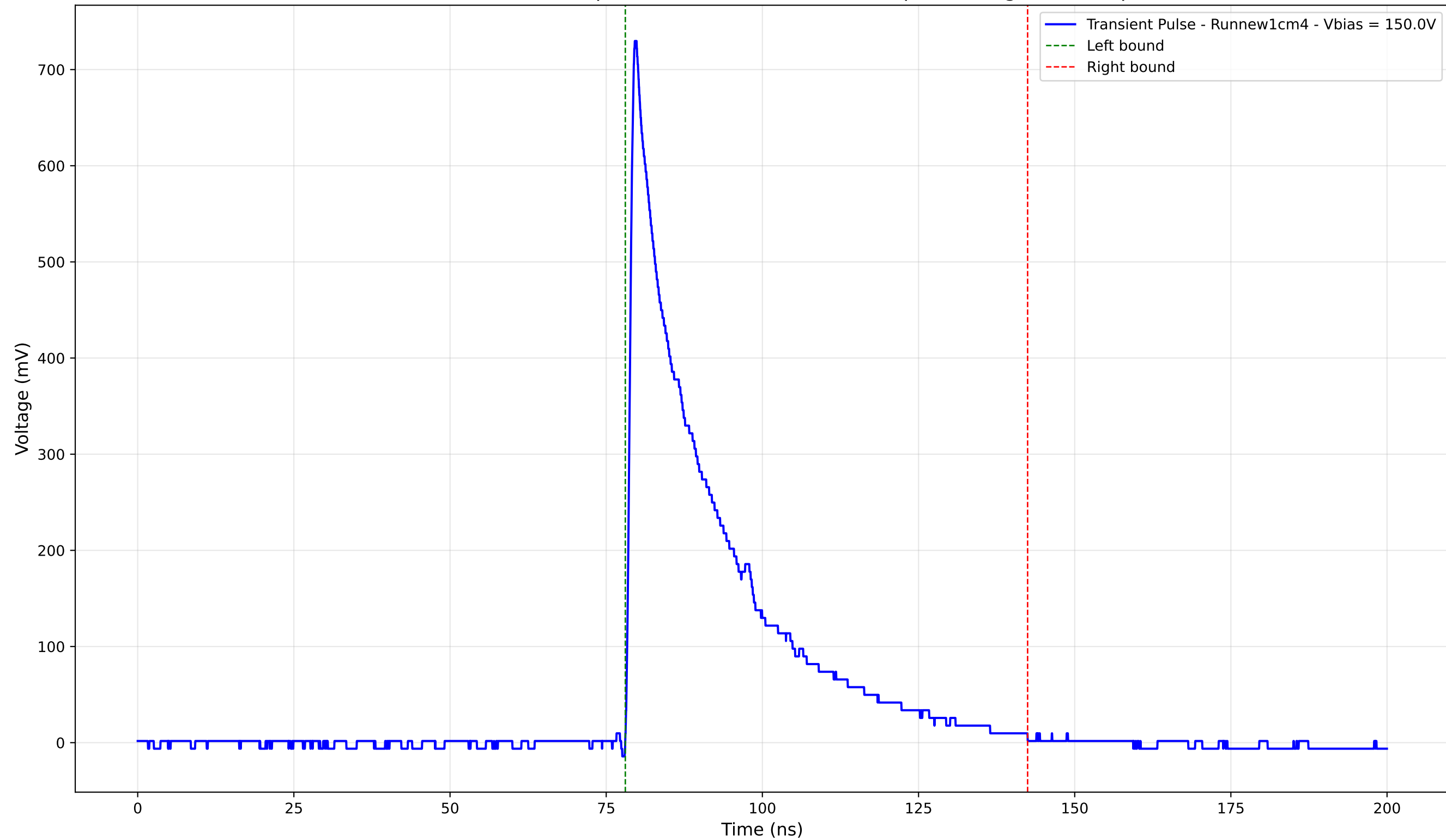
Transient Pulse - Sample: new1cm - Position: 800.0 \mu\text{m} - Charge: 188.48 pC
