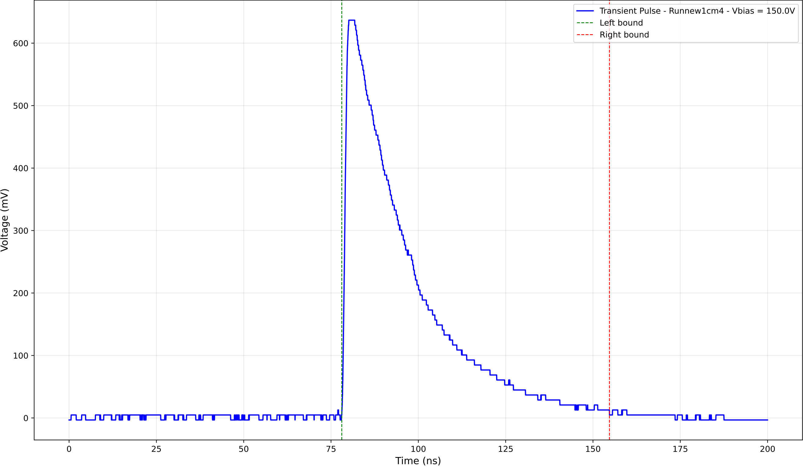
Transient Pulse - Sample: new1cm - Position: 3855.0 \mu\text{m} - Charge: 254.42 pC
