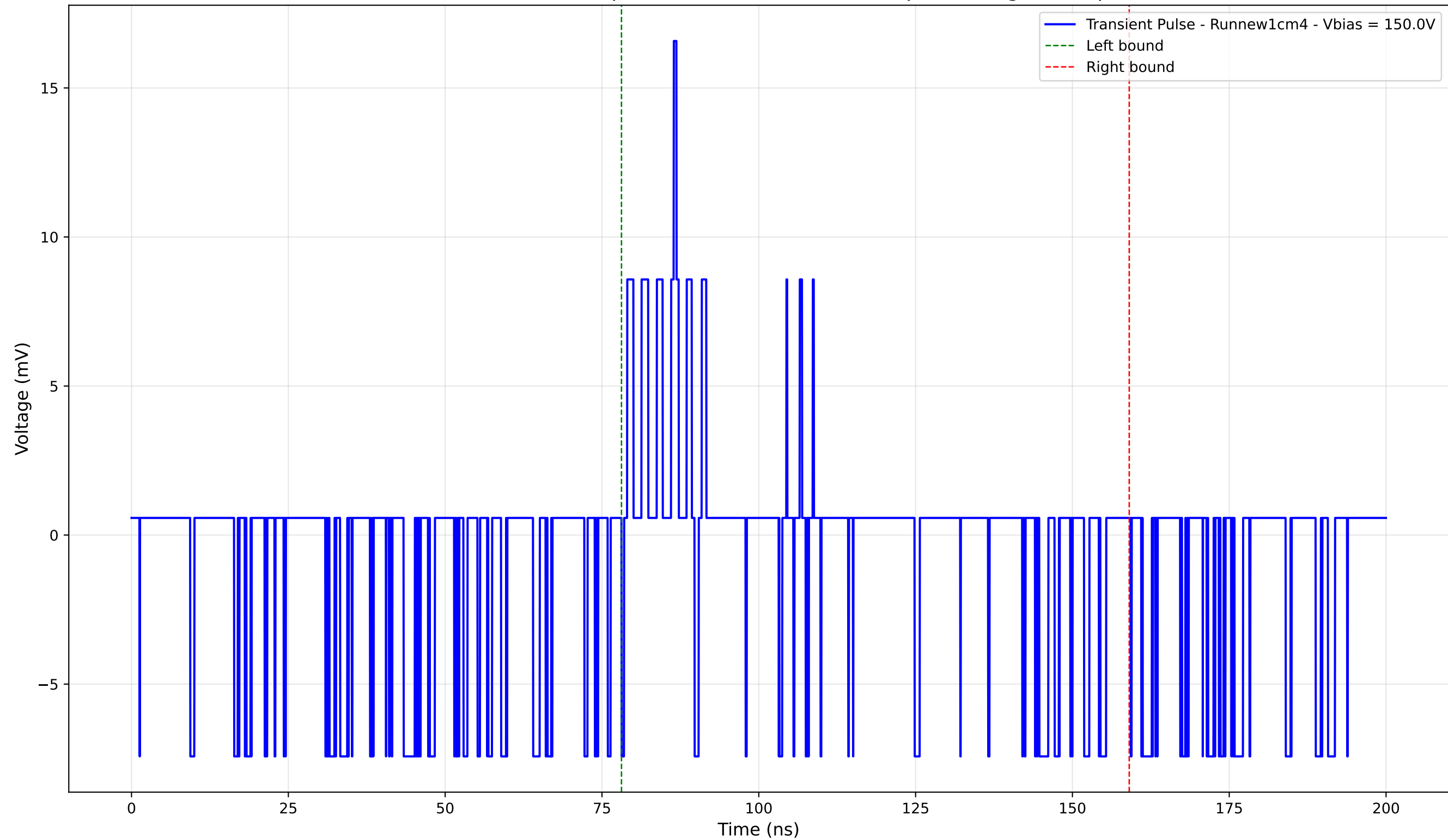
Transient Pulse - Sample: new1cm - Position: 65.0 \mu\text{m} - Charge: 0.73 pC
