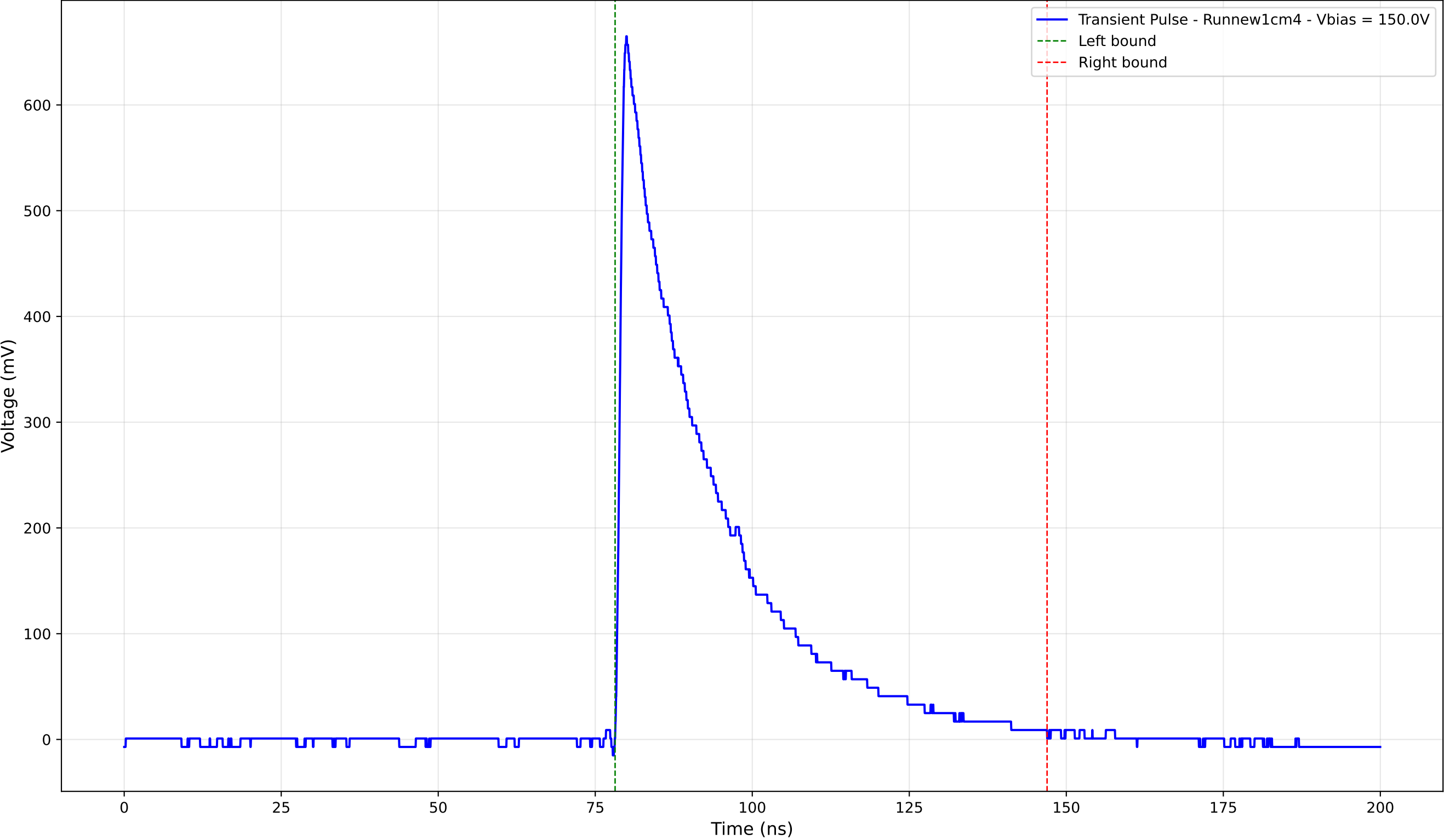
Transient Pulse - Sample: new1cm - Position: 1050.0 \mu\text{m} - Charge: 198.45 pC
