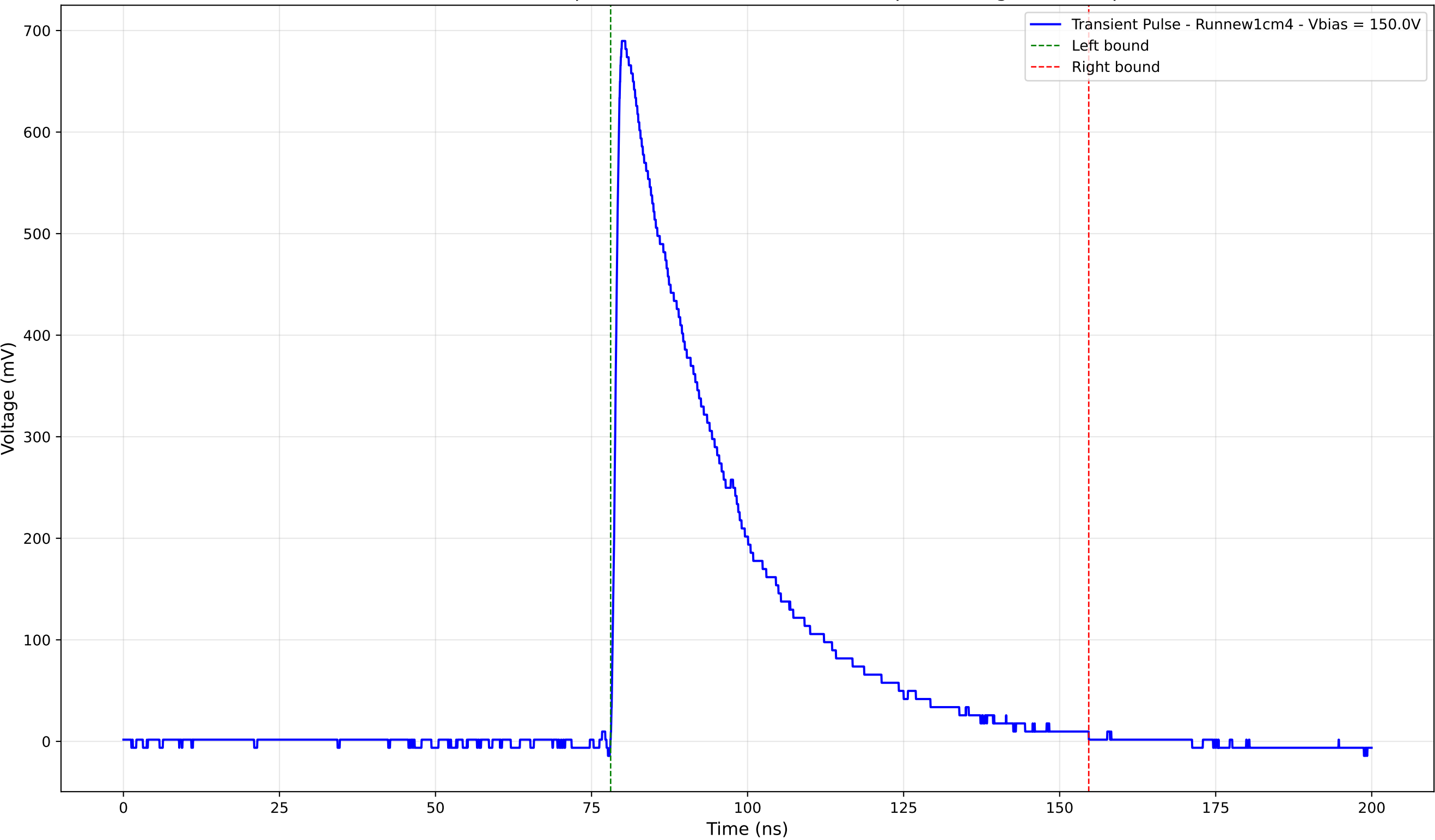
Transient Pulse - Sample: new1cm - Position: 4080.0 \mu\text{m} - Charge: 246.97 pC
