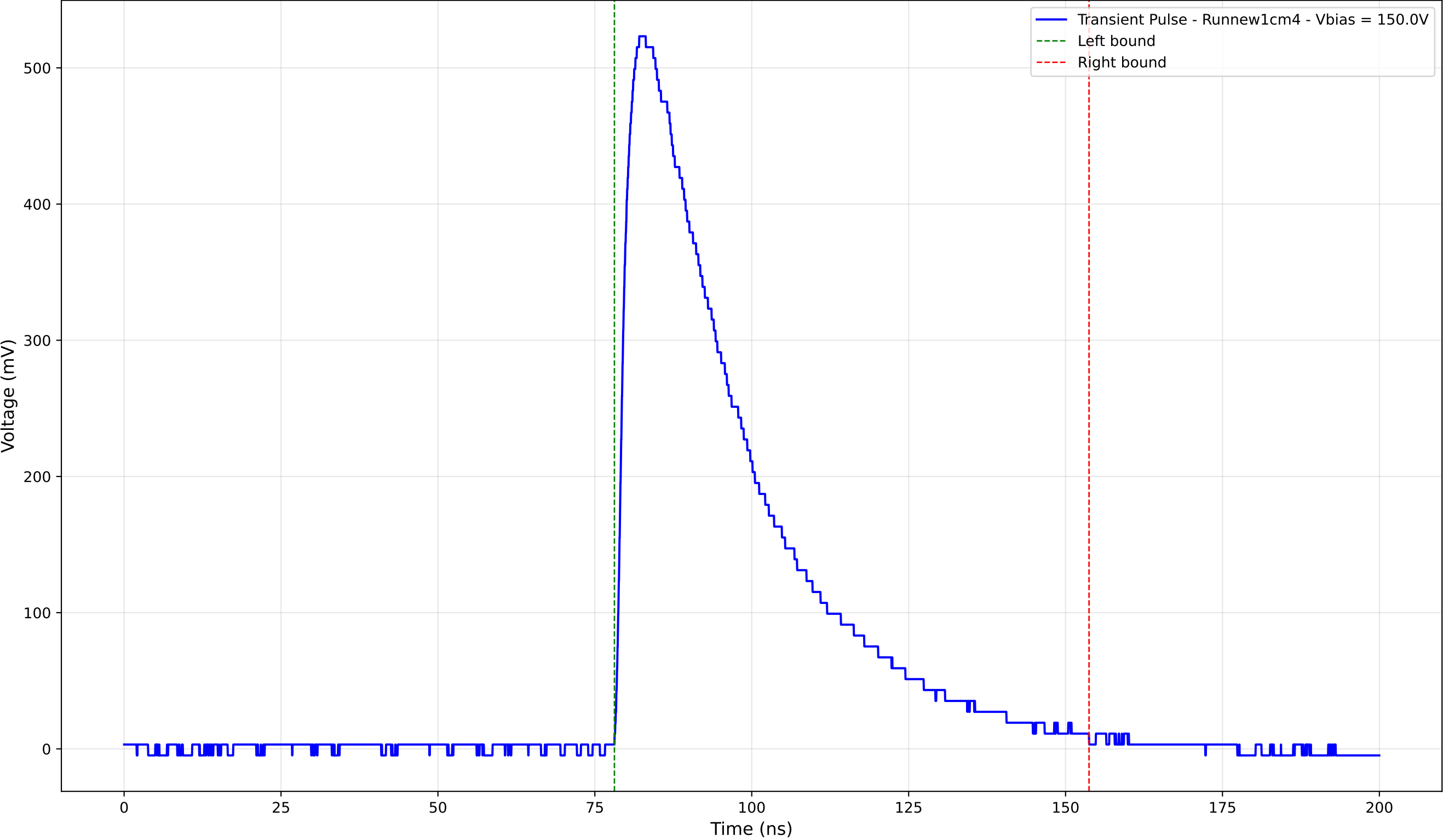
Transient Pulse - Sample: new1cm - Position: 3000.0 \mu\text{m} - Charge: 231.32 pC
