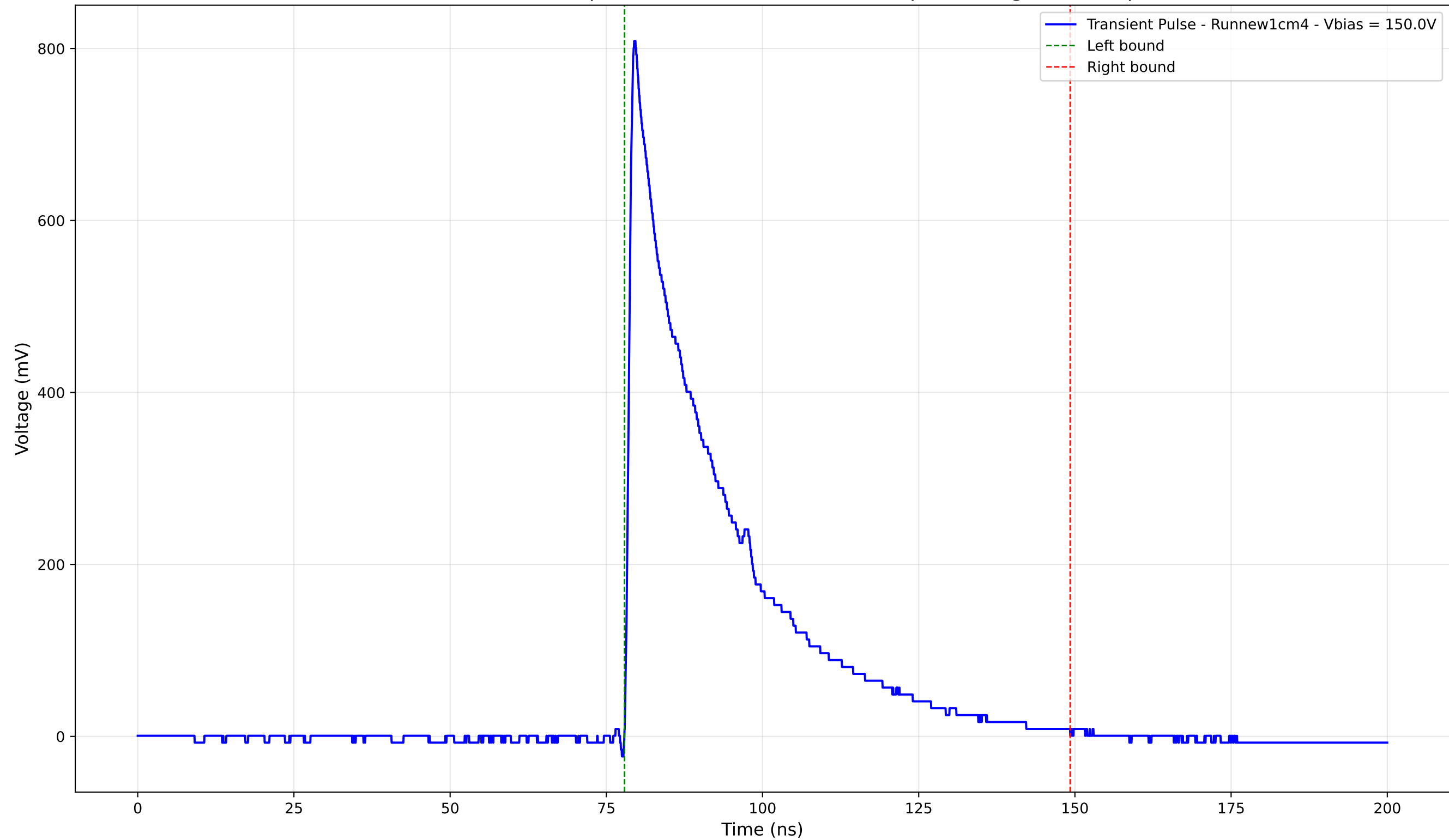
Transient Pulse - Sample: new1cm - Position: 4500.0 \mu\text{m} - Charge: 233.57 pC
