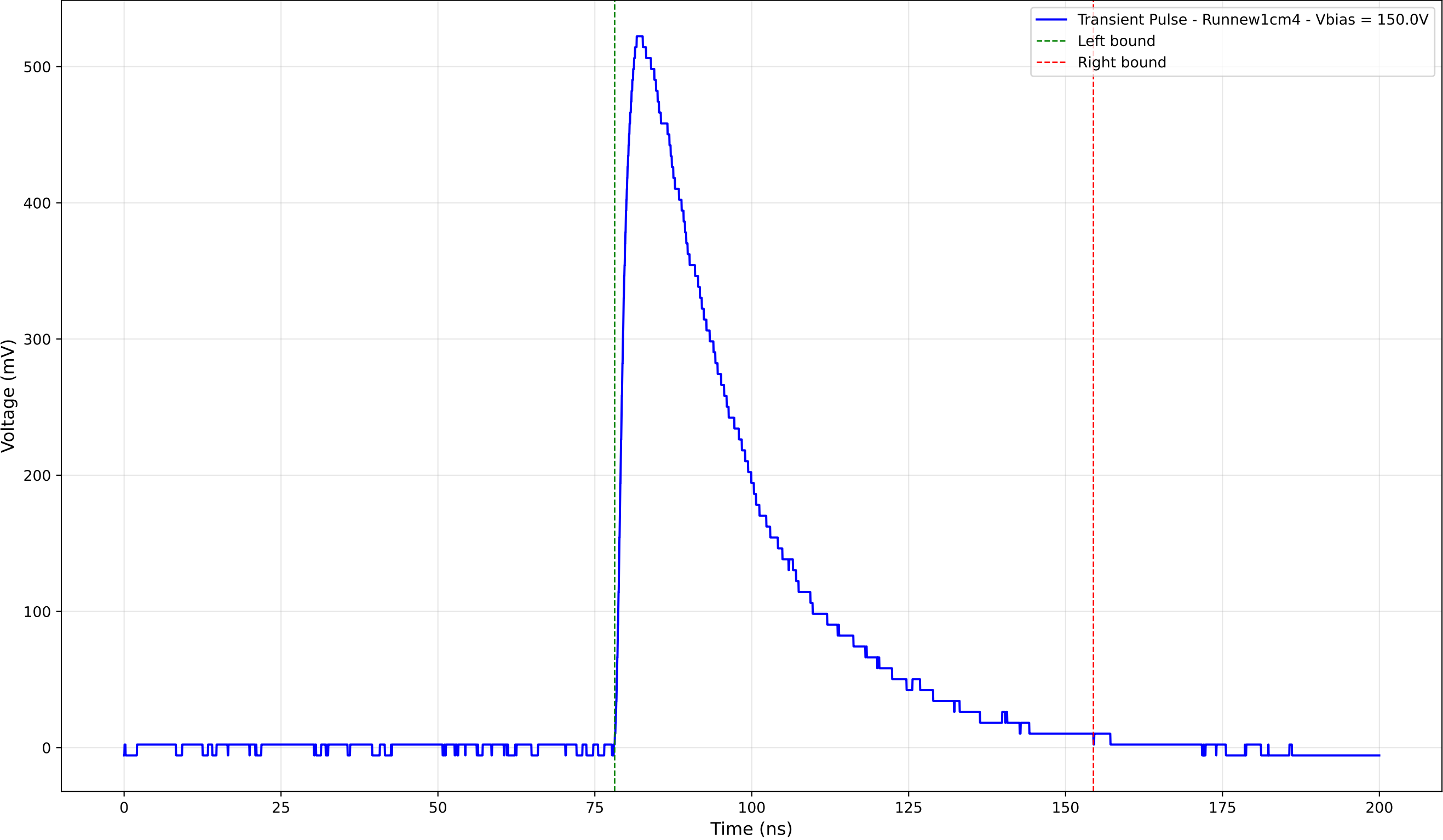
Transient Pulse - Sample: new1cm - Position: 2070.0 \mu\text{m} - Charge: 218.07 pC
