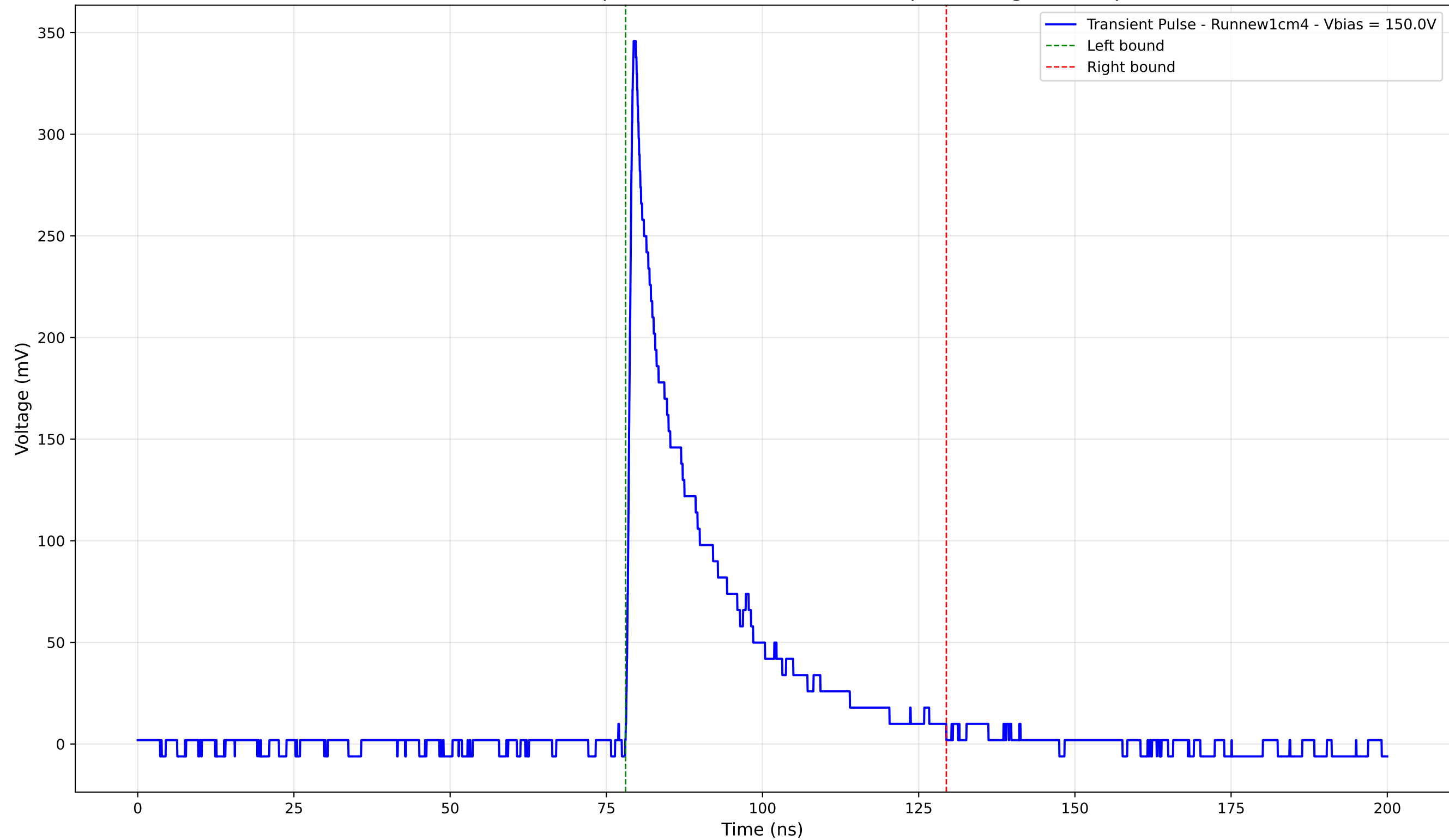
Transient Pulse - Sample: new1cm - Position: 655.0 \mu\text{m} - Charge: 72.16 pC
