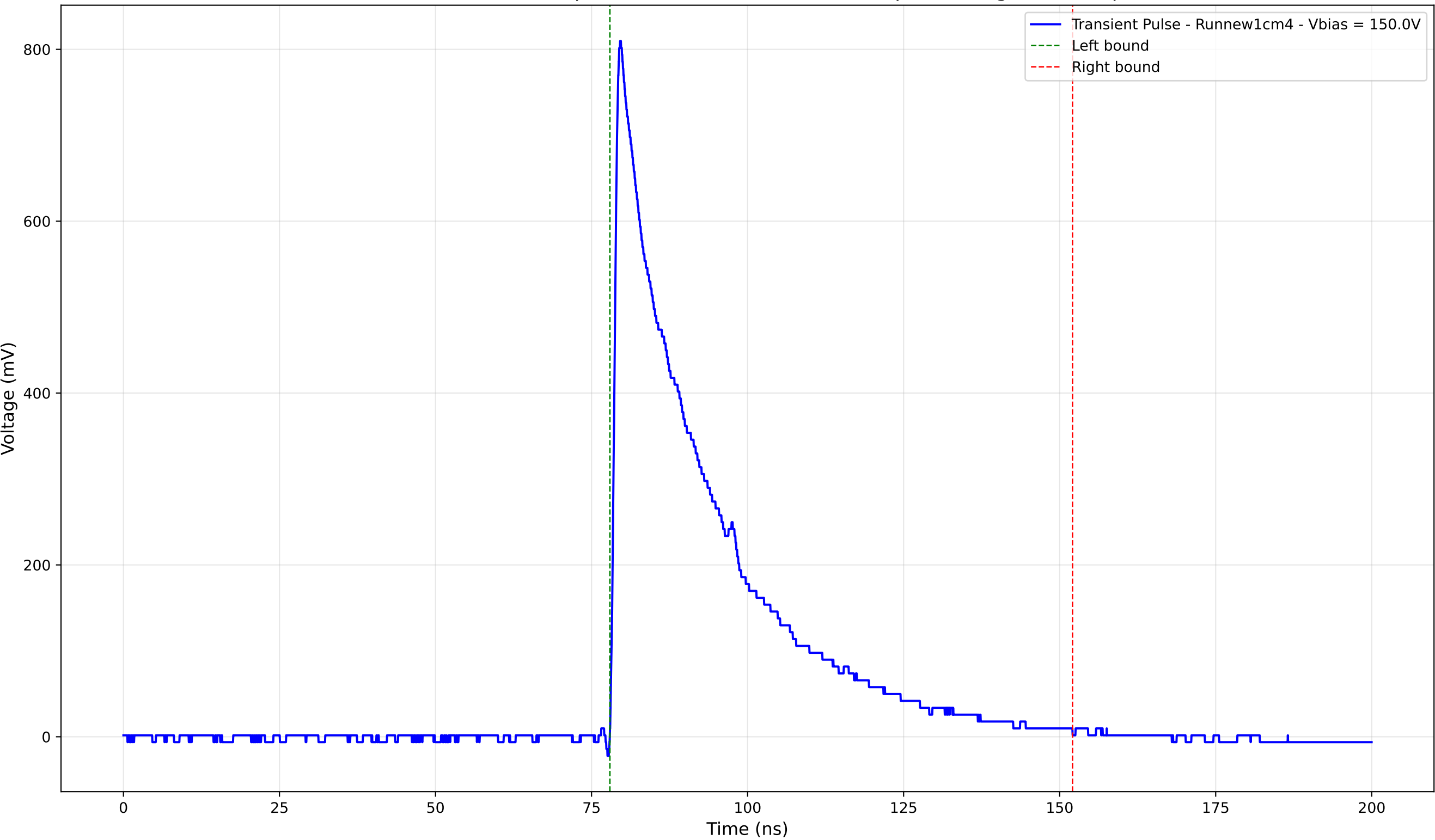
Transient Pulse - Sample: new1cm - Position: 4435.0 \mu\text{m} - Charge: 241.61 pC
