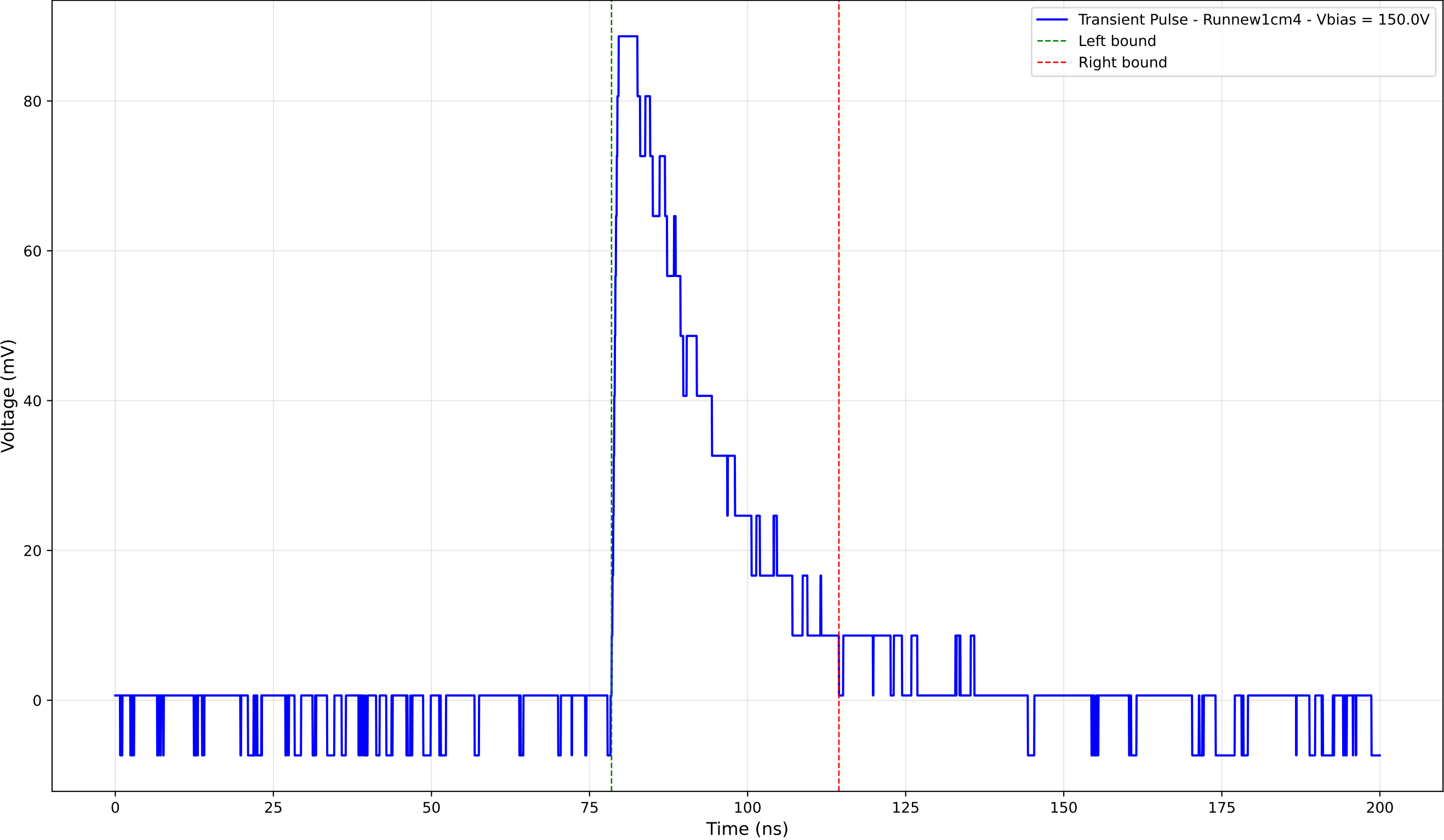
Transient Pulse - Sample: new1cm - Position: 1190.0 \mu\text{m} - Charge: 27.29 pC
