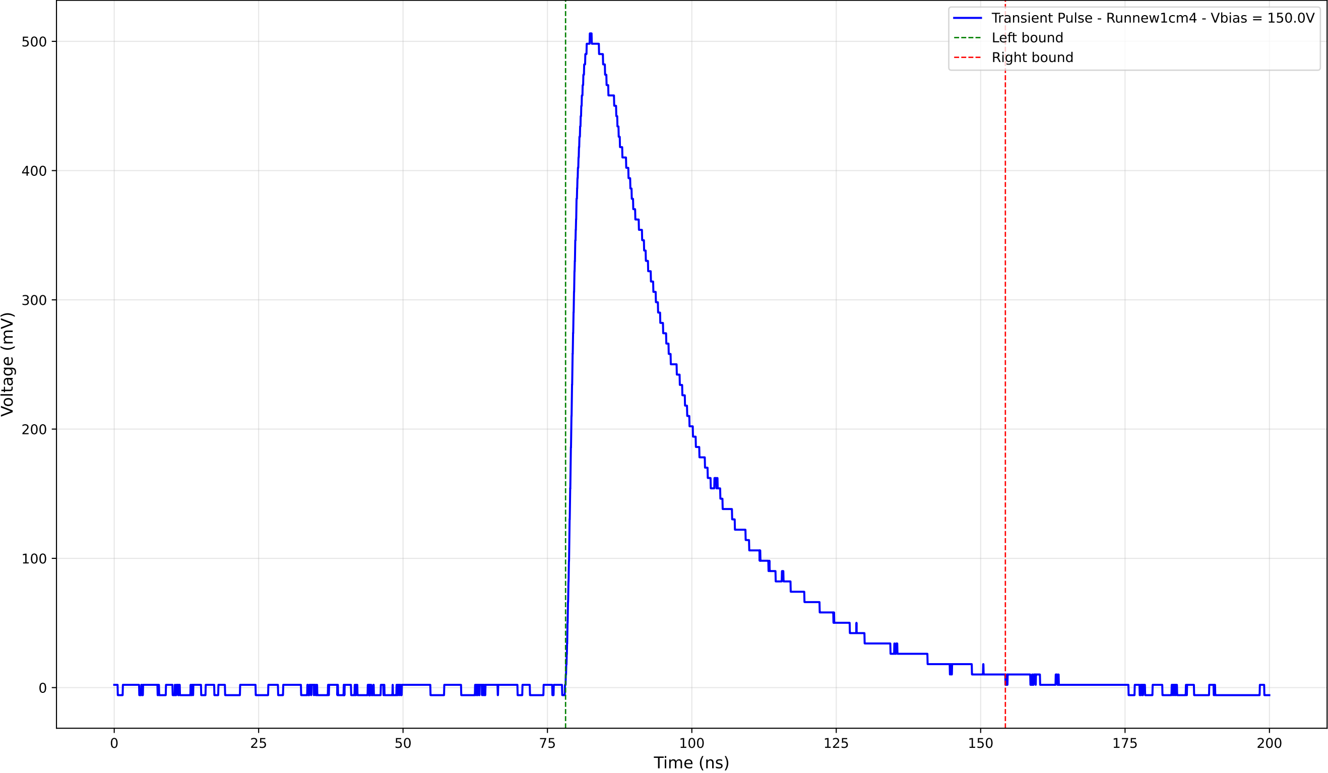
Transient Pulse - Sample: new1cm - Position: 2890.0 \mu\text{m} - Charge: 222.27 pC
