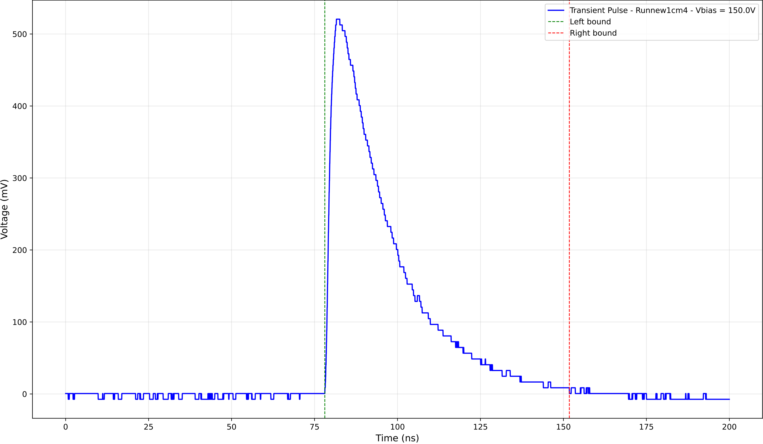
Transient Pulse - Sample: new1cm - Position: 2085.0 \mu\text{m} - Charge: 215.28 pC
