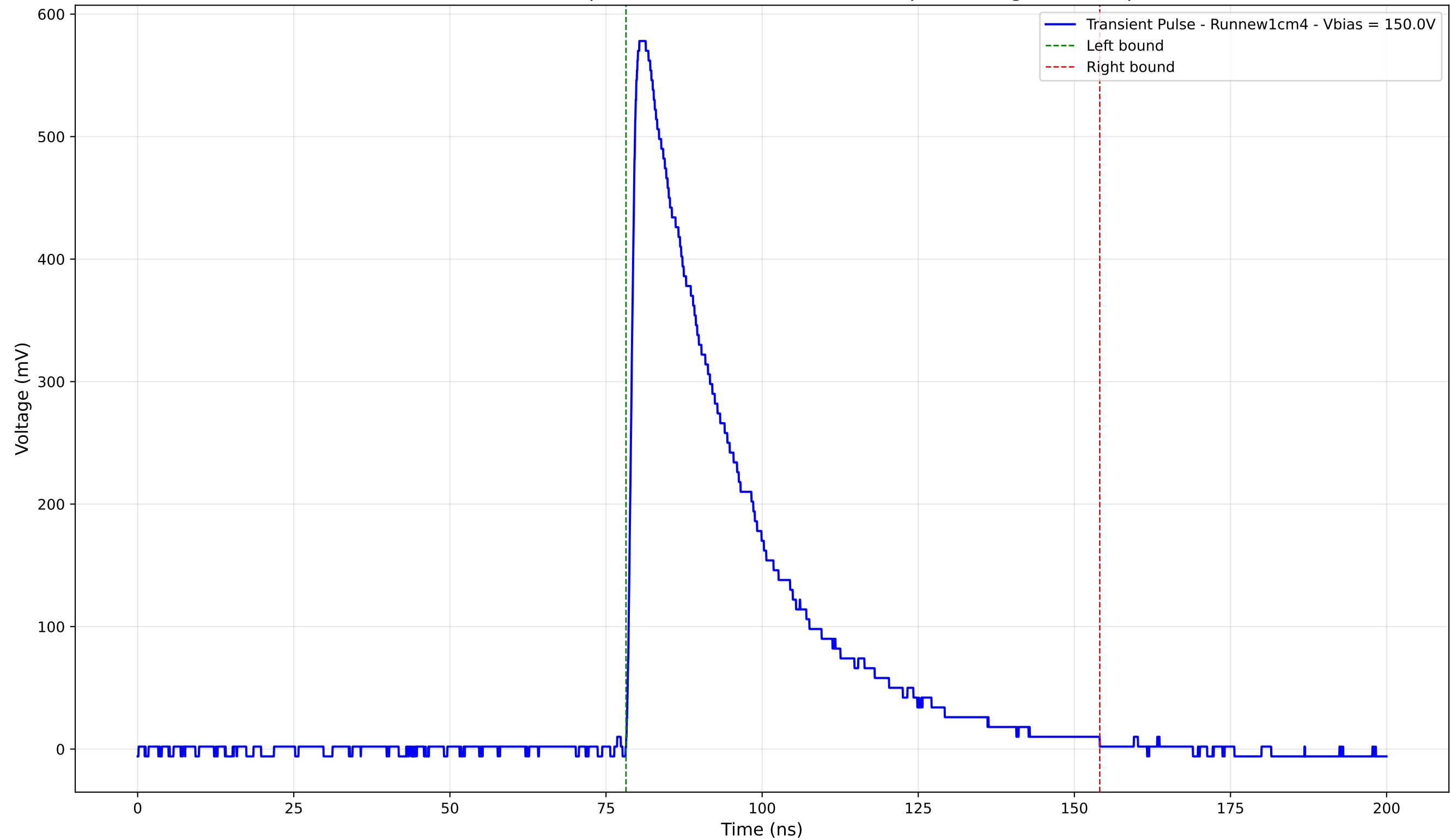
Transient Pulse - Sample: new1cm - Position: 1370.0 \mu\text{m} - Charge: 208.43 pC
