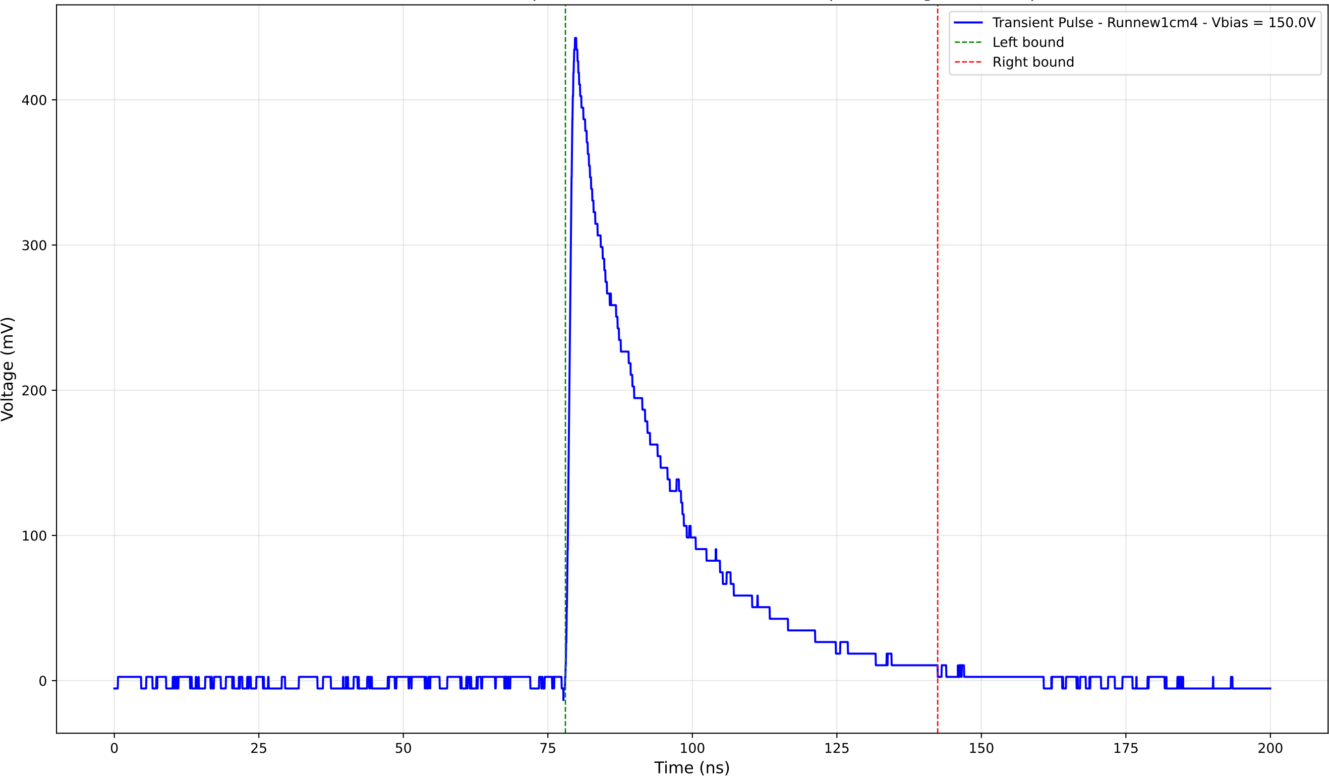
Transient Pulse - Sample: new1cm - Position: 4285.0 \mu\text{m} - Charge: 130.76 pC
