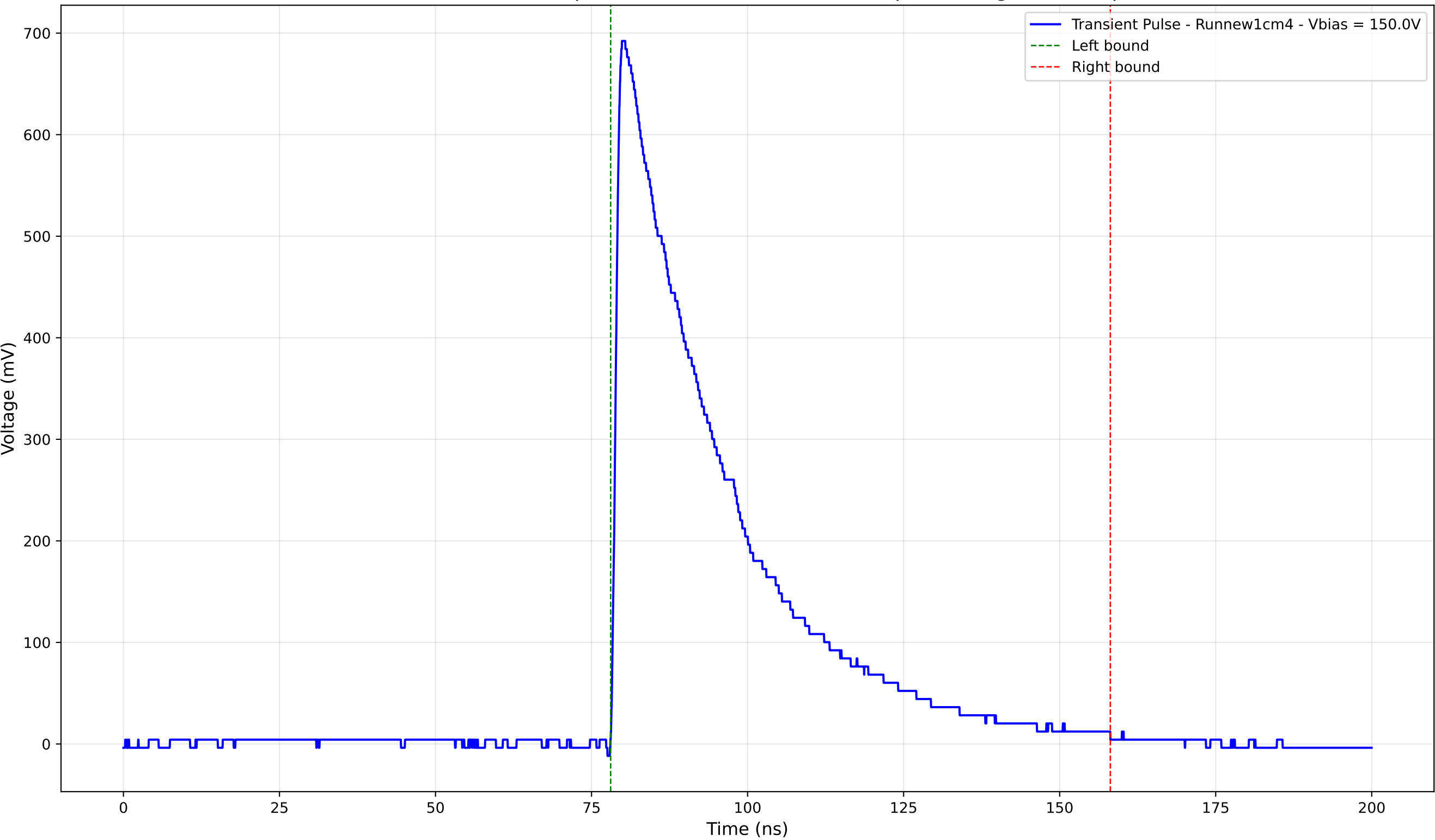
Transient Pulse - Sample: new1cm - Position: 4070.0 \mu\text{m} - Charge: 253.14 pC
