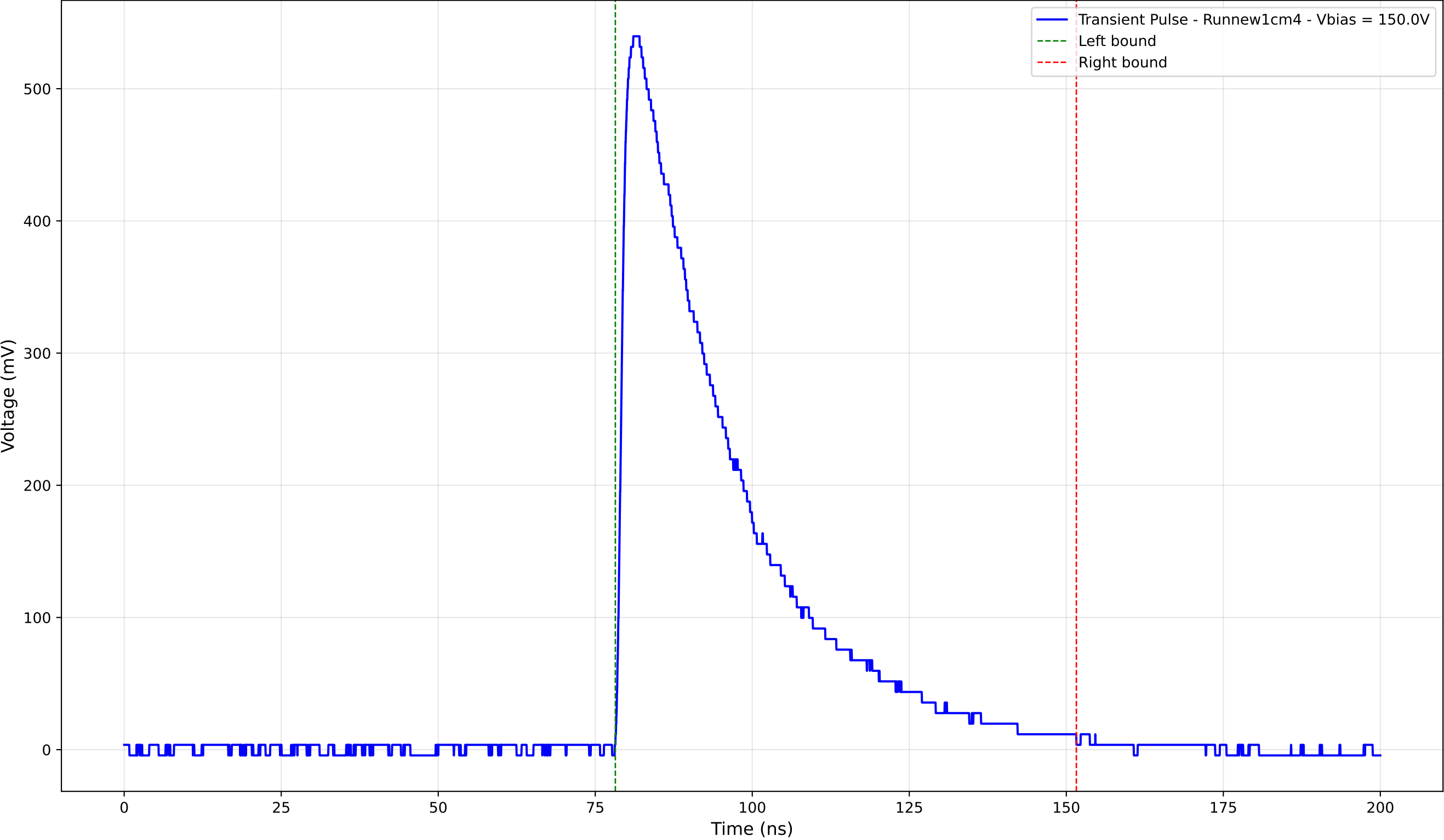
Transient Pulse - Sample: new1cm - Position: 1600.0 \mu\text{m} - Charge: 207.95 pC
