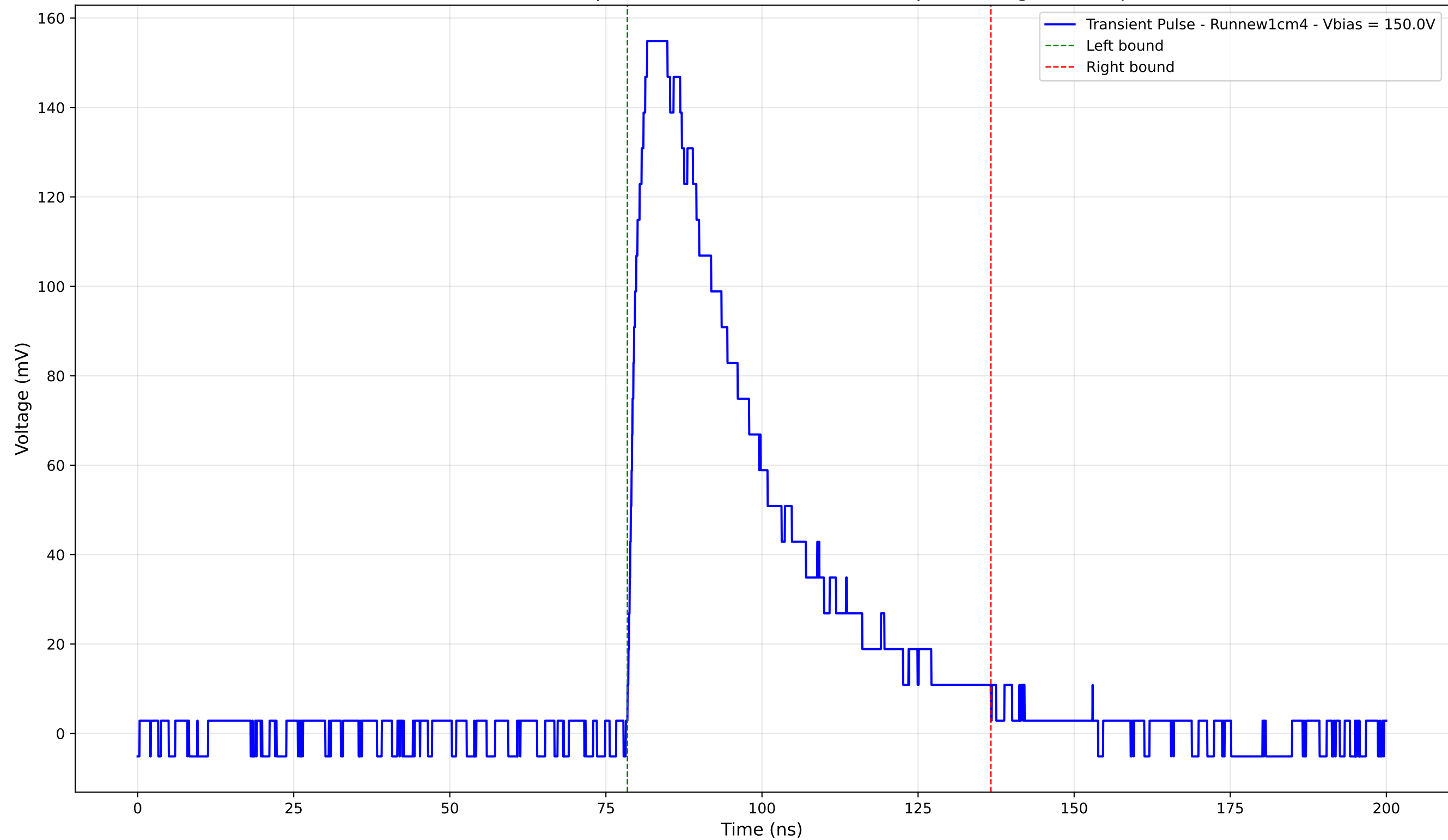
Transient Pulse - Sample: new1cm - Position: 2685.0 \mu\text{m} - Charge: 65.61 pC
