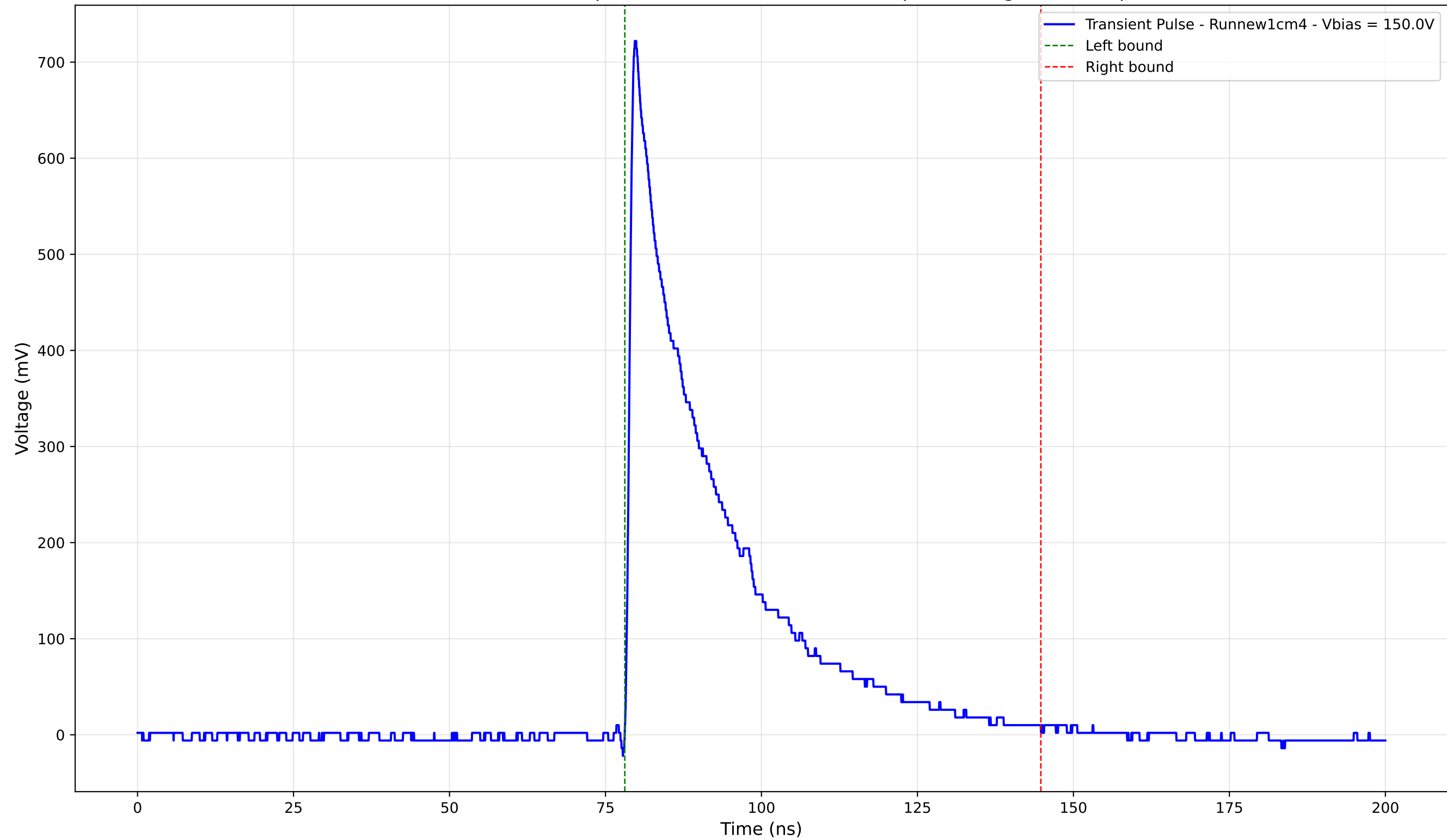
Transient Pulse - Sample: new1cm - Position: 890.0 \mu\text{m} - Charge: 197.89 pC
