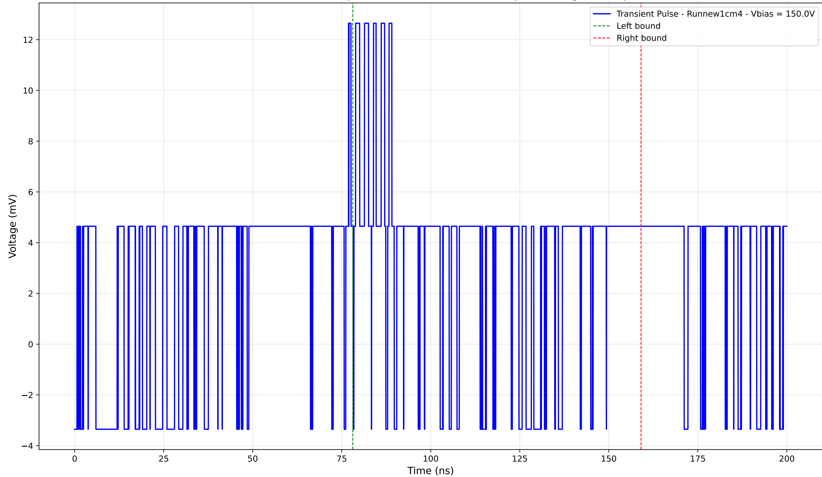
Transient Pulse - Sample: new1cm - Position: 60.0 \mu\text{m} - Charge: 6.13 pC
