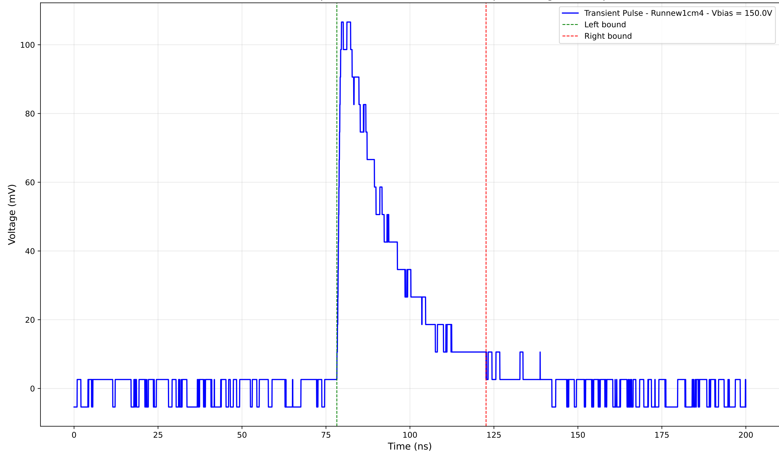
Transient Pulse - Sample: new1cm - Position: 4230.0 \mu\text{m} - Charge: 34.81 pC
