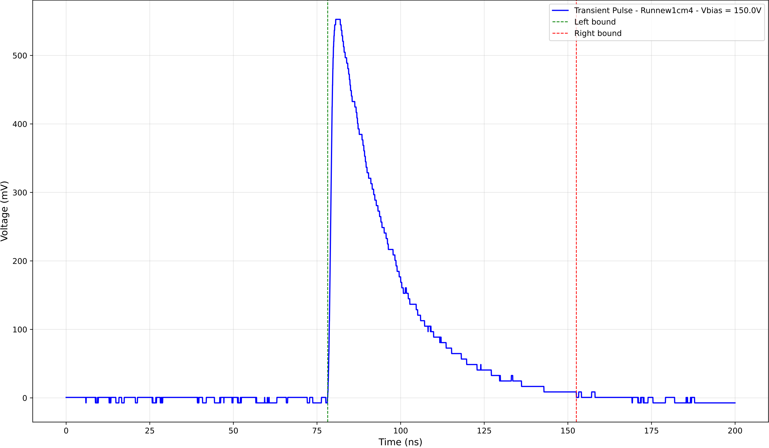
Transient Pulse - Sample: new1cm - Position: 1485.0 \mu\text{m} - Charge: 205.90 pC
