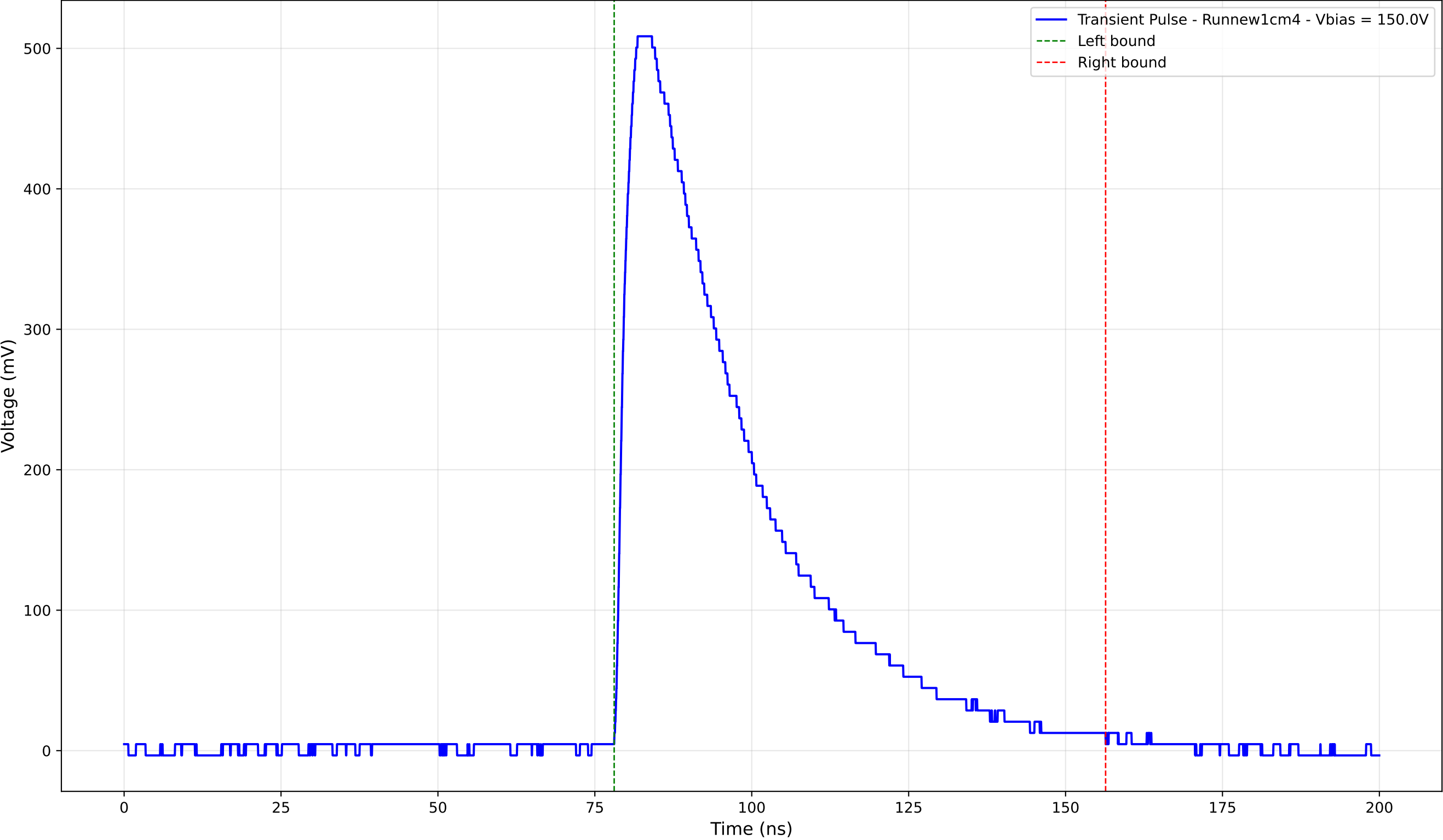
Transient Pulse - Sample: new1cm - Position: 2580.0 \mu\text{m} - Charge: 227.26 pC
