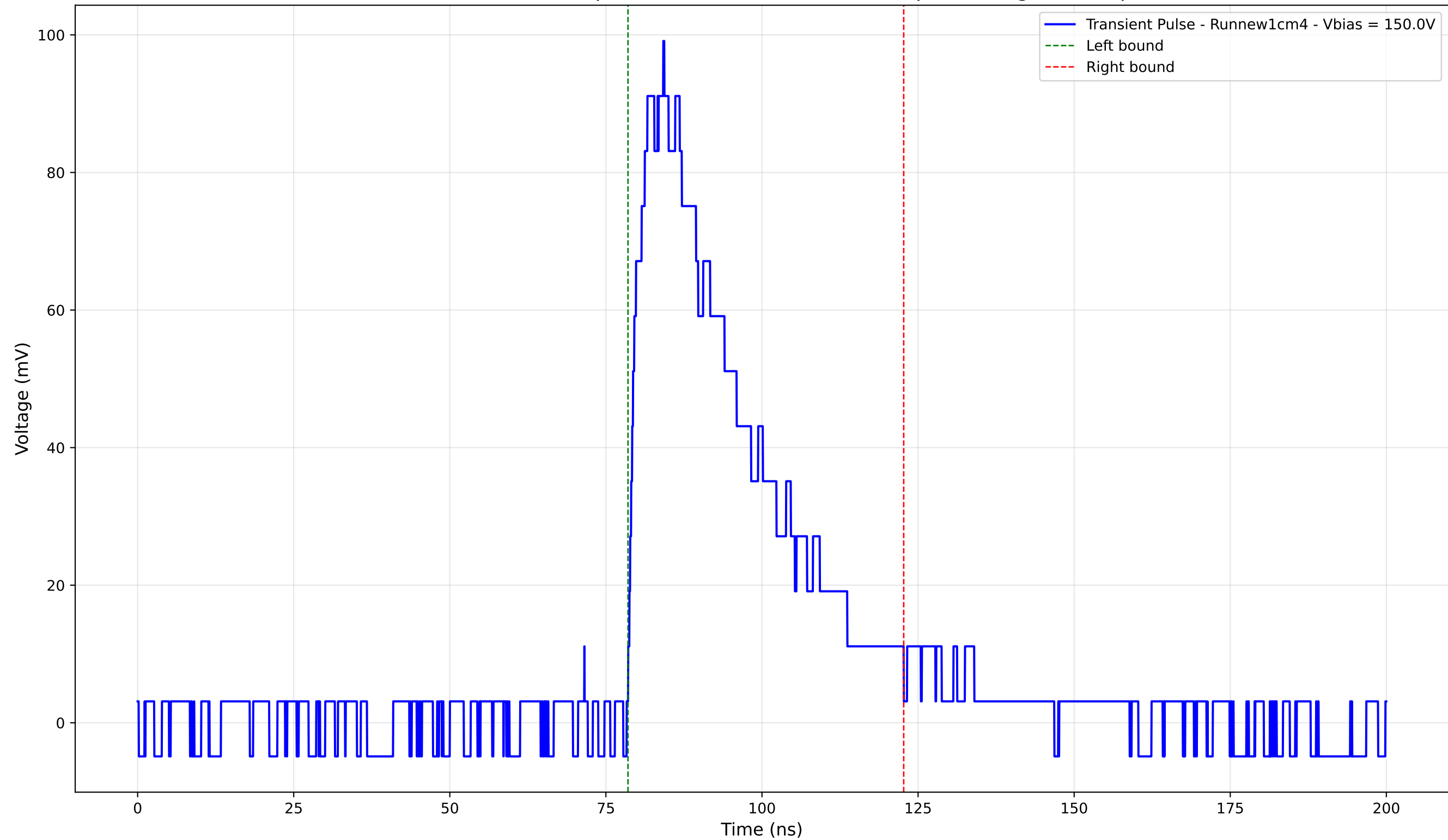
Transient Pulse - Sample: new1cm - Position: 2215.0 \mu\text{m} - Charge: 36.76 pC
