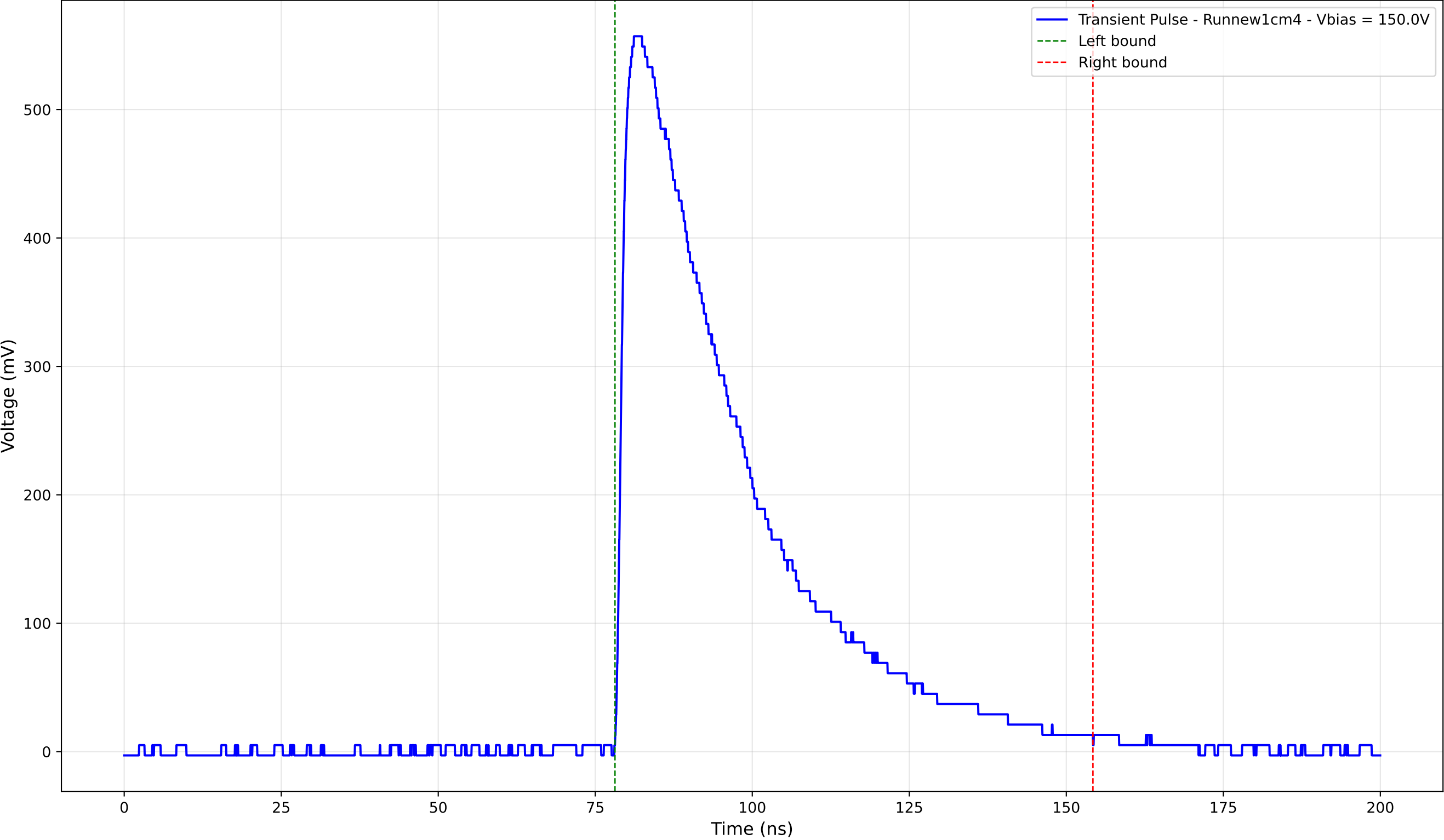
Transient Pulse - Sample: new1cm - Position: 3480.0 \mu\text{m} - Charge: 239.53 pC
