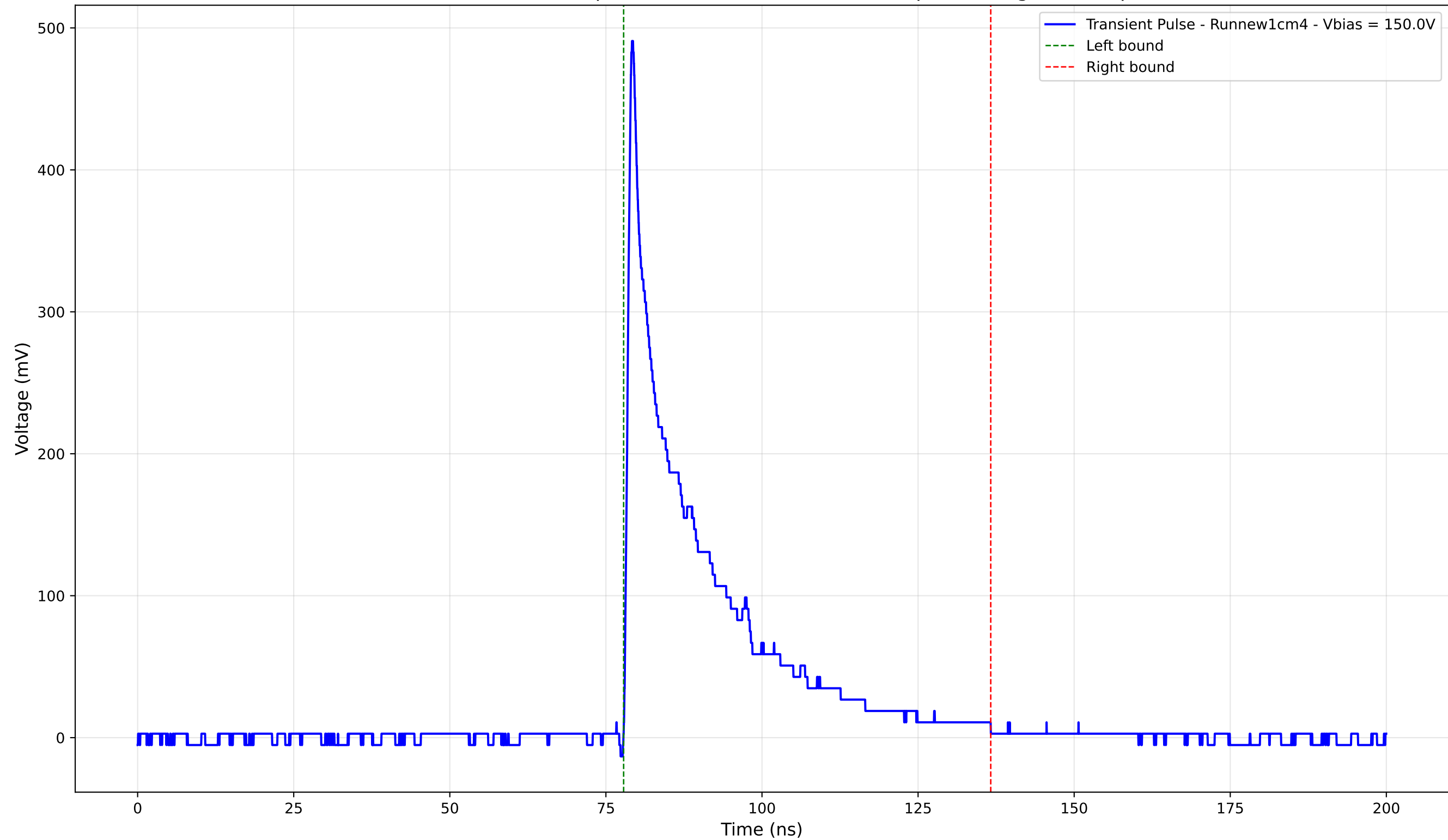
Transient Pulse - Sample: new1cm - Position: 4780.0 \mu\text{m} - Charge: 96.09 pC
