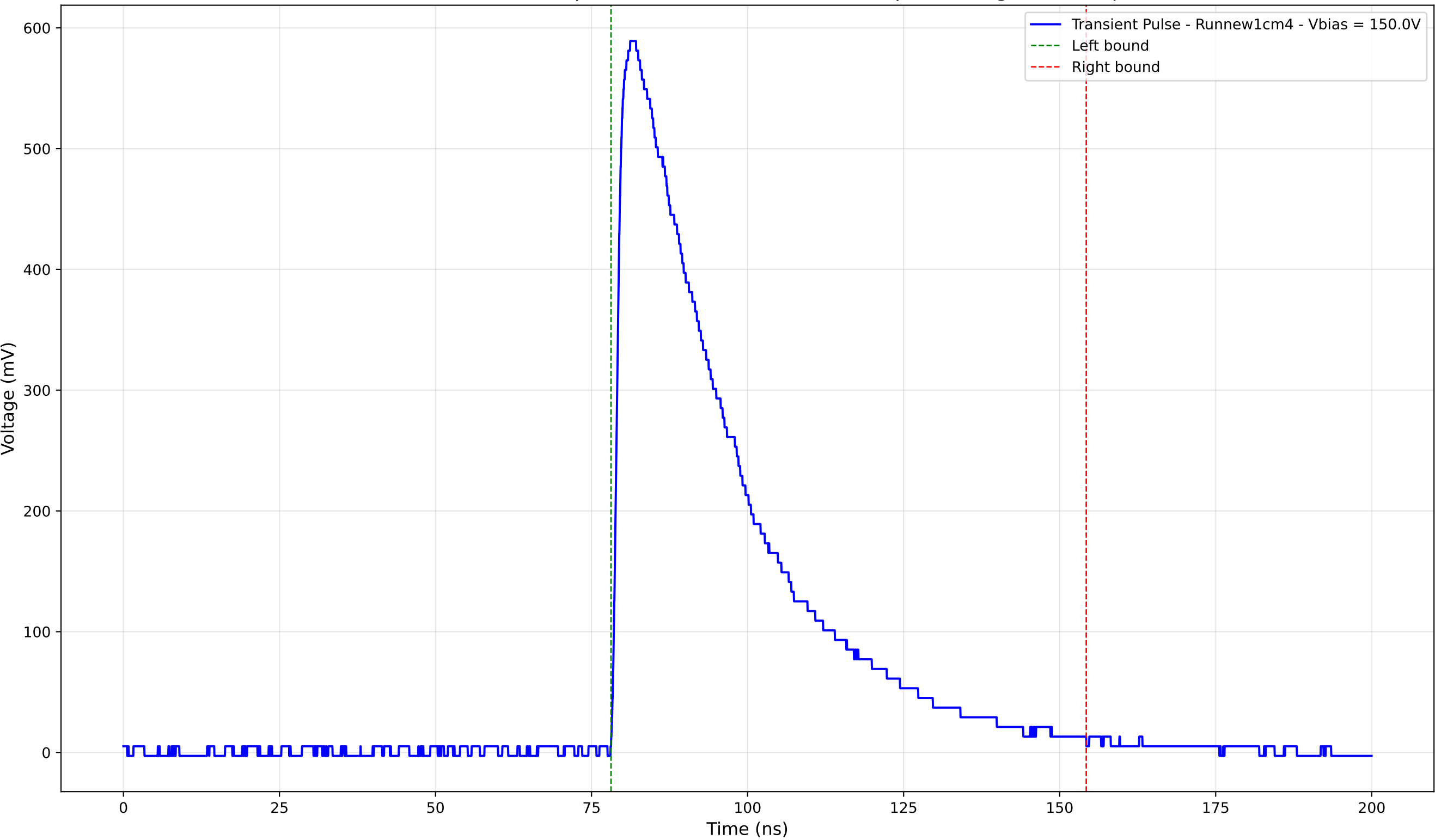
Transient Pulse - Sample: new1cm - Position: 3615.0 \mu\text{m} - Charge: 245.50 pC
