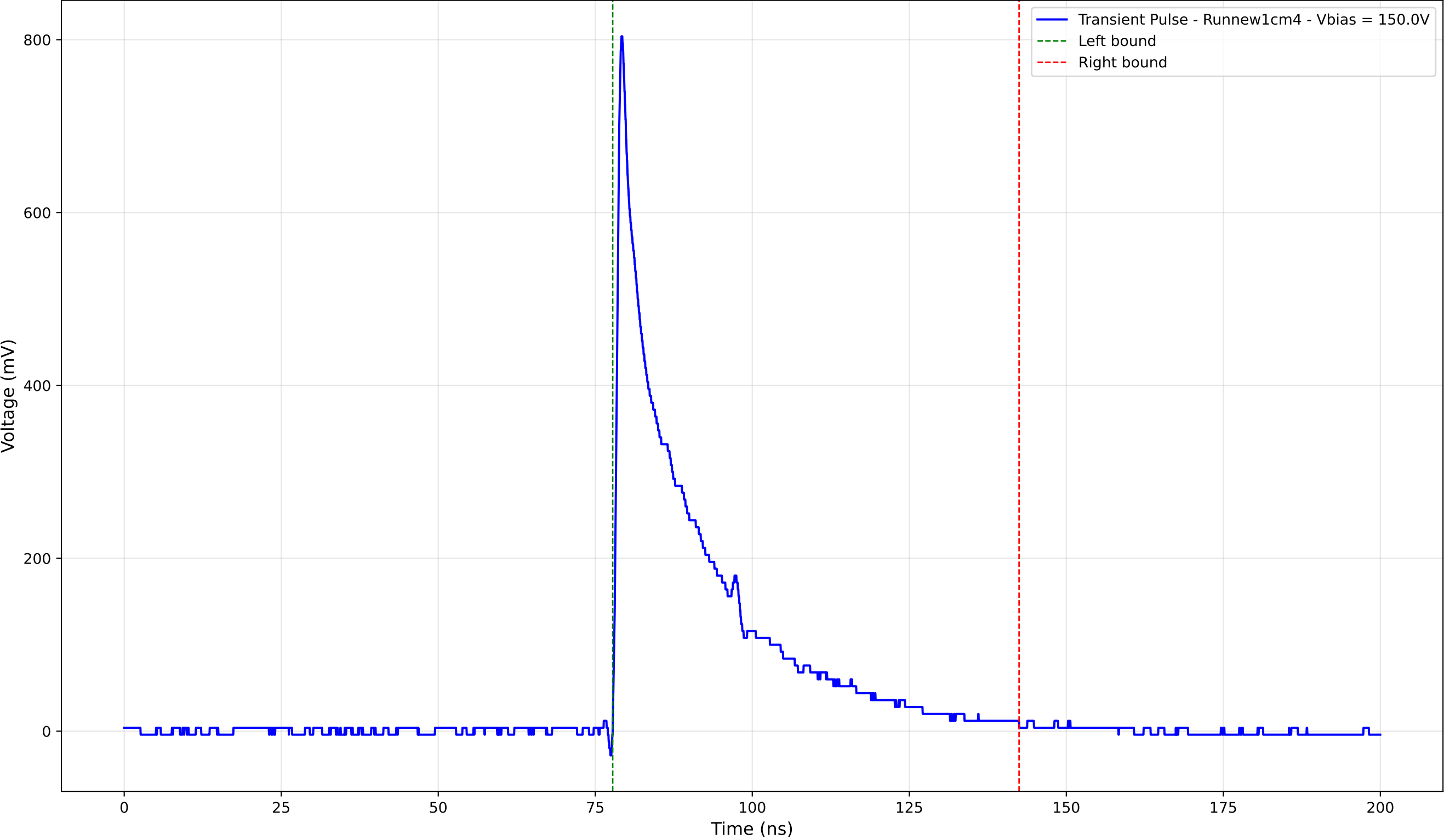
Transient Pulse - Sample: new1cm - Position: 4825.0 \mu\text{m} - Charge: 175.03 pC
