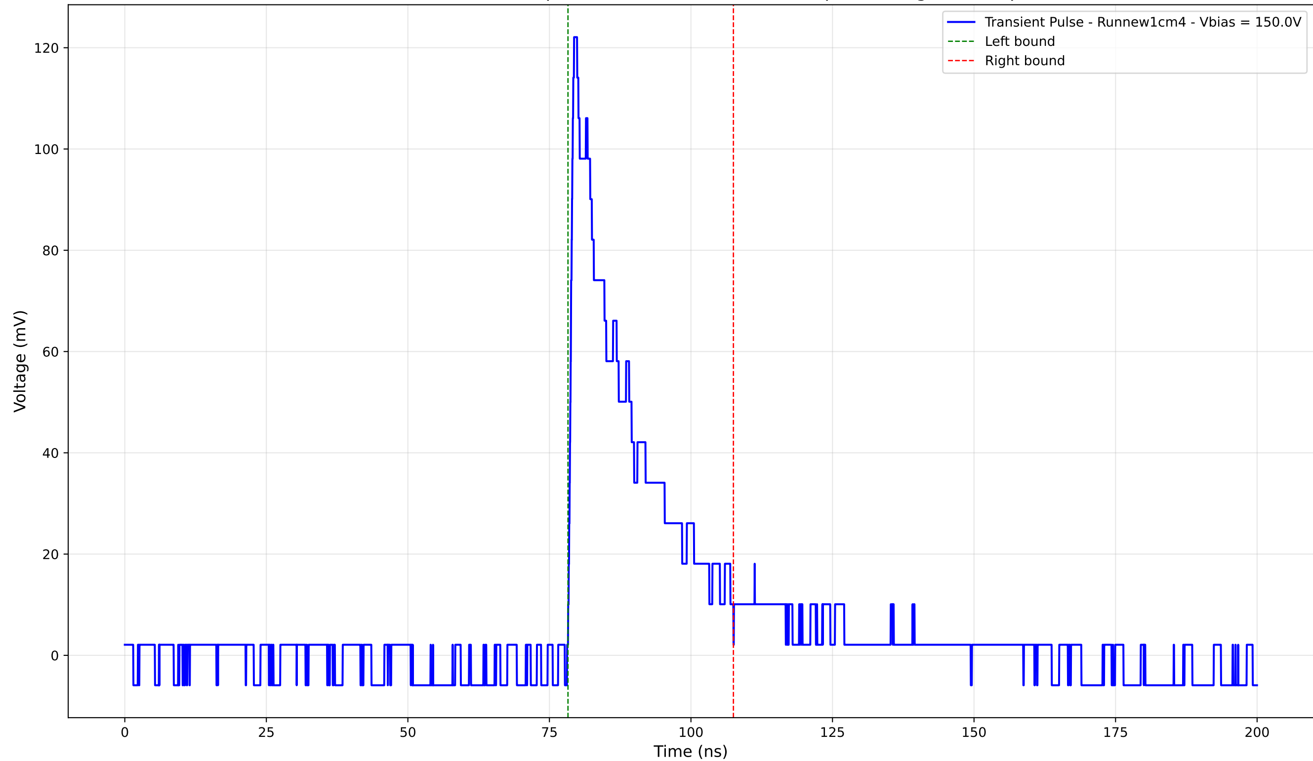
Transient Pulse - Sample: new1cm - Position: 685.0 \mu\text{m} - Charge: 25.77 pC
