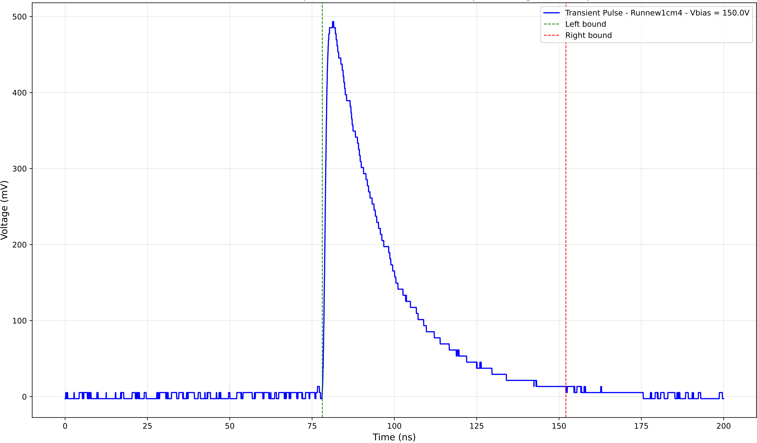
Transient Pulse - Sample: new1cm - Position: 3800.0 \mu\text{m} - Charge: 193.42 pC
