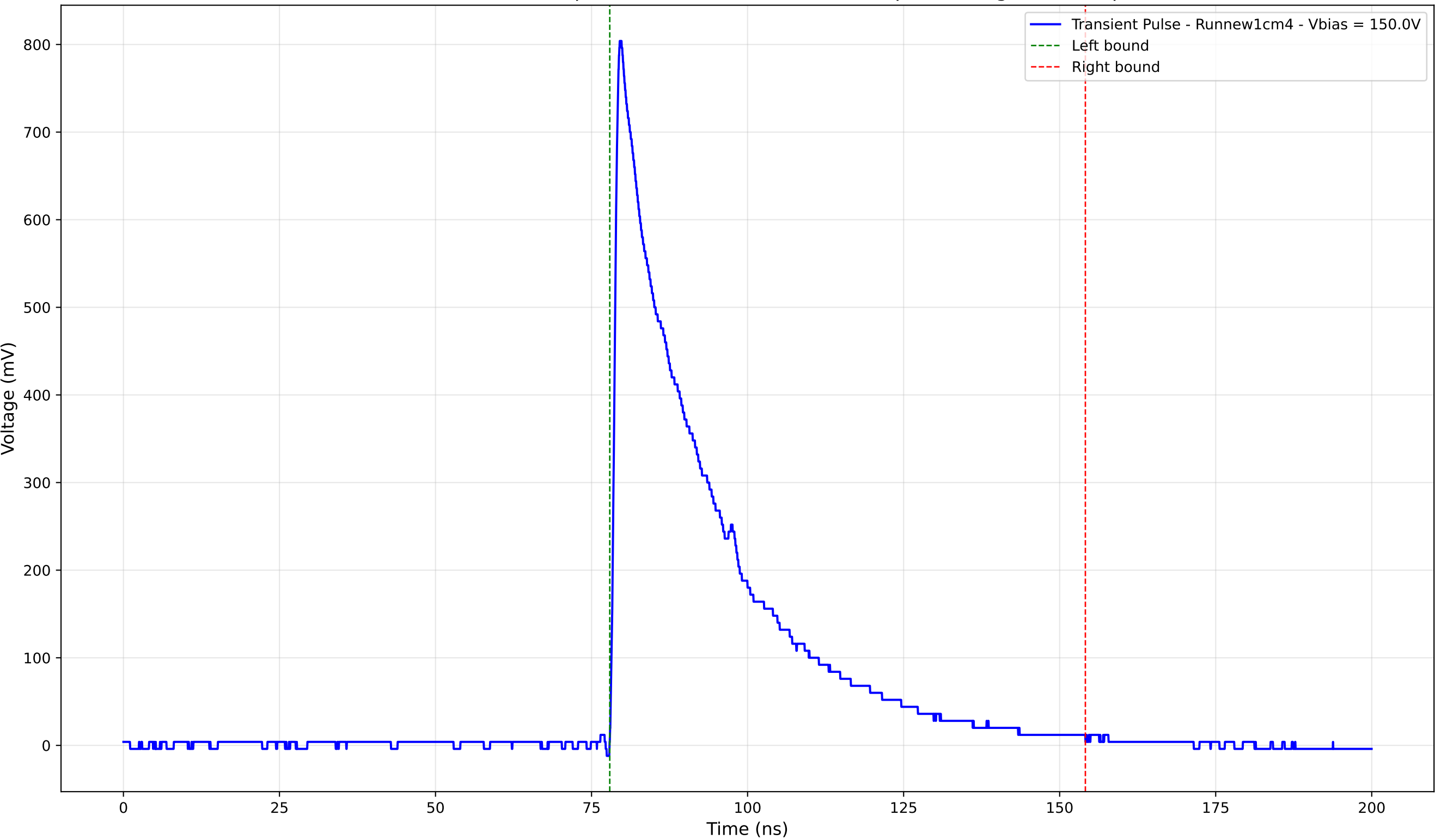
Transient Pulse - Sample: new1cm - Position: 4415.0 \mu\text{m} - Charge: 245.76 pC
