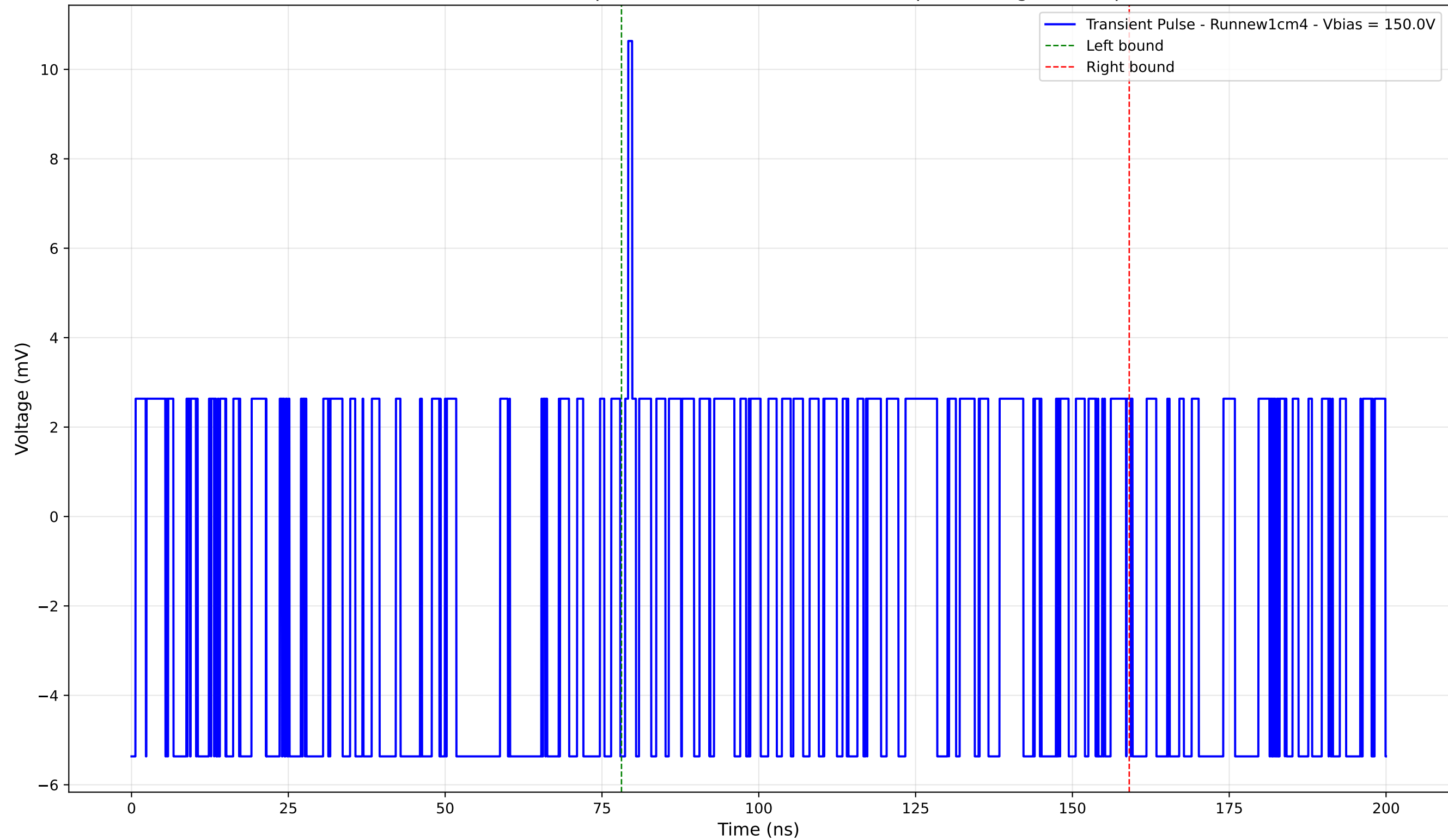
Transient Pulse - Sample: new1cm - Position: 5200.0 \mu\text{m} - Charge: -0.14 pC
