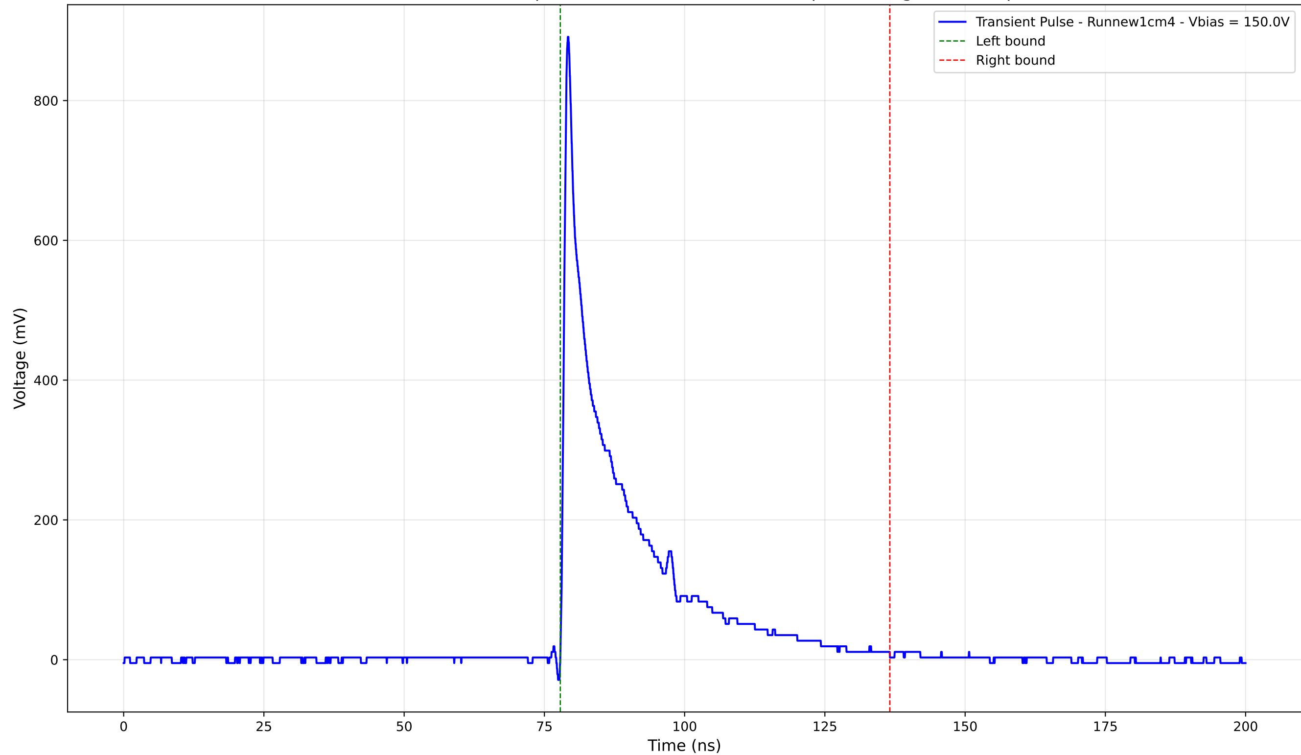
Transient Pulse - Sample: new1cm - Position: 280.0 \mu\text{m} - Charge: 157.01 pC
