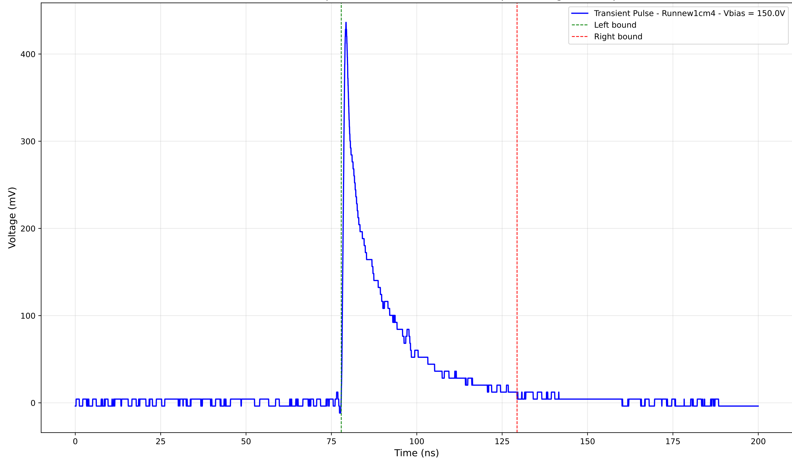
Transient Pulse - Sample: new1cm - Position: 4775.0 \mu\text{m} - Charge: 84.35 pC
