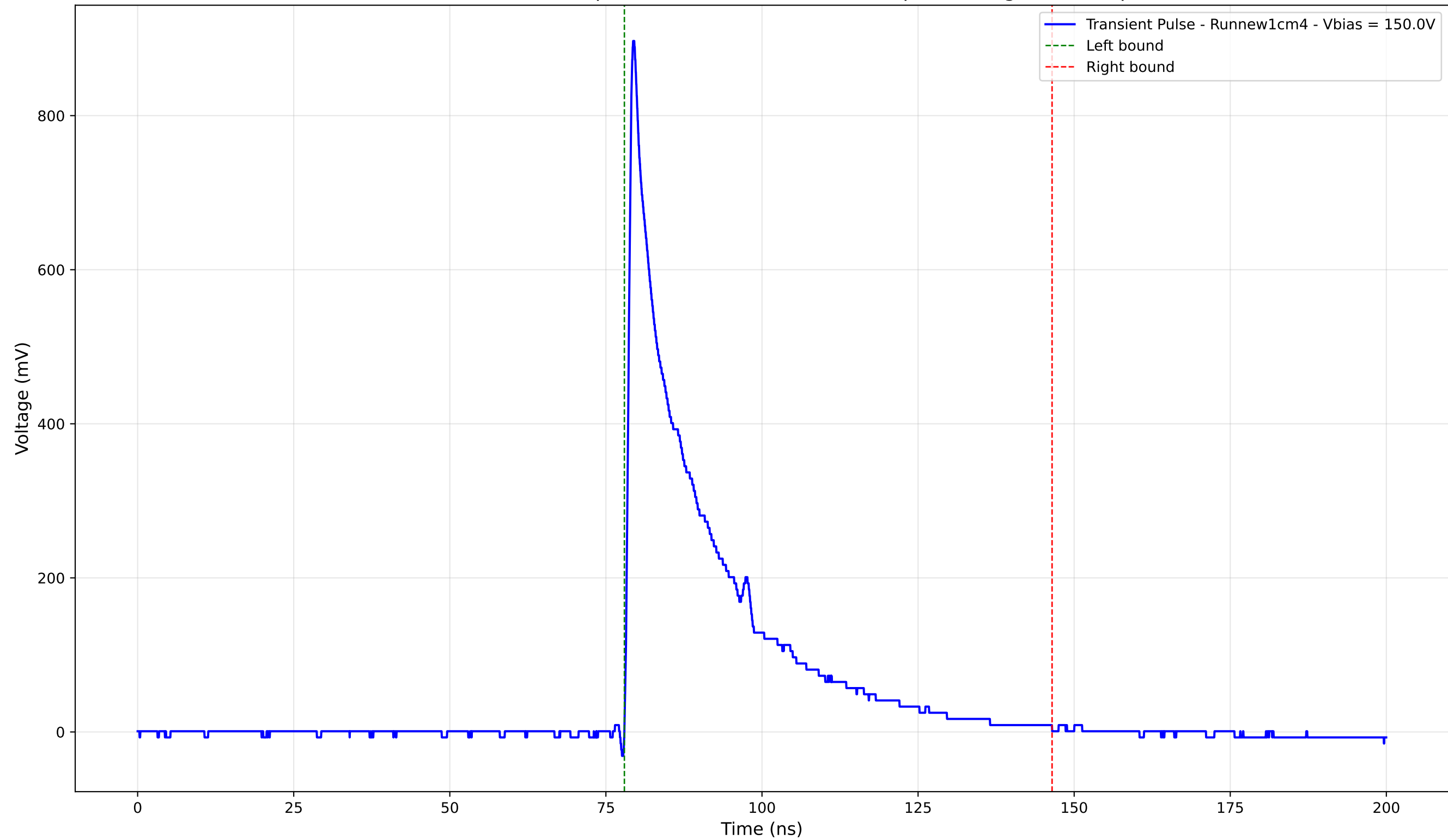
Transient Pulse - Sample: new1cm - Position: 530.0 \mu\text{m} - Charge: 199.39 pC
