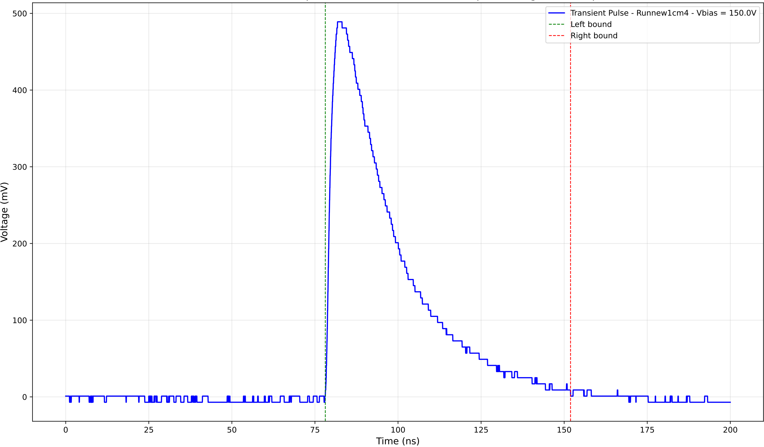
Transient Pulse - Sample: new1cm - Position: 2825.0 \mu\text{m} - Charge: 215.08 pC
