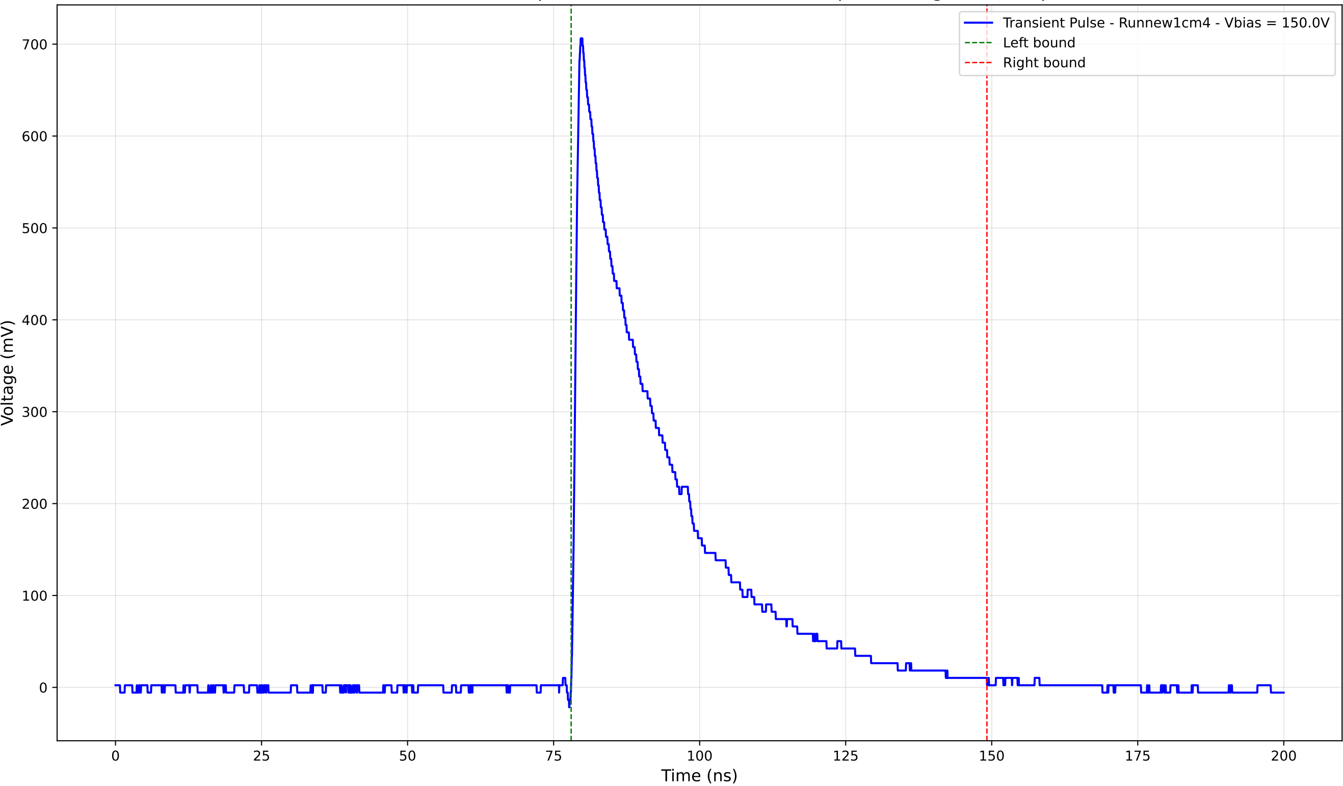
Transient Pulse - Sample: new1cm - Position: 4325.0 \mu\text{m} - Charge: 217.26 pC
