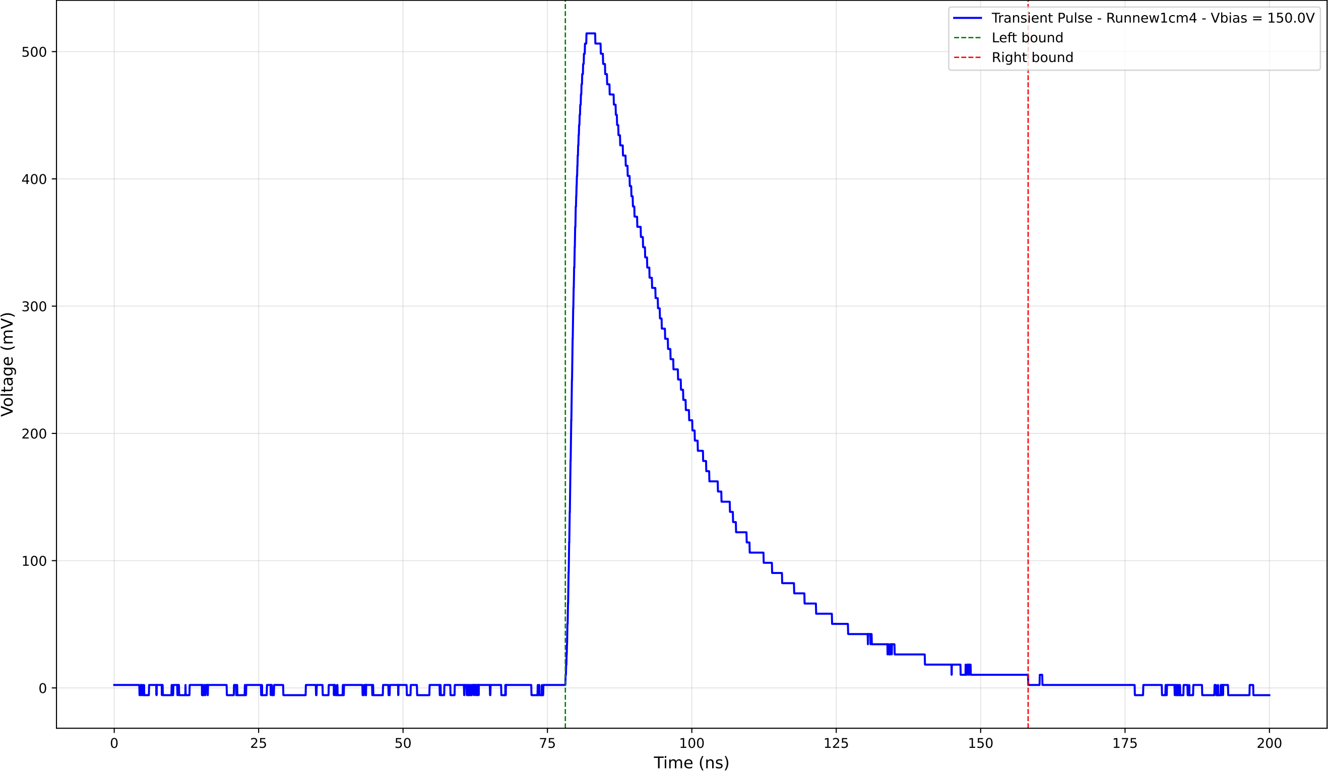
Transient Pulse - Sample: new1cm - Position: 3035.0 \mu\text{m} - Charge: 227.78 pC
