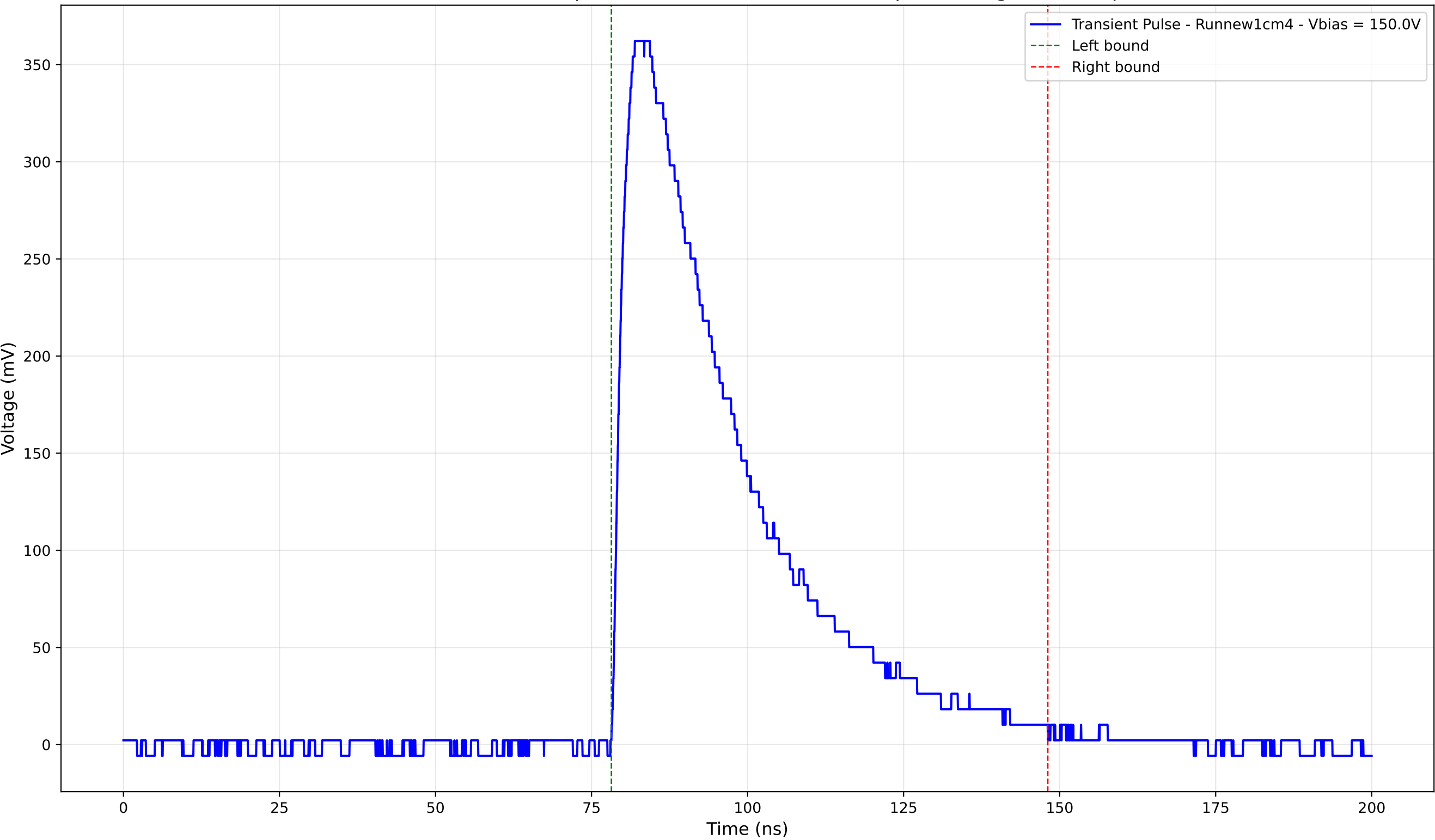
Transient Pulse - Sample: new1cm - Position: 2650.0 \mu\text{m} - Charge: 154.82 pC
