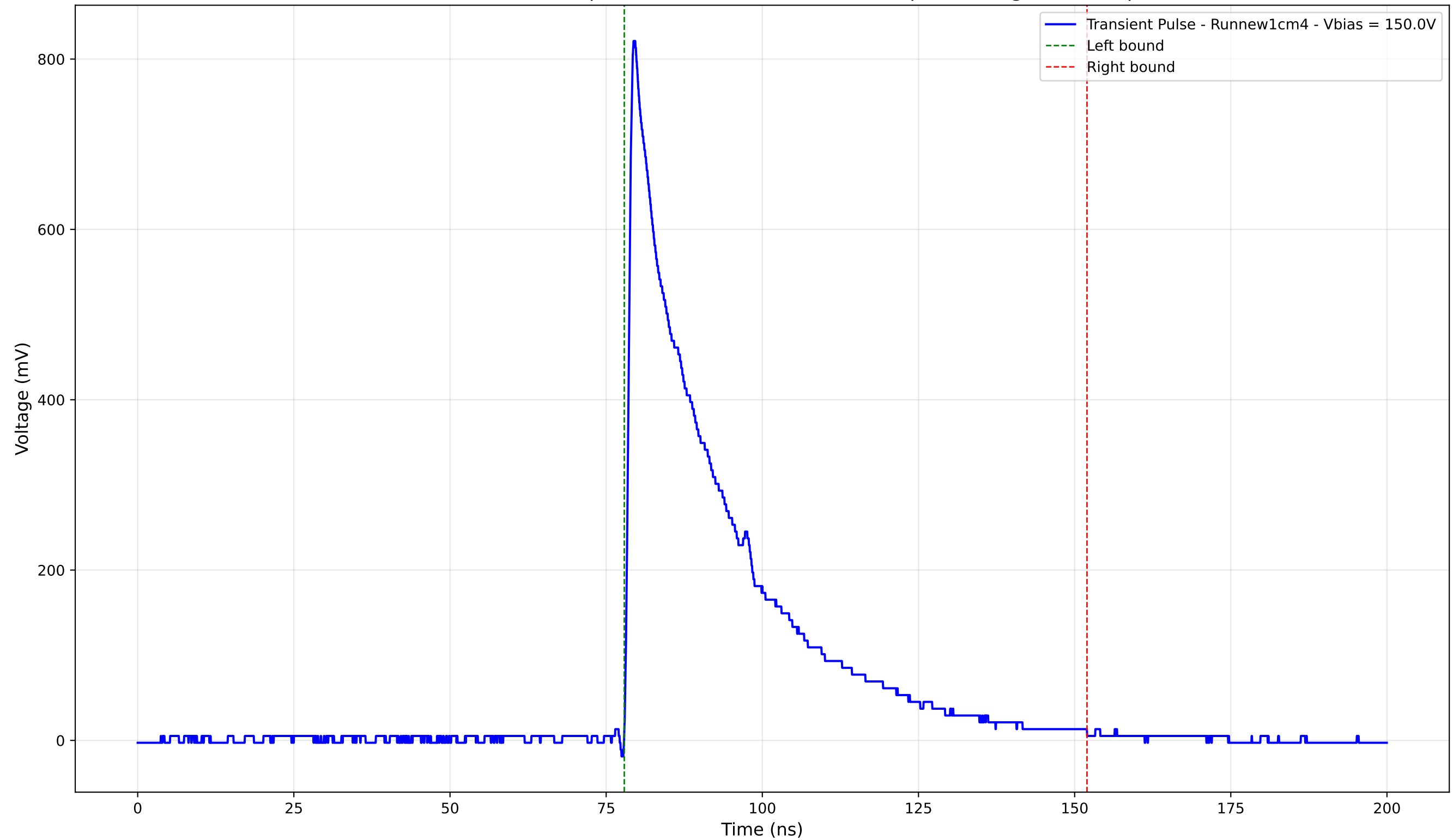
Transient Pulse - Sample: new1cm - Position: 4525.0 \mu\text{m} - Charge: 240.63 pC
