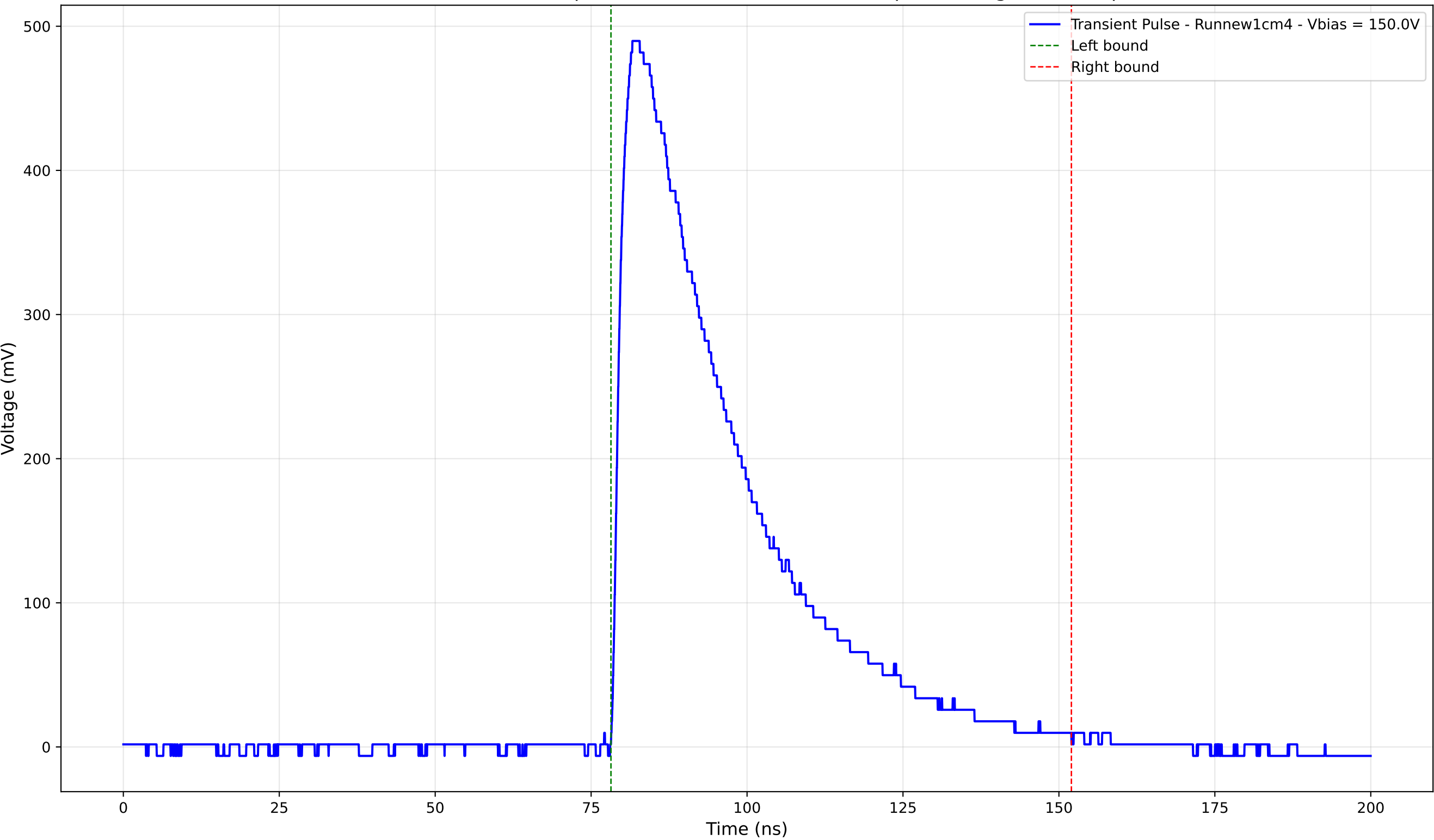
Transient Pulse - Sample: new1cm - Position: 2115.0 \mu\text{m} - Charge: 204.18 pC
