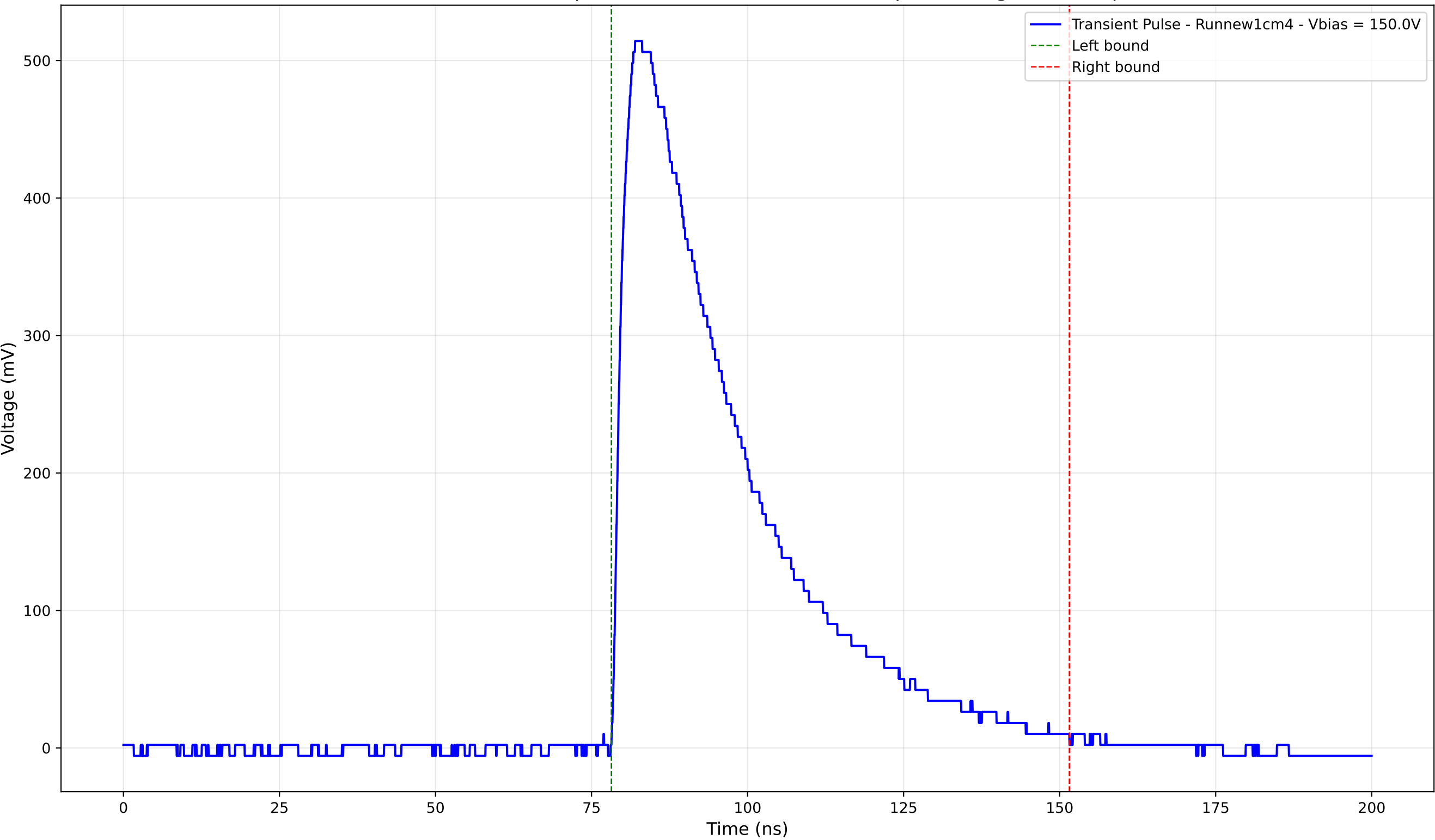
Transient Pulse - Sample: new1cm - Position: 2480.0 \mu\text{m} - Charge: 222.73 pC
