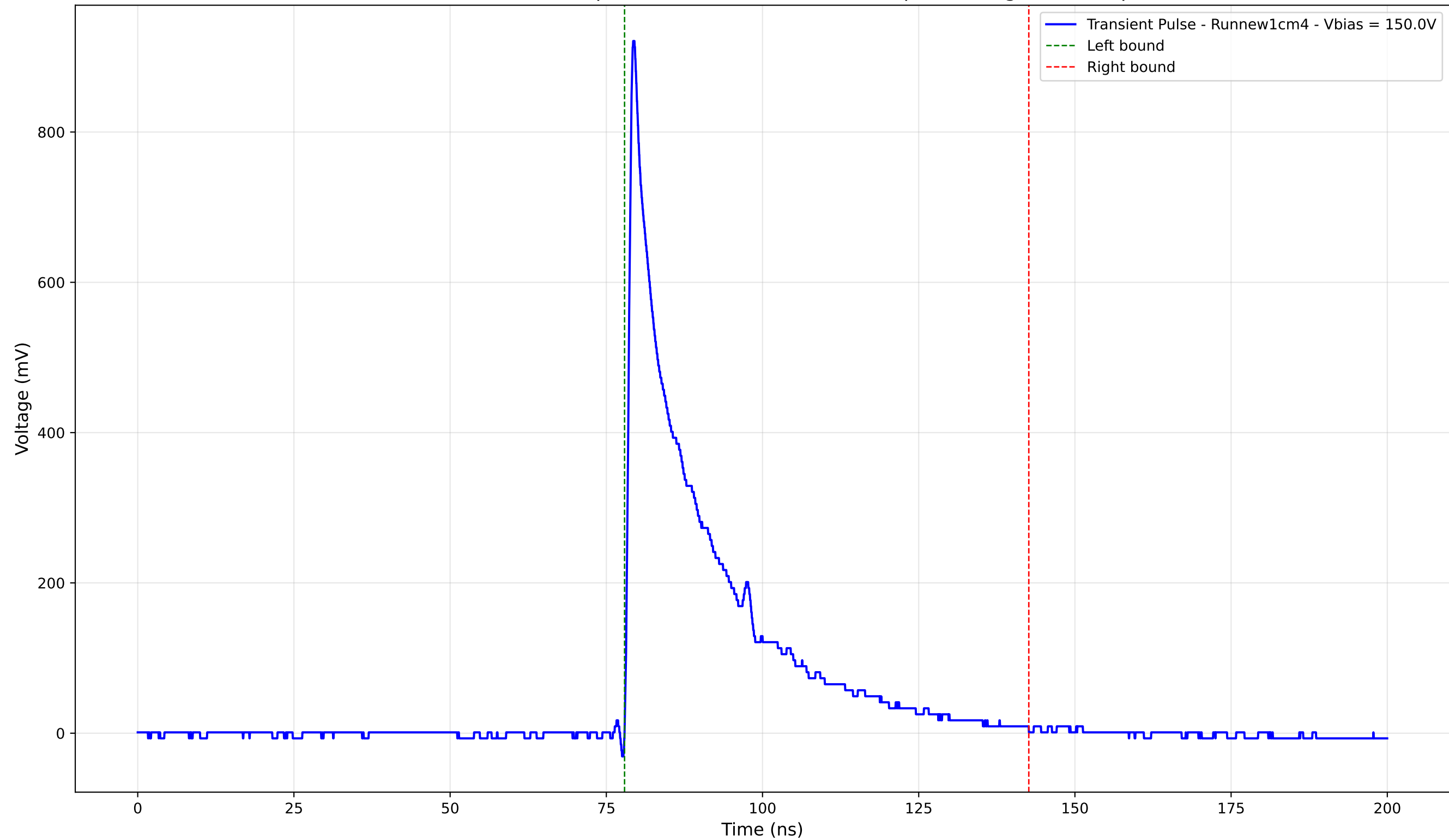
Transient Pulse - Sample: new1cm - Position: 465.0 \mu\text{m} - Charge: 198.41 pC
