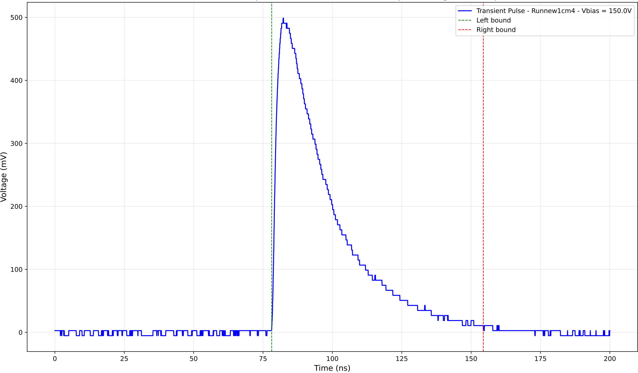
Transient Pulse - Sample: new1cm - Position: 2905.0 \mu\text{m} - Charge: 220.55 pC
