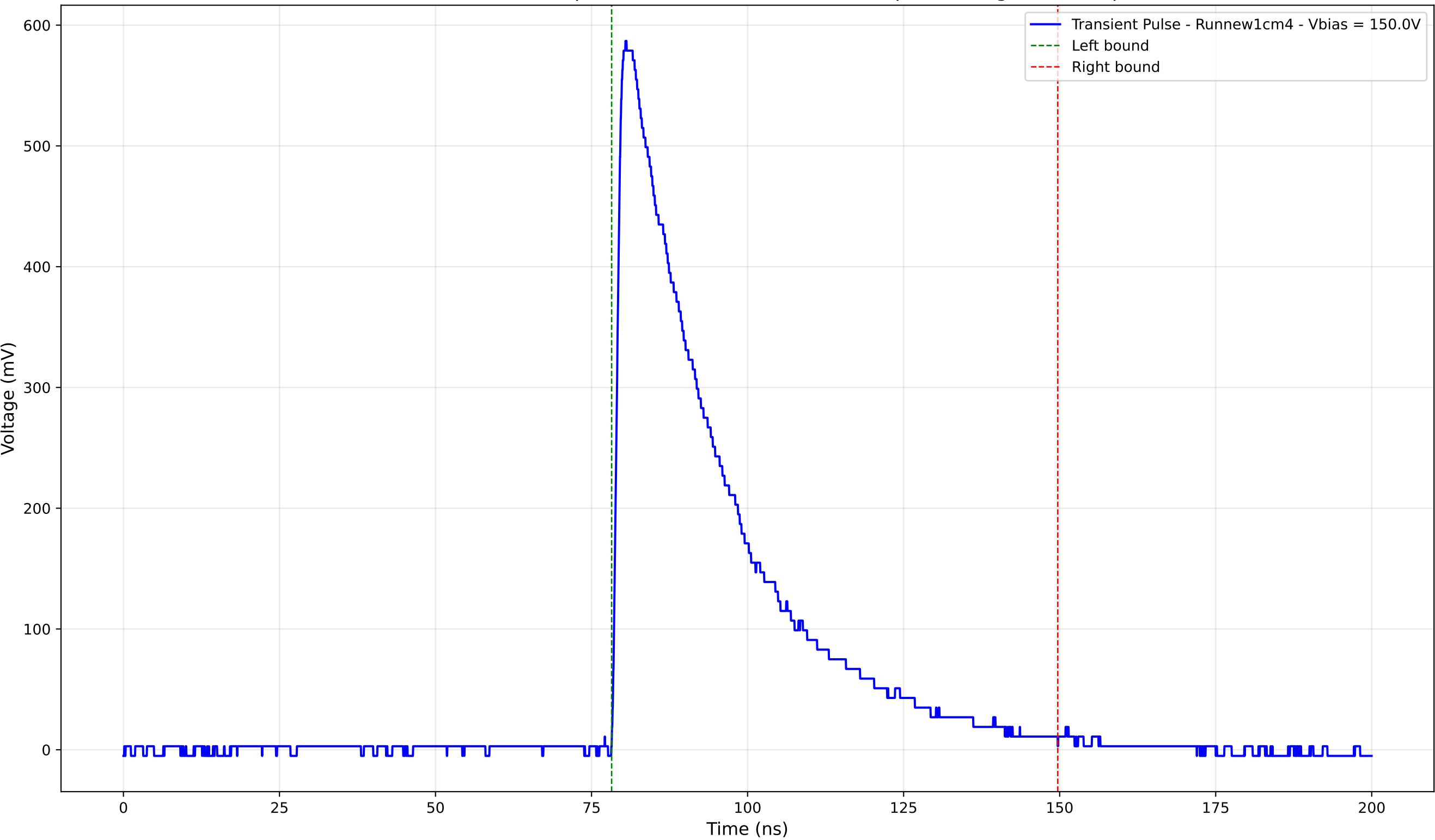
Transient Pulse - Sample: new1cm - Position: 1365.0 \mu\text{m} - Charge: 209.98 pC
