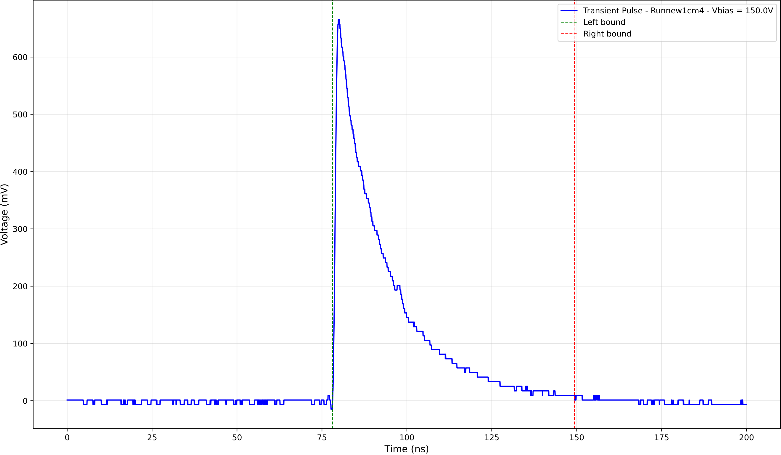
Transient Pulse - Sample: new1cm - Position: 1030.0 \mu\text{m} - Charge: 199.69 pC
