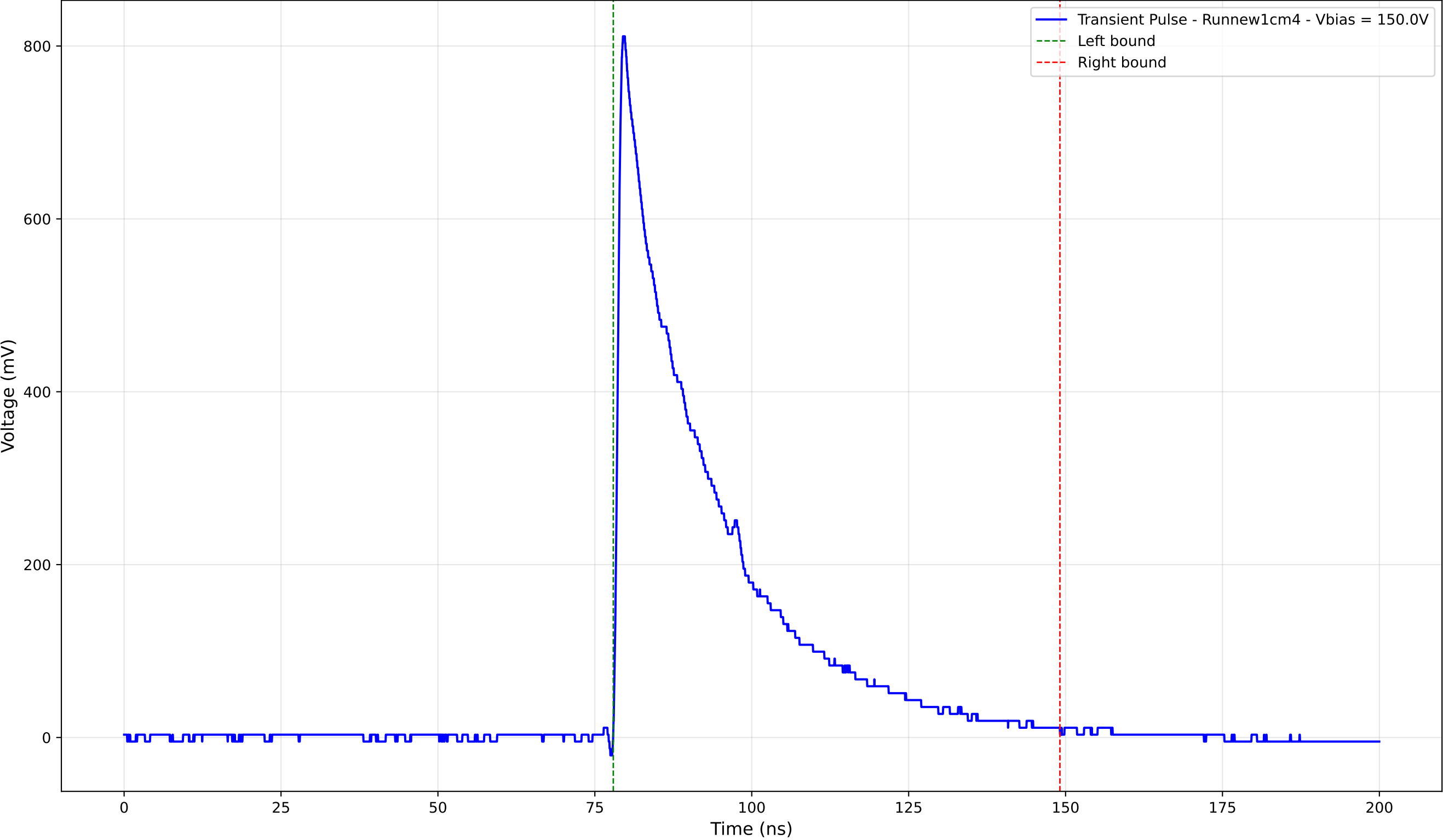
Transient Pulse - Sample: new1cm - Position: 4450.0 \mu\text{m} - Charge: 241.62 pC
