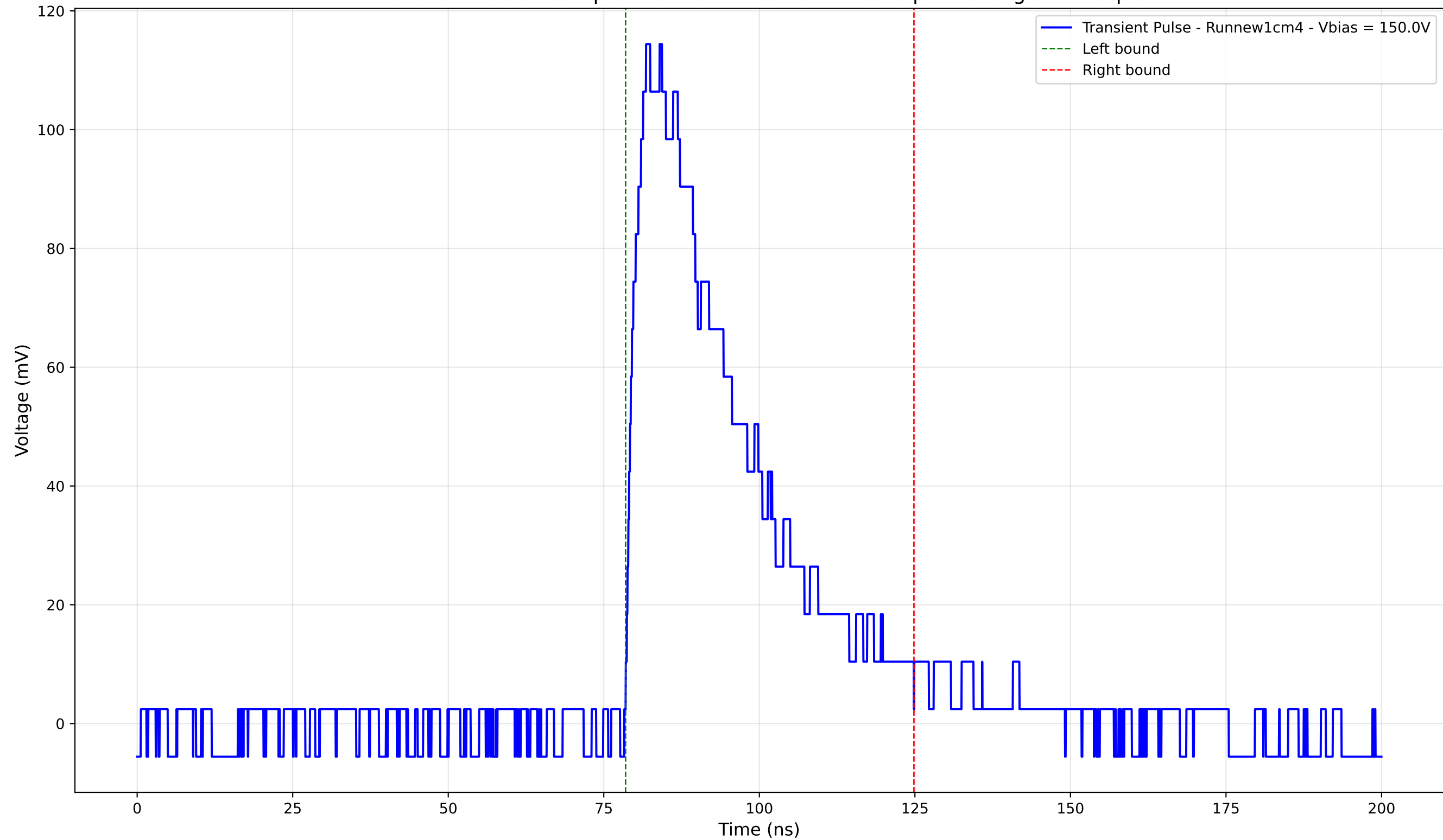
Transient Pulse - Sample: new1cm - Position: 2185.0 \mu\text{m} - Charge: 42.75 pC
