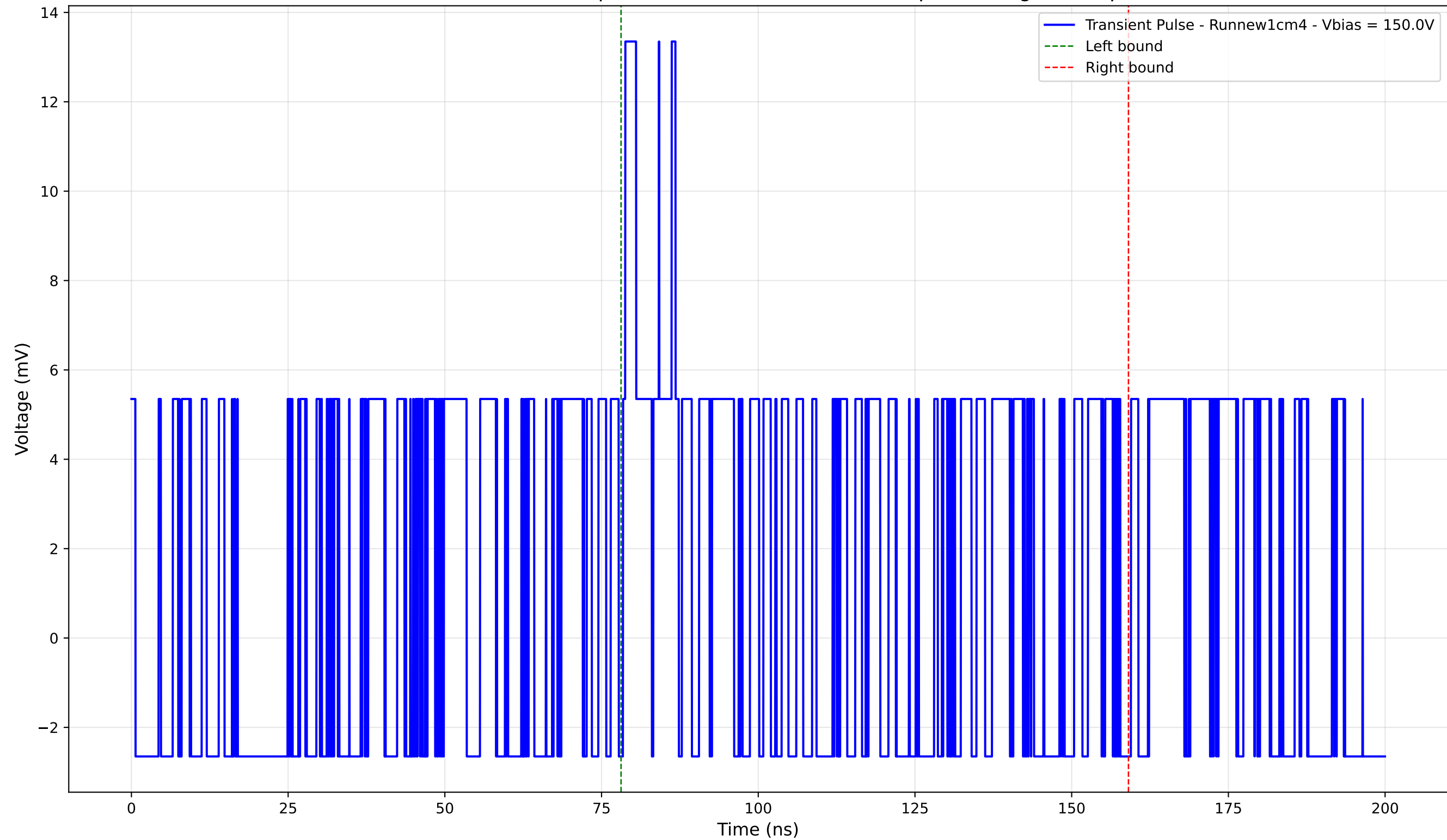
Transient Pulse - Sample: new1cm - Position: 5115.0 \mu\text{m} - Charge: 3.34 pC
