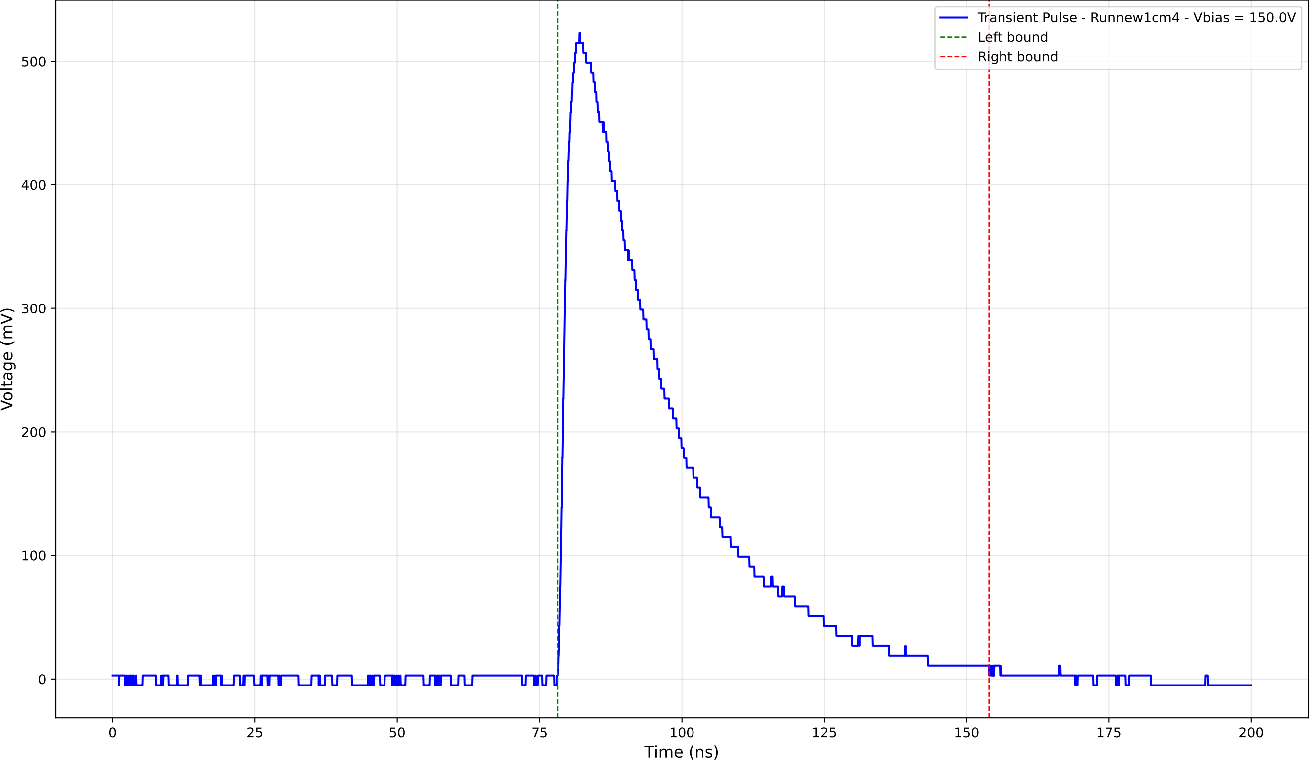
Transient Pulse - Sample: new1cm - Position: 1950.0 \mu\text{m} - Charge: 213.25 pC
