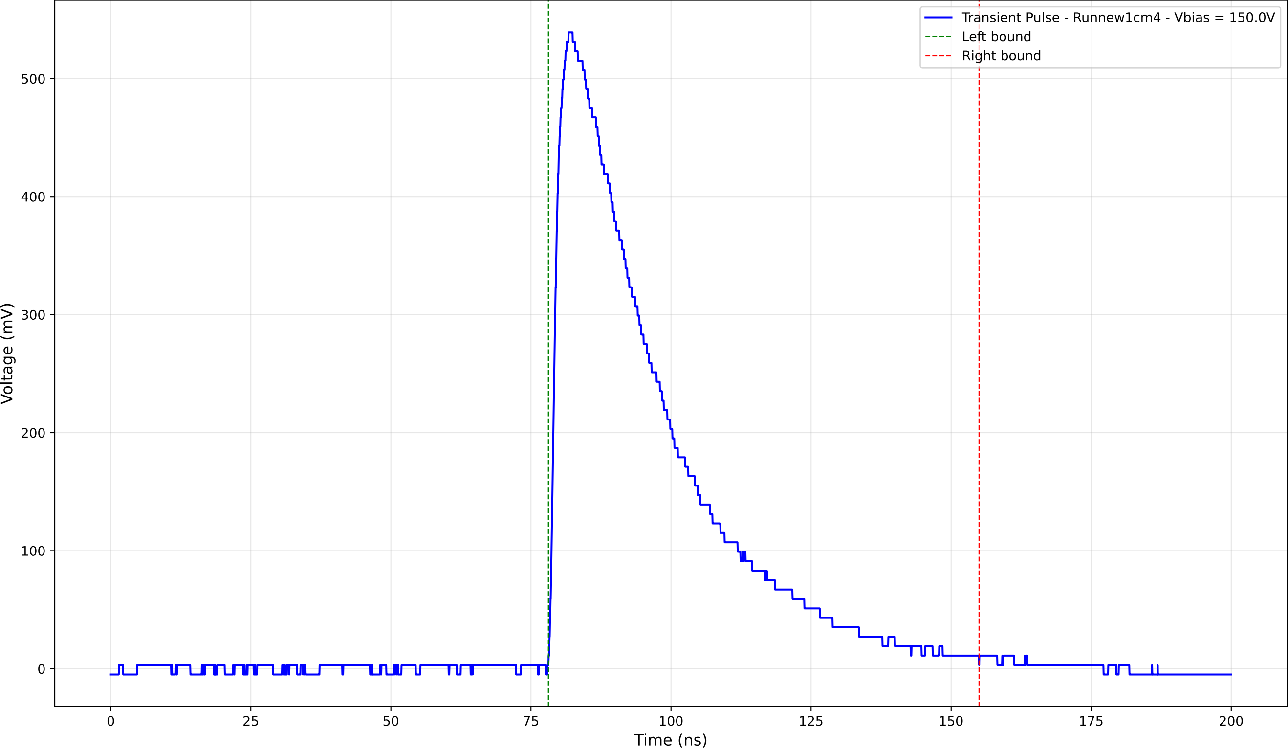
Transient Pulse - Sample: new1cm - Position: 3325.0 \mu\text{m} - Charge: 228.73 pC
