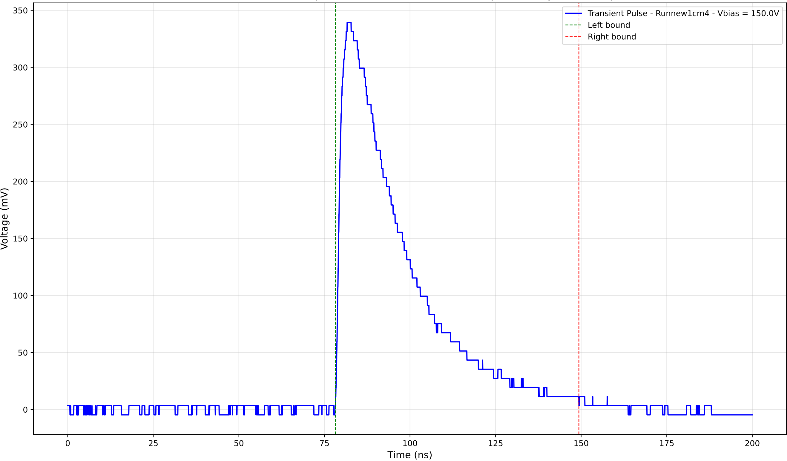
Transient Pulse - Sample: new1cm - Position: 3280.0 \mu\text{m} - Charge: 141.89 pC
