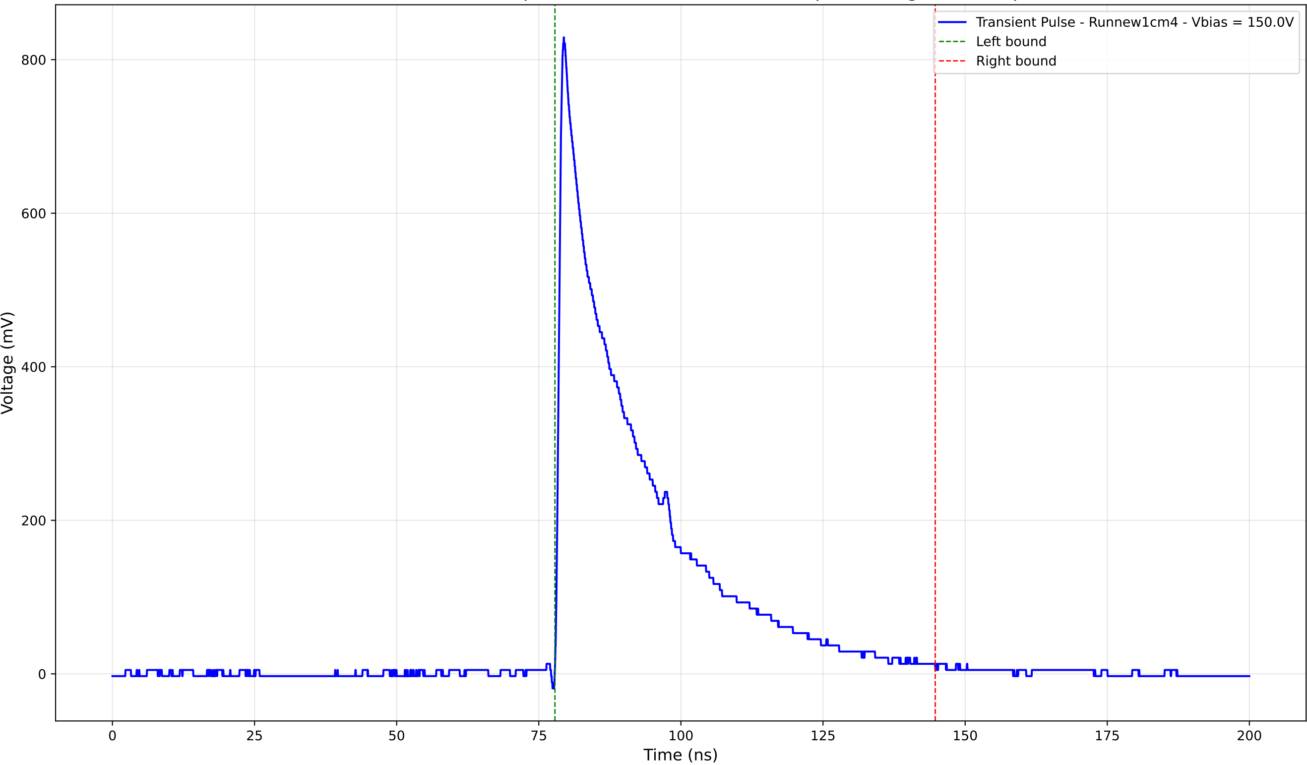
Transient Pulse - Sample: new1cm - Position: 4605.0 \mu\text{m} - Charge: 228.78 pC
