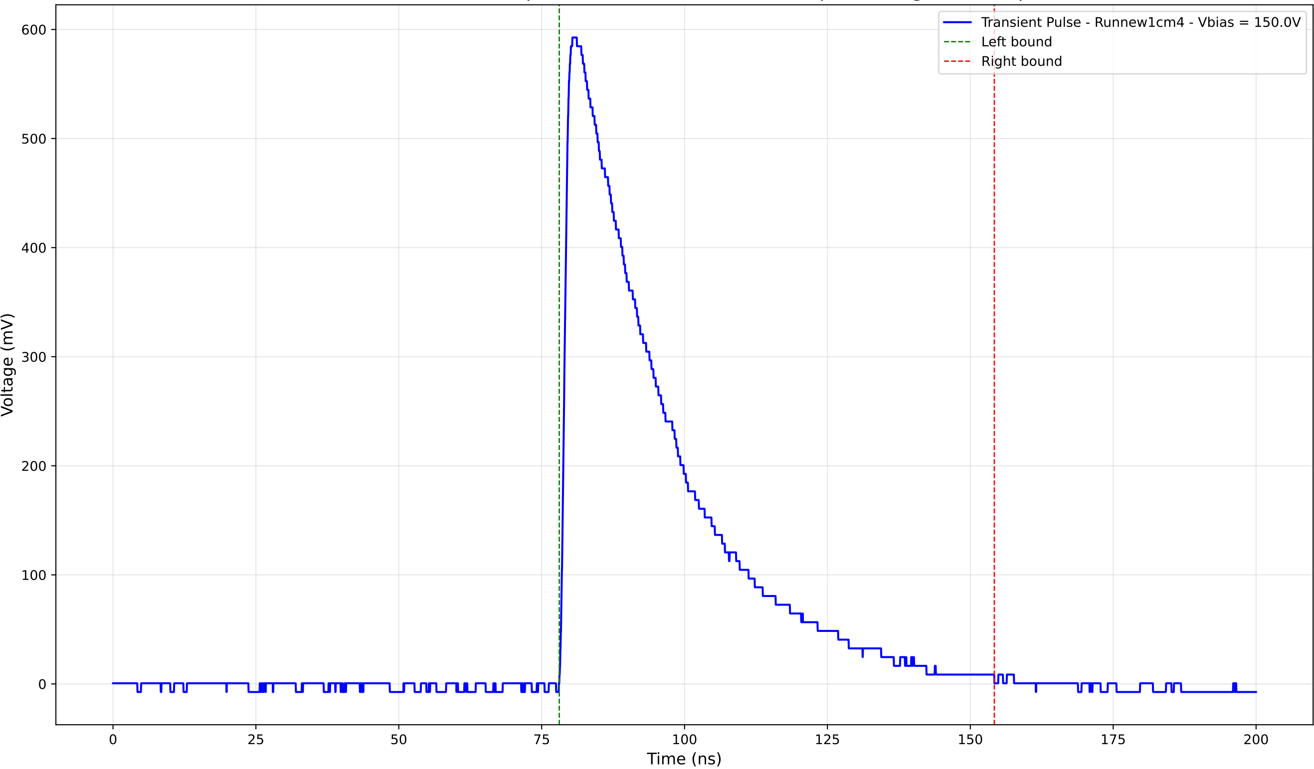
Transient Pulse - Sample: new1cm - Position: 3825.0 \mu\text{m} - Charge: 229.52 pC
