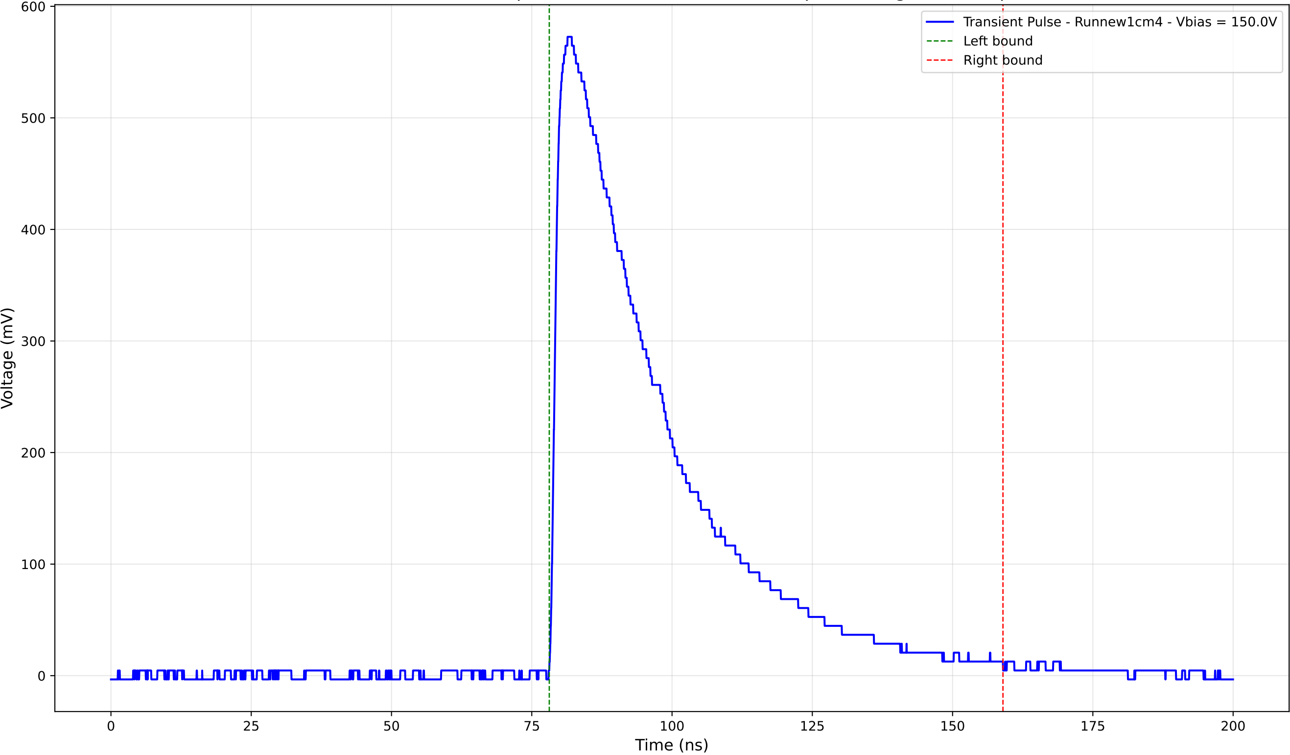
Transient Pulse - Sample: new1cm - Position: 3540.0 \mu\text{m} - Charge: 243.30 pC
