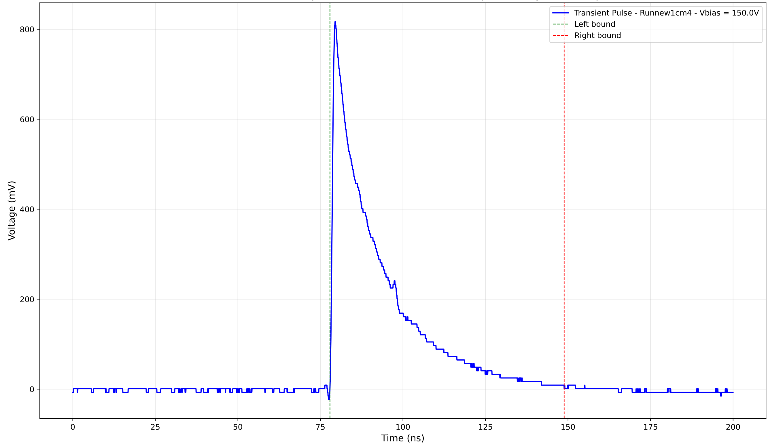
Transient Pulse - Sample: new1cm - Position: 4540.0 \mu\text{m} - Charge: 230.73 pC
