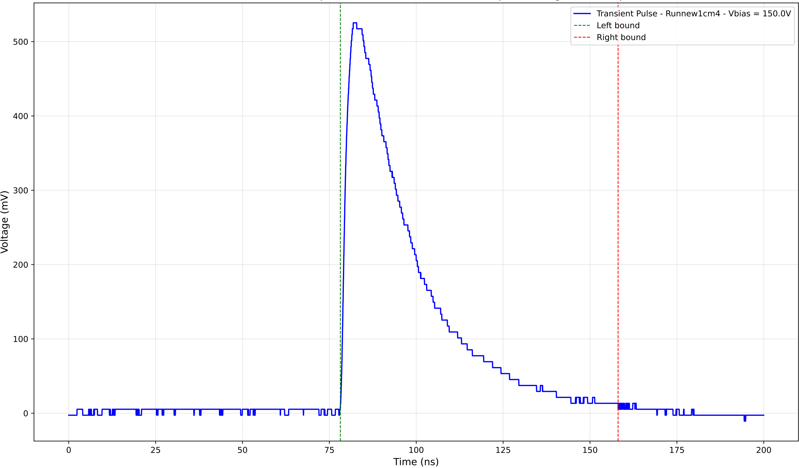
Transient Pulse - Sample: new1cm - Position: 2370.0 \mu\text{m} - Charge: 231.07 pC
