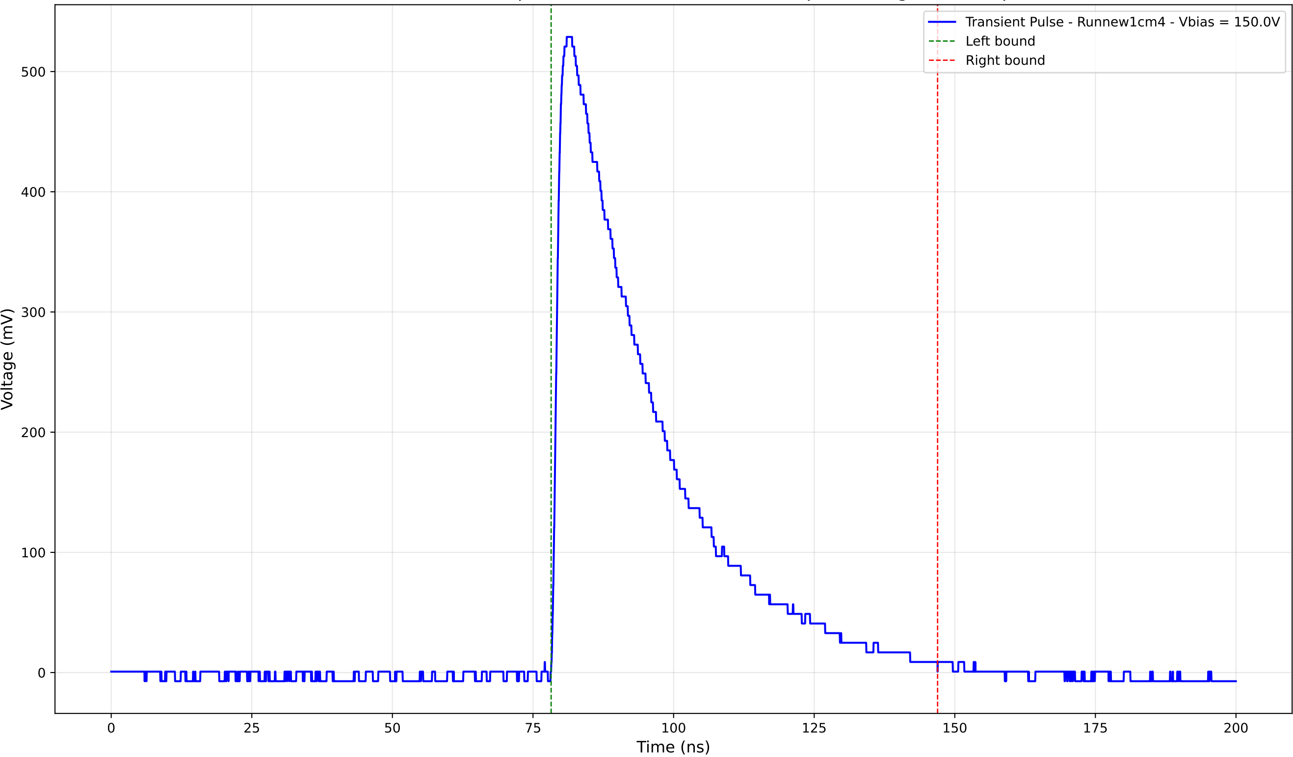
Transient Pulse - Sample: new1cm - Position: 1605.0 \mu\text{m} - Charge: 200.44 pC
