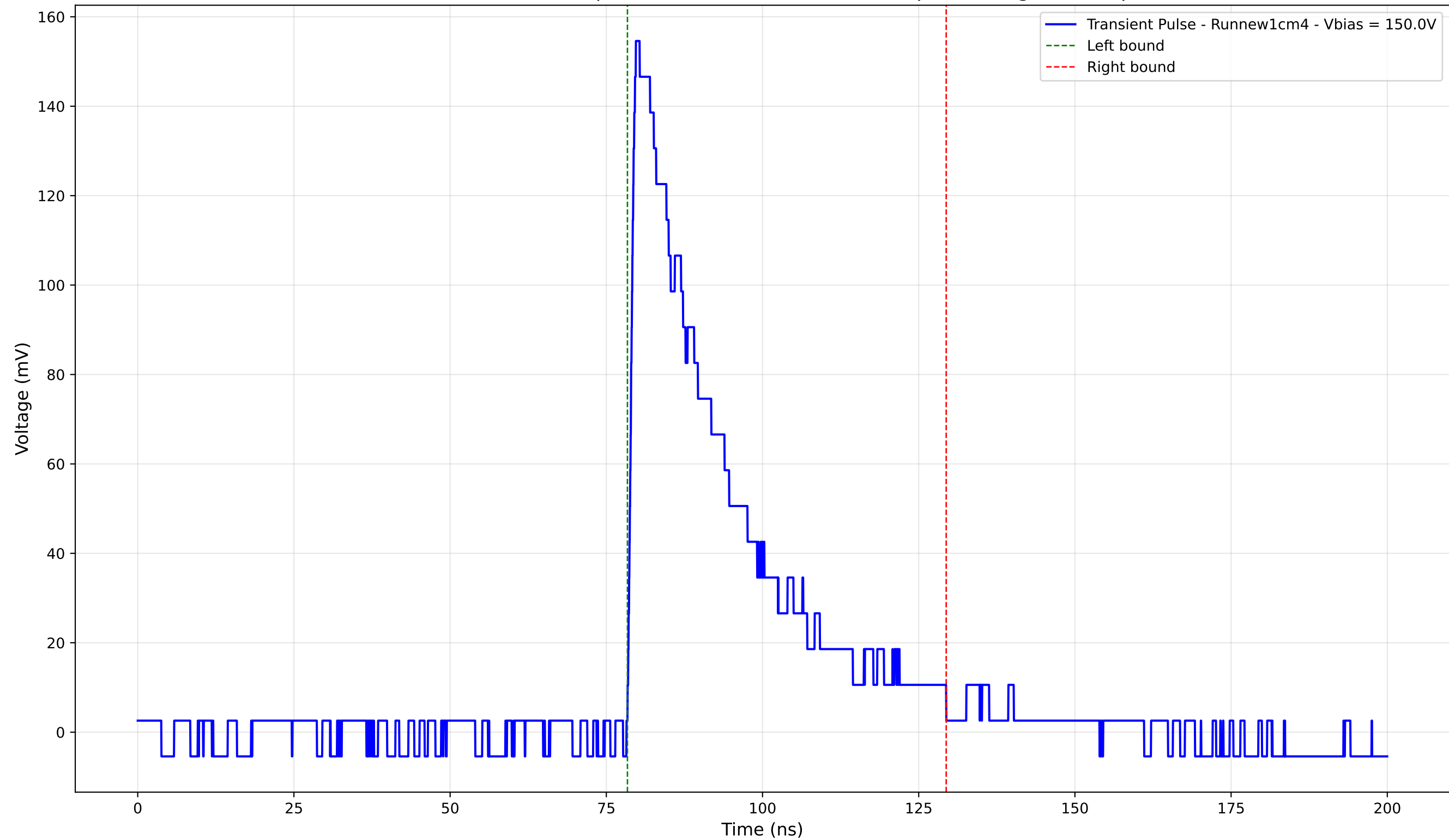
Transient Pulse - Sample: new1cm - Position: 1175.0 \mu\text{m} - Charge: 48.16 pC
