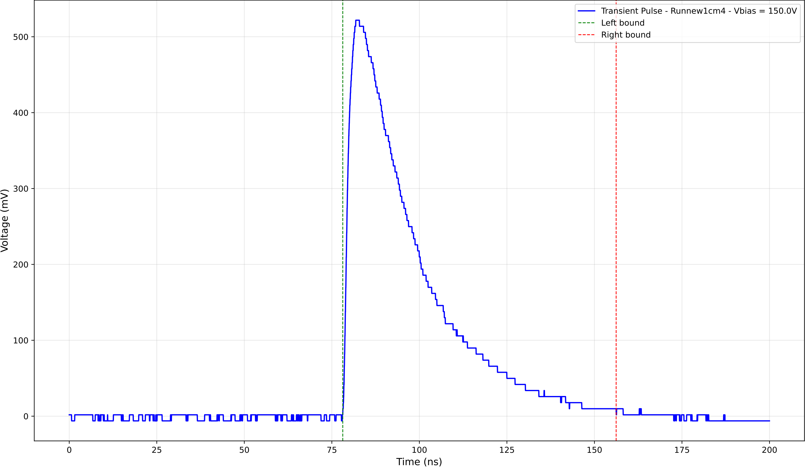
Transient Pulse - Sample: new1cm - Position: 3020.0 \mu\text{m} - Charge: 229.17 pC
