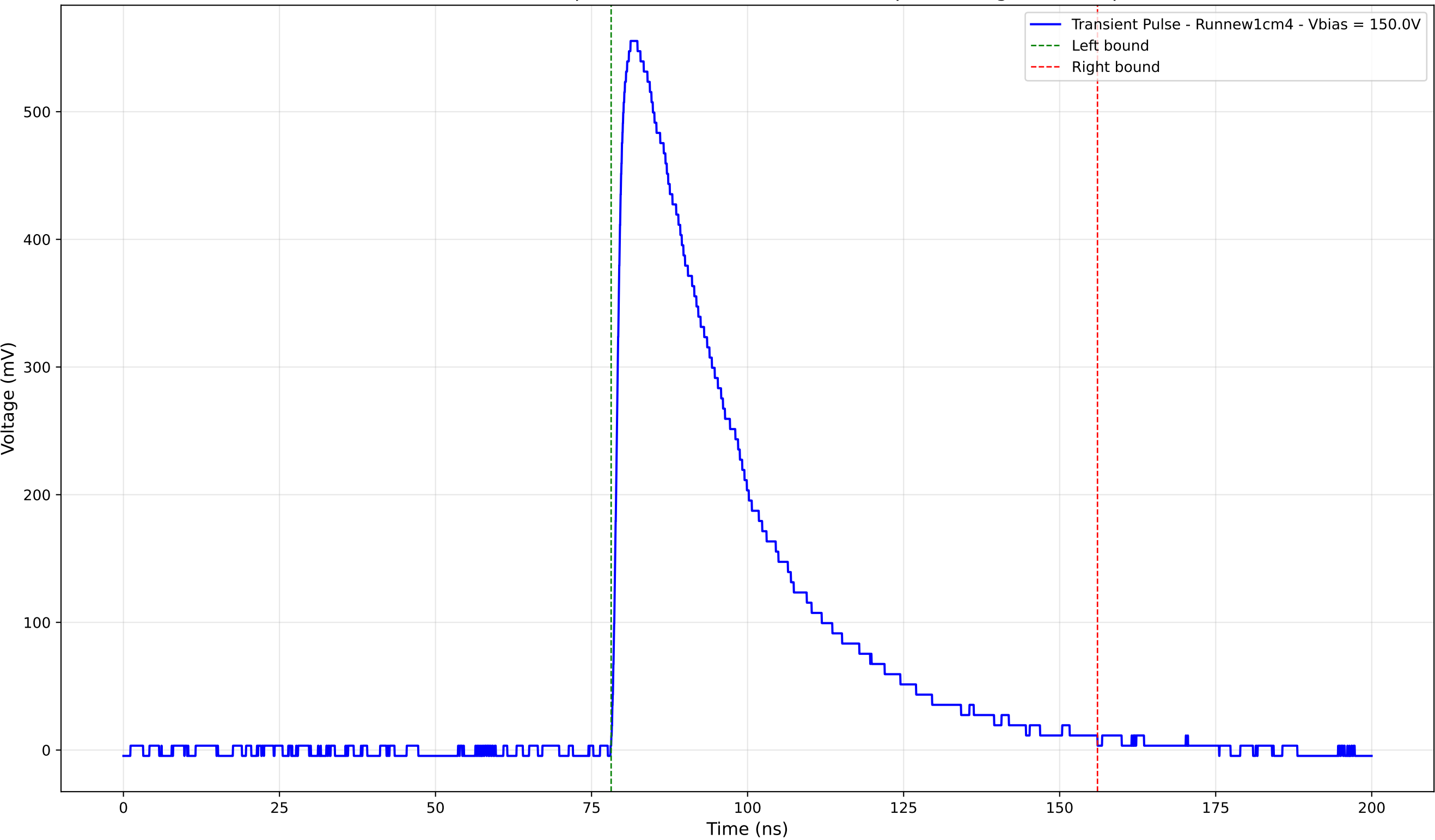
Transient Pulse - Sample: new1cm - Position: 3485.0 \mu\text{m} - Charge: 236.62 pC
