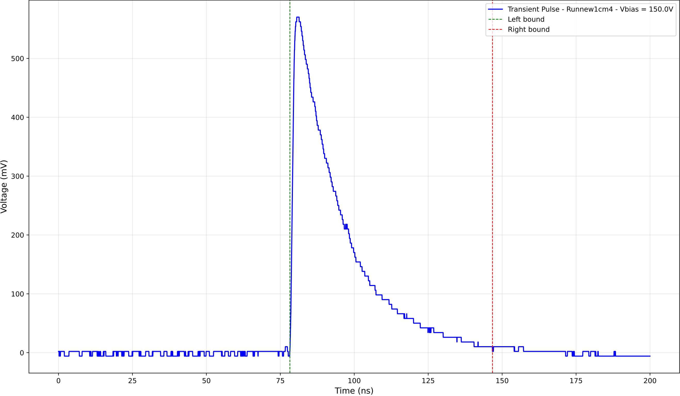
Transient Pulse - Sample: new1cm - Position: 1425.0 \mu\text{m} - Charge: 205.33 pC
