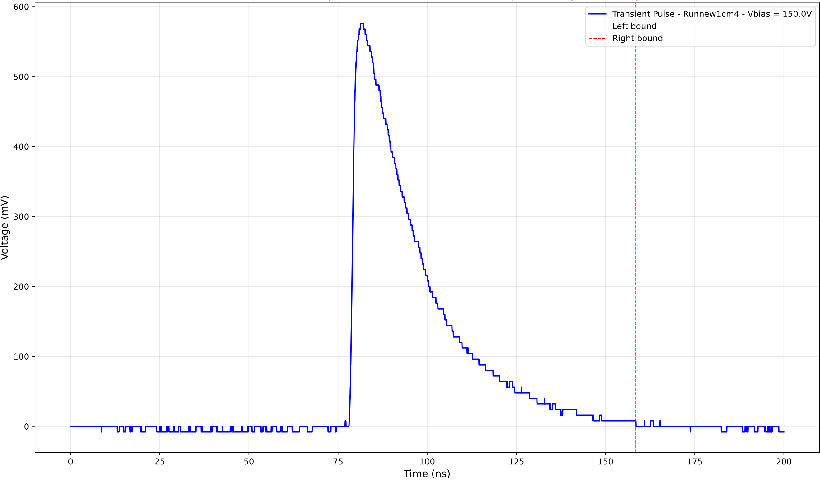
Transient Pulse - Sample: new1cm - Position: 3550.0 \mu\text{m} - Charge: 240.49 pC
