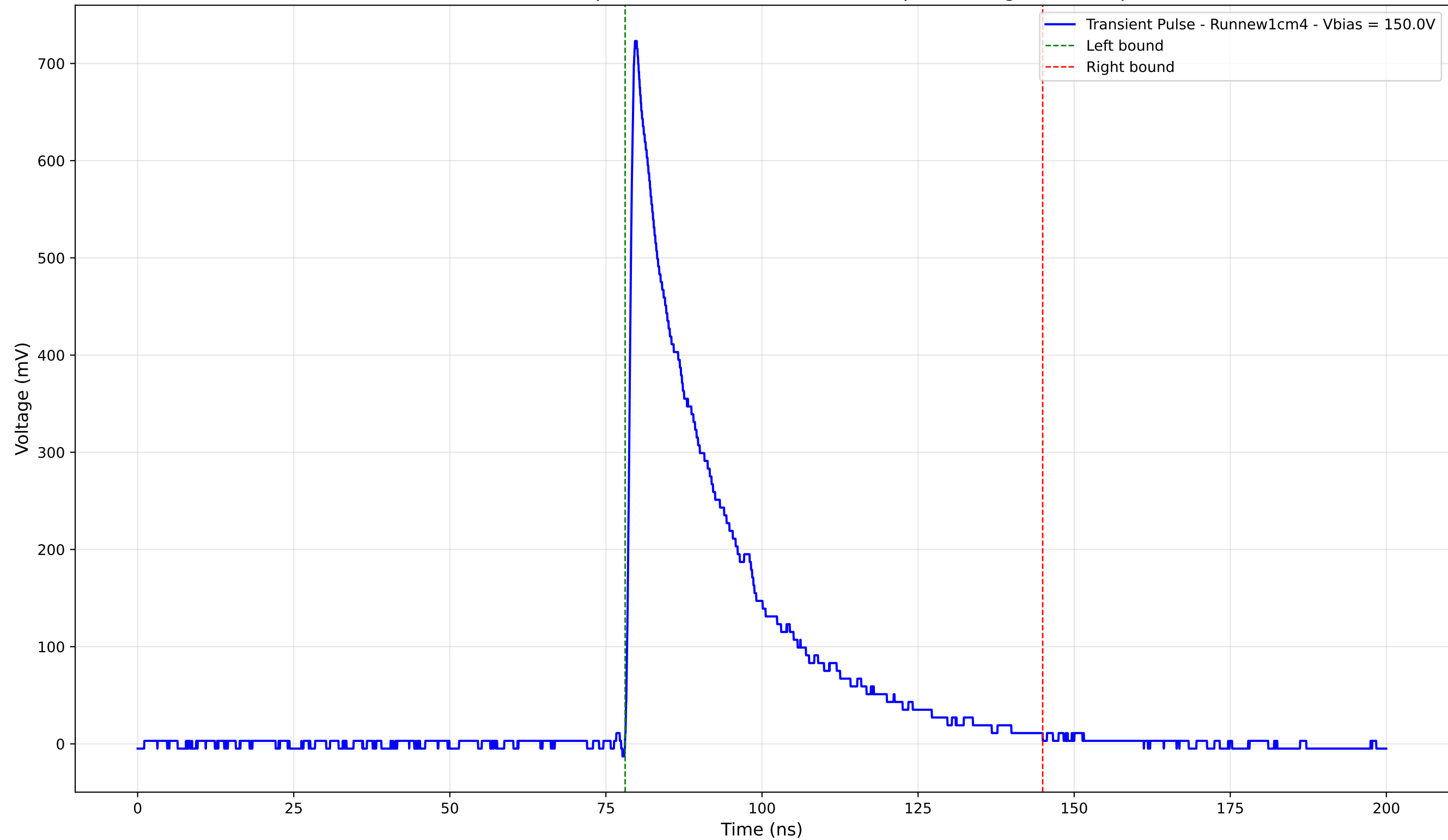
Transient Pulse - Sample: new1cm - Position: 885.0 \mu\text{m} - Charge: 200.36 pC
