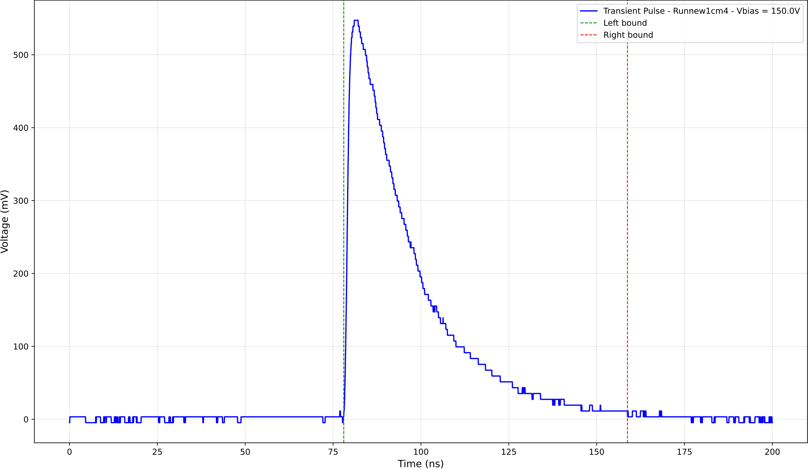
Transient Pulse - Sample: new1cm - Position: 3640.0 \mu\text{m} - Charge: 226.57 pC
