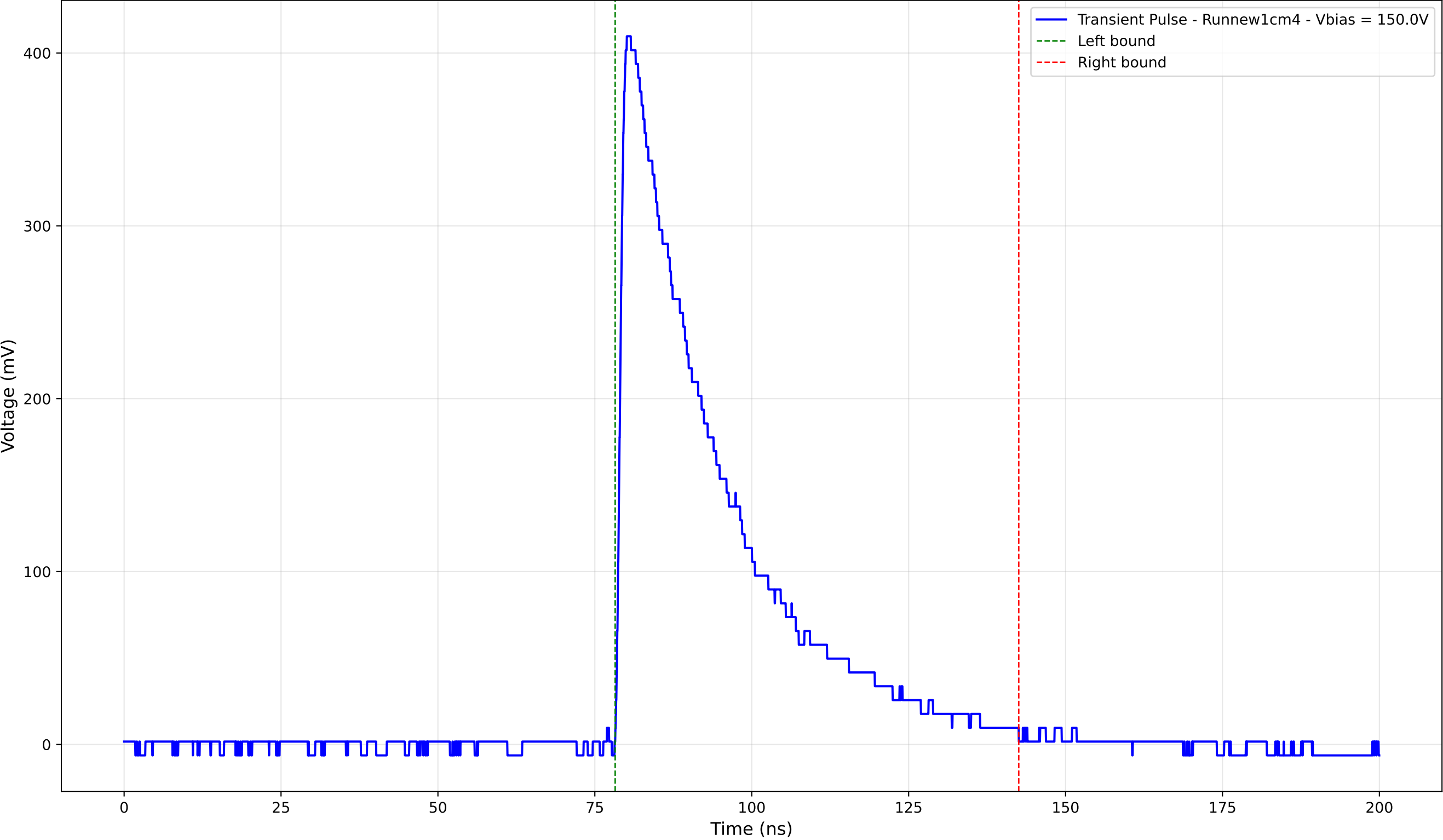
Transient Pulse - Sample: new1cm - Position: 1265.0 \mu\text{m} - Charge: 137.76 pC
