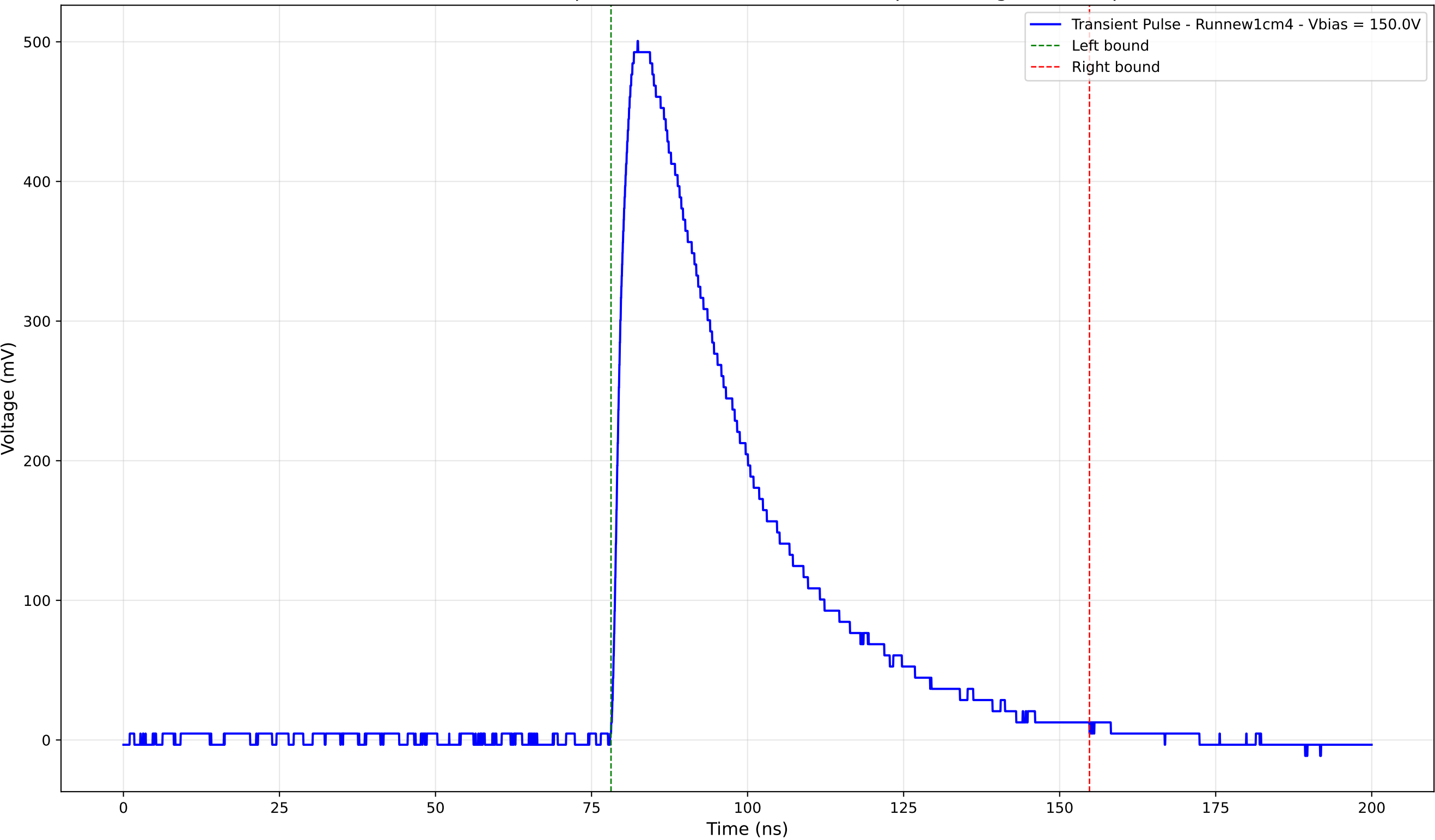
Transient Pulse - Sample: new1cm - Position: 2610.0 \mu\text{m} - Charge: 221.44 pC
