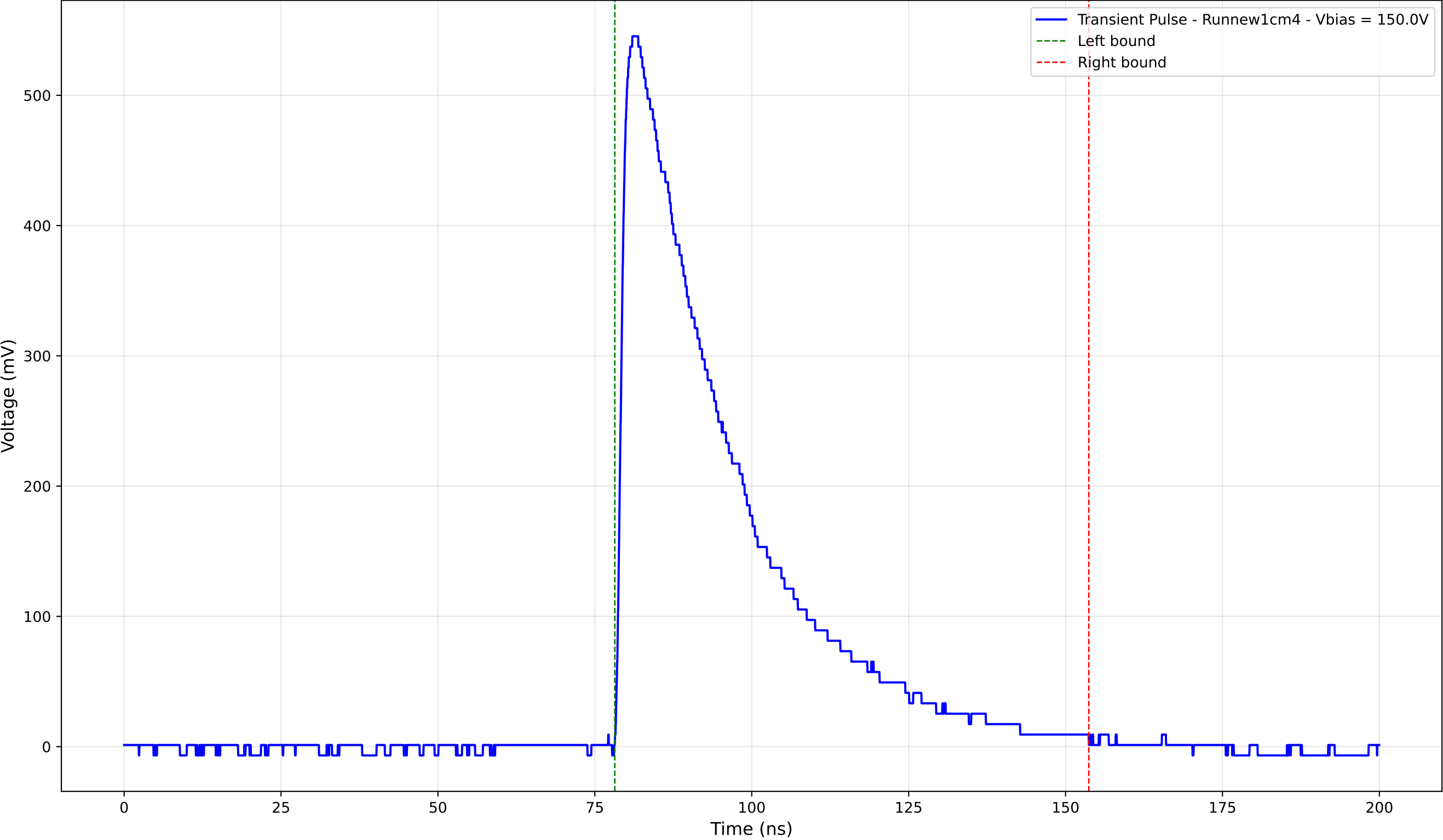
Transient Pulse - Sample: new1cm - Position: 1590.0 \mu\text{m} - Charge: 207.93 pC
