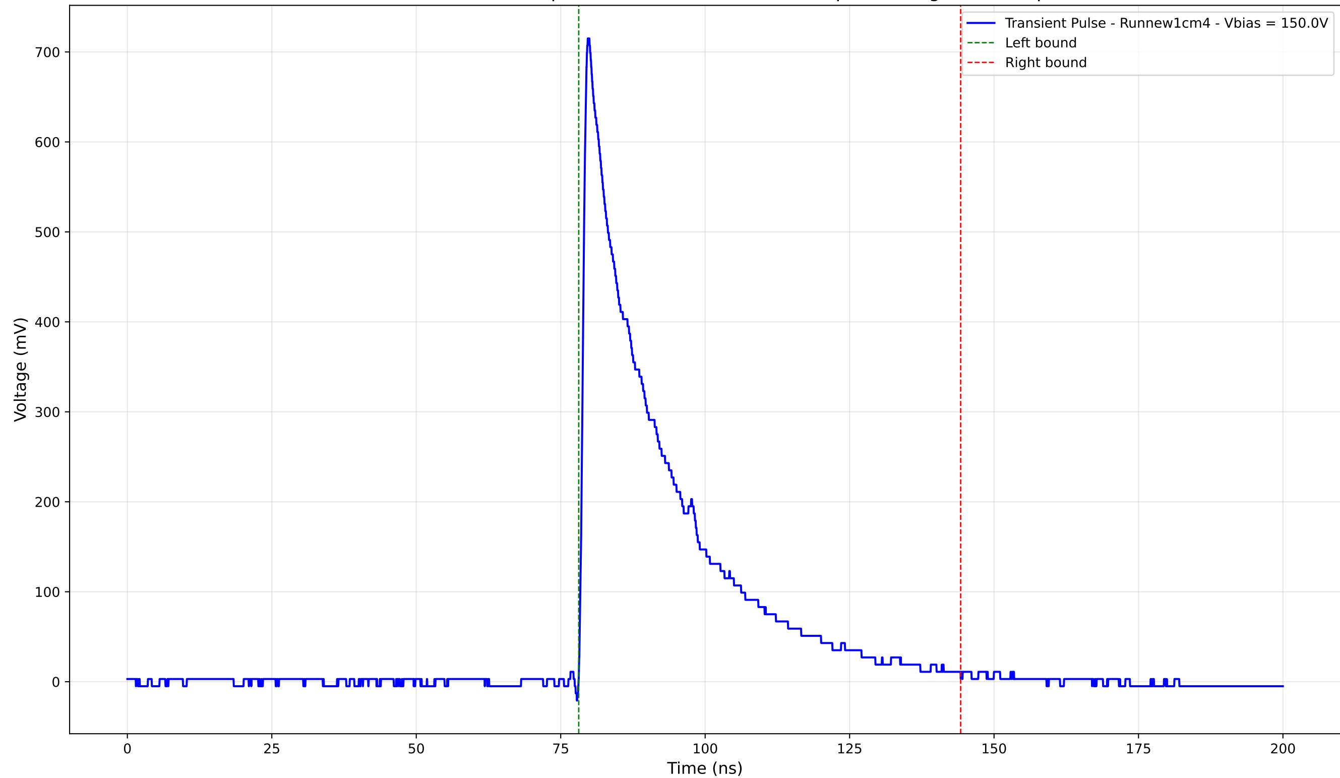
Transient Pulse - Sample: new1cm - Position: 900.0 \mu\text{m} - Charge: 198.46 pC
