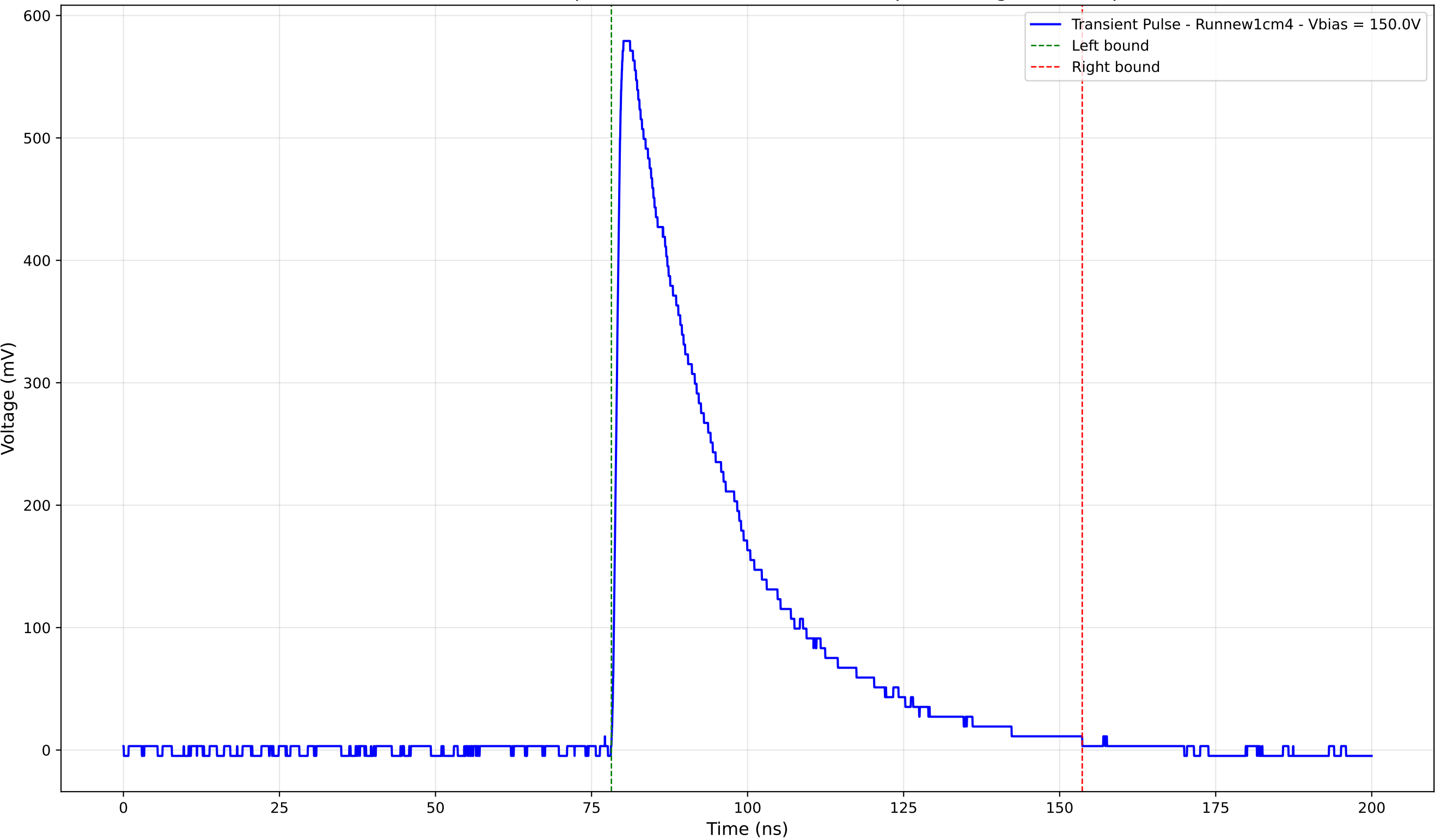
Transient Pulse - Sample: new1cm - Position: 1330.0 \mu\text{m} - Charge: 207.50 pC
