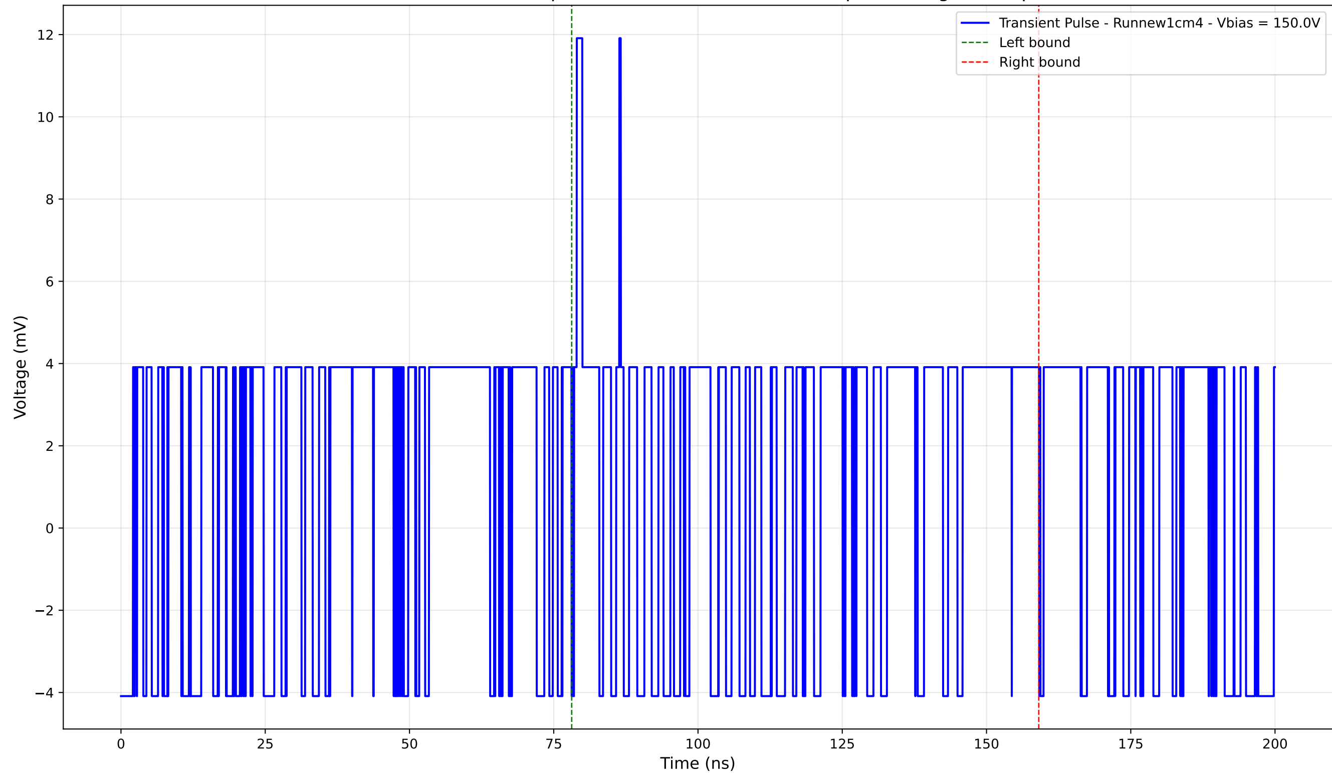
Transient Pulse - Sample: new1cm - Position: 5170.0 \mu\text{m} - Charge: 2.71 pC
