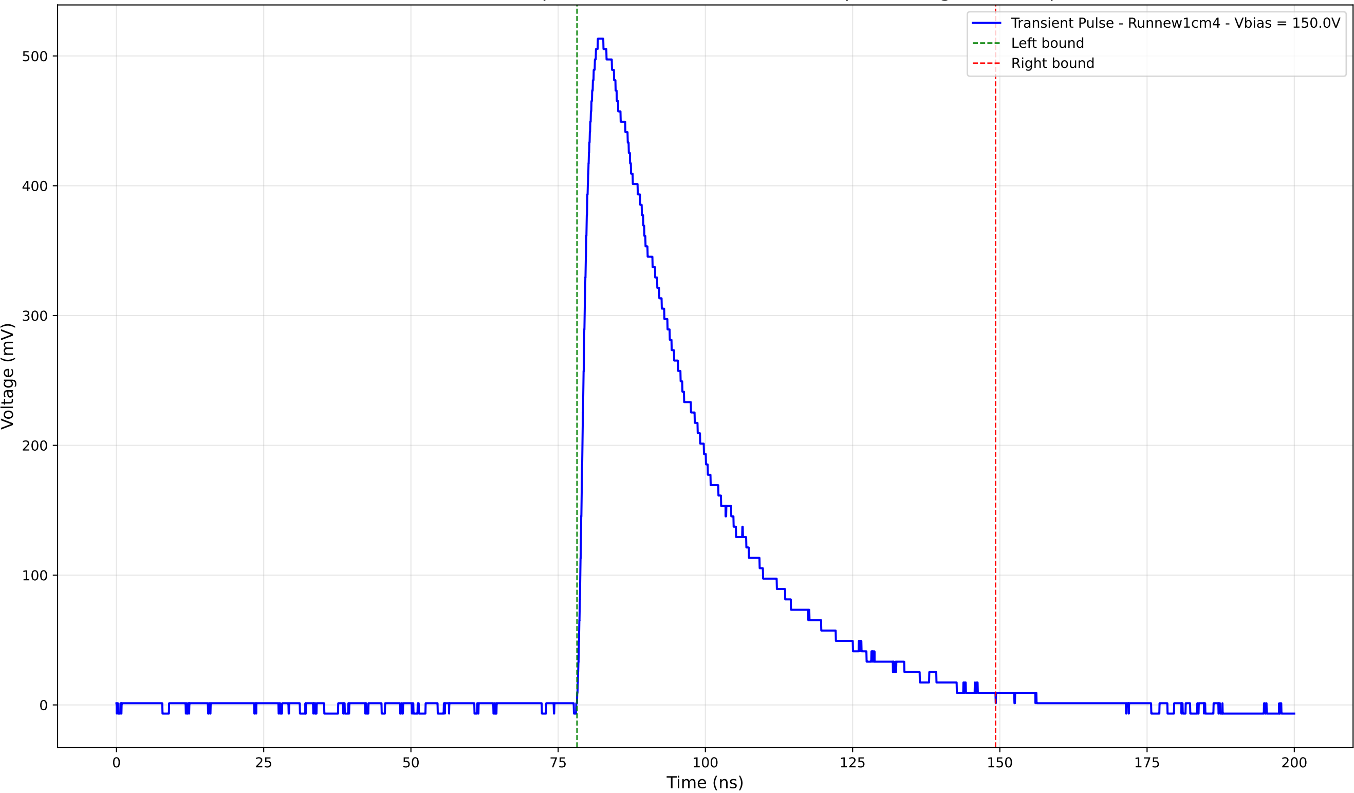
Transient Pulse - Sample: new1cm - Position: 2030.0 \mu\text{m} - Charge: 211.76 pC
