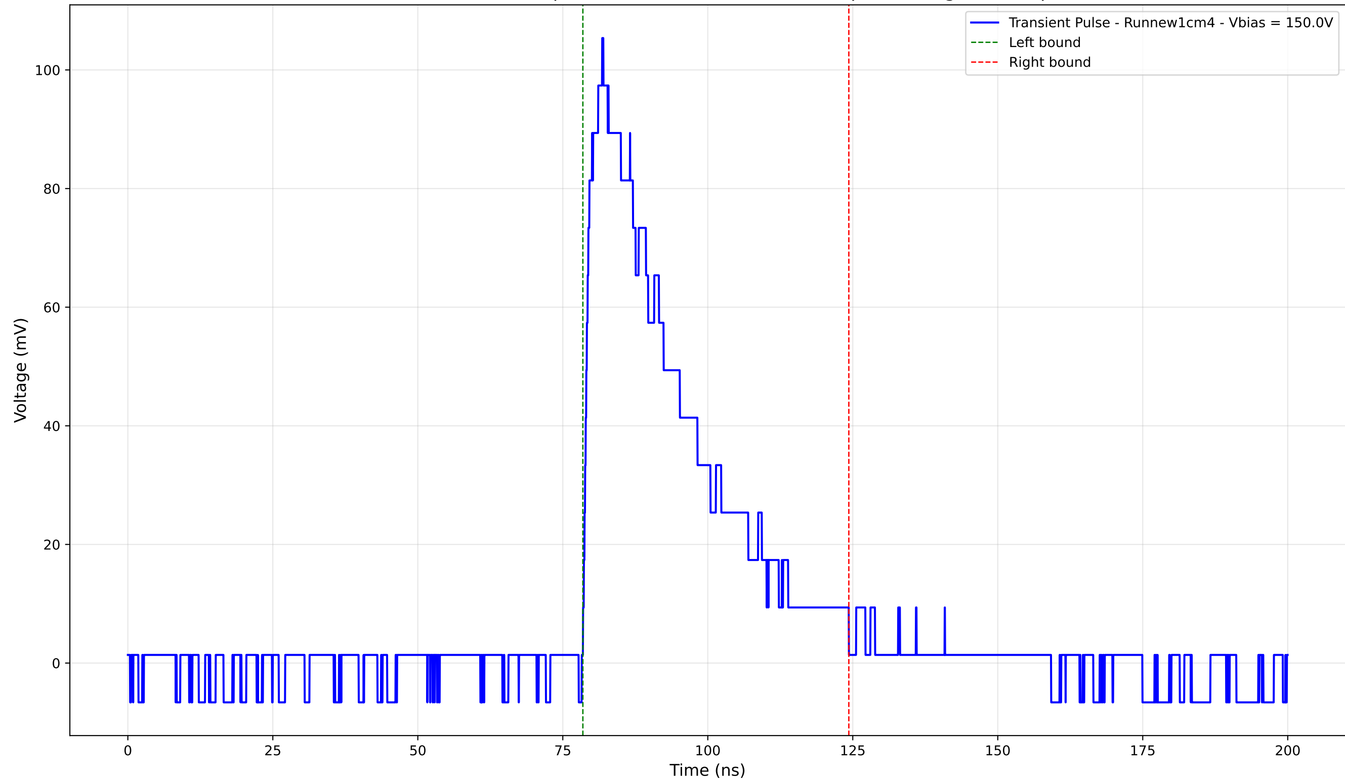
Transient Pulse - Sample: new1cm - Position: 3735.0 \mu\text{m} - Charge: 35.72 pC
