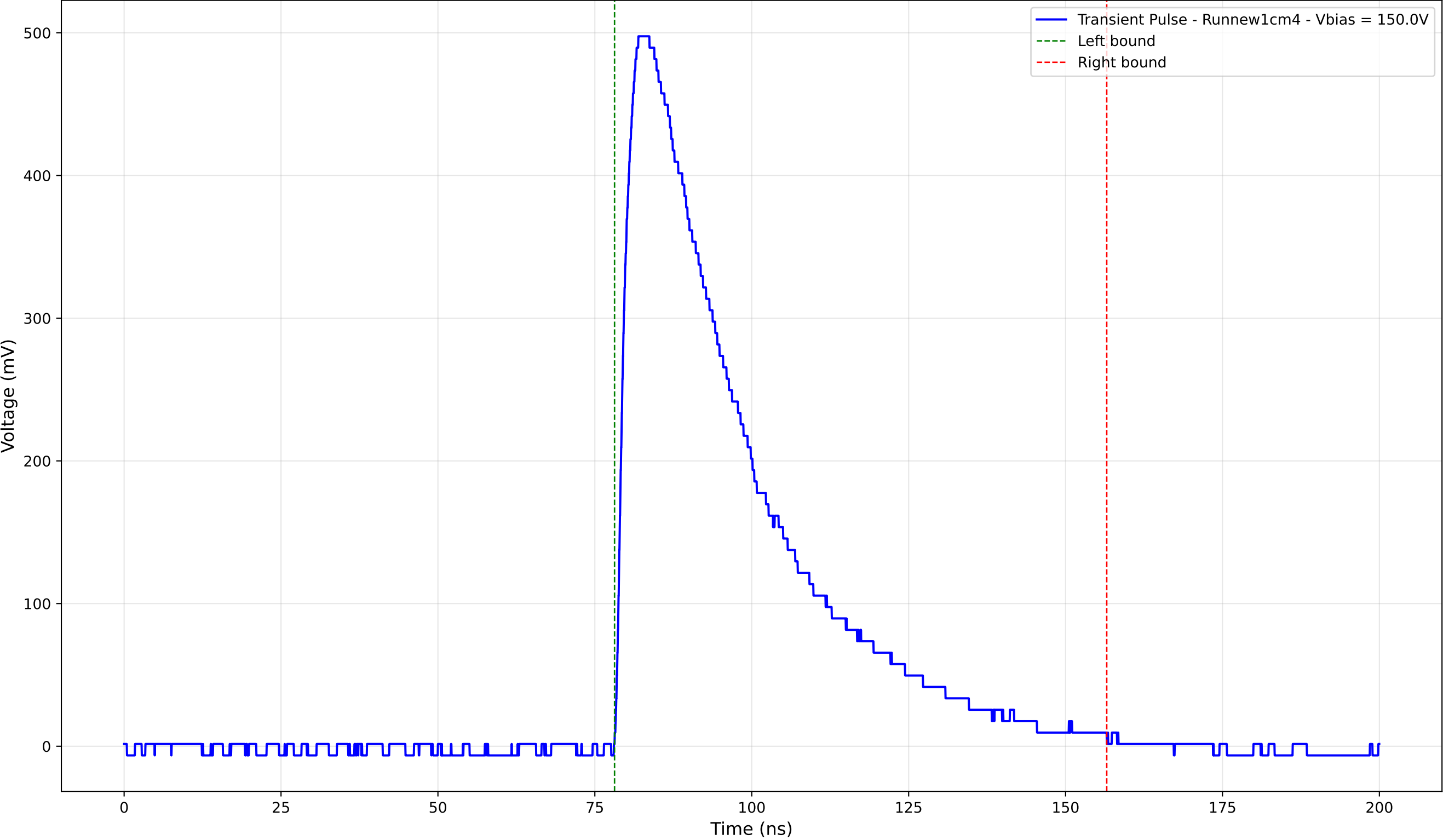
Transient Pulse - Sample: new1cm - Position: 2565.0 \mu\text{m} - Charge: 219.87 pC
