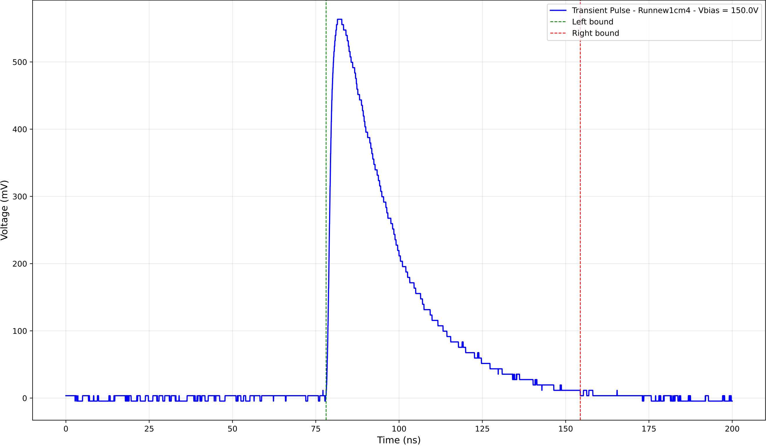
Transient Pulse - Sample: new1cm - Position: 3345.0 \mu\text{m} - Charge: 243.93 pC
