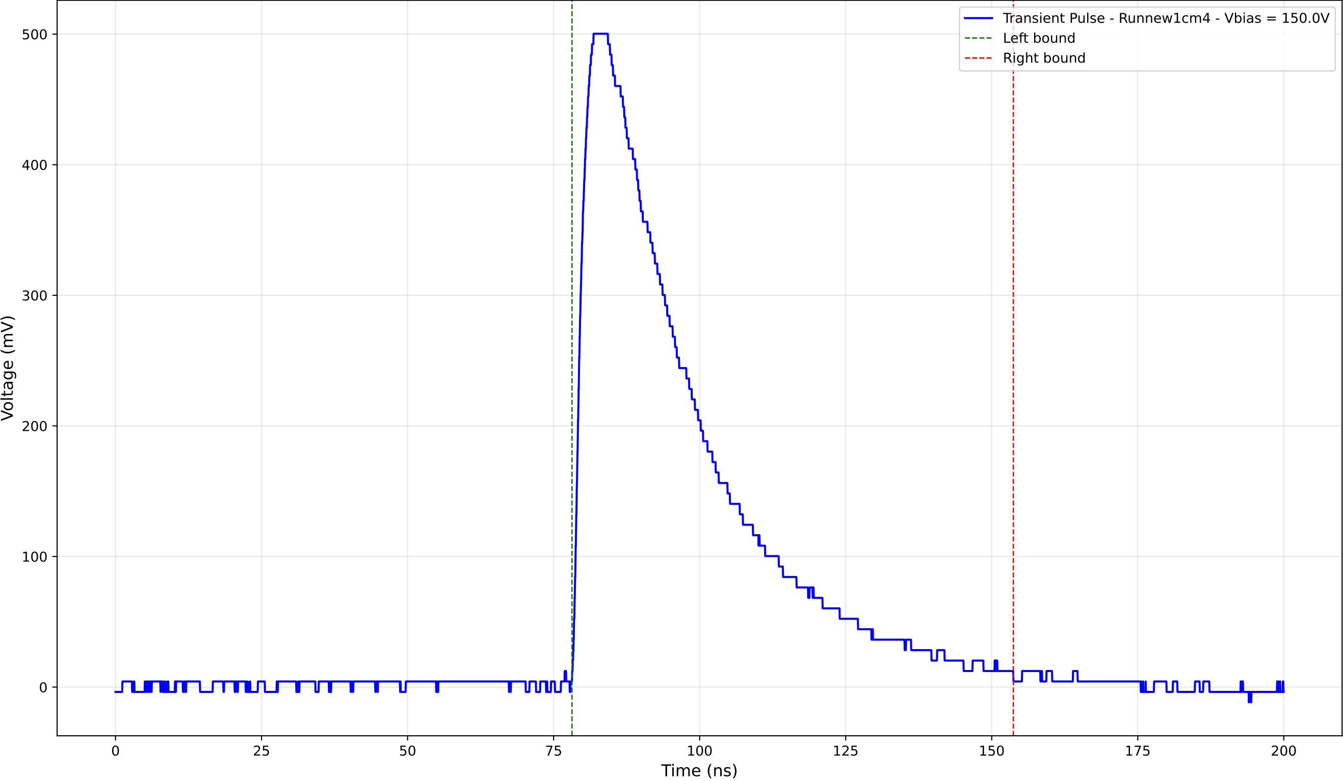
Transient Pulse - Sample: new1cm - Position: 2485.0 \mu\text{m} - Charge: 223.35 pC
