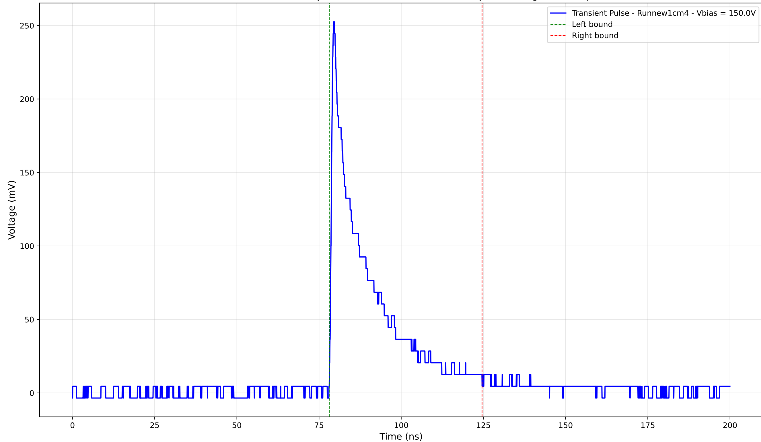
Transient Pulse - Sample: new1cm - Position: 665.0 \mu\text{m} - Charge: 53.33 pC
