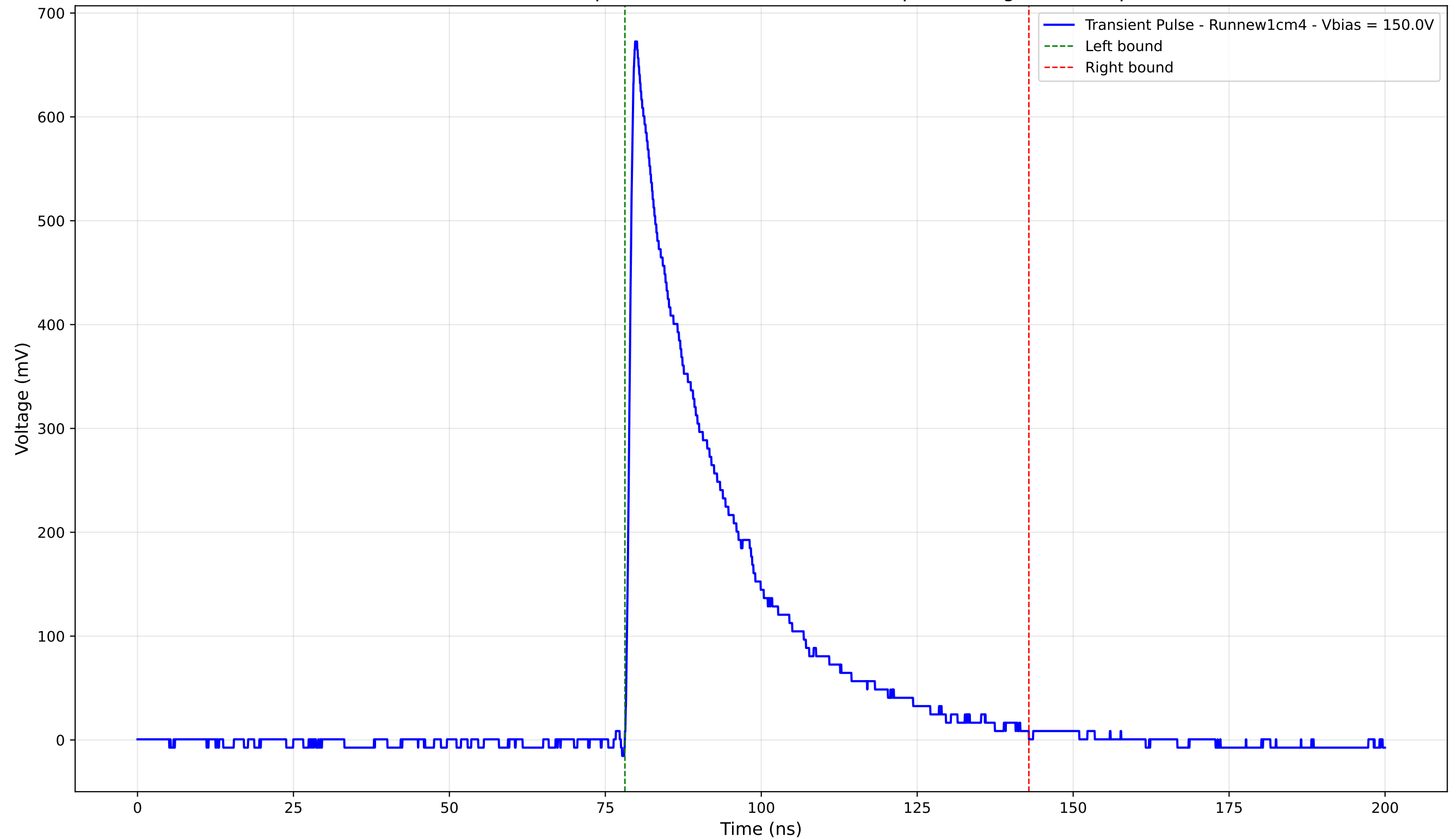
Transient Pulse - Sample: new1cm - Position: 990.0 \mu\text{m} - Charge: 194.81 pC
