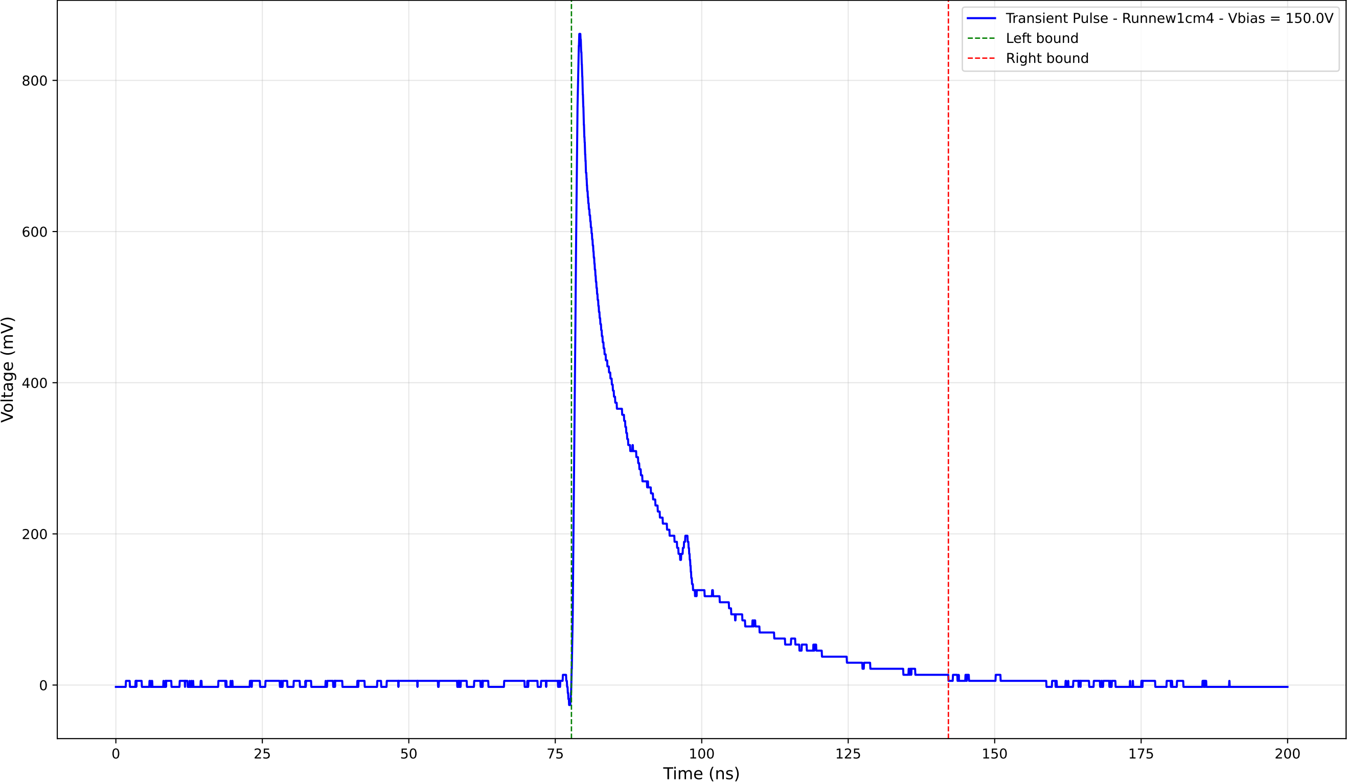
Transient Pulse - Sample: new1cm - Position: 4870.0 \mu\text{m} - Charge: 192.81 pC
