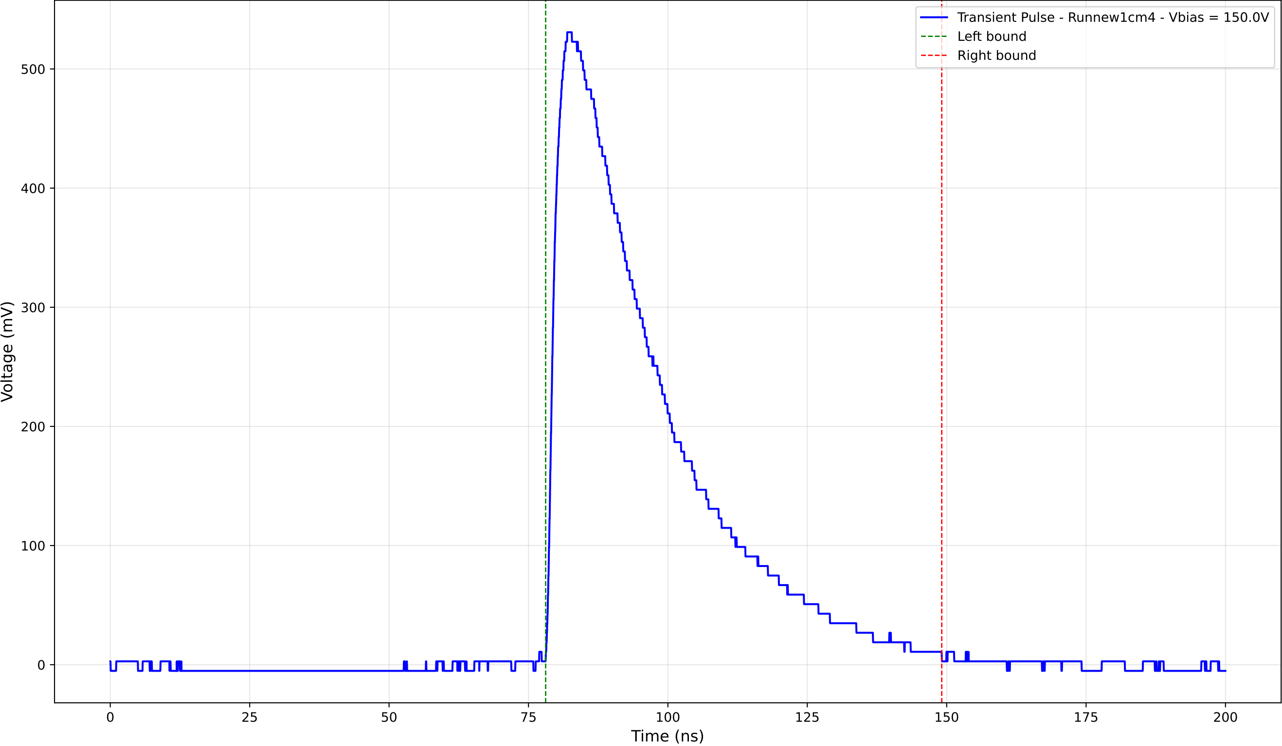
Transient Pulse - Sample: new1cm - Position: 3015.0 \mu\text{m} - Charge: 230.44 pC
