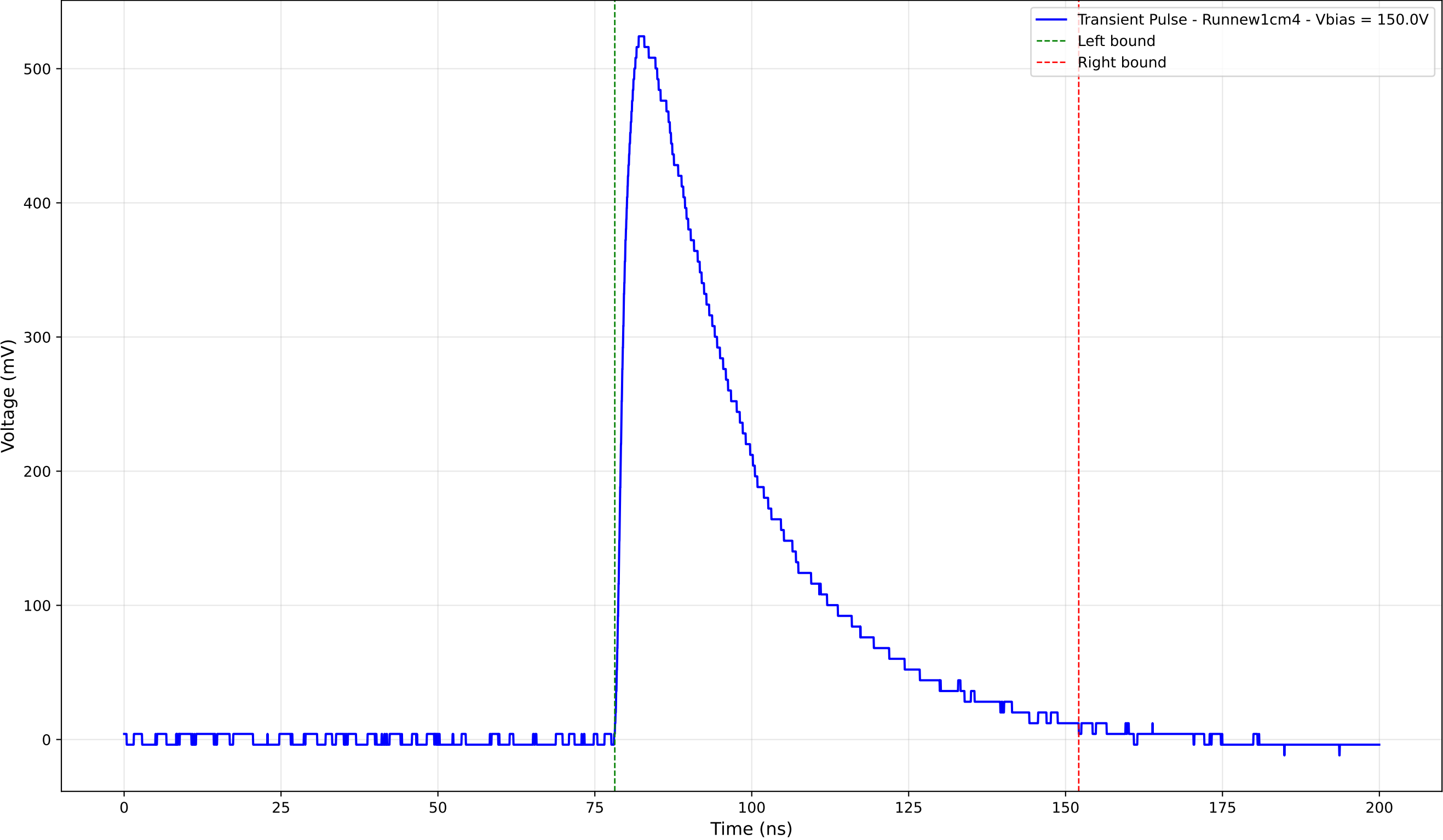
Transient Pulse - Sample: new1cm - Position: 2995.0 \mu\text{m} - Charge: 229.97 pC
