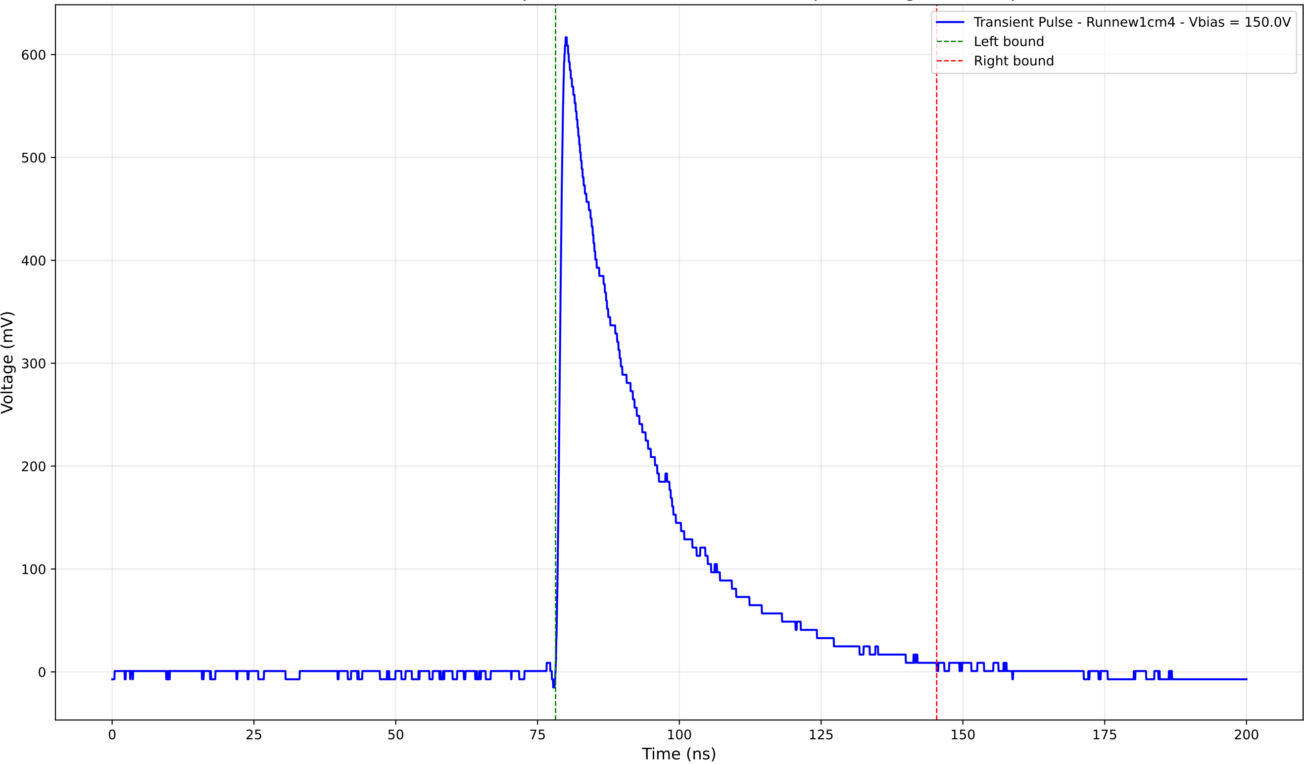
Transient Pulse - Sample: new1cm - Position: 1105.0 \mu\text{m} - Charge: 188.57 pC
