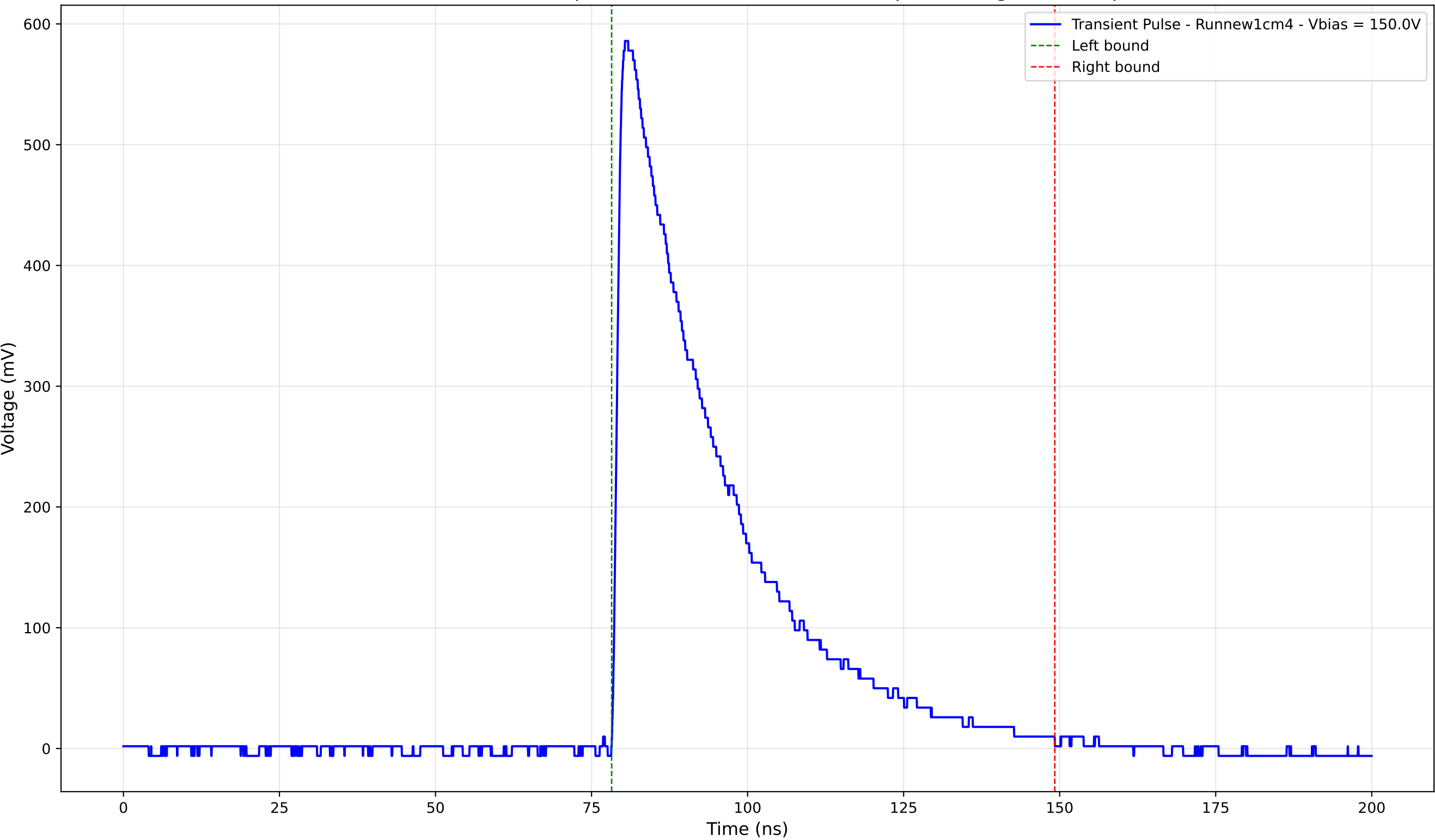
Transient Pulse - Sample: new1cm - Position: 1385.0 \mu\text{m} - Charge: 209.26 pC
