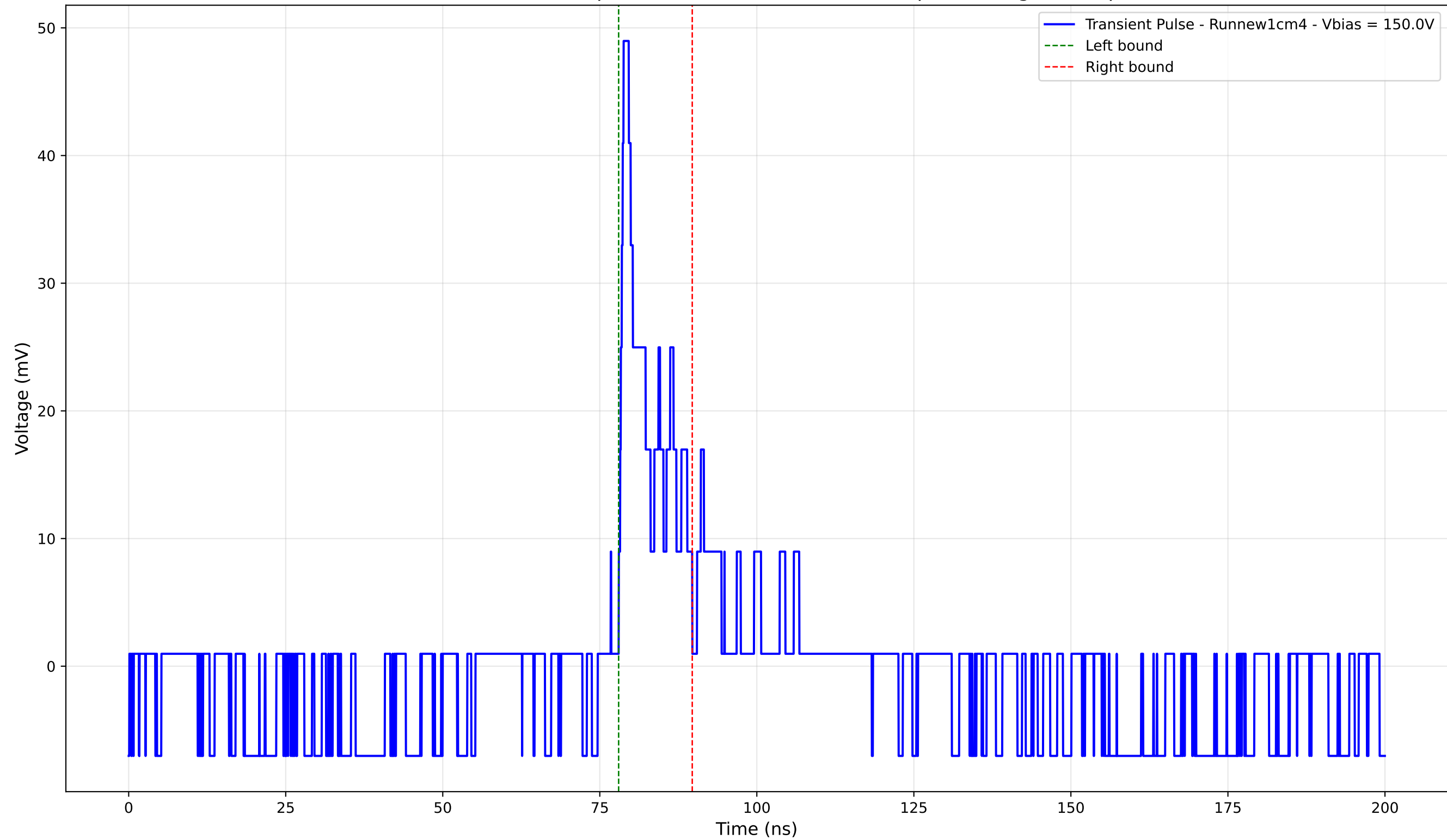
Transient Pulse - Sample: new1cm -Position: 5080.0 \mu\text{m} - Charge: 4.89 pC
