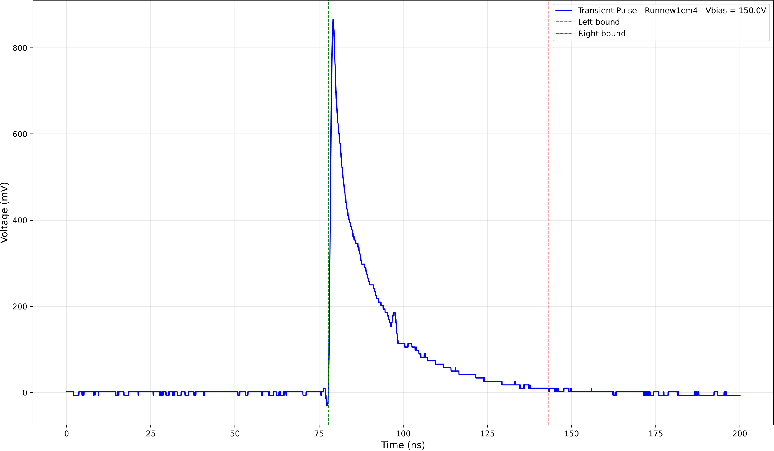
Transient Pulse - Sample: new1cm - Position: 4920.0 \mu\text{m} - Charge: 182.94 pC
