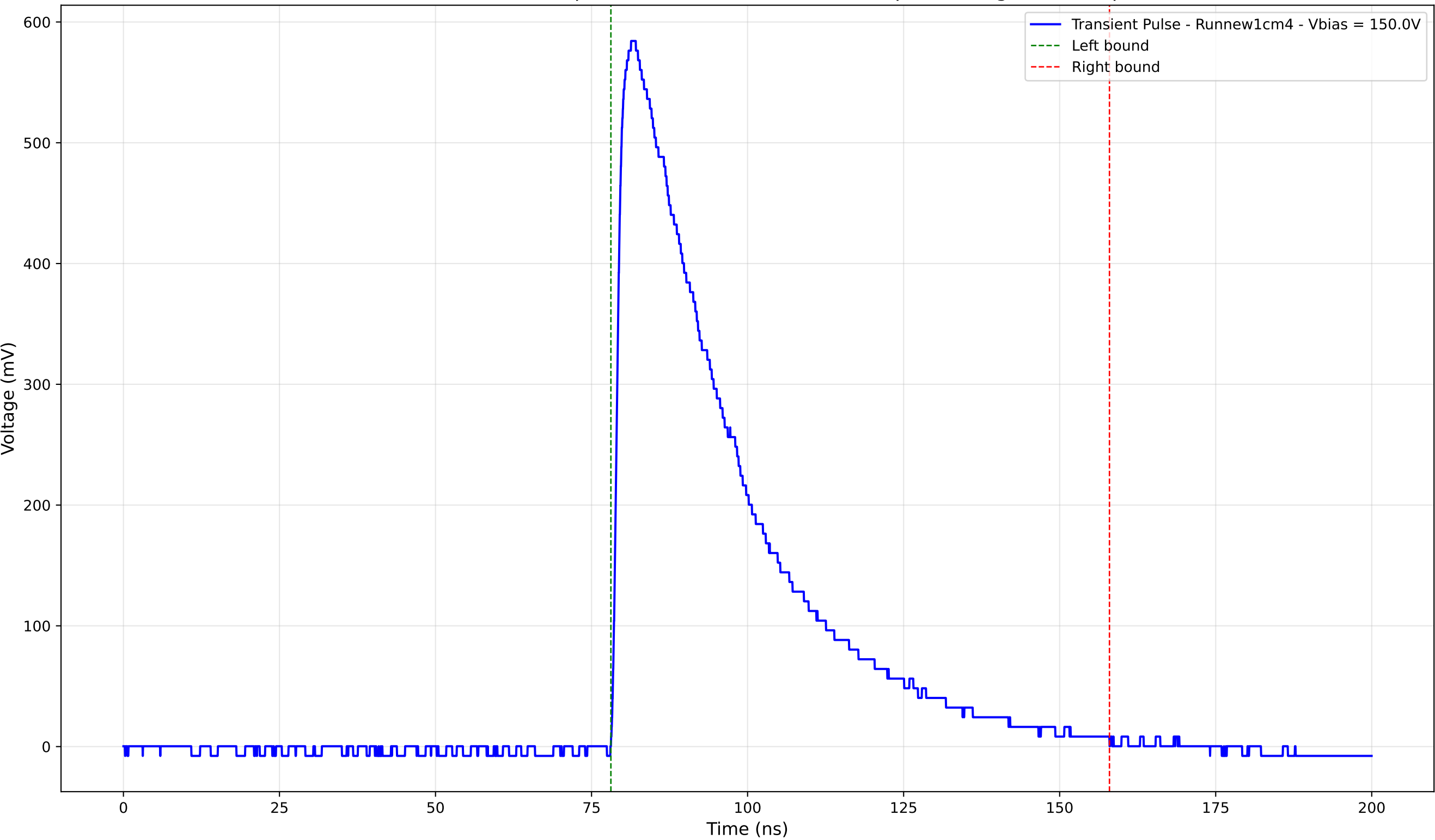
Transient Pulse - Sample: new1cm - Position: 3590.0 \mu\text{m} - Charge: 241.19 pC
