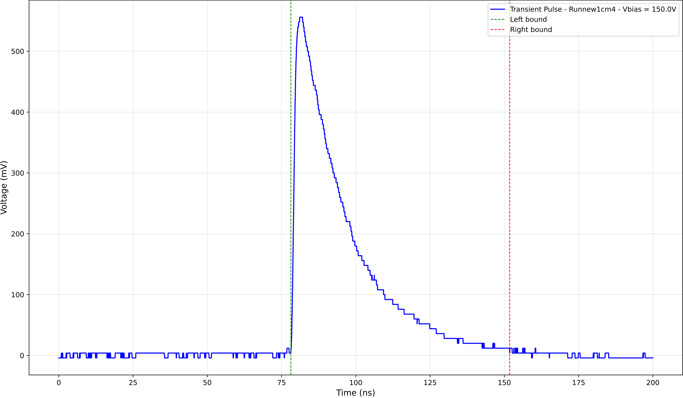
Transient Pulse - Sample: new1cm - Position: 1585.0 \mu\text{m} - Charge: 214.51 pC
