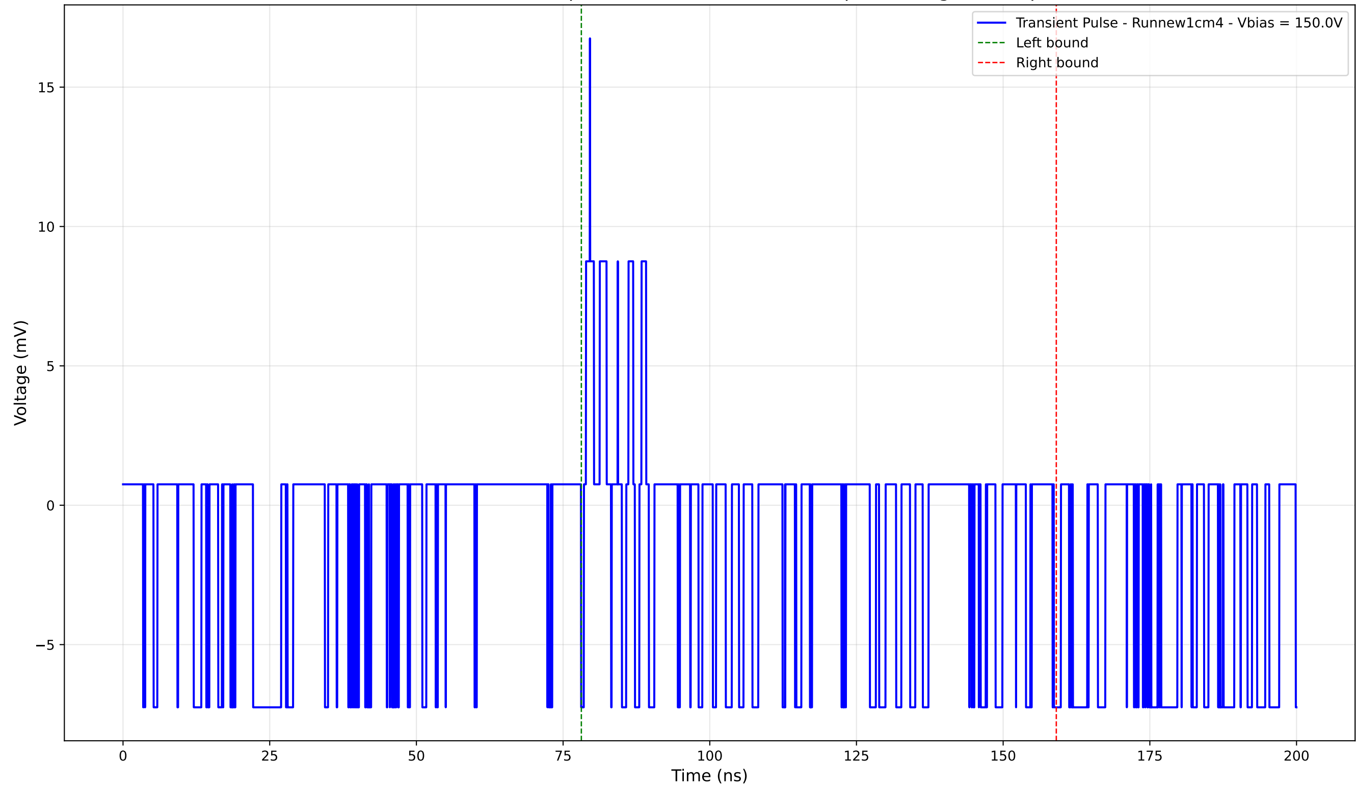
Transient Pulse - Sample: new1cm - Position: 25.0 \mu\text{m} - Charge: -1.07 pC
