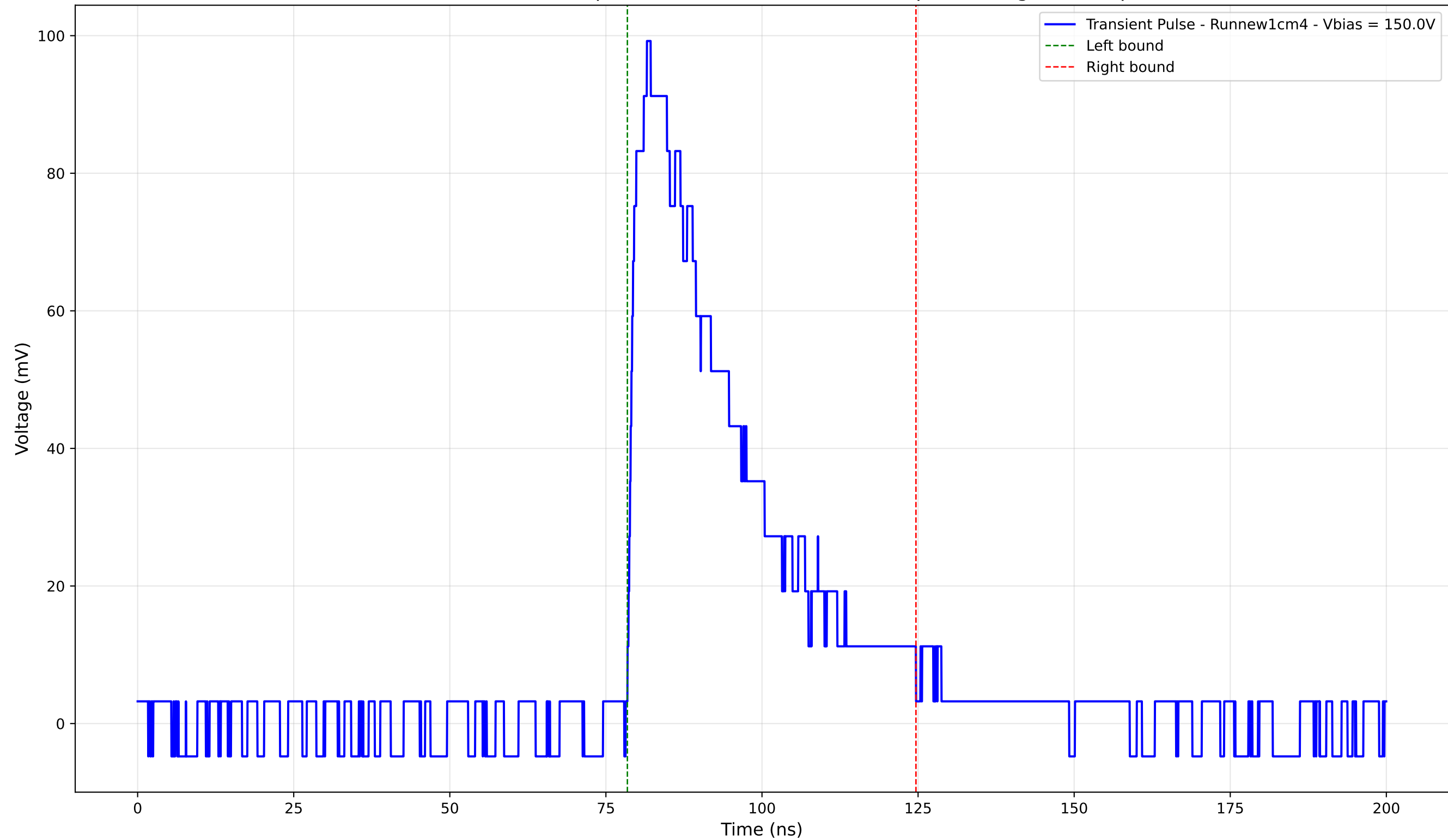
Transient Pulse - Sample: new1cm - Position: 3725.0 \mu\text{m} - Charge: 35.48 pC
