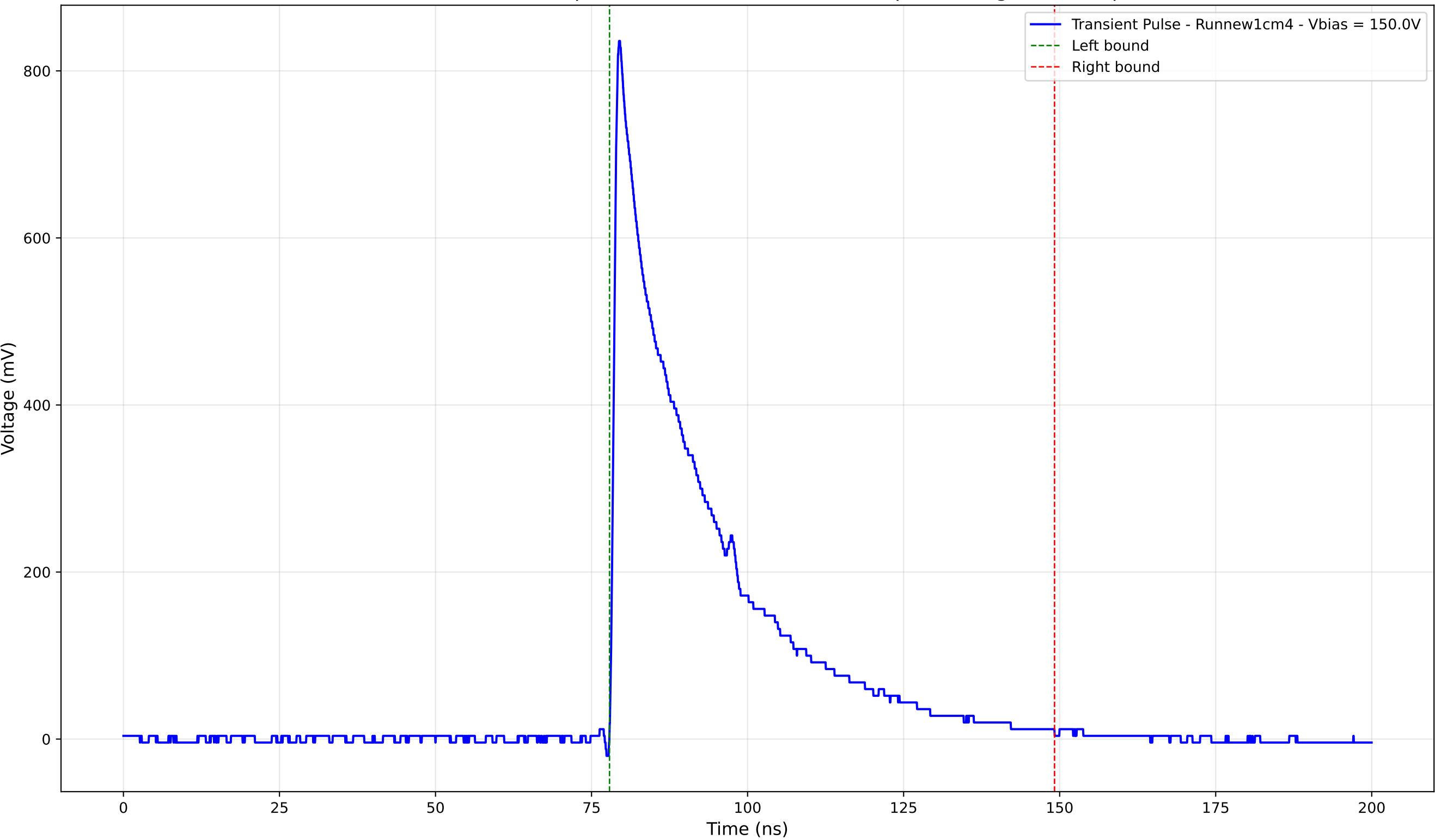
Transient Pulse - Sample: new1cm - Position: 4565.0 \mu\text{m} - Charge: 237.03 pC
