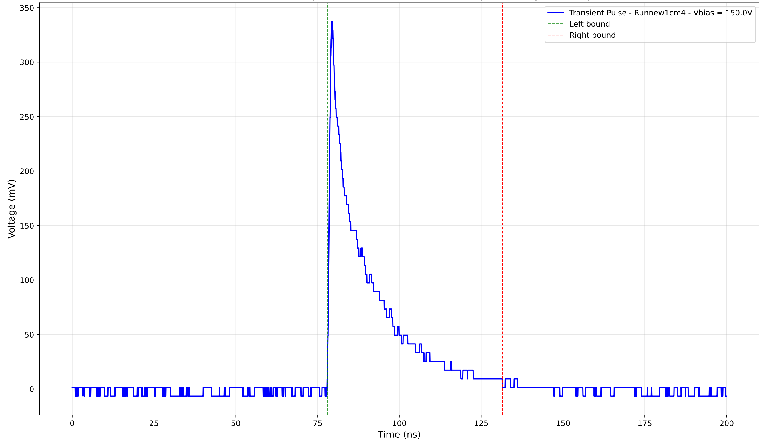
Transient Pulse - Sample: new1cm - Position: 4700.0 \mu\text{m} - Charge: 73.21 pC
