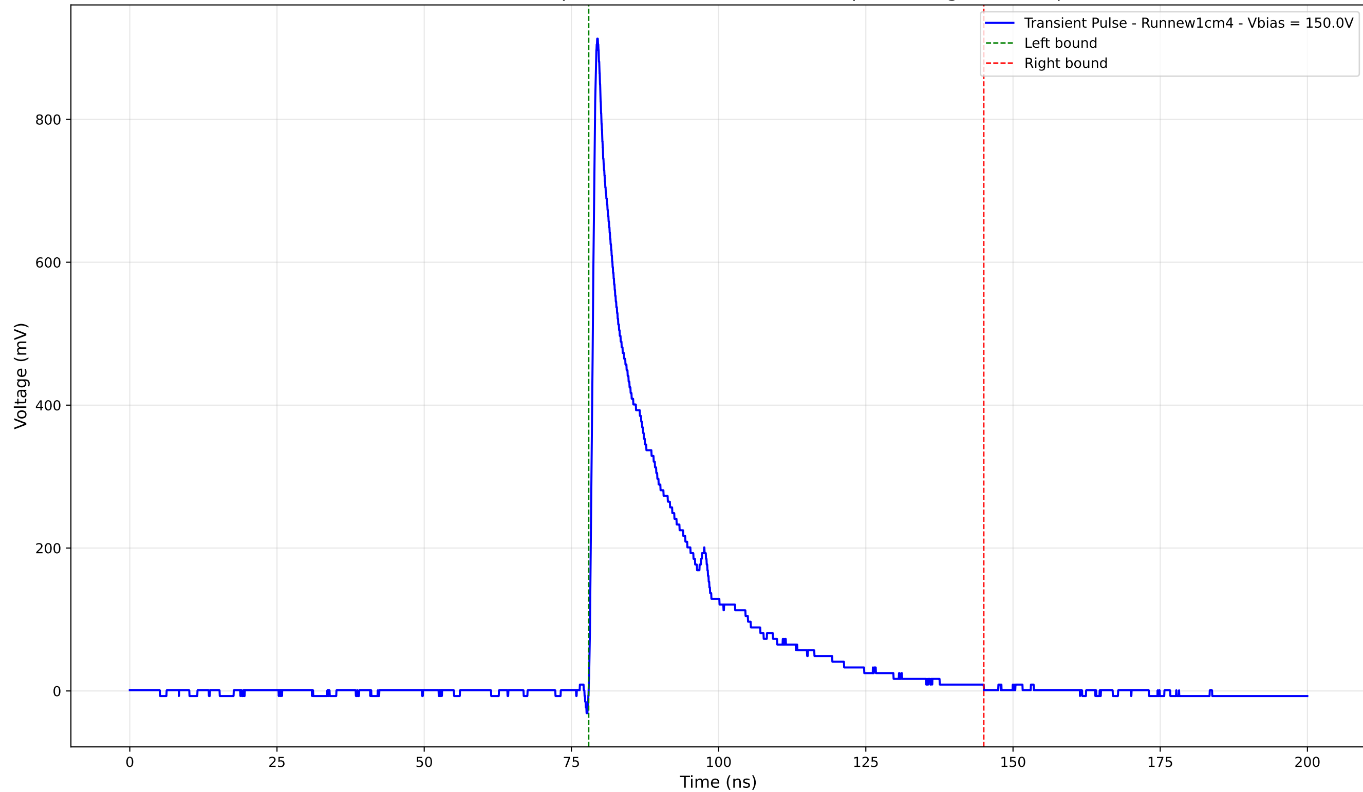
Transient Pulse - Sample: new1cm - Position: 505.0 \mu\text{m} - Charge: 200.29 pC
