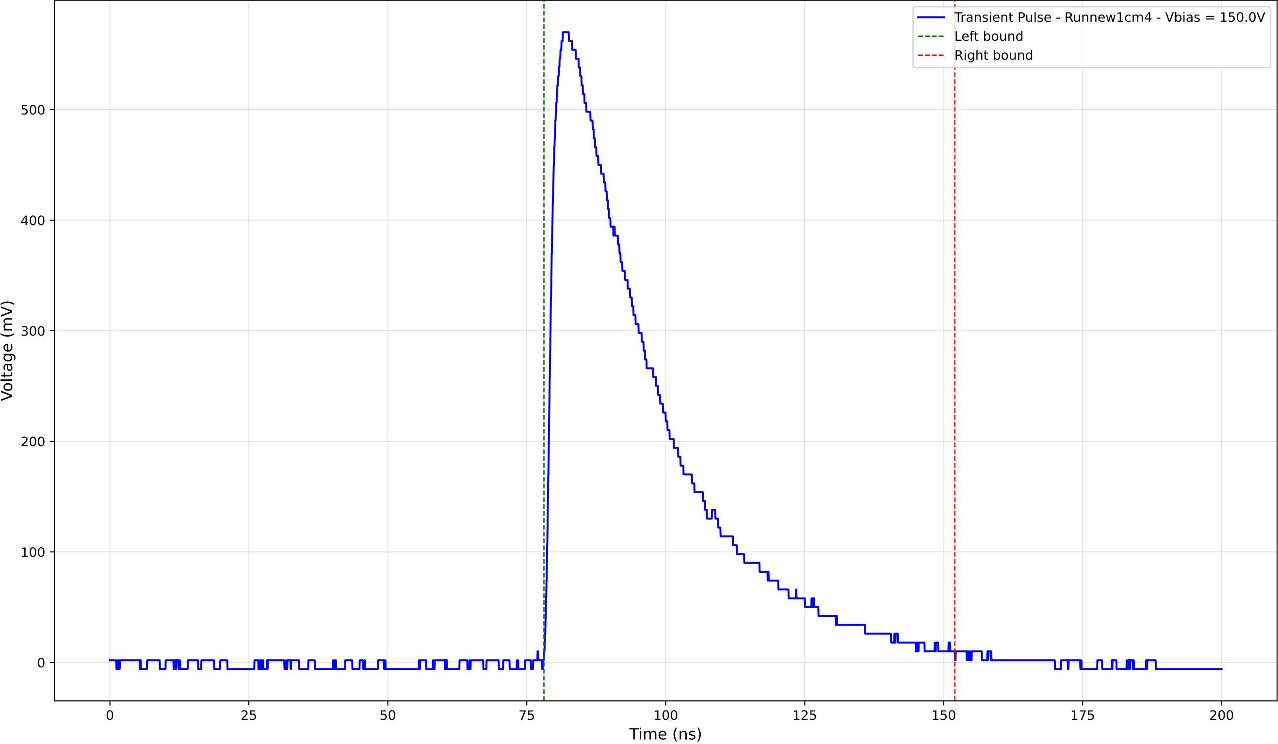
Transient Pulse - Sample: new1cm - Position: 3360.0 \mu\text{m} - Charge: 243.65 pC
