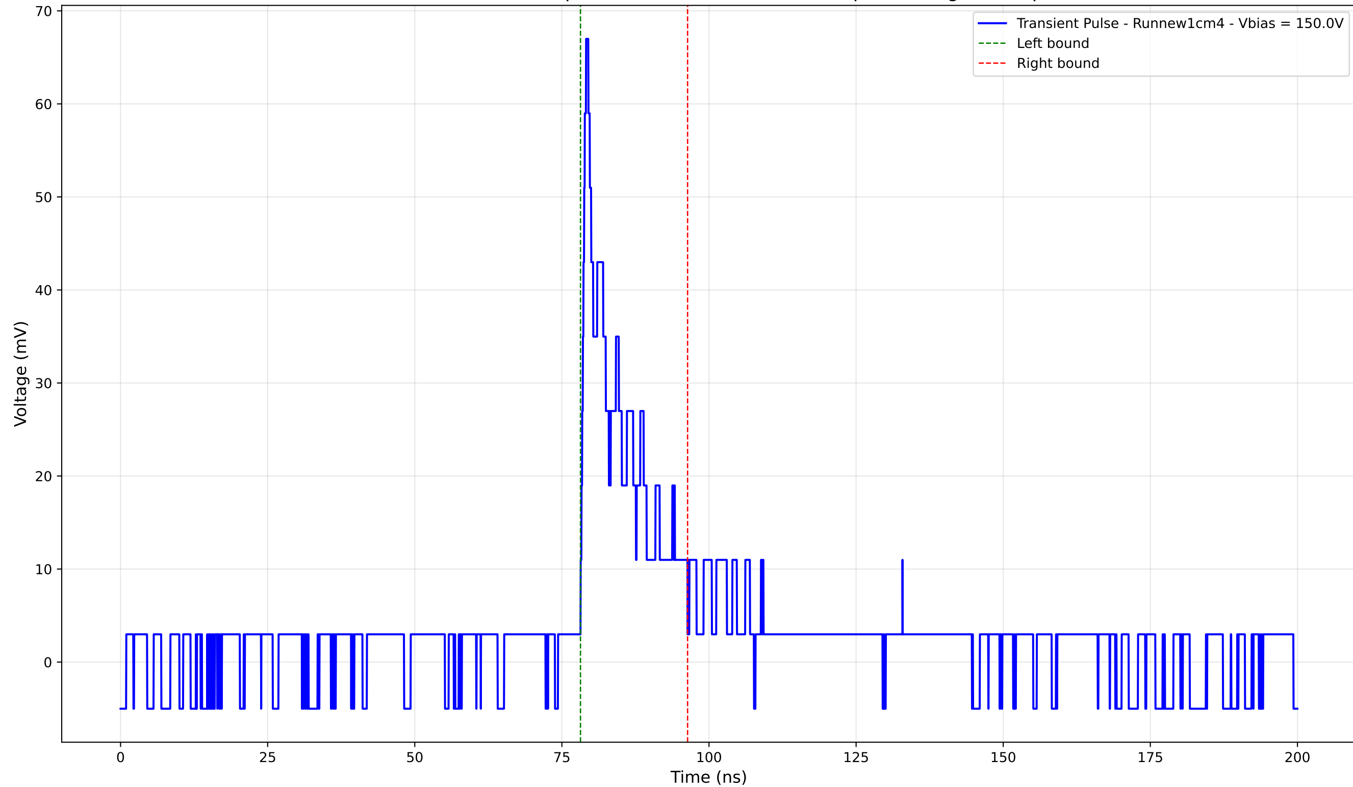
Transient Pulse - Sample: new1cm - Position: 180.0 \mu\text{m} - Charge: 8.76 pC
