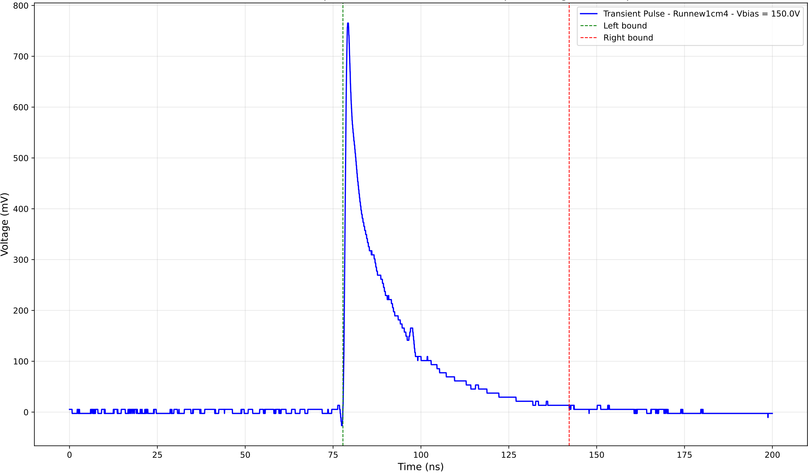
Transient Pulse - Sample: new1cm - Position: 4815.0 \mu\text{m} - Charge: 166.11 pC
