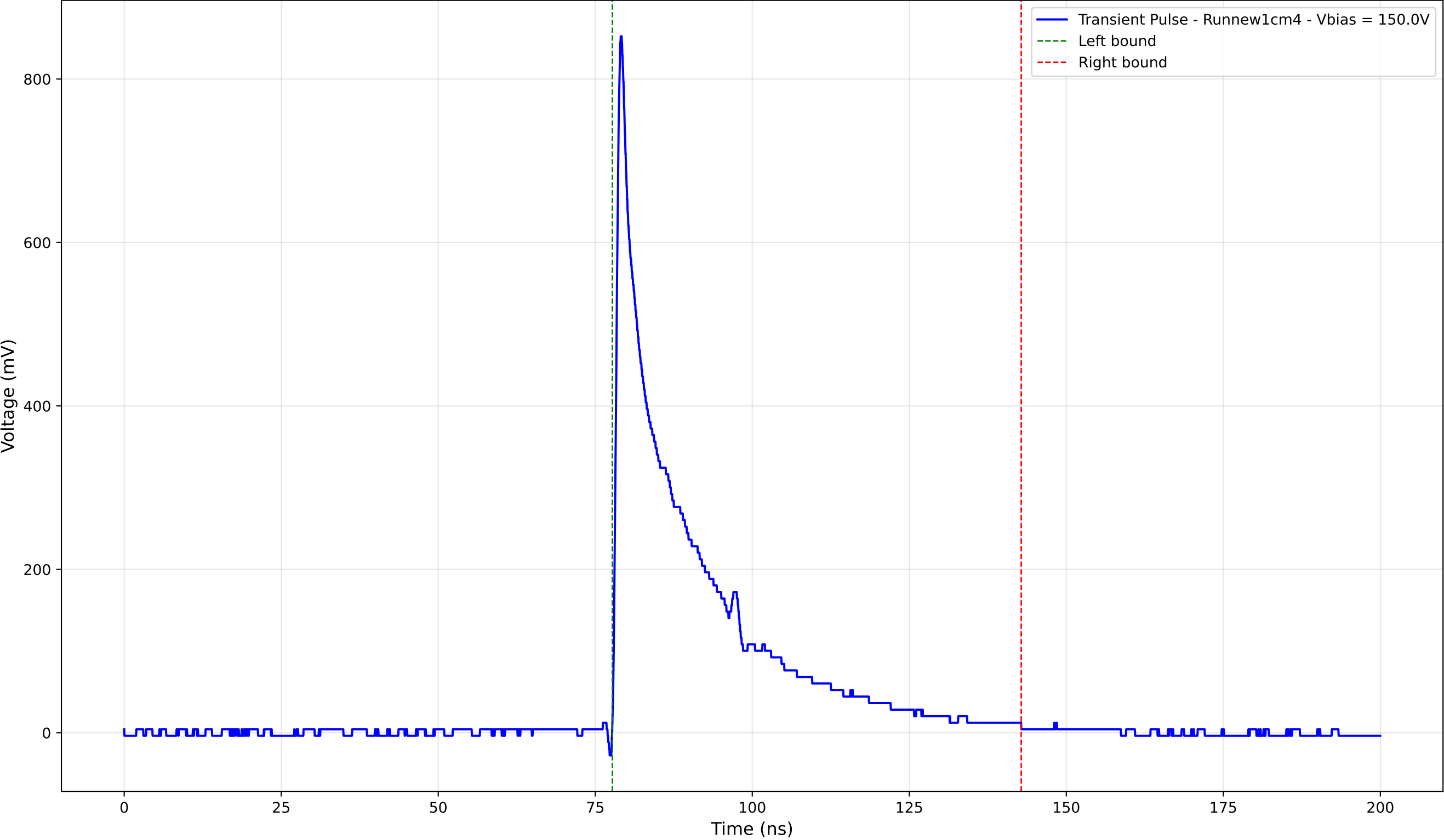
Transient Pulse - Sample: new1cm - Position: 4970.0 \mu\text{m} - Charge: 171.49 pC
