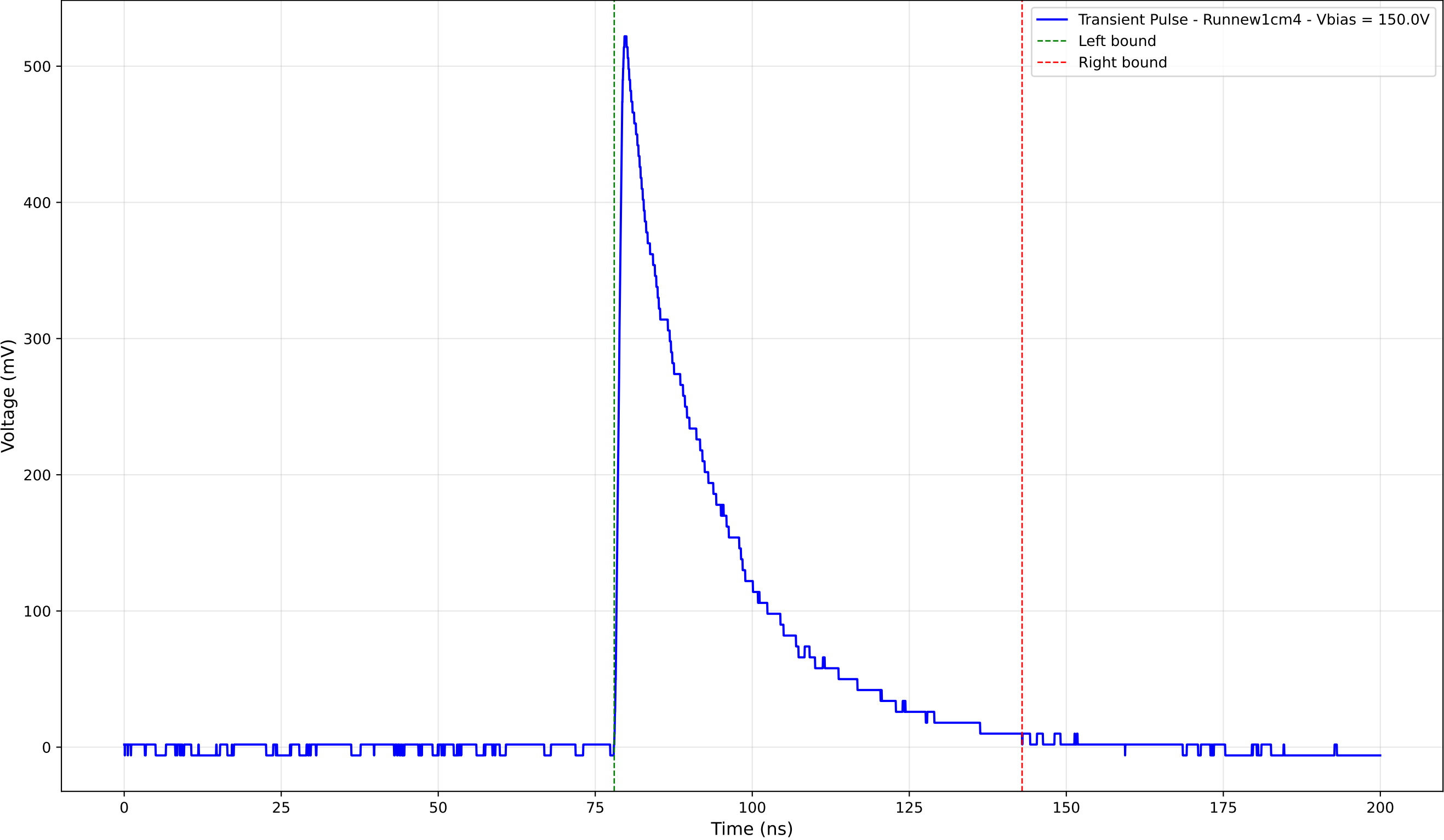
Transient Pulse - Sample: new1cm - Position: 4295.0 \mu\text{m} - Charge: 155.06 pC
