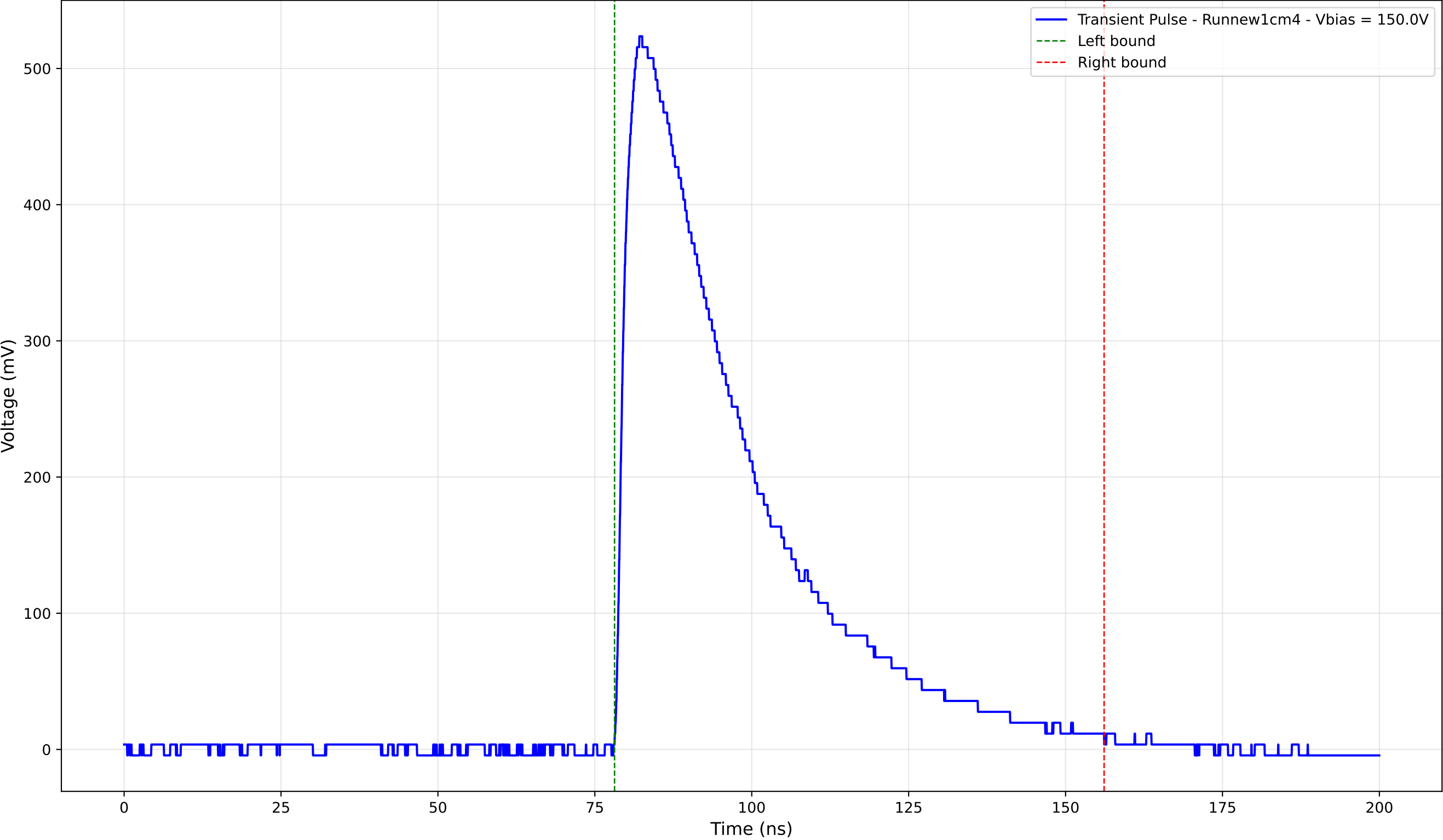
Transient Pulse - Sample: new1cm - Position: 3010.0 \mu\text{m} - Charge: 230.34 pC
