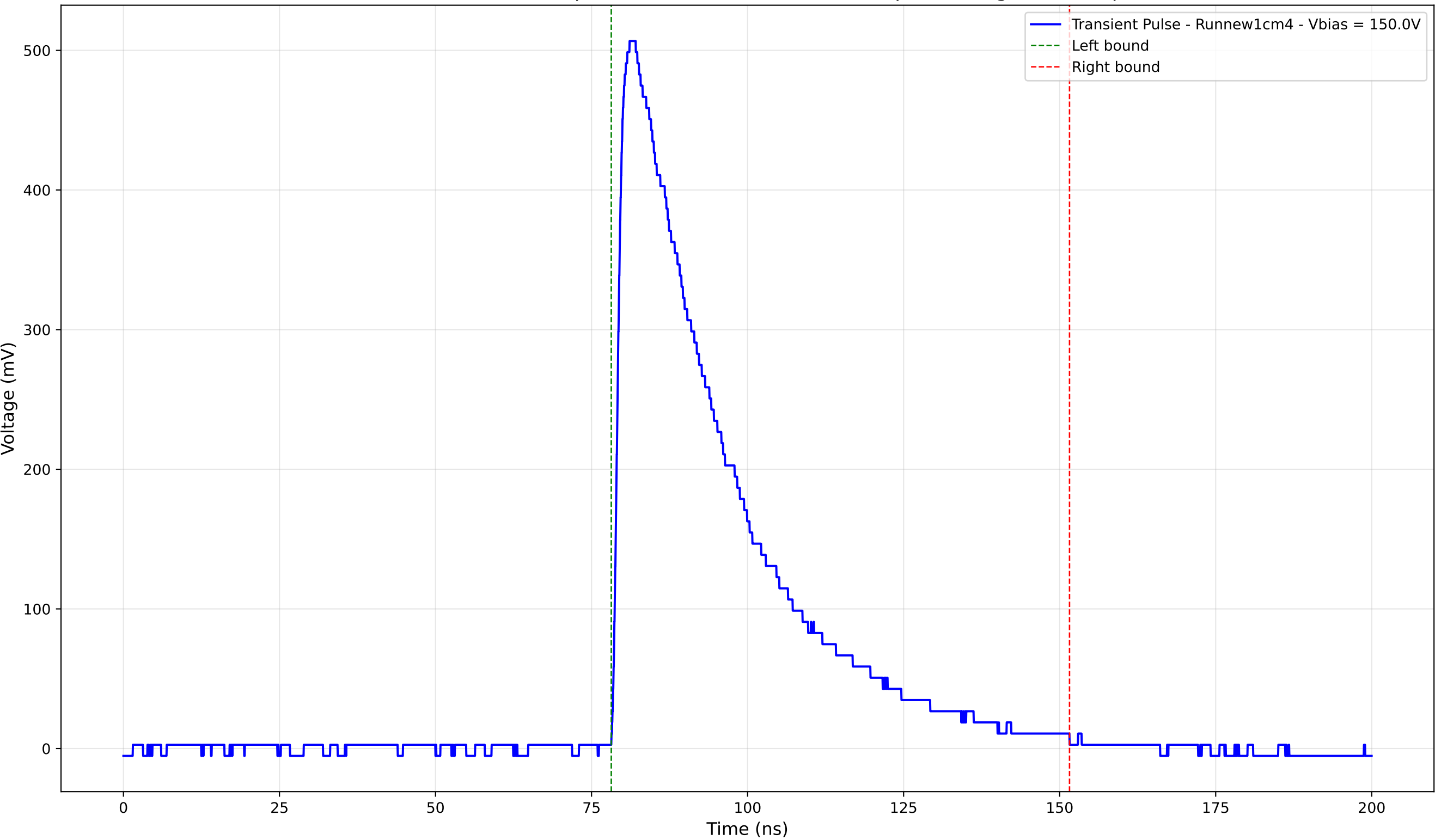
Transient Pulse - Sample: new1cm - Position: 1615.0 \mu\text{m} - Charge: 194.16 pC
