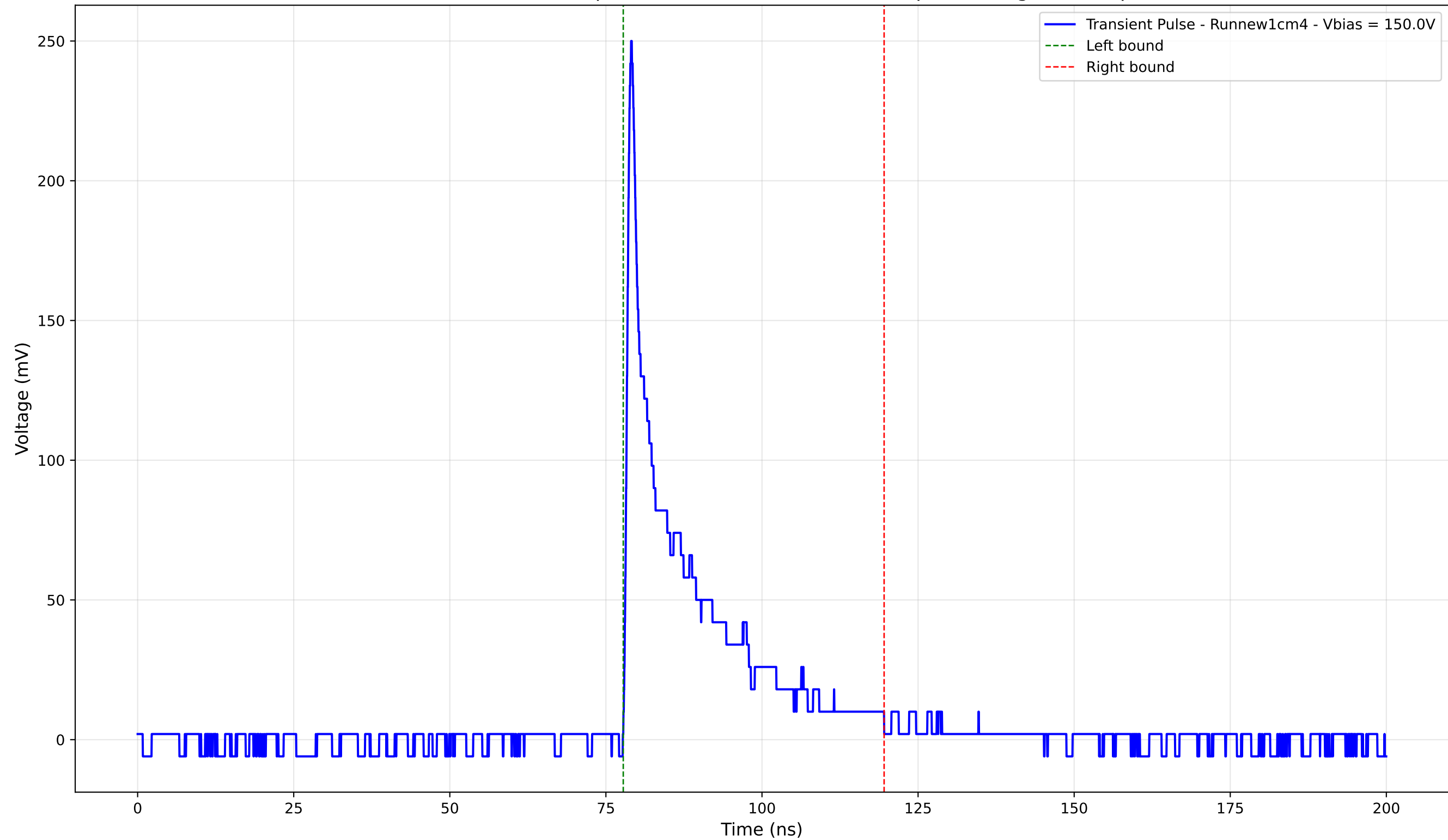
Transient Pulse - Sample: new1cm - Position: 5050.0 \mu\text{m} - Charge: 37.22 pC
