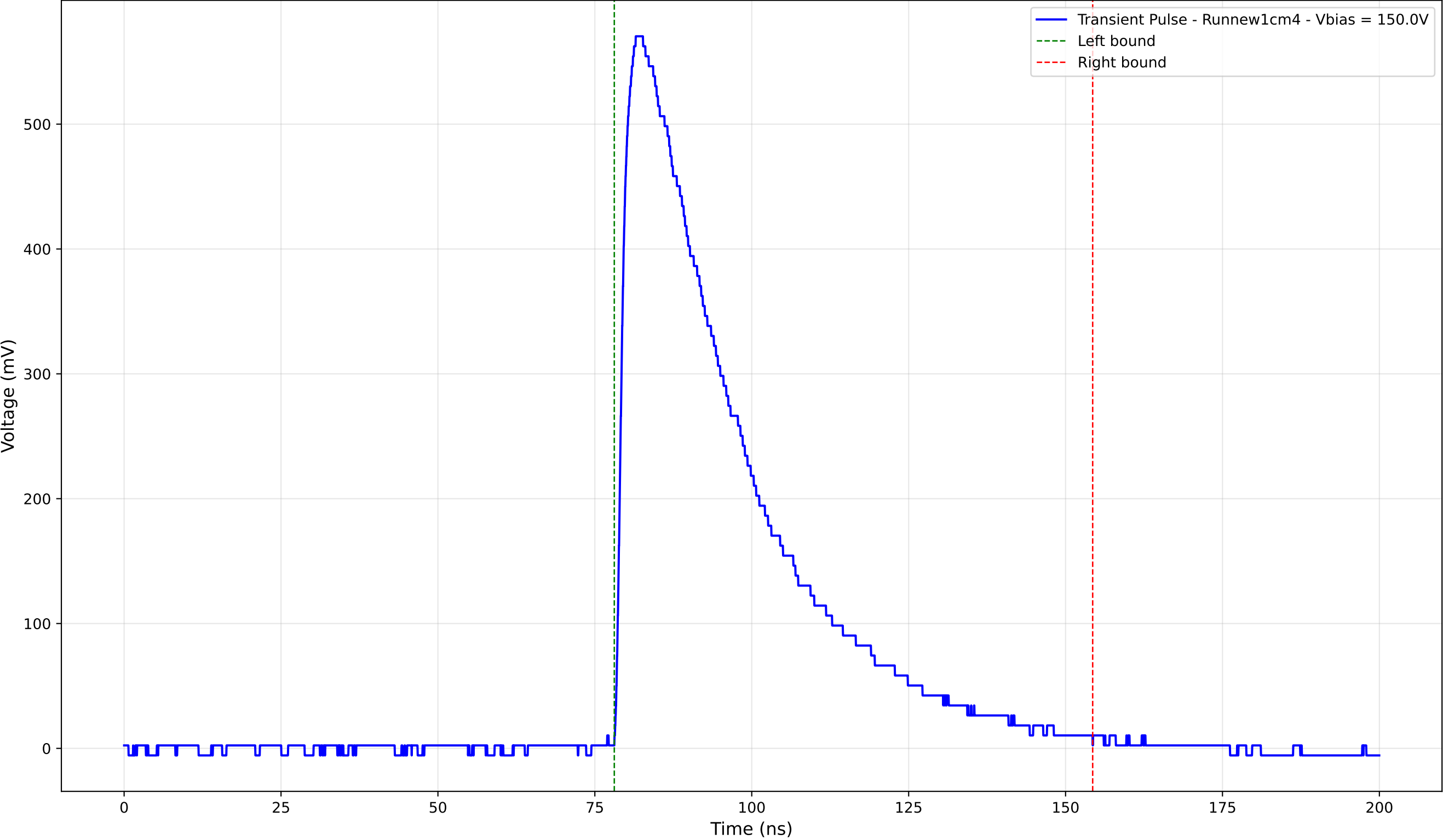
Transient Pulse - Sample: new1cm - Position: 3355.0 \mu\text{m} - Charge: 244.20 pC
