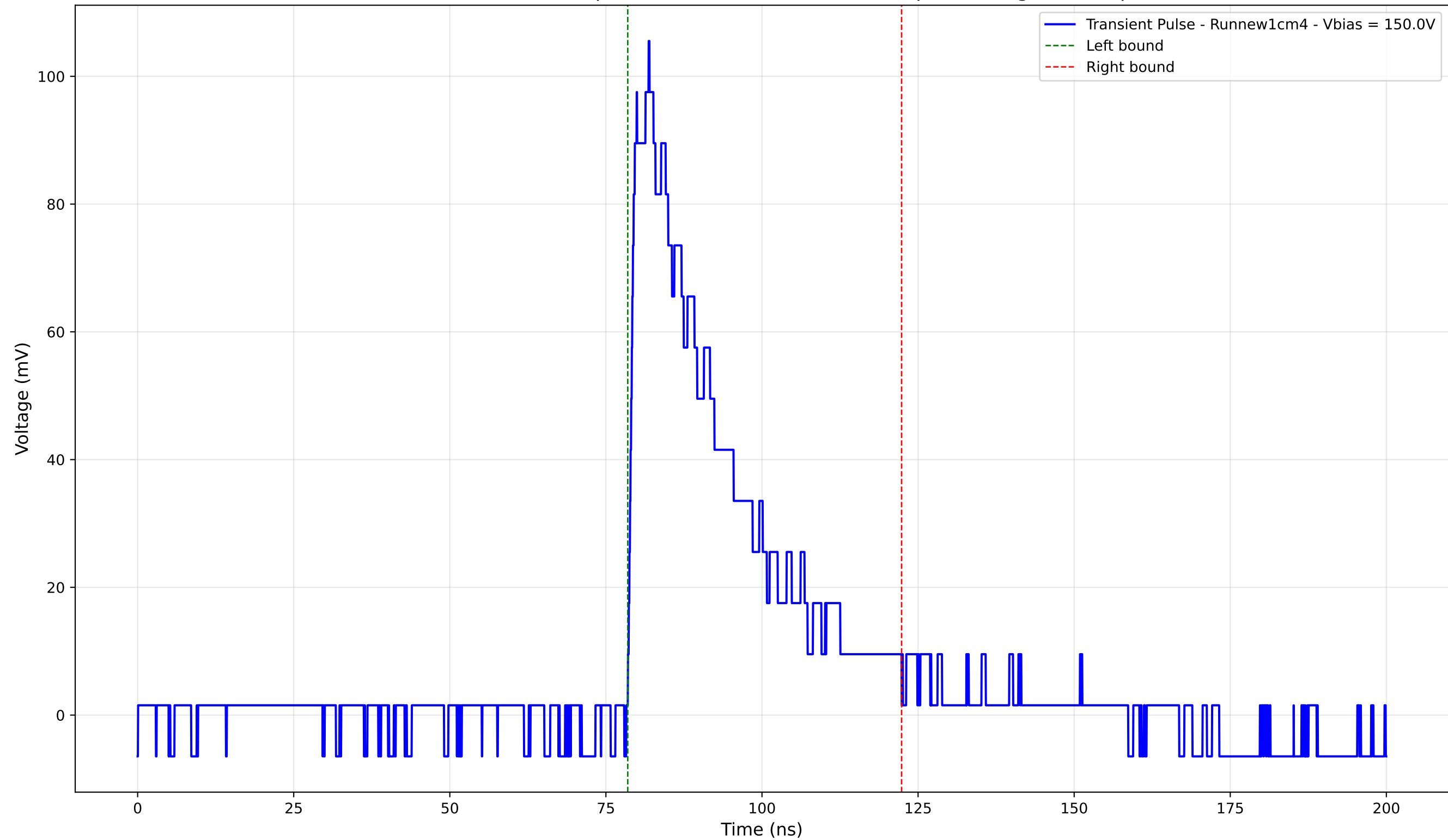
Transient Pulse - Sample: new1cm - Position: 1210.0 \mu\text{m} - Charge: 31.80 pC
