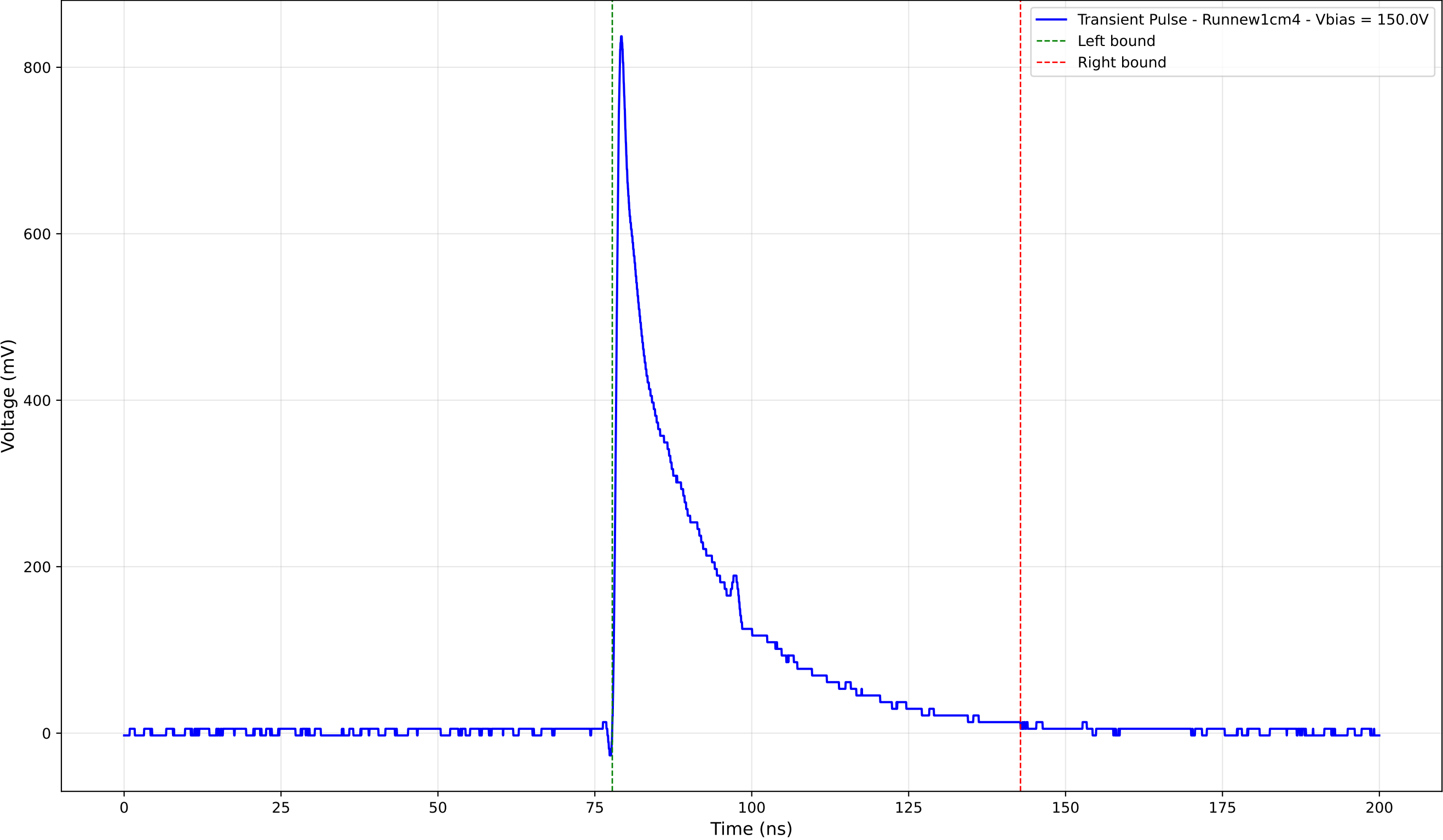
Transient Pulse - Sample: new1cm - Position: 4840.0 \mu\text{m} - Charge: 186.23 pC
