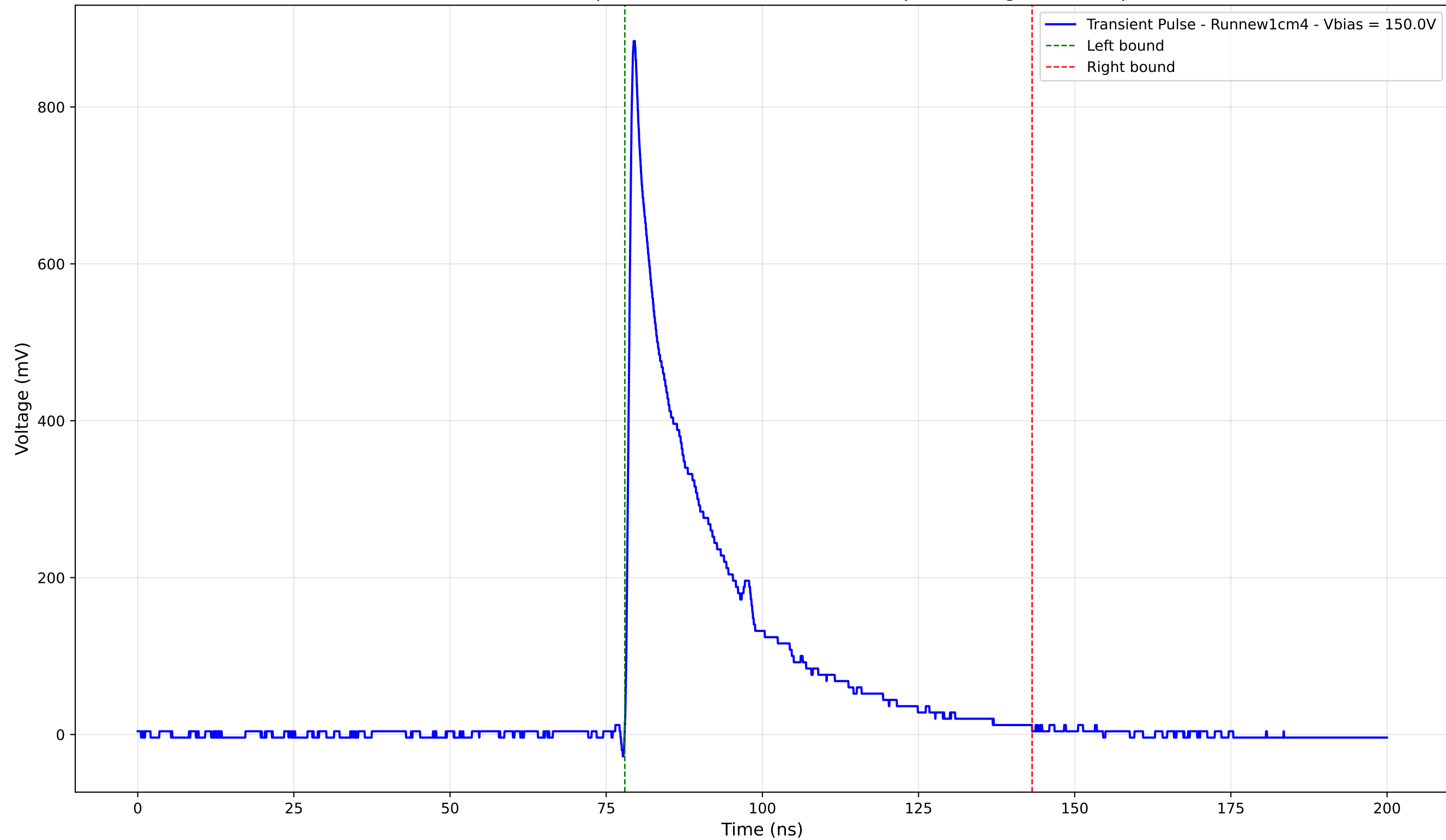
Transient Pulse - Sample: new1cm - Position: 560.0 \mu\text{m} - Charge: 201.60 pC
