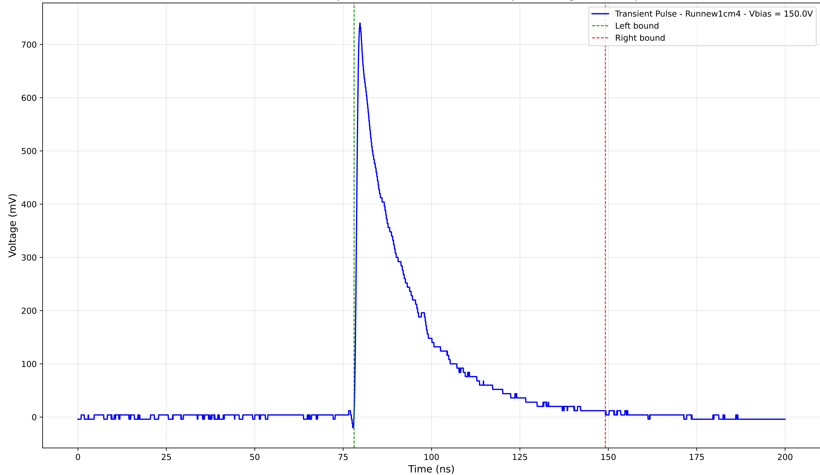
Transient Pulse - Sample: new1cm - Position: 875.0 \mu\text{m} - Charge: 203.03 pC
