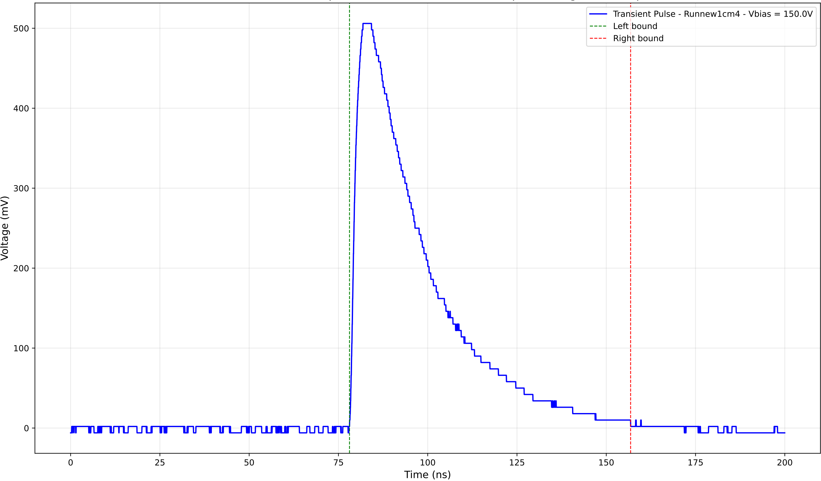
Transient Pulse - Sample: new1cm - Position: 2585.0 \mu\text{m} - Charge: 224.88 pC
