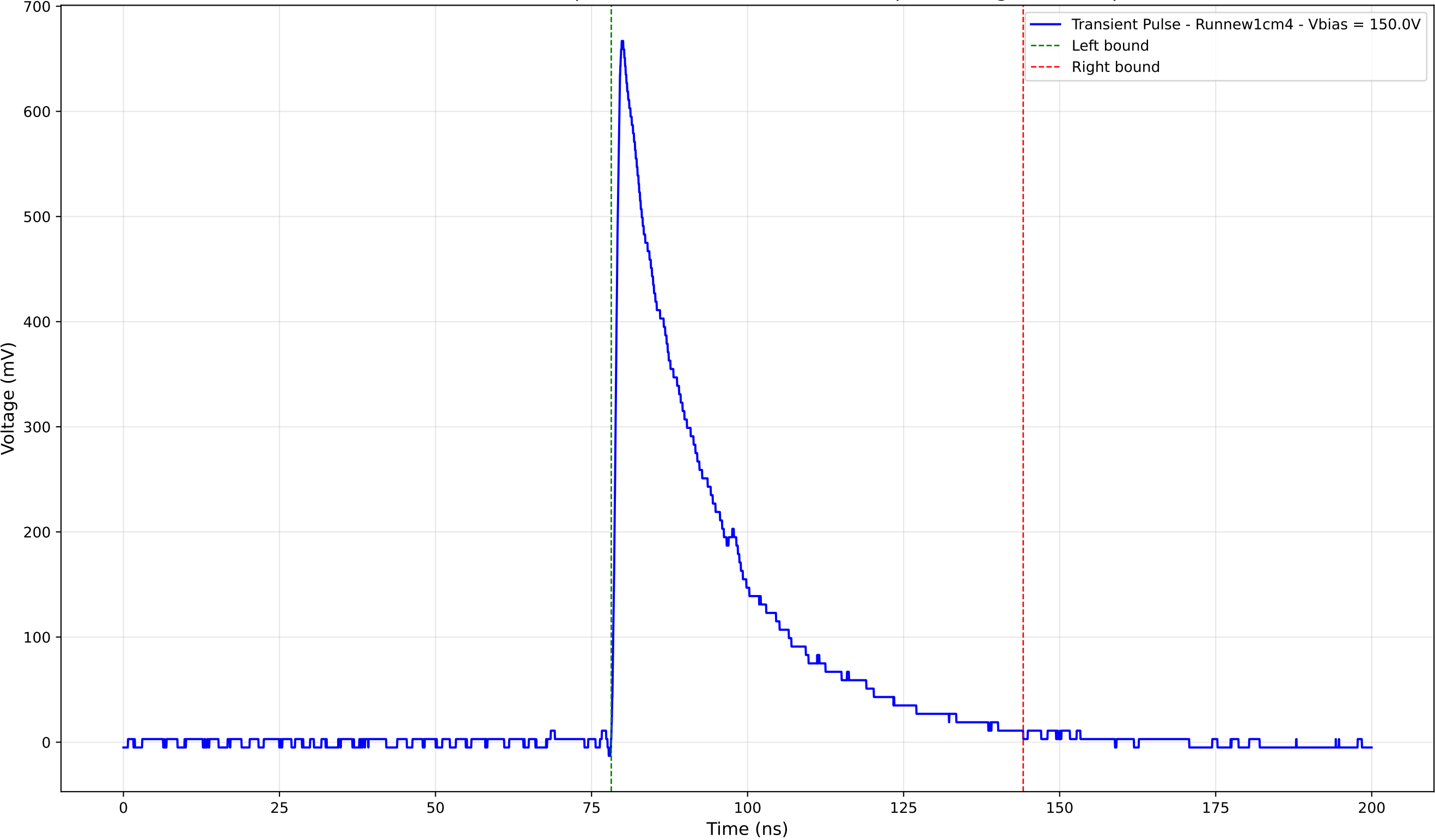
Transient Pulse - Sample: new1cm - Position: 1015.0 \mu\text{m} - Charge: 198.29 pC
