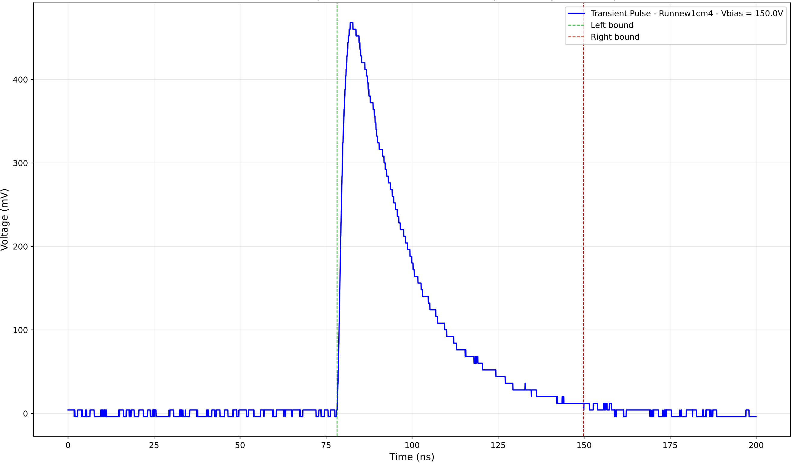
Transient Pulse - Sample: new1cm - Position: 2290.0 \mu\text{m} - Charge: 198.07 pC
