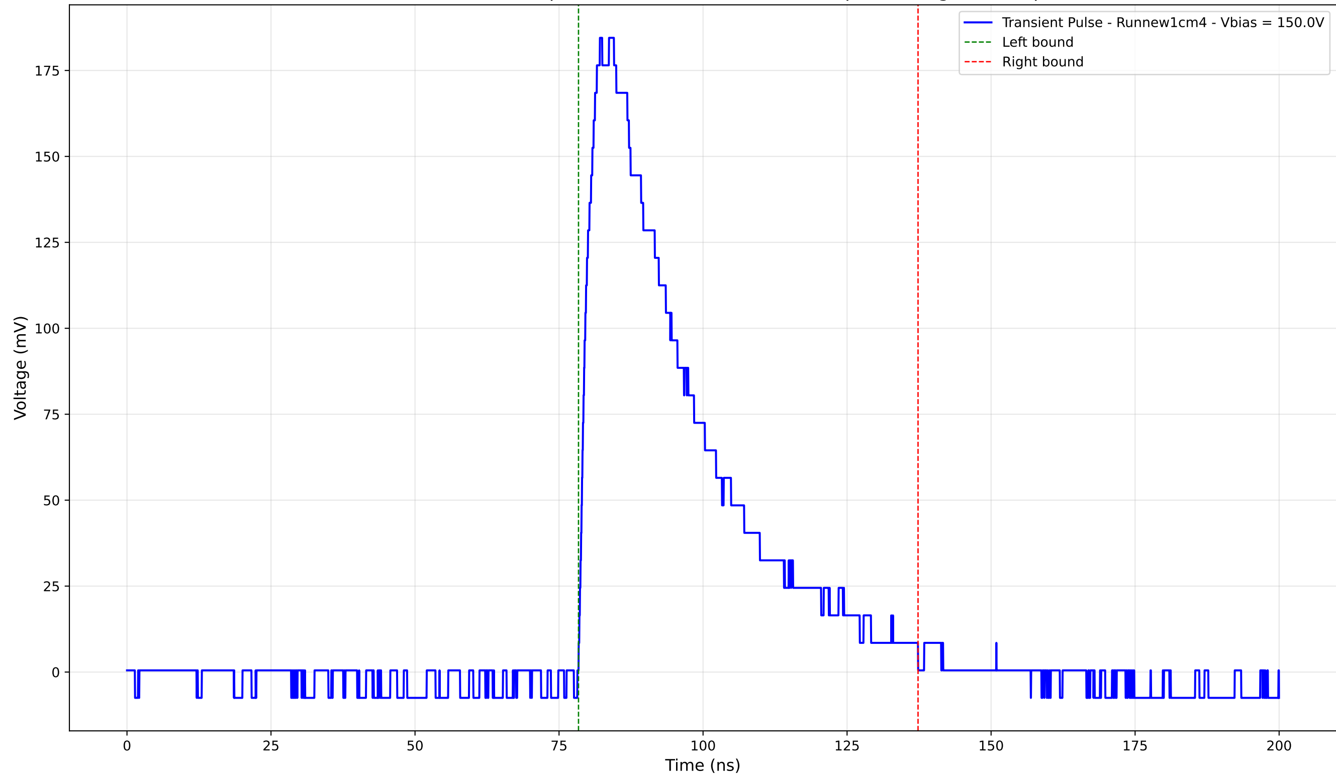
Transient Pulse - Sample: new1cm - Position: 2750.0 \mu\text{m} - Charge: 75.02 pC
