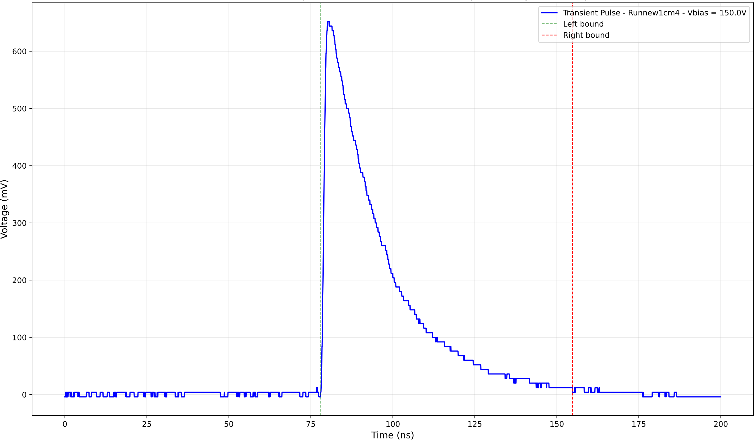
Transient Pulse - Sample: new1cm - Position: 3910.0 \mu\text{m} - Charge: 251.73 pC
