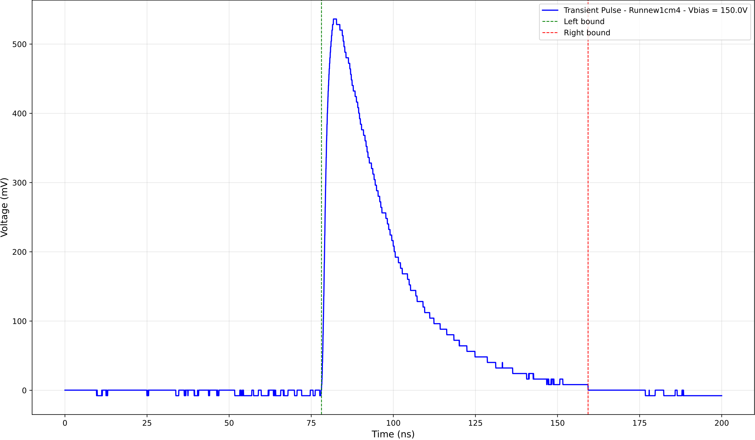
Transient Pulse - Sample: new1cm - Position: 3115.0 \mu\text{m} - Charge: 233.08 pC
