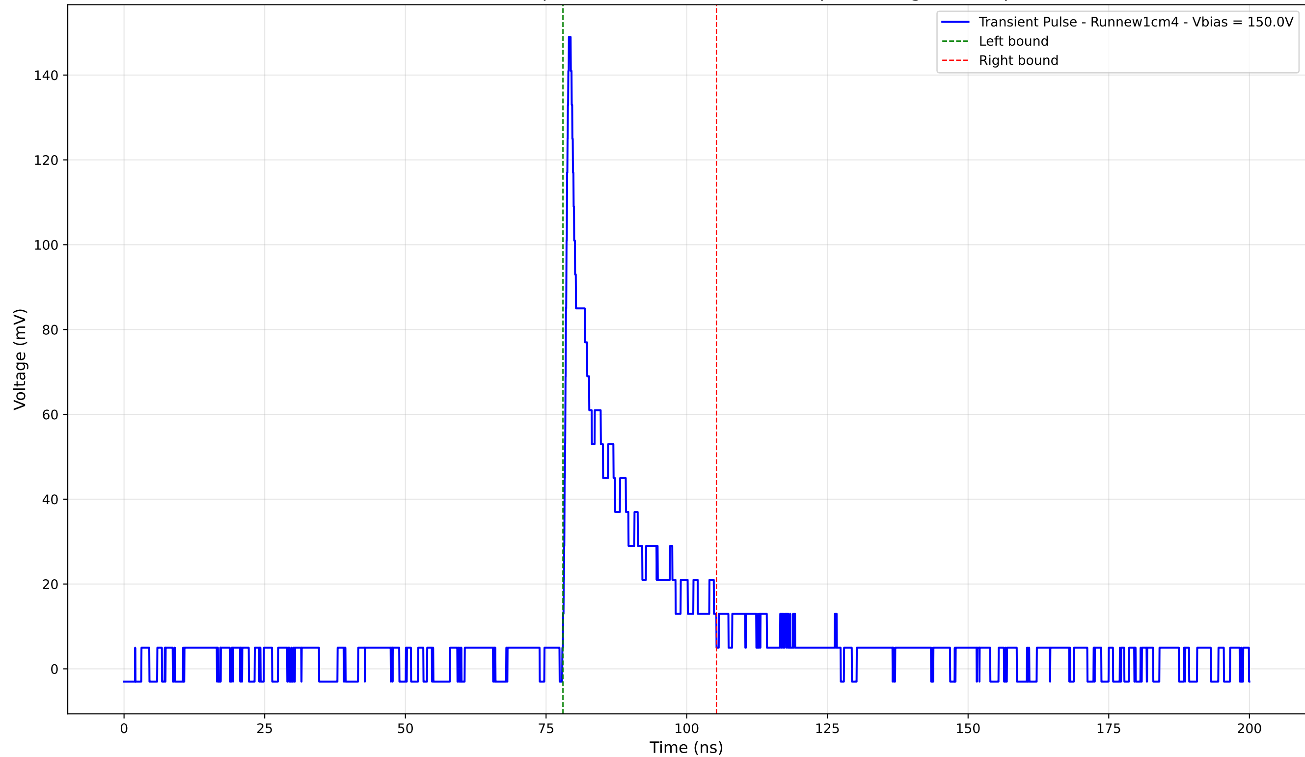
Transient Pulse - Sample: new1cm - Position: 200.0 \mu\text{m} - Charge: 22.16 pC
