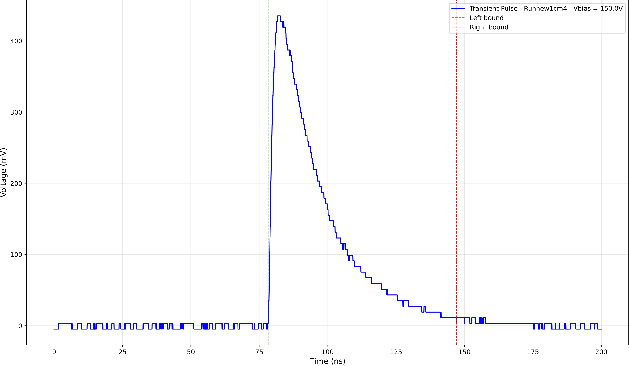
Transient Pulse - Sample: new1cm - Position: 2130.0 \mu\text{m} - Charge: 180.72 pC
