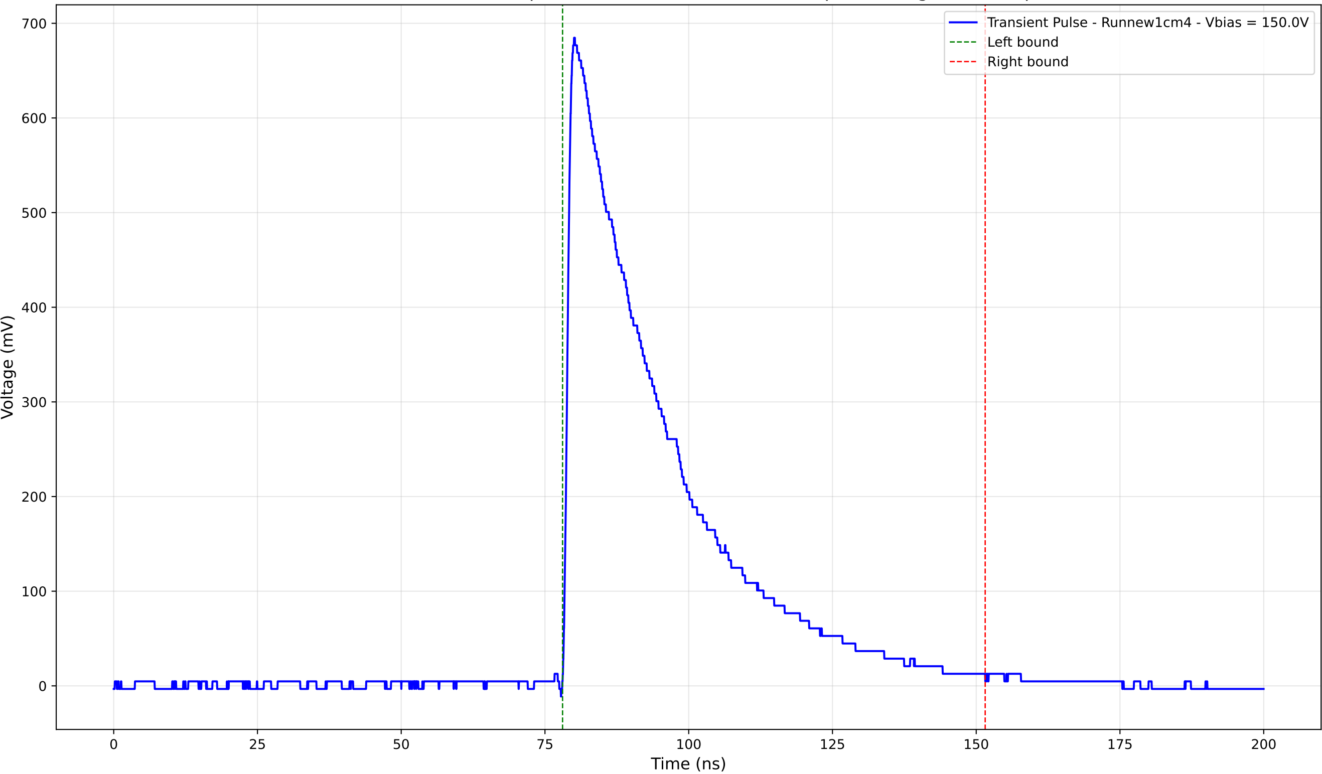
Transient Pulse - Sample: new1cm - Position: 4030.0 \mu\text{m} - Charge: 250.34 pC
