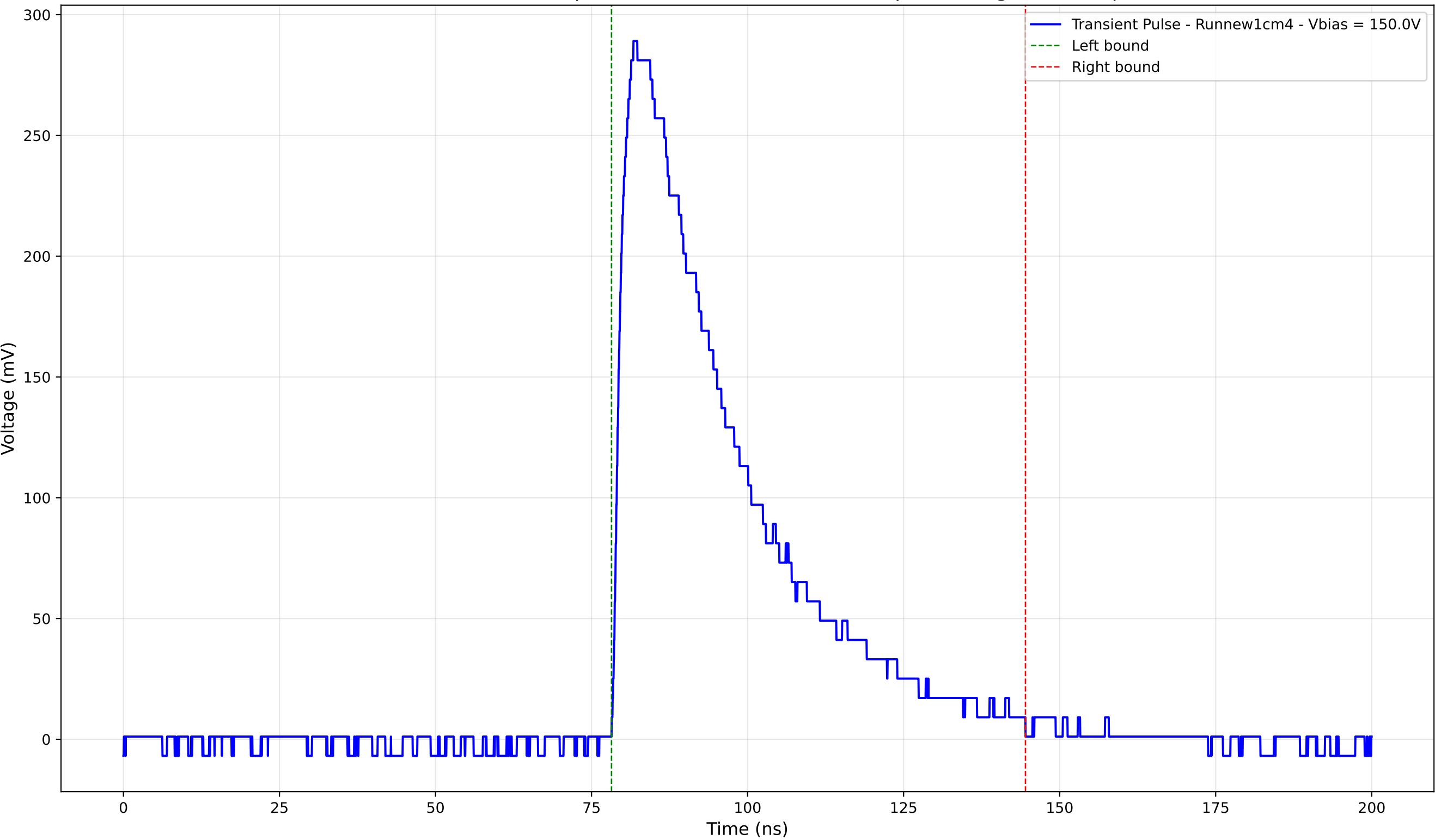
Transient Pulse - Sample: new1cm - Position: 3175.0 \mu\text{m} - Charge: 119.46 pC
