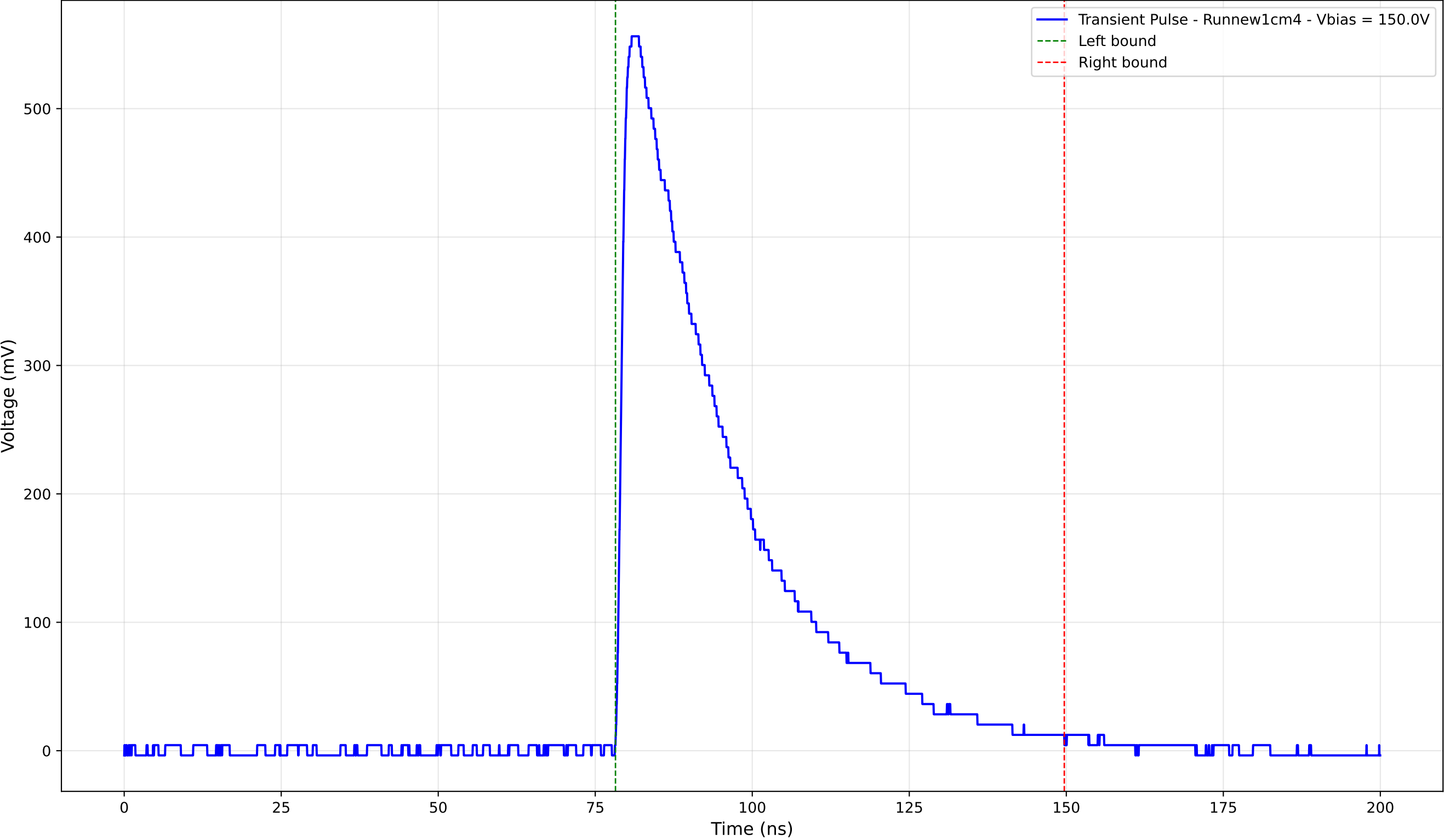
Transient Pulse - Sample: new1cm - Position: 1535.0 \mu\text{m} - Charge: 212.23 pC
