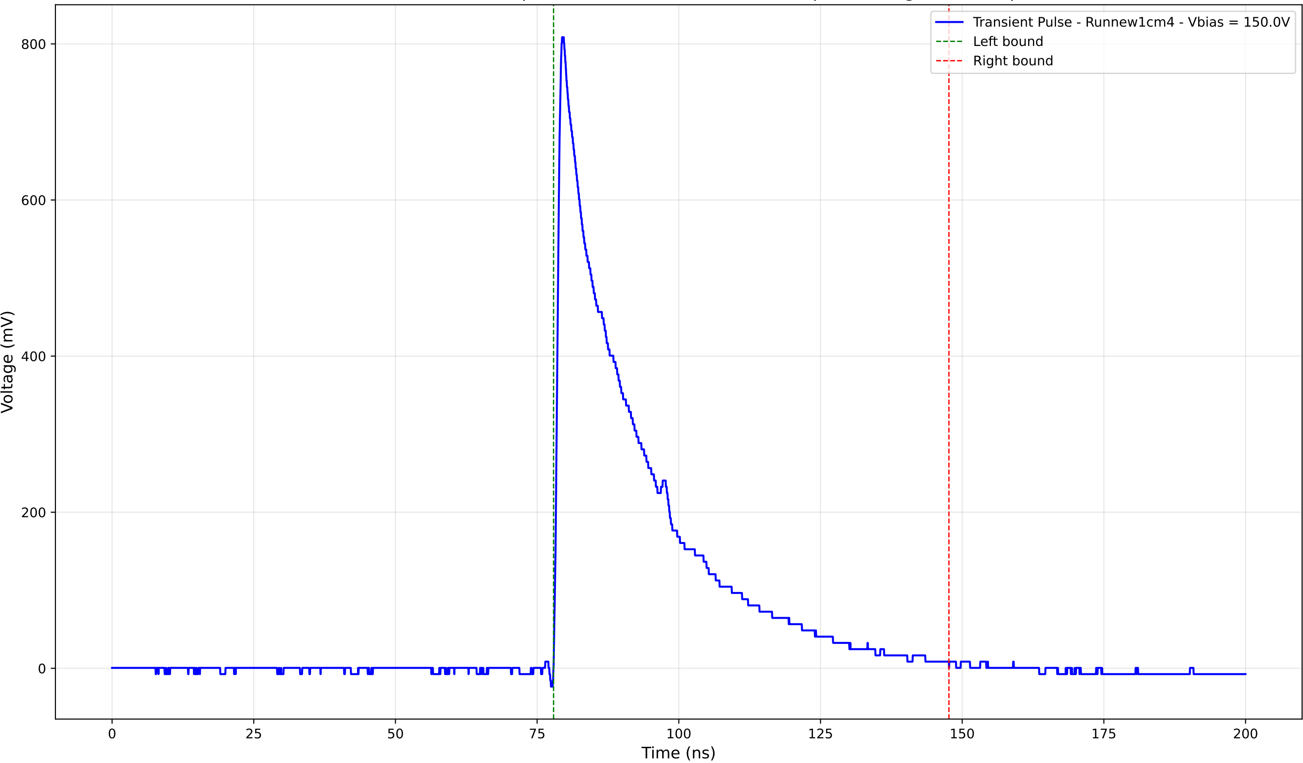
Transient Pulse - Sample: new1cm - Position: 4515.0 \mu\text{m} - Charge: 232.54 pC
