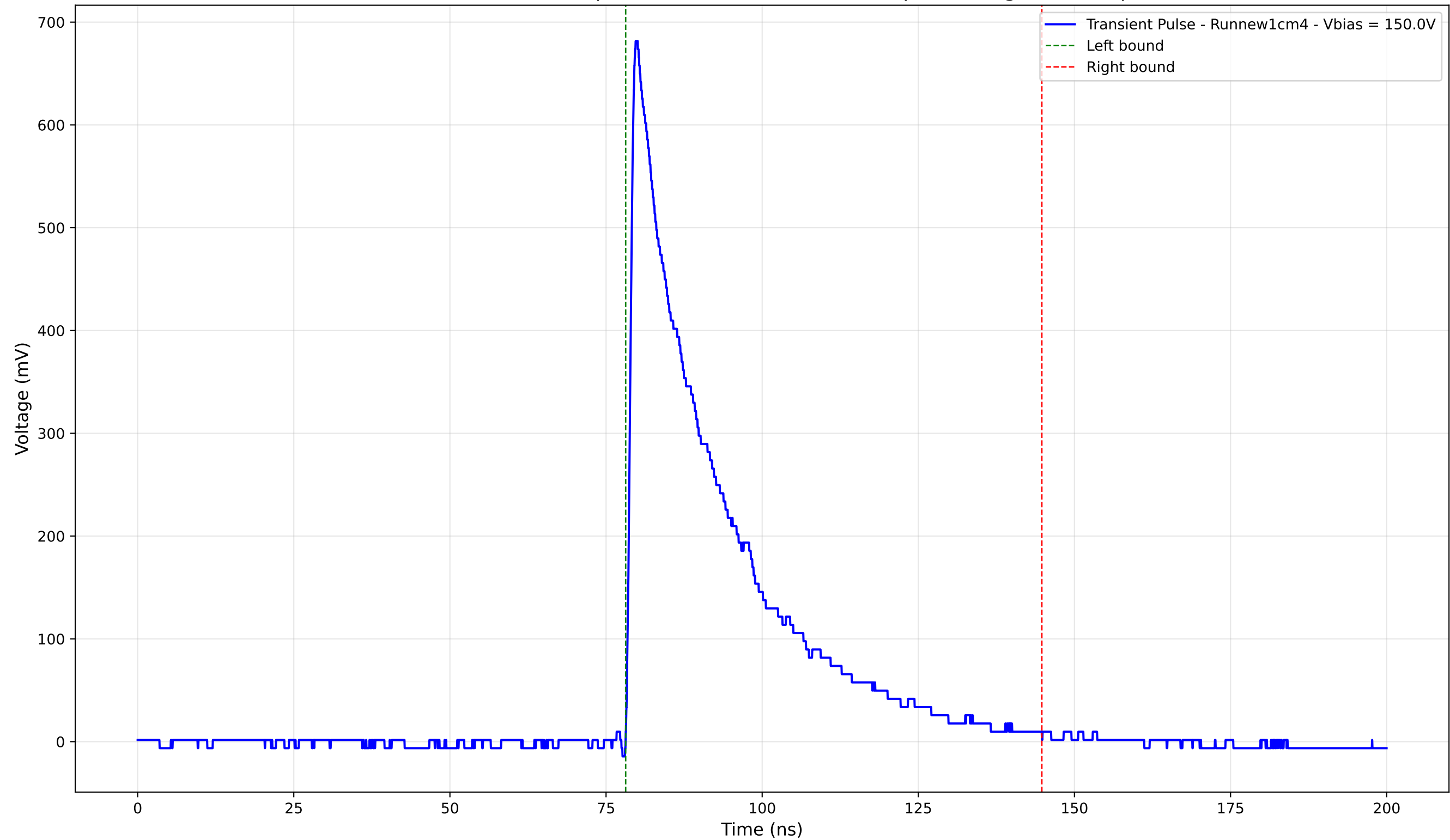
Transient Pulse - Sample: new1cm - Position: 955.0 \mu\text{m} - Charge: 195.24 pC
