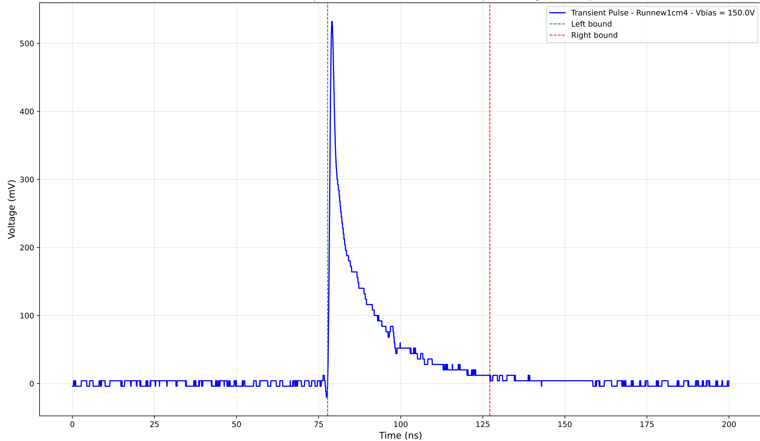
Transient Pulse - Sample: new1cm - Position: 5025.0 \mu\text{m} - Charge: 86.13 pC
