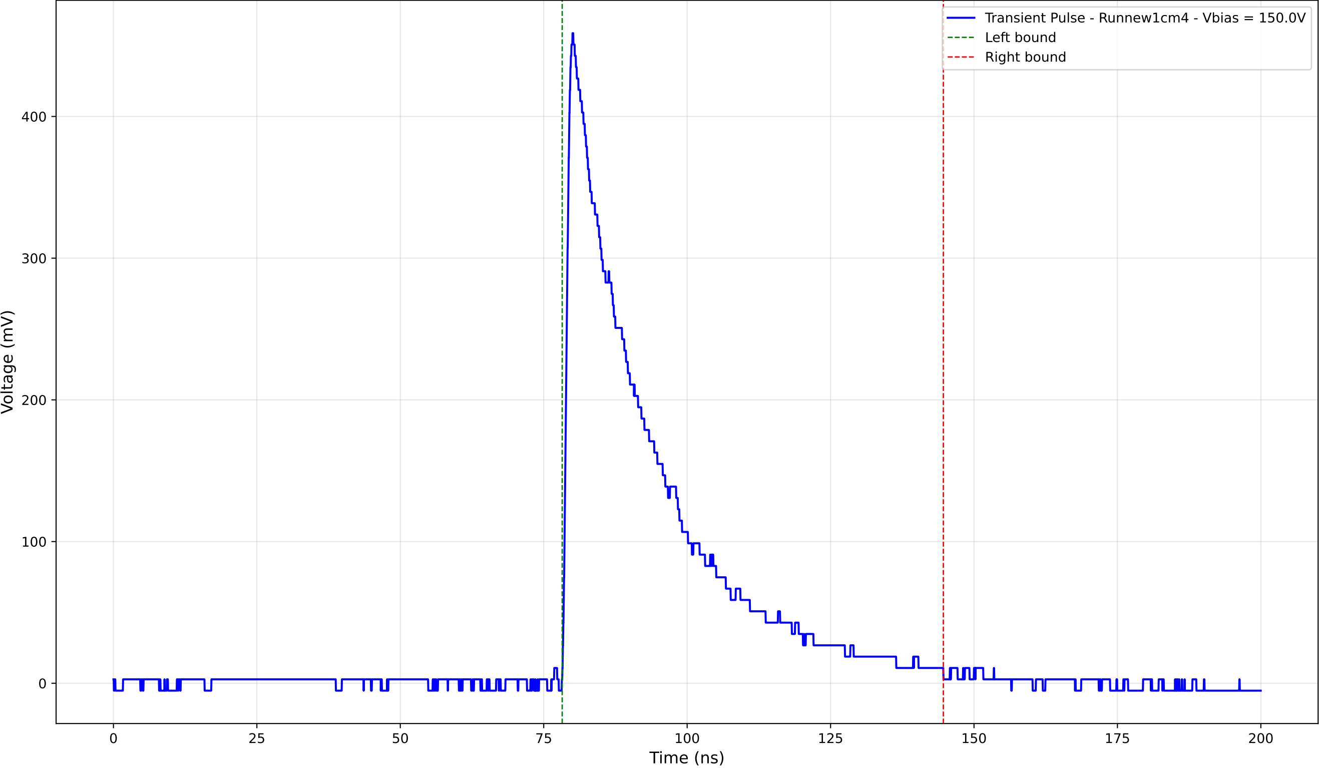
Transient Pulse - Sample: new1cm - Position: 1135.0 \mu\text{m} - Charge: 139.63 pC
