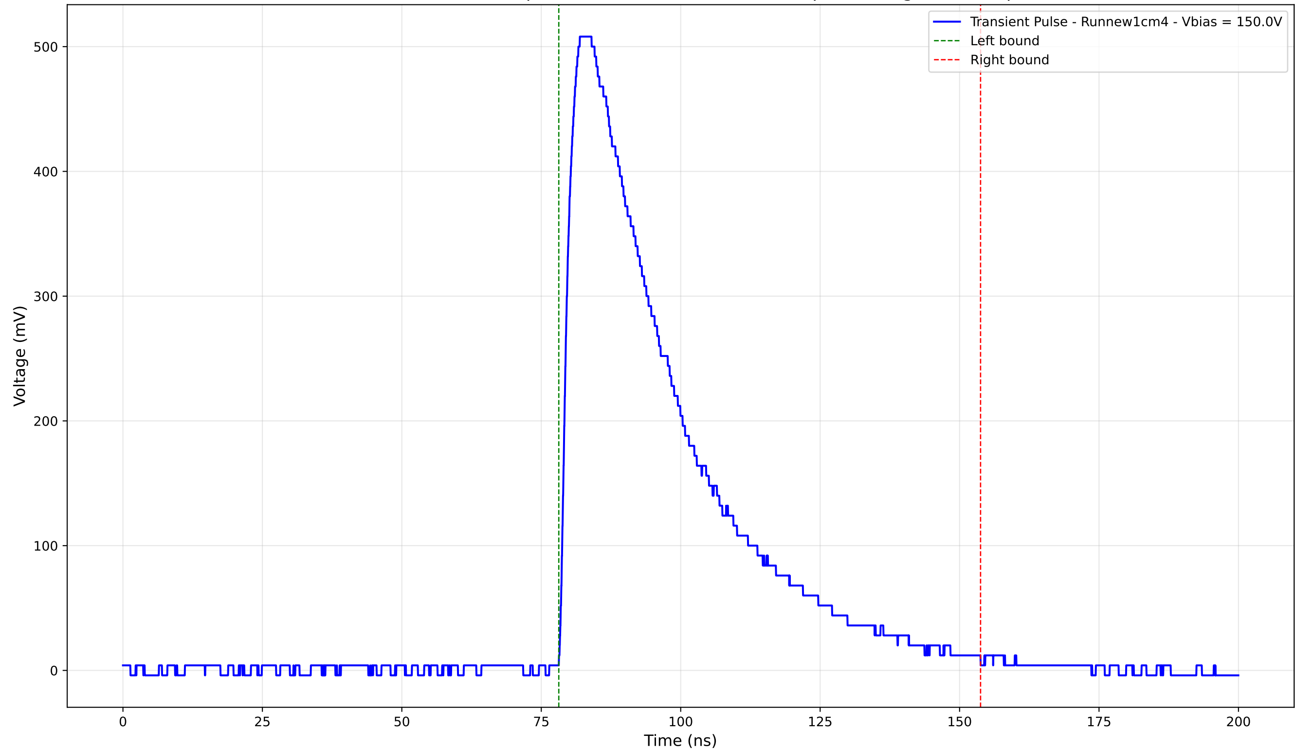
Transient Pulse - Sample: new1cm - Position: 2520.0 \mu\text{m} - Charge: 226.71 pC
