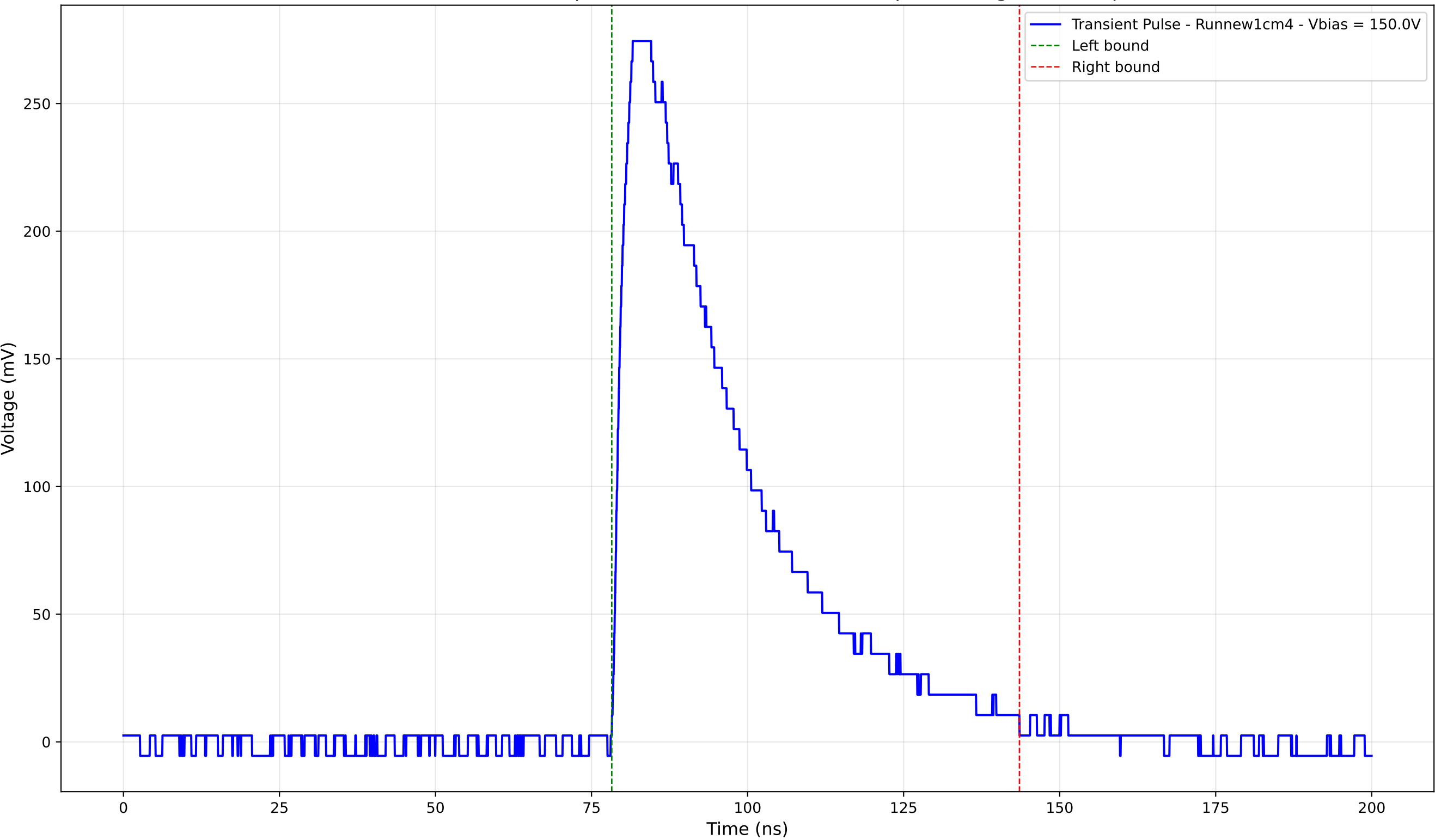
Transient Pulse - Sample: new1cm - Position: 2665.0 \mu\text{m} - Charge: 118.27 pC
