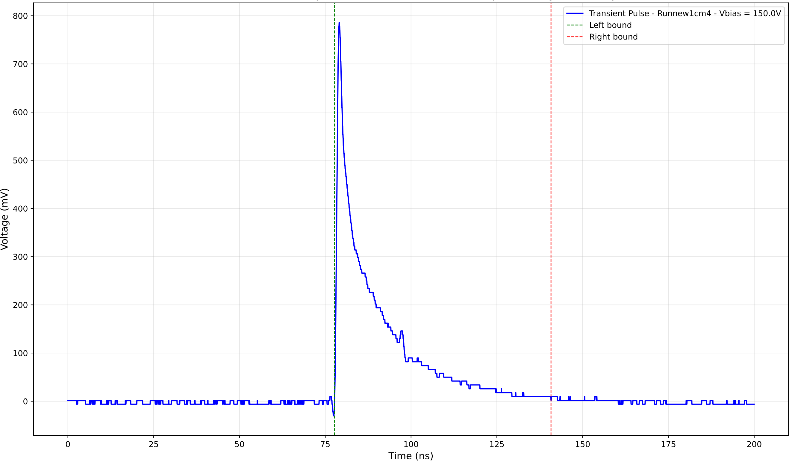
Transient Pulse - Sample: new1cm - Position: 4995.0 \mu\text{m} - Charge: 143.81 pC
