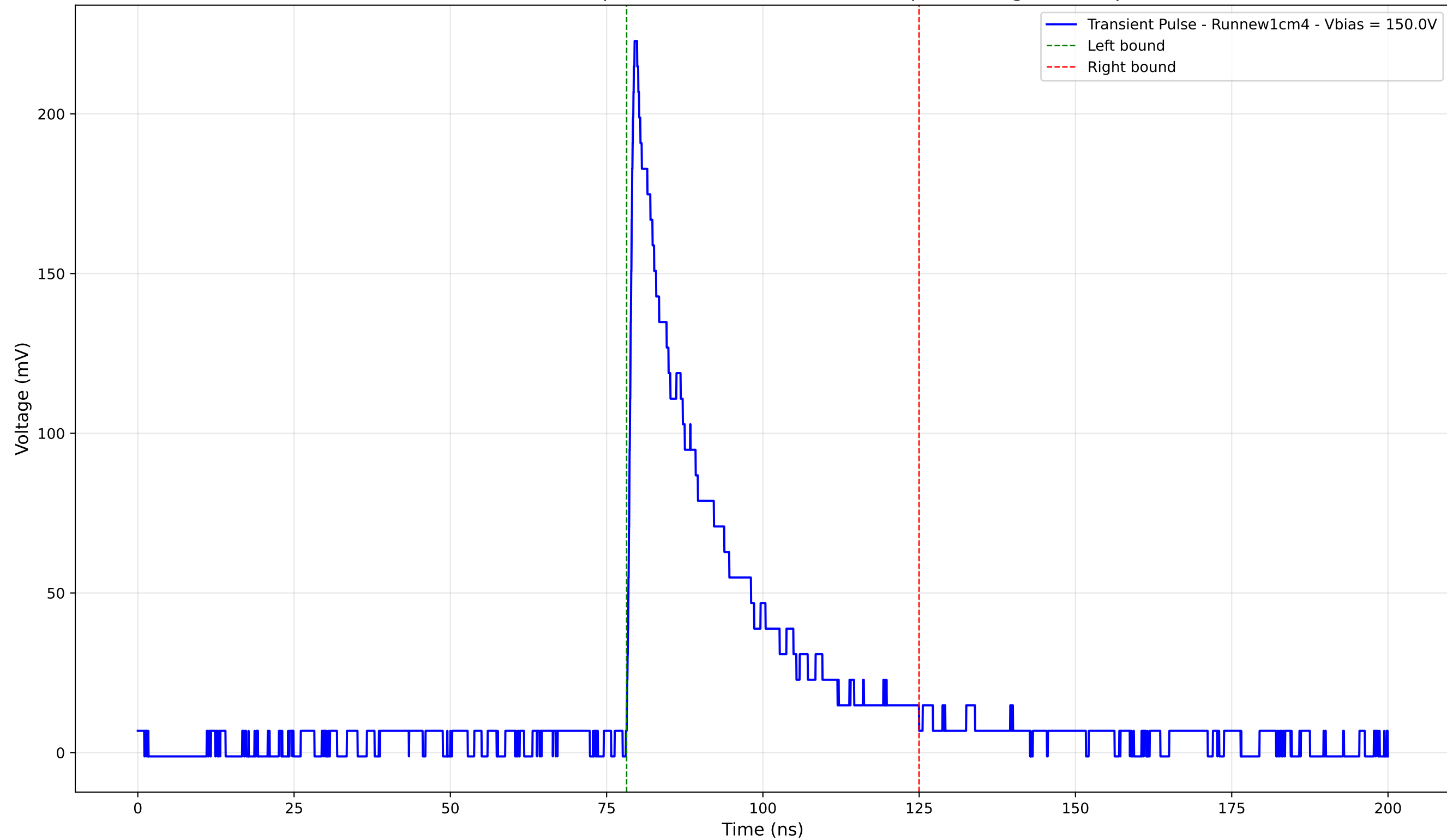
Transient Pulse - Sample: new1cm - Position: 720.0 \mu\text{m} - Charge: 55.21 pC
