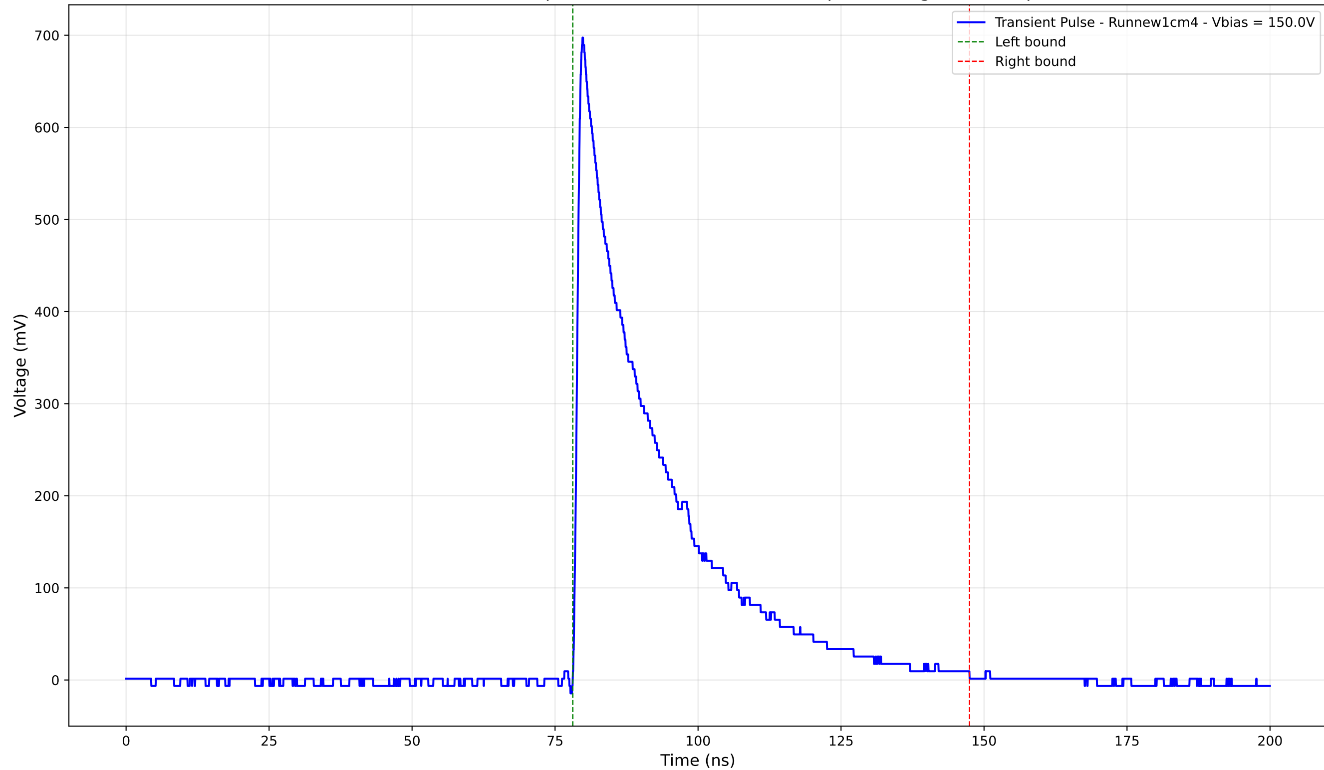
Transient Pulse - Sample: new1cm - Position: 945.0 \mu\text{m} - Charge: 196.62 pC
