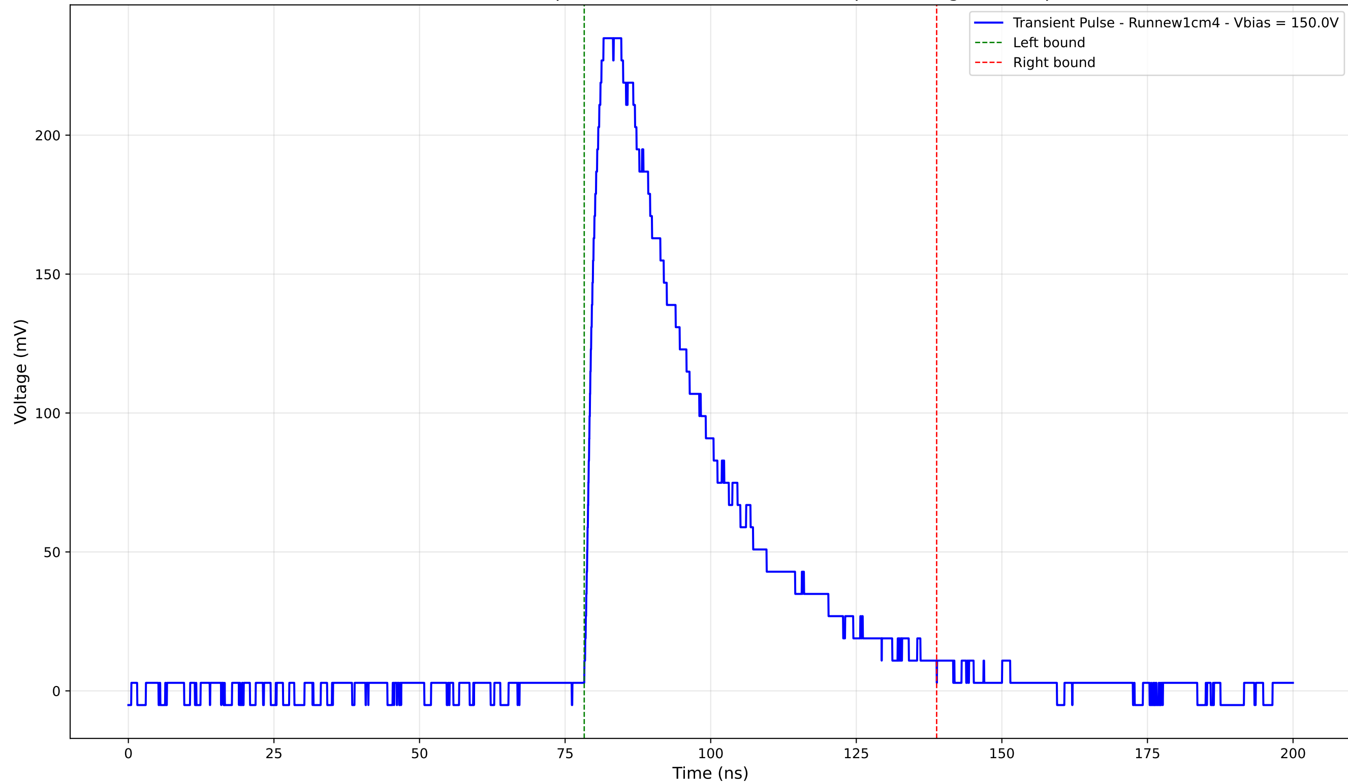
Transient Pulse - Sample: new1cm - Position: 2245.0 \mu\text{m} - Charge: 98.38 pC
