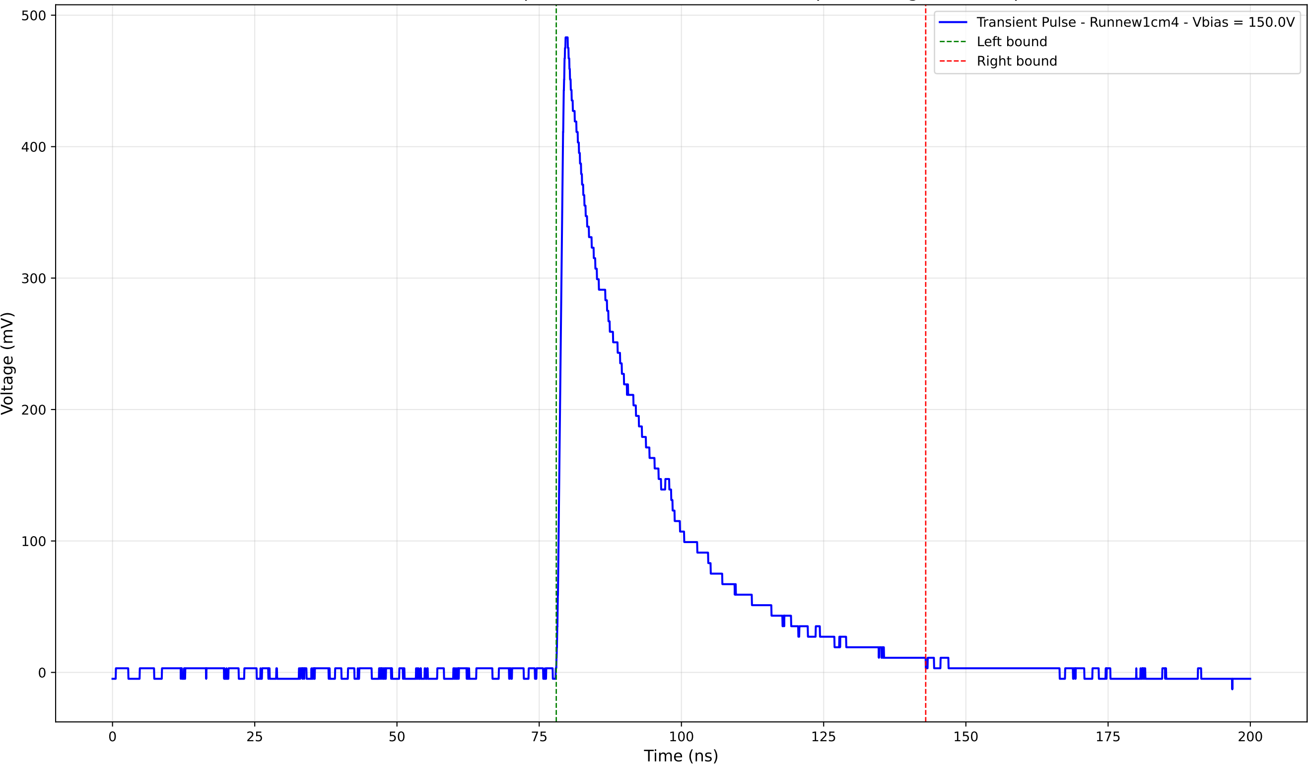
Transient Pulse - Sample: new1cm - Position: 4290.0 \mu\text{m} - Charge: 145.03 pC
