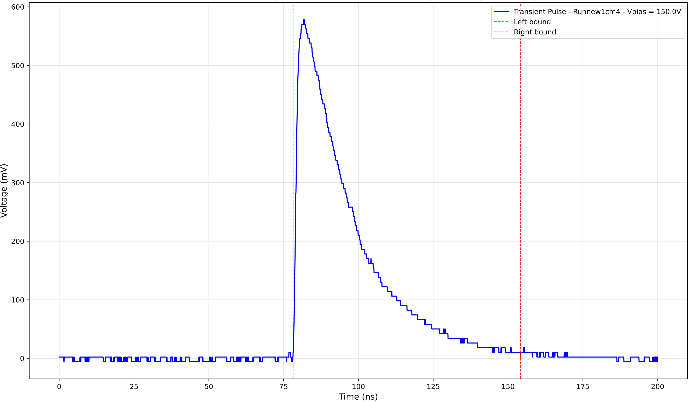
Transient Pulse - Sample: new1cm - Position: 3535.0 \mu\text{m} - Charge: 240.11 pC
