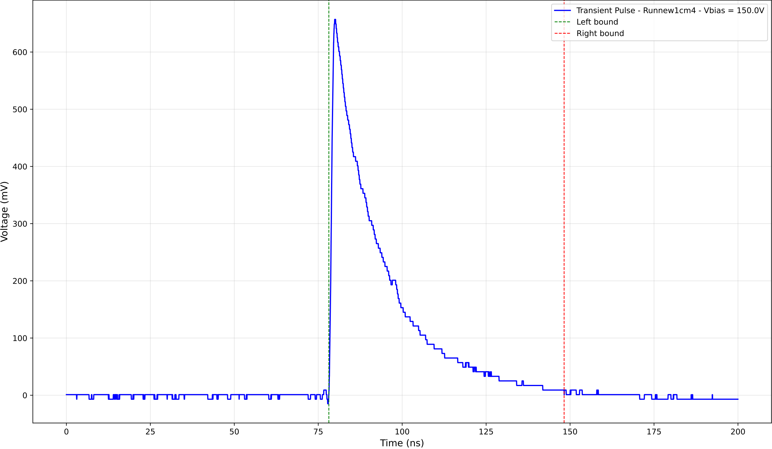
Transient Pulse - Sample: new1cm - Position: 1075.0 \mu\text{m} - Charge: 201.33 pC
