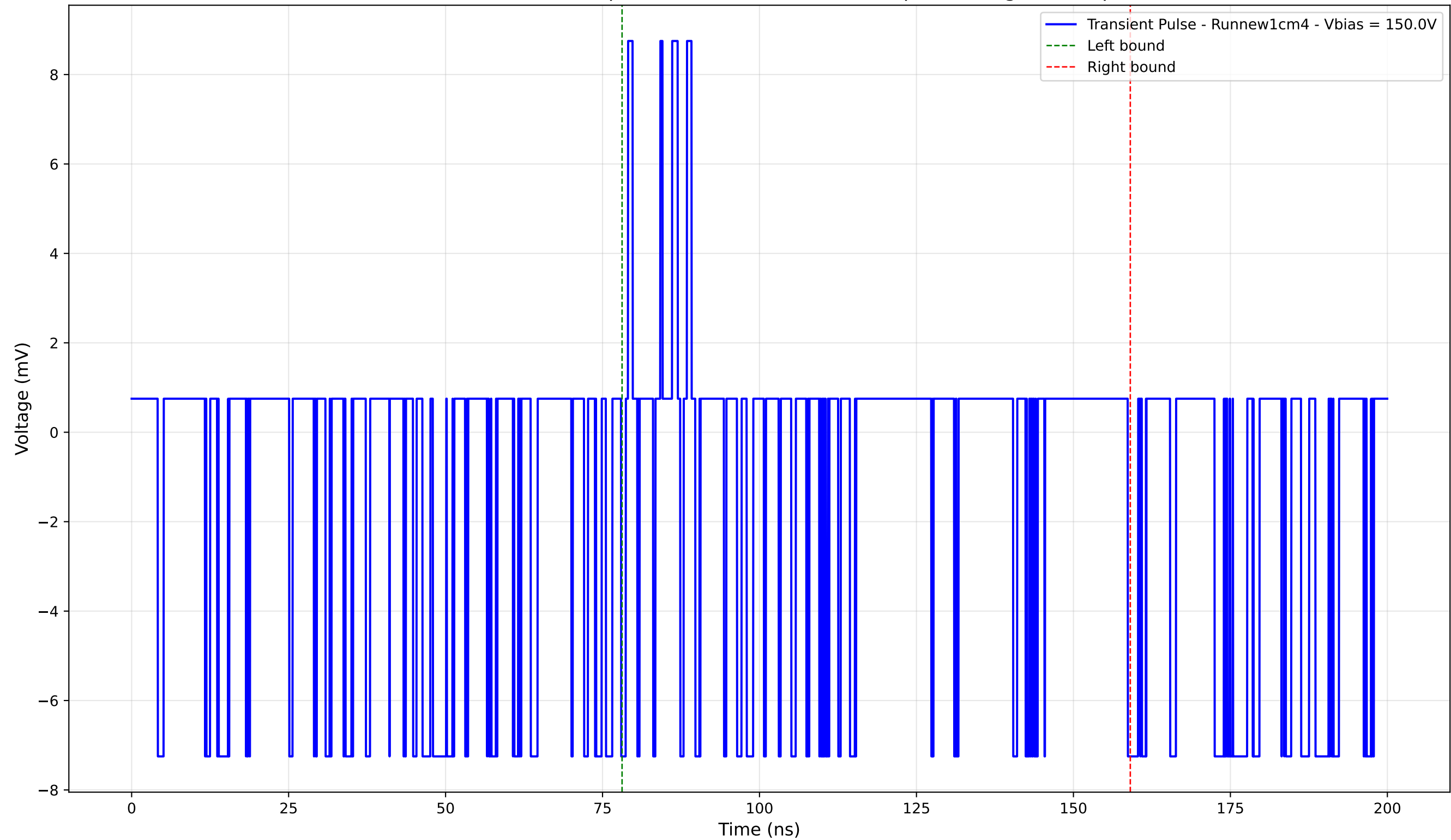
Transient Pulse - Sample: new1cm - Position: 10.0 \mu\text{m} - Charge: -0.28 pC
