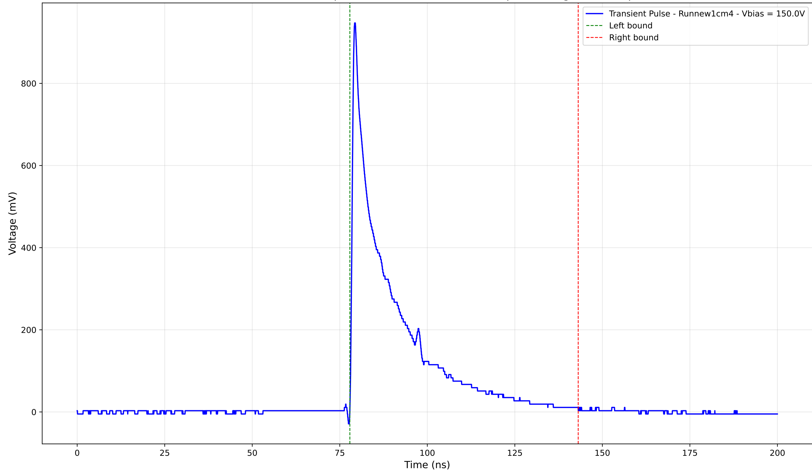
Transient Pulse - Sample: new1cm - Position: 395.0 \mu\text{m} - Charge: 199.05 pC
