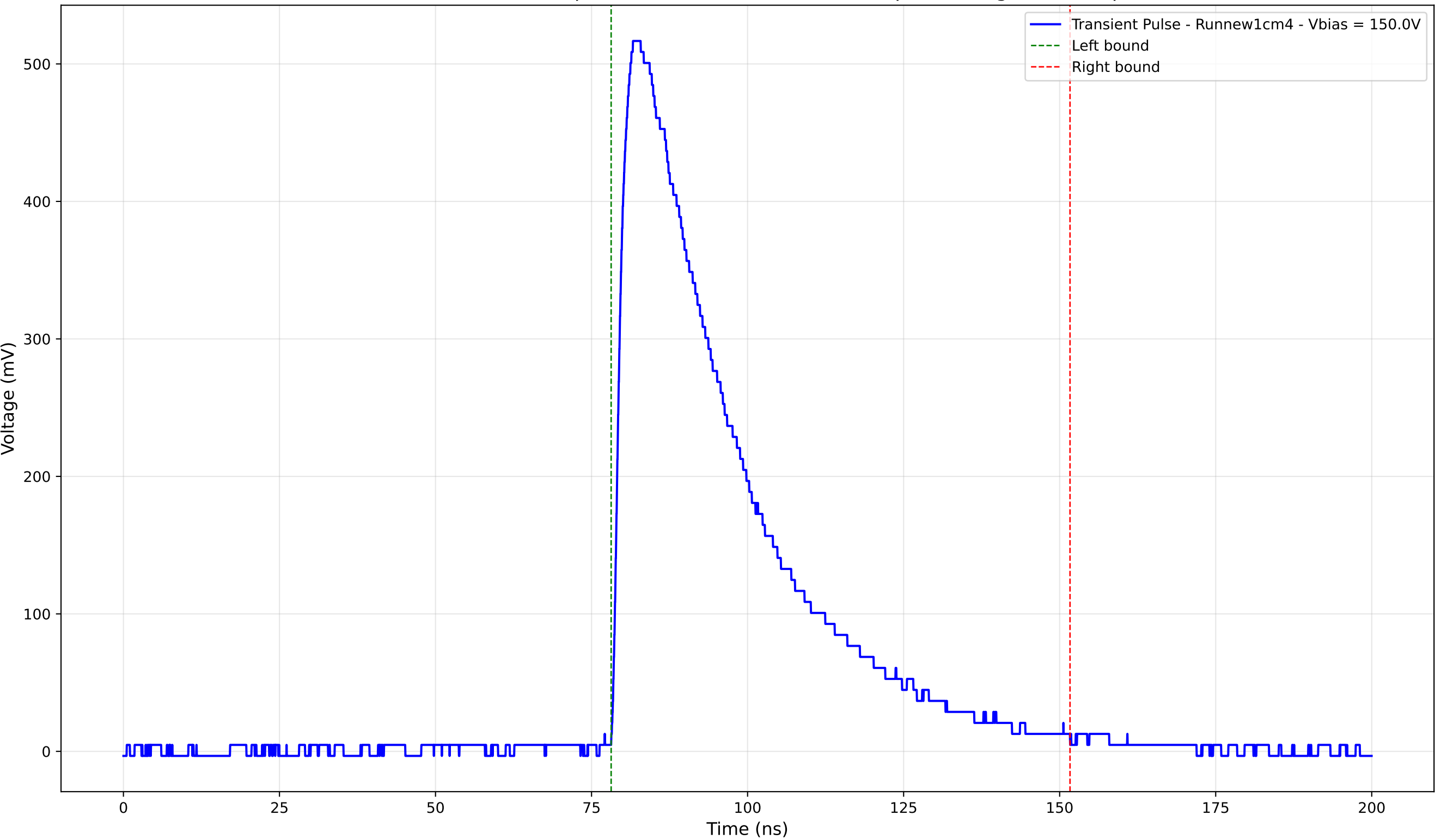
Transient Pulse - Sample: new1cm - Position: 2100.0 \mu\text{m} - Charge: 218.93 pC
