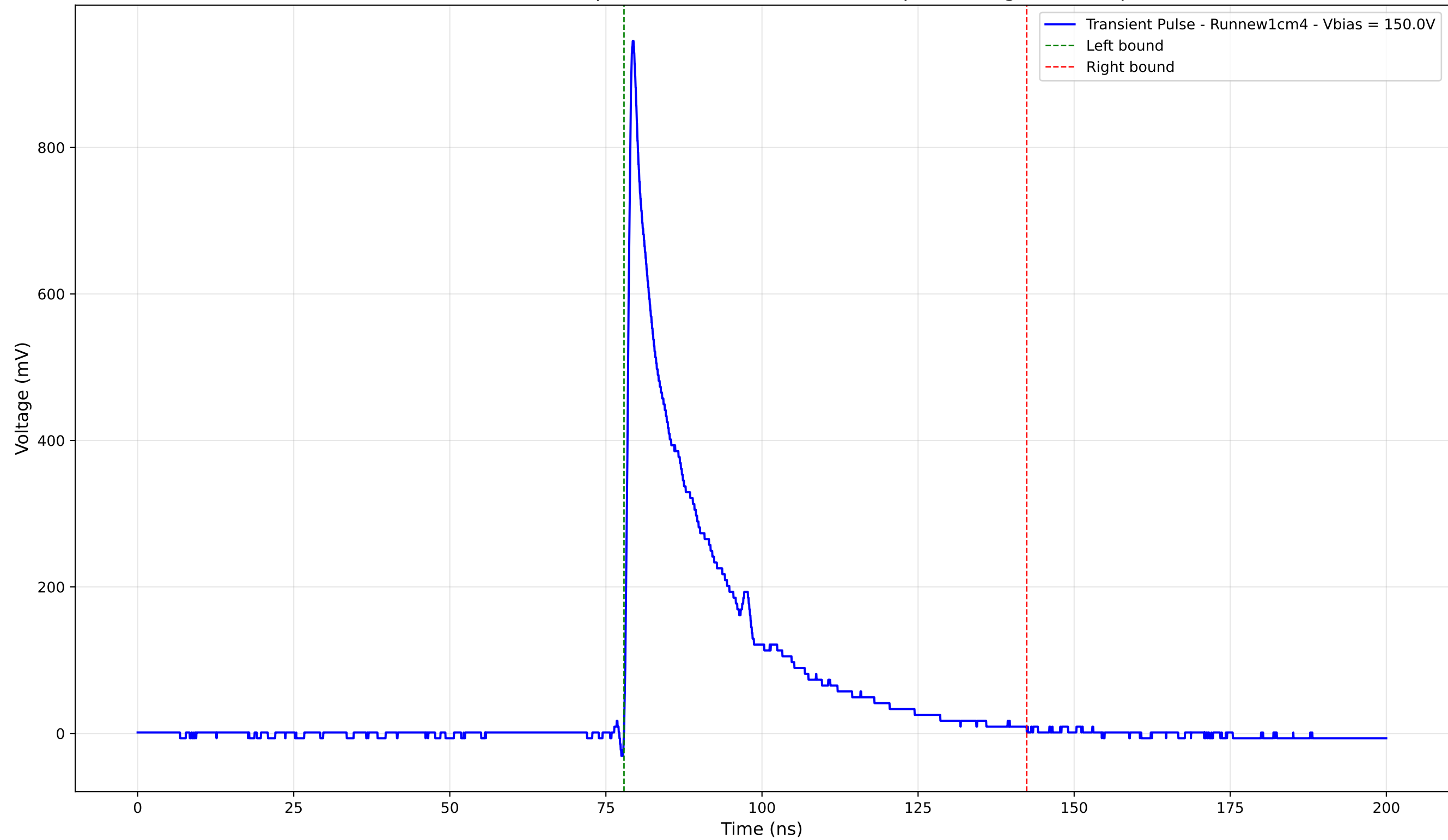
Transient Pulse - Sample: new1cm - Position: 415.0 \mu\text{m} - Charge: 197.66 pC
