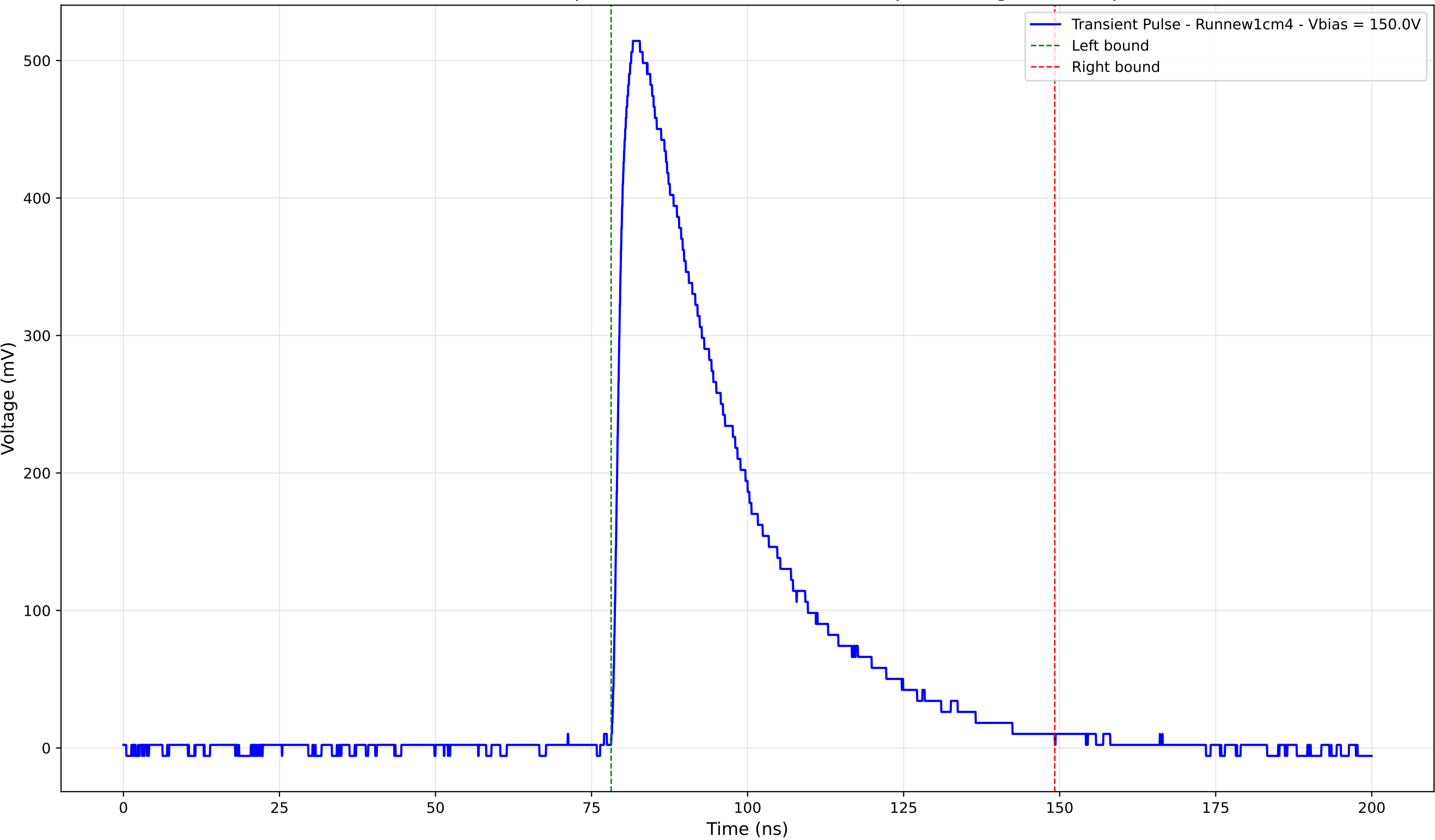
Transient Pulse - Sample: new1cm - Position: 1965.0 \mu\text{m} - Charge: 211.19 pC
