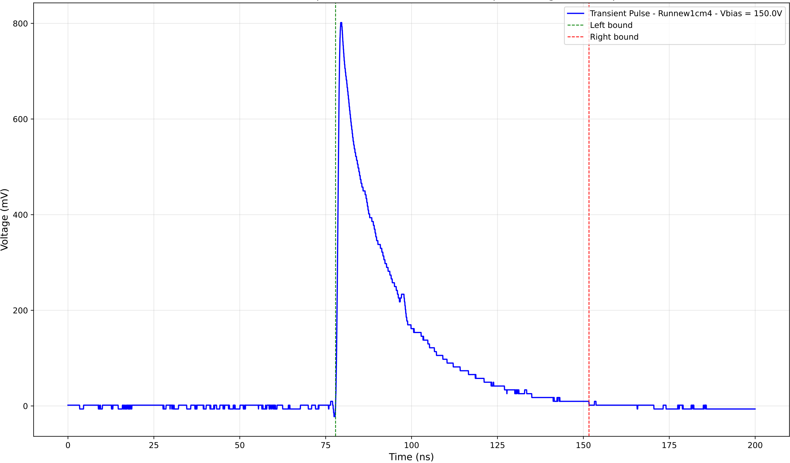
Transient Pulse - Sample: new1cm - Position: 4535.0 \mu\text{m} - Charge: 231.50 pC
