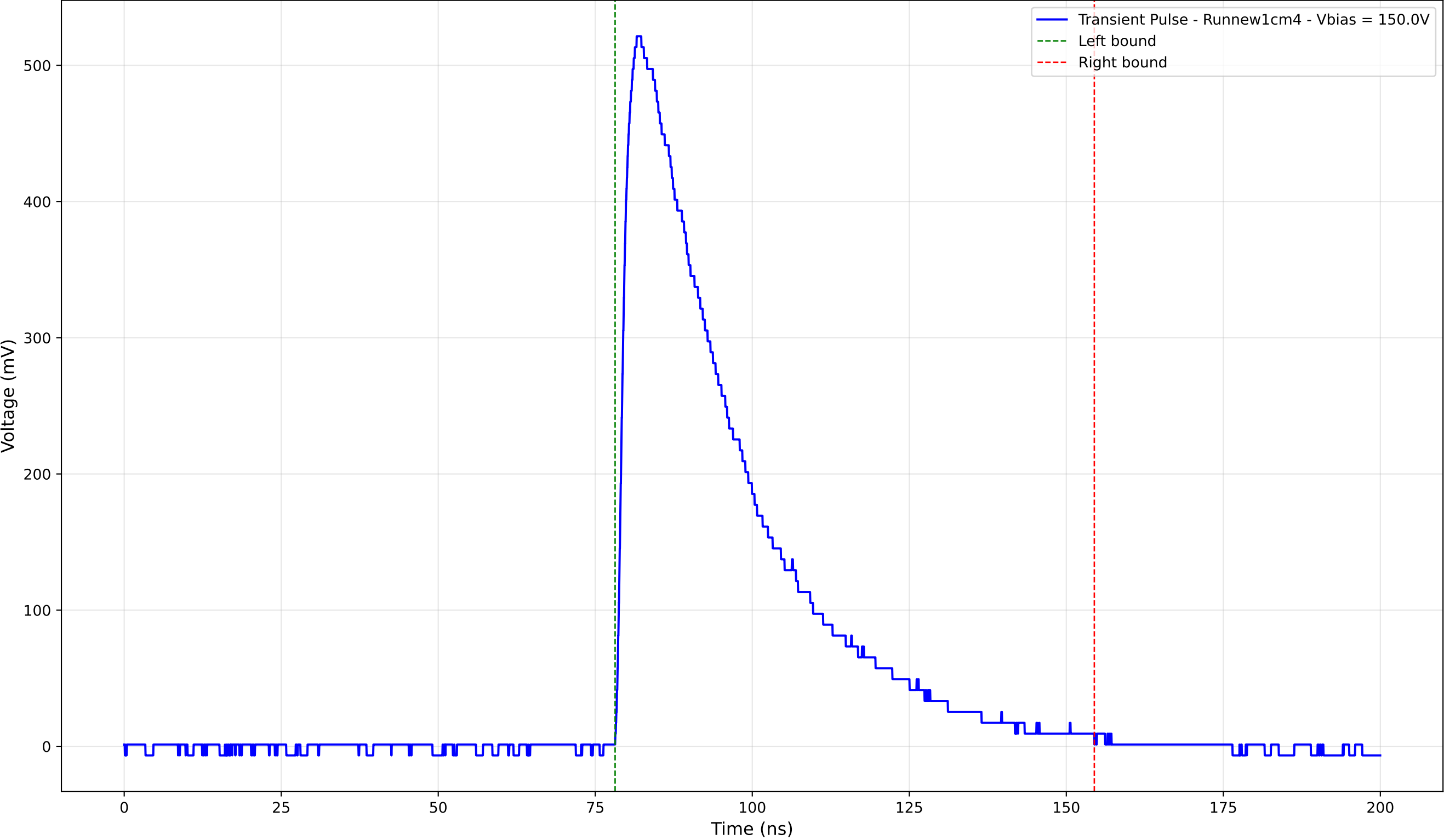
Transient Pulse - Sample: new1cm - Position: 1920.0 \mu\text{m} - Charge: 211.85 pC
