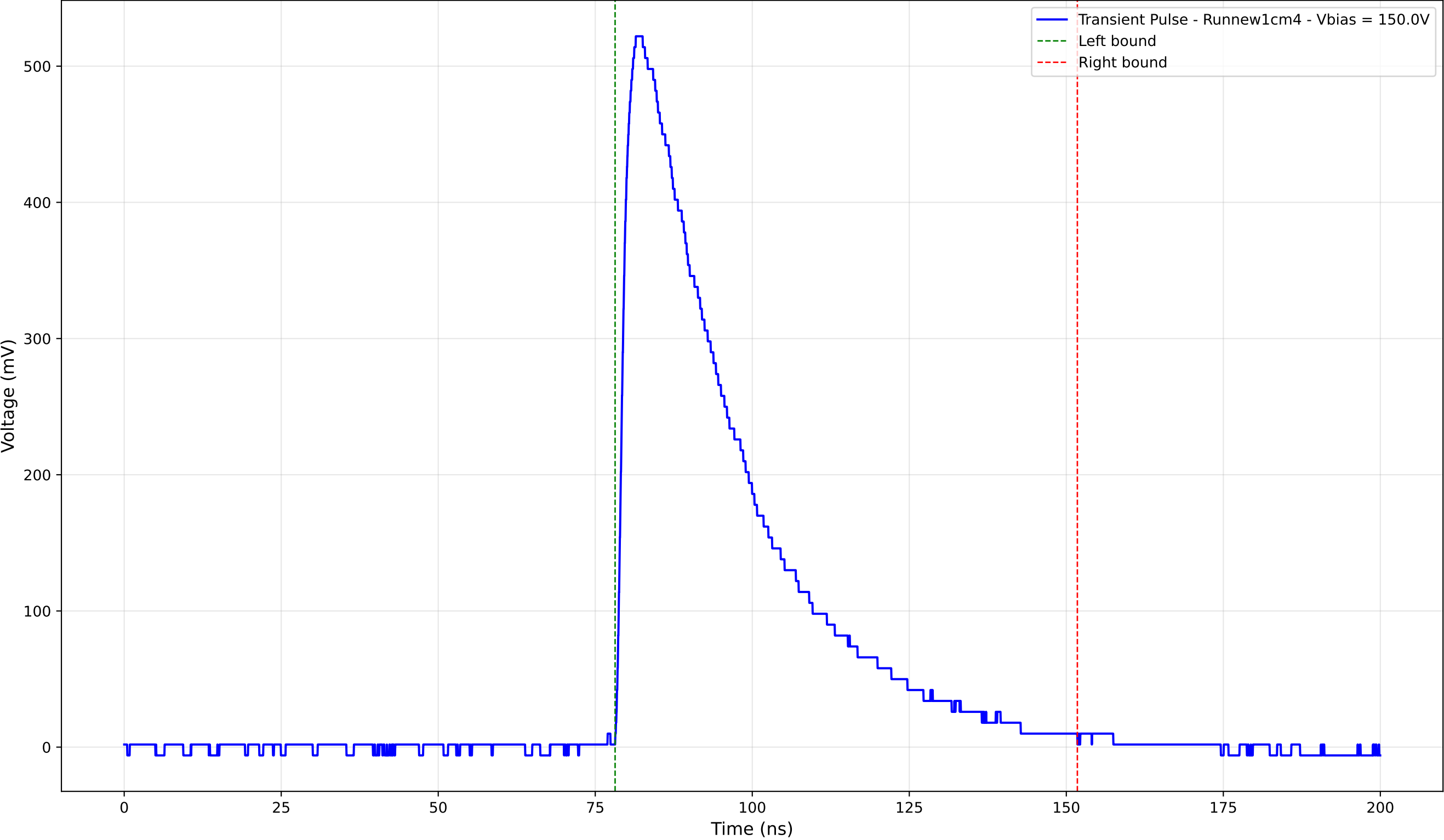
Transient Pulse - Sample: new1cm - Position: 1905.0 \mu\text{m} - Charge: 212.78 pC
