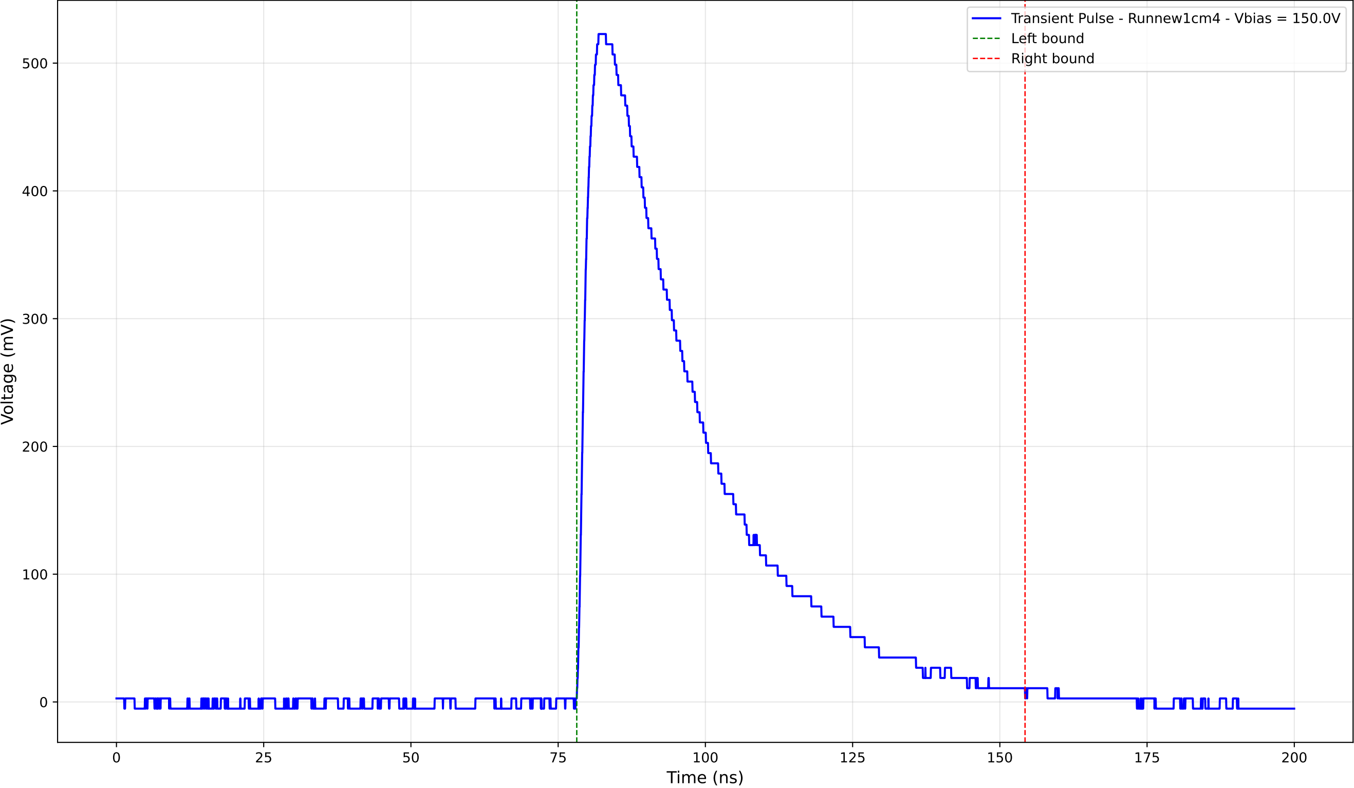
Transient Pulse - Sample: new1cm - Position: 3005.0 \mu\text{m} - Charge: 229.02 pC
