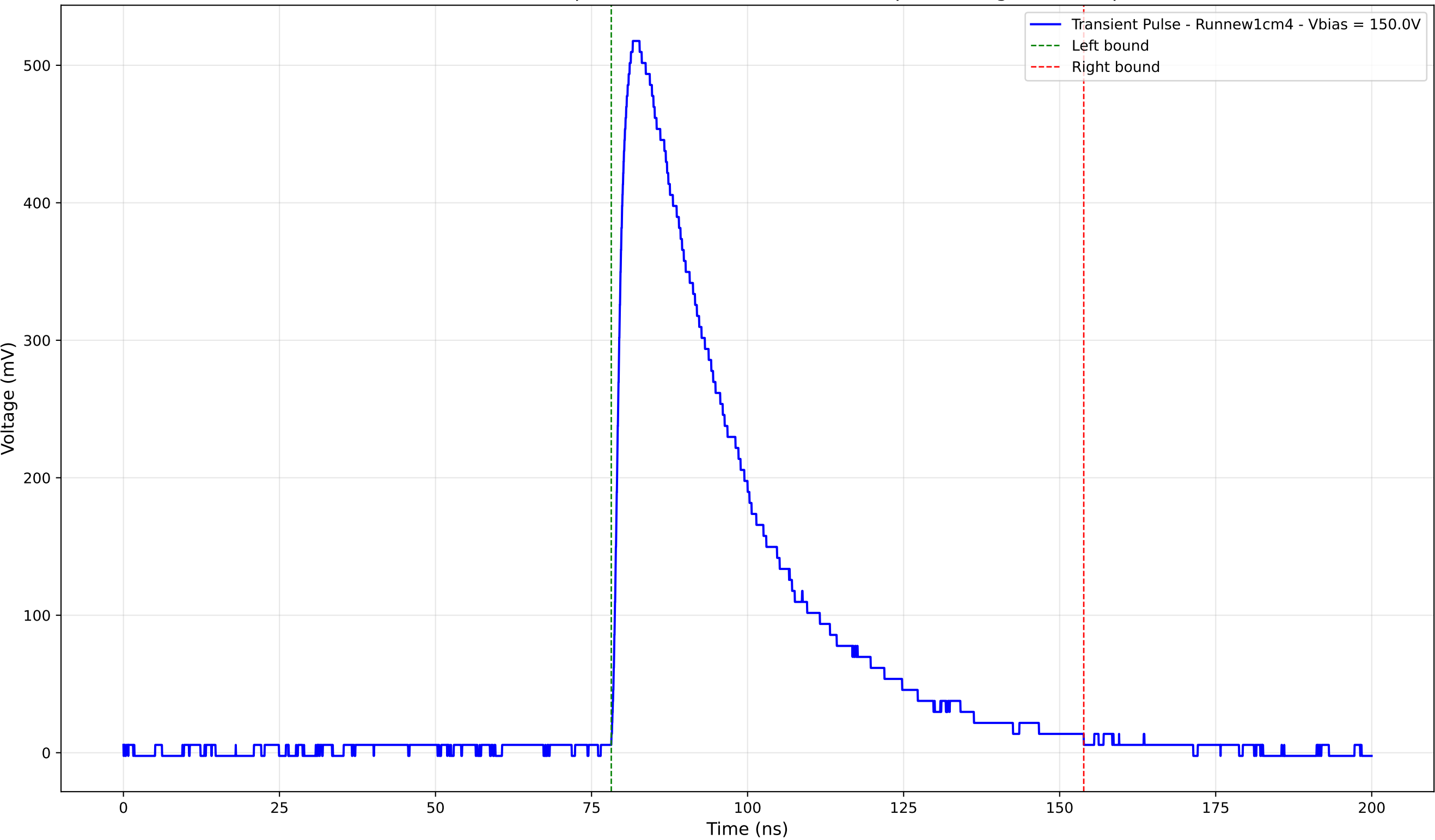
Transient Pulse - Sample: new1cm - Position: 1945.0 \mu\text{m} - Charge: 217.15 pC
