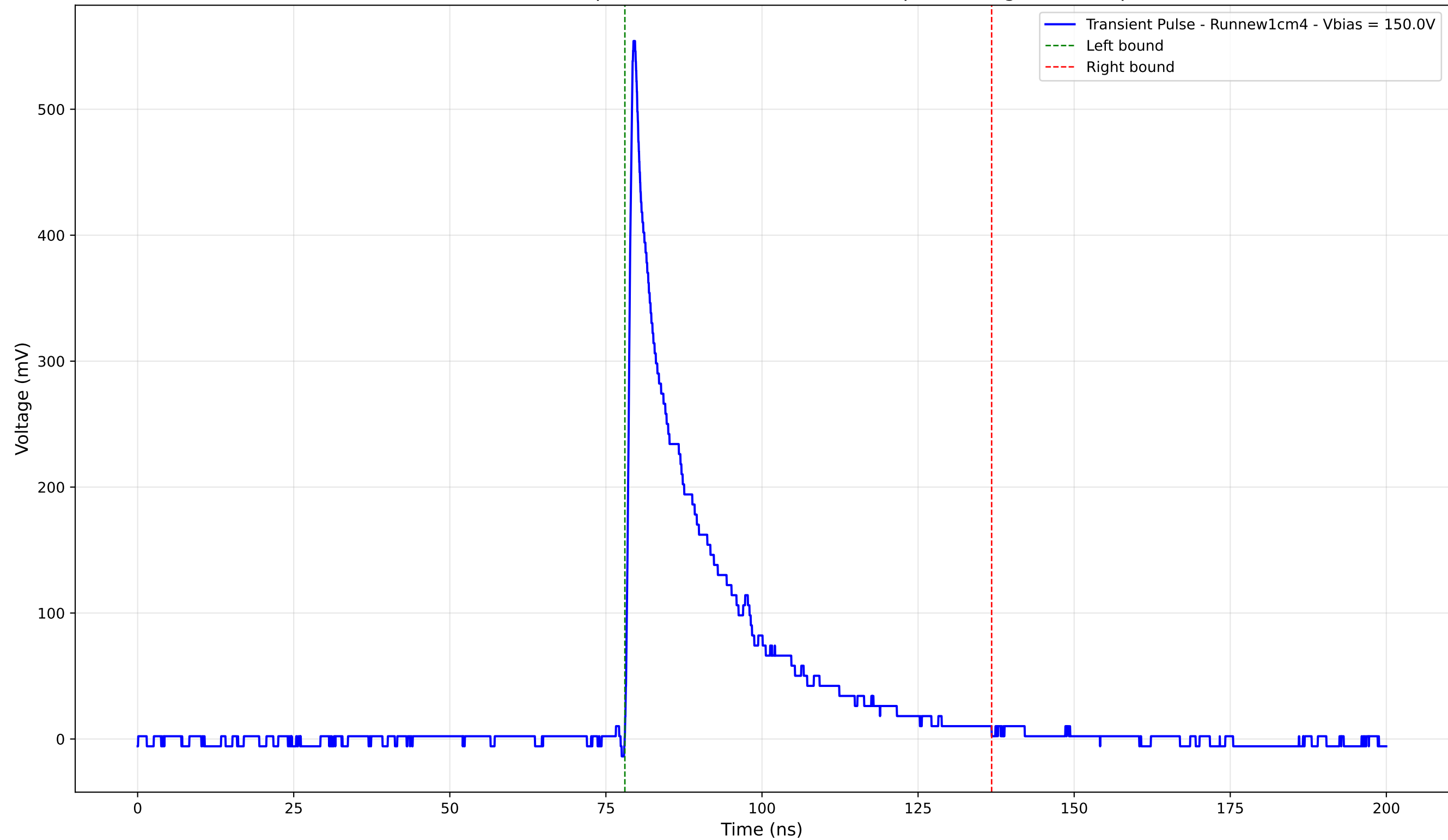
Transient Pulse - Sample: new1cm - Position: 635.0 \mu\text{m} - Charge: 115.97 pC
