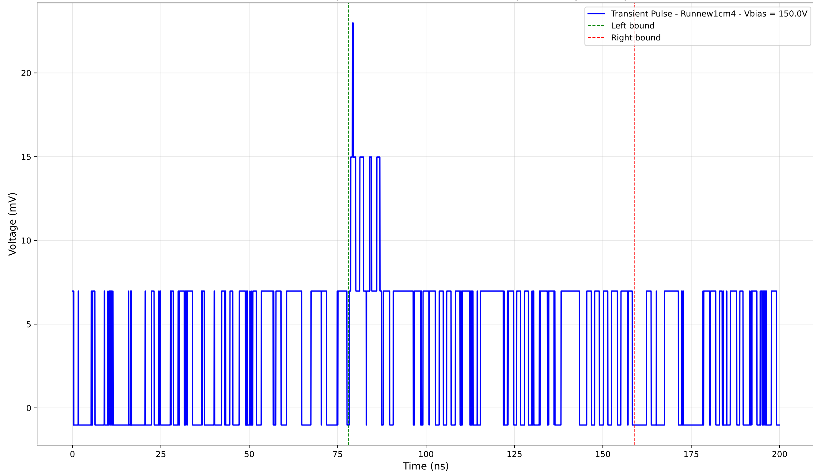
Transient Pulse - Sample: new1cm -Position: 5125.0 \mu\text{m} - Charge: 8.11 pC
