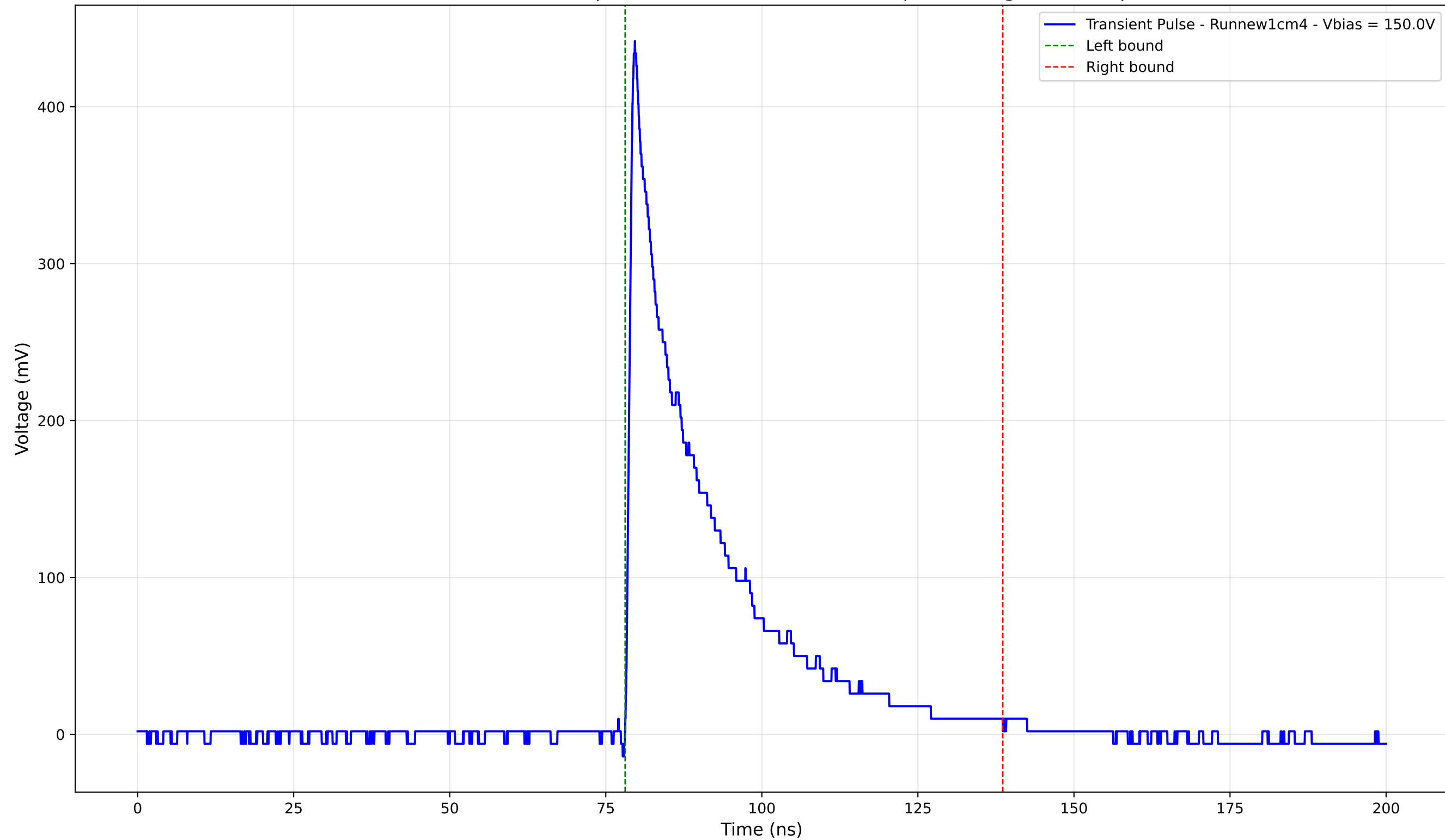
Transient Pulse - Sample: new1cm - Position: 745.0 \mu\text{m} - Charge: 105.07 pC
