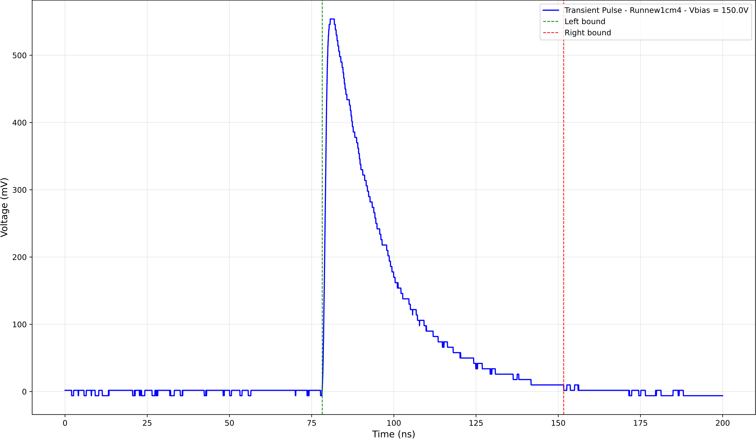
Transient Pulse - Sample: new1cm - Position: 1495.0 \mu\text{m} - Charge: 208.07 pC
