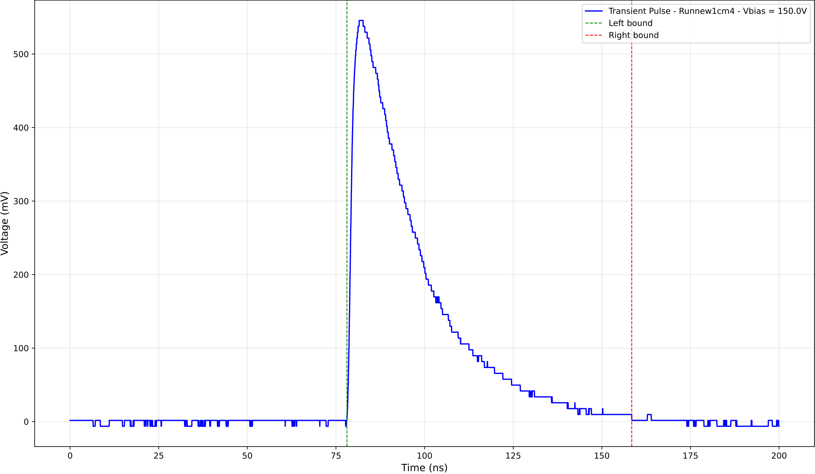
Transient Pulse - Sample: new1cm - Position: 3330.0 \mu\text{m} - Charge: 233.70 pC
