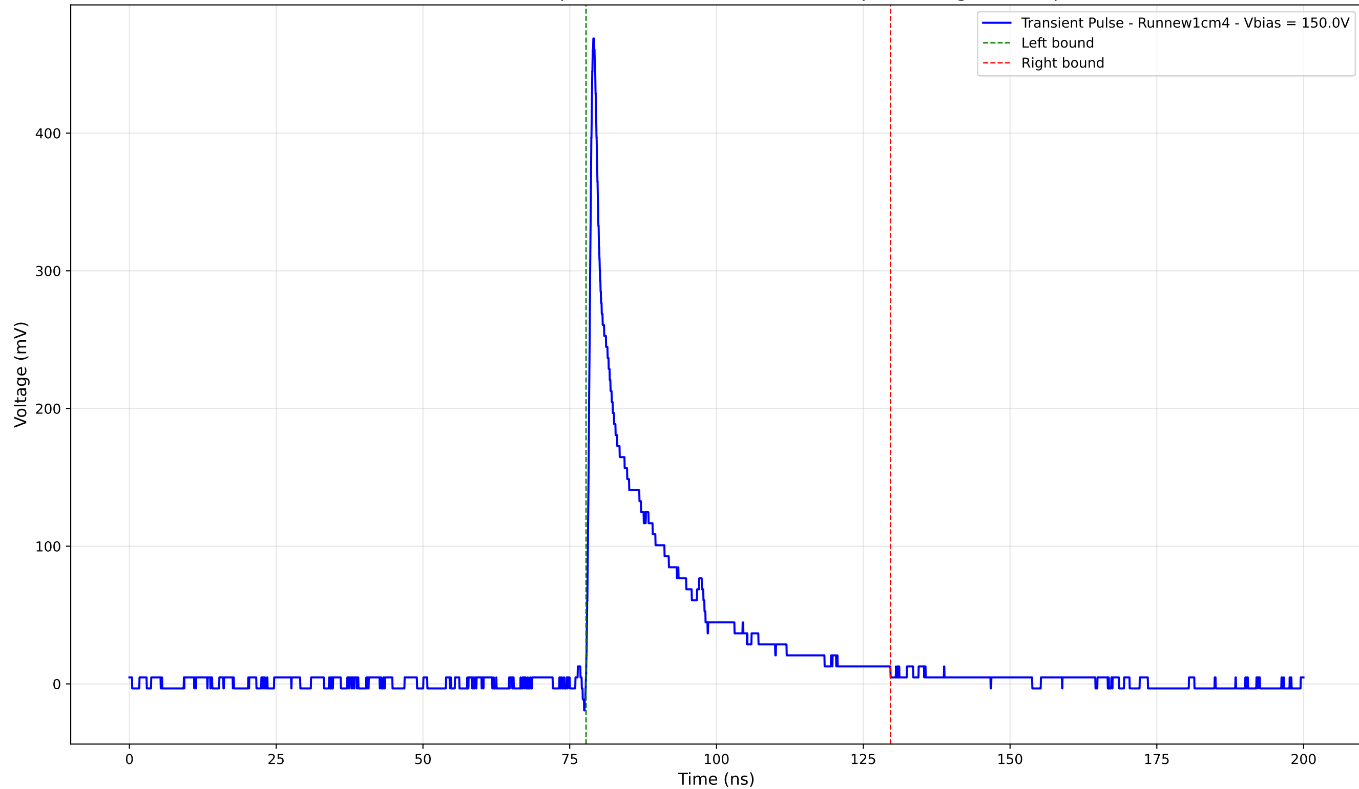
Transient Pulse - Sample: new1cm - Position: 5030.0 \mu\text{m} - Charge: 75.85 pC
