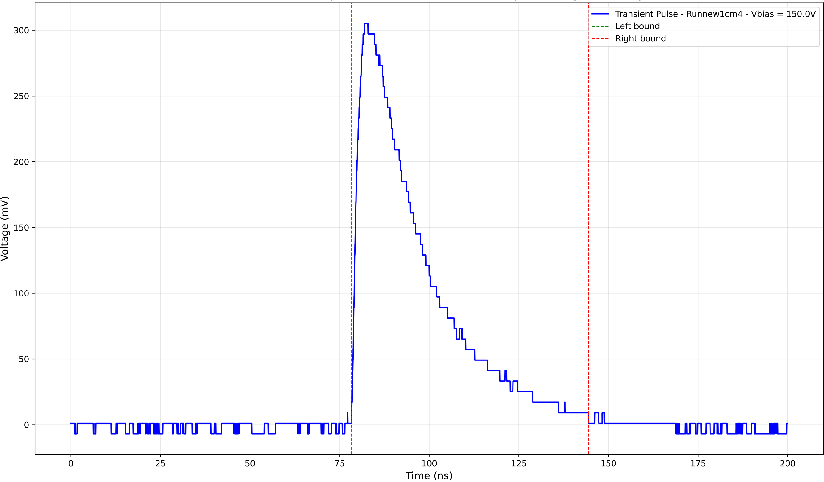
Transient Pulse - Sample: new1cm - Position: 2660.0 \mu\text{m} - Charge: 126.86 pC
