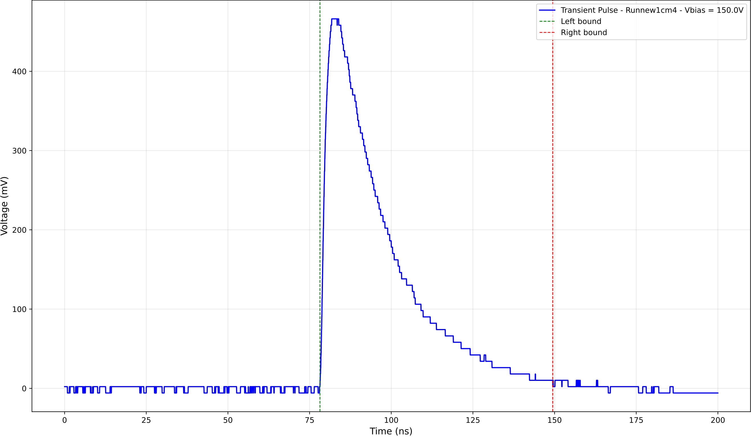
Transient Pulse - Sample: new1cm - Position: 2295.0 \mu\text{m} - Charge: 197.87 pC
