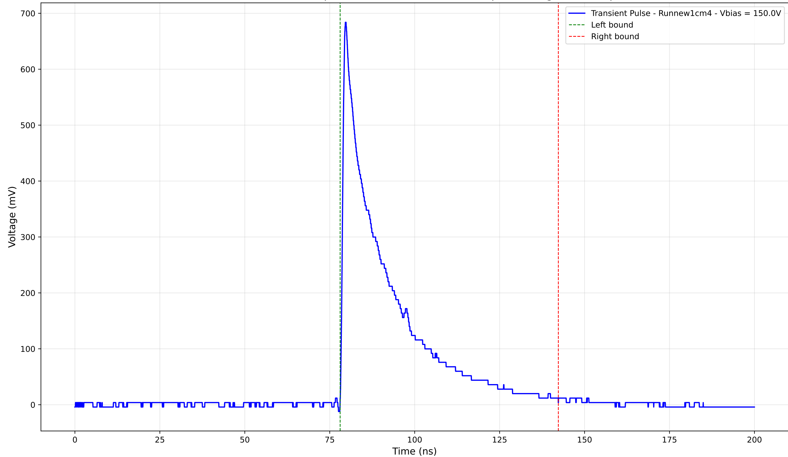
Transient Pulse - Sample: new1cm - Position: 780.0 \mu\text{m} - Charge: 174.73 pC
