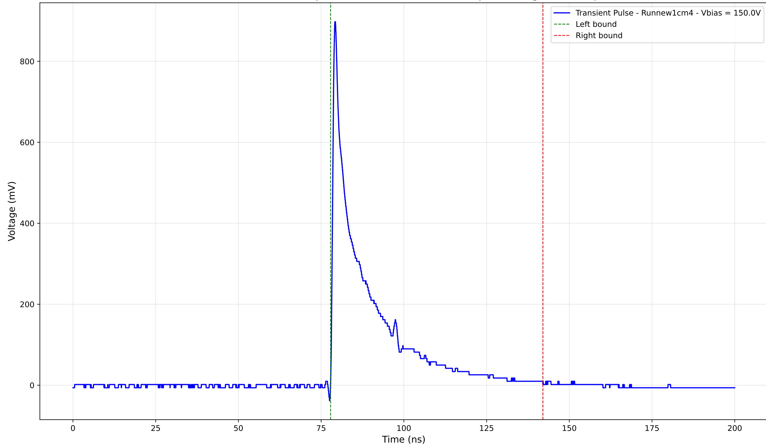
Transient Pulse - Sample: new1cm - Position: 285.0 \mu\text{m} - Charge: 160.20 pC
