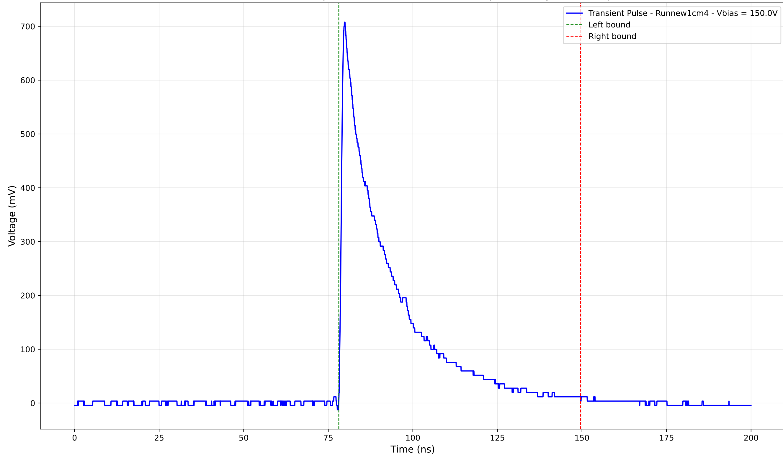
Transient Pulse - Sample: new1cm - Position: 925.0 \mu\text{m} - Charge: 201.02 pC
