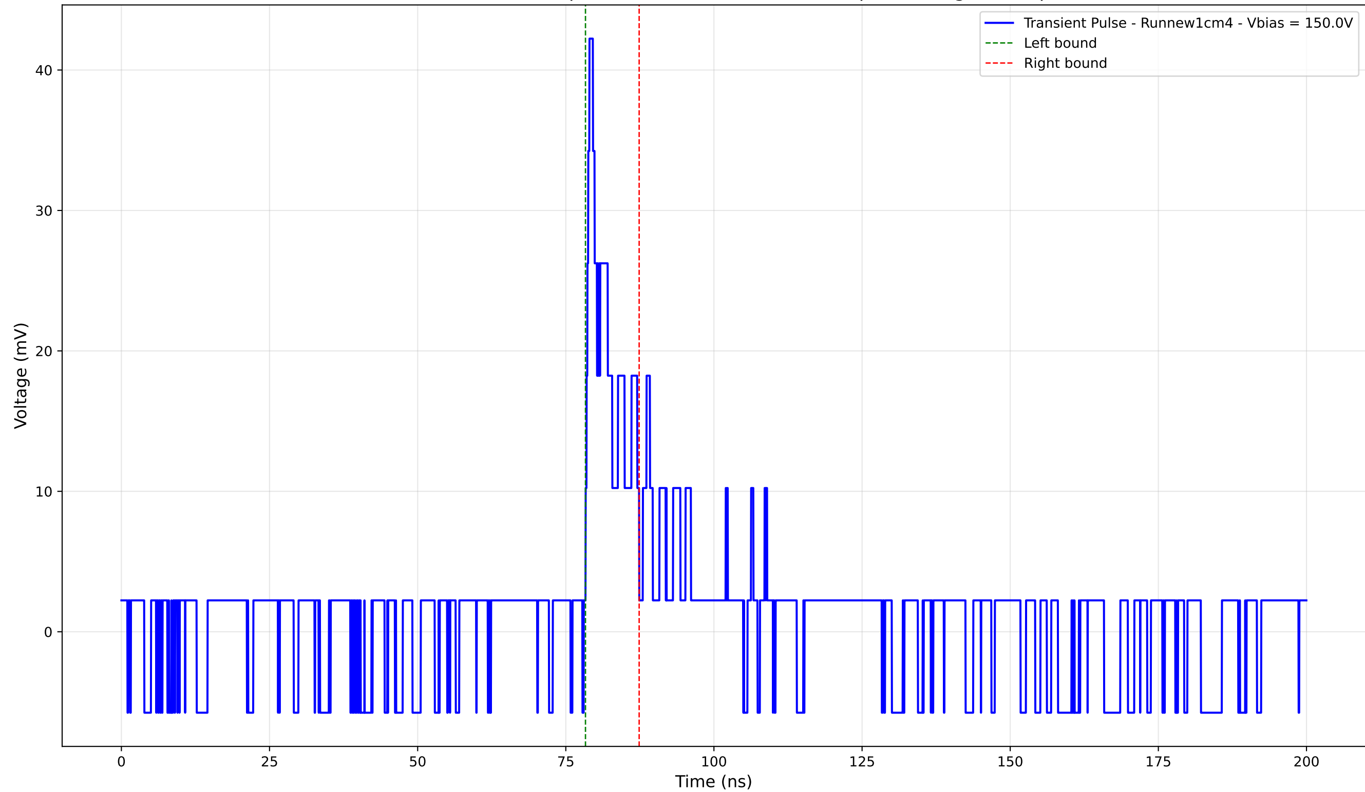
Transient Pulse - Sample: new1cm - Position: 160.0 \mu\text{m} - Charge: 3.64 pC
