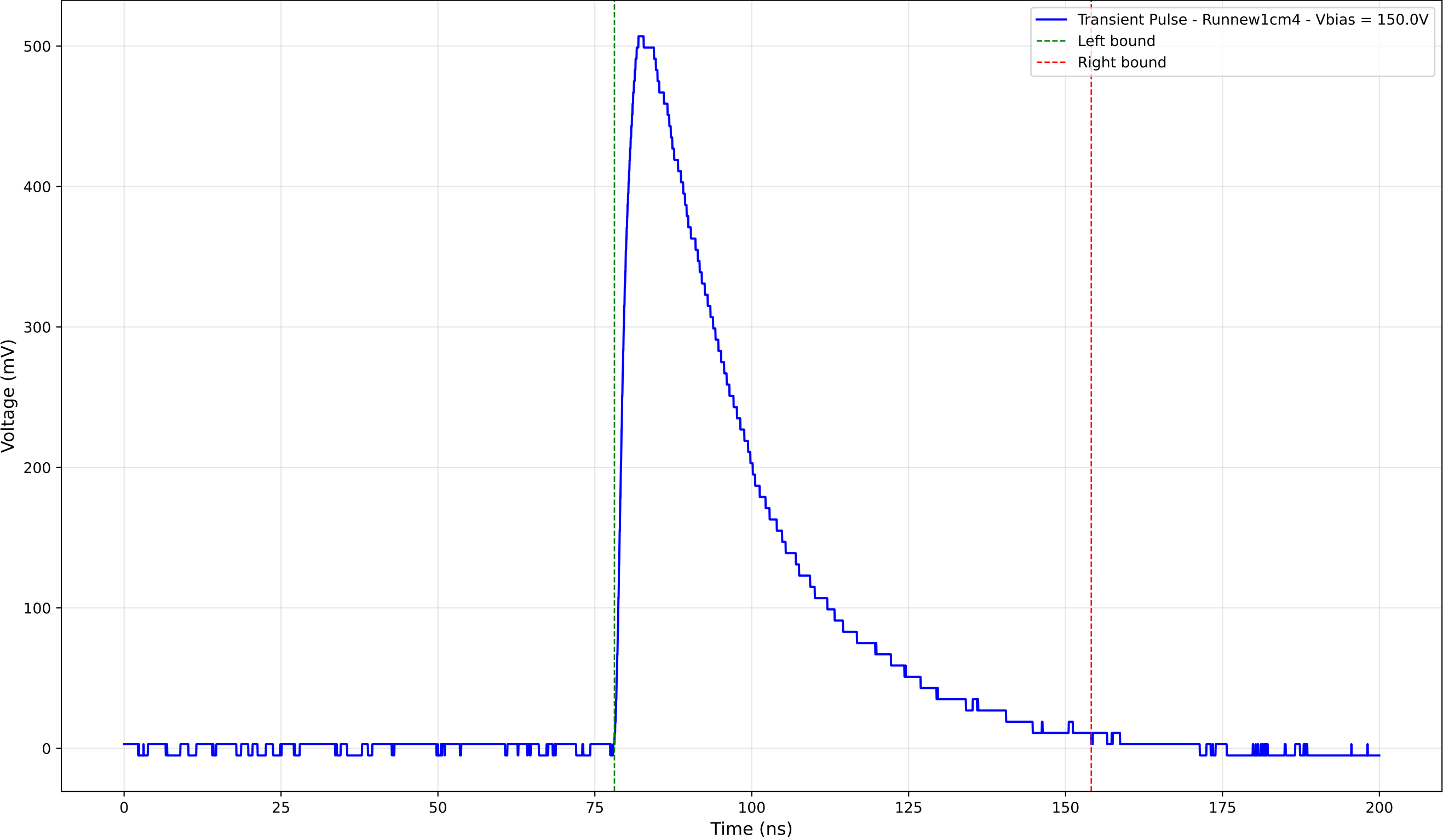
Transient Pulse - Sample: new1cm - Position: 2575.0 \mu\text{m} - Charge: 223.10 pC
