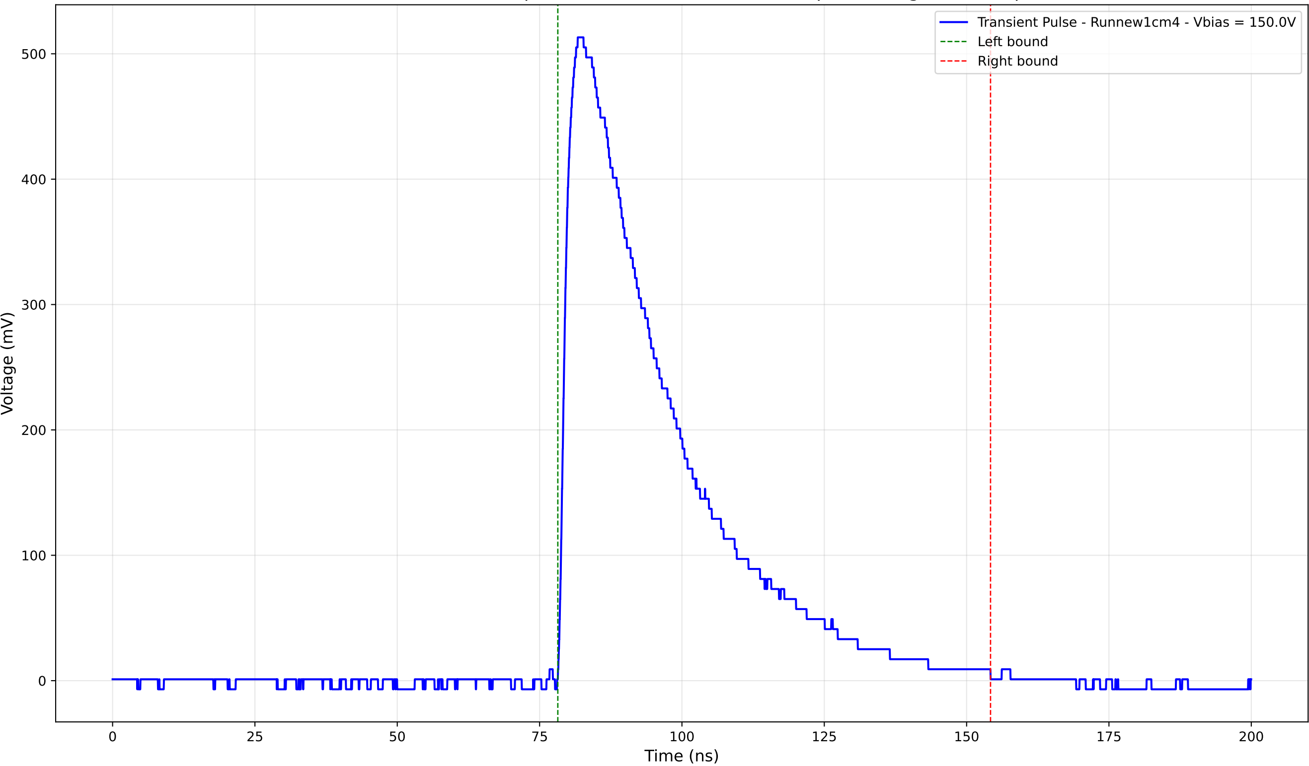
Transient Pulse - Sample: new1cm - Position: 2015.0 \mu\text{m} - Charge: 211.39 pC
