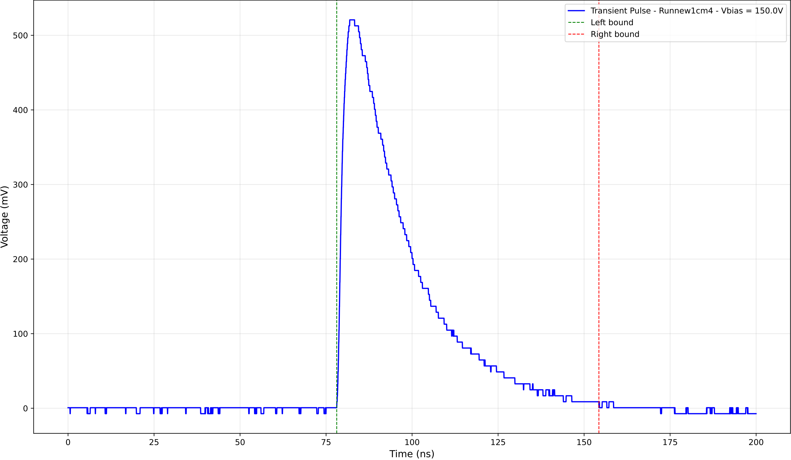
Transient Pulse - Sample: new1cm - Position: 2350.0 \mu\text{m} - Charge: 223.87 pC
