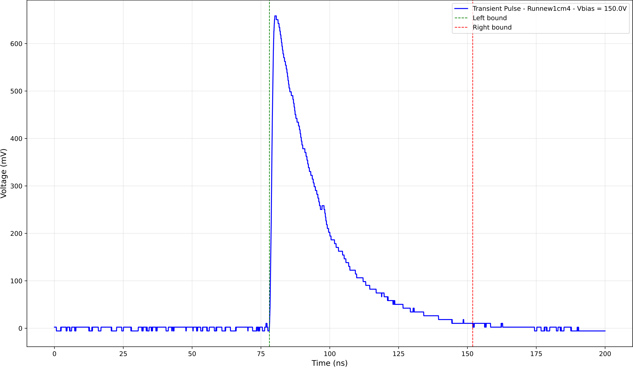
Transient Pulse - Sample: new1cm - Position: 3970.0 \mu\text{m} - Charge: 245.22 pC
