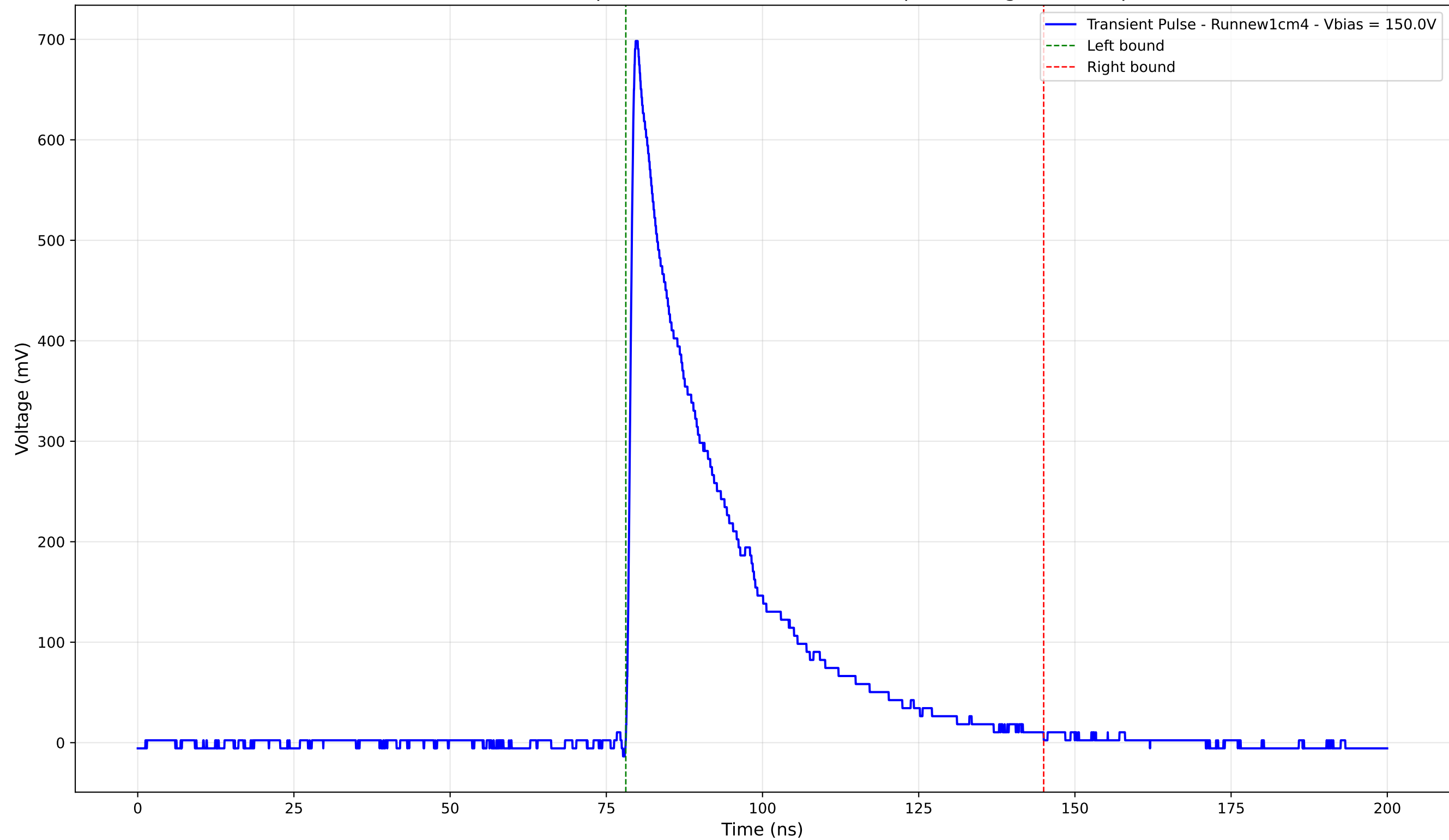
Transient Pulse - Sample: new1cm - Position: 930.0 \mu\text{m} - Charge: 197.50 pC
