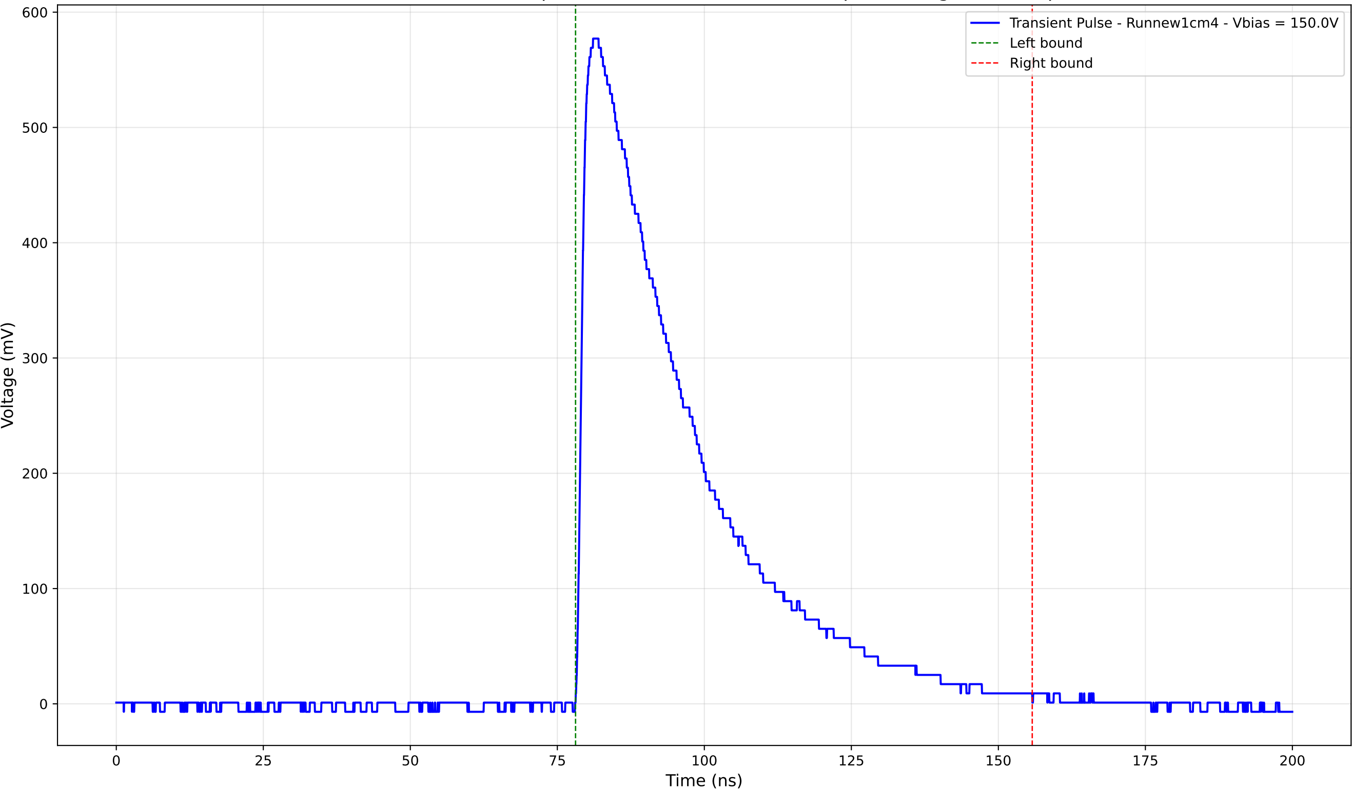
Transient Pulse - Sample: new1cm - Position: 3620.0 \mu\text{m} - Charge: 236.59 pC
