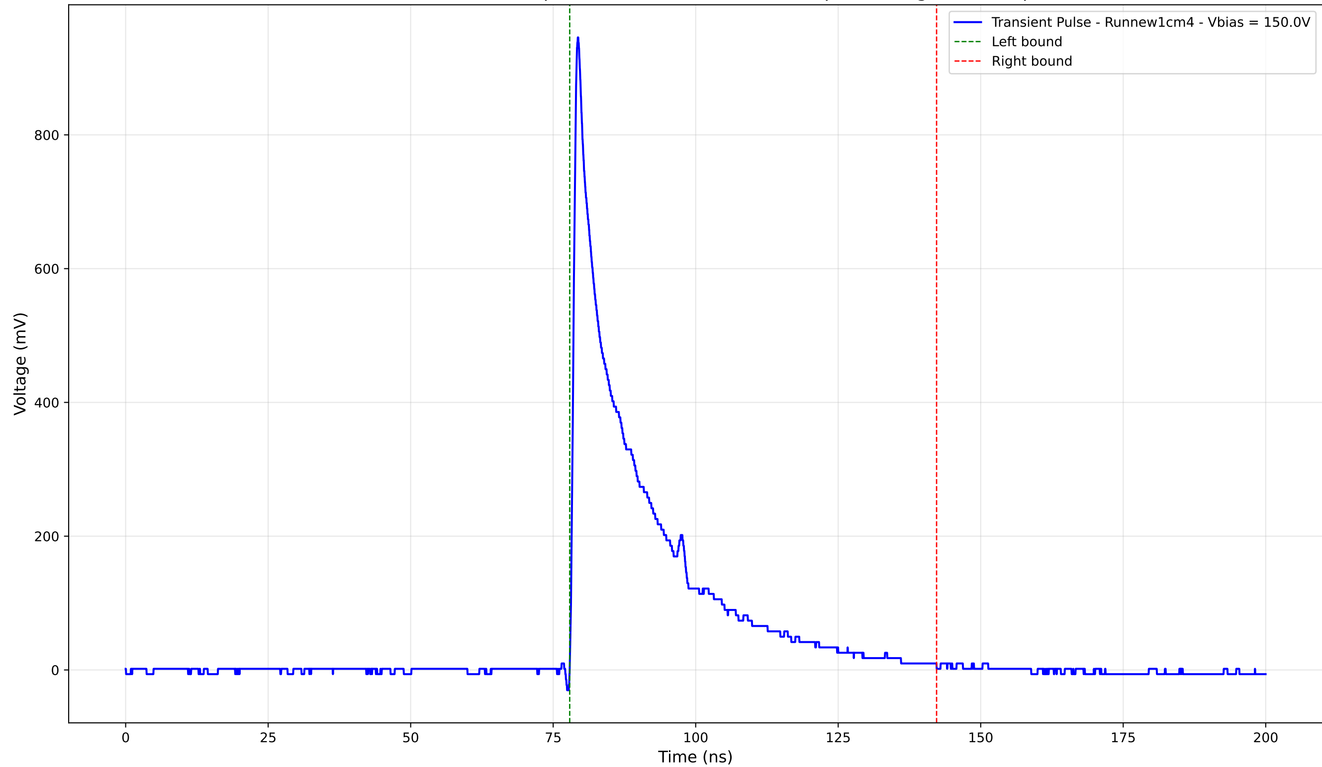
Transient Pulse - Sample: new1cm - Position: 420.0 \mu\text{m} - Charge: 198.92 pC
