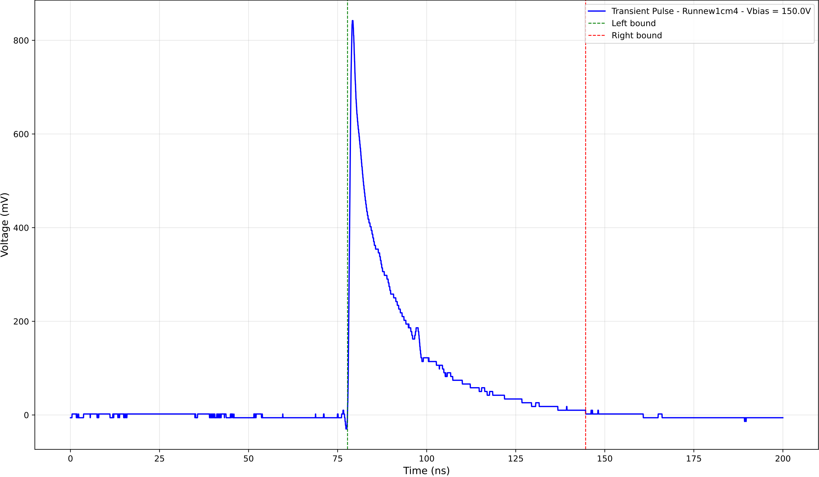
Transient Pulse - Sample: new1cm - Position: 4860.0 \mu\text{m} - Charge: 186.54 pC
