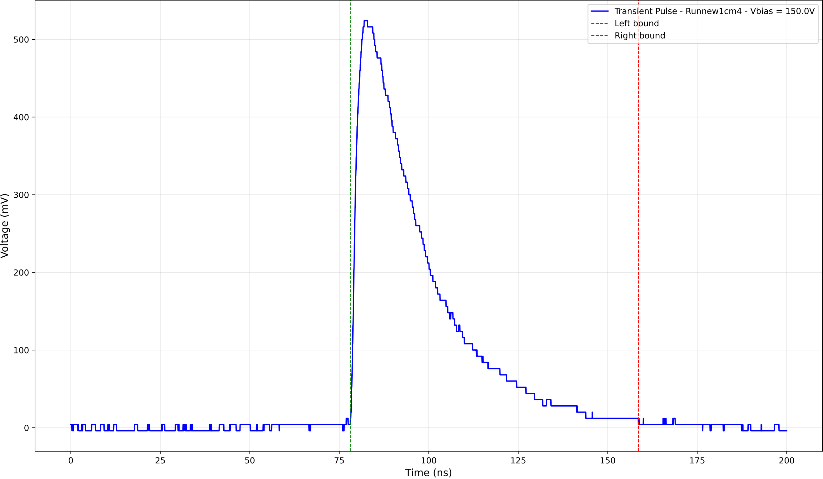
Transient Pulse - Sample: new1cm - Position: 2925.0 \mu\text{m} - Charge: 232.04 pC
