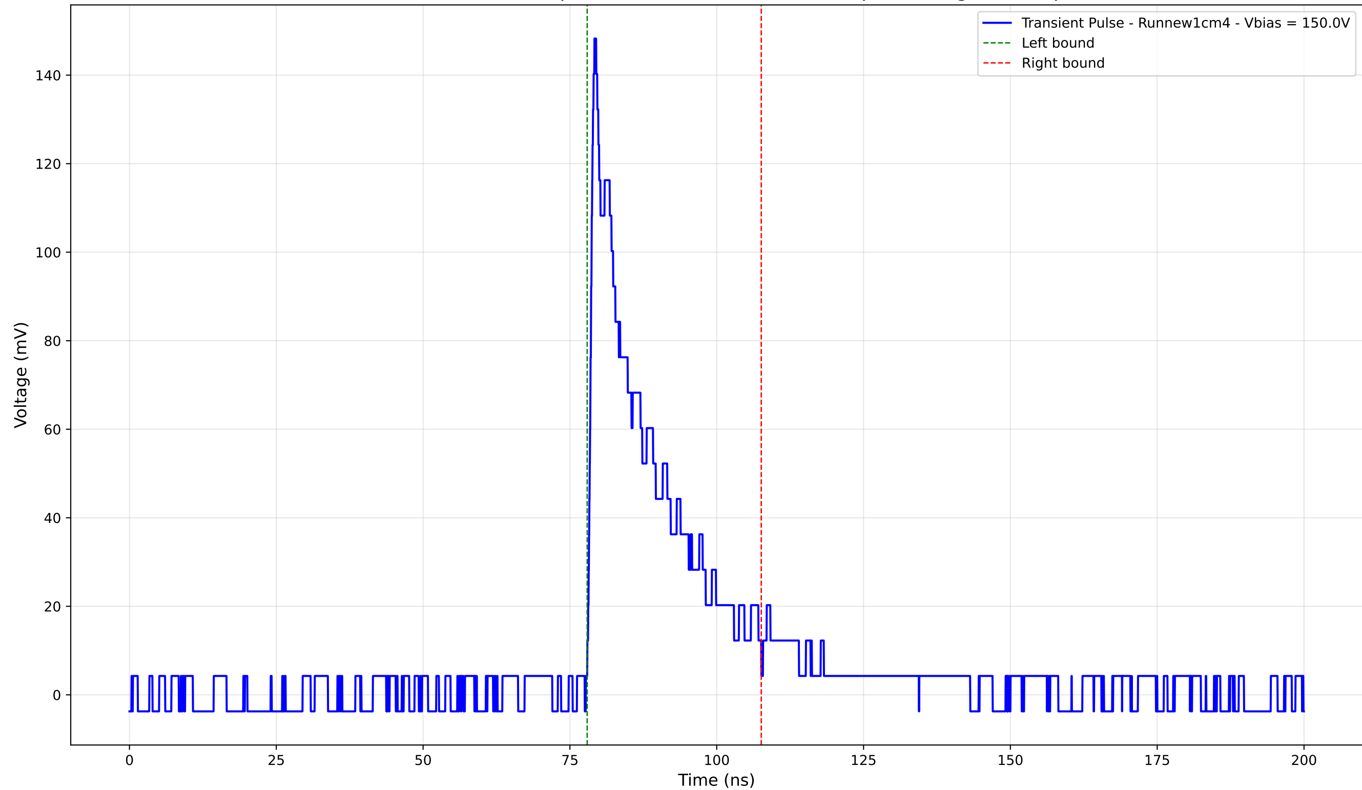
Transient Pulse - Sample: new1cm - Position: 4740.0 \mu\text{m} - Charge: 29.36 pC
