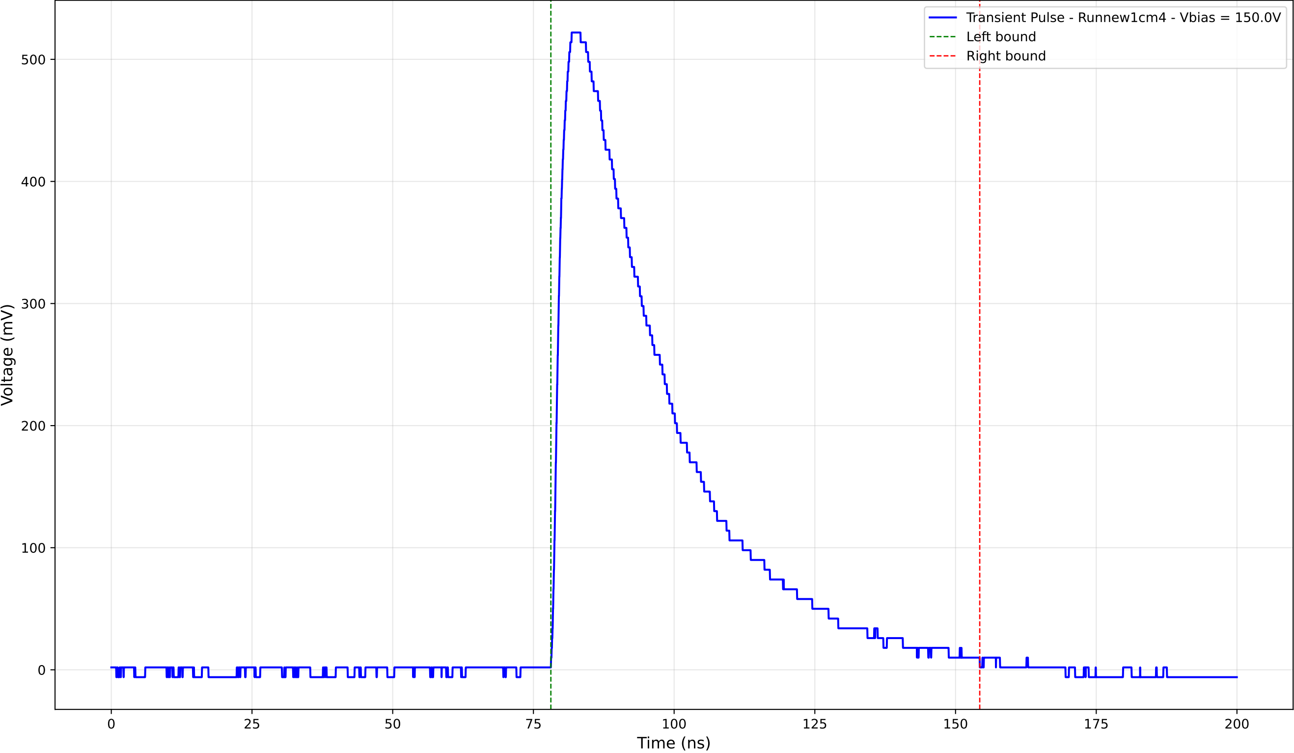
Transient Pulse - Sample: new1cm - Position: 2990.0 \mu\text{m} - Charge: 228.96 pC
