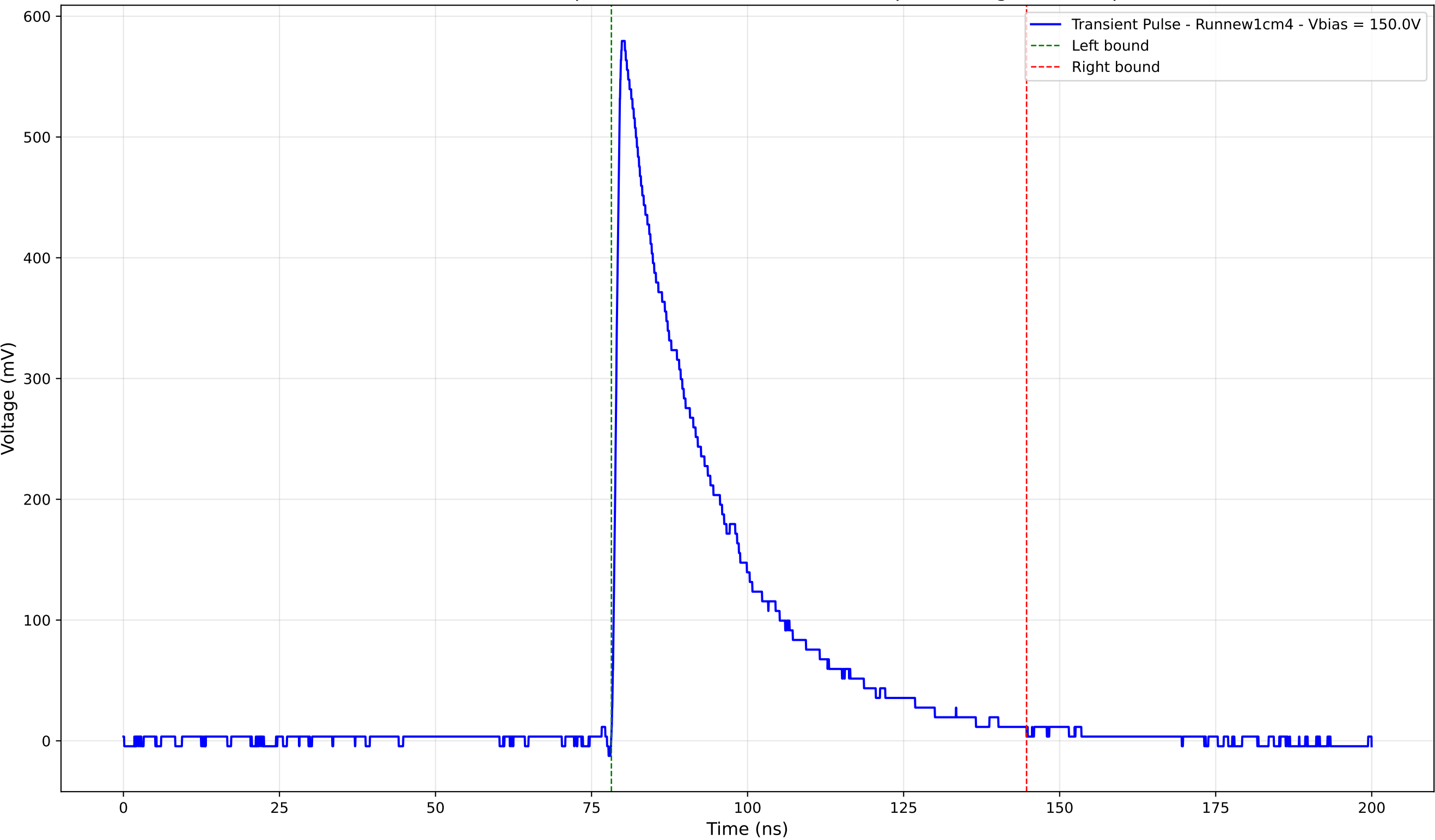
Transient Pulse - Sample: new1cm - Position: 1115.0 \mu\text{m} - Charge: 180.17 pC
