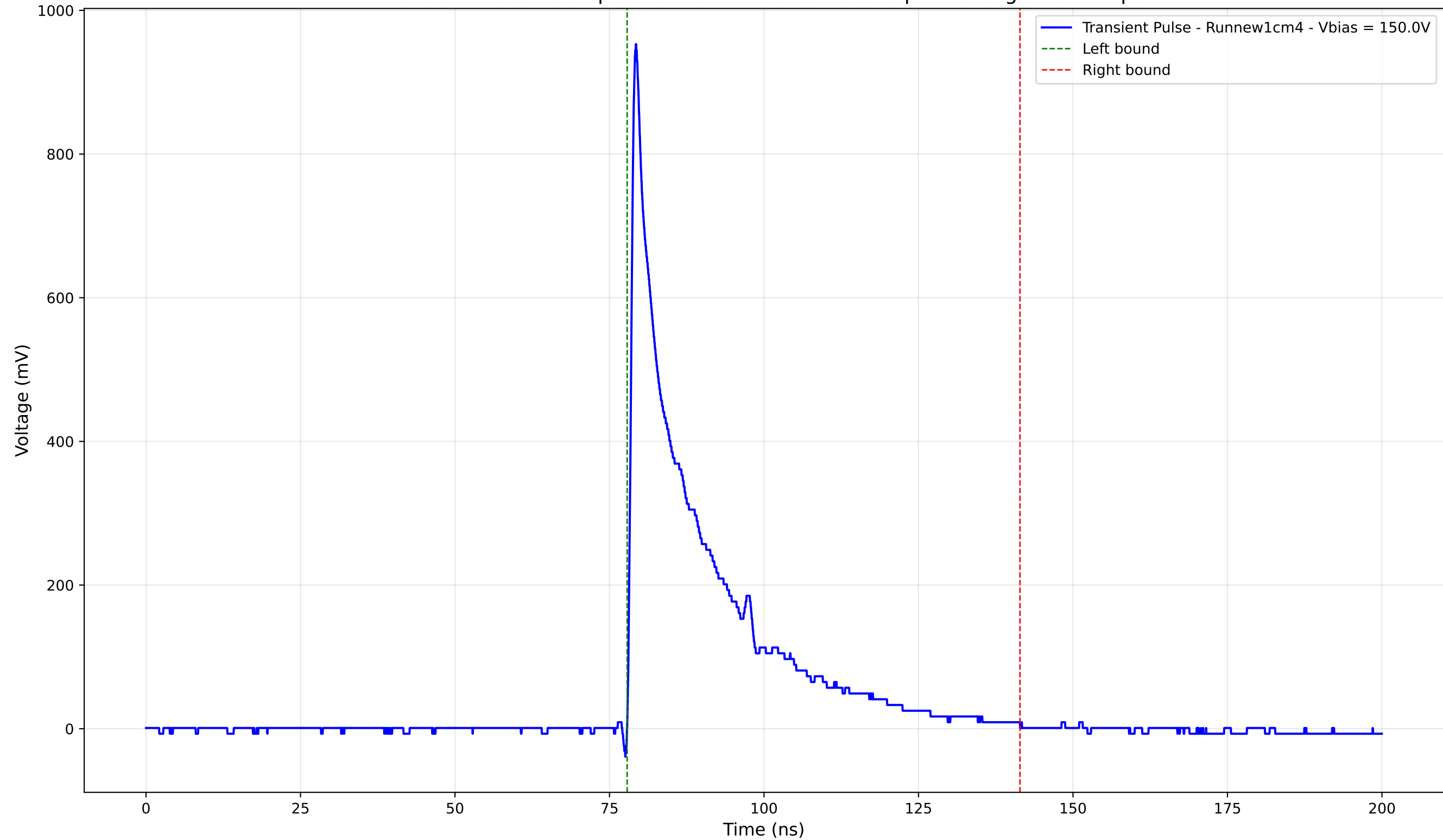
Transient Pulse - Sample: new1cm - Position: 335.0 \mu\text{m} - Charge: 187.41 pC
