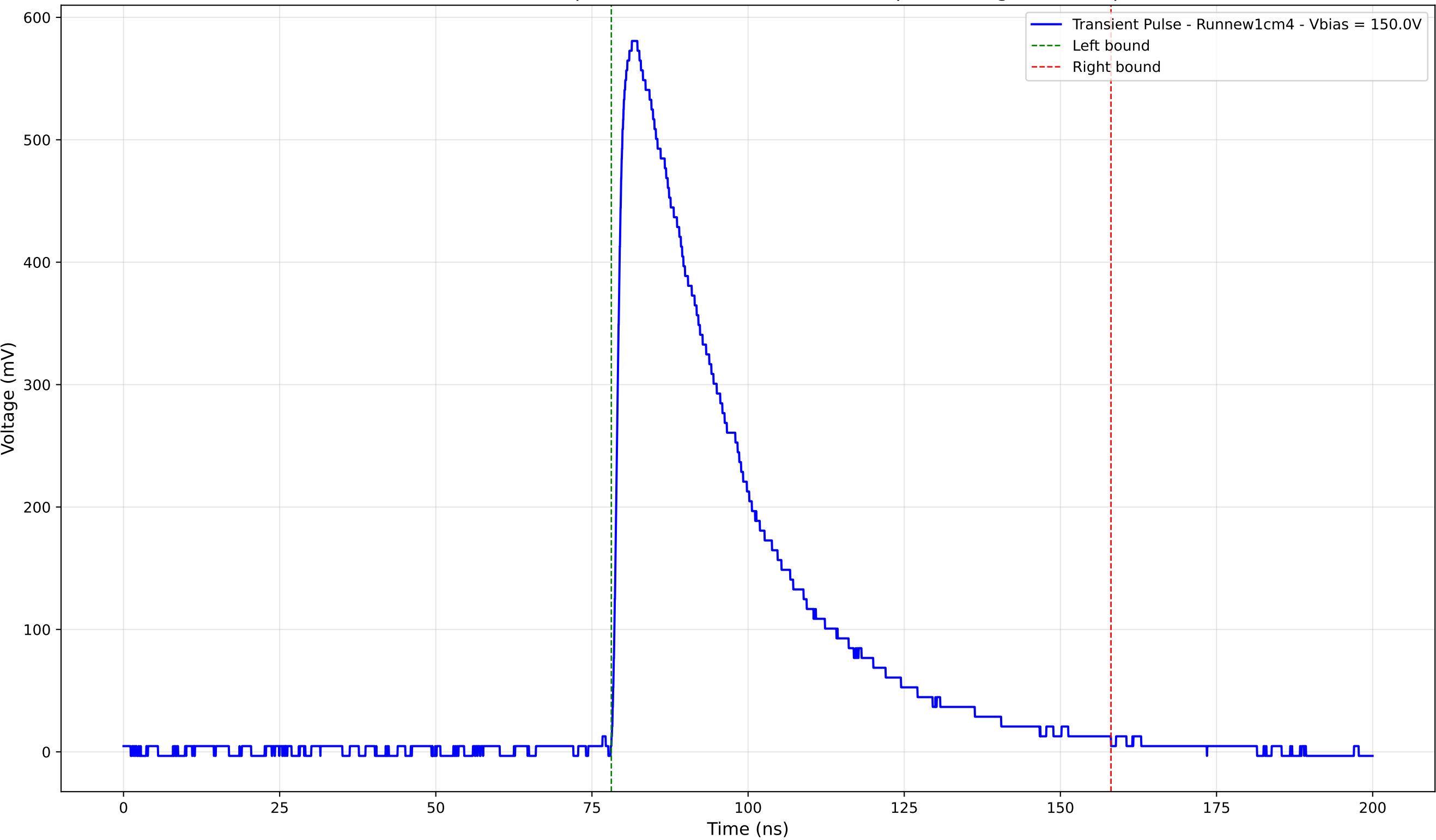
Transient Pulse - Sample: new1cm - Position: 3565.0 \mu\text{m} - Charge: 245.31 pC
