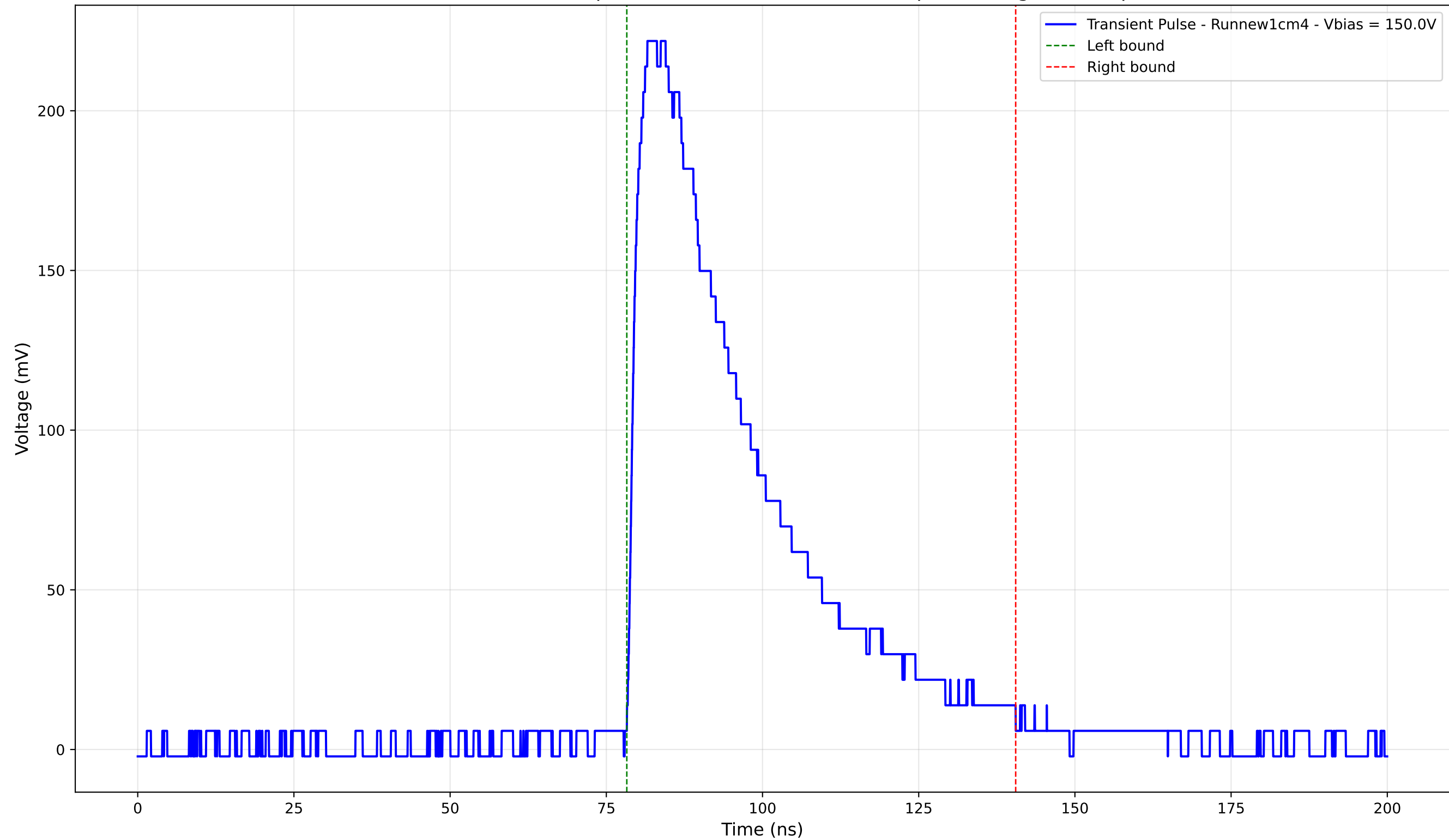
Transient Pulse - Sample: new1cm - Position: 3185.0 \mu\text{m} - Charge: 96.05 pC
