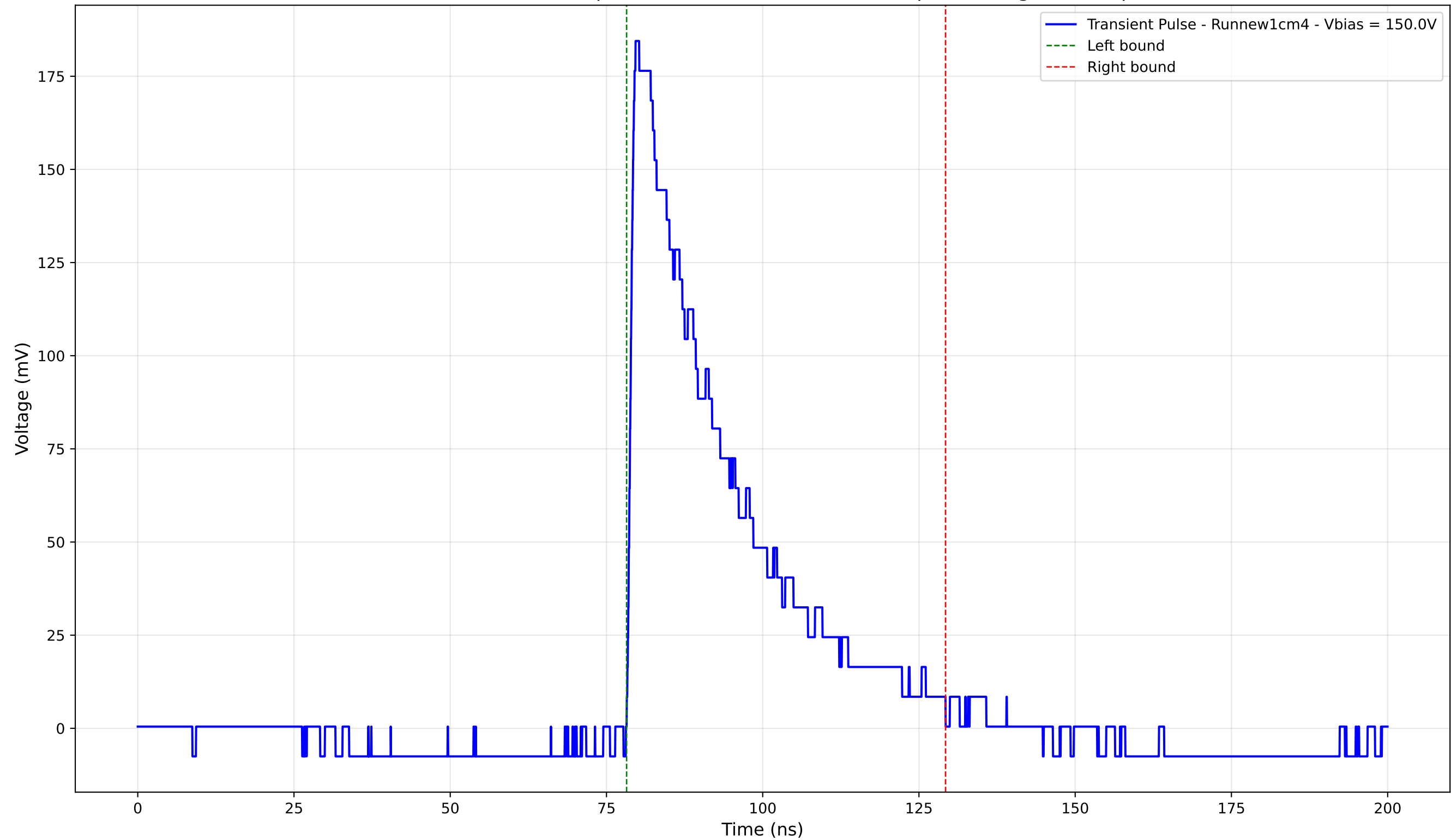
Transient Pulse - Sample: new1cm - Position: 4210.0 \mu\text{m} - Charge: 58.50 pC
