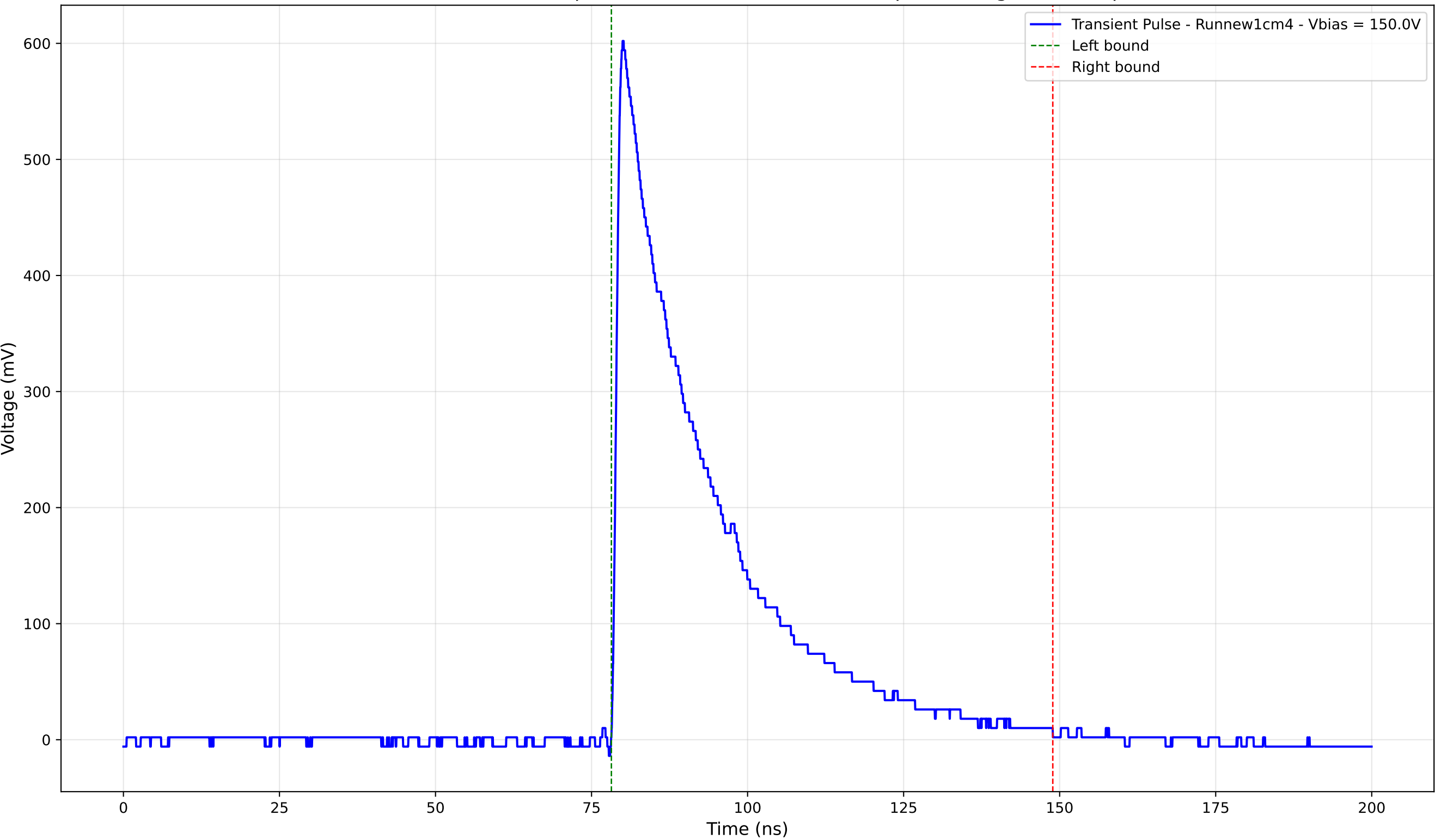
Transient Pulse - Sample: new1cm - Position: 1110.0 \mu\text{m} - Charge: 185.11 pC
