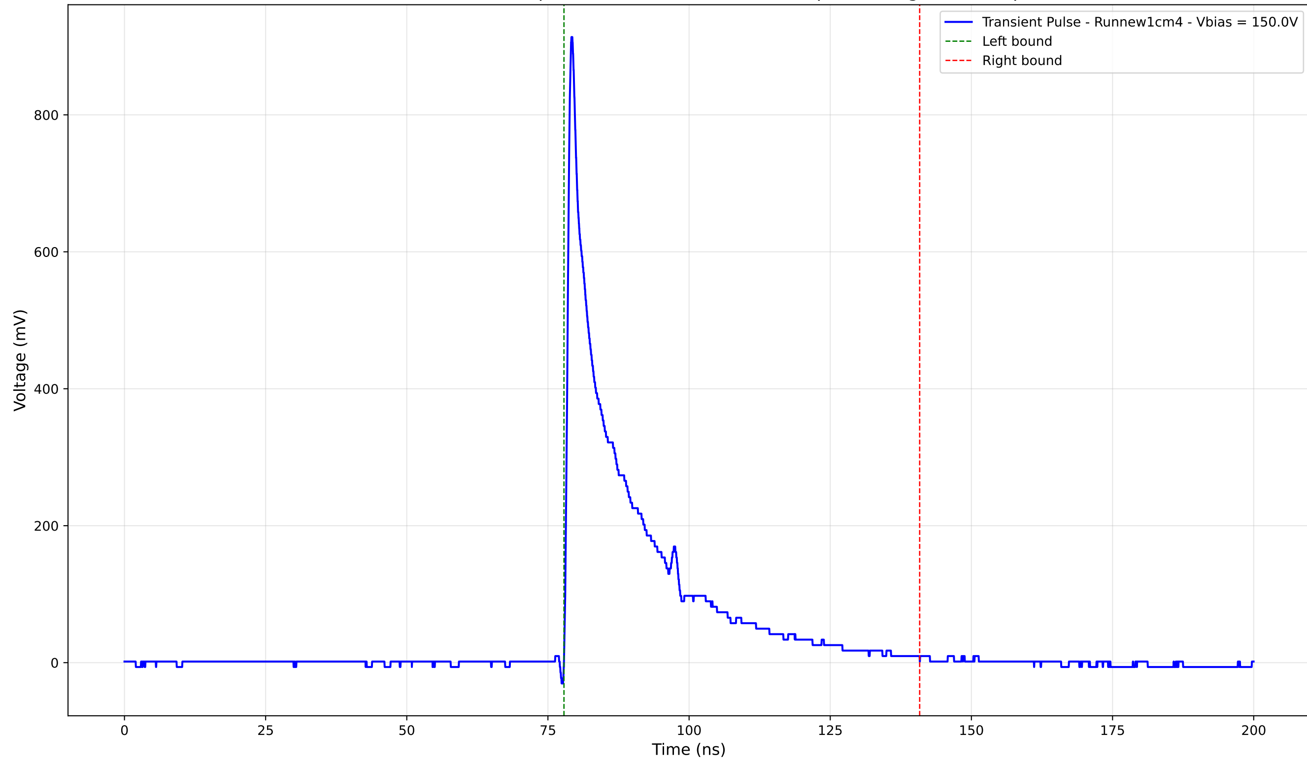
Transient Pulse - Sample: new1cm - Position: 290.0 \mu\text{m} - Charge: 169.21 pC
