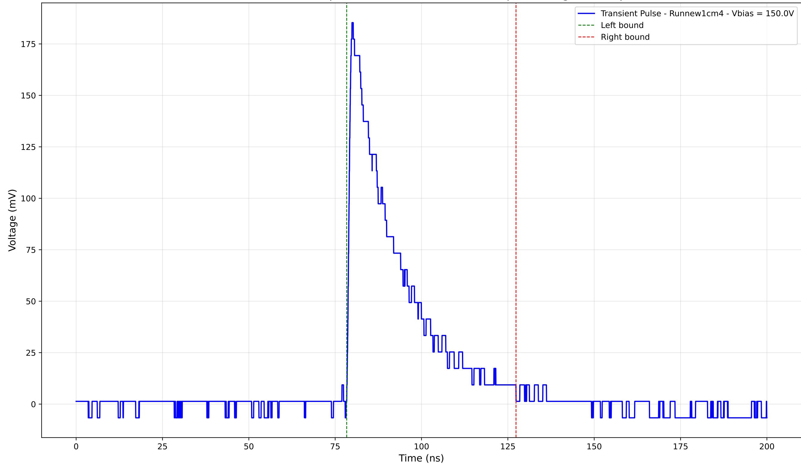
Transient Pulse - Sample: new1cm - Position: 1170.0 \mu\text{m} - Charge: 53.38 pC
