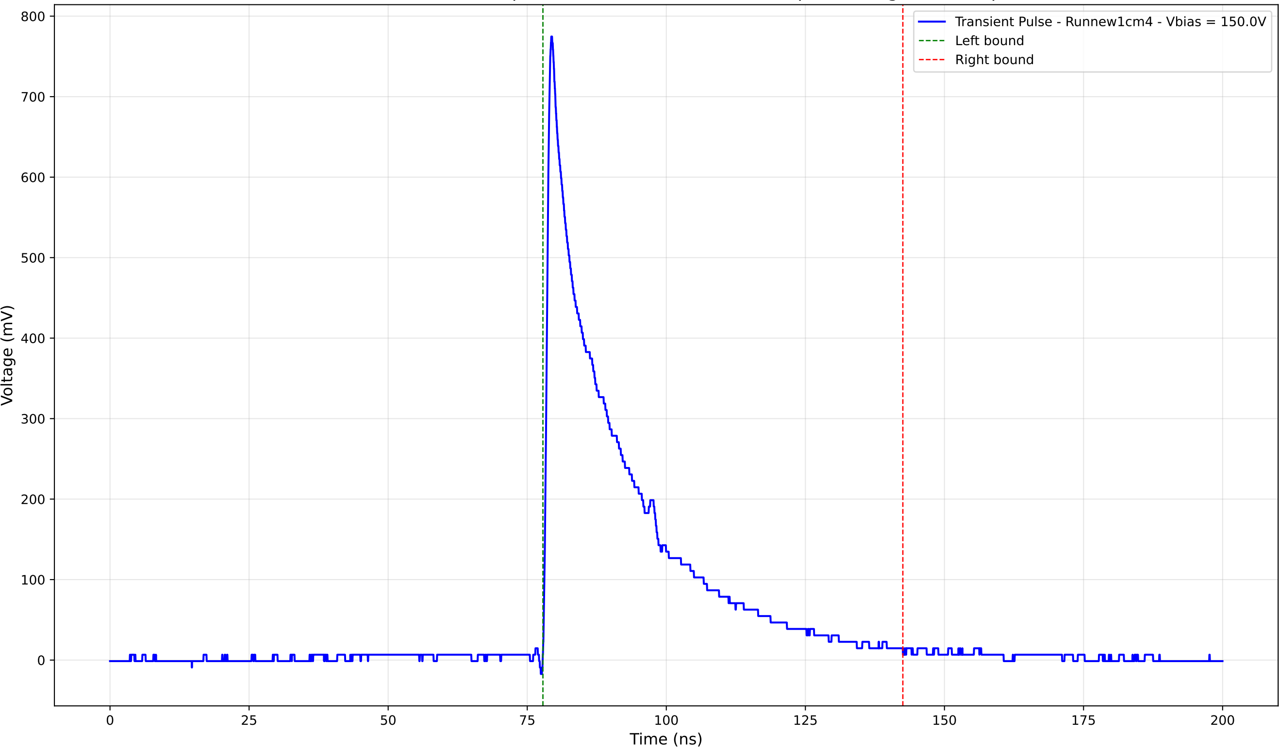
Transient Pulse - Sample: new1cm - Position: 4650.0 \mu\text{m} - Charge: 197.47 pC
