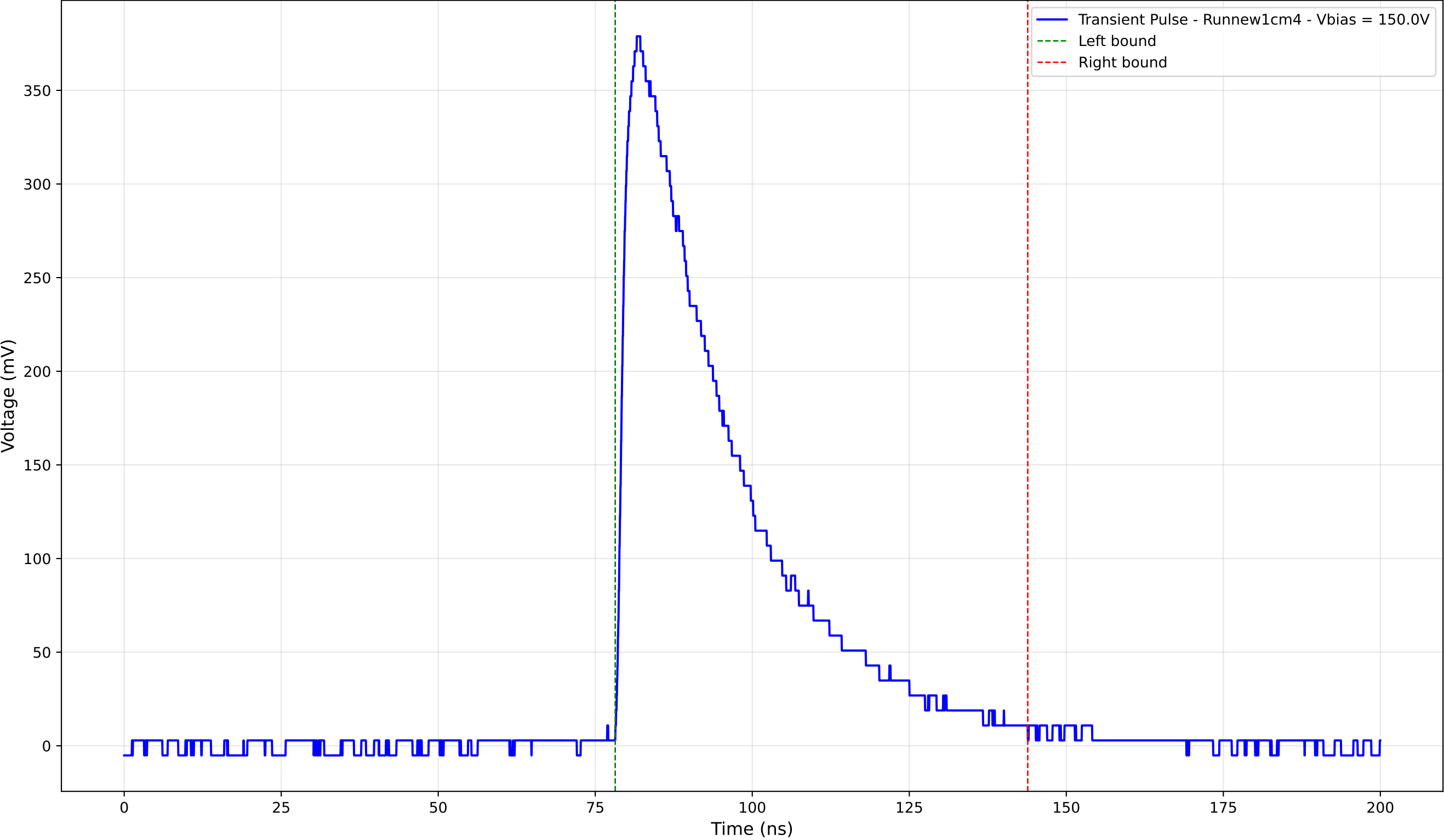
Transient Pulse - Sample: new1cm - Position: 1770.0 \mu\text{m} - Charge: 146.76 pC
