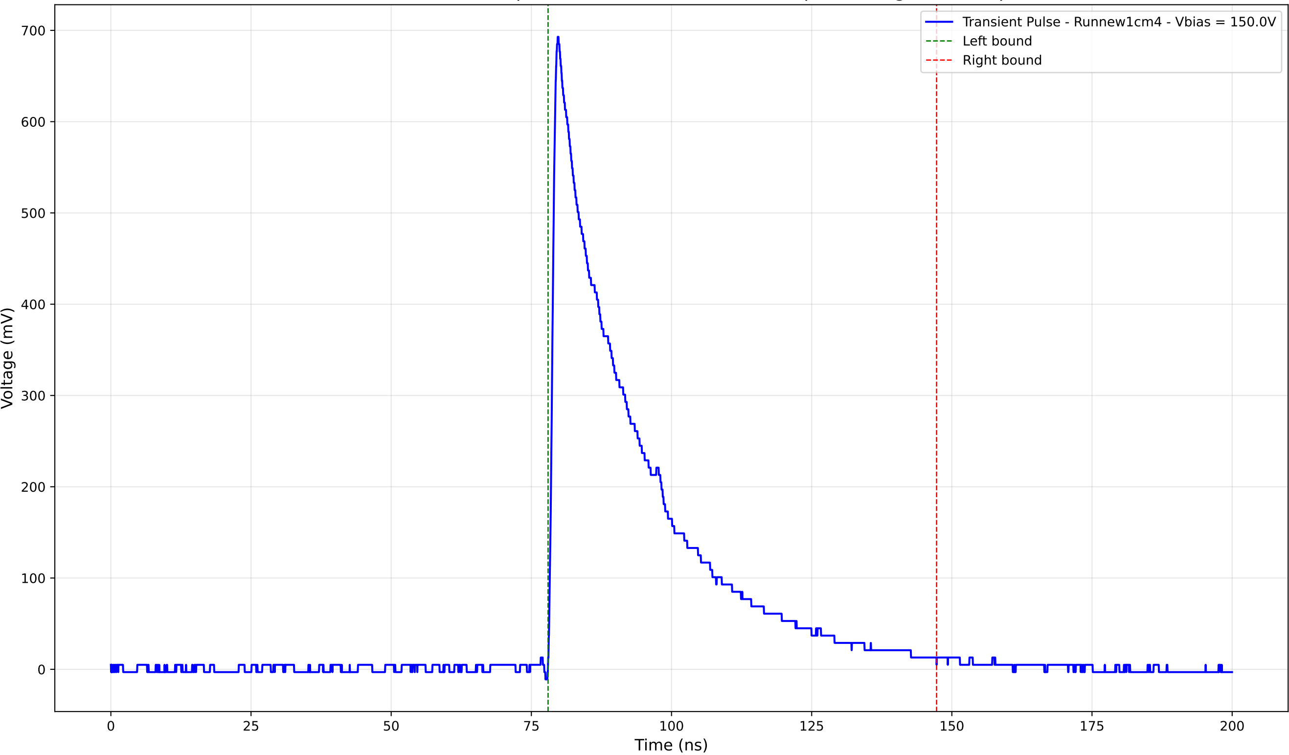
Transient Pulse - Sample: new1cm - Position: 4320.0 \mu\text{m} - Charge: 213.68 pC
