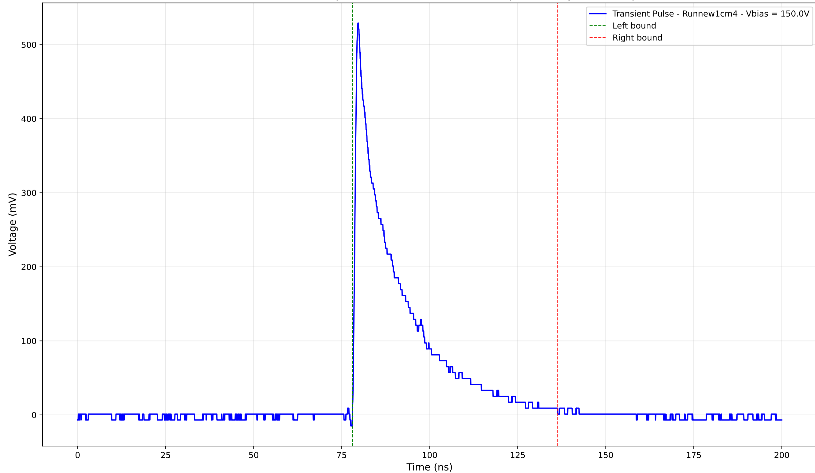
Transient Pulse - Sample: new1cm - Position: 755.0 \mu\text{m} - Charge: 126.56 pC
