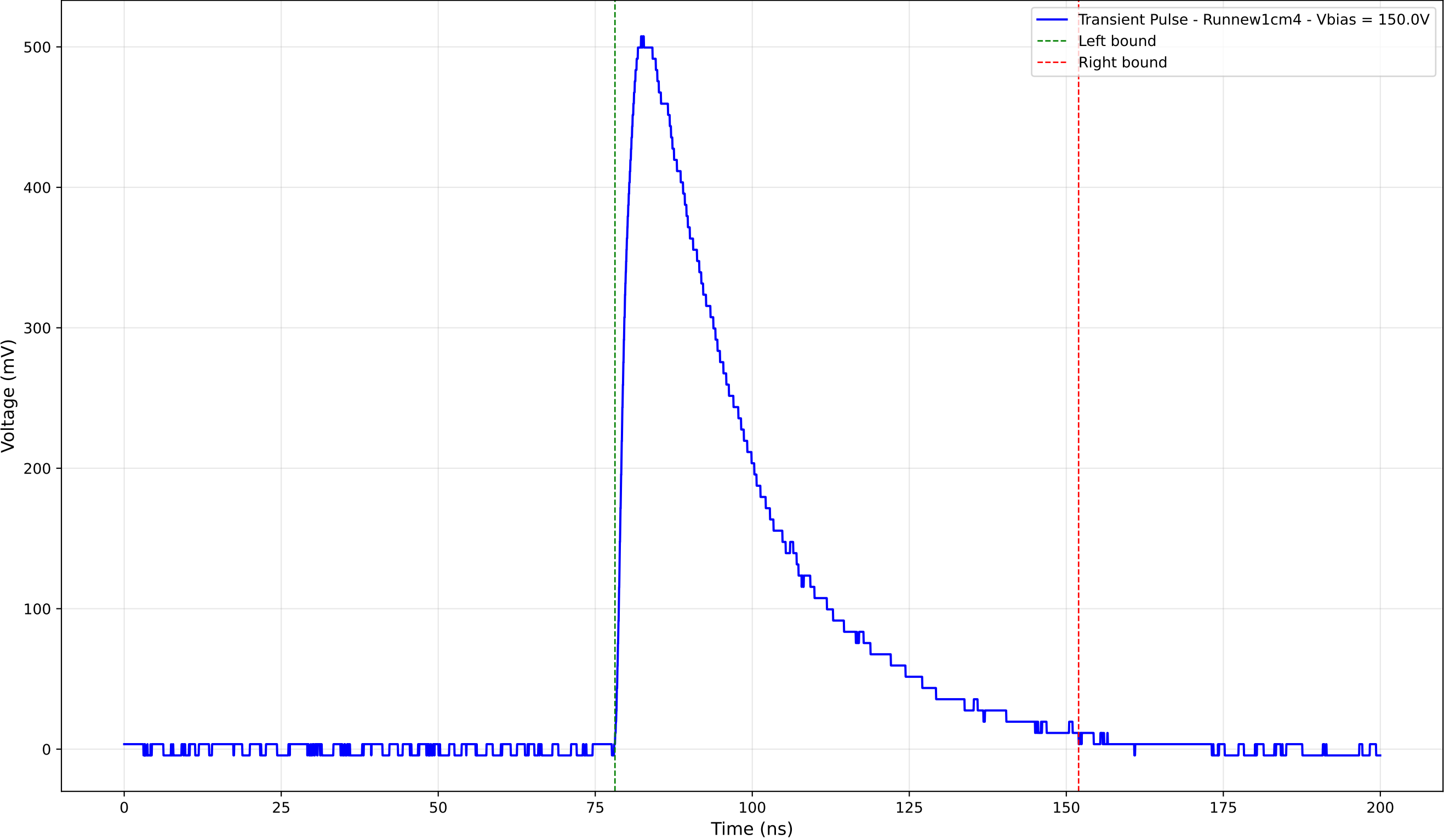
Transient Pulse - Sample: new1cm - Position: 2605.0 \mu\text{m} - Charge: 222.13 pC
