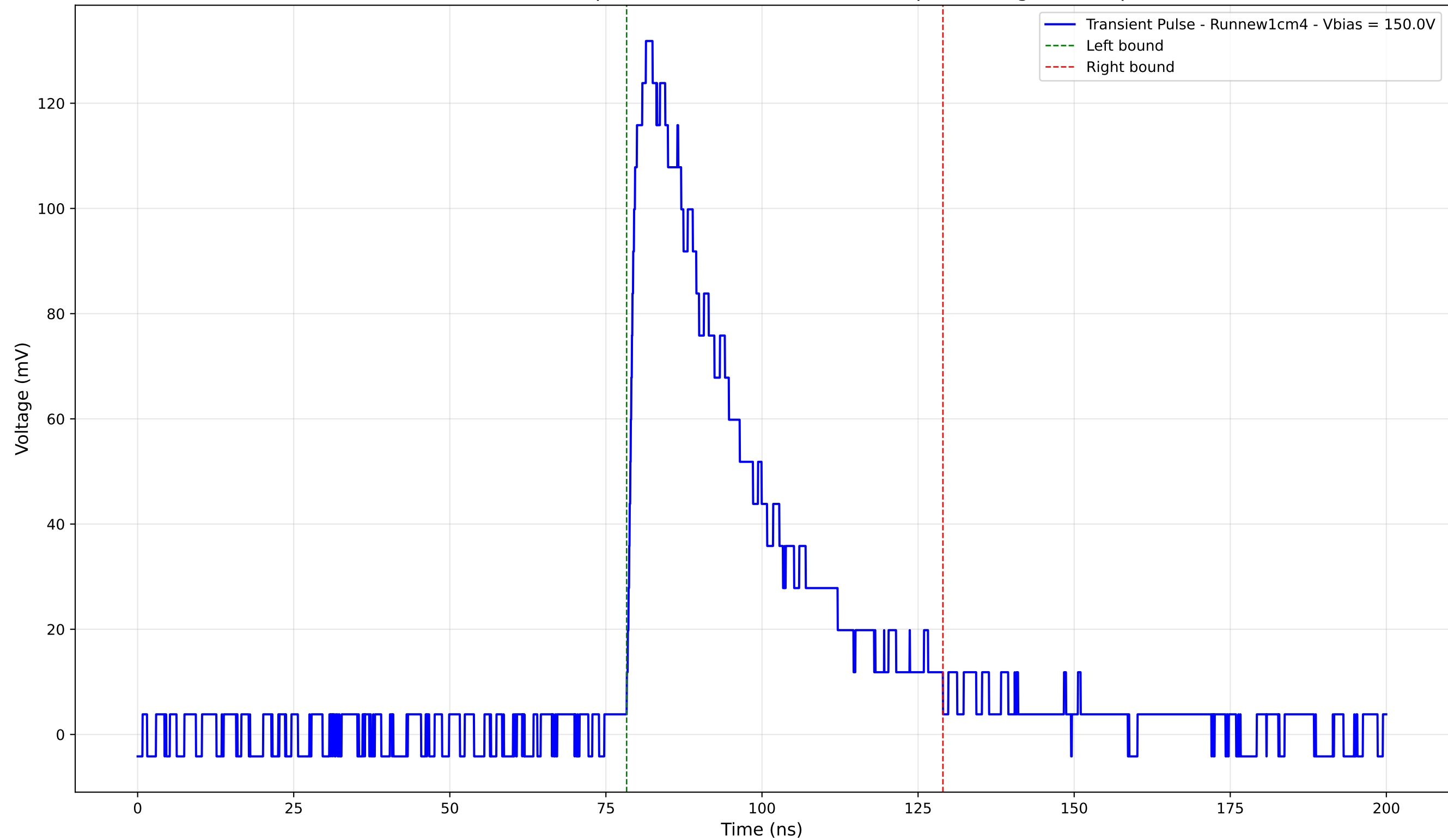
Transient Pulse - Sample: new1cm - Position: 3710.0 \mu\text{m} - Charge: 50.27 pC
