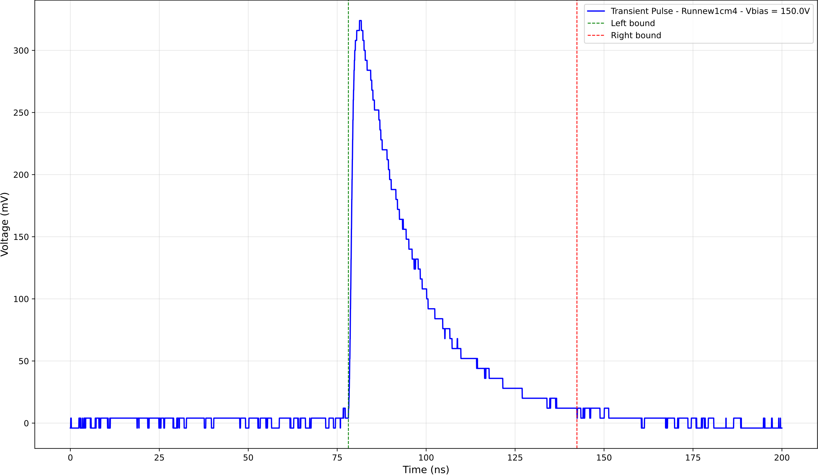
Transient Pulse - Sample: new1cm - Position: 3775.0 \mu\text{m} - Charge: 122.46 pC
