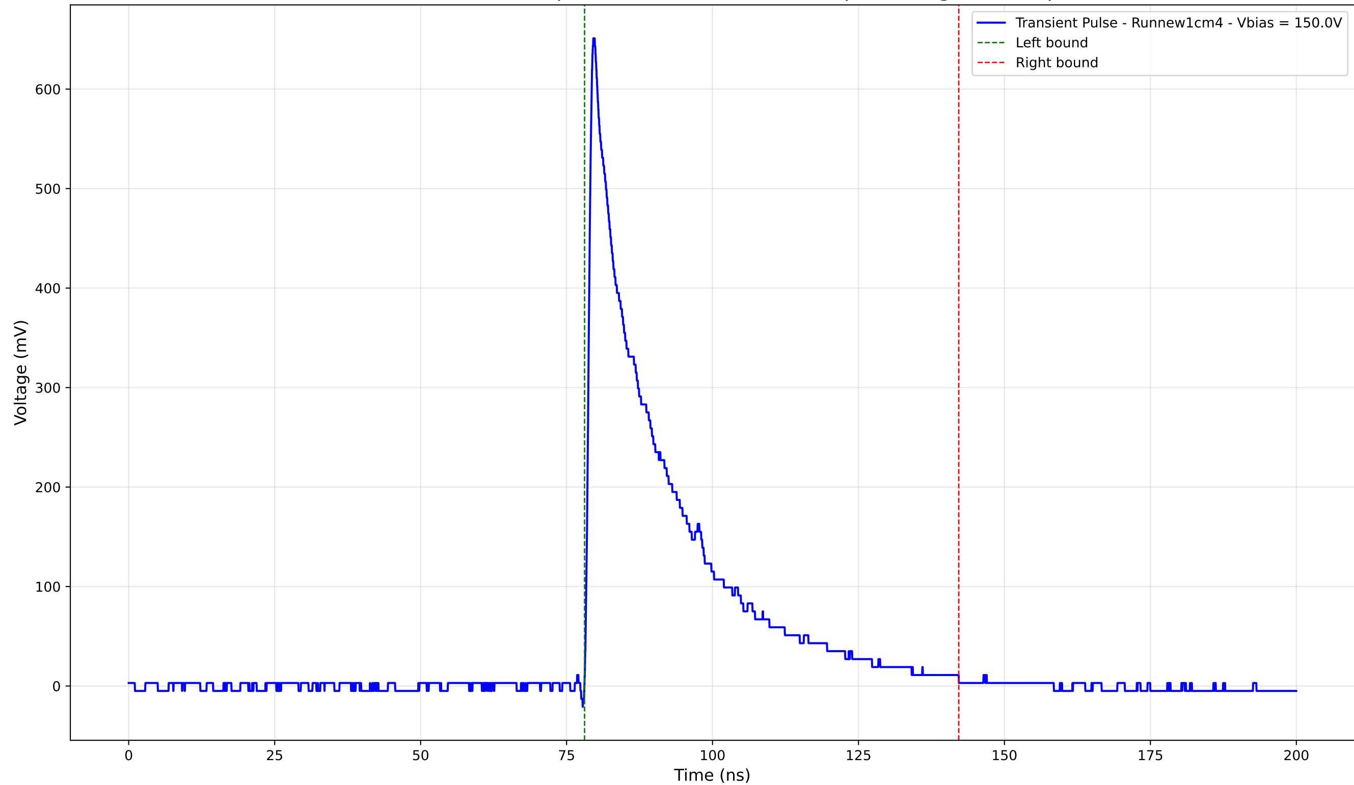
Transient Pulse - Sample: new1cm - Position: 775.0 \mu\text{m} - Charge: 163.87 pC
