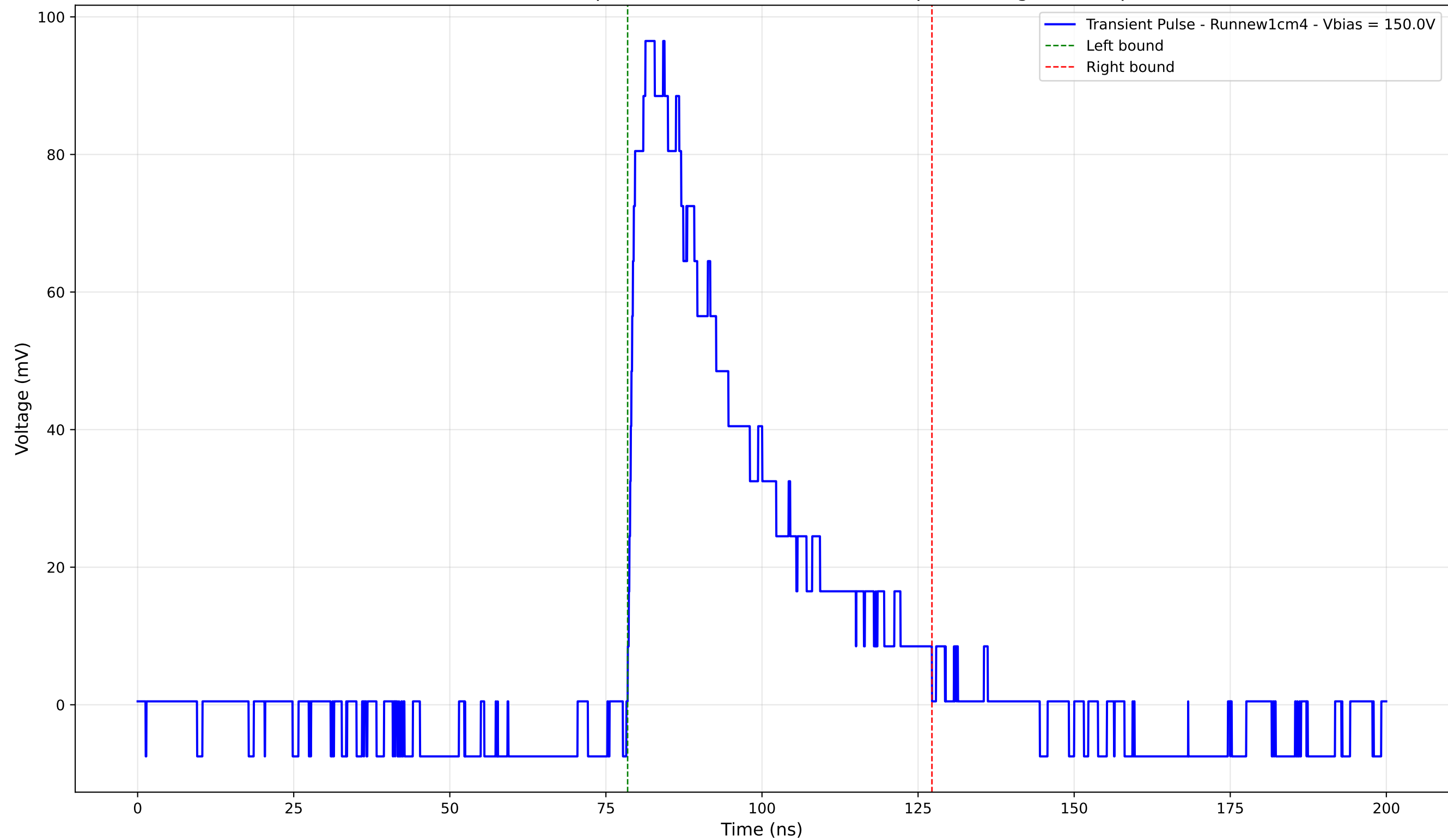
Transient Pulse - Sample: new1cm - Position: 3720.0 \mu\text{m} - Charge: 36.51 pC
