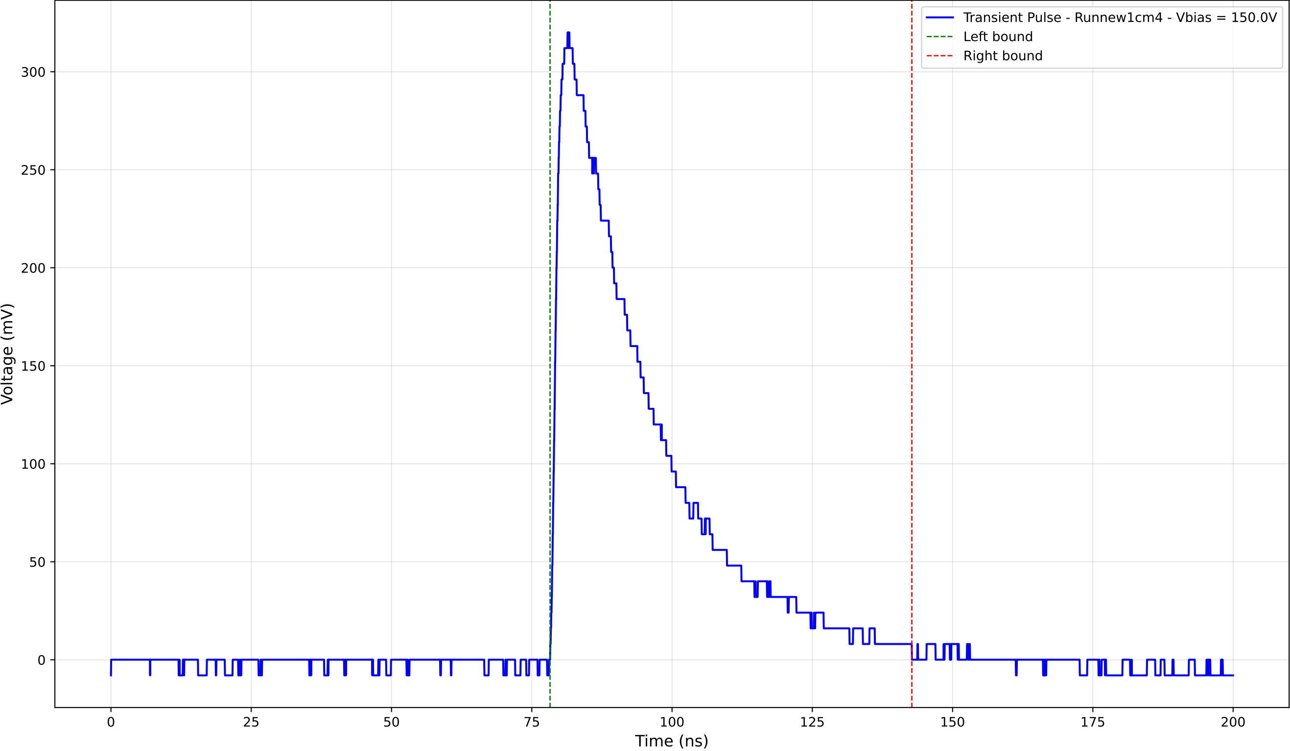
Transient Pulse - Sample: new1cm - Position: 1650.0 \mu\text{m} - Charge: 115.79 pC
