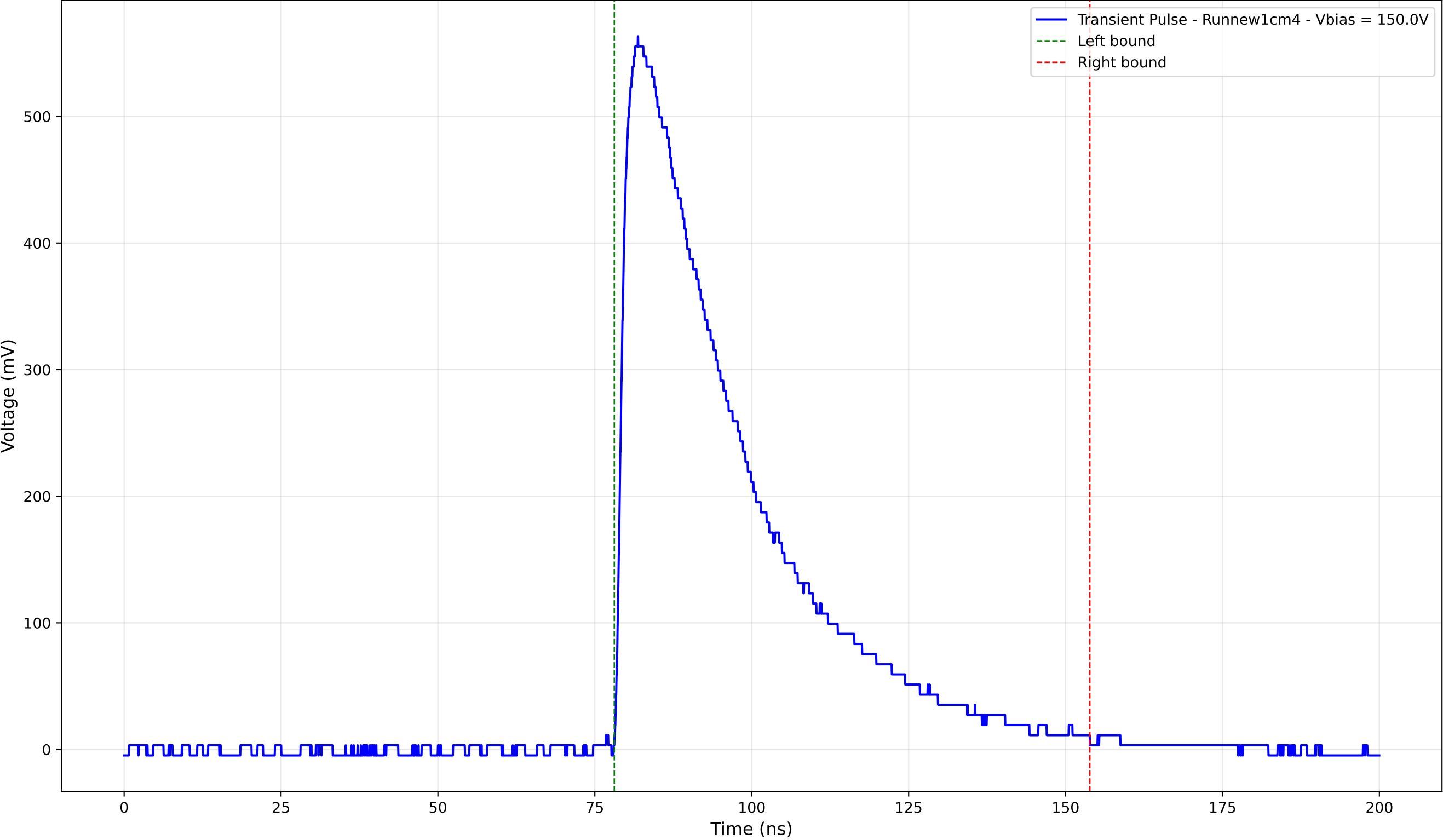
Transient Pulse - Sample: new1cm - Position: 3340.0 \mu\text{m} - Charge: 238.86 pC
