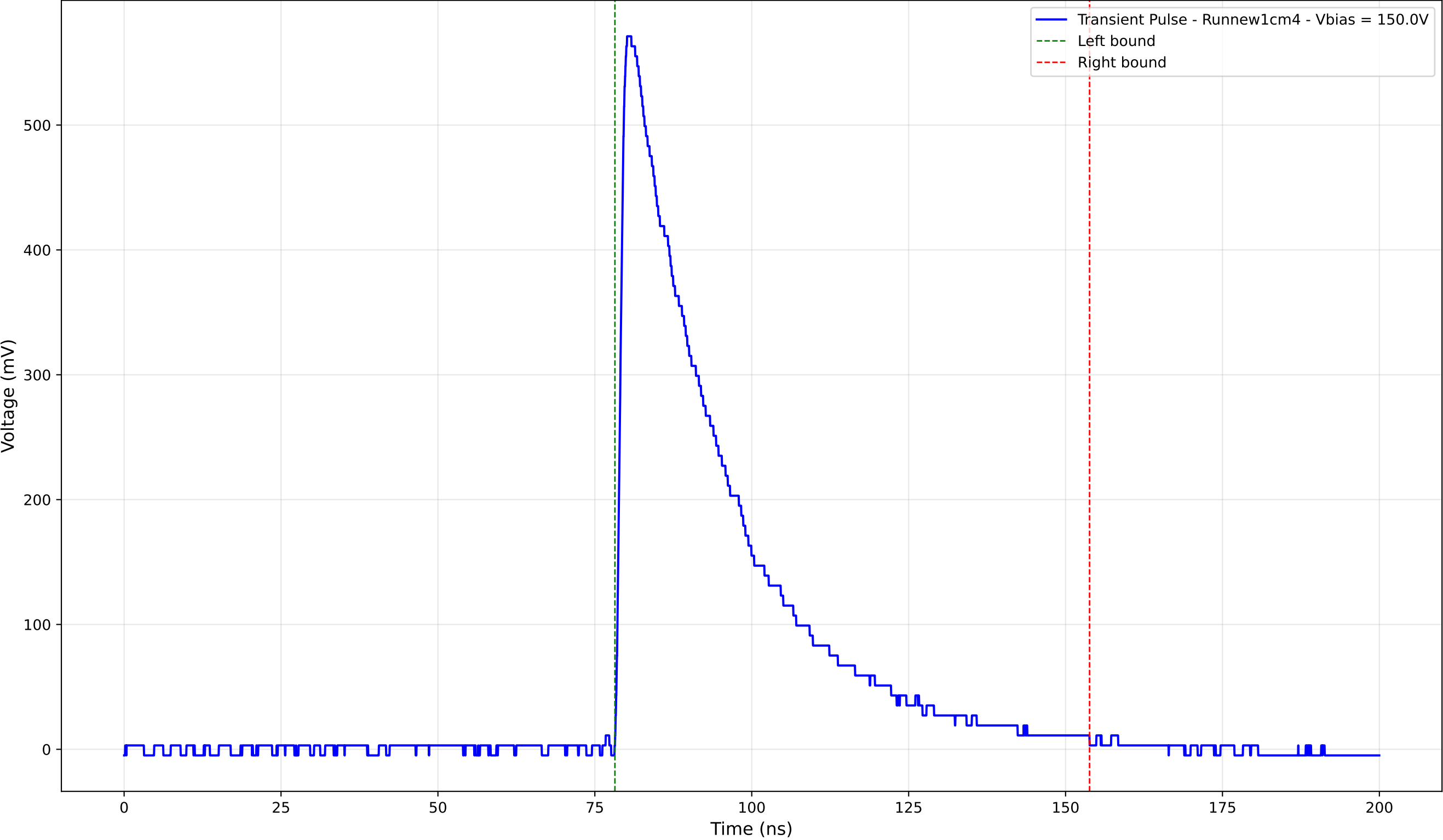
Transient Pulse - Sample: new1cm - Position: 1315.0 \mu\text{m} - Charge: 201.90 pC
