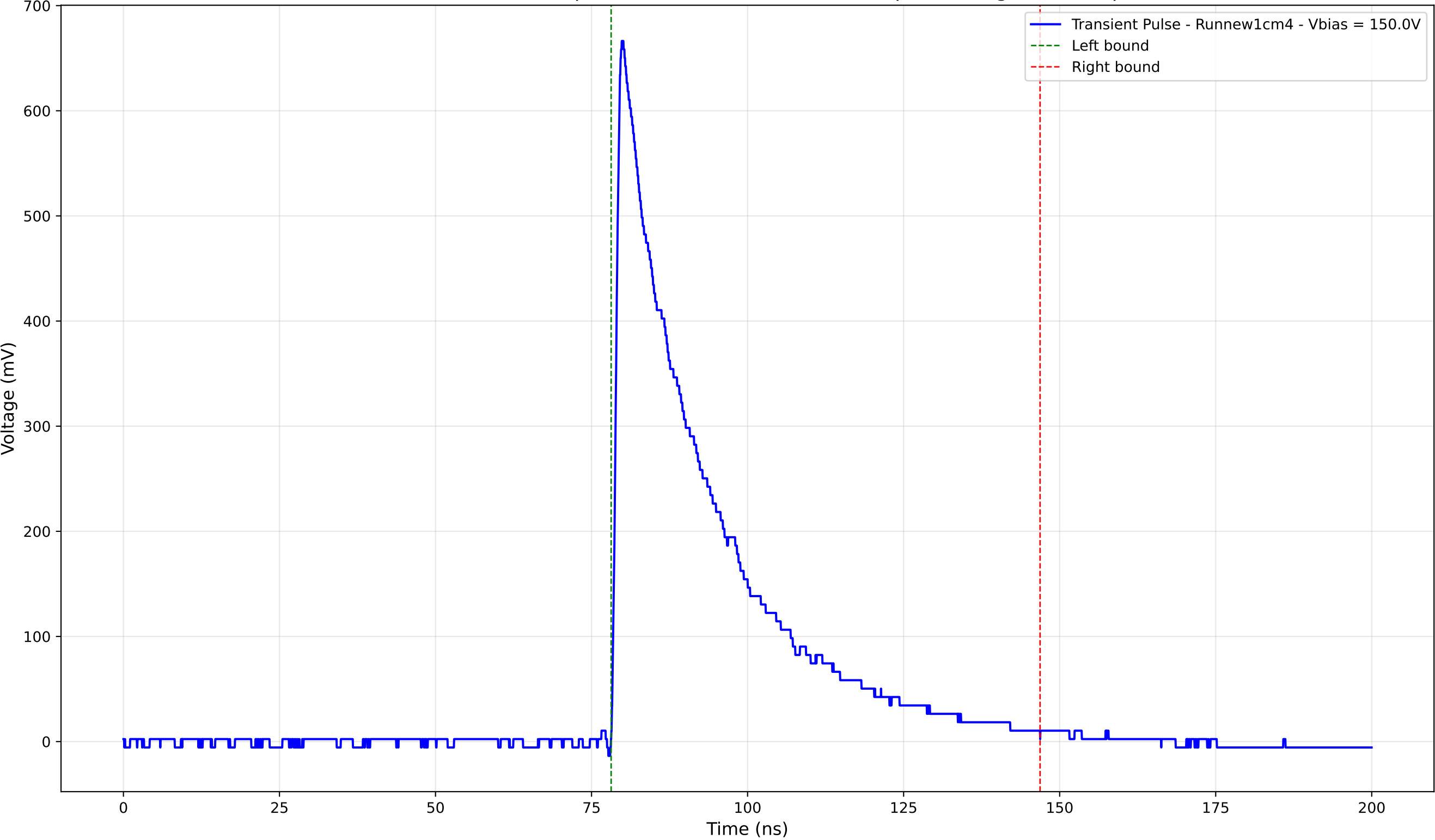
Transient Pulse - Sample: new1cm - Position: 1020.0 \mu\text{m} - Charge: 199.38 pC
