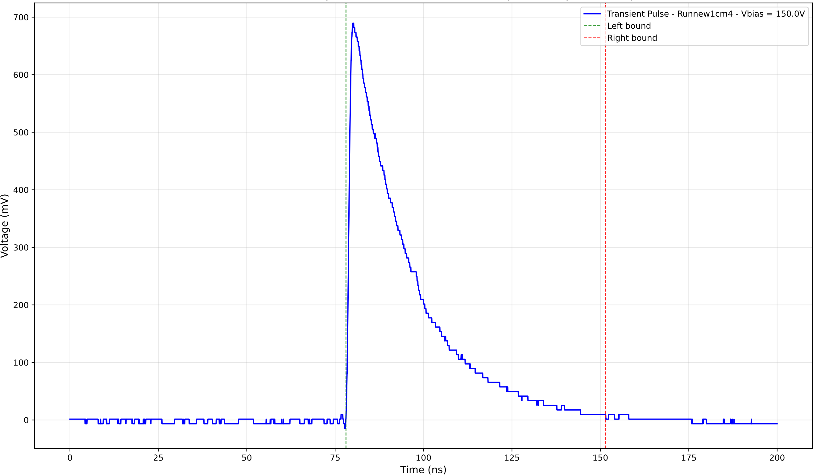
Transient Pulse - Sample: new1cm - Position: 4055.0 \mu\text{m} - Charge: 247.21 pC
