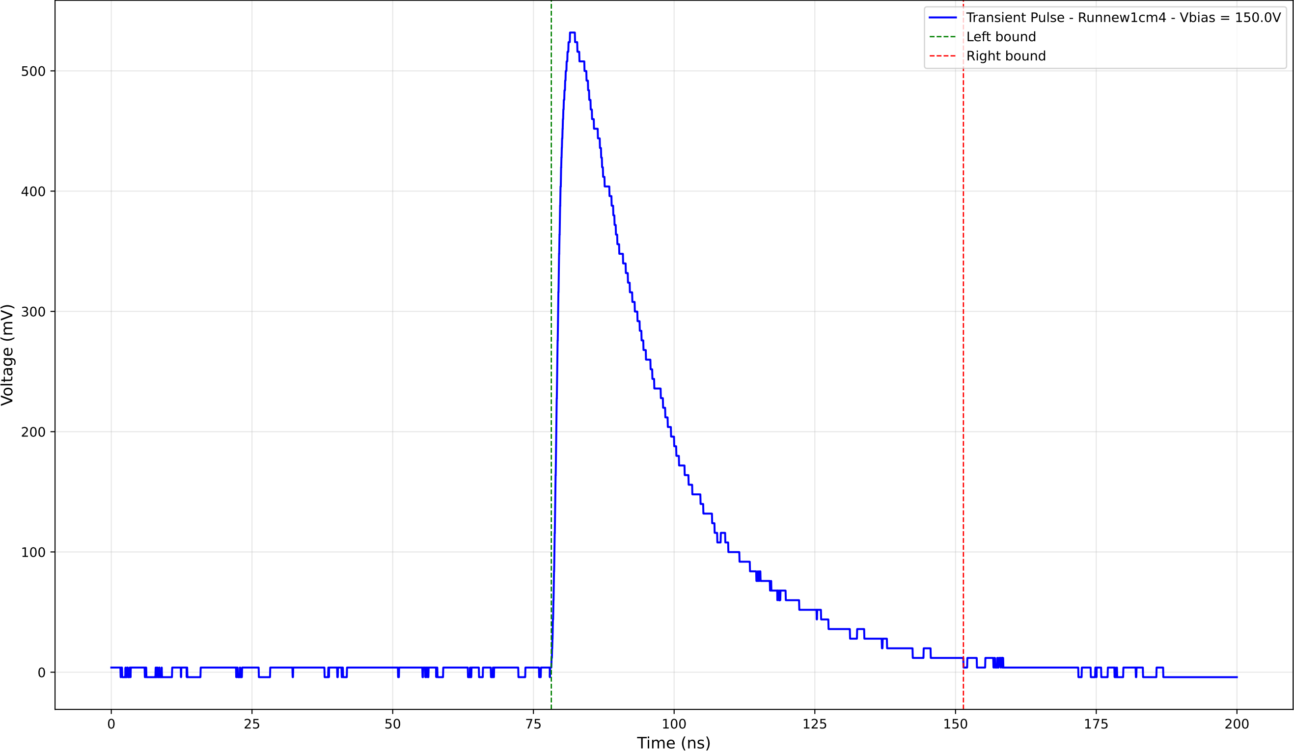
Transient Pulse - Sample: new1cm - Position: 1880.0 \mu\text{m} - Charge: 217.11 pC
