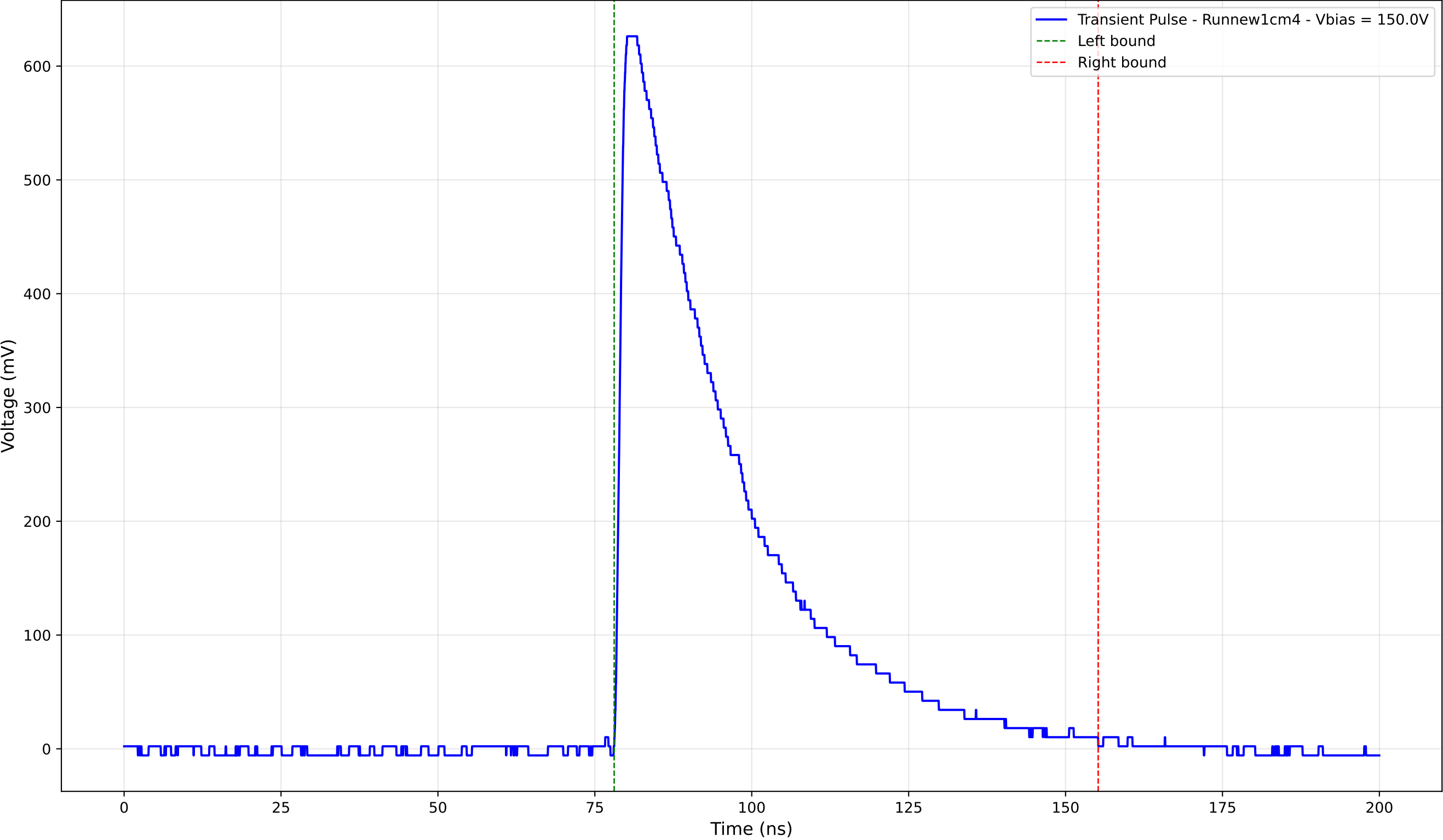
Transient Pulse - Sample: new1cm - Position: 3845.0 \mu\text{m} - Charge: 247.04 pC
