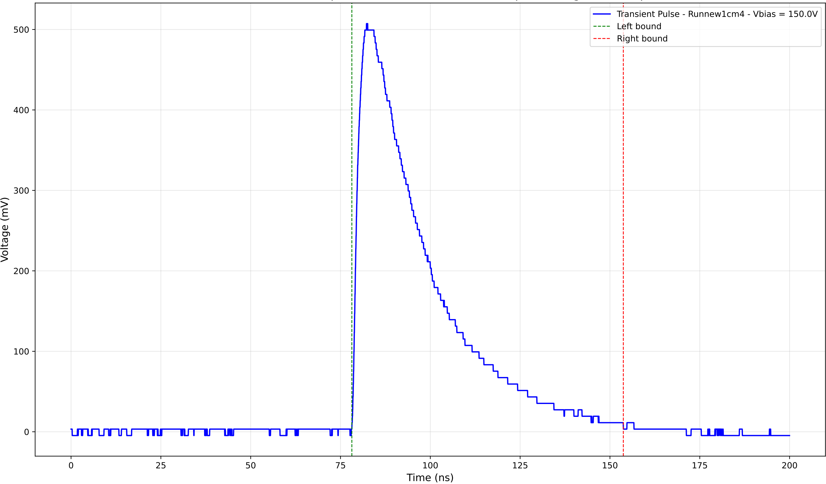
Transient Pulse - Sample: new1cm - Position: 2570.0 \mu\text{m} - Charge: 222.26 pC
