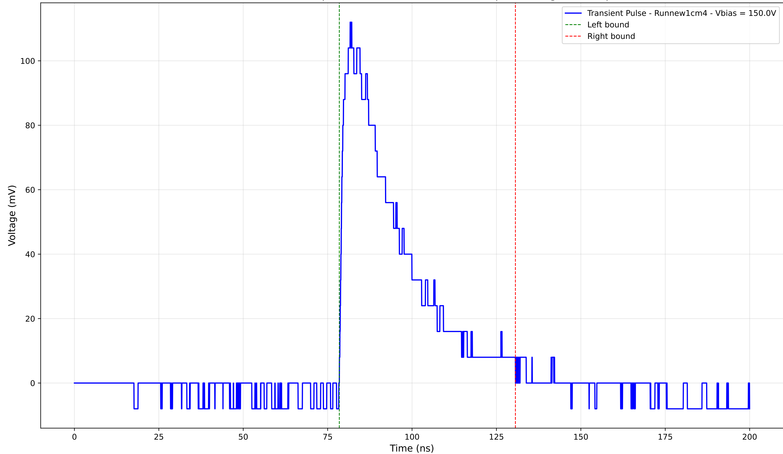
Transient Pulse - Sample: new1cm - Position: 3715.0 \mu\text{m} - Charge: 39.63 pC
