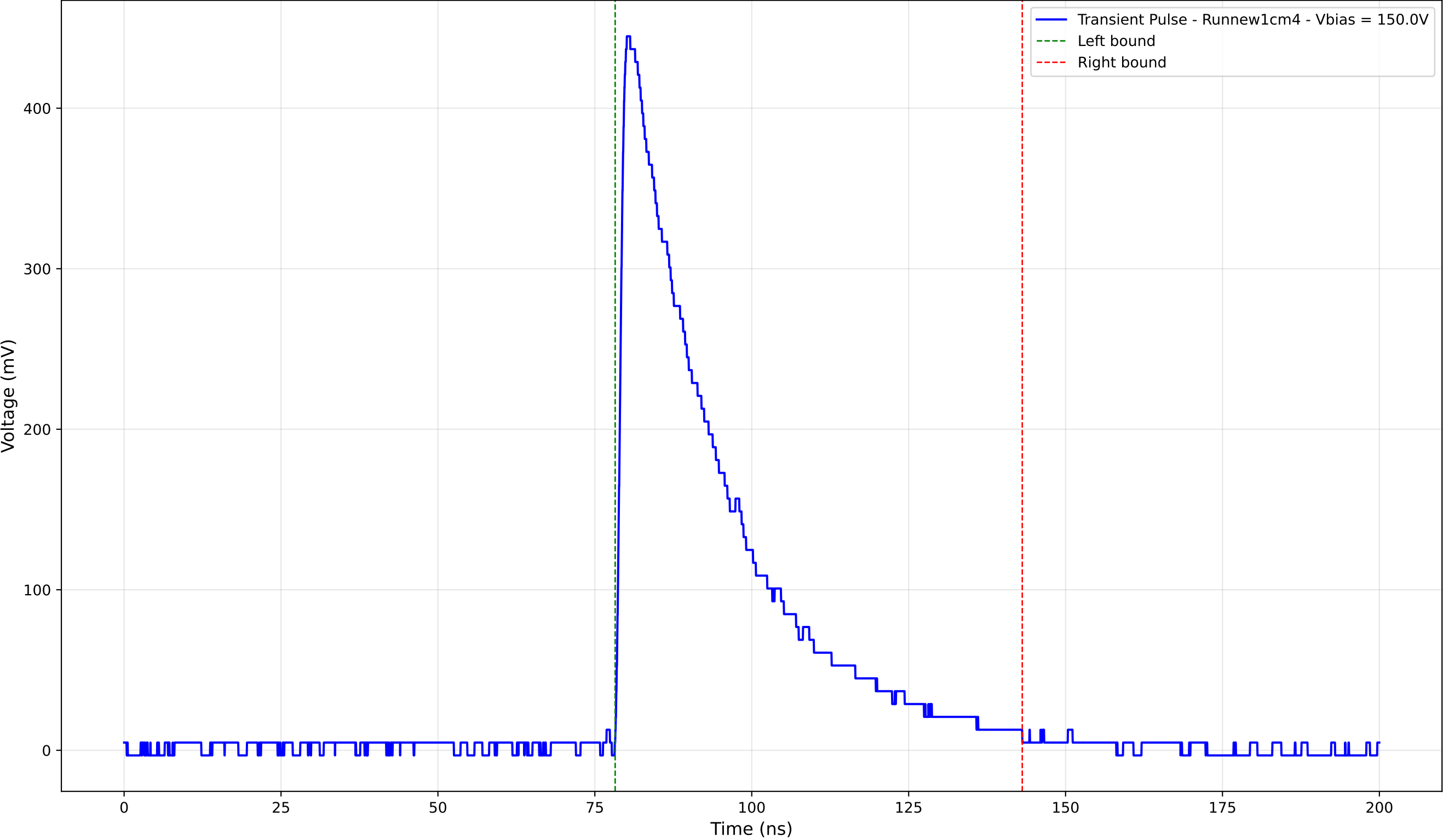
Transient Pulse - Sample: new1cm - Position: 1270.0 \mu\text{m} - Charge: 151.98 pC
