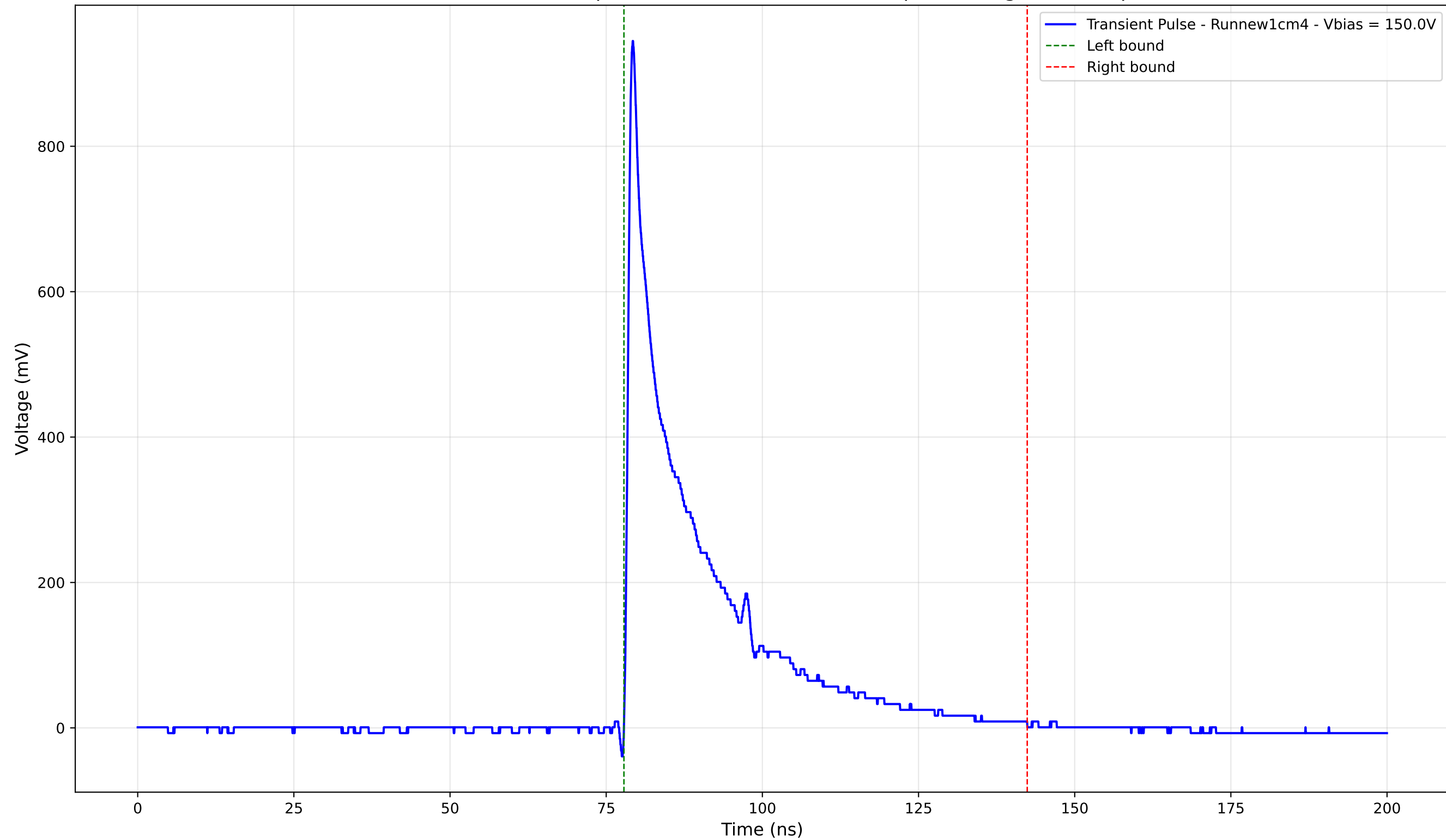
Transient Pulse - Sample: new1cm - Position: 315.0 \mu\text{m} - Charge: 180.94 pC
