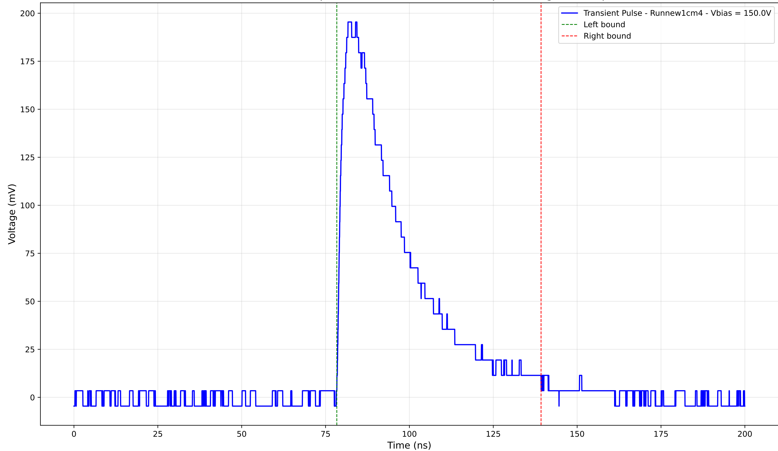
Transient Pulse - Sample: new1cm - Position: 3190.0 \mu\text{m} - Charge: 80.55 pC
