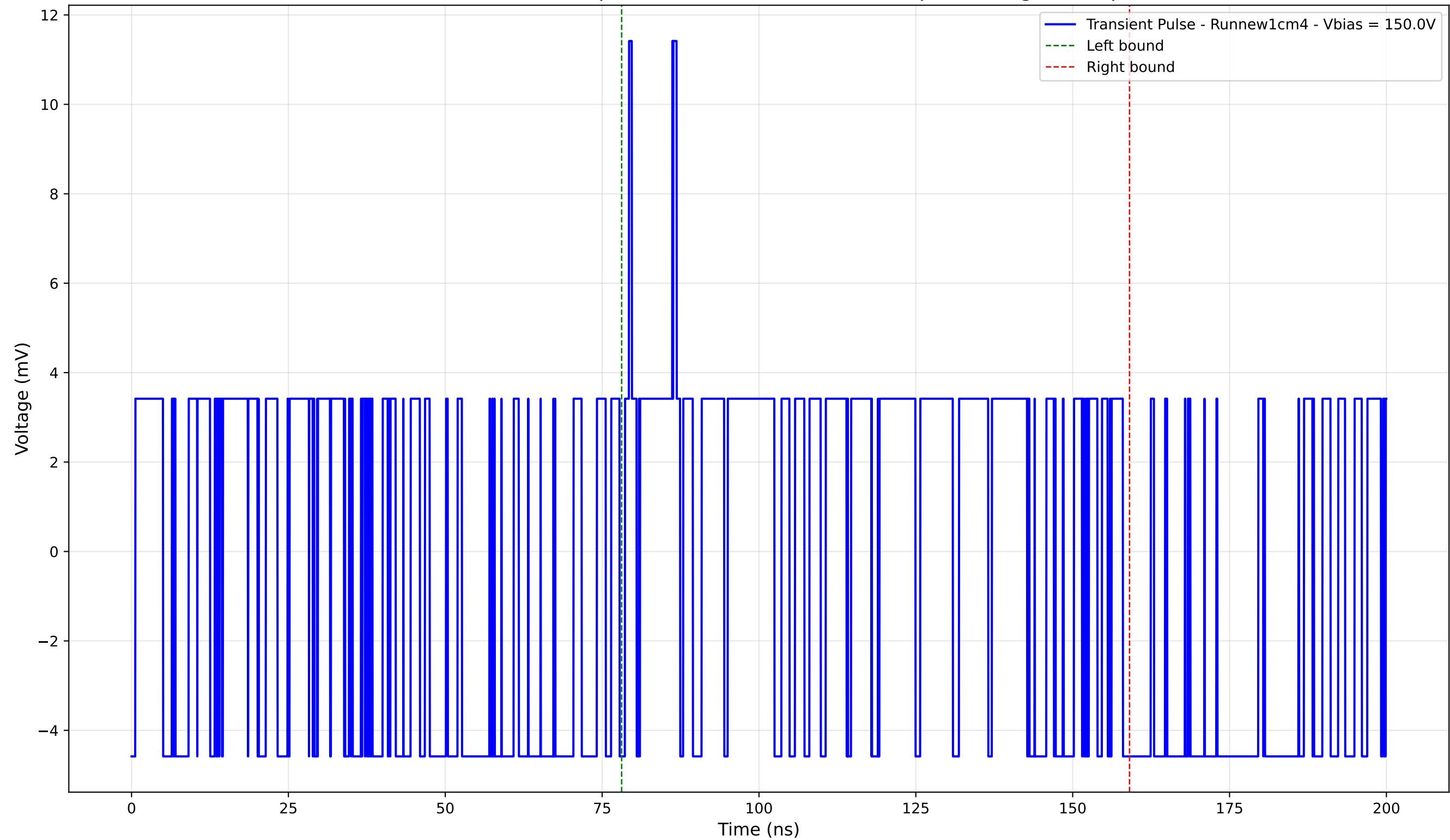
Transient Pulse - Sample: new1cm - Position: 5190.0 \mu\text{m} - Charge: 2.52 pC
