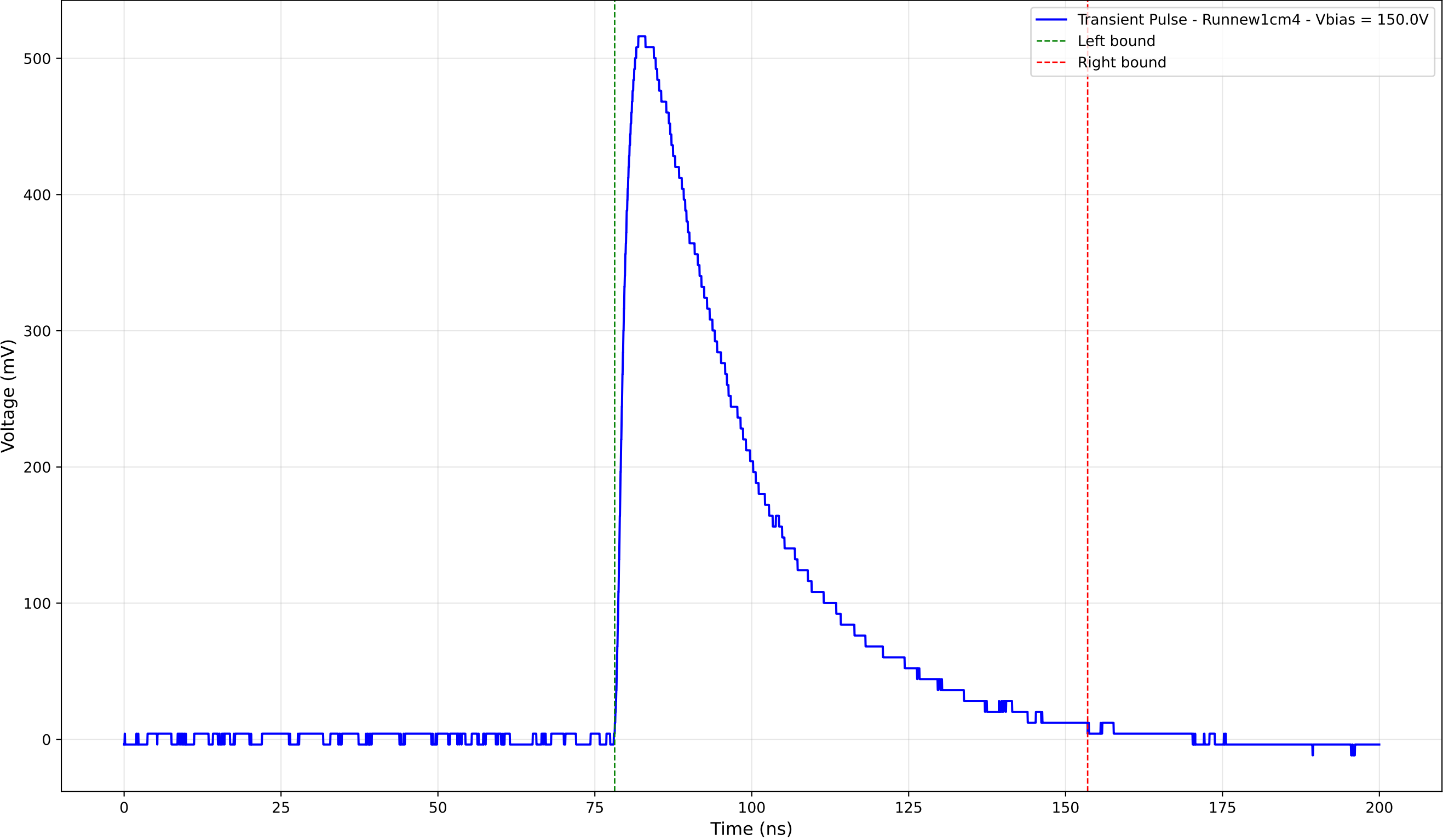
Transient Pulse - Sample: new1cm - Position: 2330.0 \mu\text{m} - Charge: 224.59 pC
