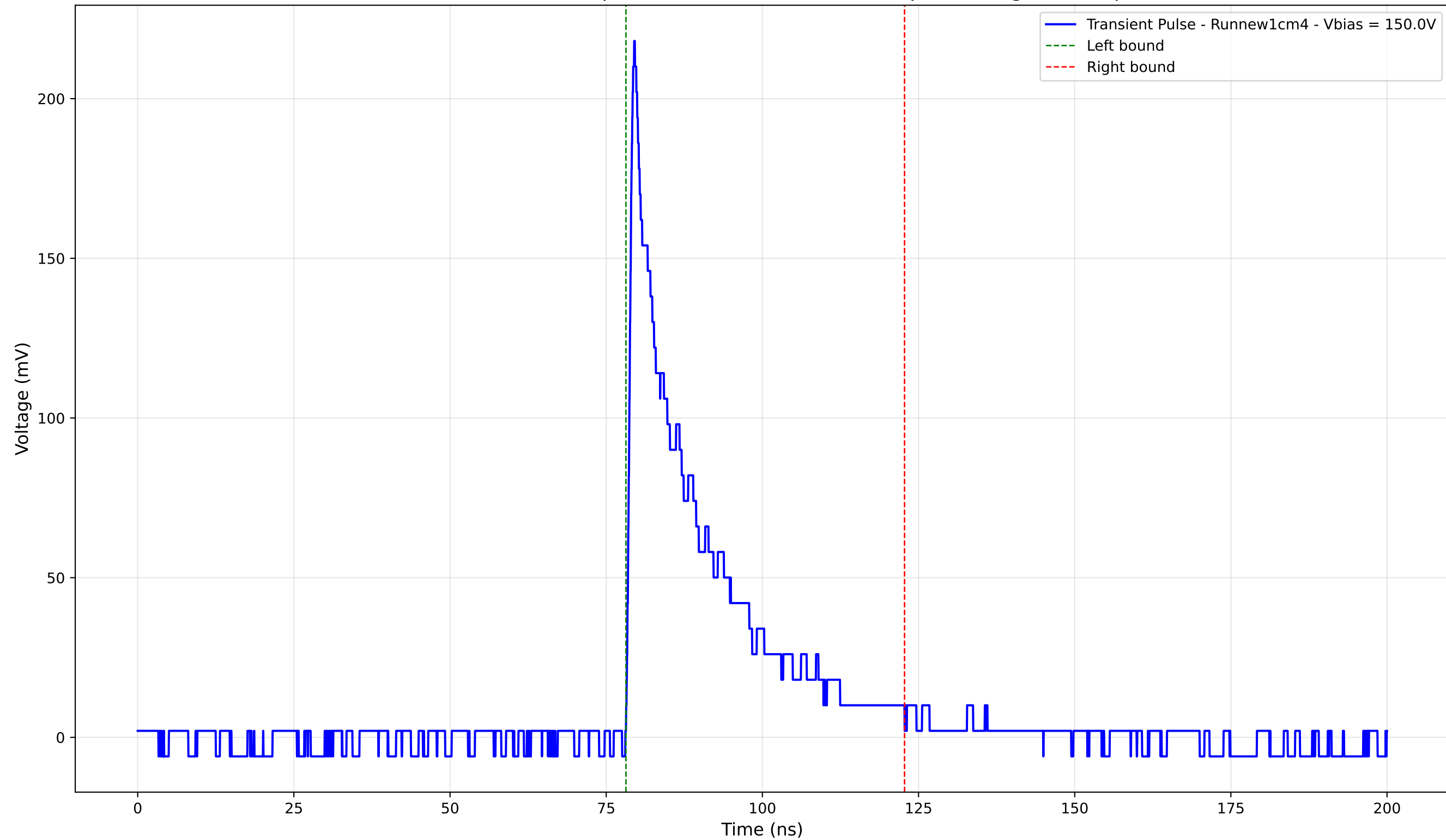
Transient Pulse - Sample: new1cm - Position: 670.0 \mu\text{m} - Charge: 43.80 pC
