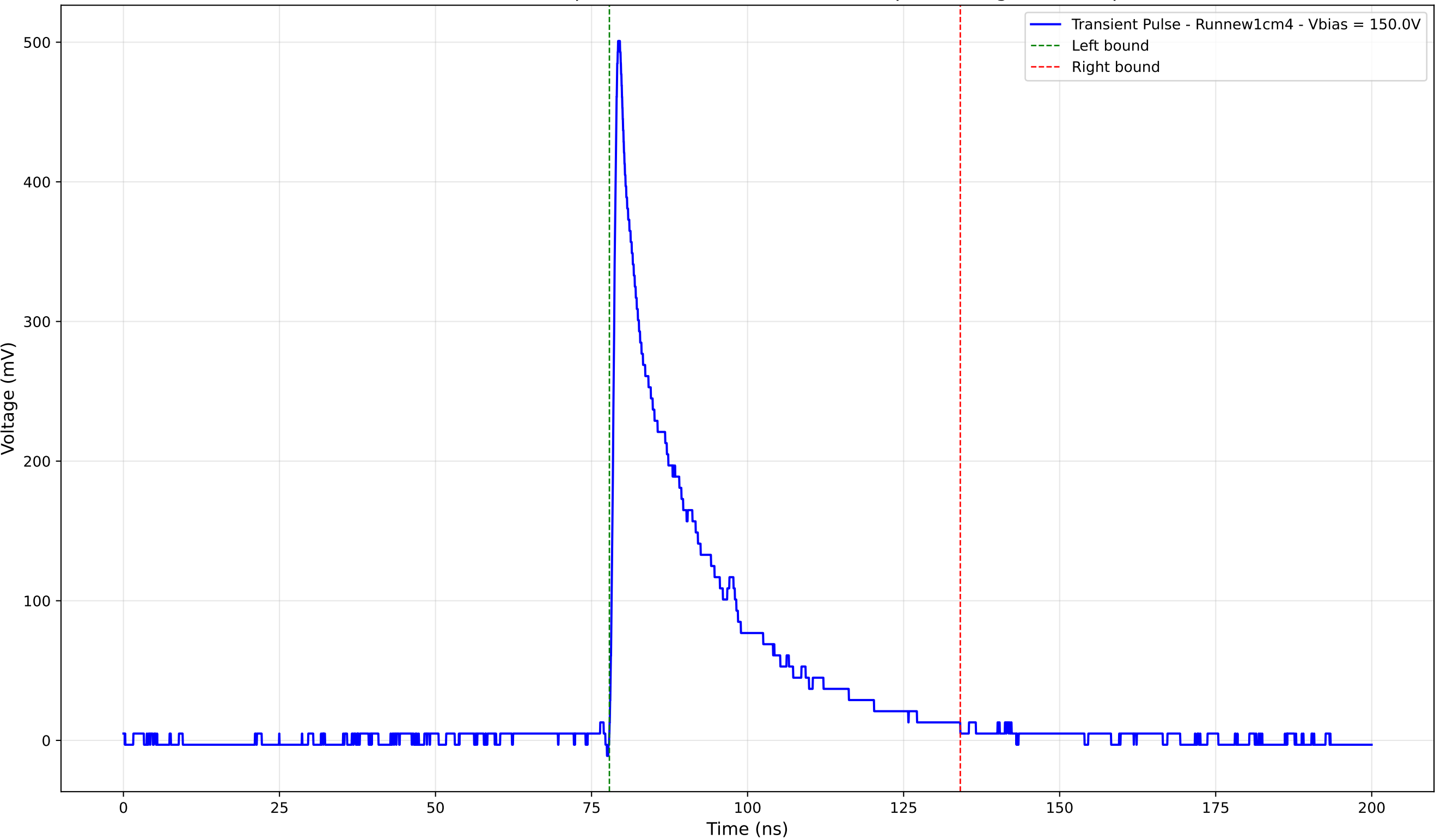
Transient Pulse - Sample: new1cm - Position: 4685.0 \mu\text{m} - Charge: 114.13 pC
