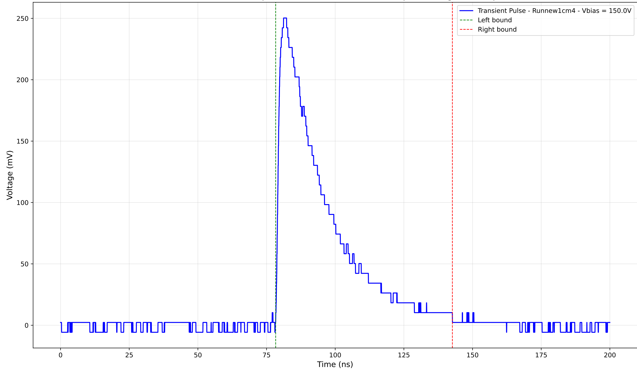
Transient Pulse - Sample: new1cm - Position: 1660.0 \mu\text{m} - Charge: 93.23 pC
