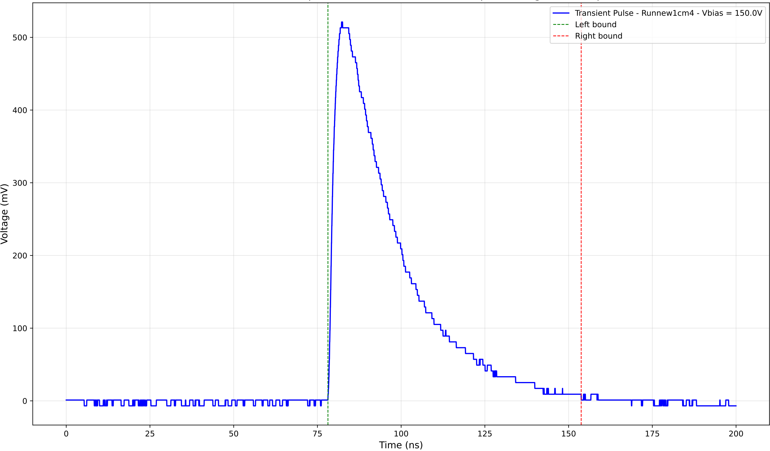
Transient Pulse - Sample: new1cm - Position: 2450.0 \mu\text{m} - Charge: 222.19 pC
