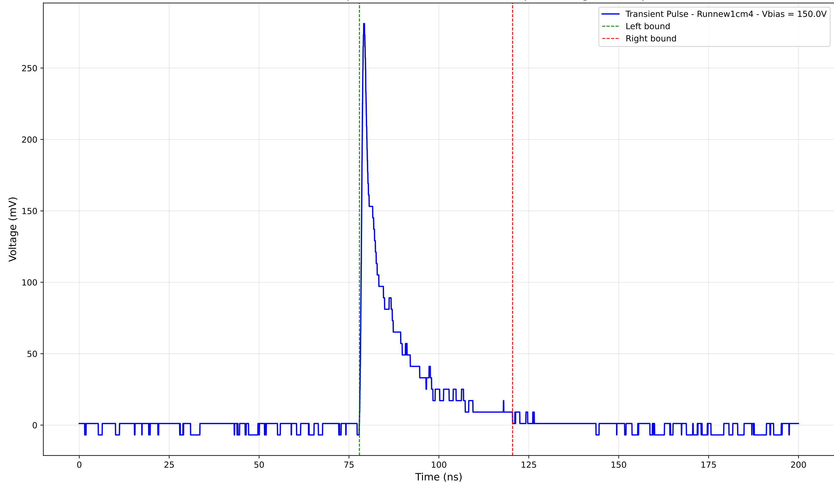
Transient Pulse - Sample: new1cm - Position: 215.0 \mu\text{m} - Charge: 40.53 pC
