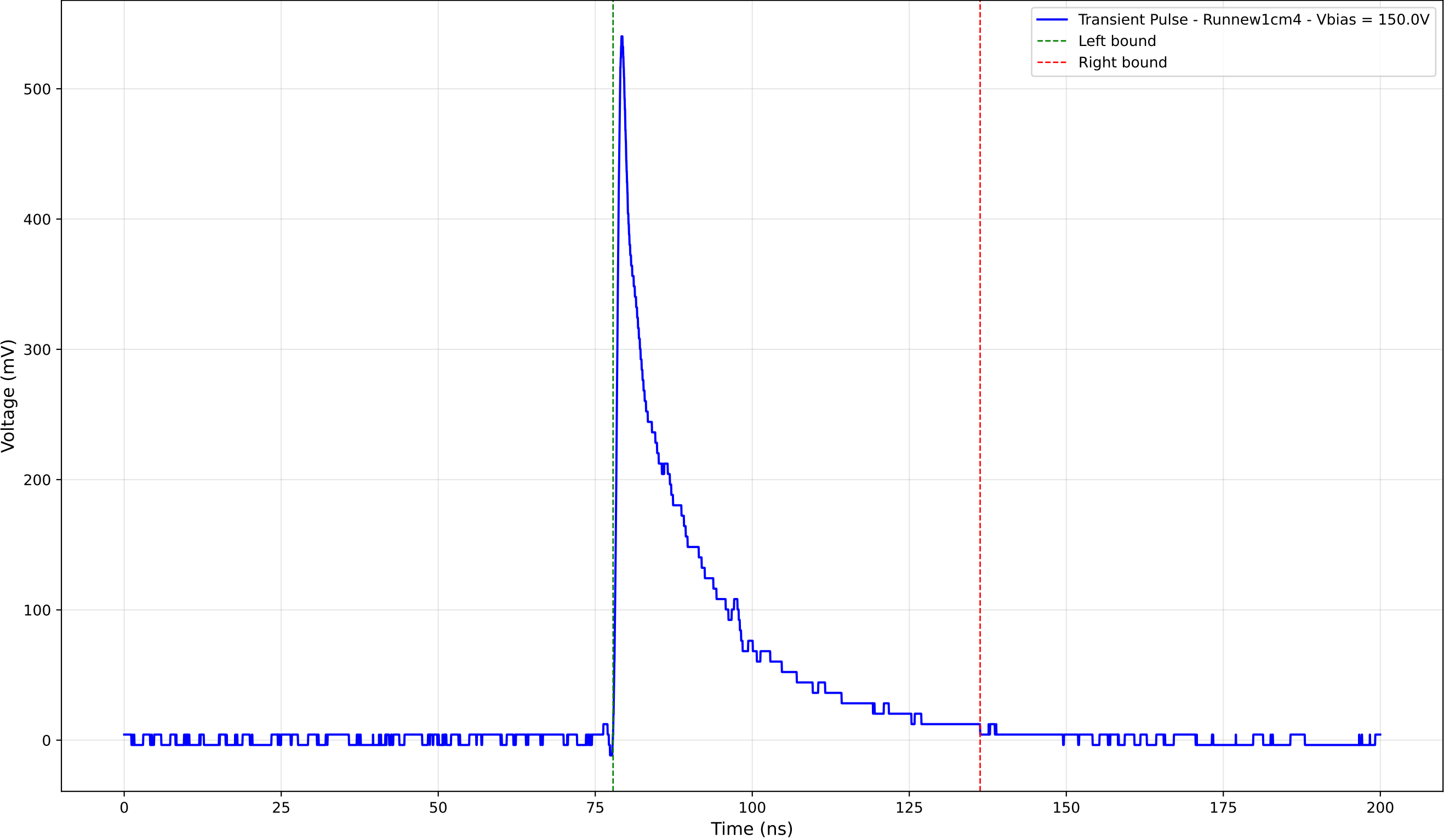
Transient Pulse - Sample: new1cm - Position: 4785.0 \mu\text{m} - Charge: 108.99 pC
