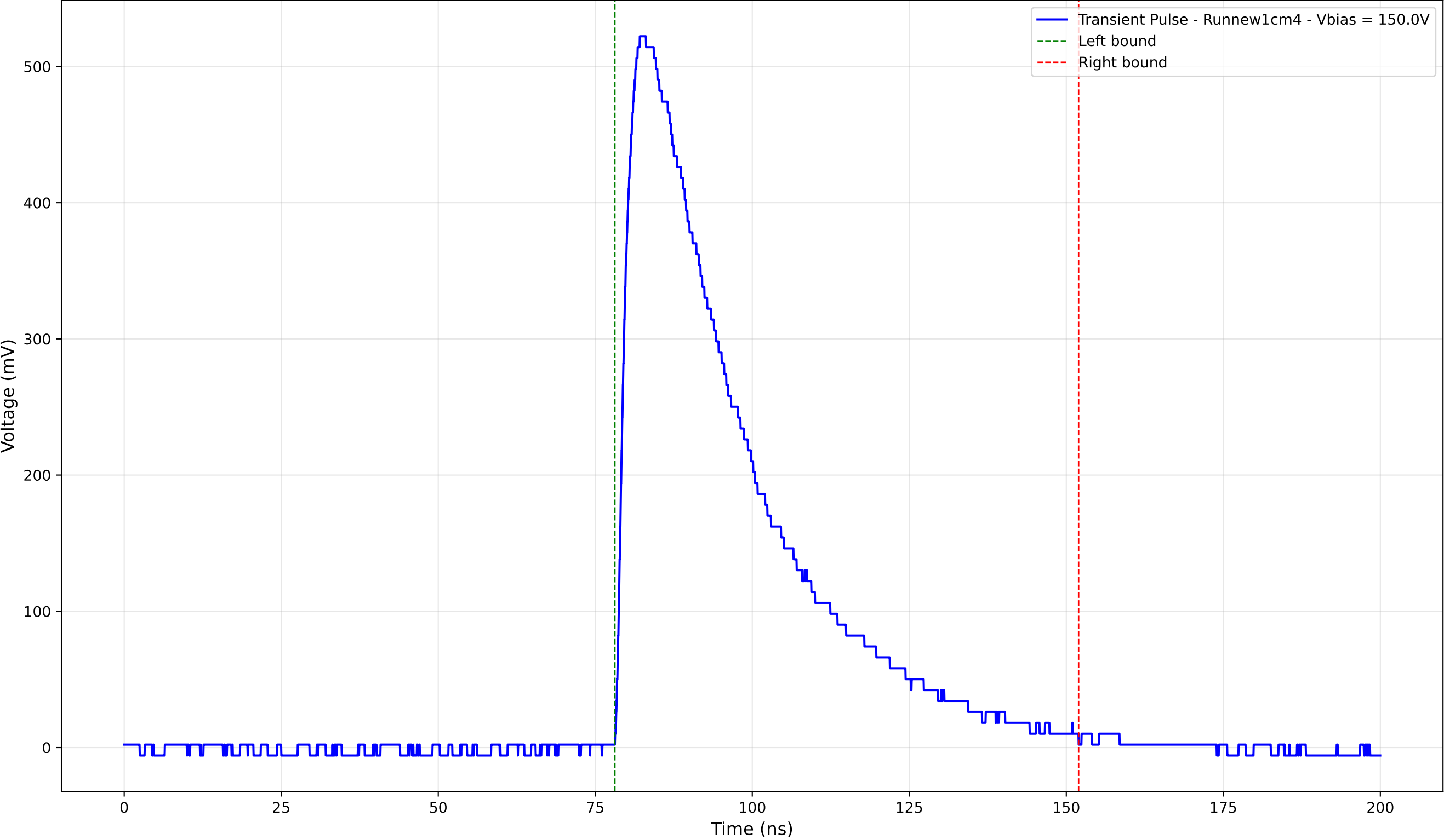
Transient Pulse - Sample: new1cm - Position: 2530.0 \mu\text{m} - Charge: 226.72 pC
