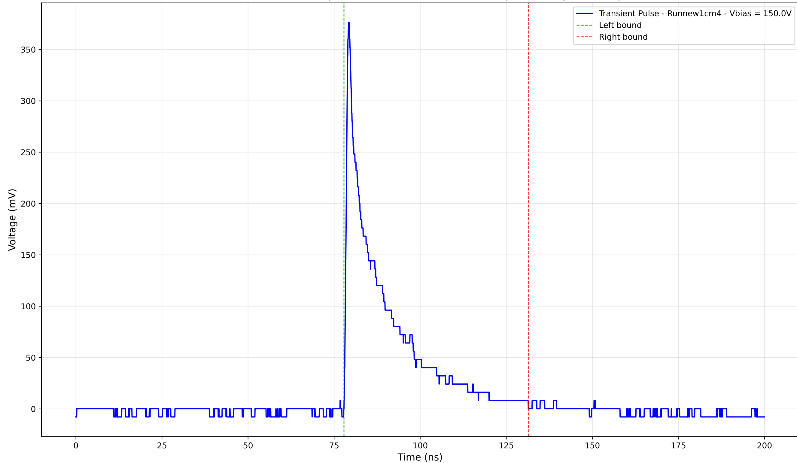
Transient Pulse - Sample: new1cm - Position: 4770.0 \mu\text{m} - Charge: 71.35 pC
