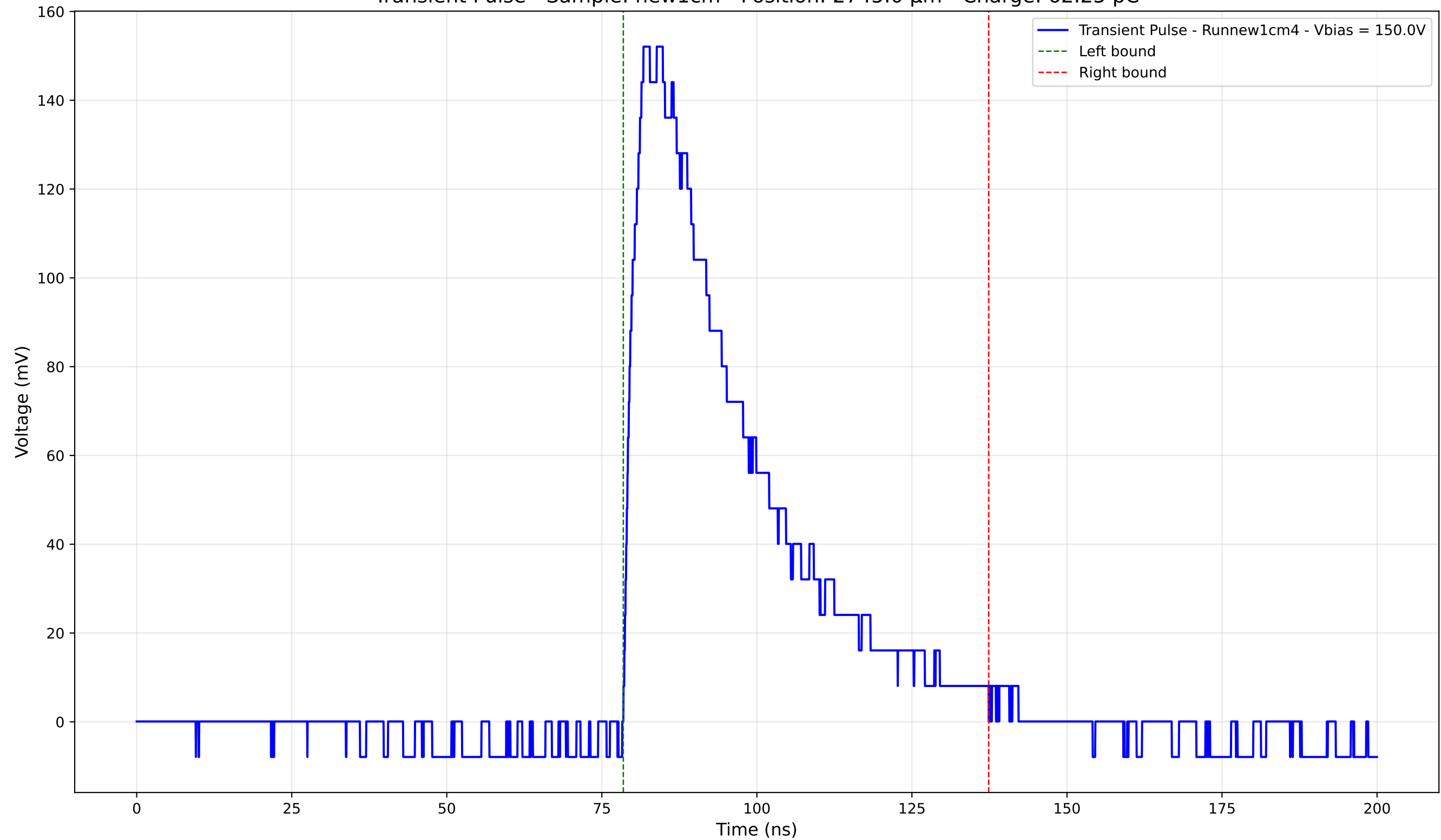
Transient Pulse - Sample: new1cm - Position: 2745.0 \mu\text{m} - Charge: 62.25 pC
