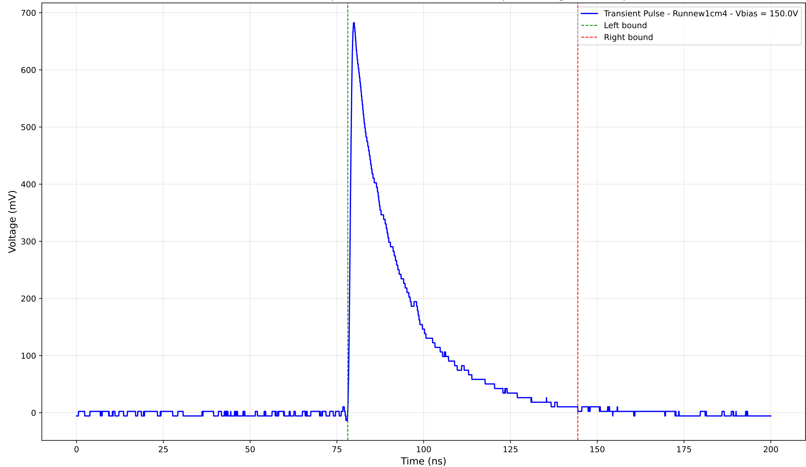
Transient Pulse - Sample: new1cm - Position: 965.0 \mu\text{m} - Charge: 195.32 pC
