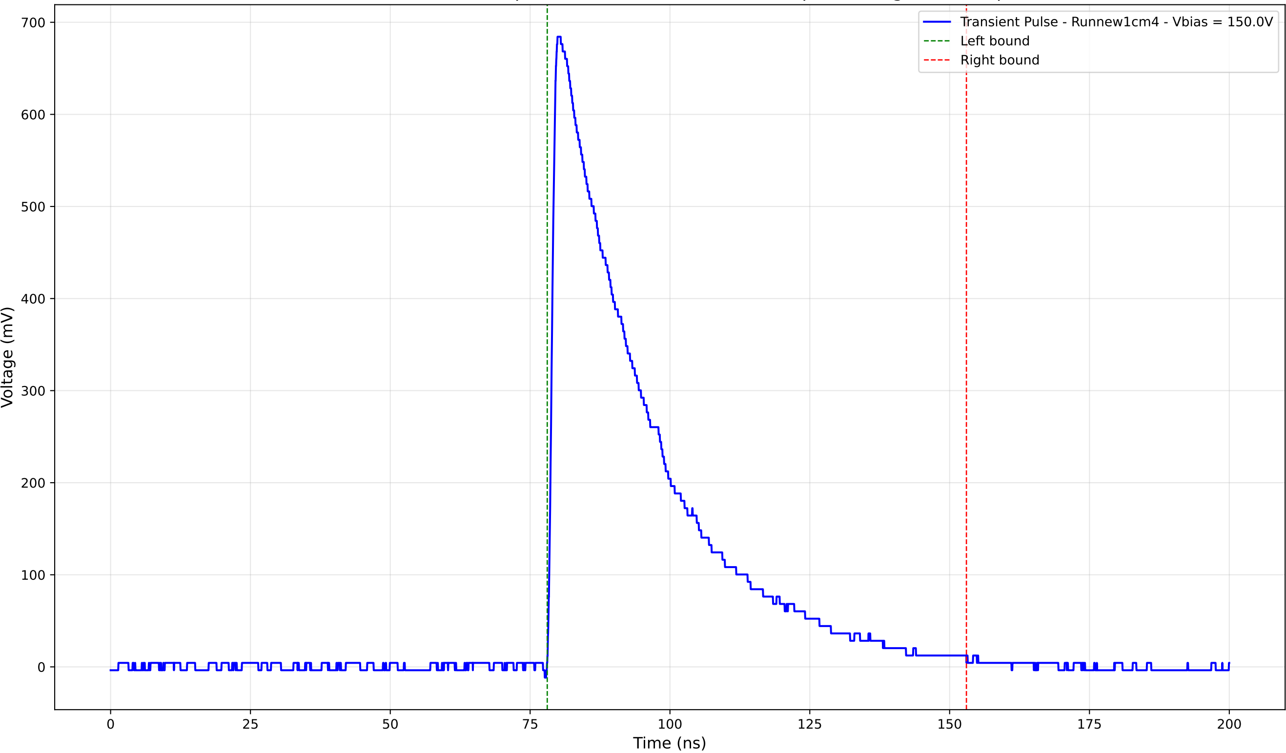
Transient Pulse - Sample: new1cm - Position: 4045.0 \mu\text{m} - Charge: 251.75 pC
