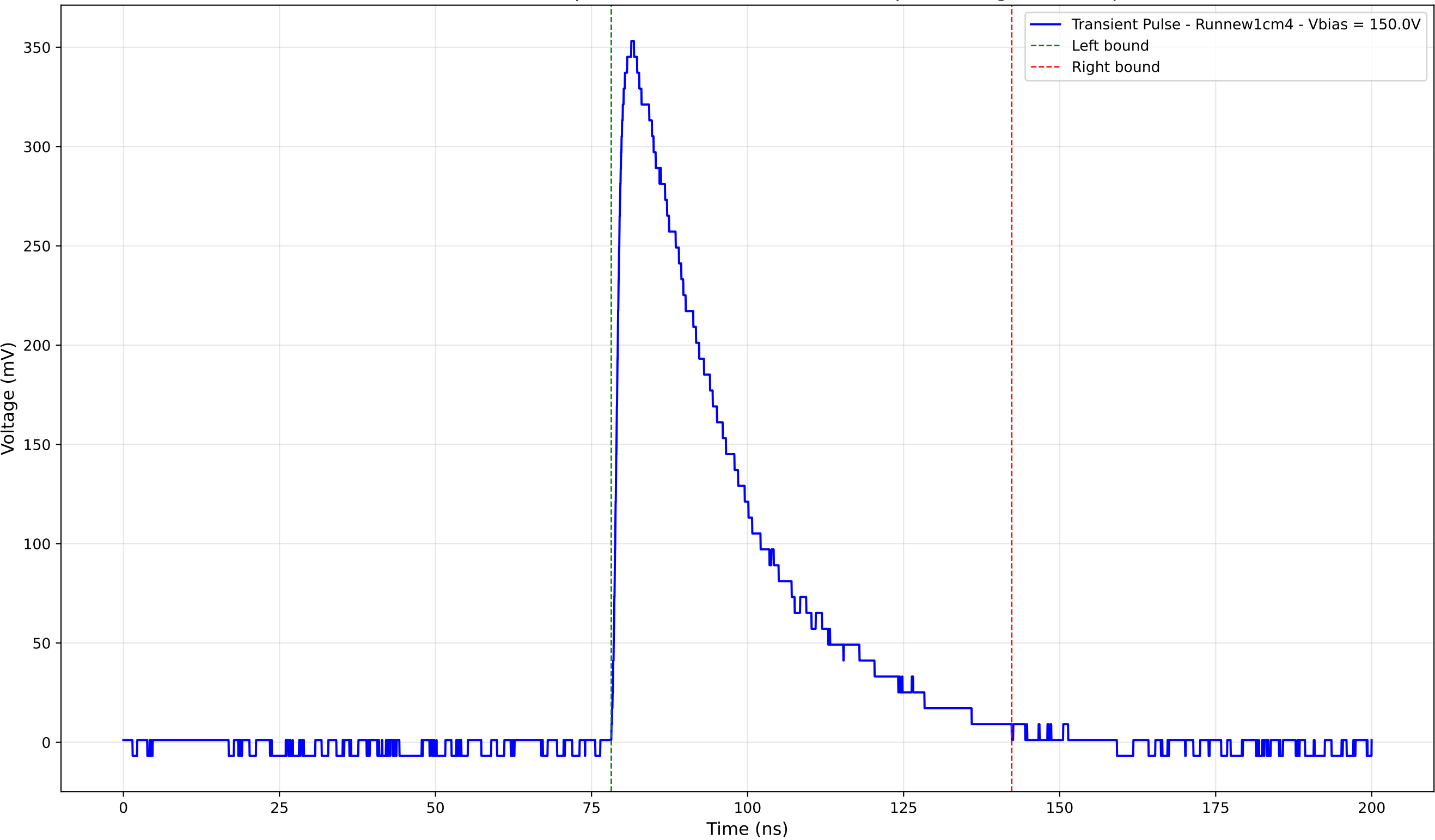
Transient Pulse - Sample: new1cm - Position: 3675.0 \mu\text{m} - Charge: 135.79 pC
