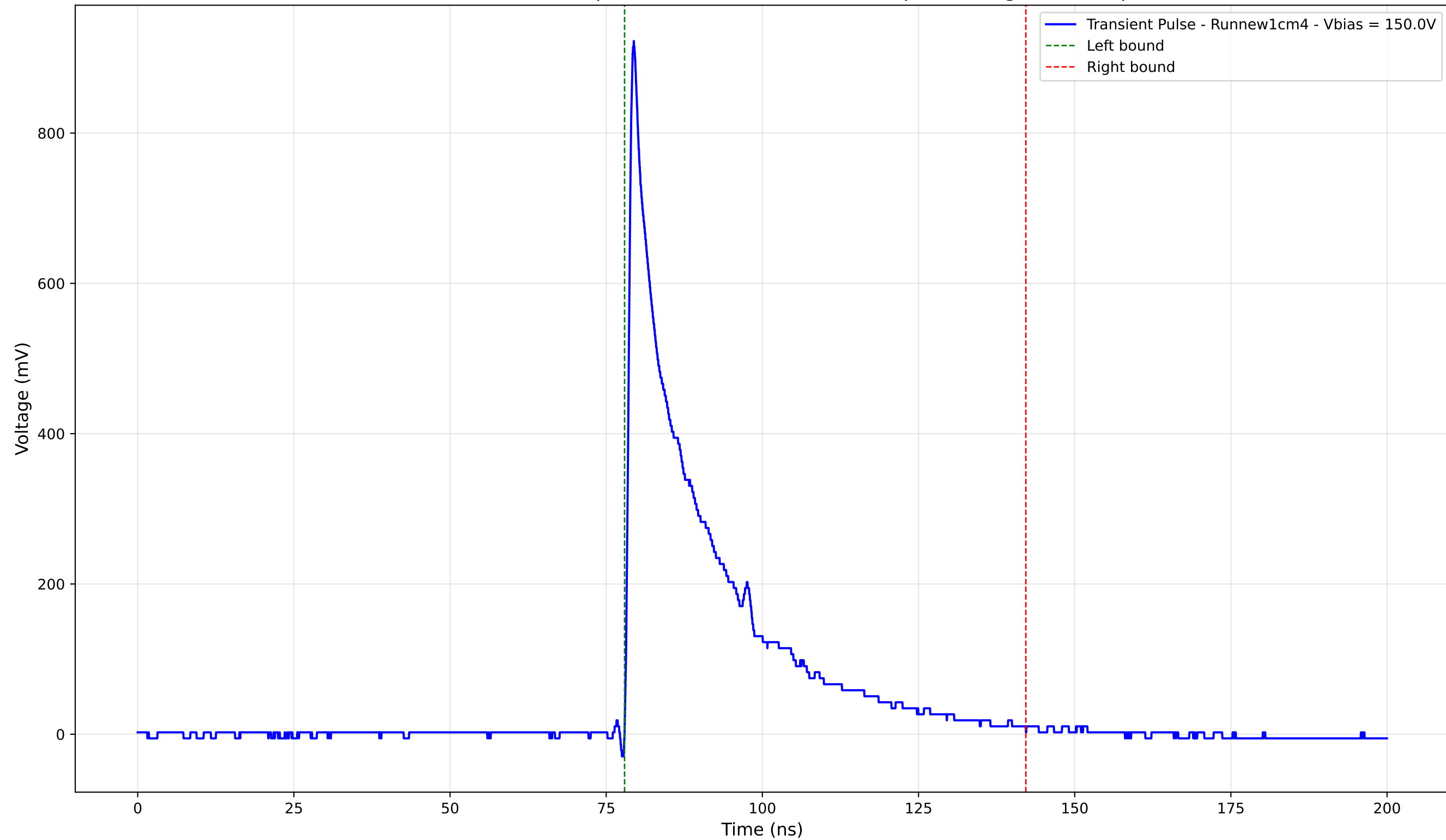
Transient Pulse - Sample: new1cm - Position: 490.0 \mu\text{m} - Charge: 201.71 pC
