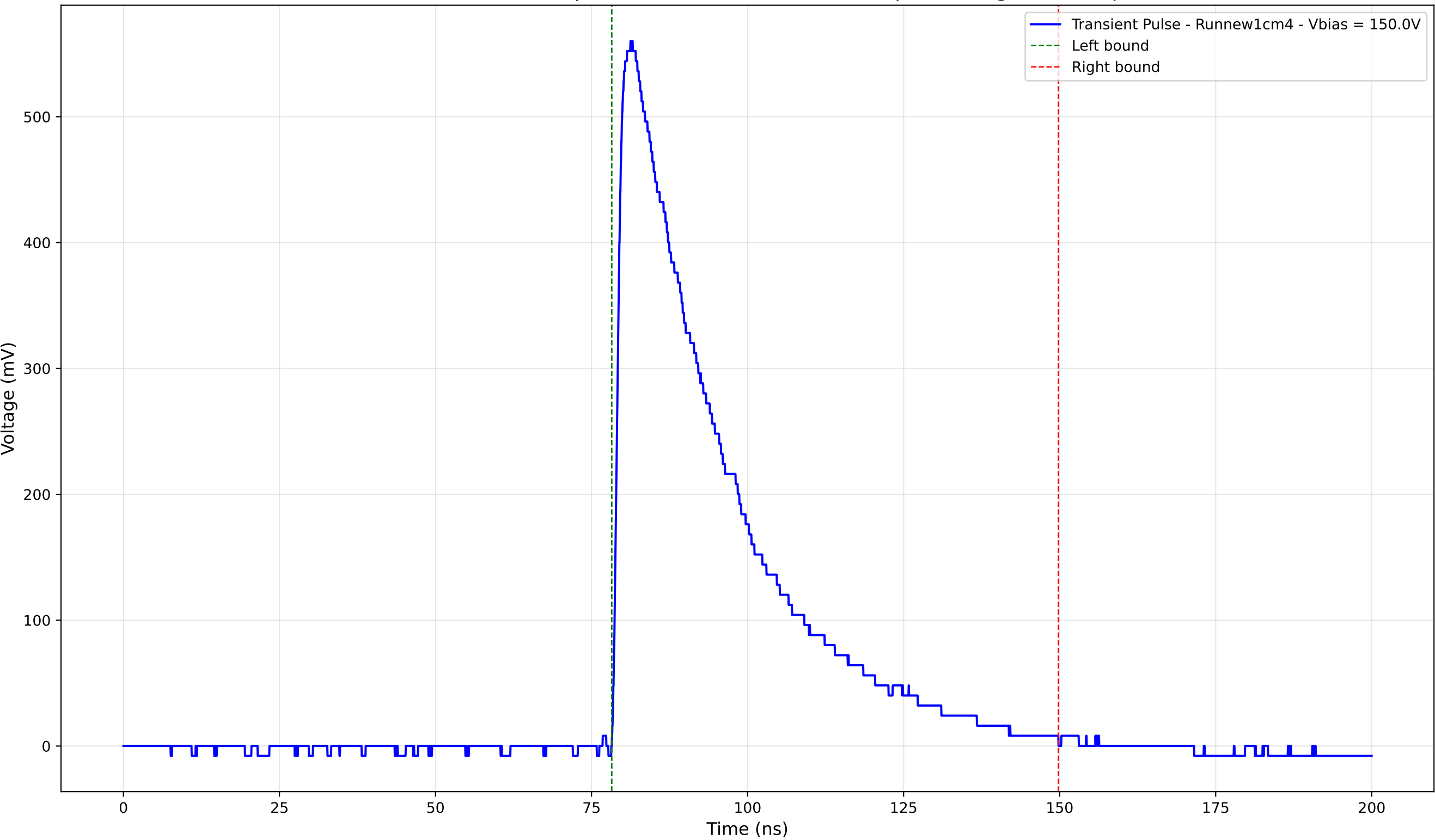
Transient Pulse - Sample: new1cm - Position: 1510.0 \mu\text{m} - Charge: 206.64 pC
