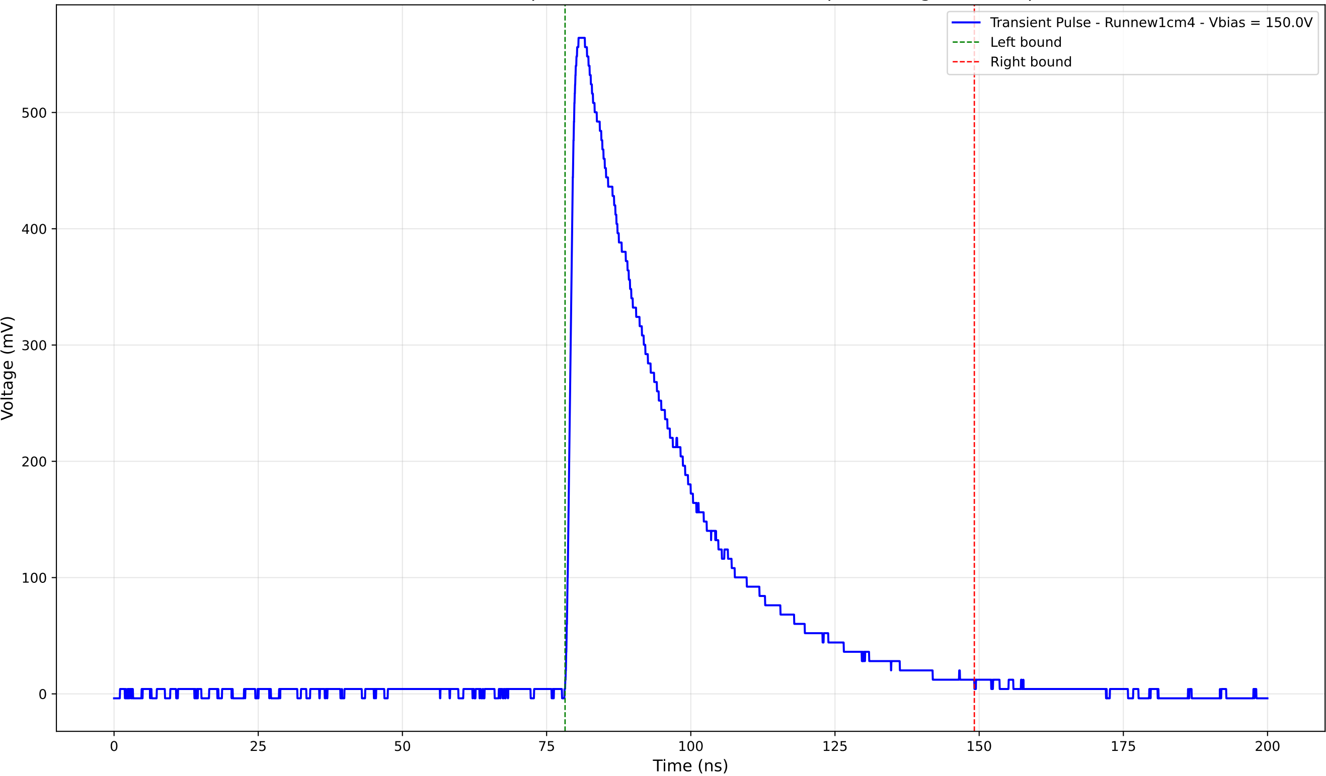
Transient Pulse - Sample: new1cm - Position: 1455.0 \mu\text{m} - Charge: 209.92 pC
