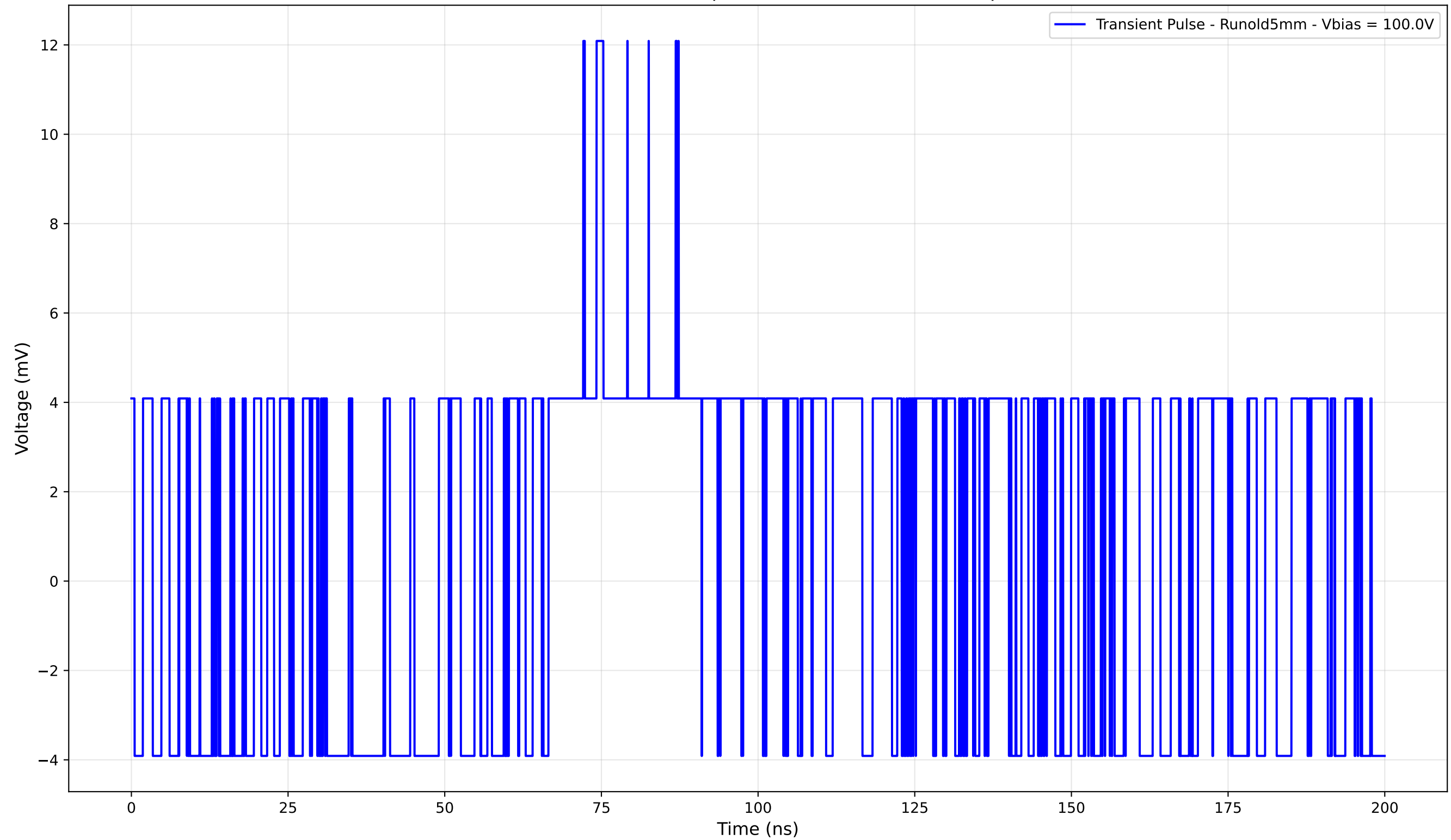
Transient Pulse - Sample: old5 - Position: 1970.0 \mu\text{m}
