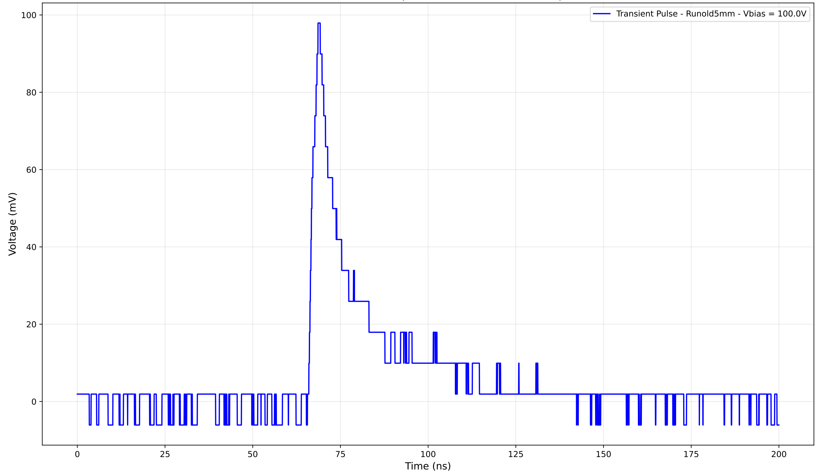
Transient Pulse - Sample: old5 - Position: 4085.0 \mu\text{m}
