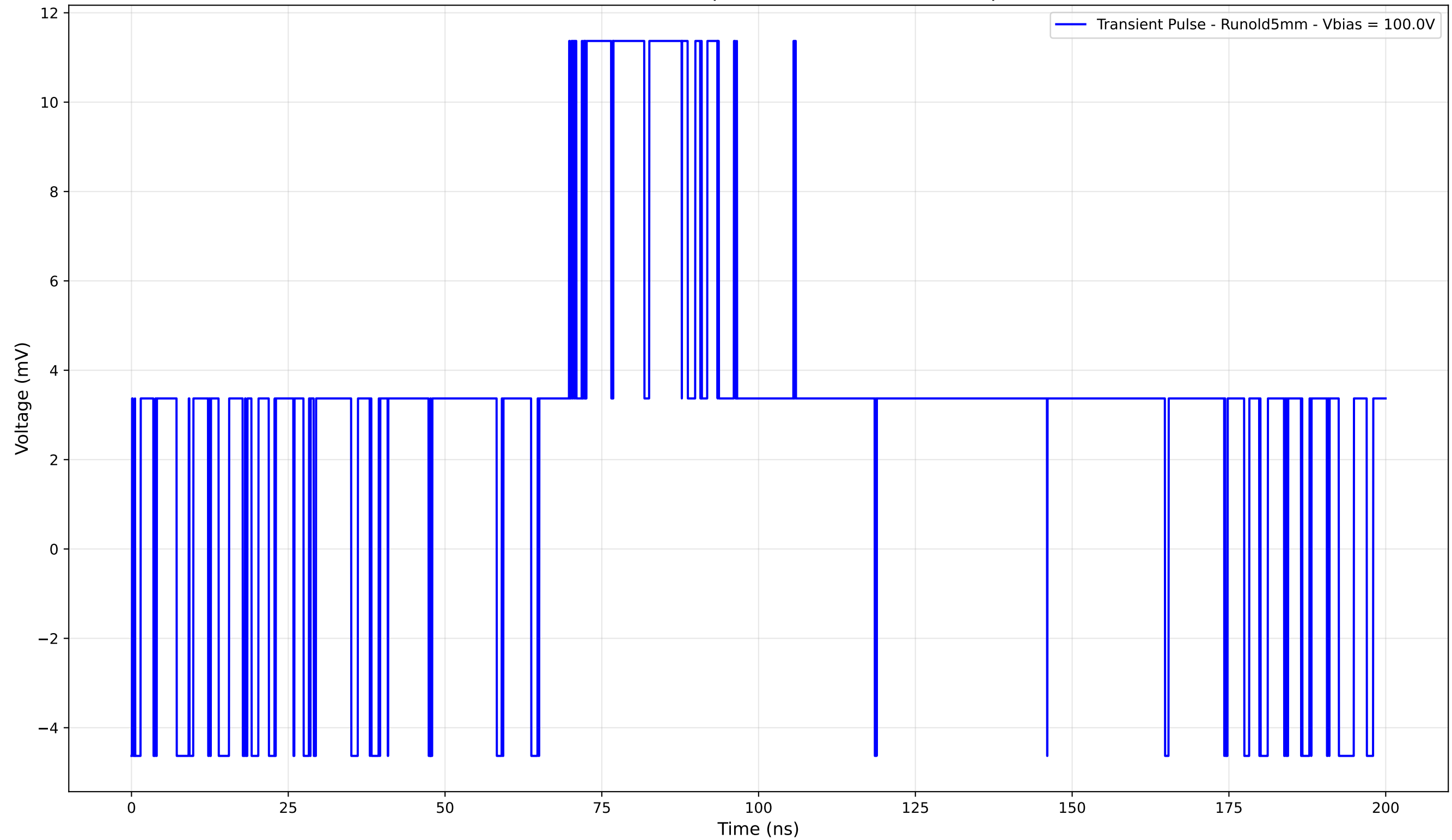
Transient Pulse - Sample: old5 - Position: 1405.0 \mu\text{m}
