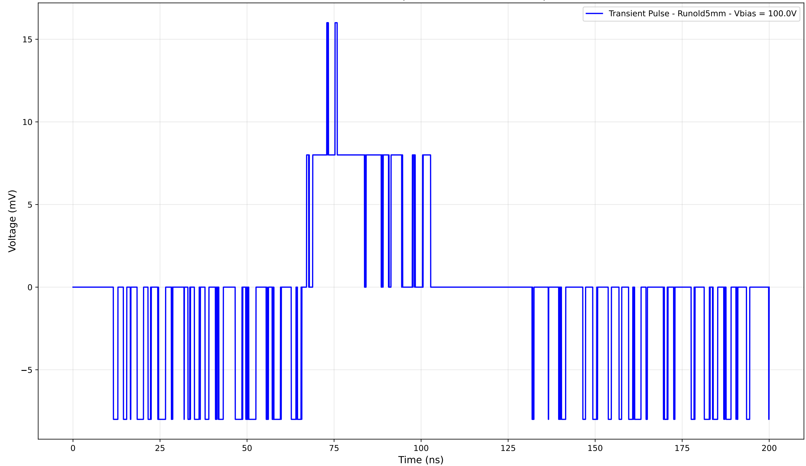
Transient Pulse - Sample: old5 - Position: 70.0 \mu\text{m}
