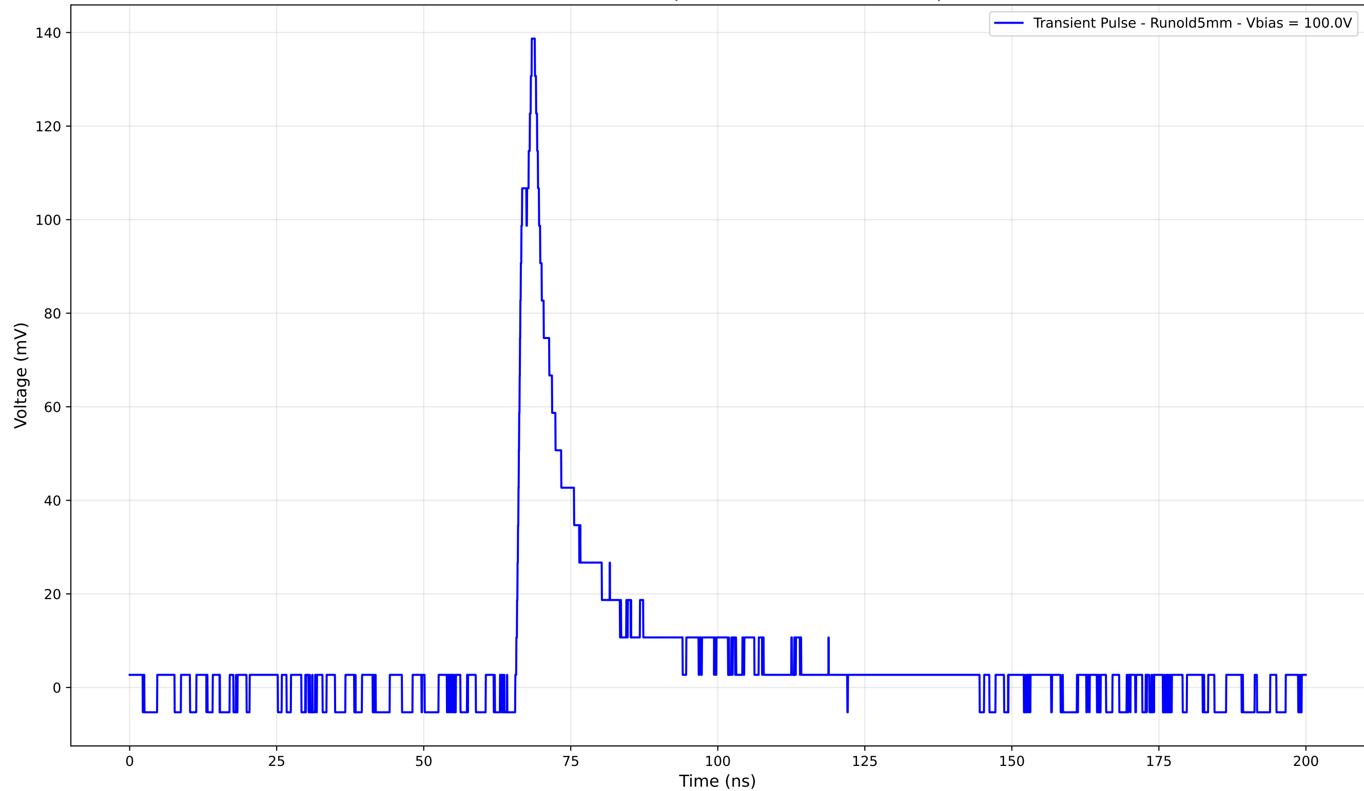
Transient Pulse - Sample: old5 - Position: 2910.0 \mu\text{m}
