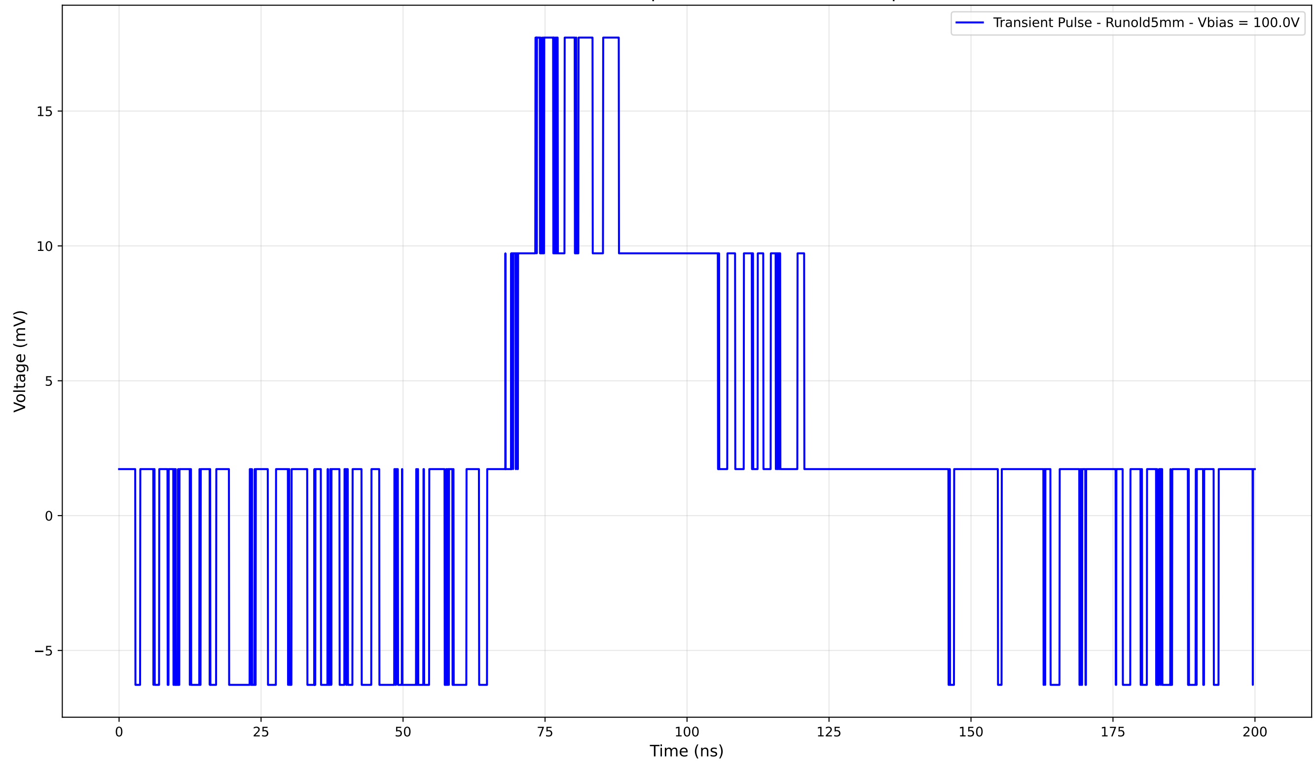
Transient Pulse - Sample: old5 - Position: 545.0 \mu\text{m}
