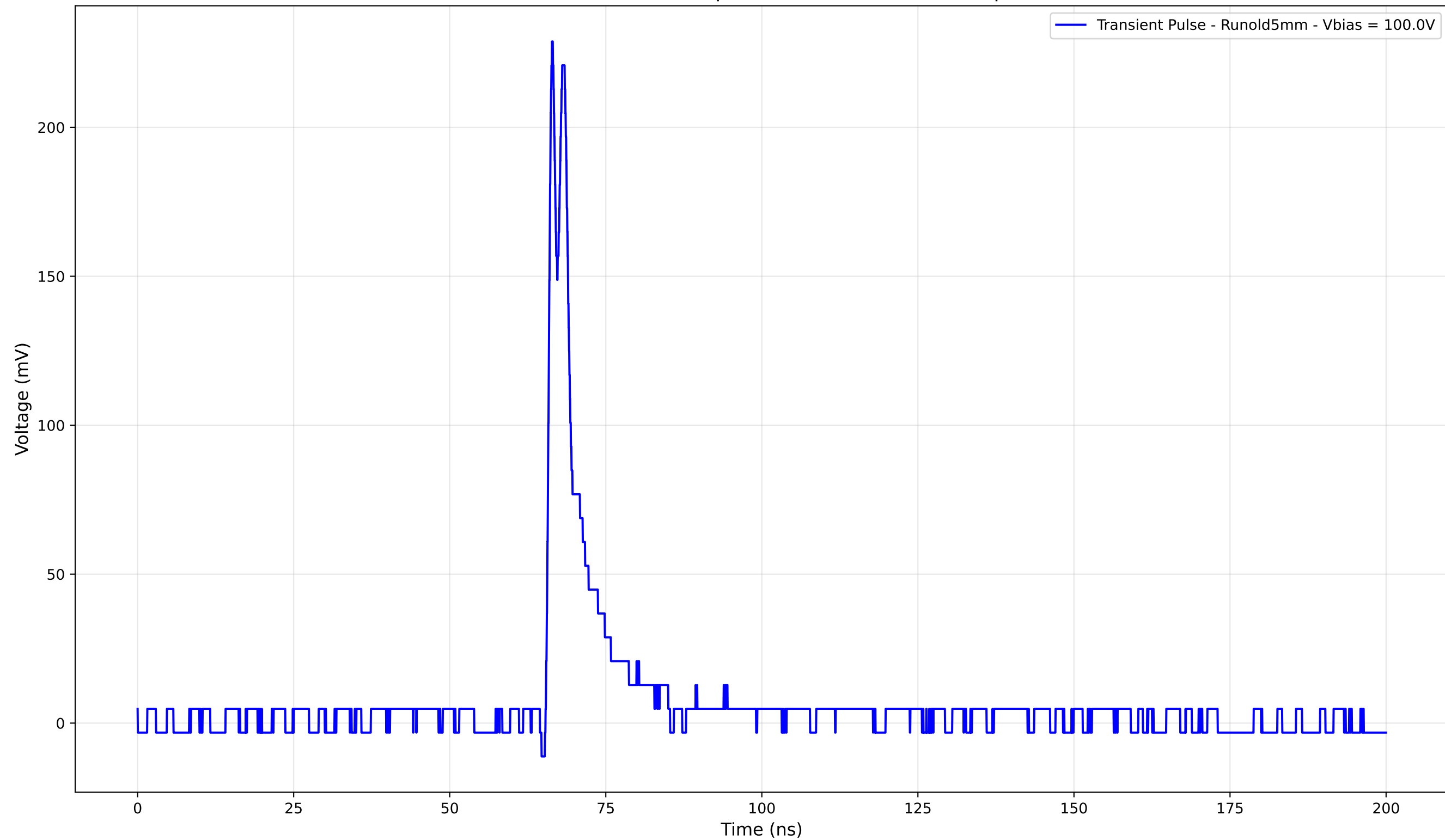
Transient Pulse - Sample: old5 - Position: 3470.0 \mu\text{m}
