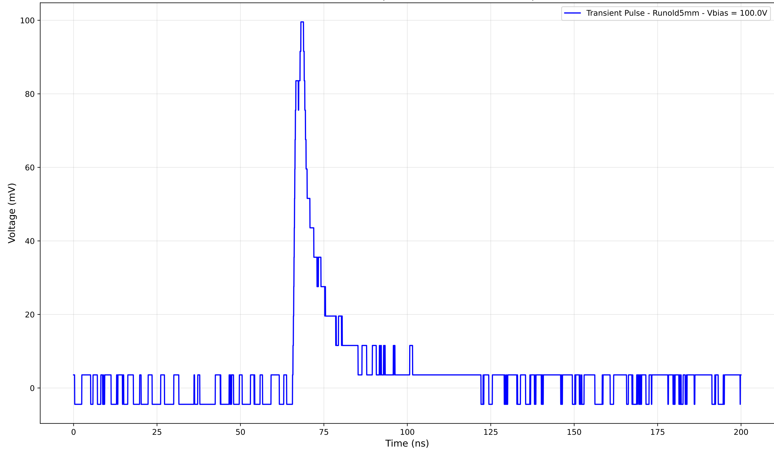
Transient Pulse - Sample: old5 - Position: 2985.0 \mu\text{m}
