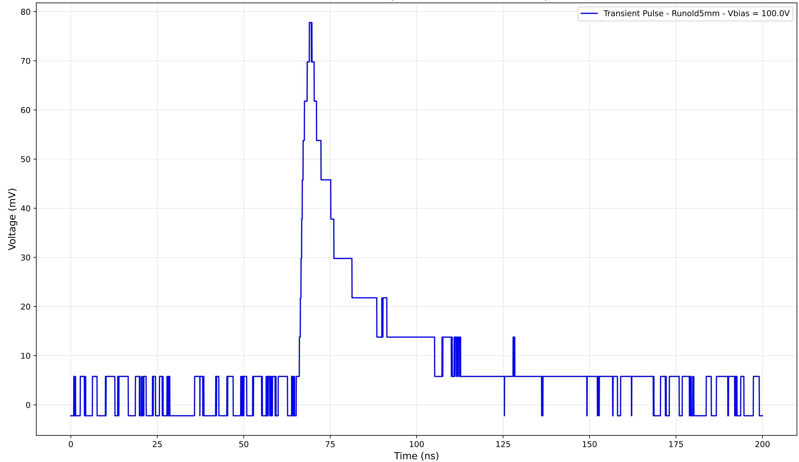
Transient Pulse - Sample: old5 - Position: 4180.0 \mu\text{m}
