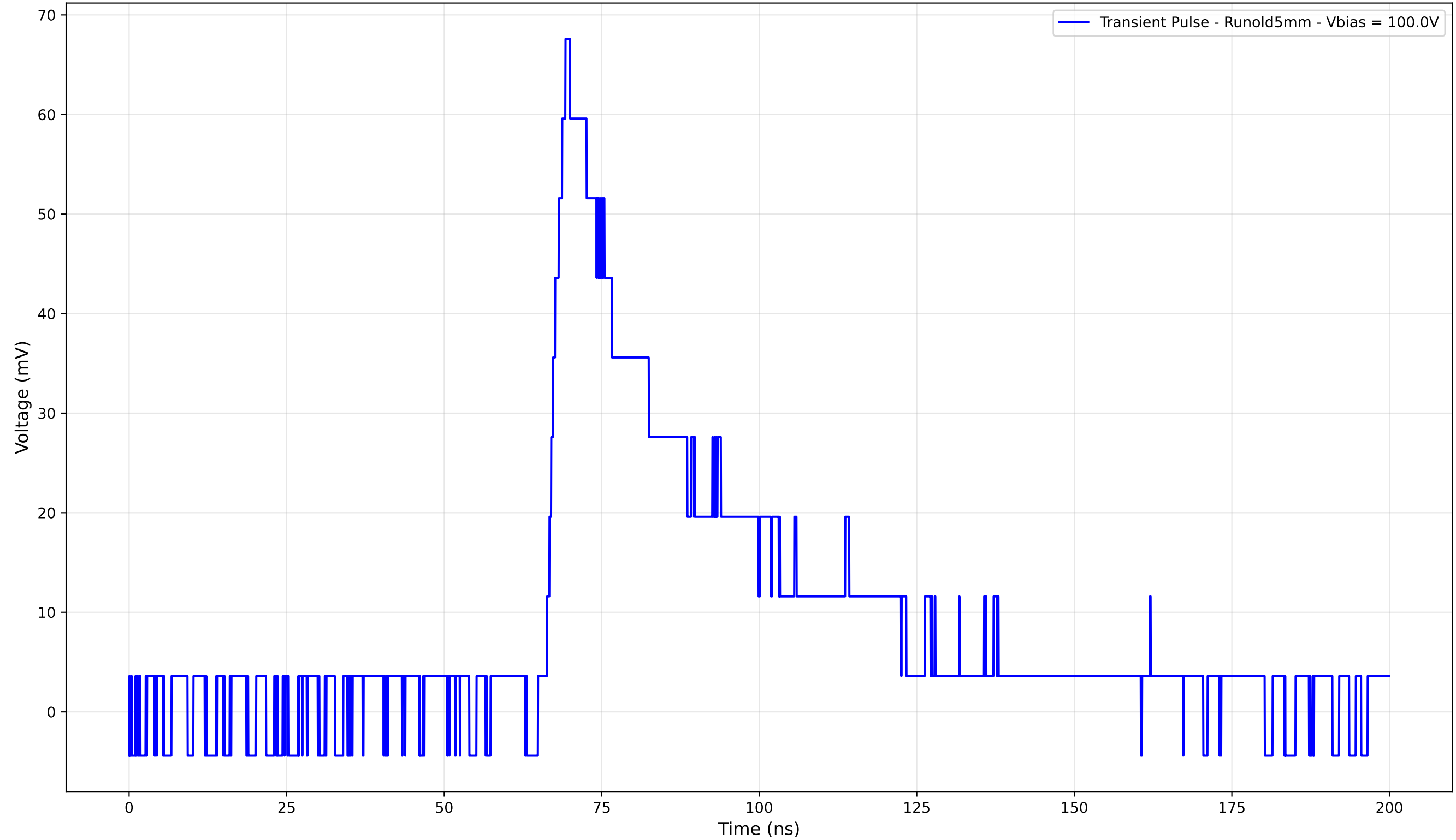
Transient Pulse - Sample: old5 - Position: 4470.0 \mu\text{m}
