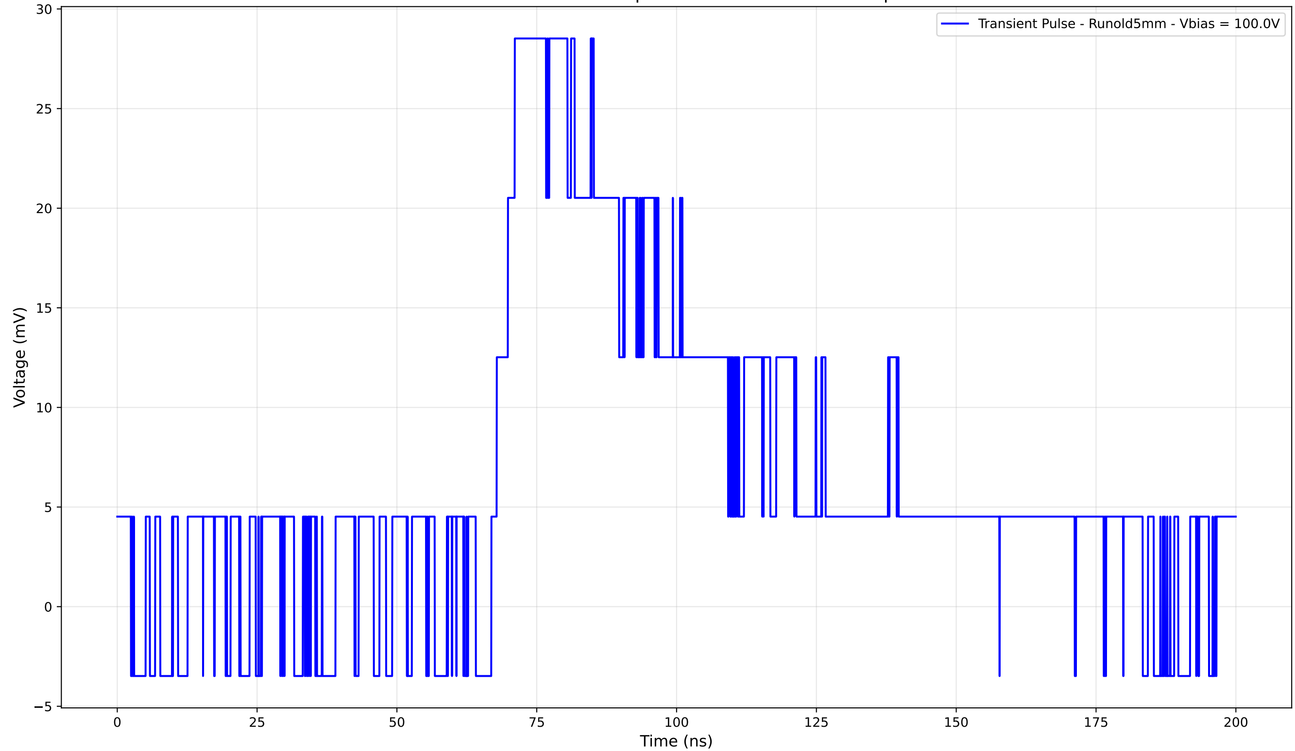
Transient Pulse - Sample: old5 - Position: 1685.0 \mu\text{m}
