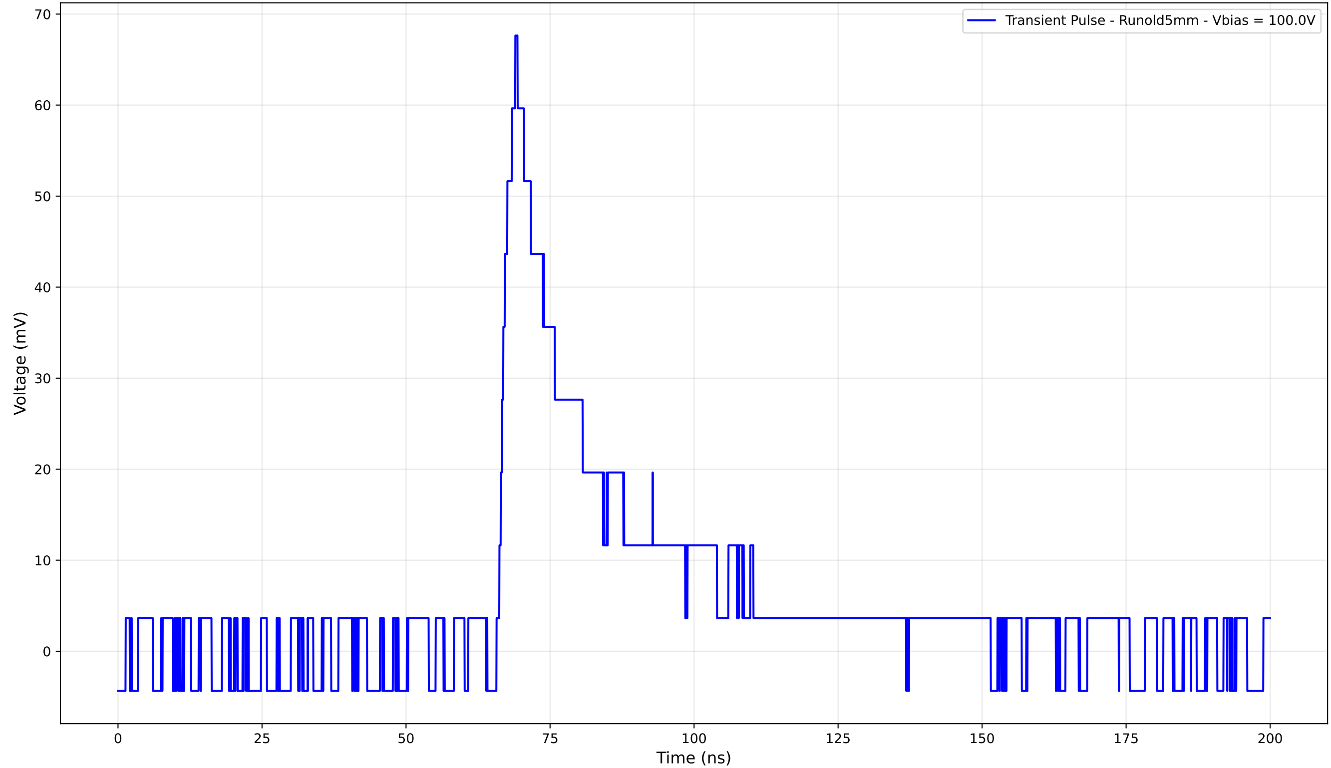
Transient Pulse - Sample: old5 - Position: 2560.0 \mu\text{m}
