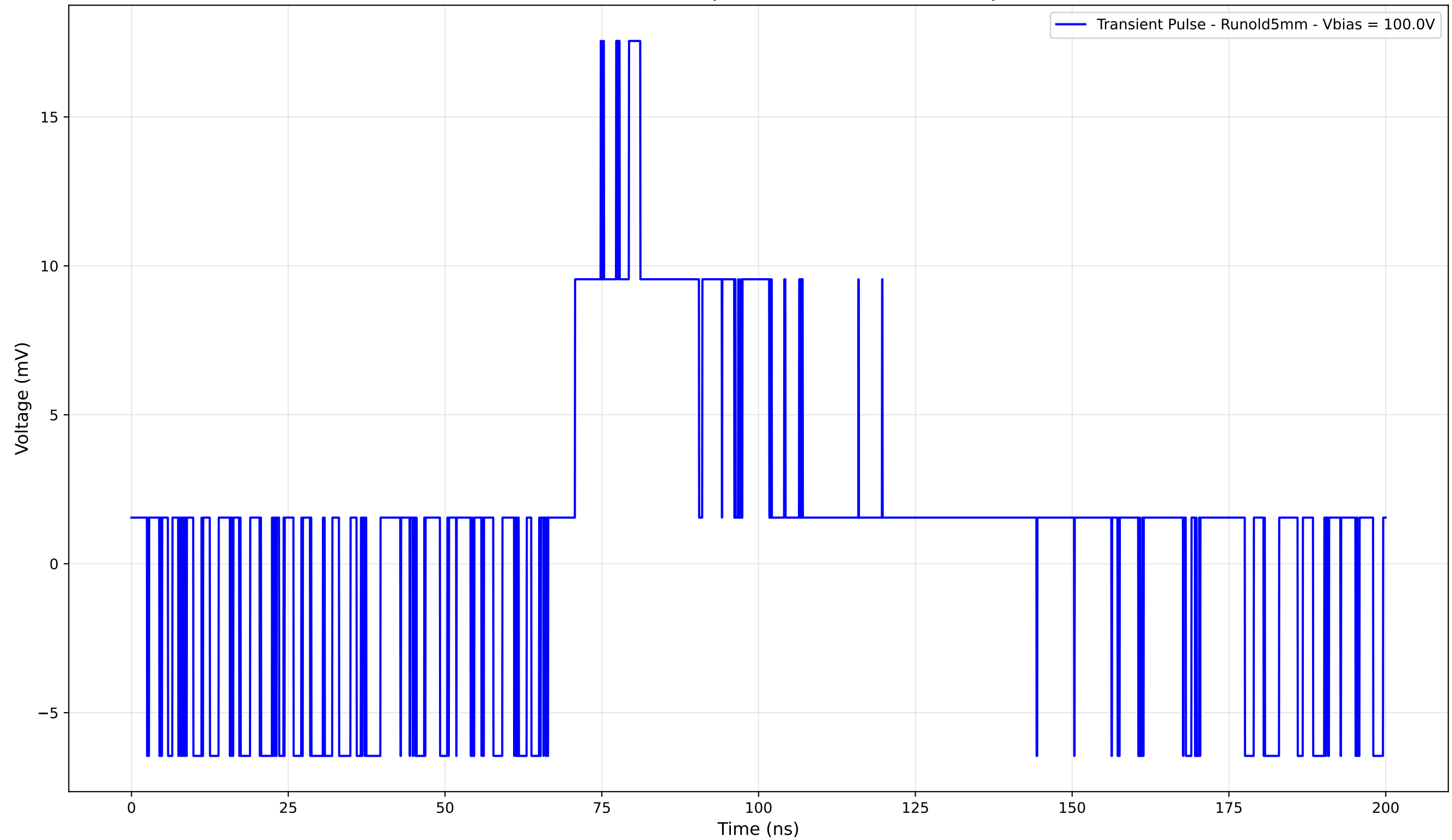
Transient Pulse - Sample: old5 - Position: 1015.0 \mu\text{m}
