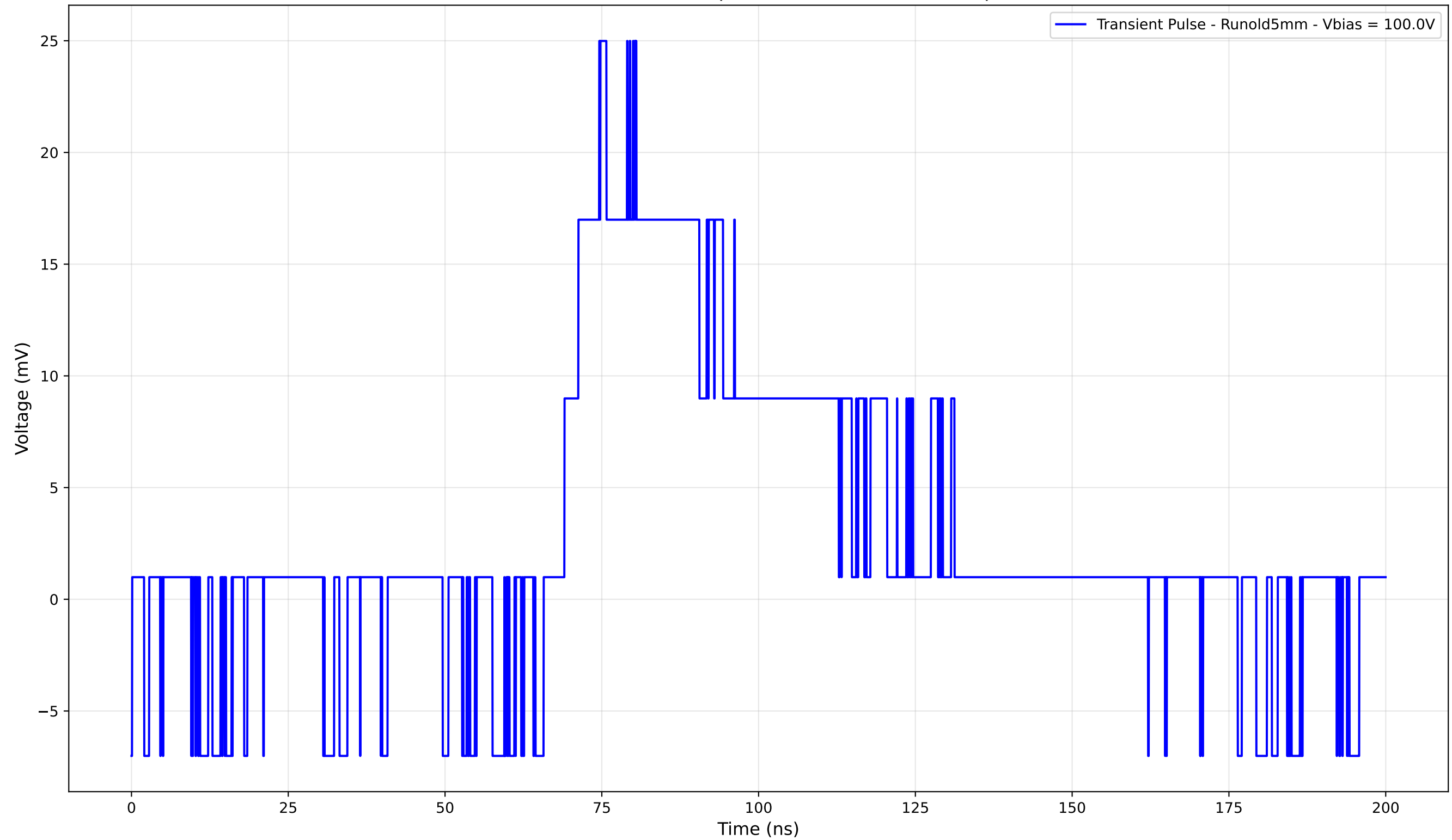
Transient Pulse - Sample: old5 - Position: 890.0 \mu\text{m}
