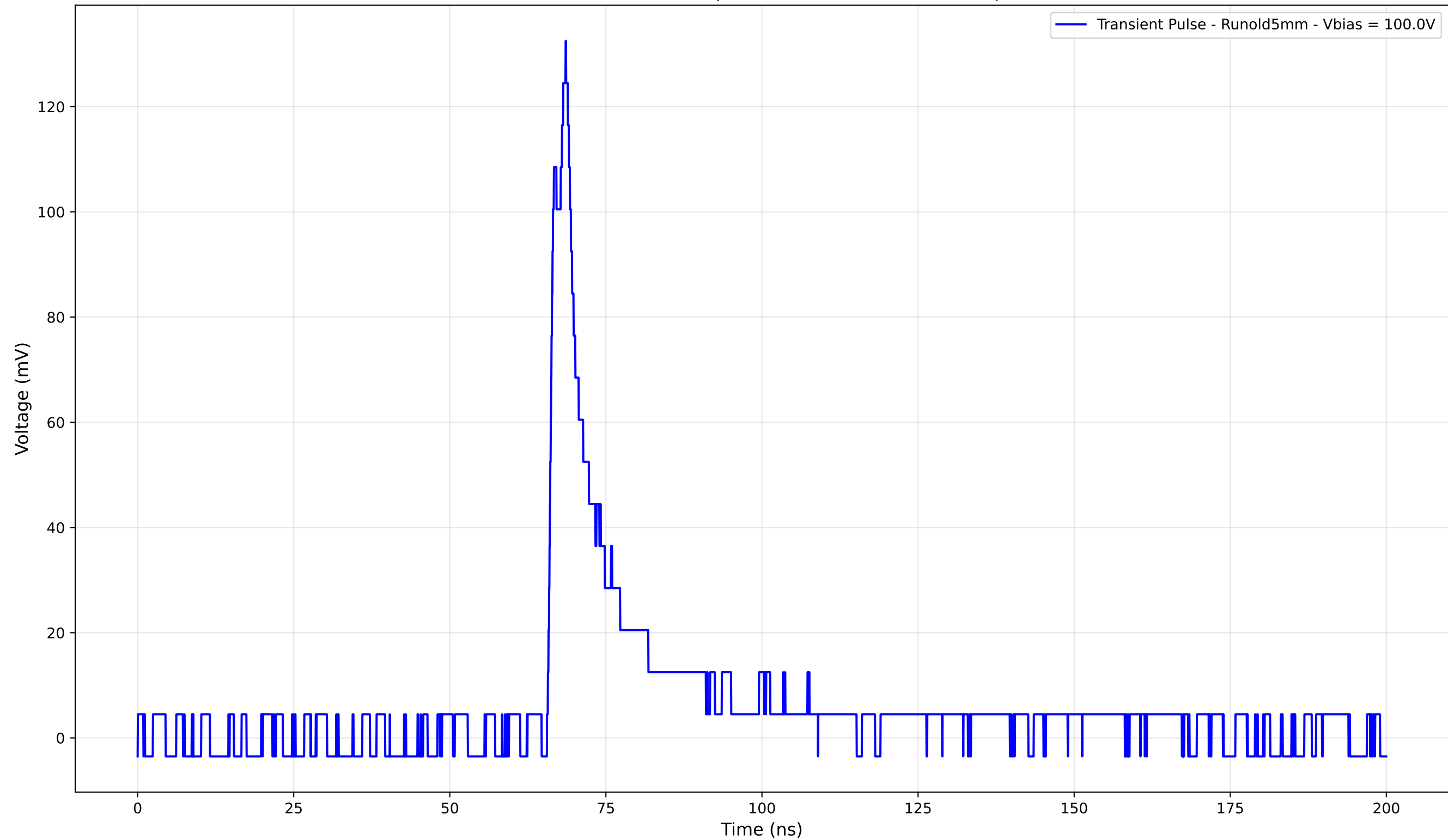
Transient Pulse - Sample: old5 - Position: 2970.0 \mu\text{m}
