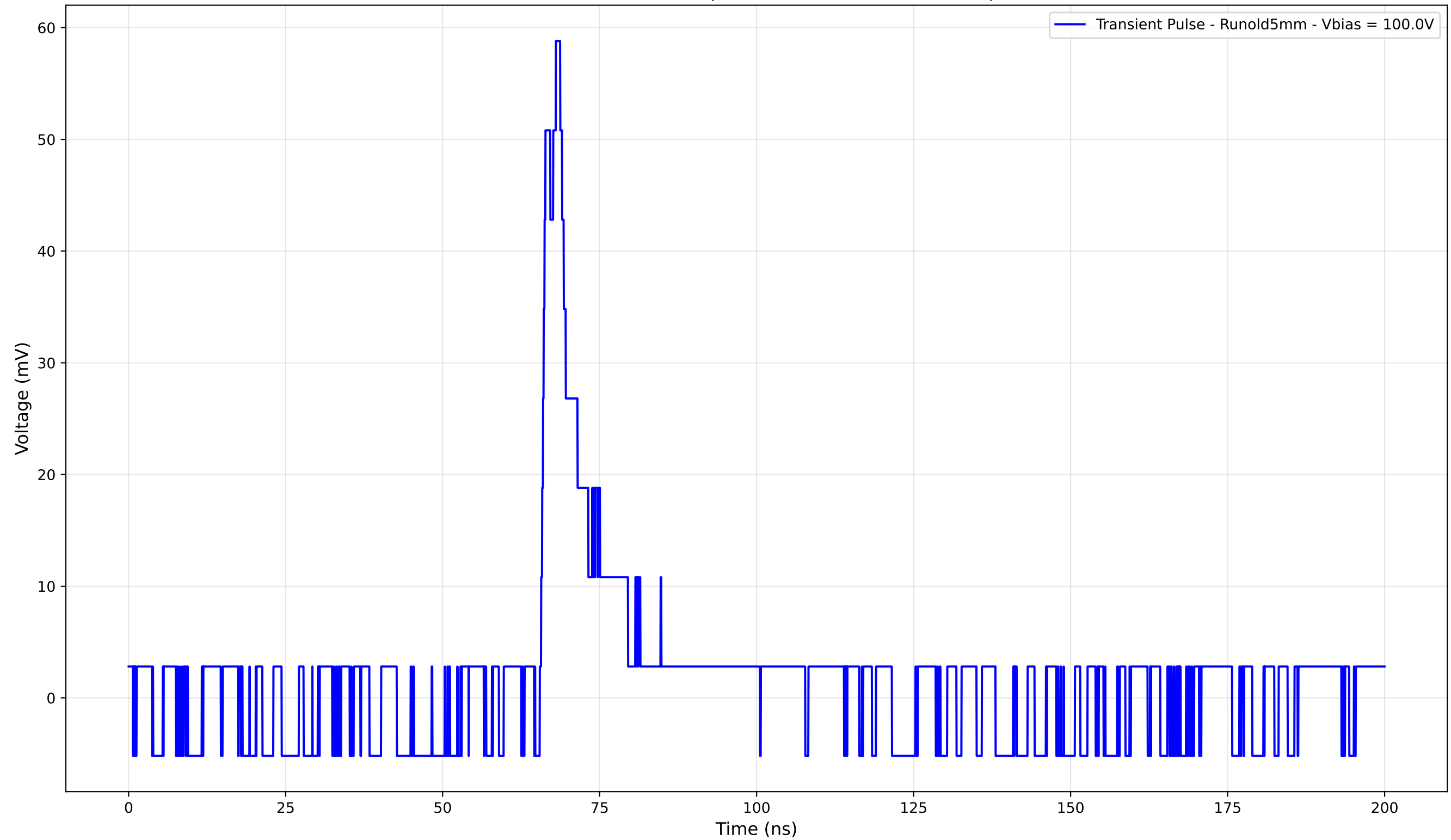
Transient Pulse - Sample: old5 - Position: 3620.0 \mu\text{m}
