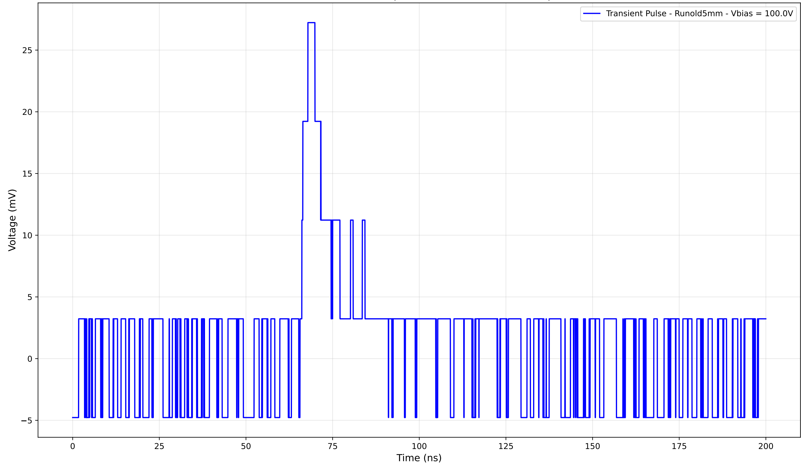
Transient Pulse - Sample: old5 - Position: 3920.0 \mu\text{m}
