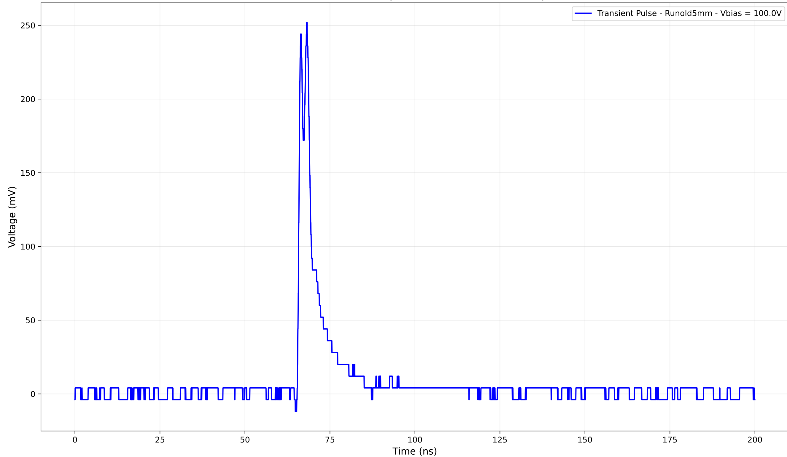
Transient Pulse - Sample: old5 - Position: 3490.0 \mu\text{m}
