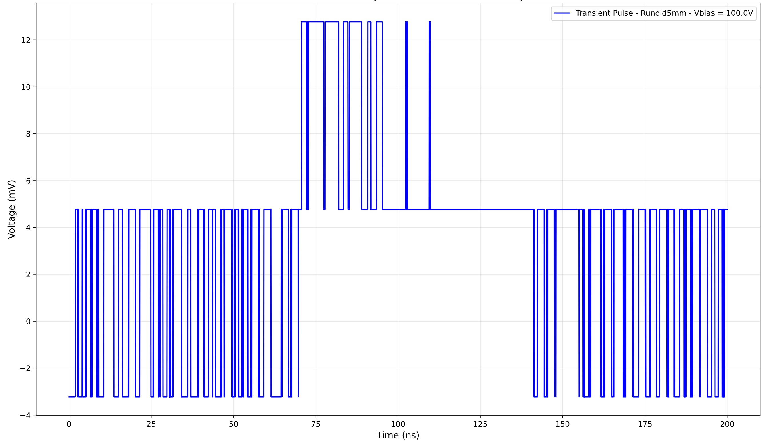
Transient Pulse - Sample: old5 - Position: 1335.0 \mu\text{m}
