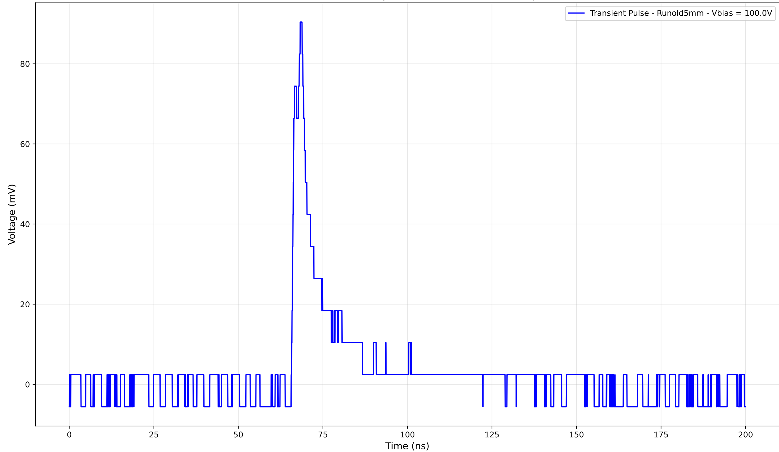
Transient Pulse - Sample: old5 - Position: 2990.0 \mu\text{m}
