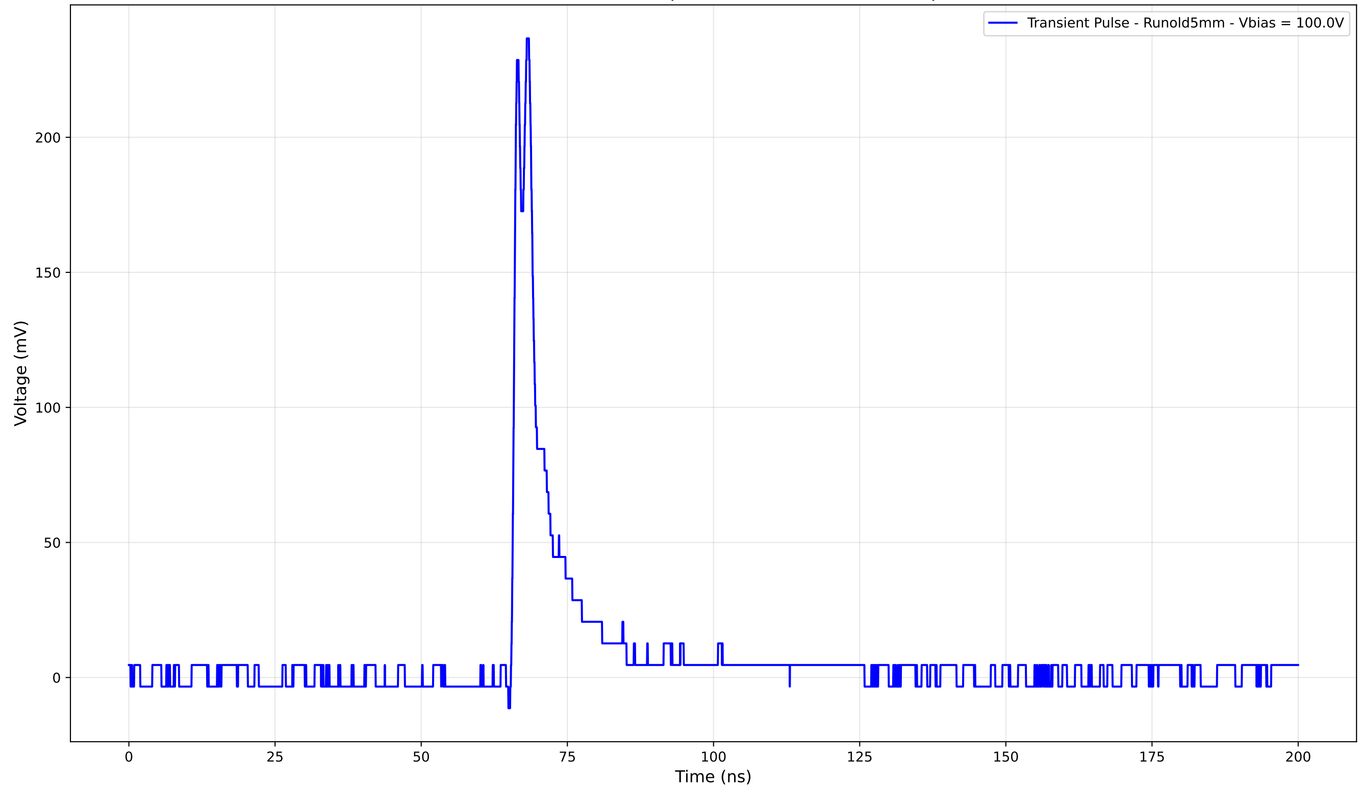
Transient Pulse - Sample: old5 - Position: 3510.0 \mu\text{m}
