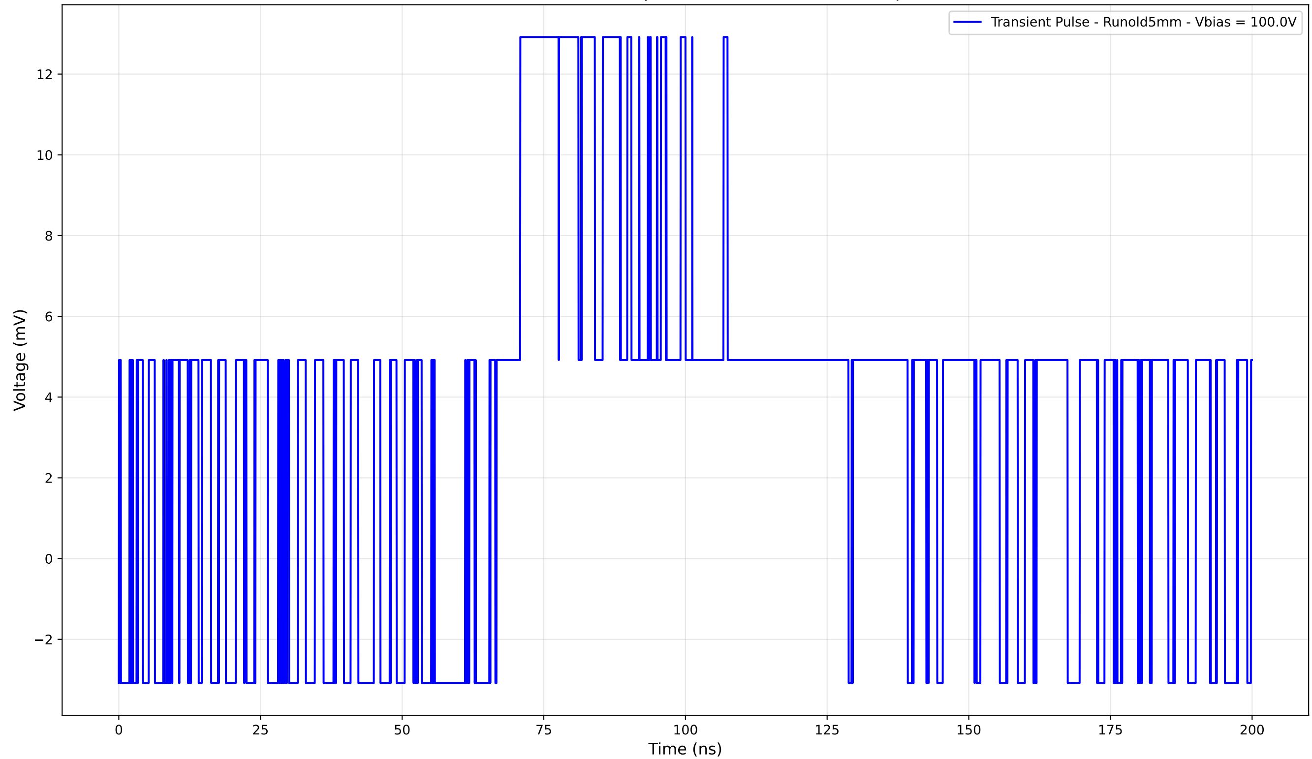
Transient Pulse - Sample: old5 - Position: 1210.0 \mu\text{m}
