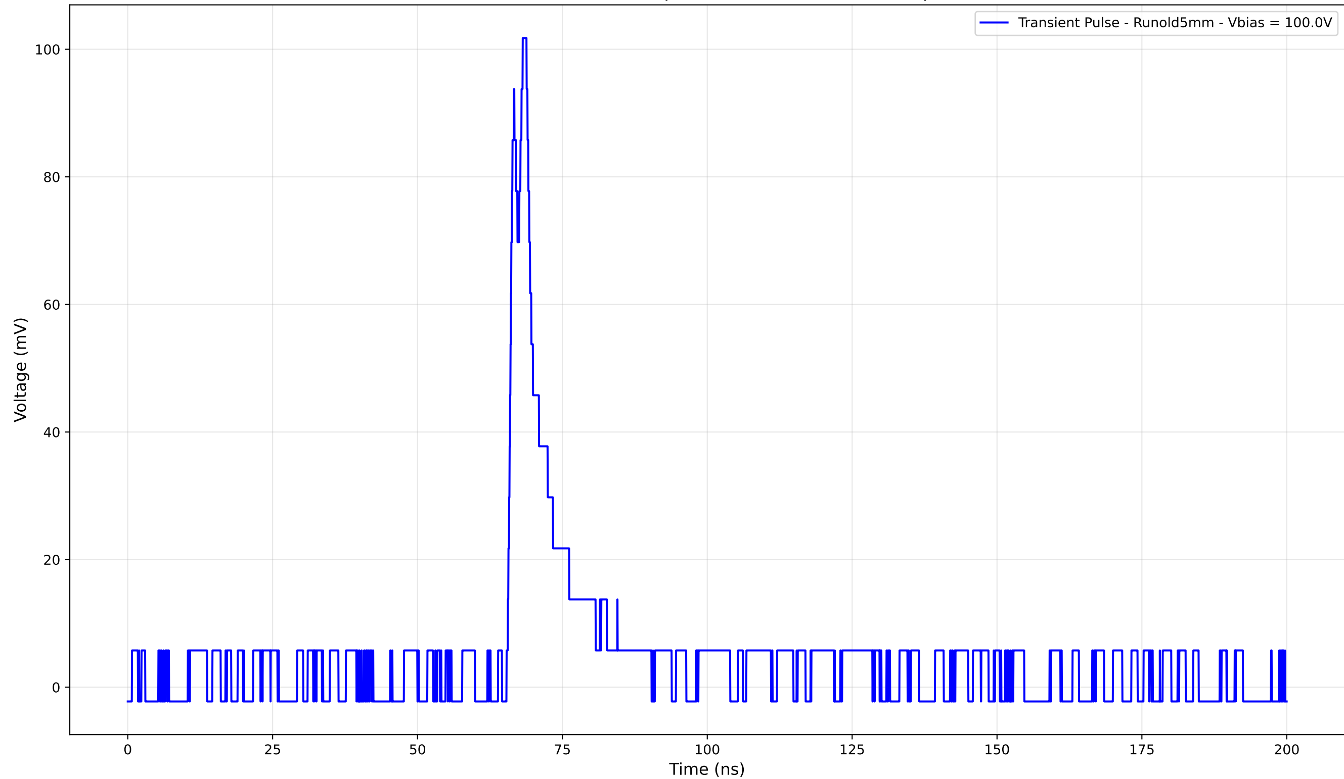
Transient Pulse - Sample: old5 - Position: 3135.0 \mu\text{m}
