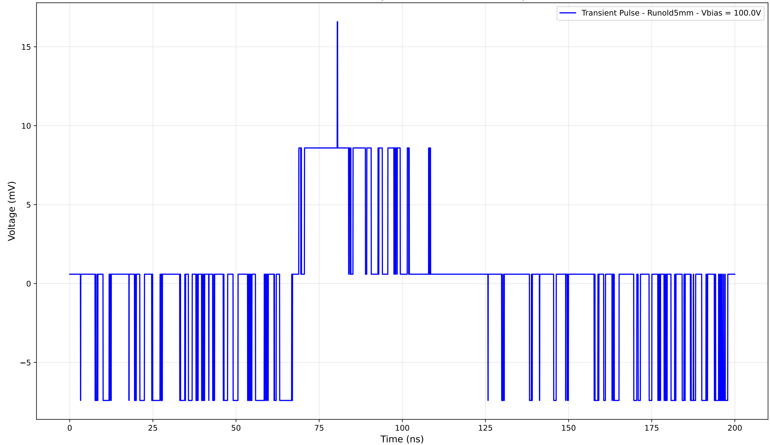
Transient Pulse - Sample: old5 - Position: 370.0 \mu\text{m}
