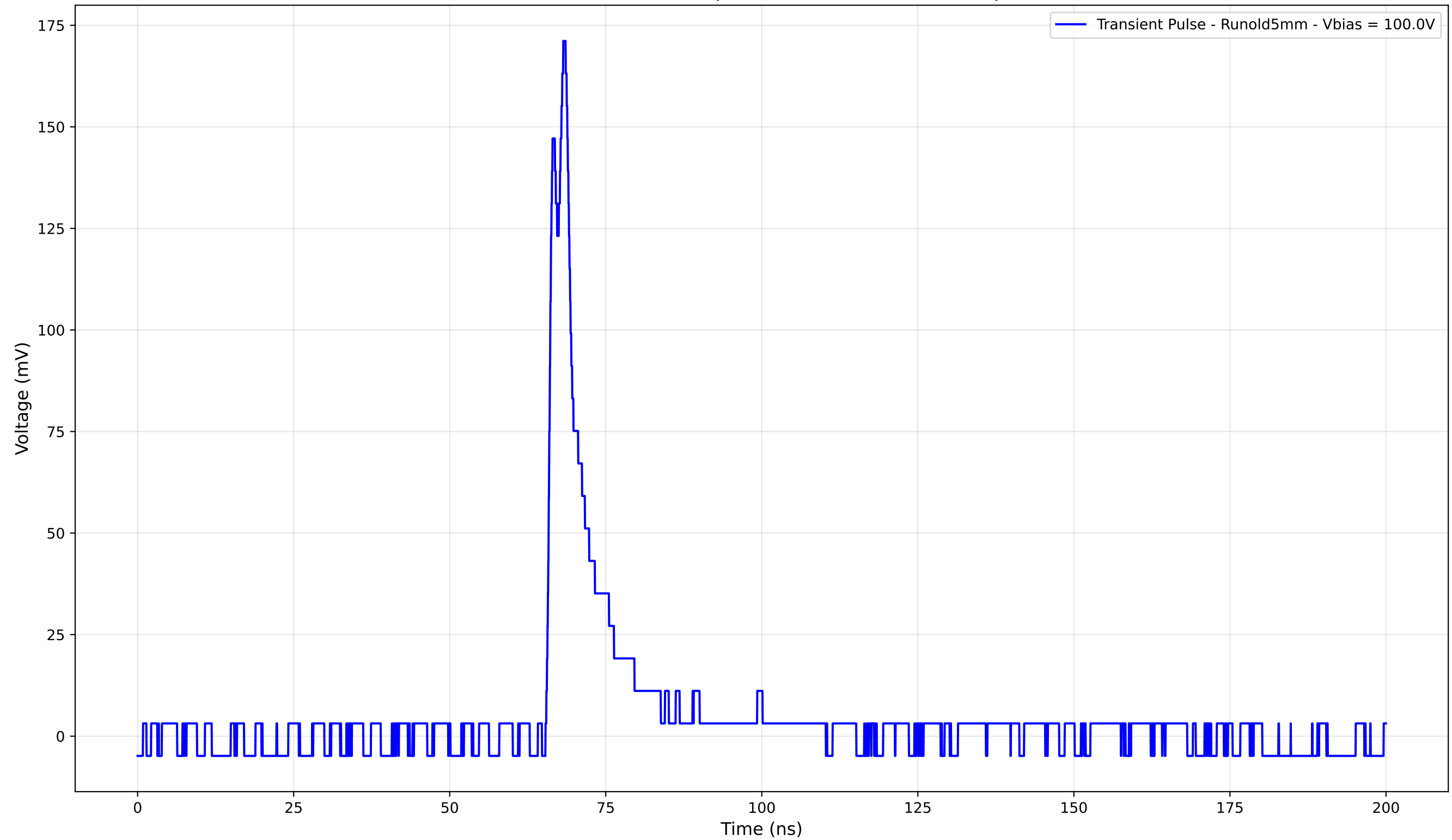
Transient Pulse - Sample: old5 - Position: 3160.0 \mu\text{m}
