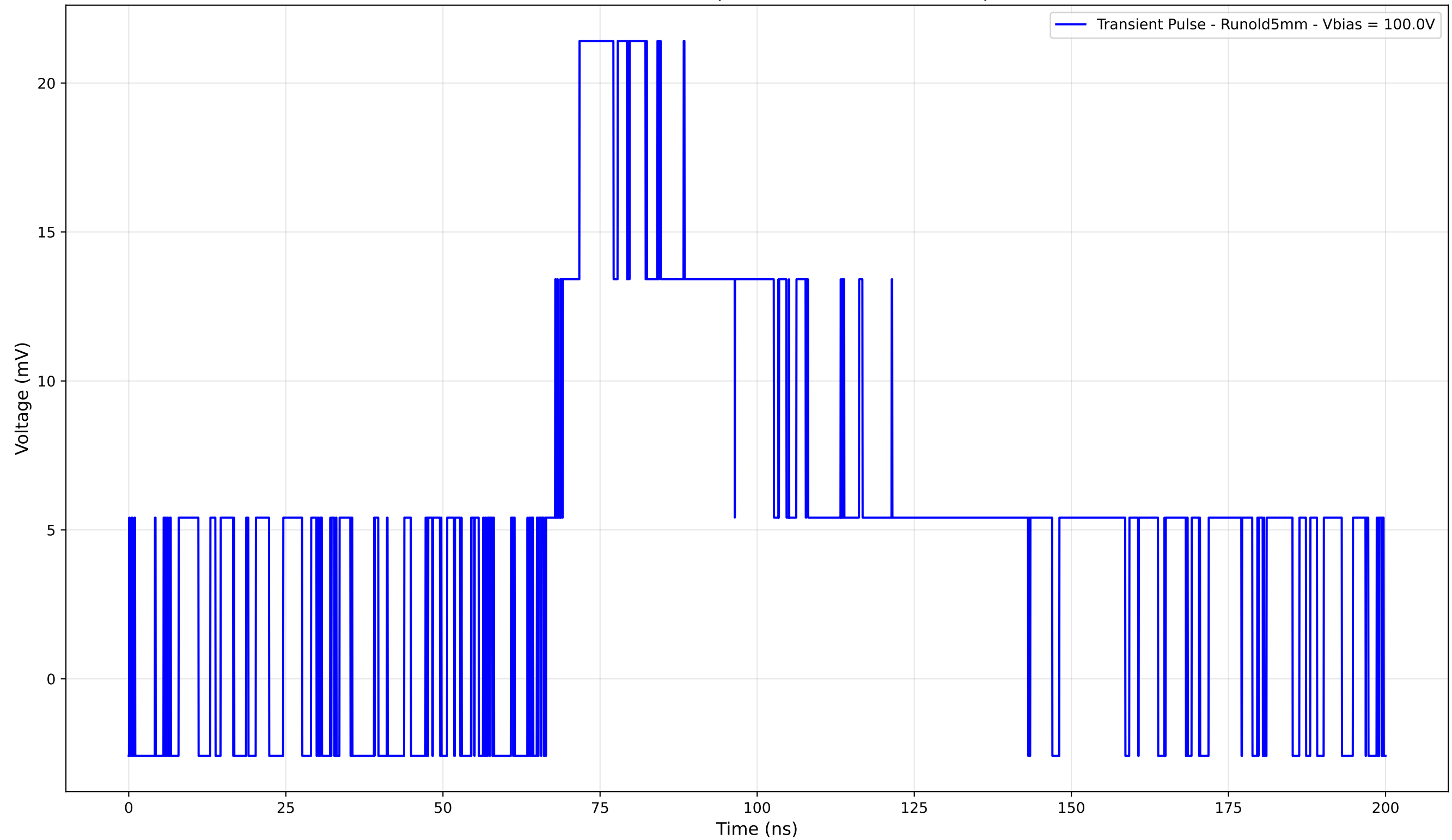
Transient Pulse - Sample: old5 - Position: 445.0 \mu\text{m}
