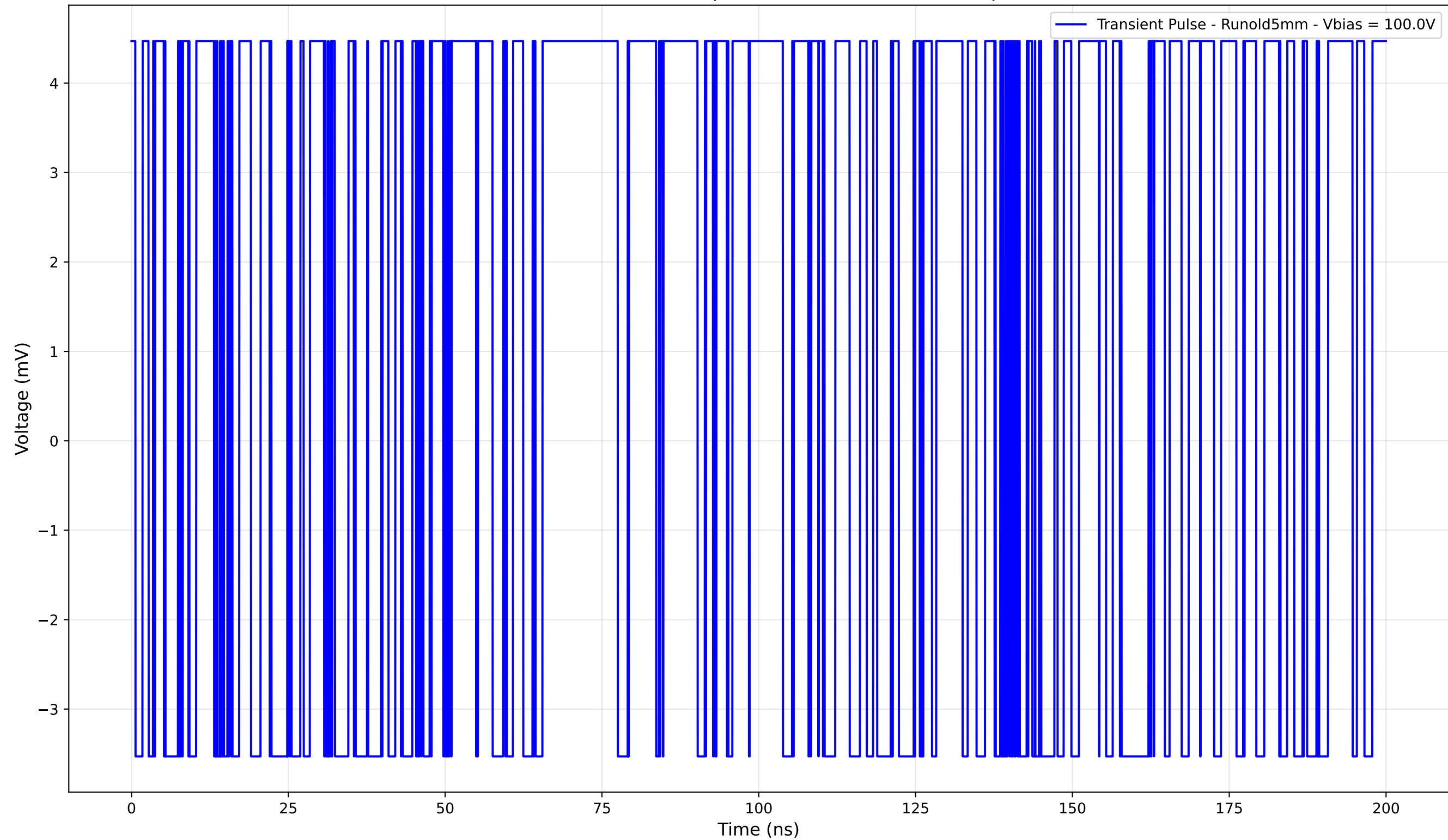
Transient Pulse - Sample: old5 - Position: 2745.0 \mu\text{m}
