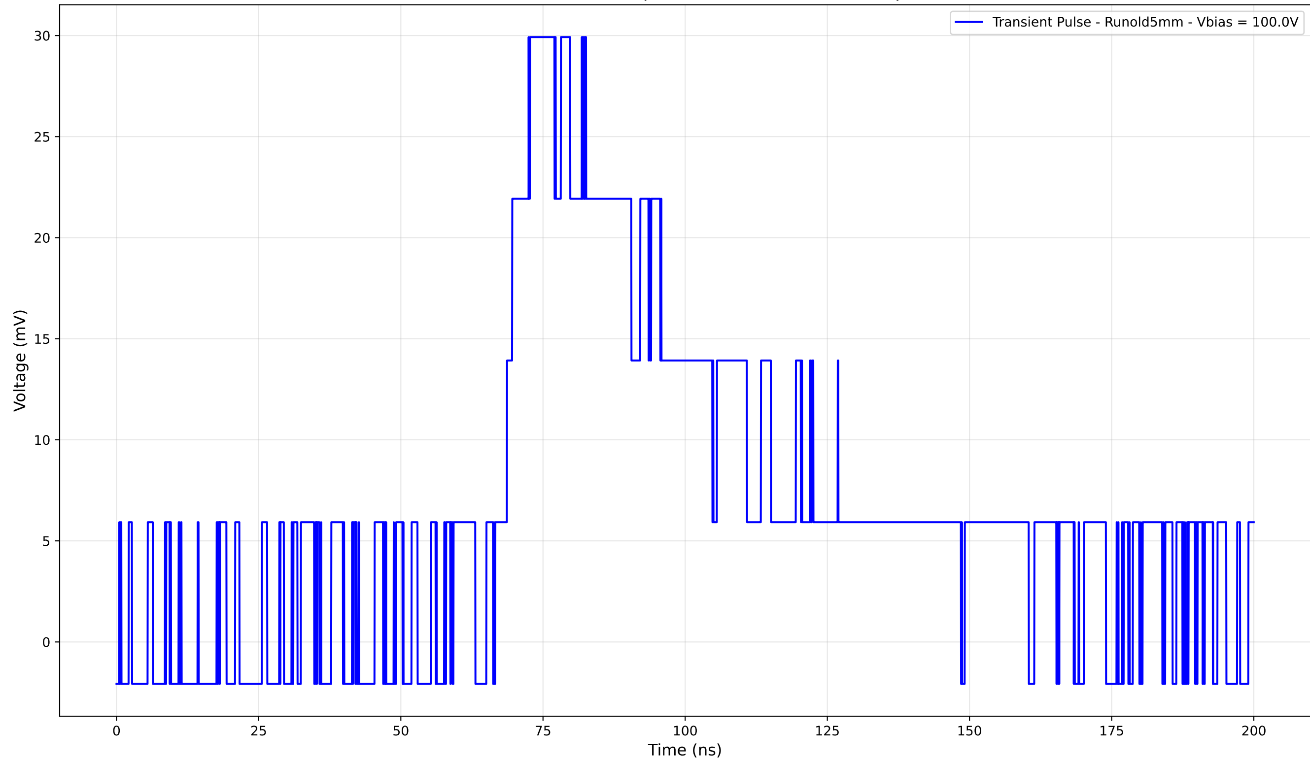
Transient Pulse - Sample: old5 - Position: 1660.0 \mu\text{m}
