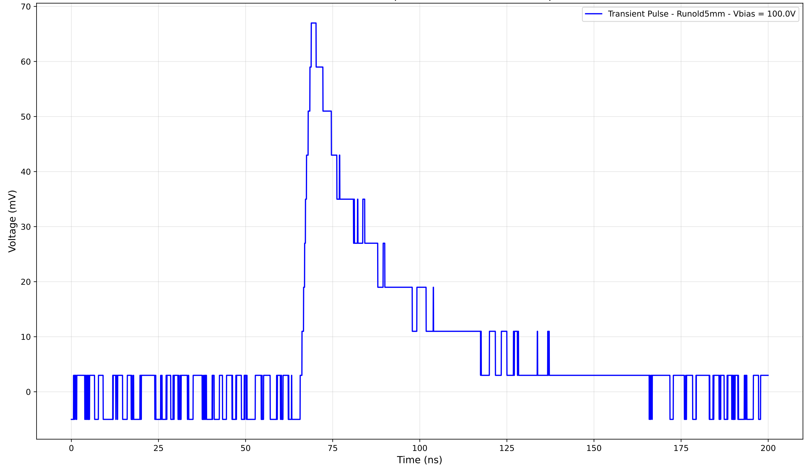
Transient Pulse - Sample: old5 - Position: 4450.0 \mu\text{m}
