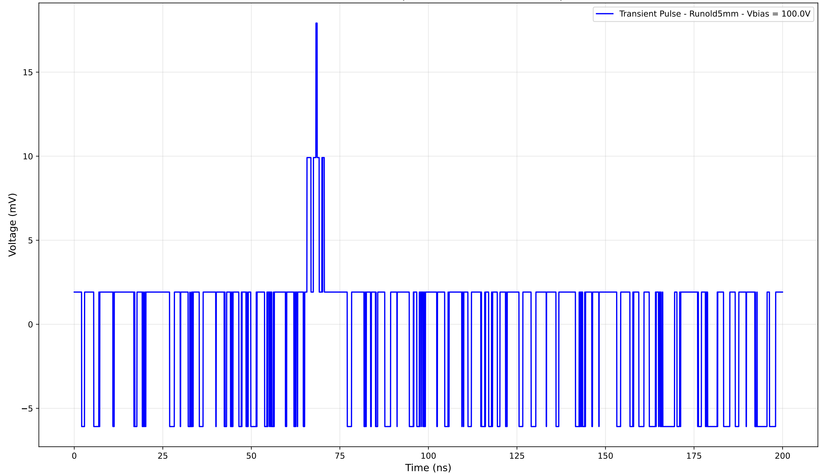
Transient Pulse - Sample: old5 - Position: 3355.0 \mu\text{m}
