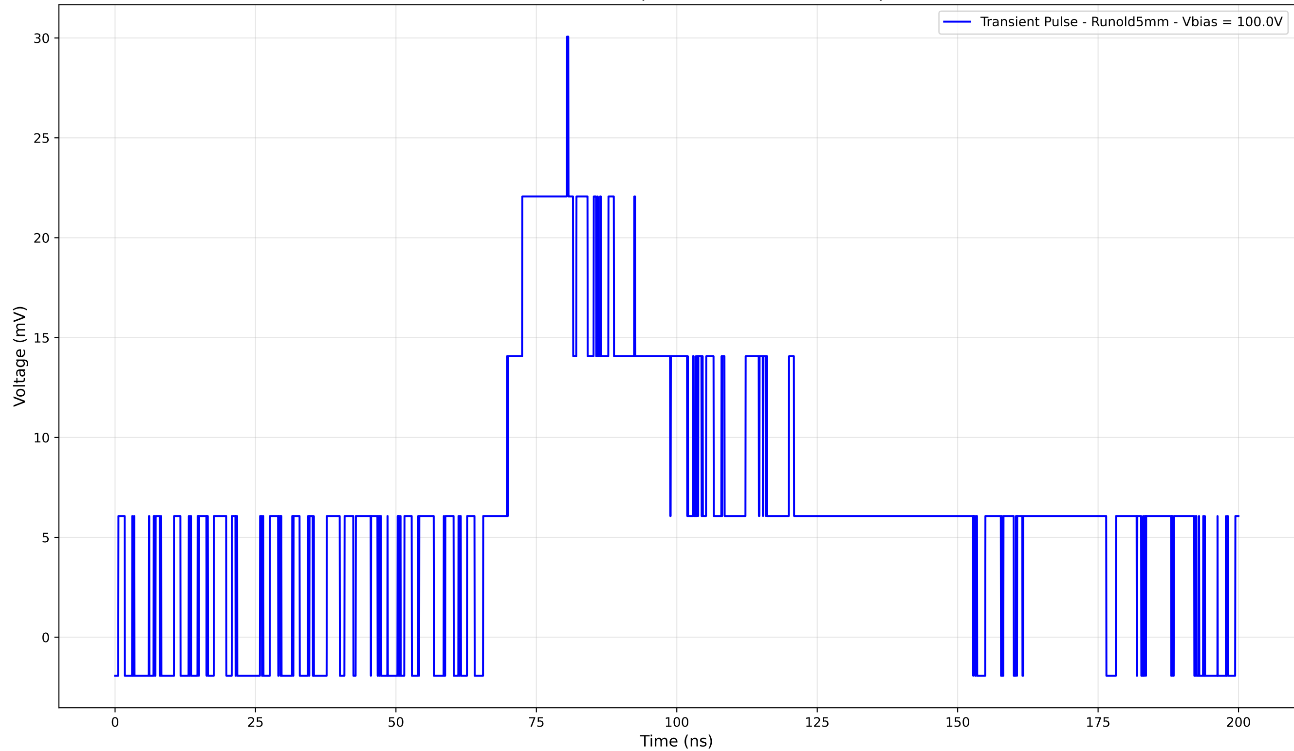
Transient Pulse - Sample: old5 - Position: 825.0 \mu\text{m}
