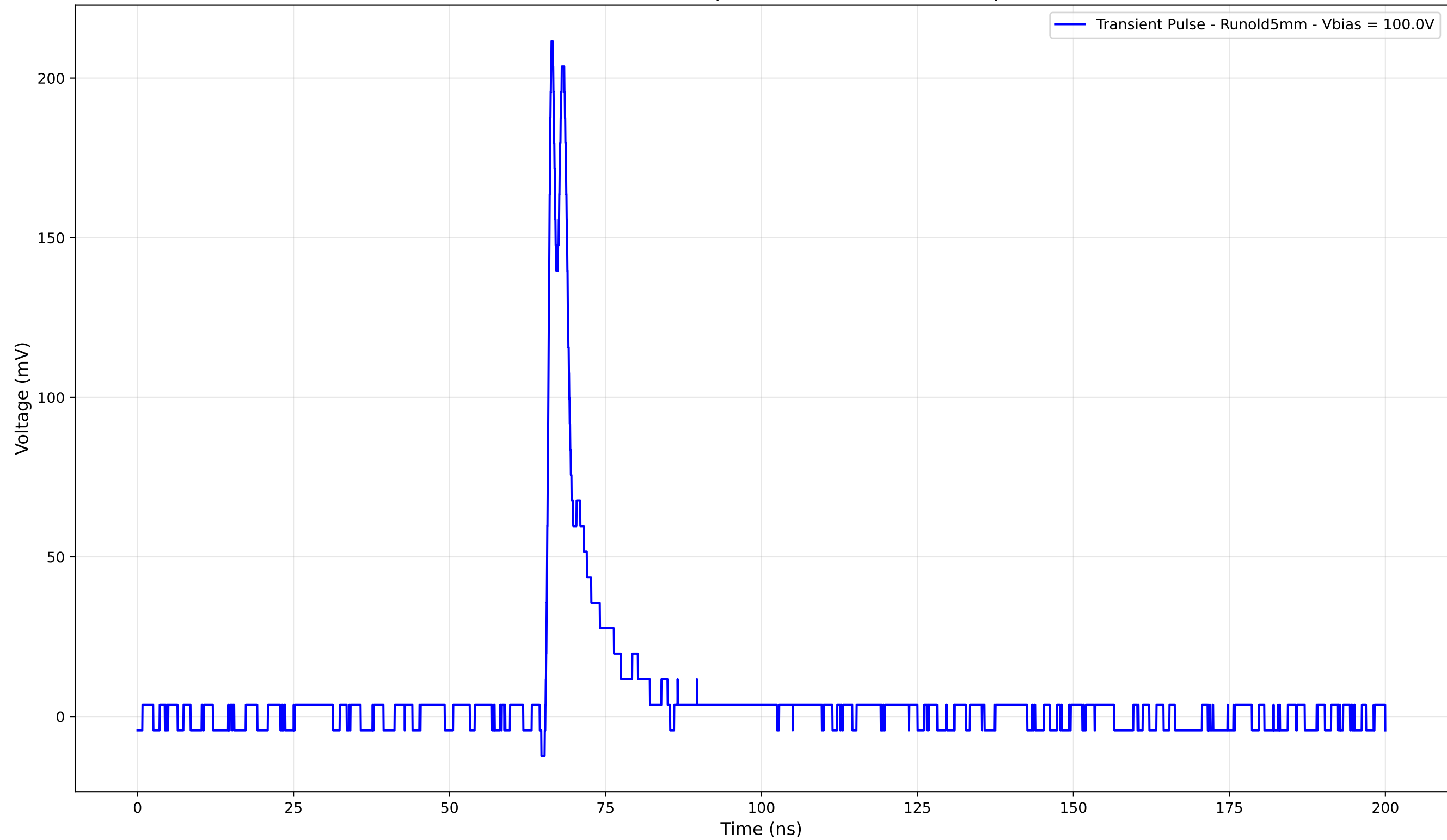
Transient Pulse - Sample: old5 - Position: 3460.0 \mu\text{m}
