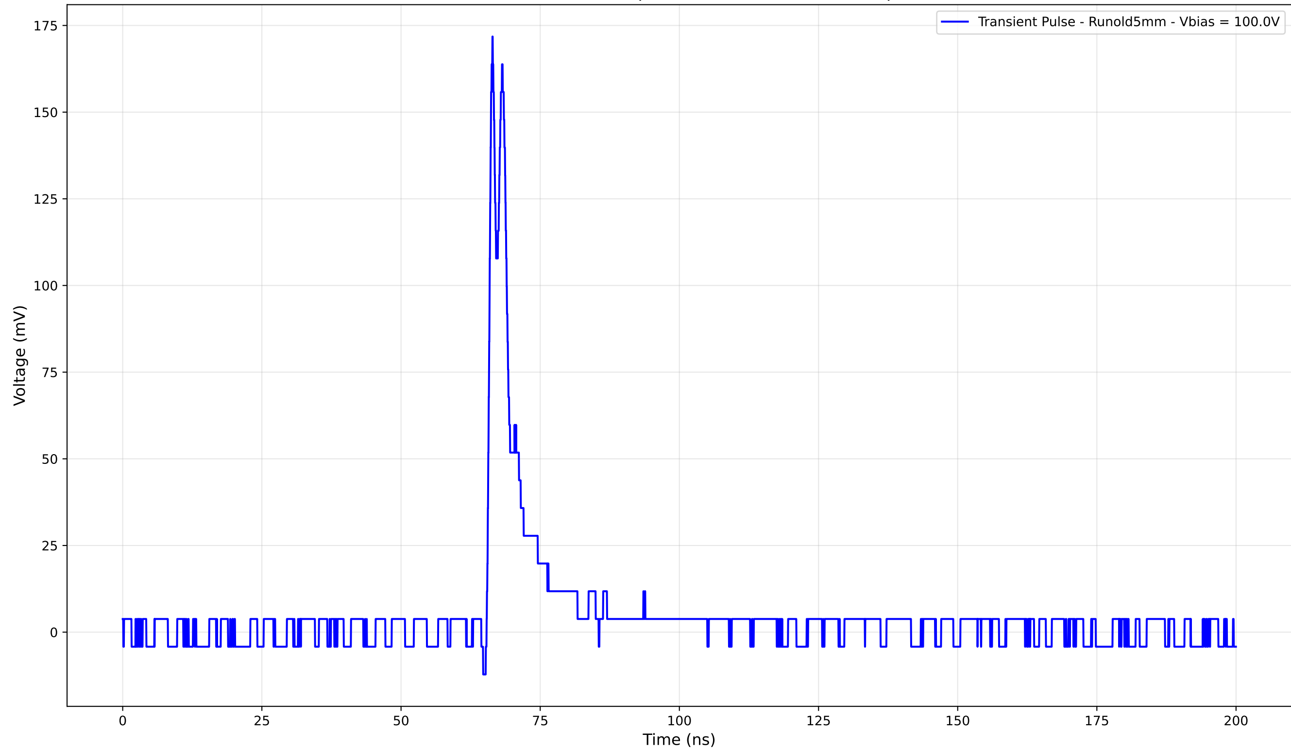
Transient Pulse - Sample: old5 - Position: 3445.0 \mu\text{m}
