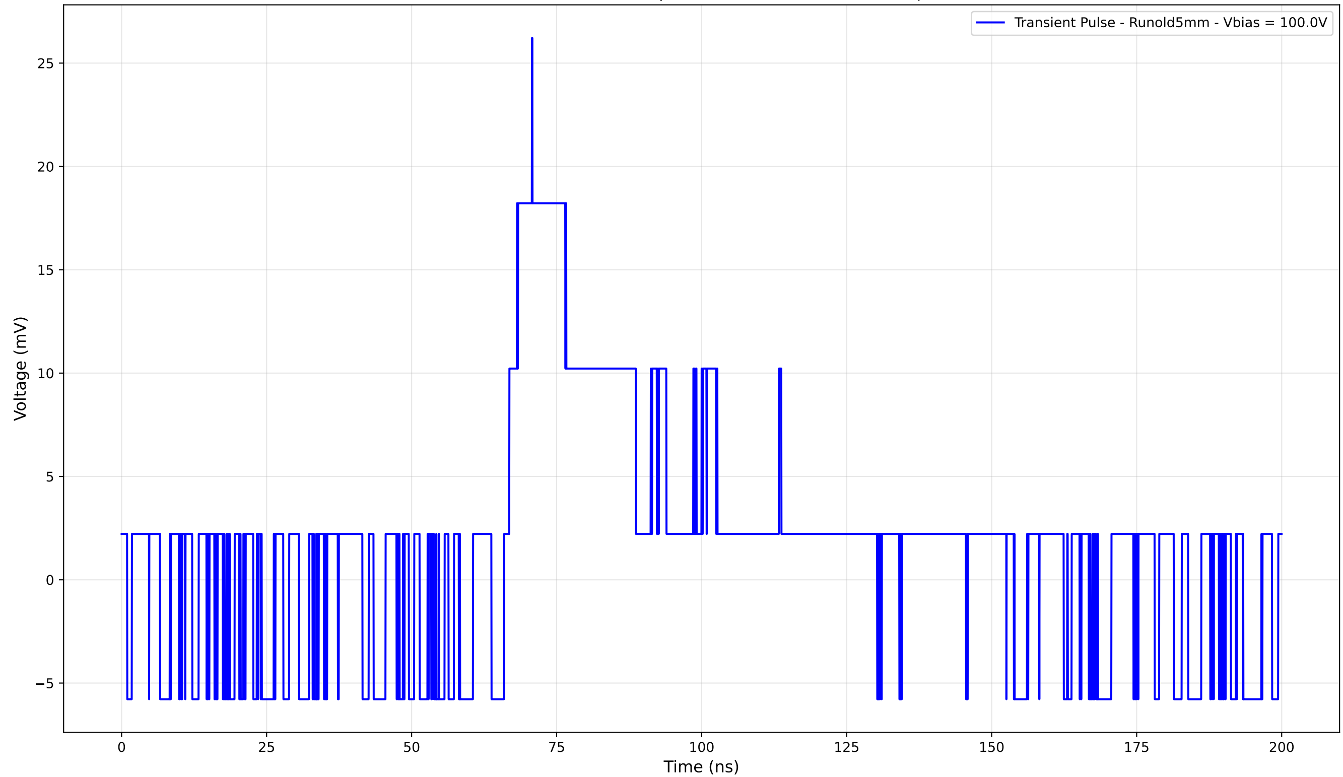
Transient Pulse - Sample: old5 - Position: 2225.0 \mu\text{m}
