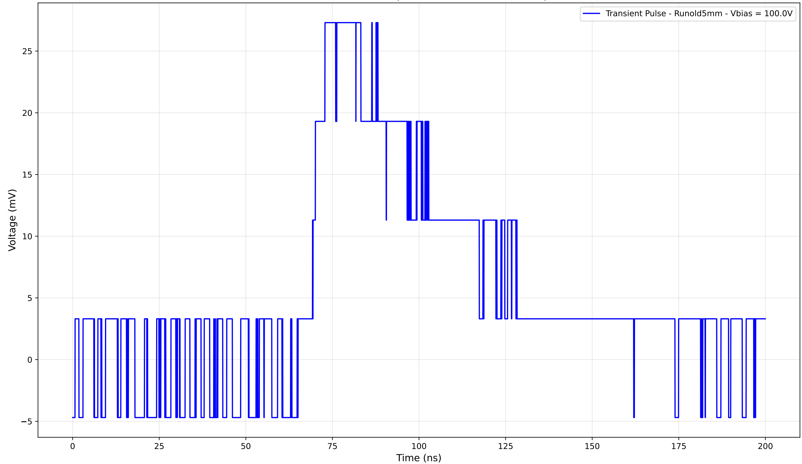
Transient Pulse - Sample: old5 - Position: 860.0 \mu\text{m}
