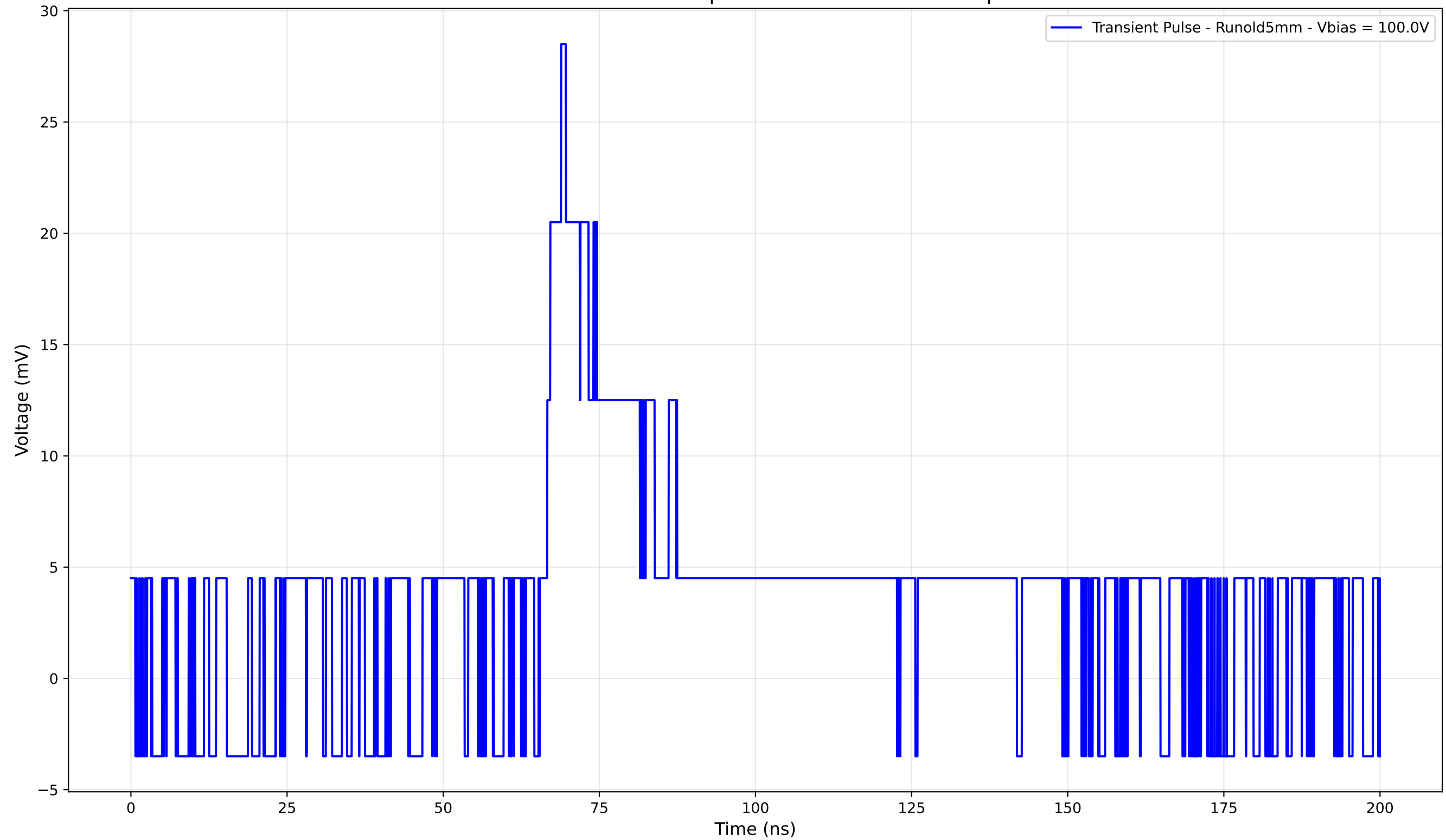
Transient Pulse - Sample: old5 - Position: 4225.0 \mu\text{m}
