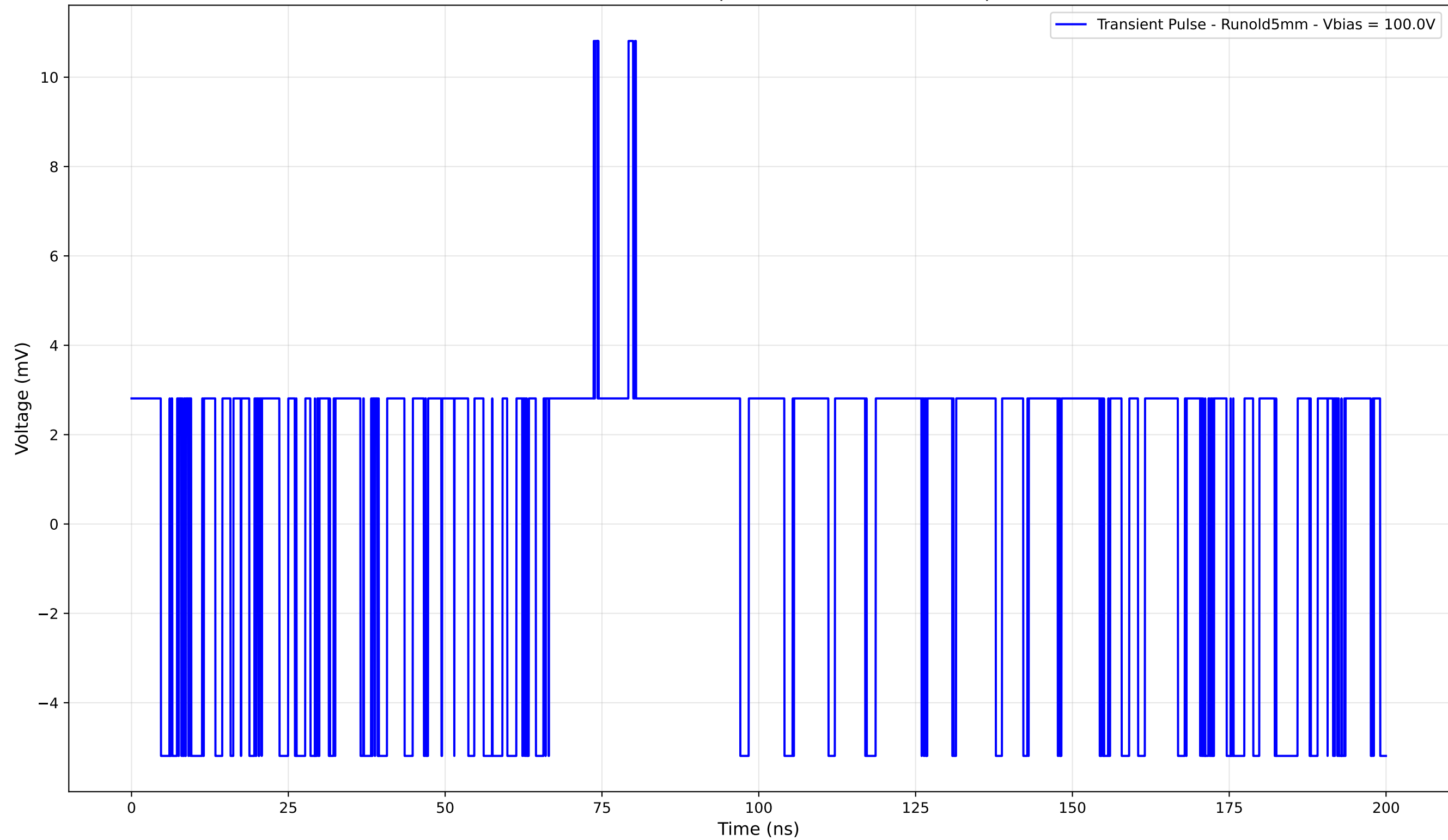
Transient Pulse - Sample: old5 - Position: 985.0 \mu\text{m}
