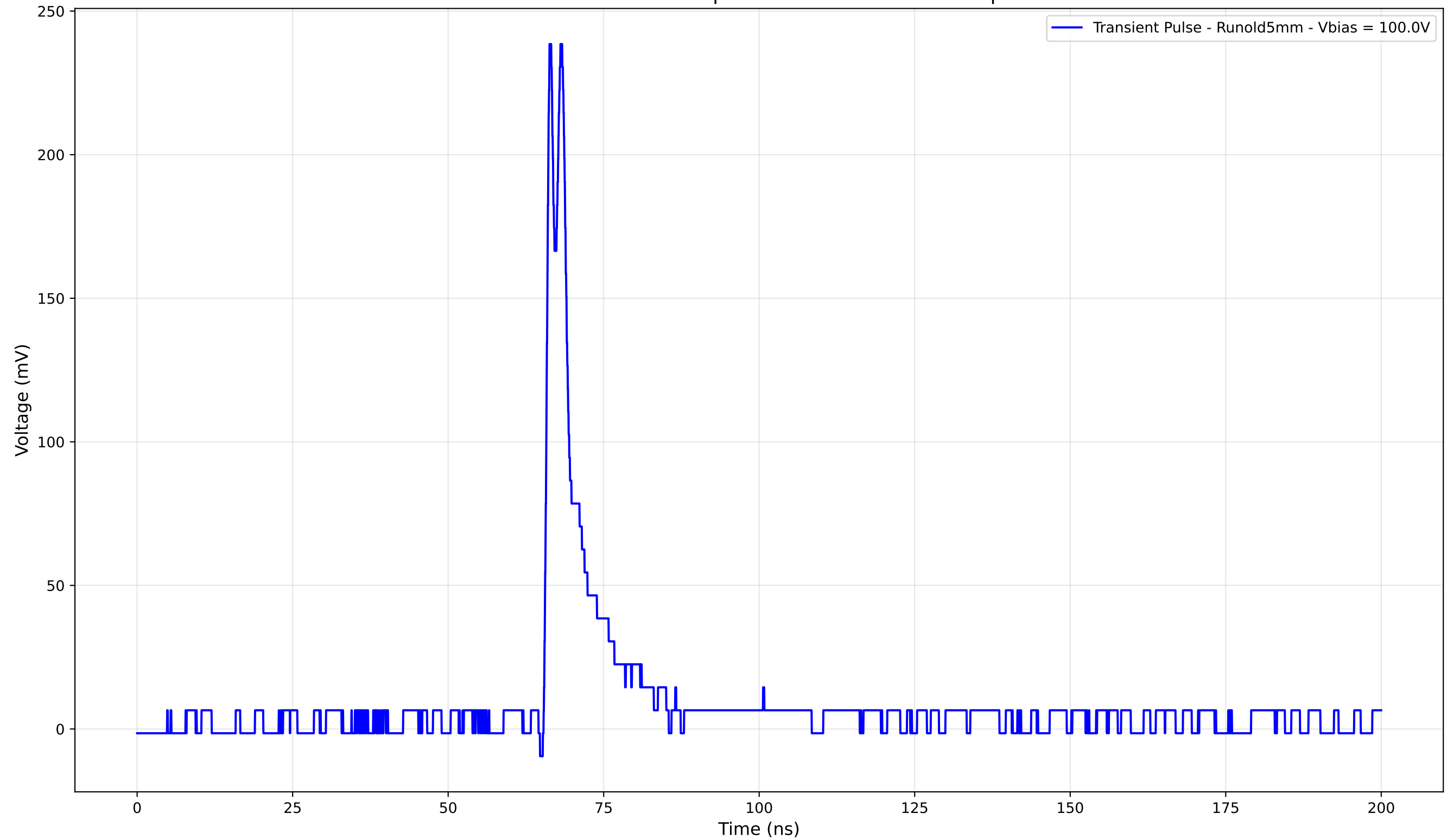
Transient Pulse - Sample: old5 - Position: 3260.0 \mu\text{m}
