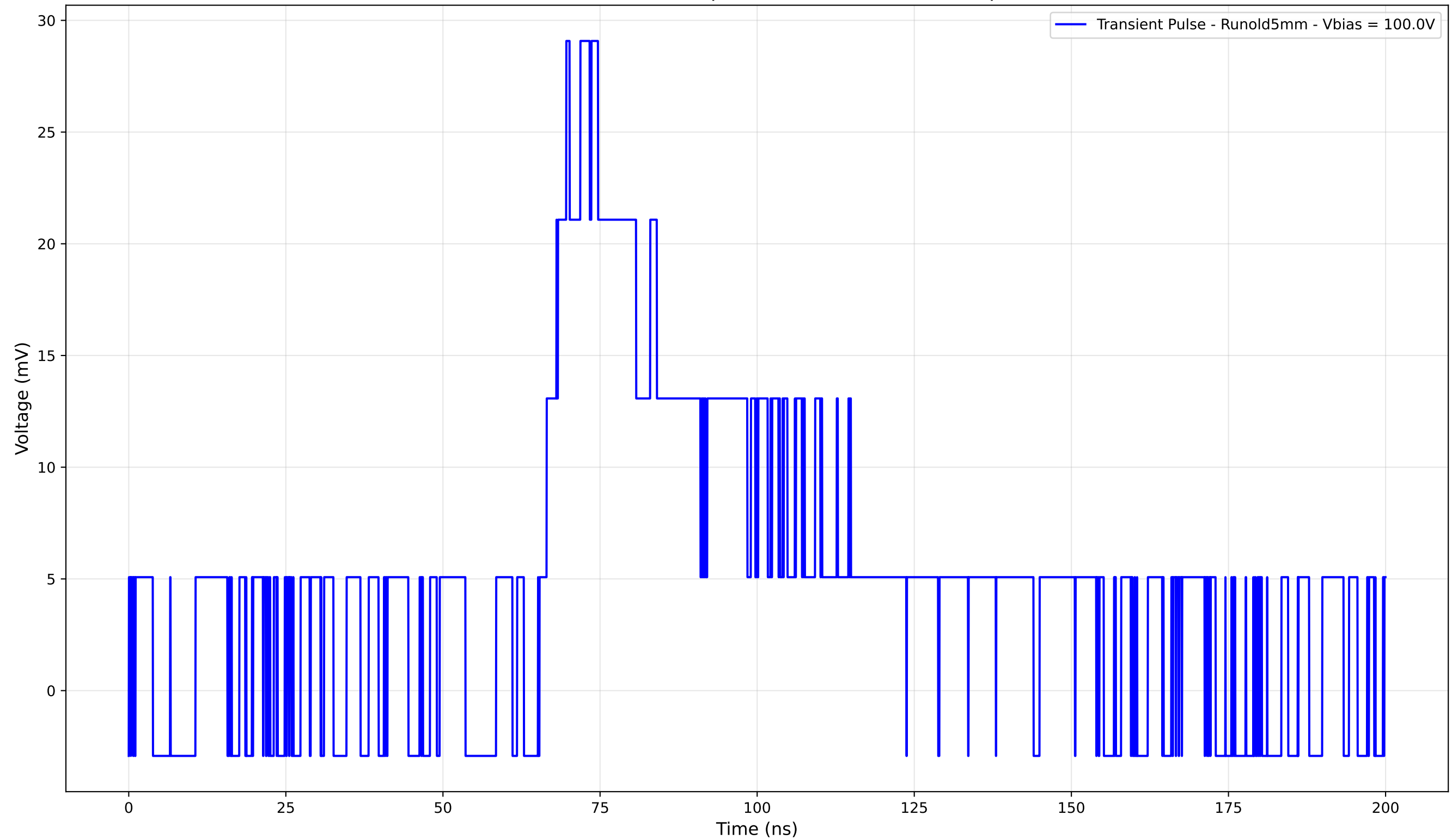
Transient Pulse - Sample: old5 - Position: 4670.0 \mu\text{m}
