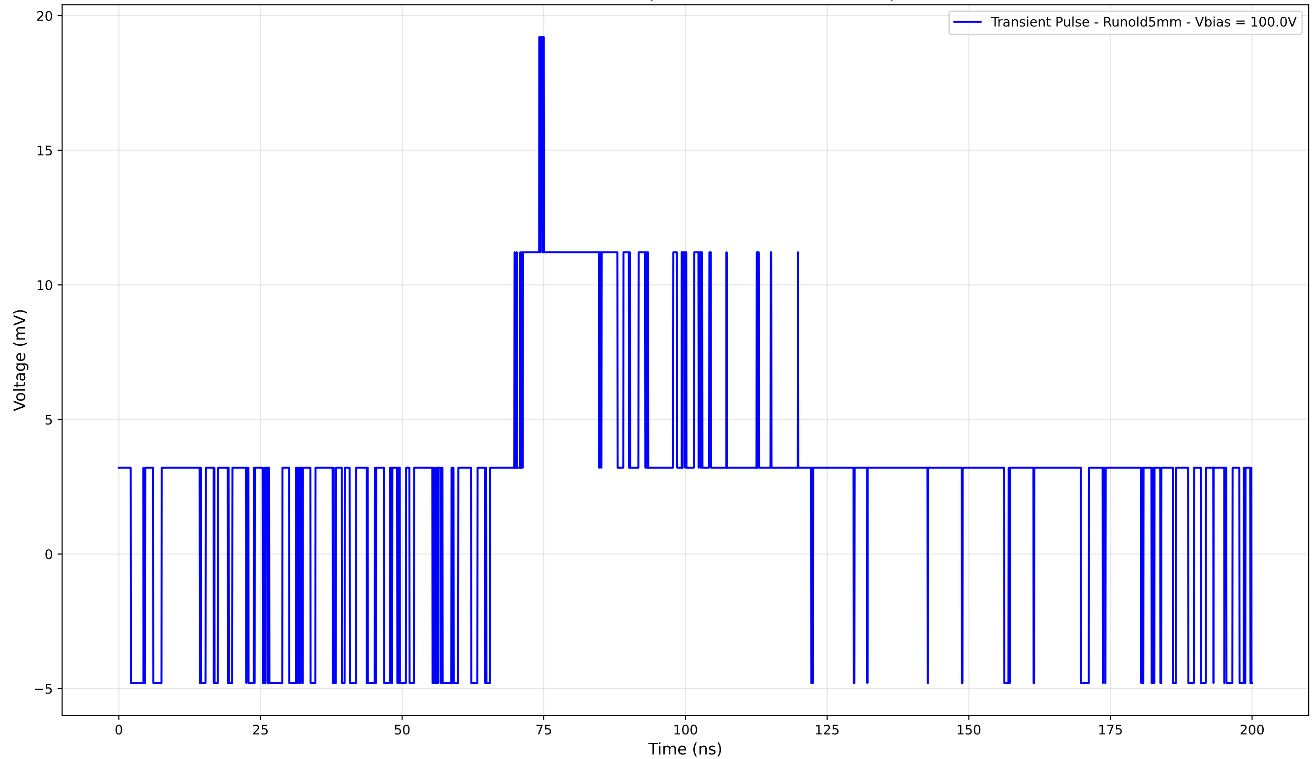
Transient Pulse - Sample: old5 - Position: 380.0 \mu\text{m}
