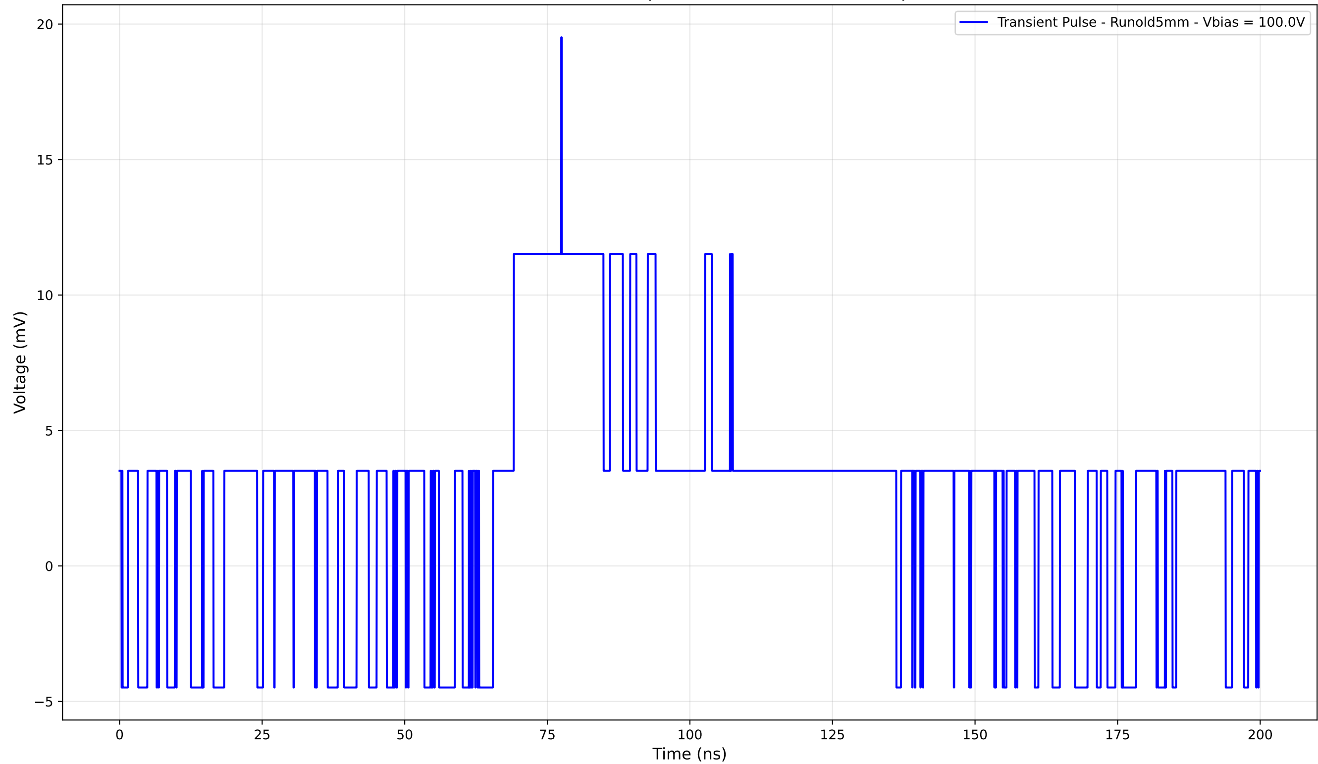
Transient Pulse - Sample: old5 - Position: 1940.0 \mu\text{m}
