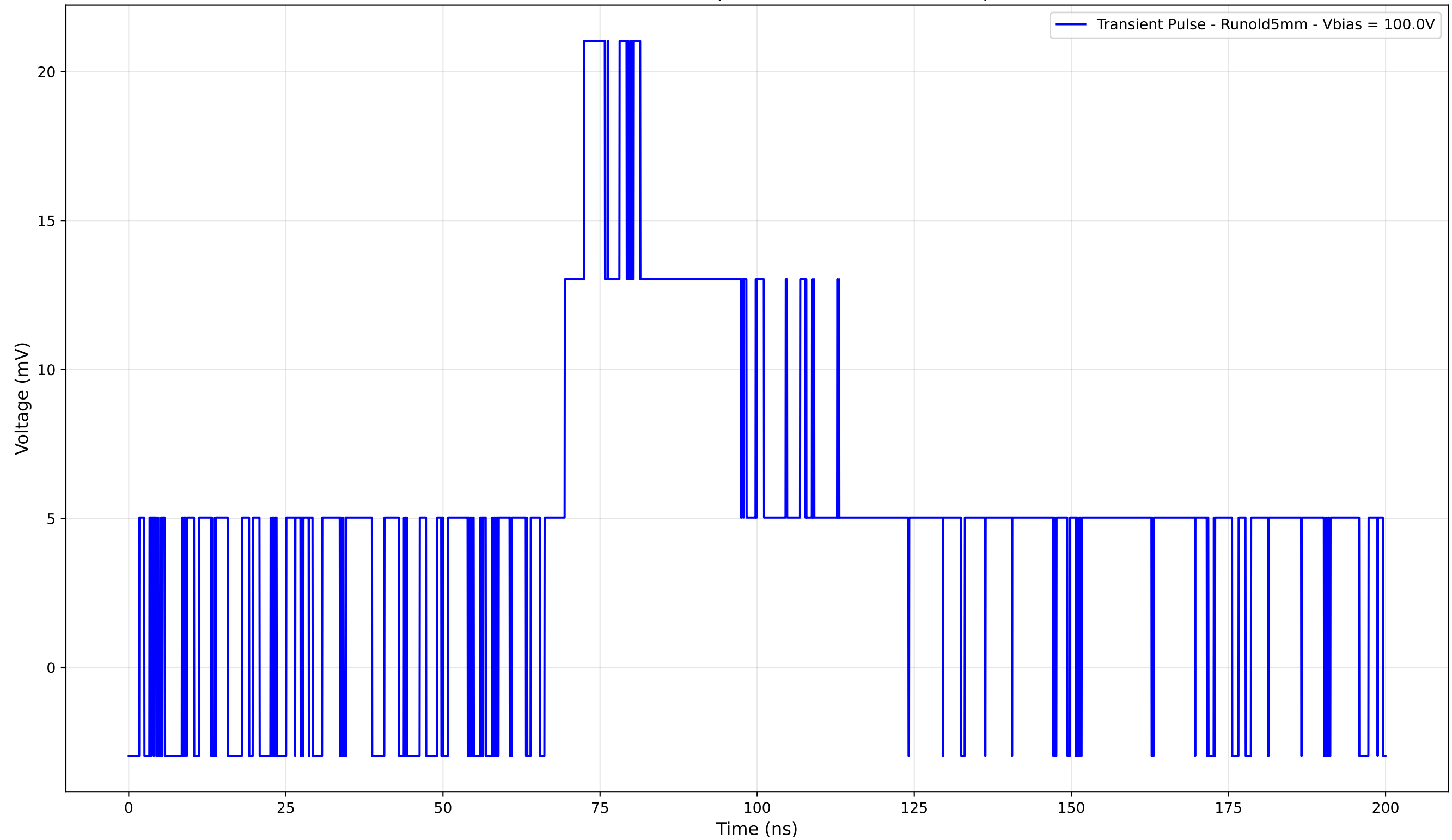
Transient Pulse - Sample: old5 - Position: 360.0 \mu\text{m}
