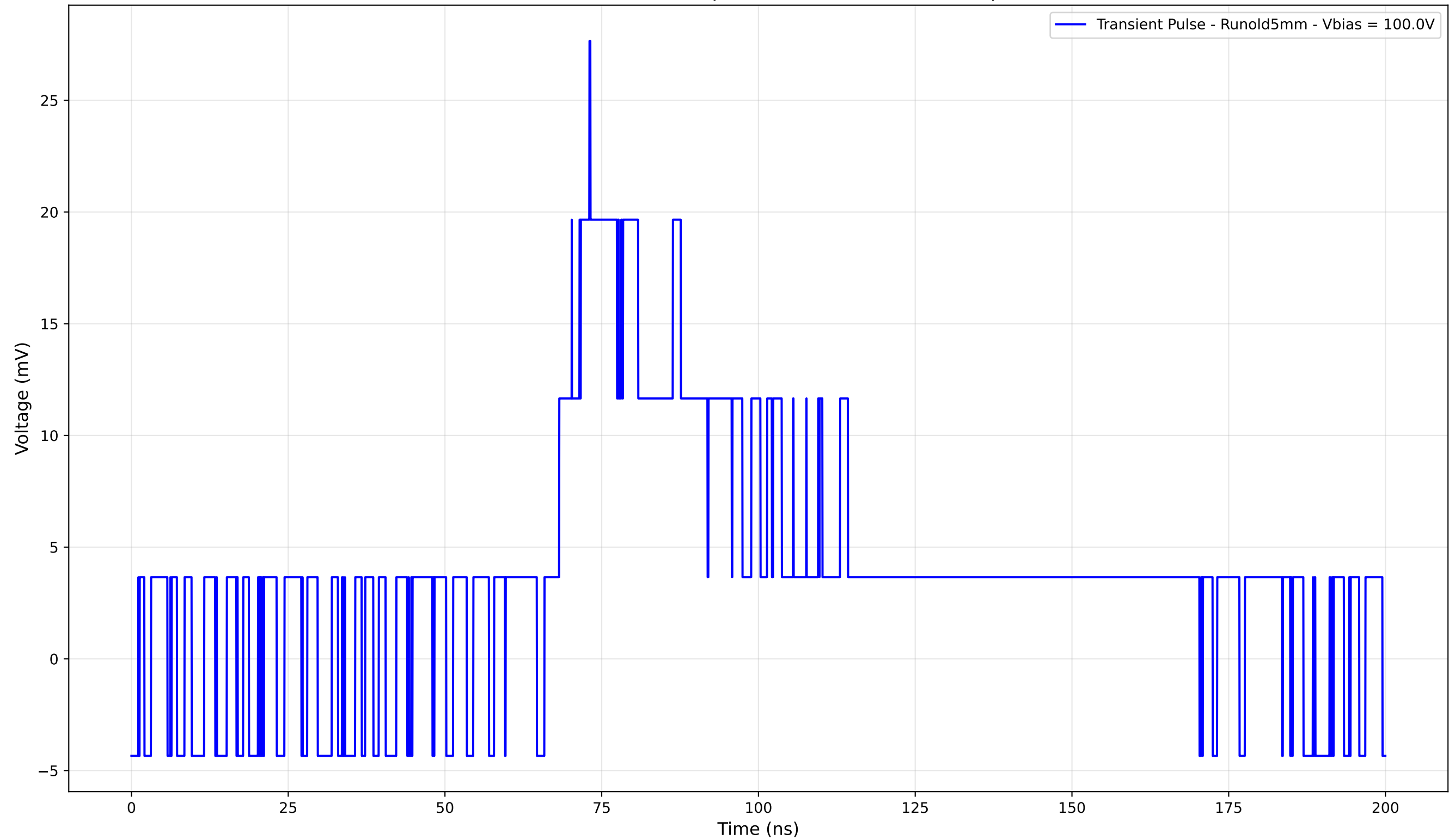
Transient Pulse - Sample: old5 - Position: 1825.0 \mu\text{m}
