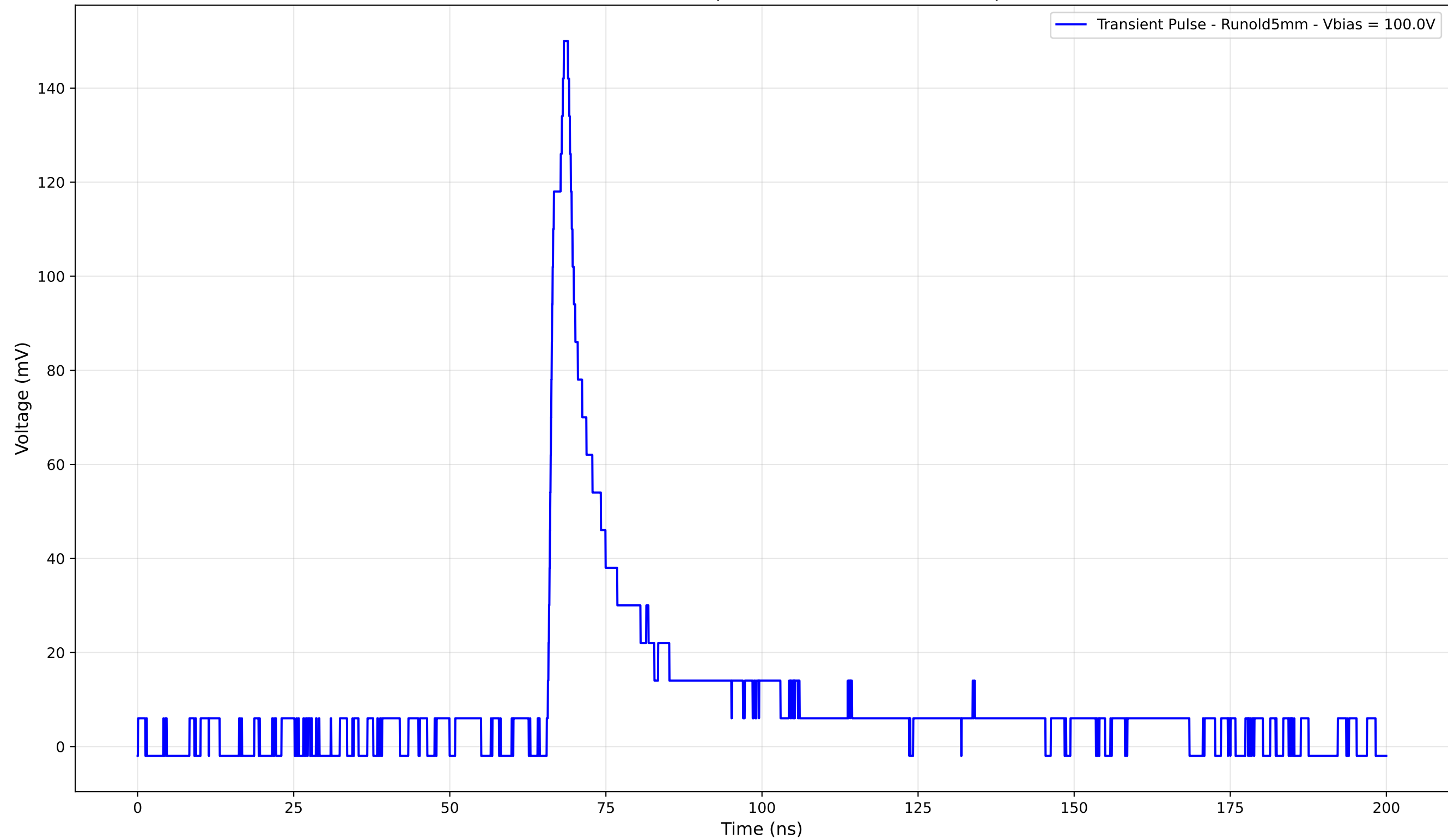
Transient Pulse - Sample: old5 - Position: 3800.0 \mu\text{m}
