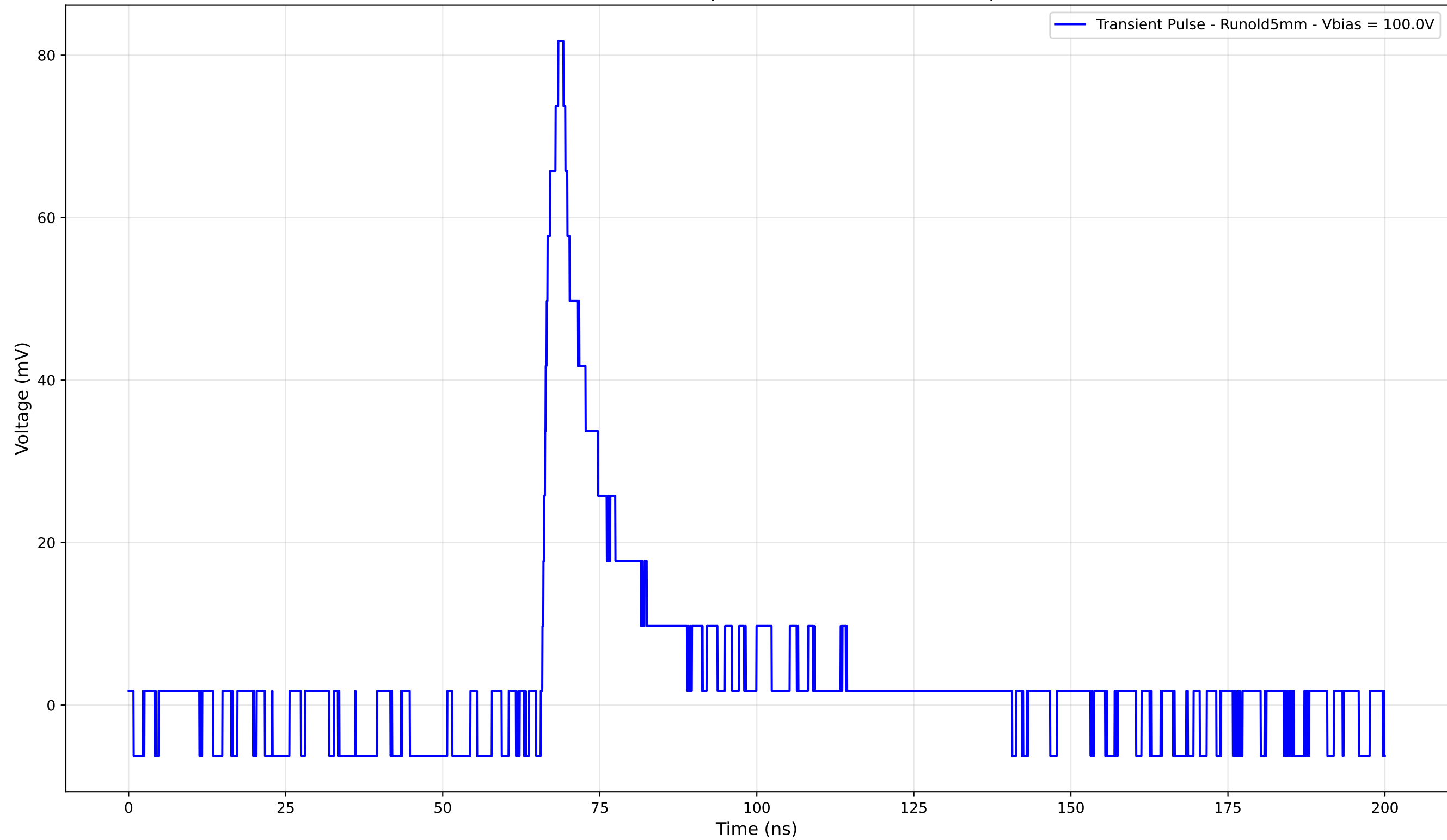
Transient Pulse - Sample: old5 - Position: 2845.0 \mu\text{m}
