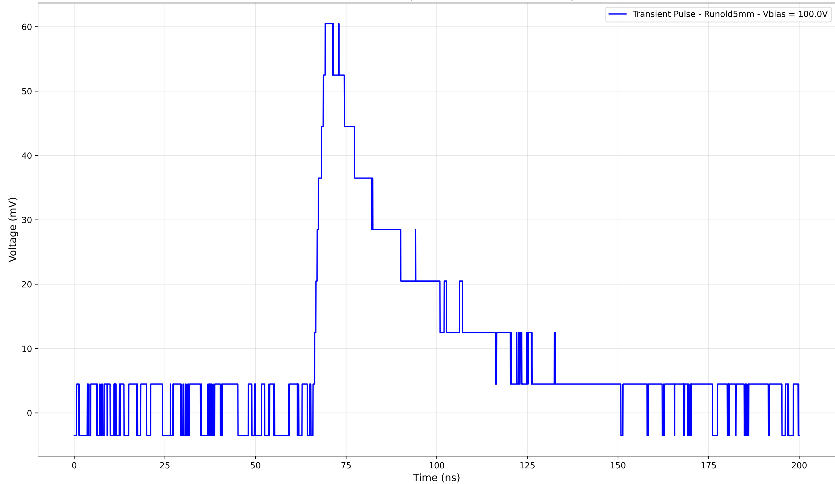
Transient Pulse - Sample: old5 - Position: 4545.0 \mu\text{m}
