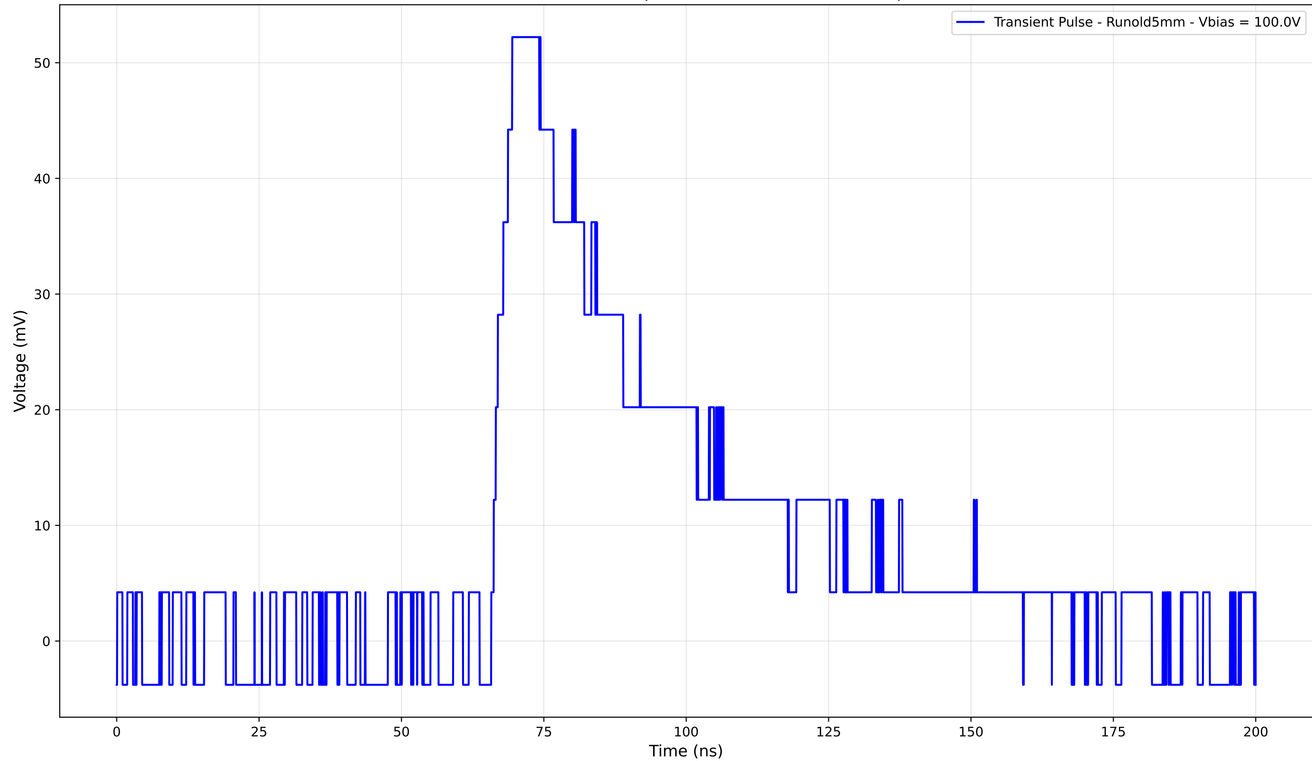
Transient Pulse - Sample: old5 - Position: 4610.0 \mu\text{m}
