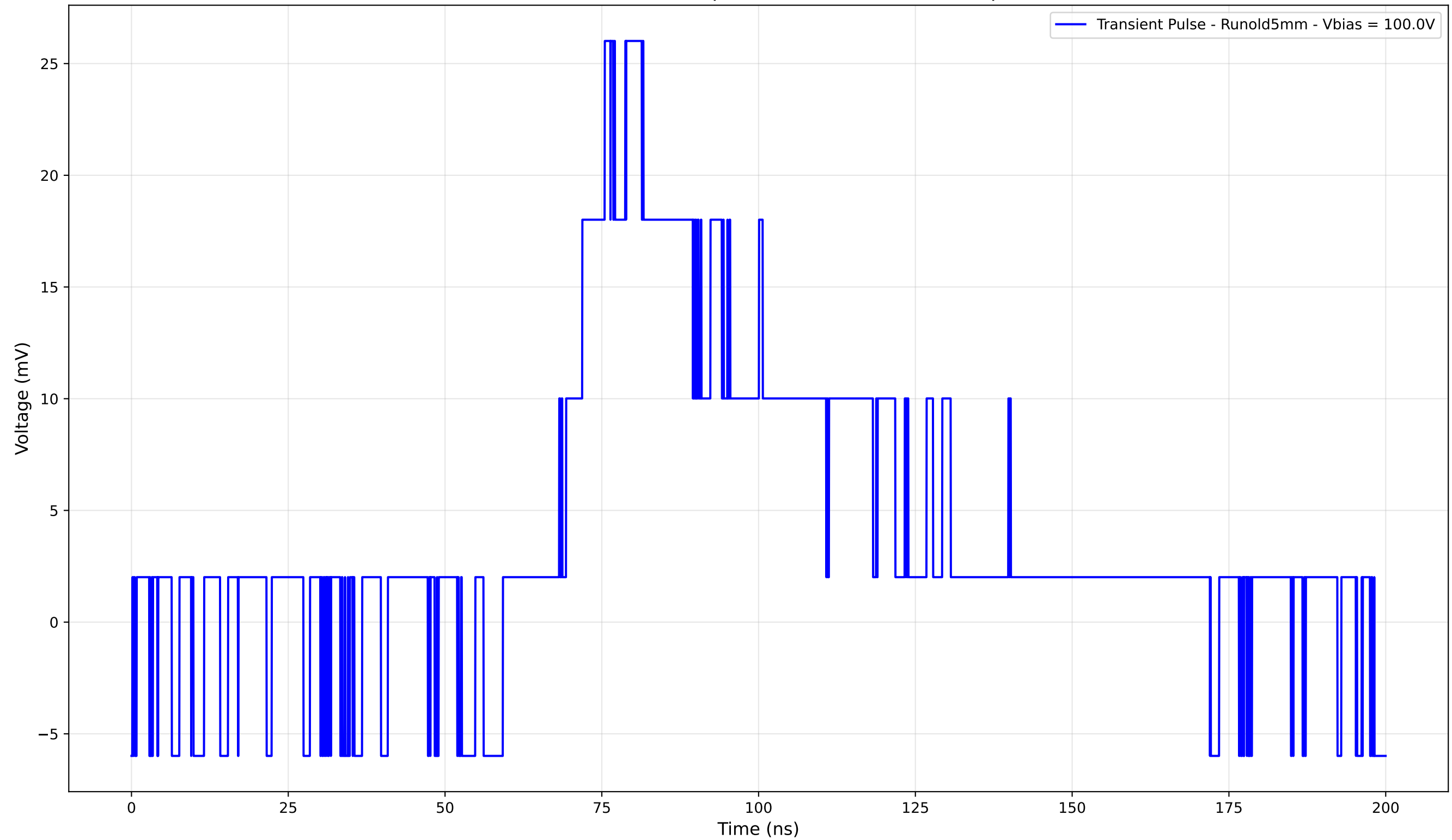
Transient Pulse - Sample: old5 - Position: 1295.0 \mu\text{m}
