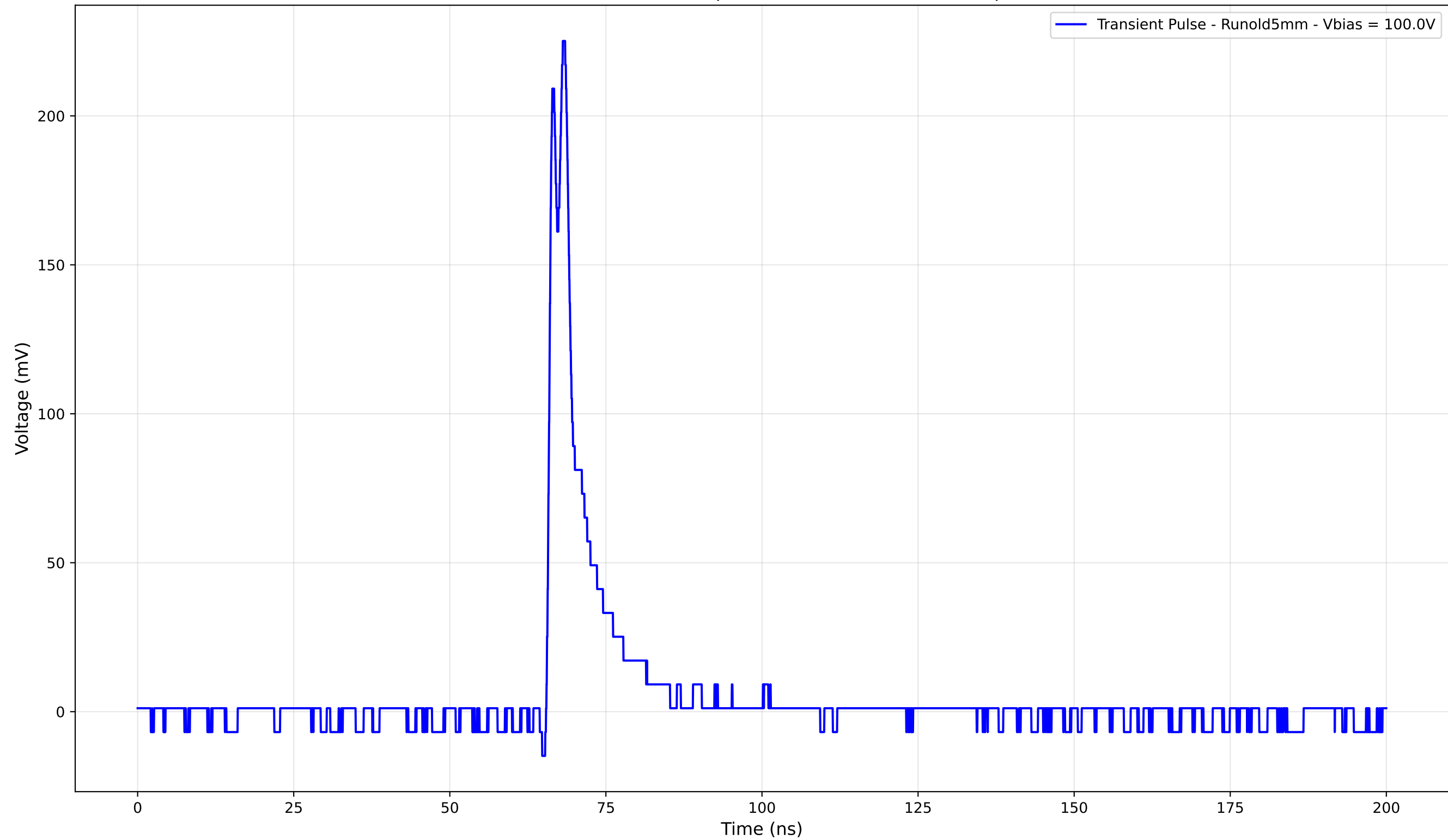
Transient Pulse - Sample: old5 - Position: 3535.0 \mu\text{m}
