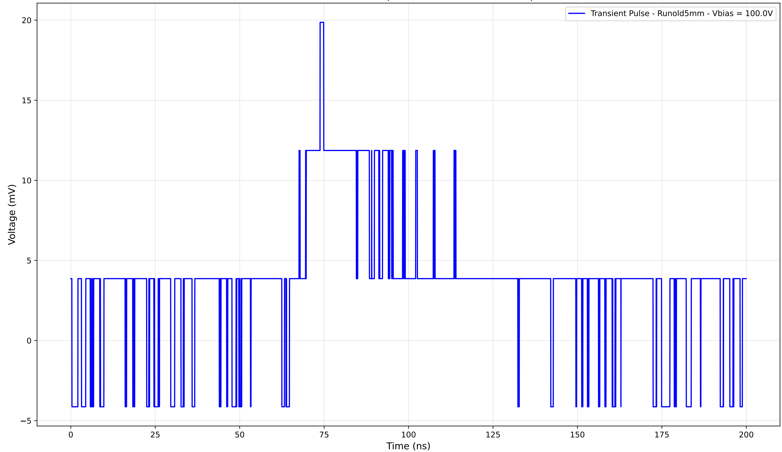
Transient Pulse - Sample: old5 - Position: 185.0 \mu\text{m}
