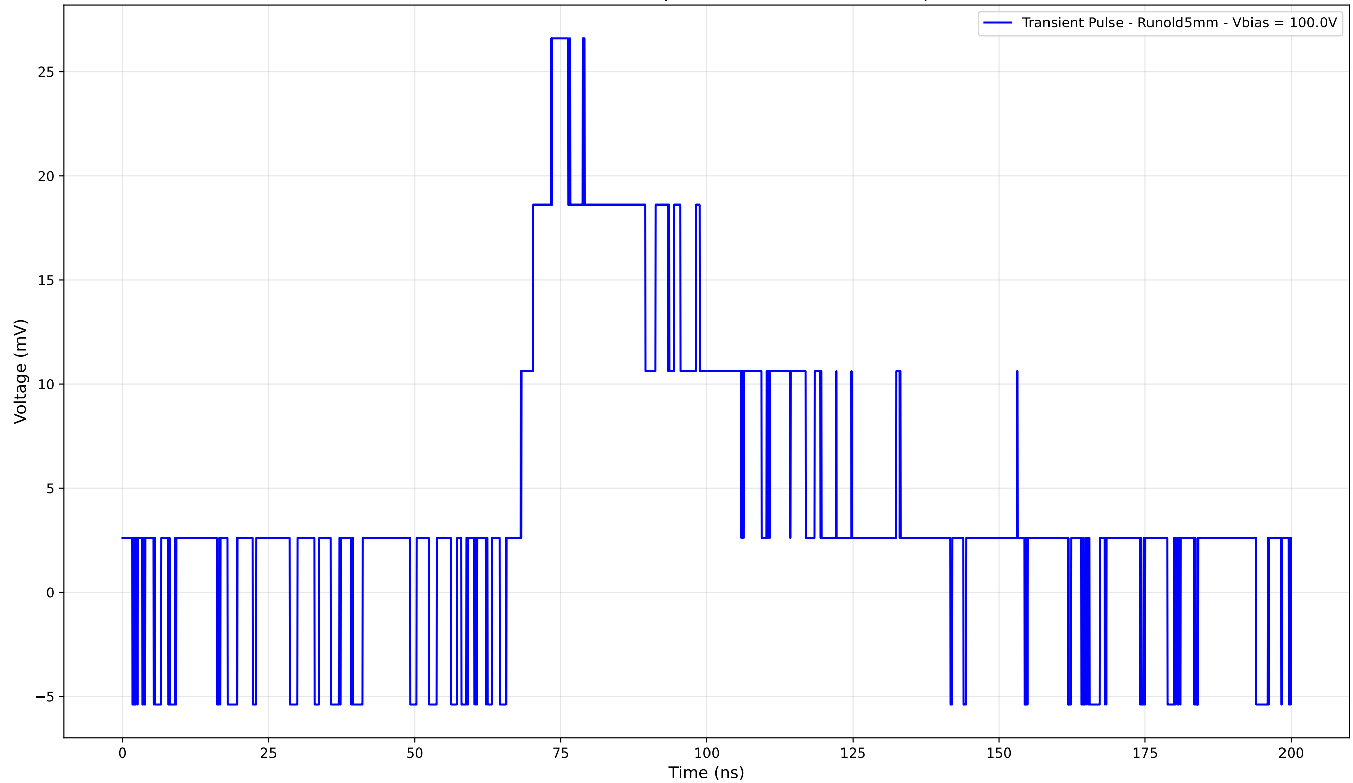
Transient Pulse - Sample: old5 - Position: 1645.0 \mu\text{m}
