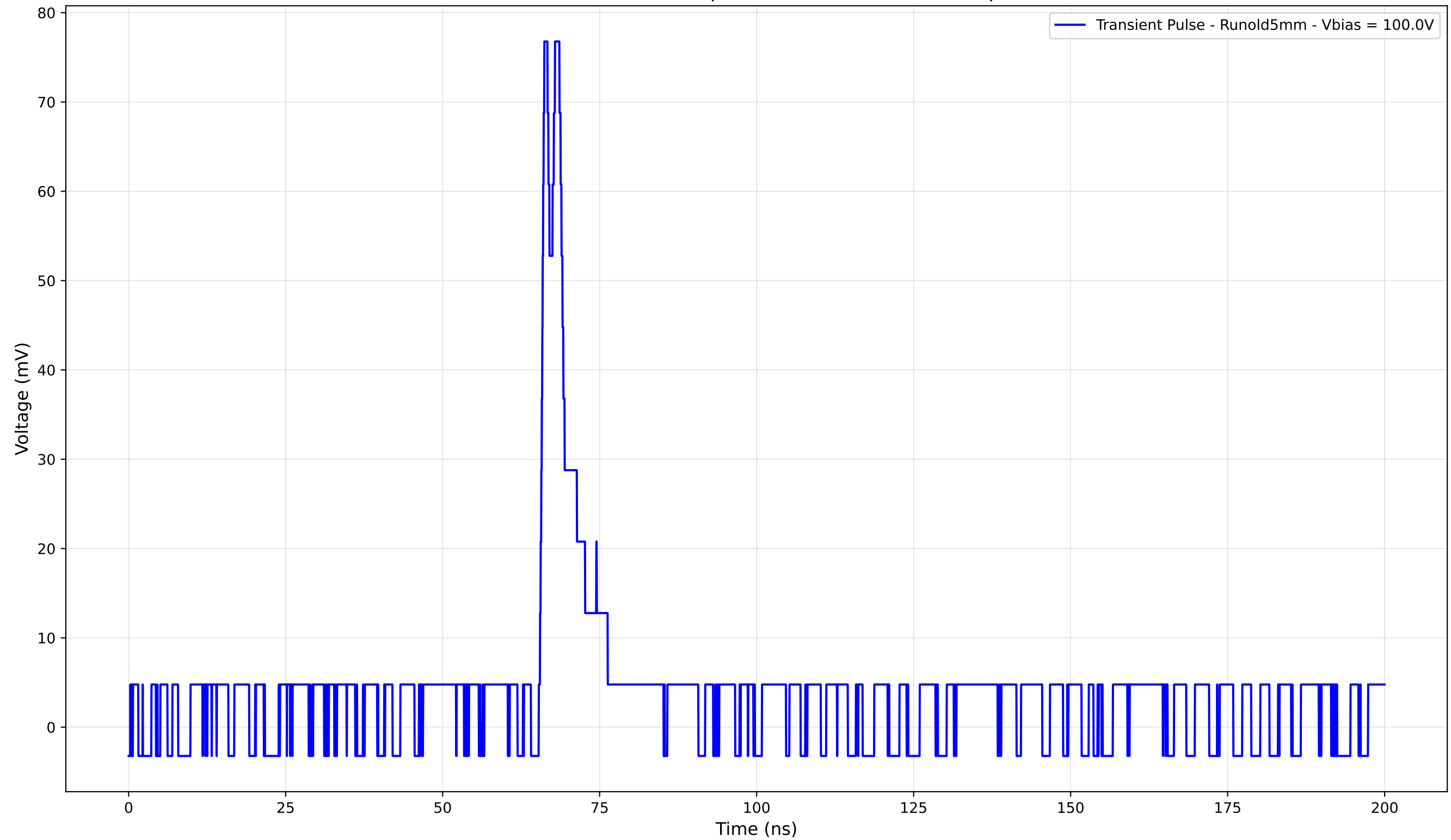
Transient Pulse - Sample: old5 - Position: 3420.0 \mu\text{m}
