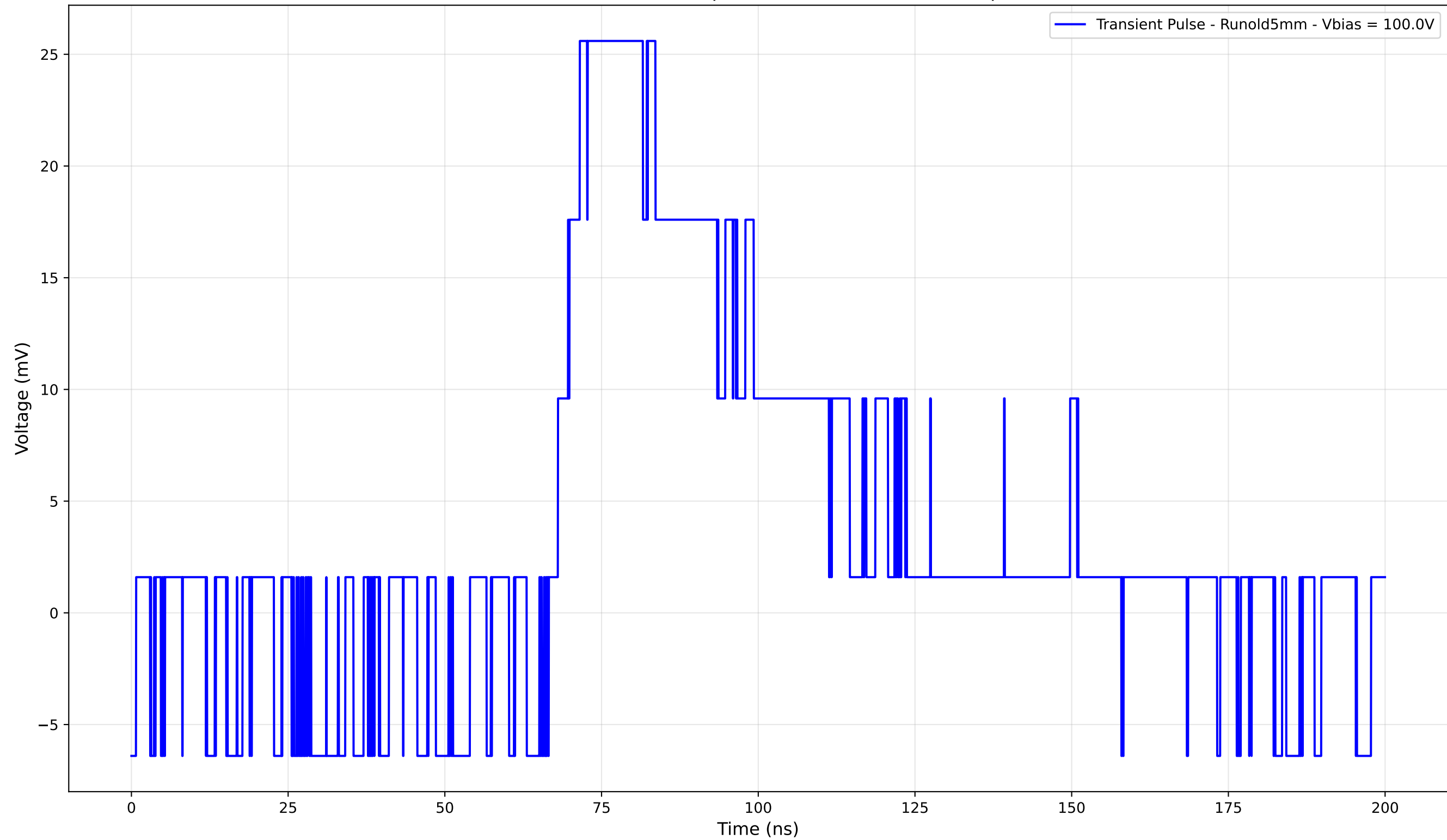
Transient Pulse - Sample: old5 - Position: 1675.0 \mu\text{m}
