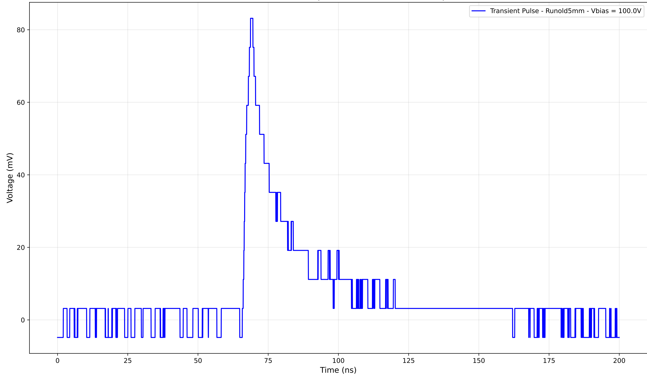
Transient Pulse - Sample: old5 - Position: 2600.0 \mu\text{m}
