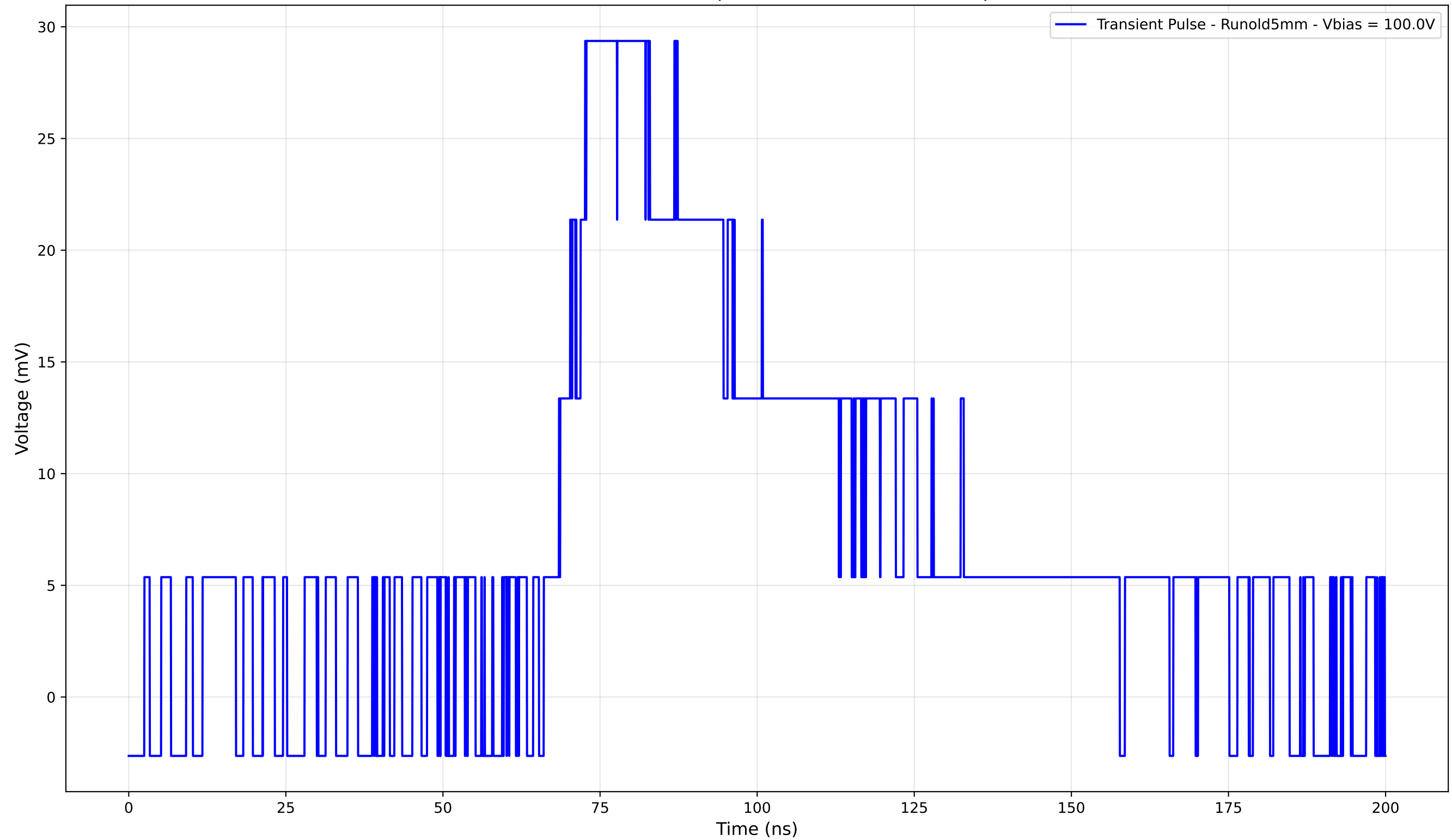
Transient Pulse - Sample: old5 - Position: 865.0 \mu\text{m}
