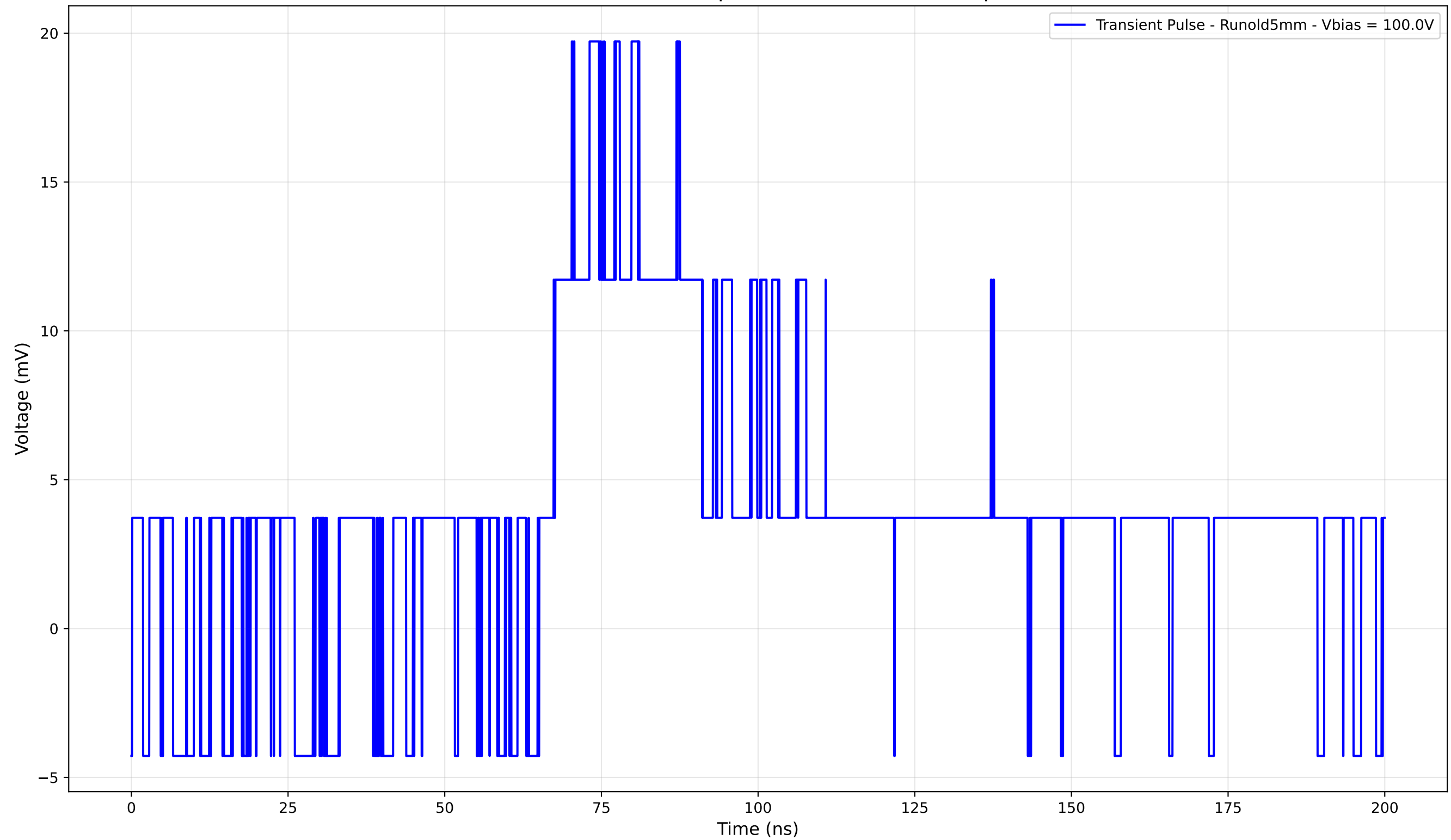
Transient Pulse - Sample: old5 - Position: 310.0 \mu\text{m}
