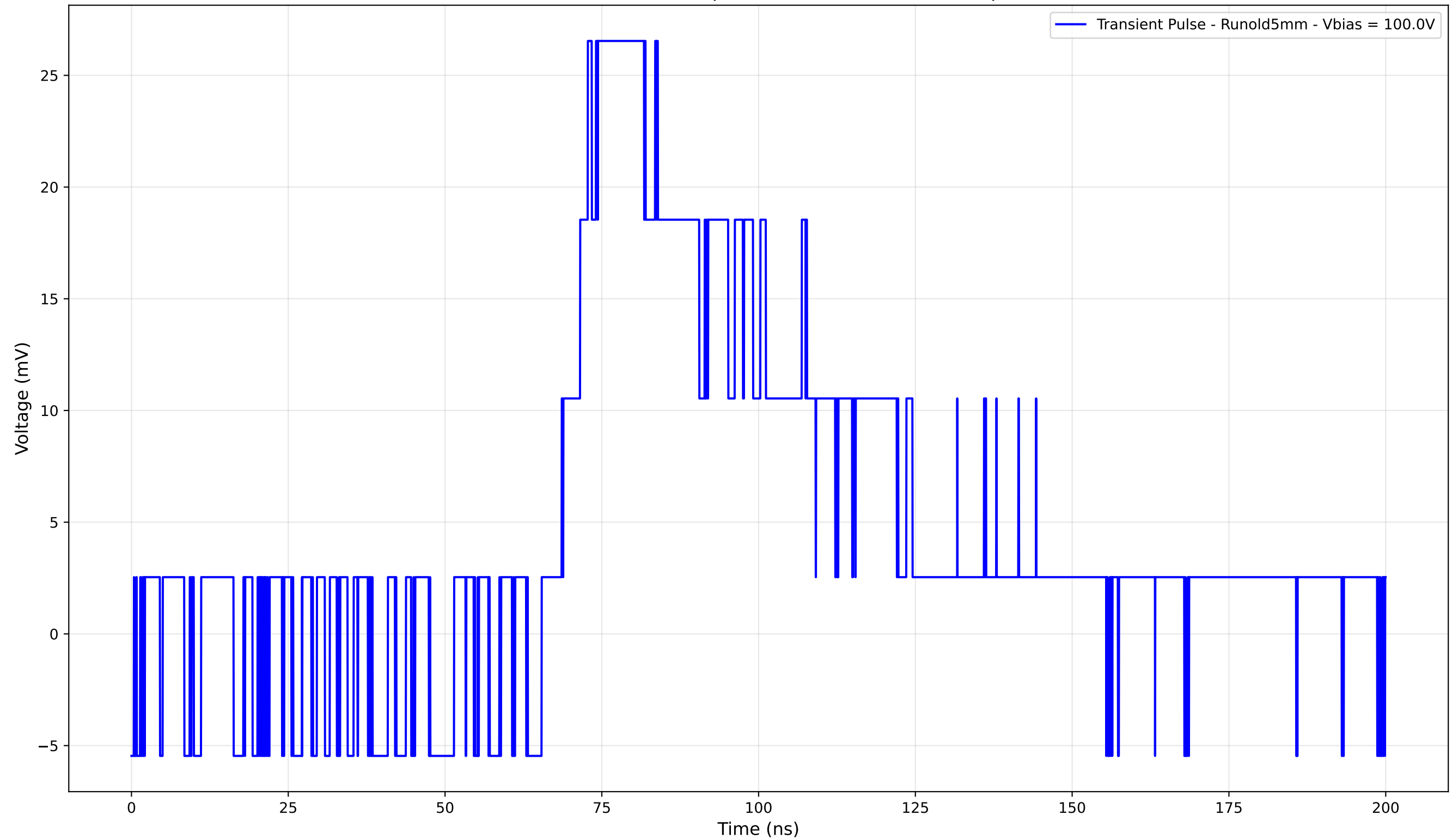
Transient Pulse - Sample: old5 - Position: 1265.0 \mu\text{m}
