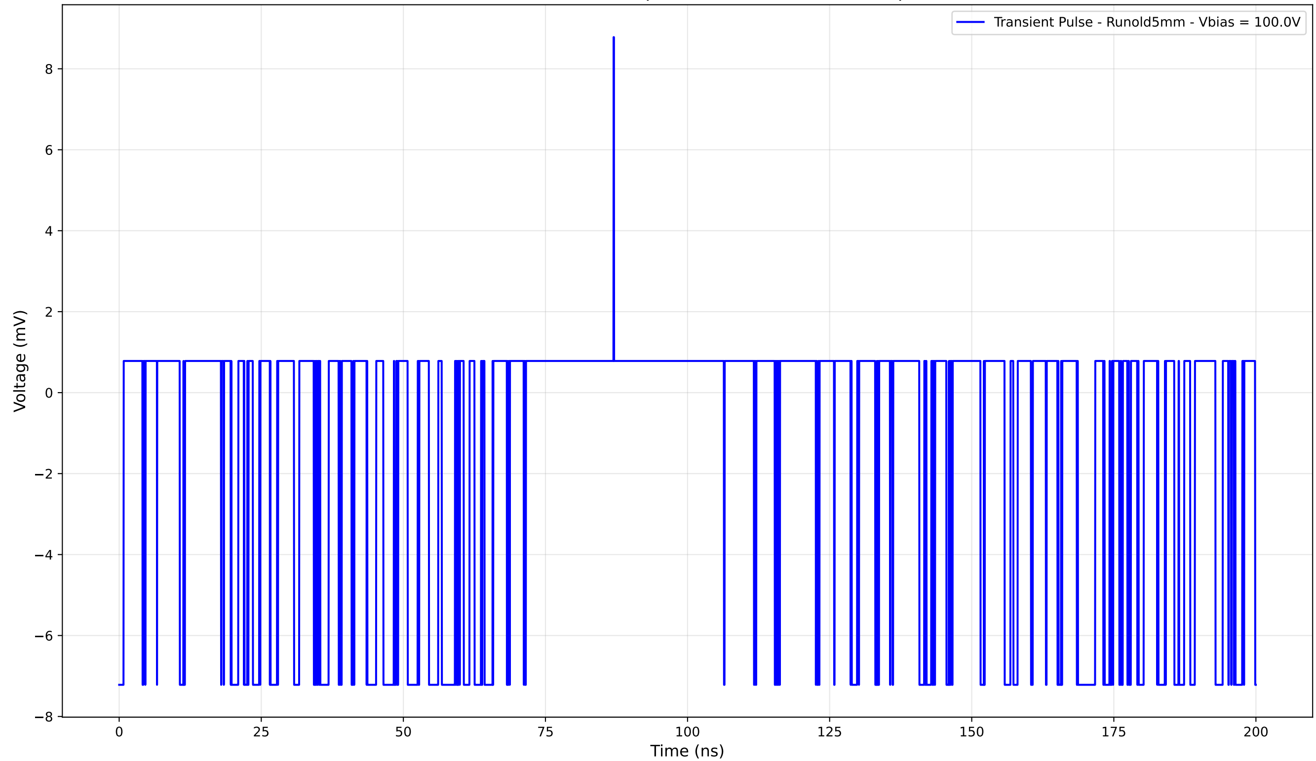
Transient Pulse - Sample: old5 - Position: 1360.0 \mu\text{m}
