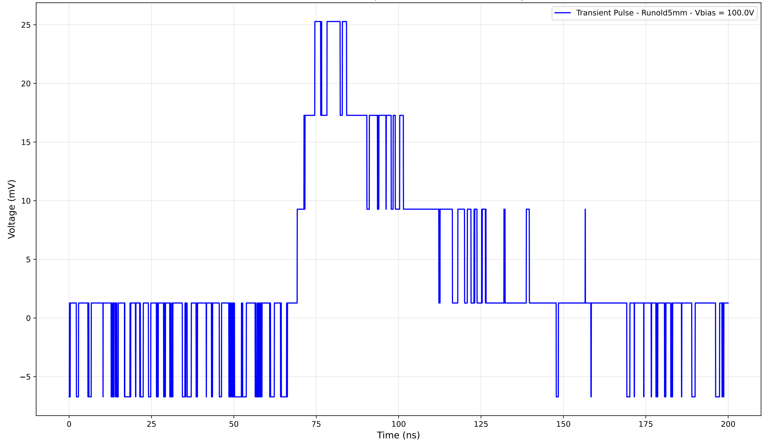
Transient Pulse - Sample: old5 - Position: 1070.0 \mu\text{m}
