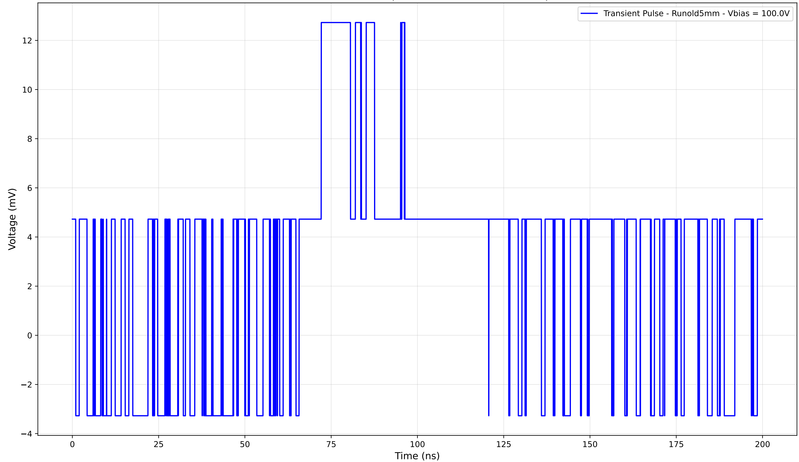
Transient Pulse - Sample: old5 - Position: 1540.0 \mu\text{m}
