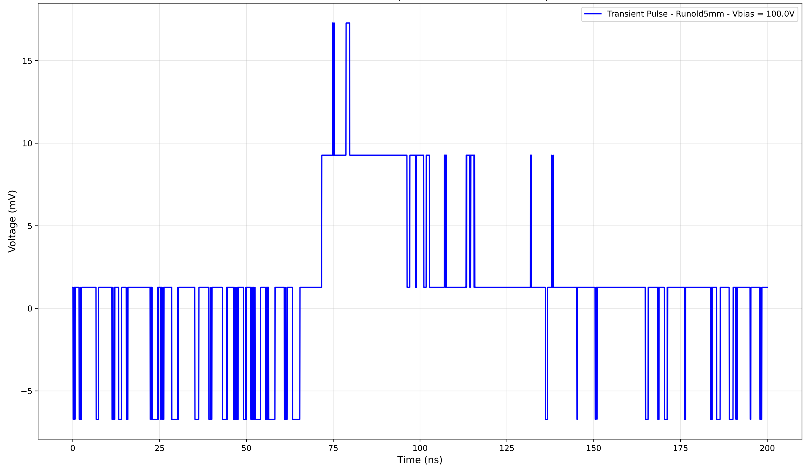
Transient Pulse - Sample: old5 - Position: 805.0 \mu\text{m}
