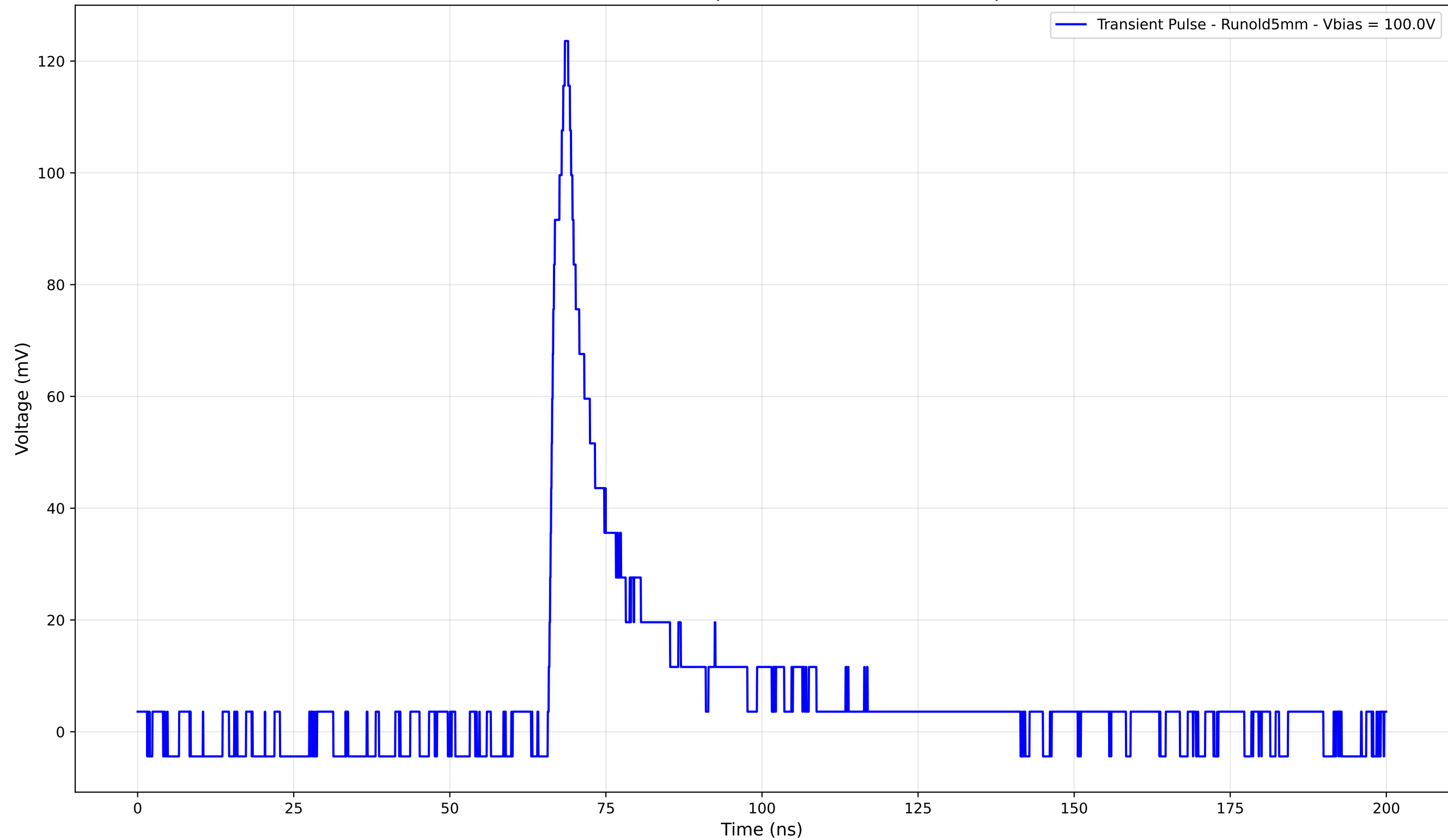
Transient Pulse - Sample: old5 - Position: 3860.0 \mu\text{m}
