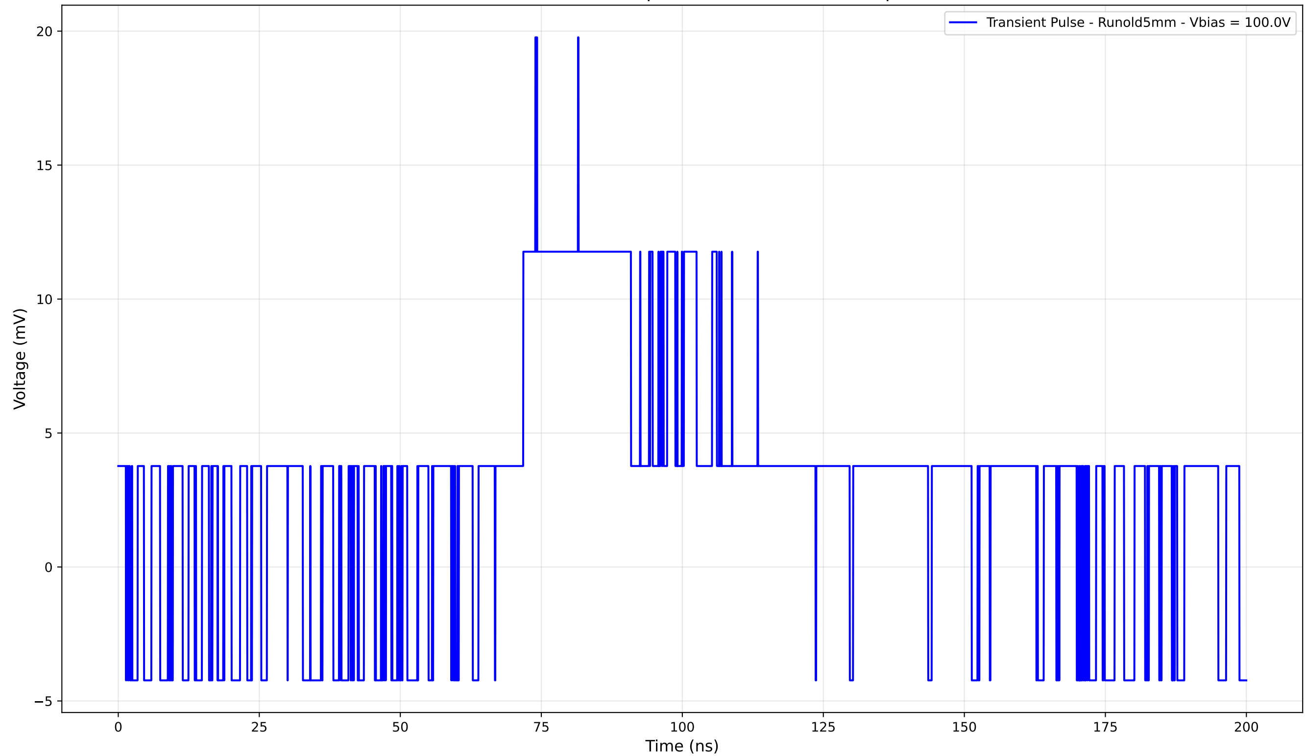
Transient Pulse - Sample: old5 - Position: 575.0 \mu\text{m}
