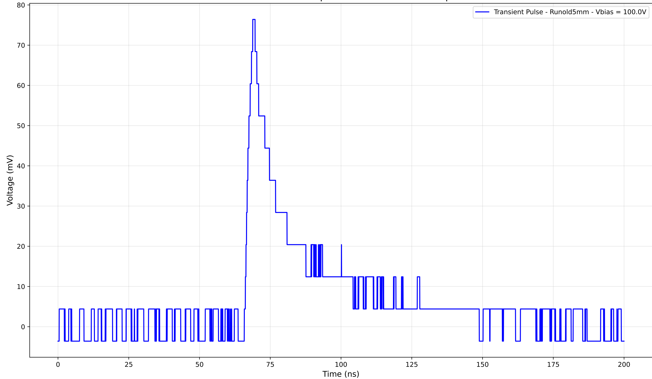
Transient Pulse - Sample: old5 - Position: 2570.0 \mu\text{m}
