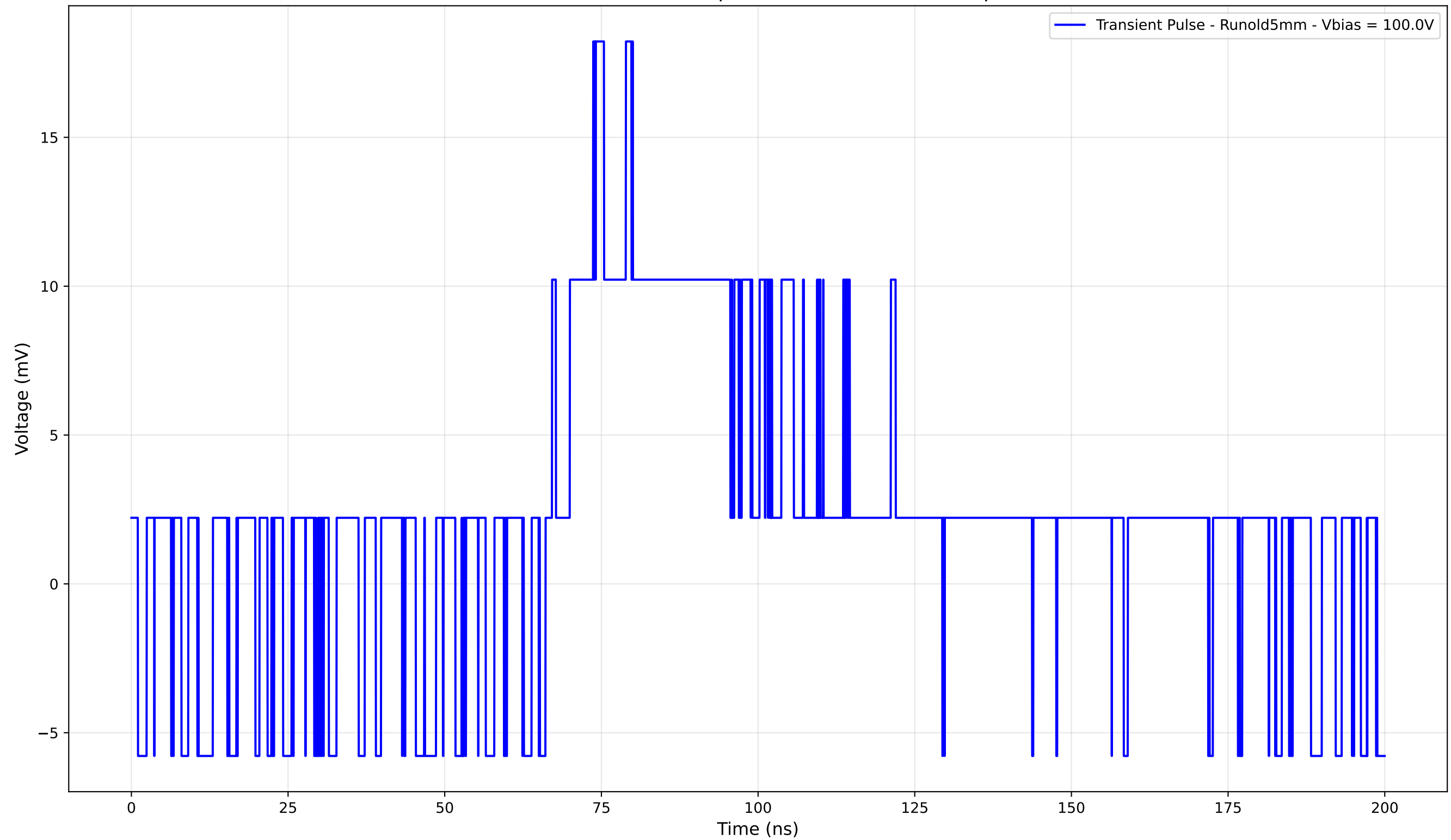
Transient Pulse - Sample: old5 - Position: 415.0 \mu\text{m}
