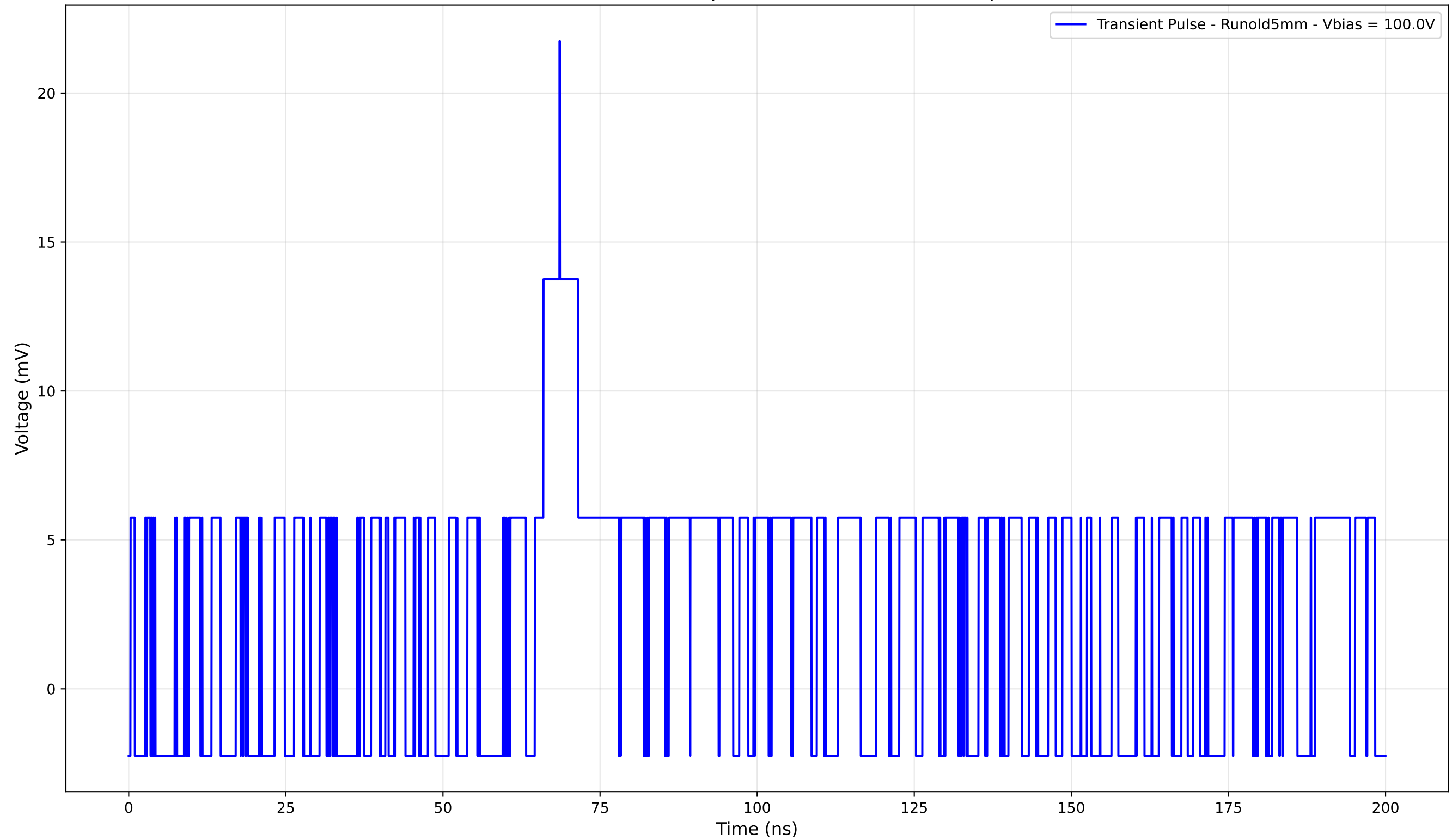
Transient Pulse - Sample: old5 - Position: 3695.0 \mu\text{m}
