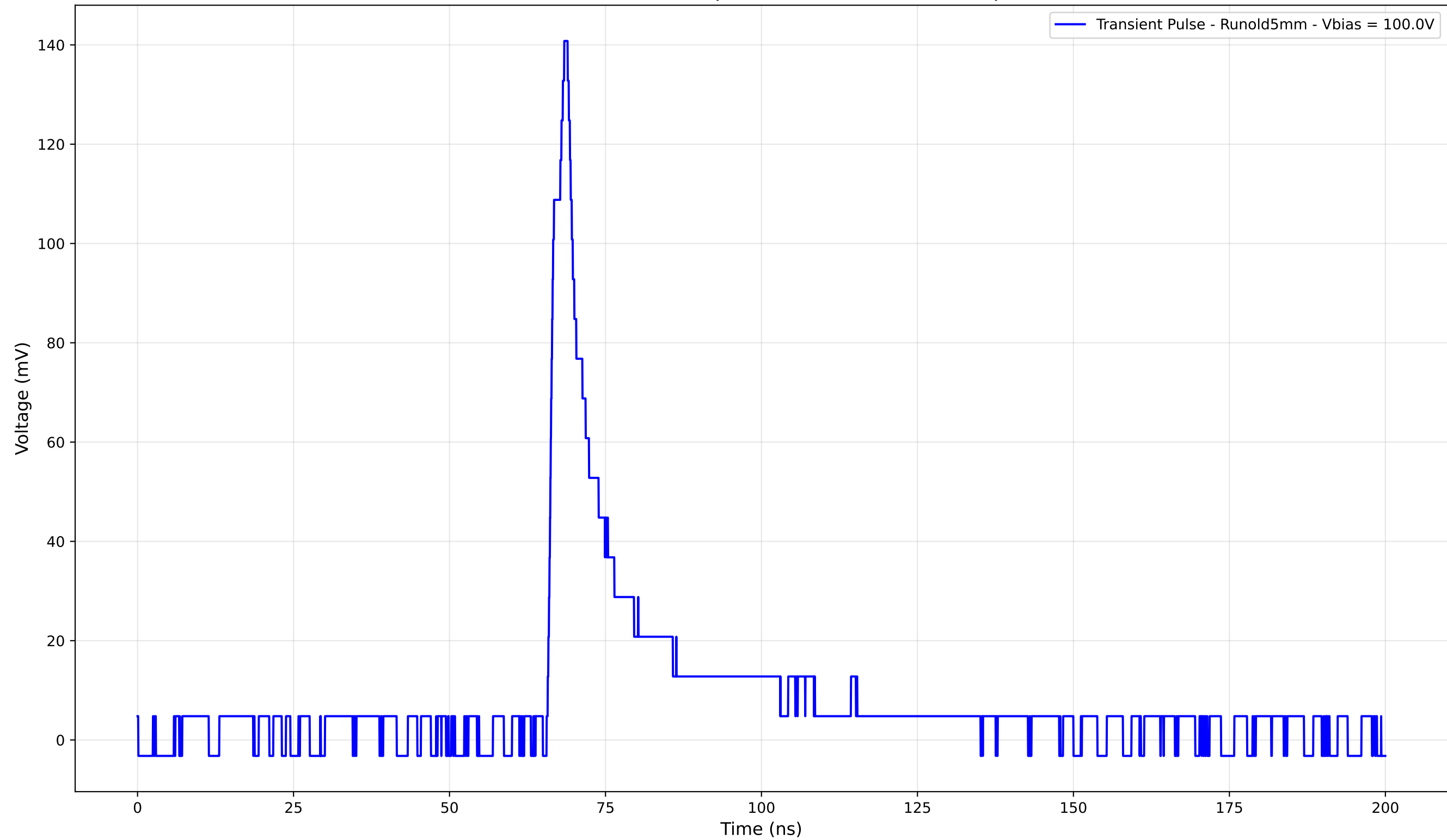
Transient Pulse - Sample: old5 - Position: 2915.0 \mu\text{m}
