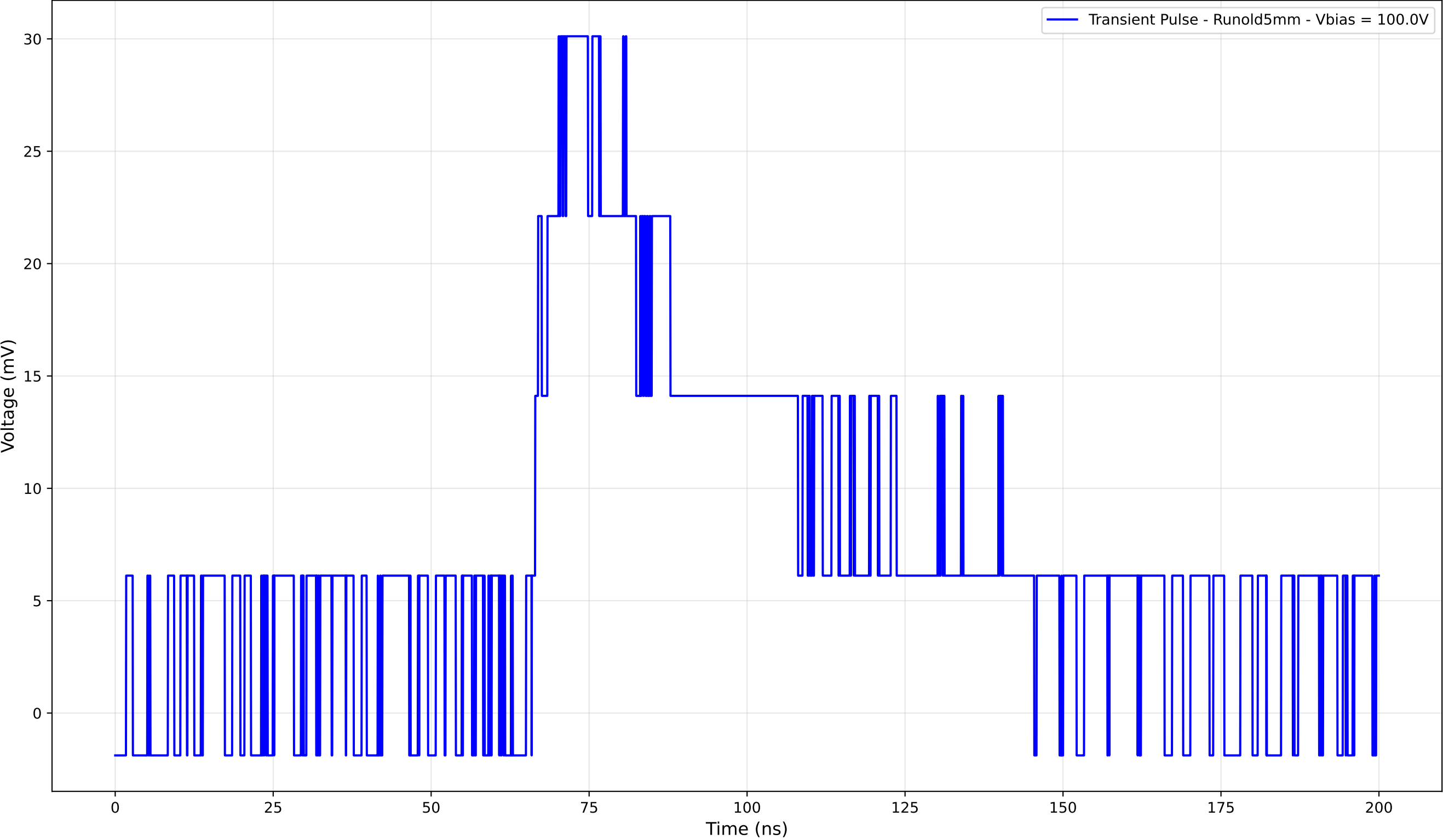
Transient Pulse - Sample: old5 - Position: 15.0 \mu\text{m}
