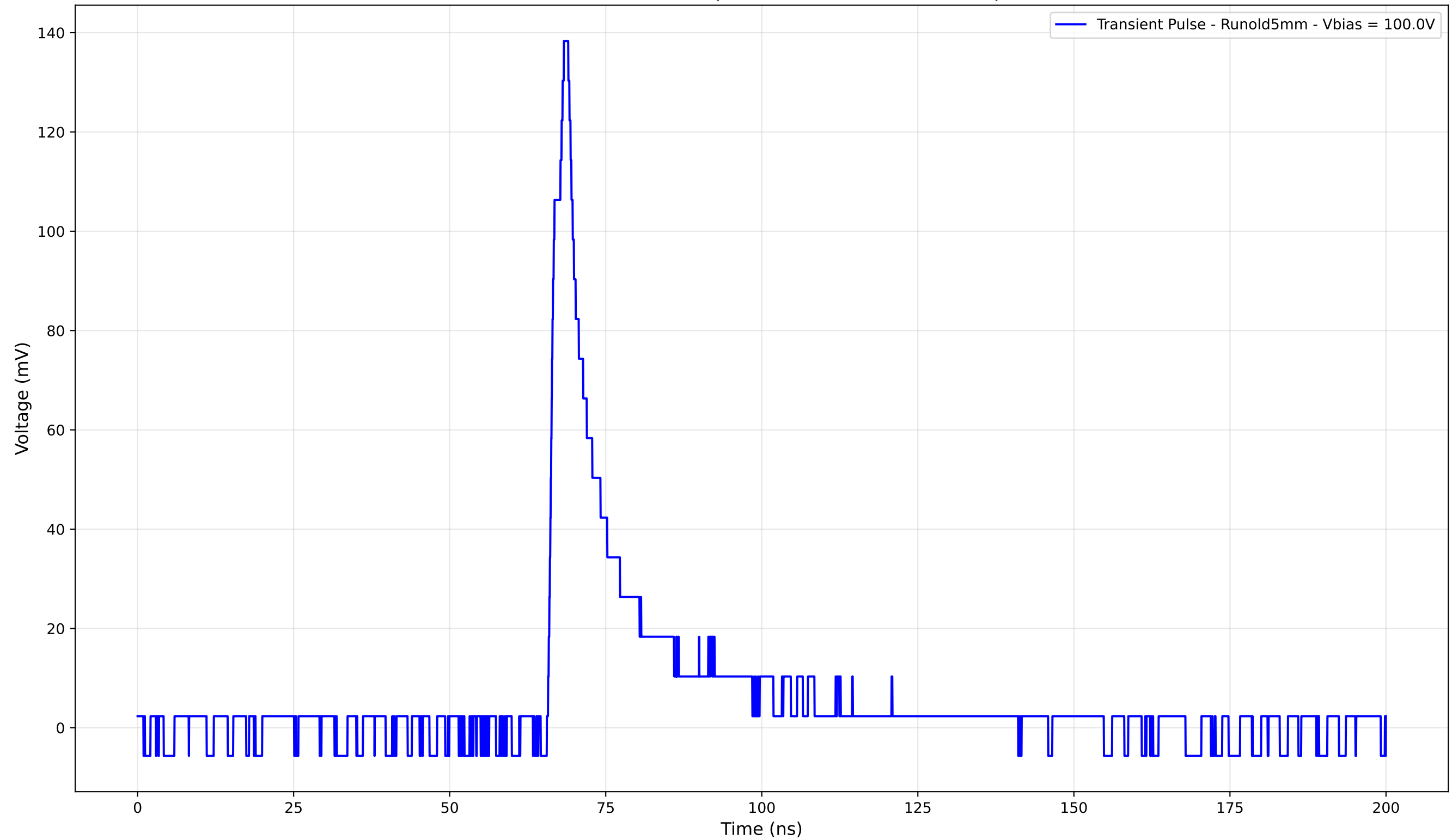
Transient Pulse - Sample: old5 - Position: 3830.0 \mu\text{m}
