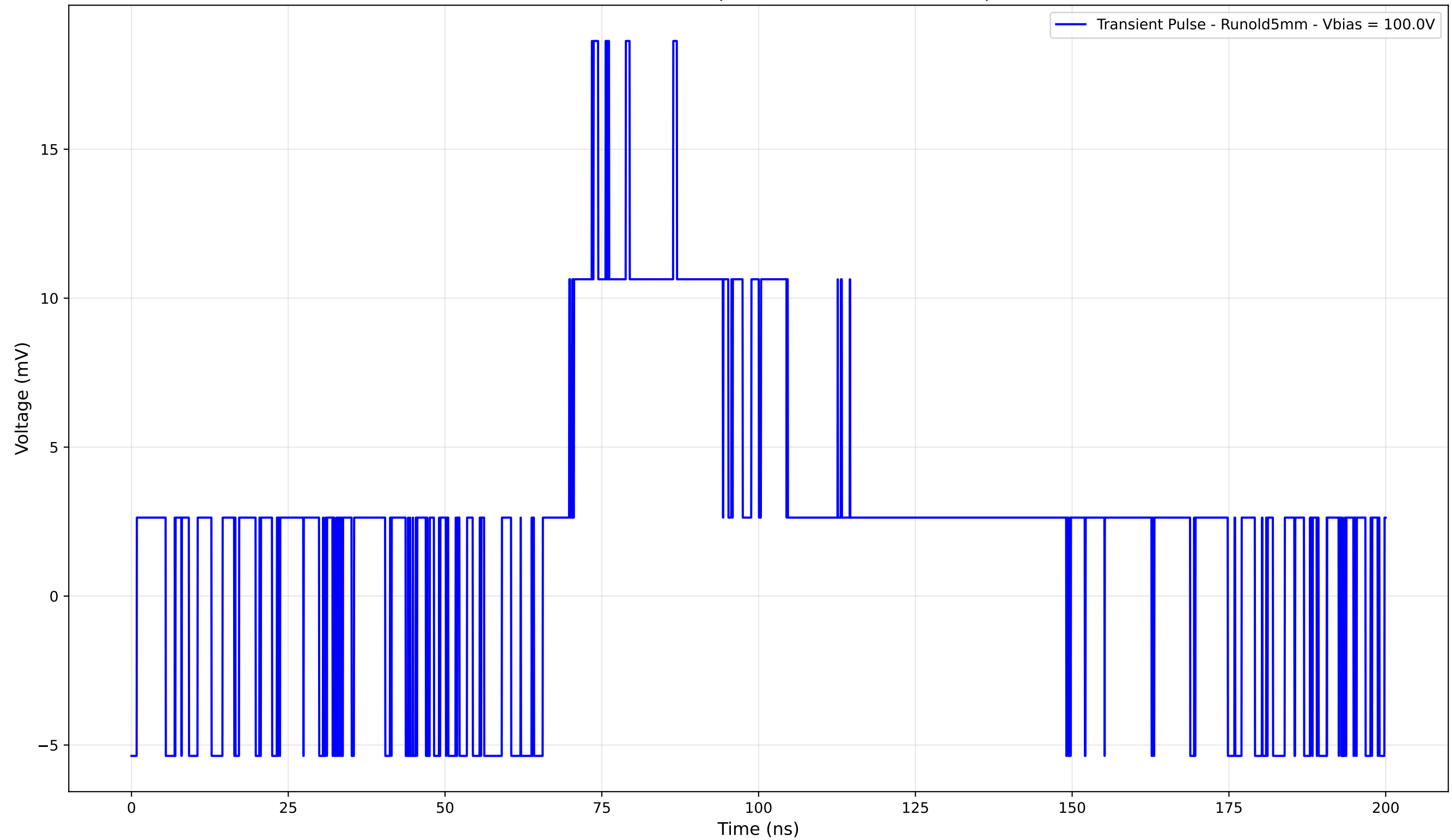
Transient Pulse - Sample: old5 - Position: 715.0 \mu\text{m}
