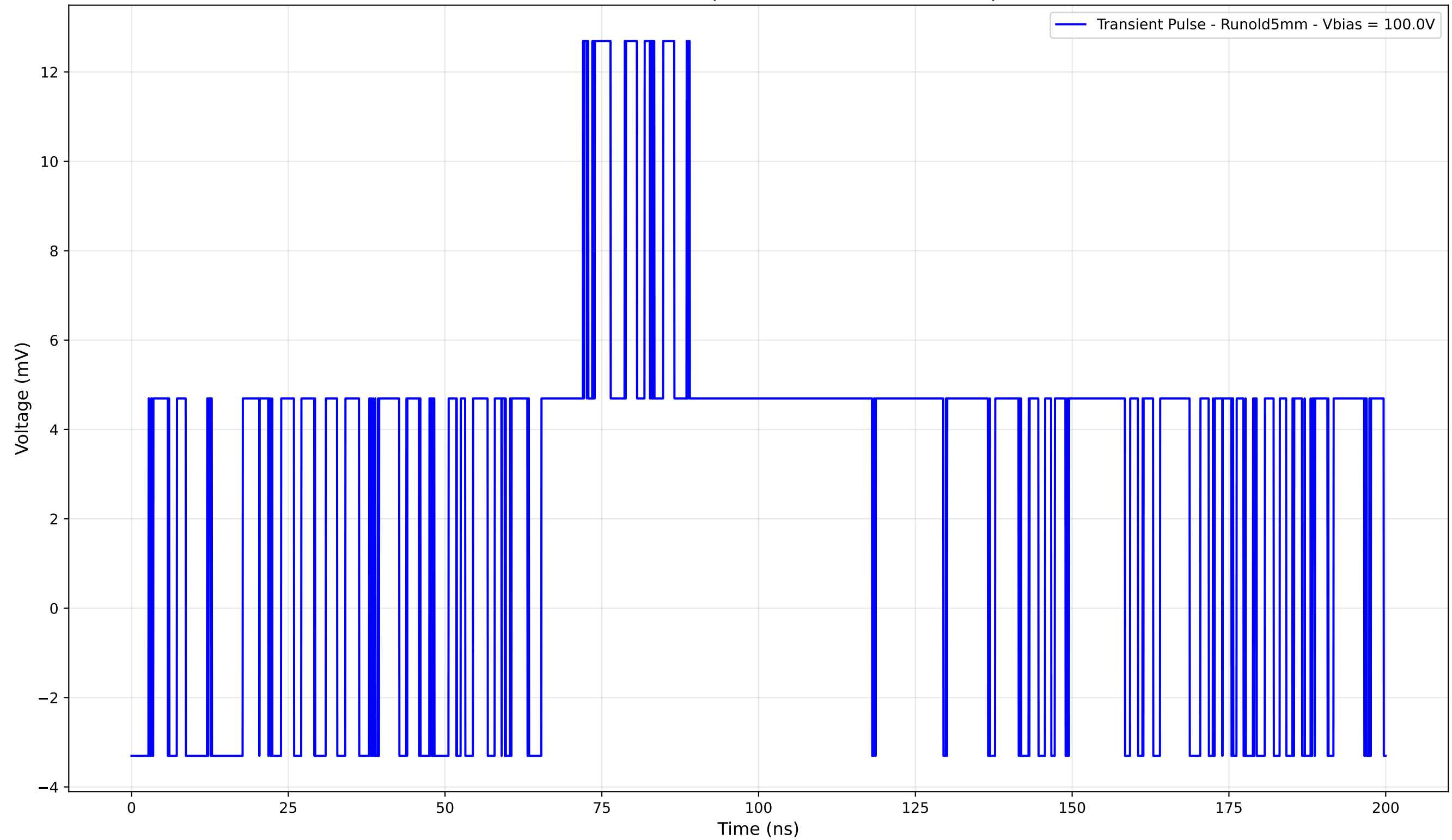
Transient Pulse - Sample: old5 - Position: 1750.0 \mu\text{m}
