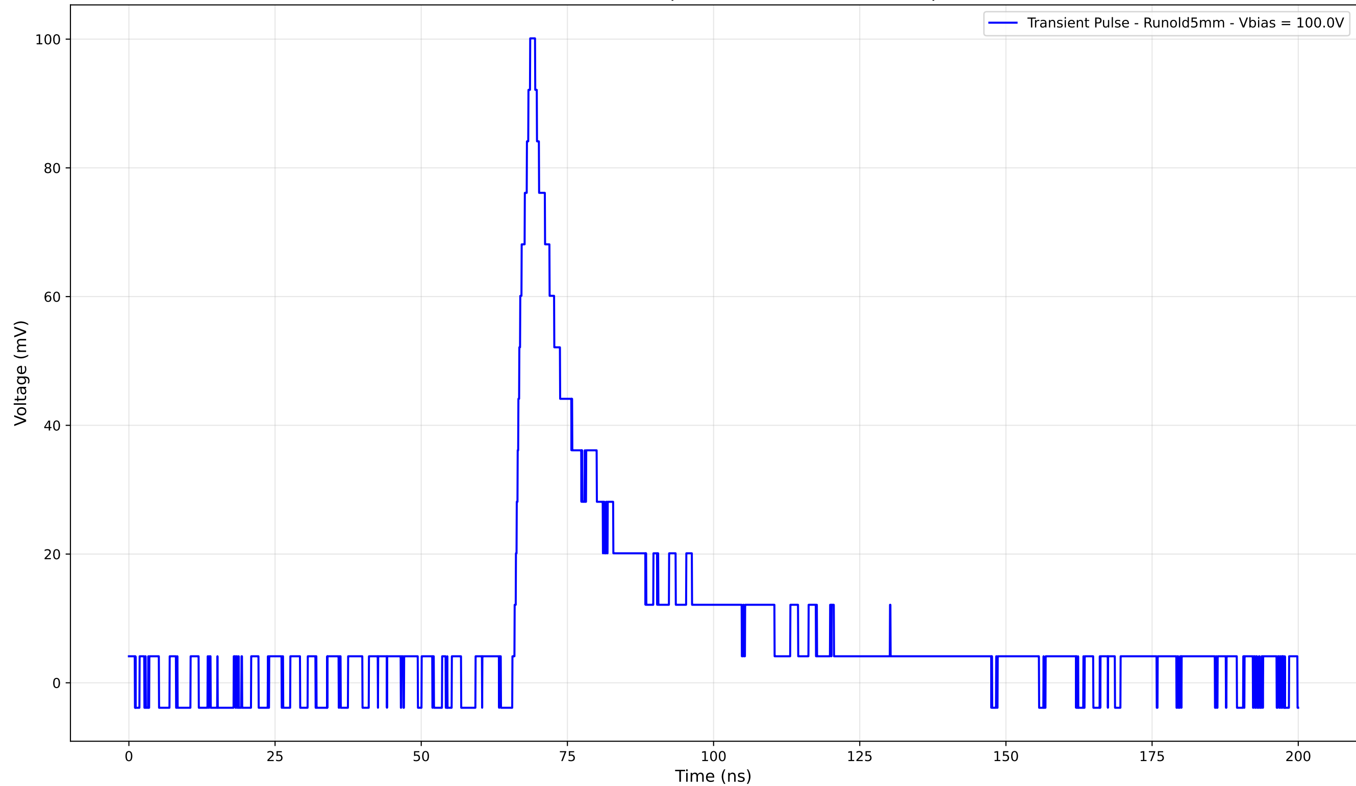
Transient Pulse - Sample: old5 - Position: 4105.0 \mu\text{m}
