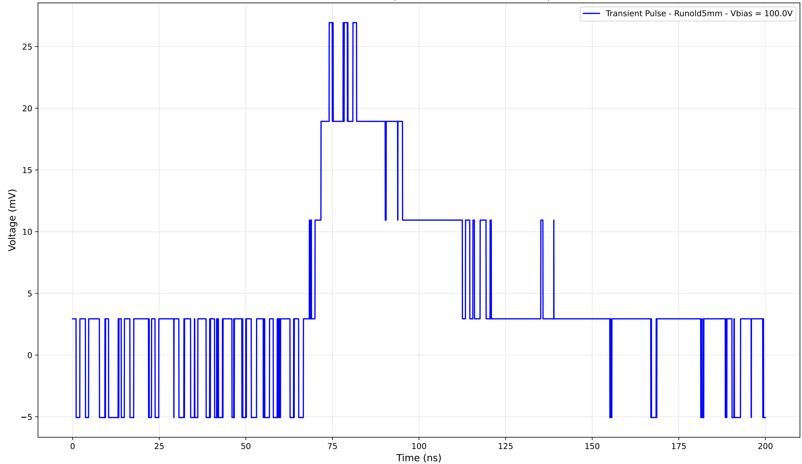
Transient Pulse - Sample: old5 - Position: 1045.0 \mu\text{m}
