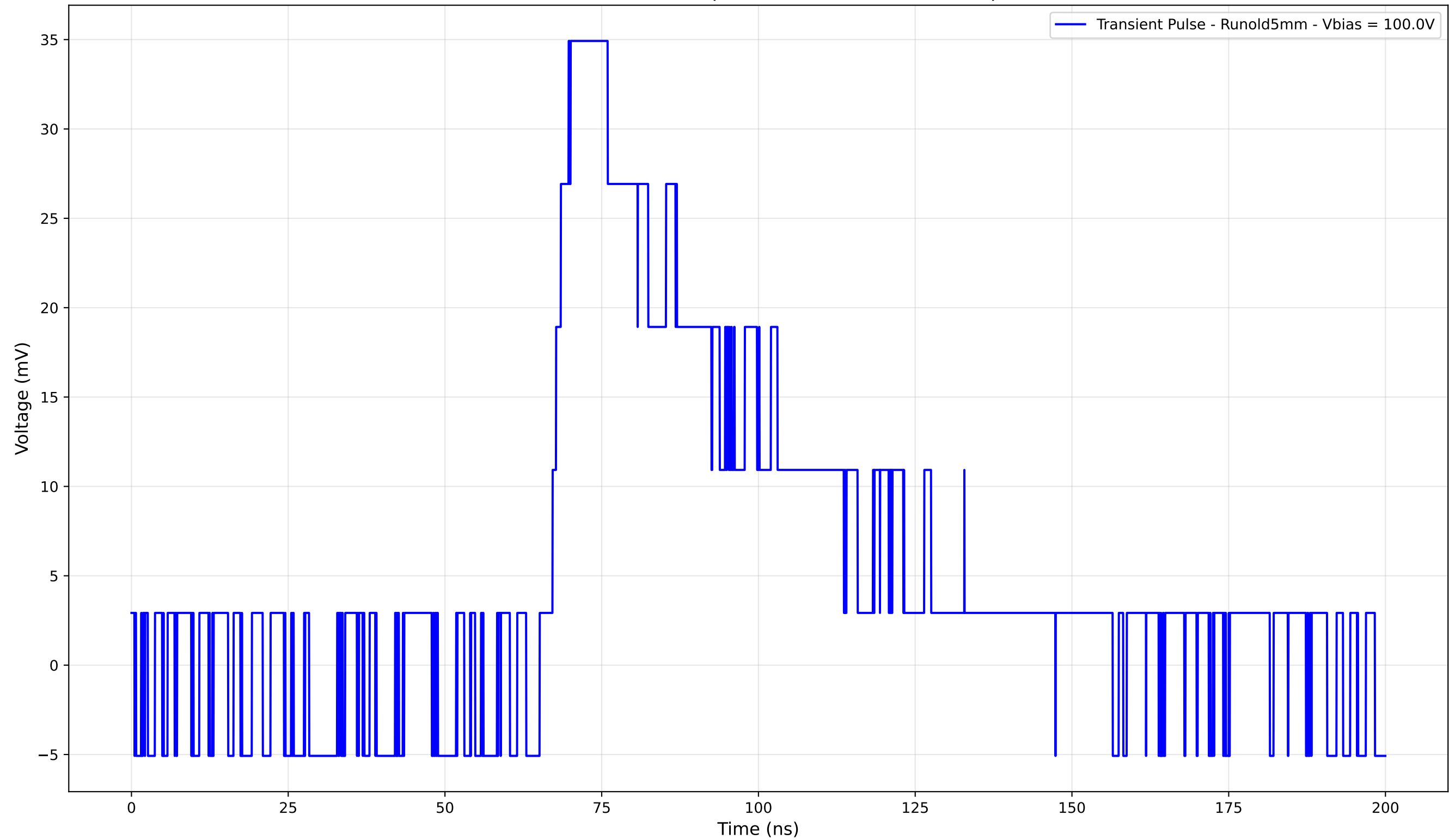
Transient Pulse - Sample: old5 - Position: 2075.0 \mu\text{m}
