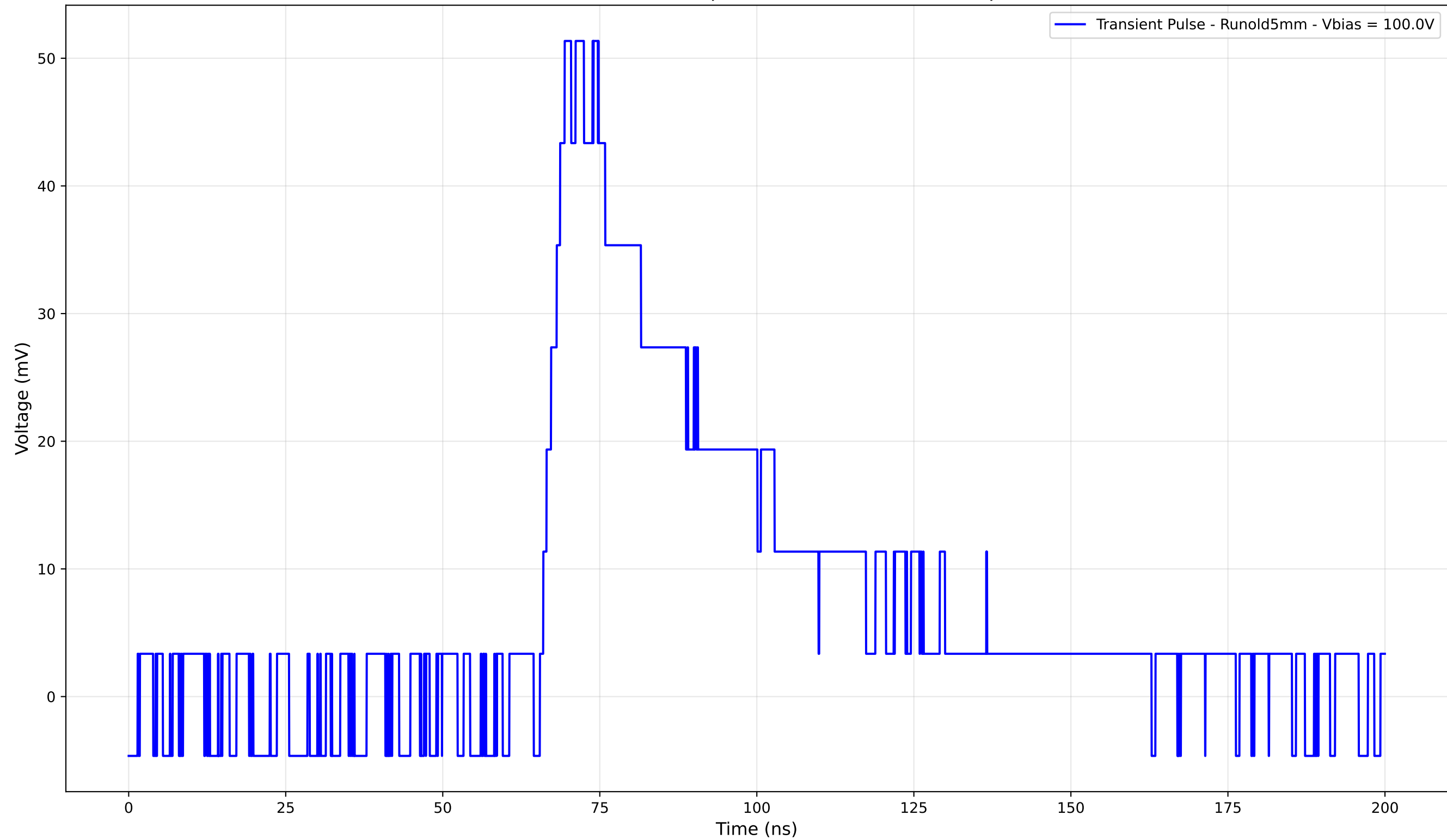
Transient Pulse - Sample: old5 - Position: 4620.0 \mu\text{m}
