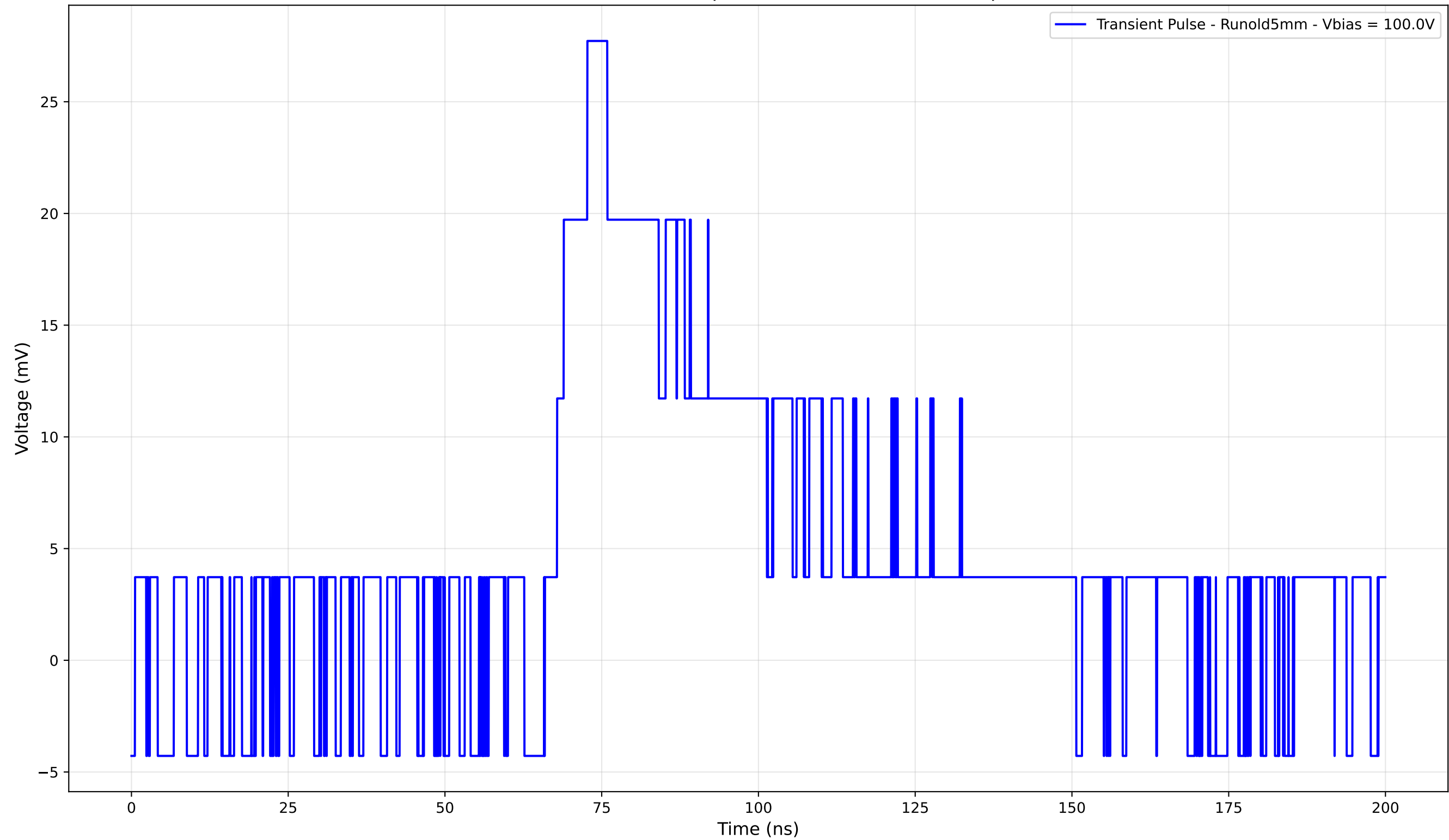
Transient Pulse - Sample: old5 - Position: 1915.0 \mu\text{m}
