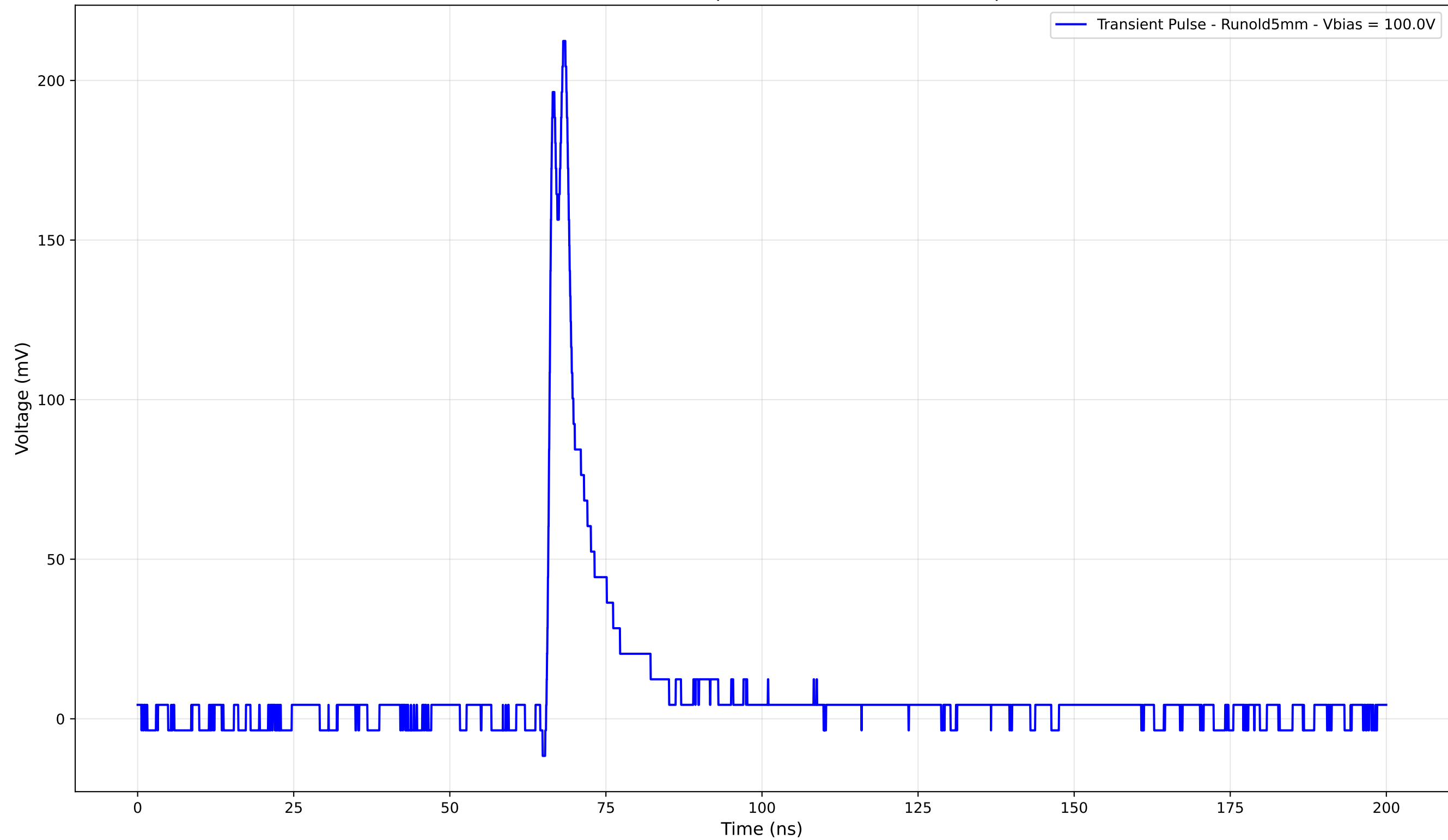
Transient Pulse - Sample: old5 - Position: 3560.0 \mu\text{m}
