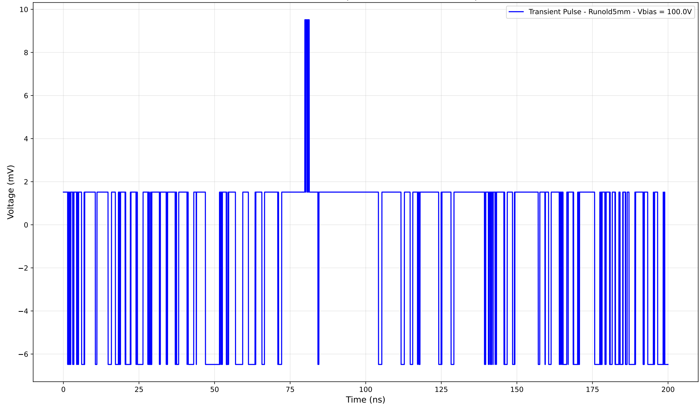
Transient Pulse - Sample: old5 - Position: 980.0 \mu\text{m}
