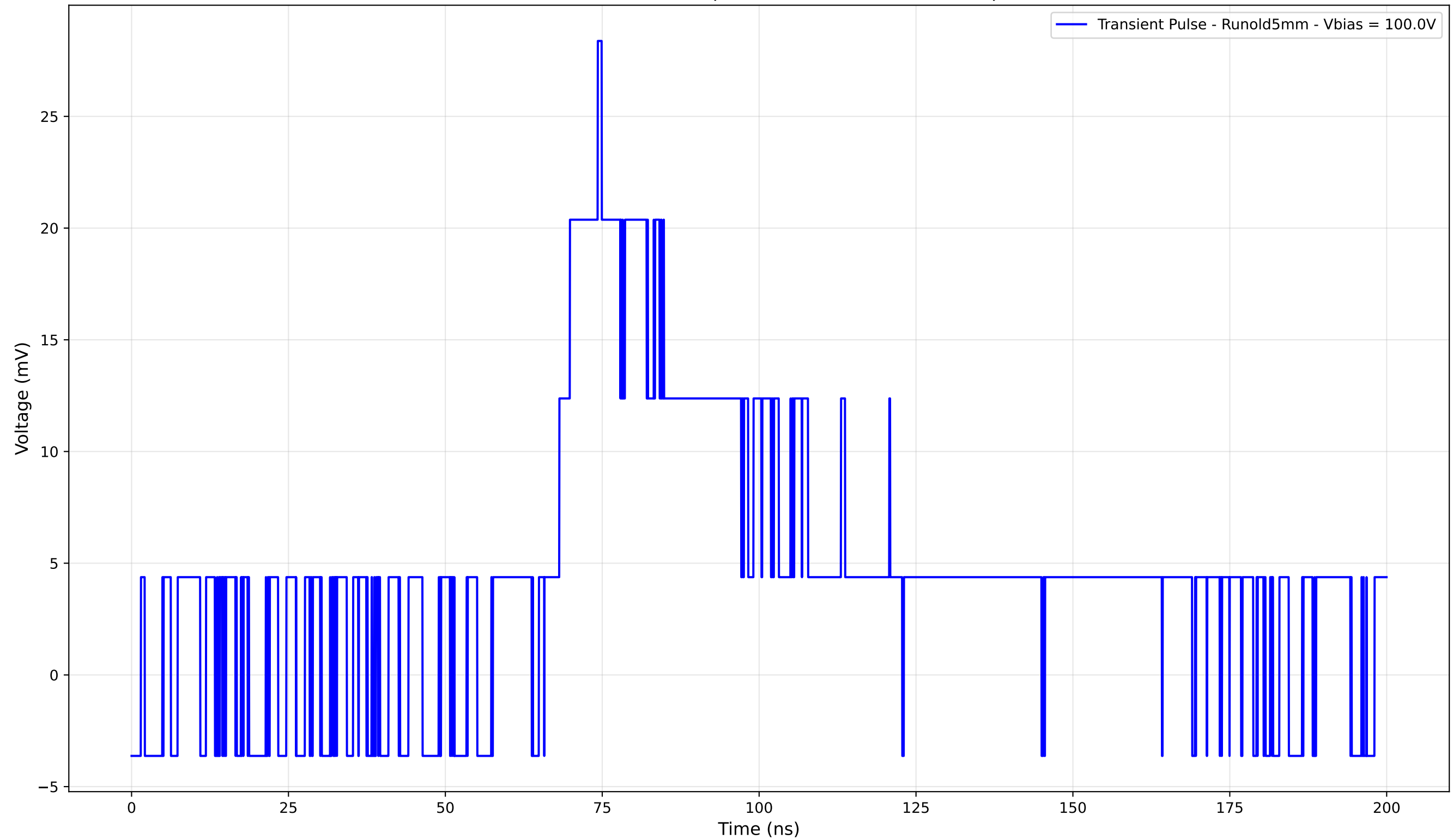
Transient Pulse - Sample: old5 - Position: 1925.0 \mu\text{m}
