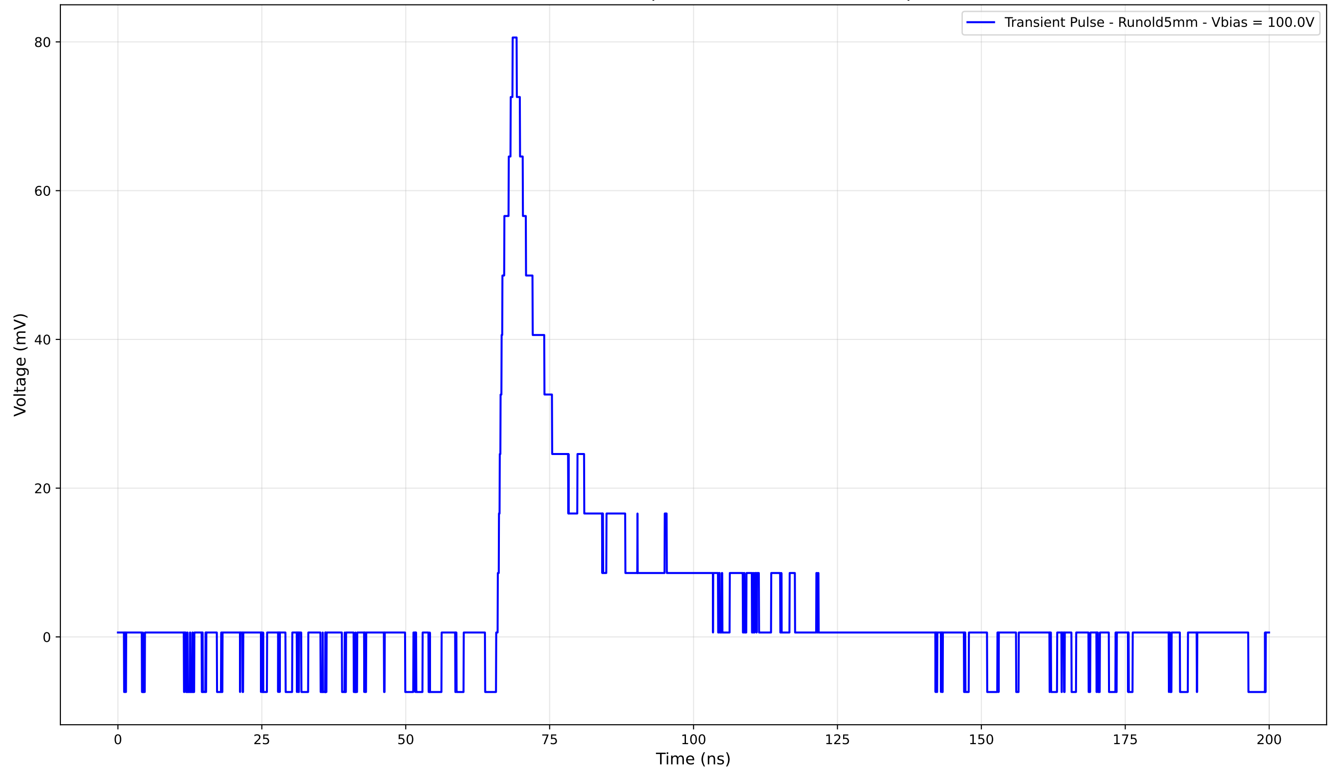
Transient Pulse - Sample: old5 - Position: 4065.0 \mu\text{m}
