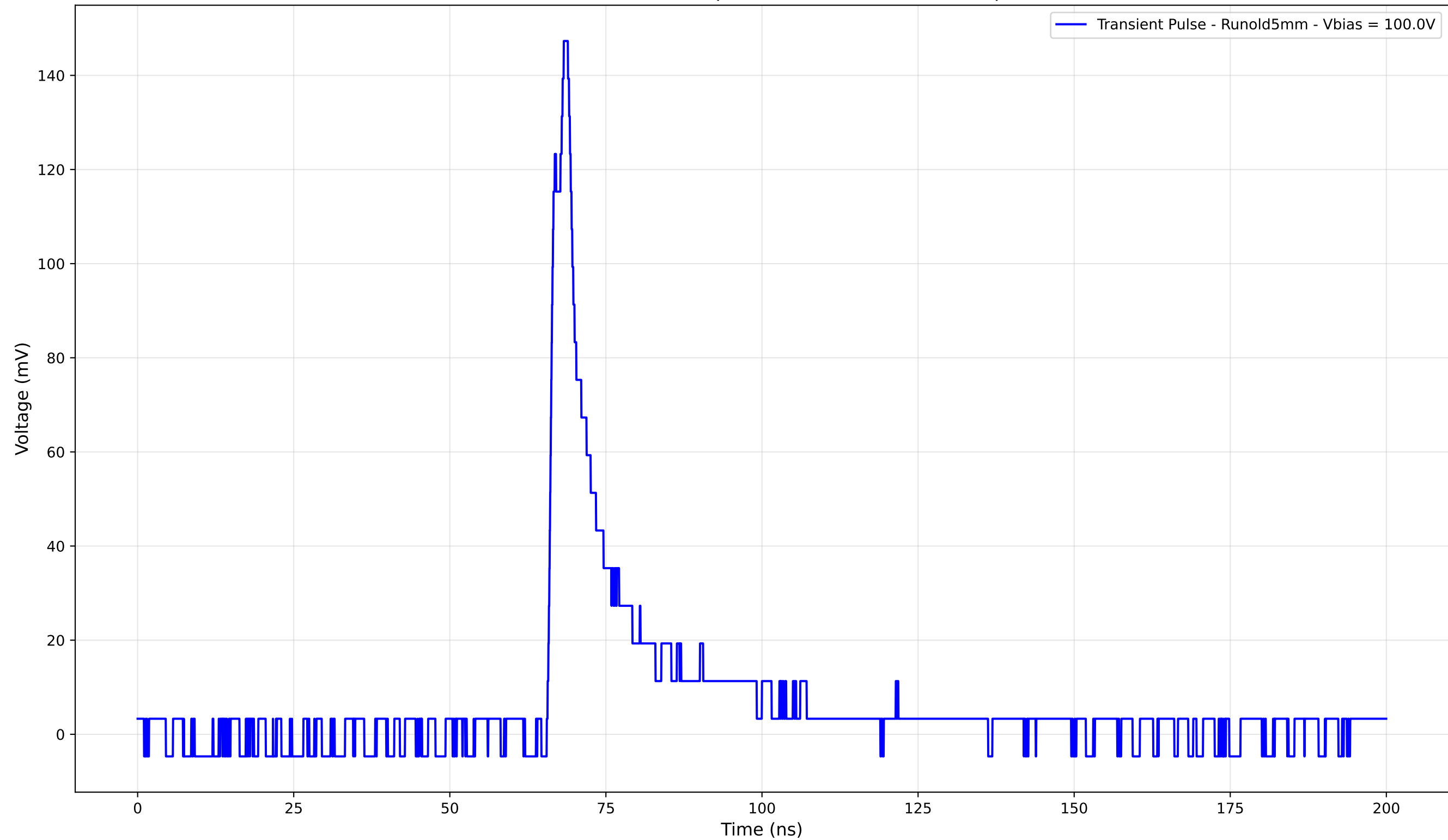
Transient Pulse - Sample: old5 - Position: 3785.0 \mu\text{m}
