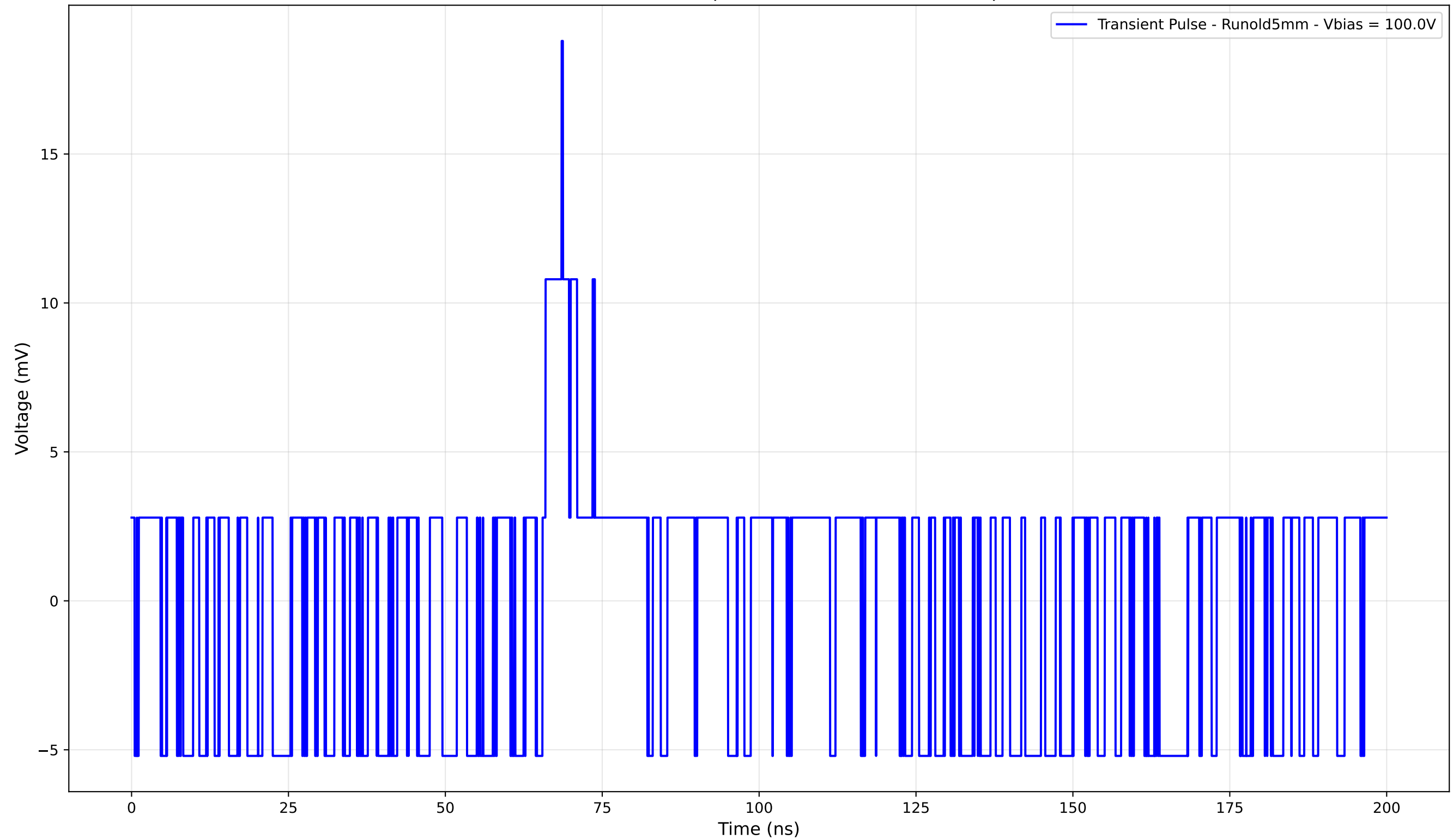
Transient Pulse - Sample: old5 - Position: 3380.0 \mu\text{m}
