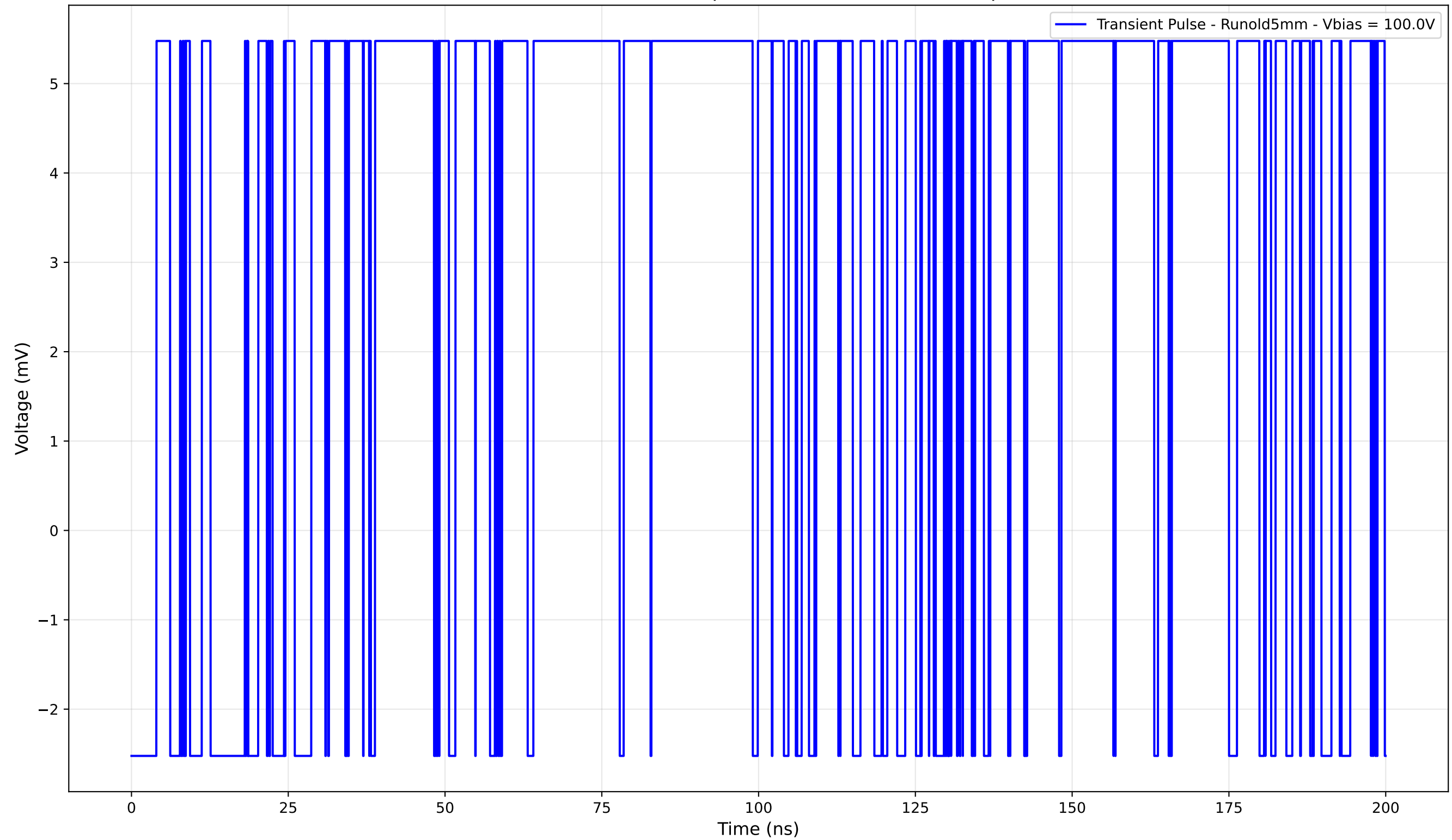
Transient Pulse - Sample: old5 - Position: 1575.0 \mu\text{m}
