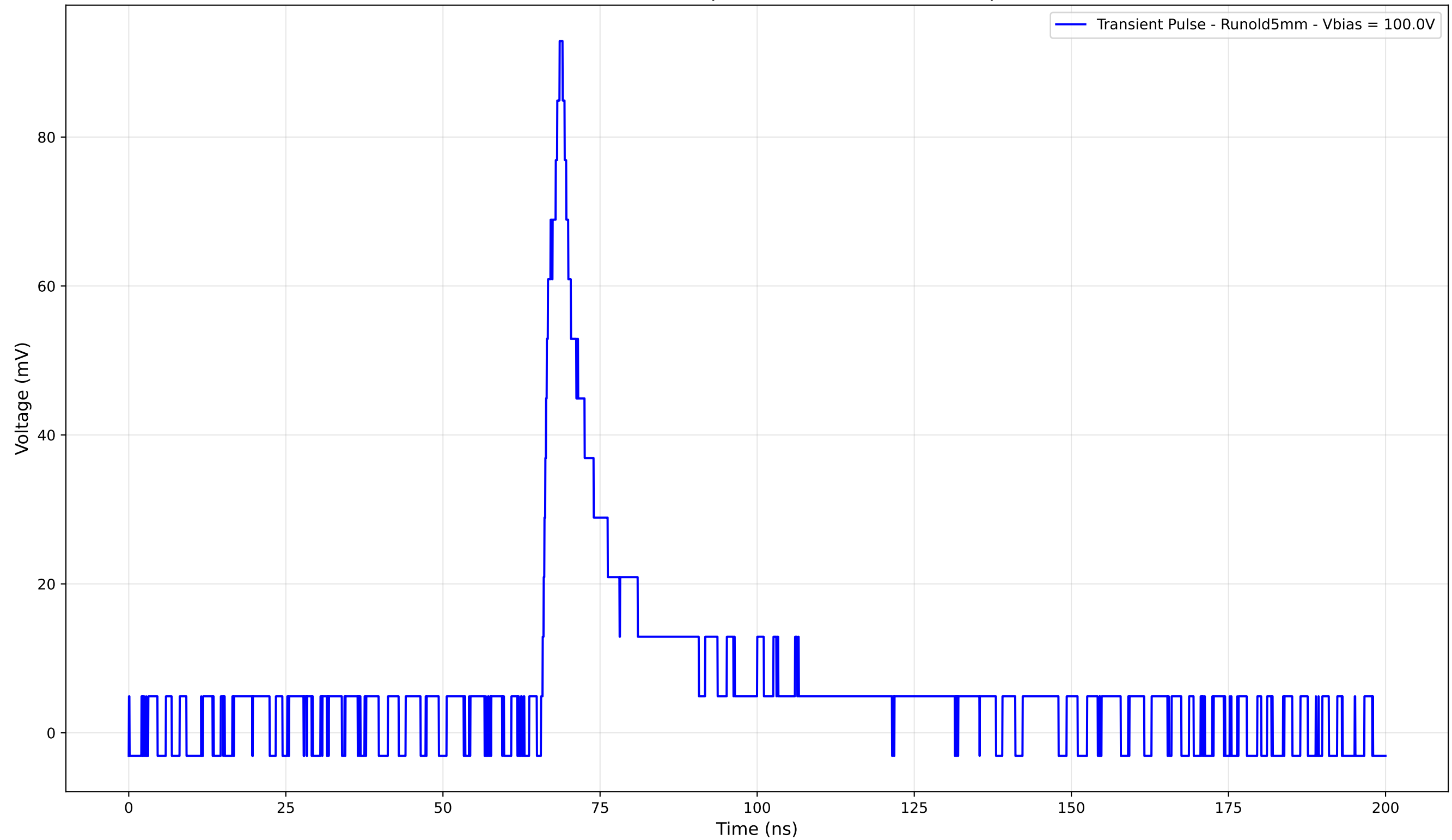
Transient Pulse - Sample: old5 - Position: 3885.0 \mu\text{m}
