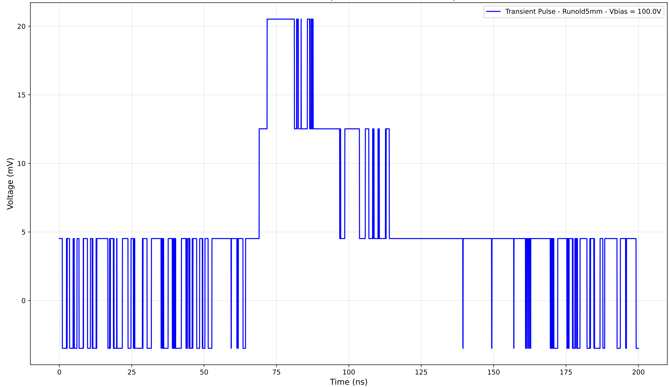
Transient Pulse - Sample: old5 - Position: 450.0 \mu\text{m}
