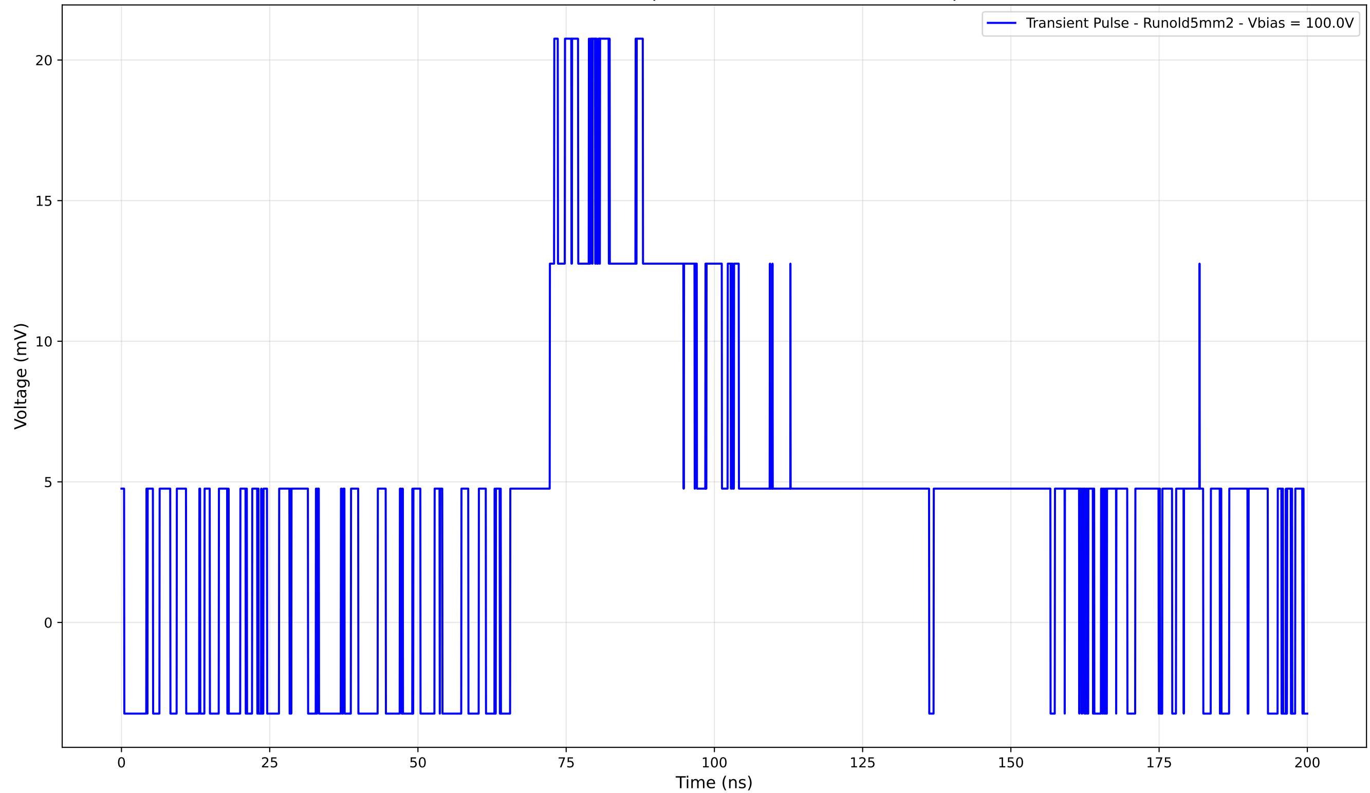
Transient Pulse - Sample: old5mm - Position: 1330.0 \mu\text{m}
