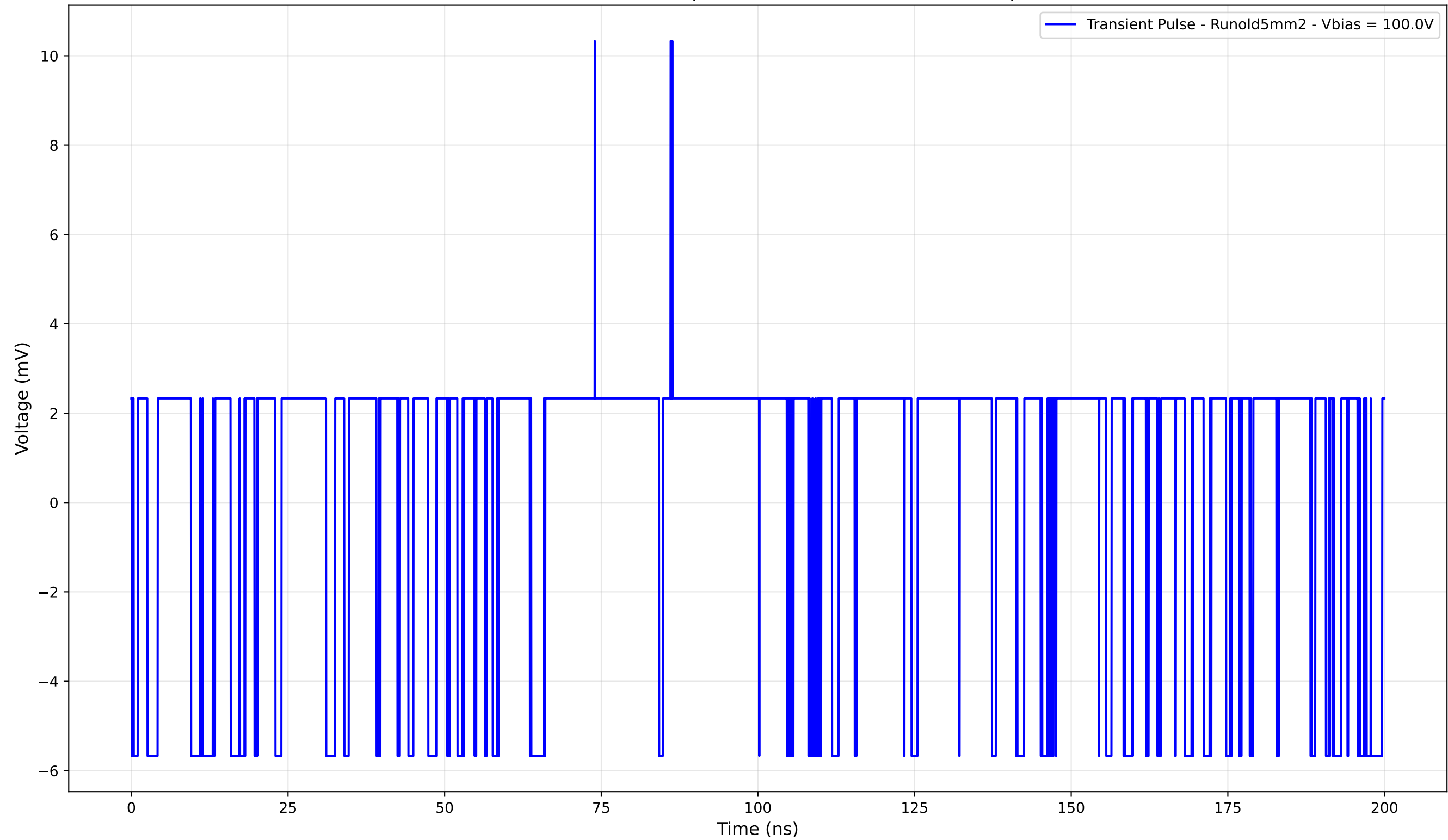
Transient Pulse - Sample: old5mm - Position: 1270.0 \mu\text{m}
