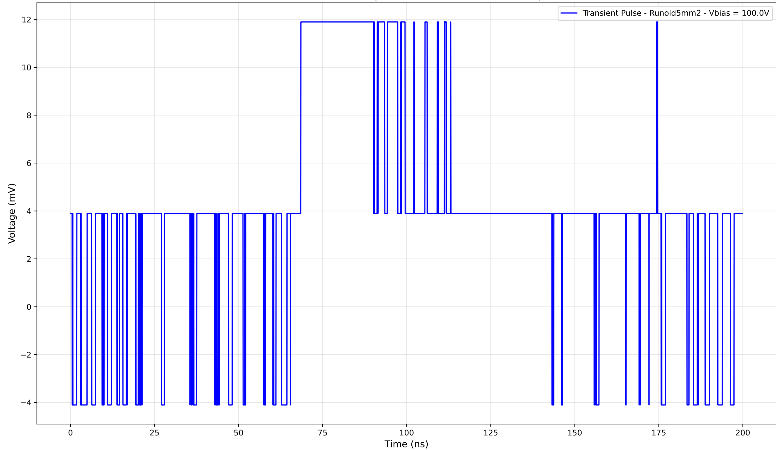
Transient Pulse - Sample: old5mm - Position: 730.0 \mu\text{m}
