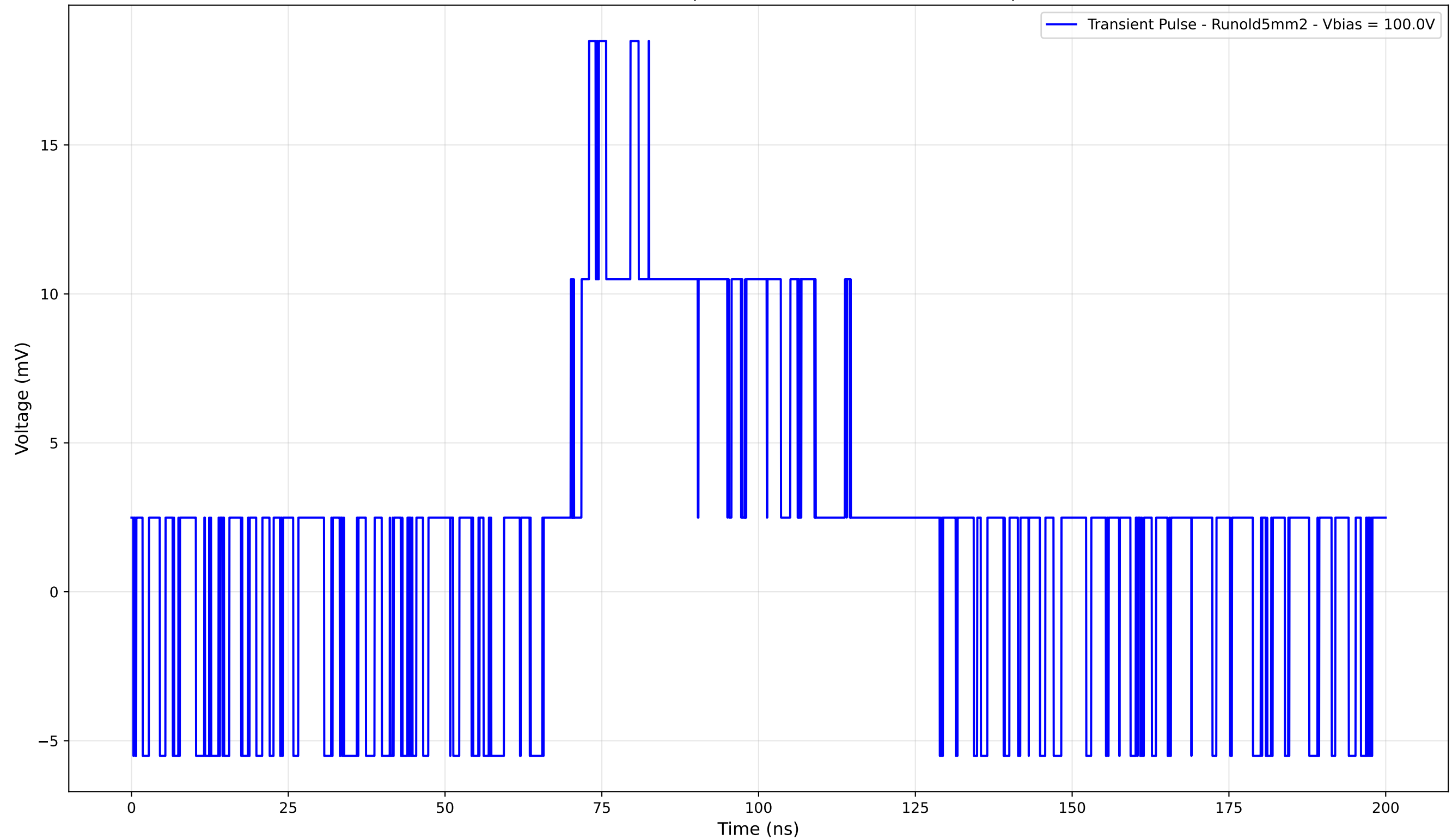
Transient Pulse - Sample: old5mm - Position: 1800.0 \mu\text{m}
