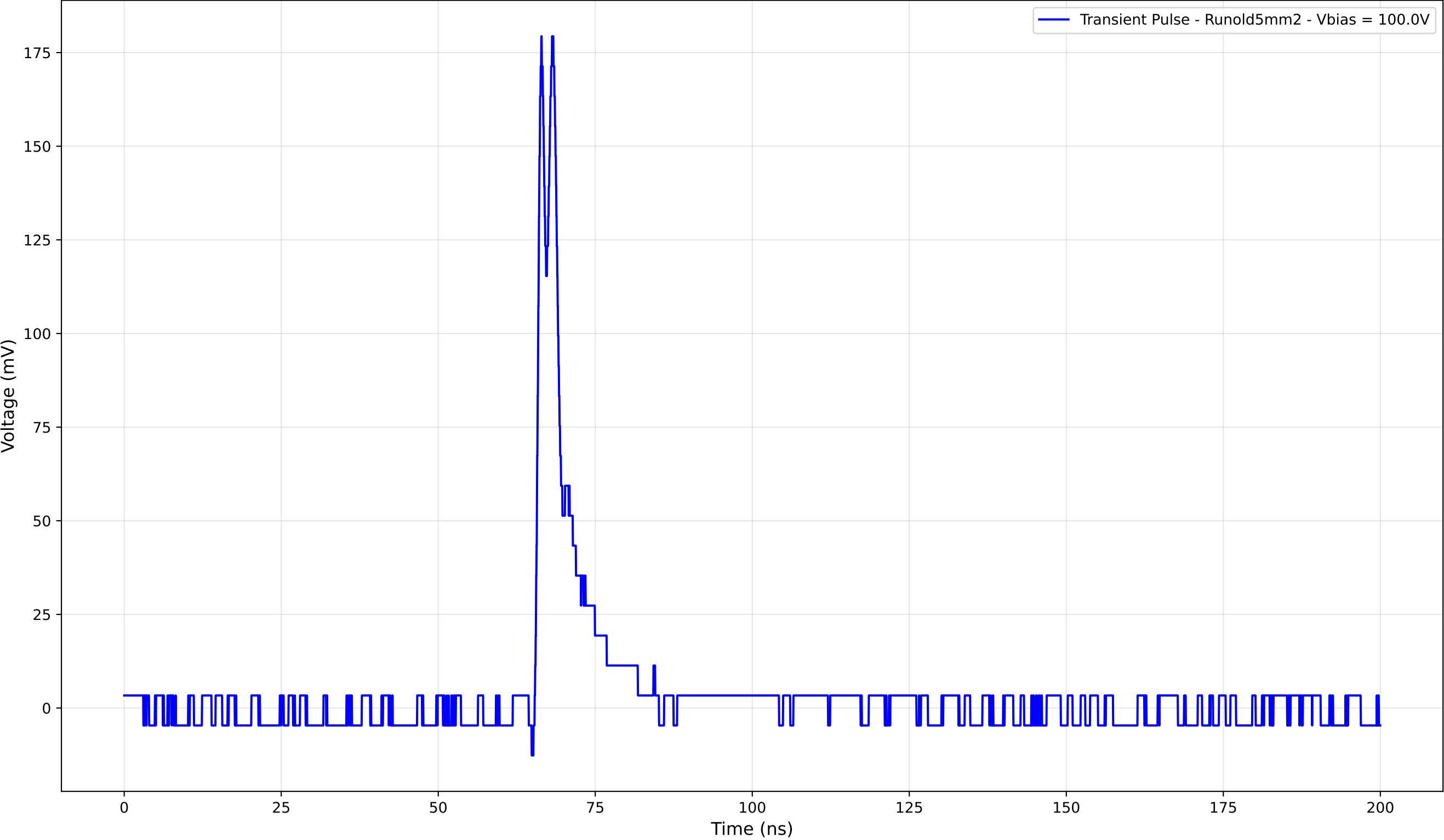
Transient Pulse - Sample: old5mm - Position: 3545.0 \mu\text{m}
