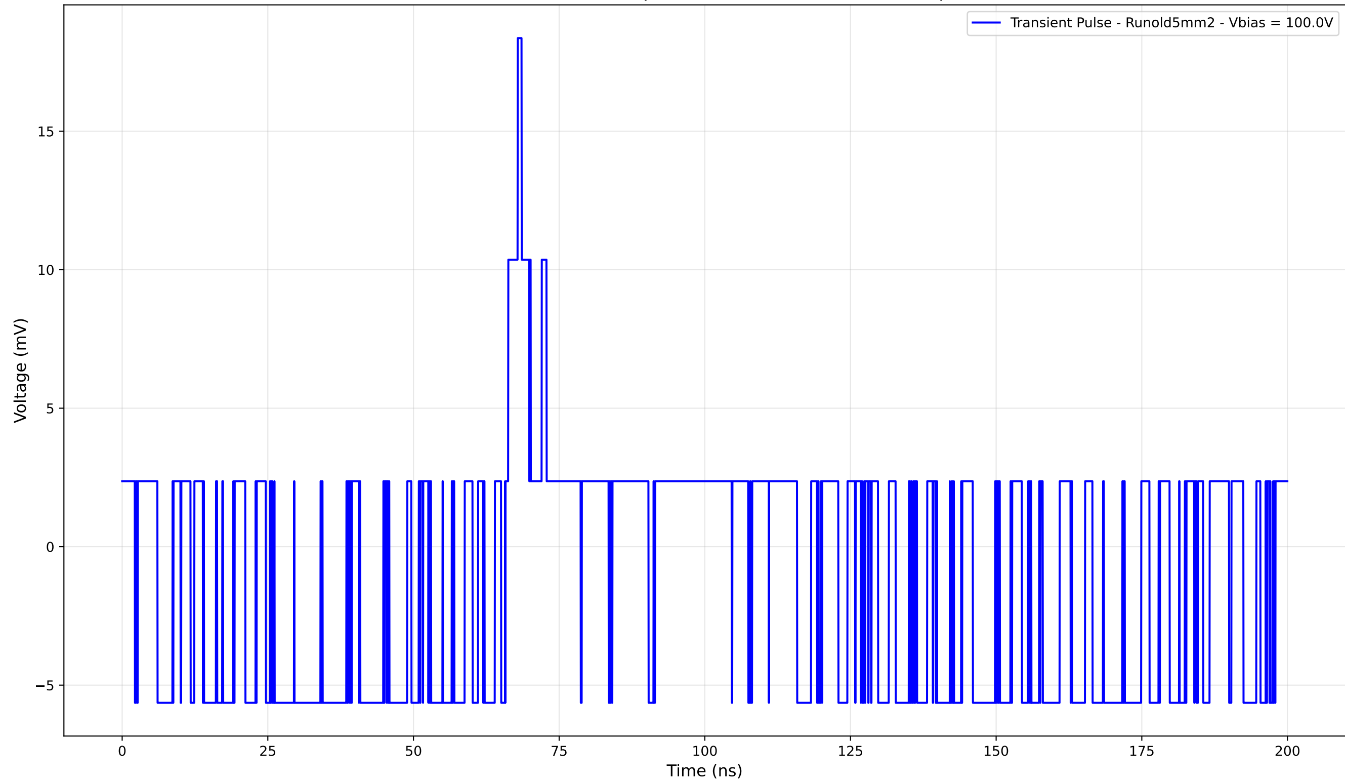
Transient Pulse - Sample: old5mm - Position: 3320.0 \mu\text{m}
