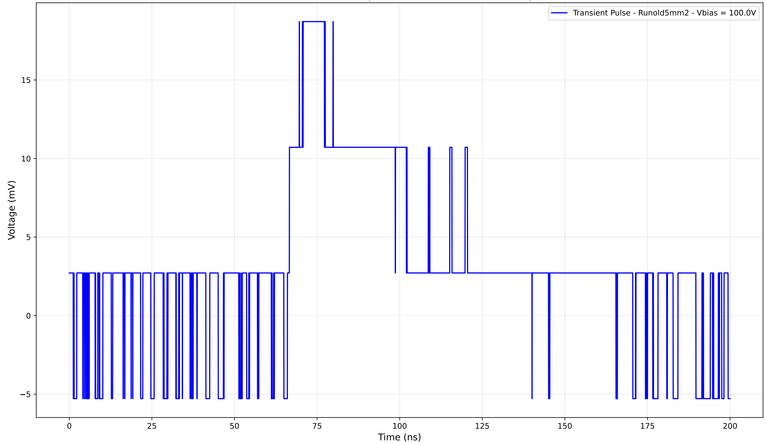
Transient Pulse - Sample: old5mm - Position: 285.0 \mu\text{m}
