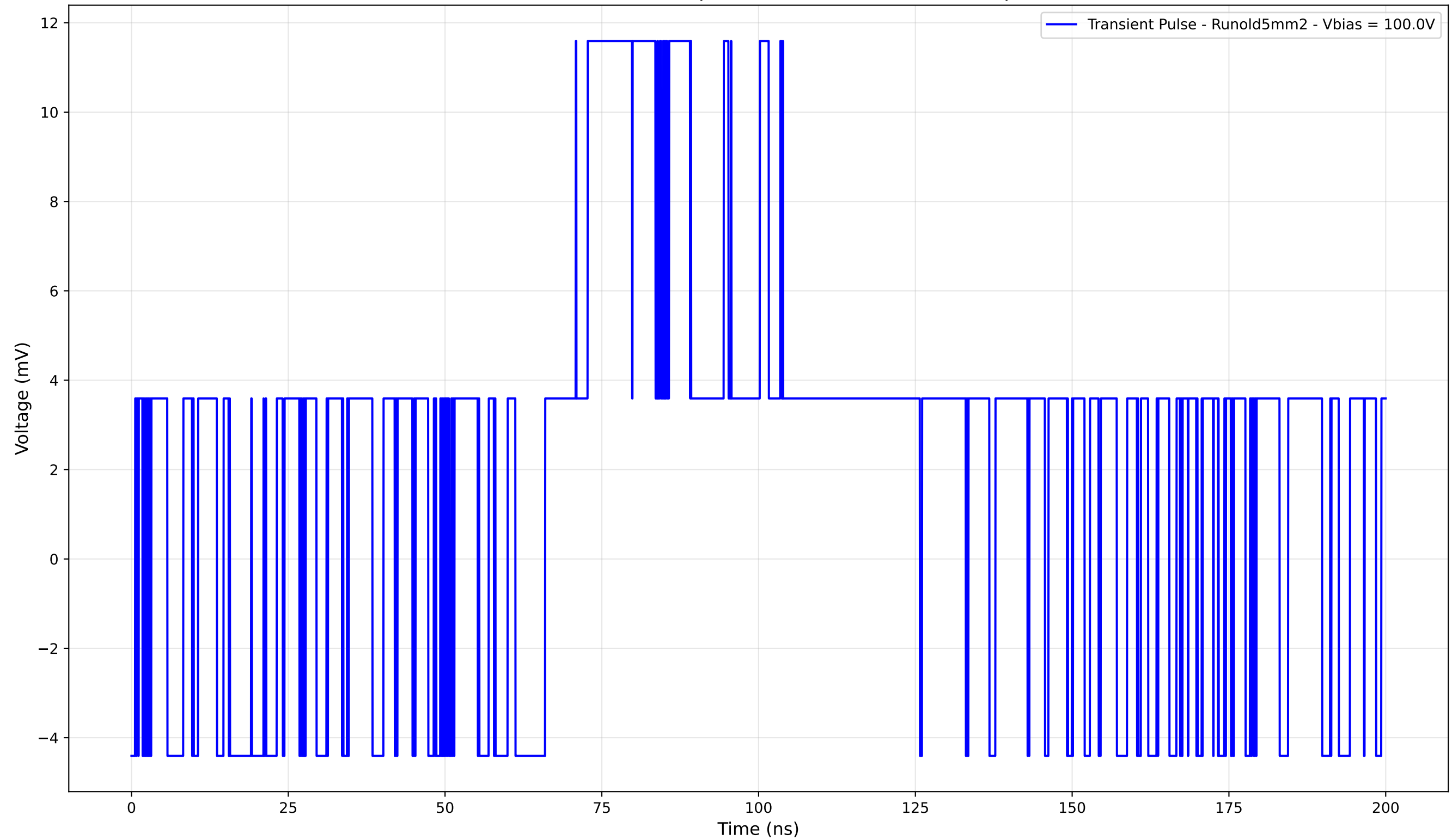
Transient Pulse - Sample: old5mm - Position: 805.0 \mu\text{m}
