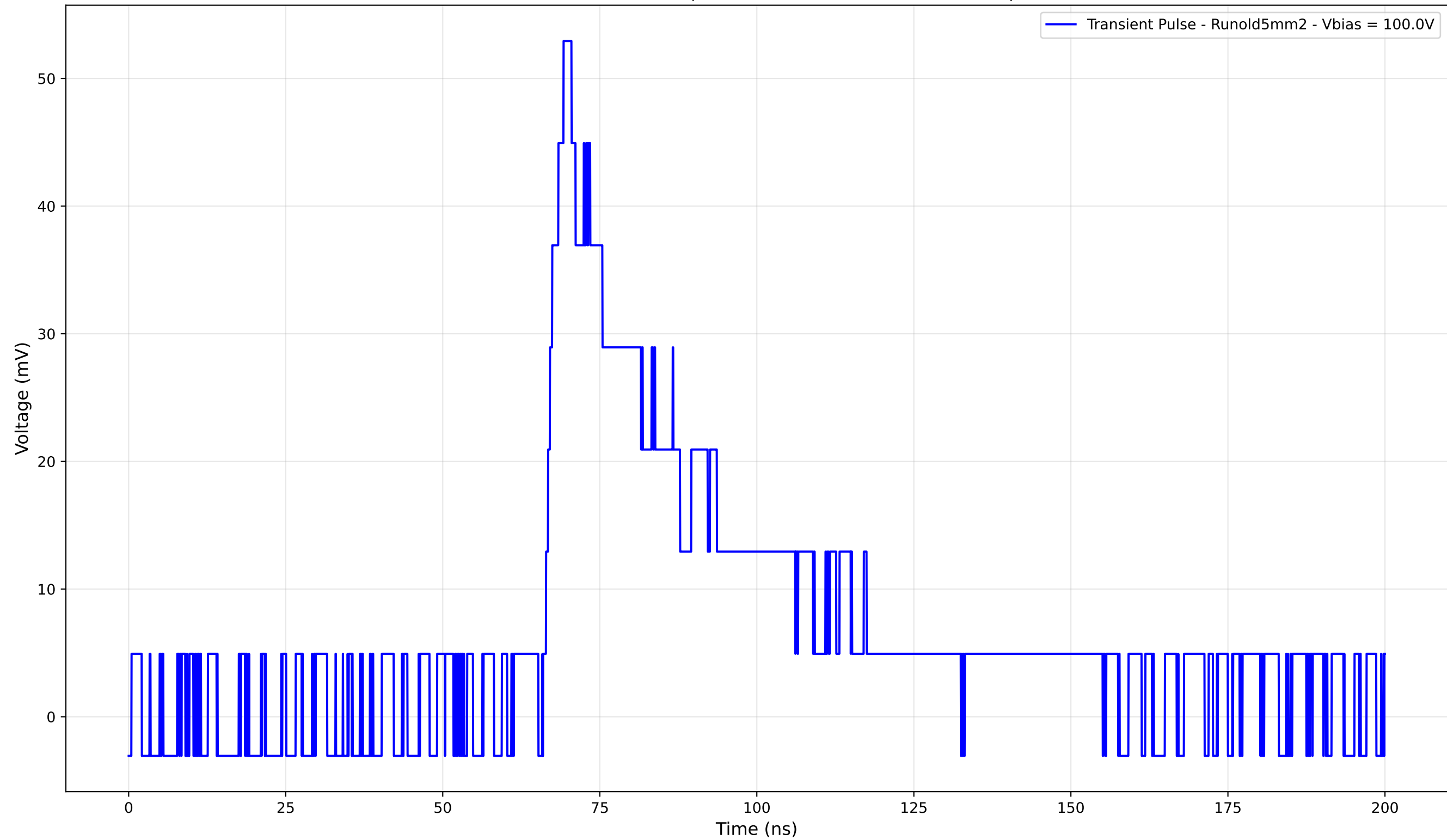
Transient Pulse - Sample: old5mm - Position: 4715.0 \mu\text{m}
