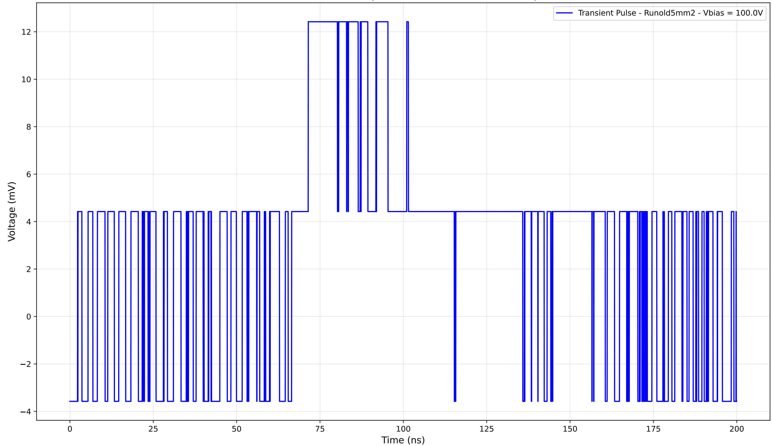
Transient Pulse - Sample: old5mm - Position: 855.0 \mu\text{m}
