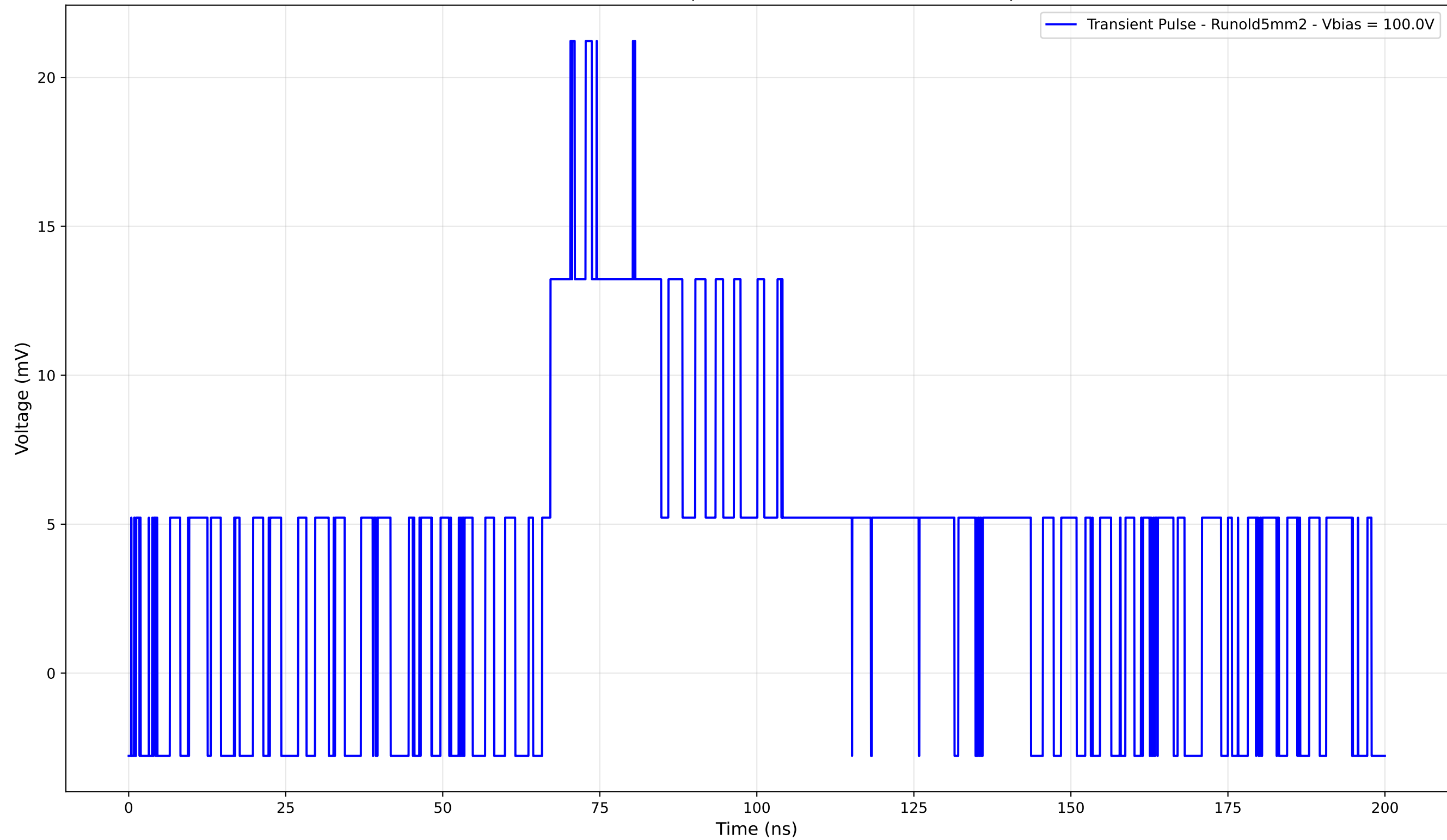
Transient Pulse - Sample: old5mm - Position: 2425.0 \mu\text{m}
