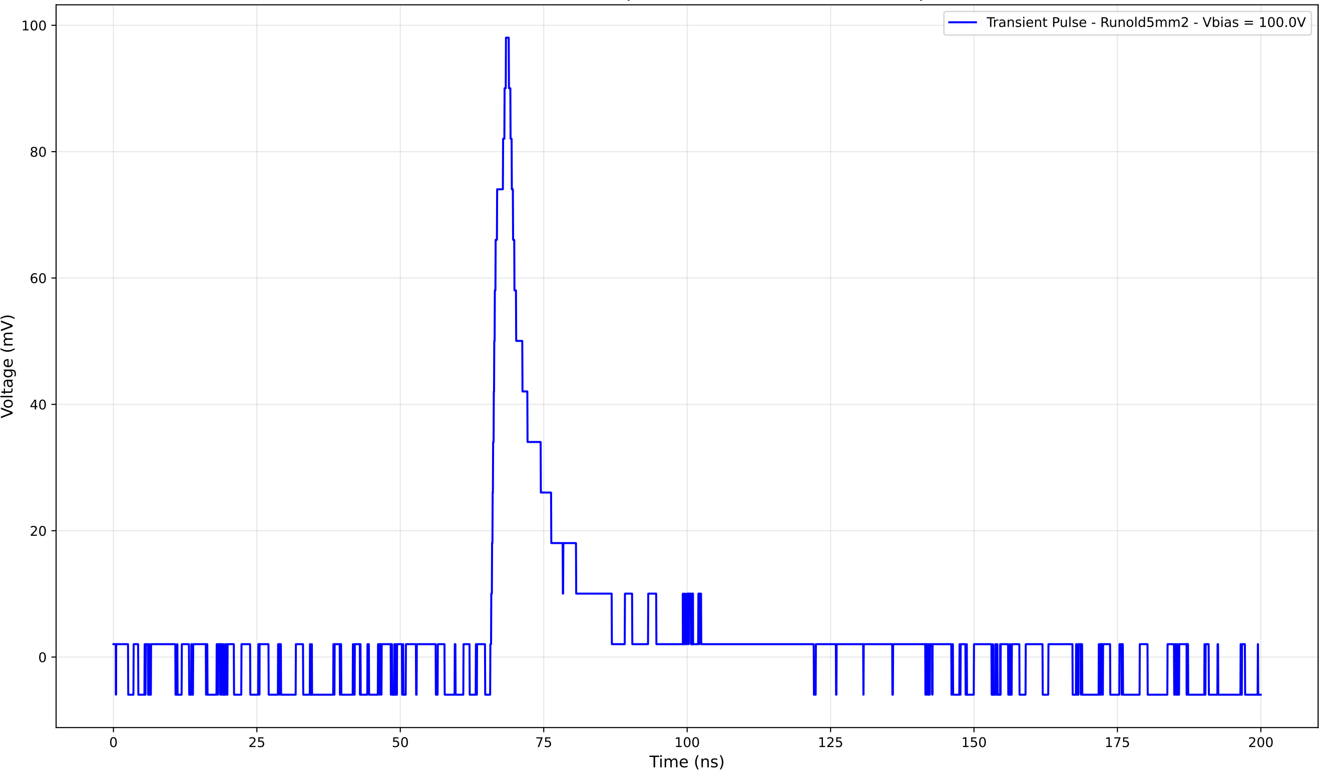
Transient Pulse - Sample: old5mm - Position: 3190.0 \mu\text{m}
