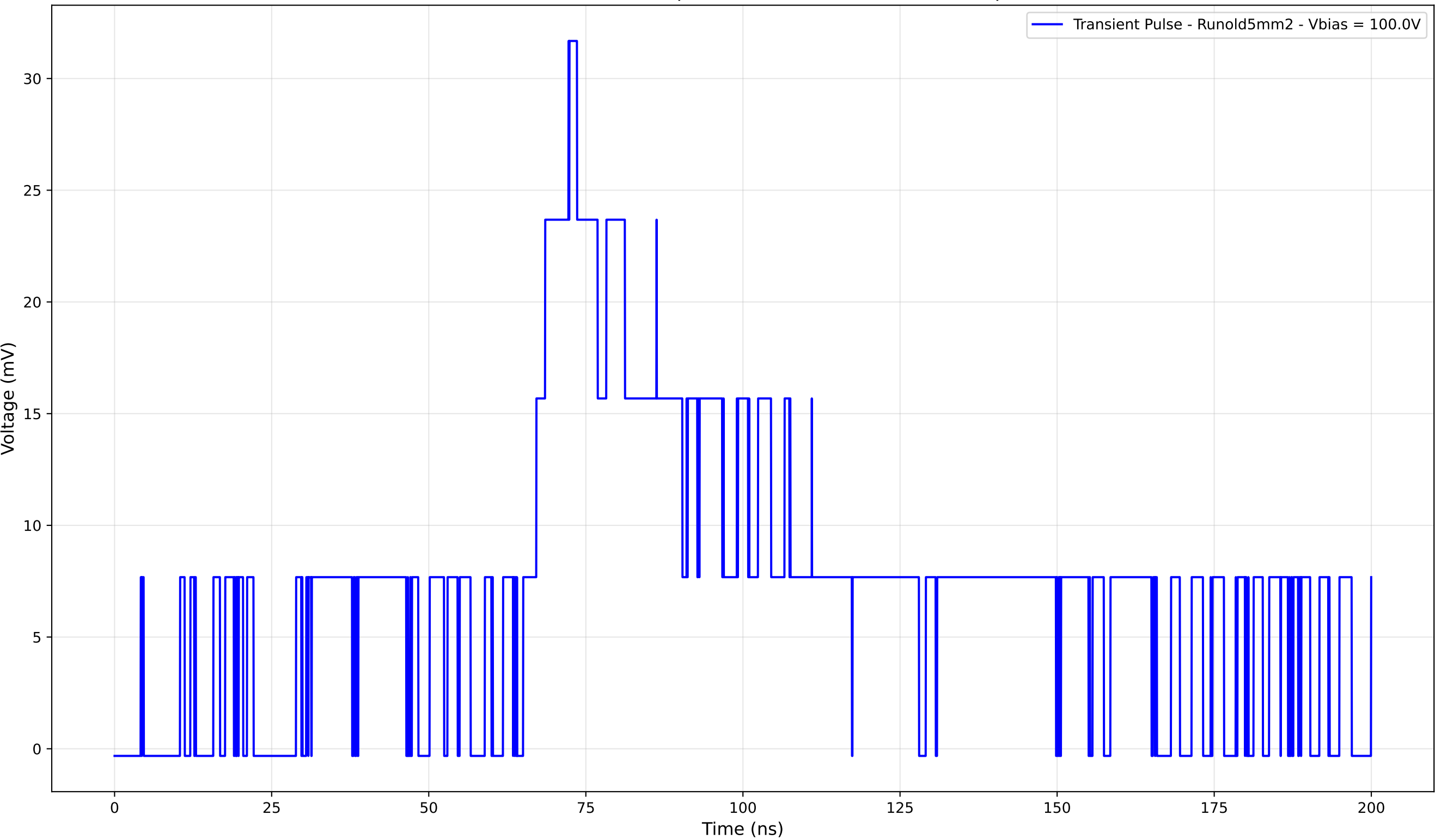
Transient Pulse - Sample: old5mm - Position: 2400.0 \mu\text{m}
