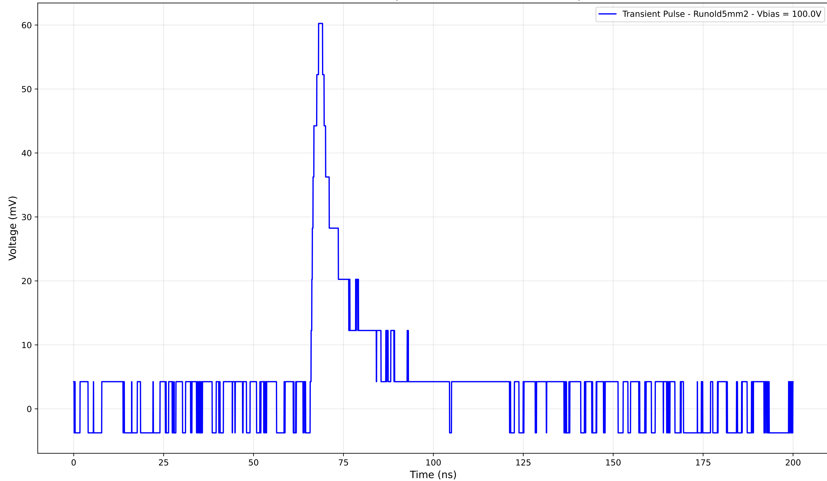
Transient Pulse - Sample: old5mm - Position: 4180.0 \mu\text{m}
