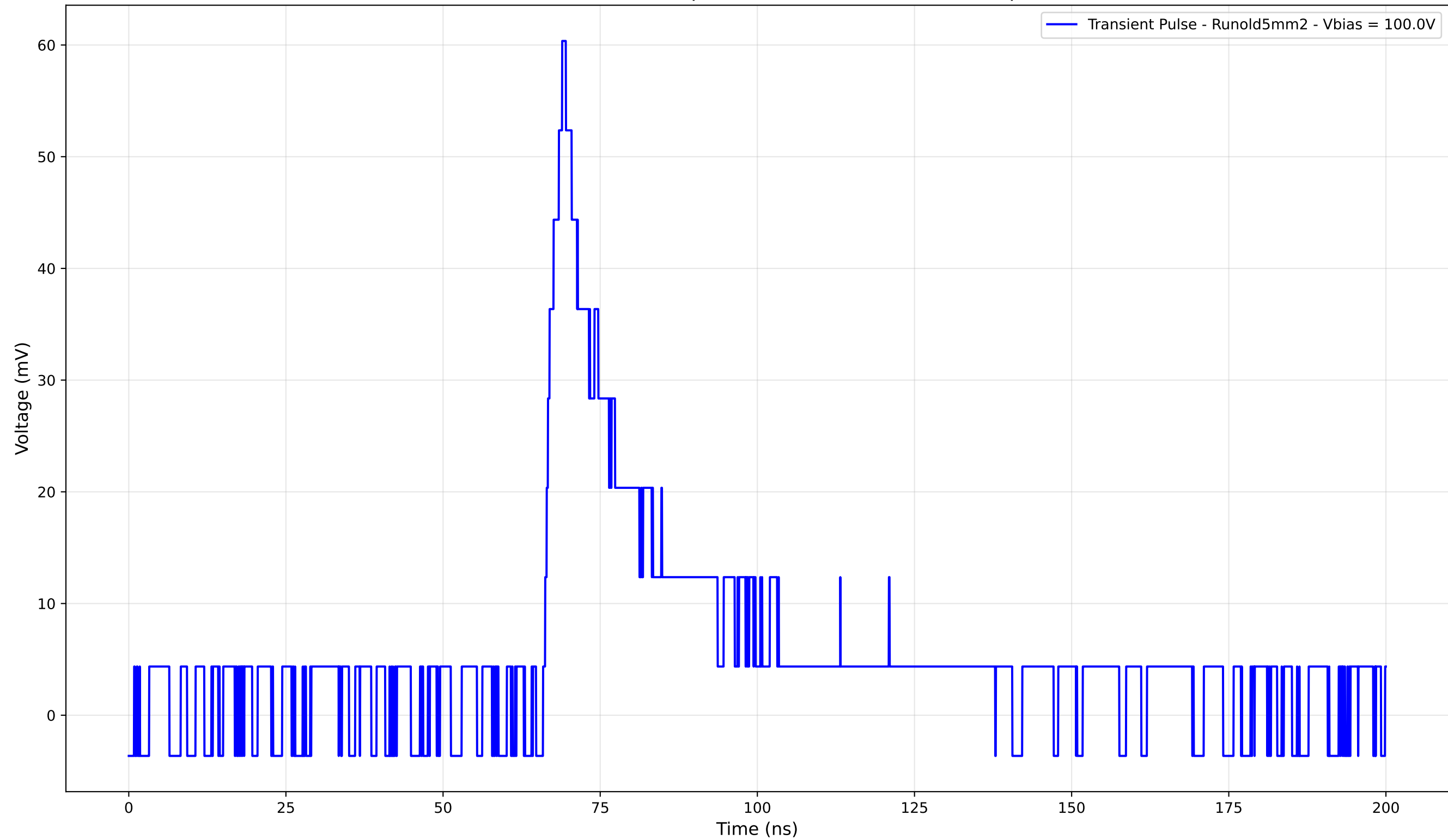
Transient Pulse - Sample: old5mm - Position: 4465.0 \mu\text{m}
