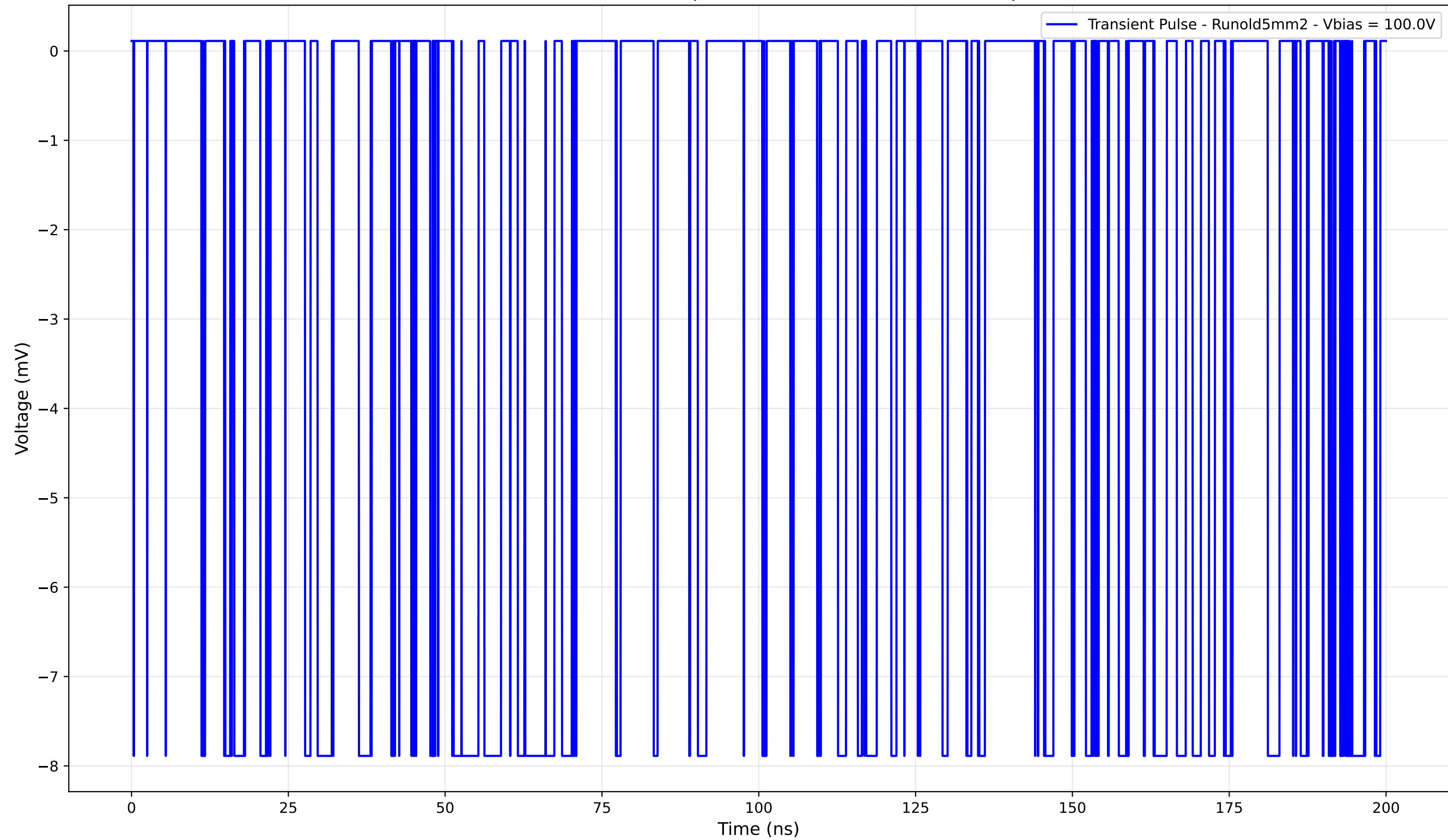
Transient Pulse - Sample: old5mm - Position: 1655.0 \mu\text{m}
