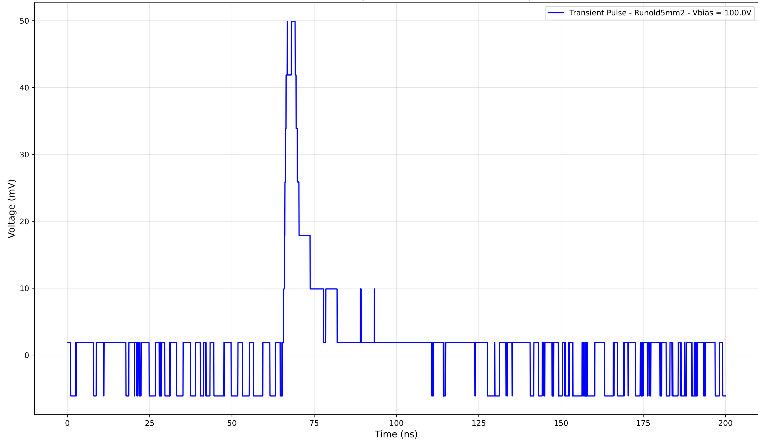
Transient Pulse - Sample: old5mm - Position: 4025.0 \mu\text{m}
