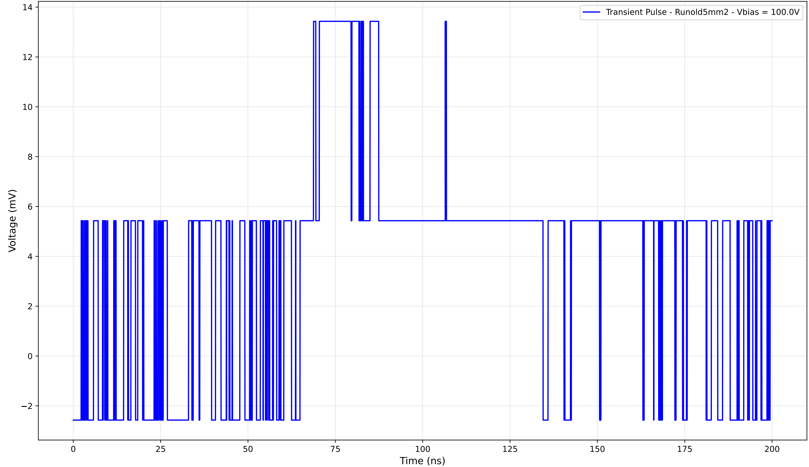
Transient Pulse - Sample: old5mm - Position: 360.0 \mu\text{m}
