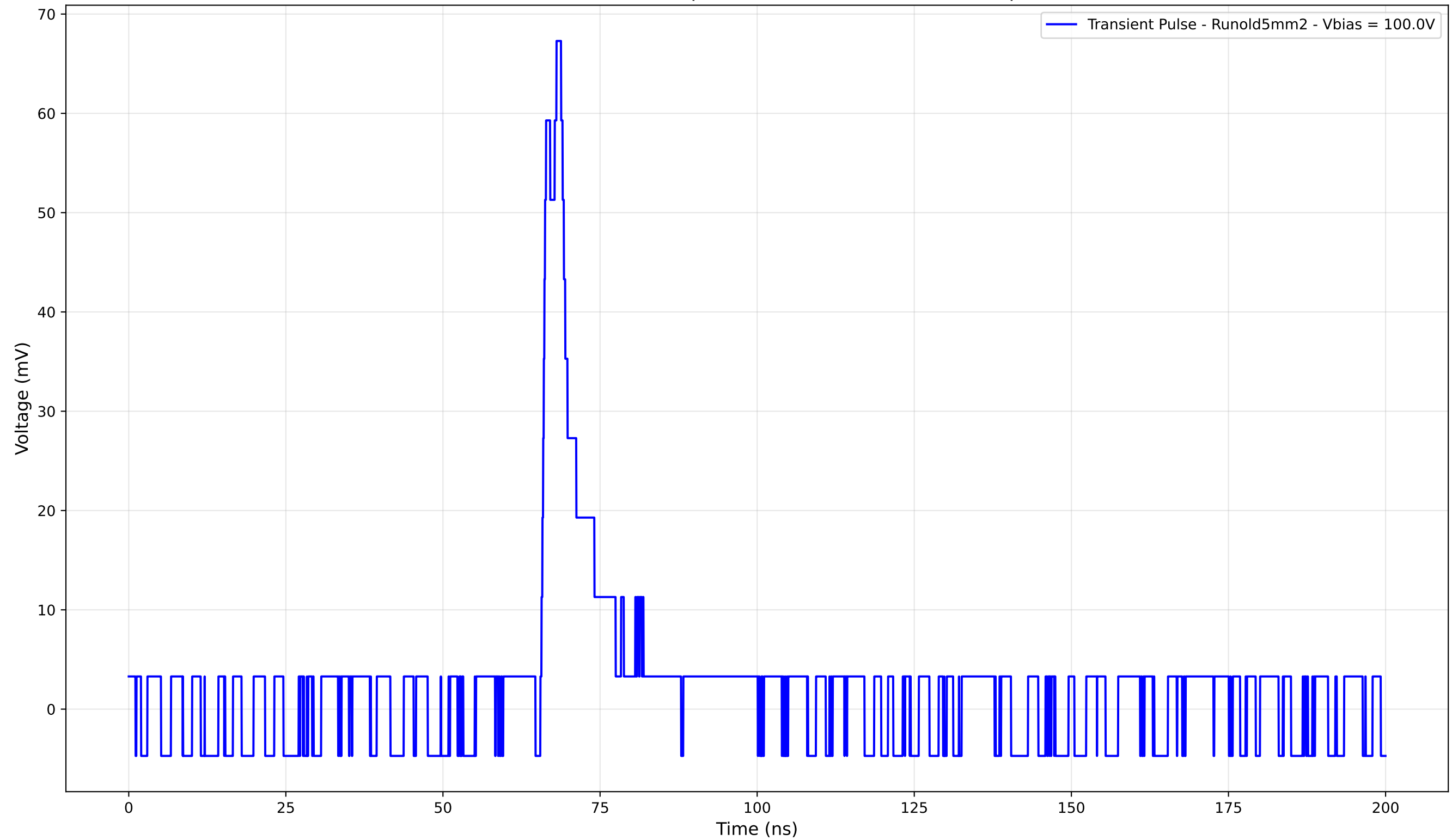
Transient Pulse - Sample: old5mm - Position: 3895.0 \mu\text{m}
