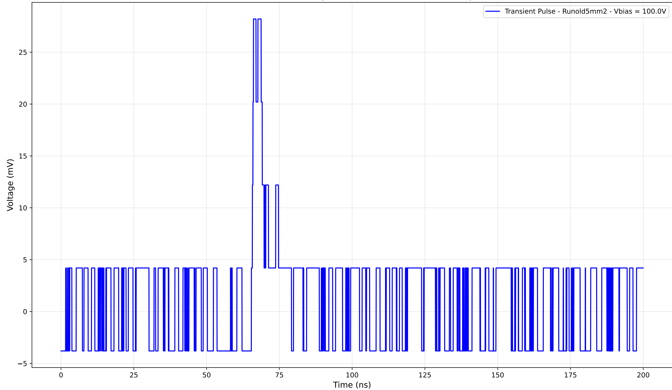
Transient Pulse - Sample: old5mm - Position: 3620.0 \mu\text{m}
