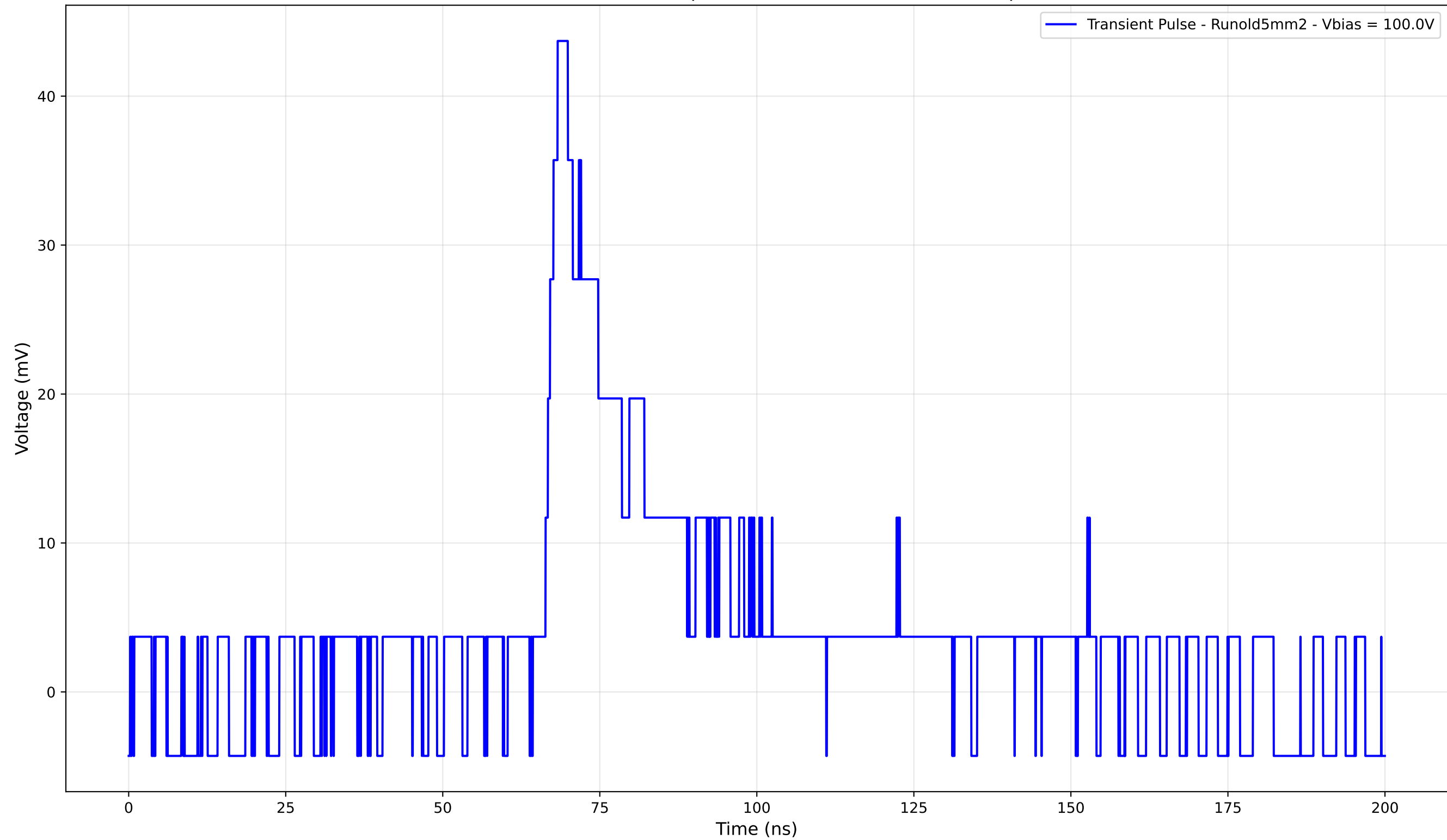
Transient Pulse - Sample: old5mm - Position: 4485.0 \mu\text{m}
