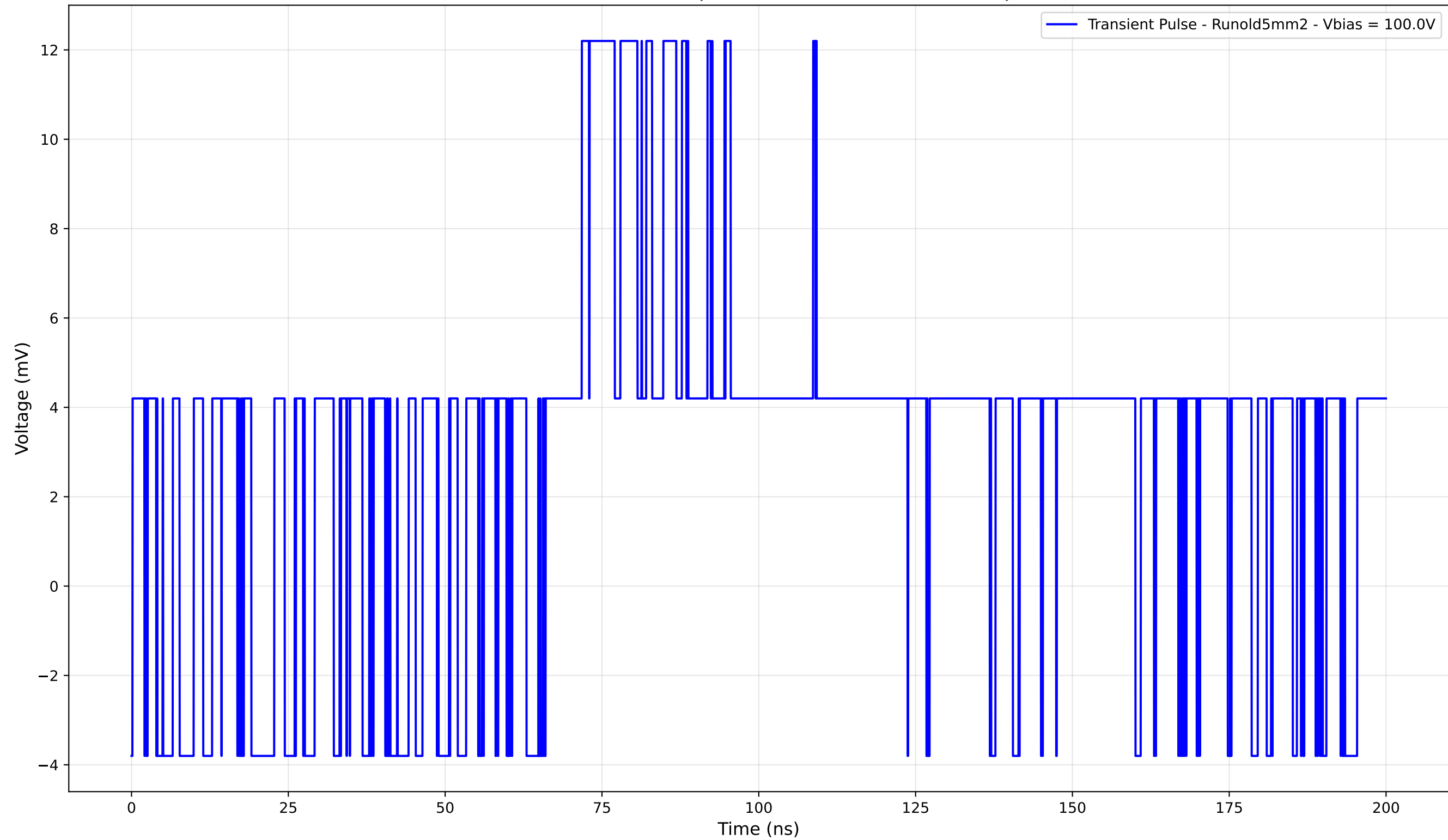
Transient Pulse - Sample: old5mm - Position: 965.0 \mu\text{m}
