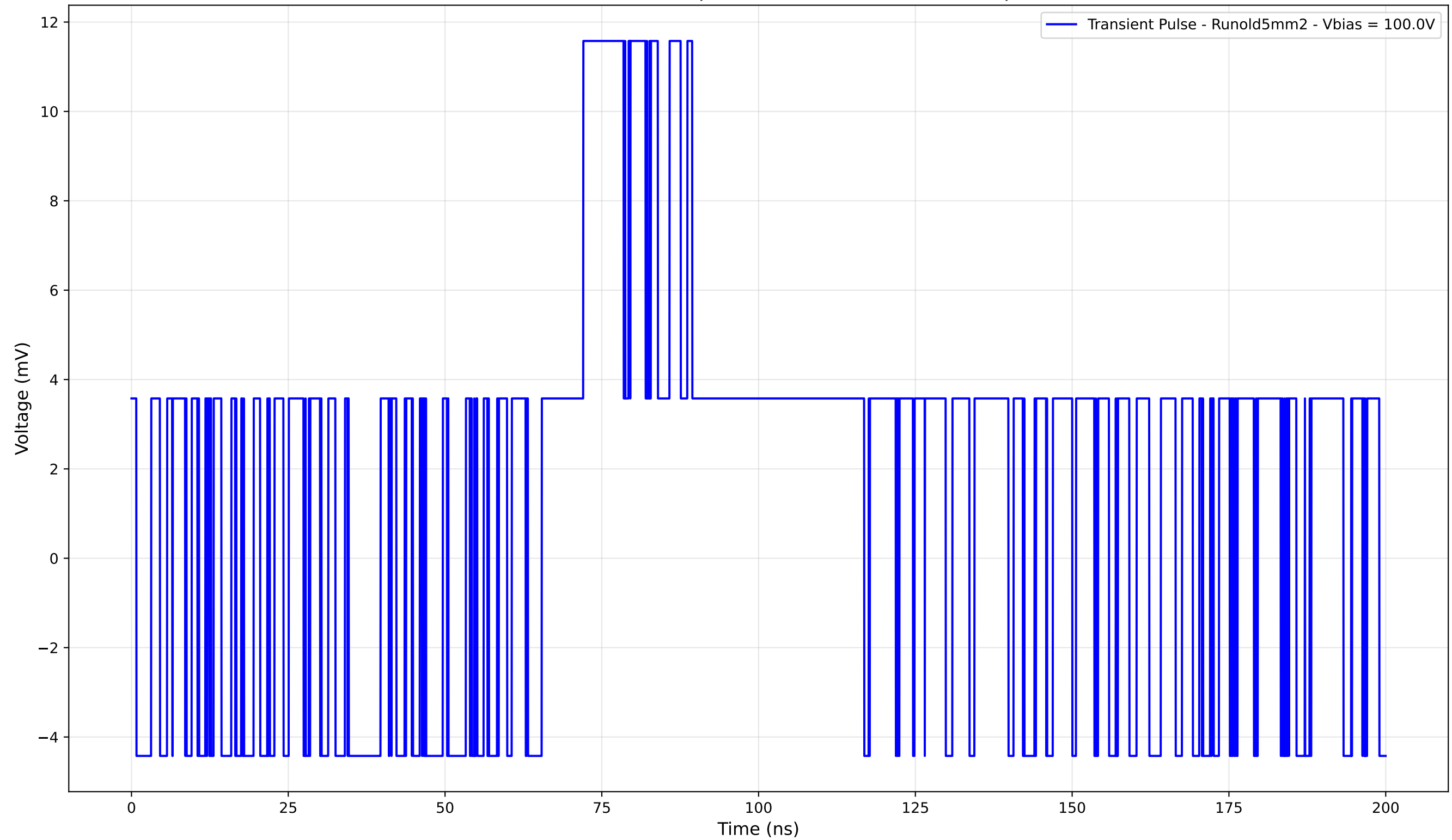
Transient Pulse - Sample: old5mm - Position: 685.0 \mu\text{m}
