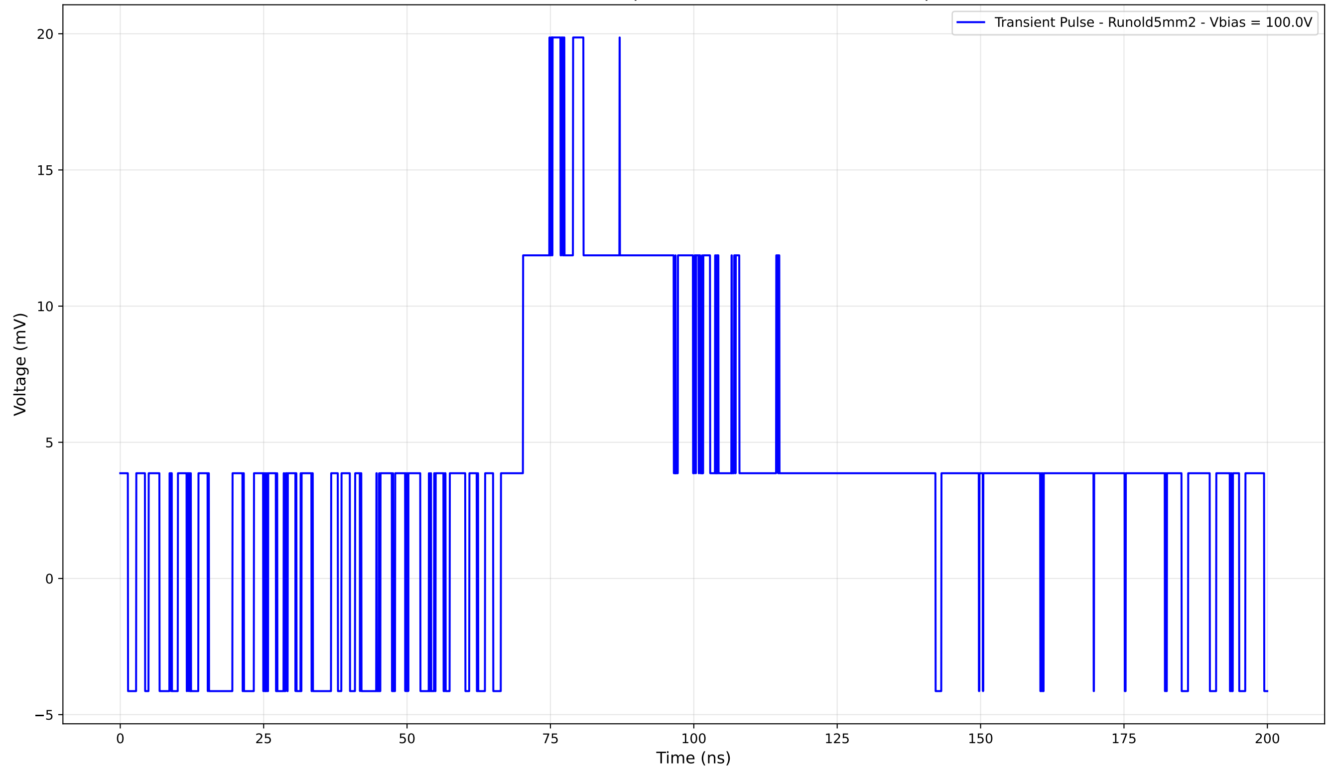
Transient Pulse - Sample: old5mm - Position: 1530.0 \mu\text{m}
