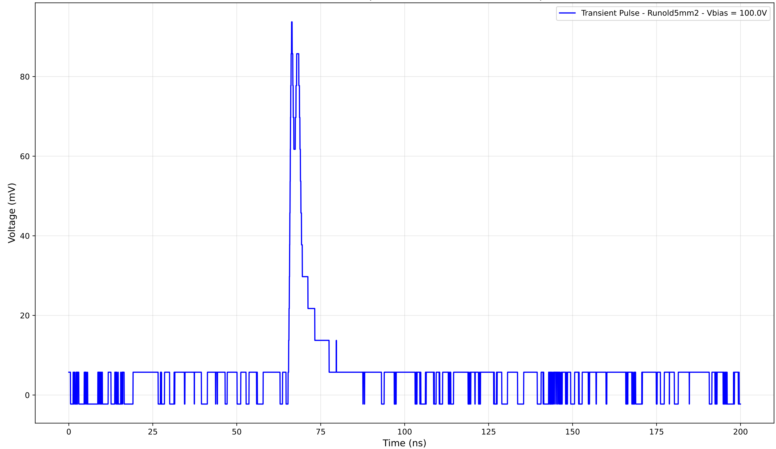
Transient Pulse - Sample: old5mm - Position: 3720.0 \mu\text{m}
