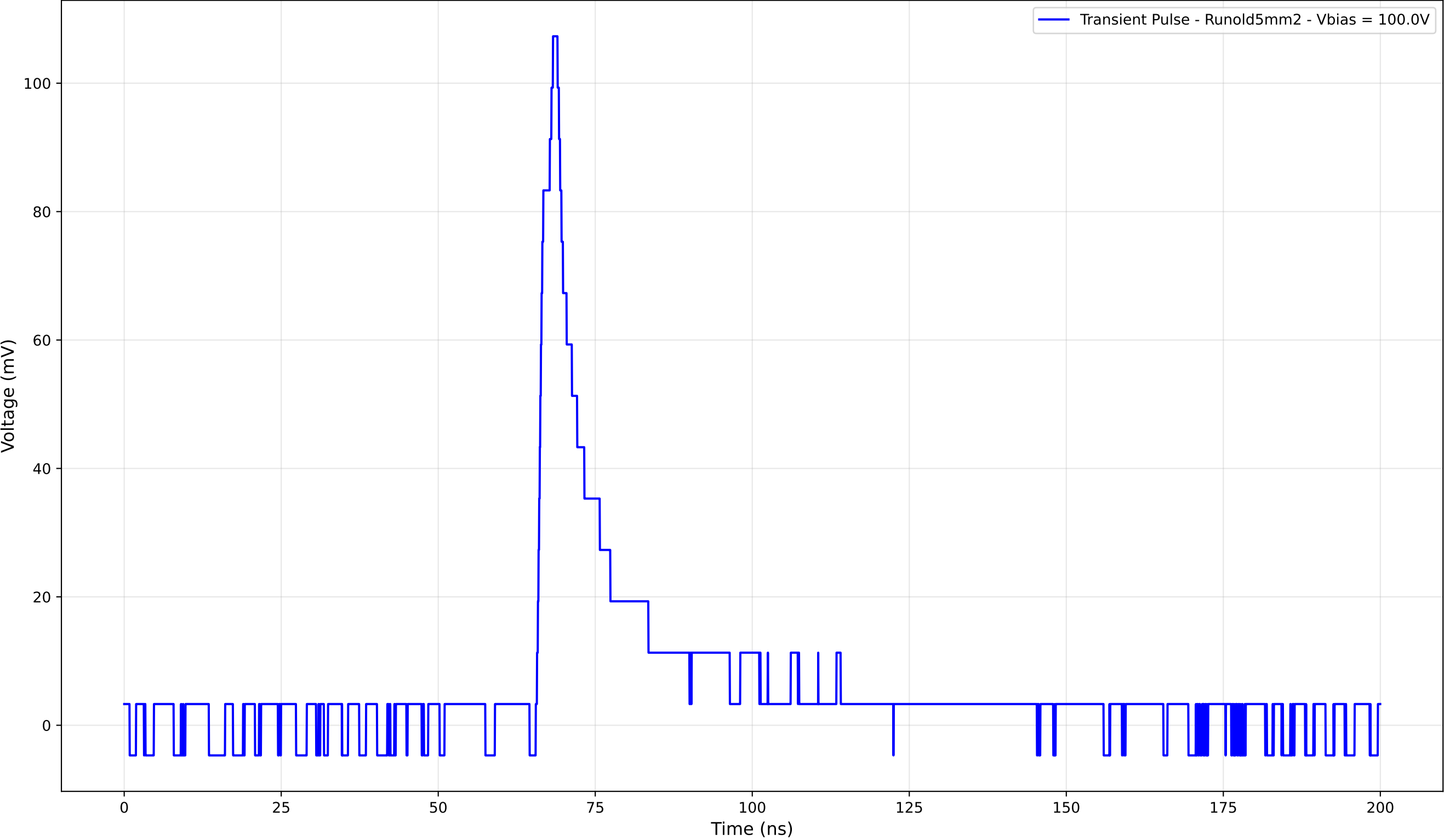
Transient Pulse - Sample: old5mm - Position: 4115.0 \mu\text{m}
