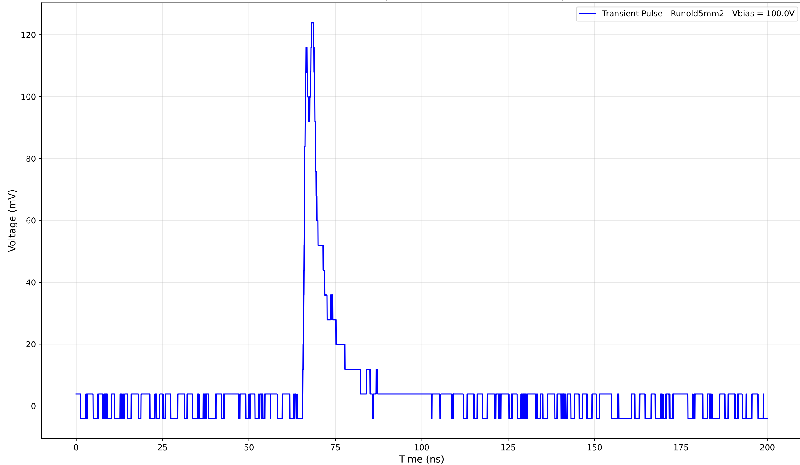
Transient Pulse - Sample: old5mm - Position: 3450.0 \mu\text{m}
