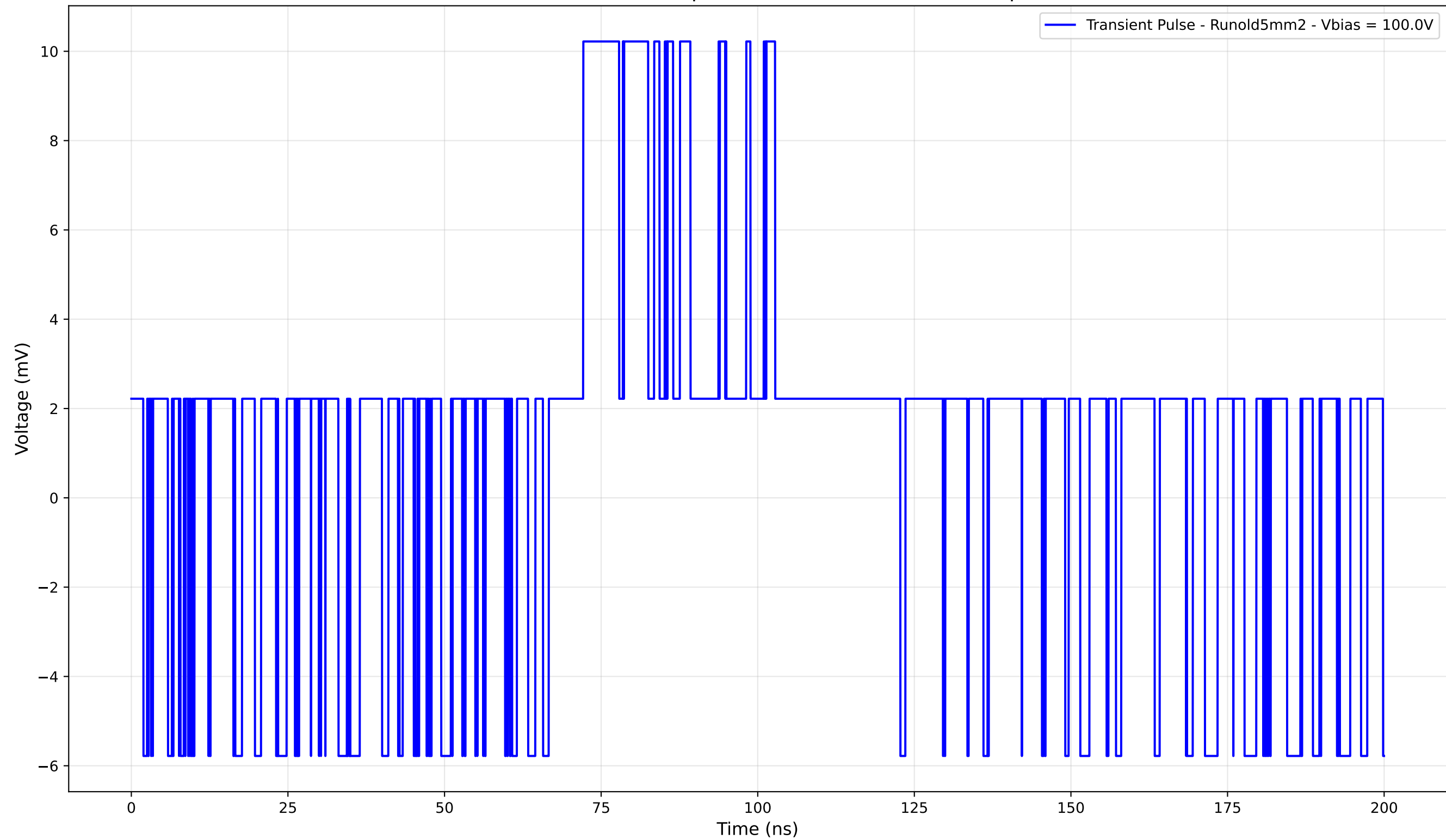
Transient Pulse - Sample: old5mm - Position: 1620.0 \mu\text{m}
