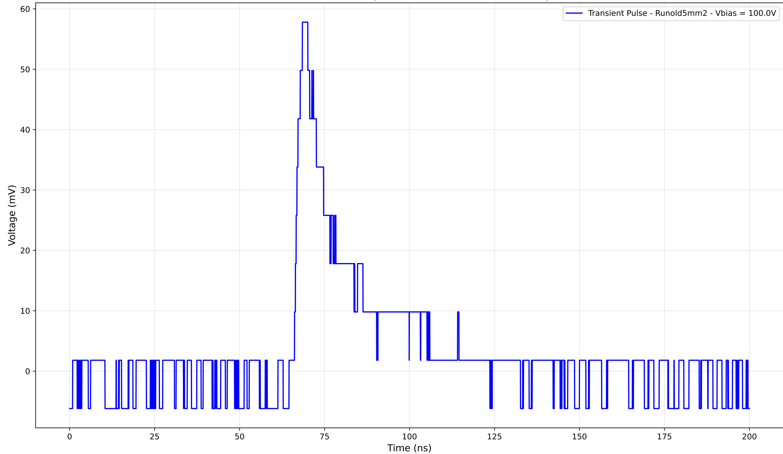
Transient Pulse - Sample: old5mm - Position: 4455.0 \mu\text{m}
