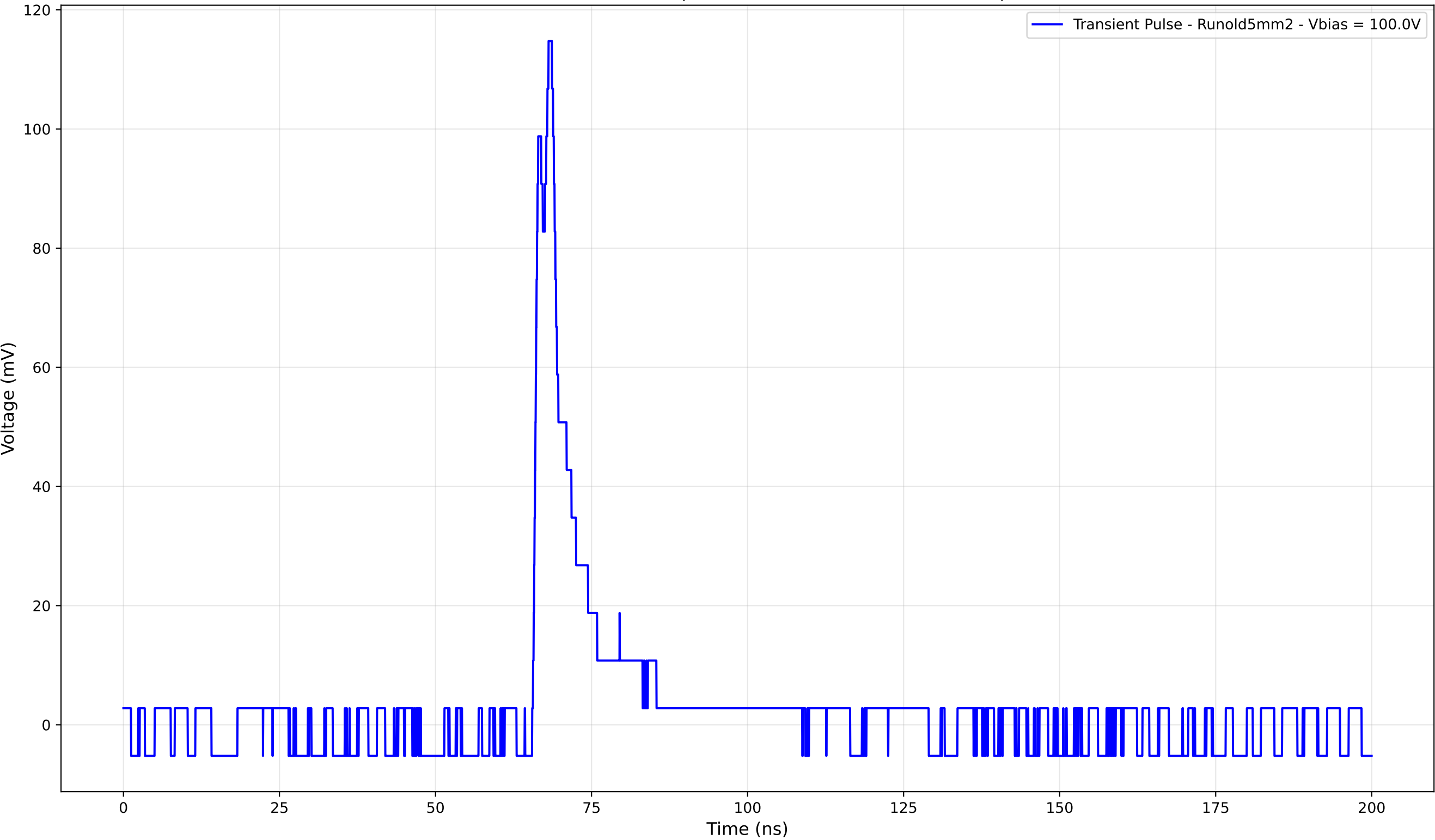
Transient Pulse - Sample: old5mm - Position: 3445.0 \mu\text{m}
