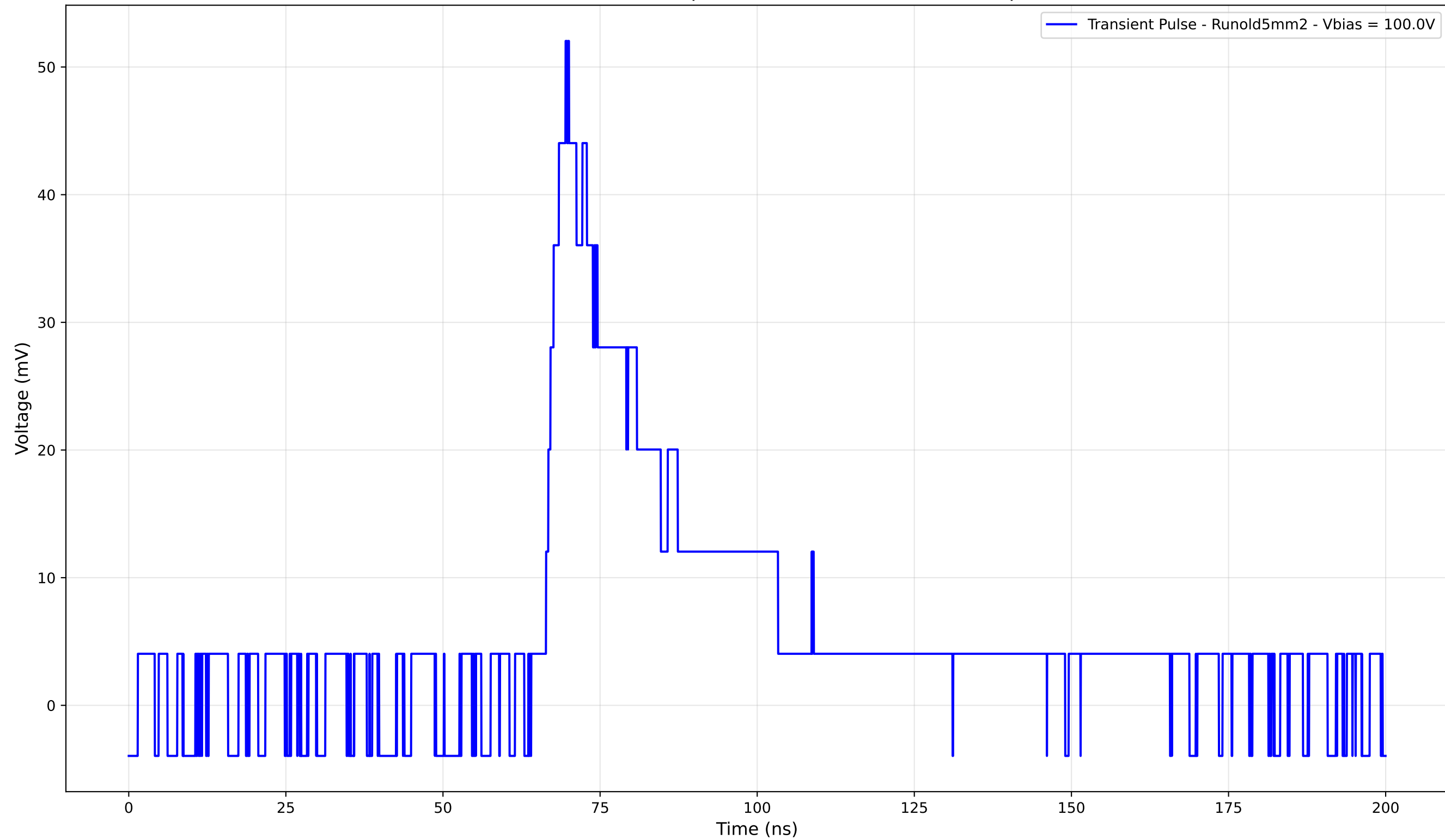
Transient Pulse - Sample: old5mm - Position: 4685.0 \mu\text{m}
