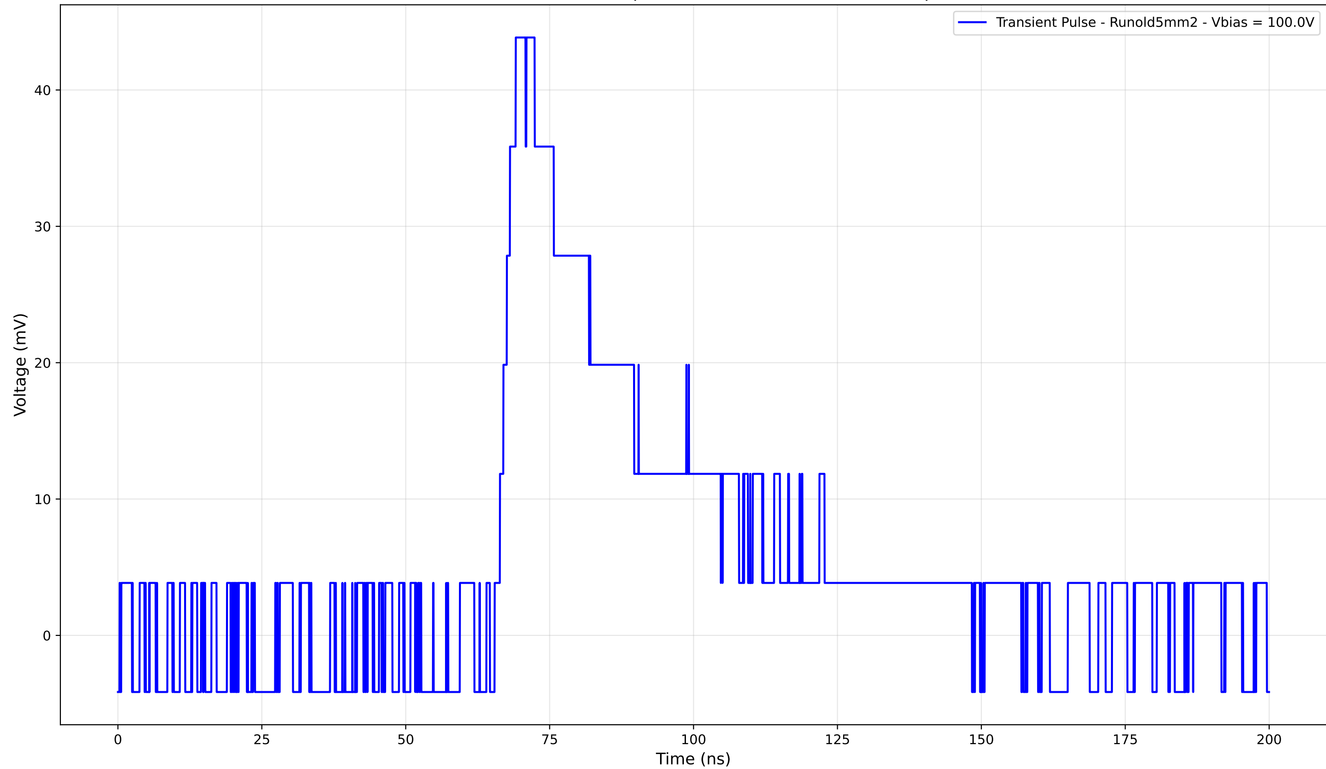
Transient Pulse - Sample: old5mm - Position: 4775.0 \mu\text{m}
