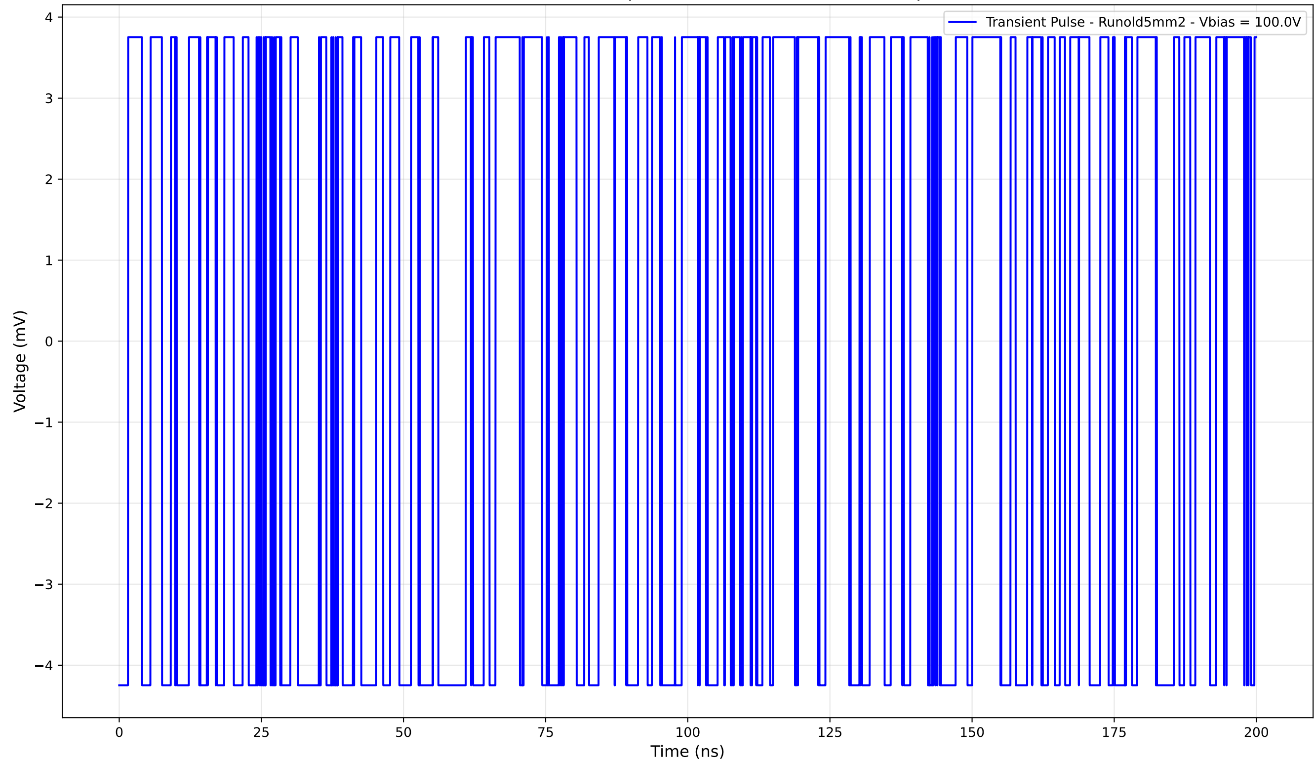
Transient Pulse - Sample: old5mm - Position: 3965.0 \mu\text{m}
