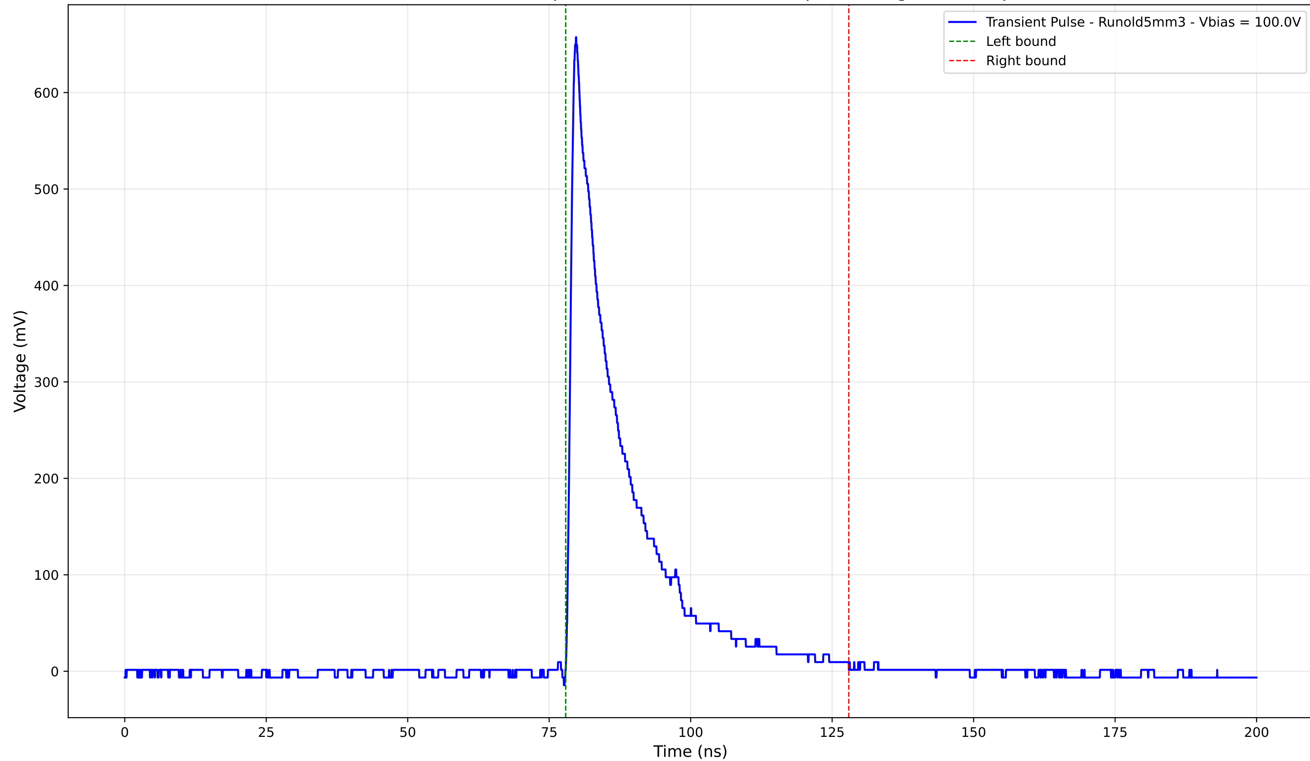
Transient Pulse - Sample: old5 - Position: 4650.0 \mu\text{m} - Charge: 125.12 pC
