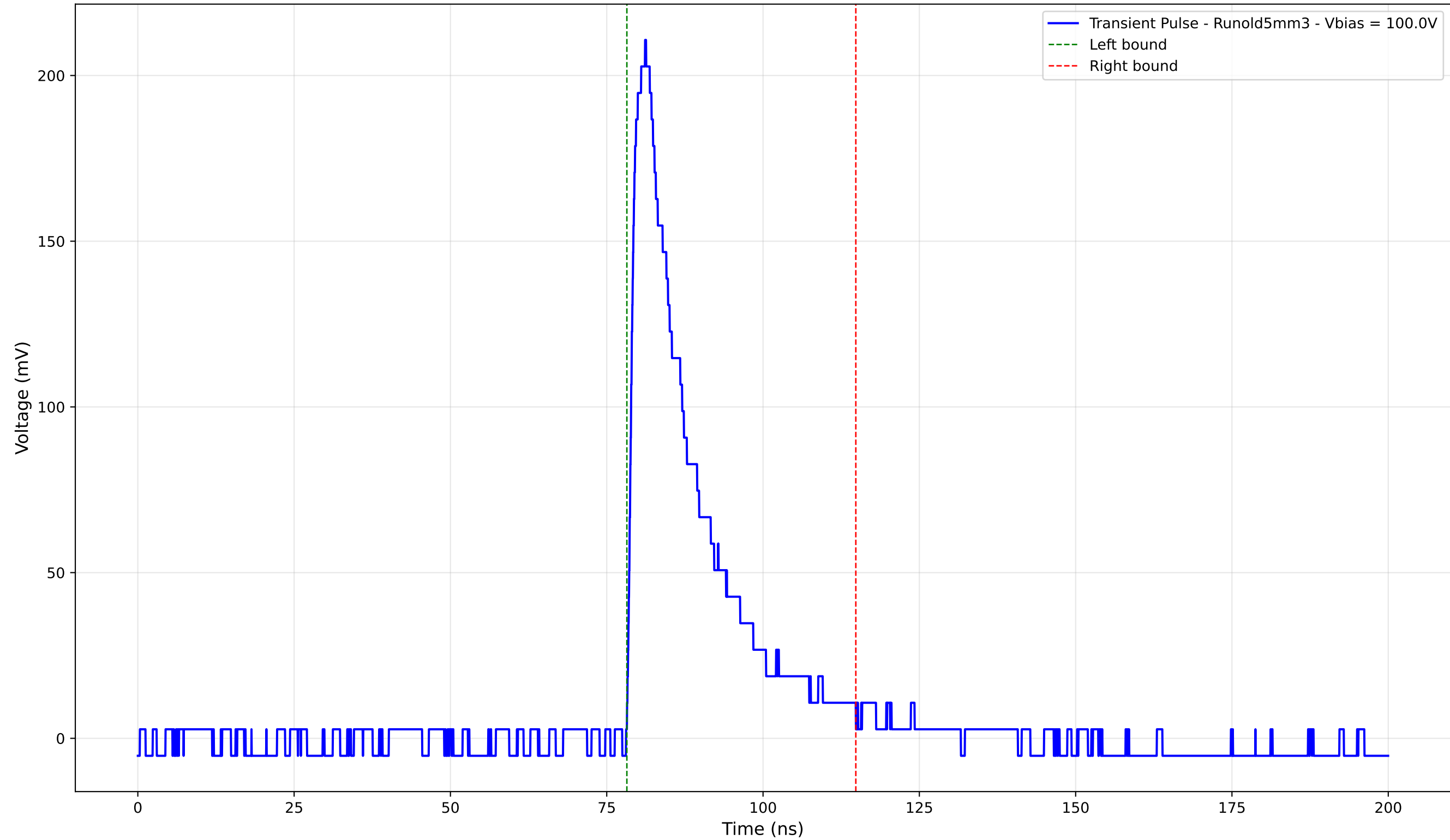
Transient Pulse - Sample: old5 - Position: 4245.0 \mu\text{m} - Charge: 45.01 pC
