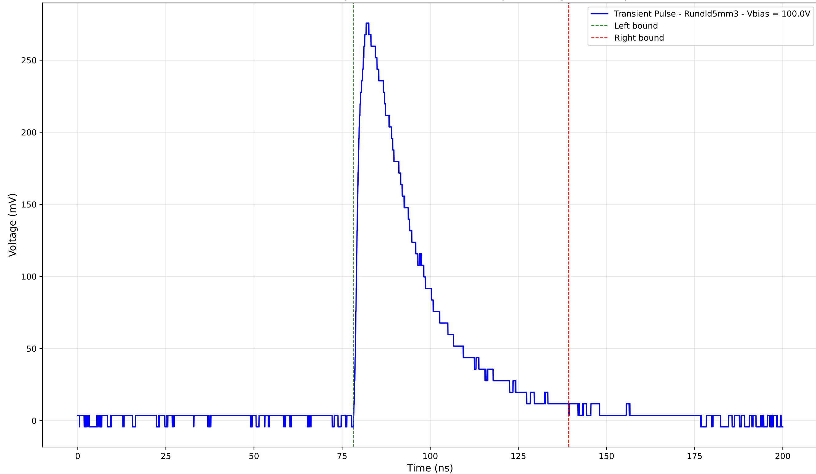
Transient Pulse - Sample: old5 - Position: 2535.0 \mu\text{m} - Charge: 103.89 pC
