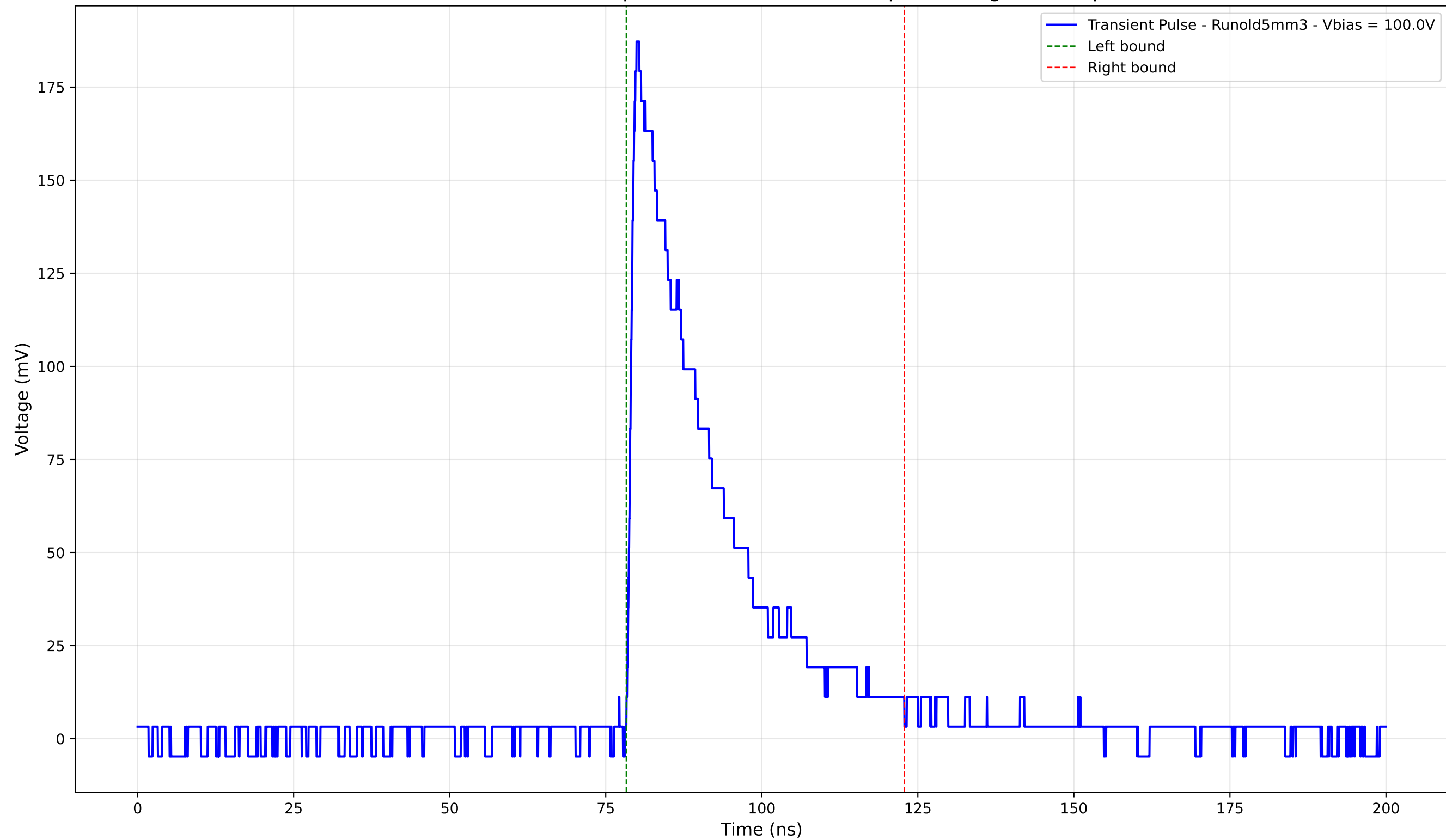
Transient Pulse - Sample: old5 - Position: 775.0 \mu\text{m} - Charge: 50.71 pC
