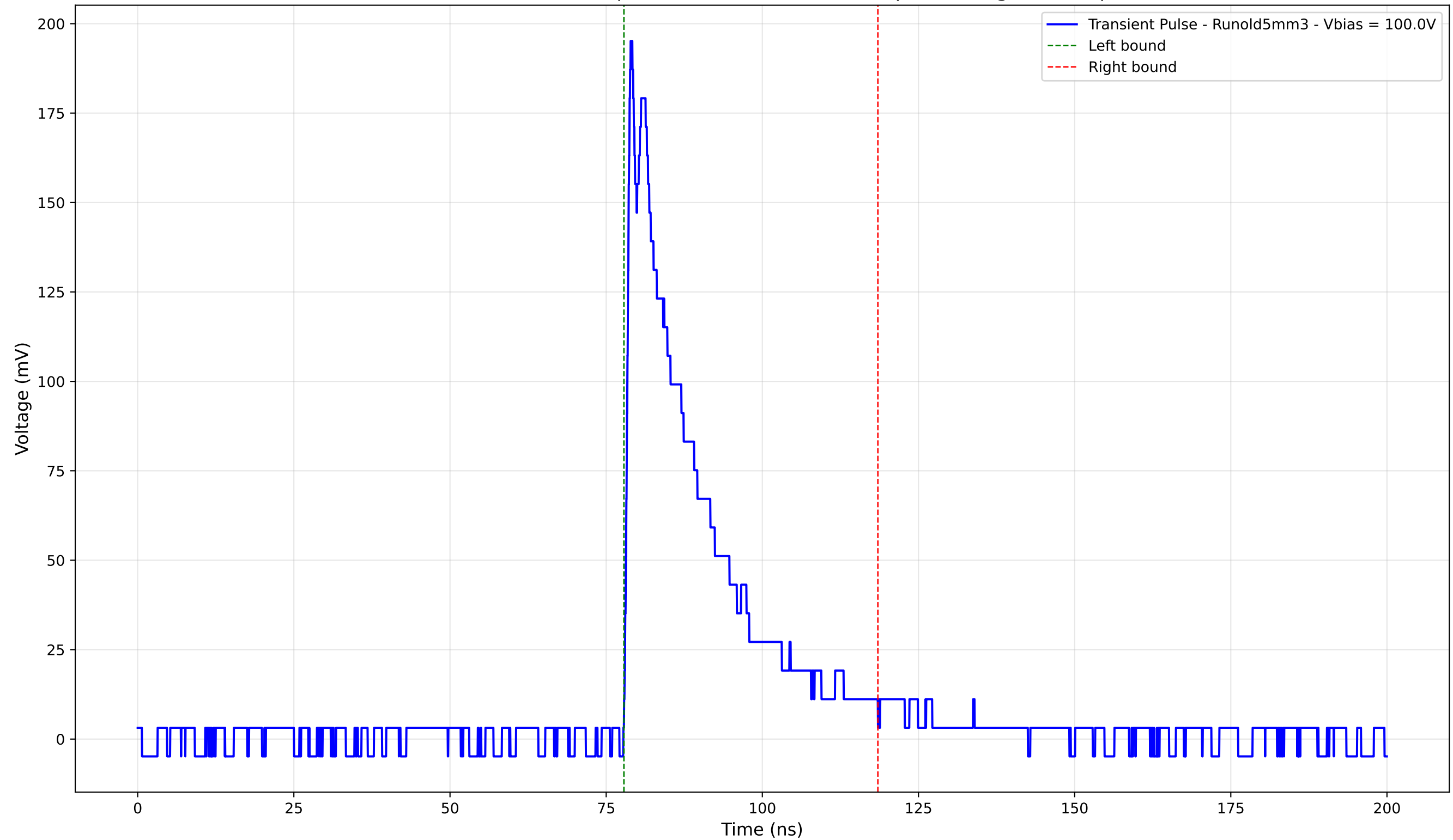
Transient Pulse - Sample: old5 - Position: 3215.0 \mu\text{m} - Charge: 44.48 pC
