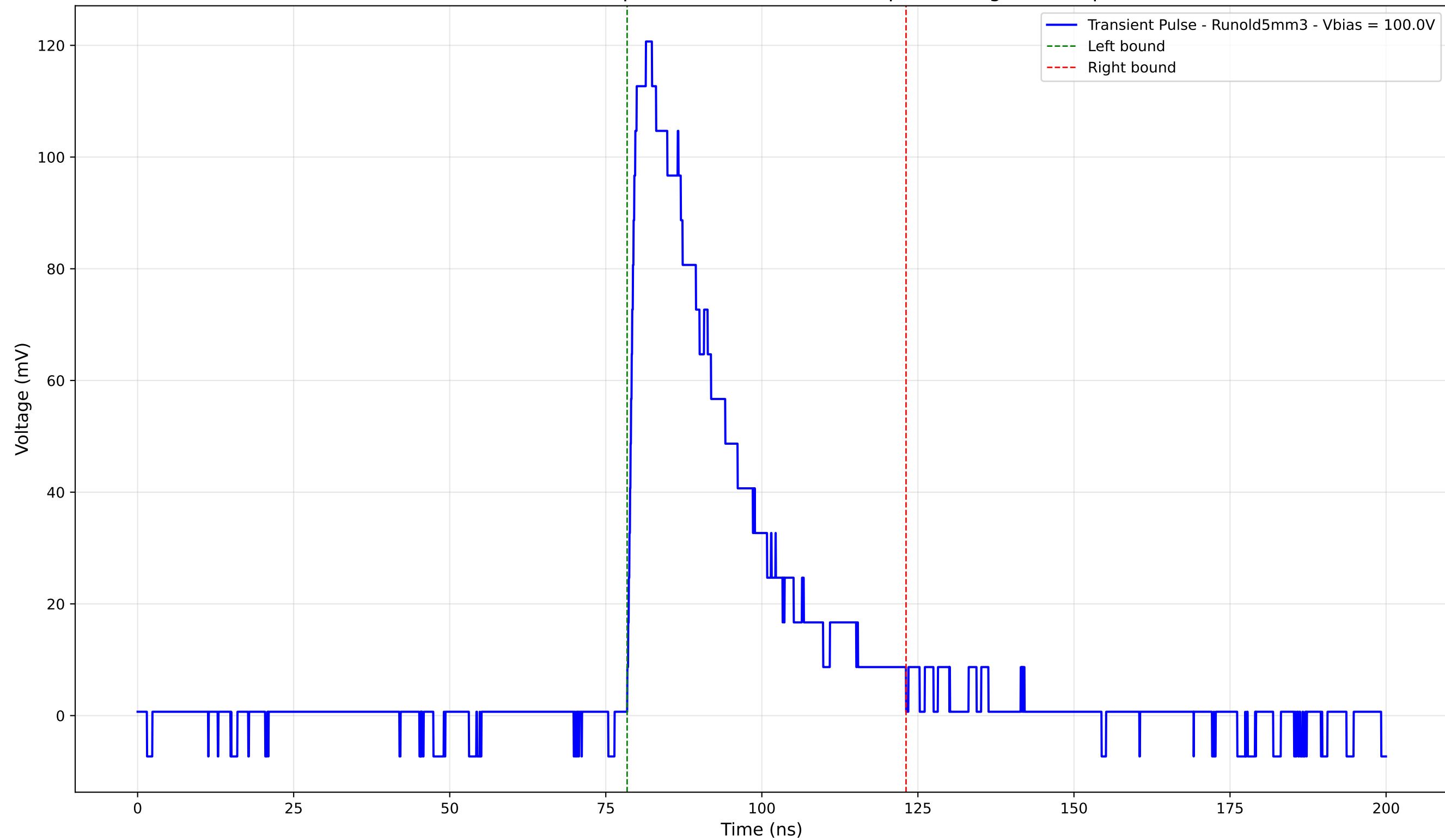
Transient Pulse - Sample: old5 - Position: 995.0 \mu\text{m} - Charge: 39.02 pC
