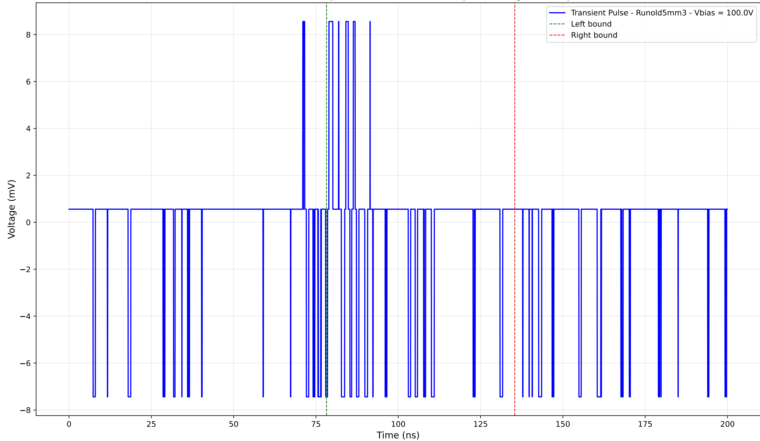
Transient Pulse - Sample: old5 - Position: 65.0 \mu\text{m} - Charge: -0.24 pC
