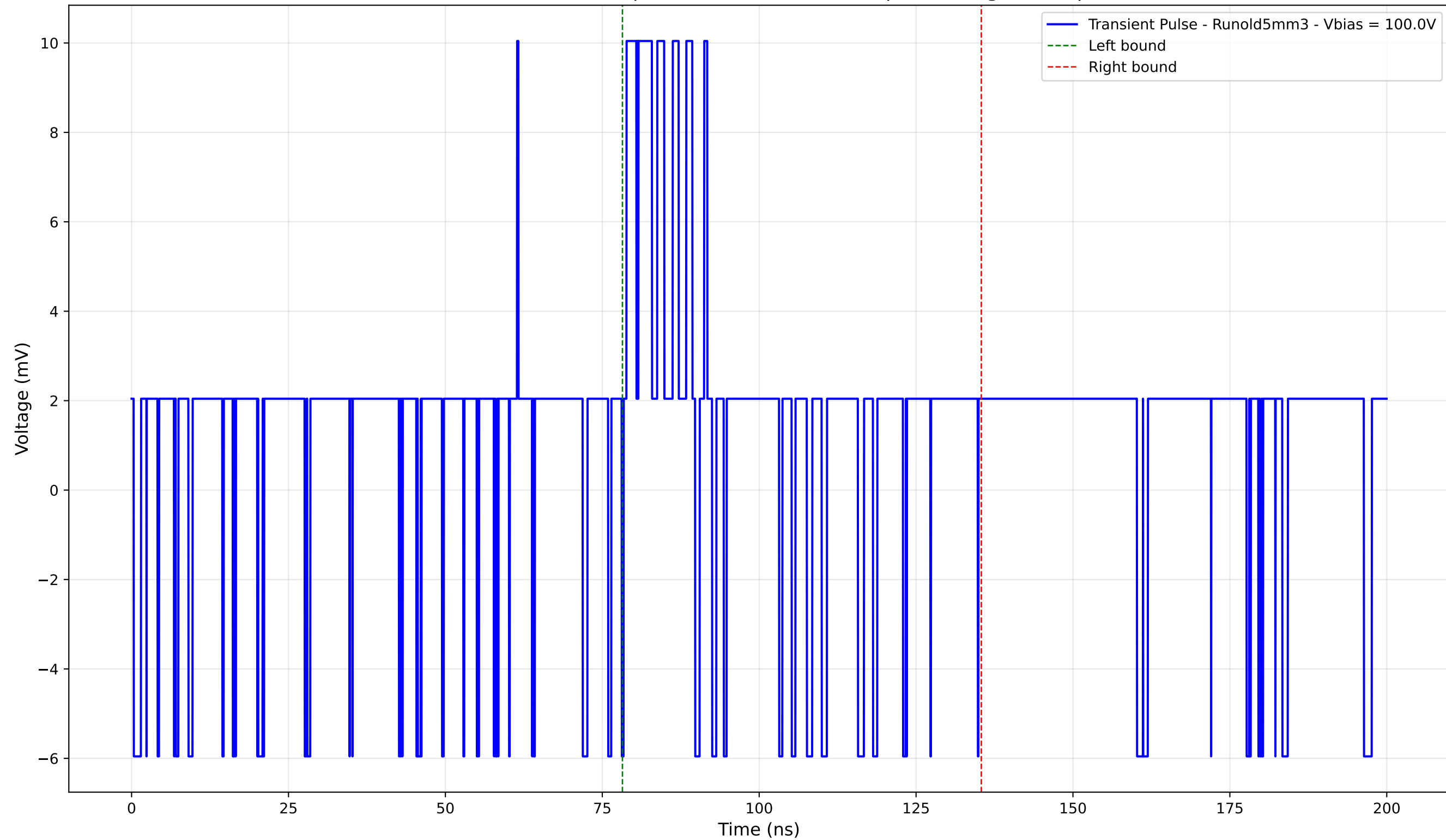
Transient Pulse - Sample: old5 - Position: 90.0 \mu\text{m} - Charge: 2.38 pC
