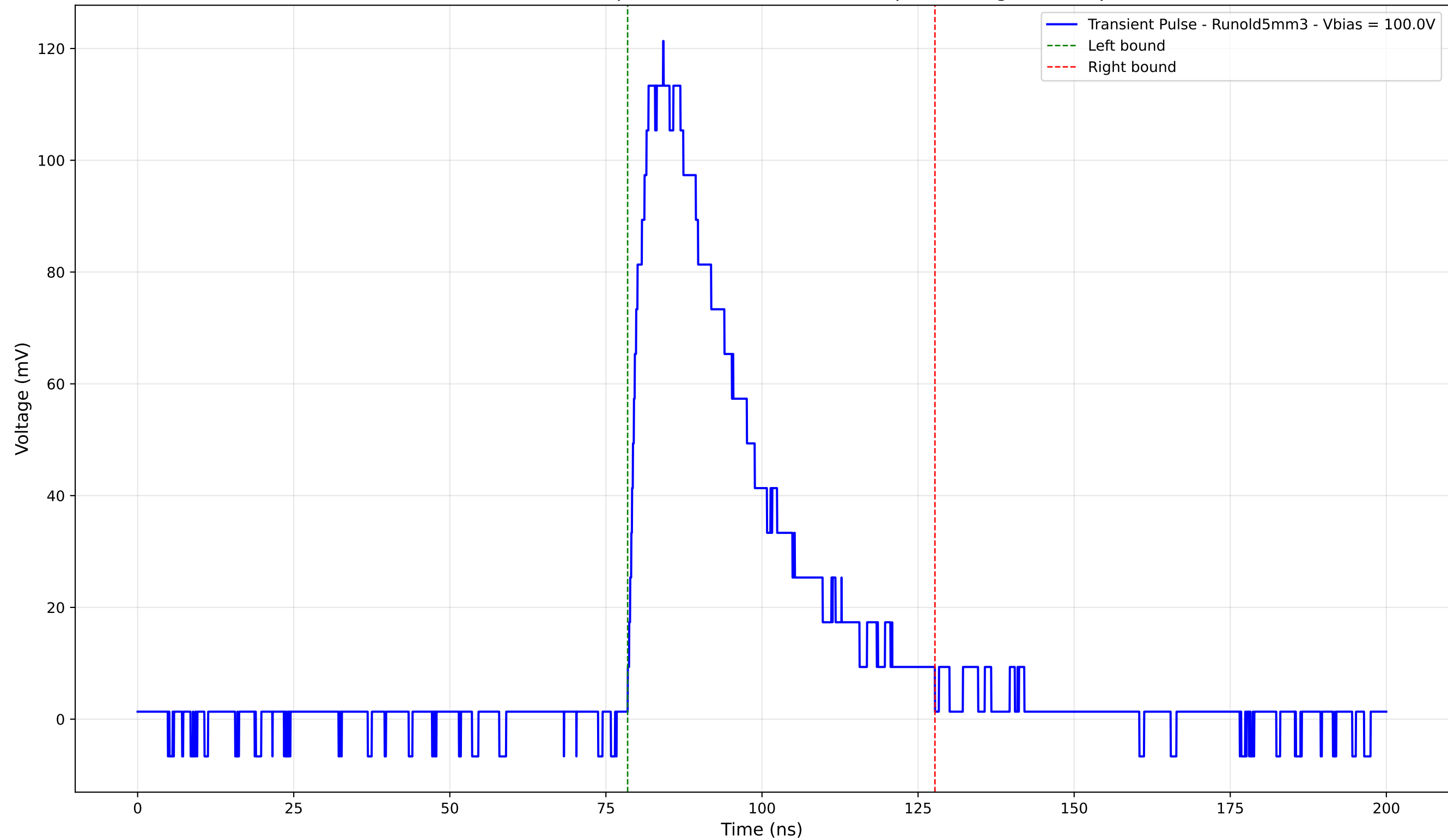
Transient Pulse - Sample: old5 - Position: 1835.0 \mu\text{m} - Charge: 45.39 pC
