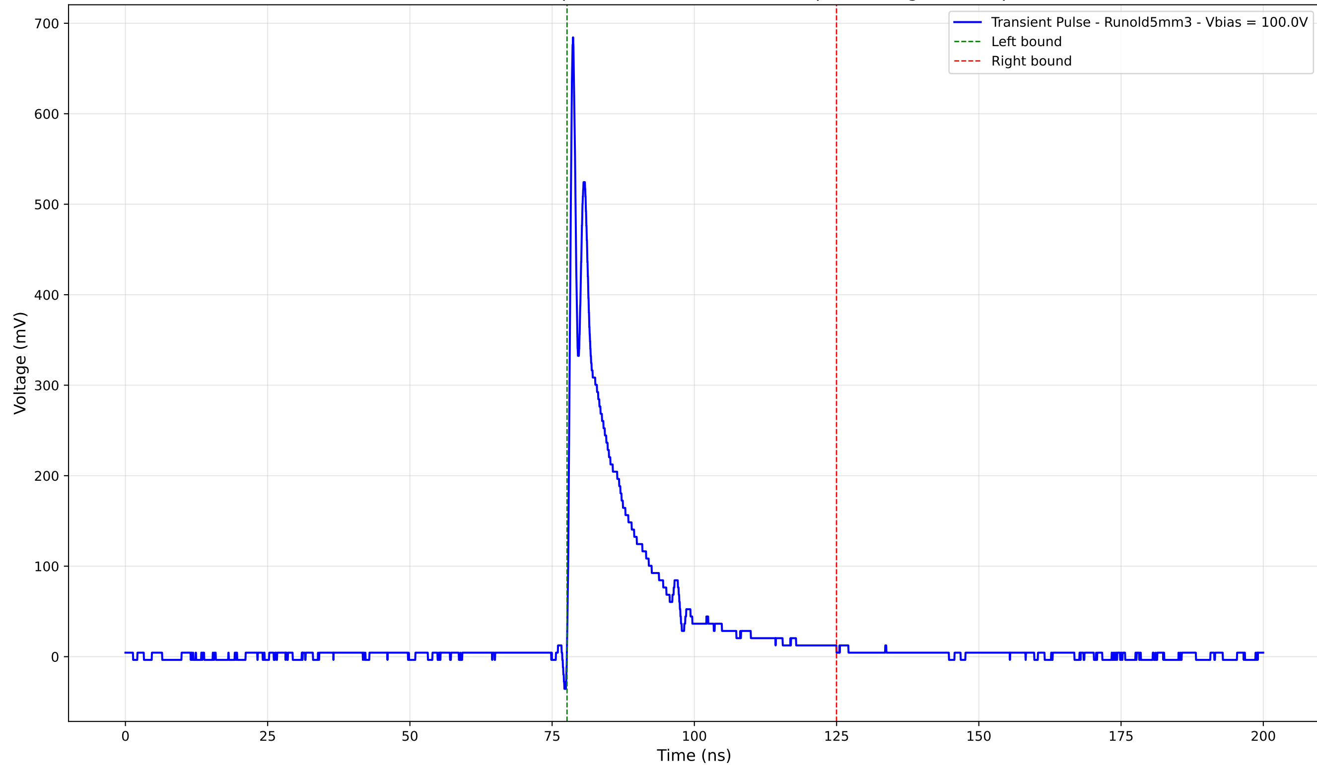
Transient Pulse - Sample: old5 - Position: 3685.0 \mu\text{m} - Charge: 97.74 pC
