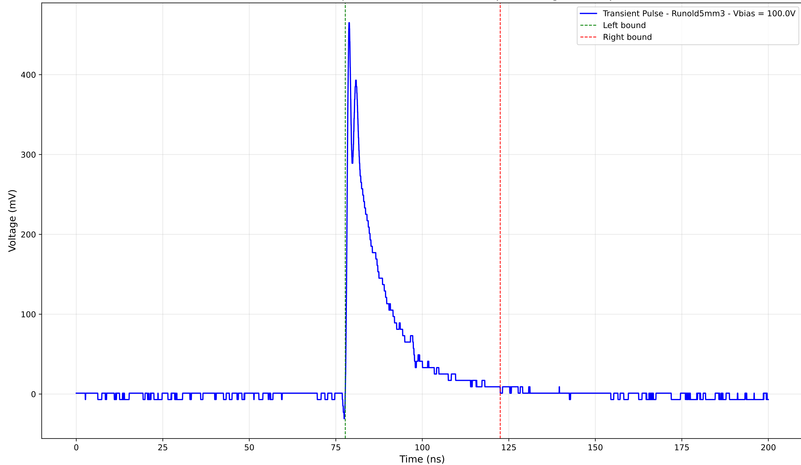
Transient Pulse - Sample: old5 - Position: 3370.0 \mu\text{m} - Charge: 80.26 pC
