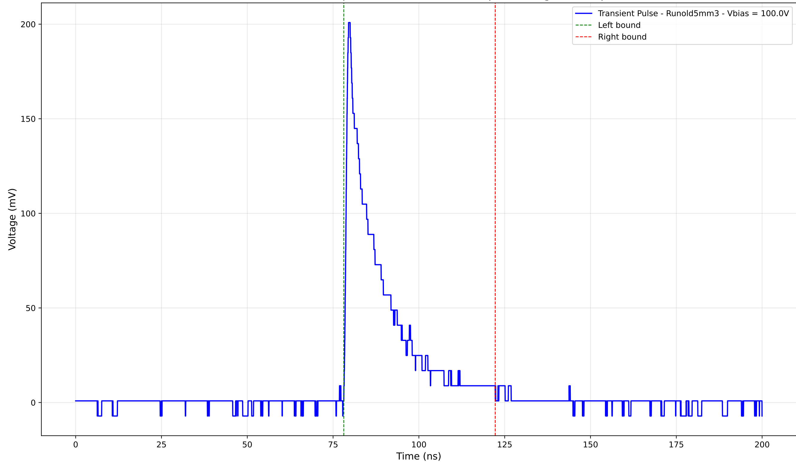
Transient Pulse - Sample: old5 - Position: 485.0 \mu\text{m} - Charge: 39.18 pC
