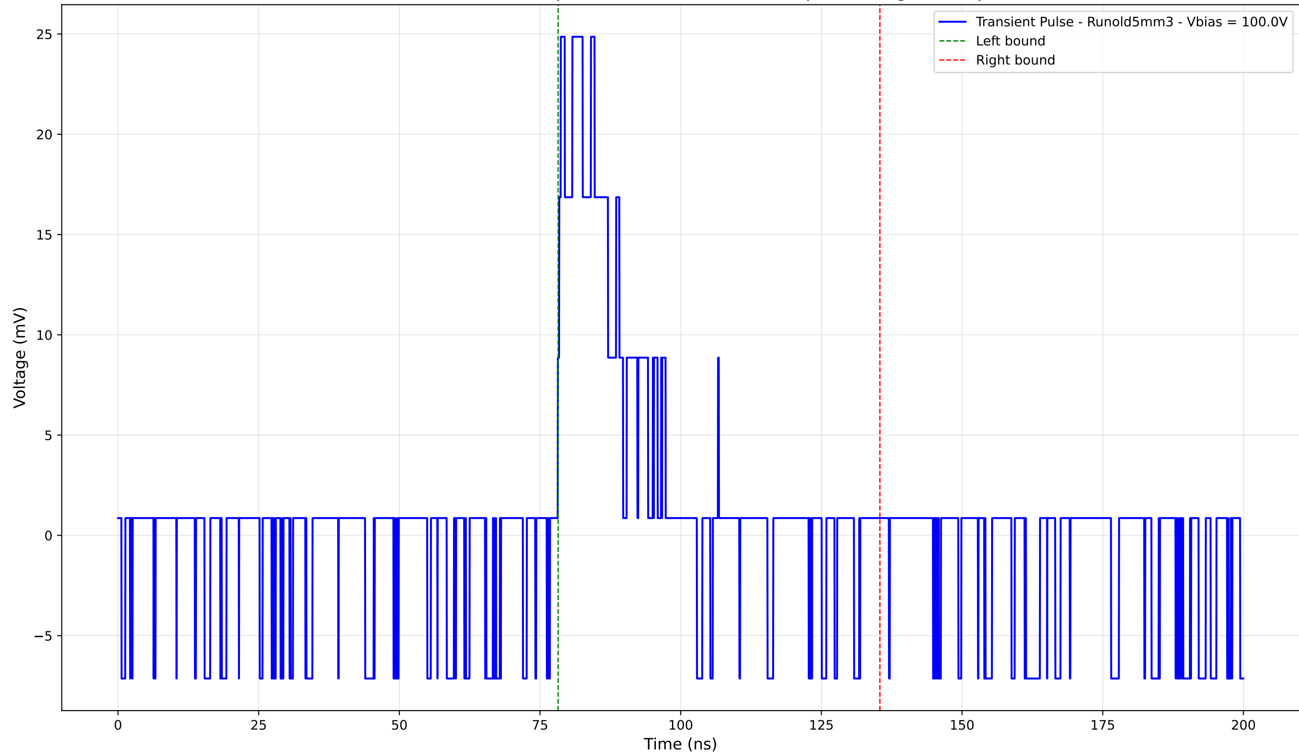
Transient Pulse - Sample: old5 - Position: 3890.0 \mu\text{m} - Charge: 4.84 pC
