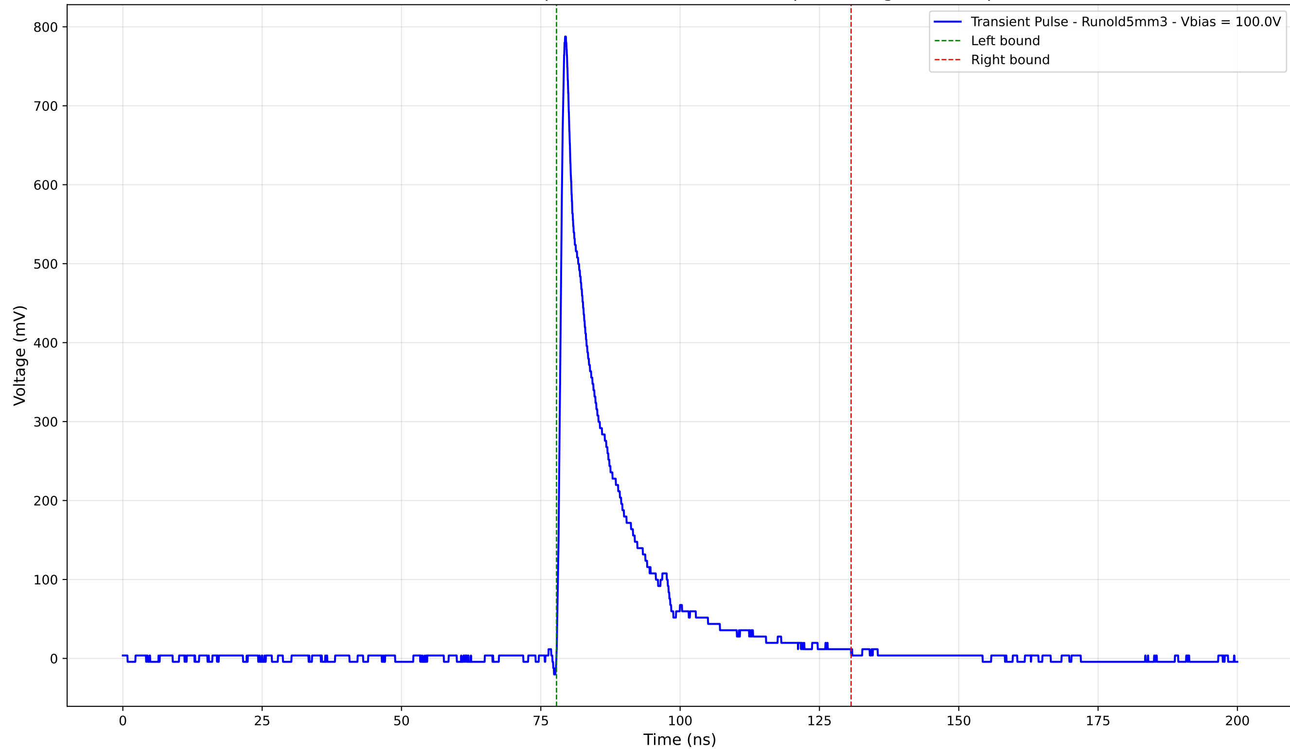
Transient Pulse - Sample: old5 - Position: 4760.0 \mu\text{m} - Charge: 134.18 pC
