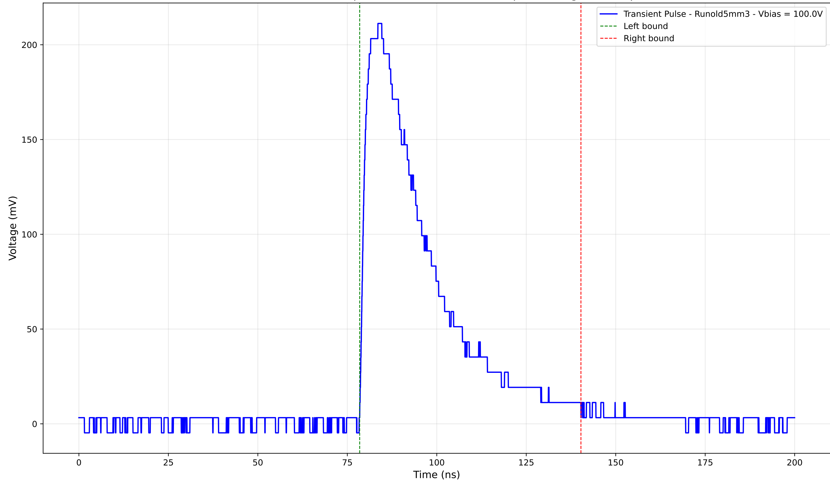
Transient Pulse - Sample: old5 - Position: 1480.0 \mu\text{m} - Charge: 85.56 pC
