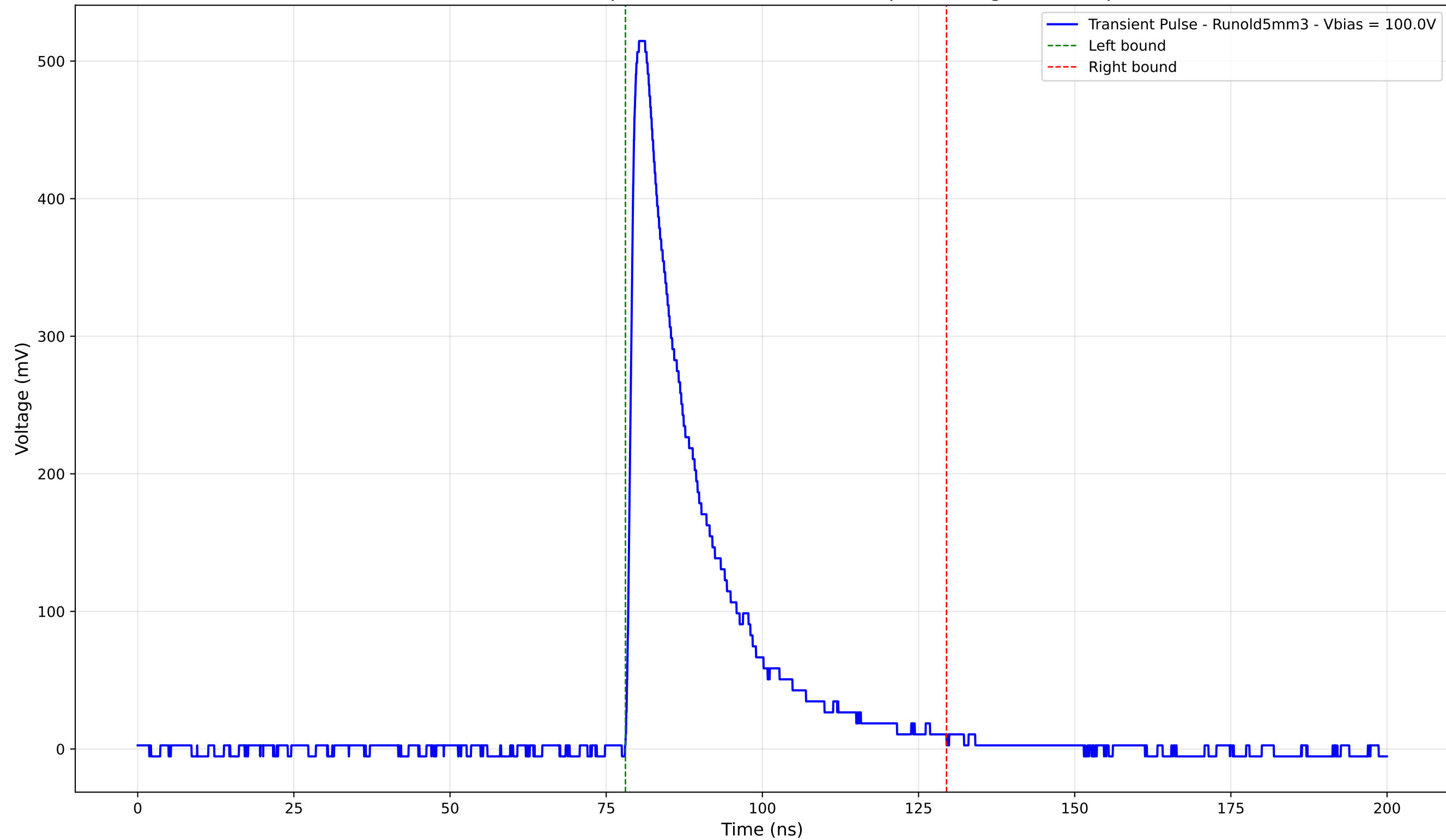
Transient Pulse - Sample: old5 - Position: 4320.0 \mu\text{m} - Charge: 118.39 pC
