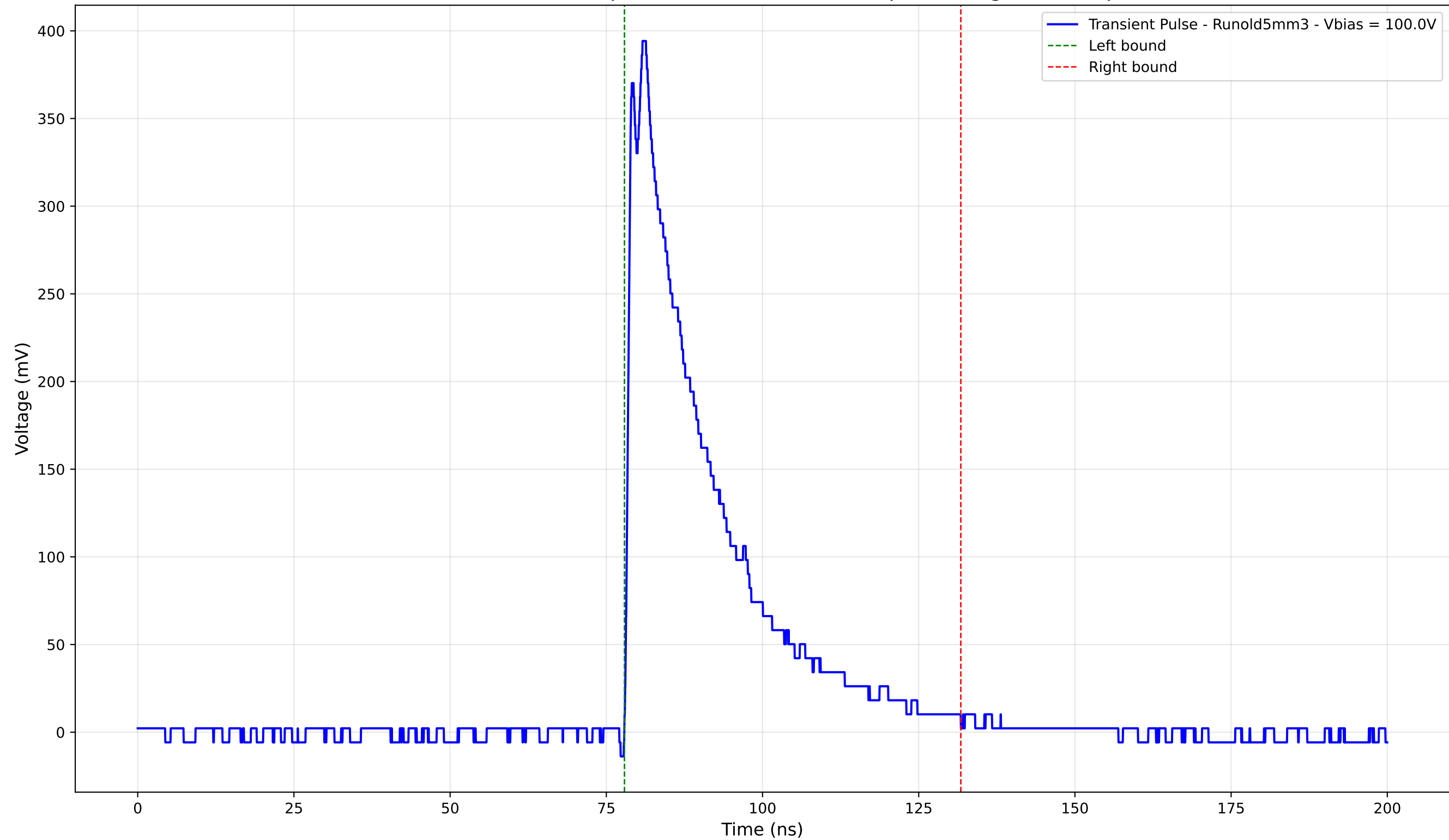
Transient Pulse - Sample: old5 - Position: 3120.0 \mu\text{m} - Charge: 107.00 pC
