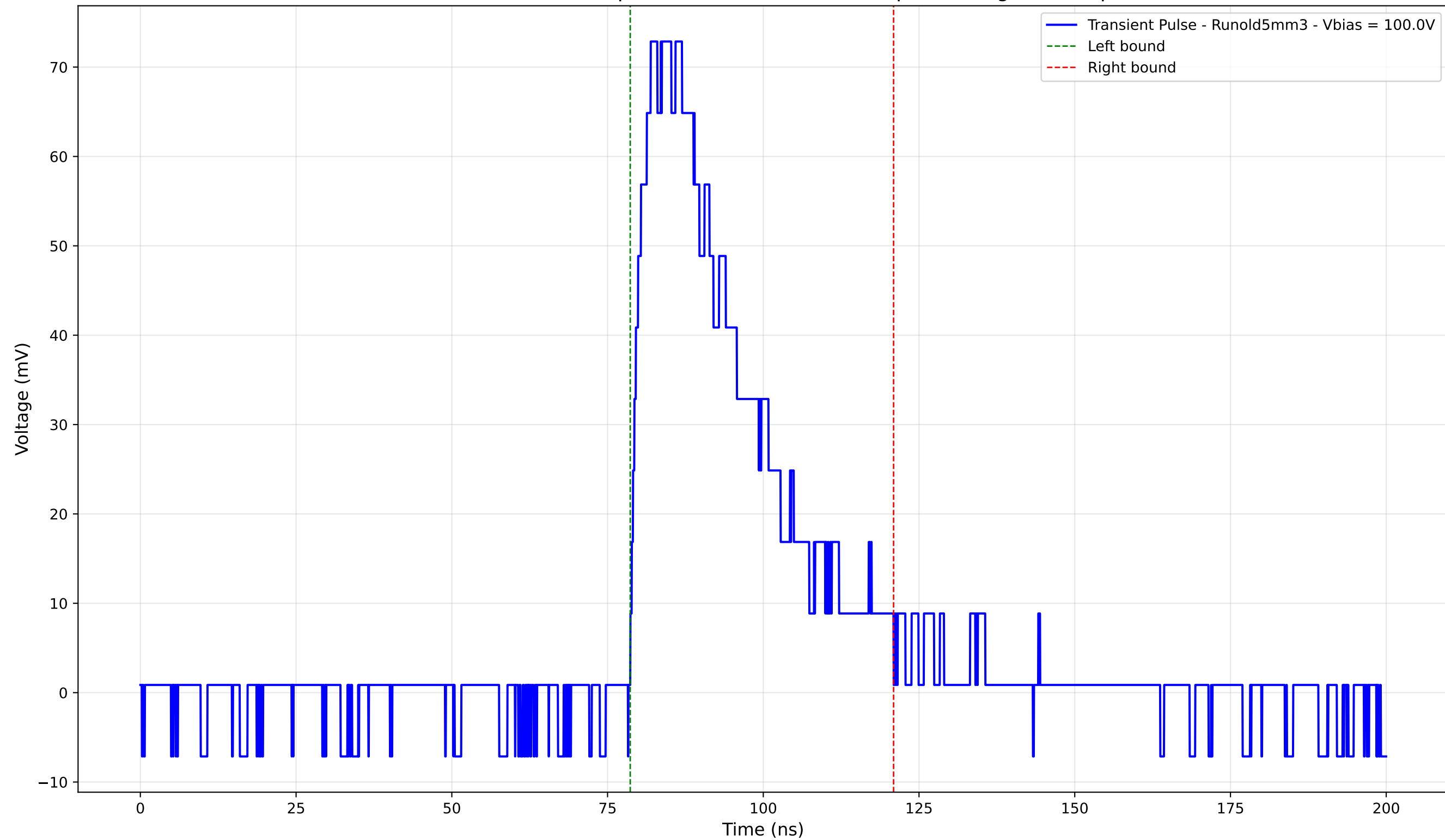
Transient Pulse - Sample: old5 - Position: 1960.0 \mu\text{m} - Charge: 28.03 pC
