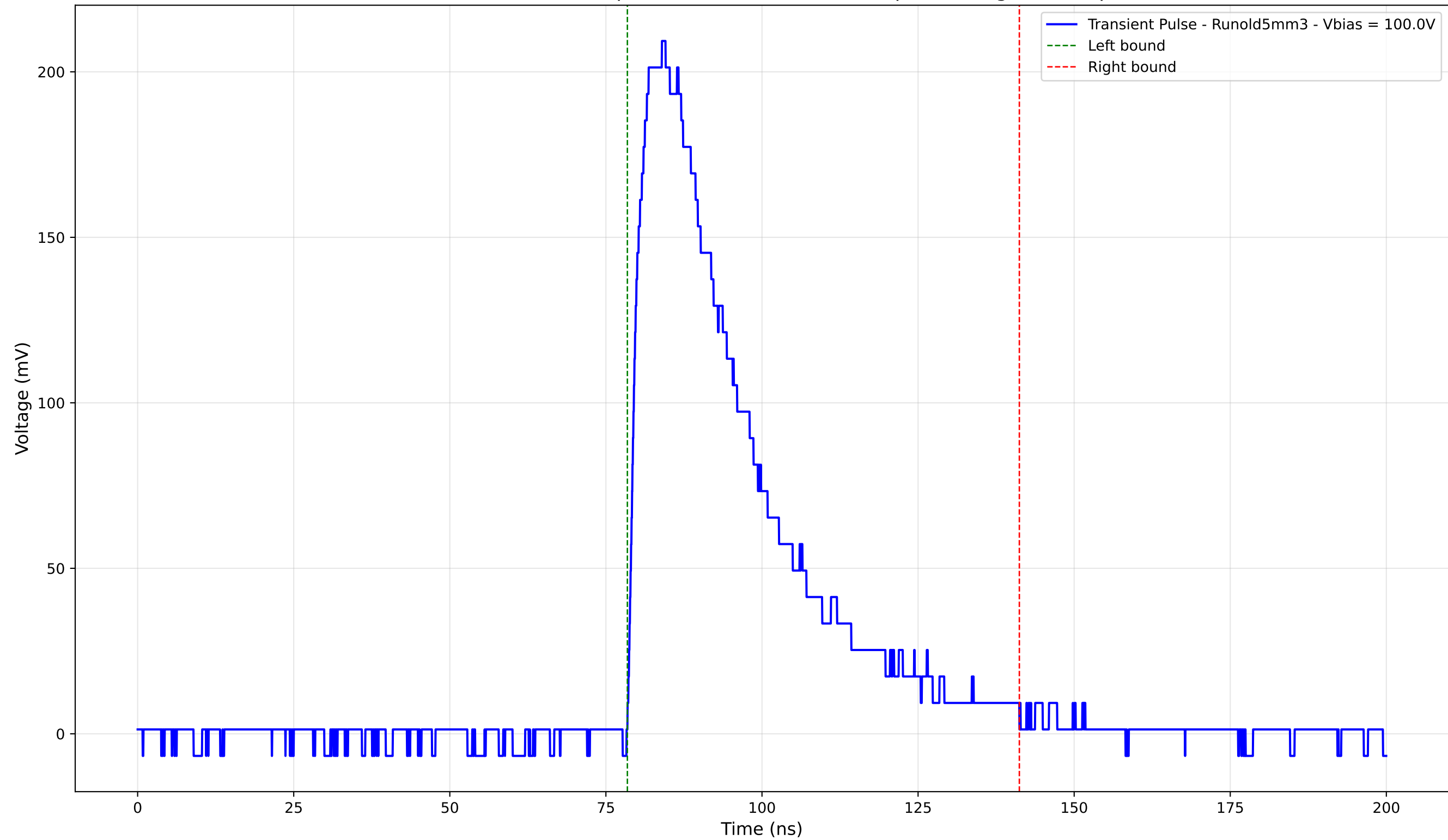
Transient Pulse - Sample: old5 - Position: 2070.0 \mu\text{m} - Charge: 84.30 pC
