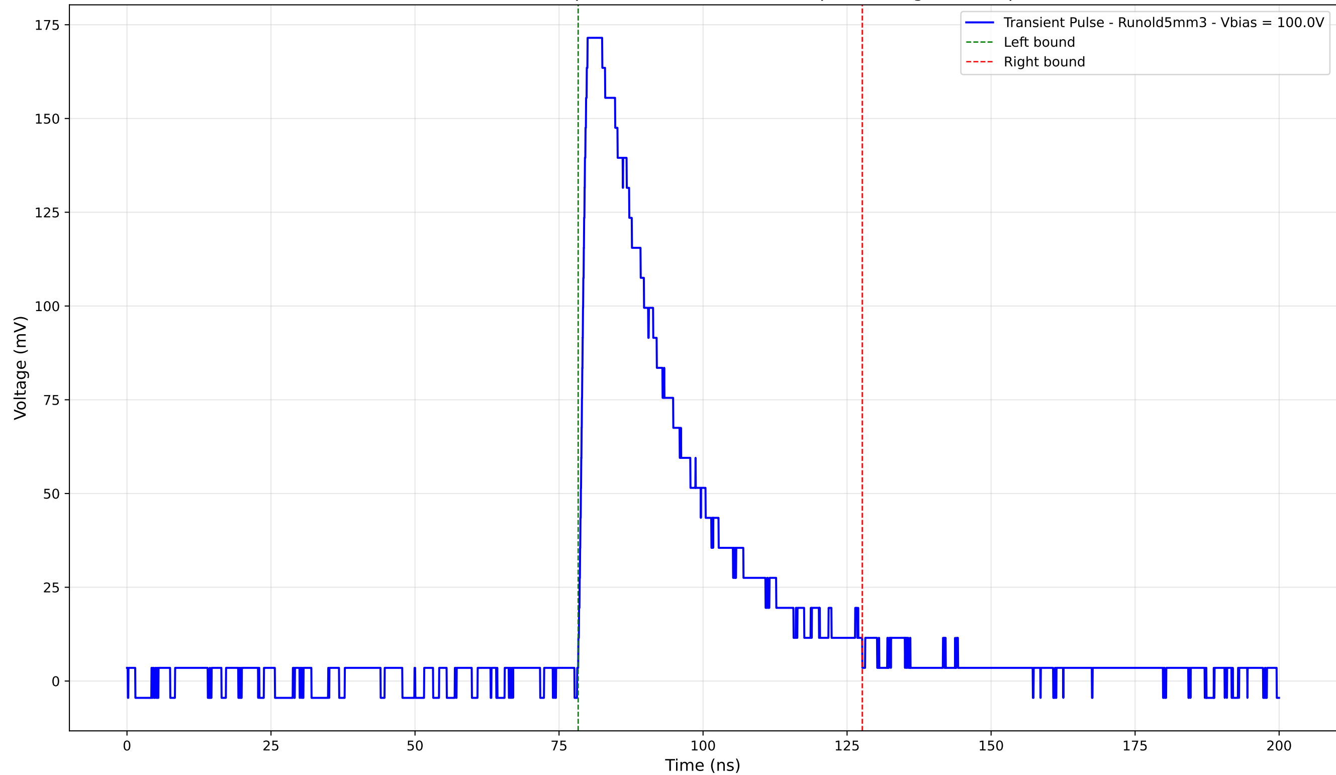
Transient Pulse - Sample: old5 - Position: 965.0 \mu\text{m} - Charge: 59.19 pC
