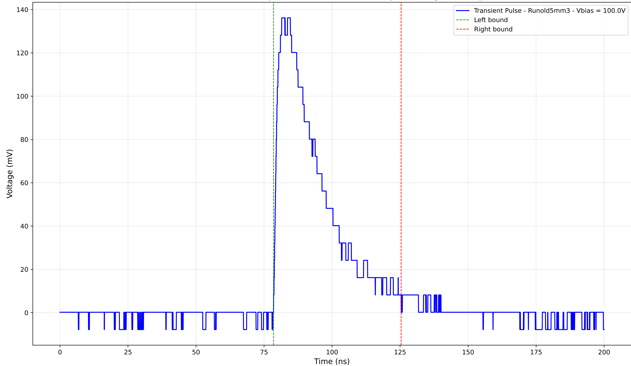
Transient Pulse - Sample: old5 - Position: 1235.0 \mu\text{m} - Charge: 49.68 pC
