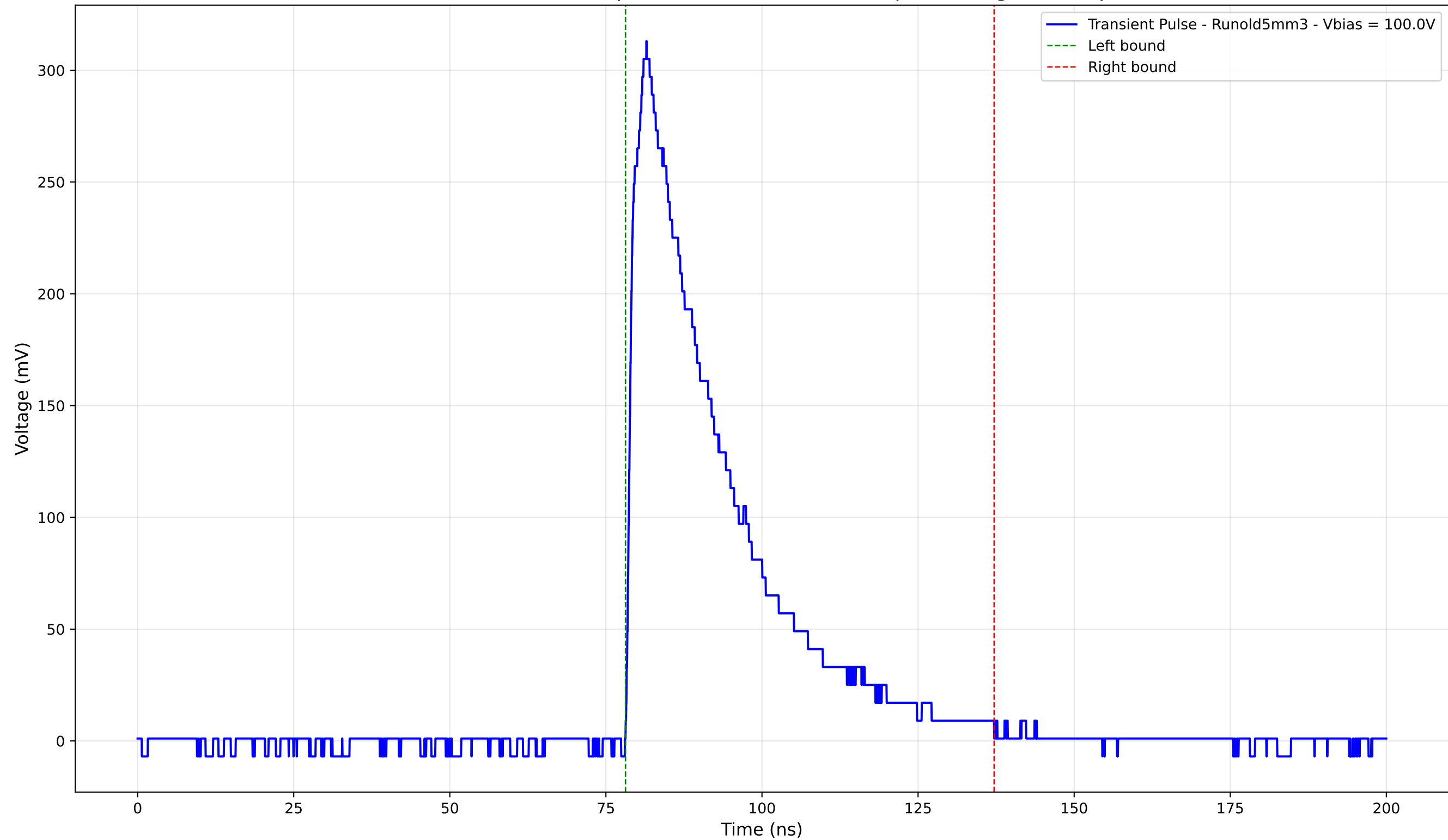
Transient Pulse - Sample: old5 - Position: 2865.0 \mu\text{m} - Charge: 98.76 pC
