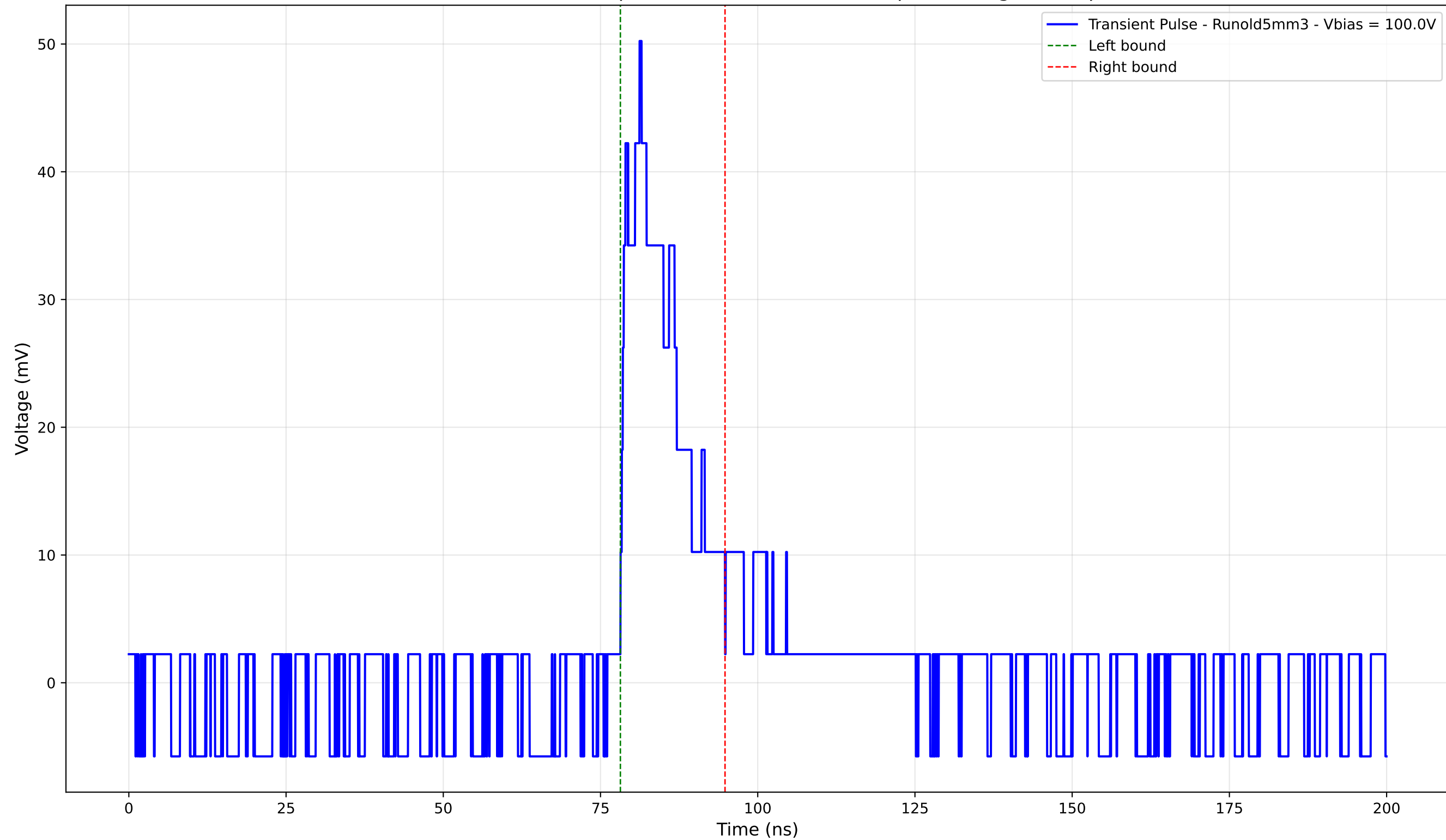
Transient Pulse - Sample: old5 - Position: 3910.0 \mu\text{m} - Charge: 8.20 pC
