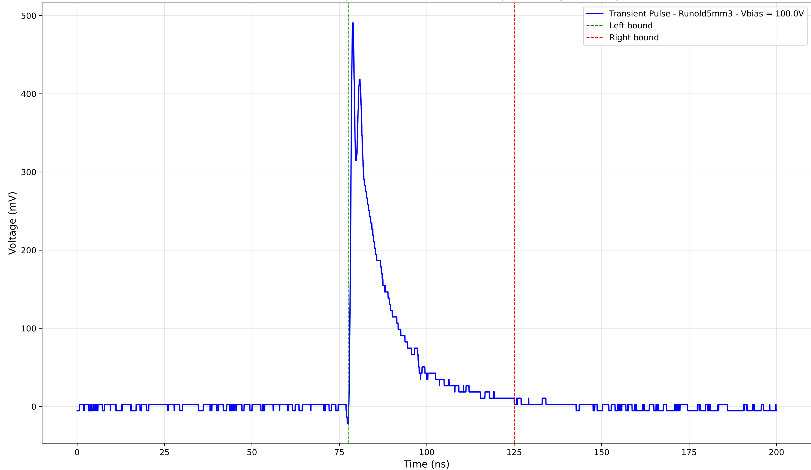
Transient Pulse - Sample: old5 - Position: 3375.0 \mu\text{m} - Charge: 87.08 pC
