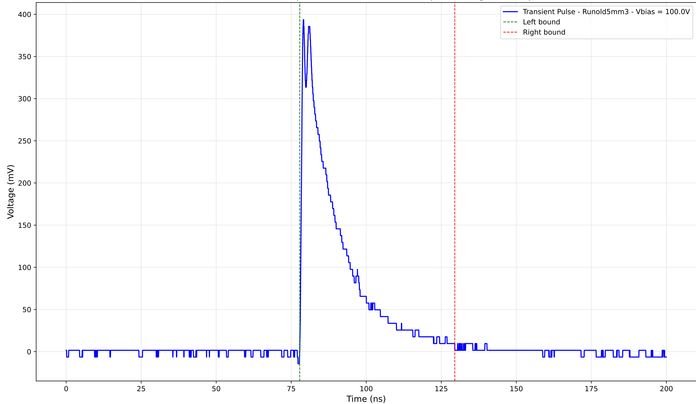
Transient Pulse - Sample: old5 - Position: 3170.0 \mu\text{m} - Charge: 97.90 pC
