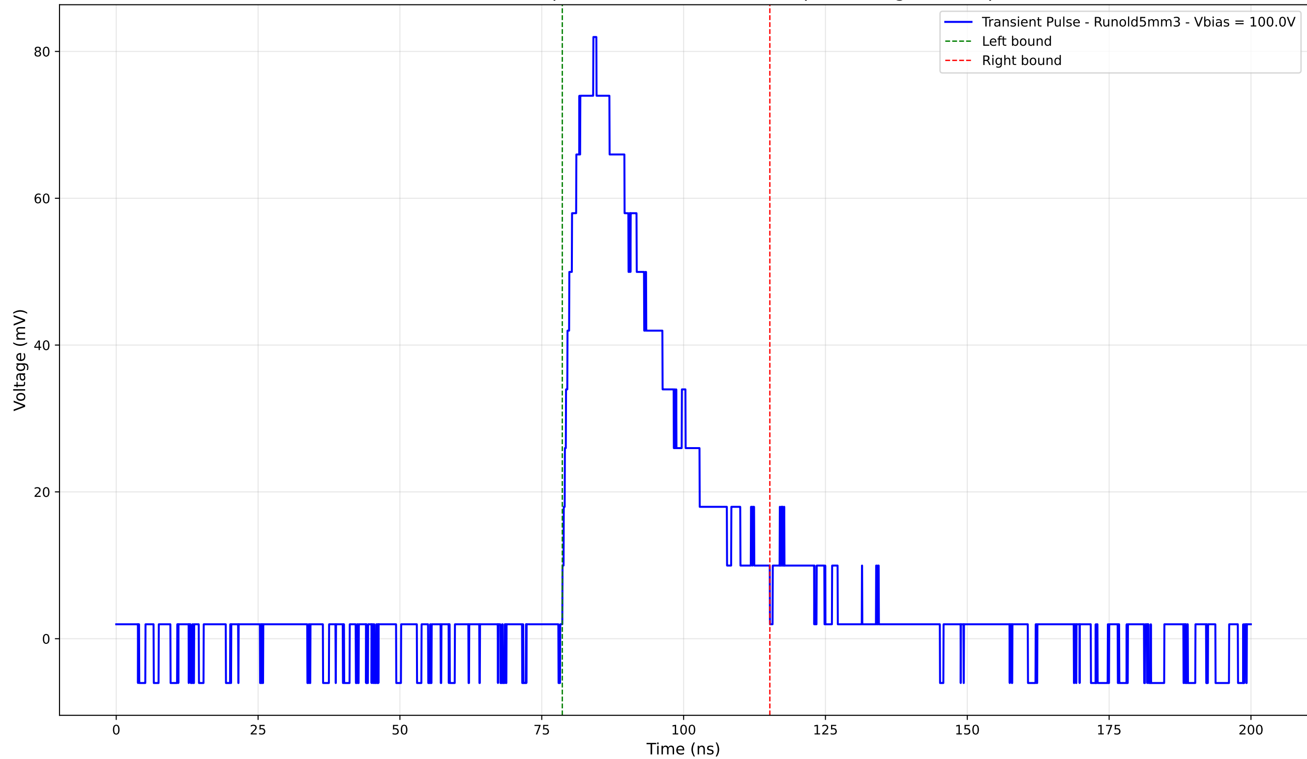
Transient Pulse - Sample: old5 - Position: 2020.0 \mu\text{m} - Charge: 28.08 pC
