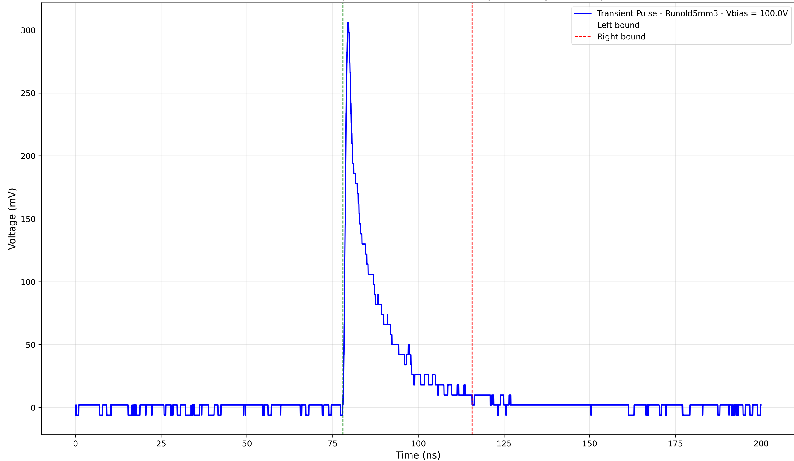
Transient Pulse - Sample: old5 - Position: 370.0 \mu\text{m} - Charge: 48.05 pC
