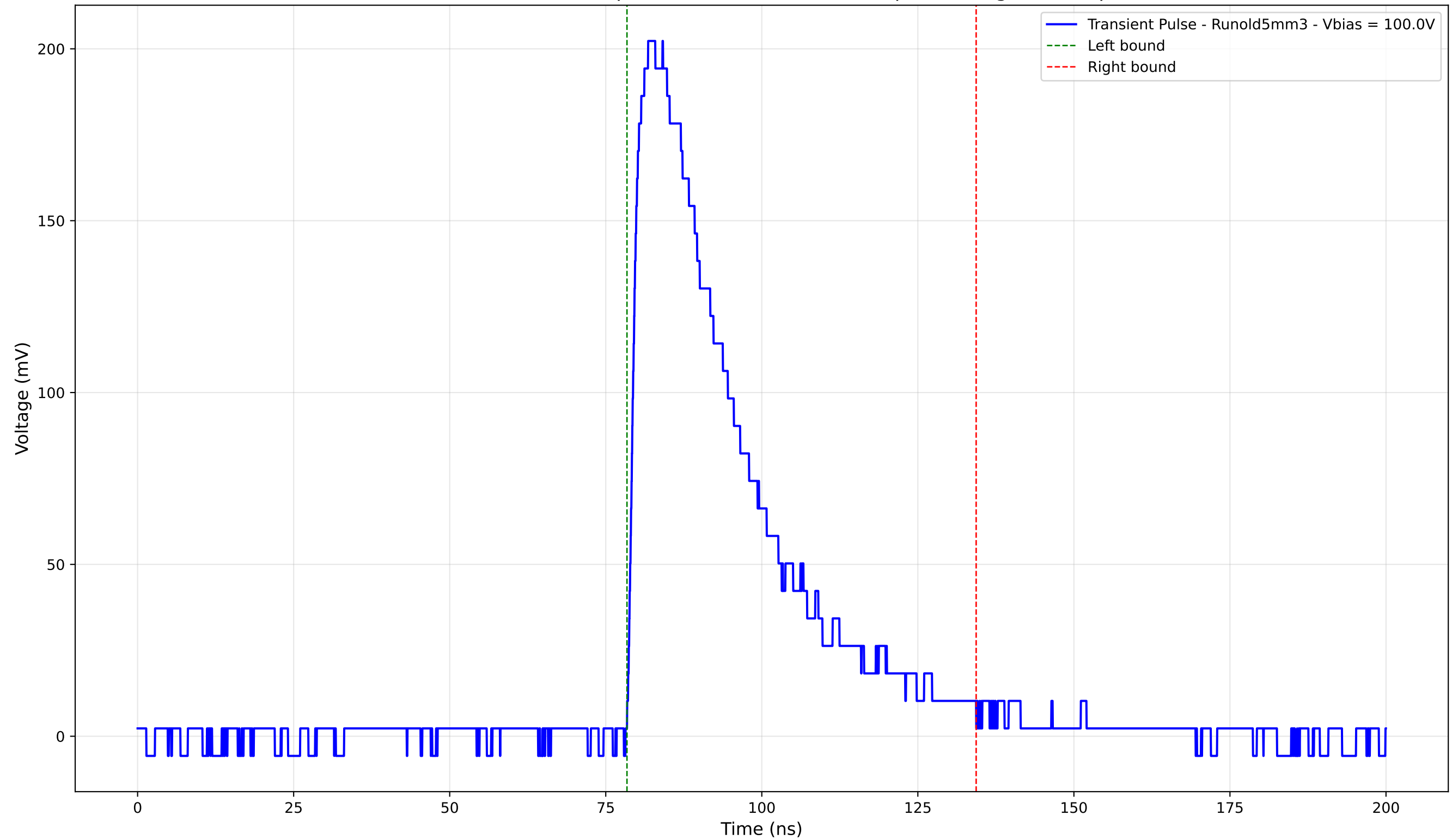
Transient Pulse - Sample: old5 - Position: 1265.0 \mu\text{m} - Charge: 76.59 pC
