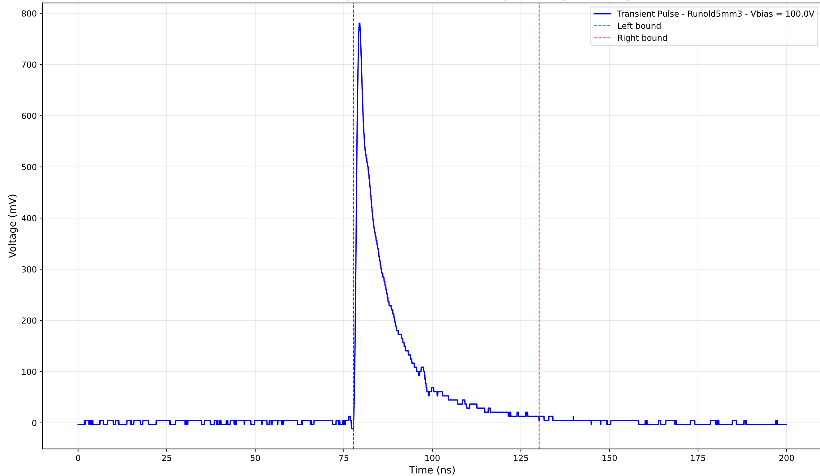
Transient Pulse - Sample: old5 - Position: 4755.0 \mu\text{m} - Charge: 134.84 pC
