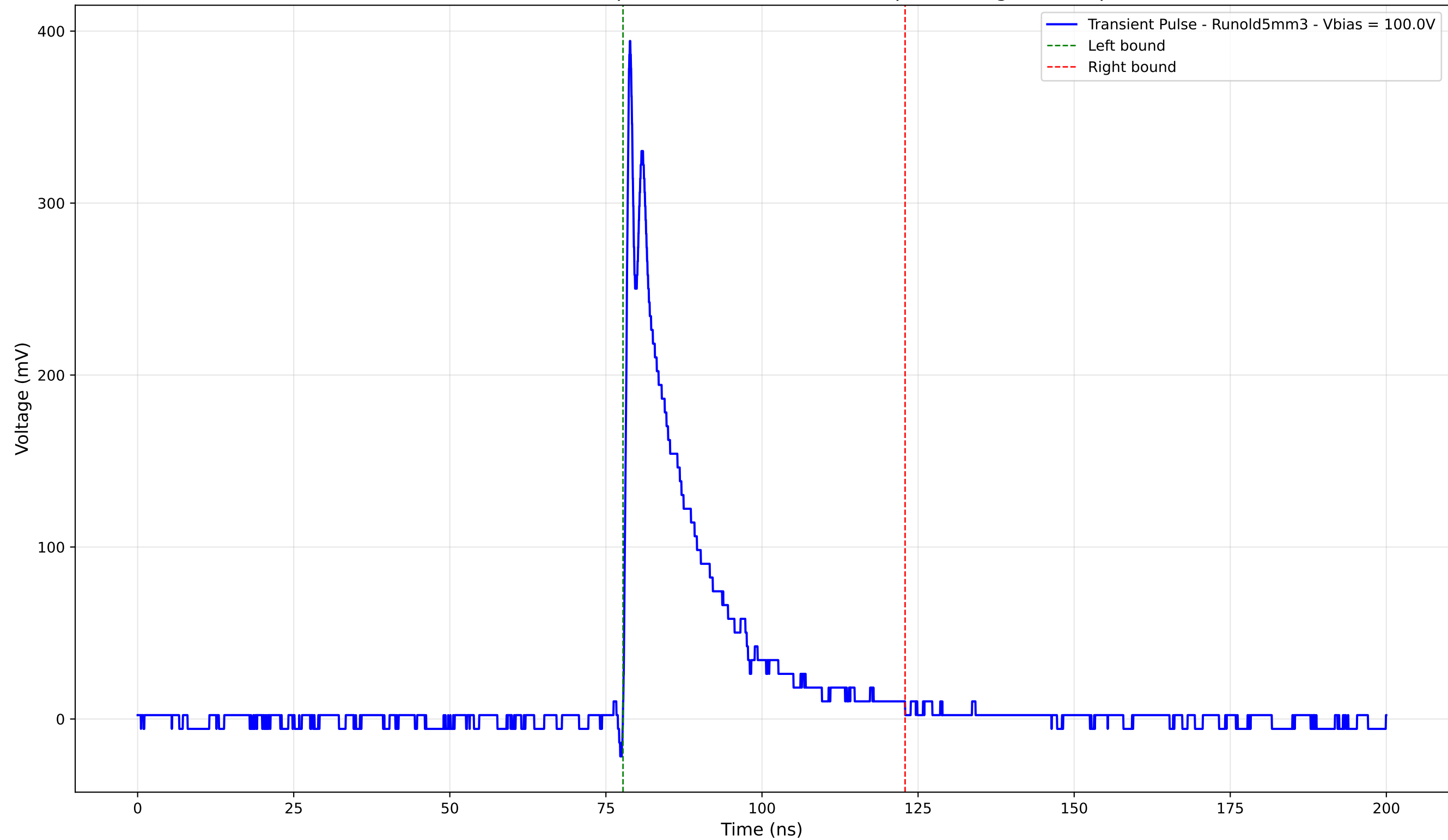
Transient Pulse - Sample: old5 - Position: 3360.0 \mu\text{m} - Charge: 68.86 pC
