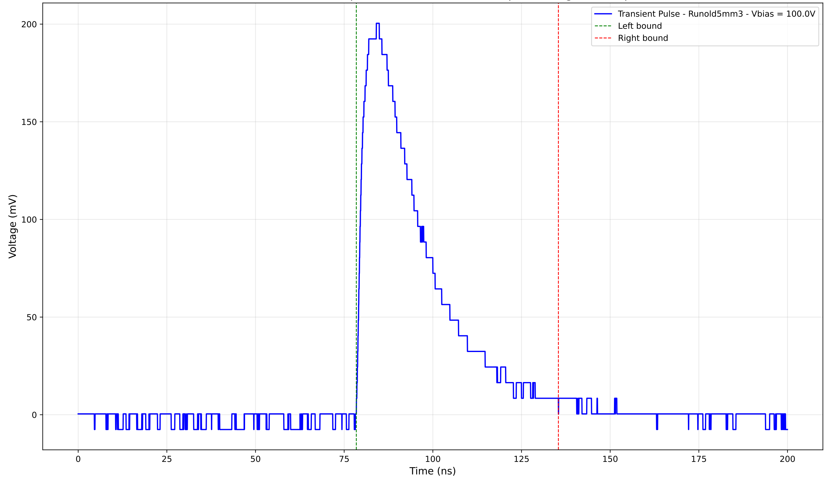
Transient Pulse - Sample: old5 - Position: 1705.0 \mu\text{m} - Charge: 79.25 pC
