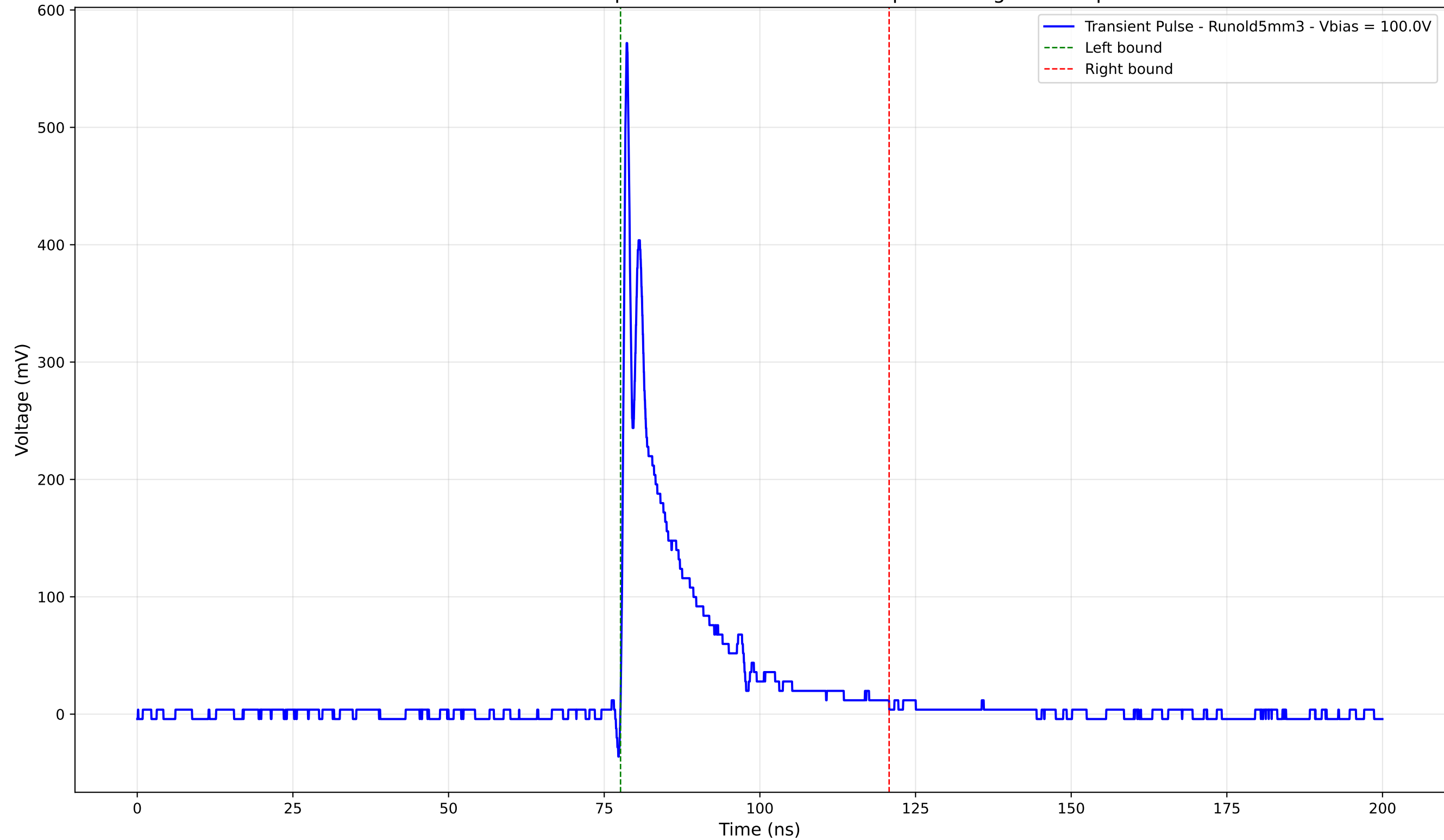
Transient Pulse - Sample: old5 - Position: 3500.0 \mu\text{m} - Charge: 73.49 pC
