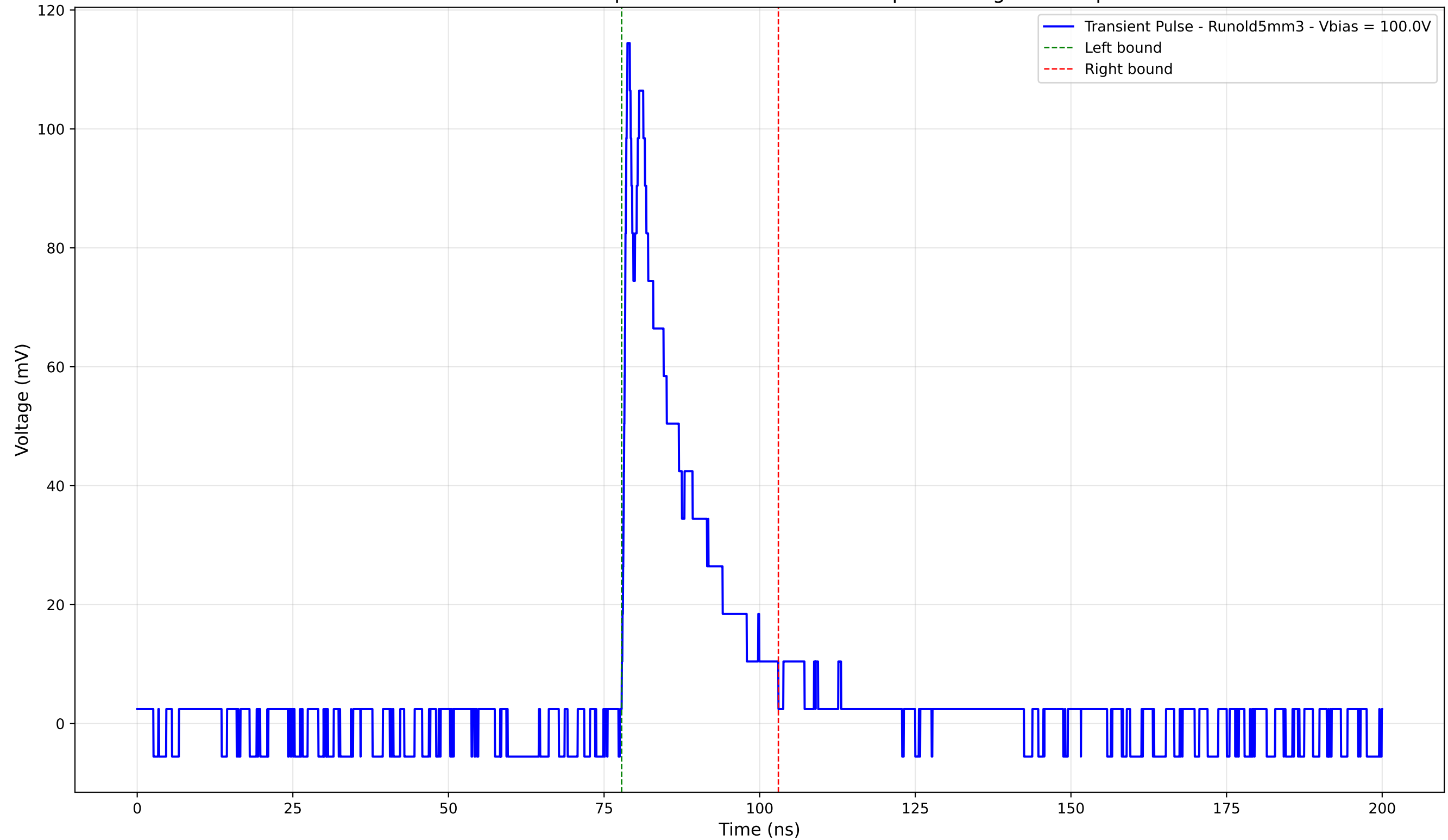
Transient Pulse - Sample: old5 - Position: 3325.0 \mu\text{m} - Charge: 20.65 pC
