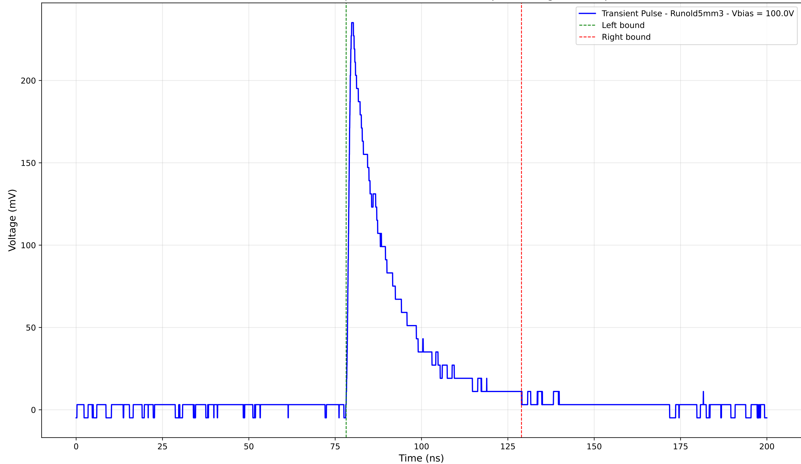
Transient Pulse - Sample: old5 - Position: 635.0 \mu\text{m} - Charge: 57.08 pC
