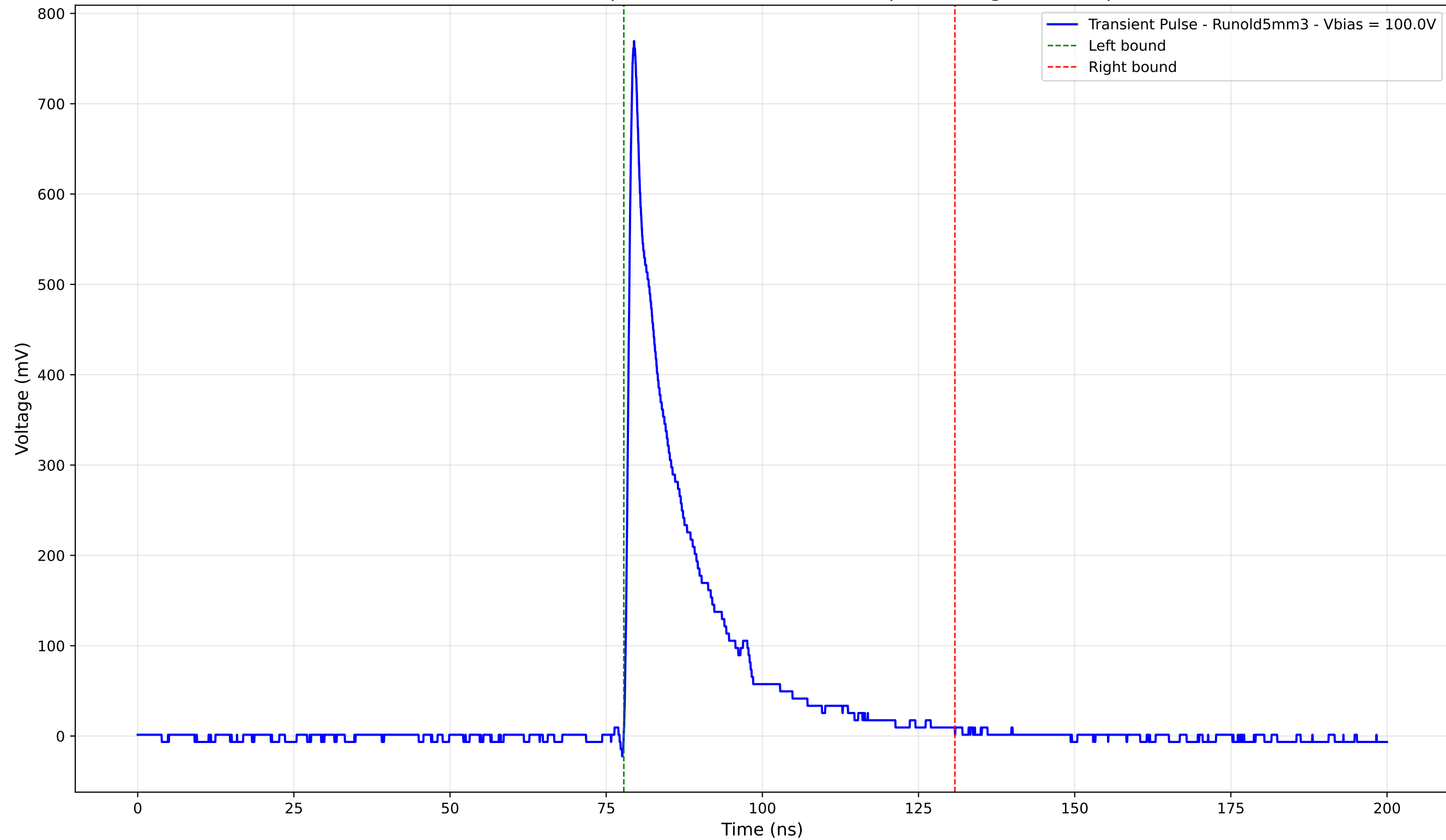
Transient Pulse - Sample: old5 - Position: 4745.0 \mu\text{m} - Charge: 131.47 pC
