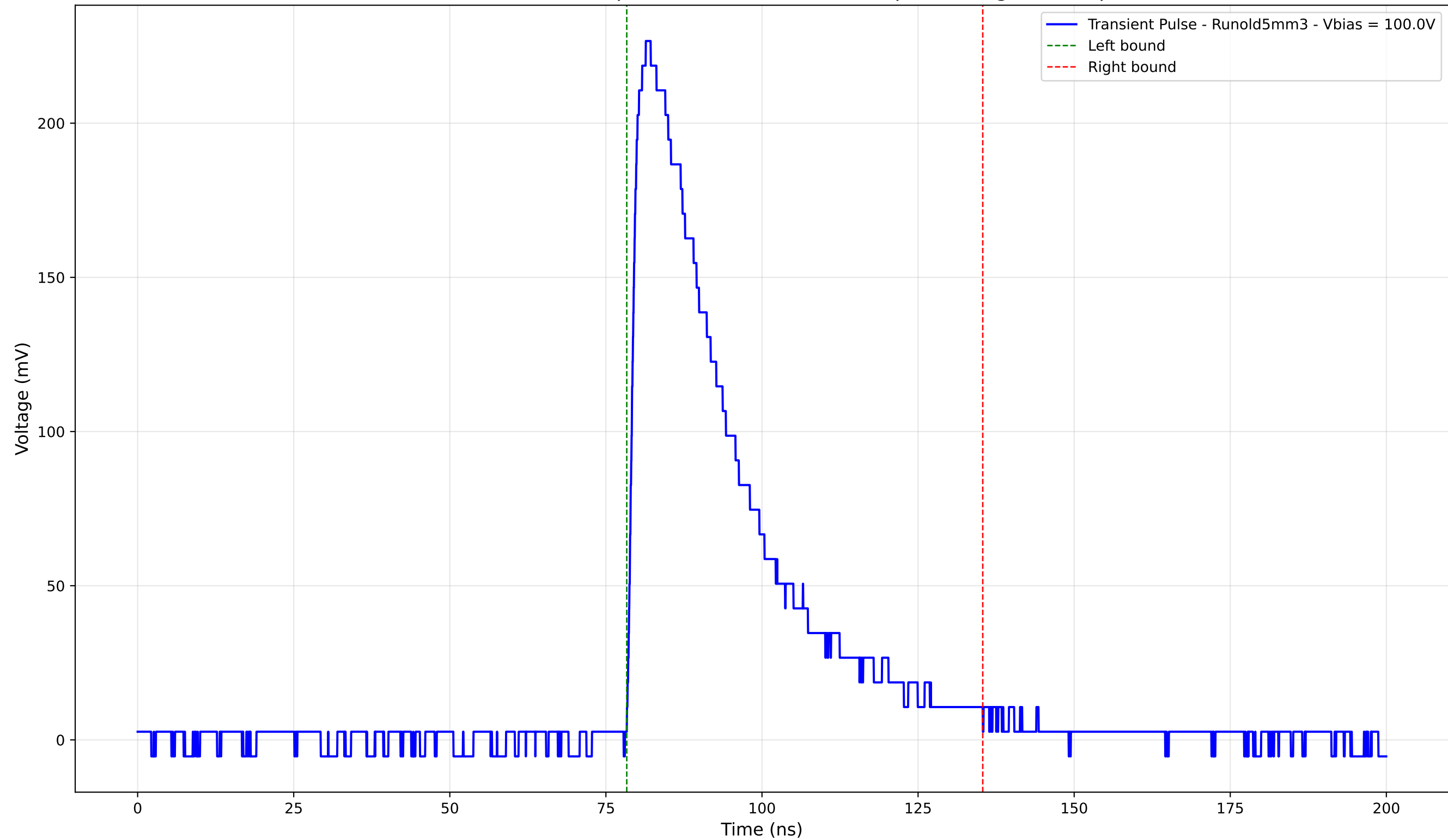
Transient Pulse - Sample: old5 - Position: 1100.0 \mu\text{m} - Charge: 81.17 pC
