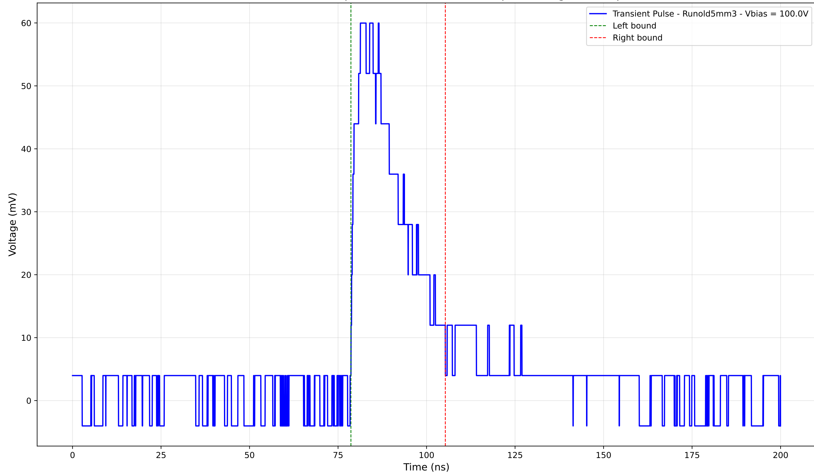
Transient Pulse - Sample: old5 - Position: 2715.0 \mu\text{m} - Charge: 17.90 pC
