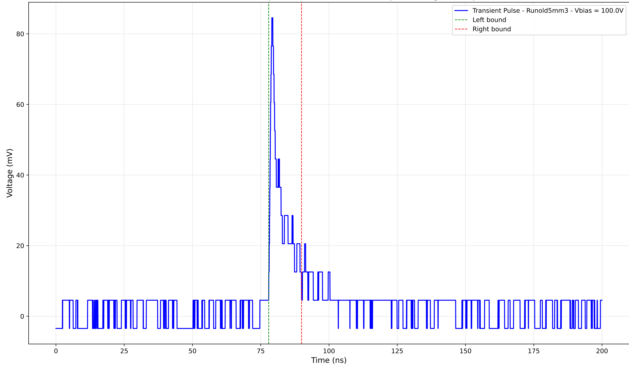
Transient Pulse - Sample: old5 - Position: 4925.0 \mu\text{m} - Charge: 7.67 pC
