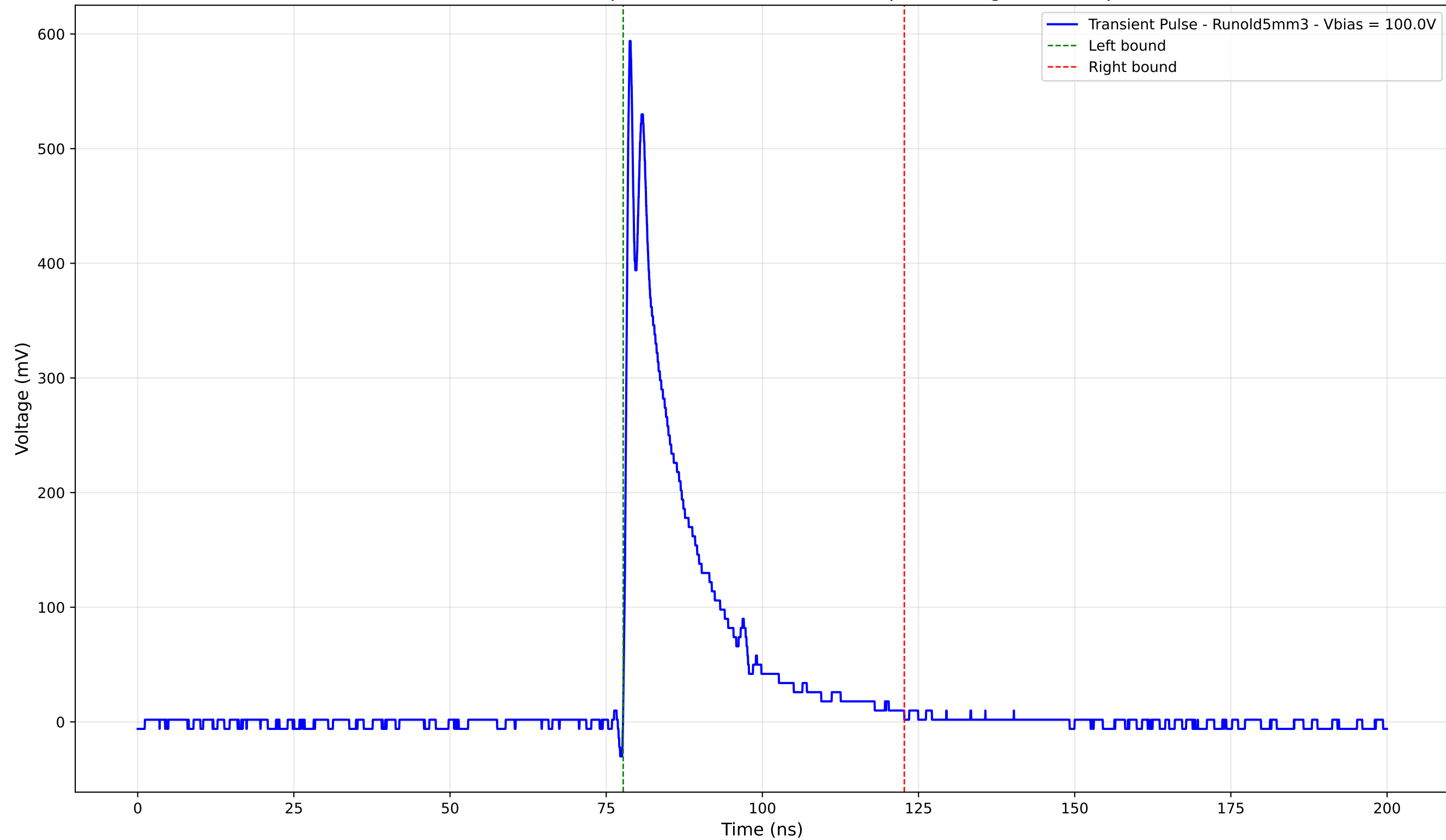
Transient Pulse - Sample: old5 - Position: 3775.0 \mu\text{m} - Charge: 102.46 pC
