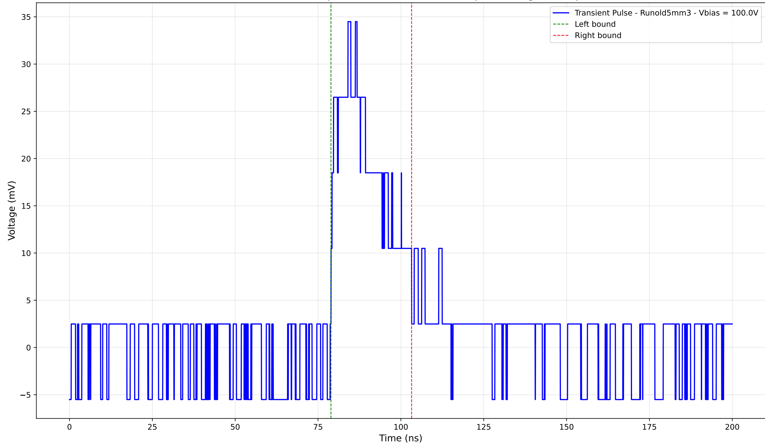
Transient Pulse - Sample: old5 - Position: 1180.0 \mu\text{m} - Charge: 9.47 pC
