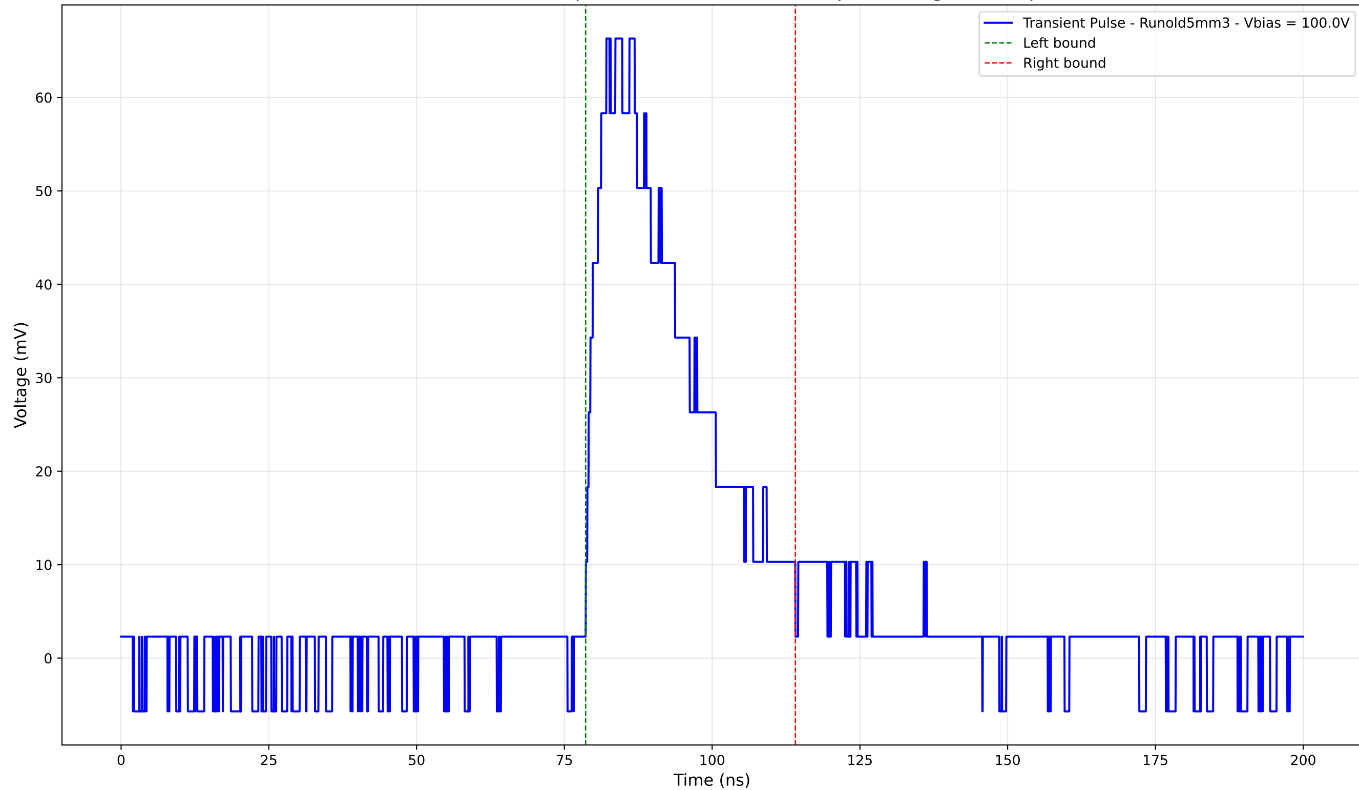
Transient Pulse - Sample: old5 - Position: 1965.0 \mu\text{m} - Charge: 23.24 pC
