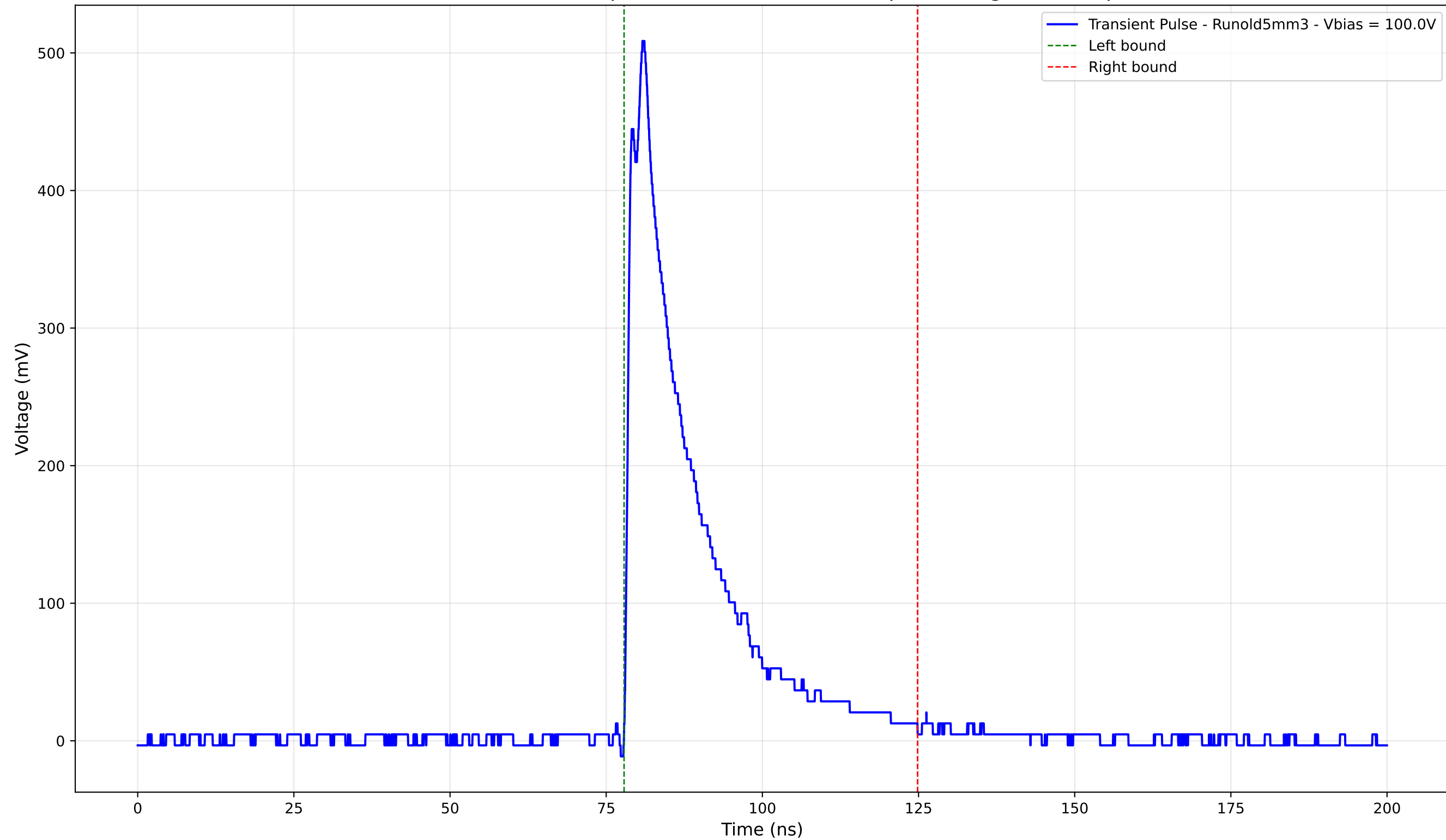
Transient Pulse - Sample: old5 - Position: 4005.0 \mu\text{m} - Charge: 111.83 pC
