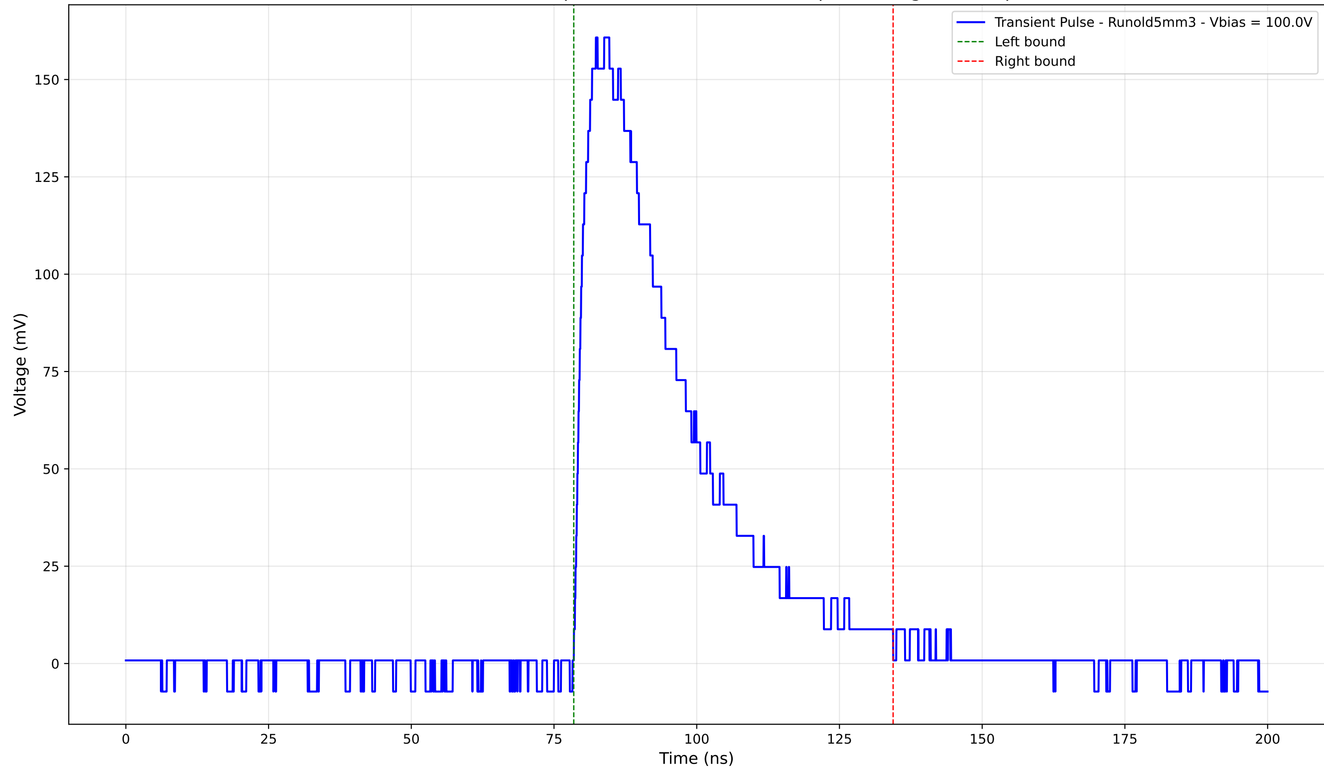
Transient Pulse - Sample: old5 - Position: 1725.0 \mu\text{m} - Charge: 63.14 pC
