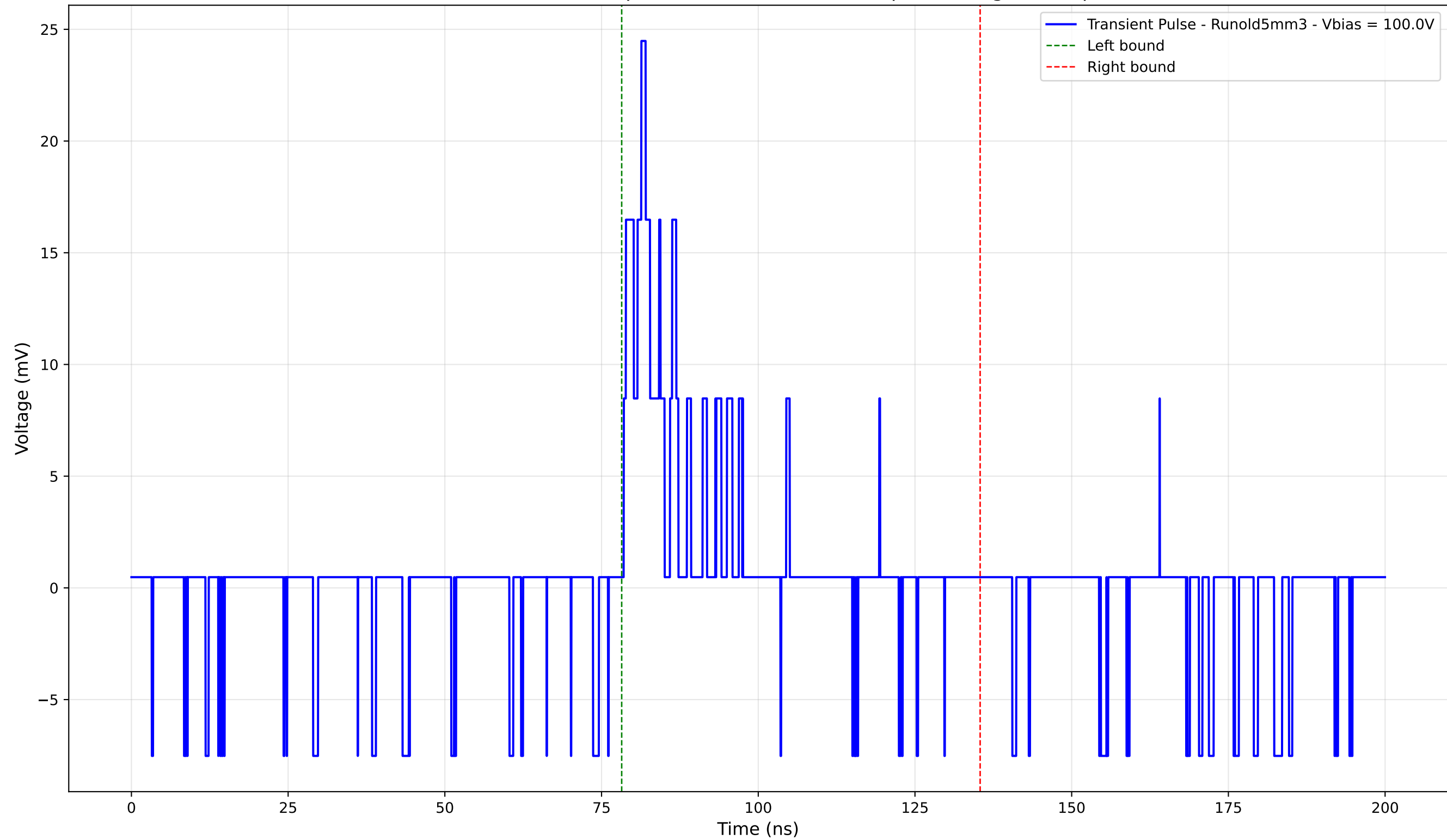
Transient Pulse - Sample: old5 - Position: 110.0 \mu\text{m} - Charge: 3.03 pC
