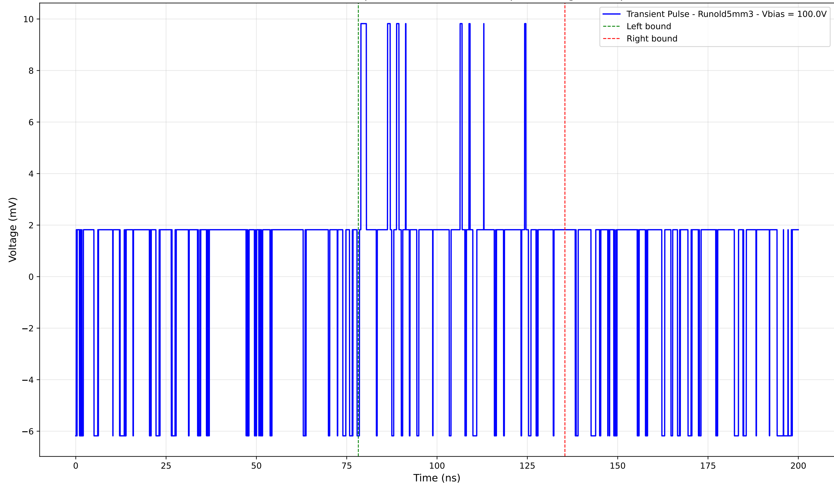
Transient Pulse - Sample: old5 - Position: 20.0 \mu\text{m} - Charge: 1.73 pC
