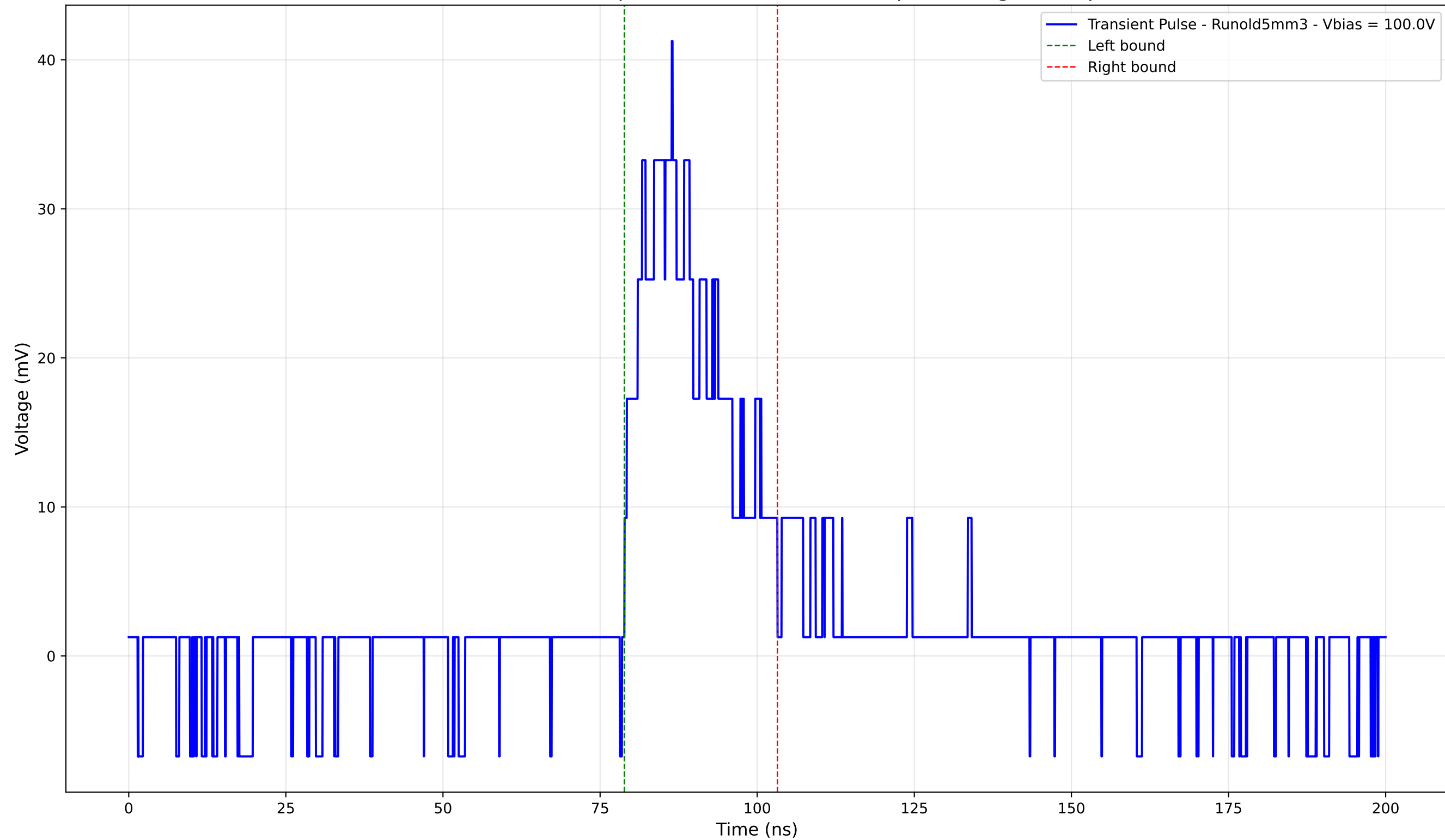
Transient Pulse - Sample: old5 - Position: 1995.0 \mu\text{m} - Charge: 9.92 pC
