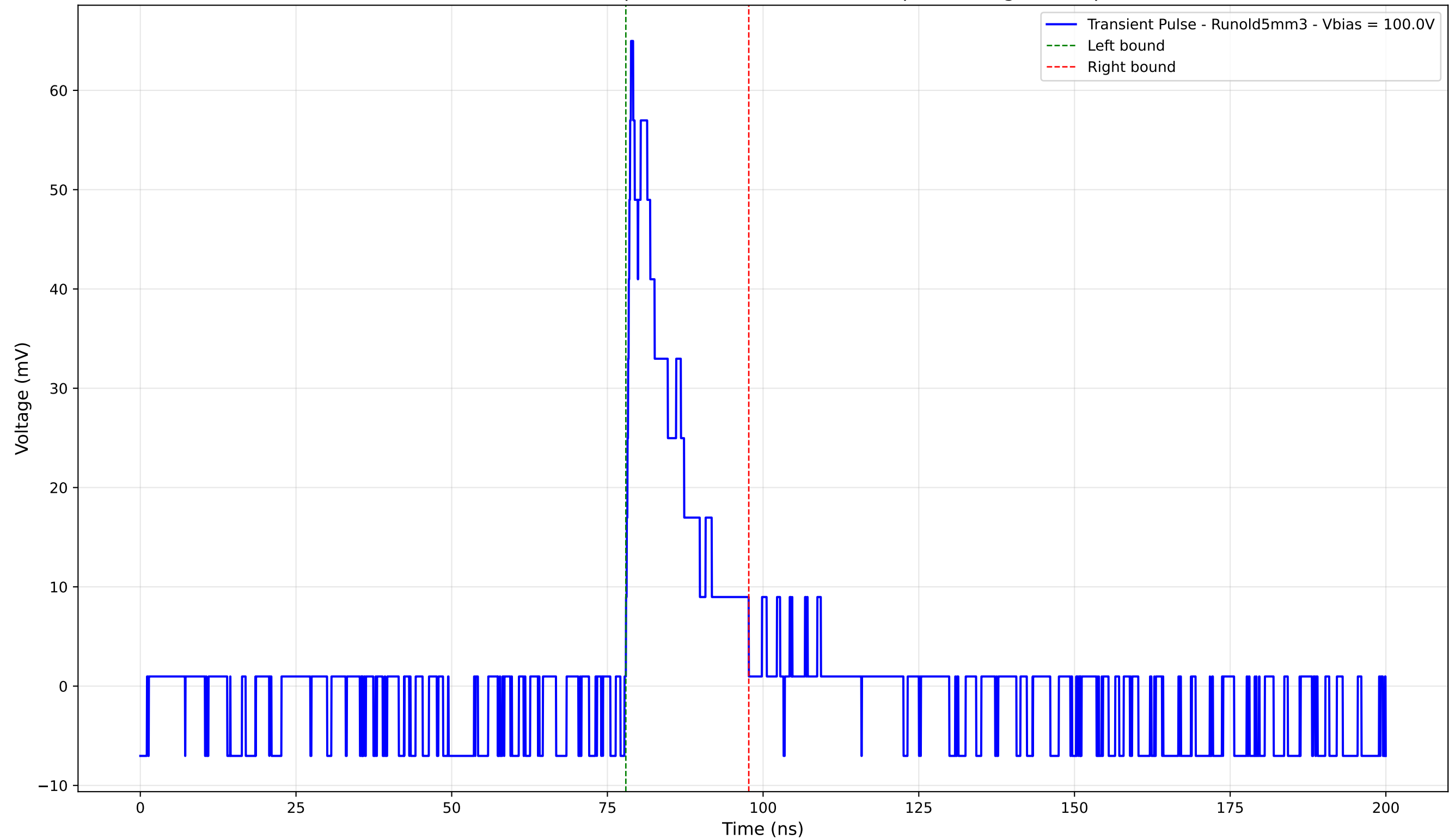
Transient Pulse - Sample: old5 - Position: 3855.0 \mu\text{m} - Charge: 9.72 pC
