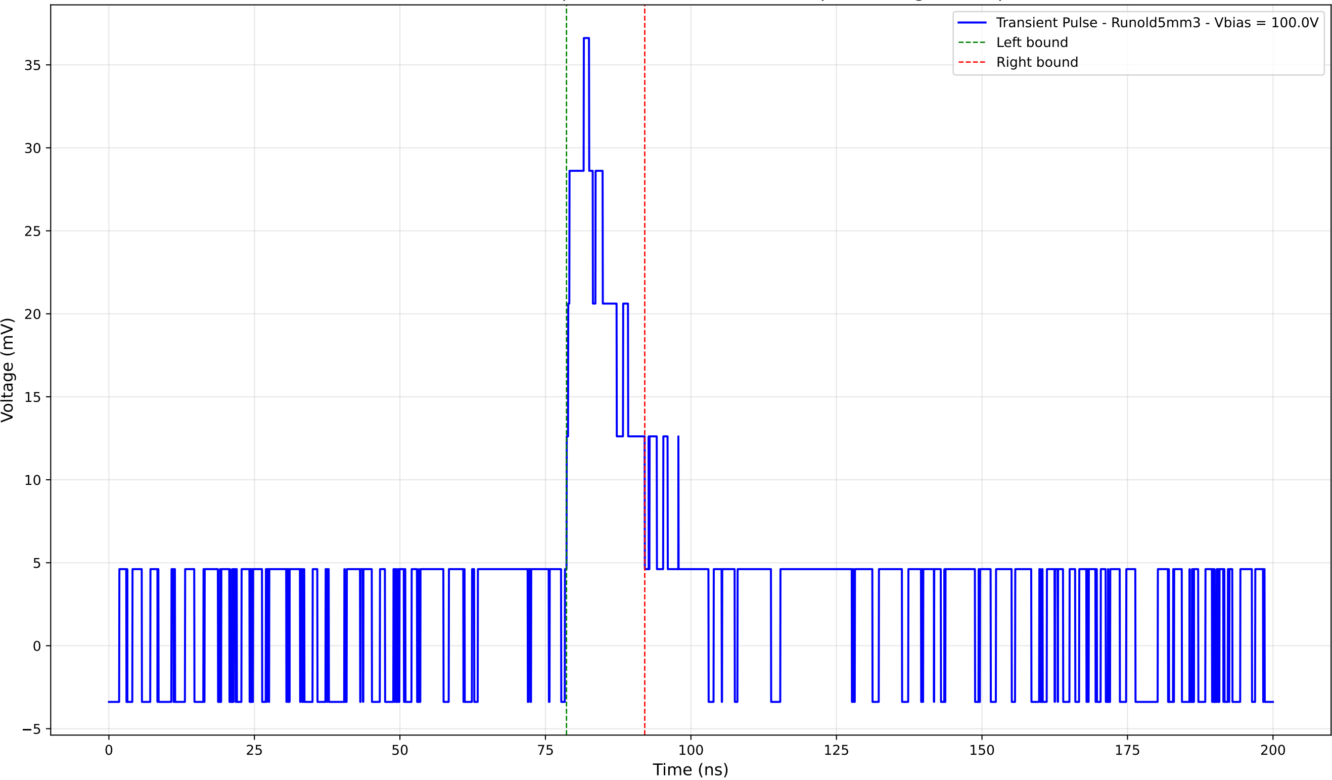
Transient Pulse - Sample: old5 - Position: 4495.0 \mu\text{m} - Charge: 5.85 pC
