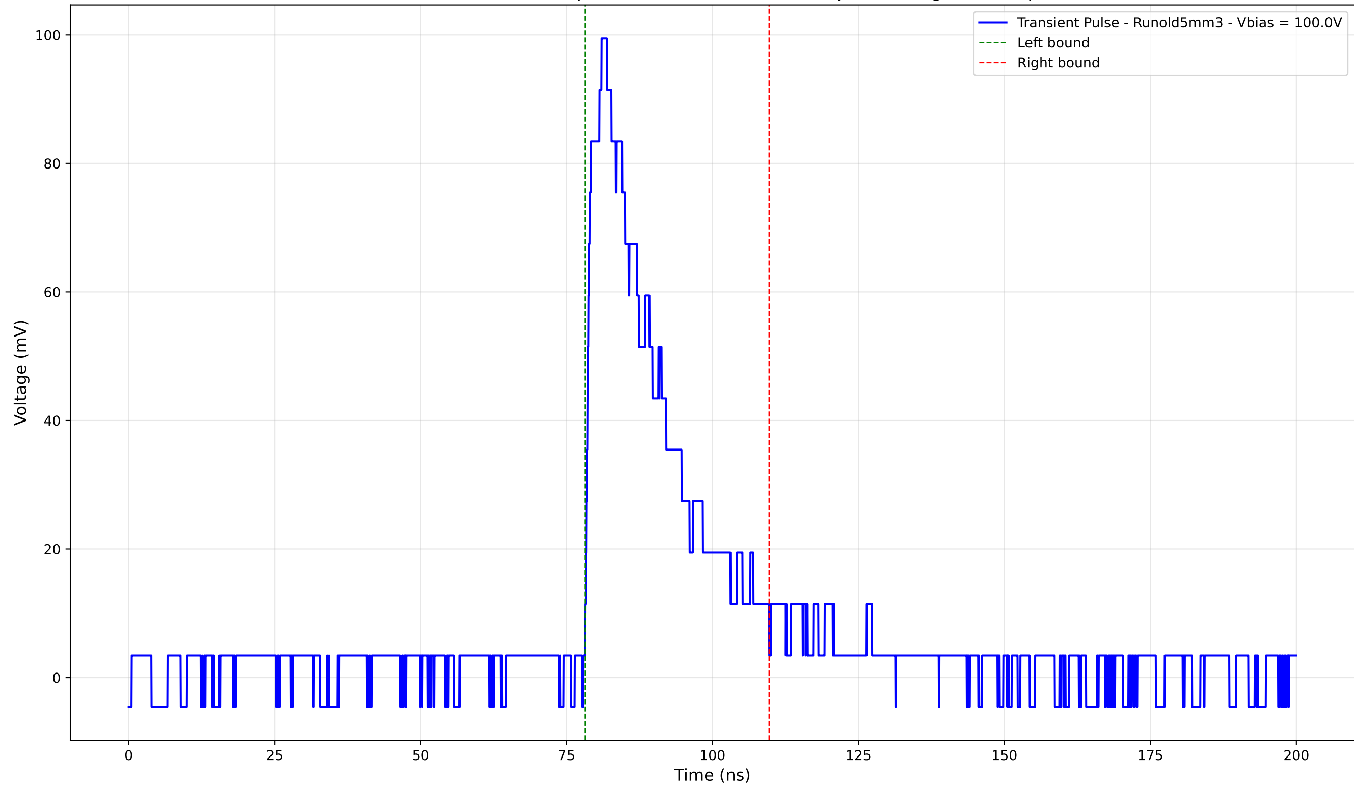
Transient Pulse - Sample: old5 - Position: 3025.0 \mu\text{m} - Charge: 26.15 pC
