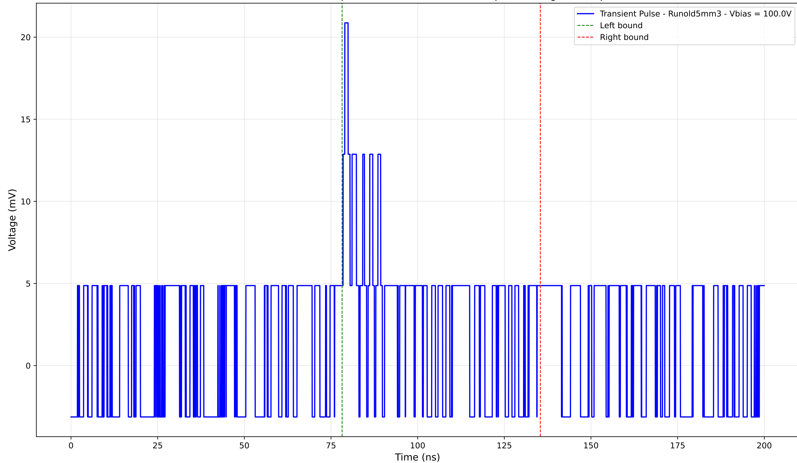
Transient Pulse - Sample: old5 - Position: 4960.0 \mu\text{m} - Charge: 4.21 pC
