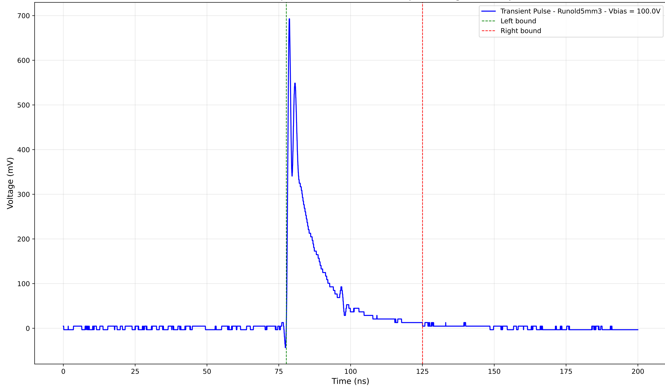
Transient Pulse - Sample: old5 - Position: 3690.0 \mu\text{m} - Charge: 101.43 pC
