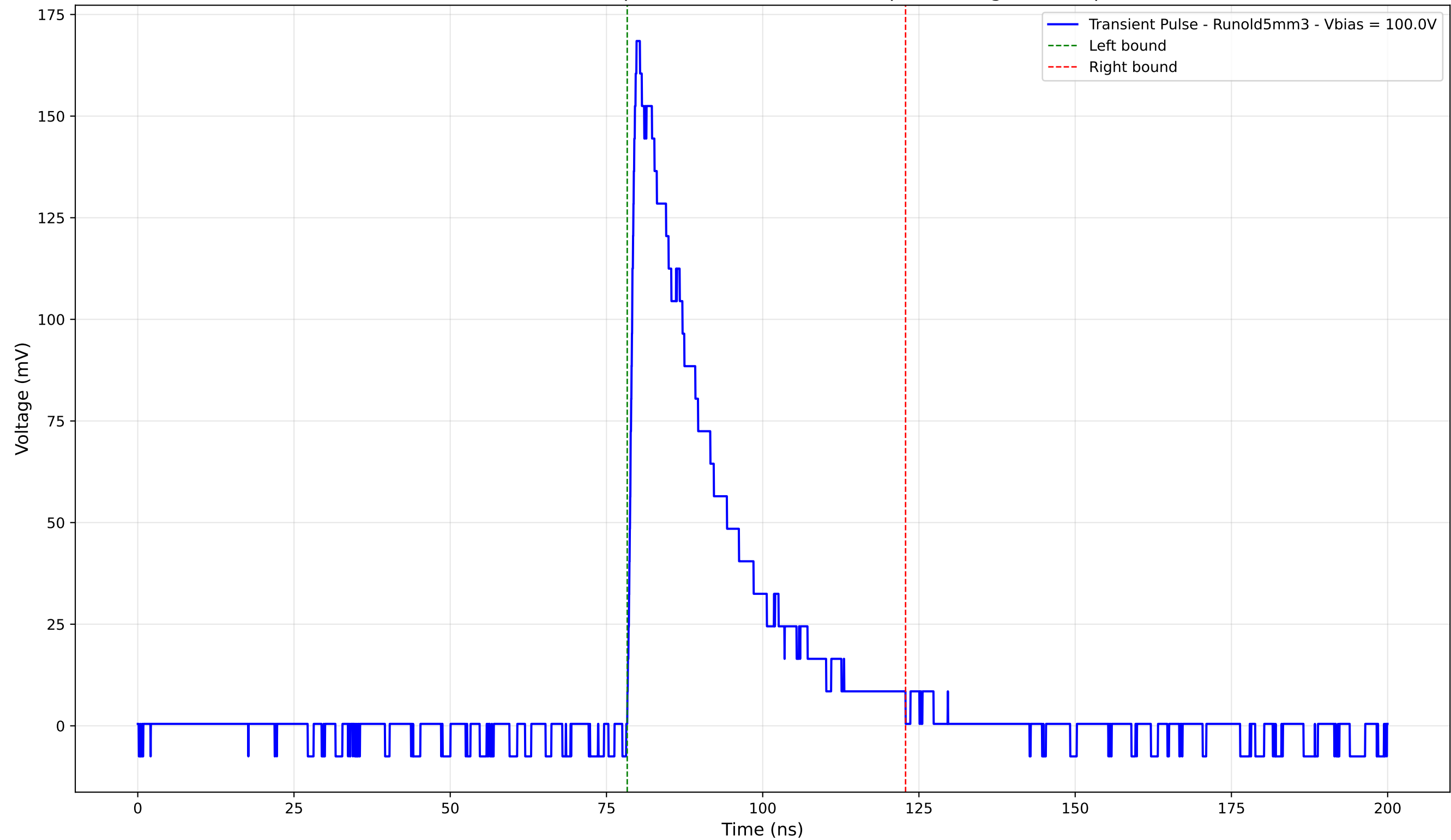
Transient Pulse - Sample: old5 - Position: 780.0 \mu\text{m} - Charge: 44.23 pC
