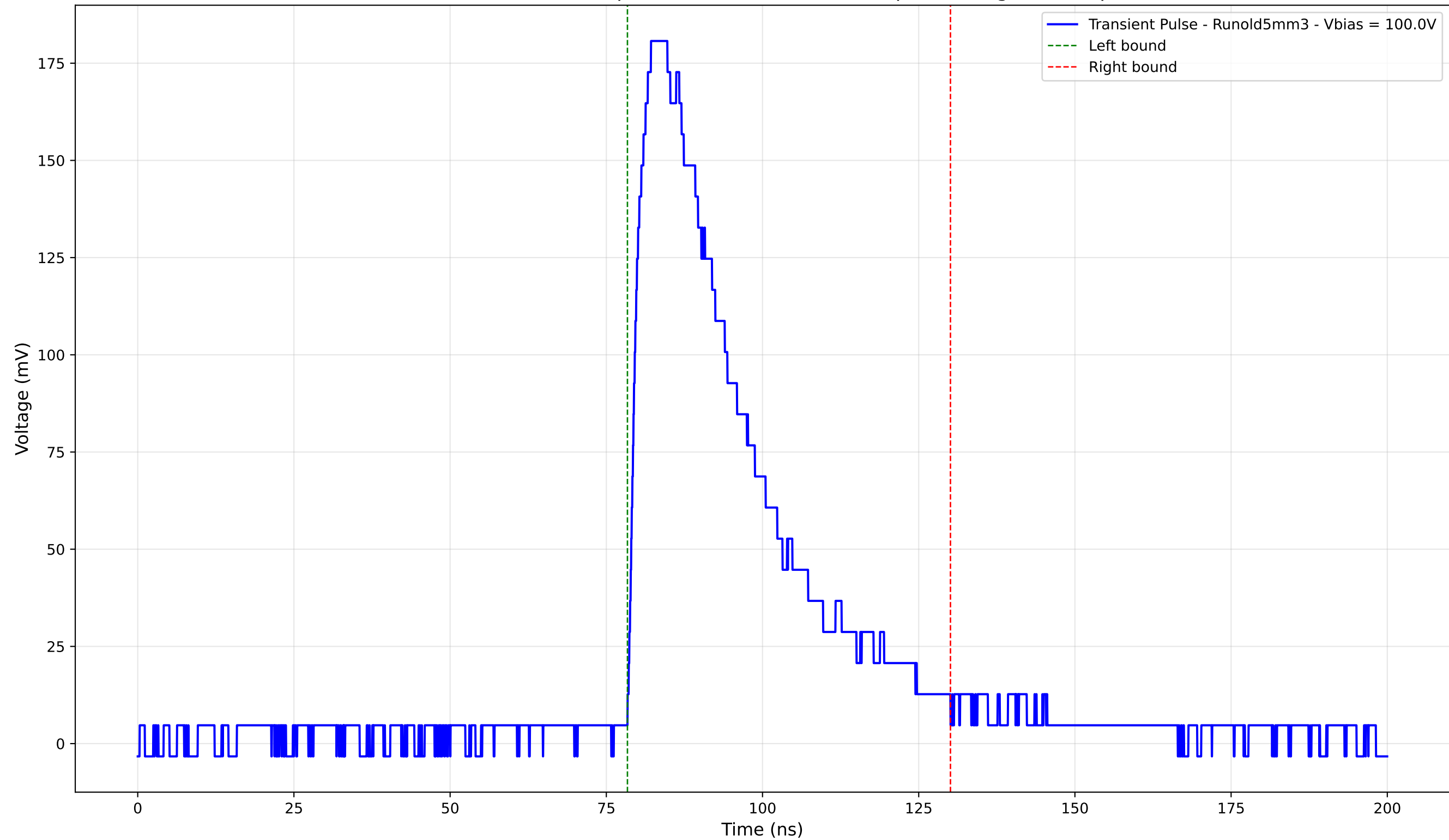
Transient Pulse - Sample: old5 - Position: 2255.0 \mu\text{m} - Charge: 72.41 pC
