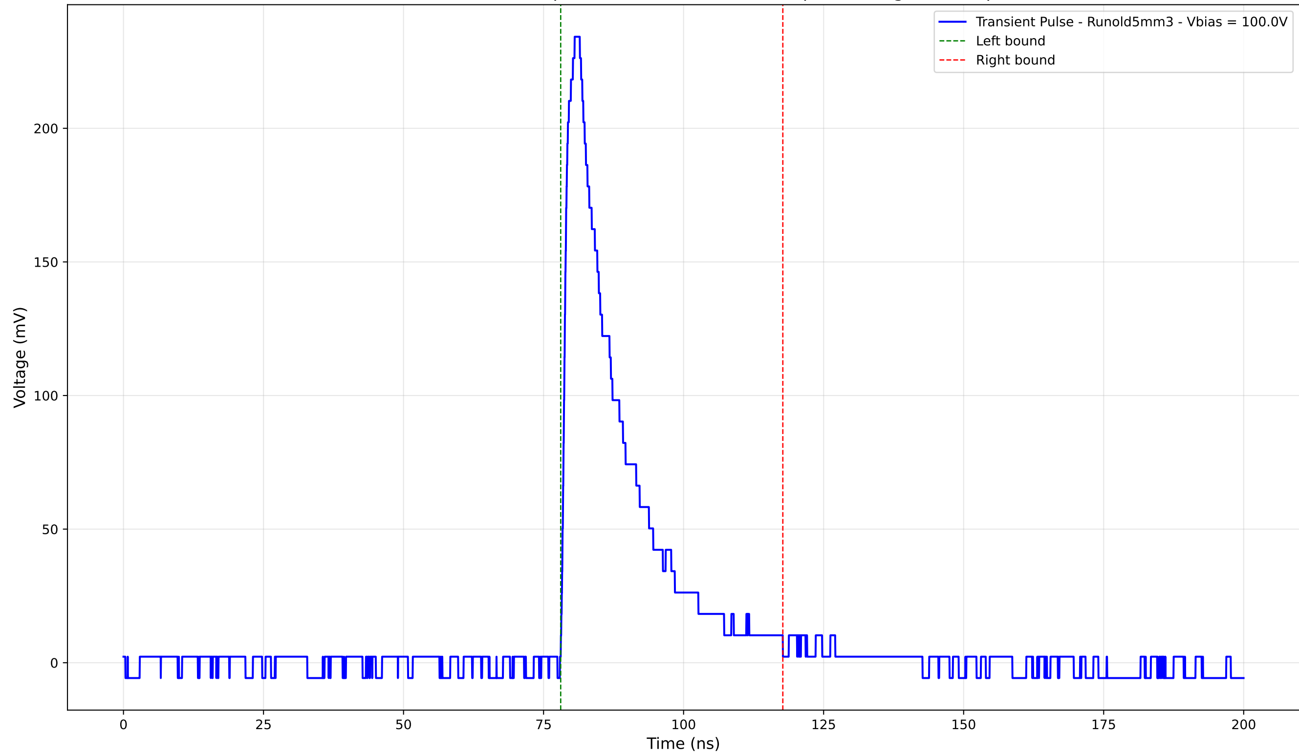
Transient Pulse - Sample: old5 - Position: 4115.0 \mu\text{m} - Charge: 50.27 pC
