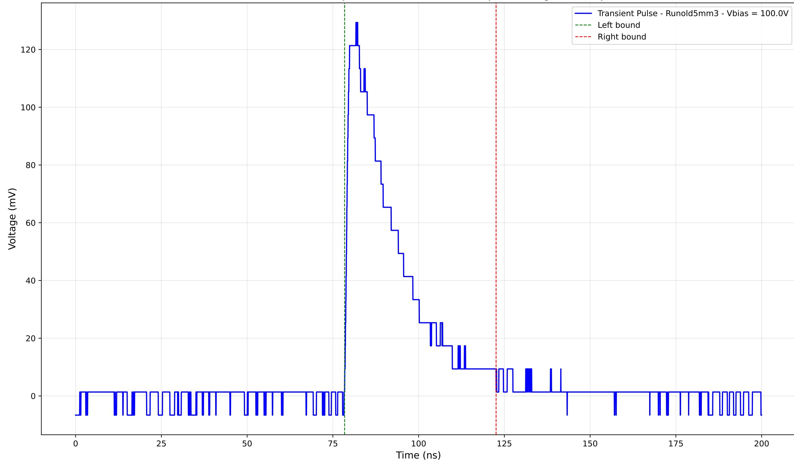
Transient Pulse - Sample: old5 - Position: 915.0 \mu\text{m} - Charge: 39.12 pC
