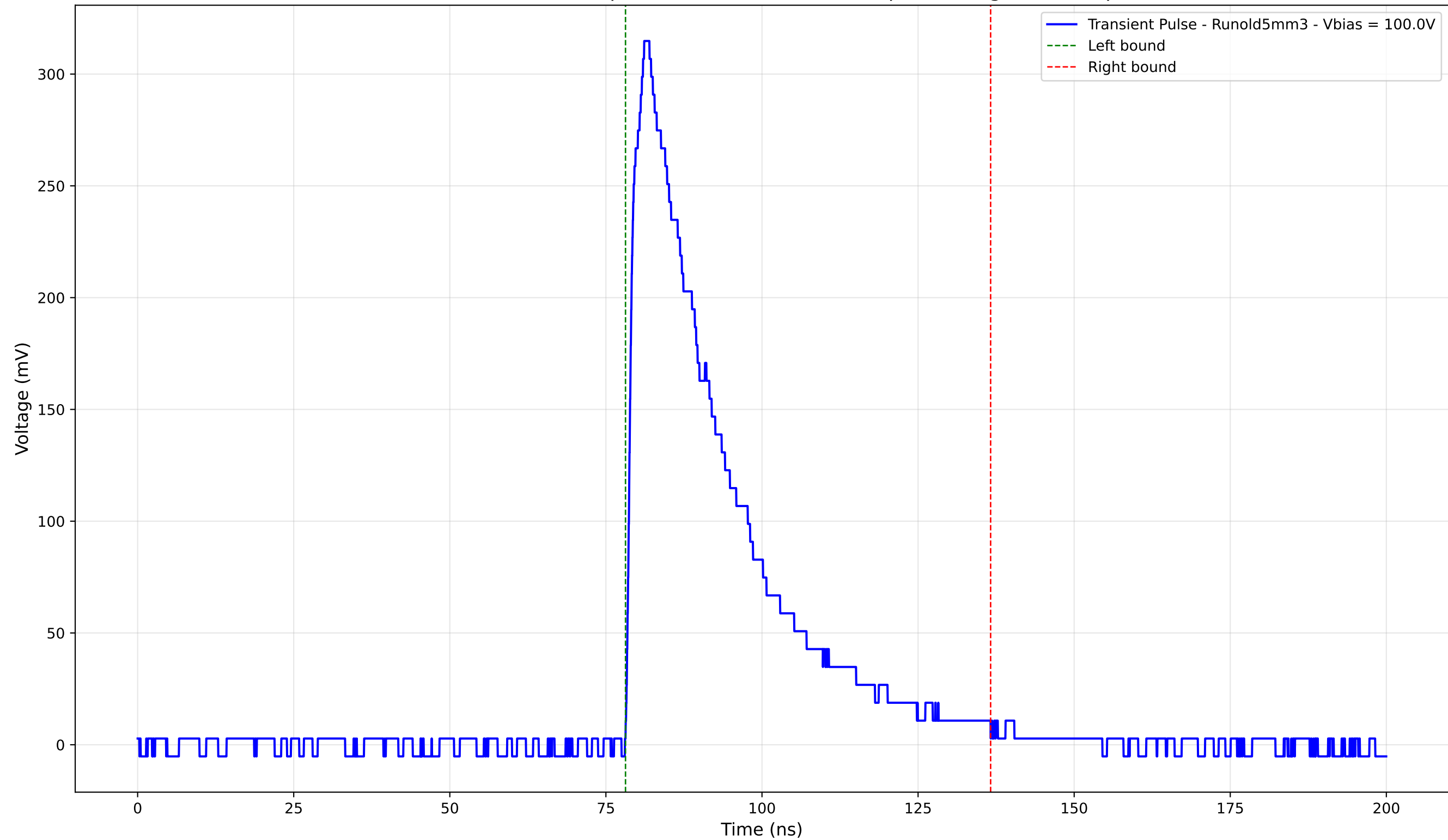
Transient Pulse - Sample: old5 - Position: 2860.0 \mu\text{m} - Charge: 102.24 pC
