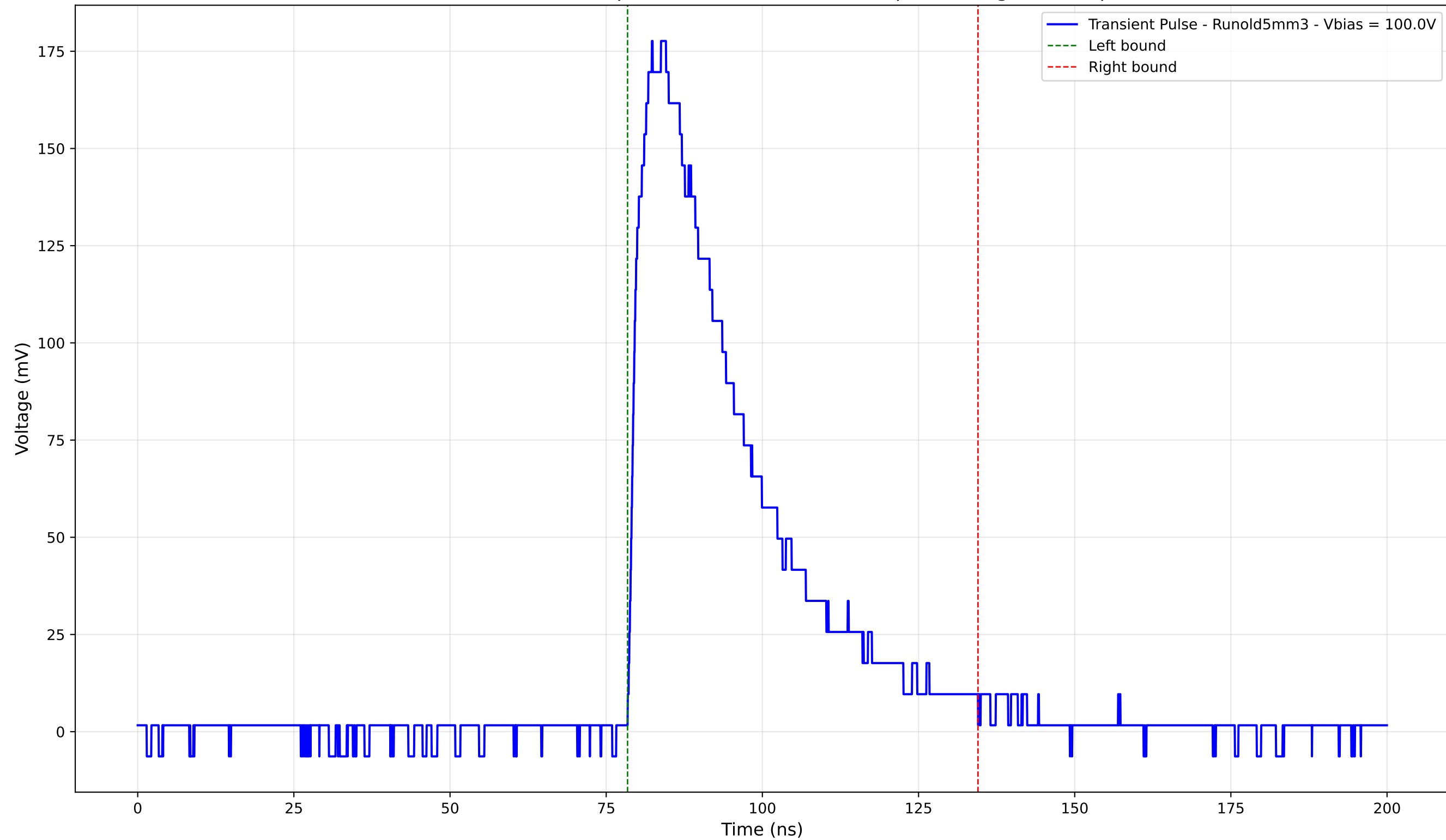
Transient Pulse - Sample: old5 - Position: 2335.0 \mu\text{m} - Charge: 68.36 pC
