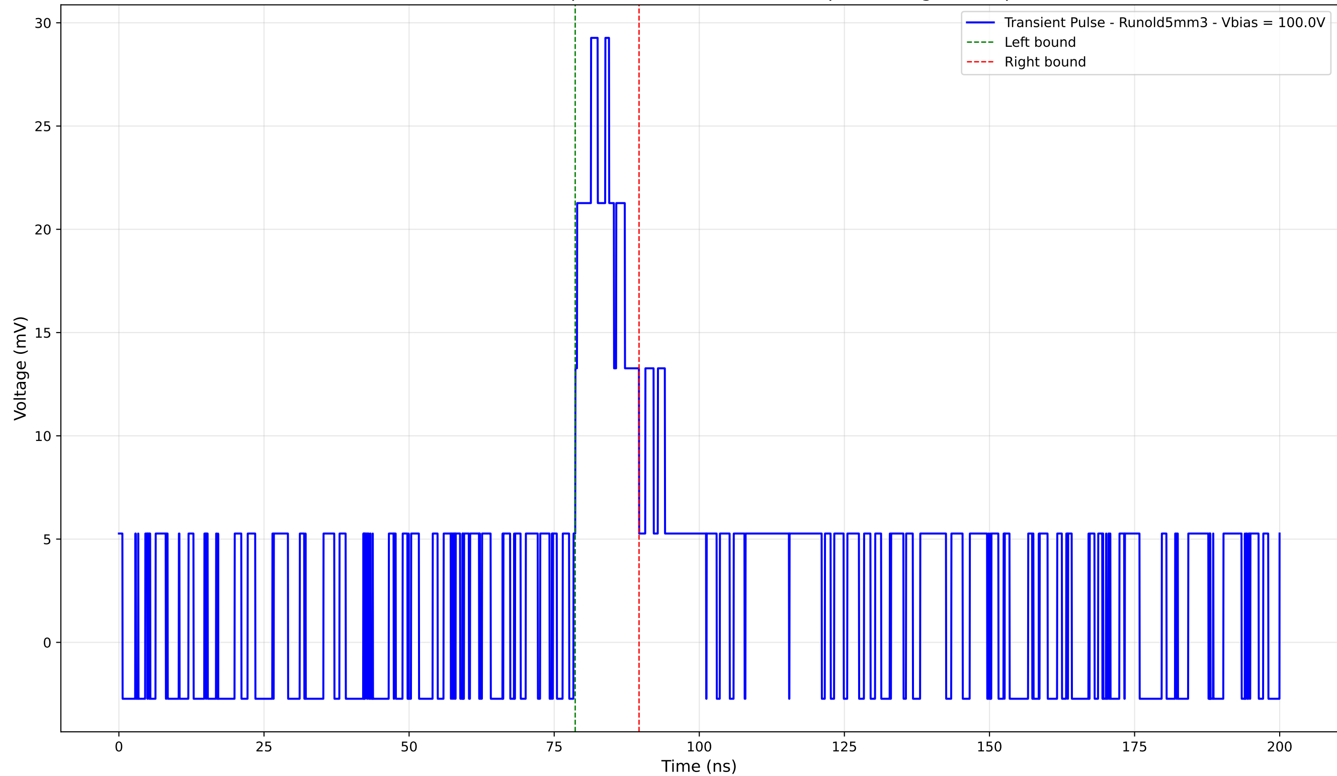
Transient Pulse - Sample: old5 - Position: 4175.0 \mu\text{m} - Charge: 4.46 pC
