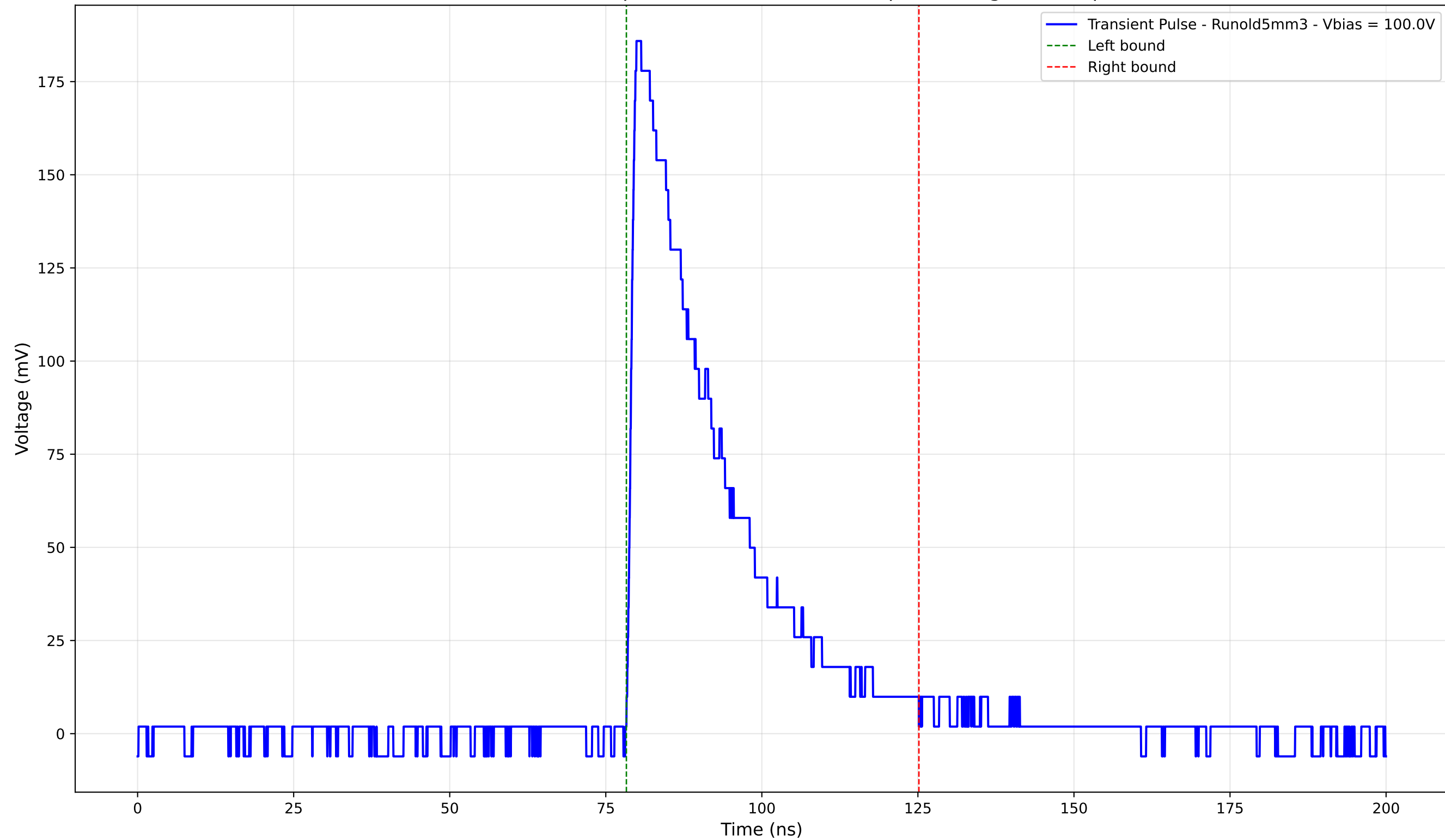
Transient Pulse - Sample: old5 - Position: 865.0 \mu\text{m} - Charge: 55.34 pC
