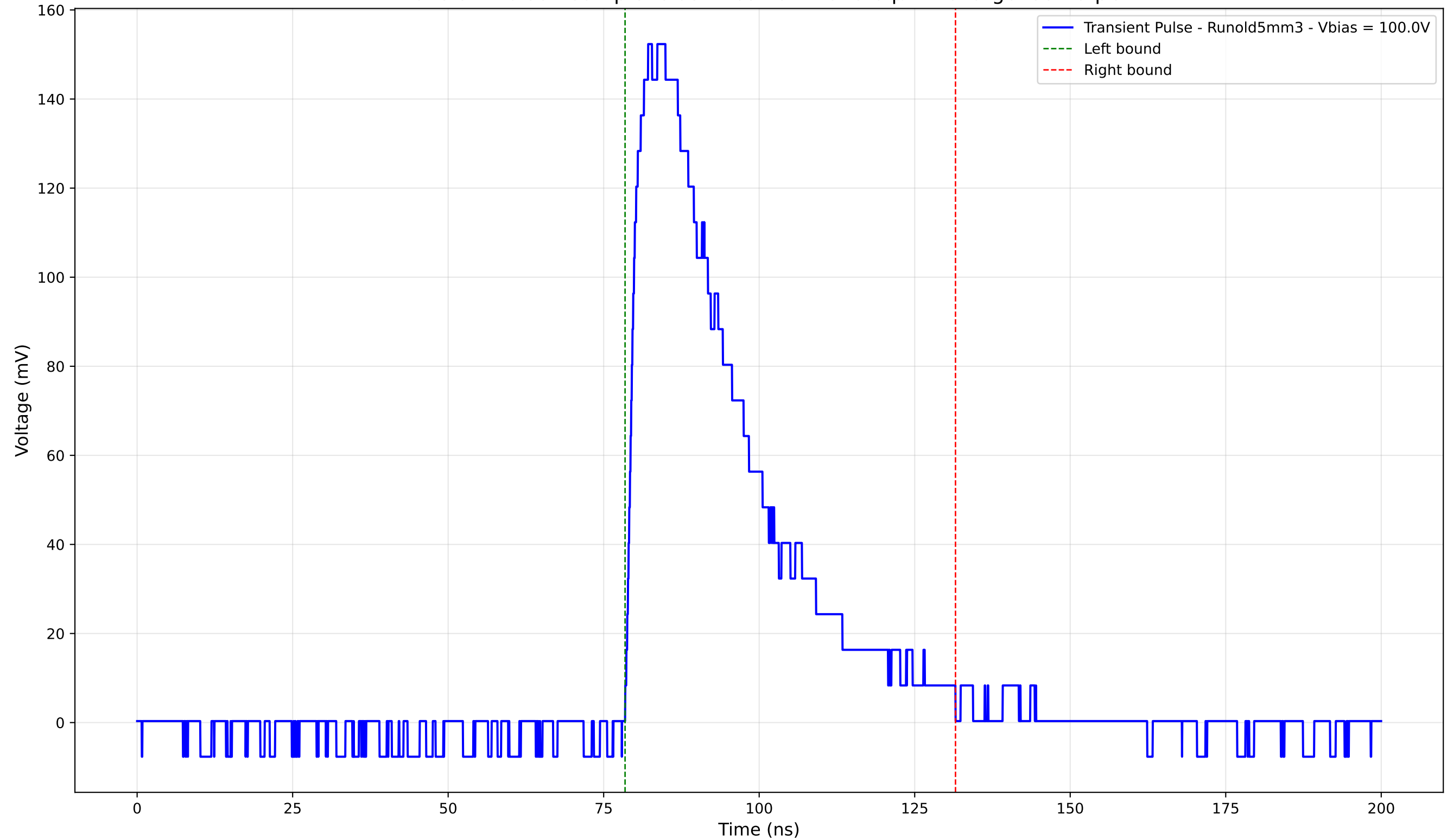
Transient Pulse - Sample: old5 - Position: 1525.0 \mu\text{m} - Charge: 59.19 pC
