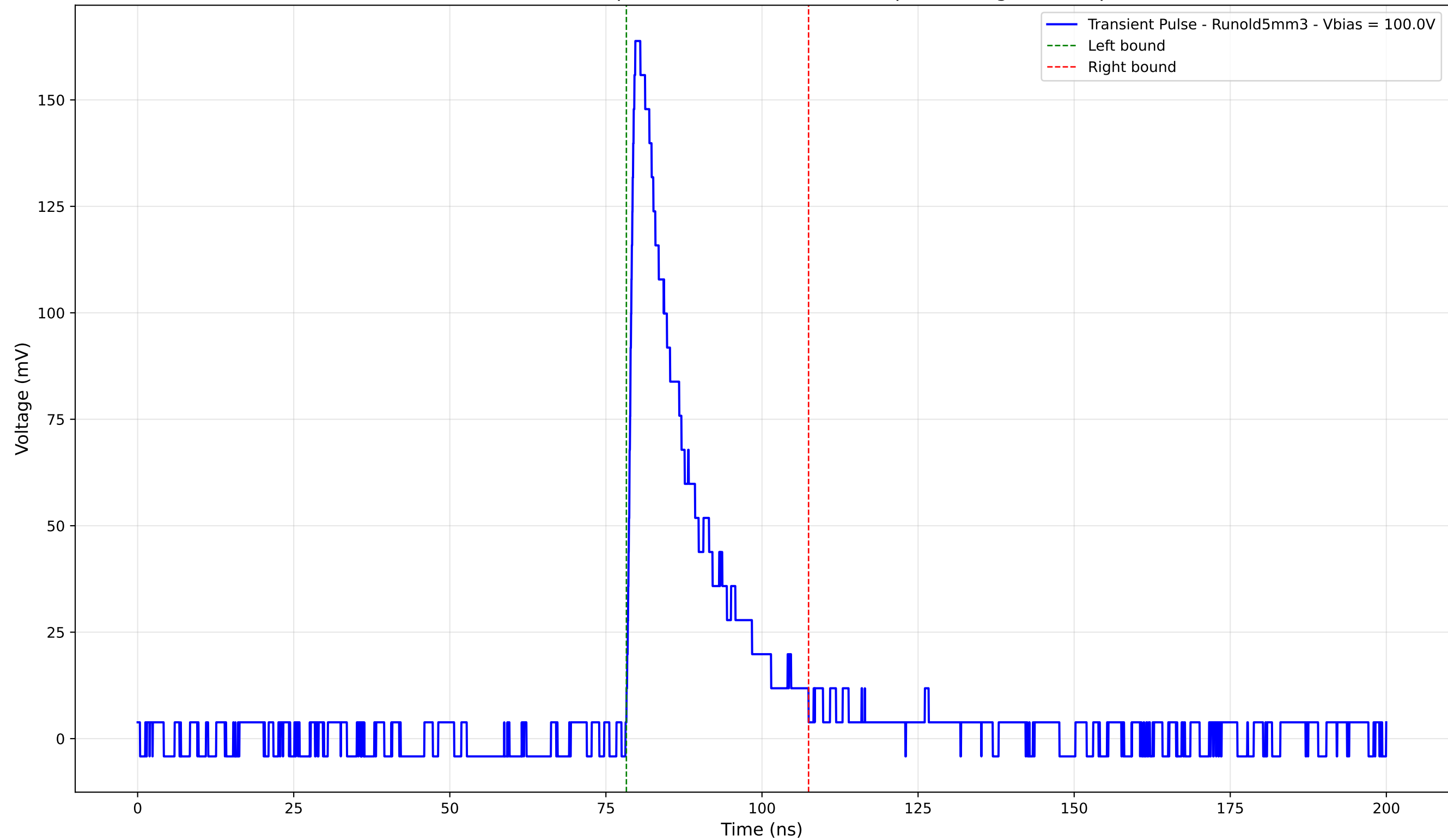
Transient Pulse - Sample: old5 - Position: 4440.0 \mu\text{m} - Charge: 32.19 pC
