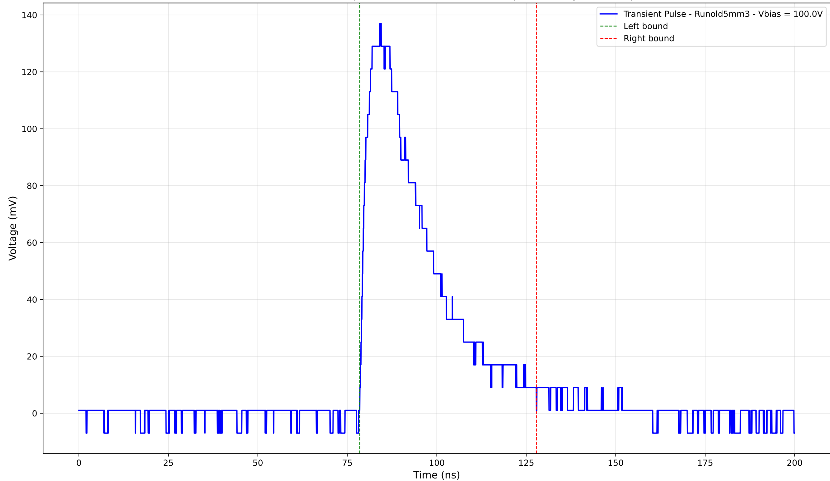
Transient Pulse - Sample: old5 - Position: 1840.0 \mu\text{m} - Charge: 52.02 pC
