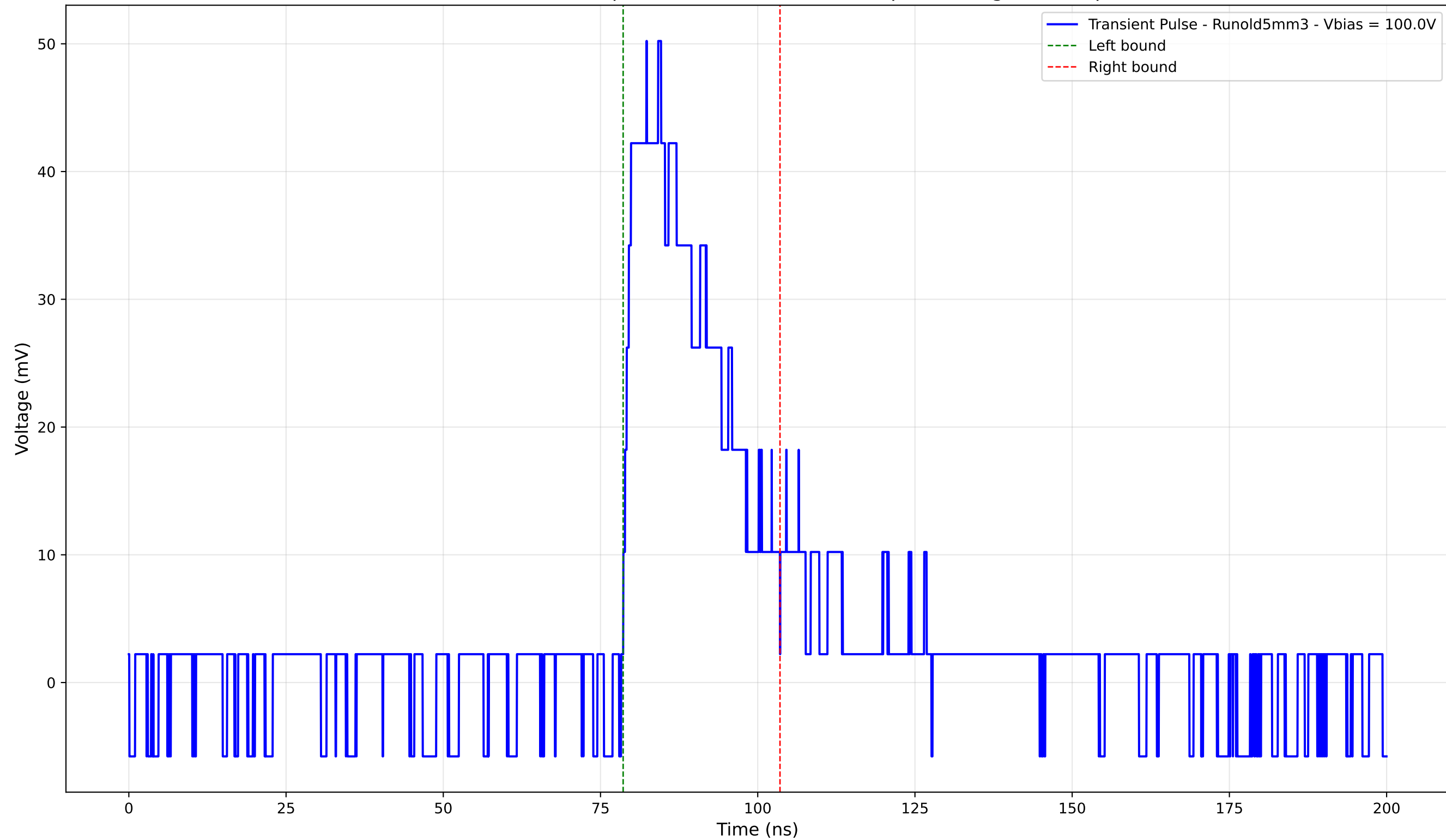
Transient Pulse - Sample: old5 - Position: 1165.0 \mu\text{m} - Charge: 13.69 pC
