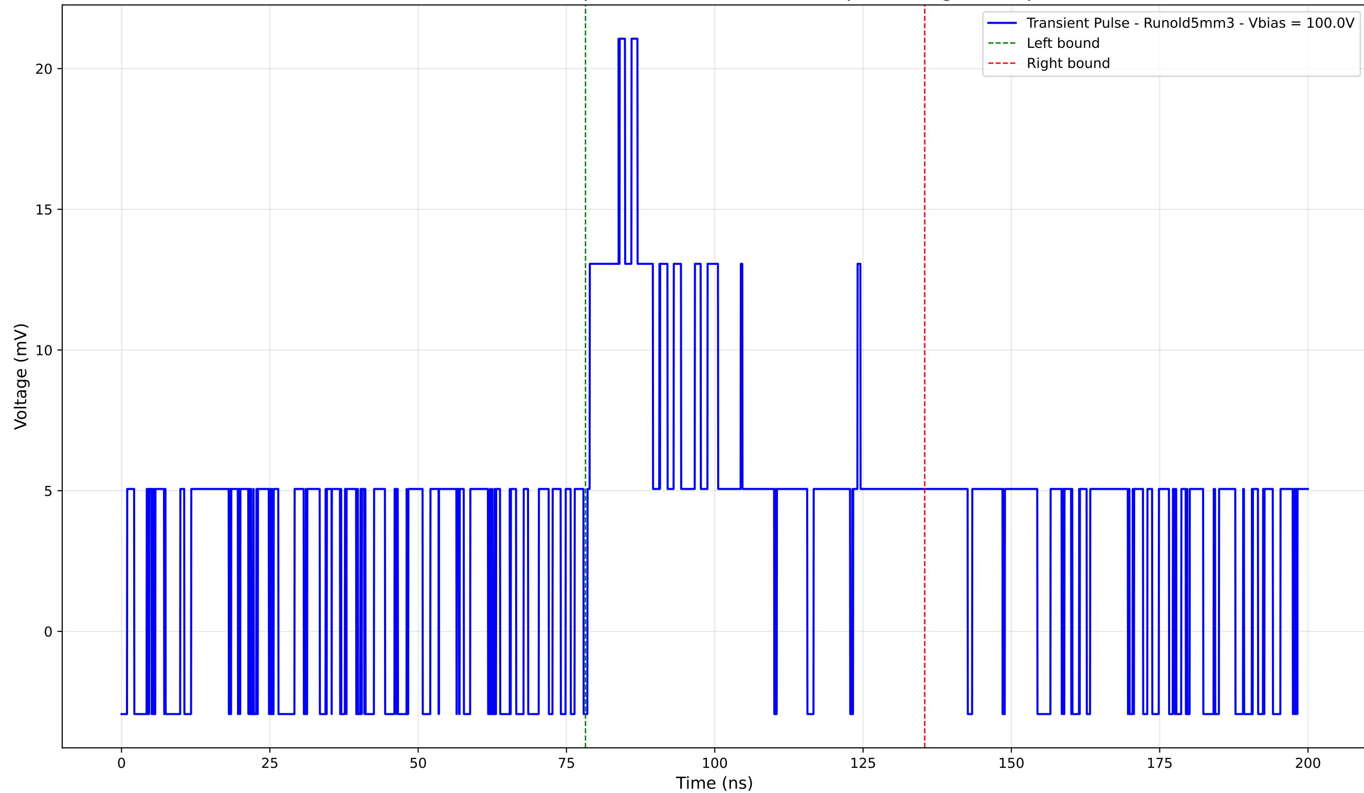
Transient Pulse - Sample: old5 - Position: 2675.0 \mu\text{m} - Charge: 8.44 pC
