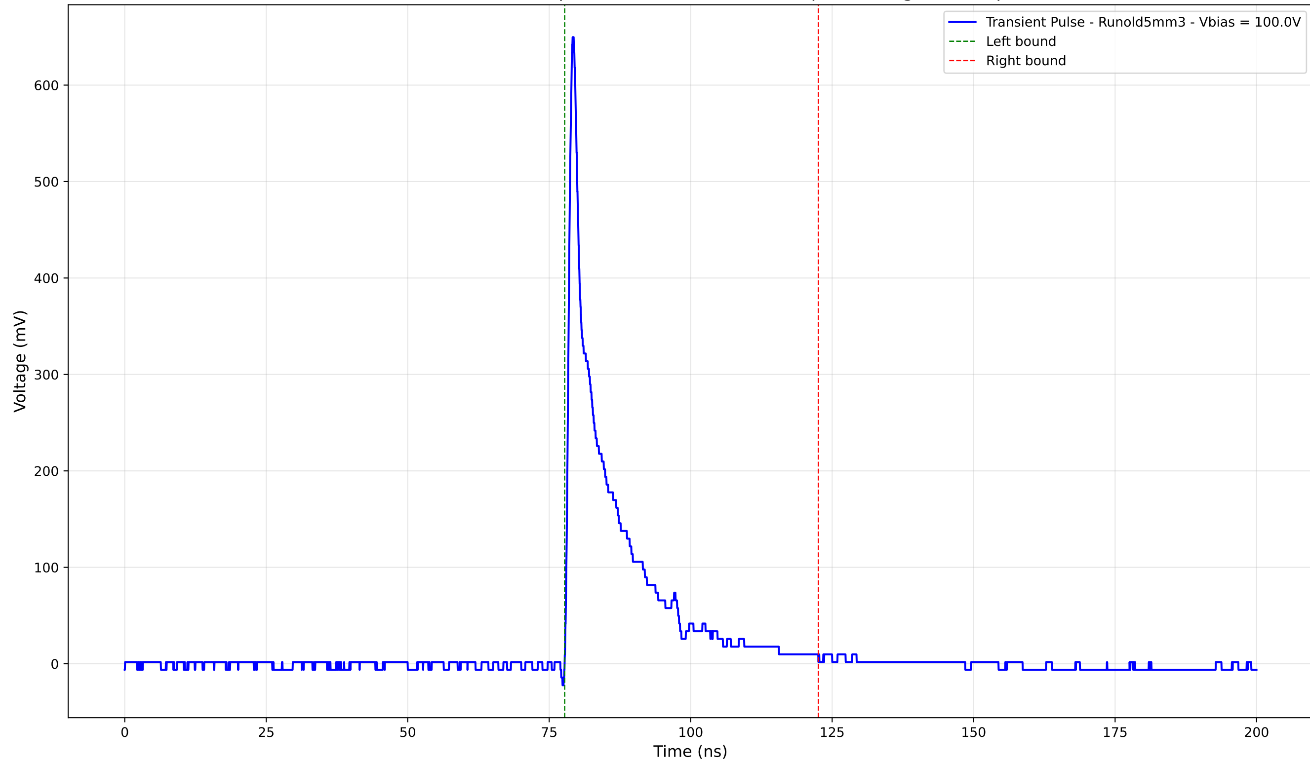
Transient Pulse - Sample: old5 - Position: 4865.0 \mu\text{m} - Charge: 85.80 pC
