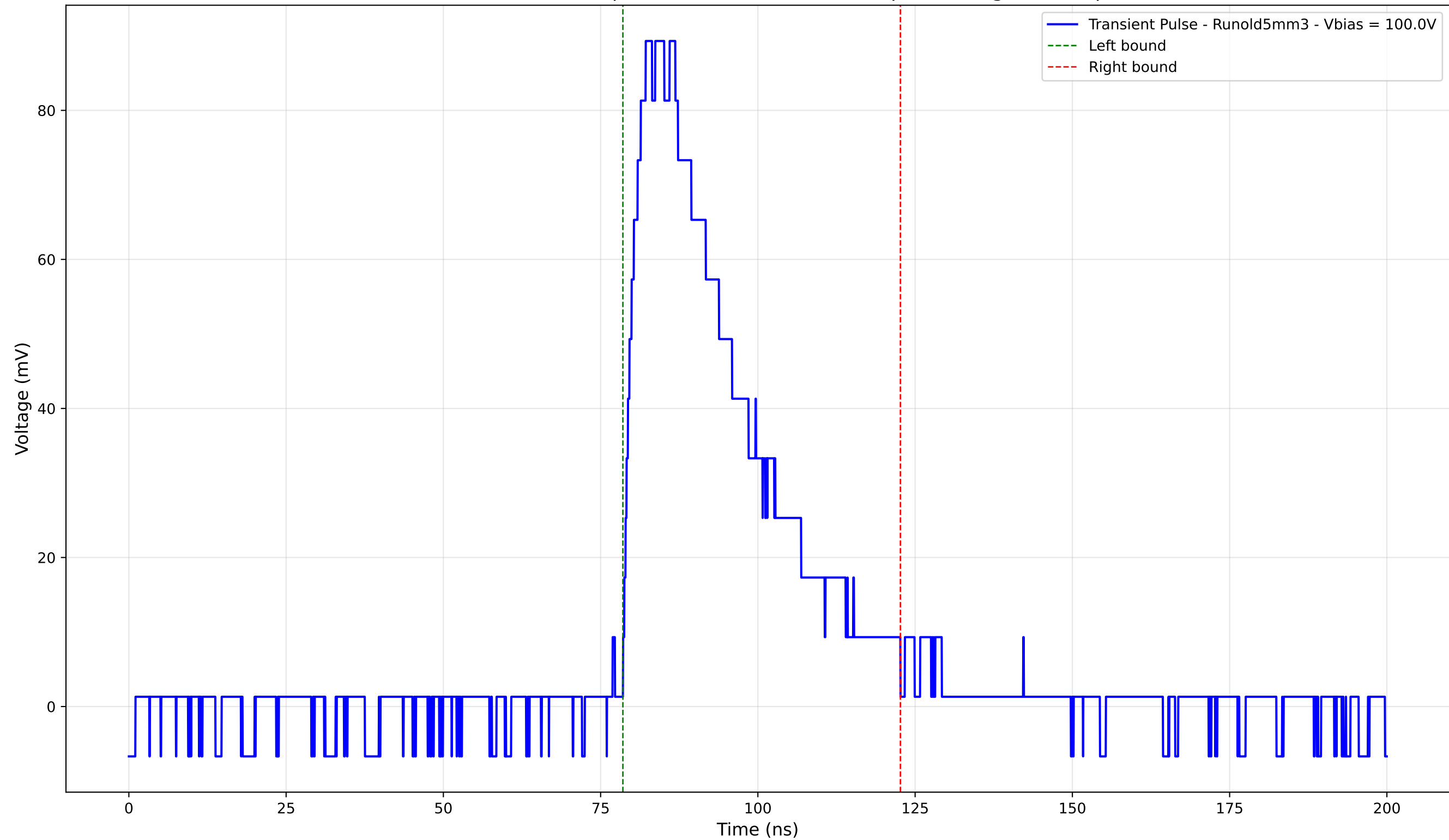
Transient Pulse - Sample: old5 - Position: 2025.0 \mu\text{m} - Charge: 34.66 pC
