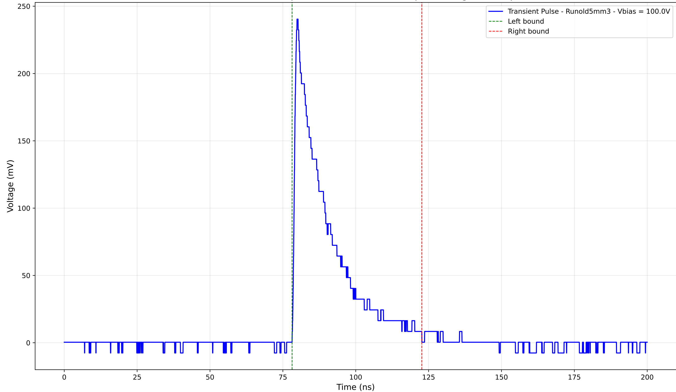
Transient Pulse - Sample: old5 - Position: 655.0 \mu\text{m} - Charge: 56.28 pC
