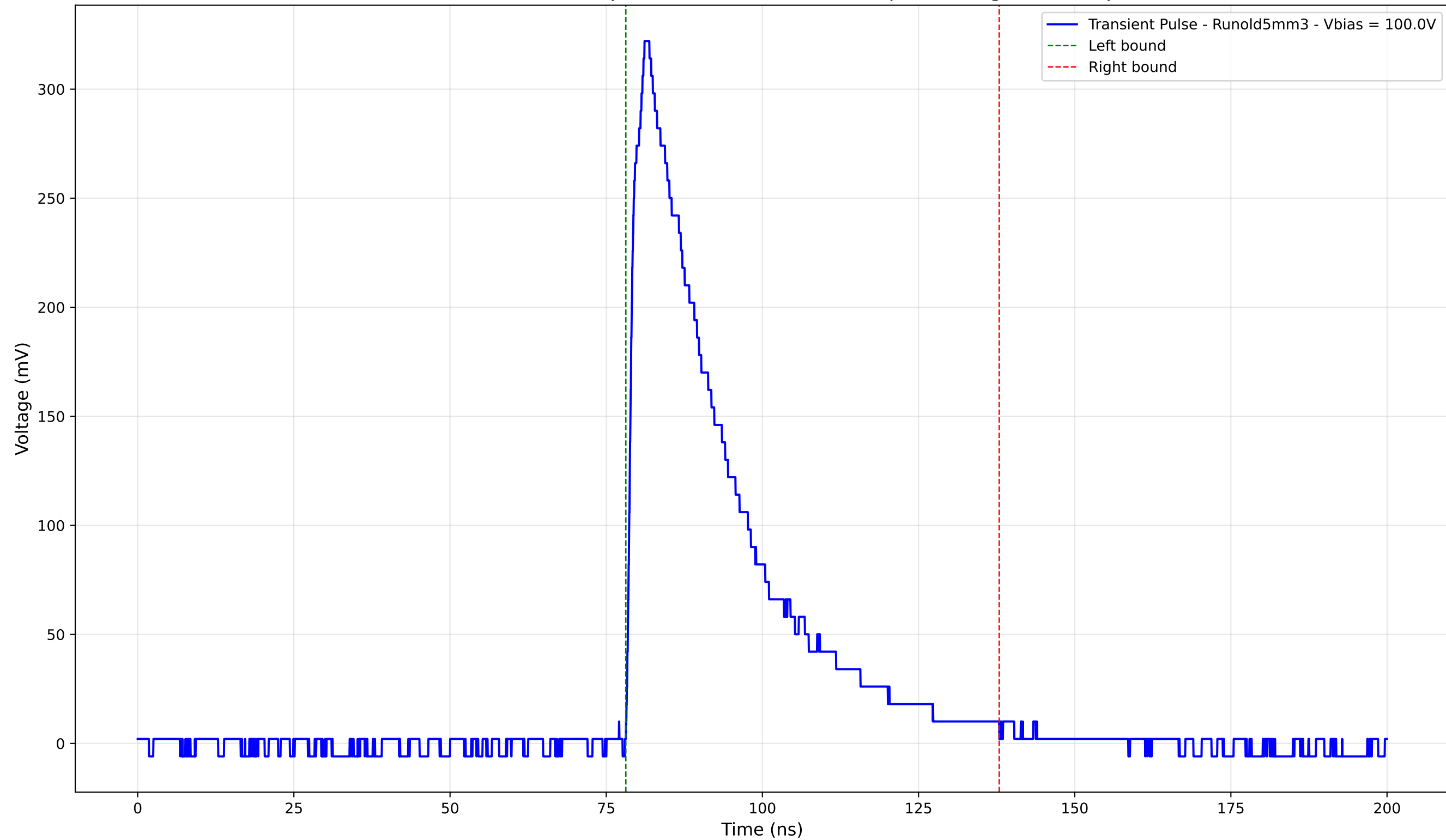
Transient Pulse - Sample: old5 - Position: 2845.0 \mu\text{m} - Charge: 105.30 pC
