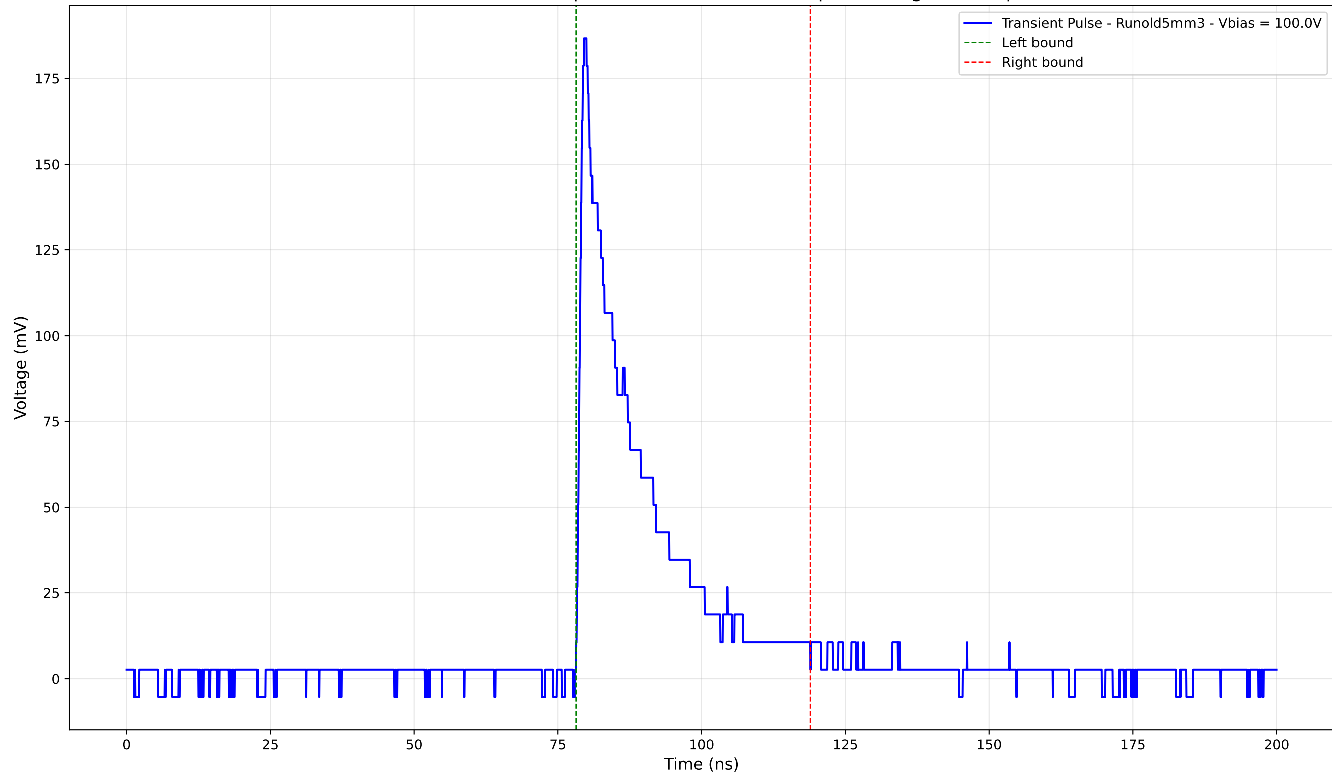
Transient Pulse - Sample: old5 - Position: 500.0 \mu\text{m} - Charge: 37.43 pC
