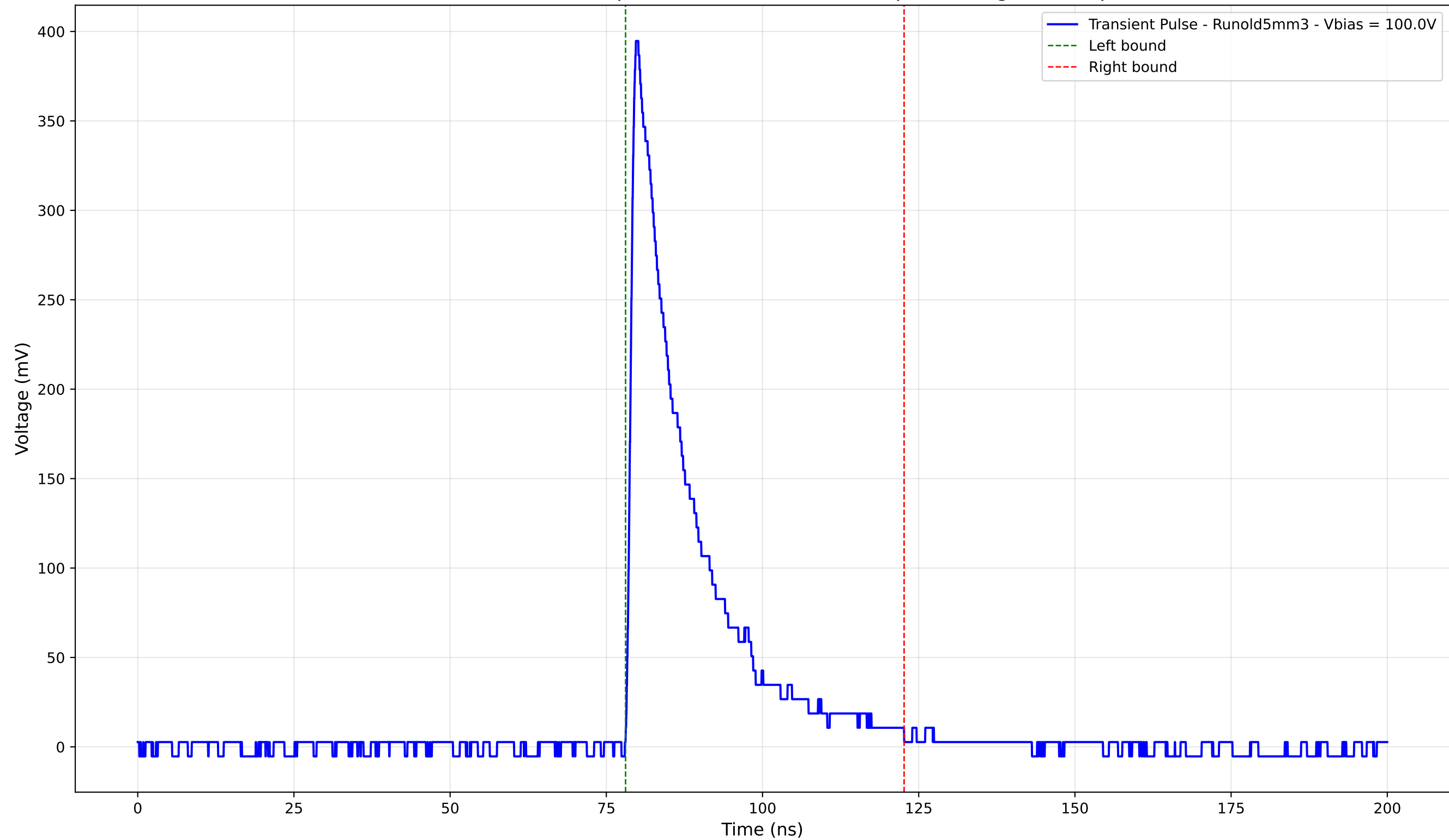
Transient Pulse - Sample: old5 - Position: 4570.0 \mu\text{m} - Charge: 78.33 pC
