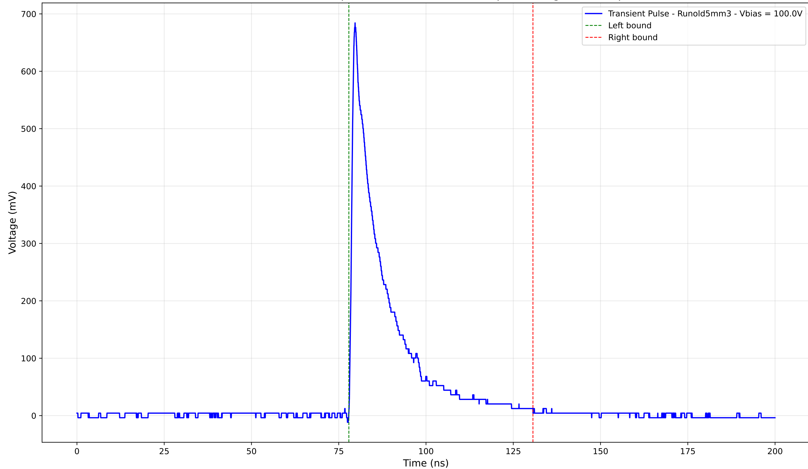
Transient Pulse - Sample: old5 - Position: 4665.0 \mu\text{m} - Charge: 130.99 pC
