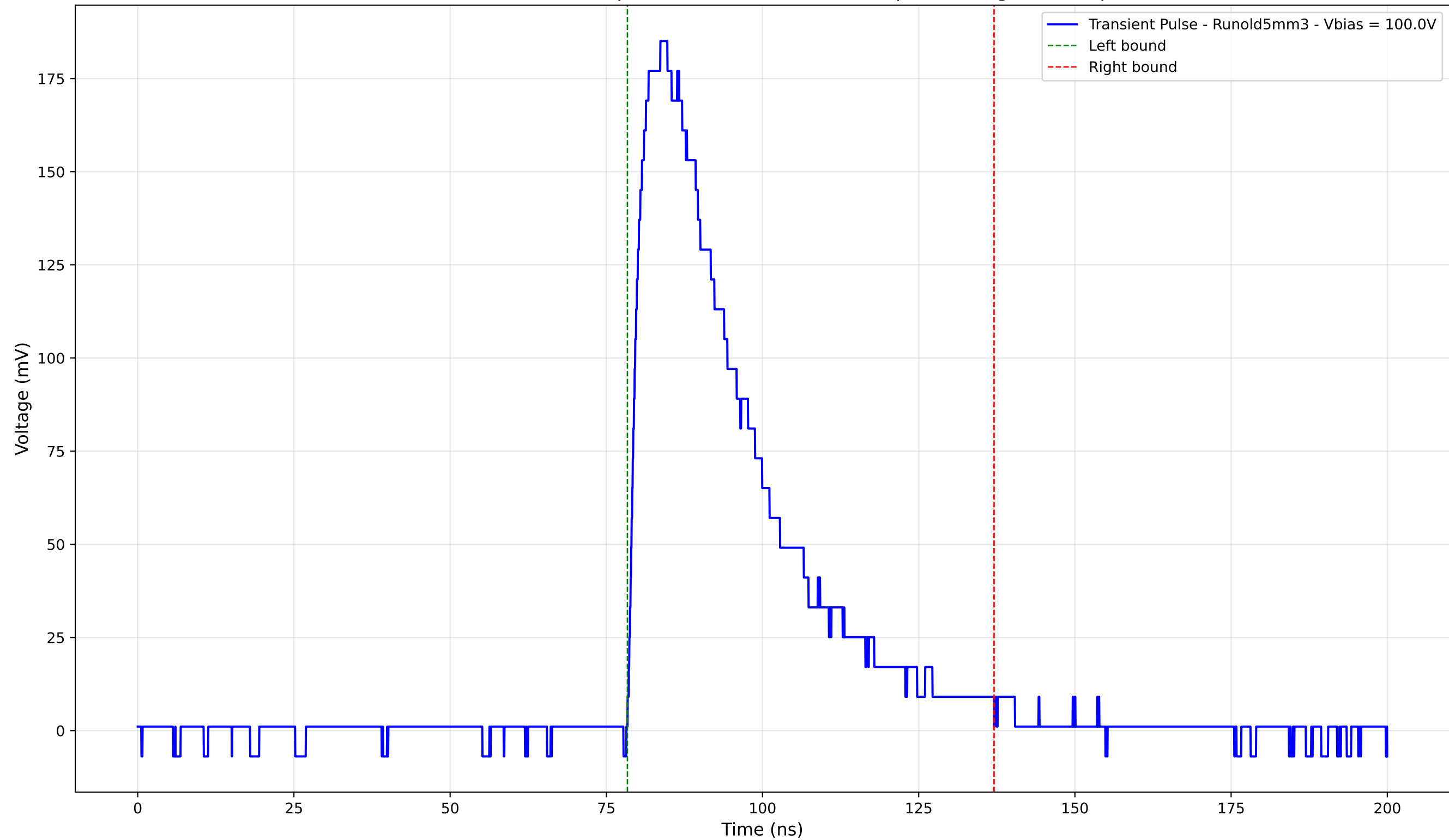
Transient Pulse - Sample: old5 - Position: 1660.0 \mu\text{m} - Charge: 73.87 pC
