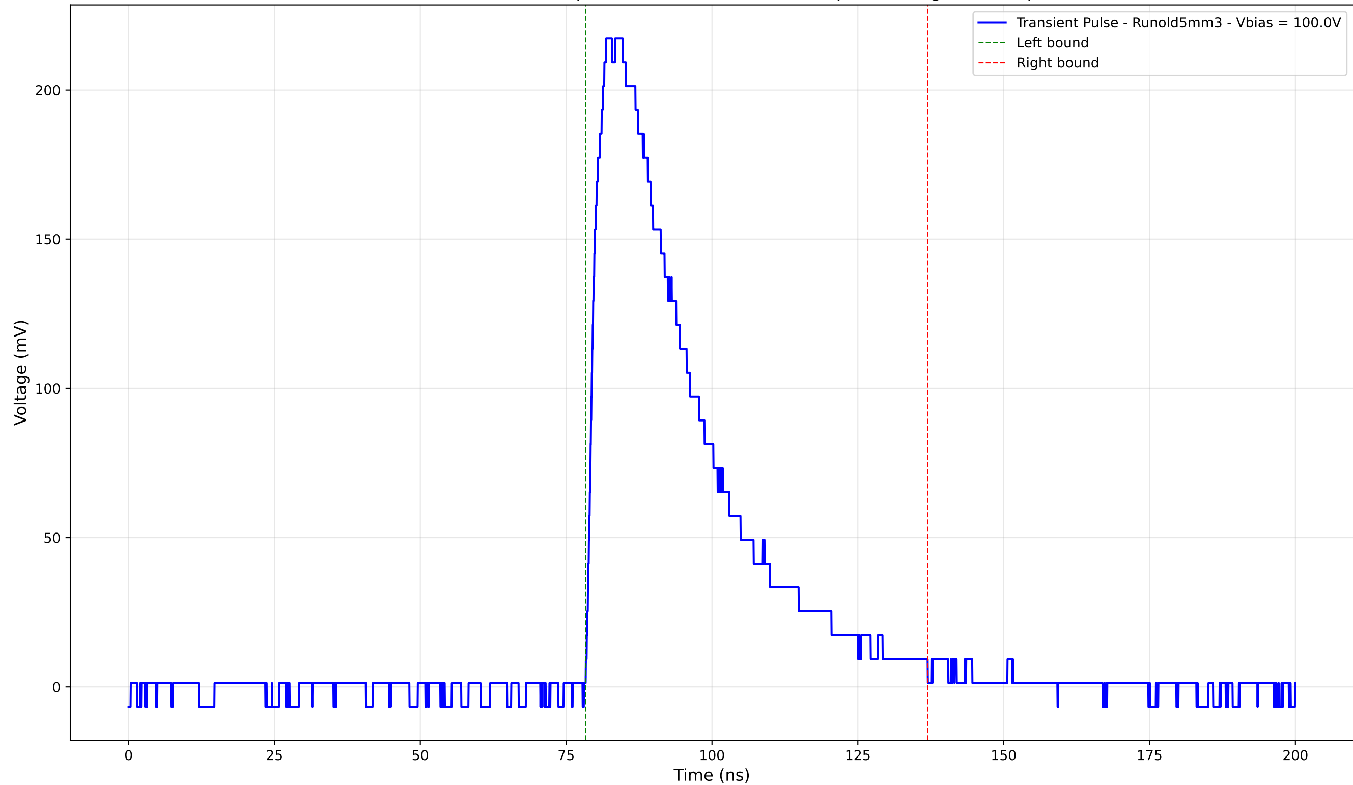
Transient Pulse - Sample: old5 - Position: 2275.0 \mu\text{m} - Charge: 85.96 pC
