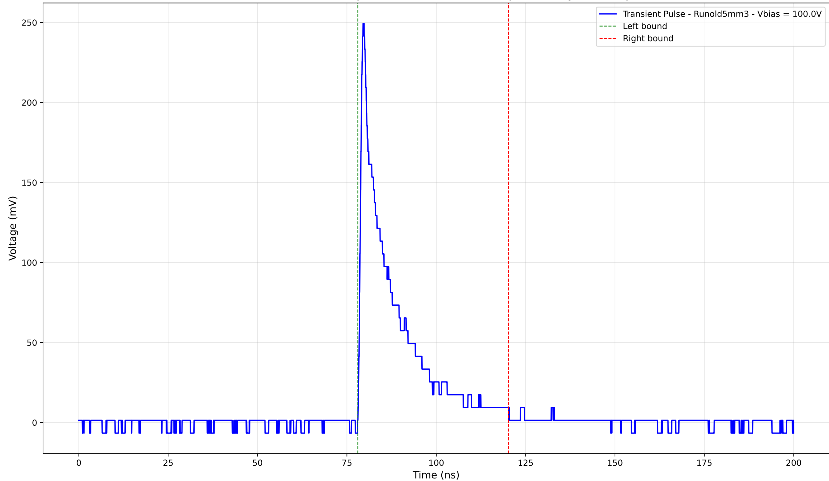
Transient Pulse - Sample: old5 - Position: 420.0 \mu\text{m} - Charge: 43.37 pC
