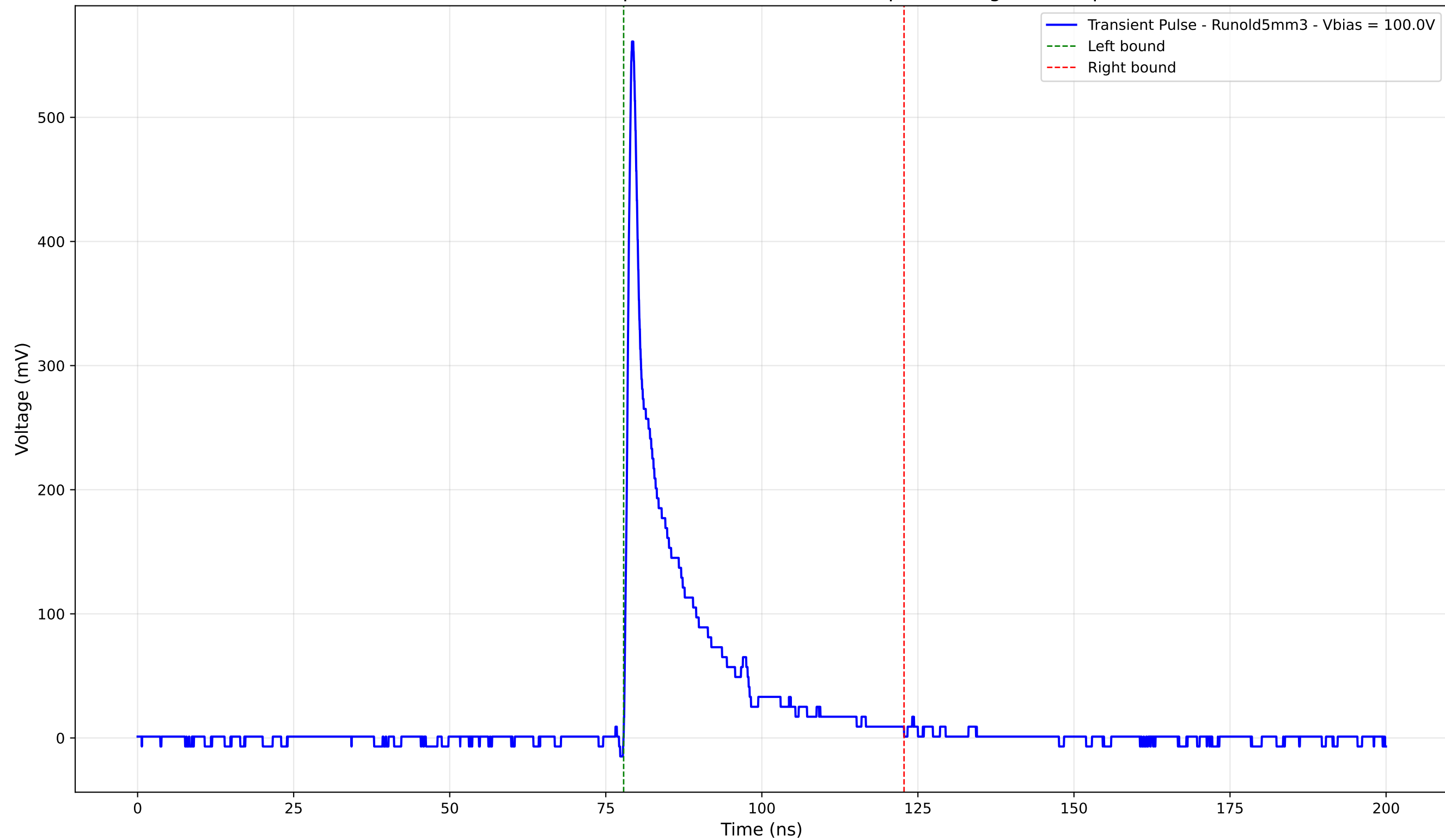
Transient Pulse - Sample: old5 - Position: 215.0 \mu\text{m} - Charge: 72.47 pC
