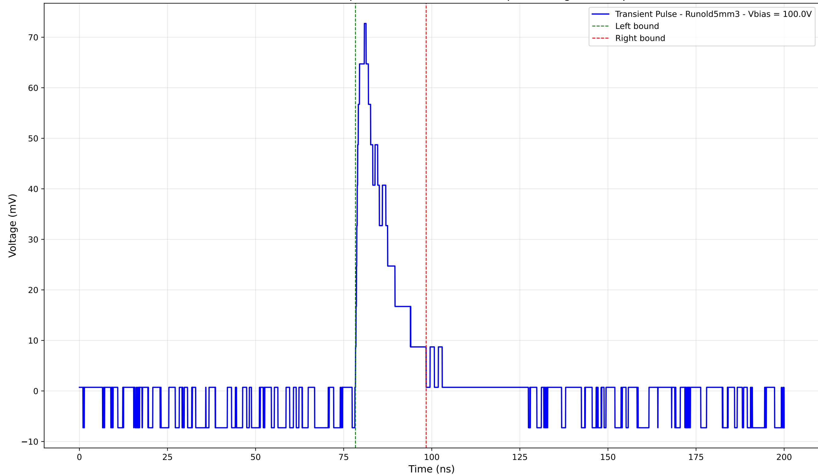
Transient Pulse - Sample: old5 - Position: 4145.0 \mu\text{m} - Charge: 12.14 pC
