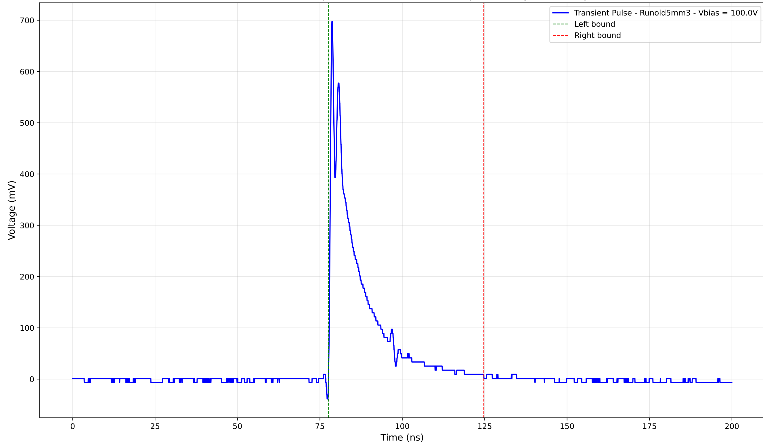
Transient Pulse - Sample: old5 - Position: 3720.0 \mu\text{m} - Charge: 107.85 pC
