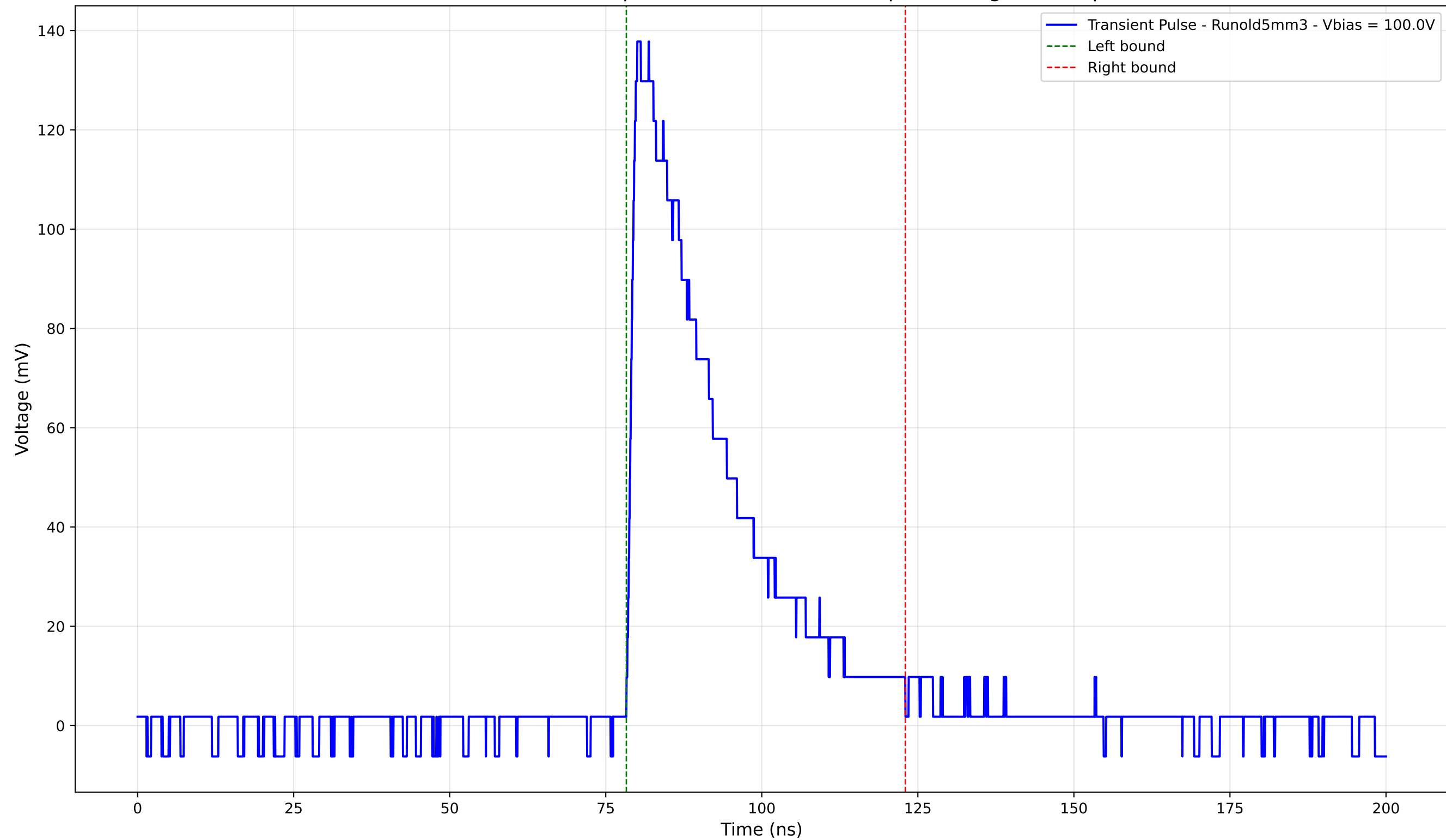
Transient Pulse - Sample: old5 - Position: 920.0 \mu\text{m} - Charge: 42.53 pC
