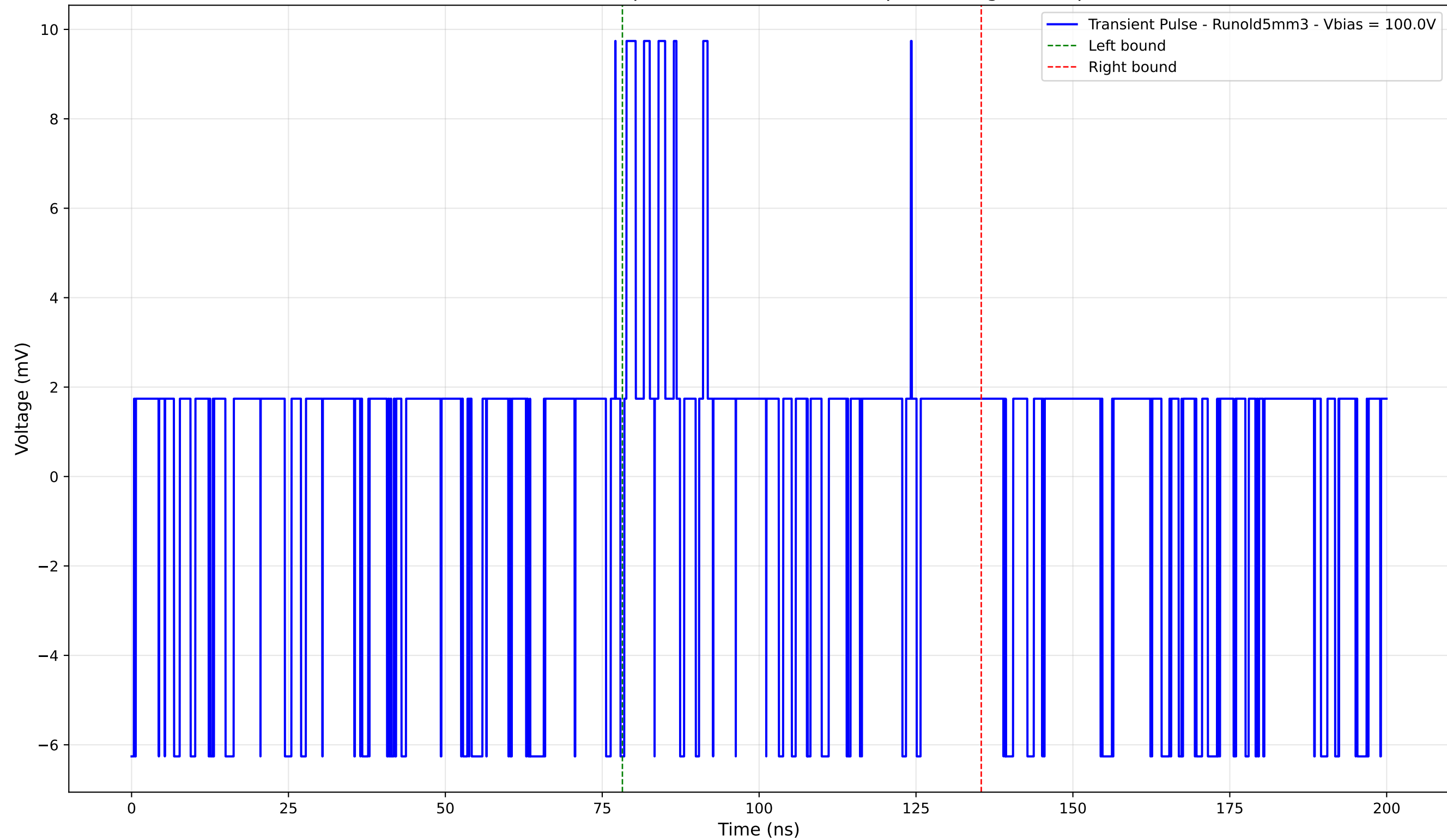
Transient Pulse - Sample: old5 - Position: 75.0 \mu\text{m} - Charge: 1.69 pC
