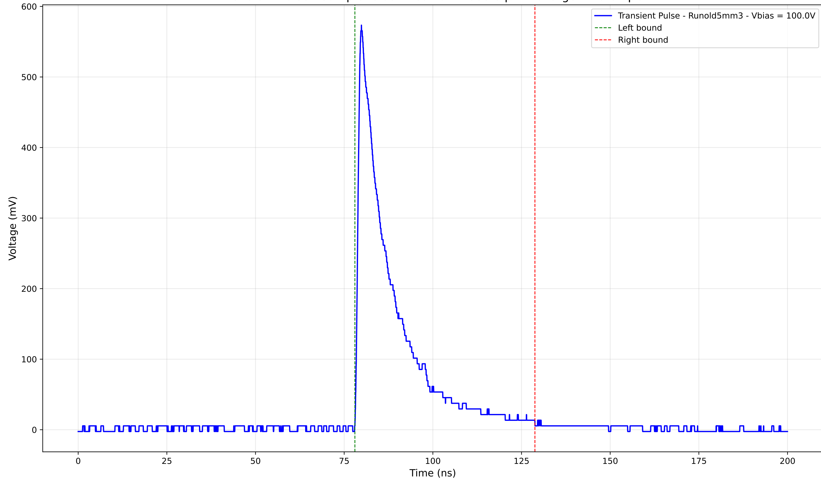
Transient Pulse - Sample: old5 - Position: 4600.0 \mu\text{m} - Charge: 115.61 pC
