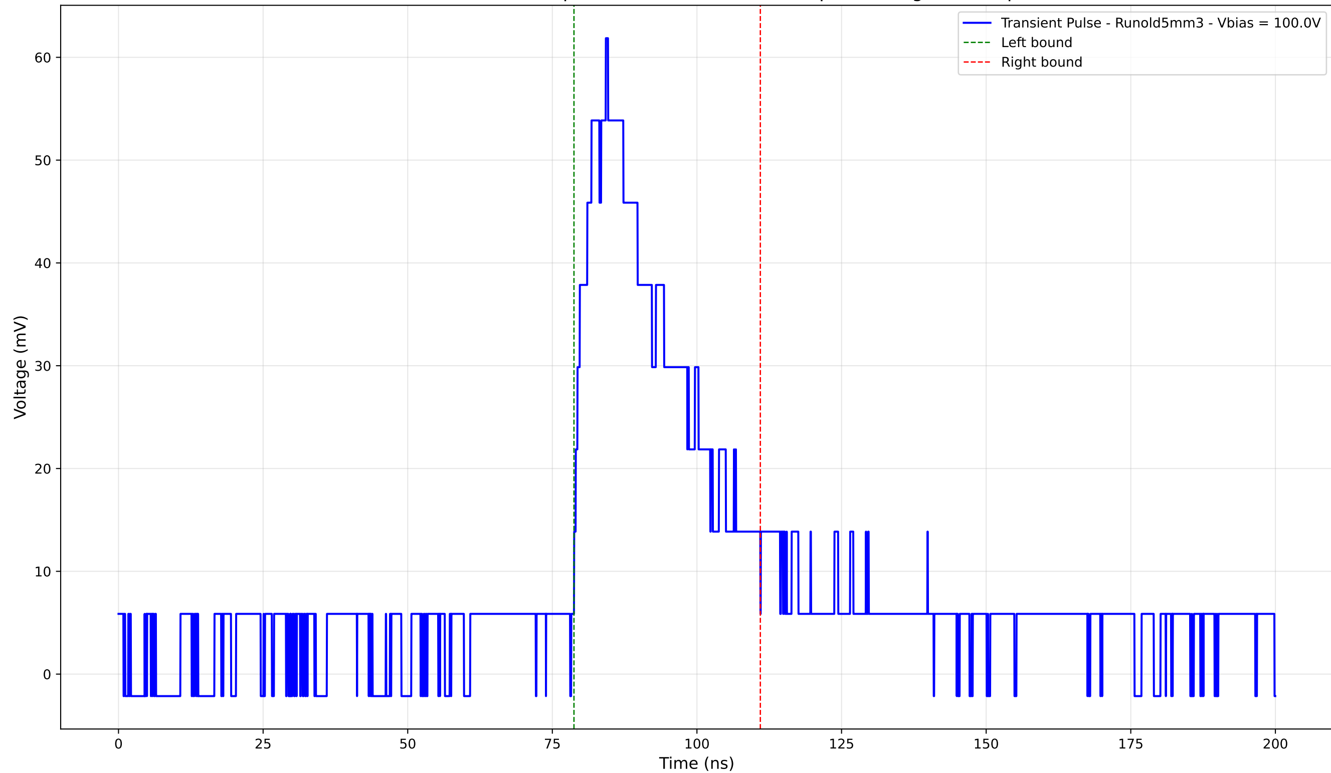
Transient Pulse - Sample: old5 - Position: 1810.0 \mu\text{m} - Charge: 20.62 pC
