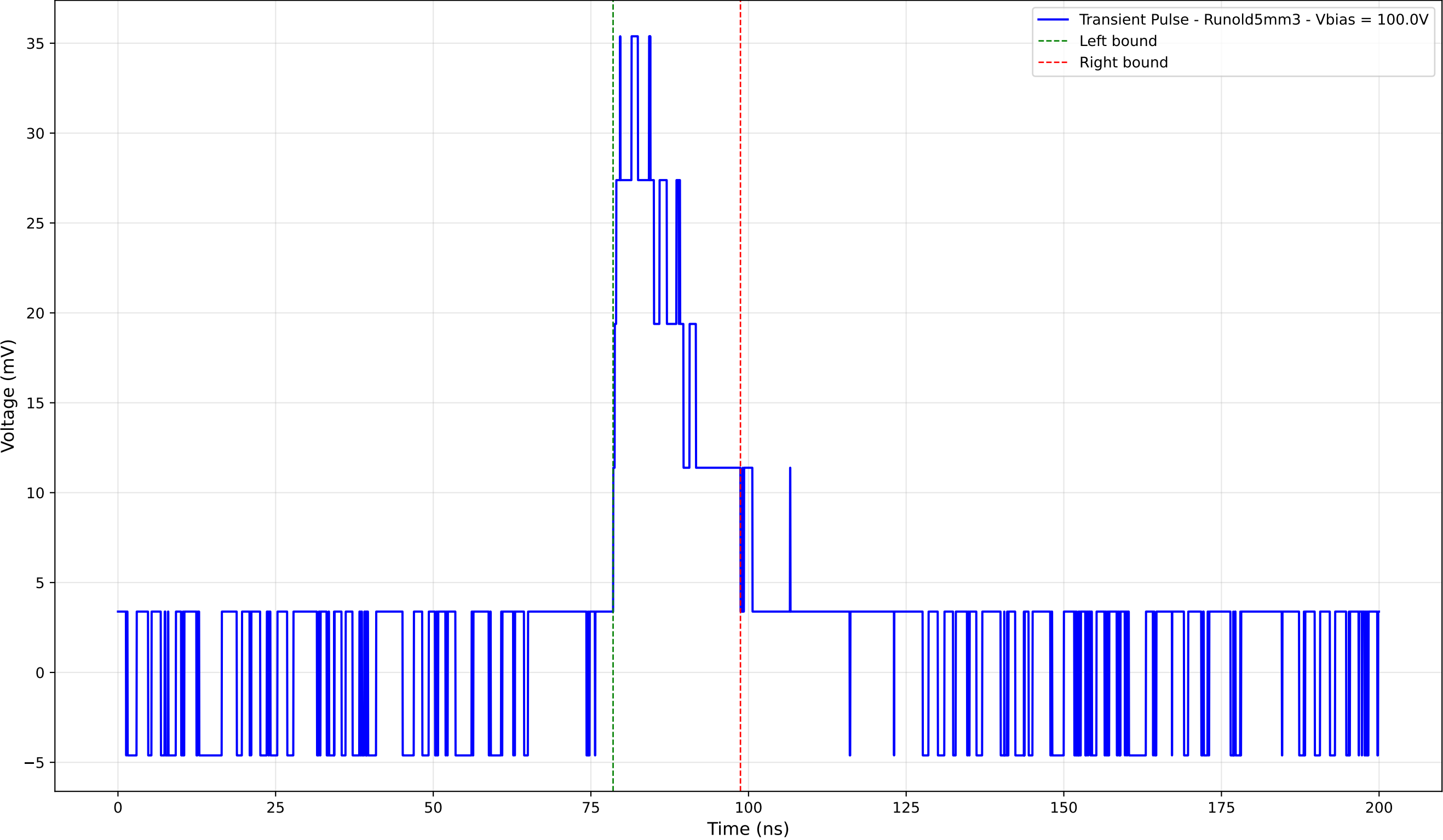
Transient Pulse - Sample: old5 - Position: 2950.0 \mu\text{m} - Charge: 7.93 pC
