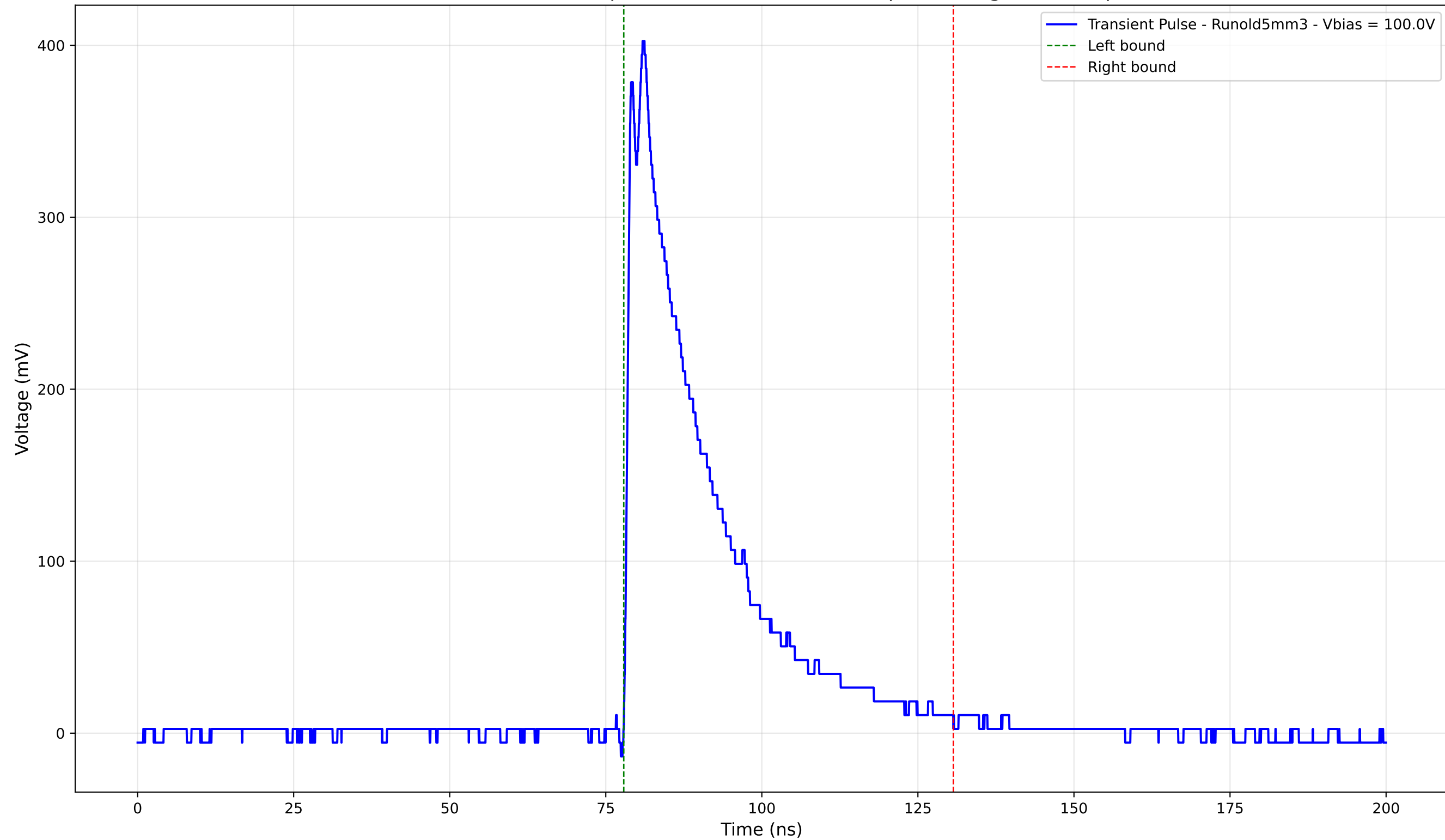
Transient Pulse - Sample: old5 - Position: 3125.0 \mu\text{m} - Charge: 106.87 pC
