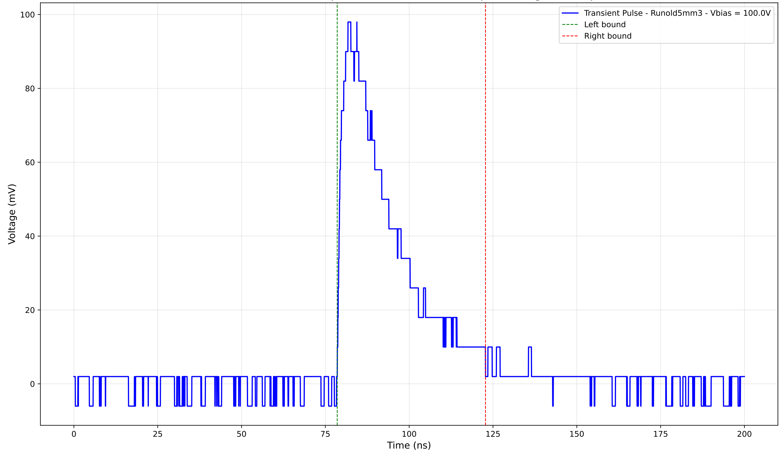
Transient Pulse - Sample: old5 - Position: 2615.0 \mu\text{m} - Charge: 33.72 pC
