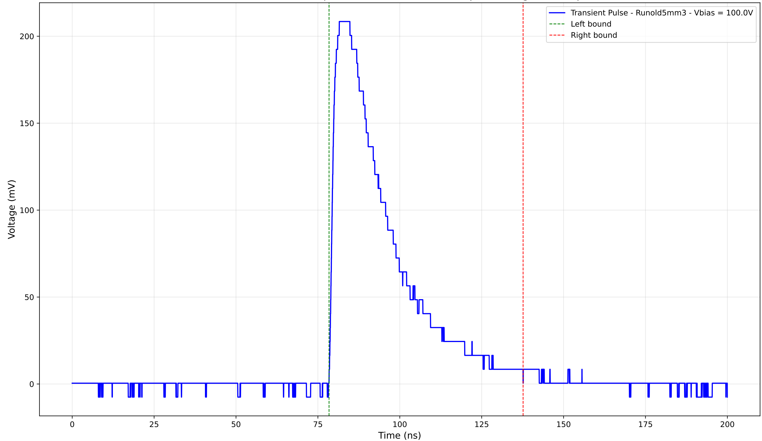
Transient Pulse - Sample: old5 - Position: 1295.0 \mu\text{m} - Charge: 81.05 pC
