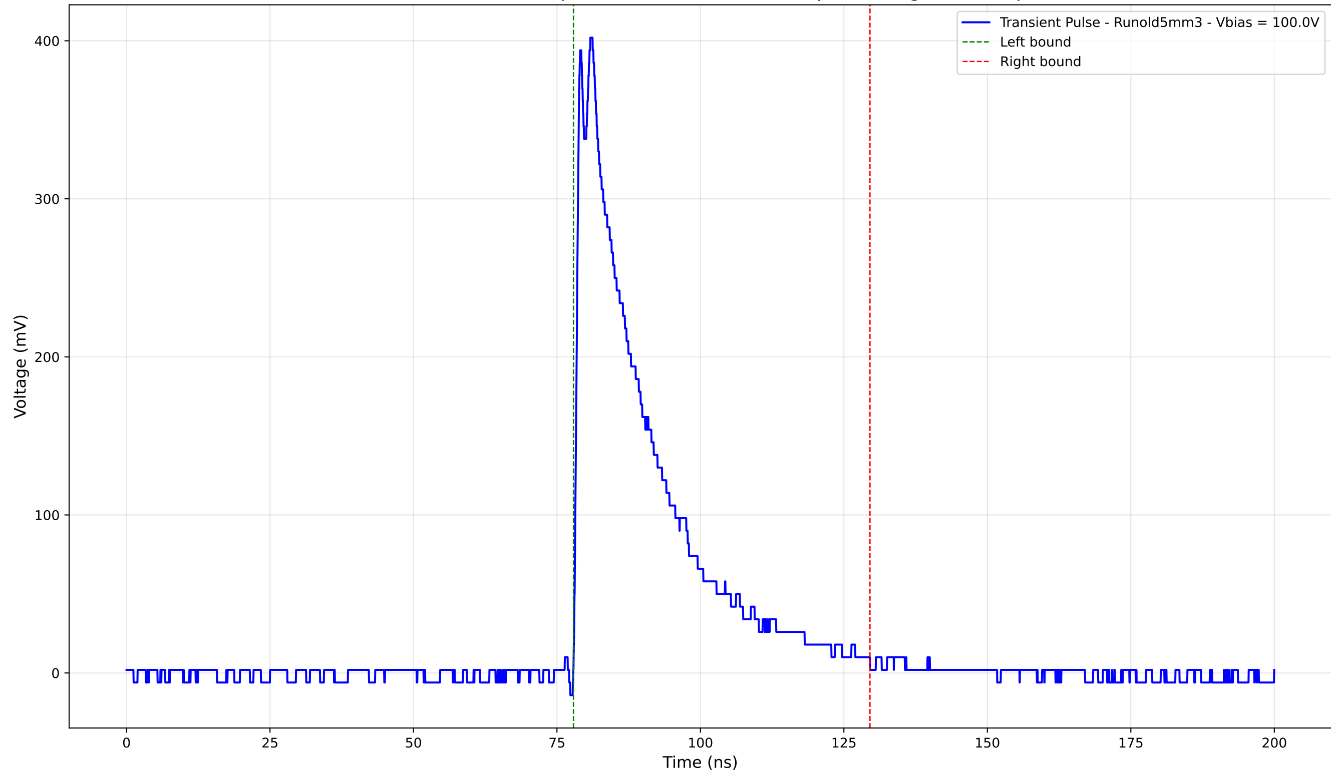
Transient Pulse - Sample: old5 - Position: 3145.0 \mu\text{m} - Charge: 105.07 pC
