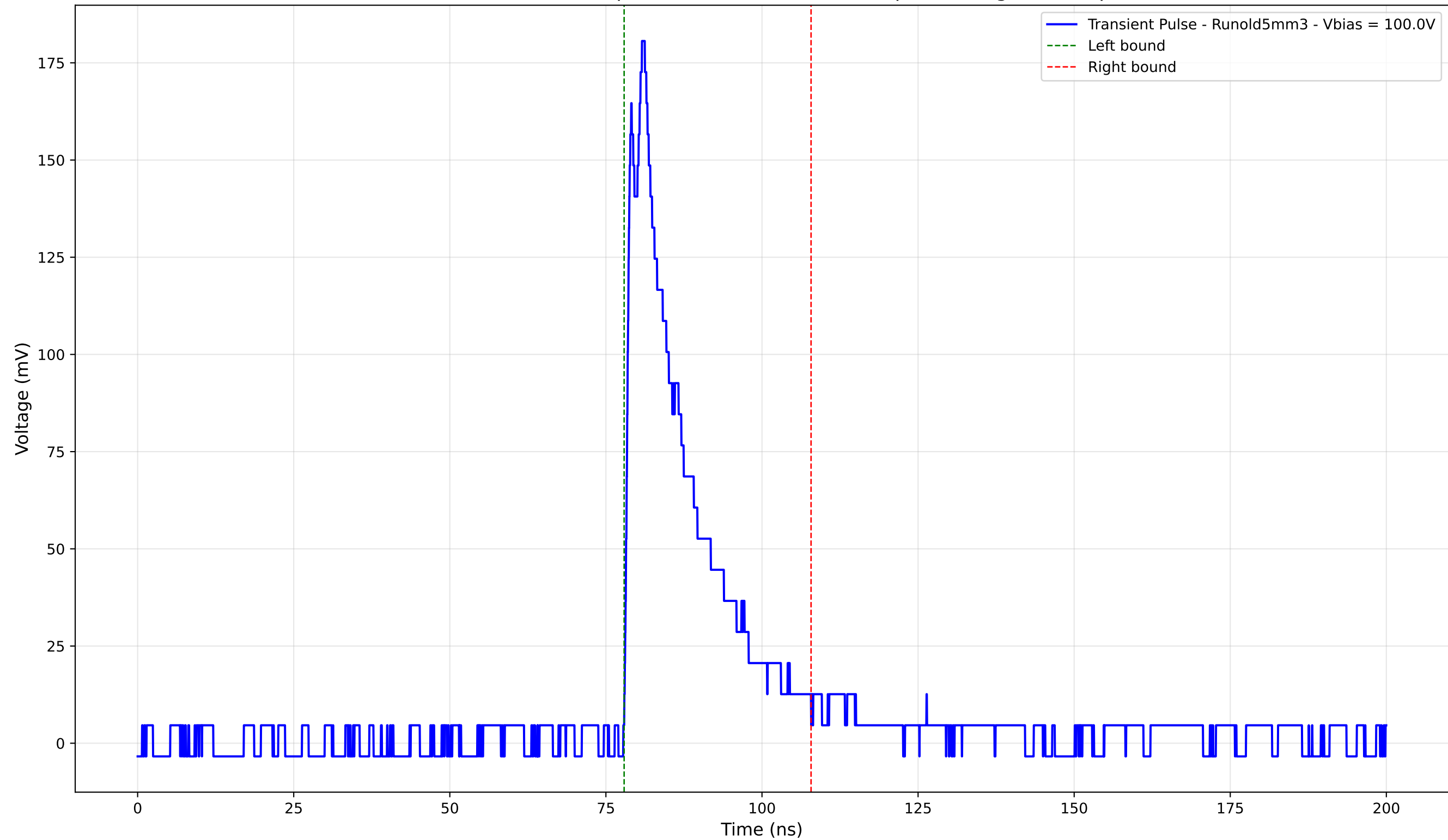
Transient Pulse - Sample: old5 - Position: 3940.0 \mu\text{m} - Charge: 36.08 pC
