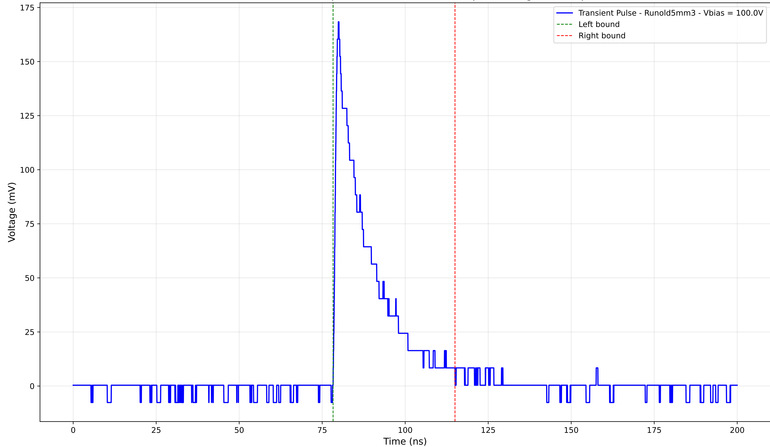
Transient Pulse - Sample: old5 - Position: 595.0 \mu\text{m} - Charge: 34.39 pC
