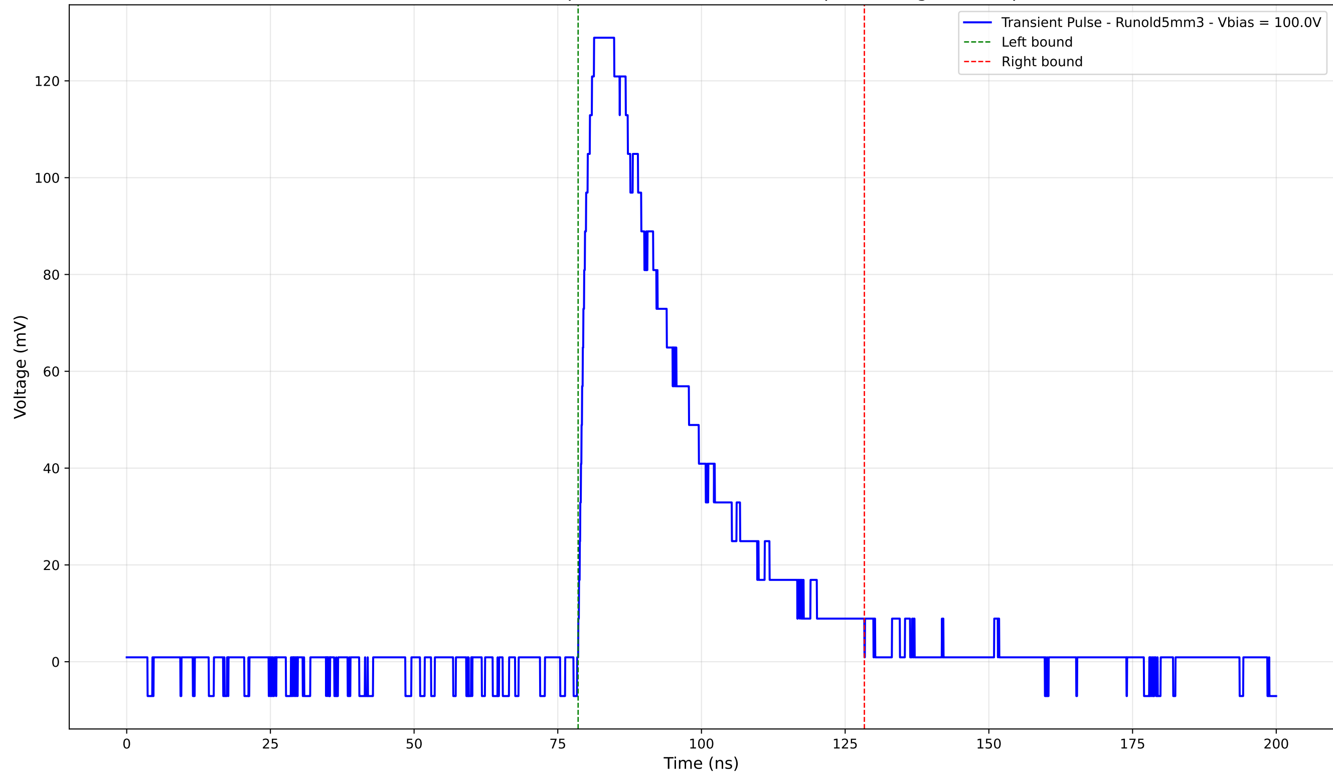
Transient Pulse - Sample: old5 - Position: 2440.0 \mu\text{m} - Charge: 48.74 pC
