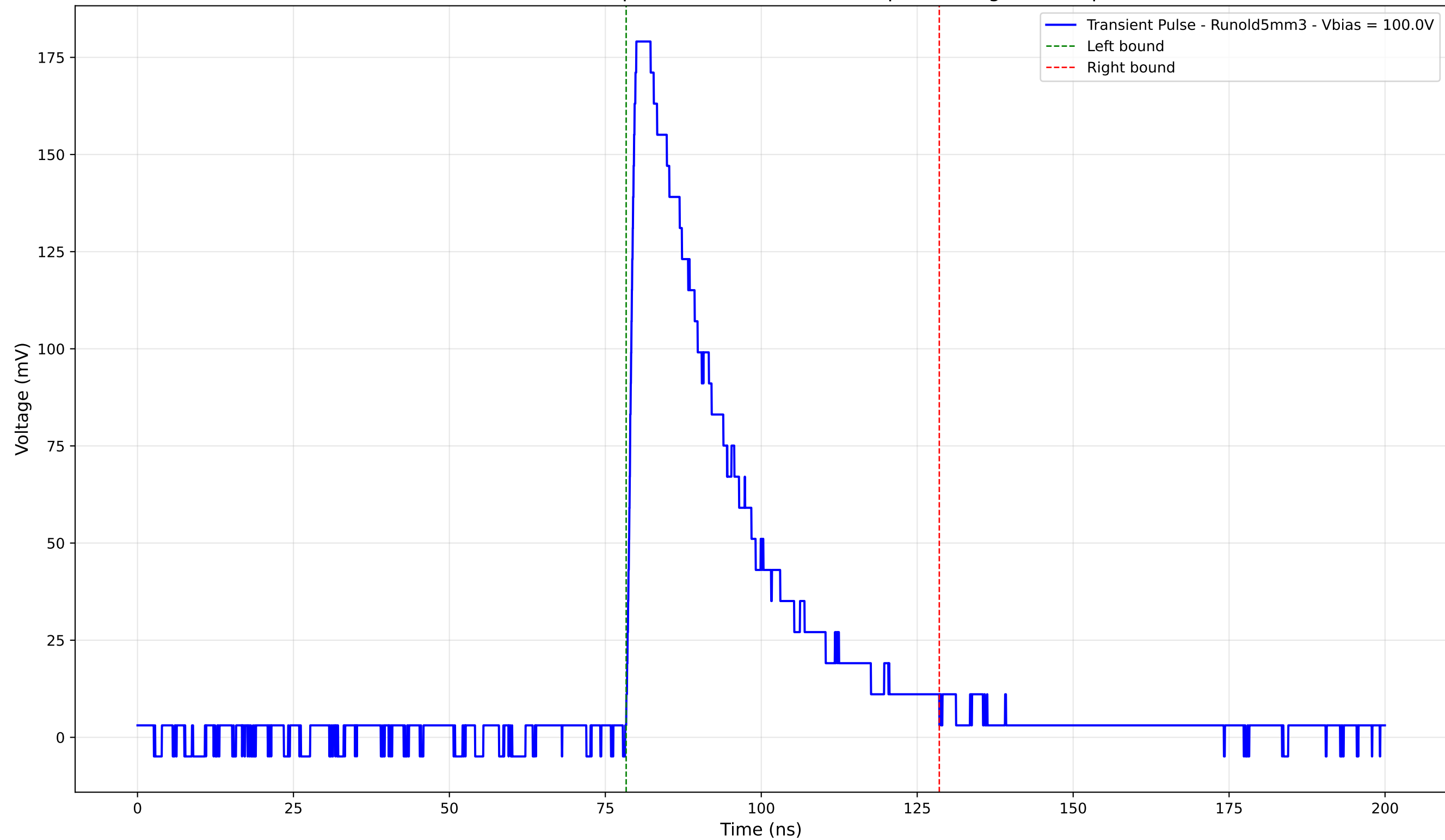
Transient Pulse - Sample: old5 - Position: 945.0 \mu\text{m} - Charge: 59.56 pC
