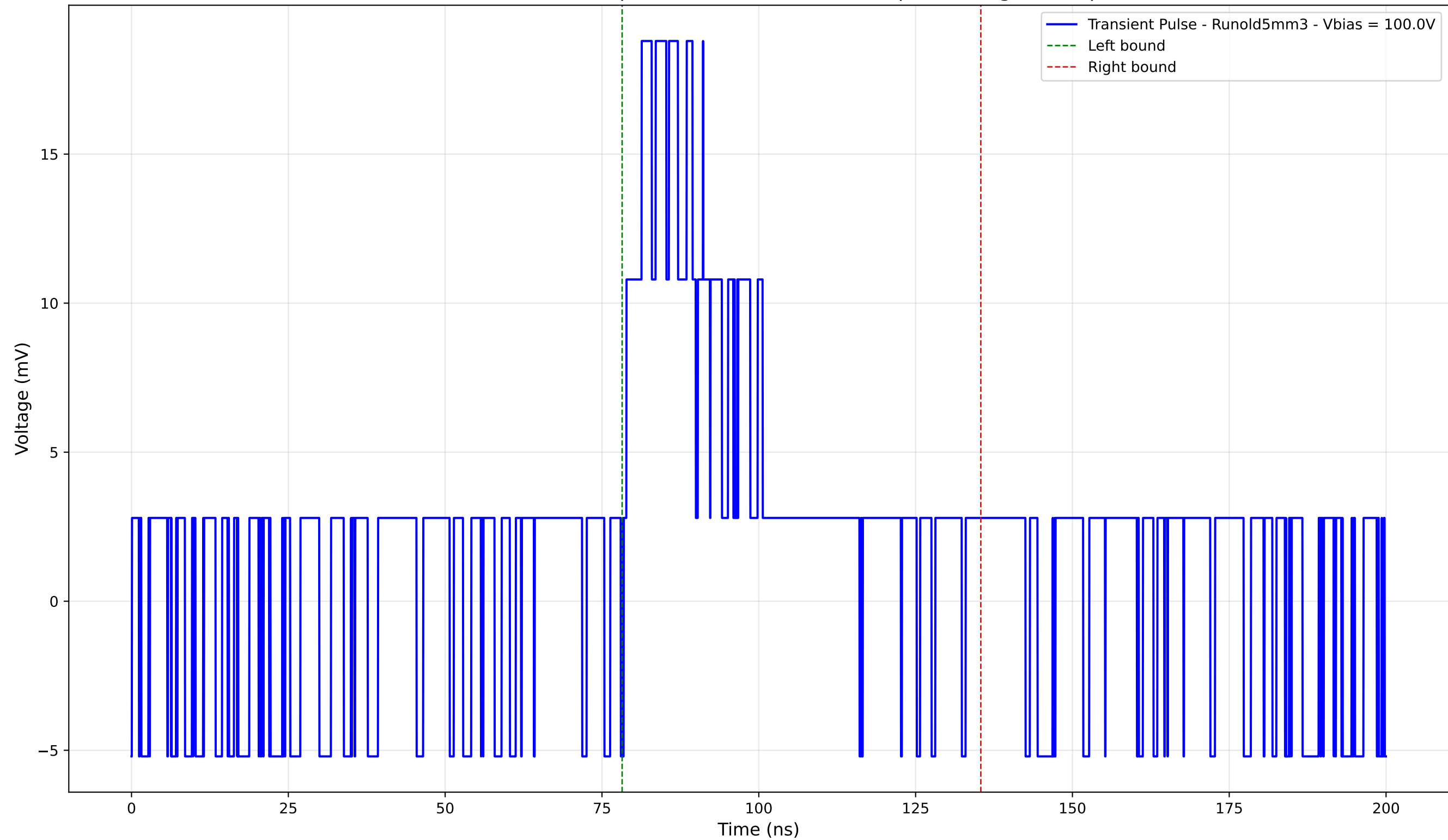
Transient Pulse - Sample: old5 - Position: 2655.0 \mu\text{m} - Charge: 6.70 pC
