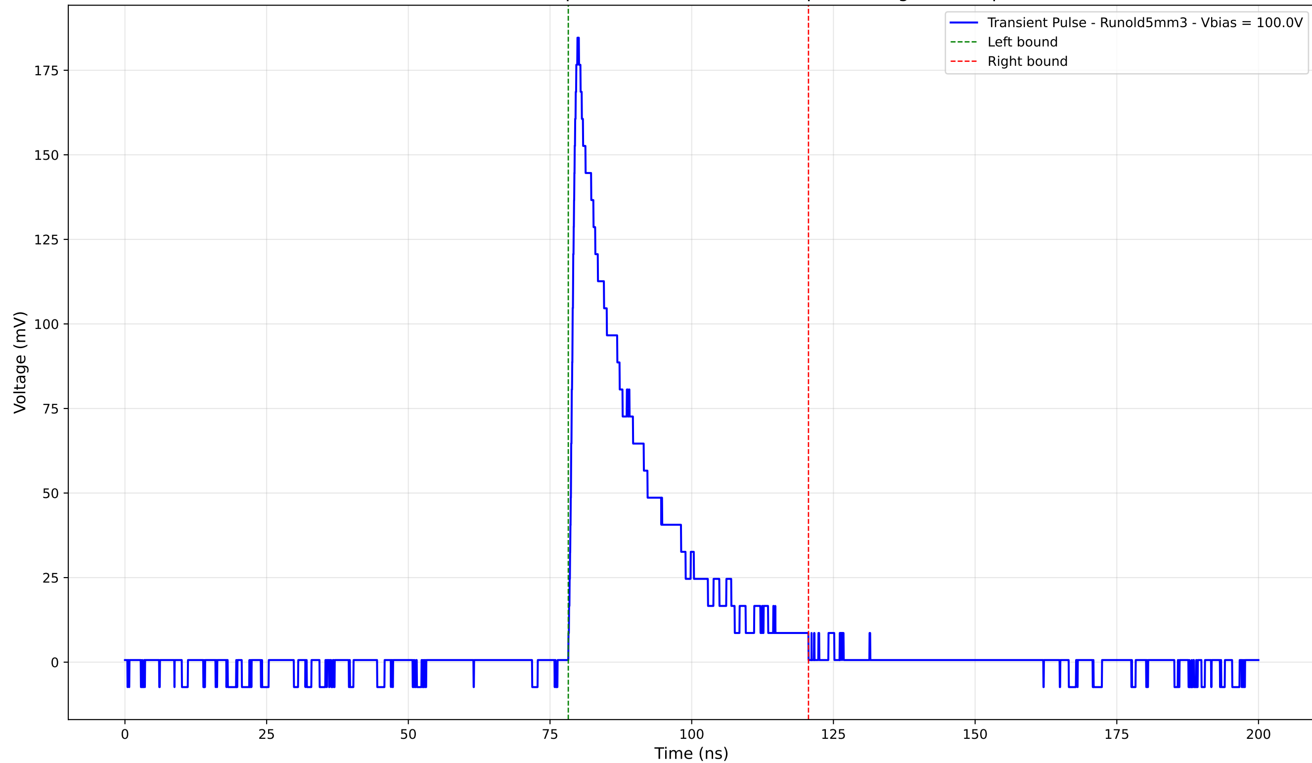
Transient Pulse - Sample: old5 - Position: 615.0 \mu\text{m} - Charge: 40.84 pC
