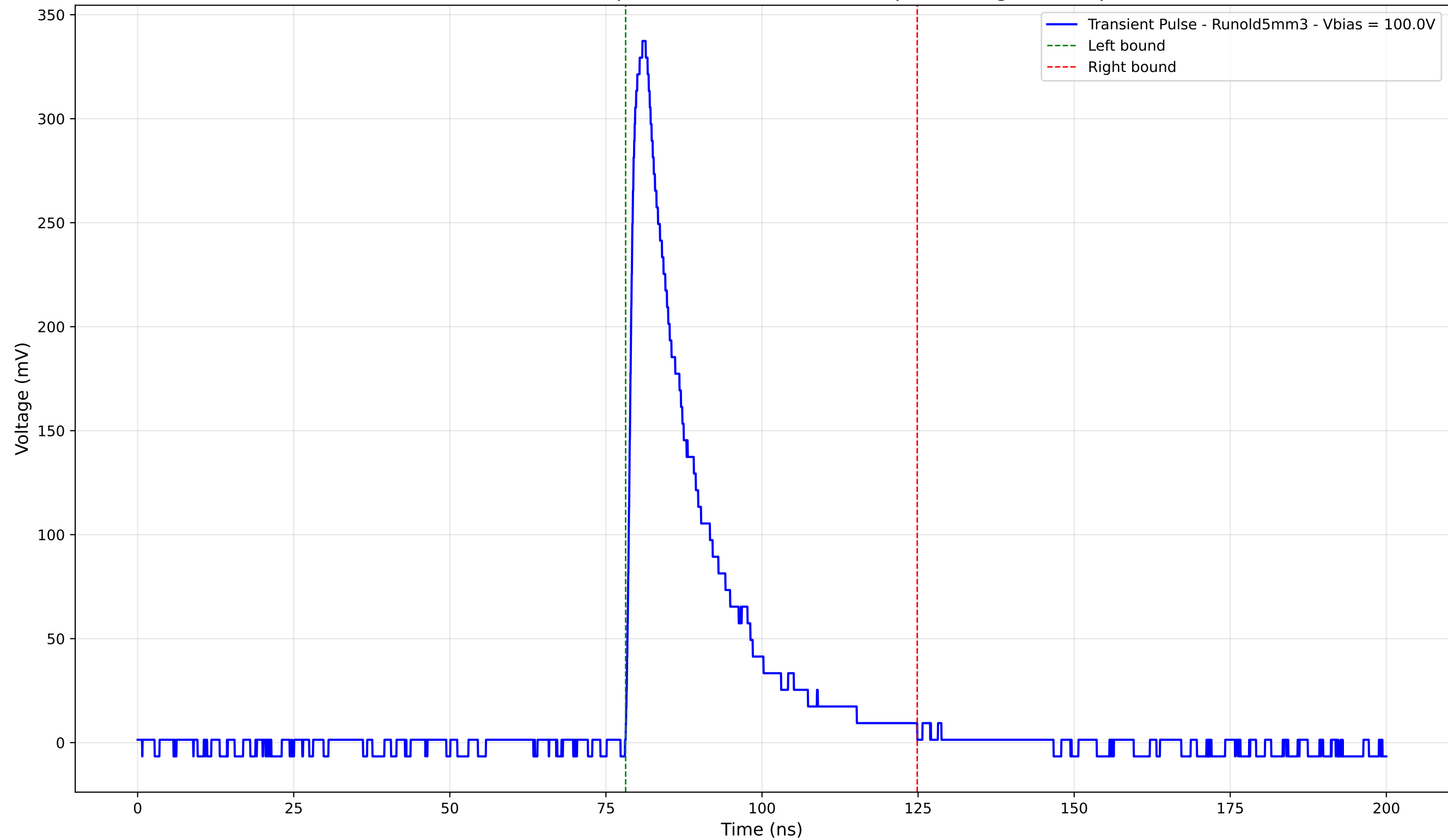
Transient Pulse - Sample: old5 - Position: 4265.0 \mu\text{m} - Charge: 74.33 pC
