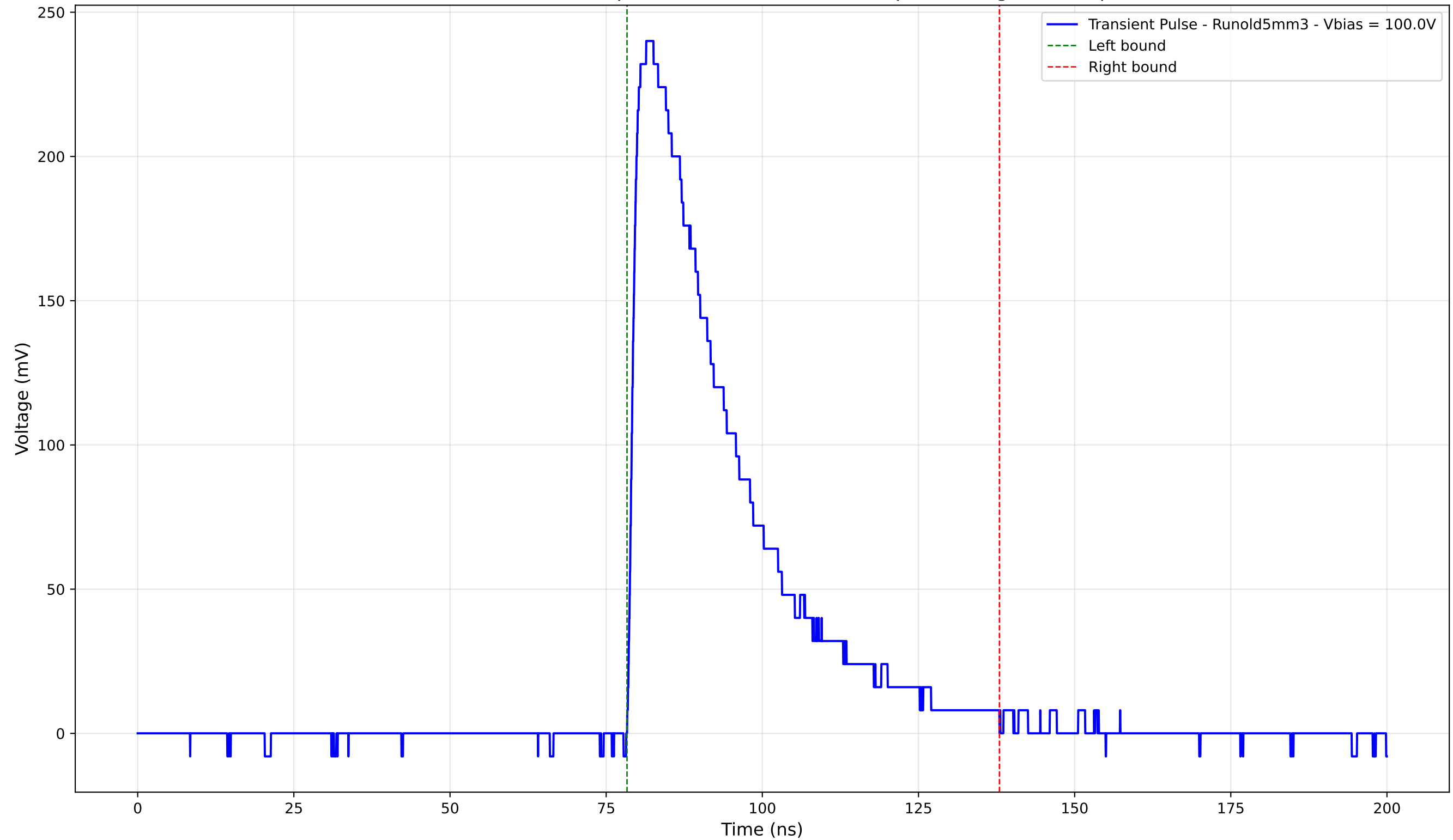
Transient Pulse - Sample: old5 - Position: 1090.0 \mu\text{m} - Charge: 84.61 pC
