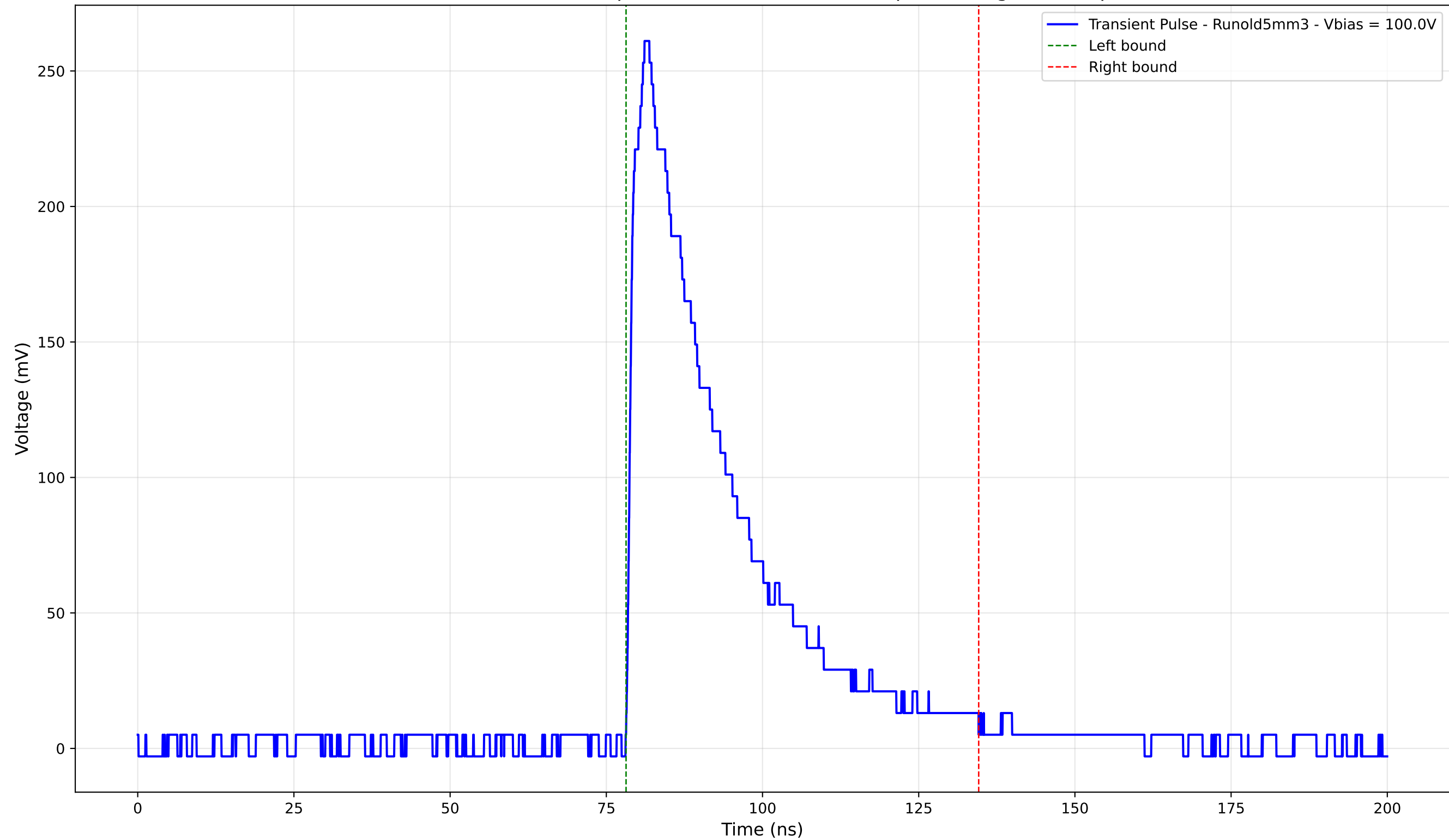
Transient Pulse - Sample: old5 - Position: 2885.0 \mu\text{m} - Charge: 84.78 pC
