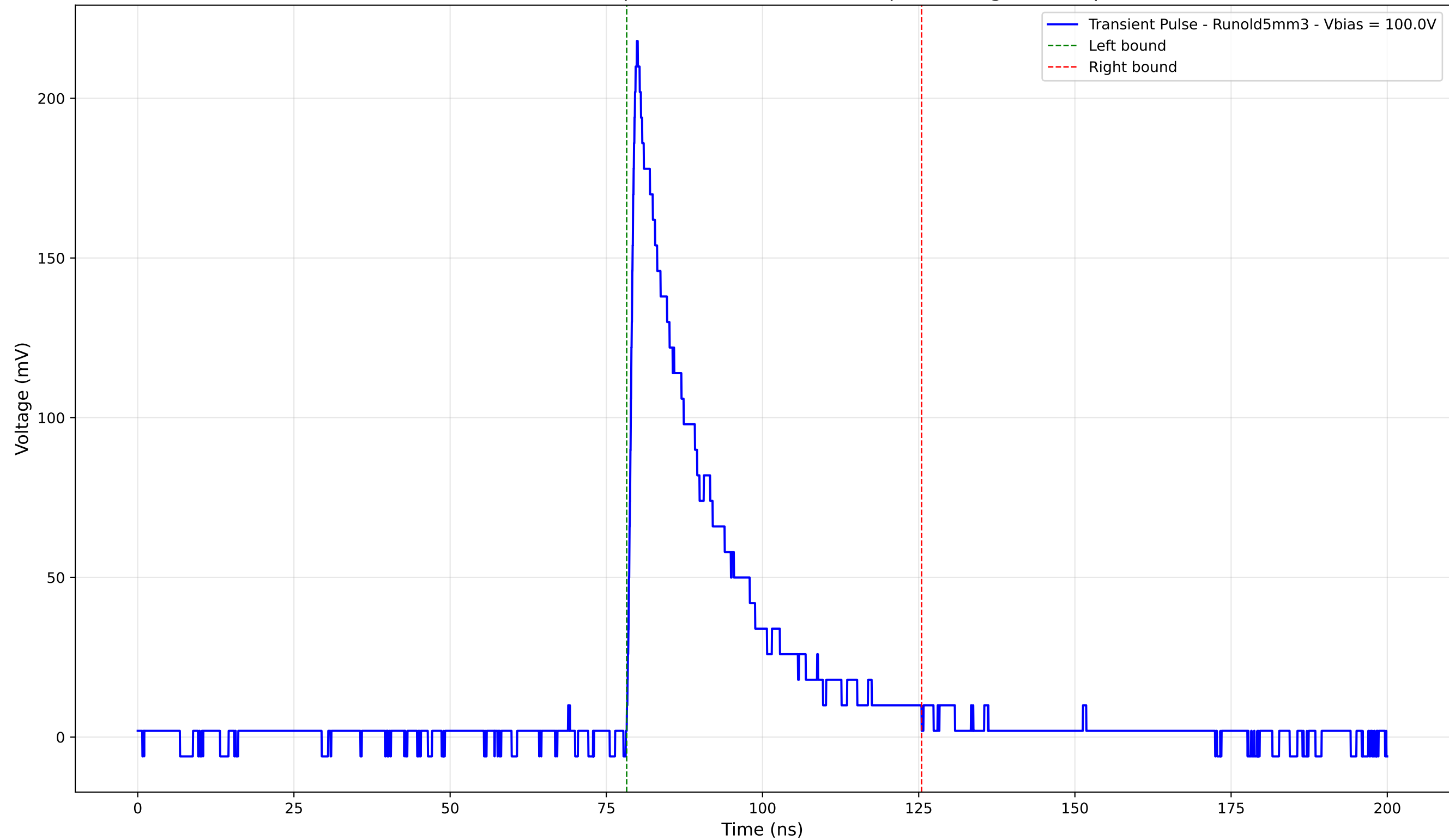
Transient Pulse - Sample: old5 - Position: 670.0 \mu\text{m} - Charge: 51.45 pC
