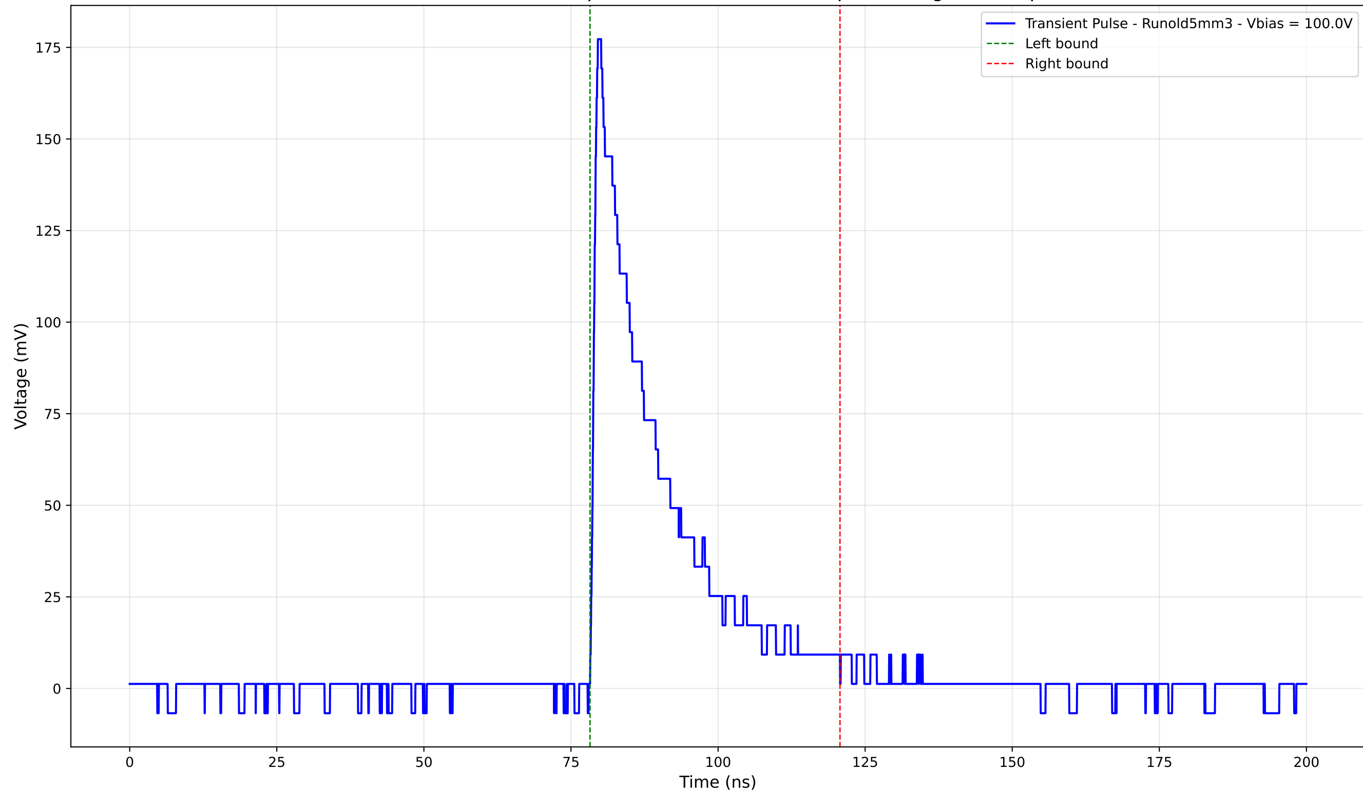
Transient Pulse - Sample: old5 - Position: 585.0 \mu\text{m} - Charge: 39.38 pC
