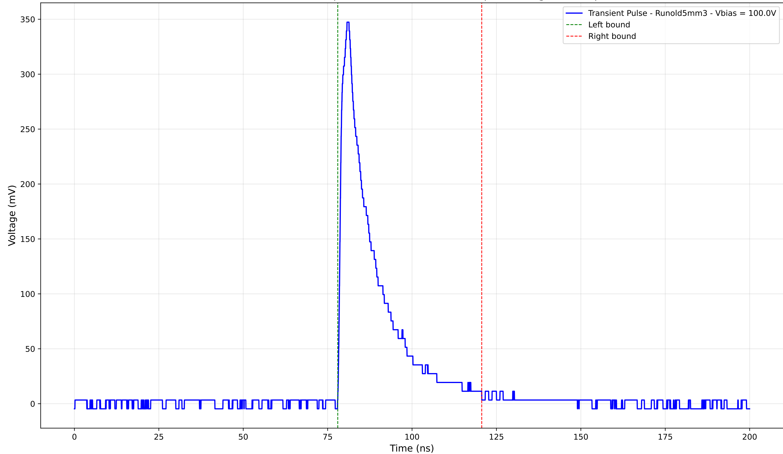
Transient Pulse - Sample: old5 - Position: 4100.0 \mu\text{m} - Charge: 74.99 pC
