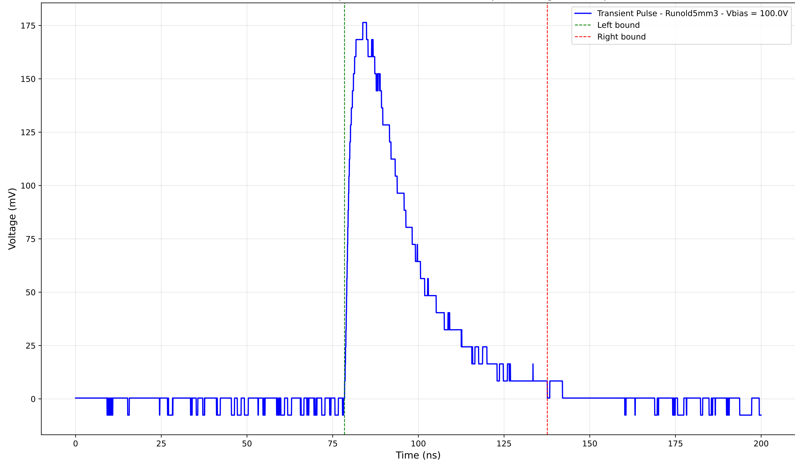
Transient Pulse - Sample: old5 - Position: 2055.0 \mu\text{m} - Charge: 70.28 pC
