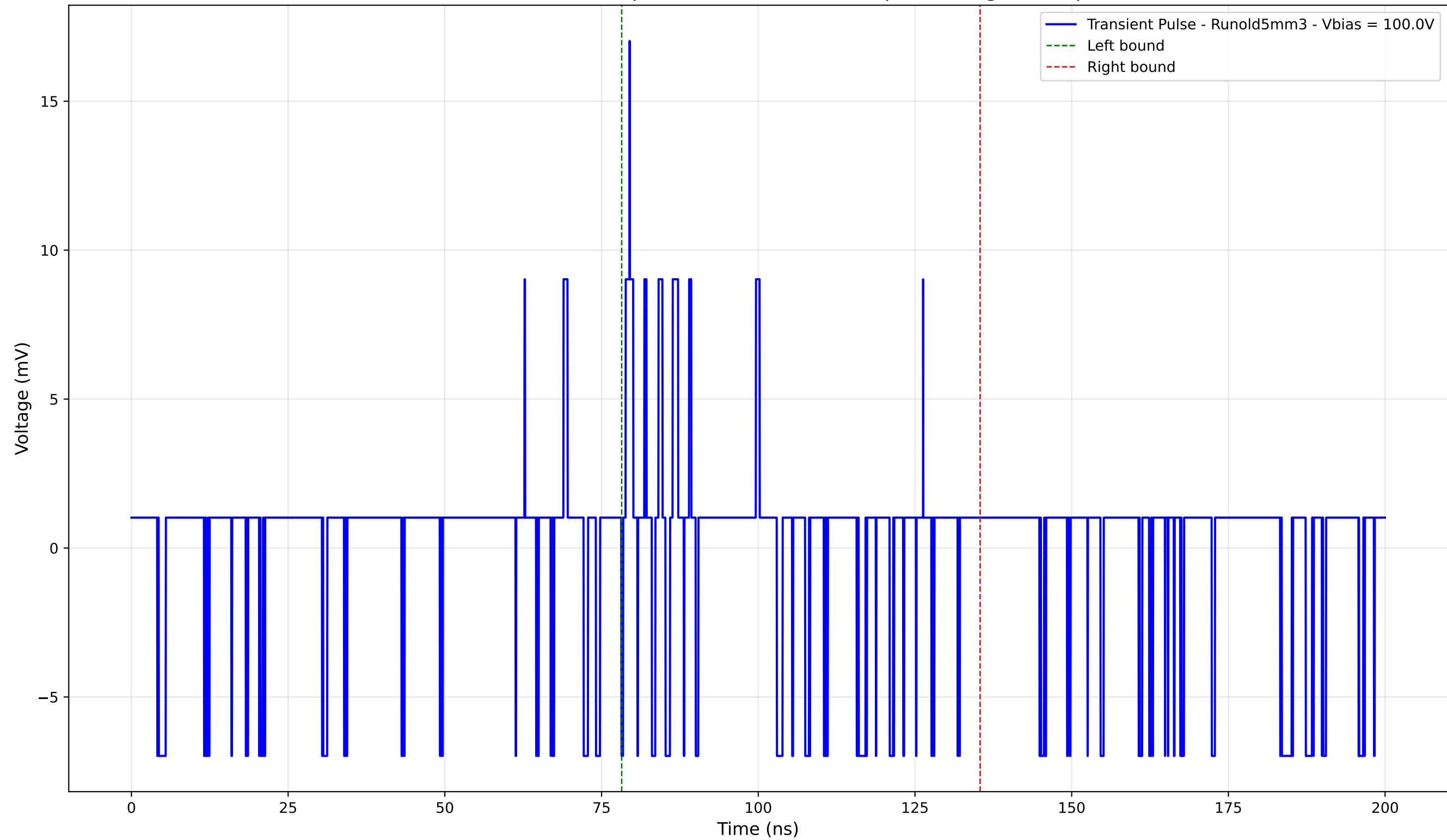
Transient Pulse - Sample: old5 - Position: 55.0 \mu\text{m} - Charge: 0.68 pC
