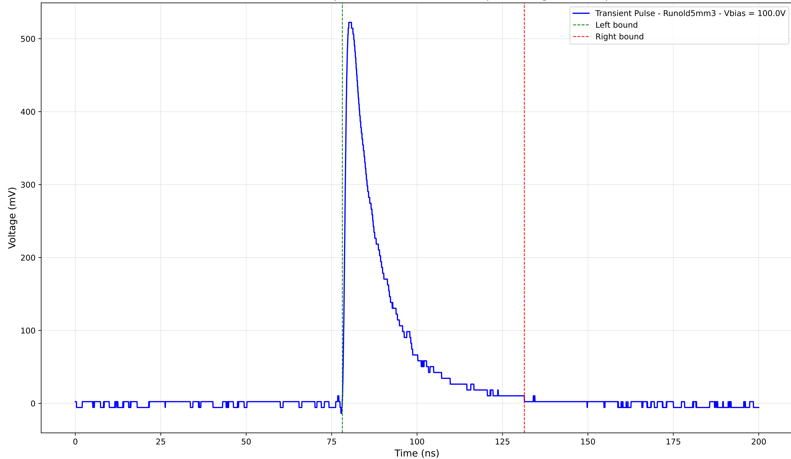
Transient Pulse - Sample: old5 - Position: 4350.0 \mu\text{m} - Charge: 118.37 pC
