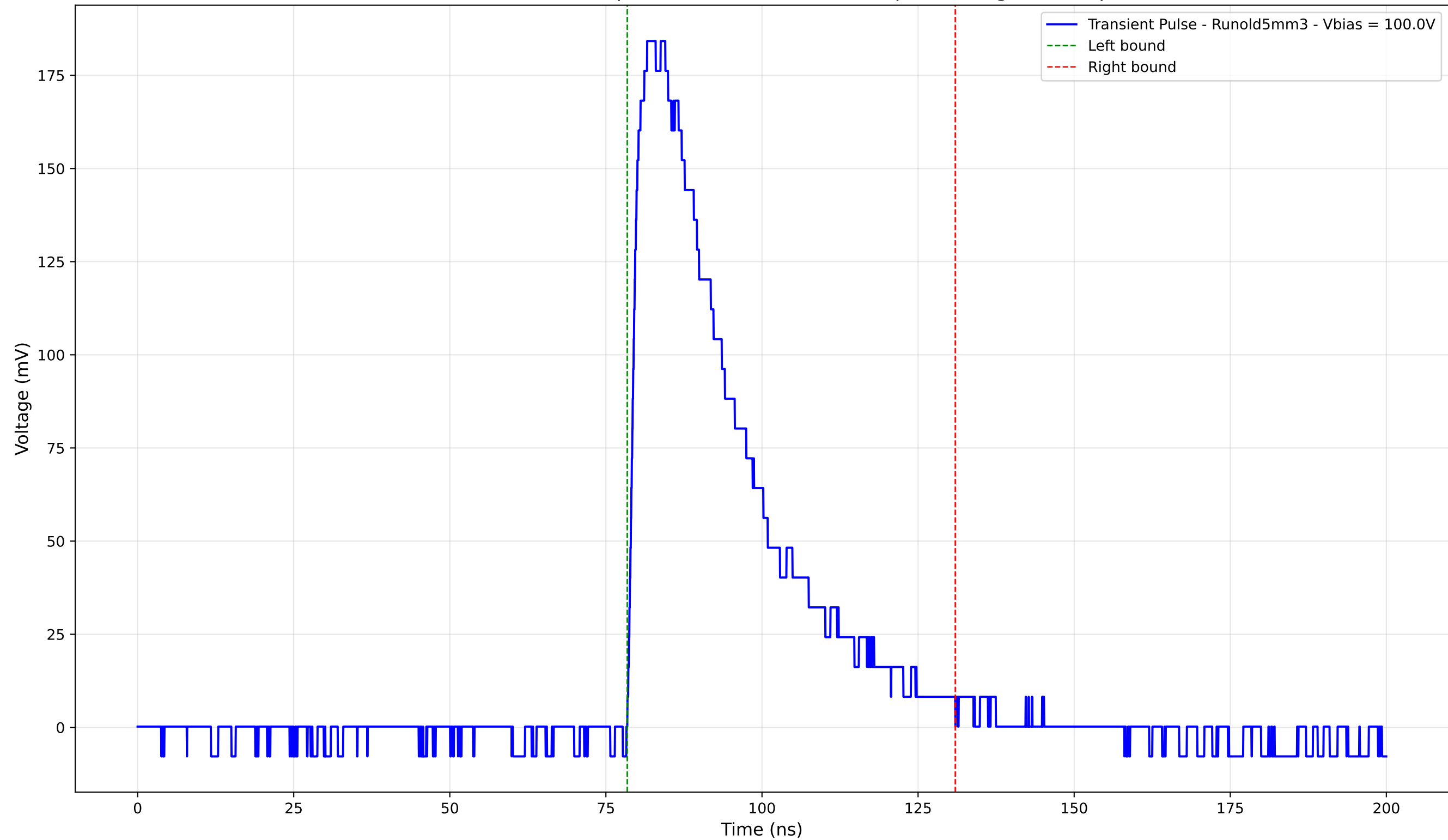
Transient Pulse - Sample: old5 - Position: 1255.0 \mu\text{m} - Charge: 68.62 pC
