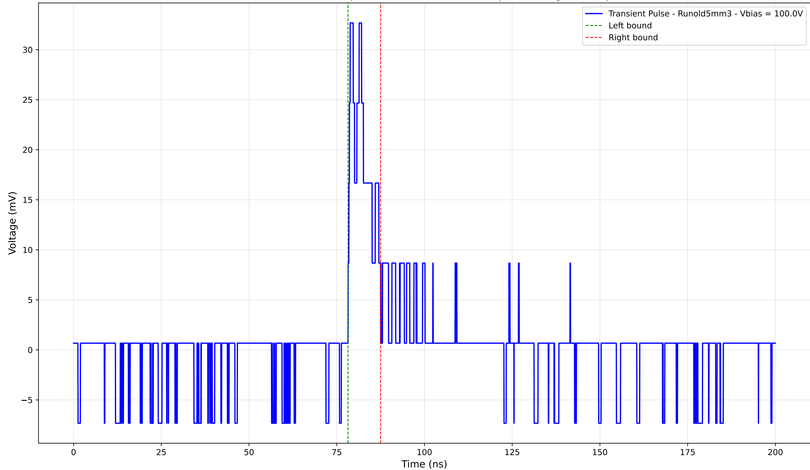
Transient Pulse - Sample: old5 - Position: 125.0 \mu\text{m} - Charge: 3.61 pC
