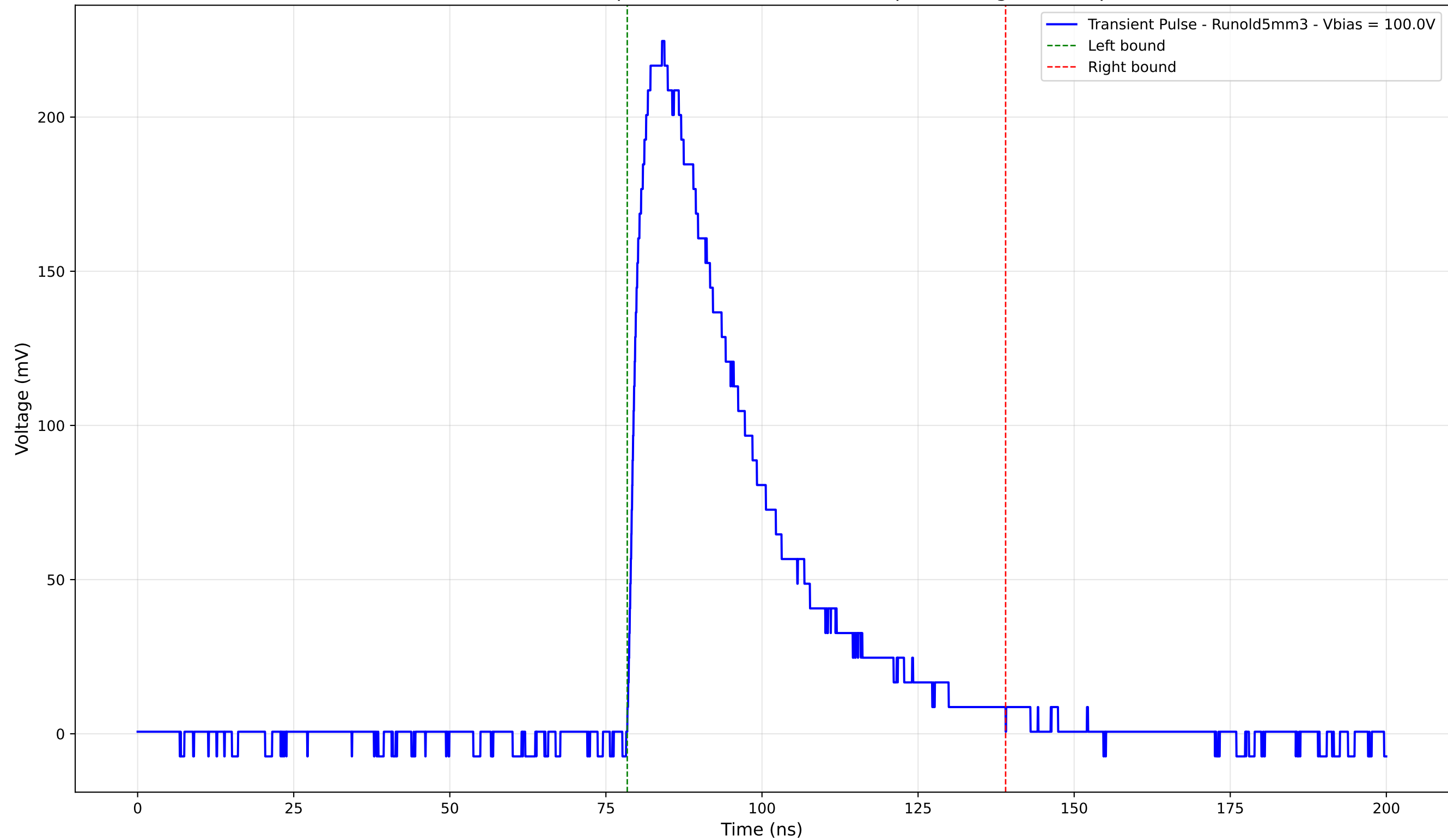
Transient Pulse - Sample: old5 - Position: 2080.0 \mu\text{m} - Charge: 88.61 pC
