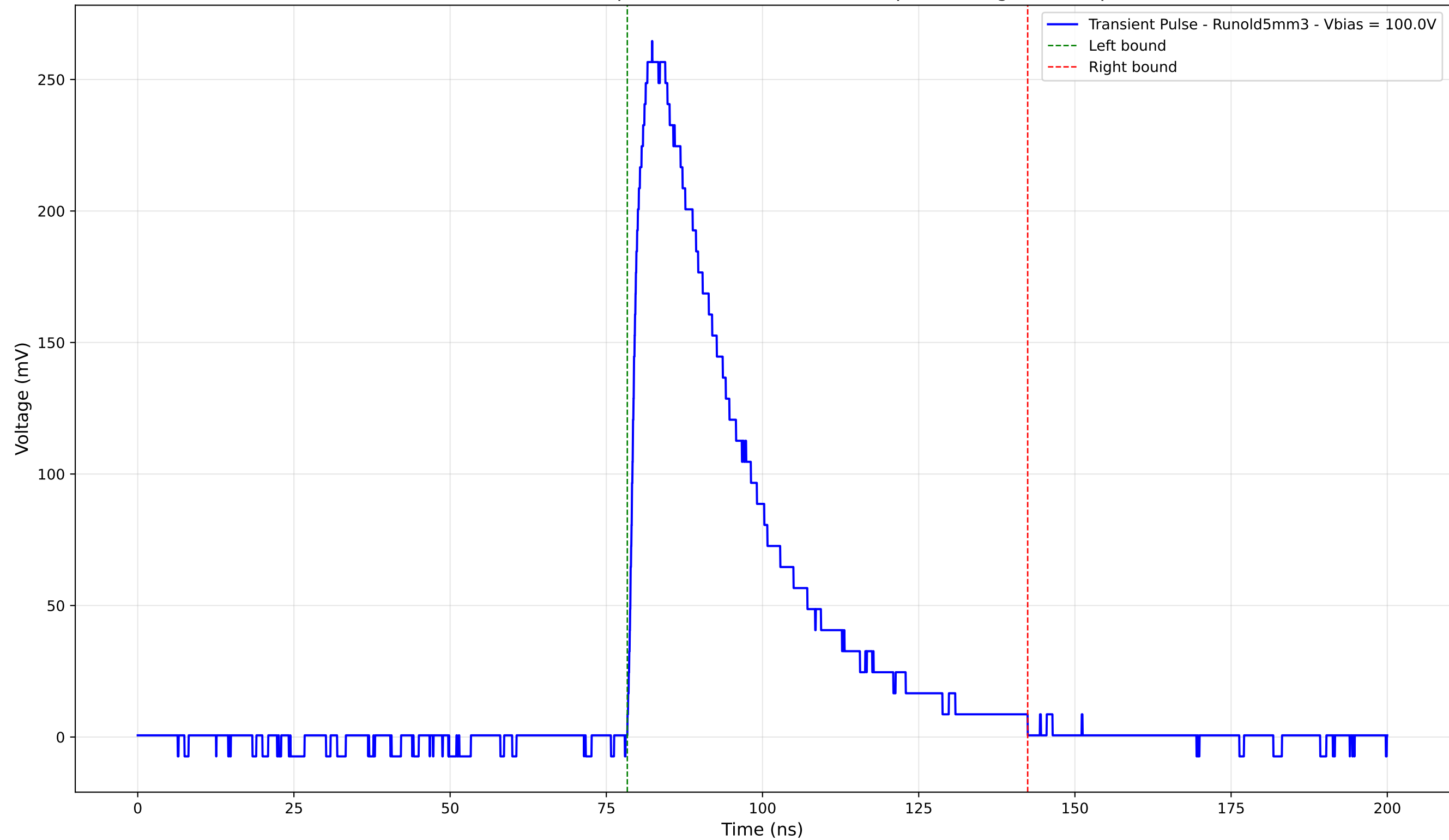
Transient Pulse - Sample: old5 - Position: 2490.0 \mu\text{m} - Charge: 98.82 pC
