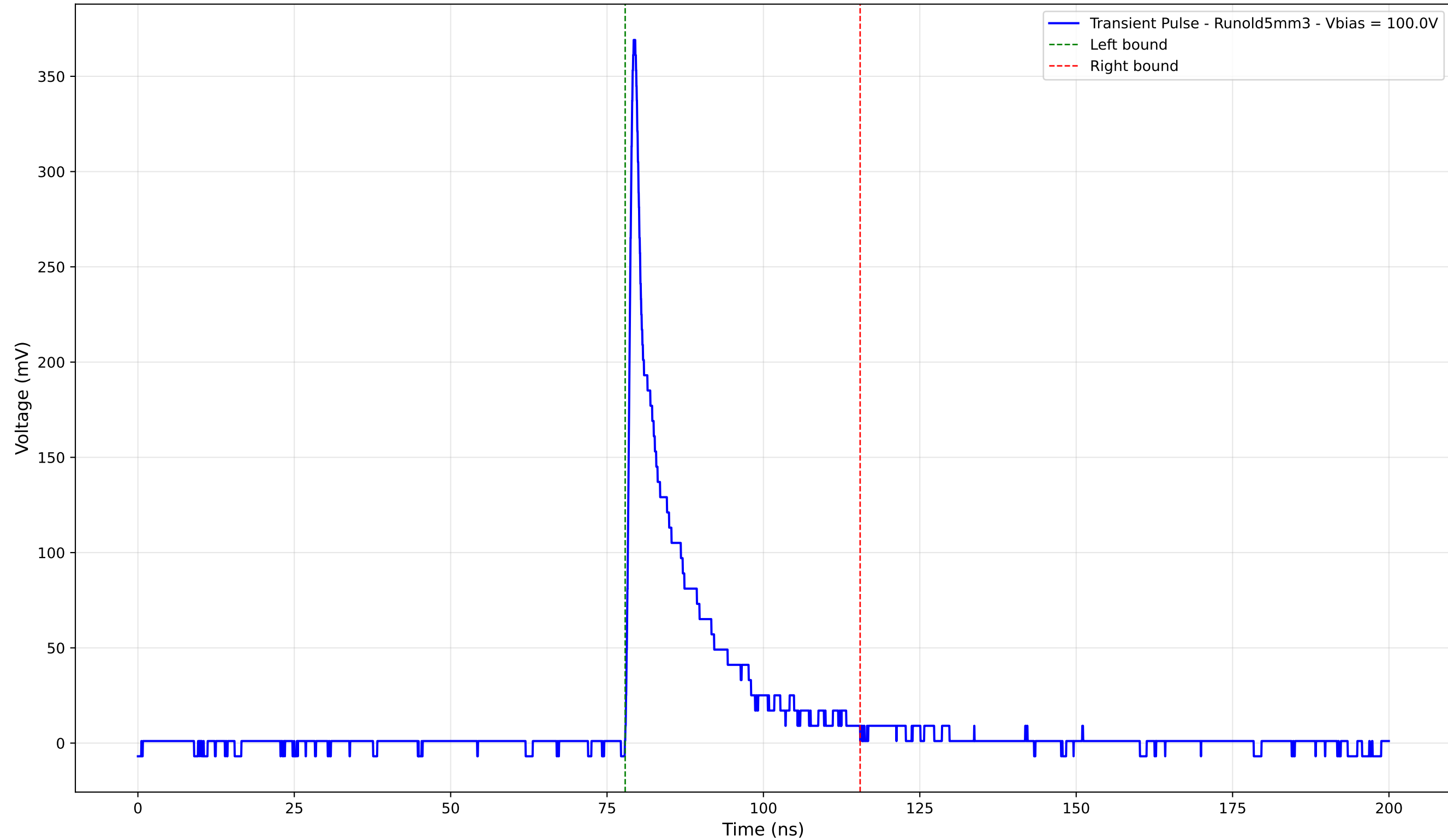
Transient Pulse - Sample: old5 - Position: 270.0 \mu\text{m} - Charge: 49.64 pC
