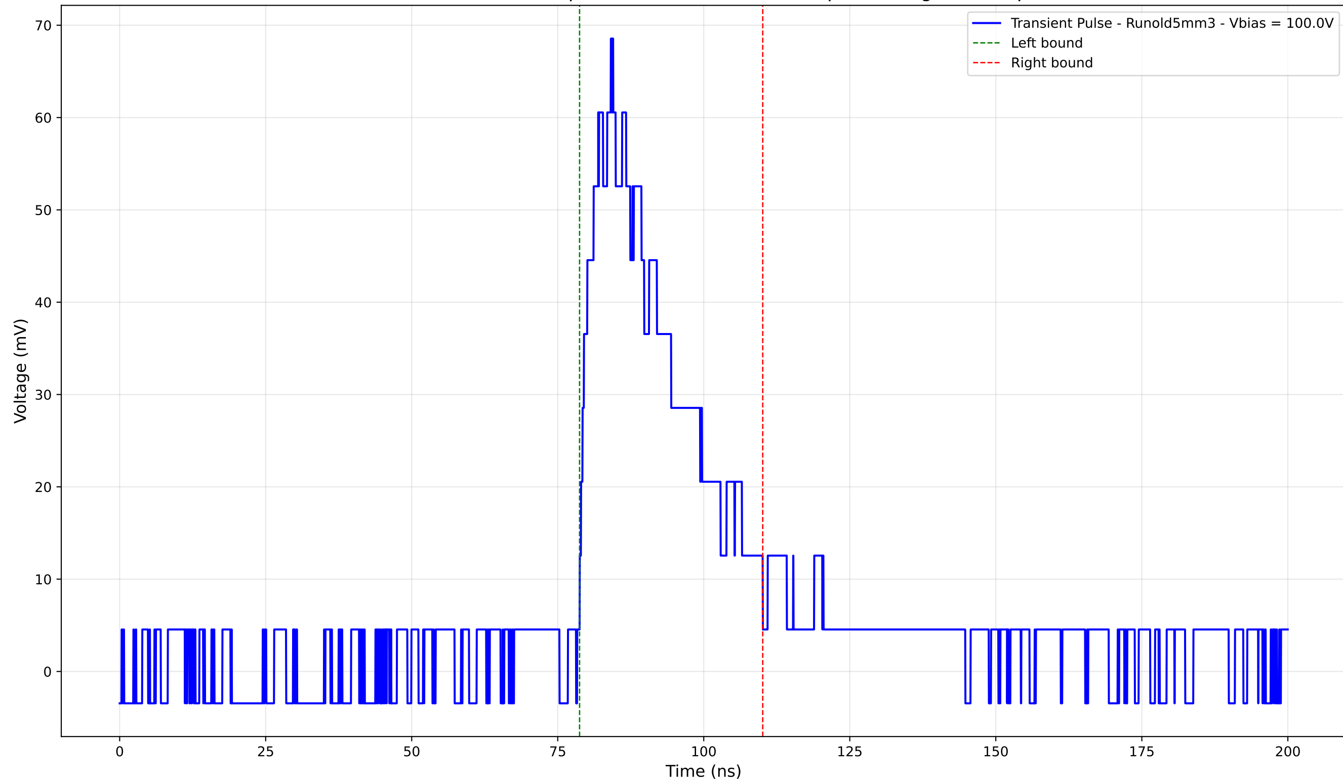
Transient Pulse - Sample: old5 - Position: 1765.0 \mu\text{m} - Charge: 21.27 pC
