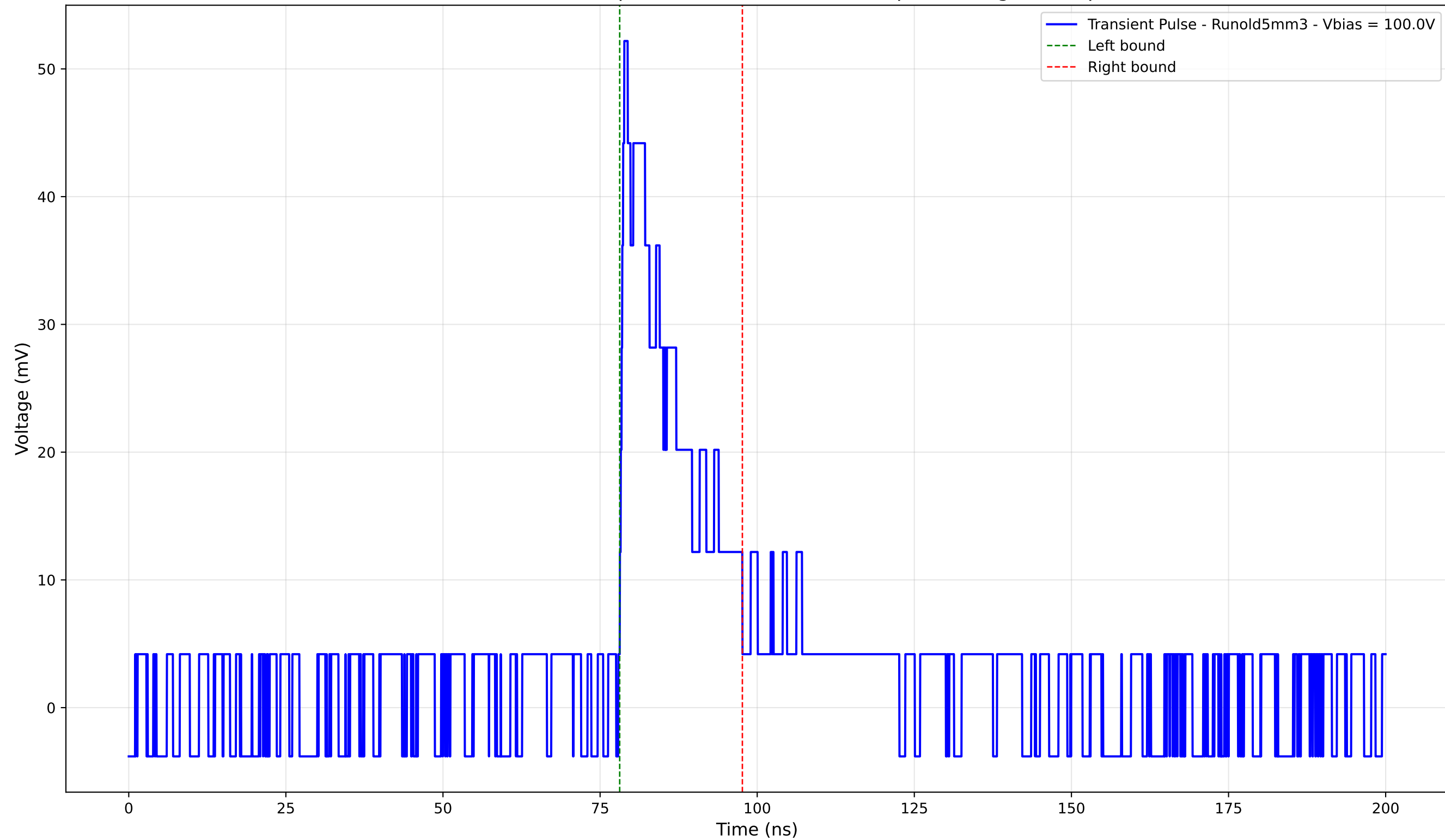
Transient Pulse - Sample: old5 - Position: 3250.0 \mu\text{m} - Charge: 9.56 pC
