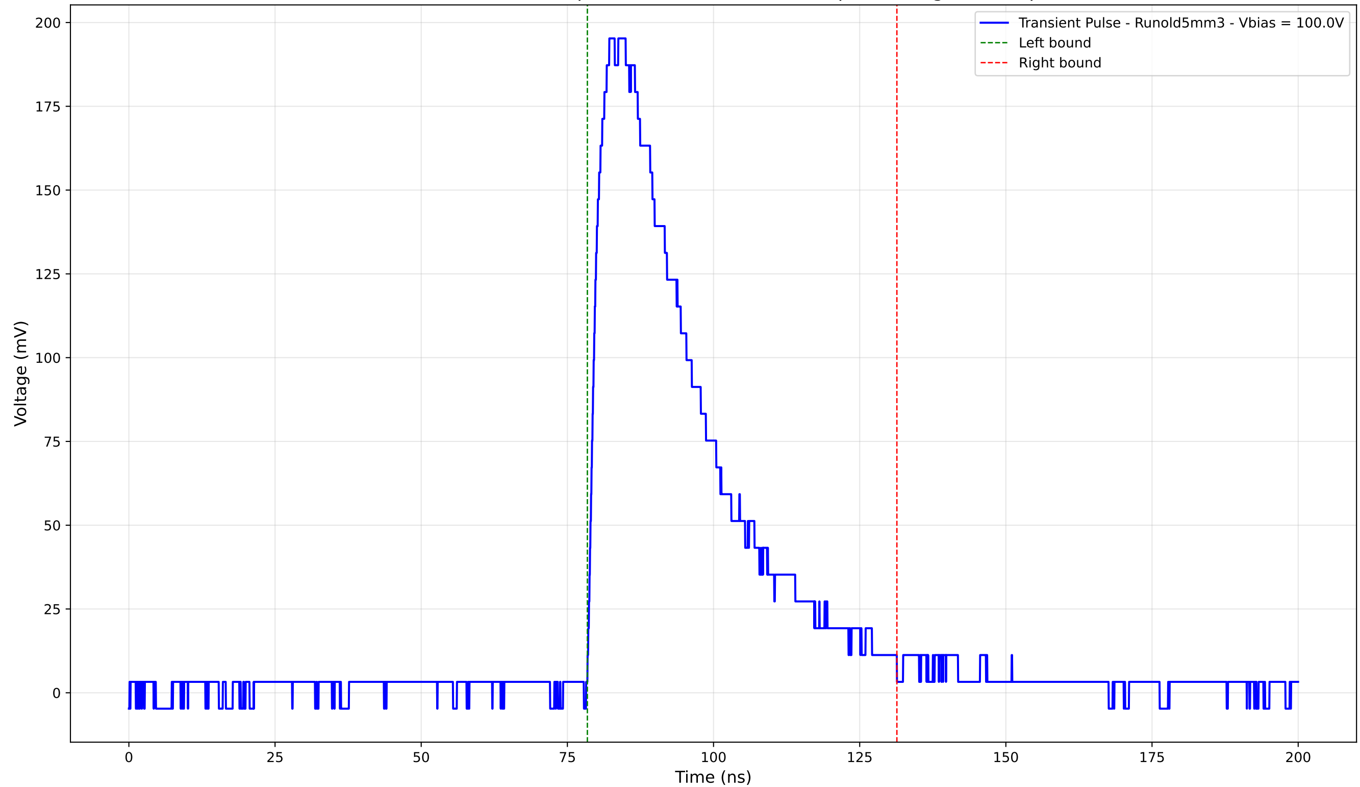
Transient Pulse - Sample: old5 - Position: 1665.0 \mu\text{m} - Charge: 78.46 pC
