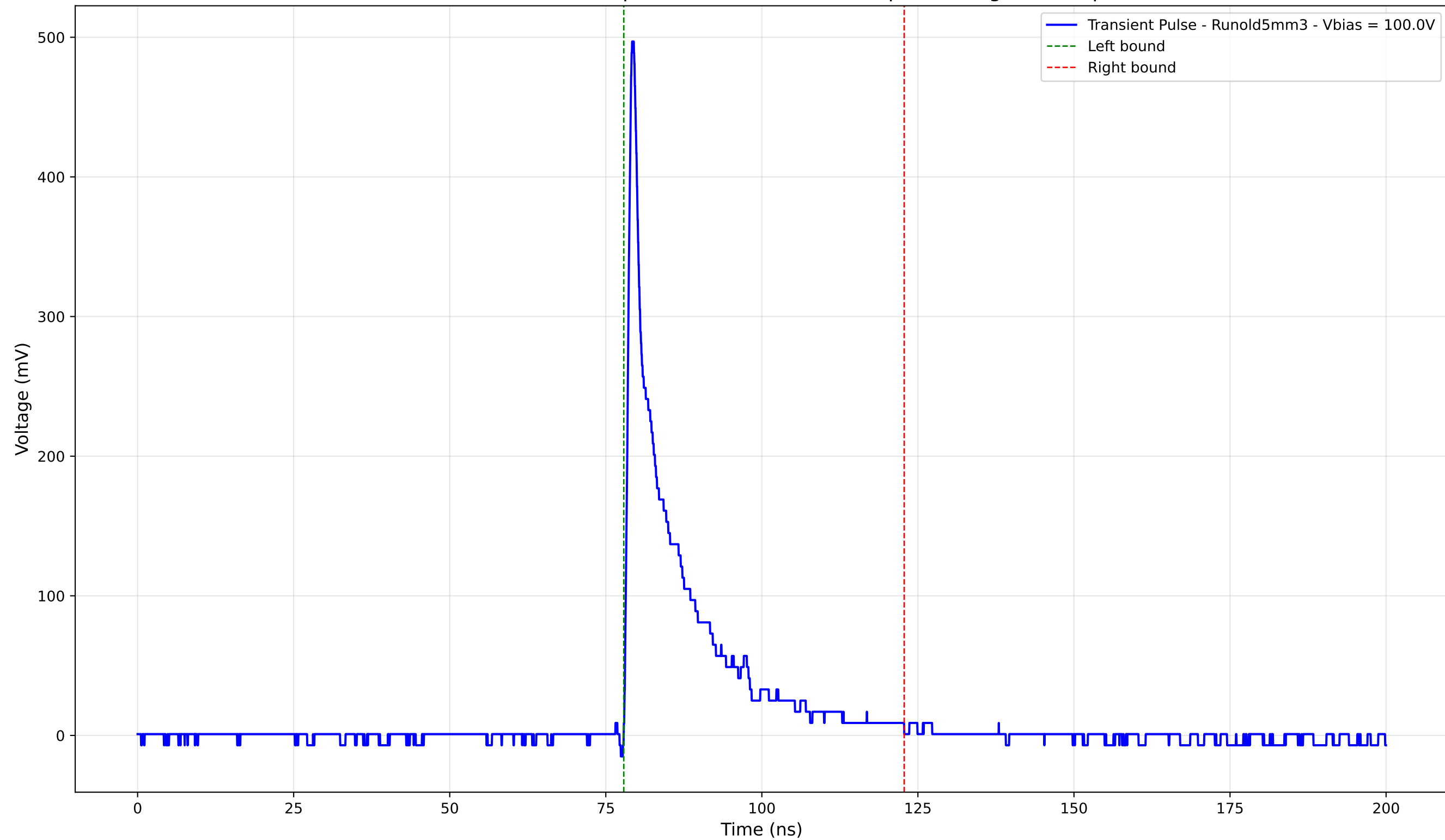
Transient Pulse - Sample: old5 - Position: 250.0 \mu\text{m} - Charge: 65.58 pC
