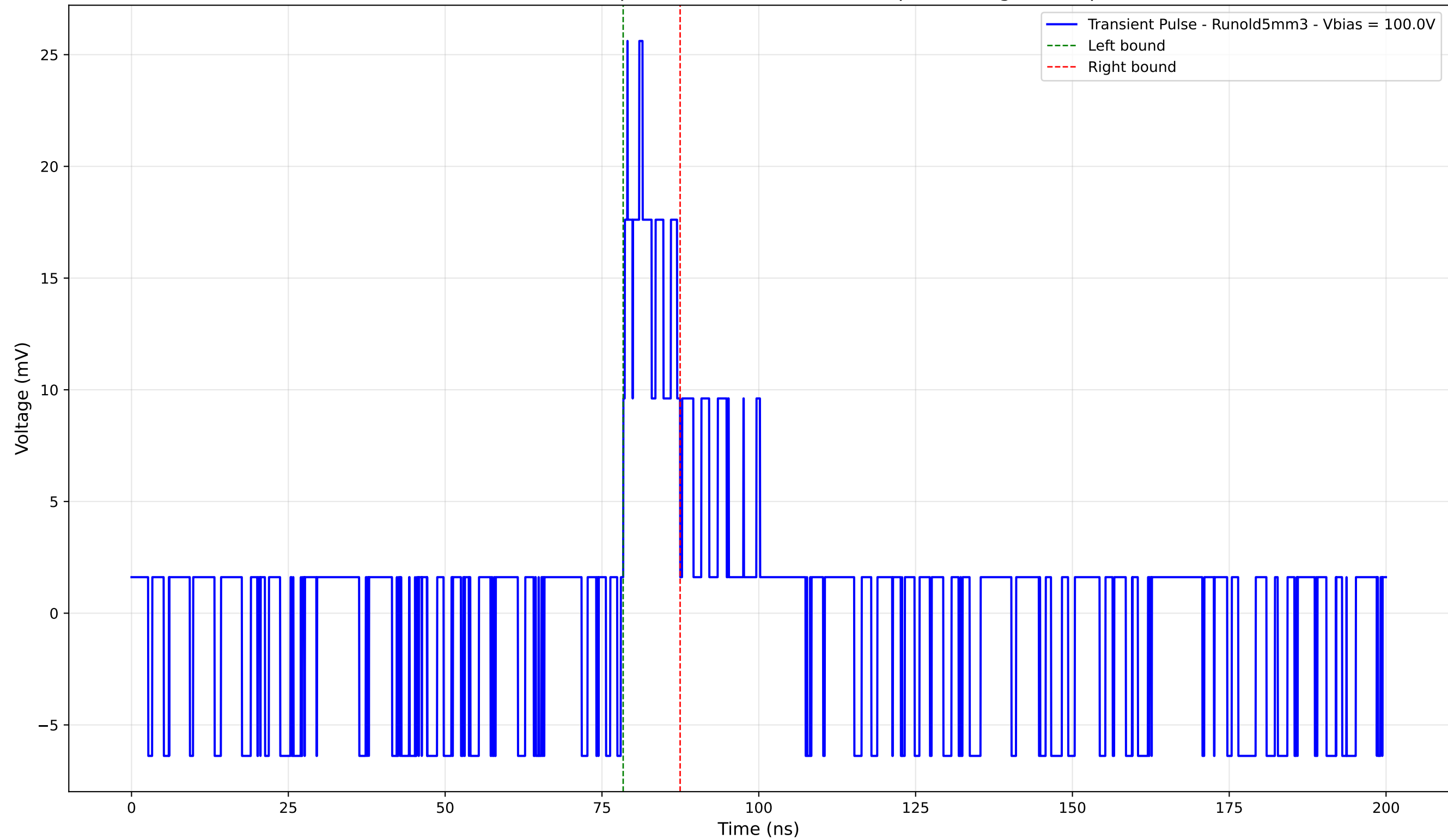
Transient Pulse - Sample: old5 - Position: 3280.0 \mu\text{m} - Charge: 2.88 pC
