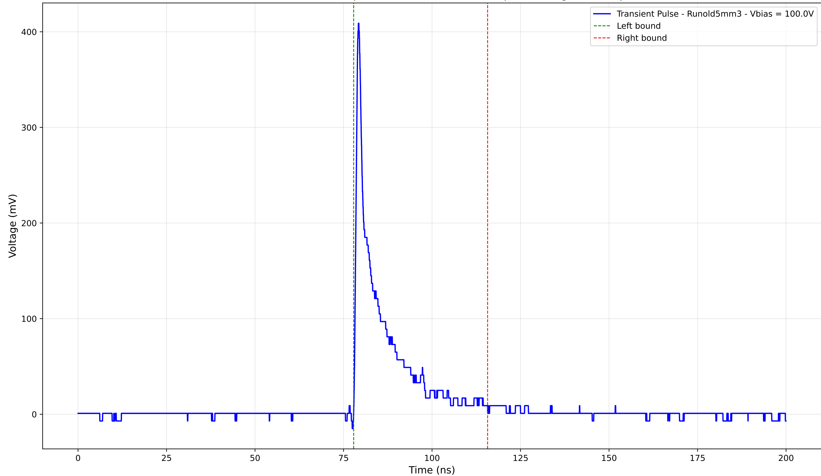
Transient Pulse - Sample: old5 - Position: 185.0 \mu\text{m} - Charge: 49.23 pC
