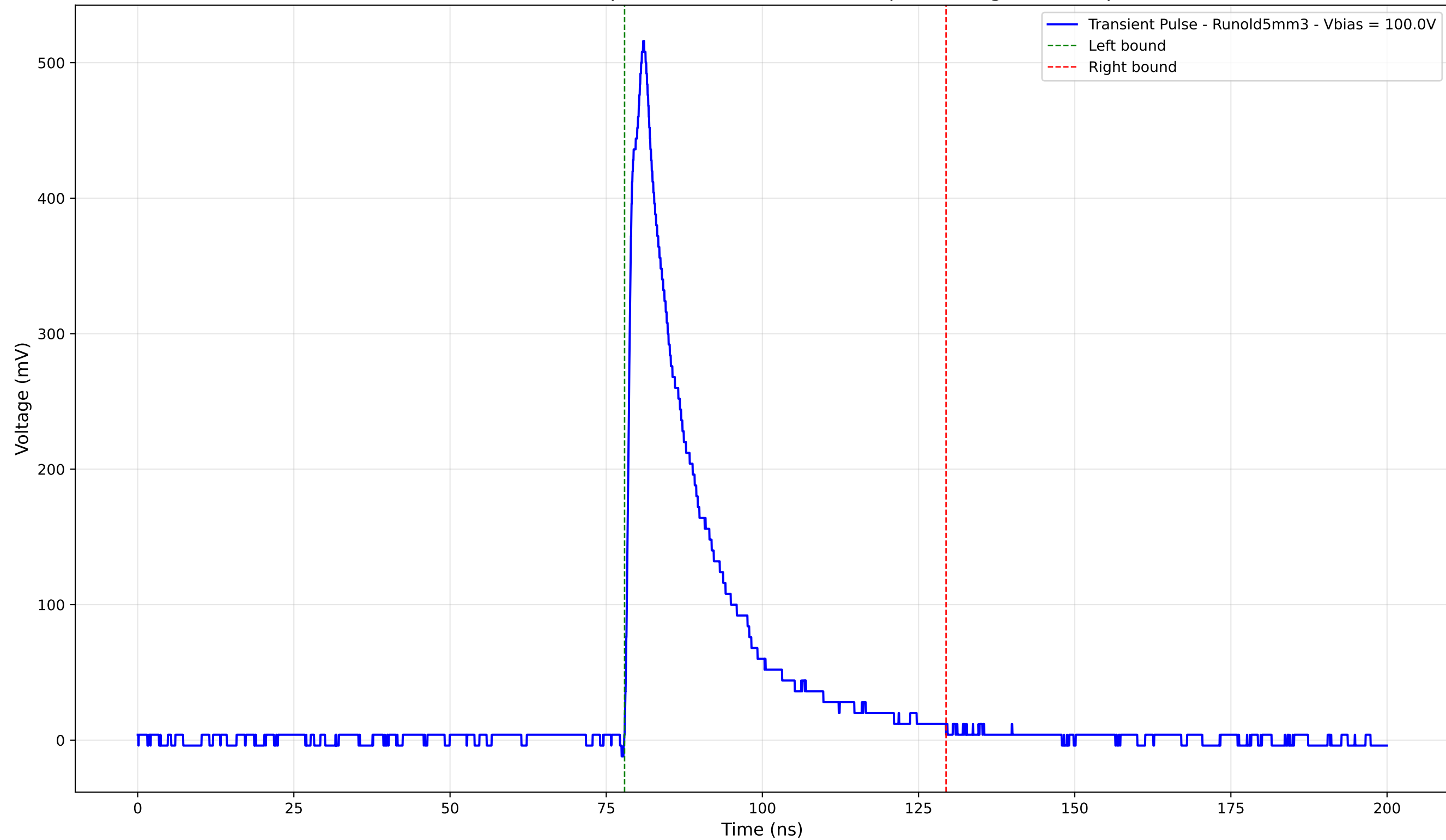
Transient Pulse - Sample: old5 - Position: 4060.0 \mu\text{m} - Charge: 114.40 pC
