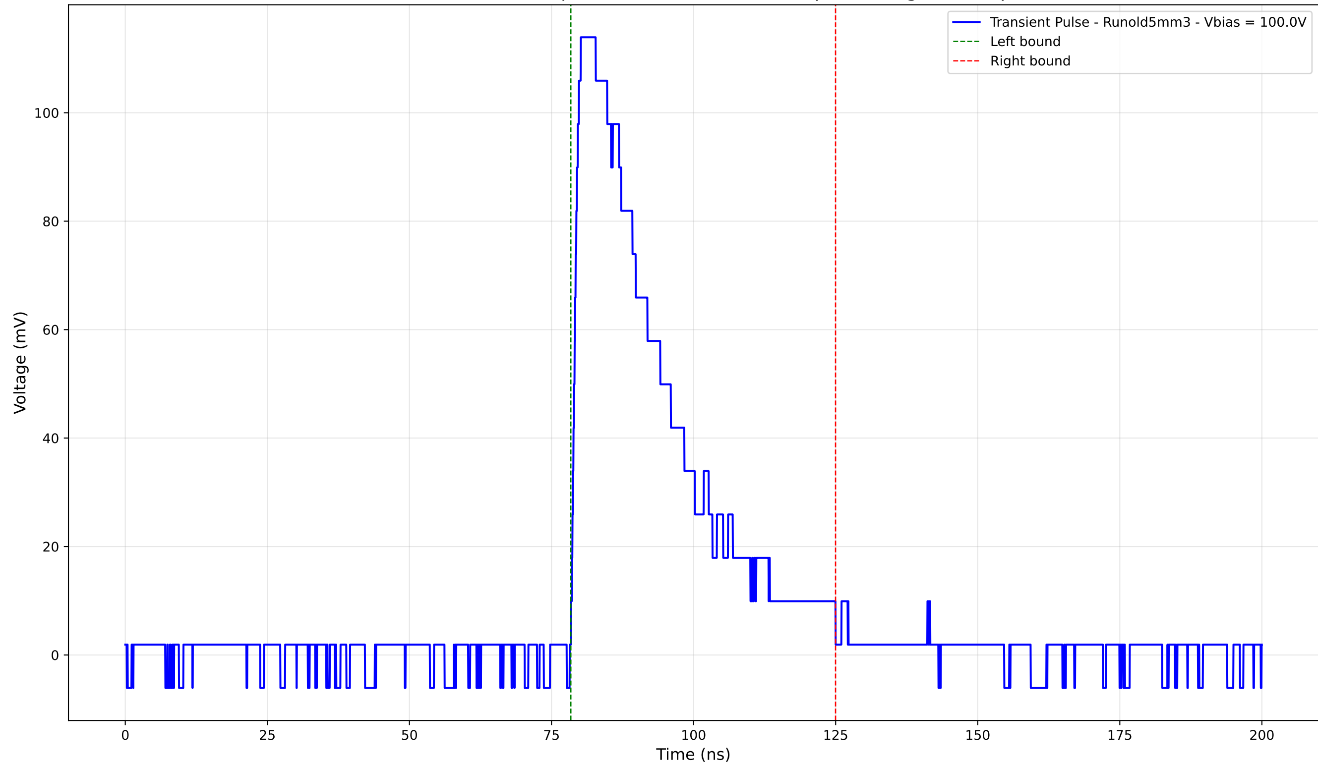
Transient Pulse - Sample: old5 - Position: 1000.0 \mu\text{m} - Charge: 39.68 pC
