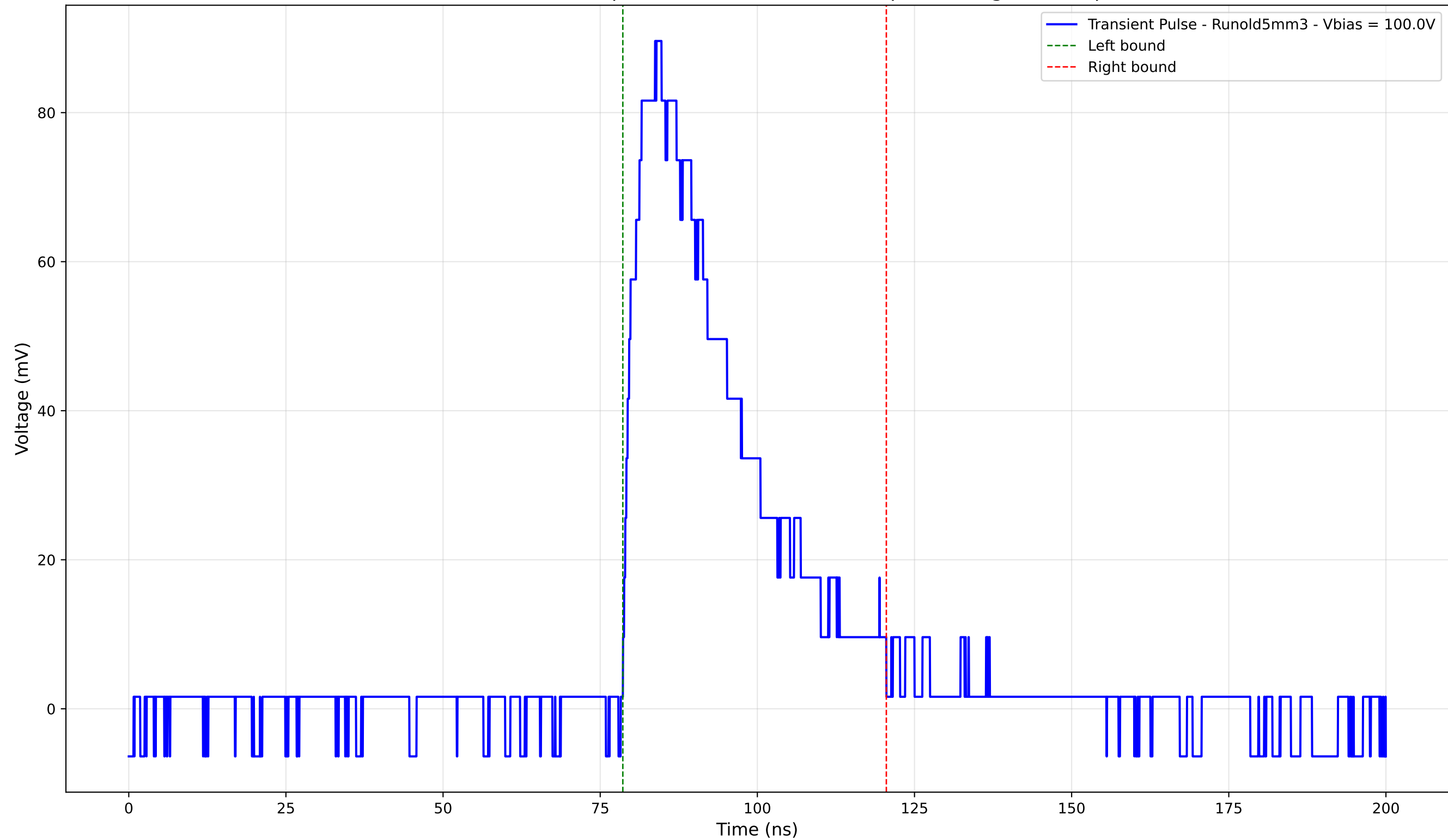
Transient Pulse - Sample: old5 - Position: 1955.0 \mu\text{m} - Charge: 32.27 pC
