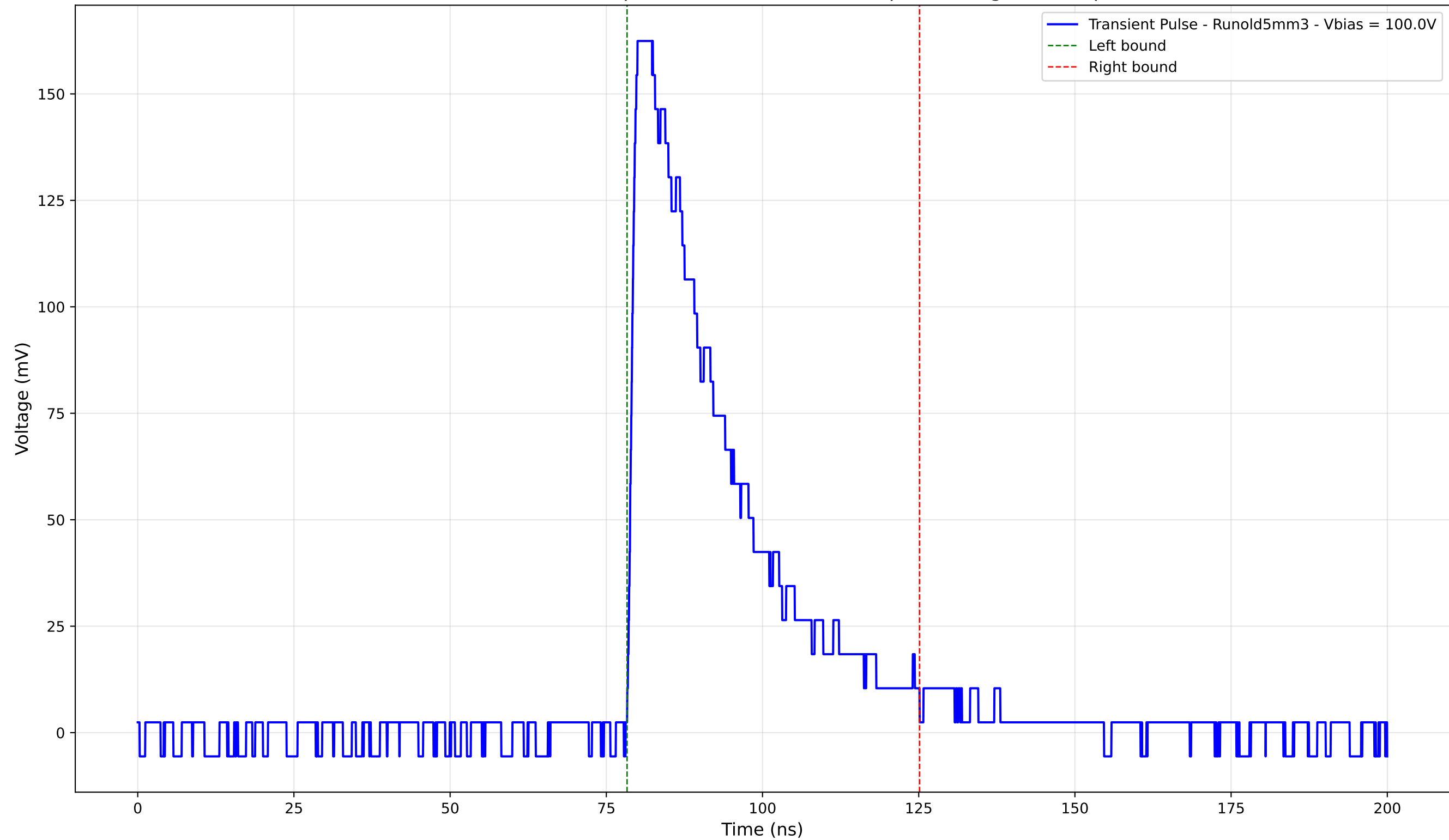
Transient Pulse - Sample: old5 - Position: 935.0 \mu\text{m} - Charge: 53.57 pC
