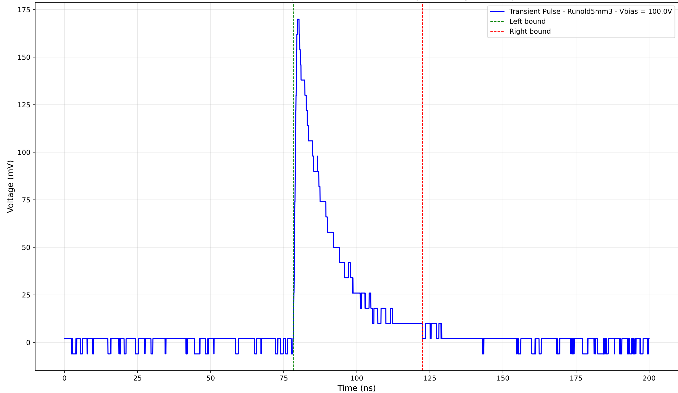
Transient Pulse - Sample: old5 - Position: 610.0 \mu\text{m} - Charge: 39.47 pC
