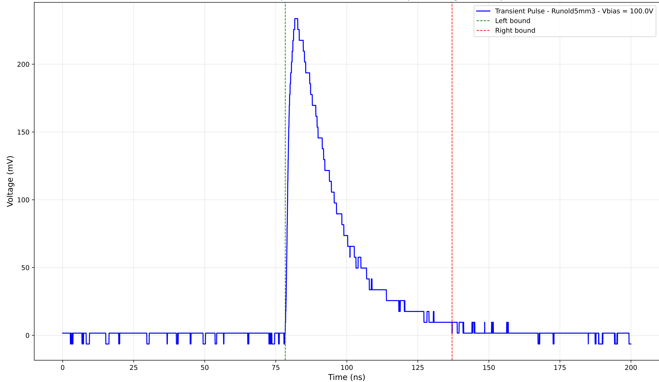
Transient Pulse - Sample: old5 - Position: 2575.0 \mu\text{m} - Charge: 85.16 pC
