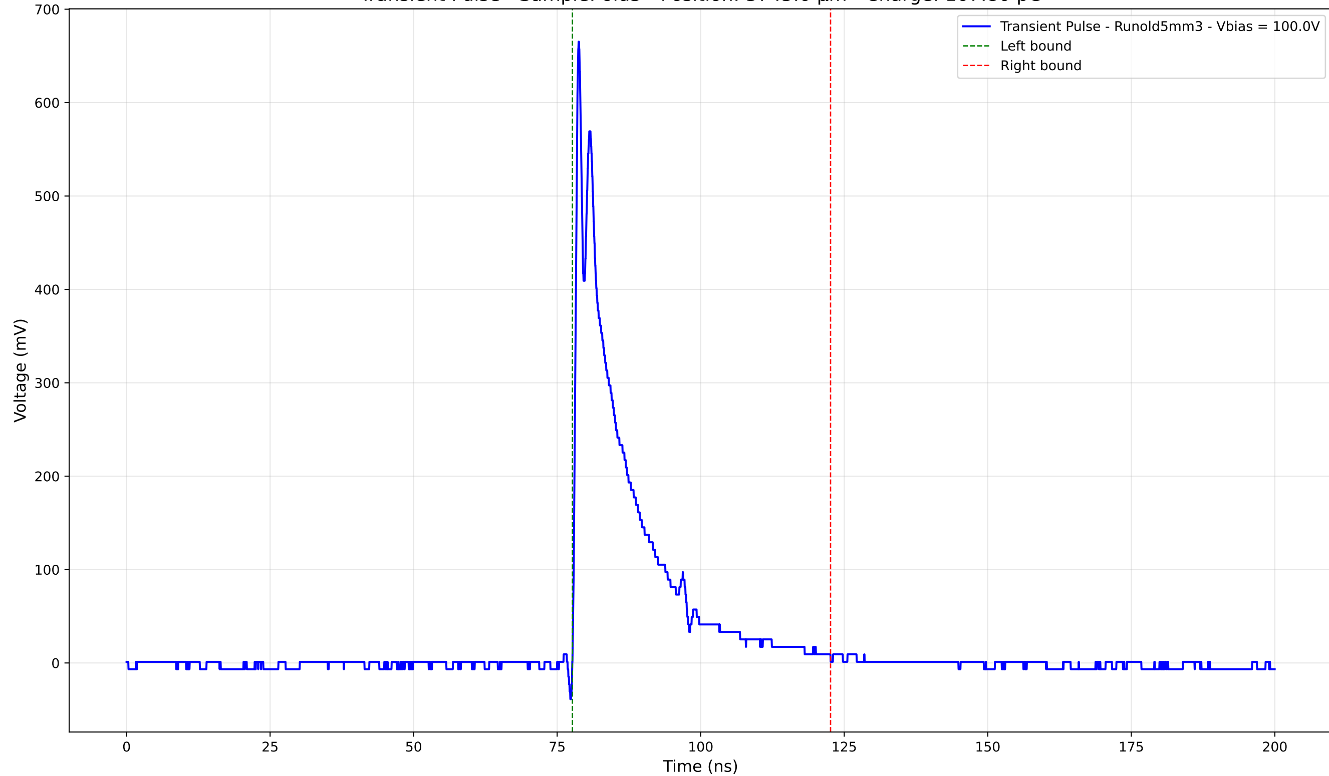
Transient Pulse - Sample: old5 - Position: 3745.0 \mu\text{m} - Charge: 107.80 pC
