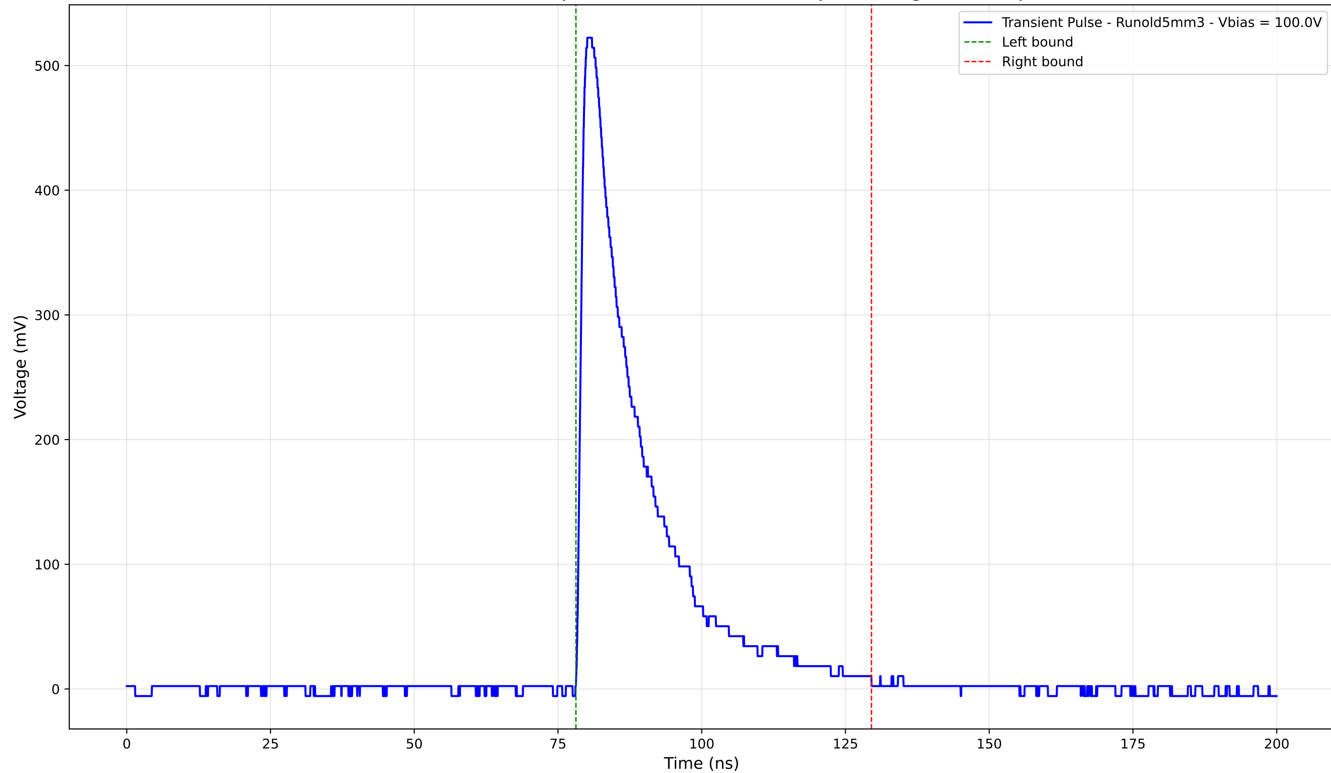
Transient Pulse - Sample: old5 - Position: 4335.0 \mu\text{m} - Charge: 119.55 pC
