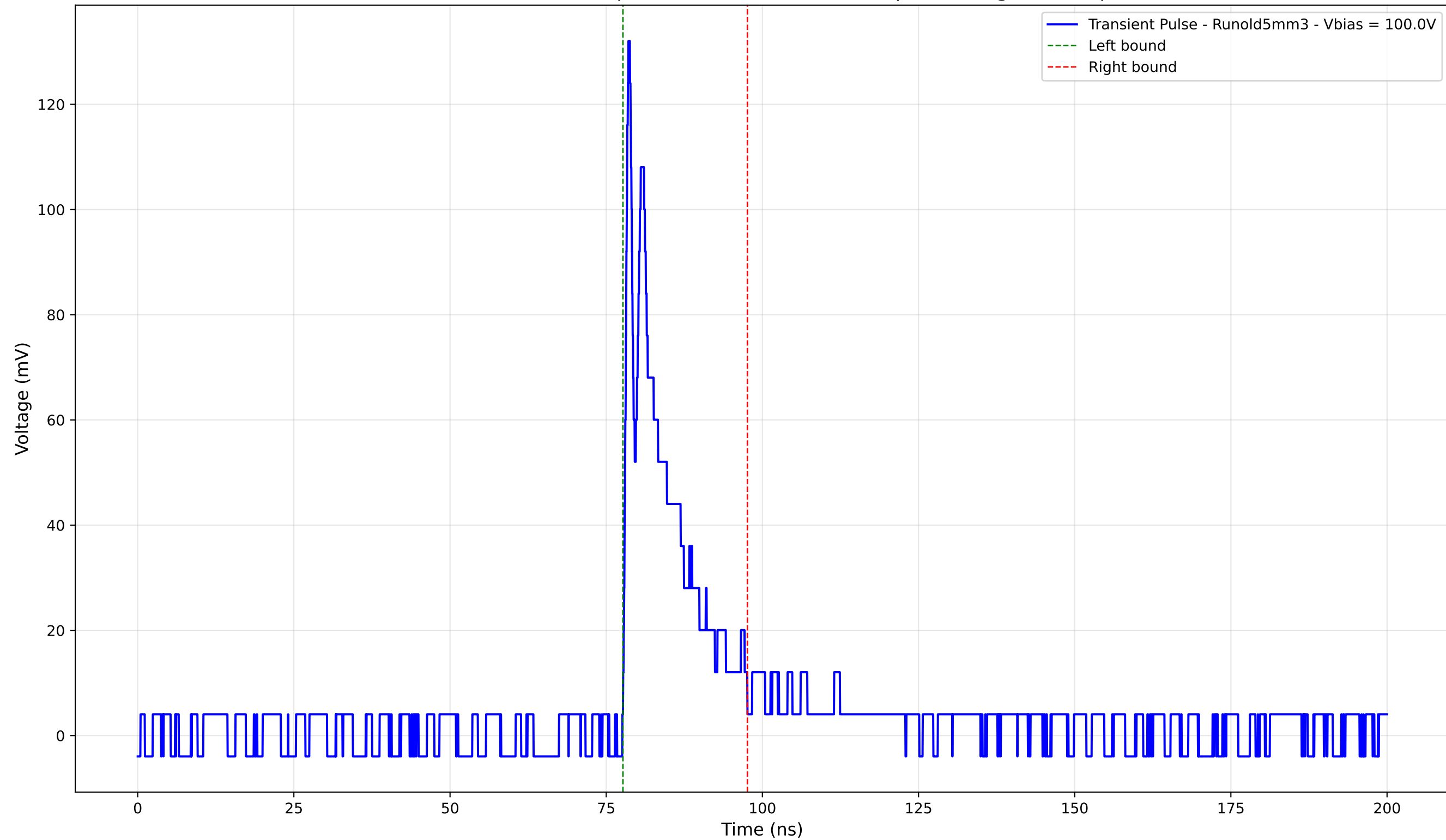
Transient Pulse - Sample: old5 - Position: 3620.0 \mu\text{m} - Charge: 16.70 pC
