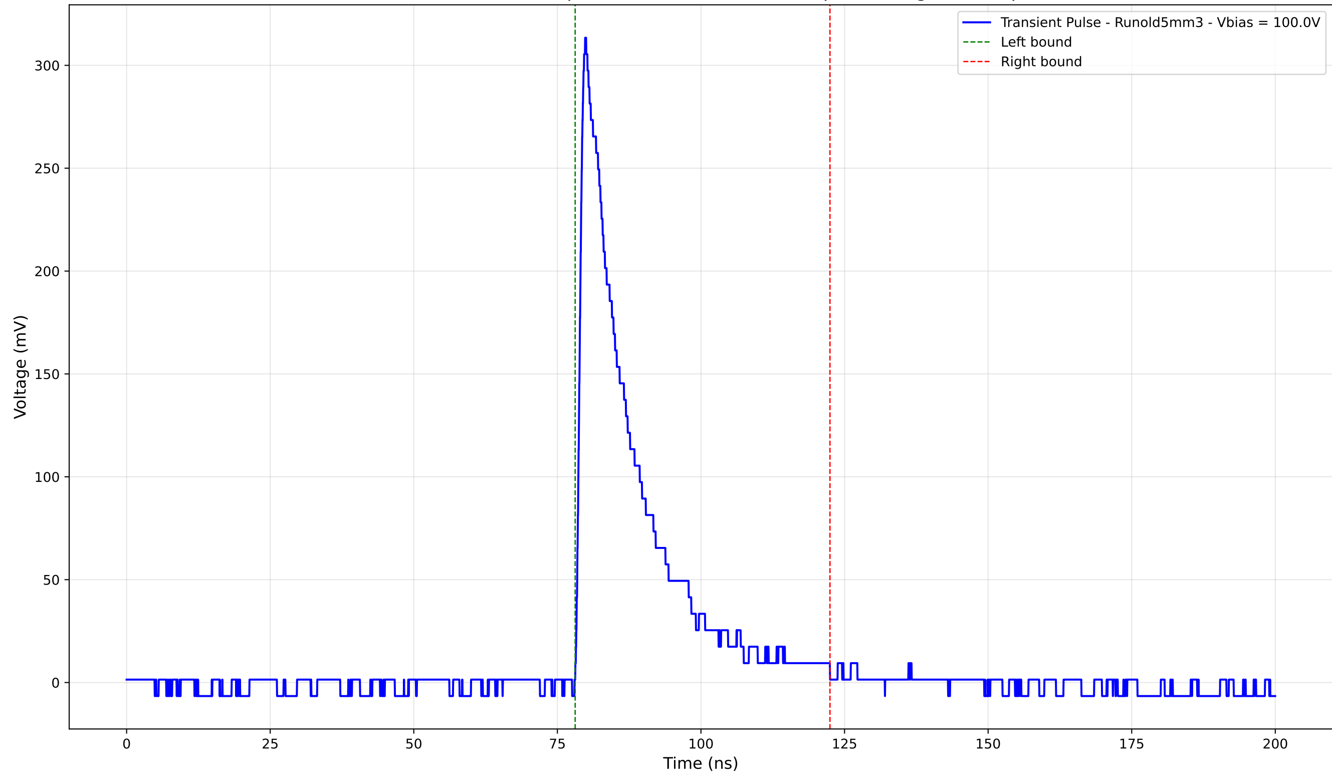
Transient Pulse - Sample: old5 - Position: 4560.0 \mu\text{m} - Charge: 60.92 pC
