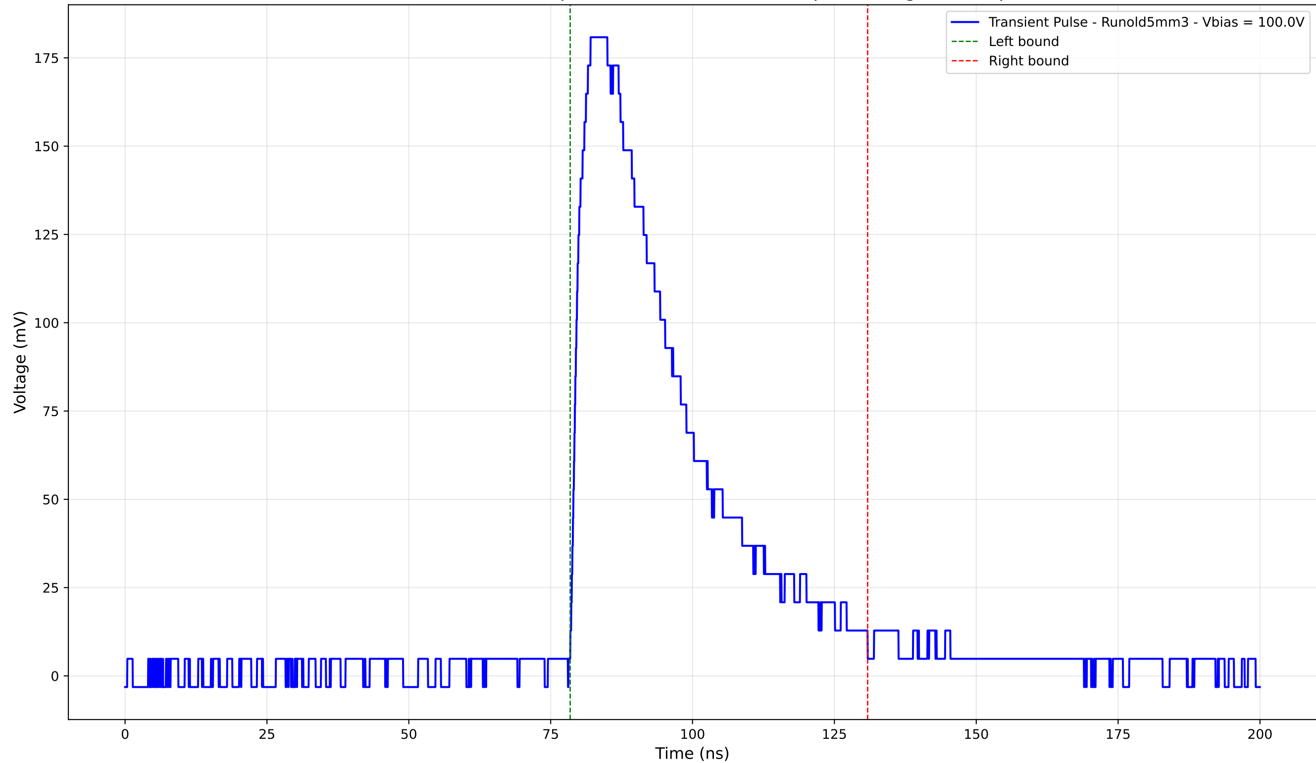
Transient Pulse - Sample: old5 - Position: 2125.0 \mu\text{m} - Charge: 74.64 pC
