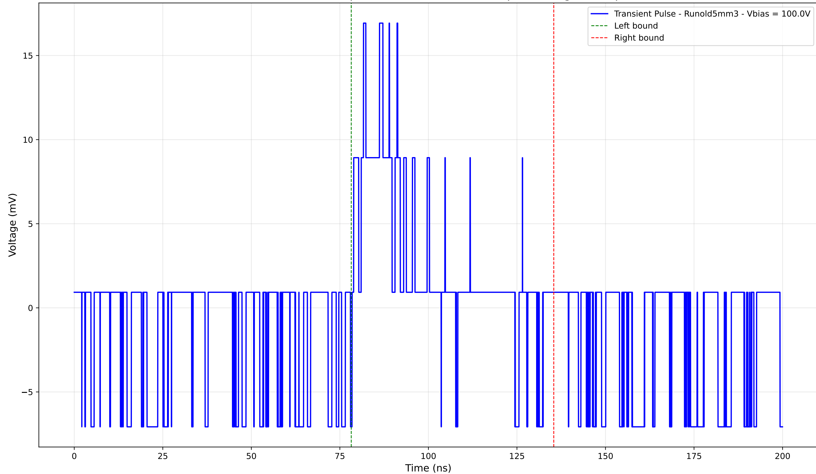
Transient Pulse - Sample: old5 - Position: 2670.0 \mu\text{m} - Charge: 3.08 pC
