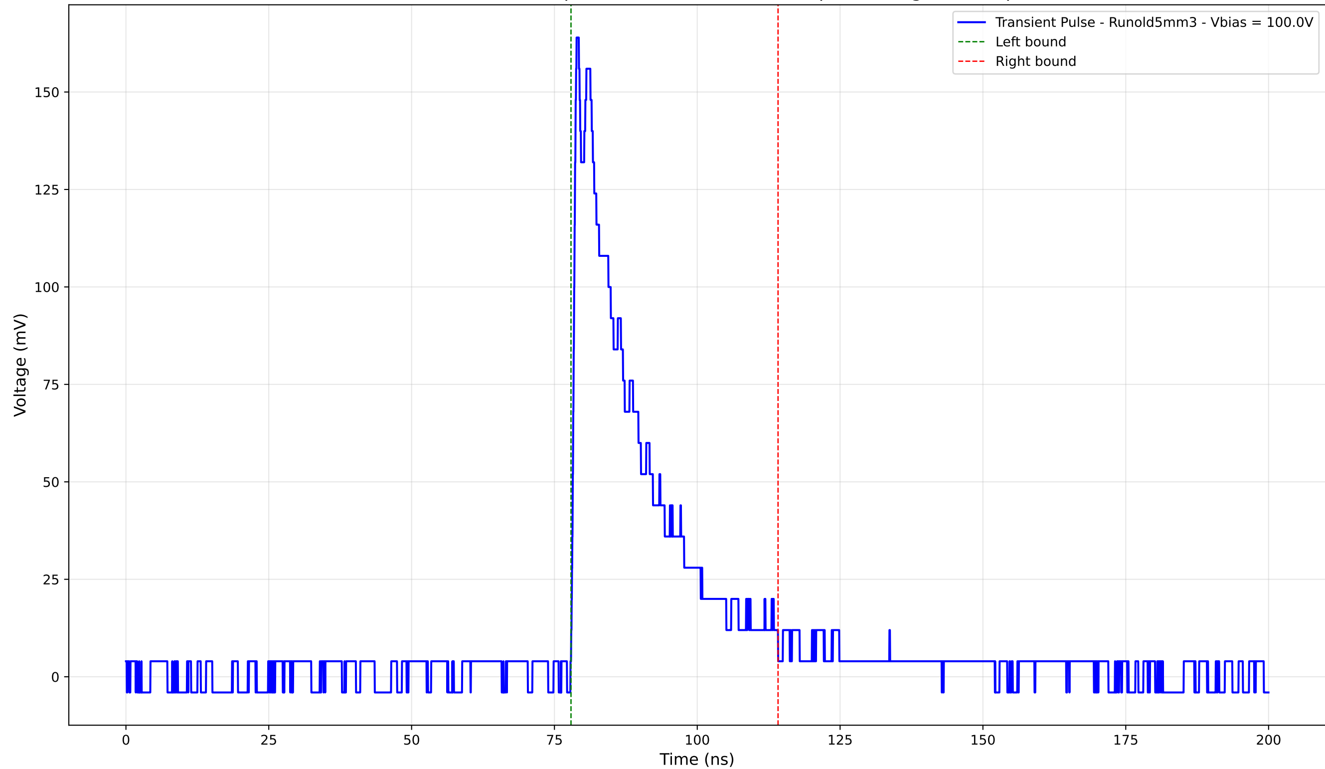
Transient Pulse - Sample: old5 - Position: 3220.0 \mu\text{m} - Charge: 37.73 pC
