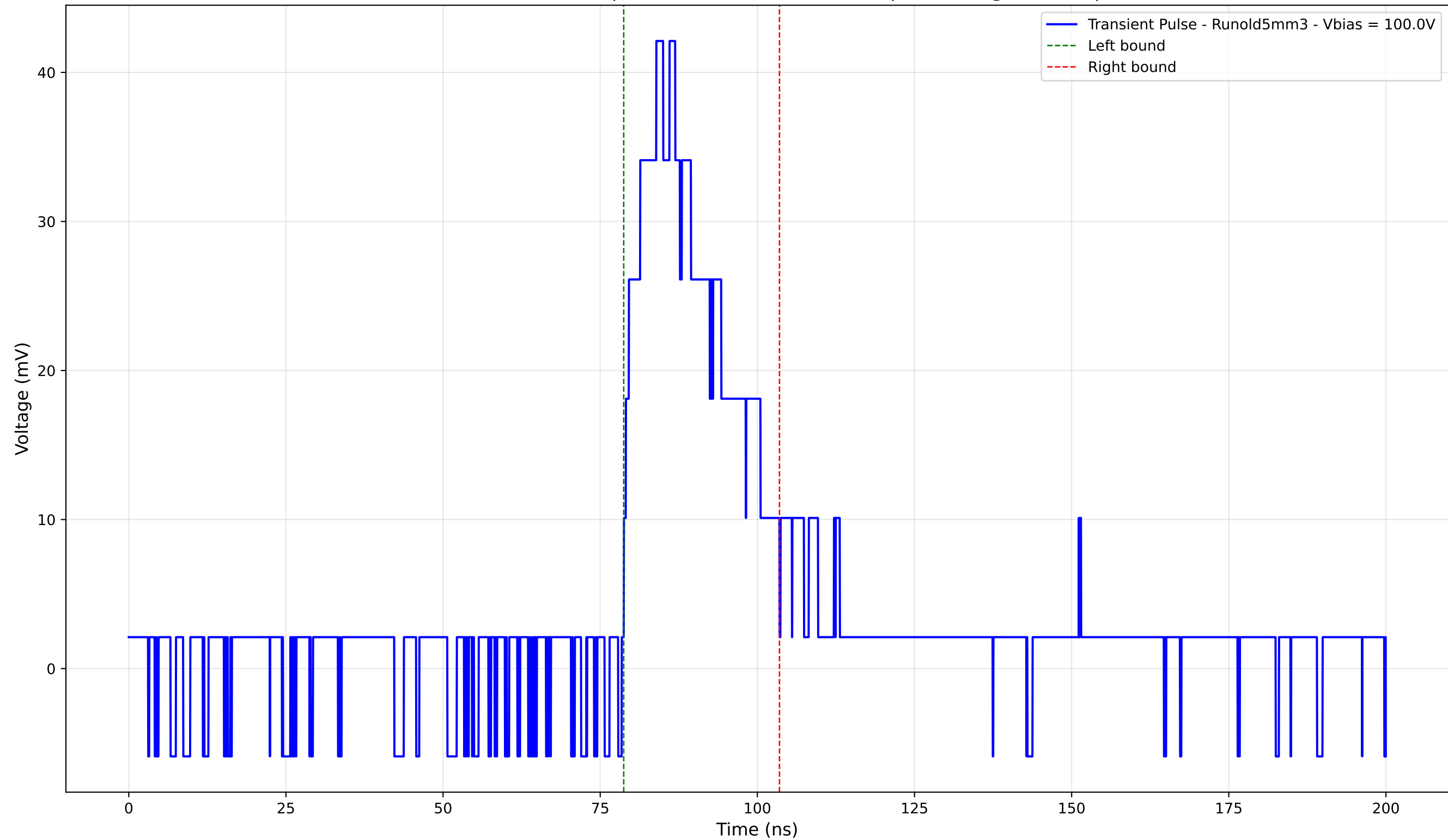
Transient Pulse - Sample: old5 - Position: 1980.0 \mu\text{m} - Charge: 12.31 pC
