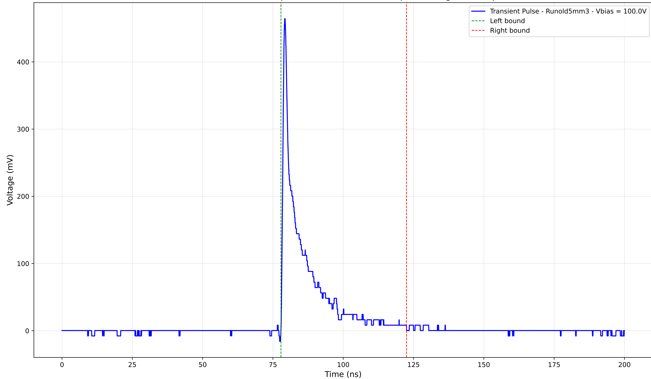
Transient Pulse - Sample: old5 - Position: 195.0 \mu\text{m} - Charge: 57.35 pC
