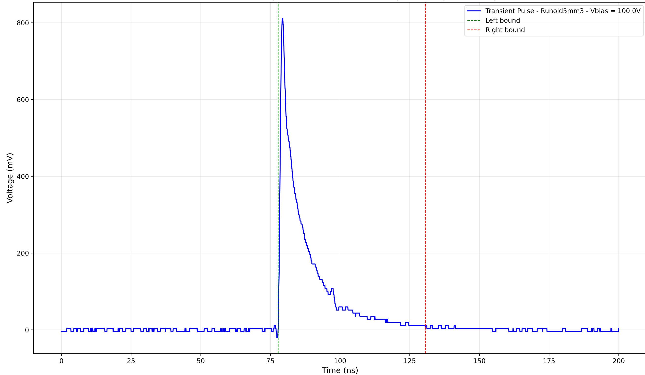
Transient Pulse - Sample: old5 - Position: 4790.0 \mu\text{m} - Charge: 132.38 pC
