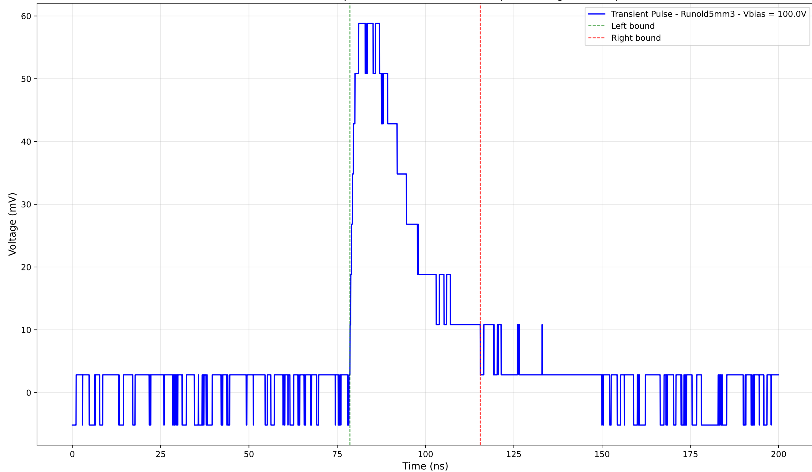
Transient Pulse - Sample: old5 - Position: 1360.0 \mu\text{m} - Charge: 21.86 pC
