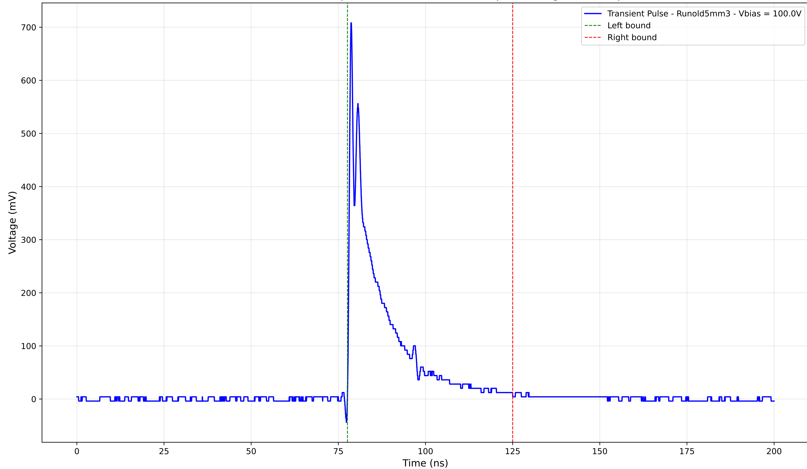
Transient Pulse - Sample: old5 - Position: 3460.0 \mu\text{m} - Charge: 106.81 pC
