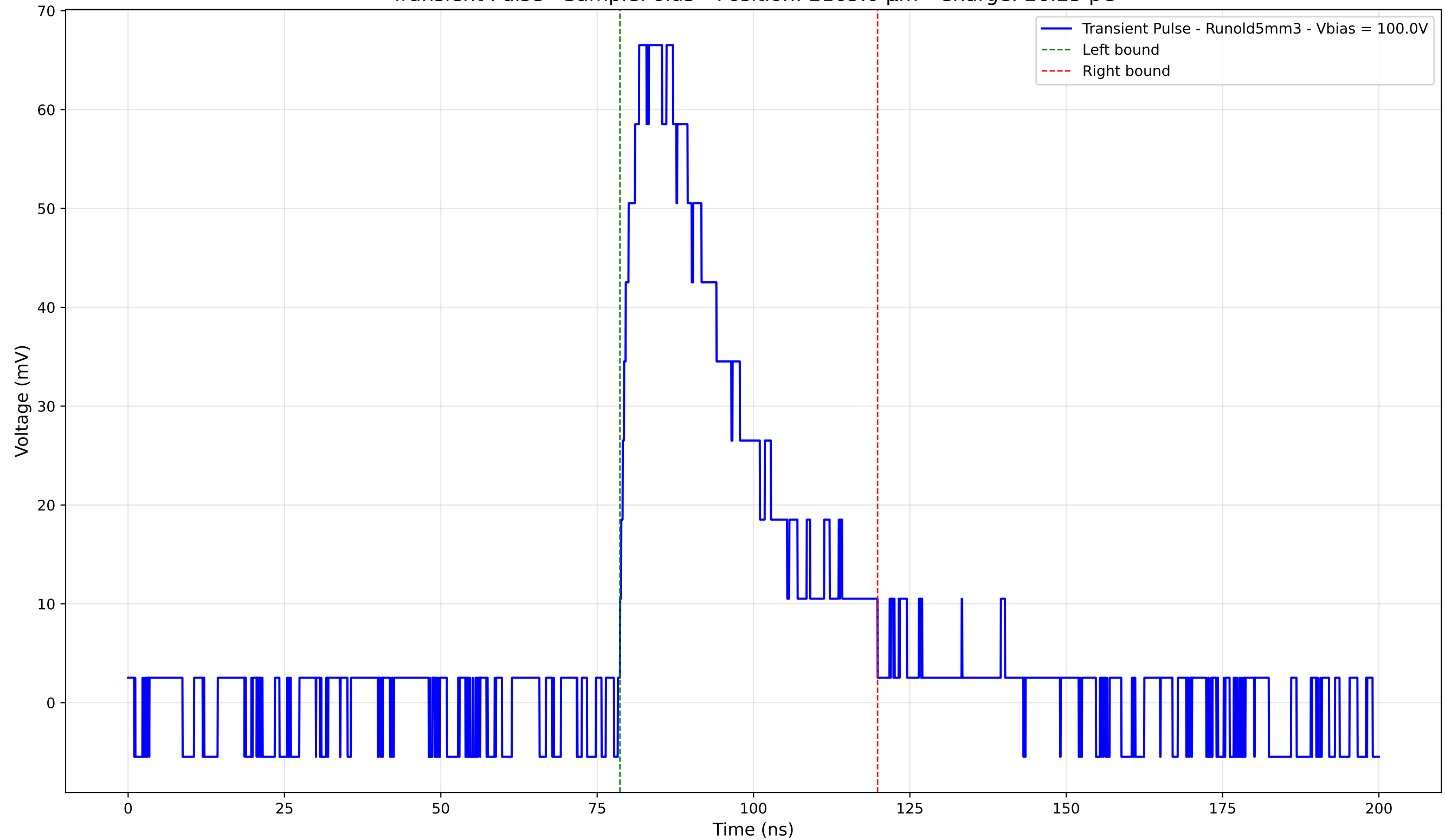
Transient Pulse - Sample: old5 - Position: 2165.0 \mu\text{m} - Charge: 26.25 pC
