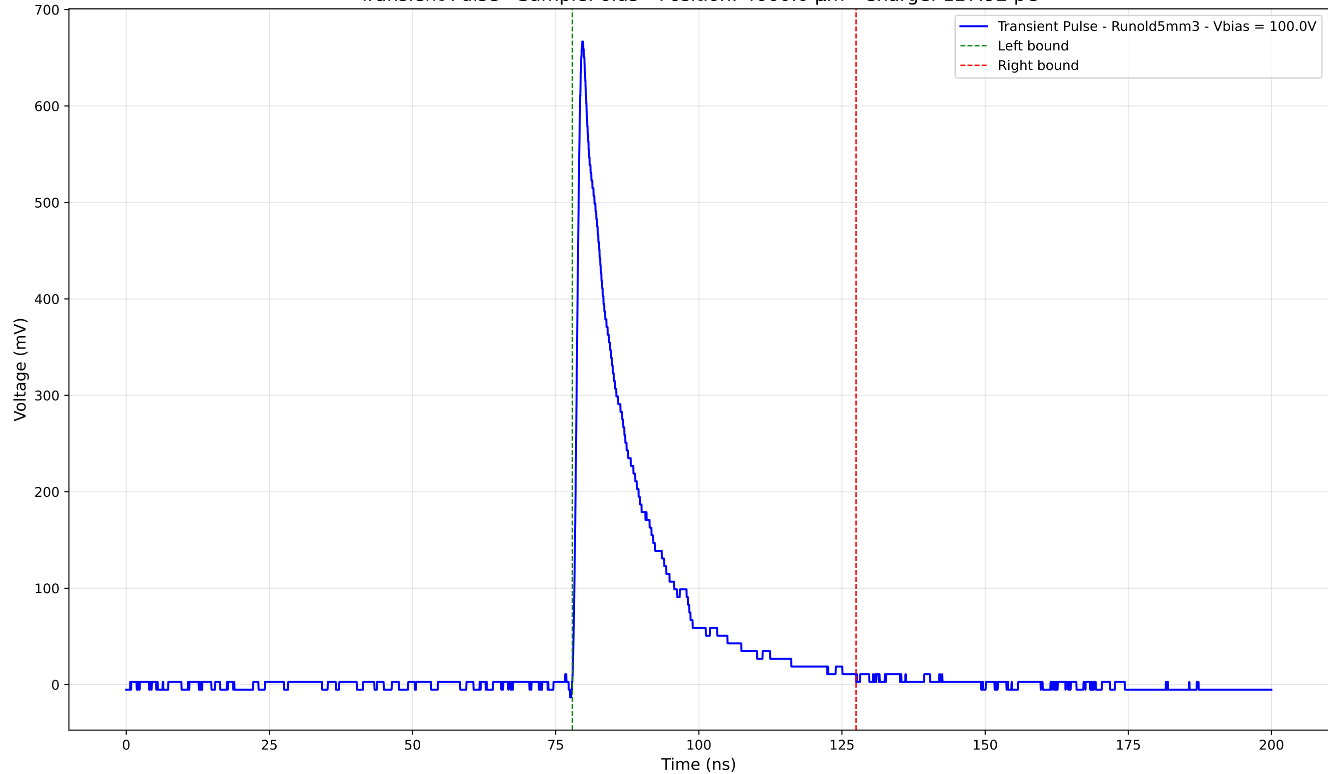
Transient Pulse - Sample: old5 - Position: 4660.0 \mu\text{m} - Charge: 127.92 pC
