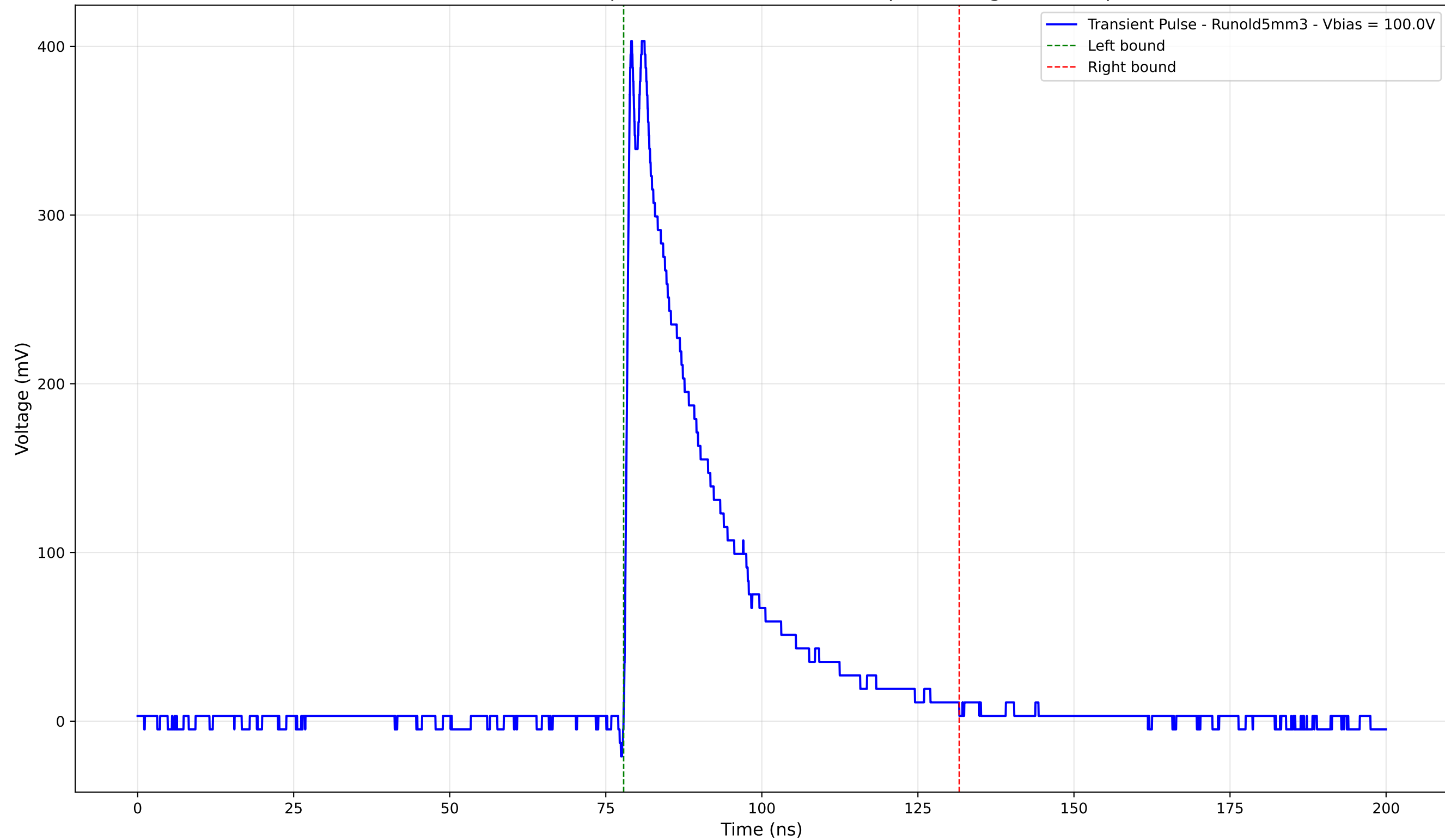
Transient Pulse - Sample: old5 - Position: 3150.0 \mu\text{m} - Charge: 106.30 pC
