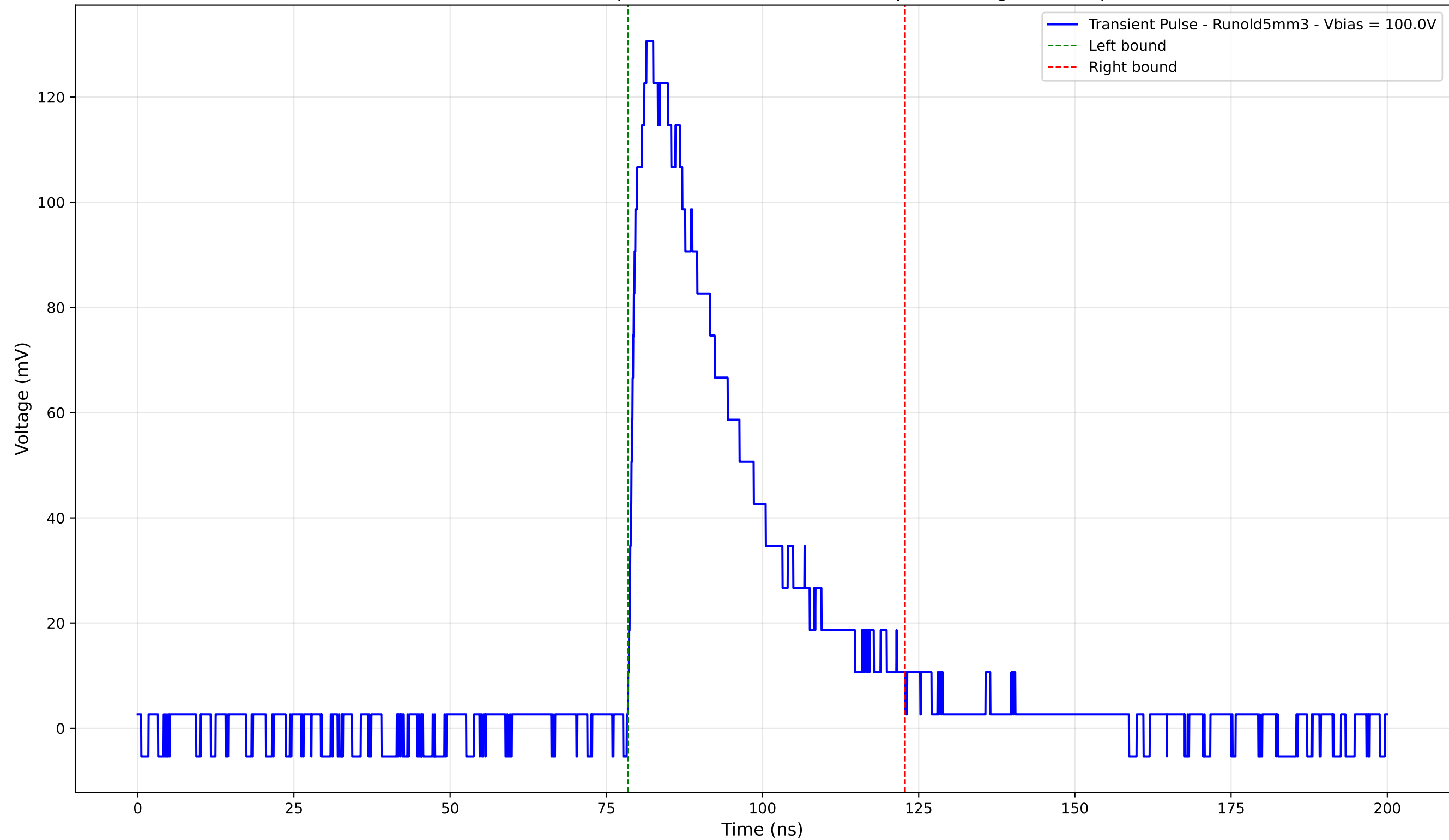
Transient Pulse - Sample: old5 - Position: 2605.0 \mu\text{m} - Charge: 45.99 pC
