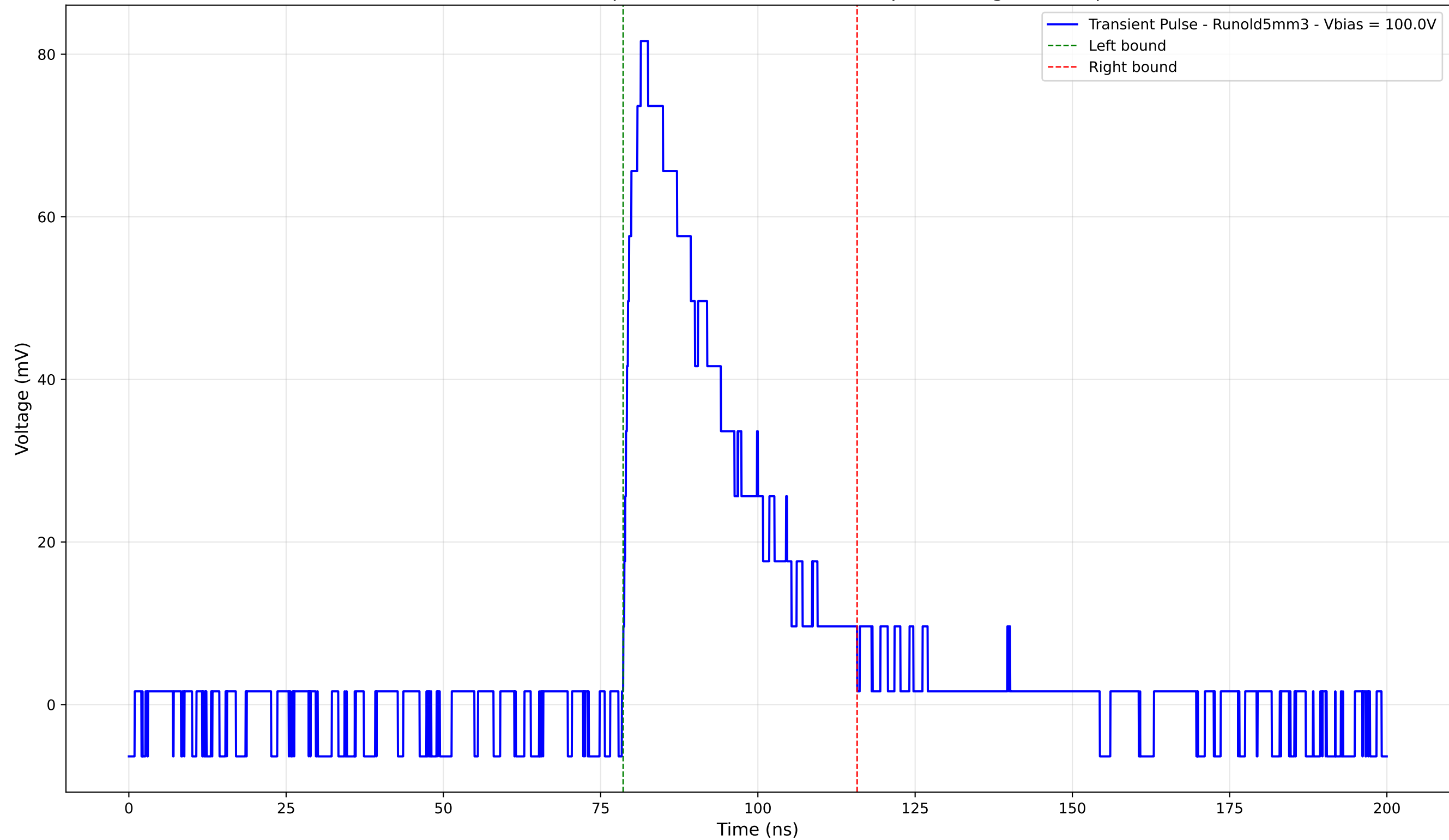
Transient Pulse - Sample: old5 - Position: 2620.0 \mu\text{m} - Charge: 26.14 pC
