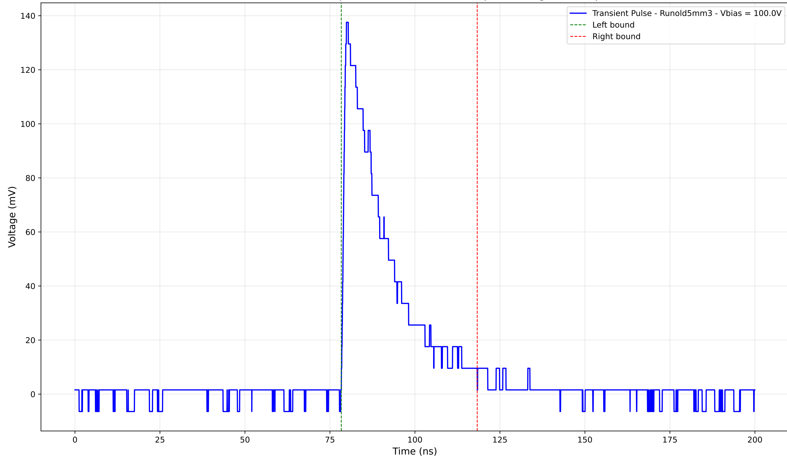
Transient Pulse - Sample: old5 - Position: 795.0 \mu\text{m} - Charge: 36.61 pC
