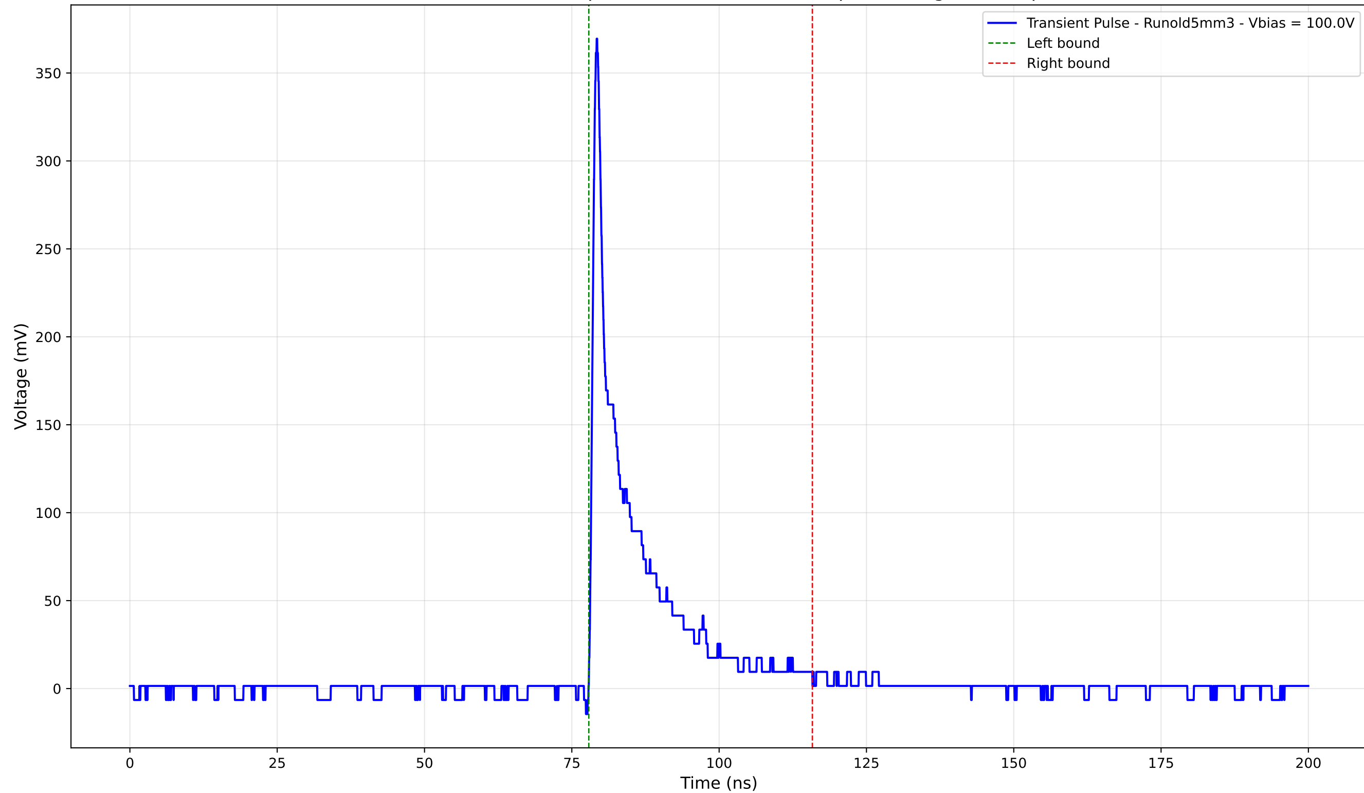
Transient Pulse - Sample: old5 - Position: 180.0 \mu\text{m} - Charge: 43.46 pC
