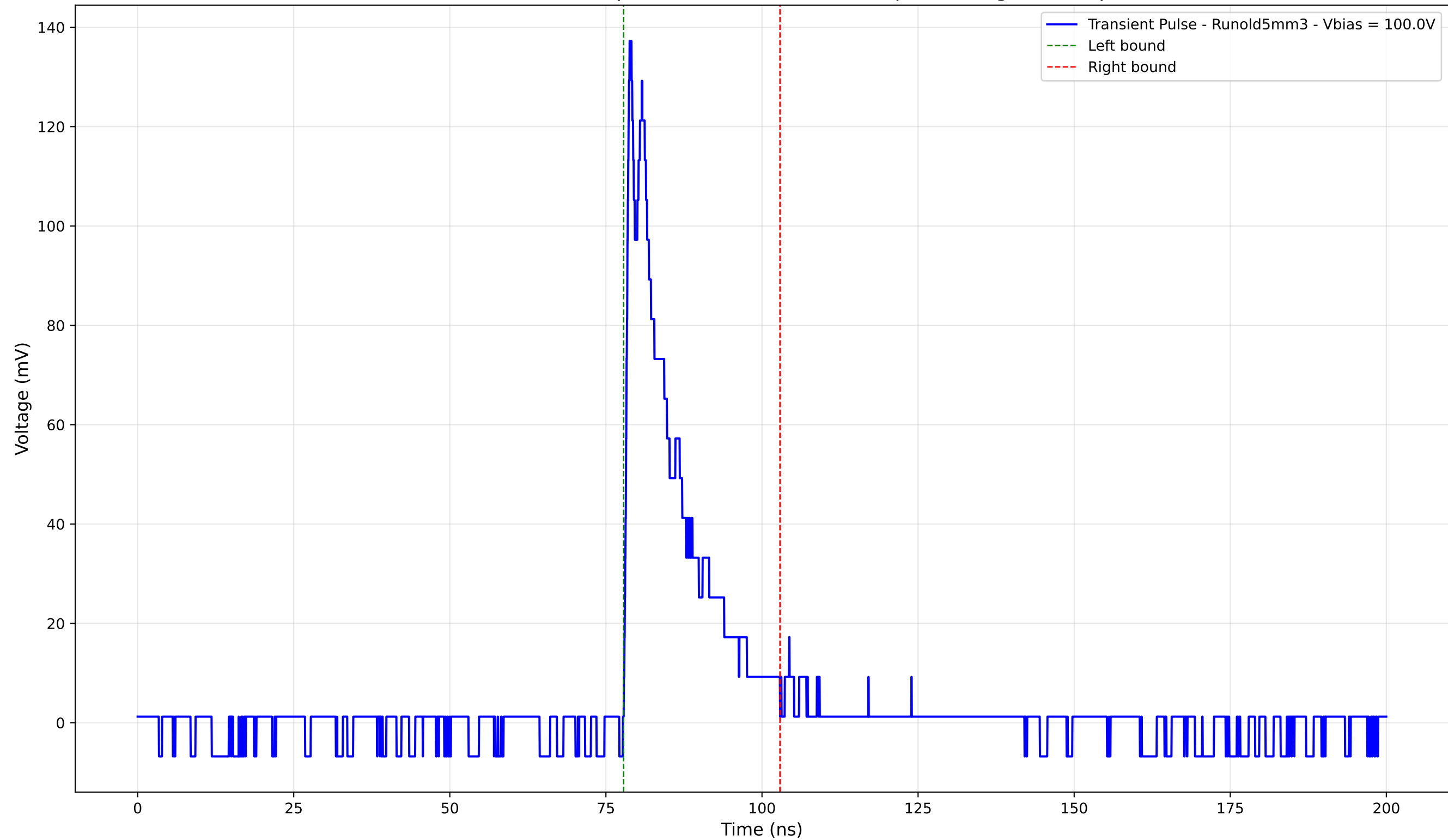
Transient Pulse - Sample: old5 - Position: 3840.0 \mu\text{m} - Charge: 21.67 pC
