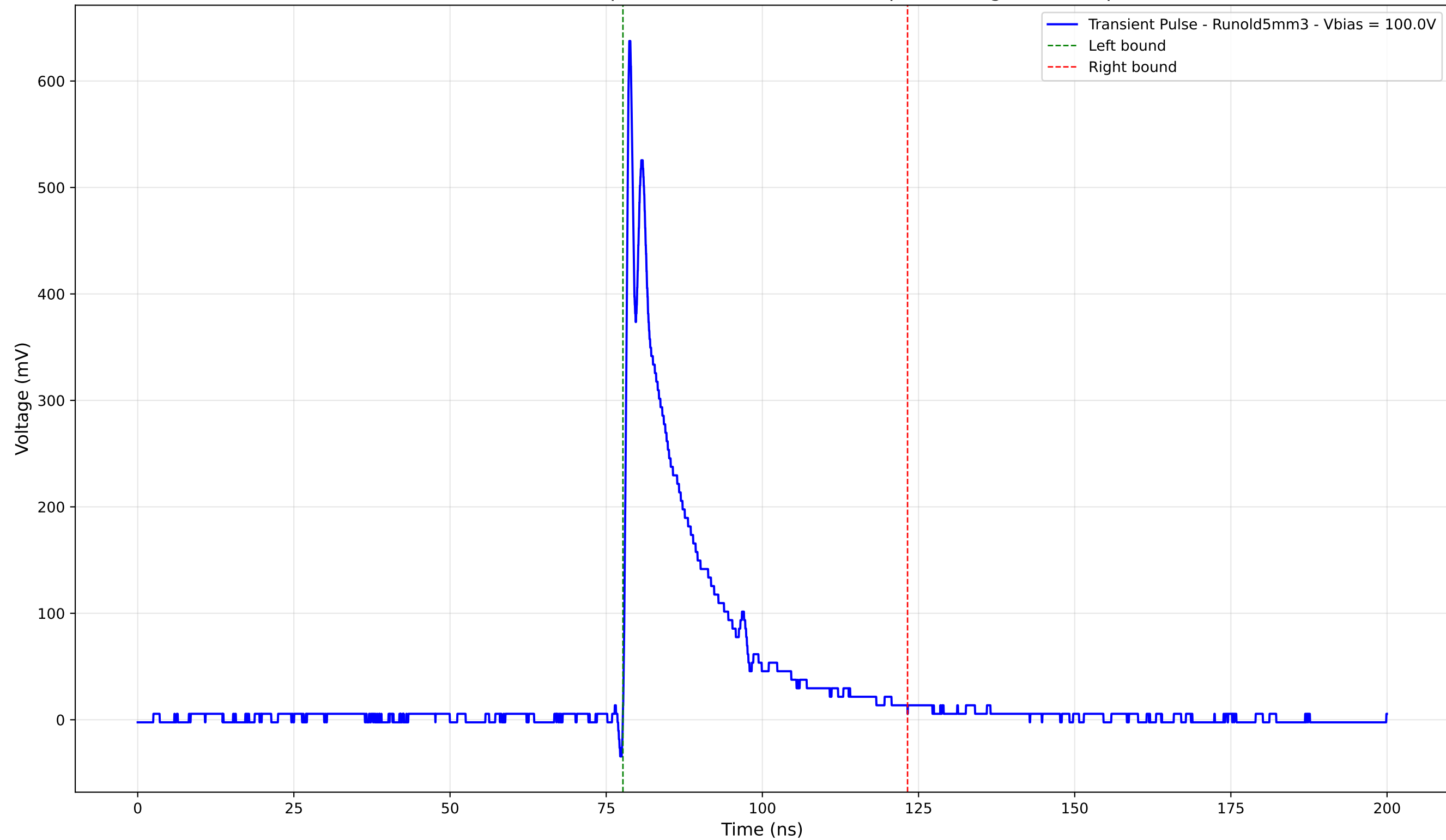
Transient Pulse - Sample: old5 - Position: 3410.0 \mu\text{m} - Charge: 108.14 pC
