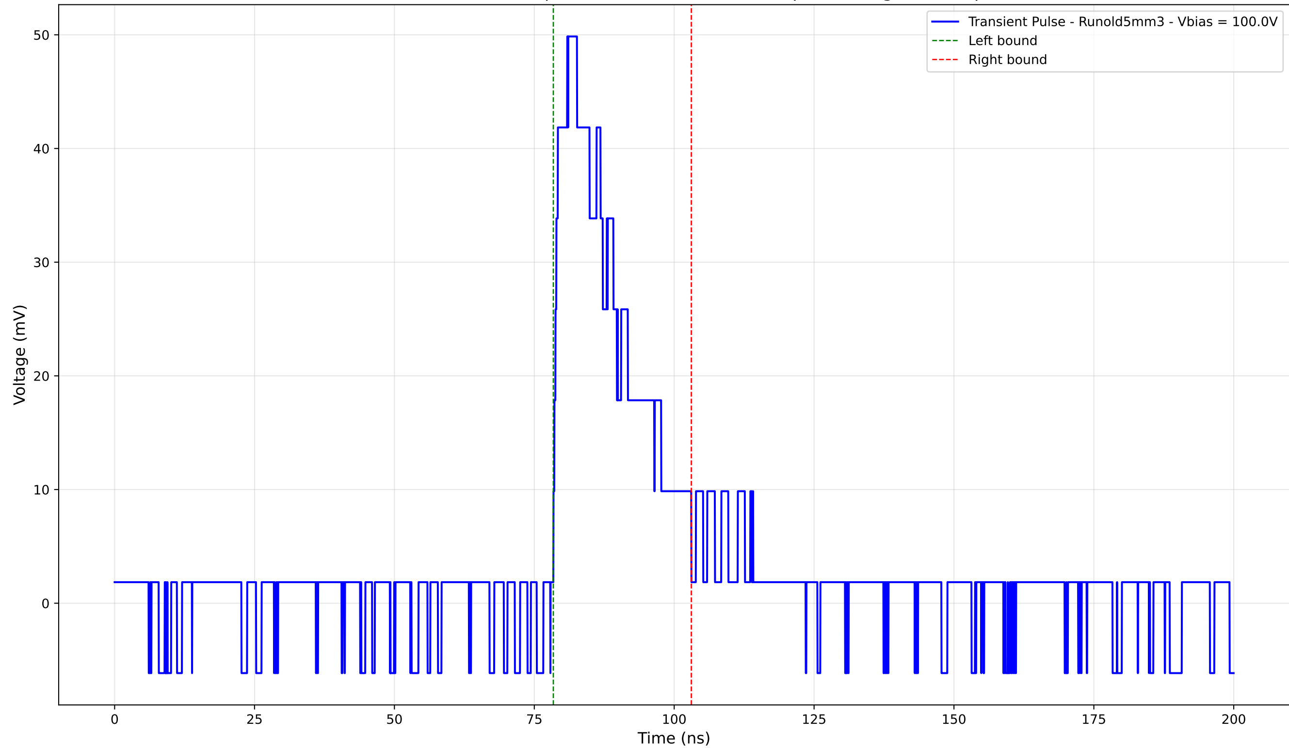
Transient Pulse - Sample: old5 - Position: 2940.0 \mu\text{m} - Charge: 12.67 pC
