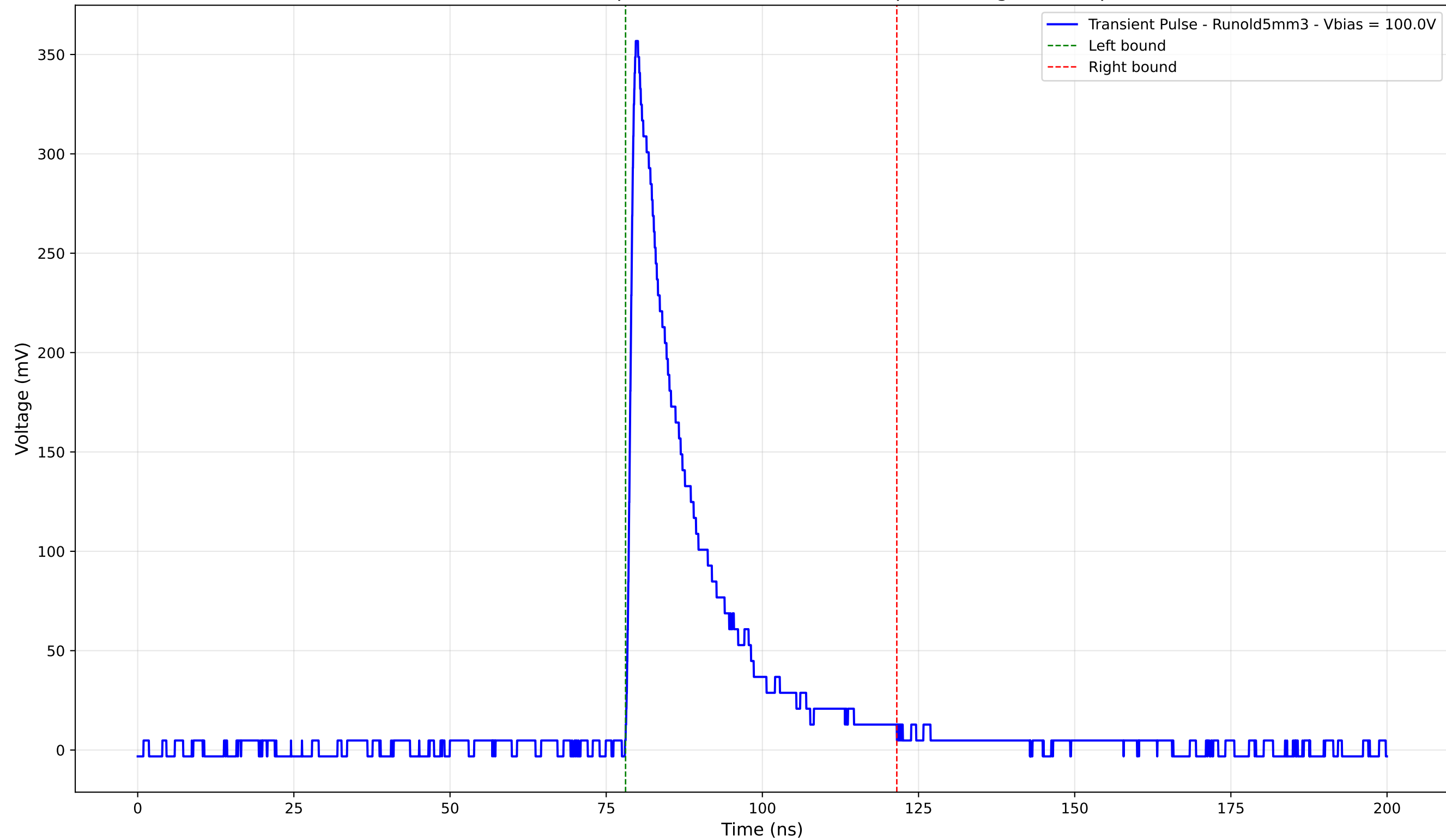
Transient Pulse - Sample: old5 - Position: 4565.0 \mu\text{m} - Charge: 71.58 pC
