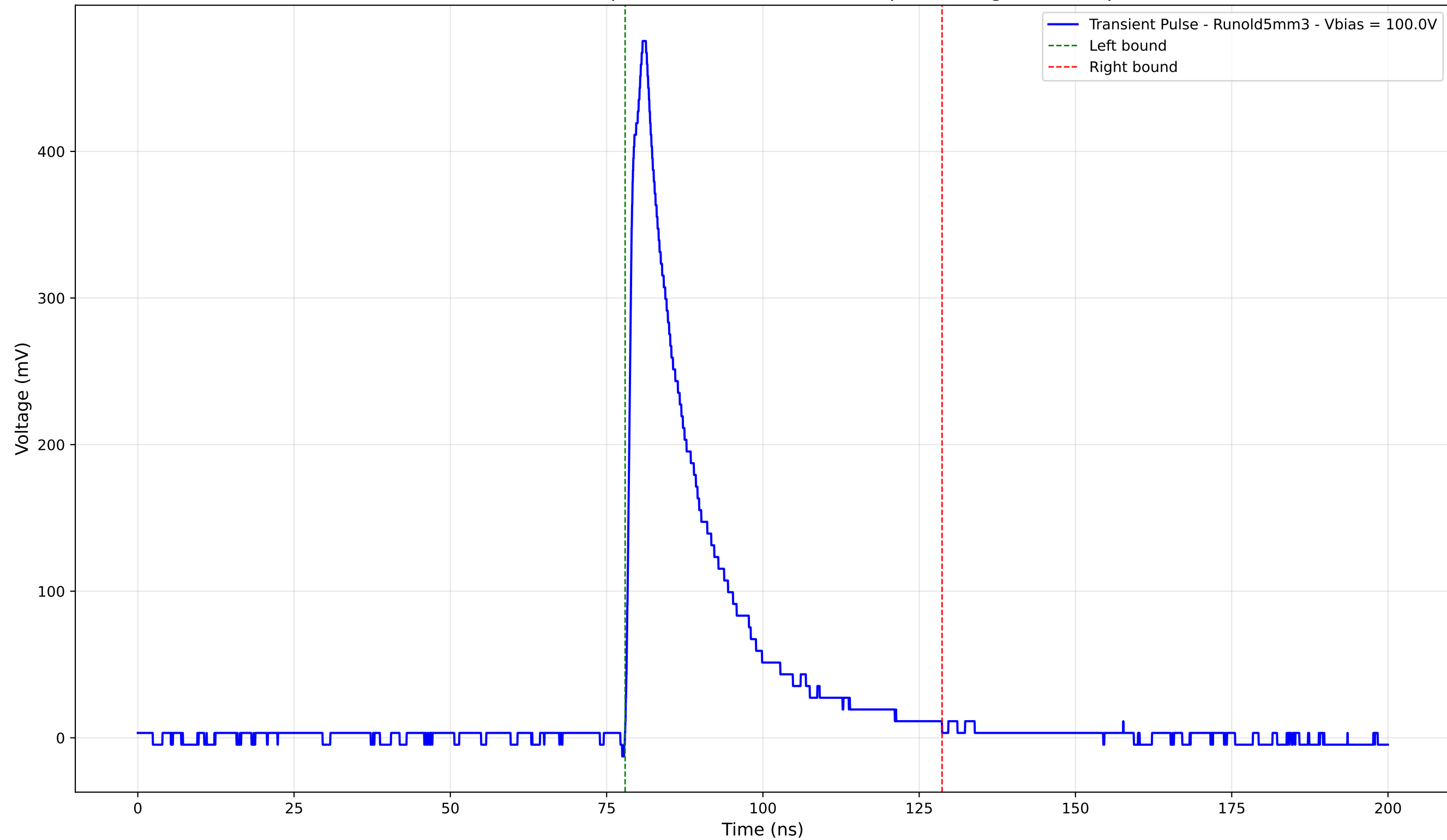
Transient Pulse - Sample: old5 - Position: 4075.0 \mu\text{m} - Charge: 105.91 pC
