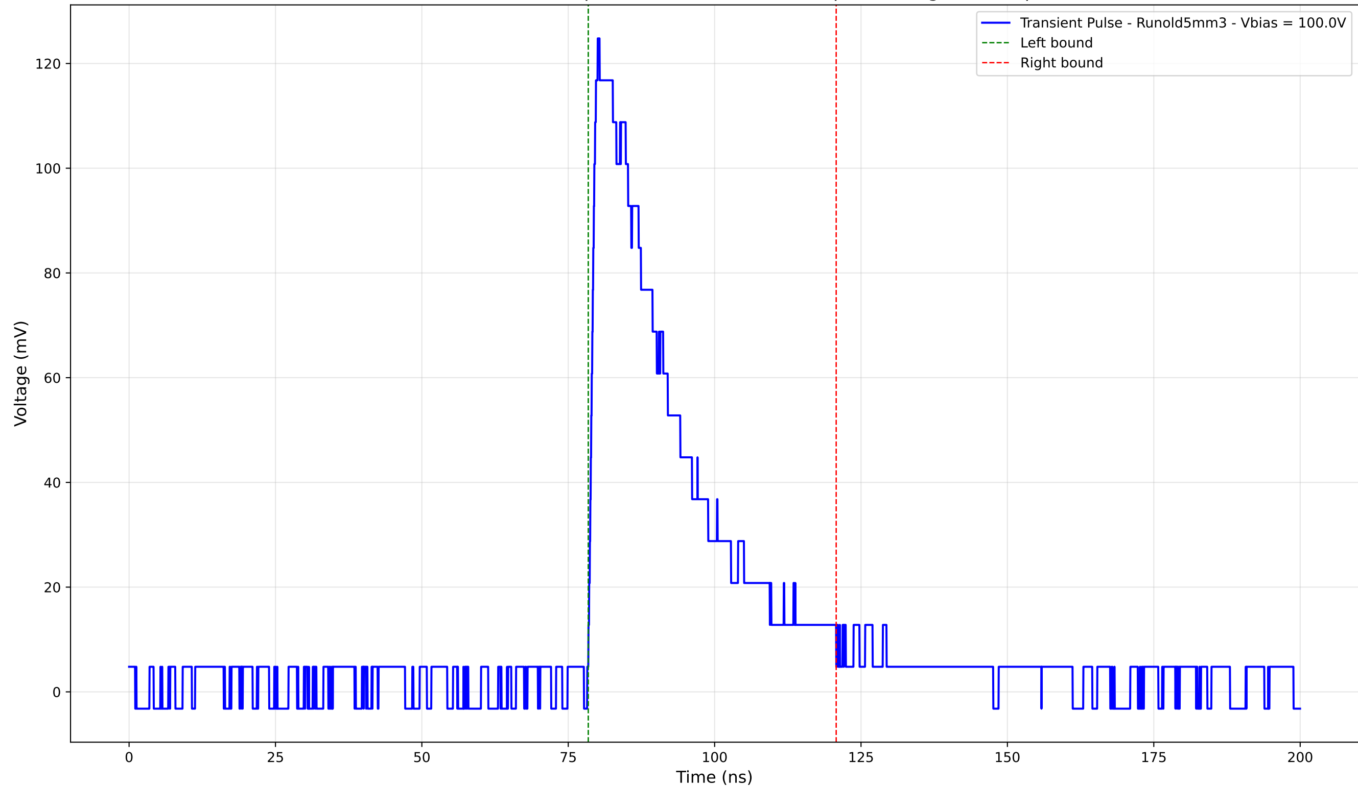
Transient Pulse - Sample: old5 - Position: 900.0 \mu\text{m} - Charge: 38.57 pC
