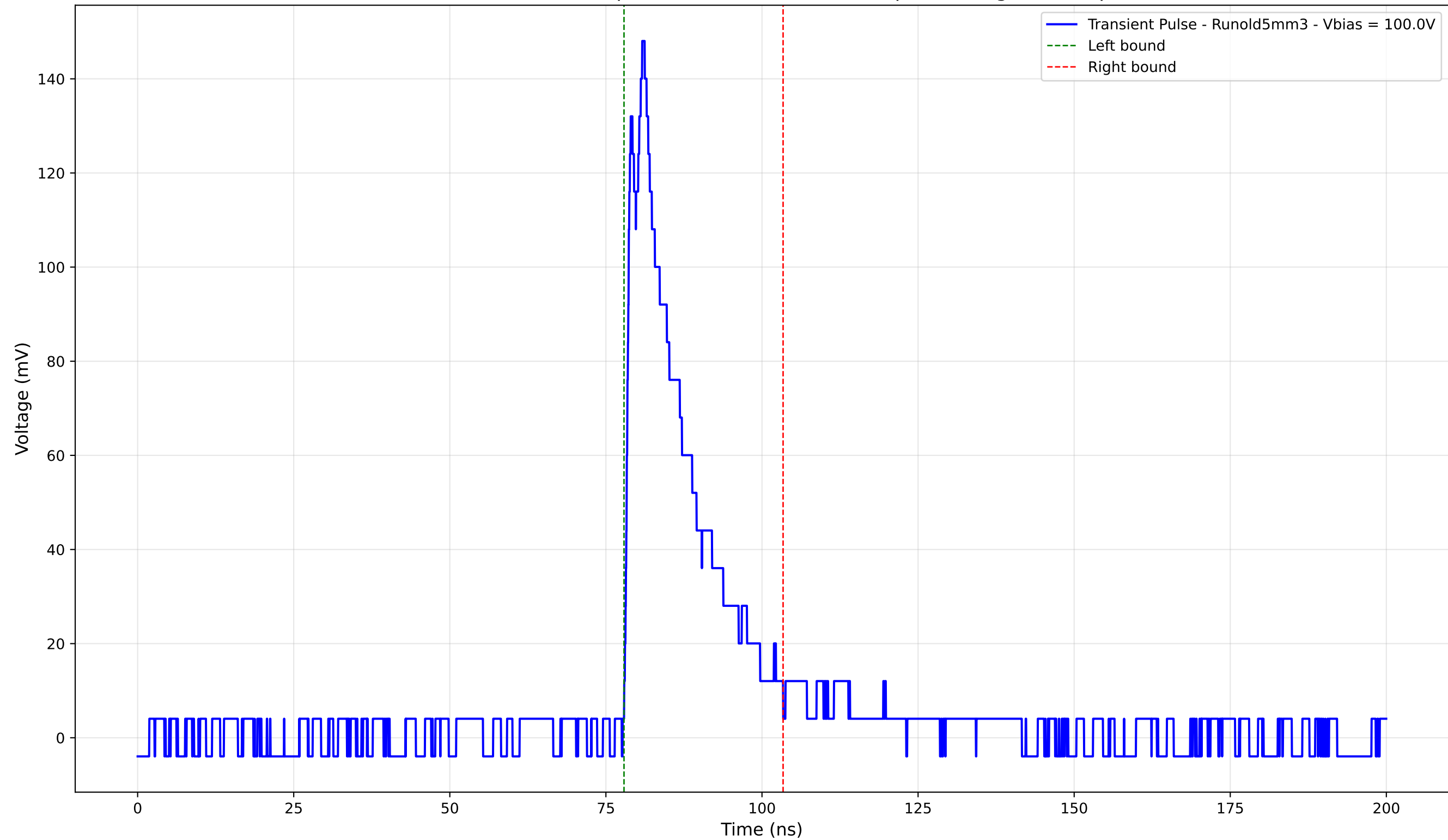
Transient Pulse - Sample: old5 - Position: 3935.0 \mu\text{m} - Charge: 28.55 pC
