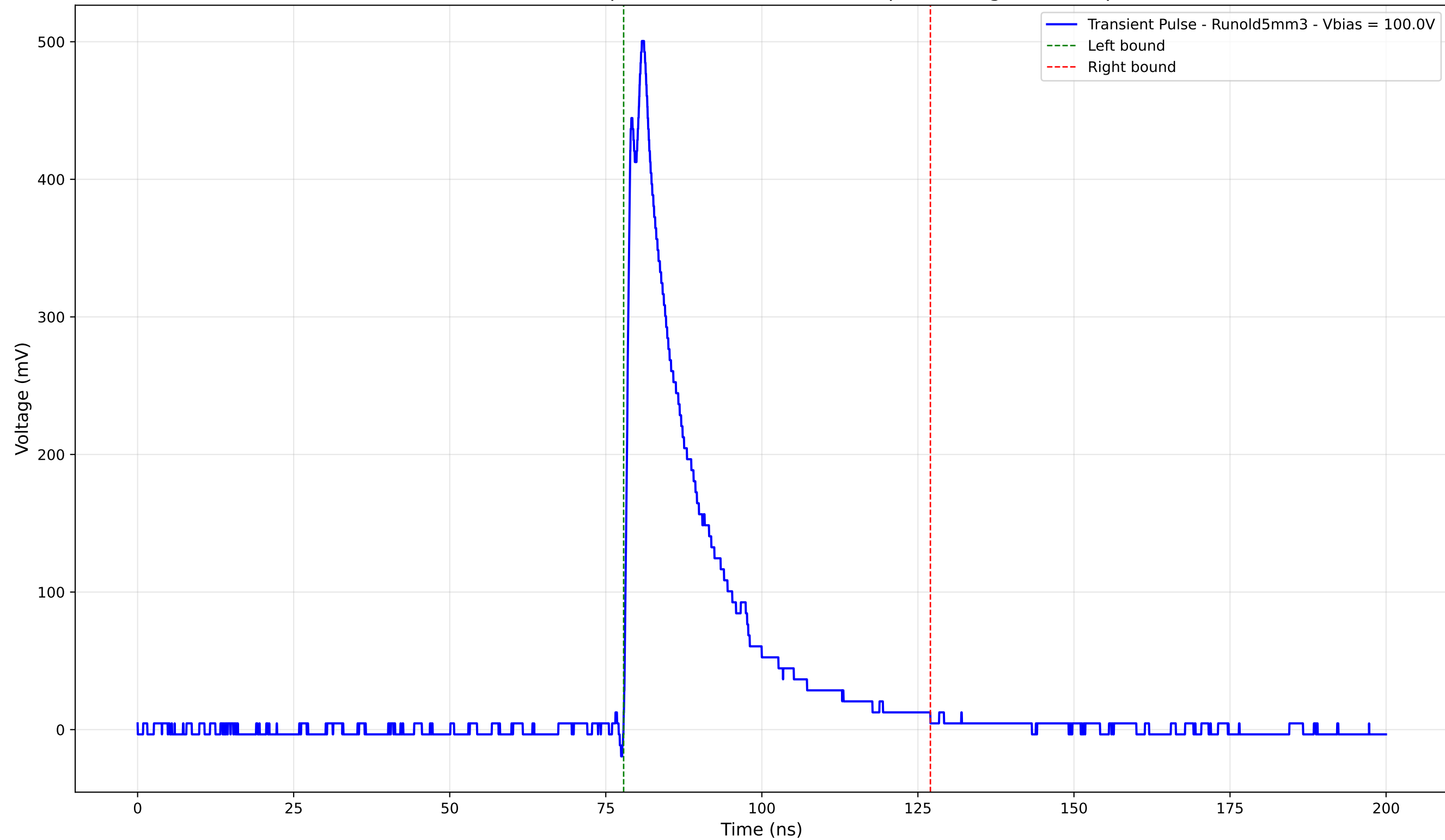
Transient Pulse - Sample: old5 - Position: 4000.0 \mu\text{m} - Charge: 109.55 pC
