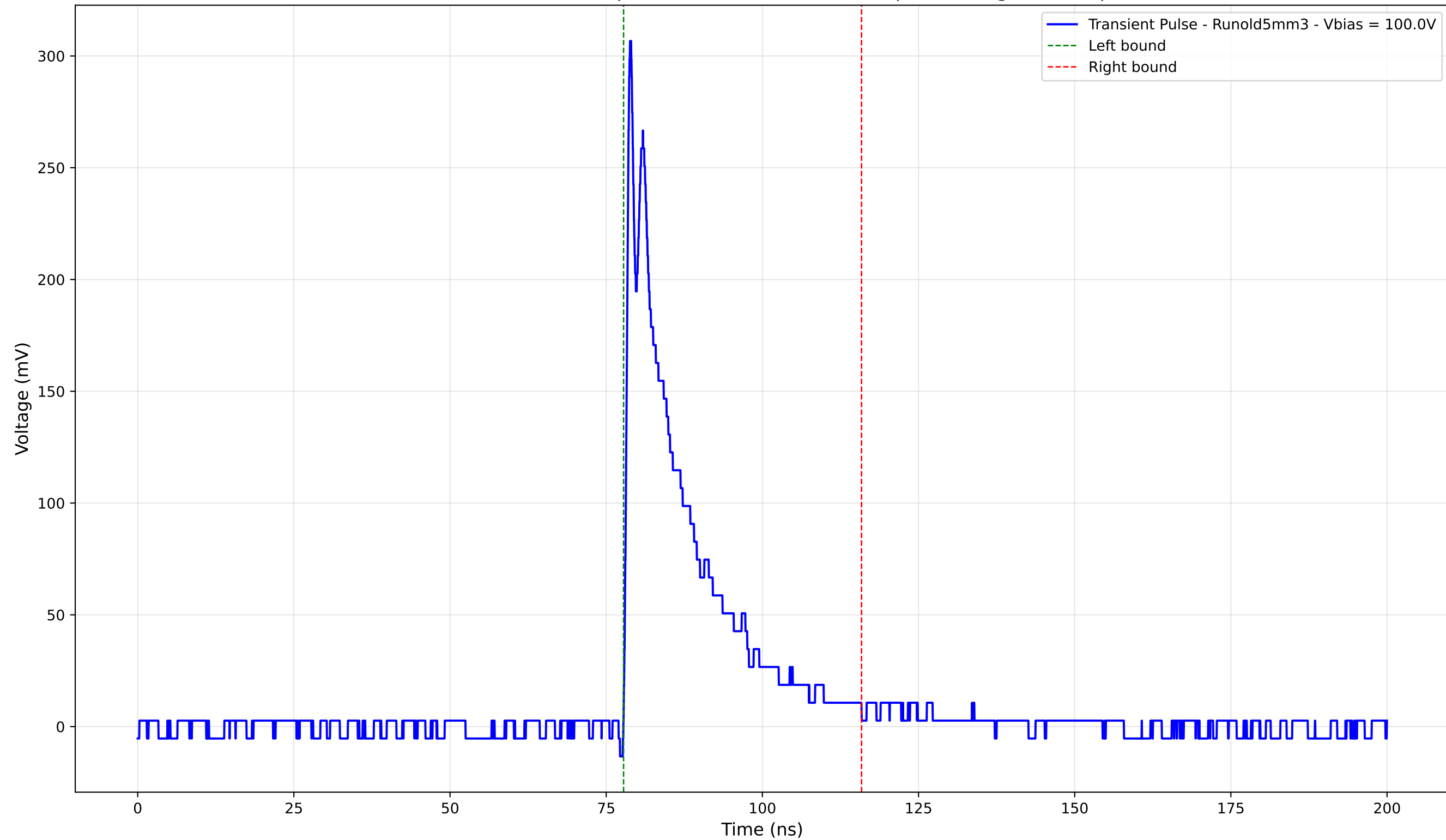
Transient Pulse - Sample: old5 - Position: 3350.0 \mu\text{m} - Charge: 53.33 pC
