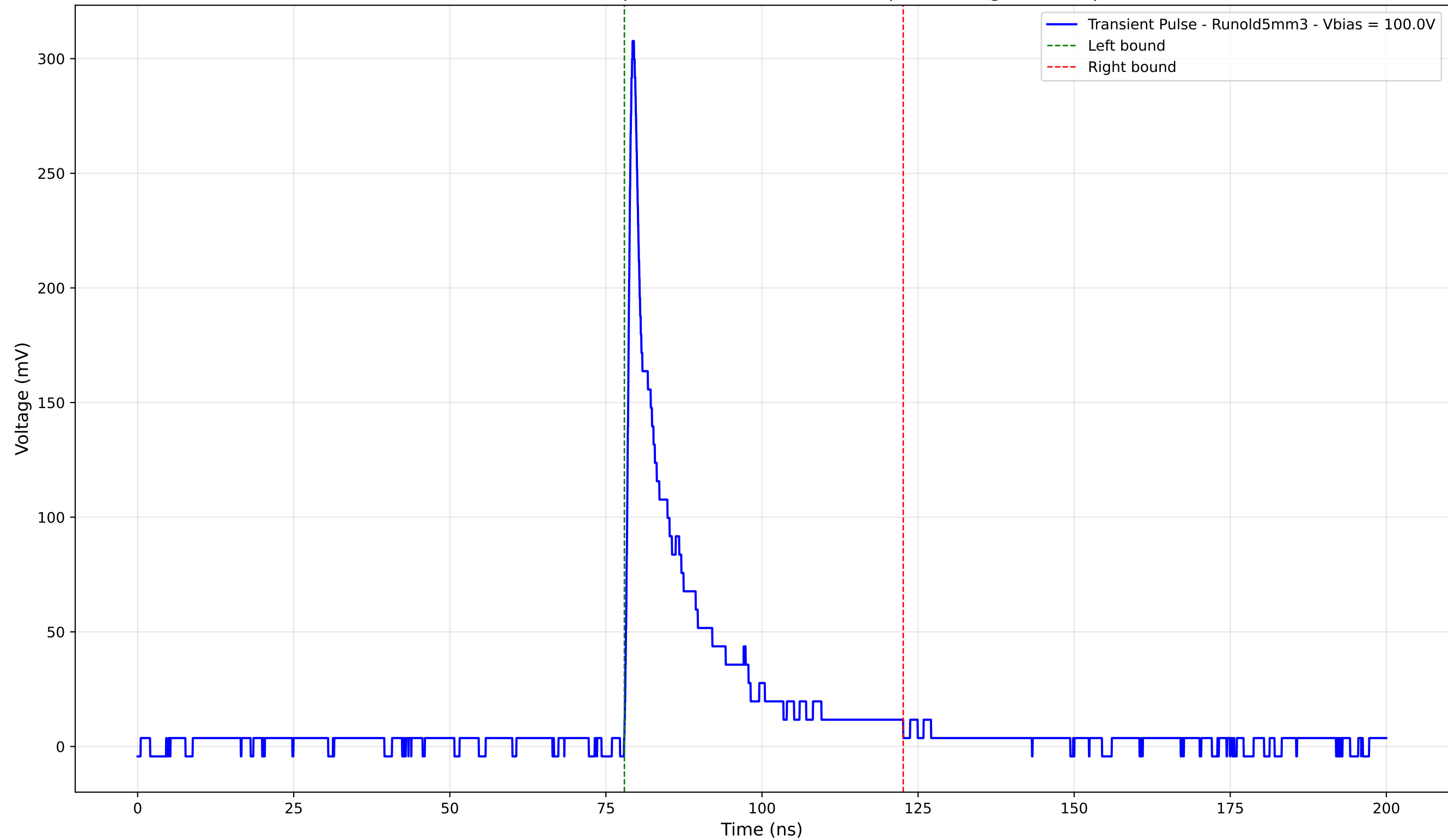
Transient Pulse - Sample: old5 - Position: 280.0 \mu\text{m} - Charge: 44.41 pC
