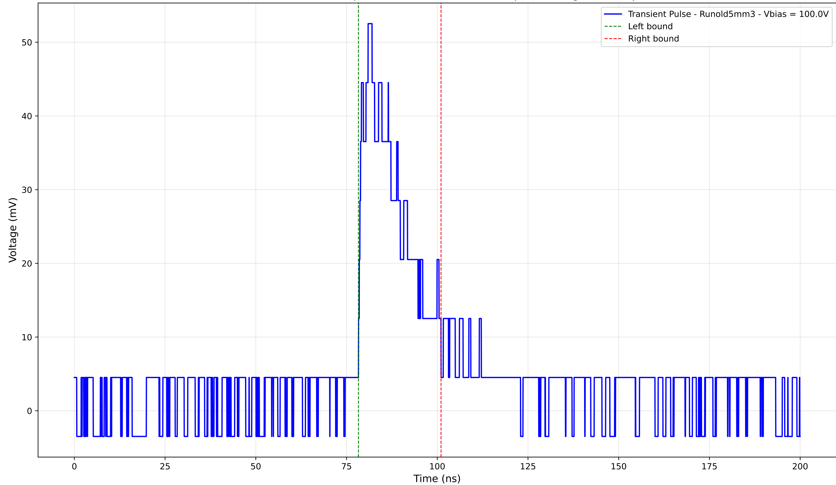
Transient Pulse - Sample: old5 - Position: 3010.0 \mu\text{m} - Charge: 12.67 pC
