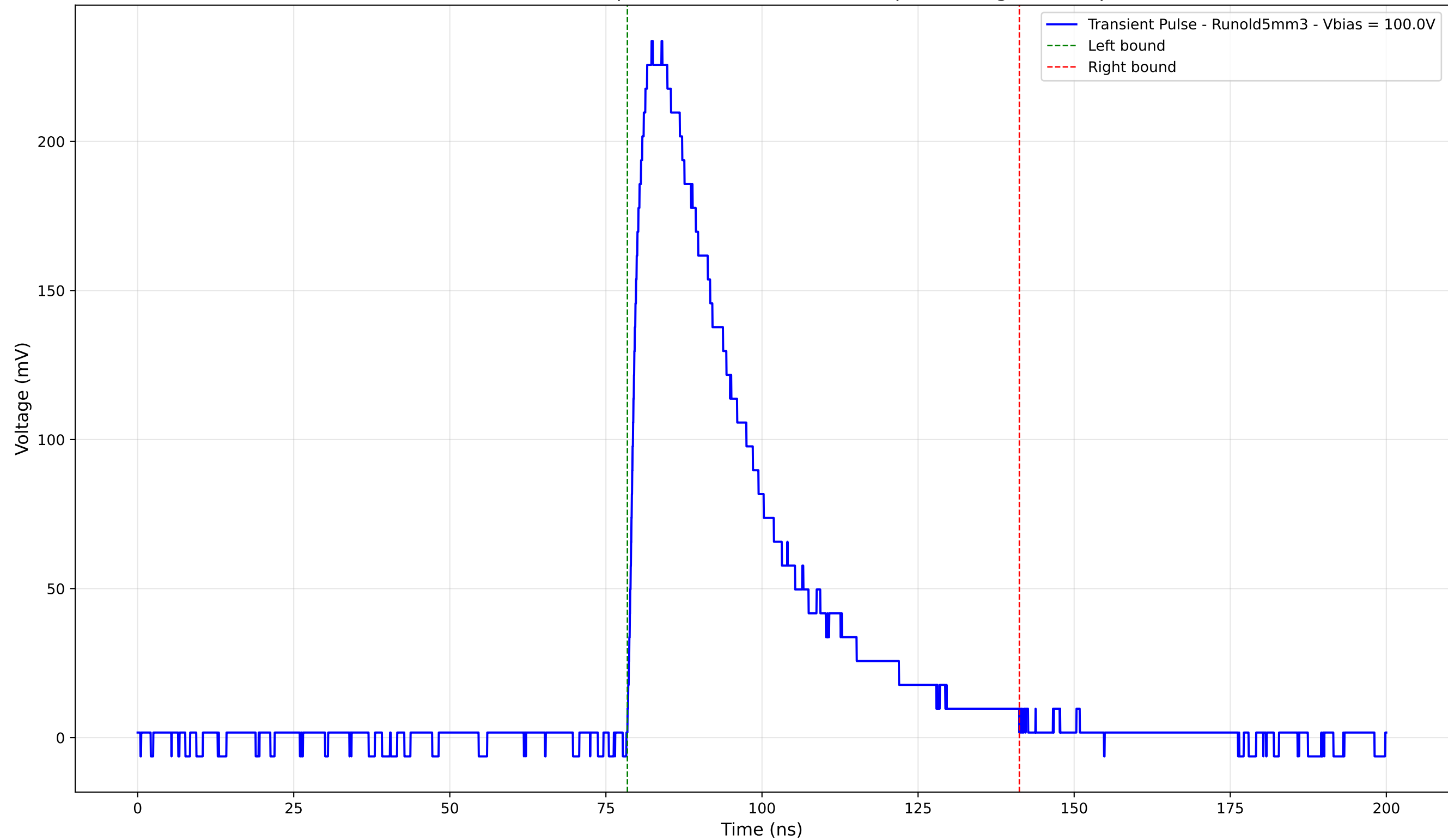
Transient Pulse - Sample: old5 - Position: 2310.0 \mu\text{m} - Charge: 91.53 pC
