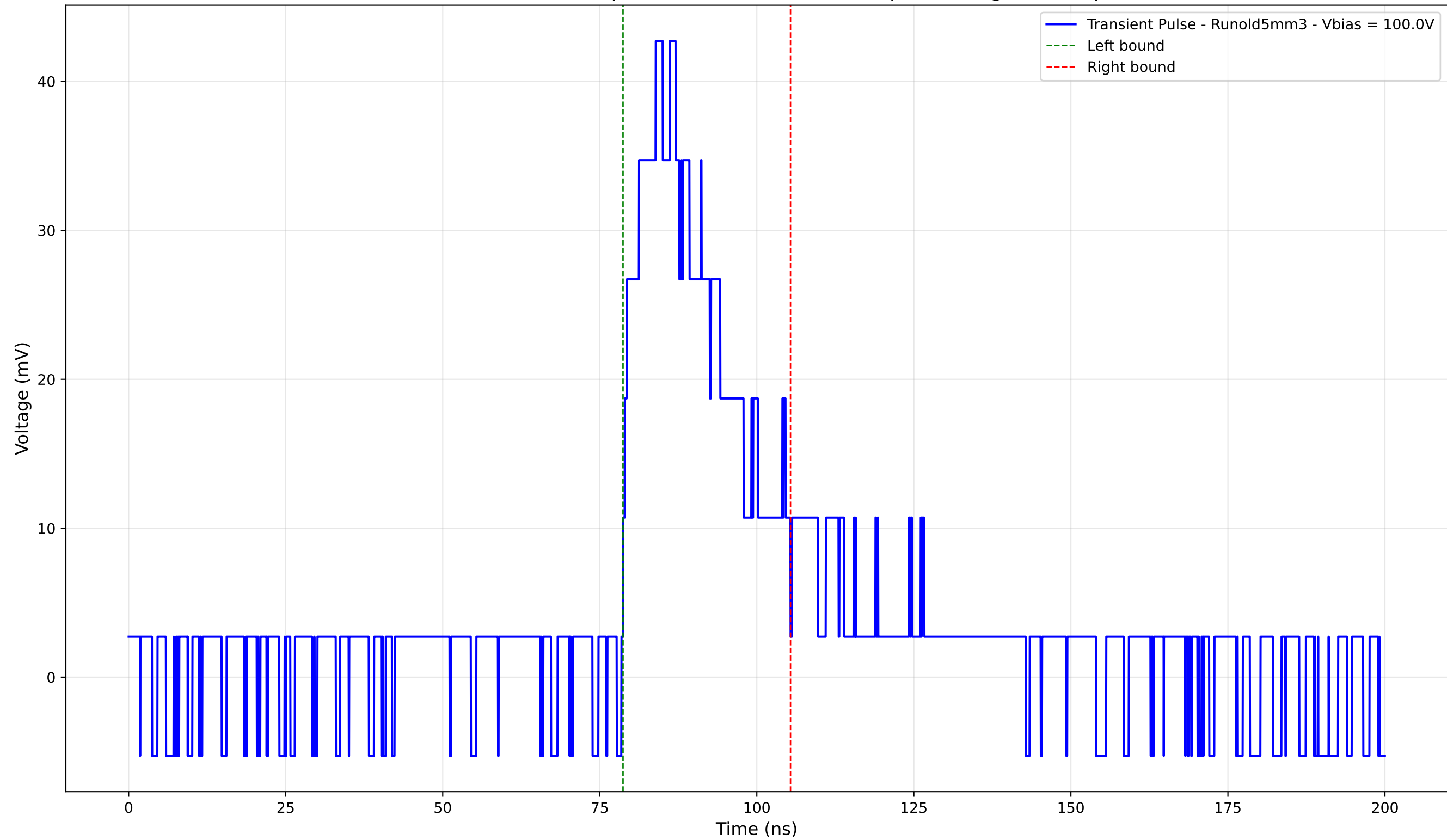
Transient Pulse - Sample: old5 - Position: 2390.0 \mu\text{m} - Charge: 12.85 pC
