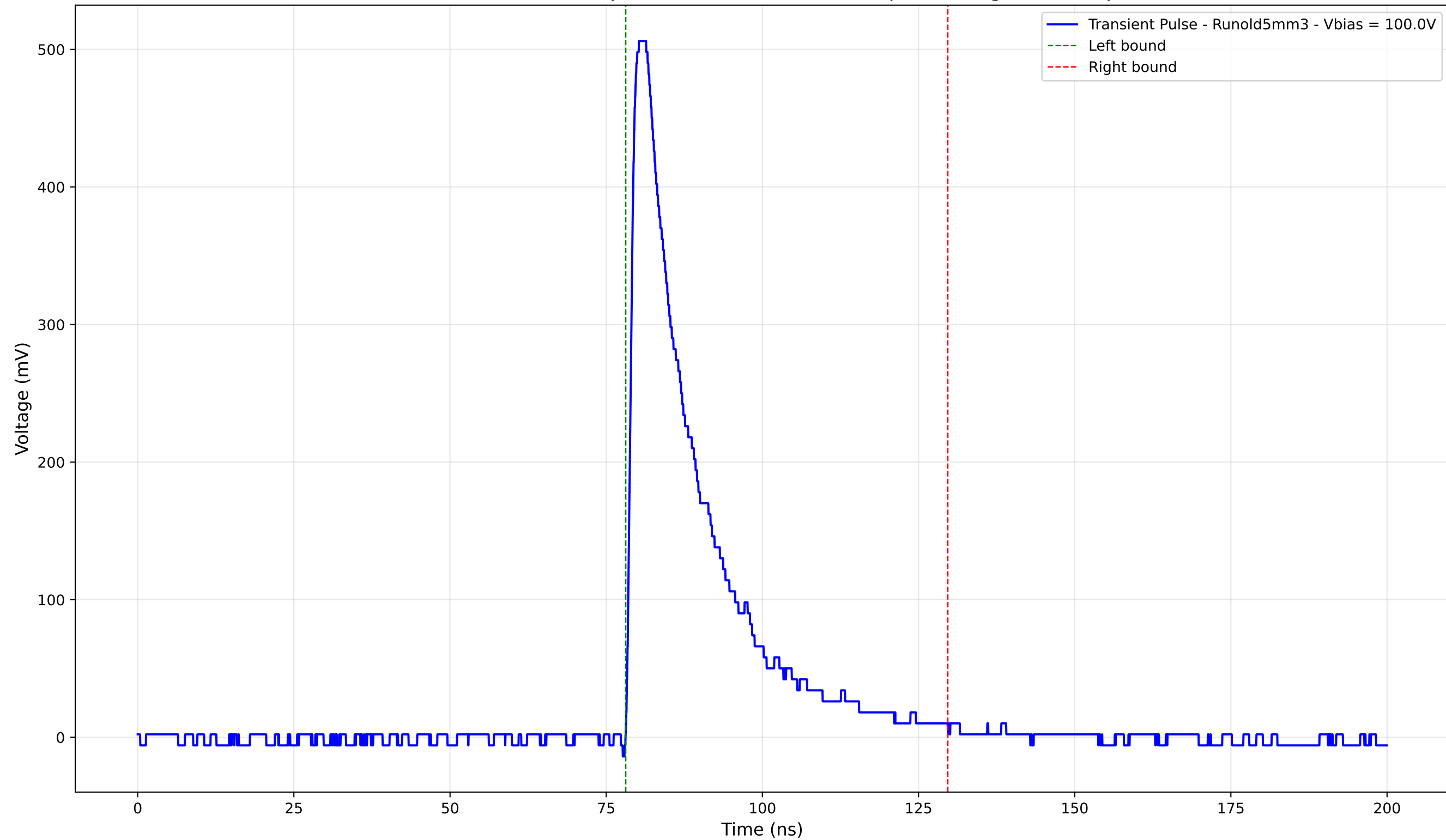
Transient Pulse - Sample: old5 - Position: 4315.0 \mu\text{m} - Charge: 116.54 pC
