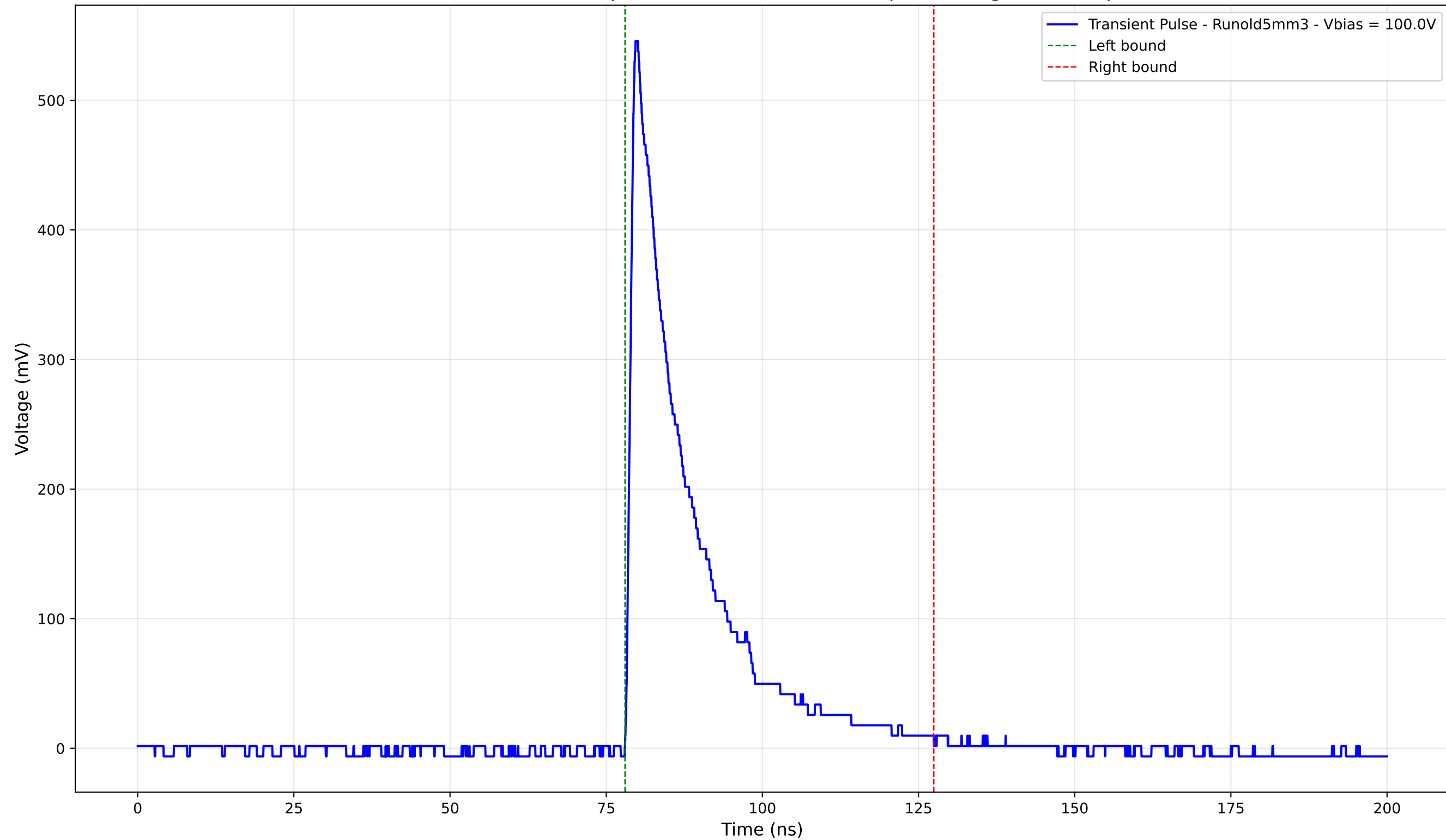
Transient Pulse - Sample: old5 - Position: 4595.0 \mu\text{m} - Charge: 108.29 pC
