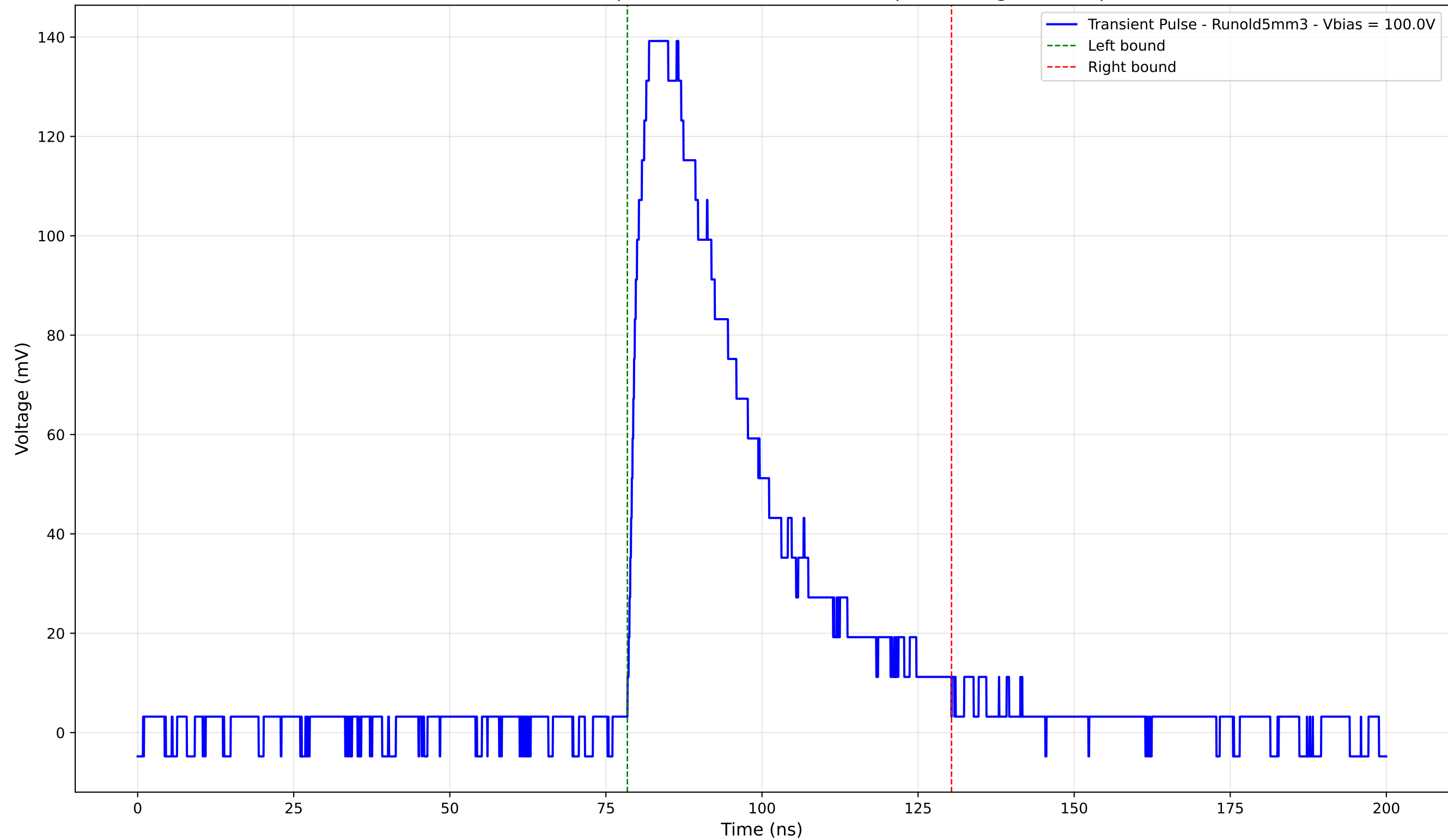
Transient Pulse - Sample: old5 - Position: 2140.0 \mu\text{m} - Charge: 56.62 pC
