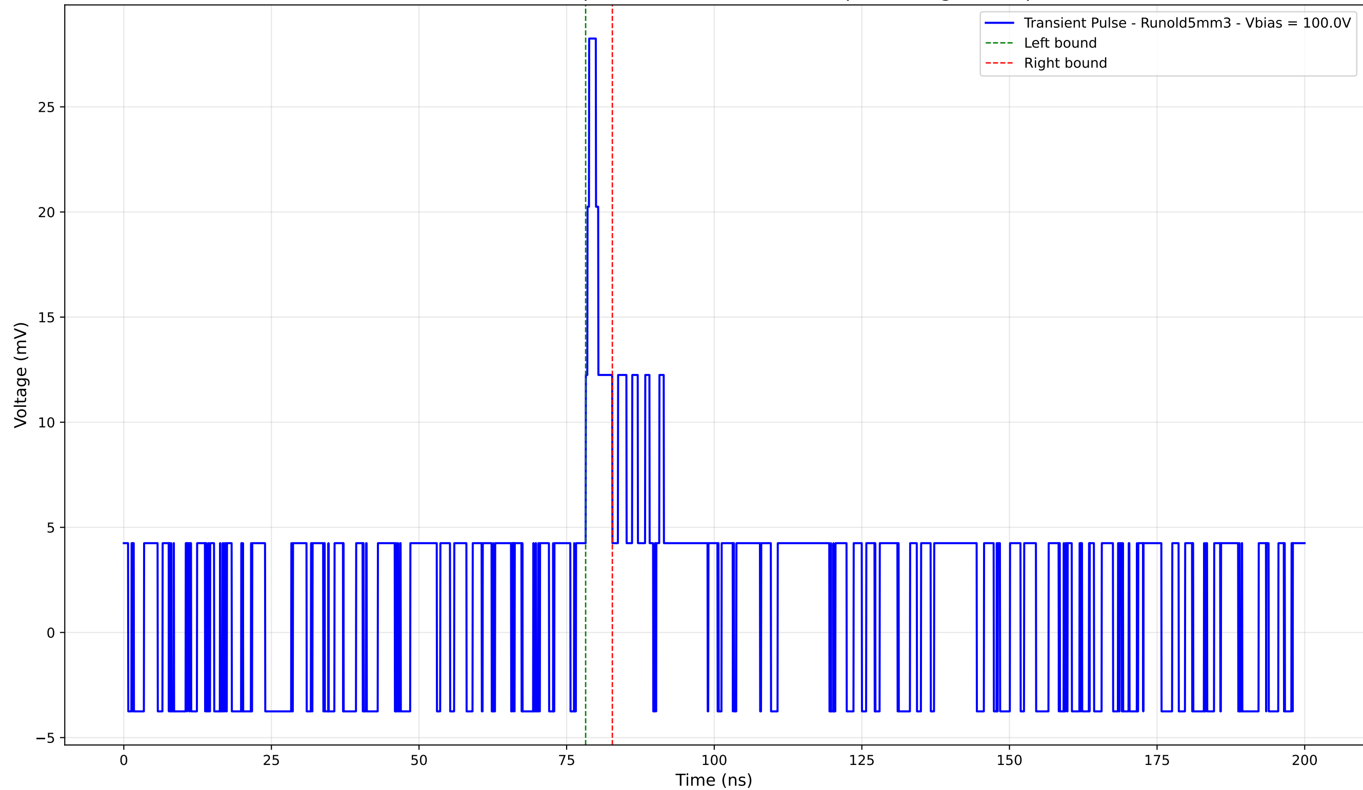
Transient Pulse - Sample: old5 - Position: 4945.0 \mu\text{m} - Charge: 1.58 pC
