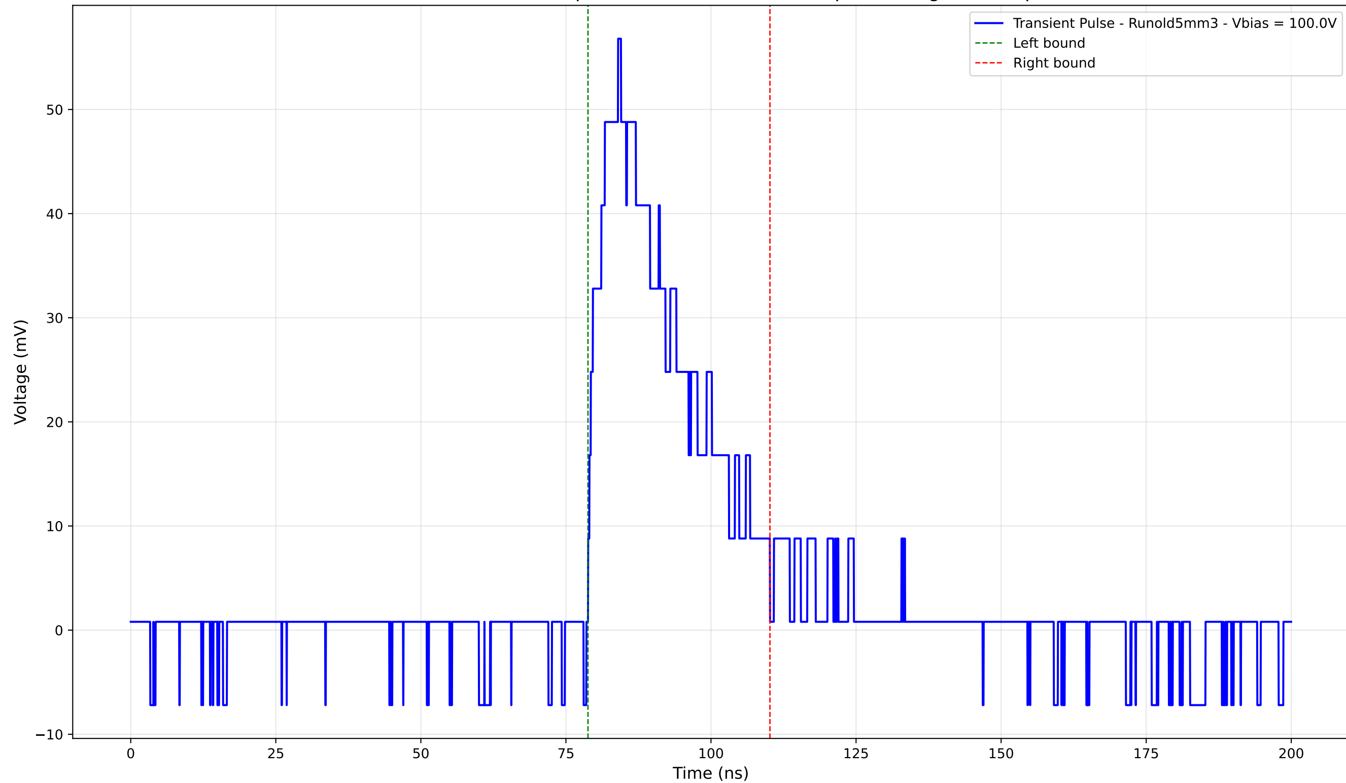
Transient Pulse - Sample: old5 - Position: 2210.0 \mu\text{m} - Charge: 17.12 pC
