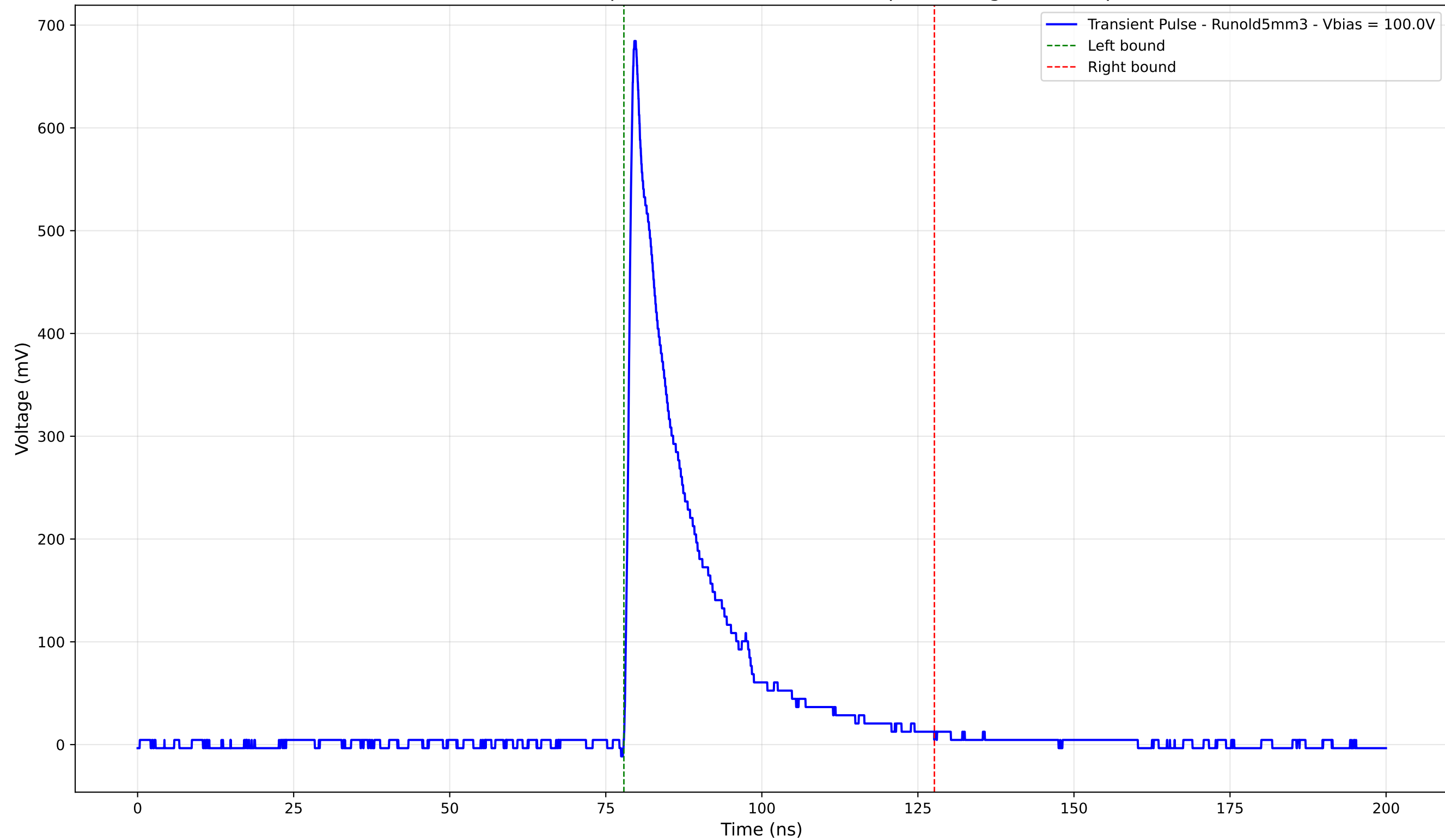
Transient Pulse - Sample: old5 - Position: 4670.0 \mu\text{m} - Charge: 130.17 pC
