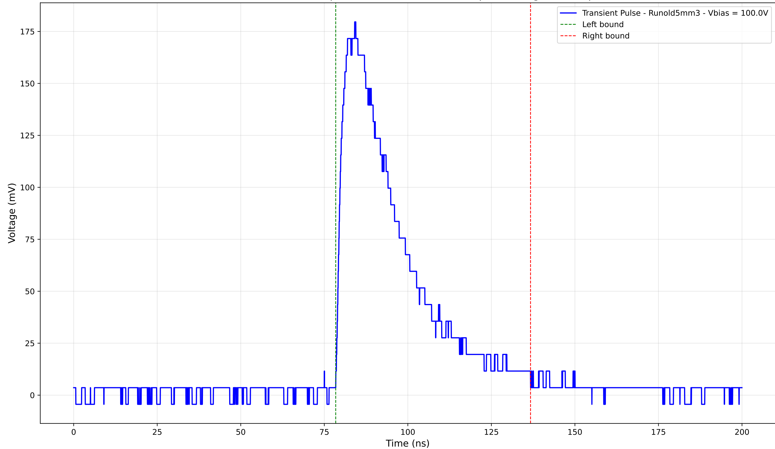
Transient Pulse - Sample: old5 - Position: 1720.0 \mu\text{m} - Charge: 72.41 pC
