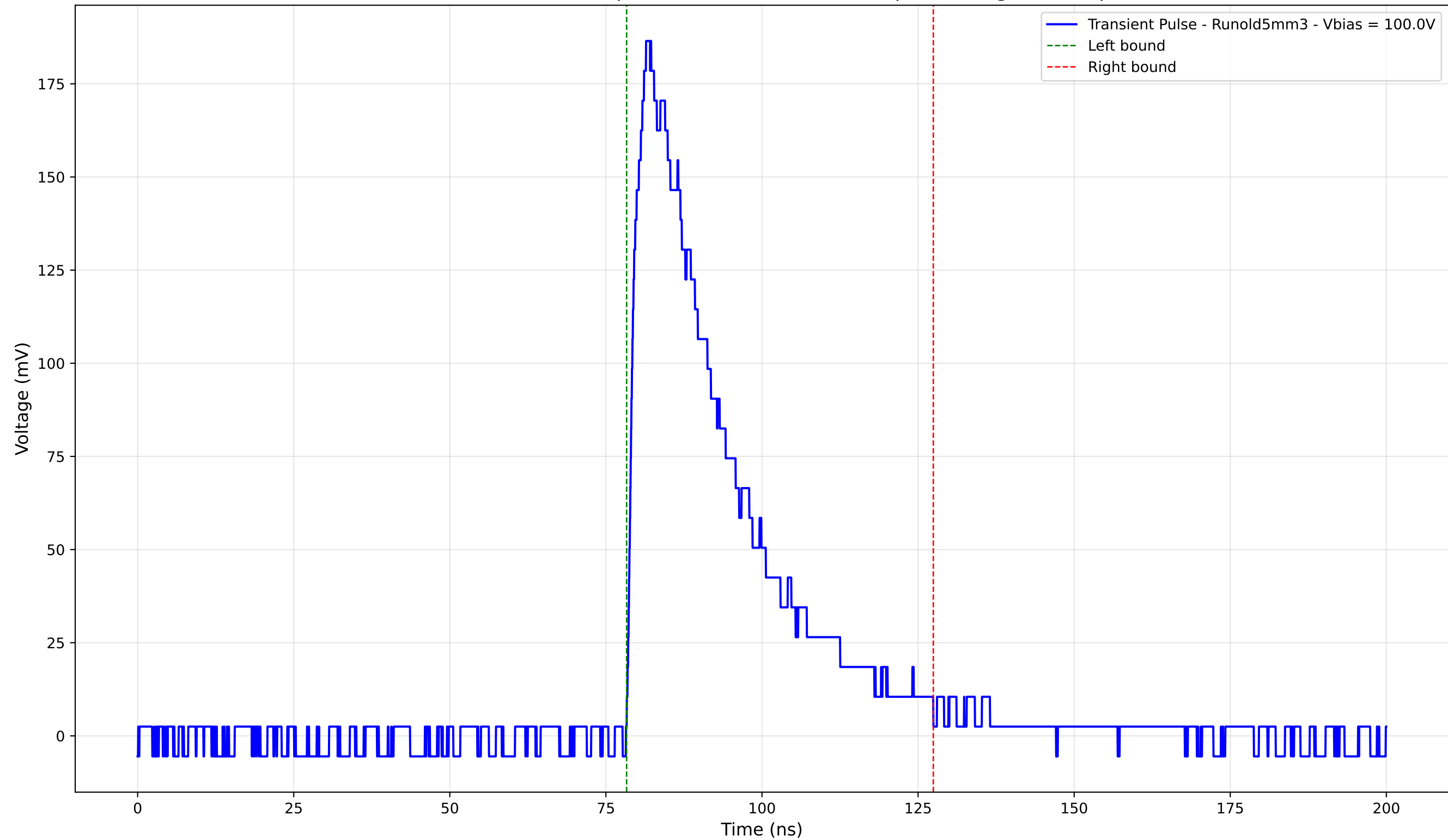
Transient Pulse - Sample: old5 - Position: 2750.0 \mu\text{m} - Charge: 61.08 pC
