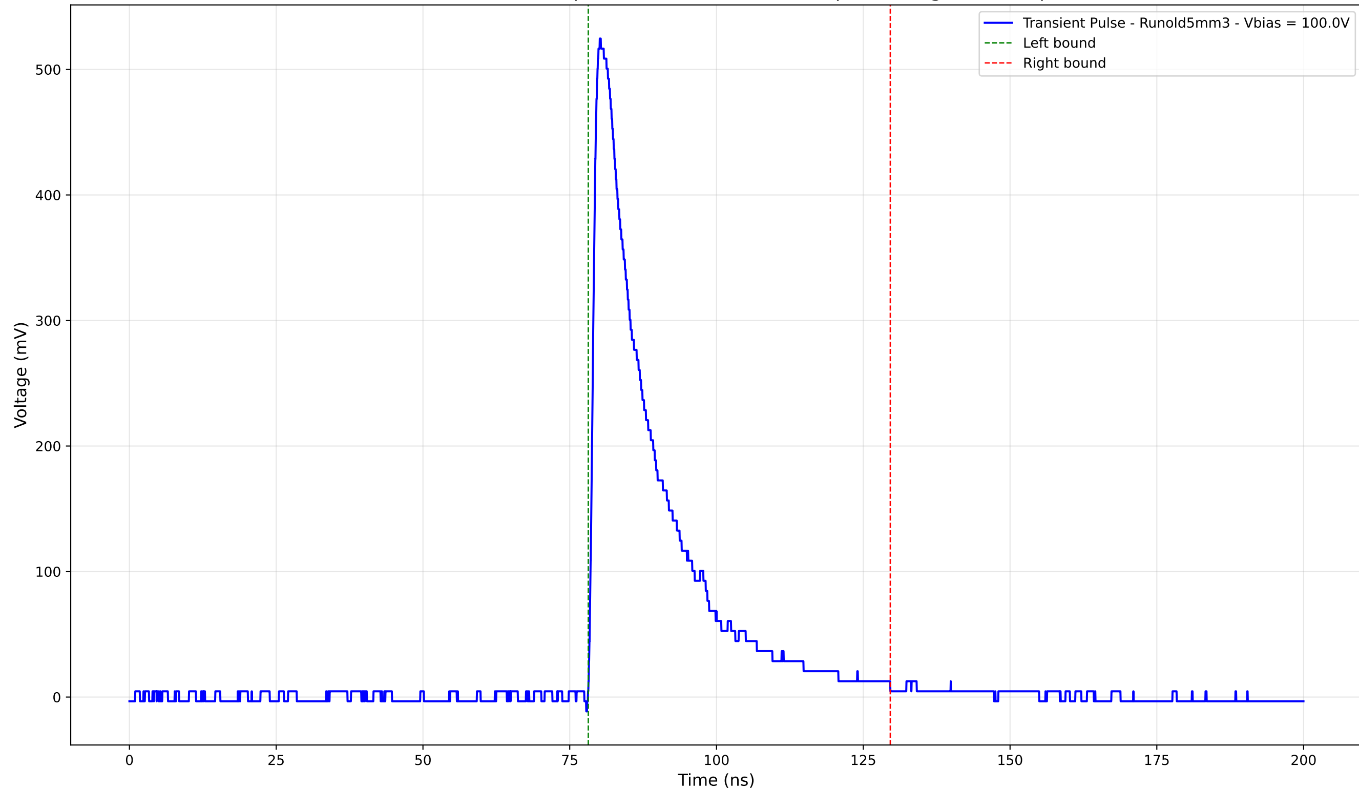
Transient Pulse - Sample: old5 - Position: 4360.0 \mu\text{m} - Charge: 118.57 pC
