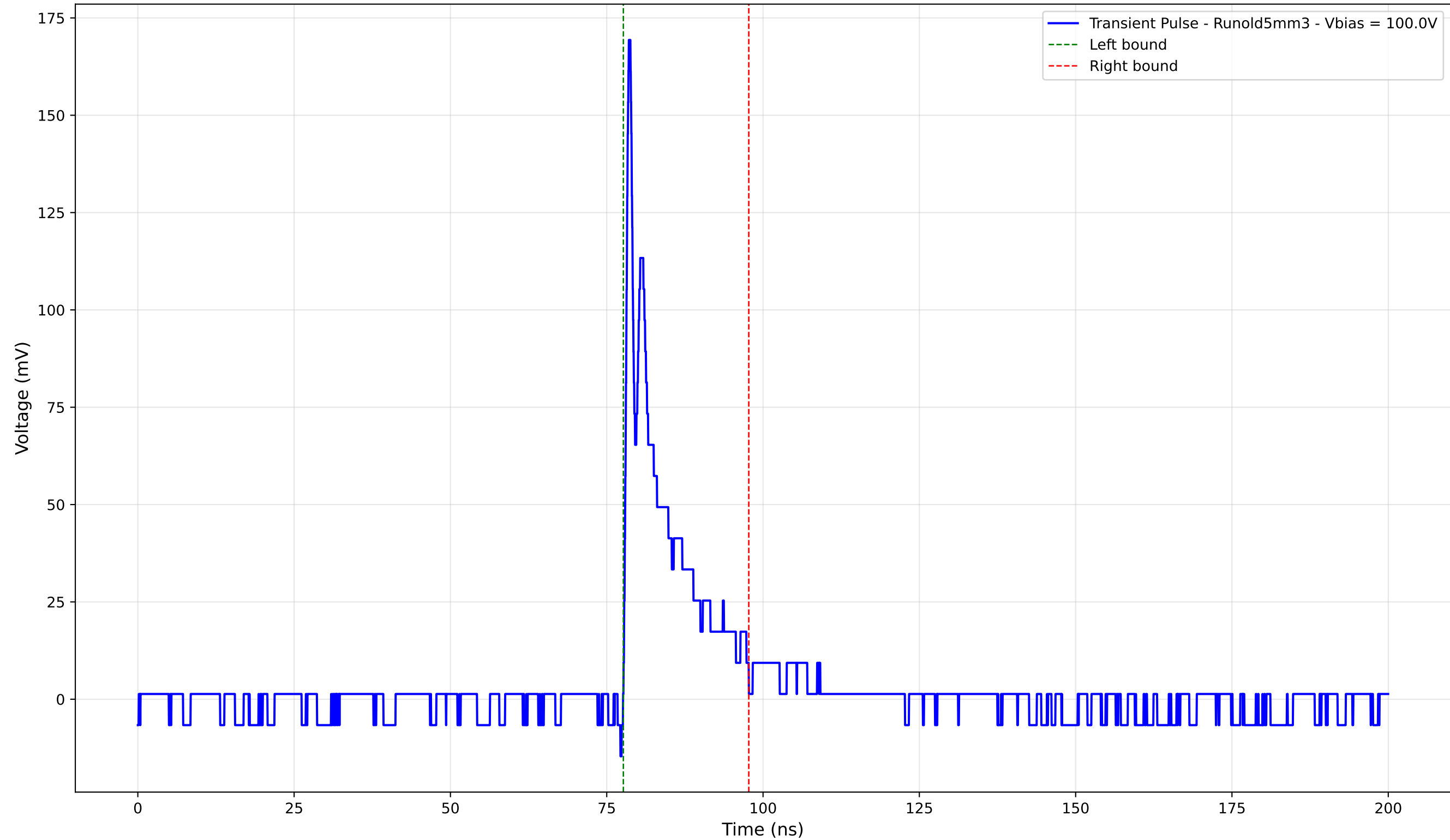
Transient Pulse - Sample: old5 - Position: 3540.0 \mu\text{m} - Charge: 17.68 pC
