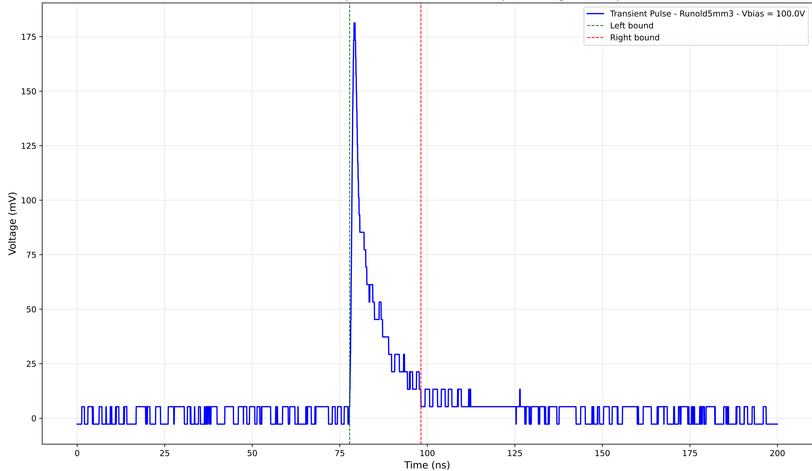
Transient Pulse - Sample: old5 - Position: 4910.0 \mu\text{m} - Charge: 20.14 pC
