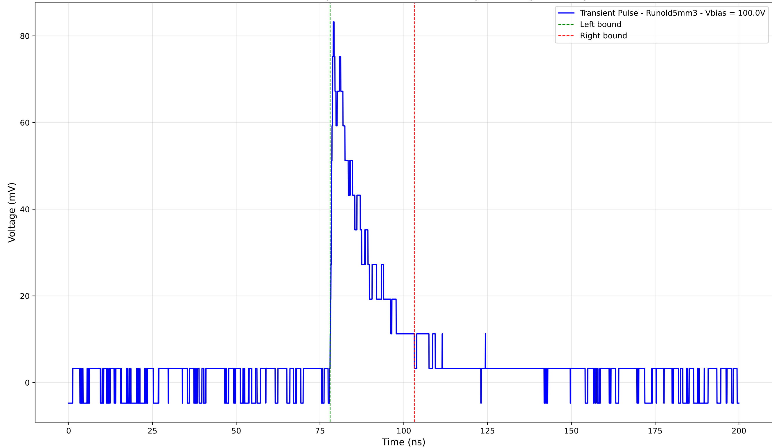
Transient Pulse - Sample: old5 - Position: 3240.0 \mu\text{m} - Charge: 15.96 pC
