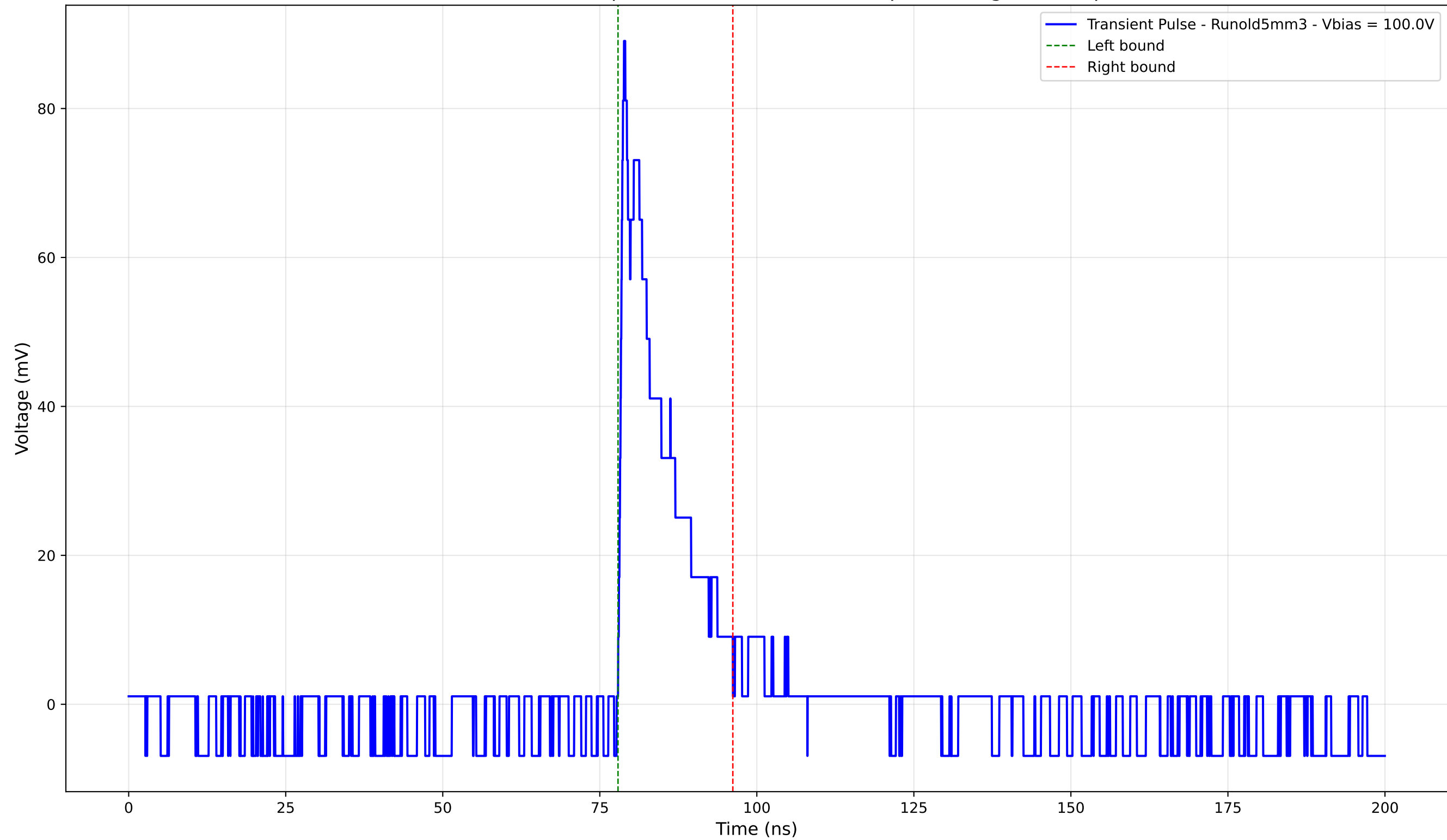
Transient Pulse - Sample: old5 - Position: 3850.0 \mu\text{m} - Charge: 12.34 pC
