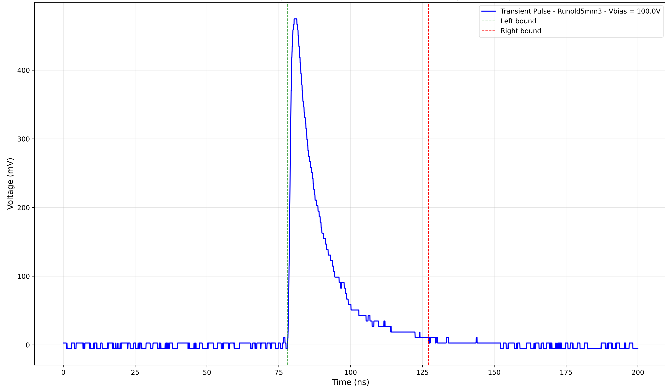
Transient Pulse - Sample: old5 - Position: 4295.0 \mu\text{m} - Charge: 108.65 pC
