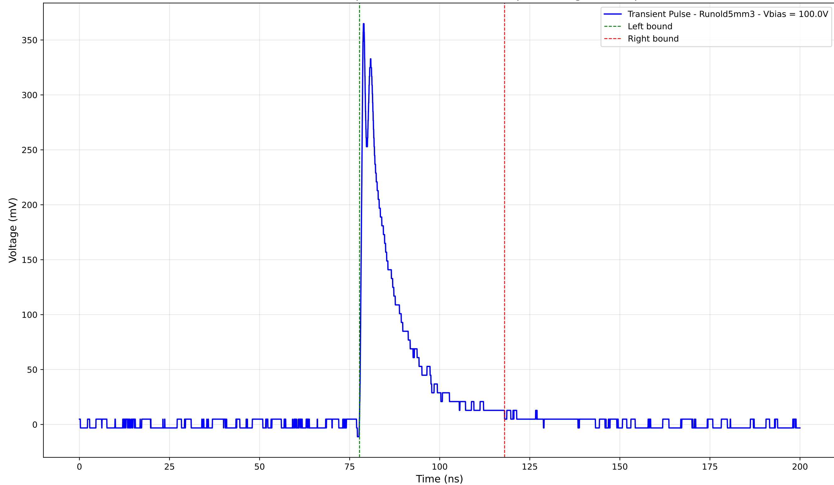
Transient Pulse - Sample: old5 - Position: 3810.0 \mu\text{m} - Charge: 64.13 pC
