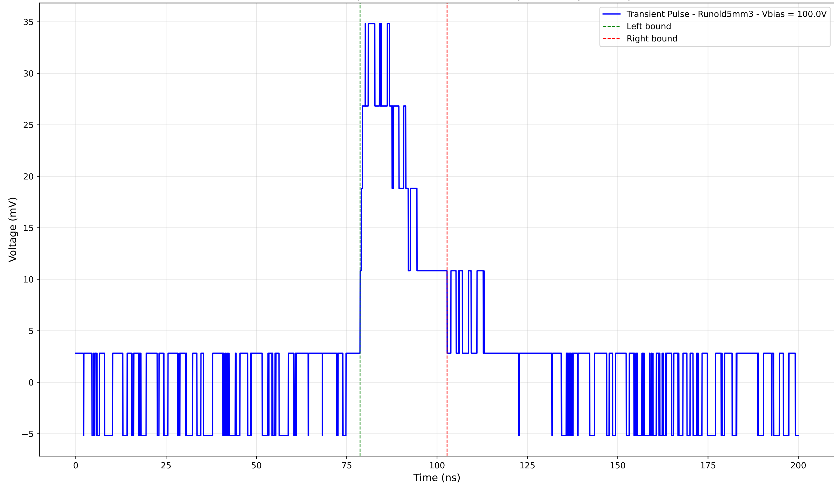
Transient Pulse - Sample: old5 - Position: 2640.0 \mu\text{m} - Charge: 9.70 pC
