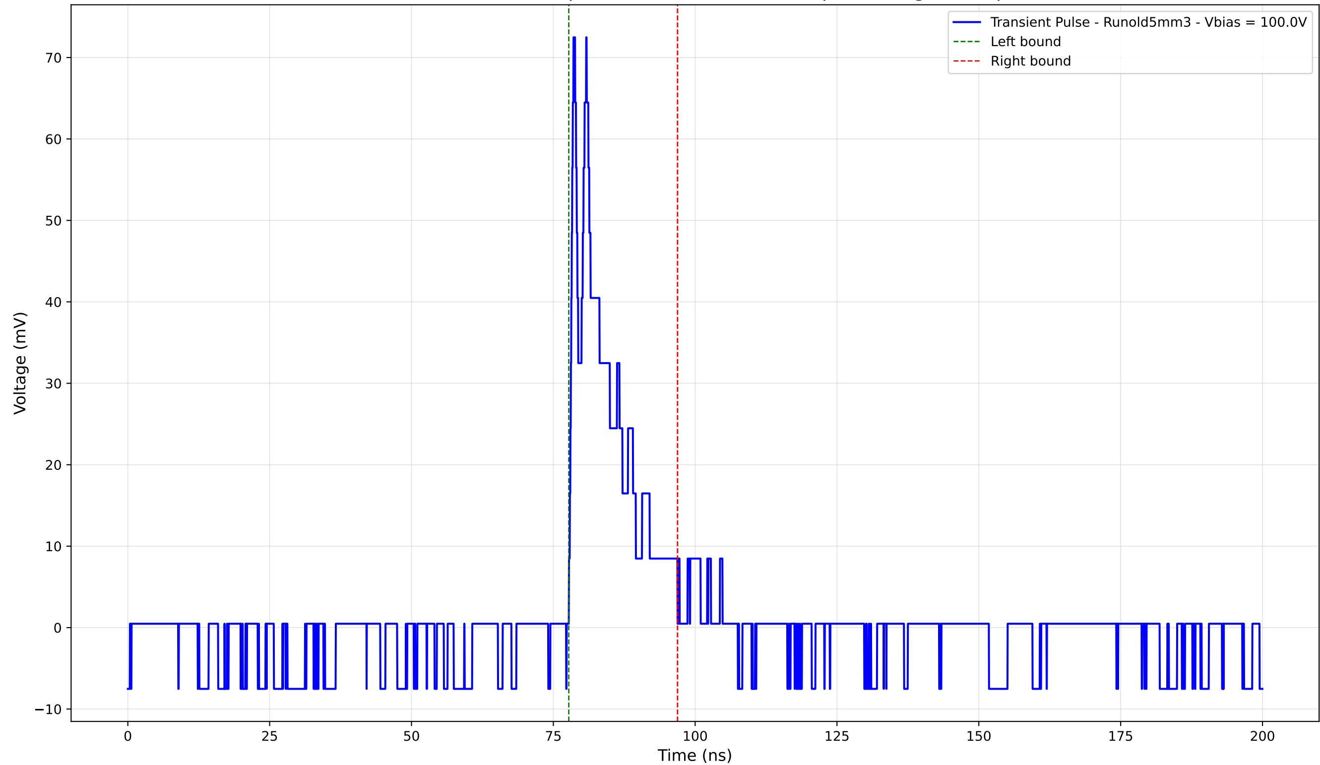
Transient Pulse - Sample: old5 - Position: 3610.0 \mu\text{m} - Charge: 9.74 pC
