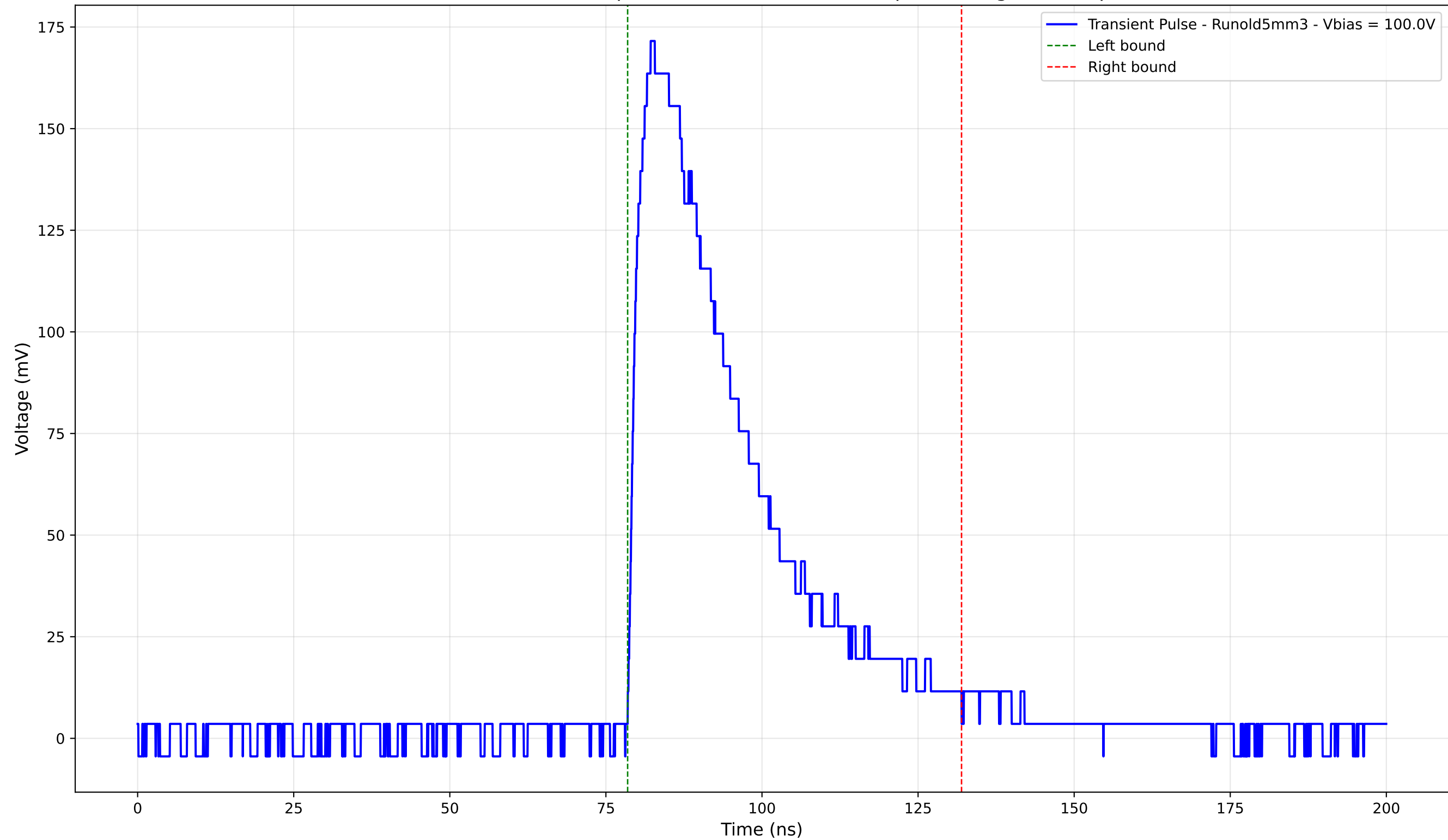
Transient Pulse - Sample: old5 - Position: 1450.0 \mu\text{m} - Charge: 66.77 pC
