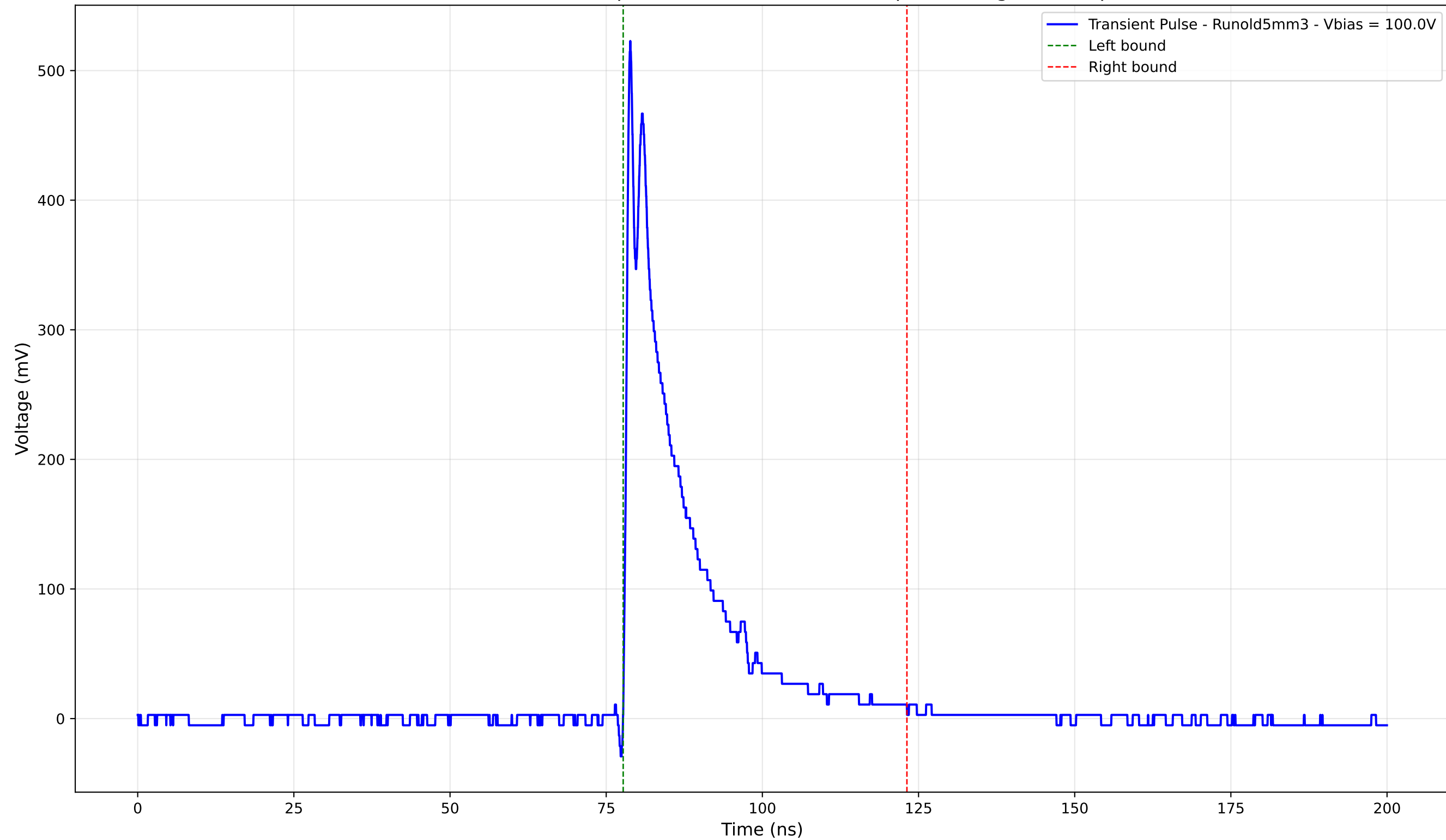
Transient Pulse - Sample: old5 - Position: 3790.0 \mu\text{m} - Charge: 89.77 pC
