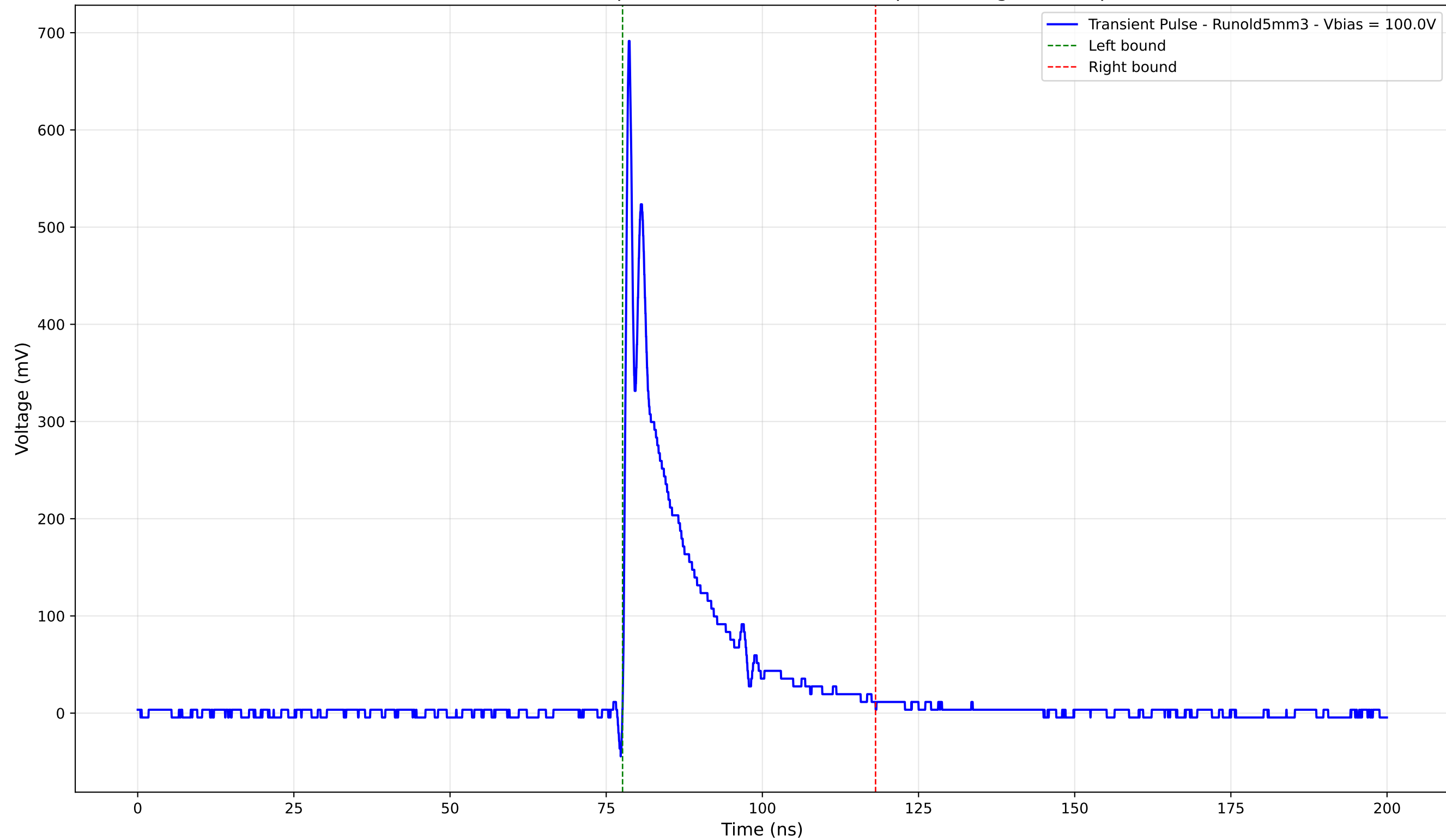
Transient Pulse - Sample: old5 - Position: 3475.0 \mu\text{m} - Charge: 96.72 pC
