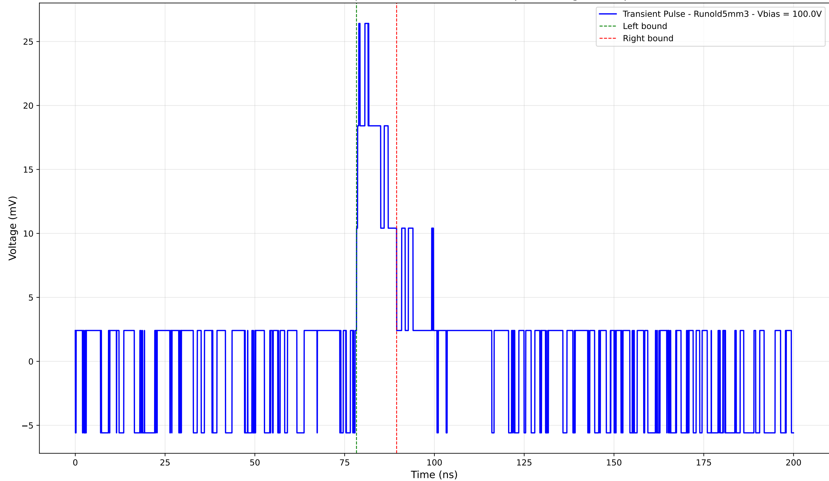
Transient Pulse - Sample: old5 - Position: 3880.0 \mu\text{m} - Charge: 3.75 pC
