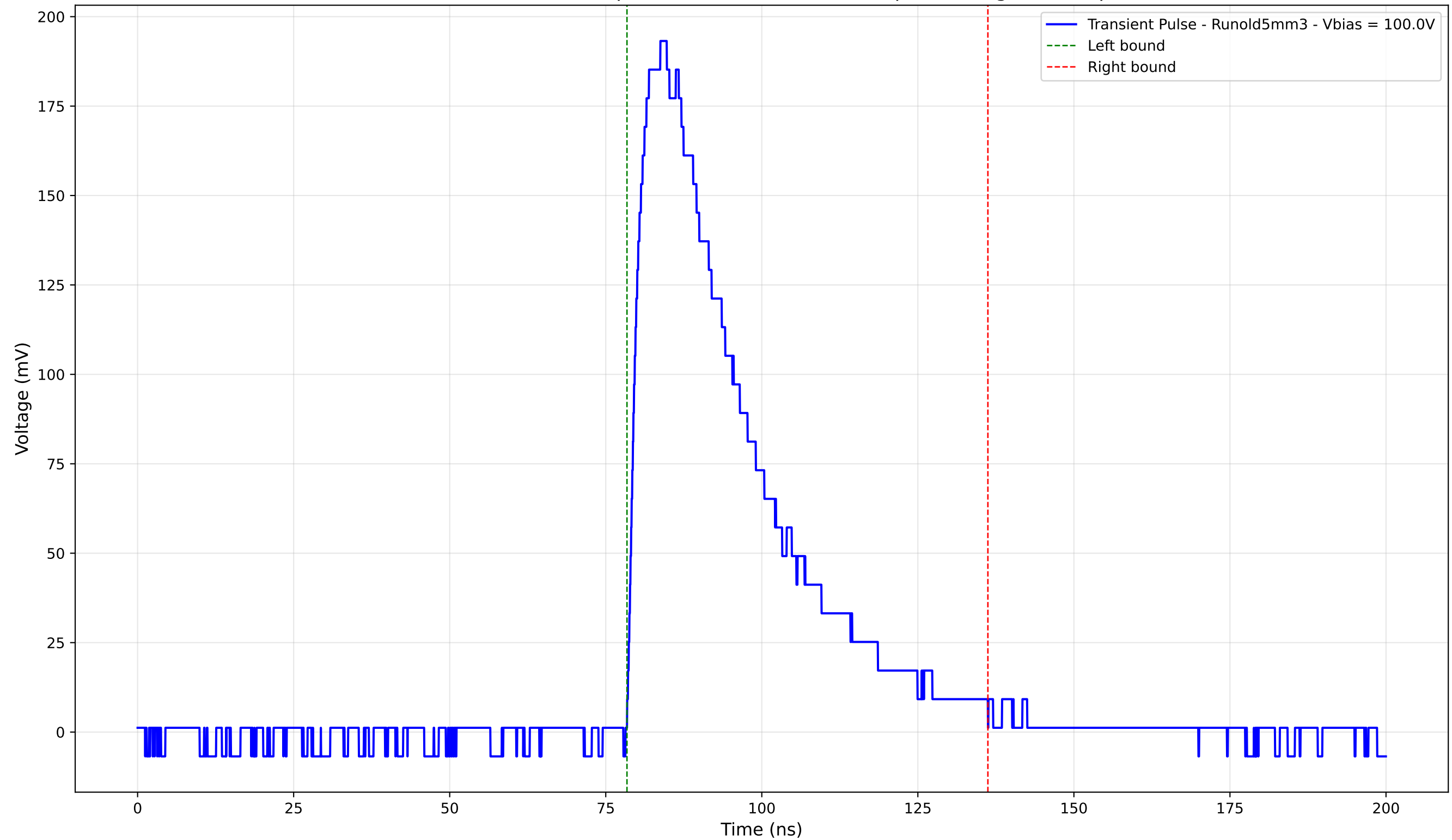
Transient Pulse - Sample: old5 - Position: 1865.0 \mu\text{m} - Charge: 77.23 pC
