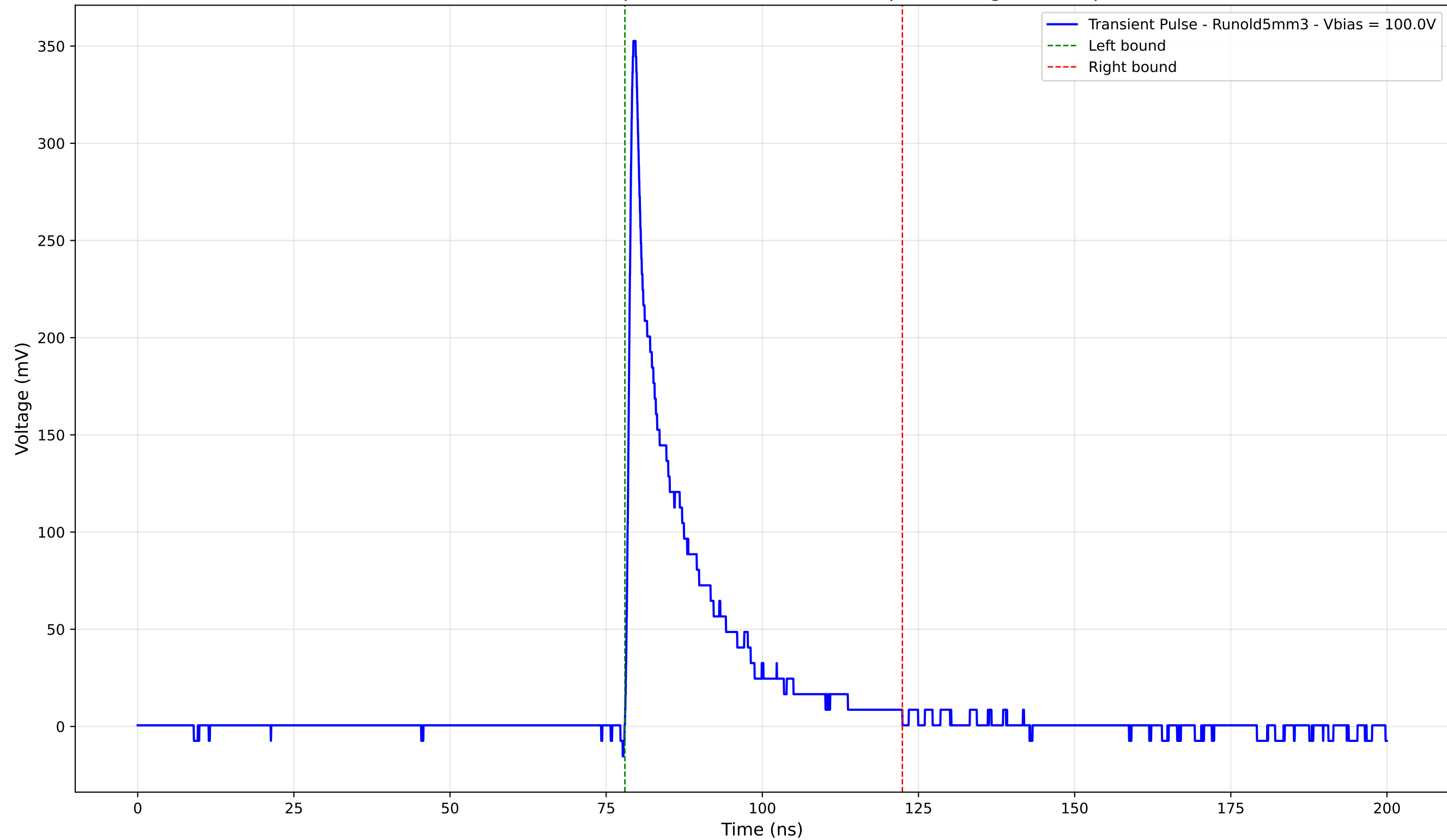
Transient Pulse - Sample: old5 - Position: 340.0 \mu\text{m} - Charge: 55.16 pC
