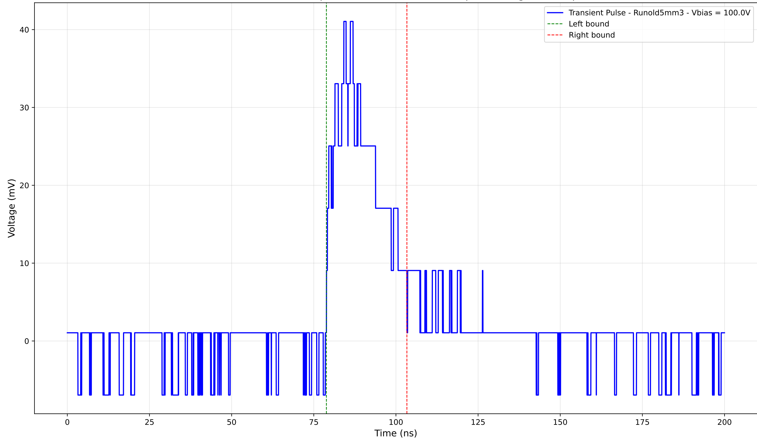
Transient Pulse - Sample: old5 - Position: 1595.0 \mu\text{m} - Charge: 11.11 pC
