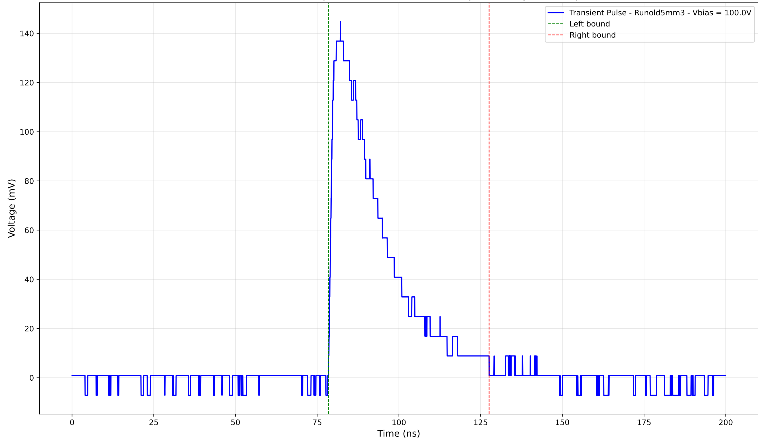
Transient Pulse - Sample: old5 - Position: 1130.0 \mu\text{m} - Charge: 47.90 pC
