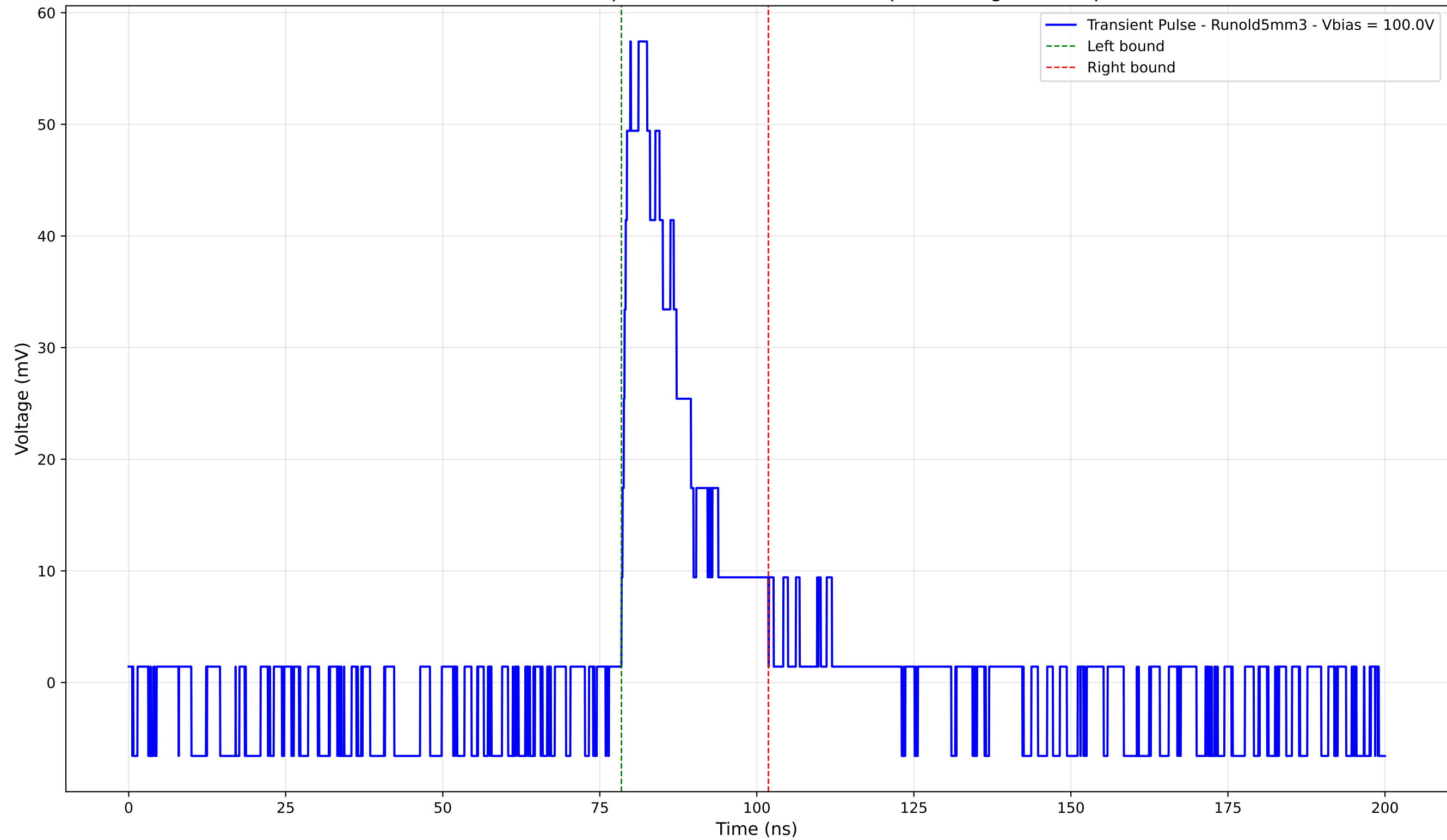
Transient Pulse - Sample: old5 - Position: 4520.0 \mu\text{m} - Charge: 11.71 pC
