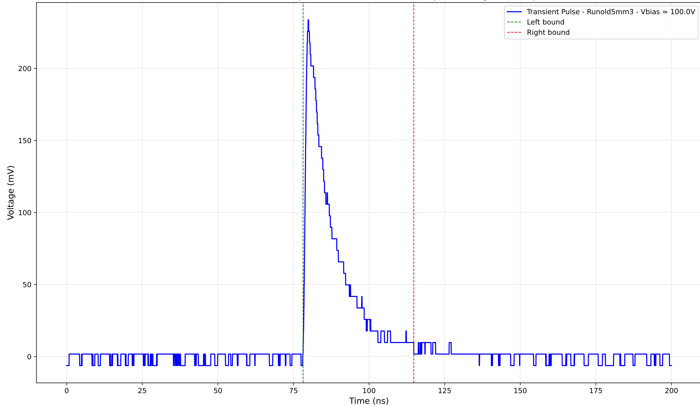
Transient Pulse - Sample: old5 - Position: 4550.0 \mu\text{m} - Charge: 44.35 pC
