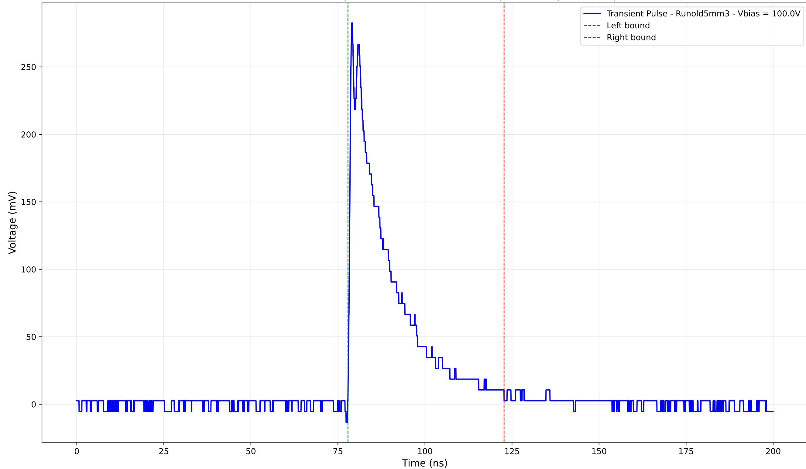
Transient Pulse - Sample: old5 - Position: 3200.0 \mu\text{m} - Charge: 64.64 pC
