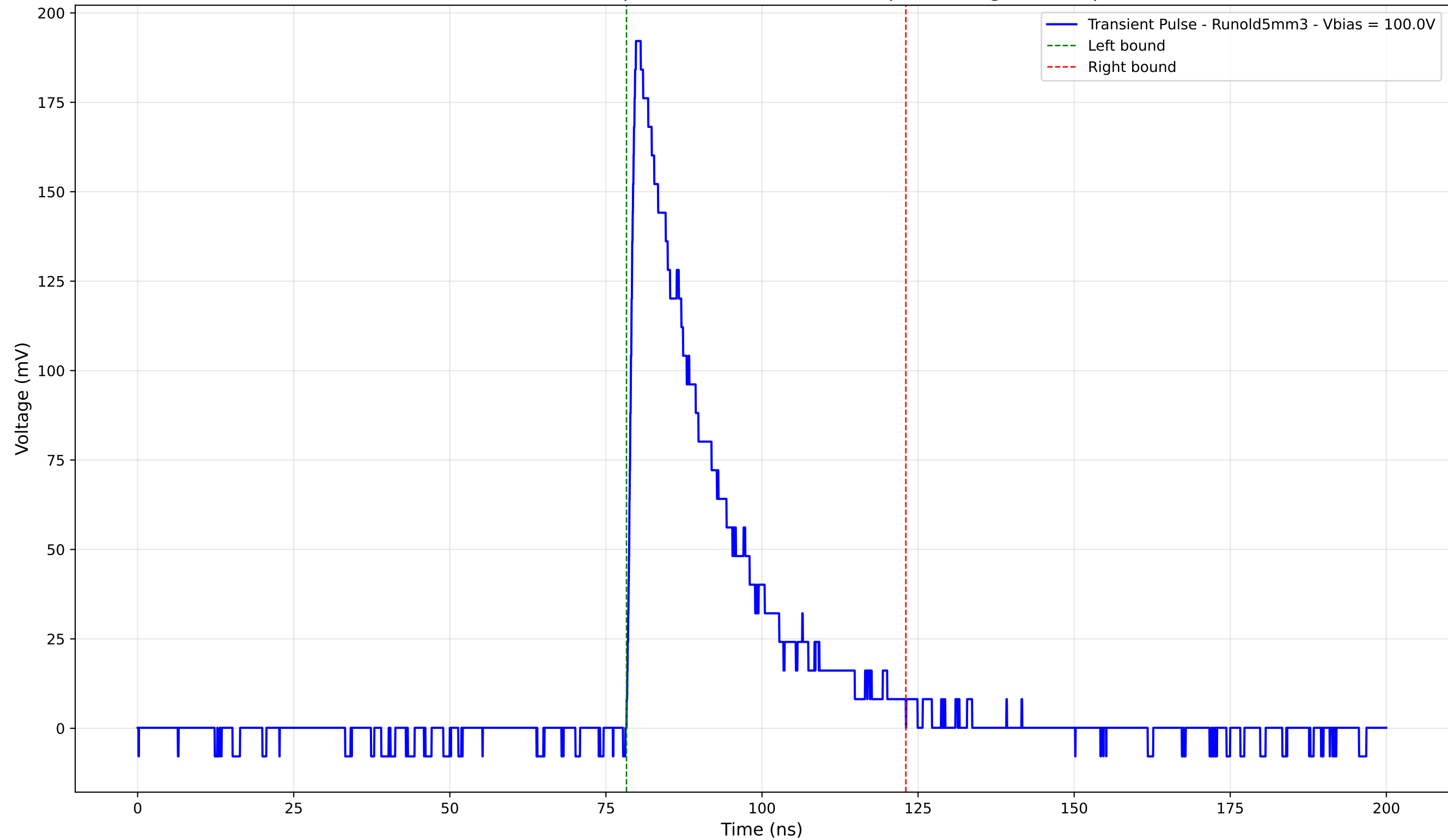
Transient Pulse - Sample: old5 - Position: 770.0 \mu\text{m} - Charge: 50.58 pC
