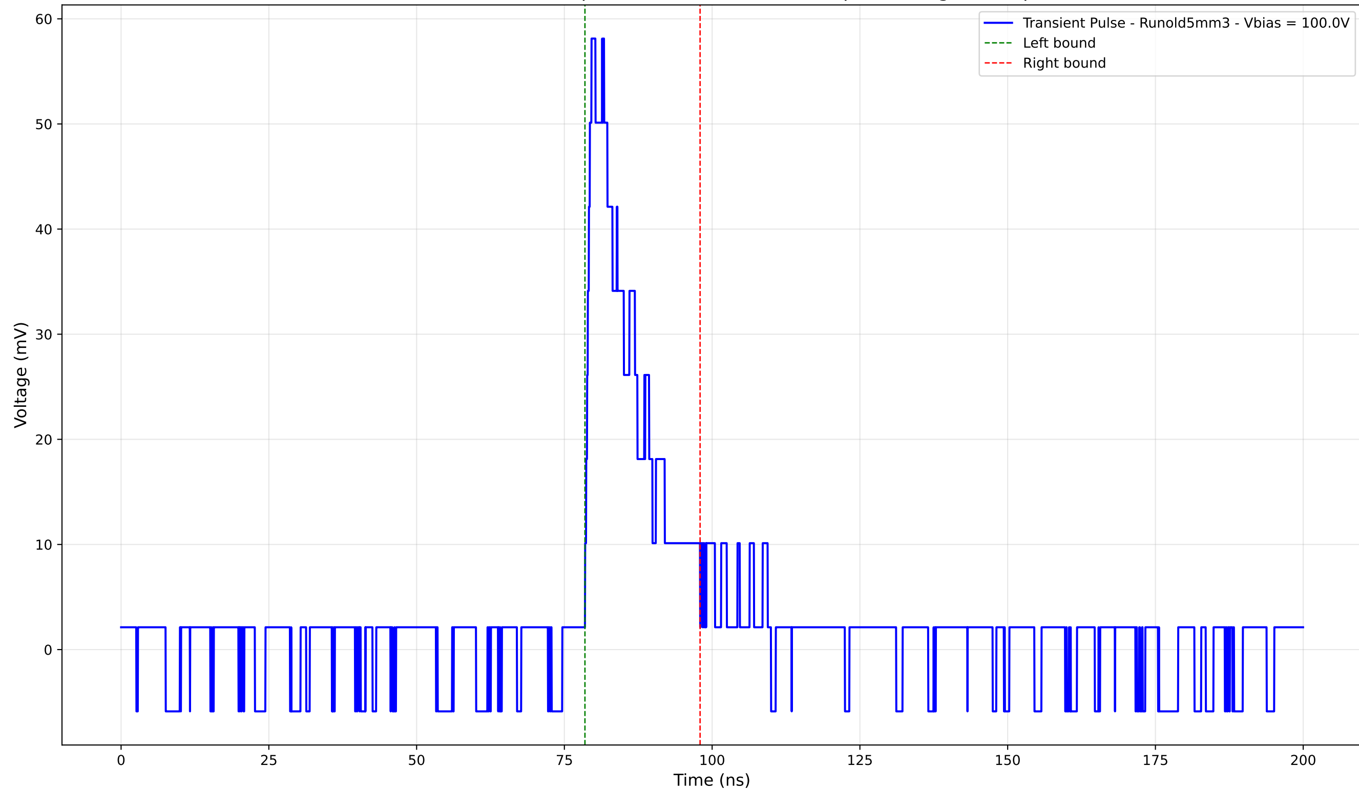
Transient Pulse - Sample: old5 - Position: 4465.0 \mu\text{m} - Charge: 9.85 pC
