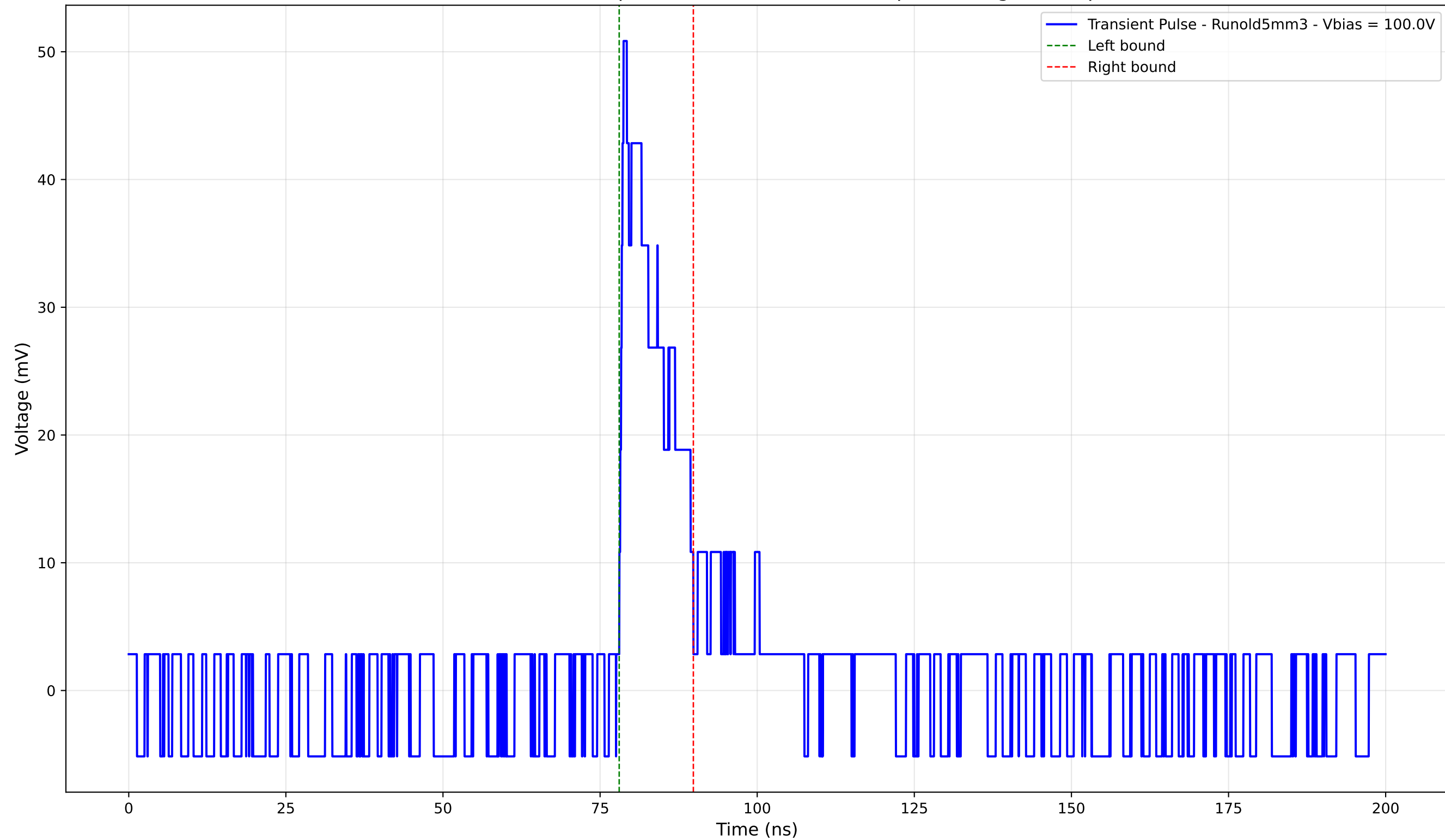
Transient Pulse - Sample: old5 - Position: 3860.0 \mu\text{m} - Charge: 6.80 pC
