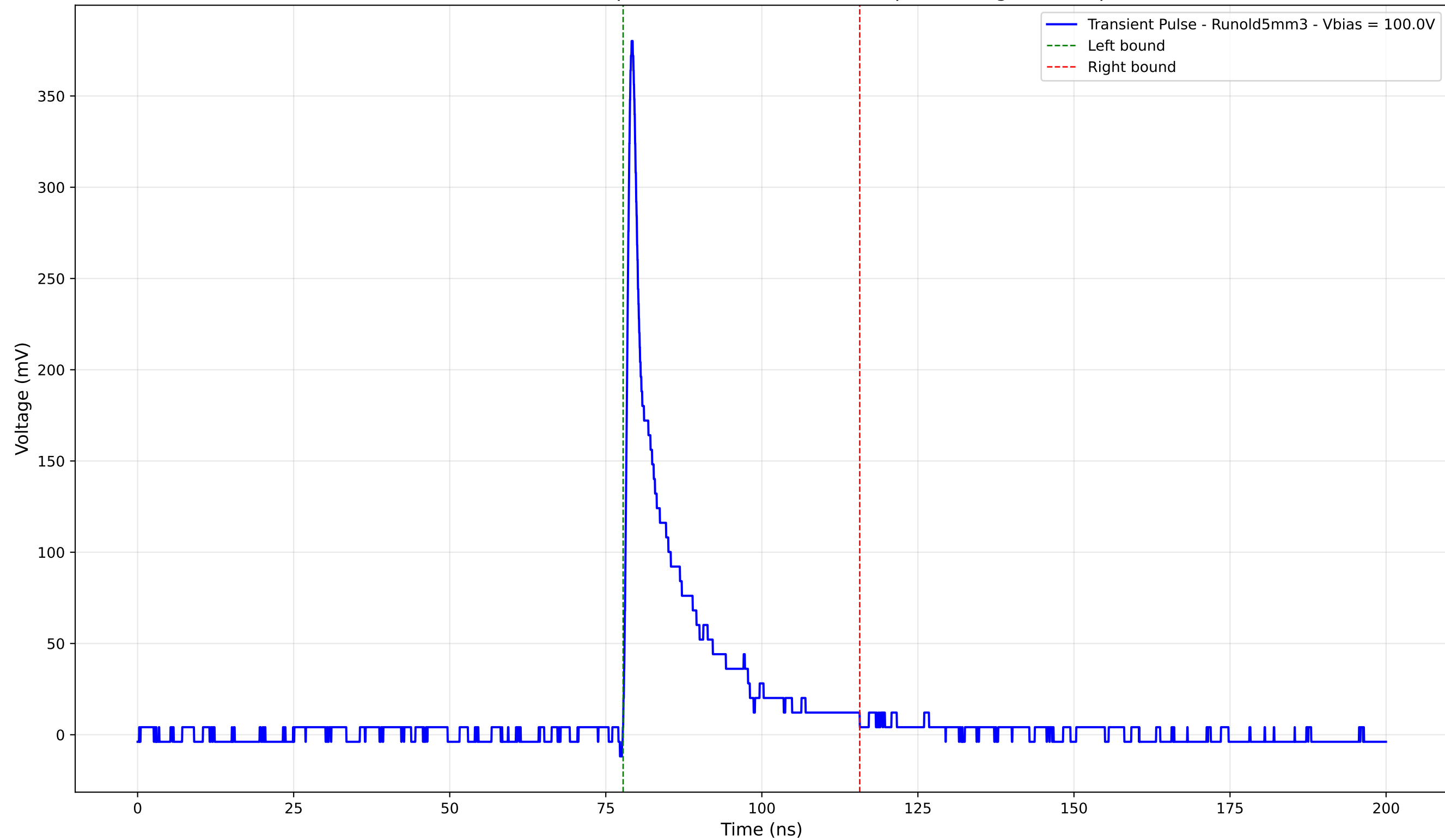
Transient Pulse - Sample: old5 - Position: 4890.0 \mu\text{m} - Charge: 47.31 pC
