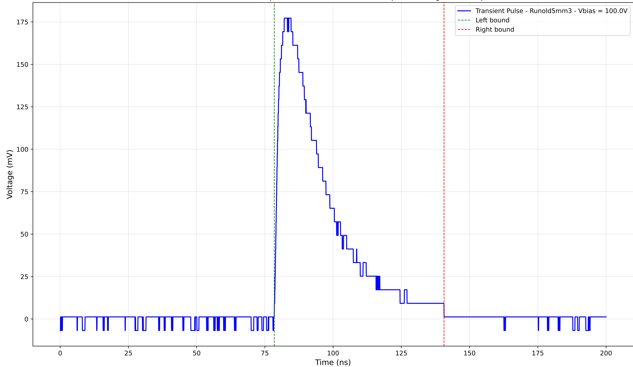
Transient Pulse - Sample: old5 - Position: 1455.0 \mu\text{m} - Charge: 70.69 pC
