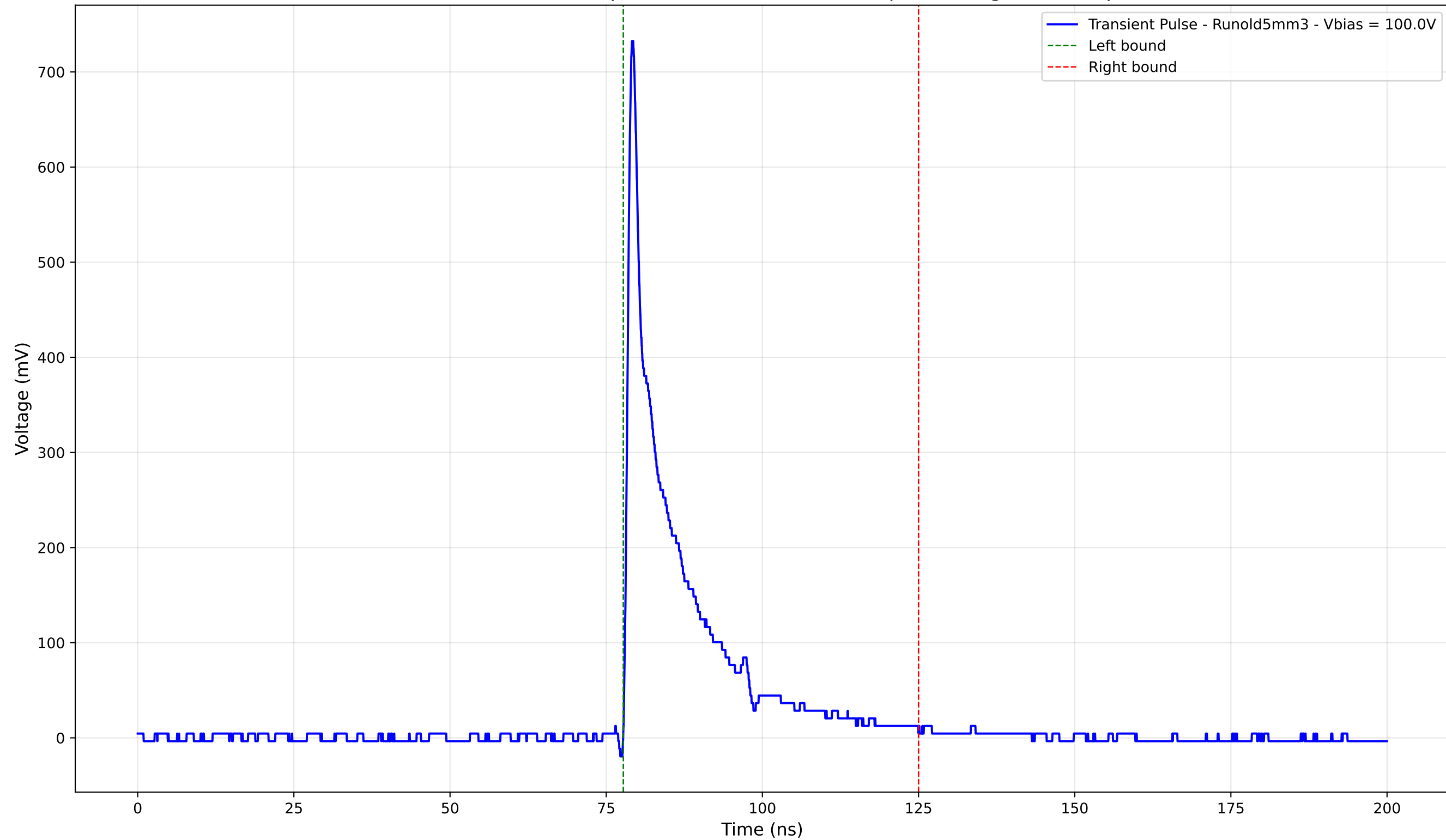
Transient Pulse - Sample: old5 - Position: 4855.0 \mu\text{m} - Charge: 101.94 pC
