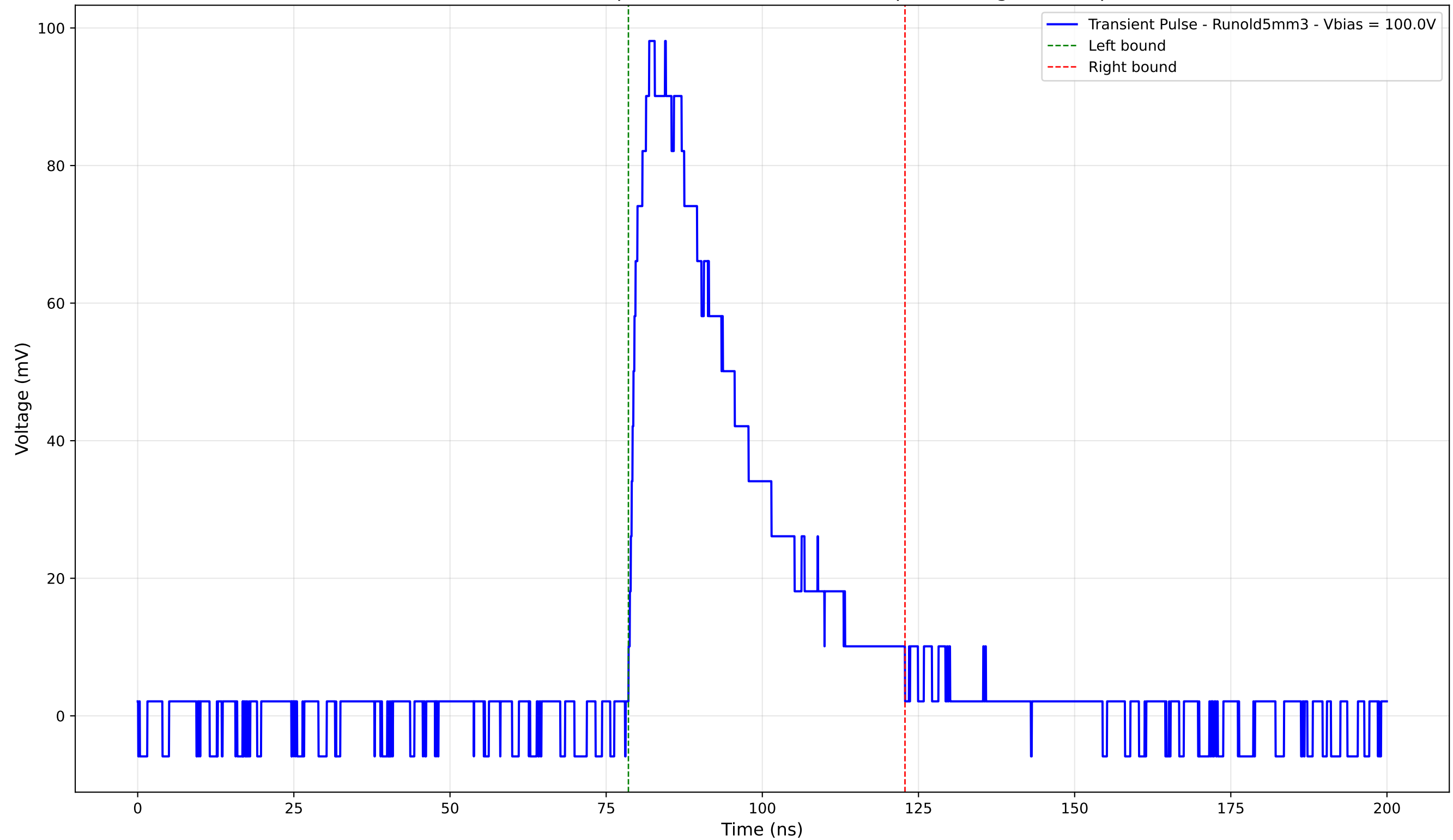
Transient Pulse - Sample: old5 - Position: 2360.0 \mu\text{m} - Charge: 35.57 pC
