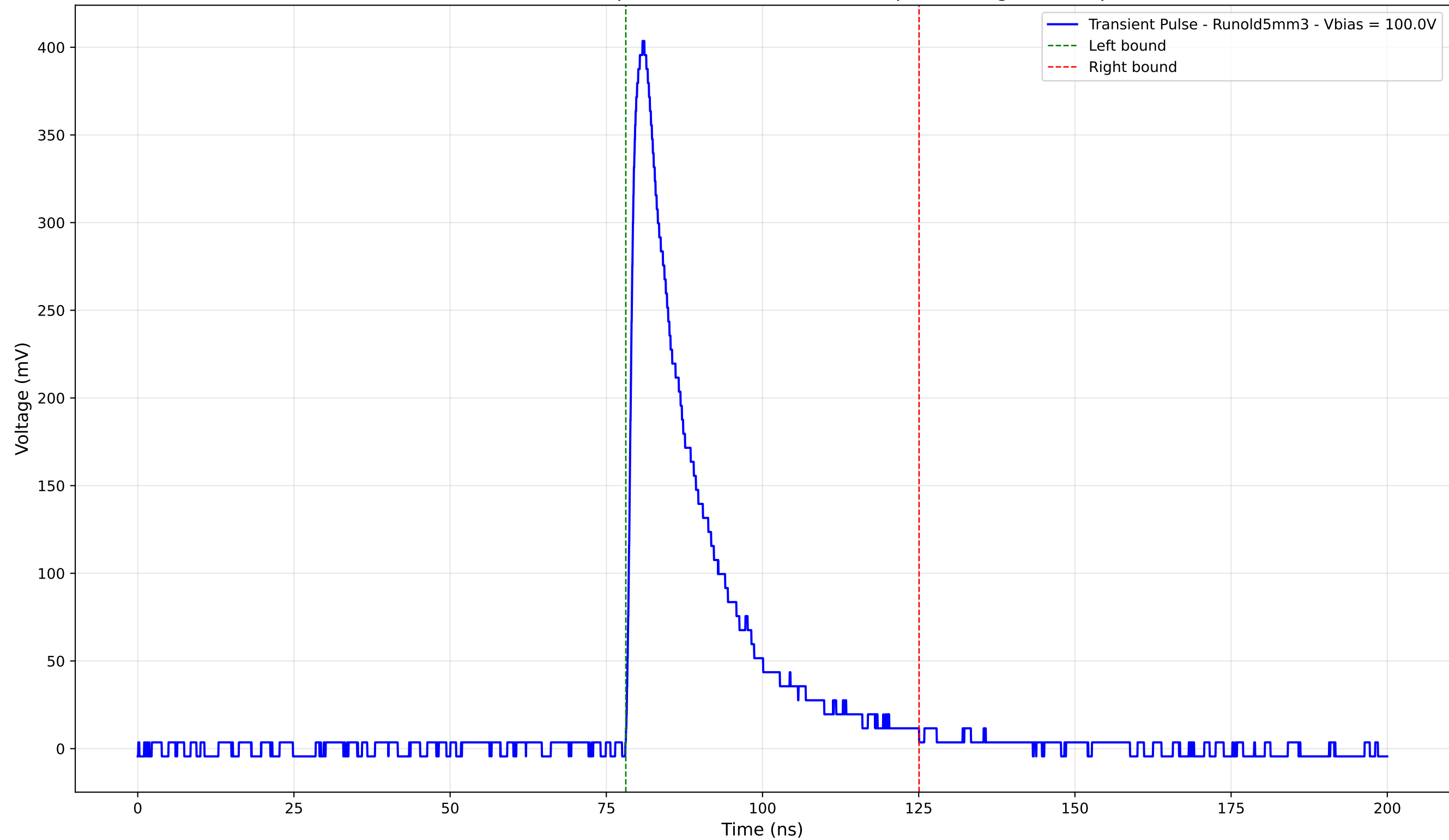
Transient Pulse - Sample: old5 - Position: 4275.0 \mu\text{m} - Charge: 90.14 pC
