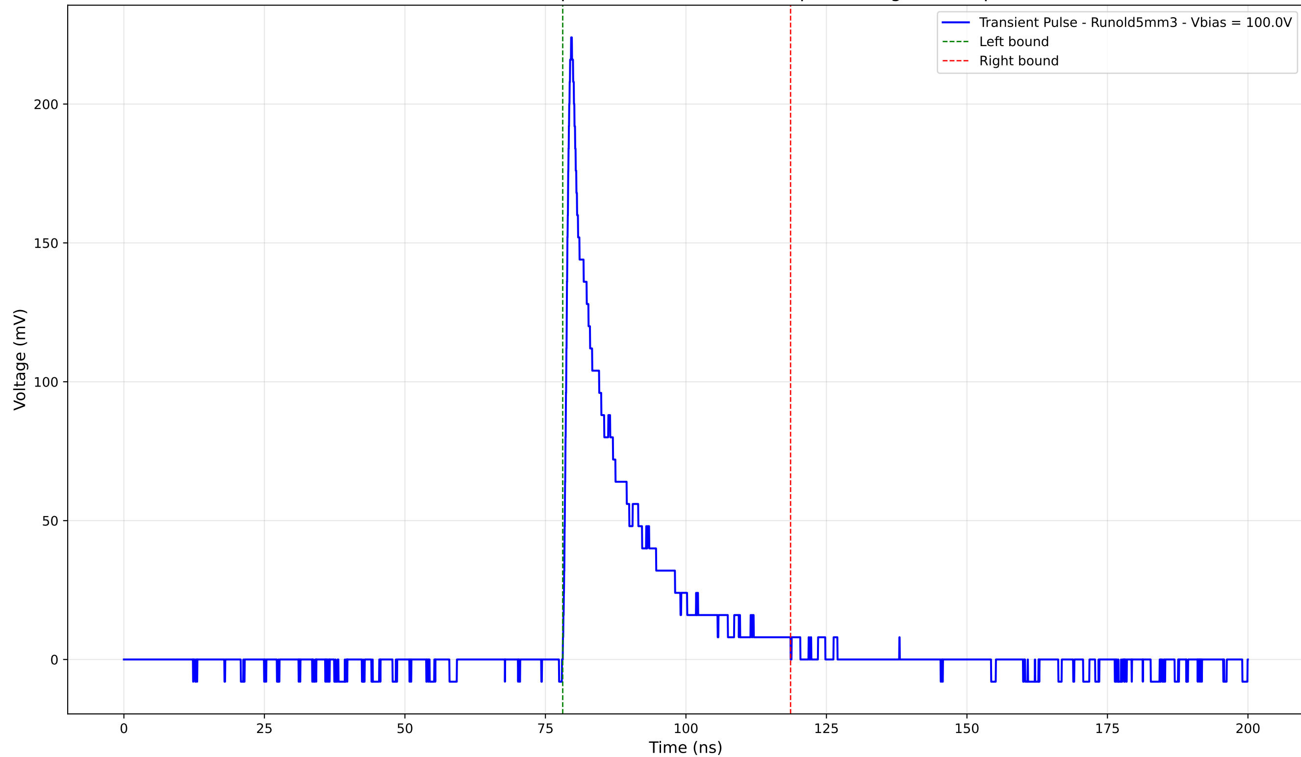
Transient Pulse - Sample: old5 - Position: 410.0 \mu\text{m} - Charge: 37.49 pC
