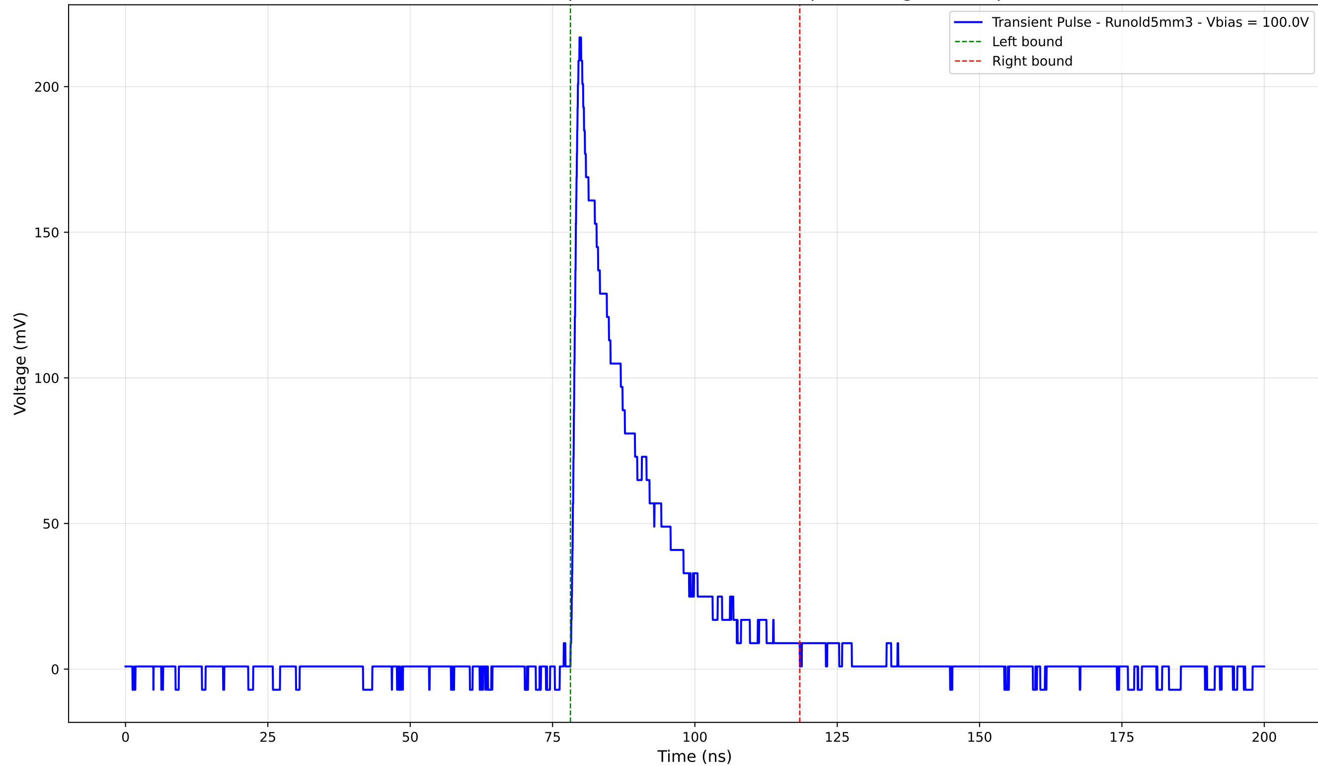
Transient Pulse - Sample: old5 - Position: 575.0 \mu\text{m} - Charge: 44.74 pC
