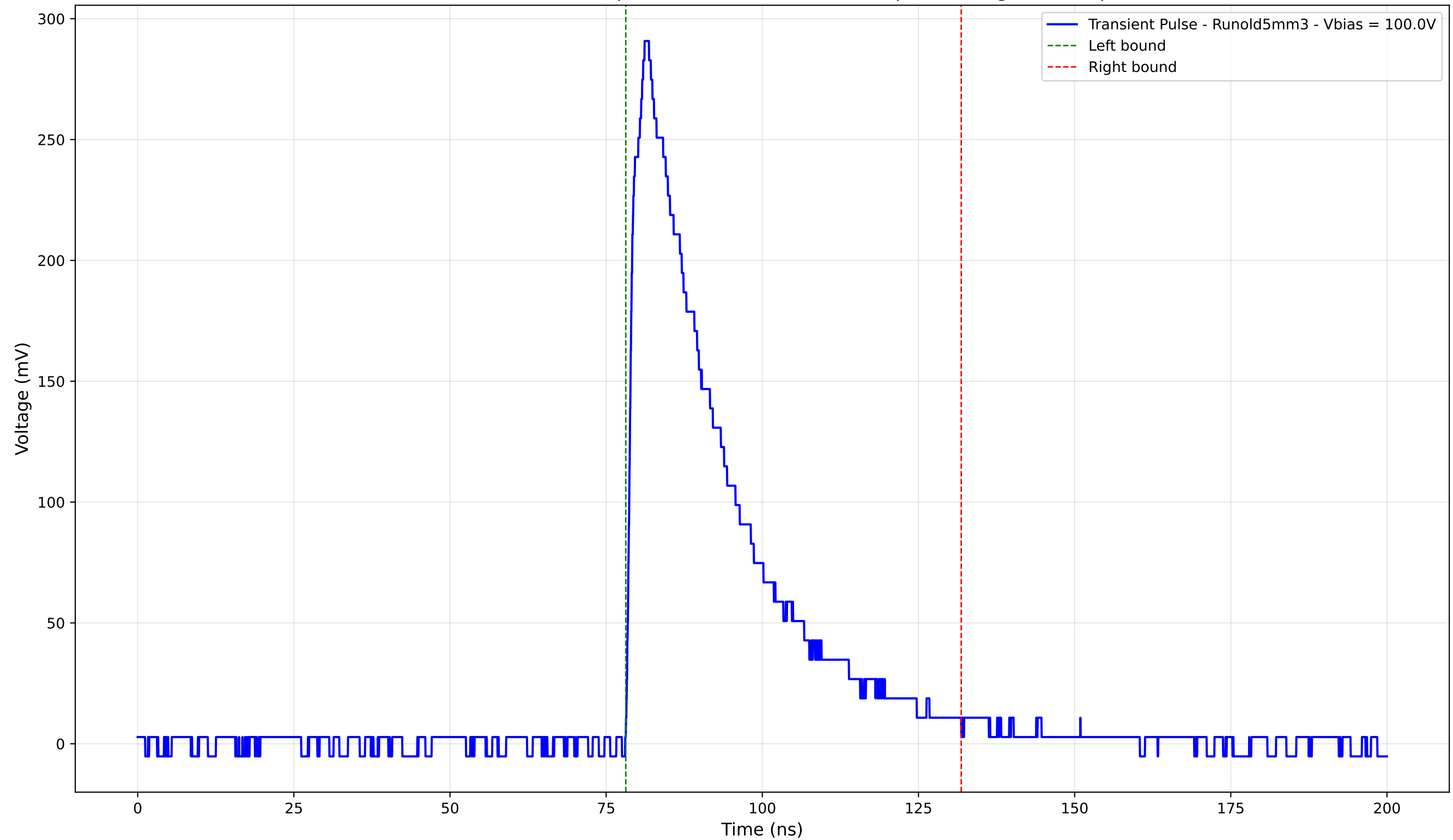
Transient Pulse - Sample: old5 - Position: 2875.0 \mu\text{m} - Charge: 92.80 pC
