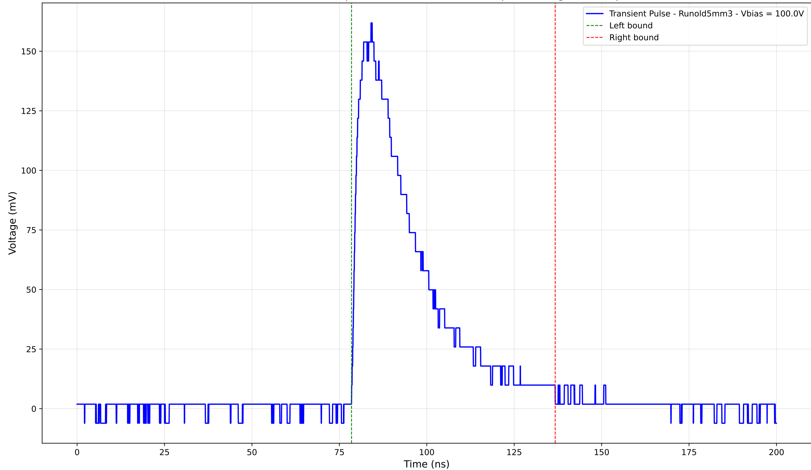
Transient Pulse - Sample: old5 - Position: 1445.0 \mu\text{m} - Charge: 61.54 pC
