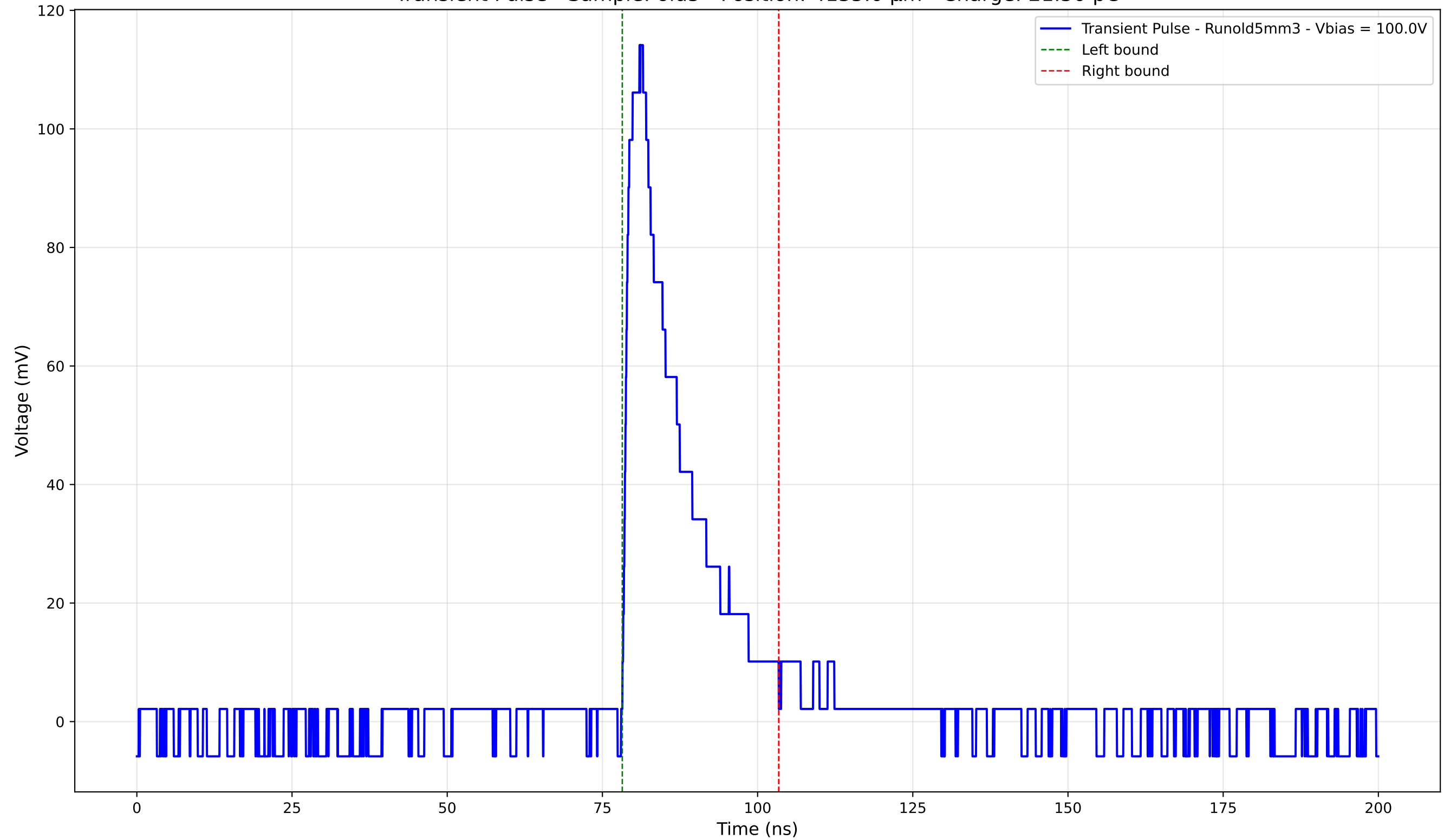
Transient Pulse - Sample: old5 - Position: 4135.0 \mu\text{m} - Charge: 21.50 pC
