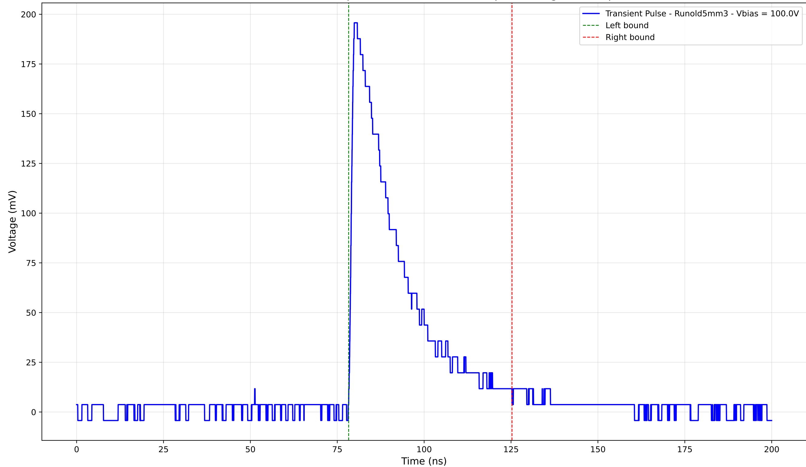
Transient Pulse - Sample: old5 - Position: 845.0 \mu\text{m} - Charge: 58.63 pC
