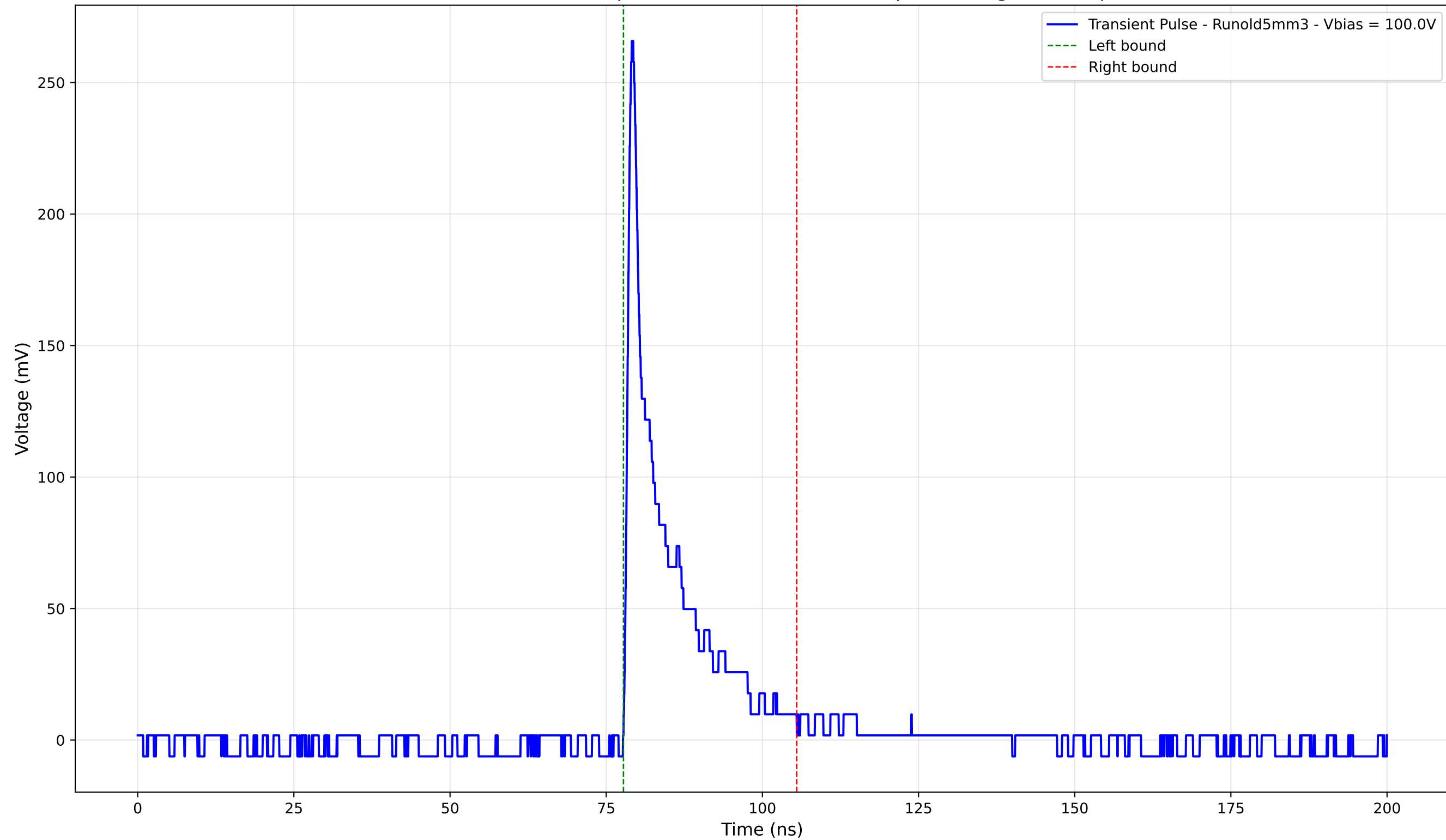
Transient Pulse - Sample: old5 - Position: 4900.0 \mu\text{m} - Charge: 30.78 pC
