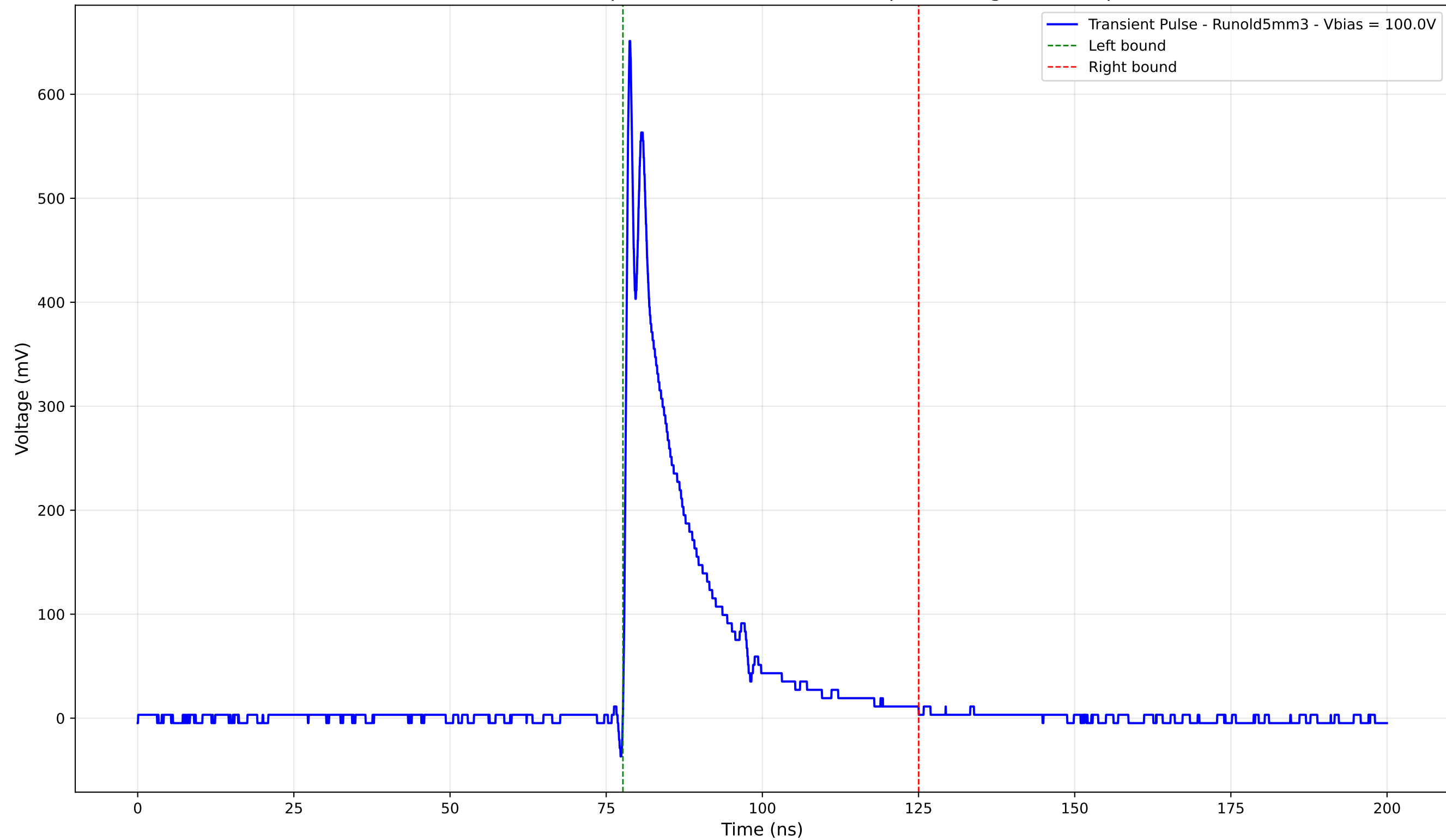
Transient Pulse - Sample: old5 - Position: 3755.0 \mu\text{m} - Charge: 109.10 pC
