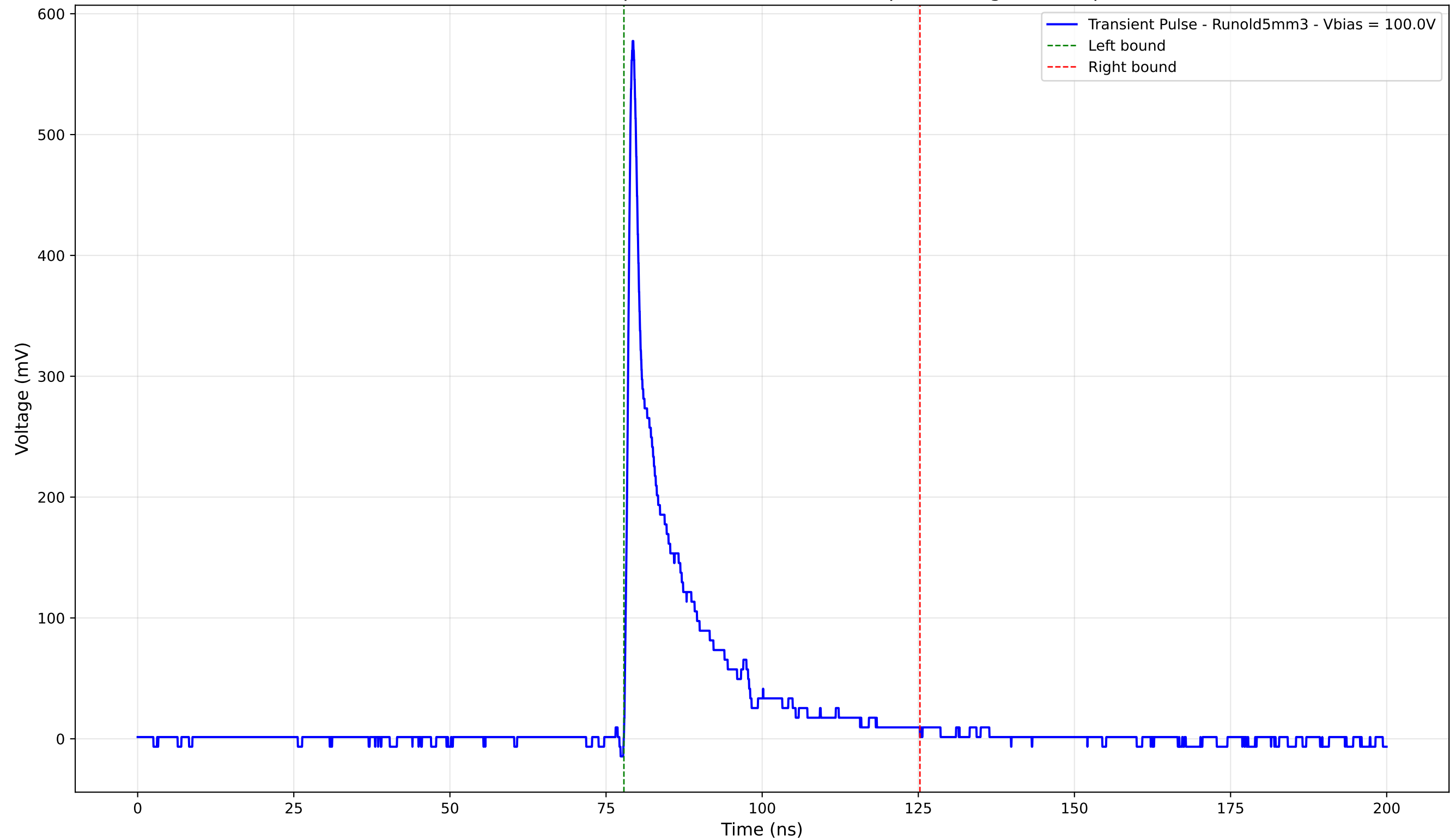
Transient Pulse - Sample: old5 - Position: 225.0 \mu\text{m} - Charge: 75.46 pC
