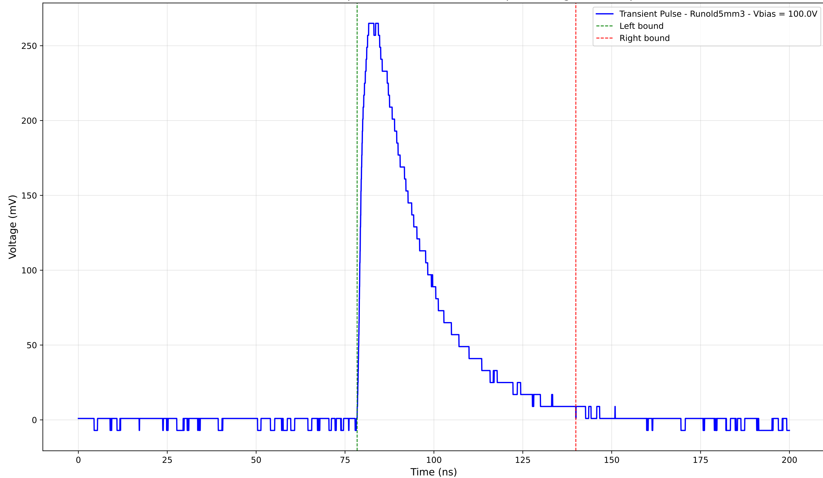
Transient Pulse - Sample: old5 - Position: 2500.0 \mu\text{m} - Charge: 100.83 pC
