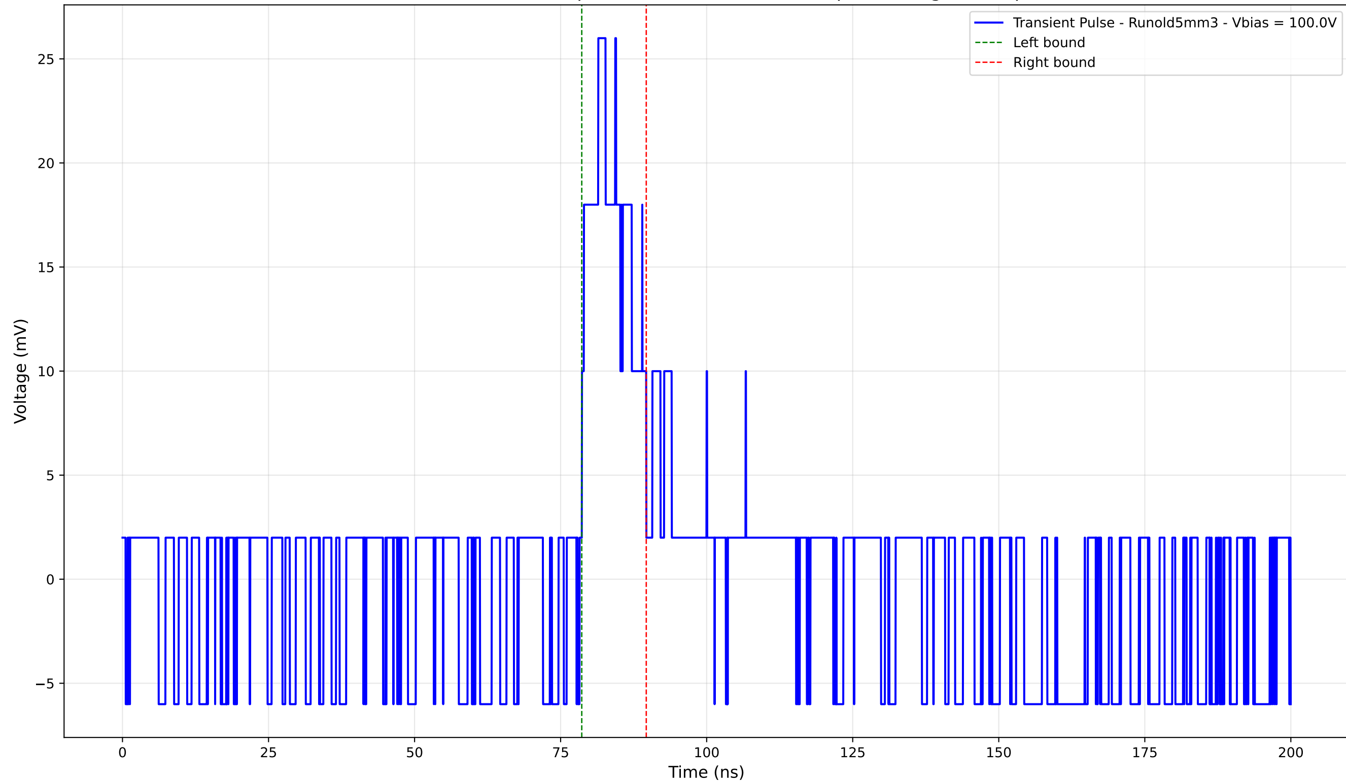
Transient Pulse - Sample: old5 - Position: 4180.0 \mu\text{m} - Charge: 3.69 pC
