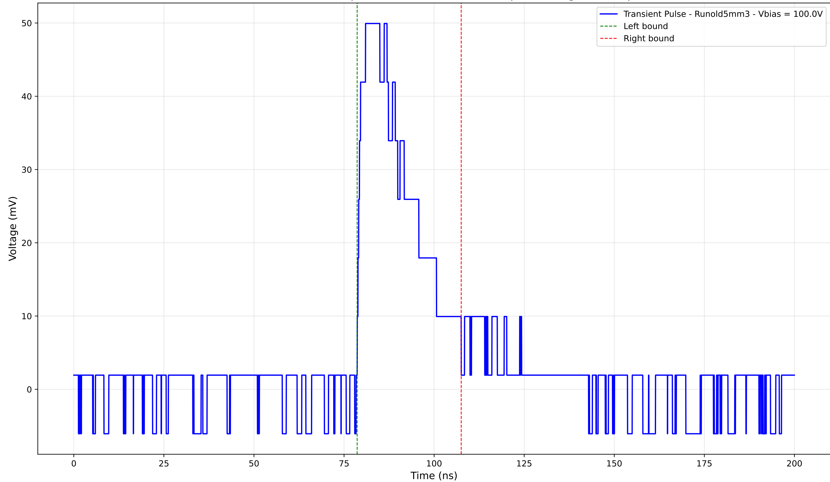
Transient Pulse - Sample: old5 - Position: 2630.0 \mu\text{m} - Charge: 15.91 pC
