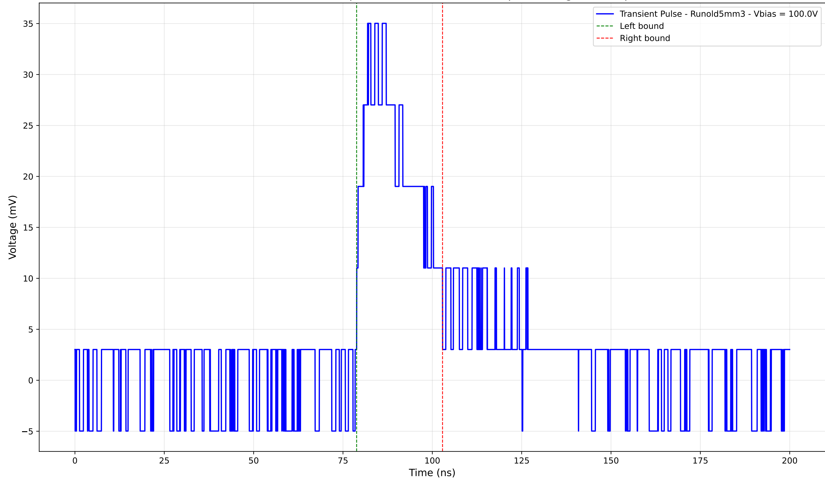
Transient Pulse - Sample: old5 - Position: 1795.0 \mu\text{m} - Charge: 10.46 pC
