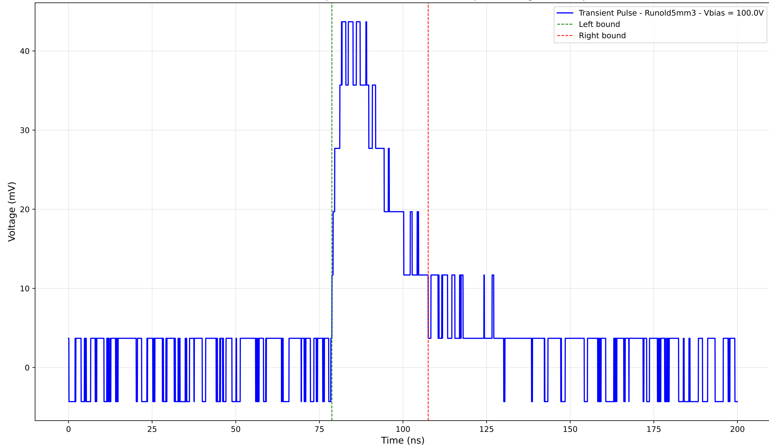
Transient Pulse - Sample: old5 - Position: 1600.0 \mu\text{m} - Charge: 14.86 pC
