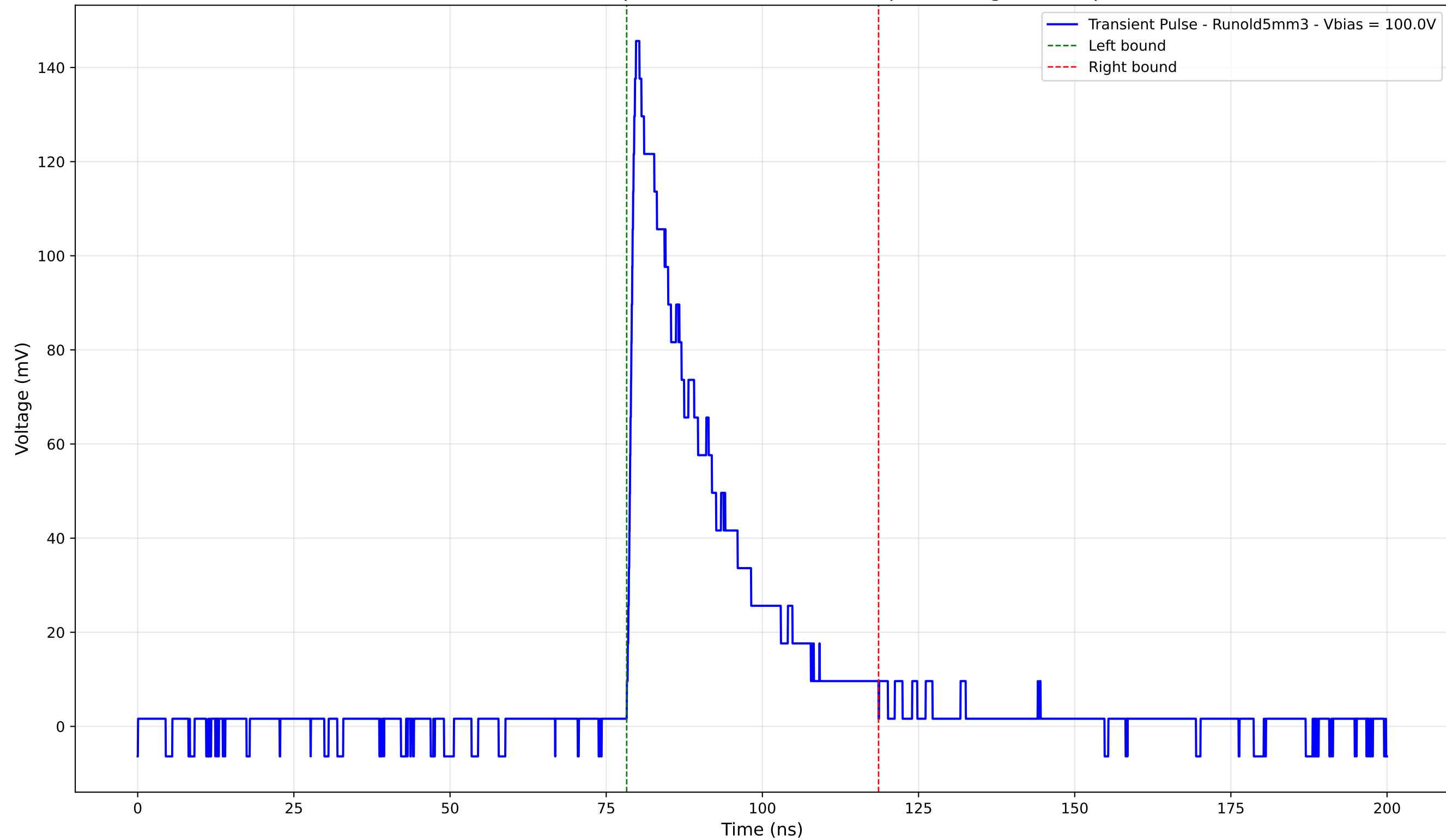
Transient Pulse - Sample: old5 - Position: 700.0 \mu\text{m} - Charge: 35.88 pC
