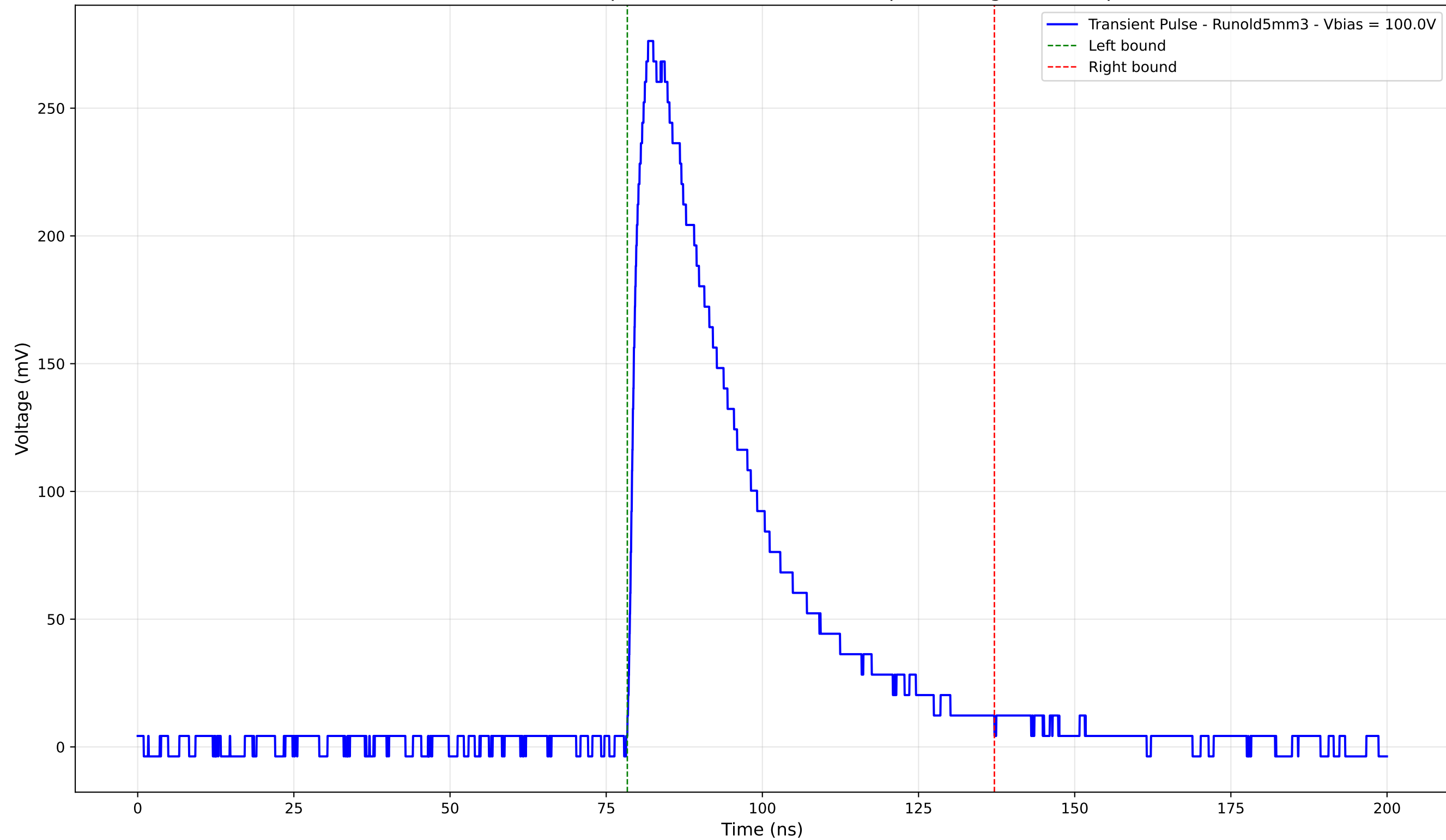
Transient Pulse - Sample: old5 - Position: 2520.0 \mu\text{m} - Charge: 104.18 pC
