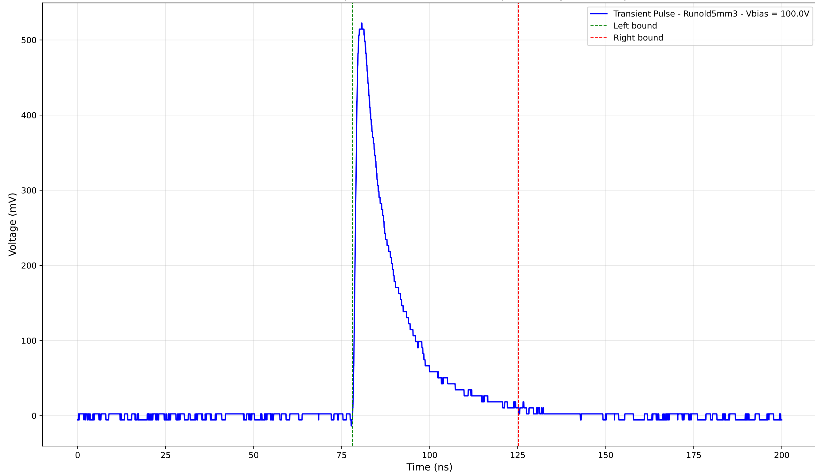
Transient Pulse - Sample: old5 - Position: 4330.0 \mu\text{m} - Charge: 117.86 pC
