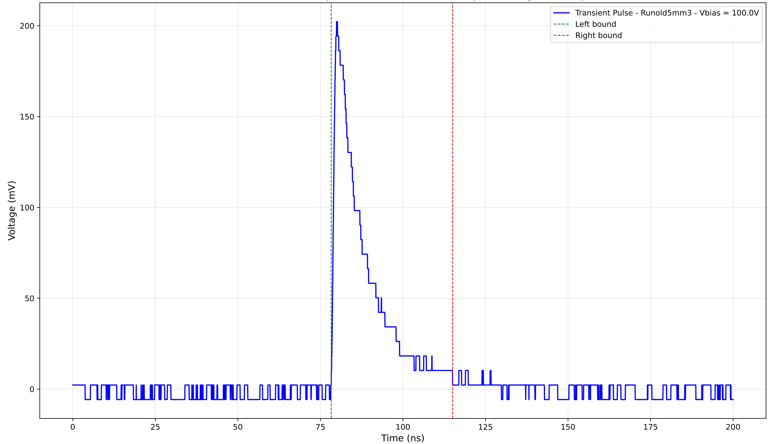
Transient Pulse - Sample: old5 - Position: 4435.0 \mu\text{m} - Charge: 39.86 pC
