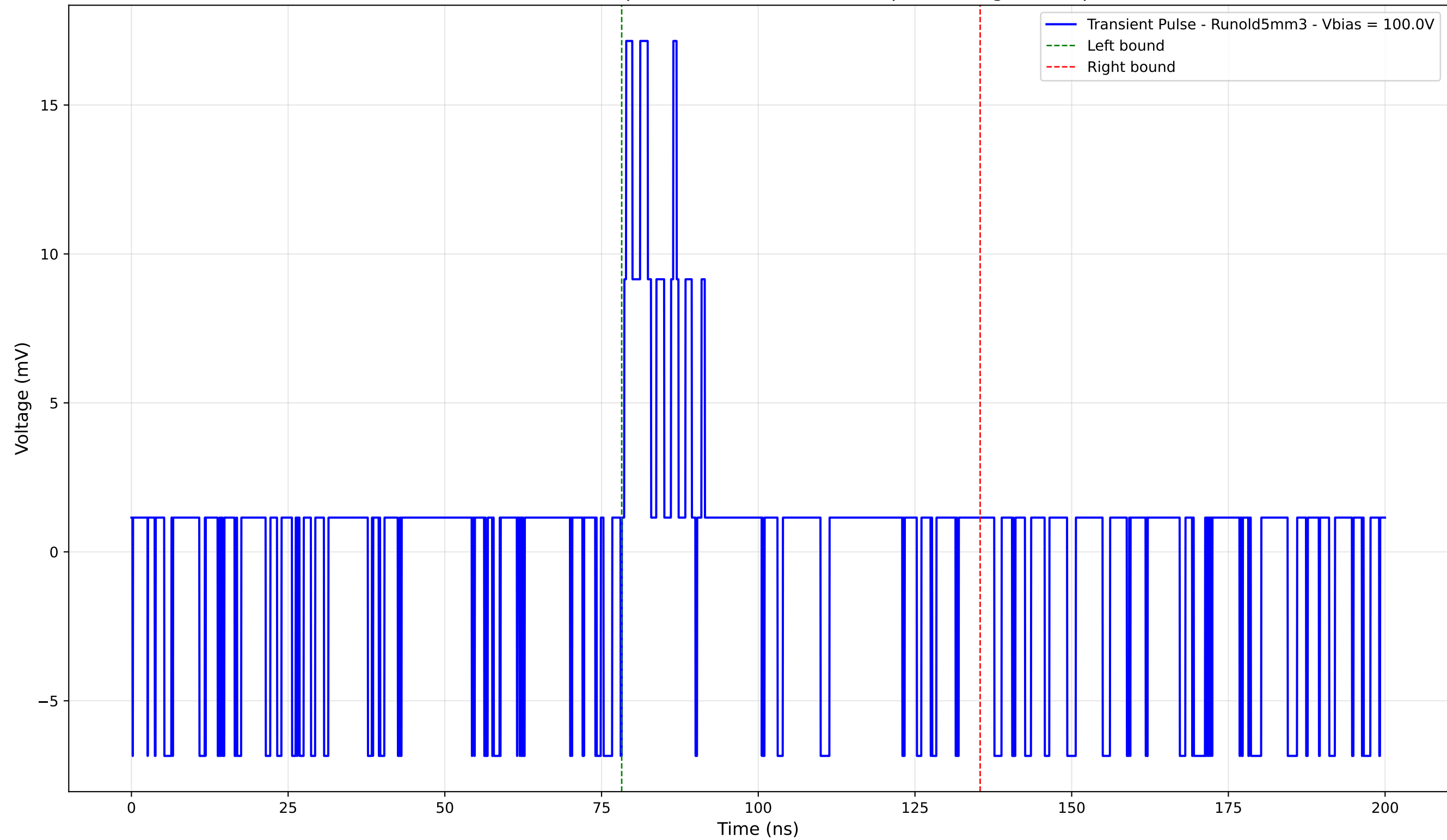
Transient Pulse - Sample: old5 - Position: 105.0 \mu\text{m} - Charge: 2.28 pC
