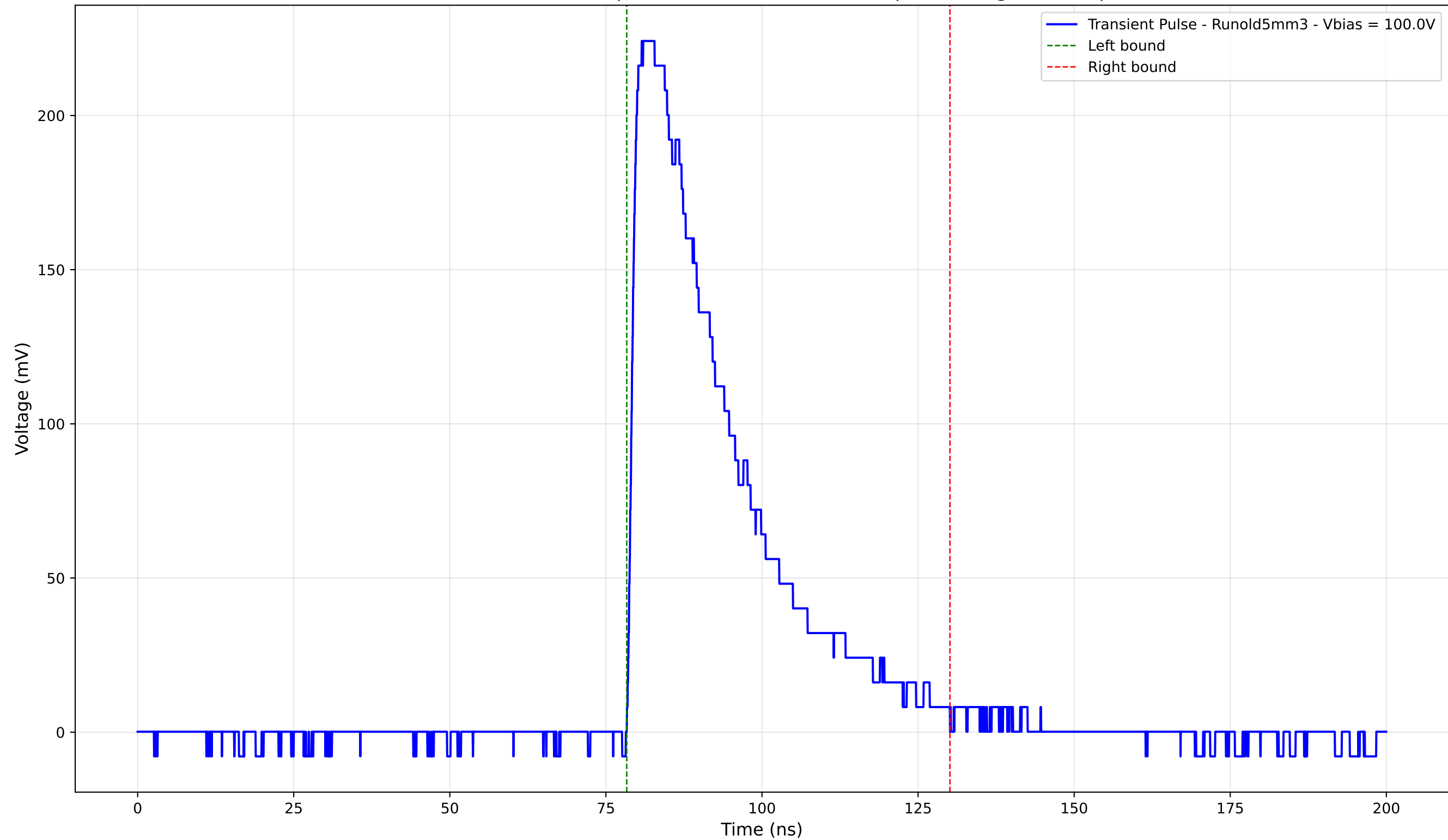
Transient Pulse - Sample: old5 - Position: 1060.0 \mu\text{m} - Charge: 79.05 pC
