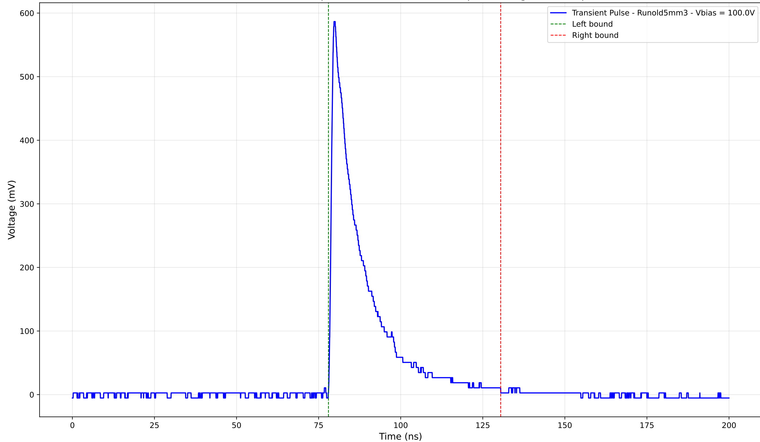
Transient Pulse - Sample: old5 - Position: 4605.0 \mu\text{m} - Charge: 117.58 pC
