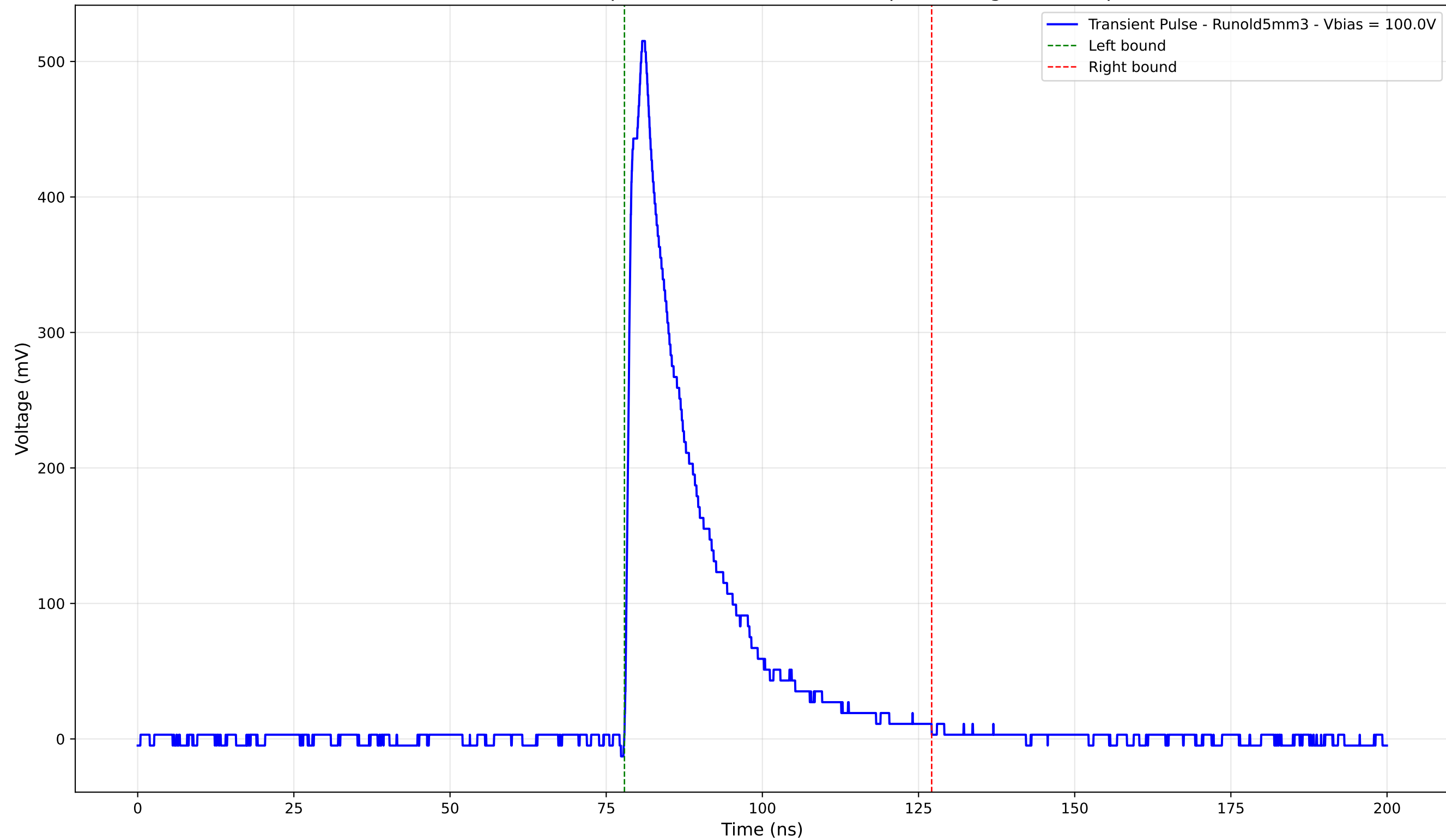
Transient Pulse - Sample: old5 - Position: 4045.0 \mu\text{m} - Charge: 112.95 pC
