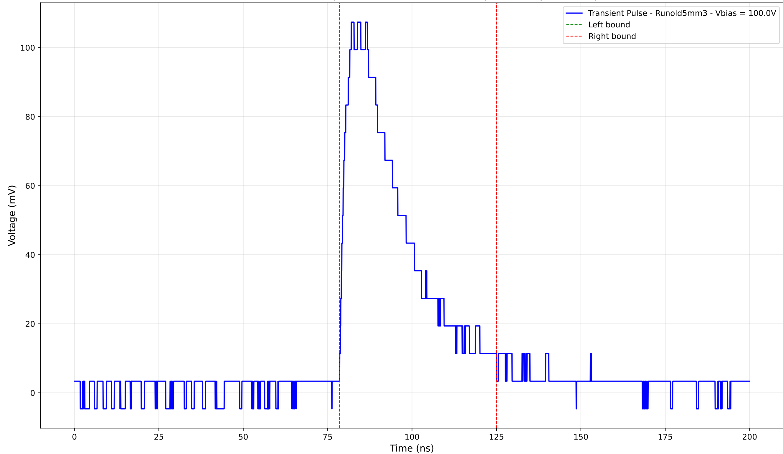
Transient Pulse - Sample: old5 - Position: 1745.0 \mu\text{m} - Charge: 42.69 pC
