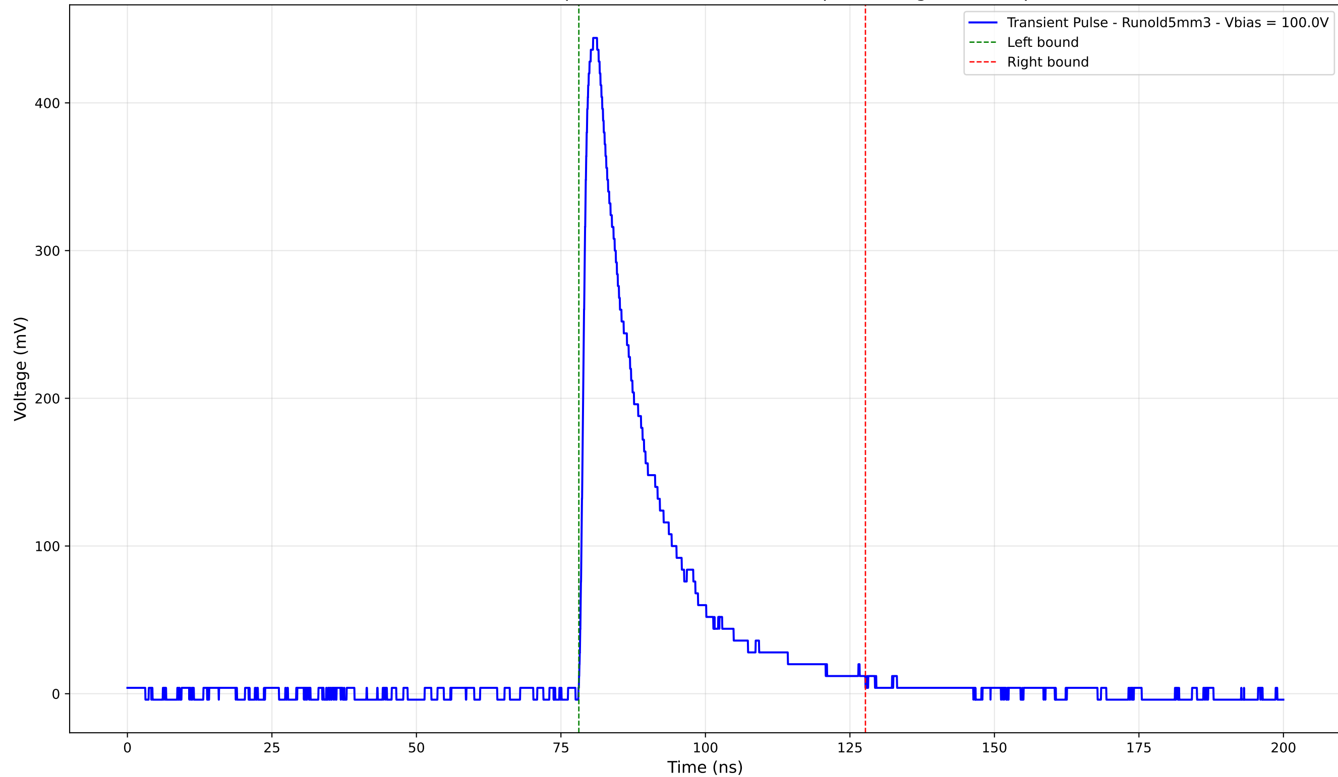
Transient Pulse - Sample: old5 - Position: 4285.0 \mu\text{m} - Charge: 102.72 pC
