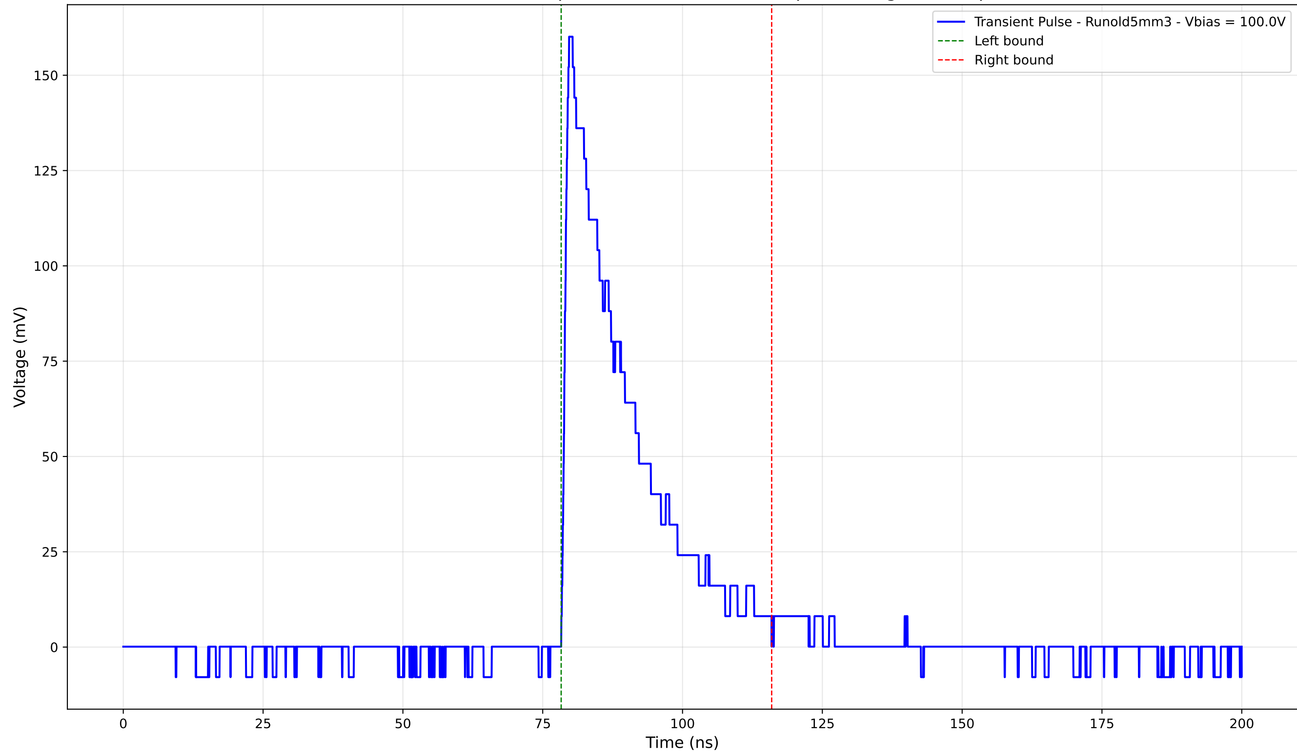
Transient Pulse - Sample: old5 - Position: 685.0 \mu\text{m} - Charge: 37.93 pC
