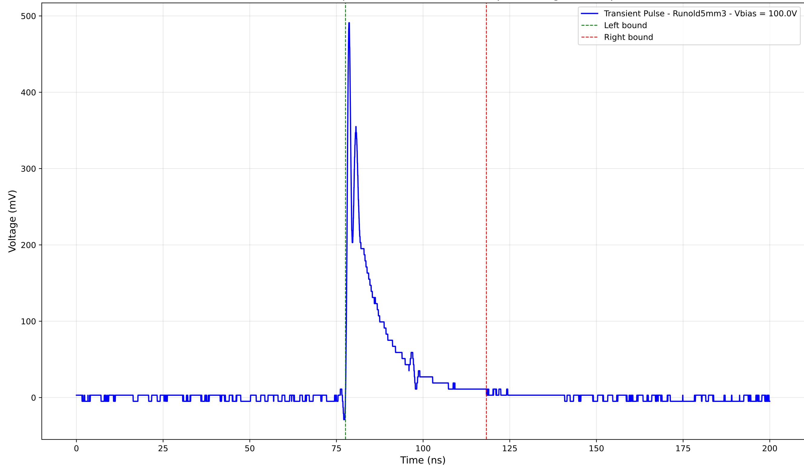
Transient Pulse - Sample: old5 - Position: 3655.0 \mu\text{m} - Charge: 61.87 pC
