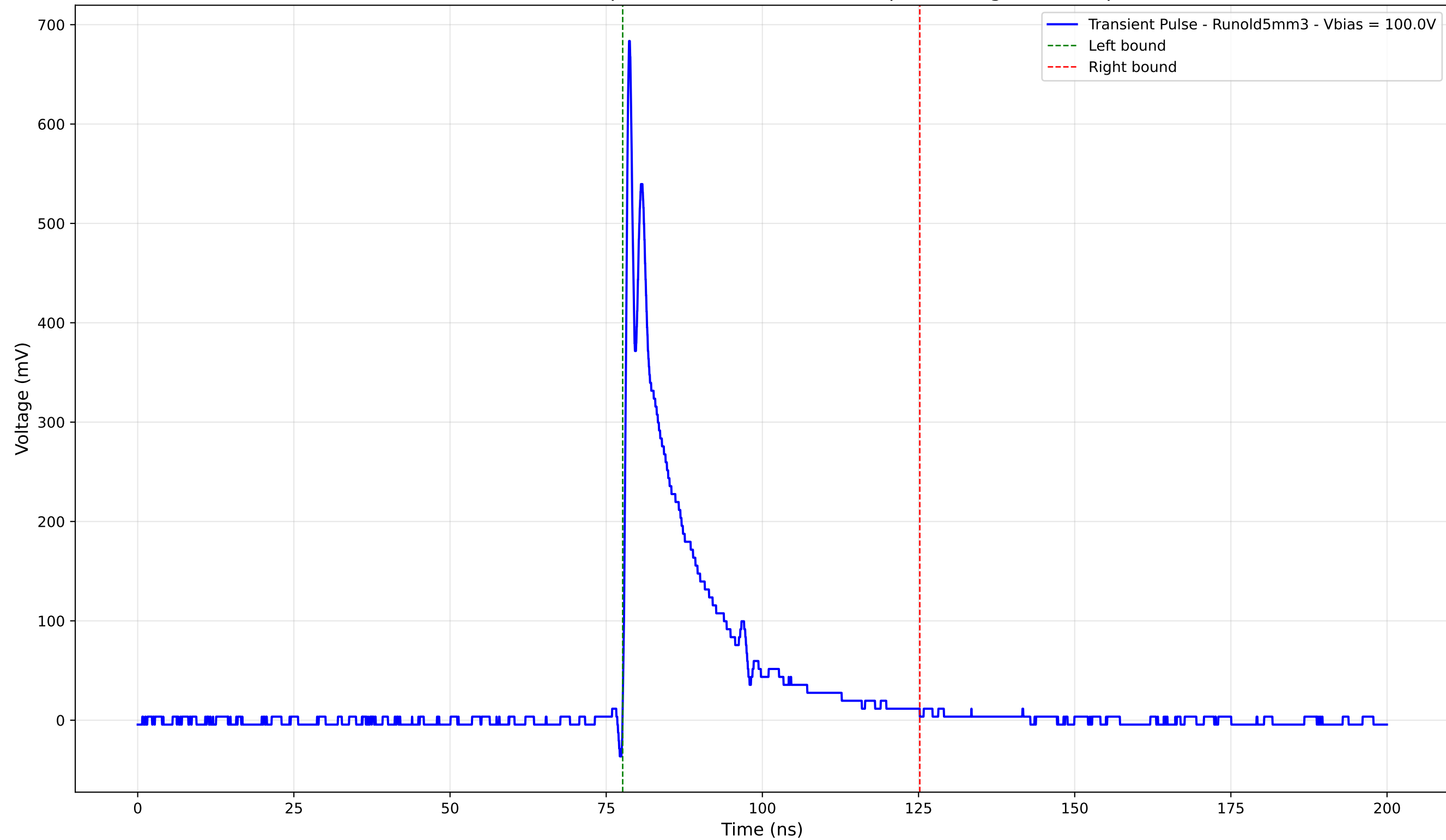
Transient Pulse - Sample: old5 - Position: 3440.0 \mu\text{m} - Charge: 106.80 pC
