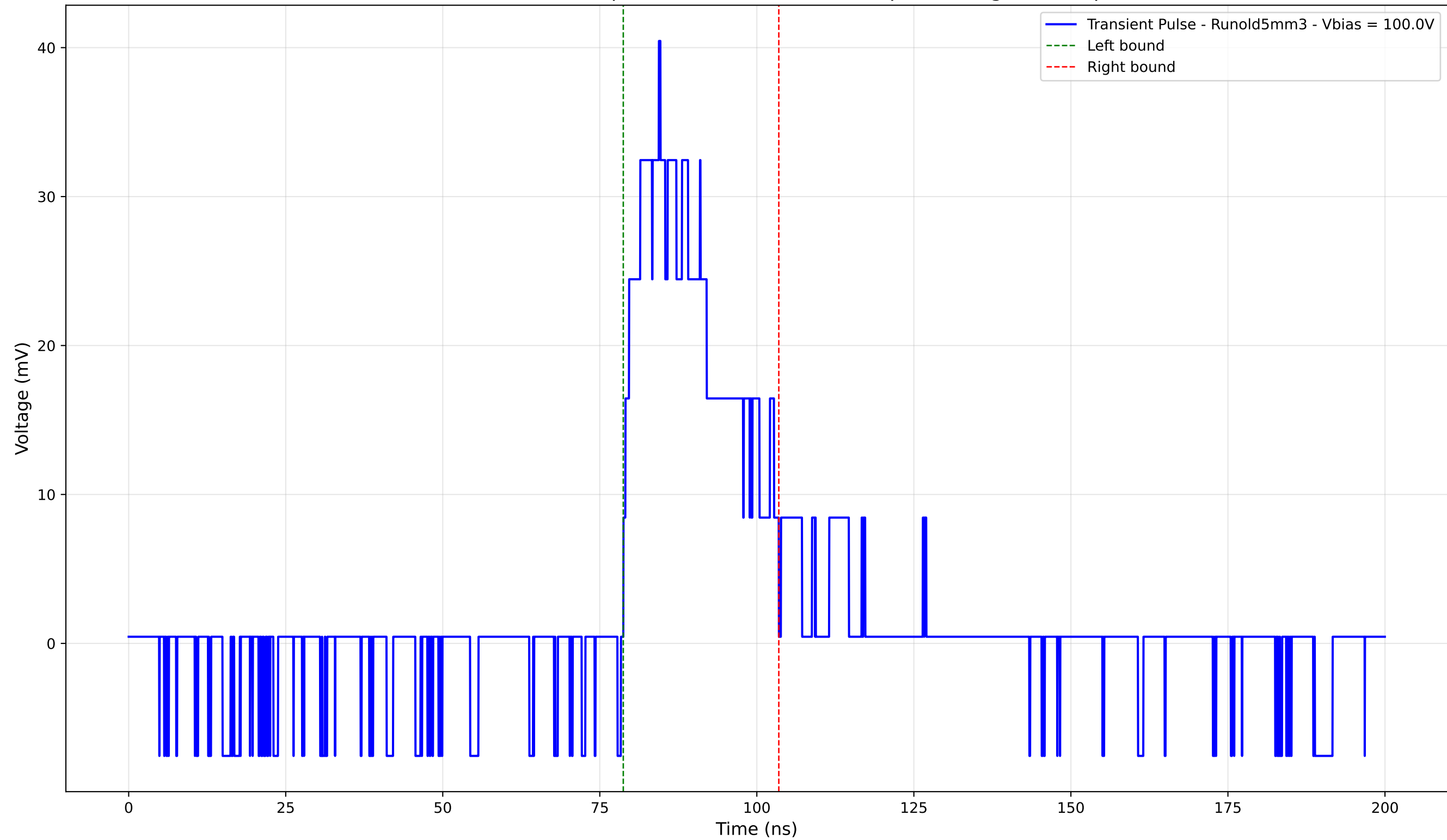
Transient Pulse - Sample: old5 - Position: 1375.0 \mu\text{m} - Charge: 10.69 pC
