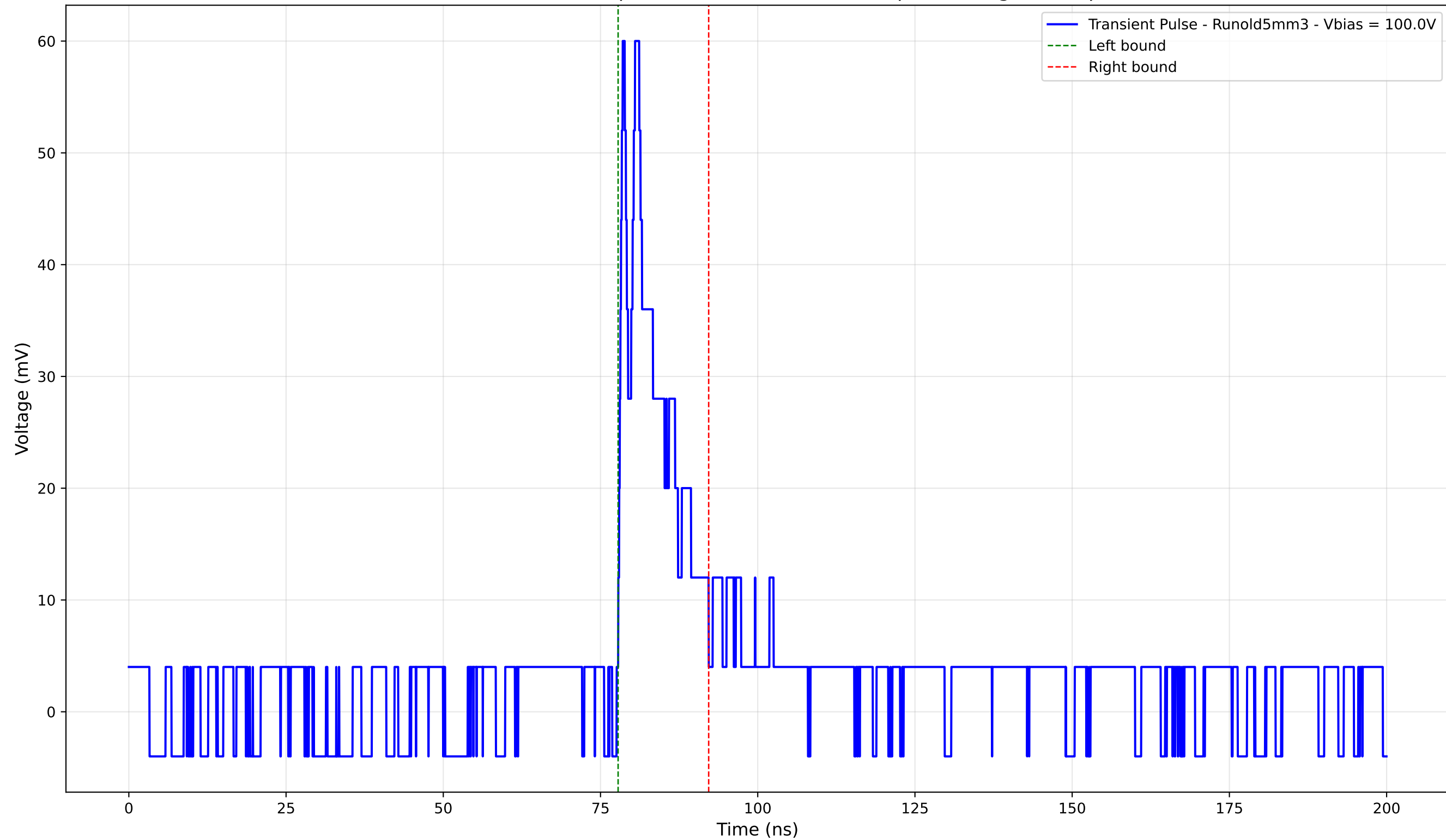
Transient Pulse - Sample: old5 - Position: 3605.0 \mu\text{m} - Charge: 8.07 pC
