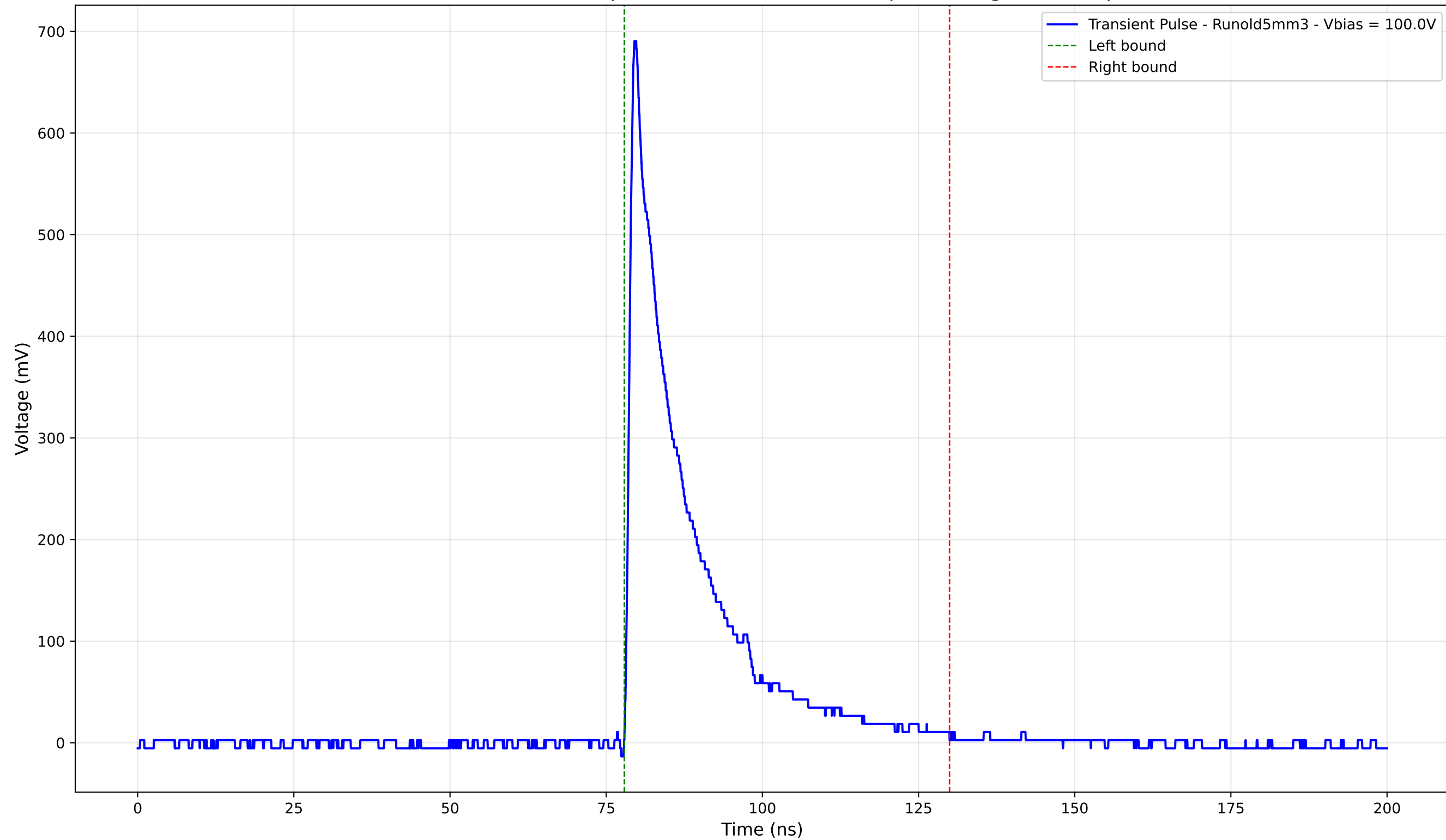
Transient Pulse - Sample: old5 - Position: 4680.0 \mu\text{m} - Charge: 130.21 pC
