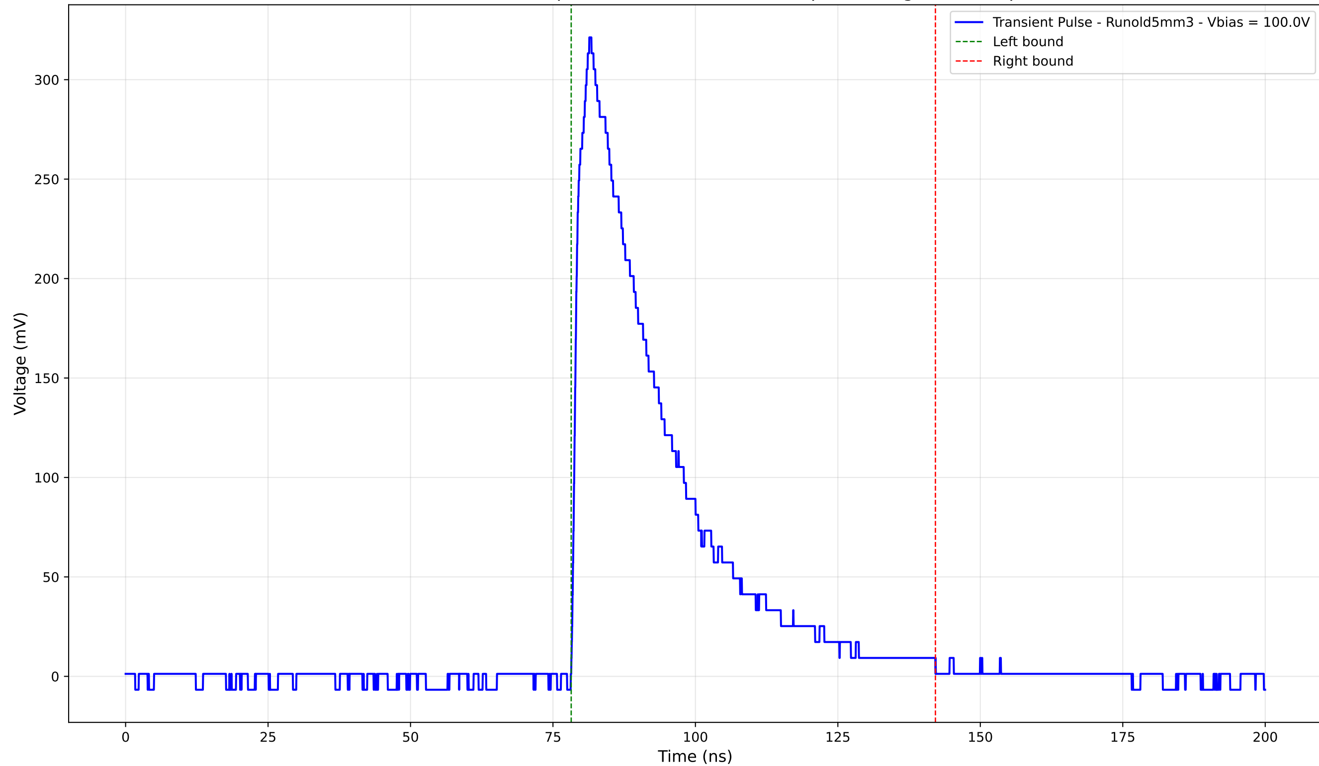
Transient Pulse - Sample: old5 - Position: 2830.0 \mu\text{m} - Charge: 105.88 pC
