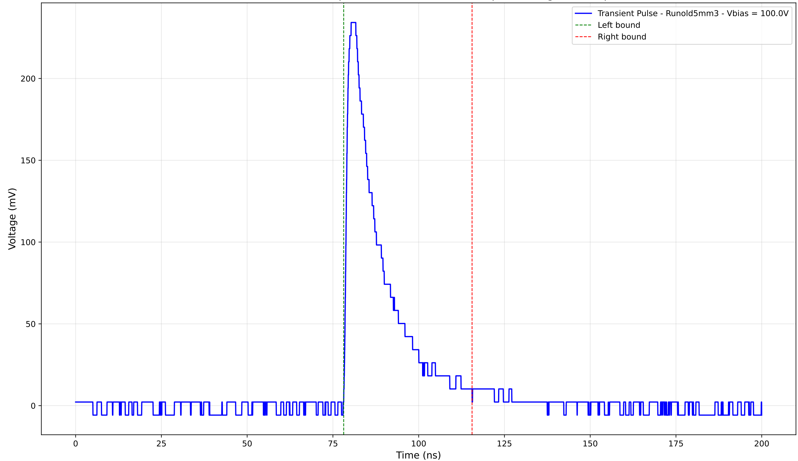
Transient Pulse - Sample: old5 - Position: 4250.0 \mu\text{m} - Charge: 51.97 pC
