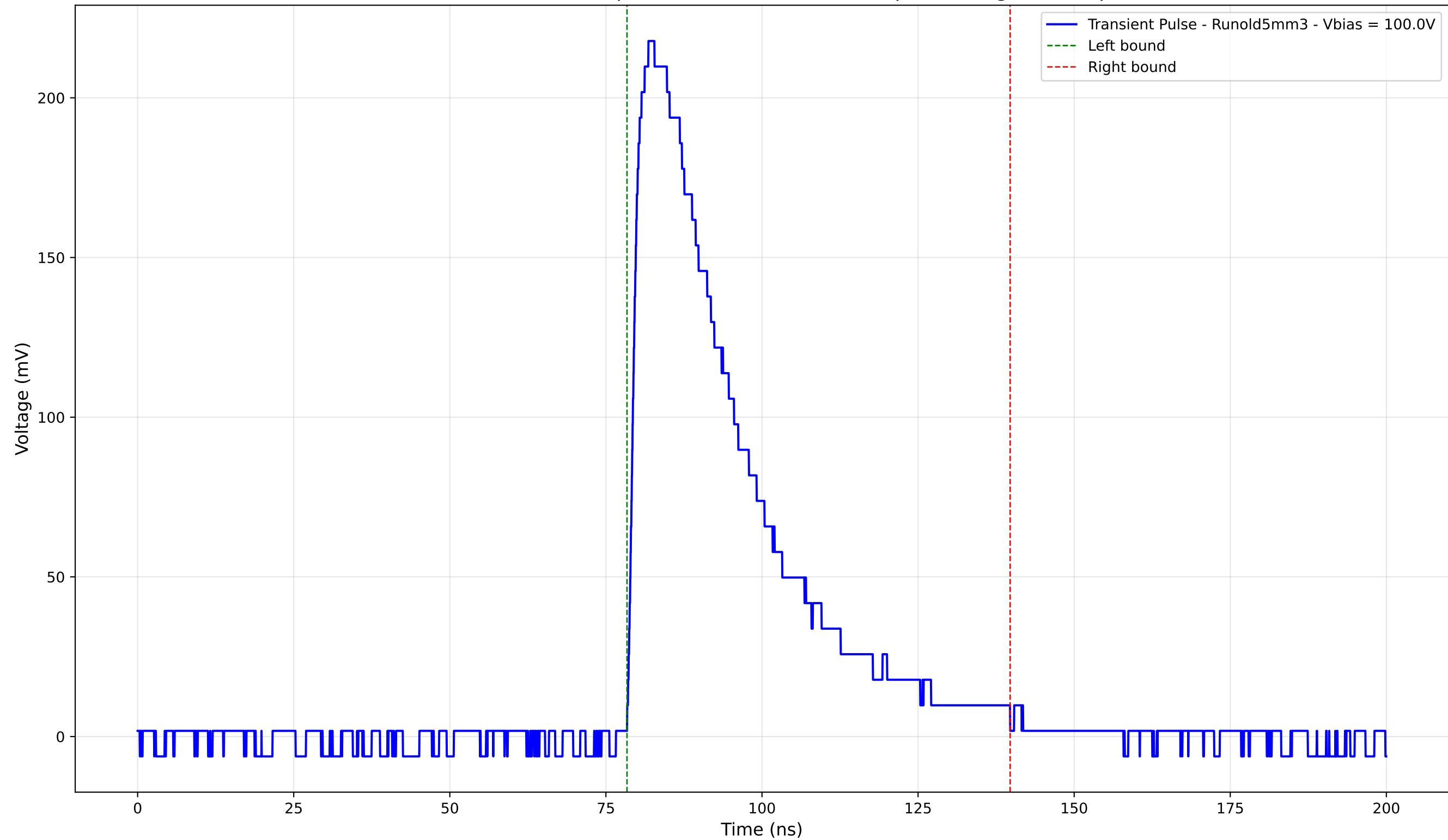
Transient Pulse - Sample: old5 - Position: 1285.0 \mu\text{m} - Charge: 83.25 pC
