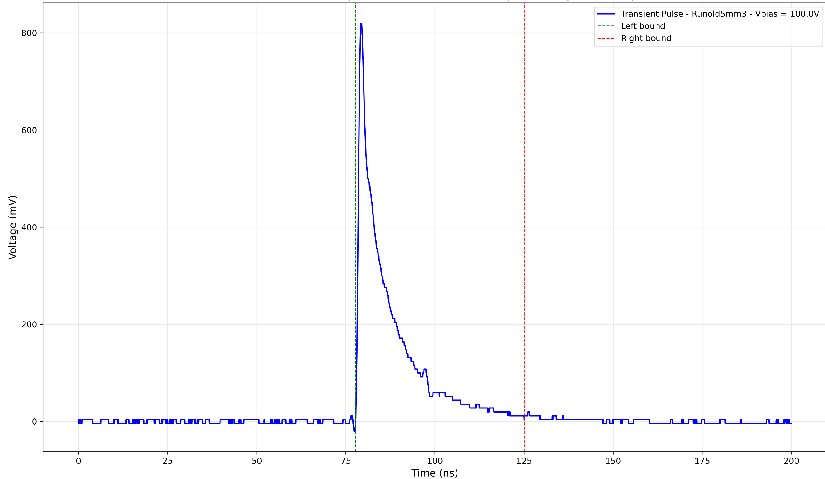
Transient Pulse - Sample: old5 - Position: 4800.0 \mu\text{m} - Charge: 130.30 pC
