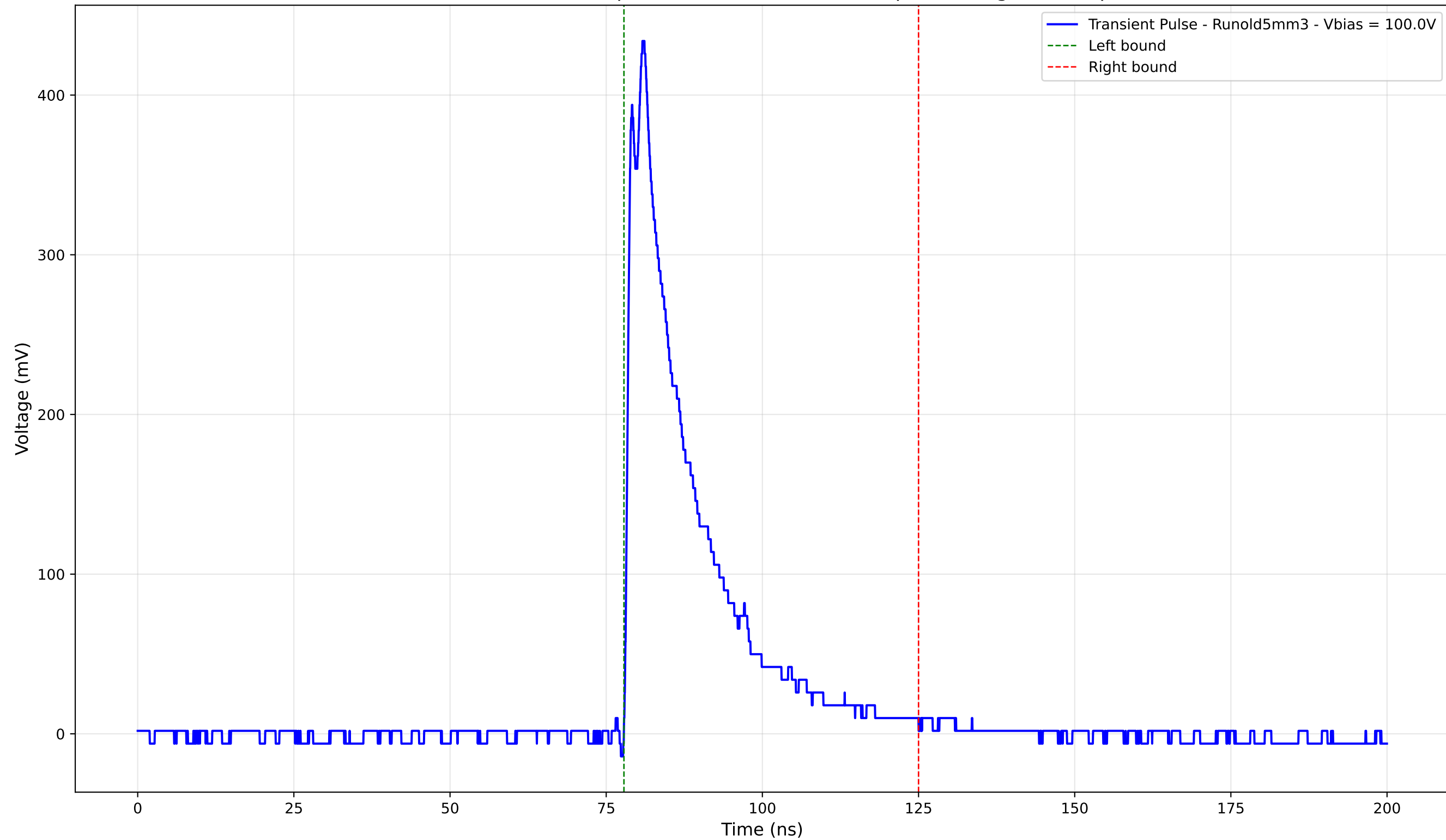
Transient Pulse - Sample: old5 - Position: 3980.0 \mu\text{m} - Charge: 92.24 pC
