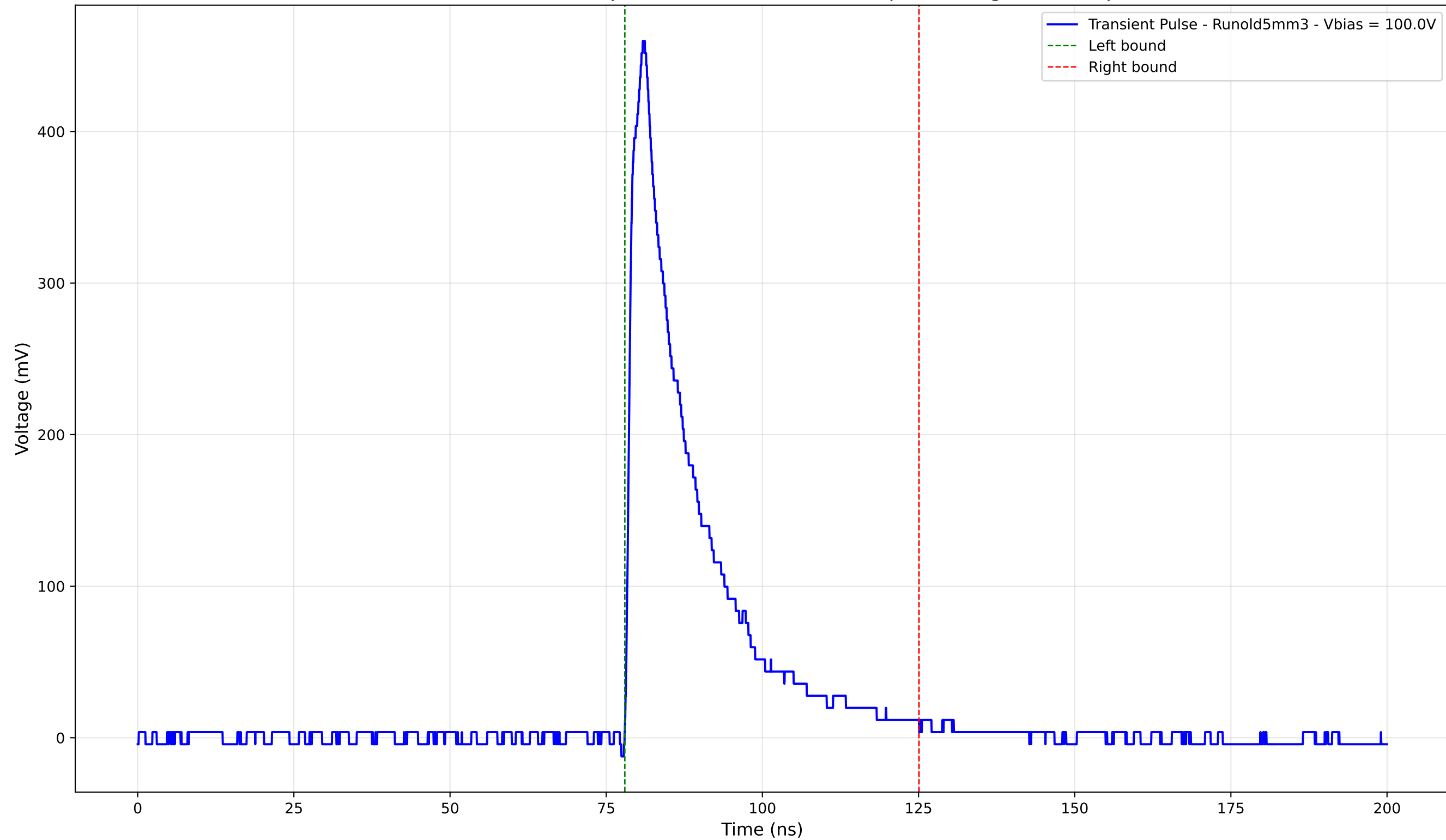
Transient Pulse - Sample: old5 - Position: 4080.0 \mu\text{m} - Charge: 100.10 pC
