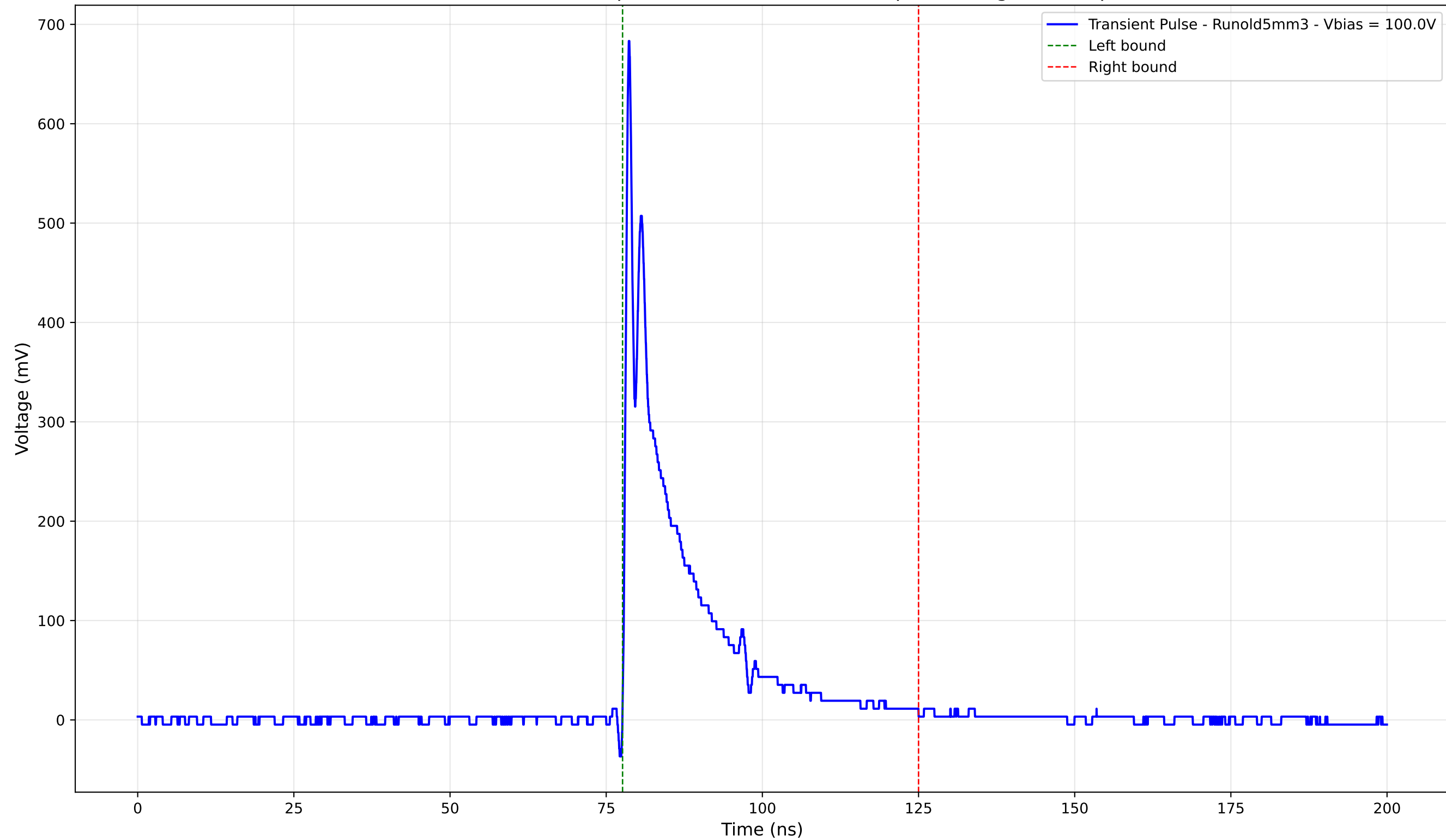
Transient Pulse - Sample: old5 - Position: 3480.0 \mu\text{m} - Charge: 95.19 pC
