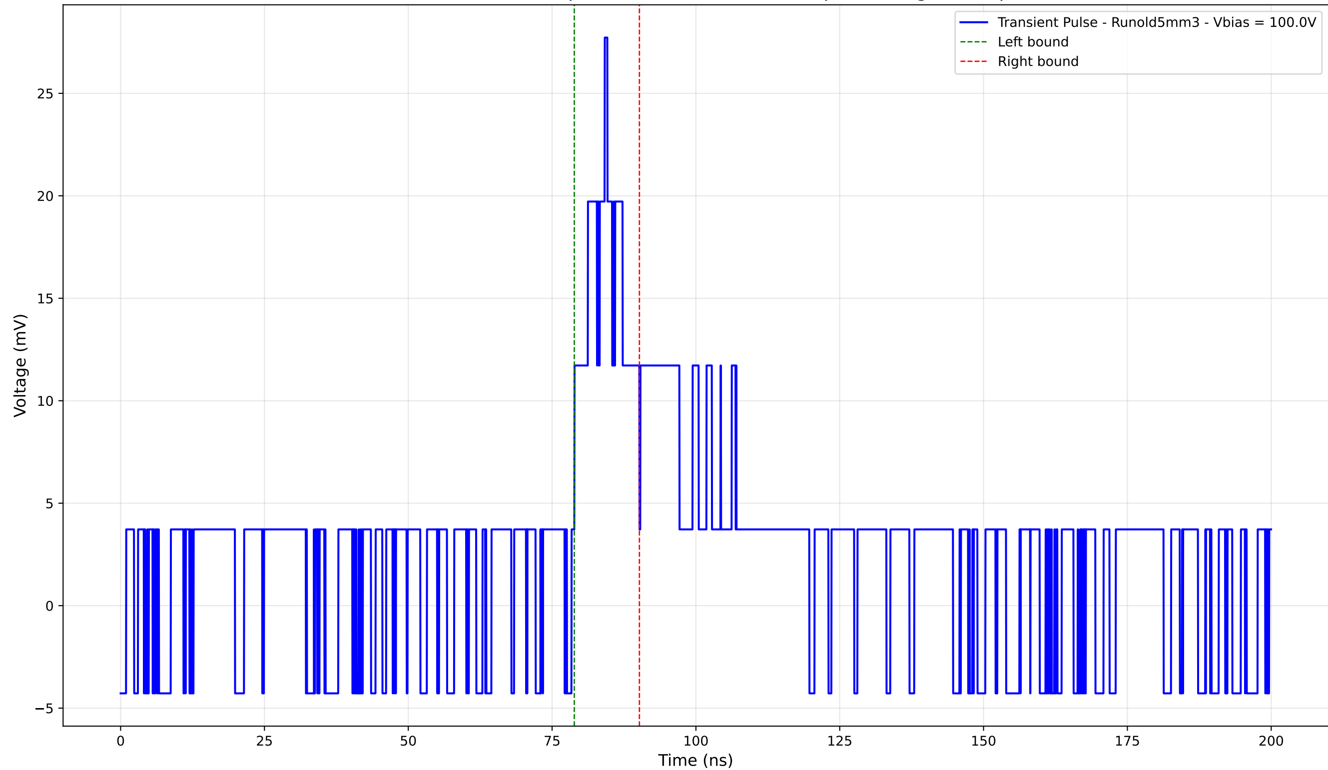
Transient Pulse - Sample: old5 - Position: 2685.0 \mu\text{m} - Charge: 3.59 pC
