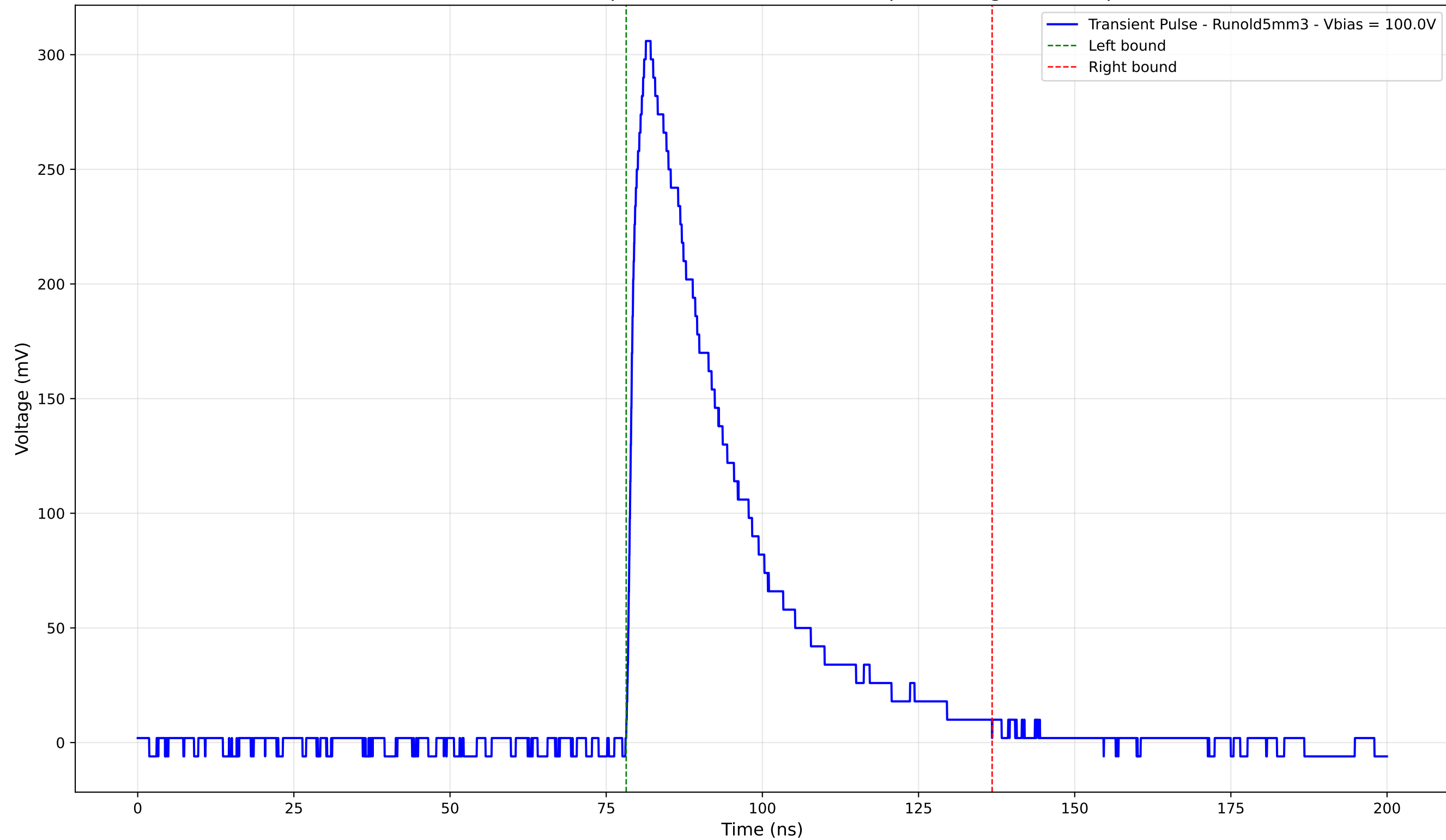
Transient Pulse - Sample: old5 - Position: 2795.0 \mu\text{m} - Charge: 102.36 pC
