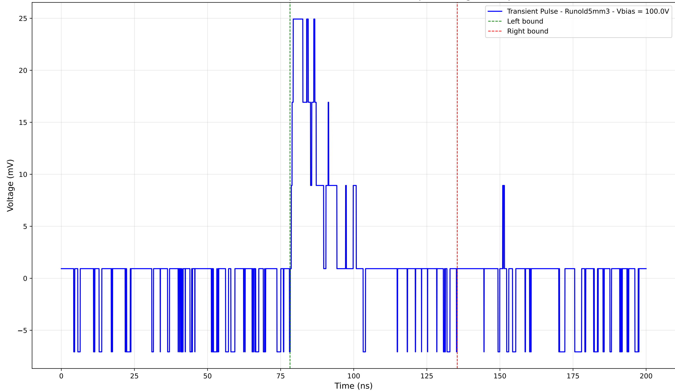
Transient Pulse - Sample: old5 - Position: 4165.0 \mu\text{m} - Charge: 5.08 pC
