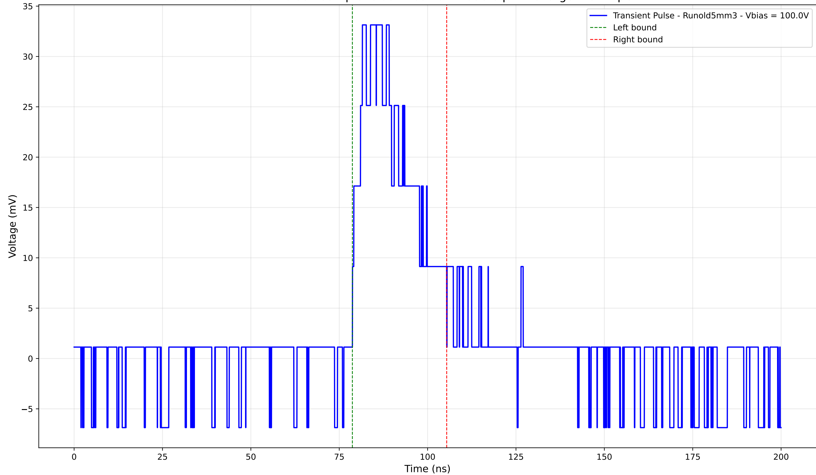
Transient Pulse - Sample: old5 - Position: 1990.0 \mu\text{m} - Charge: 10.47 pC
