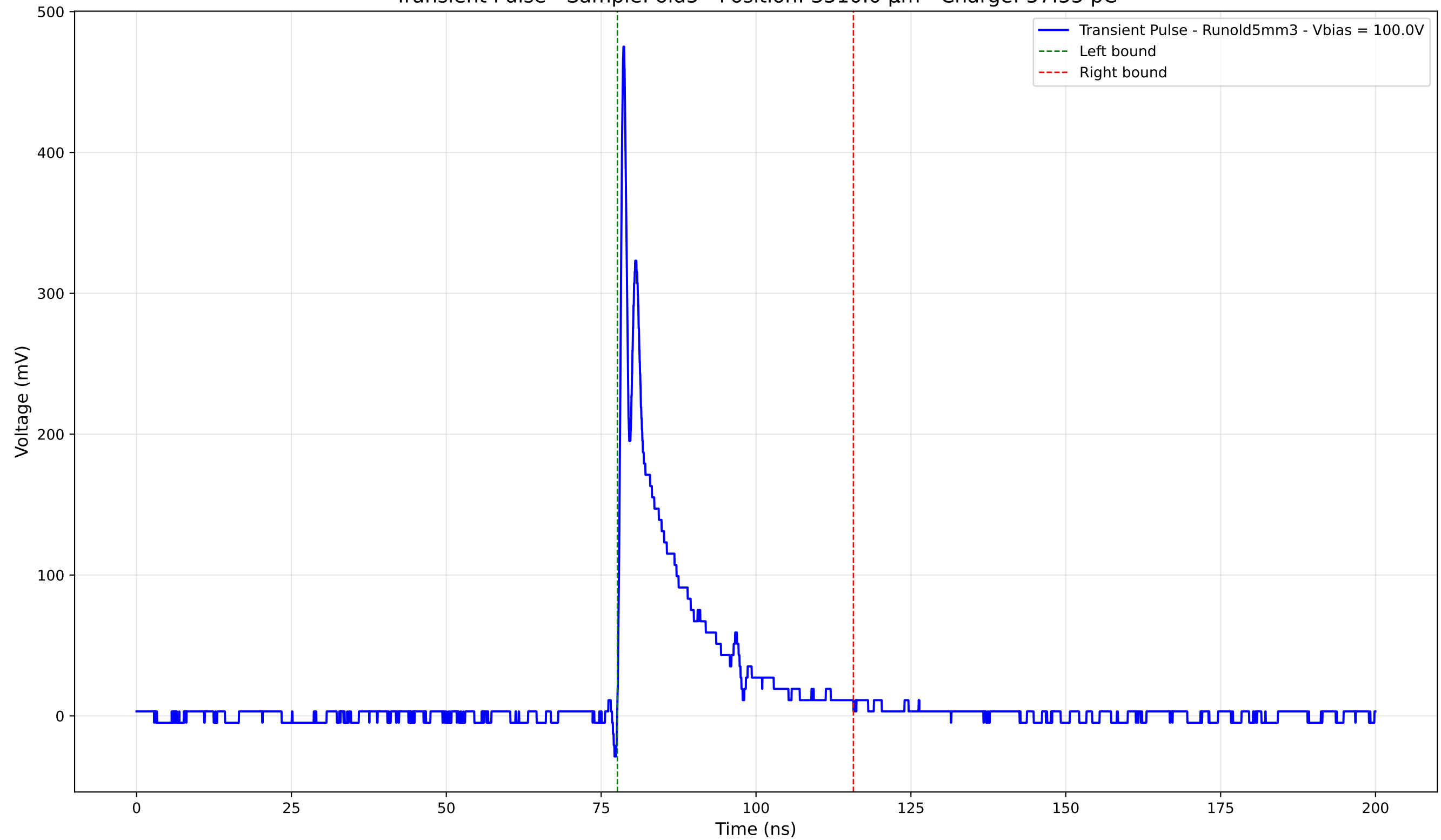
Transient Pulse - Sample: old5 - Position: 3510.0 \mu\text{m} - Charge: 57.55 pC
