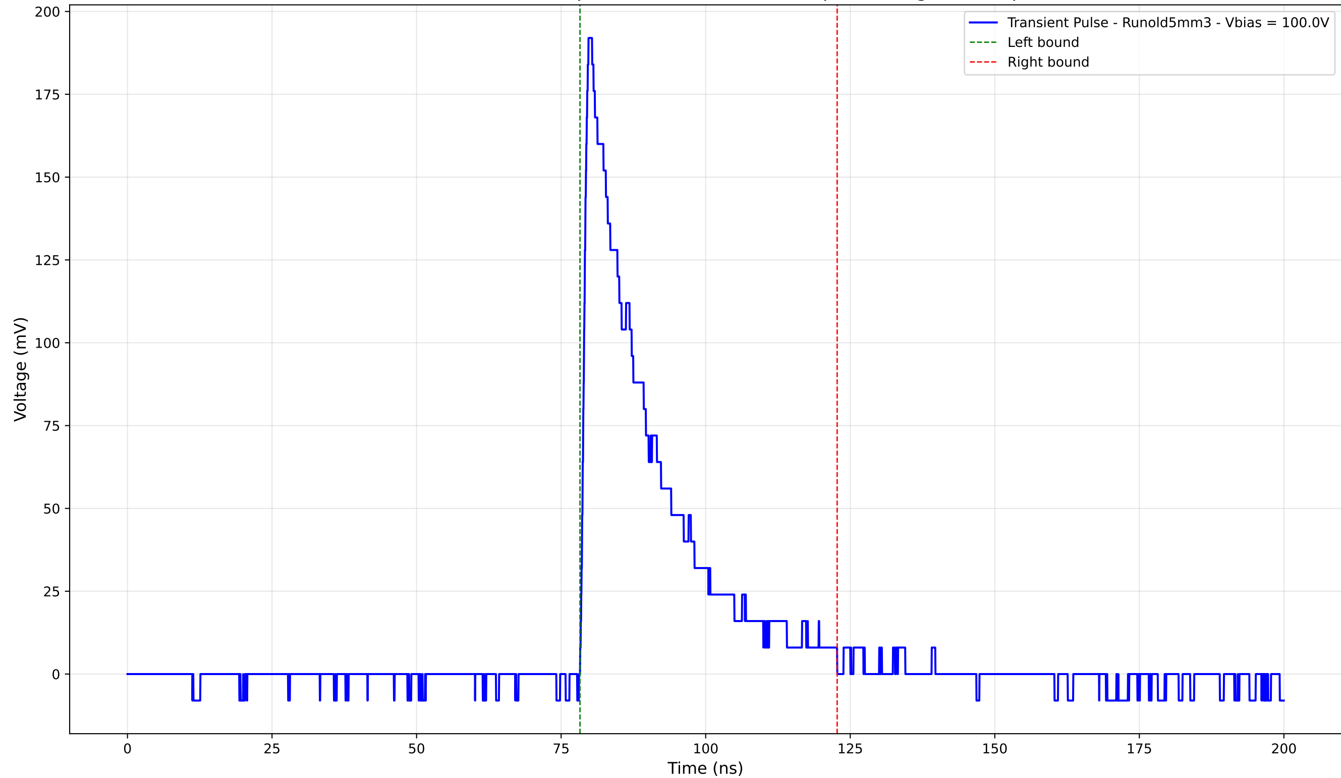
Transient Pulse - Sample: old5 - Position: 675.0 \mu\text{m} - Charge: 45.51 pC
