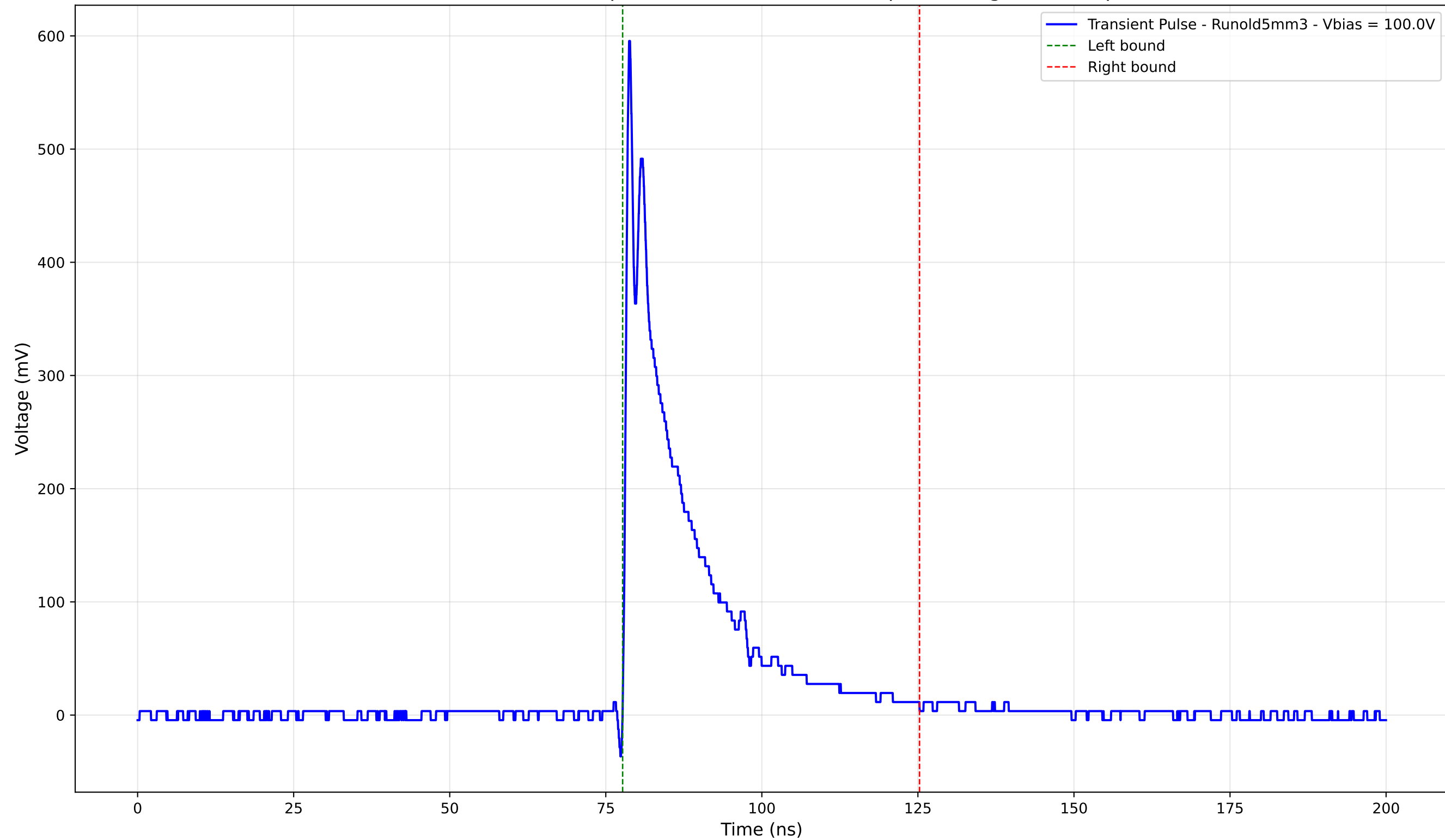
Transient Pulse - Sample: old5 - Position: 3395.0 \mu\text{m} - Charge: 102.99 pC
