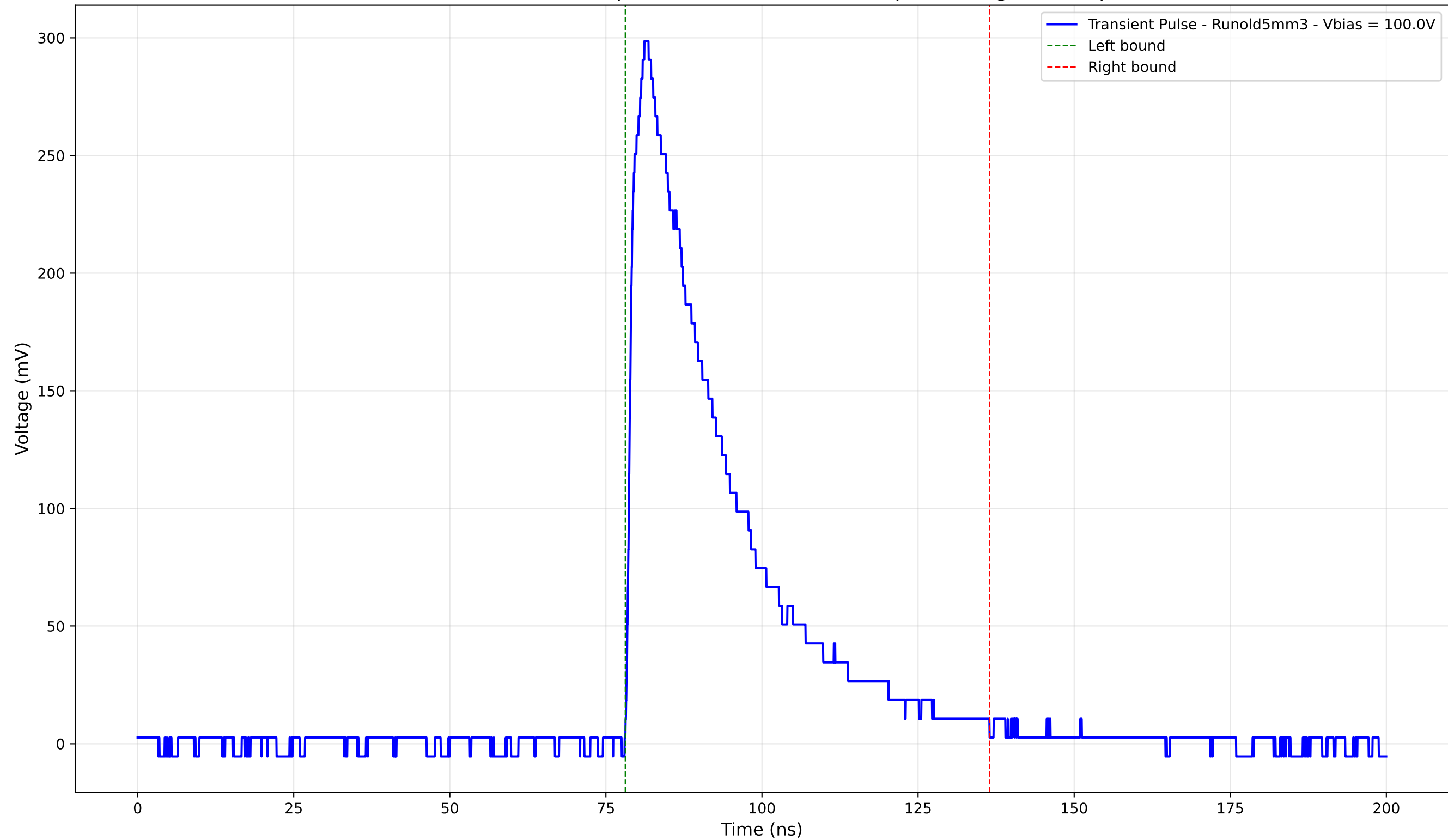
Transient Pulse - Sample: old5 - Position: 2870.0 \mu\text{m} - Charge: 97.47 pC
