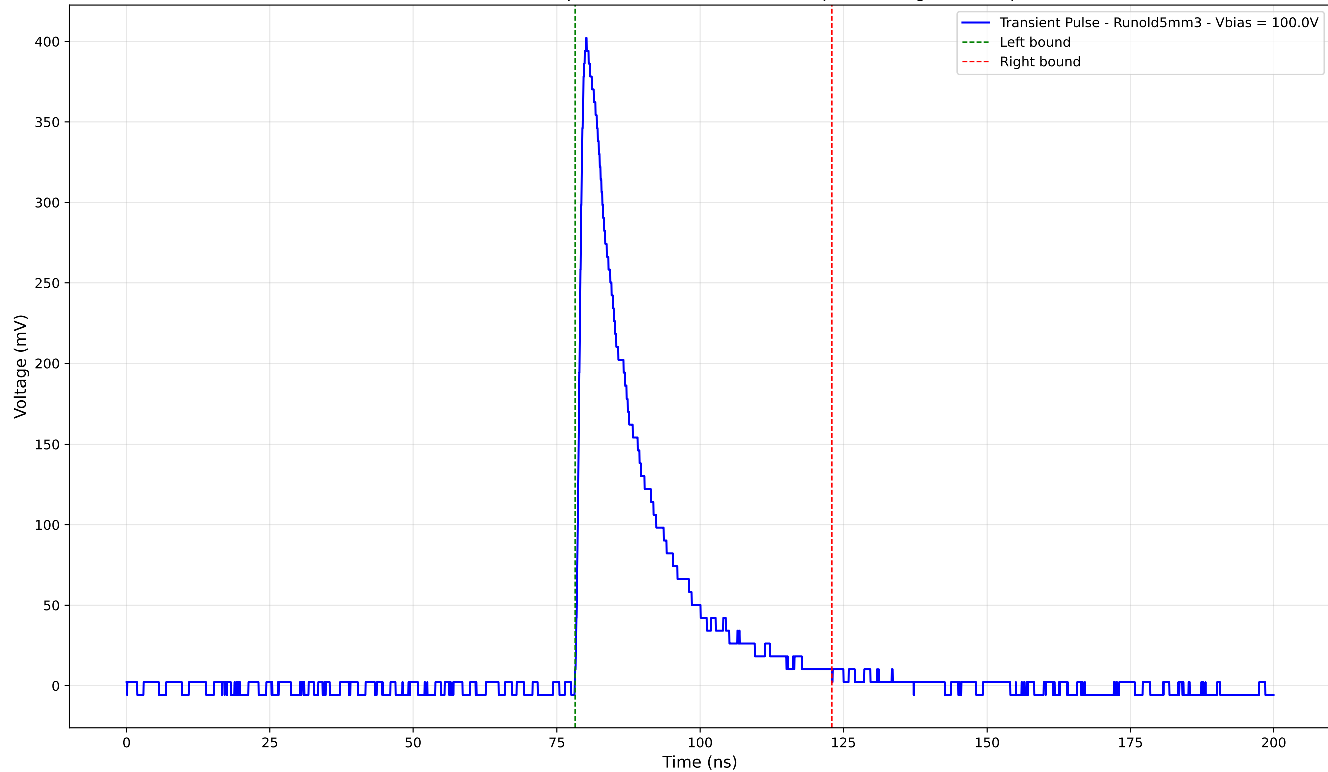
Transient Pulse - Sample: old5 - Position: 4405.0 \mu\text{m} - Charge: 84.70 pC
