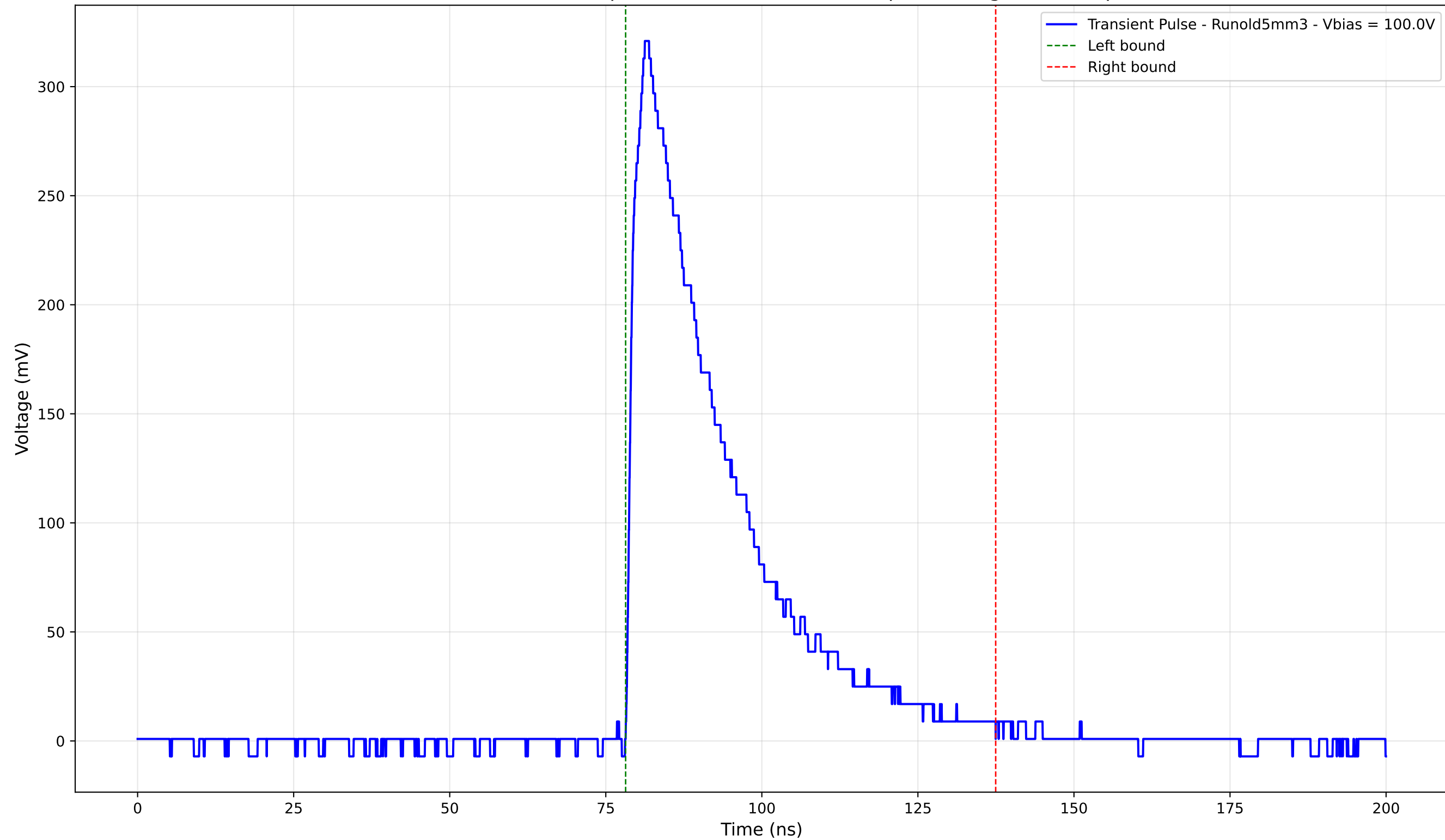
Transient Pulse - Sample: old5 - Position: 2825.0 \mu\text{m} - Charge: 104.83 pC
