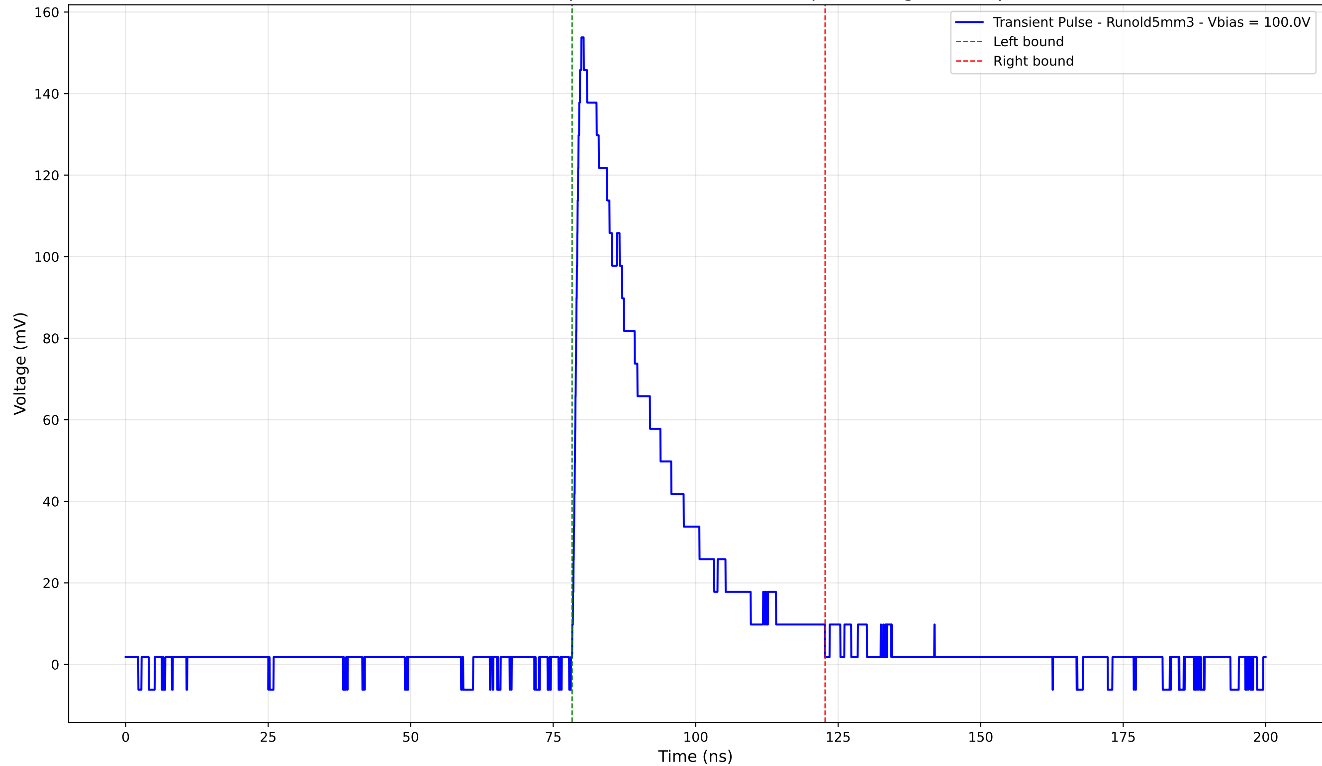
Transient Pulse - Sample: old5 - Position: 785.0 \mu\text{m} - Charge: 42.02 pC
