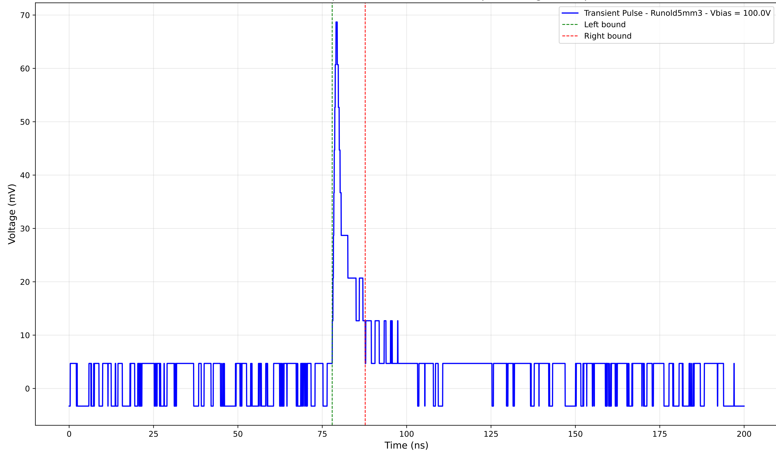
Transient Pulse - Sample: old5 - Position: 4930.0 \mu\text{m} - Charge: 5.48 pC
