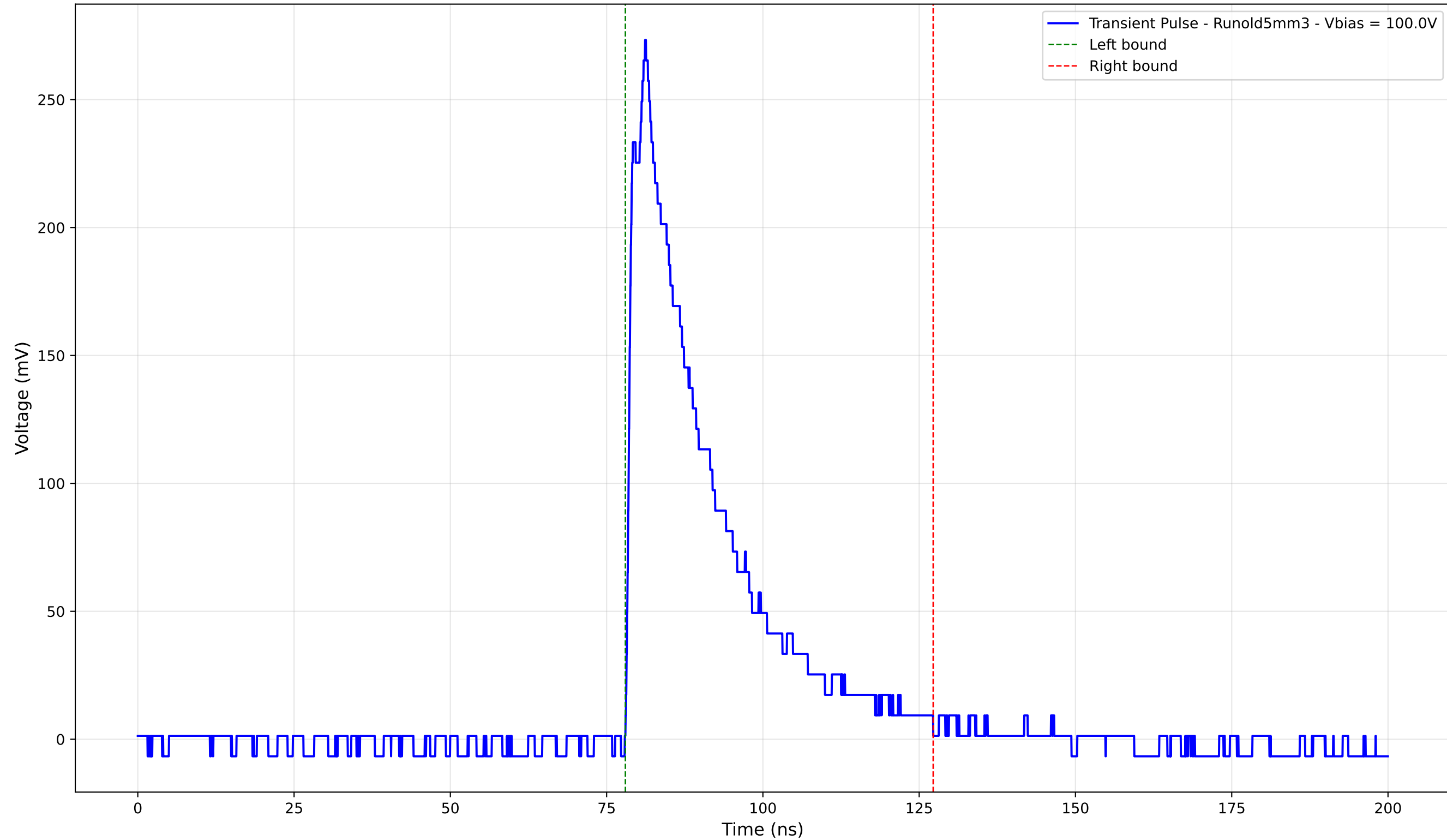
Transient Pulse - Sample: old5 - Position: 3060.0 \mu\text{m} - Charge: 72.20 pC
