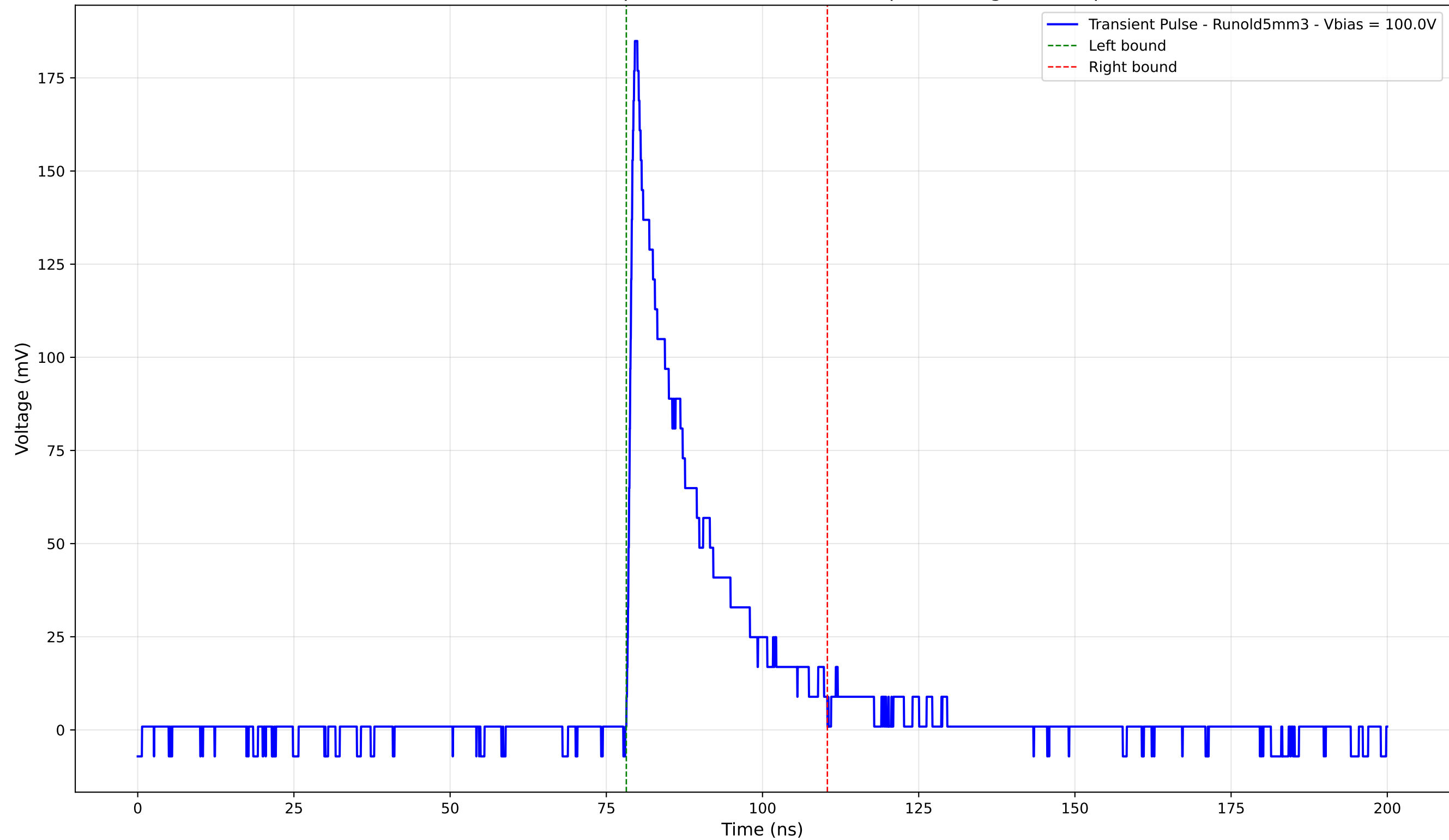
Transient Pulse - Sample: old5 - Position: 505.0 \mu\text{m} - Charge: 34.96 pC
