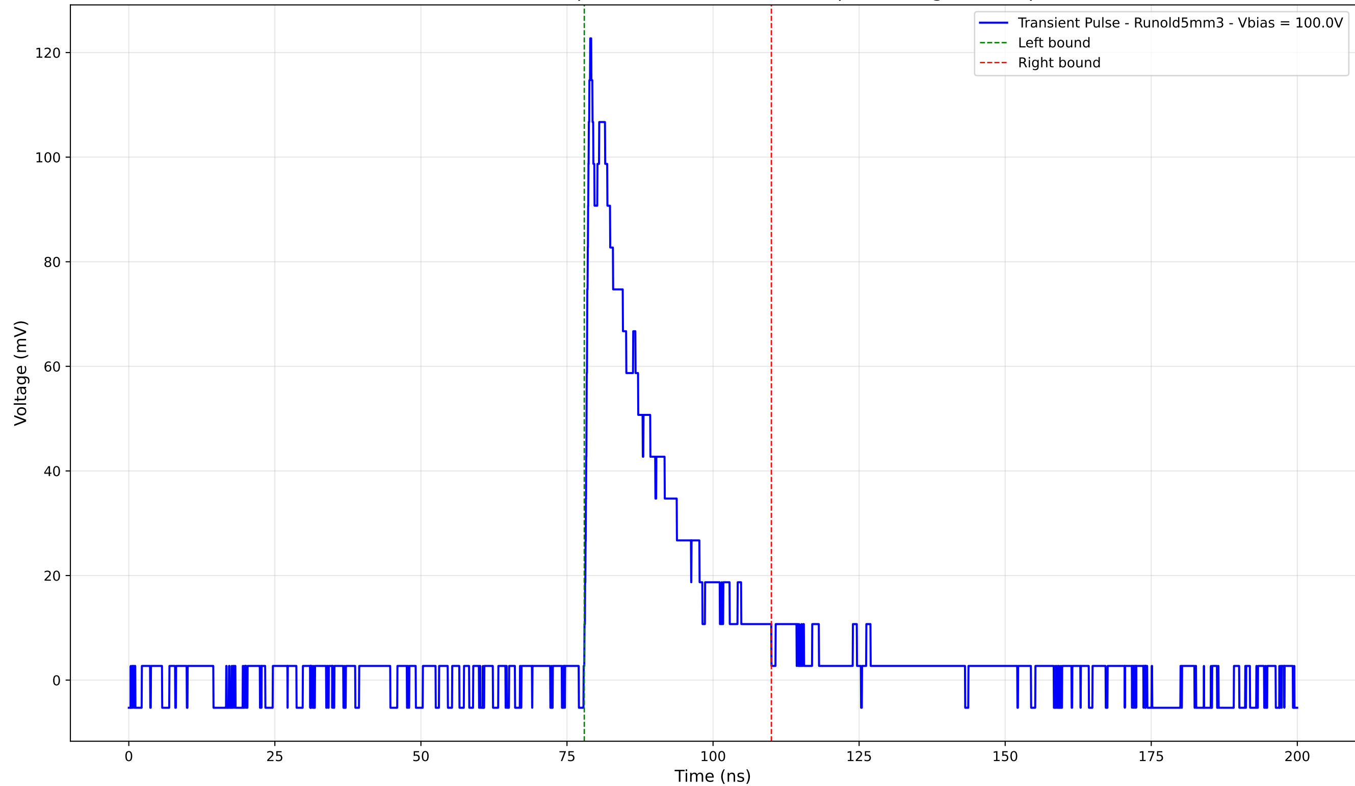
Transient Pulse - Sample: old5 - Position: 3230.0 \mu\text{m} - Charge: 25.89 pC
