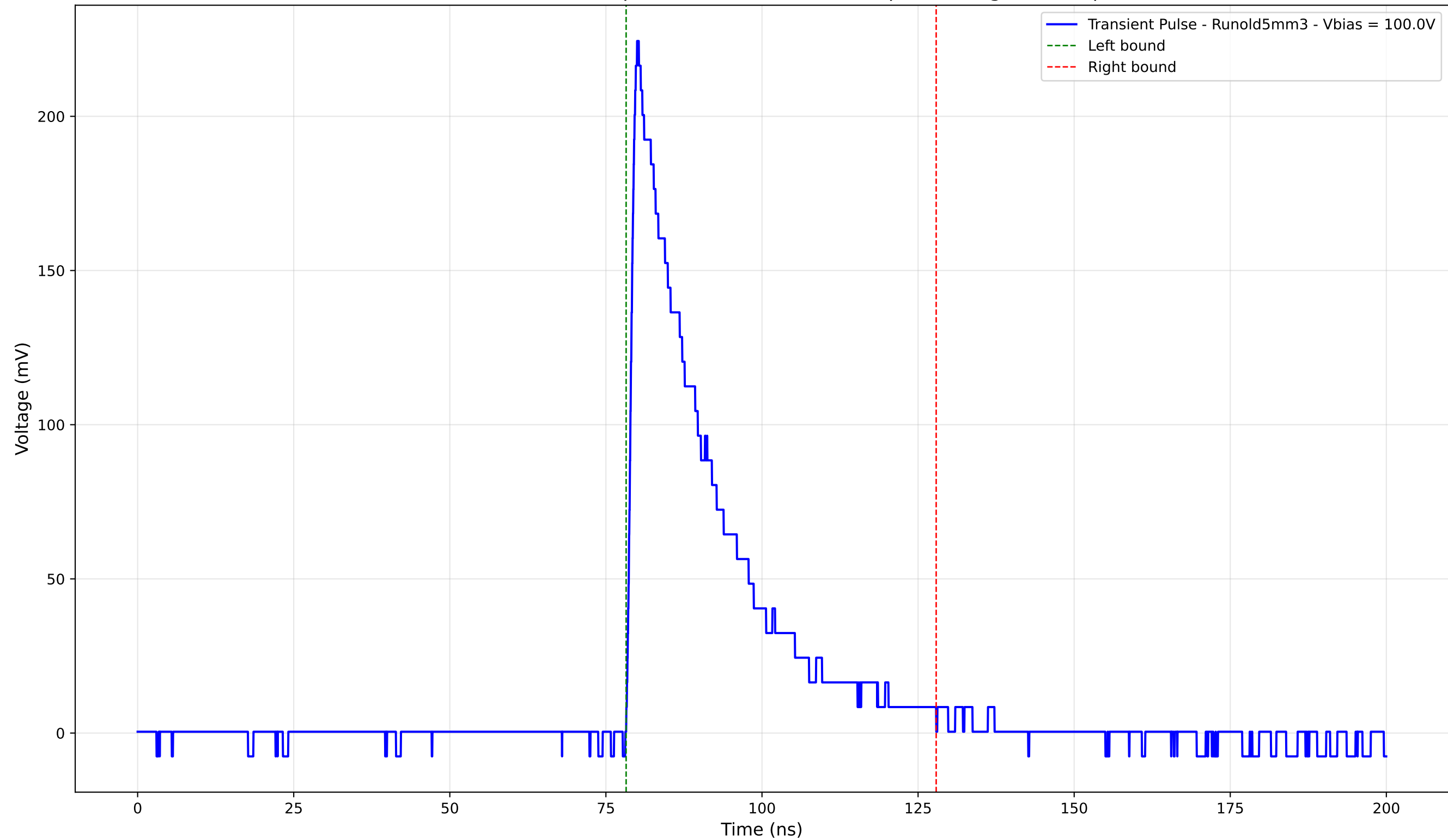
Transient Pulse - Sample: old5 - Position: 750.0 \mu\text{m} - Charge: 57.93 pC
