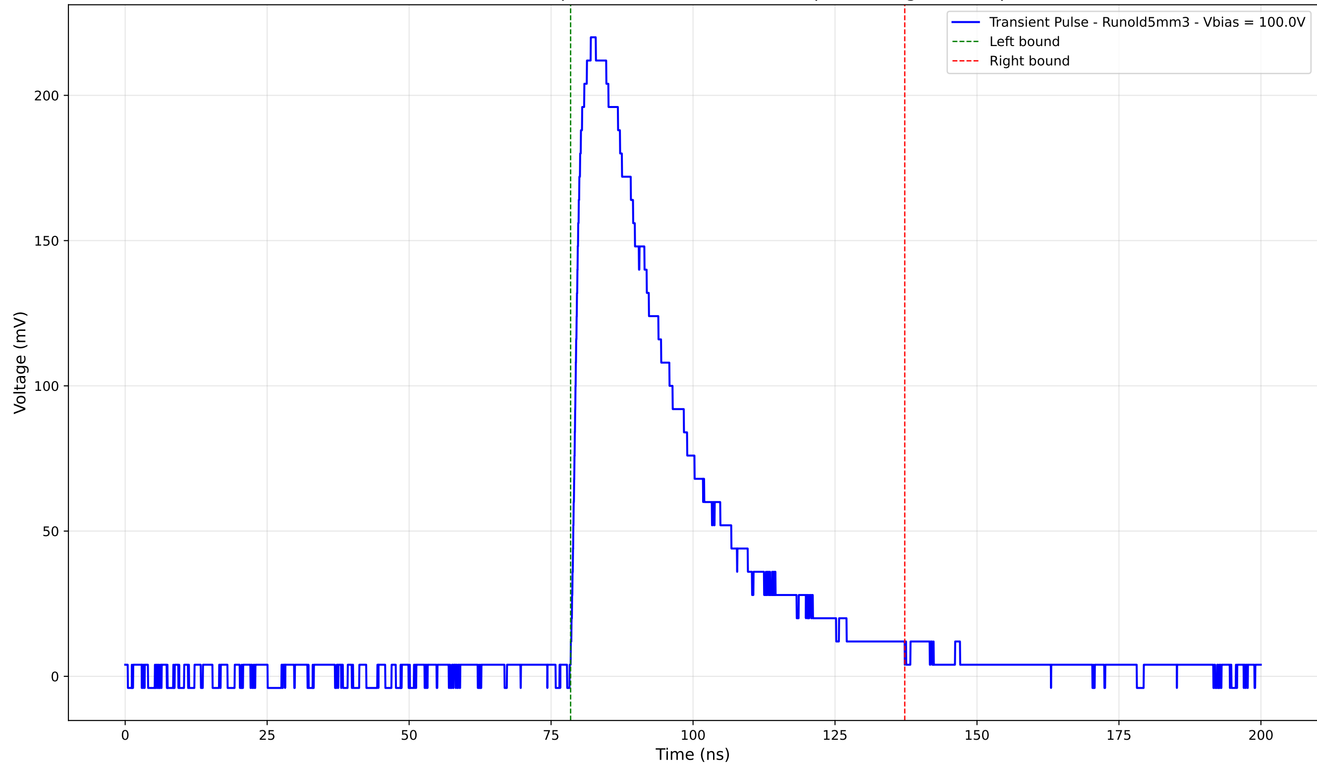
Transient Pulse - Sample: old5 - Position: 1290.0 \mu\text{m} - Charge: 85.84 pC
