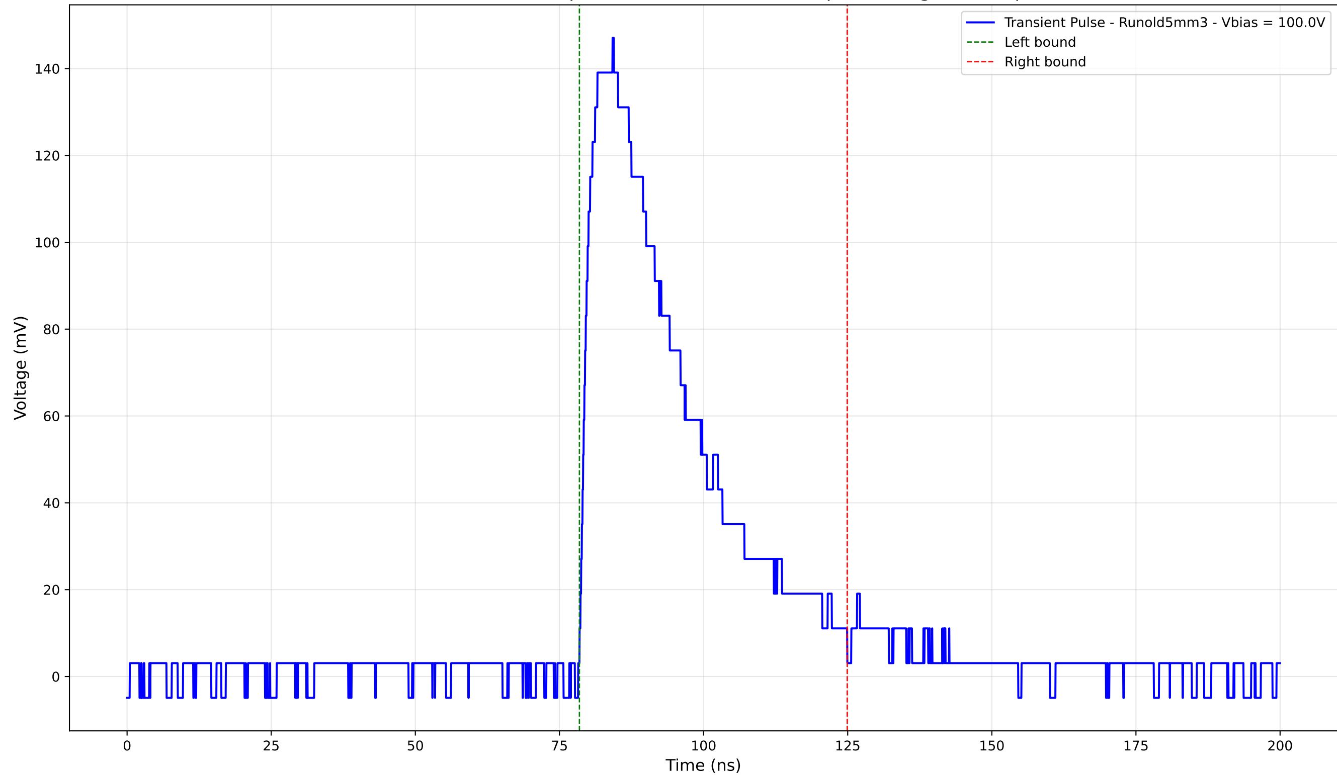
Transient Pulse - Sample: old5 - Position: 1440.0 \mu\text{m} - Charge: 55.28 pC
