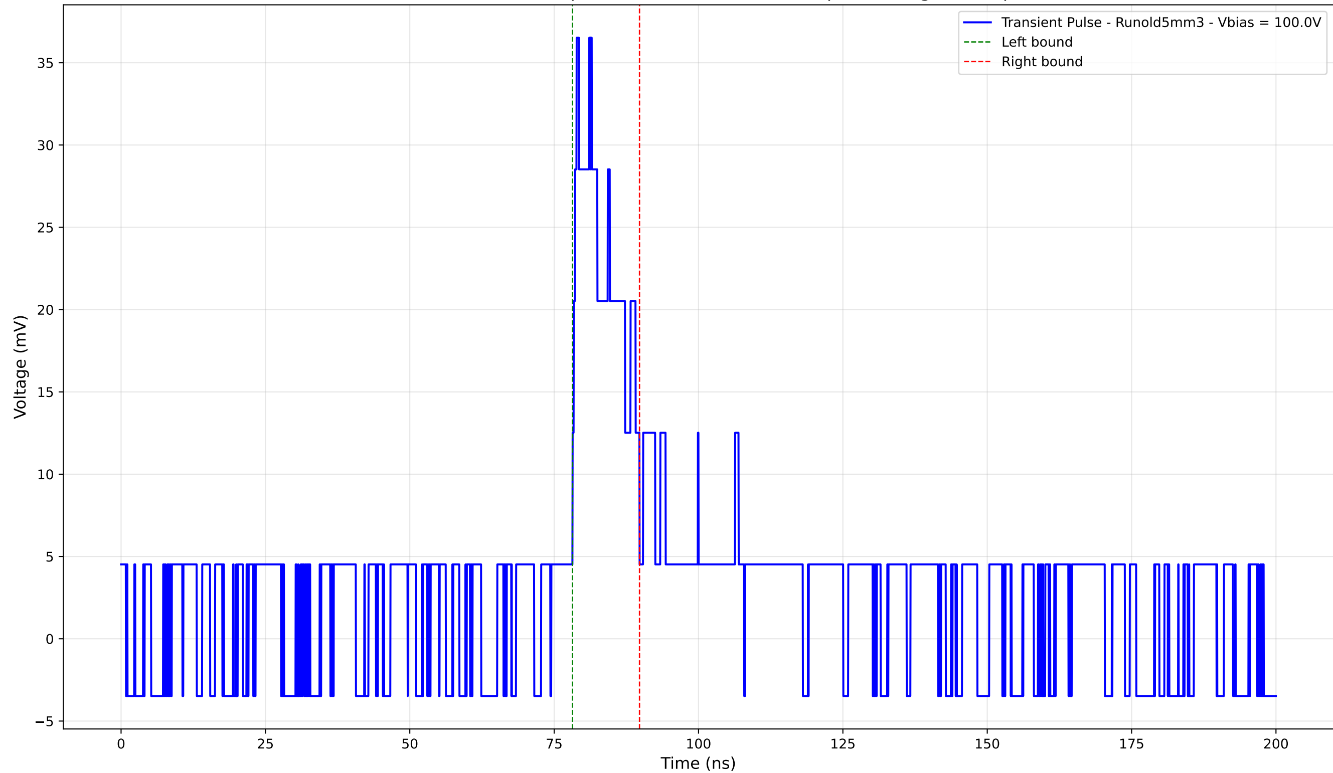
Transient Pulse - Sample: old5 - Position: 3260.0 \mu\text{m} - Charge: 5.28 pC
