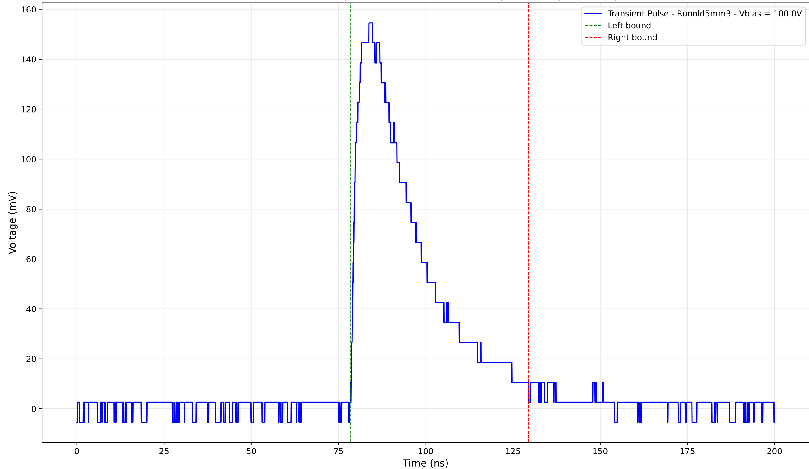
Transient Pulse - Sample: old5 - Position: 2135.0 \mu\text{m} - Charge: 61.26 pC
