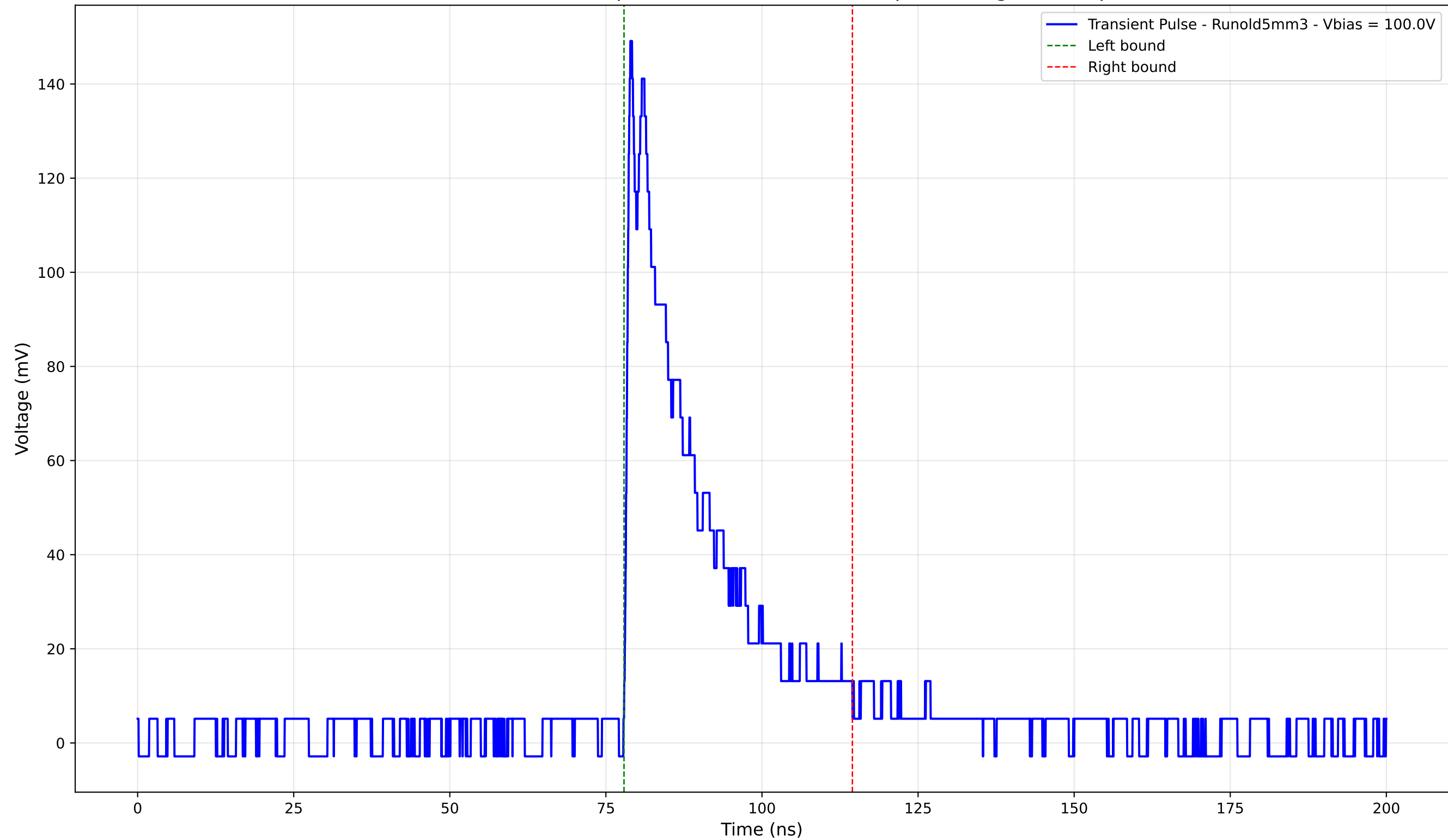
Transient Pulse - Sample: old5 - Position: 3225.0 \mu\text{m} - Charge: 33.66 pC
