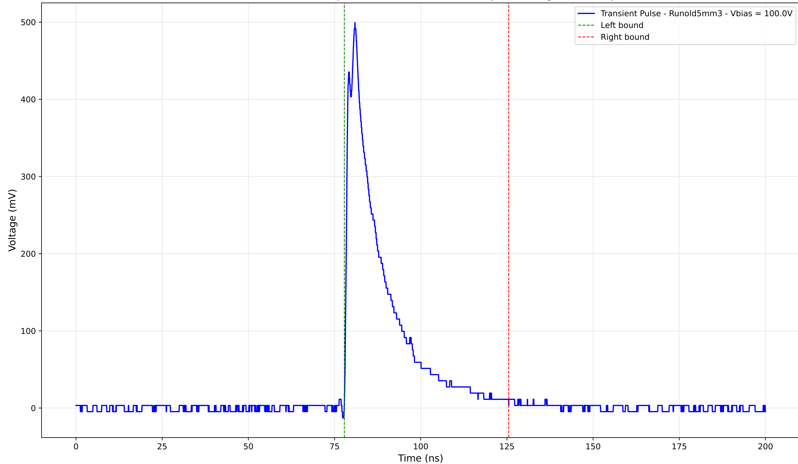
Transient Pulse - Sample: old5 - Position: 3995.0 \mu\text{m} - Charge: 107.27 pC
