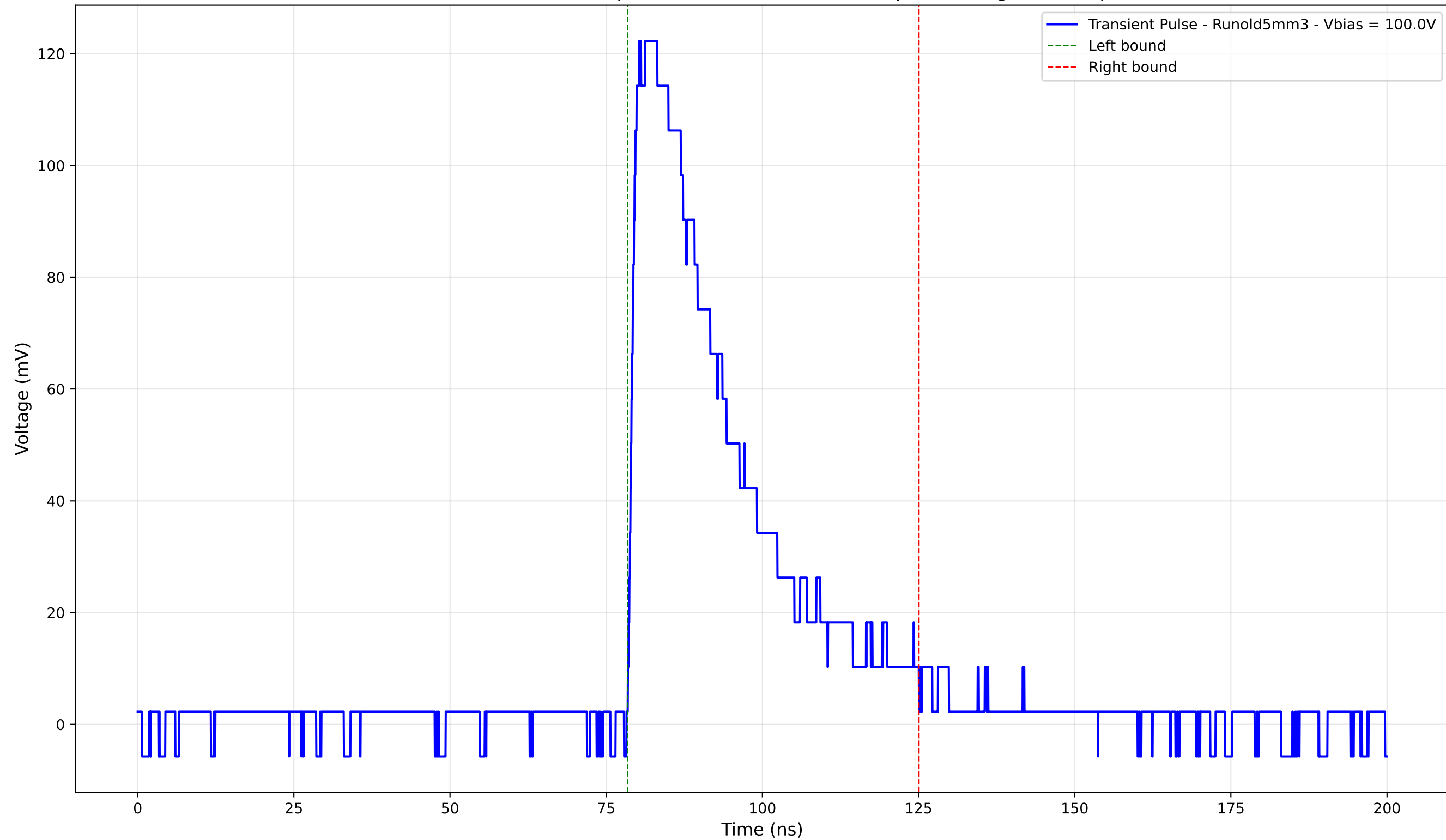
Transient Pulse - Sample: old5 - Position: 1015.0 \mu\text{m} - Charge: 43.35 pC
