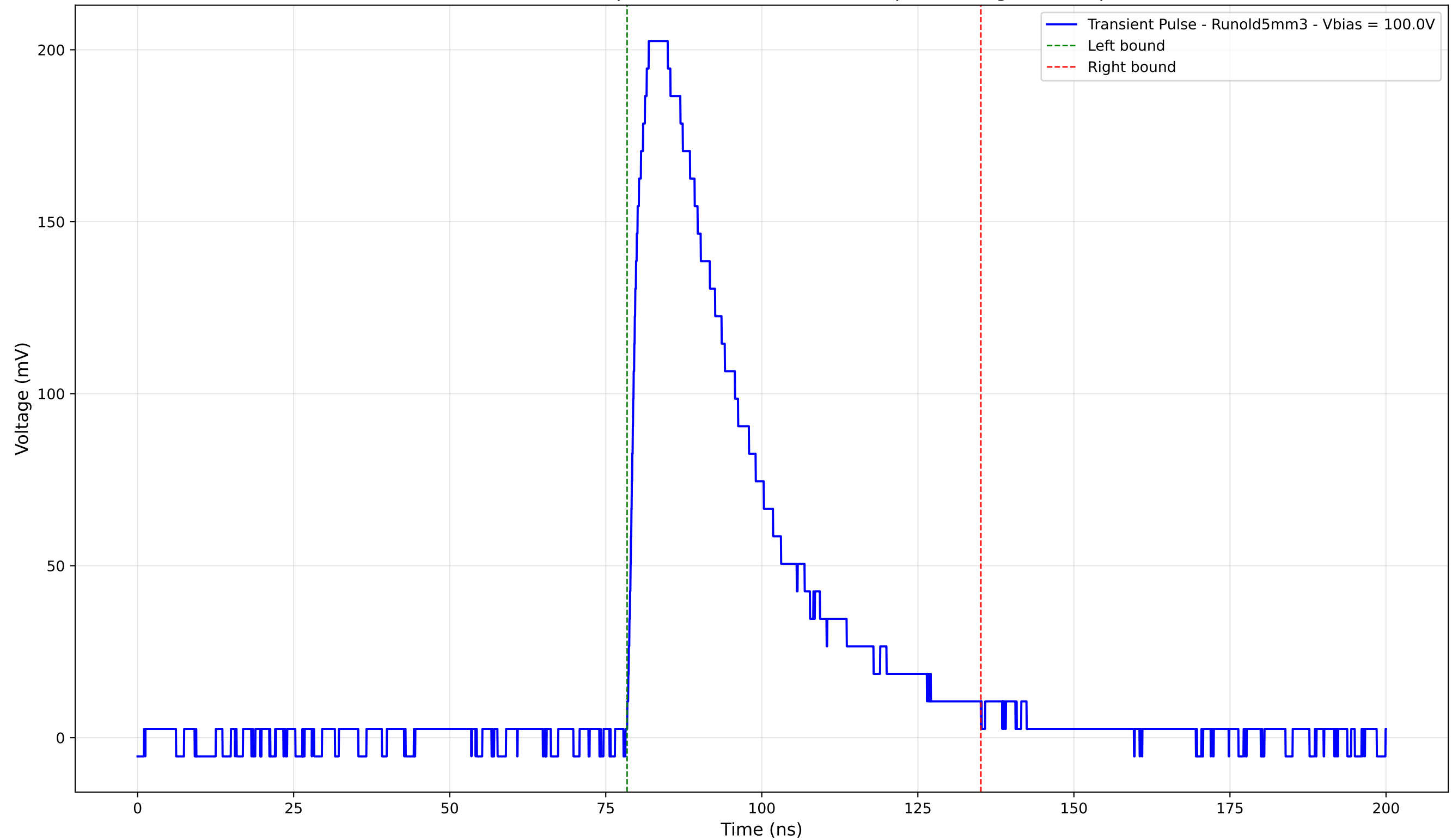
Transient Pulse - Sample: old5 - Position: 2265.0 \mu\text{m} - Charge: 80.55 pC
