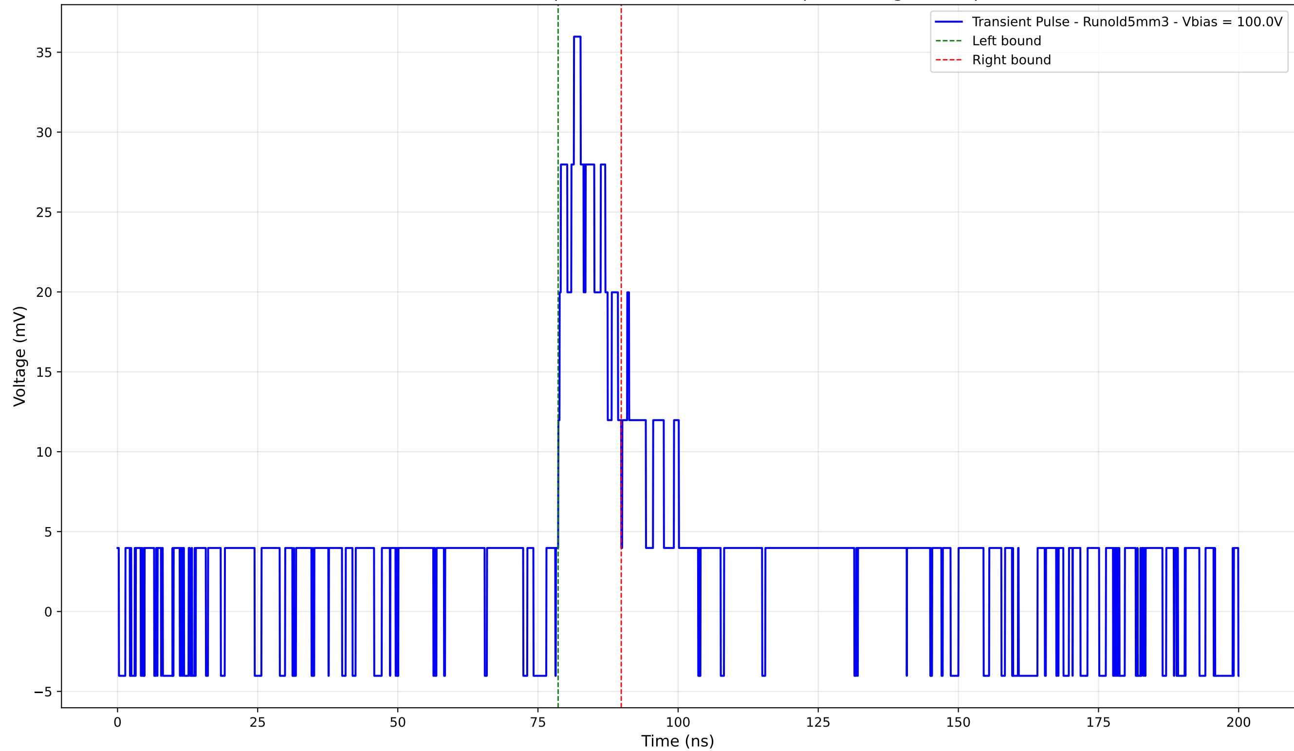
Transient Pulse - Sample: old5 - Position: 4500.0 \mu\text{m} - Charge: 5.38 pC
