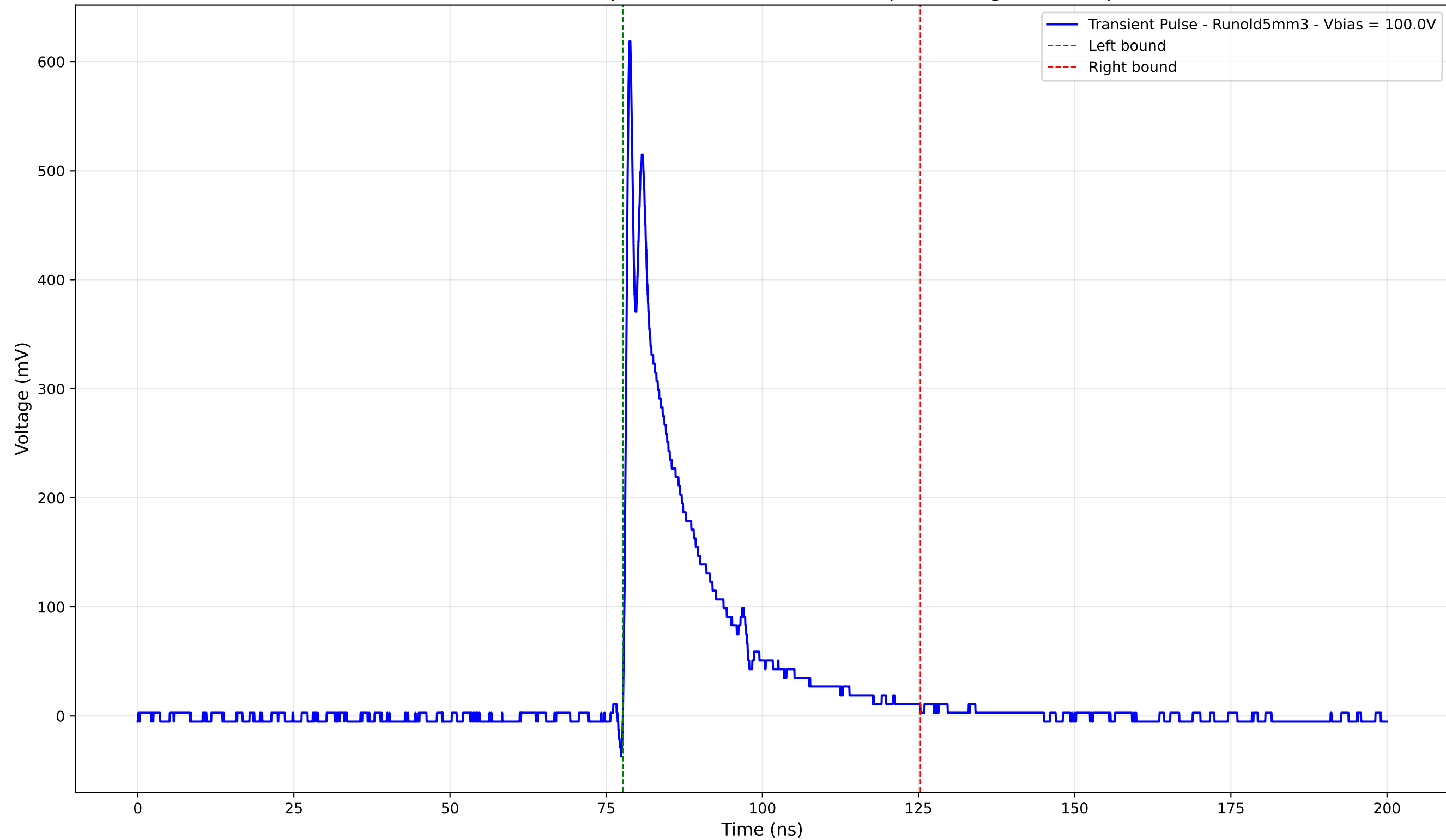
Transient Pulse - Sample: old5 - Position: 3405.0 \mu\text{m} - Charge: 104.82 pC
