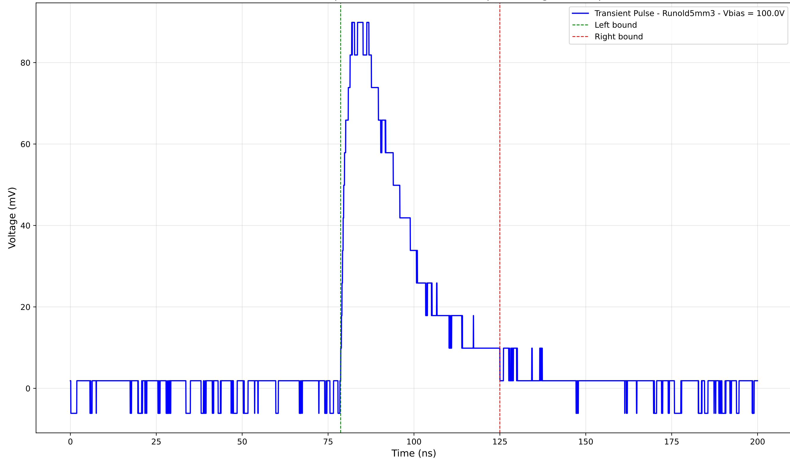
Transient Pulse - Sample: old5 - Position: 1825.0 \mu\text{m} - Charge: 35.00 pC
