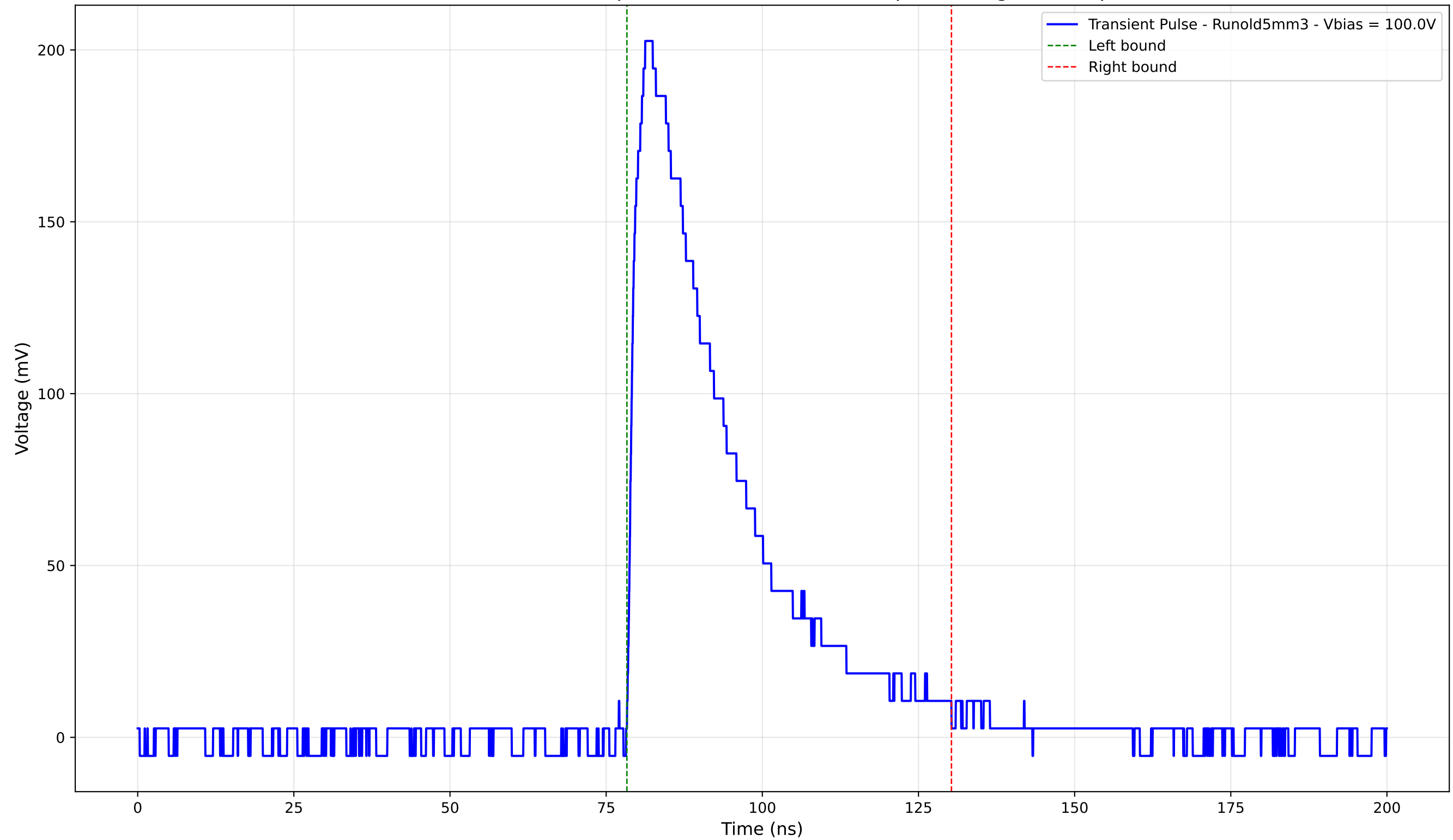
Transient Pulse - Sample: old5 - Position: 2755.0 \mu\text{m} - Charge: 68.84 pC
