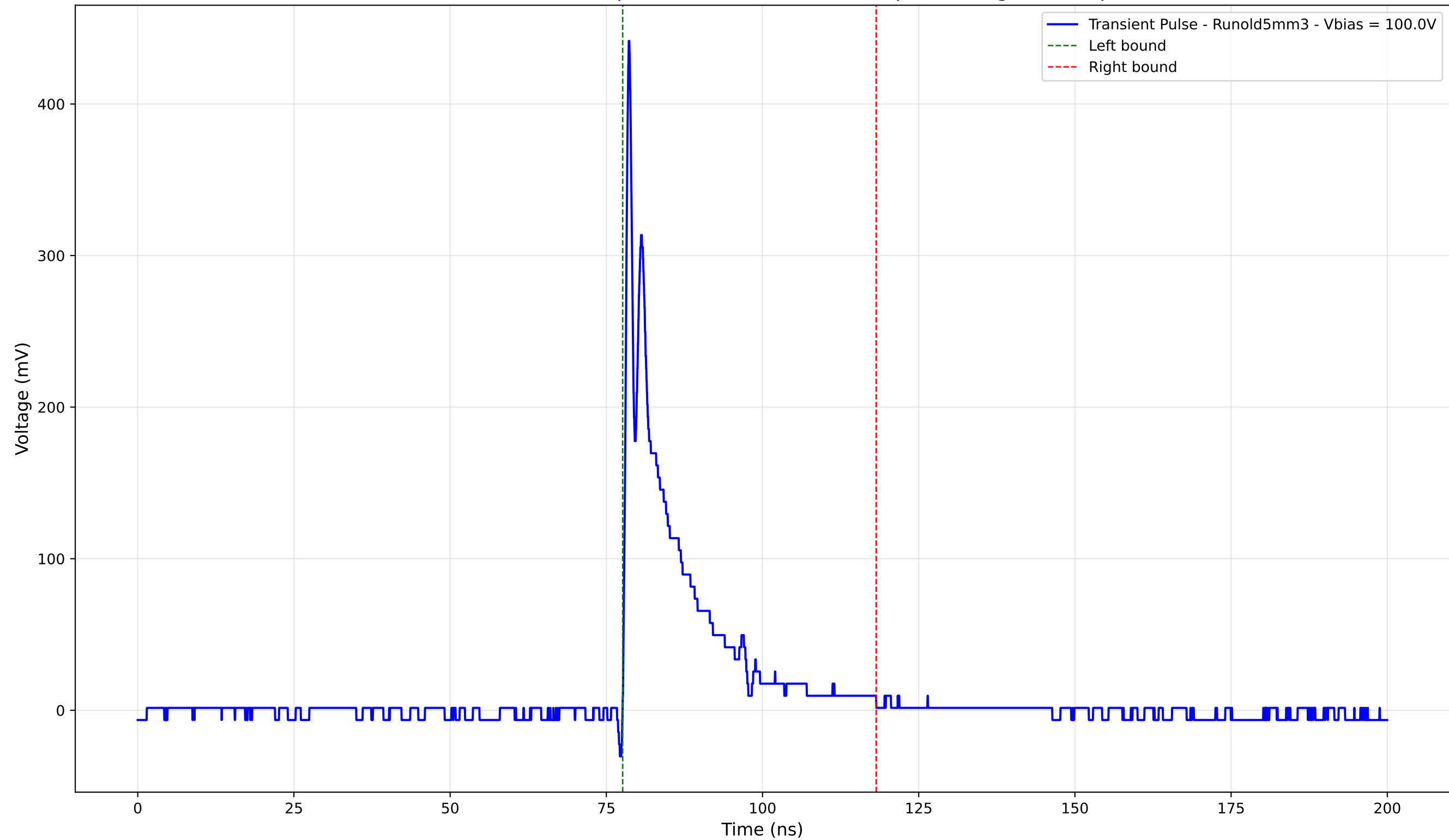
Transient Pulse - Sample: old5 - Position: 3650.0 \mu\text{m} - Charge: 53.73 pC
