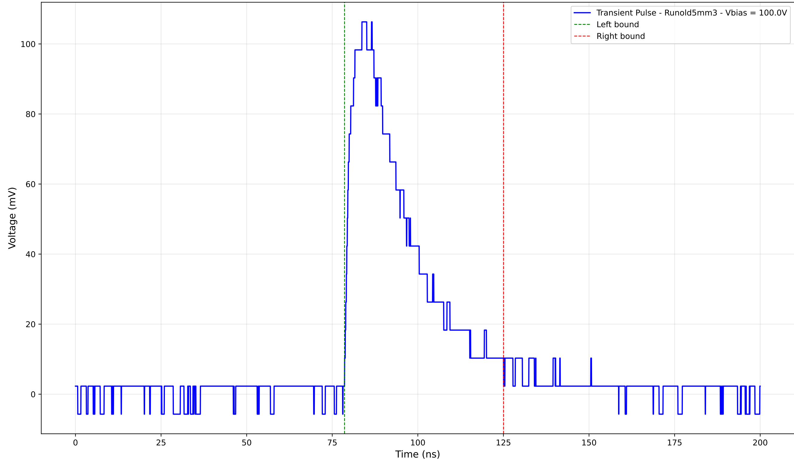
Transient Pulse - Sample: old5 - Position: 2030.0 \mu\text{m} - Charge: 40.91 pC
