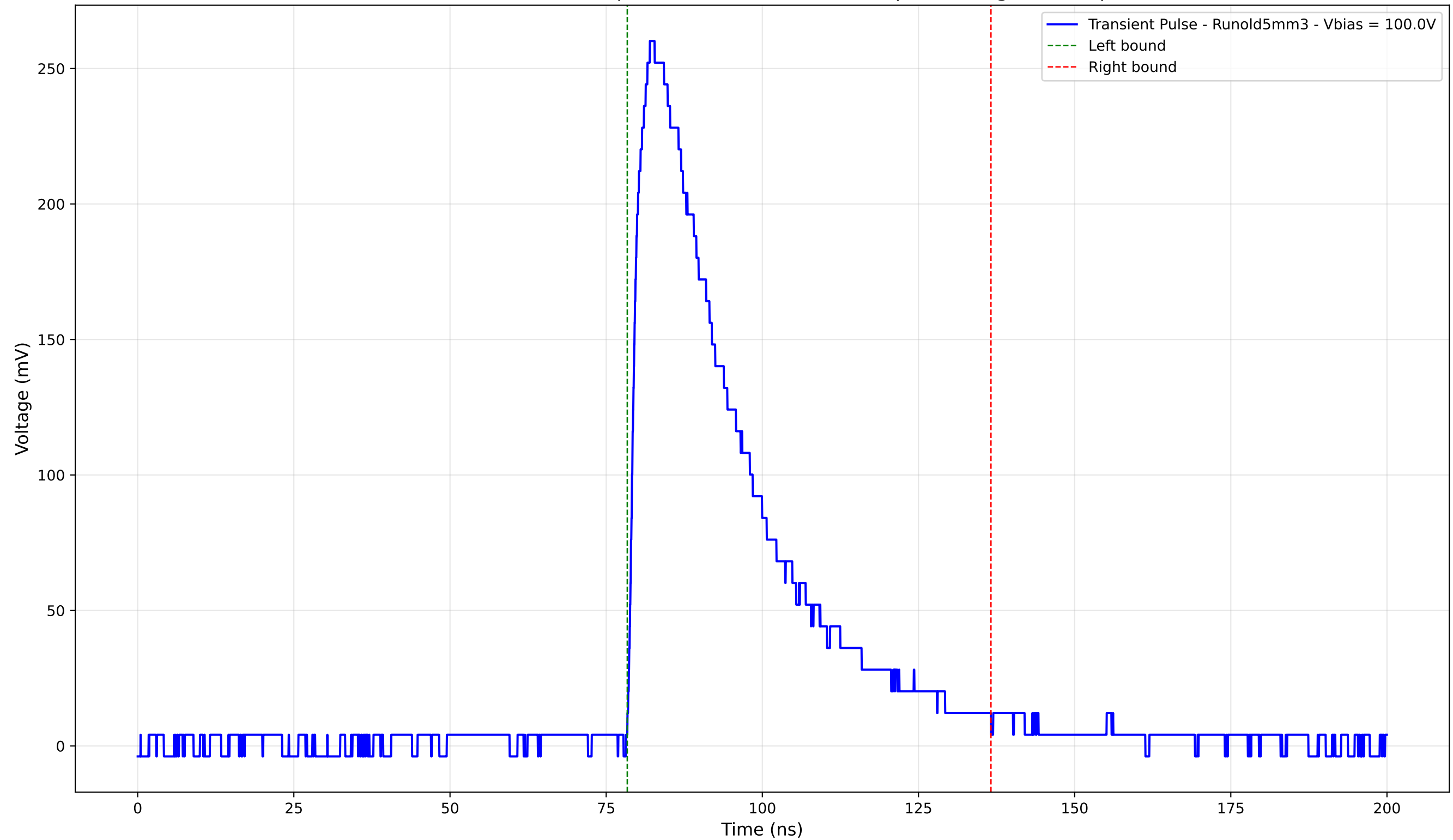
Transient Pulse - Sample: old5 - Position: 2485.0 \mu\text{m} - Charge: 99.03 pC
