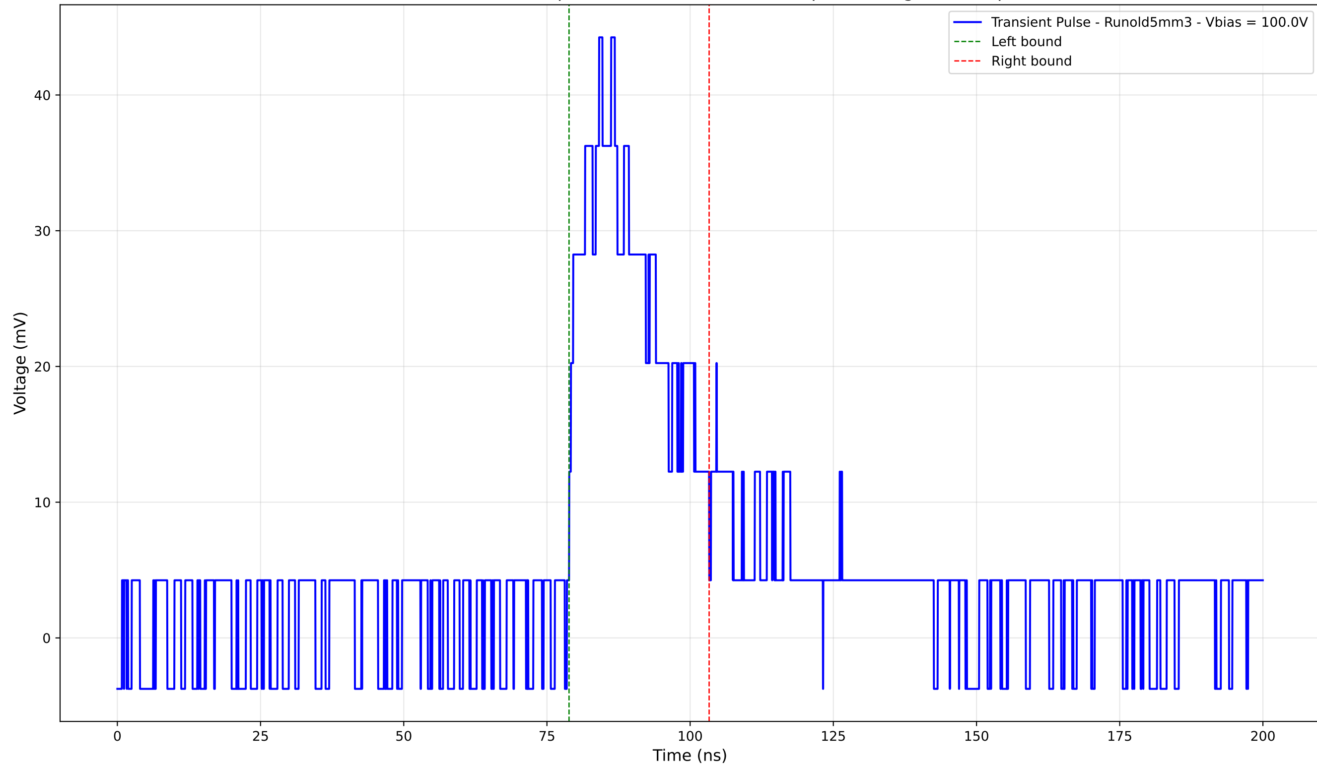
Transient Pulse - Sample: old5 - Position: 1575.0 \mu\text{m} - Charge: 12.58 pC
