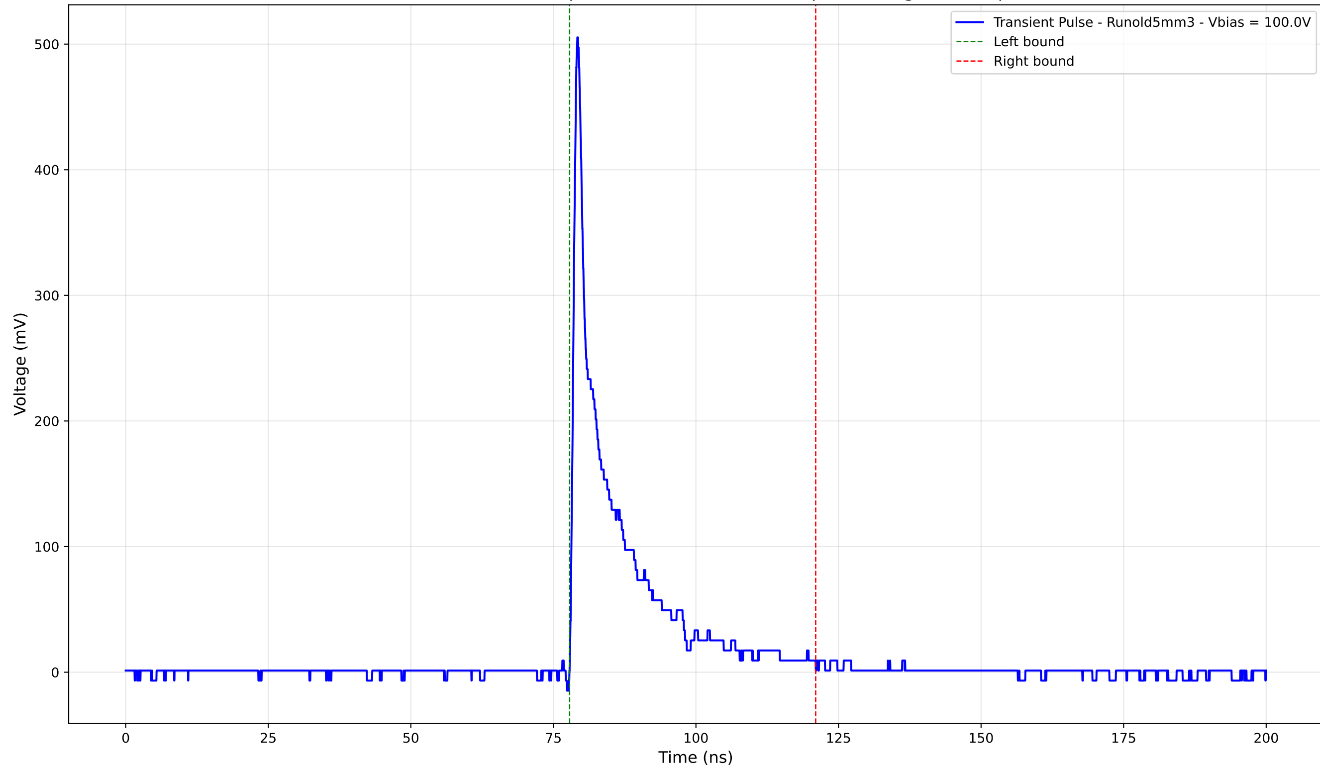
Transient Pulse - Sample: old5 - Position: 200.0 \mu\text{m} - Charge: 62.96 pC
