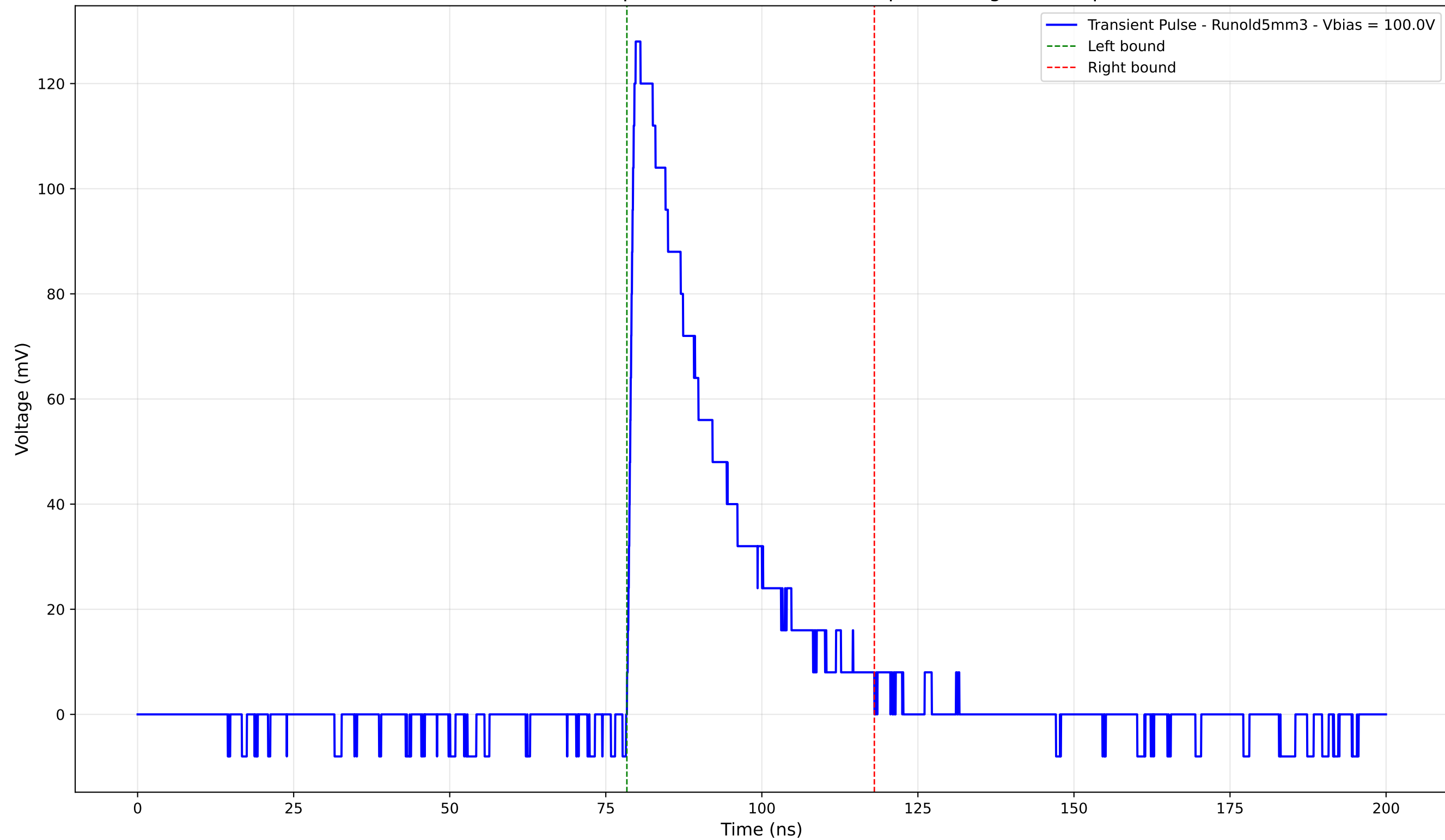
Transient Pulse - Sample: old5 - Position: 805.0 \mu\text{m} - Charge: 35.19 pC
