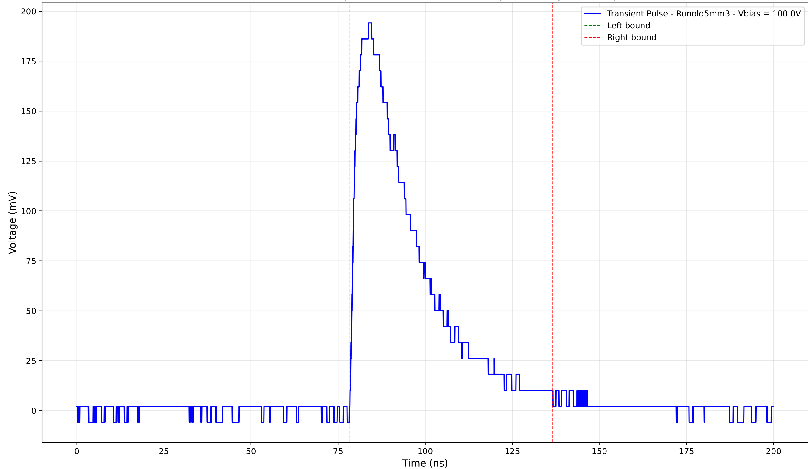
Transient Pulse - Sample: old5 - Position: 2260.0 \mu\text{m} - Charge: 76.24 pC
