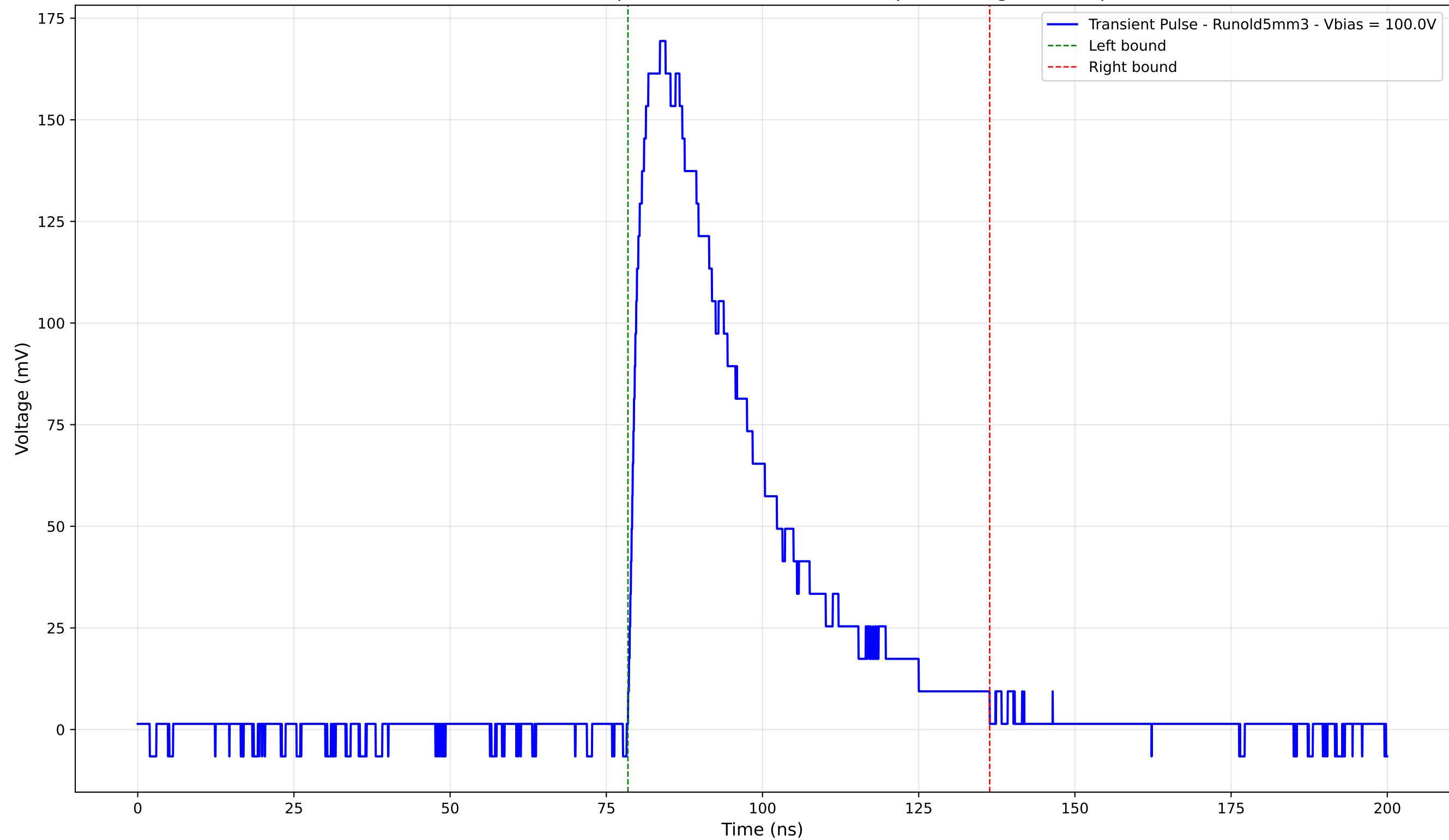
Transient Pulse - Sample: old5 - Position: 2130.0 \mu\text{m} - Charge: 67.80 pC
