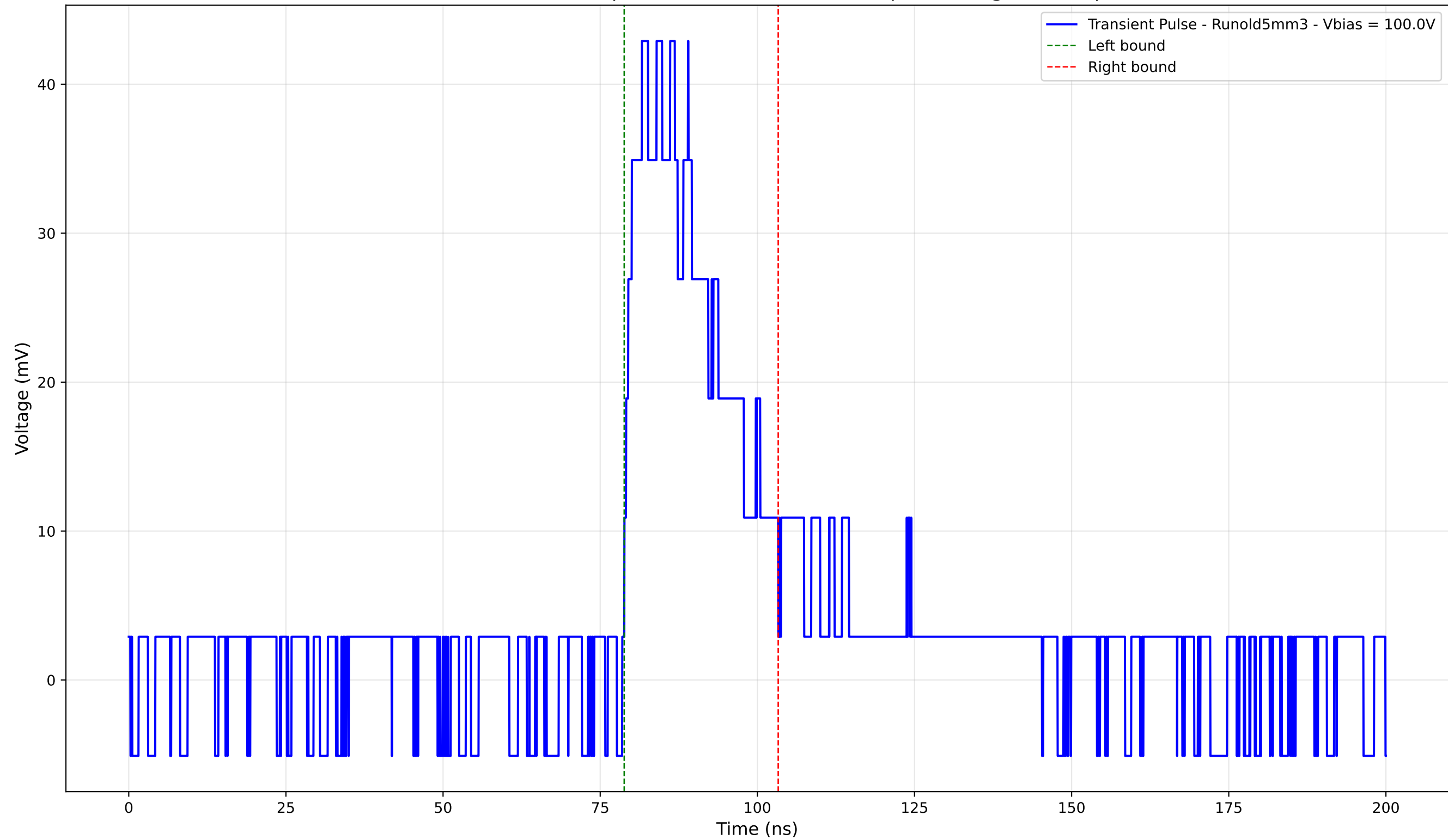
Transient Pulse - Sample: old5 - Position: 1195.0 \mu\text{m} - Charge: 12.45 pC
