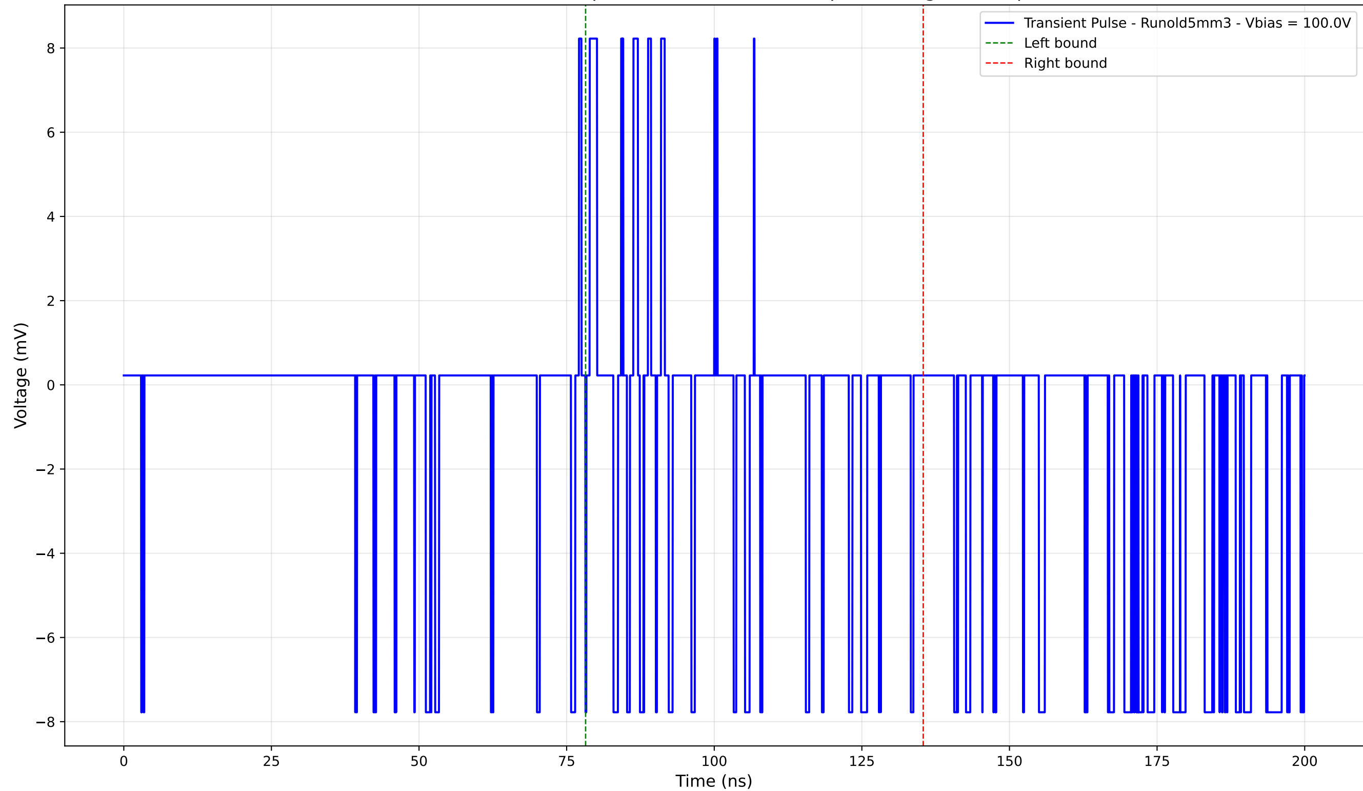
Transient Pulse - Sample: old5 - Position: 25.0 \mu\text{m} - Charge: -0.42 pC
