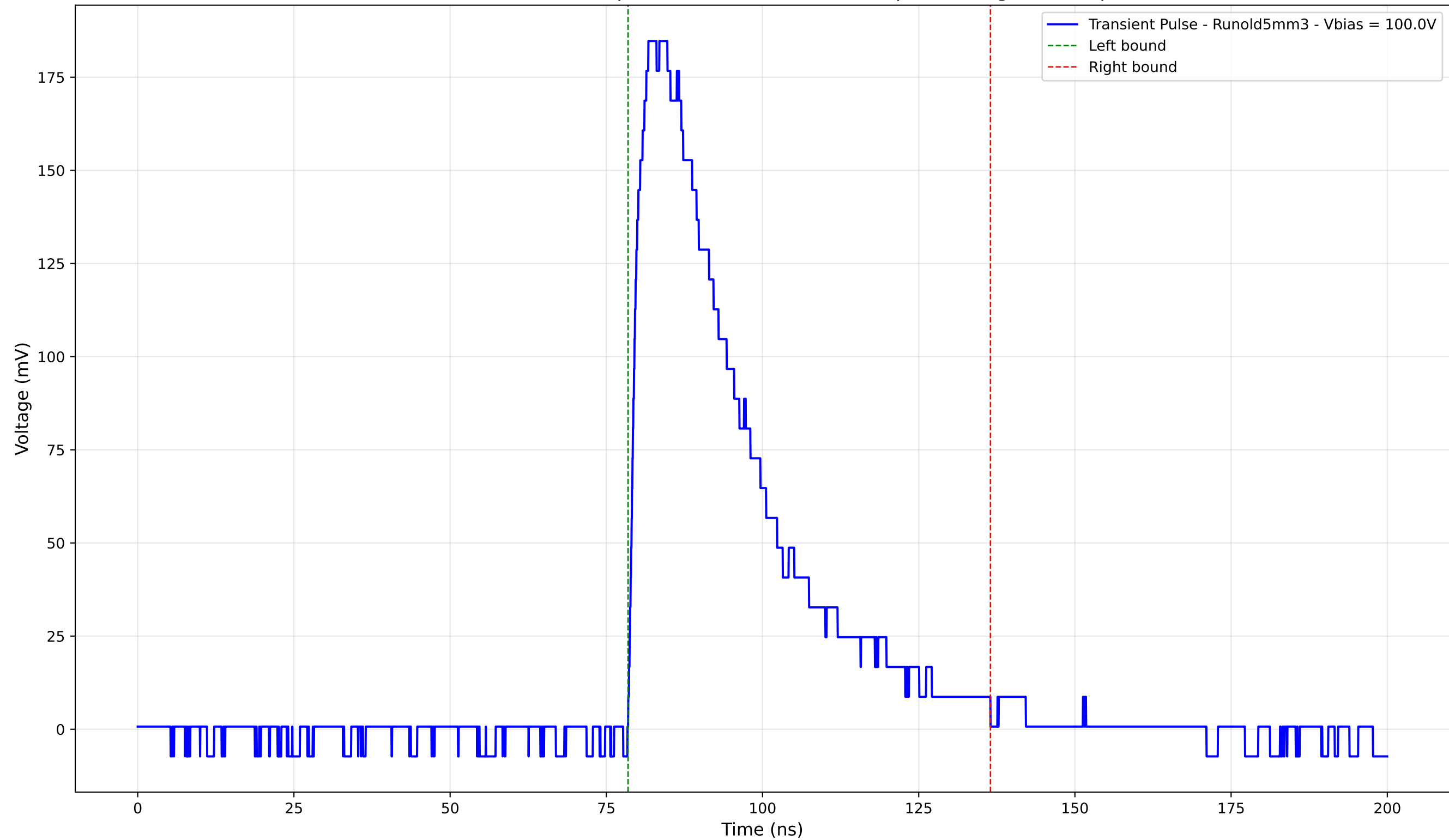
Transient Pulse - Sample: old5 - Position: 2330.0 \mu\text{m} - Charge: 72.58 pC
