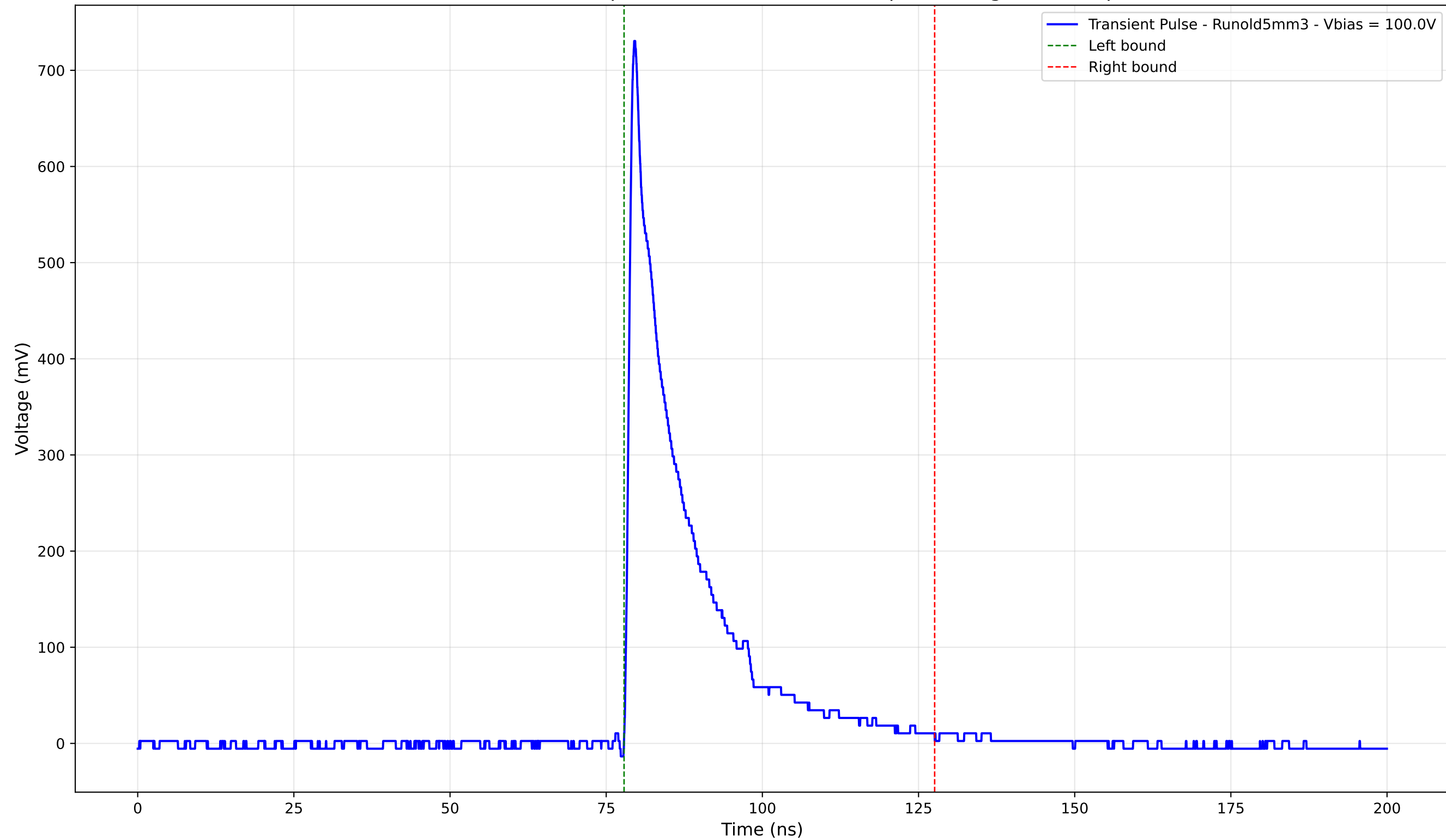
Transient Pulse - Sample: old5 - Position: 4710.0 \mu\text{m} - Charge: 131.73 pC
