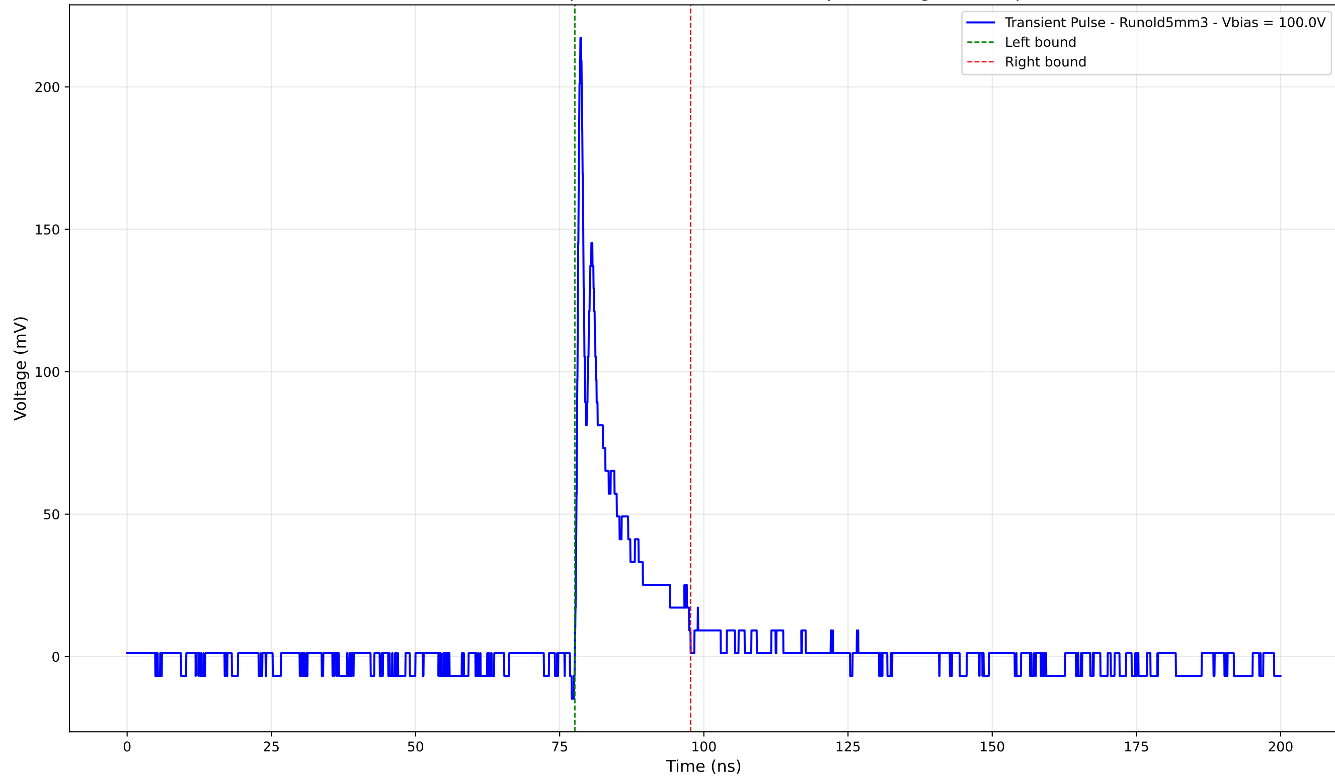
Transient Pulse - Sample: old5 - Position: 3535.0 \mu\text{m} - Charge: 21.57 pC
