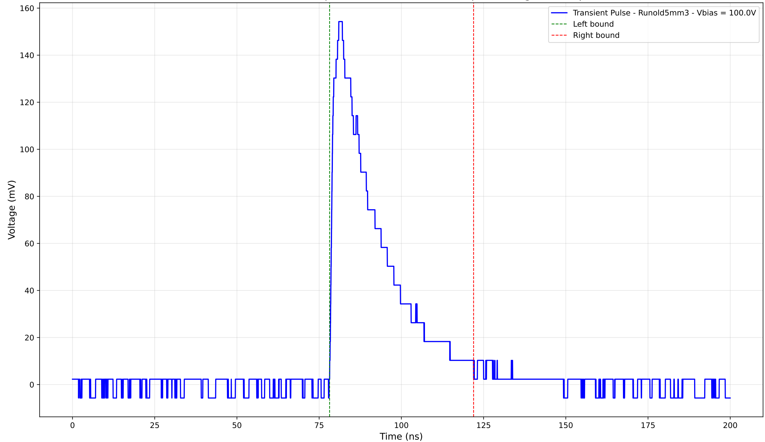
Transient Pulse - Sample: old5 - Position: 2910.0 \mu\text{m} - Charge: 46.89 pC
