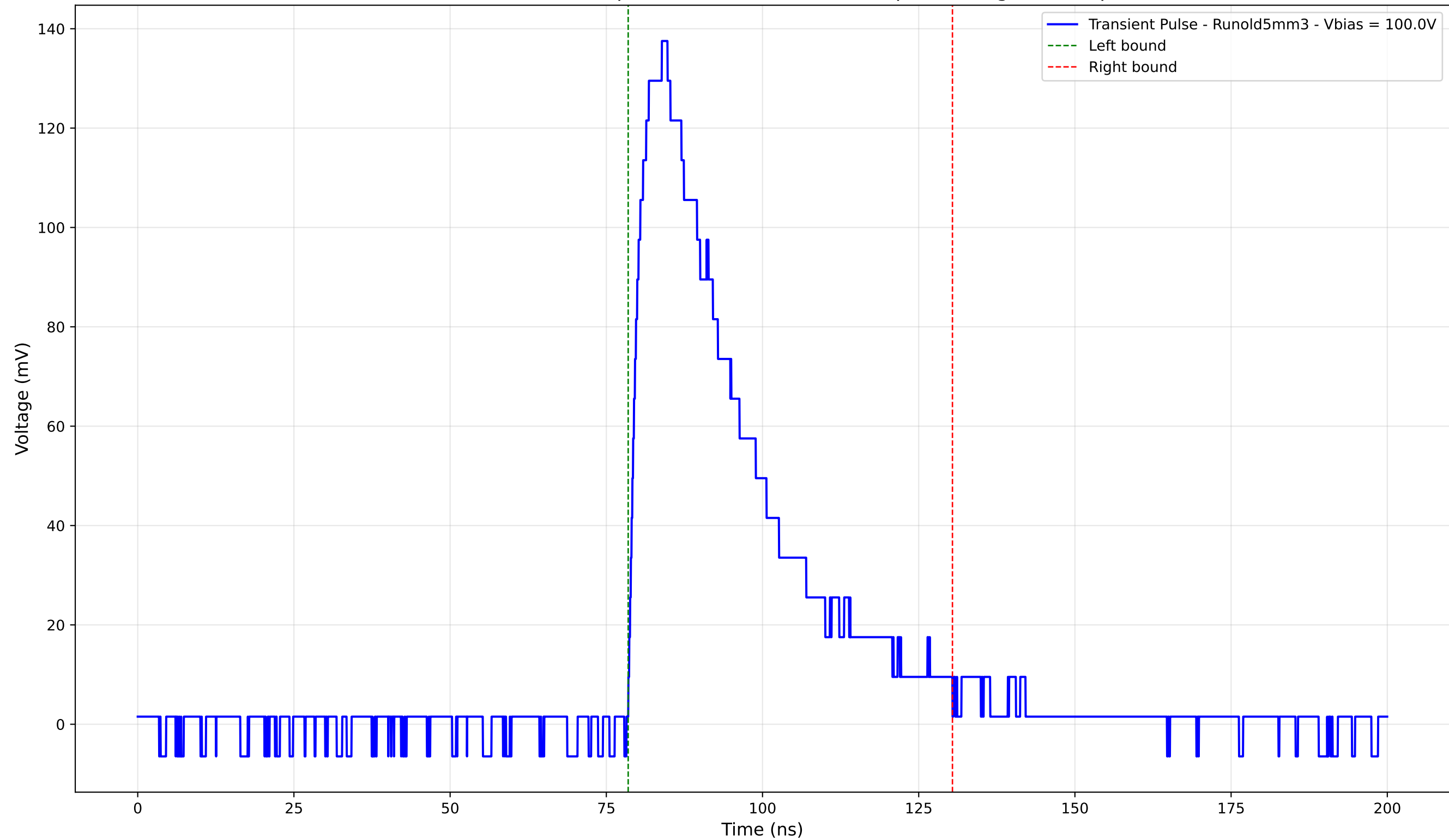
Transient Pulse - Sample: old5 - Position: 2240.0 \mu\text{m} - Charge: 51.87 pC
