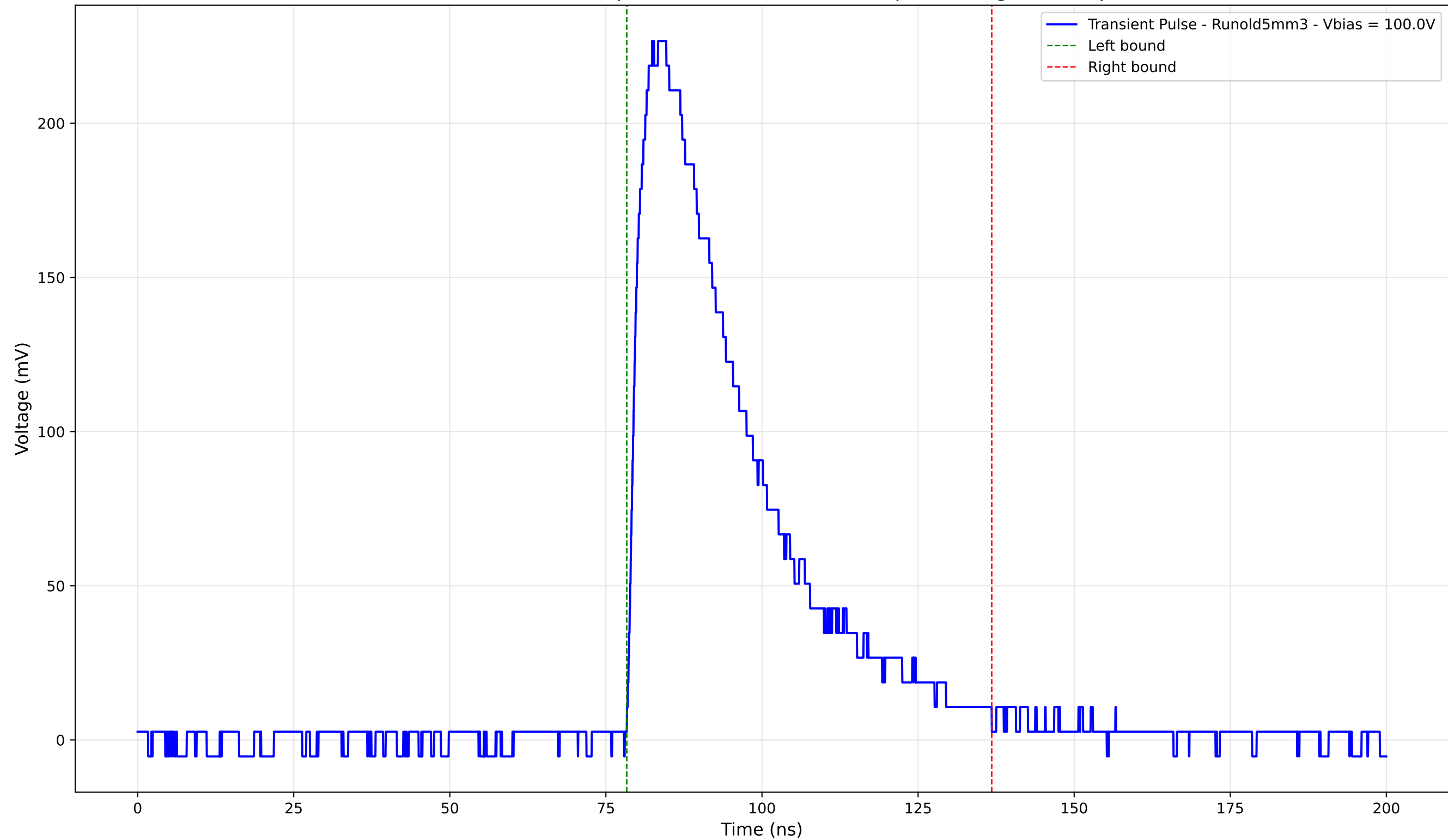
Transient Pulse - Sample: old5 - Position: 2085.0 \mu\text{m} - Charge: 91.92 pC
