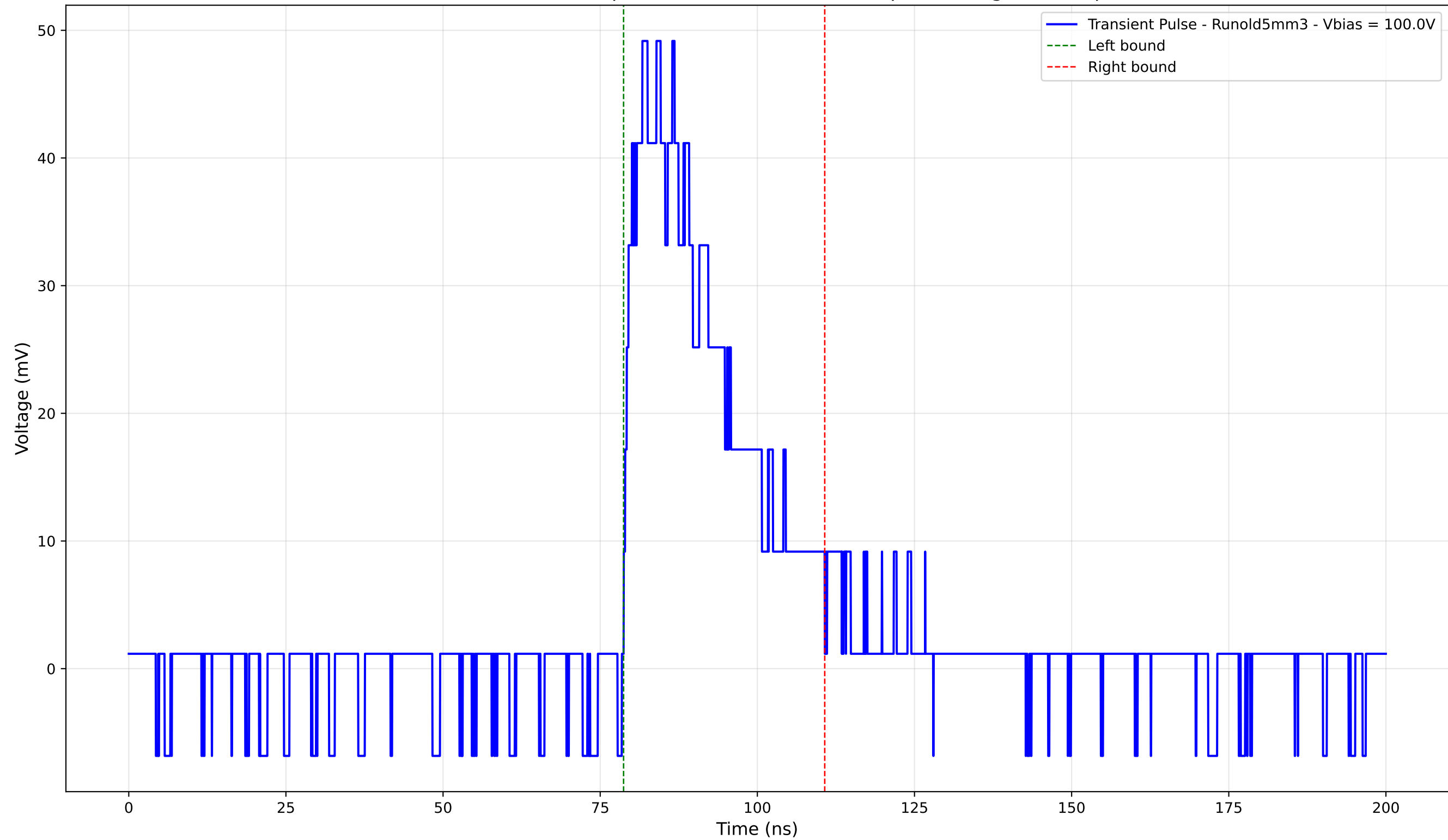
Transient Pulse - Sample: old5 - Position: 1200.0 \mu\text{m} - Charge: 15.41 pC
