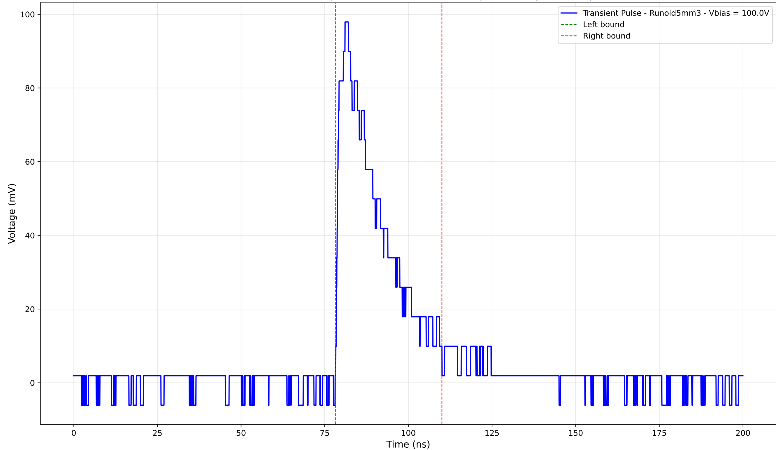
Transient Pulse - Sample: old5 - Position: 2925.0 \mu\text{m} - Charge: 27.22 pC
