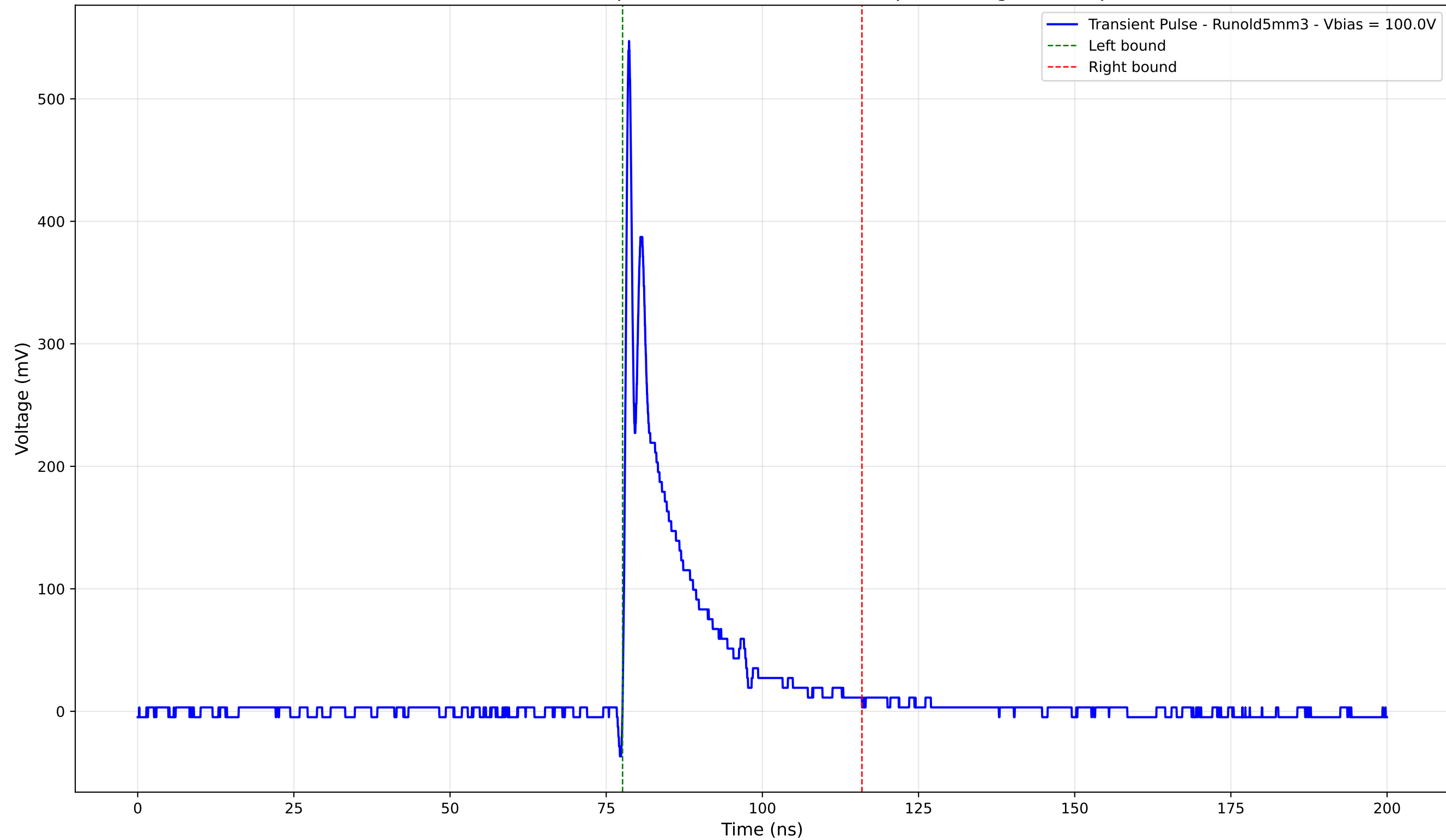
Transient Pulse - Sample: old5 - Position: 3660.0 \mu\text{m} - Charge: 68.38 pC
