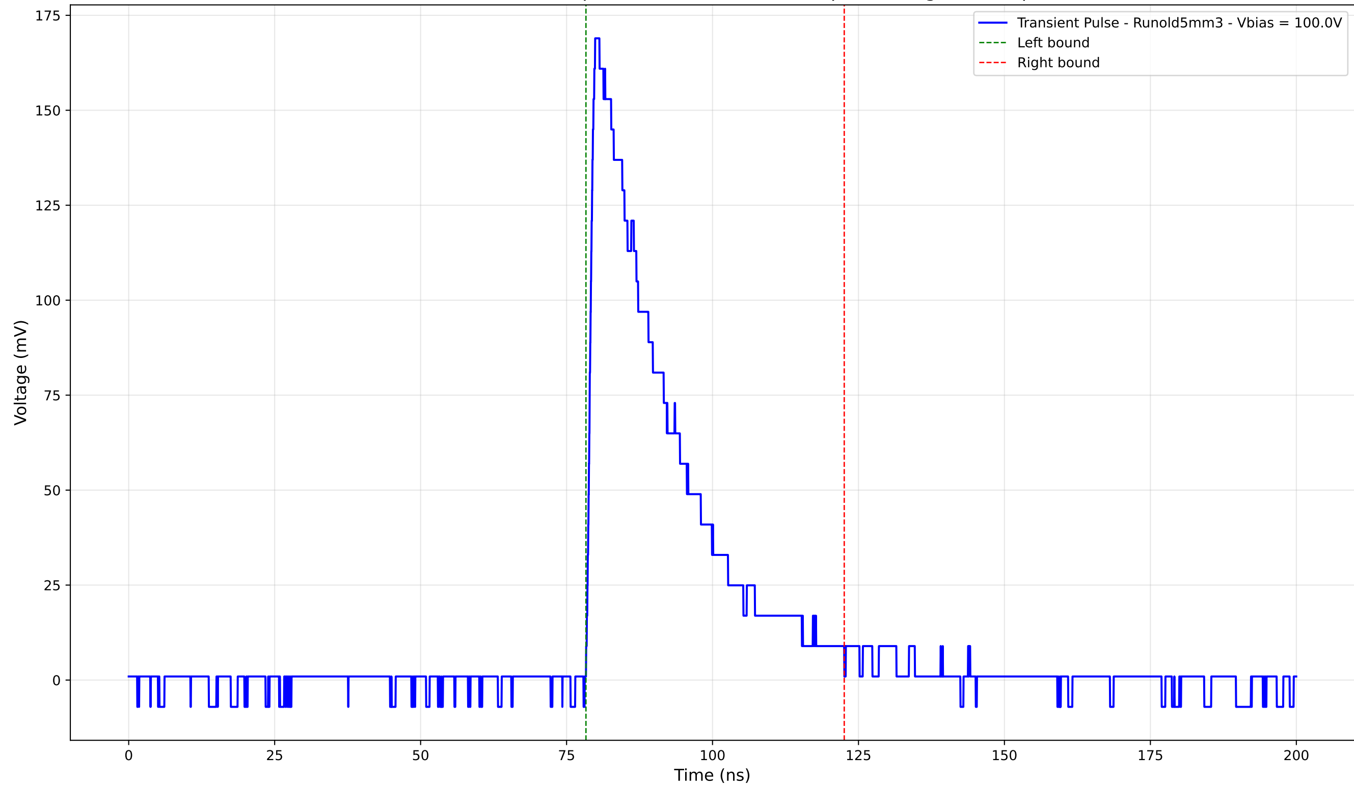
Transient Pulse - Sample: old5 - Position: 830.0 \mu\text{m} - Charge: 48.09 pC
