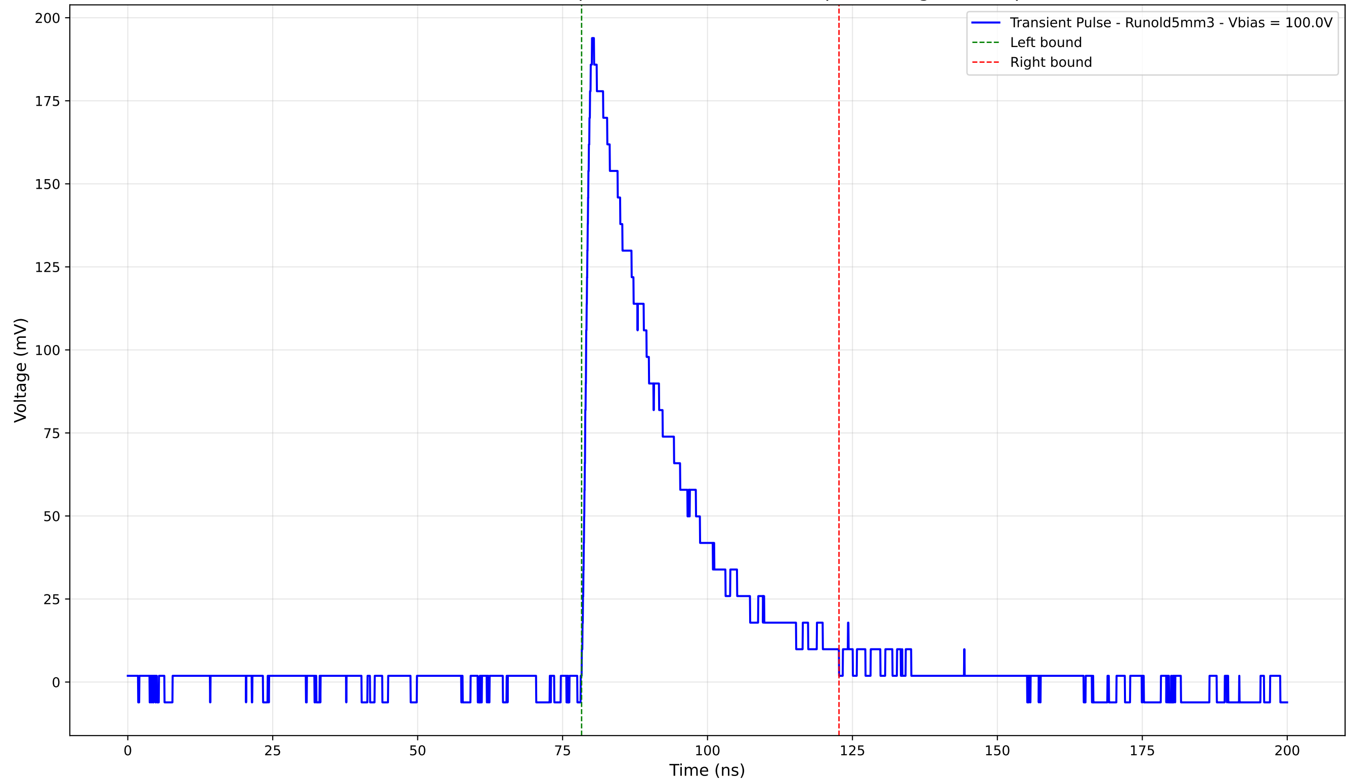
Transient Pulse - Sample: old5 - Position: 840.0 \mu\text{m} - Charge: 54.75 pC
