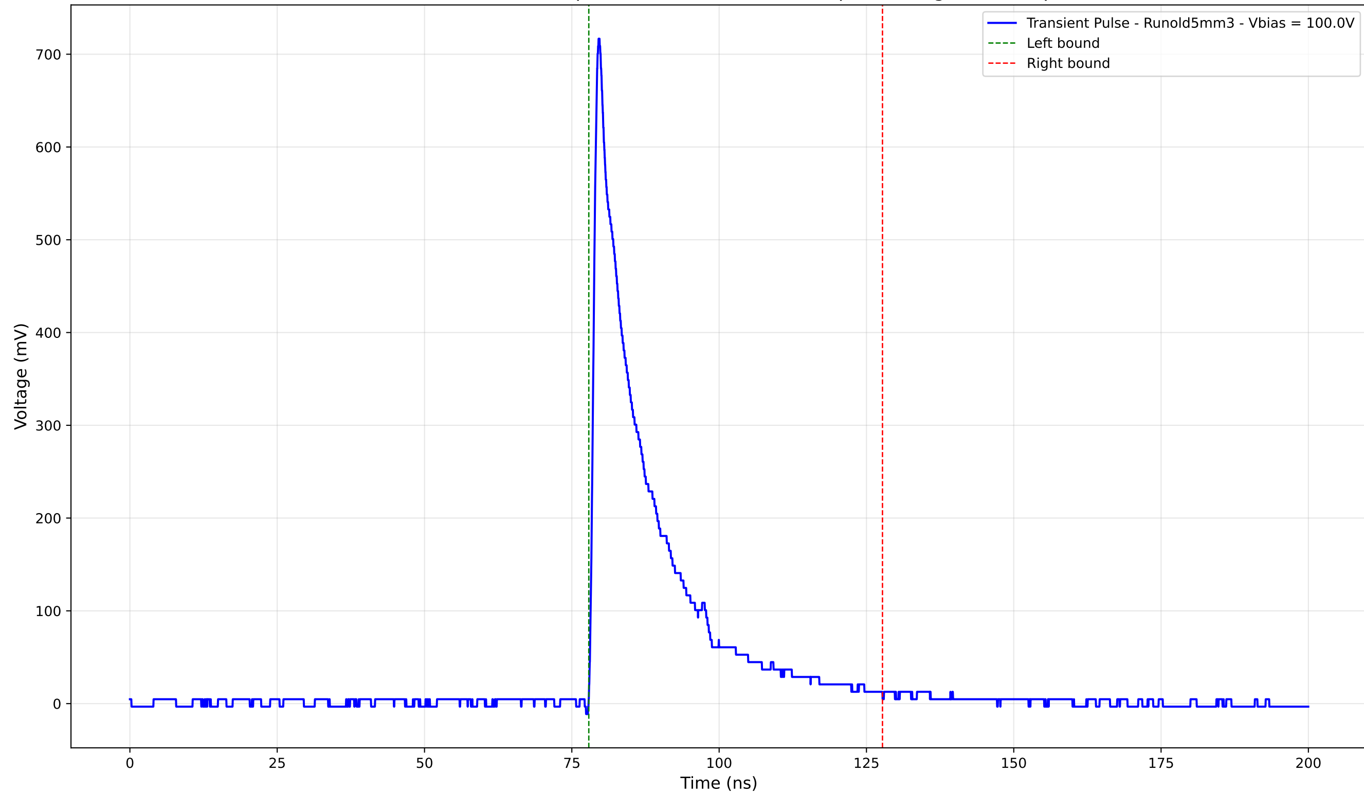
Transient Pulse - Sample: old5 - Position: 4695.0 \mu\text{m} - Charge: 133.27 pC
