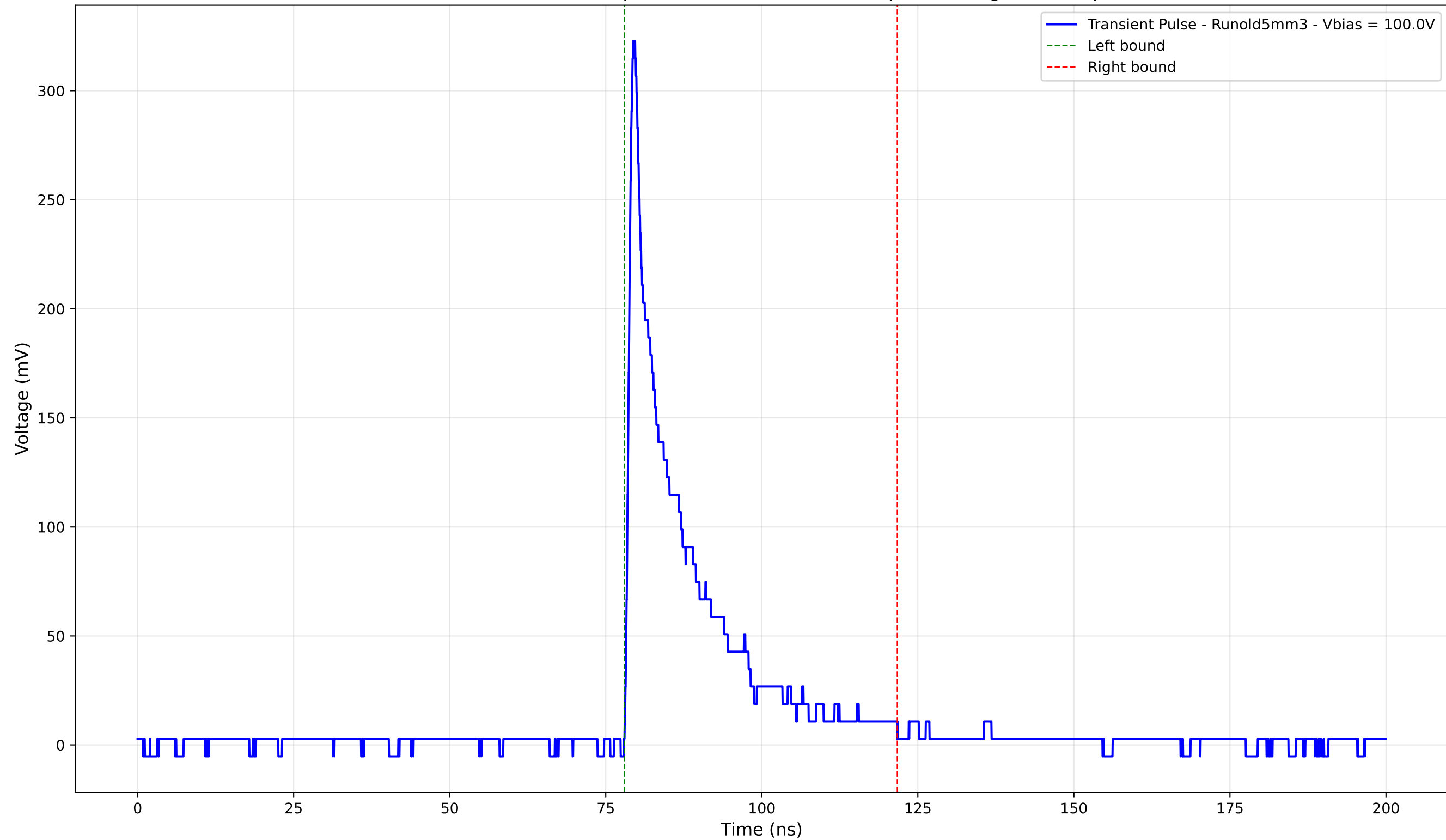
Transient Pulse - Sample: old5 - Position: 365.0 \mu\text{m} - Charge: 52.43 pC
