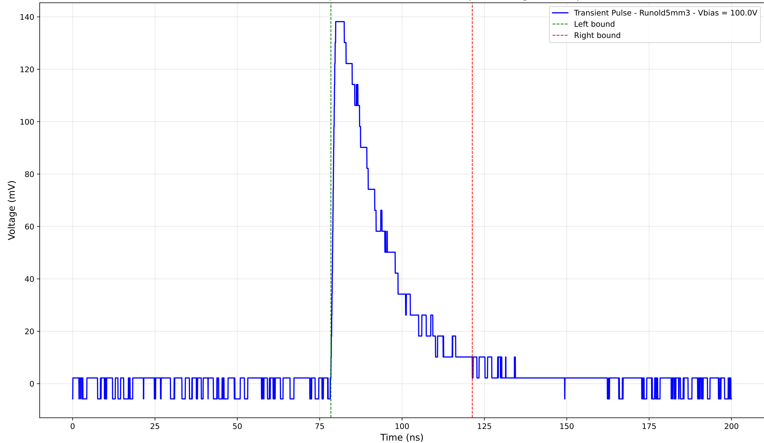
Transient Pulse - Sample: old5 - Position: 925.0 \mu\text{m} - Charge: 44.18 pC
