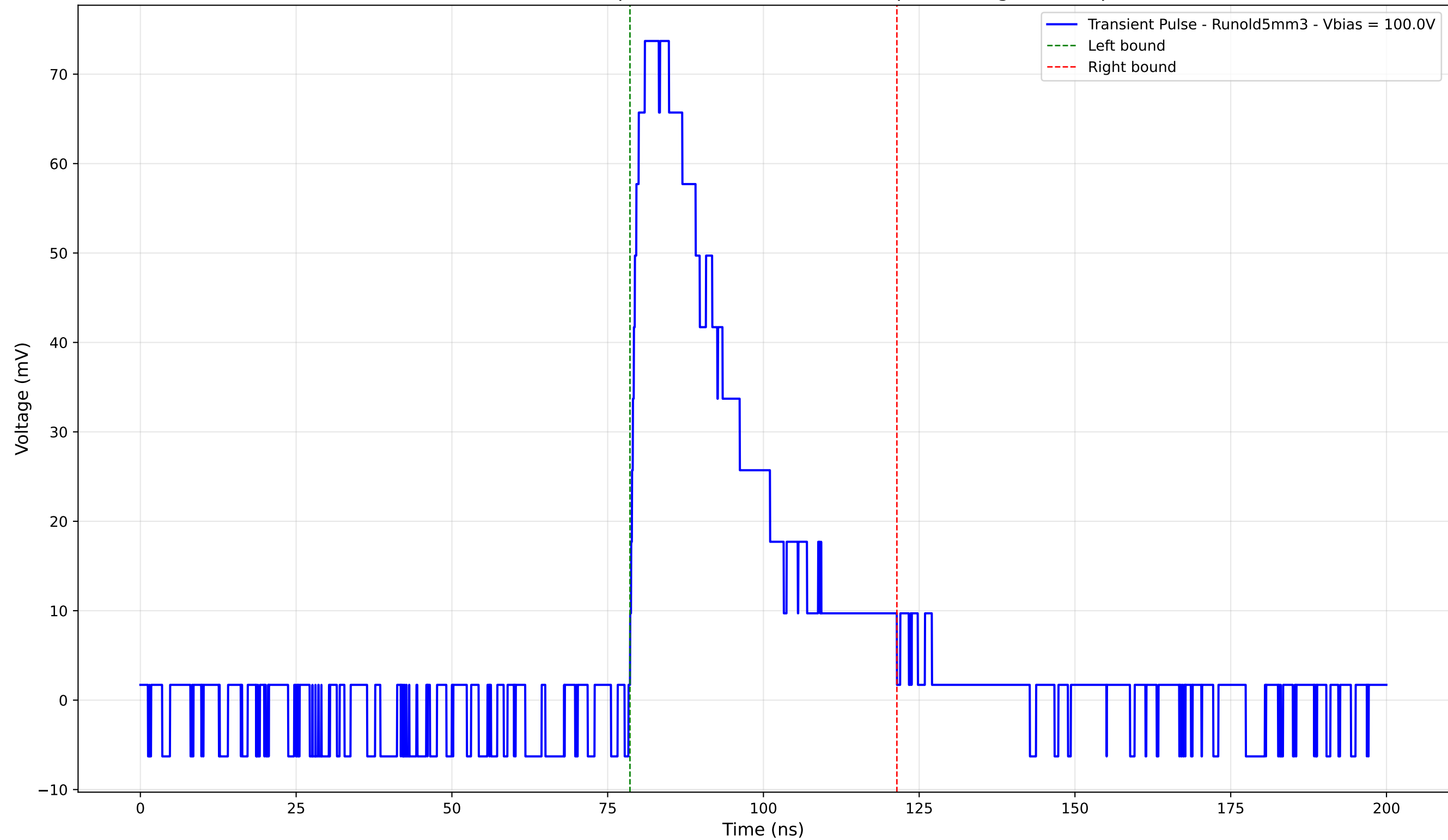
Transient Pulse - Sample: old5 - Position: 1150.0 \mu\text{m} - Charge: 26.41 pC
