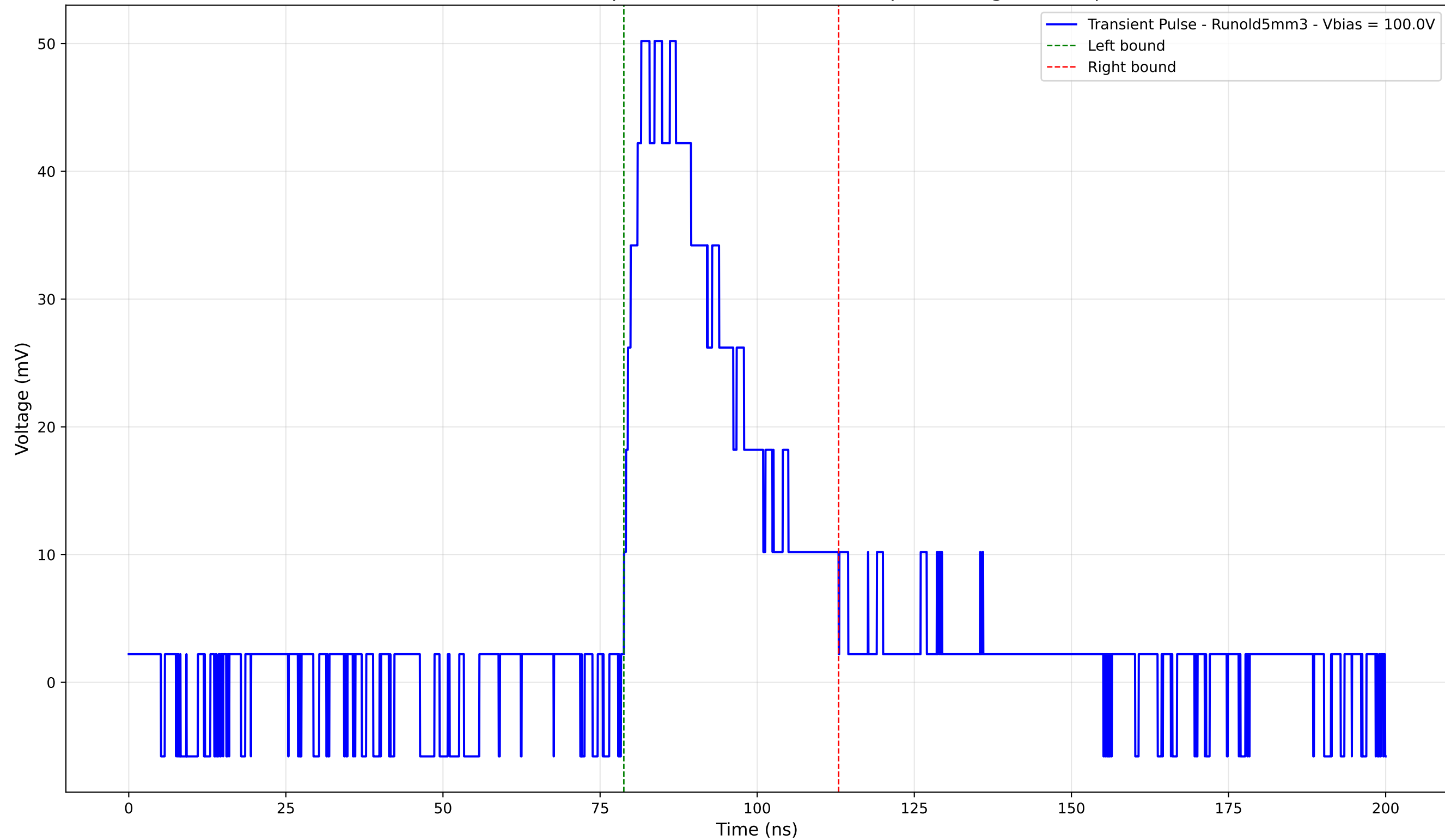
Transient Pulse - Sample: old5 - Position: 1405.0 \mu\text{m} - Charge: 17.74 pC
