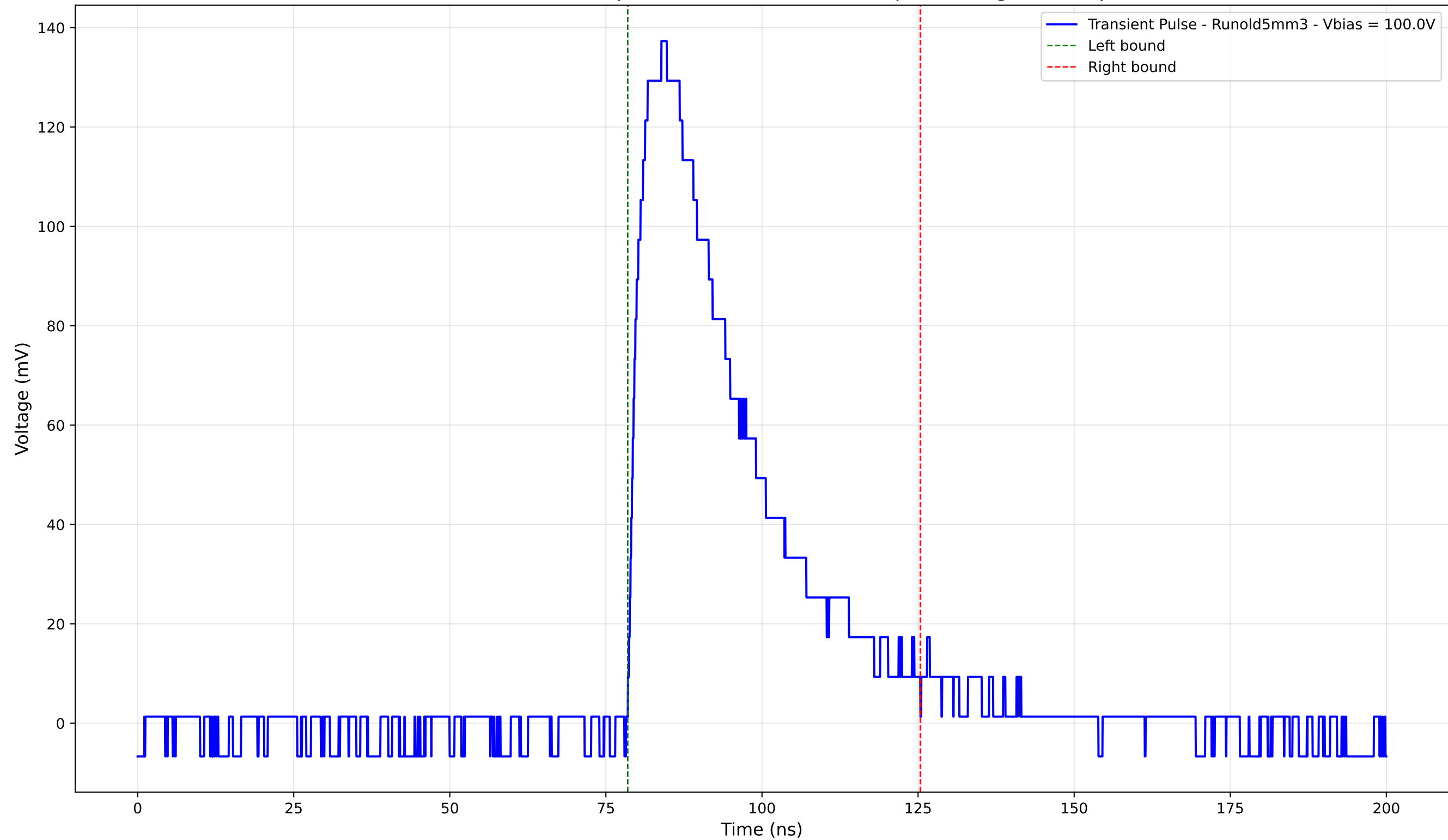
Transient Pulse - Sample: old5 - Position: 2040.0 \mu\text{m} - Charge: 51.90 pC
