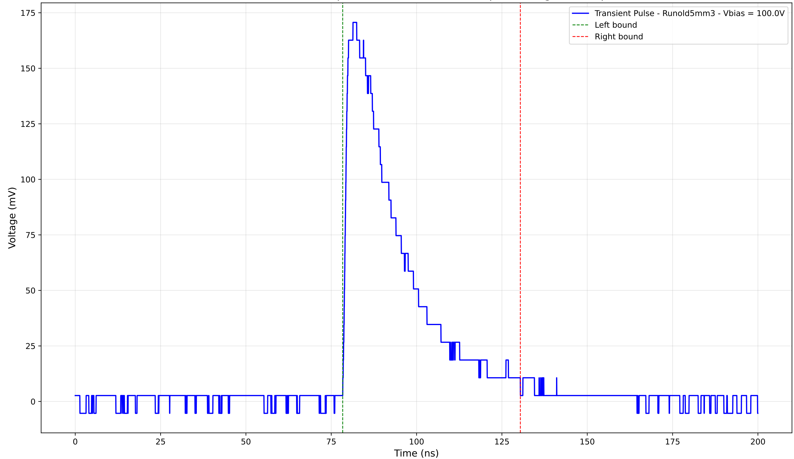
Transient Pulse - Sample: old5 - Position: 1035.0 \mu\text{m} - Charge: 60.30 pC
