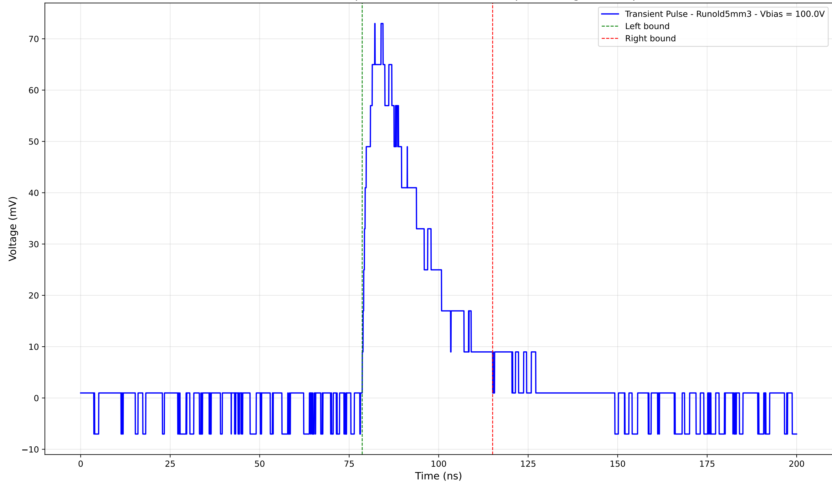
Transient Pulse - Sample: old5 - Position: 2420.0 \mu\text{m} - Charge: 23.29 pC
