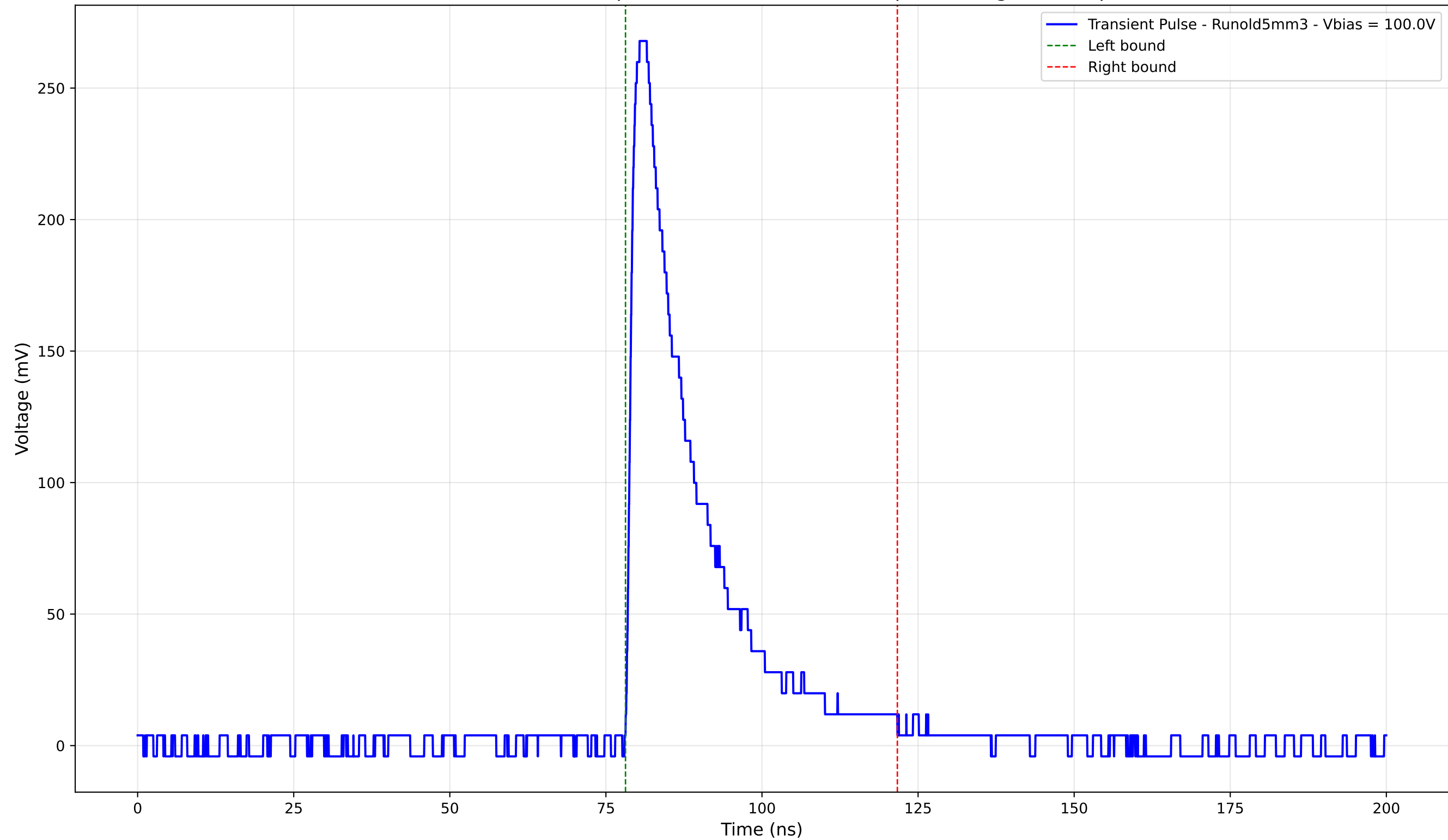
Transient Pulse - Sample: old5 - Position: 4255.0 \mu\text{m} - Charge: 60.72 pC
