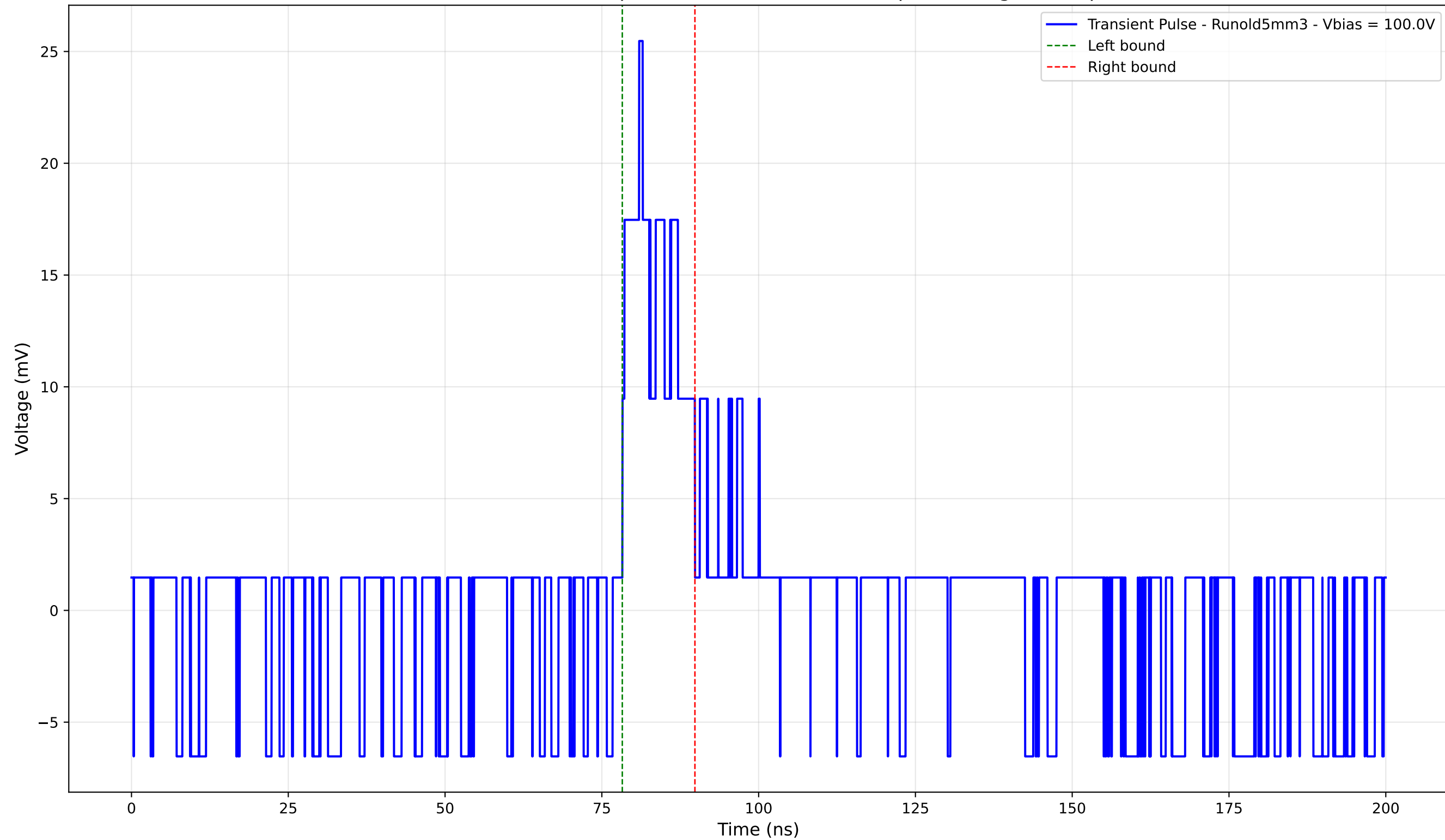
Transient Pulse - Sample: old5 - Position: 3270.0 \mu\text{m} - Charge: 3.36 pC
