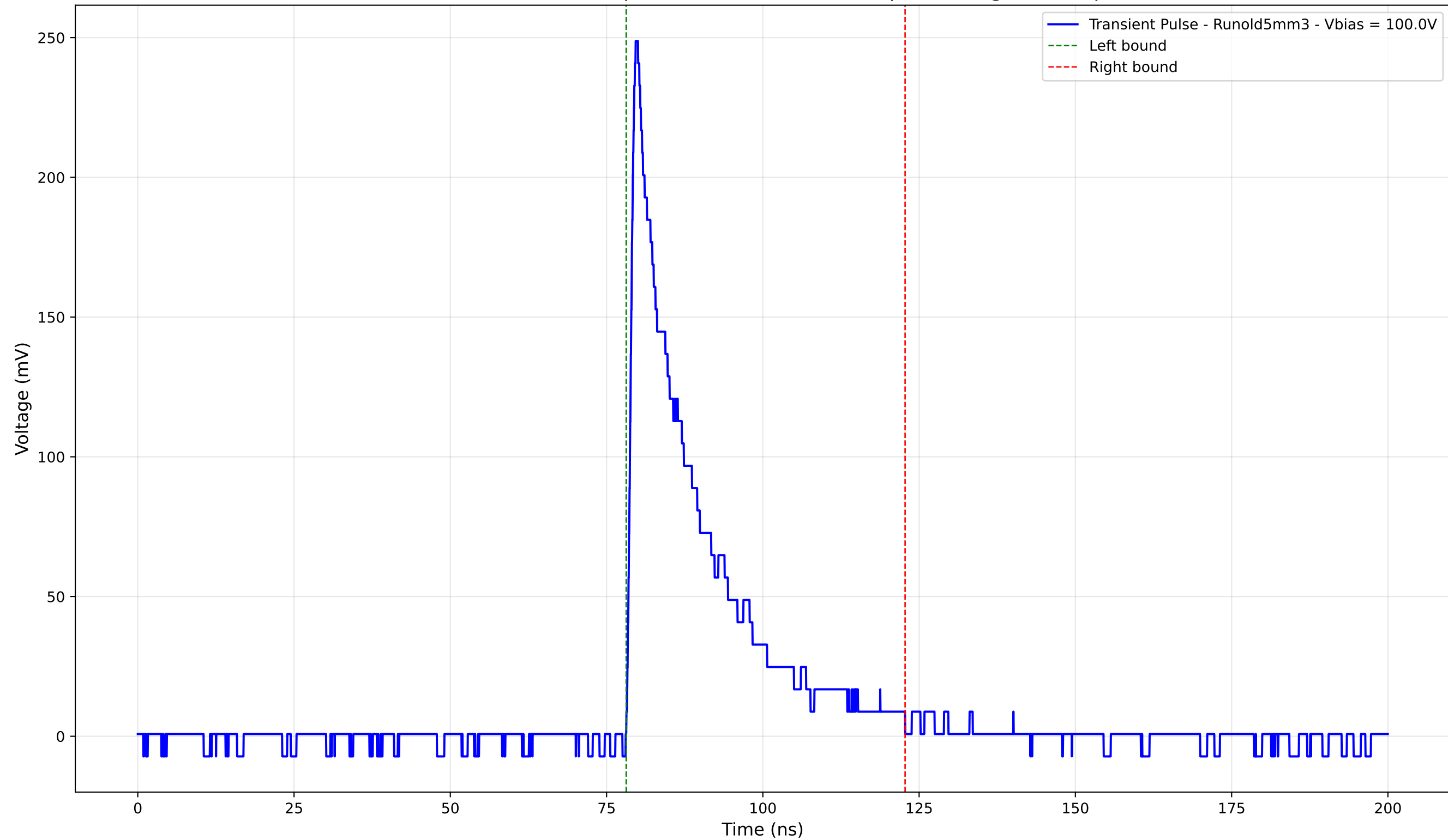
Transient Pulse - Sample: old5 - Position: 530.0 \mu\text{m} - Charge: 50.87 pC
