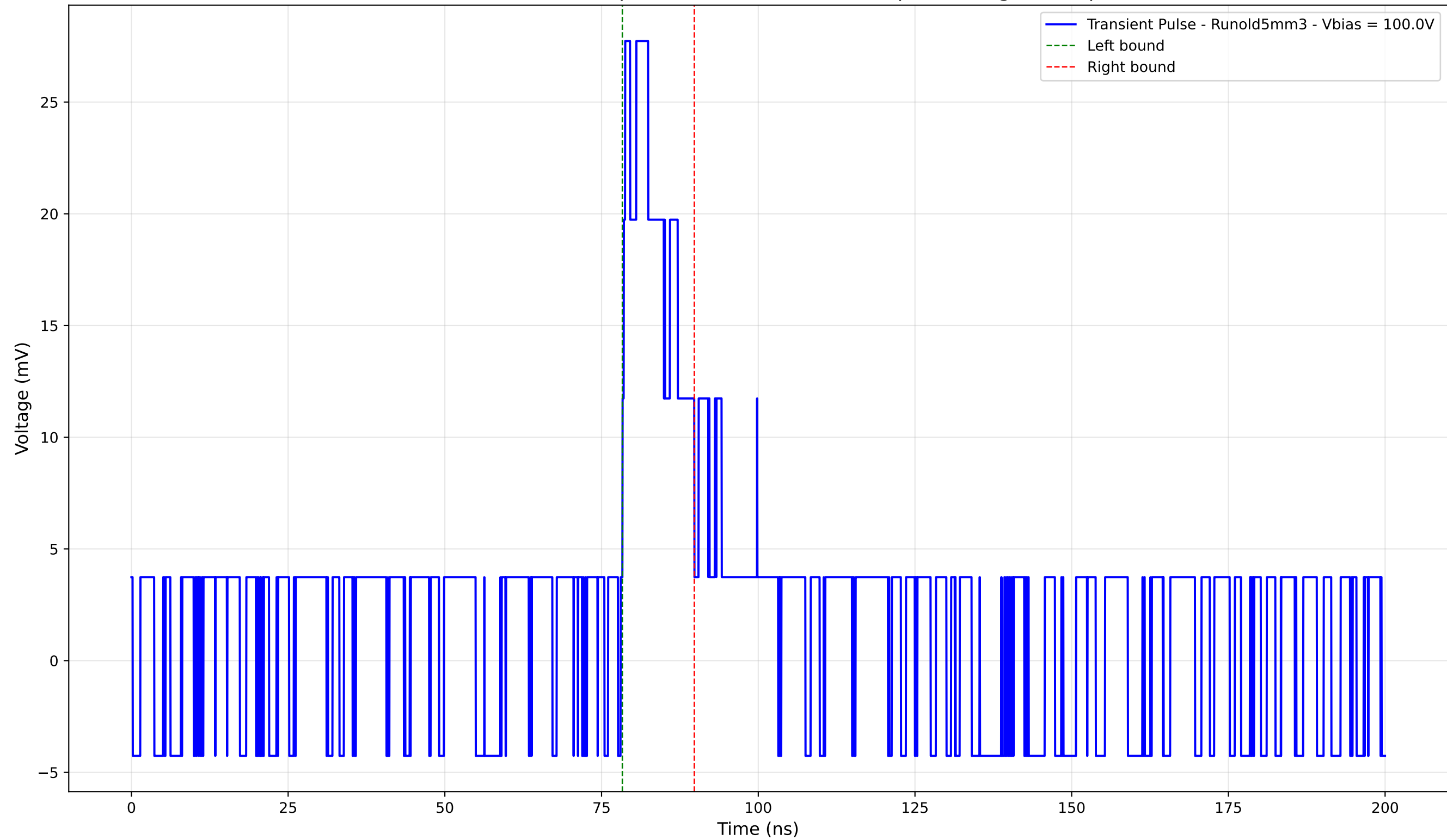
Transient Pulse - Sample: old5 - Position: 3265.0 \mu\text{m} - Charge: 4.37 pC
