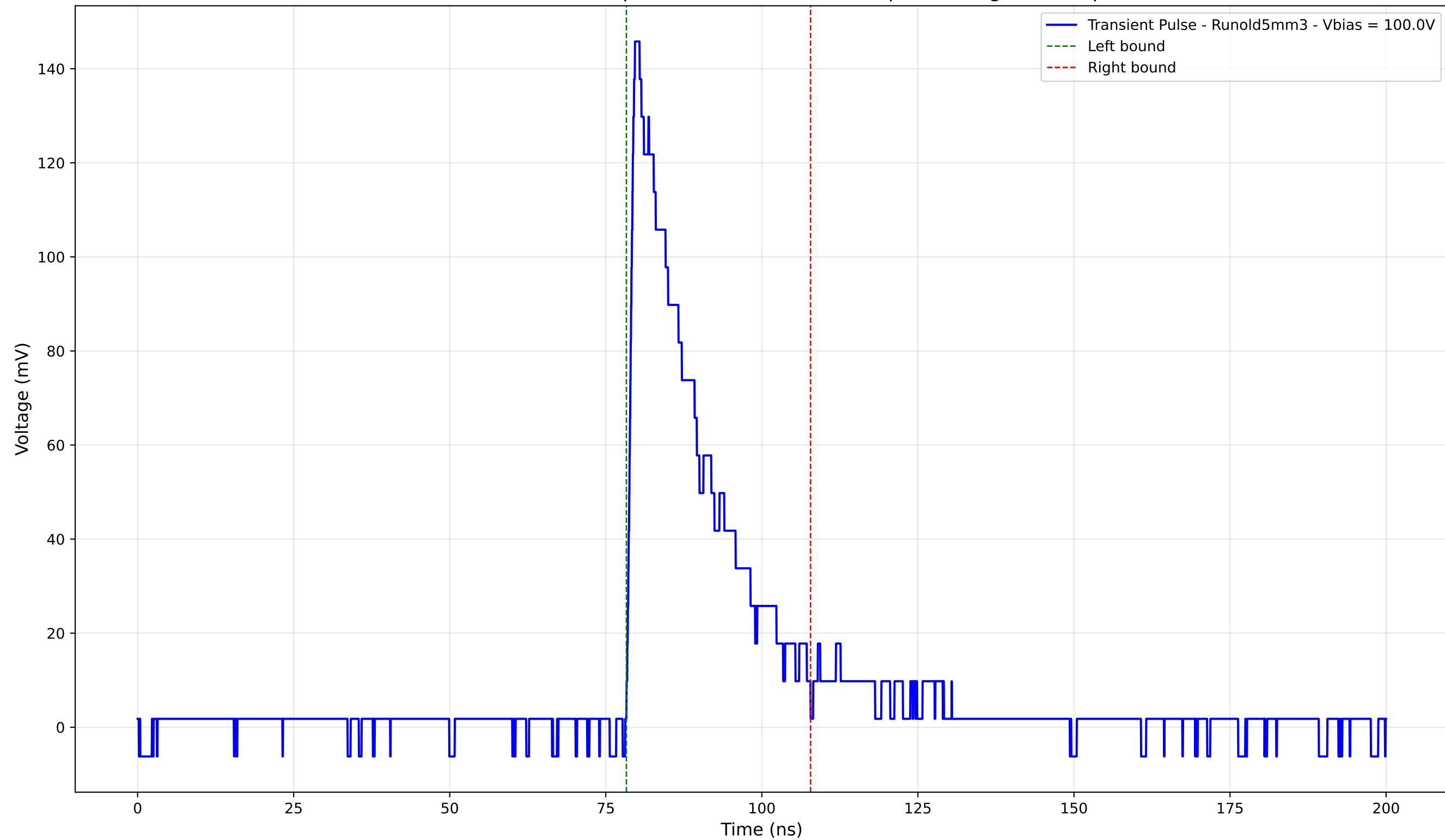
Transient Pulse - Sample: old5 - Position: 695.0 \mu\text{m} - Charge: 33.62 pC
