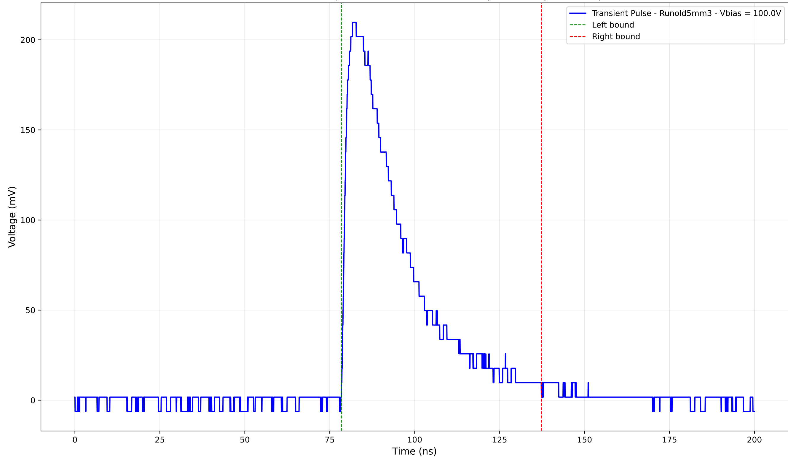
Transient Pulse - Sample: old5 - Position: 1300.0 \mu\text{m} - Charge: 79.95 pC
