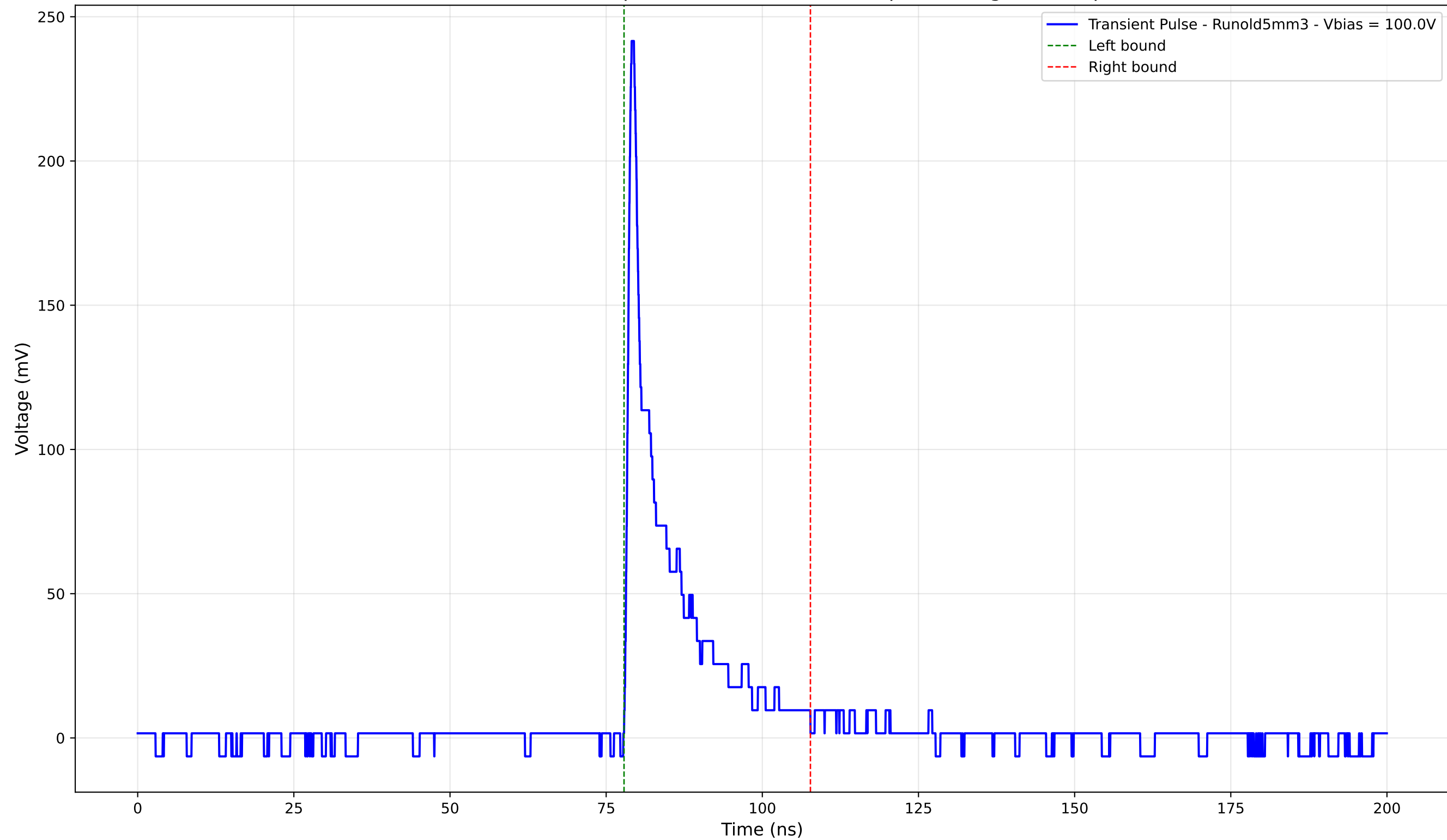
Transient Pulse - Sample: old5 - Position: 165.0 \mu\text{m} - Charge: 27.84 pC
