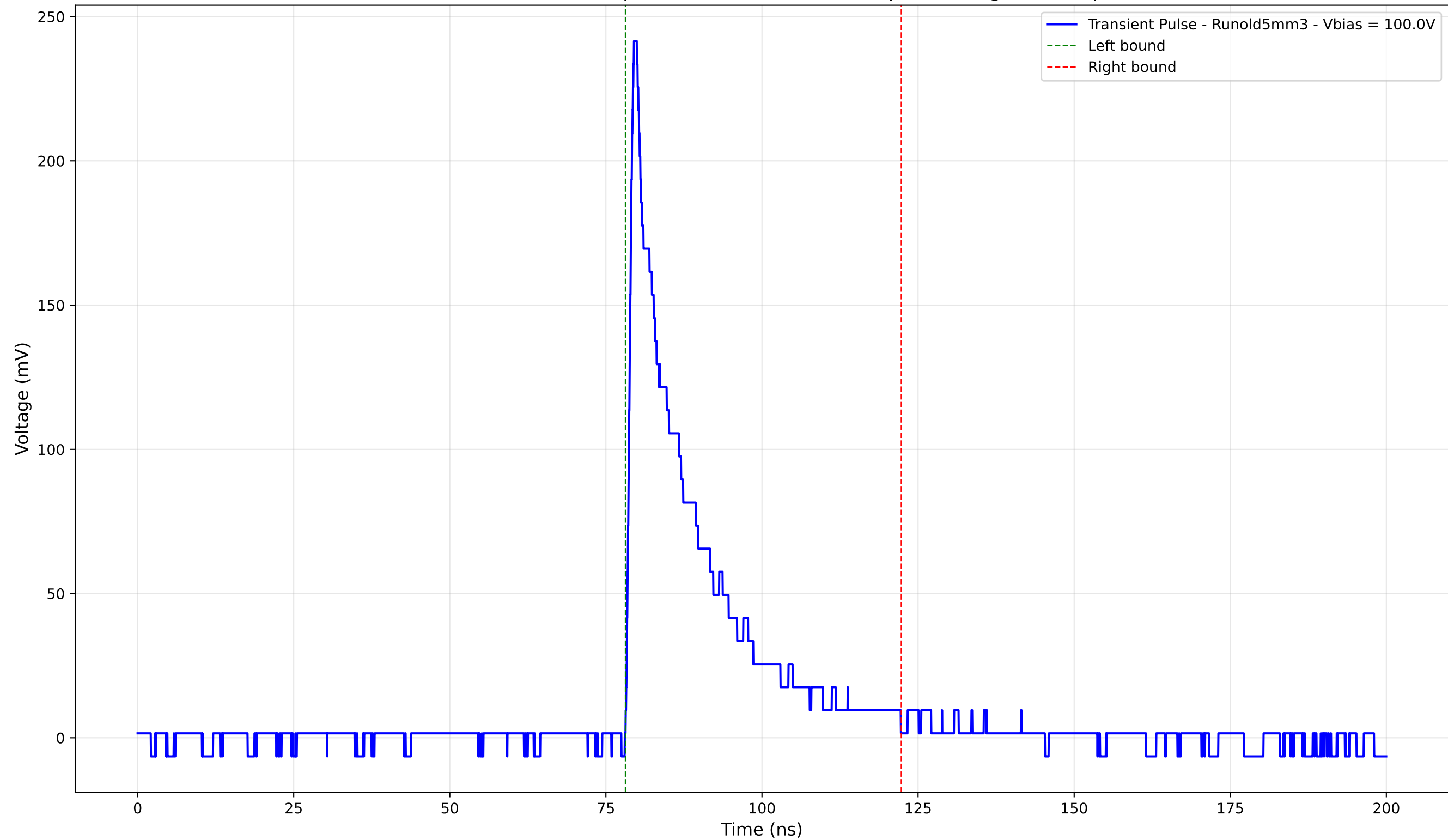
Transient Pulse - Sample: old5 - Position: 475.0 \mu\text{m} - Charge: 45.71 pC
