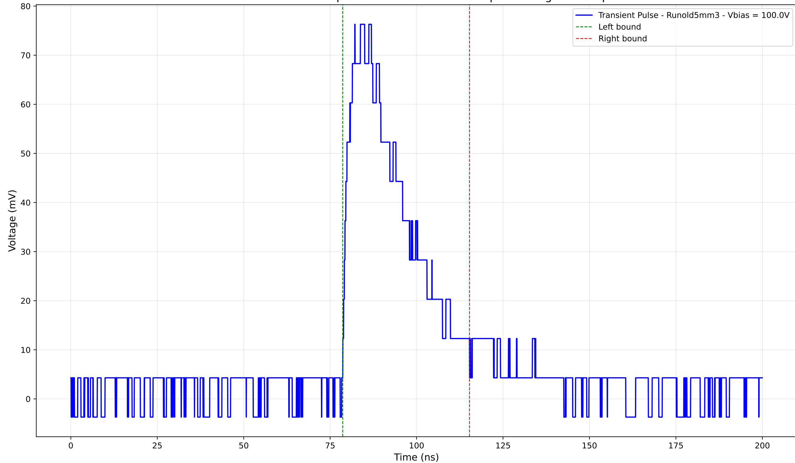
Transient Pulse - Sample: old5 - Position: 1615.0 \mu\text{m} - Charge: 28.33 pC
