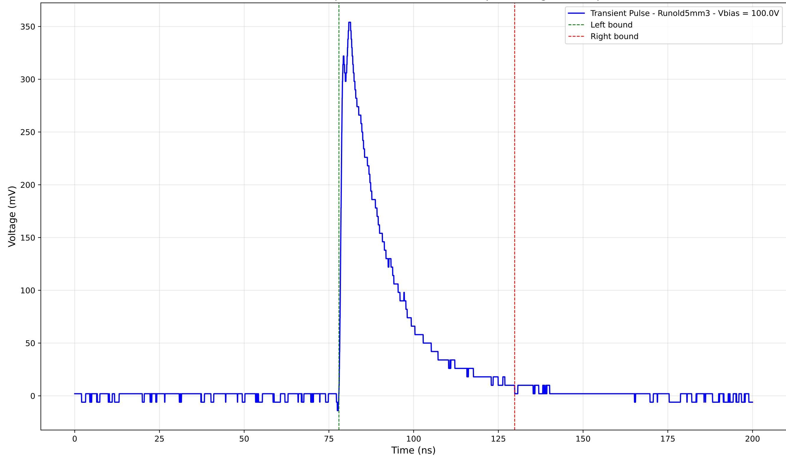
Transient Pulse - Sample: old5 - Position: 3085.0 \mu\text{m} - Charge: 97.70 pC
