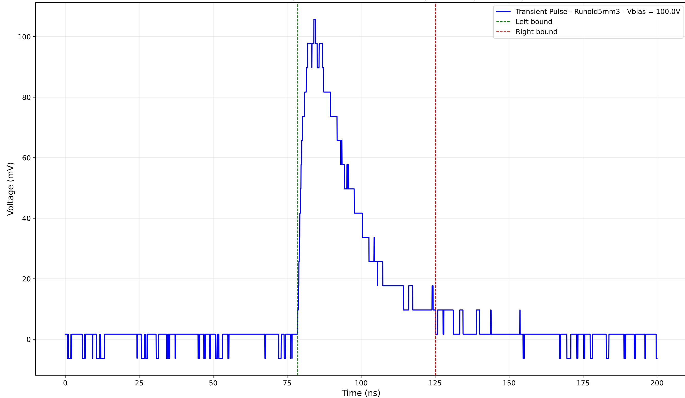
Transient Pulse - Sample: old5 - Position: 1950.0 \mu\text{m} - Charge: 39.18 pC
