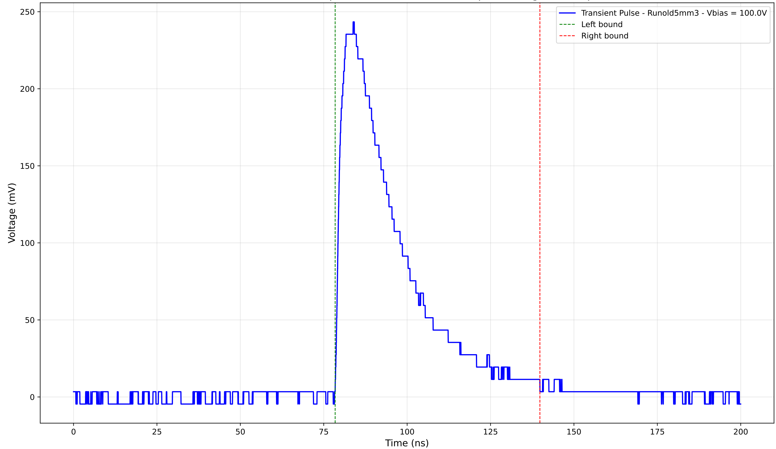
Transient Pulse - Sample: old5 - Position: 2300.0 \mu\text{m} - Charge: 95.81 pC
