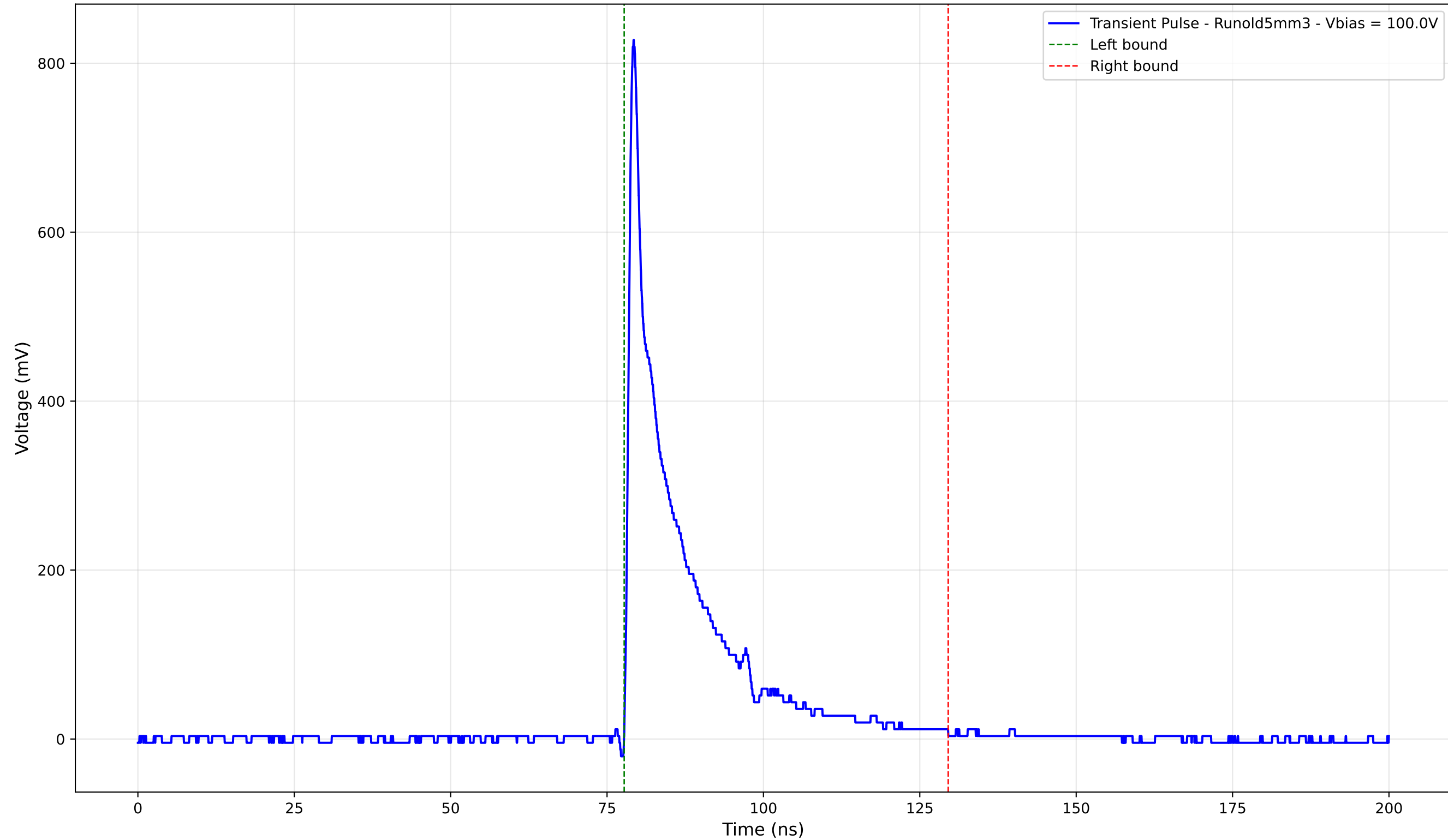
Transient Pulse - Sample: old5 - Position: 4830.0 \mu\text{m} - Charge: 124.52 pC
