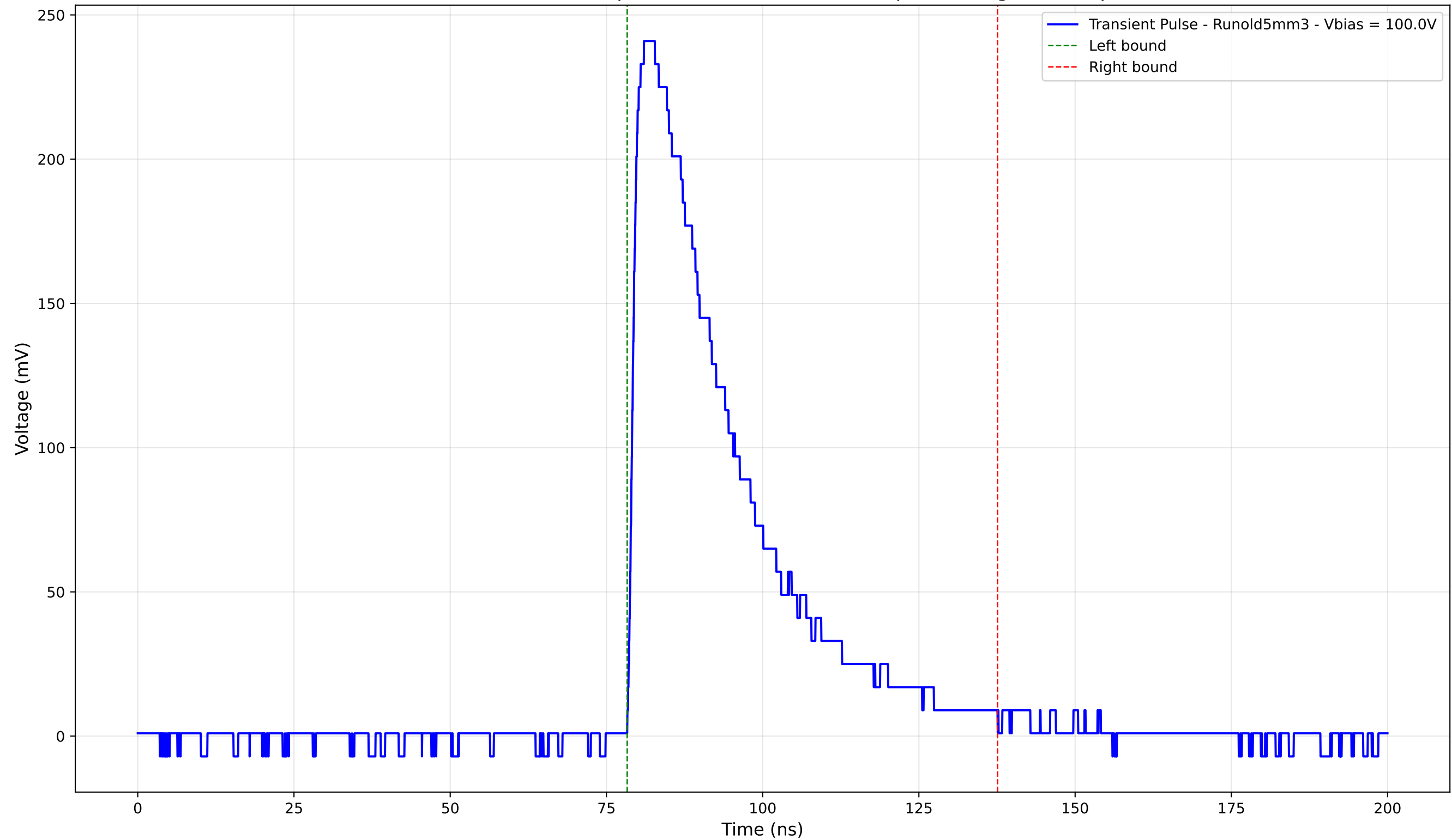
Transient Pulse - Sample: old5 - Position: 1085.0 \mu\text{m} - Charge: 86.33 pC
