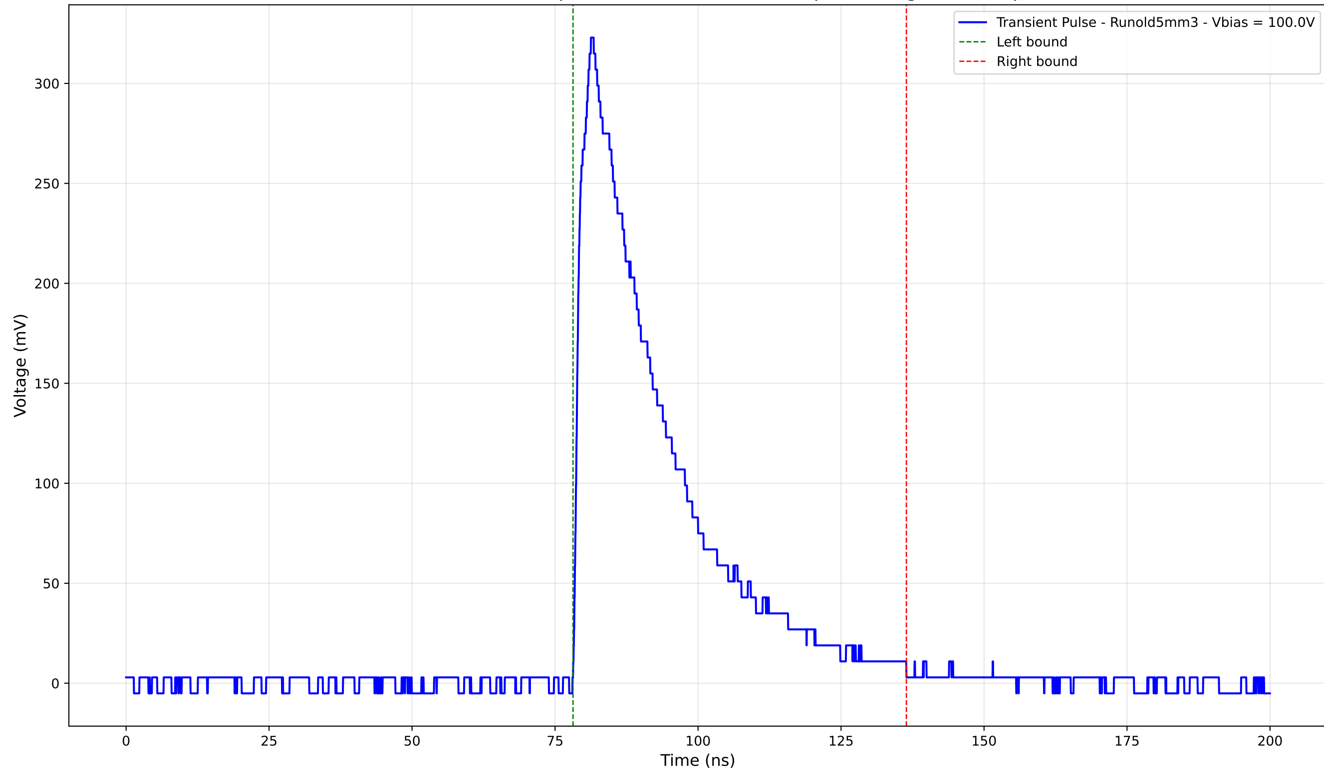
Transient Pulse - Sample: old5 - Position: 2850.0 \mu\text{m} - Charge: 104.43 pC
