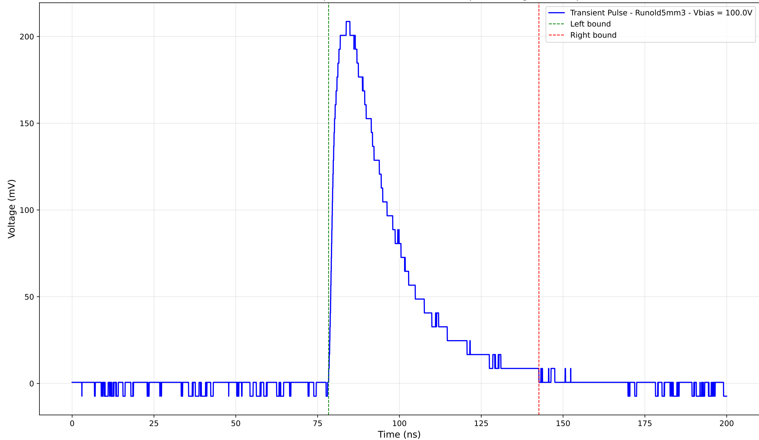
Transient Pulse - Sample: old5 - Position: 1880.0 \mu\text{m} - Charge: 84.70 pC
