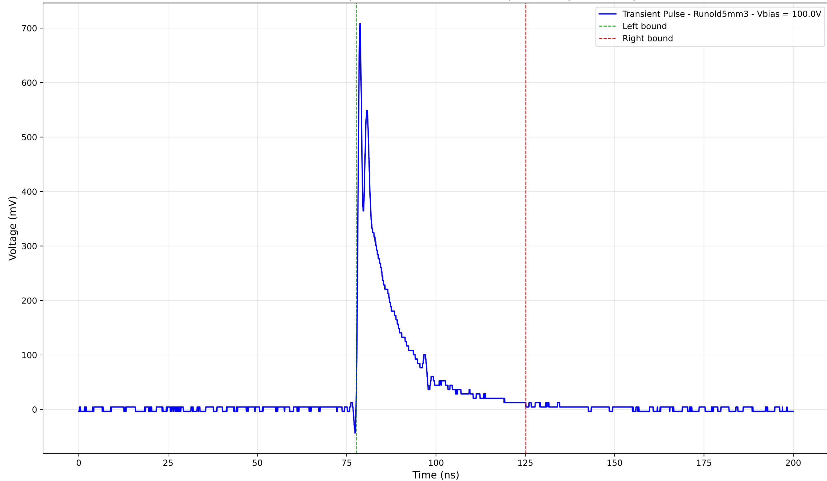
Transient Pulse - Sample: old5 - Position: 3455.0 \mu\text{m} - Charge: 107.16 pC
