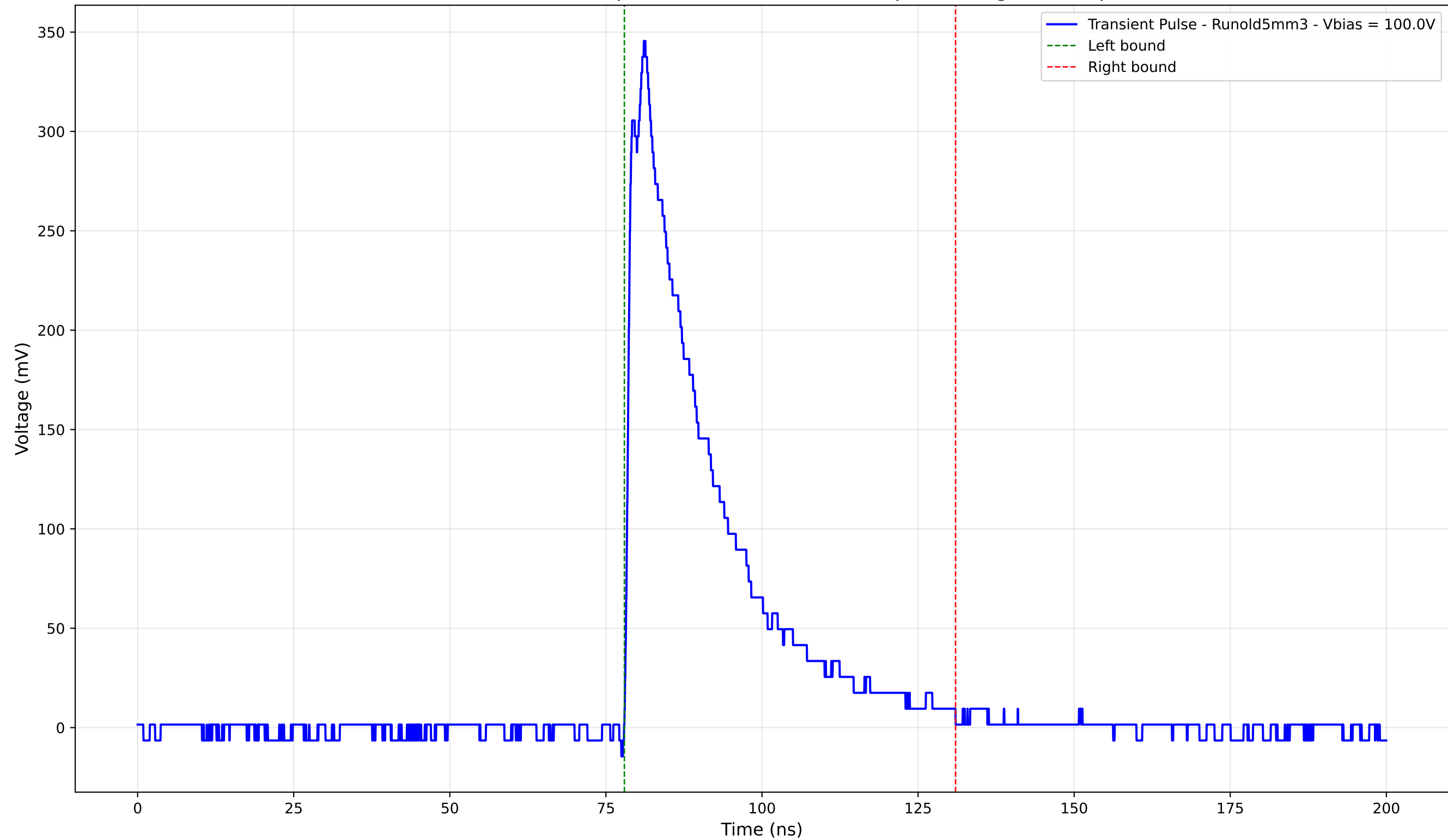
Transient Pulse - Sample: old5 - Position: 3080.0 \mu\text{m} - Charge: 94.12 pC
