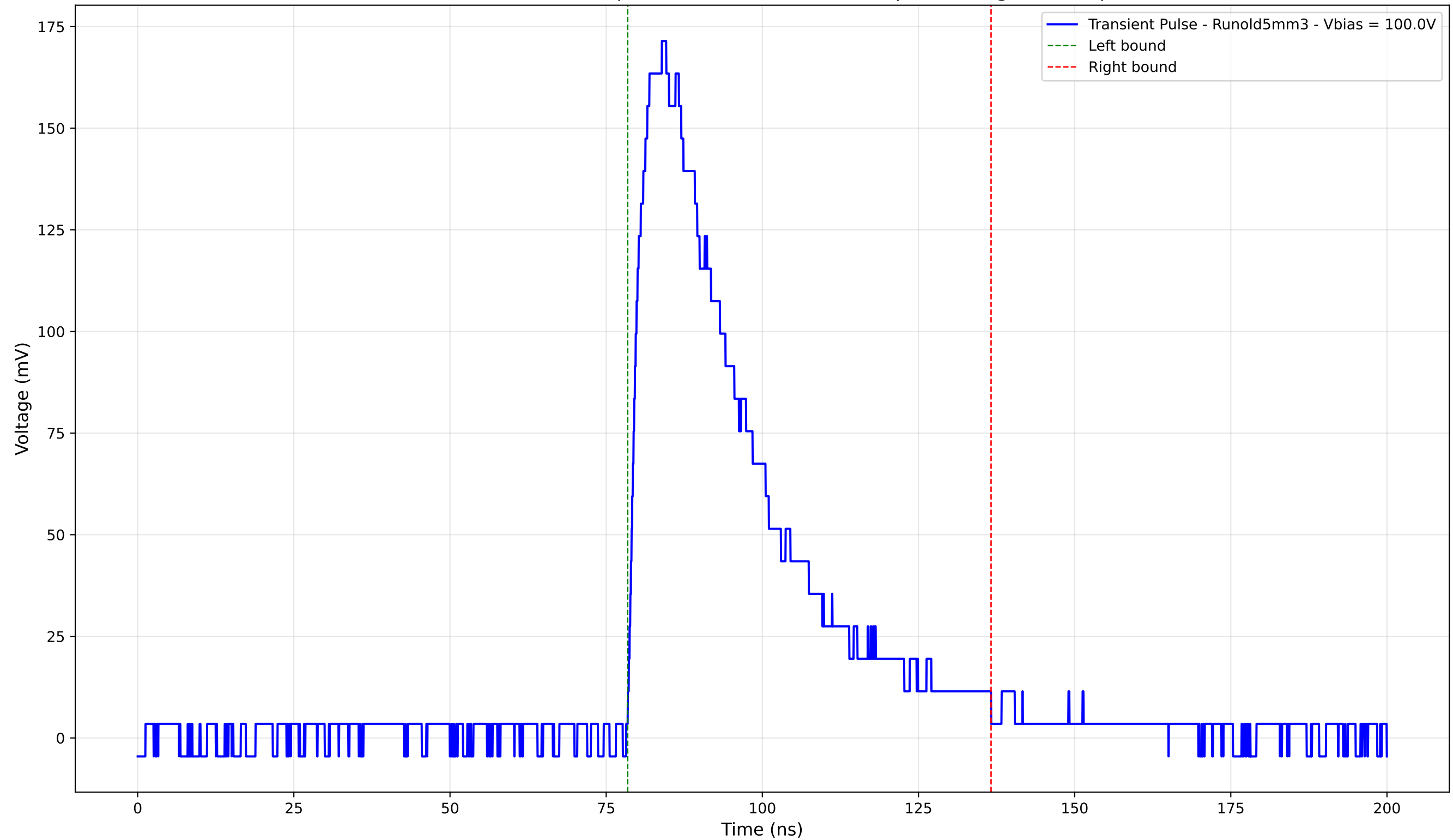
Transient Pulse - Sample: old5 - Position: 2050.0 \mu\text{m} - Charge: 68.53 pC
