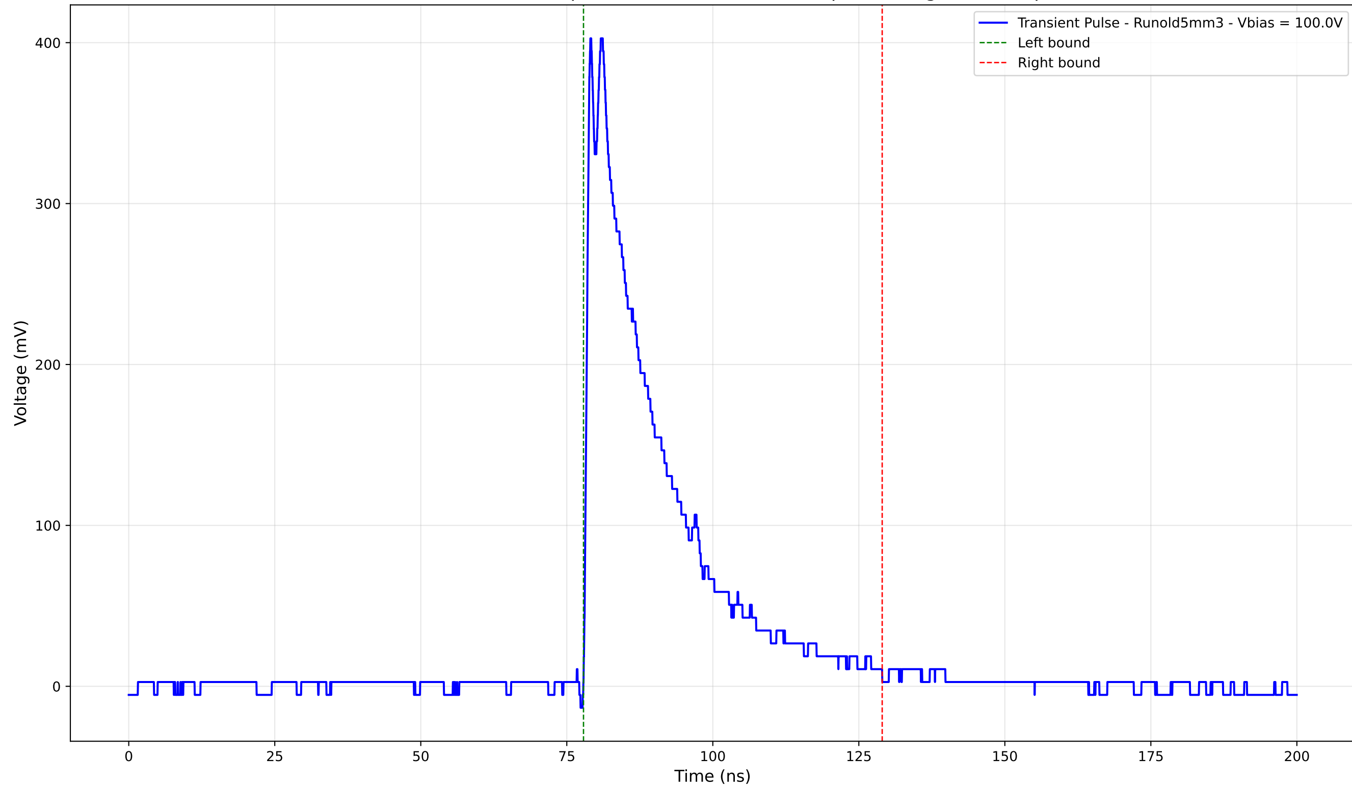
Transient Pulse - Sample: old5 - Position: 3155.0 \mu\text{m} - Charge: 103.92 pC
