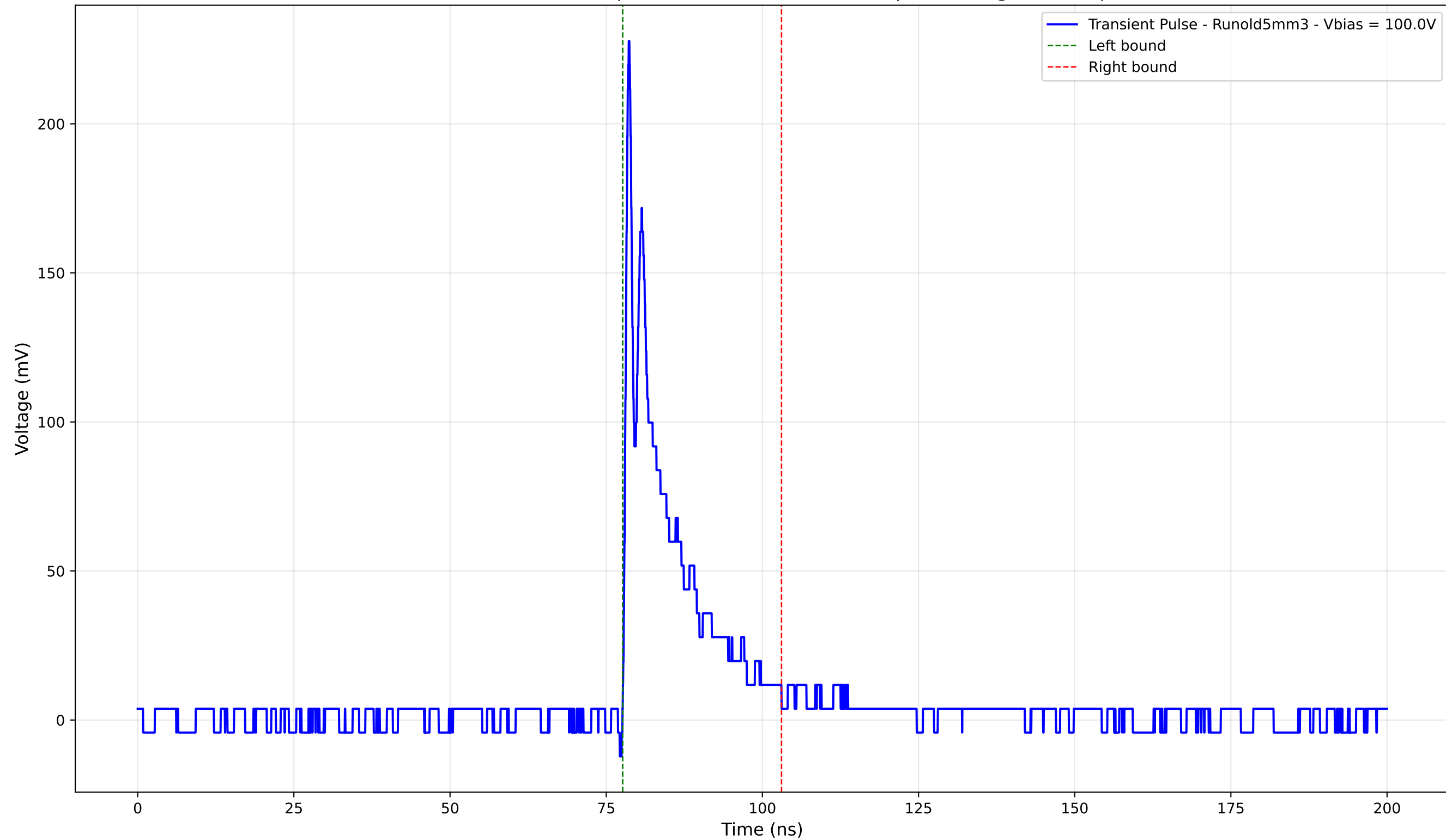
Transient Pulse - Sample: old5 - Position: 3630.0 \mu\text{m} - Charge: 27.32 pC
