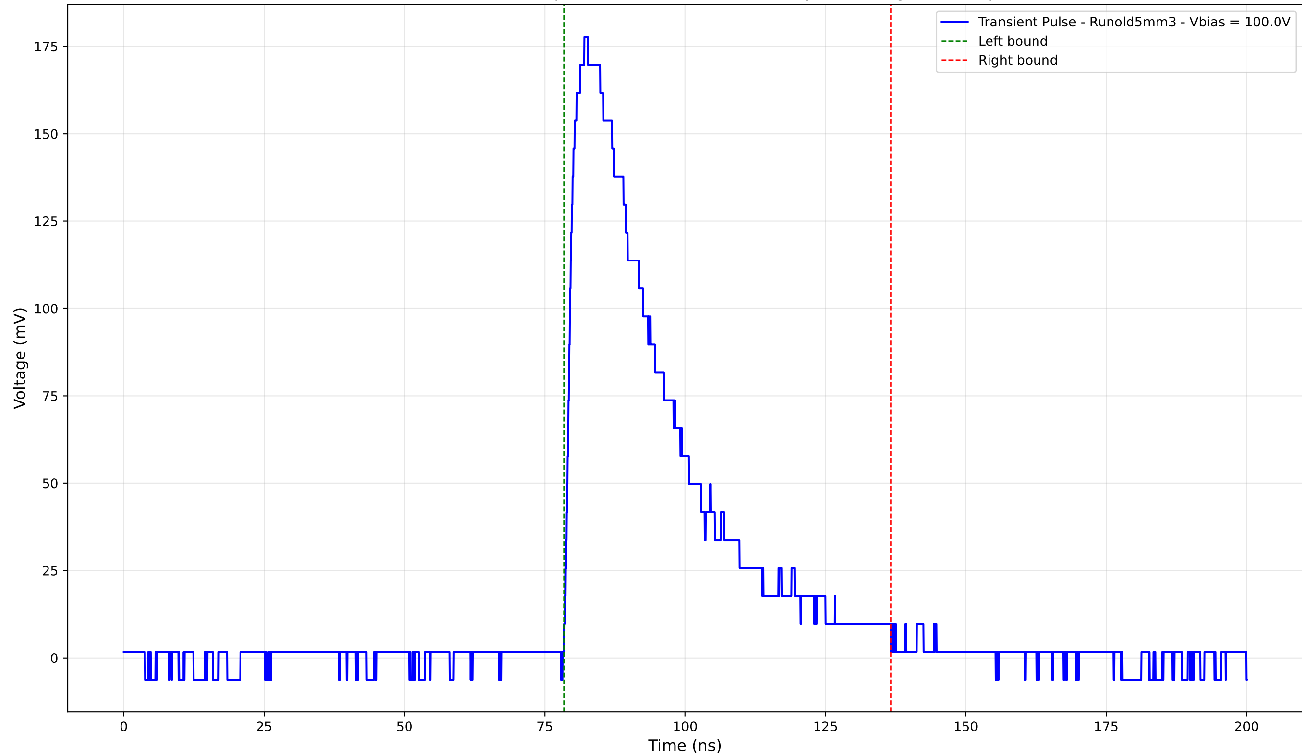
Transient Pulse - Sample: old5 - Position: 1250.0 \mu\text{m} - Charge: 67.01 pC
