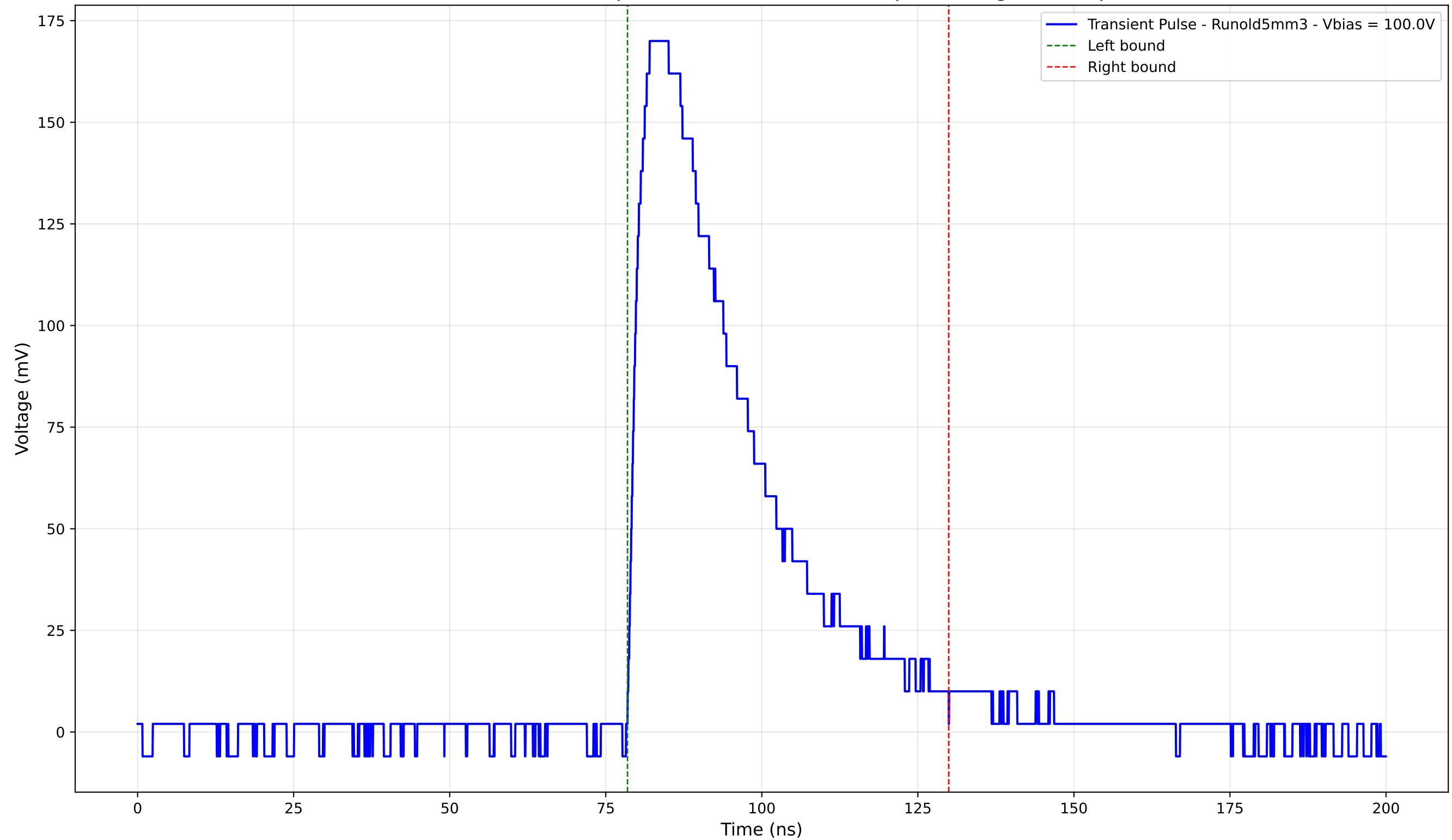
Transient Pulse - Sample: old5 - Position: 1925.0 \mu\text{m} - Charge: 68.27 pC
