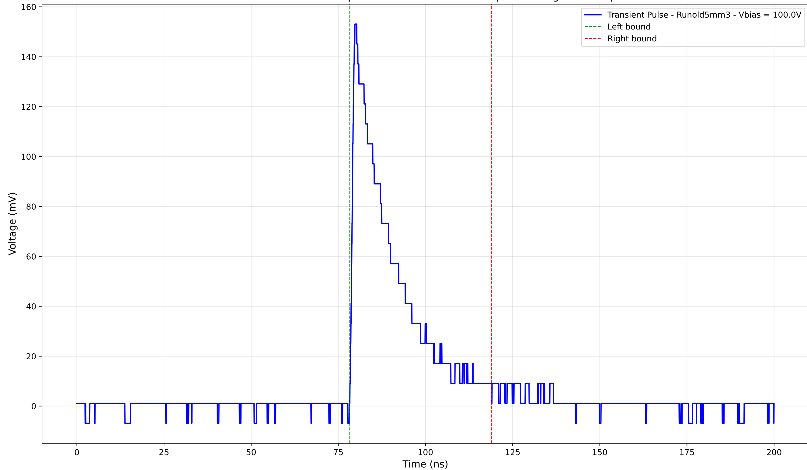
Transient Pulse - Sample: old5 - Position: 690.0 \mu\text{m} - Charge: 37.19 pC
