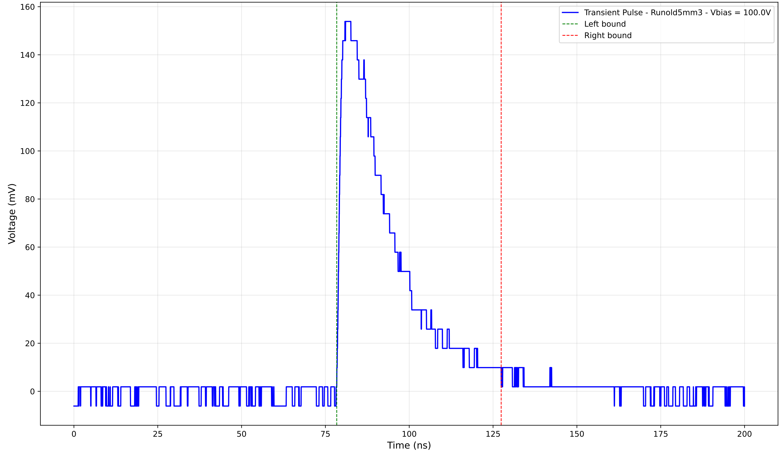
Transient Pulse - Sample: old5 - Position: 1030.0 \mu\text{m} - Charge: 53.21 pC
