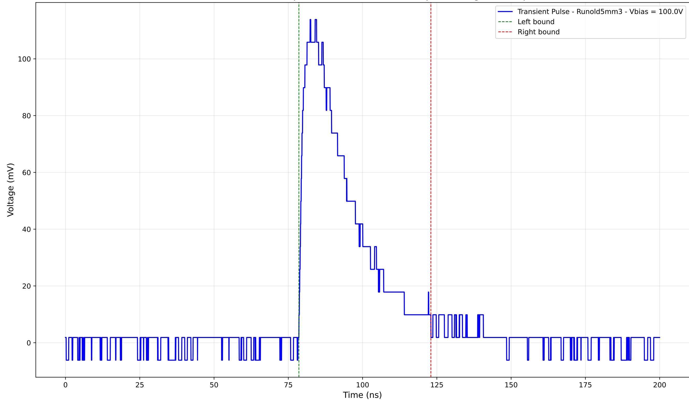
Transient Pulse - Sample: old5 - Position: 1340.0 \mu\text{m} - Charge: 40.56 pC
