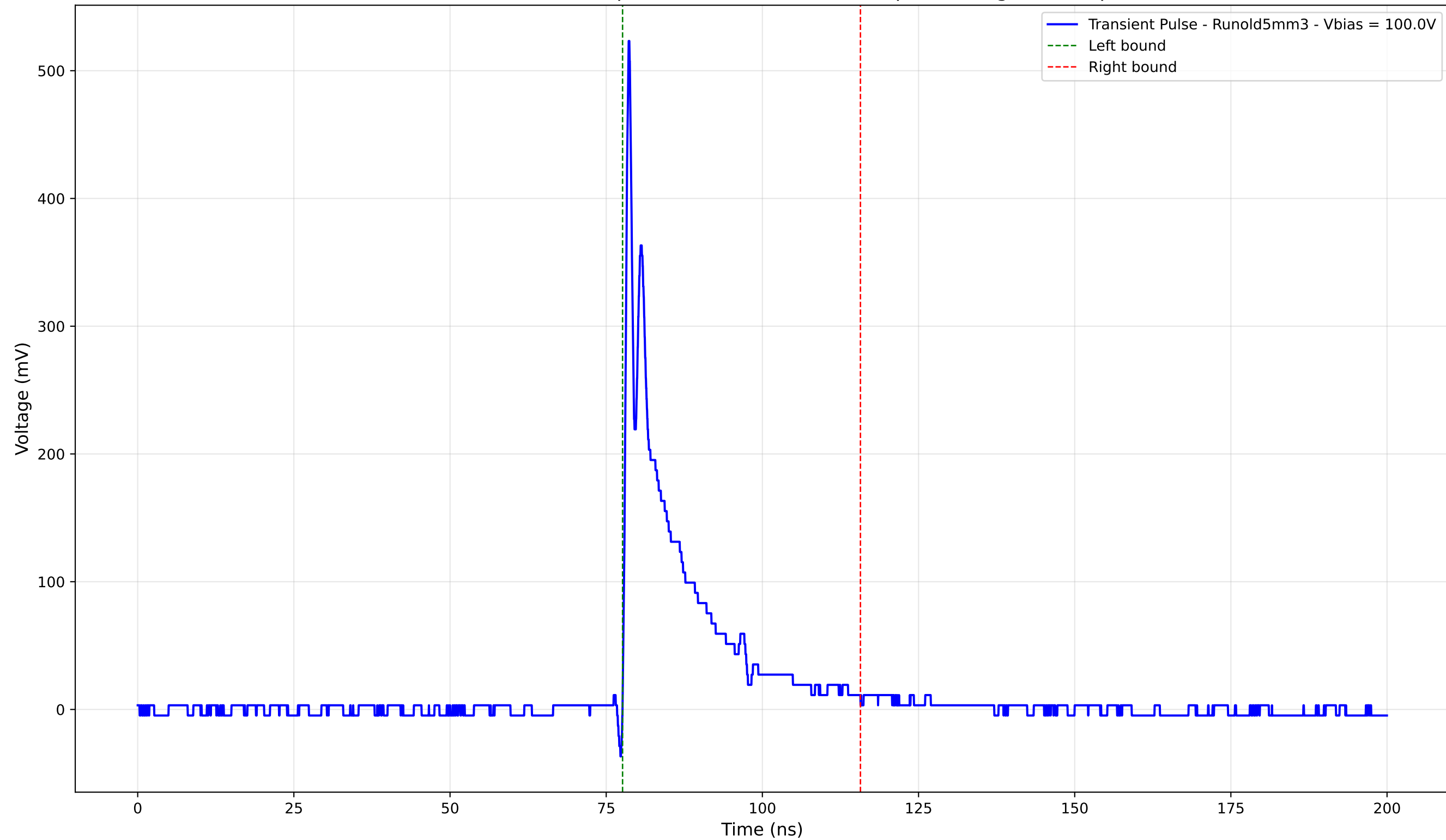
Transient Pulse - Sample: old5 - Position: 3505.0 \mu\text{m} - Charge: 64.51 pC
