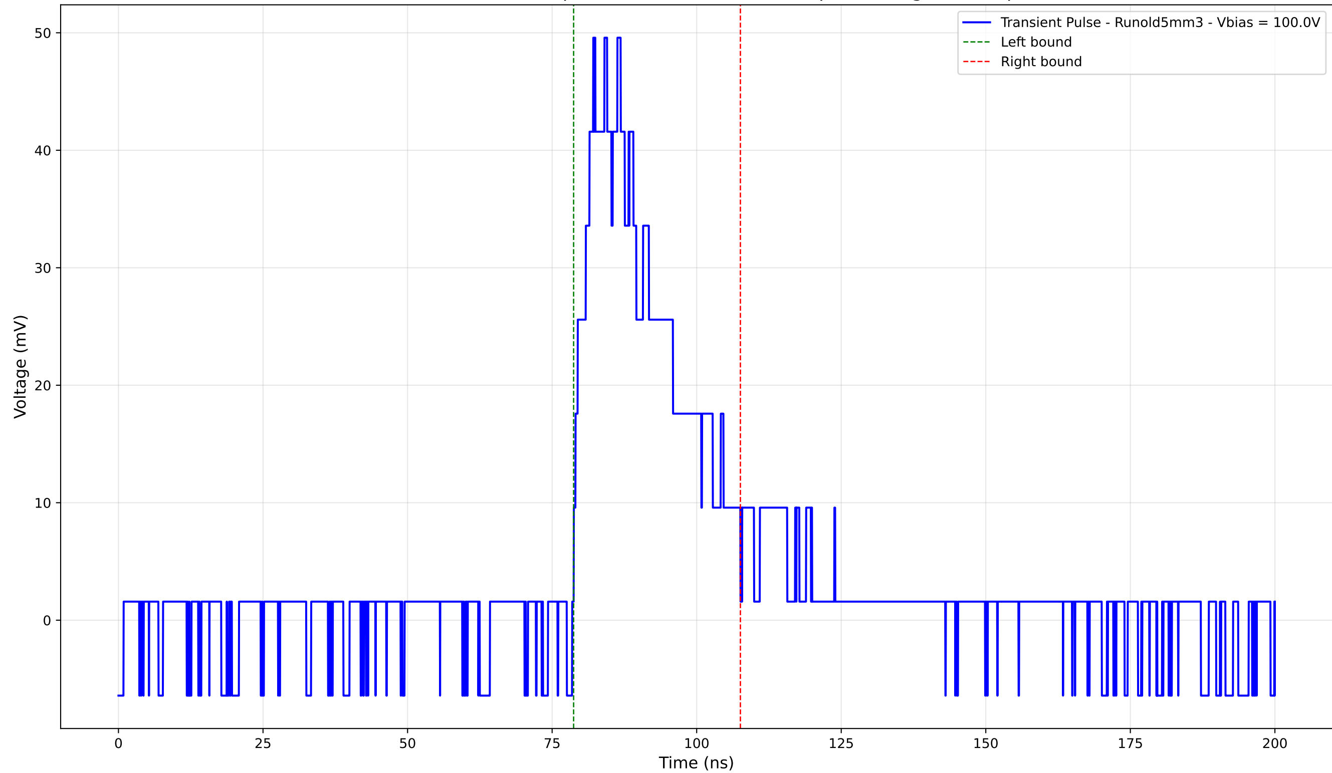
Transient Pulse - Sample: old5 - Position: 1975.0 \mu\text{m} - Charge: 14.85 pC
