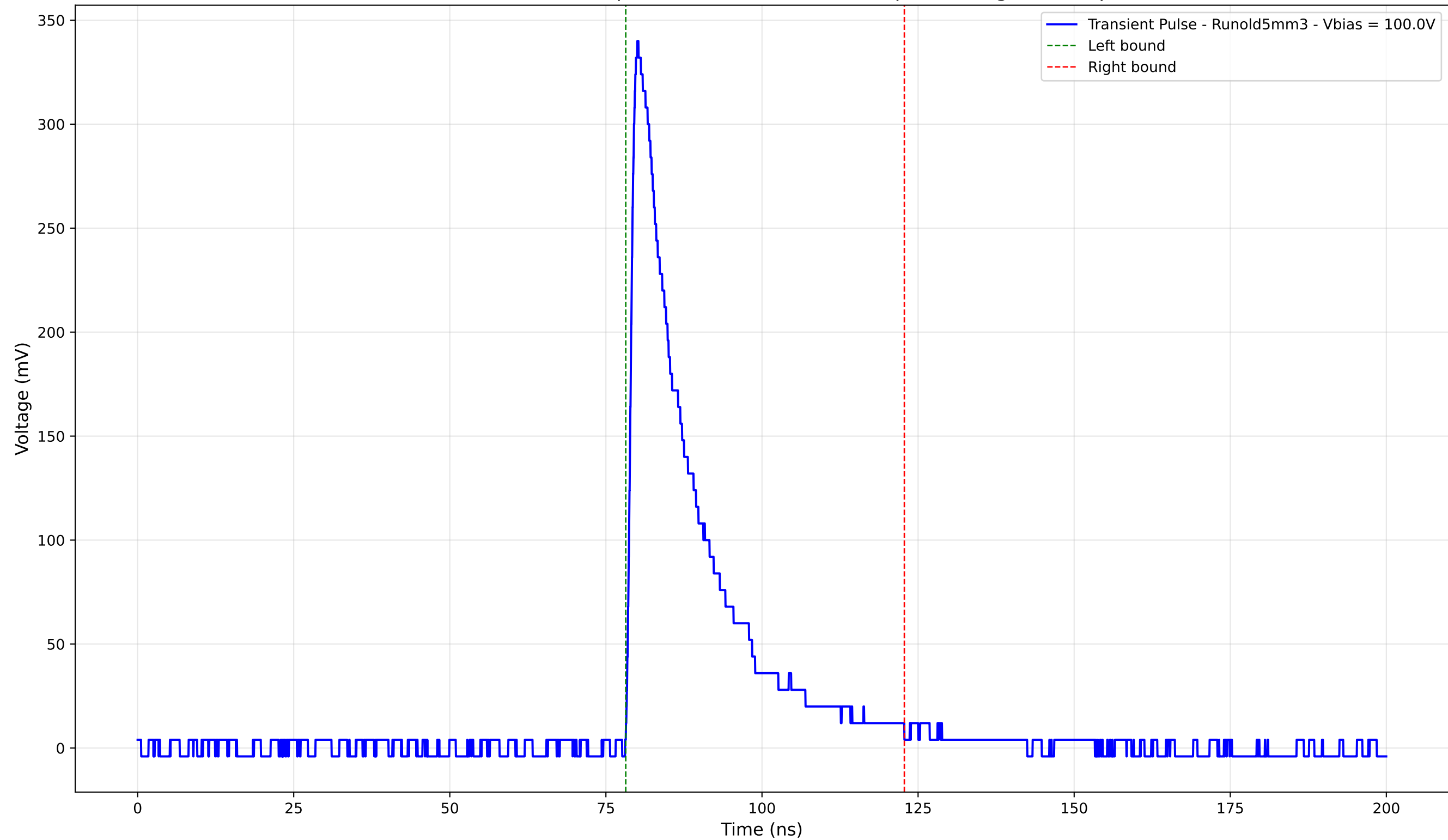
Transient Pulse - Sample: old5 - Position: 4415.0 \mu\text{m} - Charge: 72.31 pC
