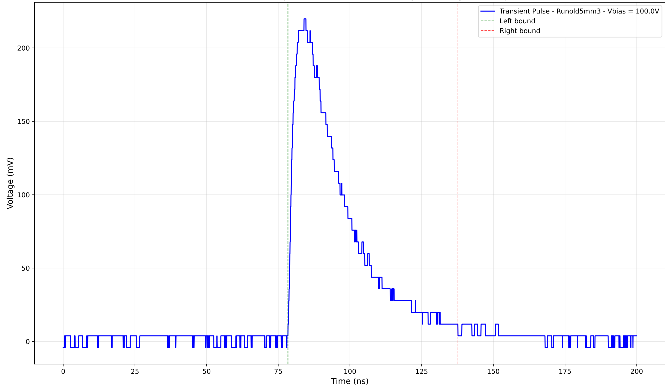
Transient Pulse - Sample: old5 - Position: 1890.0 \mu\text{m} - Charge: 89.78 pC
