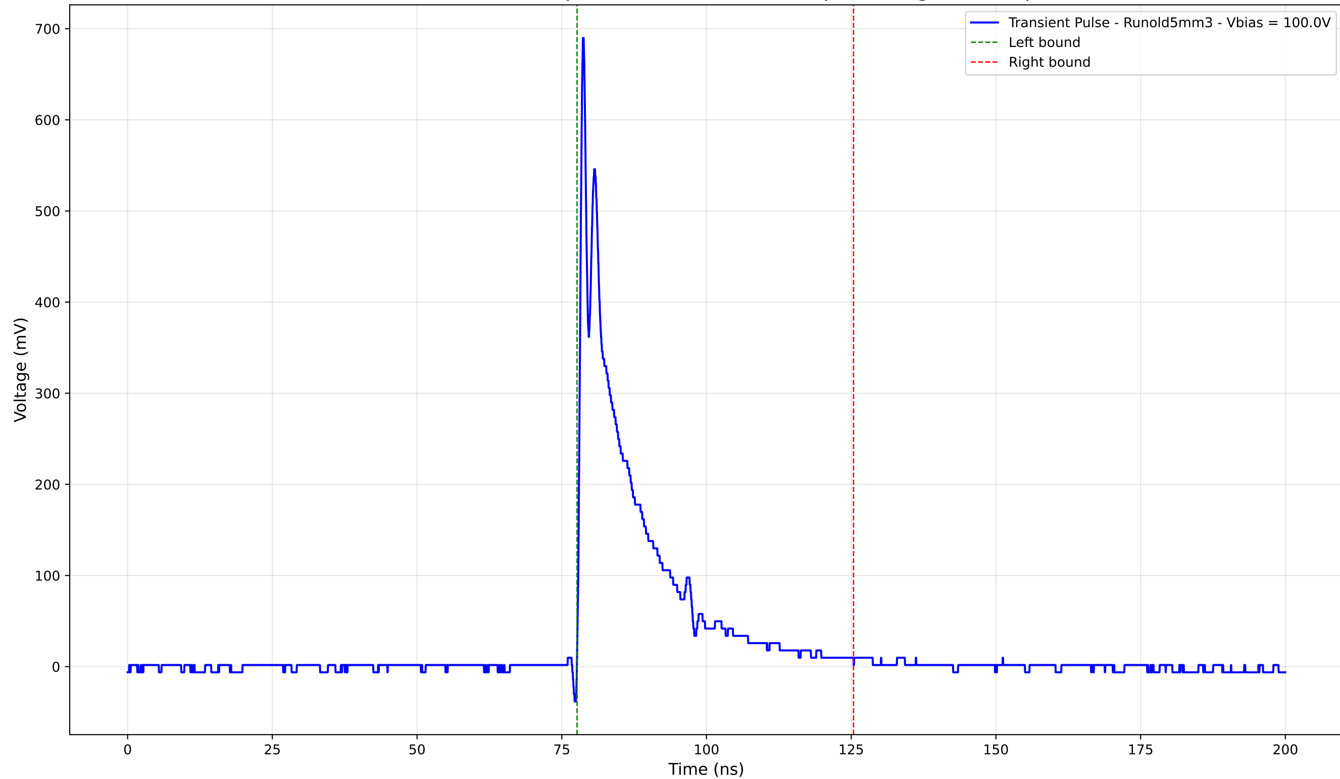
Transient Pulse - Sample: old5 - Position: 3445.0 \mu\text{m} - Charge: 105.43 pC
