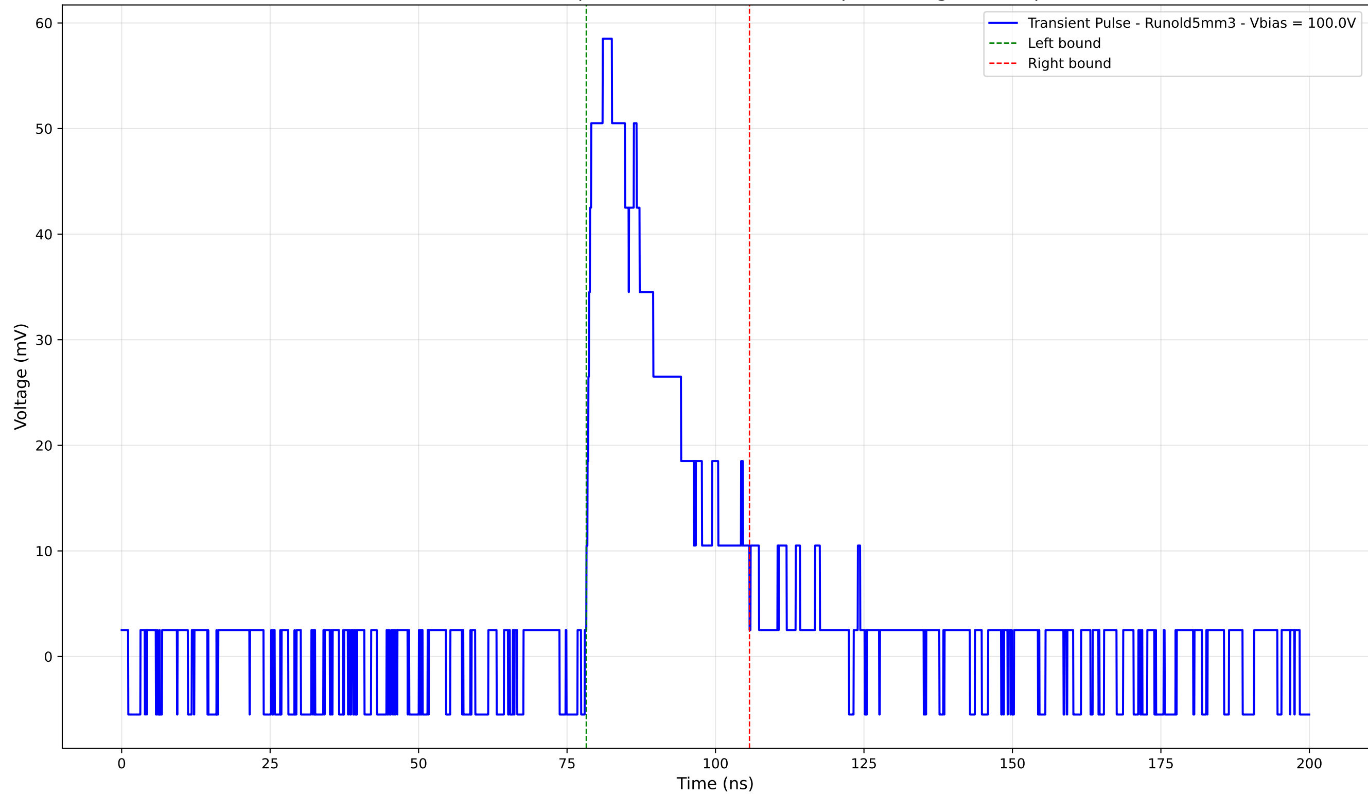
Transient Pulse - Sample: old5 - Position: 3015.0 \mu\text{m} - Charge: 15.83 pC
