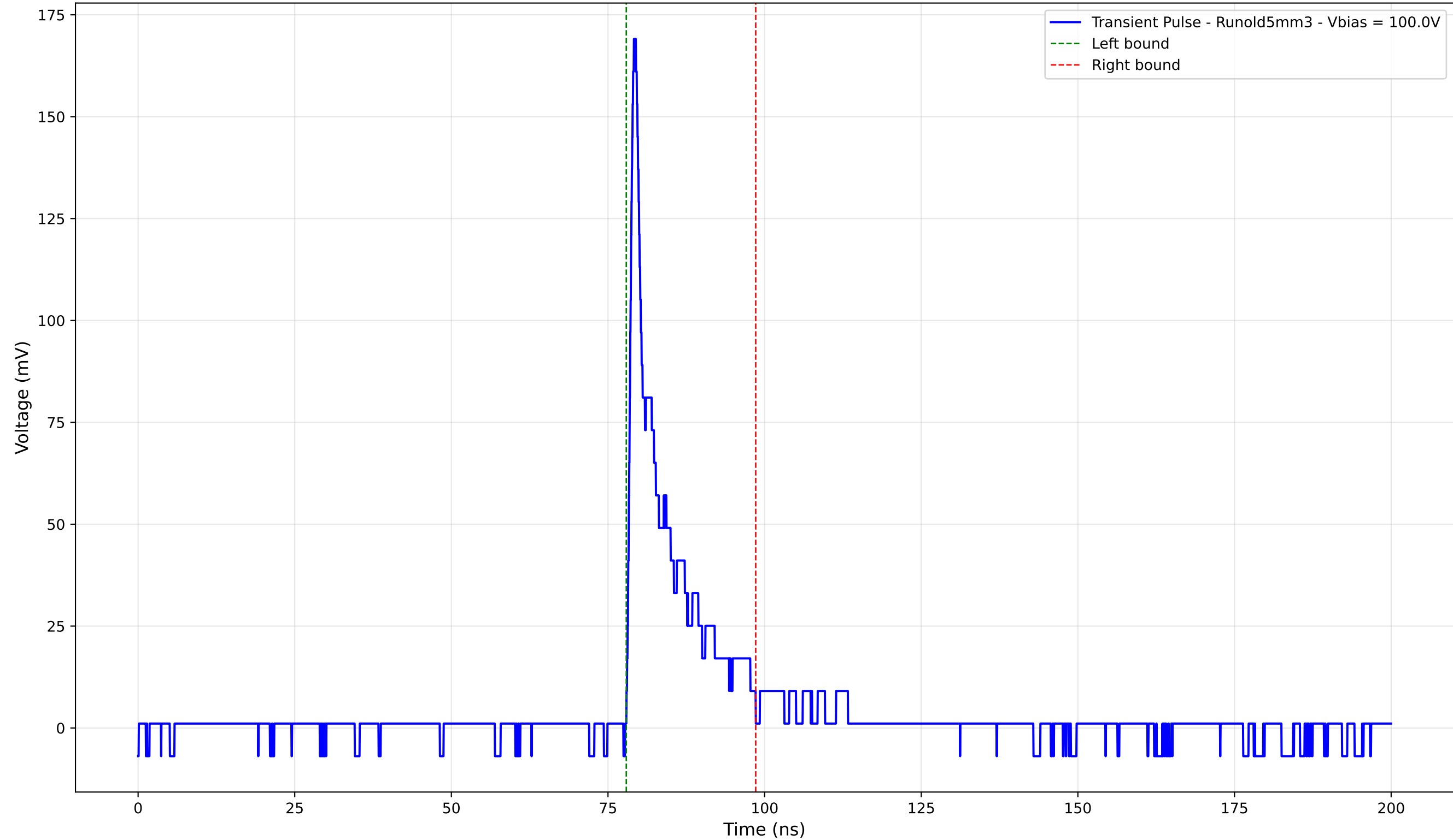
Transient Pulse - Sample: old5 - Position: 155.0 \mu\text{m} - Charge: 17.87 pC
