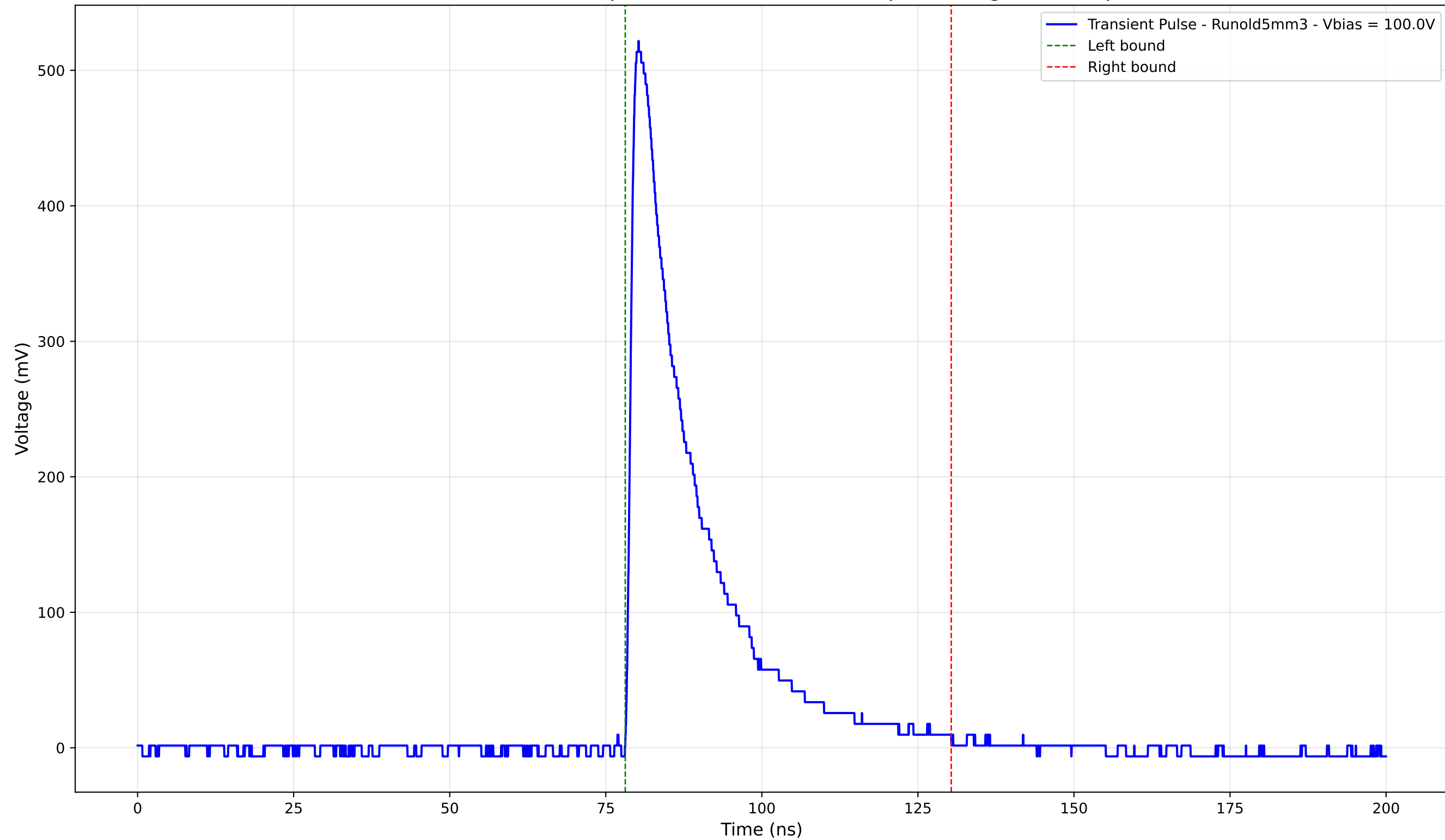
Transient Pulse - Sample: old5 - Position: 4365.0 \mu\text{m} - Charge: 115.51 pC
