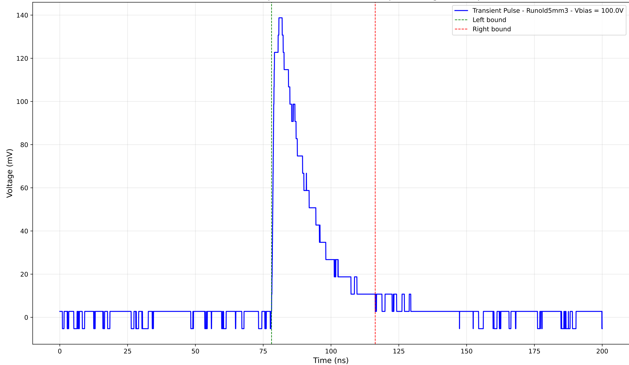
Transient Pulse - Sample: old5 - Position: 3035.0 \mu\text{m} - Charge: 37.79 pC
