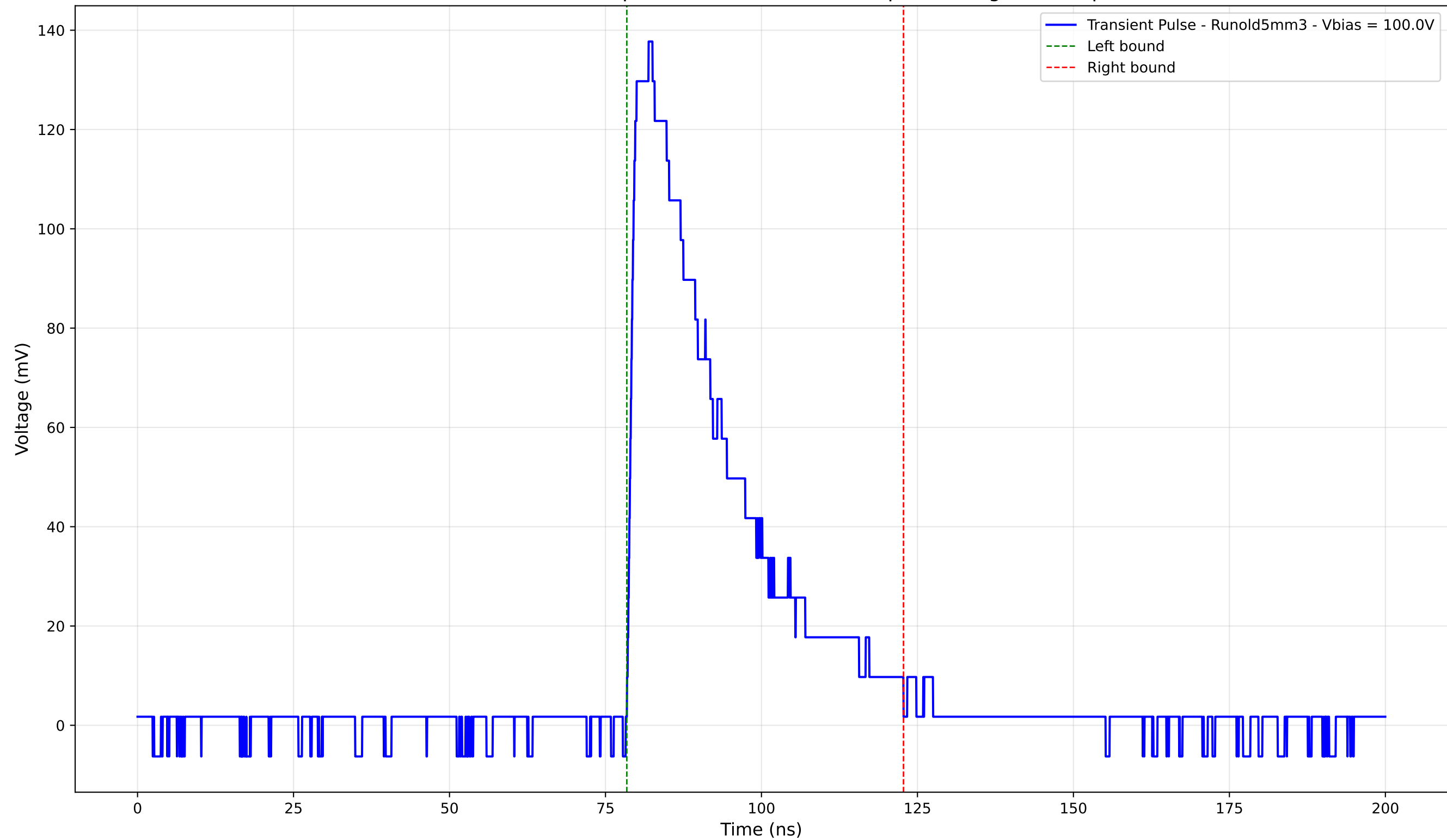
Transient Pulse - Sample: old5 - Position: 985.0 \mu\text{m} - Charge: 43.96 pC
