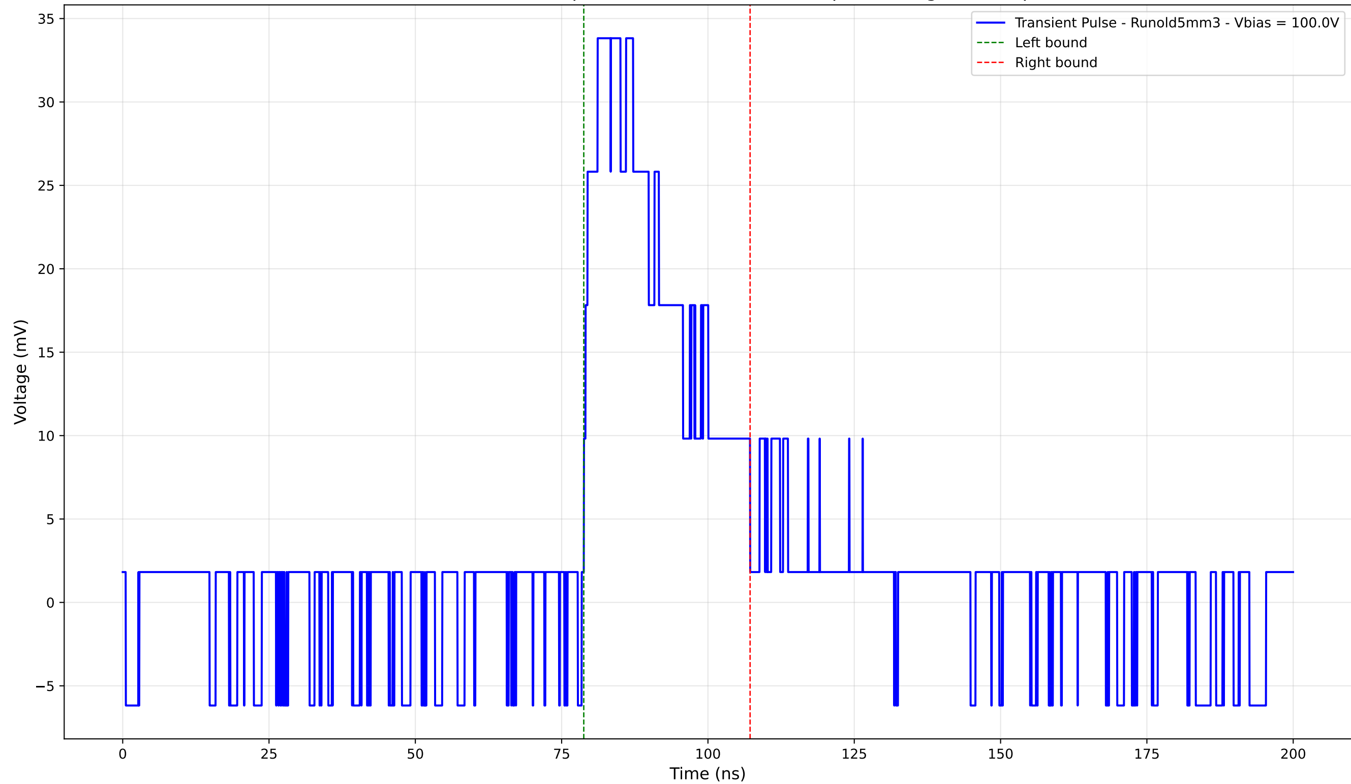
Transient Pulse - Sample: old5 - Position: 1190.0 \mu\text{m} - Charge: 11.15 pC
