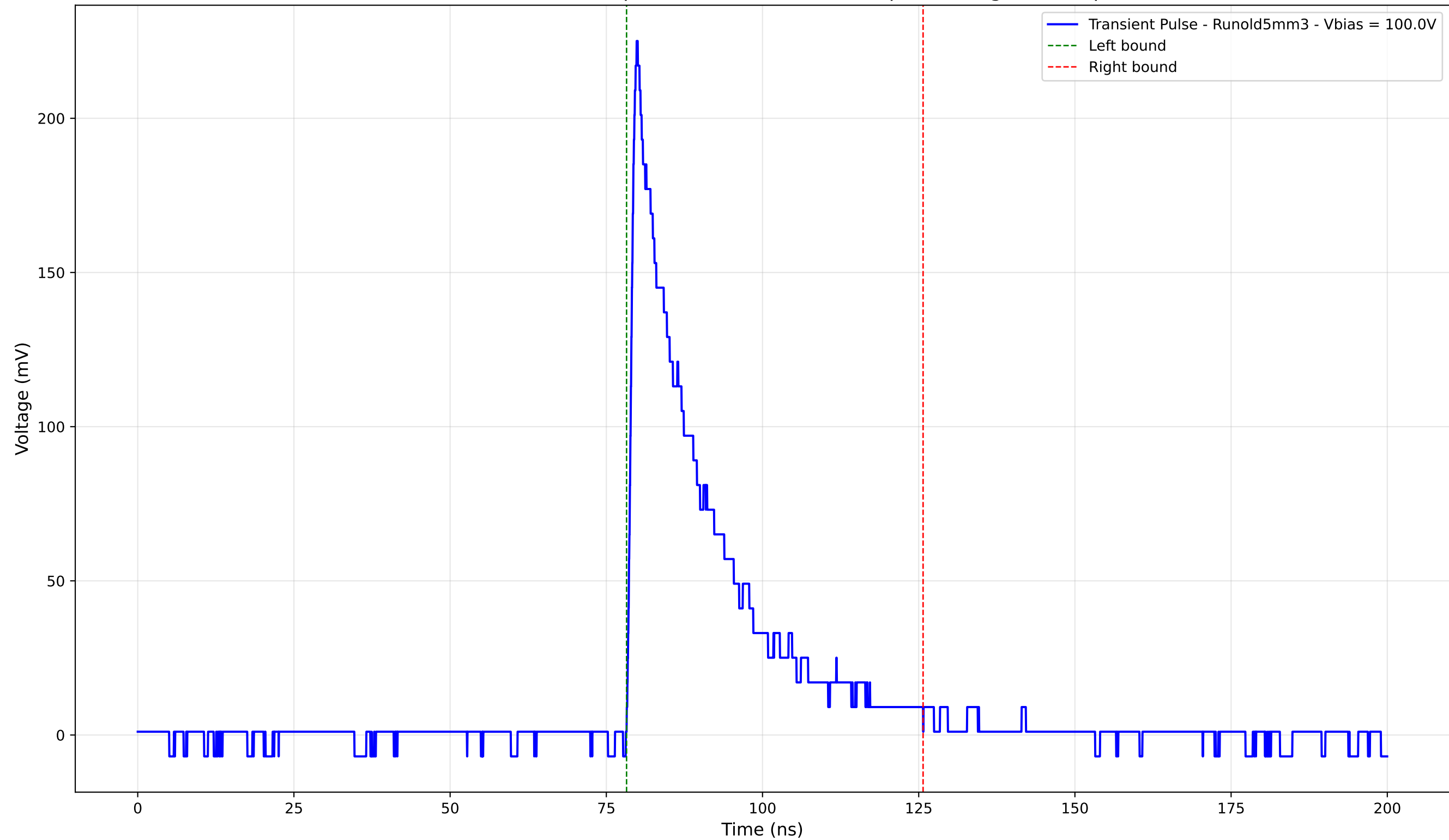
Transient Pulse - Sample: old5 - Position: 630.0 \mu\text{m} - Charge: 51.20 pC
