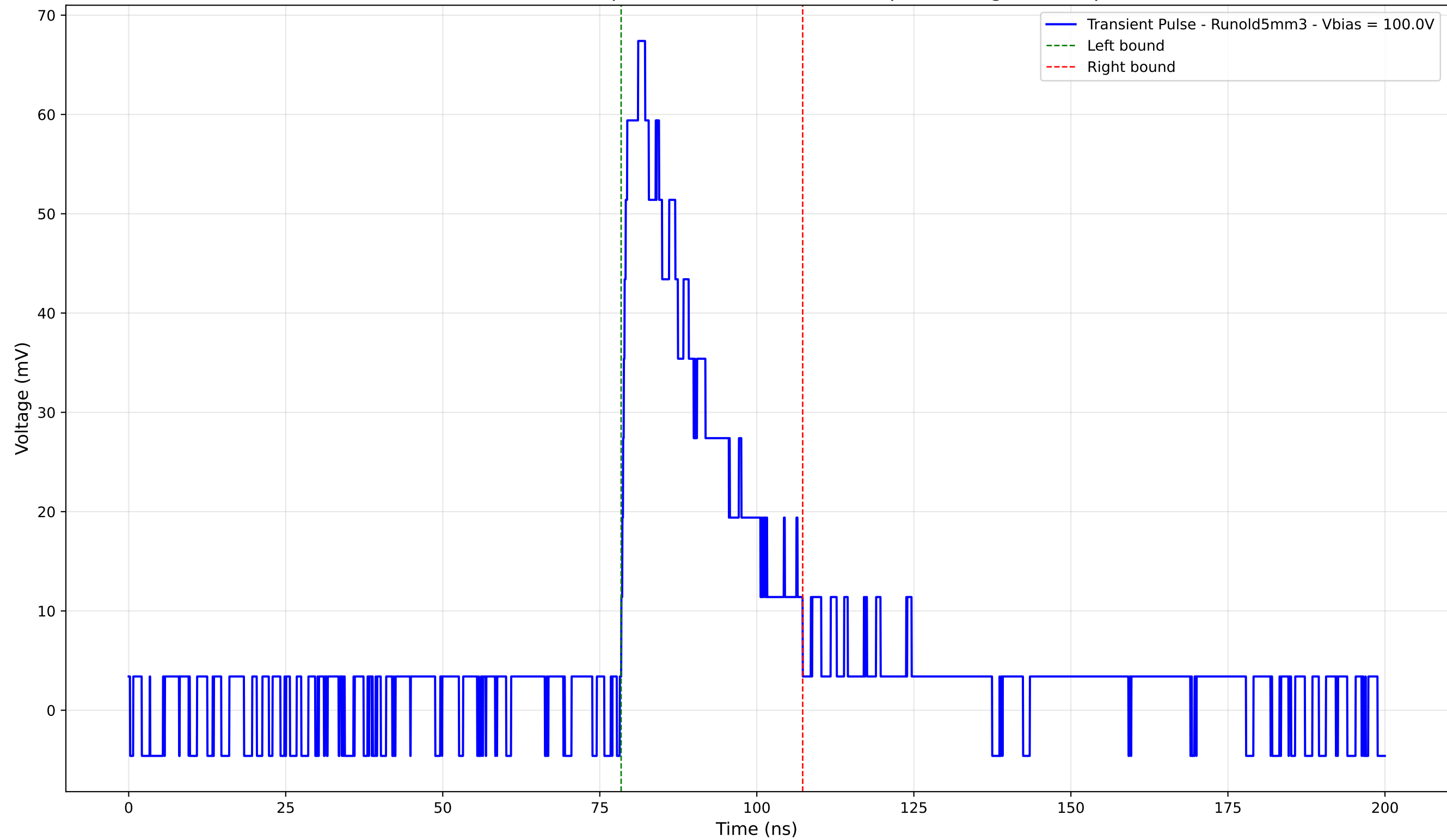
Transient Pulse - Sample: old5 - Position: 2935.0 \mu\text{m} - Charge: 18.41 pC
