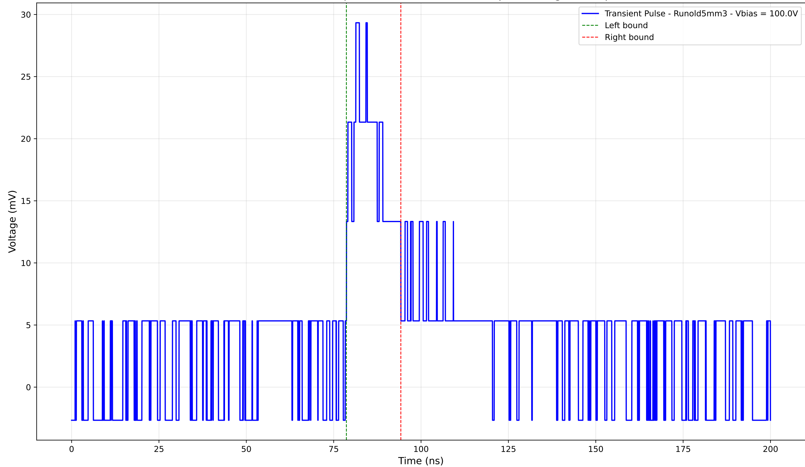
Transient Pulse - Sample: old5 - Position: 2990.0 \mu\text{m} - Charge: 5.78 pC
