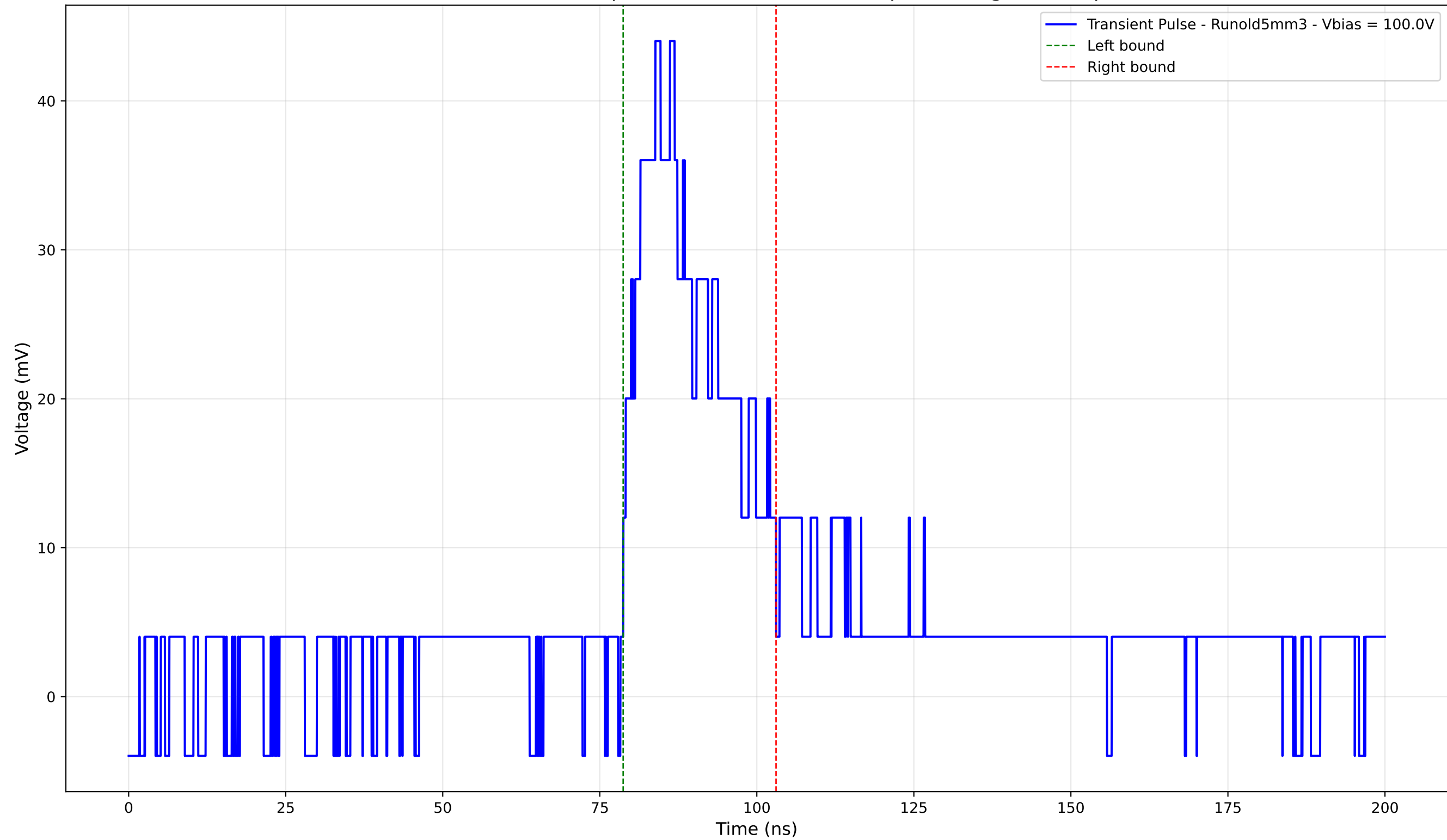
Transient Pulse - Sample: old5 - Position: 2200.0 \mu\text{m} - Charge: 12.16 pC
