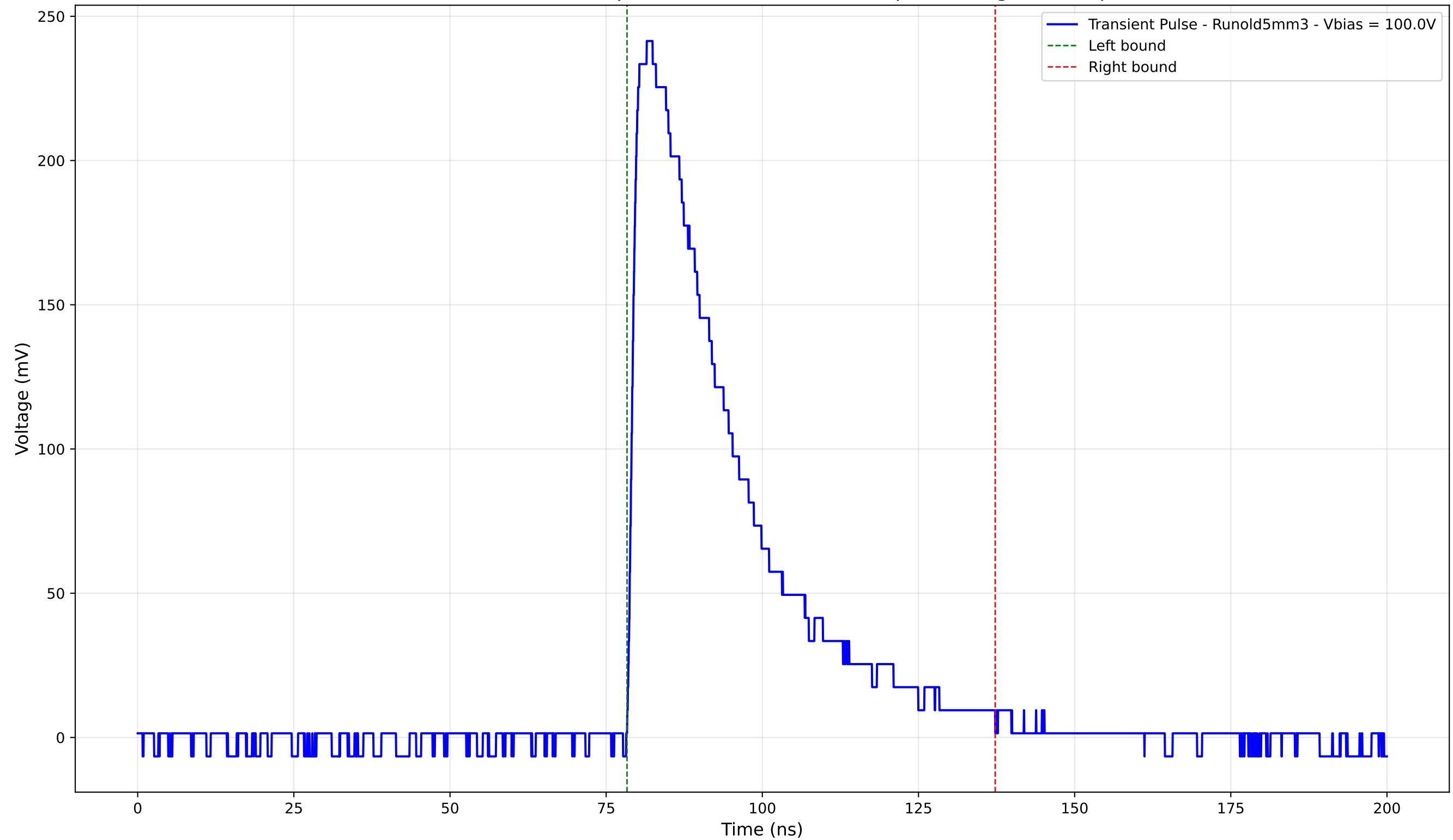
Transient Pulse - Sample: old5 - Position: 1070.0 \mu\text{m} - Charge: 86.46 pC
