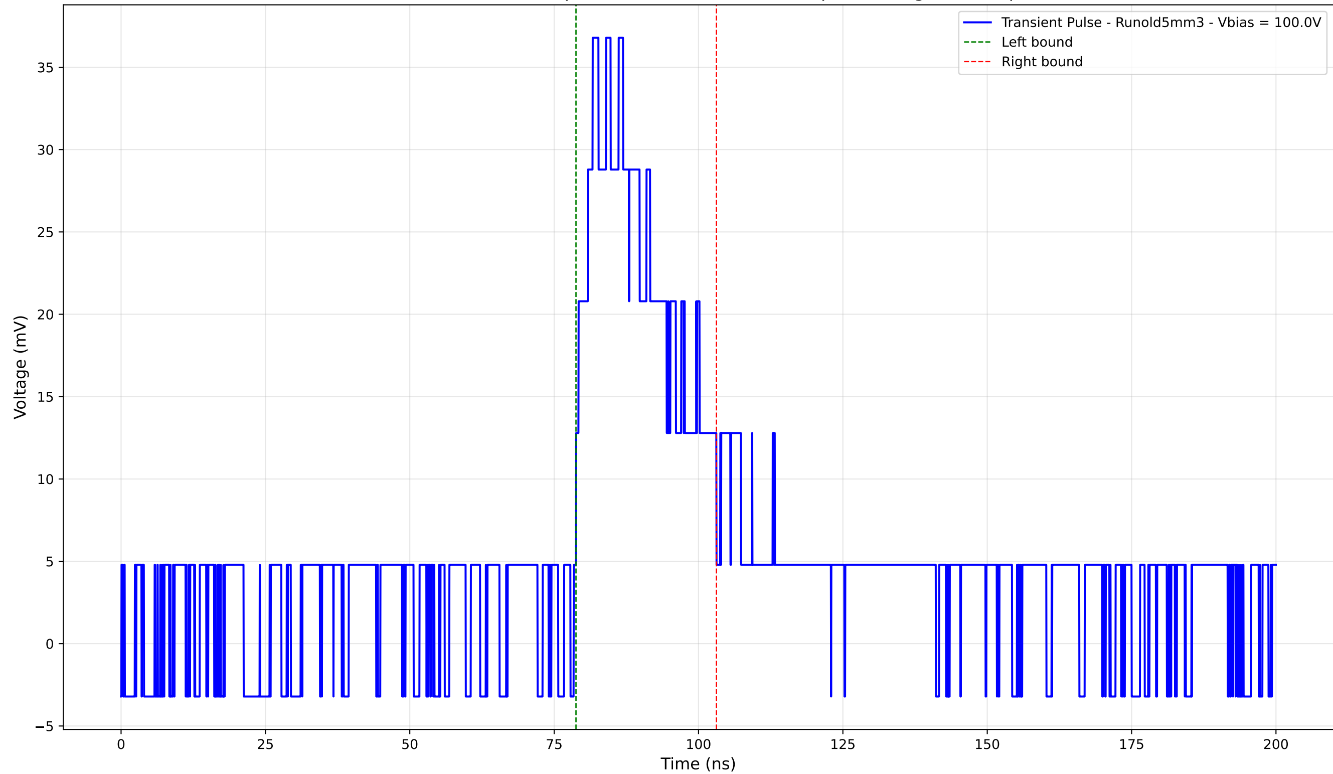
Transient Pulse - Sample: old5 - Position: 1390.0 \mu\text{m} - Charge: 10.92 pC
