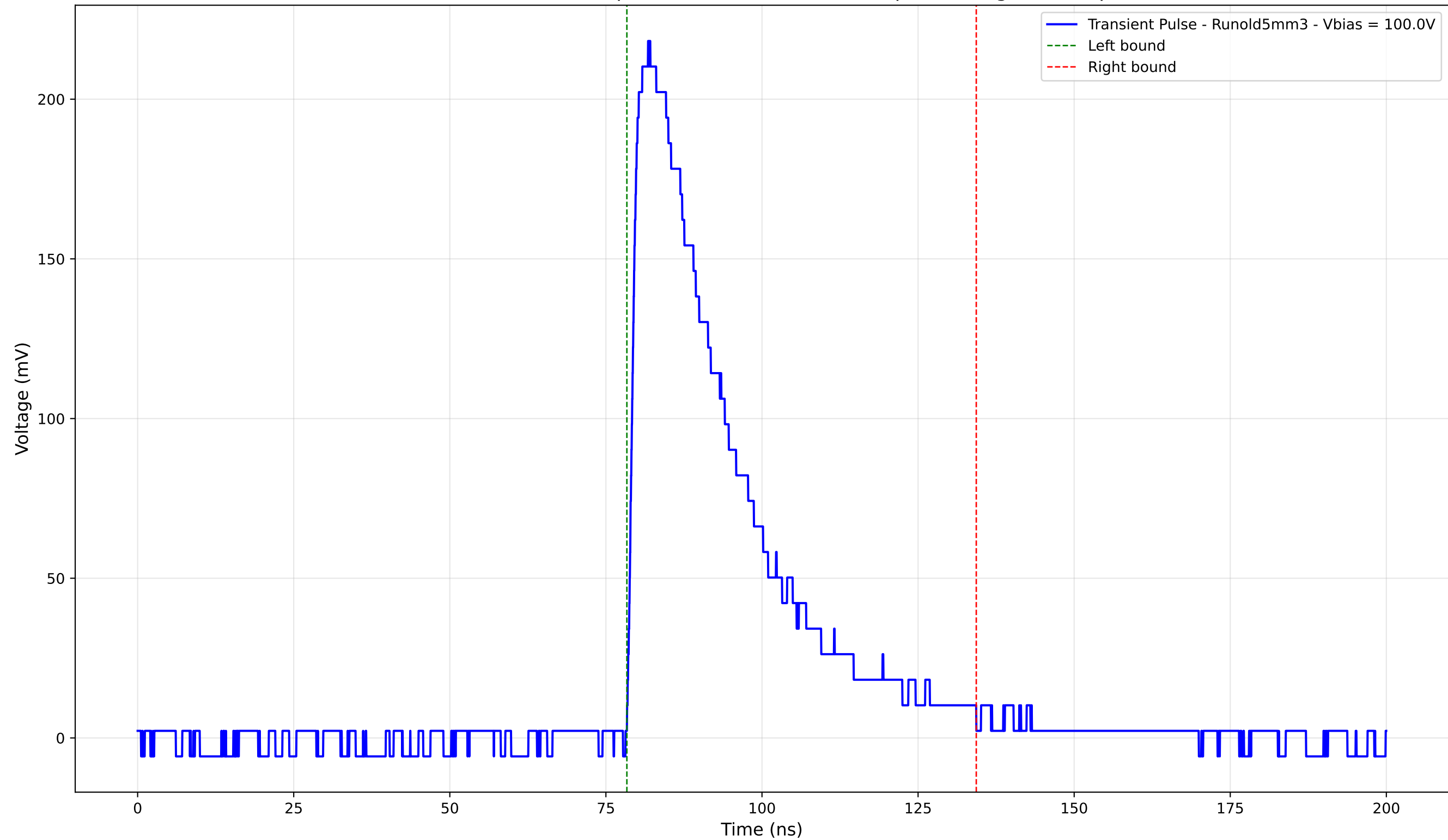
Transient Pulse - Sample: old5 - Position: 1105.0 \mu\text{m} - Charge: 76.06 pC
