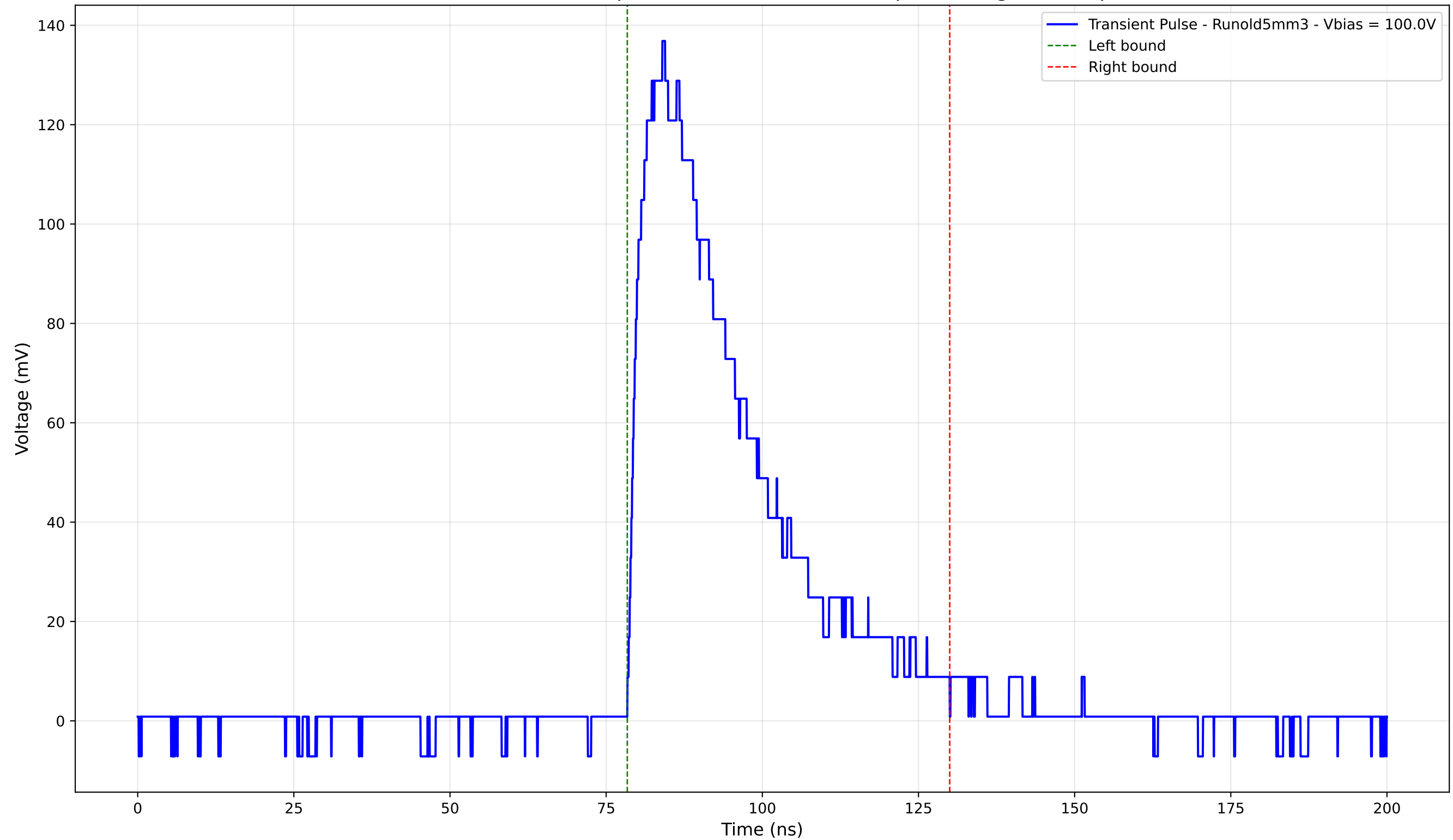
Transient Pulse - Sample: old5 - Position: 1940.0 \mu\text{m} - Charge: 52.53 pC
