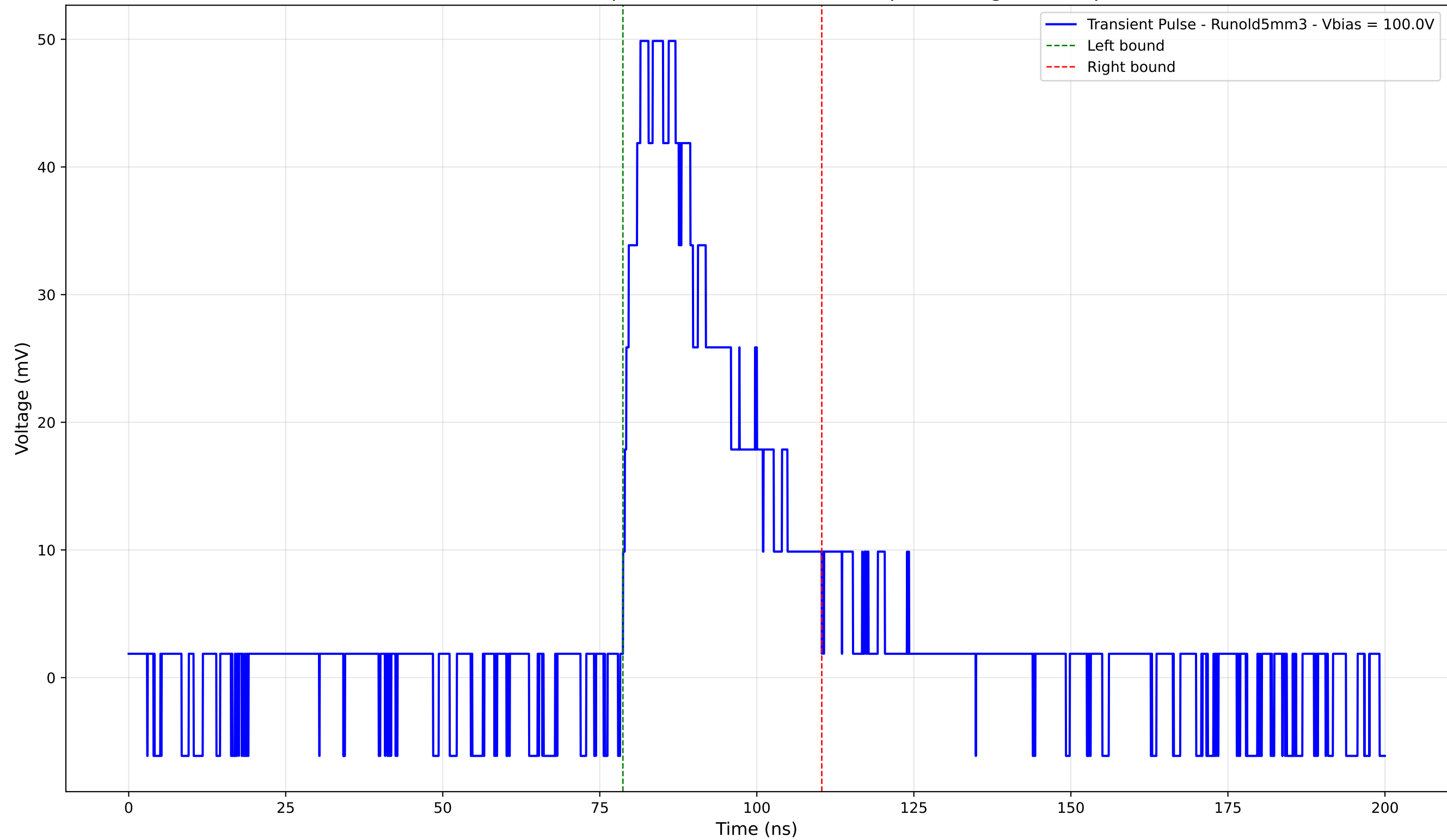
Transient Pulse - Sample: old5 - Position: 2380.0 \mu\text{m} - Charge: 16.67 pC
