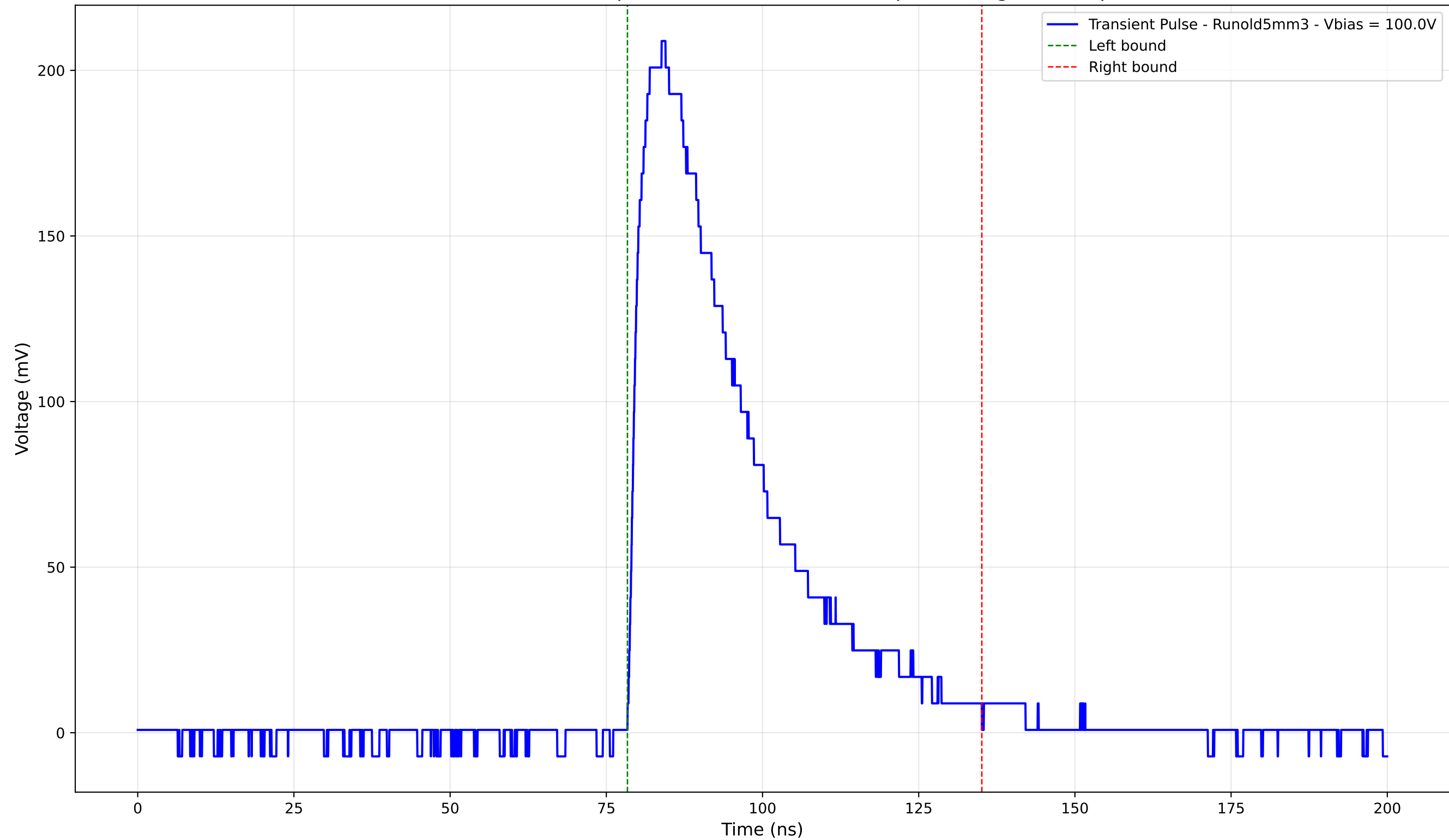
Transient Pulse - Sample: old5 - Position: 1700.0 \mu\text{m} - Charge: 82.61 pC
