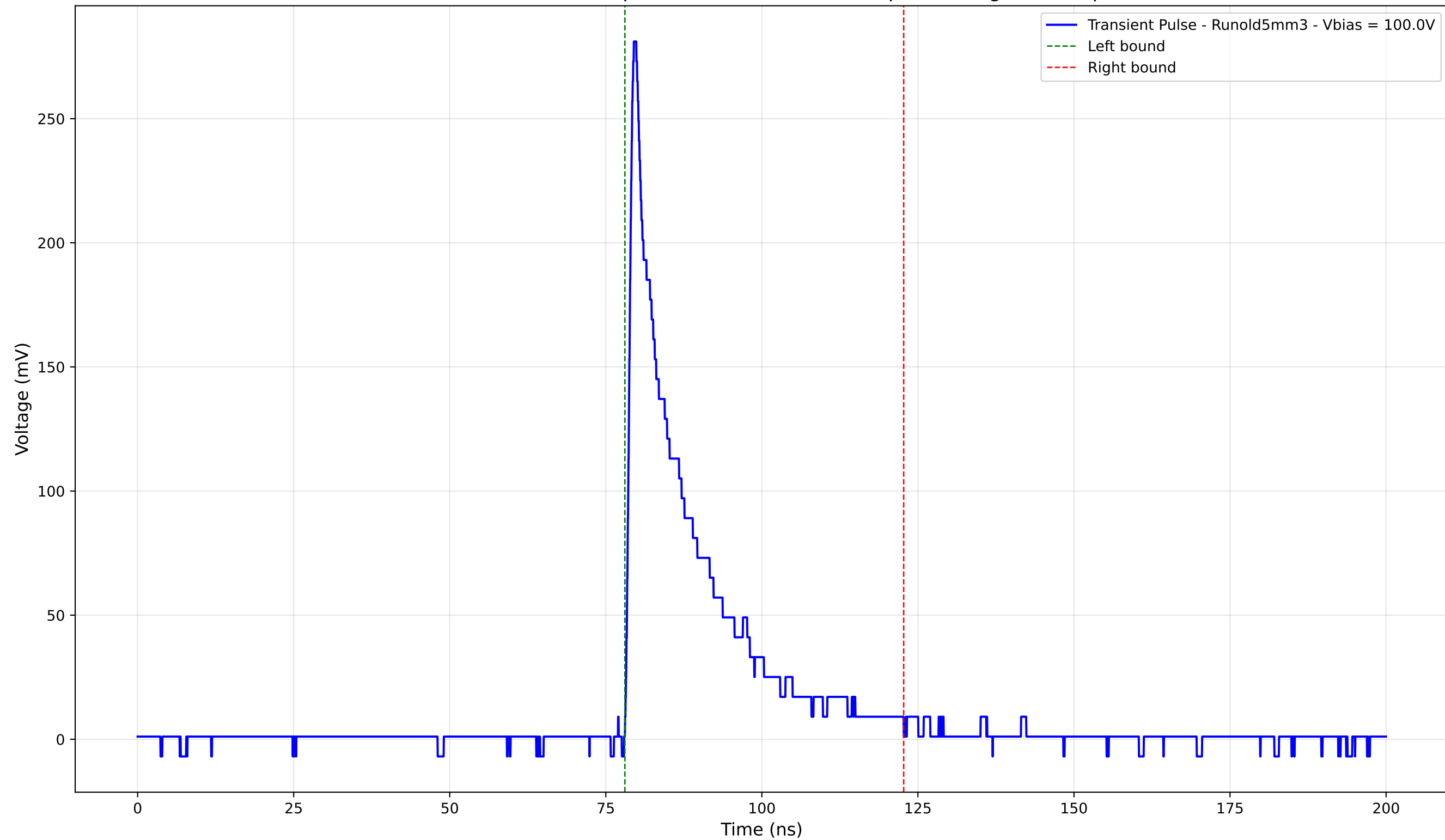
Transient Pulse - Sample: old5 - Position: 430.0 \mu\text{m} - Charge: 51.02 pC
