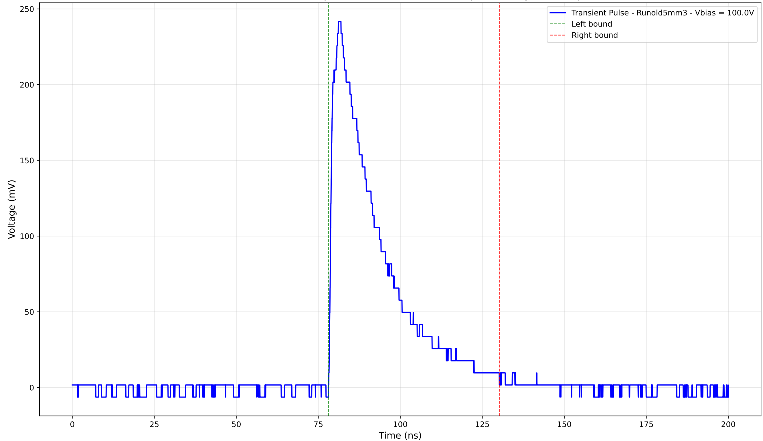
Transient Pulse - Sample: old5 - Position: 2890.0 \mu\text{m} - Charge: 76.03 pC
