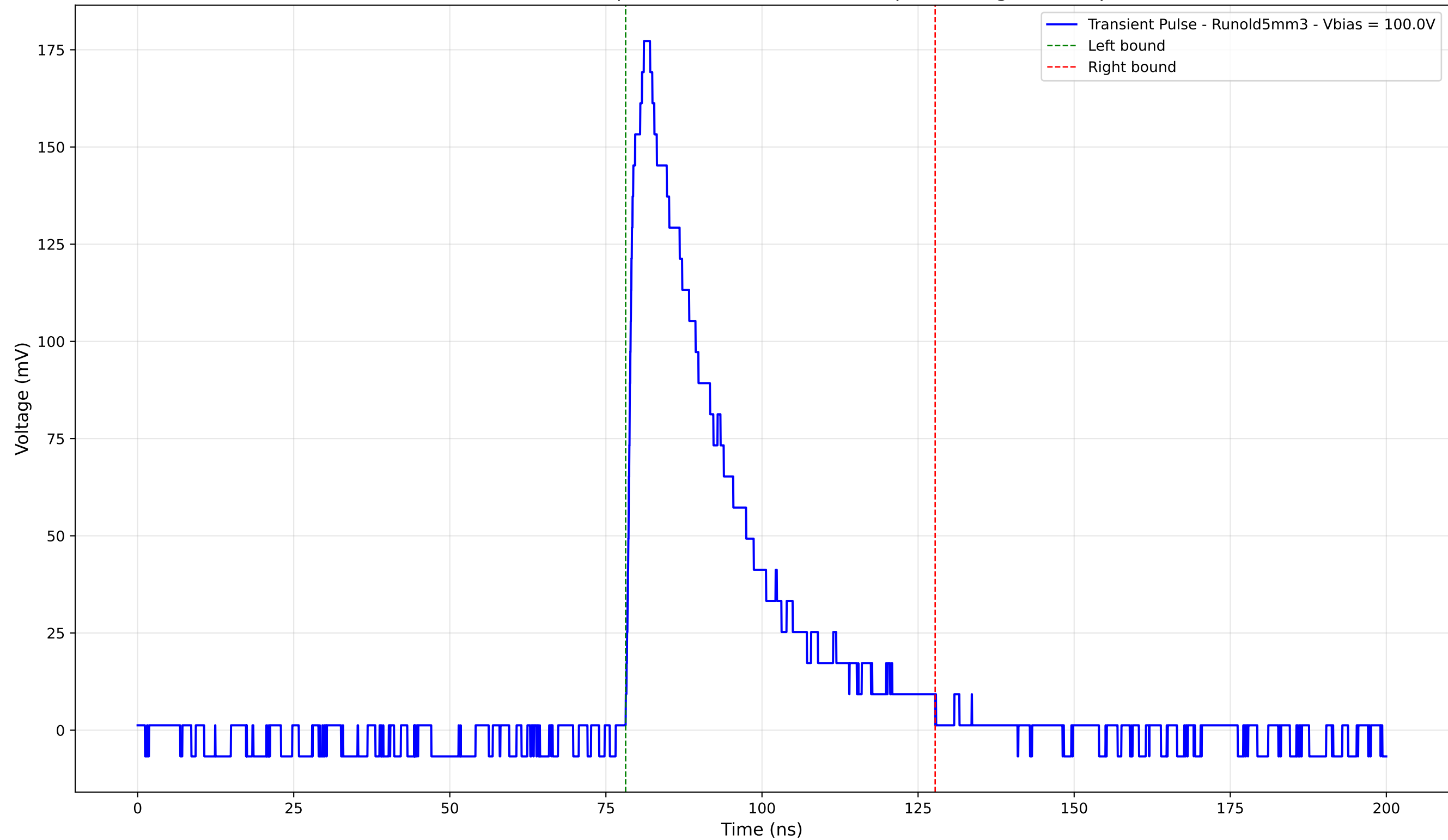
Transient Pulse - Sample: old5 - Position: 2905.0 \mu\text{m} - Charge: 54.15 pC
