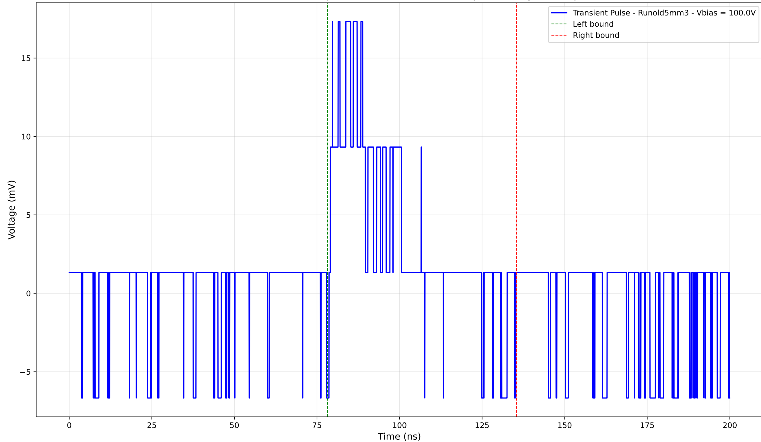
Transient Pulse - Sample: old5 - Position: 2680.0 \mu\text{m} - Charge: 4.46 pC
