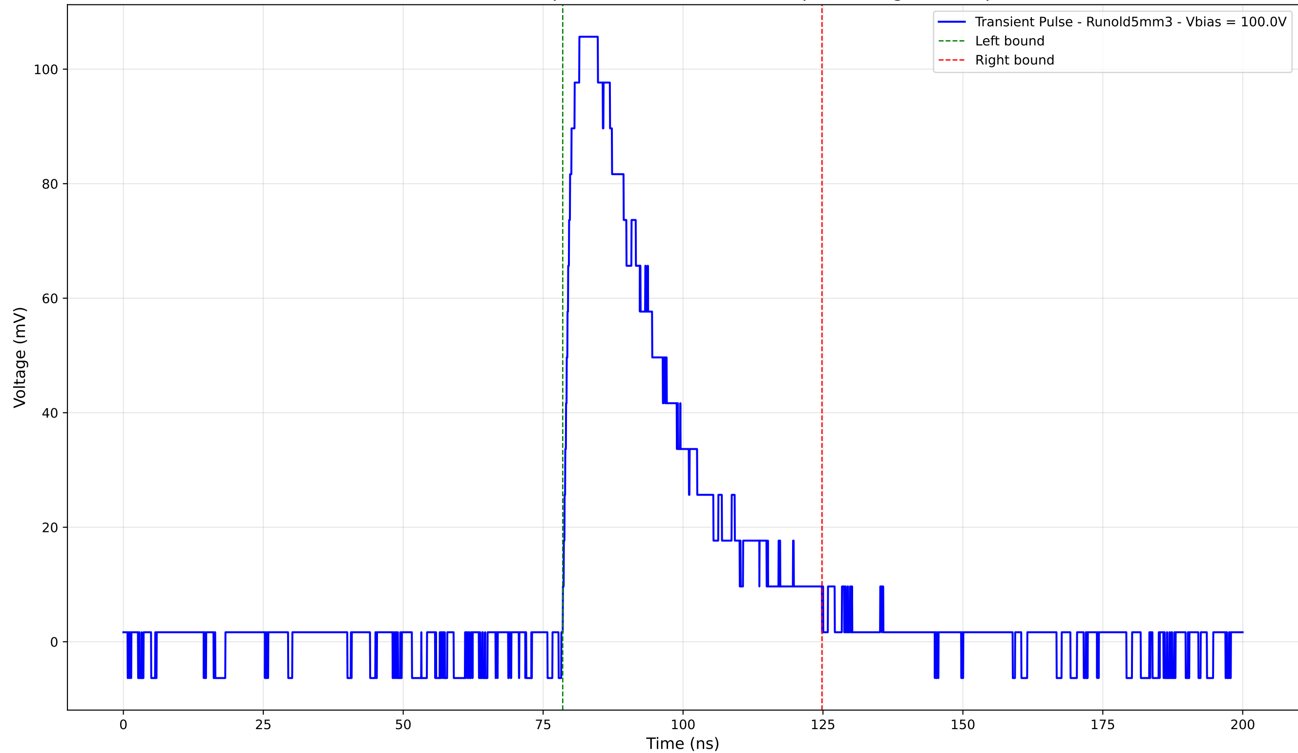
Transient Pulse - Sample: old5 - Position: 1225.0 \mu\text{m} - Charge: 39.45 pC
