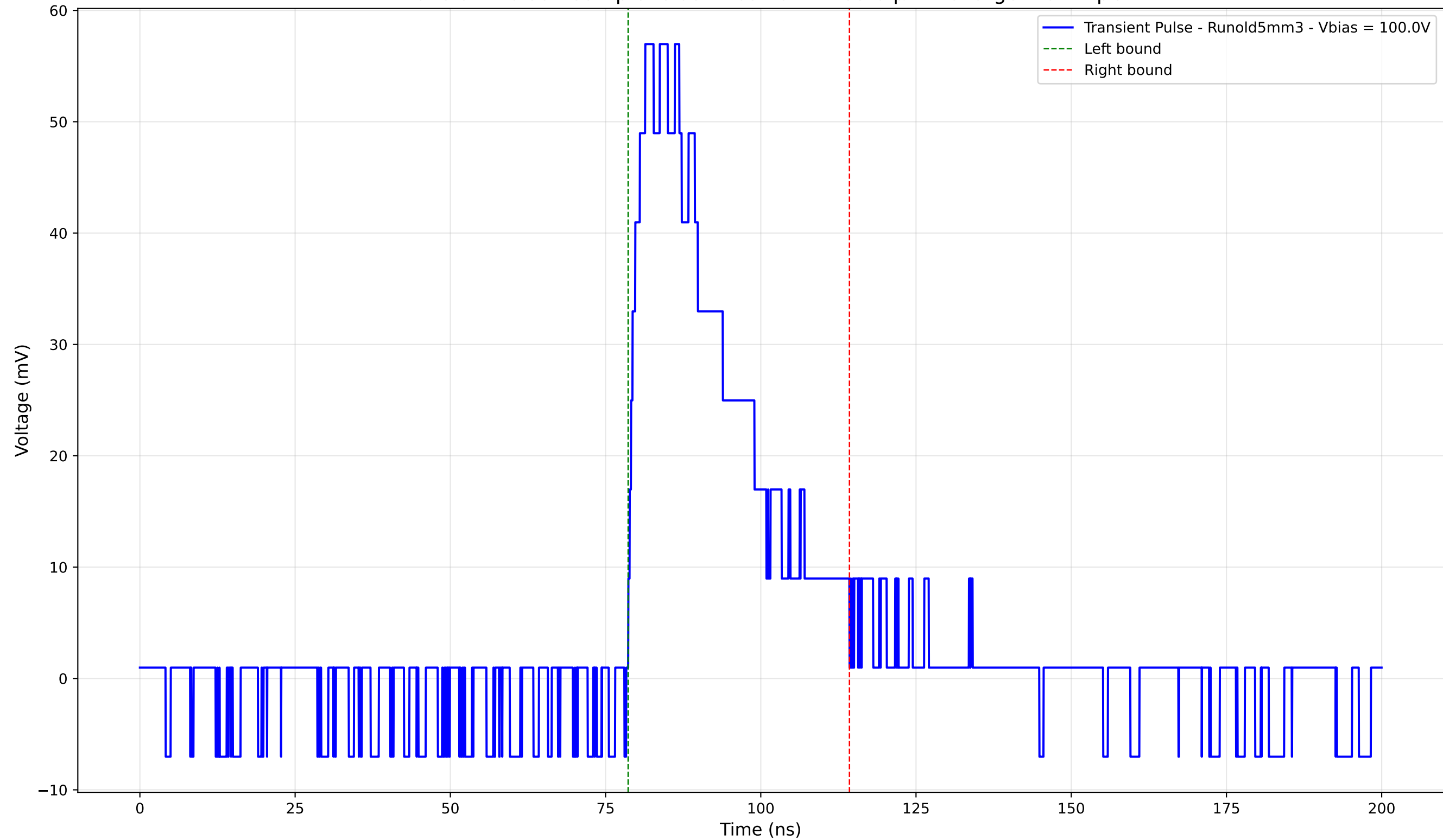
Transient Pulse - Sample: old5 - Position: 1205.0 \mu\text{m} - Charge: 19.27 pC
