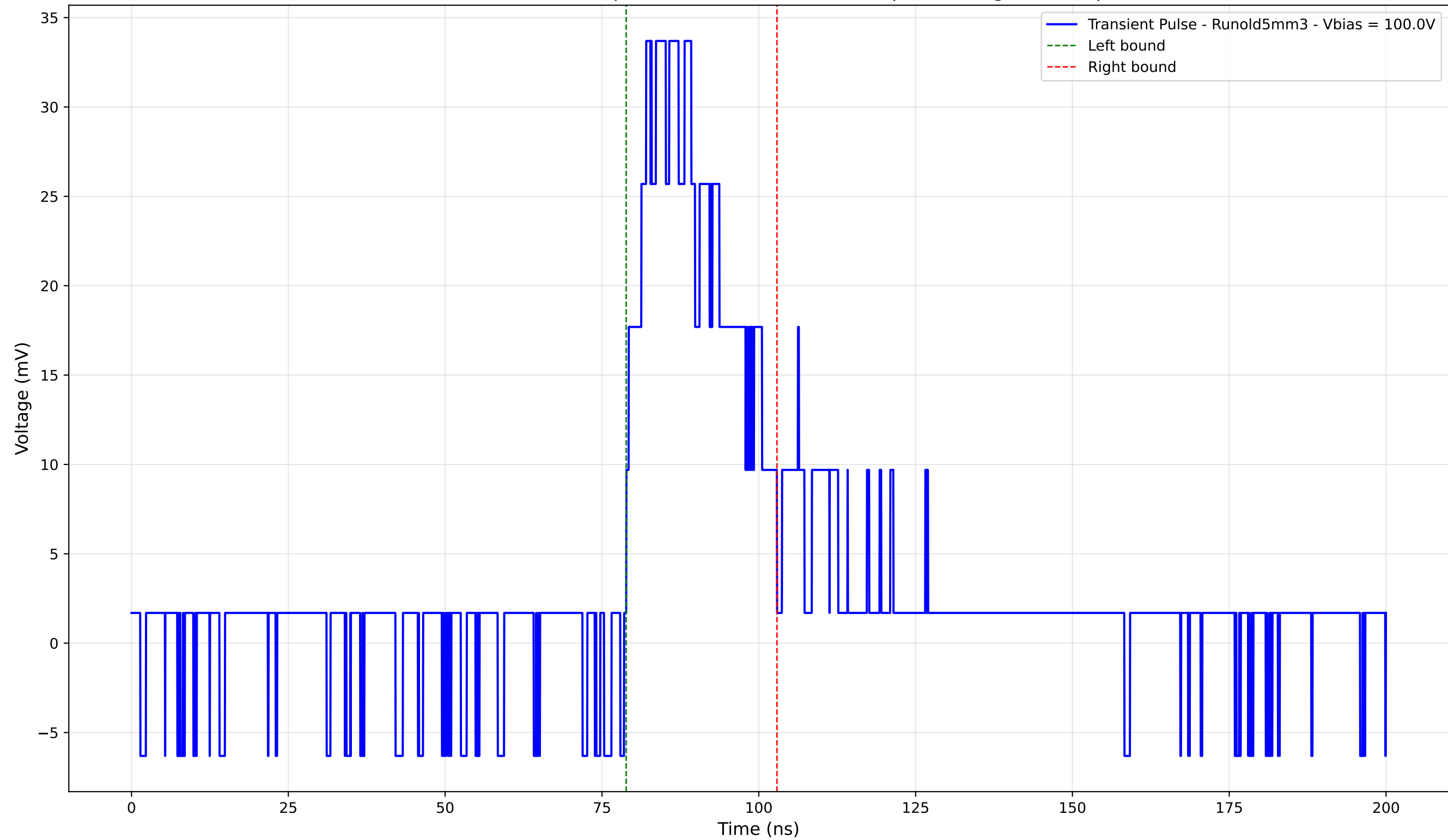
Transient Pulse - Sample: old5 - Position: 1985.0 \mu\text{m} - Charge: 10.55 pC
