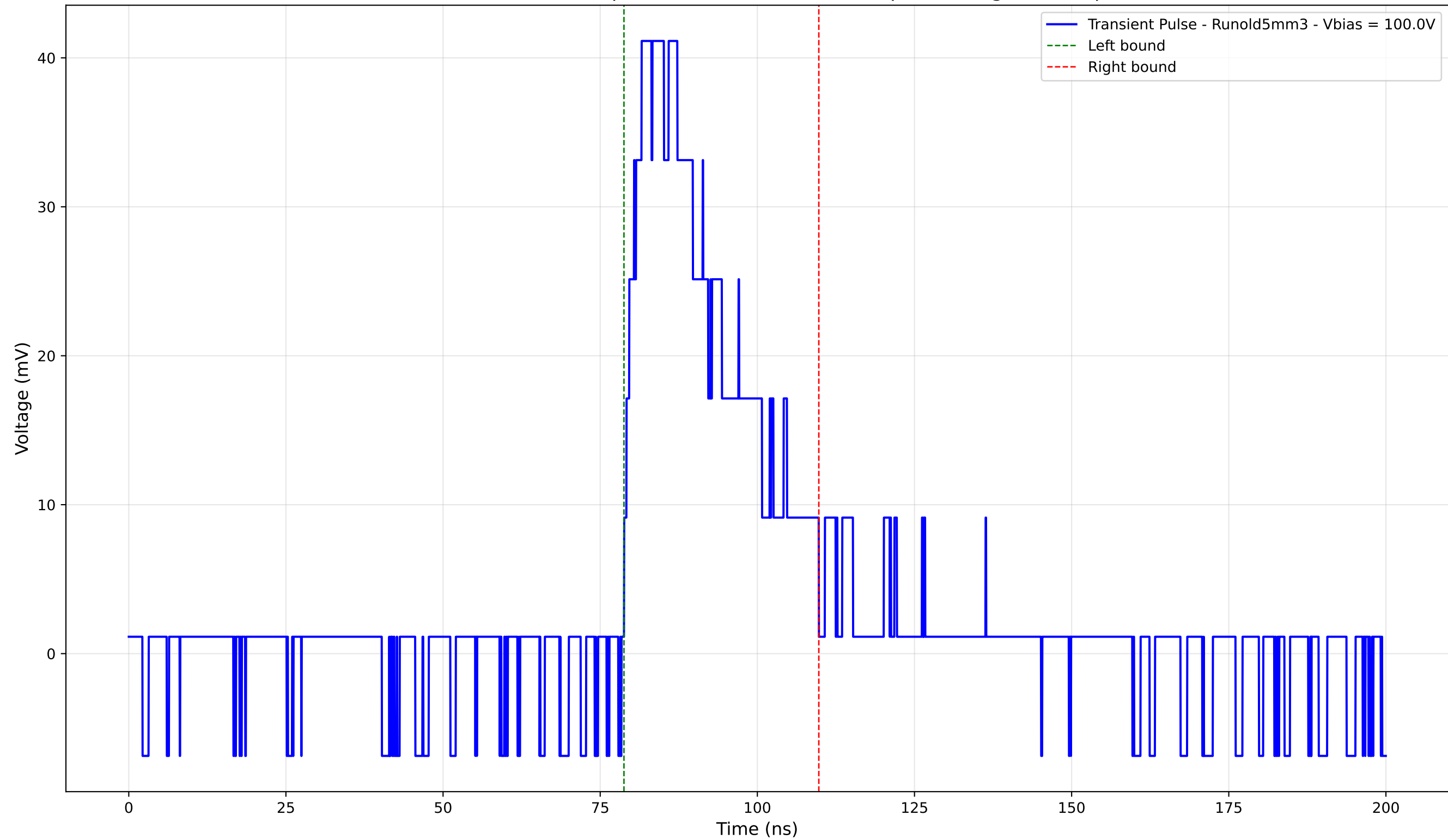
Transient Pulse - Sample: old5 - Position: 1570.0 \mu\text{m} - Charge: 13.79 pC
