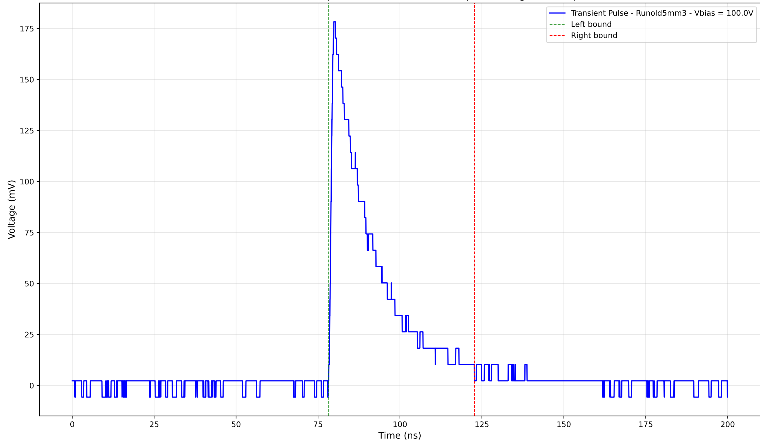
Transient Pulse - Sample: old5 - Position: 725.0 \mu\text{m} - Charge: 46.64 pC
