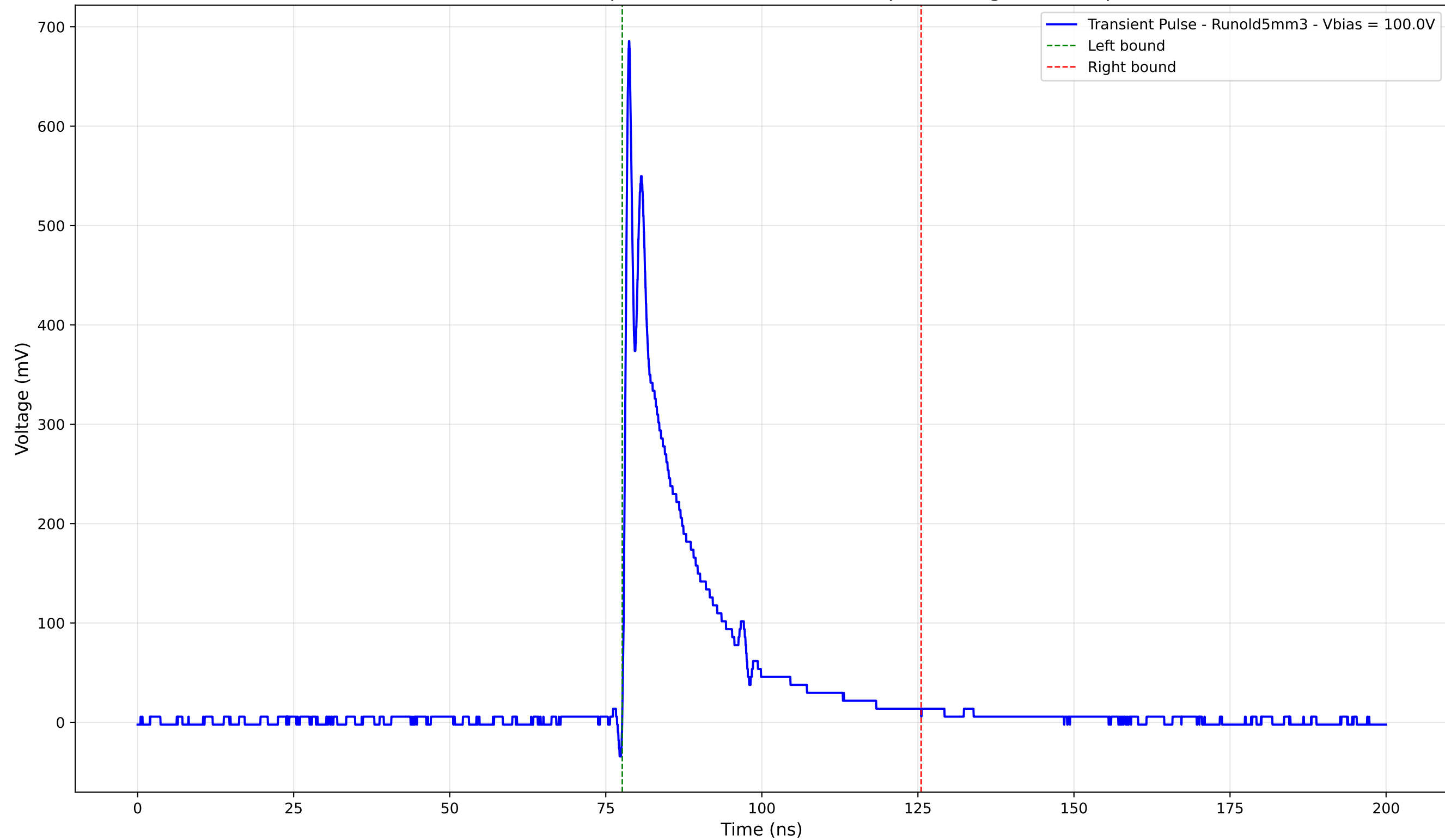
Transient Pulse - Sample: old5 - Position: 3435.0 \mu\text{m} - Charge: 109.77 pC
