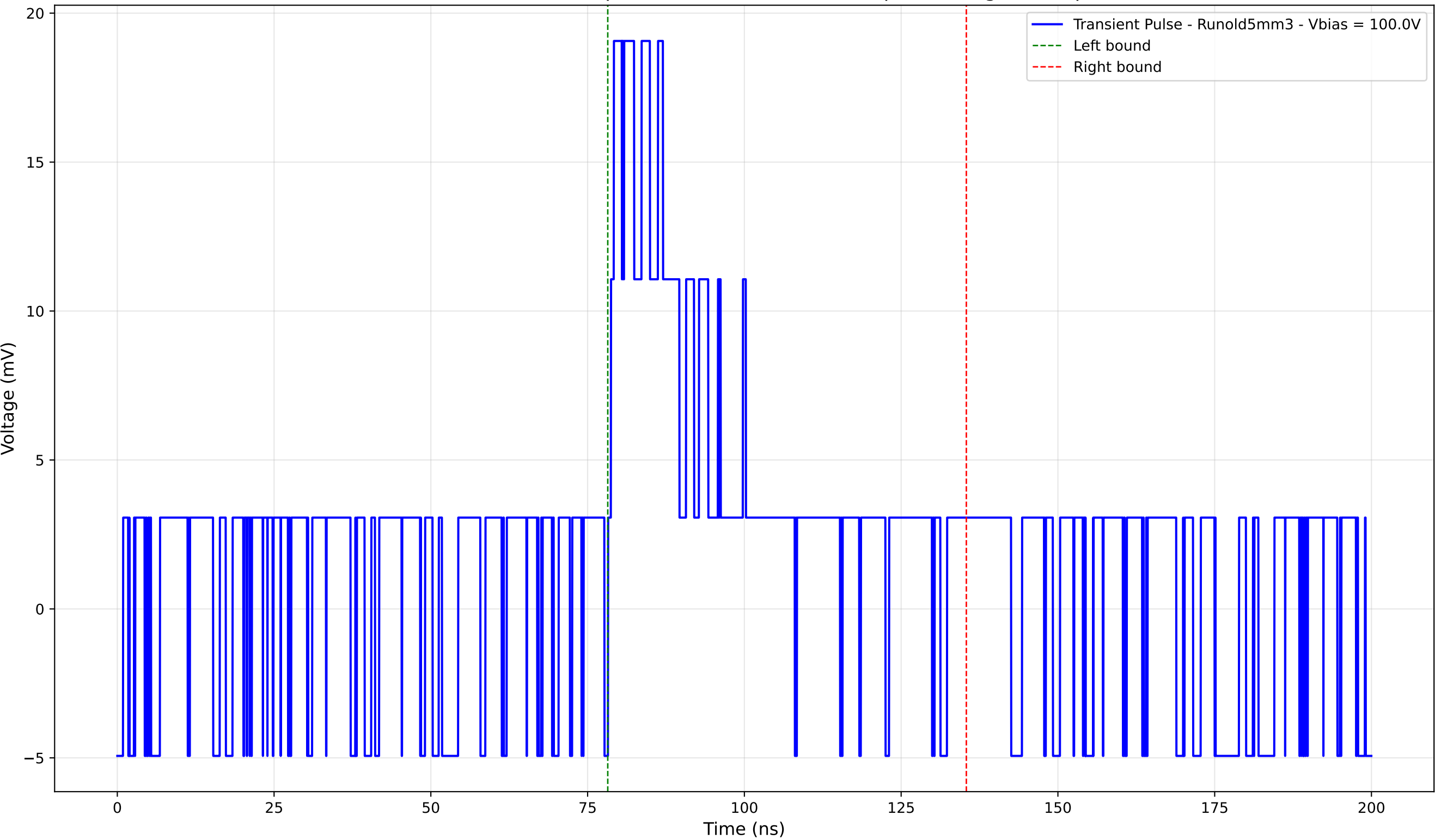
Transient Pulse - Sample: old5 - Position: 2965.0 \mu\text{m} - Charge: 6.22 pC
