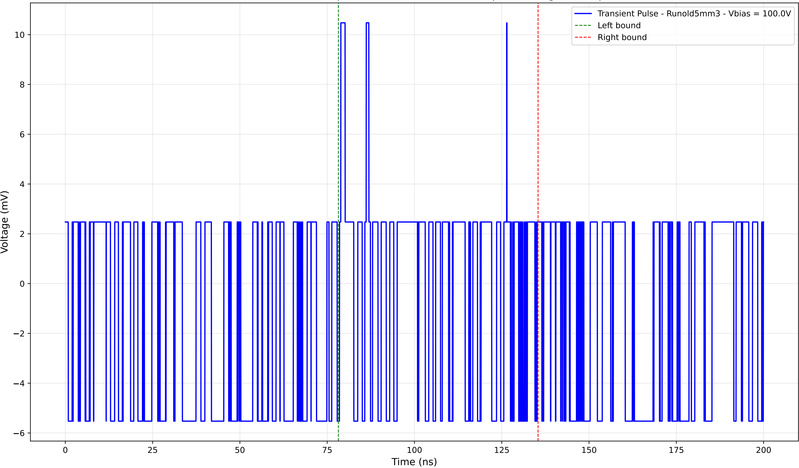
Transient Pulse - Sample: old5 - Position: 4990.0 \mu\text{m} - Charge: 0.43 pC
