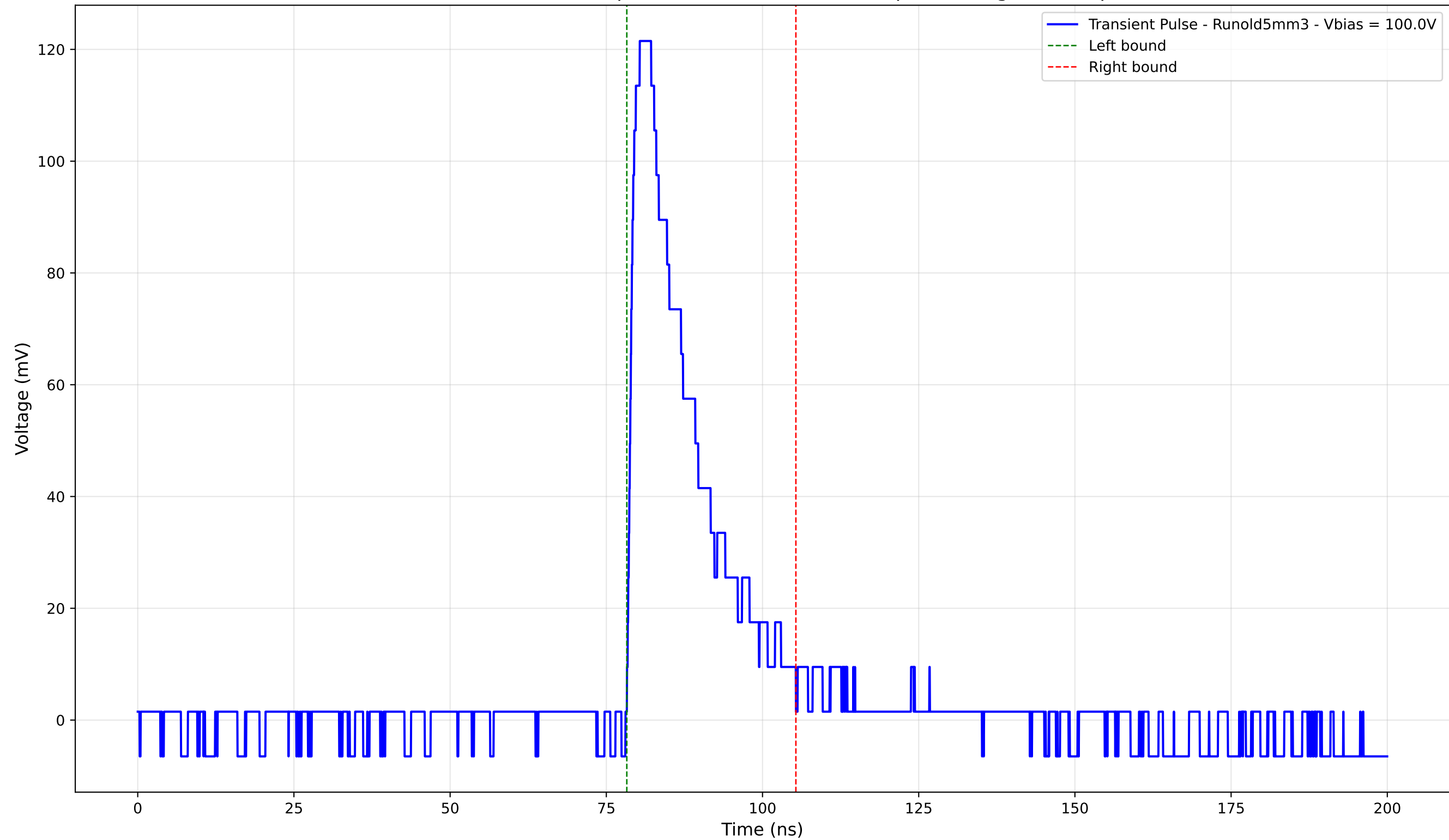
Transient Pulse - Sample: old5 - Position: 4230.0 \mu\text{m} - Charge: 26.21 pC
