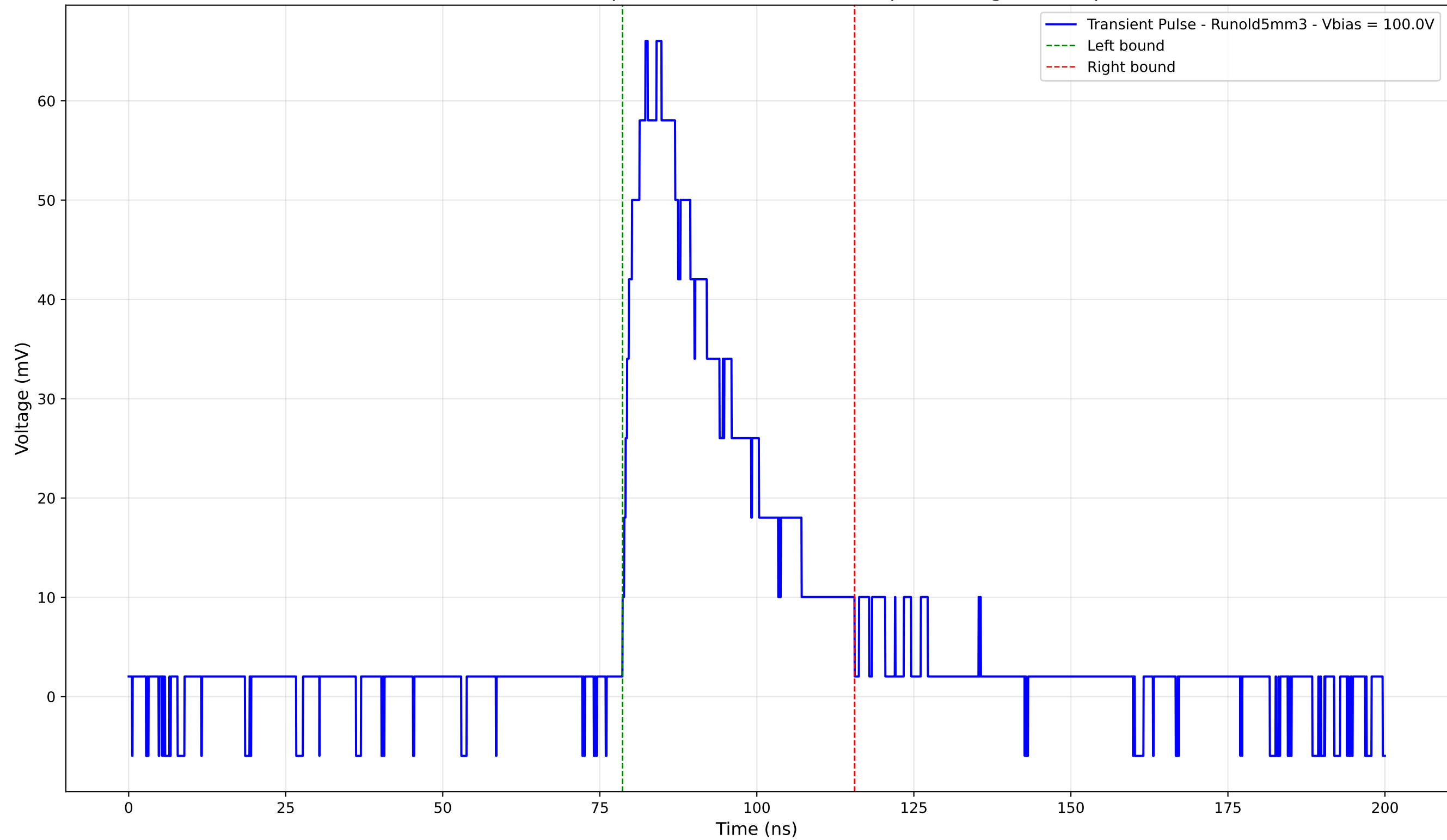
Transient Pulse - Sample: old5 - Position: 2375.0 \mu\text{m} - Charge: 22.32 pC
