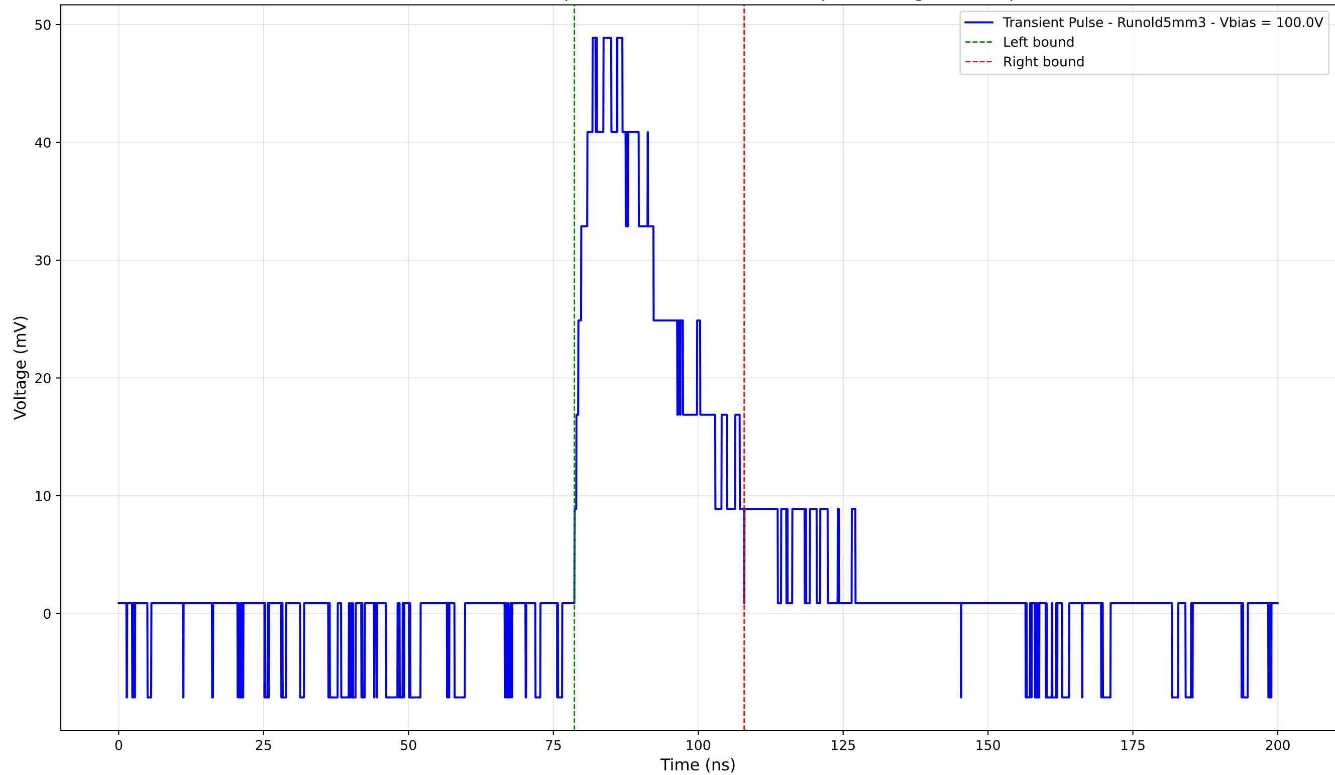
Transient Pulse - Sample: old5 - Position: 1770.0 \mu\text{m} - Charge: 16.10 pC
