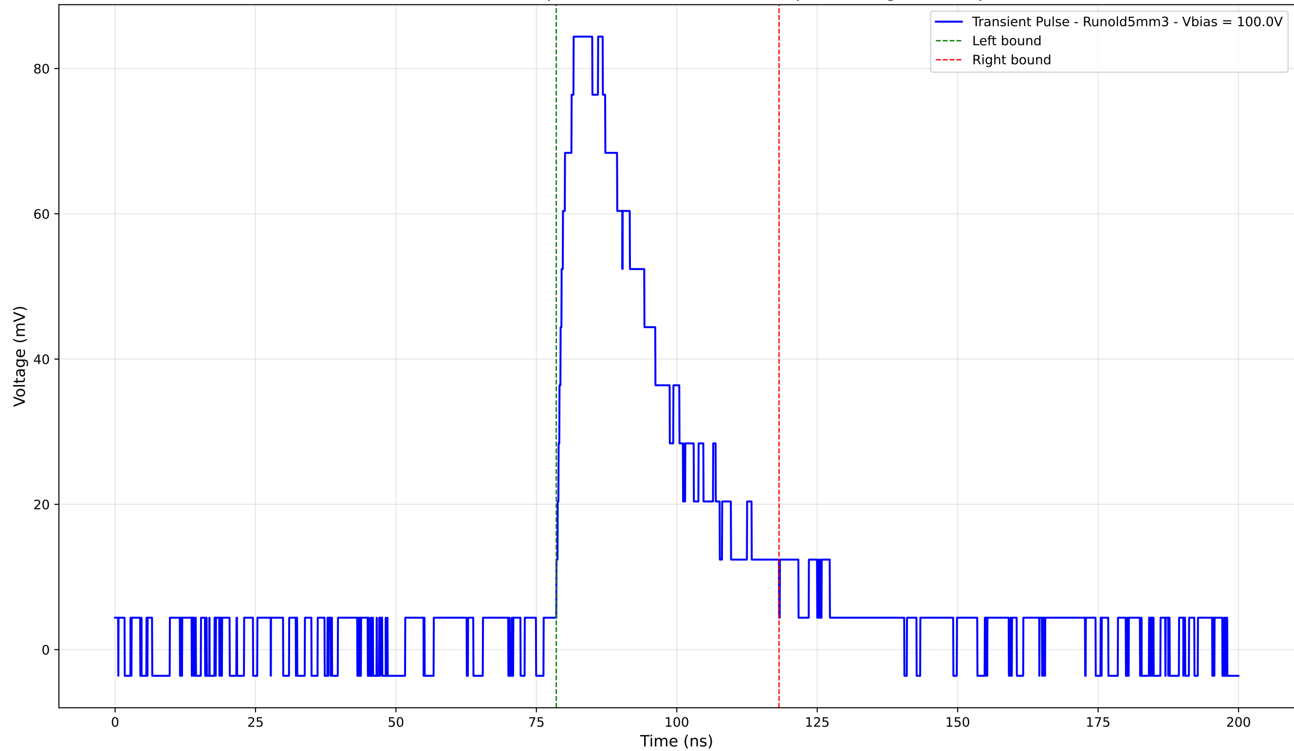
Transient Pulse - Sample: old5 - Position: 2365.0 \mu\text{m} - Charge: 32.24 pC
