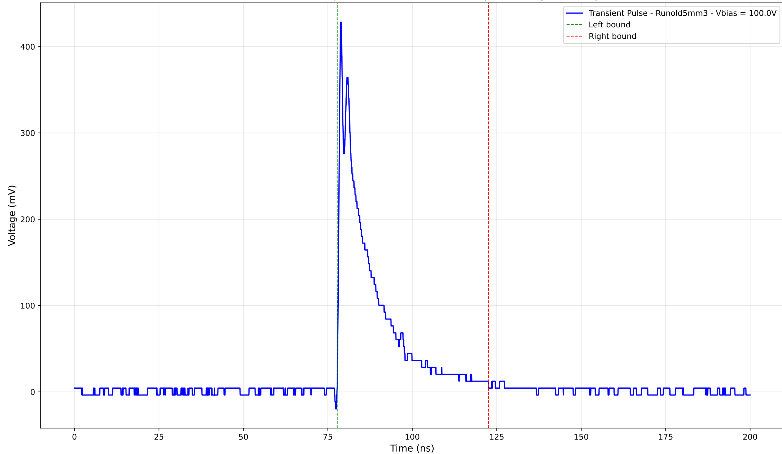
Transient Pulse - Sample: old5 - Position: 3365.0 \mu\text{m} - Charge: 77.14 pC
