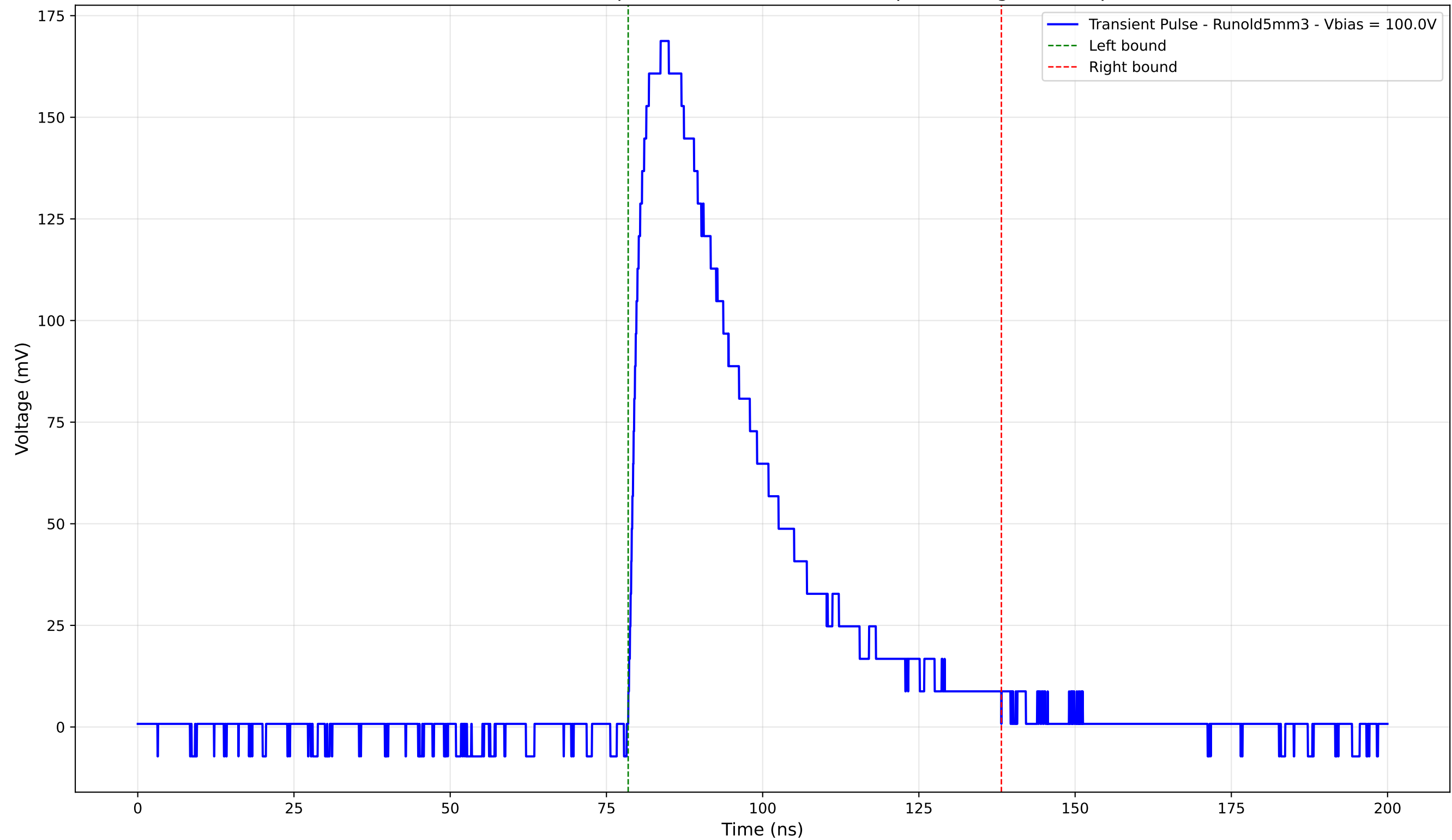
Transient Pulse - Sample: old5 - Position: 1855.0 \mu\text{m} - Charge: 68.88 pC
