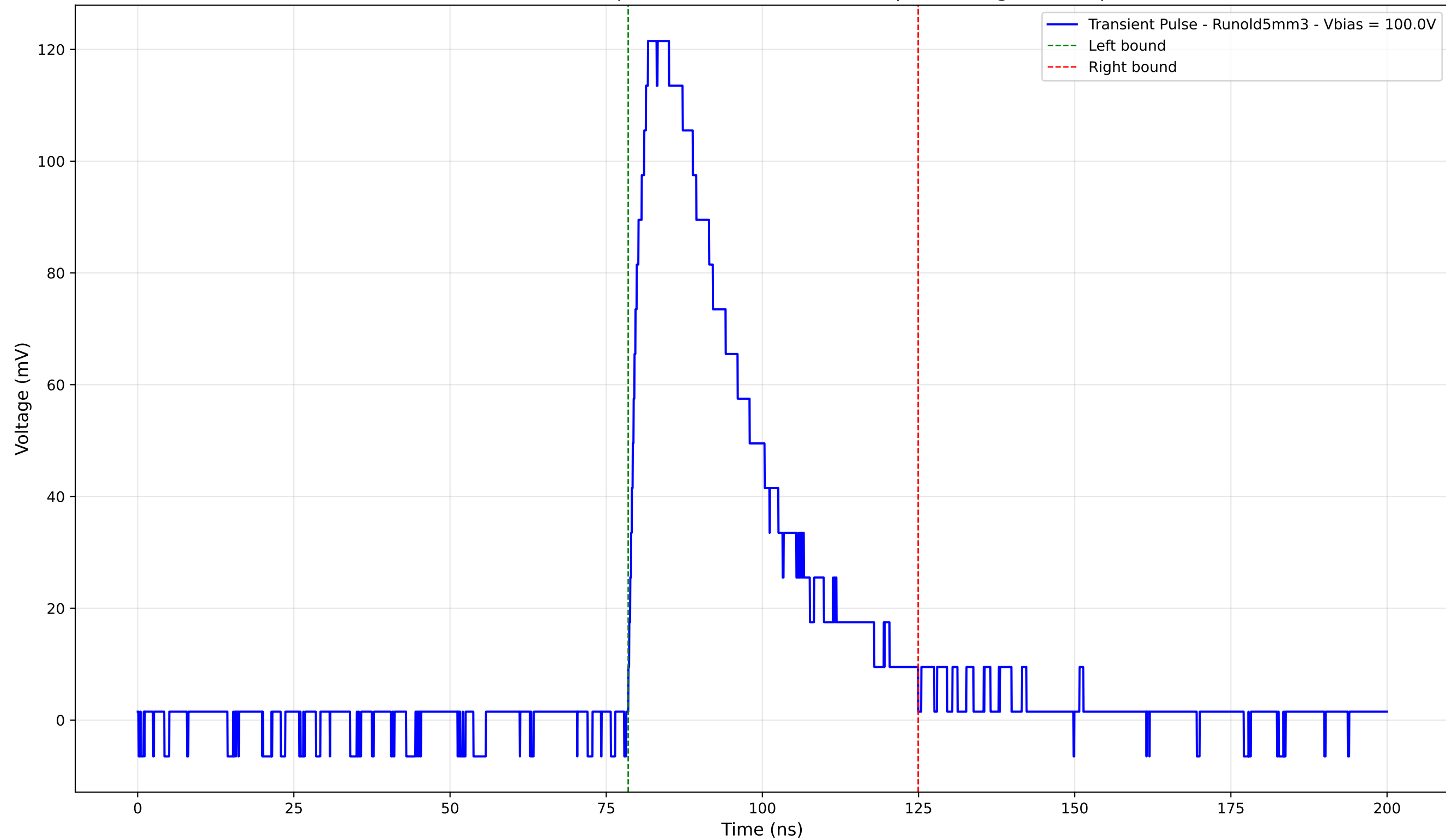
Transient Pulse - Sample: old5 - Position: 2145.0 \mu\text{m} - Charge: 47.33 pC
