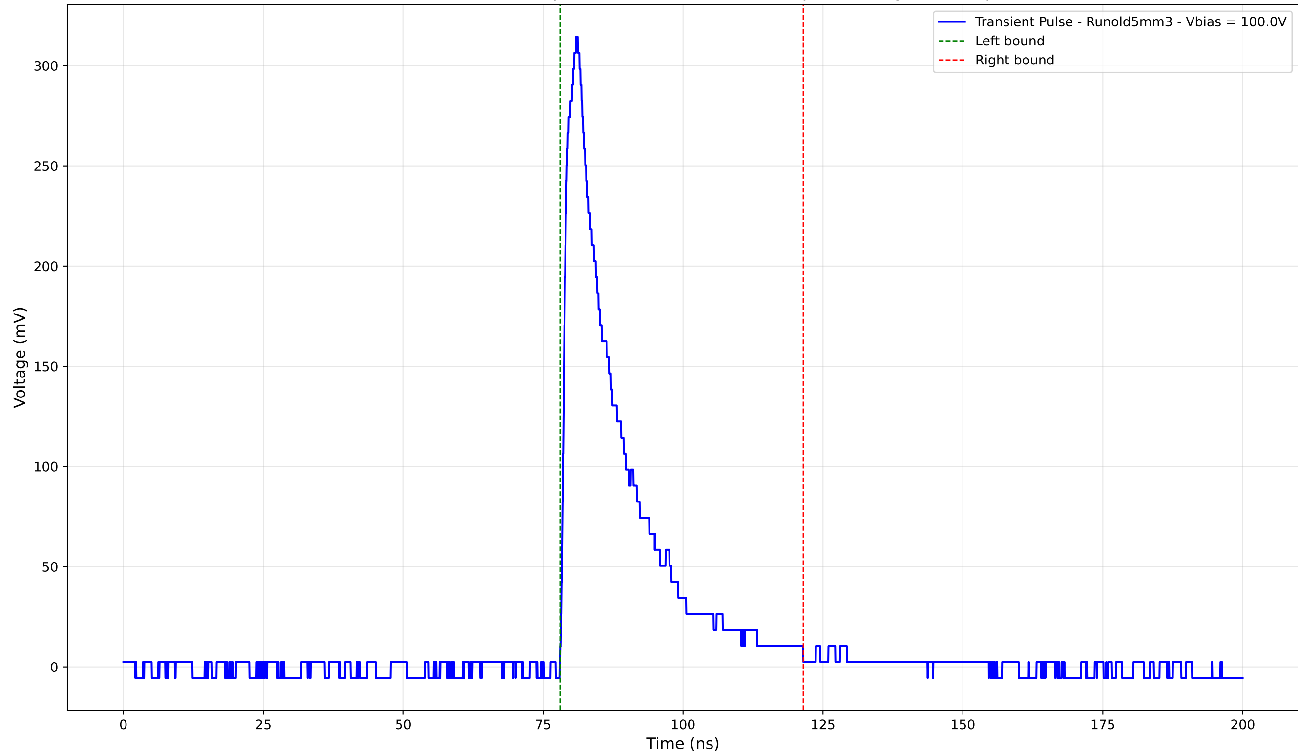
Transient Pulse - Sample: old5 - Position: 4105.0 \mu\text{m} - Charge: 66.75 pC
