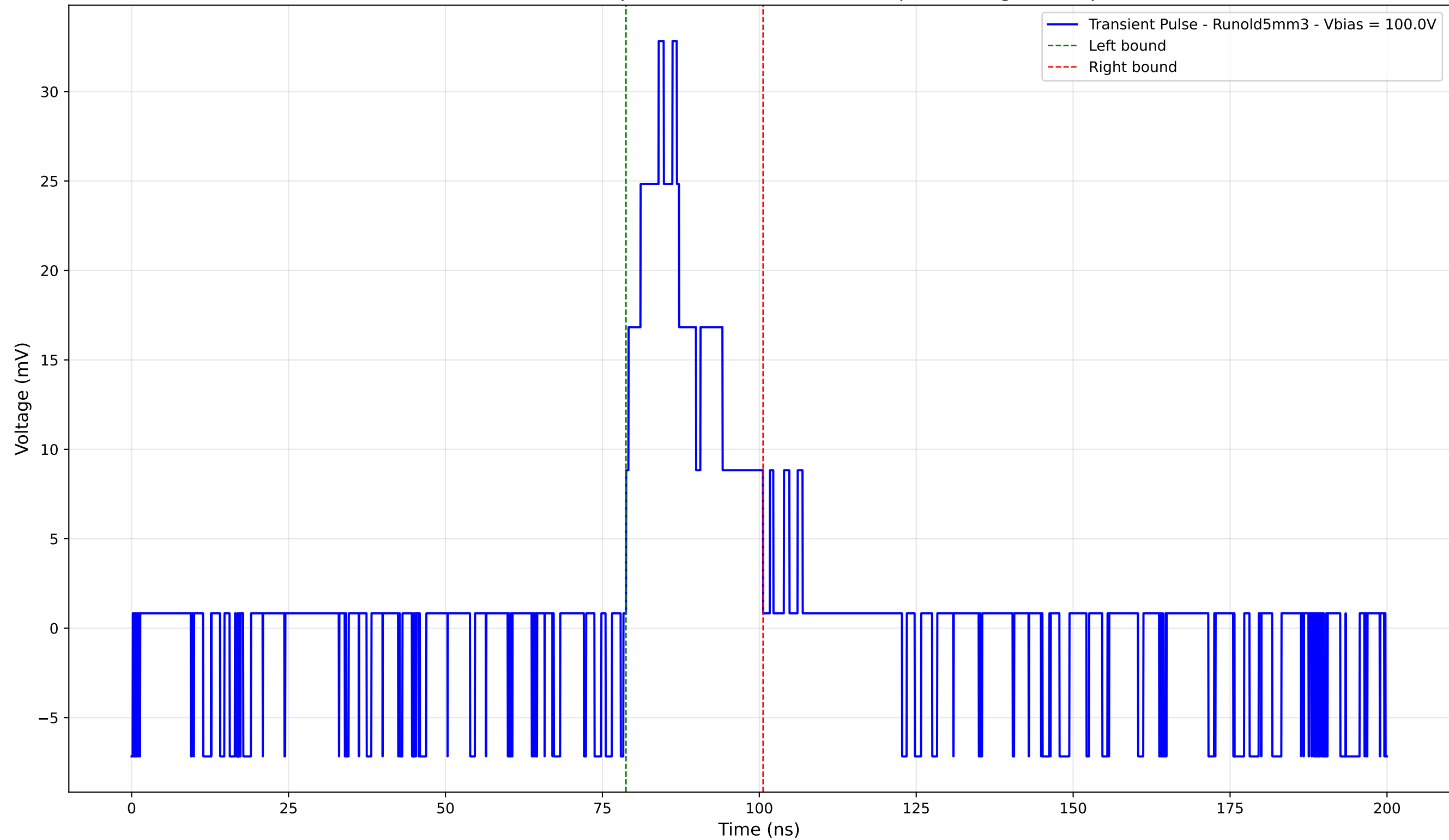
Transient Pulse - Sample: old5 - Position: 2700.0 \mu\text{m} - Charge: 7.36 pC
