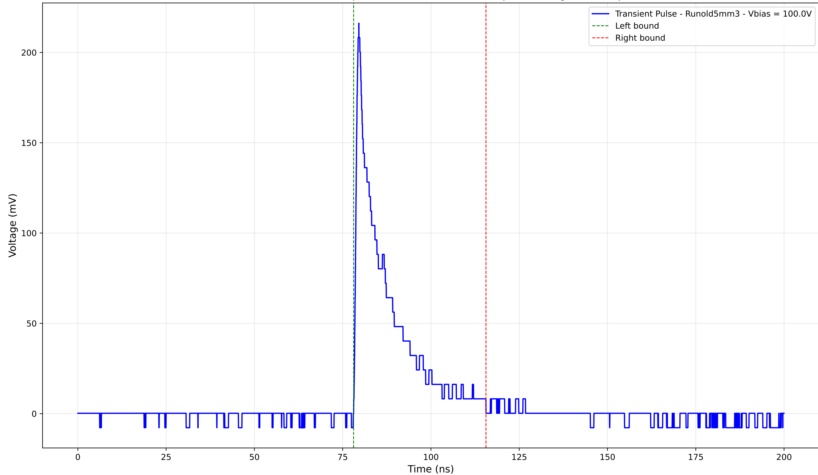
Transient Pulse - Sample: old5 - Position: 405.0 \mu\text{m} - Charge: 35.23 pC
