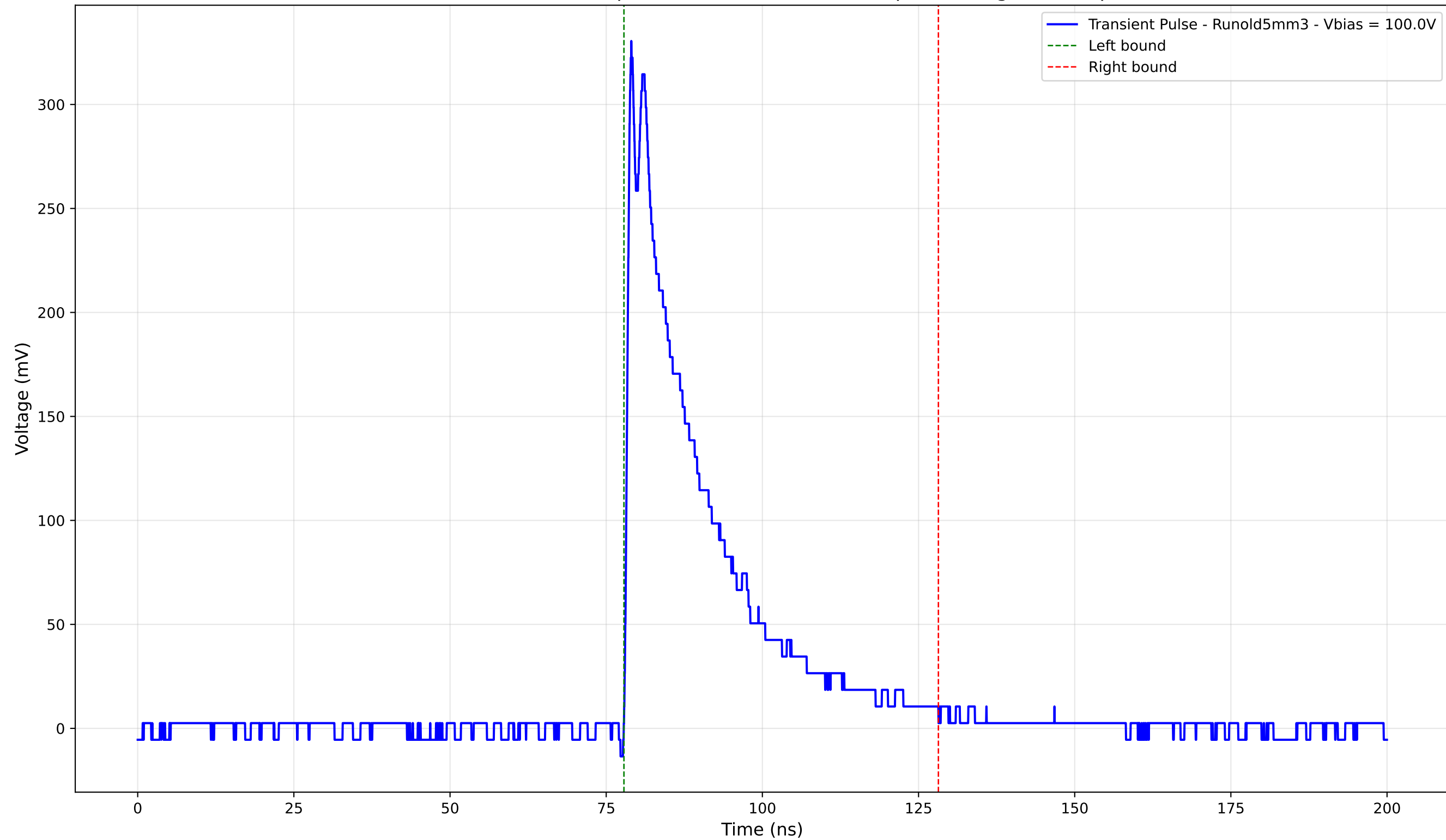
Transient Pulse - Sample: old5 - Position: 3190.0 \mu\text{m} - Charge: 78.92 pC
