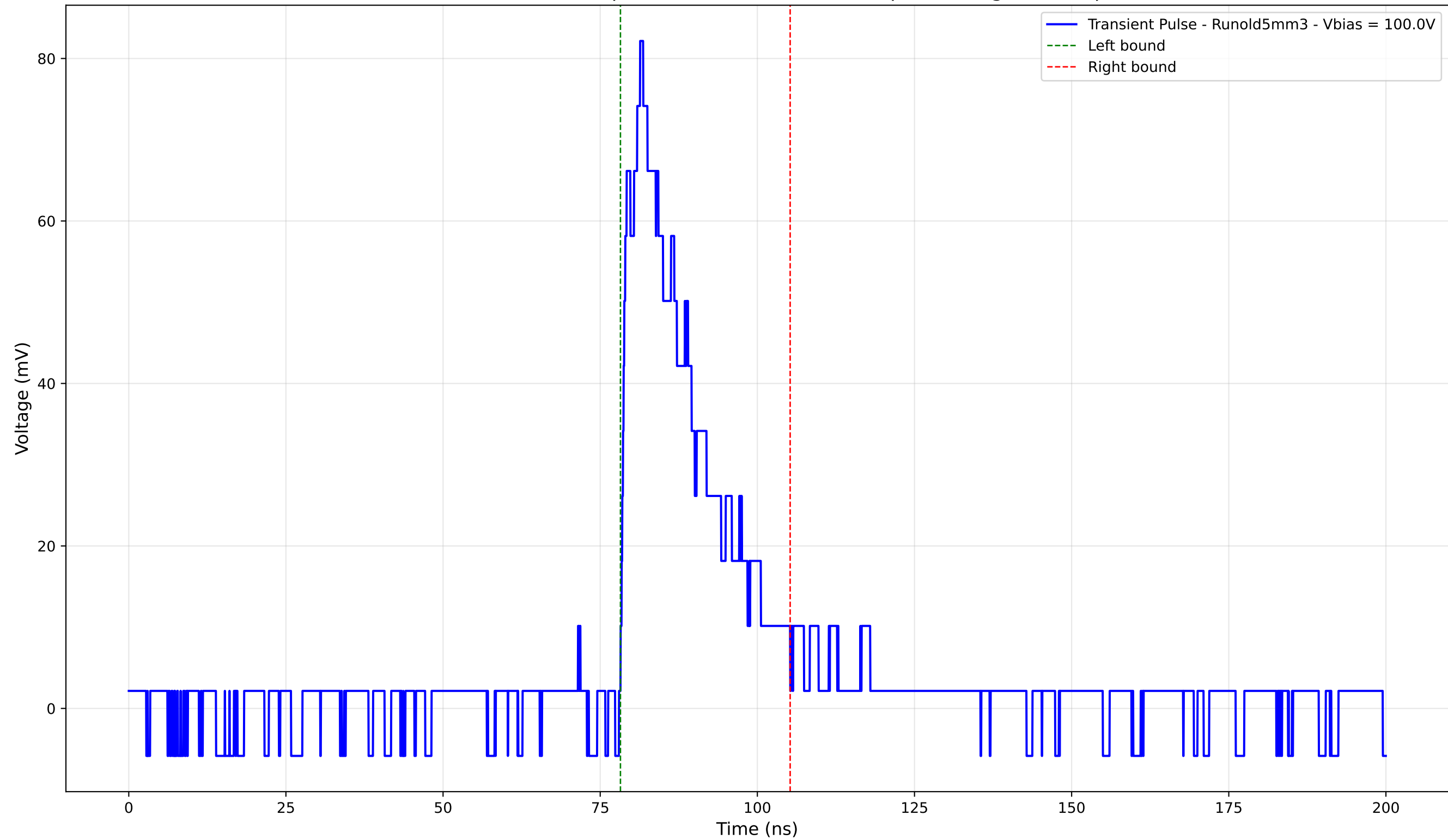
Transient Pulse - Sample: old5 - Position: 3020.0 \mu\text{m} - Charge: 18.98 pC
