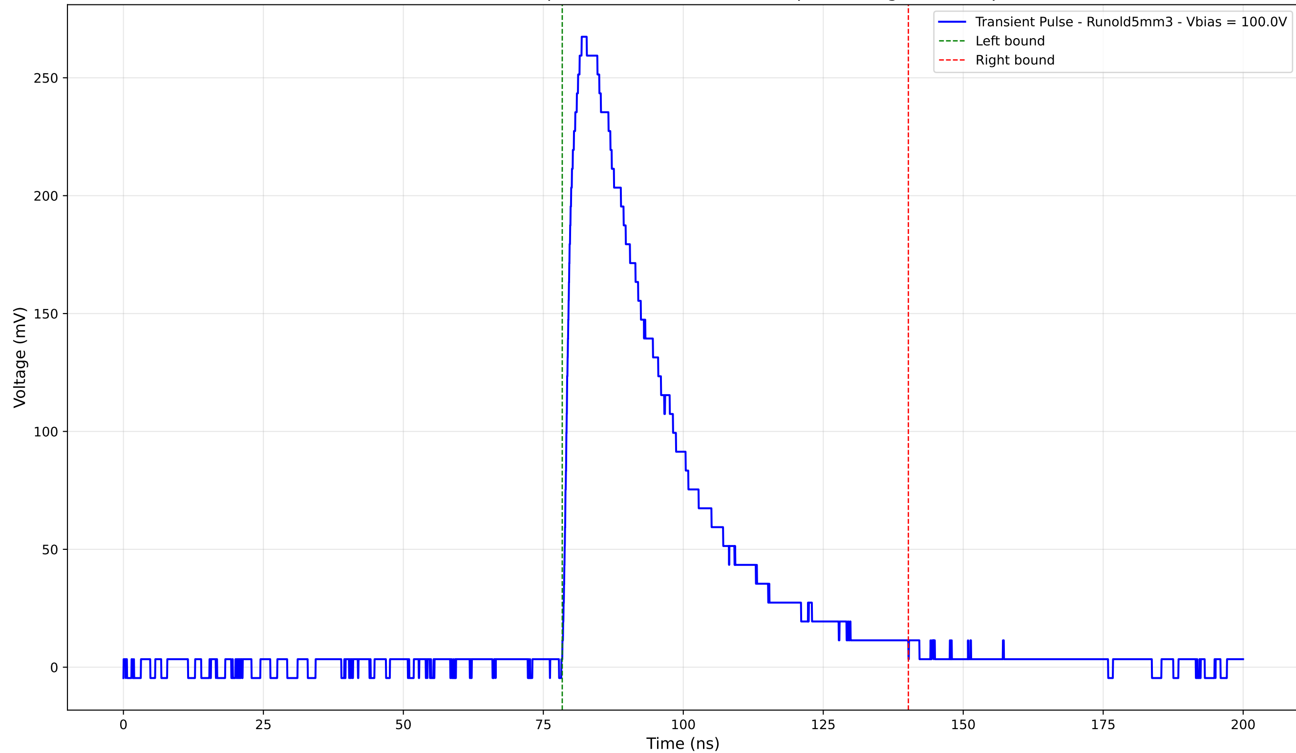
Transient Pulse - Sample: old5 - Position: 2495.0 \mu\text{m} - Charge: 102.17 pC
