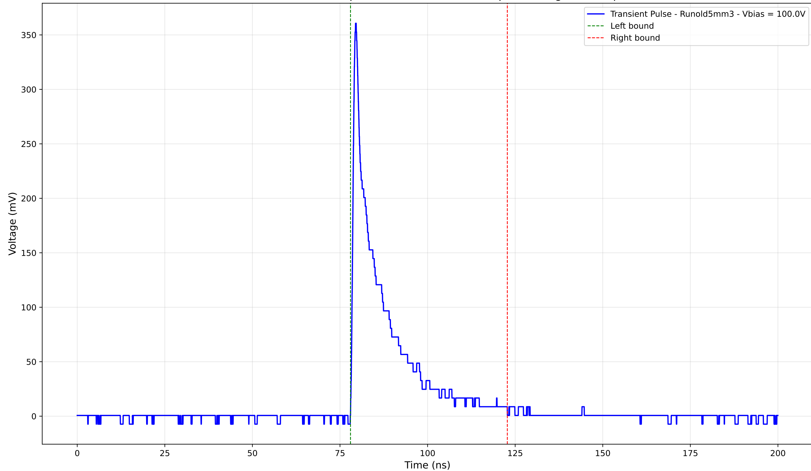
Transient Pulse - Sample: old5 - Position: 345.0 \mu\text{m} - Charge: 56.21 pC
