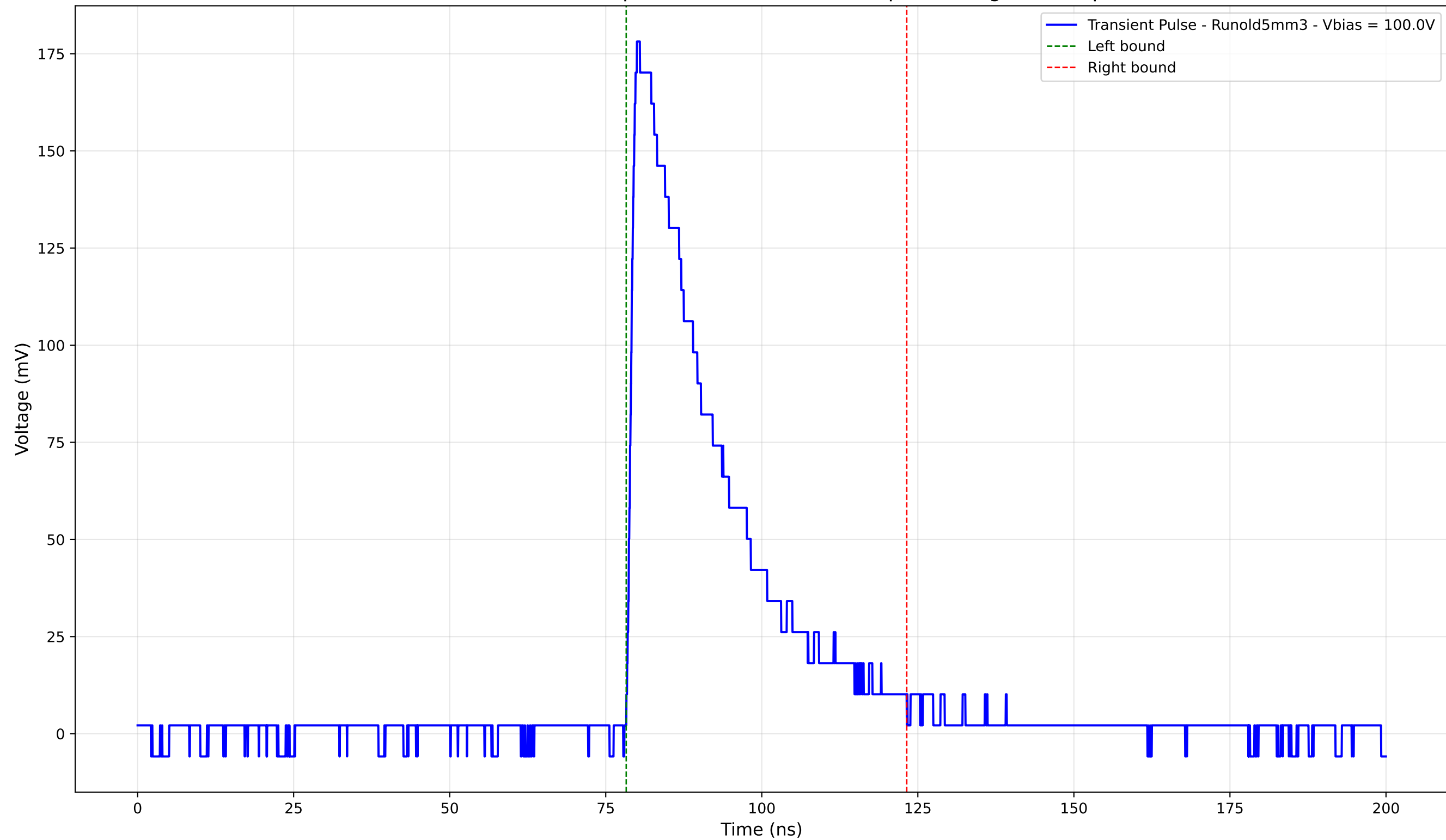
Transient Pulse - Sample: old5 - Position: 870.0 \mu\text{m} - Charge: 52.80 pC
