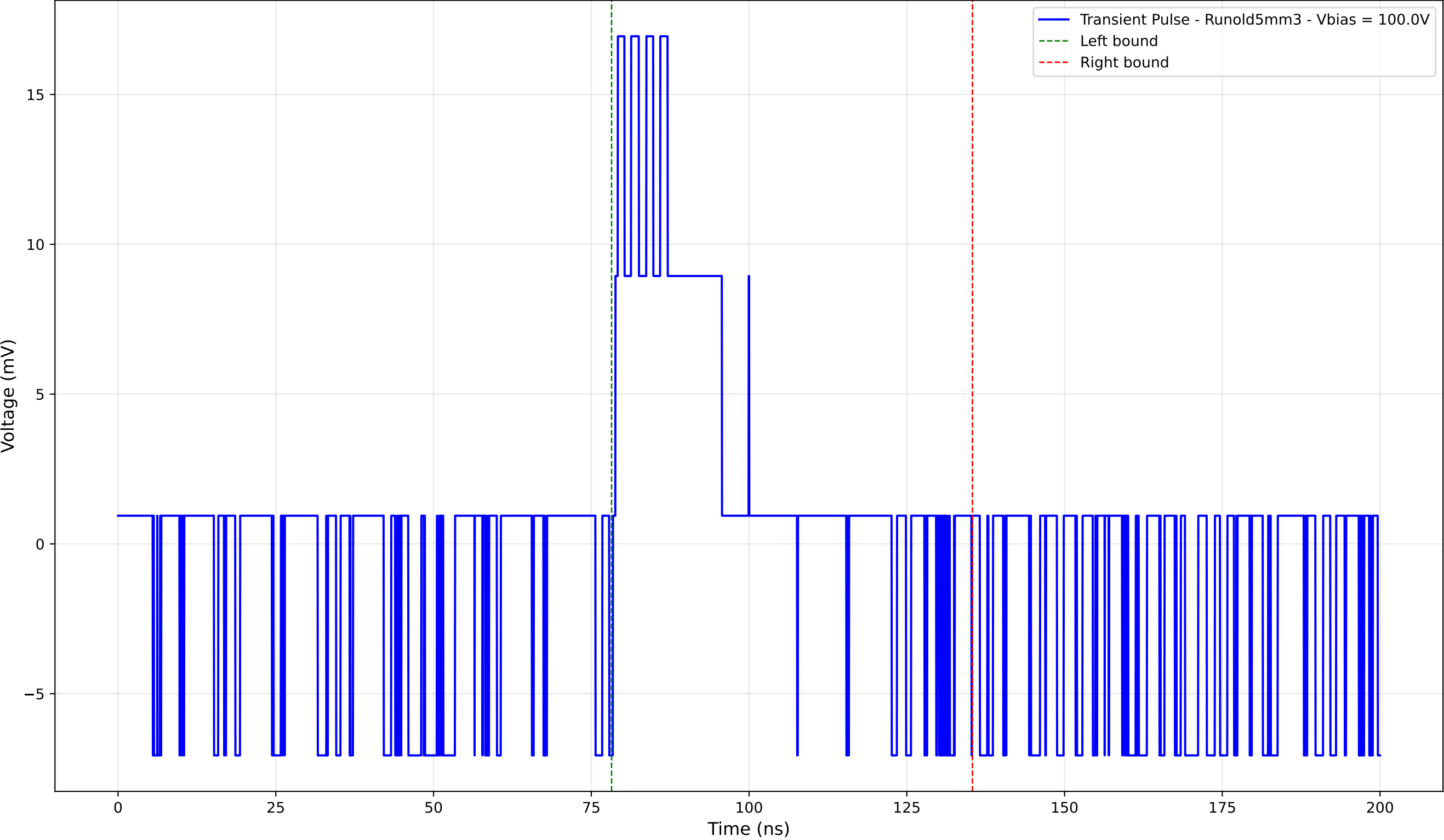
Transient Pulse - Sample: old5 - Position: 2660.0 \mu\text{m} - Charge: 3.82 pC
