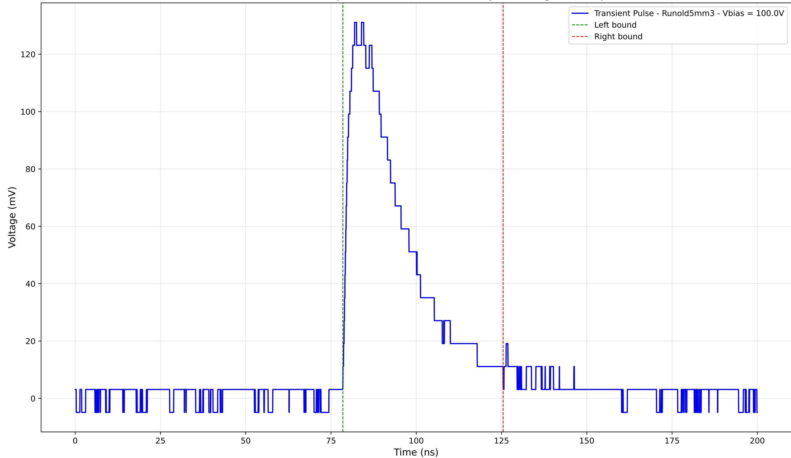
Transient Pulse - Sample: old5 - Position: 1435.0 \mu\text{m} - Charge: 49.28 pC
