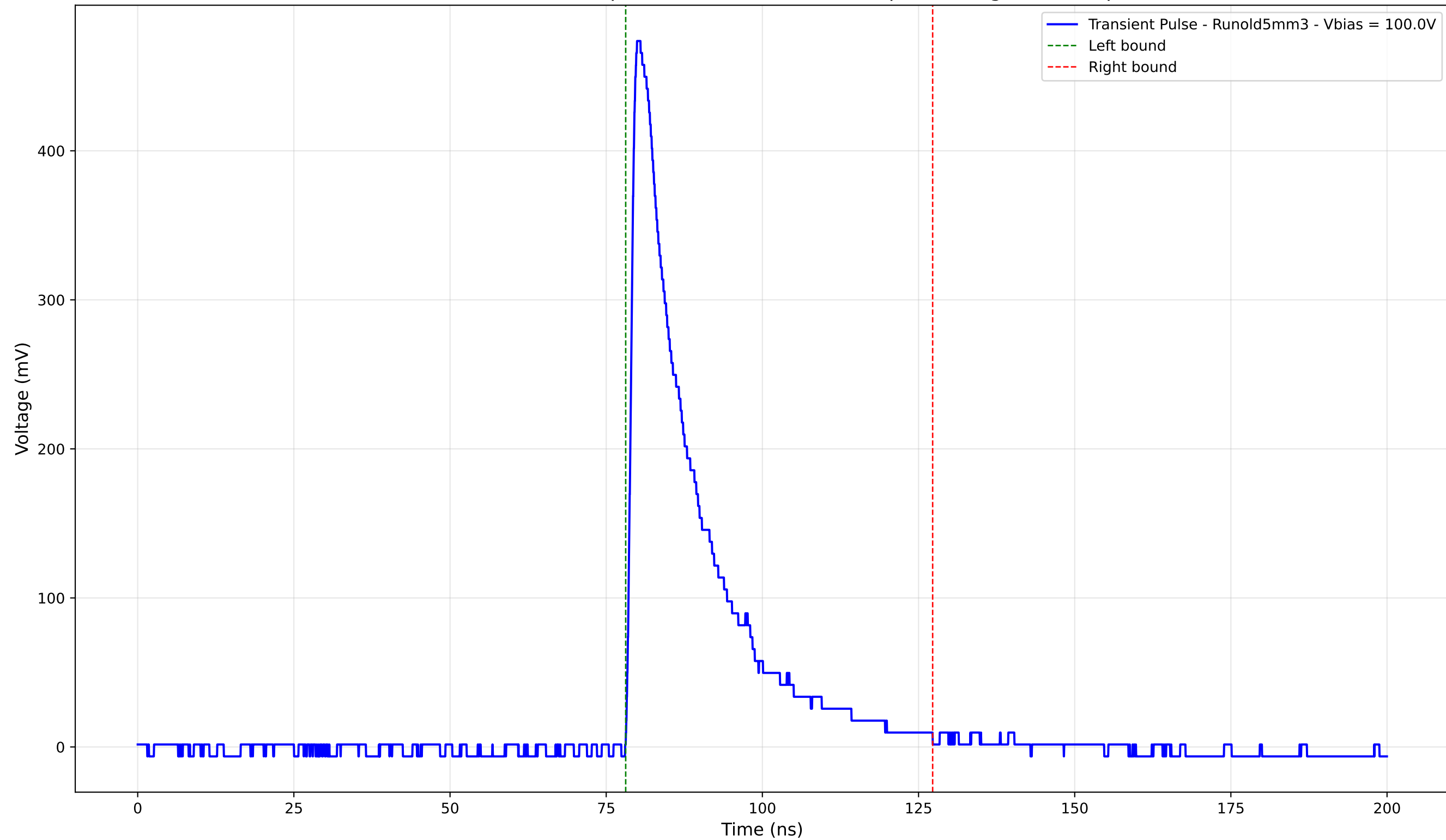
Transient Pulse - Sample: old5 - Position: 4390.0 \mu\text{m} - Charge: 103.54 pC
