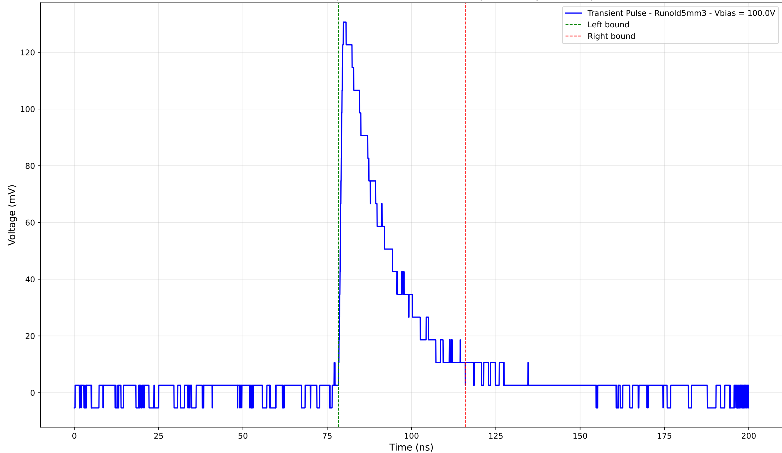
Transient Pulse - Sample: old5 - Position: 800.0 \mu\text{m} - Charge: 36.35 pC
