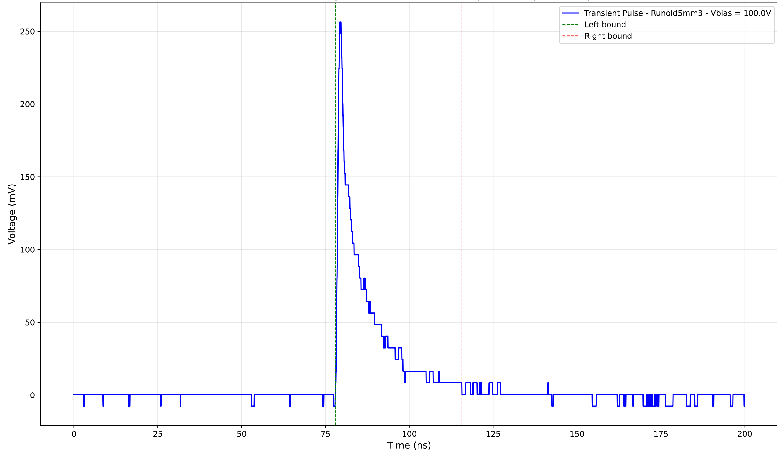
Transient Pulse - Sample: old5 - Position: 295.0 \mu\text{m} - Charge: 36.17 pC
