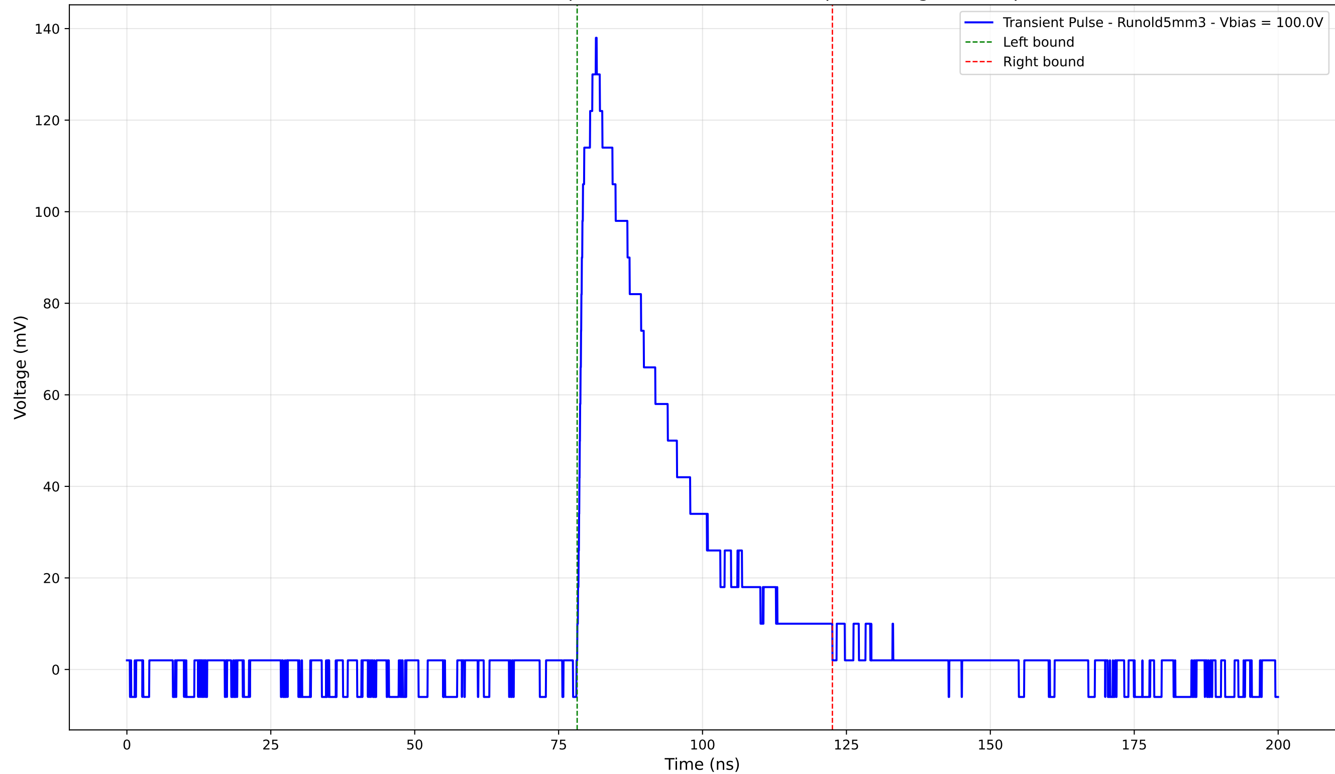
Transient Pulse - Sample: old5 - Position: 2915.0 \mu\text{m} - Charge: 40.68 pC
