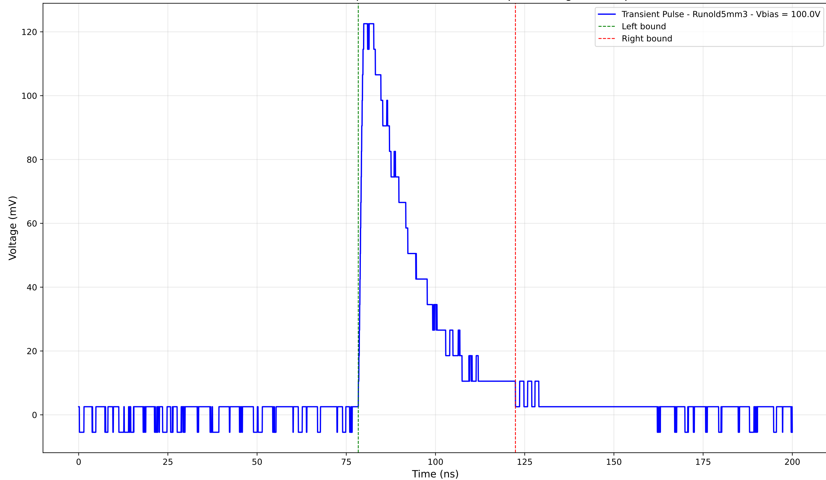
Transient Pulse - Sample: old5 - Position: 895.0 \mu\text{m} - Charge: 38.25 pC
