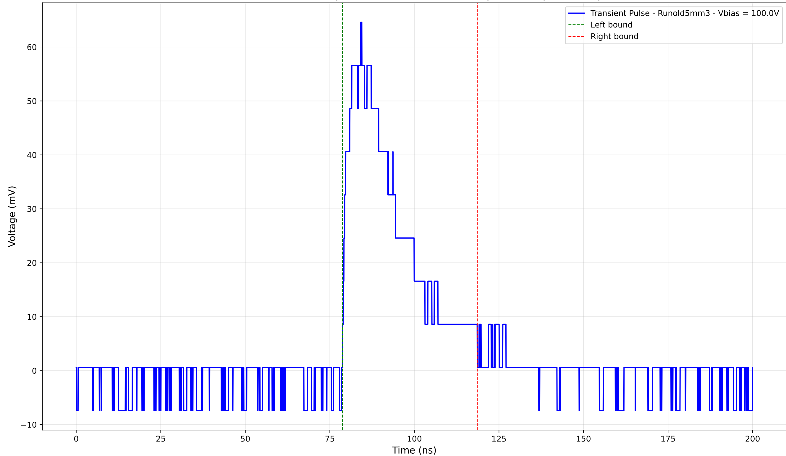
Transient Pulse - Sample: old5 - Position: 1410.0 \mu\text{m} - Charge: 21.00 pC
