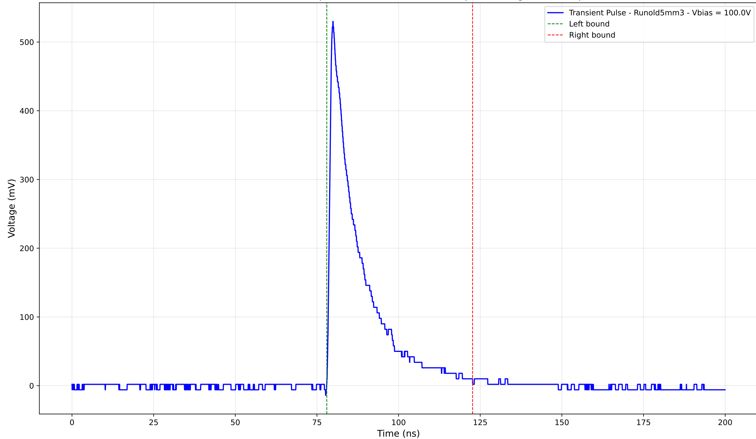
Transient Pulse - Sample: old5 - Position: 4590.0 \mu\text{m} - Charge: 102.81 pC
