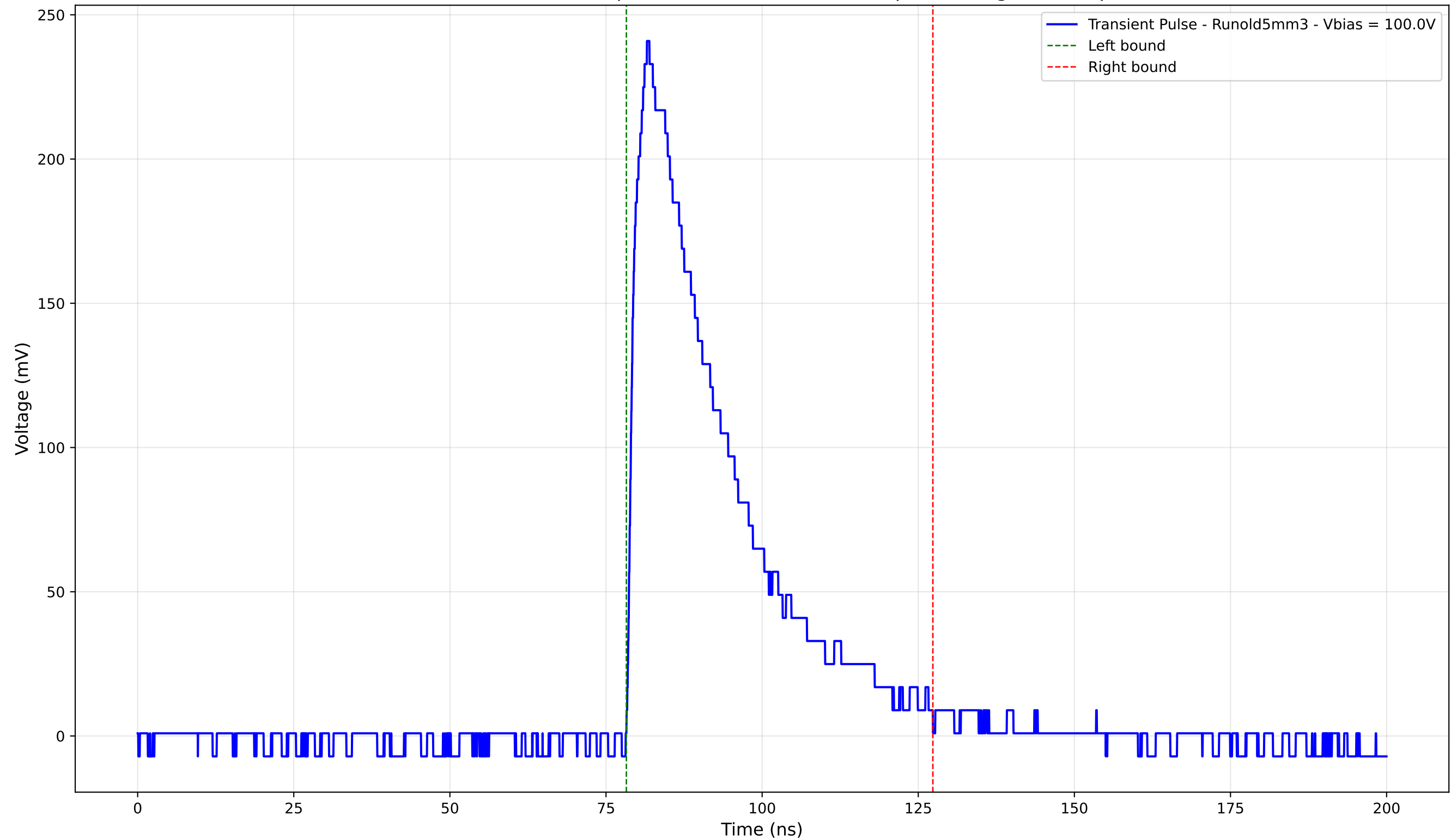
Transient Pulse - Sample: old5 - Position: 2765.0 \mu\text{m} - Charge: 77.56 pC
