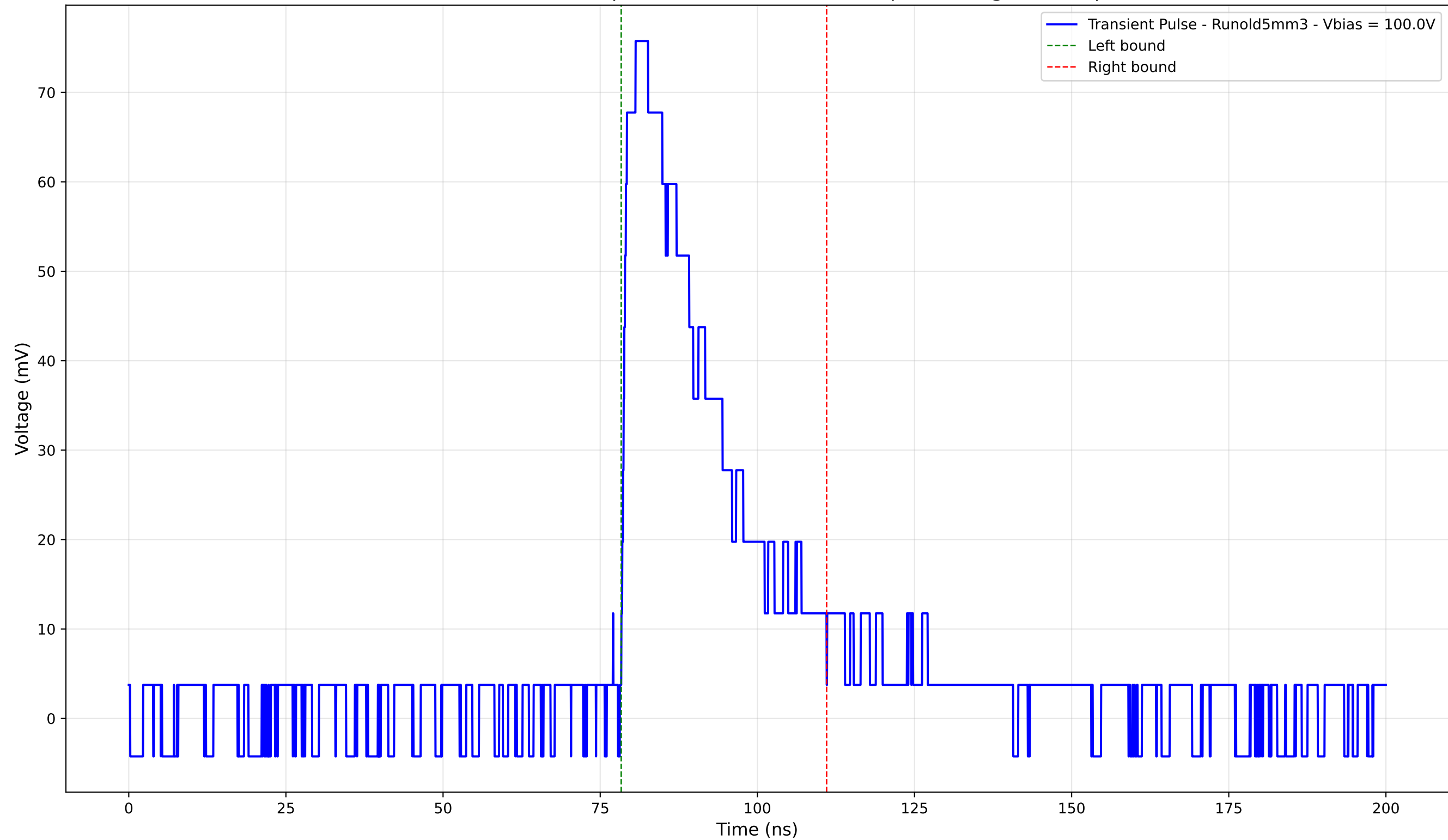
Transient Pulse - Sample: old5 - Position: 2930.0 \mu\text{m} - Charge: 23.24 pC
