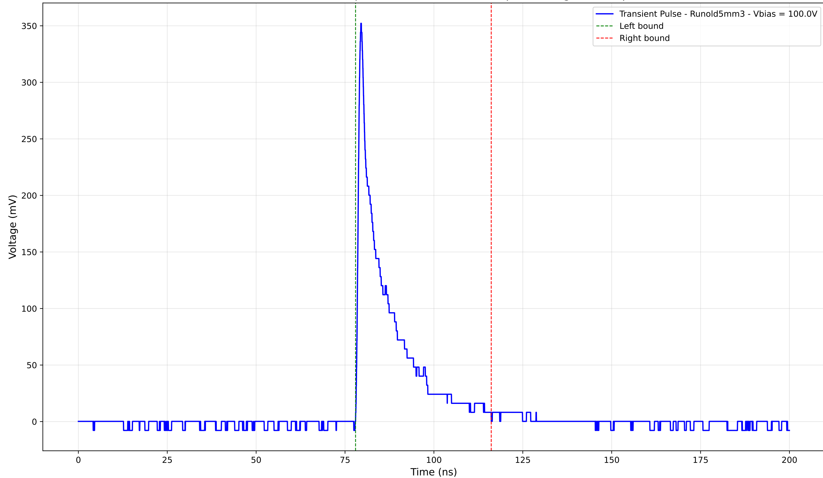
Transient Pulse - Sample: old5 - Position: 350.0 \mu\text{m} - Charge: 53.45 pC
