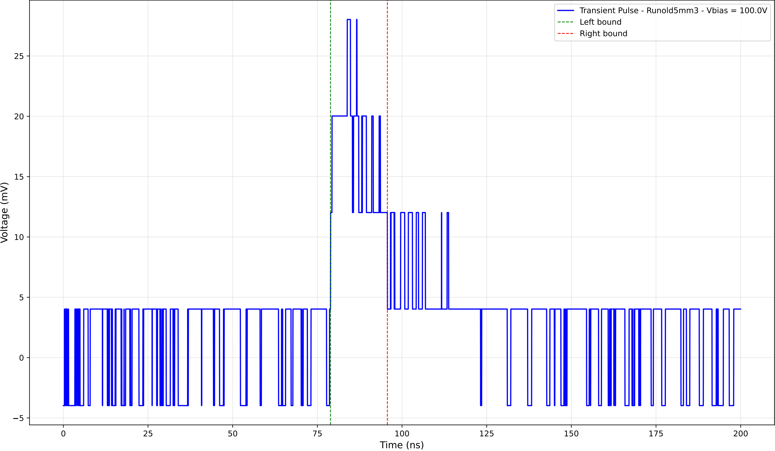
Transient Pulse - Sample: old5 - Position: 2650.0 \mu\text{m} - Charge: 5.74 pC
