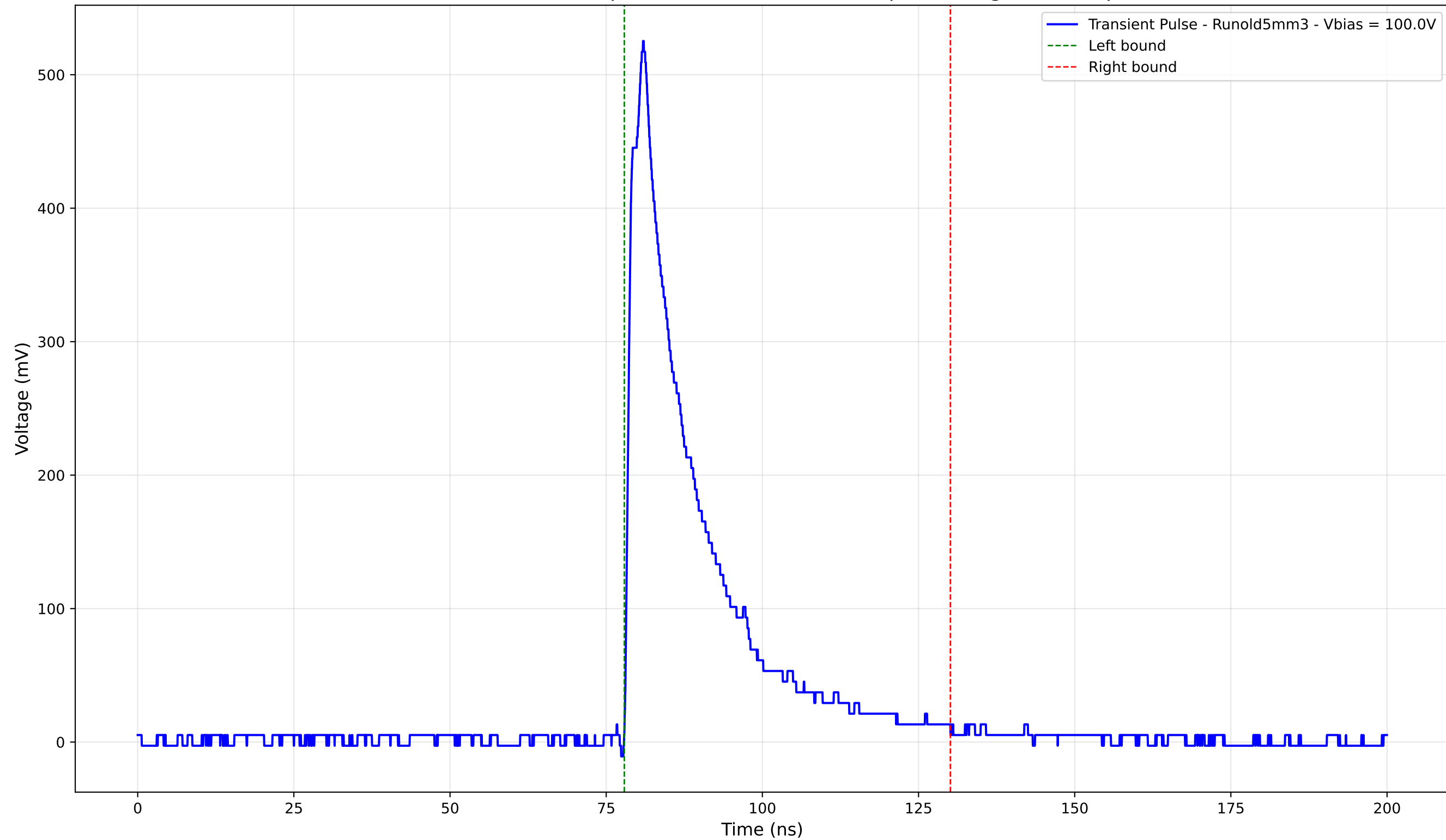
Transient Pulse - Sample: old5 - Position: 4040.0 \mu\text{m} - Charge: 117.44 pC
