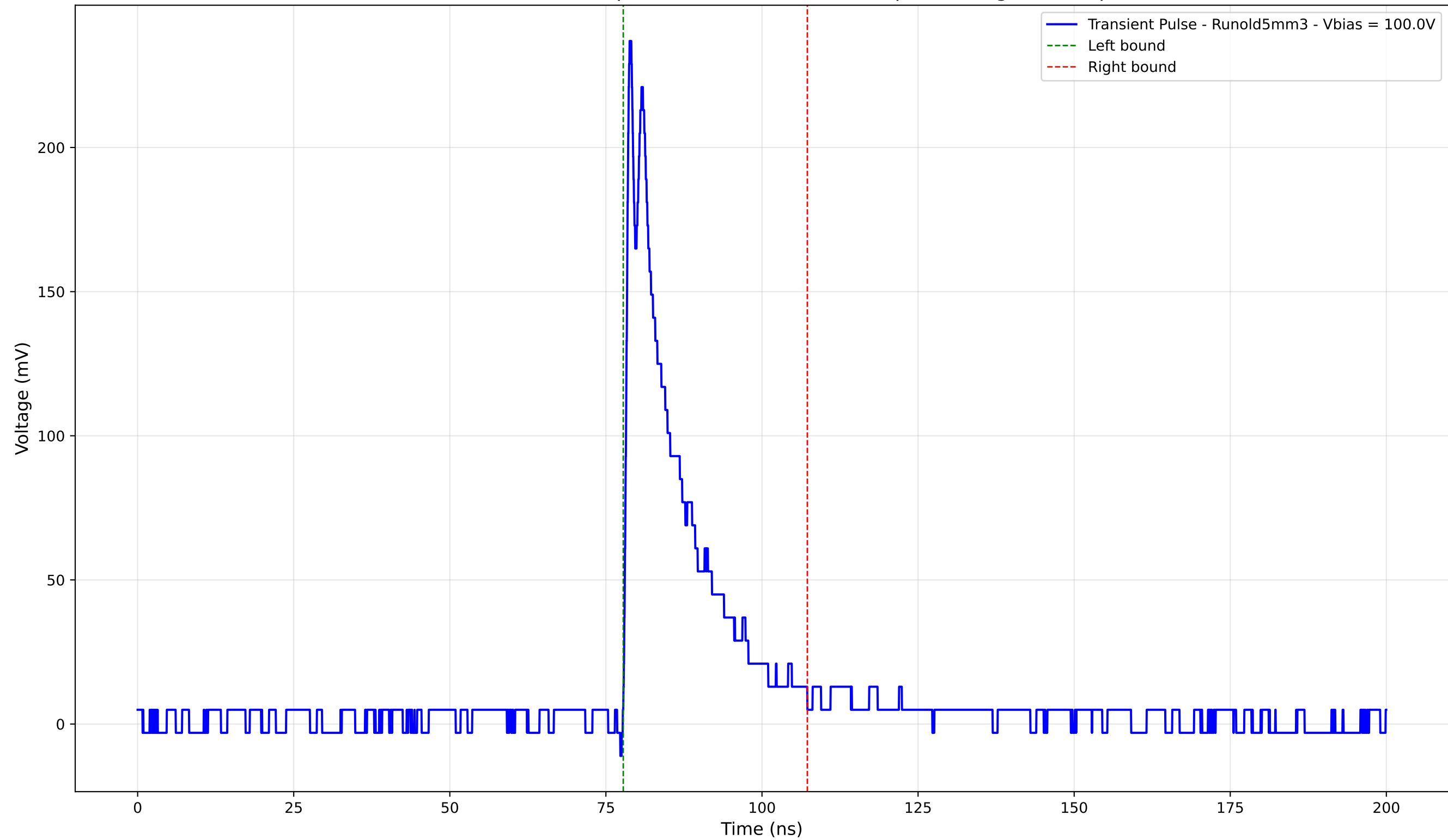
Transient Pulse - Sample: old5 - Position: 3825.0 \mu\text{m} - Charge: 40.30 pC
