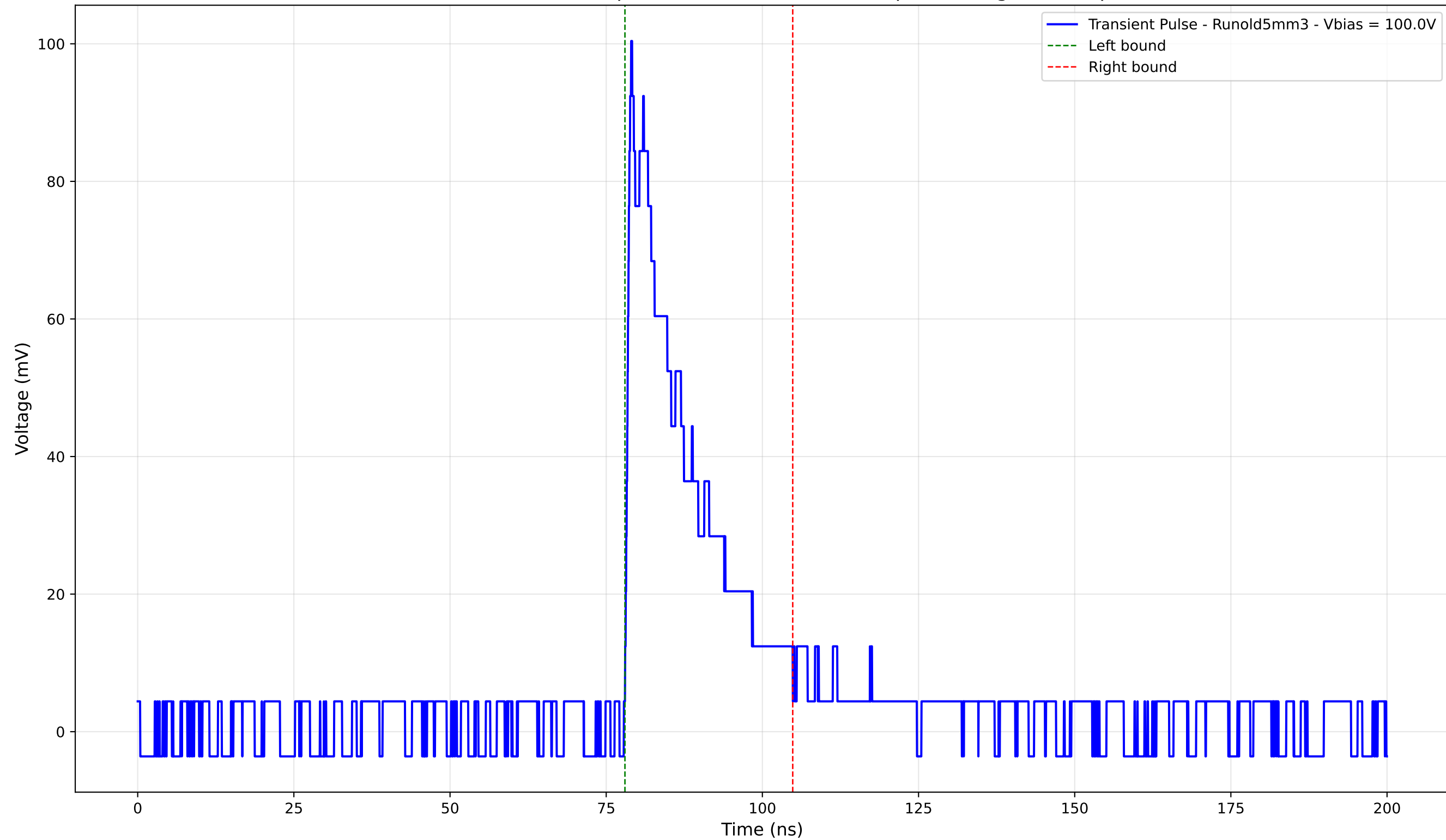
Transient Pulse - Sample: old5 - Position: 3235.0 \mu\text{m} - Charge: 19.91 pC
