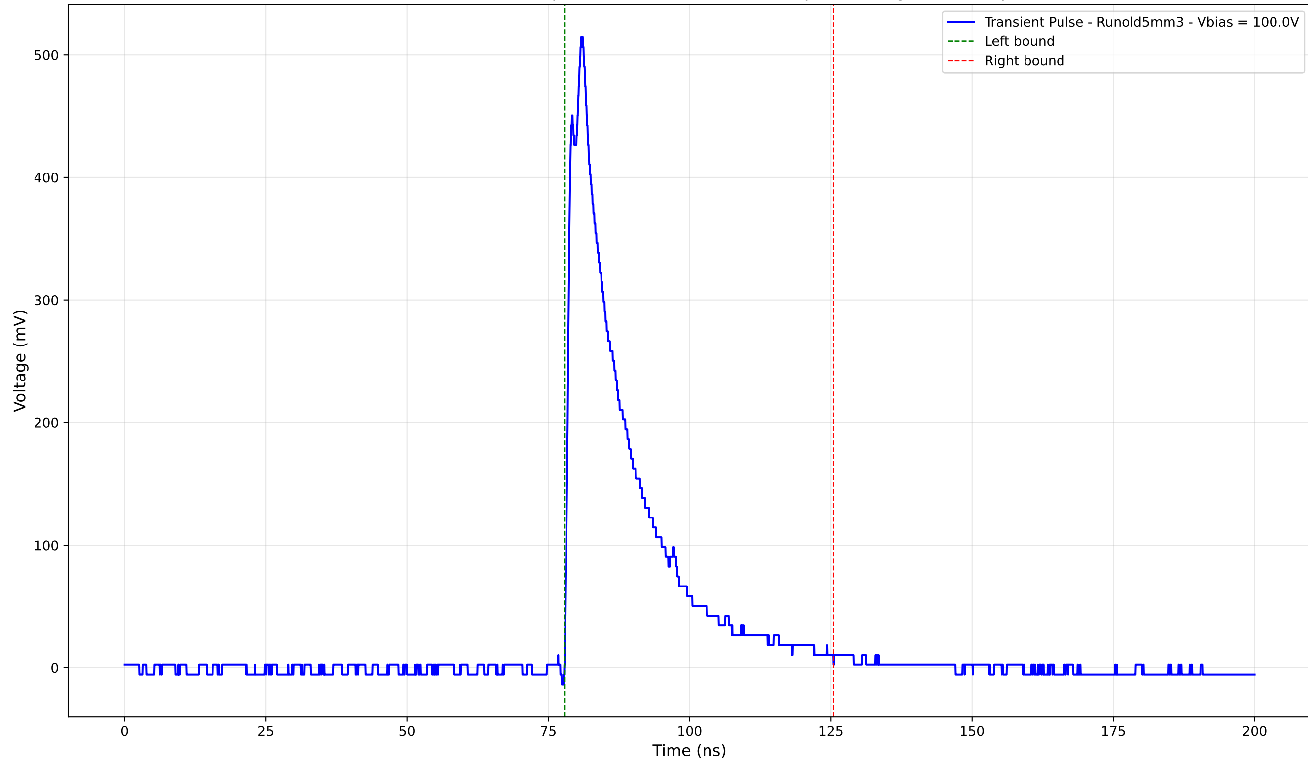
Transient Pulse - Sample: old5 - Position: 4010.0 \mu\text{m} - Charge: 111.61 pC
