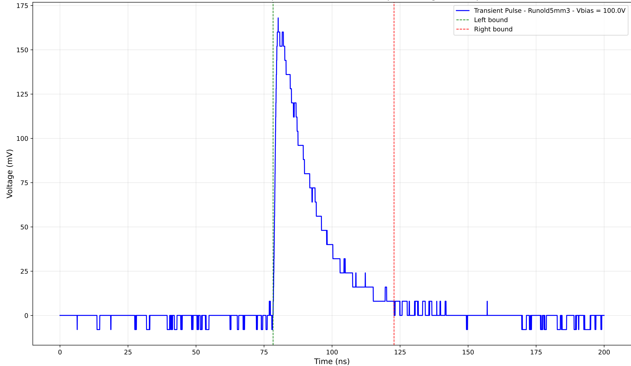
Transient Pulse - Sample: old5 - Position: 875.0 \mu\text{m} - Charge: 47.94 pC
