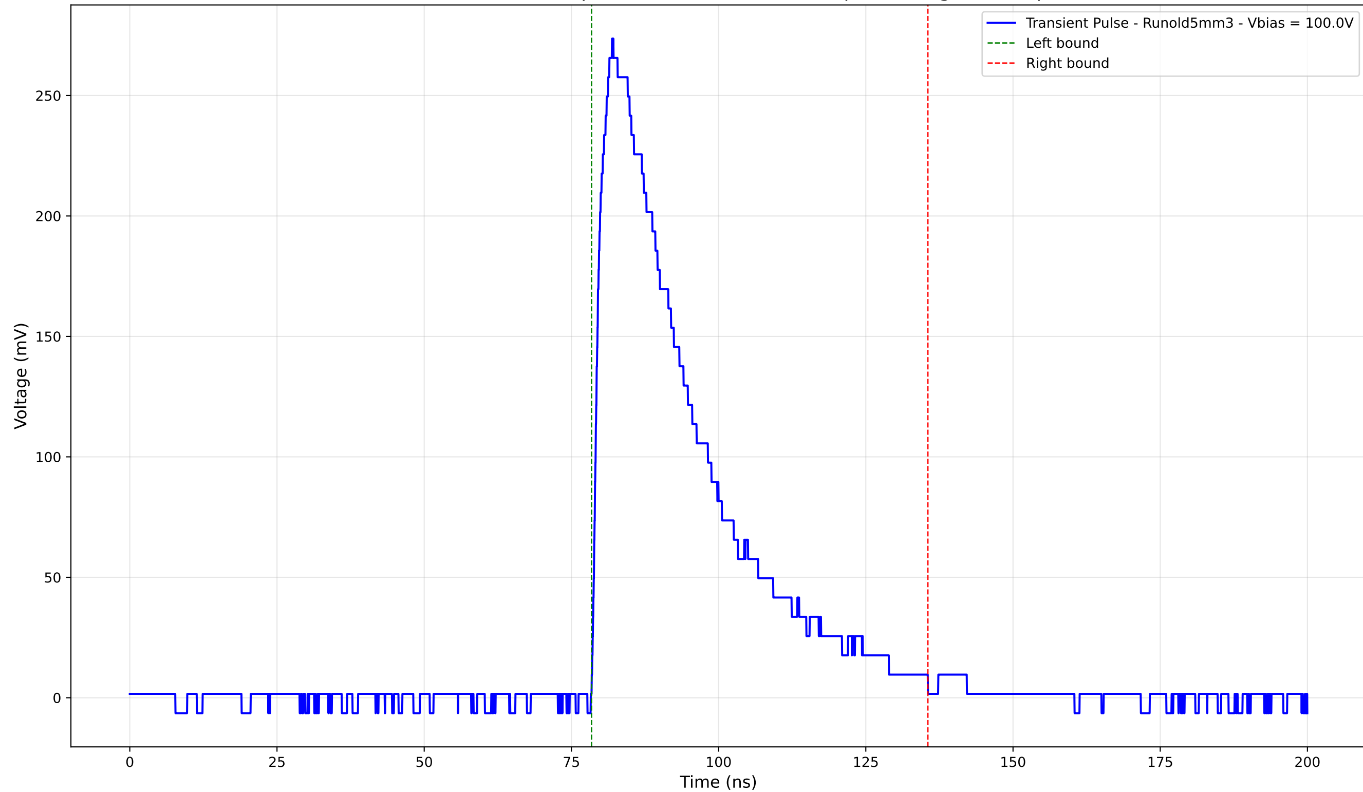
Transient Pulse - Sample: old5 - Position: 2550.0 \mu\text{m} - Charge: 98.79 pC
