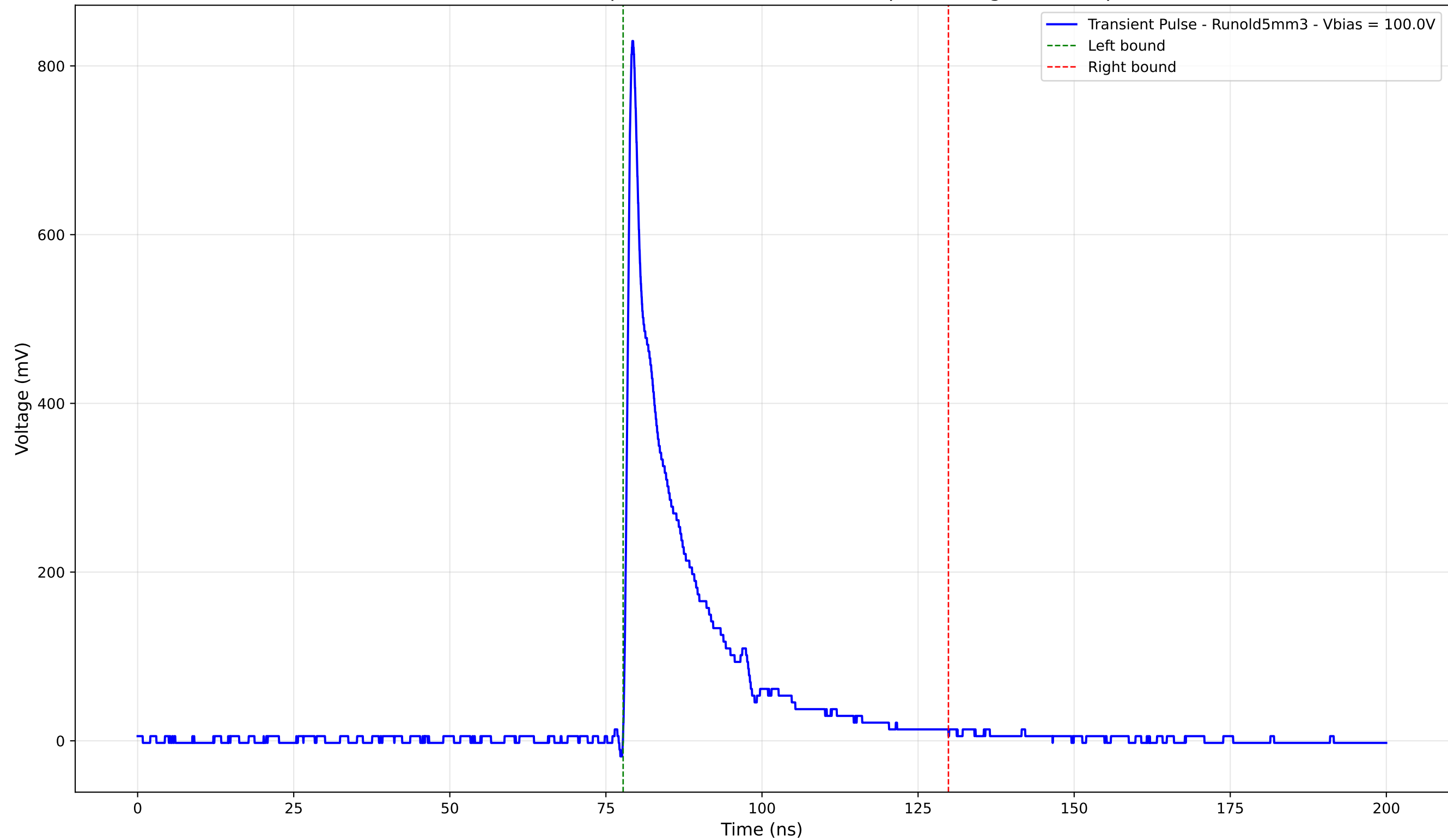
Transient Pulse - Sample: old5 - Position: 4815.0 \mu\text{m} - Charge: 130.62 pC
