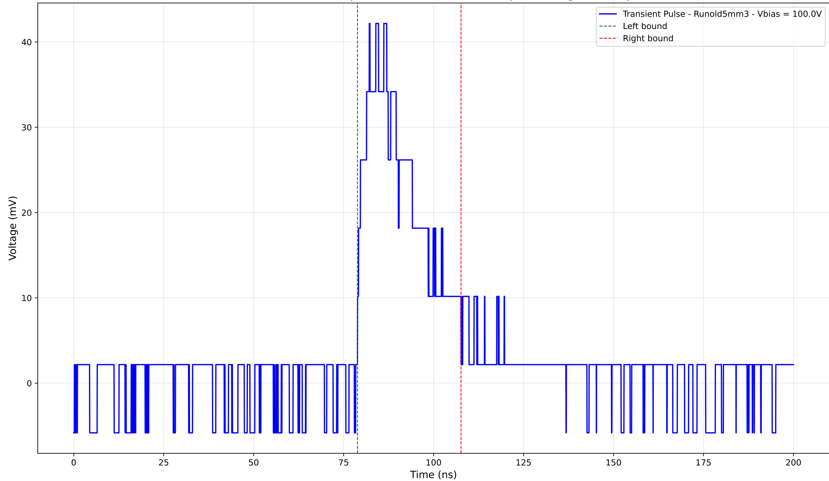
Transient Pulse - Sample: old5 - Position: 2185.0 \mu\text{m} - Charge: 12.88 pC
