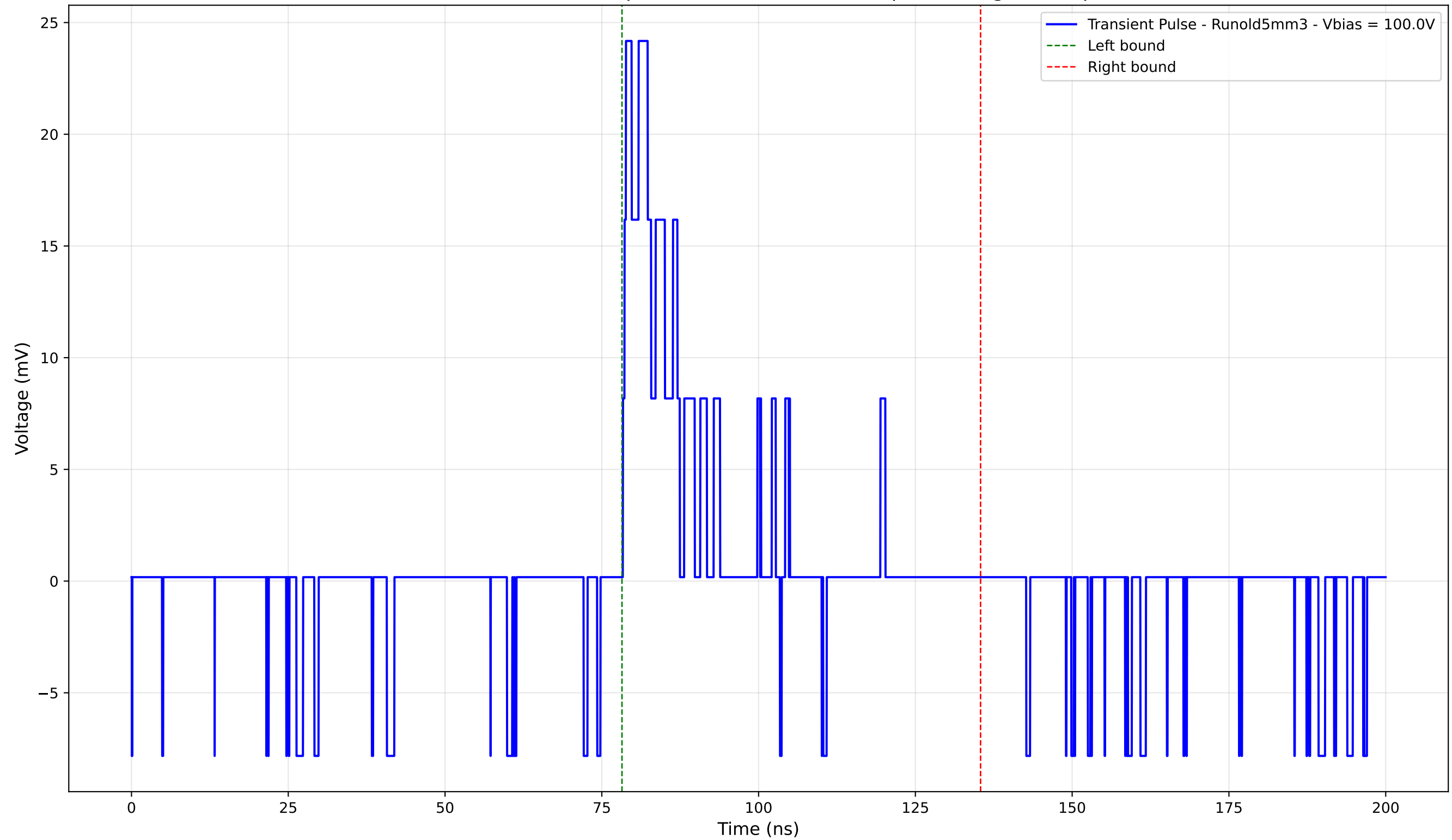
Transient Pulse - Sample: old5 - Position: 120.0 \mu\text{m} - Charge: 3.93 pC
