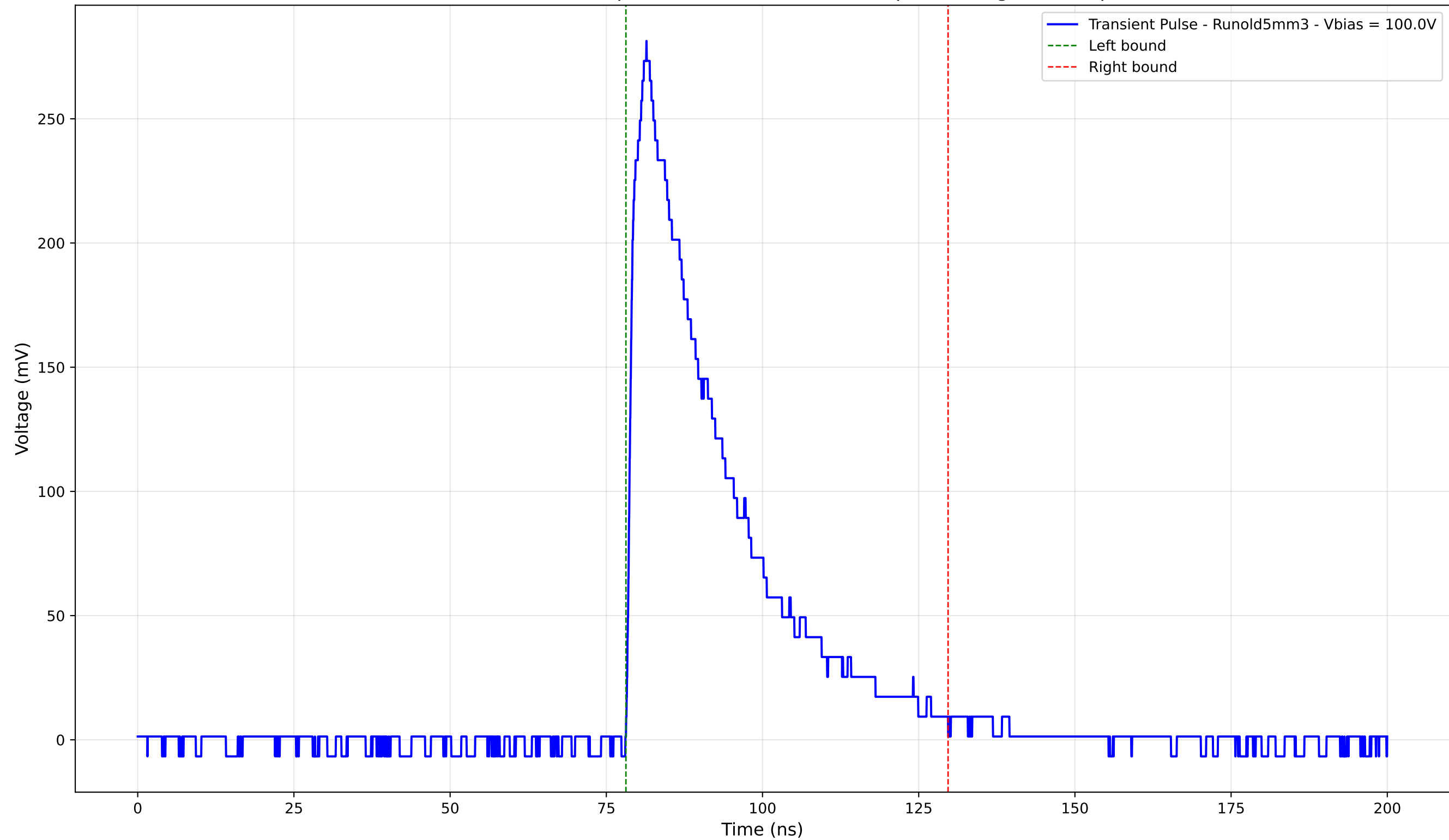
Transient Pulse - Sample: old5 - Position: 2880.0 \mu\text{m} - Charge: 87.44 pC
