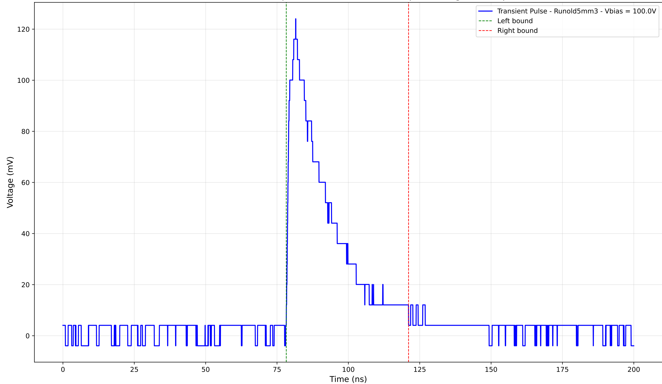
Transient Pulse - Sample: old5 - Position: 2920.0 \mu\text{m} - Charge: 36.24 pC
