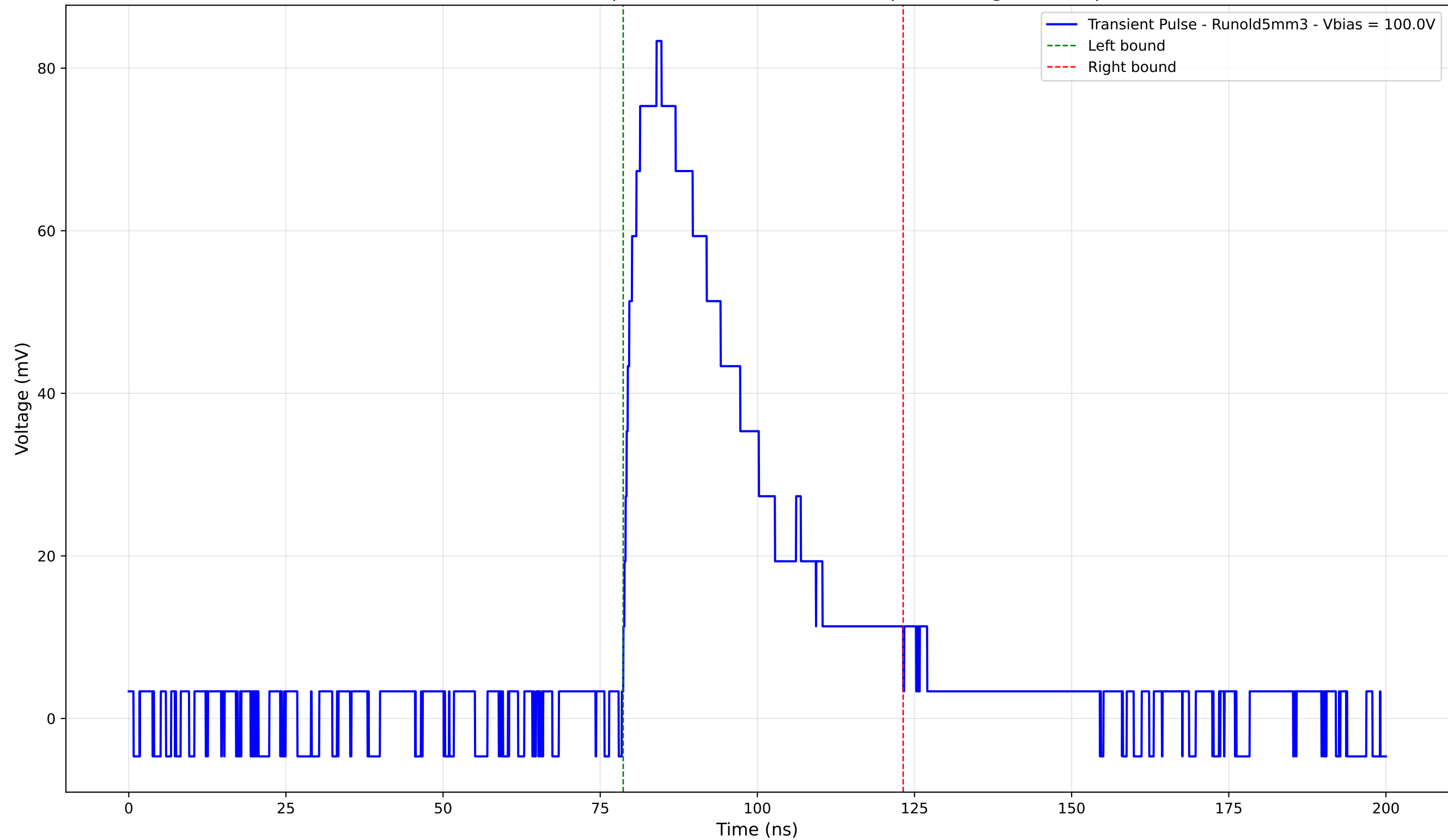
Transient Pulse - Sample: old5 - Position: 1755.0 \mu\text{m} - Charge: 31.98 pC
