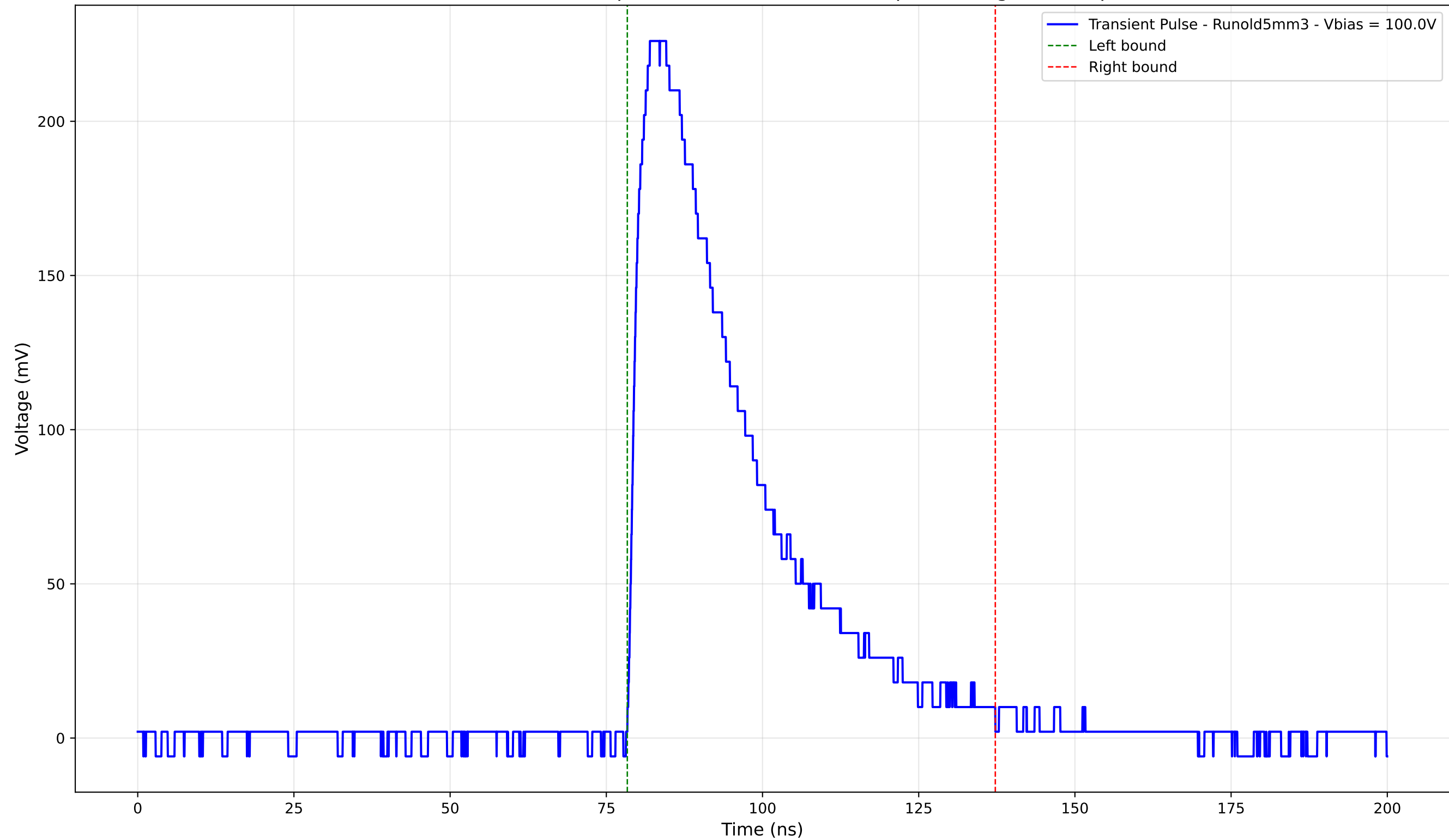
Transient Pulse - Sample: old5 - Position: 2280.0 \mu\text{m} - Charge: 90.77 pC
