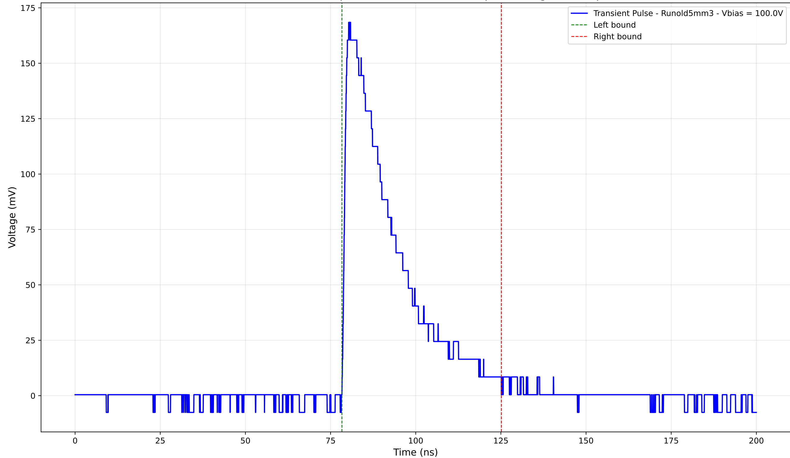
Transient Pulse - Sample: old5 - Position: 970.0 \mu\text{m} - Charge: 53.38 pC
