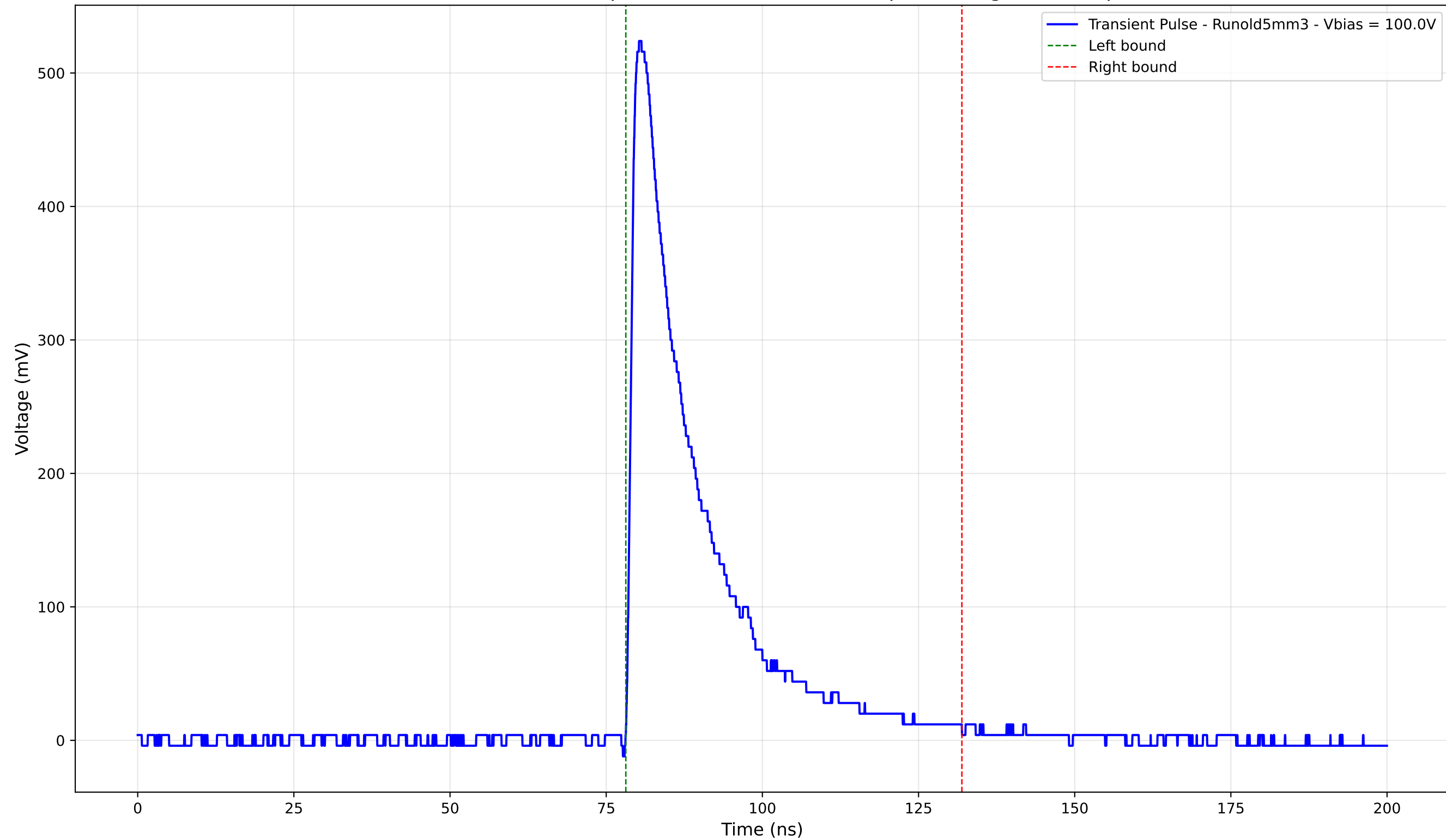
Transient Pulse - Sample: old5 - Position: 4340.0 \mu\text{m} - Charge: 120.19 pC
