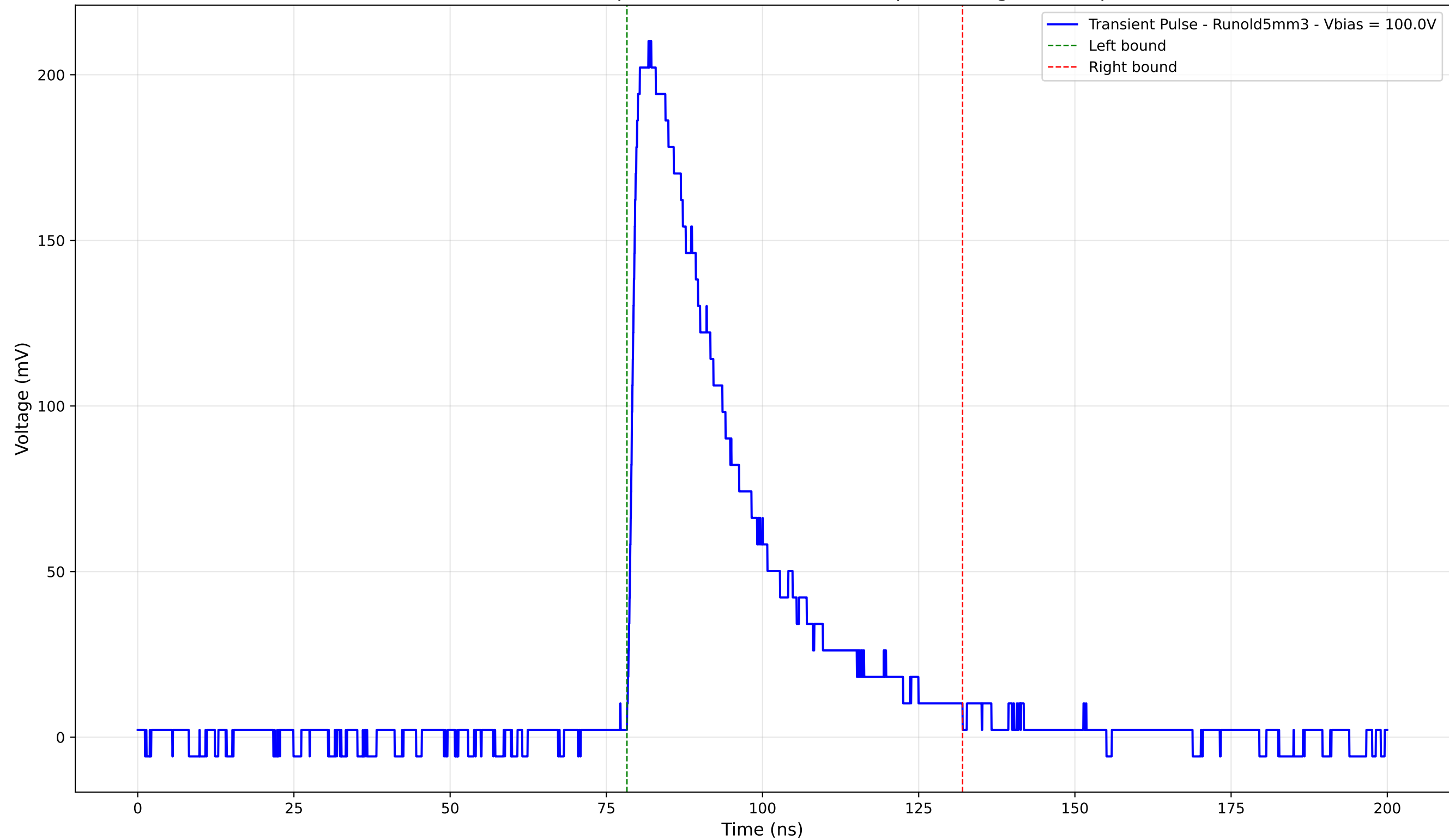
Transient Pulse - Sample: old5 - Position: 1050.0 \mu\text{m} - Charge: 73.07 pC
