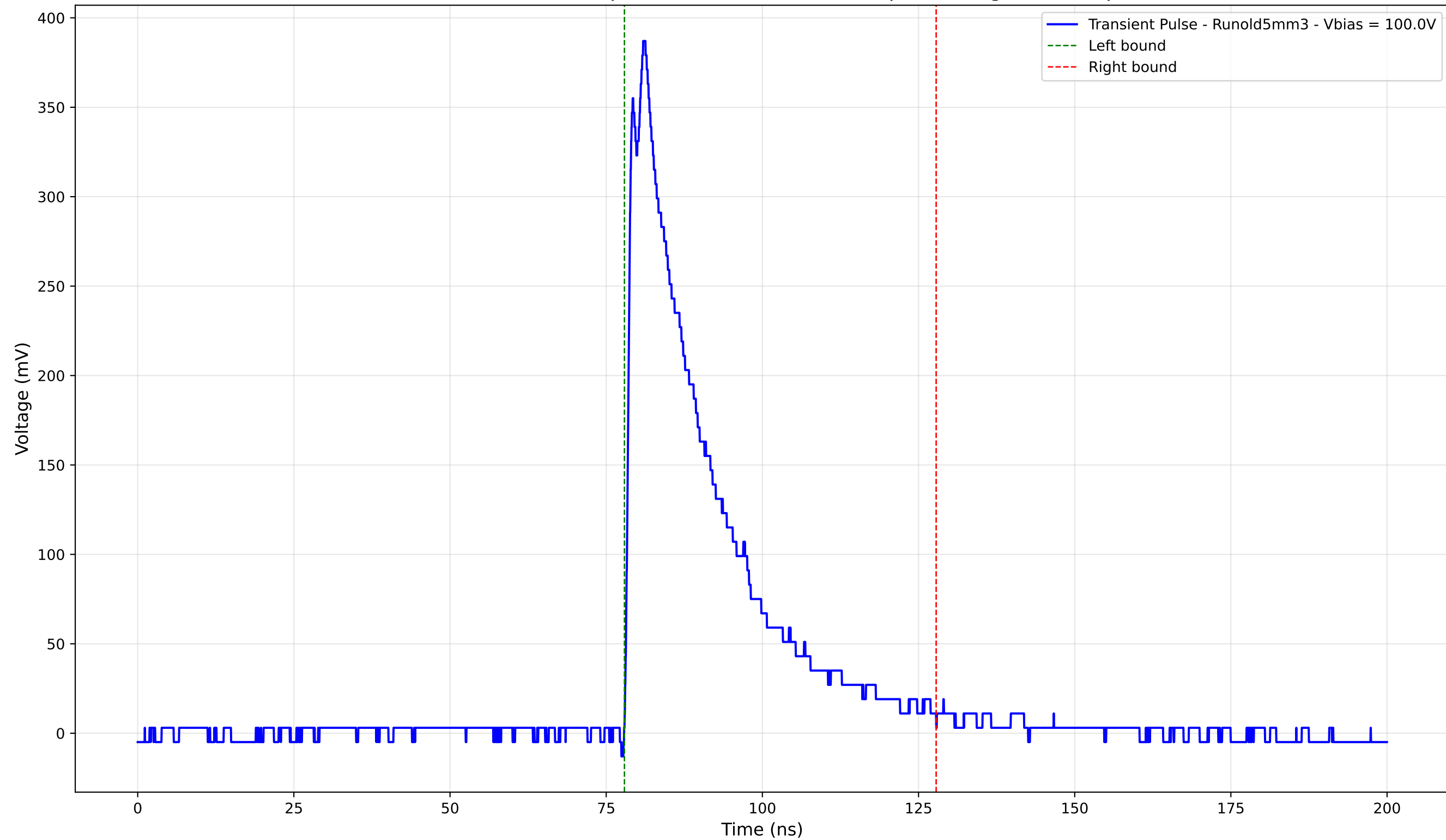
Transient Pulse - Sample: old5 - Position: 3100.0 \mu\text{m} - Charge: 104.52 pC
