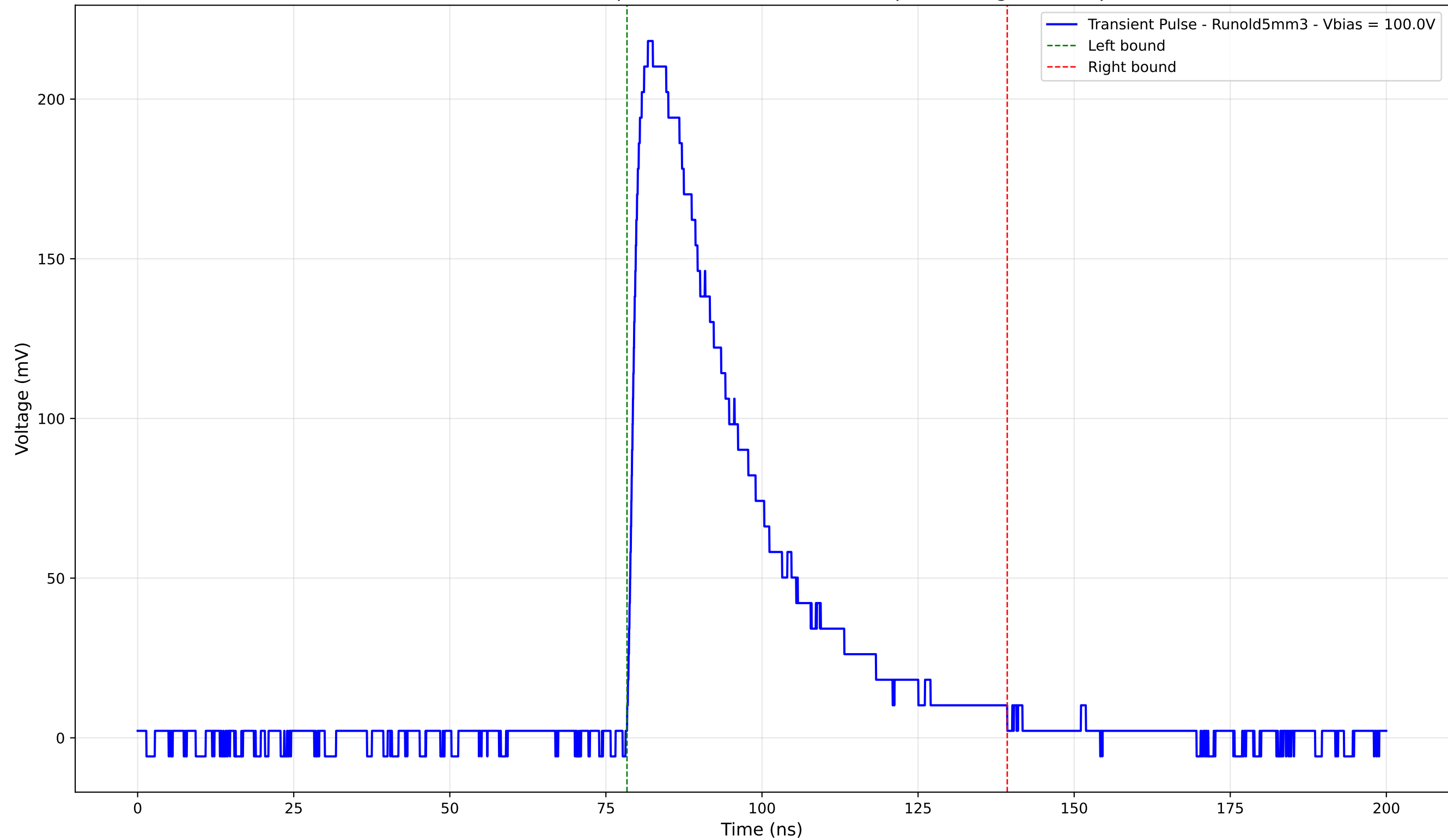
Transient Pulse - Sample: old5 - Position: 1275.0 \mu\text{m} - Charge: 82.58 pC
