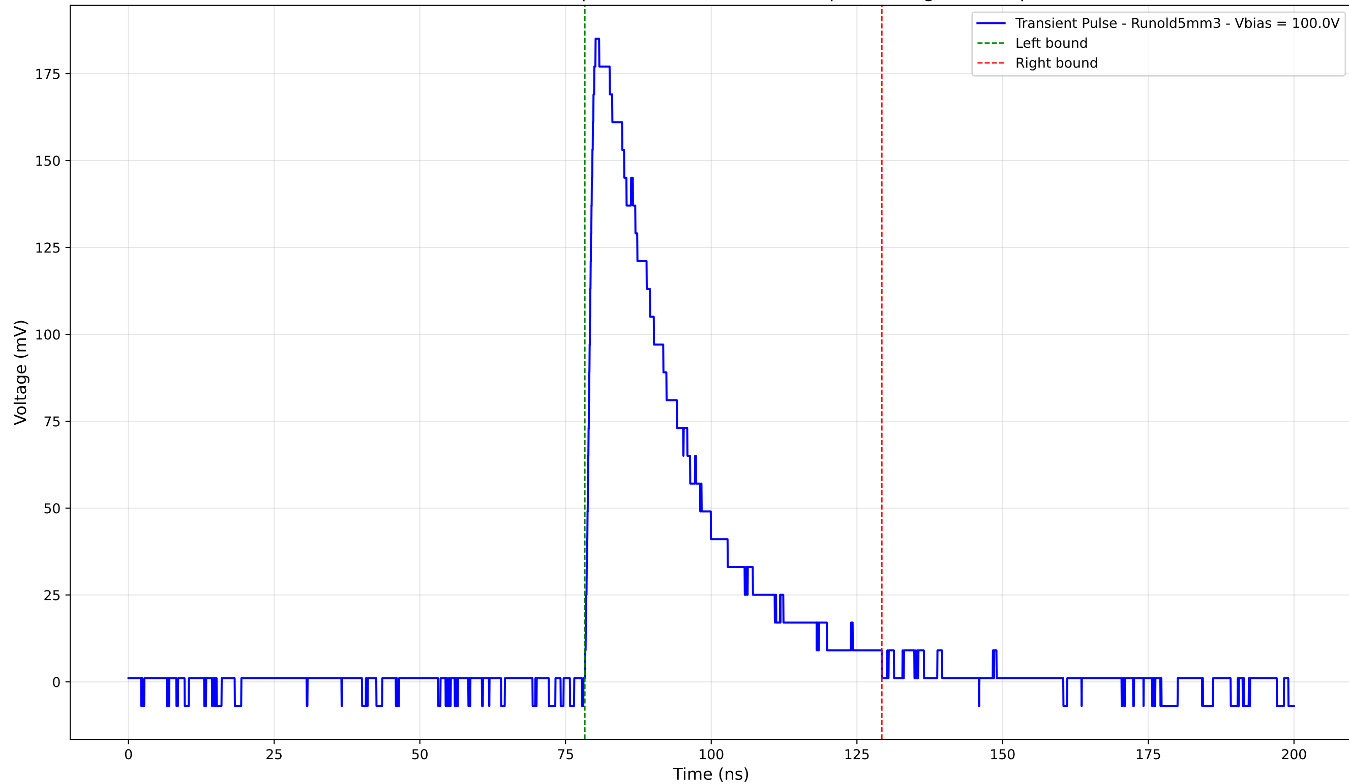
Transient Pulse - Sample: old5 - Position: 955.0 \mu\text{m} - Charge: 59.27 pC
