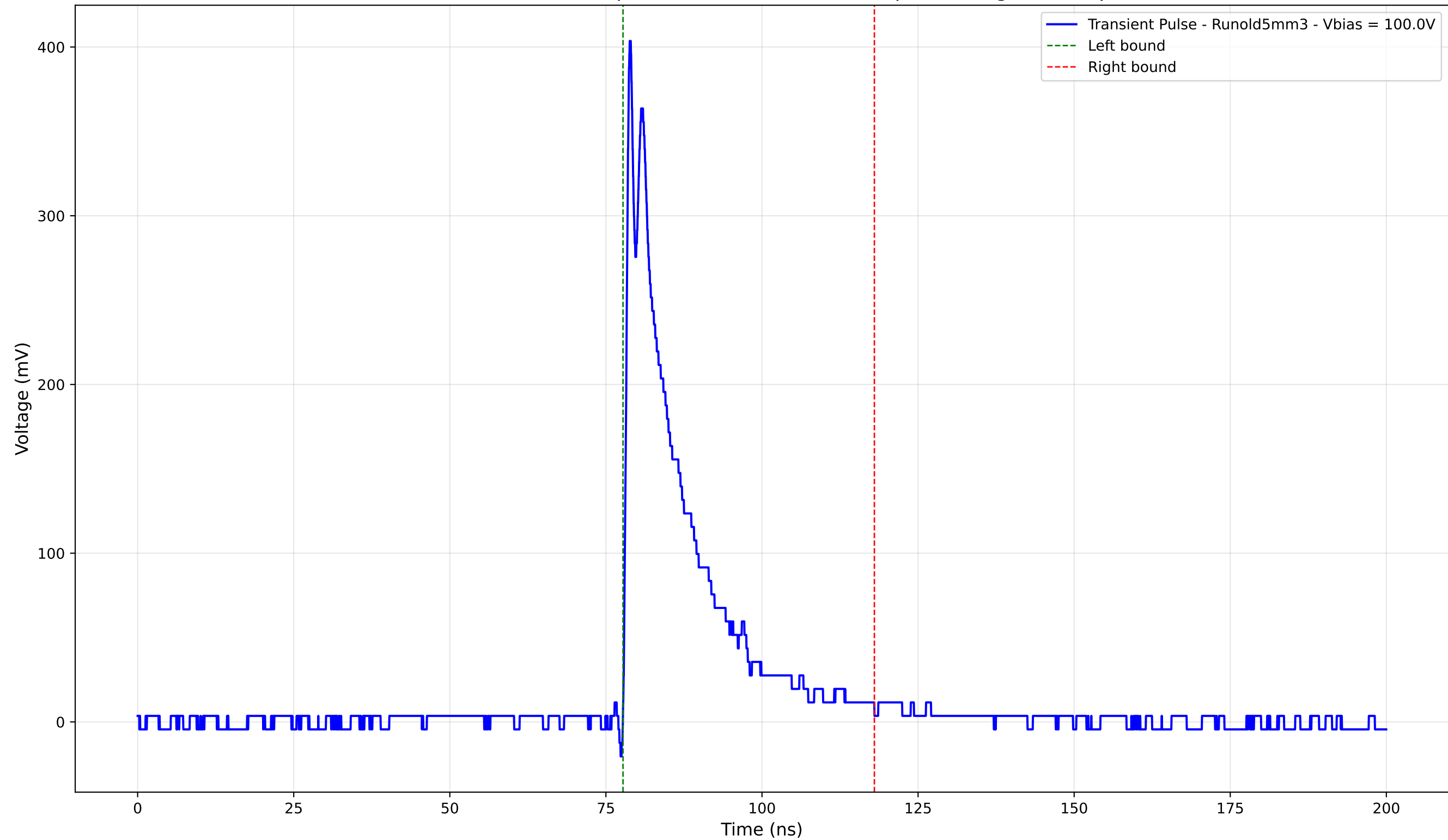
Transient Pulse - Sample: old5 - Position: 3805.0 \mu\text{m} - Charge: 70.25 pC
