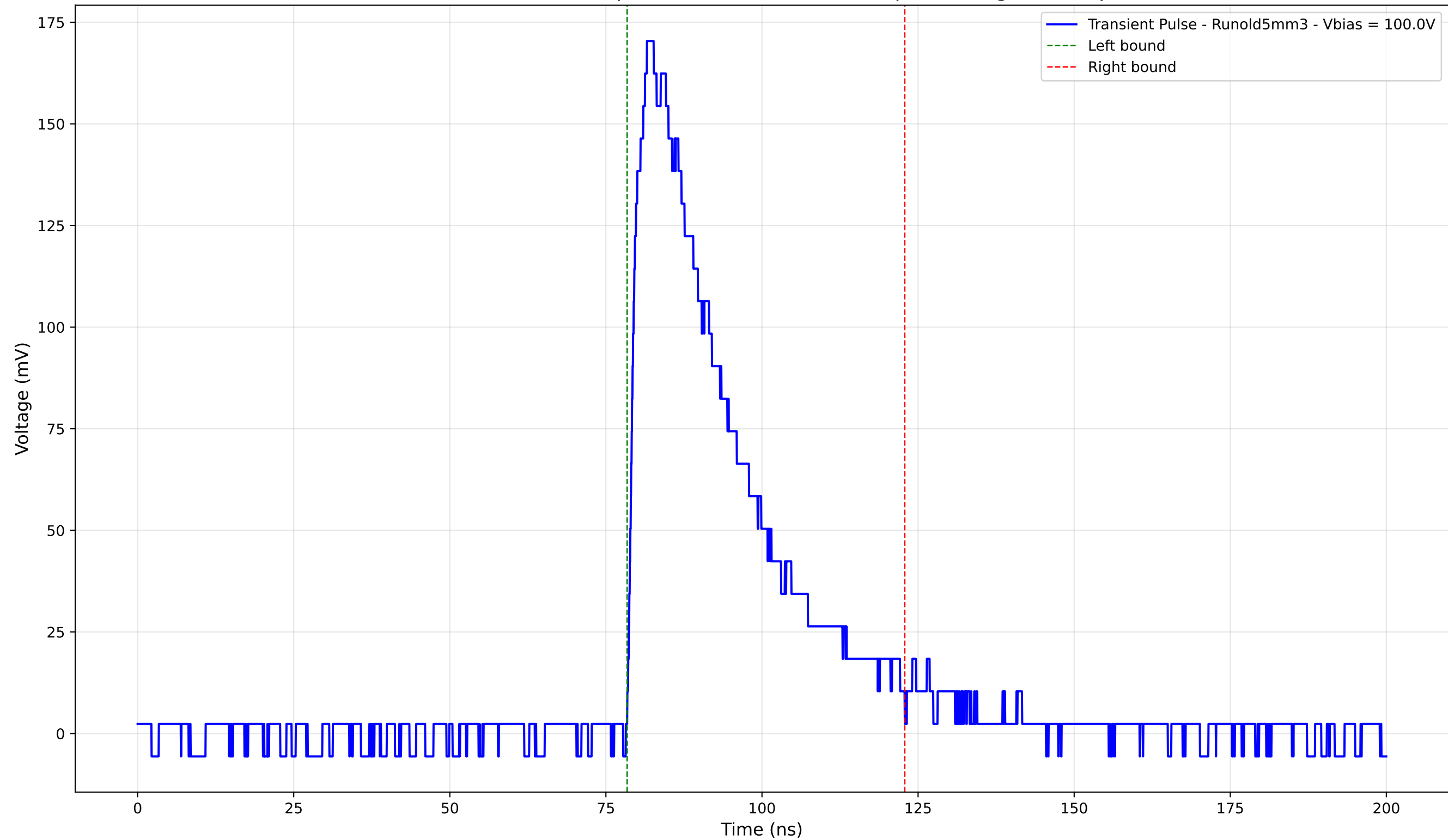
Transient Pulse - Sample: old5 - Position: 2595.0 \mu\text{m} - Charge: 59.25 pC
