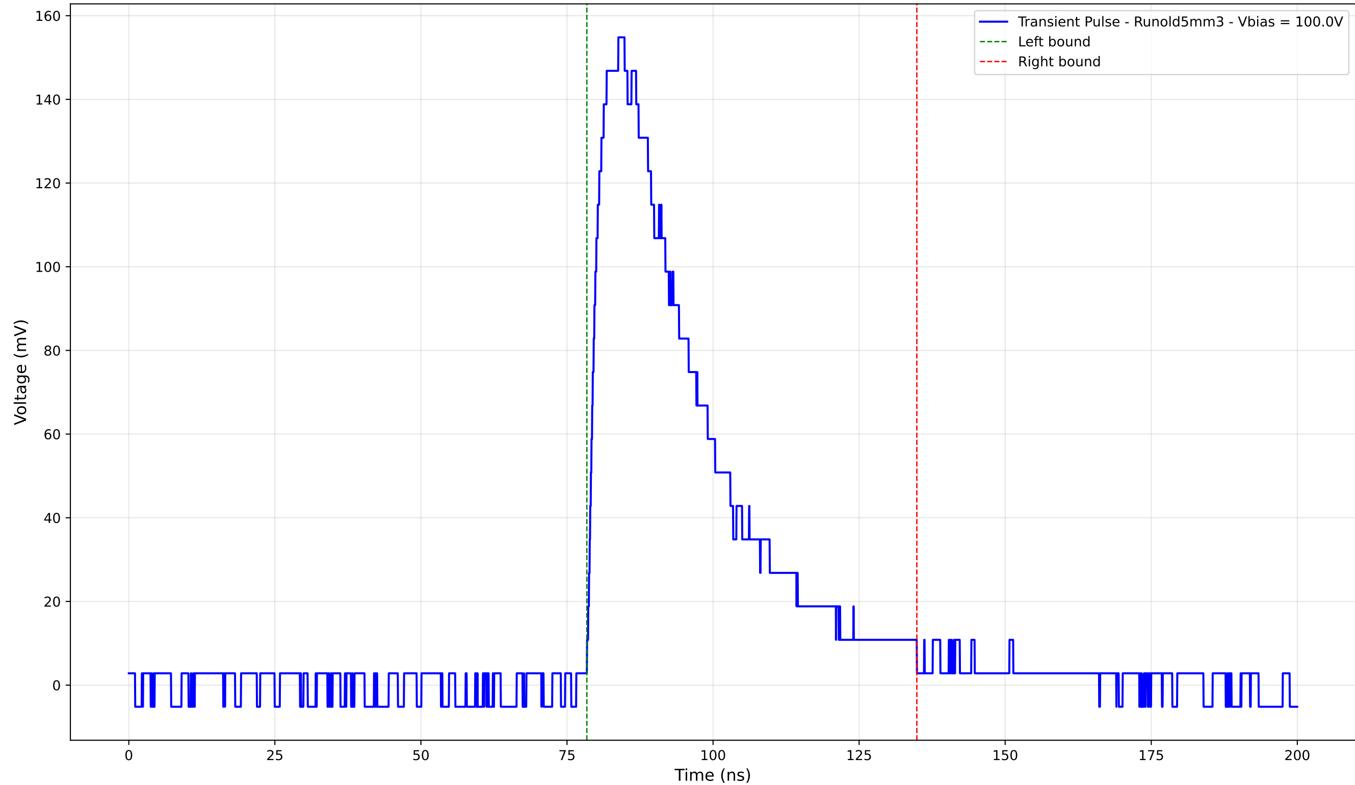
Transient Pulse - Sample: old5 - Position: 1645.0 \mu\text{m} - Charge: 62.02 pC
