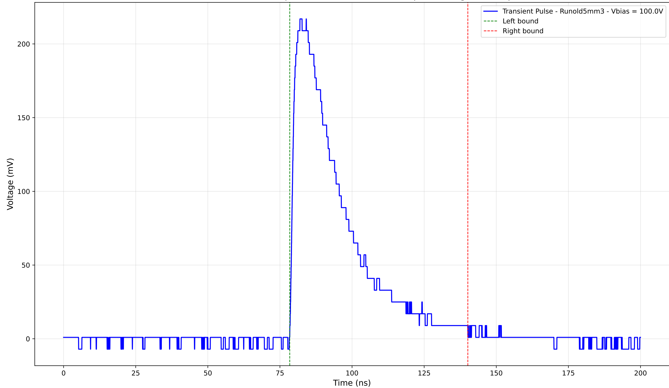
Transient Pulse - Sample: old5 - Position: 1280.0 \mu\text{m} - Charge: 82.38 pC
