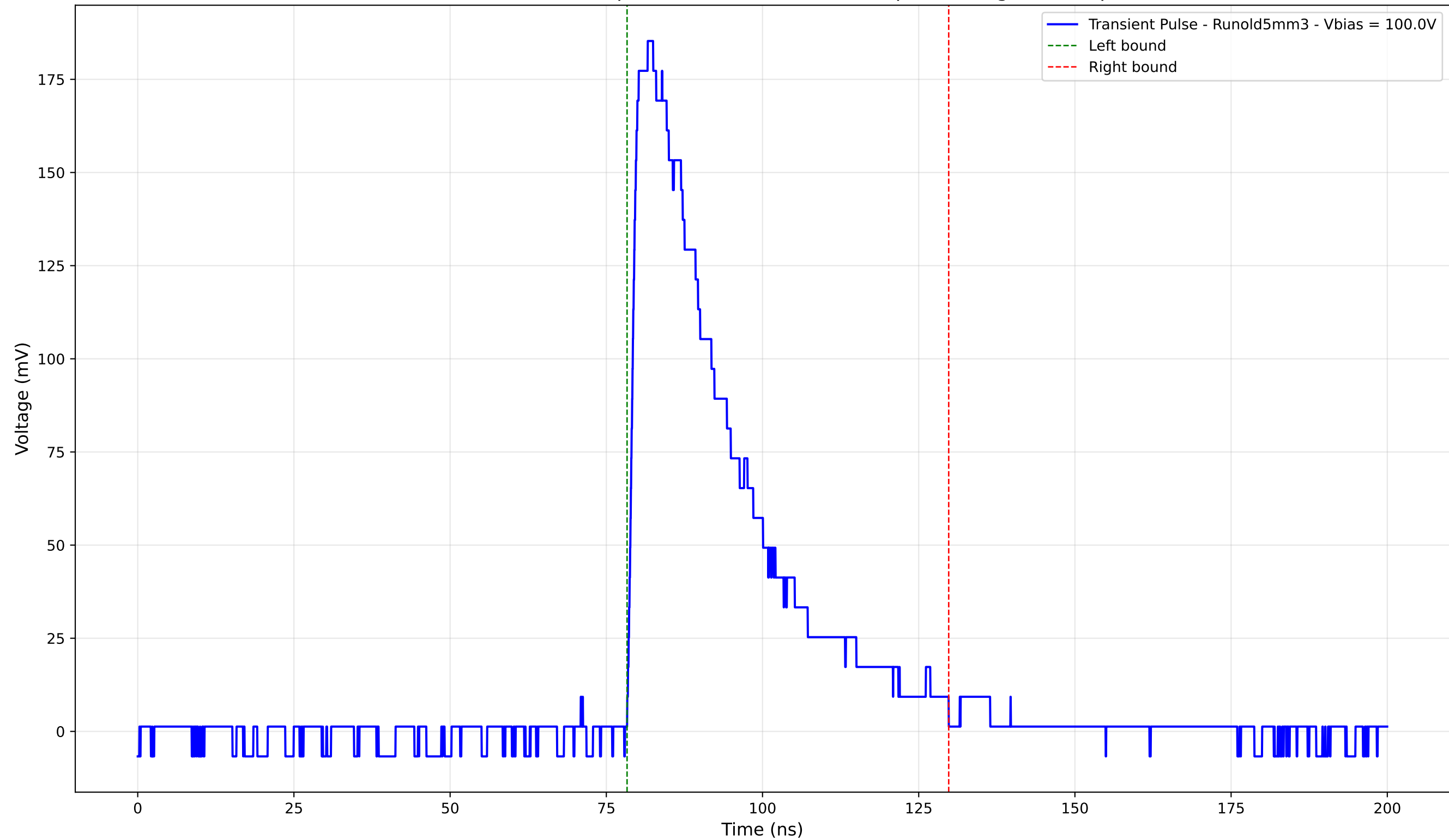
Transient Pulse - Sample: old5 - Position: 1040.0 \mu\text{m} - Charge: 64.09 pC
