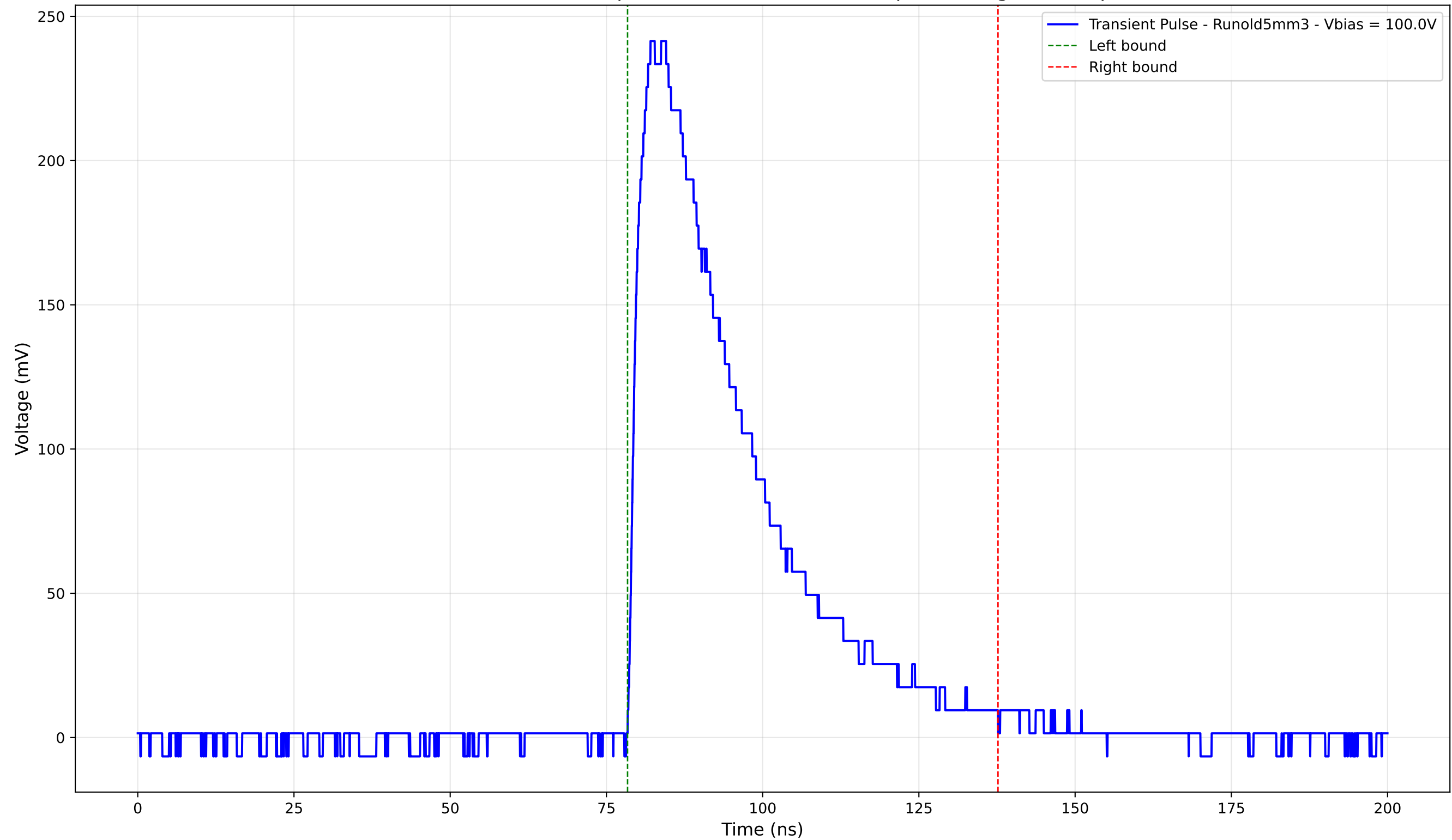
Transient Pulse - Sample: old5 - Position: 2295.0 \mu\text{m} - Charge: 94.77 pC
