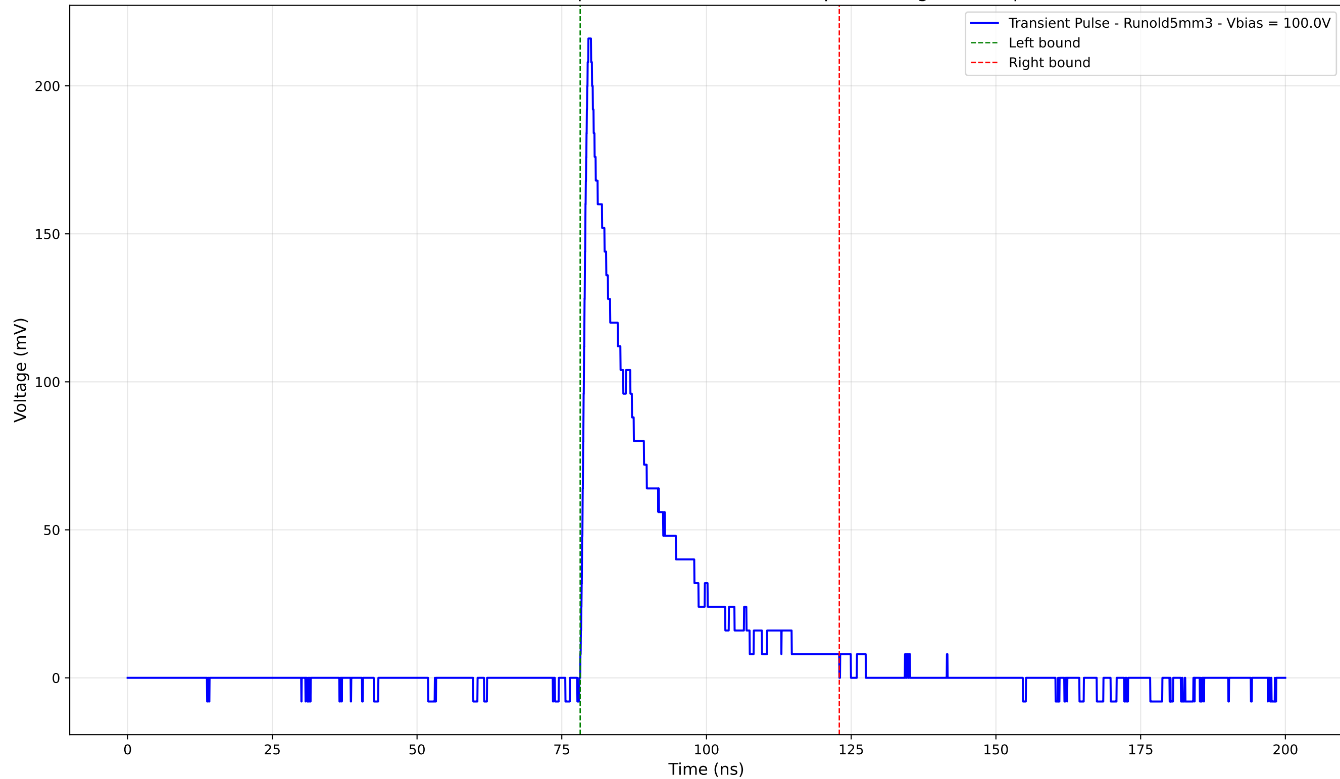
Transient Pulse - Sample: old5 - Position: 520.0 \mu\text{m} - Charge: 43.89 pC
