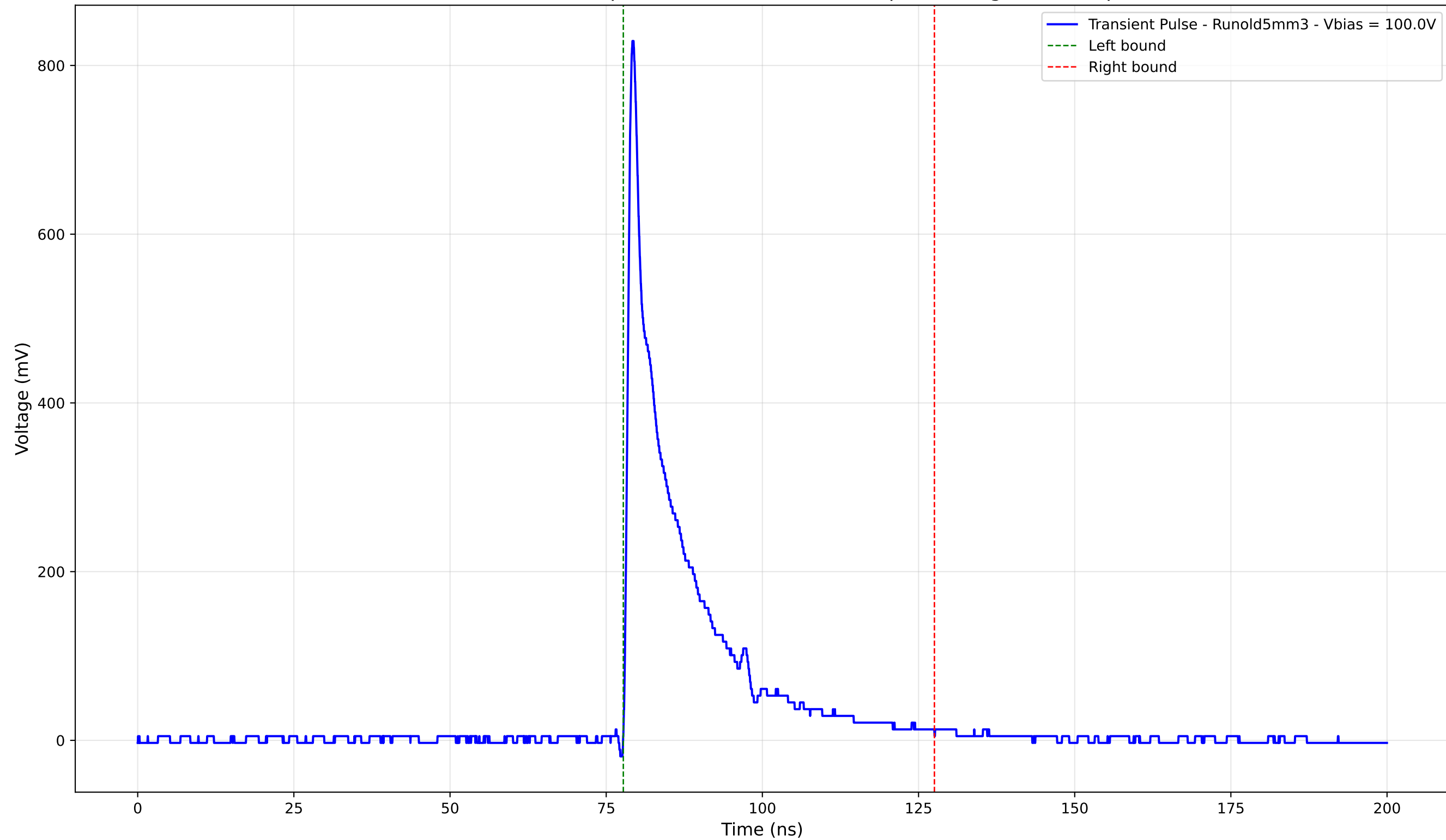
Transient Pulse - Sample: old5 - Position: 4820.0 \mu\text{m} - Charge: 127.77 pC
