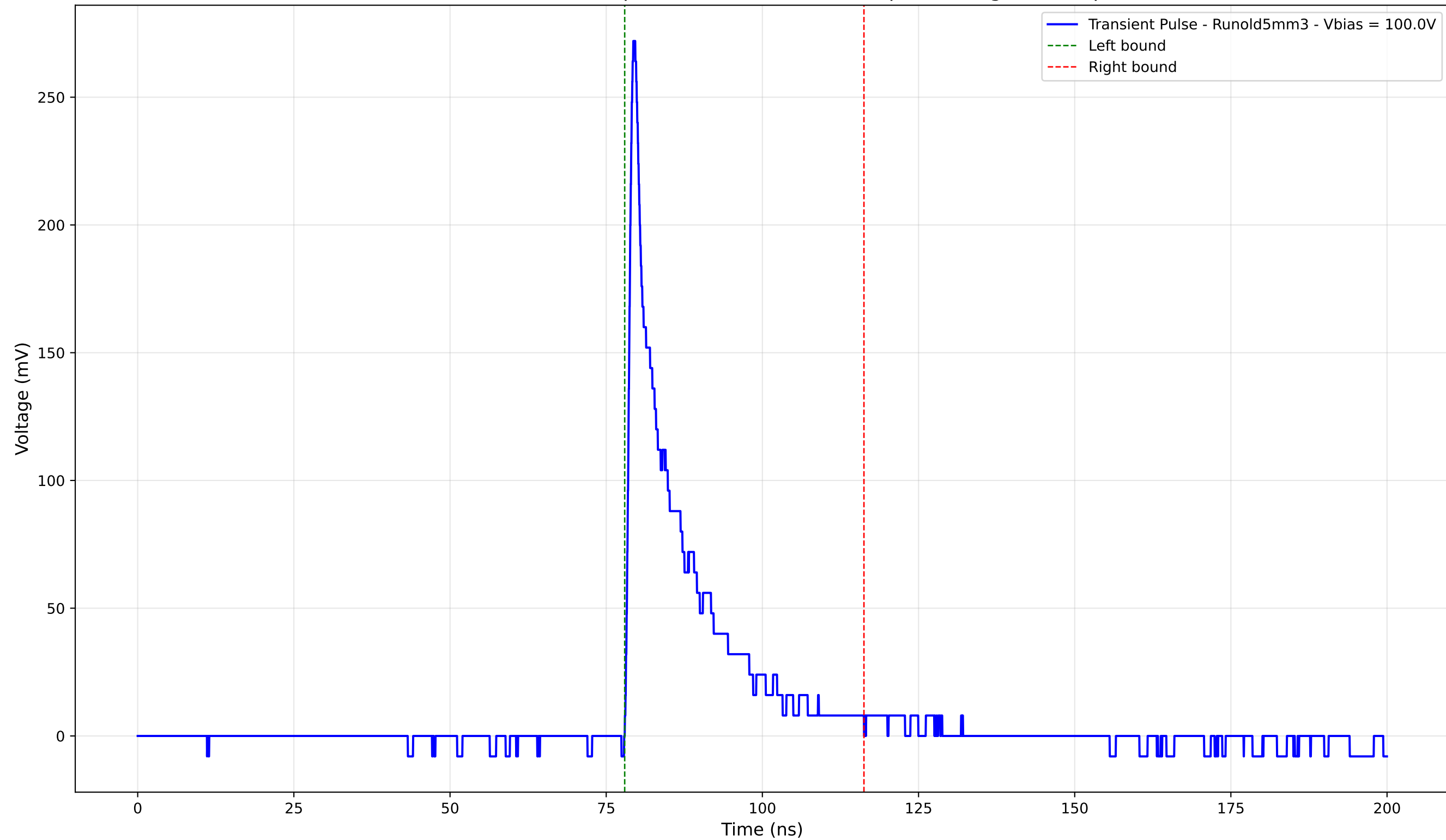
Transient Pulse - Sample: old5 - Position: 315.0 \mu\text{m} - Charge: 39.92 pC
