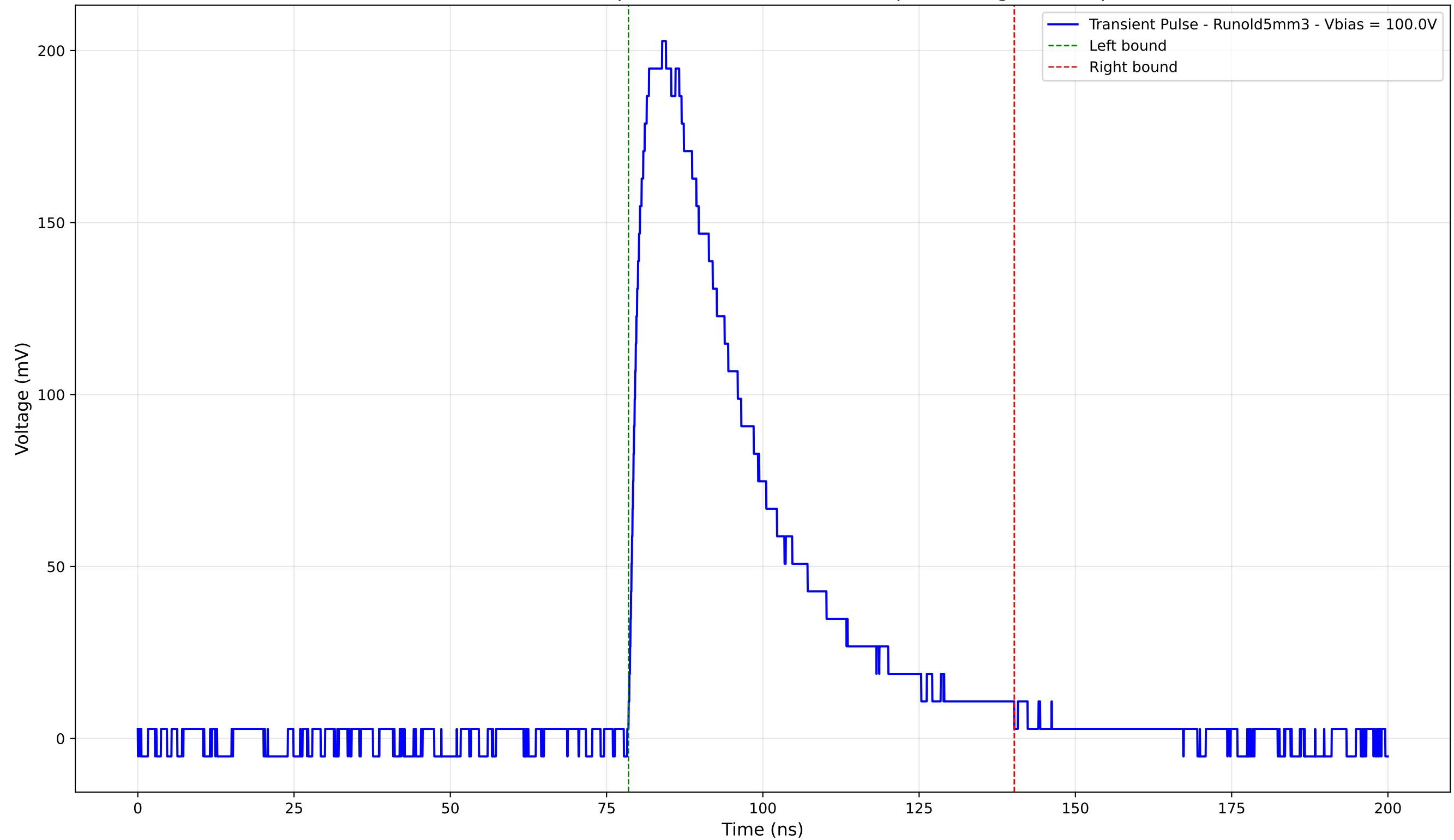
Transient Pulse - Sample: old5 - Position: 1670.0 \mu\text{m} - Charge: 82.67 pC
