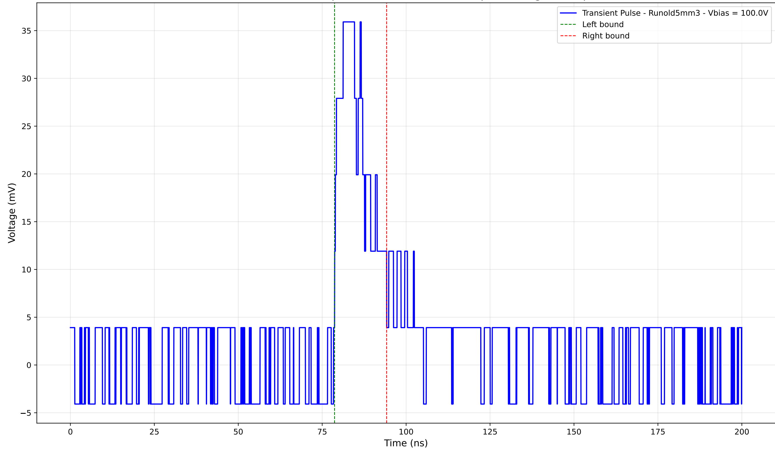
Transient Pulse - Sample: old5 - Position: 4200.0 \mu\text{m} - Charge: 7.20 pC
