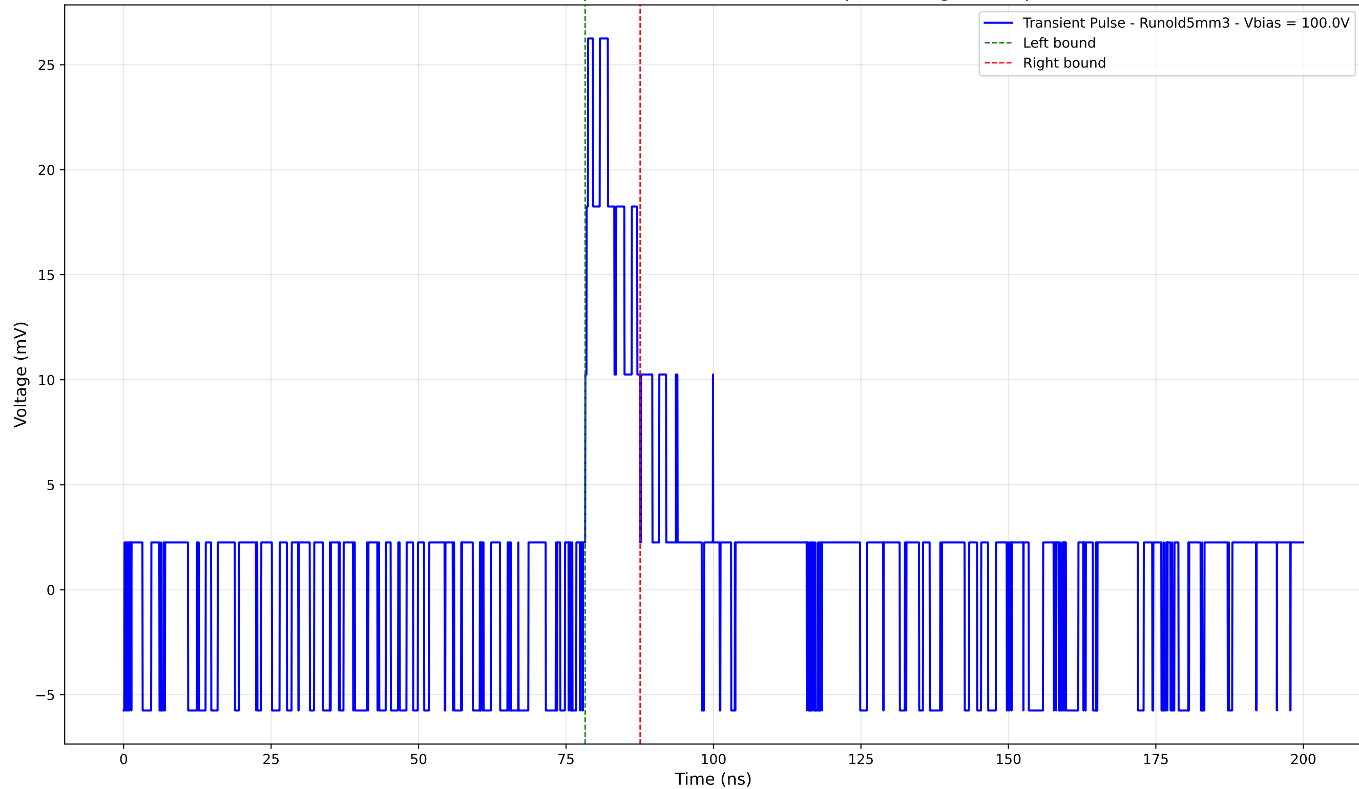
Transient Pulse - Sample: old5 - Position: 3875.0 \mu\text{m} - Charge: 3.40 pC
