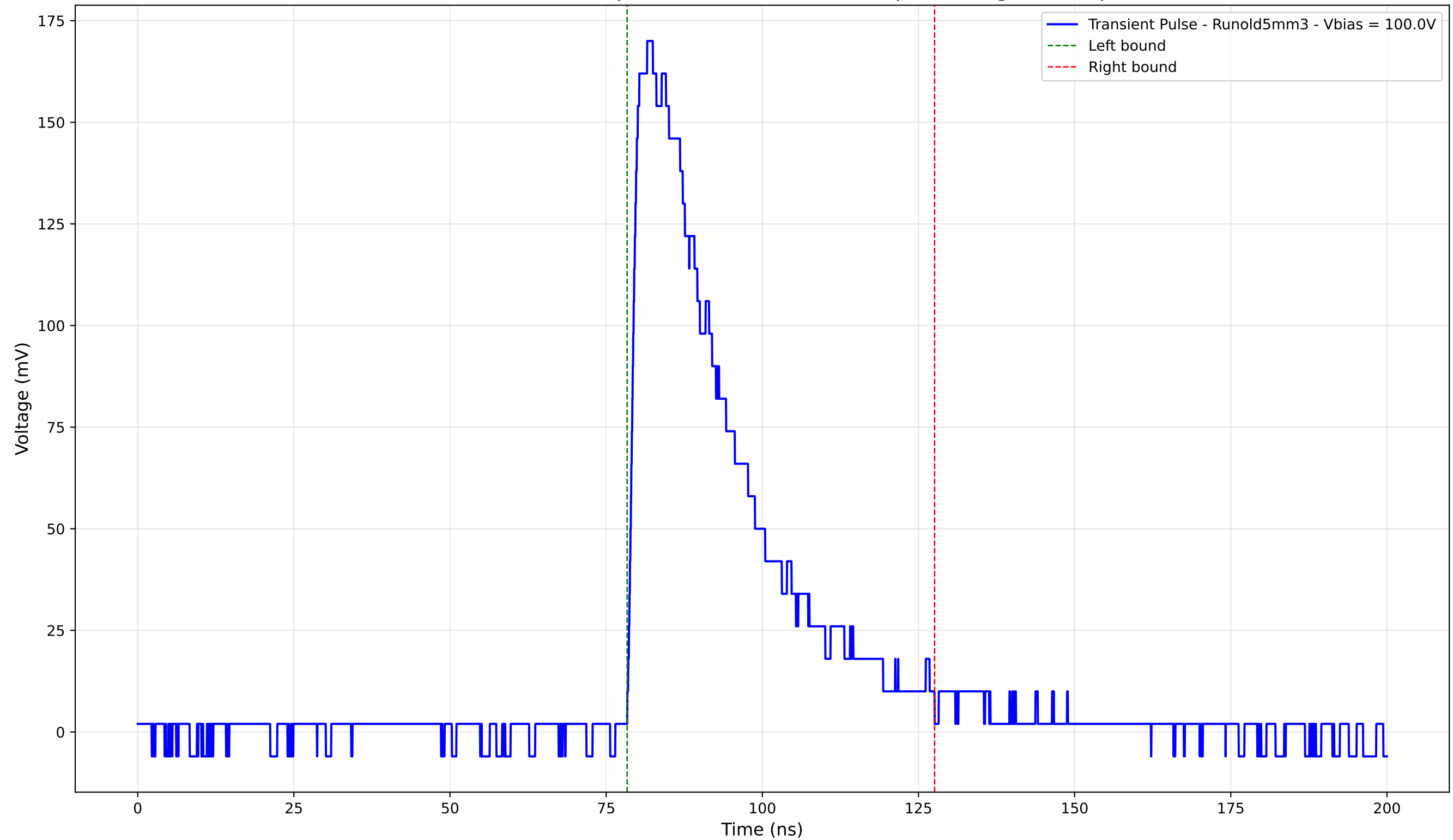
Transient Pulse - Sample: old5 - Position: 1120.0 \mu\text{m} - Charge: 59.37 pC
