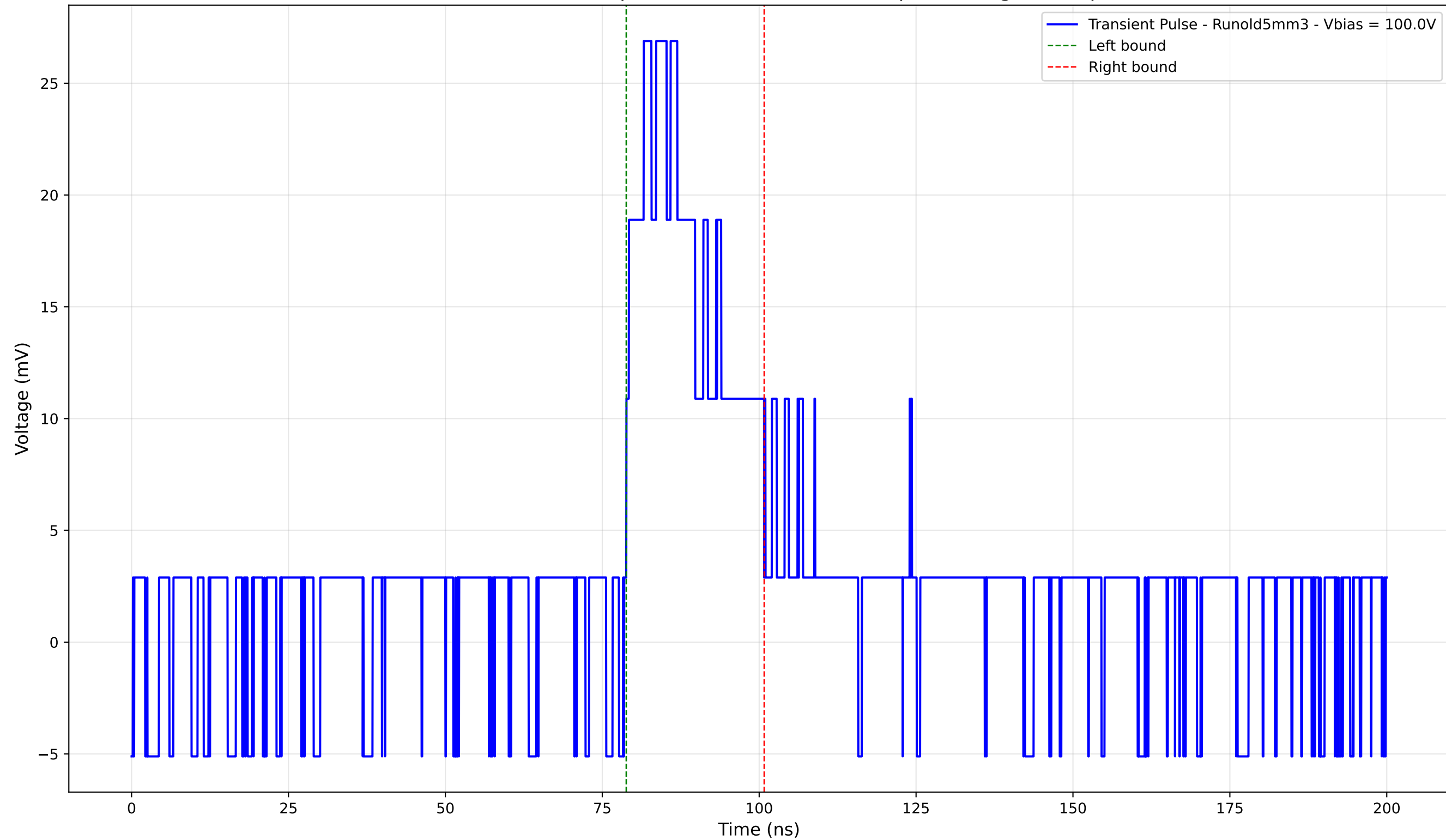
Transient Pulse - Sample: old5 - Position: 2695.0 \mu\text{m} - Charge: 7.34 pC
