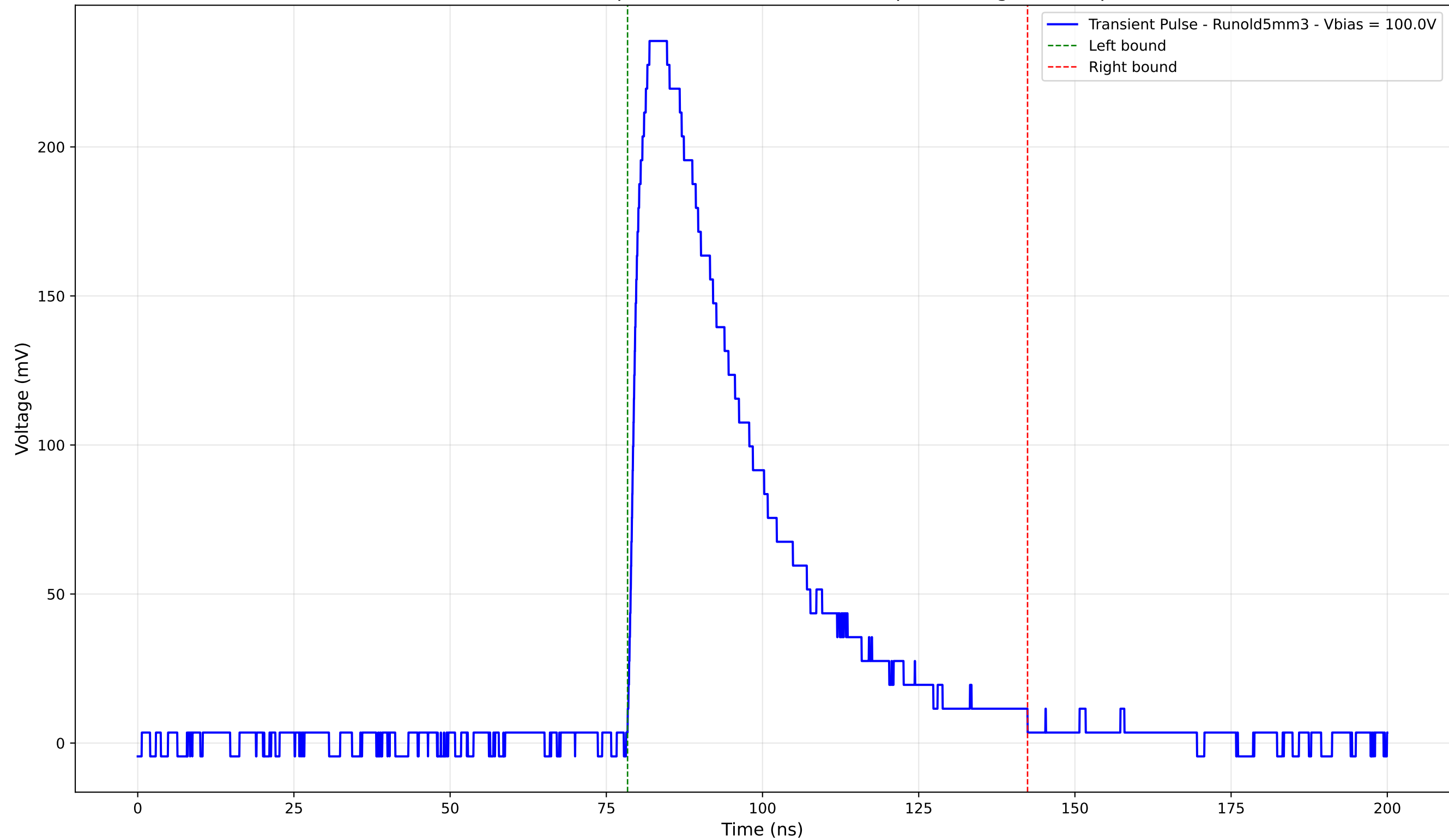
Transient Pulse - Sample: old5 - Position: 2290.0 \mu\text{m} - Charge: 96.84 pC
