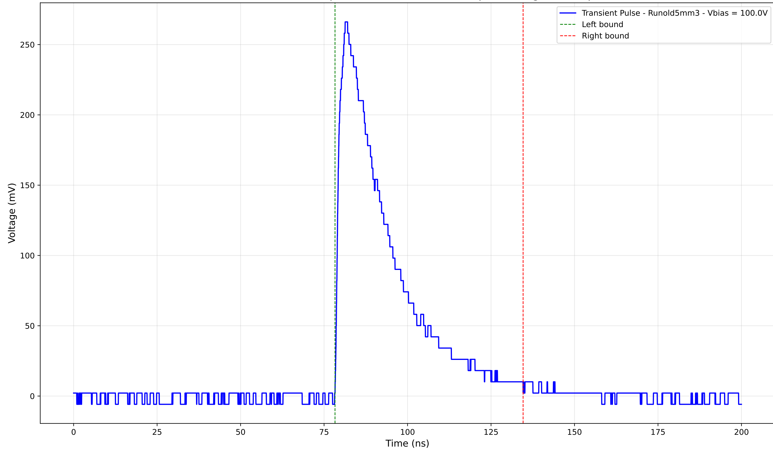
Transient Pulse - Sample: old5 - Position: 2775.0 \mu\text{m} - Charge: 89.47 pC
