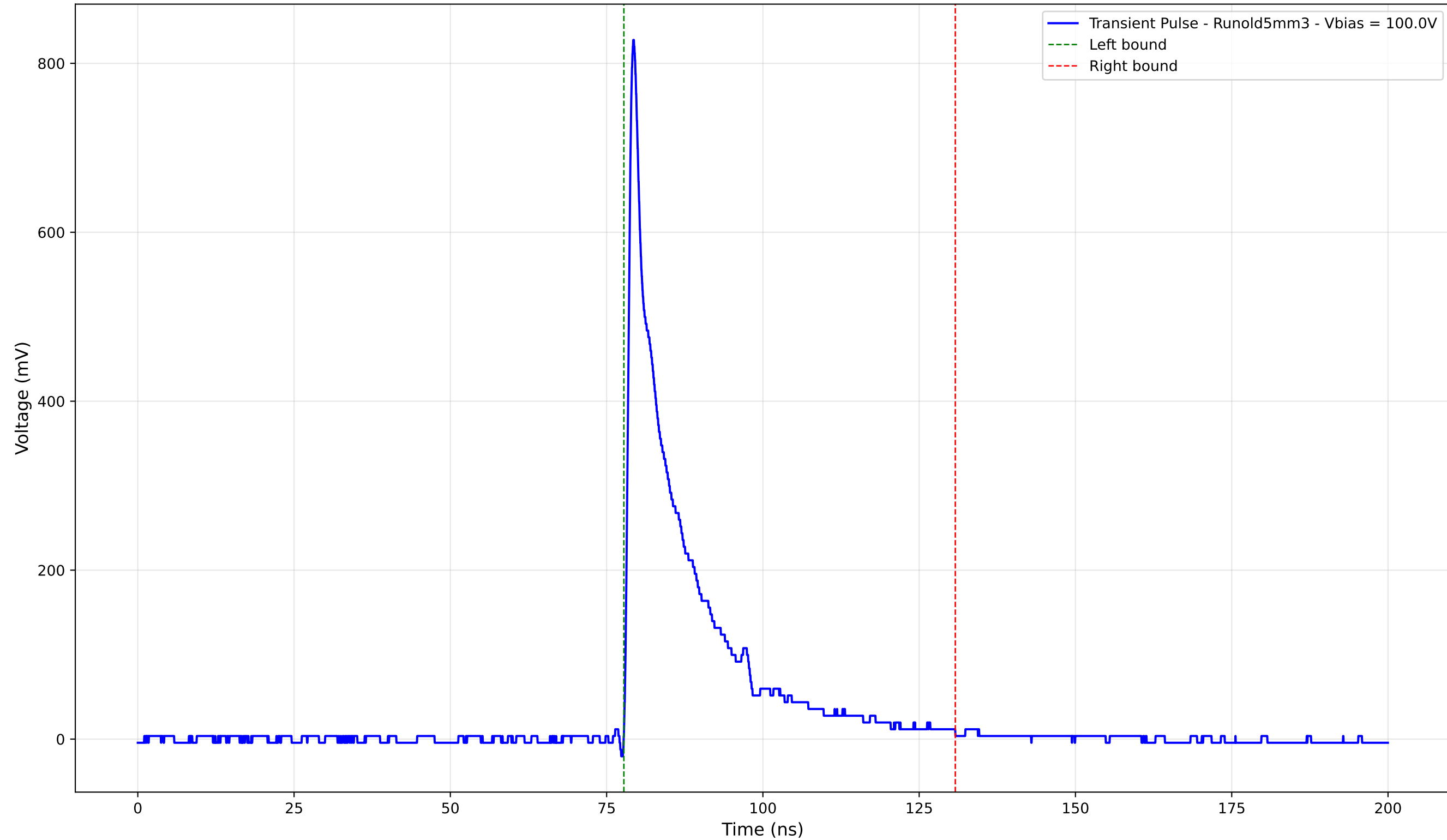
Transient Pulse - Sample: old5 - Position: 4805.0 \mu\text{m} - Charge: 130.81 pC
