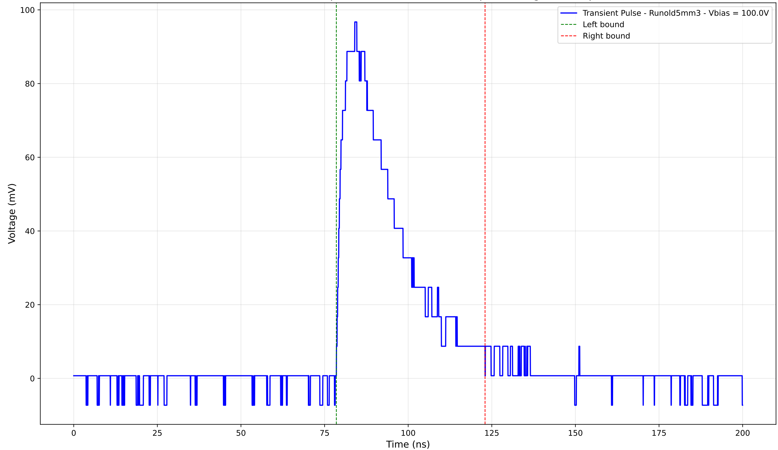
Transient Pulse - Sample: old5 - Position: 2155.0 \mu\text{m} - Charge: 34.57 pC
