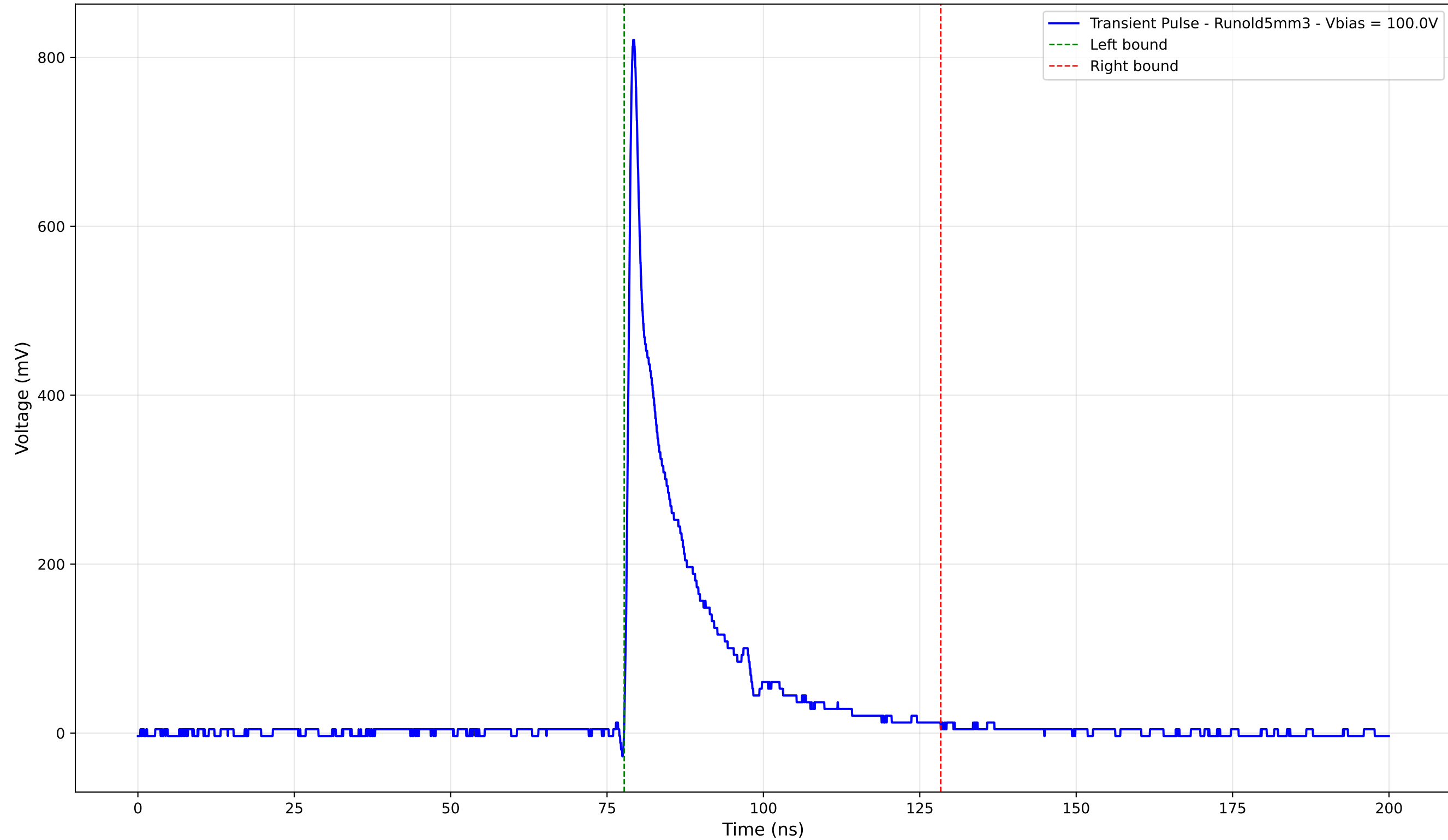
Transient Pulse - Sample: old5 - Position: 4835.0 \mu\text{m} - Charge: 123.04 pC
