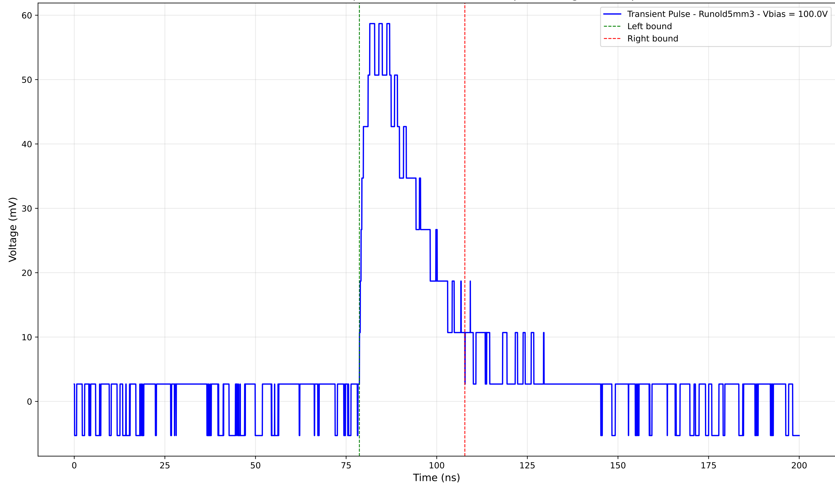
Transient Pulse - Sample: old5 - Position: 2415.0 \mu\text{m} - Charge: 19.07 pC
