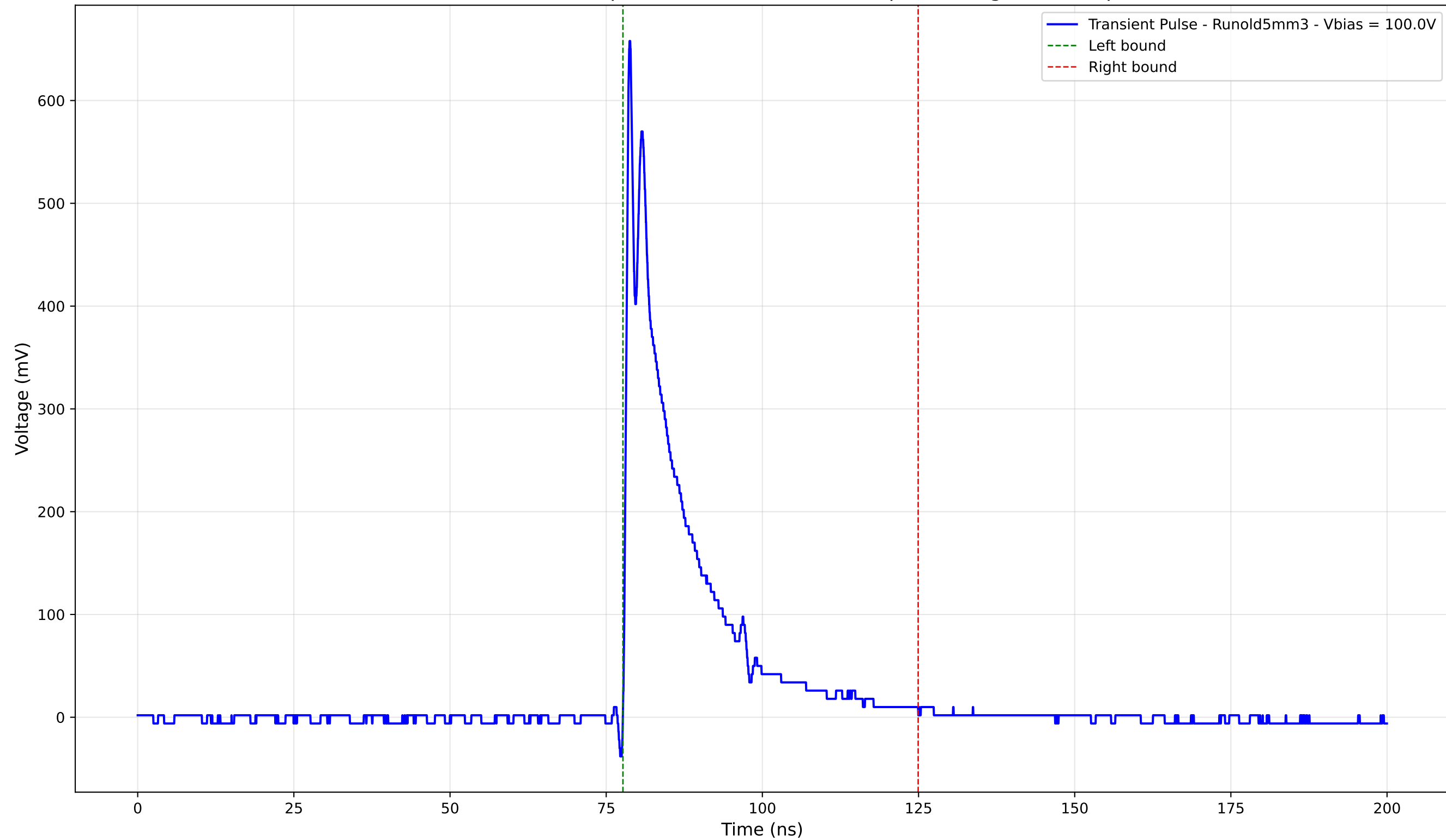
Transient Pulse - Sample: old5 - Position: 3750.0 \mu\text{m} - Charge: 108.76 pC
