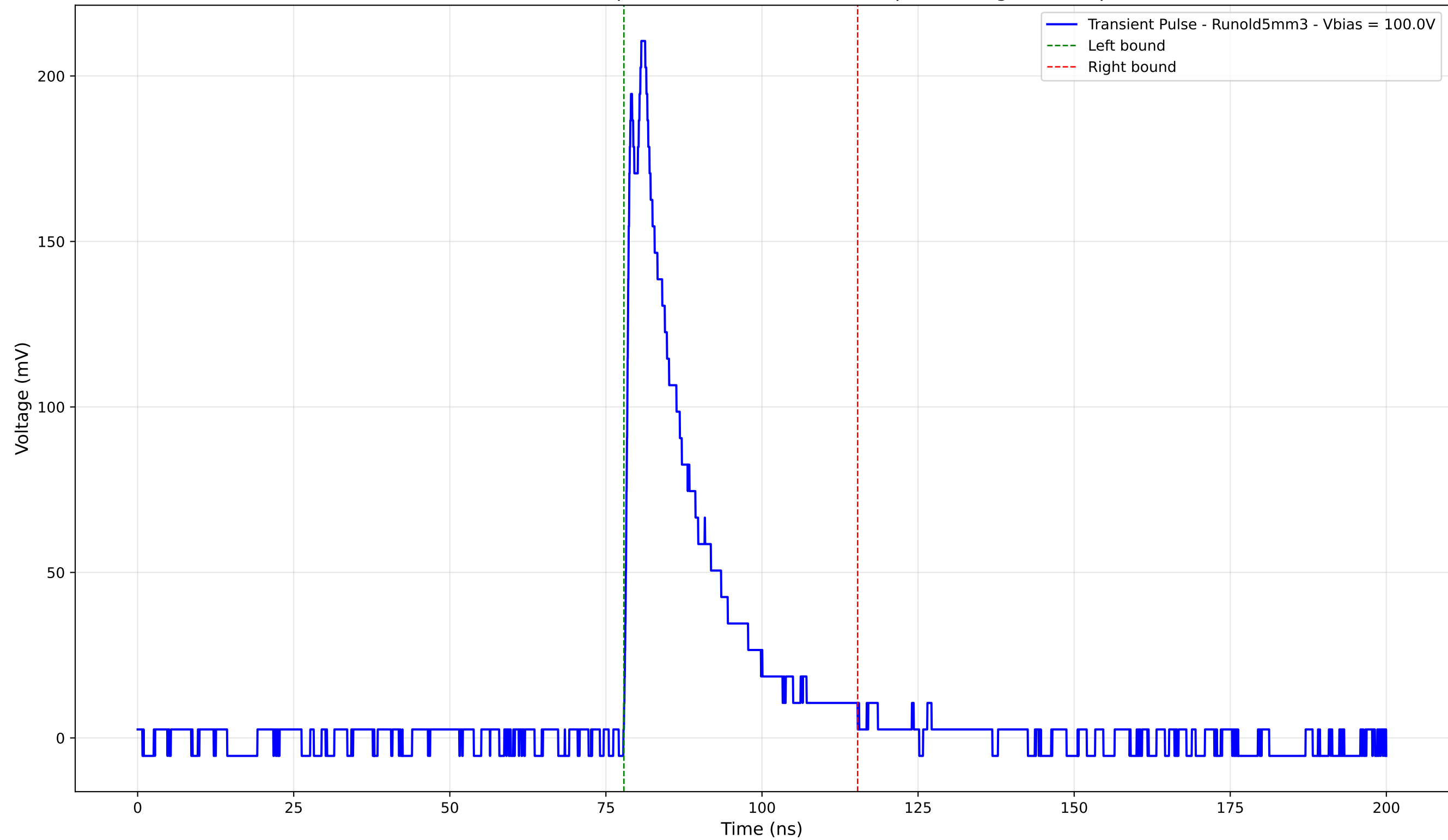
Transient Pulse - Sample: old5 - Position: 3945.0 \mu\text{m} - Charge: 43.09 pC
