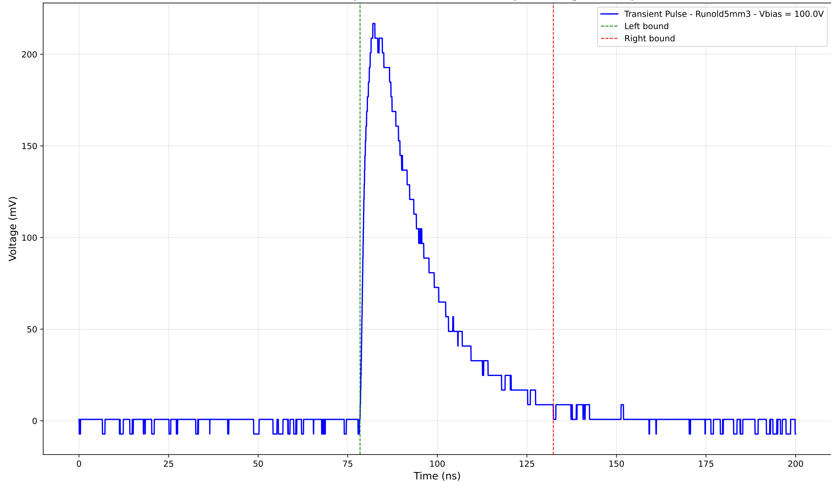
Transient Pulse - Sample: old5 - Position: 2465.0 \mu\text{m} - Charge: 79.81 pC
