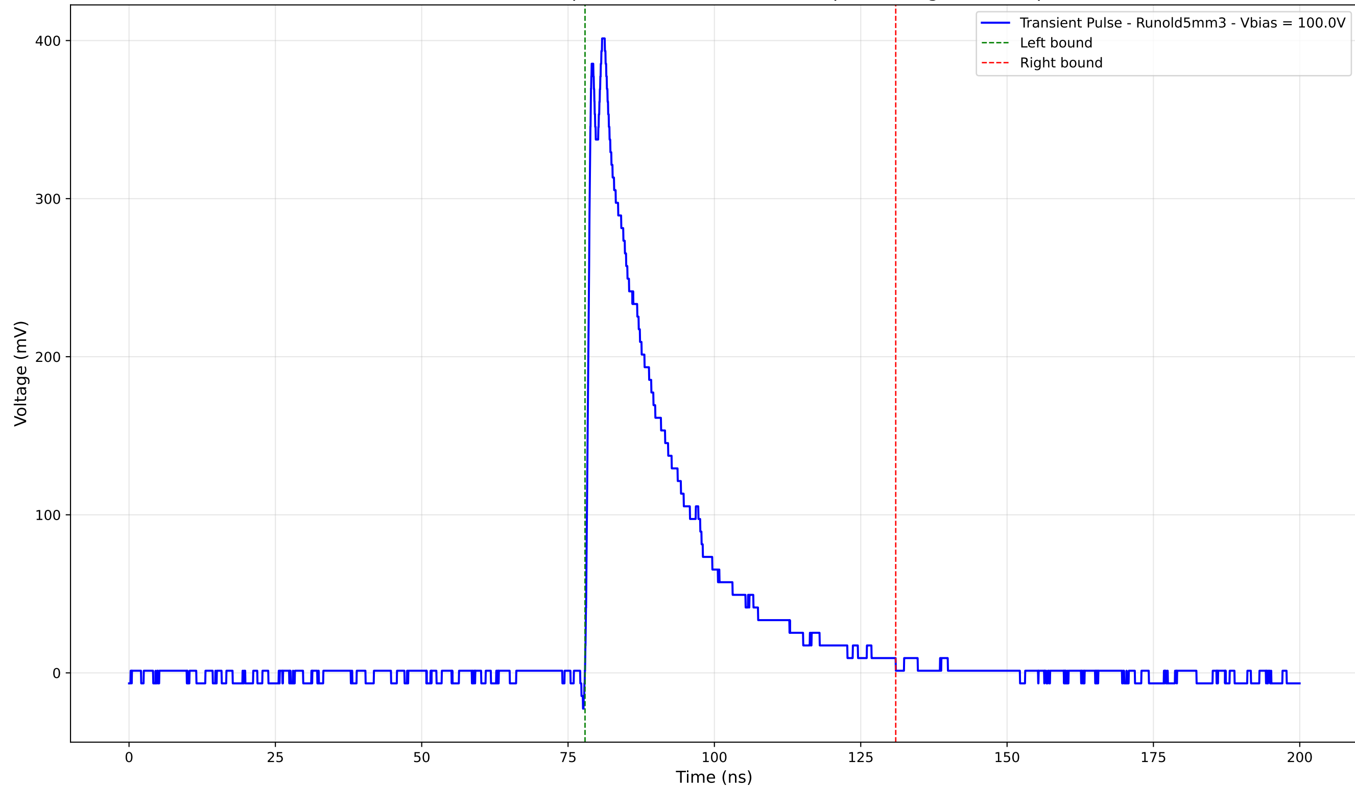
Transient Pulse - Sample: old5 - Position: 3135.0 \mu\text{m} - Charge: 105.16 pC
