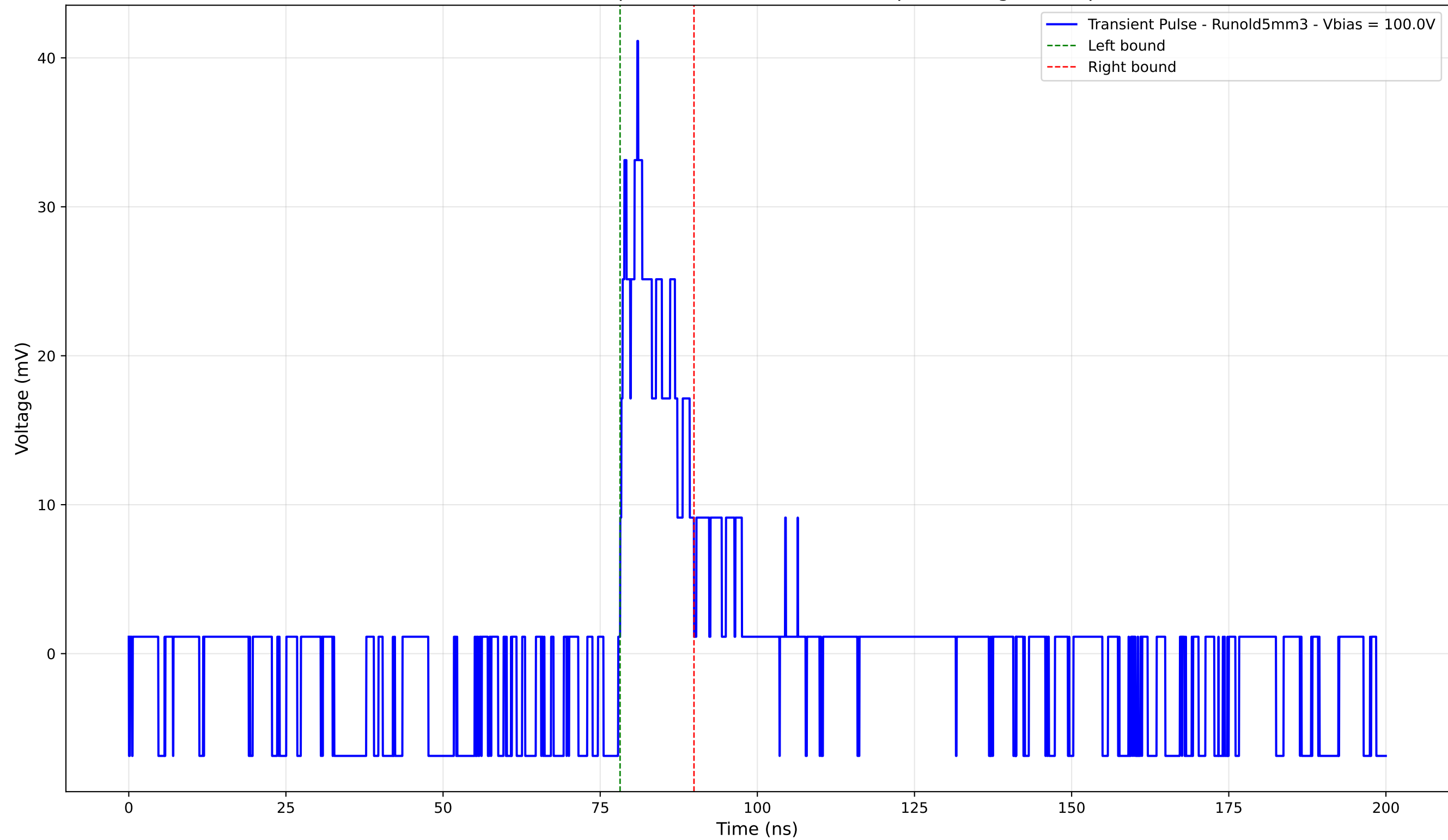
Transient Pulse - Sample: old5 - Position: 3300.0 \mu\text{m} - Charge: 5.03 pC
