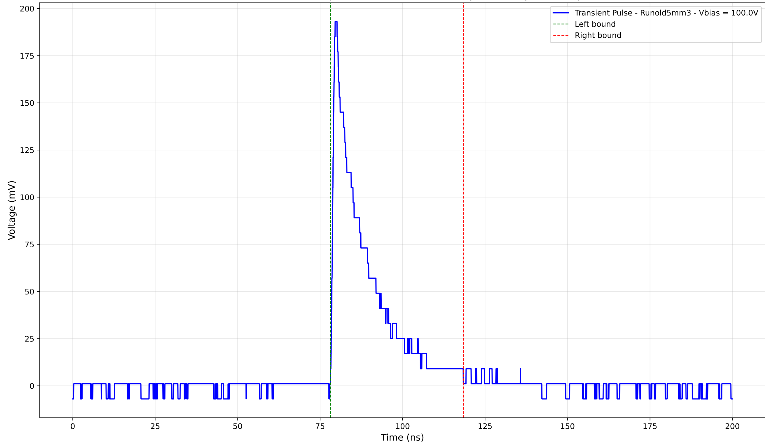
Transient Pulse - Sample: old5 - Position: 510.0 \mu\text{m} - Charge: 38.48 pC
