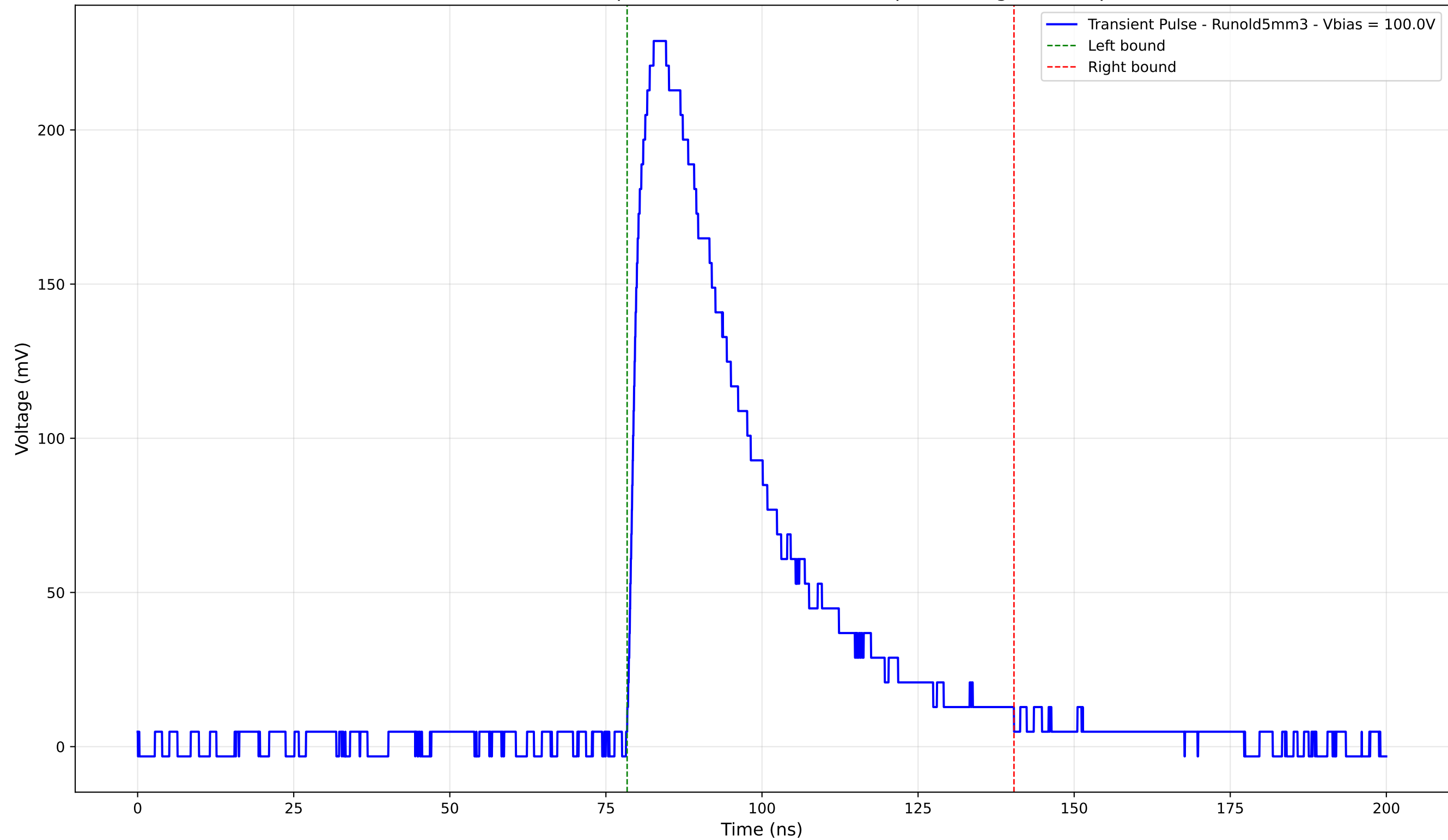
Transient Pulse - Sample: old5 - Position: 2090.0 \mu\text{m} - Charge: 95.29 pC
