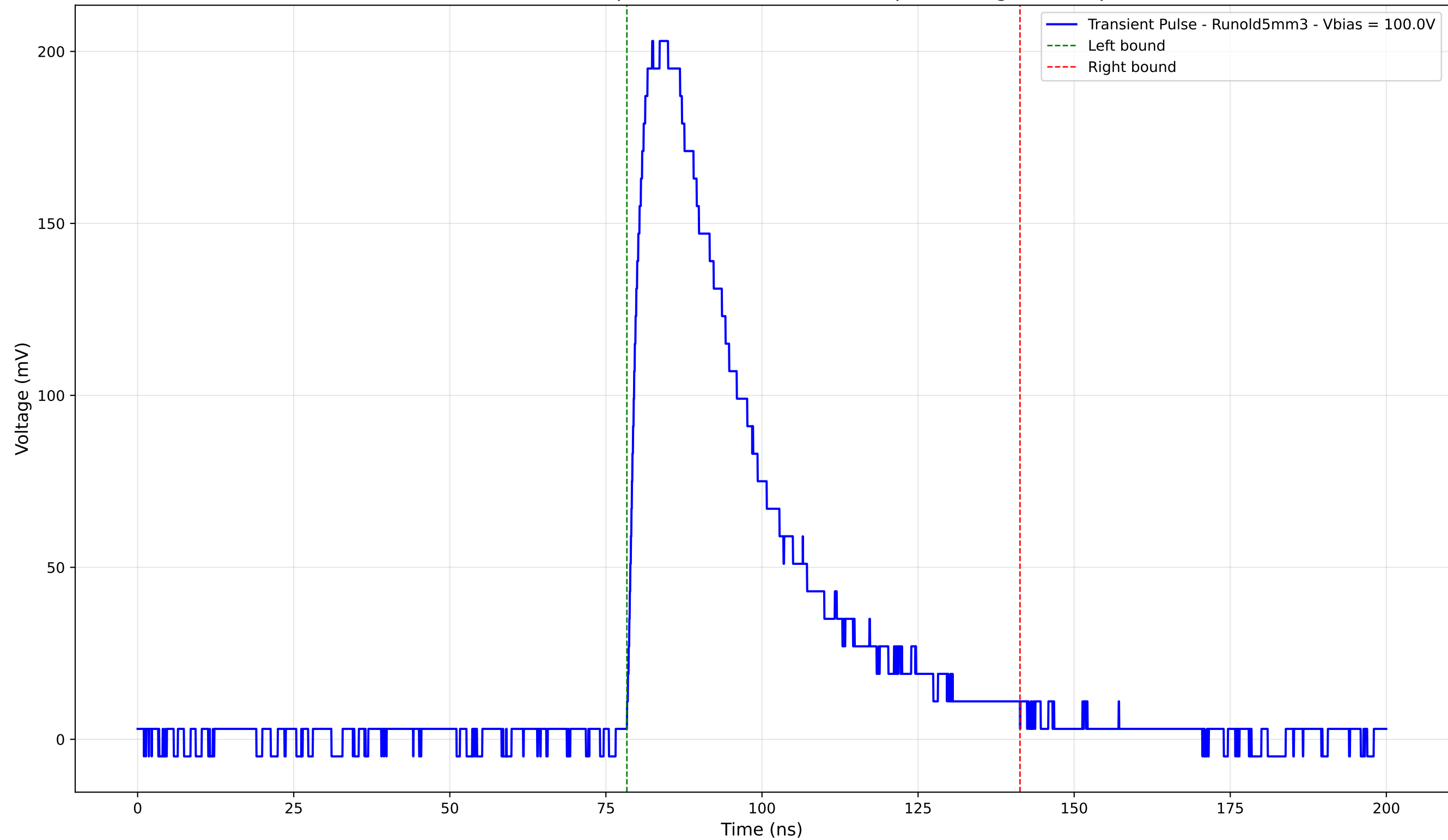
Transient Pulse - Sample: old5 - Position: 1910.0 \mu\text{m} - Charge: 85.40 pC
