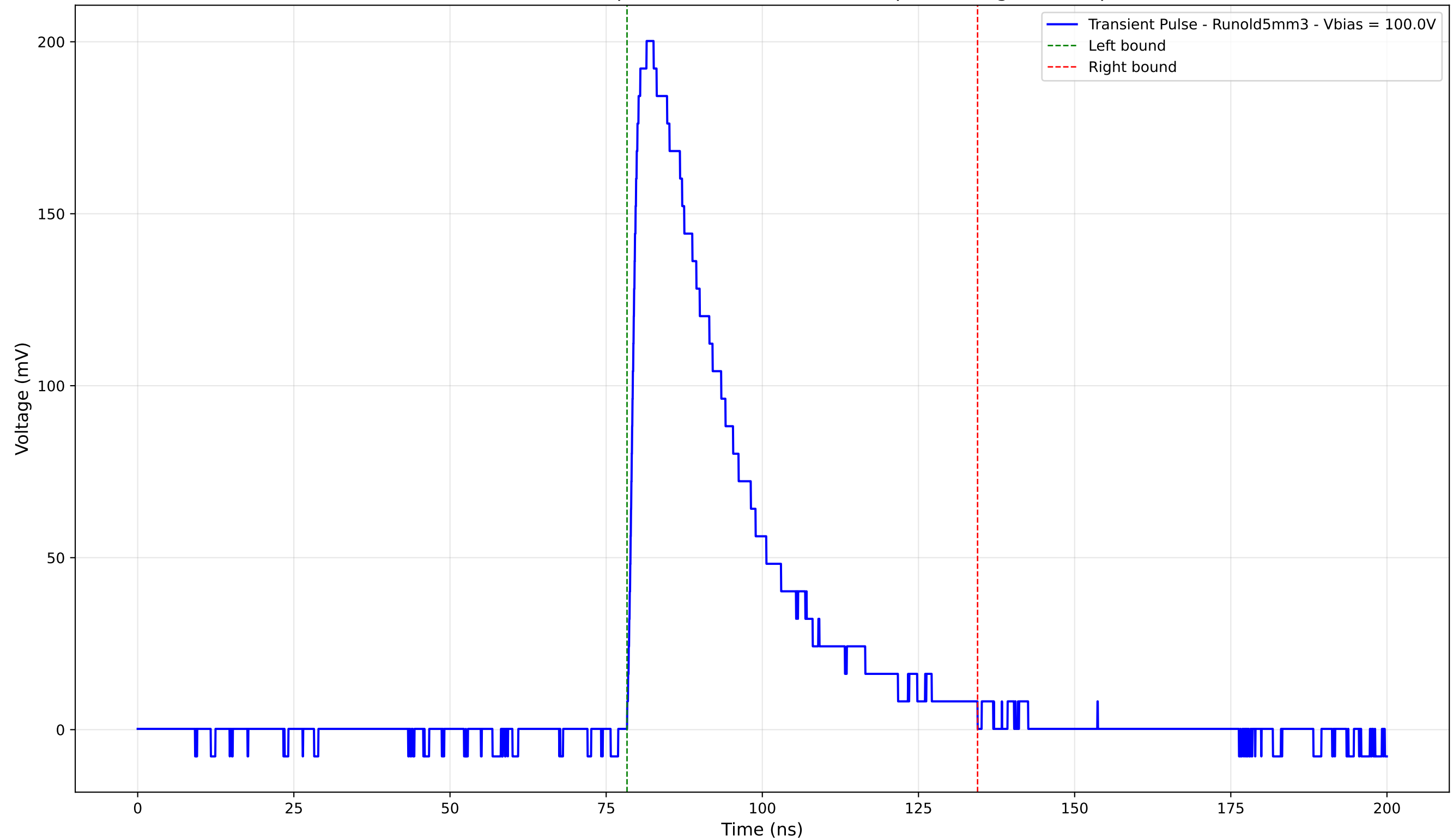
Transient Pulse - Sample: old5 - Position: 1110.0 \mu\text{m} - Charge: 69.73 pC
