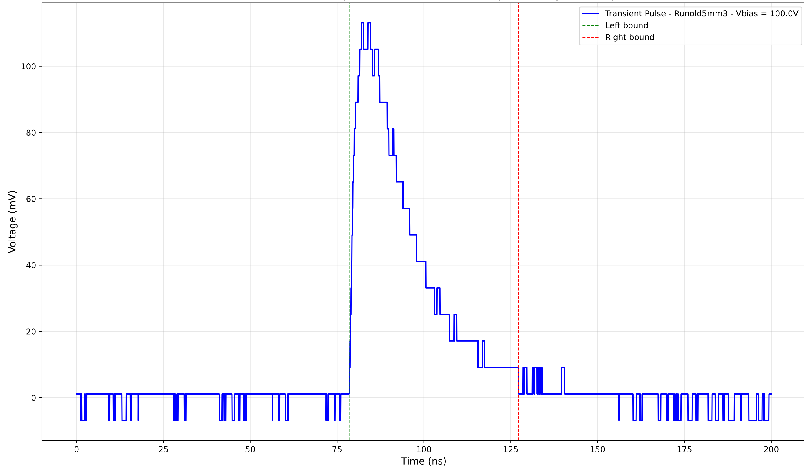
Transient Pulse - Sample: old5 - Position: 1430.0 \mu\text{m} - Charge: 41.97 pC
