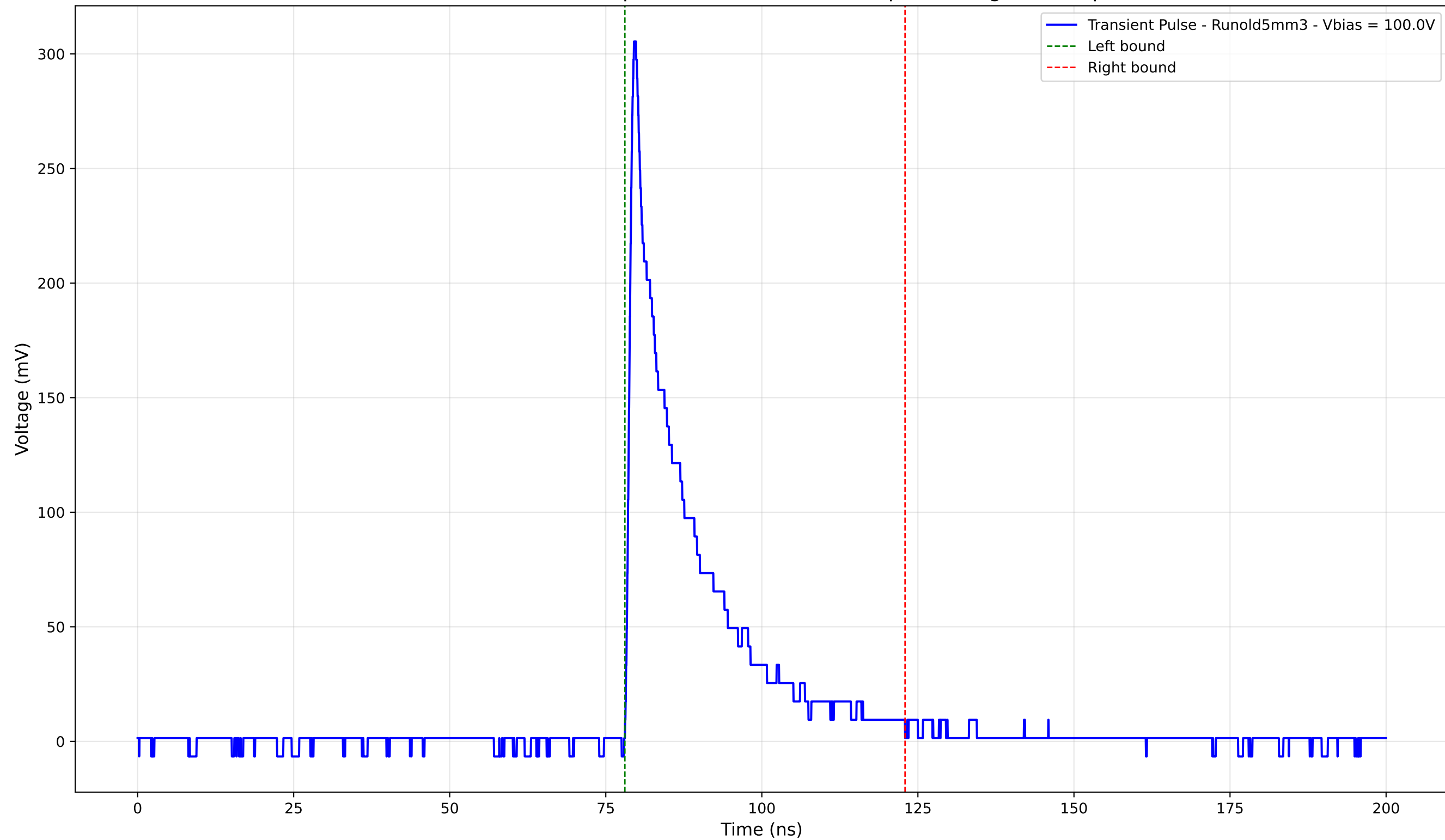
Transient Pulse - Sample: old5 - Position: 455.0 \mu\text{m} - Charge: 55.81 pC
