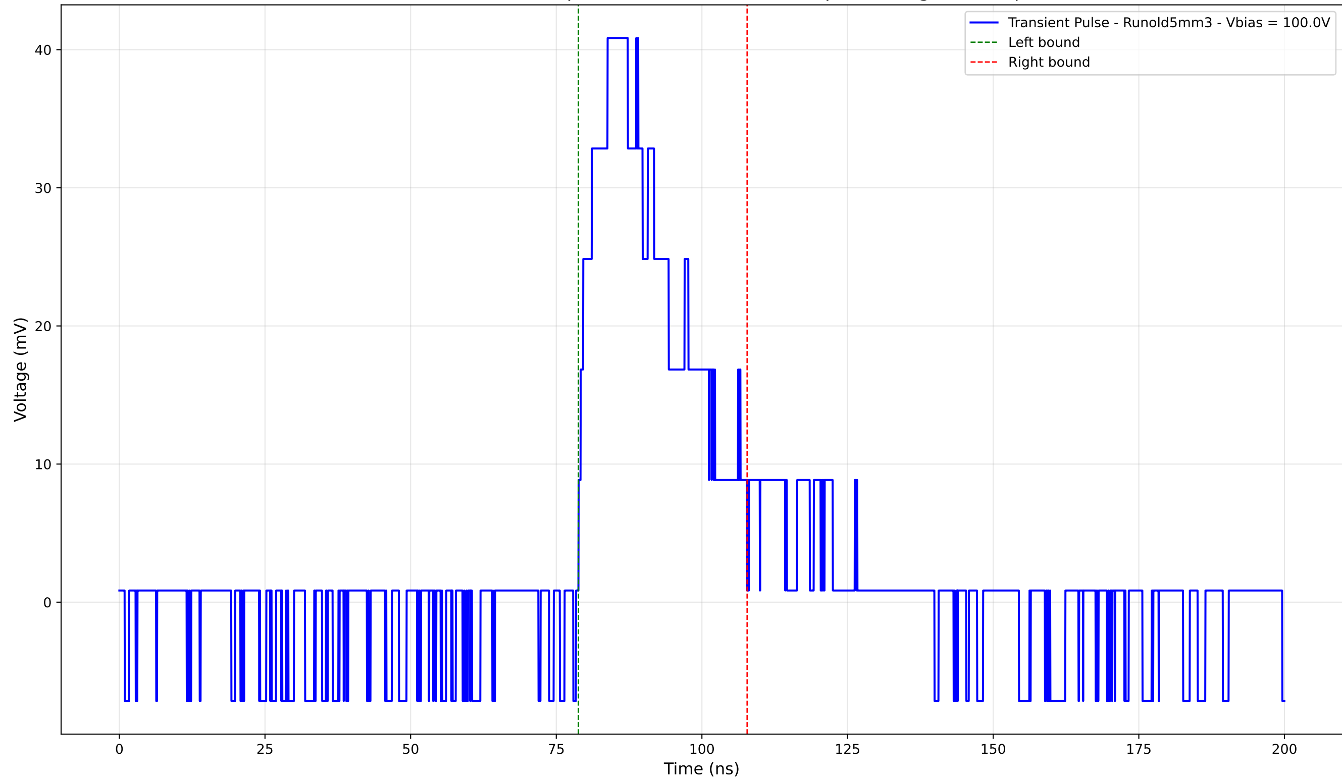
Transient Pulse - Sample: old5 - Position: 1775.0 \mu\text{m} - Charge: 13.41 pC
