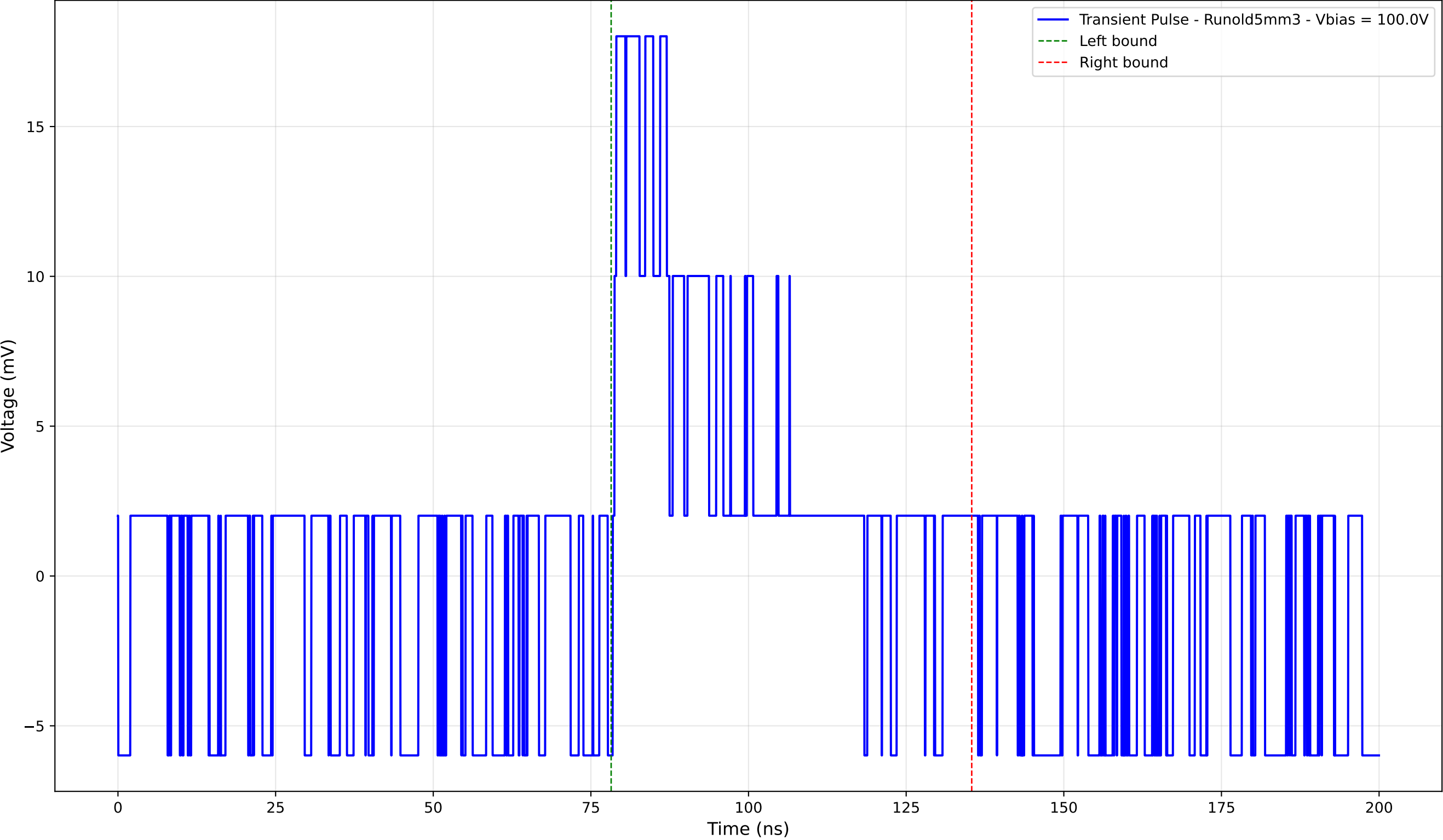
Transient Pulse - Sample: old5 - Position: 2960.0 \mu\text{m} - Charge: 5.41 pC
