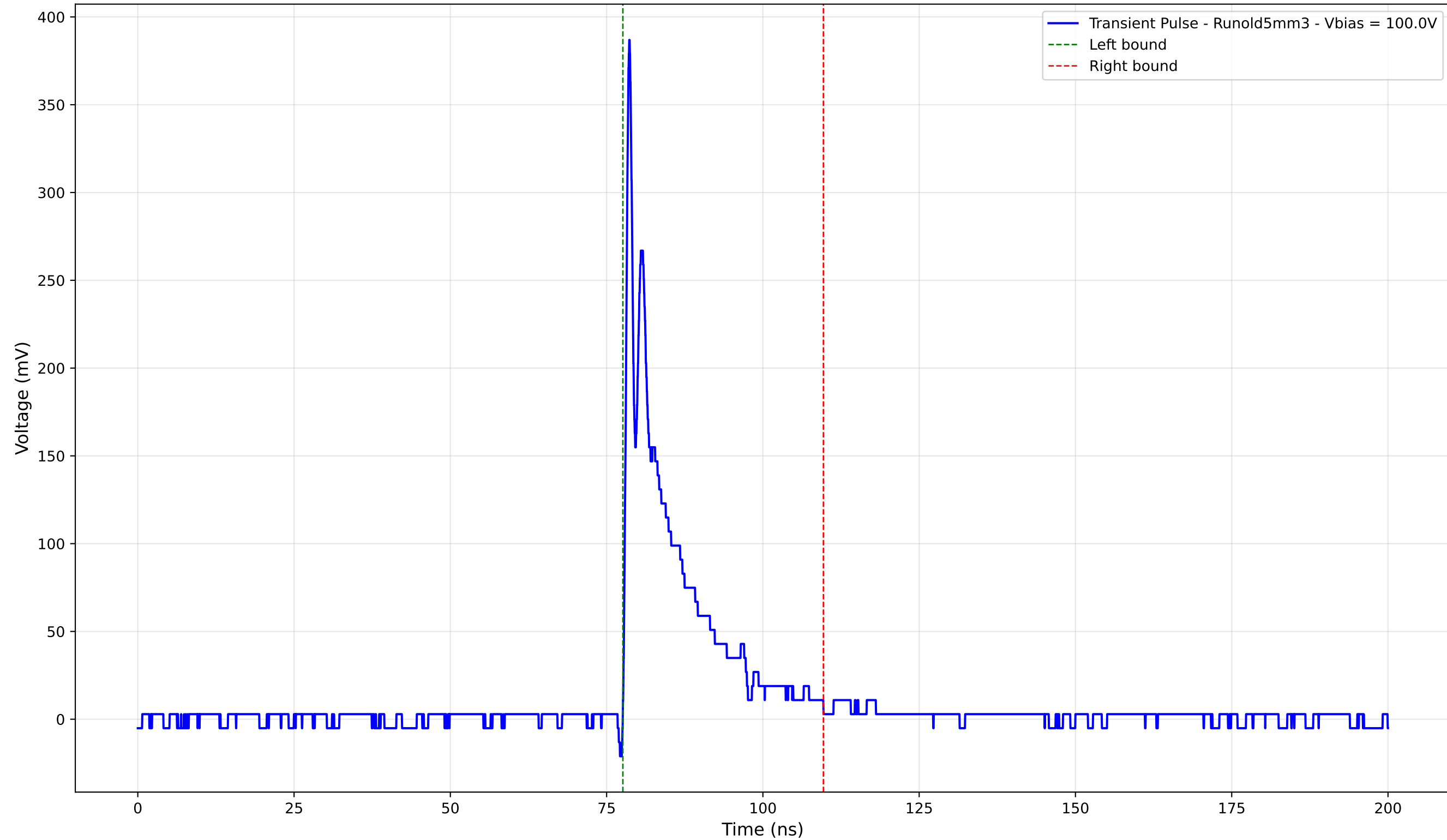
Transient Pulse - Sample: old5 - Position: 3645.0 \mu\text{m} - Charge: 46.34 pC
