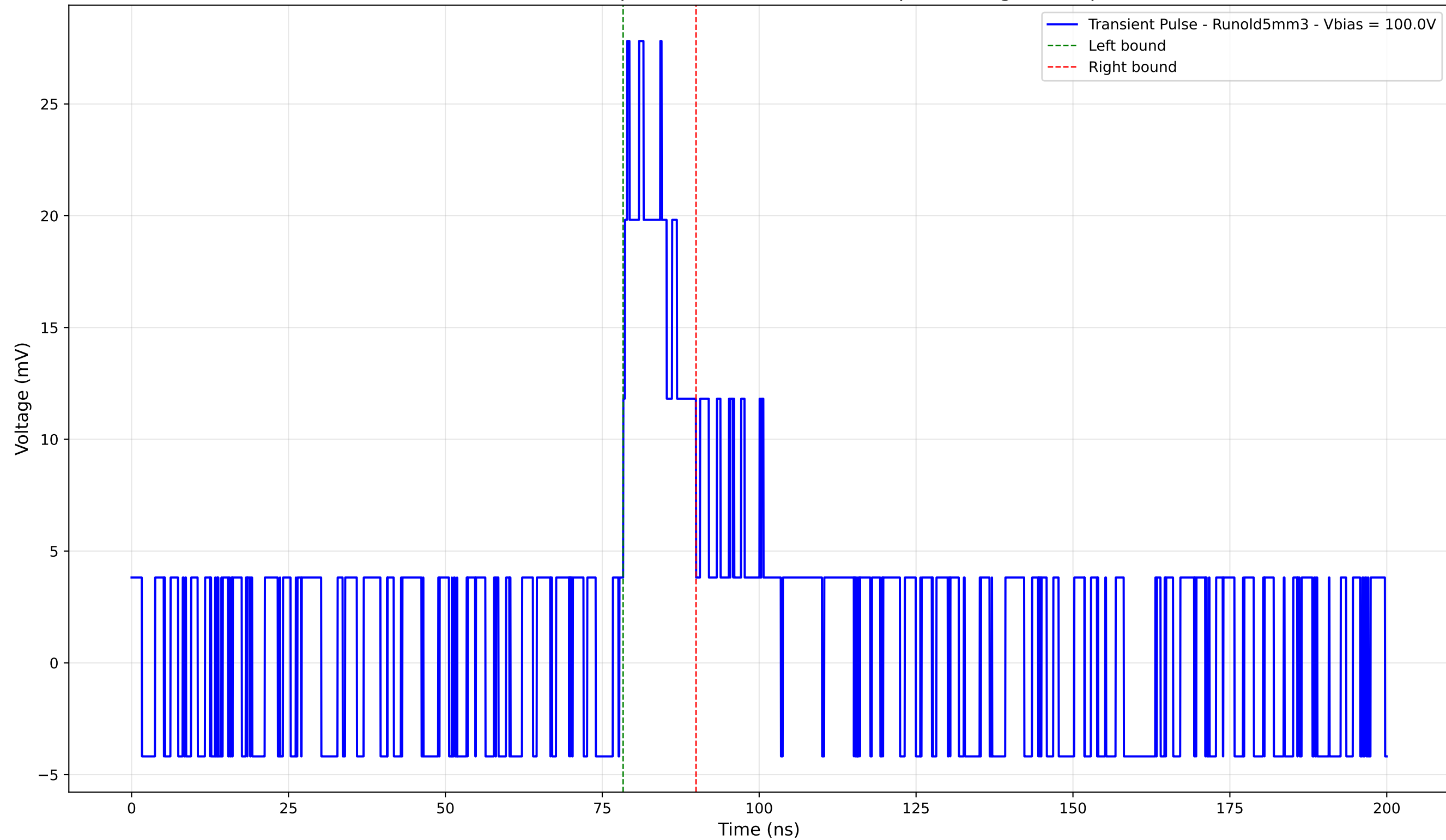
Transient Pulse - Sample: old5 - Position: 3885.0 \mu\text{m} - Charge: 4.14 pC
