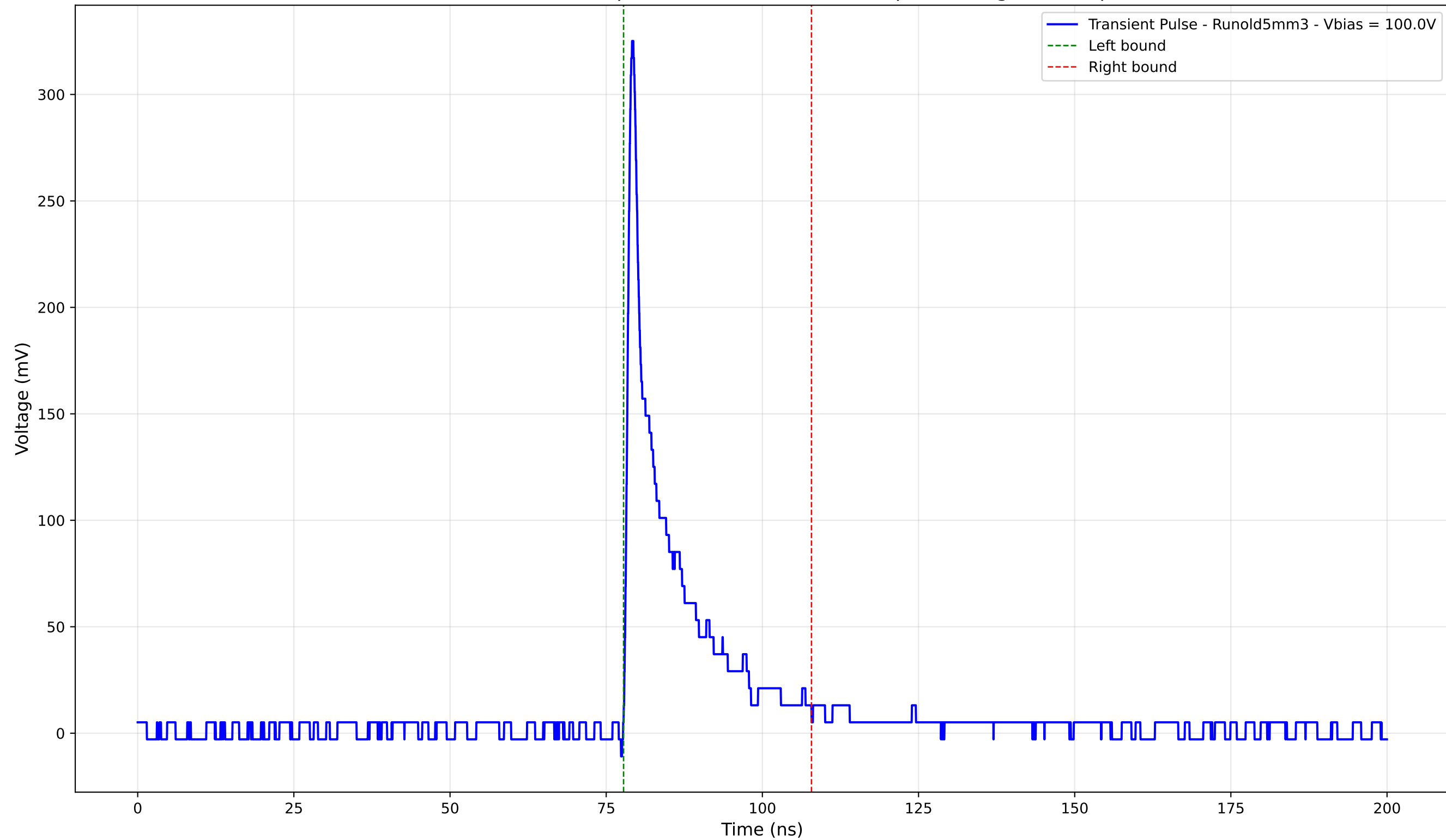
Transient Pulse - Sample: old5 - Position: 4895.0 \mu\text{m} - Charge: 39.24 pC
