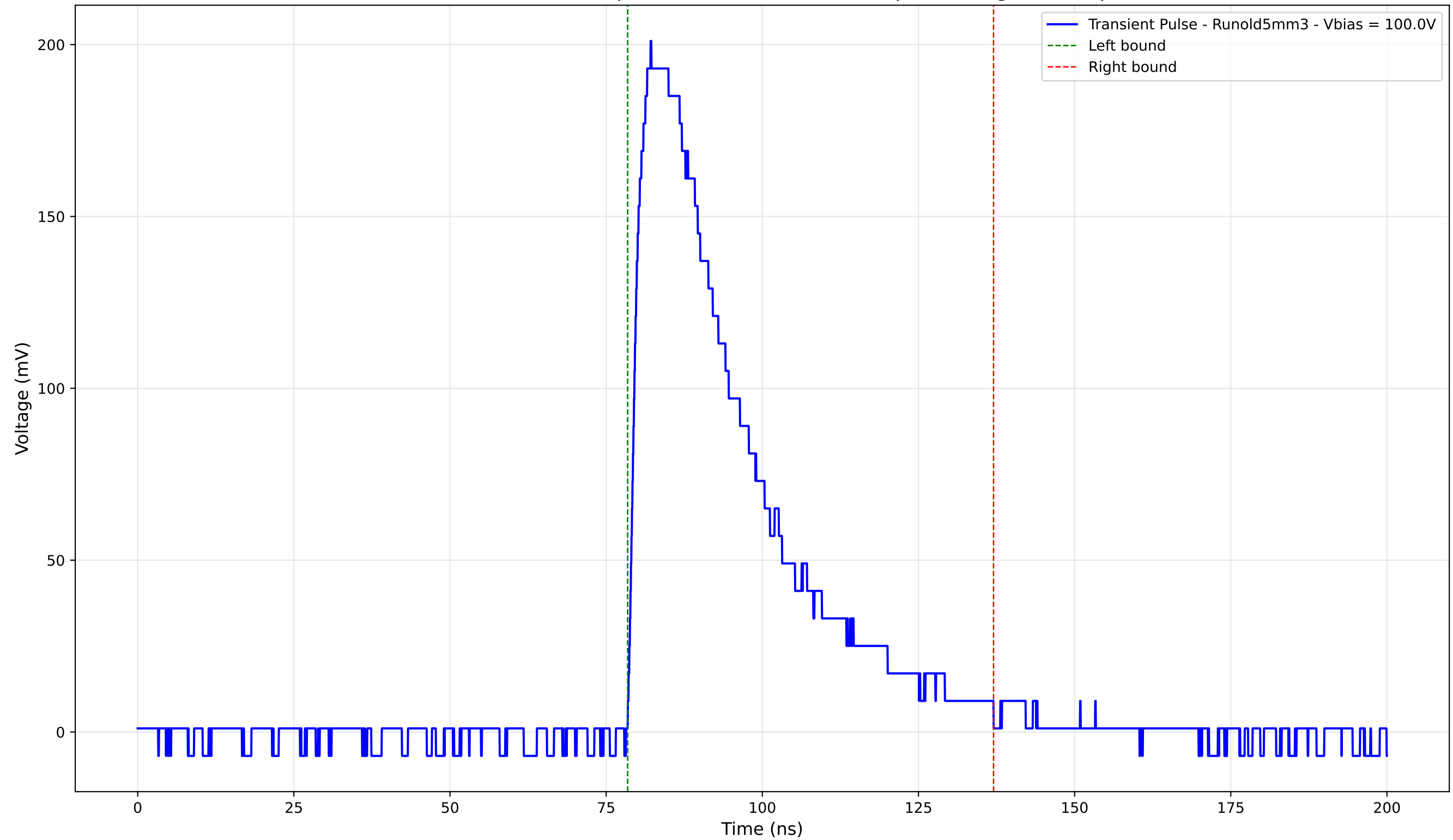
Transient Pulse - Sample: old5 - Position: 1505.0 \mu\text{m} - Charge: 78.51 pC
