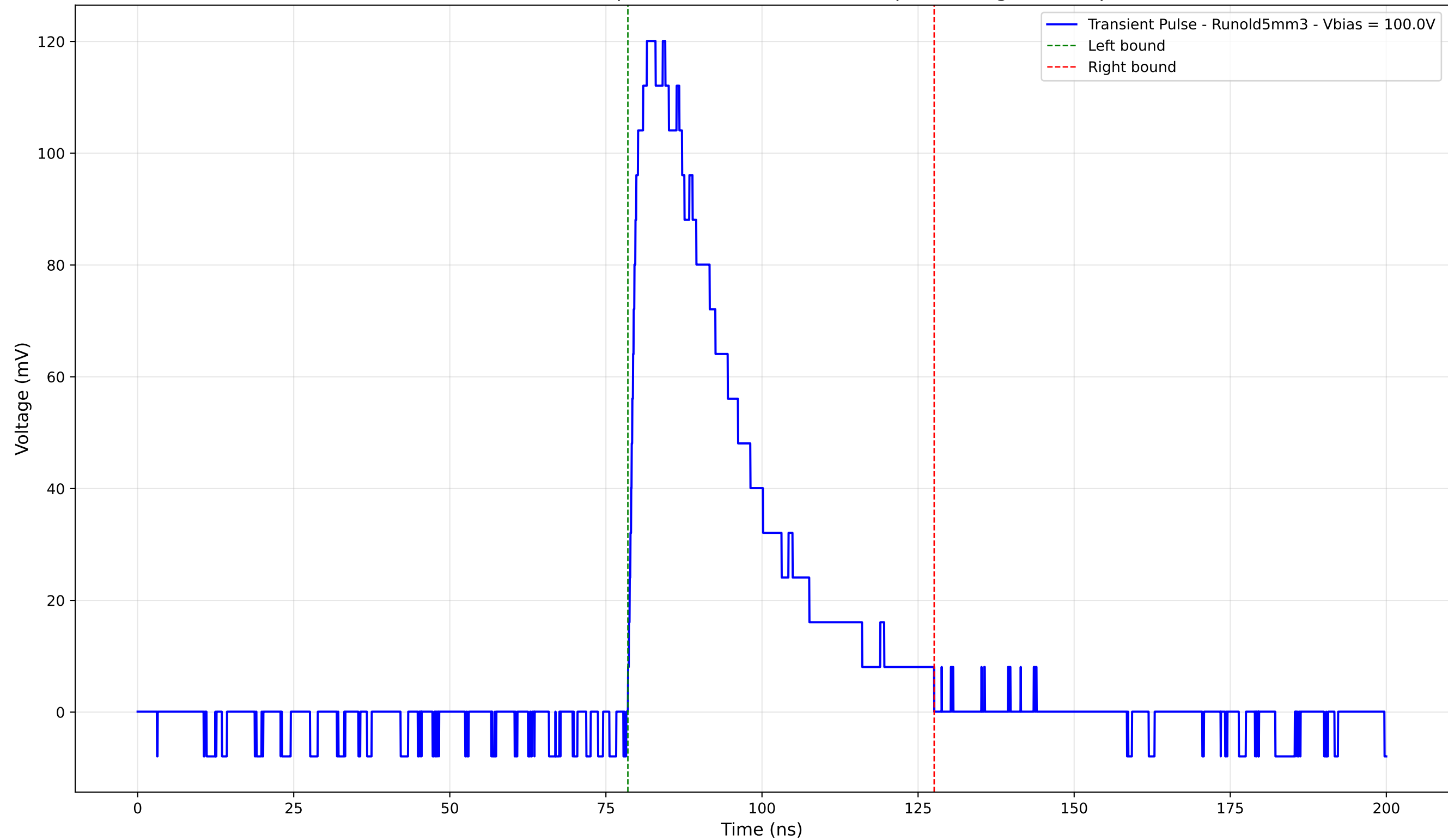
Transient Pulse - Sample: old5 - Position: 1230.0 \mu\text{m} - Charge: 43.21 pC
