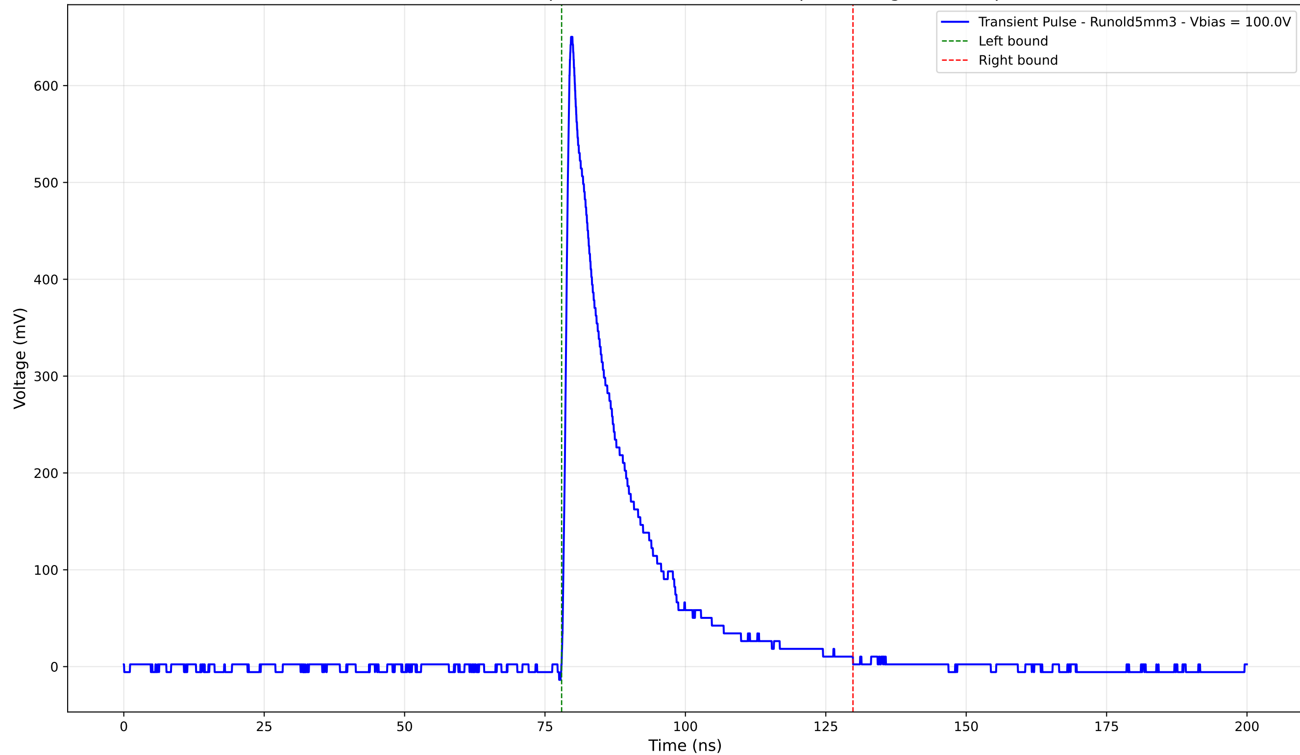
Transient Pulse - Sample: old5 - Position: 4645.0 \mu\text{m} - Charge: 126.17 pC
