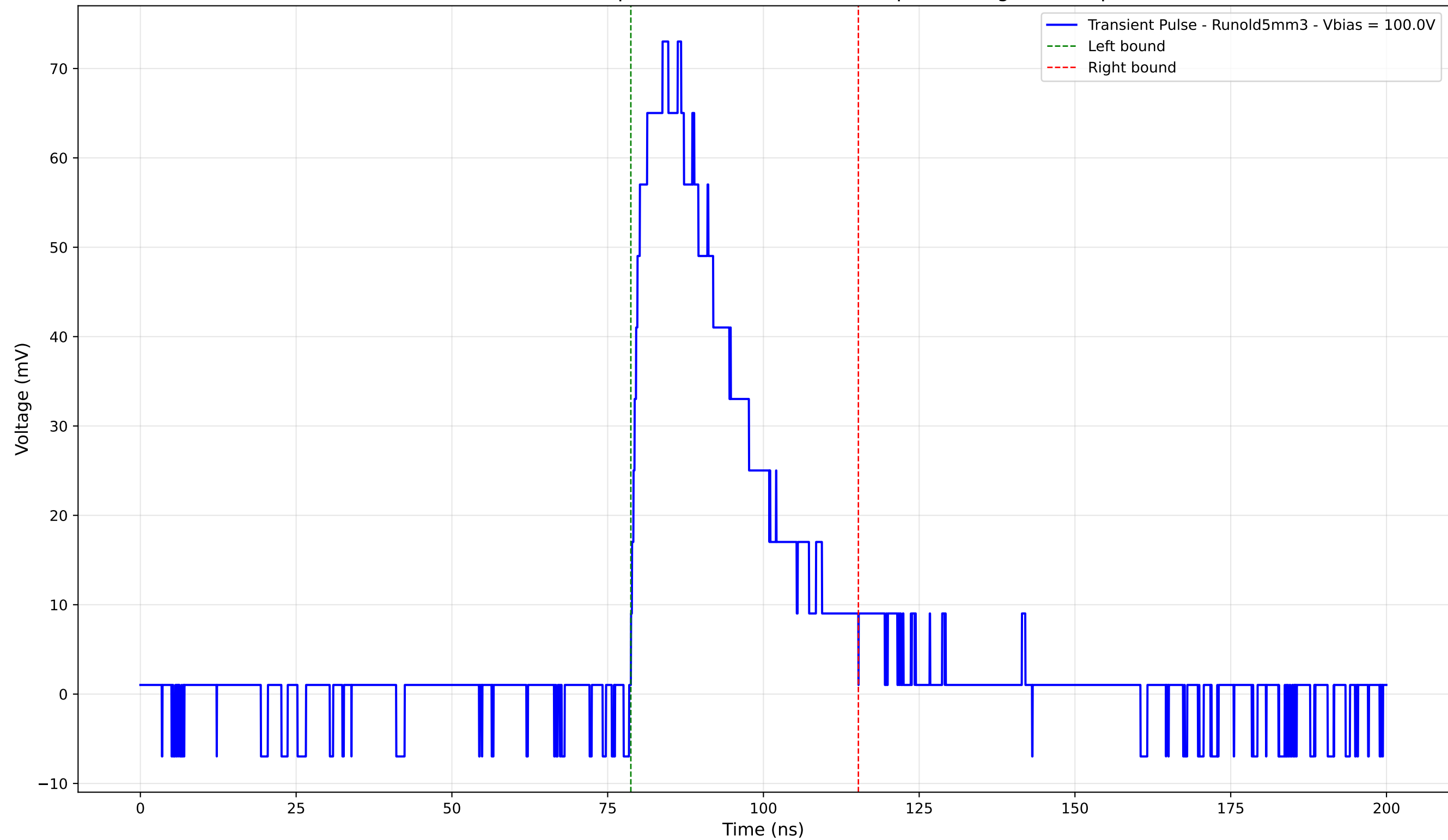
Transient Pulse - Sample: old5 - Position: 1415.0 \mu\text{m} - Charge: 24.82 pC
