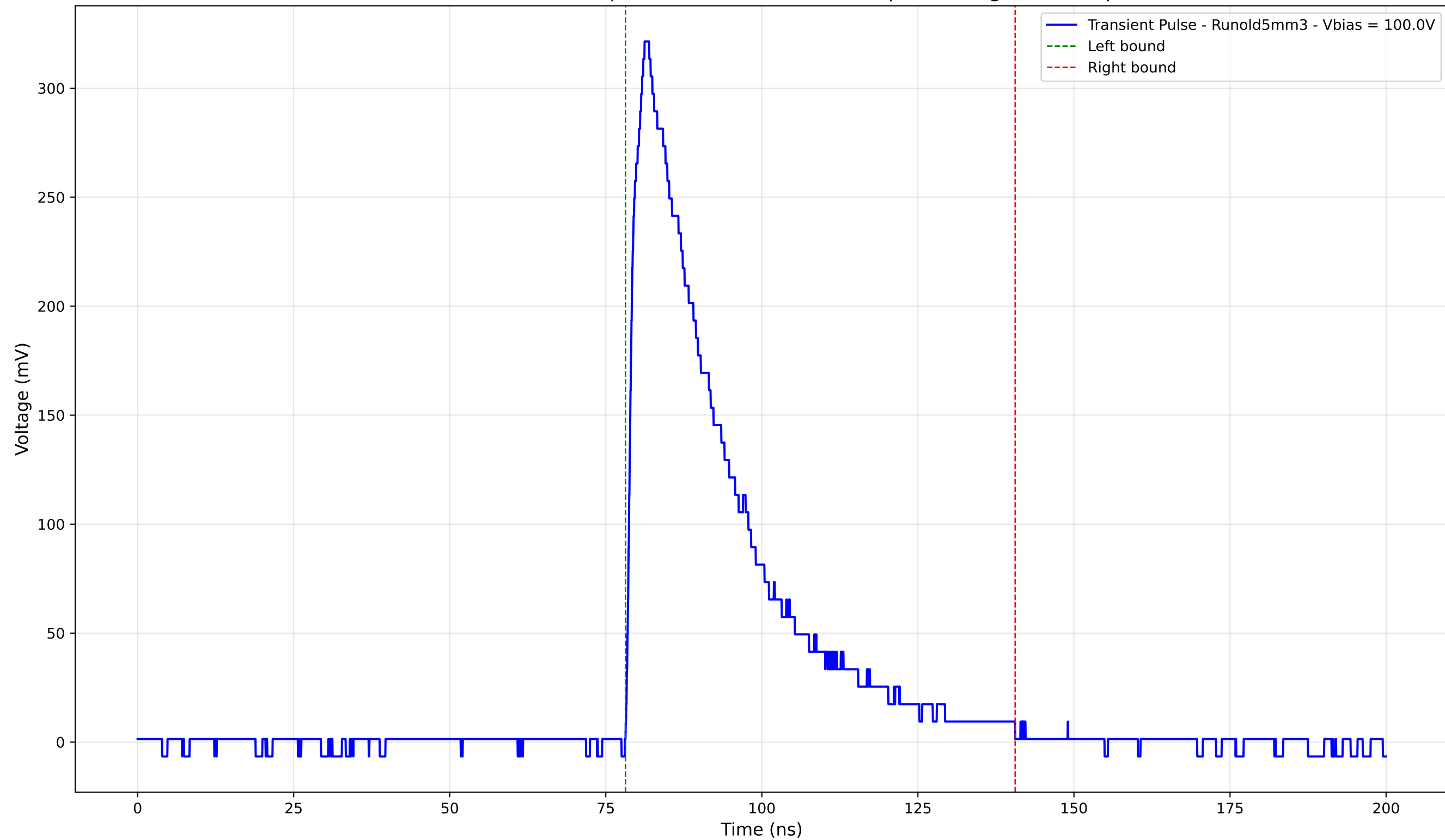
Transient Pulse - Sample: old5 - Position: 2835.0 \mu\text{m} - Charge: 104.94 pC
