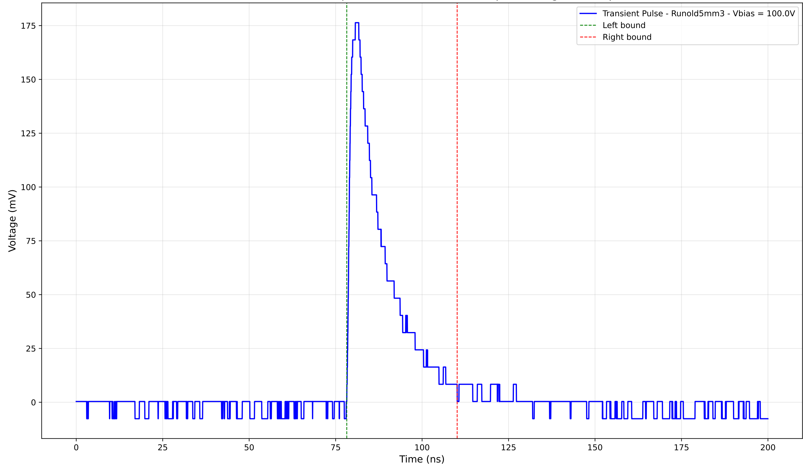
Transient Pulse - Sample: old5 - Position: 4240.0 \mu\text{m} - Charge: 37.45 pC
