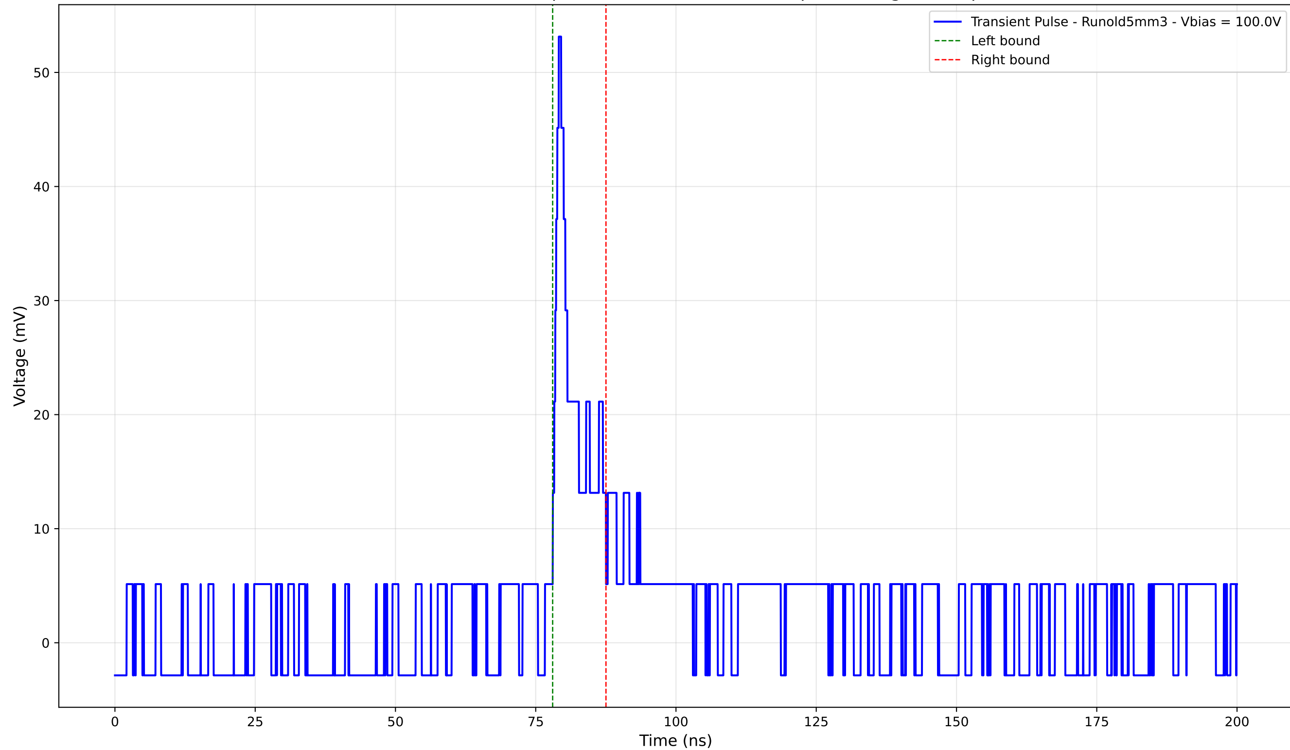
Transient Pulse - Sample: old5 - Position: 4935.0 \mu\text{m} - Charge: 4.28 pC
