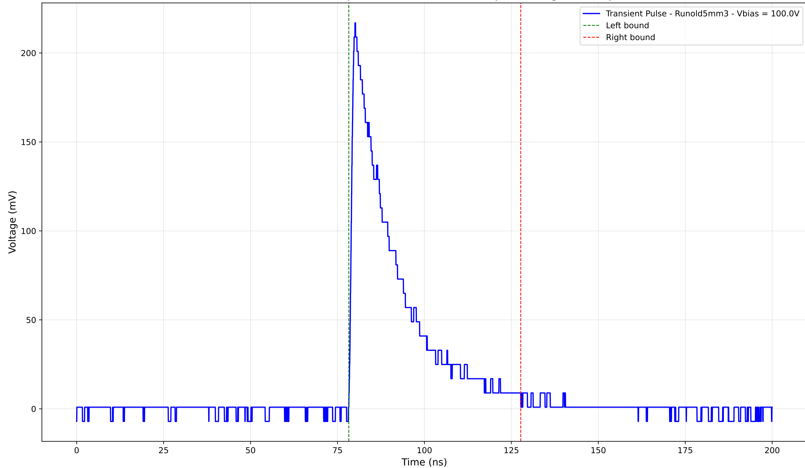
Transient Pulse - Sample: old5 - Position: 740.0 \mu\text{m} - Charge: 56.69 pC
