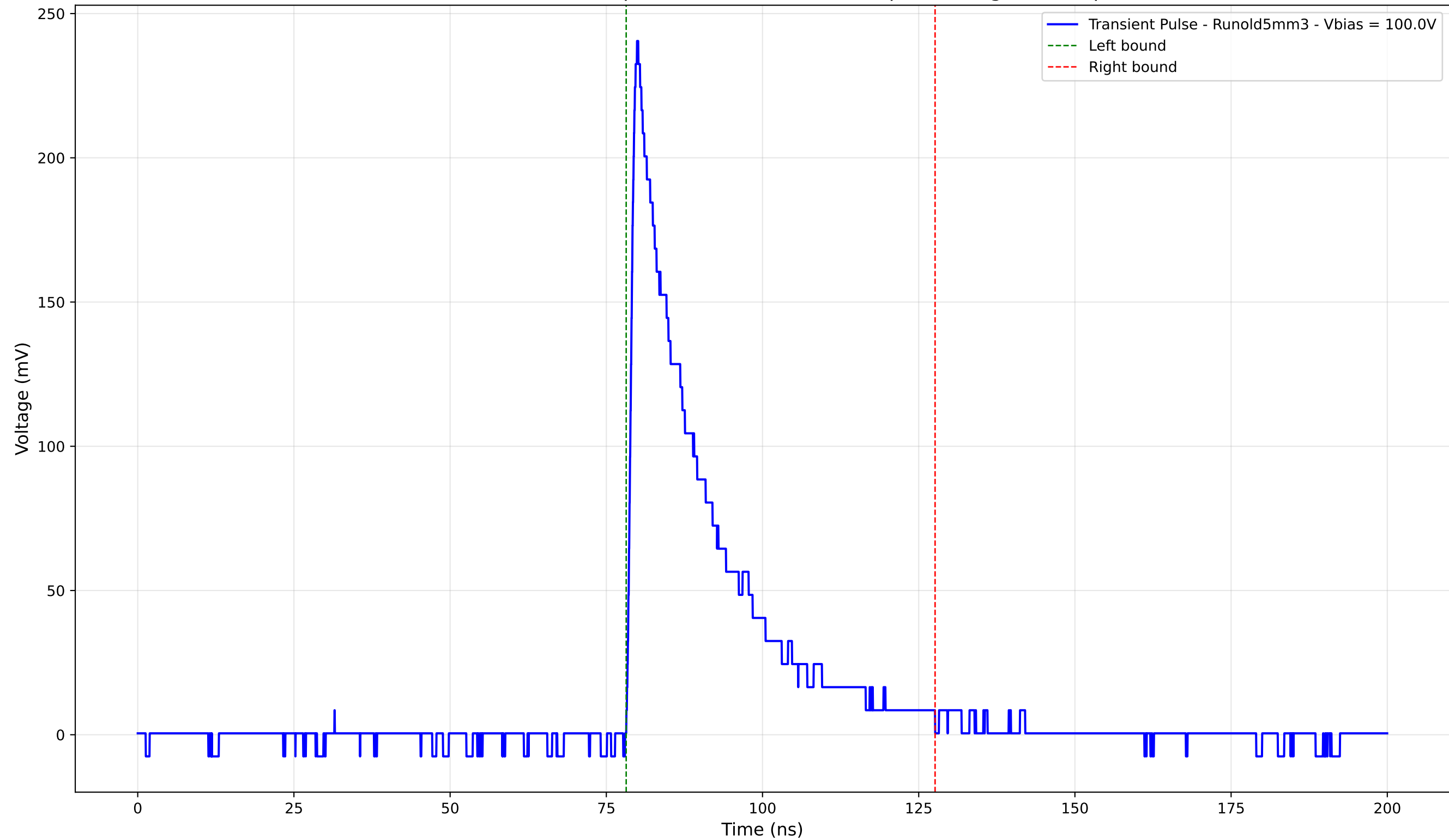
Transient Pulse - Sample: old5 - Position: 640.0 \mu\text{m} - Charge: 56.09 pC
