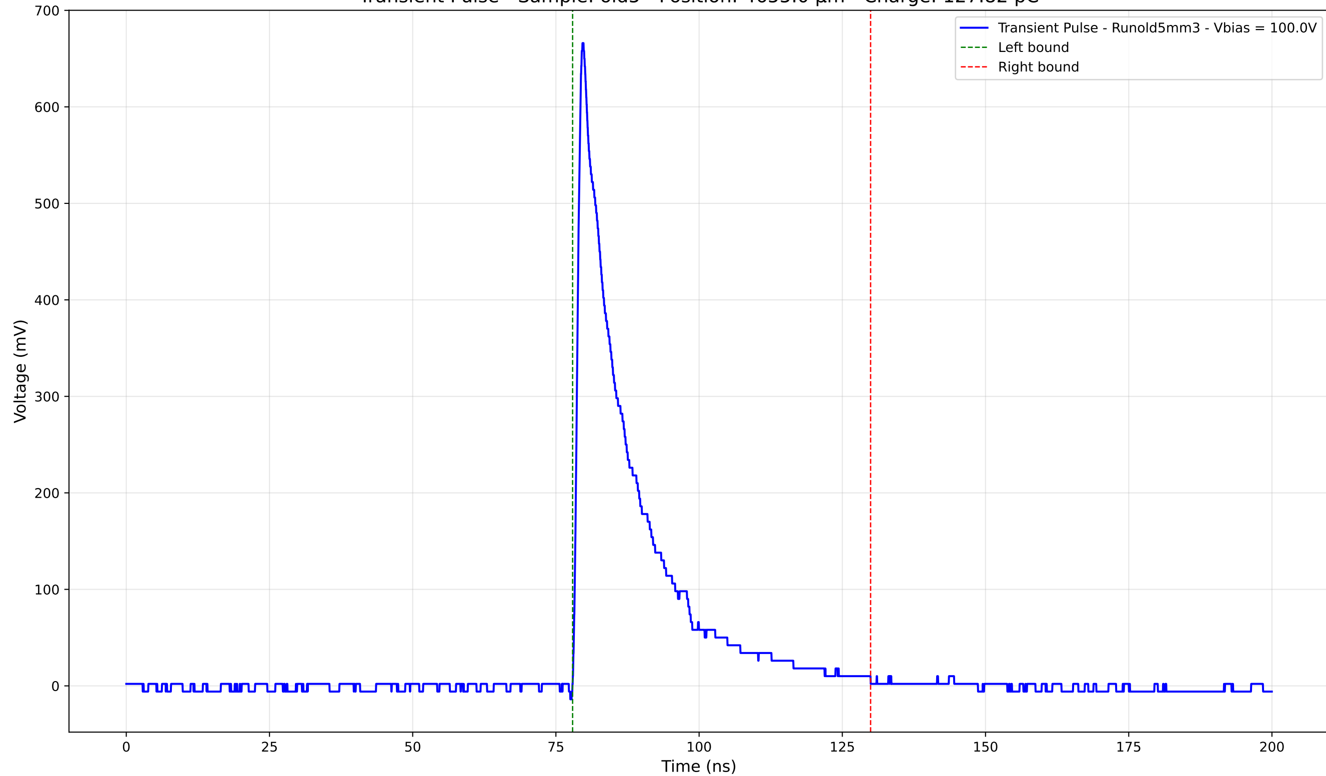
Transient Pulse - Sample: old5 - Position: 4655.0 \mu\text{m} - Charge: 127.82 pC
