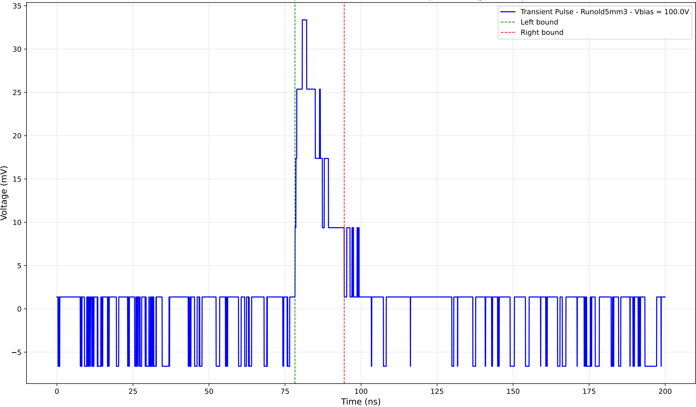
Transient Pulse - Sample: old5 - Position: 3900.0 \mu\text{m} - Charge: 5.89 pC
