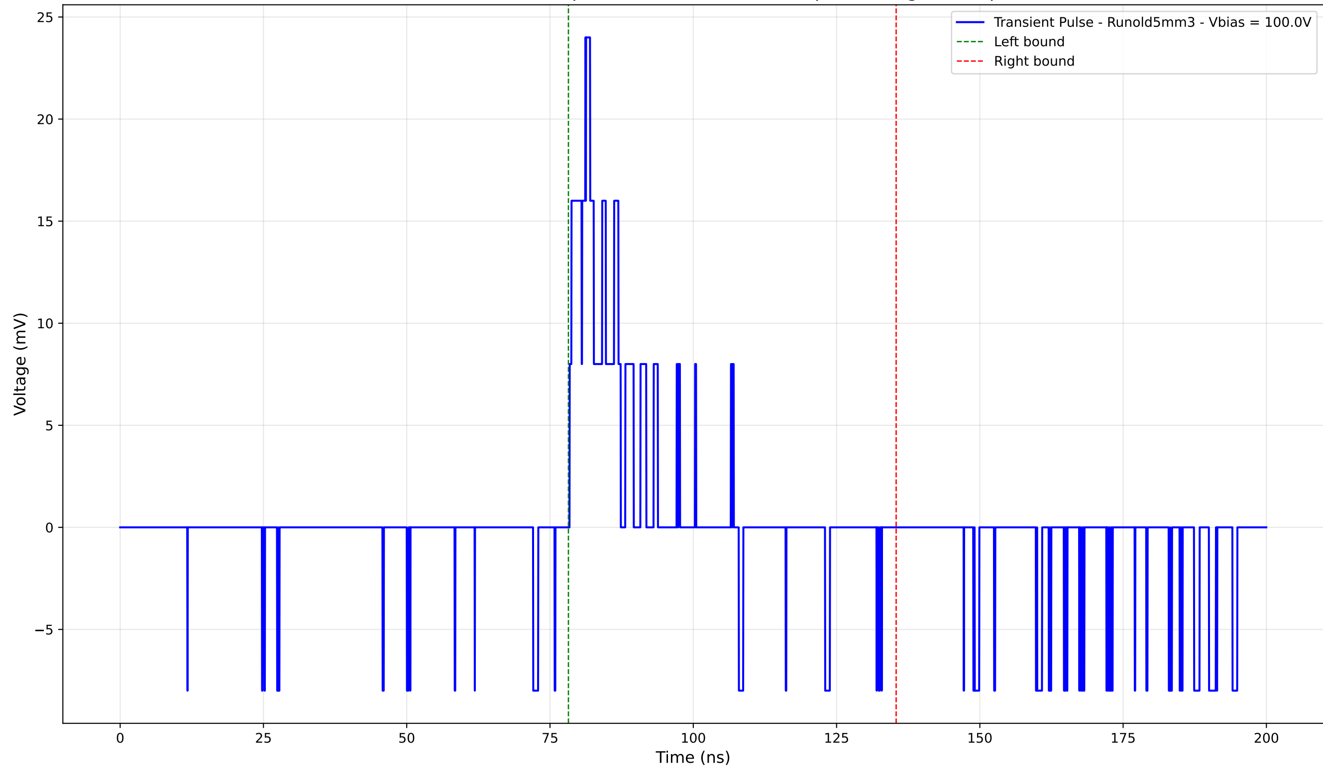
Transient Pulse - Sample: old5 - Position: 115.0 \mu\text{m} - Charge: 2.75 pC
