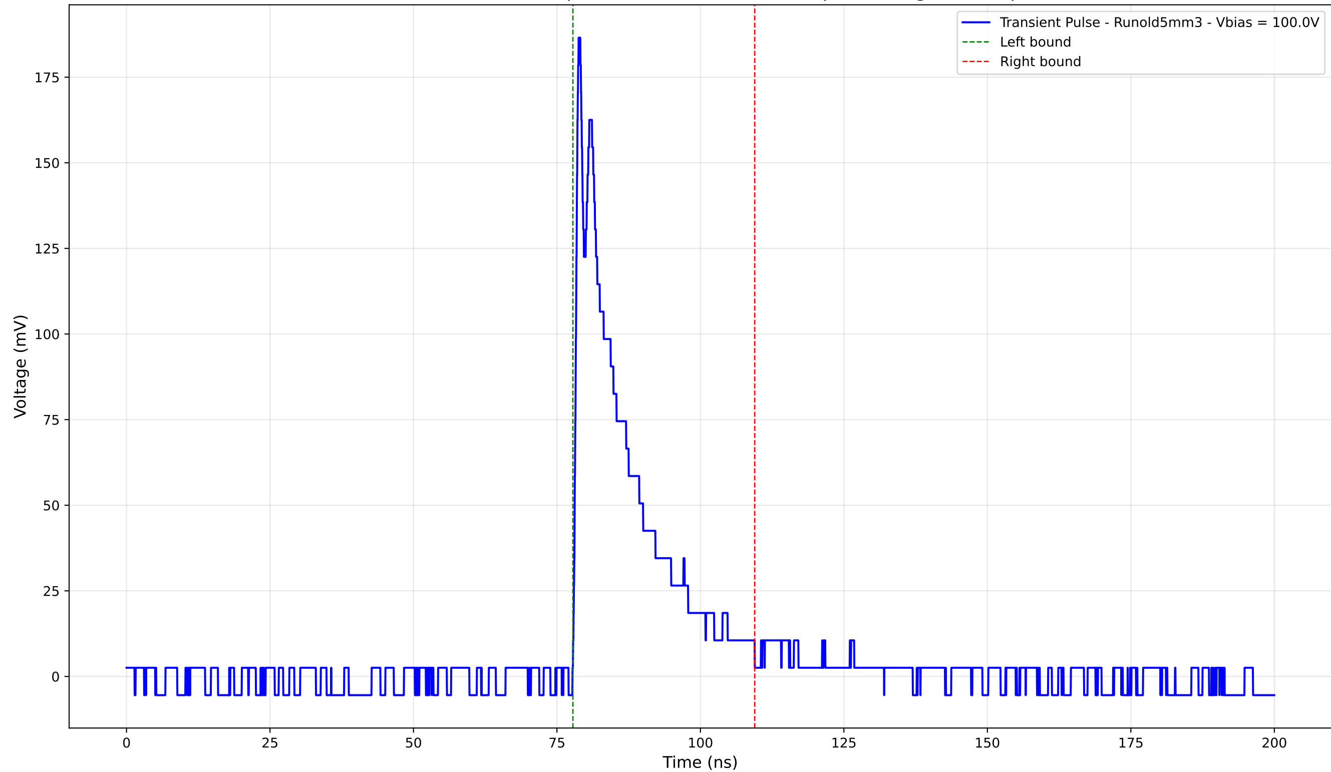
Transient Pulse - Sample: old5 - Position: 3335.0 \mu\text{m} - Charge: 32.62 pC
