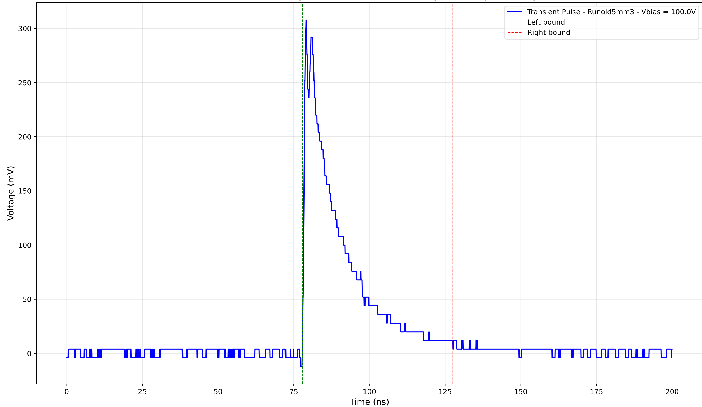
Transient Pulse - Sample: old5 - Position: 3195.0 \mu\text{m} - Charge: 74.17 pC
