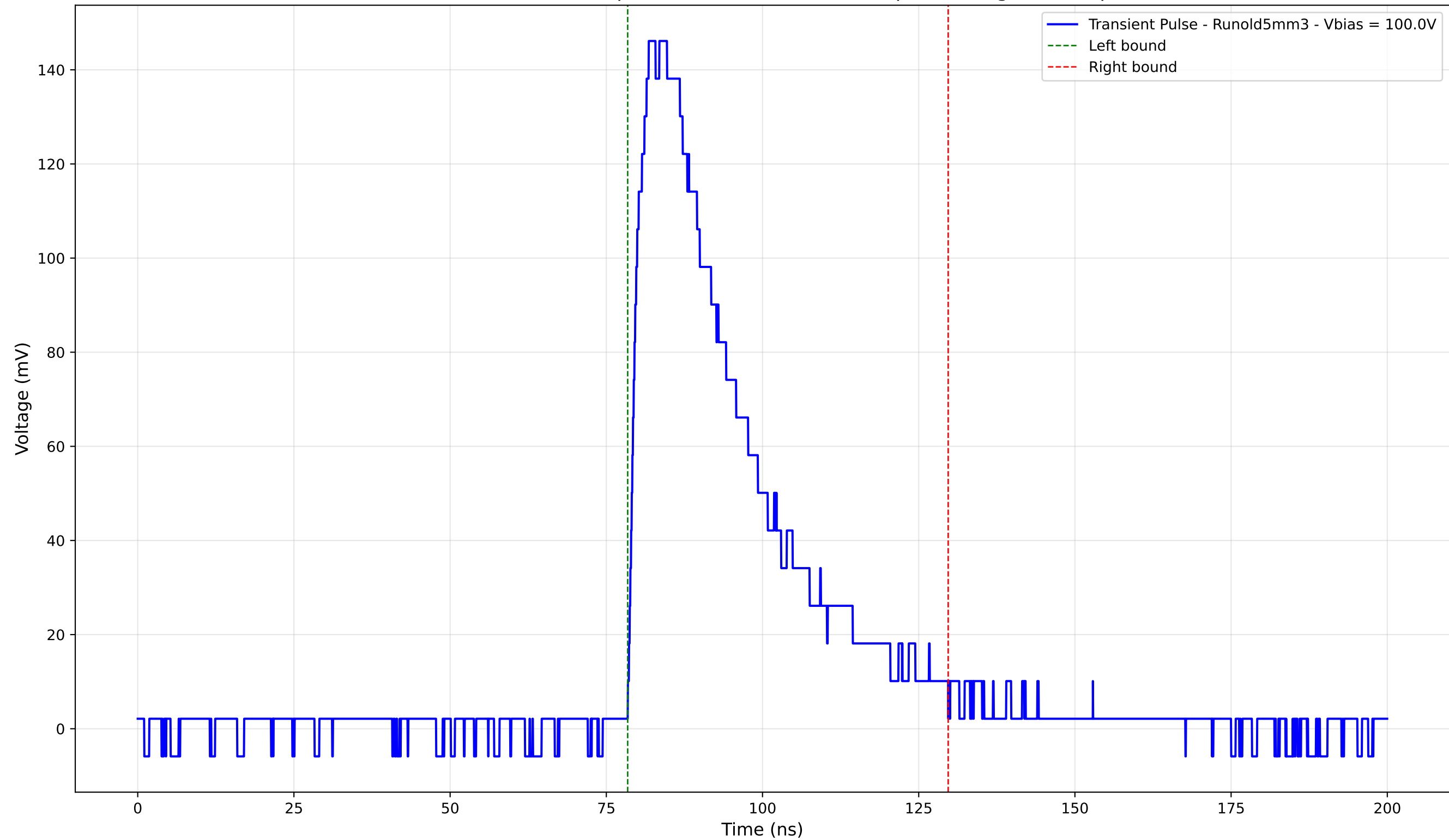
Transient Pulse - Sample: old5 - Position: 2345.0 \mu\text{m} - Charge: 56.84 pC
