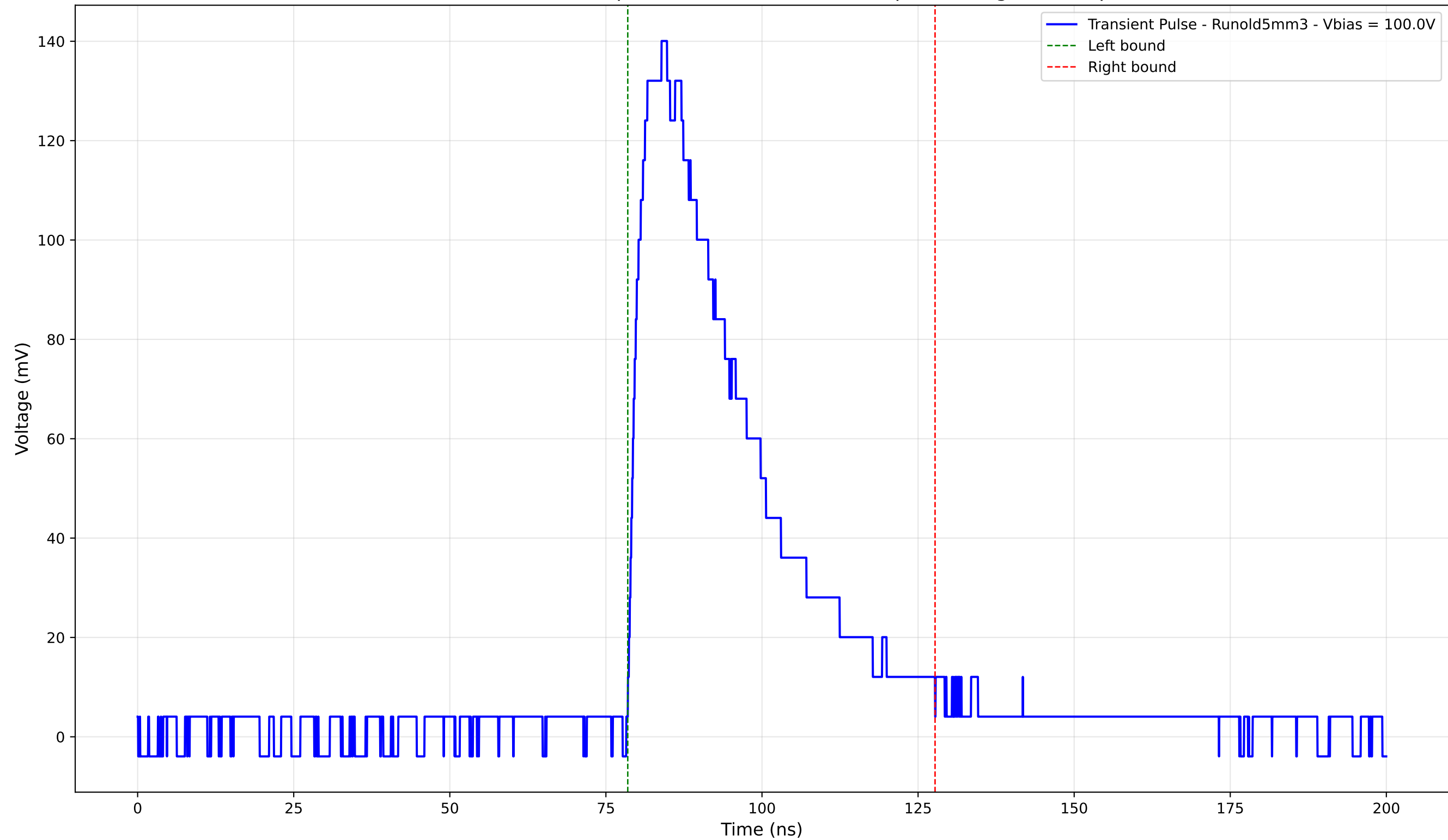
Transient Pulse - Sample: old5 - Position: 1735.0 \mu\text{m} - Charge: 54.62 pC
