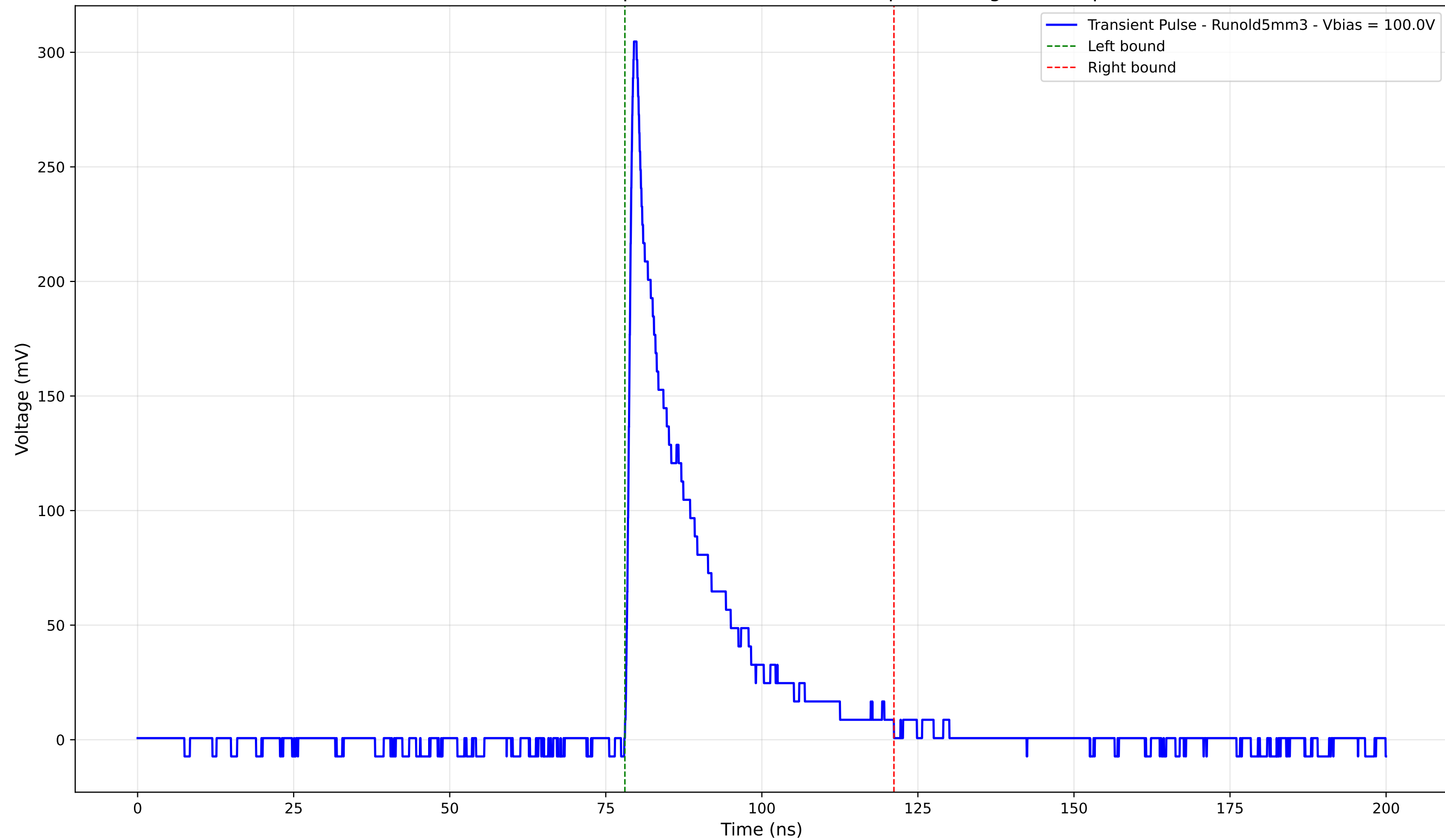
Transient Pulse - Sample: old5 - Position: 450.0 \mu\text{m} - Charge: 55.43 pC
