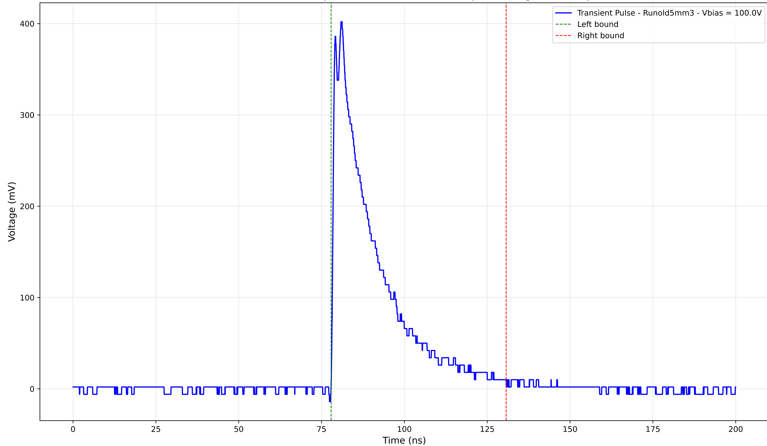
Transient Pulse - Sample: old5 - Position: 3130.0 \mu\text{m} - Charge: 106.85 pC
