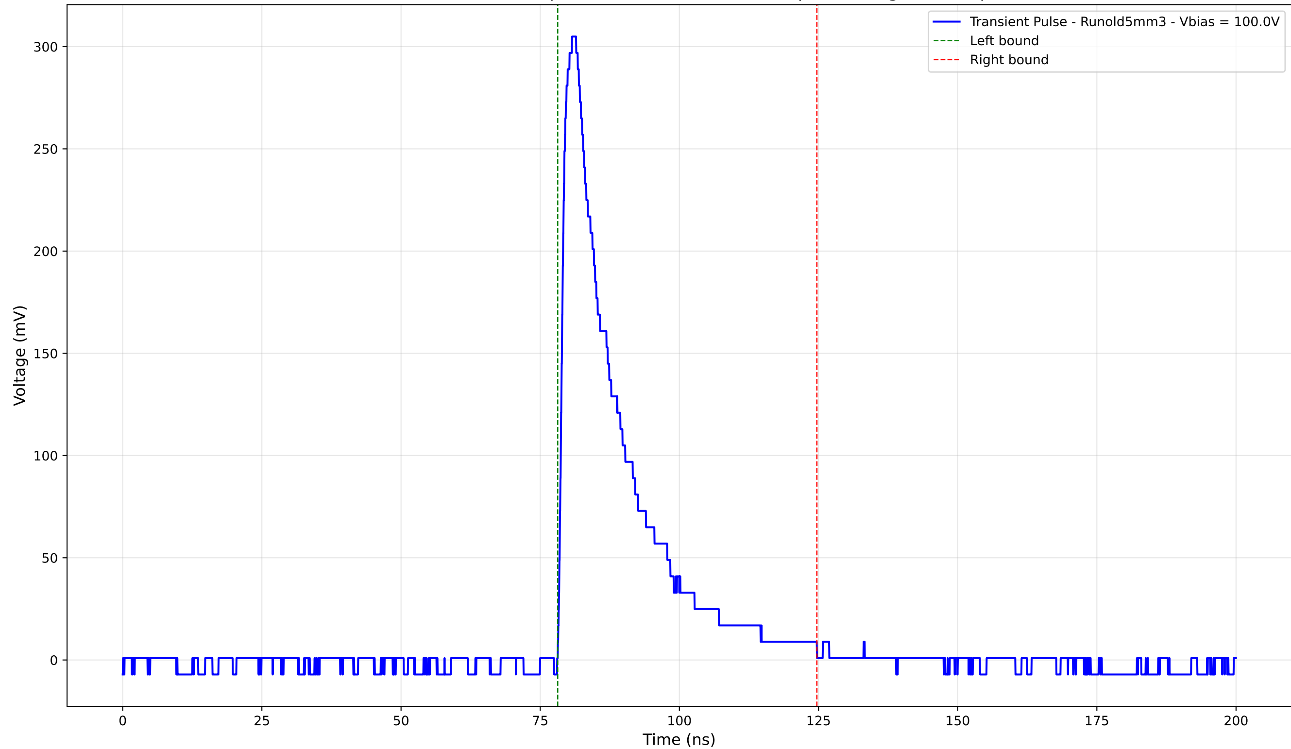
Transient Pulse - Sample: old5 - Position: 4260.0 \mu\text{m} - Charge: 67.76 pC
