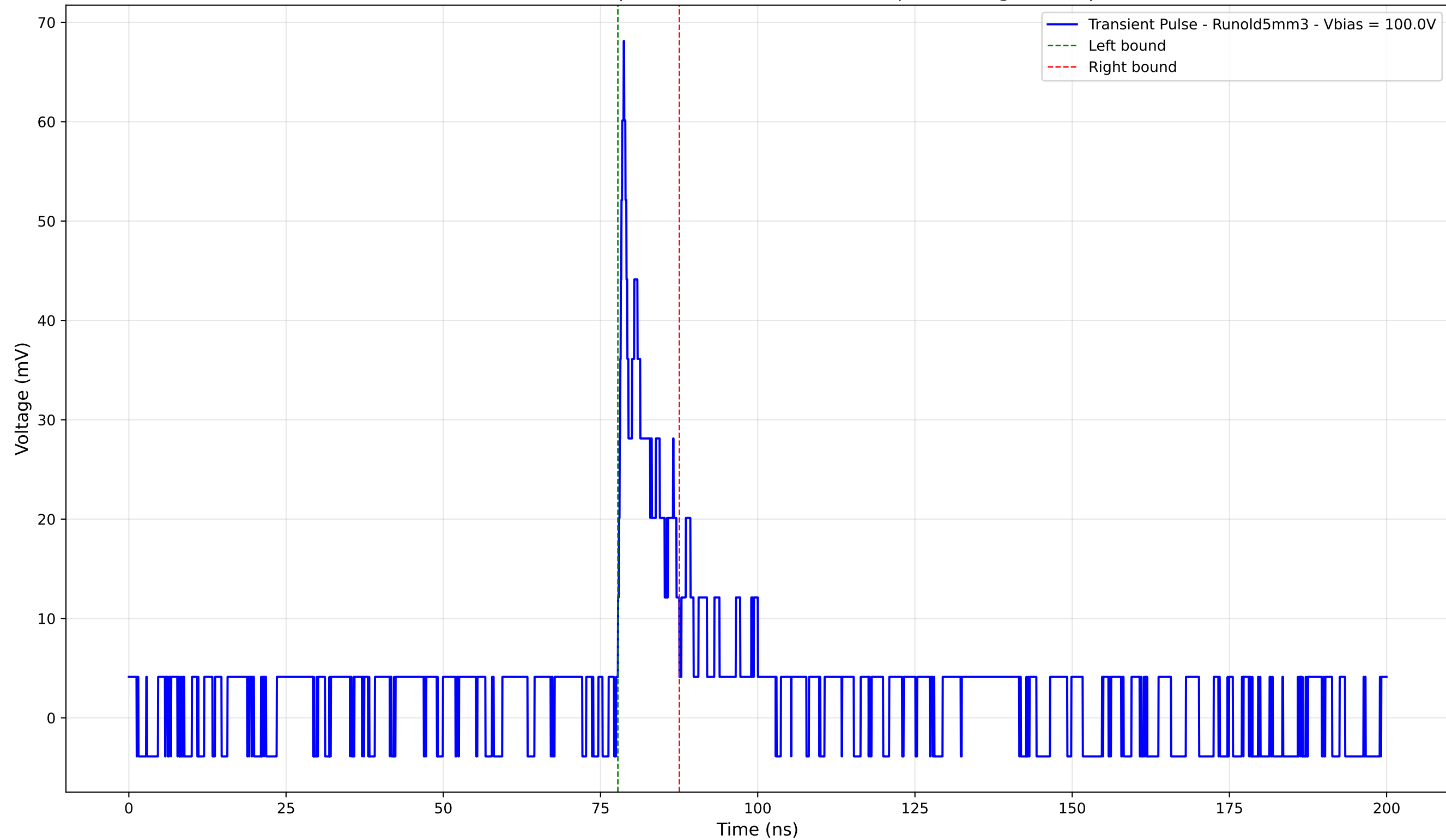
Transient Pulse - Sample: old5 - Position: 3560.0 \mu\text{m} - Charge: 5.56 pC
