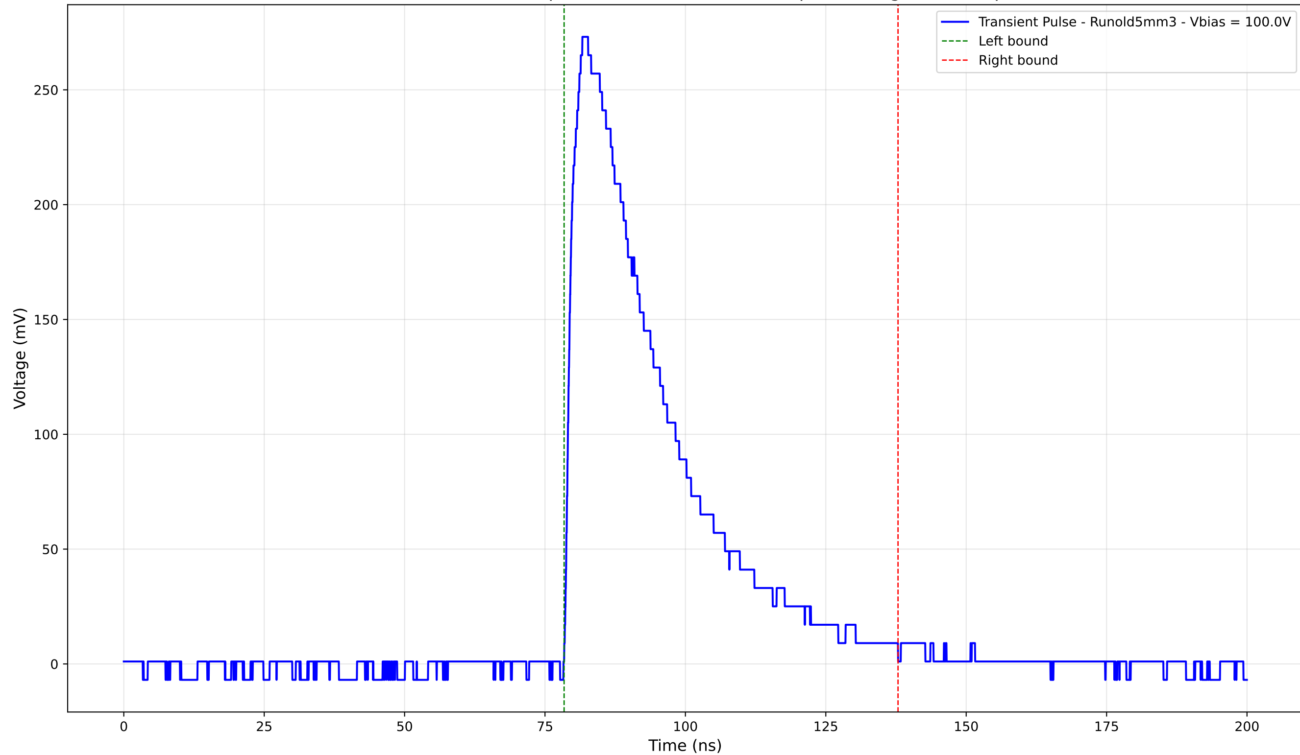
Transient Pulse - Sample: old5 - Position: 2540.0 \mu\text{m} - Charge: 100.30 pC
