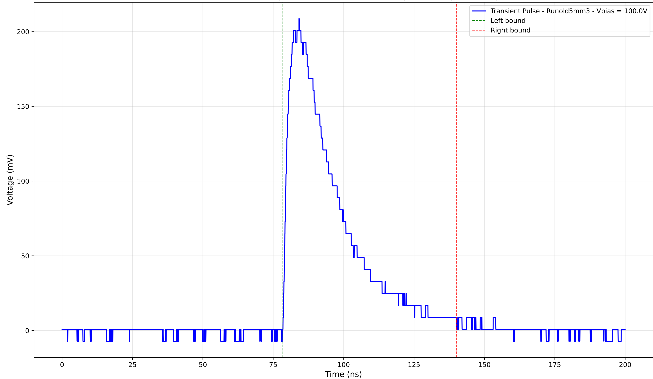
Transient Pulse - Sample: old5 - Position: 2115.0 \mu\text{m} - Charge: 81.66 pC
