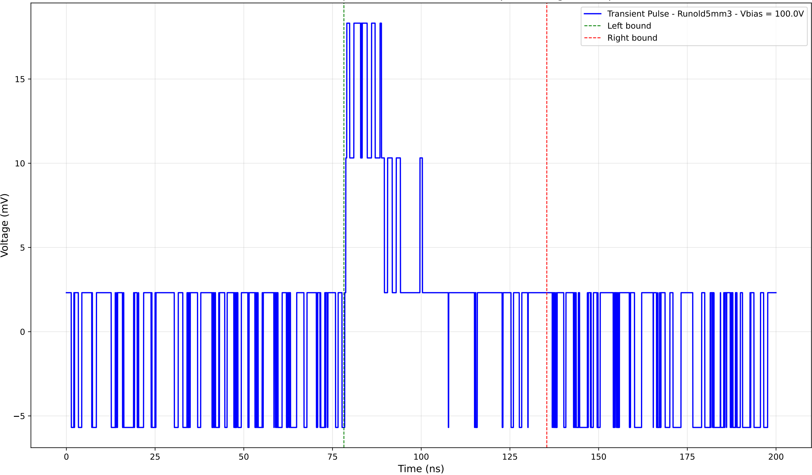
Transient Pulse - Sample: old5 - Position: 2985.0 \mu\text{m} - Charge: 5.40 pC
