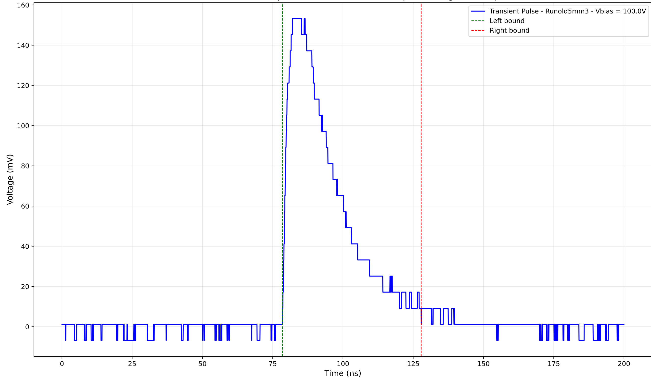
Transient Pulse - Sample: old5 - Position: 1930.0 \mu\text{m} - Charge: 61.41 pC
