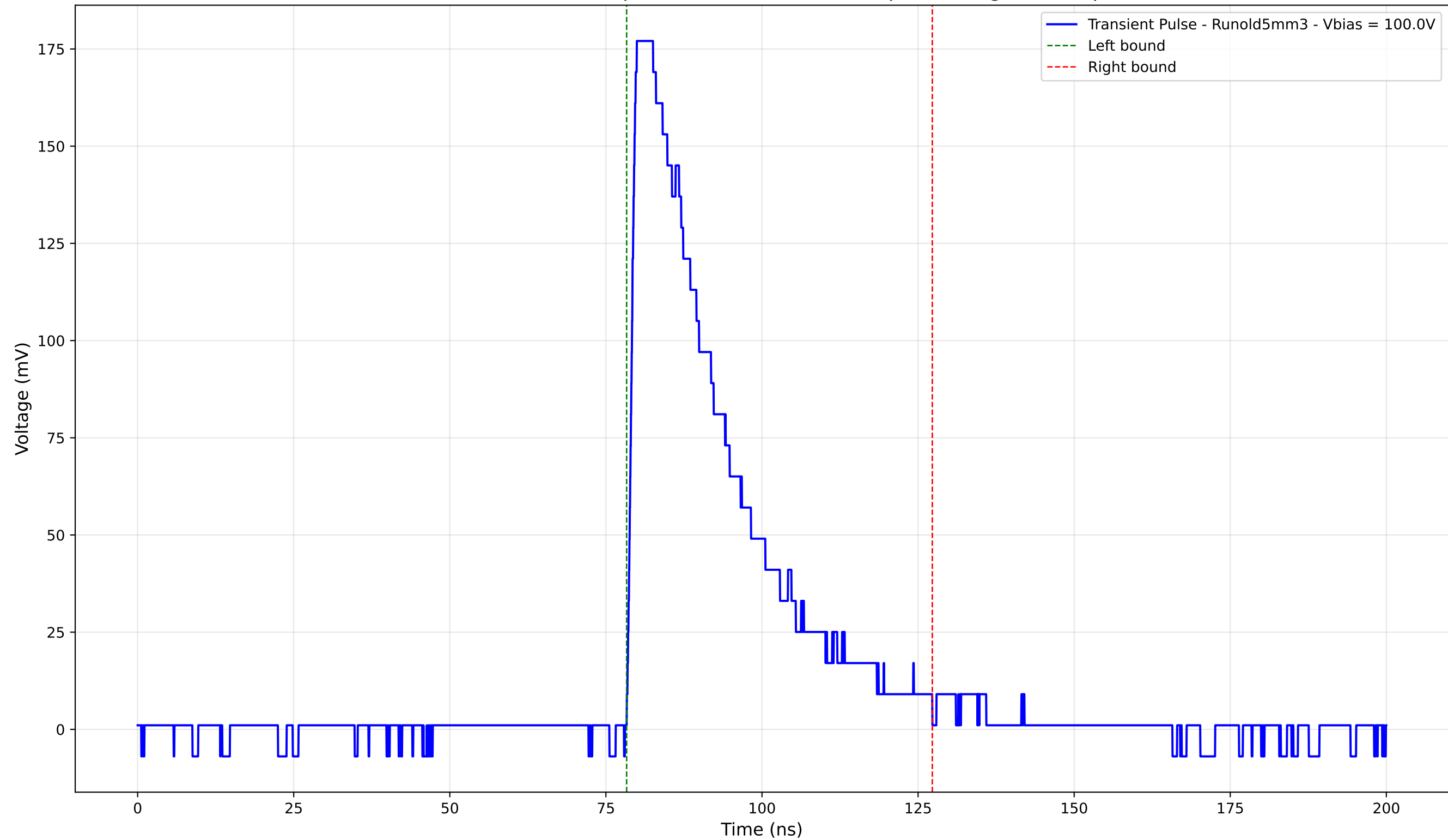
Transient Pulse - Sample: old5 - Position: 960.0 \mu\text{m} - Charge: 58.30 pC
