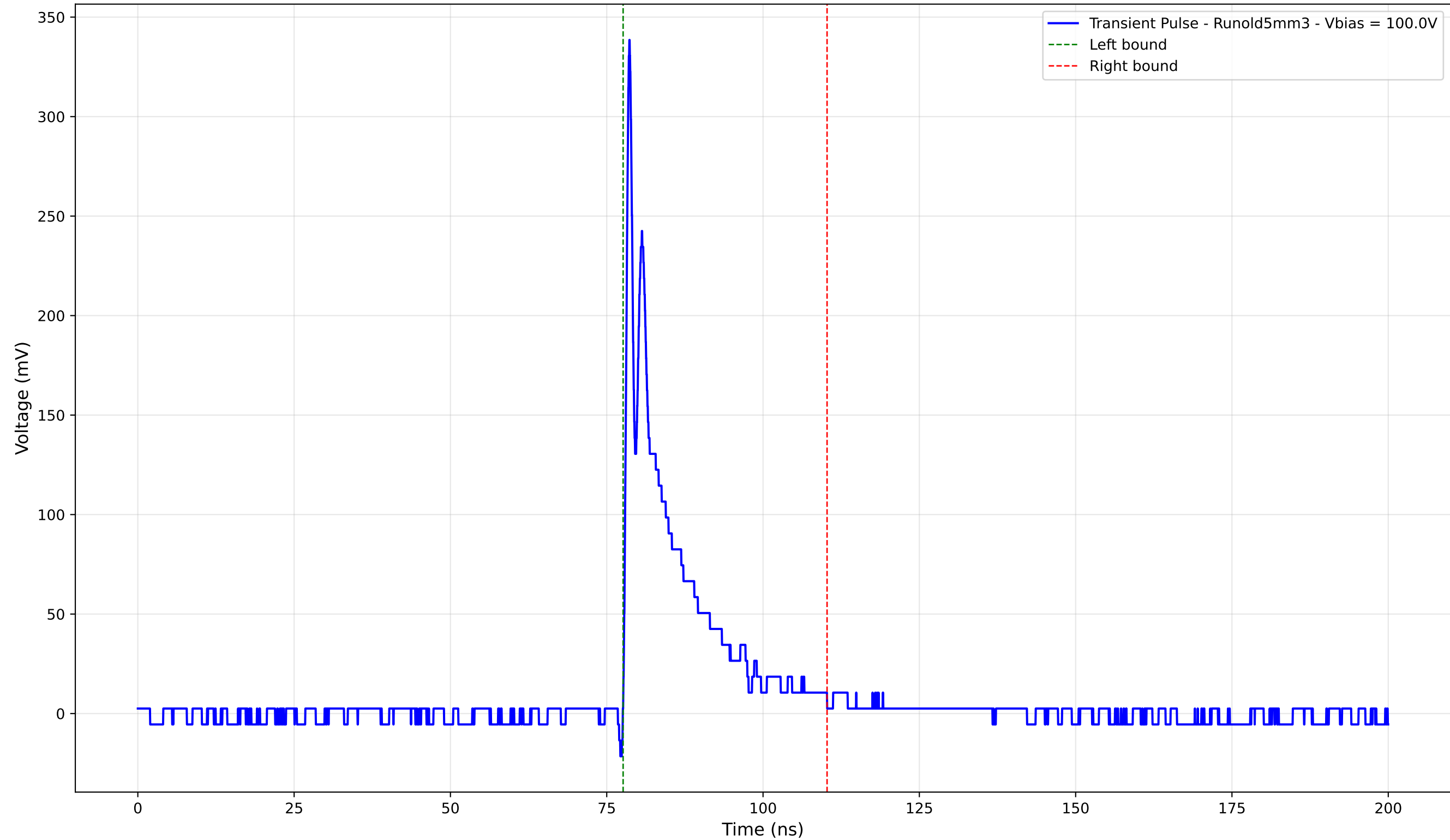
Transient Pulse - Sample: old5 - Position: 3640.0 \mu\text{m} - Charge: 40.08 pC
