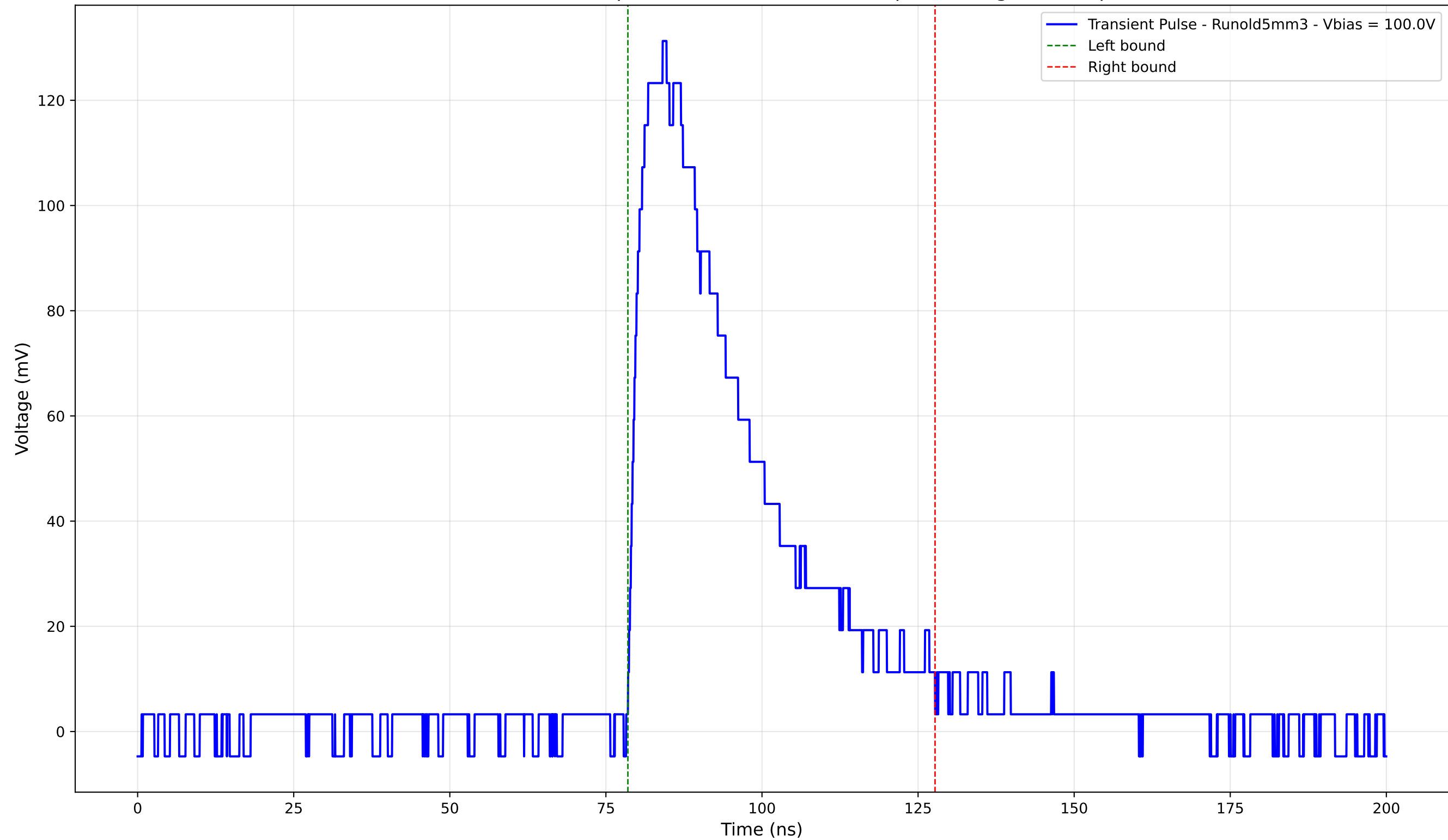
Transient Pulse - Sample: old5 - Position: 1635.0 \mu\text{m} - Charge: 51.33 pC
