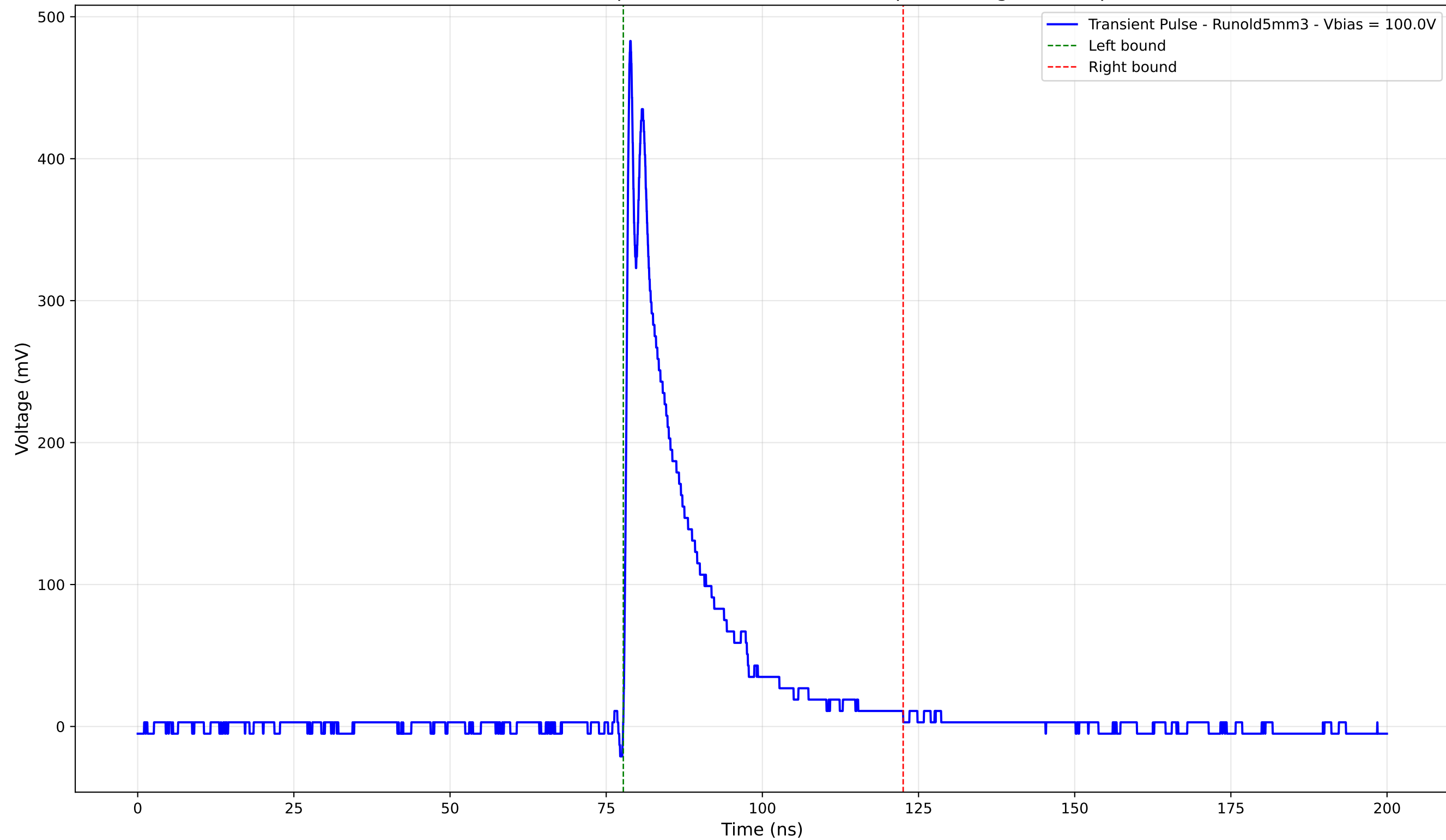
Transient Pulse - Sample: old5 - Position: 3795.0 \mu\text{m} - Charge: 83.42 pC
