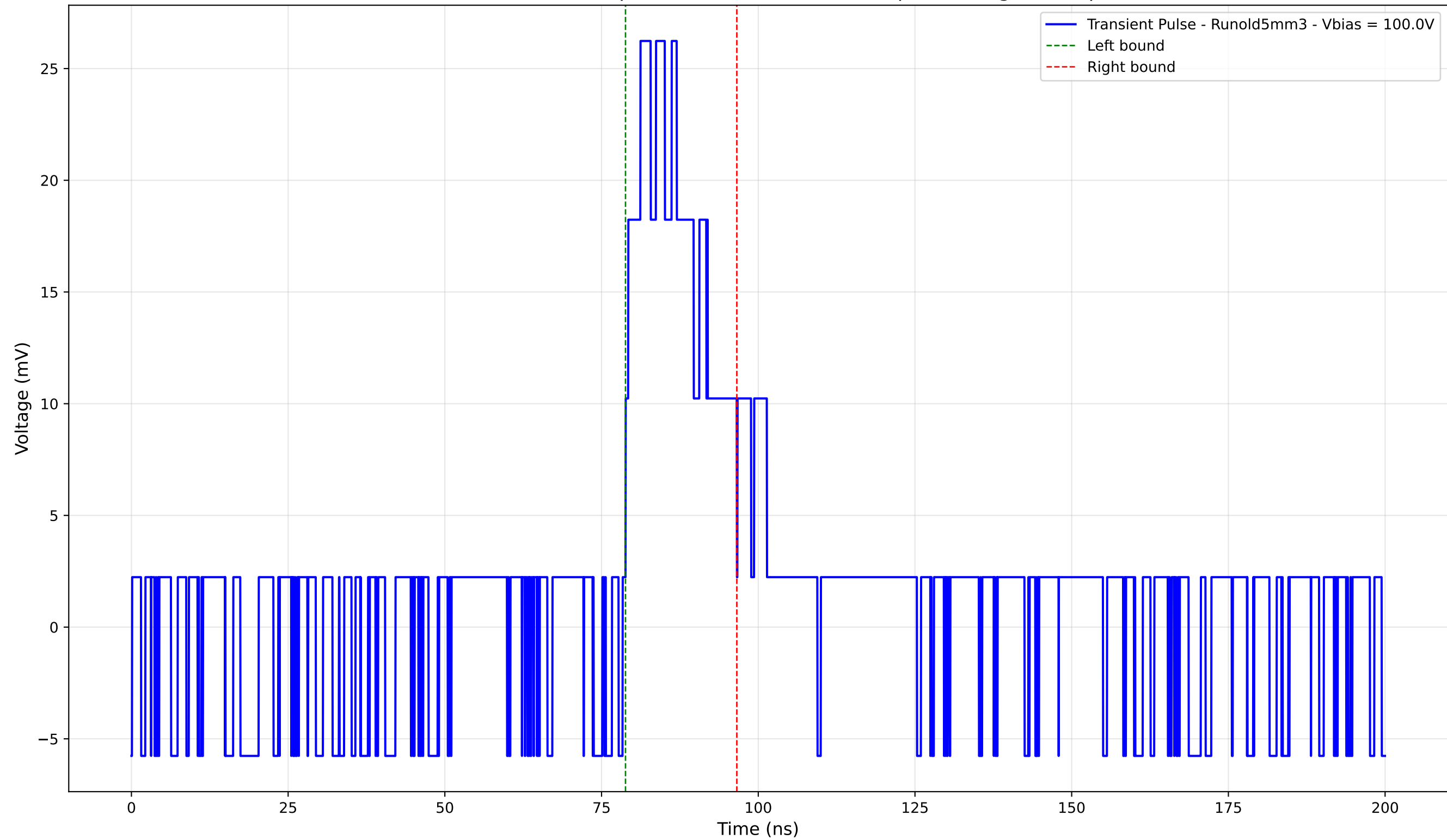
Transient Pulse - Sample: old5 - Position: 2645.0 \mu\text{m} - Charge: 6.12 pC
