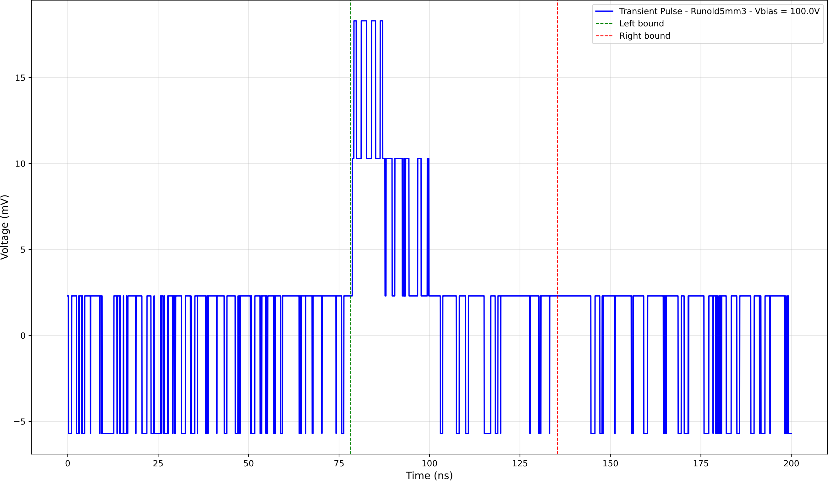
Transient Pulse - Sample: old5 - Position: 2975.0 \mu\text{m} - Charge: 4.82 pC
