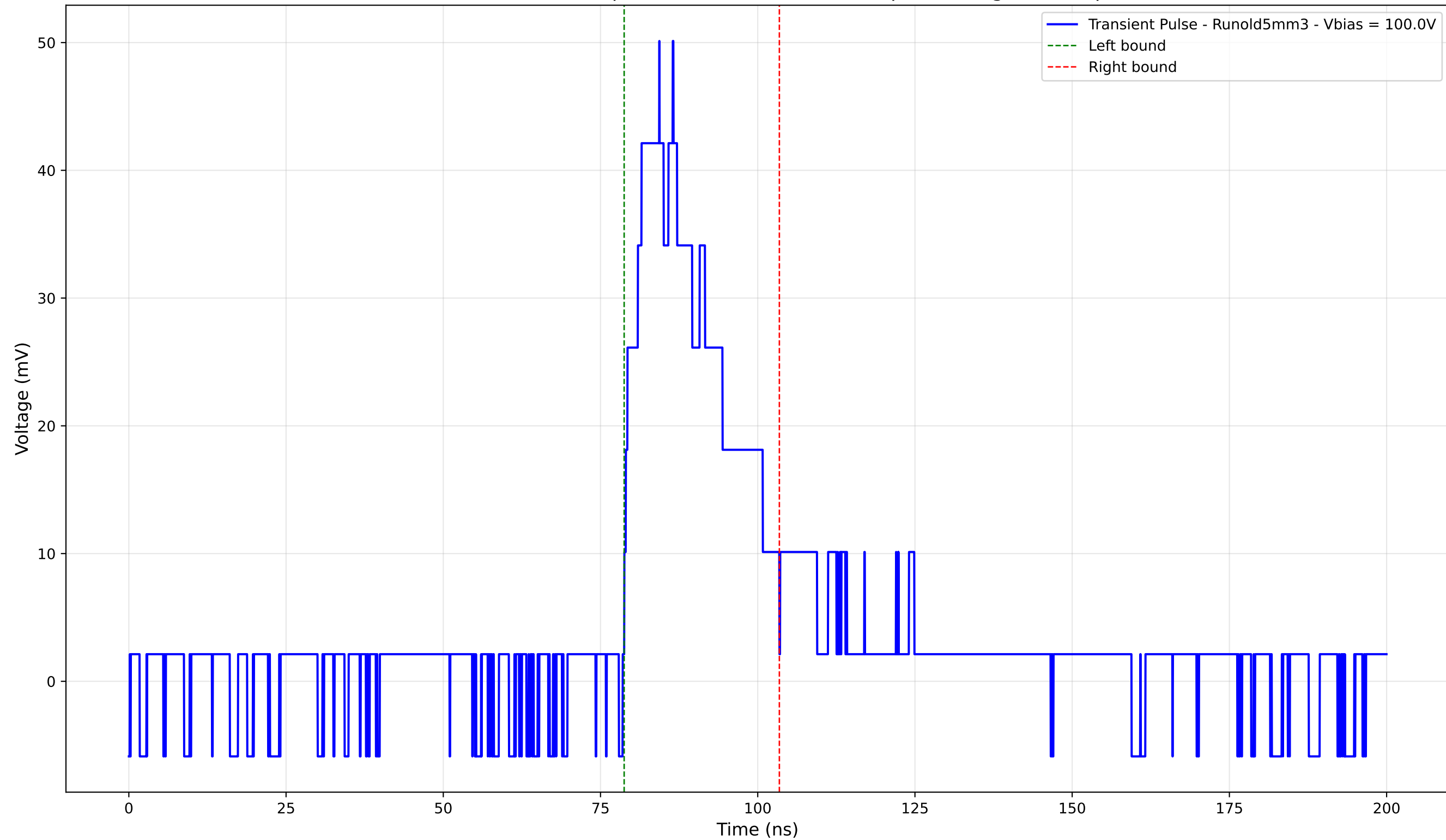
Transient Pulse - Sample: old5 - Position: 2385.0 \mu\text{m} - Charge: 13.23 pC
