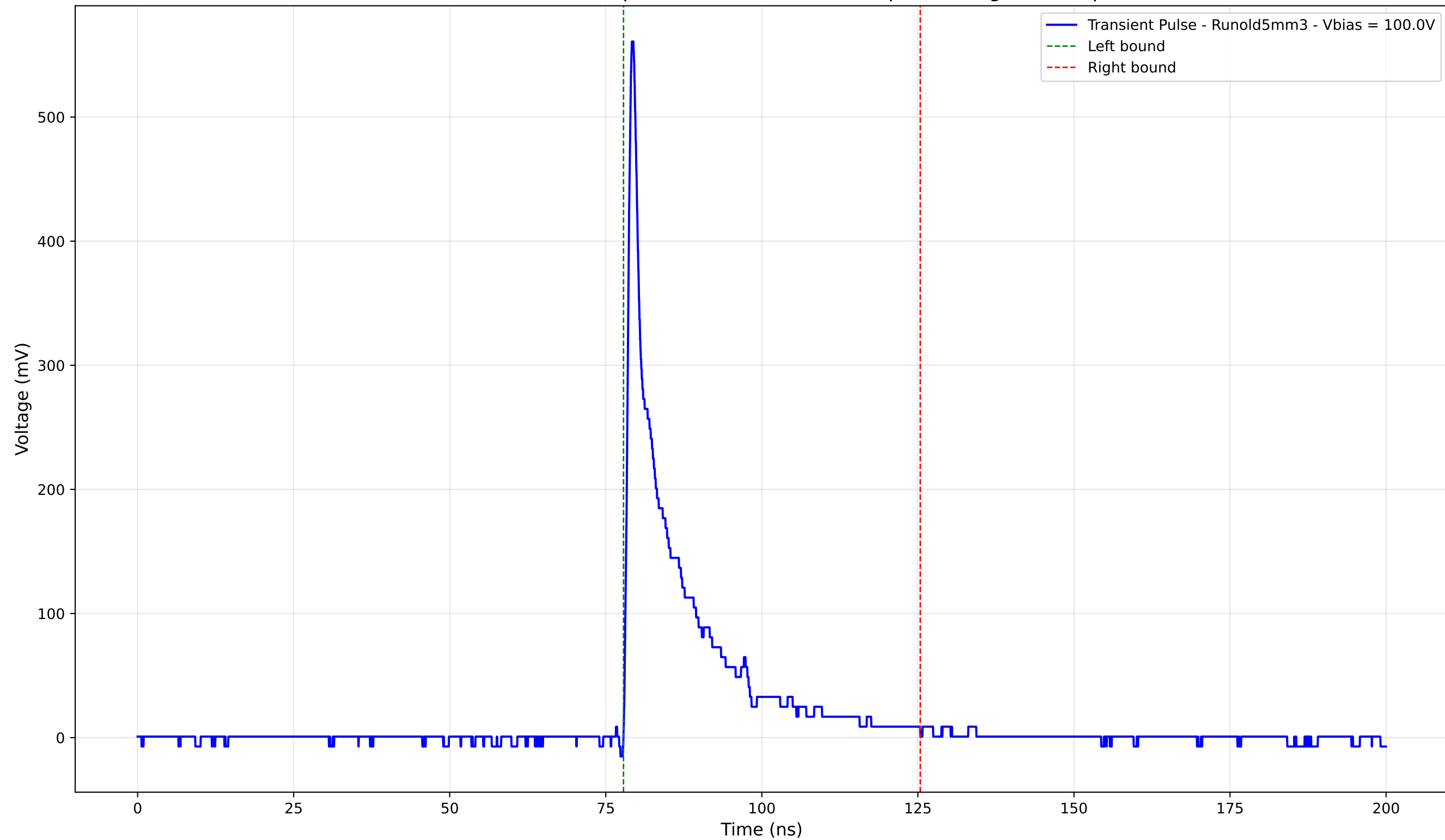
Transient Pulse - Sample: old5 - Position: 220.0 \mu\text{m} - Charge: 73.37 pC
