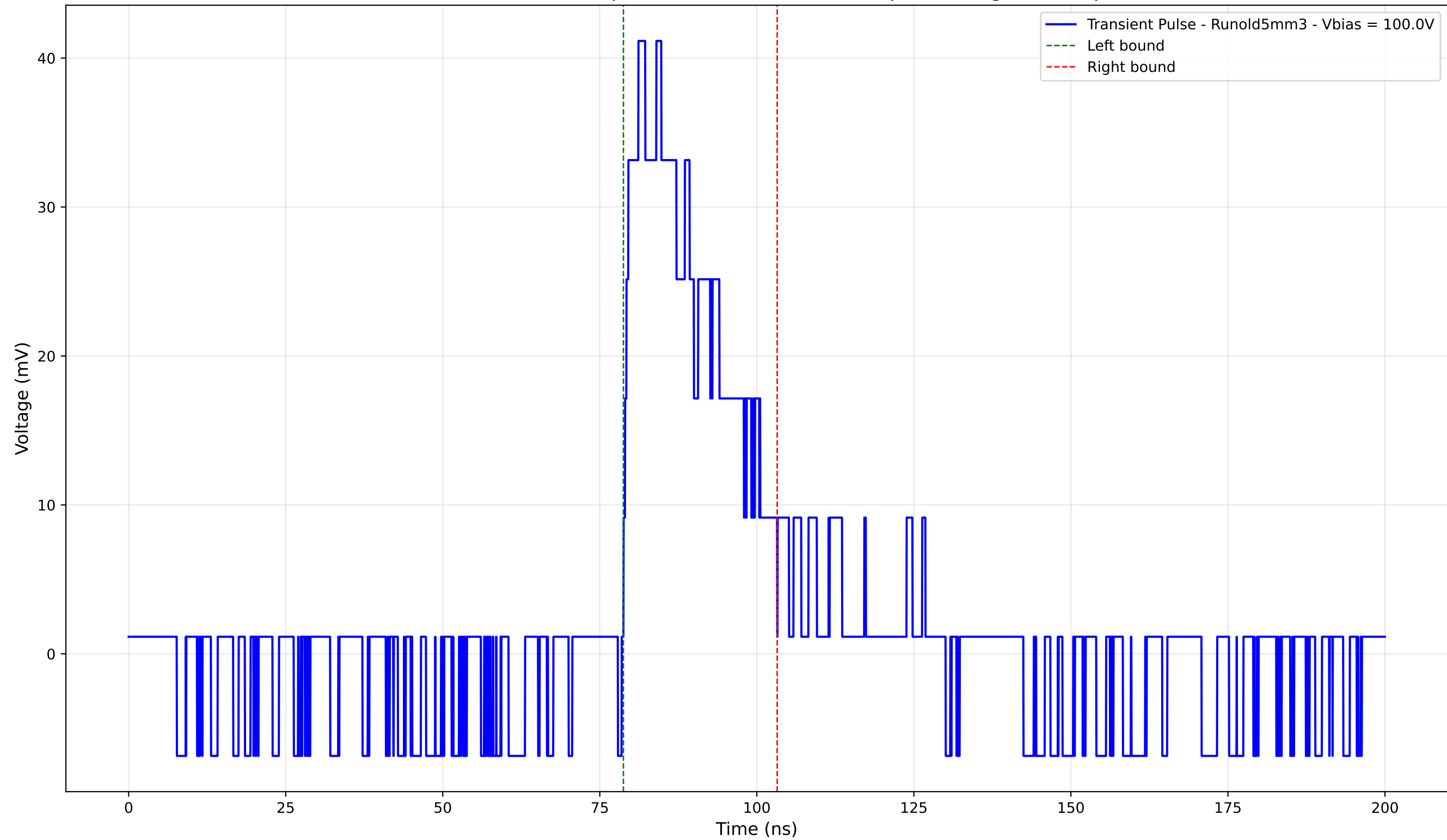
Transient Pulse - Sample: old5 - Position: 2635.0 \mu\text{m} - Charge: 11.70 pC
