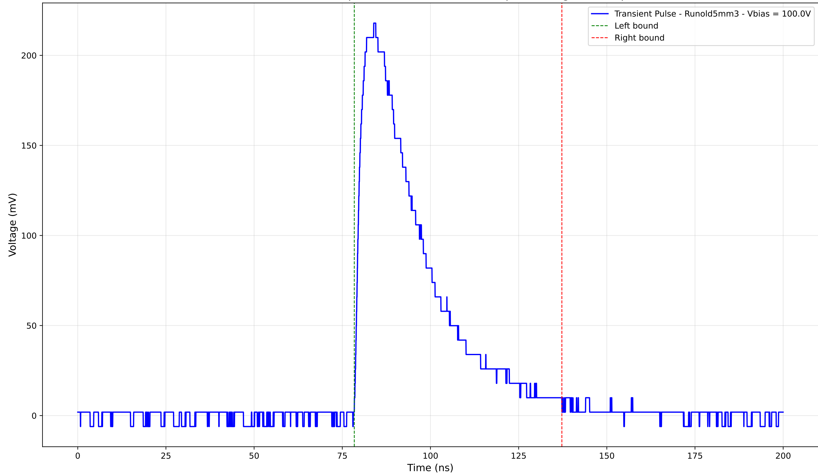
Transient Pulse - Sample: old5 - Position: 2075.0 \mu\text{m} - Charge: 86.73 pC
