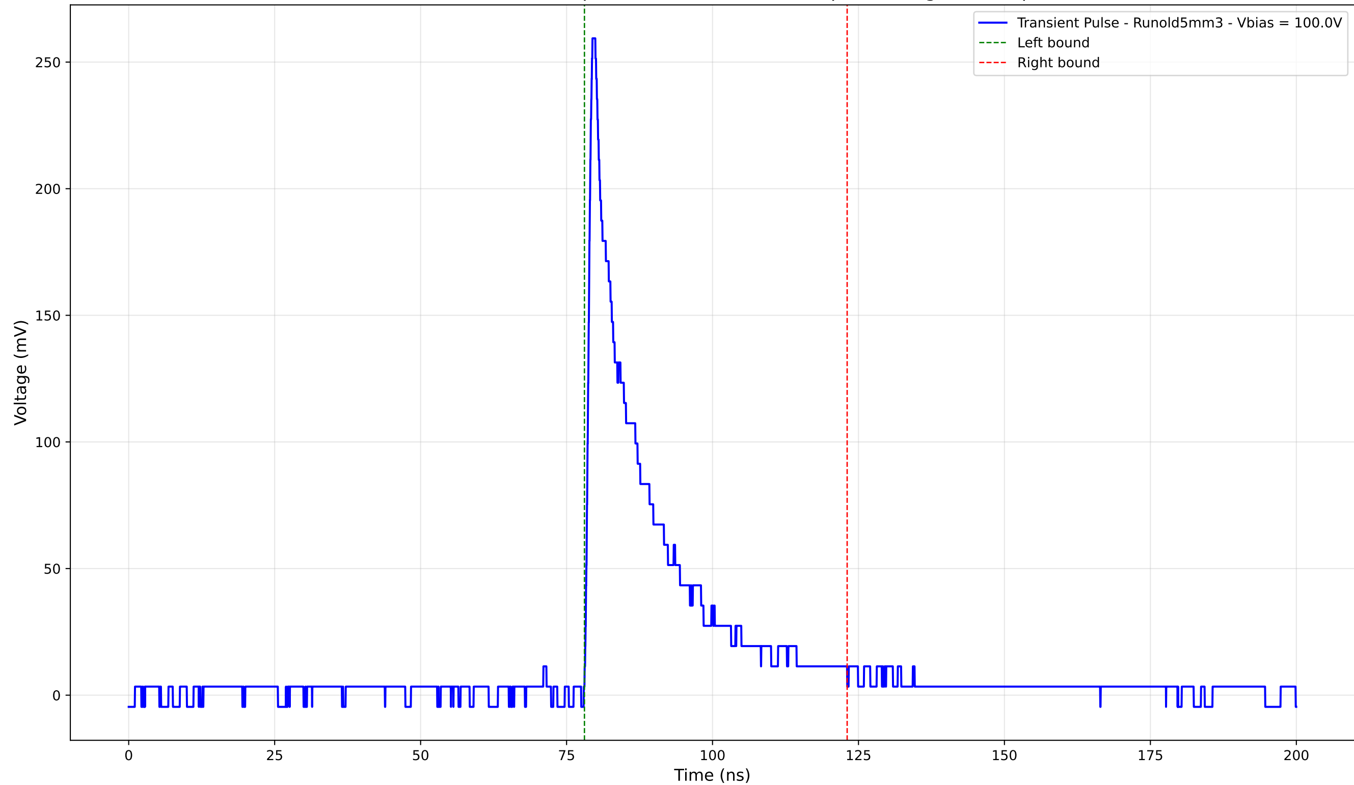
Transient Pulse - Sample: old5 - Position: 425.0 \mu\text{m} - Charge: 49.46 pC
