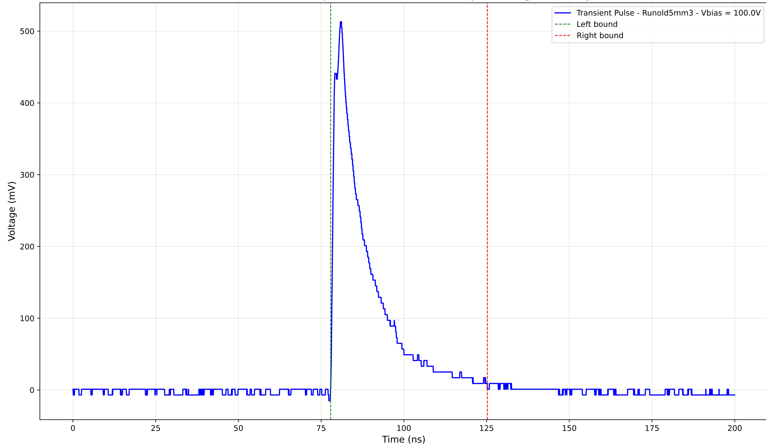
Transient Pulse - Sample: old5 - Position: 4025.0 \mu\text{m} - Charge: 111.07 pC
