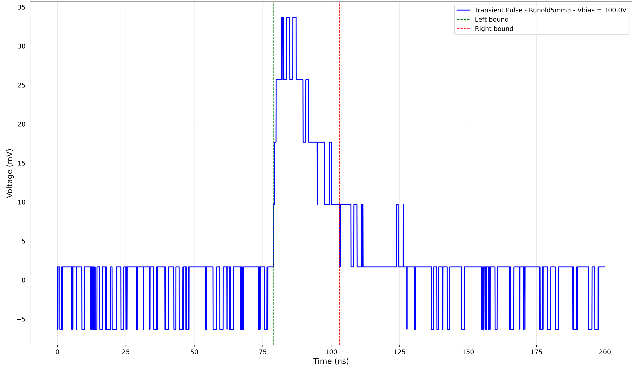
Transient Pulse - Sample: old5 - Position: 1380.0 \mu\text{m} - Charge: 9.94 pC
