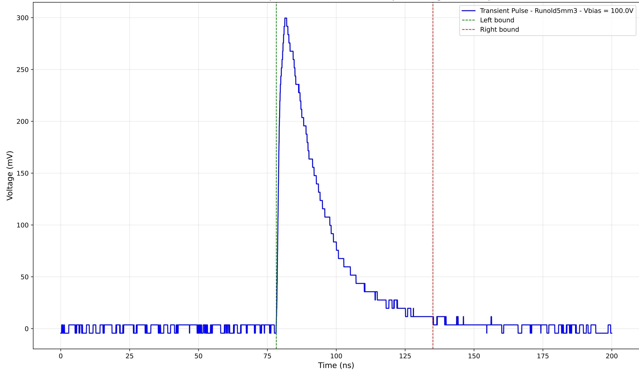
Transient Pulse - Sample: old5 - Position: 2790.0 \mu\text{m} - Charge: 100.46 pC
