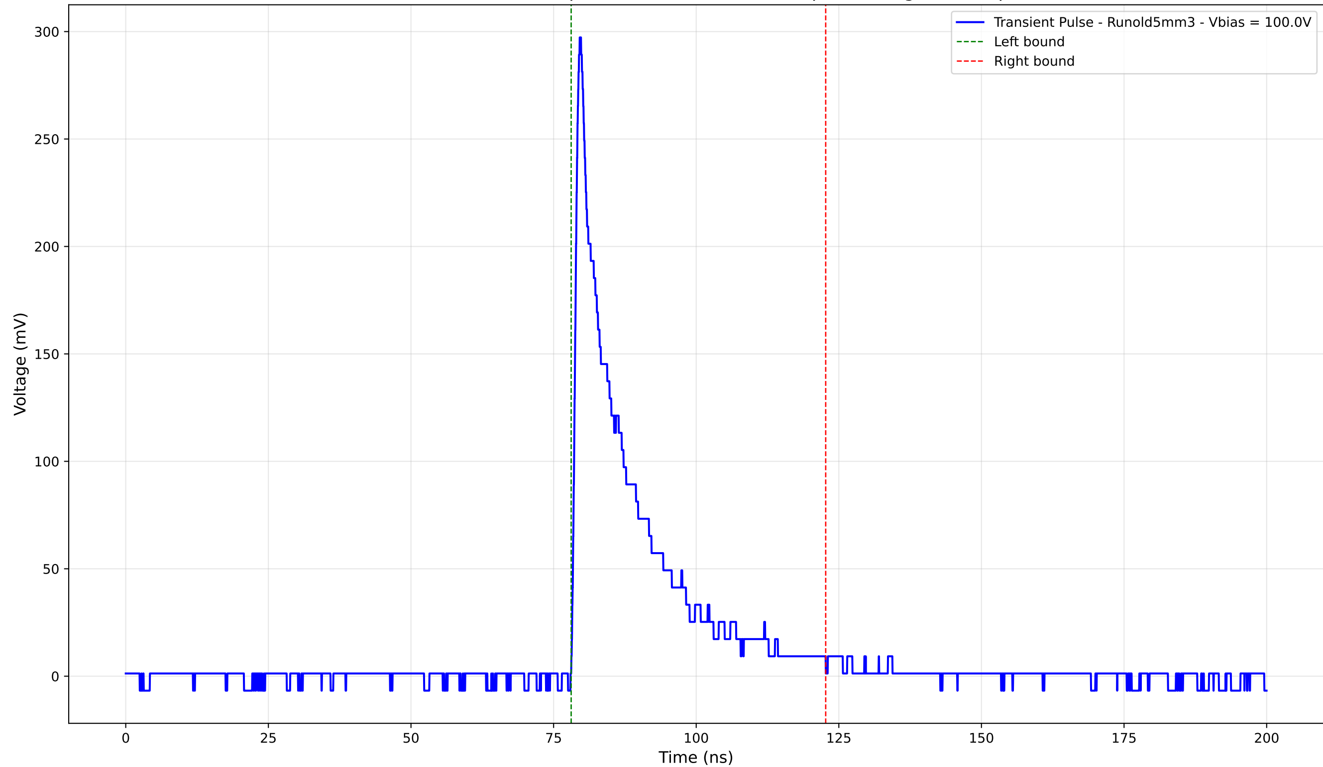
Transient Pulse - Sample: old5 - Position: 435.0 \mu\text{m} - Charge: 52.73 pC
