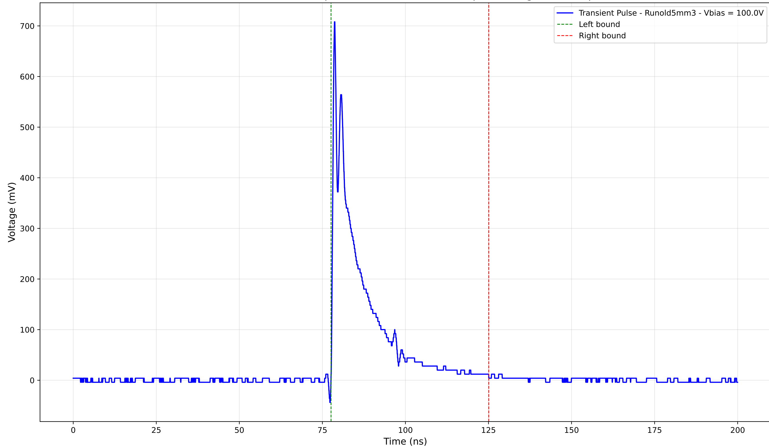
Transient Pulse - Sample: old5 - Position: 3700.0 \mu\text{m} - Charge: 105.97 pC
