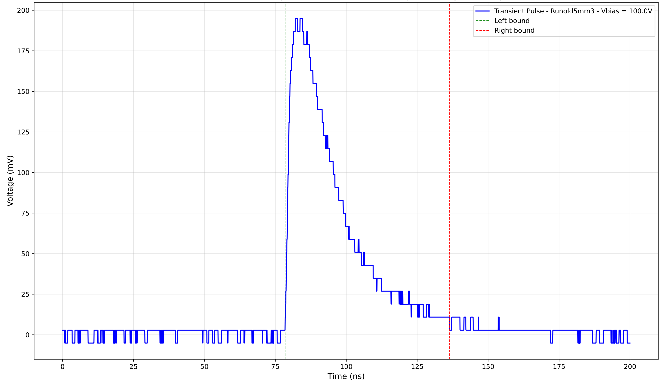
Transient Pulse - Sample: old5 - Position: 1465.0 \mu\text{m} - Charge: 78.58 pC
