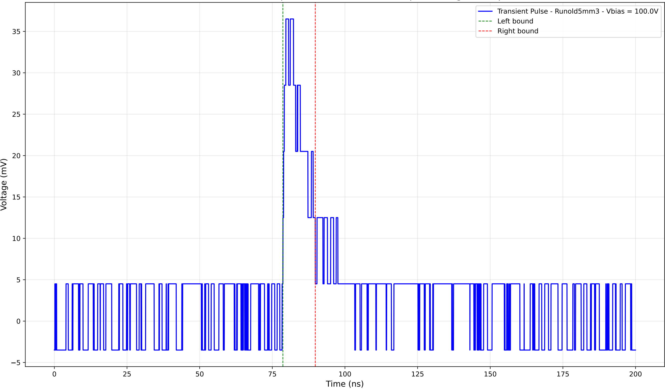
Transient Pulse - Sample: old5 - Position: 4480.0 \mu\text{m} - Charge: 5.34 pC
