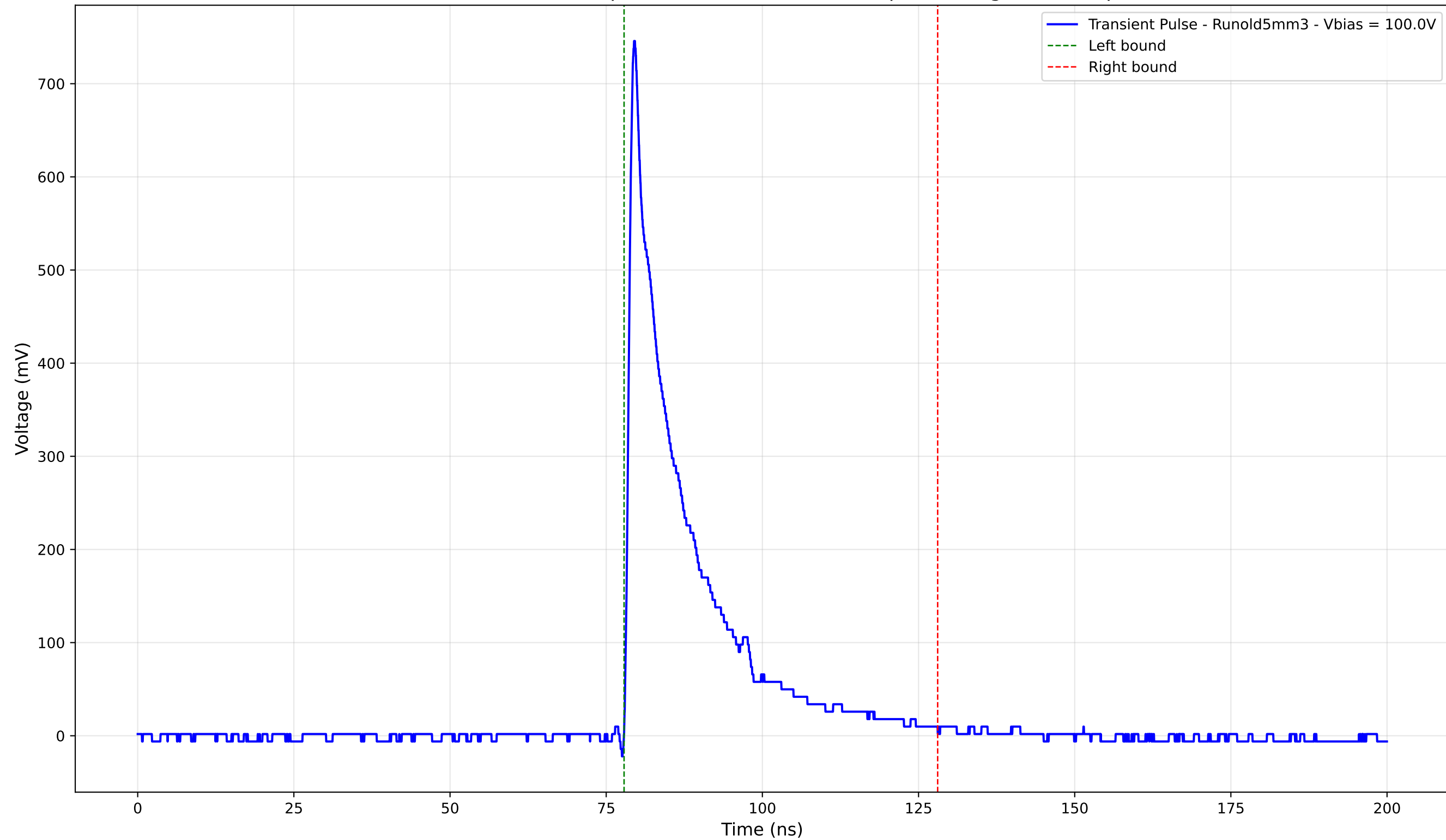
Transient Pulse - Sample: old5 - Position: 4725.0 \mu\text{m} - Charge: 131.07 pC
