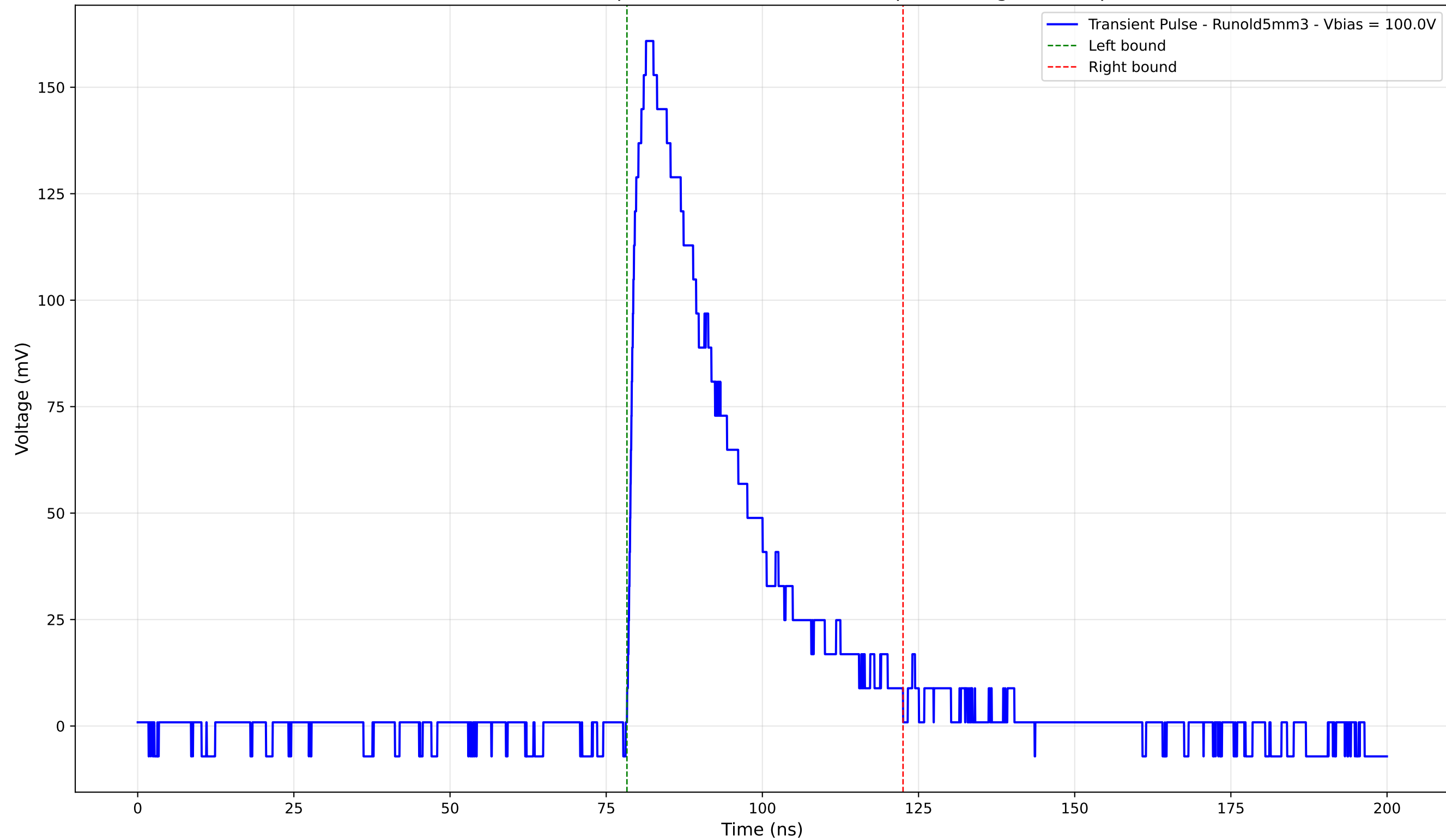
Transient Pulse - Sample: old5 - Position: 2745.0 \mu\text{m} - Charge: 52.01 pC
