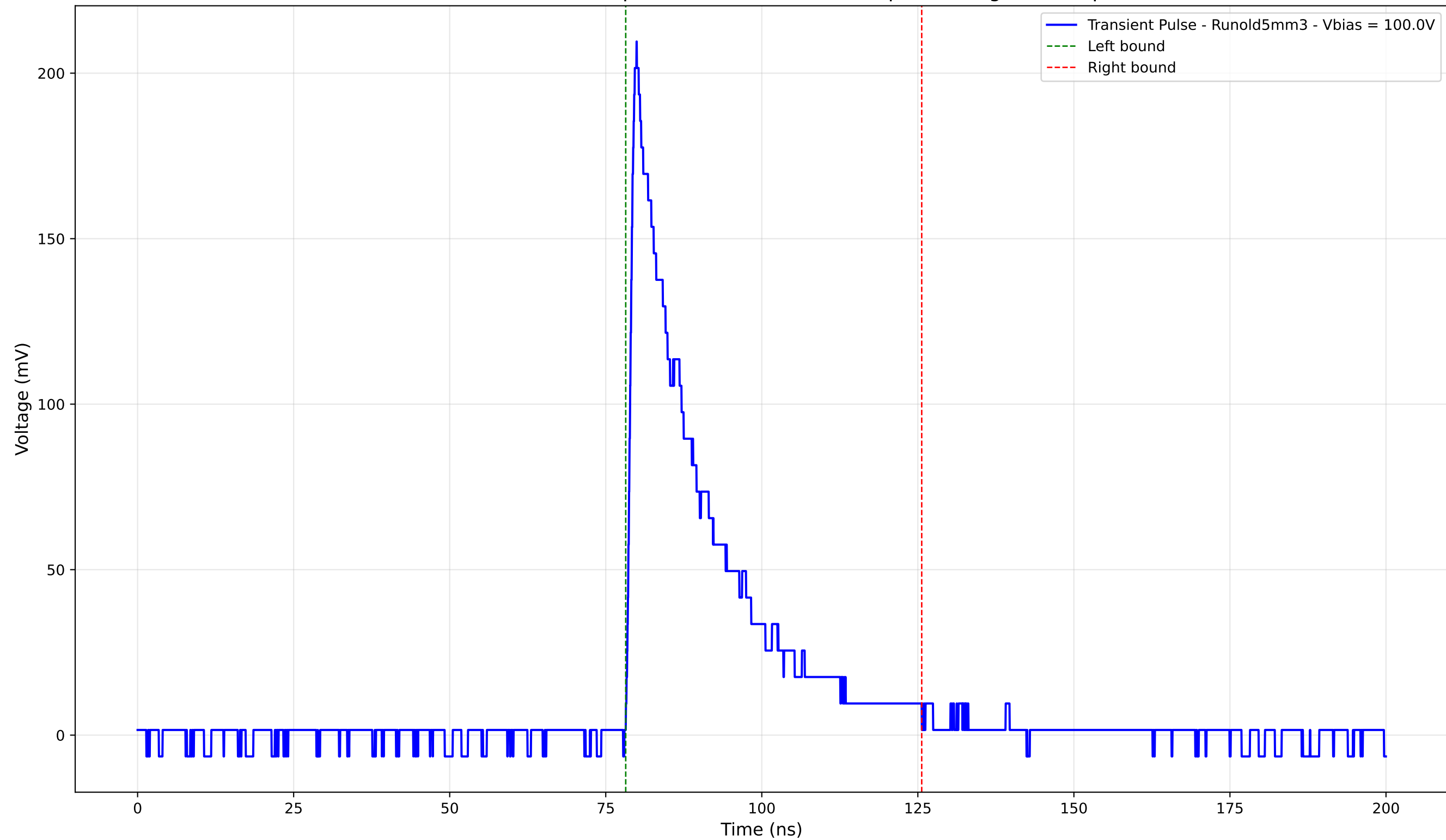
Transient Pulse - Sample: old5 - Position: 625.0 \mu\text{m} - Charge: 48.04 pC
