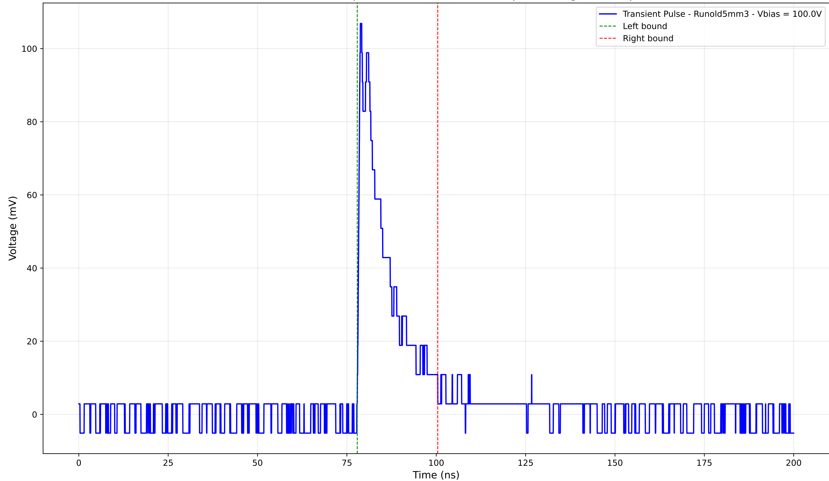
Transient Pulse - Sample: old5 - Position: 3845.0 \mu\text{m} - Charge: 17.35 pC
