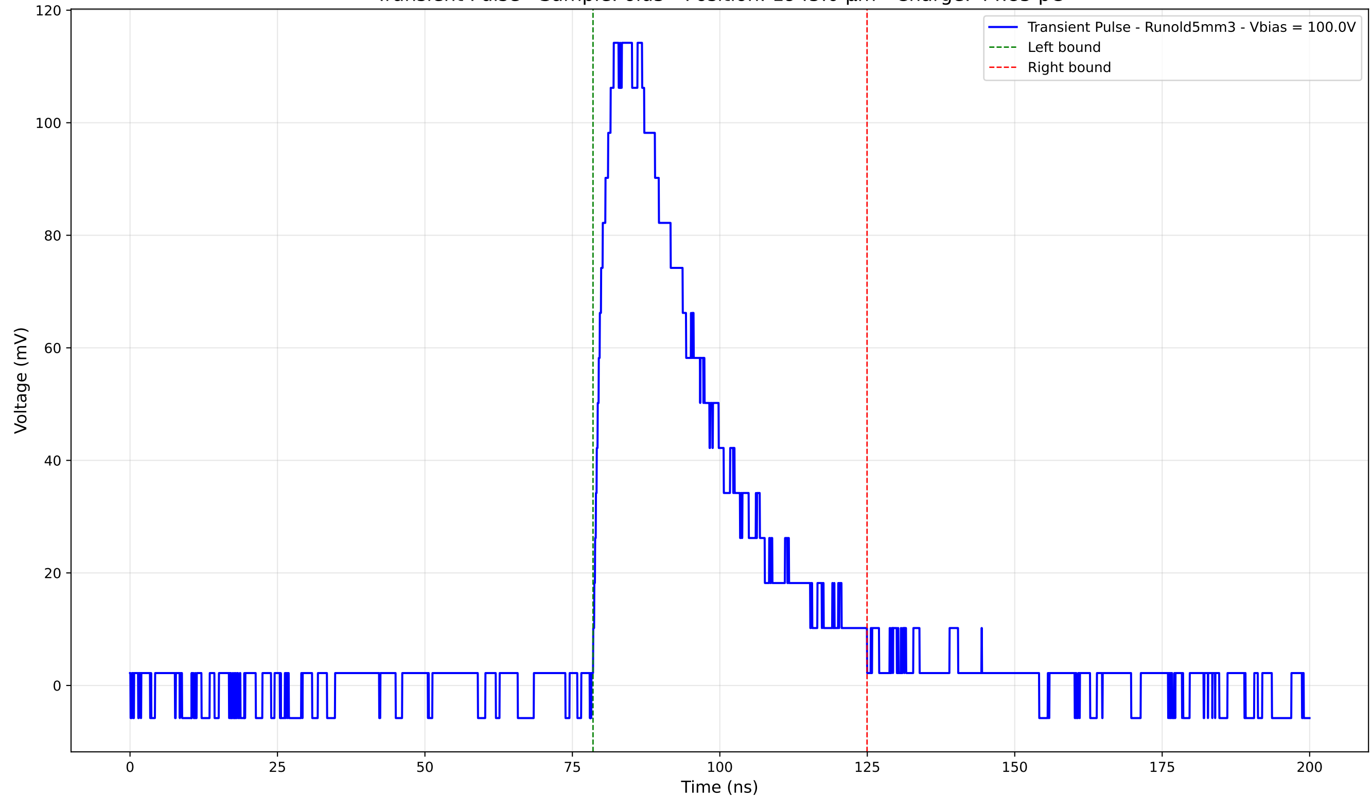
Transient Pulse - Sample: old5 - Position: 1945.0 \mu\text{m} - Charge: 44.85 pC
