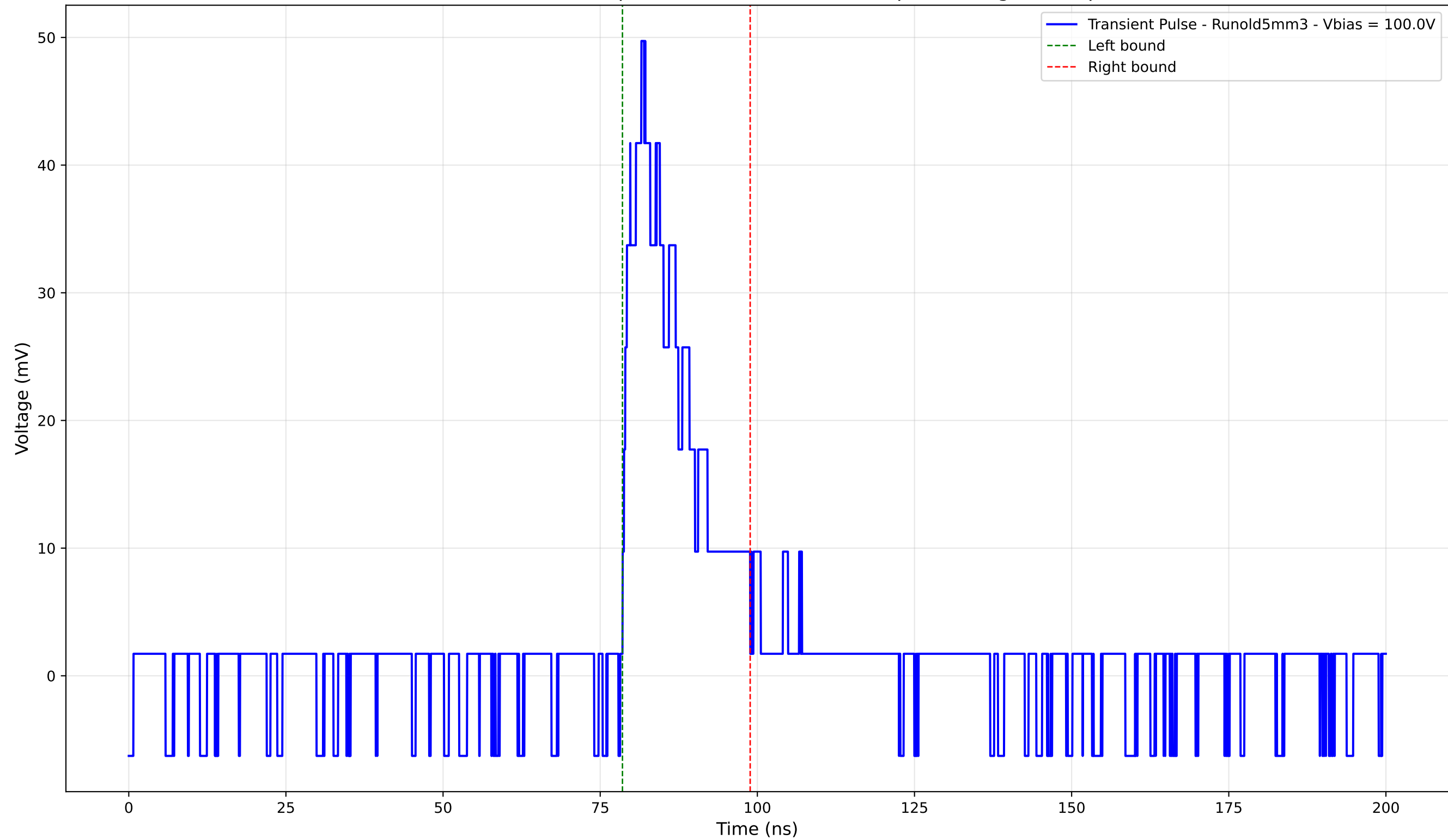
Transient Pulse - Sample: old5 - Position: 4205.0 \mu\text{m} - Charge: 9.18 pC
