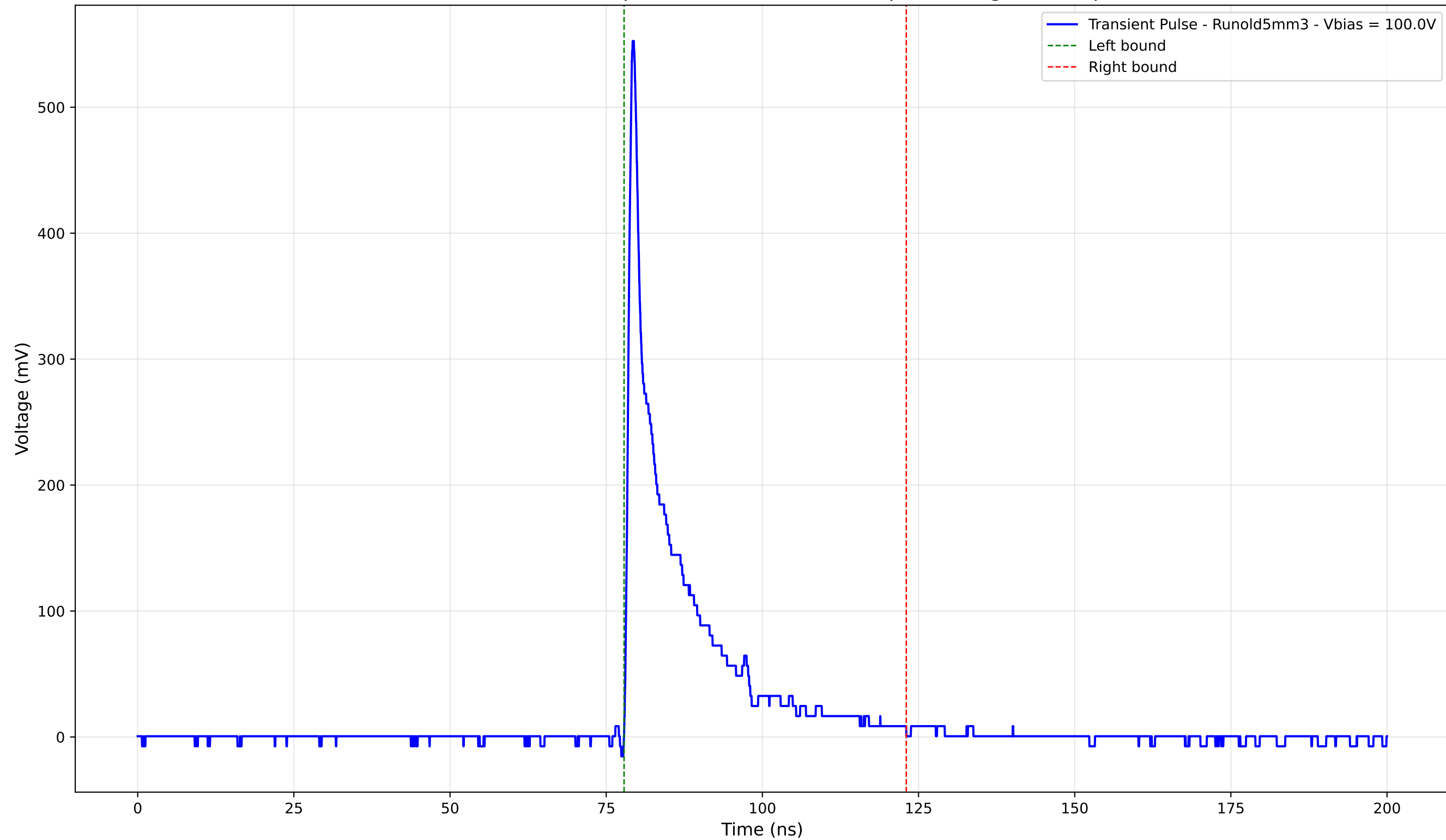
Transient Pulse - Sample: old5 - Position: 240.0 \mu\text{m} - Charge: 72.55 pC
