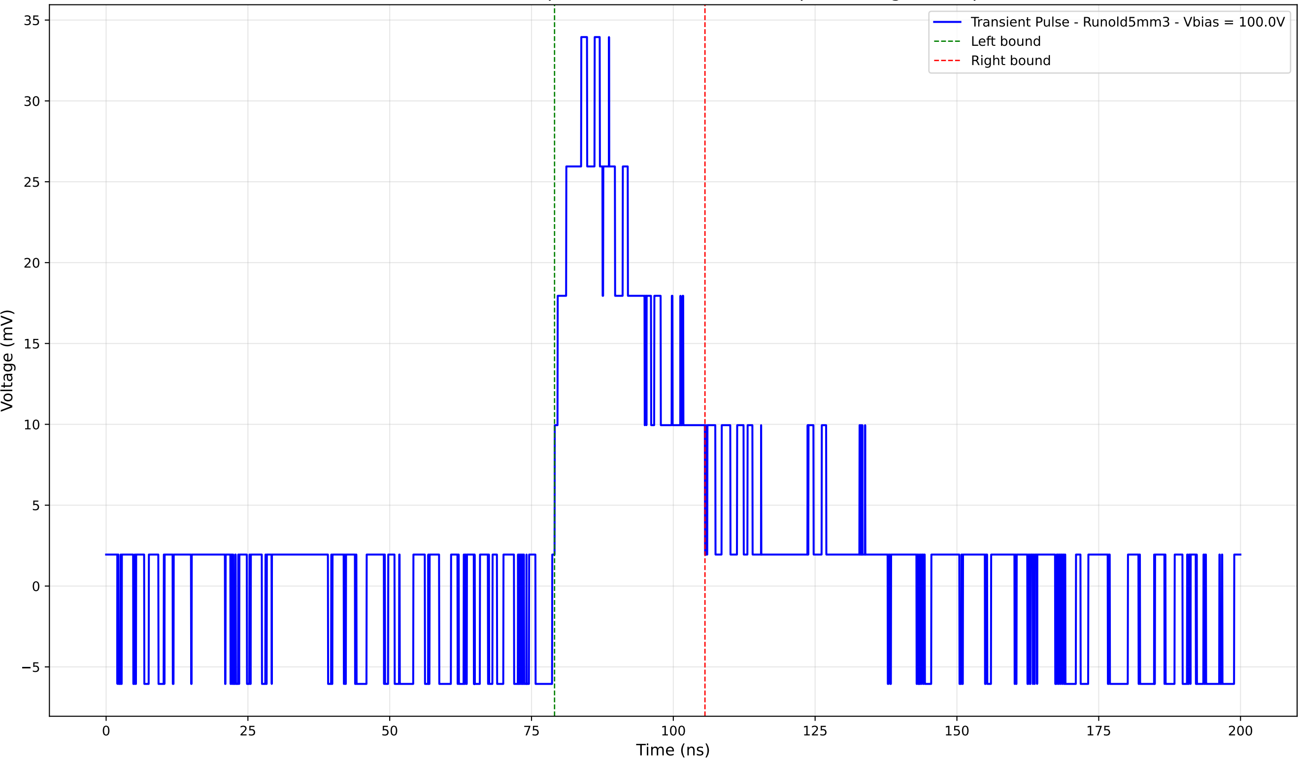
Transient Pulse - Sample: old5 - Position: 1790.0 \mu\text{m} - Charge: 9.95 pC
