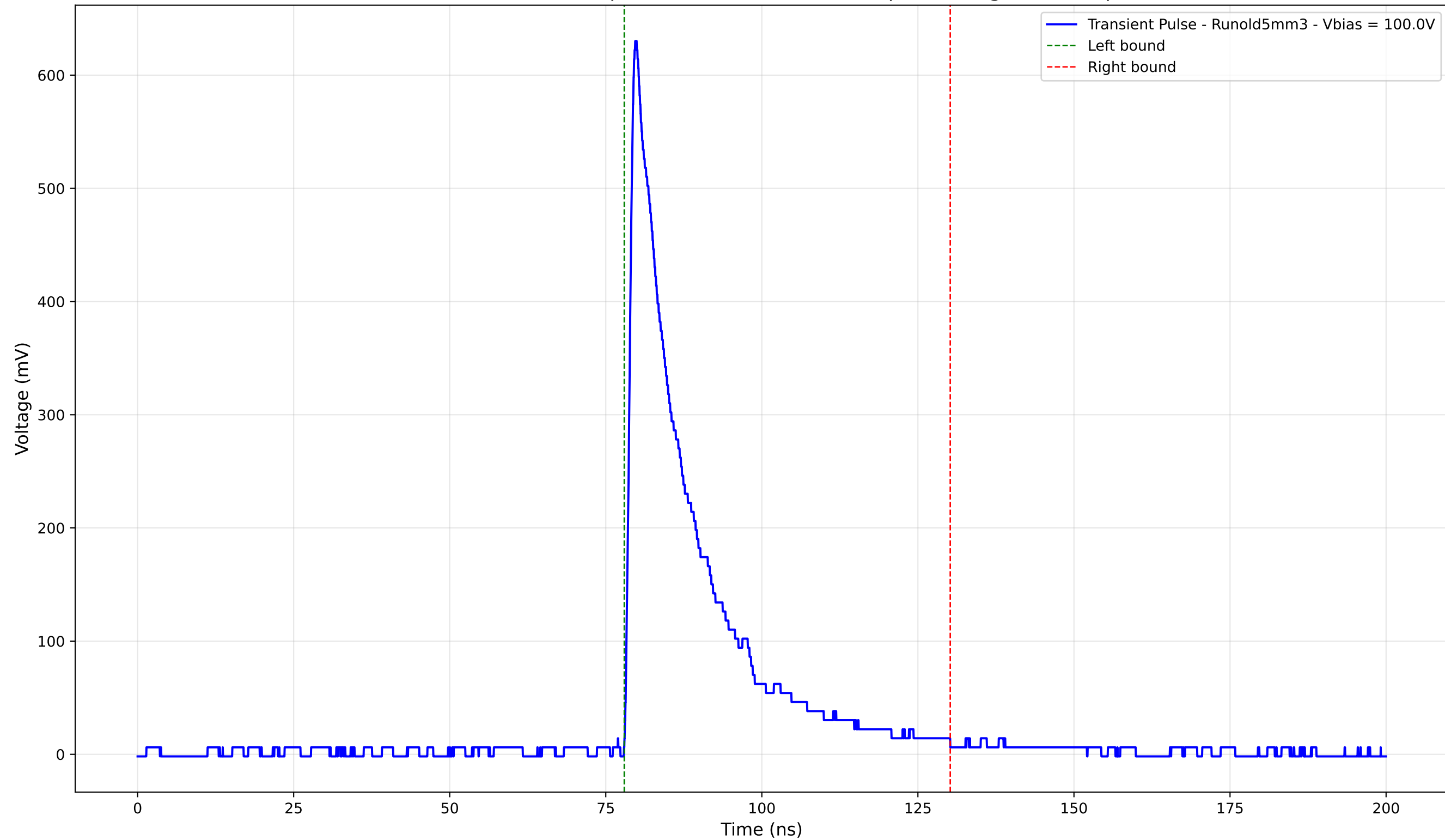
Transient Pulse - Sample: old5 - Position: 4625.0 \mu\text{m} - Charge: 127.29 pC
