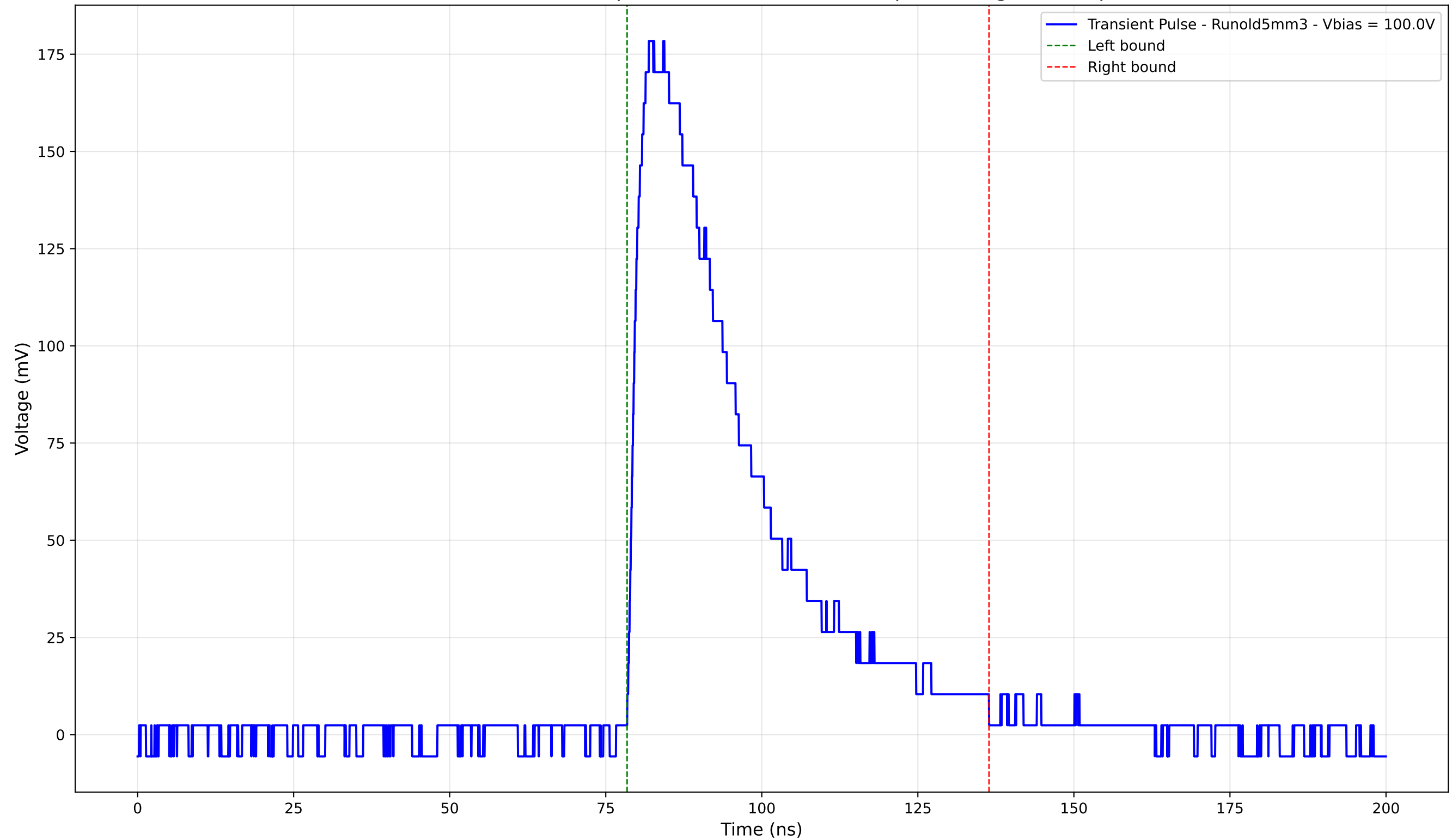
Transient Pulse - Sample: old5 - Position: 1515.0 \mu\text{m} - Charge: 70.16 pC
