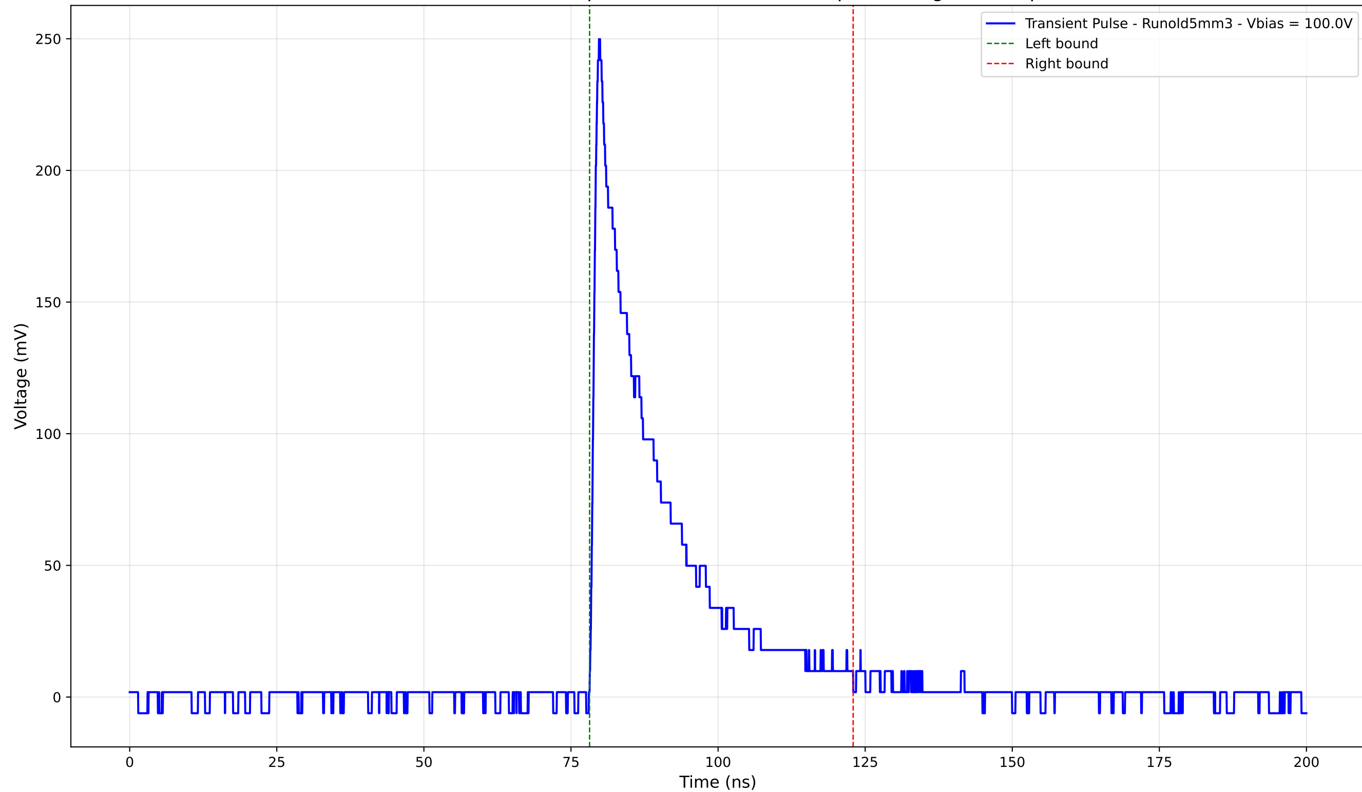
Transient Pulse - Sample: old5 - Position: 565.0 \mu\text{m} - Charge: 52.94 pC
