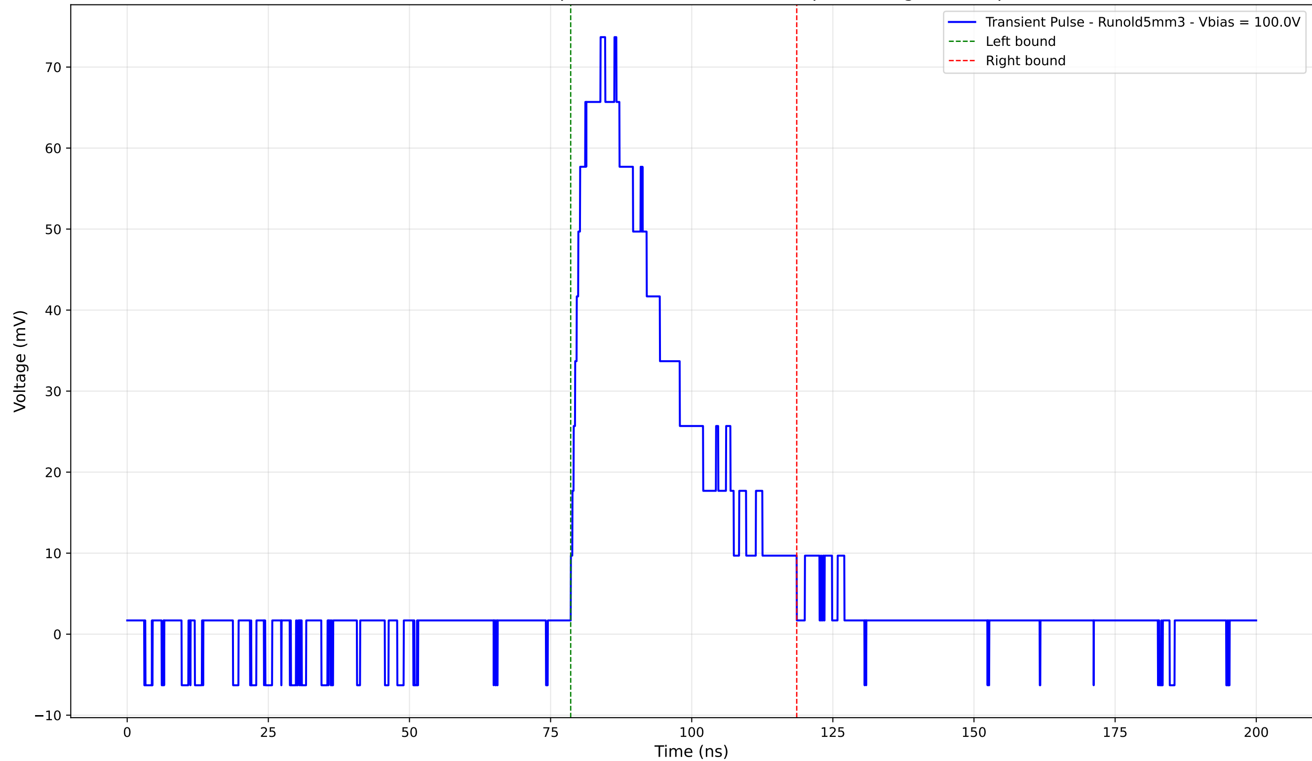
Transient Pulse - Sample: old5 - Position: 1555.0 \mu\text{m} - Charge: 26.52 pC
