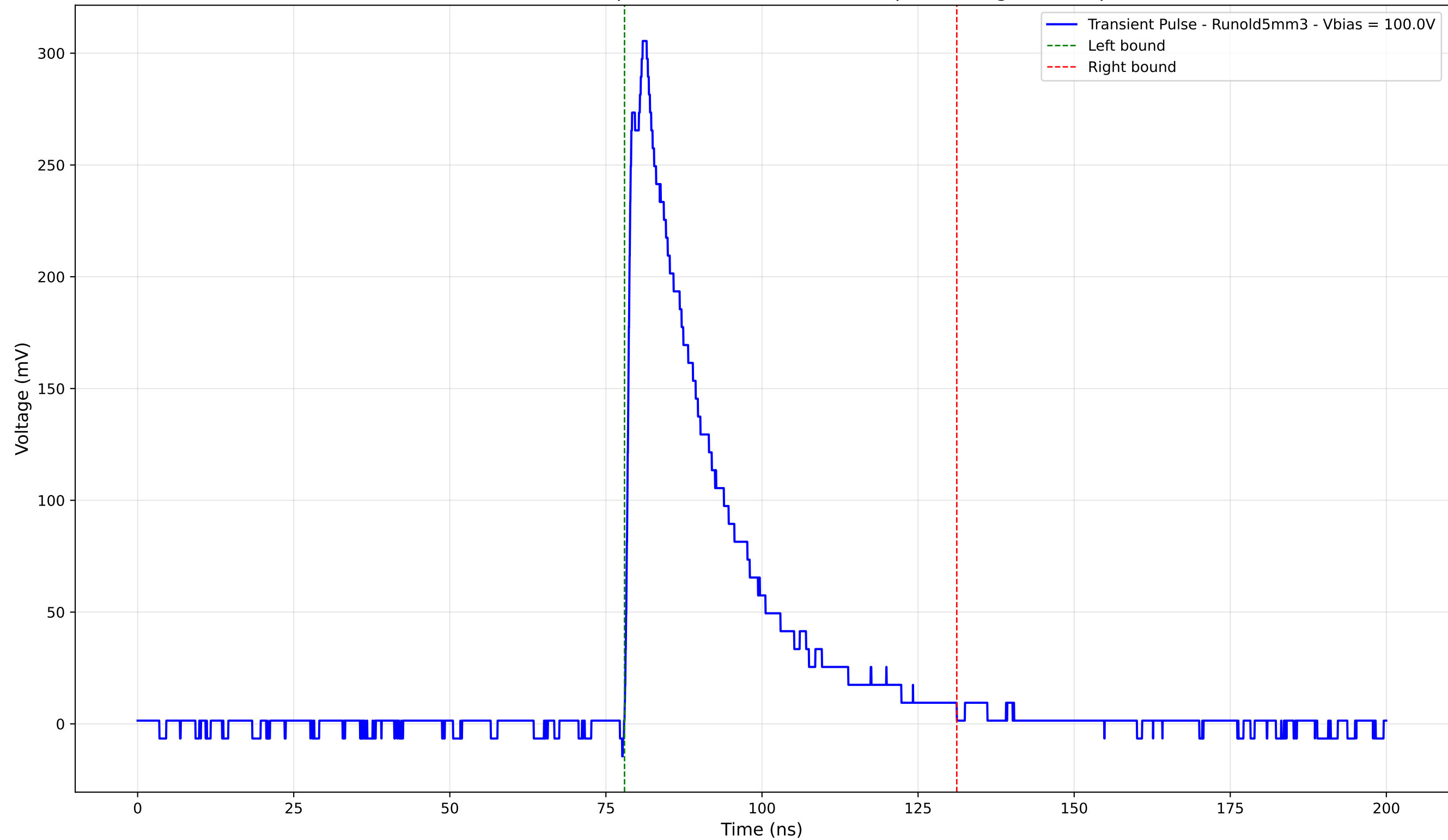
Transient Pulse - Sample: old5 - Position: 3070.0 \mu\text{m} - Charge: 84.84 pC
