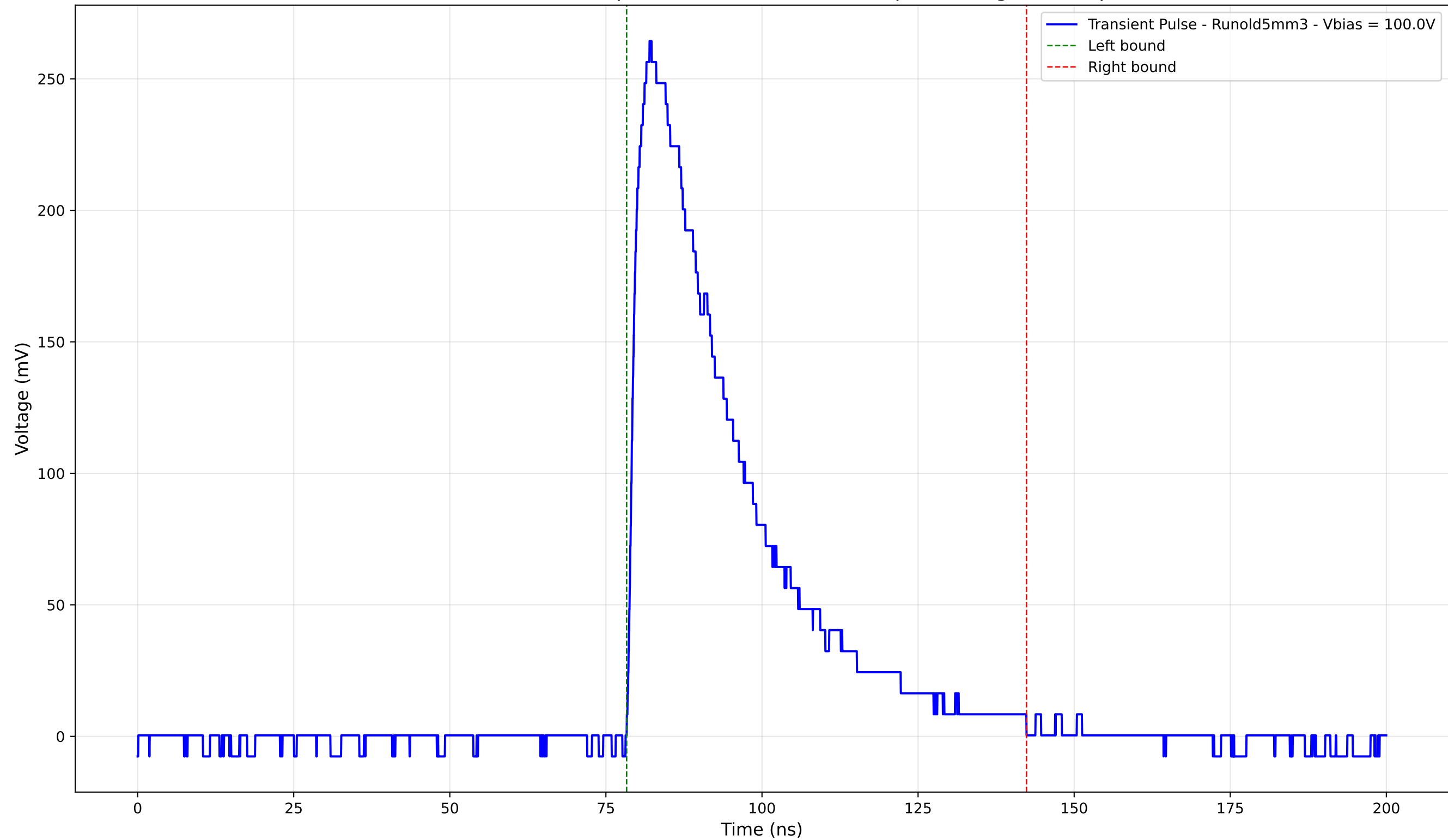
Transient Pulse - Sample: old5 - Position: 2560.0 \mu\text{m} - Charge: 96.01 pC
