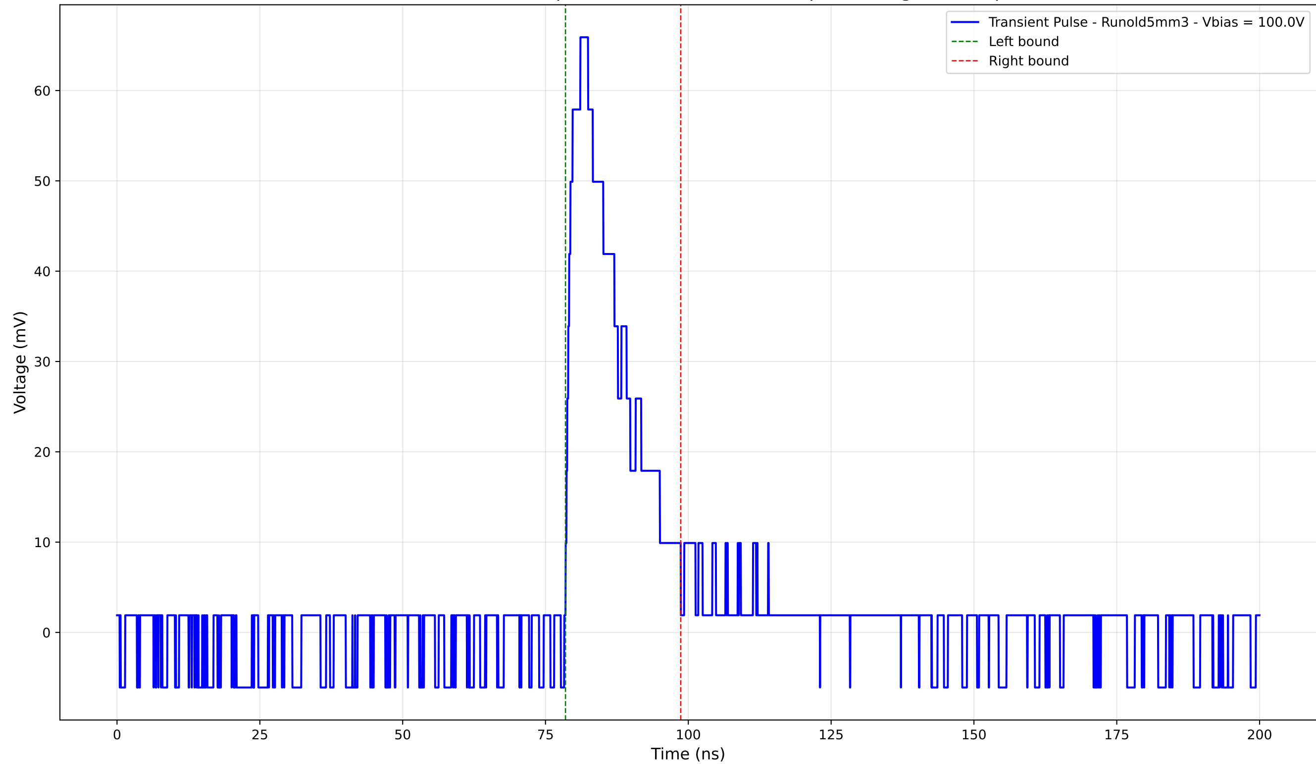
Transient Pulse - Sample: old5 - Position: 4215.0 \mu\text{m} - Charge: 13.04 pC
