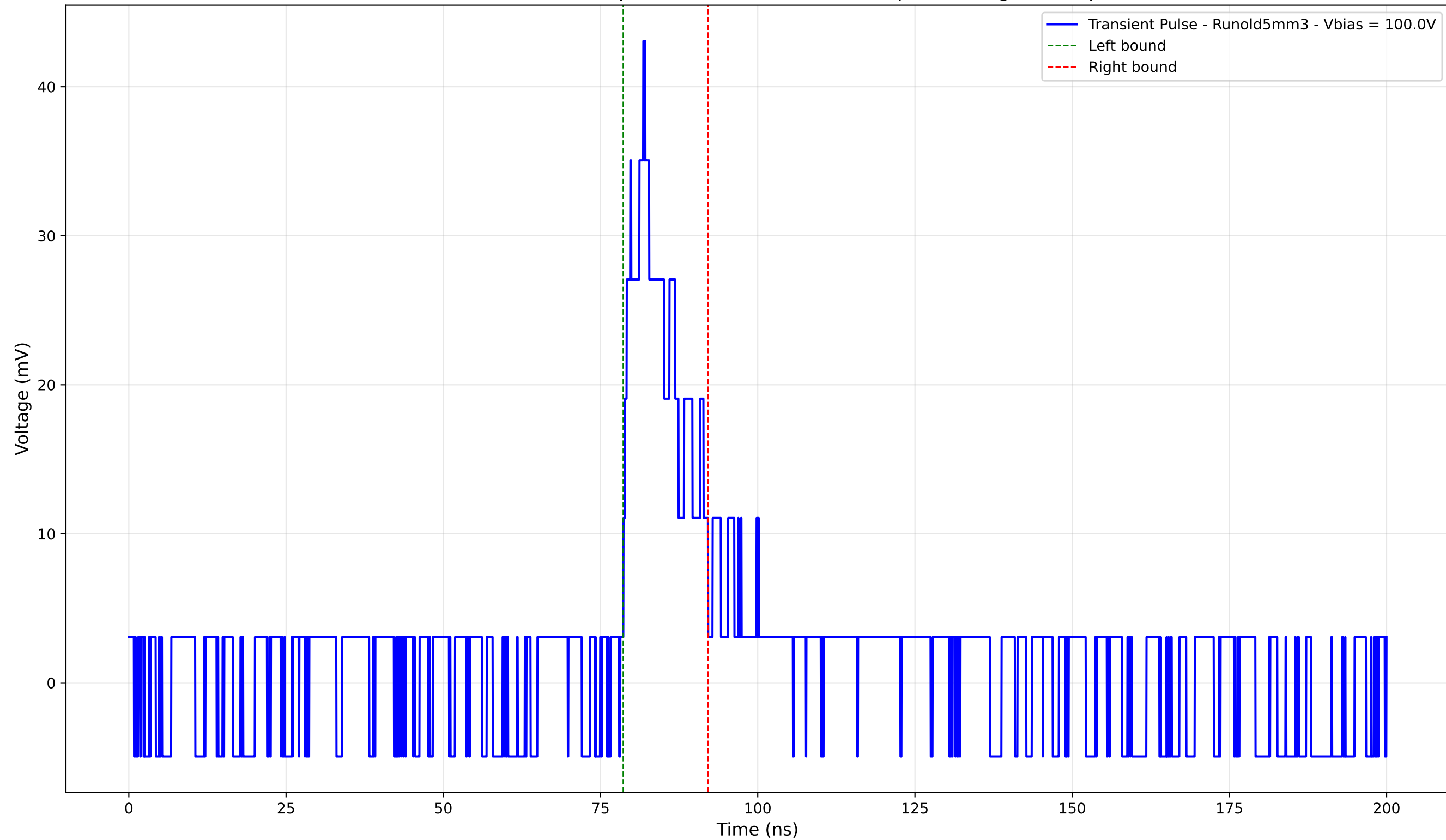
Transient Pulse - Sample: old5 - Position: 4505.0 \mu\text{m} - Charge: 6.04 pC
