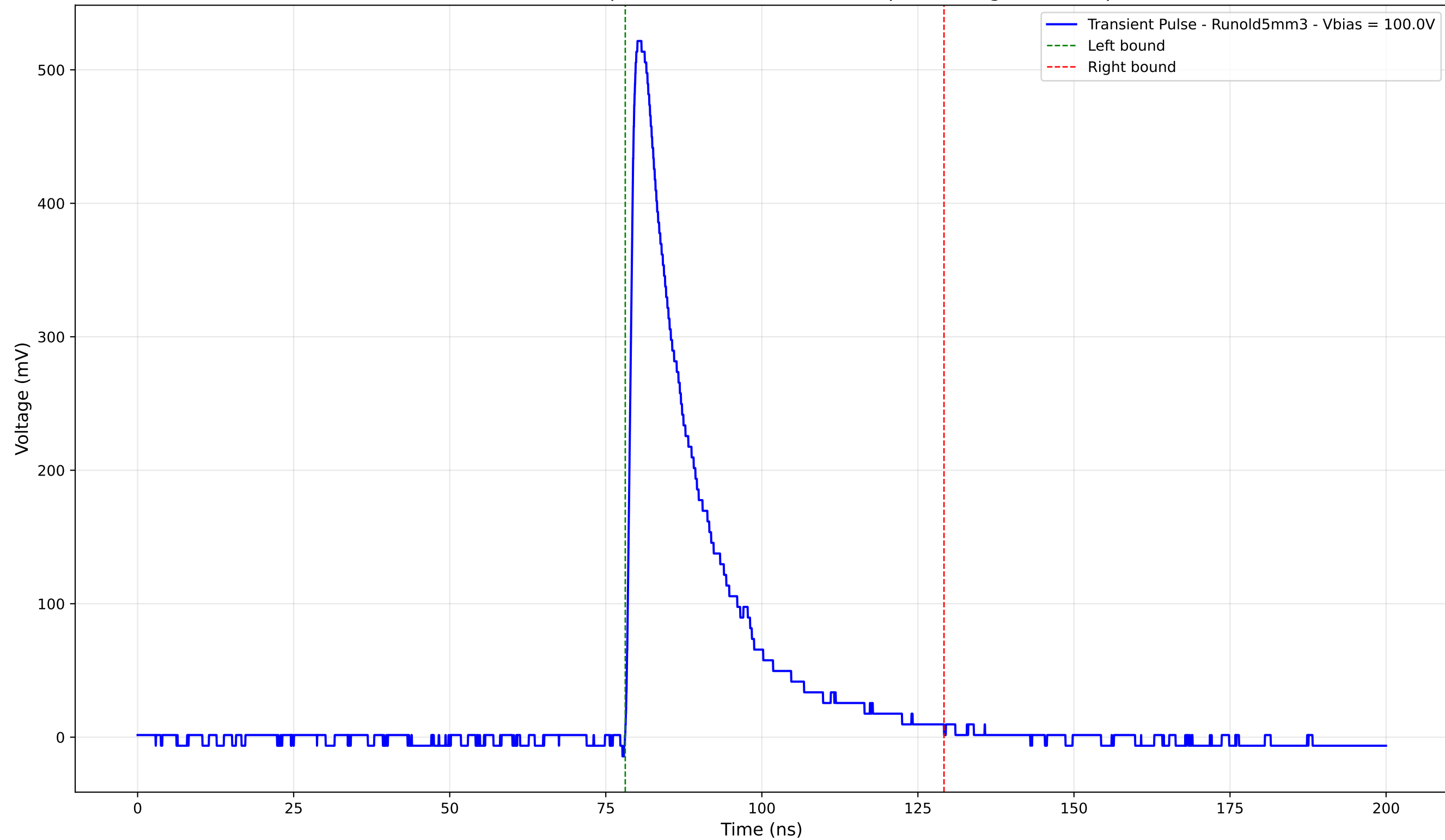
Transient Pulse - Sample: old5 - Position: 4345.0 \mu\text{m} - Charge: 117.87 pC
