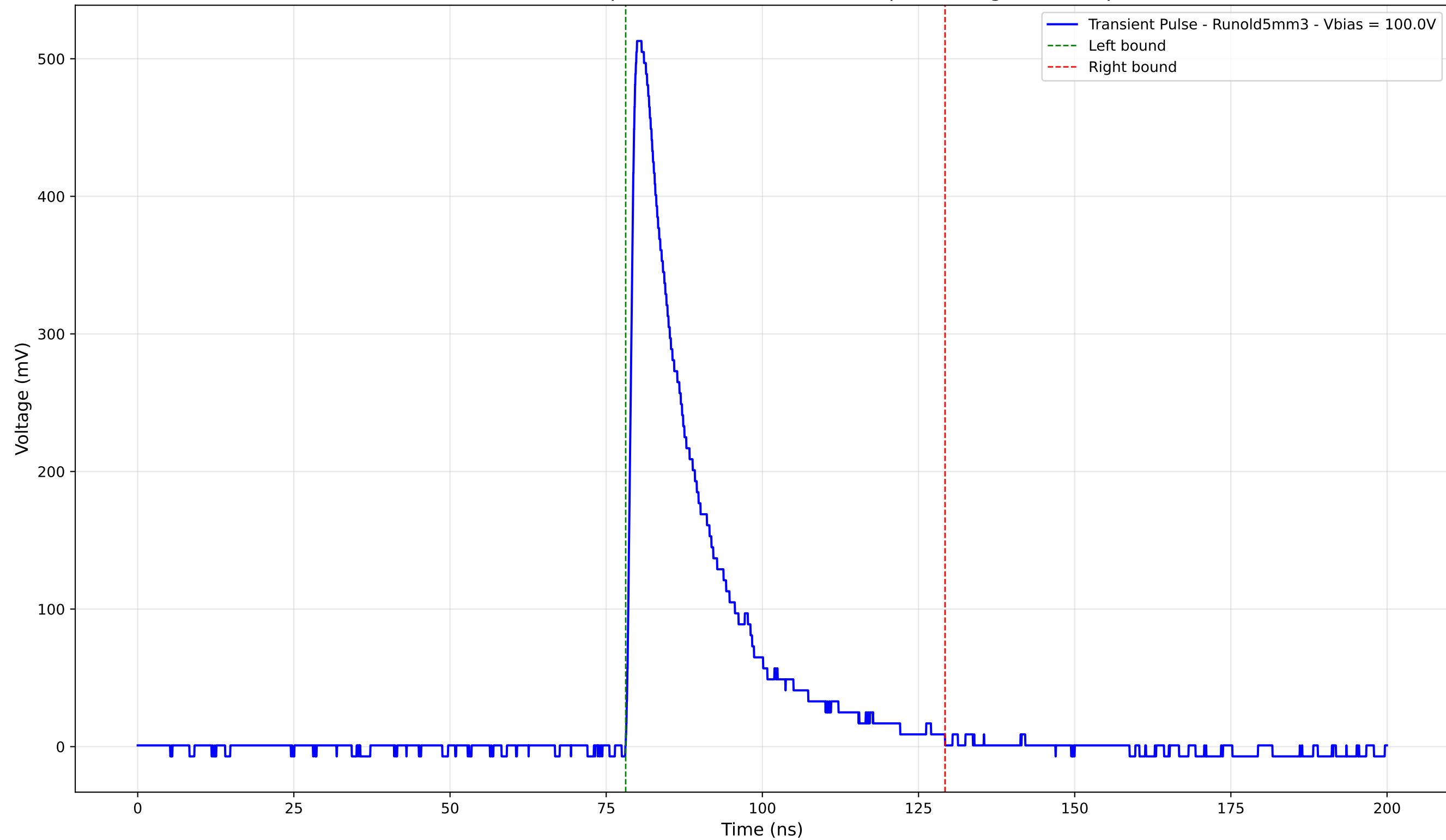
Transient Pulse - Sample: old5 - Position: 4370.0 \mu\text{m} - Charge: 114.96 pC
