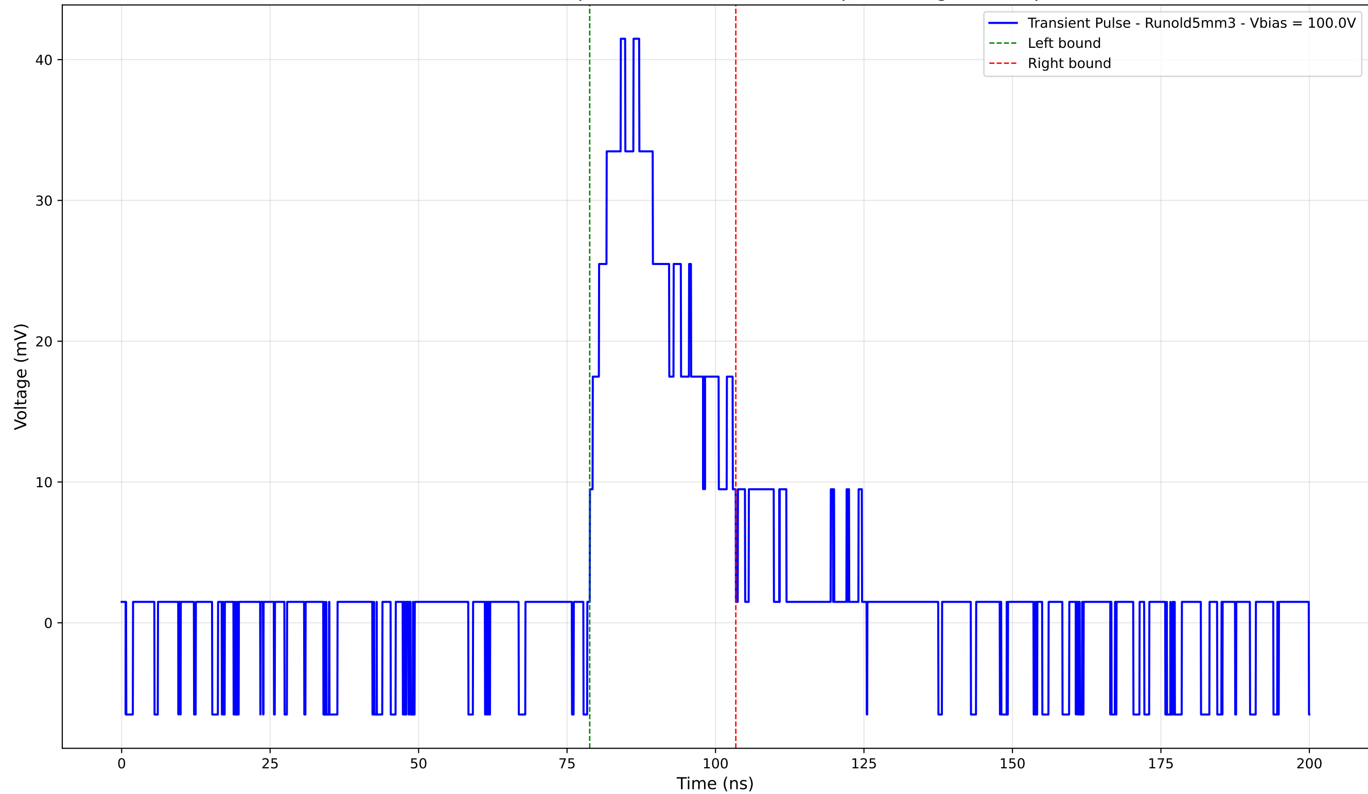
Transient Pulse - Sample: old5 - Position: 1800.0 \mu\text{m} - Charge: 11.87 pC
