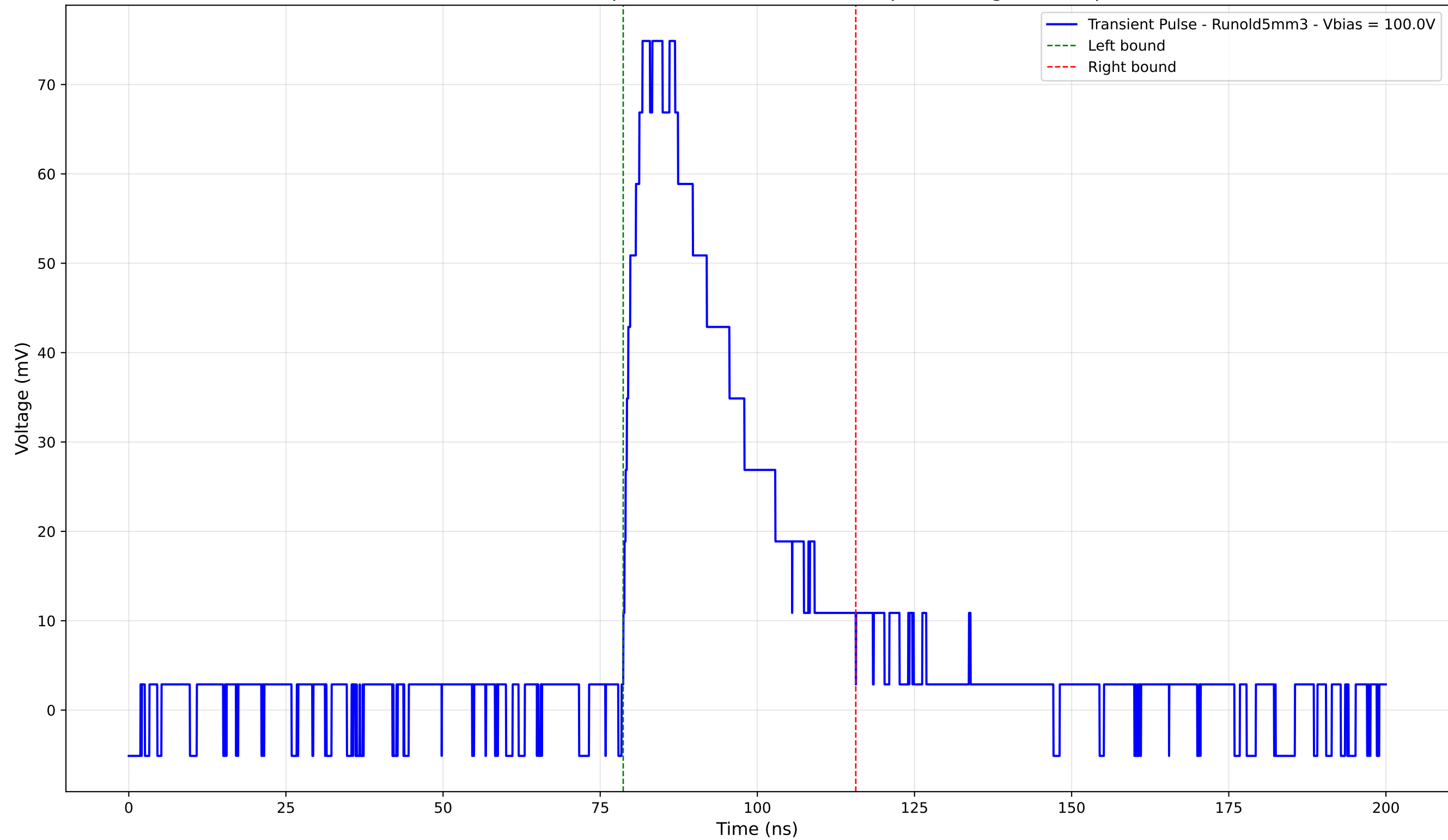
Transient Pulse - Sample: old5 - Position: 2220.0 \mu\text{m} - Charge: 27.11 pC
