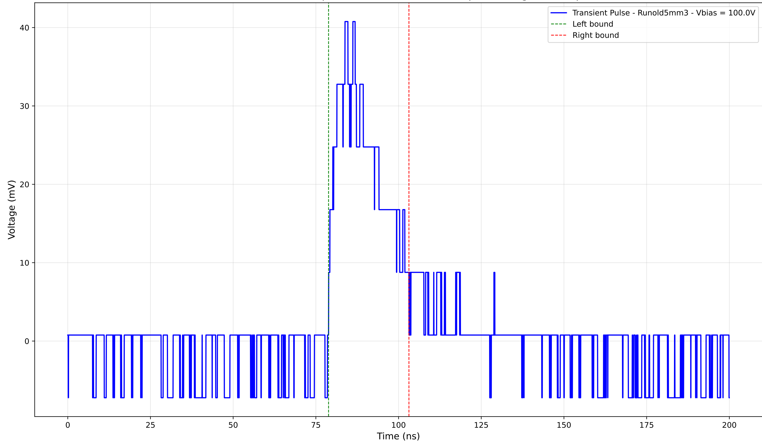
Transient Pulse - Sample: old5 - Position: 1780.0 \mu\text{m} - Charge: 11.25 pC
