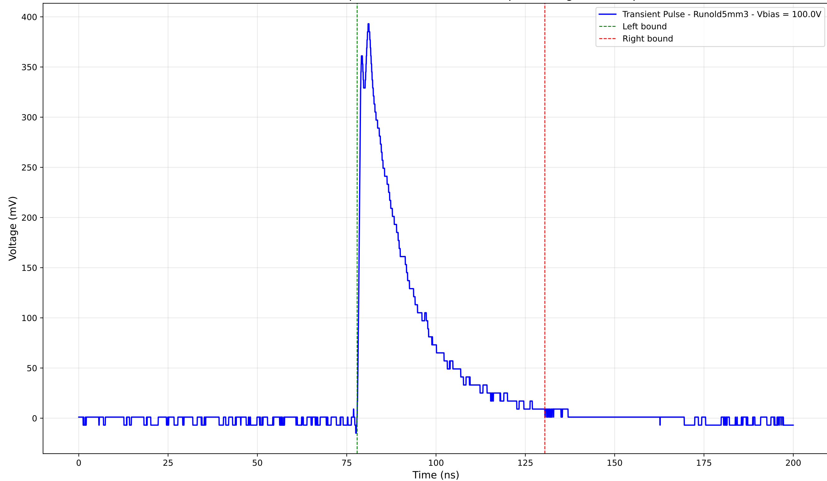
Transient Pulse - Sample: old5 - Position: 3110.0 \mu\text{m} - Charge: 105.30 pC
