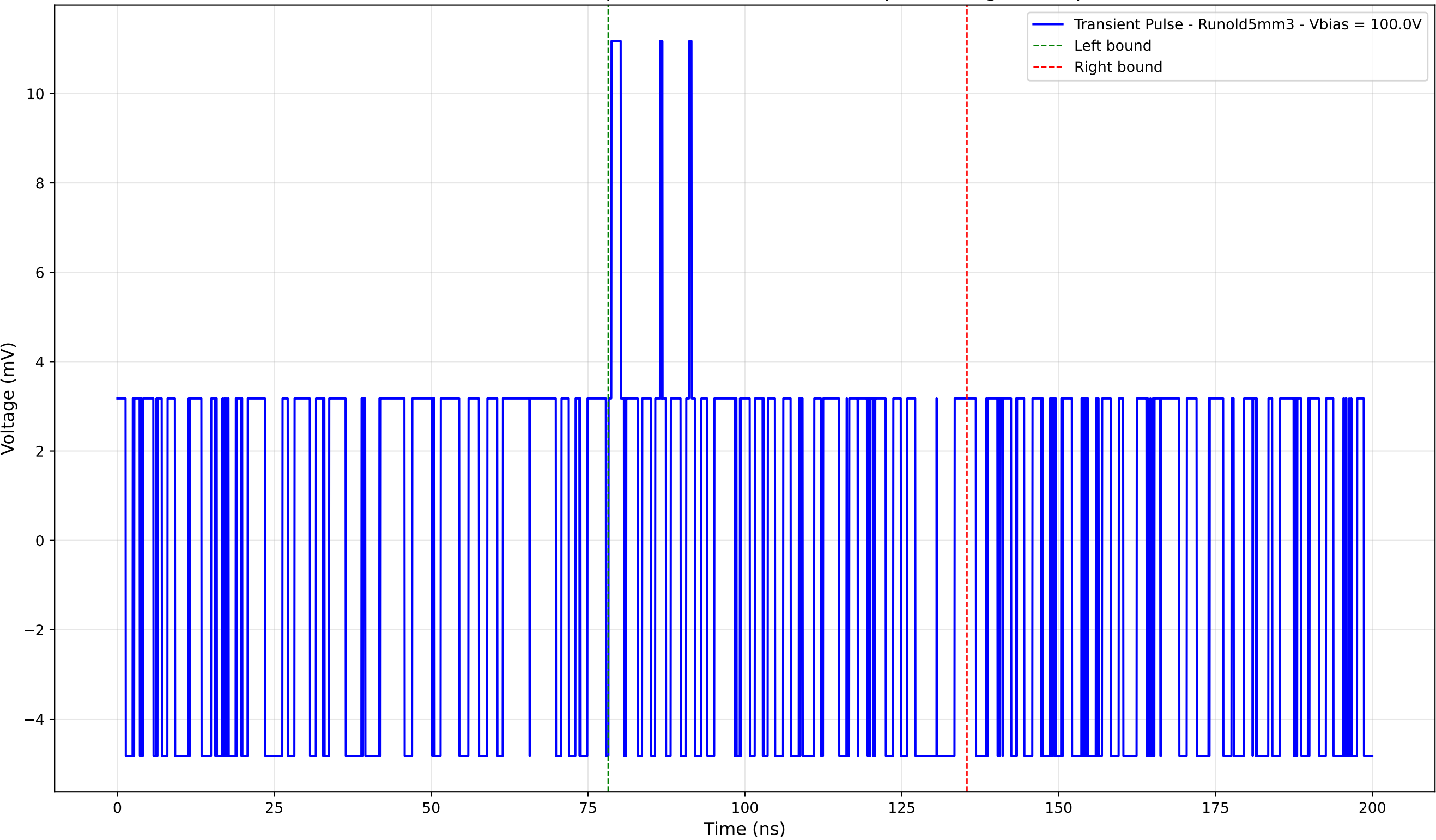
Transient Pulse - Sample: old5 - Position: 4980.0 \mu\text{m} - Charge: 0.30 pC
