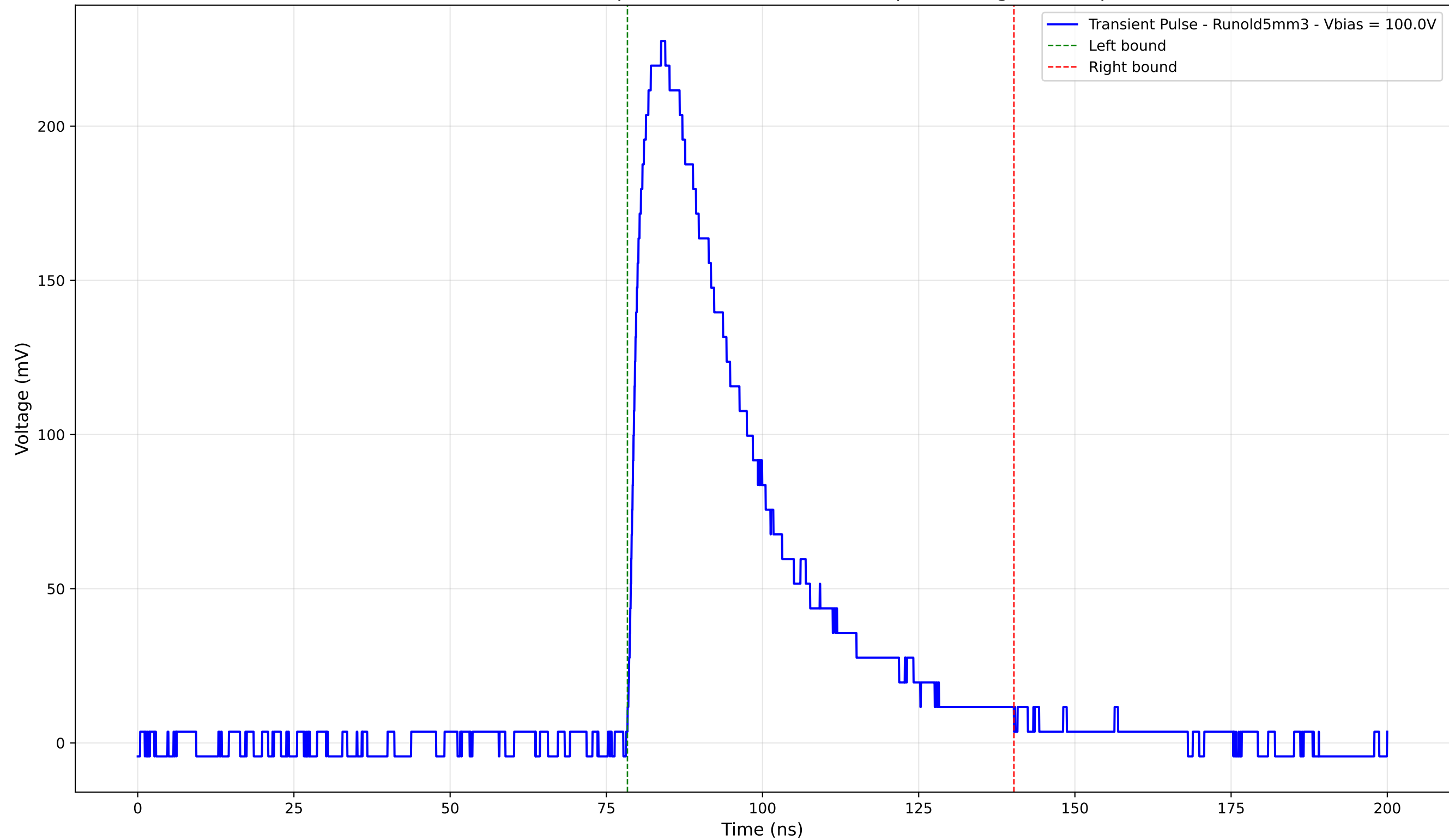
Transient Pulse - Sample: old5 - Position: 2100.0 \mu\text{m} - Charge: 92.40 pC
