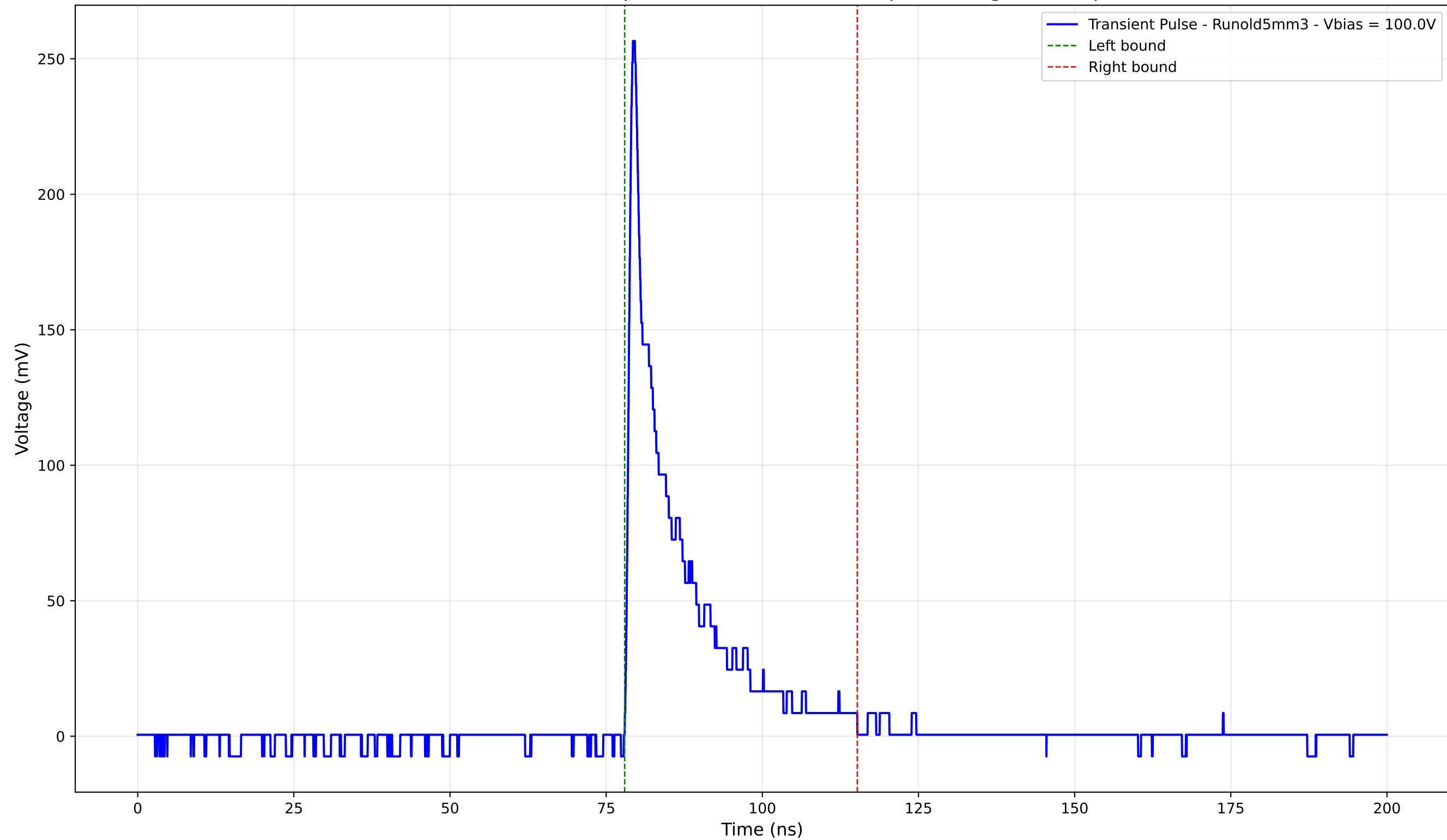
Transient Pulse - Sample: old5 - Position: 290.0 \mu\text{m} - Charge: 35.68 pC
