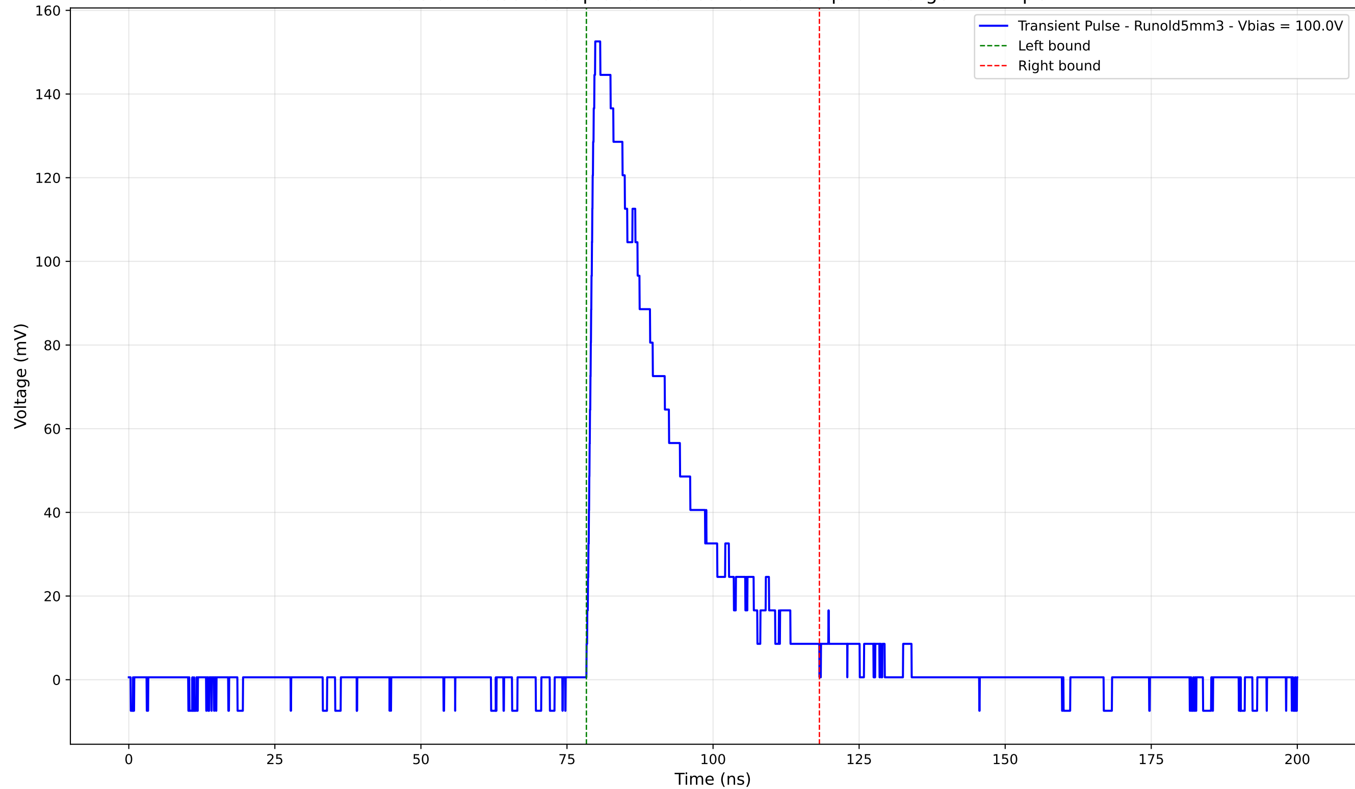
Transient Pulse - Sample: old5 - Position: 825.0 \mu\text{m} - Charge: 42.74 pC
