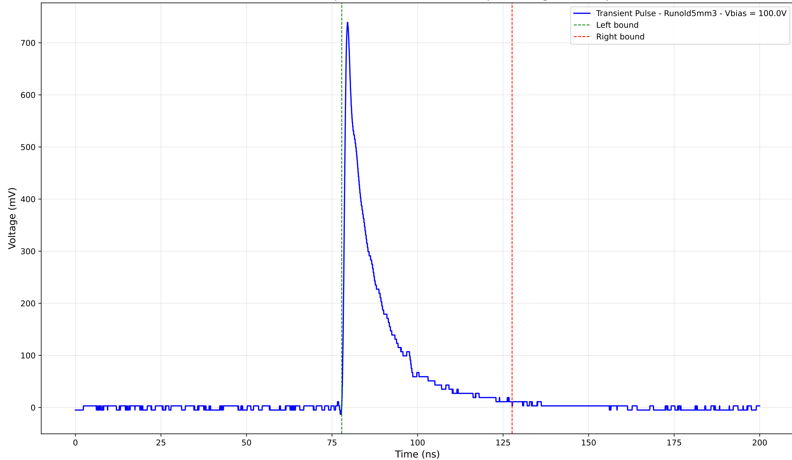
Transient Pulse - Sample: old5 - Position: 4715.0 \mu\text{m} - Charge: 132.55 pC
