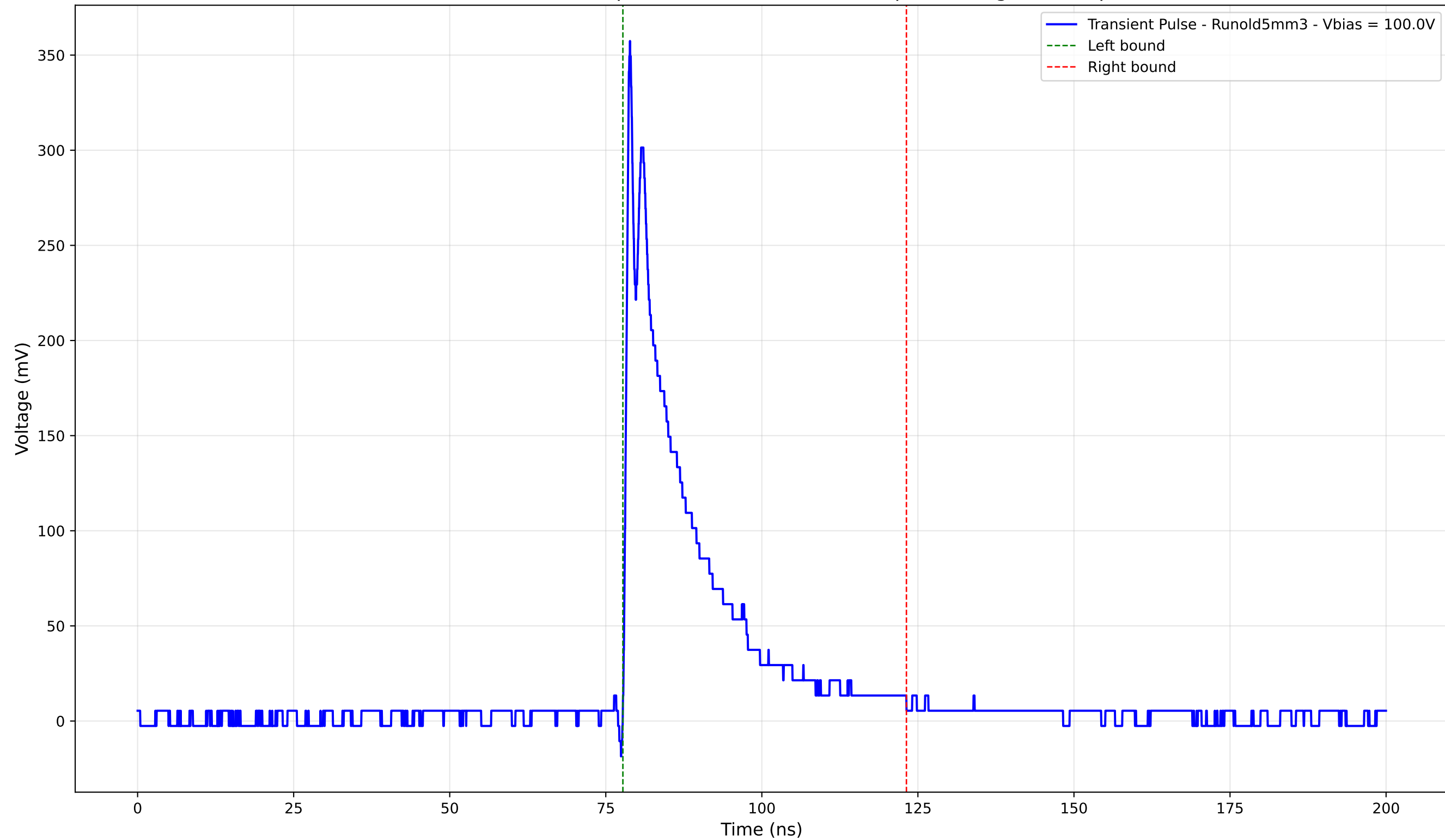
Transient Pulse - Sample: old5 - Position: 3355.0 \mu\text{m} - Charge: 65.10 pC
