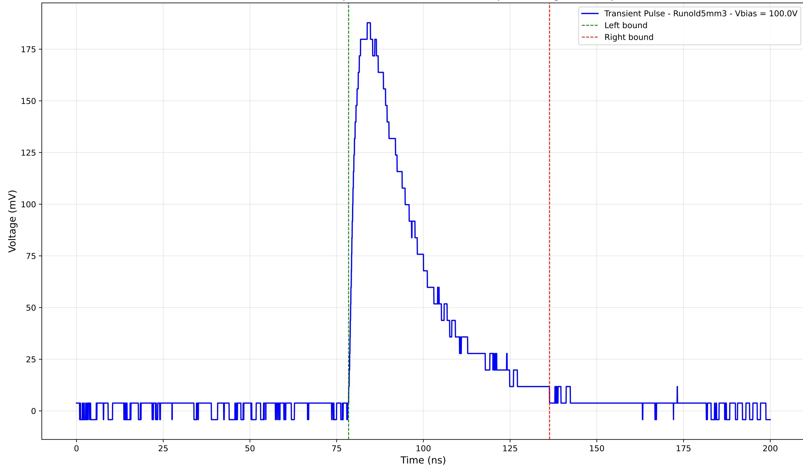
Transient Pulse - Sample: old5 - Position: 1860.0 \mu\text{m} - Charge: 77.06 pC
