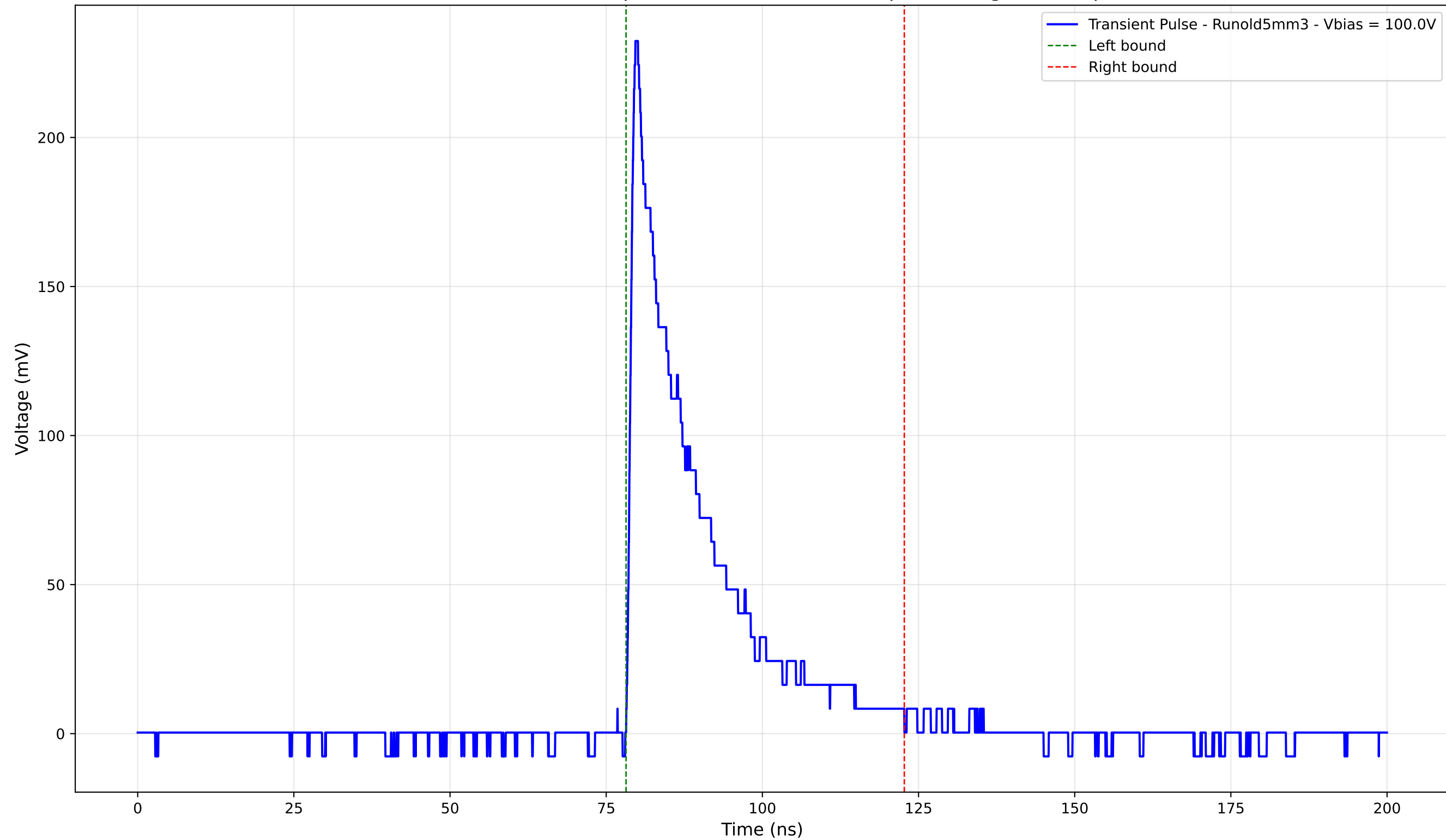
Transient Pulse - Sample: old5 - Position: 570.0 \mu\text{m} - Charge: 48.64 pC
