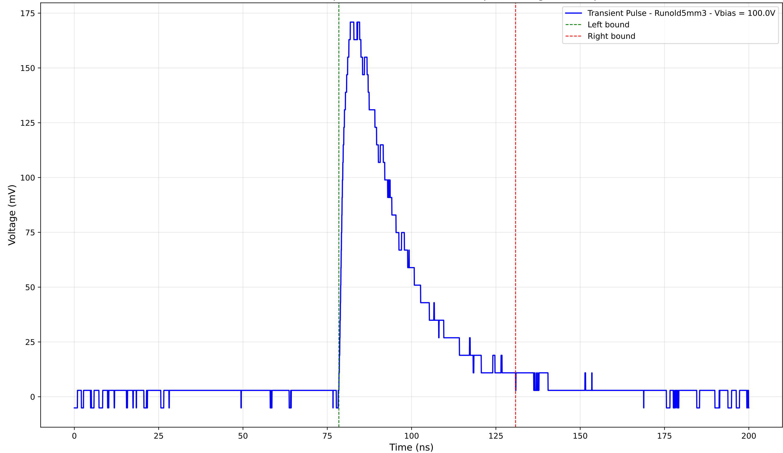
Transient Pulse - Sample: old5 - Position: 2450.0 \mu\text{m} - Charge: 64.21 pC
