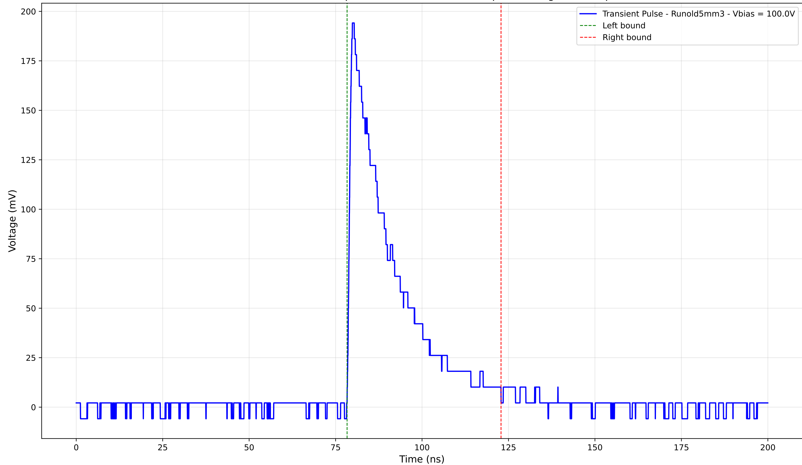
Transient Pulse - Sample: old5 - Position: 730.0 \mu\text{m} - Charge: 50.48 pC
