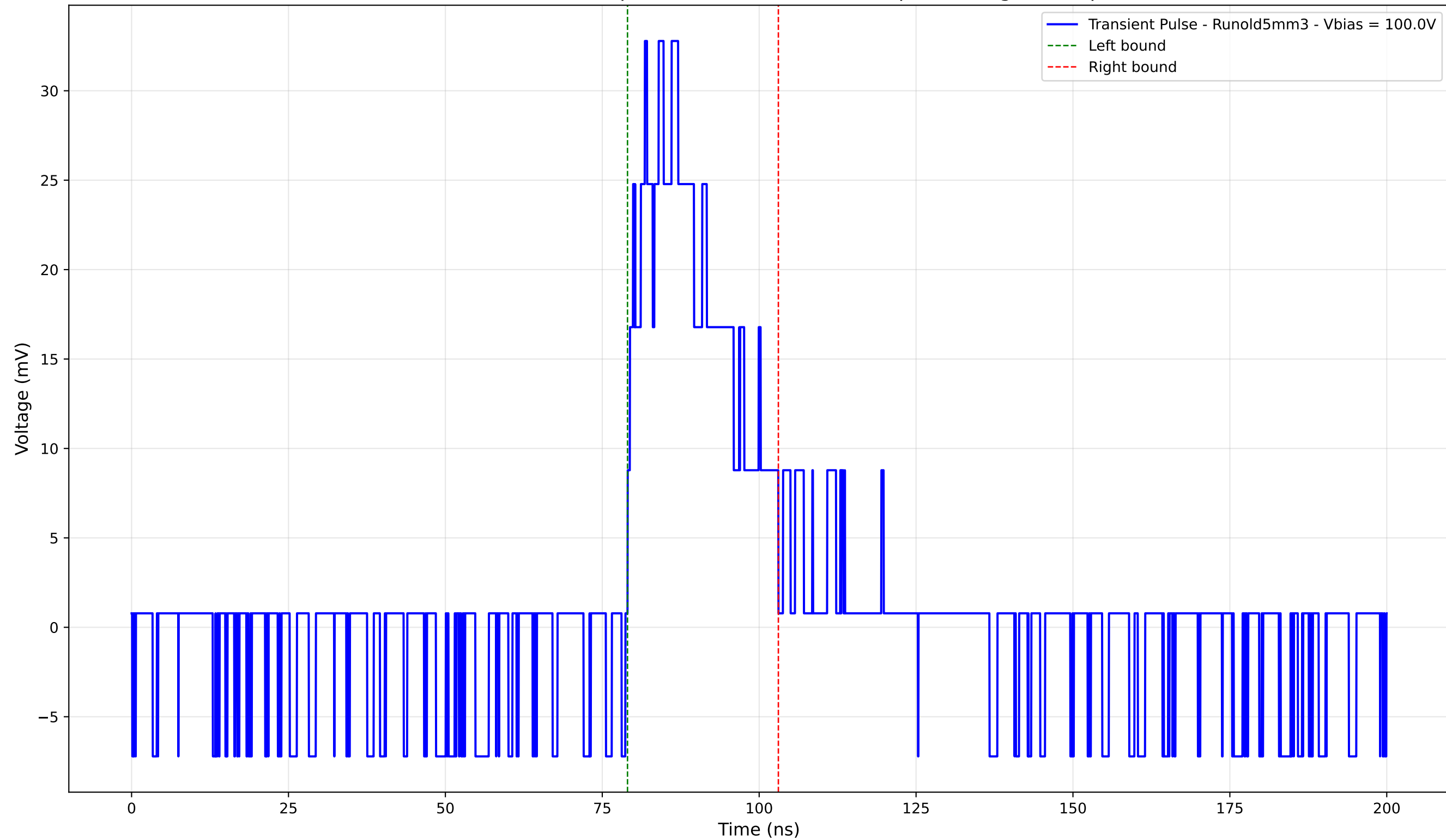
Transient Pulse - Sample: old5 - Position: 1385.0 \mu\text{m} - Charge: 8.85 pC
