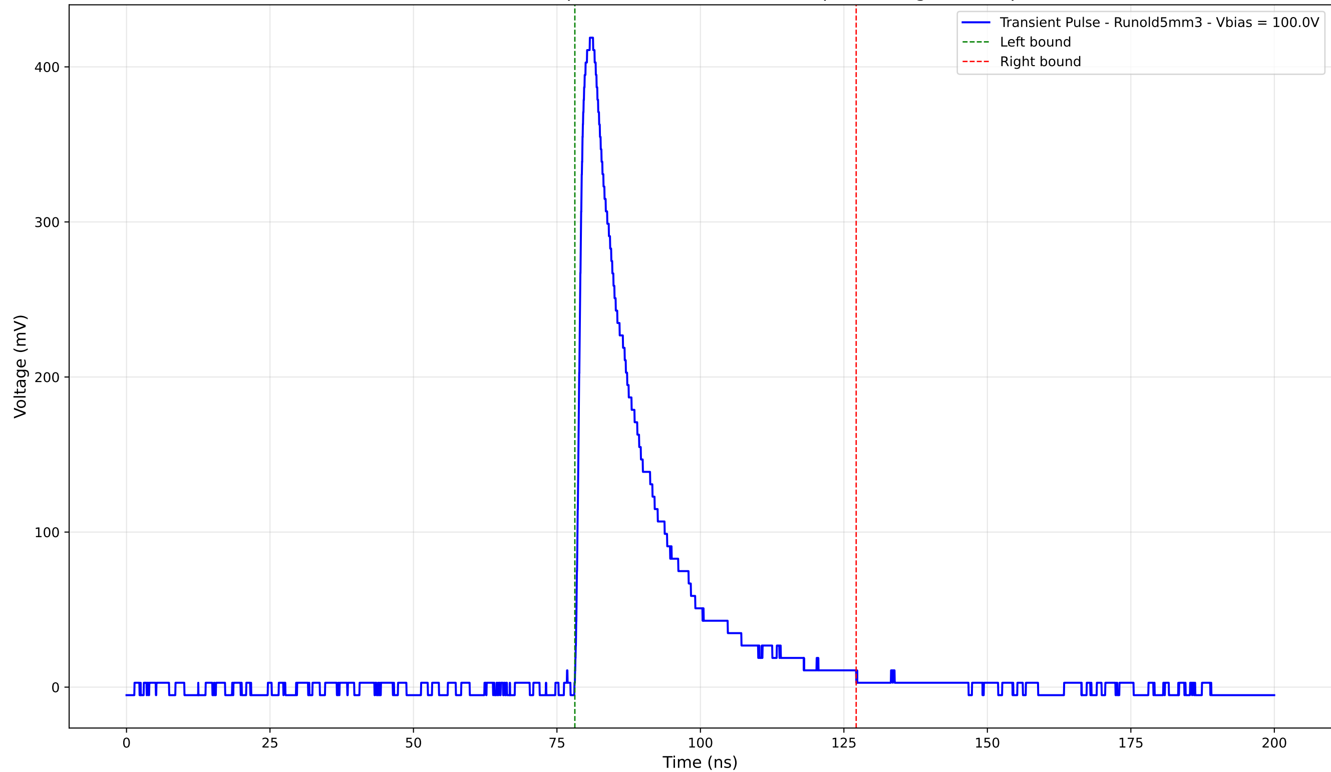
Transient Pulse - Sample: old5 - Position: 4280.0 \mu\text{m} - Charge: 94.84 pC
