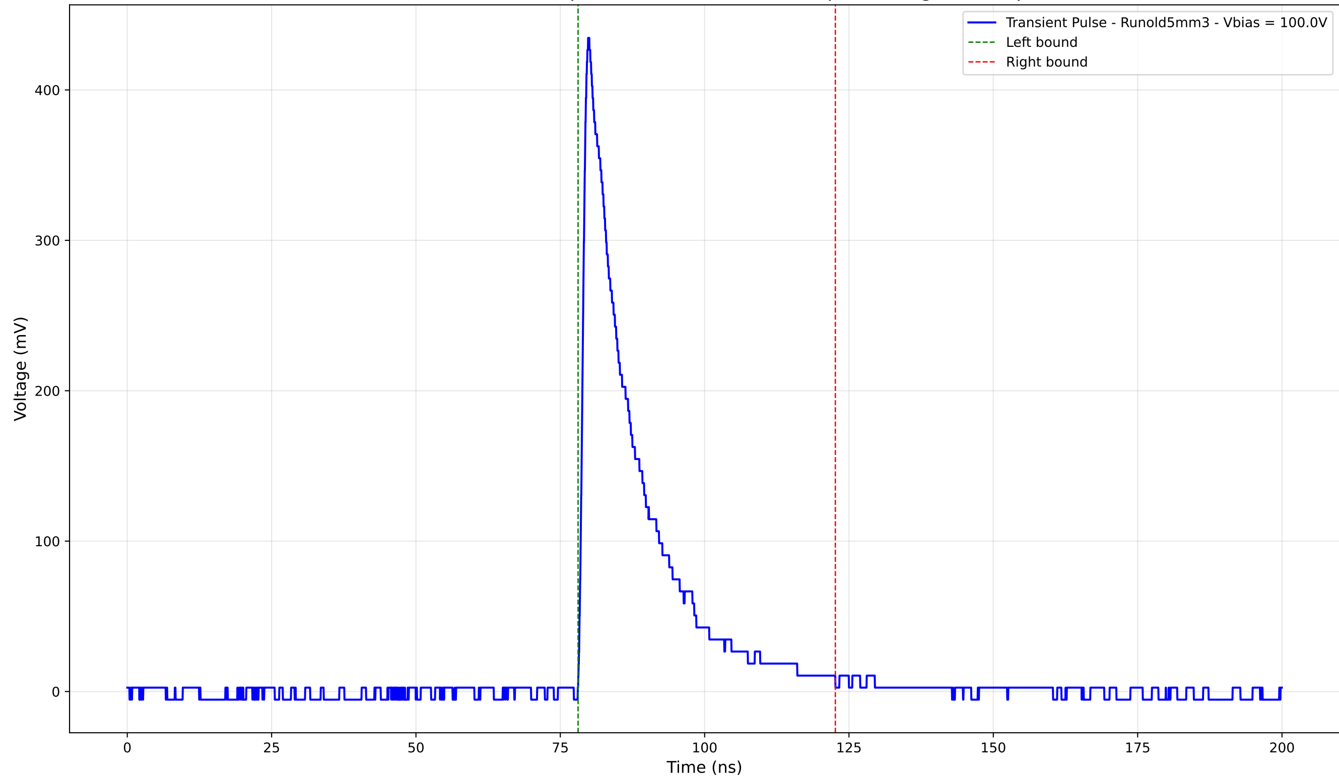
Transient Pulse - Sample: old5 - Position: 4575.0 \mu\text{m} - Charge: 84.47 pC
