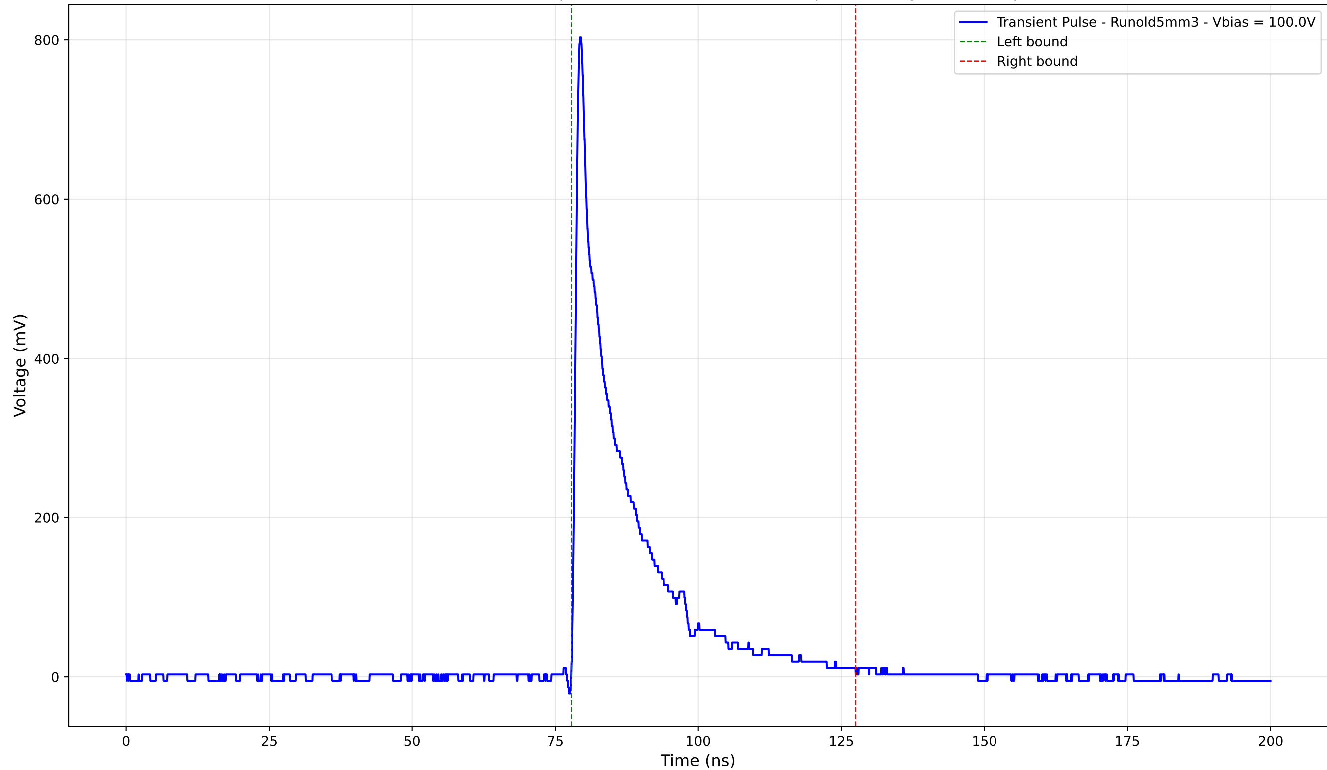
Transient Pulse - Sample: old5 - Position: 4780.0 \mu\text{m} - Charge: 131.98 pC
