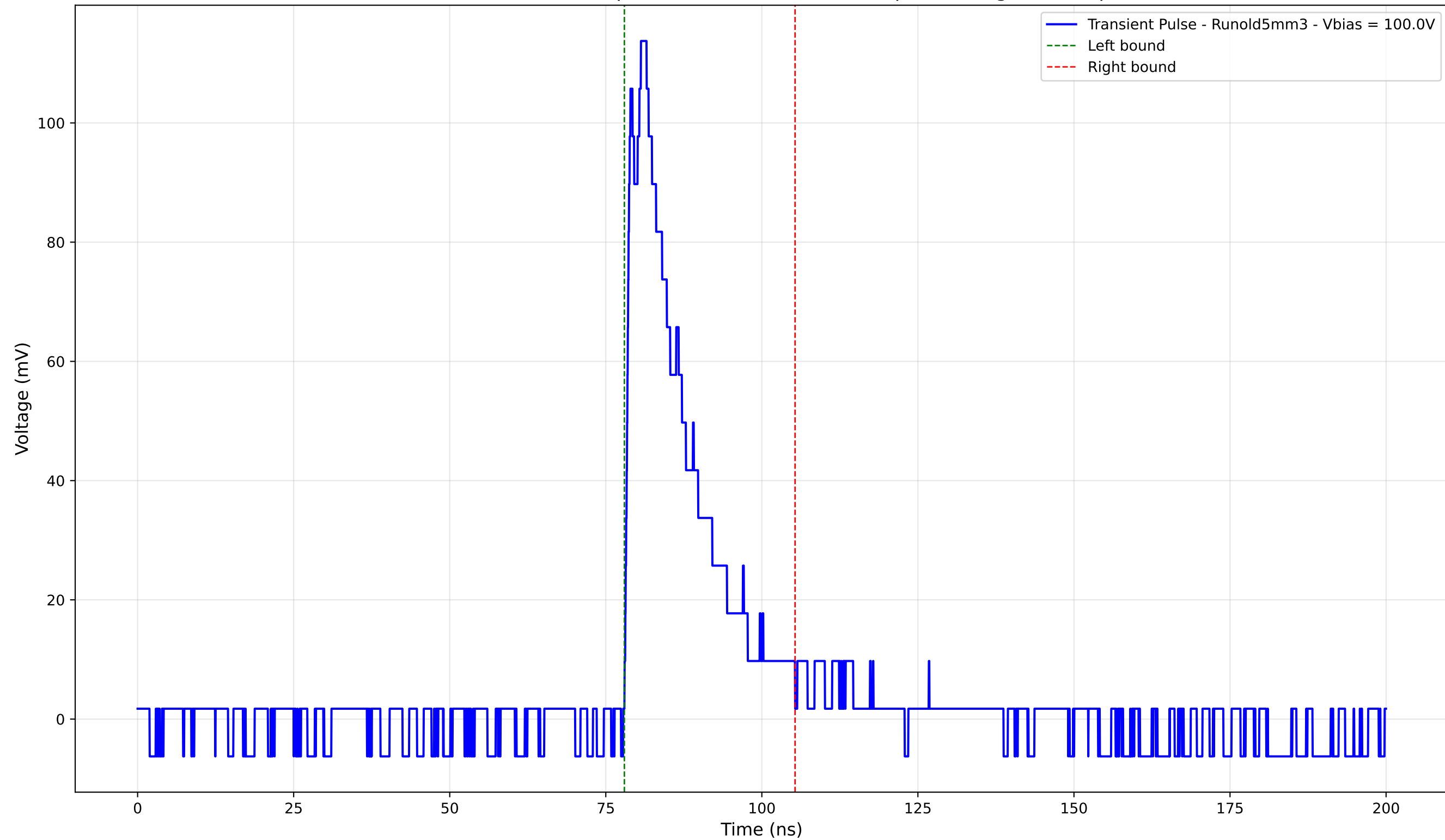
Transient Pulse - Sample: old5 - Position: 3930.0 \mu\text{m} - Charge: 22.72 pC
