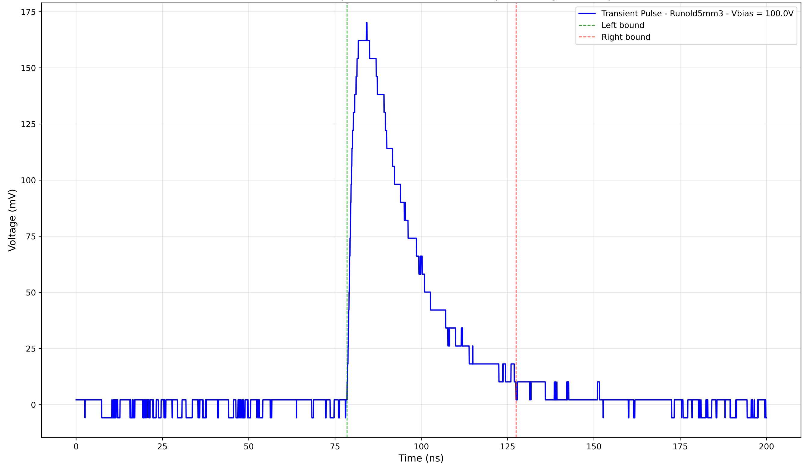
Transient Pulse - Sample: old5 - Position: 2250.0 \mu\text{m} - Charge: 64.14 pC
