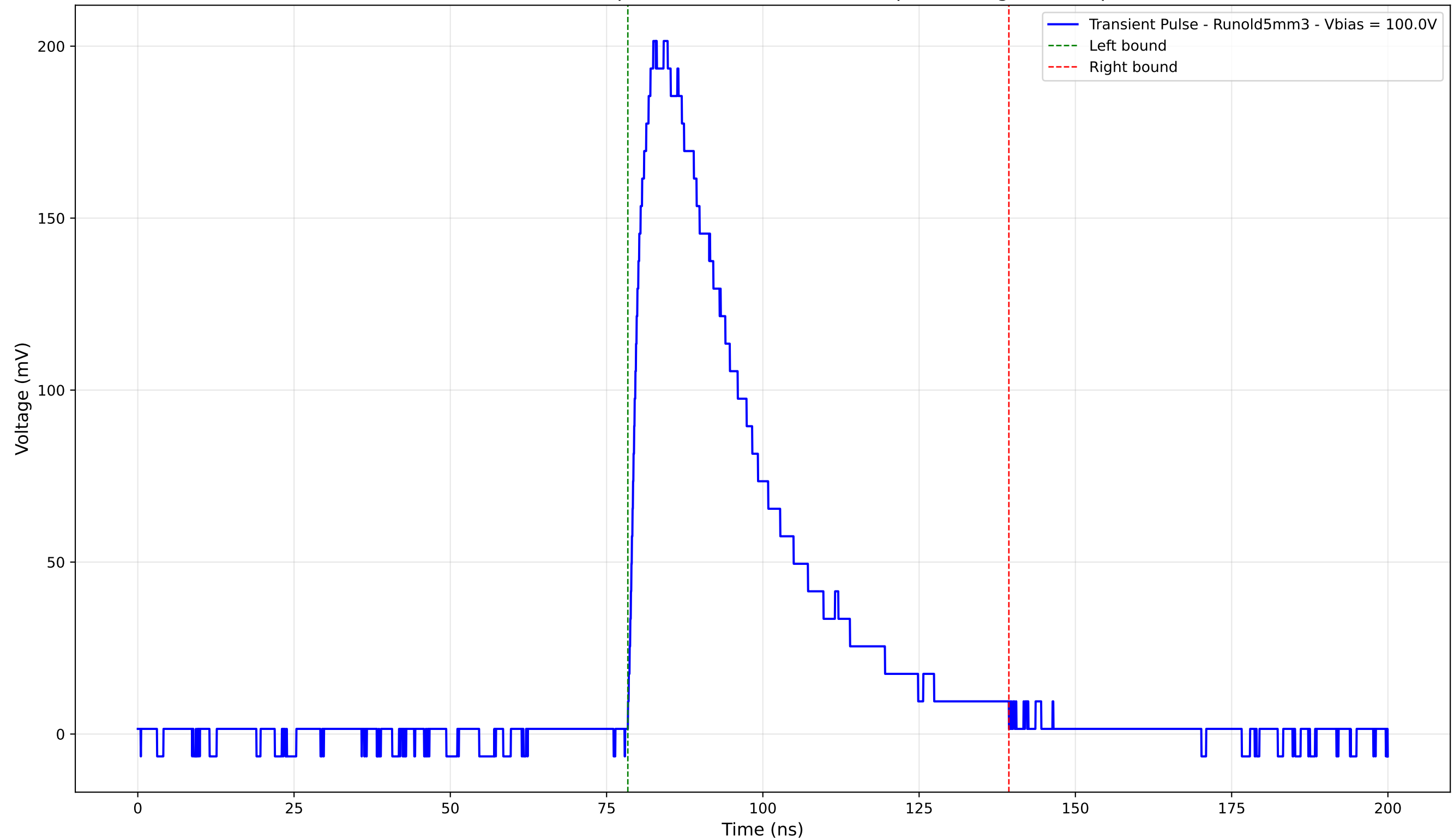
Transient Pulse - Sample: old5 - Position: 1870.0 \mu\text{m} - Charge: 81.31 pC
