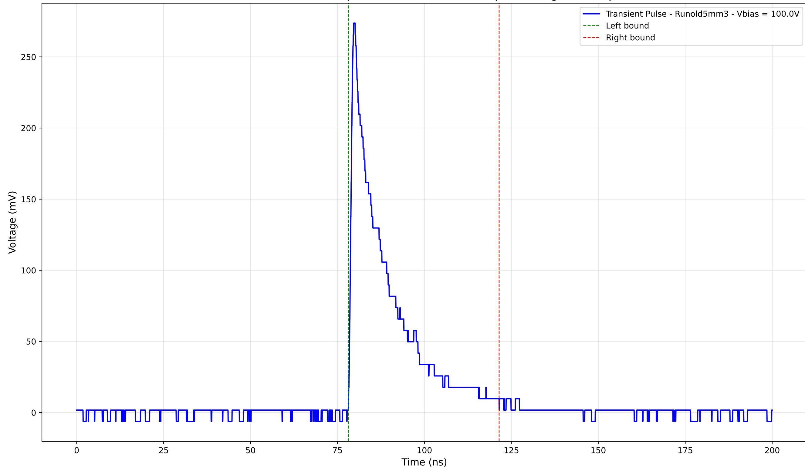
Transient Pulse - Sample: old5 - Position: 540.0 \mu\text{m} - Charge: 56.54 pC
