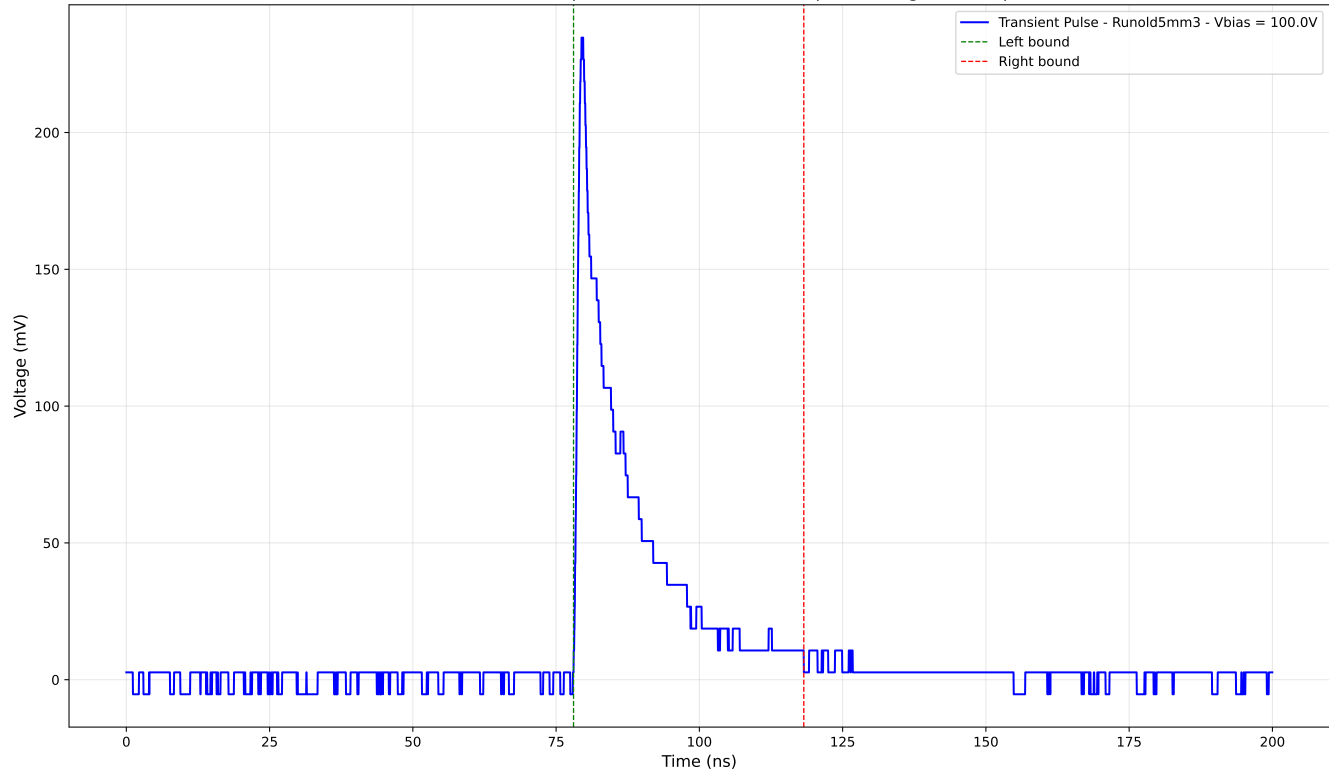
Transient Pulse - Sample: old5 - Position: 385.0 \mu\text{m} - Charge: 39.29 pC
