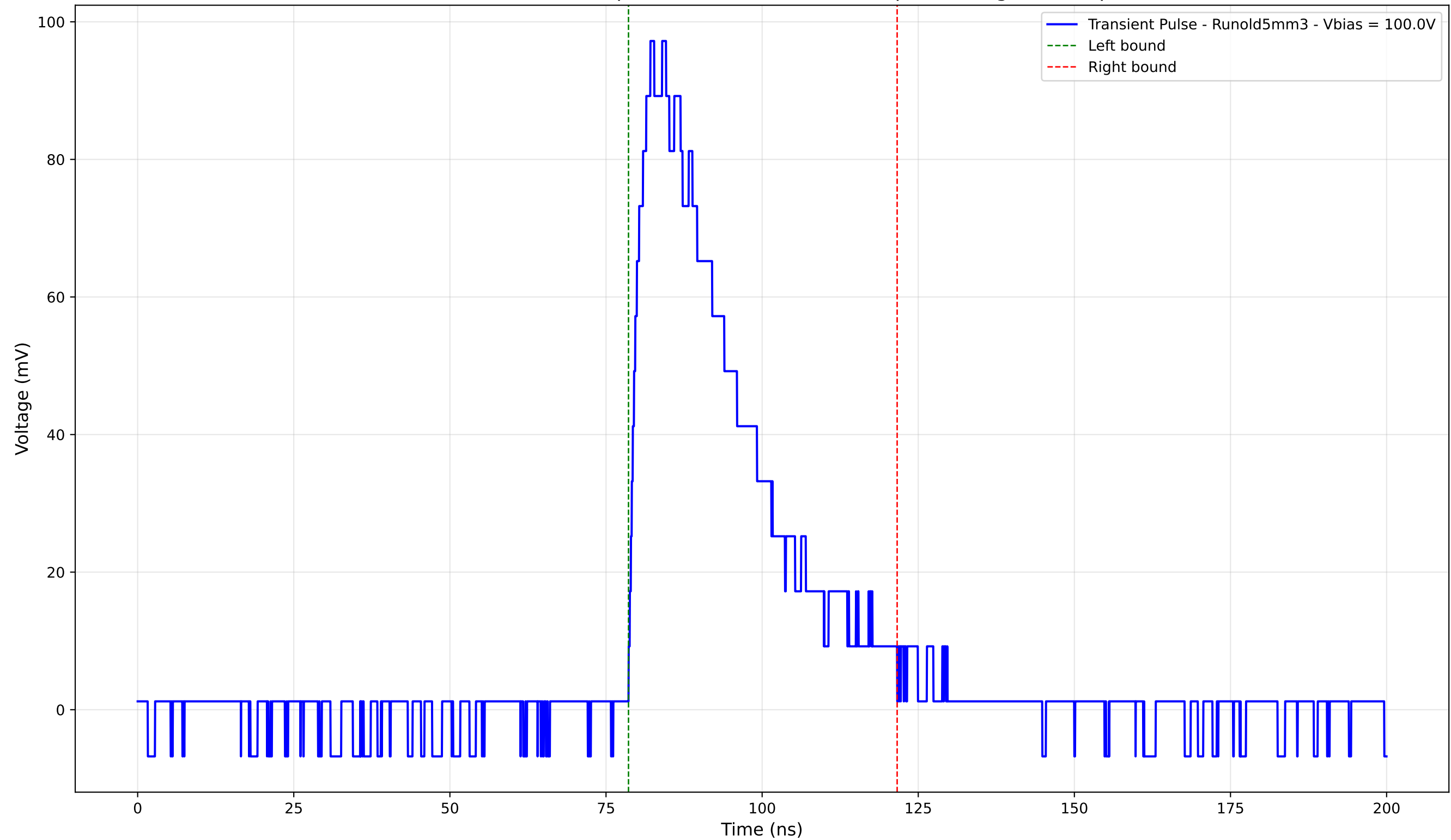
Transient Pulse - Sample: old5 - Position: 1545.0 \mu\text{m} - Charge: 34.97 pC
