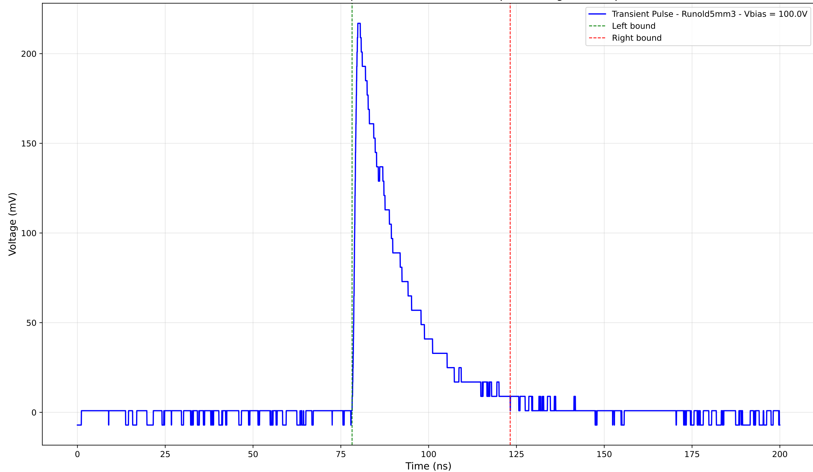
Transient Pulse - Sample: old5 - Position: 755.0 \mu\text{m} - Charge: 56.60 pC
