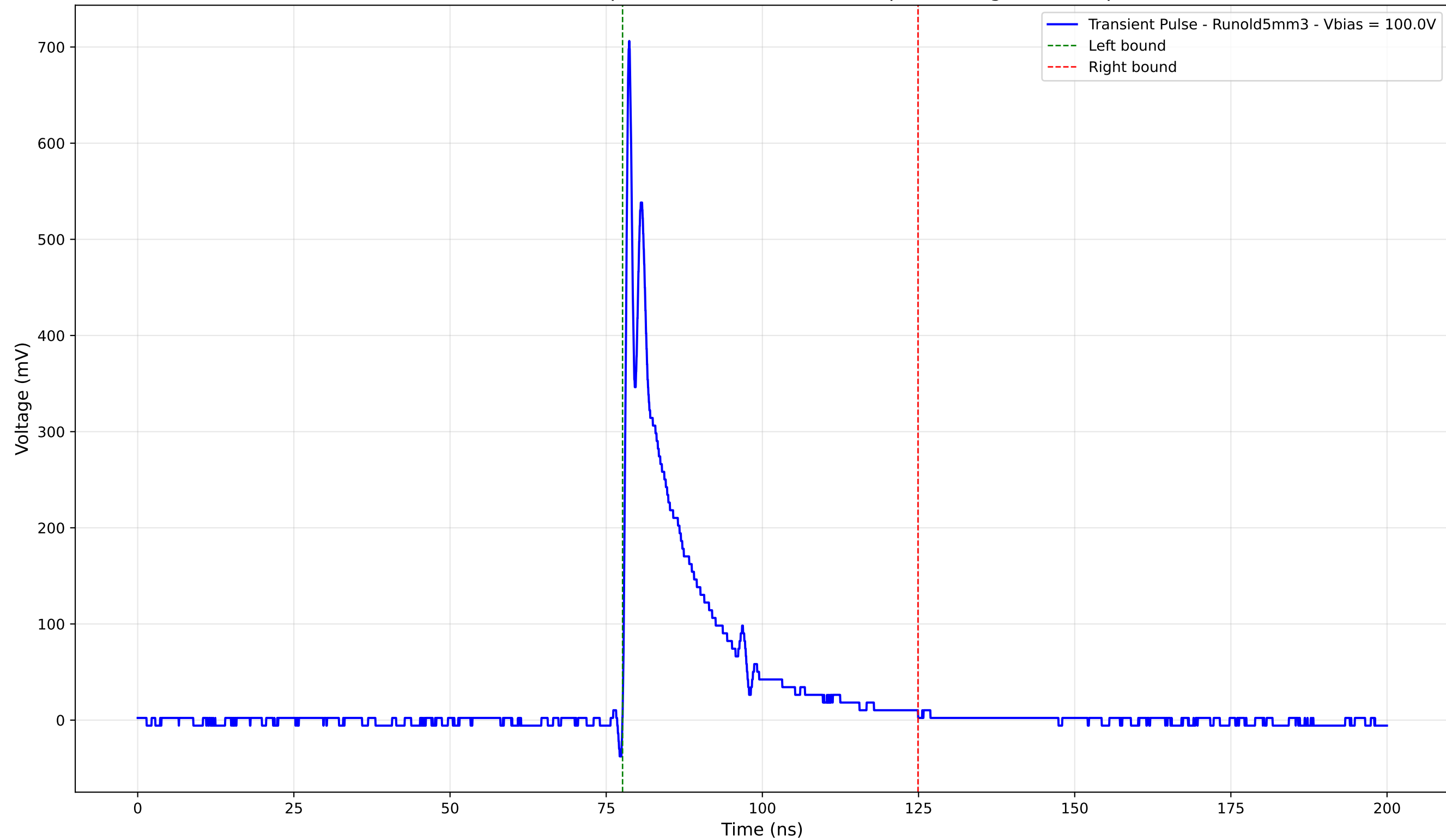
Transient Pulse - Sample: old5 - Position: 3470.0 \mu\text{m} - Charge: 100.69 pC
