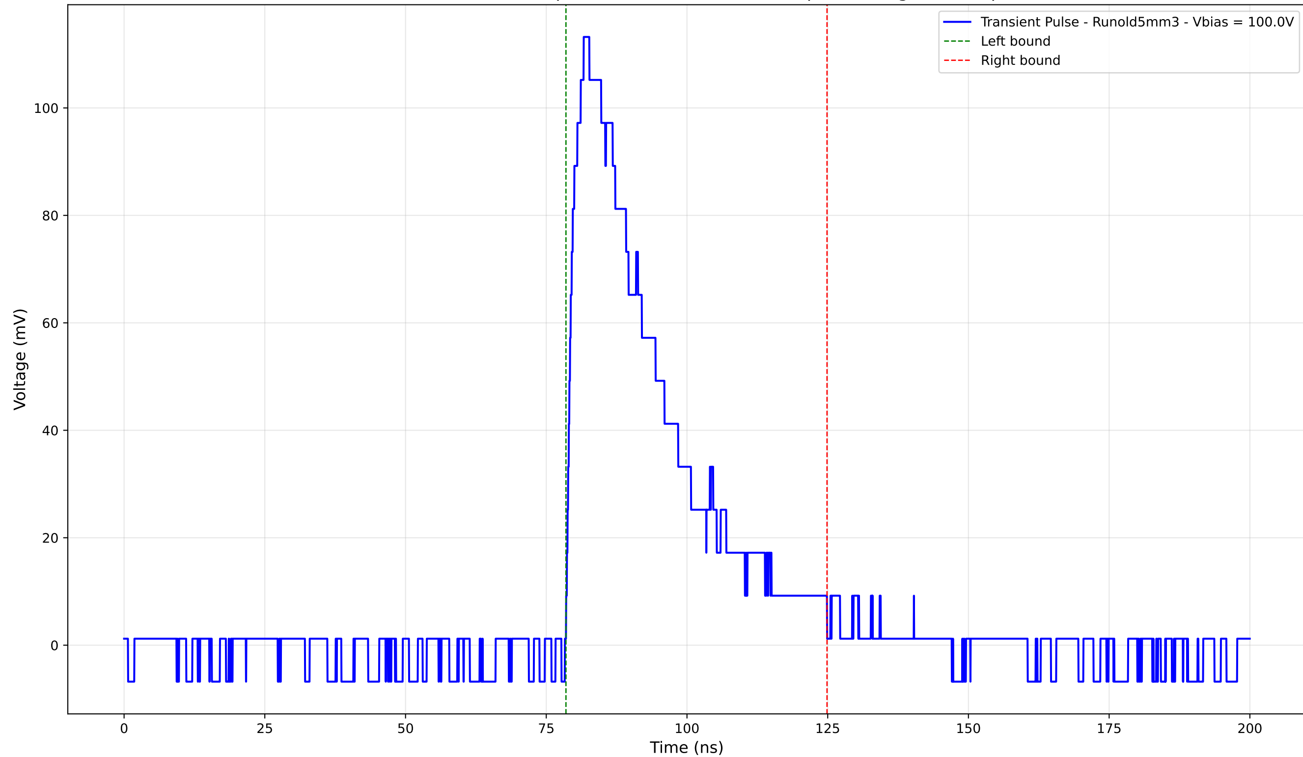
Transient Pulse - Sample: old5 - Position: 2610.0 \mu\text{m} - Charge: 38.54 pC
