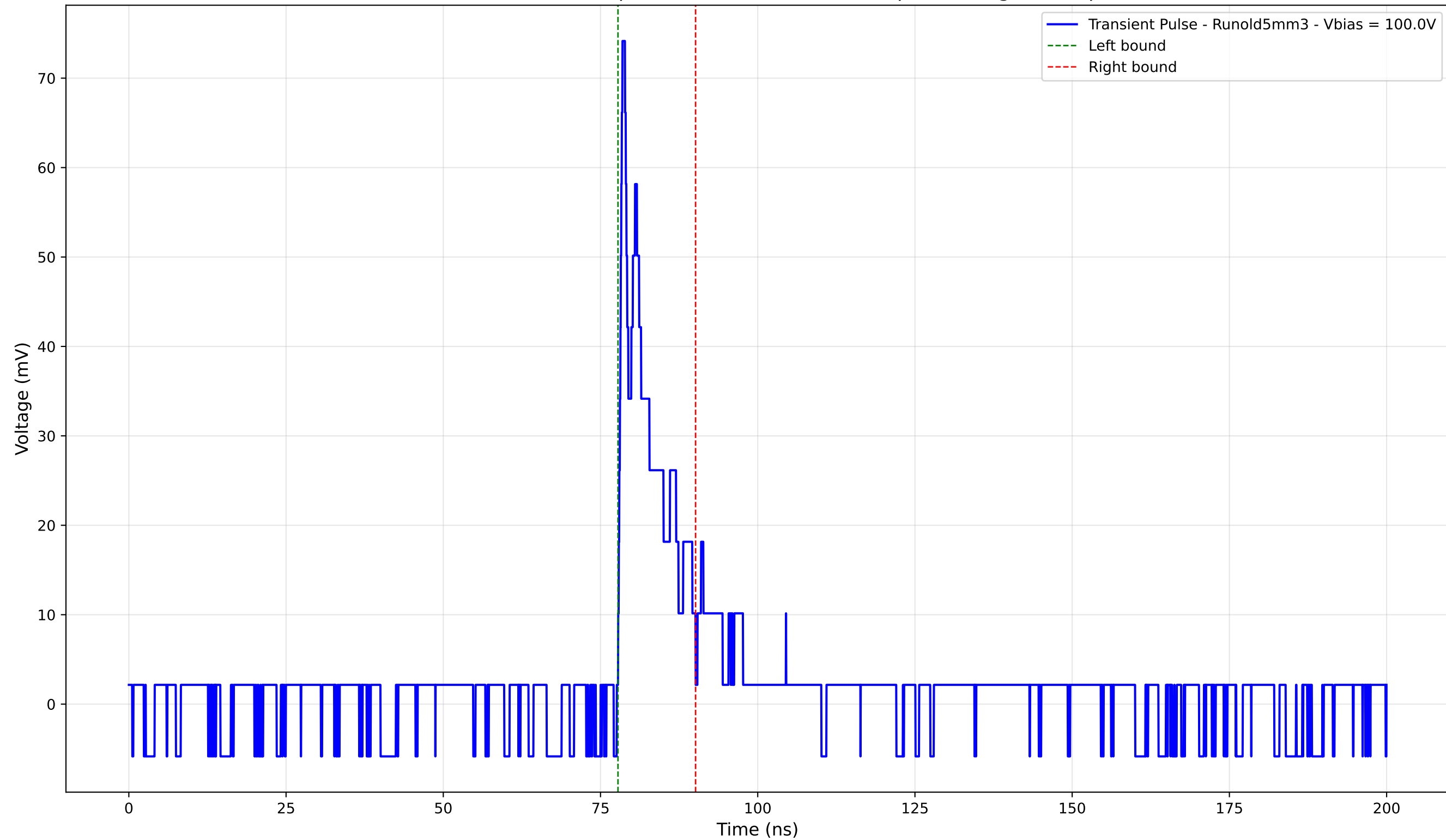
Transient Pulse - Sample: old5 - Position: 3555.0 \mu\text{m} - Charge: 7.42 pC
