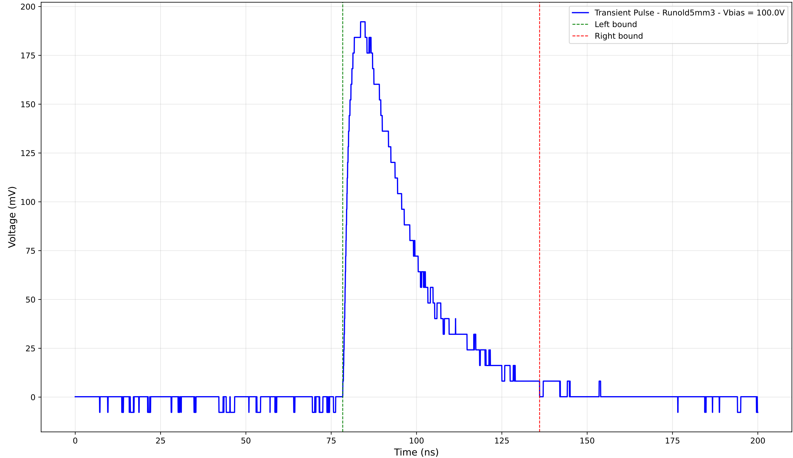
Transient Pulse - Sample: old5 - Position: 1710.0 \mu\text{m} - Charge: 77.08 pC
