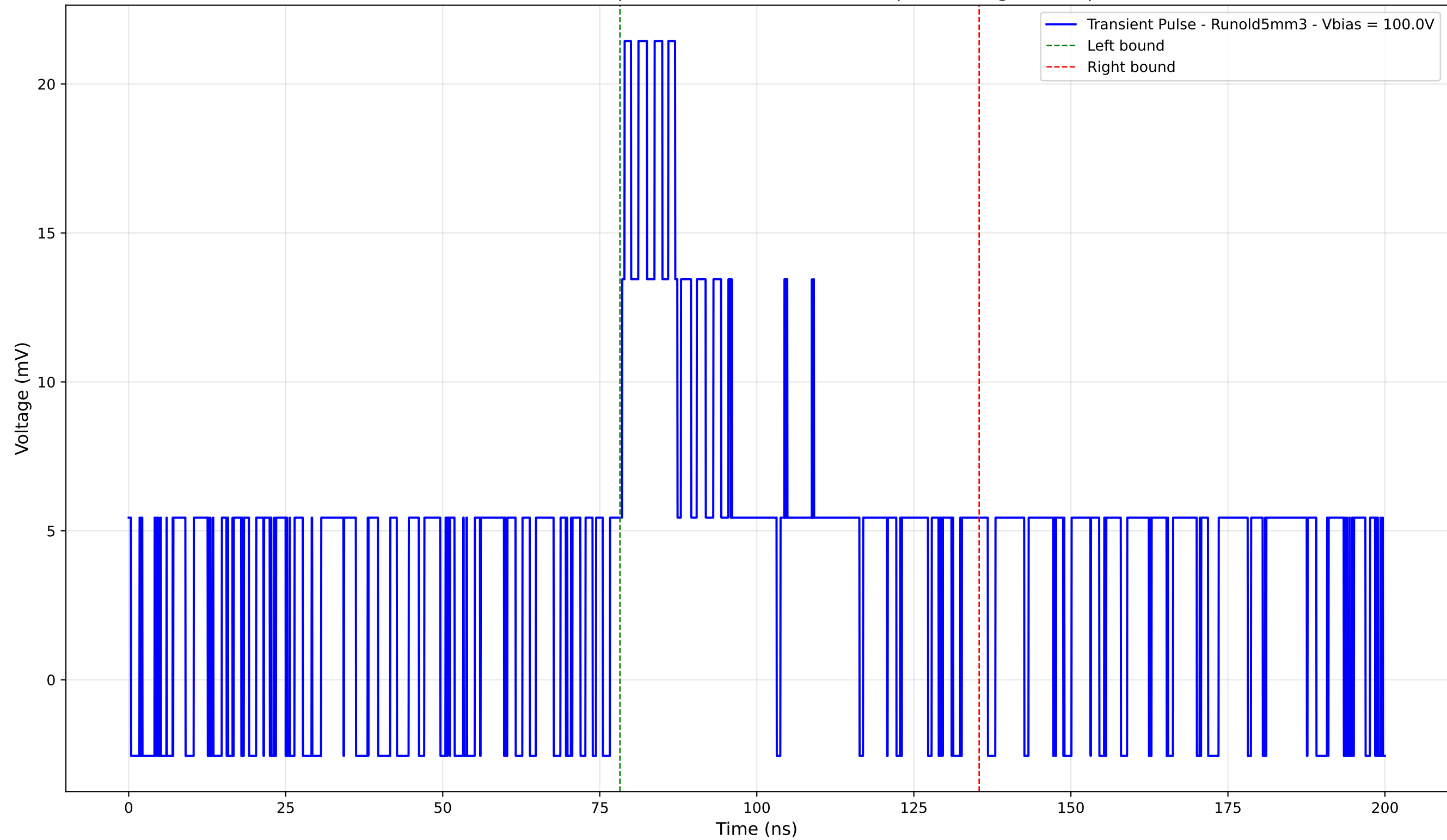
Transient Pulse - Sample: old5 - Position: 2970.0 \mu\text{m} - Charge: 8.55 pC
