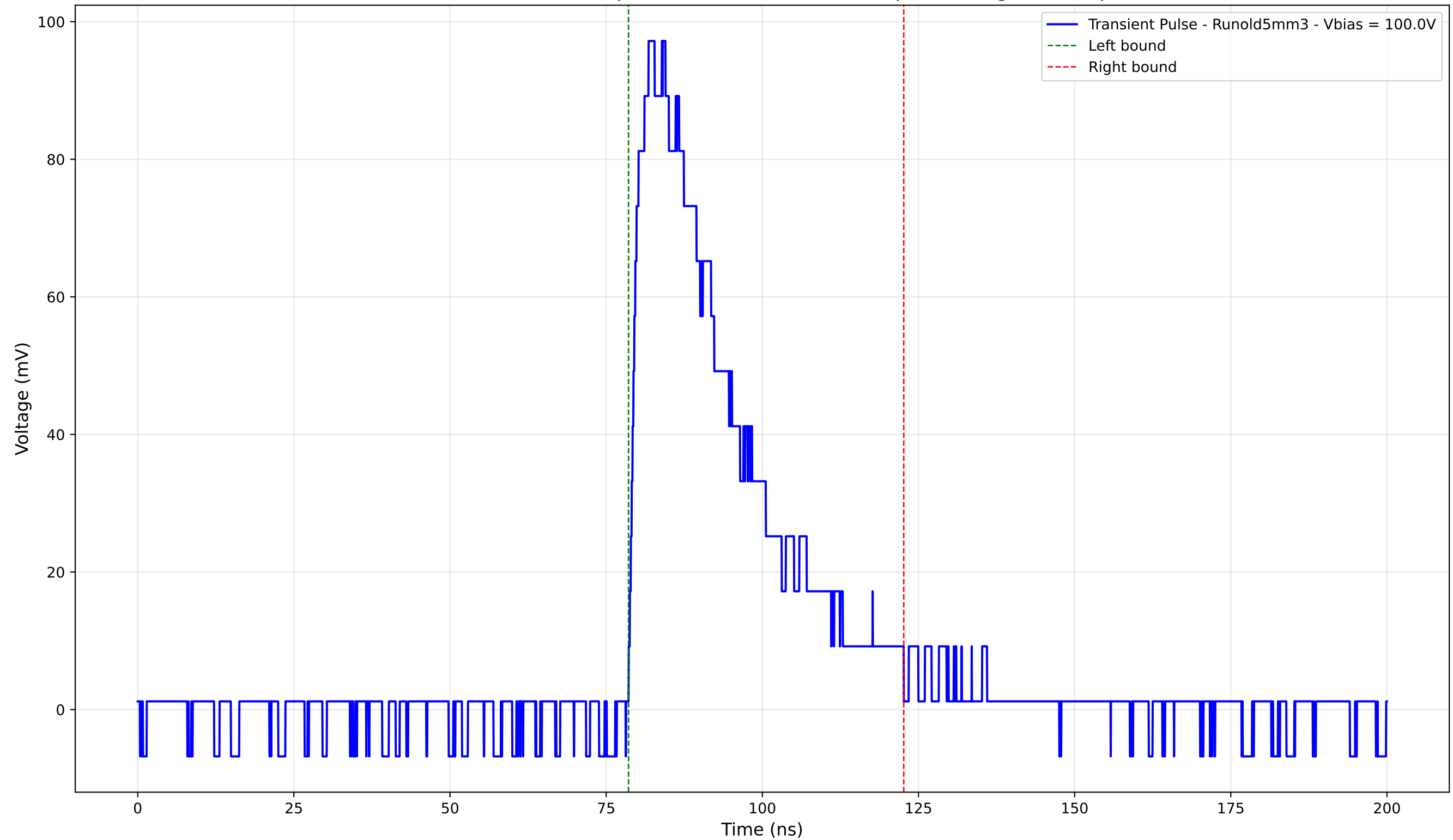
Transient Pulse - Sample: old5 - Position: 1345.0 \mu\text{m} - Charge: 34.24 pC
