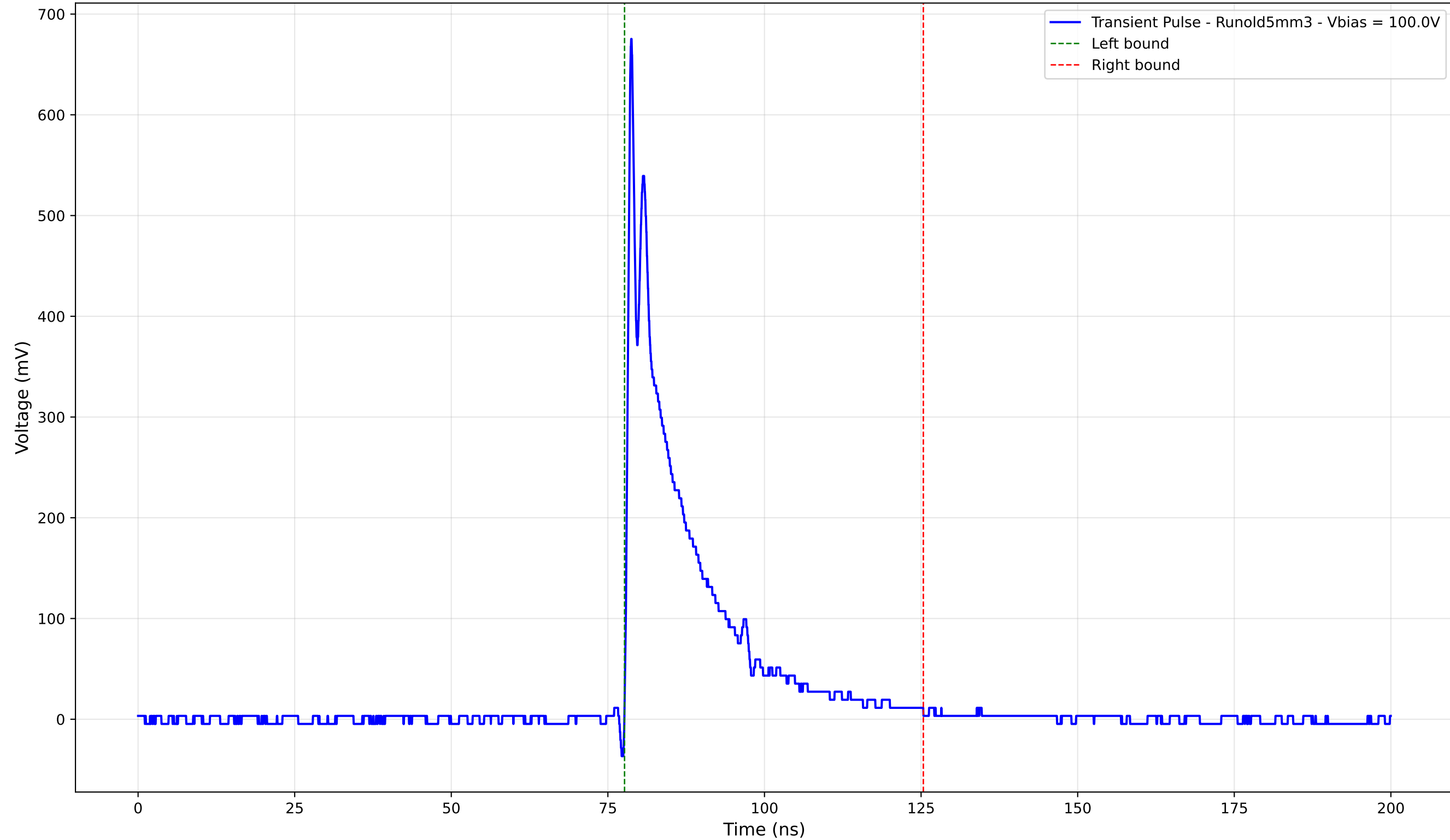
Transient Pulse - Sample: old5 - Position: 3430.0 \mu\text{m} - Charge: 107.17 pC
