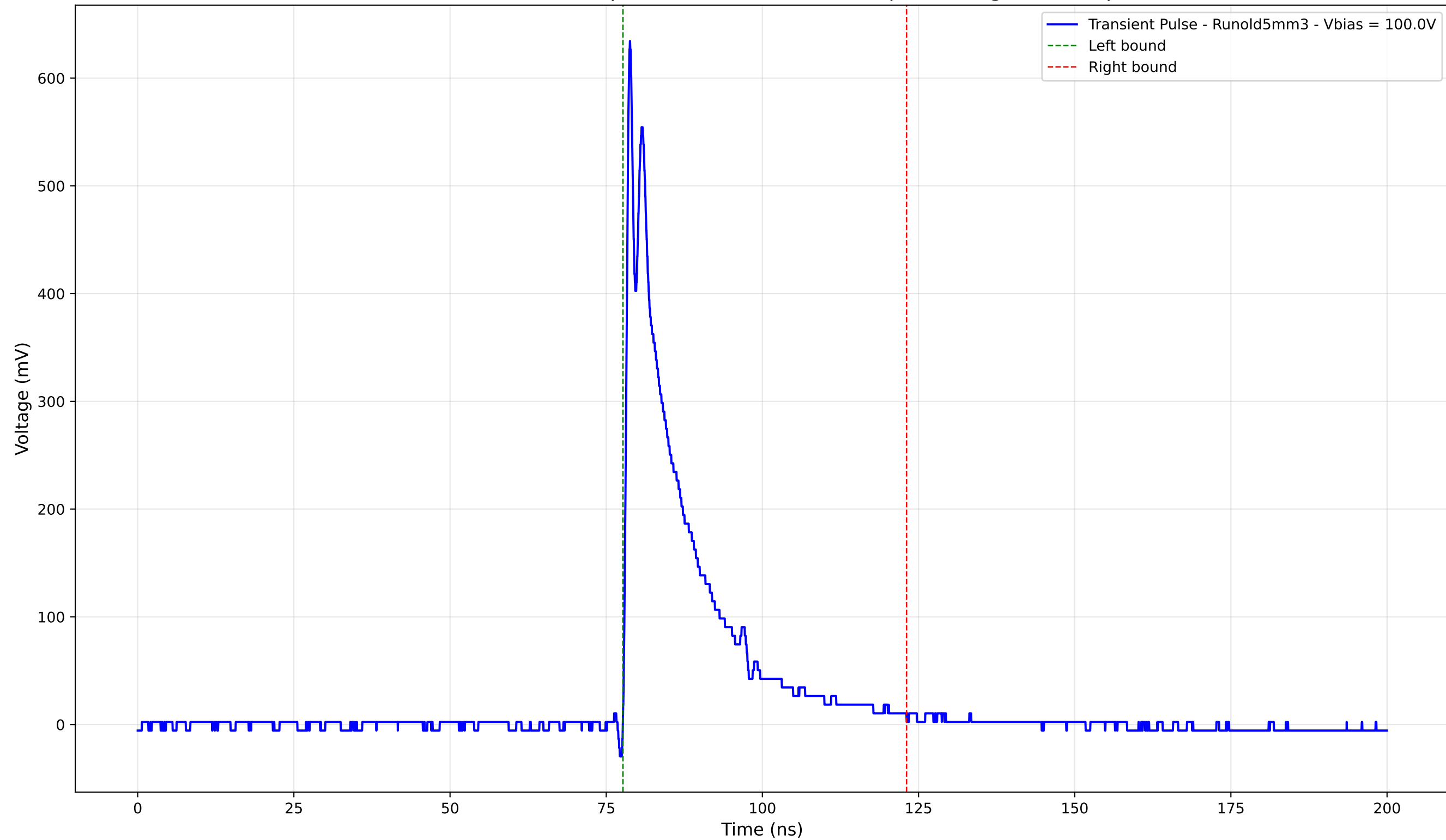
Transient Pulse - Sample: old5 - Position: 3765.0 \mu\text{m} - Charge: 106.39 pC
