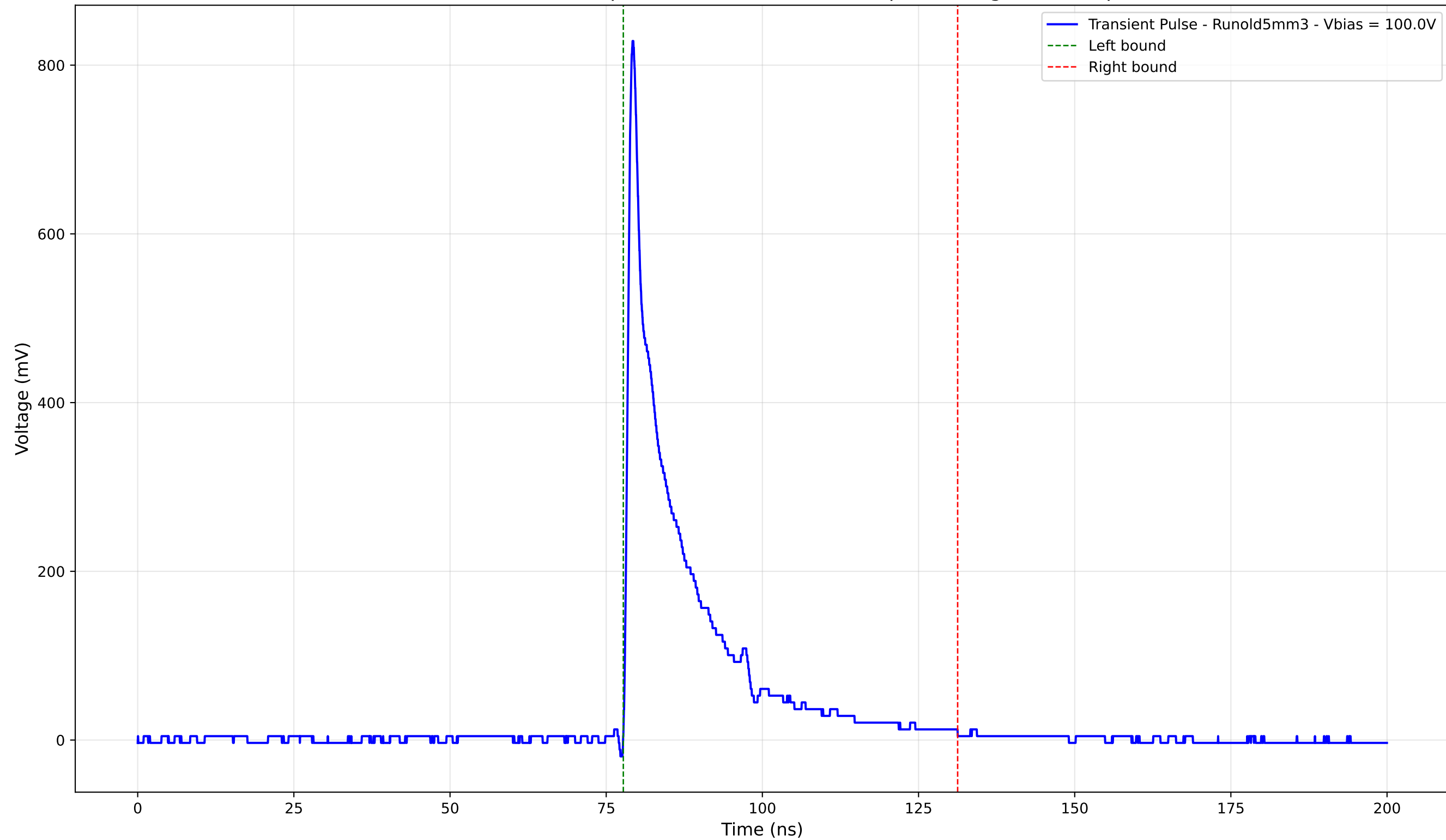
Transient Pulse - Sample: old5 - Position: 4825.0 \mu\text{m} - Charge: 127.61 pC
