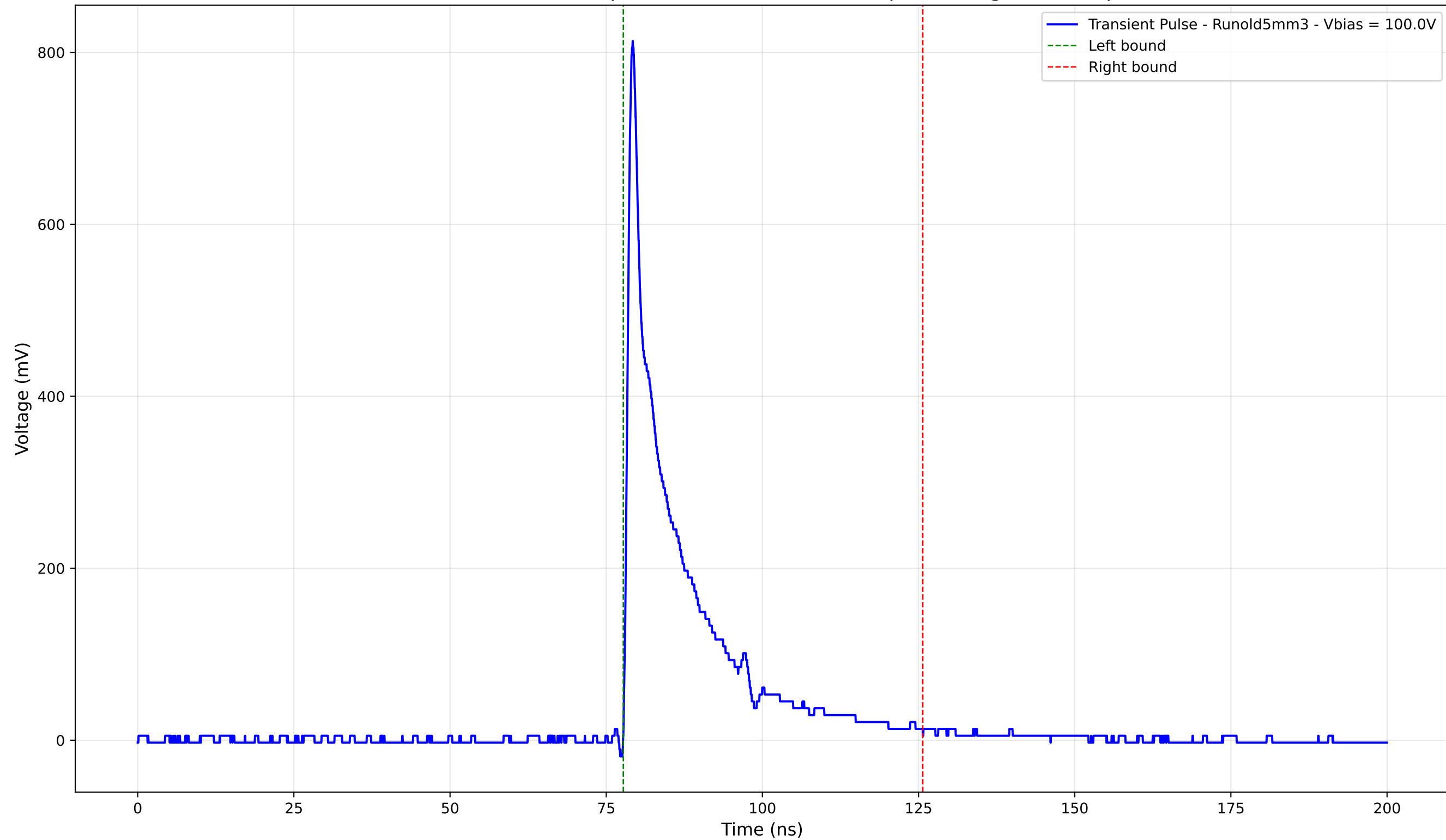
Transient Pulse - Sample: old5 - Position: 4840.0 \mu\text{m} - Charge: 119.44 pC
