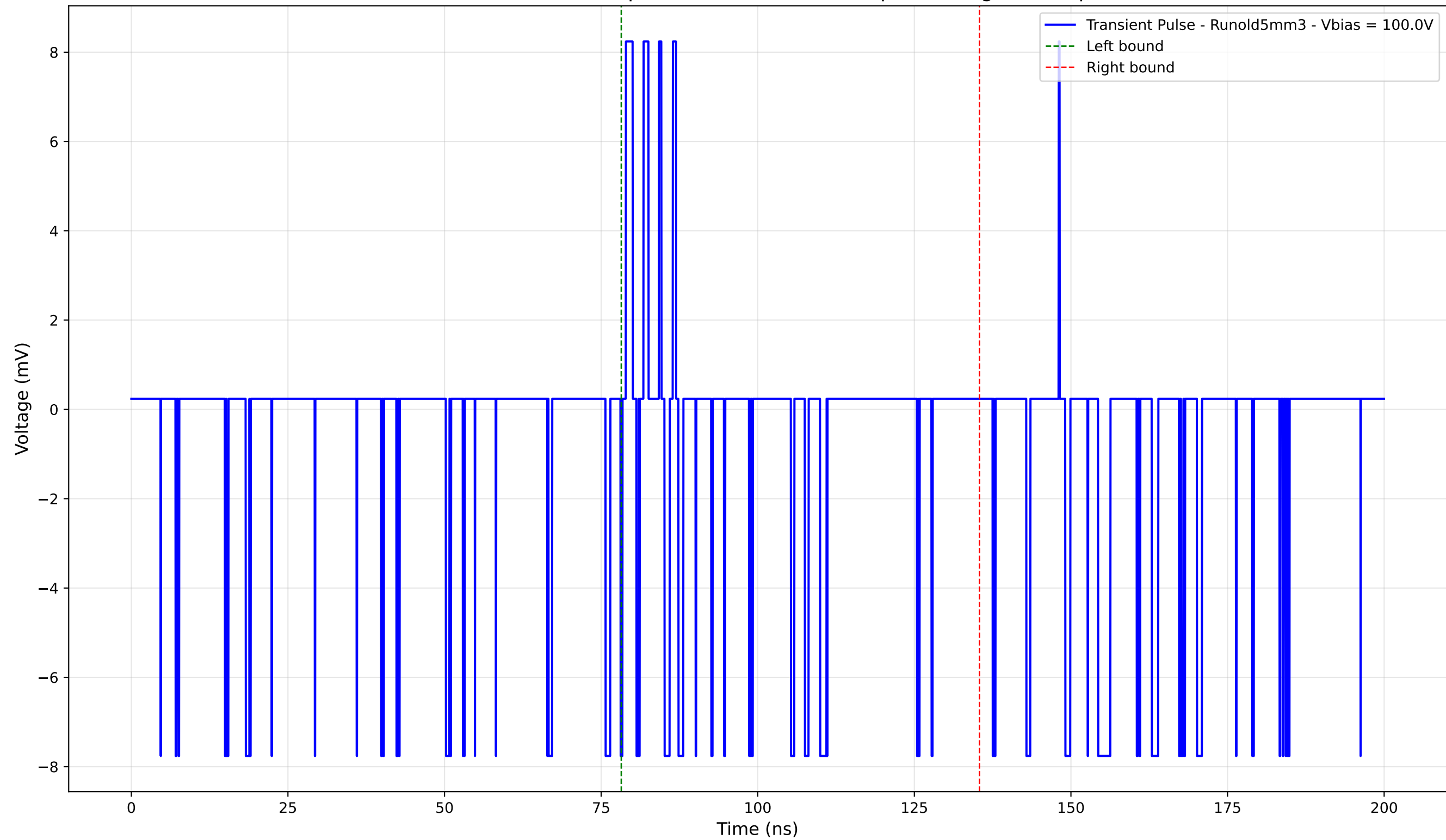
Transient Pulse - Sample: old5 - Position: 35.0 \mu\text{m} - Charge: -0.21 pC
