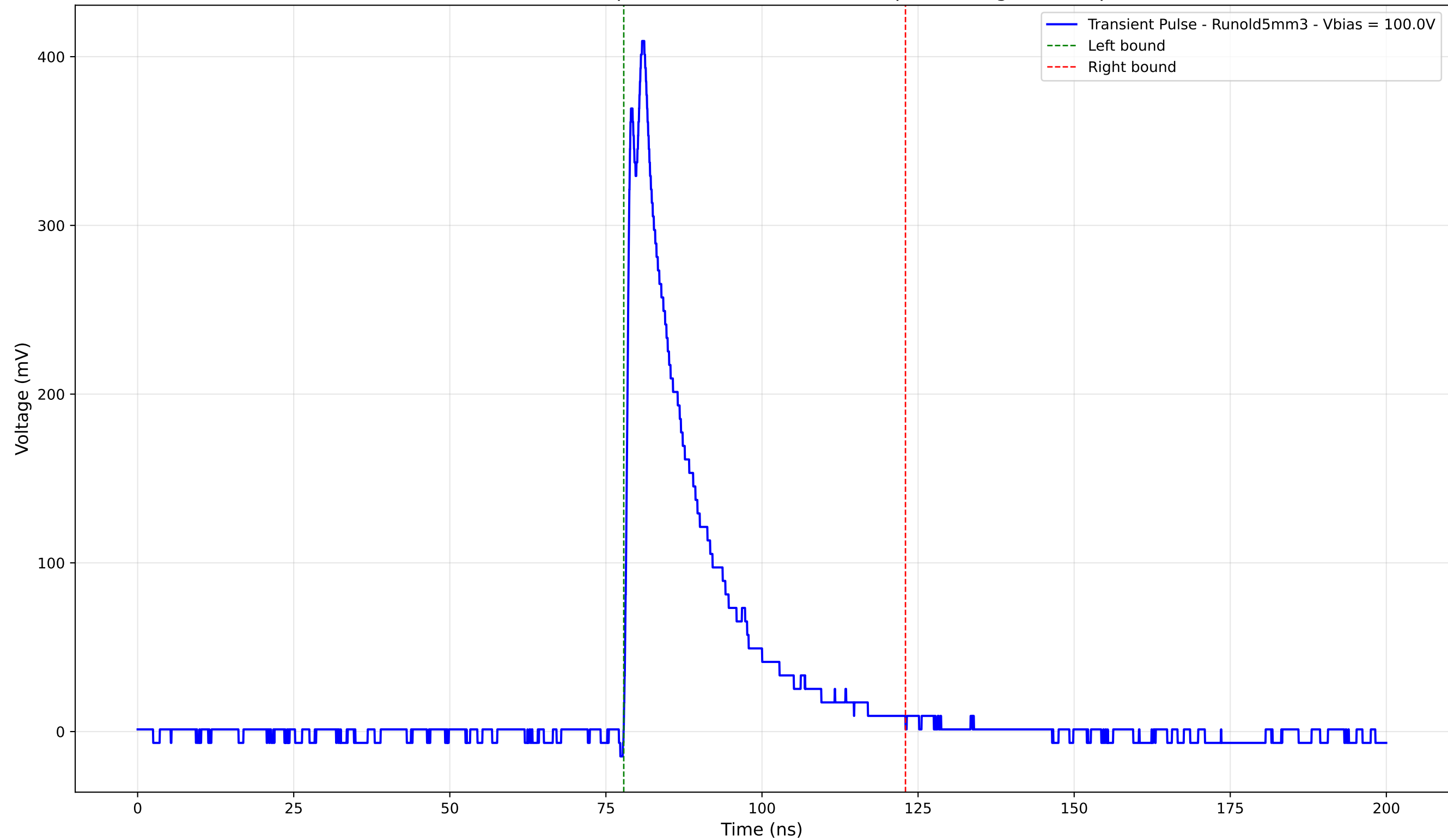
Transient Pulse - Sample: old5 - Position: 3975.0 \mu\text{m} - Charge: 86.42 pC
