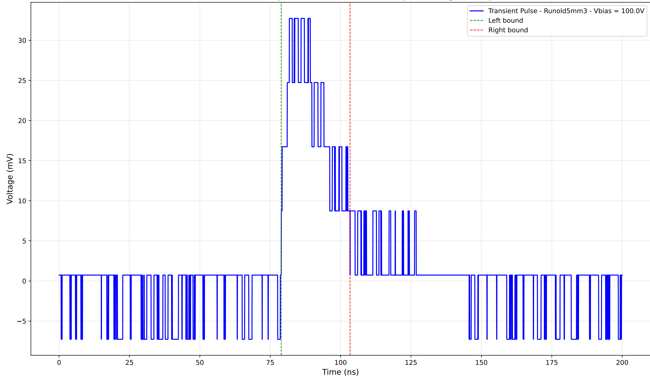
Transient Pulse - Sample: old5 - Position: 1785.0 \mu\text{m} - Charge: 9.84 pC
