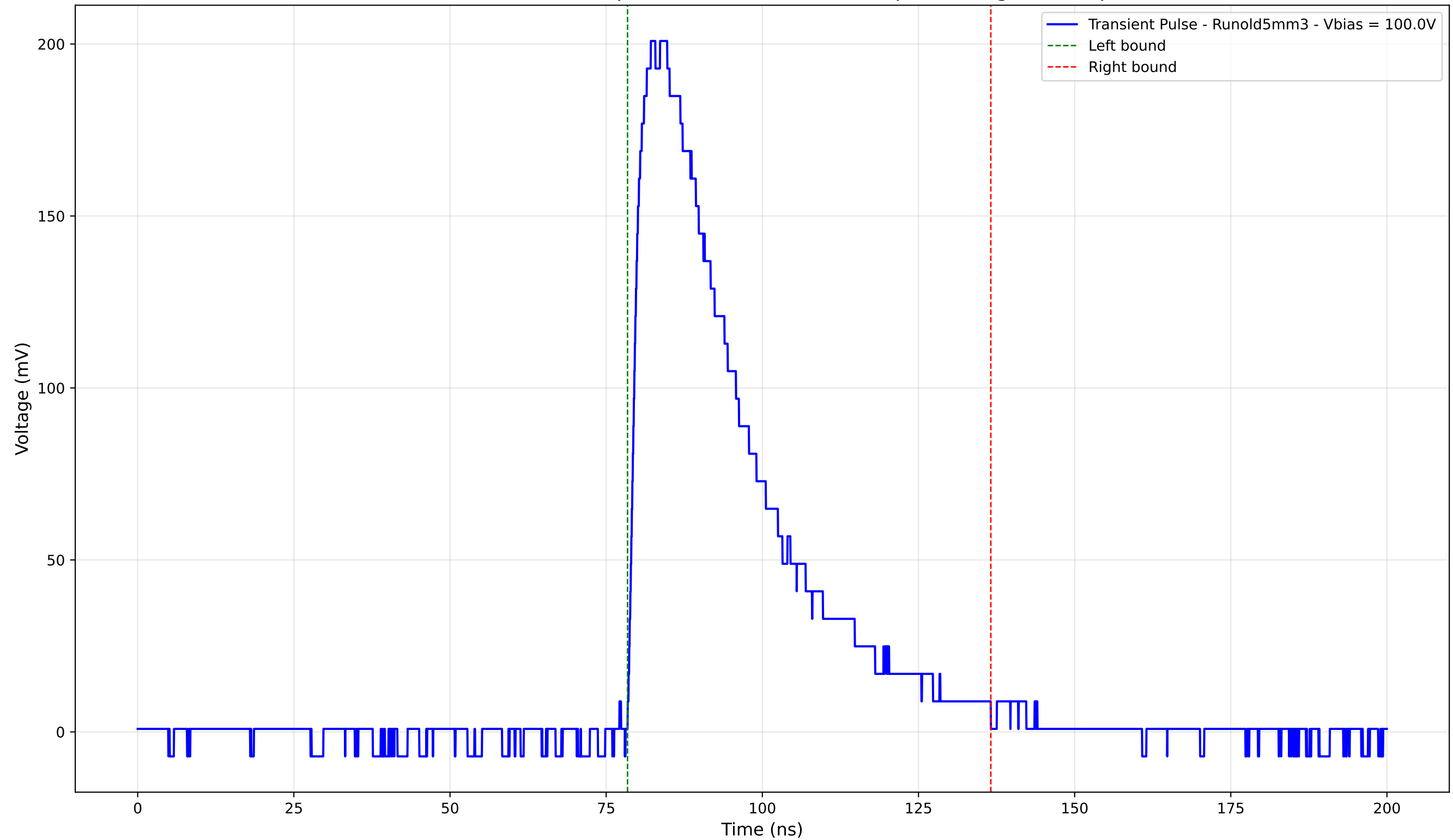
Transient Pulse - Sample: old5 - Position: 1470.0 \mu\text{m} - Charge: 79.72 pC
