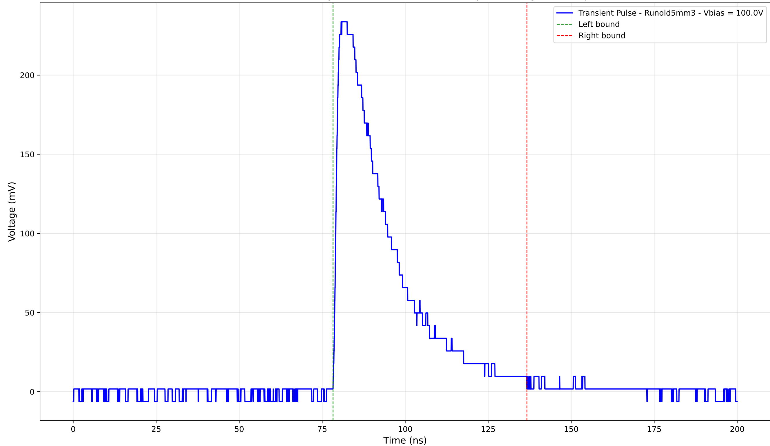
Transient Pulse - Sample: old5 - Position: 1065.0 \mu\text{m} - Charge: 83.74 pC
