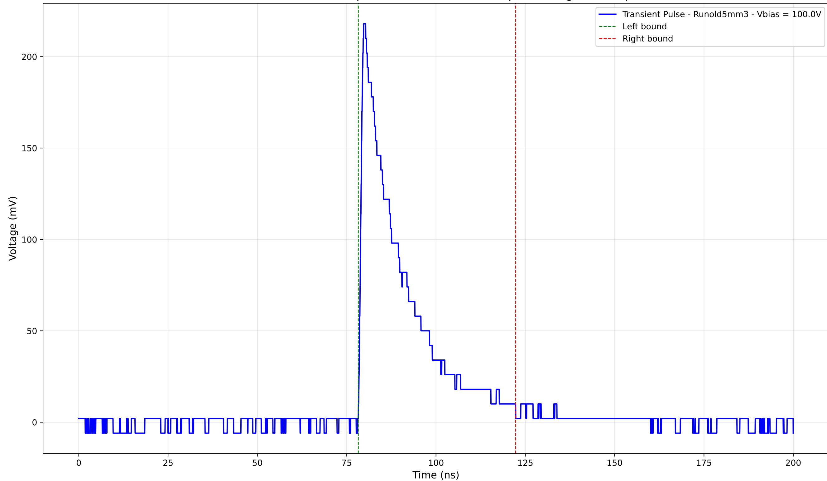
Transient Pulse - Sample: old5 - Position: 665.0 \mu\text{m} - Charge: 52.74 pC
