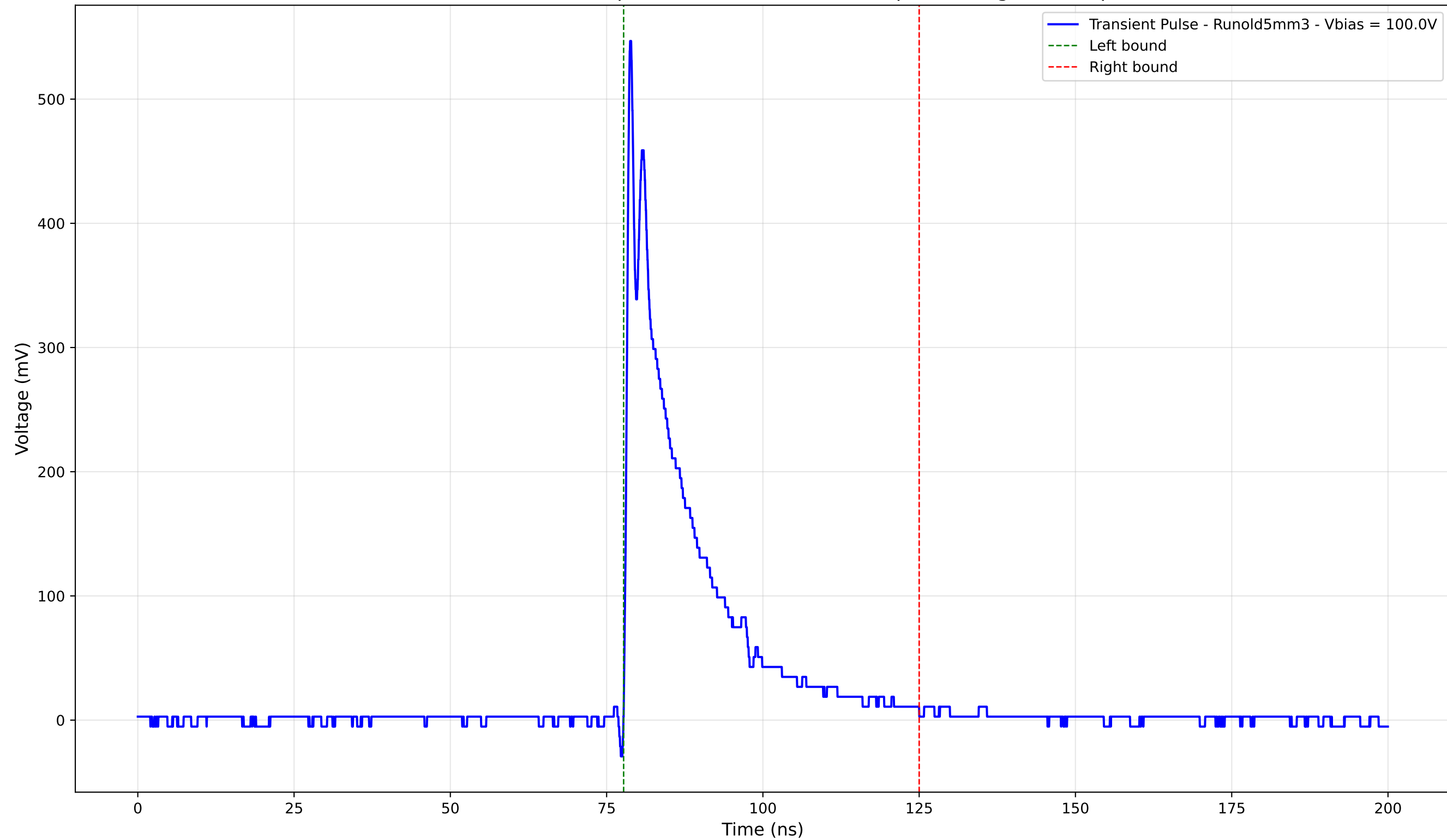
Transient Pulse - Sample: old5 - Position: 3385.0 \mu\text{m} - Charge: 95.69 pC
