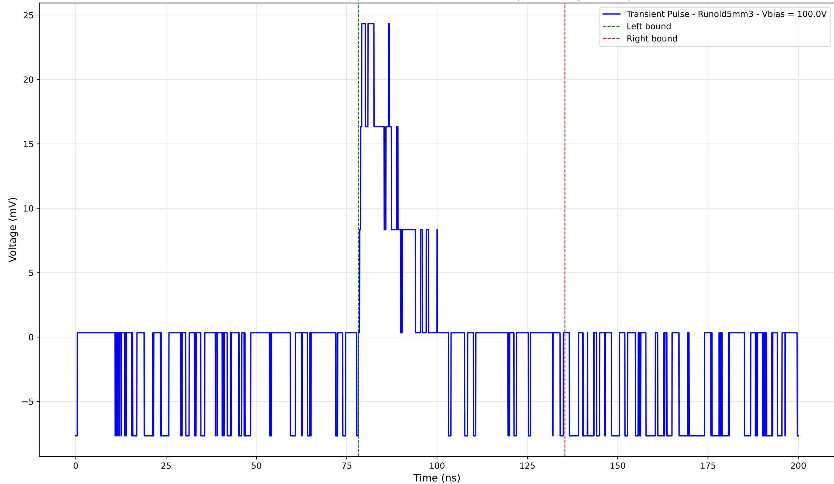
Transient Pulse - Sample: old5 - Position: 4170.0 \mu\text{m} - Charge: 4.03 pC
