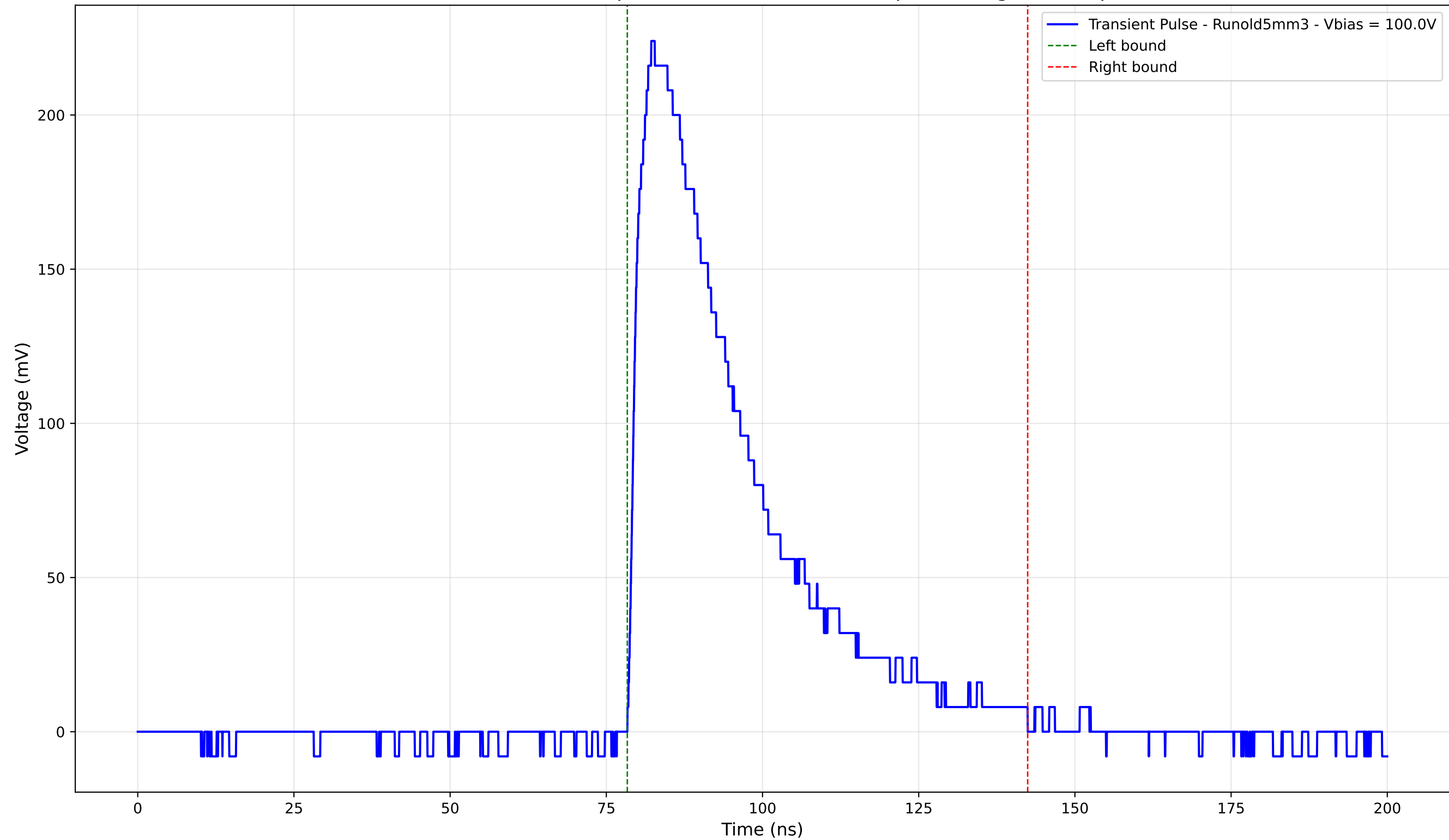
Transient Pulse - Sample: old5 - Position: 2315.0 \mu\text{m} - Charge: 86.85 pC
