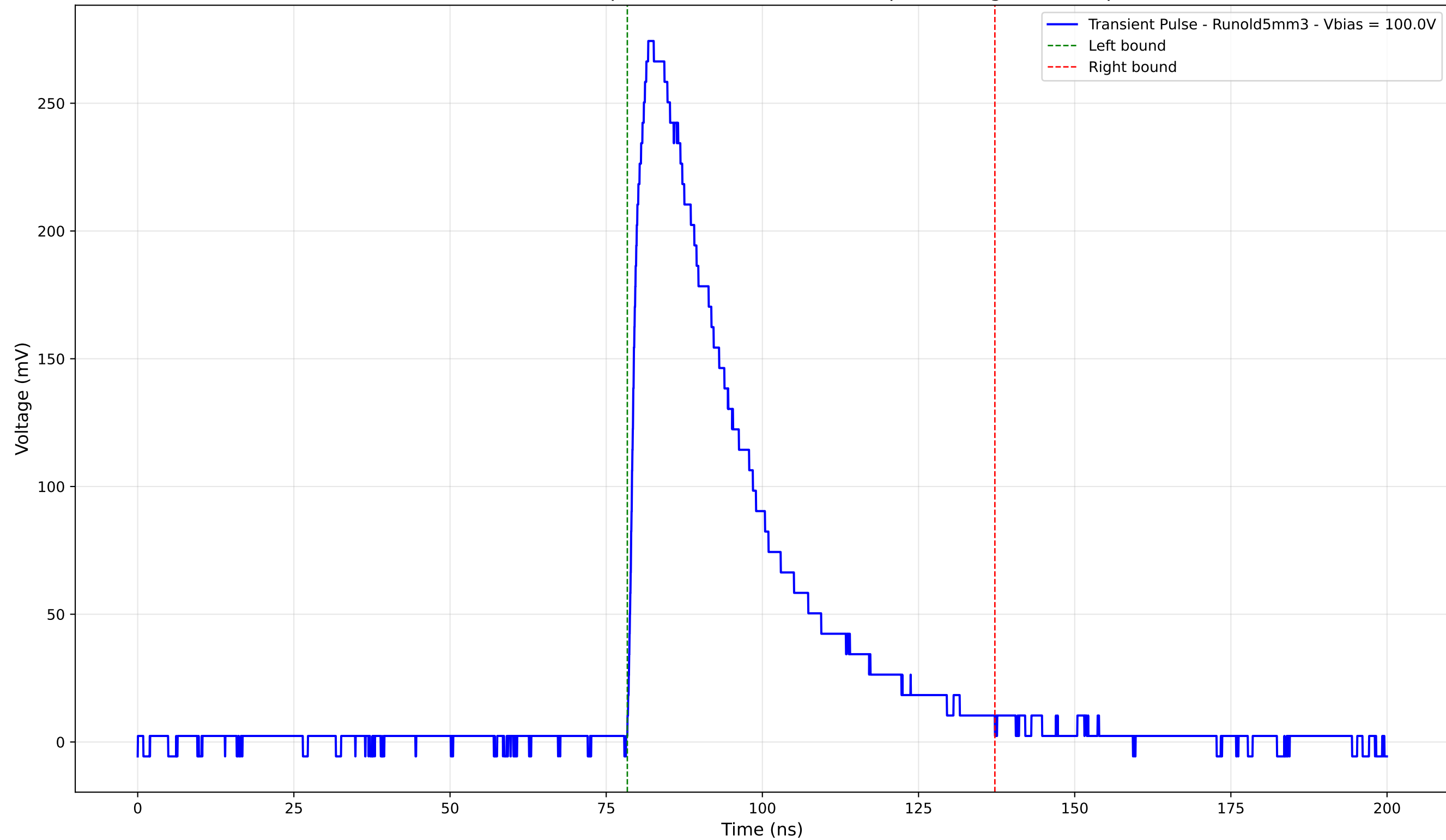
Transient Pulse - Sample: old5 - Position: 2510.0 \mu\text{m} - Charge: 103.11 pC
