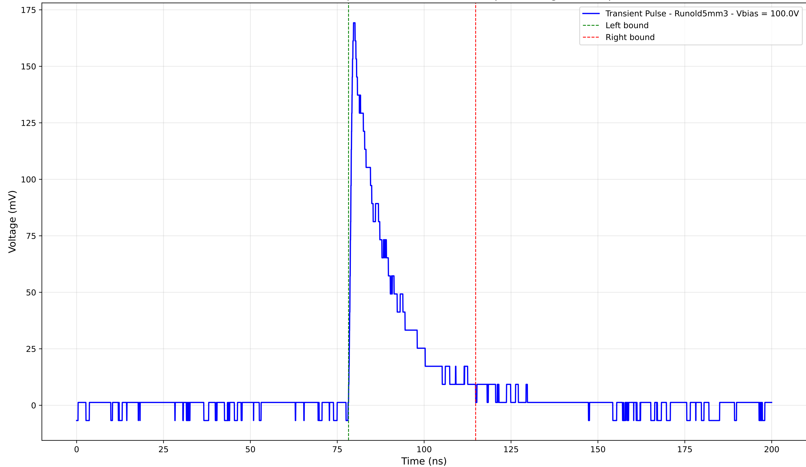
Transient Pulse - Sample: old5 - Position: 590.0 \mu\text{m} - Charge: 35.39 pC
