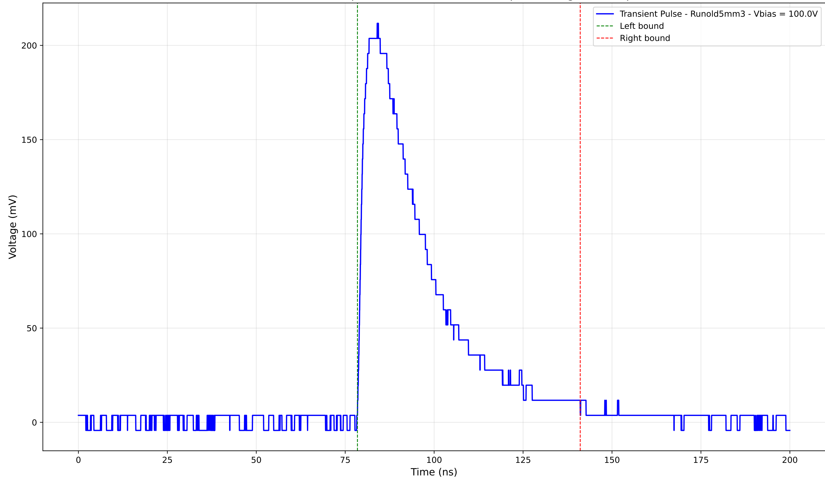
Transient Pulse - Sample: old5 - Position: 1475.0 \mu\text{m} - Charge: 85.27 pC
