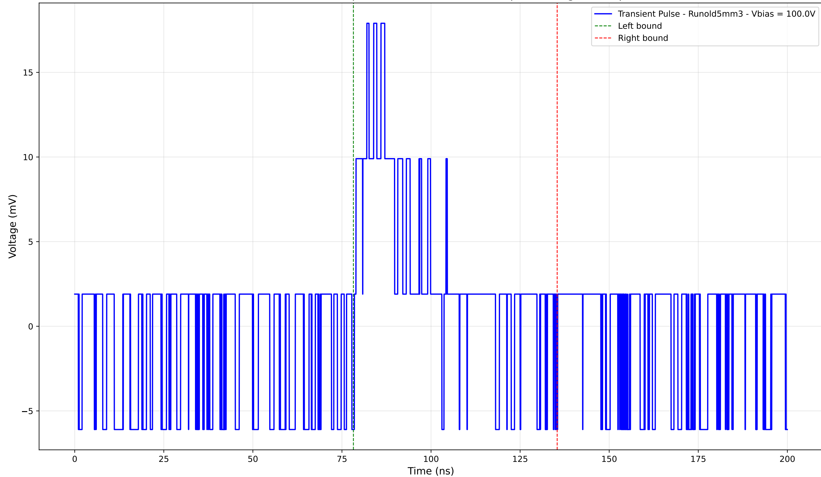
Transient Pulse - Sample: old5 - Position: 2665.0 \mu\text{m} - Charge: 4.15 pC
