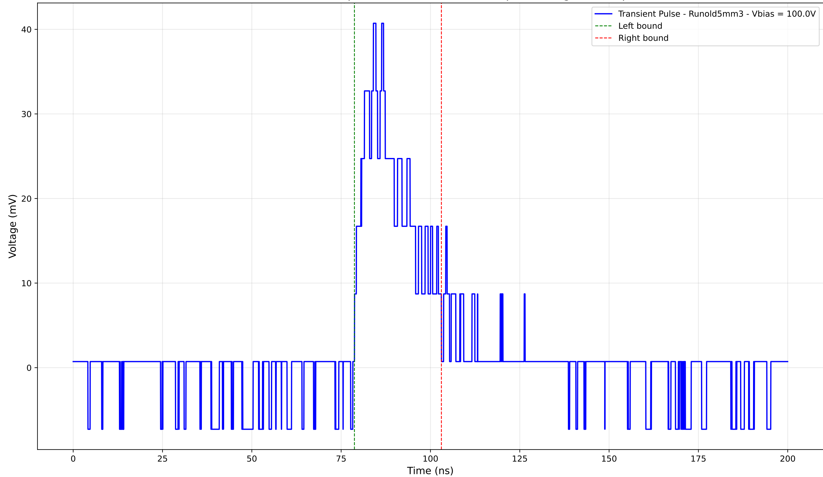
Transient Pulse - Sample: old5 - Position: 2190.0 \mu\text{m} - Charge: 10.09 pC
