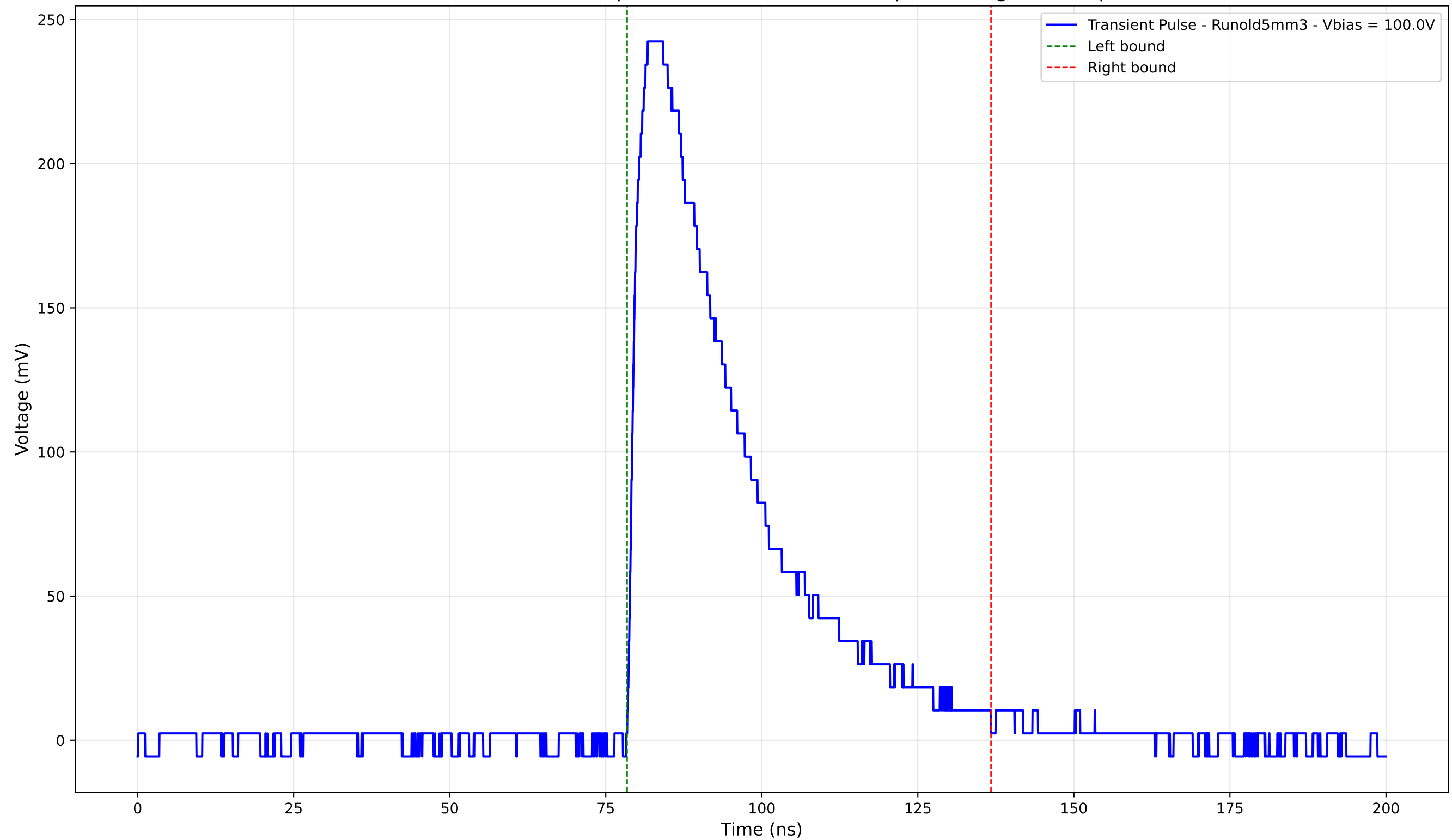
Transient Pulse - Sample: old5 - Position: 2480.0 \mu\text{m} - Charge: 94.04 pC
