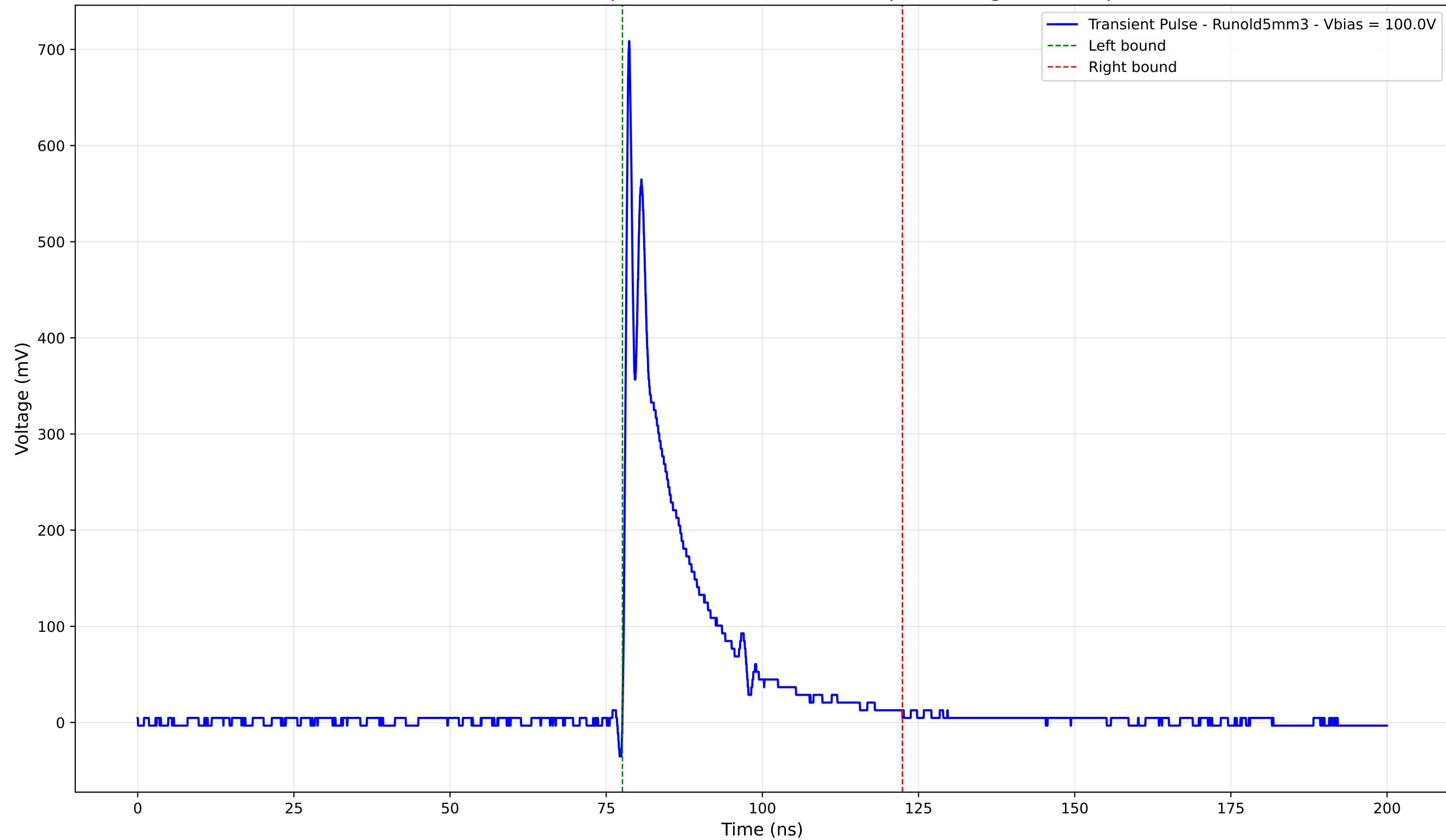
Transient Pulse - Sample: old5 - Position: 3695.0 \mu\text{m} - Charge: 103.99 pC
