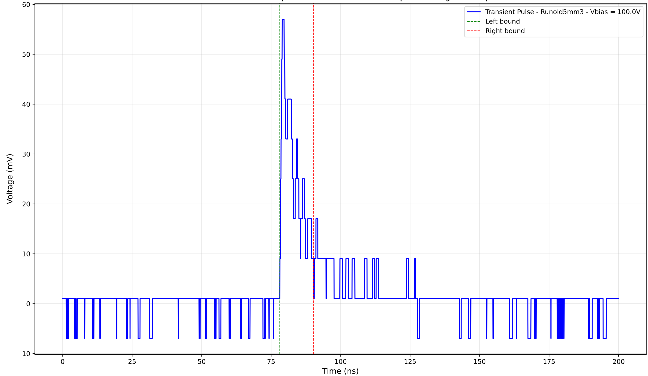
Transient Pulse - Sample: old5 - Position: 135.0 \mu\text{m} - Charge: 6.35 pC
