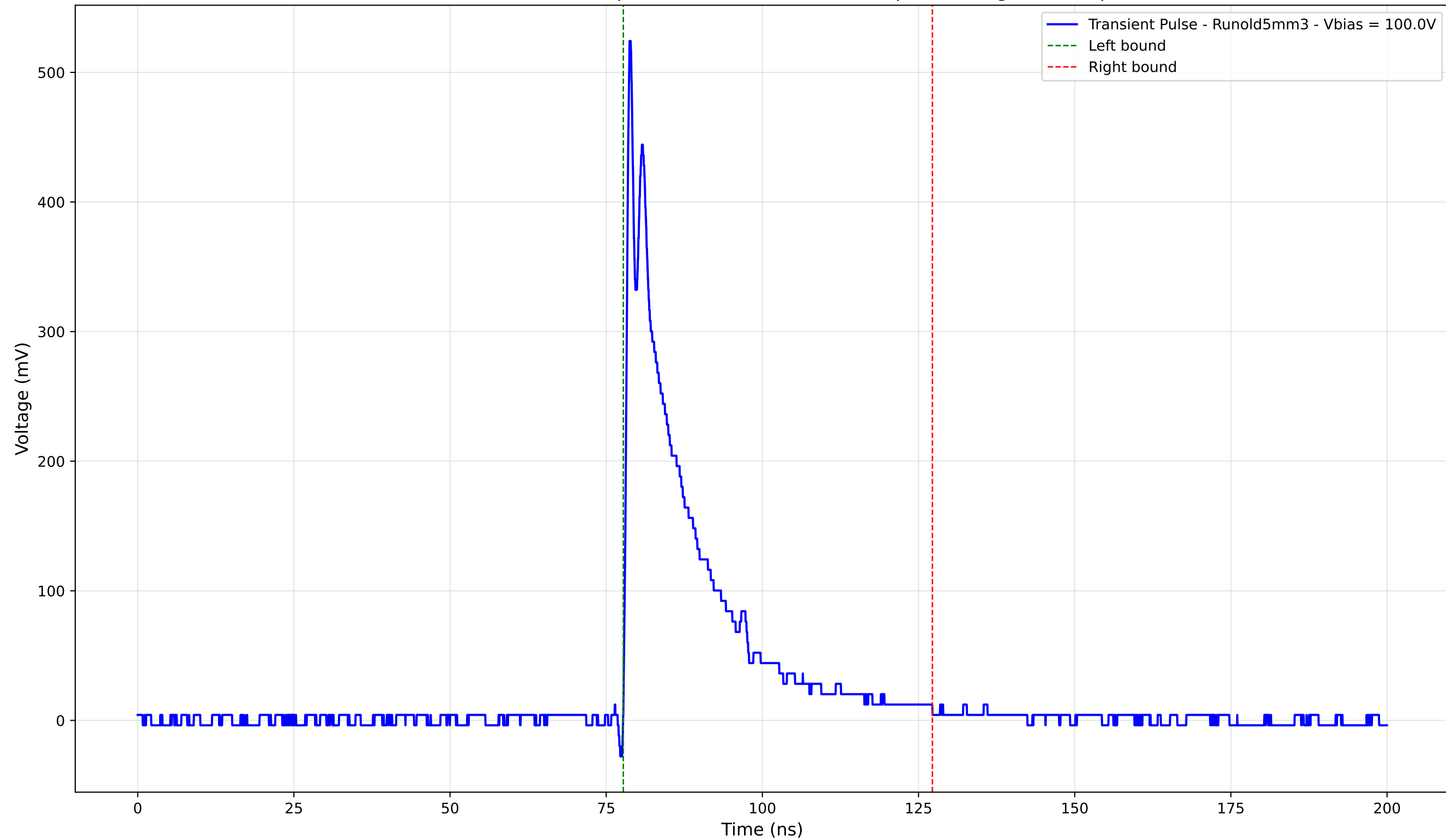
Transient Pulse - Sample: old5 - Position: 3380.0 \mu\text{m} - Charge: 93.61 pC
