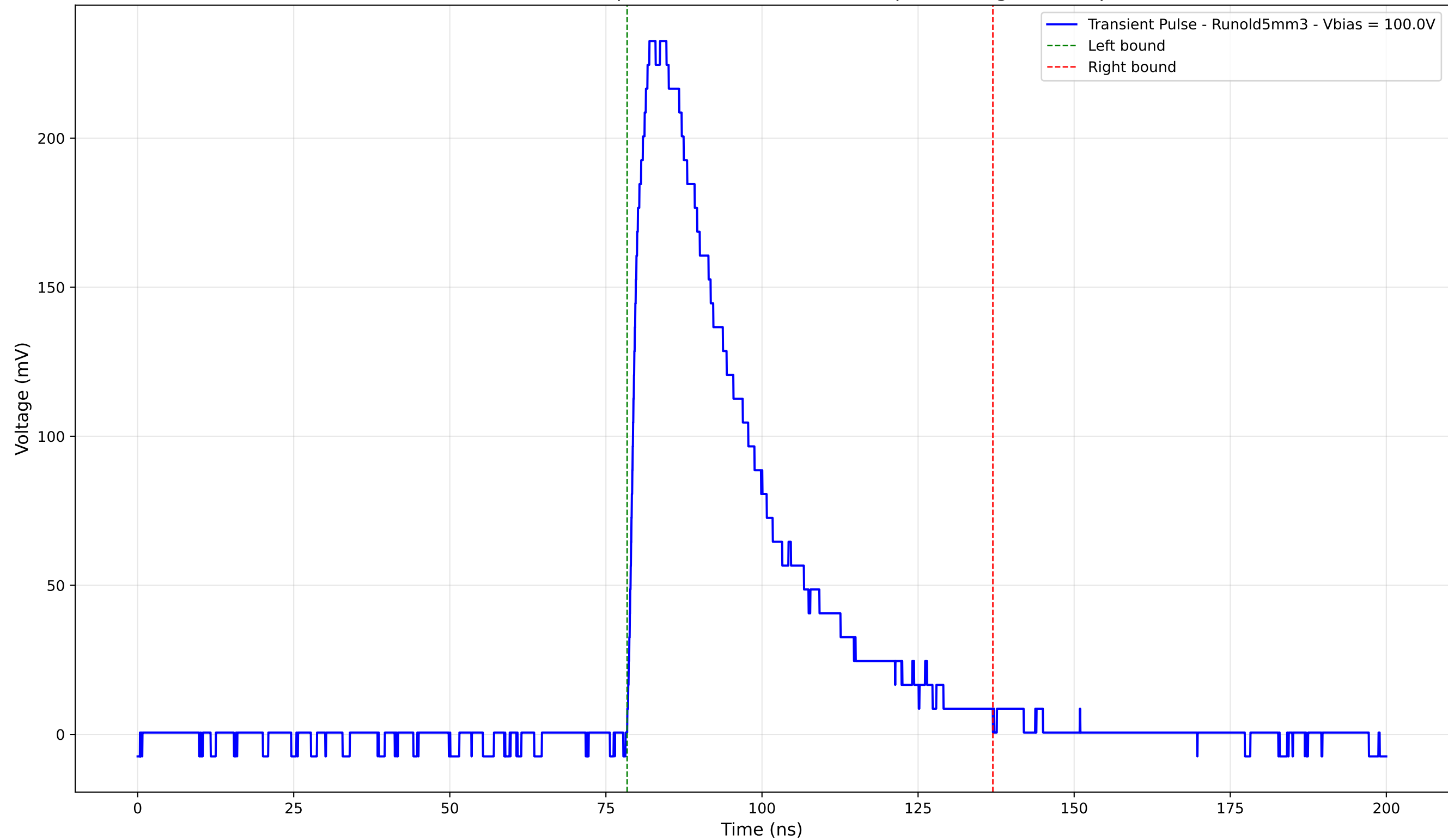
Transient Pulse - Sample: old5 - Position: 2285.0 \mu\text{m} - Charge: 91.18 pC
