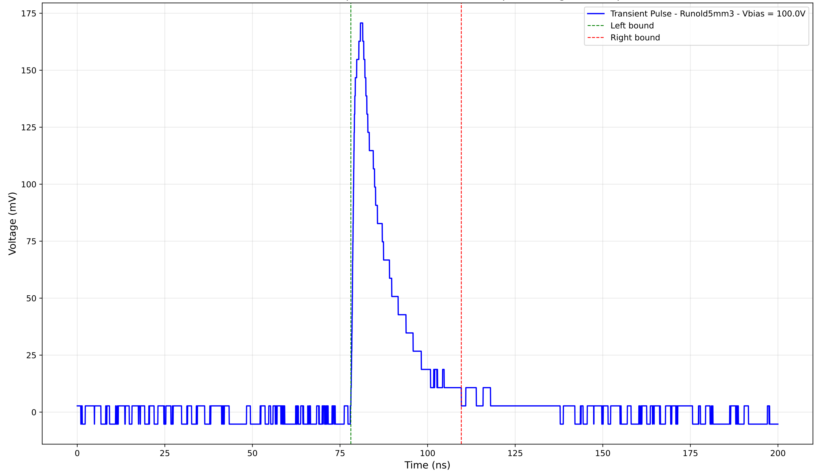
Transient Pulse - Sample: old5 - Position: 4125.0 \mu\text{m} - Charge: 34.34 pC
