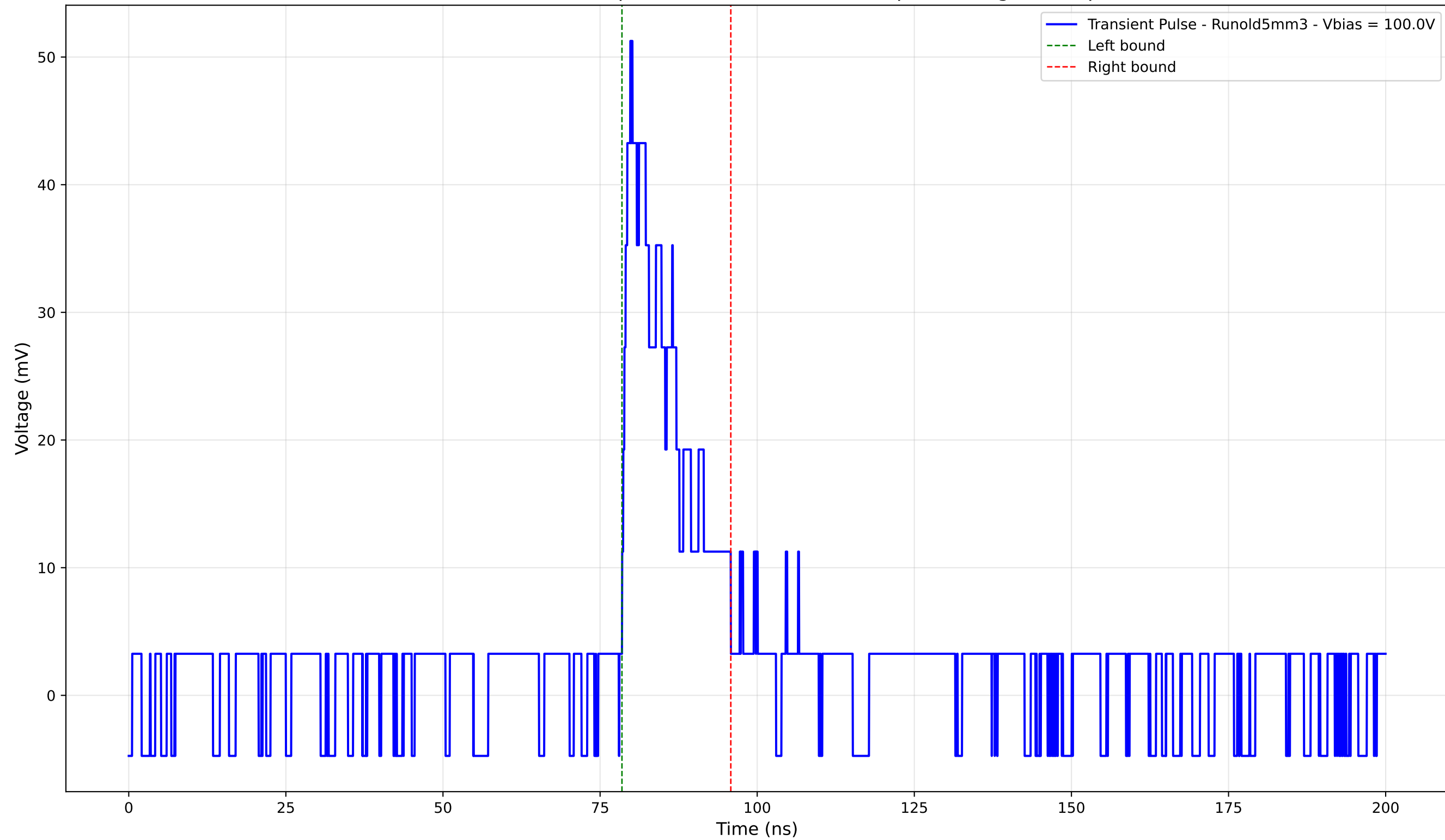
Transient Pulse - Sample: old5 - Position: 4470.0 \mu\text{m} - Charge: 8.19 pC
