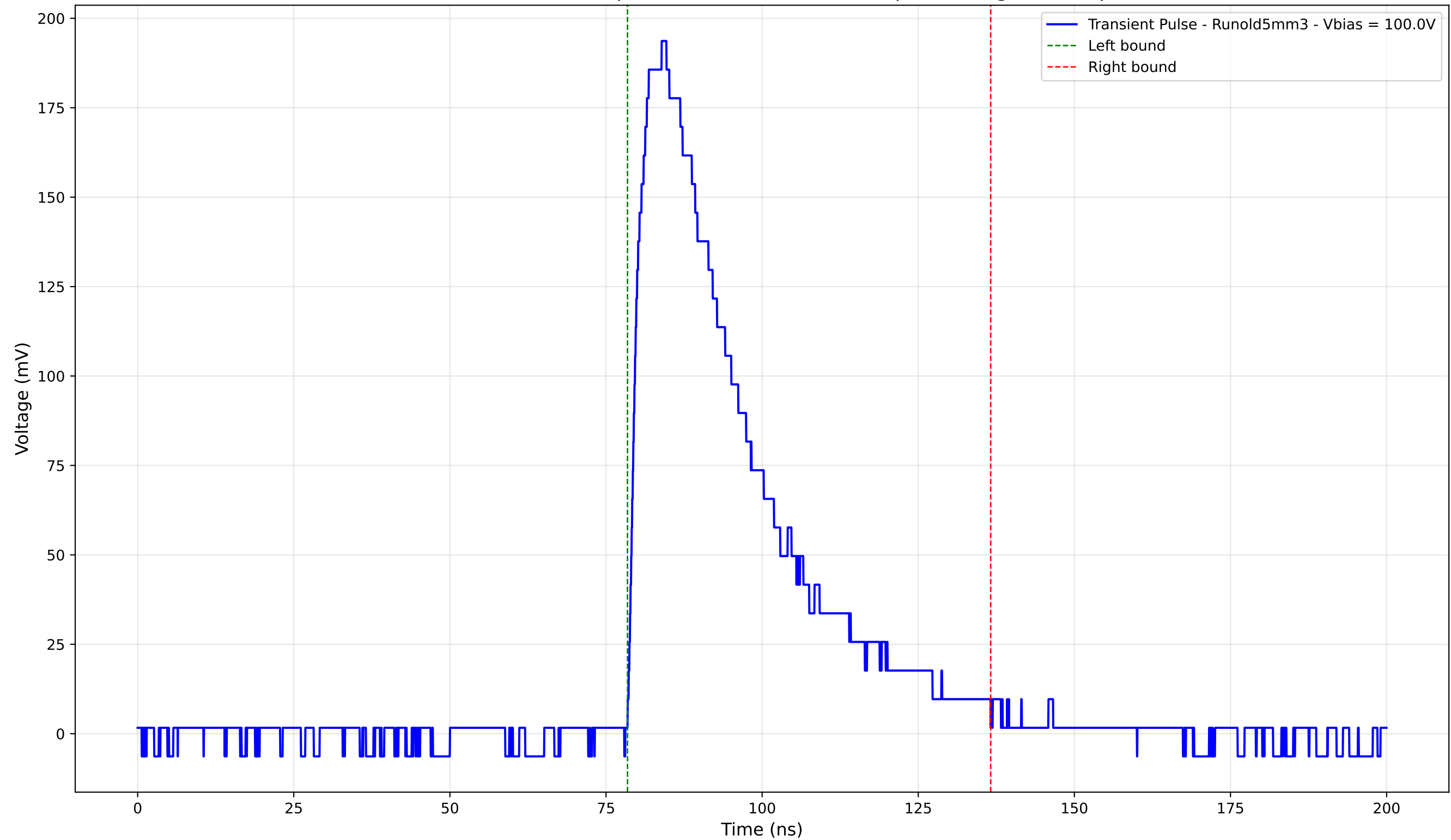
Transient Pulse - Sample: old5 - Position: 2060.0 \mu\text{m} - Charge: 76.86 pC
