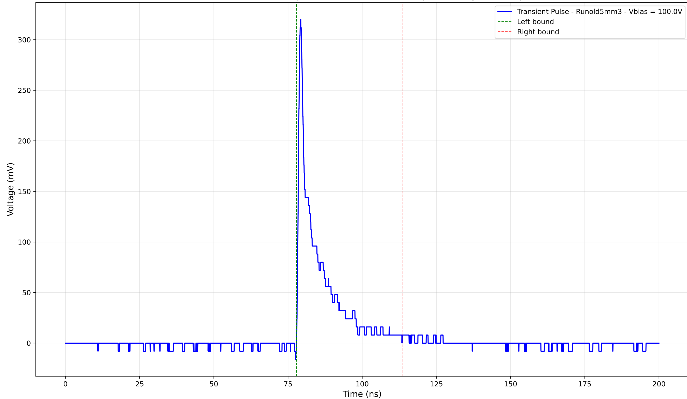
Transient Pulse - Sample: old5 - Position: 175.0 \mu\text{m} - Charge: 36.70 pC
