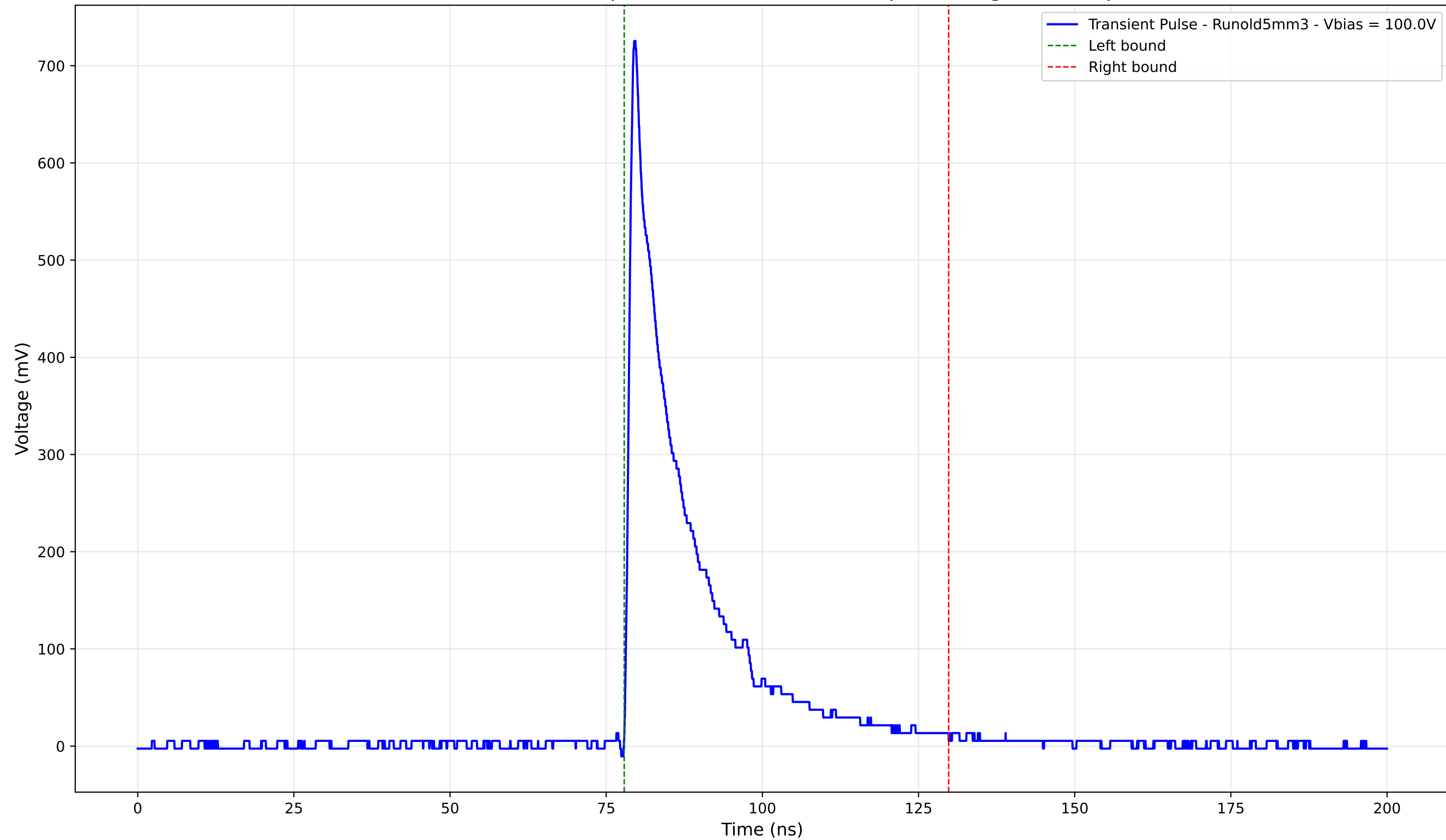
Transient Pulse - Sample: old5 - Position: 4705.0 \mu\text{m} - Charge: 133.76 pC
