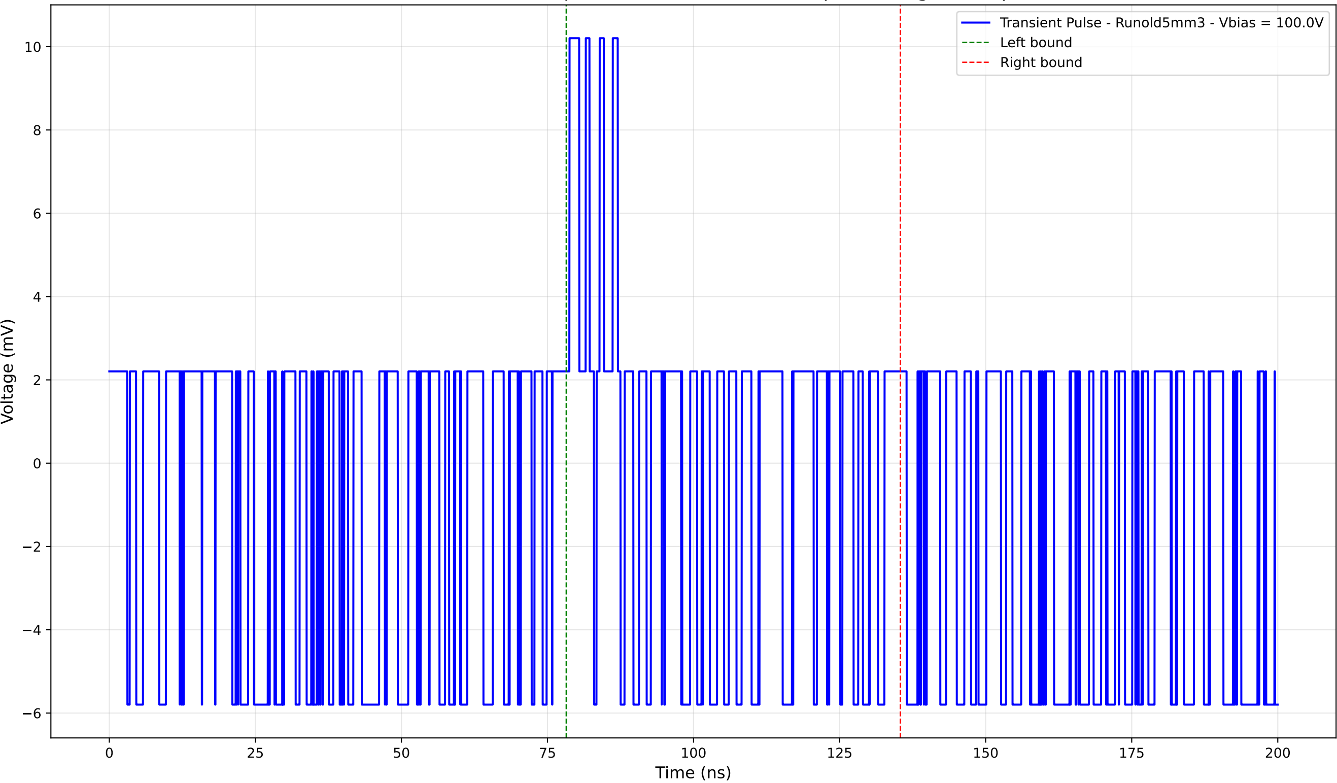
Transient Pulse - Sample: old5 - Position: 4970.0 \mu\text{m} - Charge: 0.68 pC
