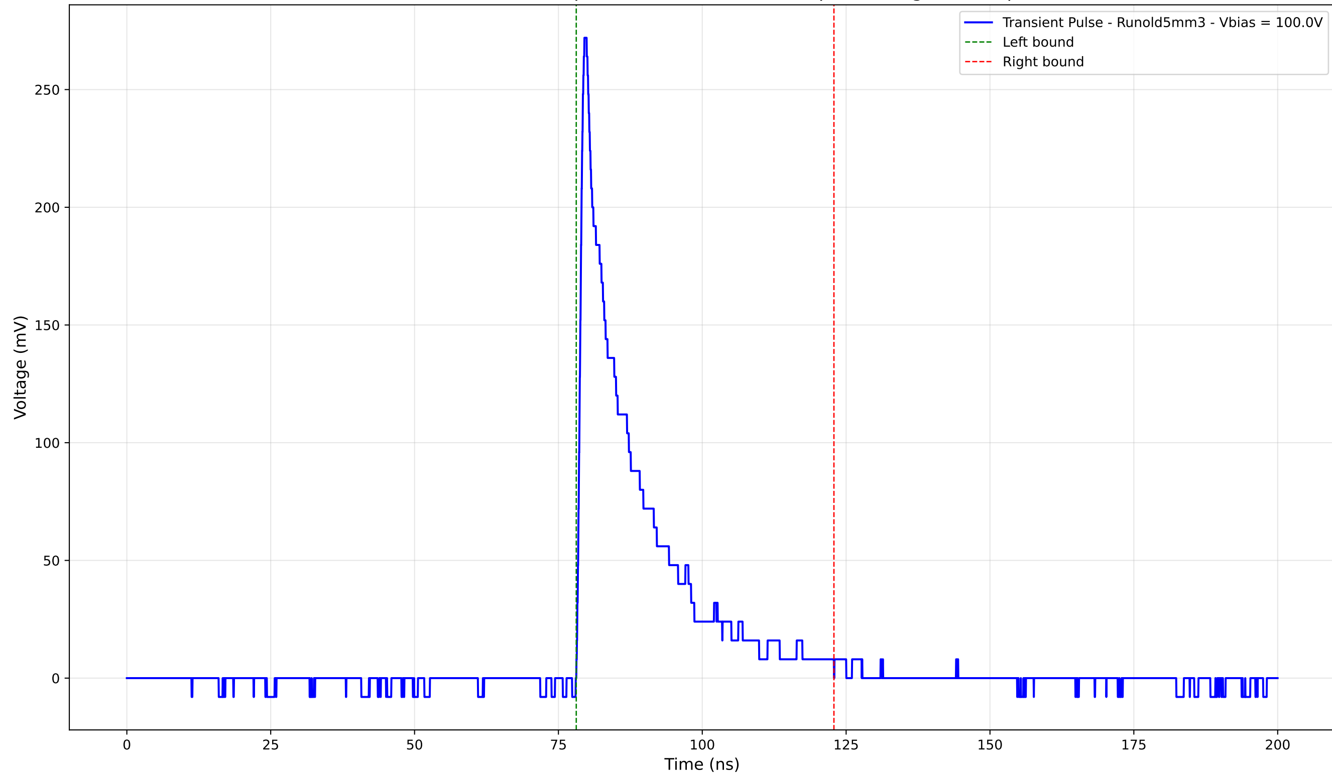
Transient Pulse - Sample: old5 - Position: 465.0 \mu\text{m} - Charge: 50.12 pC
