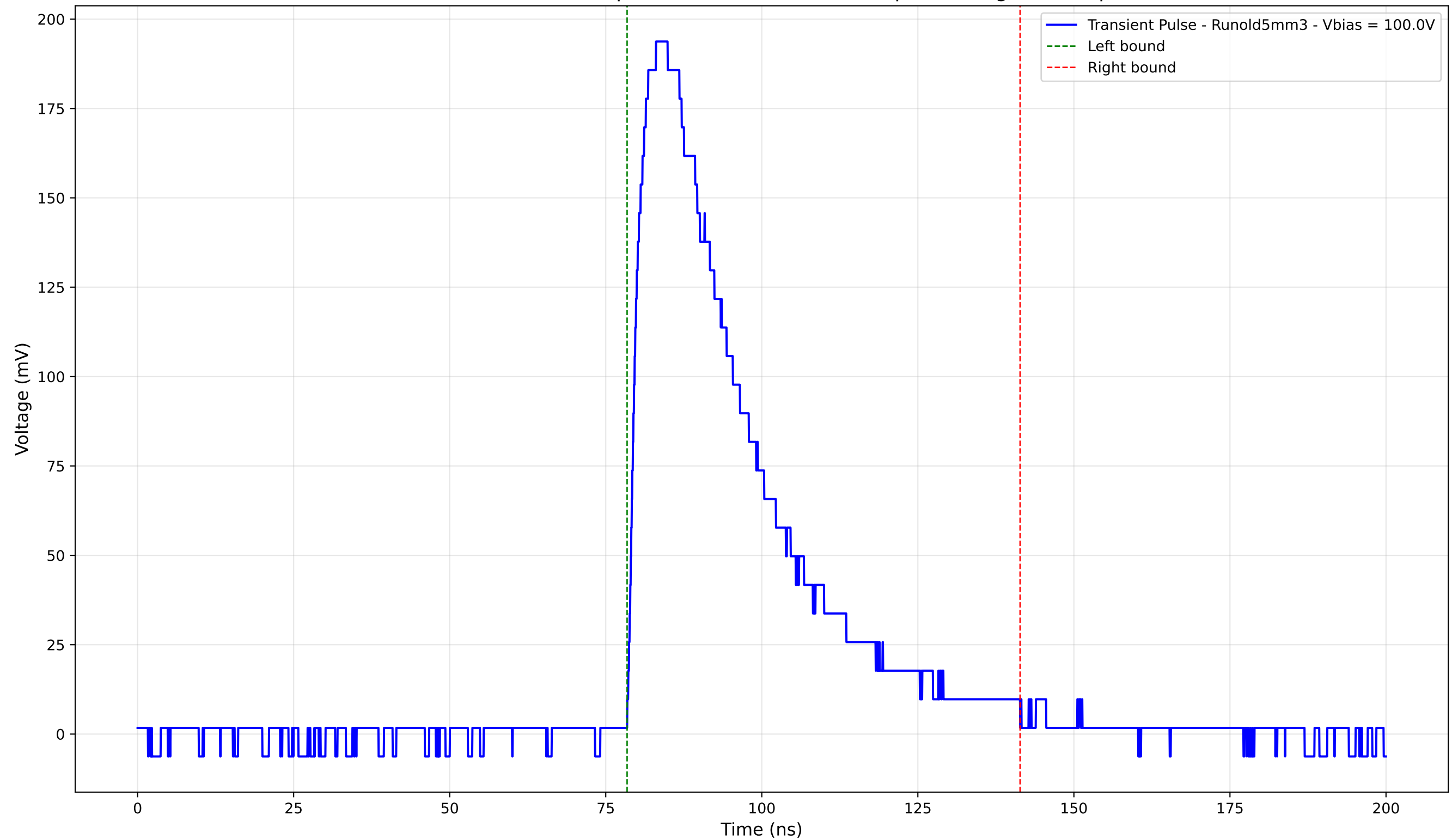
Transient Pulse - Sample: old5 - Position: 1915.0 \mu\text{m} - Charge: 79.64 pC
