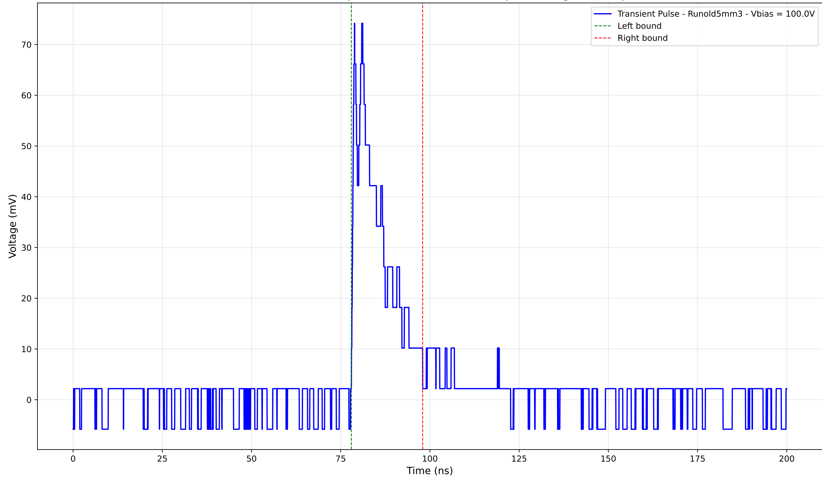
Transient Pulse - Sample: old5 - Position: 3315.0 \mu\text{m} - Charge: 12.24 pC
