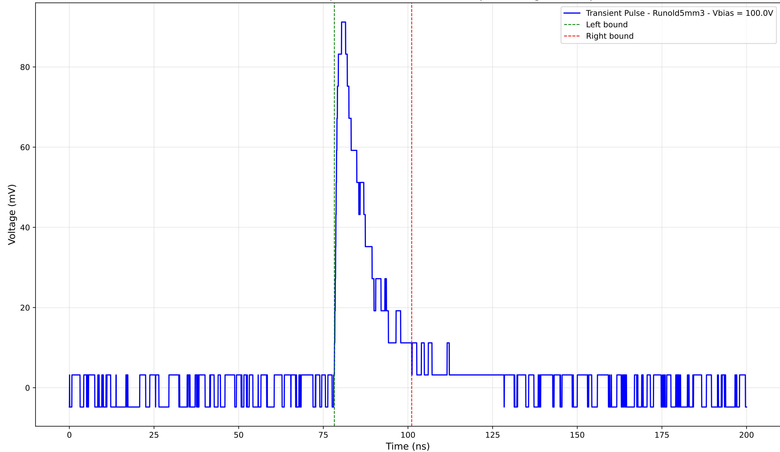
Transient Pulse - Sample: old5 - Position: 4140.0 \mu\text{m} - Charge: 17.15 pC
