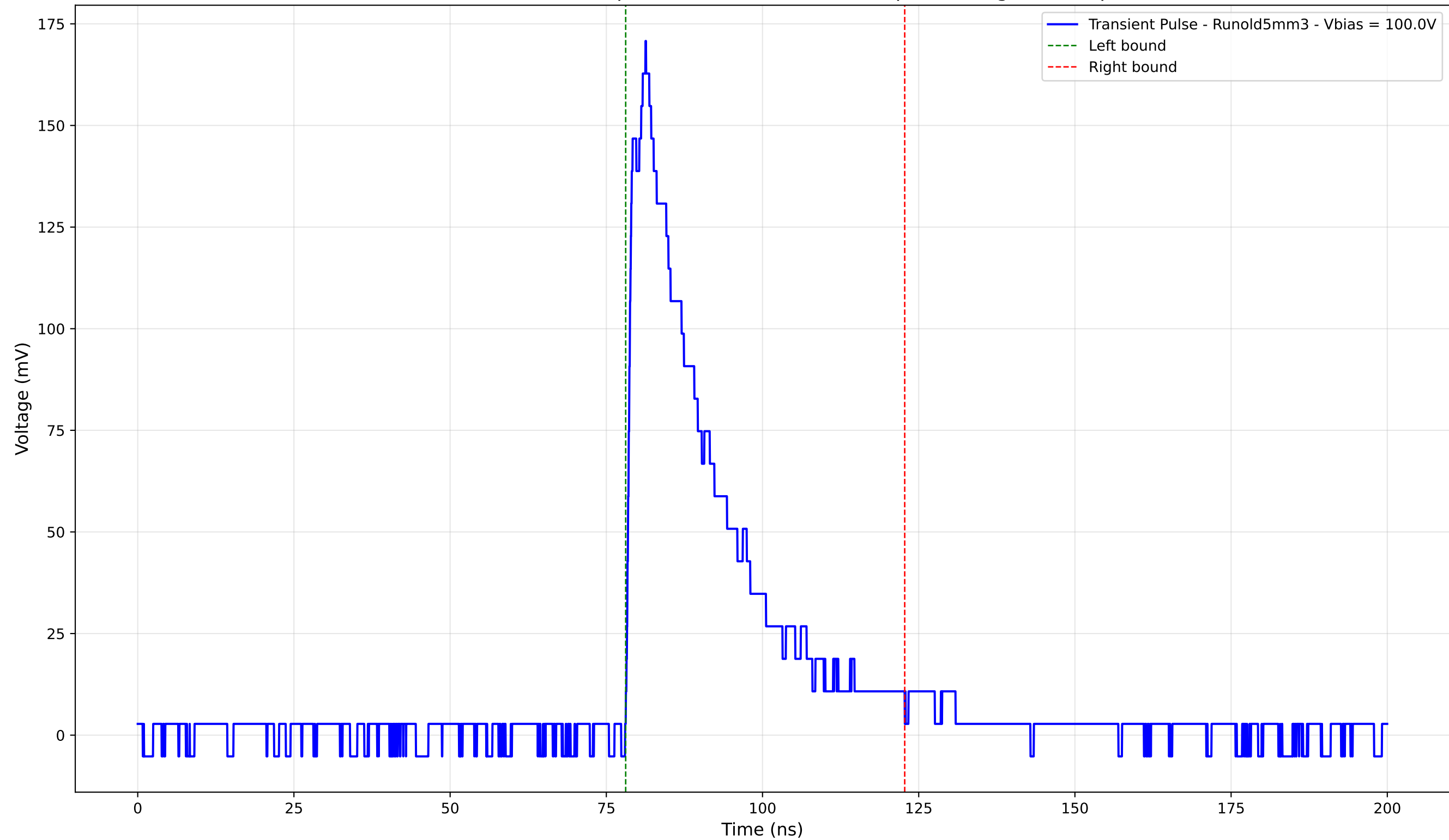
Transient Pulse - Sample: old5 - Position: 3040.0 \mu\text{m} - Charge: 46.10 pC
