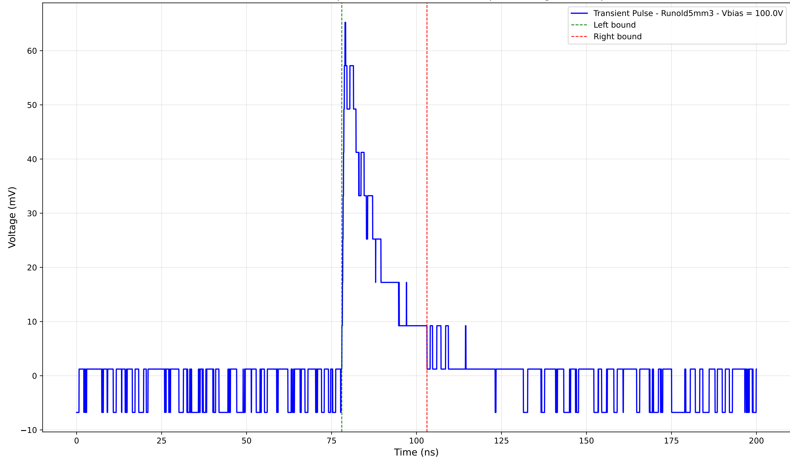
Transient Pulse - Sample: old5 - Position: 3245.0 \mu\text{m} - Charge: 12.19 pC
