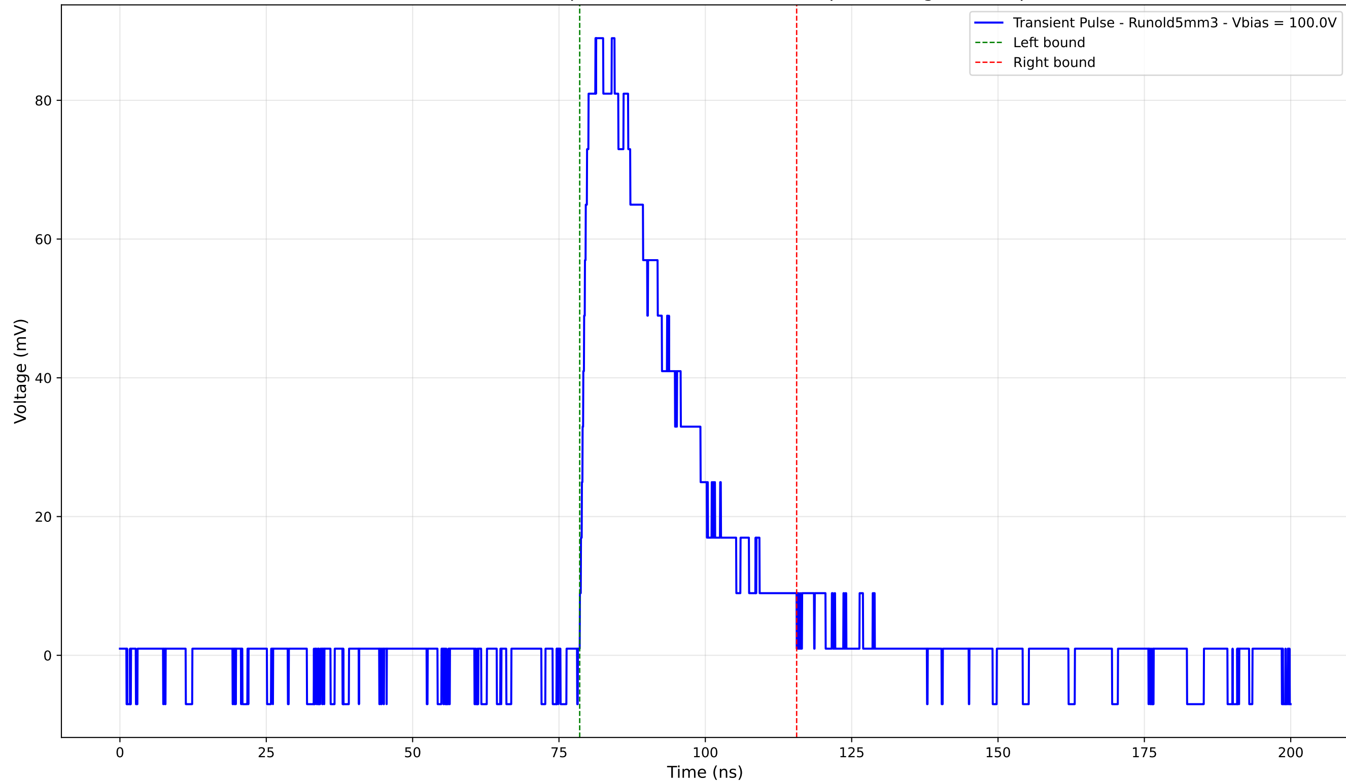
Transient Pulse - Sample: old5 - Position: 1145.0 \mu\text{m} - Charge: 28.68 pC
