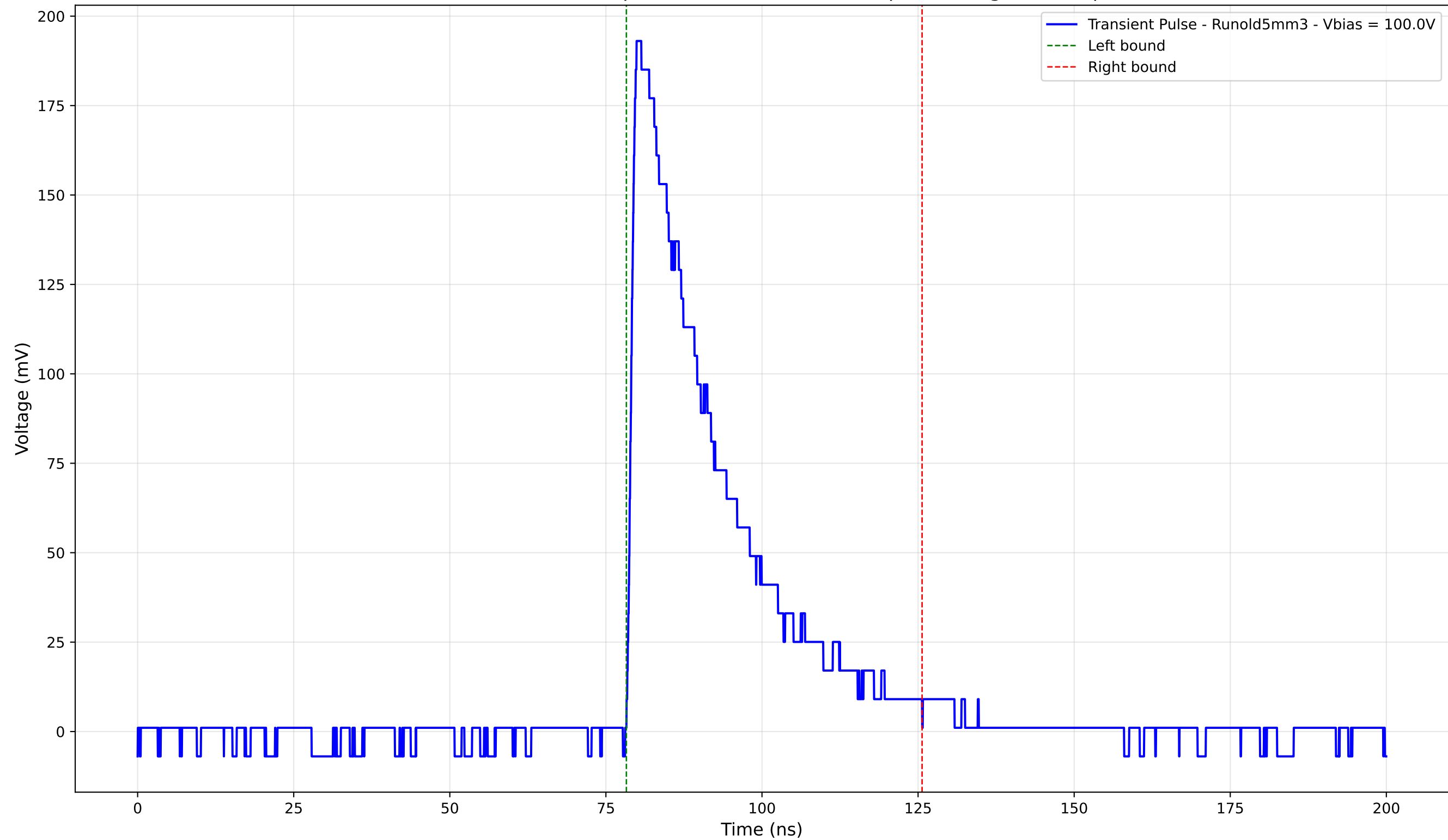
Transient Pulse - Sample: old5 - Position: 860.0 \mu\text{m} - Charge: 56.80 pC
