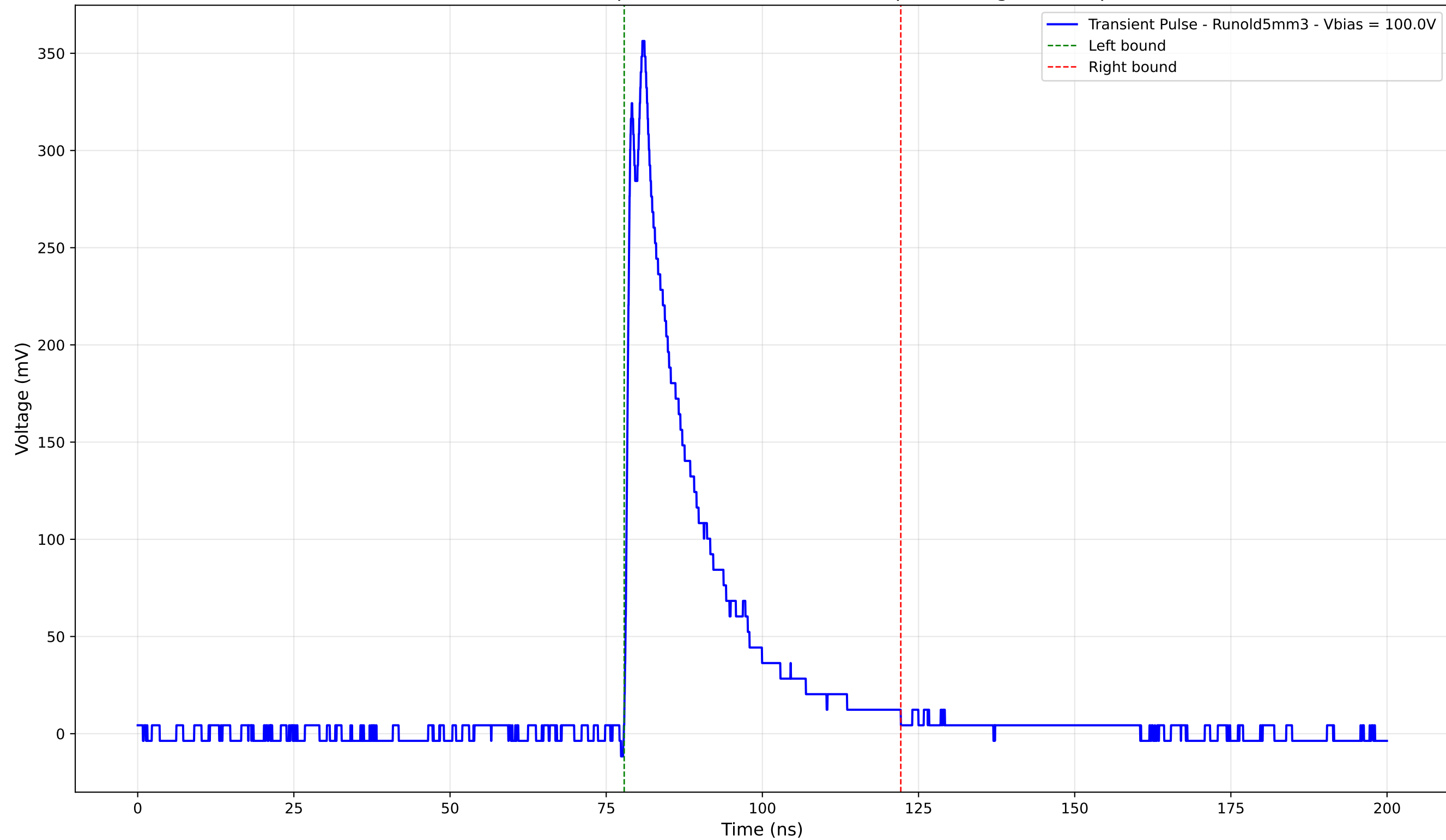
Transient Pulse - Sample: old5 - Position: 3965.0 \mu\text{m} - Charge: 75.82 pC
