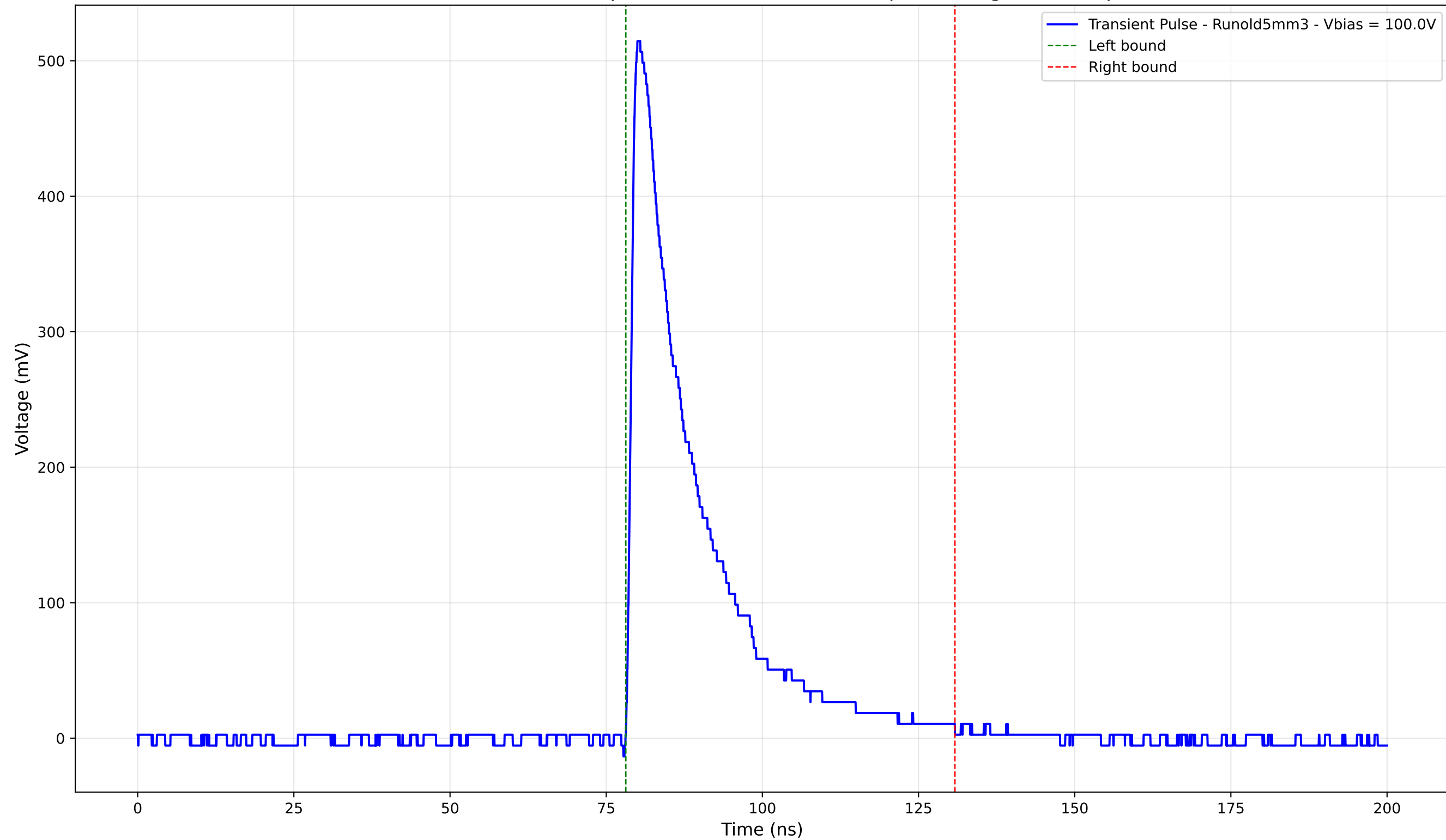
Transient Pulse - Sample: old5 - Position: 4375.0 \mu\text{m} - Charge: 114.50 pC
