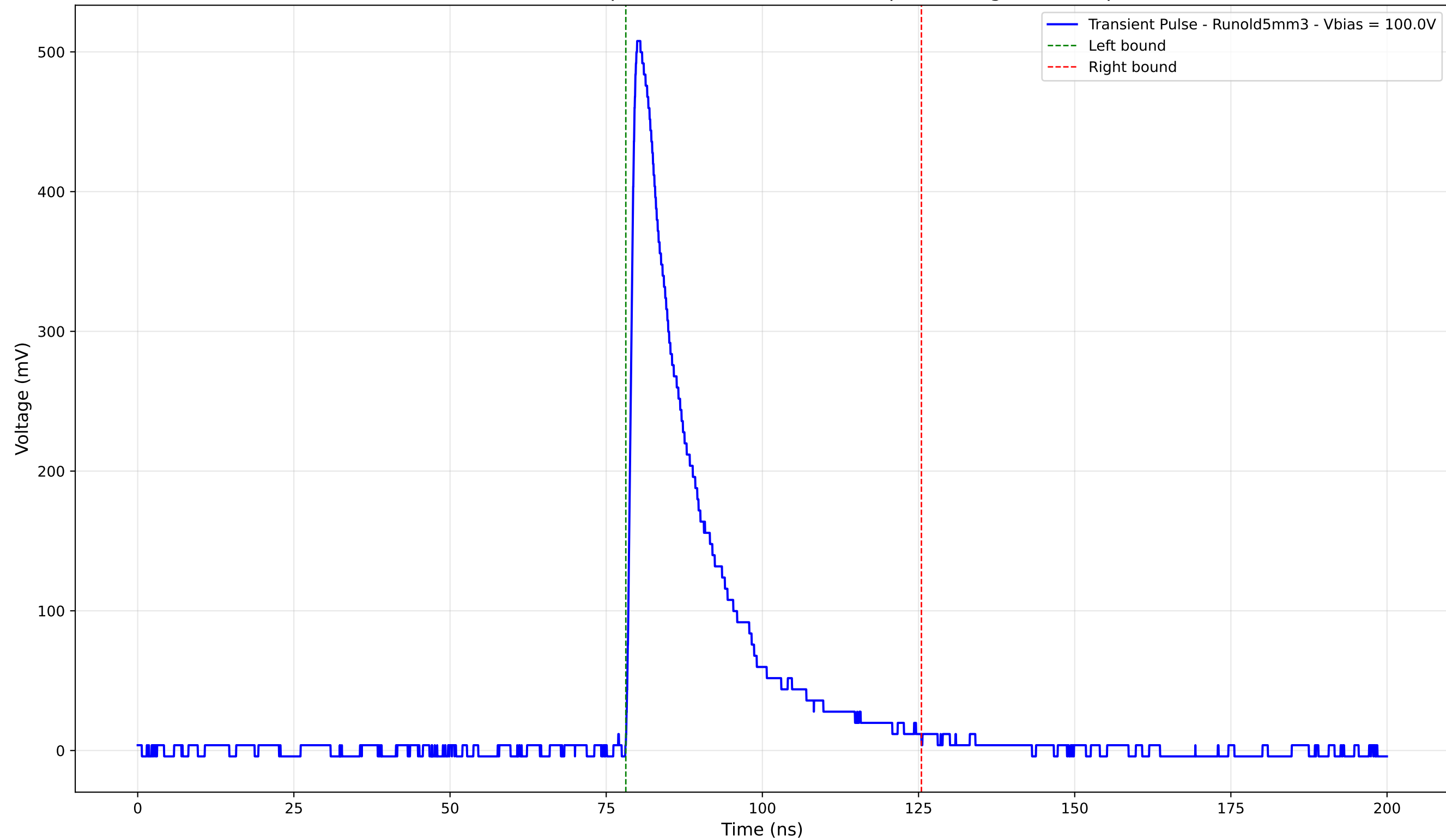
Transient Pulse - Sample: old5 - Position: 4380.0 \mu\text{m} - Charge: 112.89 pC
