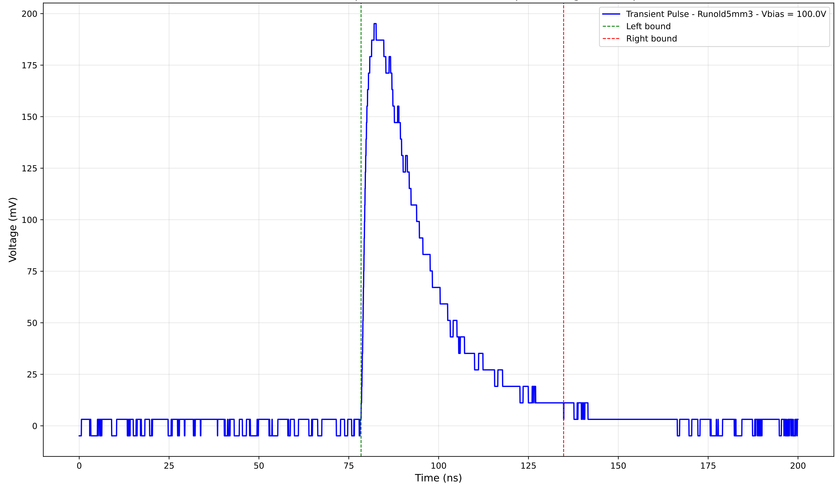
Transient Pulse - Sample: old5 - Position: 1310.0 \mu\text{m} - Charge: 74.05 pC
