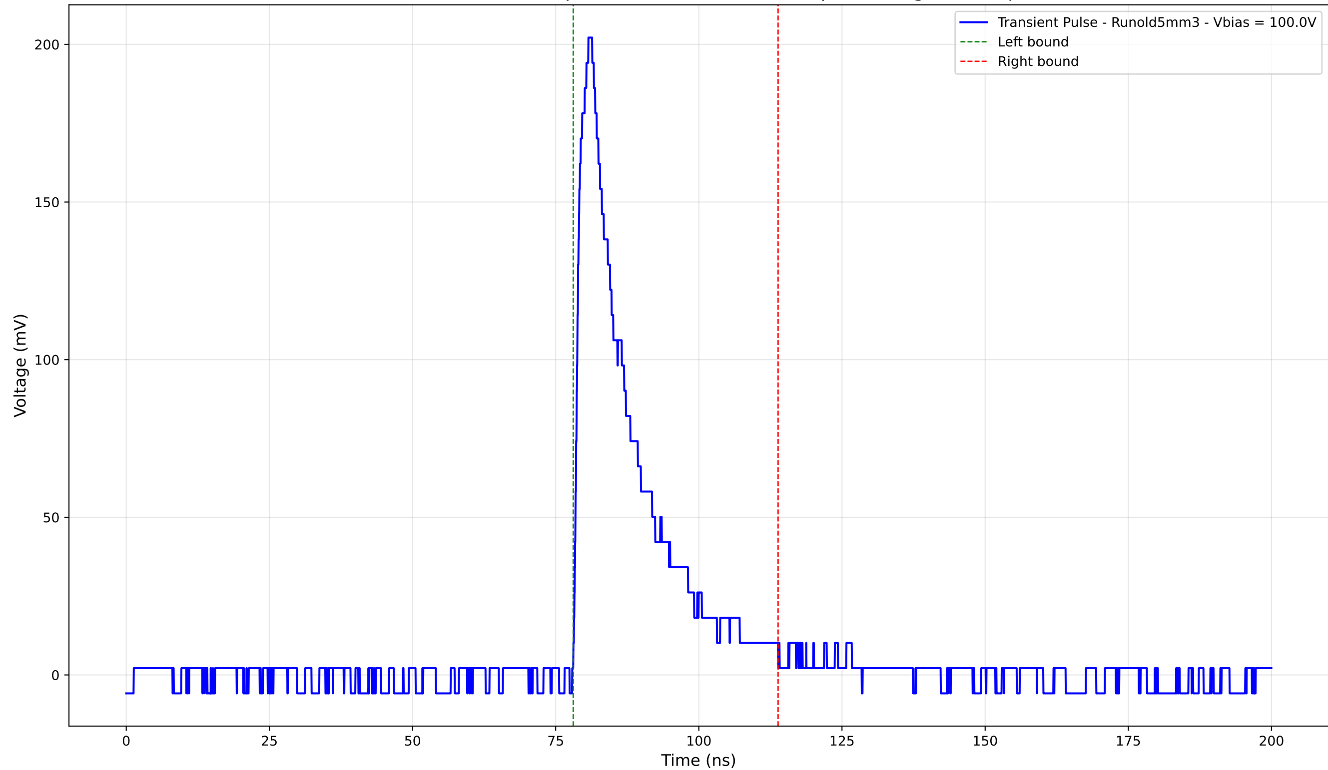
Transient Pulse - Sample: old5 - Position: 4120.0 \mu\text{m} - Charge: 41.49 pC
