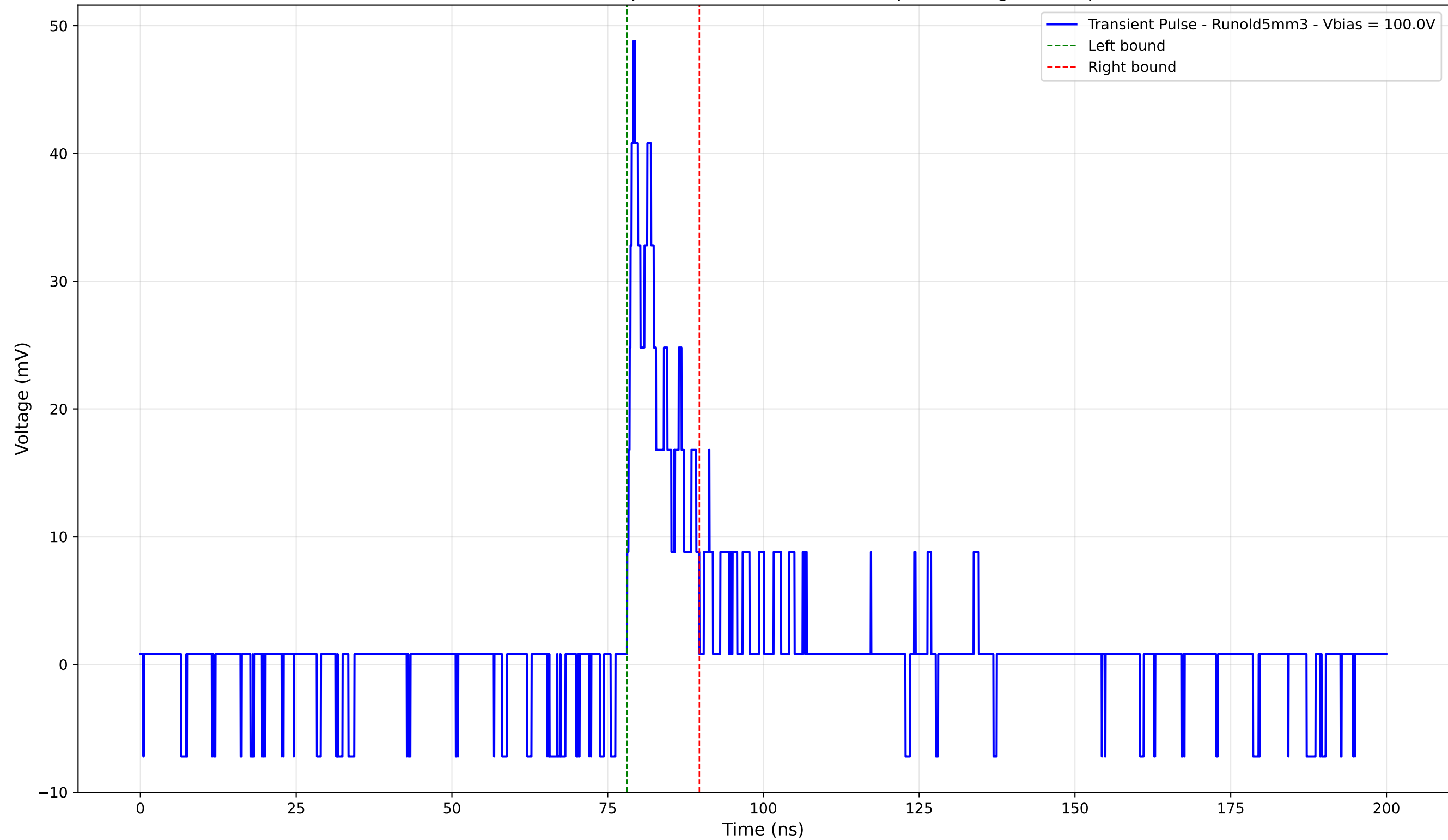
Transient Pulse - Sample: old5 - Position: 130.0 \mu\text{m} - Charge: 5.15 pC
