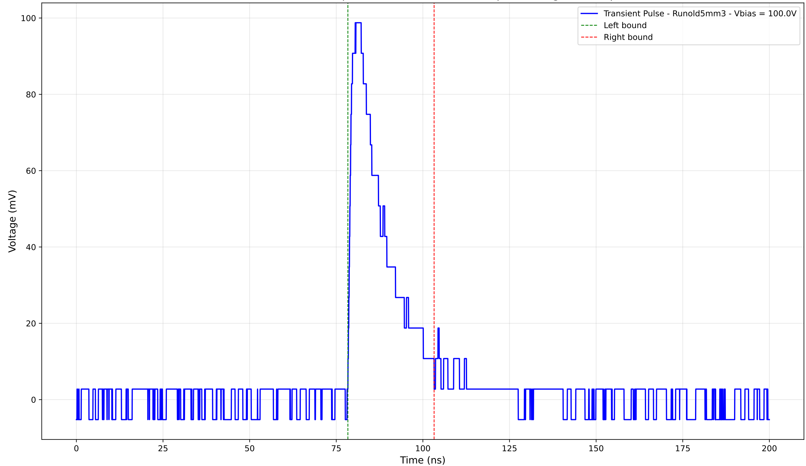
Transient Pulse - Sample: old5 - Position: 4225.0 \mu\text{m} - Charge: 21.45 pC
