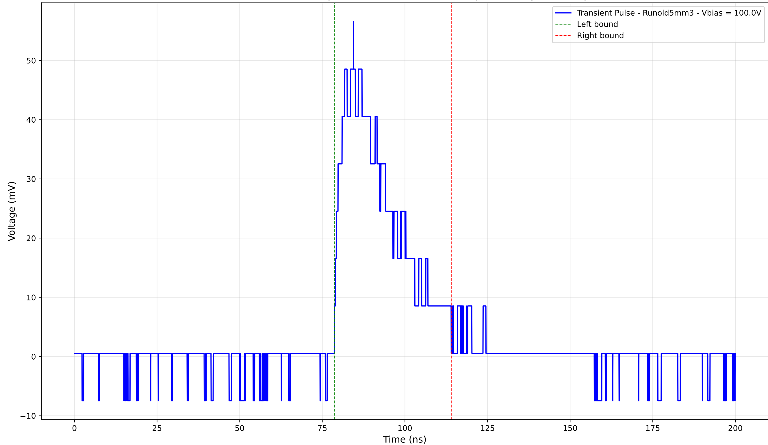
Transient Pulse - Sample: old5 - Position: 1605.0 \mu\text{m} - Charge: 17.58 pC
