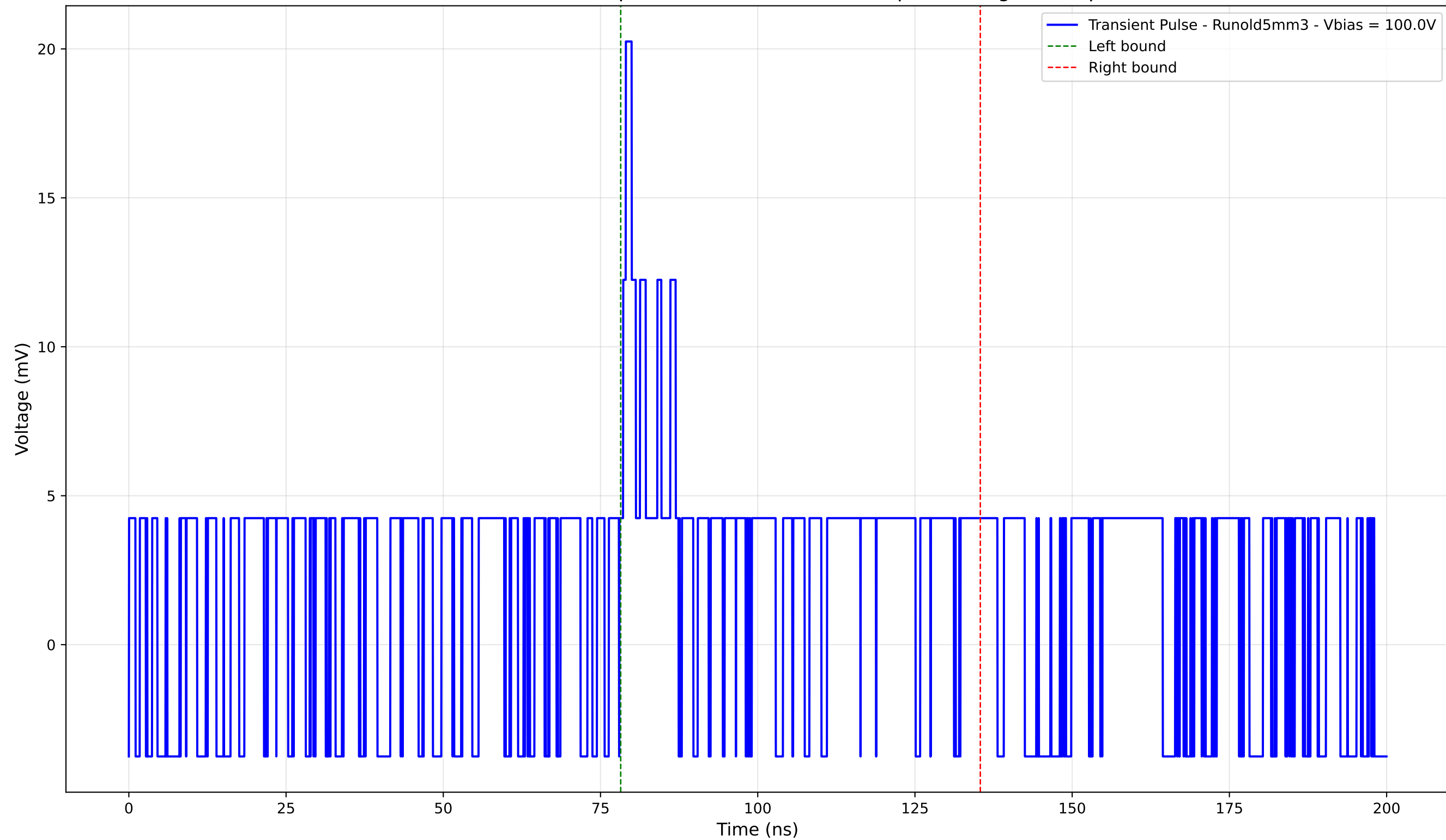
Transient Pulse - Sample: old5 - Position: 4965.0 \mu\text{m} - Charge: 4.58 pC
