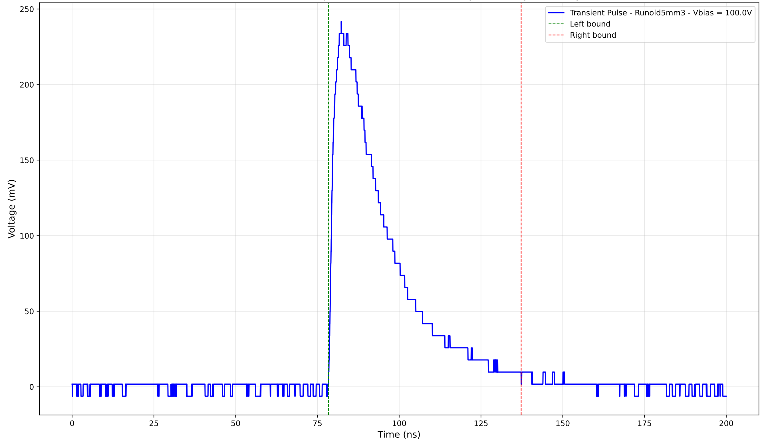
Transient Pulse - Sample: old5 - Position: 2475.0 \mu\text{m} - Charge: 89.25 pC
