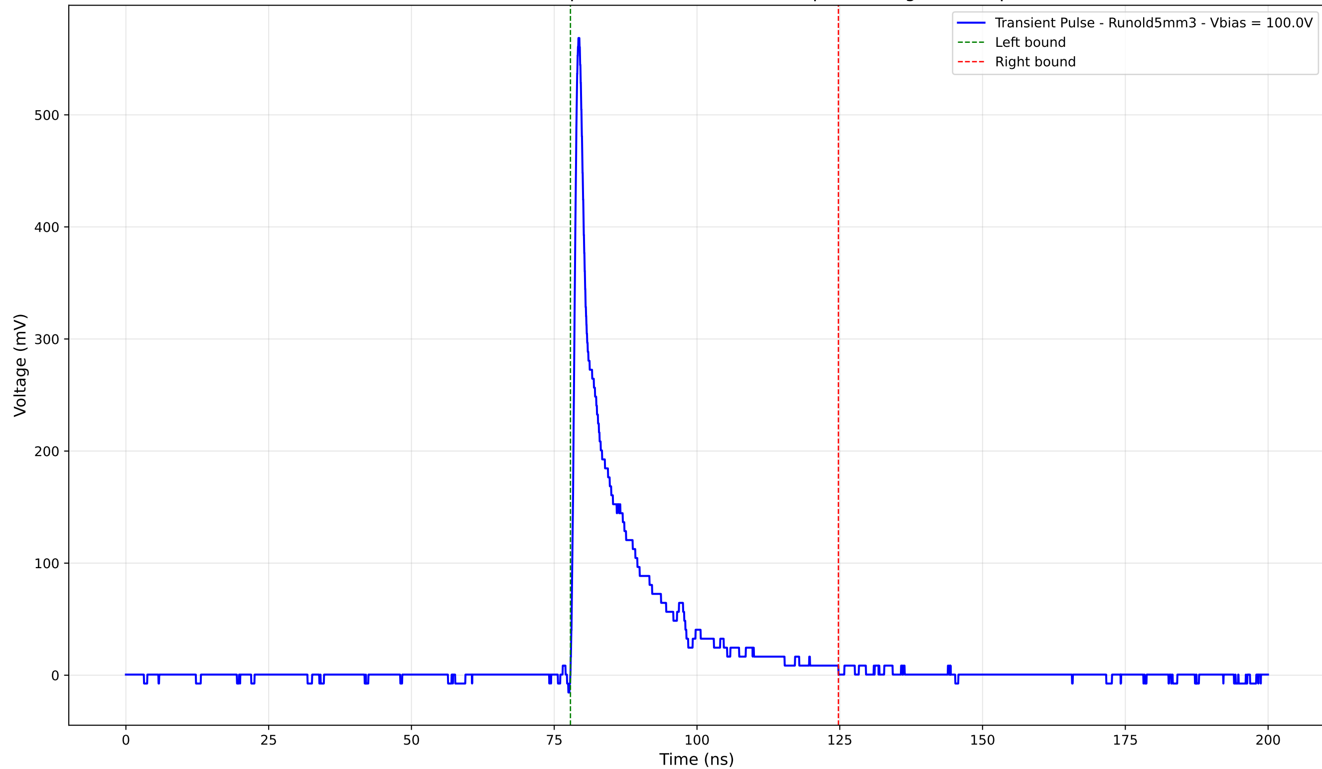
Transient Pulse - Sample: old5 - Position: 230.0 \mu\text{m} - Charge: 74.75 pC
