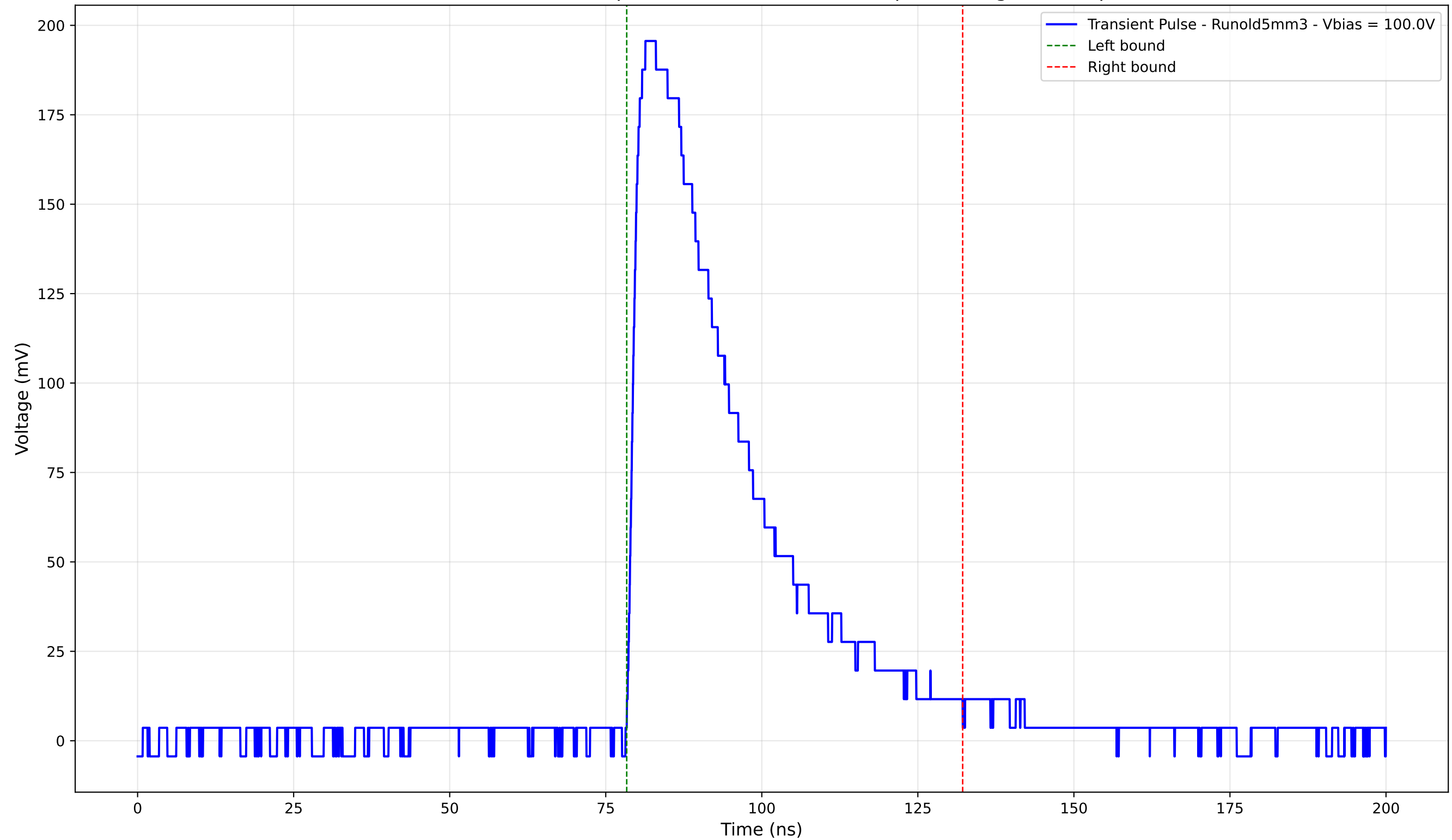
Transient Pulse - Sample: old5 - Position: 1260.0 \mu\text{m} - Charge: 75.77 pC
