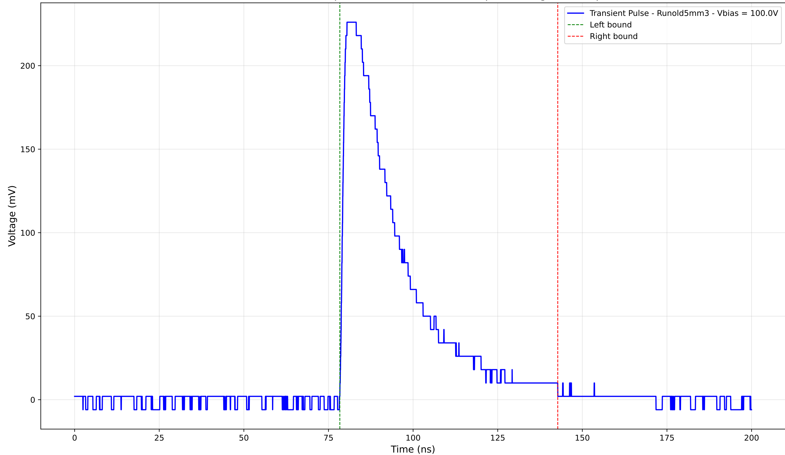
Transient Pulse - Sample: old5 - Position: 1095.0 \mu\text{m} - Charge: 84.75 pC
