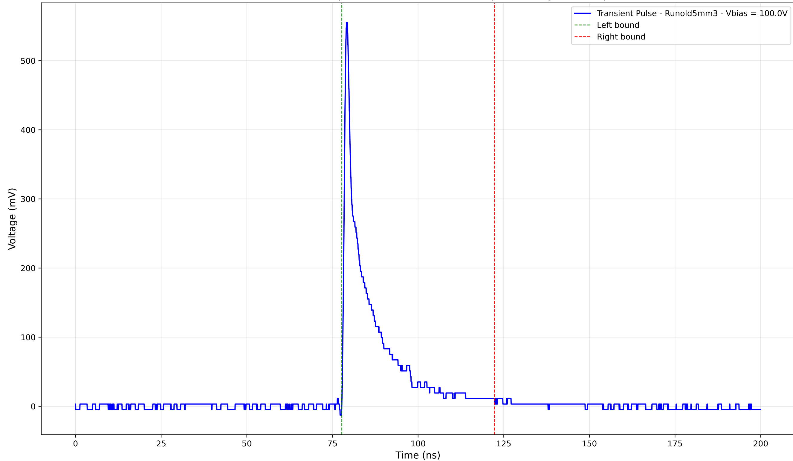
Transient Pulse - Sample: old5 - Position: 4875.0 \mu\text{m} - Charge: 72.64 pC
