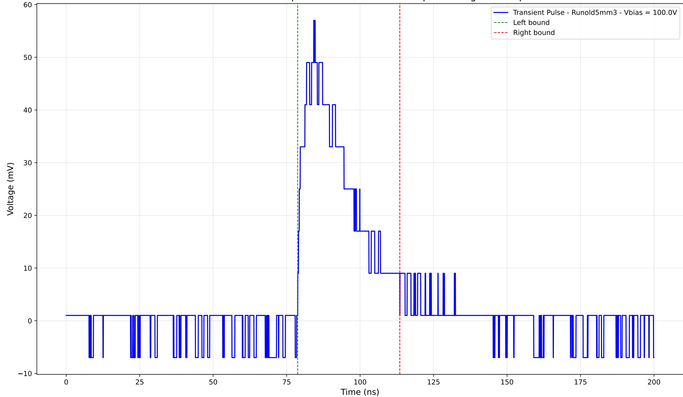
Transient Pulse - Sample: old5 - Position: 2010.0 \mu\text{m} - Charge: 18.11 pC
