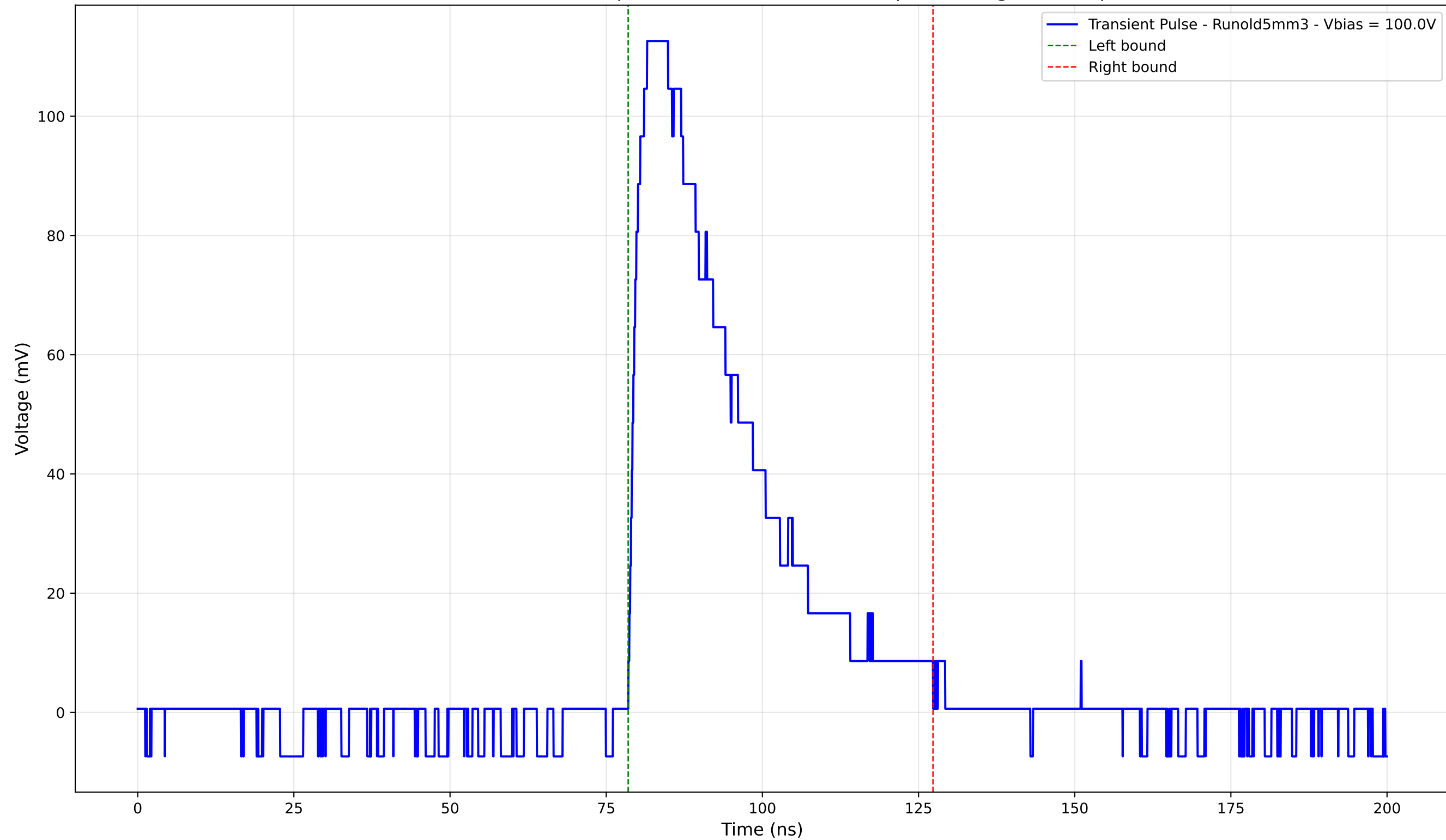
Transient Pulse - Sample: old5 - Position: 2435.0 \mu\text{m} - Charge: 41.78 pC
