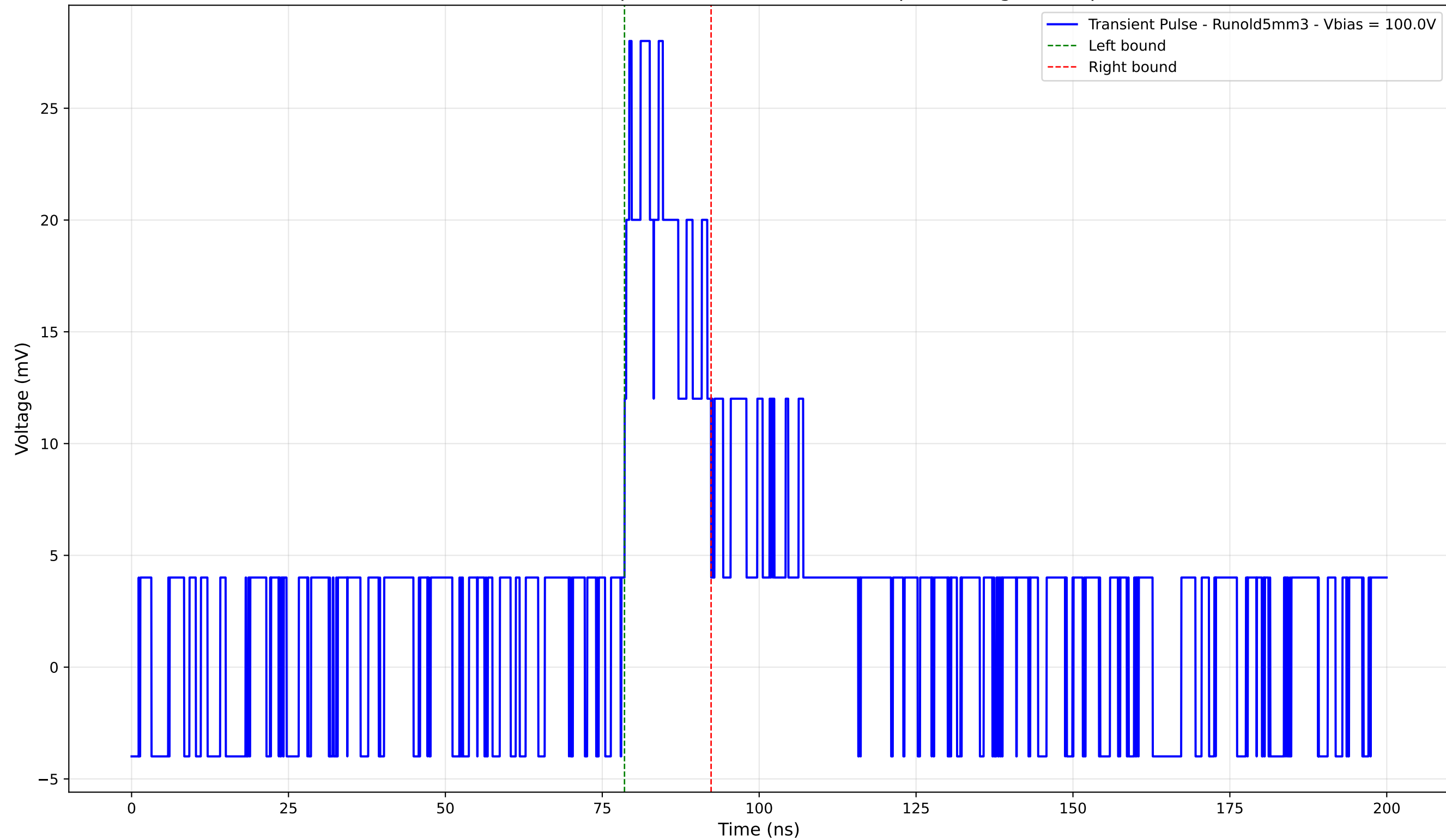
Transient Pulse - Sample: old5 - Position: 2955.0 \mu\text{m} - Charge: 5.34 pC
