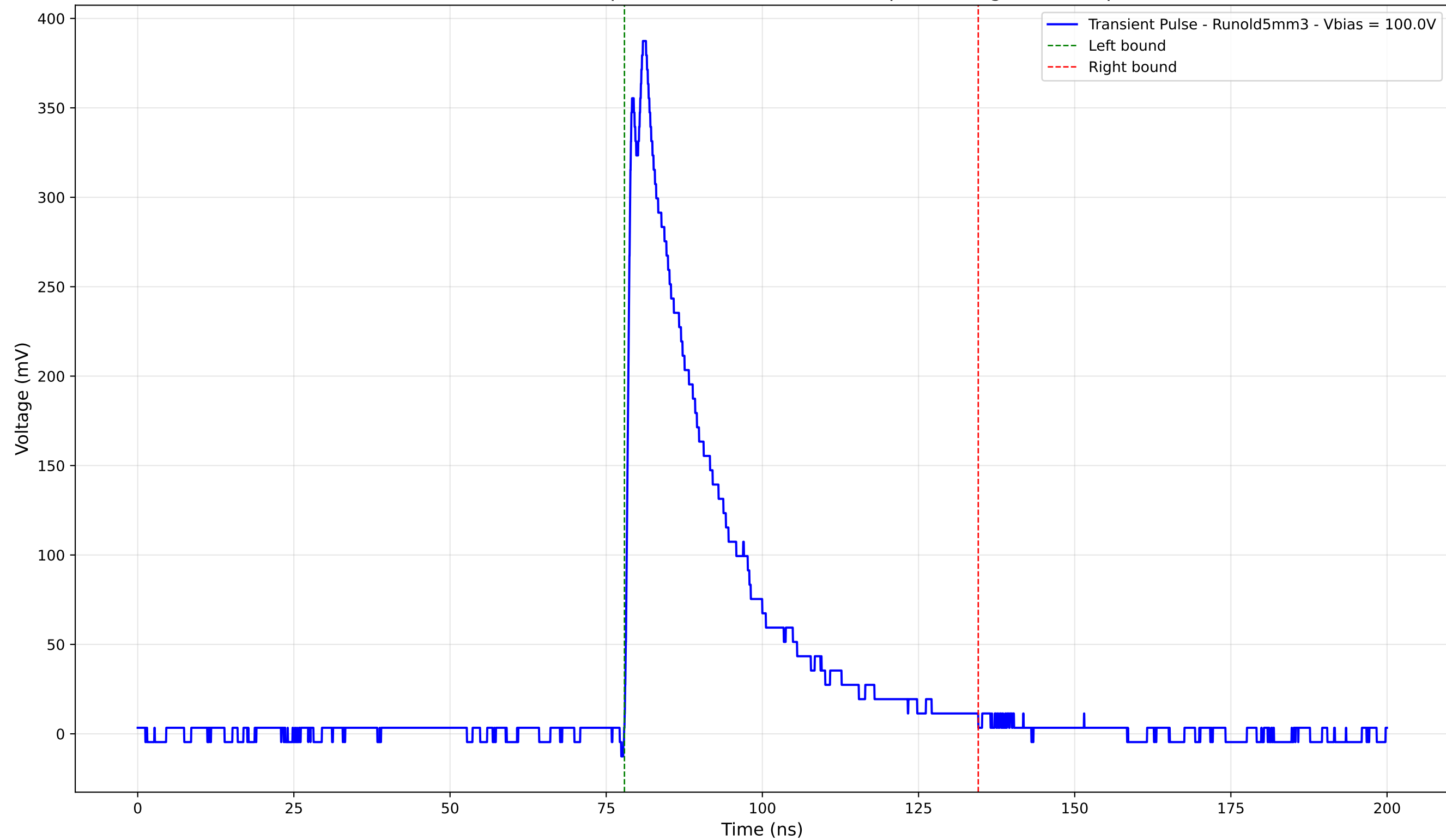
Transient Pulse - Sample: old5 - Position: 3105.0 \mu\text{m} - Charge: 106.63 pC
