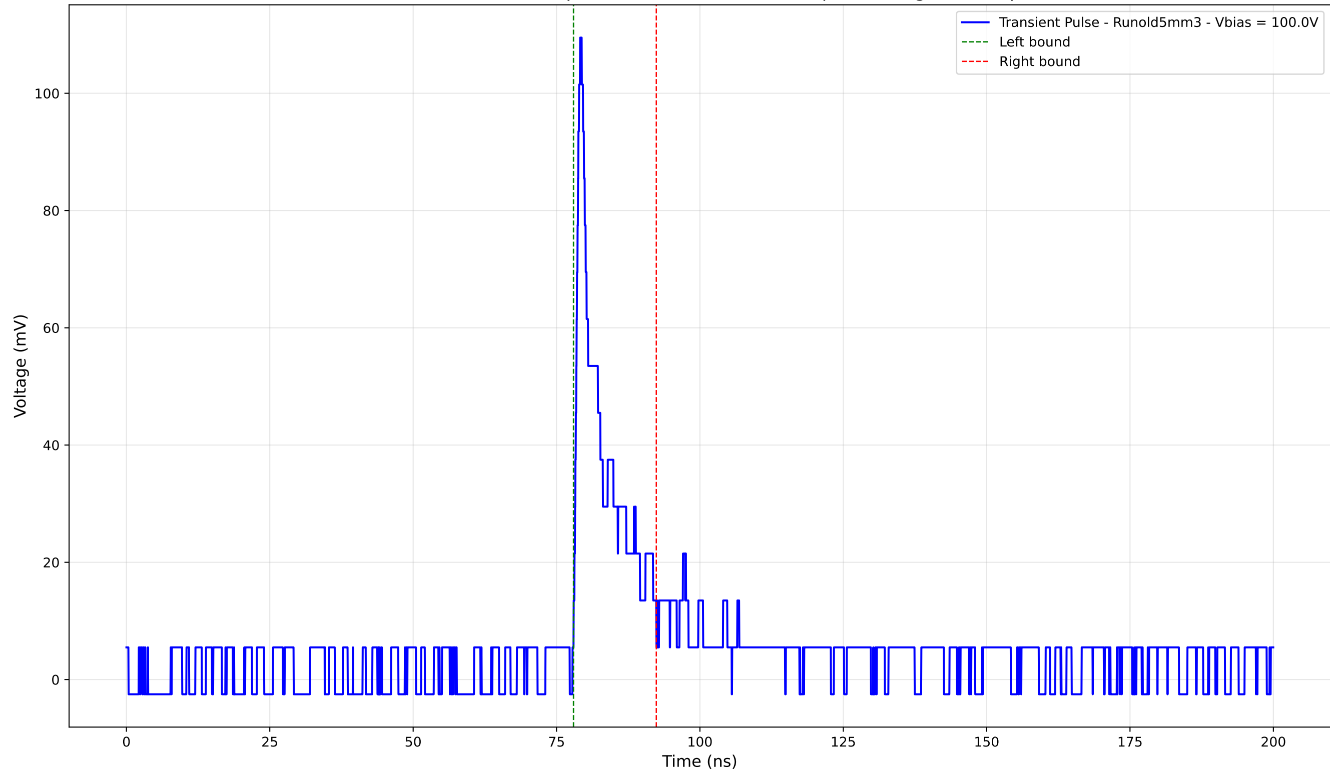
Transient Pulse - Sample: old5 - Position: 4920.0 \mu\text{m} - Charge: 10.92 pC
