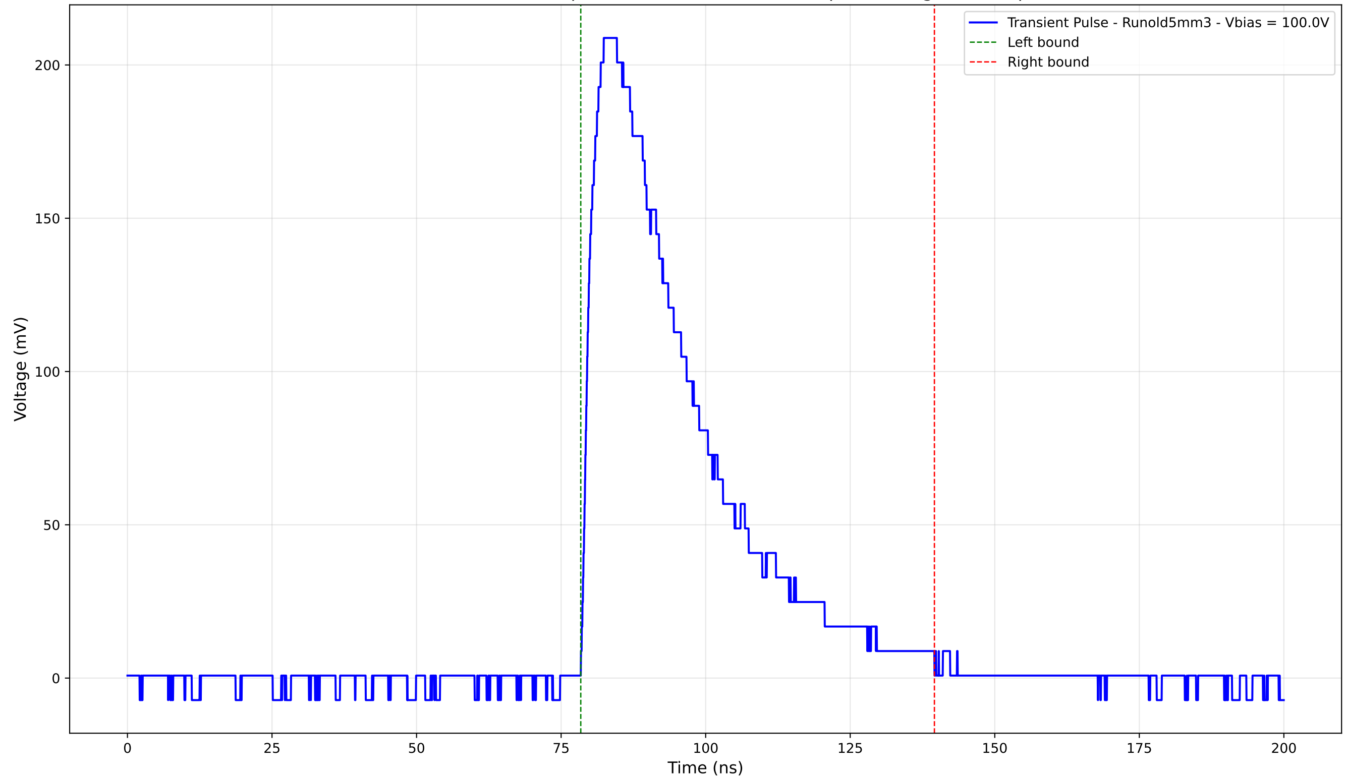
Transient Pulse - Sample: old5 - Position: 1905.0 \mu\text{m} - Charge: 84.90 pC
