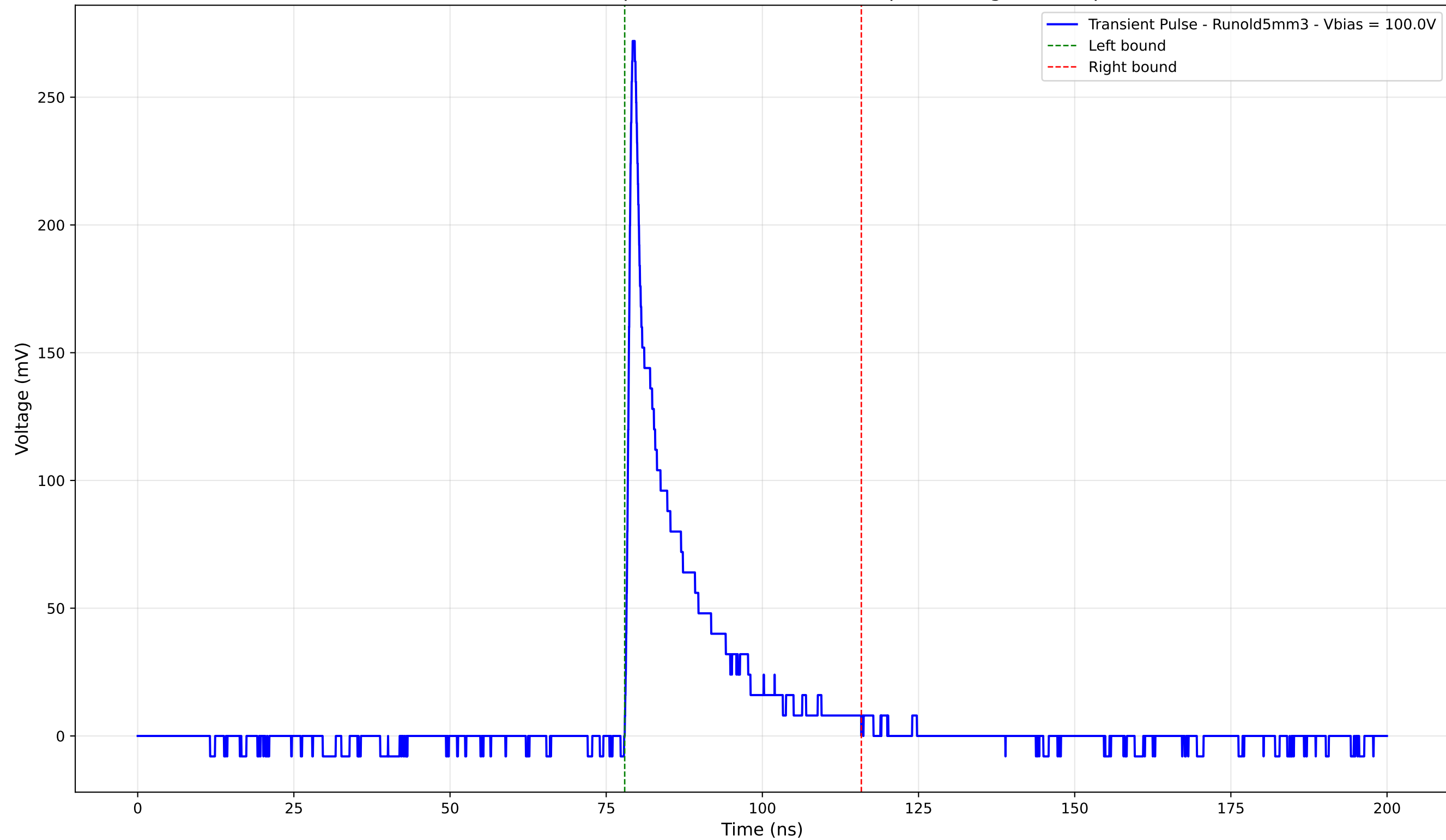
Transient Pulse - Sample: old5 - Position: 285.0 \mu\text{m} - Charge: 37.42 pC
