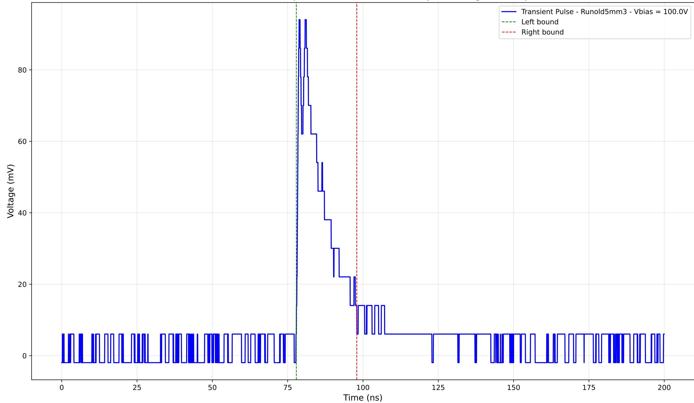
Transient Pulse - Sample: old5 - Position: 3320.0 \mu\text{m} - Charge: 17.46 pC
