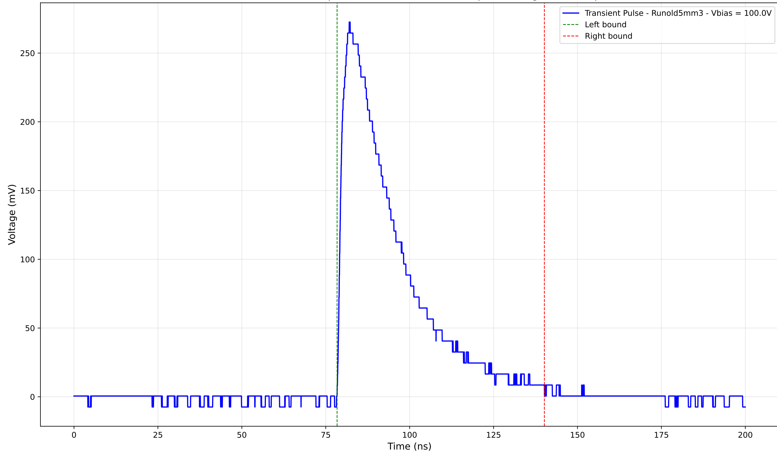
Transient Pulse - Sample: old5 - Position: 2515.0 \mu\text{m} - Charge: 100.56 pC
