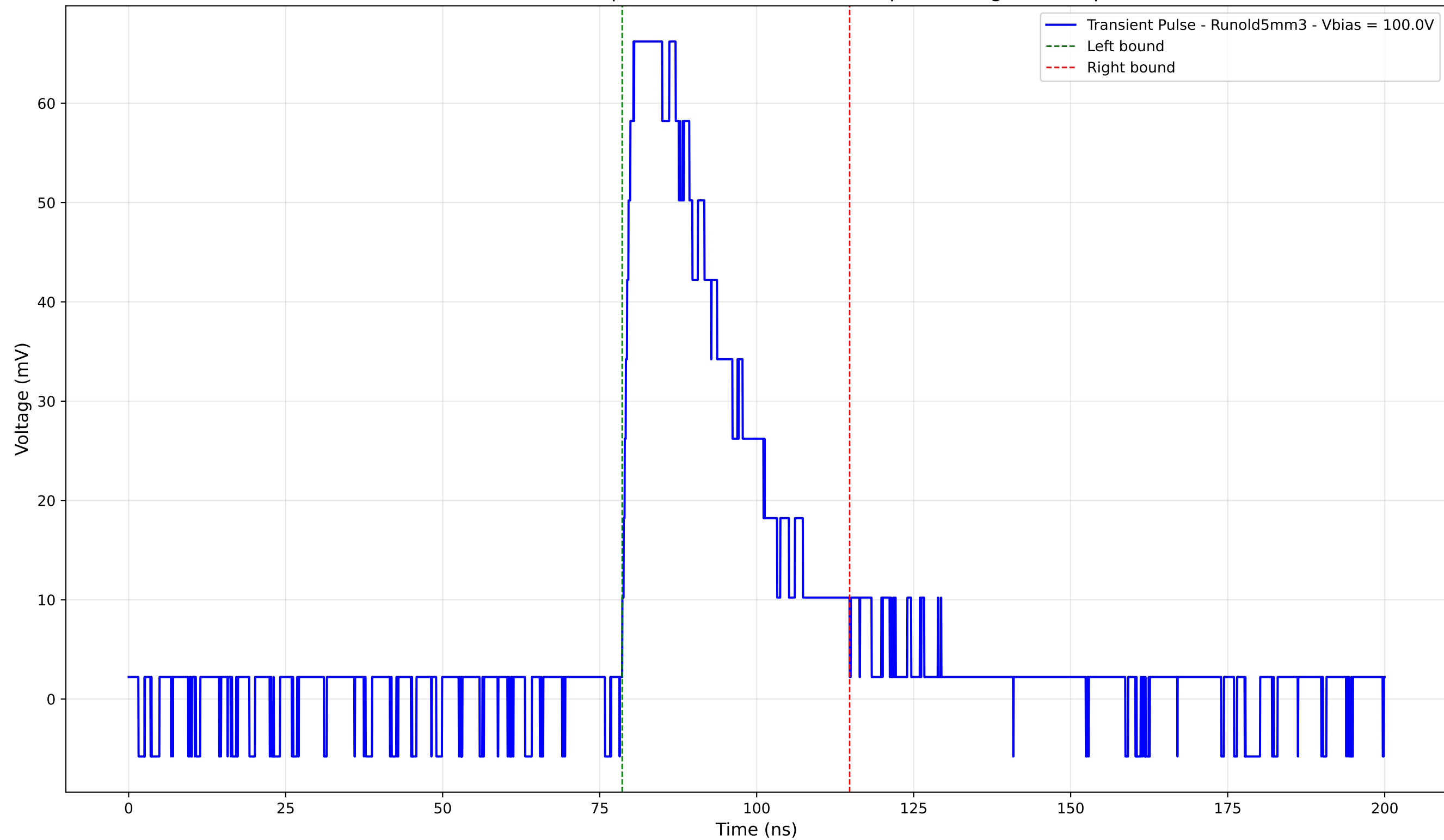
Transient Pulse - Sample: old5 - Position: 1210.0 \mu\text{m} - Charge: 24.49 pC
