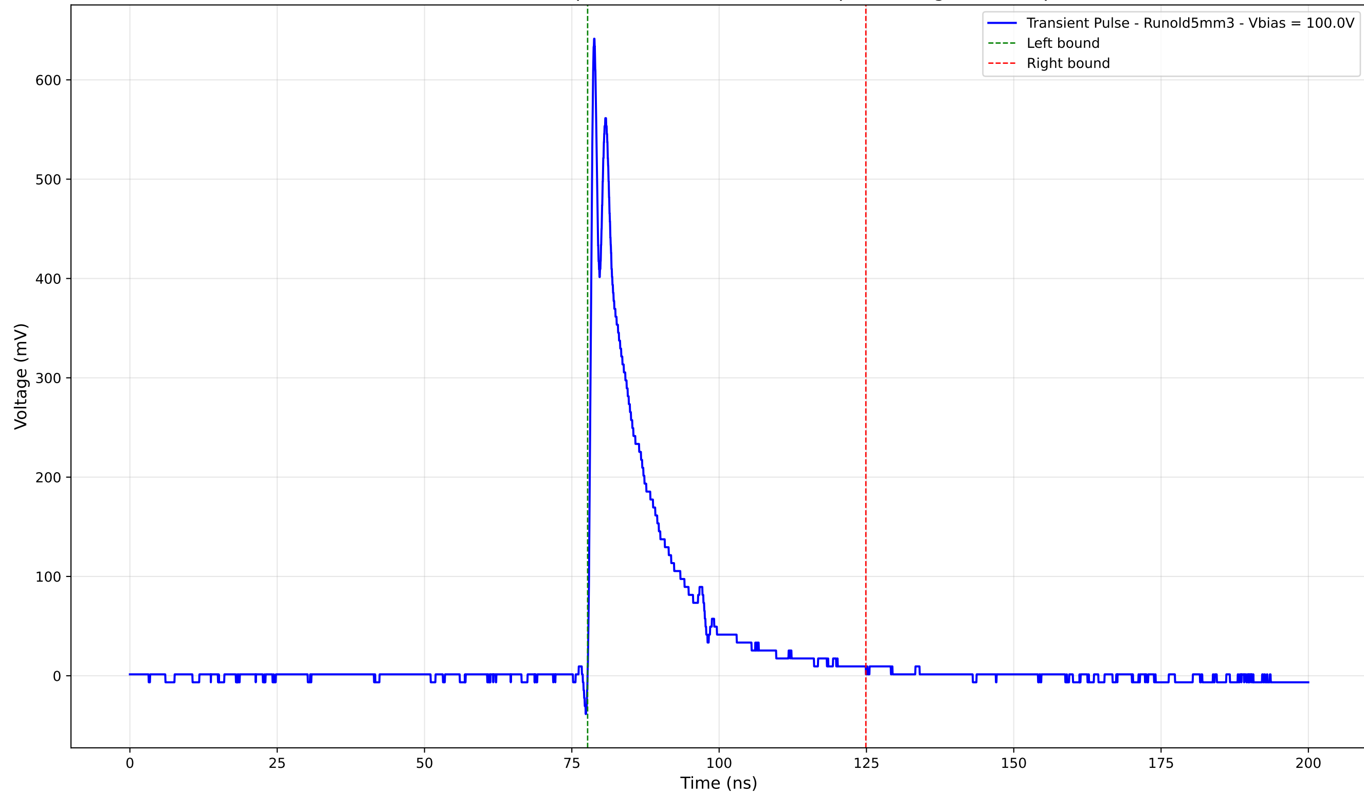
Transient Pulse - Sample: old5 - Position: 3760.0 \mu\text{m} - Charge: 106.49 pC
