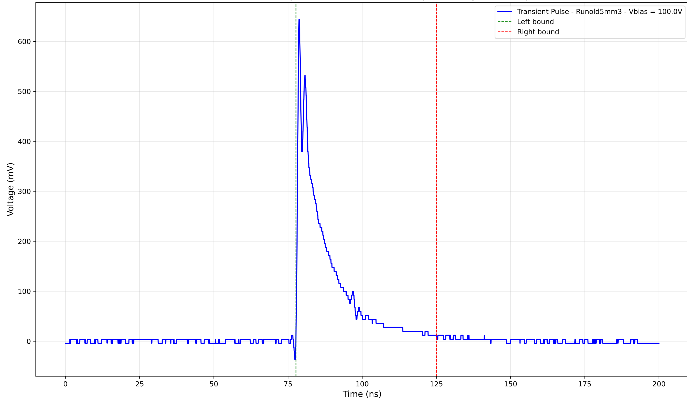
Transient Pulse - Sample: old5 - Position: 3415.0 \mu\text{m} - Charge: 107.99 pC
