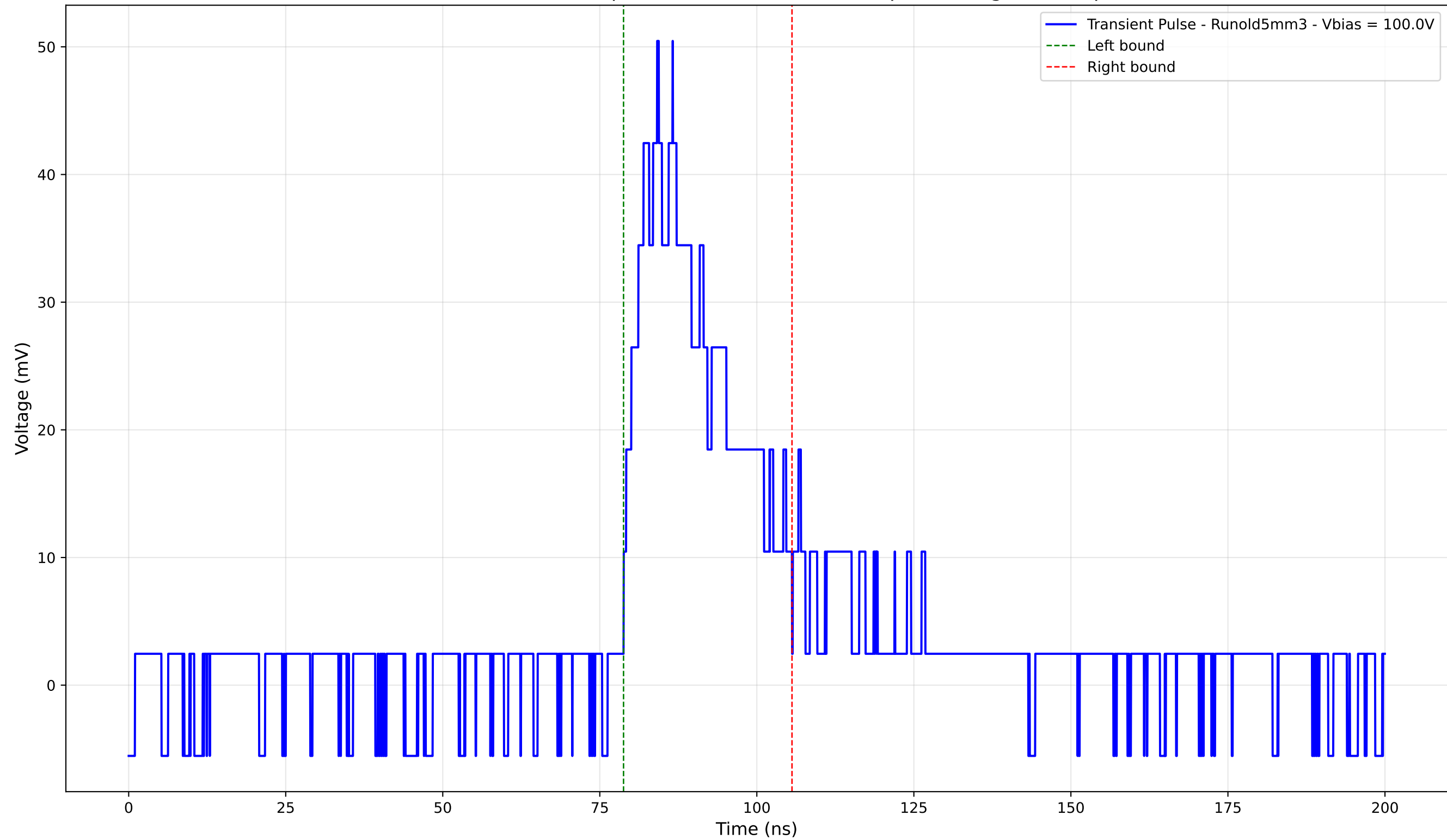
Transient Pulse - Sample: old5 - Position: 2205.0 \mu\text{m} - Charge: 13.68 pC
