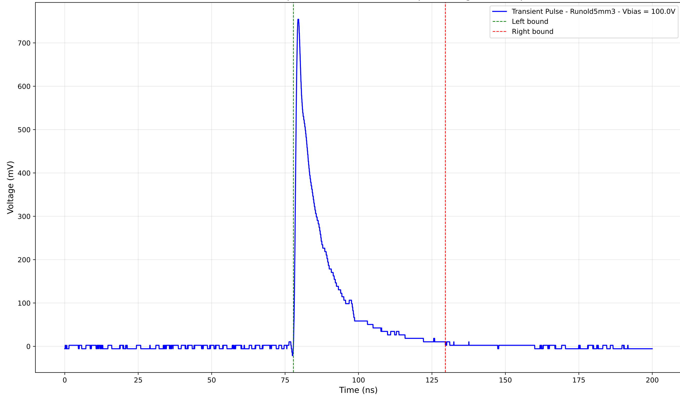
Transient Pulse - Sample: old5 - Position: 4735.0 \mu\text{m} - Charge: 132.78 pC
