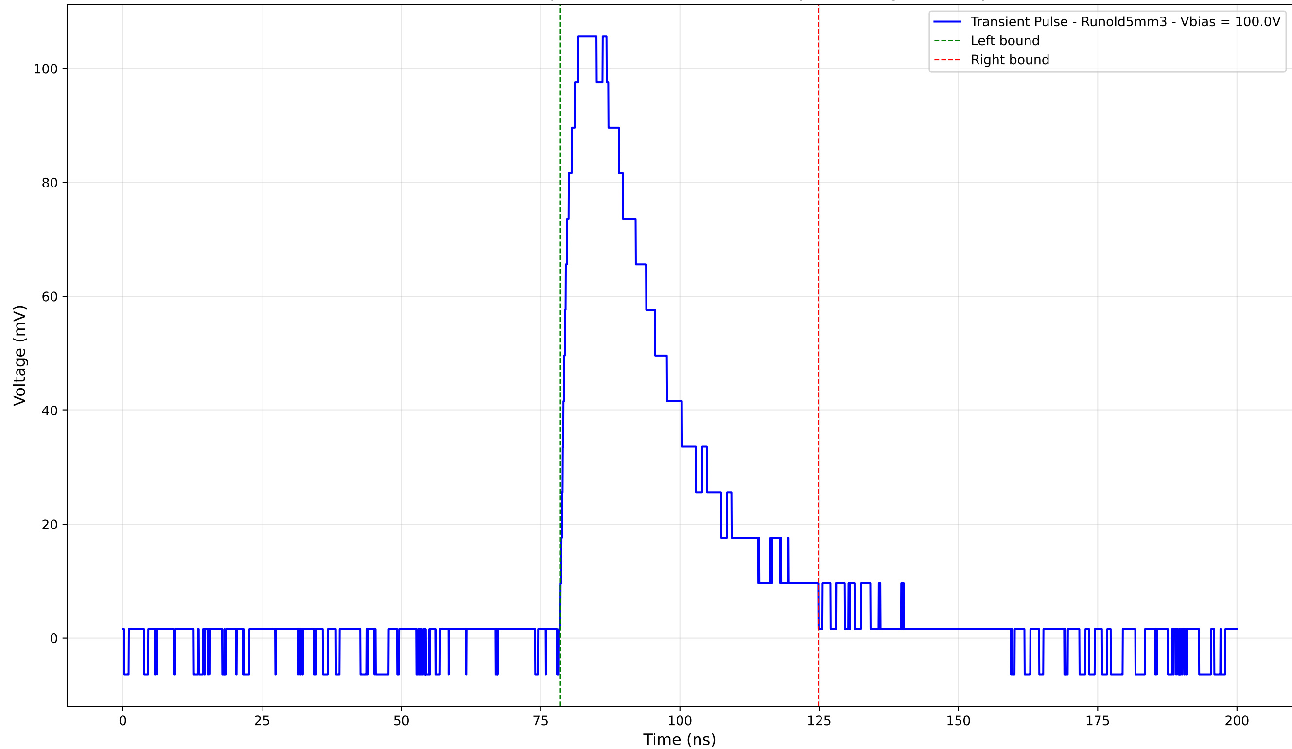
Transient Pulse - Sample: old5 - Position: 2355.0 \mu\text{m} - Charge: 41.25 pC
