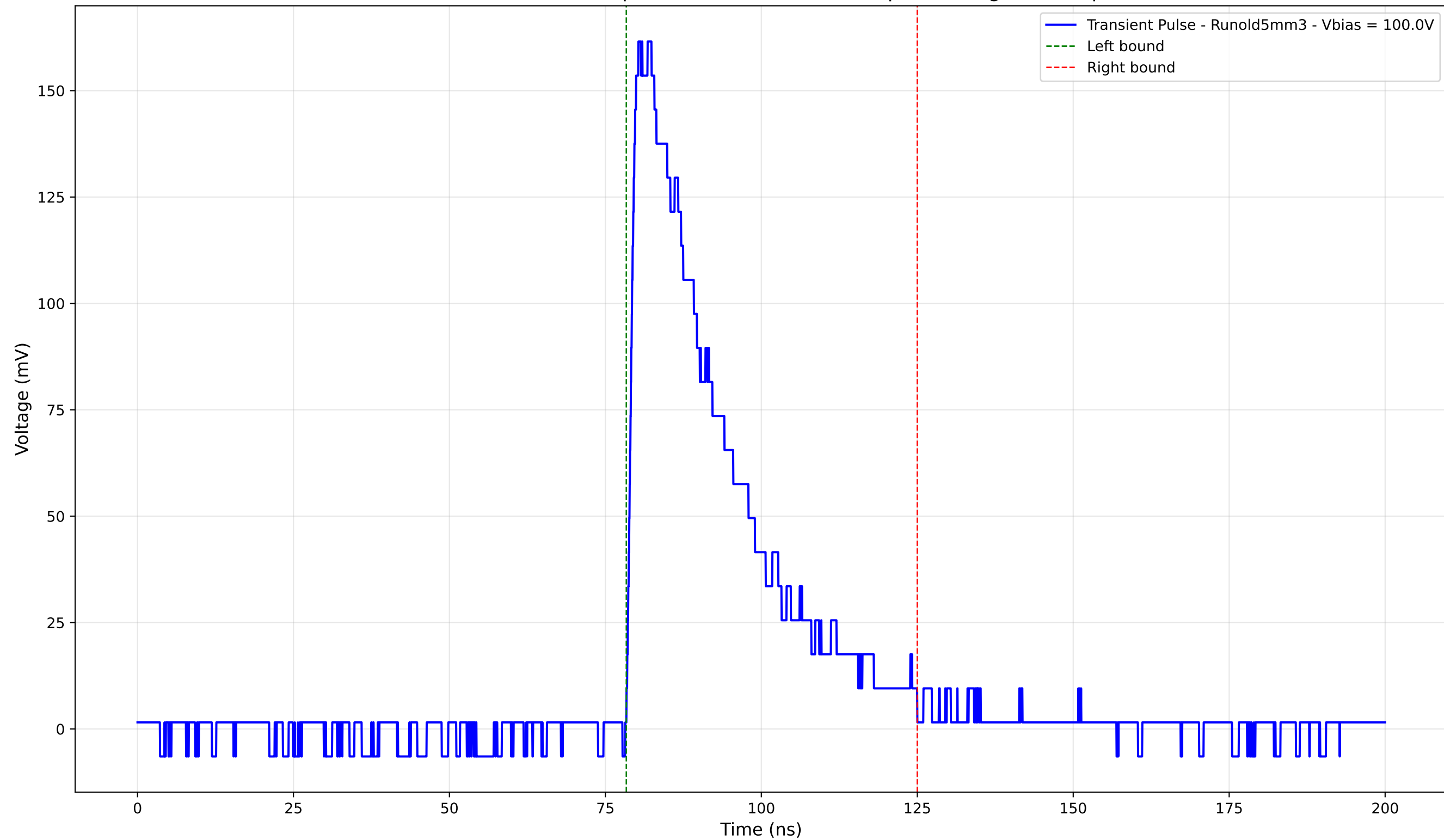
Transient Pulse - Sample: old5 - Position: 975.0 \mu\text{m} - Charge: 52.08 pC
