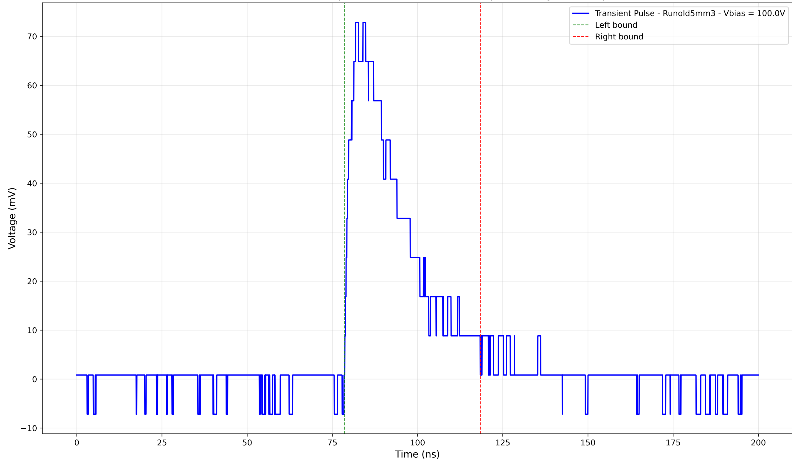
Transient Pulse - Sample: old5 - Position: 2370.0 \mu\text{m} - Charge: 24.97 pC
