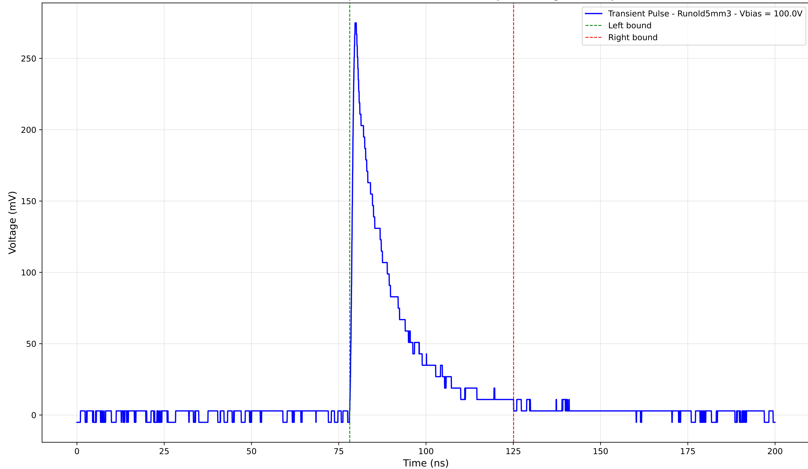
Transient Pulse - Sample: old5 - Position: 550.0 \mu\text{m} - Charge: 57.93 pC
