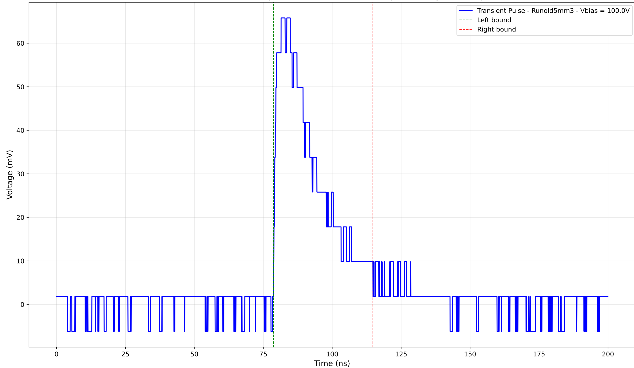
Transient Pulse - Sample: old5 - Position: 1155.0 \mu\text{m} - Charge: 21.92 pC
