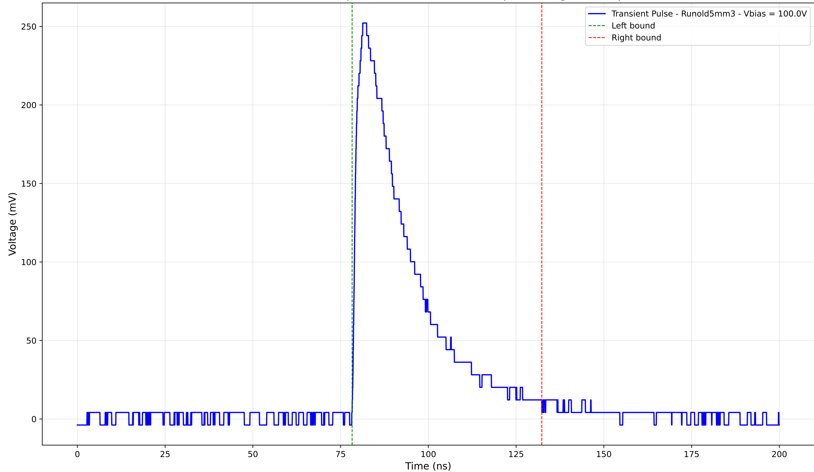
Transient Pulse - Sample: old5 - Position: 2770.0 \mu\text{m} - Charge: 86.73 pC
