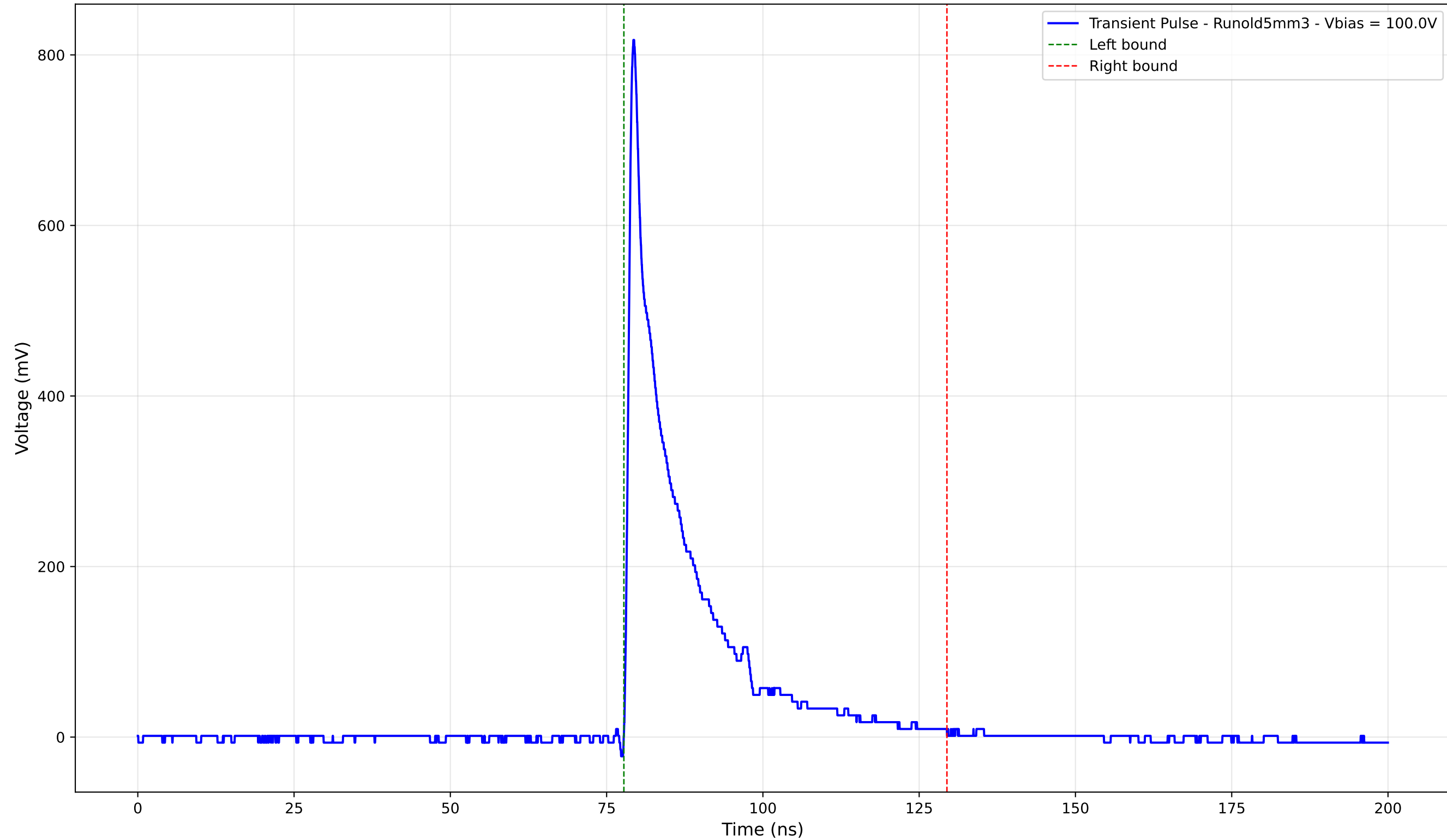
Transient Pulse - Sample: old5 - Position: 4795.0 \mu\text{m} - Charge: 129.63 pC
