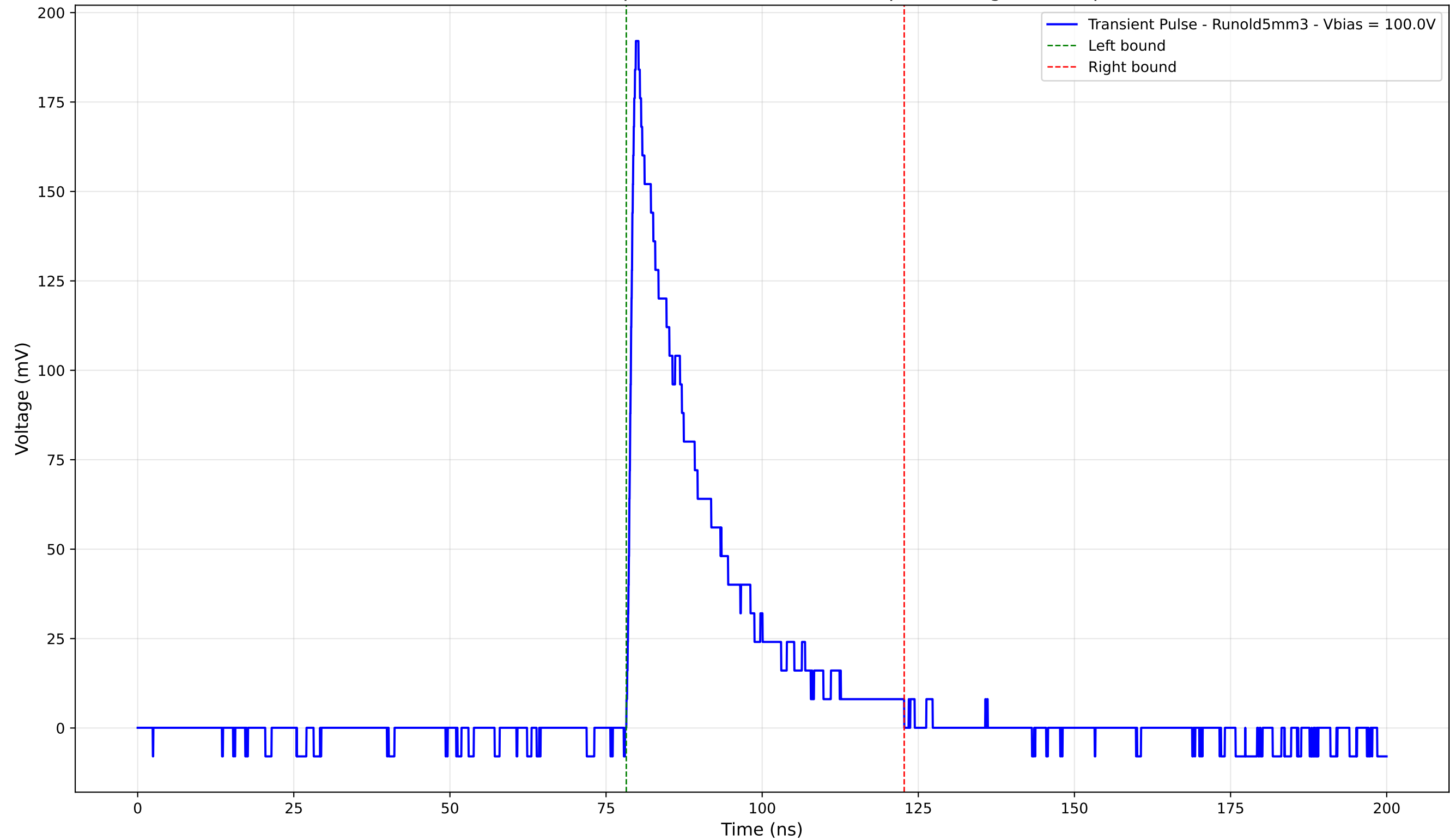
Transient Pulse - Sample: old5 - Position: 620.0 \mu\text{m} - Charge: 42.29 pC
