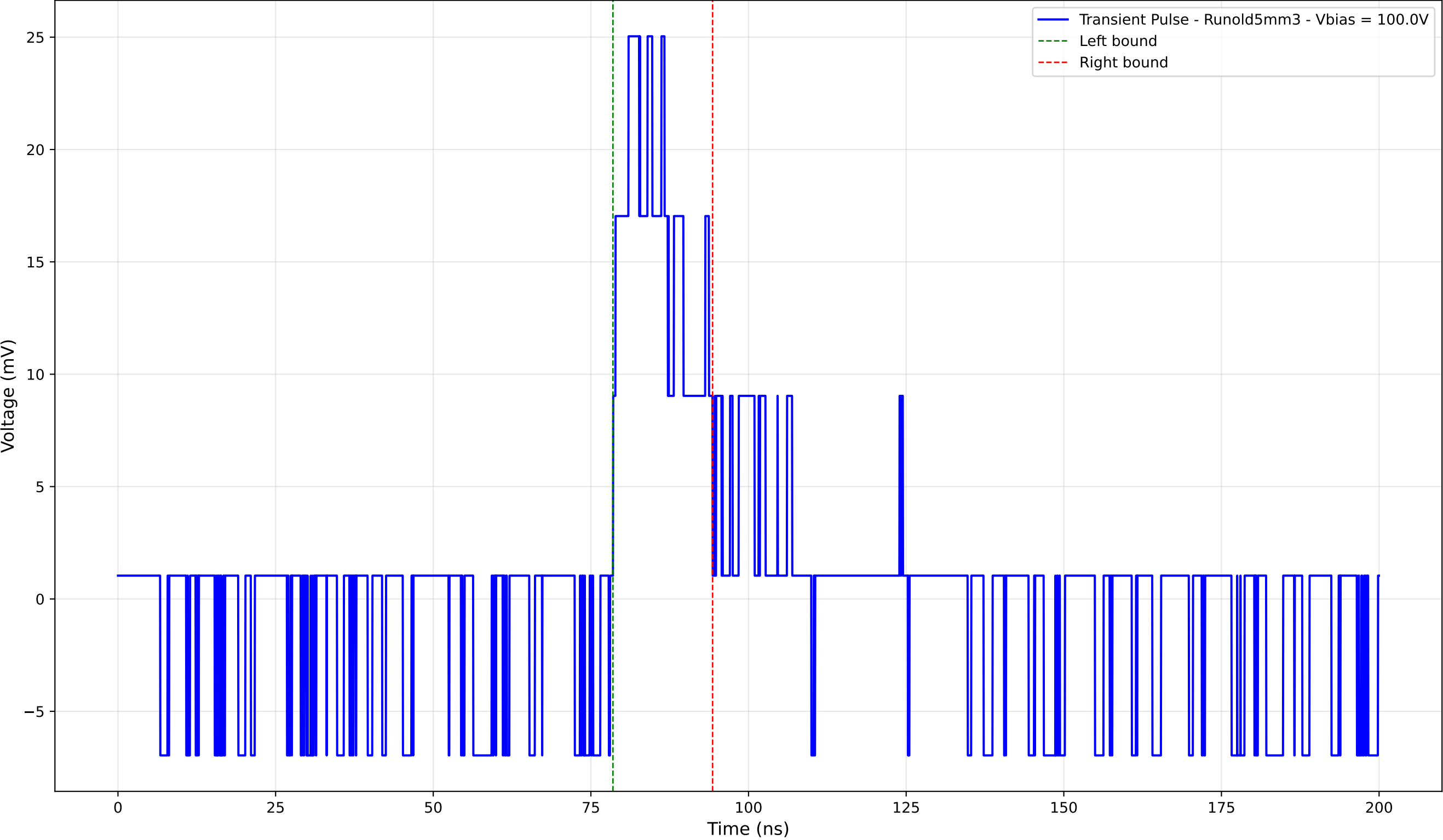
Transient Pulse - Sample: old5 - Position: 2995.0 \mu\text{m} - Charge: 5.01 pC
