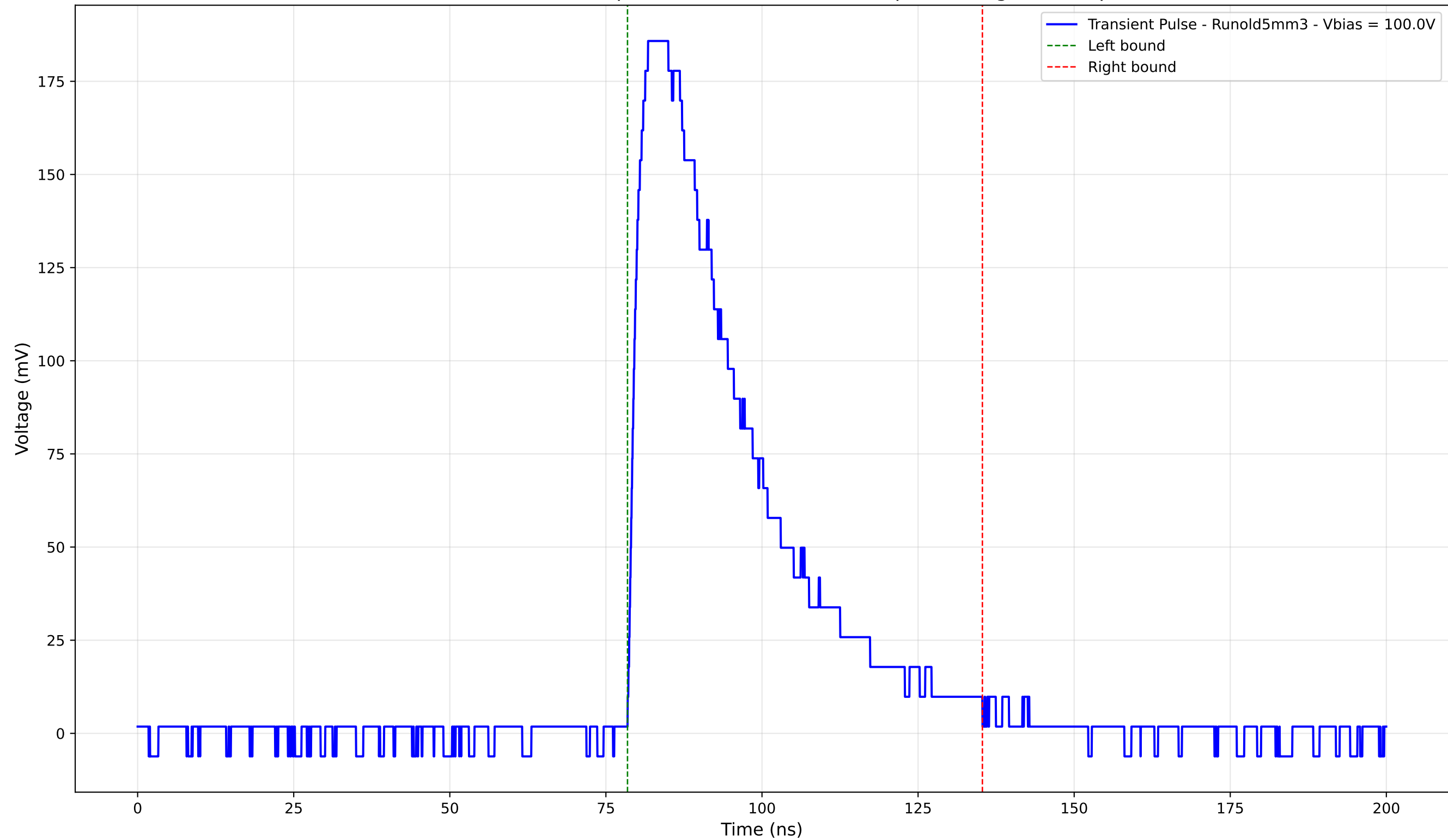
Transient Pulse - Sample: old5 - Position: 1510.0 \mu\text{m} - Charge: 74.65 pC
