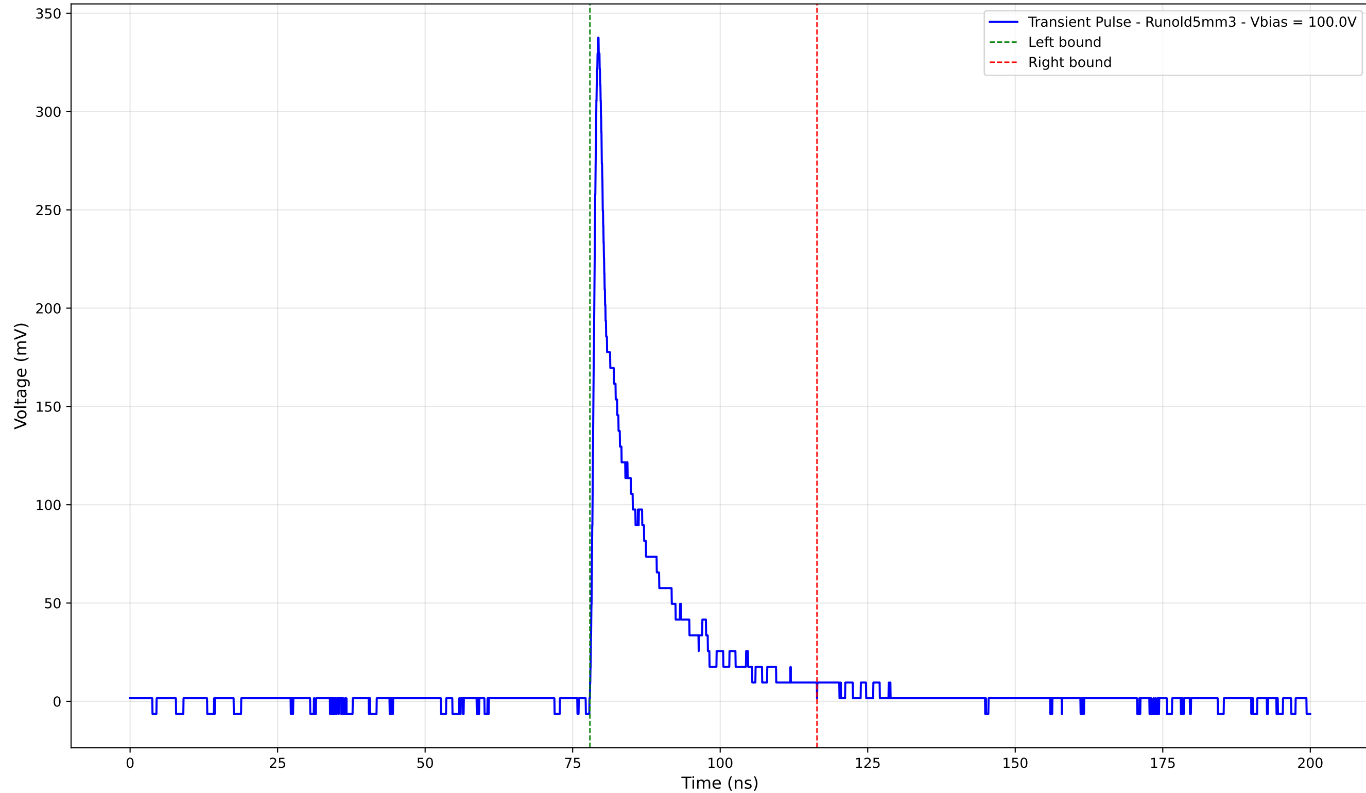
Transient Pulse - Sample: old5 - Position: 275.0 \mu\text{m} - Charge: 45.27 pC
