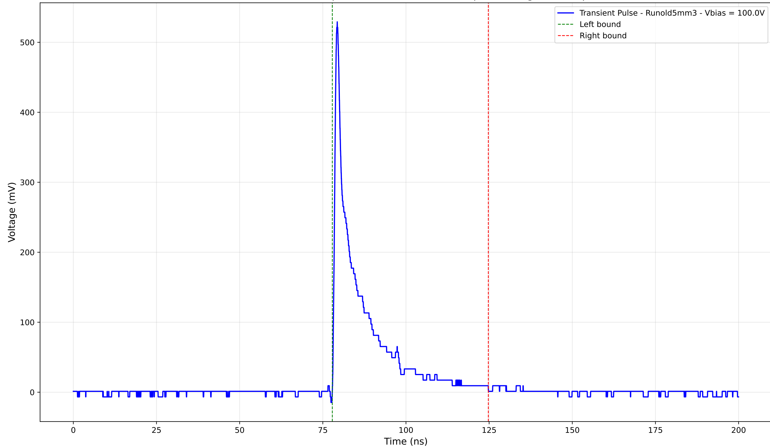
Transient Pulse - Sample: old5 - Position: 245.0 \mu\text{m} - Charge: 70.22 pC
