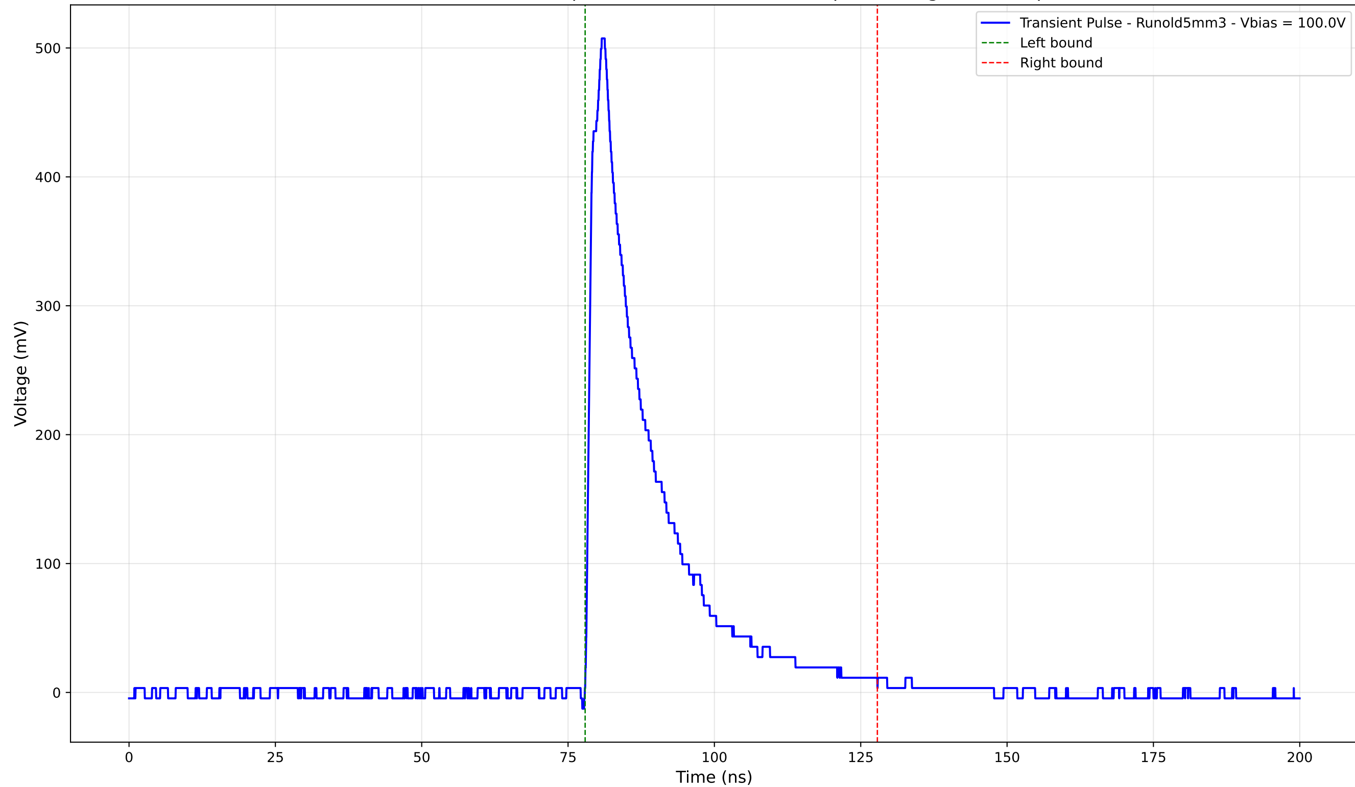
Transient Pulse - Sample: old5 - Position: 4055.0 \mu\text{m} - Charge: 112.83 pC
