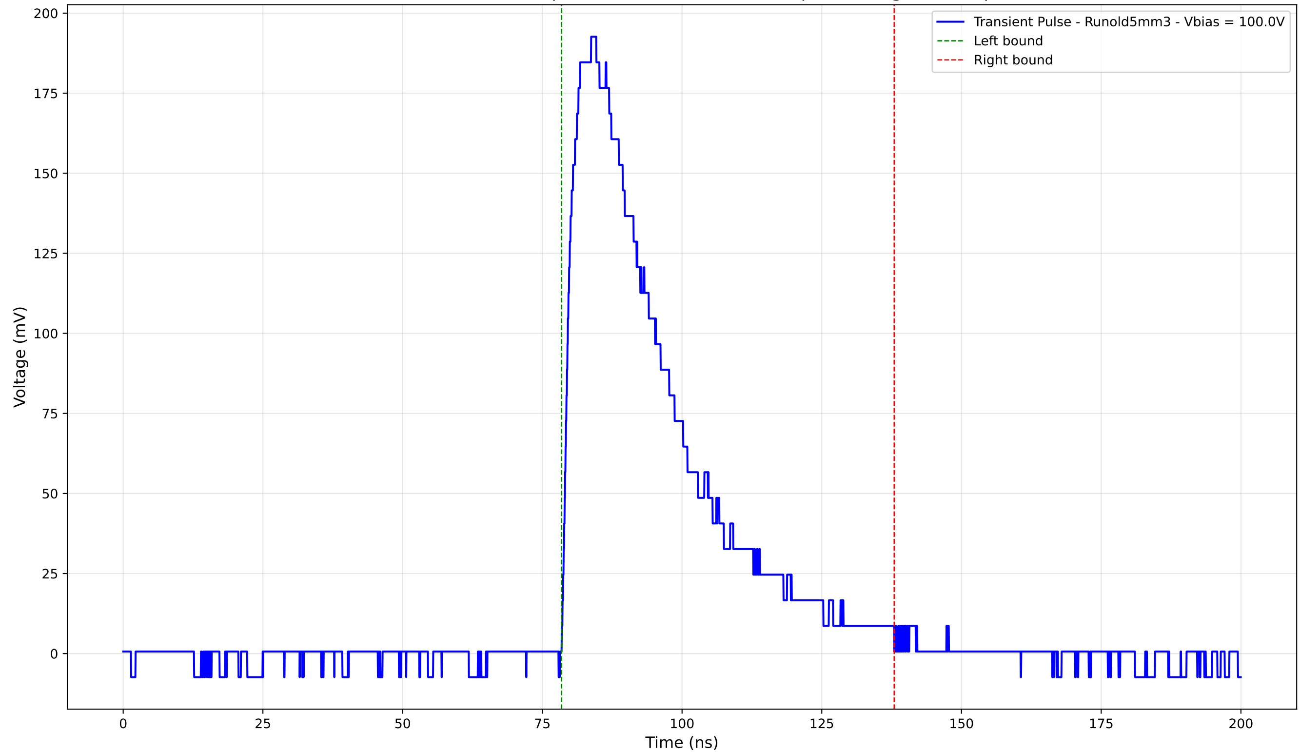
Transient Pulse - Sample: old5 - Position: 2120.0 \mu\text{m} - Charge: 75.71 pC
