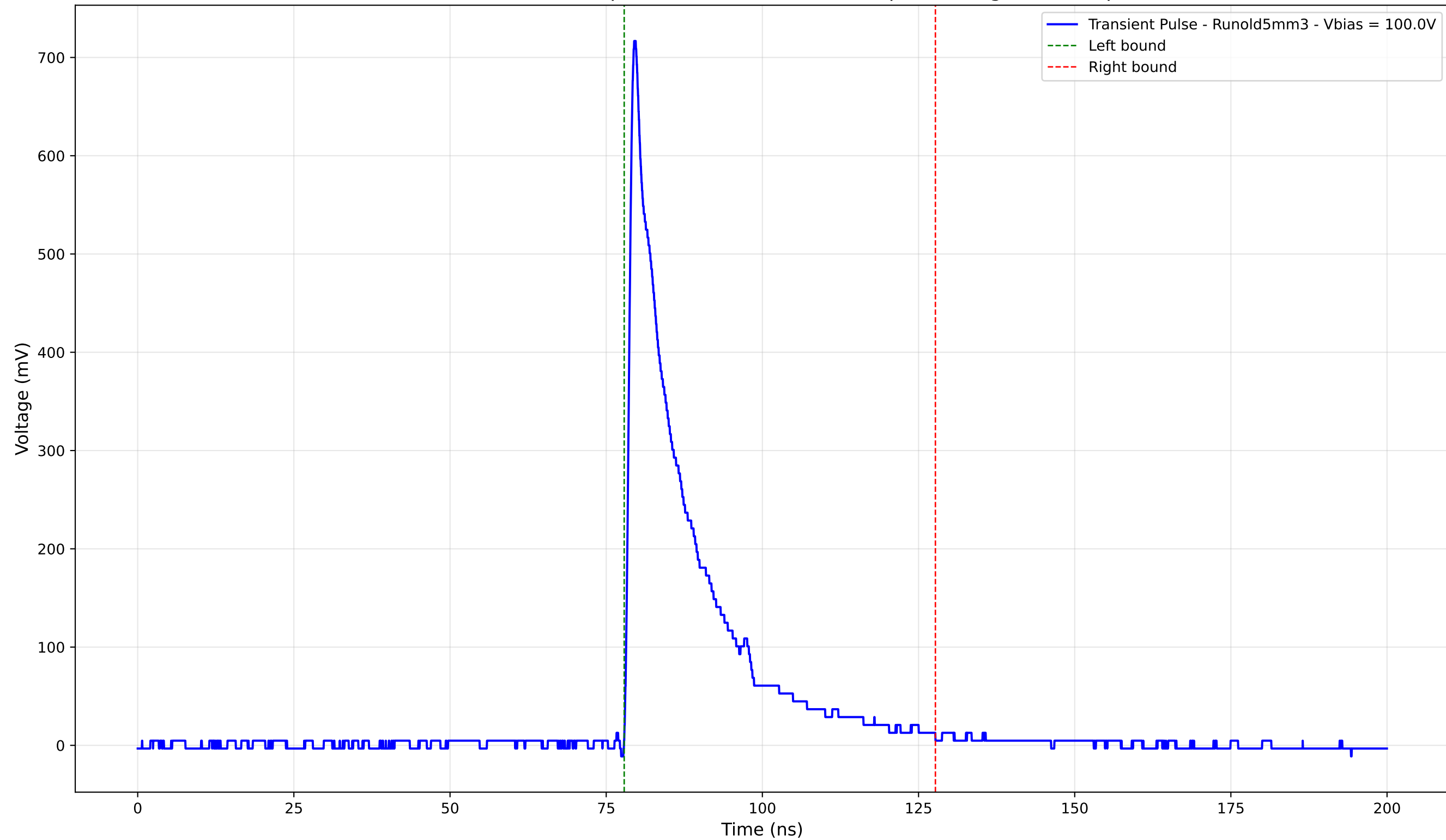
Transient Pulse - Sample: old5 - Position: 4700.0 \mu\text{m} - Charge: 132.65 pC
