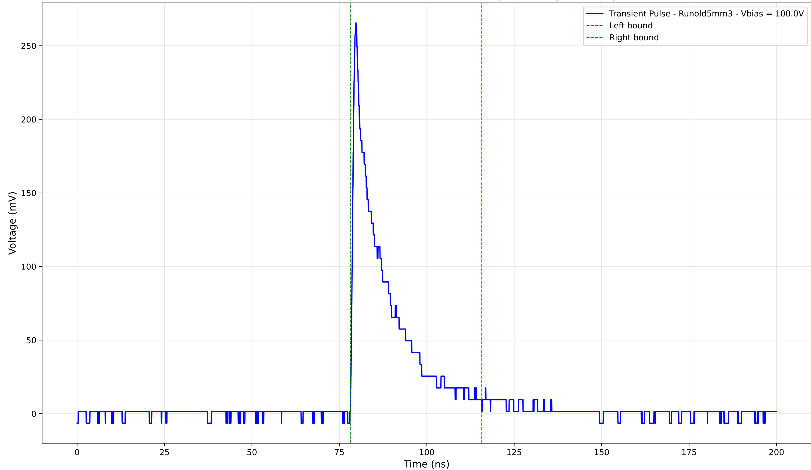
Transient Pulse - Sample: old5 - Position: 470.0 \mu\text{m} - Charge: 47.71 pC
