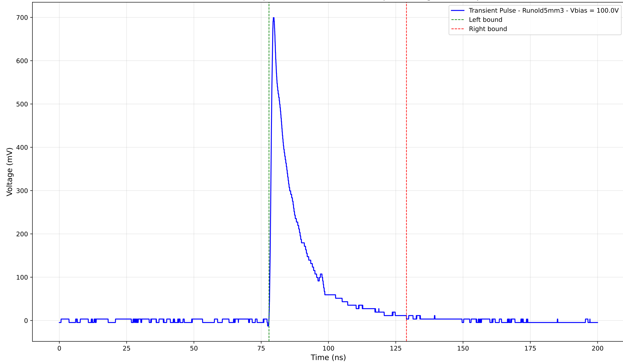
Transient Pulse - Sample: old5 - Position: 4685.0 \mu\text{m} - Charge: 130.78 pC
