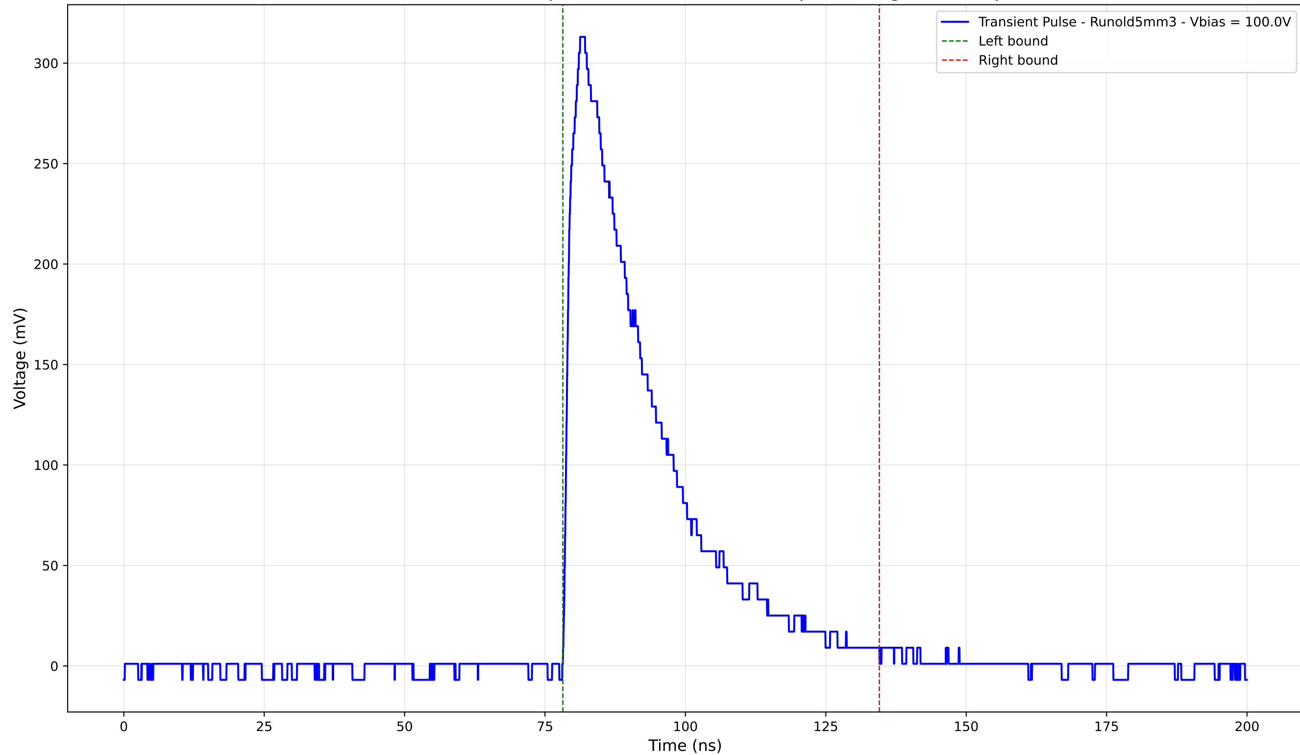
Transient Pulse - Sample: old5 - Position: 2815.0 \mu\text{m} - Charge: 102.55 pC
