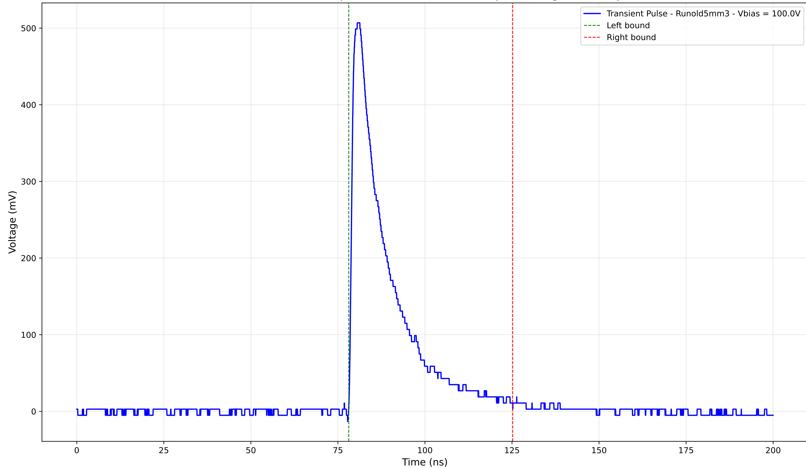
Transient Pulse - Sample: old5 - Position: 4310.0 \mu\text{m} - Charge: 115.95 pC
