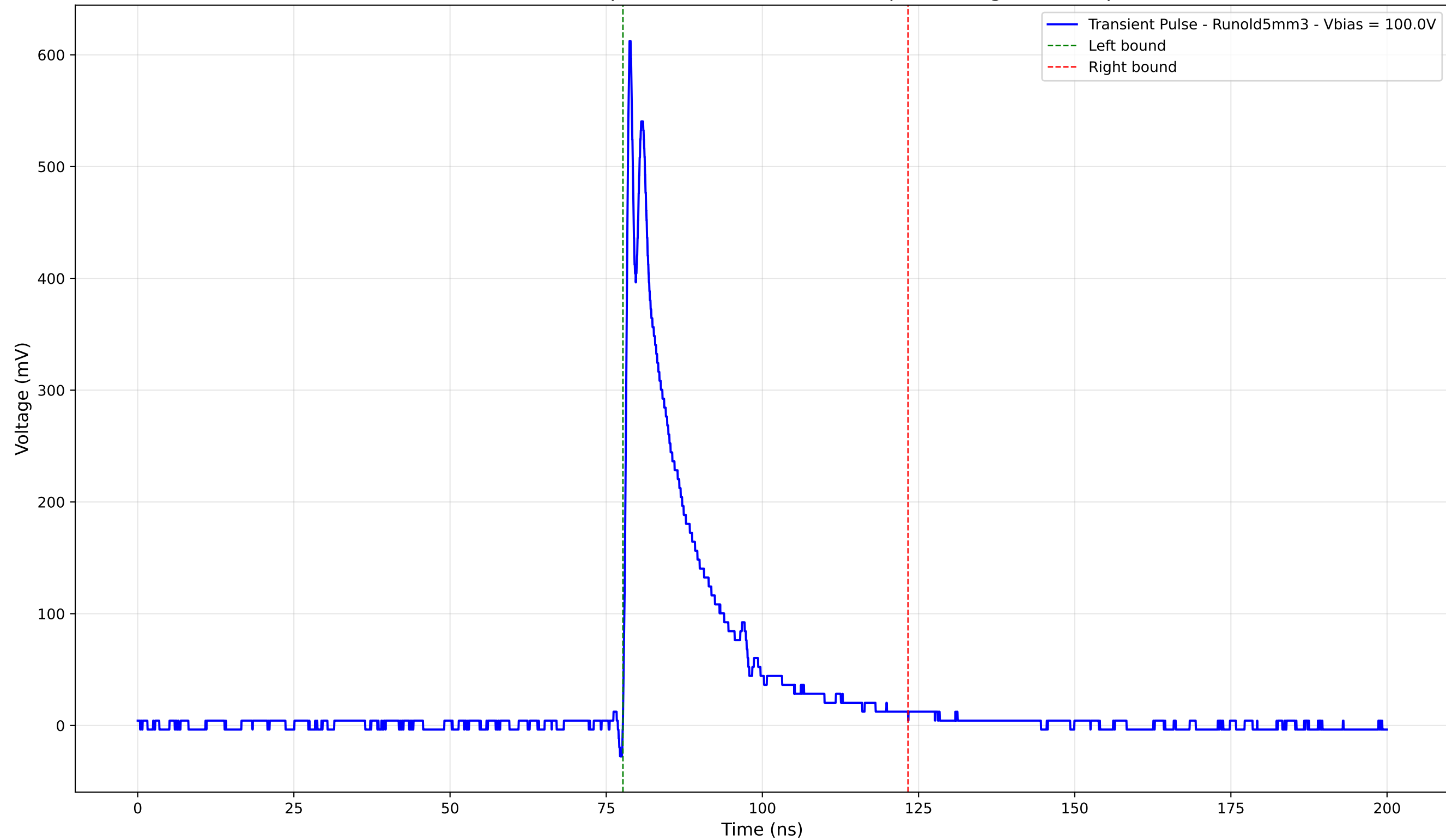
Transient Pulse - Sample: old5 - Position: 3770.0 \mu\text{m} - Charge: 106.33 pC
