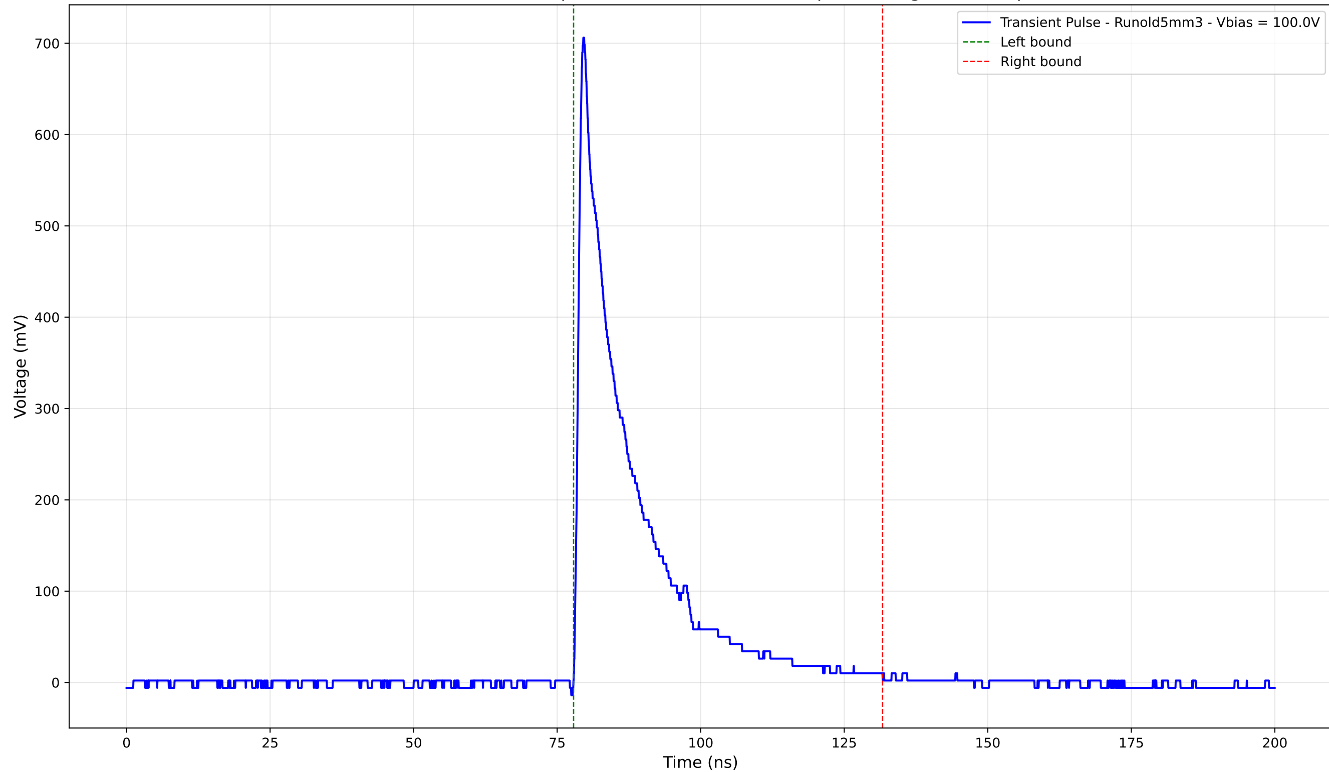
Transient Pulse - Sample: old5 - Position: 4690.0 \mu\text{m} - Charge: 130.53 pC
