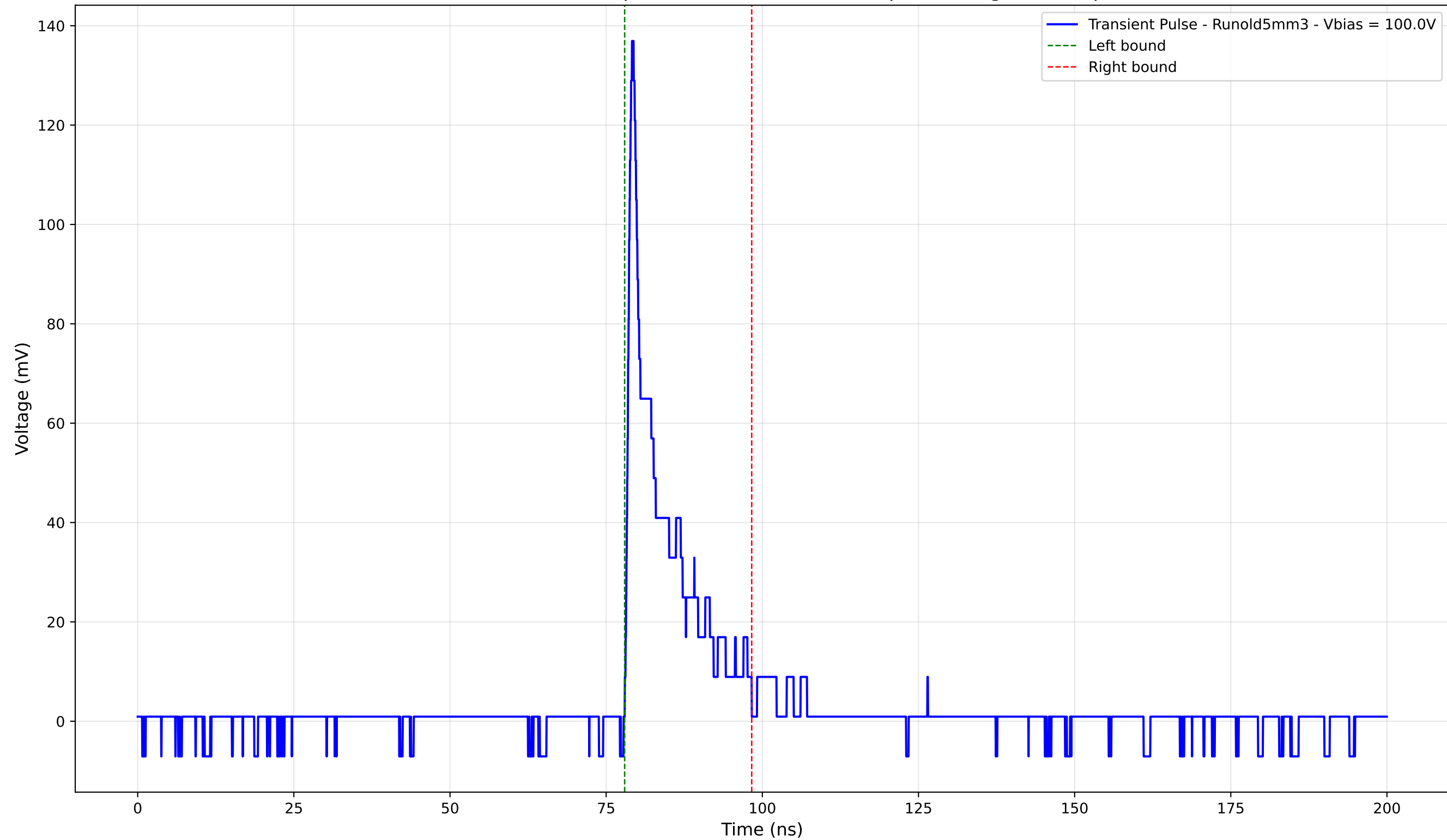
Transient Pulse - Sample: old5 - Position: 150.0 \mu\text{m} - Charge: 14.46 pC
