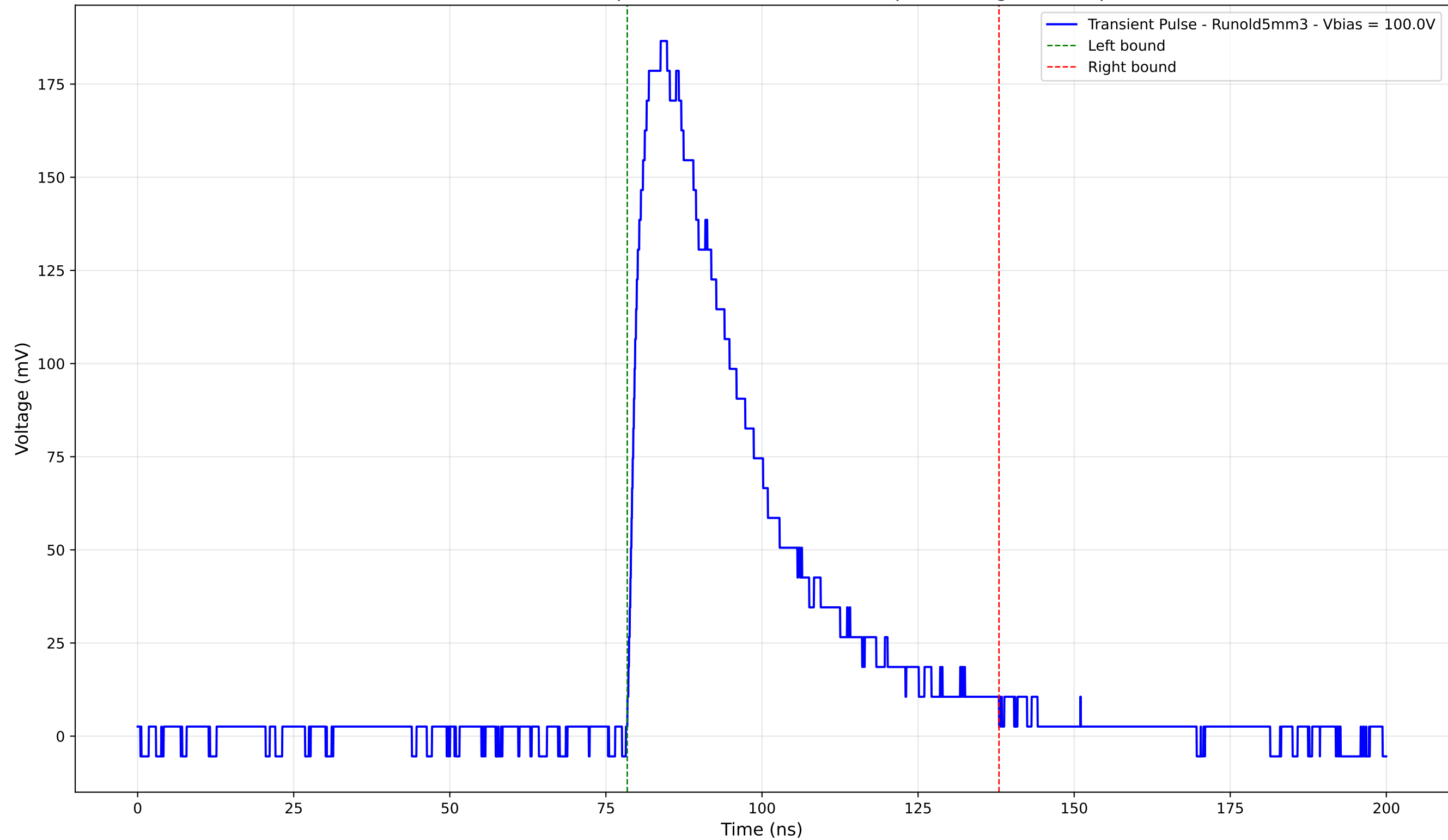
Transient Pulse - Sample: old5 - Position: 1920.0 \mu\text{m} - Charge: 75.89 pC
