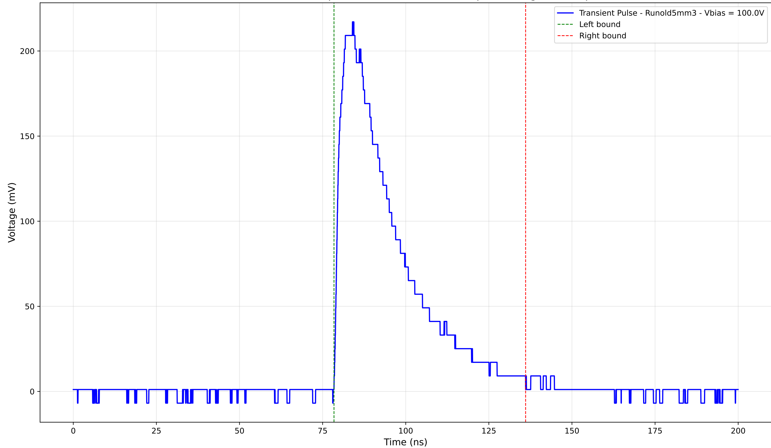
Transient Pulse - Sample: old5 - Position: 2270.0 \mu\text{m} - Charge: 83.03 pC
