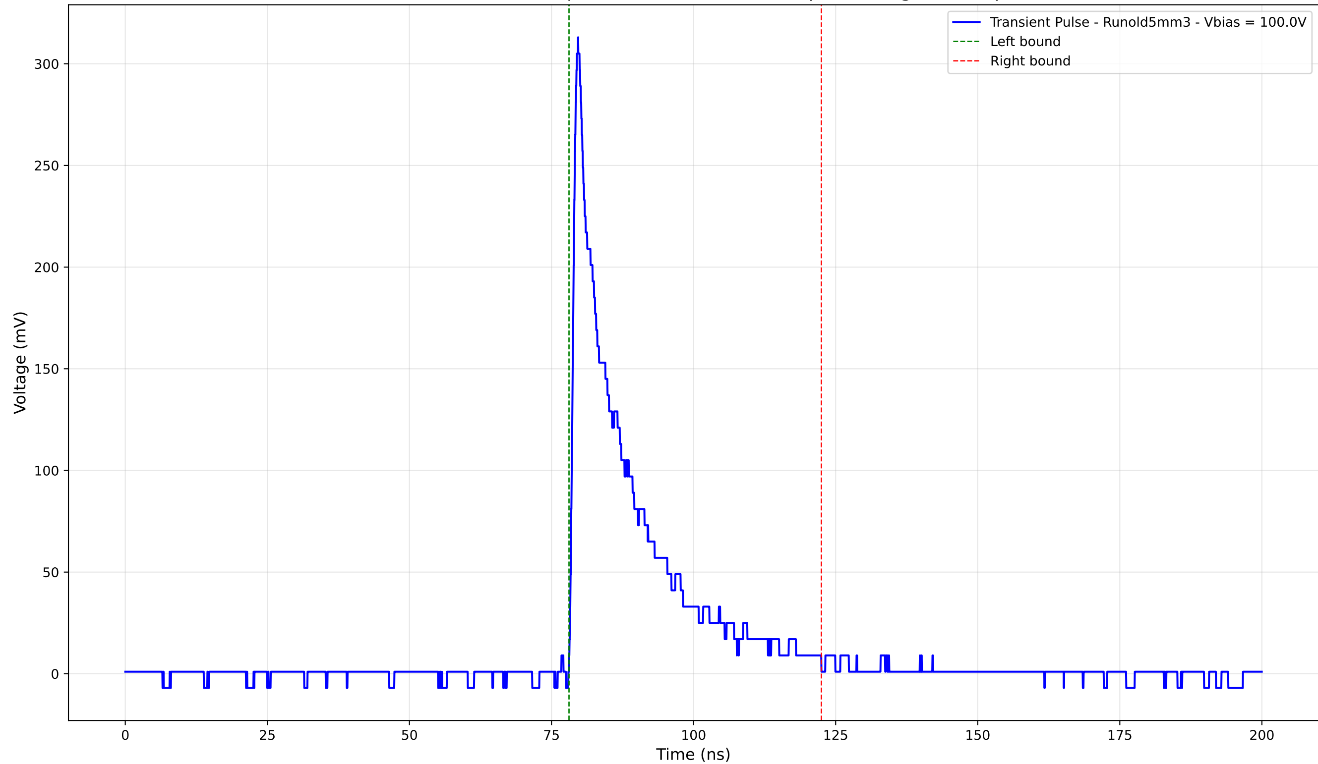
Transient Pulse - Sample: old5 - Position: 445.0 \mu\text{m} - Charge: 56.72 pC
