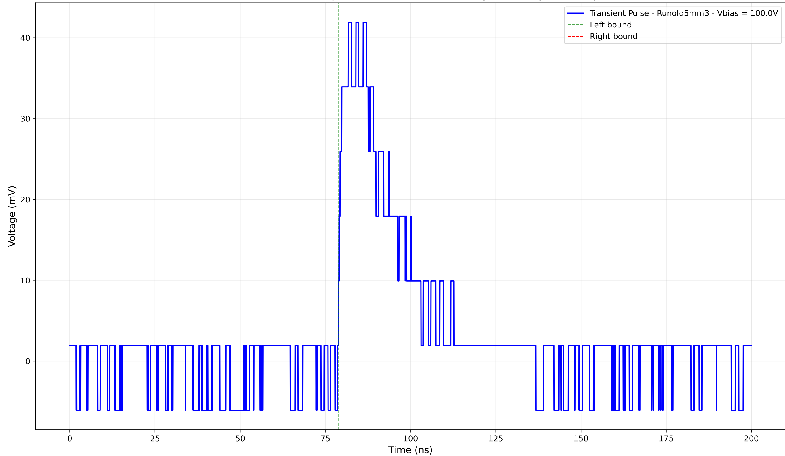
Transient Pulse - Sample: old5 - Position: 1170.0 \mu\text{m} - Charge: 11.78 pC
