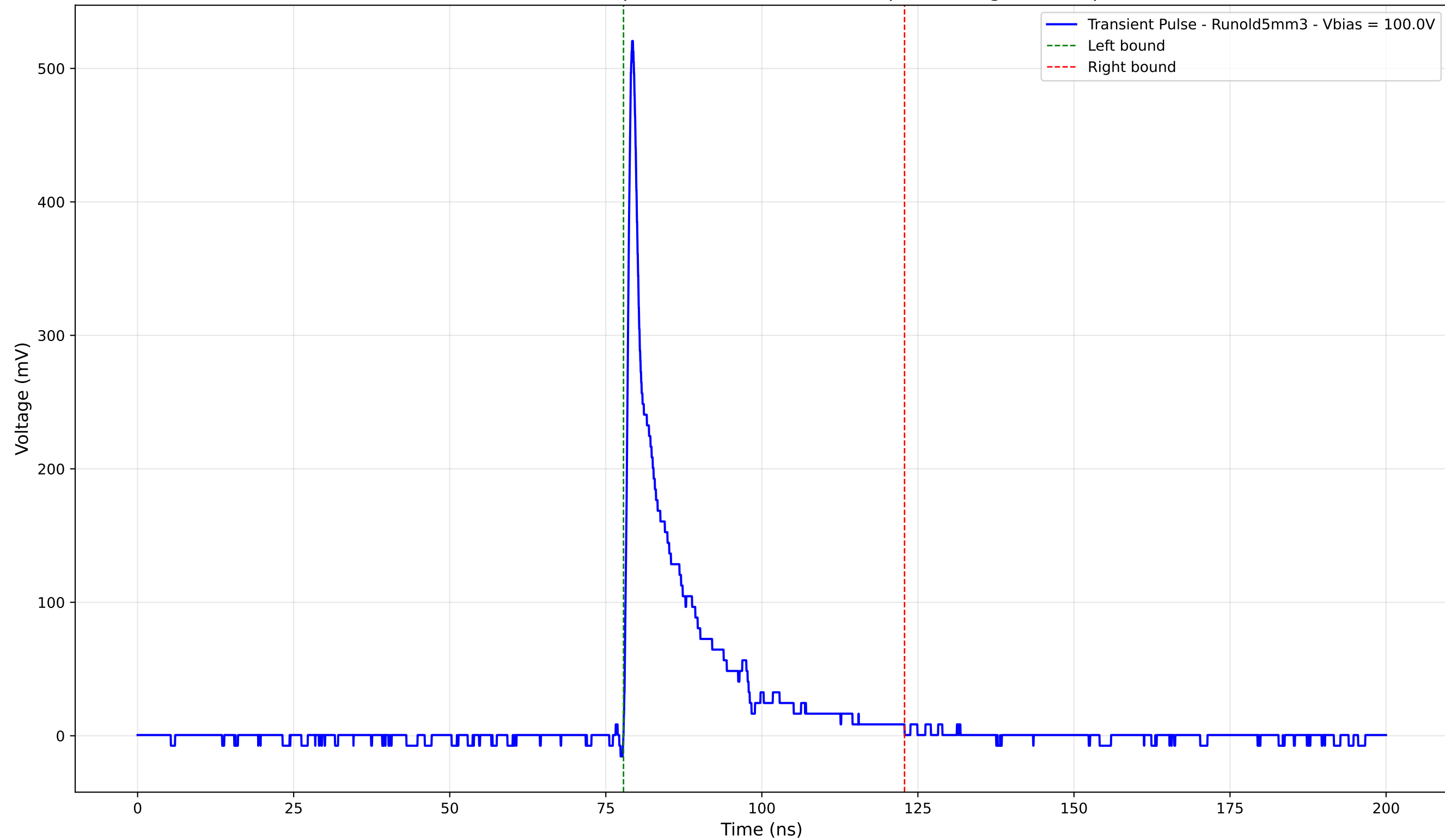
Transient Pulse - Sample: old5 - Position: 205.0 \mu\text{m} - Charge: 65.14 pC
