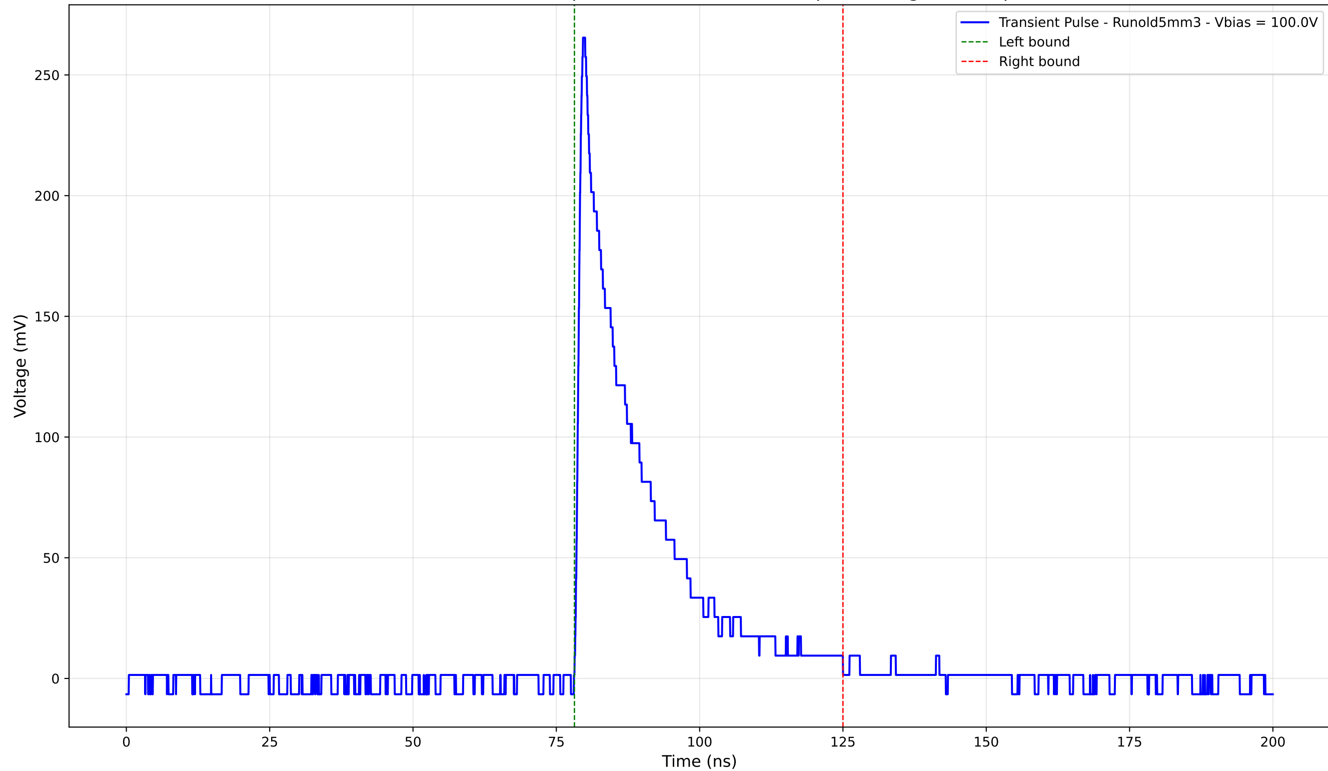
Transient Pulse - Sample: old5 - Position: 535.0 \mu\text{m} - Charge: 54.84 pC
