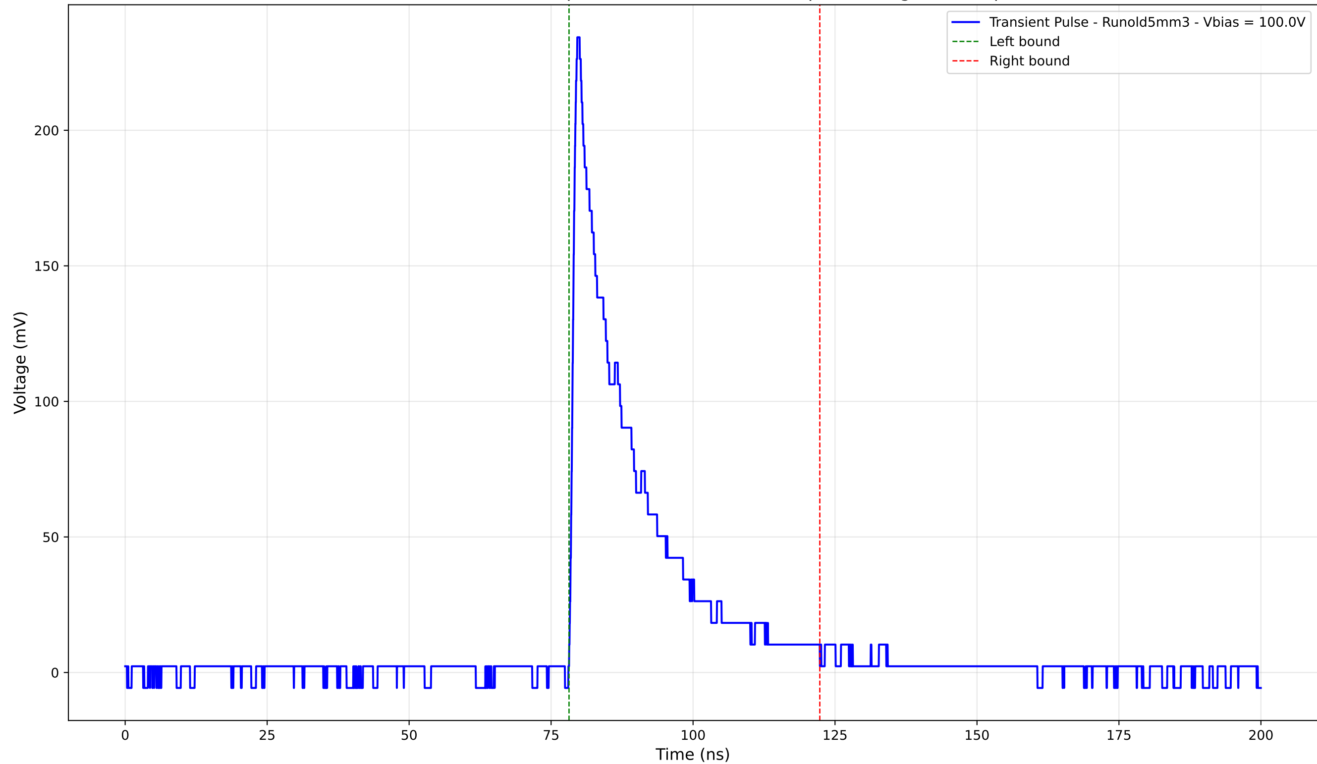
Transient Pulse - Sample: old5 - Position: 525.0 \mu\text{m} - Charge: 48.55 pC
