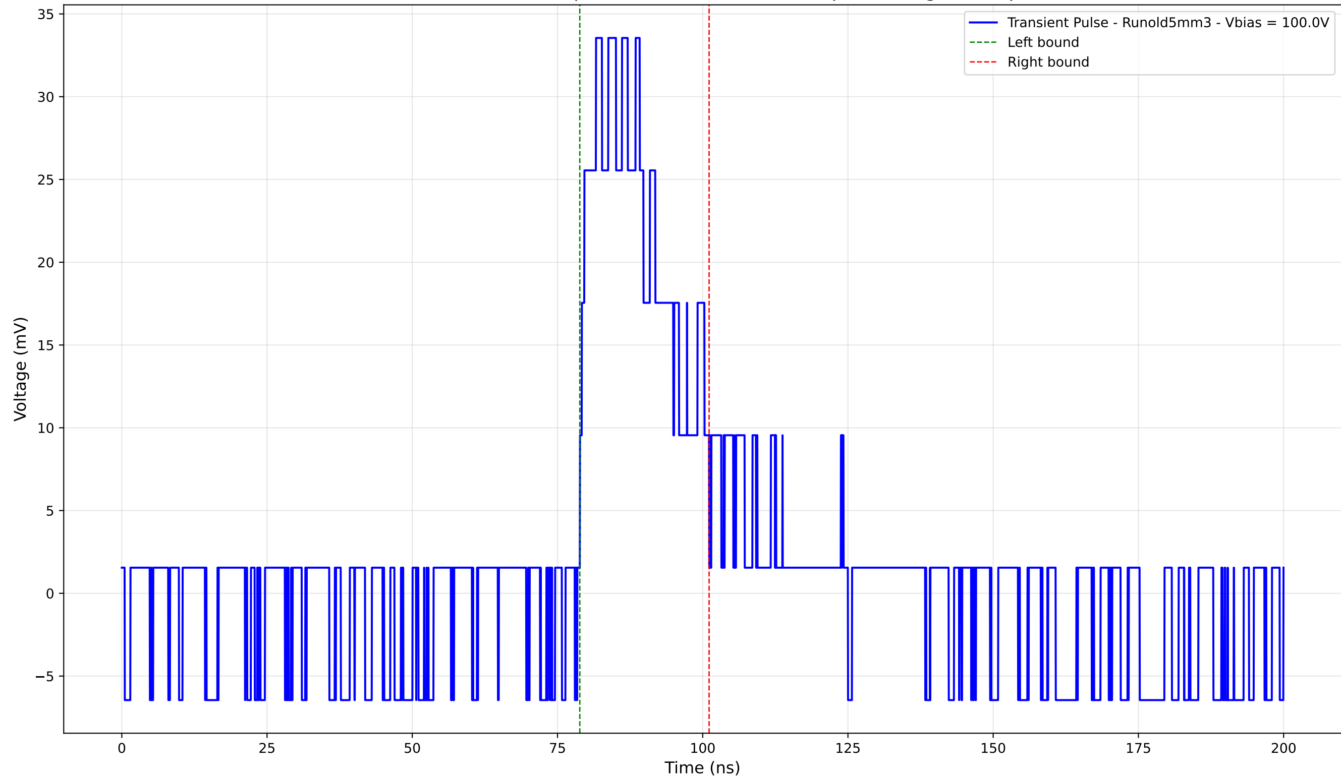
Transient Pulse - Sample: old5 - Position: 1185.0 \mu\text{m} - Charge: 9.53 pC
