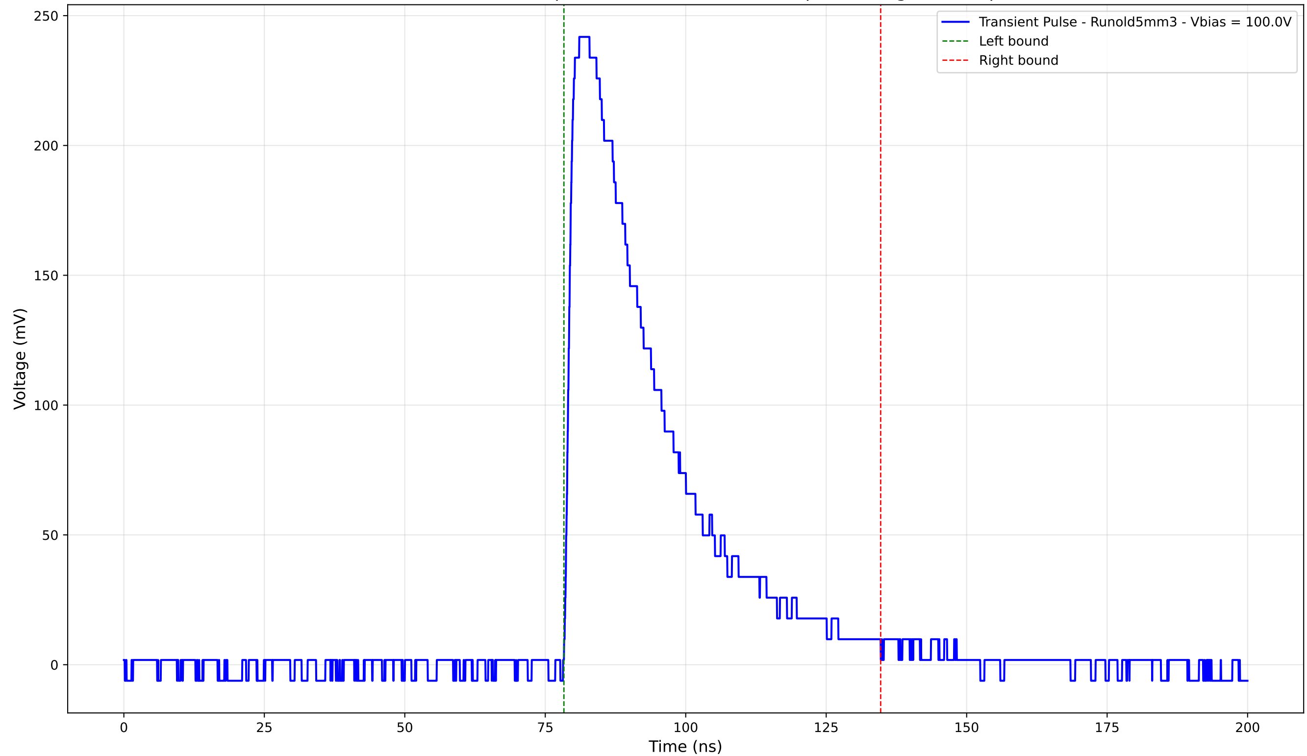
Transient Pulse - Sample: old5 - Position: 1080.0 \mu\text{m} - Charge: 86.77 pC
