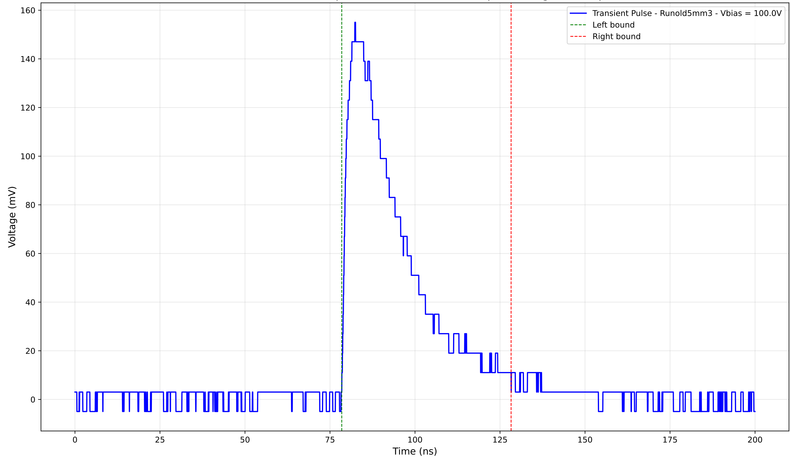
Transient Pulse - Sample: old5 - Position: 2445.0 \mu\text{m} - Charge: 56.56 pC
