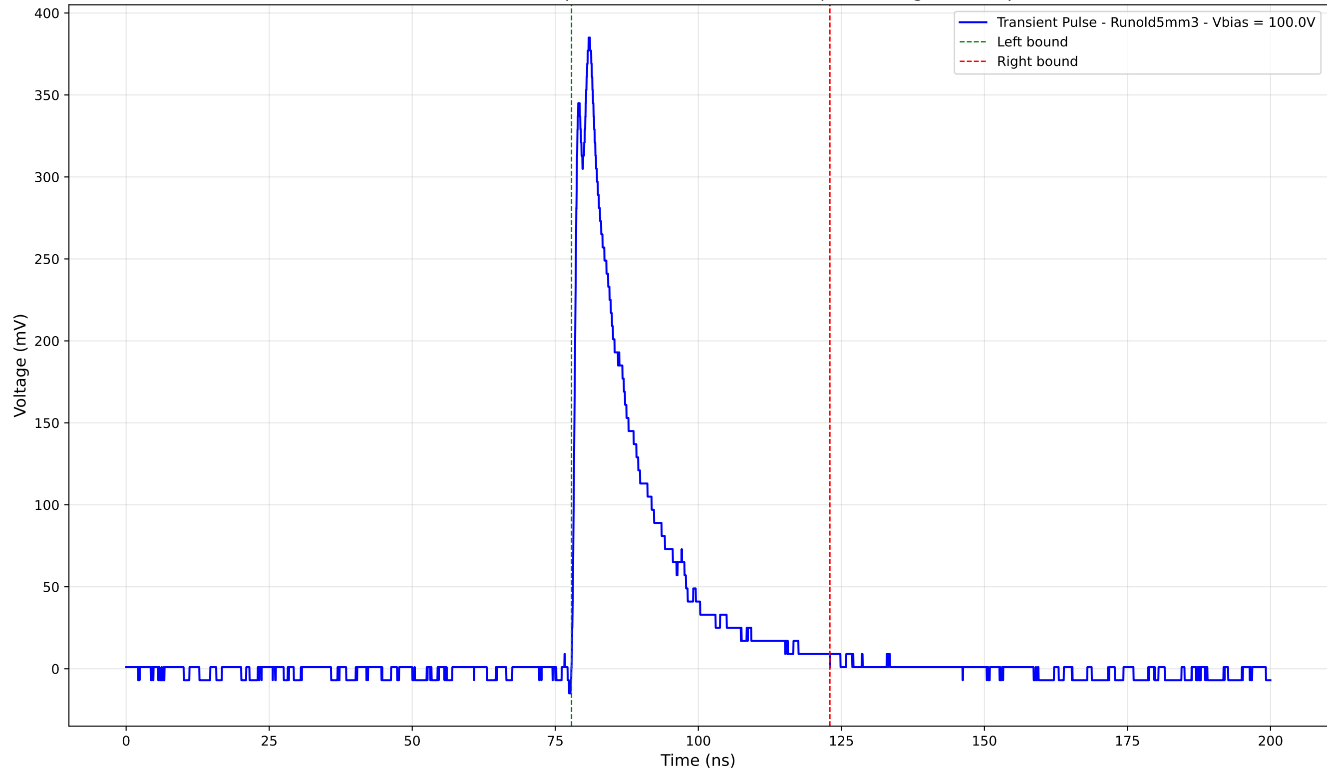
Transient Pulse - Sample: old5 - Position: 3970.0 \mu\text{m} - Charge: 80.08 pC
