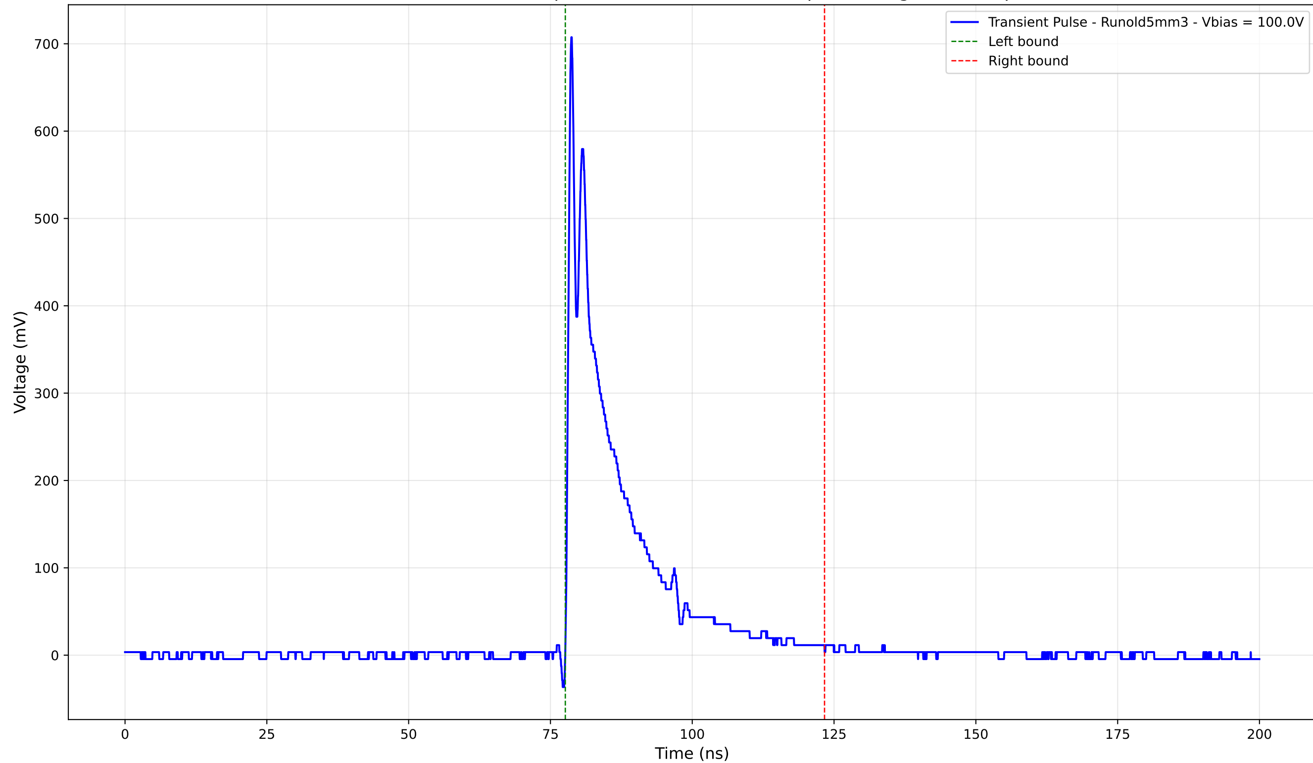
Transient Pulse - Sample: old5 - Position: 3715.0 \mu\text{m} - Charge: 108.73 pC
