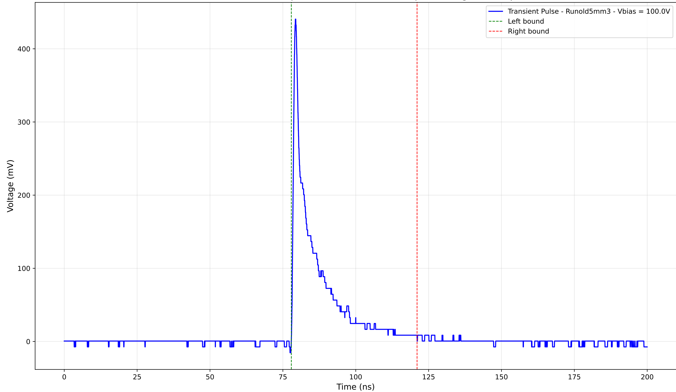
Transient Pulse - Sample: old5 - Position: 260.0 \mu\text{m} - Charge: 57.73 pC
