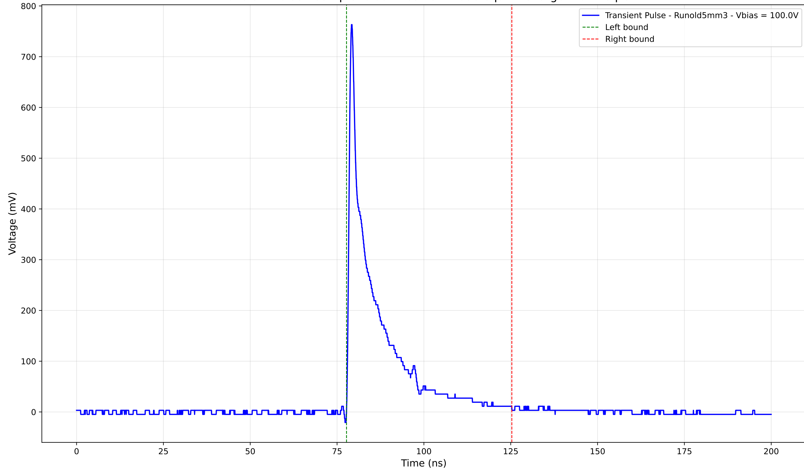
Transient Pulse - Sample: old5 - Position: 4850.0 \mu\text{m} - Charge: 107.20 pC
