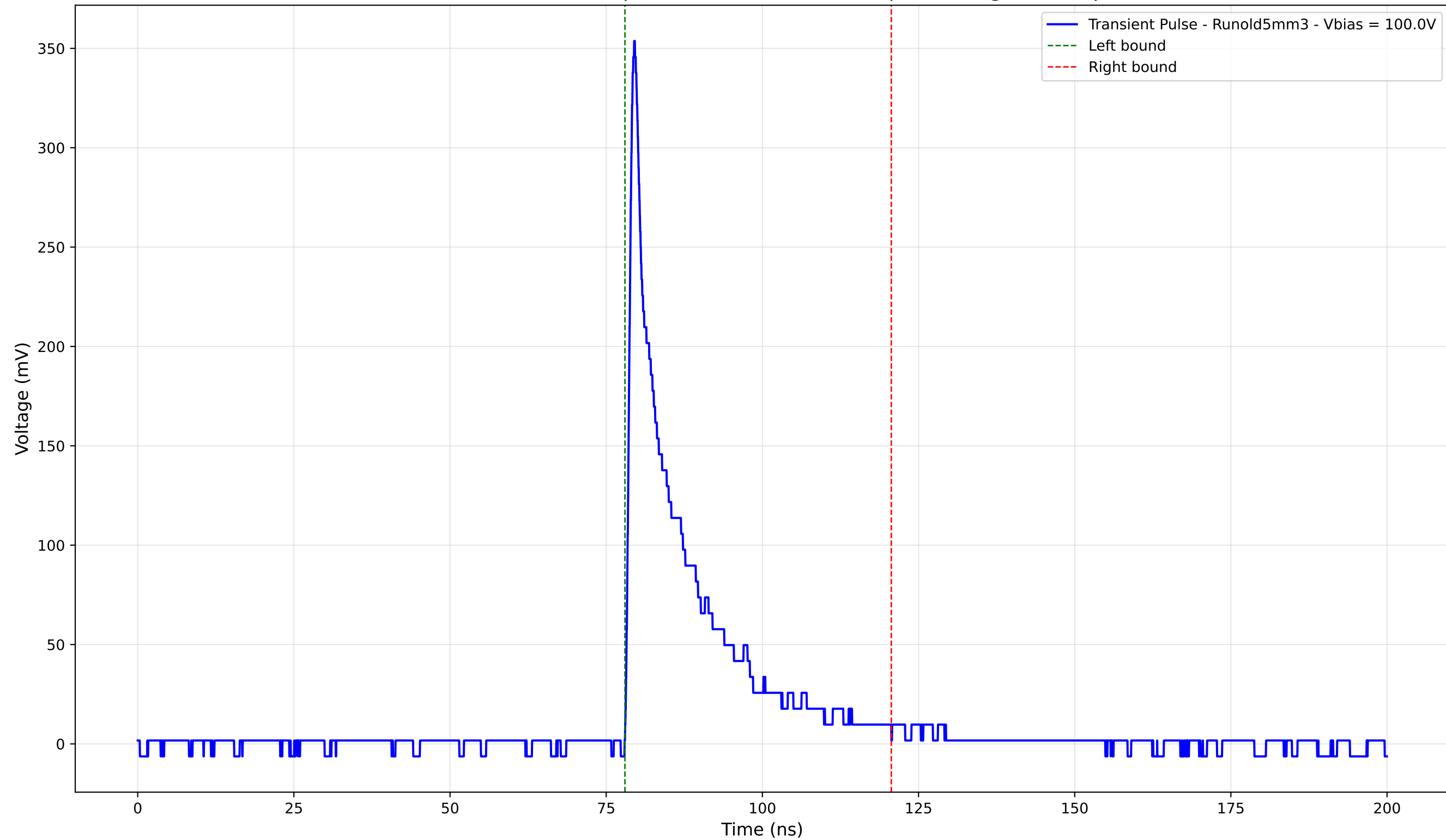
Transient Pulse - Sample: old5 - Position: 335.0 \mu\text{m} - Charge: 54.28 pC
