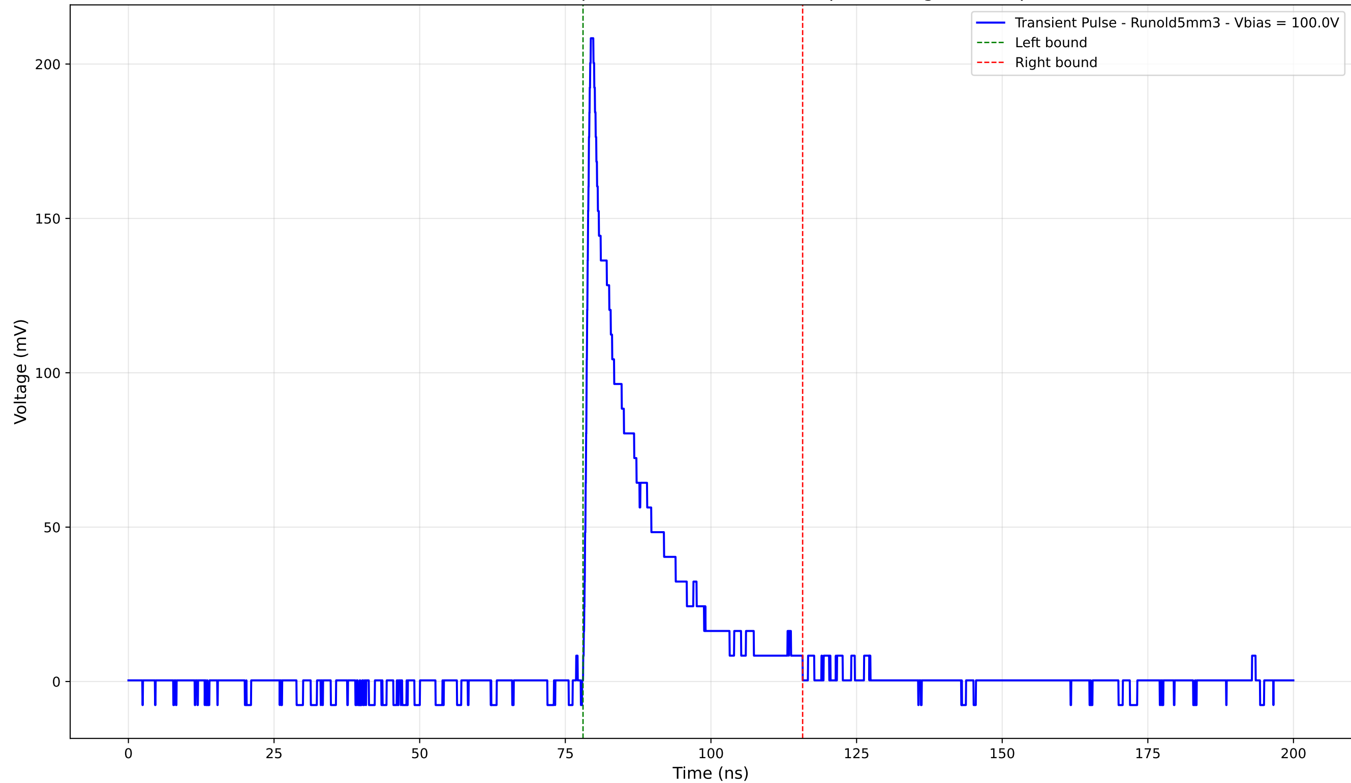
Transient Pulse - Sample: old5 - Position: 395.0 \mu\text{m} - Charge: 34.90 pC
