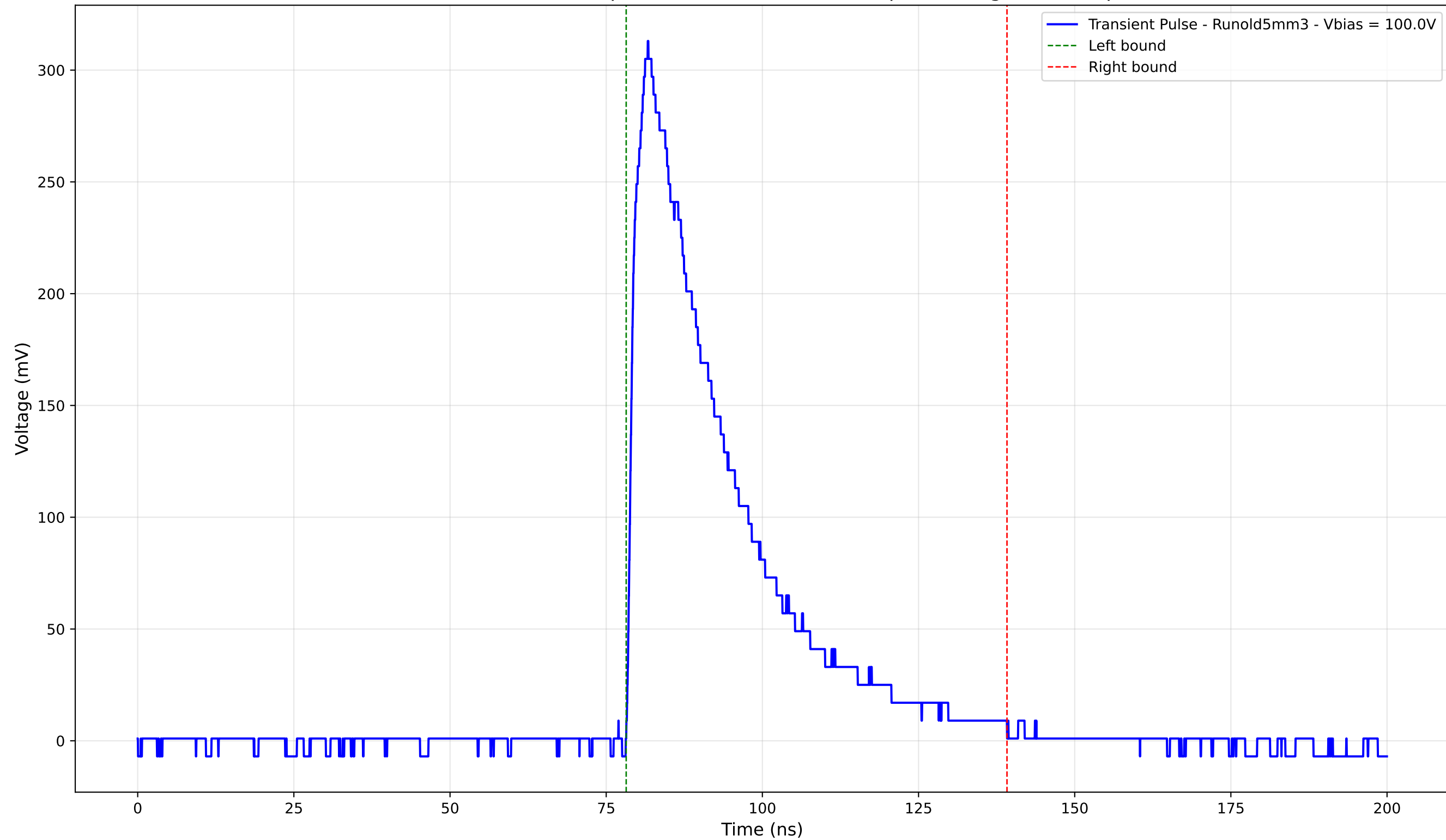
Transient Pulse - Sample: old5 - Position: 2800.0 \mu\text{m} - Charge: 102.36 pC
