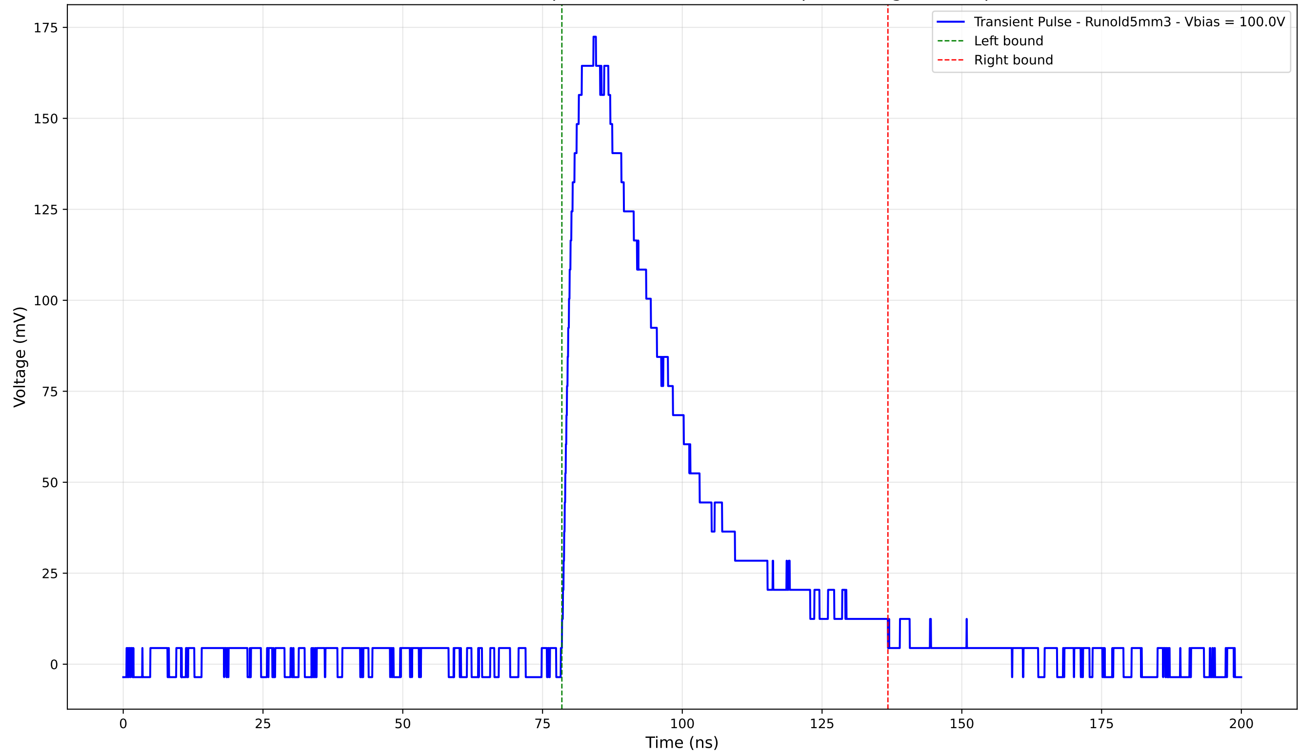
Transient Pulse - Sample: old5 - Position: 1650.0 \mu\text{m} - Charge: 70.10 pC
