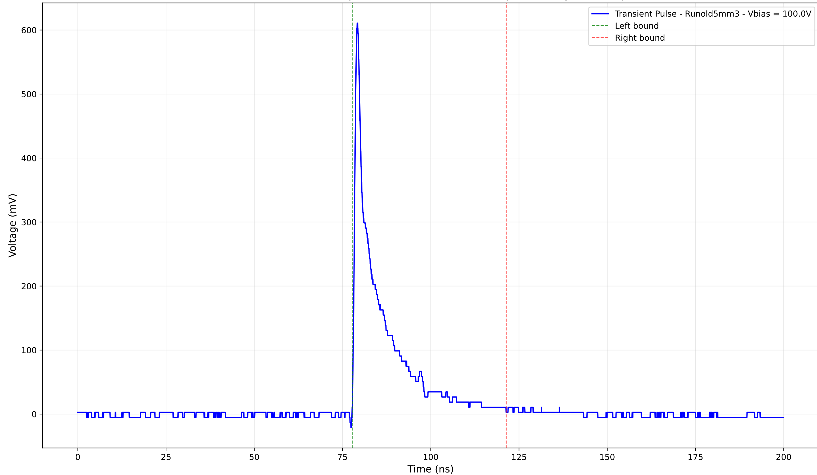
Transient Pulse - Sample: old5 - Position: 4870.0 \mu\text{m} - Charge: 79.76 pC
