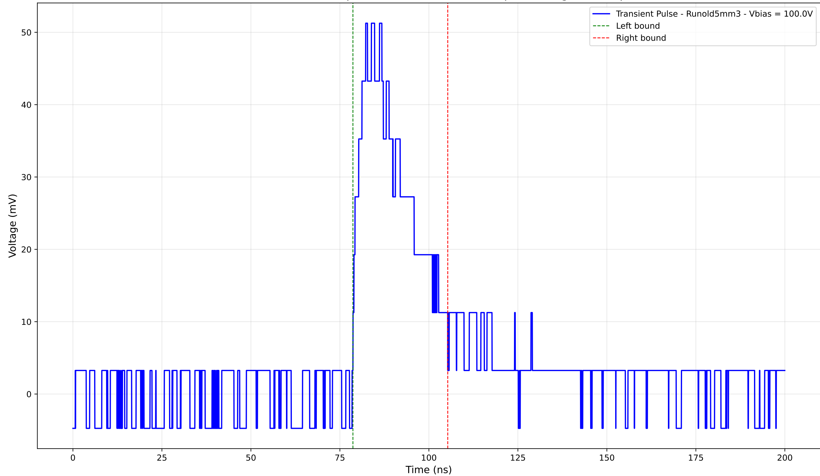
Transient Pulse - Sample: old5 - Position: 2410.0 \mu\text{m} - Charge: 15.53 pC
