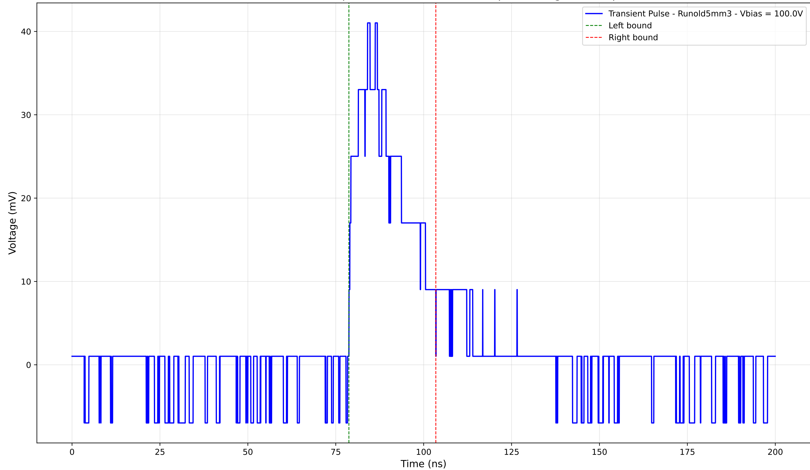
Transient Pulse - Sample: old5 - Position: 2395.0 \mu\text{m} - Charge: 11.45 pC
