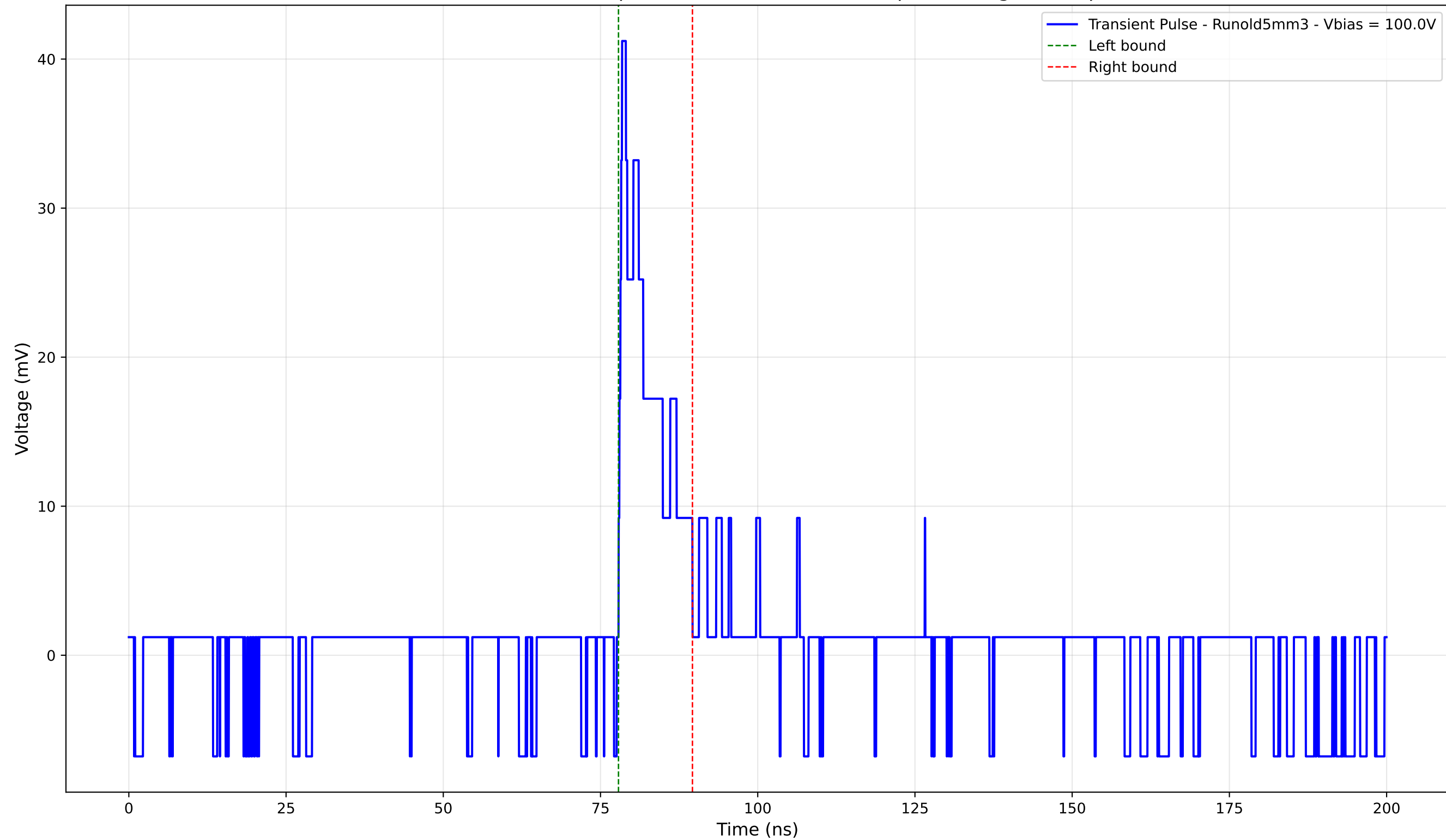
Transient Pulse - Sample: old5 - Position: 3565.0 \mu\text{m} - Charge: 4.41 pC
