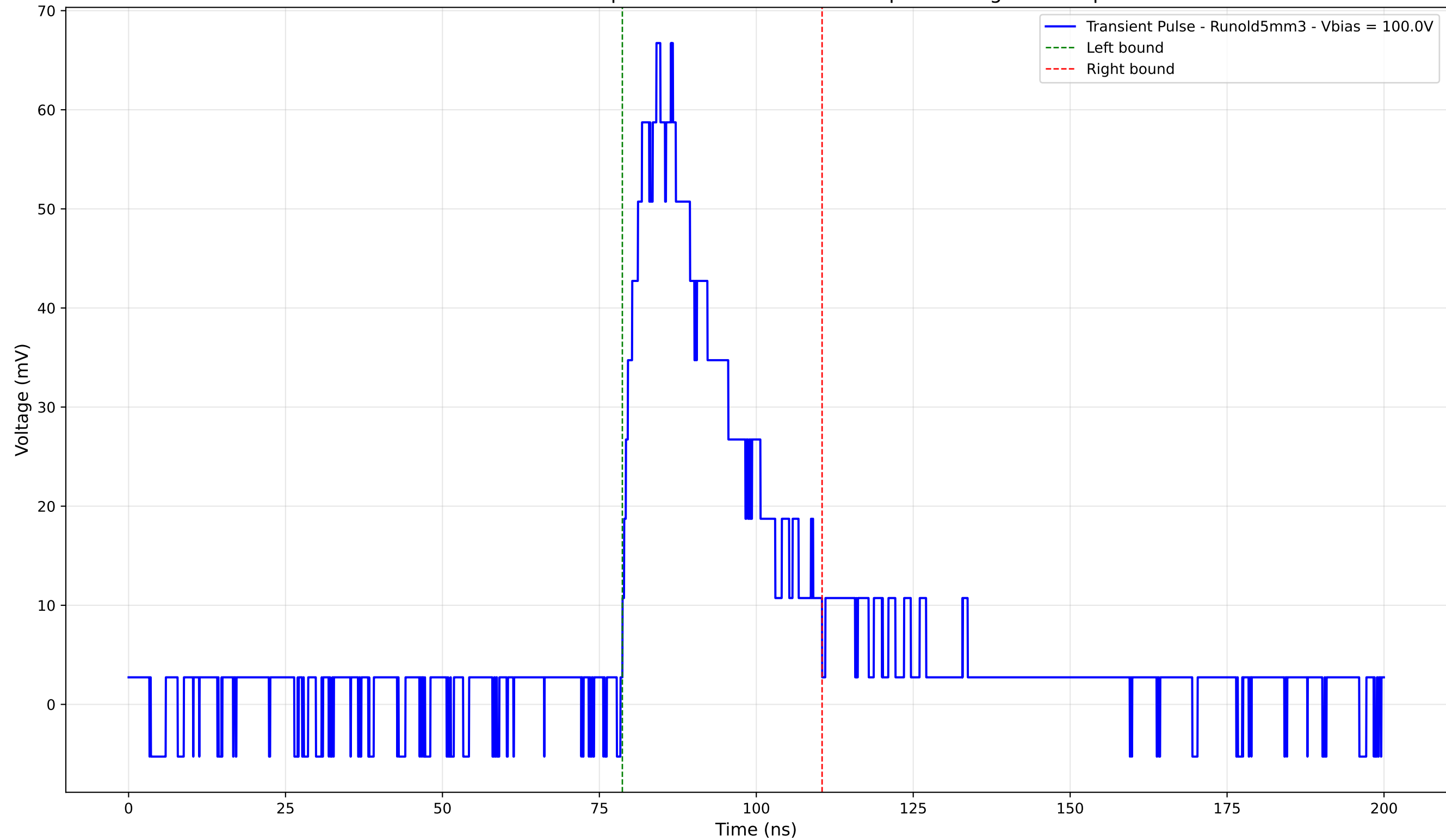
Transient Pulse - Sample: old5 - Position: 2170.0 \mu\text{m} - Charge: 21.08 pC
