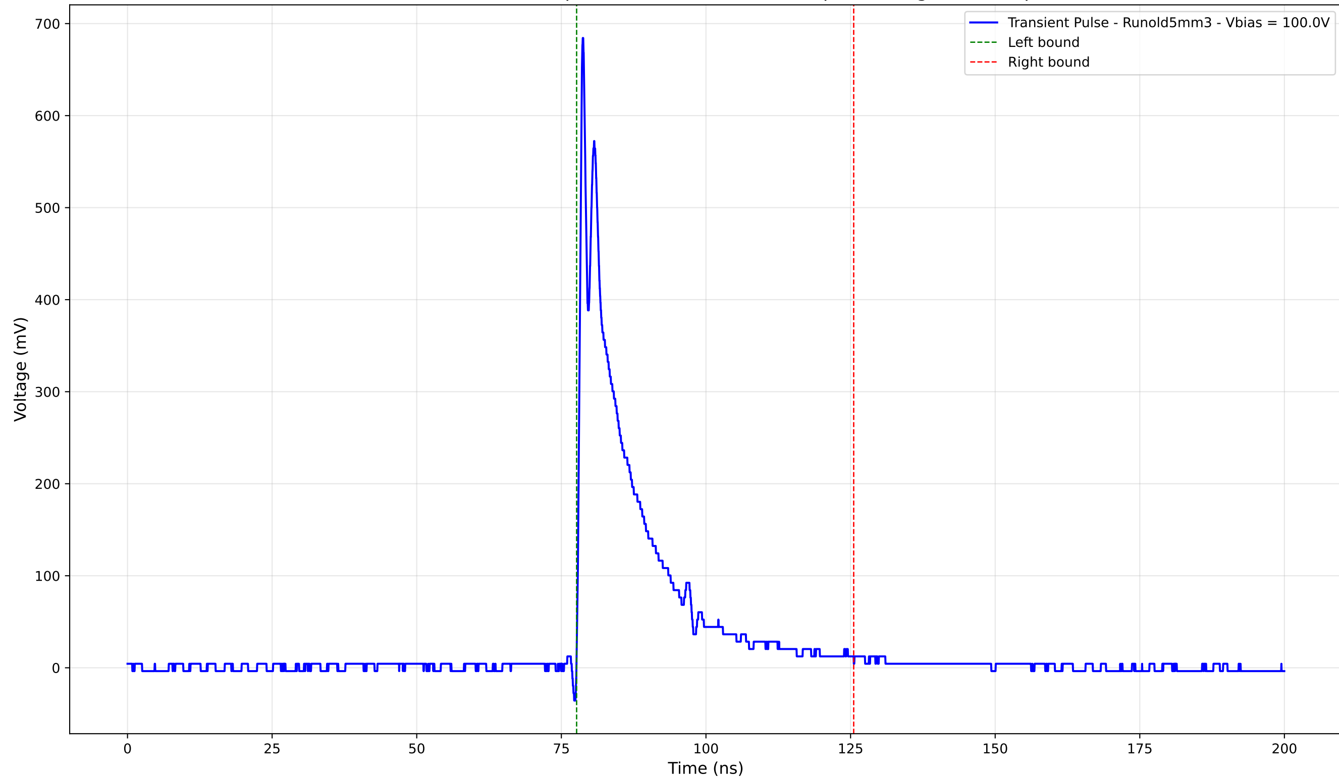
Transient Pulse - Sample: old5 - Position: 3725.0 \mu\text{m} - Charge: 109.31 pC
