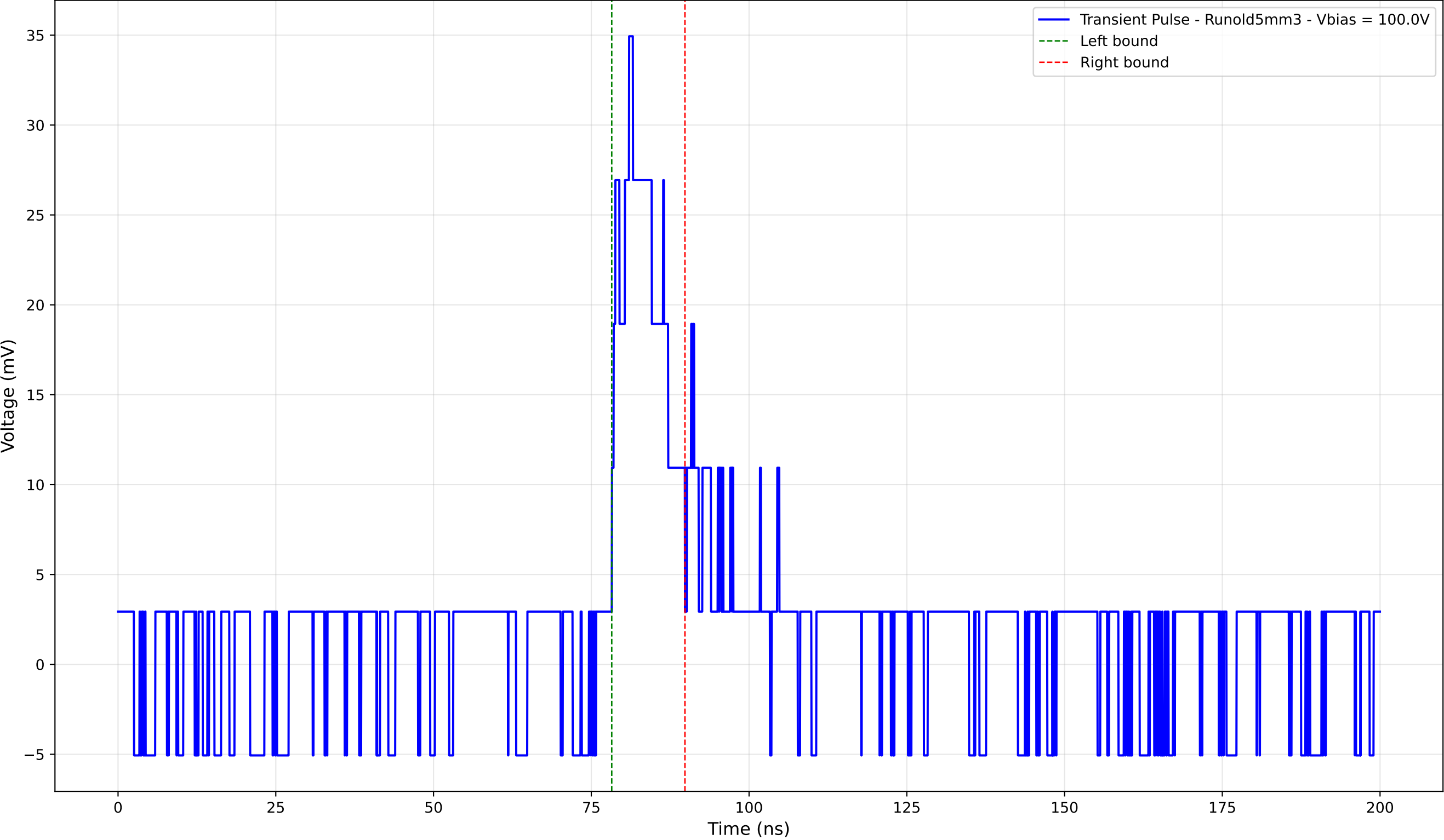
Transient Pulse - Sample: old5 - Position: 3895.0 \mu\text{m} - Charge: 4.83 pC
