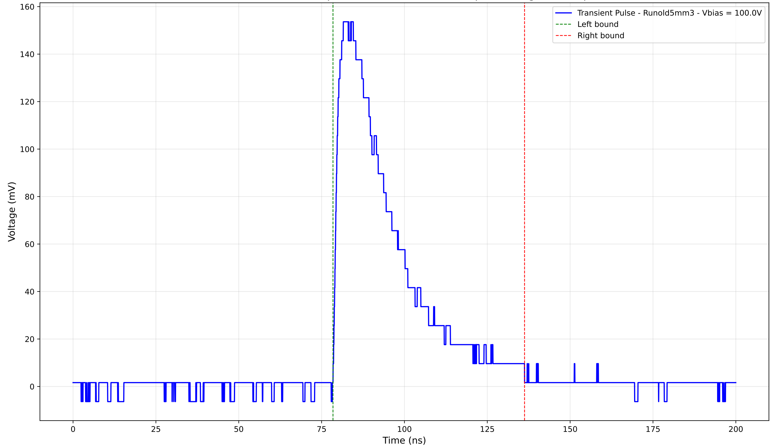
Transient Pulse - Sample: old5 - Position: 1325.0 \mu\text{m} - Charge: 59.92 pC
