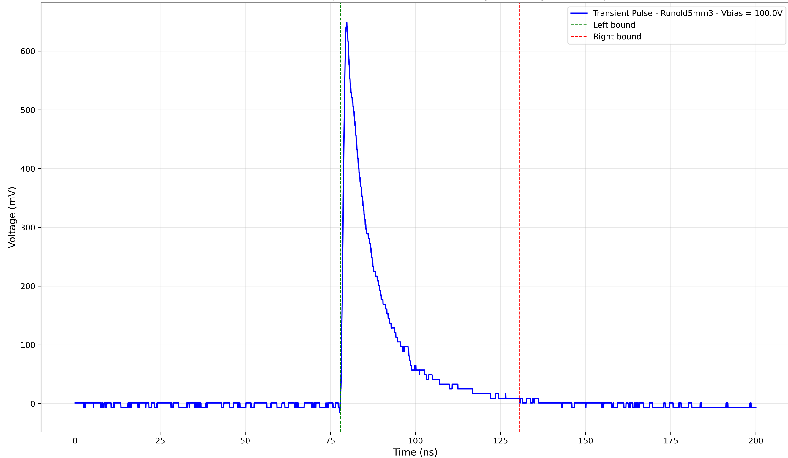
Transient Pulse - Sample: old5 - Position: 4640.0 \mu\text{m} - Charge: 124.81 pC
