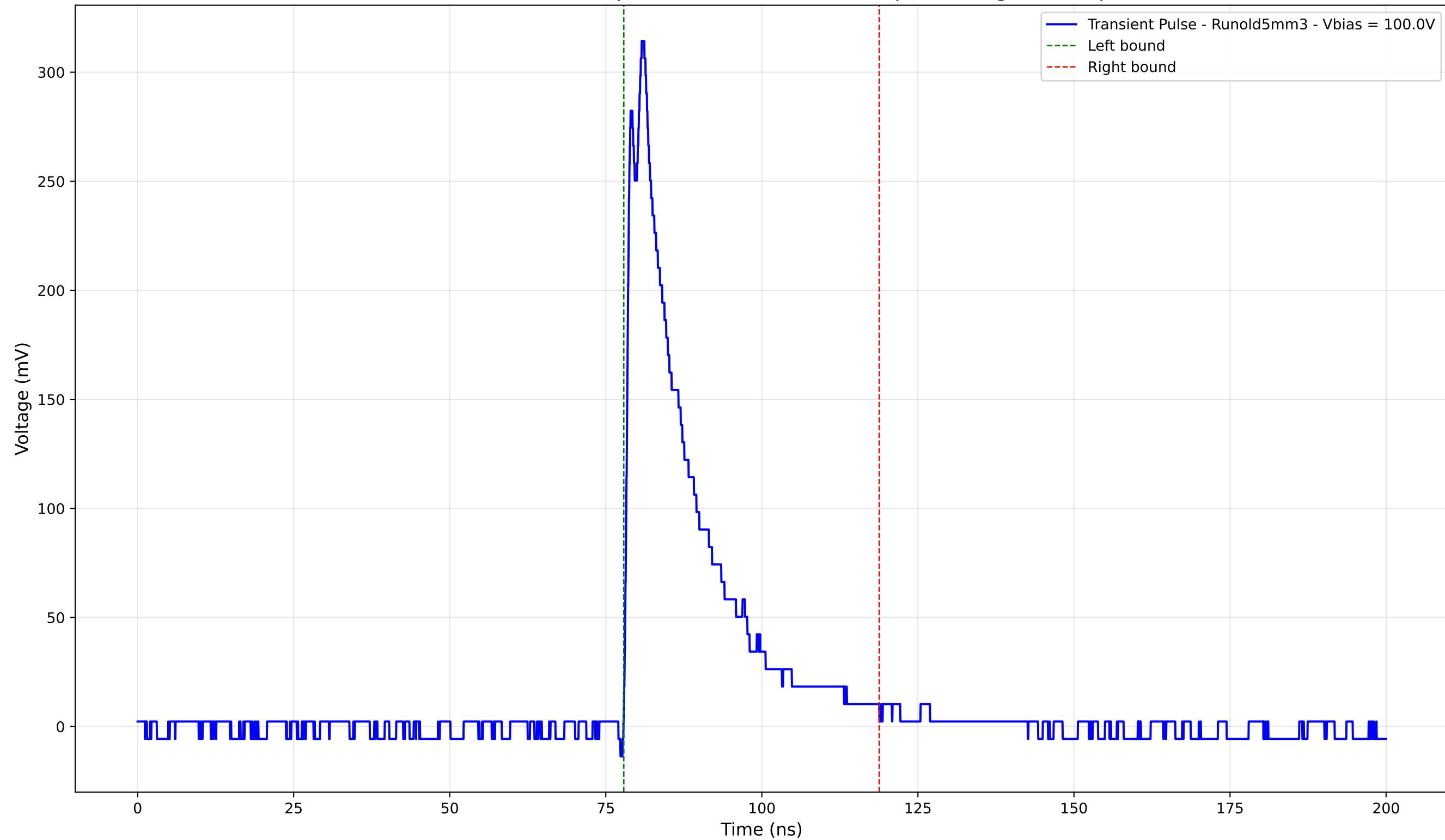
Transient Pulse - Sample: old5 - Position: 3960.0 \mu\text{m} - Charge: 65.24 pC
