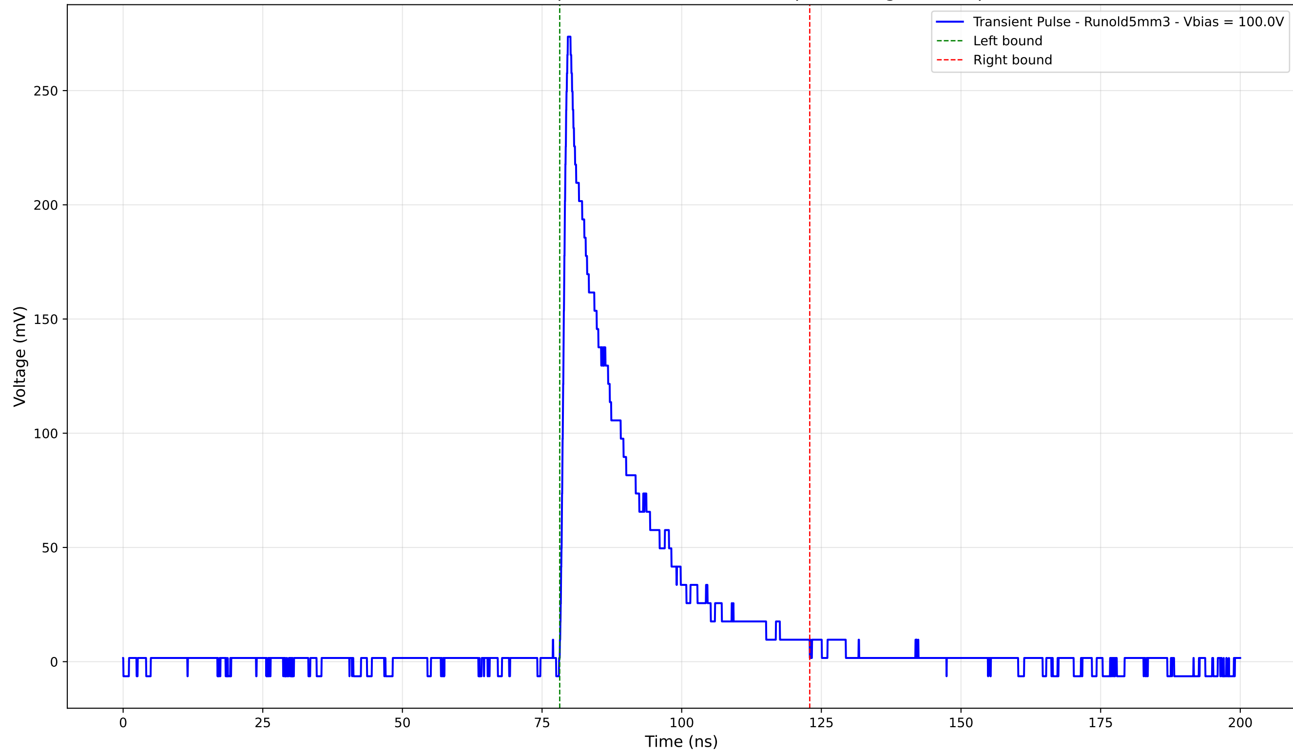
Transient Pulse - Sample: old5 - Position: 545.0 \mu\text{m} - Charge: 57.46 pC
