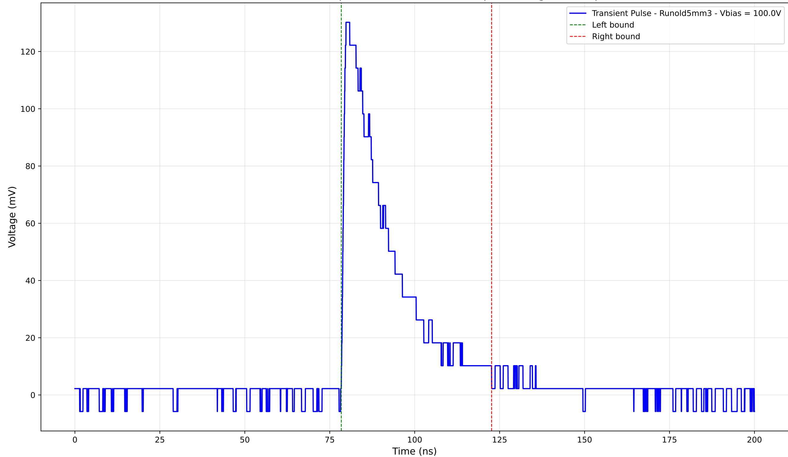
Transient Pulse - Sample: old5 - Position: 810.0 \mu\text{m} - Charge: 38.60 pC
