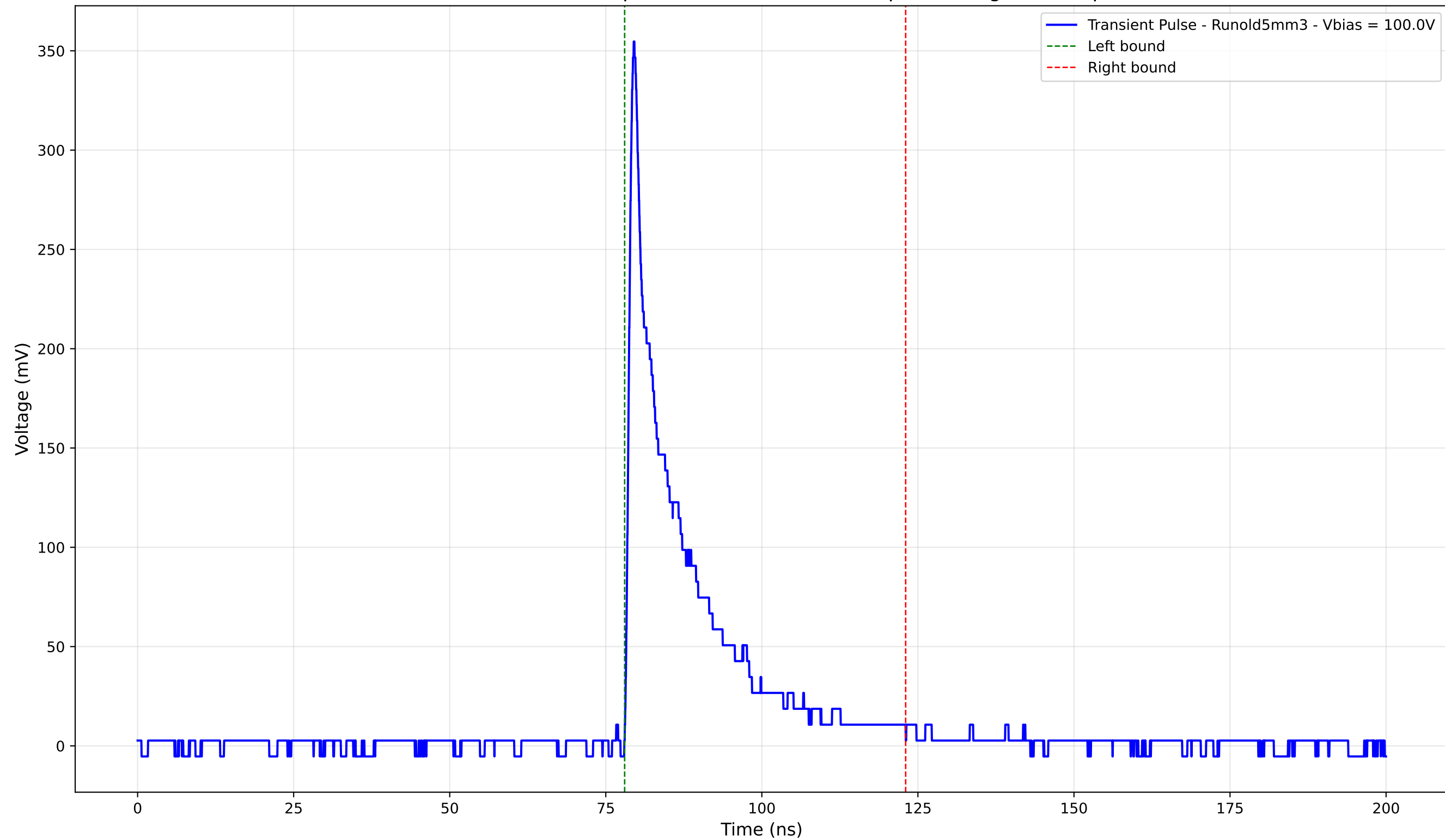
Transient Pulse - Sample: old5 - Position: 355.0 \mu\text{m} - Charge: 55.90 pC
