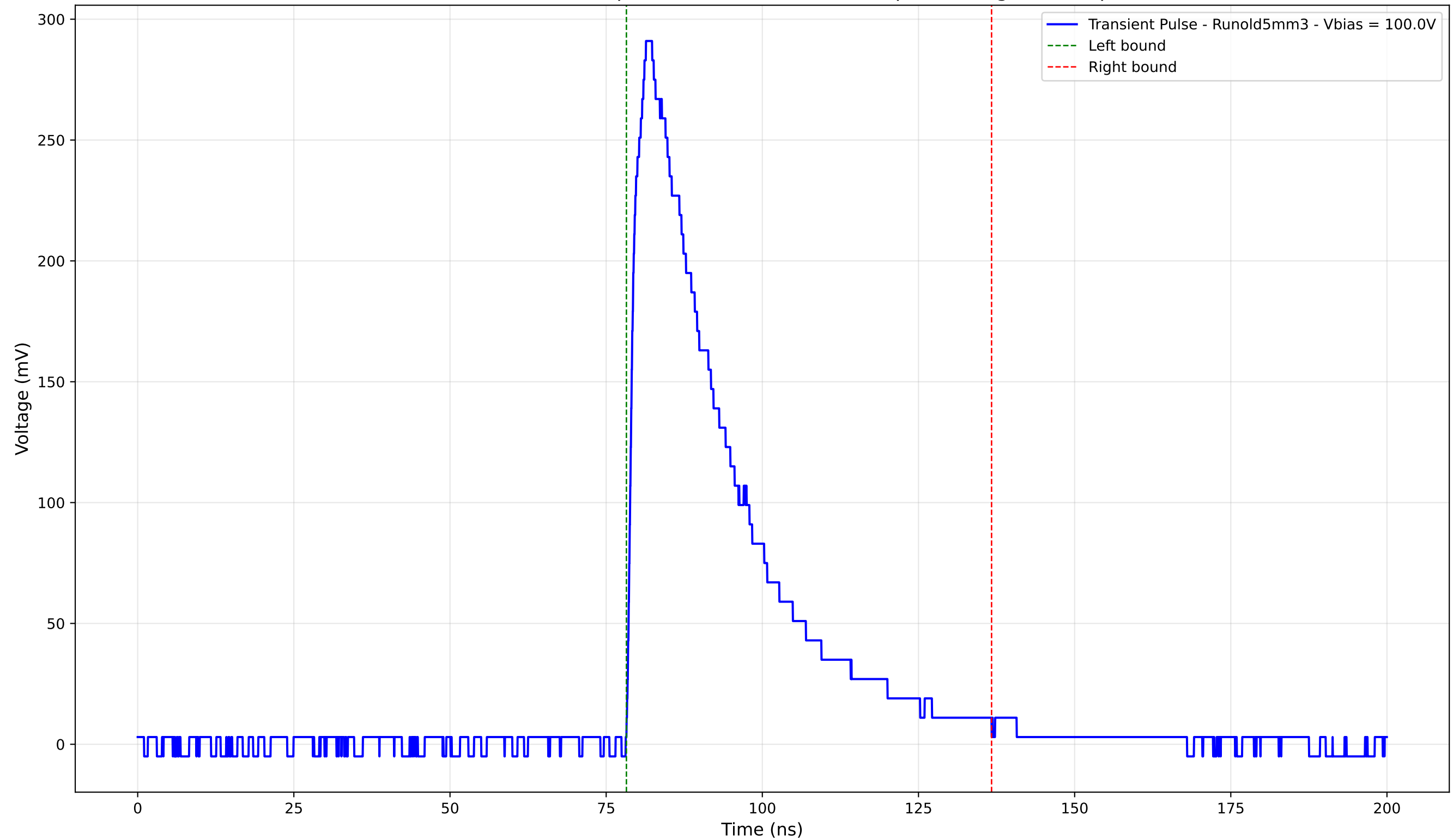
Transient Pulse - Sample: old5 - Position: 2785.0 \mu\text{m} - Charge: 98.11 pC
