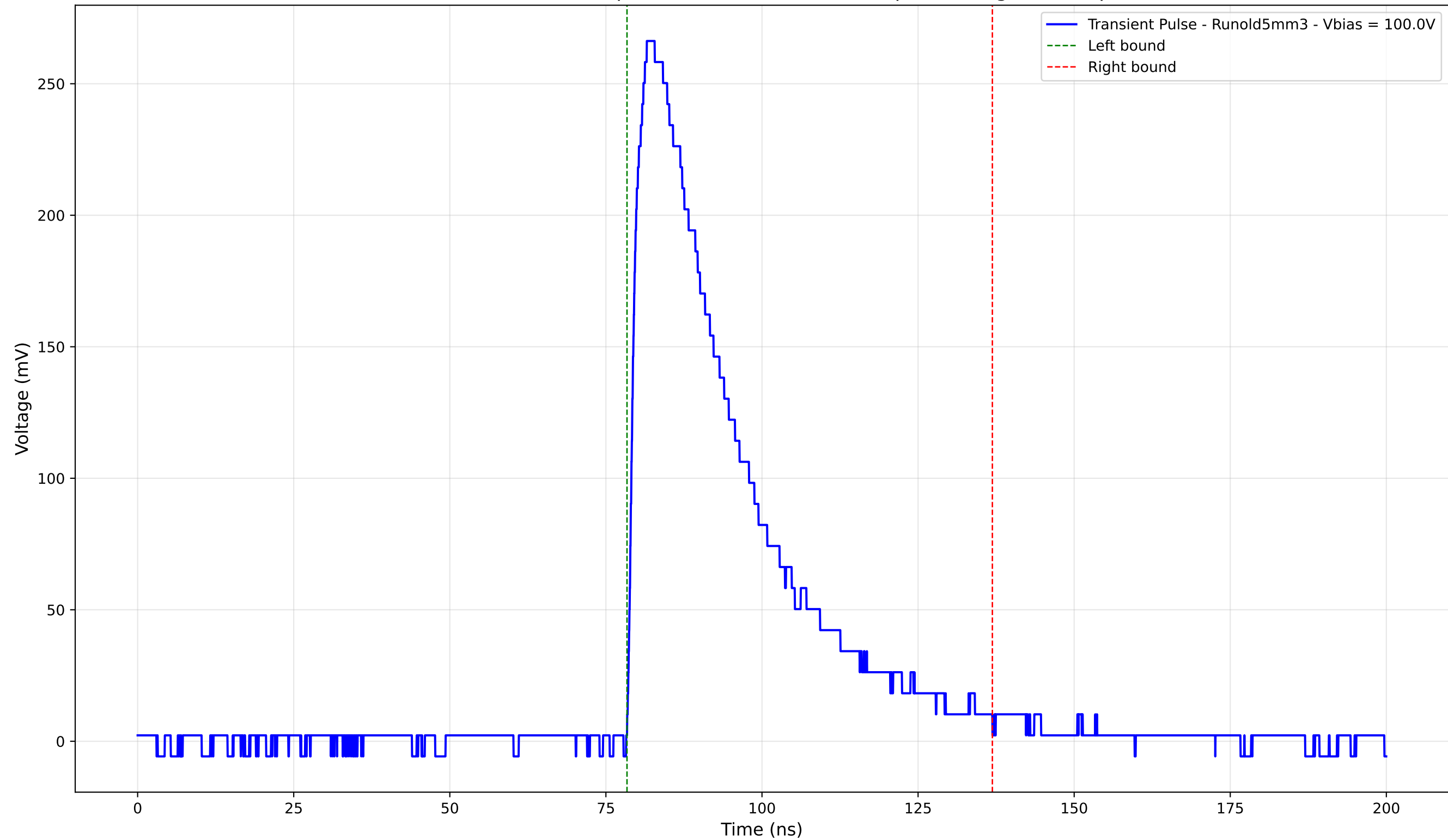
Transient Pulse - Sample: old5 - Position: 2555.0 \mu\text{m} - Charge: 99.46 pC
