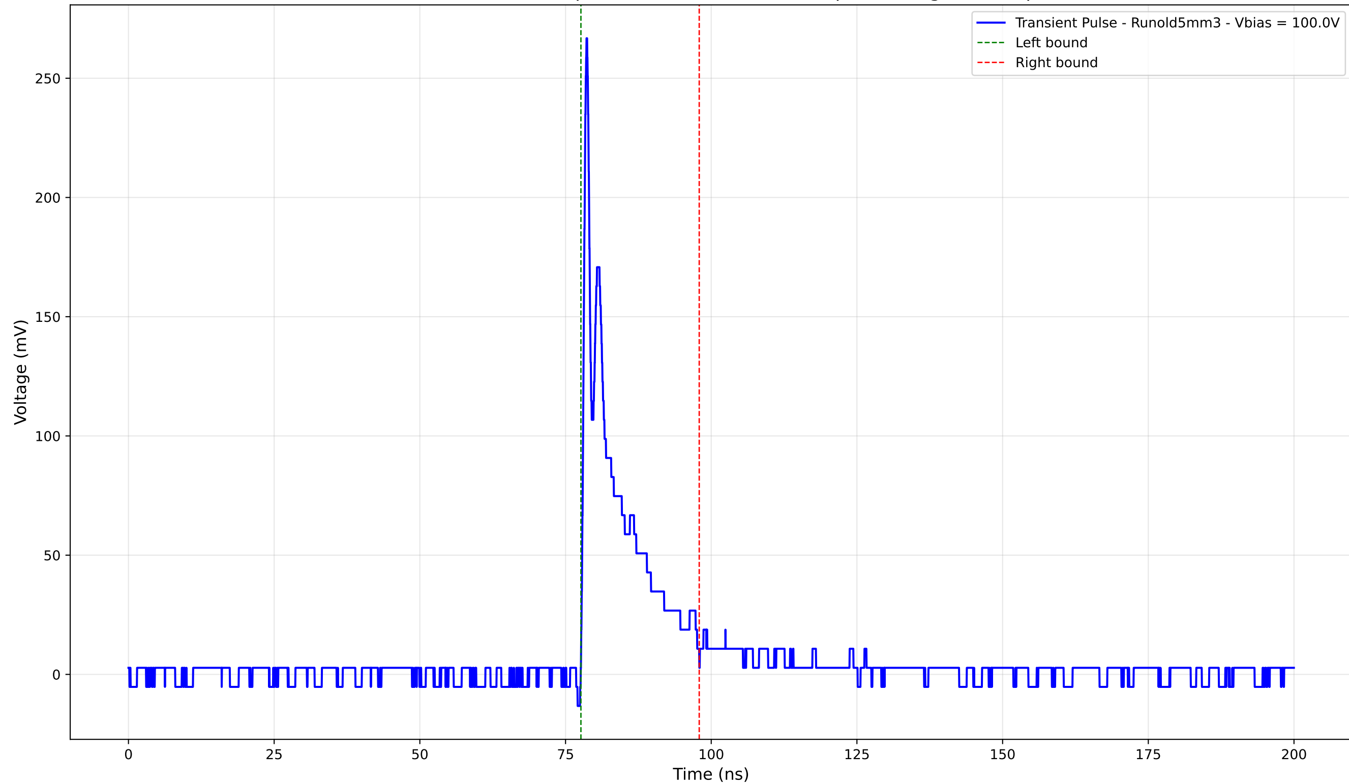
Transient Pulse - Sample: old5 - Position: 3530.0 \mu\text{m} - Charge: 27.06 pC
