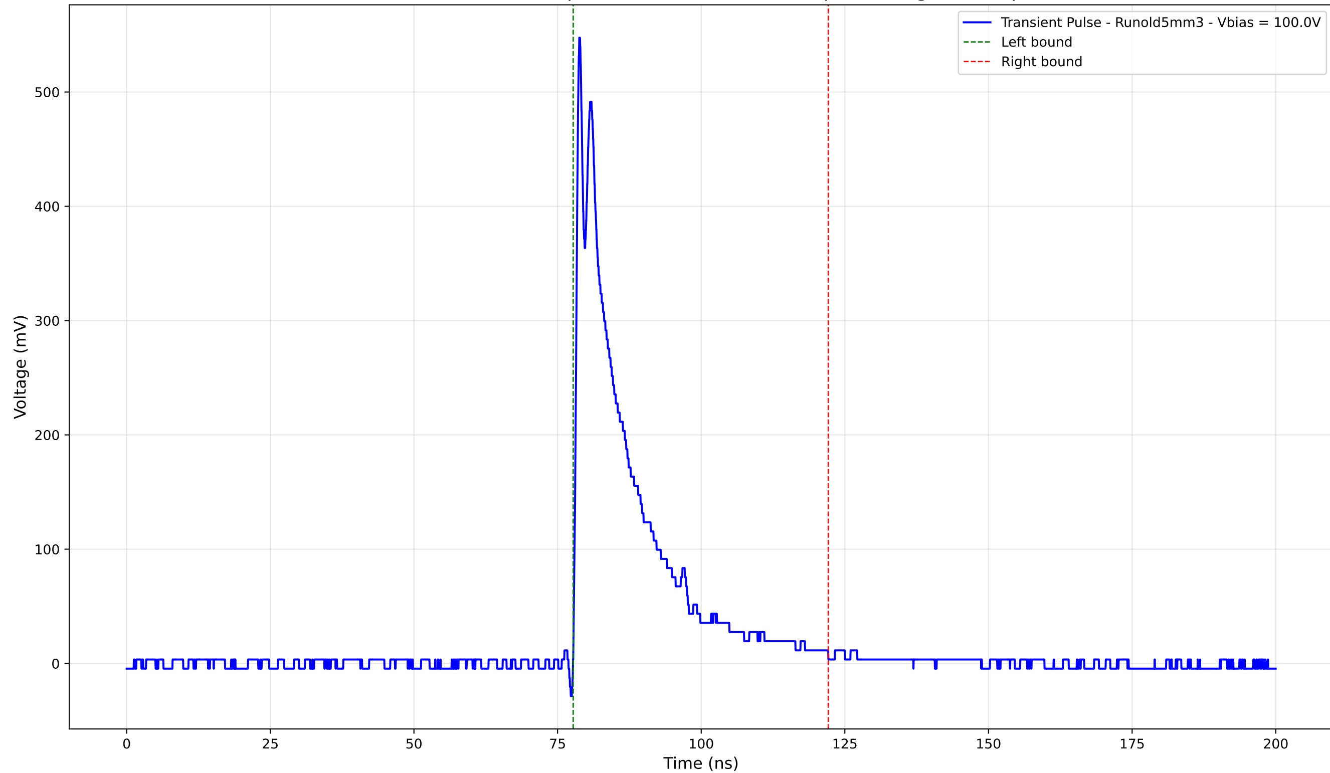
Transient Pulse - Sample: old5 - Position: 3785.0 \mu\text{m} - Charge: 96.05 pC
