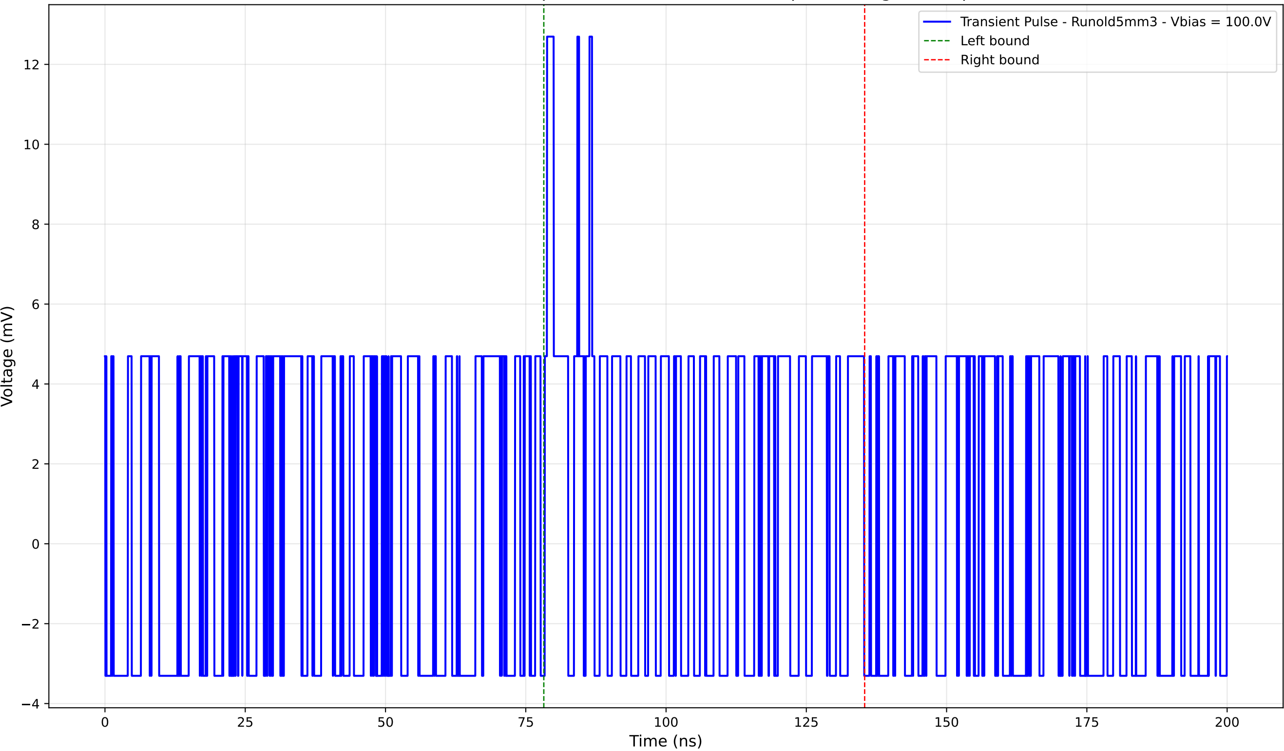
Transient Pulse - Sample: old5 - Position: 4975.0 \mu\text{m} - Charge: 2.18 pC
