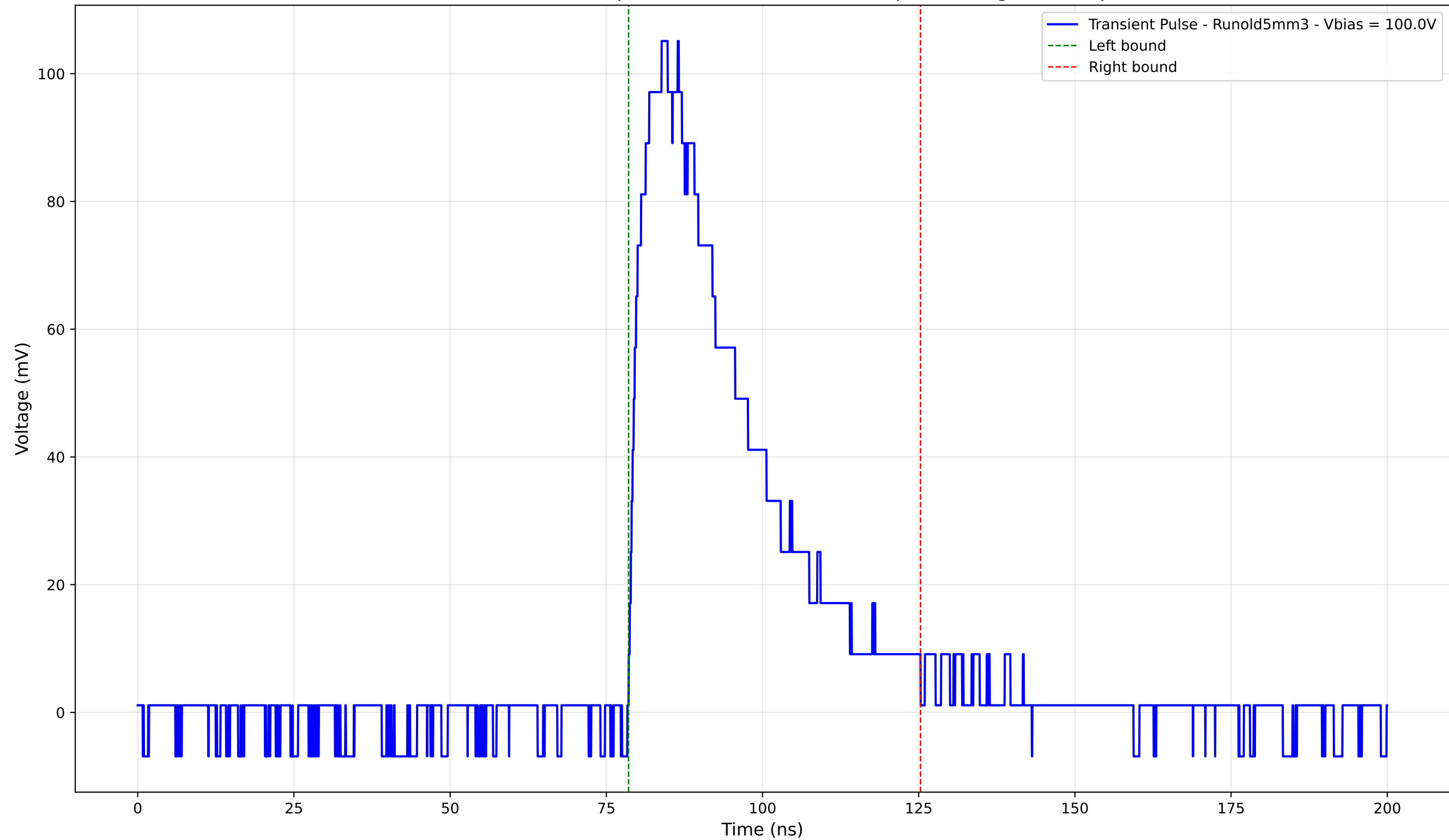
Transient Pulse - Sample: old5 - Position: 1830.0 \mu\text{m} - Charge: 39.29 pC
