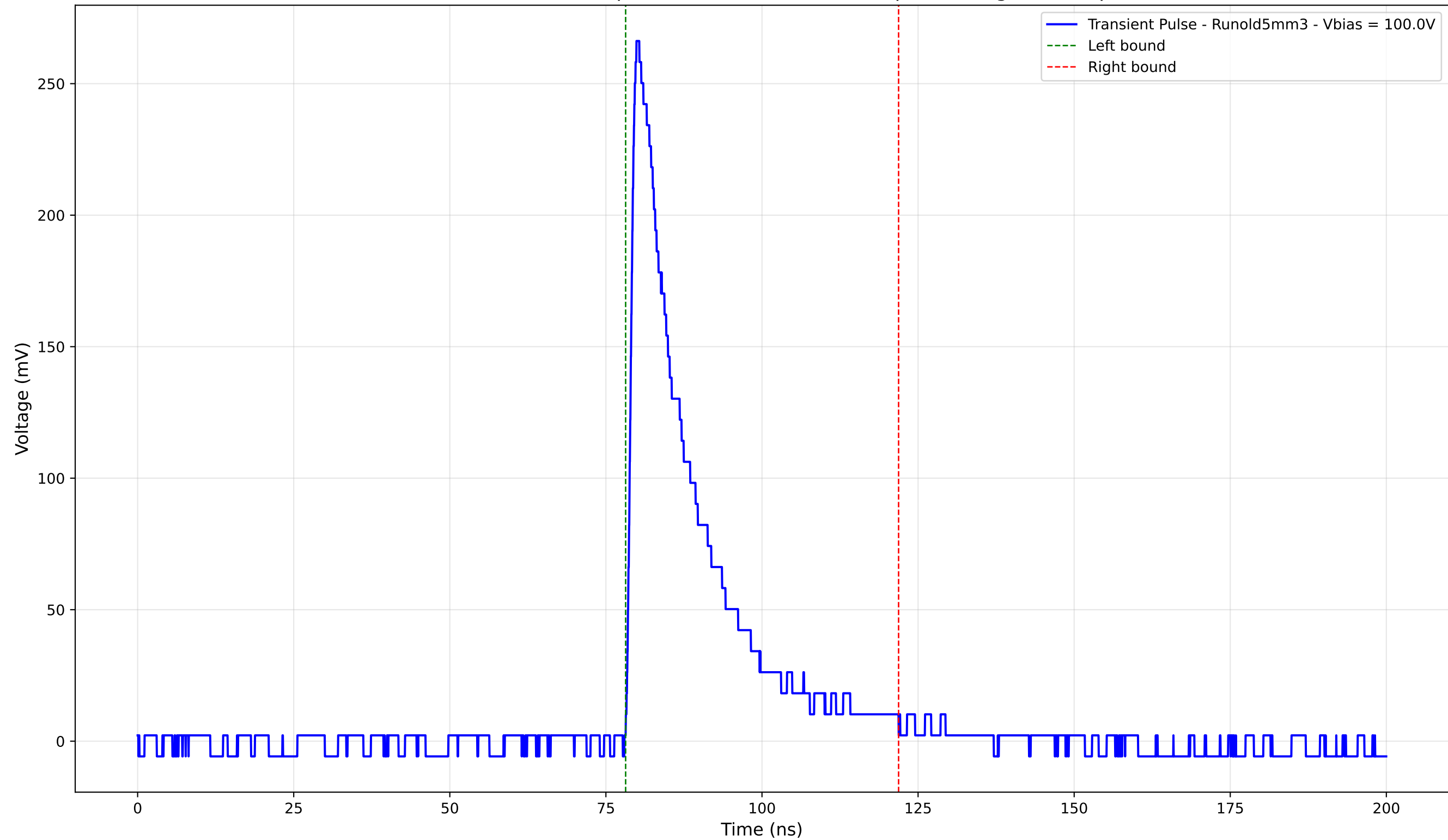
Transient Pulse - Sample: old5 - Position: 4425.0 \mu\text{m} - Charge: 55.66 pC
