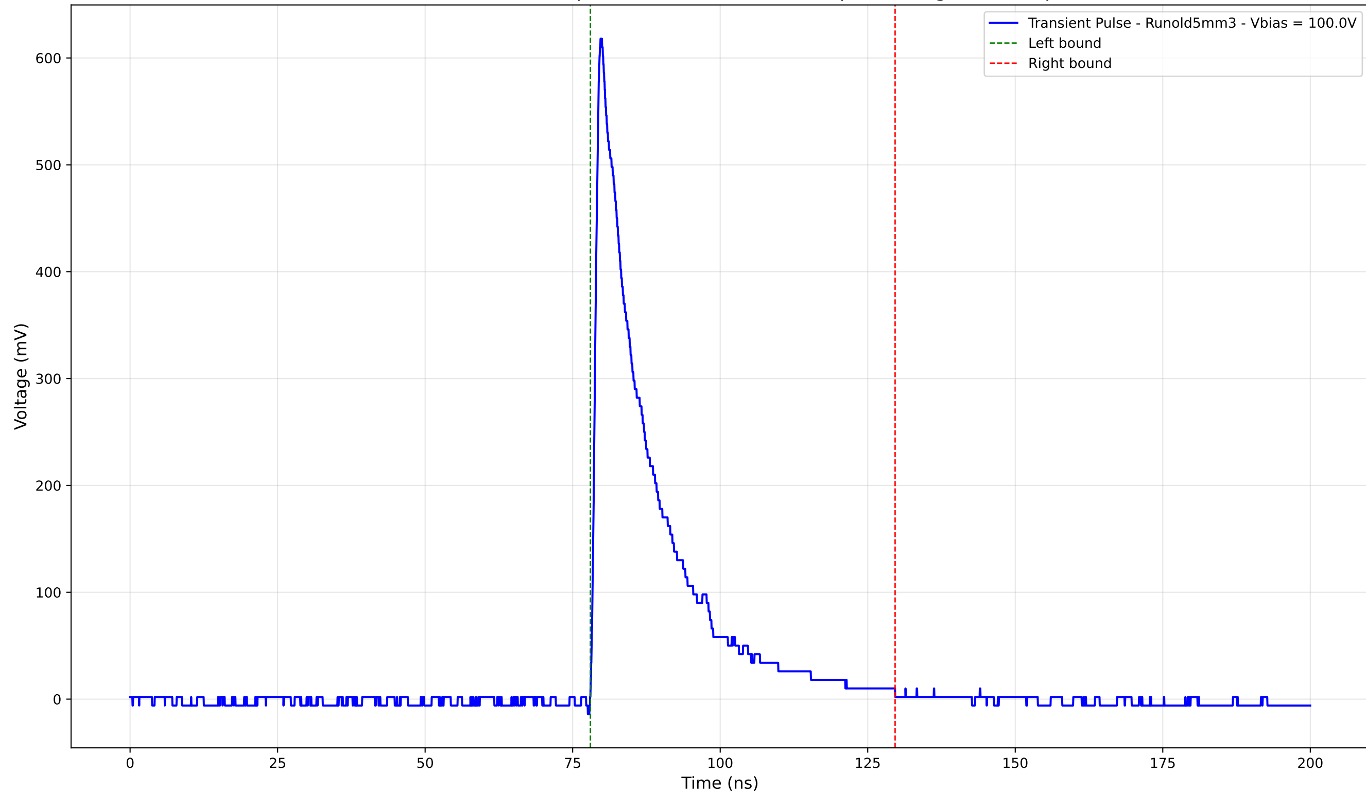
Transient Pulse - Sample: old5 - Position: 4620.0 \mu\text{m} - Charge: 121.64 pC
