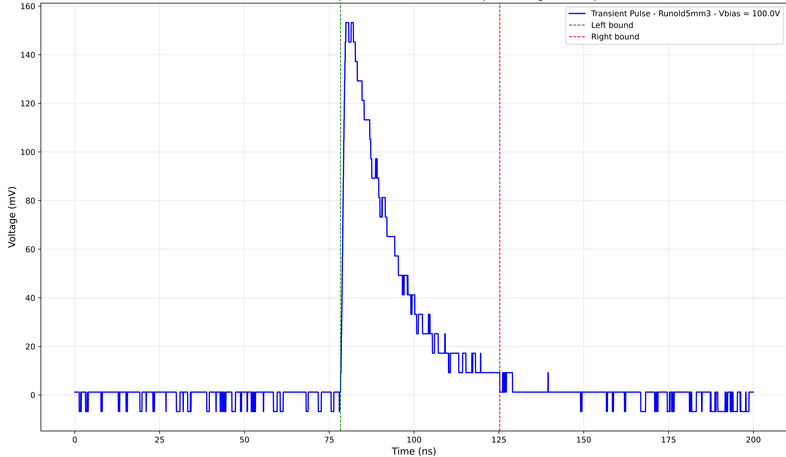
Transient Pulse - Sample: old5 - Position: 880.0 \mu\text{m} - Charge: 46.89 pC
