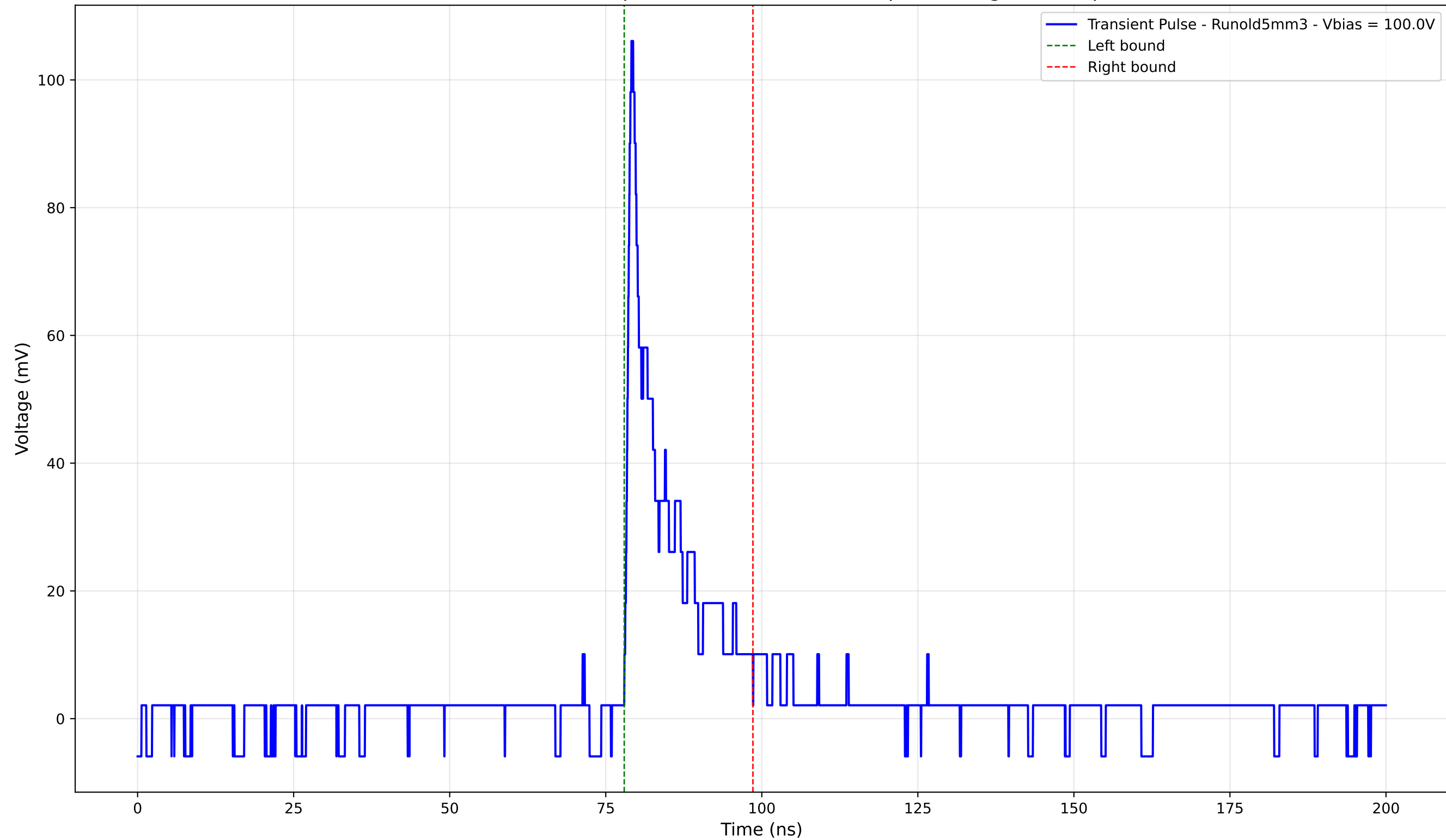
Transient Pulse - Sample: old5 - Position: 145.0 \mu\text{m} - Charge: 12.36 pC
