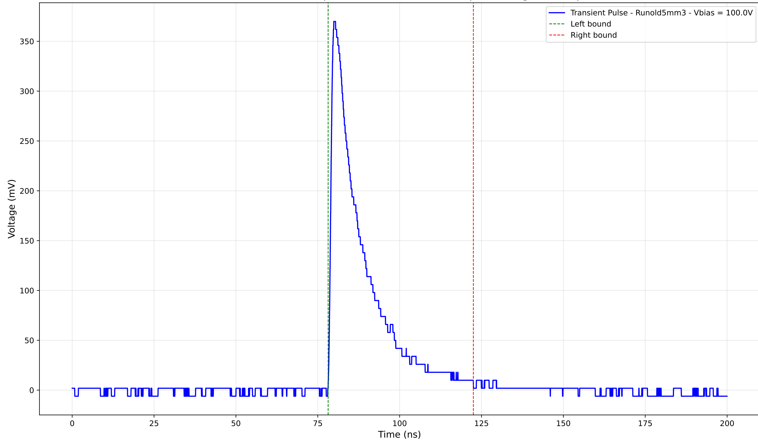
Transient Pulse - Sample: old5 - Position: 4410.0 \mu\text{m} - Charge: 78.11 pC
