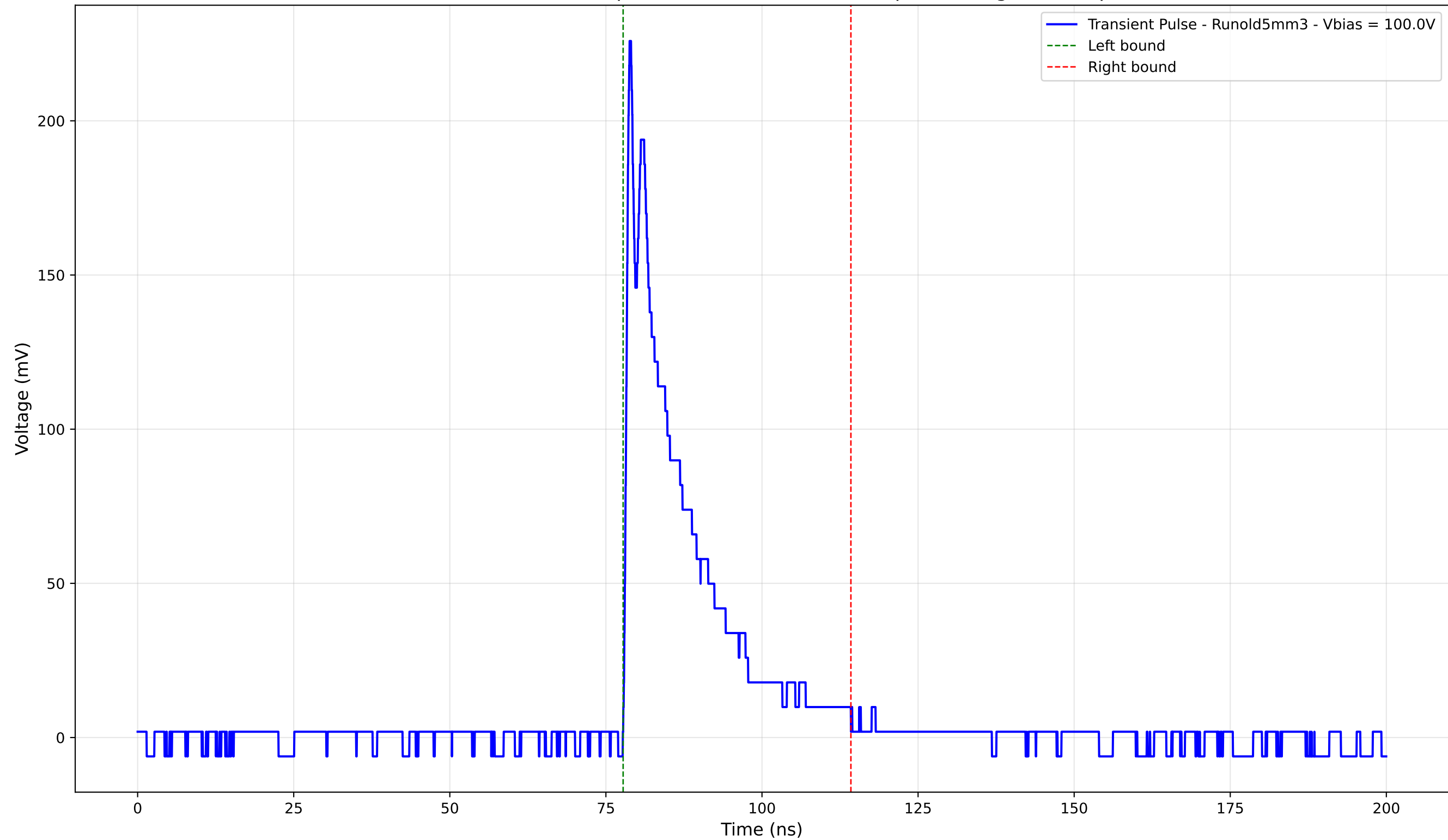
Transient Pulse - Sample: old5 - Position: 3340.0 \mu\text{m} - Charge: 39.57 pC
