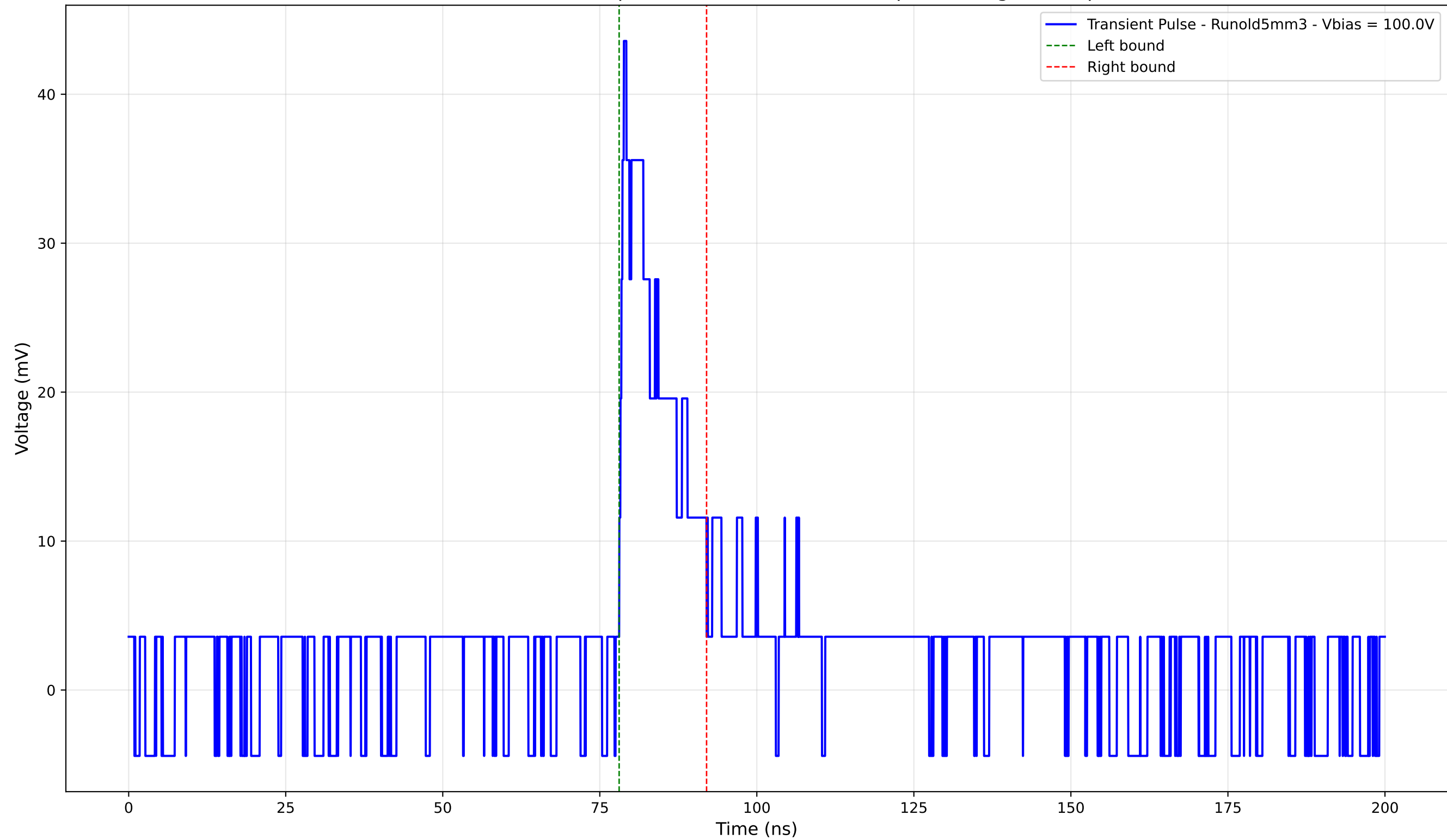
Transient Pulse - Sample: old5 - Position: 3865.0 \mu\text{m} - Charge: 6.14 pC
