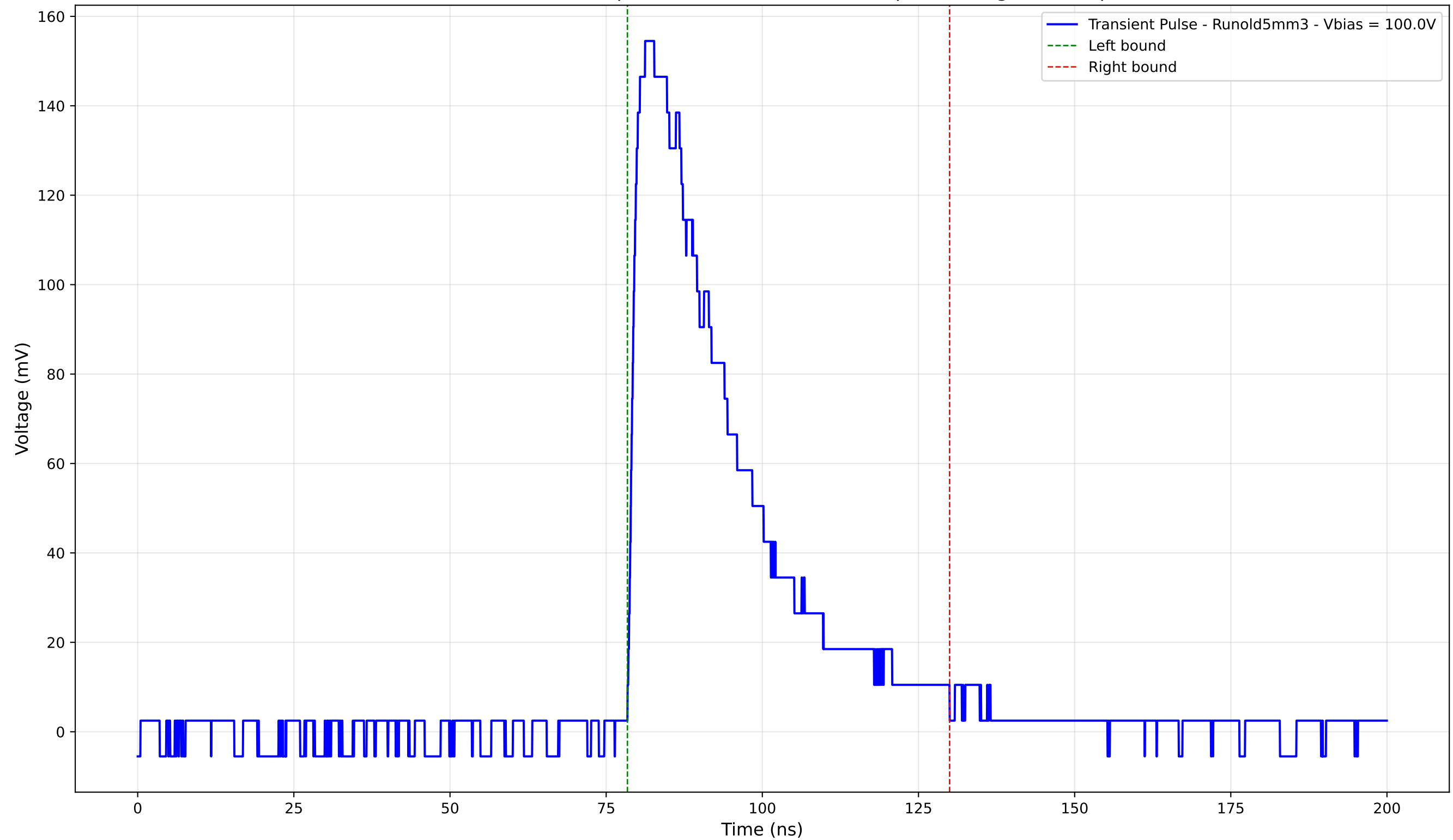
Transient Pulse - Sample: old5 - Position: 1125.0 \mu\text{m} - Charge: 55.39 pC
