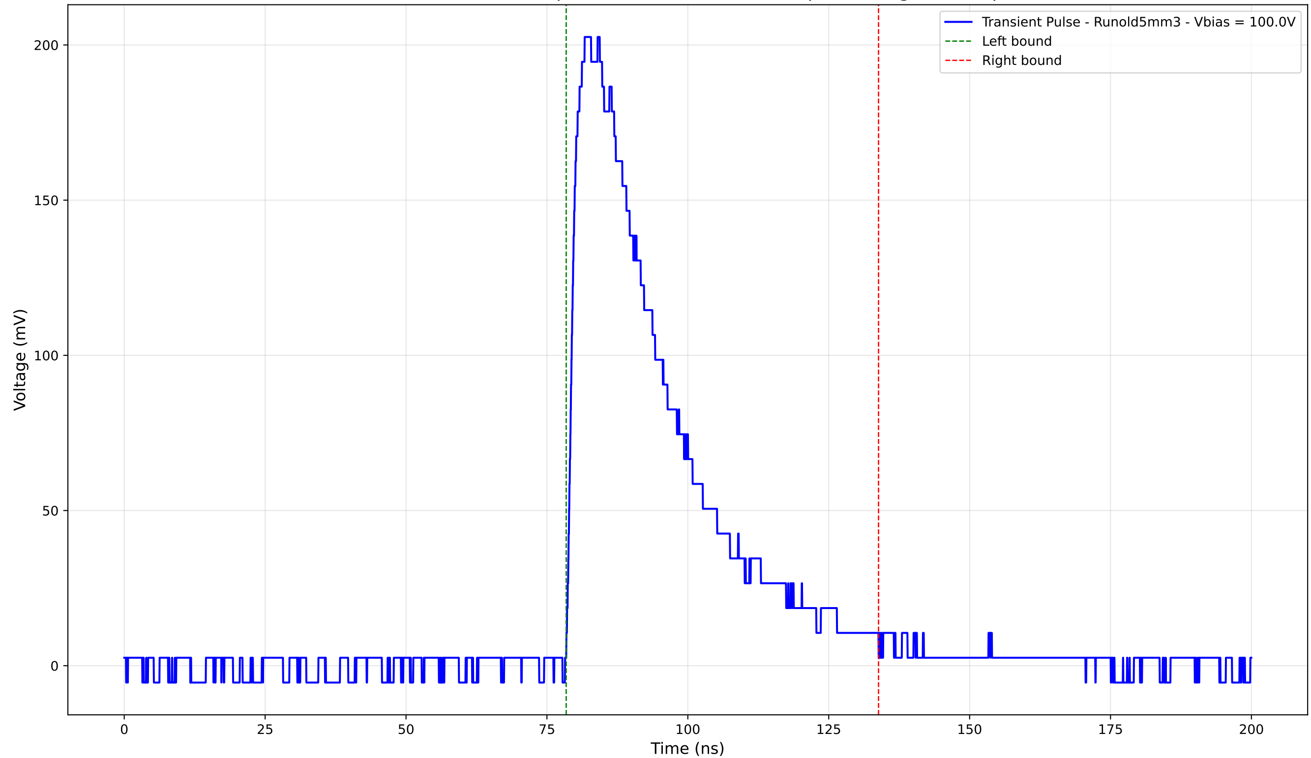
Transient Pulse - Sample: old5 - Position: 1305.0 \mu\text{m} - Charge: 77.06 pC
