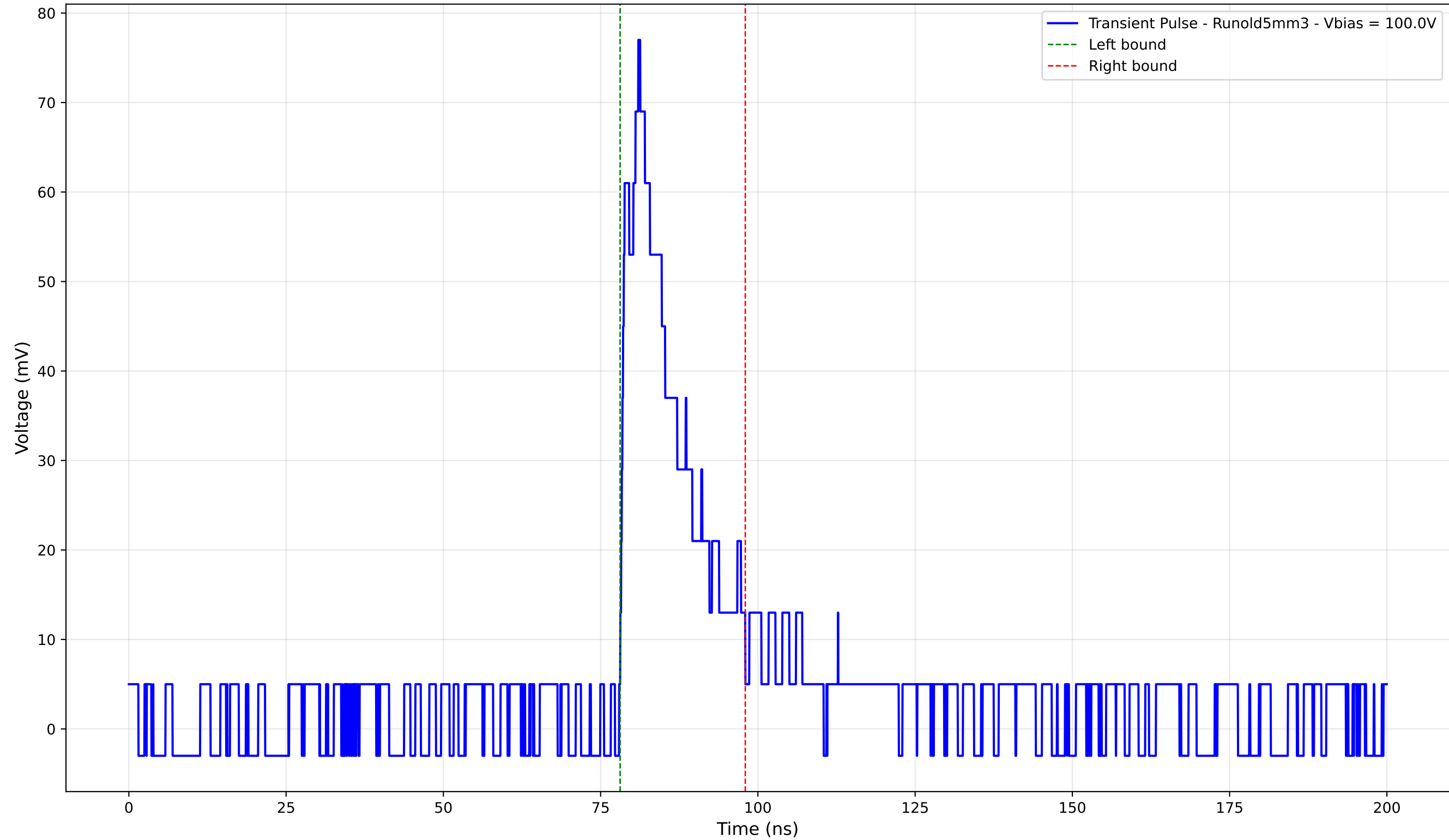
Transient Pulse - Sample: old5 - Position: 3920.0 \mu\text{m} - Charge: 13.79 pC
