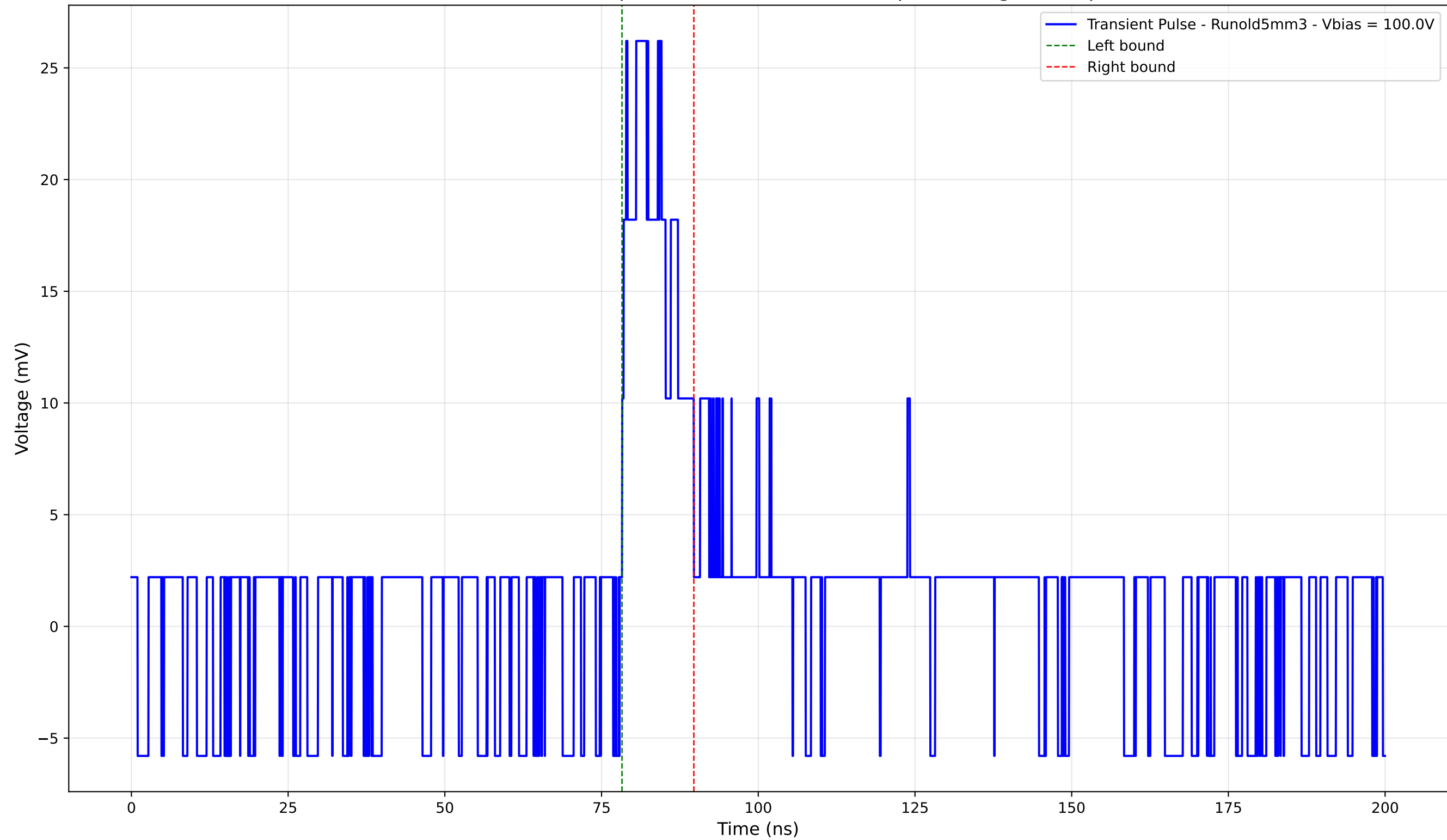
Transient Pulse - Sample: old5 - Position: 3290.0 \mu\text{m} - Charge: 3.98 pC
