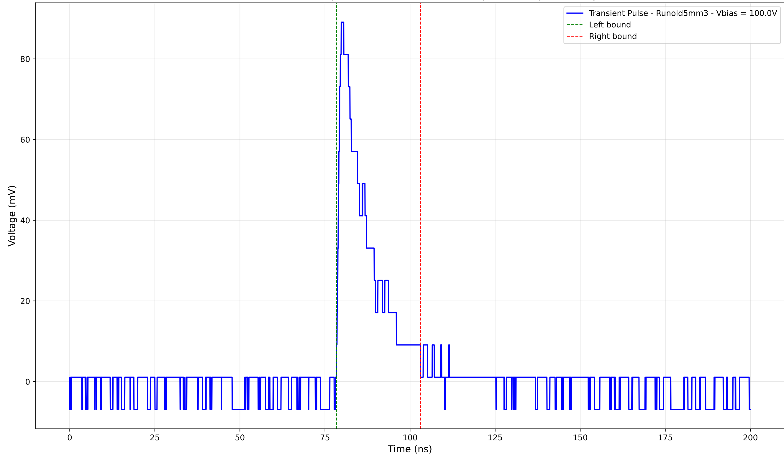
Transient Pulse - Sample: old5 - Position: 4455.0 \mu\text{m} - Charge: 16.01 pC
