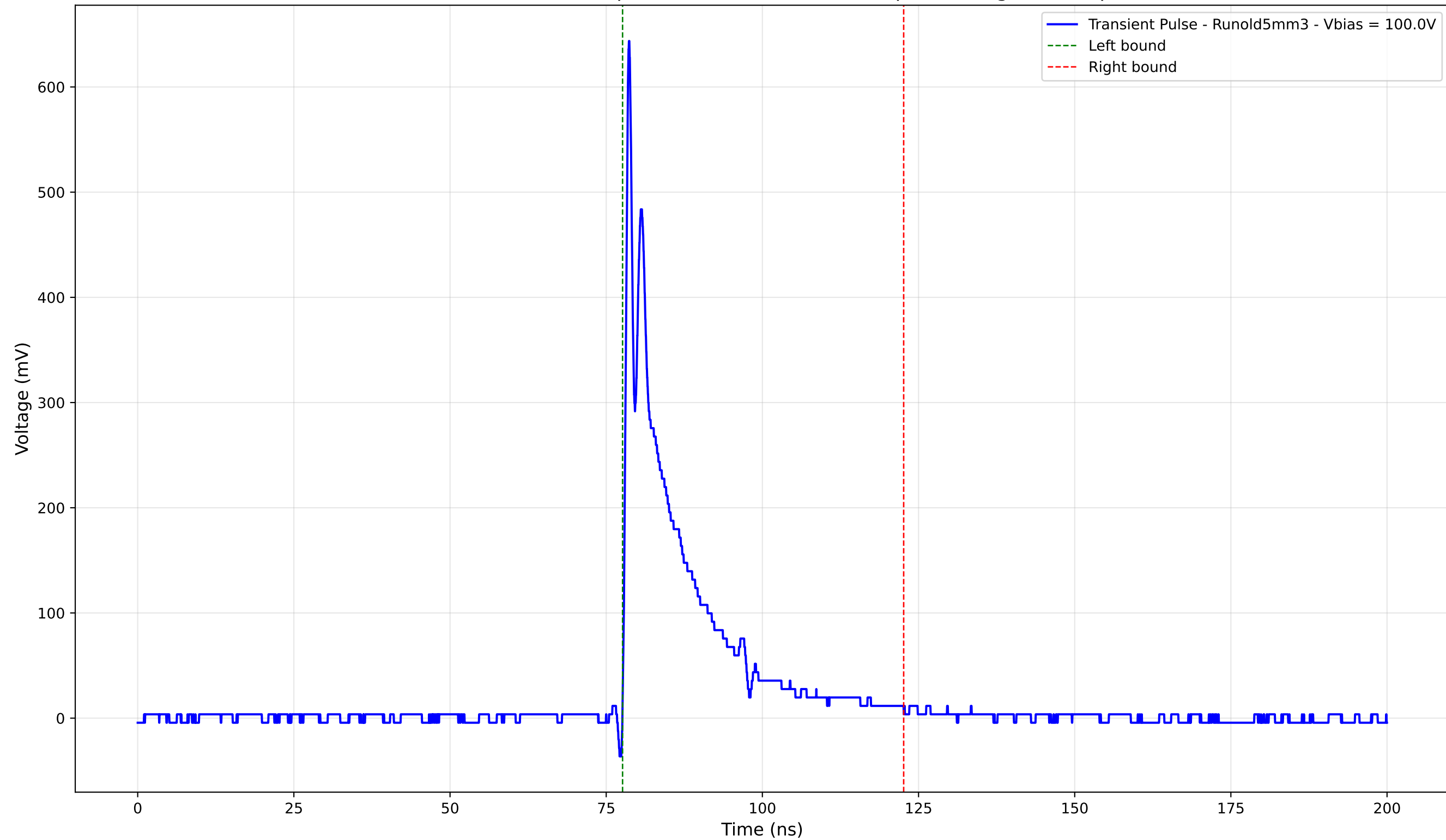
Transient Pulse - Sample: old5 - Position: 3675.0 \mu\text{m} - Charge: 87.89 pC
