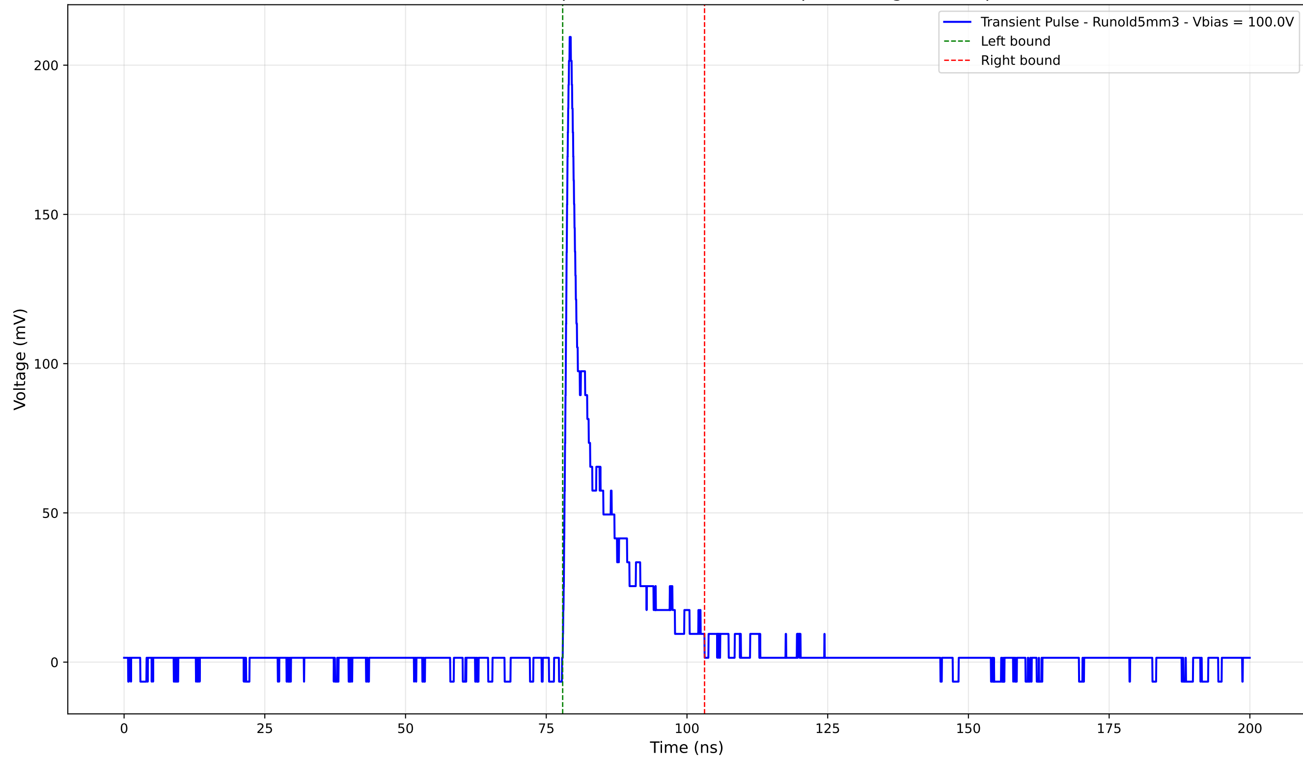
Transient Pulse - Sample: old5 - Position: 160.0 \mu\text{m} - Charge: 23.18 pC
