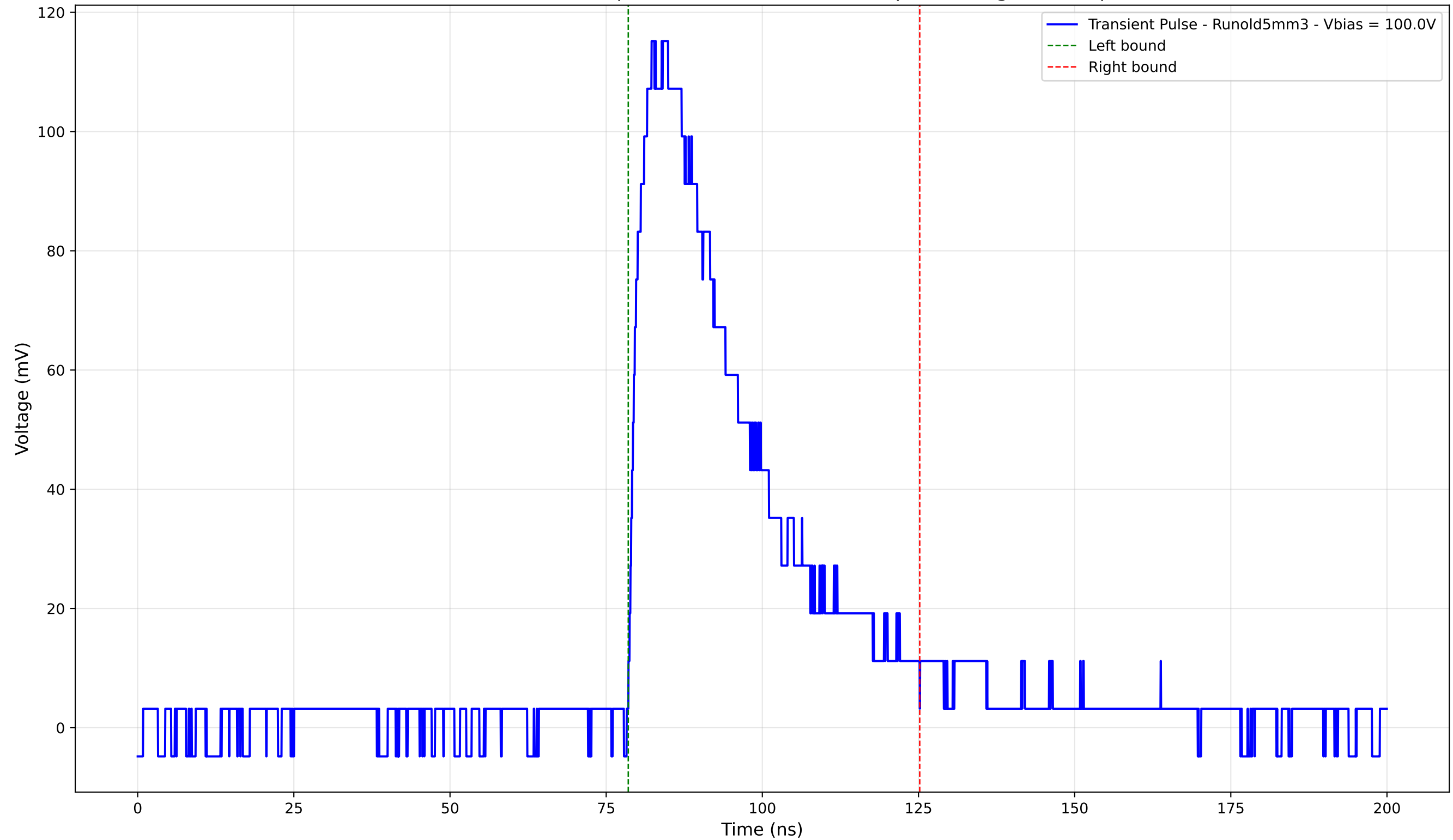
Transient Pulse - Sample: old5 - Position: 1630.0 \mu\text{m} - Charge: 44.74 pC
