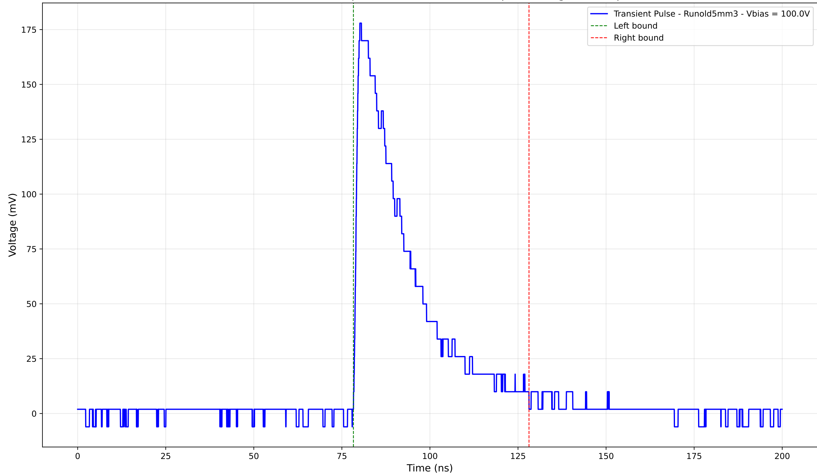
Transient Pulse - Sample: old5 - Position: 940.0 \mu\text{m} - Charge: 57.04 pC
