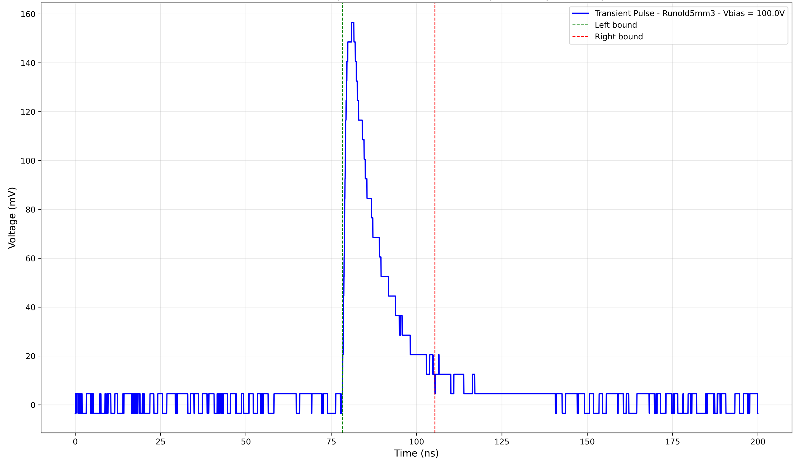
Transient Pulse - Sample: old5 - Position: 4235.0 \mu\text{m} - Charge: 32.87 pC
