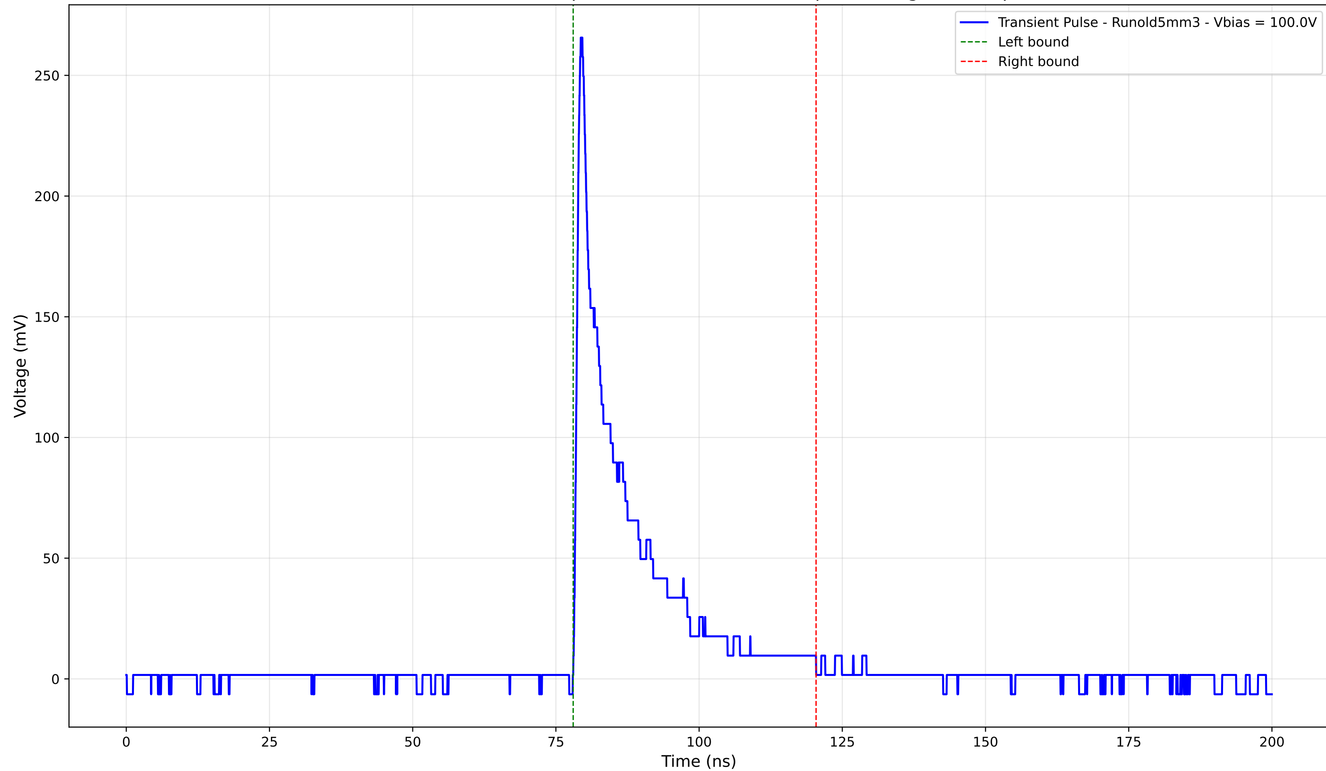
Transient Pulse - Sample: old5 - Position: 310.0 \mu\text{m} - Charge: 40.41 pC
