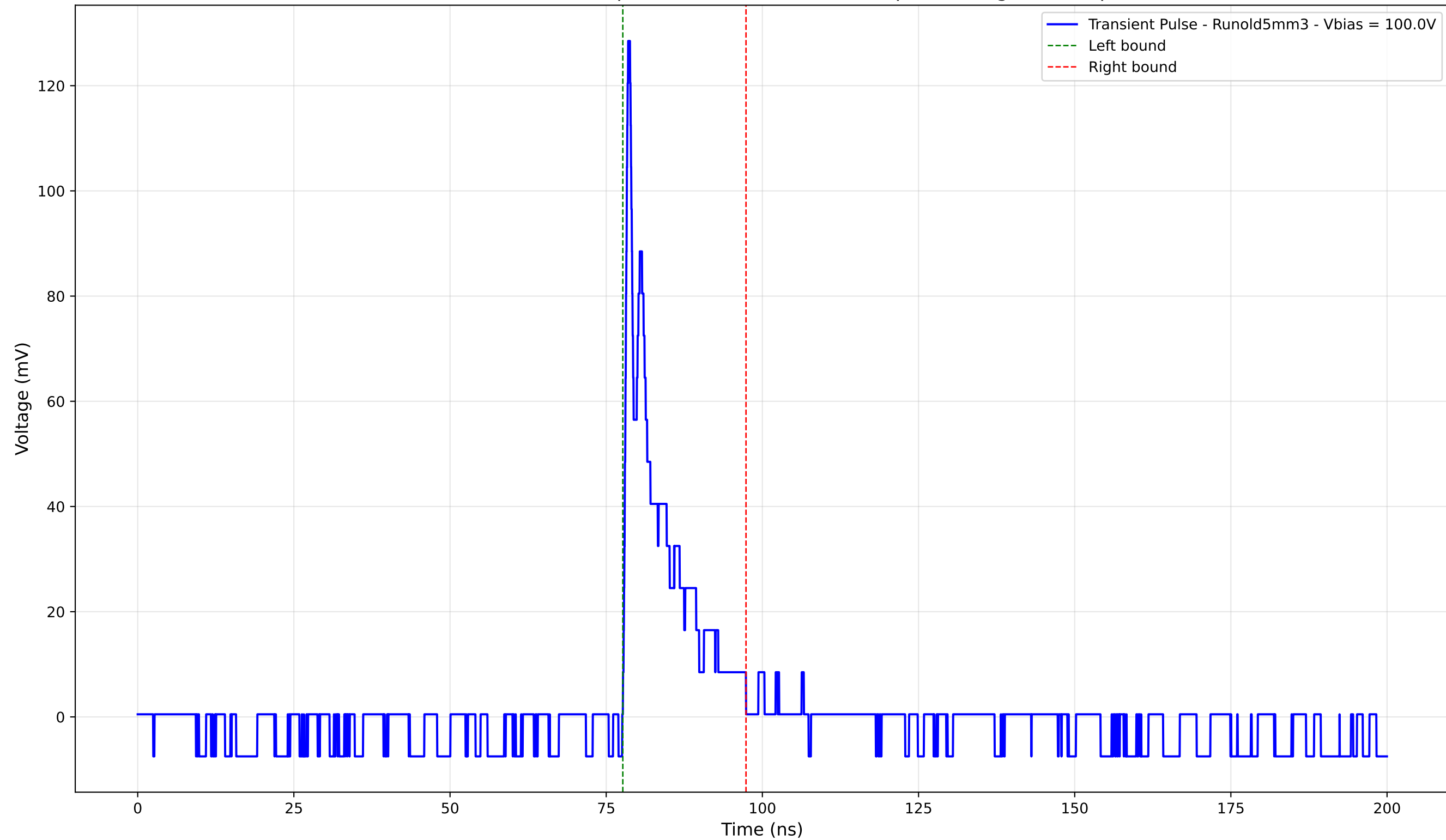
Transient Pulse - Sample: old5 - Position: 3545.0 \mu\text{m} - Charge: 12.81 pC
