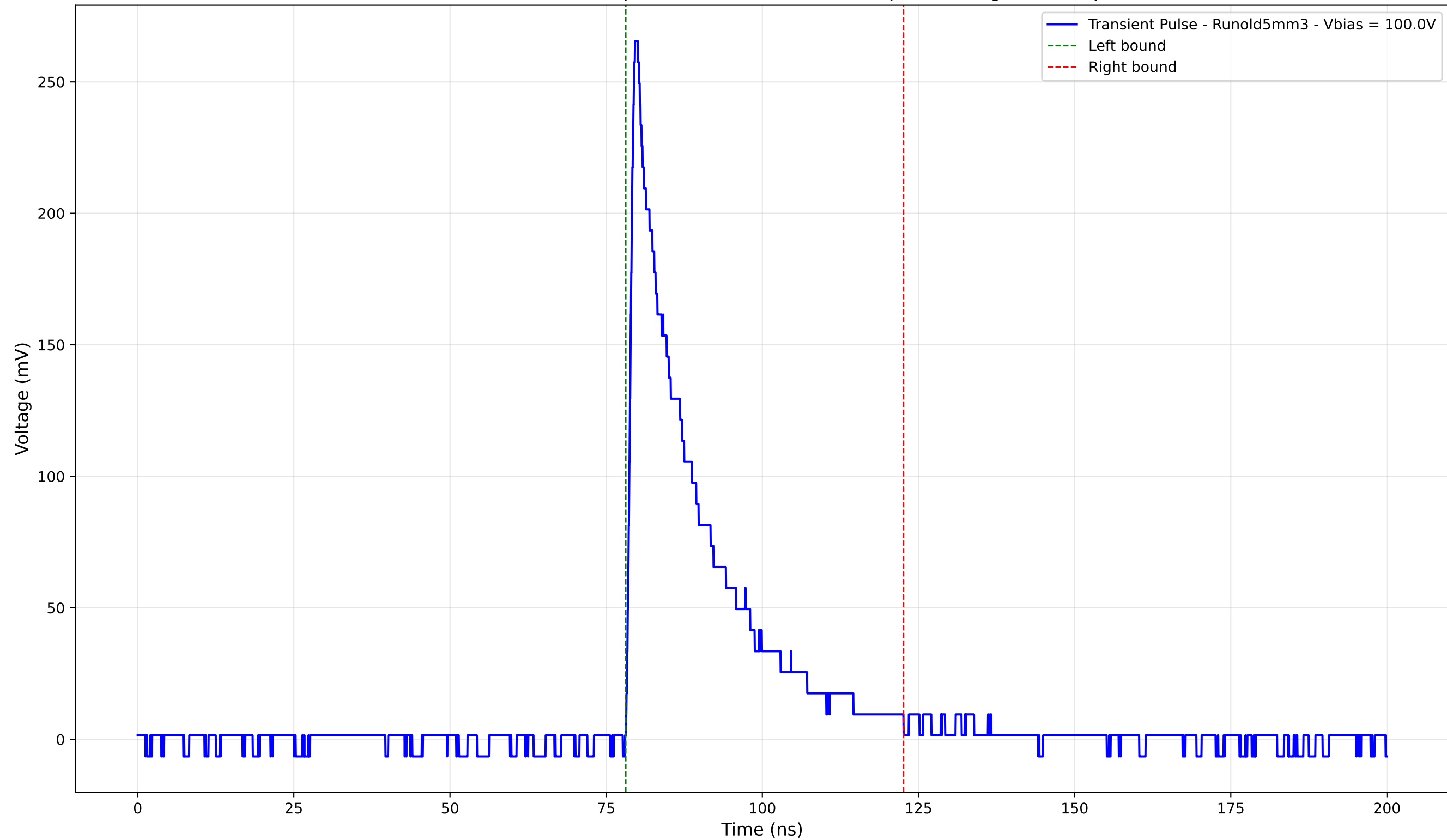
Transient Pulse - Sample: old5 - Position: 555.0 \mu\text{m} - Charge: 56.17 pC
