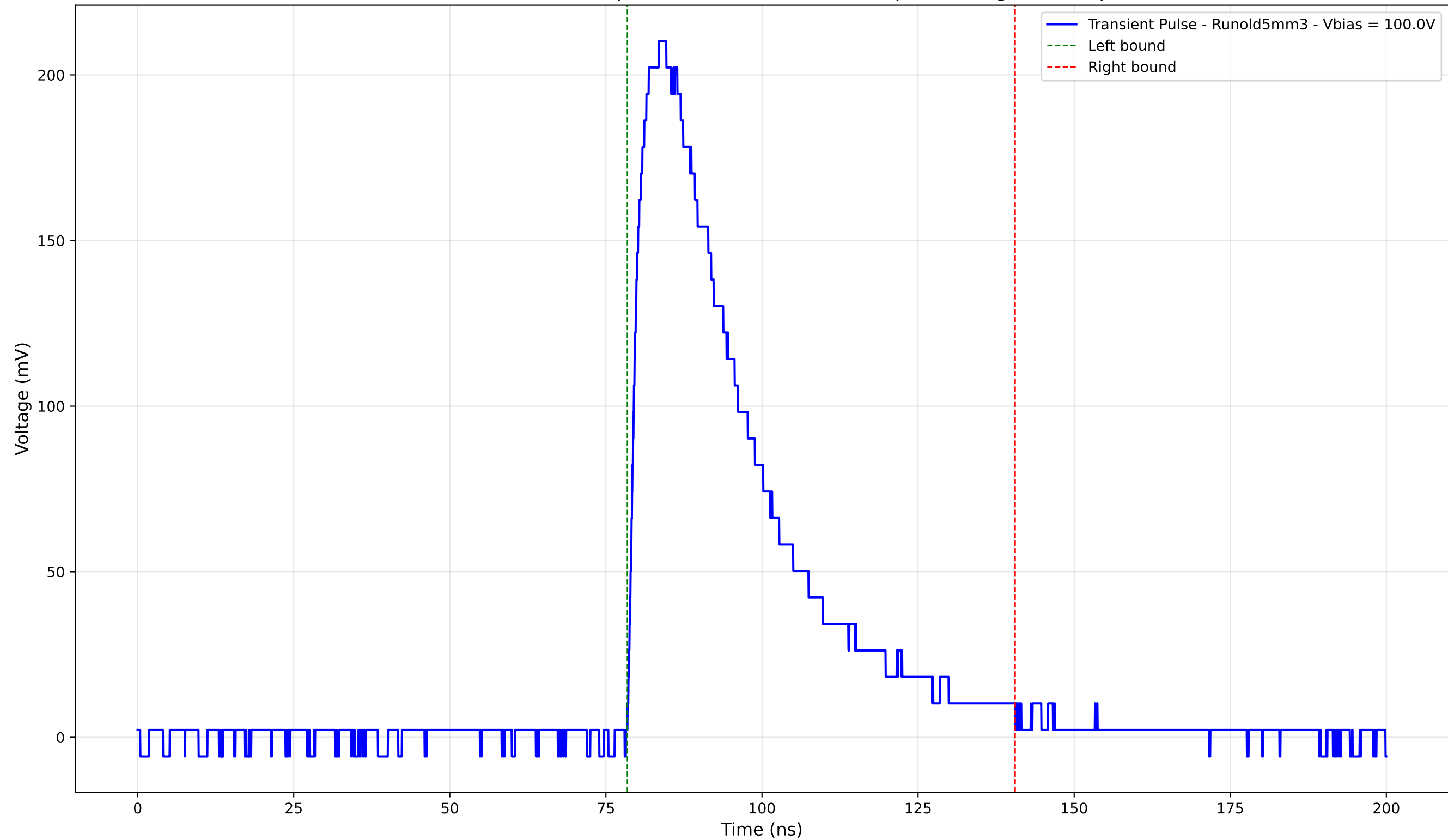
Transient Pulse - Sample: old5 - Position: 1680.0 \mu\text{m} - Charge: 85.98 pC
