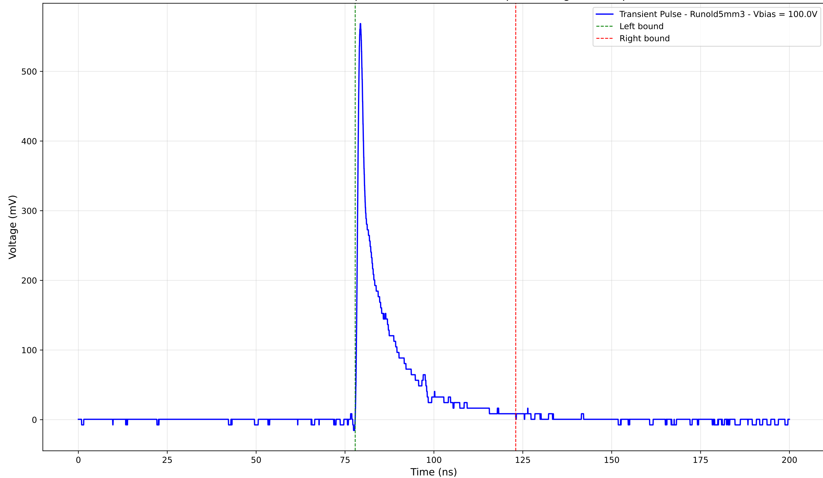
Transient Pulse - Sample: old5 - Position: 235.0 \mu\text{m} - Charge: 73.80 pC
