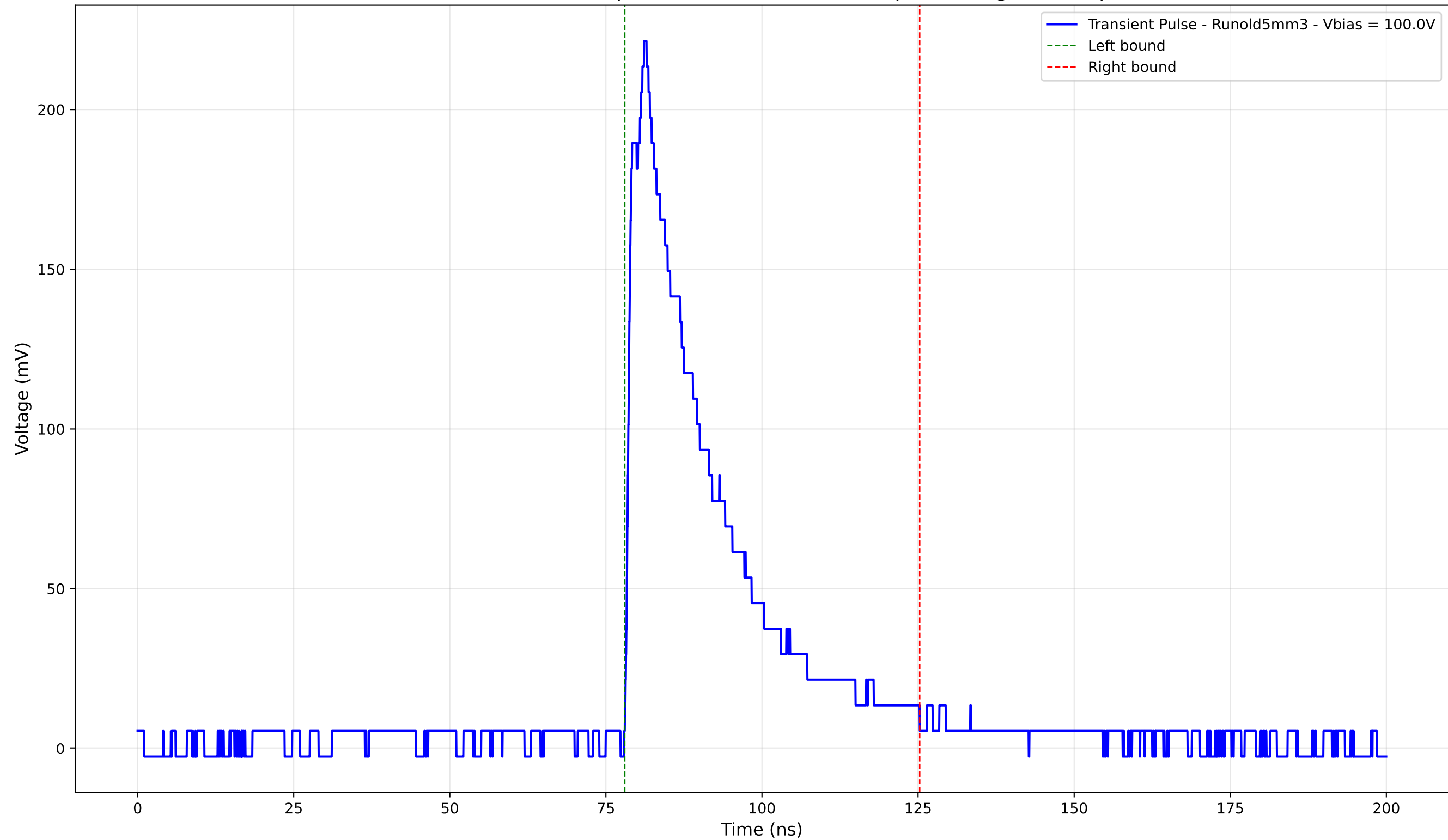
Transient Pulse - Sample: old5 - Position: 3050.0 \mu\text{m} - Charge: 61.49 pC
