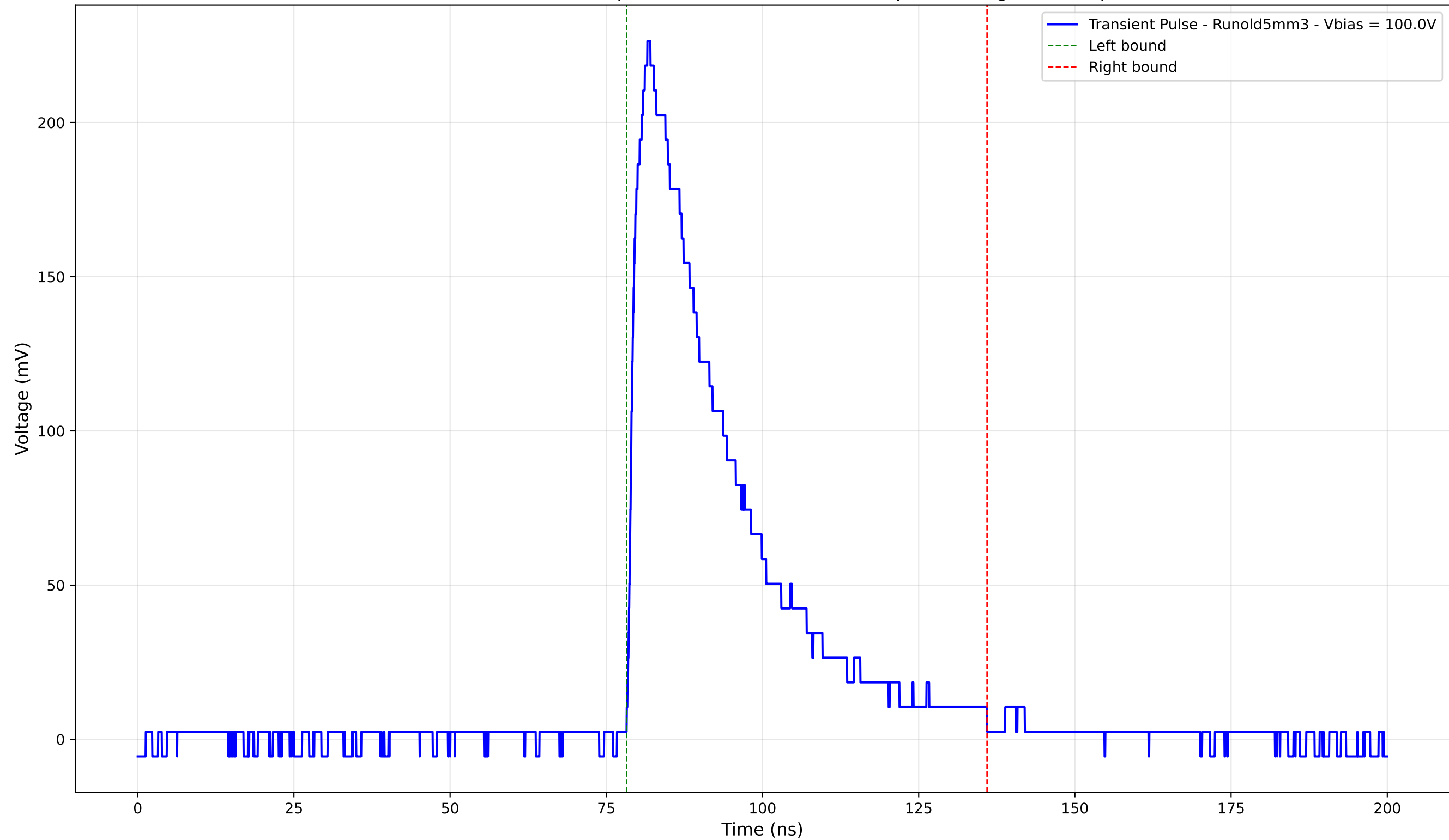
Transient Pulse - Sample: old5 - Position: 2760.0 \mu\text{m} - Charge: 75.25 pC
