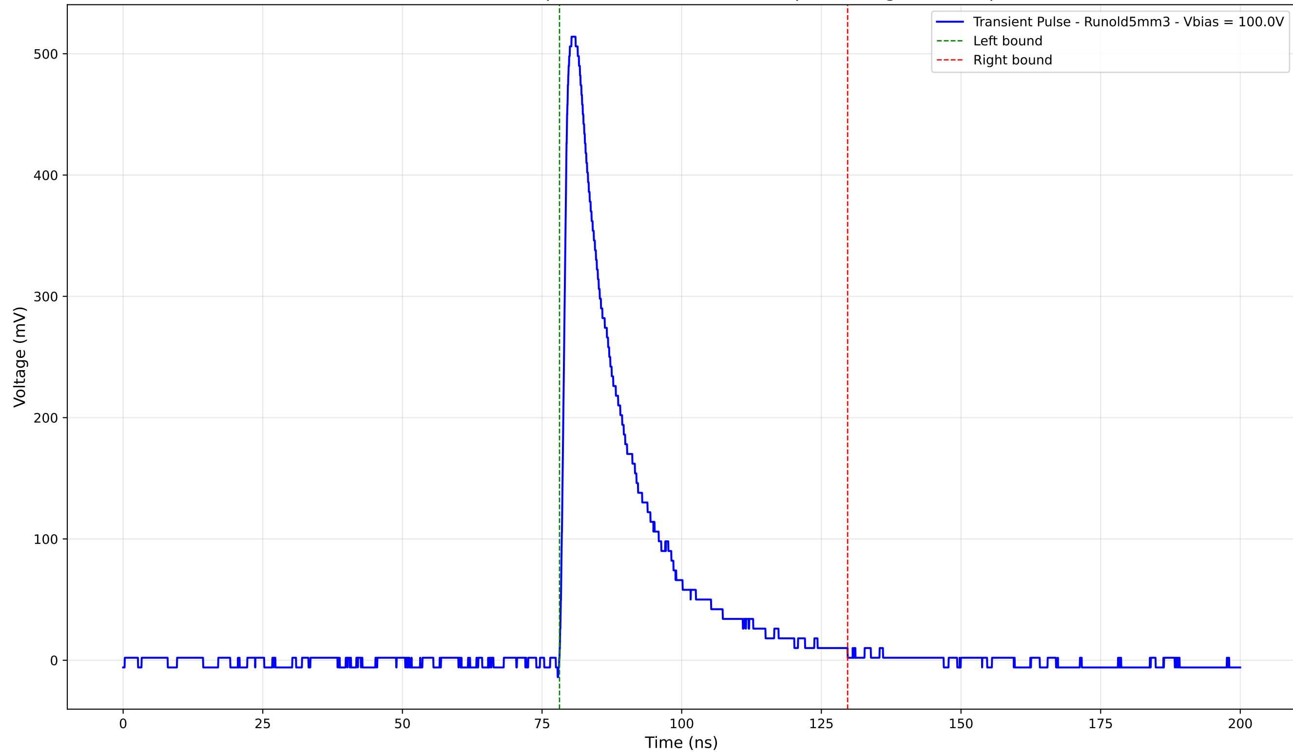
Transient Pulse - Sample: old5 - Position: 4325.0 \mu\text{m} - Charge: 117.99 pC
