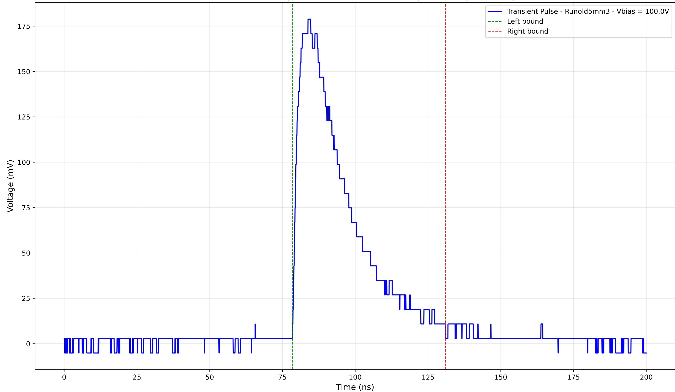
Transient Pulse - Sample: old5 - Position: 1655.0 \mu\text{m} - Charge: 70.96 pC
