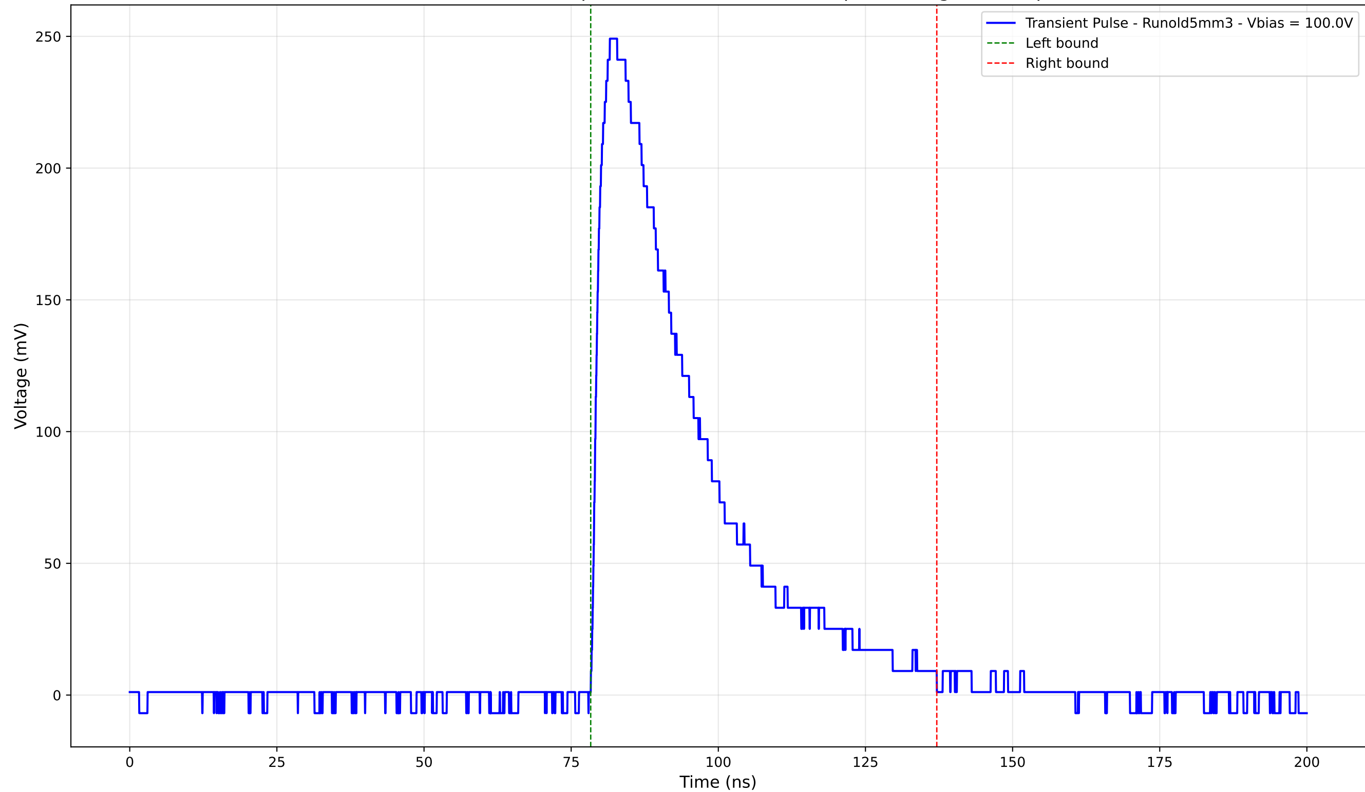
Transient Pulse - Sample: old5 - Position: 2565.0 \mu\text{m} - Charge: 92.71 pC
