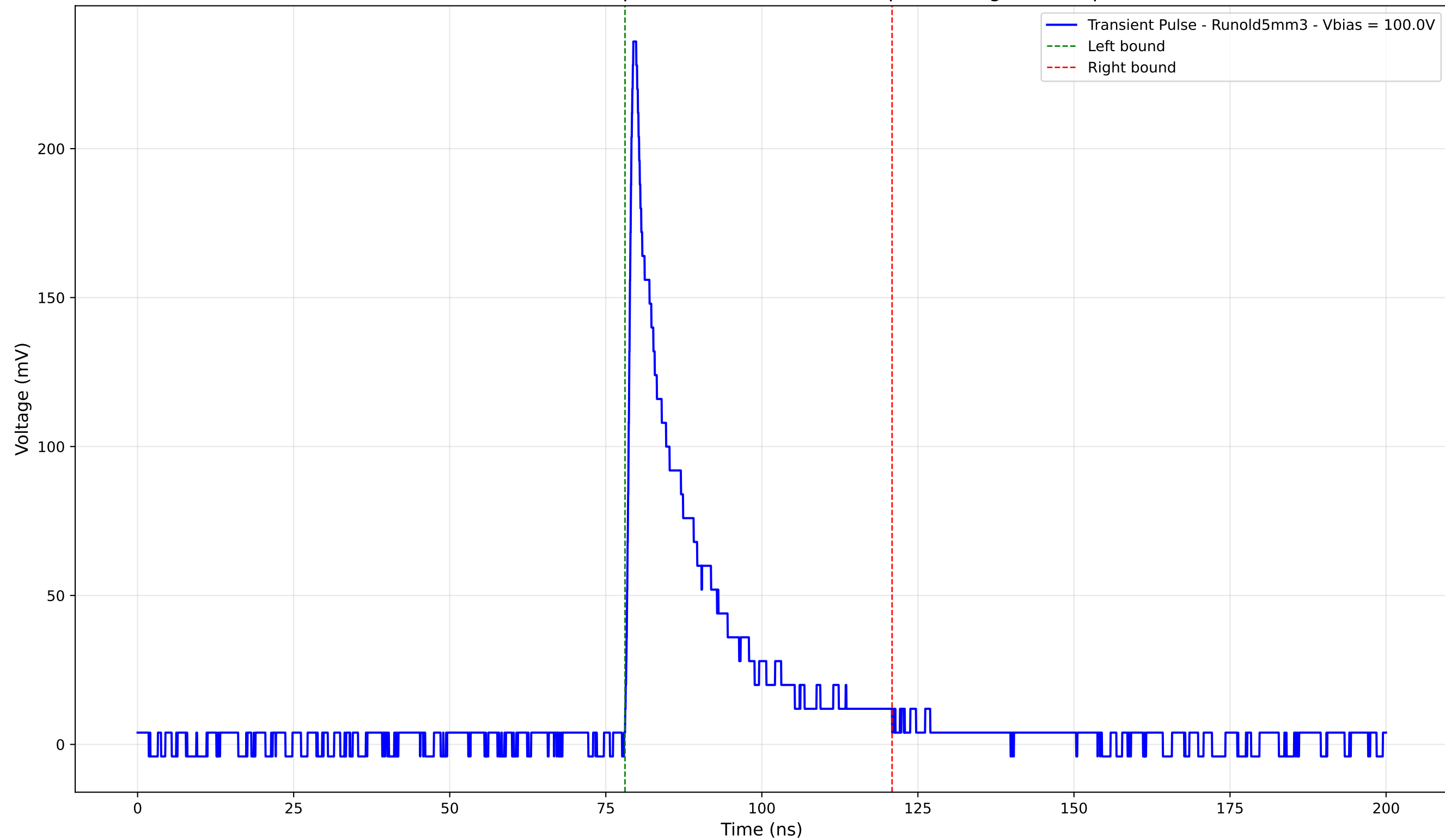
Transient Pulse - Sample: old5 - Position: 415.0 \mu\text{m} - Charge: 42.91 pC
