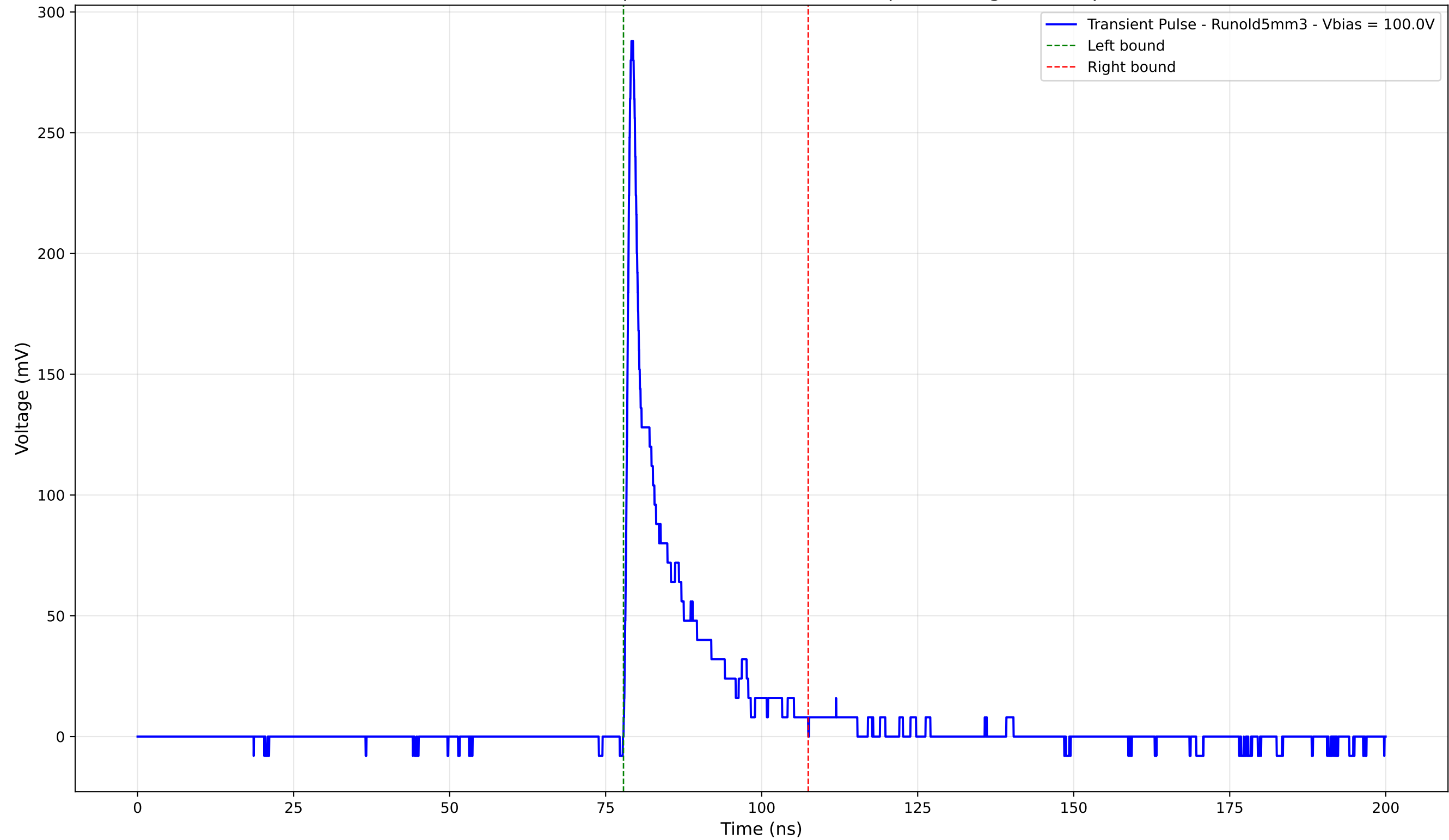
Transient Pulse - Sample: old5 - Position: 170.0 \mu\text{m} - Charge: 32.22 pC
