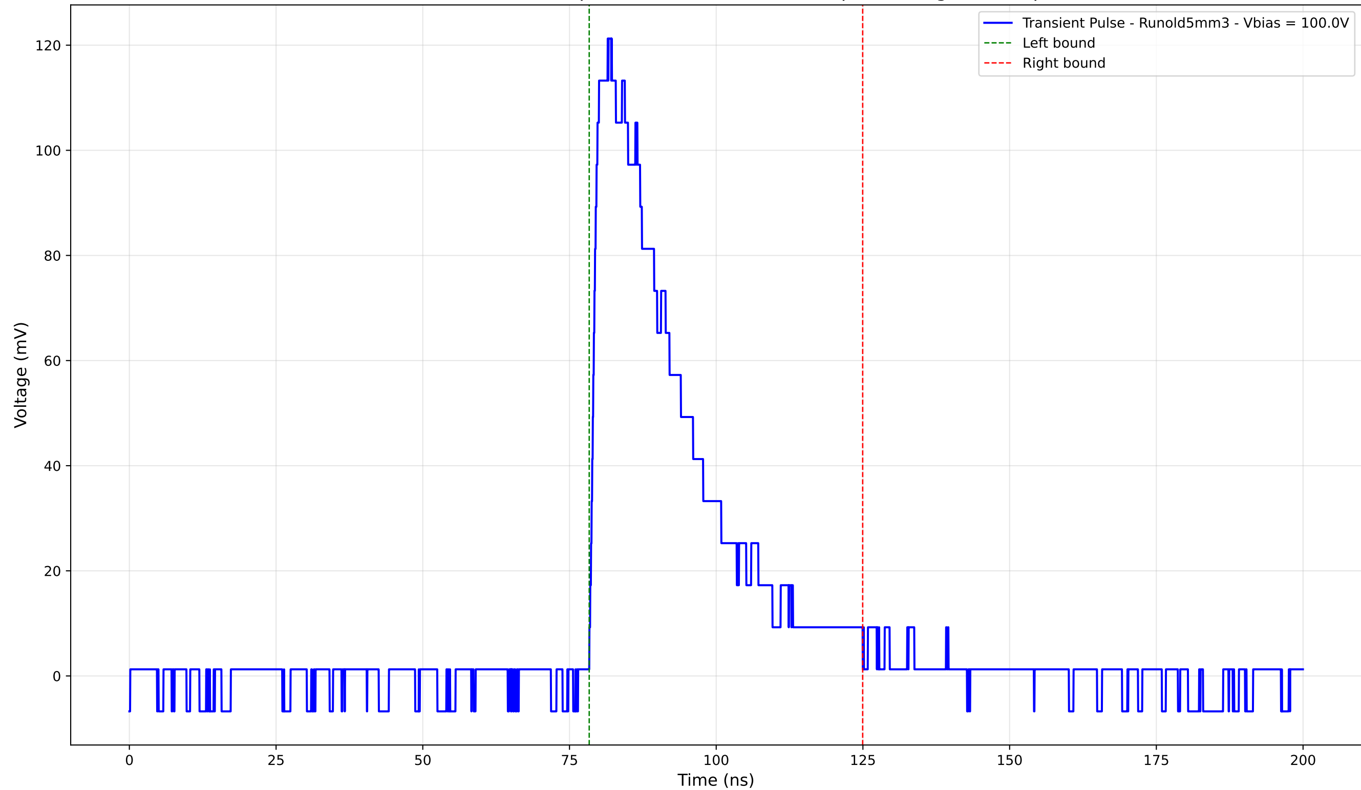
Transient Pulse - Sample: old5 - Position: 1010.0 \mu\text{m} - Charge: 39.46 pC
