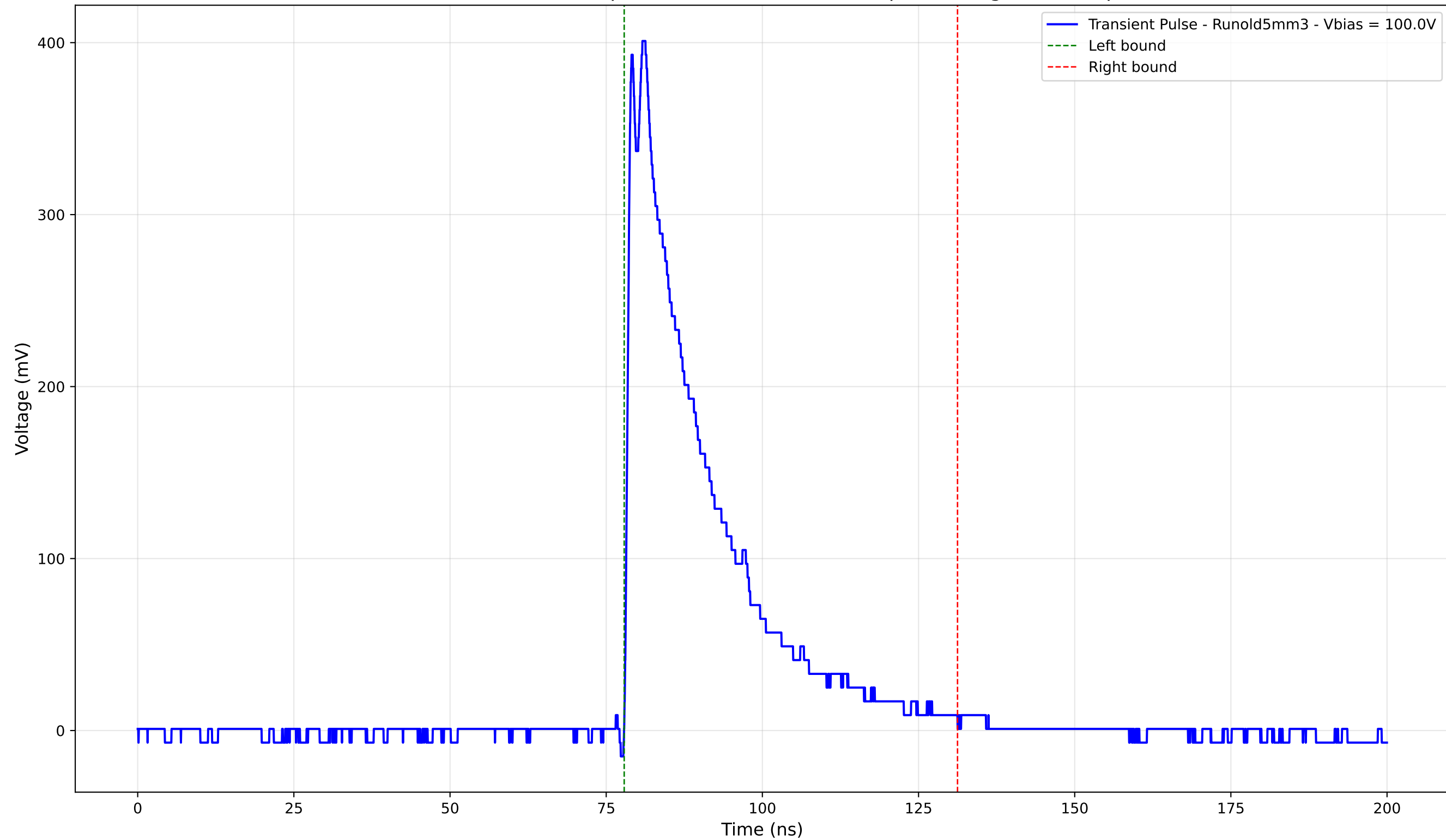
Transient Pulse - Sample: old5 - Position: 3140.0 \mu\text{m} - Charge: 104.89 pC
