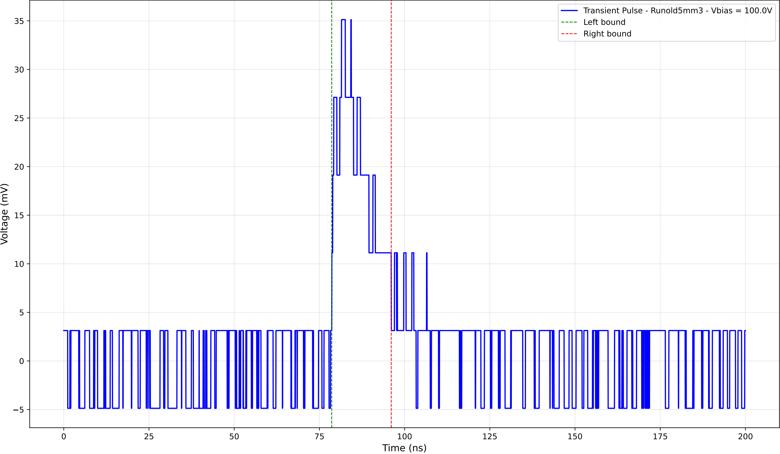
Transient Pulse - Sample: old5 - Position: 4195.0 \mu\text{m} - Charge: 6.85 pC
