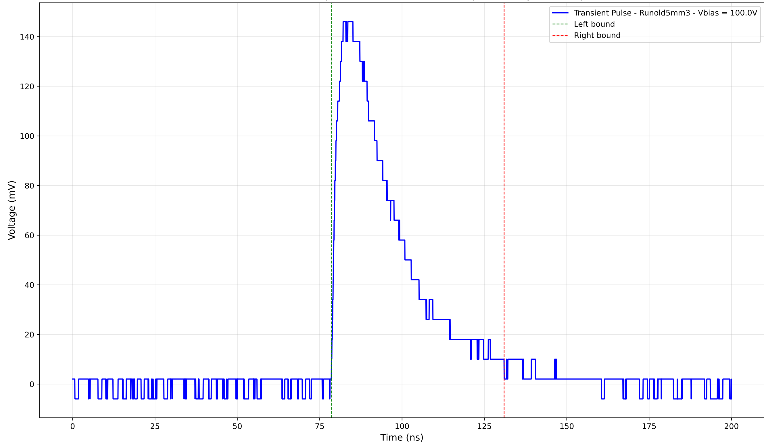
Transient Pulse - Sample: old5 - Position: 1845.0 \mu\text{m} - Charge: 59.69 pC
