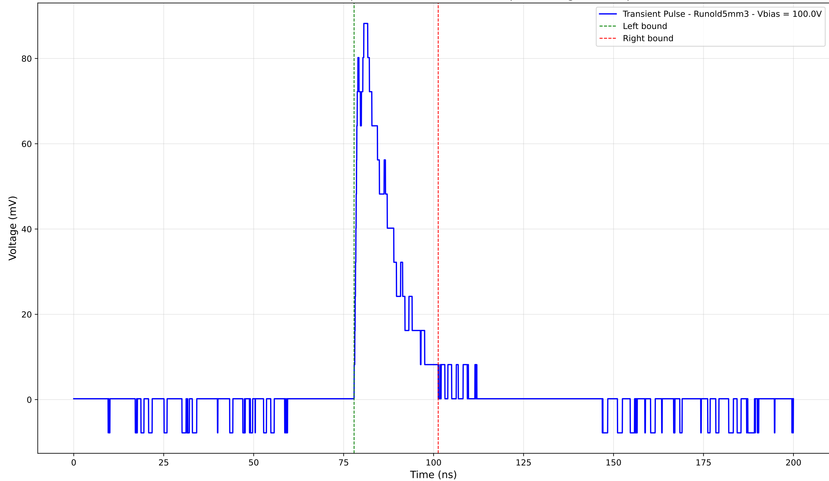
Transient Pulse - Sample: old5 - Position: 3925.0 \mu\text{m} - Charge: 17.37 pC
