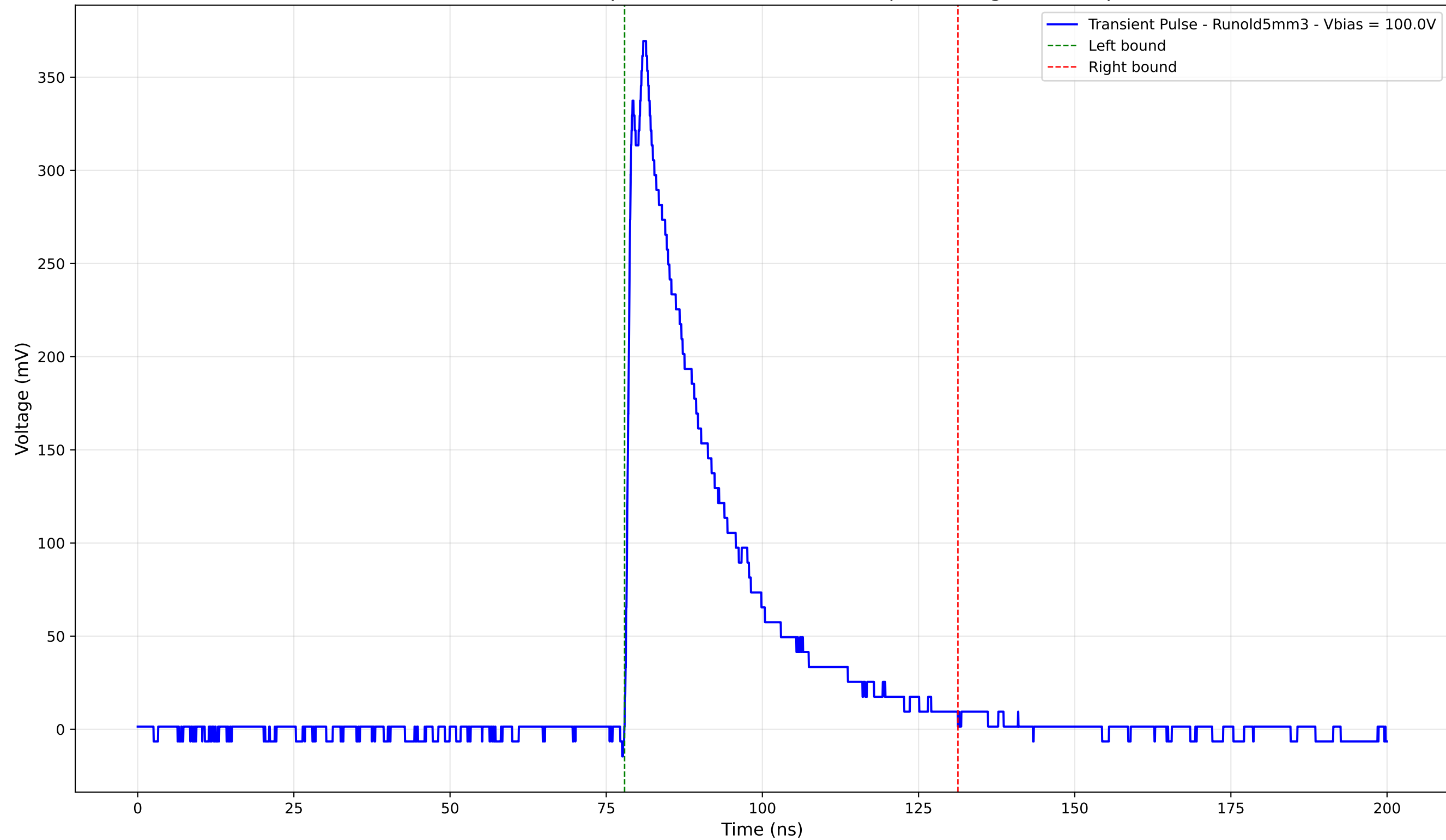
Transient Pulse - Sample: old5 - Position: 3090.0 \mu\text{m} - Charge: 100.81 pC
