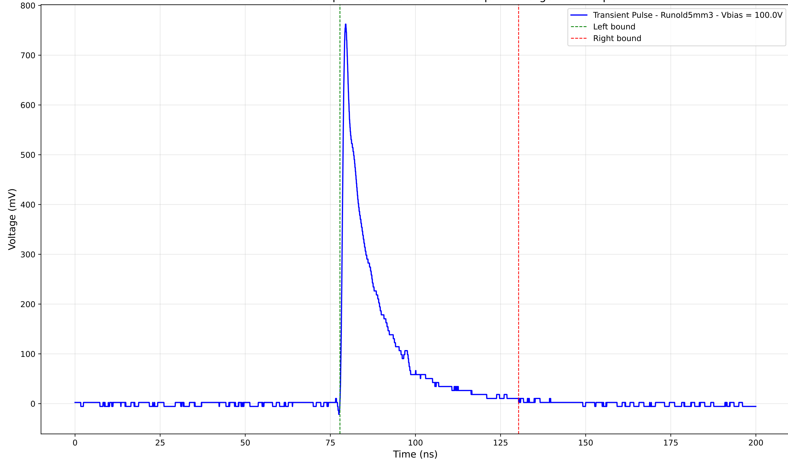
Transient Pulse - Sample: old5 - Position: 4740.0 \mu\text{m} - Charge: 132.24 pC
