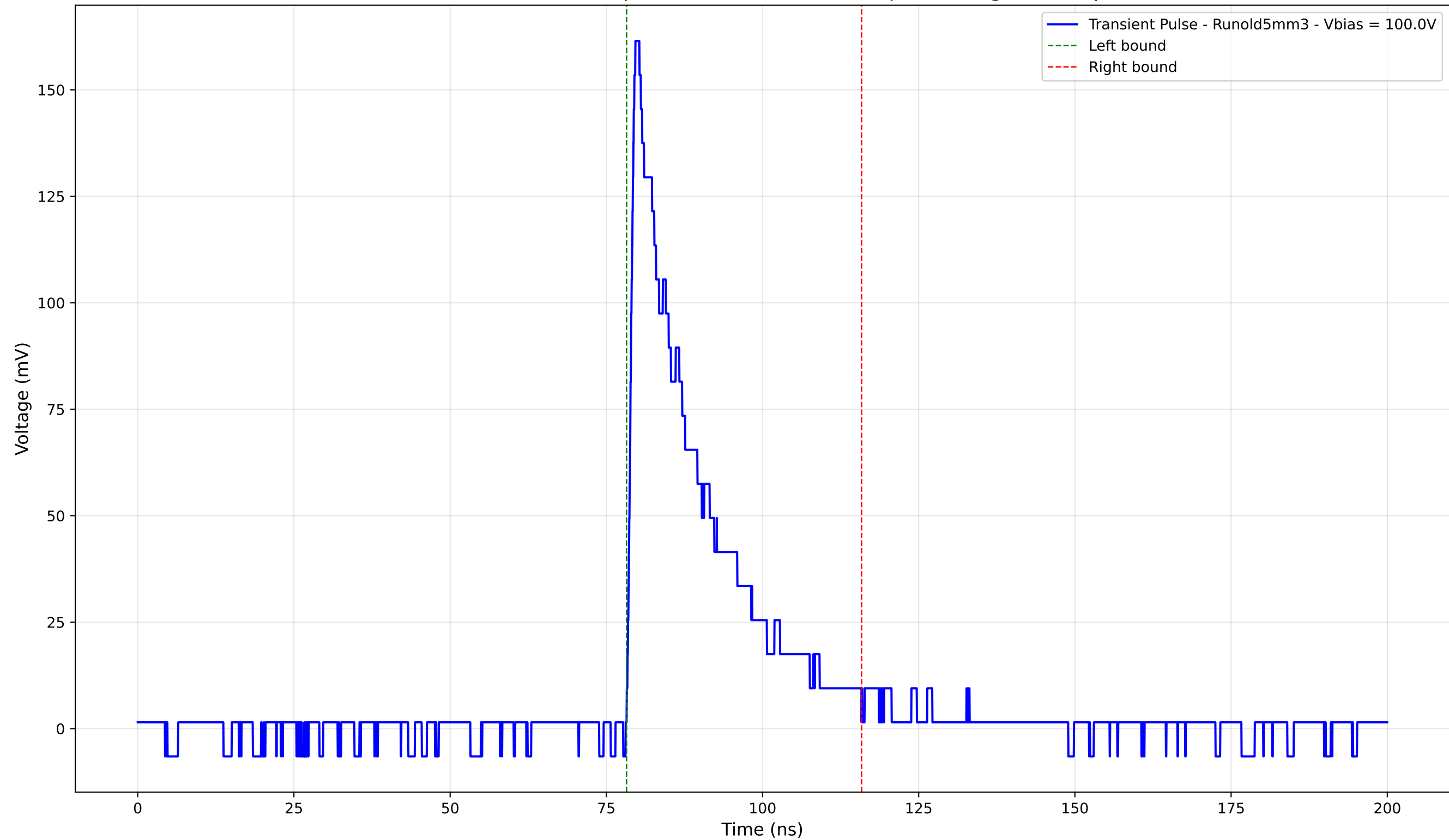
Transient Pulse - Sample: old5 - Position: 600.0 \mu\text{m} - Charge: 35.53 pC
