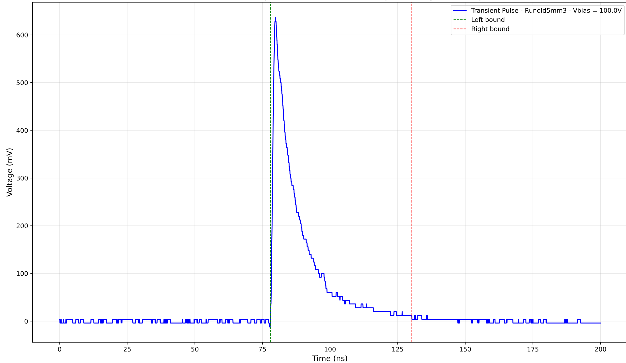
Transient Pulse - Sample: old5 - Position: 4630.0 \mu\text{m} - Charge: 125.70 pC
