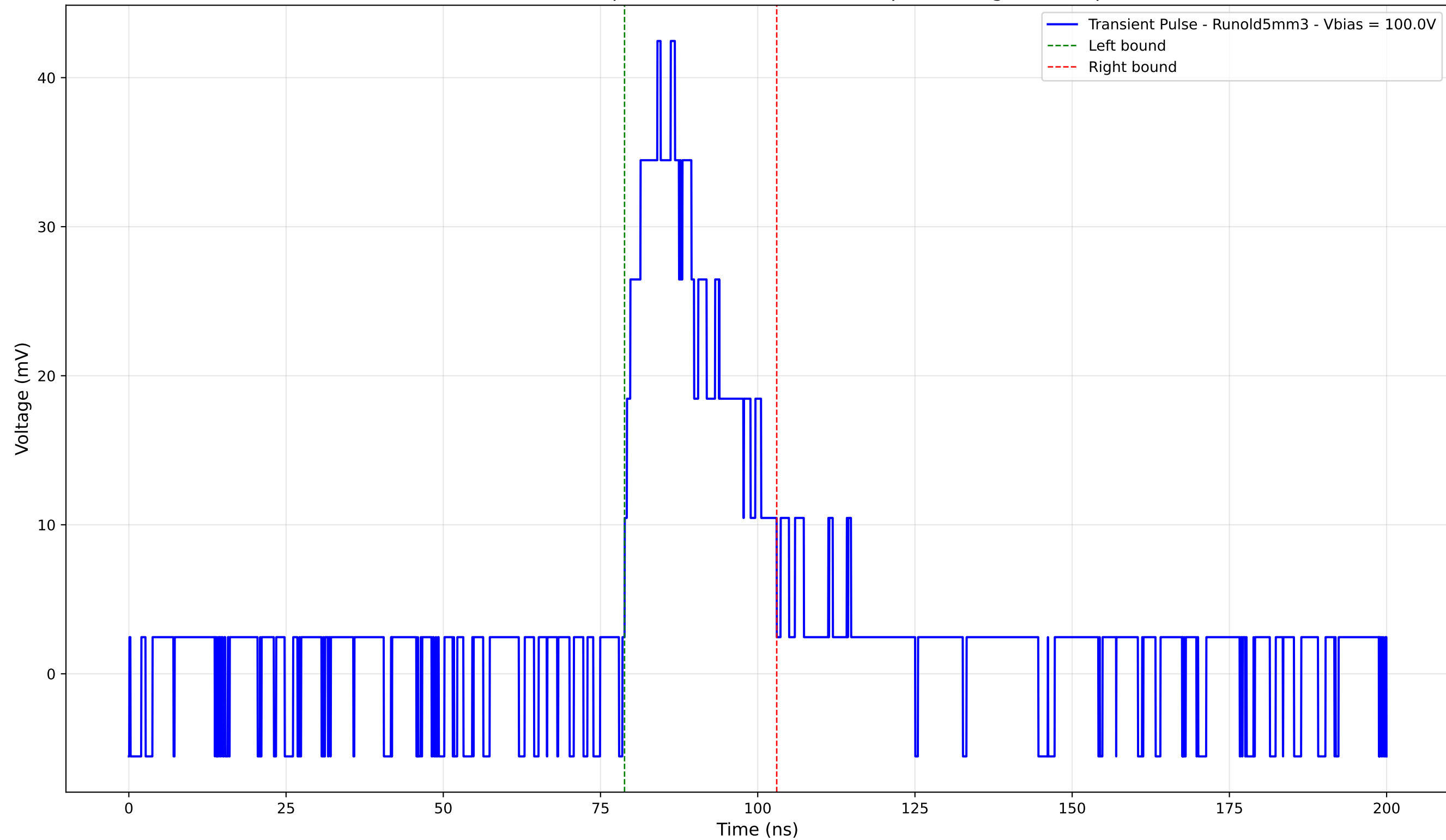
Transient Pulse - Sample: old5 - Position: 2400.0 \mu\text{m} - Charge: 11.70 pC
