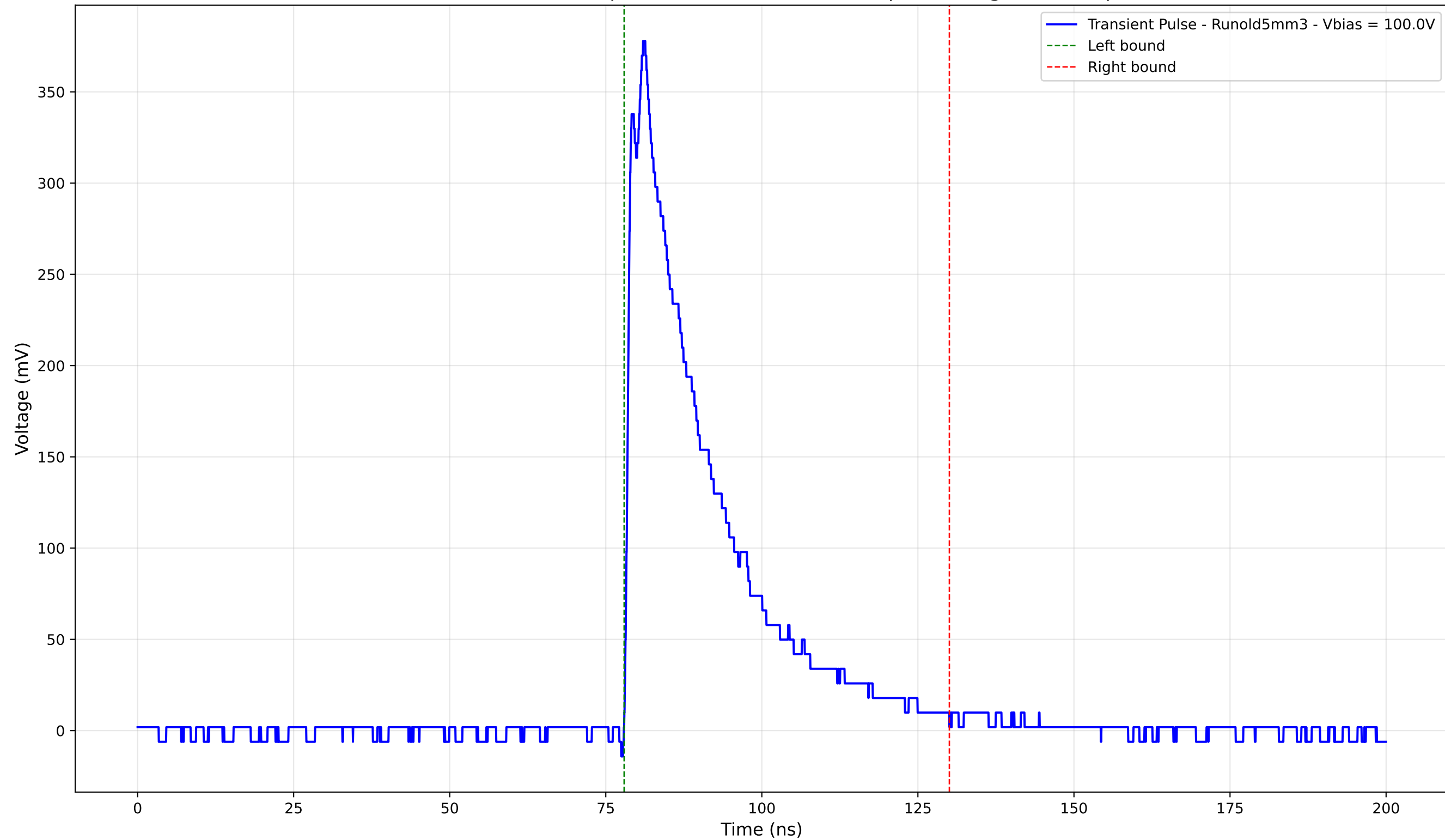
Transient Pulse - Sample: old5 - Position: 3095.0 \mu\text{m} - Charge: 102.15 pC
