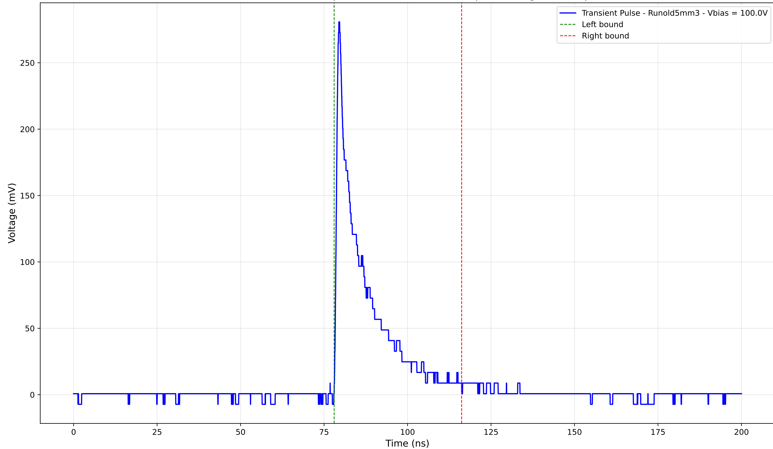
Transient Pulse - Sample: old5 - Position: 375.0 \mu\text{m} - Charge: 44.59 pC
