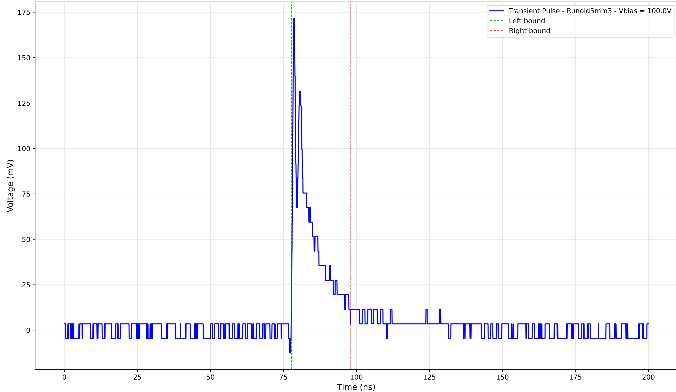
Transient Pulse - Sample: old5 - Position: 3625.0 \mu\text{m} - Charge: 20.46 pC
