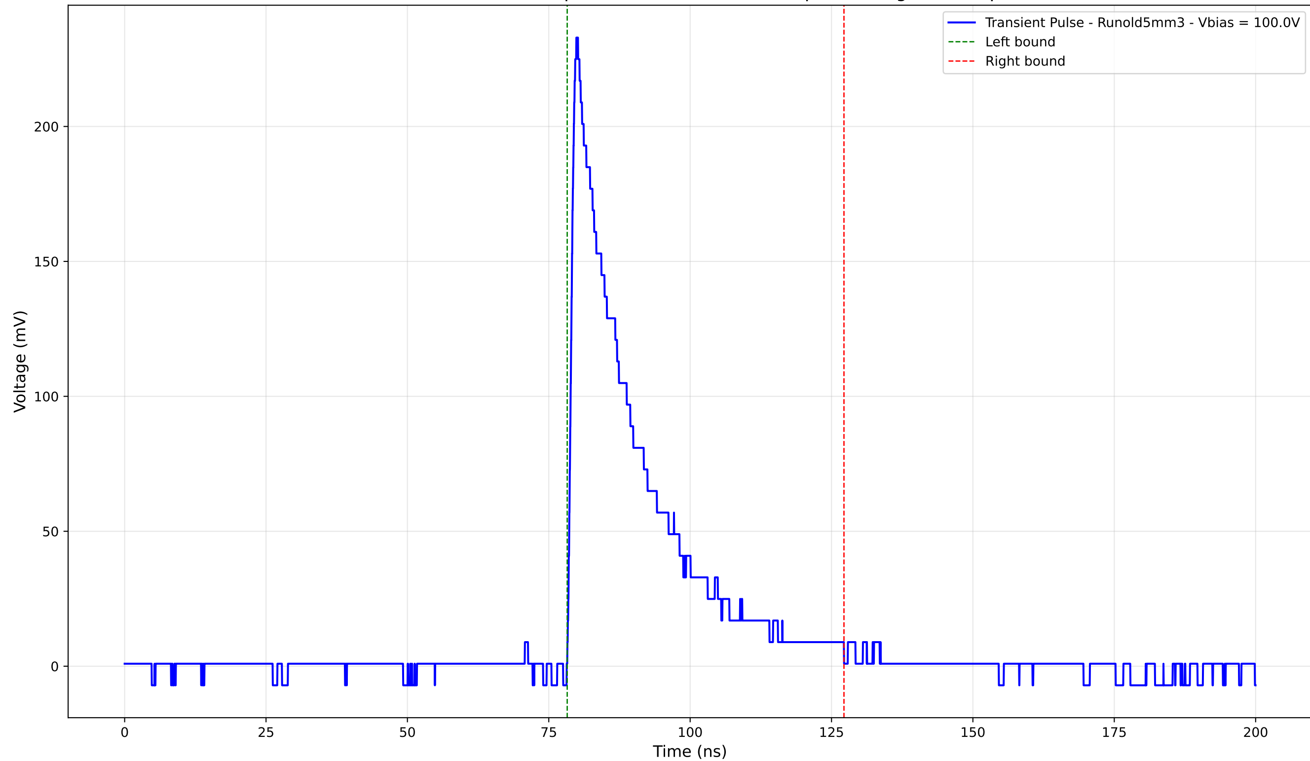
Transient Pulse - Sample: old5 - Position: 660.0 \mu\text{m} - Charge: 54.49 pC
