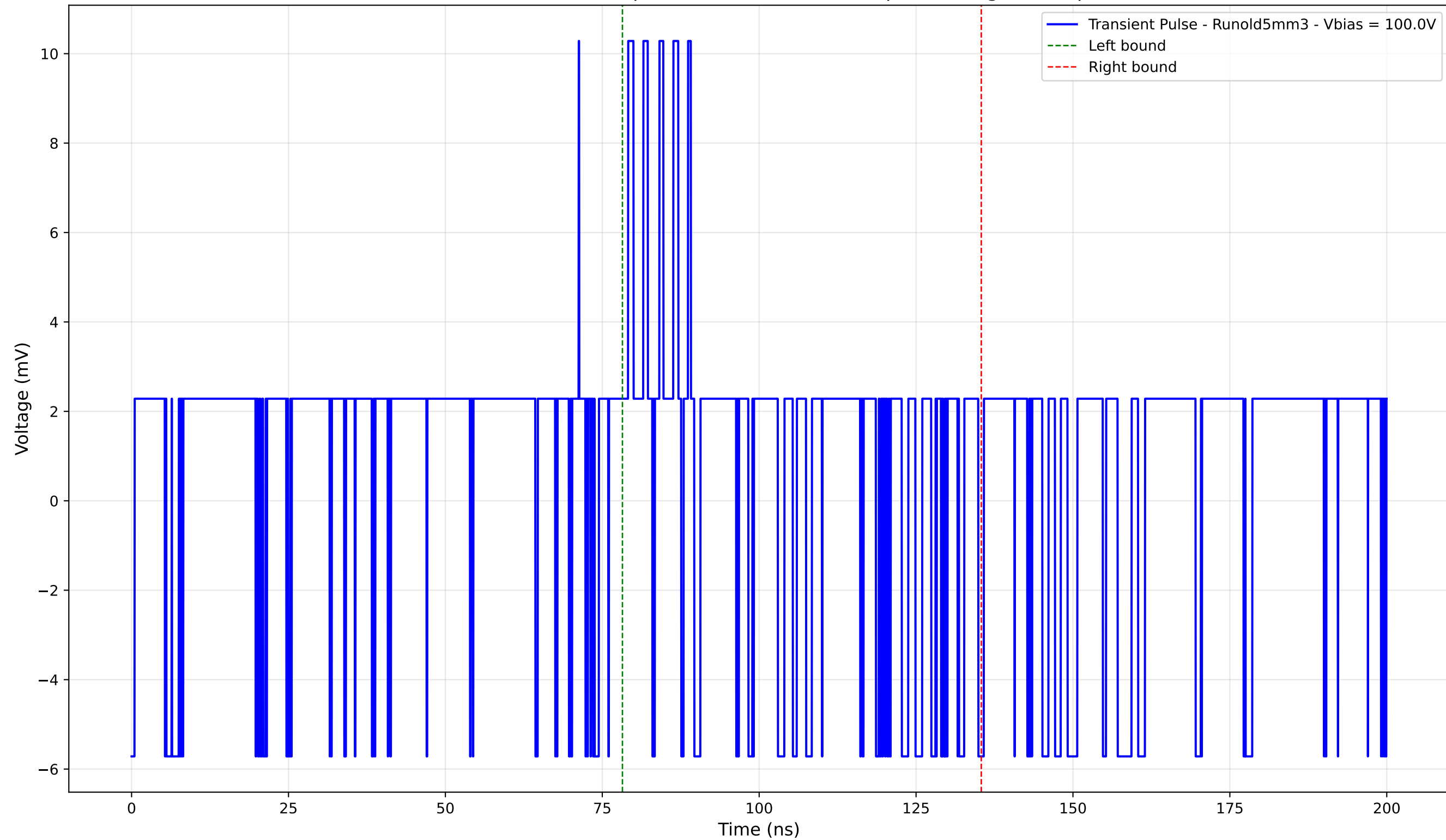
Transient Pulse - Sample: old5 - Position: 60.0 \mu\text{m} - Charge: 1.21 pC
