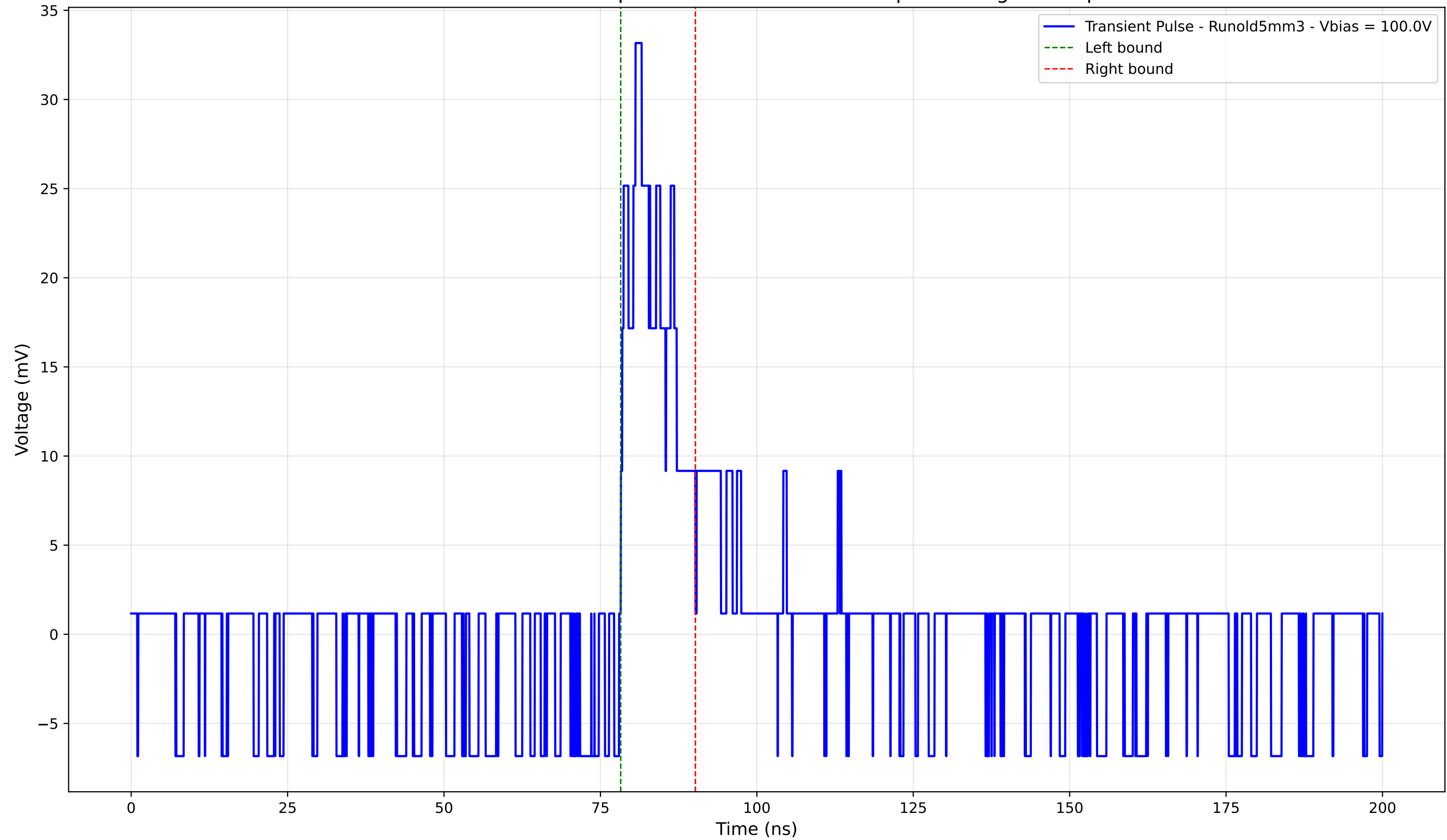
Transient Pulse - Sample: old5 - Position: 3295.0 \mu\text{m} - Charge: 4.47 pC
