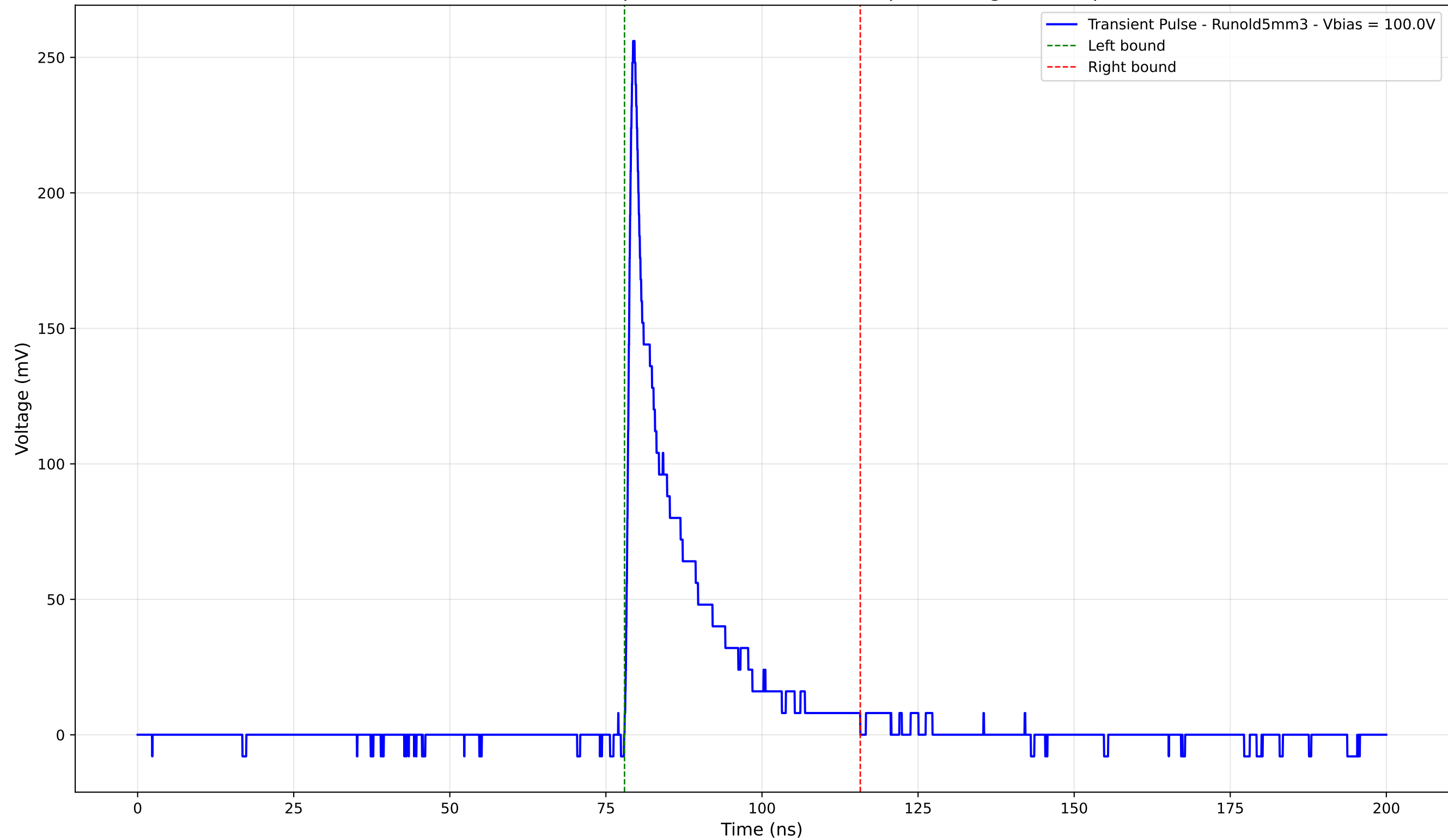
Transient Pulse - Sample: old5 - Position: 305.0 \mu\text{m} - Charge: 36.85 pC
