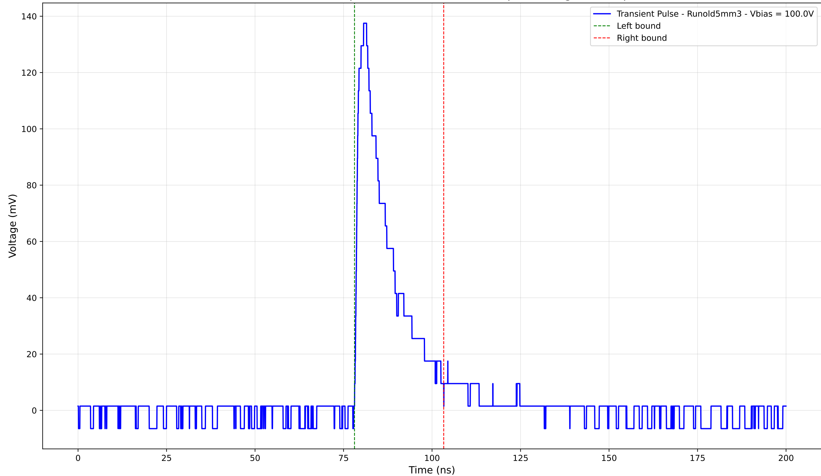
Transient Pulse - Sample: old5 - Position: 4130.0 \mu\text{m} - Charge: 27.30 pC
