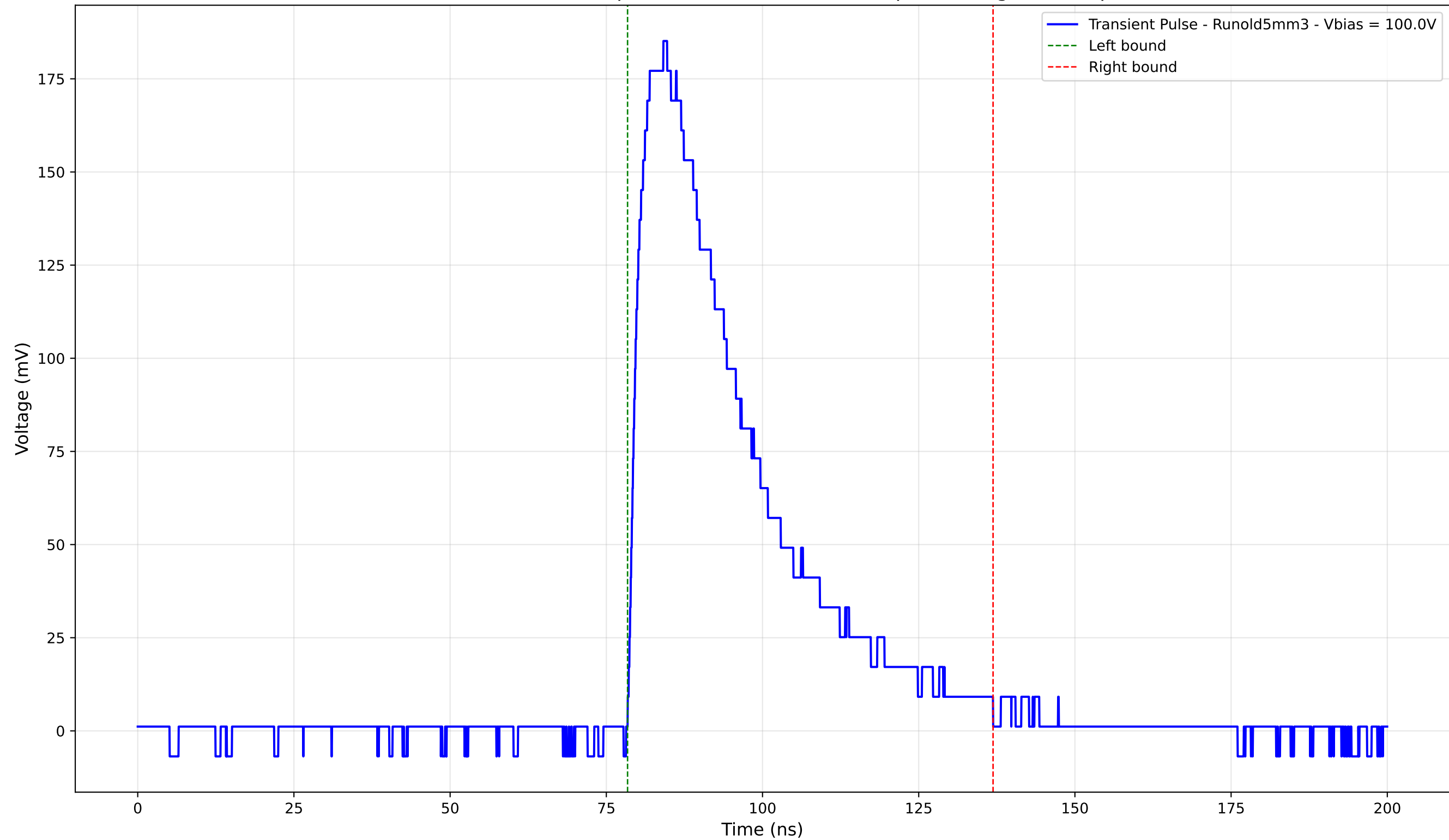
Transient Pulse - Sample: old5 - Position: 1715.0 \mu\text{m} - Charge: 73.50 pC
