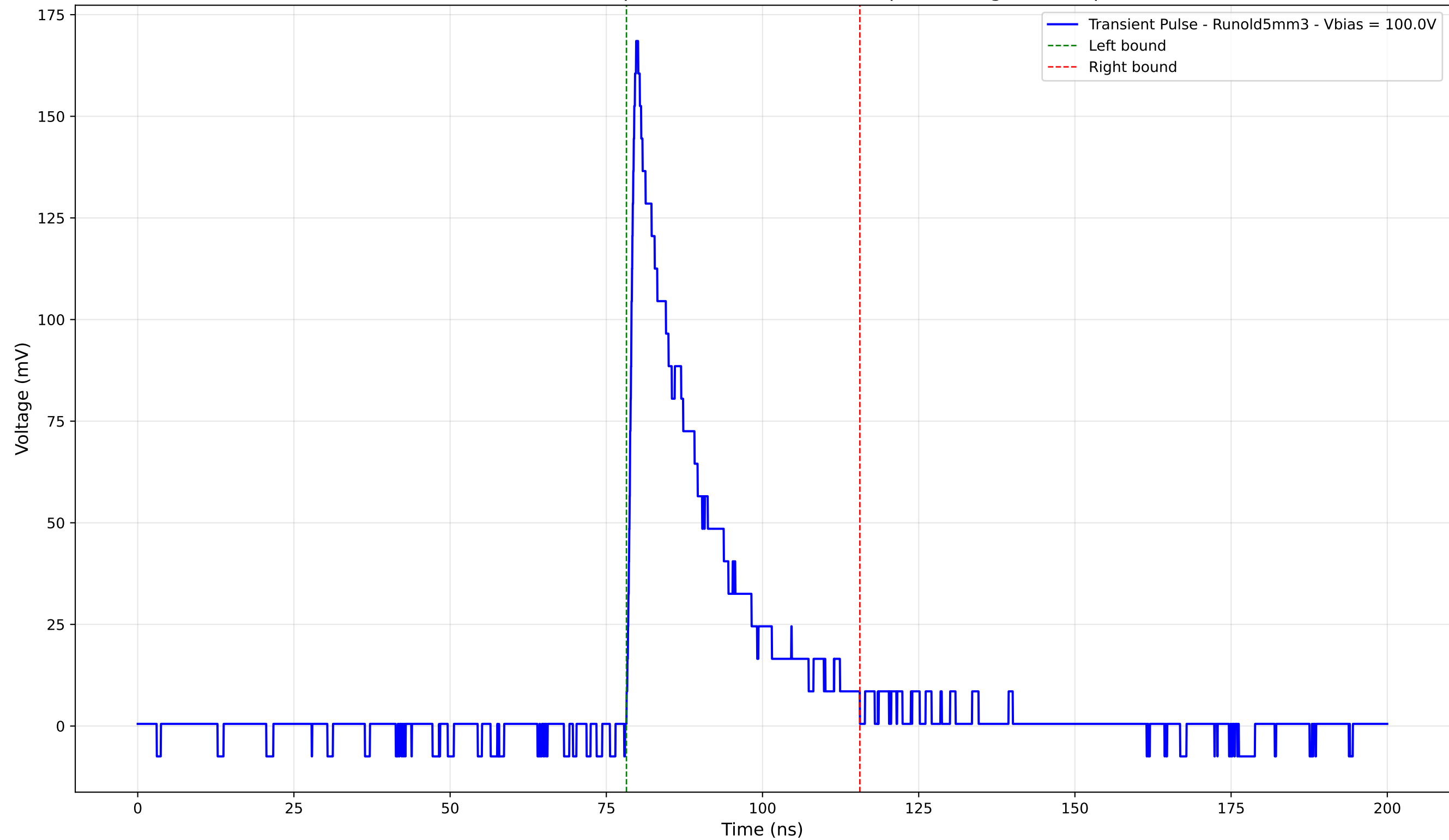
Transient Pulse - Sample: old5 - Position: 605.0 \mu\text{m} - Charge: 35.63 pC
