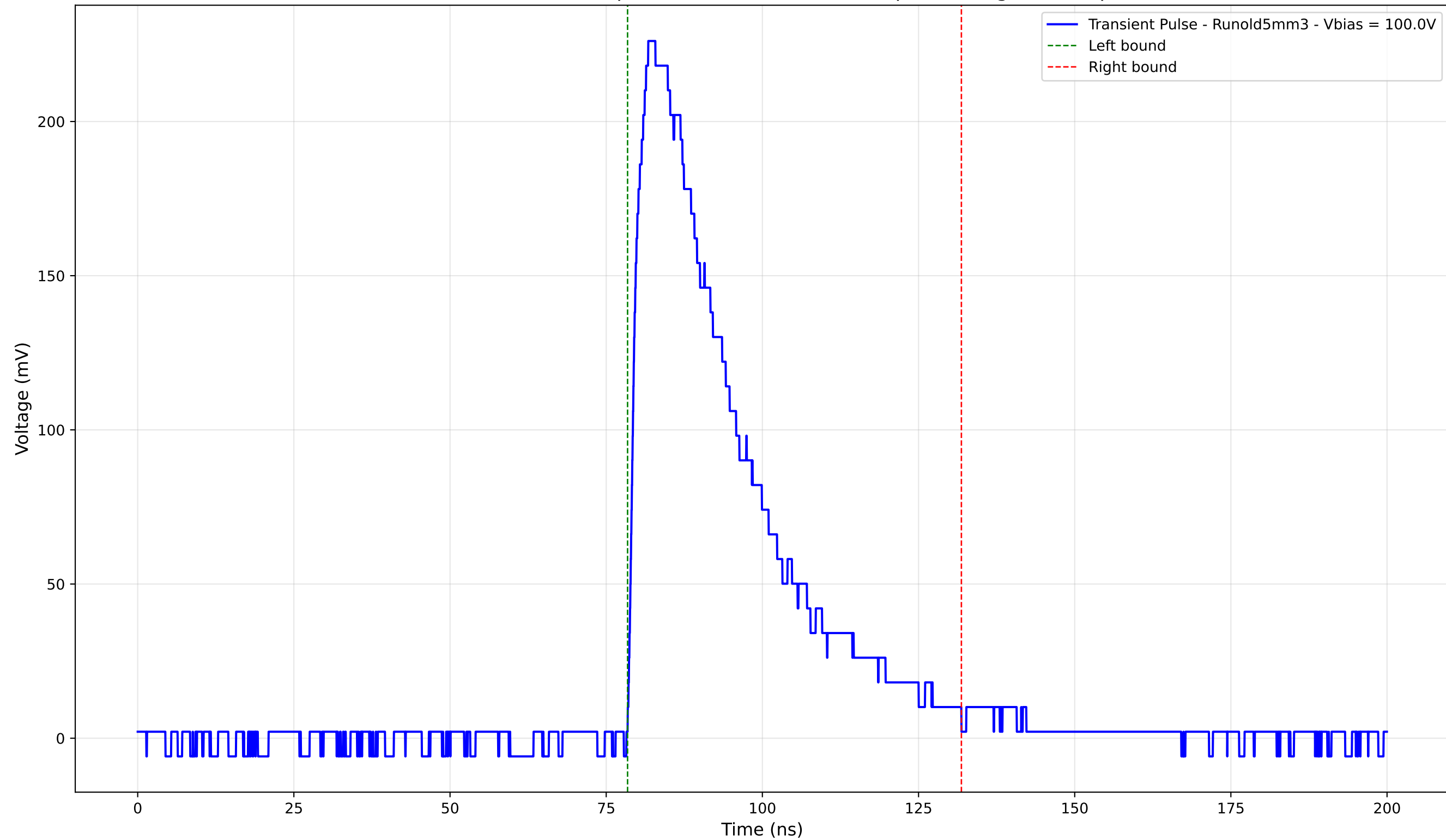
Transient Pulse - Sample: old5 - Position: 2470.0 \mu\text{m} - Charge: 84.58 pC
