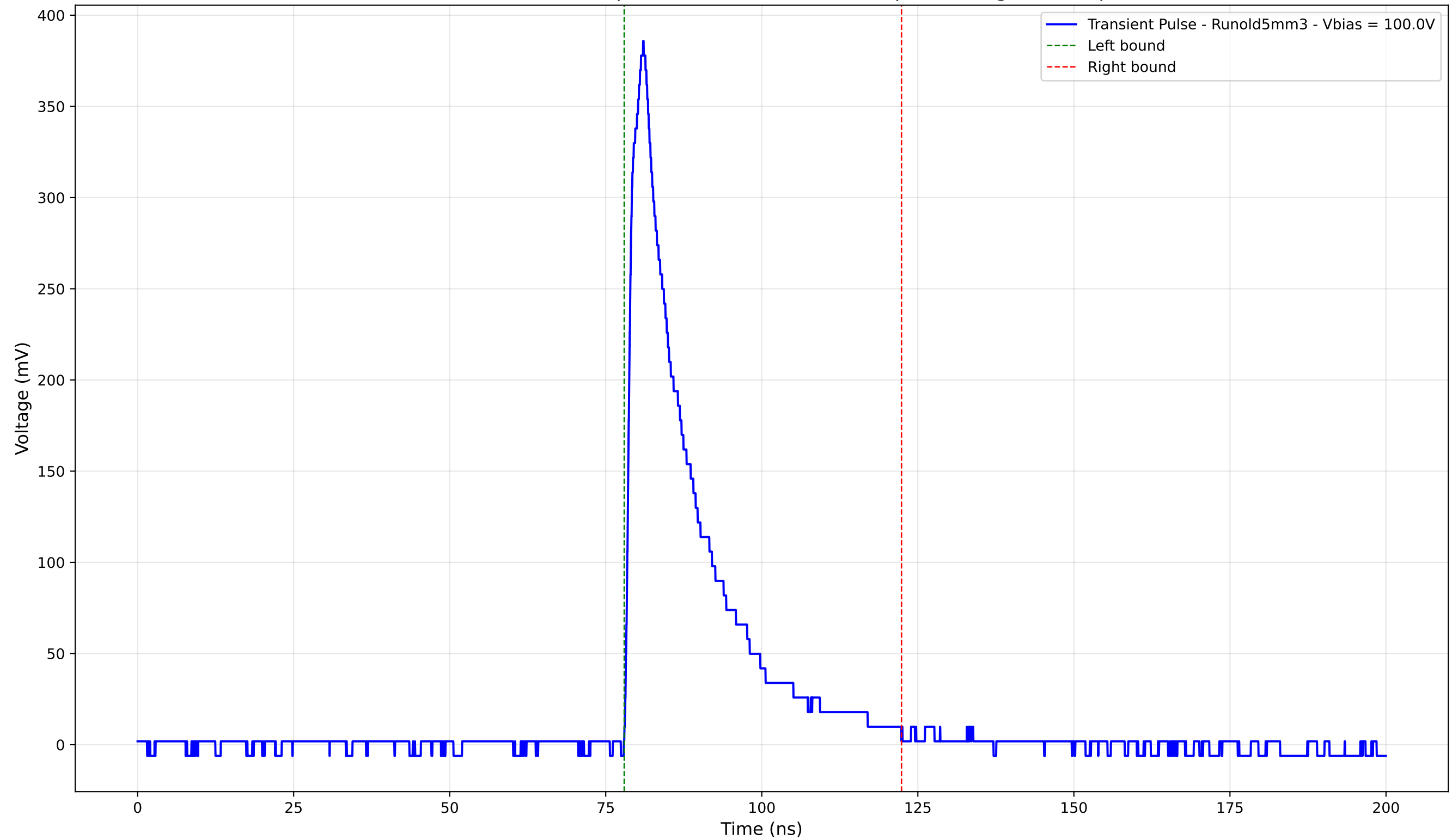
Transient Pulse - Sample: old5 - Position: 4095.0 \mu\text{m} - Charge: 81.71 pC
