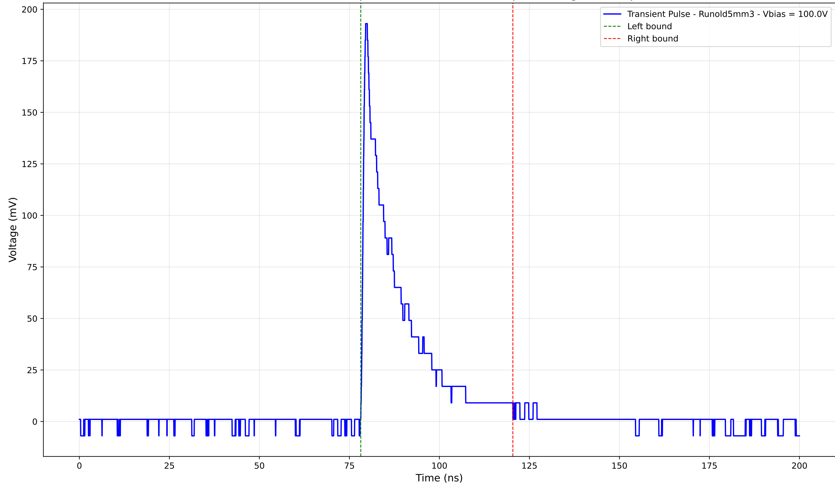
Transient Pulse - Sample: old5 - Position: 490.0 \mu\text{m} - Charge: 37.04 pC
