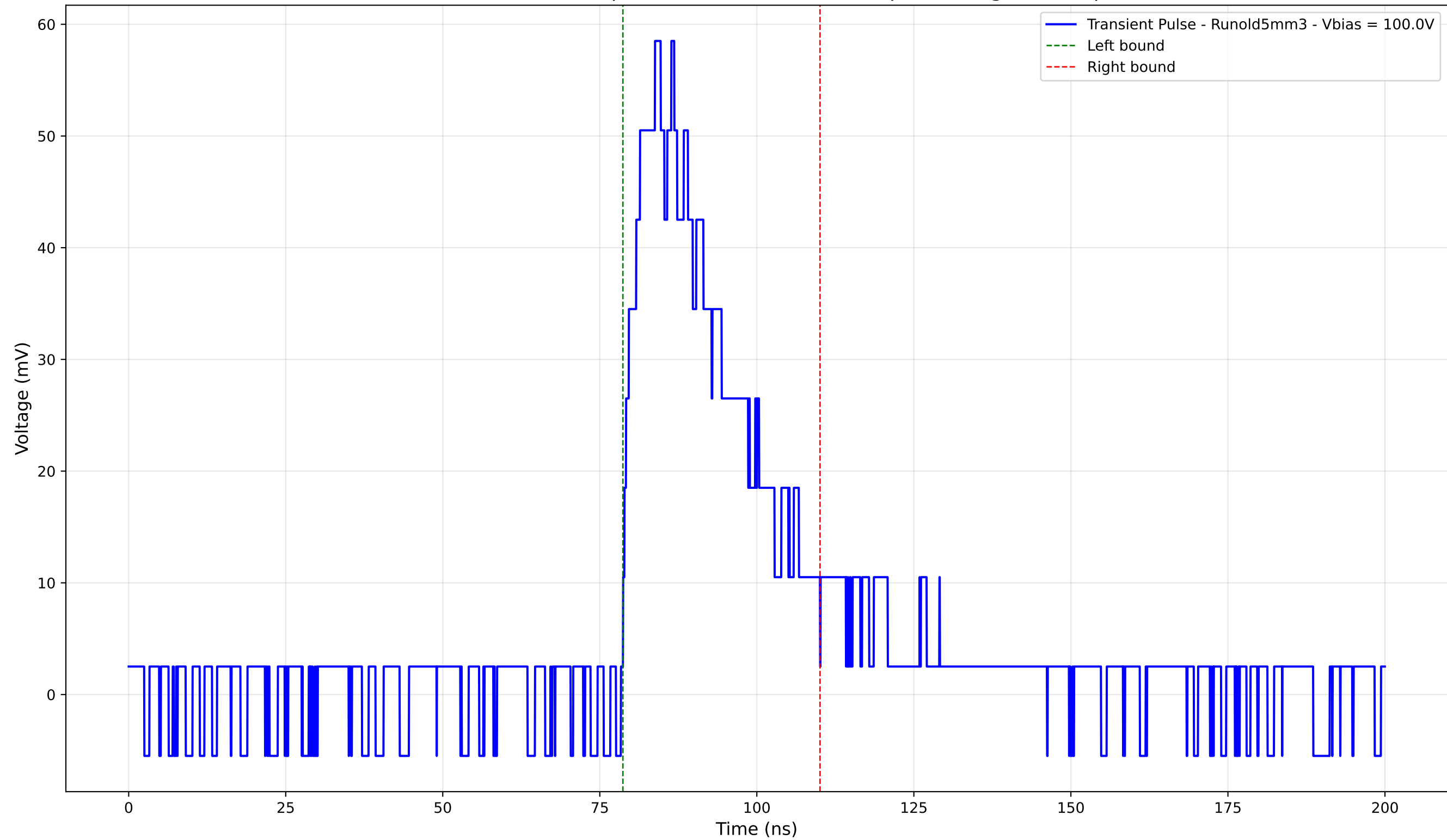
Transient Pulse - Sample: old5 - Position: 1970.0 \mu\text{m} - Charge: 19.12 pC
