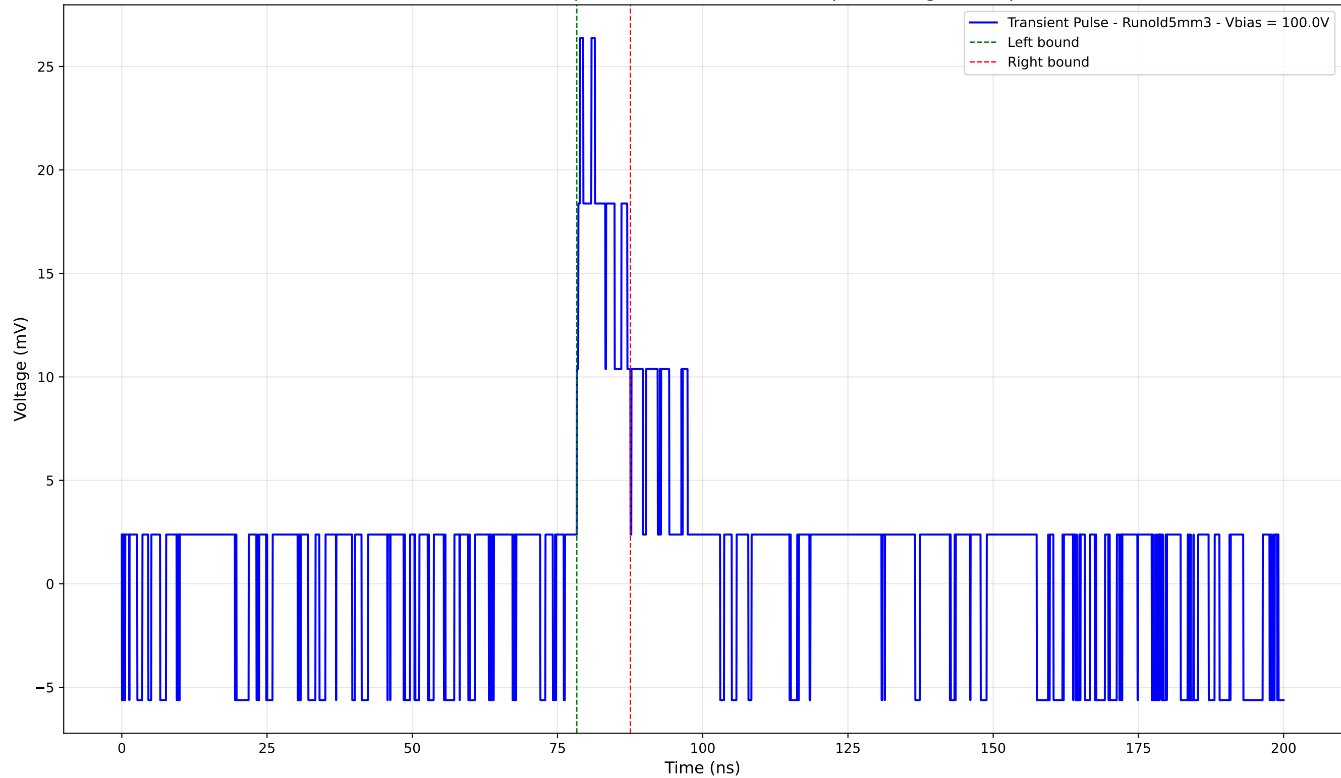
Transient Pulse - Sample: old5 - Position: 3275.0 \mu\text{m} - Charge: 3.25 pC
