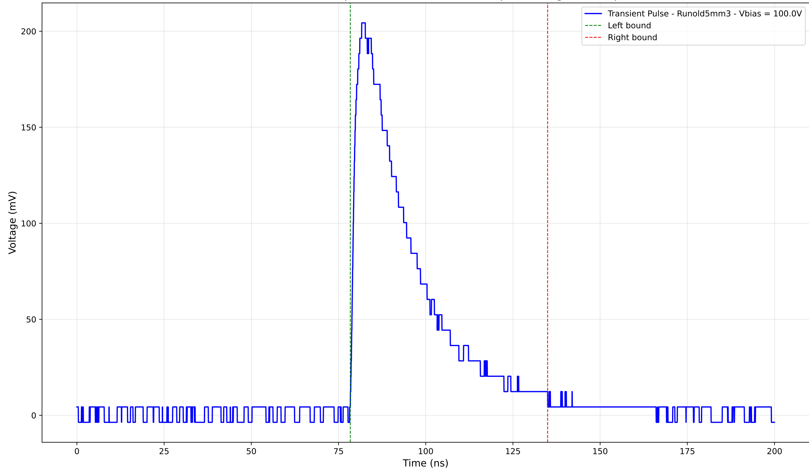
Transient Pulse - Sample: old5 - Position: 2585.0 \mu\text{m} - Charge: 75.81 pC
