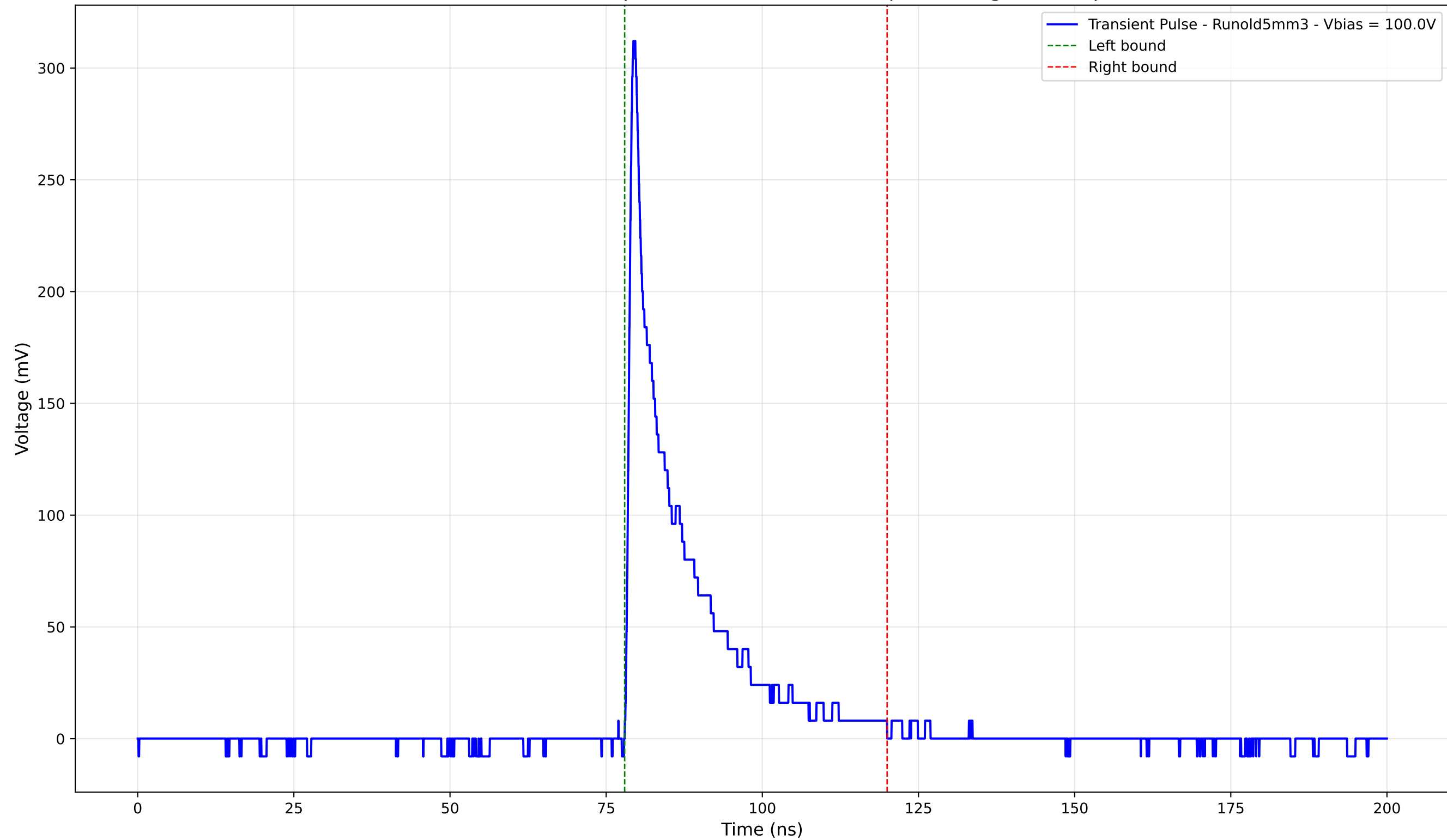
Transient Pulse - Sample: old5 - Position: 325.0 \mu\text{m} - Charge: 47.27 pC
