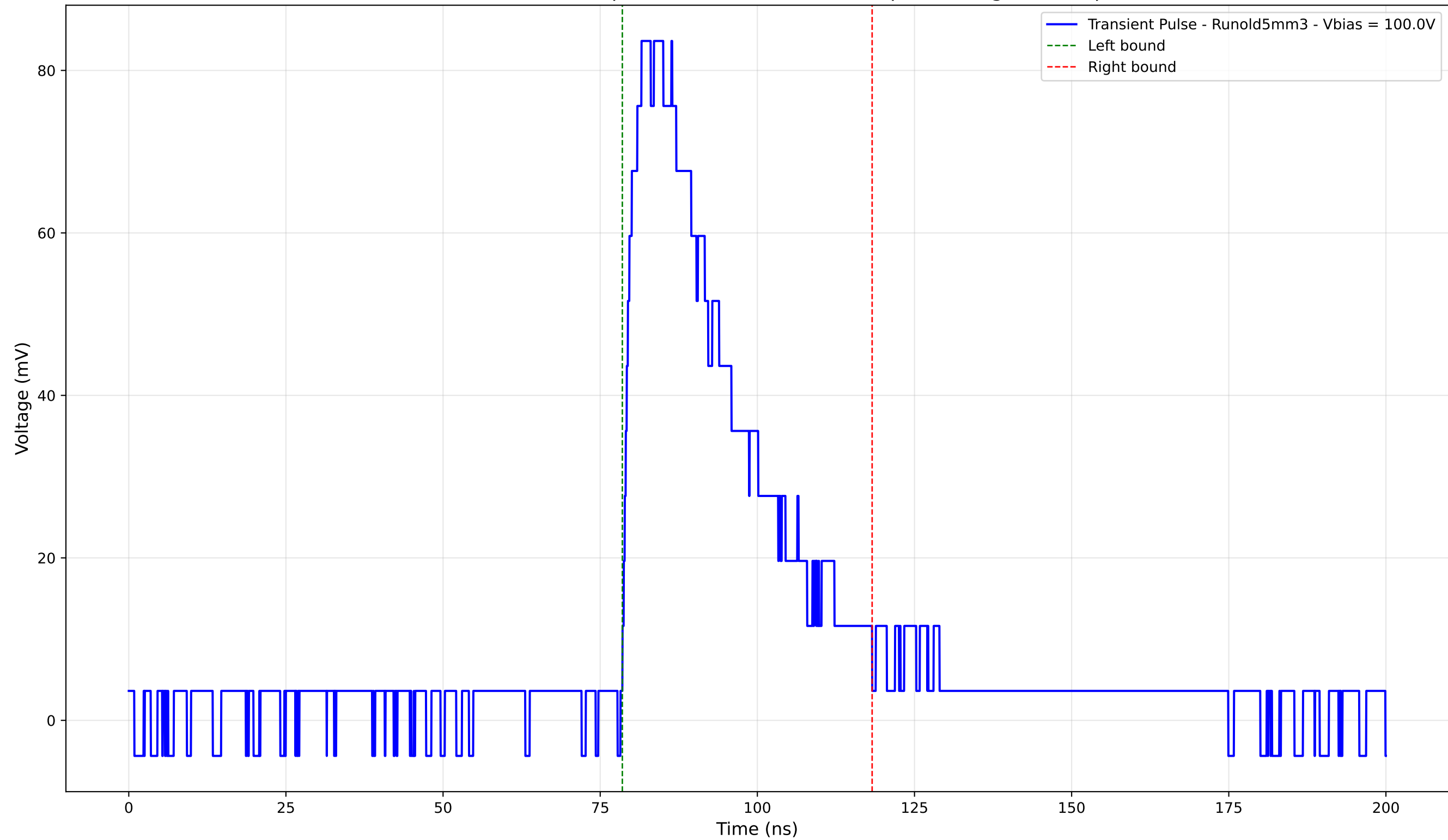
Transient Pulse - Sample: old5 - Position: 2425.0 \mu\text{m} - Charge: 31.56 pC
