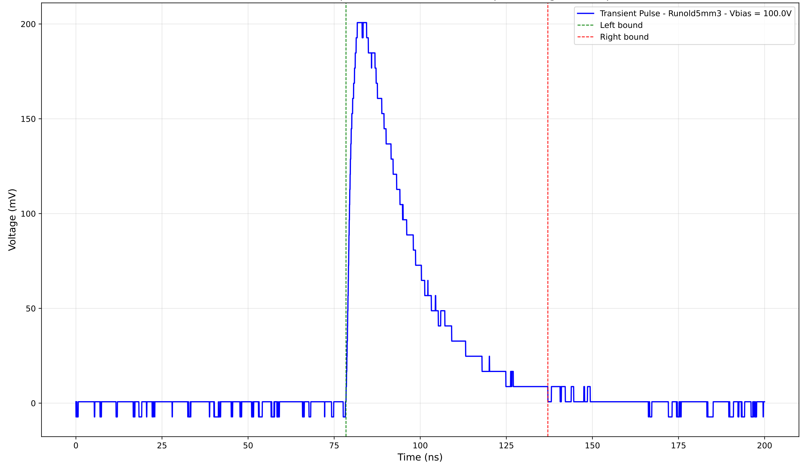
Transient Pulse - Sample: old5 - Position: 2325.0 \mu\text{m} - Charge: 77.73 pC
