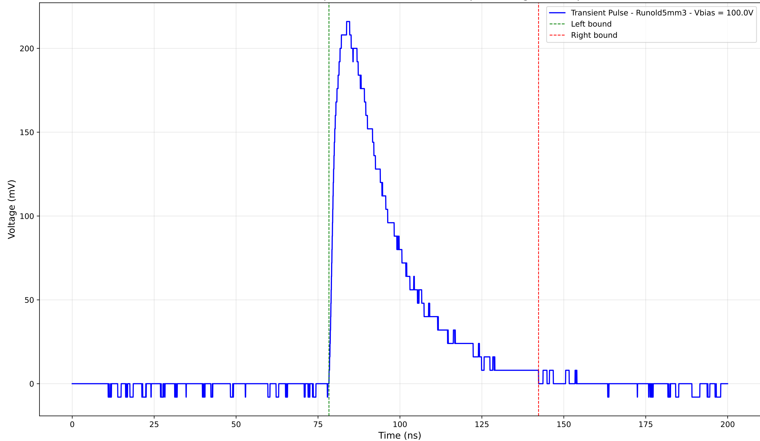
Transient Pulse - Sample: old5 - Position: 1885.0 \mu\text{m} - Charge: 85.80 pC
