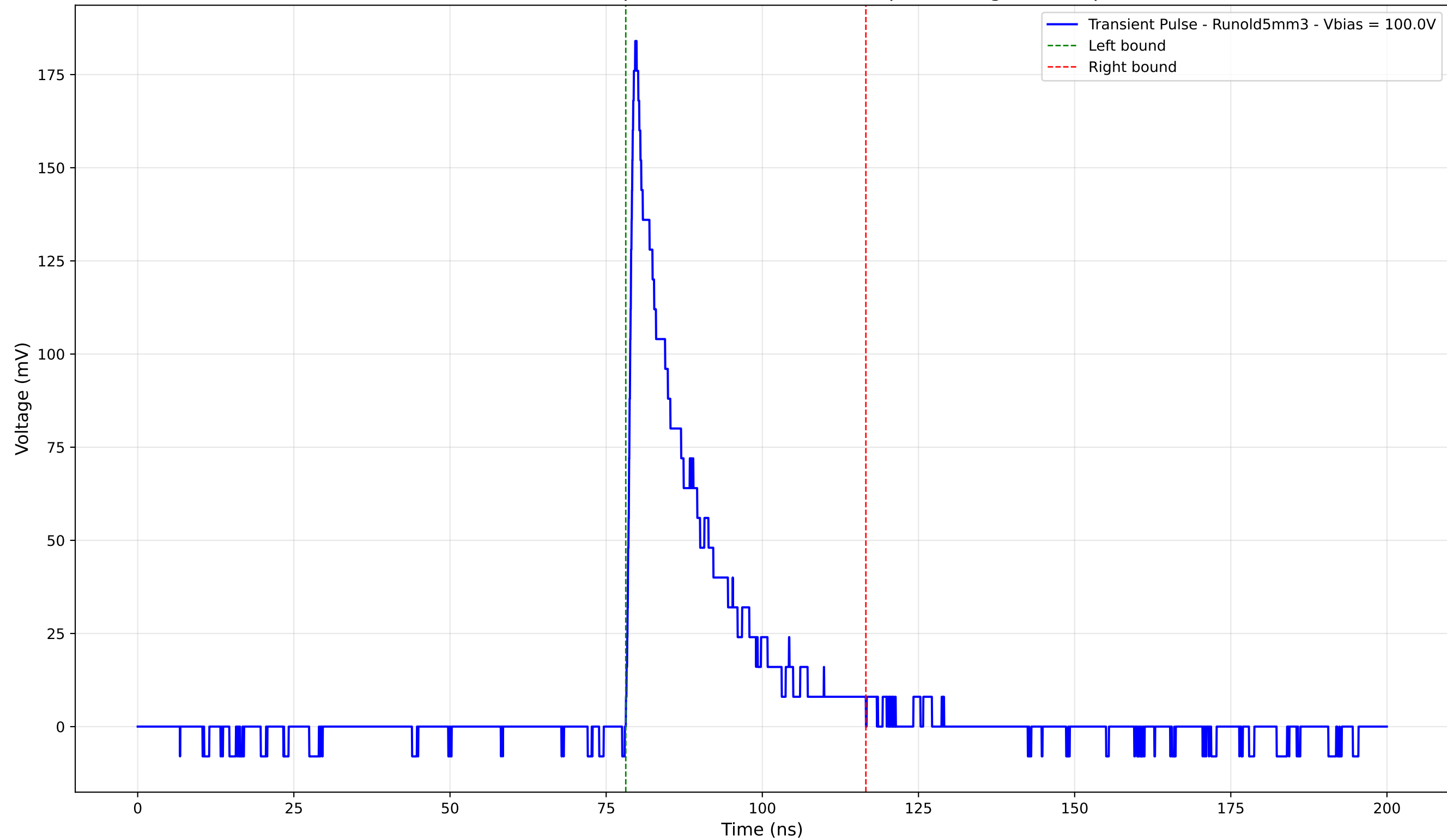
Transient Pulse - Sample: old5 - Position: 495.0 \mu\text{m} - Charge: 34.44 pC
