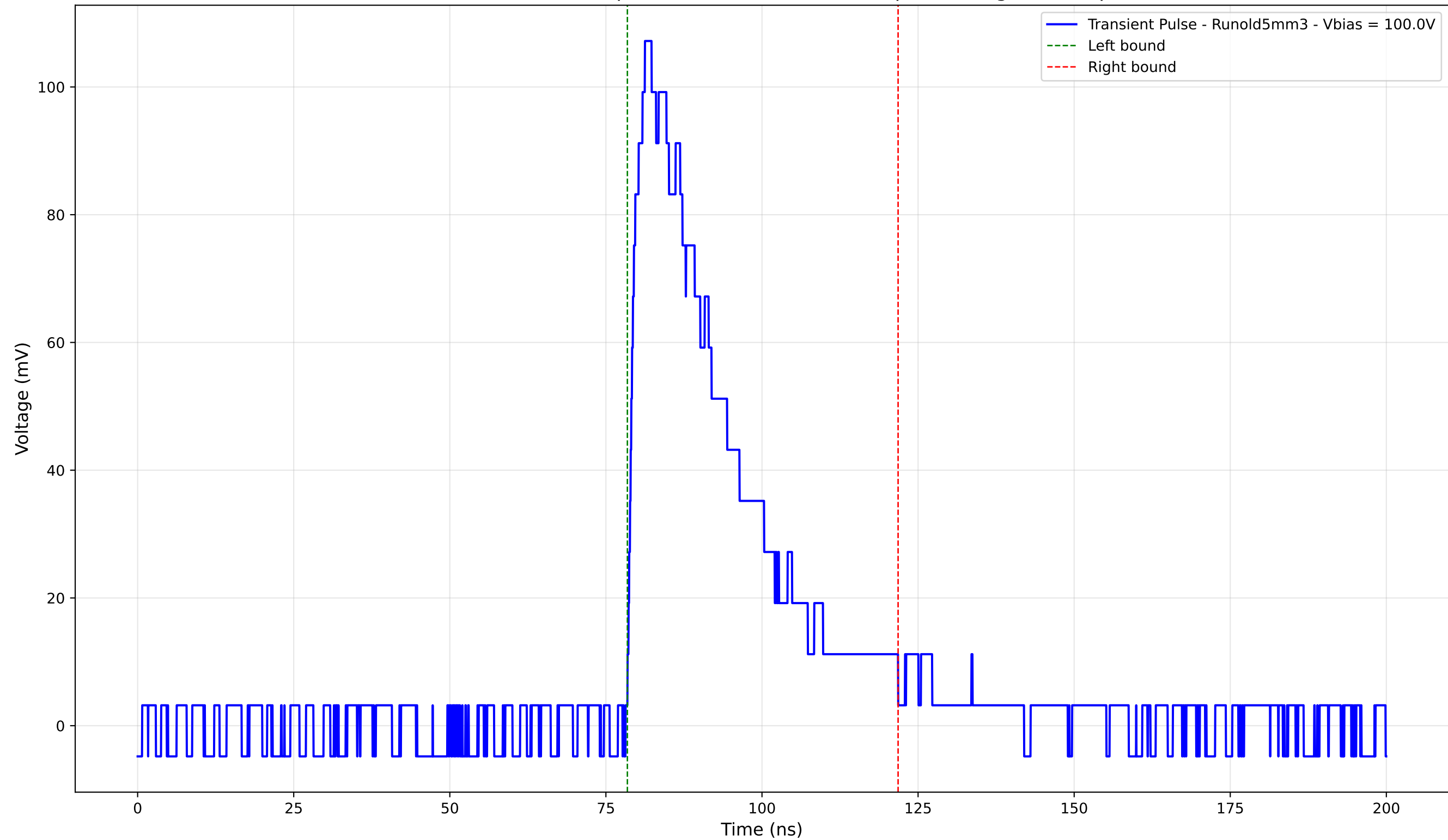
Transient Pulse - Sample: old5 - Position: 2730.0 \mu\text{m} - Charge: 35.36 pC
