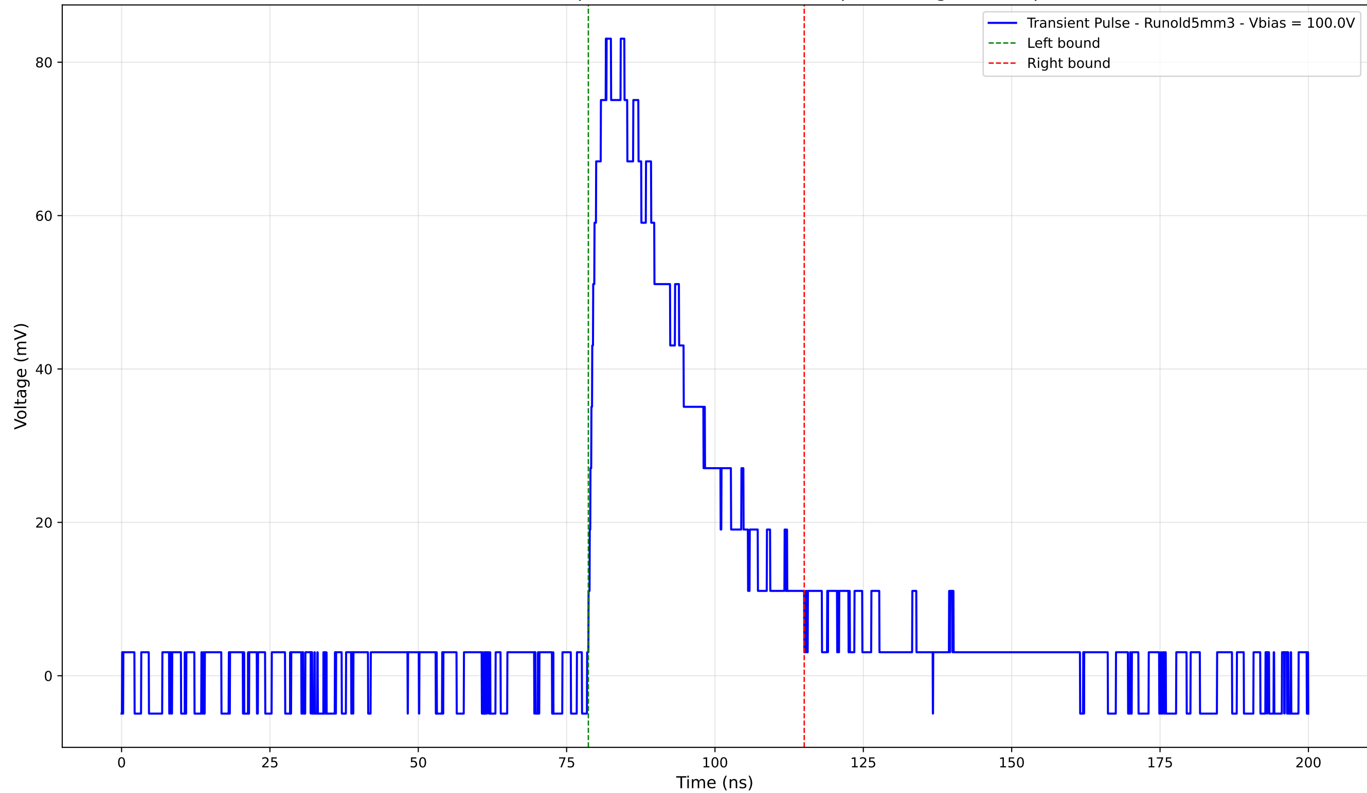
Transient Pulse - Sample: old5 - Position: 1215.0 \mu\text{m} - Charge: 28.26 pC
