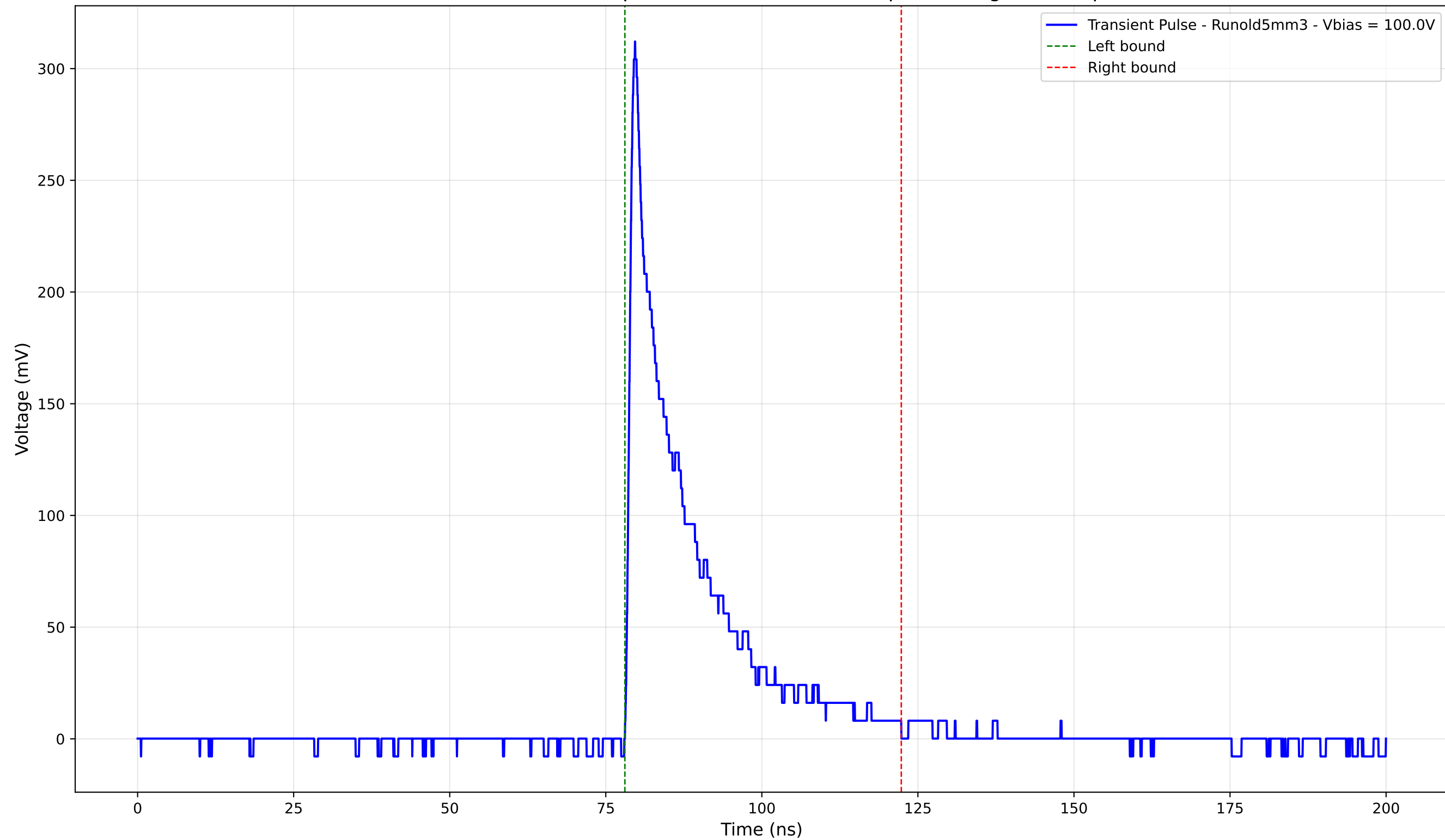
Transient Pulse - Sample: old5 - Position: 440.0 \mu\text{m} - Charge: 54.98 pC
