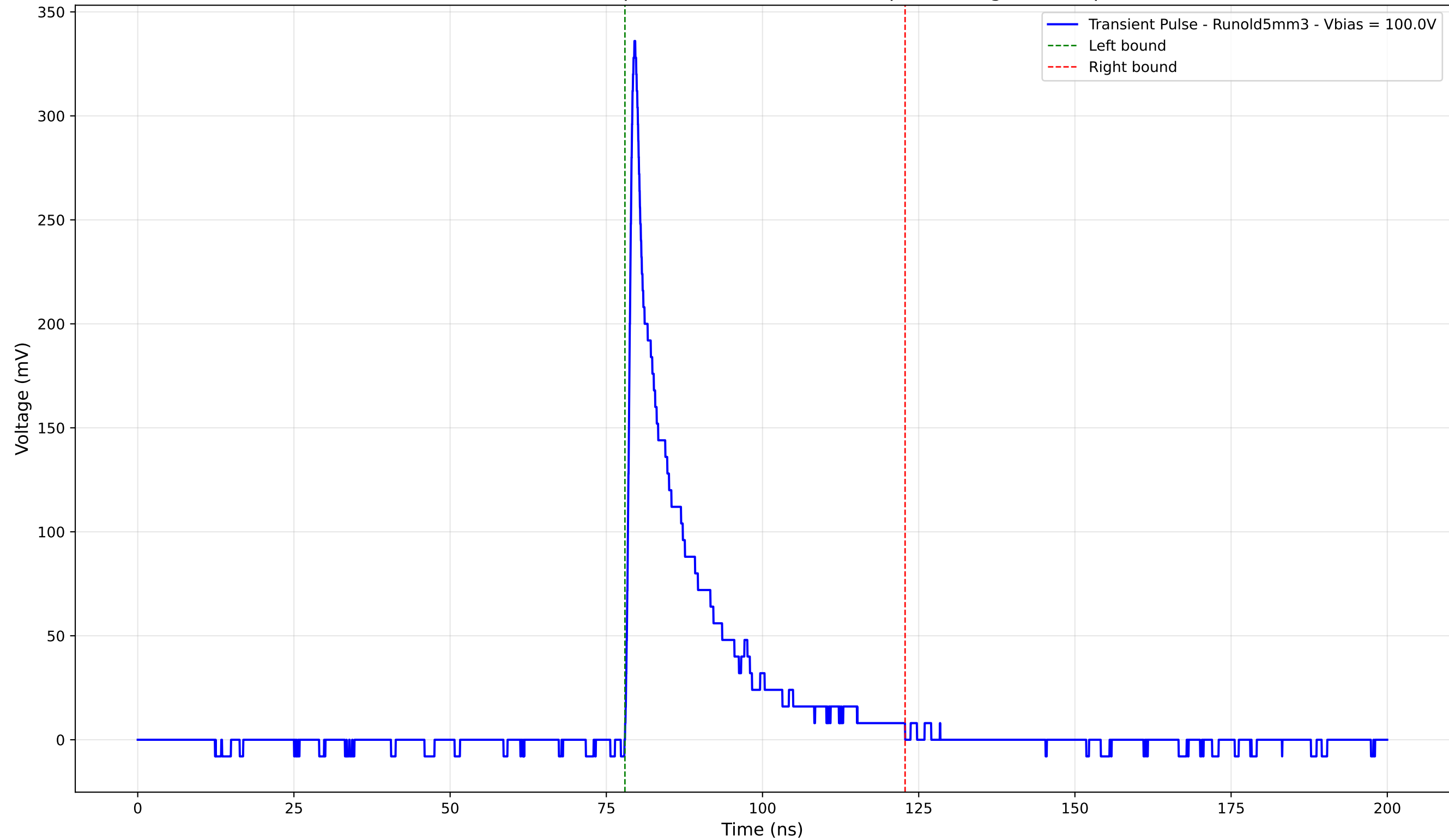
Transient Pulse - Sample: old5 - Position: 360.0 \mu\text{m} - Charge: 52.68 pC
