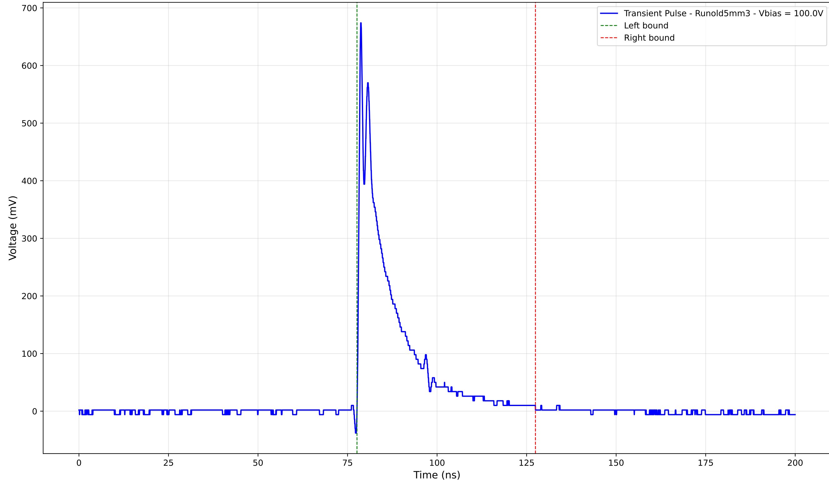
Transient Pulse - Sample: old5 - Position: 3730.0 \mu\text{m} - Charge: 108.35 pC
