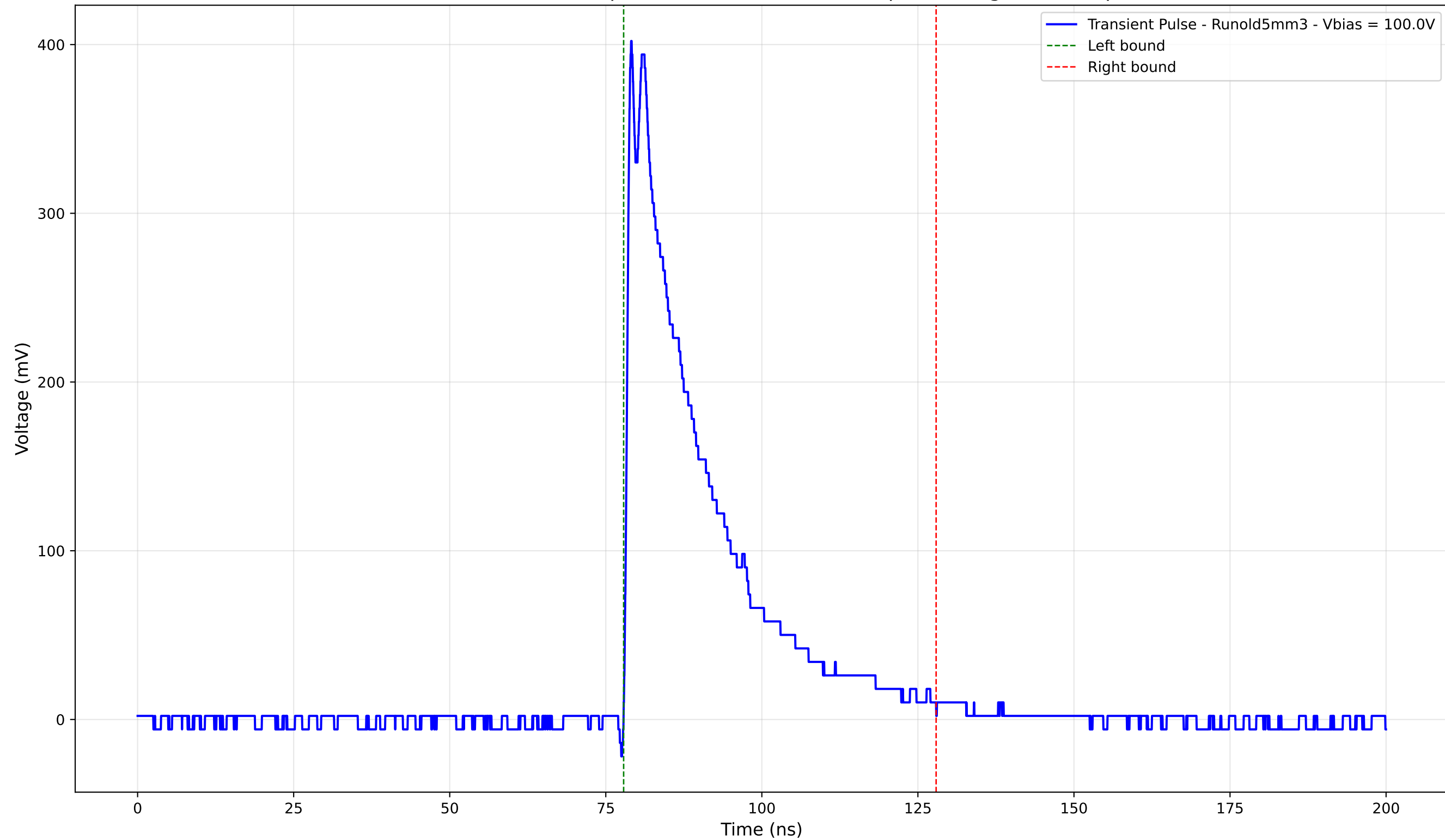
Transient Pulse - Sample: old5 - Position: 3160.0 \mu\text{m} - Charge: 101.79 pC
