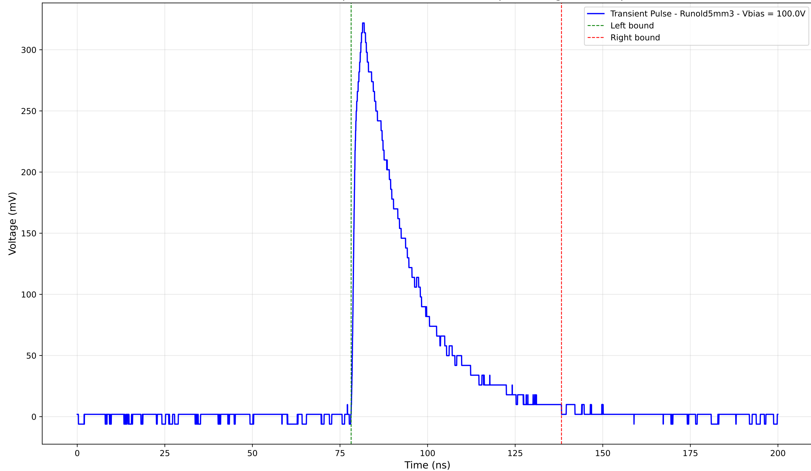
Transient Pulse - Sample: old5 - Position: 2820.0 \mu\text{m} - Charge: 105.94 pC
