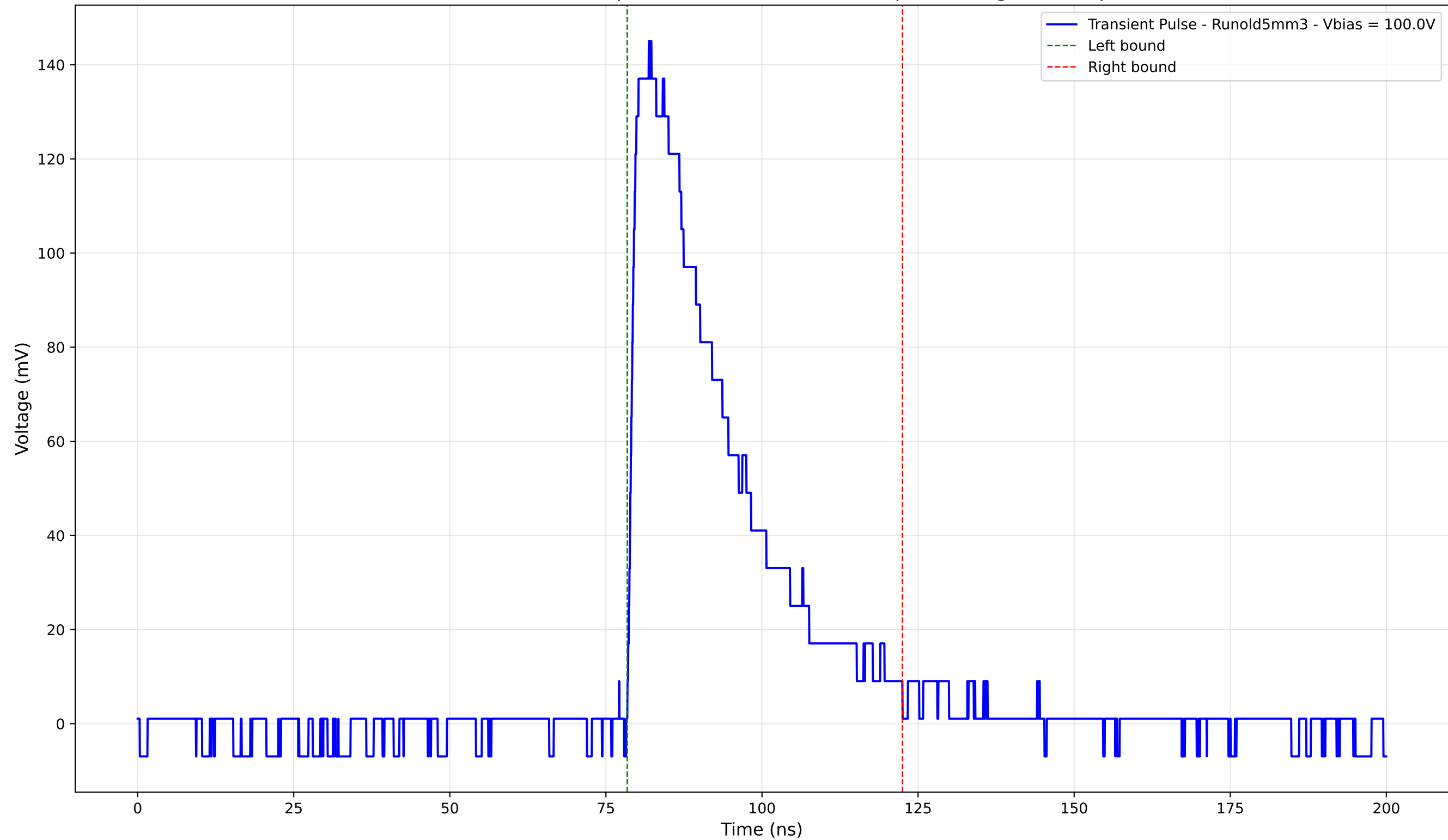
Transient Pulse - Sample: old5 - Position: 1025.0 \mu\text{m} - Charge: 47.56 pC
