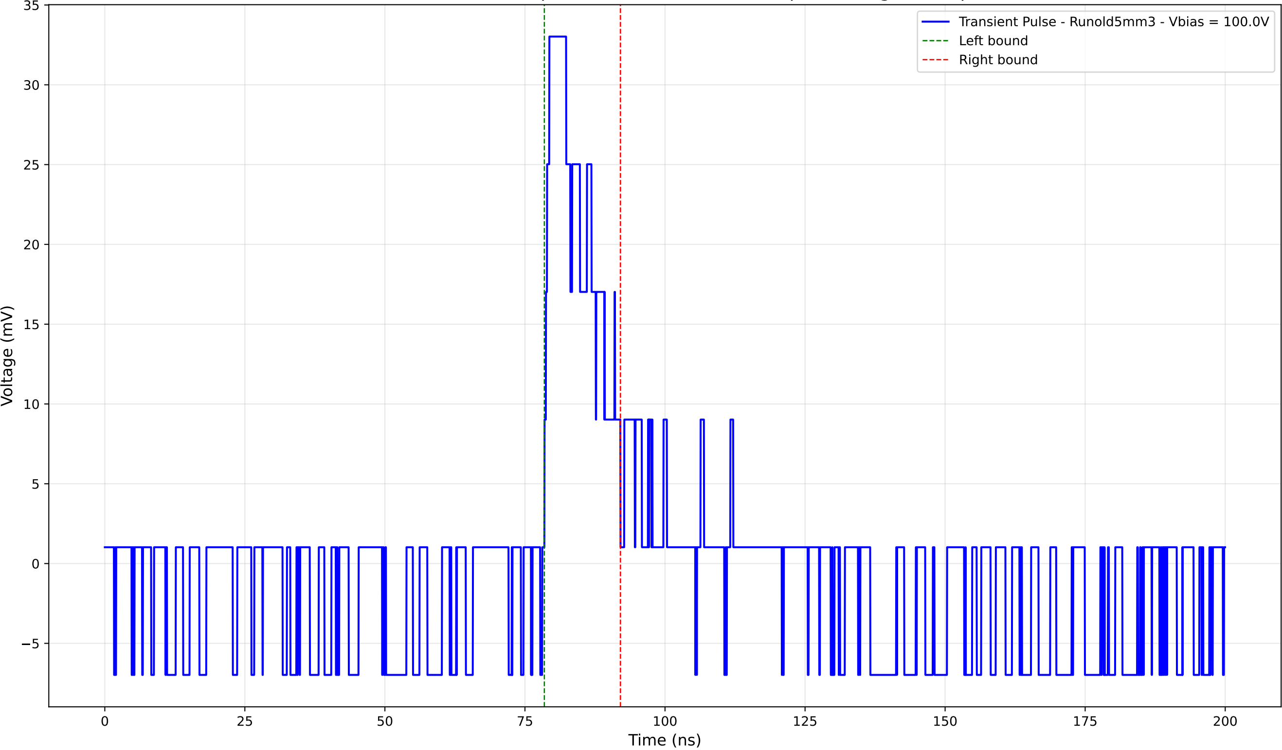
Transient Pulse - Sample: old5 - Position: 4160.0 \mu\text{m} - Charge: 5.63 pC
