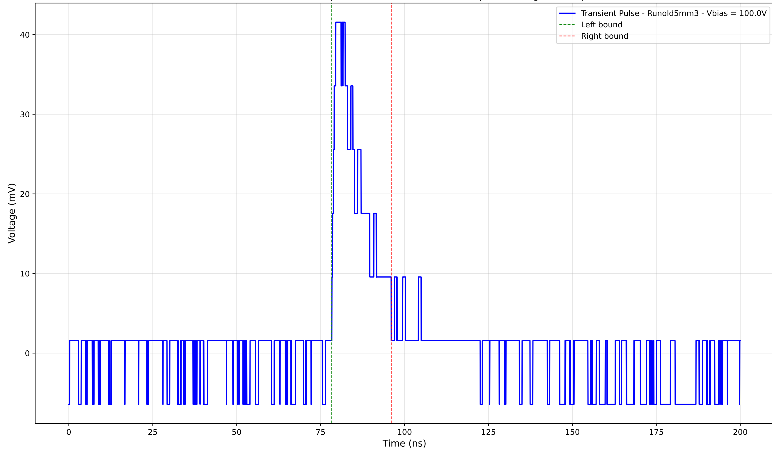
Transient Pulse - Sample: old5 - Position: 4155.0 \mu\text{m} - Charge: 7.58 pC
