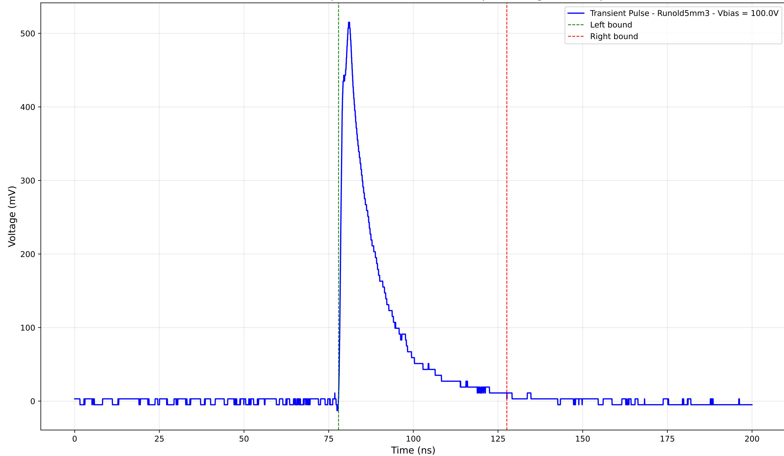
Transient Pulse - Sample: old5 - Position: 4050.0 \mu\text{m} - Charge: 112.94 pC
