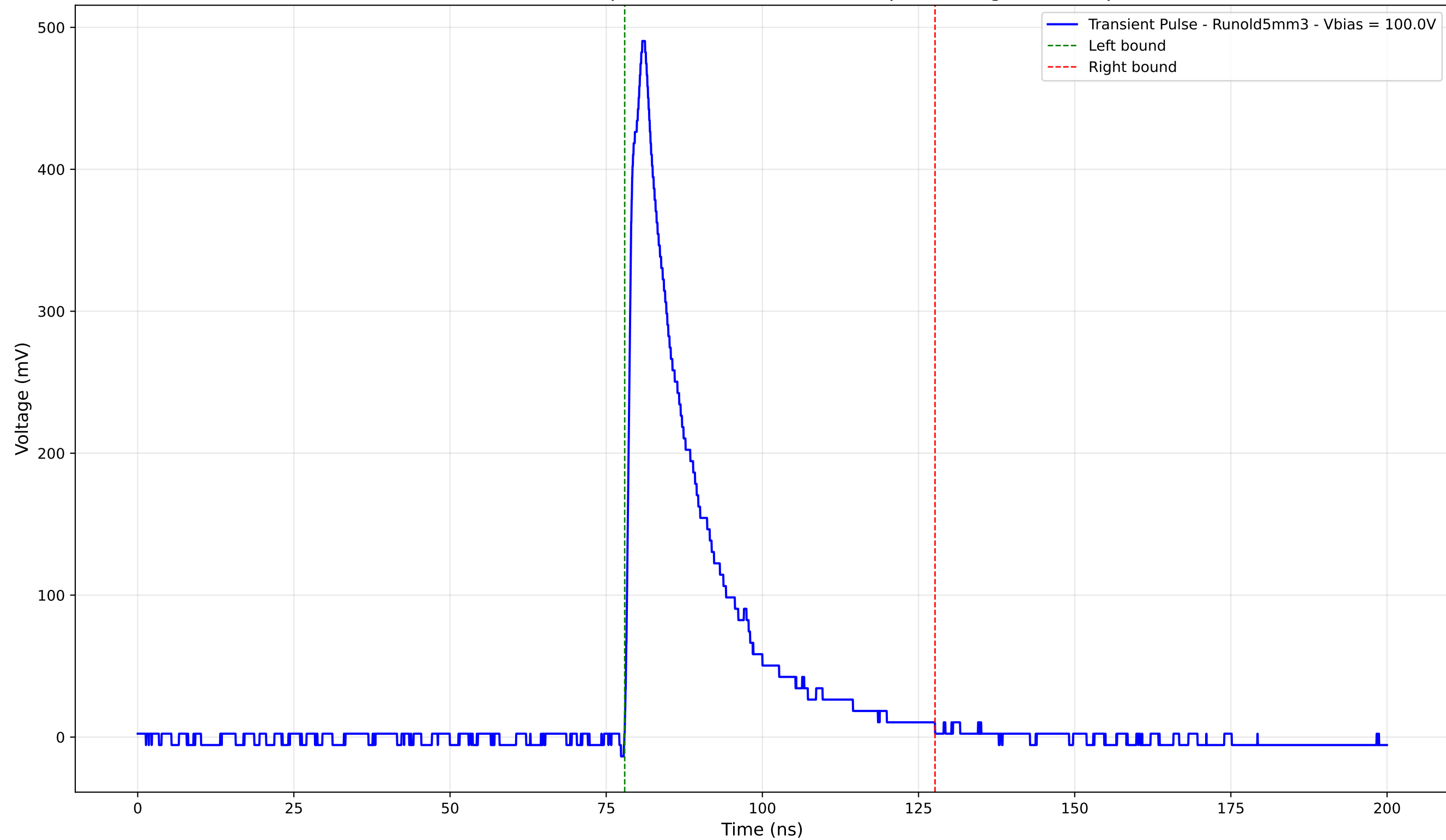
Transient Pulse - Sample: old5 - Position: 4065.0 \mu\text{m} - Charge: 107.54 pC
