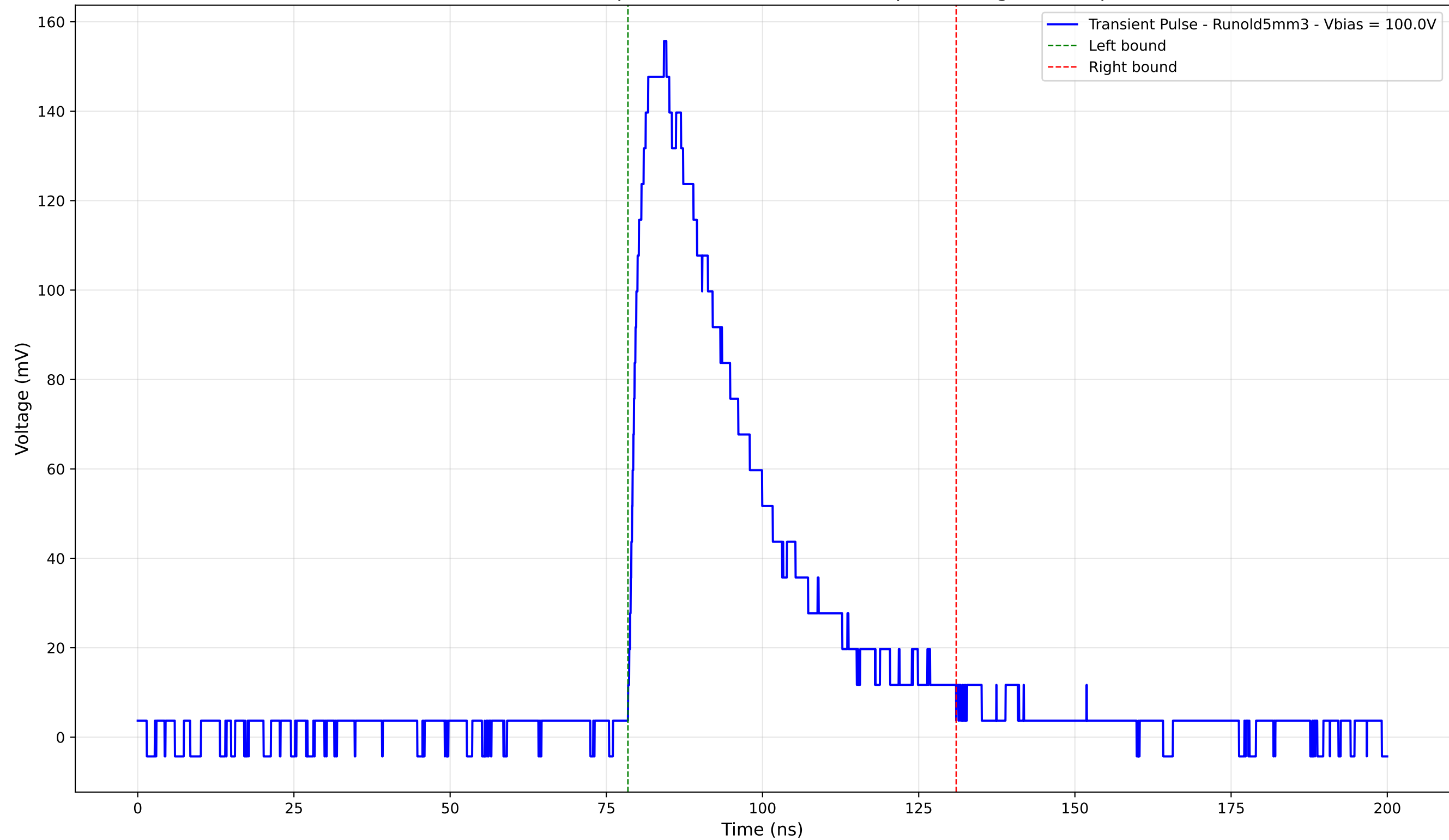
Transient Pulse - Sample: old5 - Position: 2245.0 \mu\text{m} - Charge: 59.34 pC
