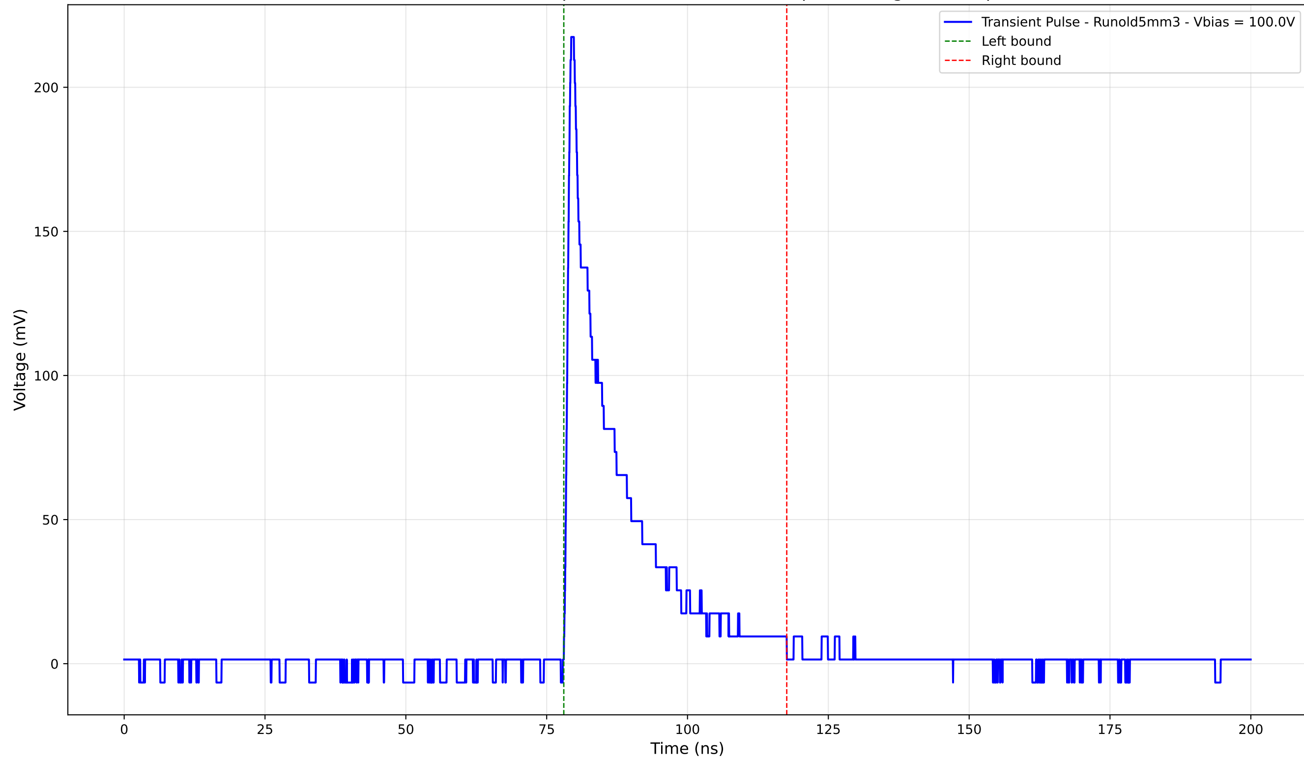
Transient Pulse - Sample: old5 - Position: 390.0 \mu\text{m} - Charge: 37.24 pC
