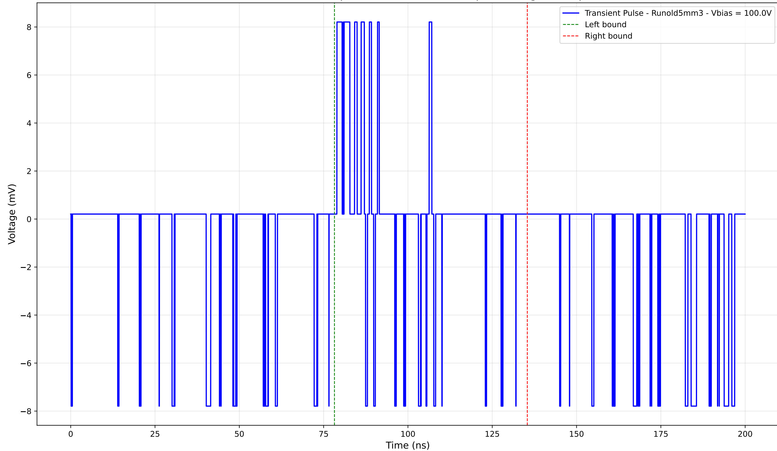
Transient Pulse - Sample: old5 - Position: 85.0 \mu\text{m} - Charge: 0.73 pC
