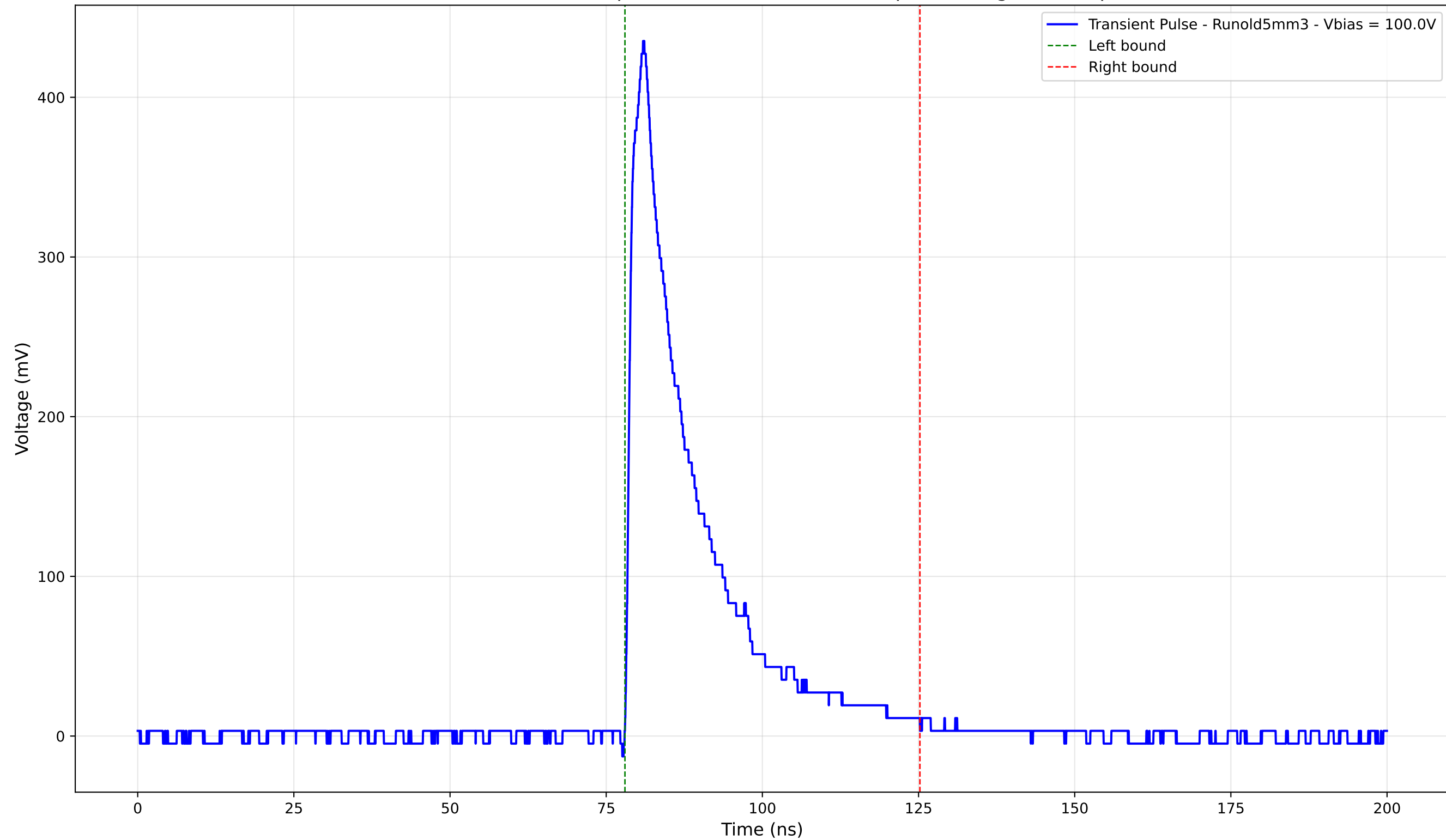
Transient Pulse - Sample: old5 - Position: 4085.0 \mu\text{m} - Charge: 94.95 pC
