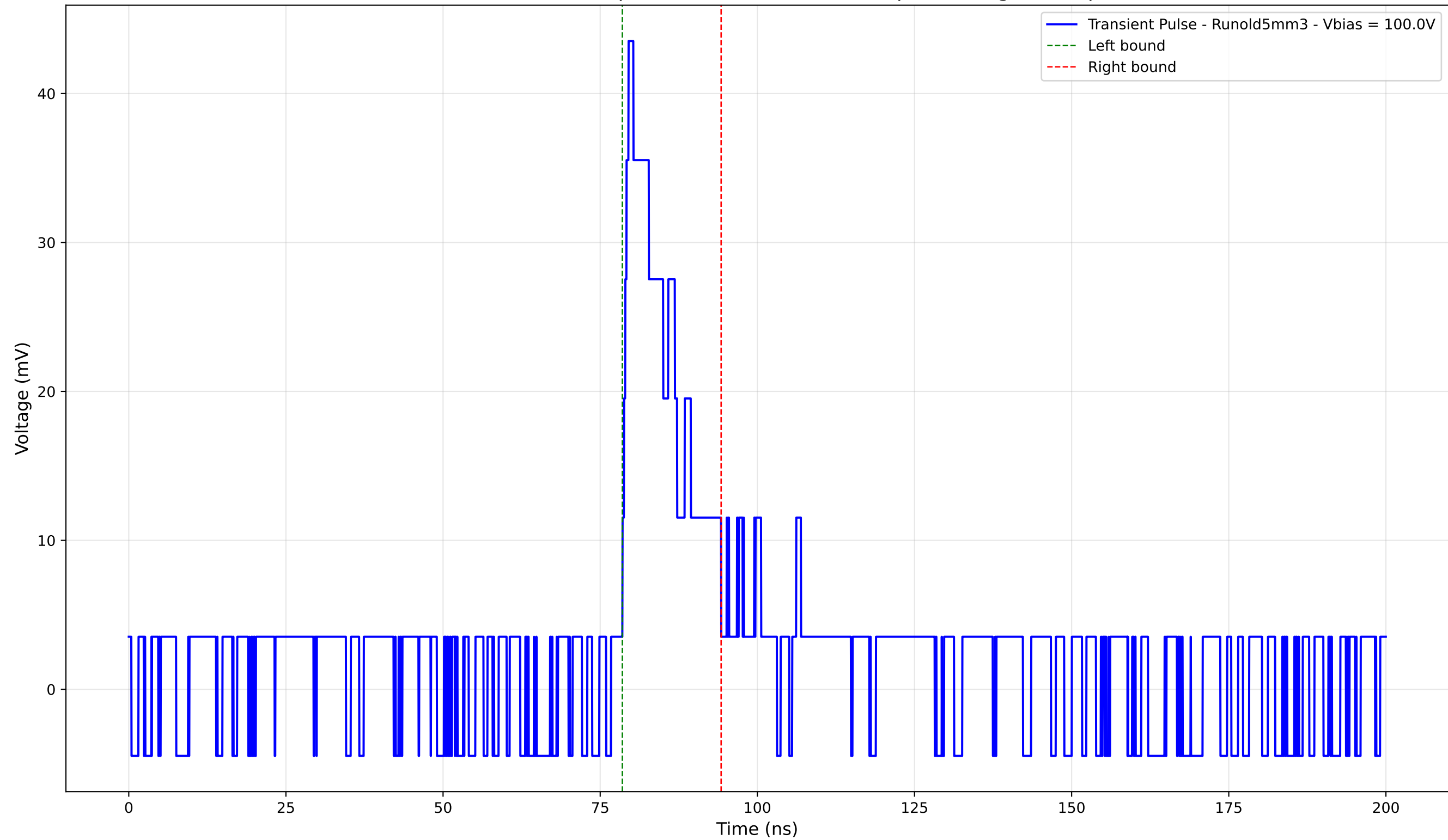
Transient Pulse - Sample: old5 - Position: 4475.0 \mu\text{m} - Charge: 6.96 pC
