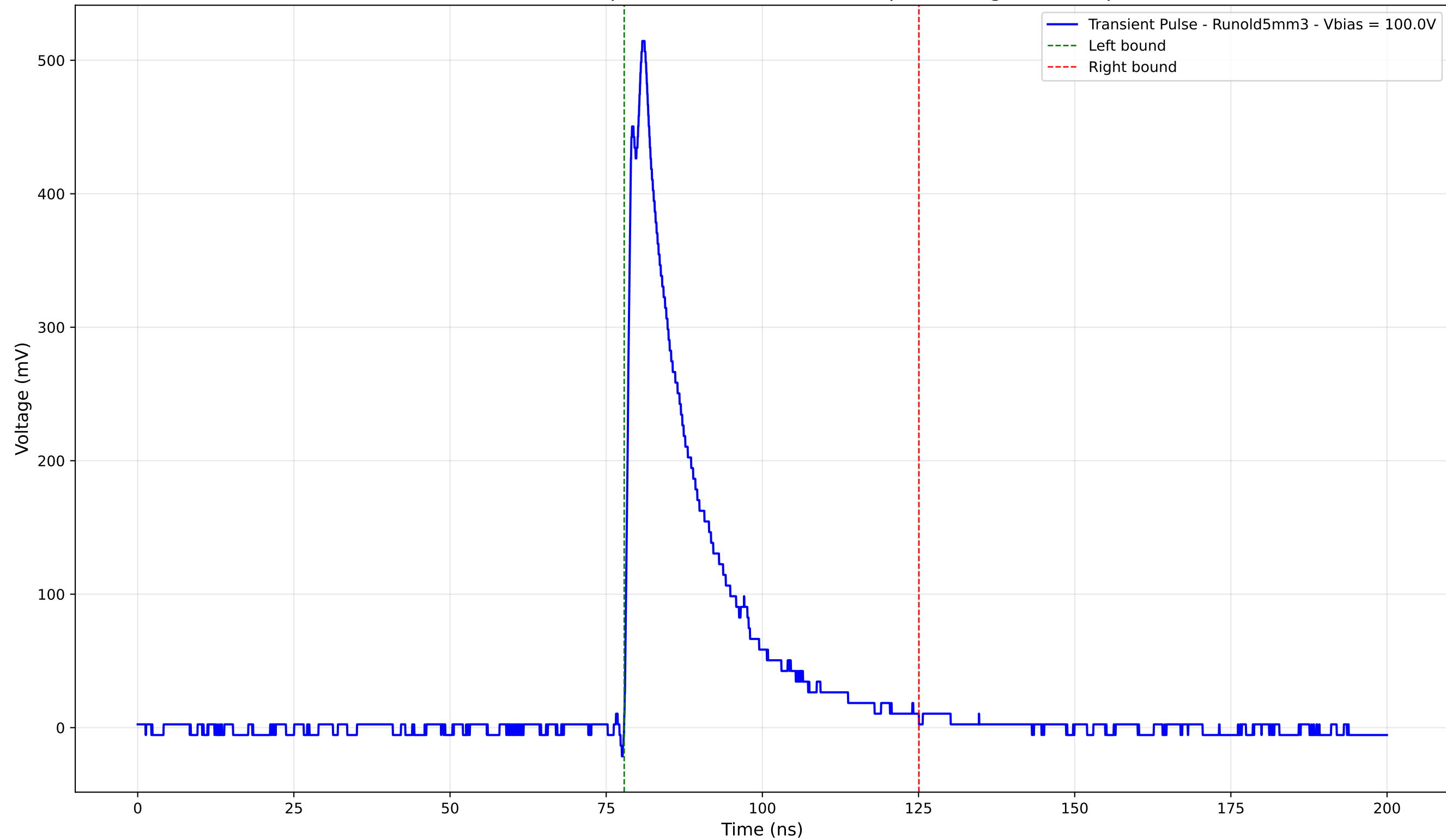
Transient Pulse - Sample: old5 - Position: 4015.0 \mu\text{m} - Charge: 111.65 pC
