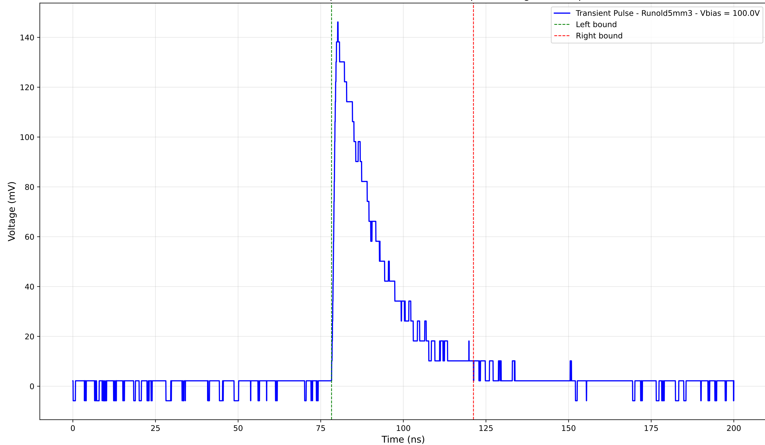
Transient Pulse - Sample: old5 - Position: 790.0 \mu\text{m} - Charge: 39.89 pC
