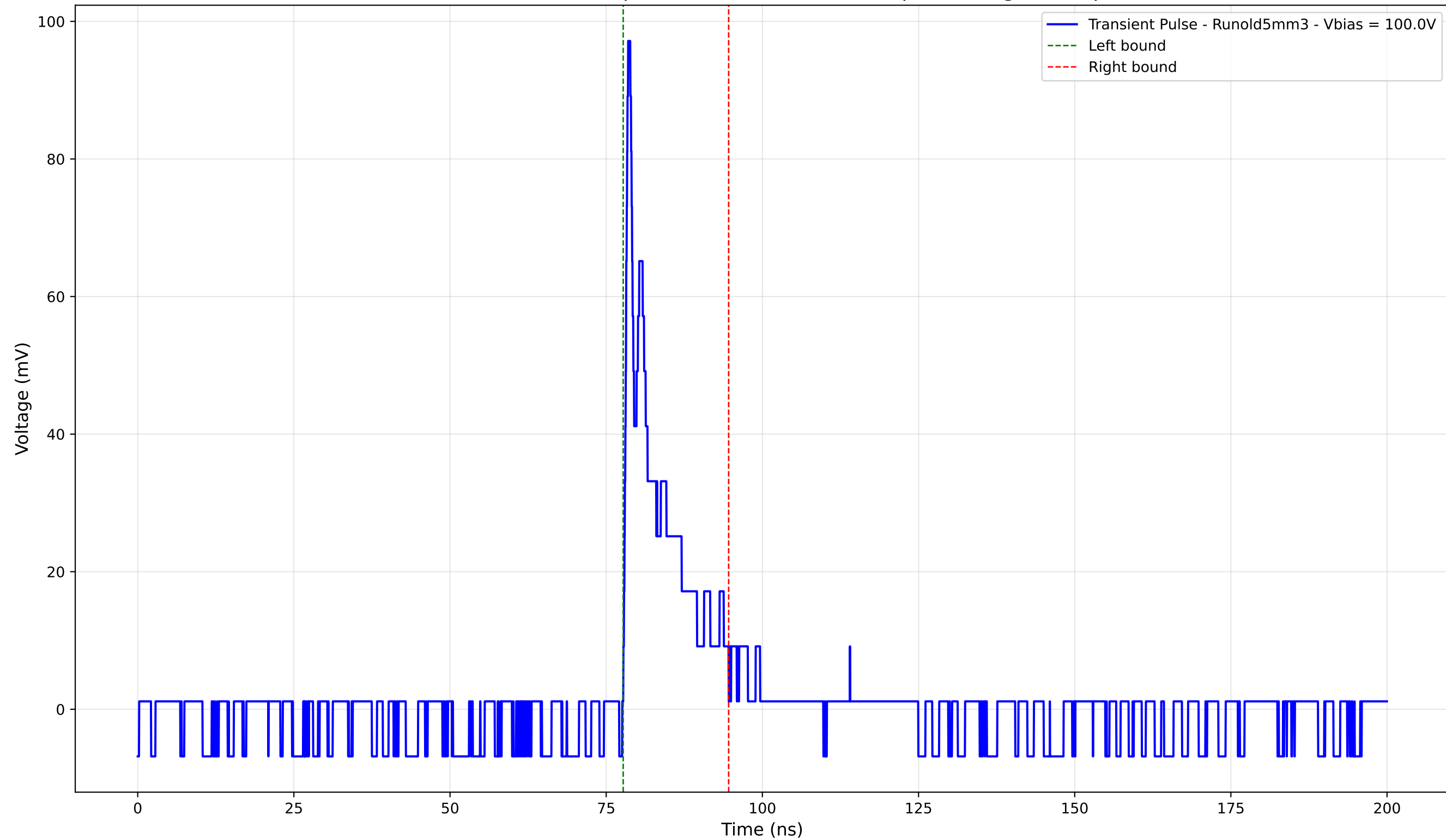
Transient Pulse - Sample: old5 - Position: 3550.0 \mu\text{m} - Charge: 9.66 pC
