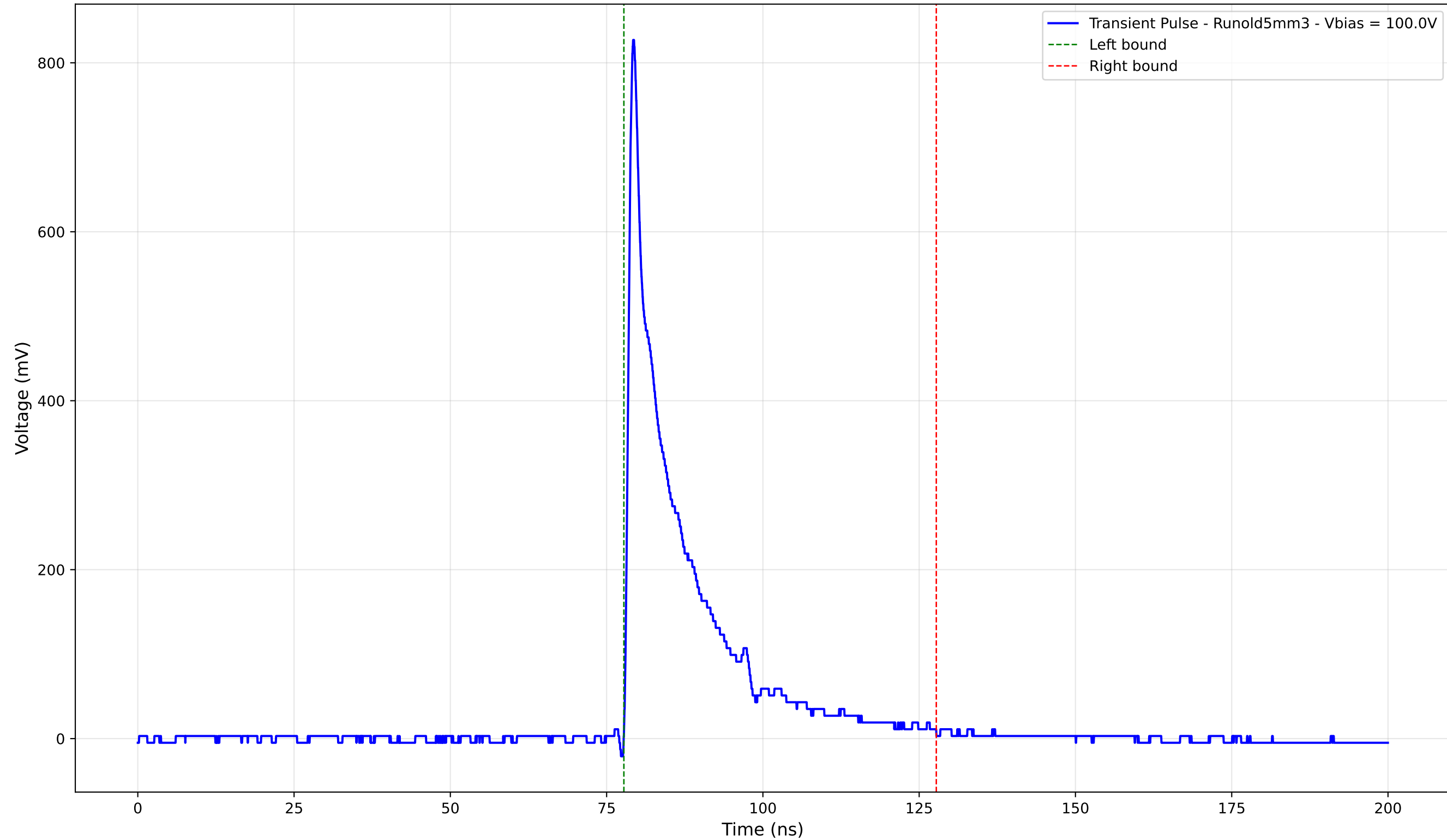
Transient Pulse - Sample: old5 - Position: 4810.0 \mu\text{m} - Charge: 128.68 pC
