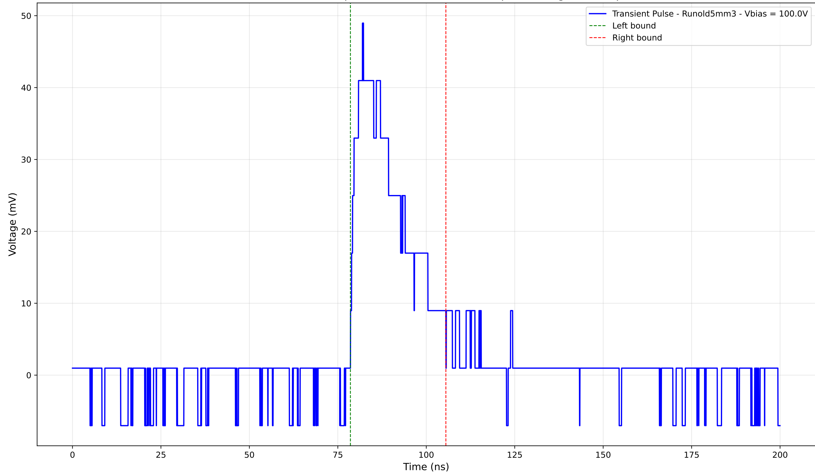
Transient Pulse - Sample: old5 - Position: 2710.0 \mu\text{m} - Charge: 13.03 pC
