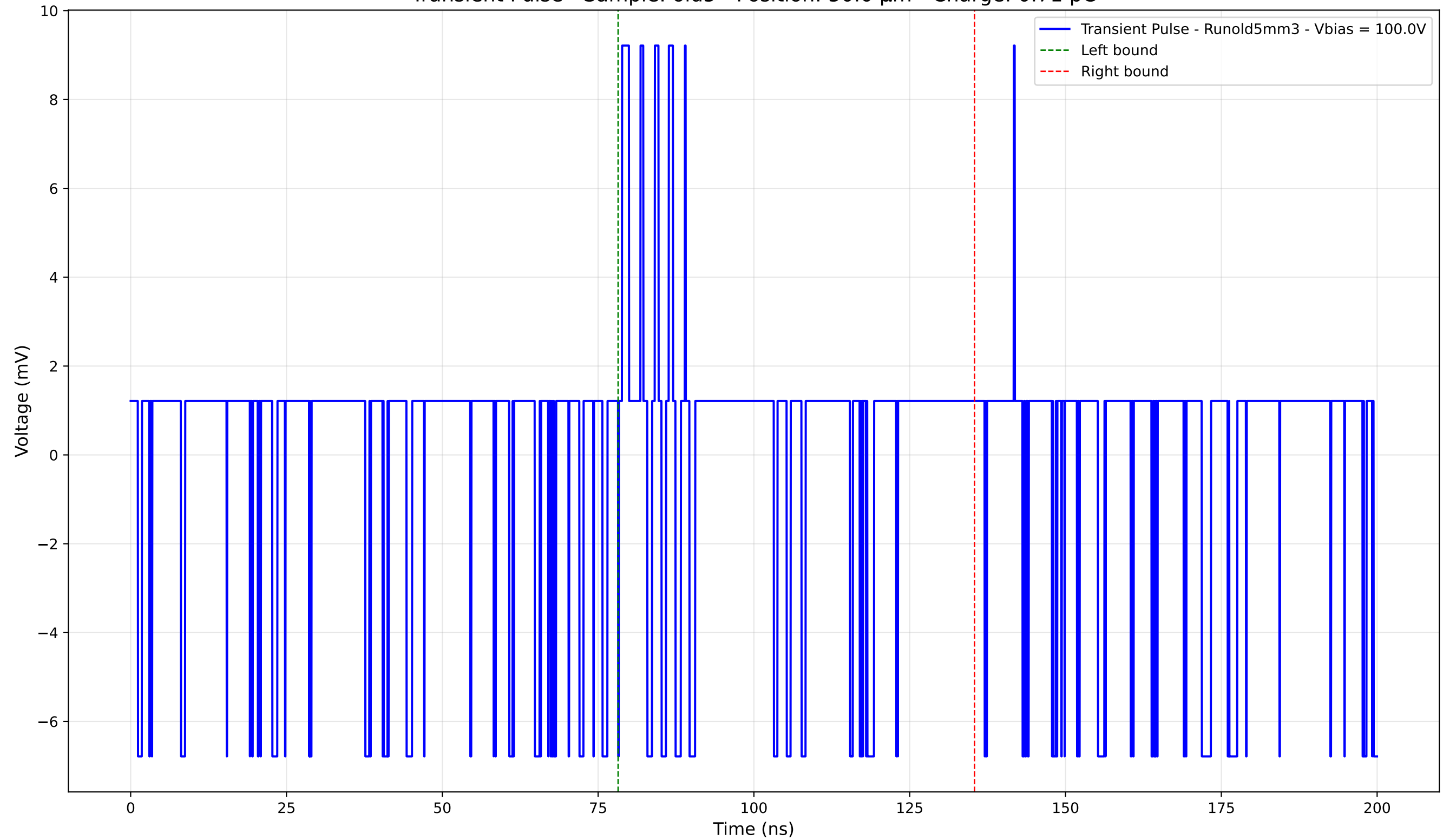
Transient Pulse - Sample: old5 - Position: 50.0 \mu\text{m} - Charge: 0.71 pC
