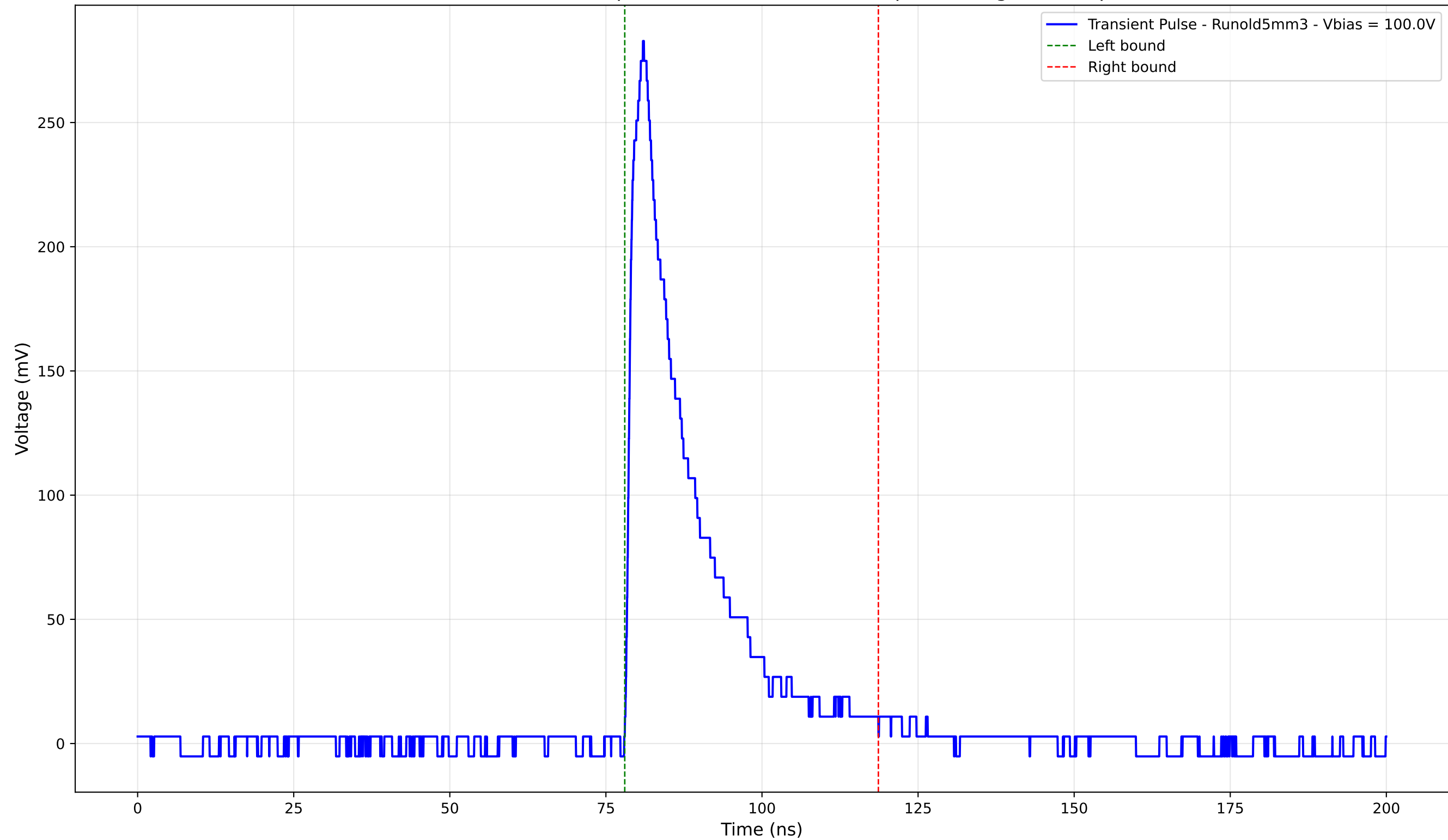
Transient Pulse - Sample: old5 - Position: 4110.0 \mu\text{m} - Charge: 59.22 pC
