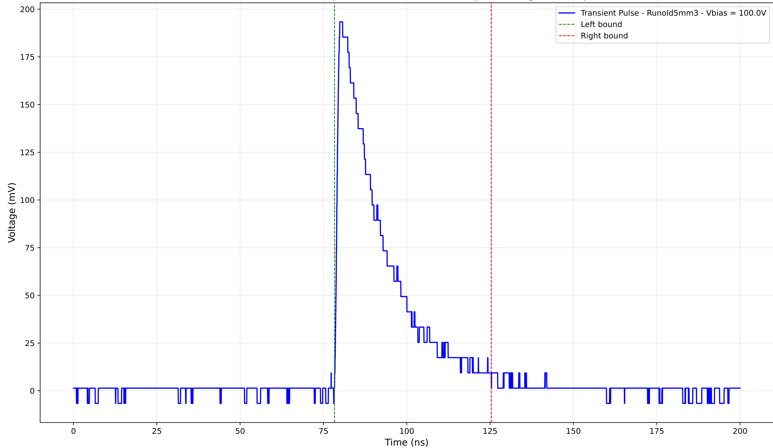
Transient Pulse - Sample: old5 - Position: 855.0 \mu\text{m} - Charge: 57.68 pC
