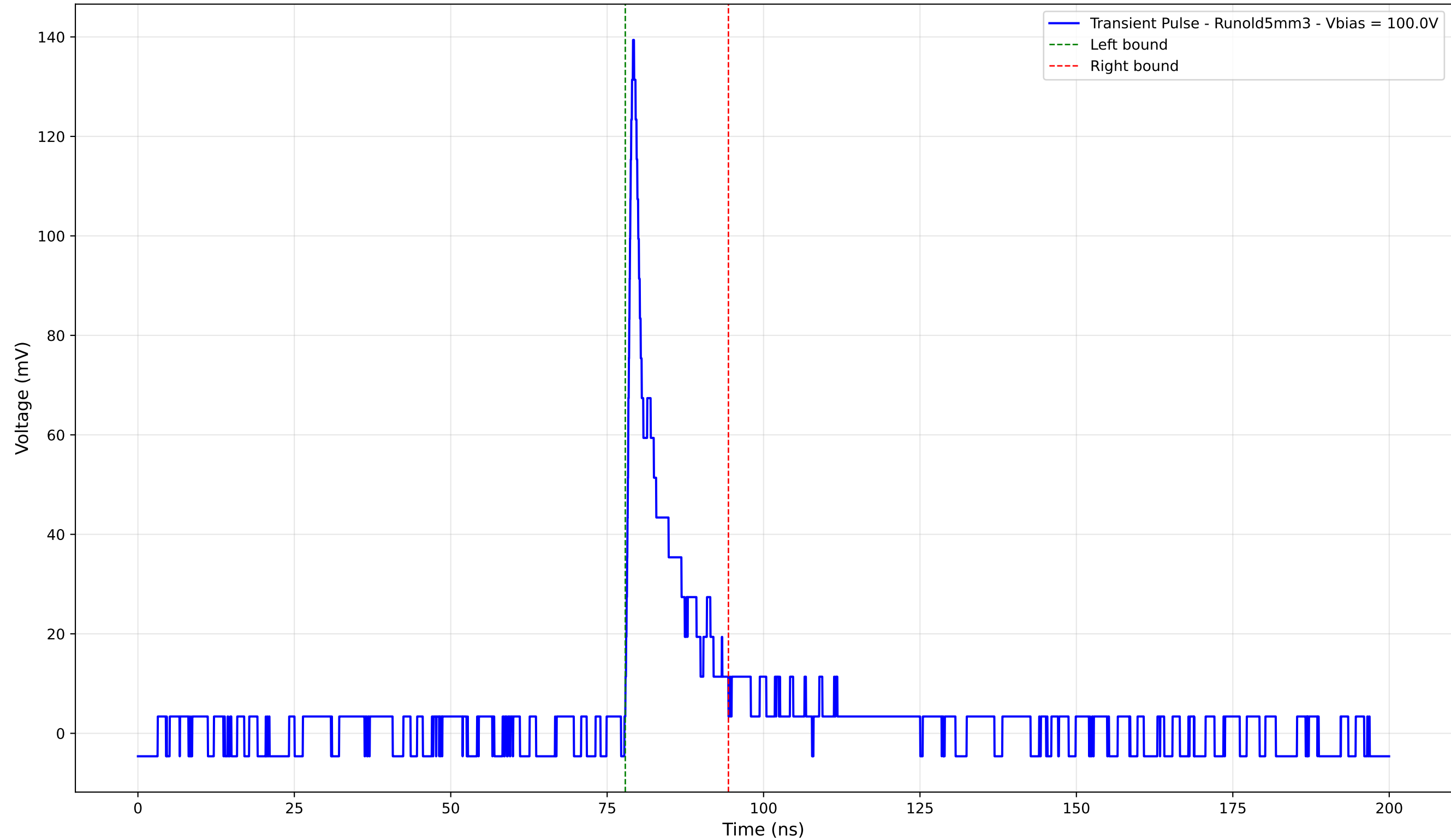
Transient Pulse - Sample: old5 - Position: 4915.0 \mu\text{m} - Charge: 13.80 pC
