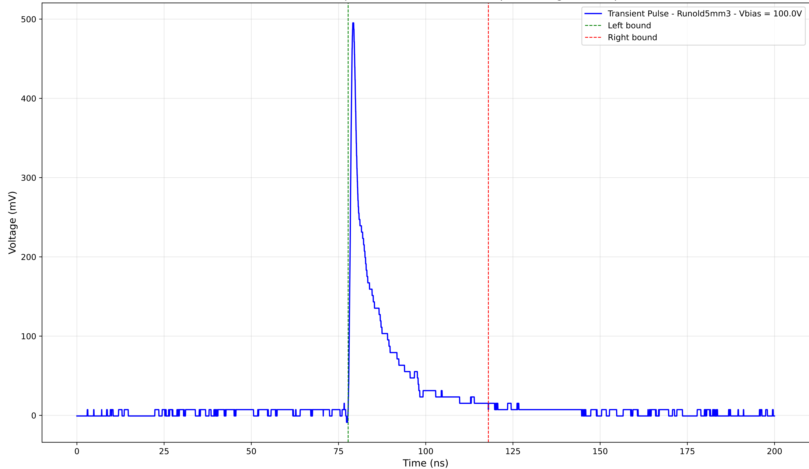
Transient Pulse - Sample: old5 - Position: 4880.0 \mu\text{m} - Charge: 66.19 pC
