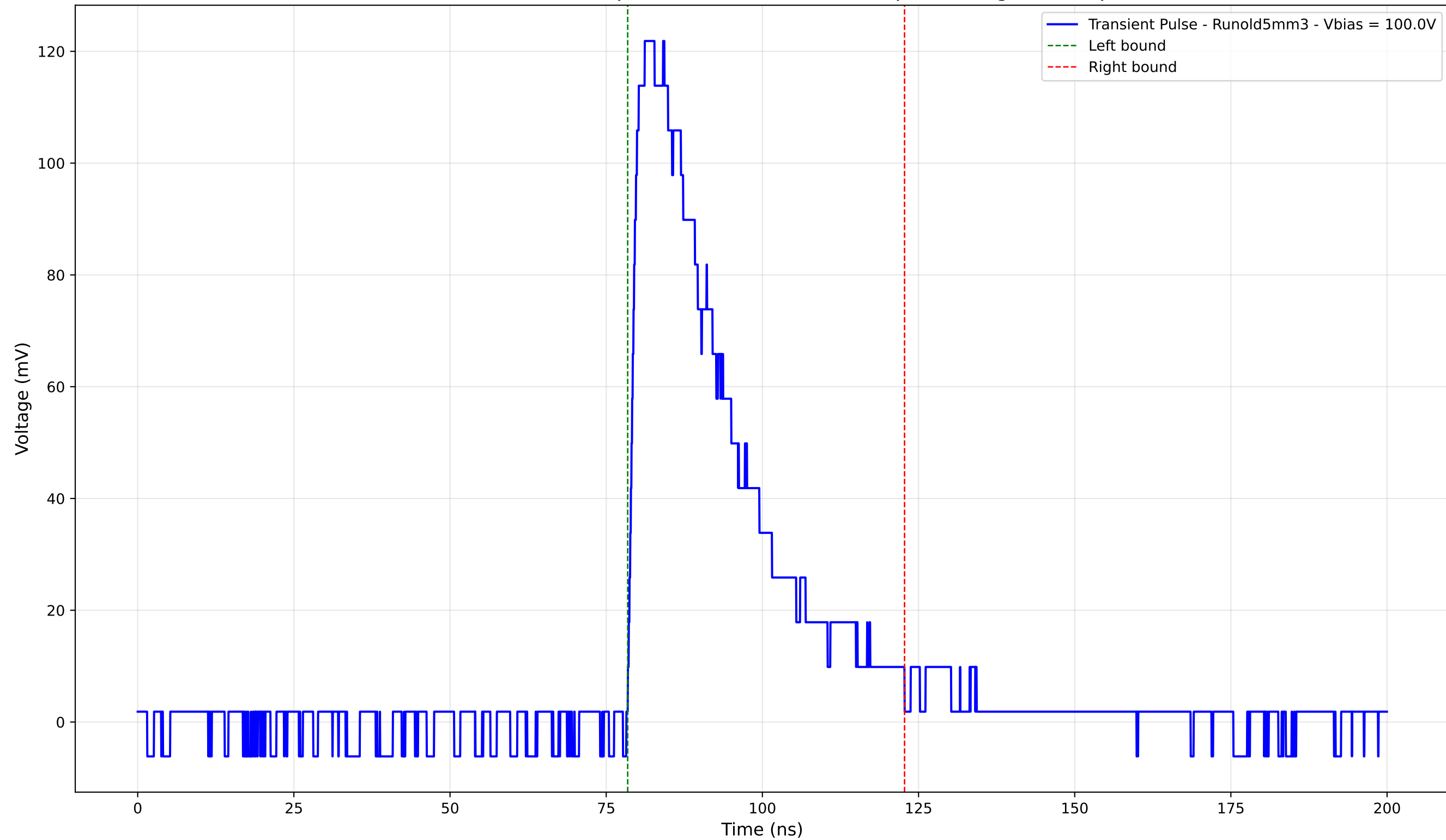
Transient Pulse - Sample: old5 - Position: 1135.0 \mu\text{m} - Charge: 41.97 pC
