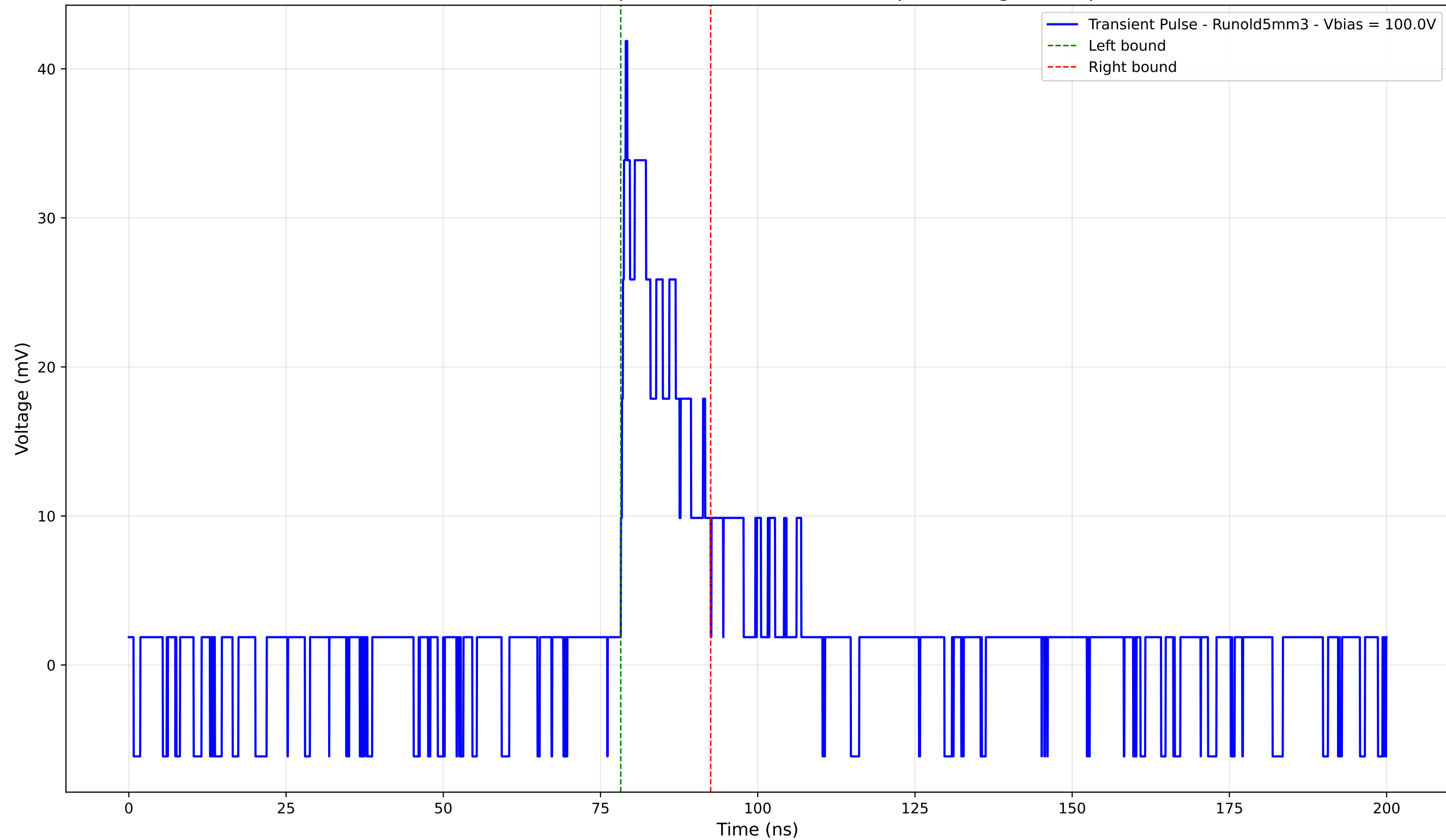
Transient Pulse - Sample: old5 - Position: 3255.0 \mu\text{m} - Charge: 6.13 pC
