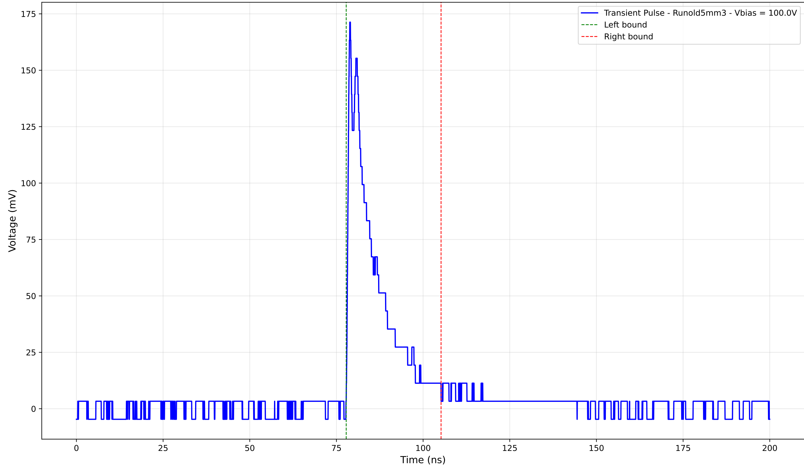
Transient Pulse - Sample: old5 - Position: 3835.0 \mu\text{m} - Charge: 27.59 pC
