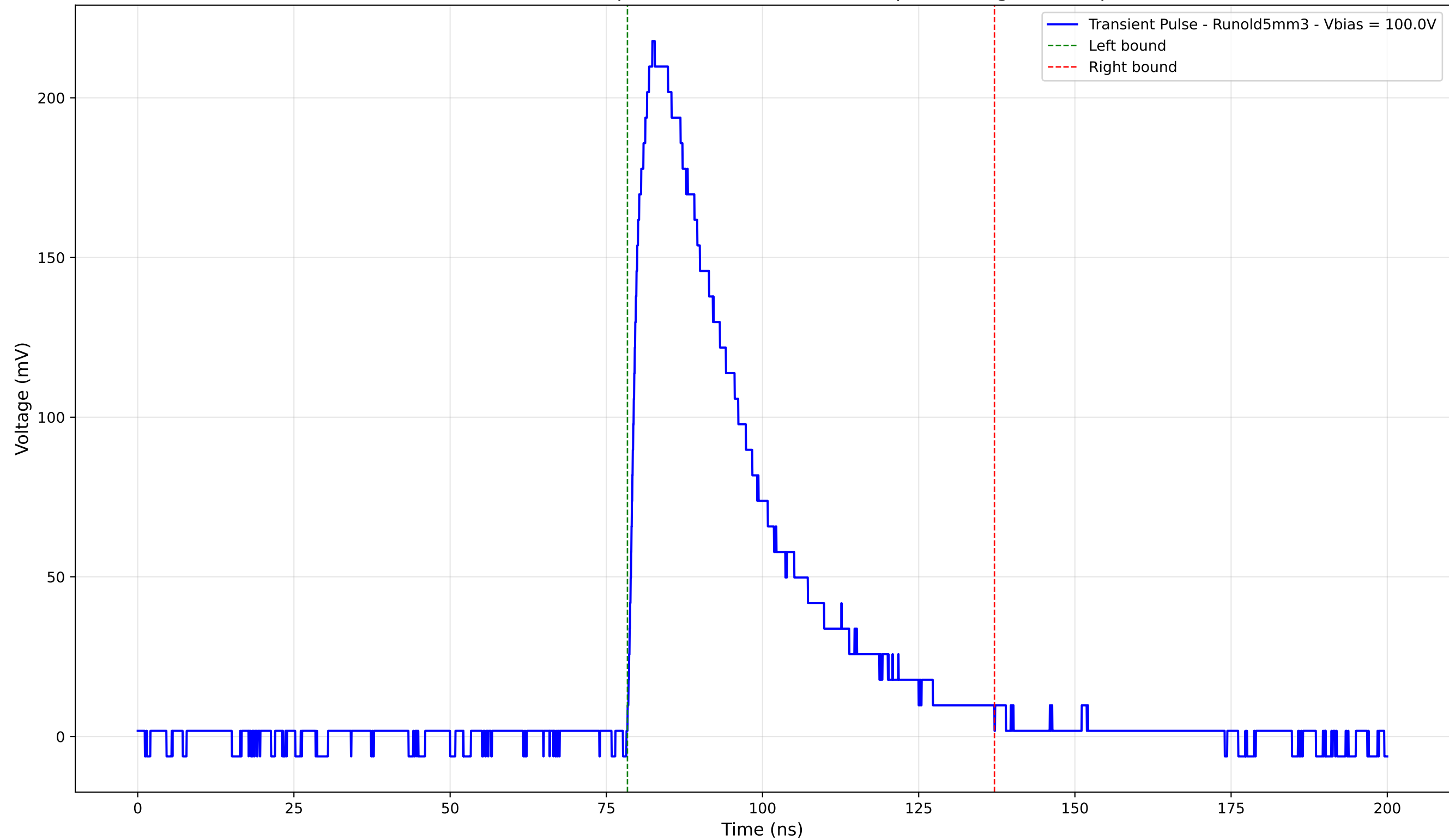
Transient Pulse - Sample: old5 - Position: 2320.0 \mu\text{m} - Charge: 83.90 pC
