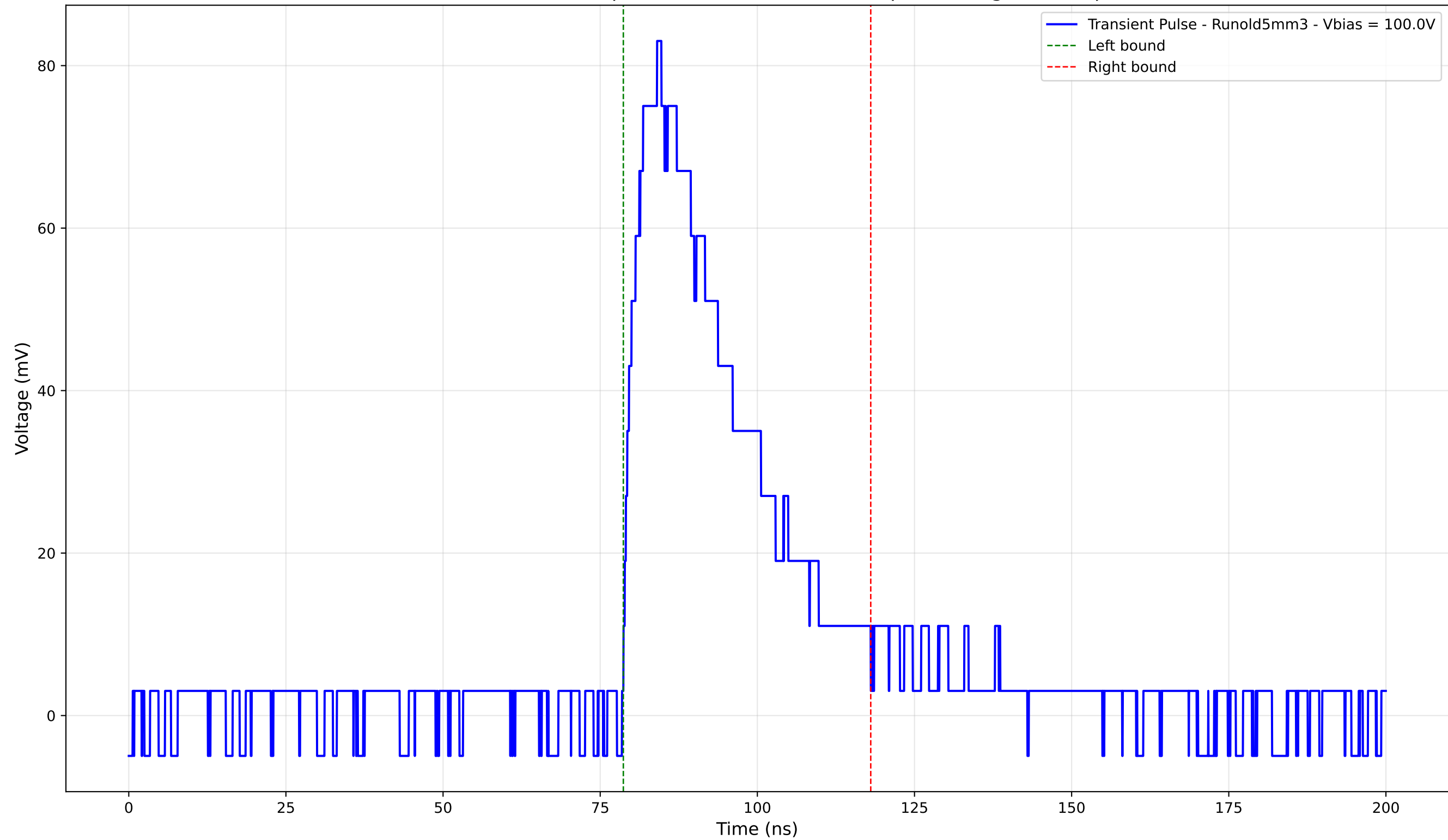
Transient Pulse - Sample: old5 - Position: 1820.0 \mu\text{m} - Charge: 29.68 pC
