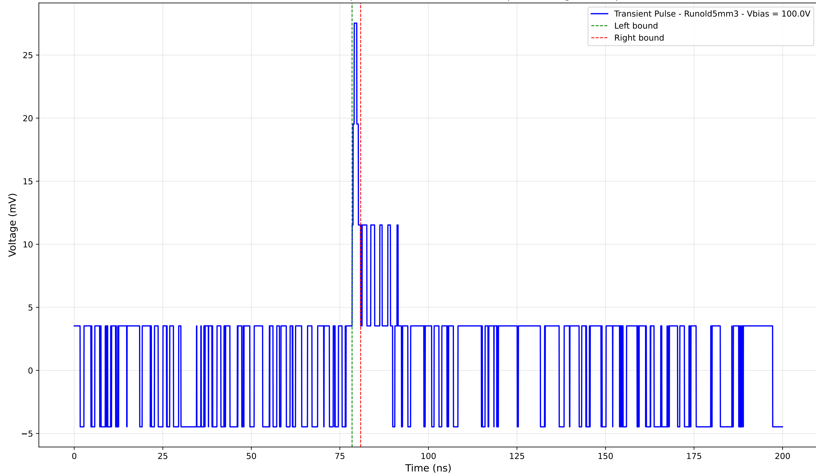
Transient Pulse - Sample: old5 - Position: 4950.0 \mu\text{m} - Charge: 0.91 pC
