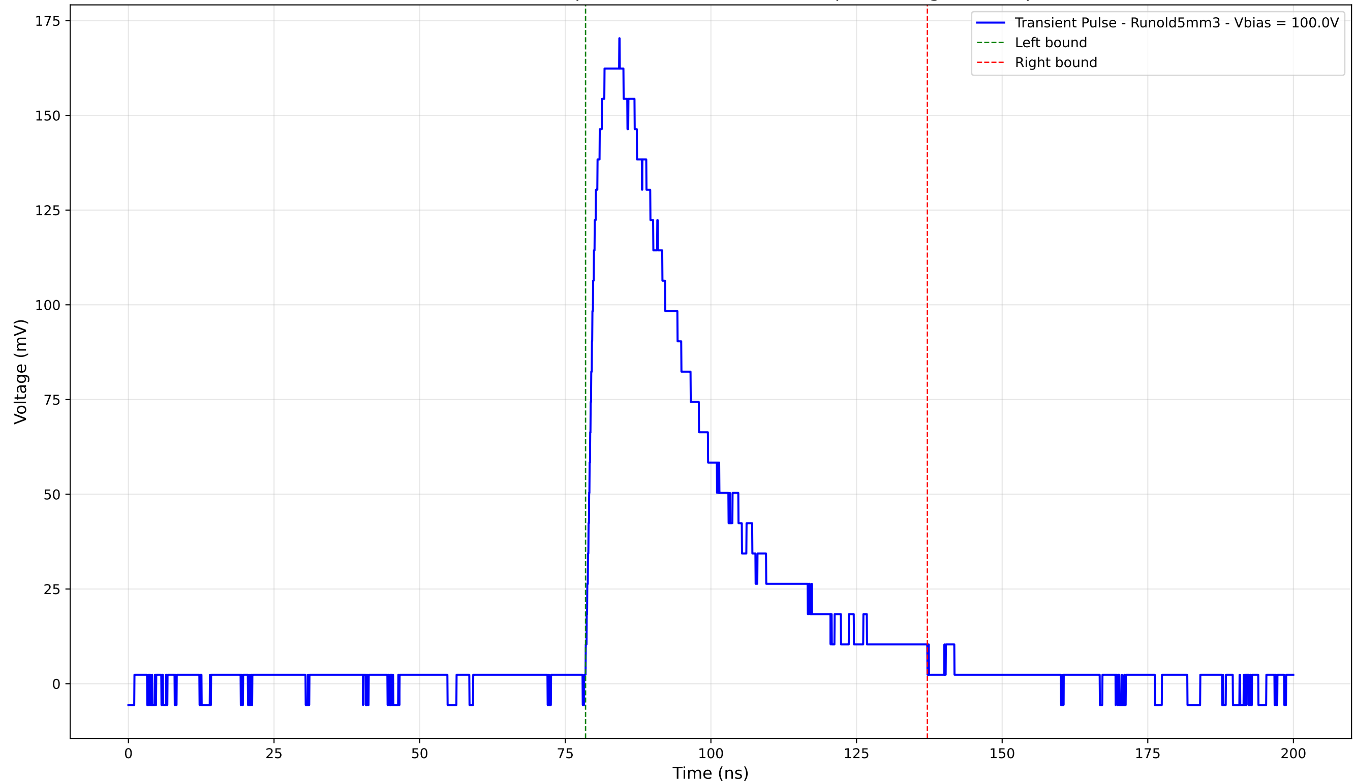
Transient Pulse - Sample: old5 - Position: 1520.0 \mu\text{m} - Charge: 66.65 pC
