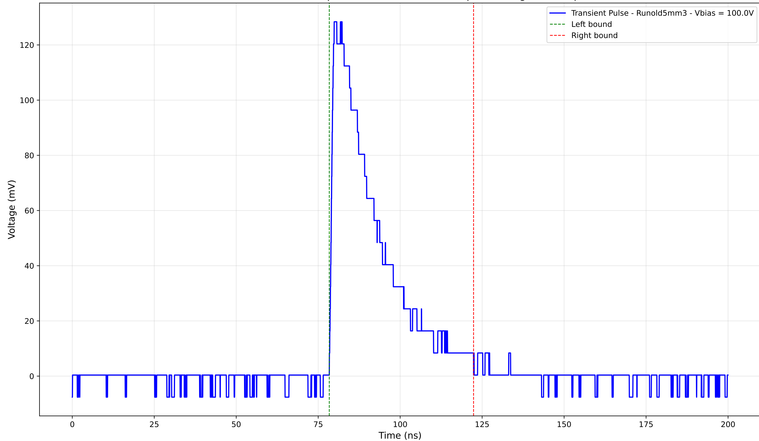
Transient Pulse - Sample: old5 - Position: 890.0 \mu\text{m} - Charge: 38.79 pC
