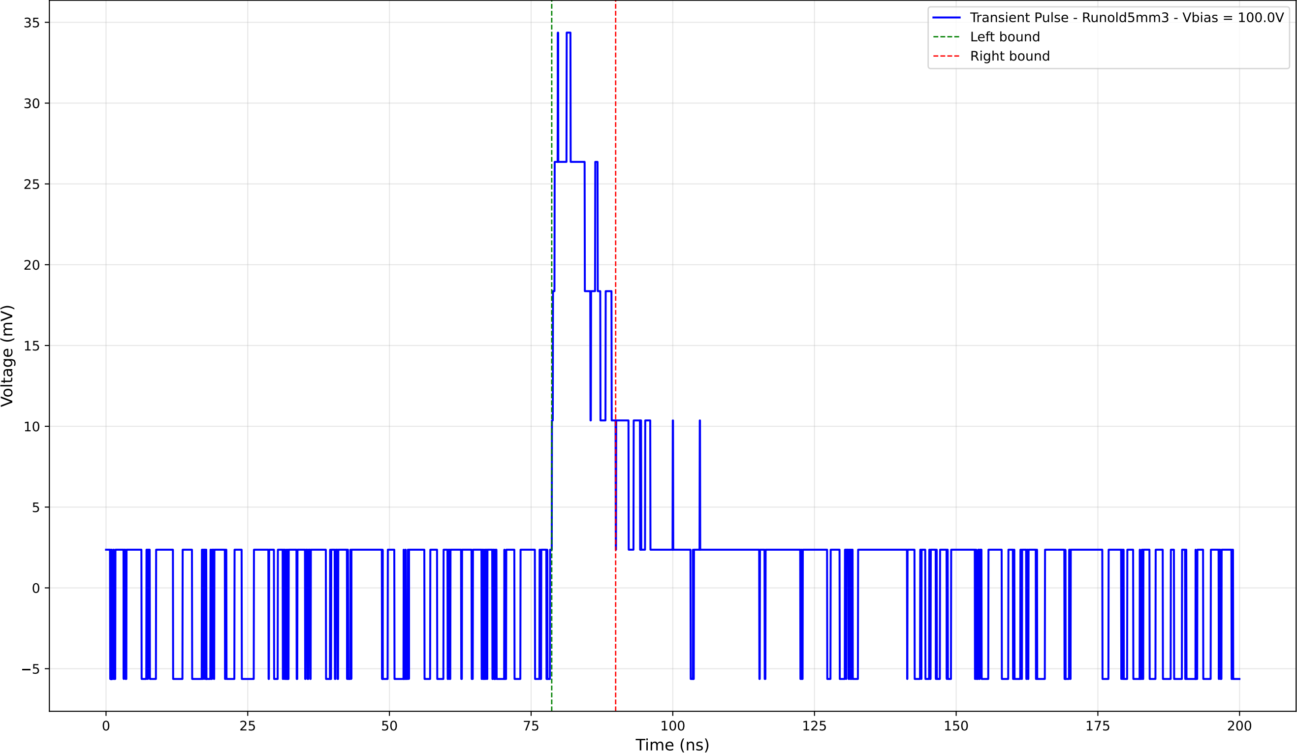
Transient Pulse - Sample: old5 - Position: 4490.0 \mu\text{m} - Charge: 4.88 pC
