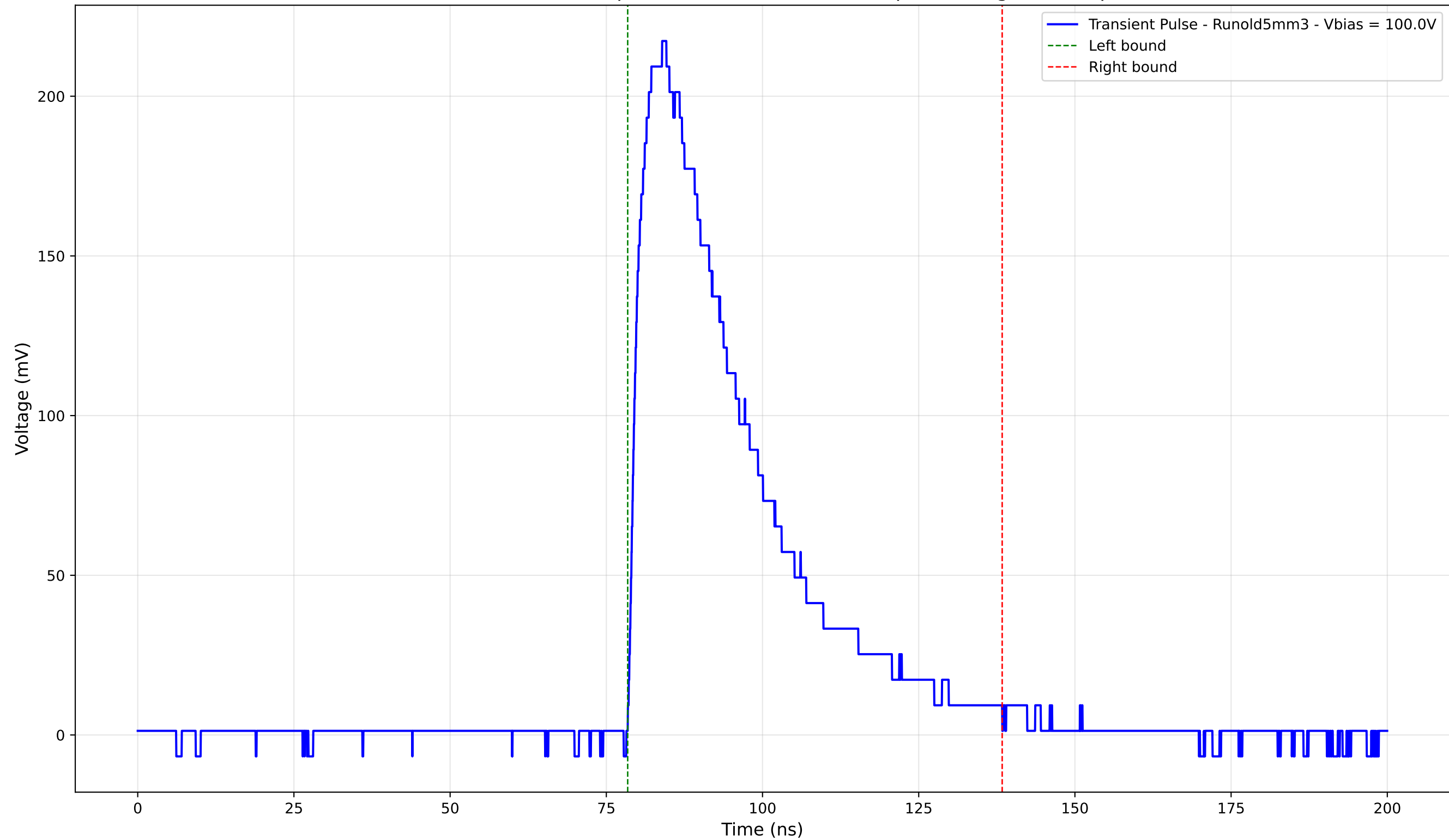
Transient Pulse - Sample: old5 - Position: 1900.0 \mu\text{m} - Charge: 85.60 pC
