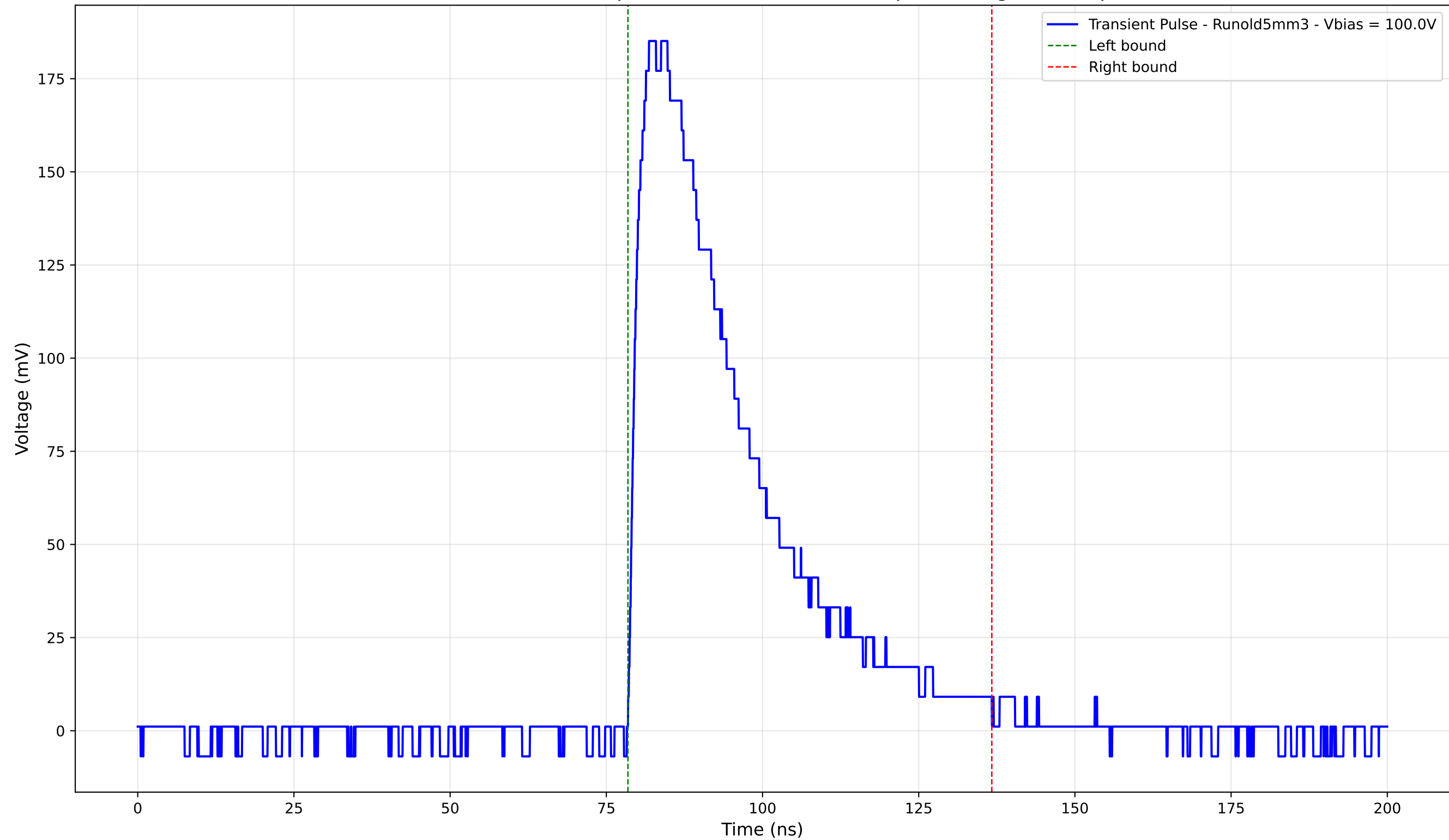
Transient Pulse - Sample: old5 - Position: 1460.0 \mu\text{m} - Charge: 73.25 pC
