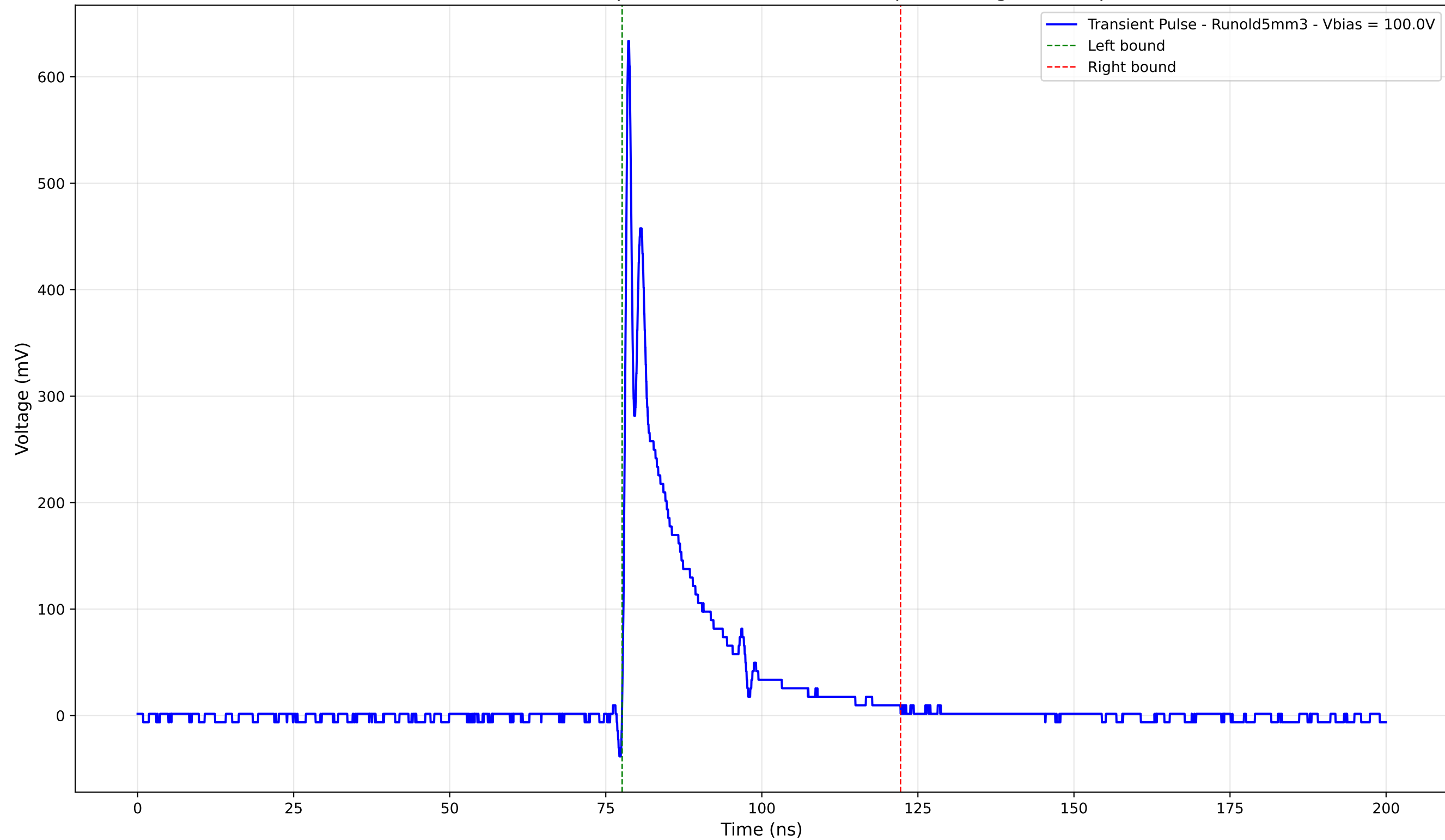
Transient Pulse - Sample: old5 - Position: 3490.0 \mu\text{m} - Charge: 83.47 pC
