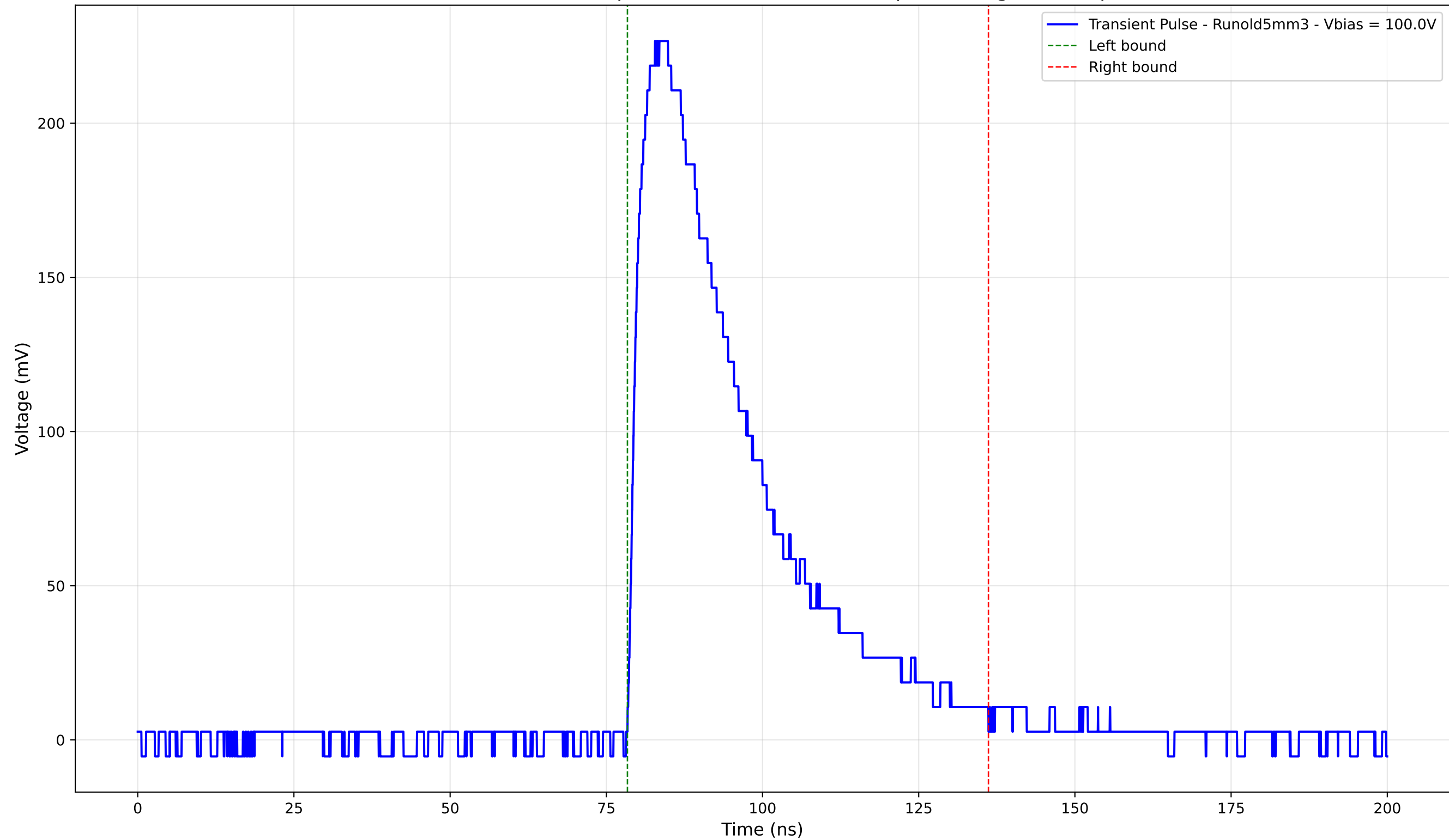
Transient Pulse - Sample: old5 - Position: 2095.0 \mu\text{m} - Charge: 91.71 pC
