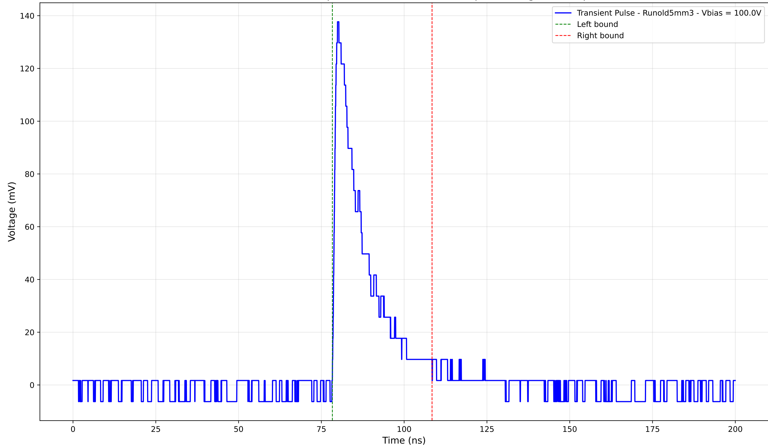
Transient Pulse - Sample: old5 - Position: 4445.0 \mu\text{m} - Charge: 26.04 pC
