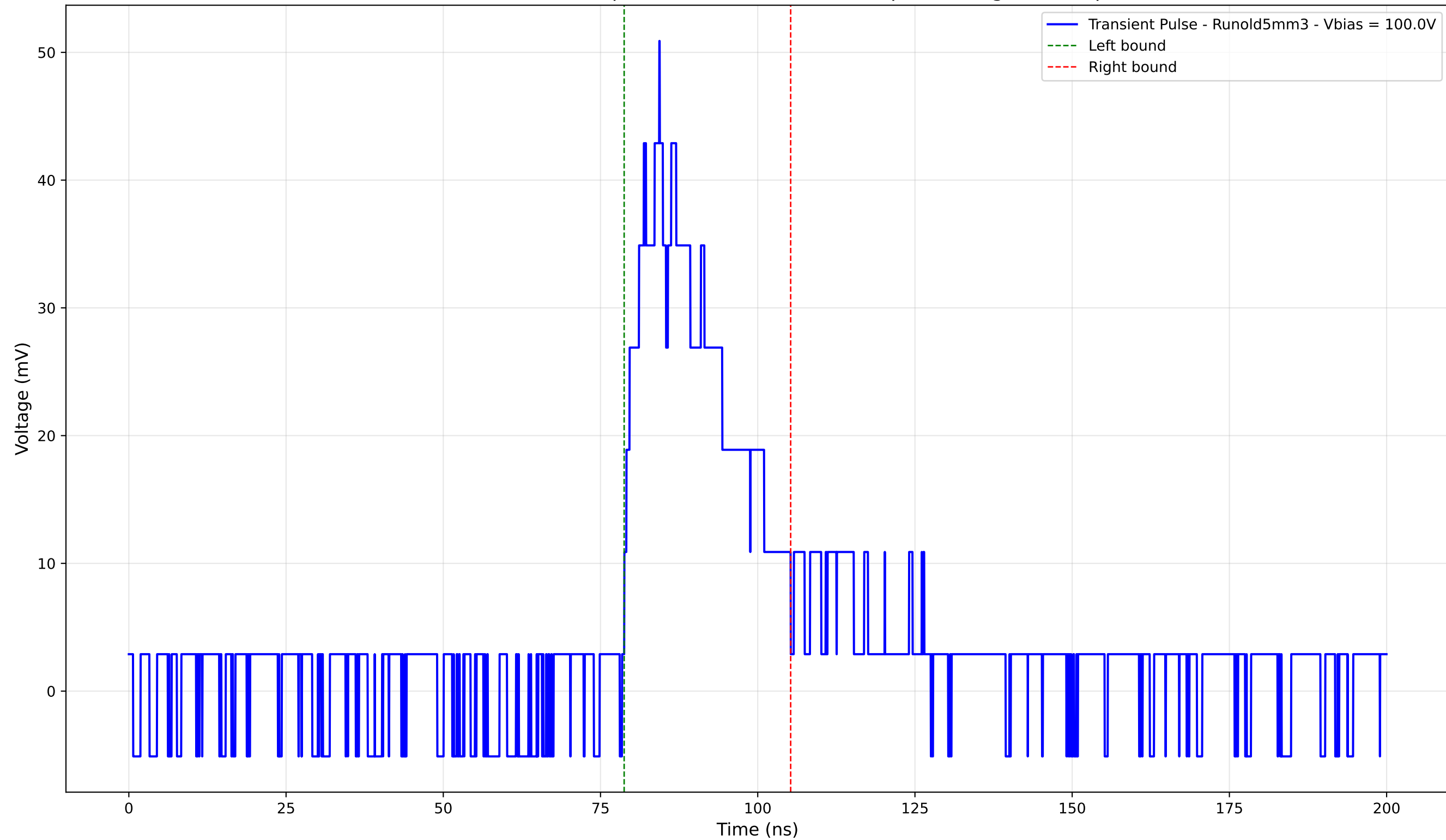
Transient Pulse - Sample: old5 - Position: 1400.0 \mu\text{m} - Charge: 13.36 pC
