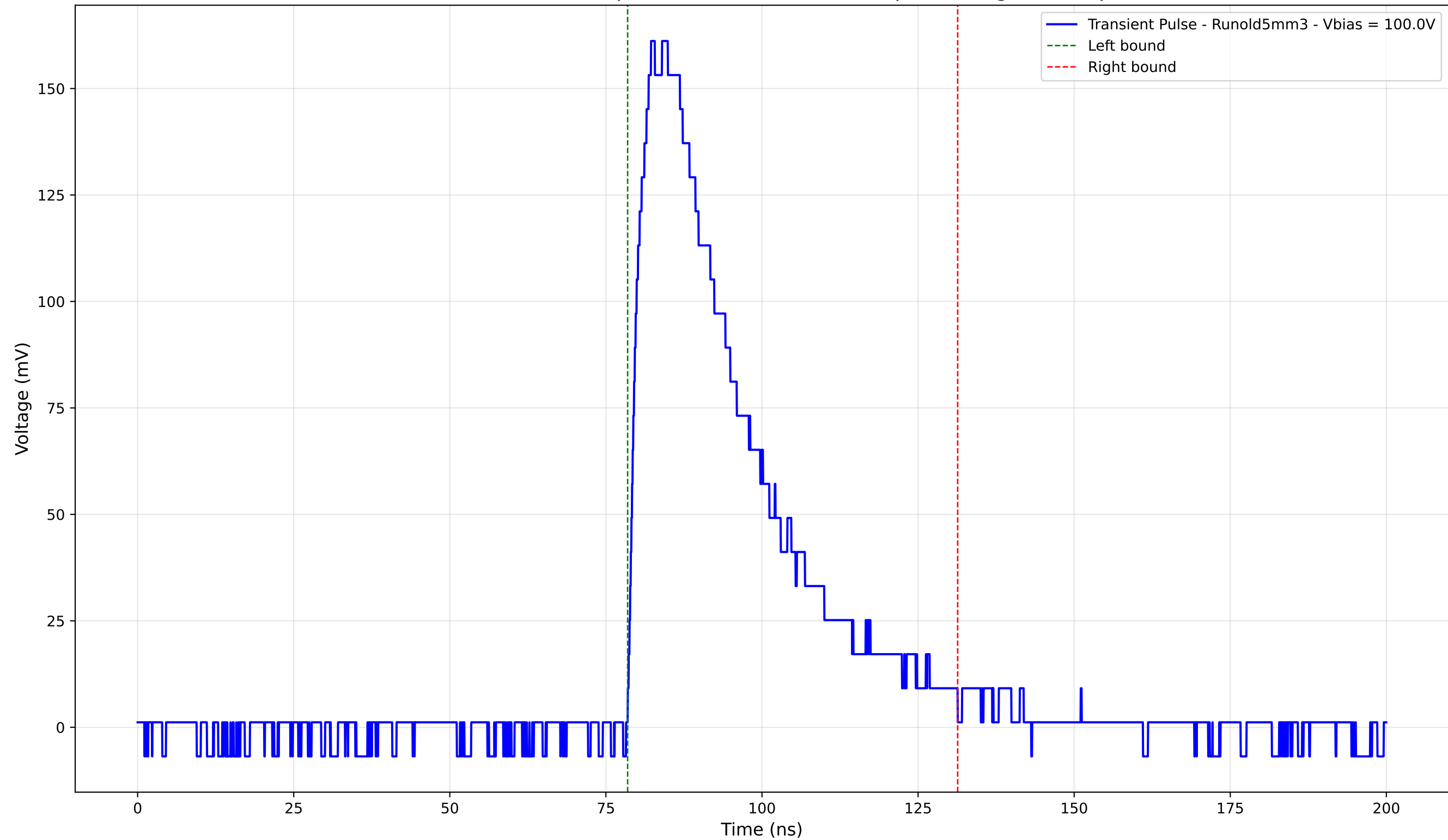
Transient Pulse - Sample: old5 - Position: 1850.0 \mu\text{m} - Charge: 63.27 pC
