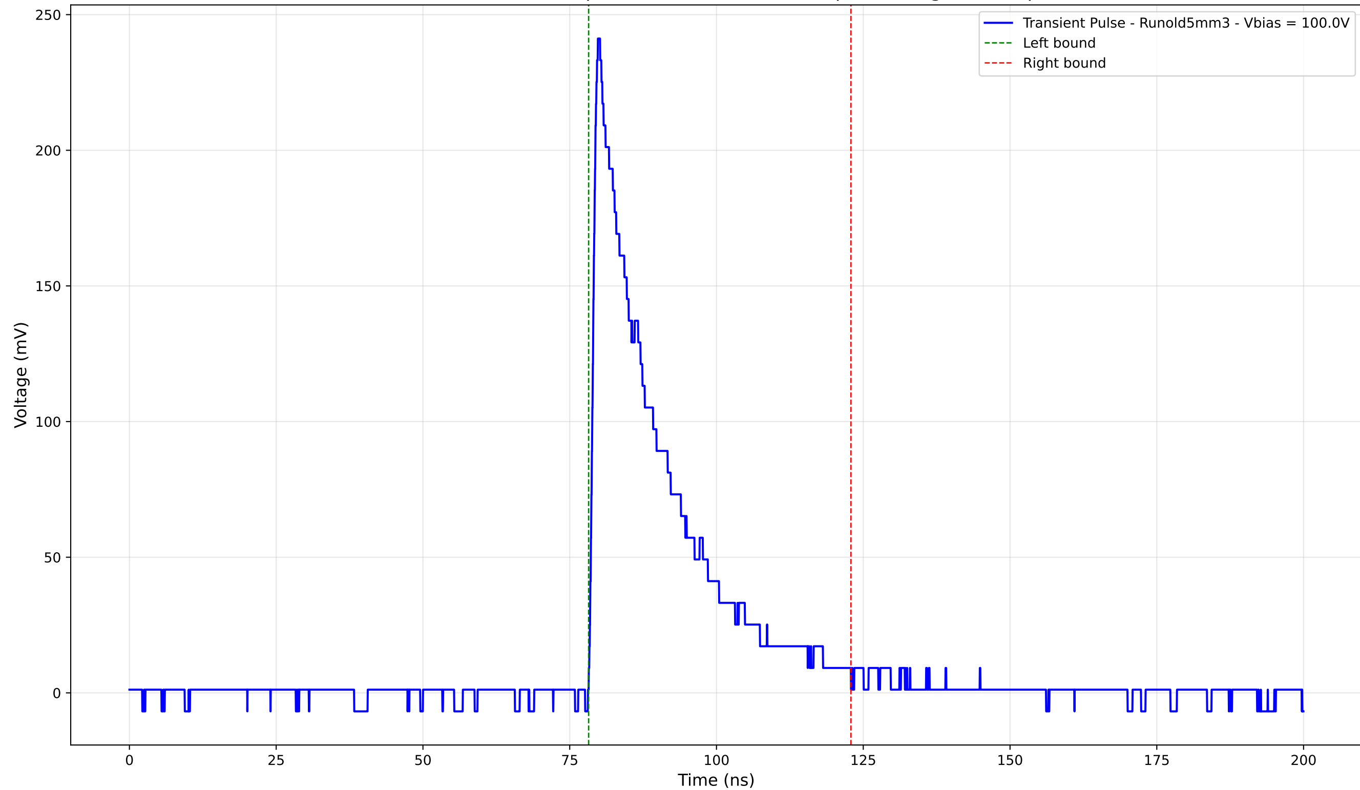
Transient Pulse - Sample: old5 - Position: 650.0 \mu\text{m} - Charge: 56.91 pC
