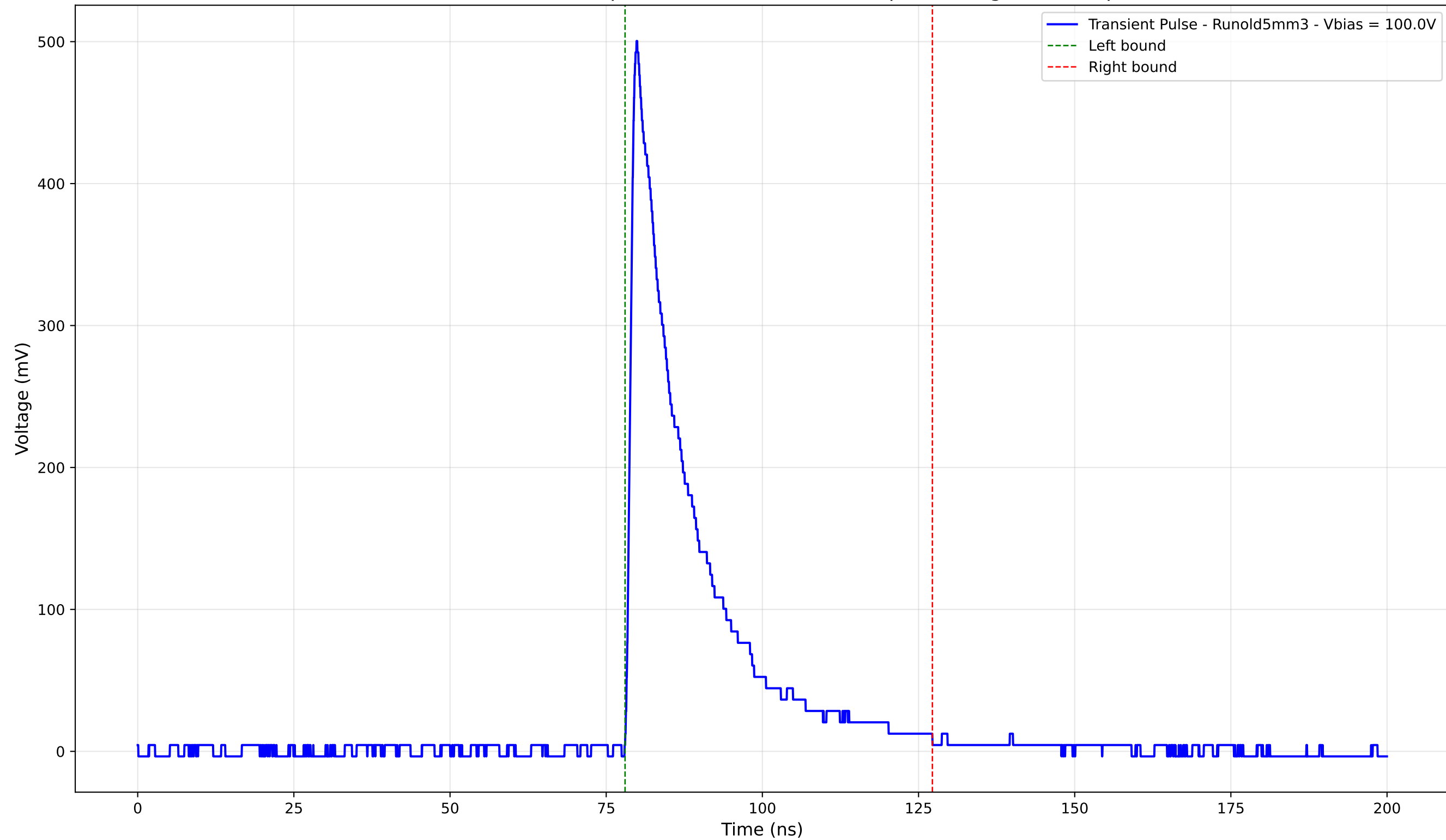
Transient Pulse - Sample: old5 - Position: 4585.0 \mu\text{m} - Charge: 100.88 pC
