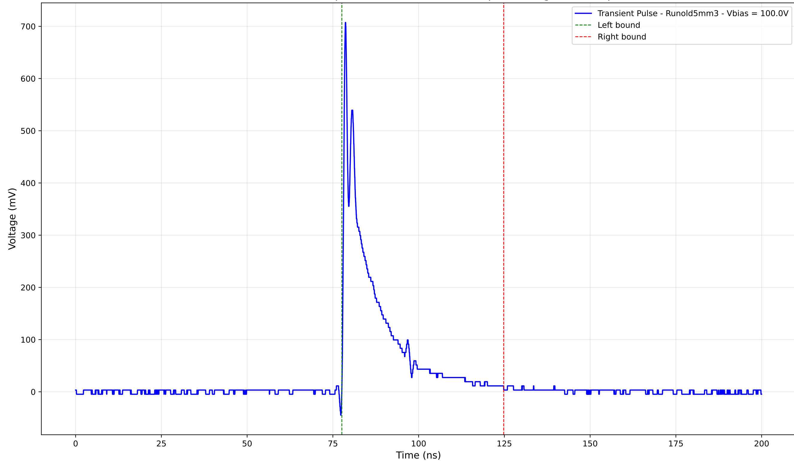
Transient Pulse - Sample: old5 - Position: 3465.0 \mu\text{m} - Charge: 103.79 pC
