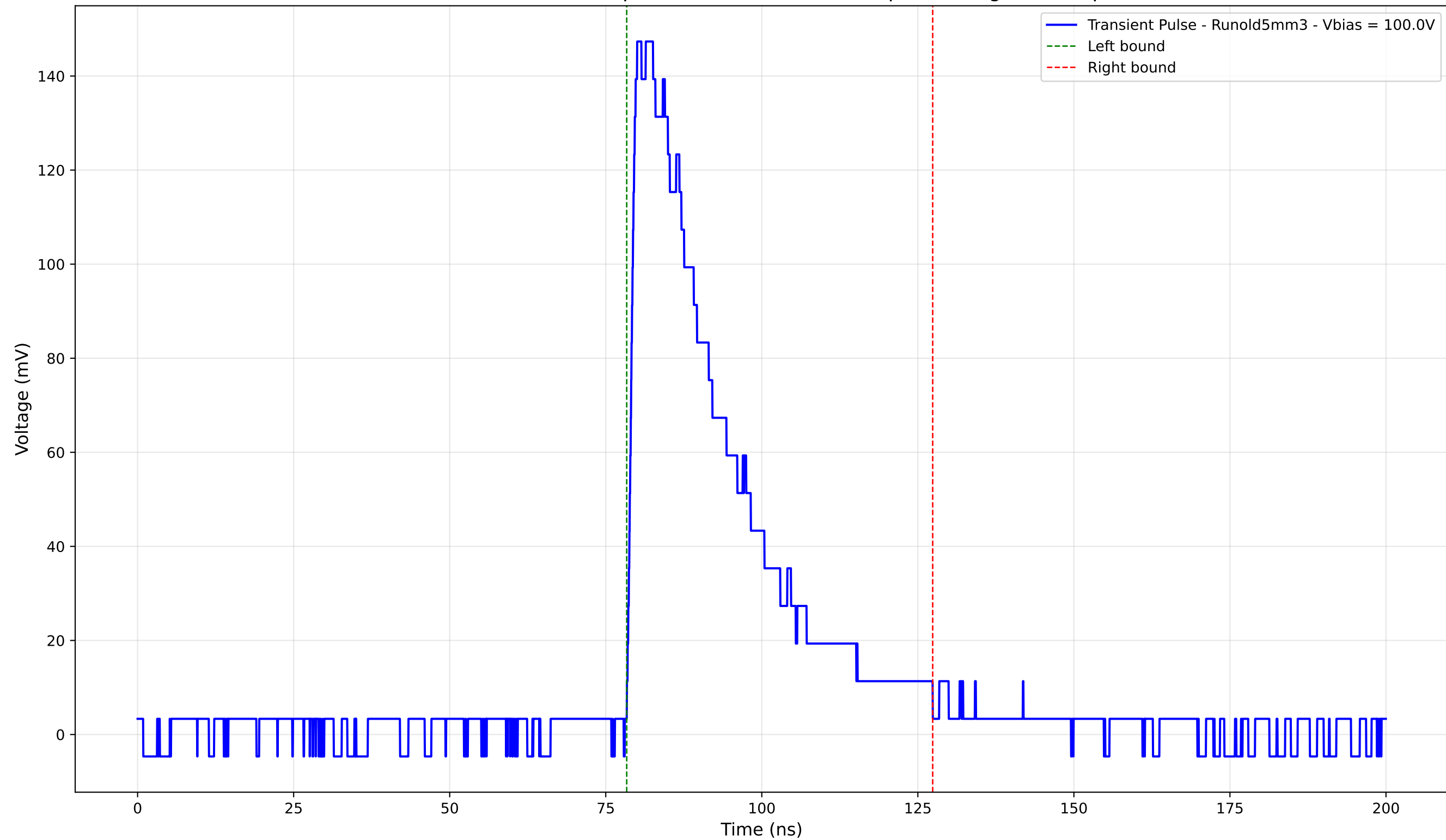
Transient Pulse - Sample: old5 - Position: 980.0 \mu\text{m} - Charge: 49.89 pC
