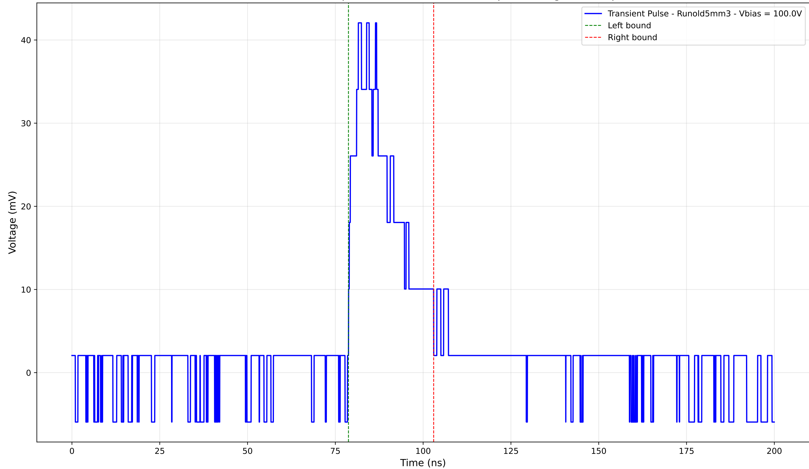
Transient Pulse - Sample: old5 - Position: 2705.0 \mu\text{m} - Charge: 10.60 pC
