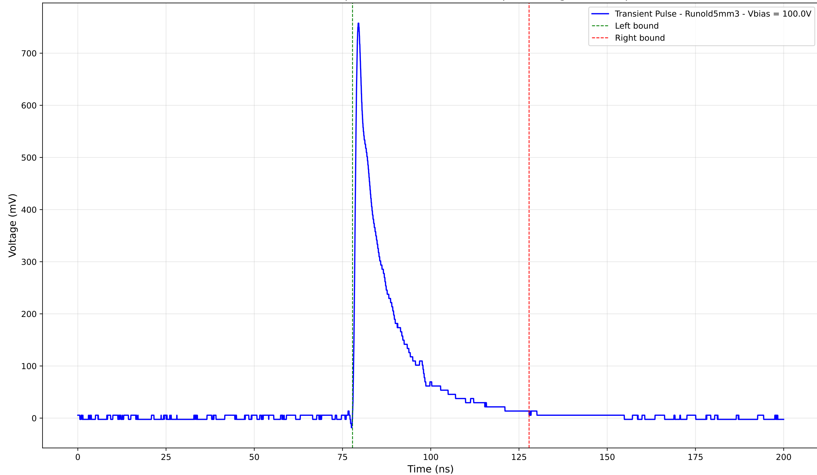
Transient Pulse - Sample: old5 - Position: 4730.0 \mu\text{m} - Charge: 134.66 pC
