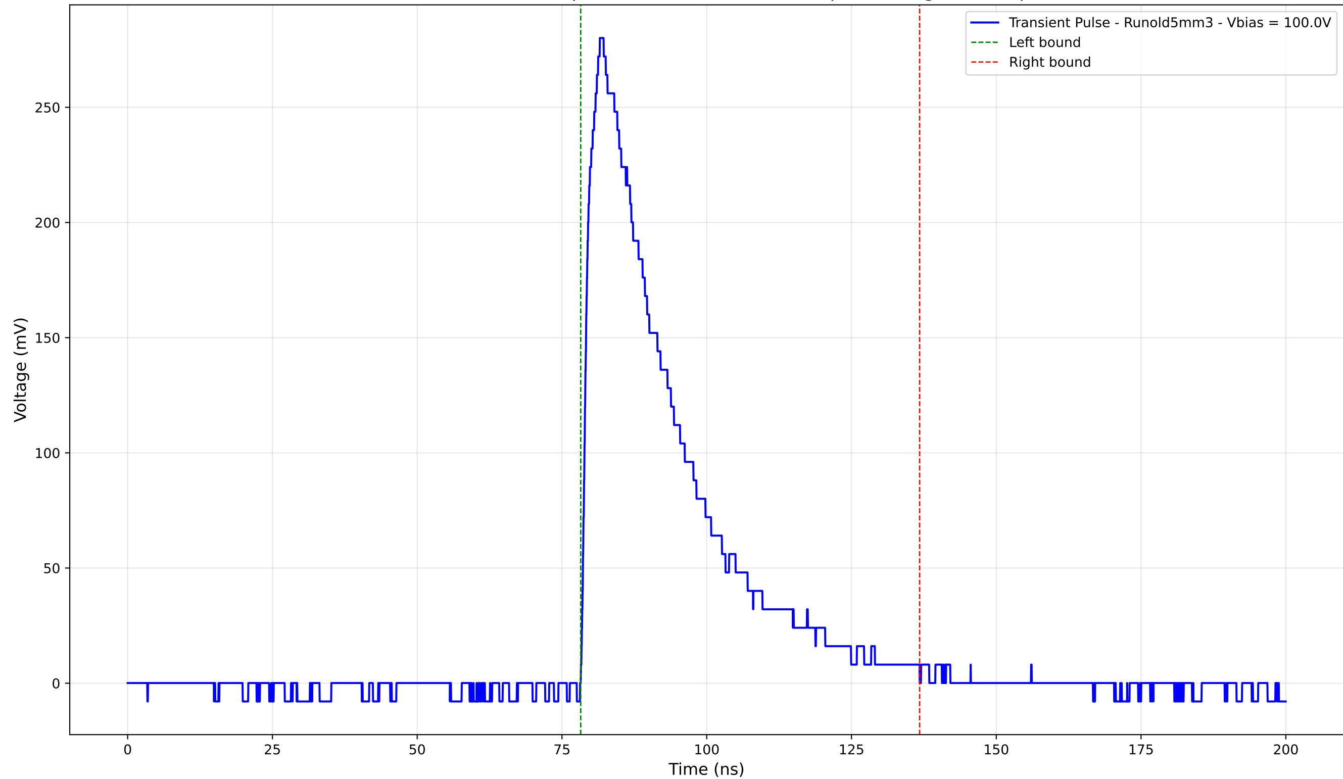
Transient Pulse - Sample: old5 - Position: 2780.0 \mu\text{m} - Charge: 92.64 pC
