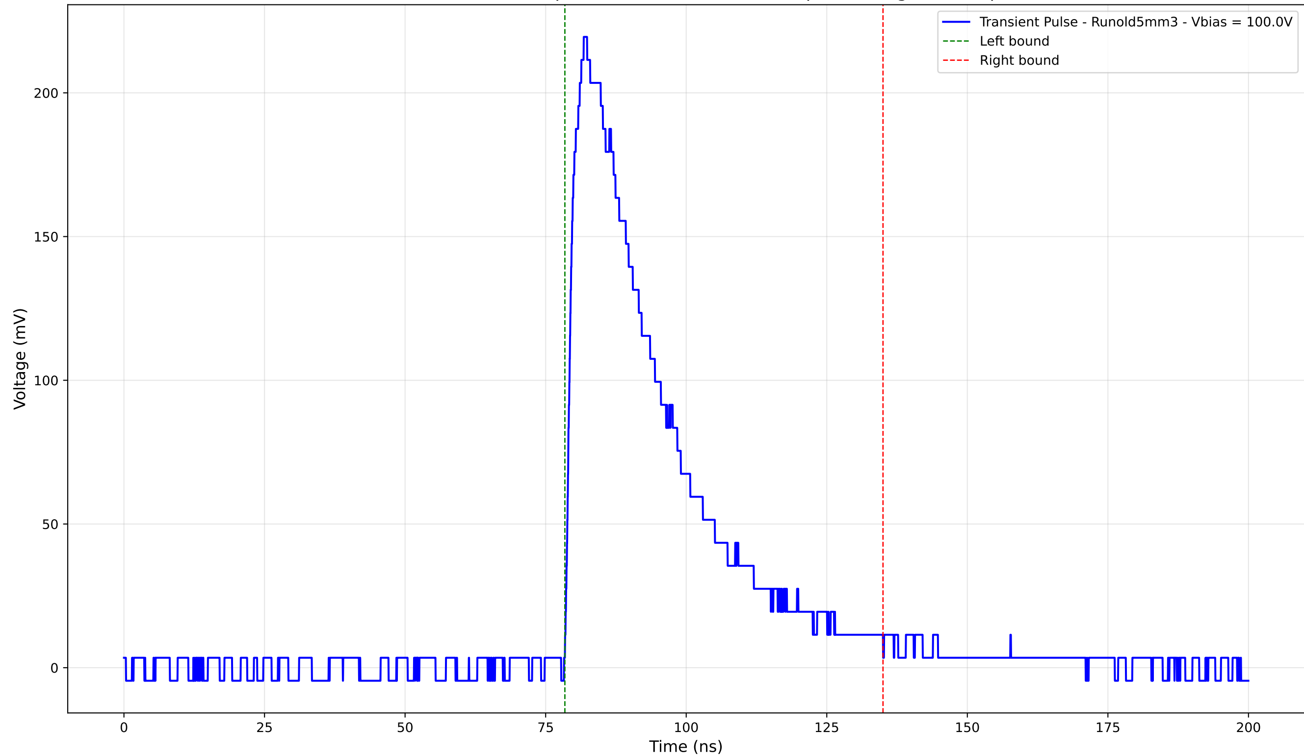
Transient Pulse - Sample: old5 - Position: 2580.0 \mu\text{m} - Charge: 79.66 pC
