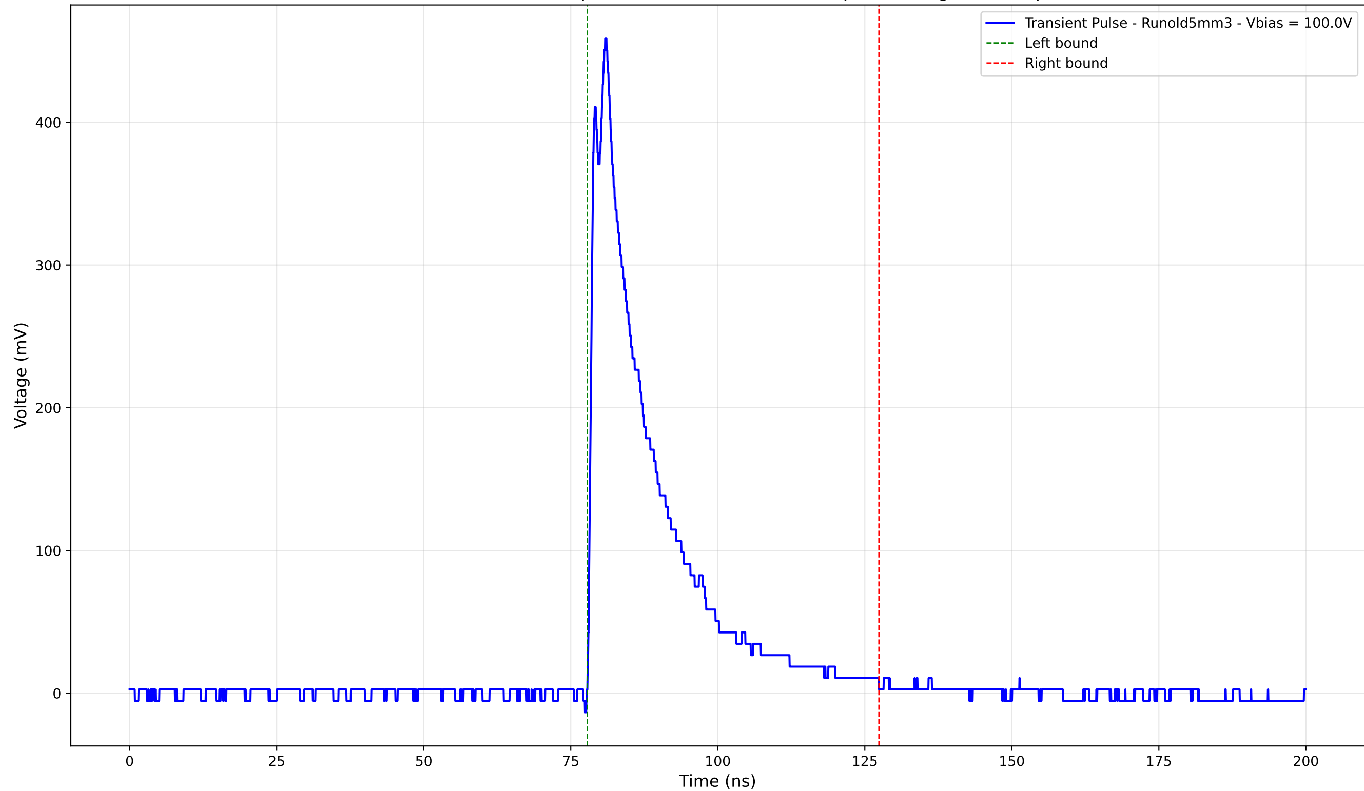
Transient Pulse - Sample: old5 - Position: 3985.0 \mu\text{m} - Charge: 99.02 pC
