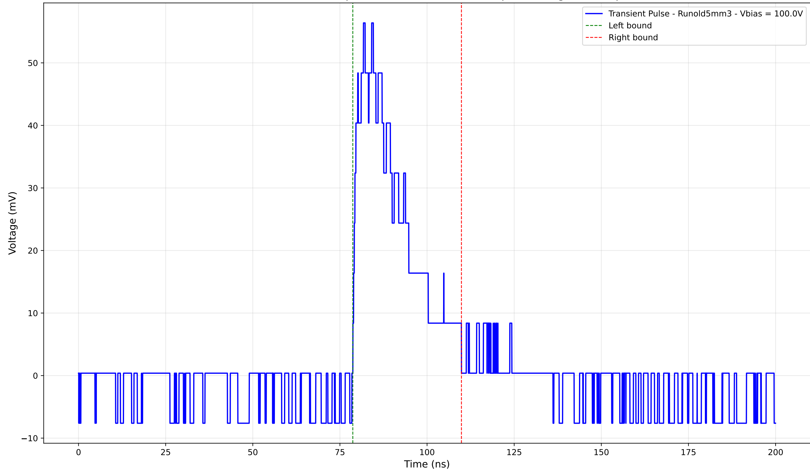
Transient Pulse - Sample: old5 - Position: 1160.0 \mu\text{m} - Charge: 15.64 pC
