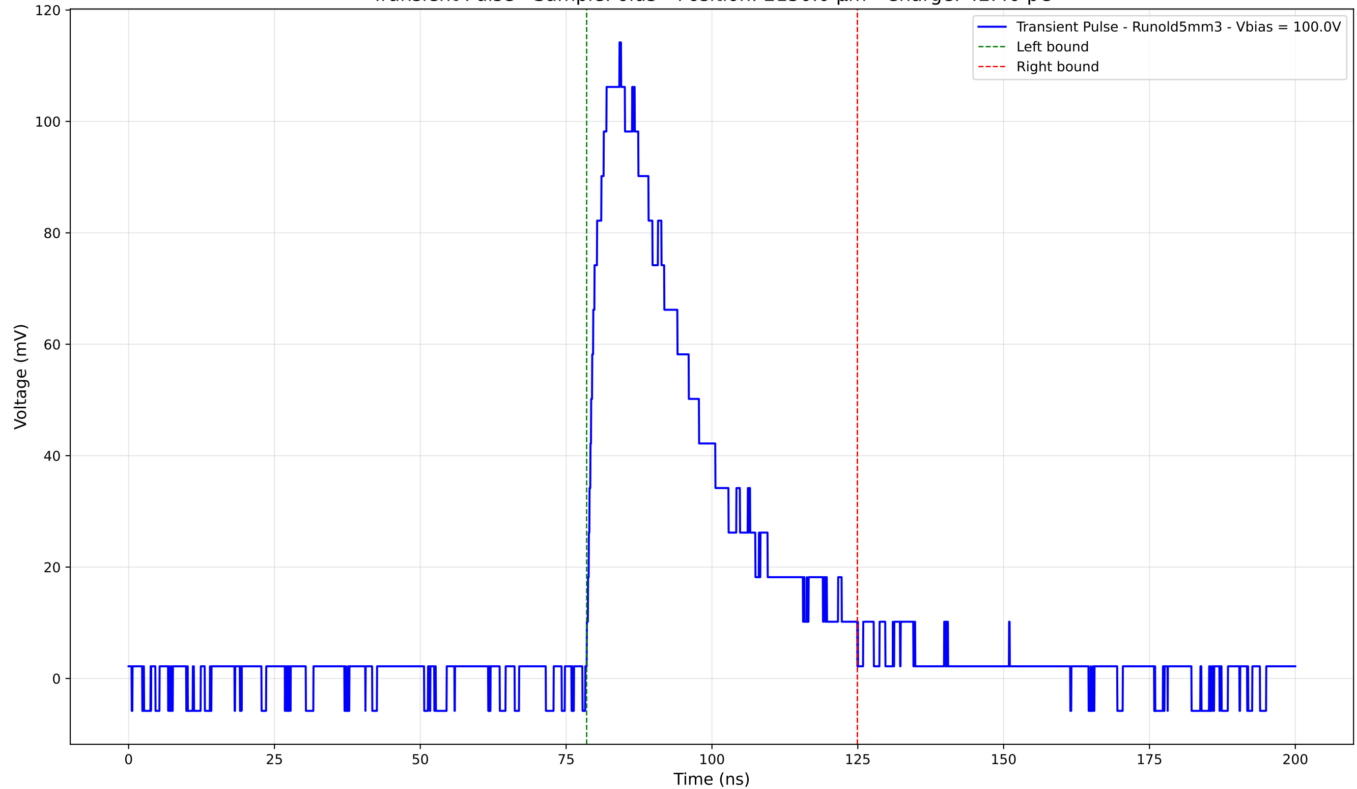
Transient Pulse - Sample: old5 - Position: 2150.0 \mu\text{m} - Charge: 42.40 pC
