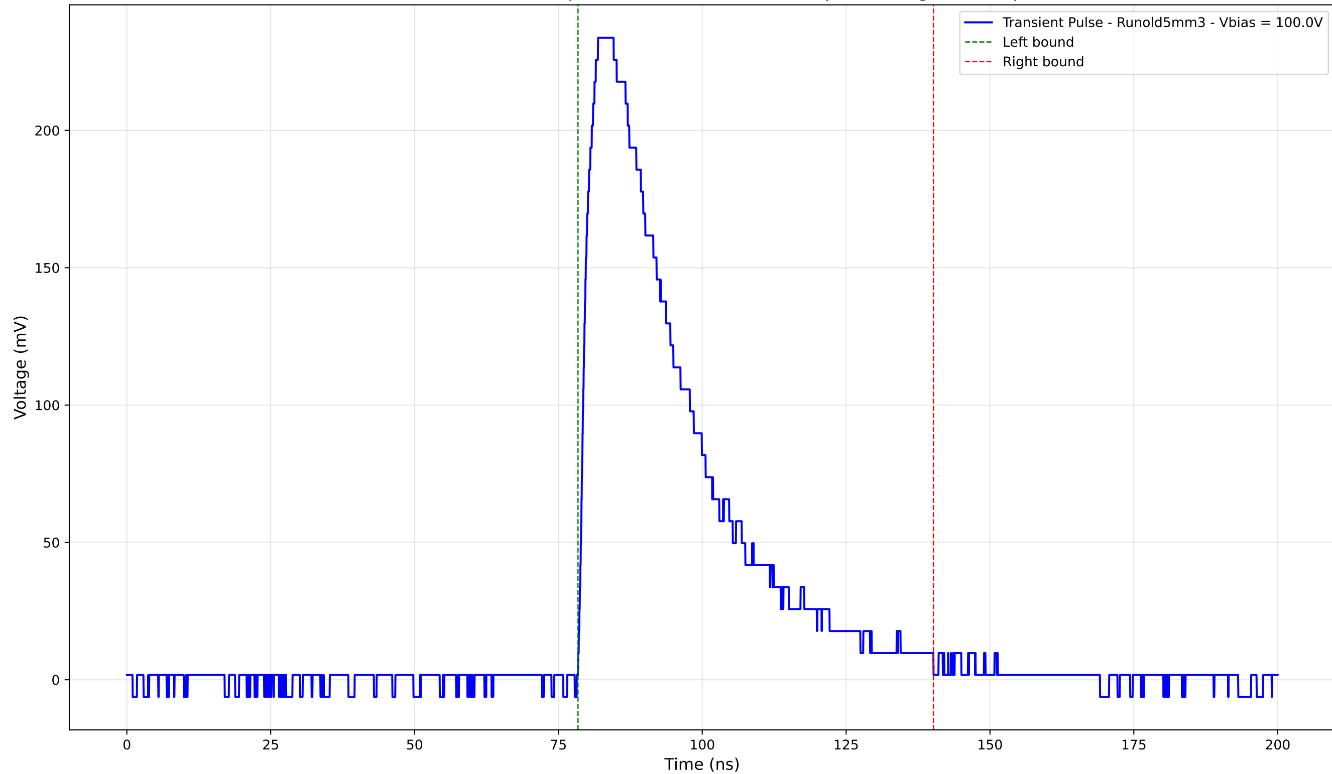
Transient Pulse - Sample: old5 - Position: 2305.0 \mu\text{m} - Charge: 93.21 pC
