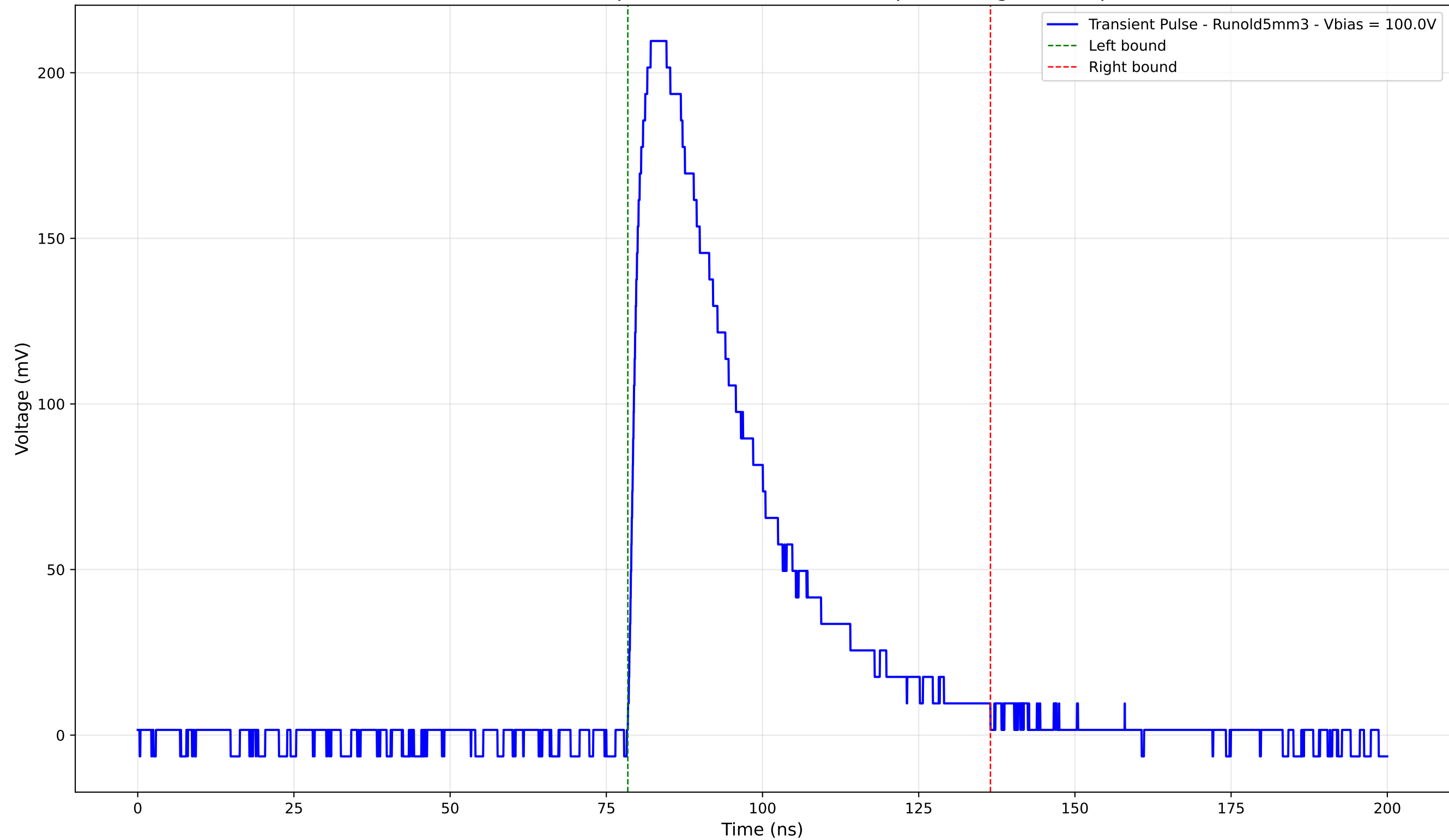
Transient Pulse - Sample: old5 - Position: 1485.0 \mu\text{m} - Charge: 82.47 pC
