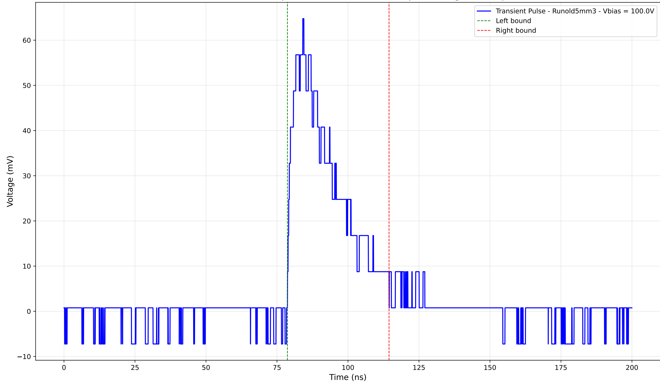
Transient Pulse - Sample: old5 - Position: 1560.0 \mu\text{m} - Charge: 20.55 pC
