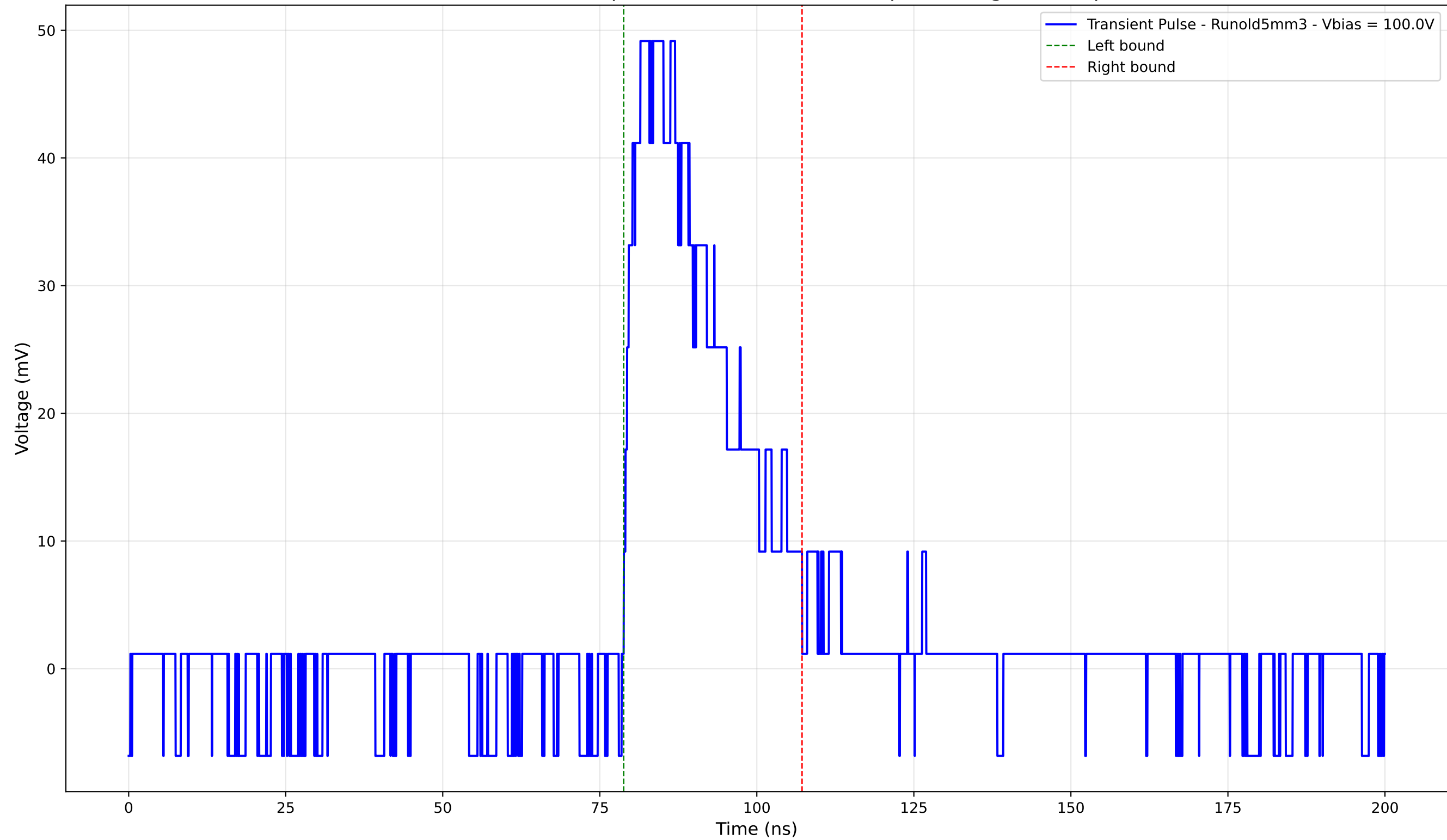
Transient Pulse - Sample: old5 - Position: 1365.0 \mu\text{m} - Charge: 15.41 pC
