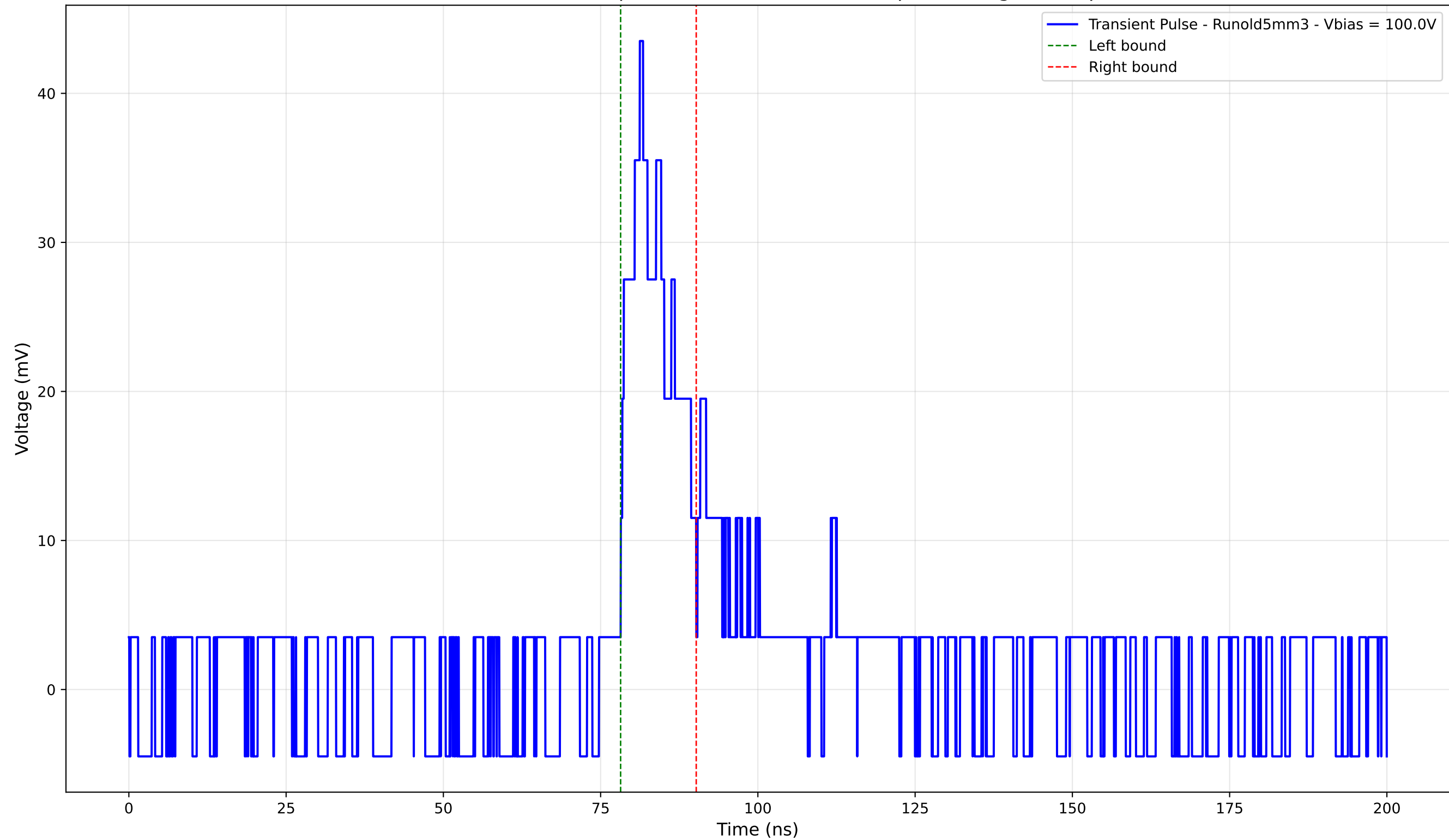
Transient Pulse - Sample: old5 - Position: 3905.0 \mu\text{m} - Charge: 6.18 pC
