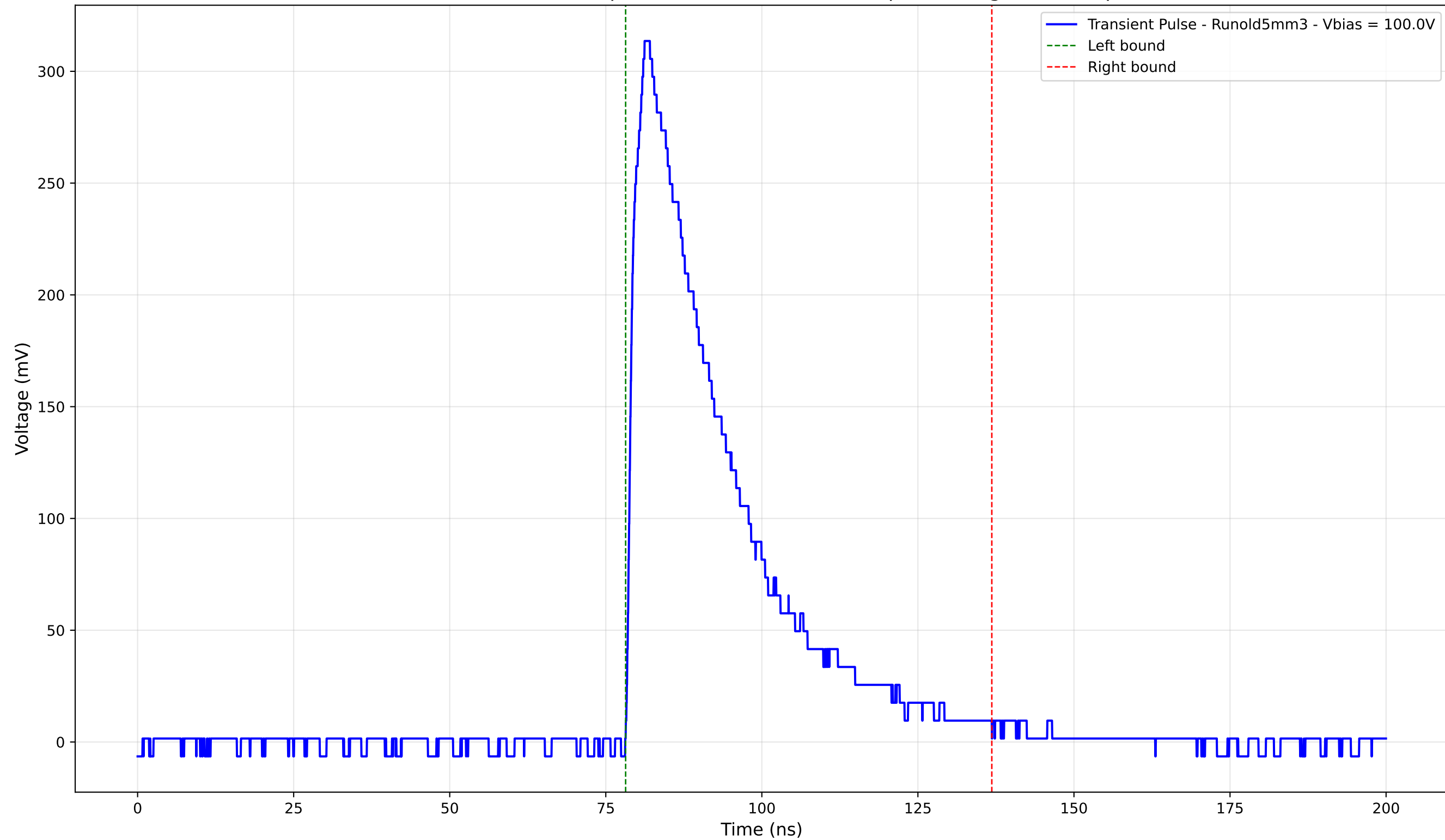
Transient Pulse - Sample: old5 - Position: 2810.0 \mu\text{m} - Charge: 103.94 pC
