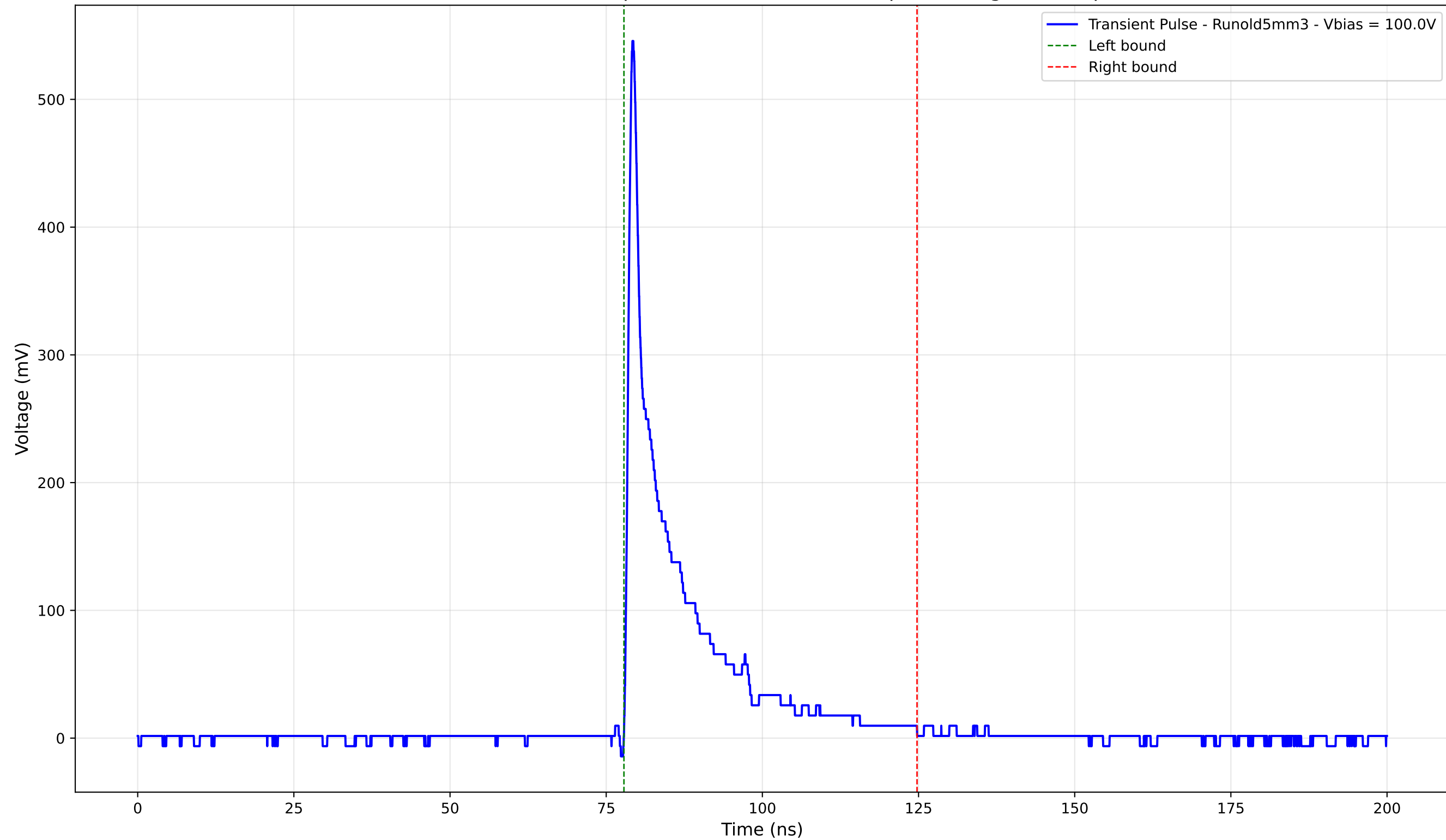
Transient Pulse - Sample: old5 - Position: 210.0 \mu\text{m} - Charge: 70.43 pC
