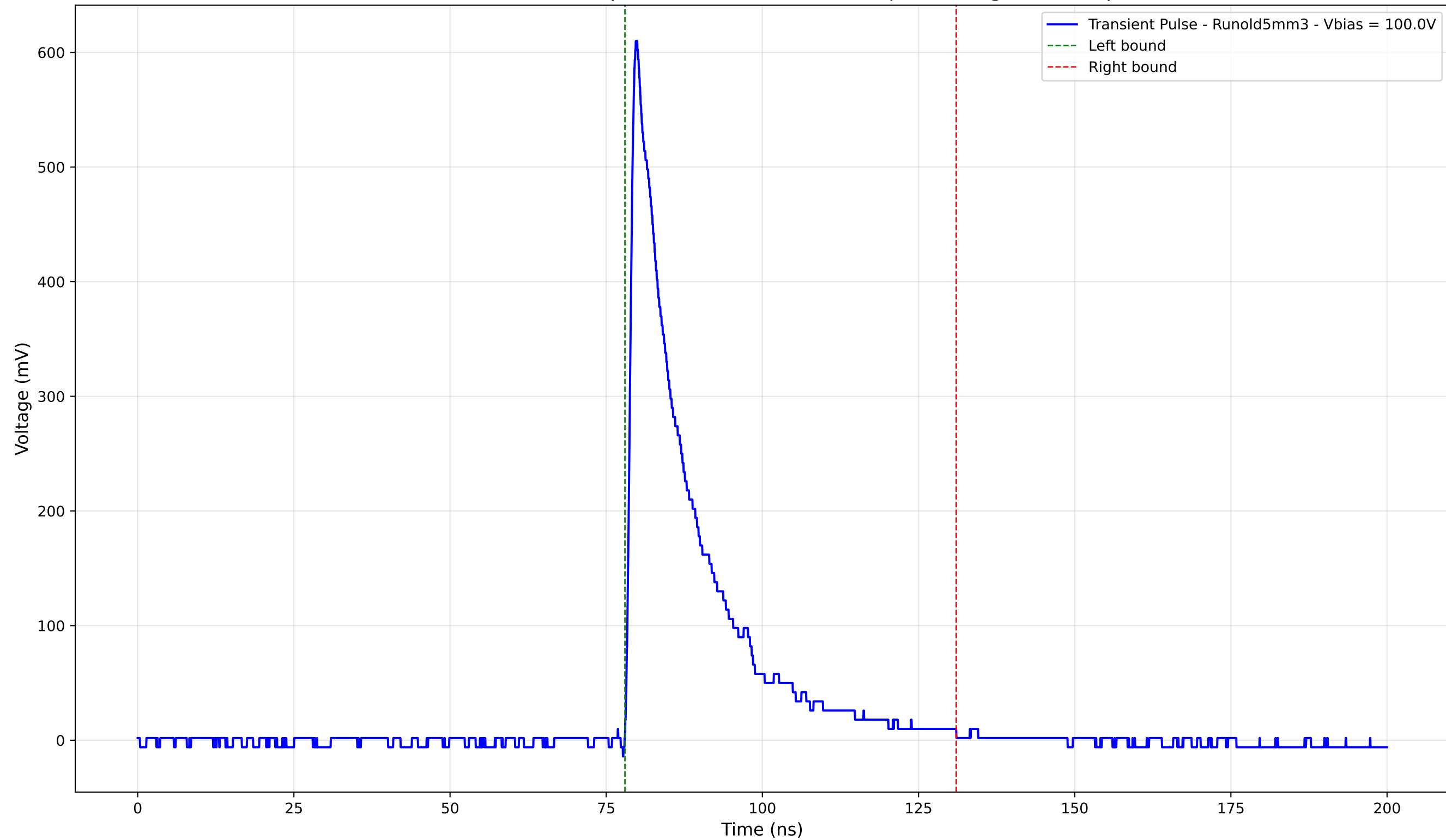
Transient Pulse - Sample: old5 - Position: 4615.0 \mu\text{m} - Charge: 120.59 pC
