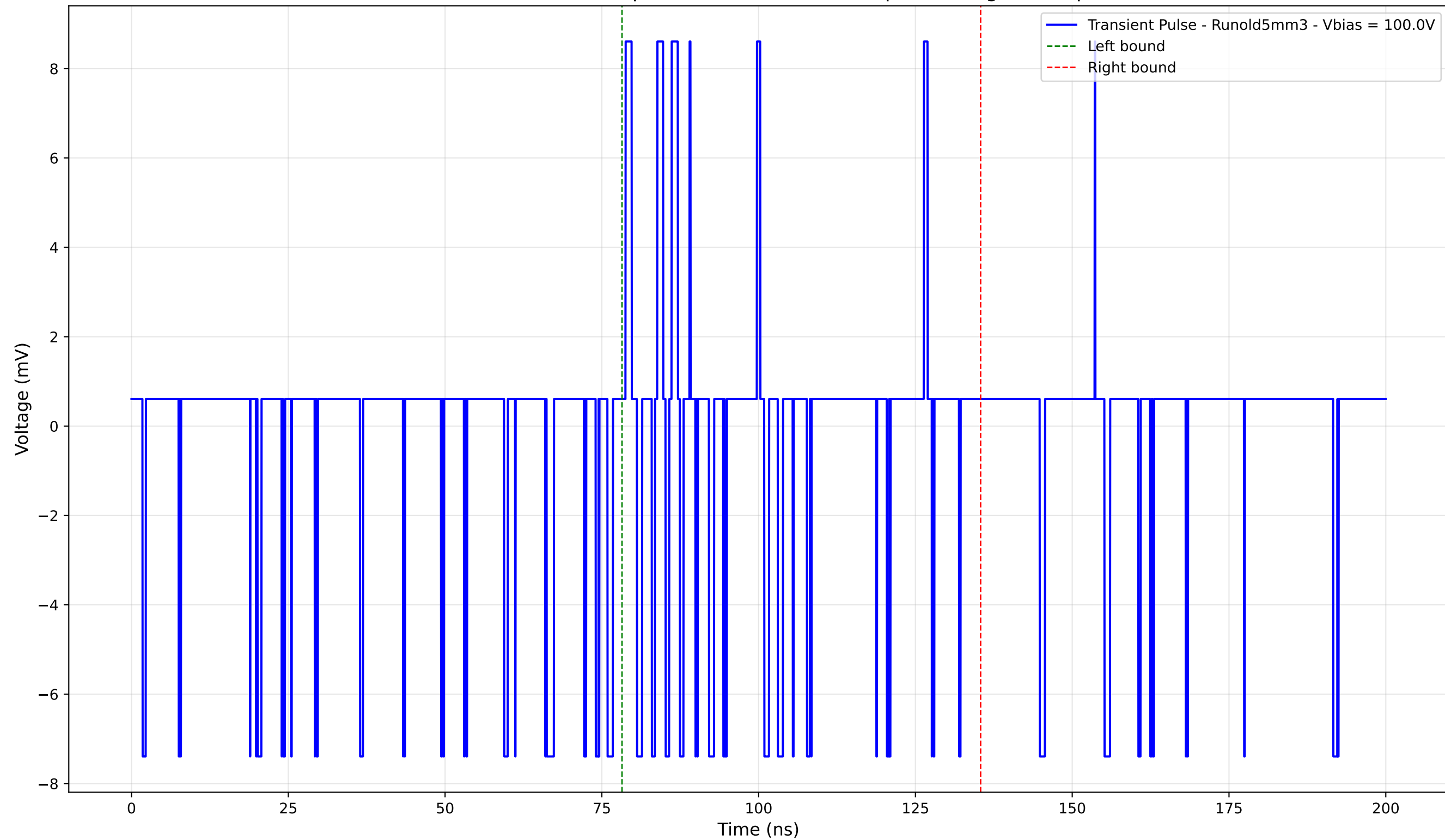
Transient Pulse - Sample: old5 - Position: 40.0 \mu\text{m} - Charge: 0.21 pC
