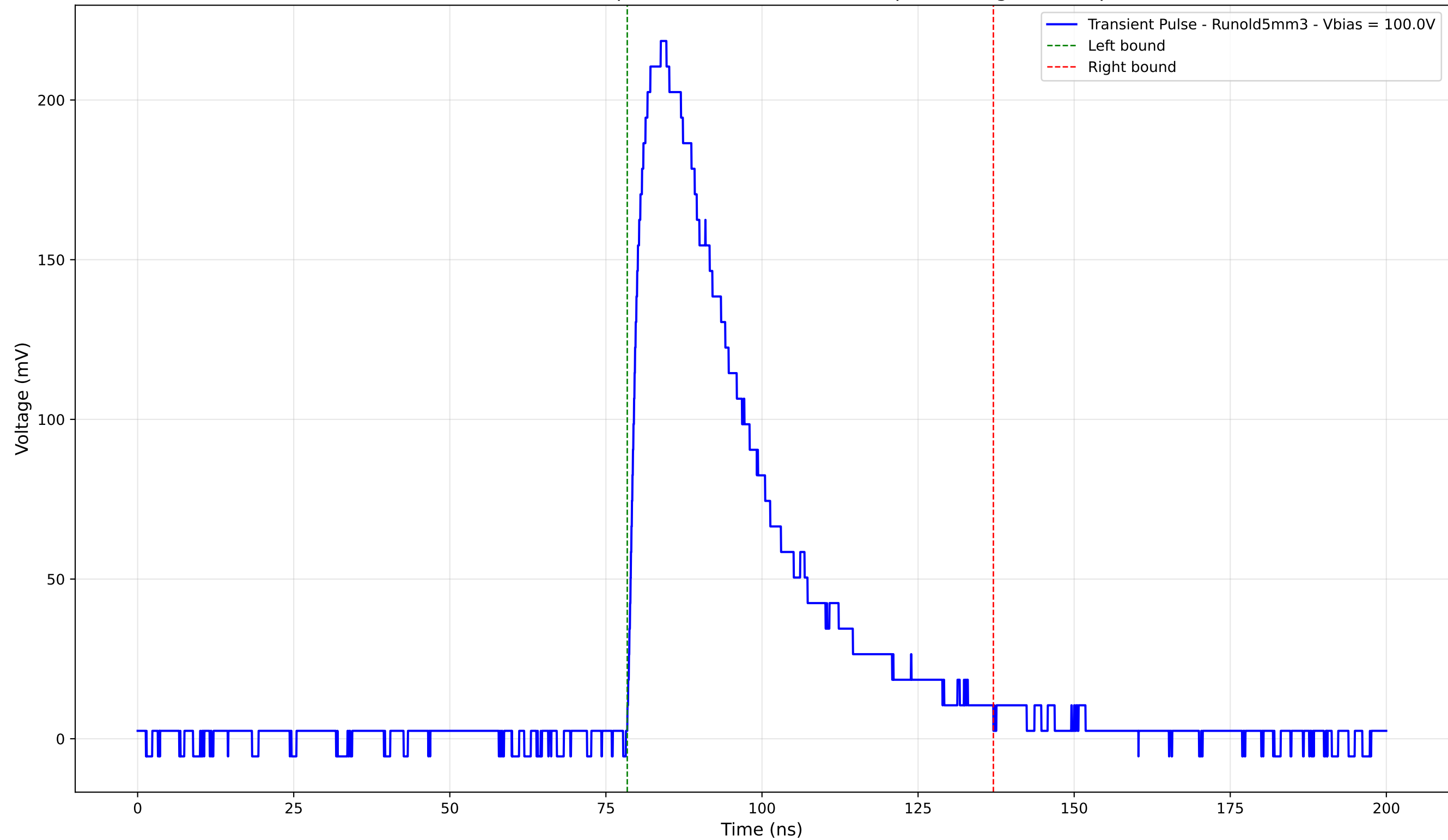
Transient Pulse - Sample: old5 - Position: 1895.0 \mu\text{m} - Charge: 88.09 pC
