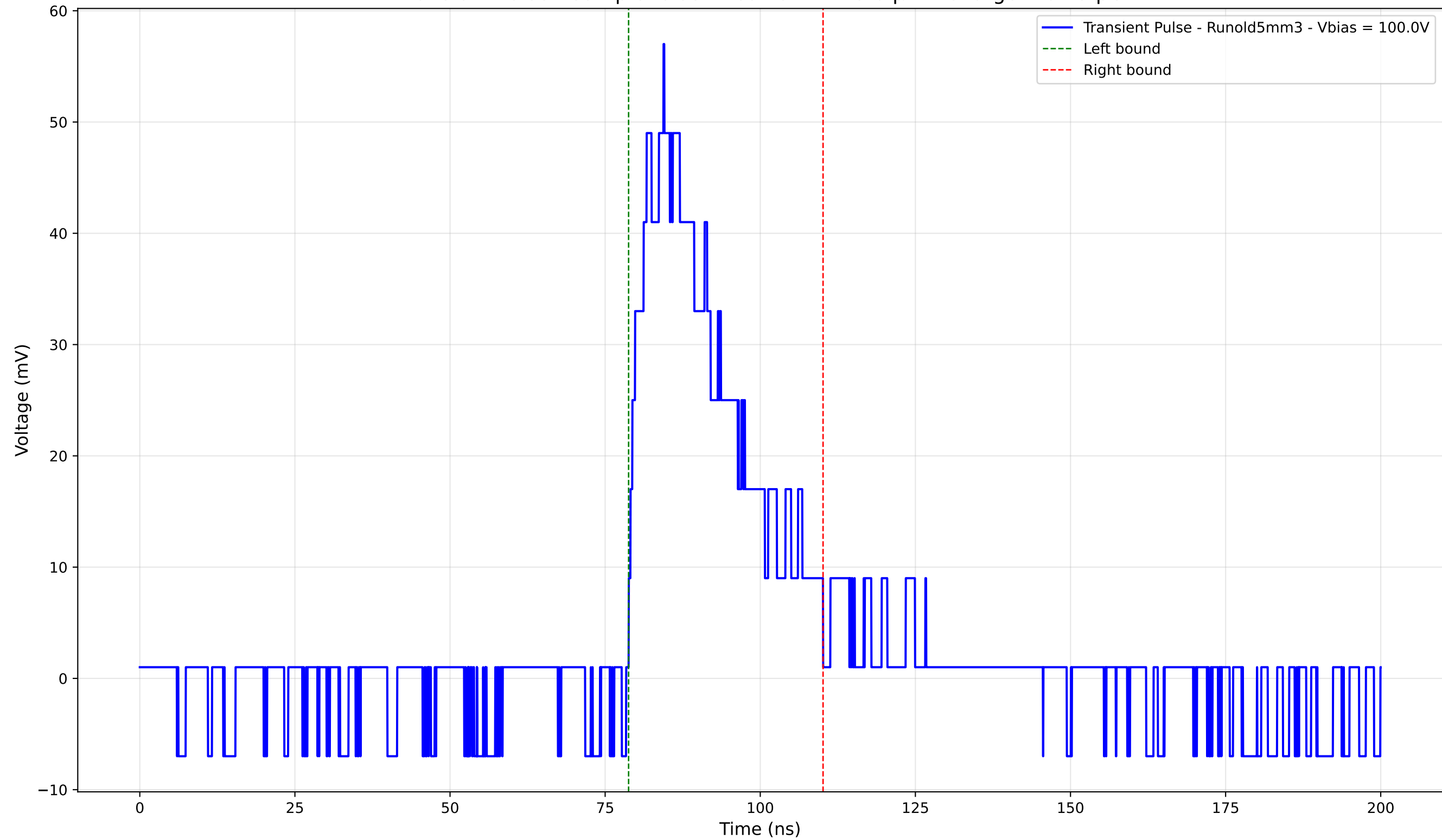
Transient Pulse - Sample: old5 - Position: 2175.0 \mu\text{m} - Charge: 16.43 pC
