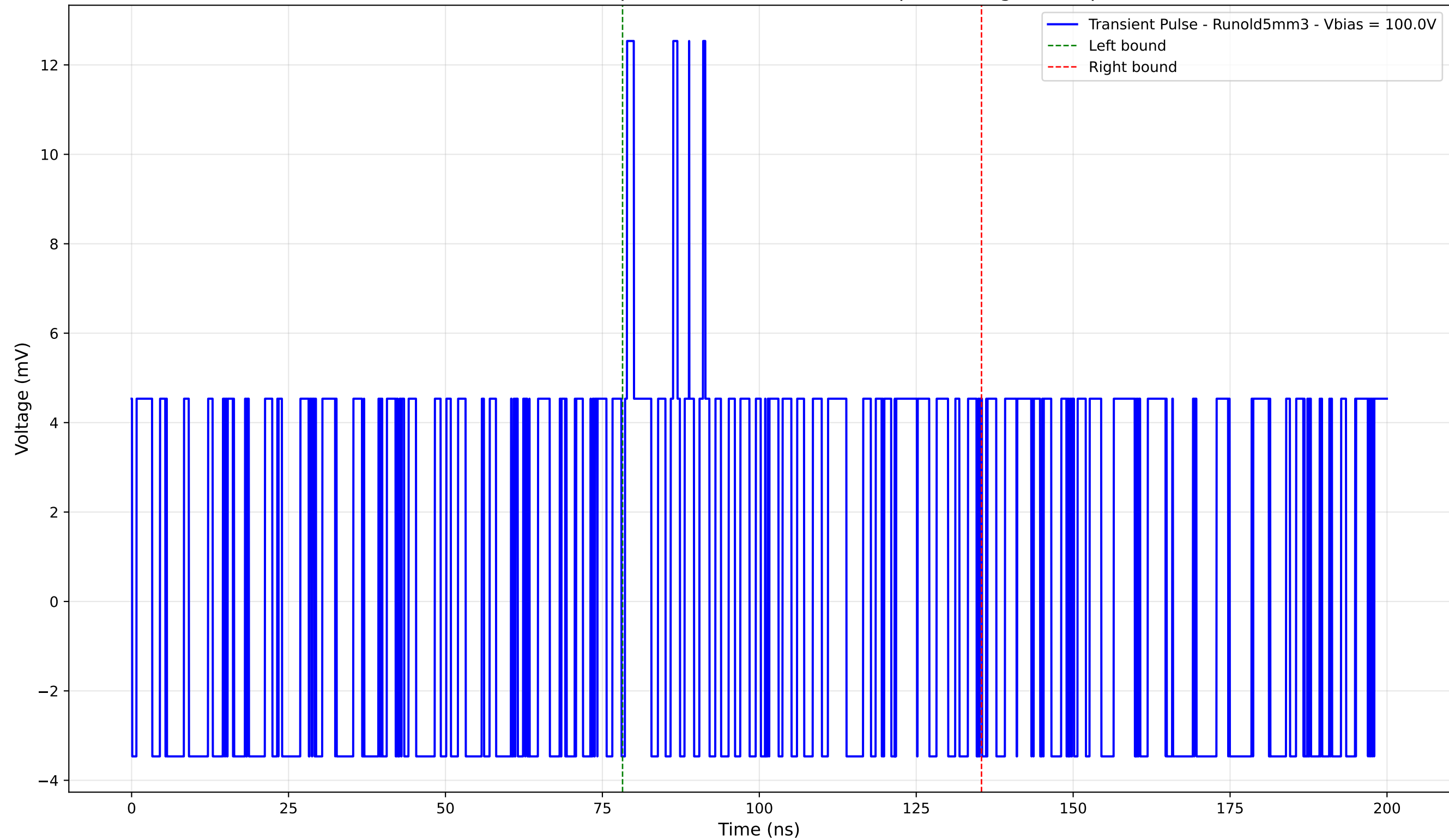
Transient Pulse - Sample: old5 - Position: 4985.0 \mu\text{m} - Charge: 2.10 pC
