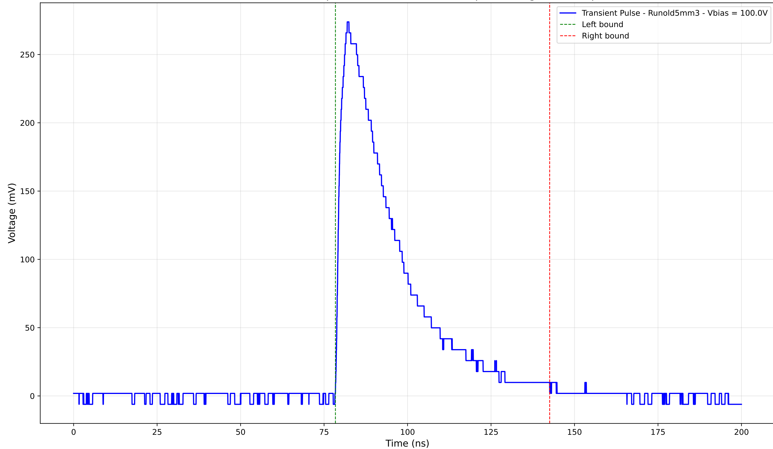
Transient Pulse - Sample: old5 - Position: 2505.0 \mu\text{m} - Charge: 102.22 pC
