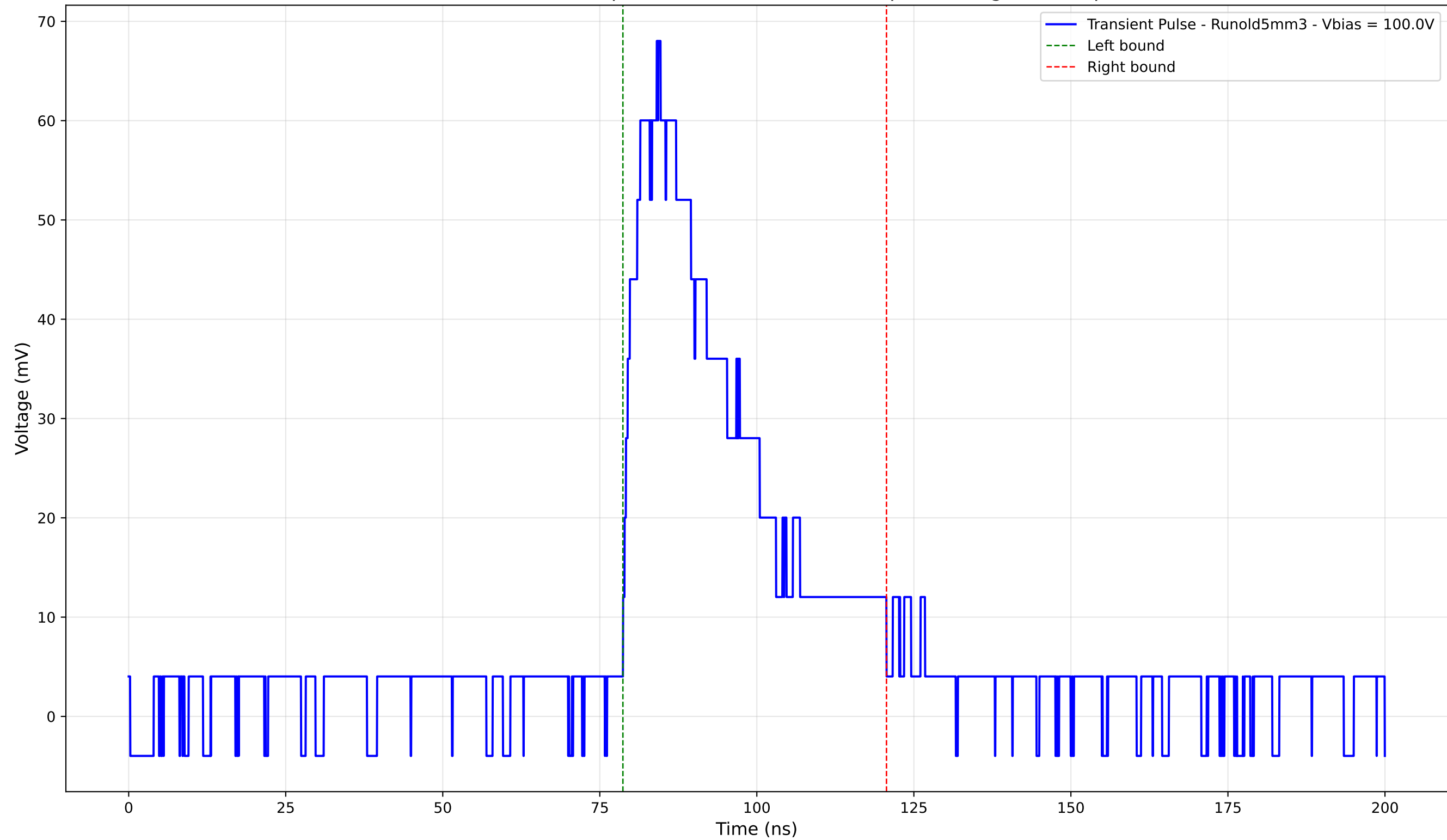
Transient Pulse - Sample: old5 - Position: 2215.0 \mu\text{m} - Charge: 24.46 pC
