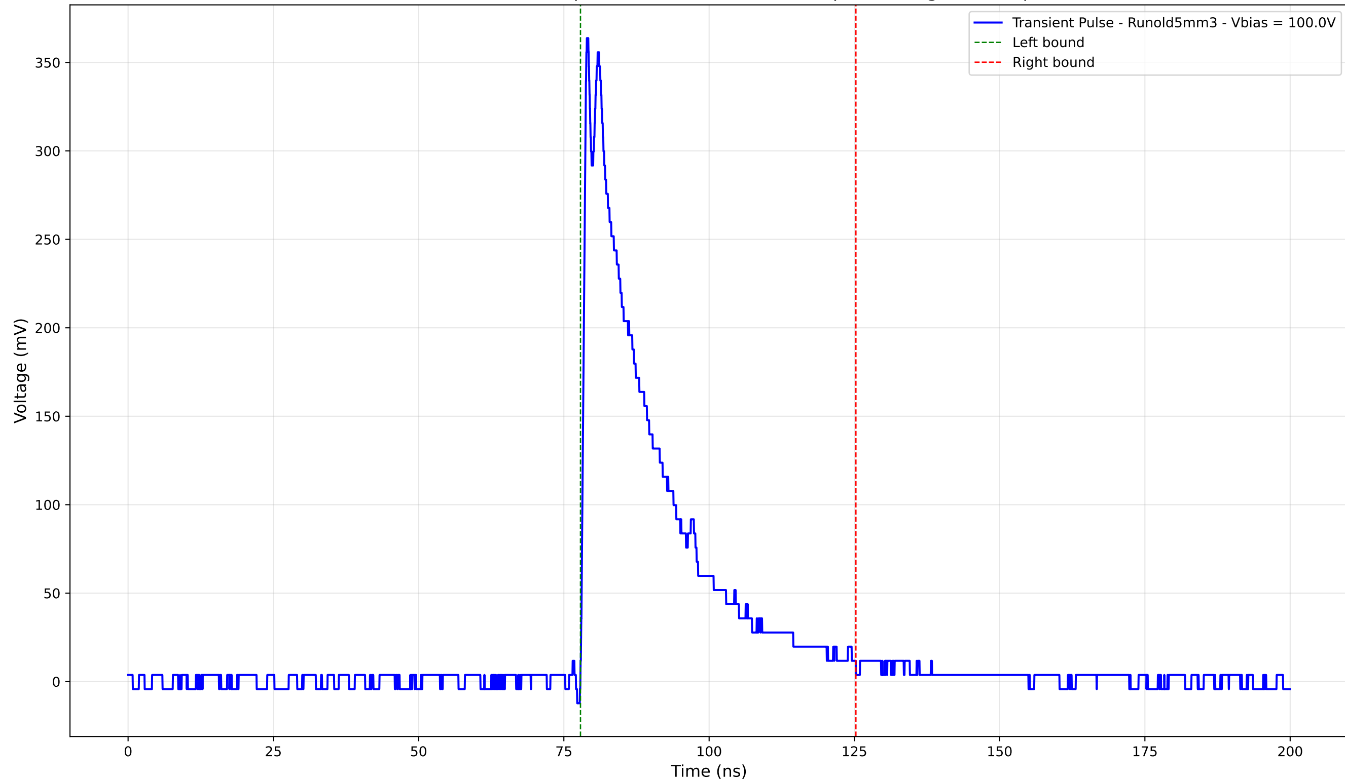
Transient Pulse - Sample: old5 - Position: 3180.0 \mu\text{m} - Charge: 90.20 pC
