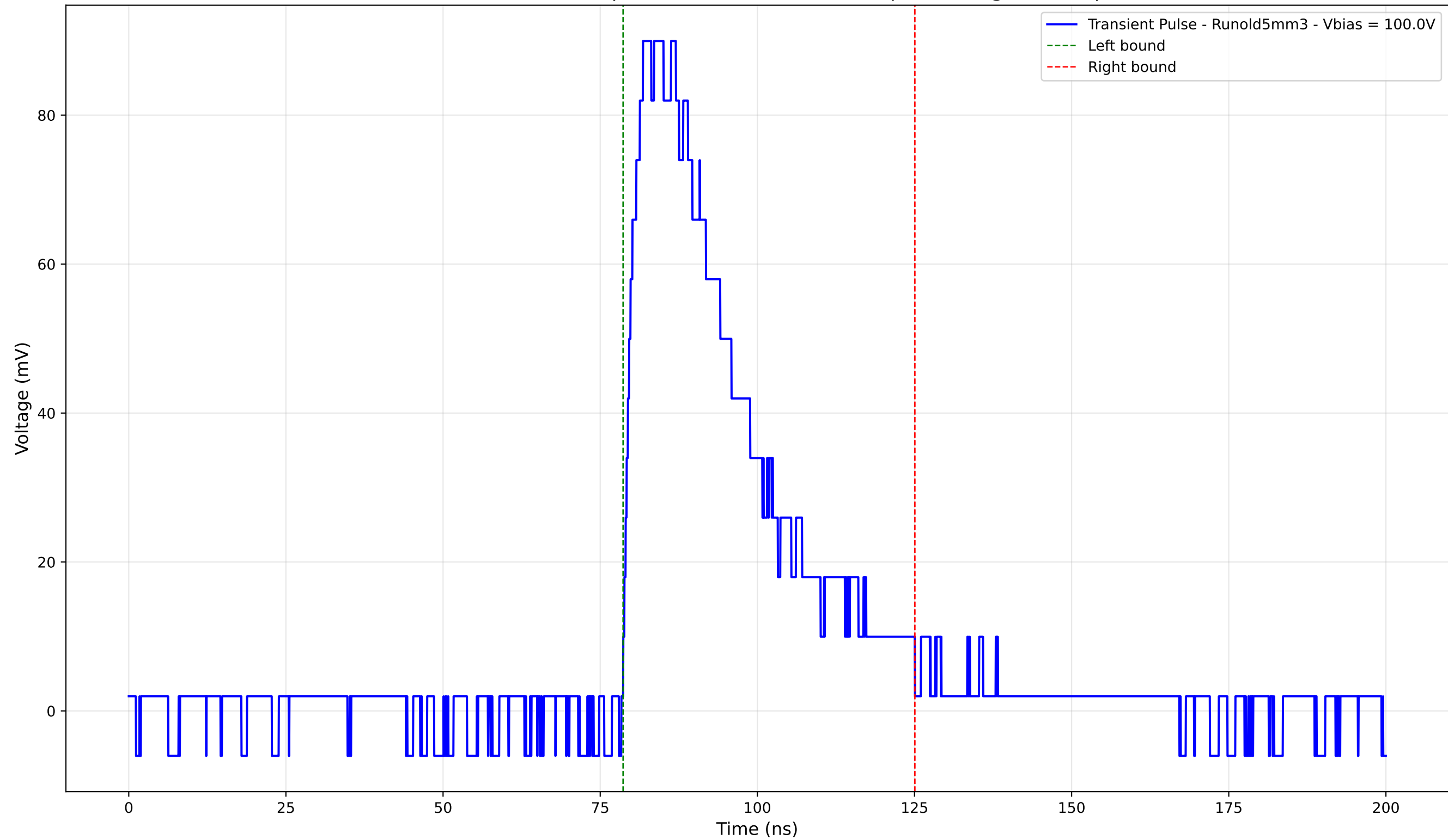
Transient Pulse - Sample: old5 - Position: 1750.0 \mu\text{m} - Charge: 36.02 pC
