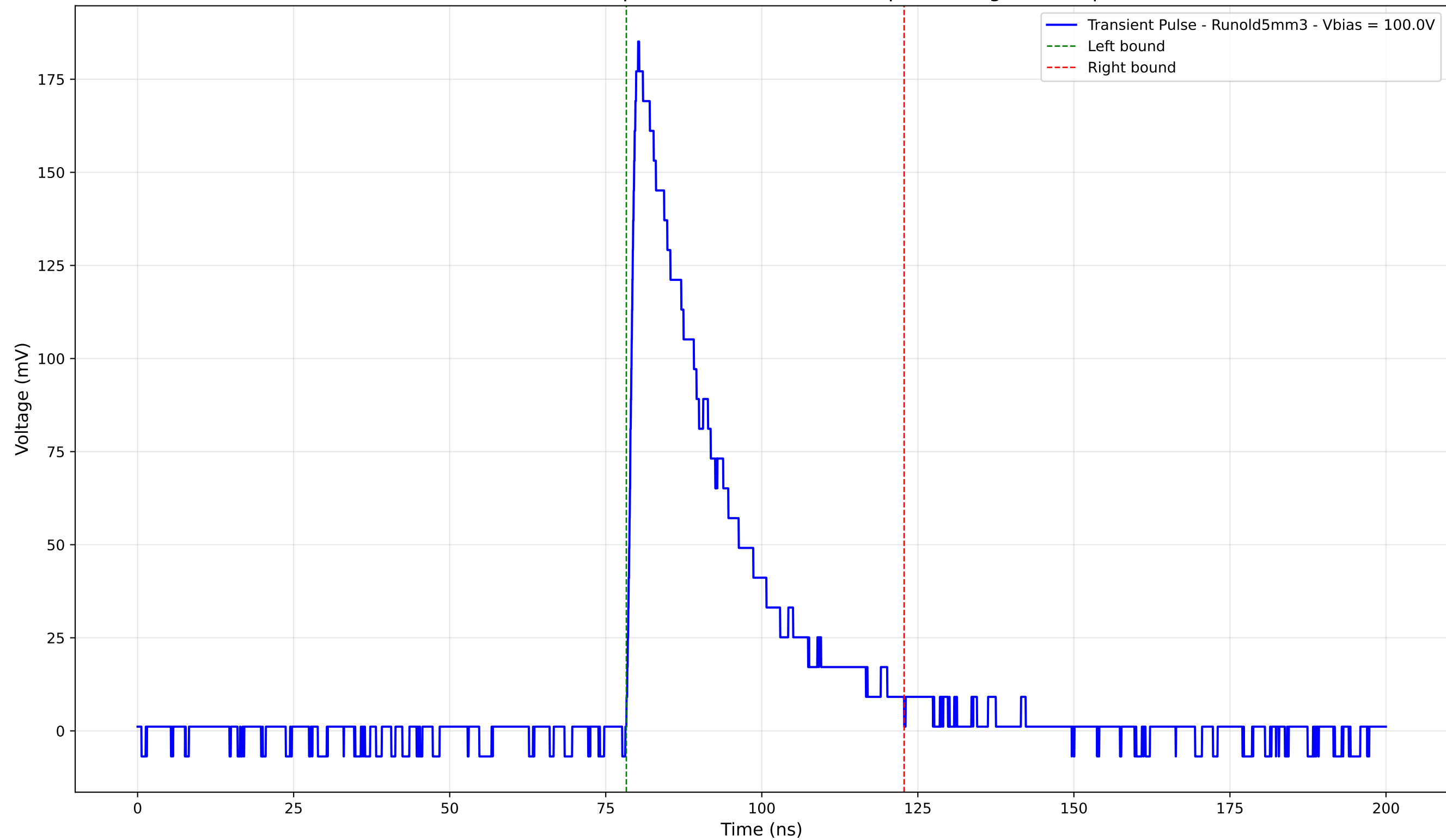
Transient Pulse - Sample: old5 - Position: 835.0 \mu\text{m} - Charge: 51.59 pC
