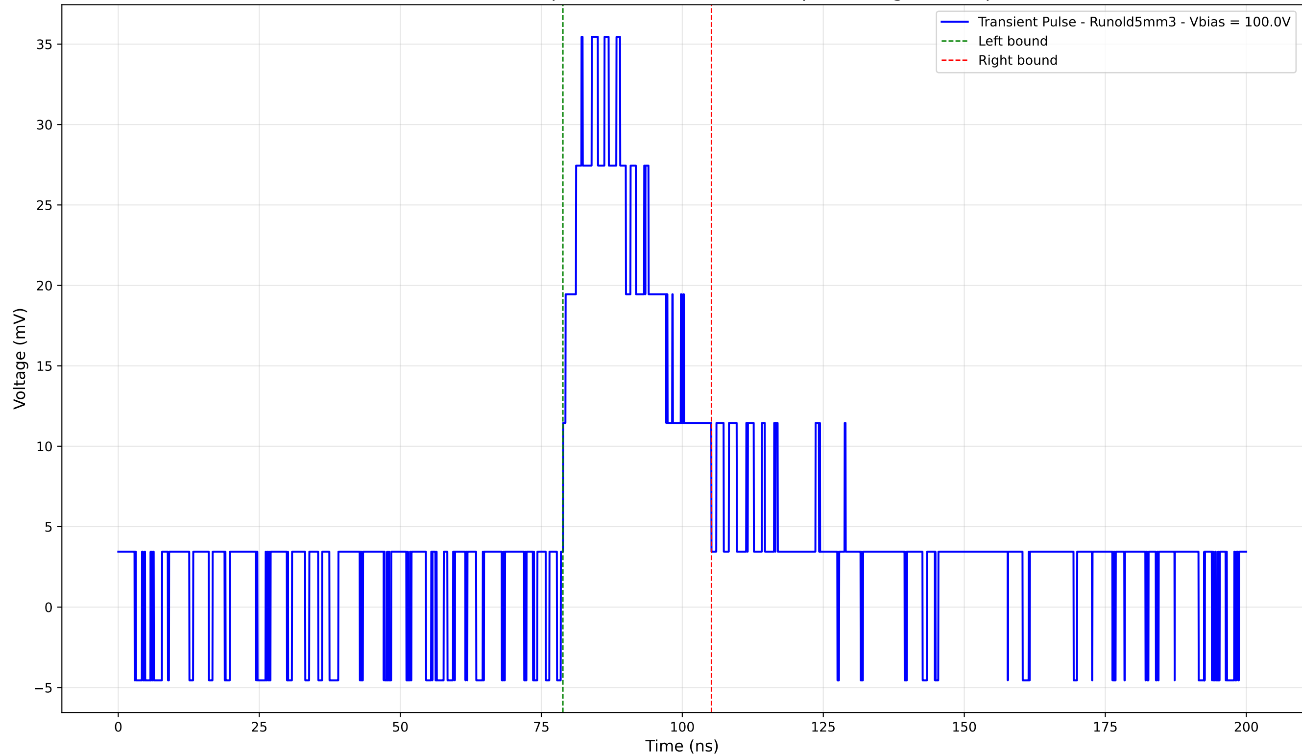
Transient Pulse - Sample: old5 - Position: 1590.0 \mu\text{m} - Charge: 11.10 pC
