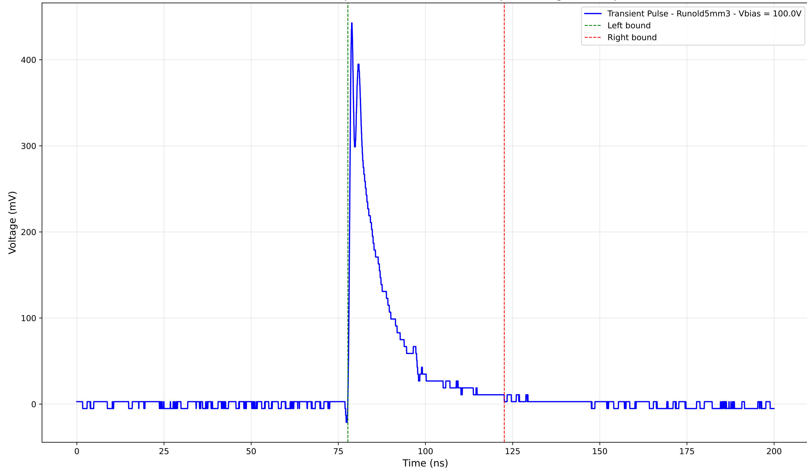
Transient Pulse - Sample: old5 - Position: 3800.0 \mu\text{m} - Charge: 77.08 pC
