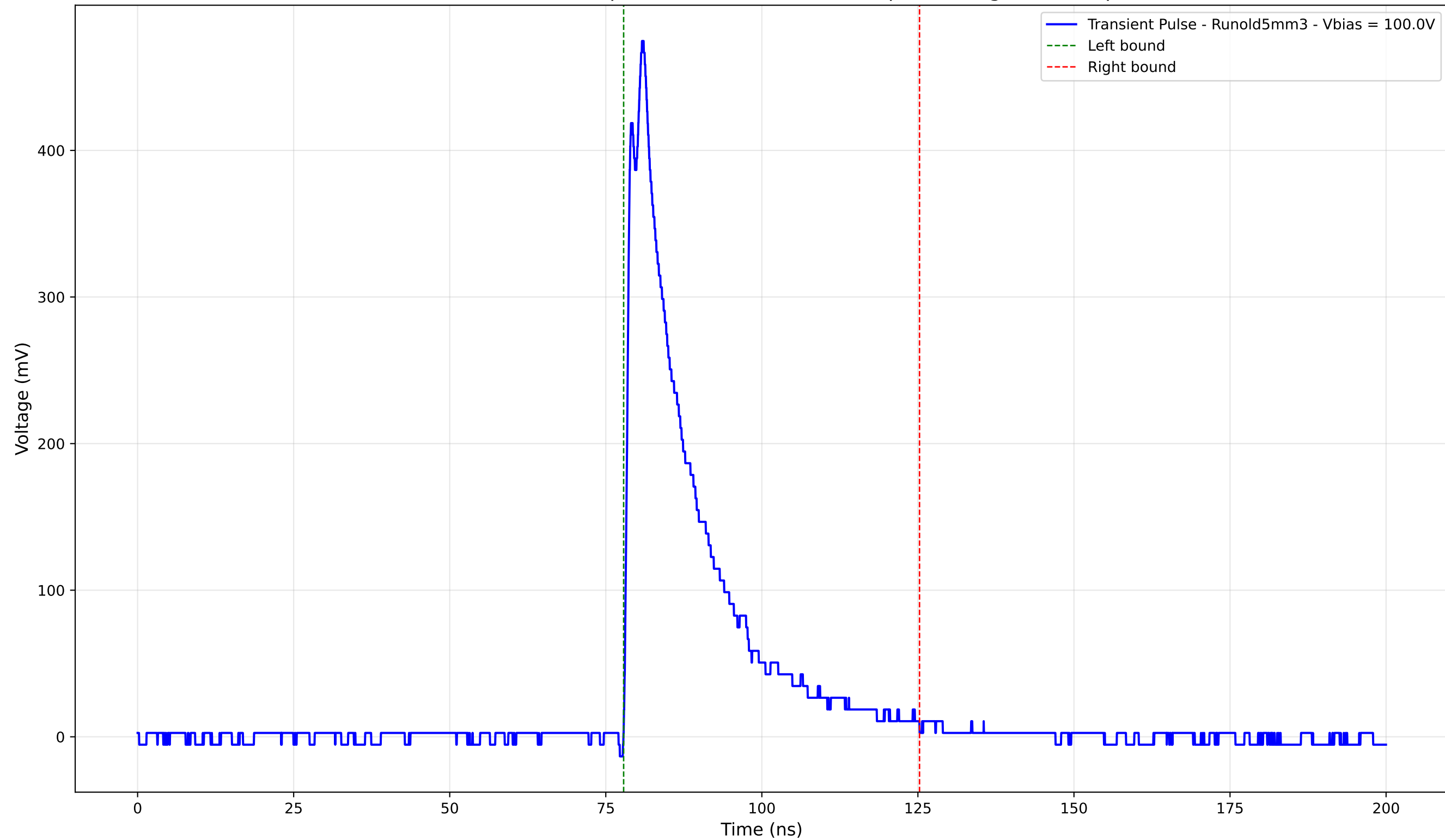
Transient Pulse - Sample: old5 - Position: 3990.0 \mu\text{m} - Charge: 102.28 pC
