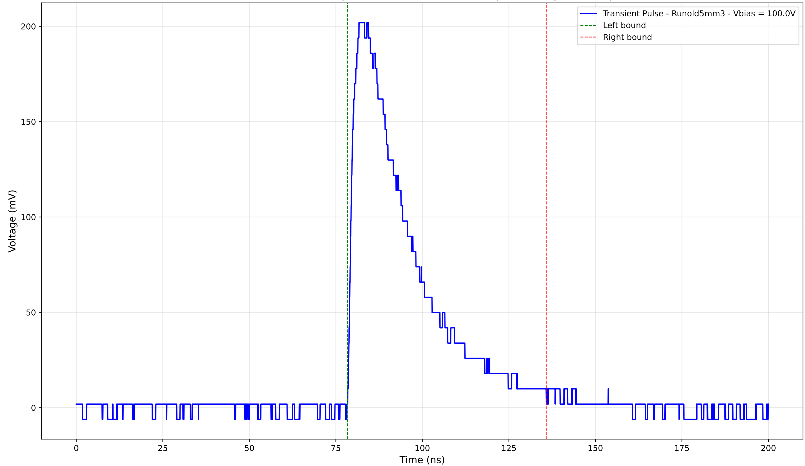
Transient Pulse - Sample: old5 - Position: 2460.0 \mu\text{m} - Charge: 77.27 pC
