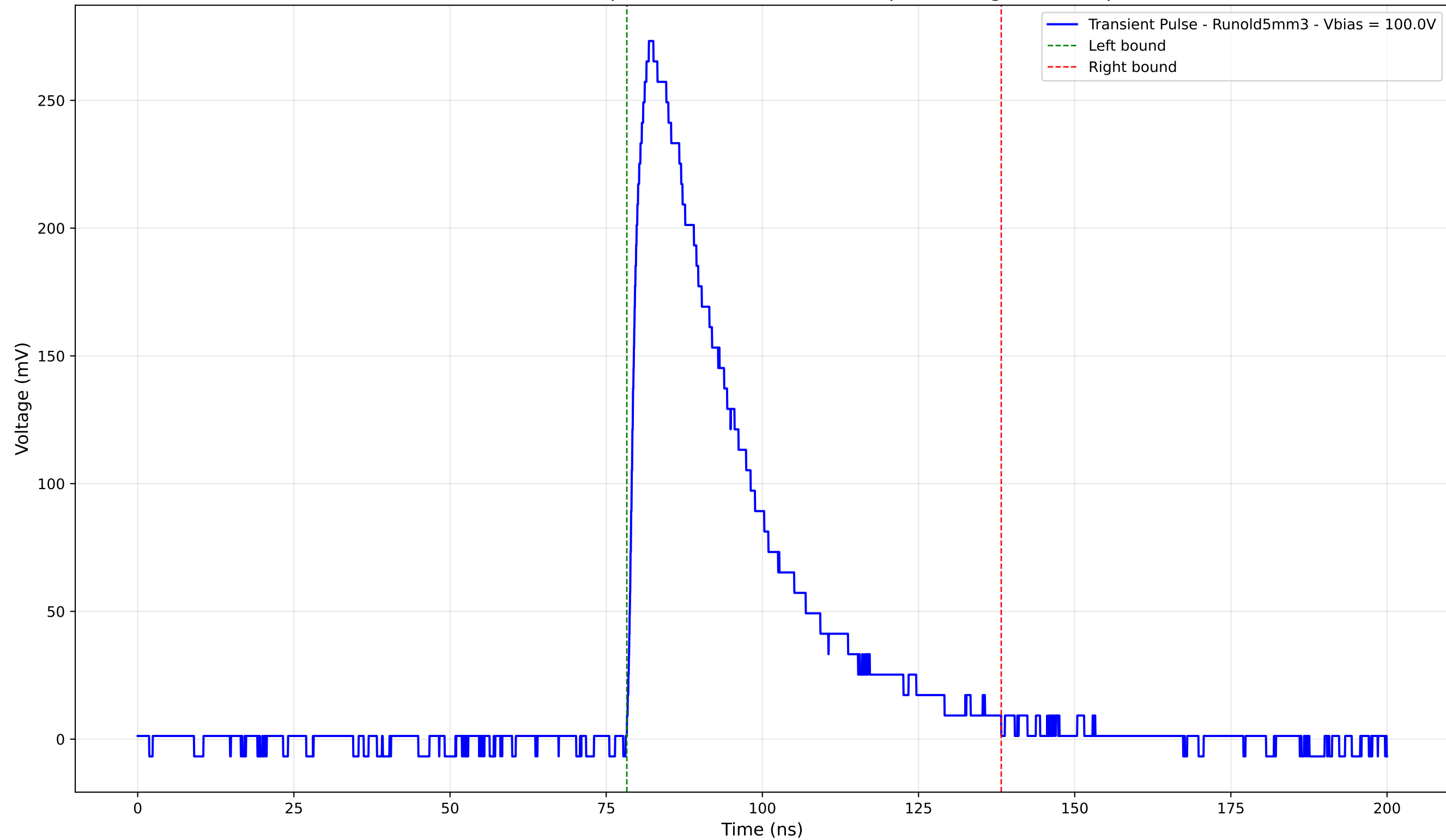
Transient Pulse - Sample: old5 - Position: 2545.0 \mu\text{m} - Charge: 100.89 pC
