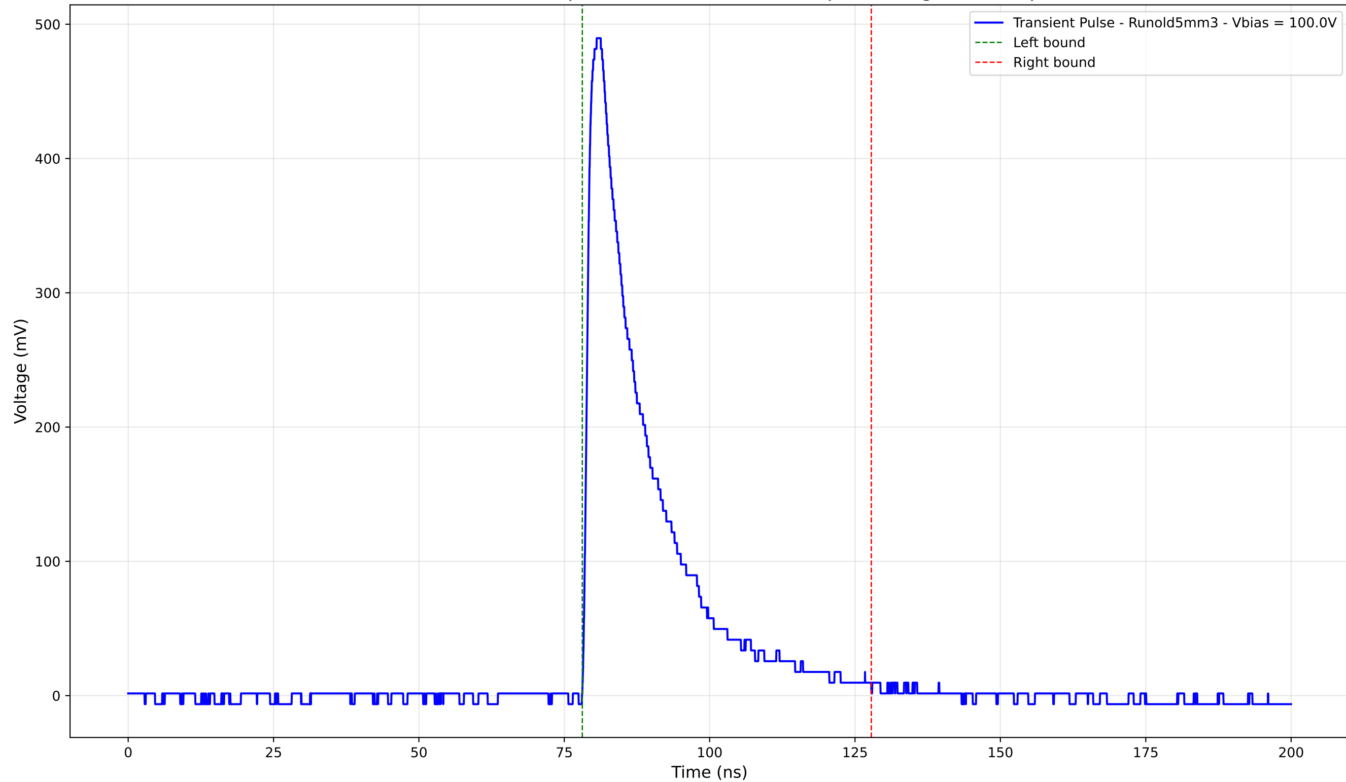
Transient Pulse - Sample: old5 - Position: 4300.0 \mu\text{m} - Charge: 110.54 pC
