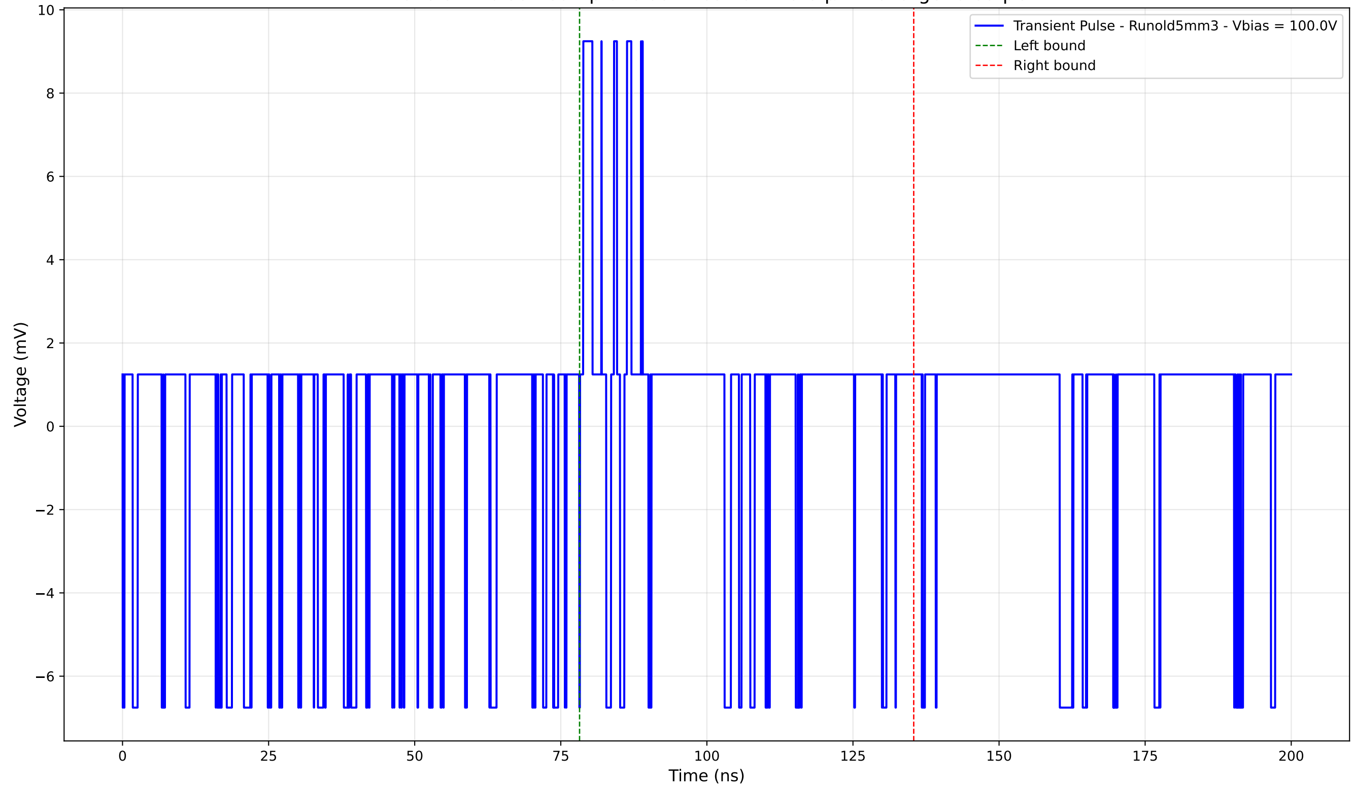
Transient Pulse - Sample: old5 - Position: 15.0 \mu\text{m} - Charge: 0.85 pC
