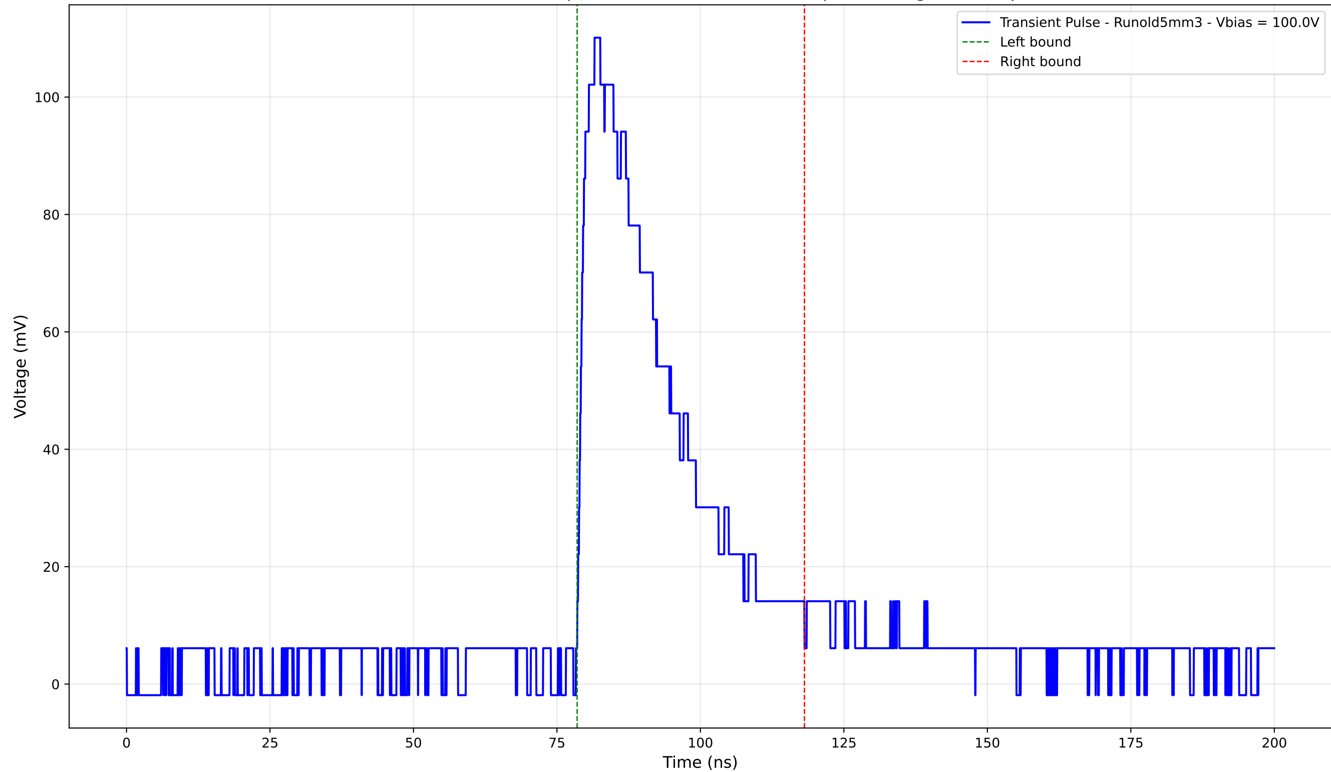
Transient Pulse - Sample: old5 - Position: 1140.0 \mu\text{m} - Charge: 37.42 pC
