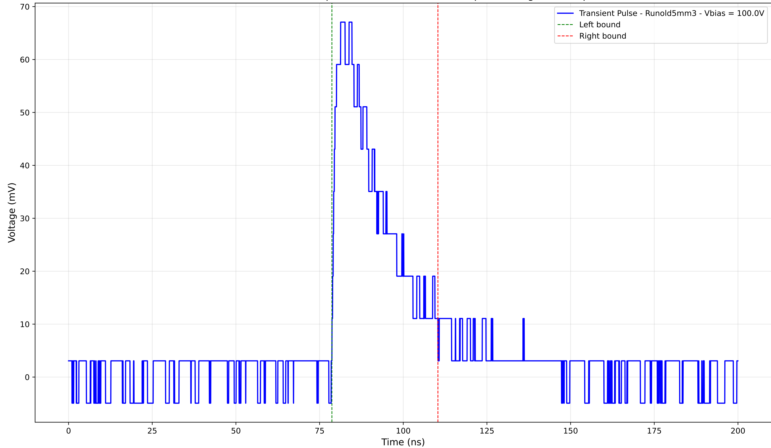
Transient Pulse - Sample: old5 - Position: 2625.0 \mu\text{m} - Charge: 21.06 pC
