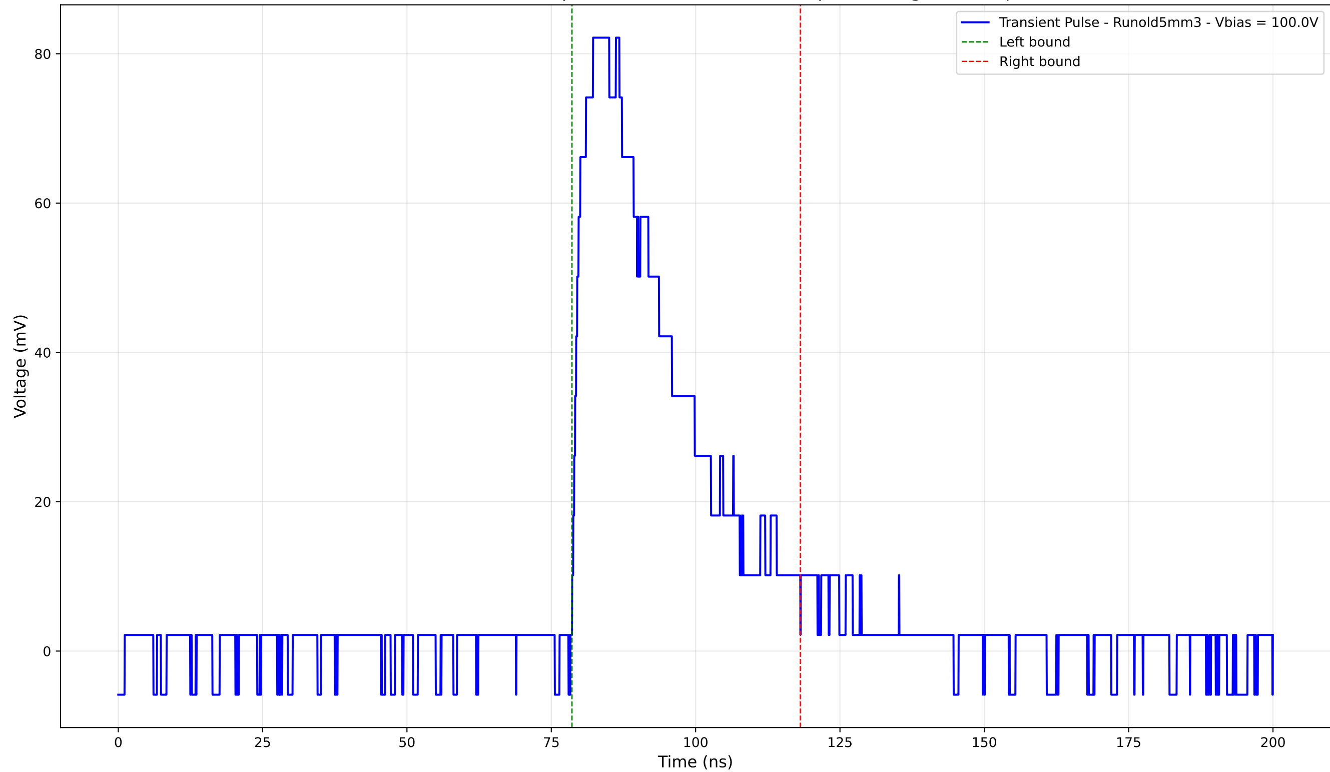
Transient Pulse - Sample: old5 - Position: 1350.0 \mu\text{m} - Charge: 30.04 pC
