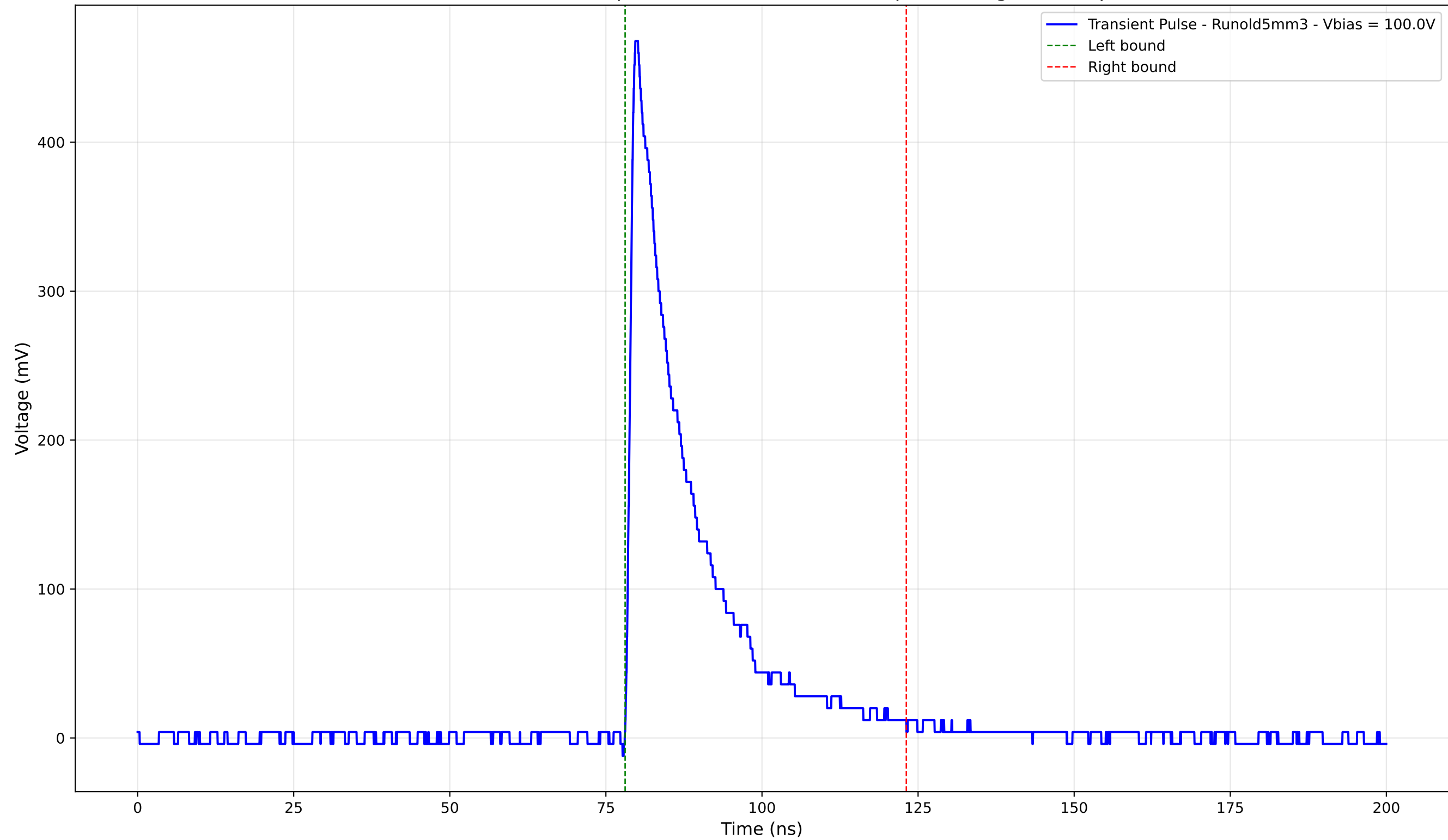
Transient Pulse - Sample: old5 - Position: 4580.0 \mu\text{m} - Charge: 93.68 pC
