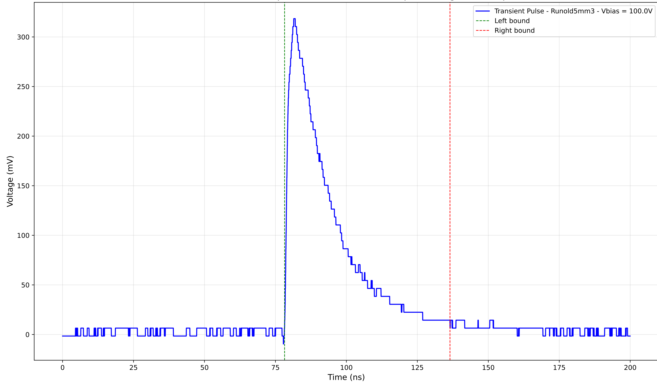
Transient Pulse - Sample: old5 - Position: 2805.0 \mu\text{m} - Charge: 108.61 pC
