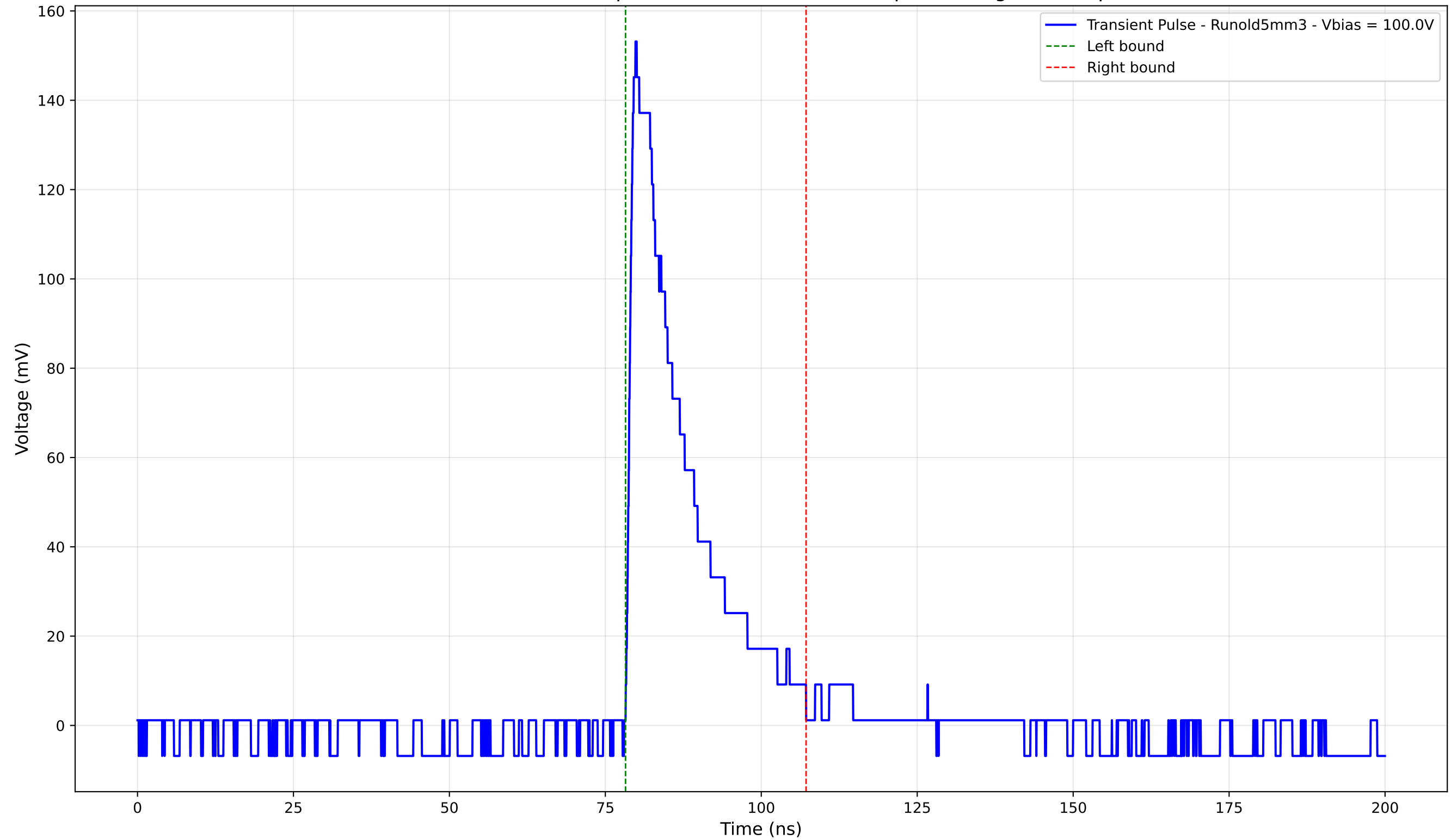
Transient Pulse - Sample: old5 - Position: 4540.0 \mu\text{m} - Charge: 29.16 pC
