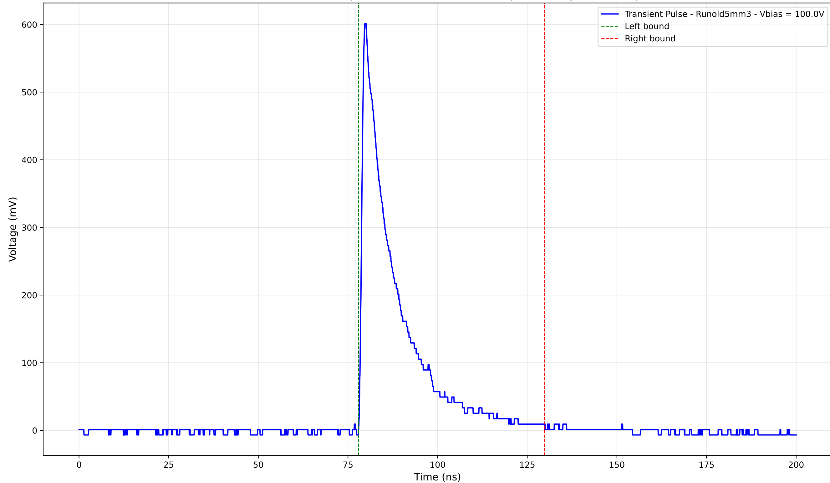
Transient Pulse - Sample: old5 - Position: 4610.0 \mu\text{m} - Charge: 118.98 pC
