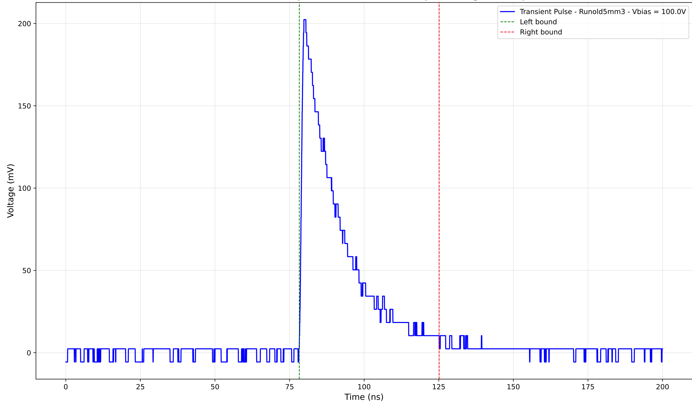
Transient Pulse - Sample: old5 - Position: 735.0 \mu\text{m} - Charge: 54.67 pC
