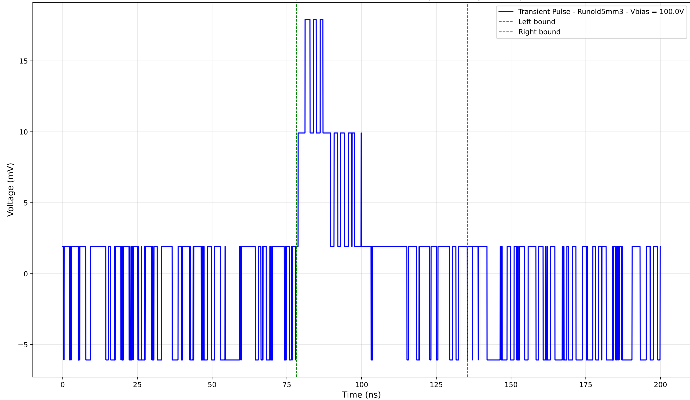
Transient Pulse - Sample: old5 - Position: 2980.0 \mu\text{m} - Charge: 4.51 pC
