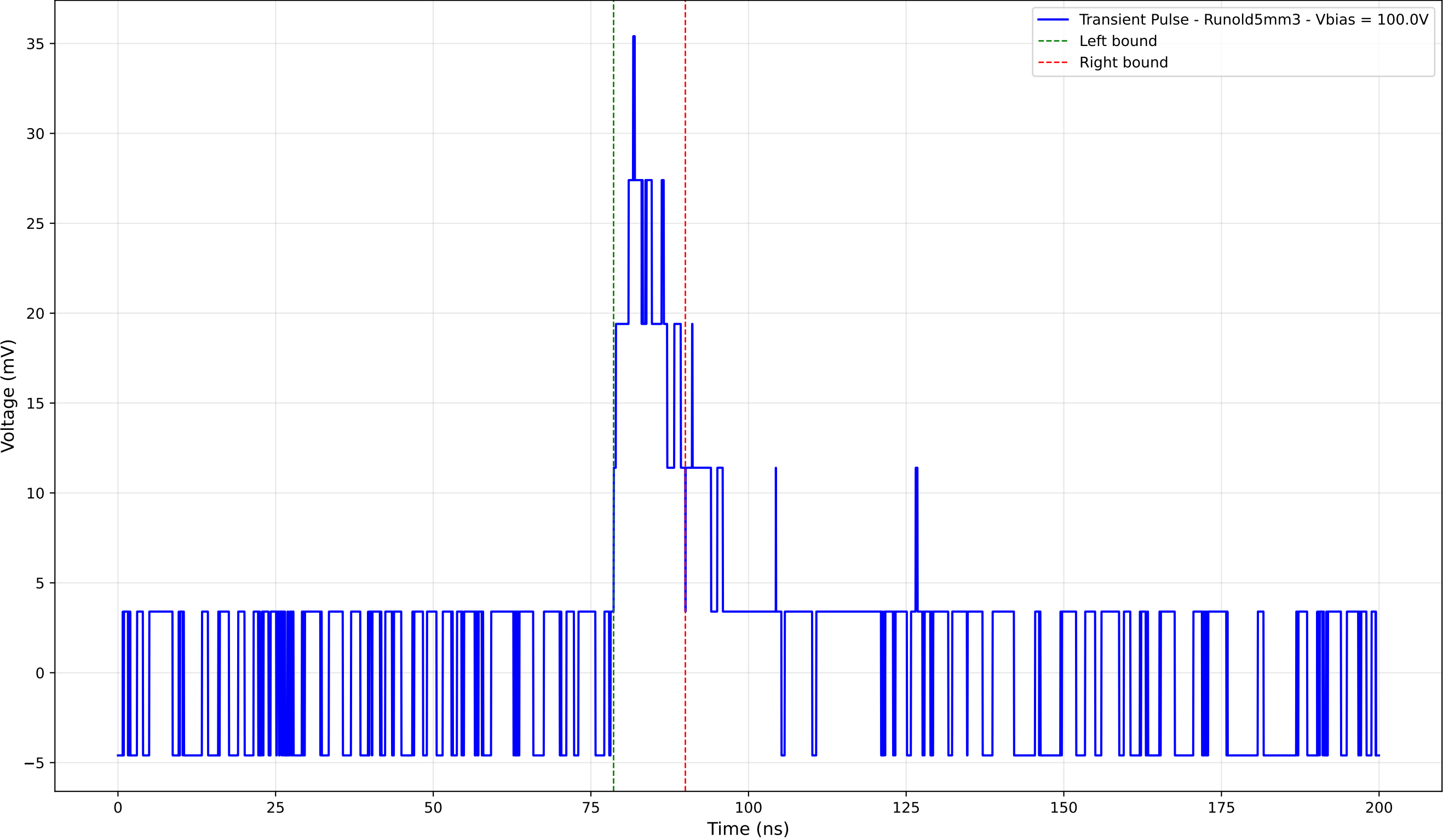
Transient Pulse - Sample: old5 - Position: 4190.0 \mu\text{m} - Charge: 4.66 pC
