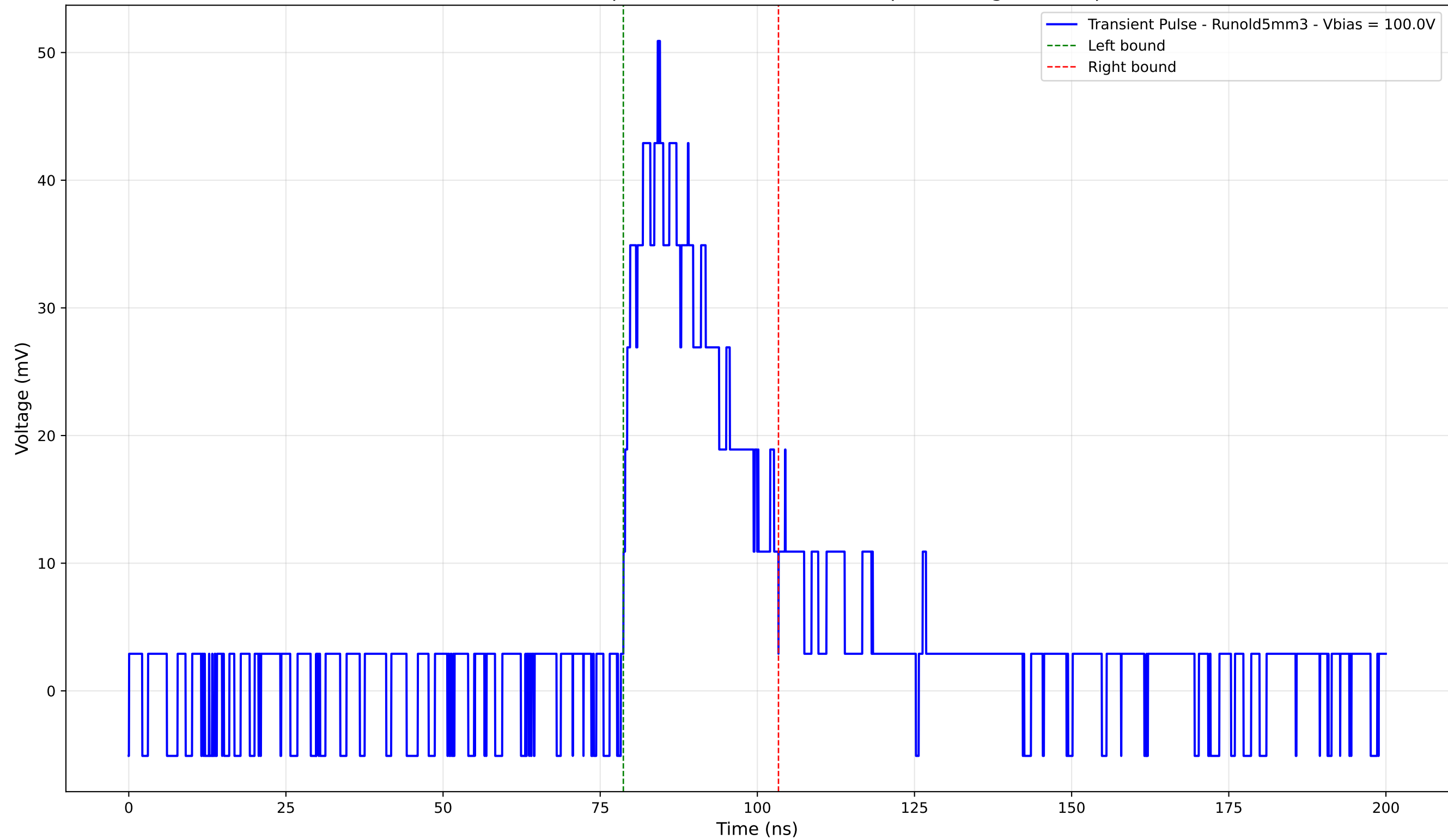
Transient Pulse - Sample: old5 - Position: 1370.0 \mu\text{m} - Charge: 13.58 pC
