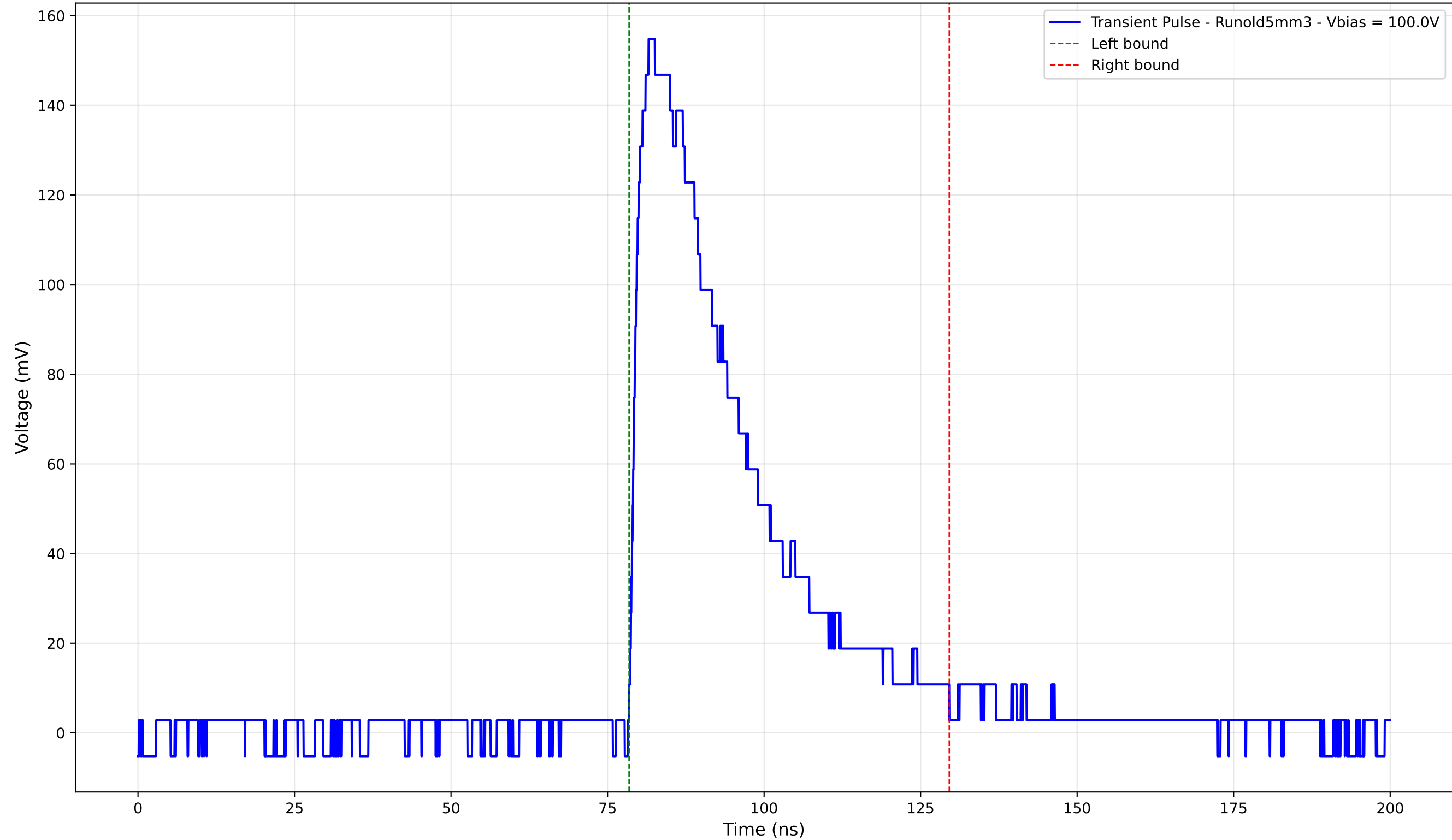
Transient Pulse - Sample: old5 - Position: 1240.0 \mu\text{m} - Charge: 57.89 pC
