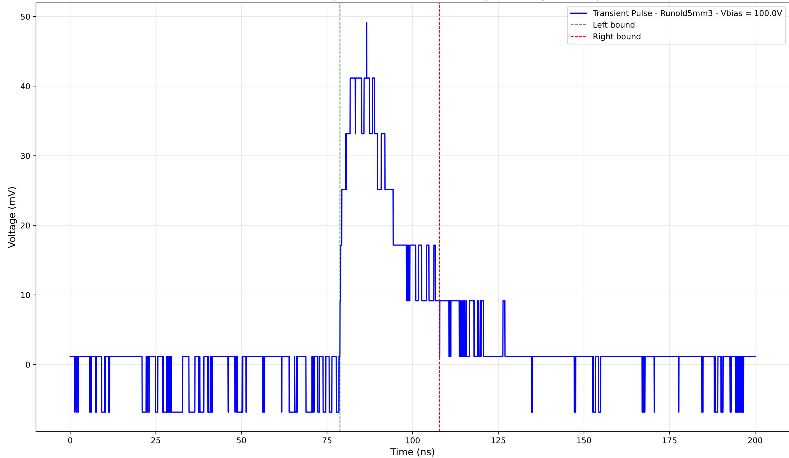
Transient Pulse - Sample: old5 - Position: 2180.0 \mu\text{m} - Charge: 13.95 pC
