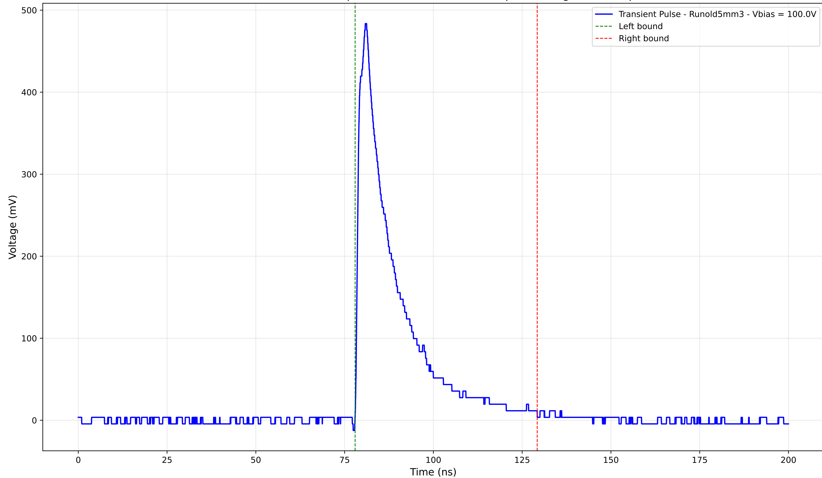
Transient Pulse - Sample: old5 - Position: 4070.0 \mu\text{m} - Charge: 108.41 pC
