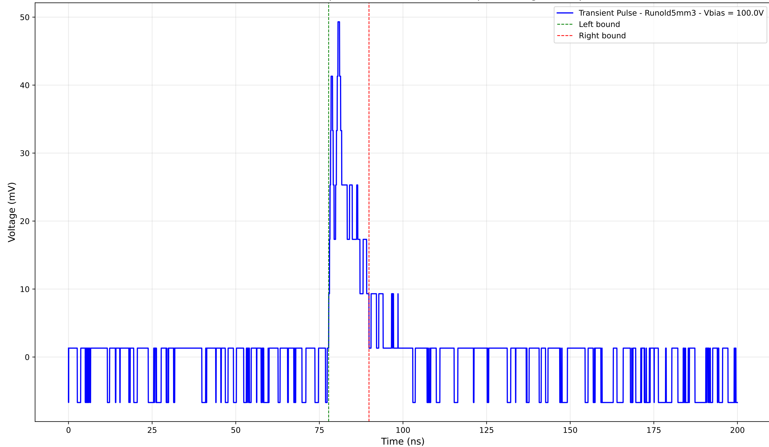
Transient Pulse - Sample: old5 - Position: 3600.0 \mu\text{m} - Charge: 5.49 pC
