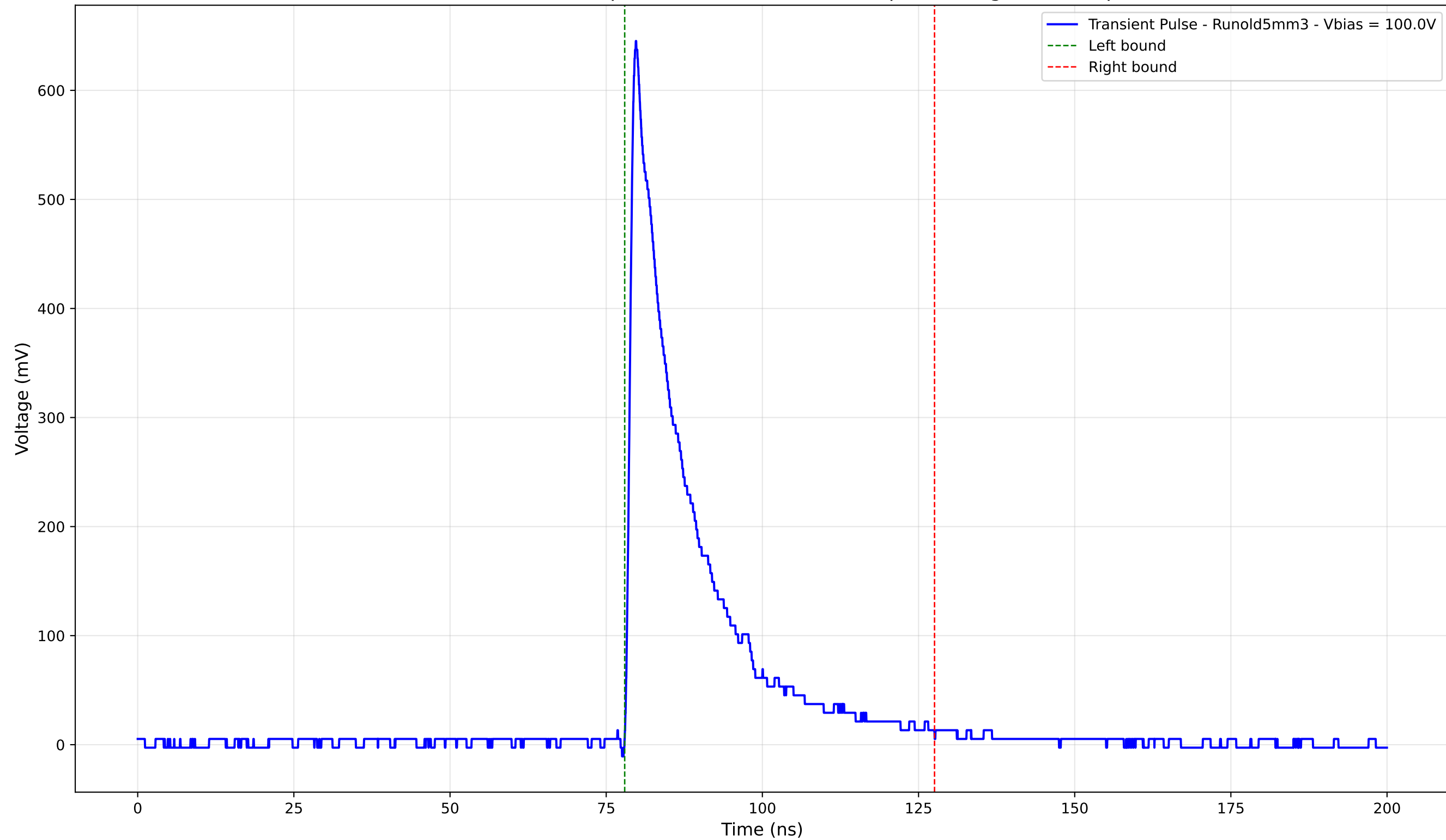
Transient Pulse - Sample: old5 - Position: 4635.0 \mu\text{m} - Charge: 127.57 pC
