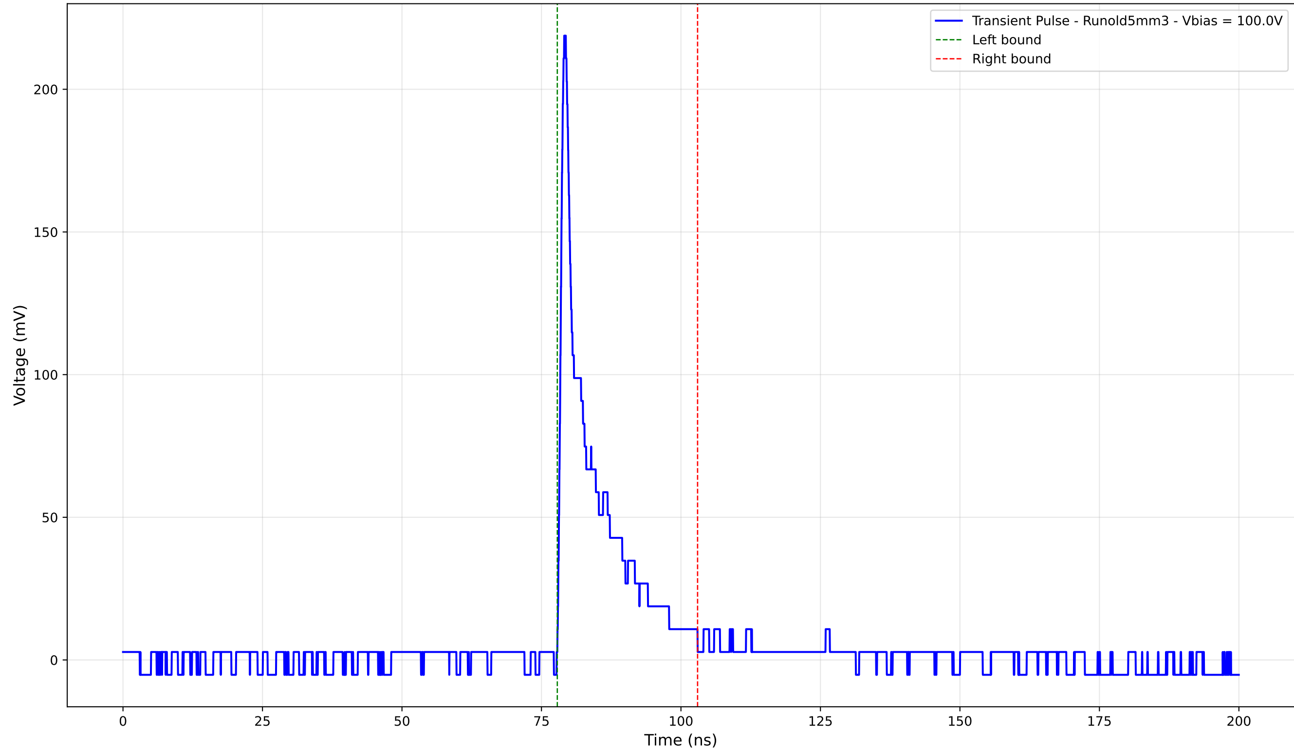
Transient Pulse - Sample: old5 - Position: 4905.0 \mu\text{m} - Charge: 24.83 pC
