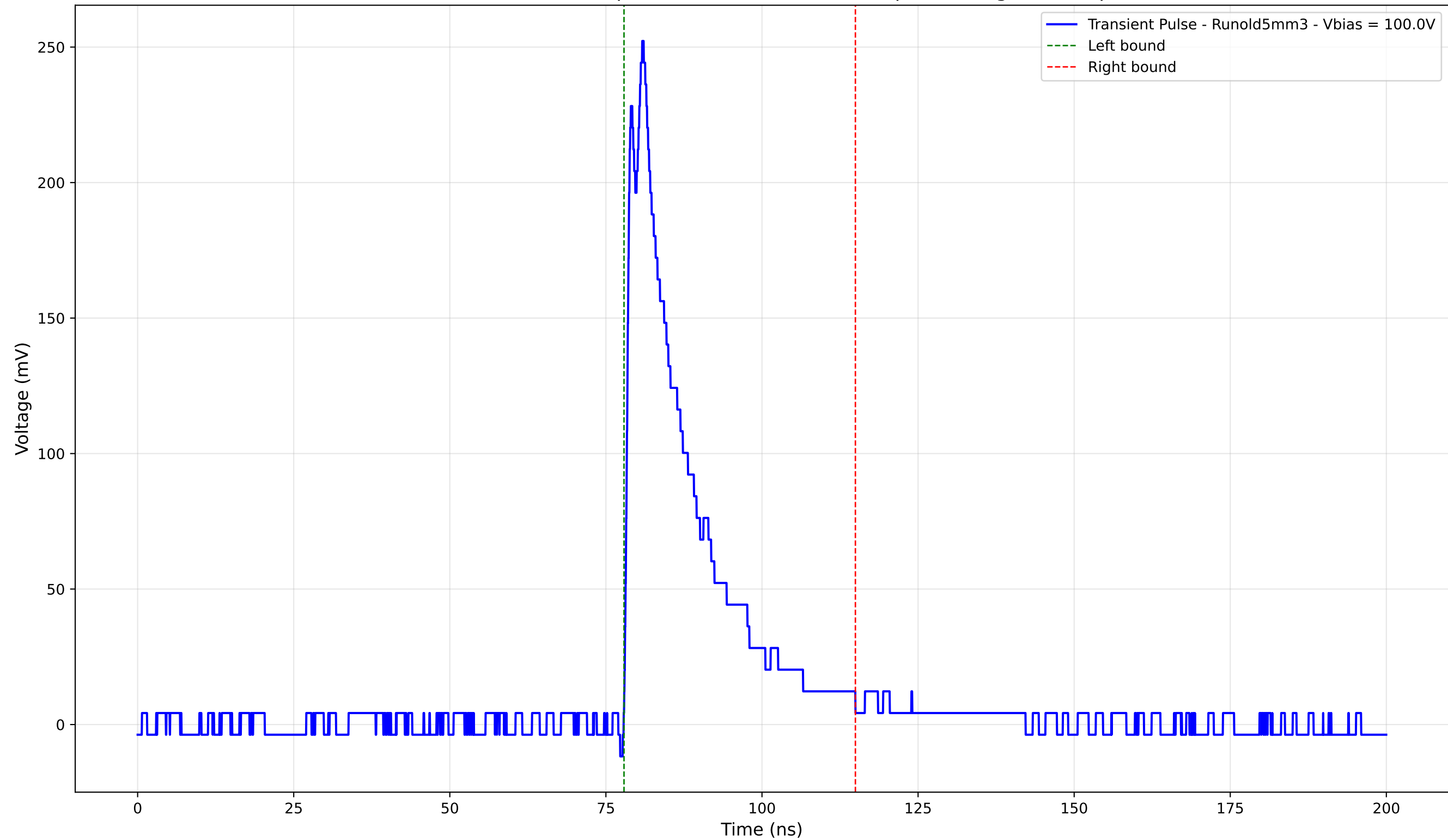
Transient Pulse - Sample: old5 - Position: 3950.0 \mu\text{m} - Charge: 51.26 pC
