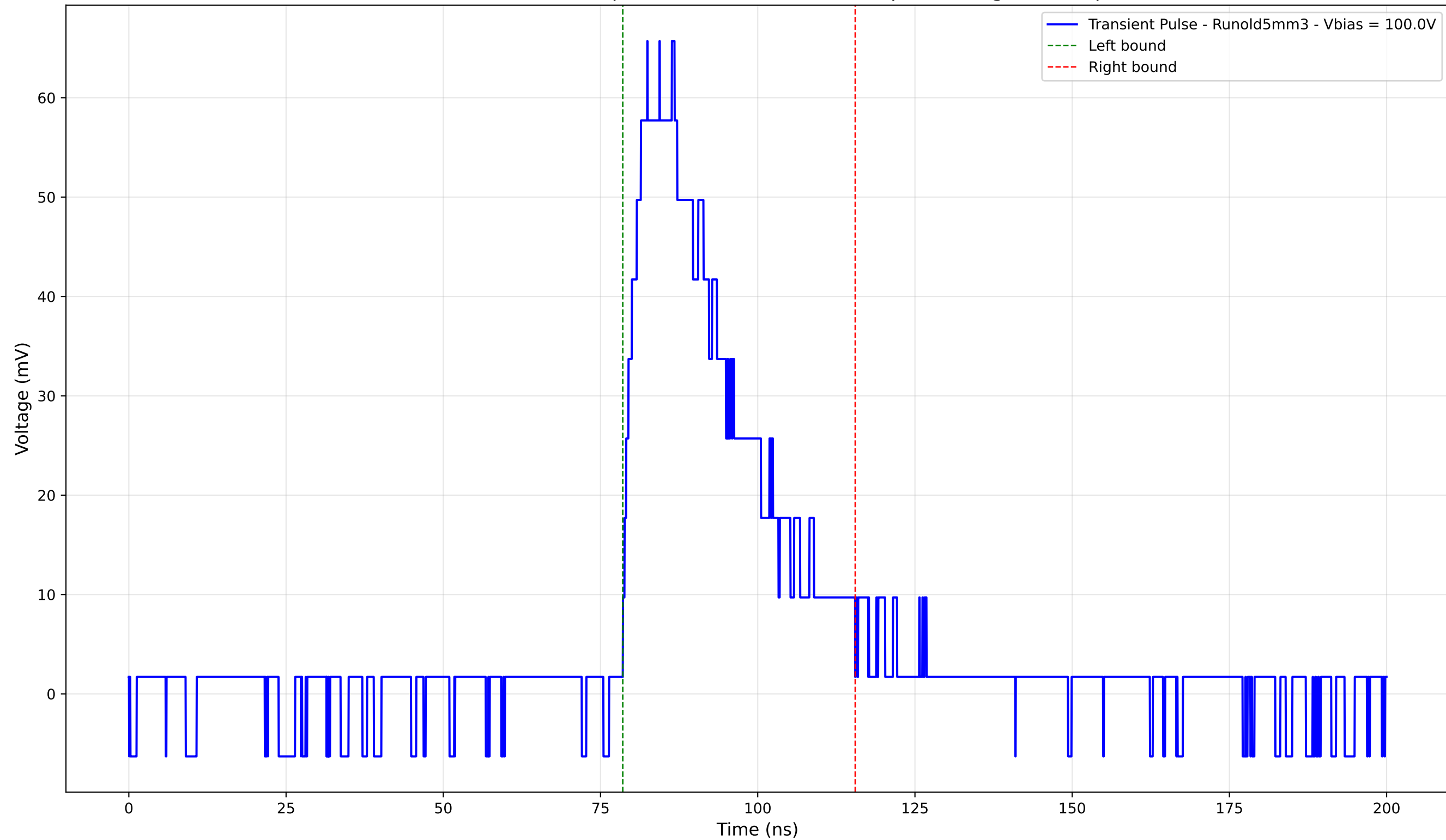
Transient Pulse - Sample: old5 - Position: 1610.0 \mu\text{m} - Charge: 22.38 pC
