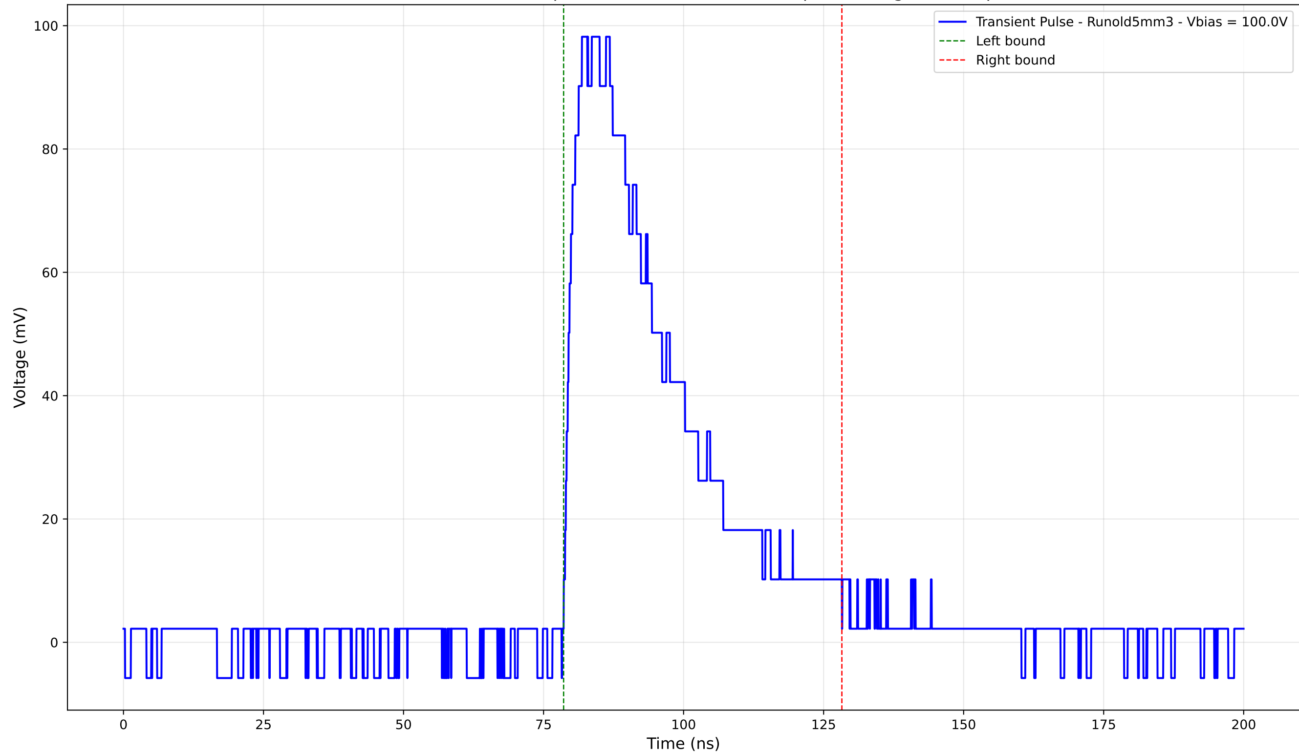
Transient Pulse - Sample: old5 - Position: 1625.0 \mu\text{m} - Charge: 39.45 pC
