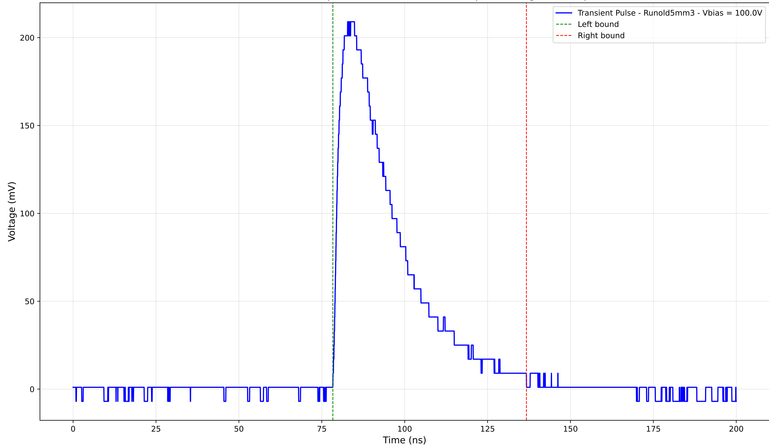
Transient Pulse - Sample: old5 - Position: 1695.0 \mu\text{m} - Charge: 83.32 pC
