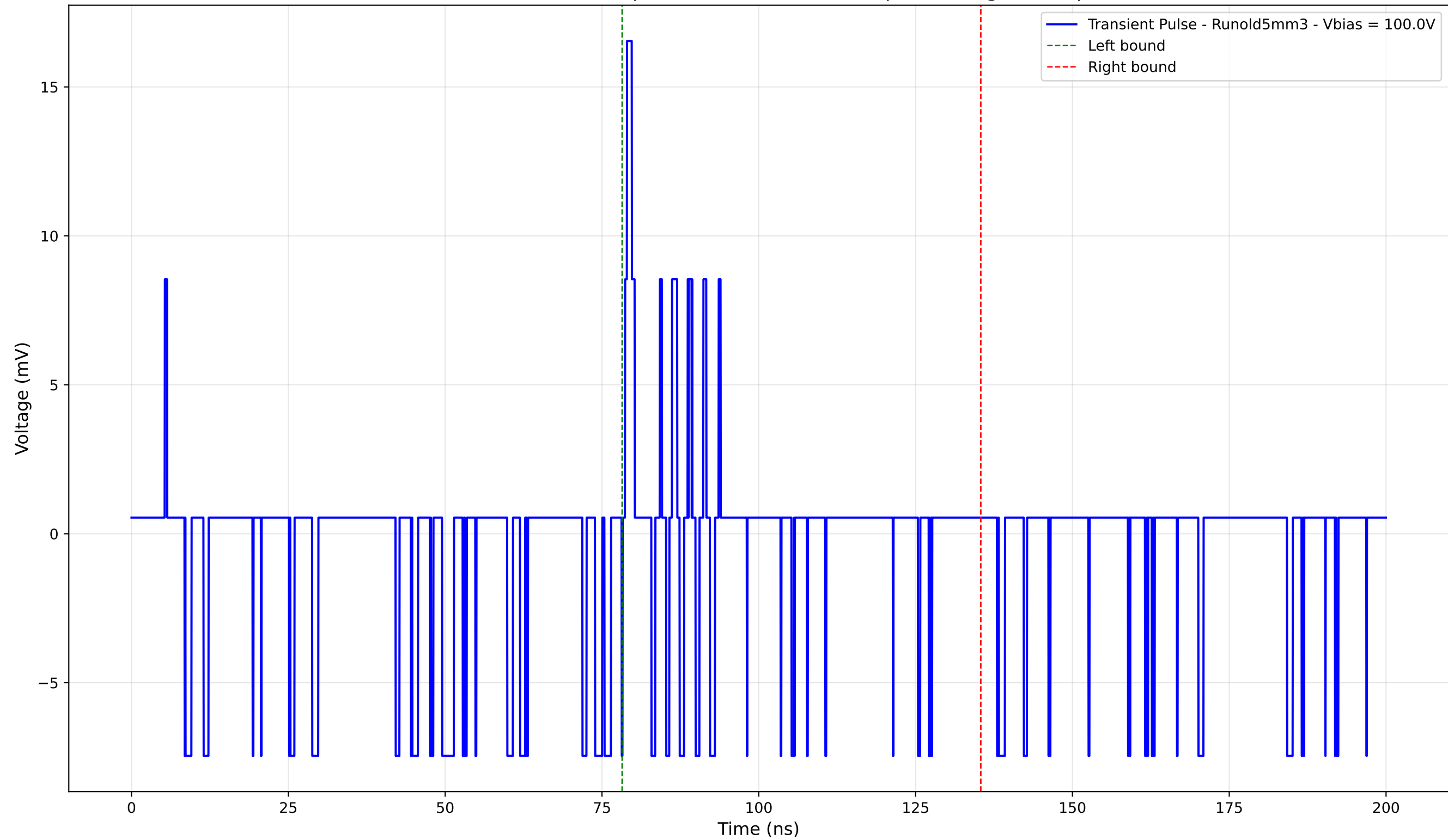
Transient Pulse - Sample: old5 - Position: 10.0 \mu\text{m} - Charge: 0.59 pC
