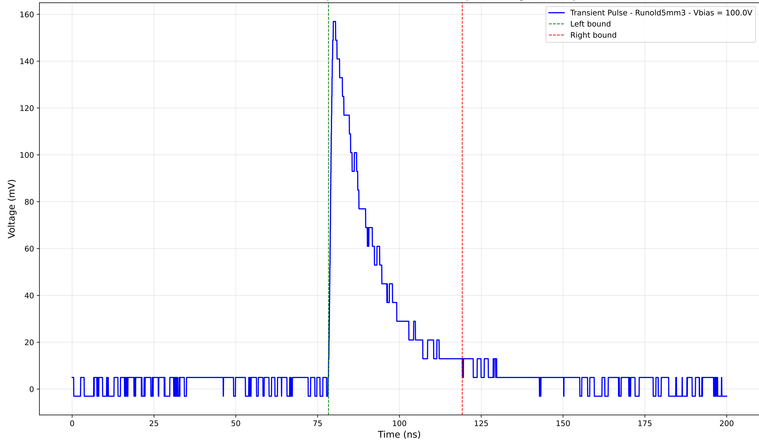
Transient Pulse - Sample: old5 - Position: 715.0 \mu\text{m} - Charge: 41.80 pC
