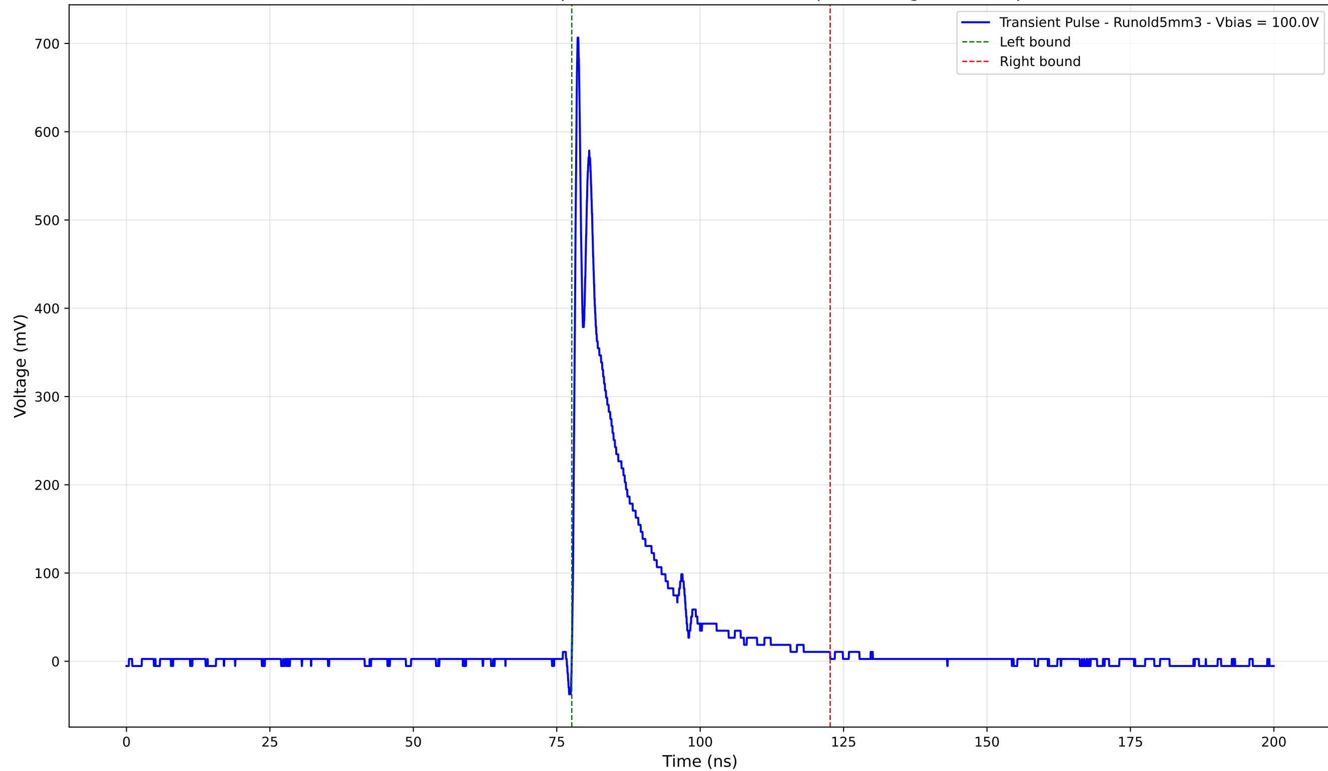
Transient Pulse - Sample: old5 - Position: 3710.0 \mu\text{m} - Charge: 106.34 pC
