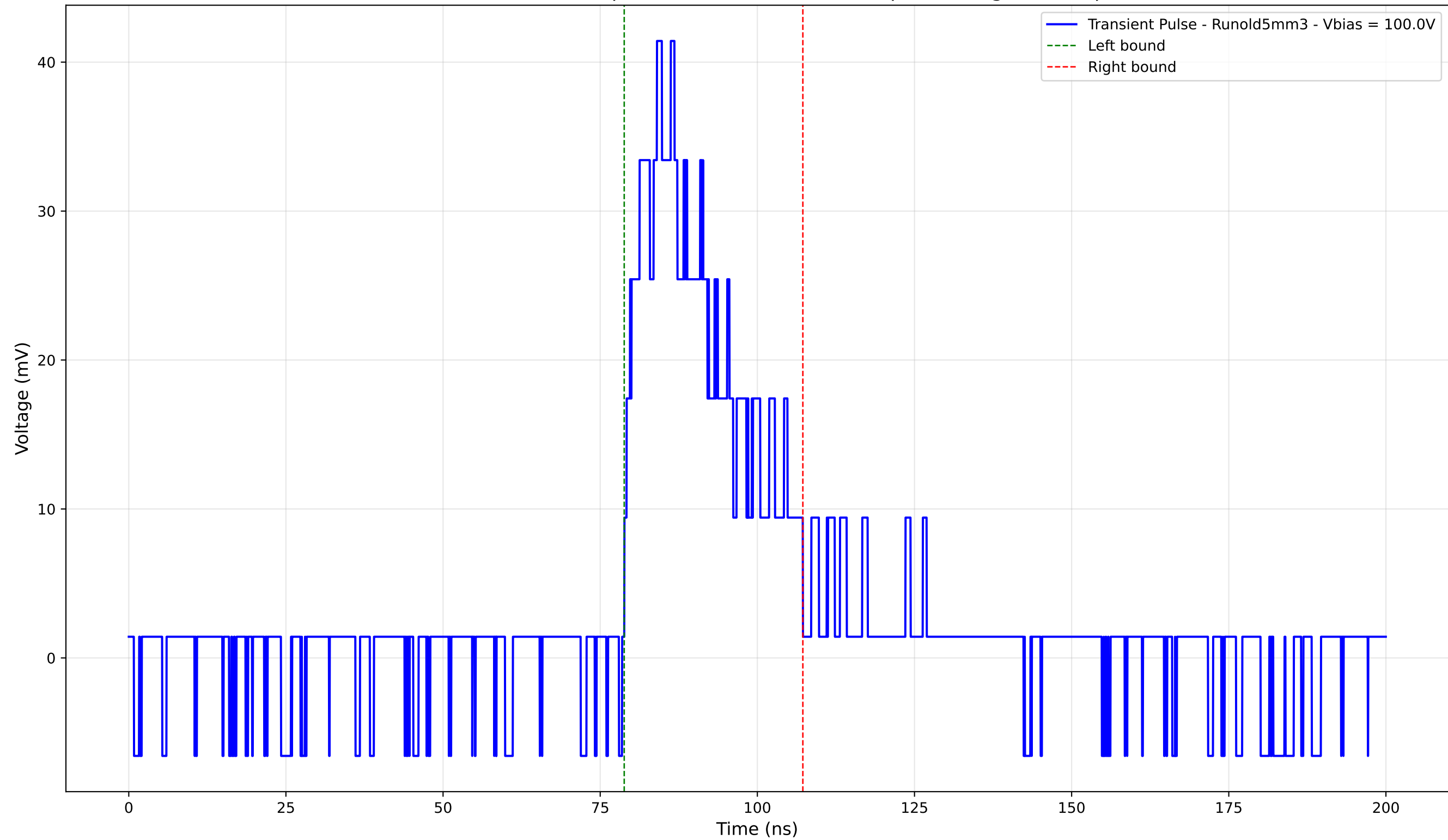
Transient Pulse - Sample: old5 - Position: 2000.0 \mu\text{m} - Charge: 12.07 pC
