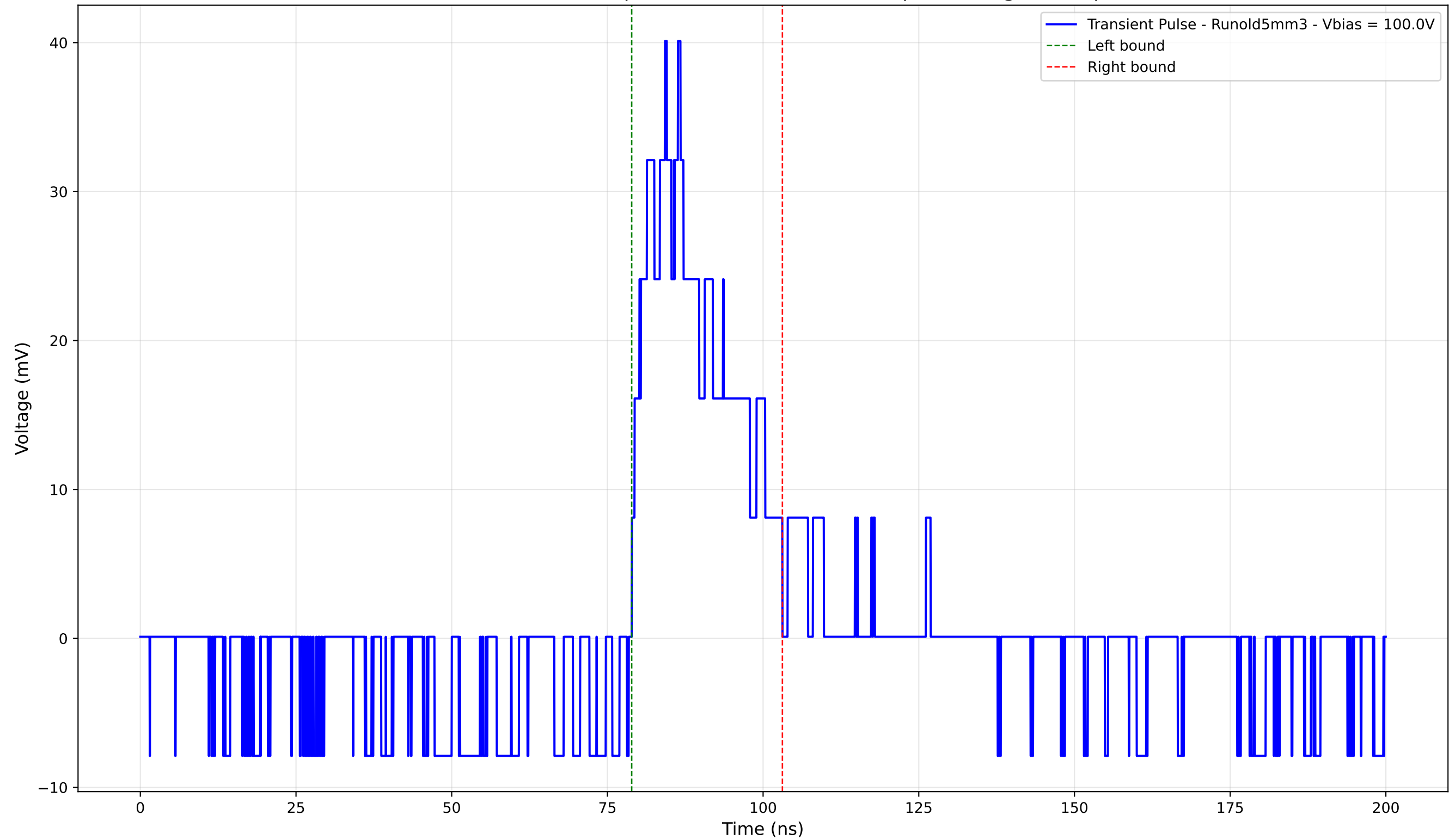
Transient Pulse - Sample: old5 - Position: 1395.0 \mu\text{m} - Charge: 9.68 pC
