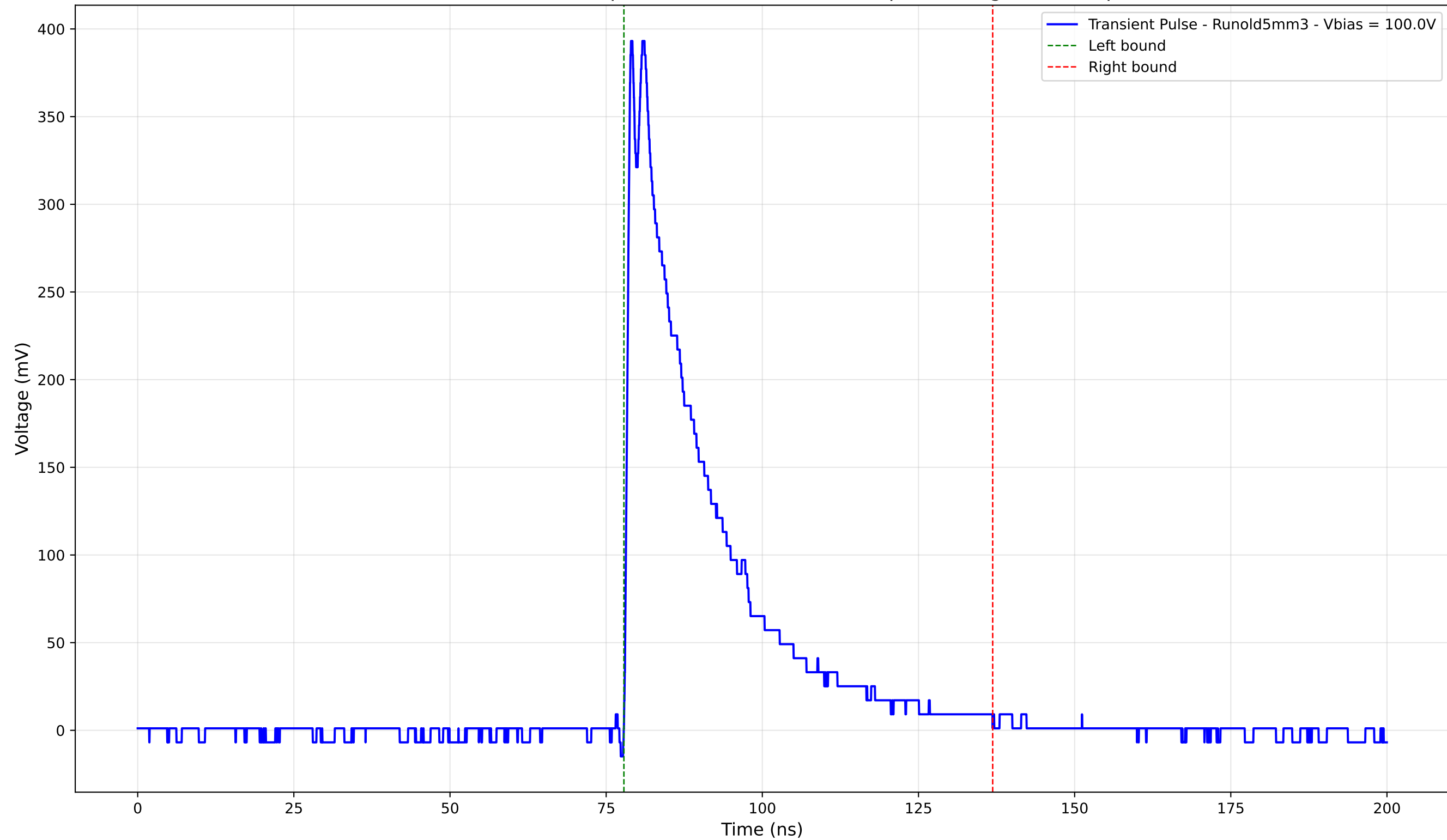
Transient Pulse - Sample: old5 - Position: 3165.0 \mu\text{m} - Charge: 101.56 pC
