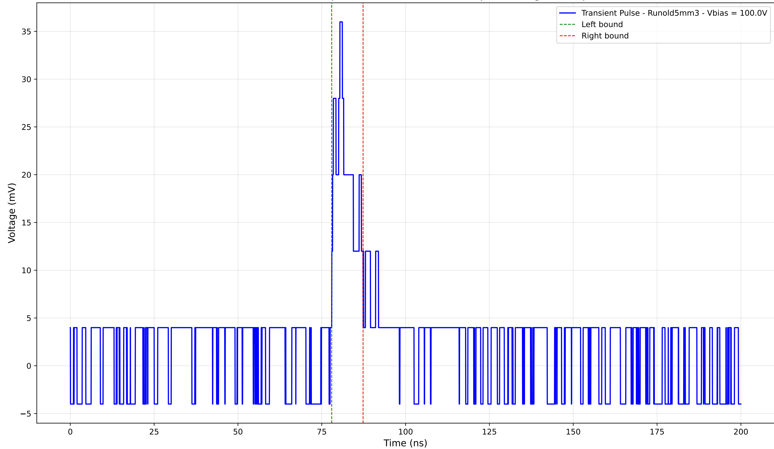
Transient Pulse - Sample: old5 - Position: 3580.0 \mu\text{m} - Charge: 3.83 pC
