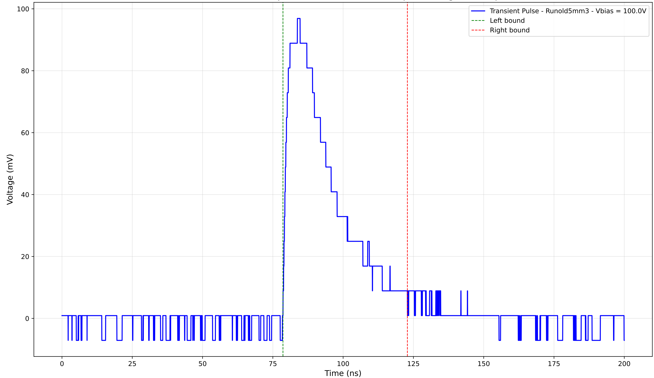
Transient Pulse - Sample: old5 - Position: 1425.0 \mu\text{m} - Charge: 35.50 pC
