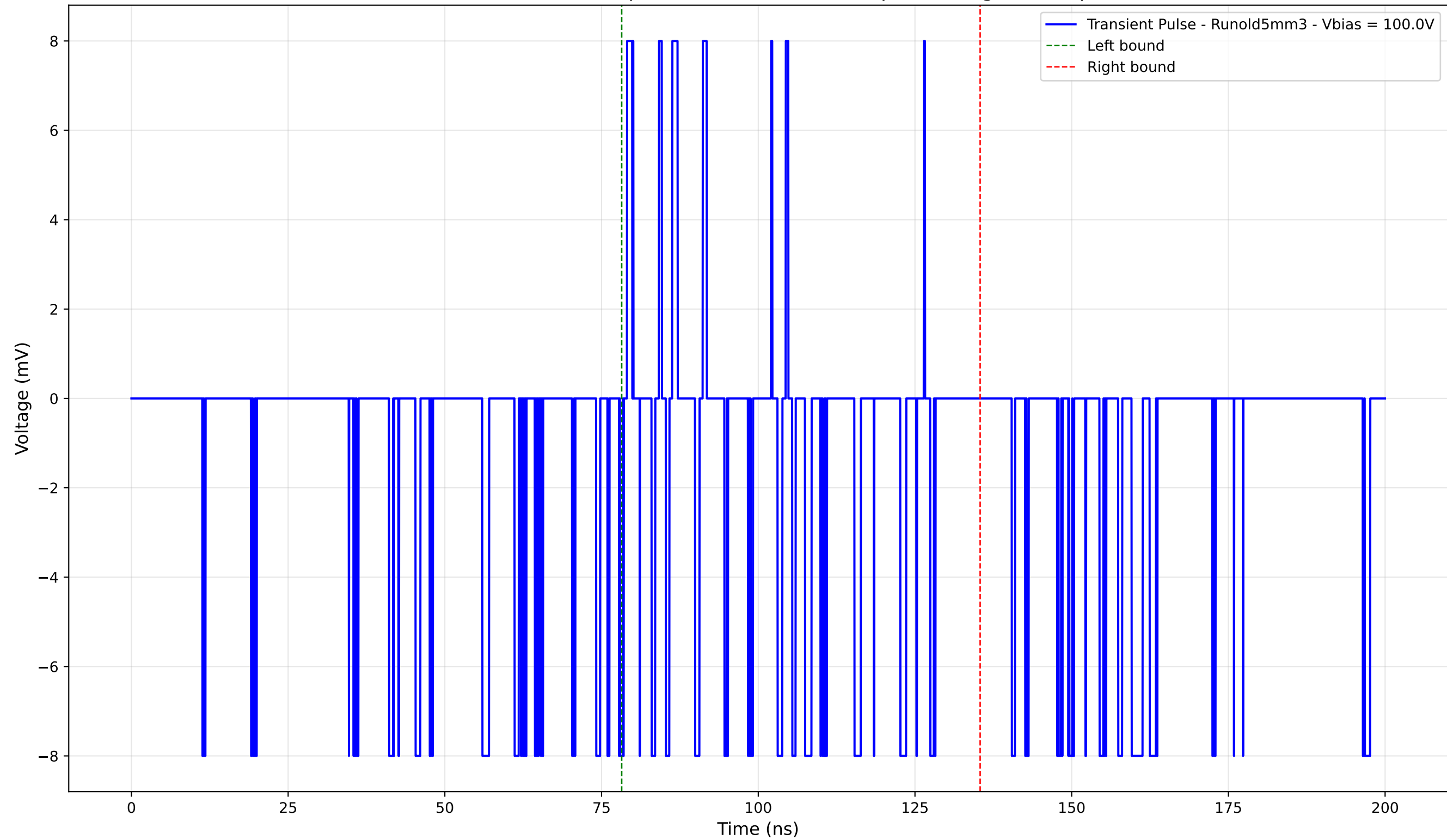
Transient Pulse - Sample: old5 - Position: 30.0 \mu\text{m} - Charge: -0.86 pC
