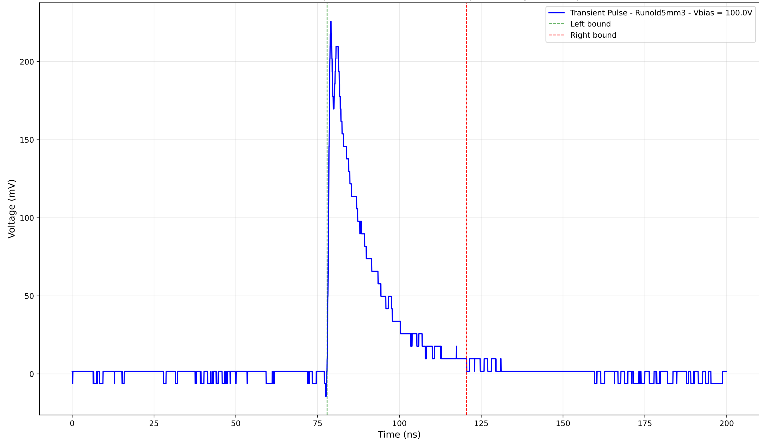
Transient Pulse - Sample: old5 - Position: 3210.0 \mu\text{m} - Charge: 50.70 pC
