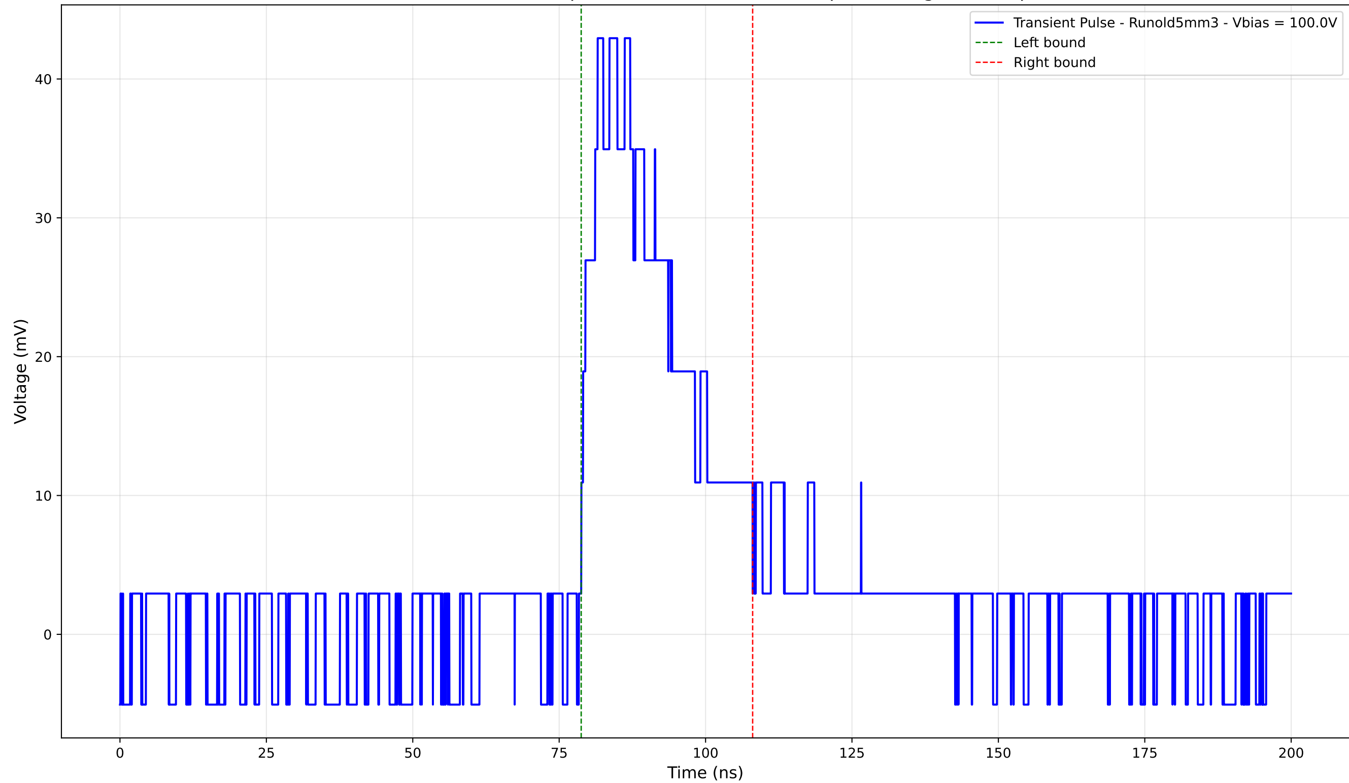
Transient Pulse - Sample: old5 - Position: 2405.0 \mu\text{m} - Charge: 13.83 pC
