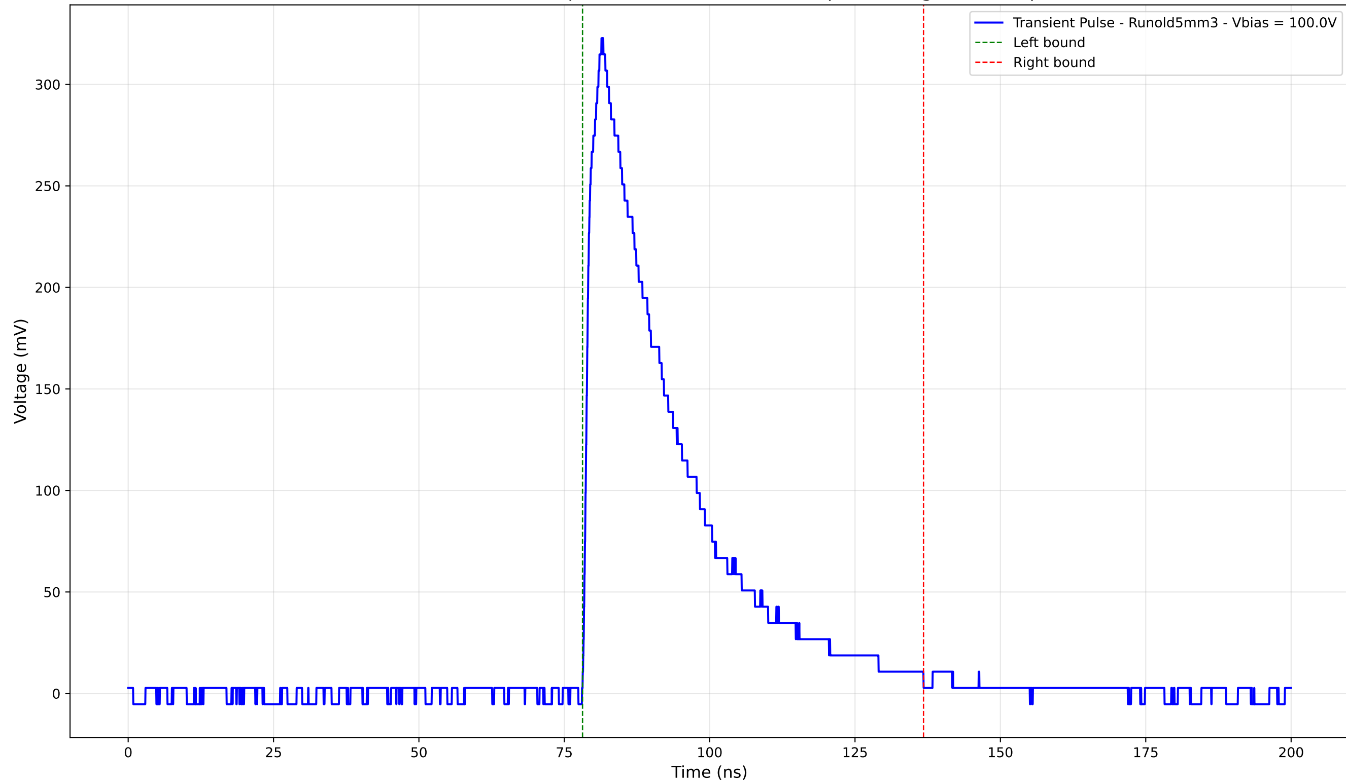
Transient Pulse - Sample: old5 - Position: 2855.0 \mu\text{m} - Charge: 104.57 pC
