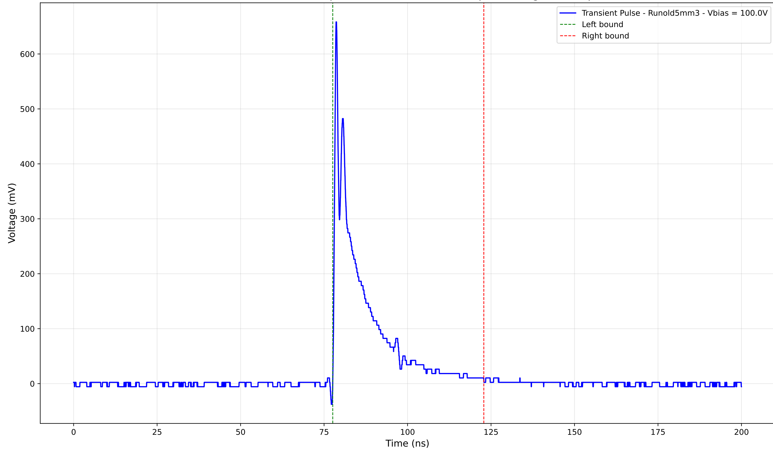
Transient Pulse - Sample: old5 - Position: 3485.0 \mu\text{m} - Charge: 89.16 pC
