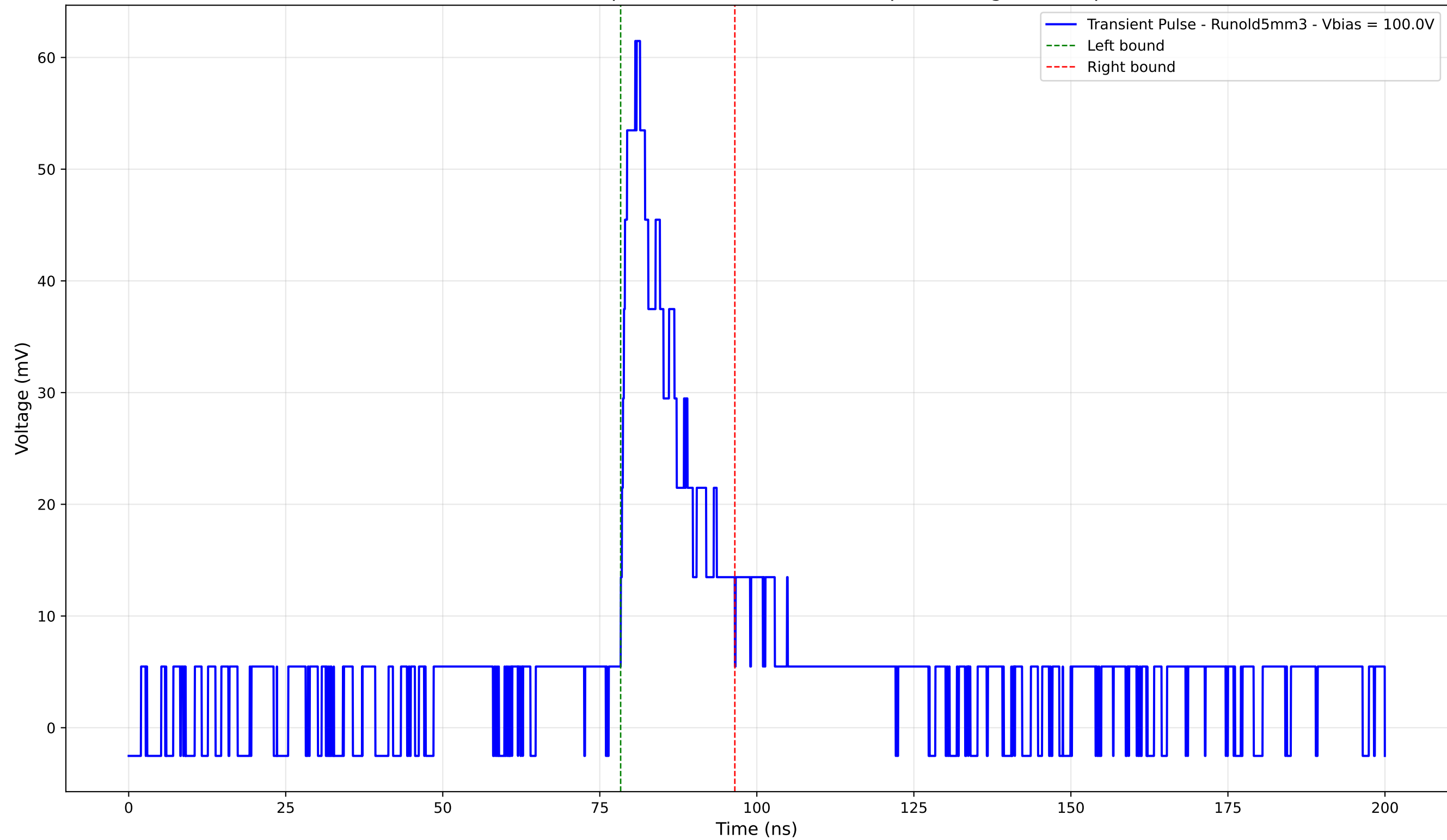
Transient Pulse - Sample: old5 - Position: 4150.0 \mu\text{m} - Charge: 10.87 pC
