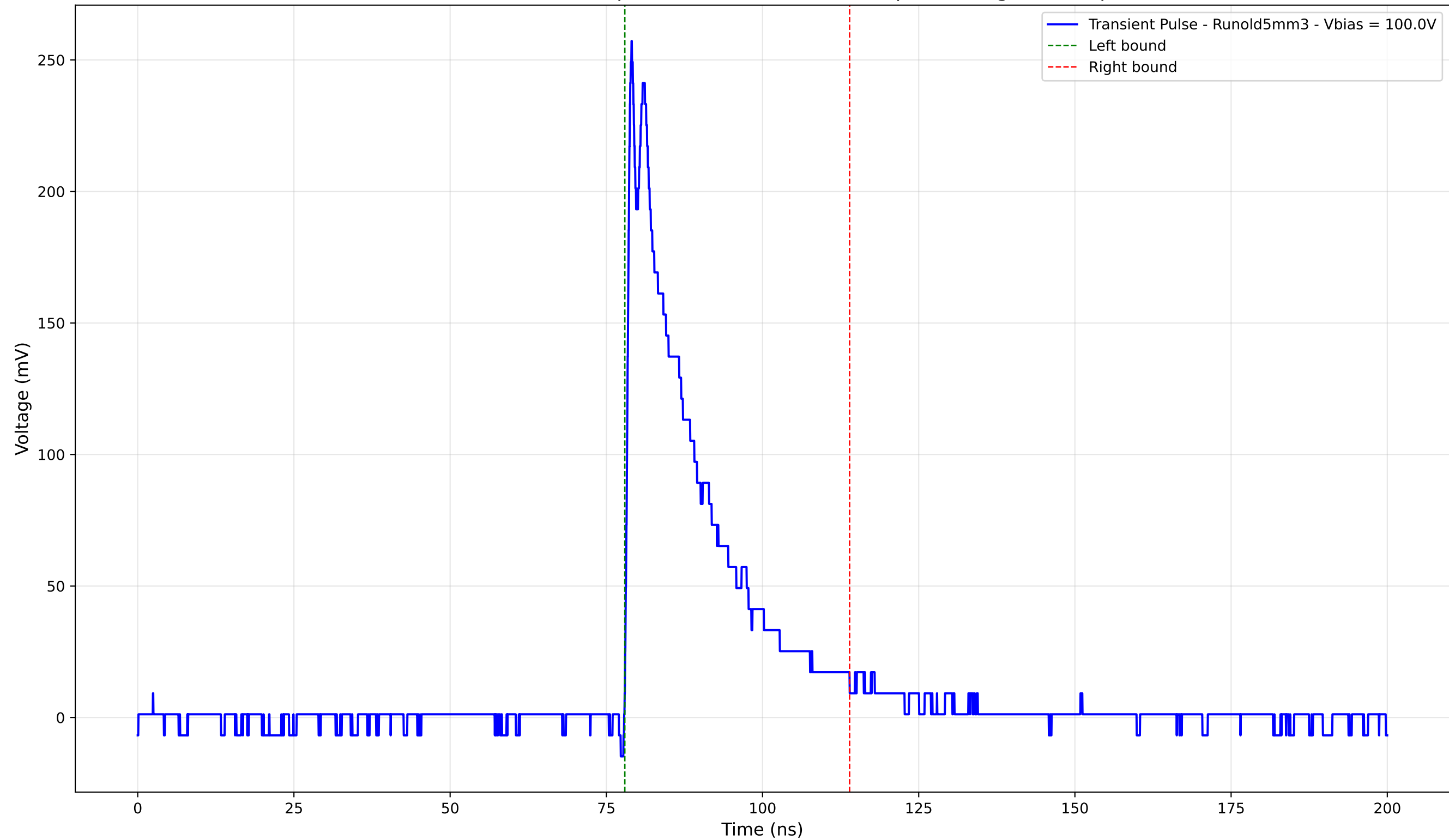
Transient Pulse - Sample: old5 - Position: 3205.0 \mu\text{m} - Charge: 56.56 pC
