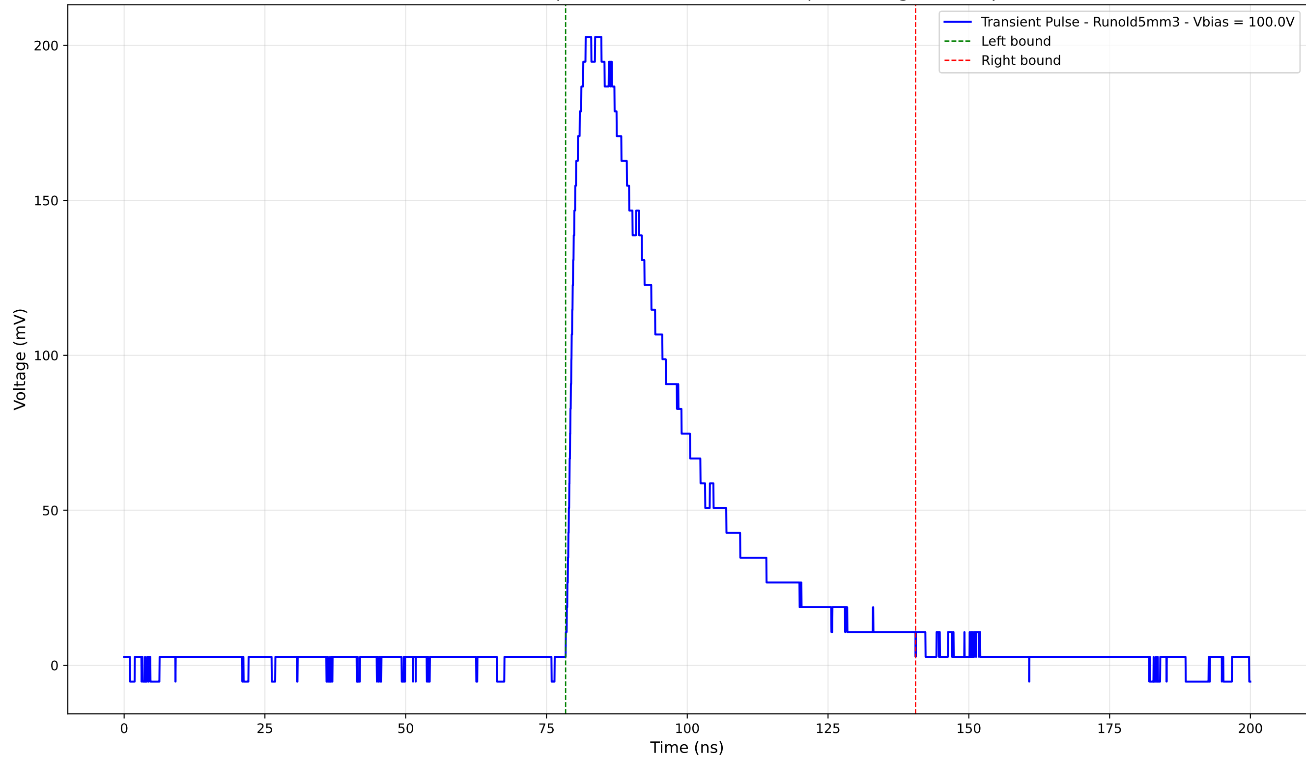
Transient Pulse - Sample: old5 - Position: 1500.0 \mu\text{m} - Charge: 82.98 pC
