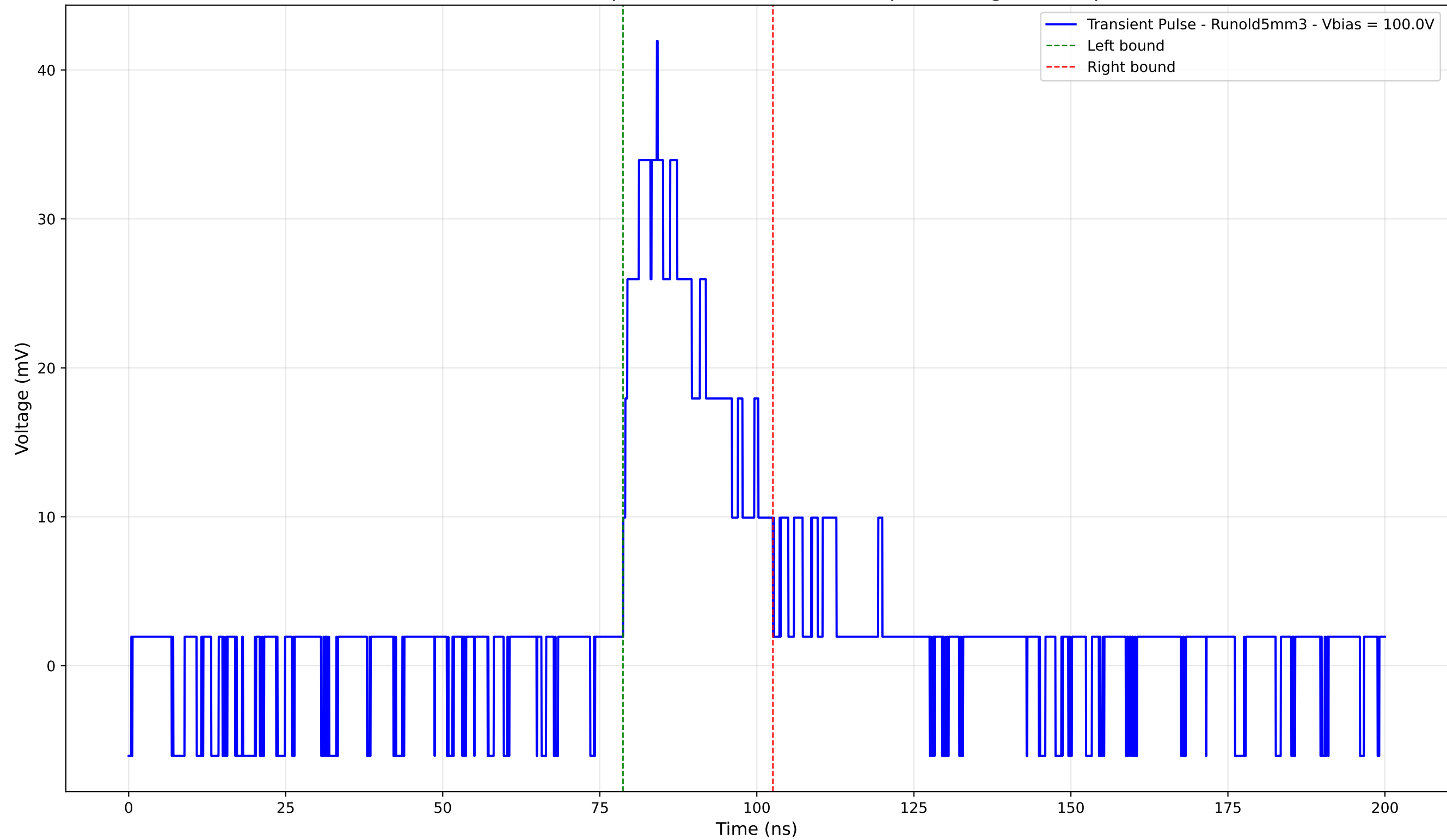
Transient Pulse - Sample: old5 - Position: 1175.0 \mu\text{m} - Charge: 10.27 pC
