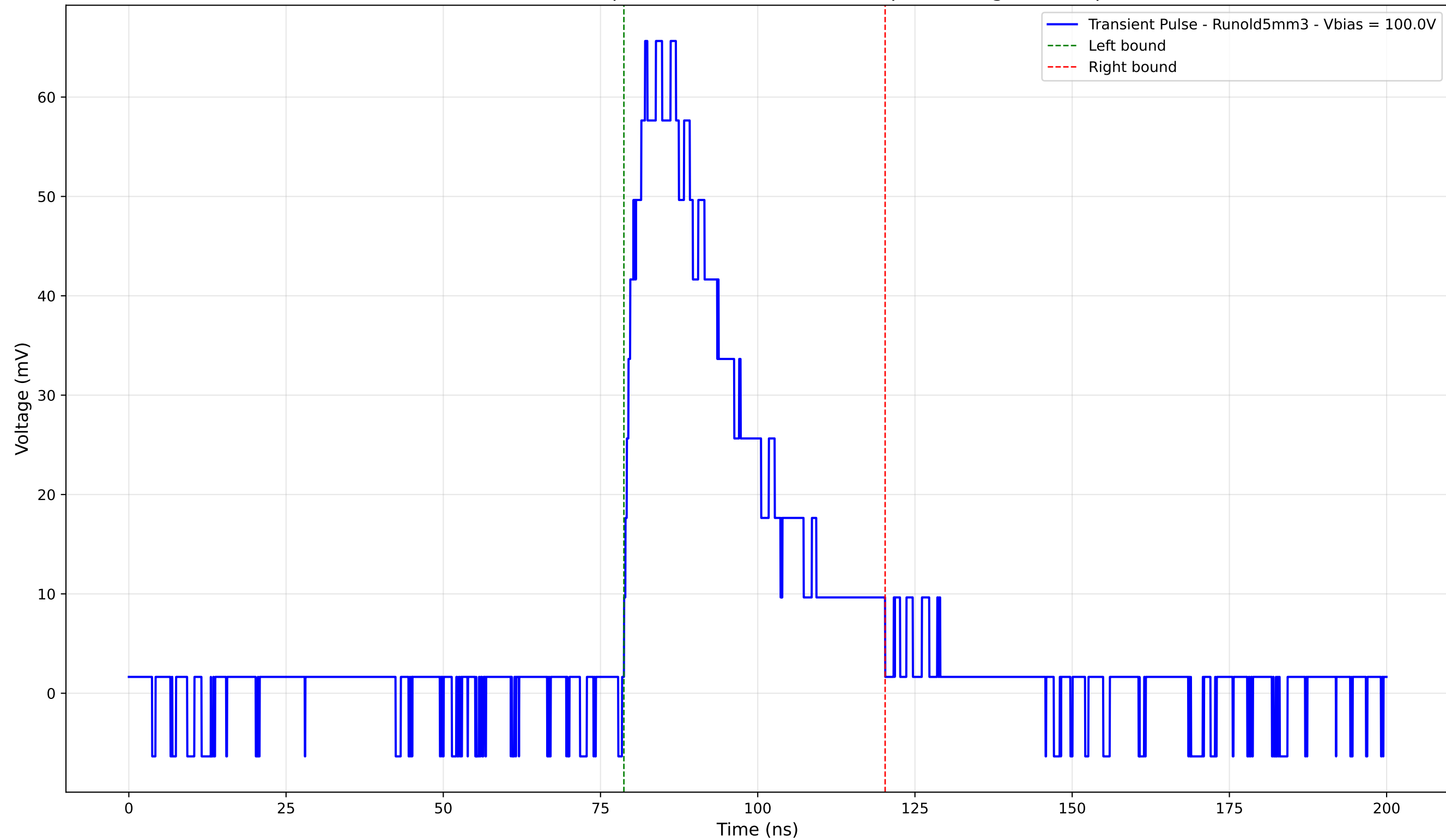
Transient Pulse - Sample: old5 - Position: 1815.0 \mu\text{m} - Charge: 24.25 pC
