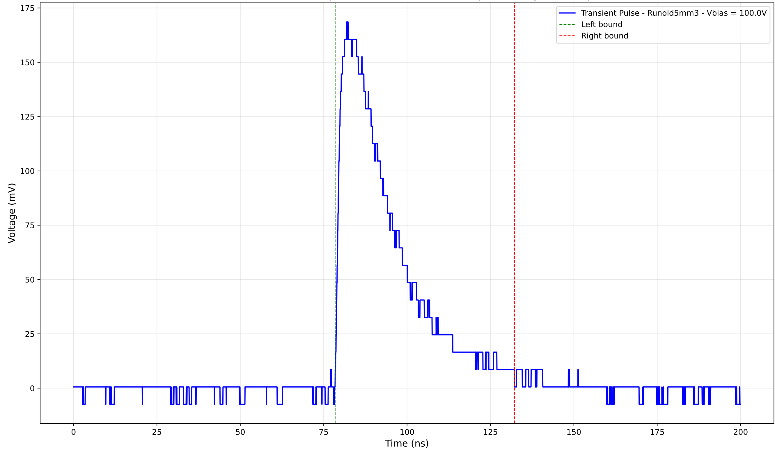
Transient Pulse - Sample: old5 - Position: 1245.0 \mu\text{m} - Charge: 61.71 pC
