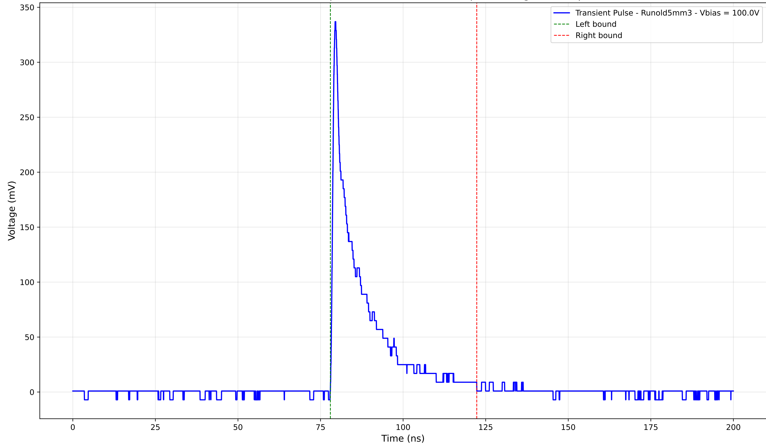
Transient Pulse - Sample: old5 - Position: 330.0 \mu\text{m} - Charge: 52.24 pC
