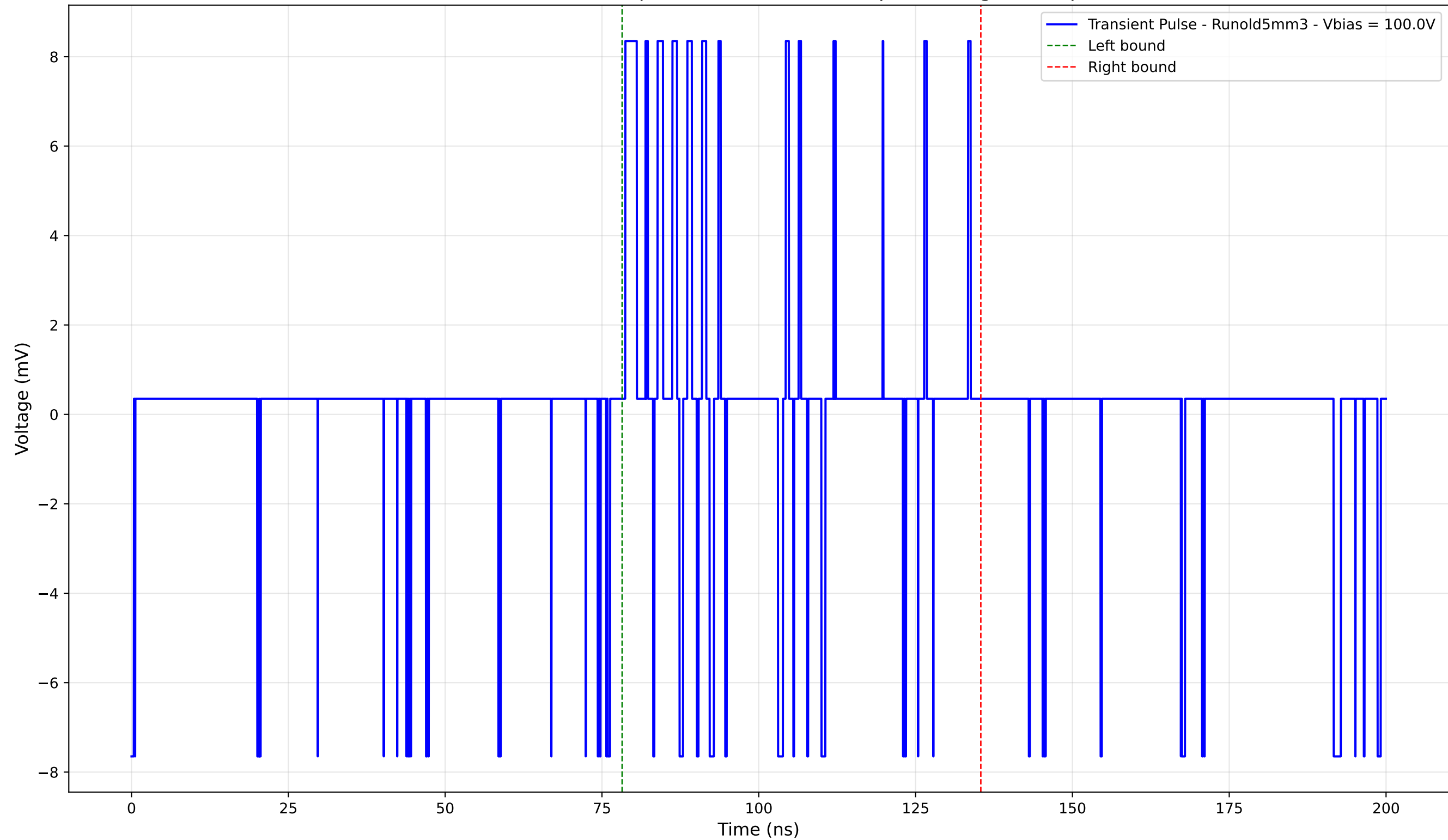
Transient Pulse - Sample: old5 - Position: 5.0 \mu\text{m} - Charge: 0.92 pC
