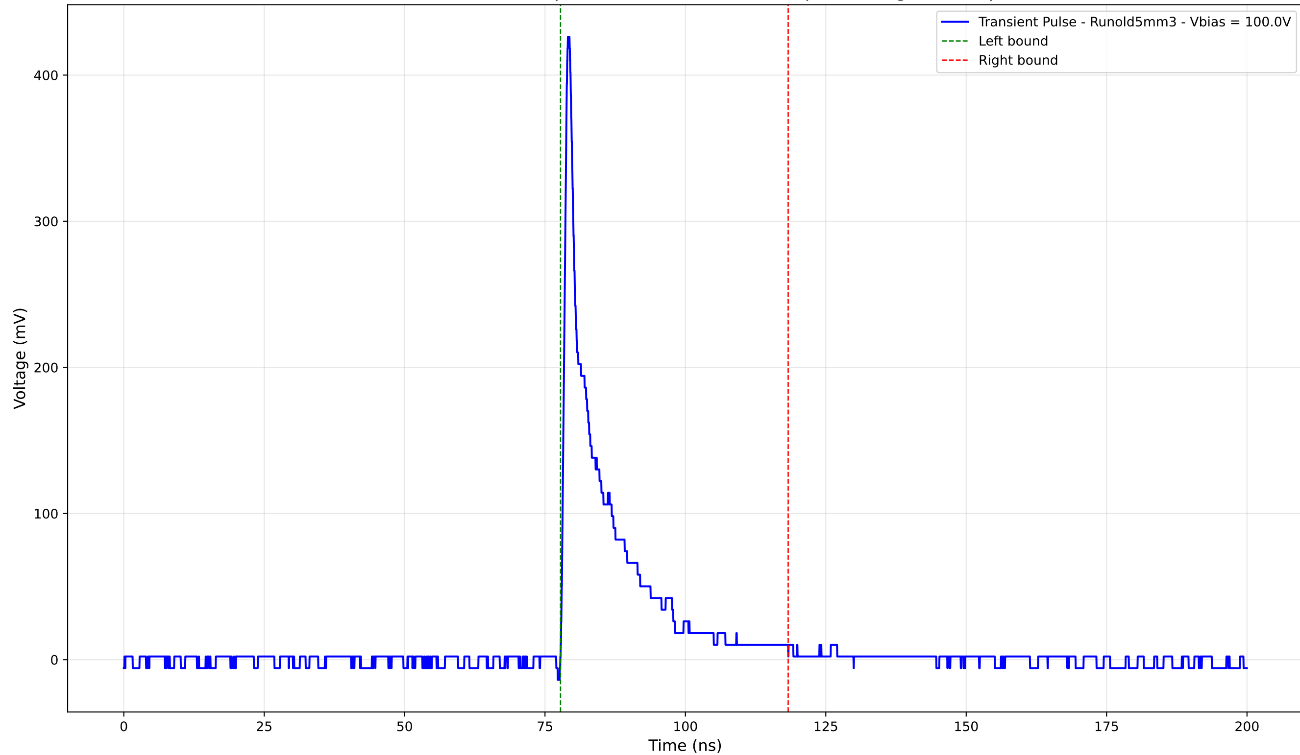
Transient Pulse - Sample: old5 - Position: 4885.0 \mu\text{m} - Charge: 53.02 pC
