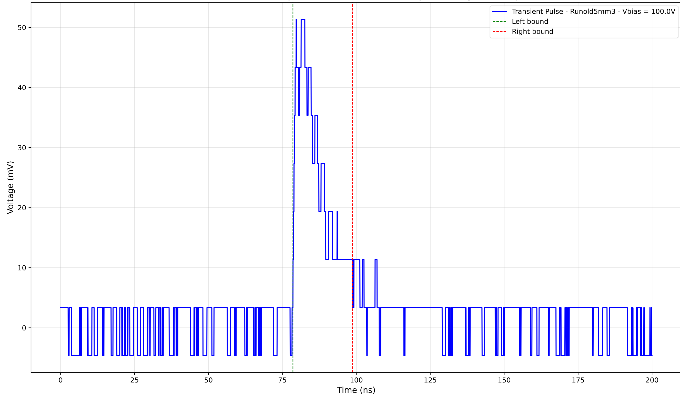
Transient Pulse - Sample: old5 - Position: 4515.0 \mu\text{m} - Charge: 10.21 pC
