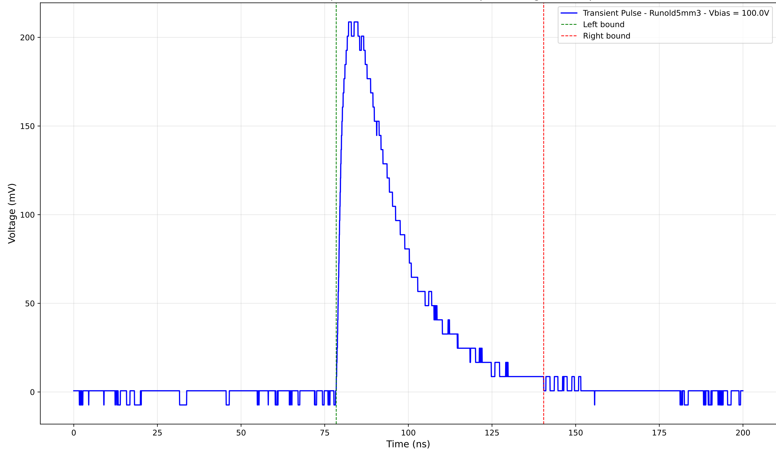
Transient Pulse - Sample: old5 - Position: 1690.0 \mu\text{m} - Charge: 84.20 pC
