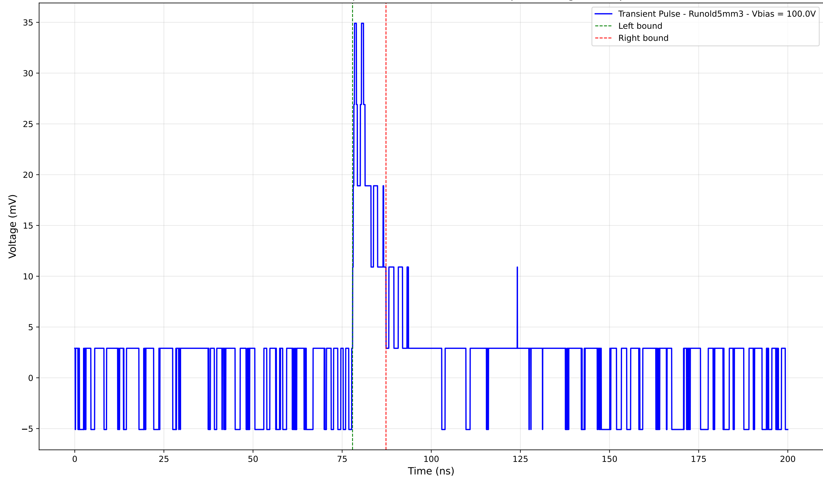
Transient Pulse - Sample: old5 - Position: 3575.0 \mu\text{m} - Charge: 3.60 pC
