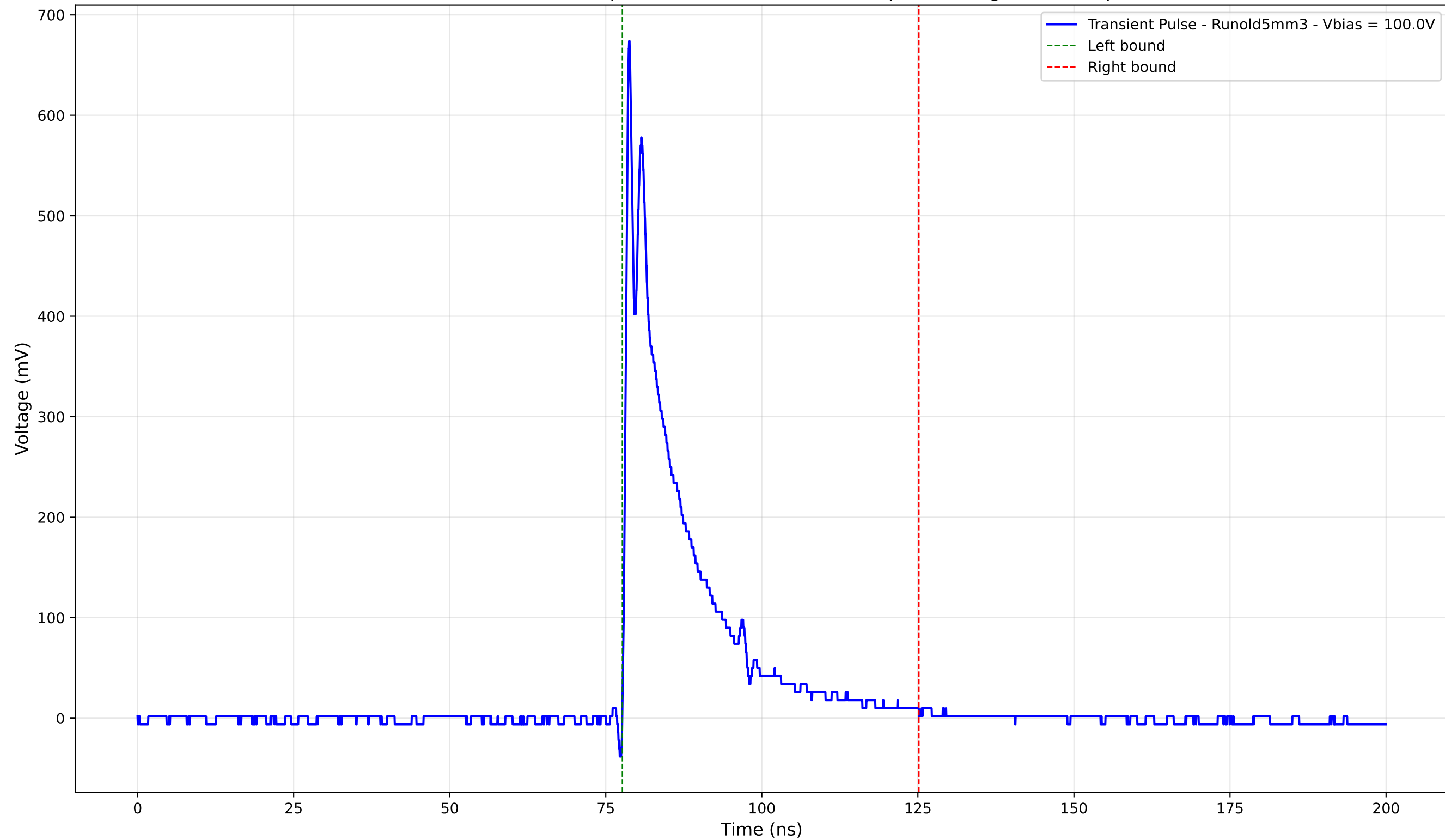
Transient Pulse - Sample: old5 - Position: 3740.0 \mu\text{m} - Charge: 108.63 pC
