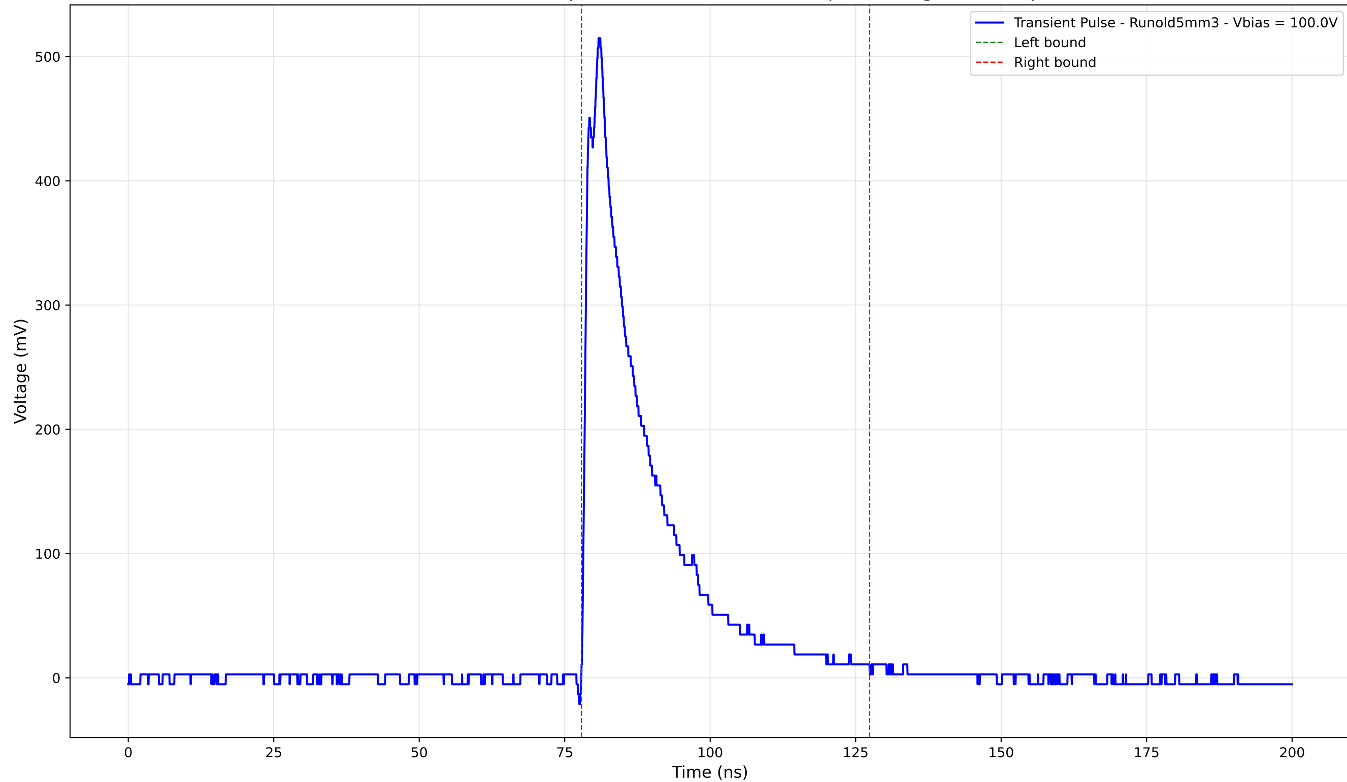
Transient Pulse - Sample: old5 - Position: 4020.0 \mu\text{m} - Charge: 112.34 pC
