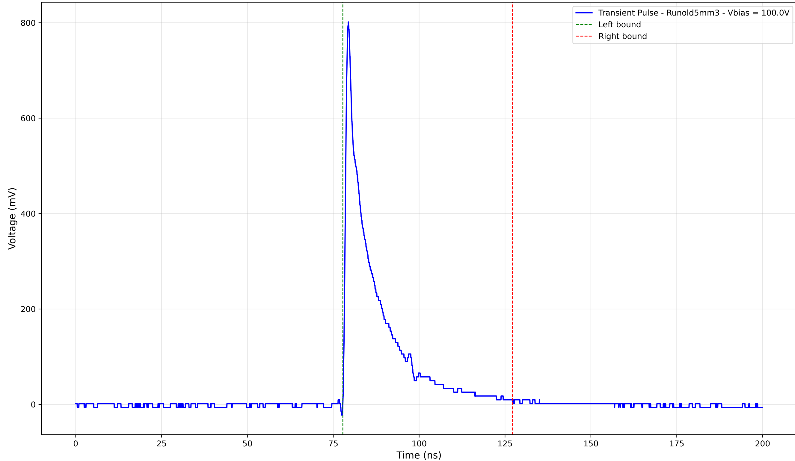
Transient Pulse - Sample: old5 - Position: 4775.0 \mu\text{m} - Charge: 130.65 pC
