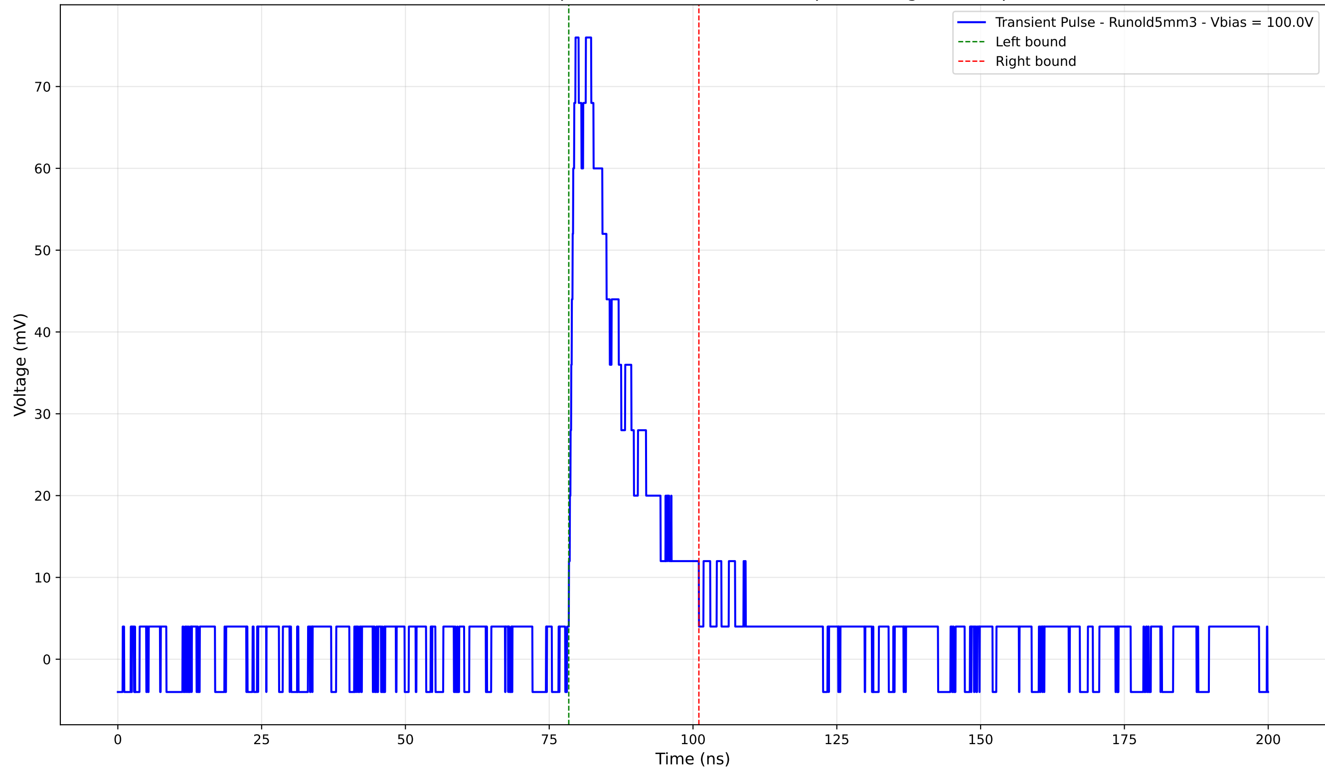
Transient Pulse - Sample: old5 - Position: 4525.0 \mu\text{m} - Charge: 15.32 pC
