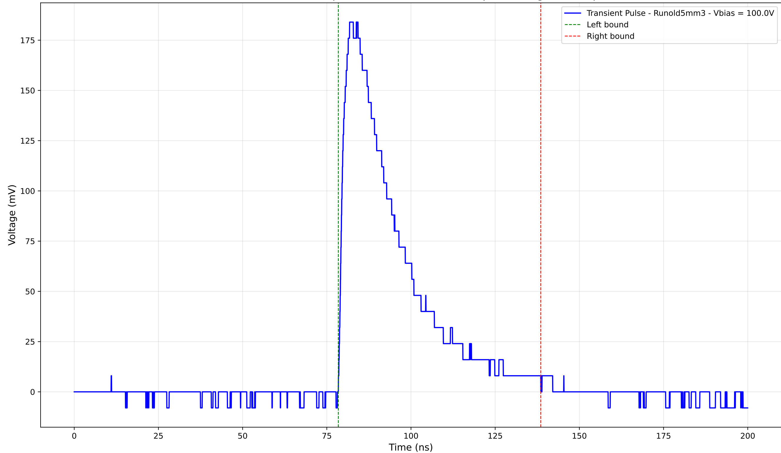
Transient Pulse - Sample: old5 - Position: 2455.0 \mu\text{m} - Charge: 68.01 pC
