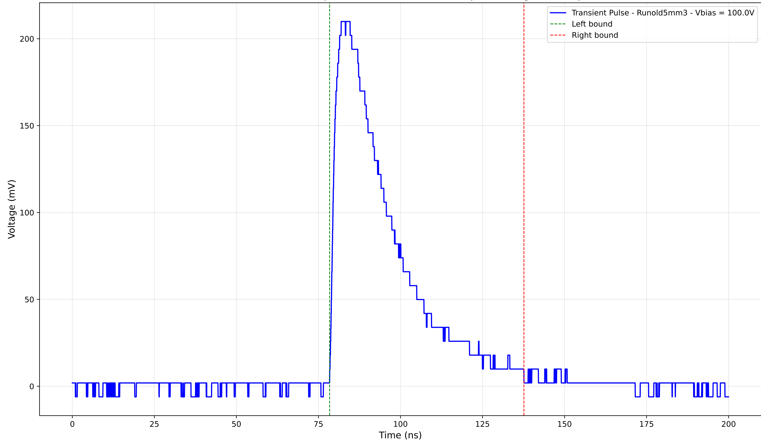
Transient Pulse - Sample: old5 - Position: 1490.0 \mu\text{m} - Charge: 84.16 pC
