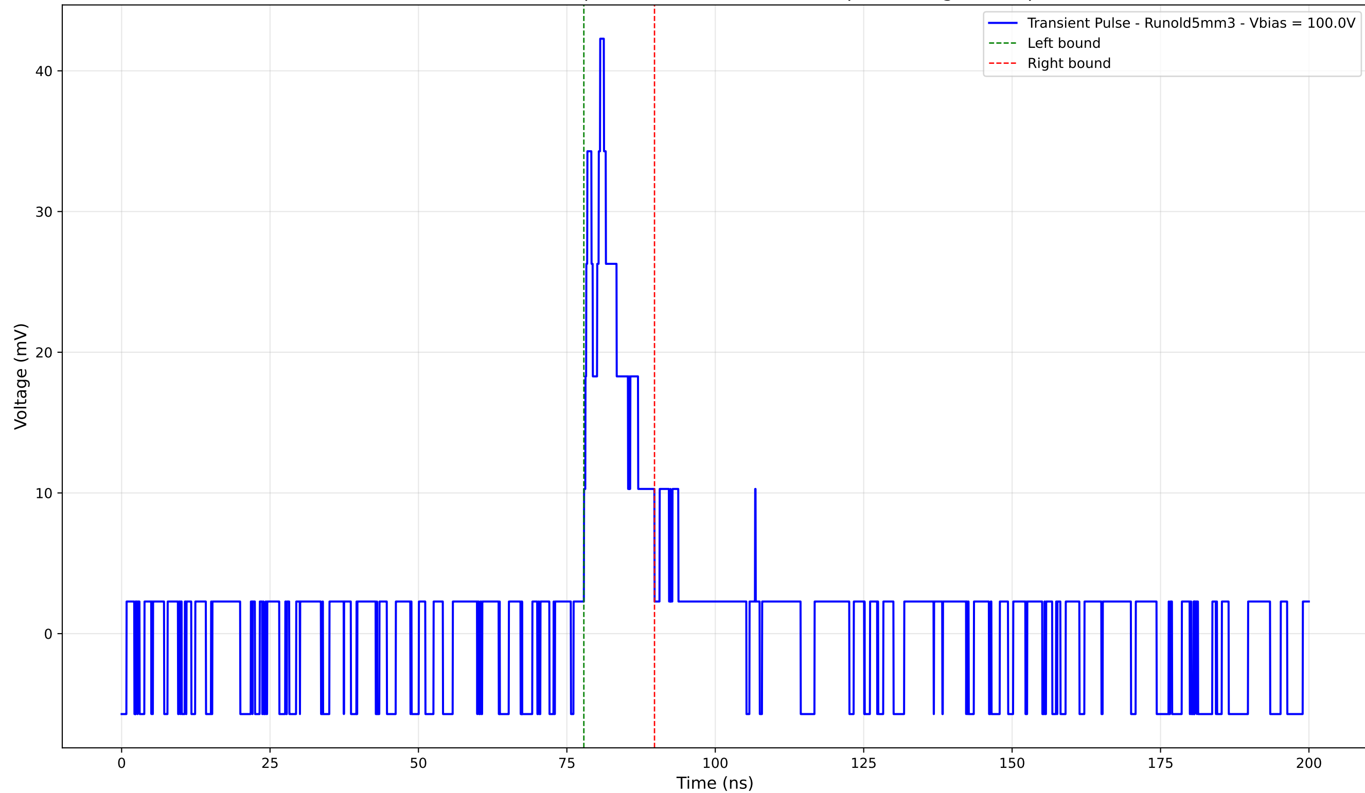
Transient Pulse - Sample: old5 - Position: 3595.0 \mu\text{m} - Charge: 4.91 pC
