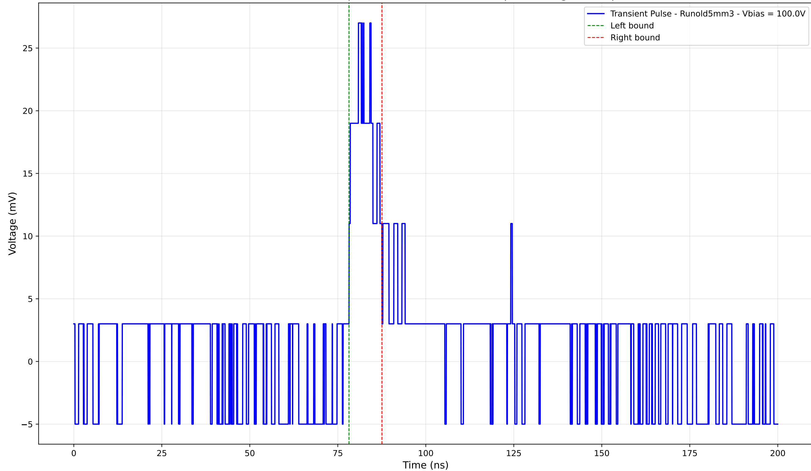
Transient Pulse - Sample: old5 - Position: 3285.0 \mu\text{m} - Charge: 3.44 pC
