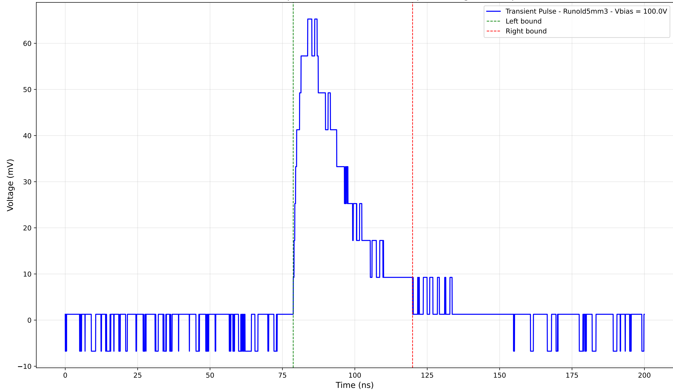
Transient Pulse - Sample: old5 - Position: 2015.0 \mu\text{m} - Charge: 23.66 pC
