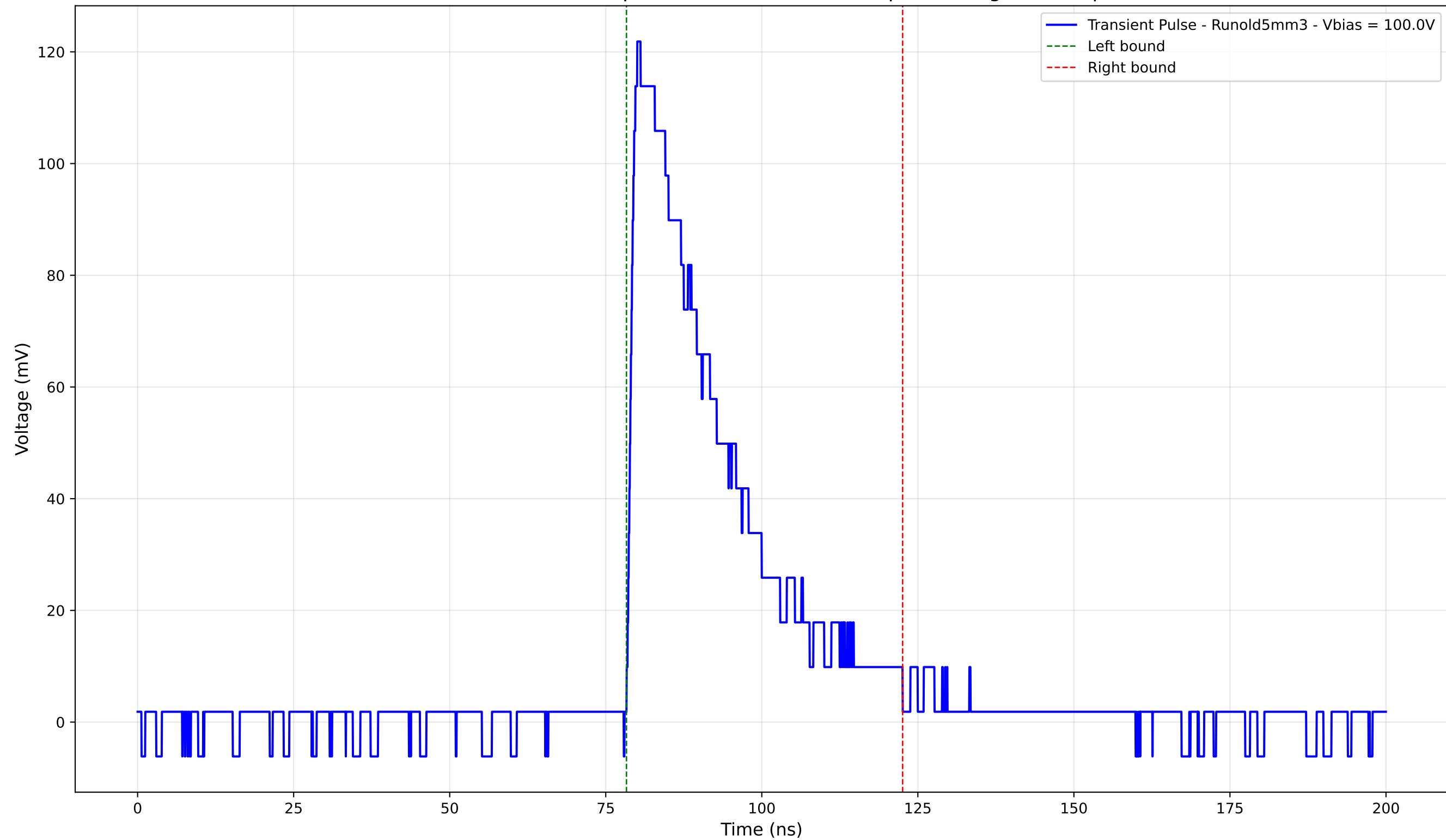
Transient Pulse - Sample: old5 - Position: 905.0 \mu\text{m} - Charge: 38.12 pC
