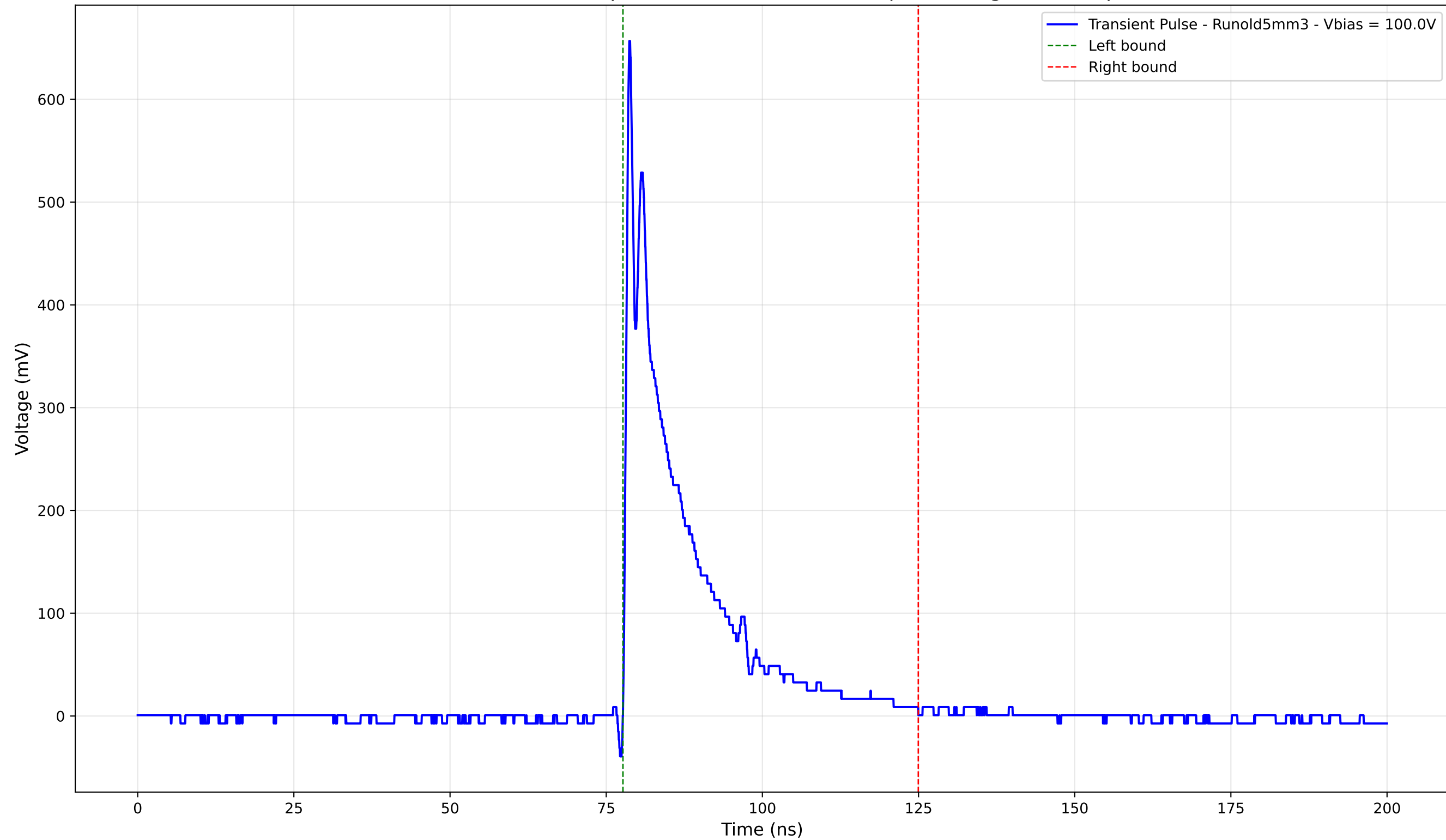
Transient Pulse - Sample: old5 - Position: 3420.0 \mu\text{m} - Charge: 105.95 pC
