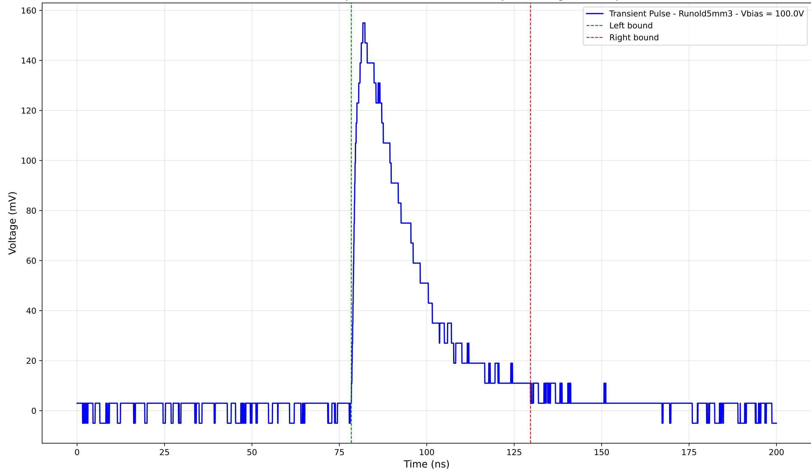
Transient Pulse - Sample: old5 - Position: 2600.0 \mu\text{m} - Charge: 53.92 pC
