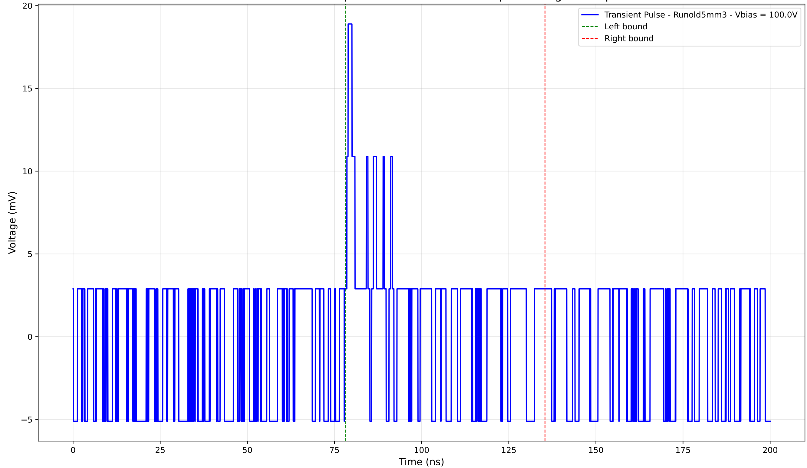
Transient Pulse - Sample: old5 - Position: 4955.0 \mu\text{m} - Charge: 2.07 pC
