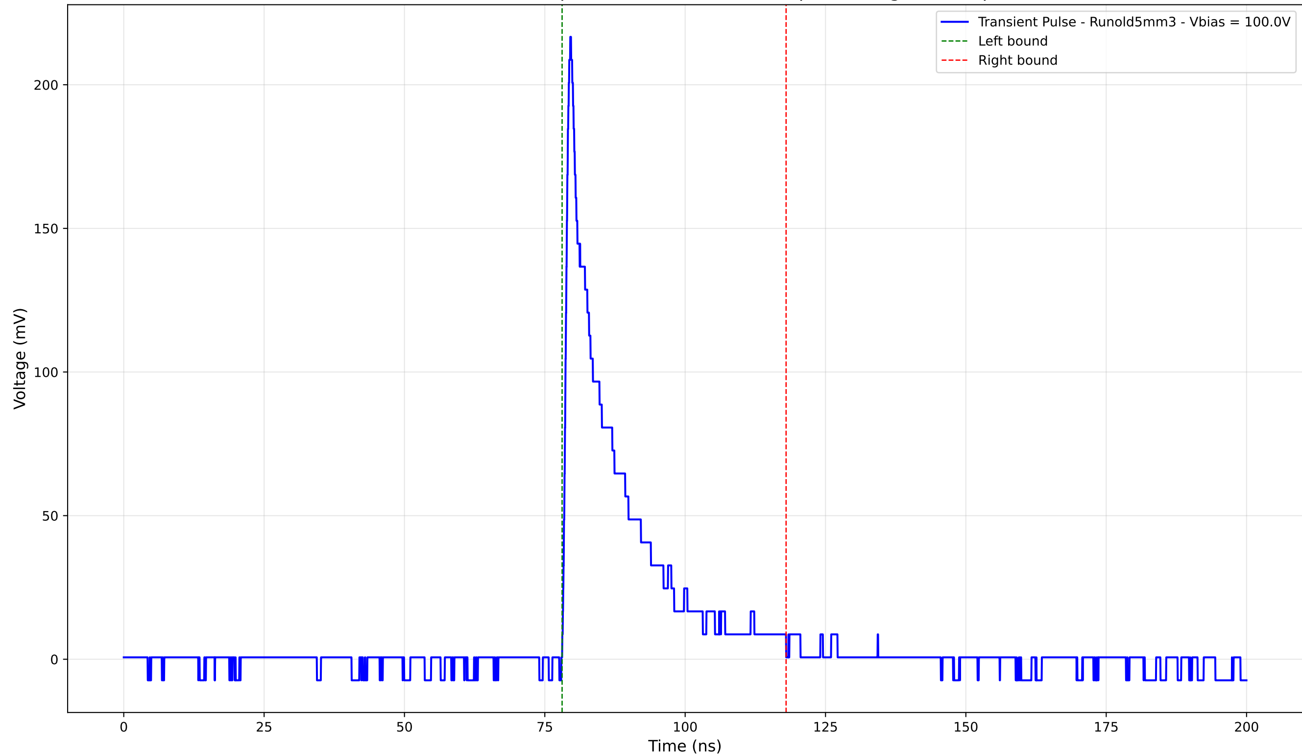
Transient Pulse - Sample: old5 - Position: 400.0 \mu\text{m} - Charge: 35.81 pC
