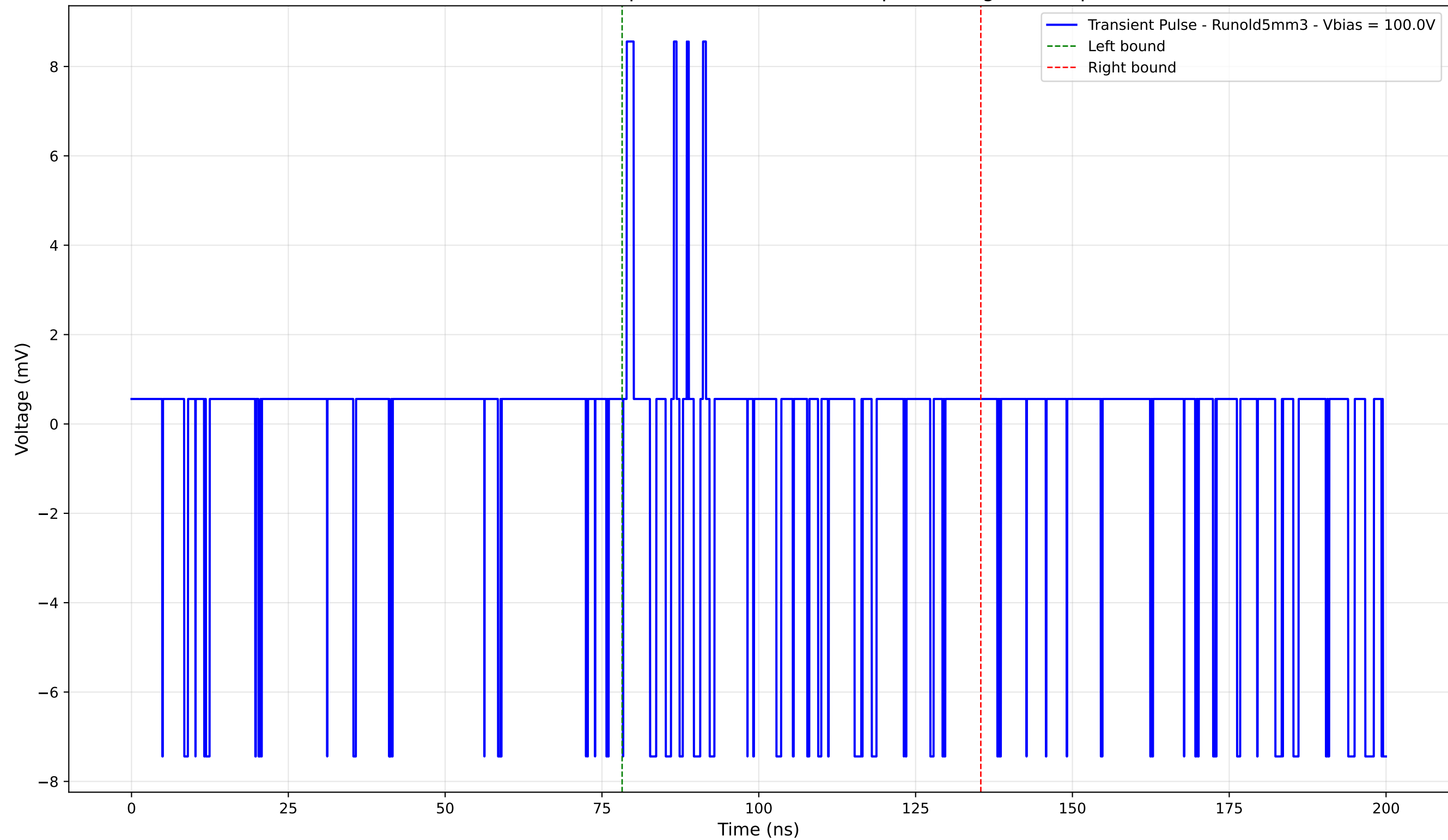
Transient Pulse - Sample: old5 - Position: 45.0 \mu\text{m} - Charge: -0.52 pC
