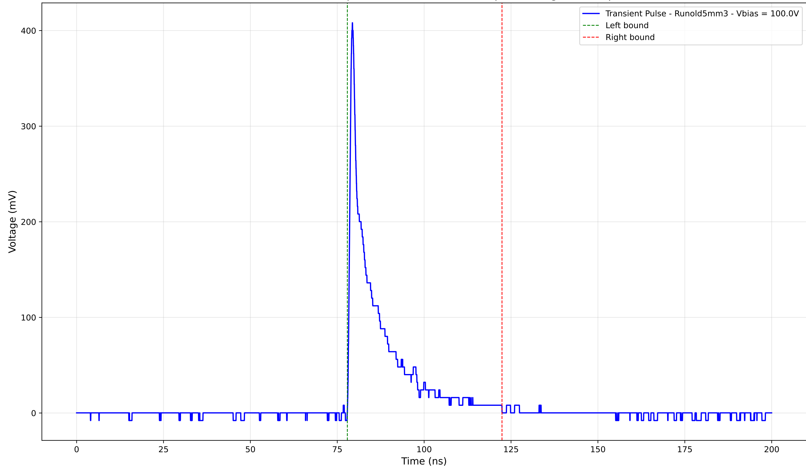
Transient Pulse - Sample: old5 - Position: 265.0 \mu\text{m} - Charge: 53.77 pC
