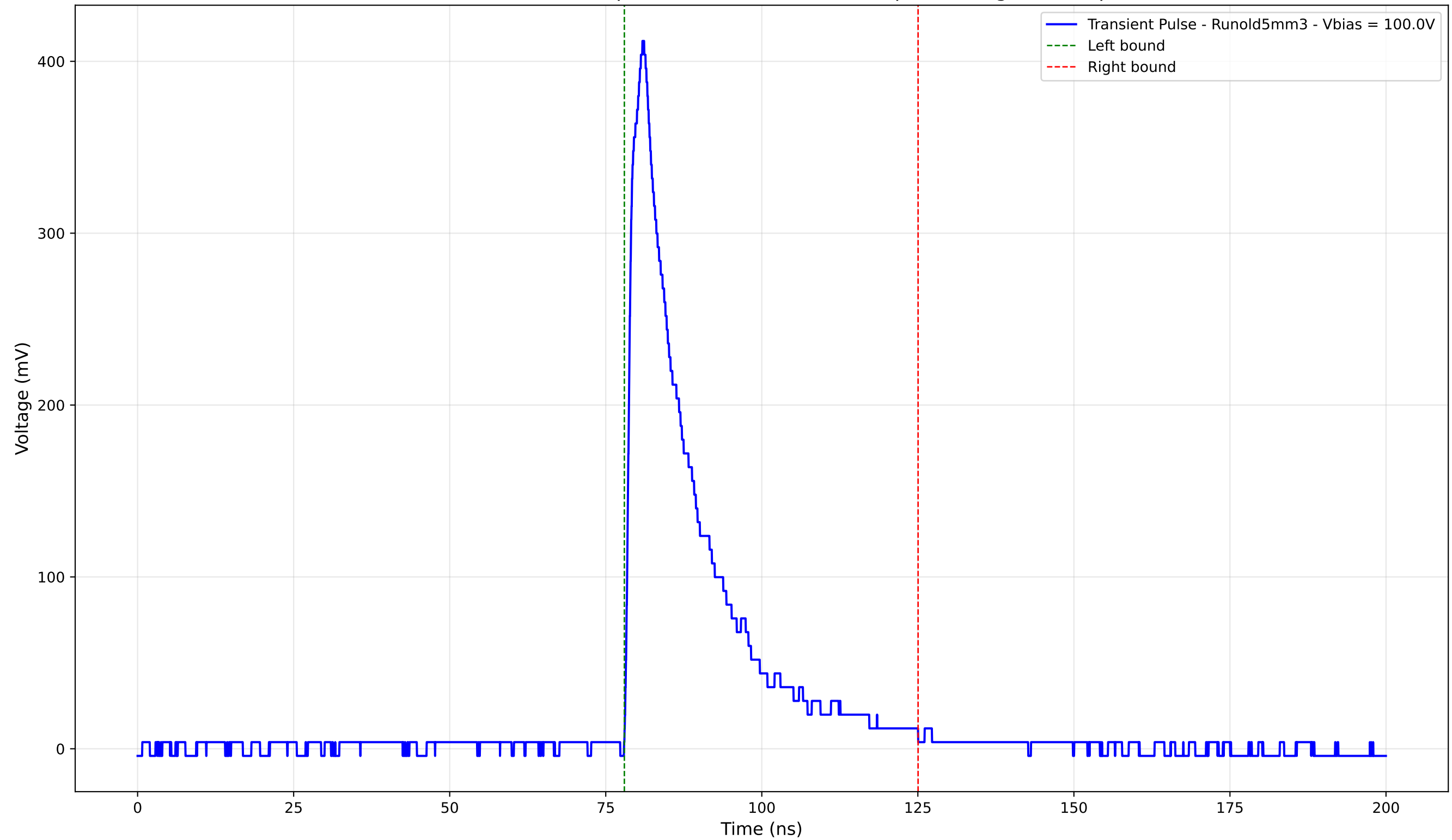
Transient Pulse - Sample: old5 - Position: 4090.0 \mu\text{m} - Charge: 89.54 pC
