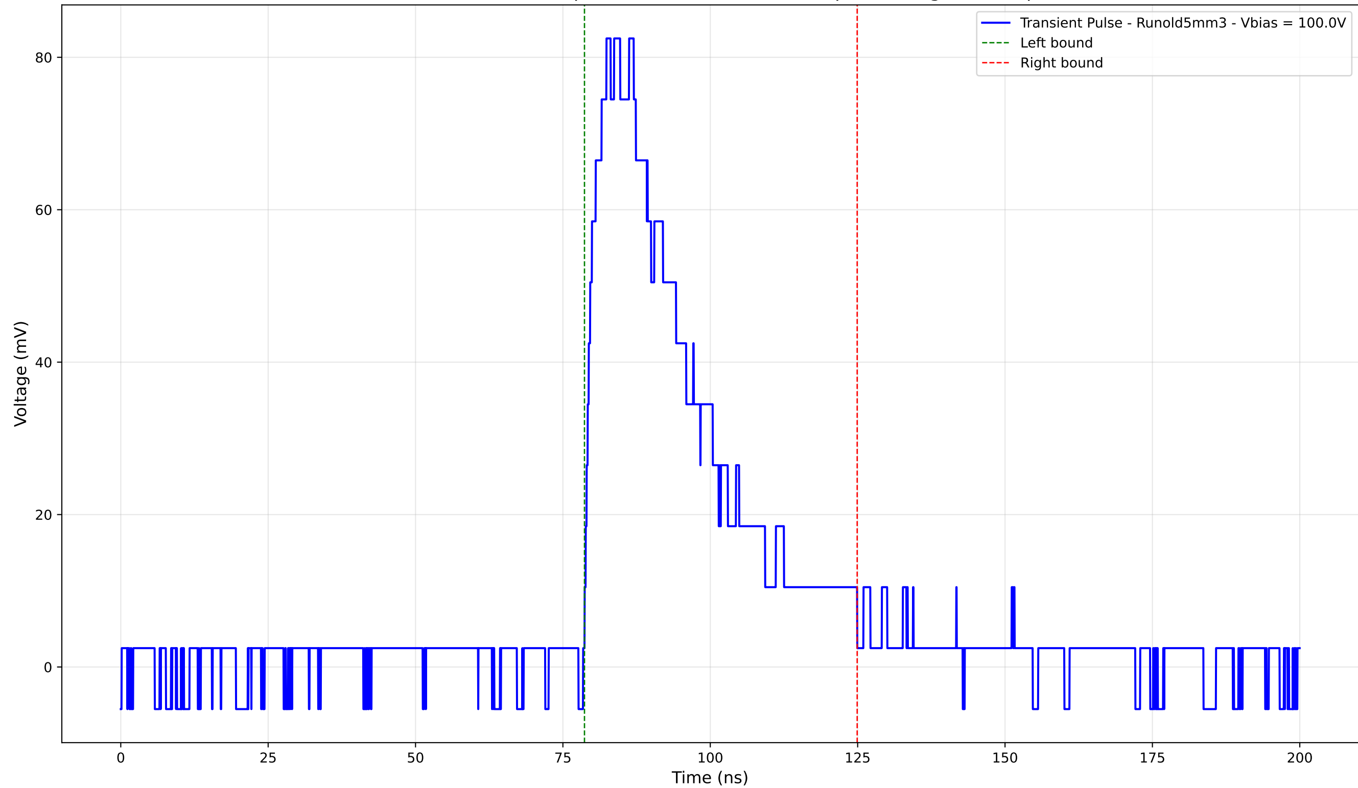
Transient Pulse - Sample: old5 - Position: 2160.0 \mu\text{m} - Charge: 31.62 pC
