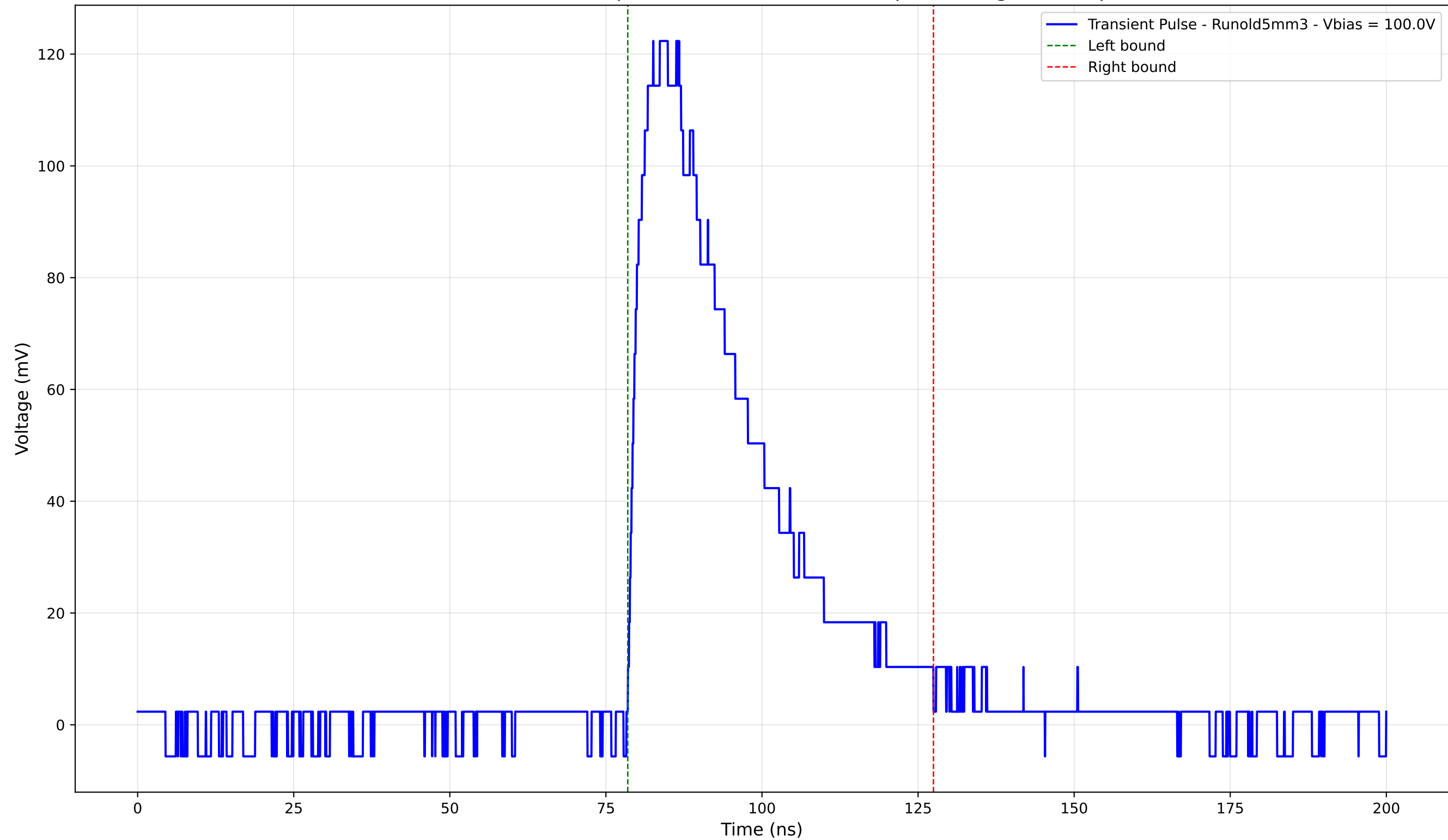
Transient Pulse - Sample: old5 - Position: 1740.0 \mu\text{m} - Charge: 48.06 pC
