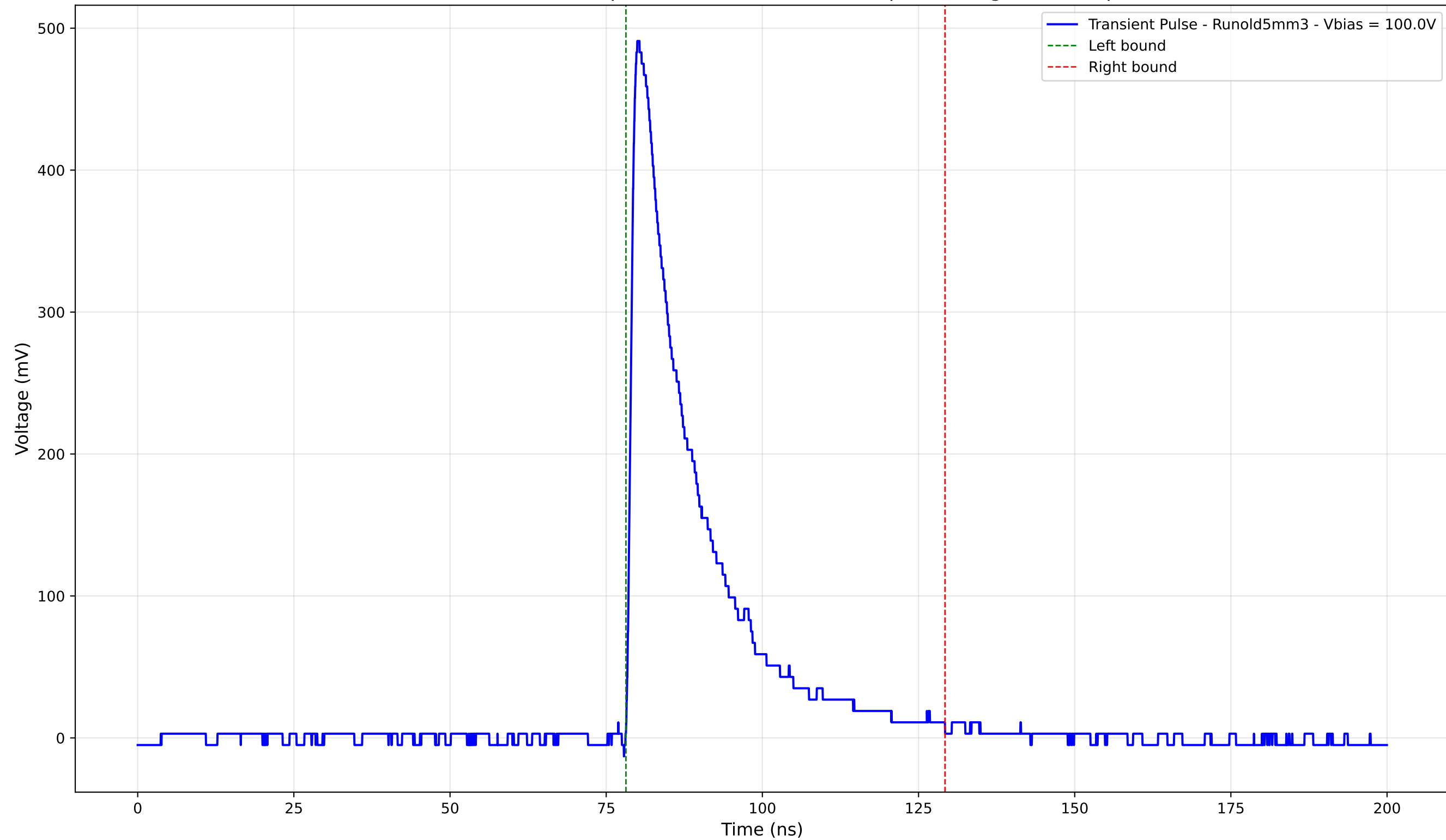
Transient Pulse - Sample: old5 - Position: 4385.0 \mu\text{m} - Charge: 108.58 pC
