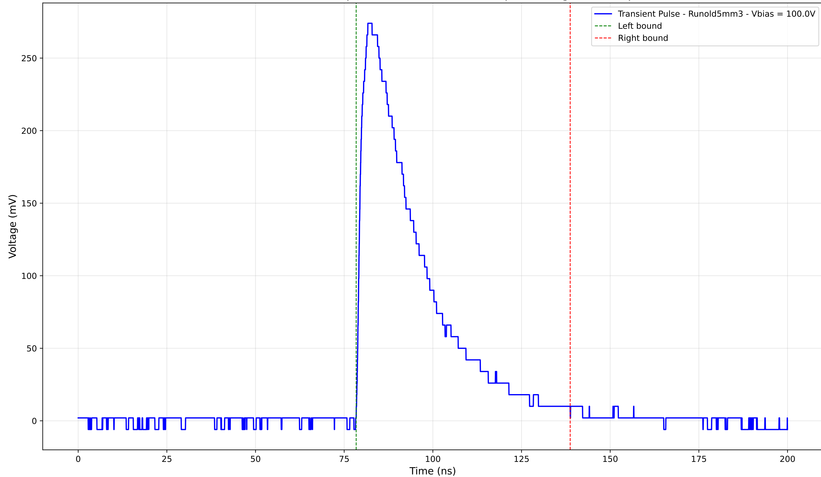
Transient Pulse - Sample: old5 - Position: 2525.0 \mu\text{m} - Charge: 101.85 pC
