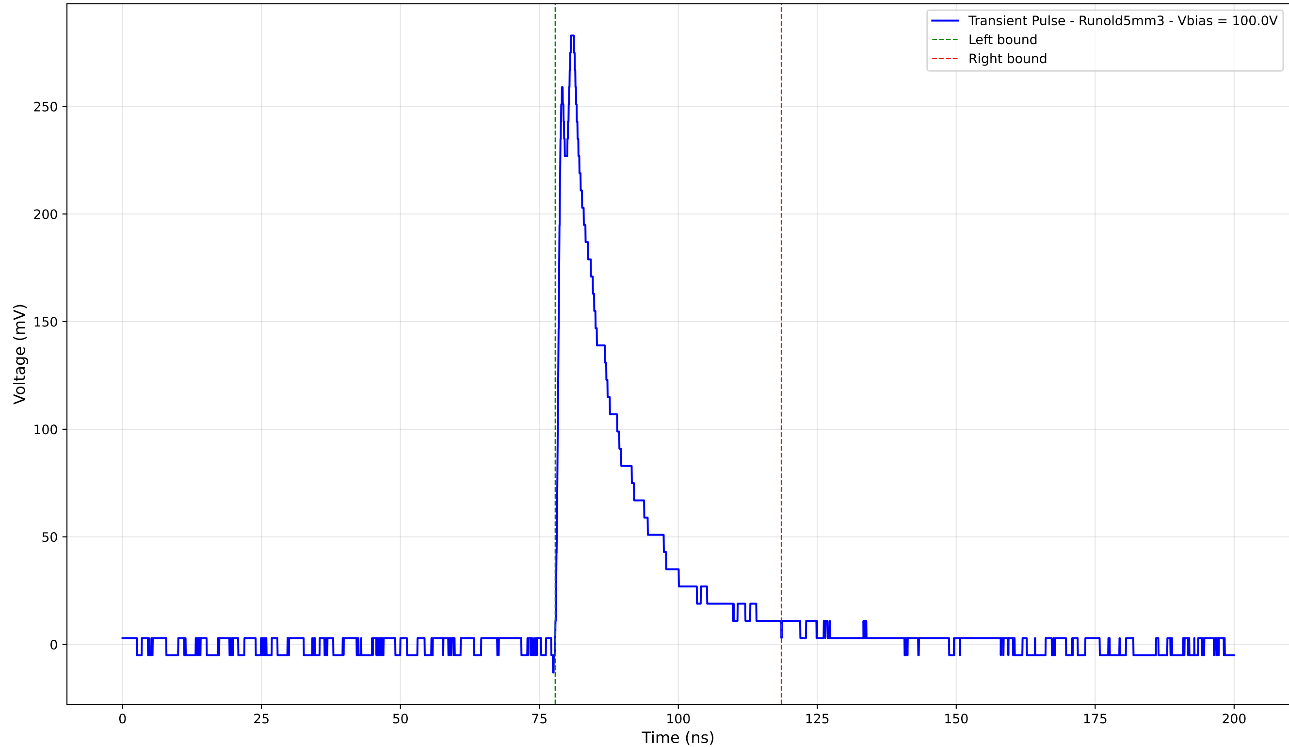
Transient Pulse - Sample: old5 - Position: 3955.0 \mu\text{m} - Charge: 59.62 pC
