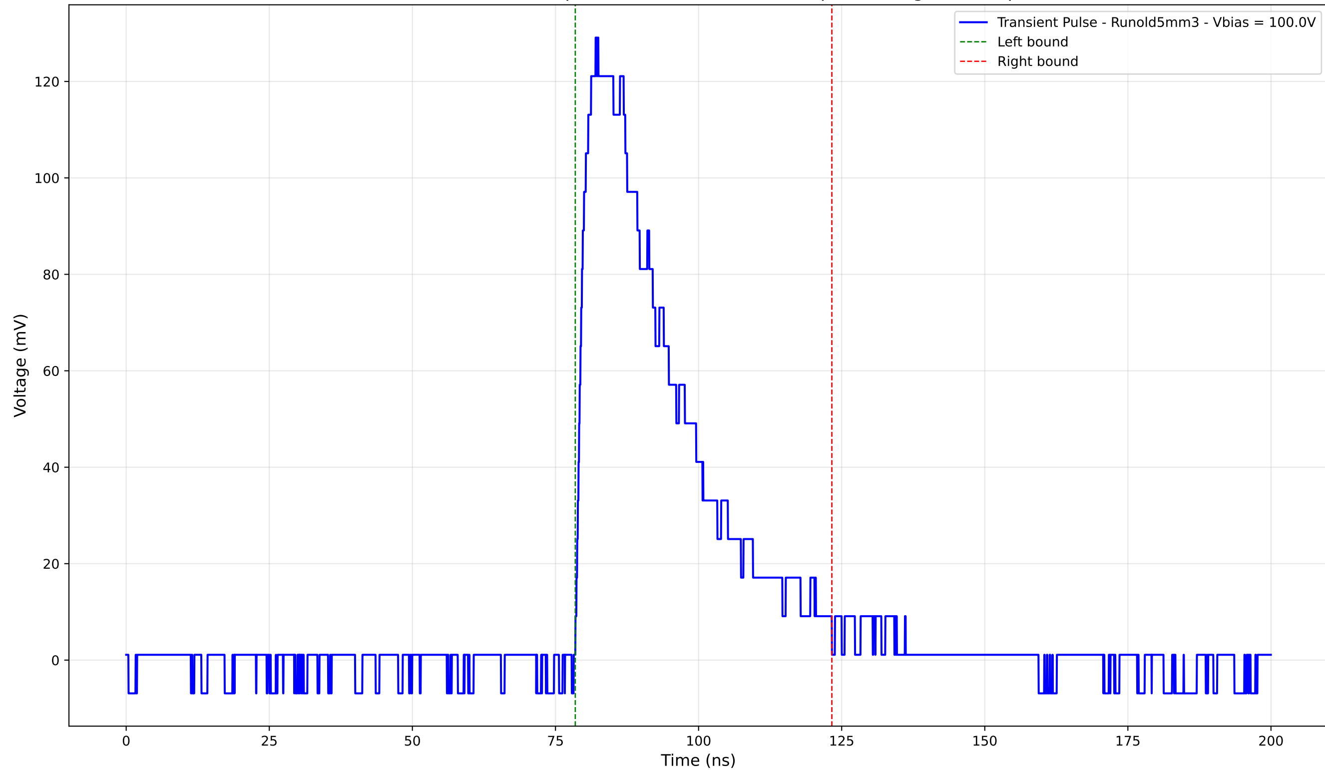
Transient Pulse - Sample: old5 - Position: 1335.0 \mu\text{m} - Charge: 45.78 pC
