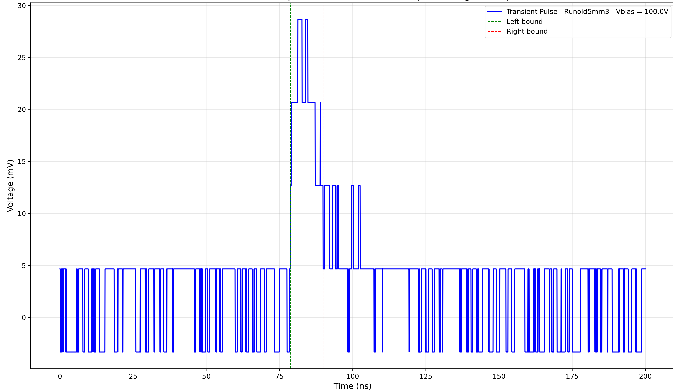
Transient Pulse - Sample: old5 - Position: 4185.0 \mu\text{m} - Charge: 4.51 pC
