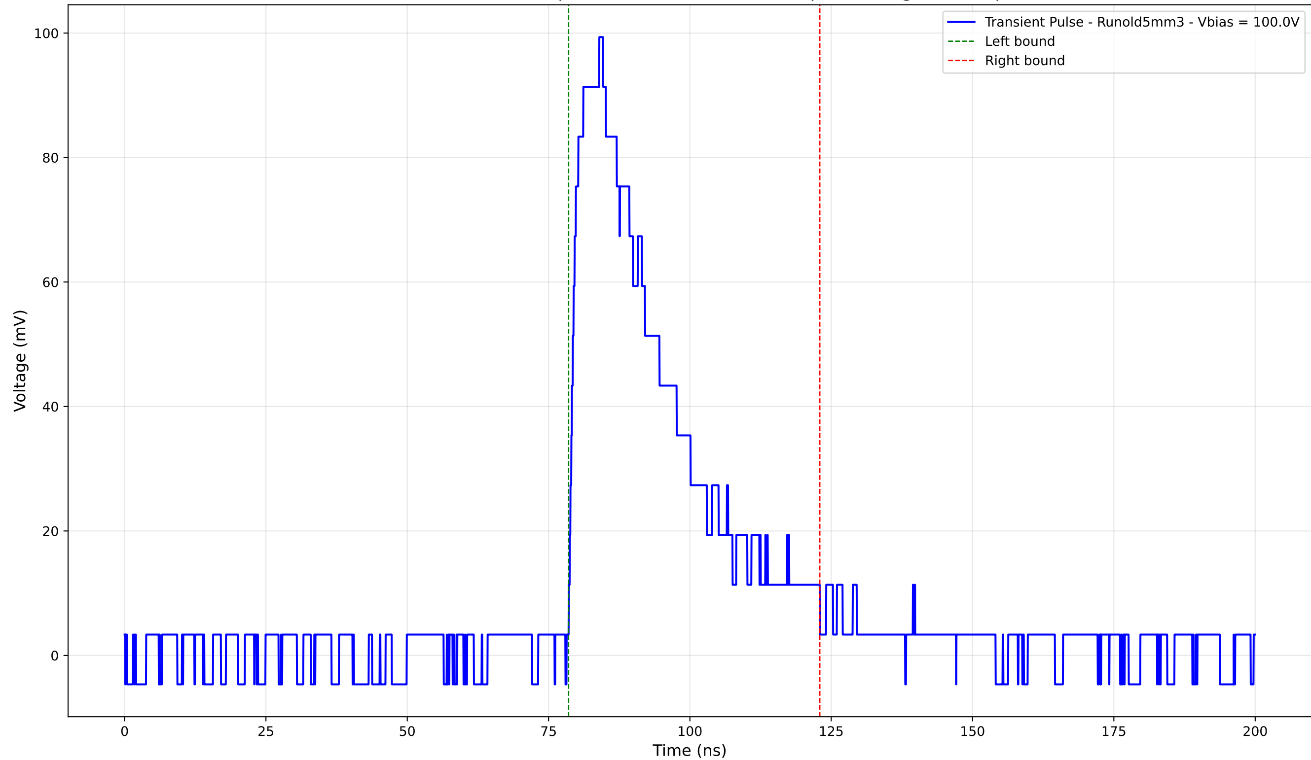
Transient Pulse - Sample: old5 - Position: 1220.0 \mu\text{m} - Charge: 35.34 pC
