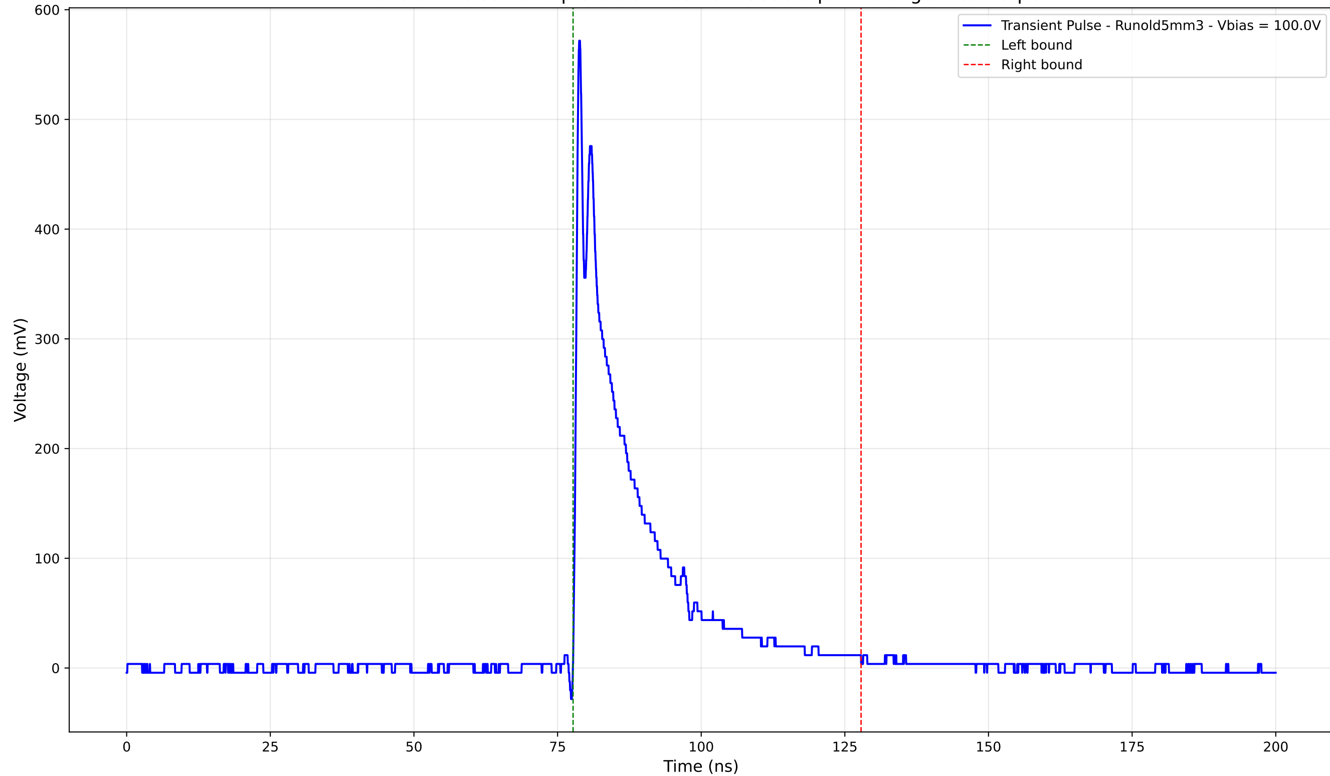
Transient Pulse - Sample: old5 - Position: 3390.0 \mu\text{m} - Charge: 100.49 pC
