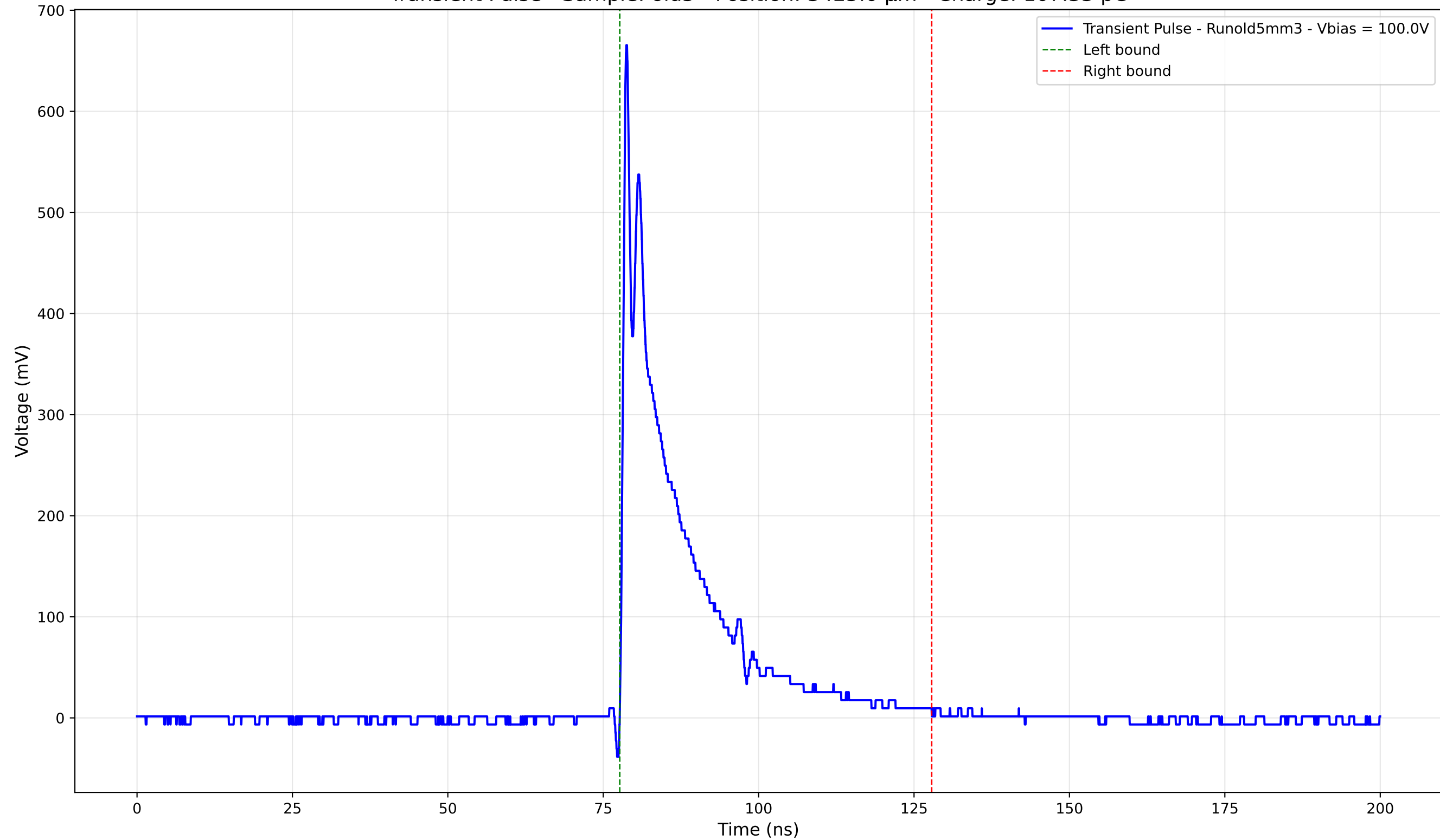
Transient Pulse - Sample: old5 - Position: 3425.0 \mu\text{m} - Charge: 107.33 pC
