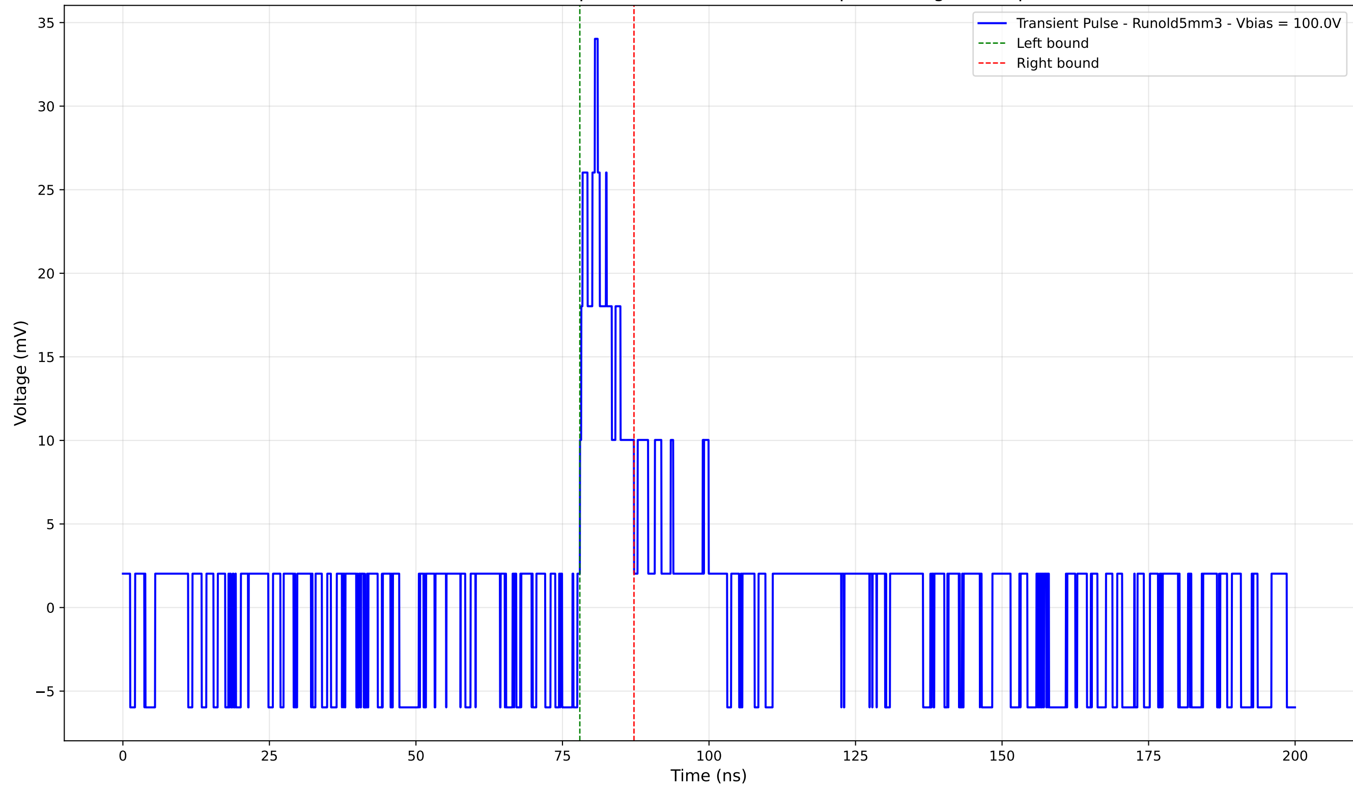
Transient Pulse - Sample: old5 - Position: 3585.0 \mu\text{m} - Charge: 3.26 pC
