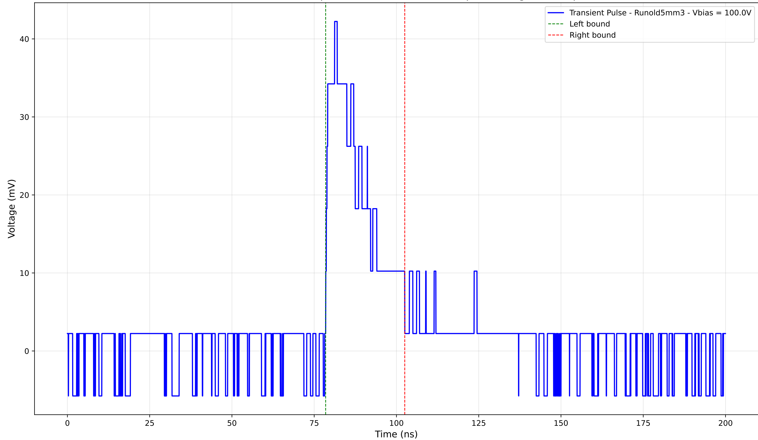
Transient Pulse - Sample: old5 - Position: 2945.0 \mu\text{m} - Charge: 10.01 pC
