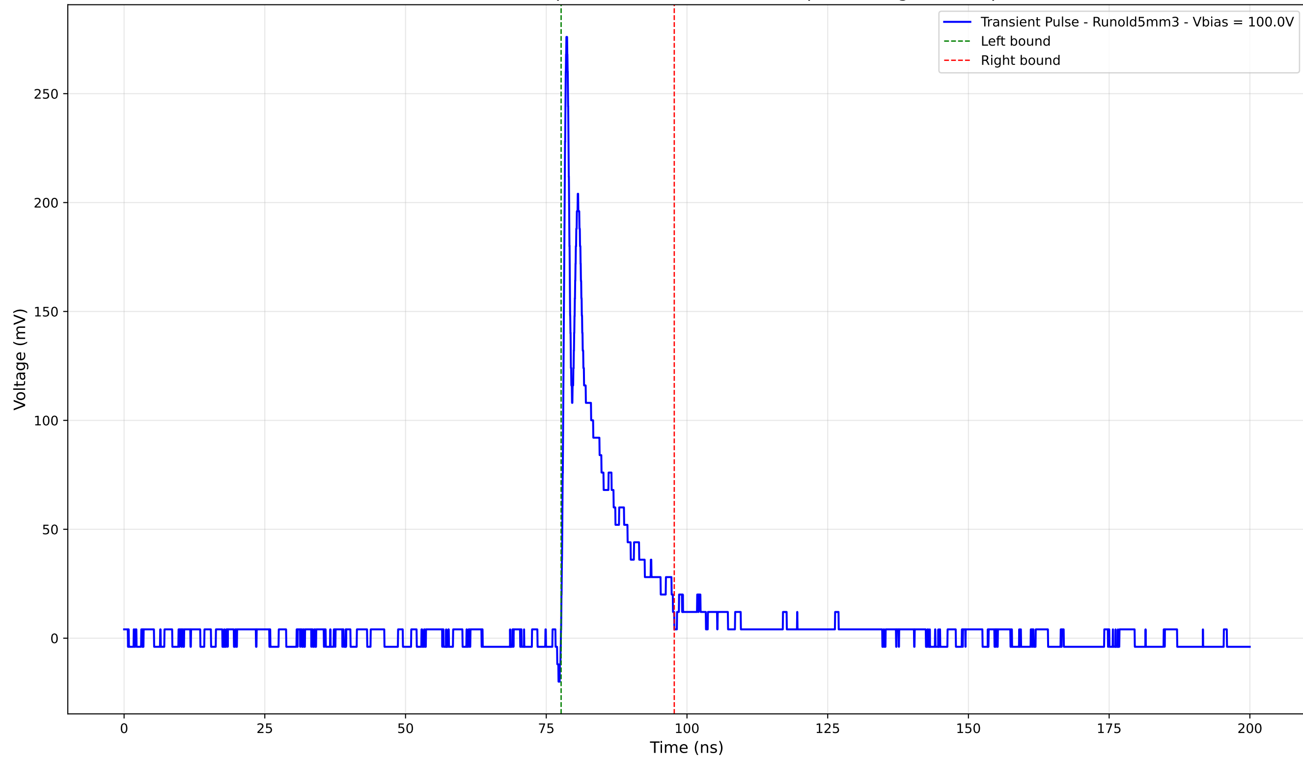
Transient Pulse - Sample: old5 - Position: 3635.0 \mu\text{m} - Charge: 30.51 pC
