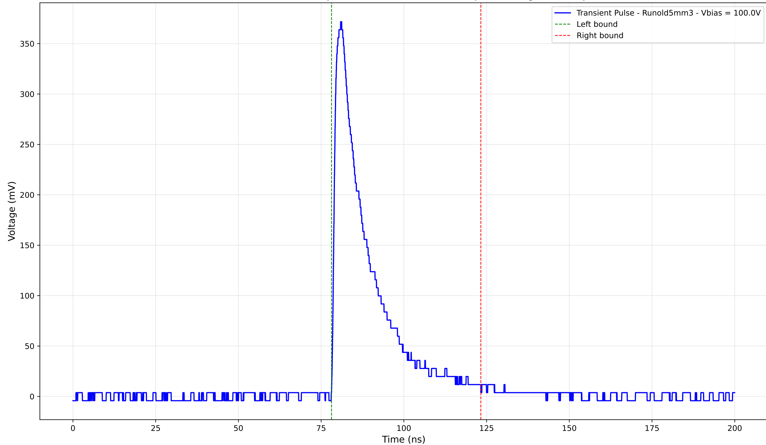
Transient Pulse - Sample: old5 - Position: 4270.0 \mu\text{m} - Charge: 83.50 pC
