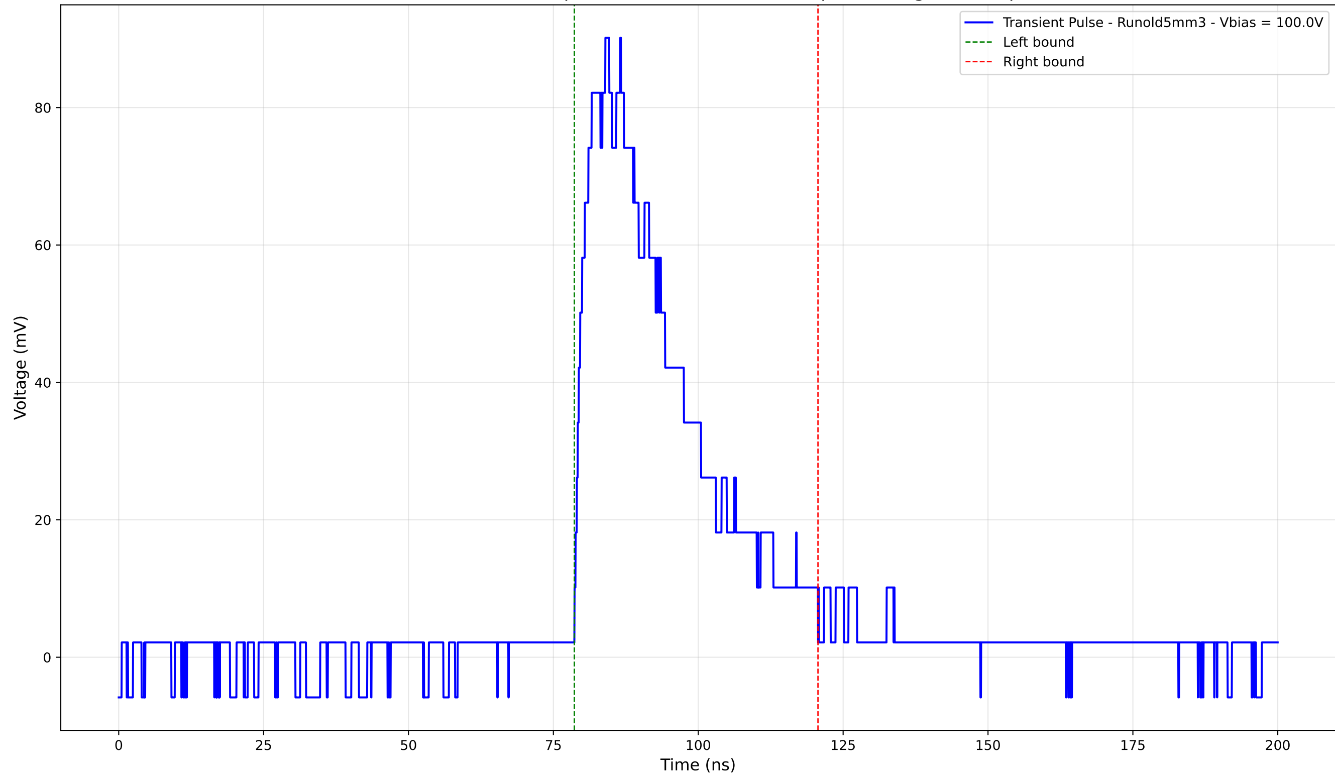
Transient Pulse - Sample: old5 - Position: 1620.0 \mu\text{m} - Charge: 32.47 pC
