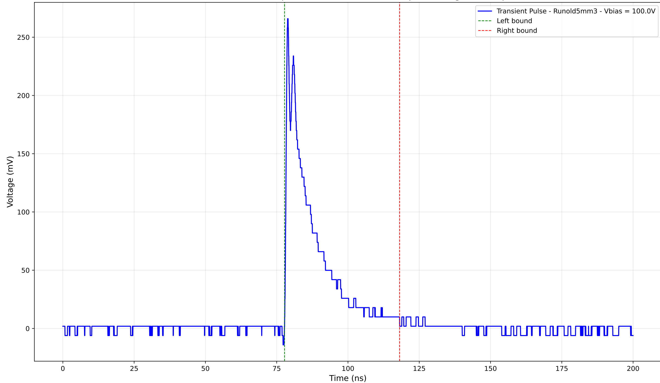
Transient Pulse - Sample: old5 - Position: 3345.0 \mu\text{m} - Charge: 47.47 pC
