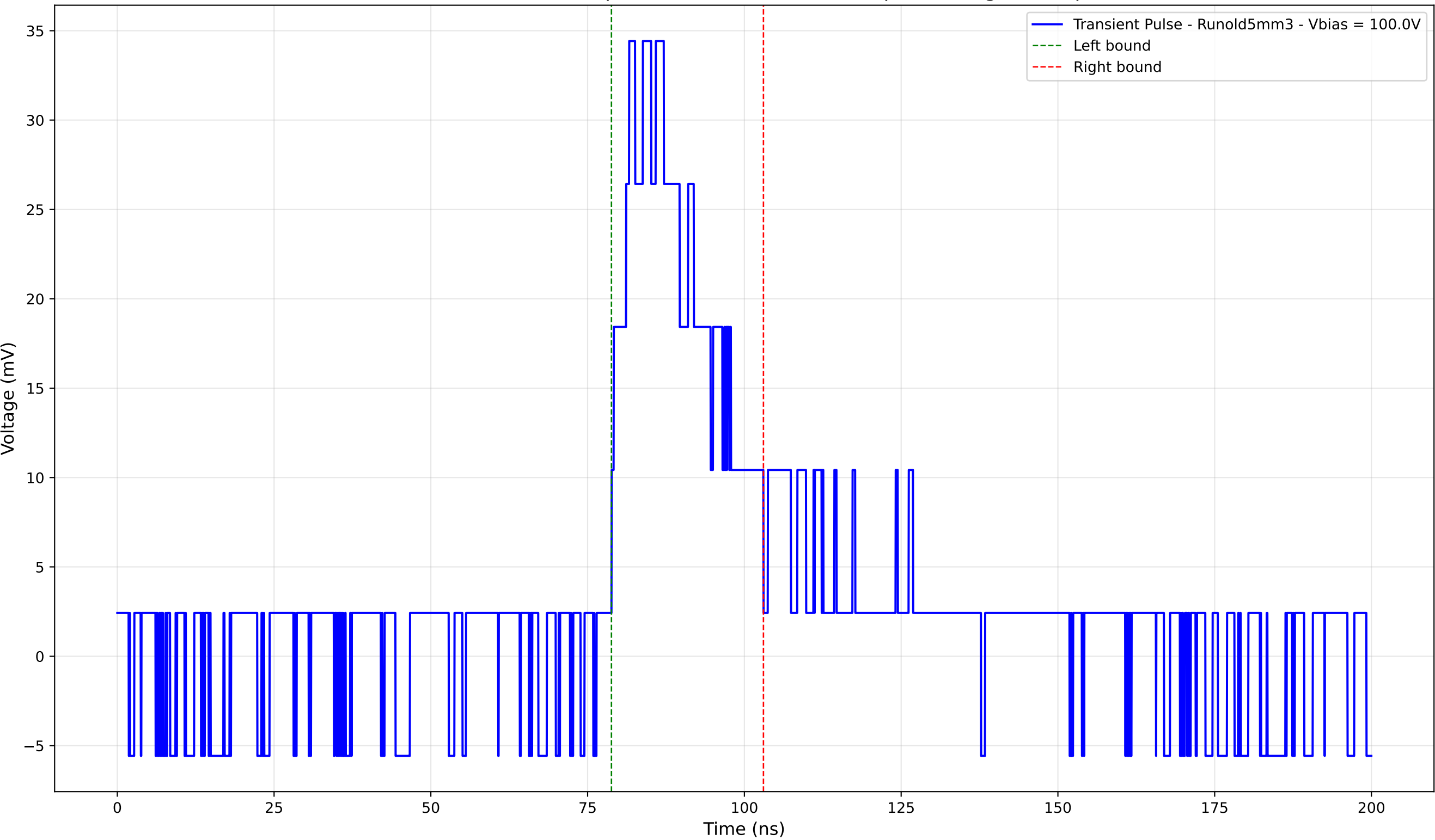
Transient Pulse - Sample: old5 - Position: 1580.0 \mu\text{m} - Charge: 9.96 pC
