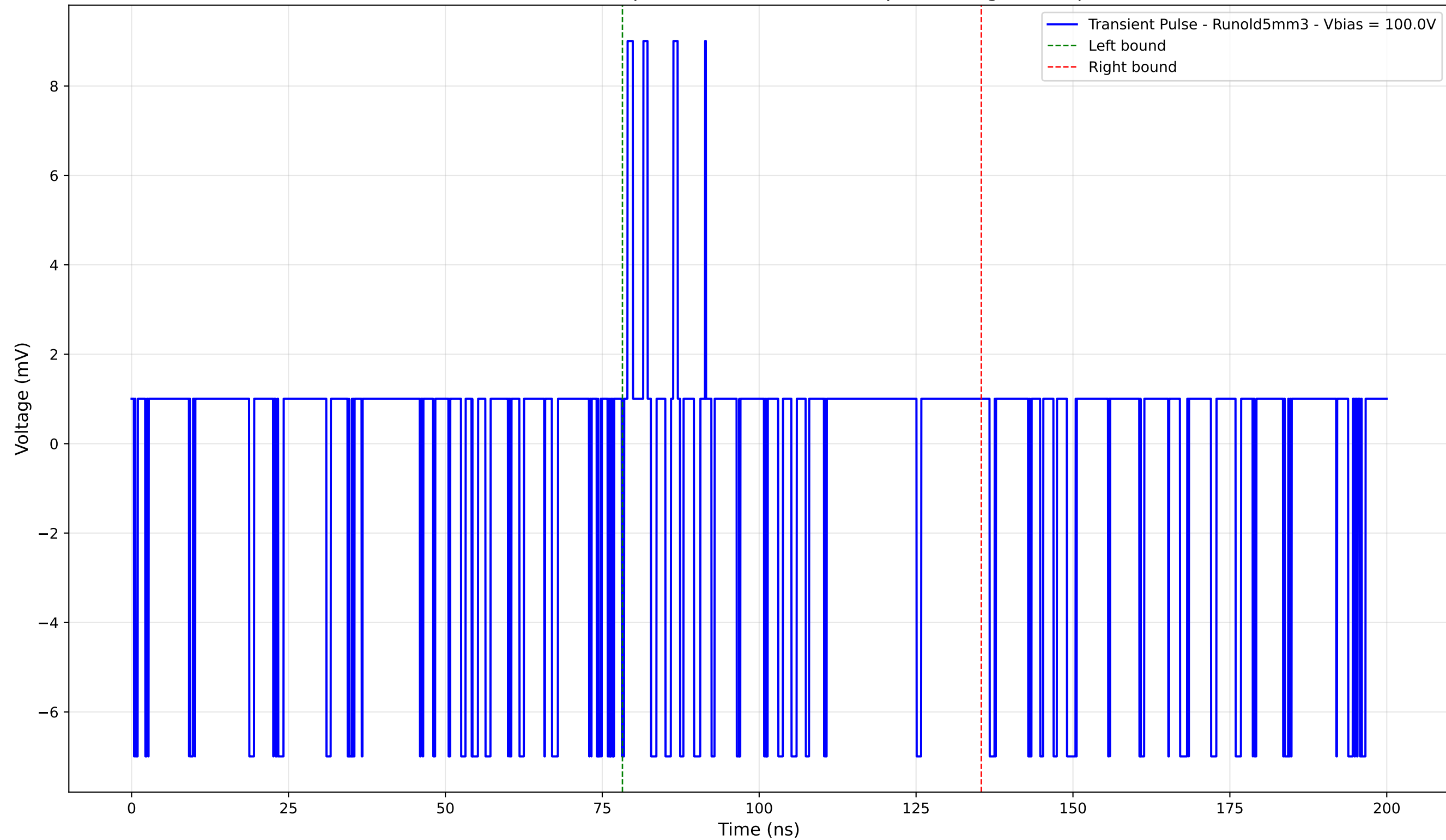
Transient Pulse - Sample: old5 - Position: 70.0 \mu\text{m} - Charge: 0.23 pC
