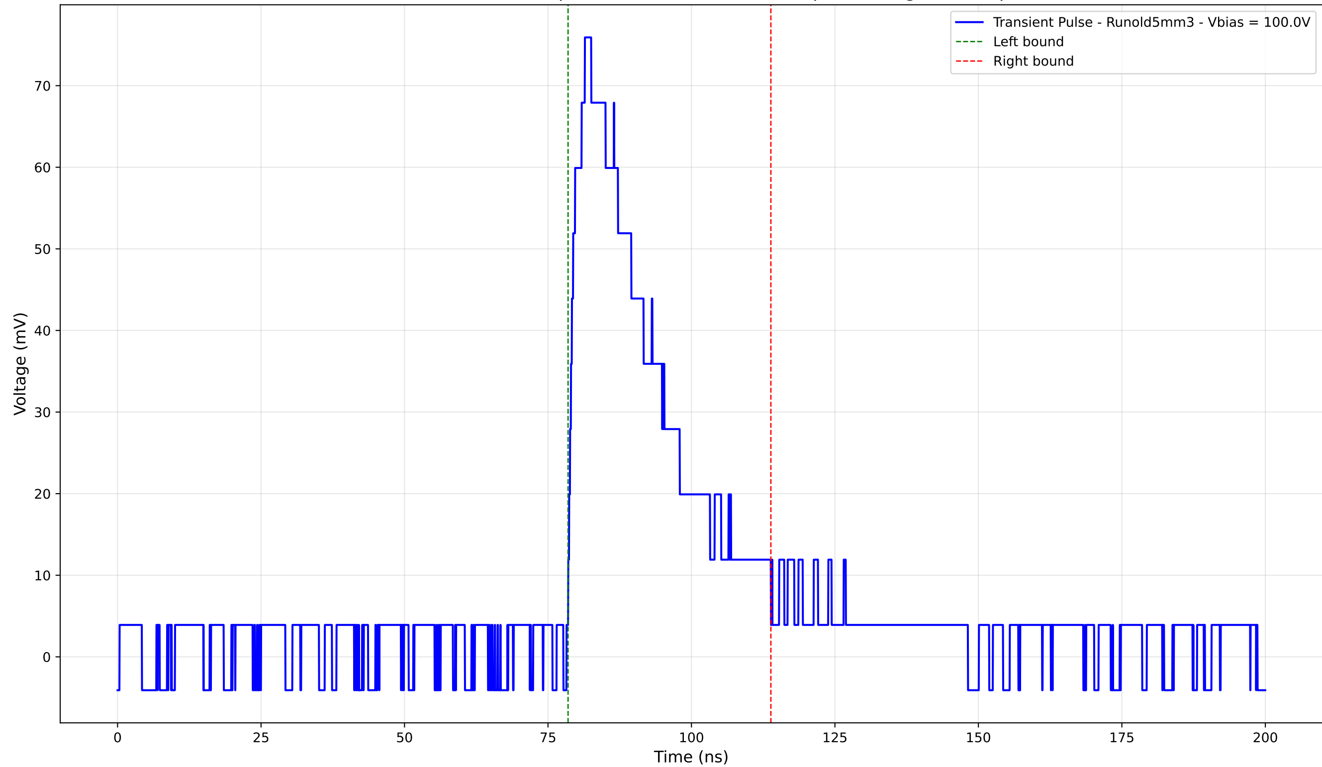
Transient Pulse - Sample: old5 - Position: 2720.0 \mu\text{m} - Charge: 23.91 pC
