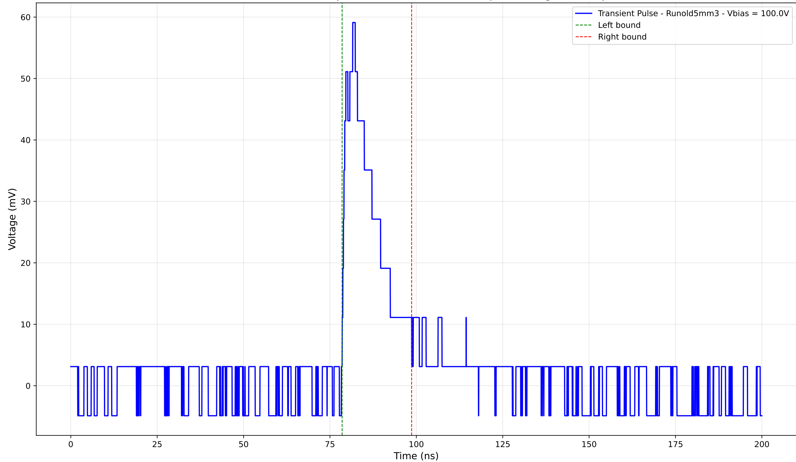
Transient Pulse - Sample: old5 - Position: 4210.0 \mu\text{m} - Charge: 11.15 pC
