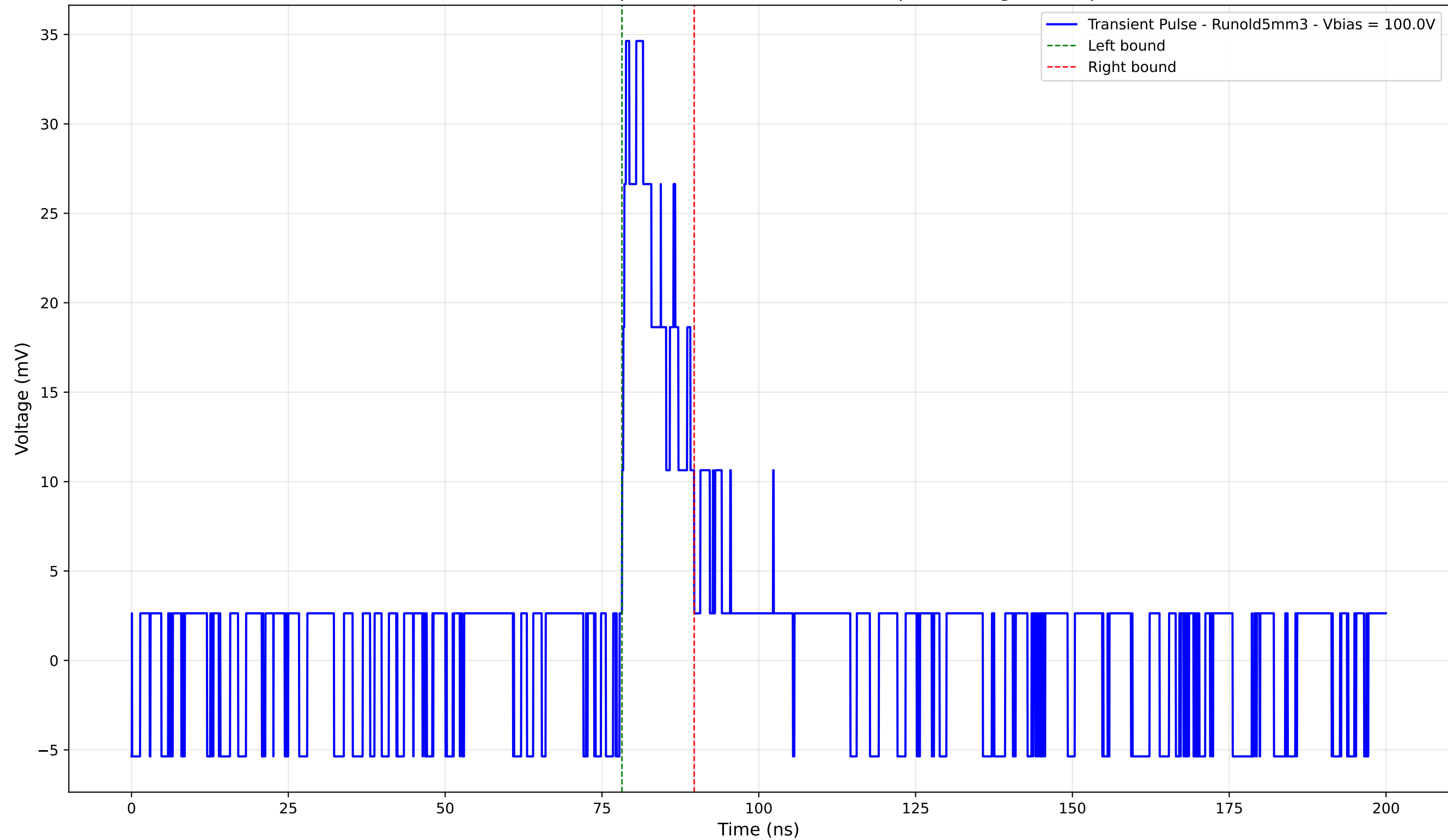
Transient Pulse - Sample: old5 - Position: 3870.0 \mu\text{m} - Charge: 4.84 pC
