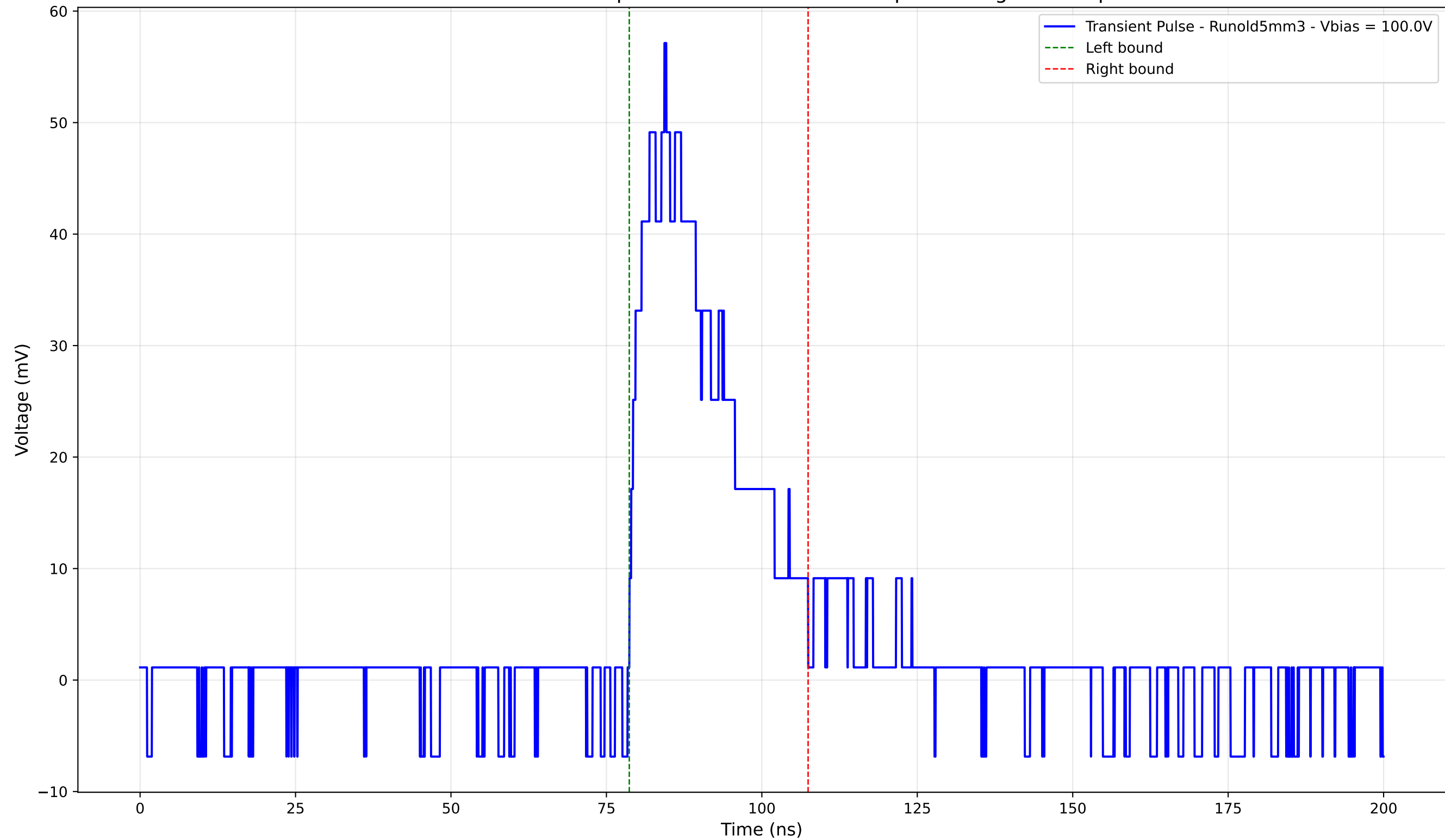
Transient Pulse - Sample: old5 - Position: 1565.0 \mu\text{m} - Charge: 15.61 pC
