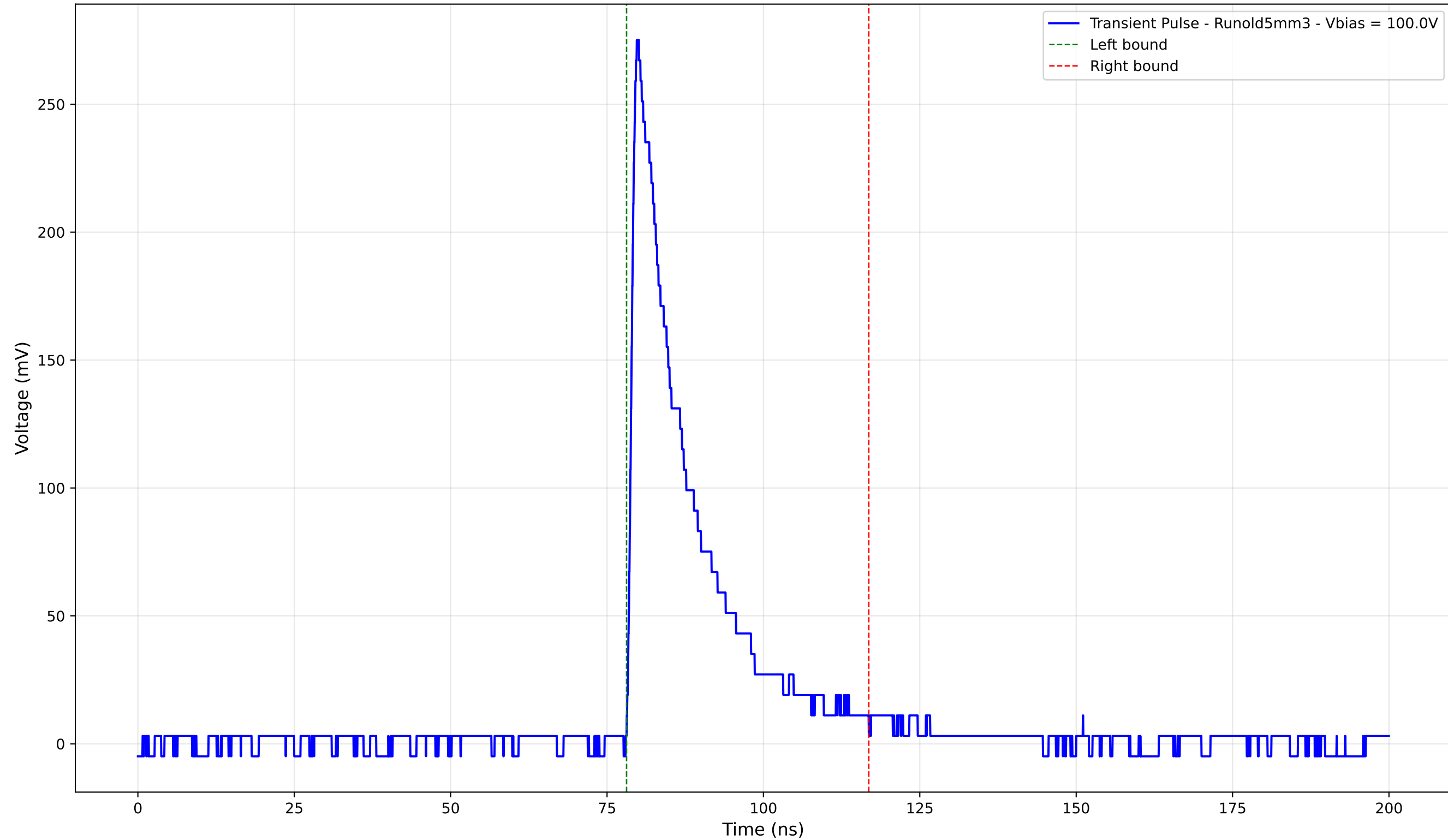
Transient Pulse - Sample: old5 - Position: 4555.0 \mu\text{m} - Charge: 54.17 pC
