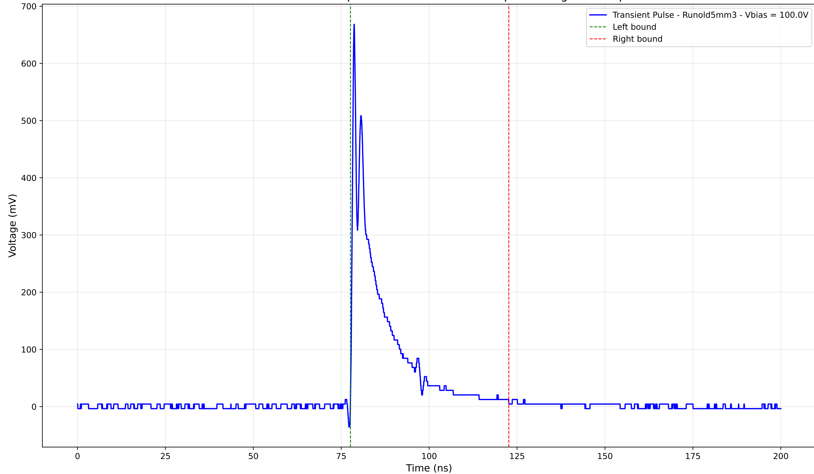
Transient Pulse - Sample: old5 - Position: 3680.0 \mu\text{m} - Charge: 92.38 pC
