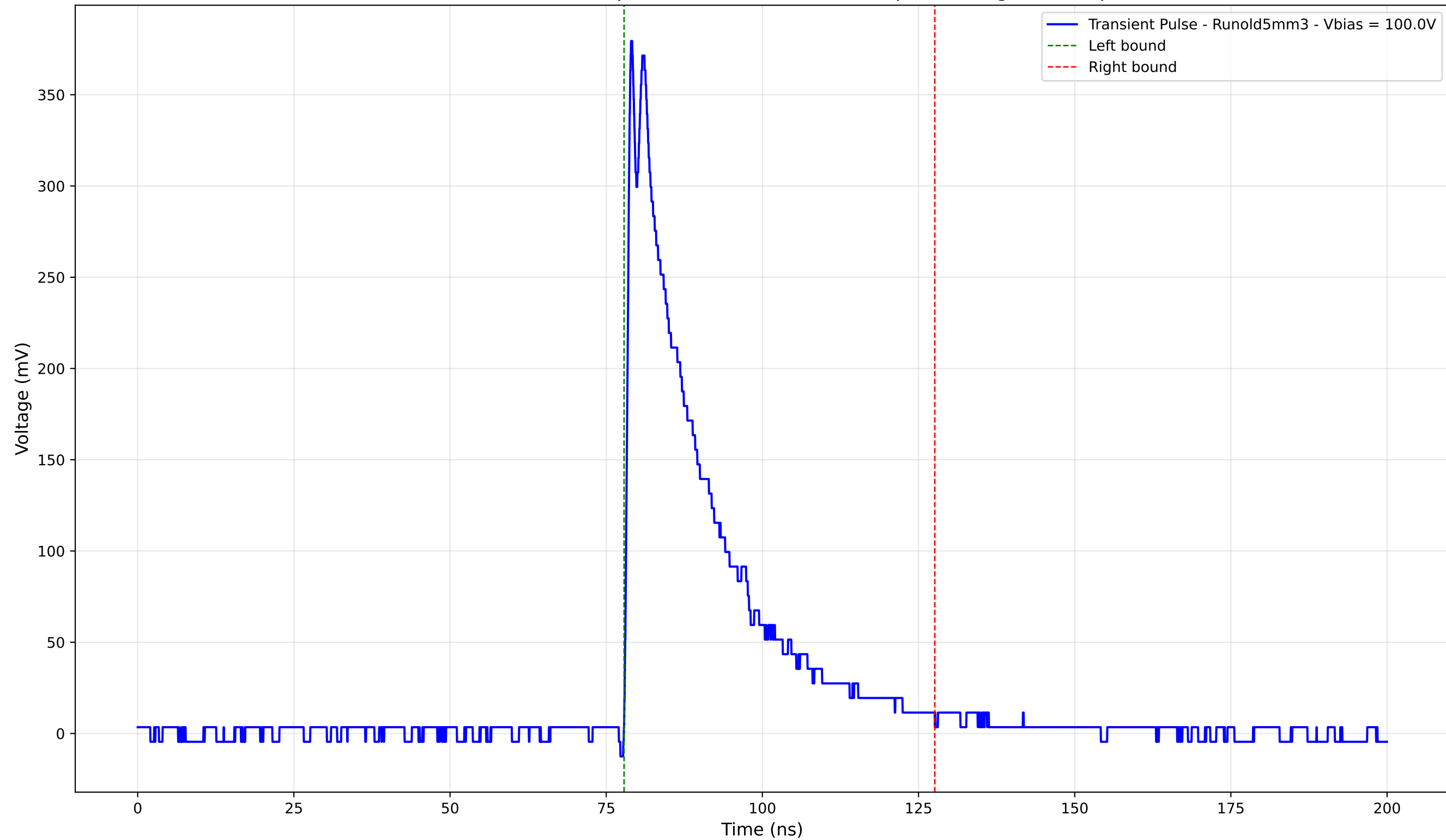
Transient Pulse - Sample: old5 - Position: 3175.0 \mu\text{m} - Charge: 94.61 pC
