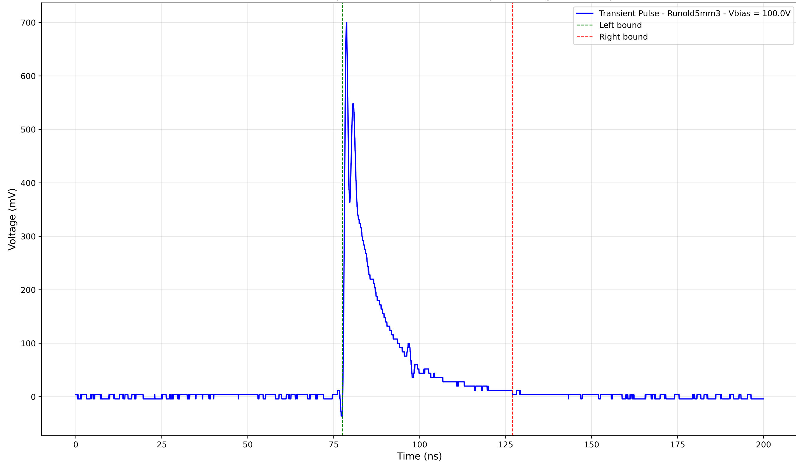
Transient Pulse - Sample: old5 - Position: 3450.0 \mu\text{m} - Charge: 107.25 pC
