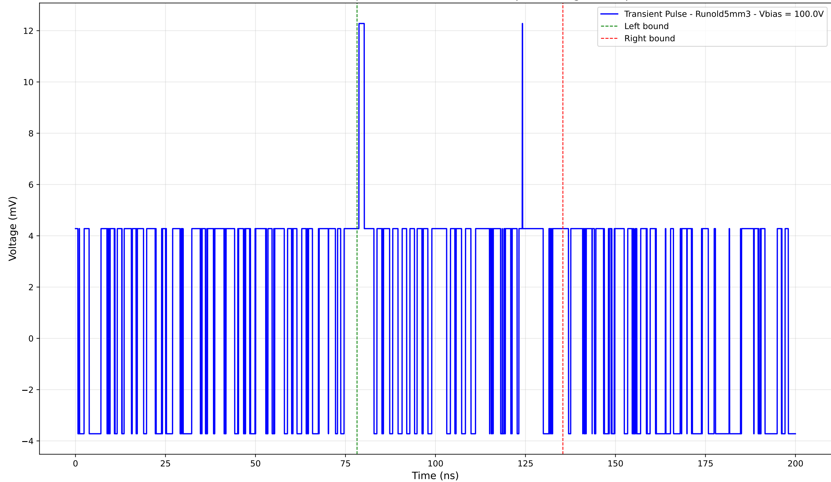
Transient Pulse - Sample: old5 - Position: 5000.0 \mu\text{m} - Charge: 2.92 pC
