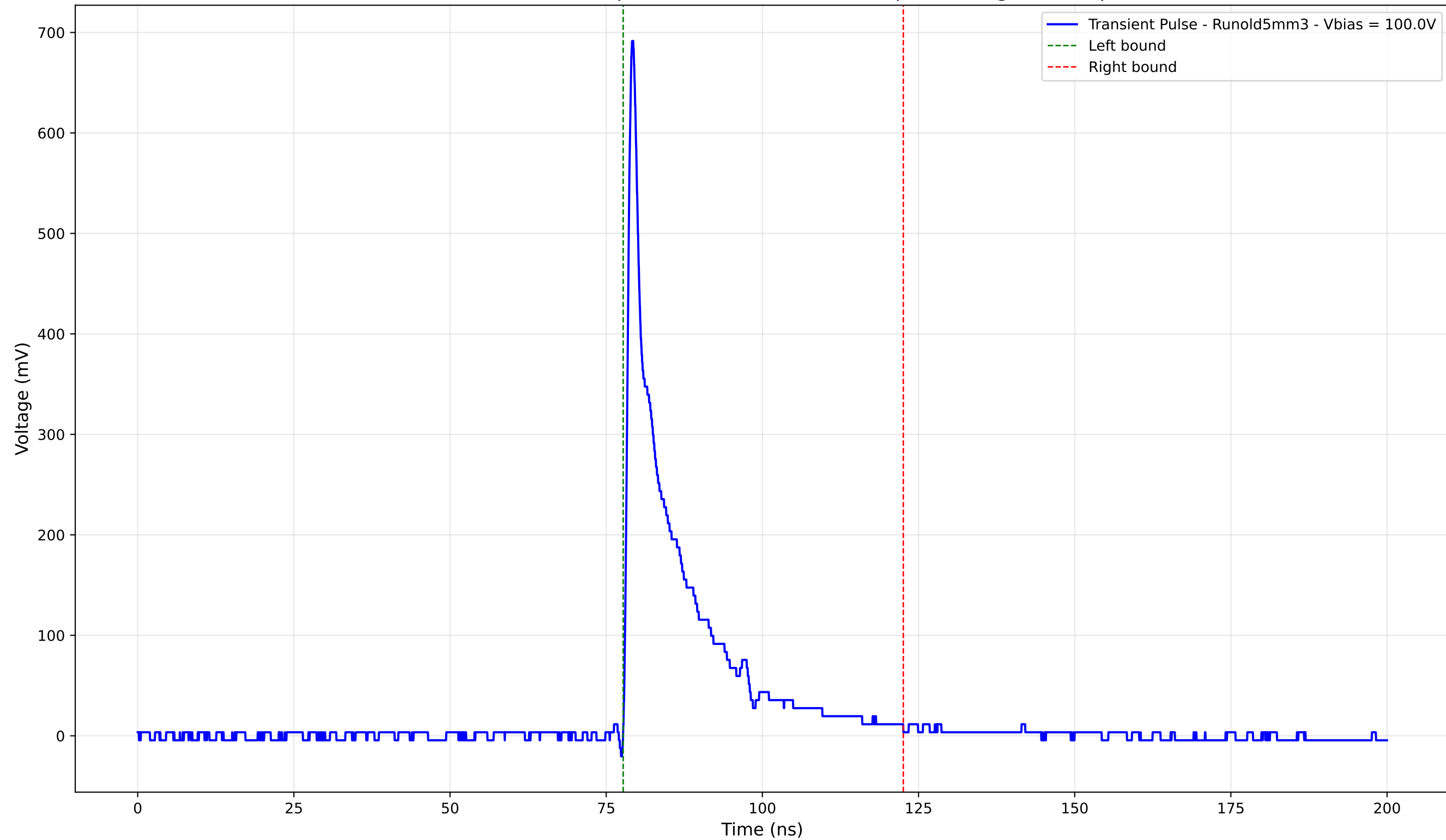
Transient Pulse - Sample: old5 - Position: 4860.0 \mu\text{m} - Charge: 93.76 pC
