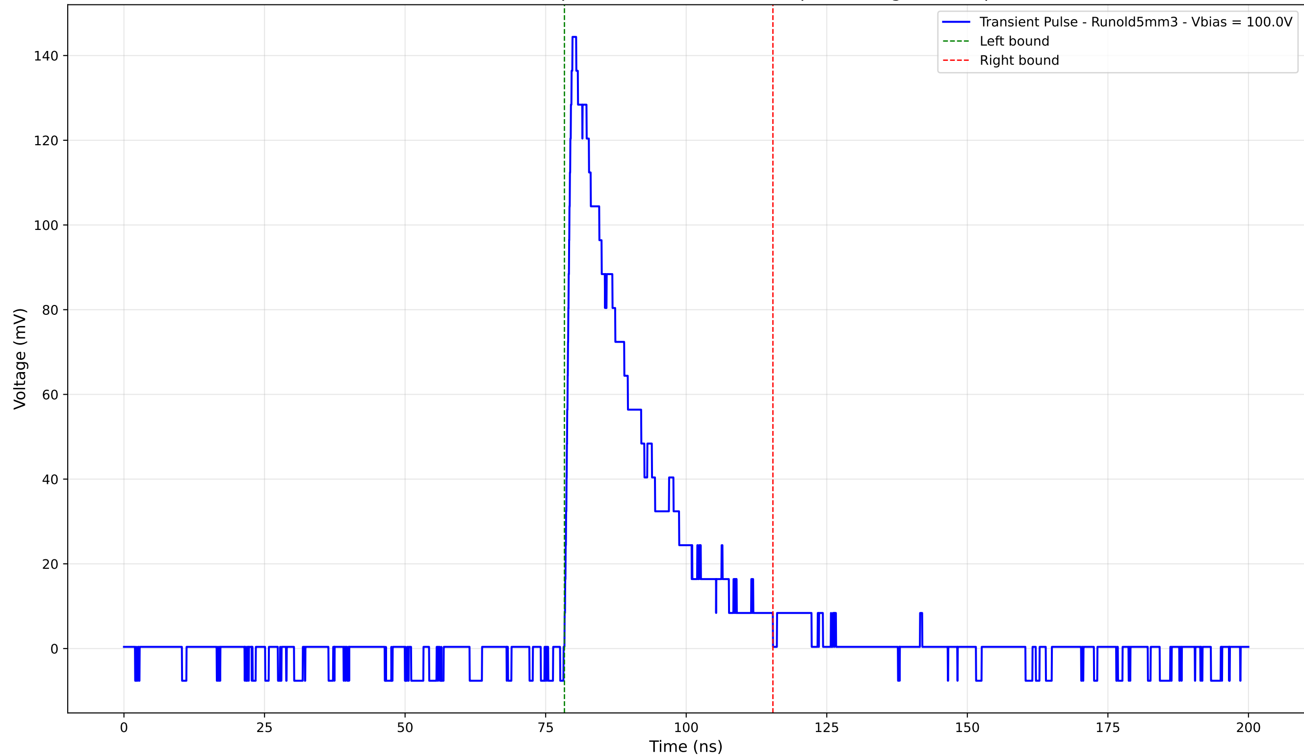
Transient Pulse - Sample: old5 - Position: 705.0 \mu\text{m} - Charge: 34.51 pC
