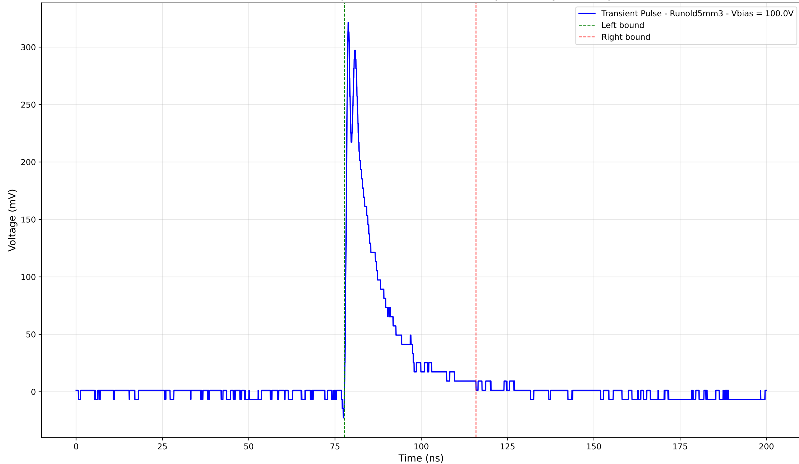
Transient Pulse - Sample: old5 - Position: 3815.0 \mu\text{m} - Charge: 54.14 pC
