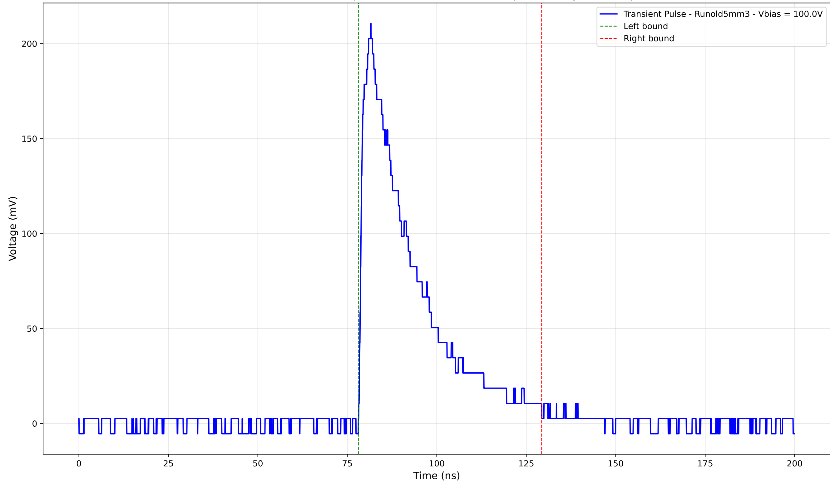
Transient Pulse - Sample: old5 - Position: 2900.0 \mu\text{m} - Charge: 64.33 pC
