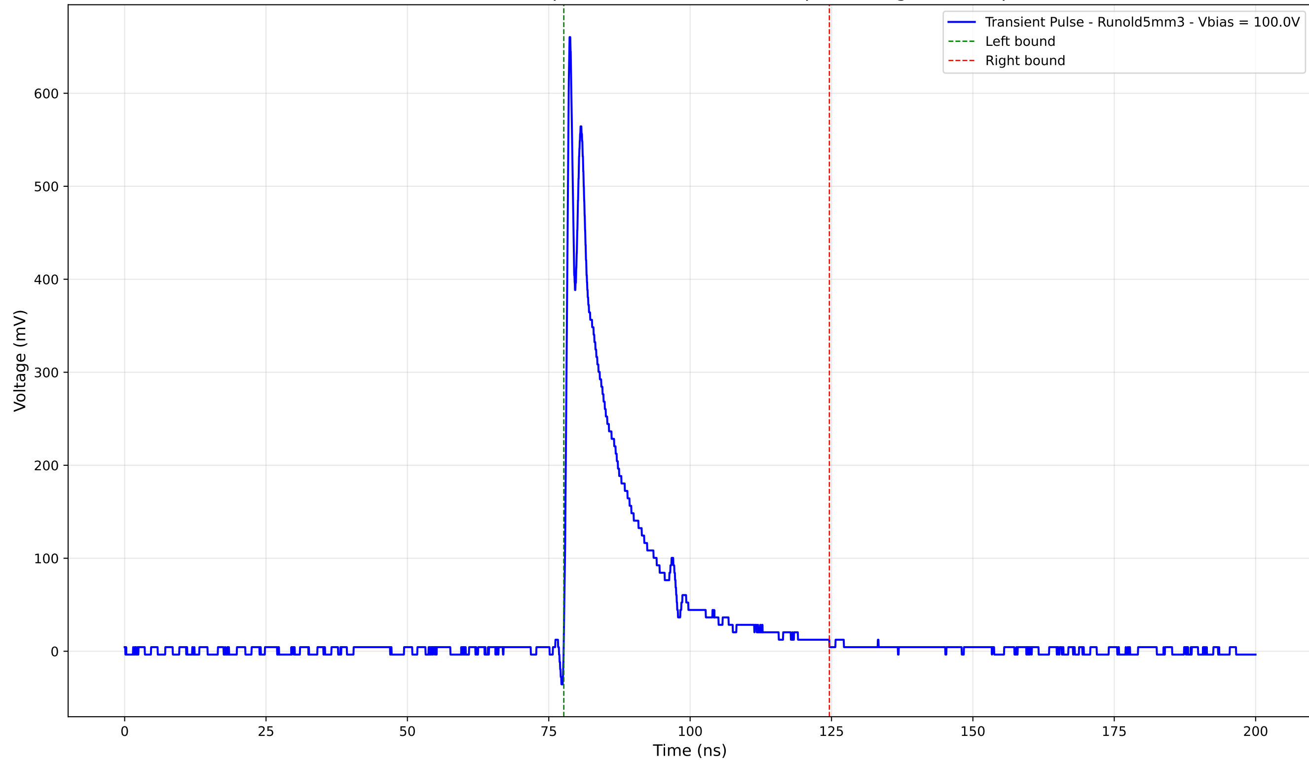
Transient Pulse - Sample: old5 - Position: 3735.0 \mu\text{m} - Charge: 108.65 pC
