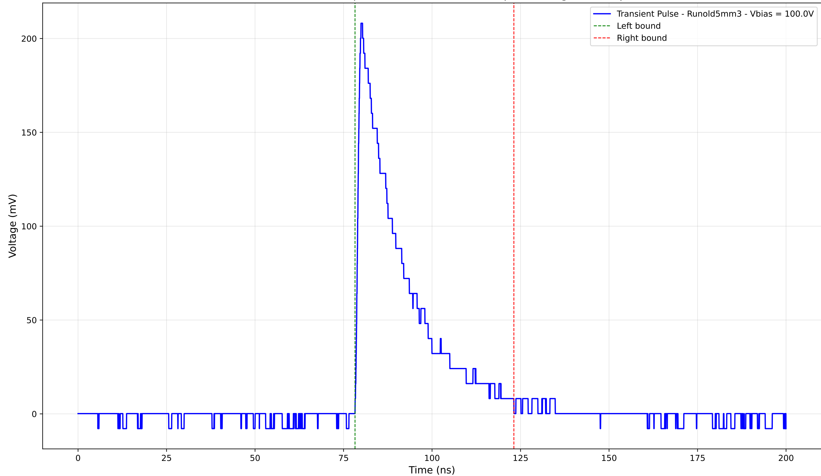
Transient Pulse - Sample: old5 - Position: 765.0 \mu\text{m} - Charge: 54.26 pC
