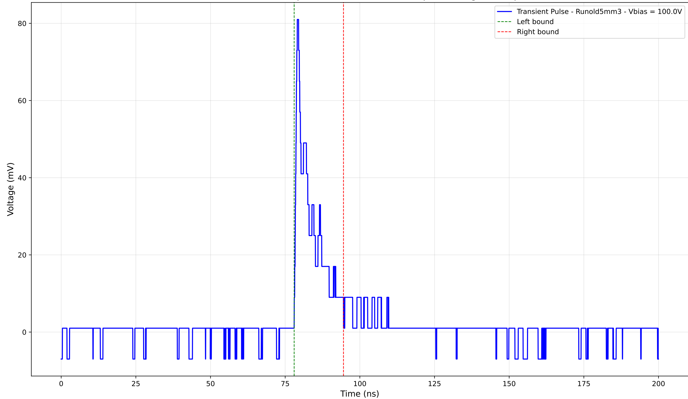
Transient Pulse - Sample: old5 - Position: 140.0 \mu\text{m} - Charge: 8.79 pC
