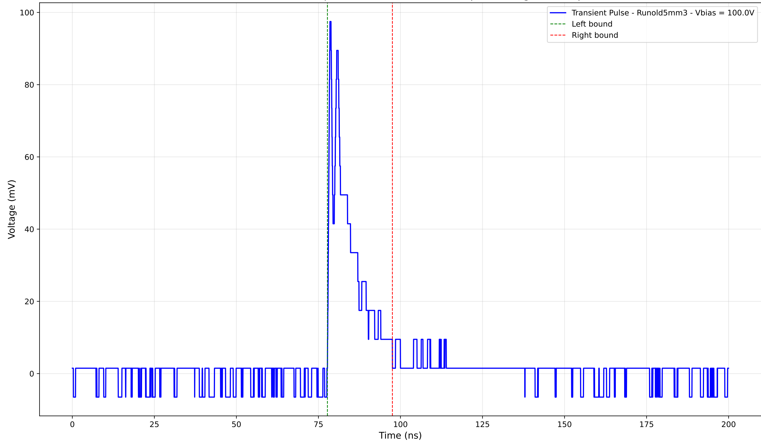
Transient Pulse - Sample: old5 - Position: 3615.0 \mu\text{m} - Charge: 12.83 pC
