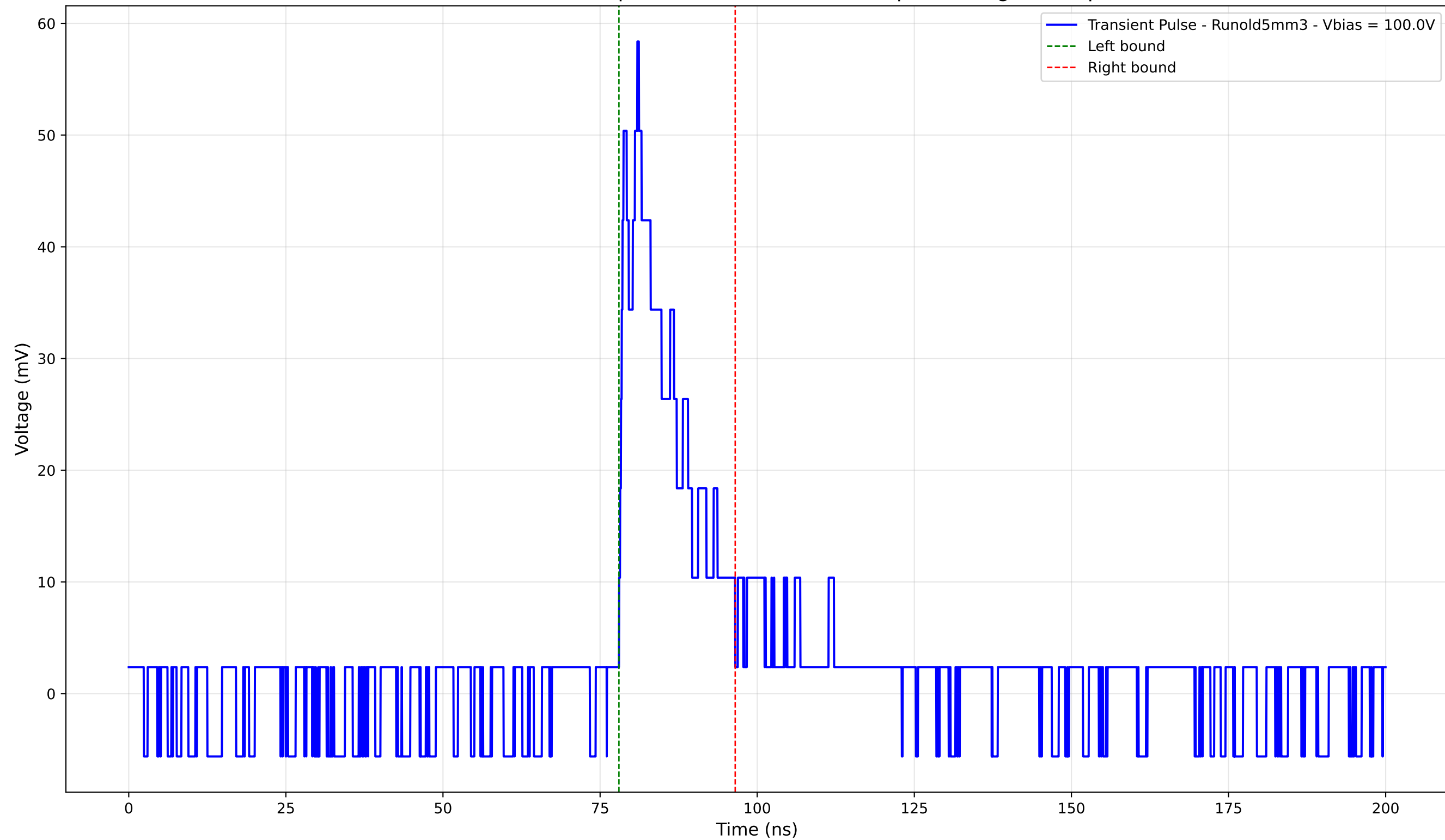
Transient Pulse - Sample: old5 - Position: 3310.0 \mu\text{m} - Charge: 9.56 pC
