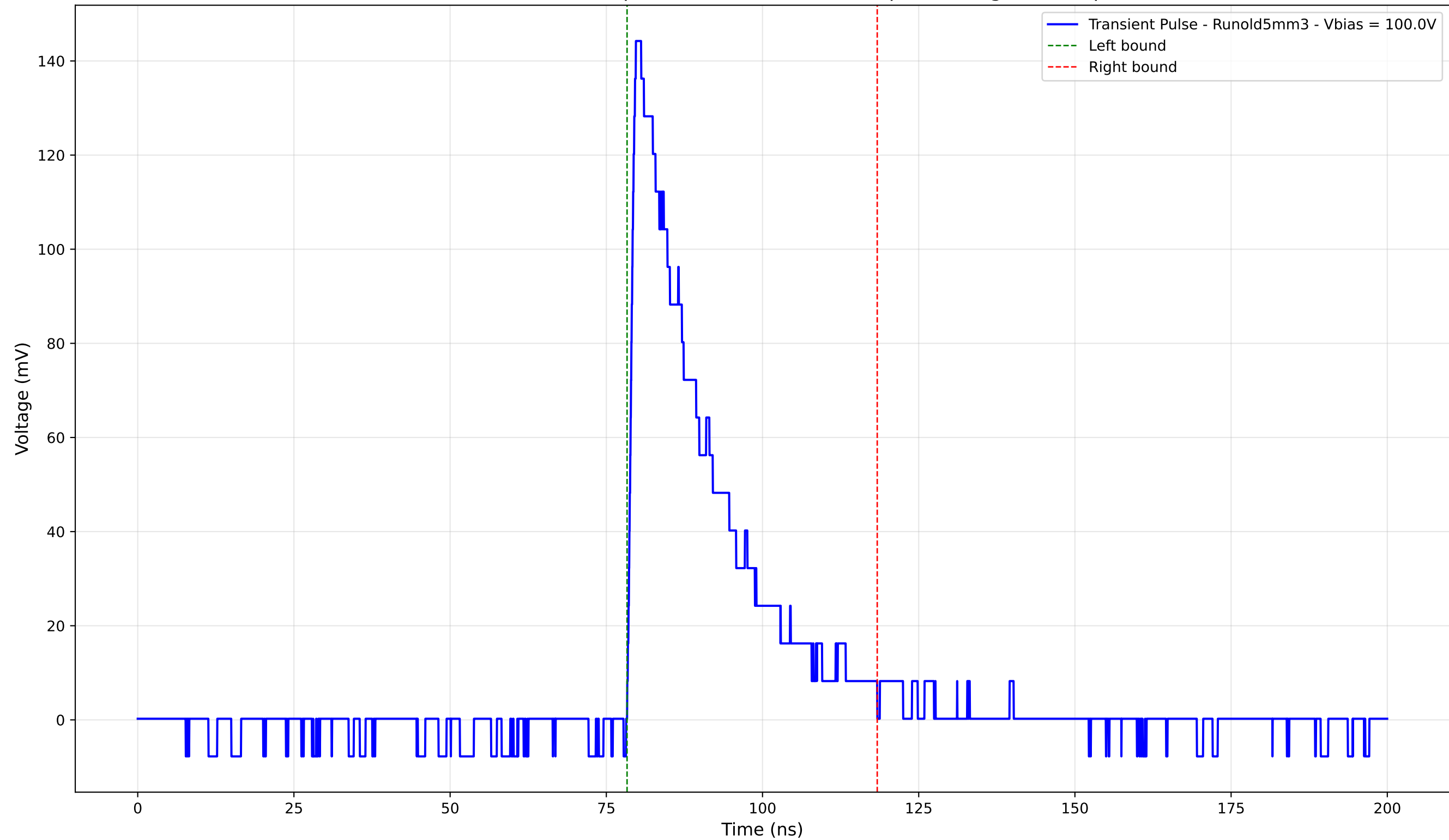
Transient Pulse - Sample: old5 - Position: 710.0 \mu\text{m} - Charge: 36.48 pC
