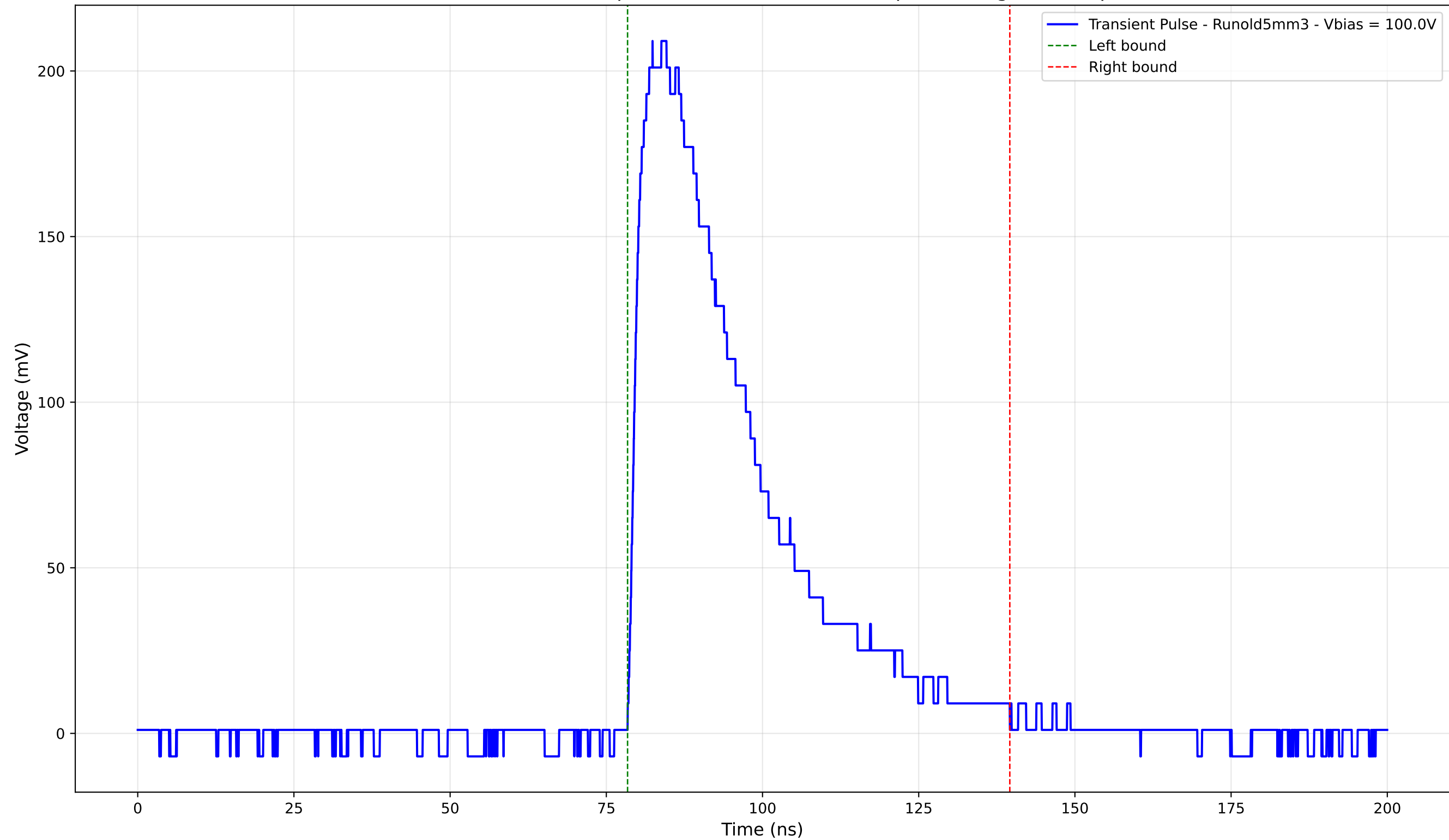
Transient Pulse - Sample: old5 - Position: 1685.0 \mu\text{m} - Charge: 84.77 pC
