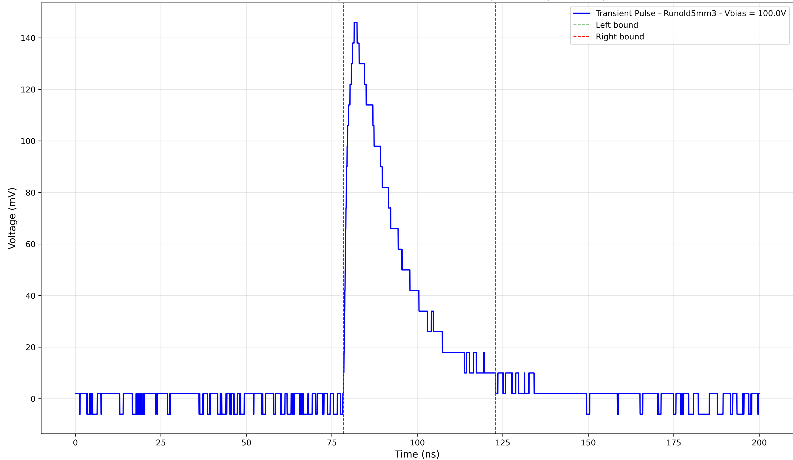
Transient Pulse - Sample: old5 - Position: 2740.0 \mu\text{m} - Charge: 46.45 pC
