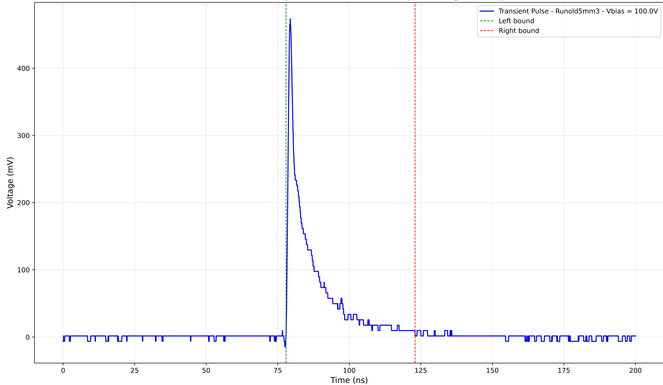
Transient Pulse - Sample: old5 - Position: 255.0 \mu\text{m} - Charge: 63.29 pC
