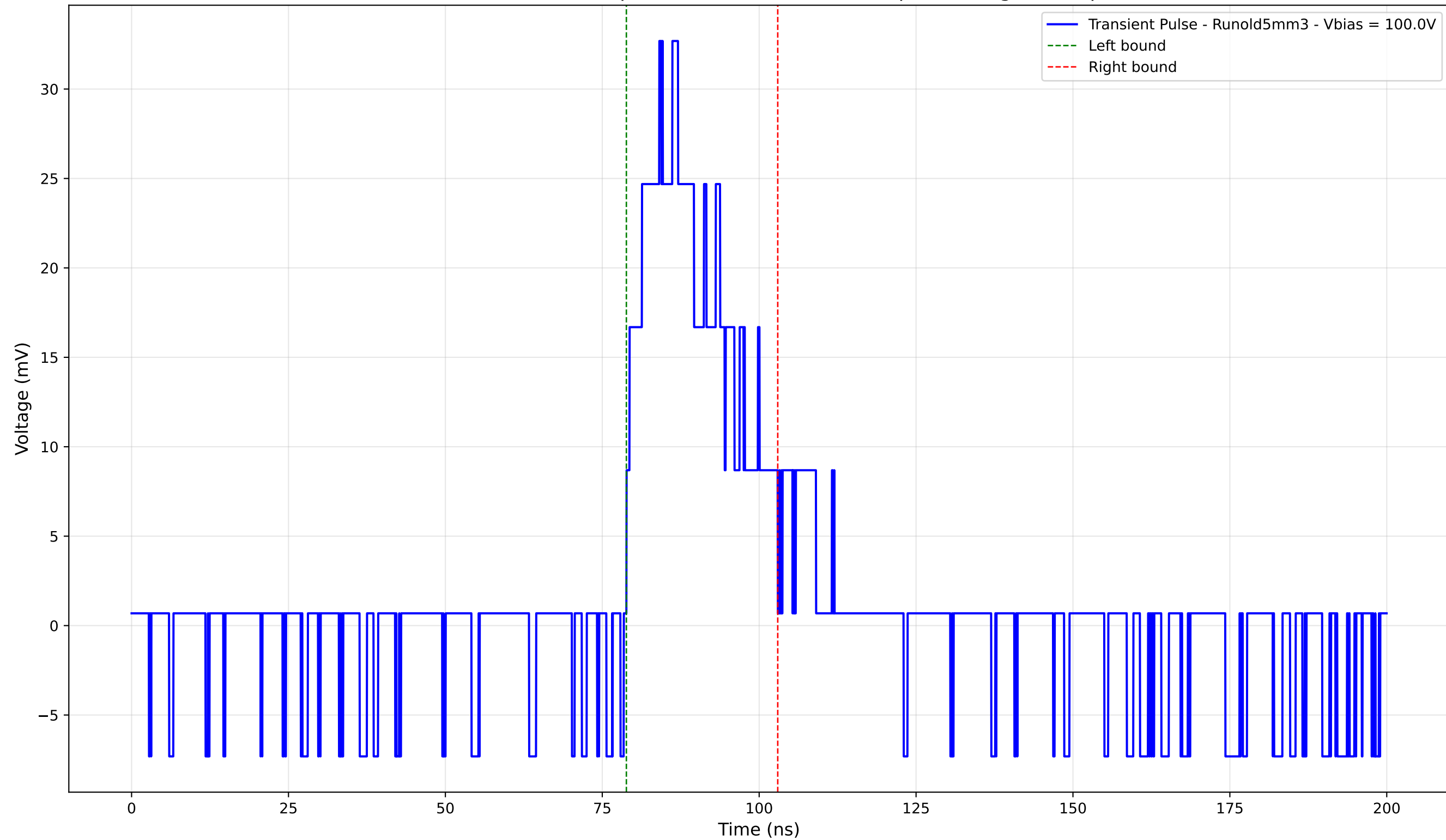
Transient Pulse - Sample: old5 - Position: 1585.0 \mu\text{m} - Charge: 8.72 pC
