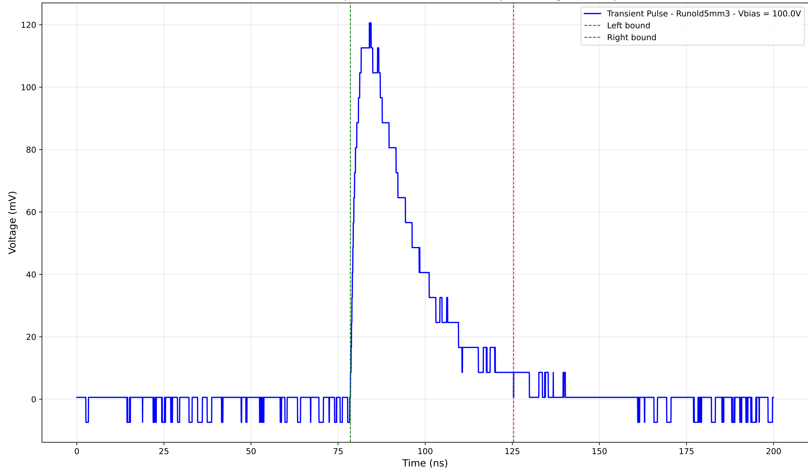
Transient Pulse - Sample: old5 - Position: 2235.0 \mu\text{m} - Charge: 42.84 pC
