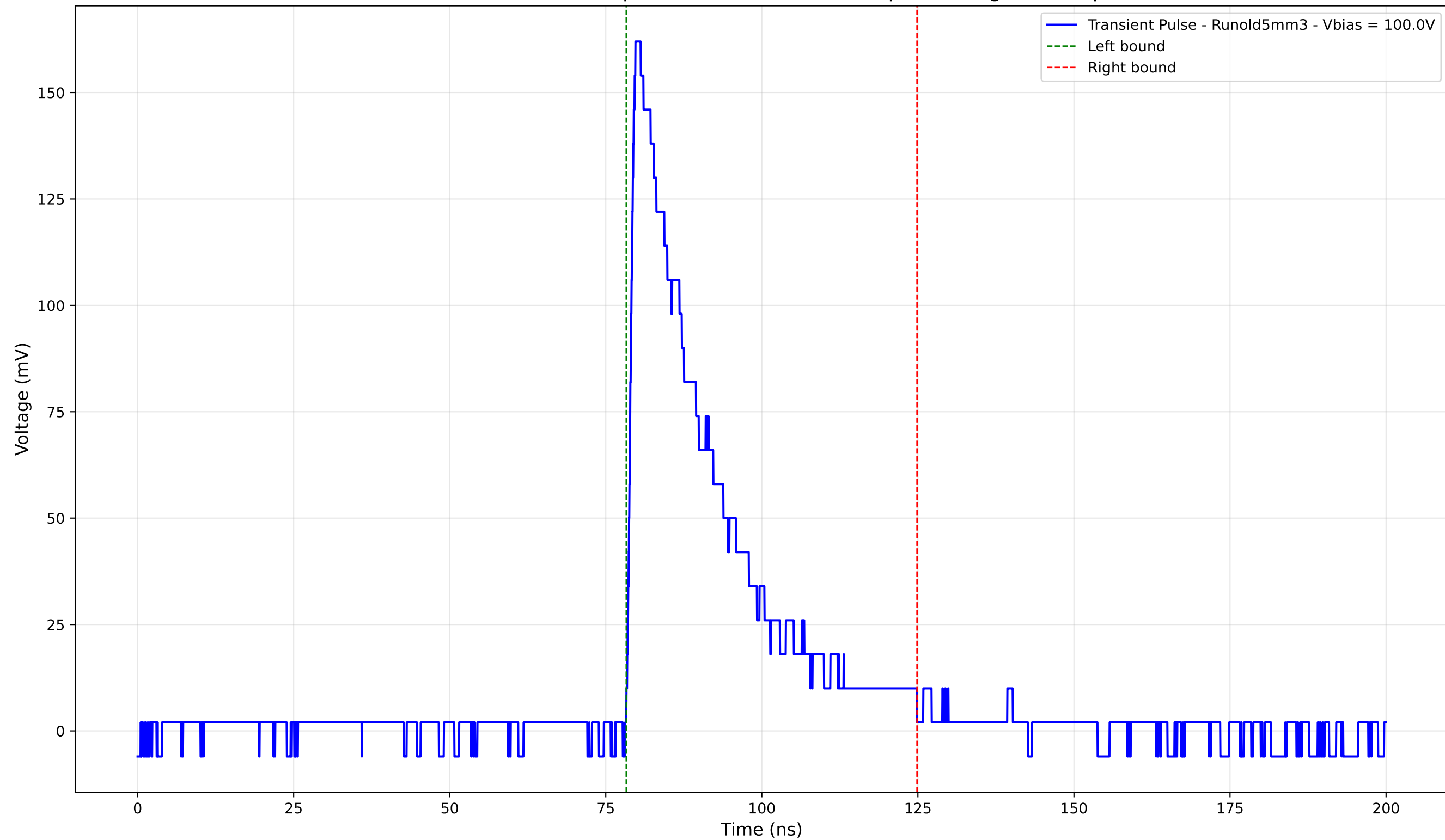
Transient Pulse - Sample: old5 - Position: 720.0 \mu\text{m} - Charge: 43.49 pC
