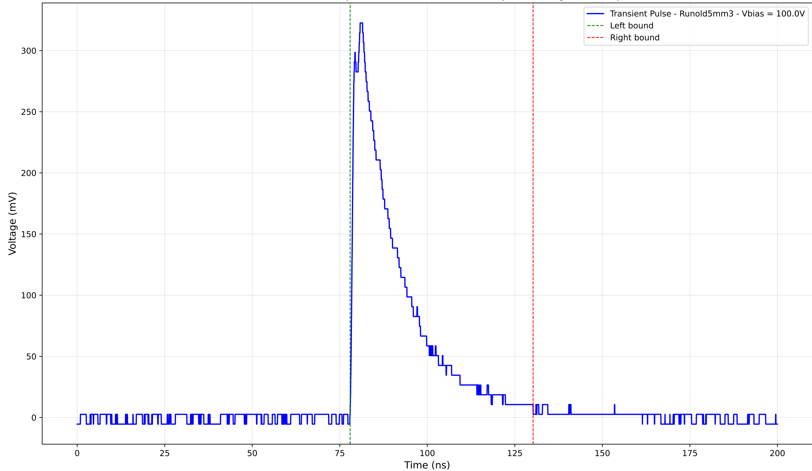
Transient Pulse - Sample: old5 - Position: 3075.0 \mu\text{m} - Charge: 89.96 pC
