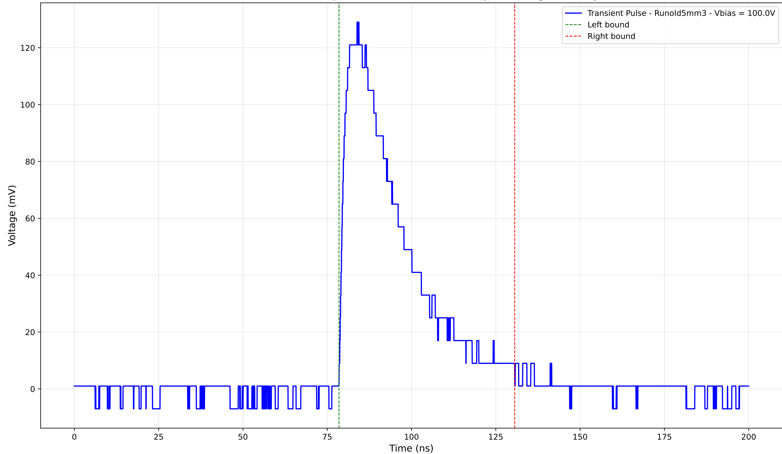
Transient Pulse - Sample: old5 - Position: 1535.0 \mu\text{m} - Charge: 48.91 pC
