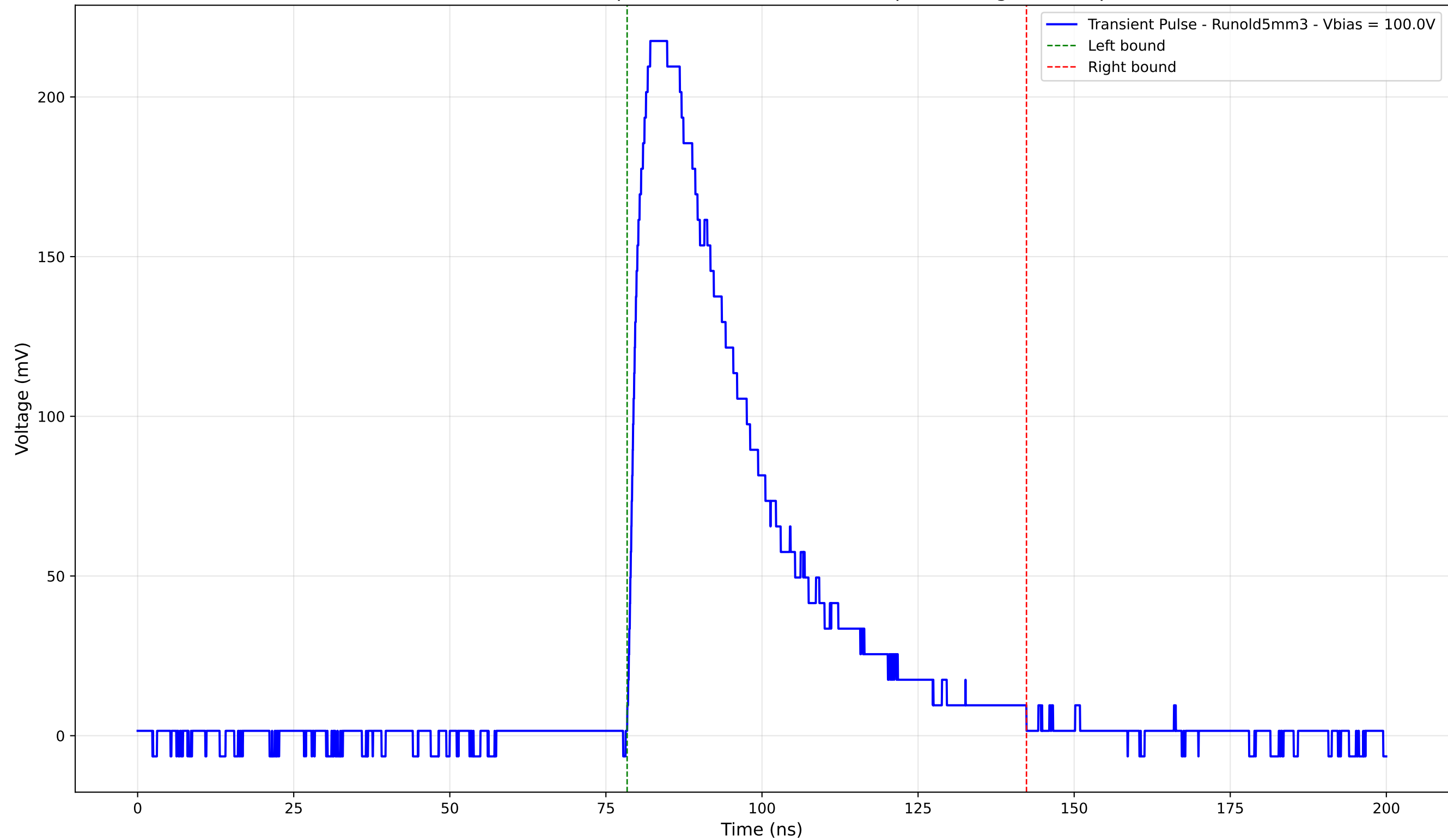
Transient Pulse - Sample: old5 - Position: 2105.0 \mu\text{m} - Charge: 89.65 pC
