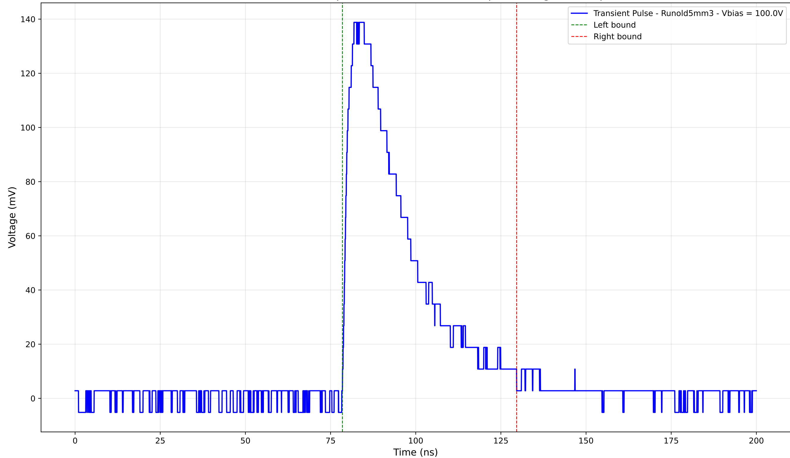
Transient Pulse - Sample: old5 - Position: 1530.0 \mu\text{m} - Charge: 55.12 pC
