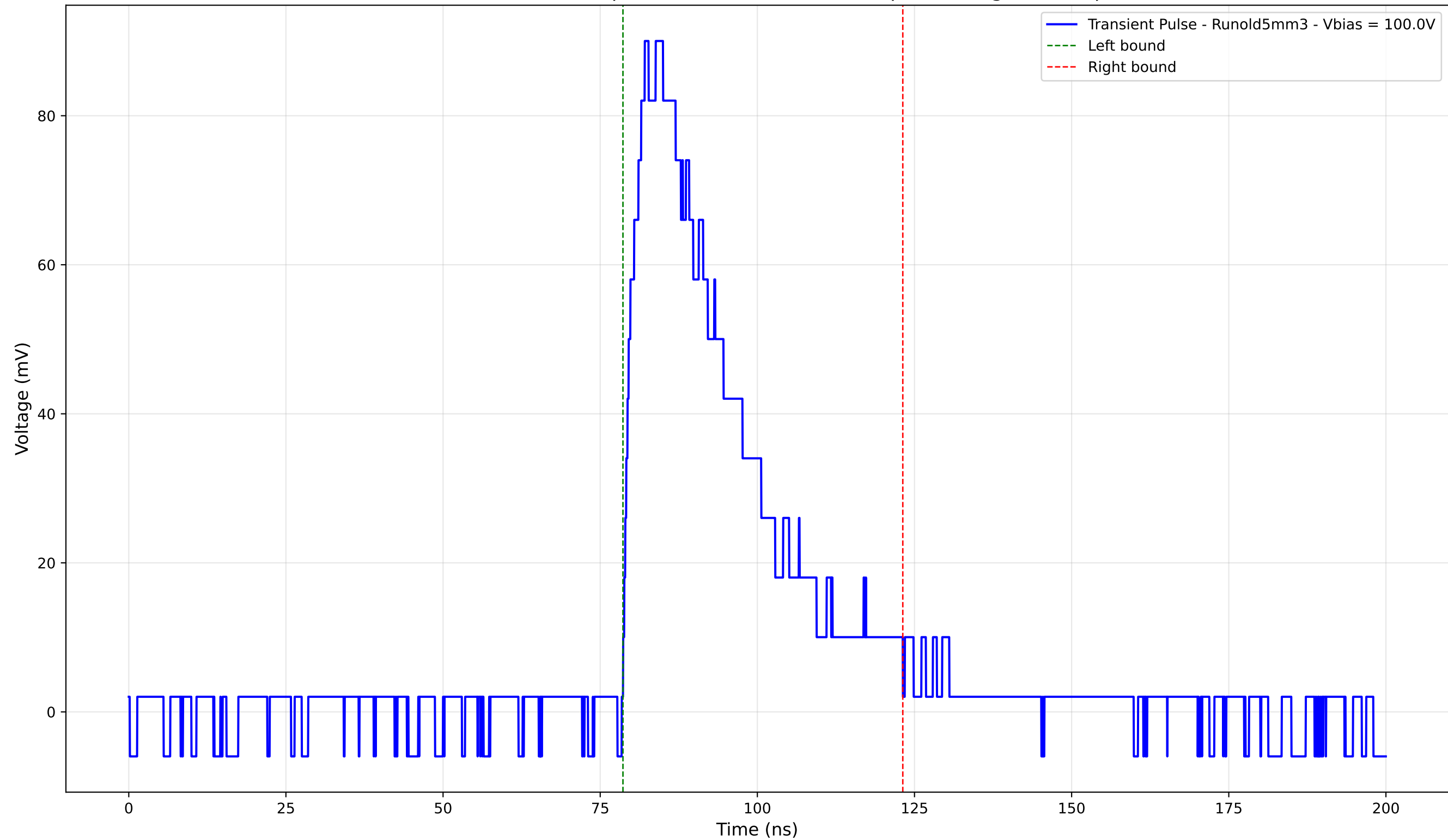
Transient Pulse - Sample: old5 - Position: 2225.0 \mu\text{m} - Charge: 32.72 pC
