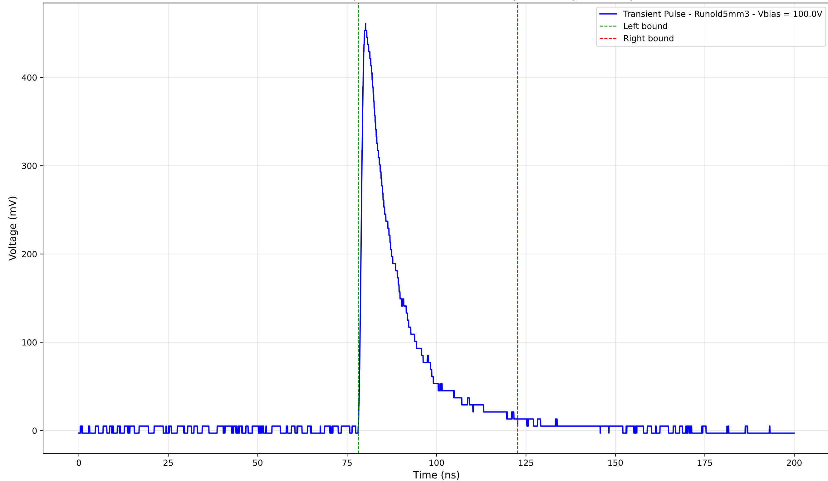
Transient Pulse - Sample: old5 - Position: 4395.0 \mu\text{m} - Charge: 99.80 pC
