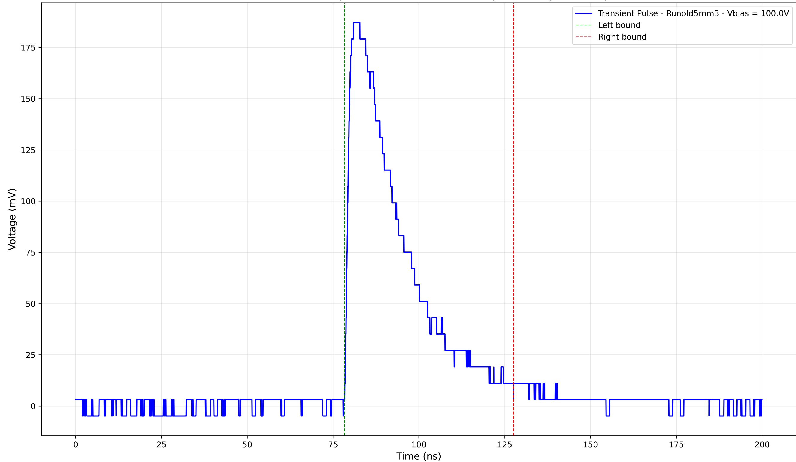
Transient Pulse - Sample: old5 - Position: 1115.0 \mu\text{m} - Charge: 66.82 pC
