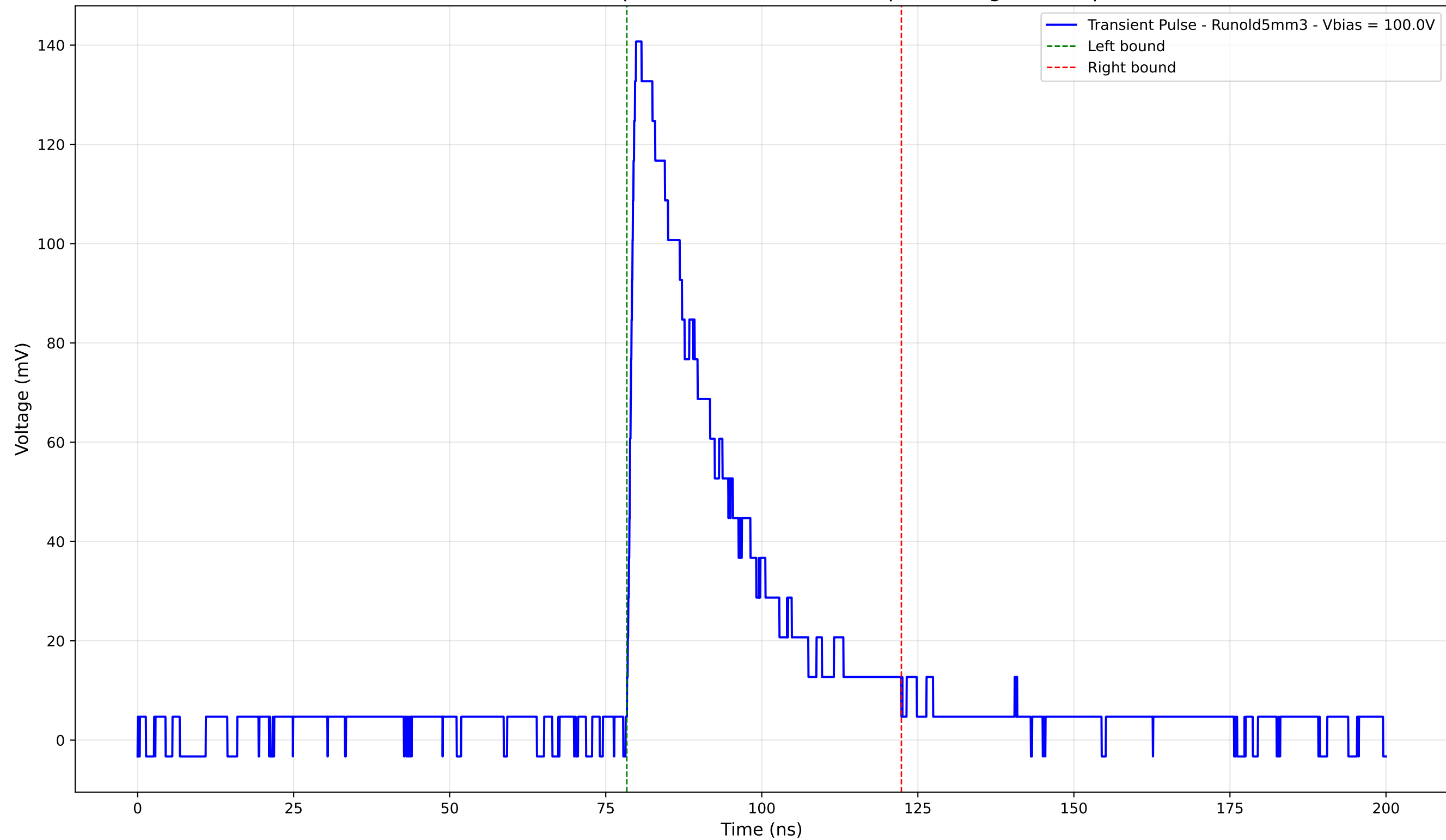
Transient Pulse - Sample: old5 - Position: 815.0 \mu\text{m} - Charge: 42.06 pC
