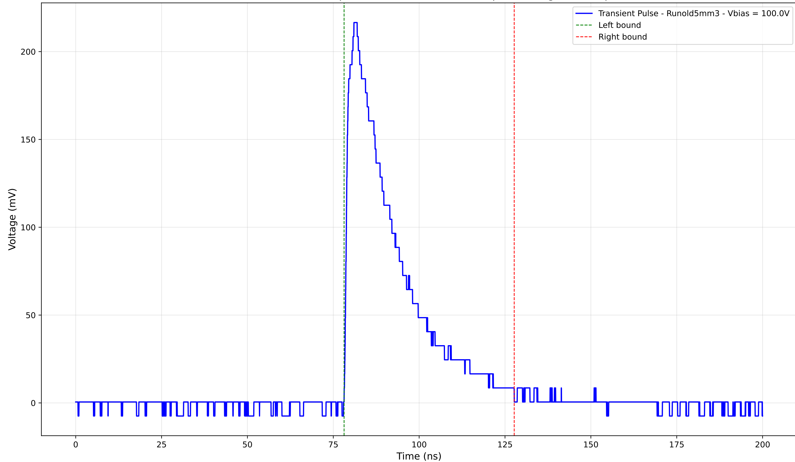
Transient Pulse - Sample: old5 - Position: 2895.0 \mu\text{m} - Charge: 67.45 pC
