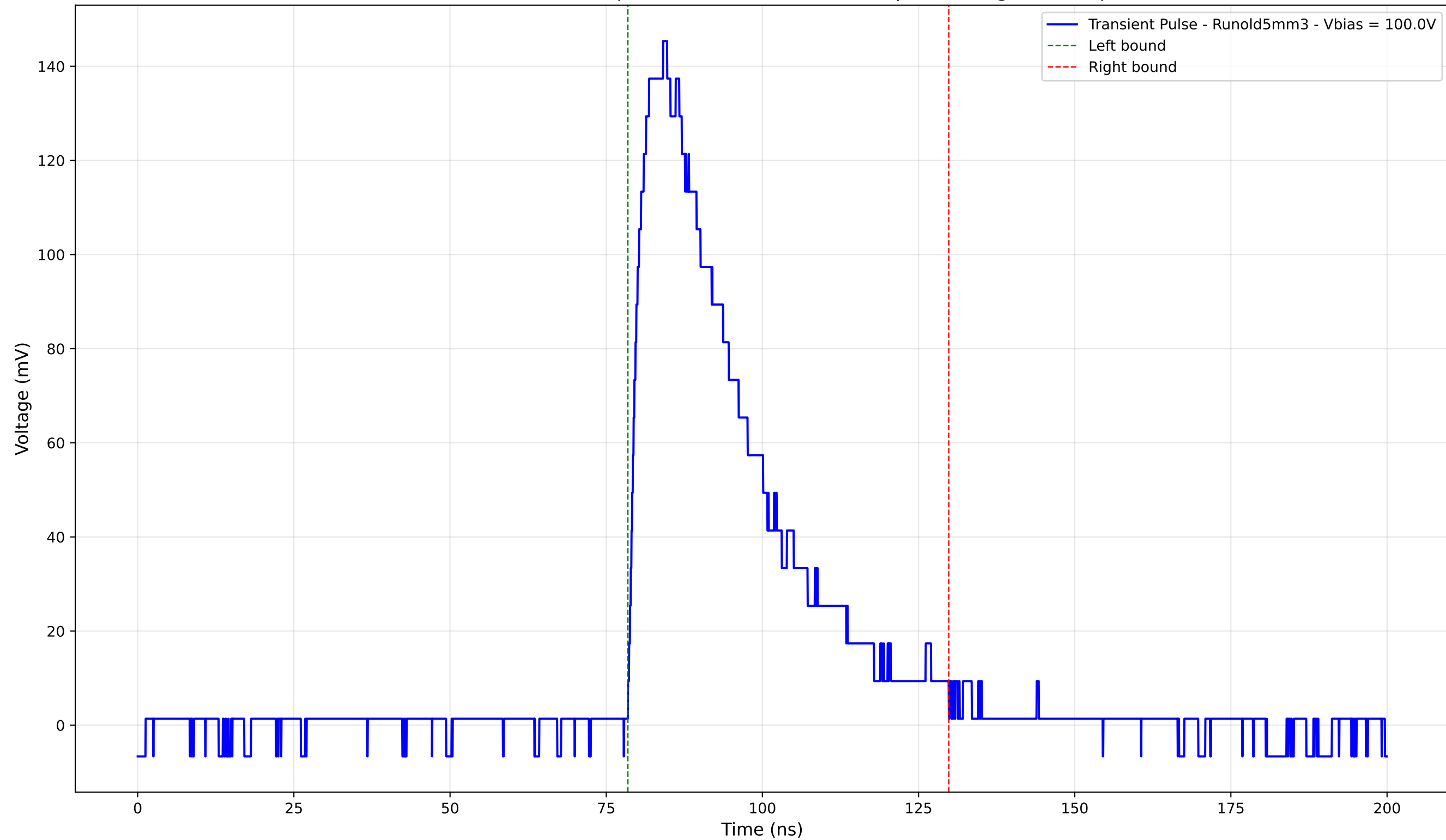
Transient Pulse - Sample: old5 - Position: 1640.0 \mu\text{m} - Charge: 55.07 pC
