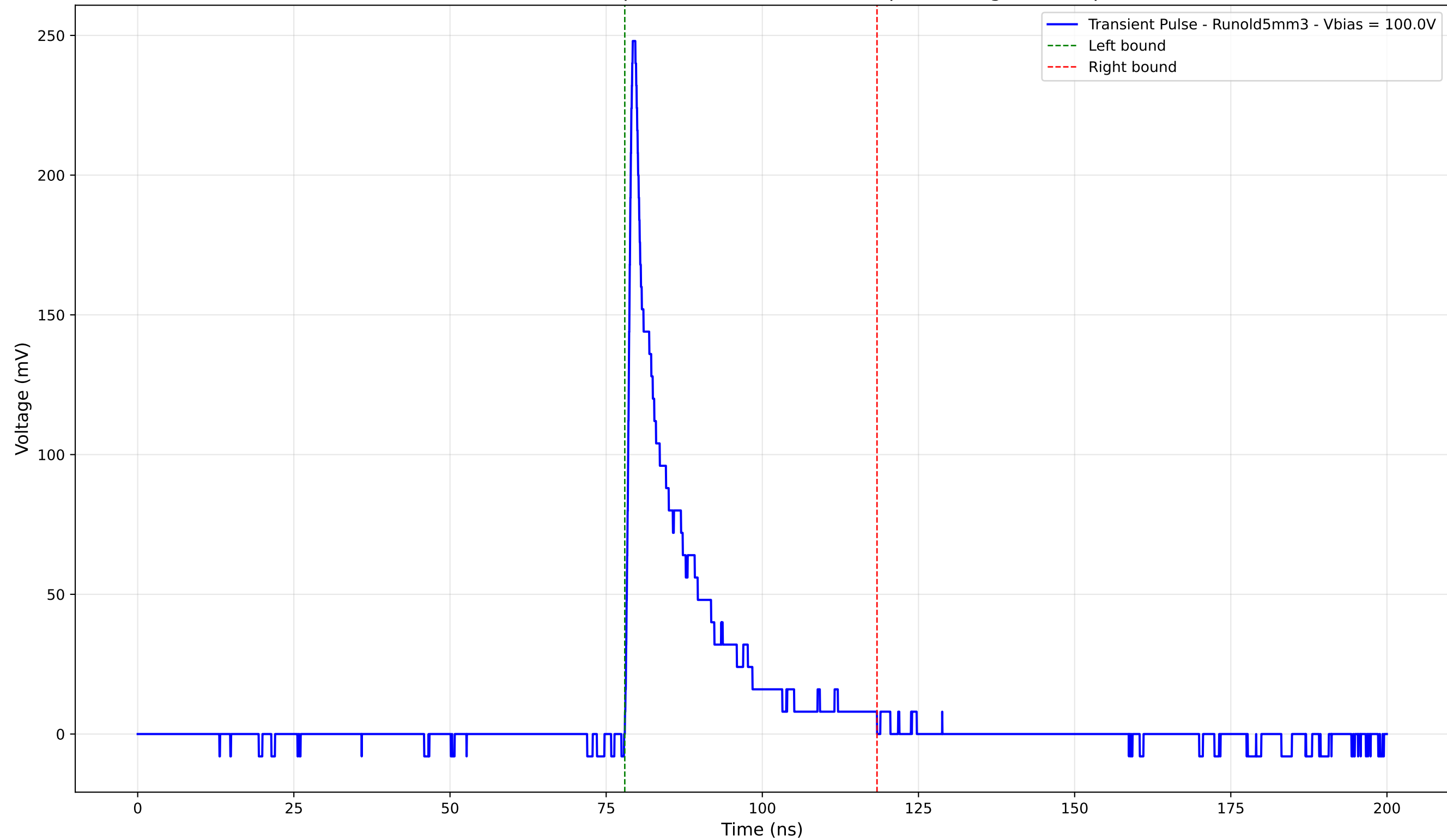
Transient Pulse - Sample: old5 - Position: 300.0 \mu\text{m} - Charge: 36.28 pC
