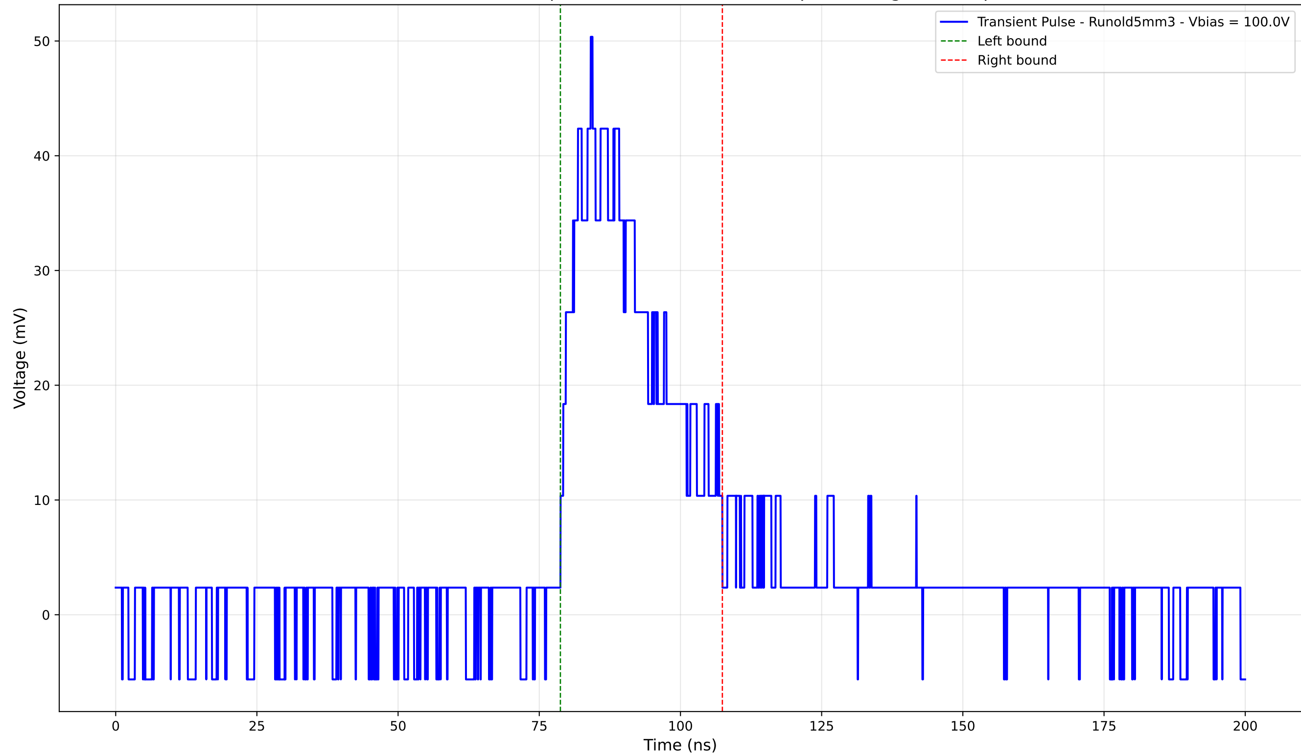
Transient Pulse - Sample: old5 - Position: 1805.0 \mu\text{m} - Charge: 14.79 pC
