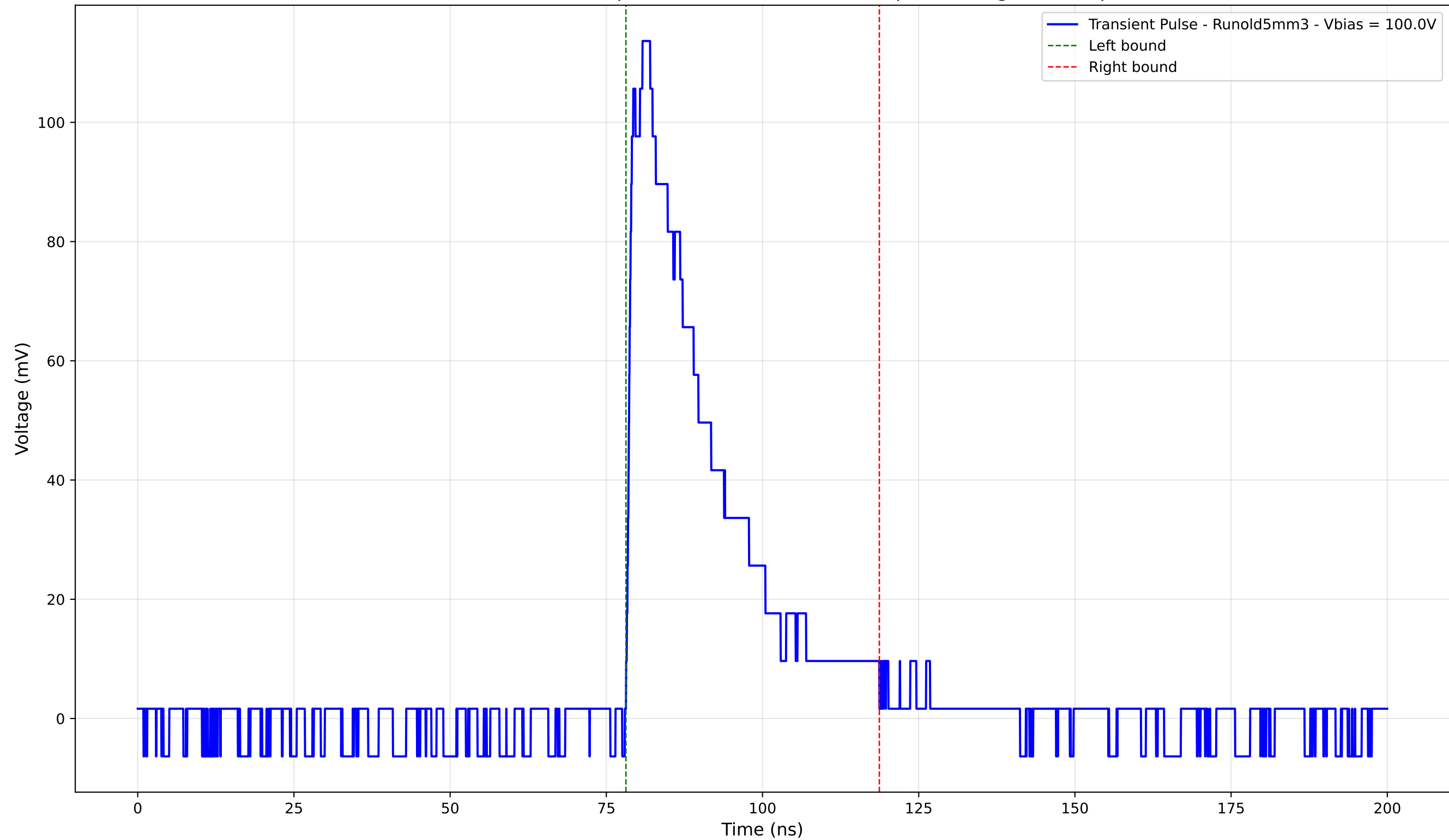
Transient Pulse - Sample: old5 - Position: 3030.0 \mu\text{m} - Charge: 31.54 pC
