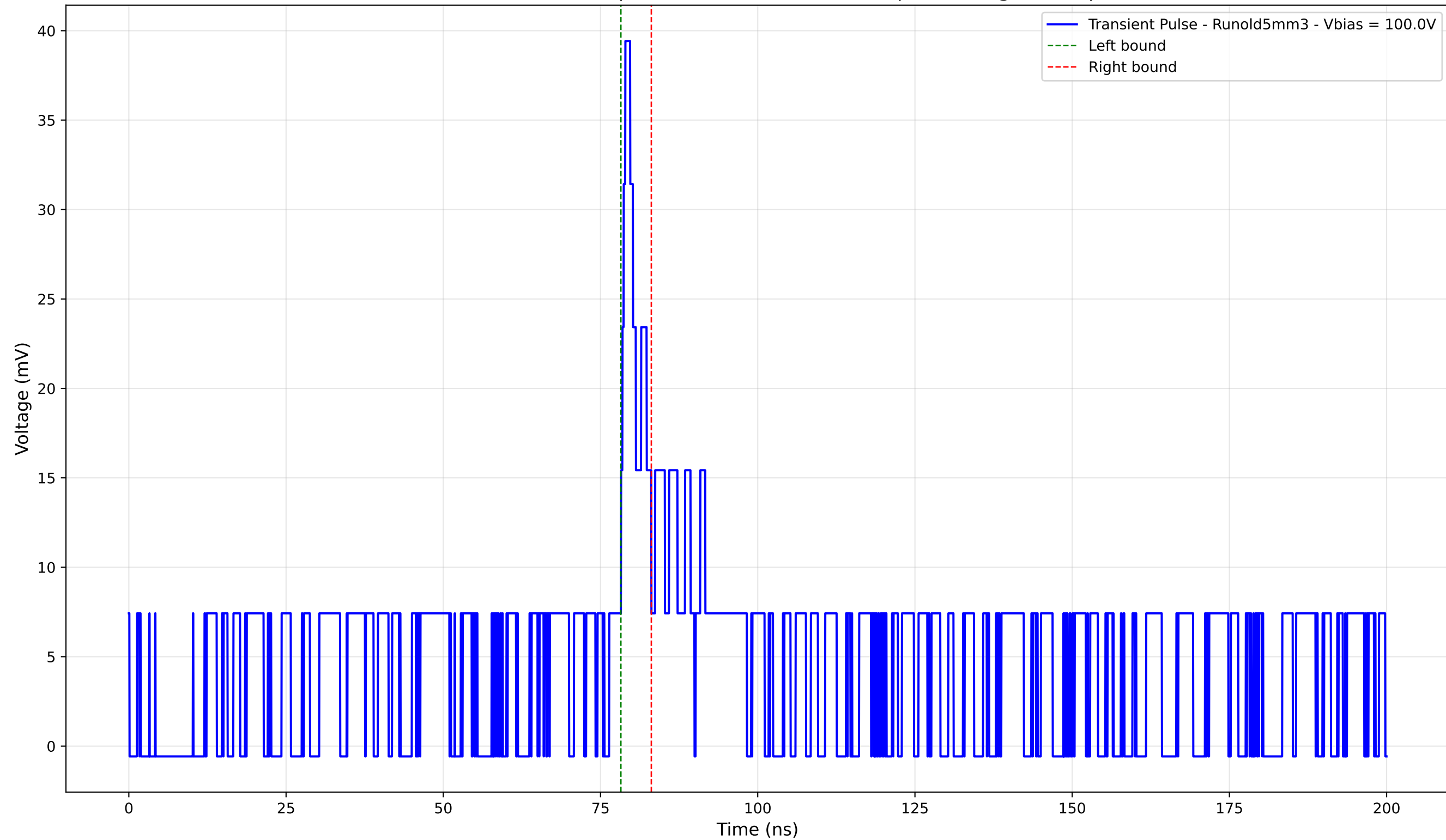
Transient Pulse - Sample: old5 - Position: 4940.0 \mu\text{m} - Charge: 2.33 pC
