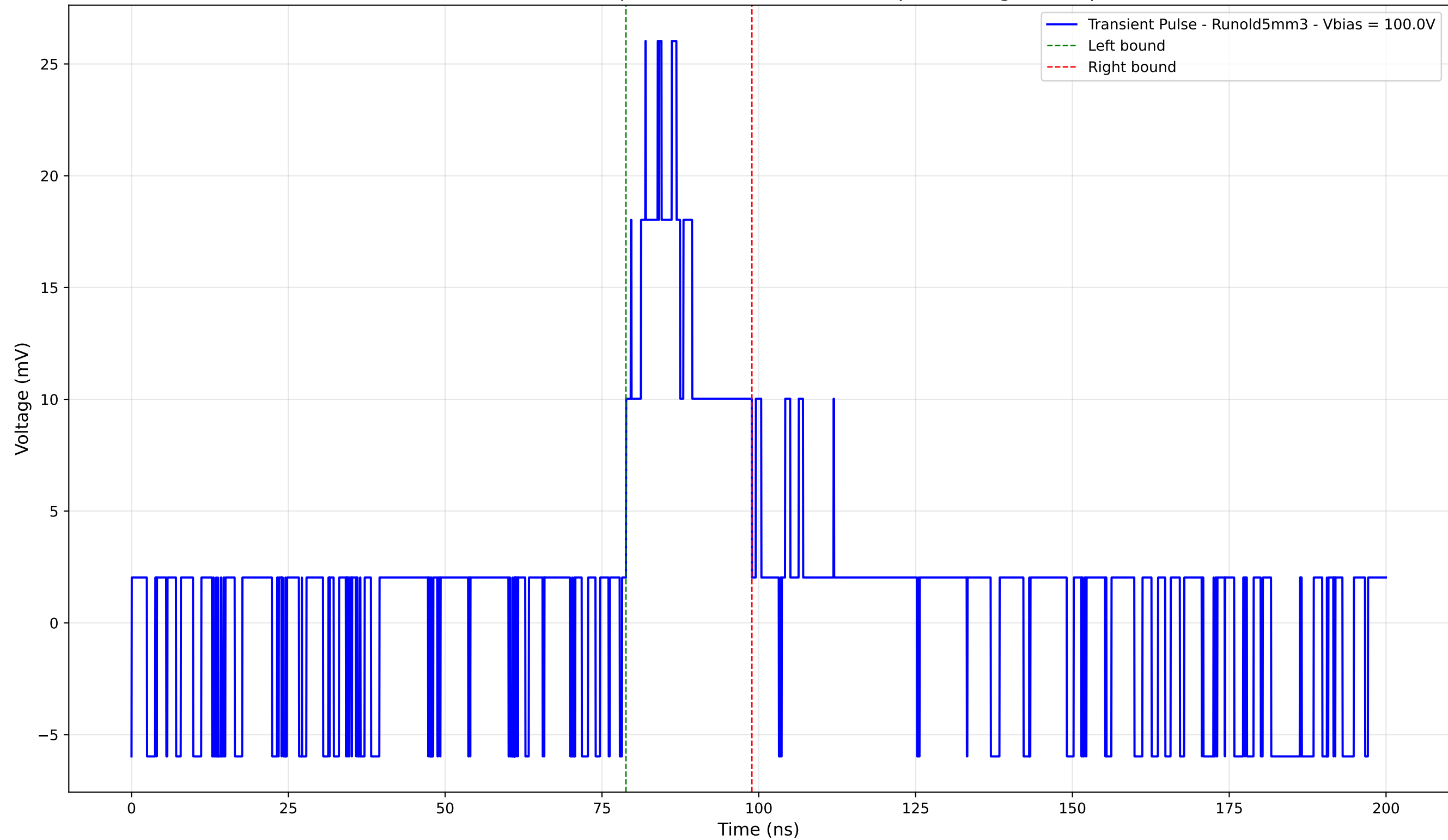
Transient Pulse - Sample: old5 - Position: 2690.0 \mu\text{m} - Charge: 5.48 pC
