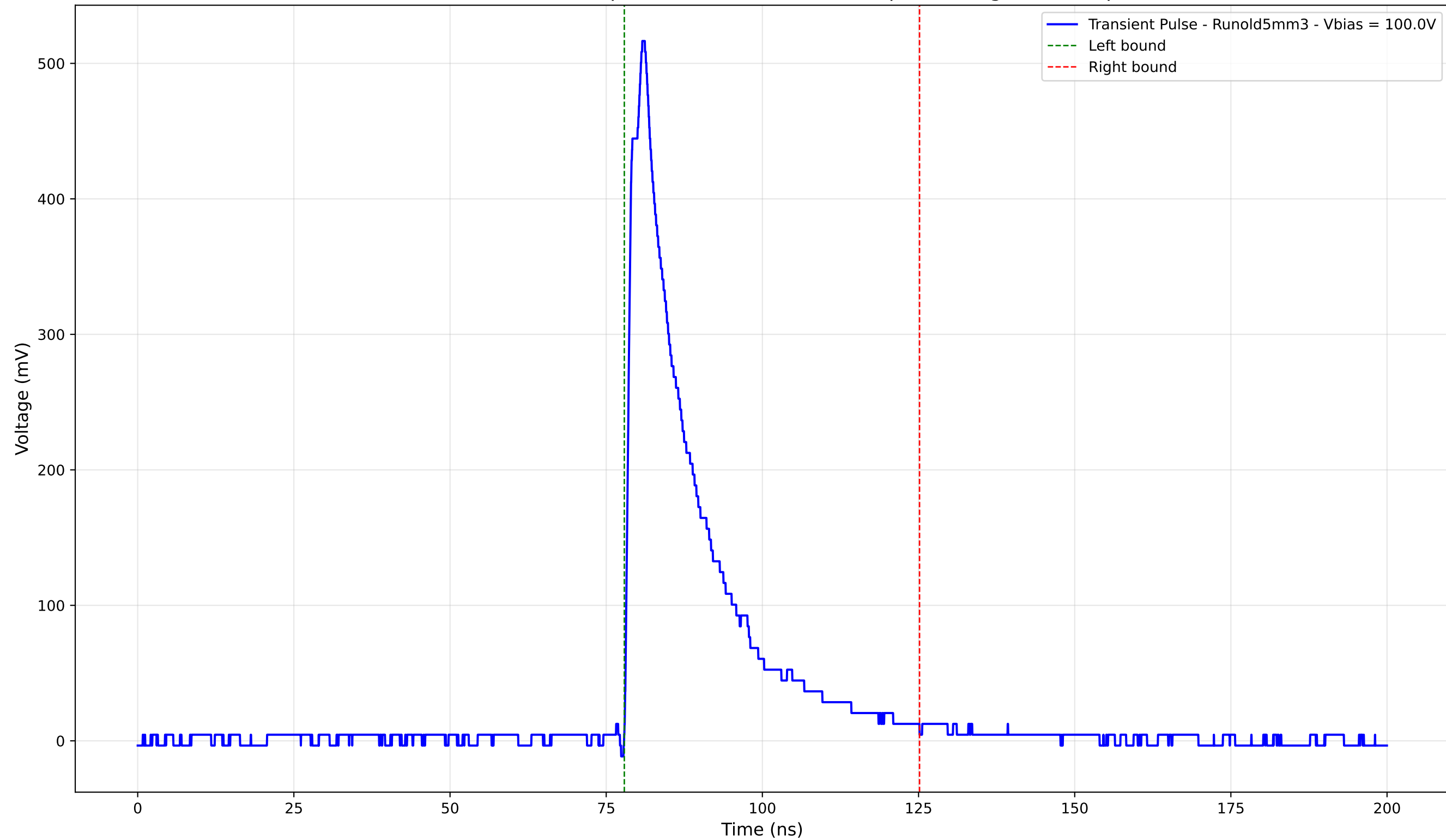
Transient Pulse - Sample: old5 - Position: 4035.0 \mu\text{m} - Charge: 114.70 pC
