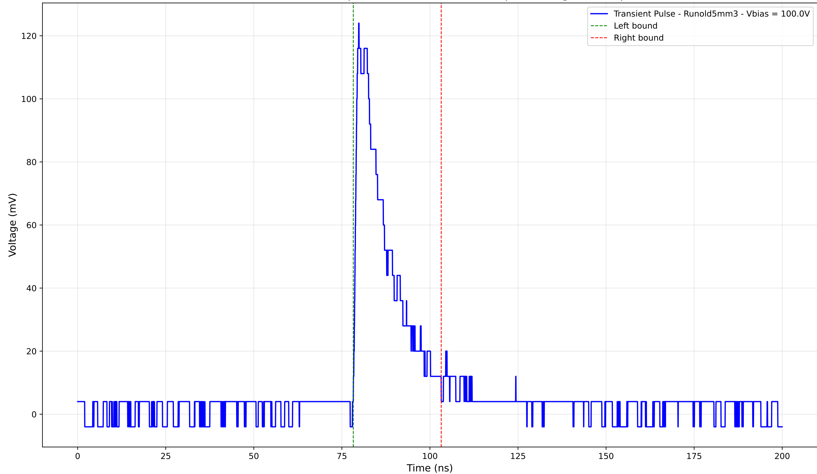
Transient Pulse - Sample: old5 - Position: 4535.0 \mu\text{m} - Charge: 24.41 pC
