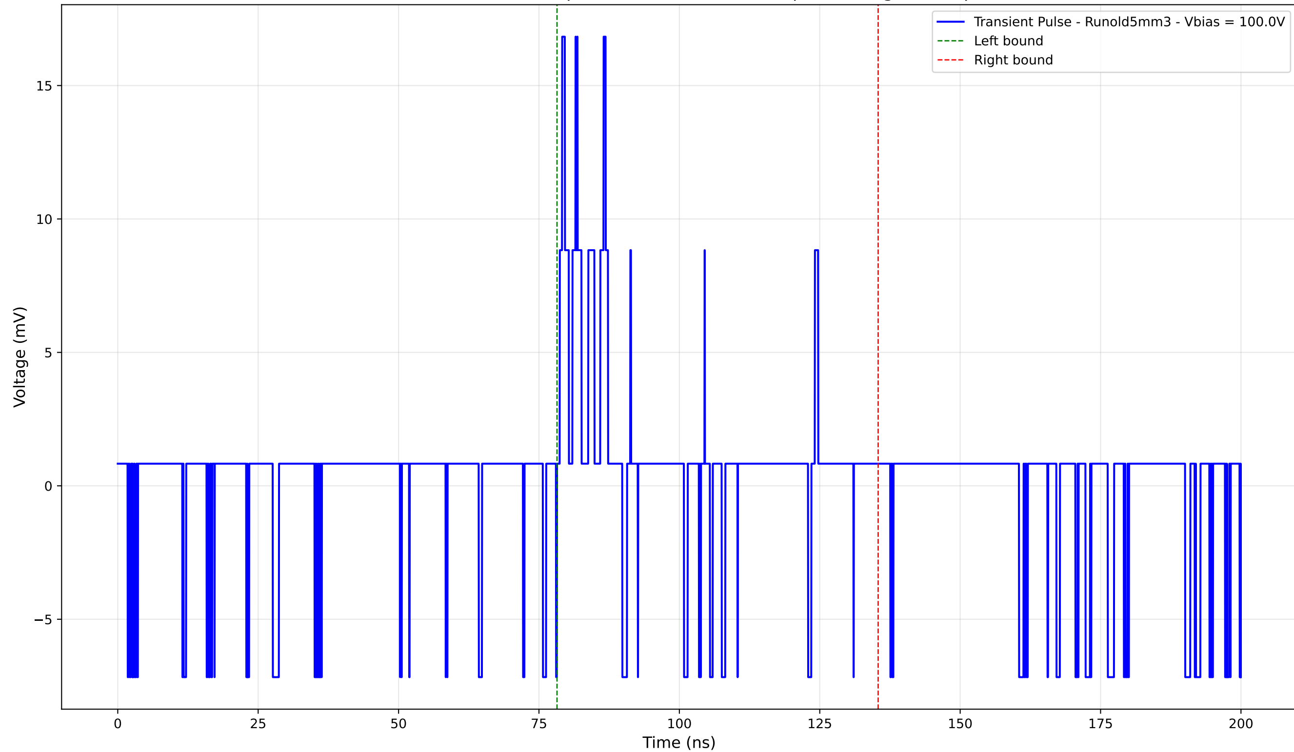
Transient Pulse - Sample: old5 - Position: 95.0 \mu\text{m} - Charge: 1.58 pC
