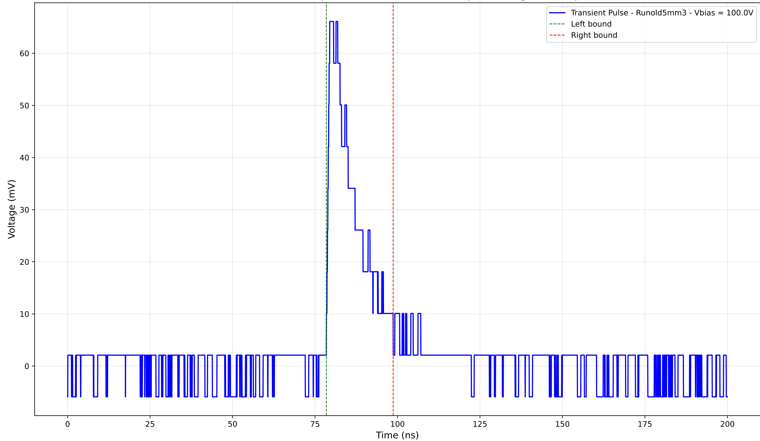
Transient Pulse - Sample: old5 - Position: 4460.0 \mu\text{m} - Charge: 12.23 pC
