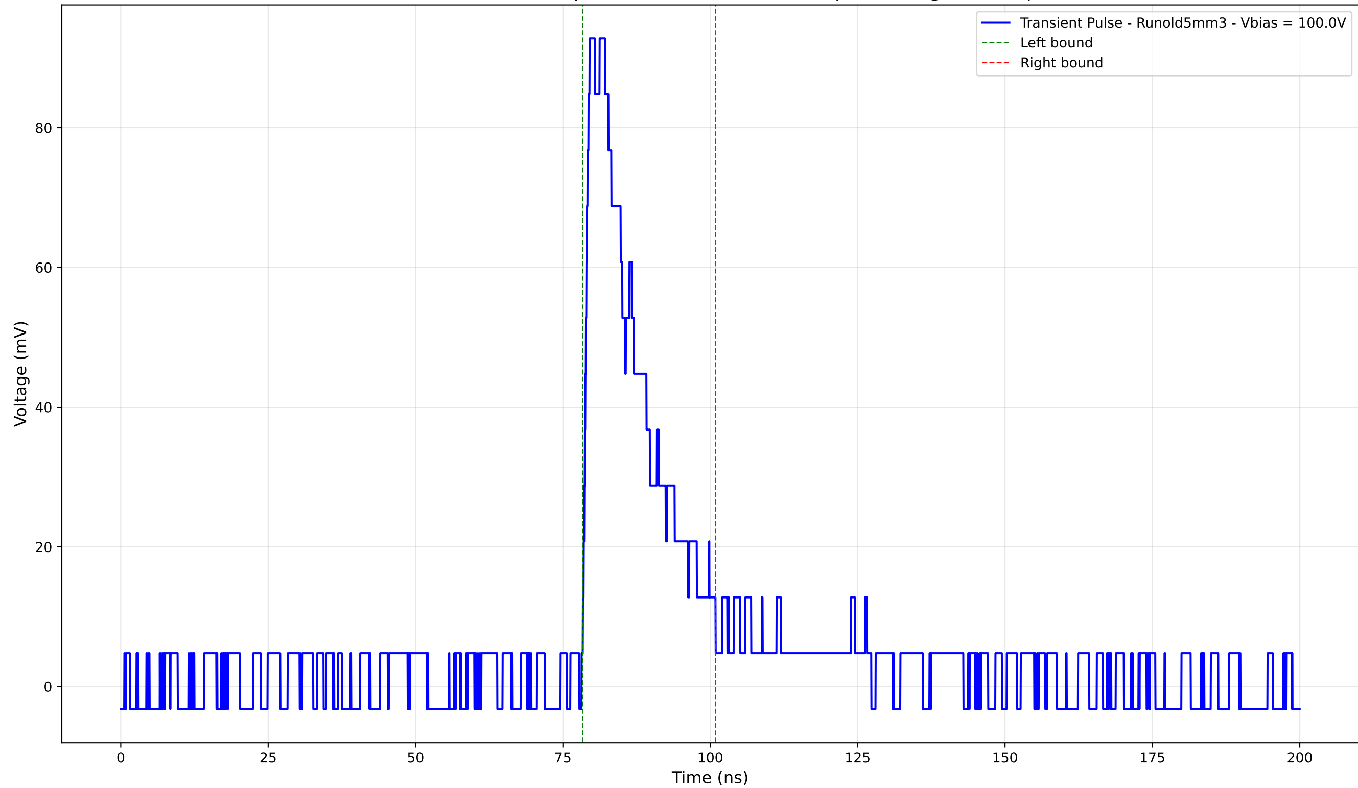
Transient Pulse - Sample: old5 - Position: 4530.0 \mu\text{m} - Charge: 19.42 pC
