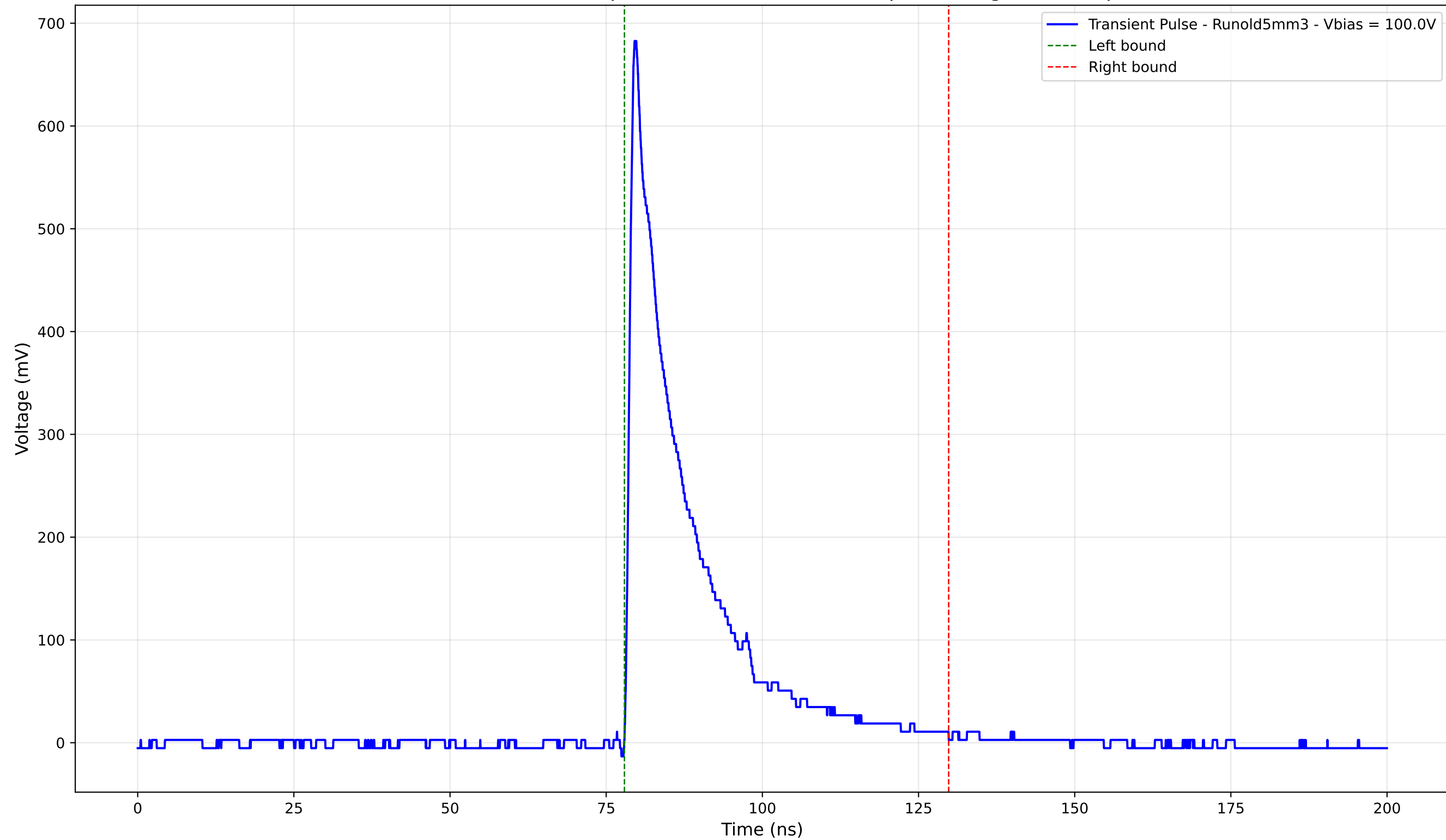
Transient Pulse - Sample: old5 - Position: 4675.0 \mu\text{m} - Charge: 128.49 pC
