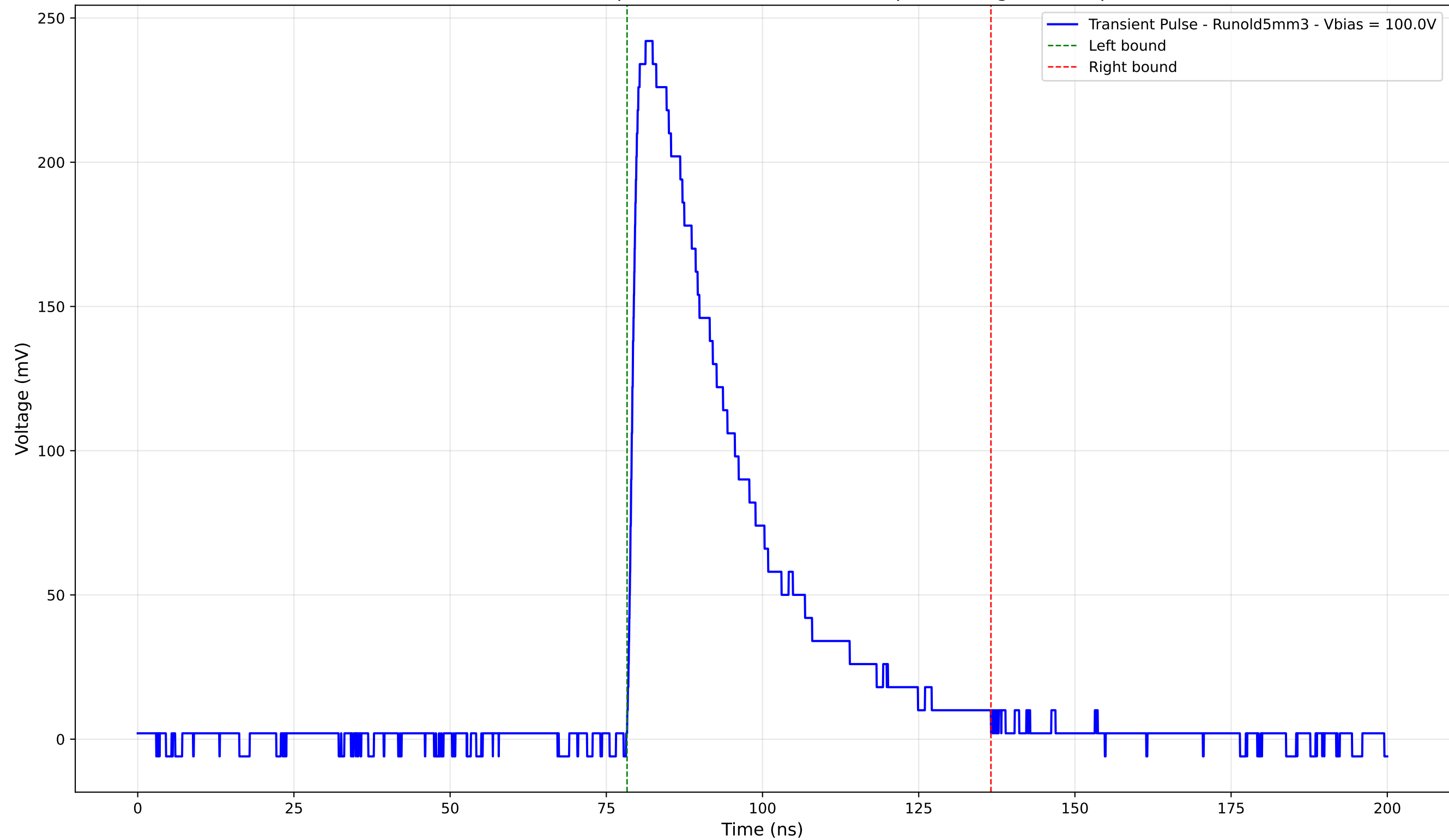
Transient Pulse - Sample: old5 - Position: 1075.0 \mu\text{m} - Charge: 86.94 pC
