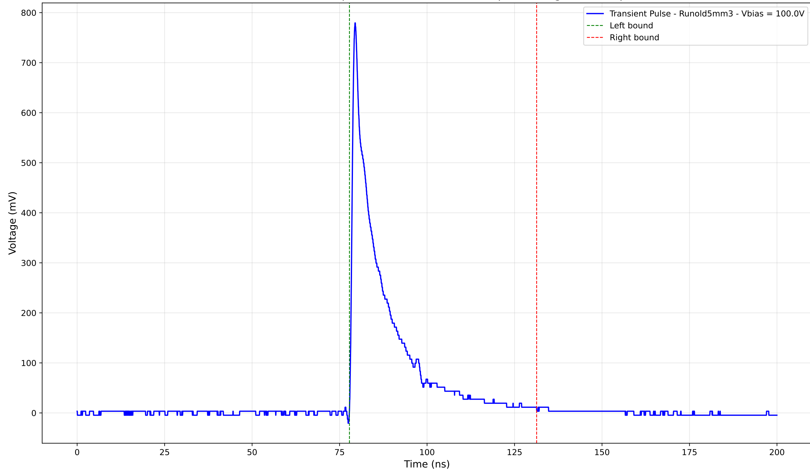
Transient Pulse - Sample: old5 - Position: 4750.0 \mu\text{m} - Charge: 134.69 pC
