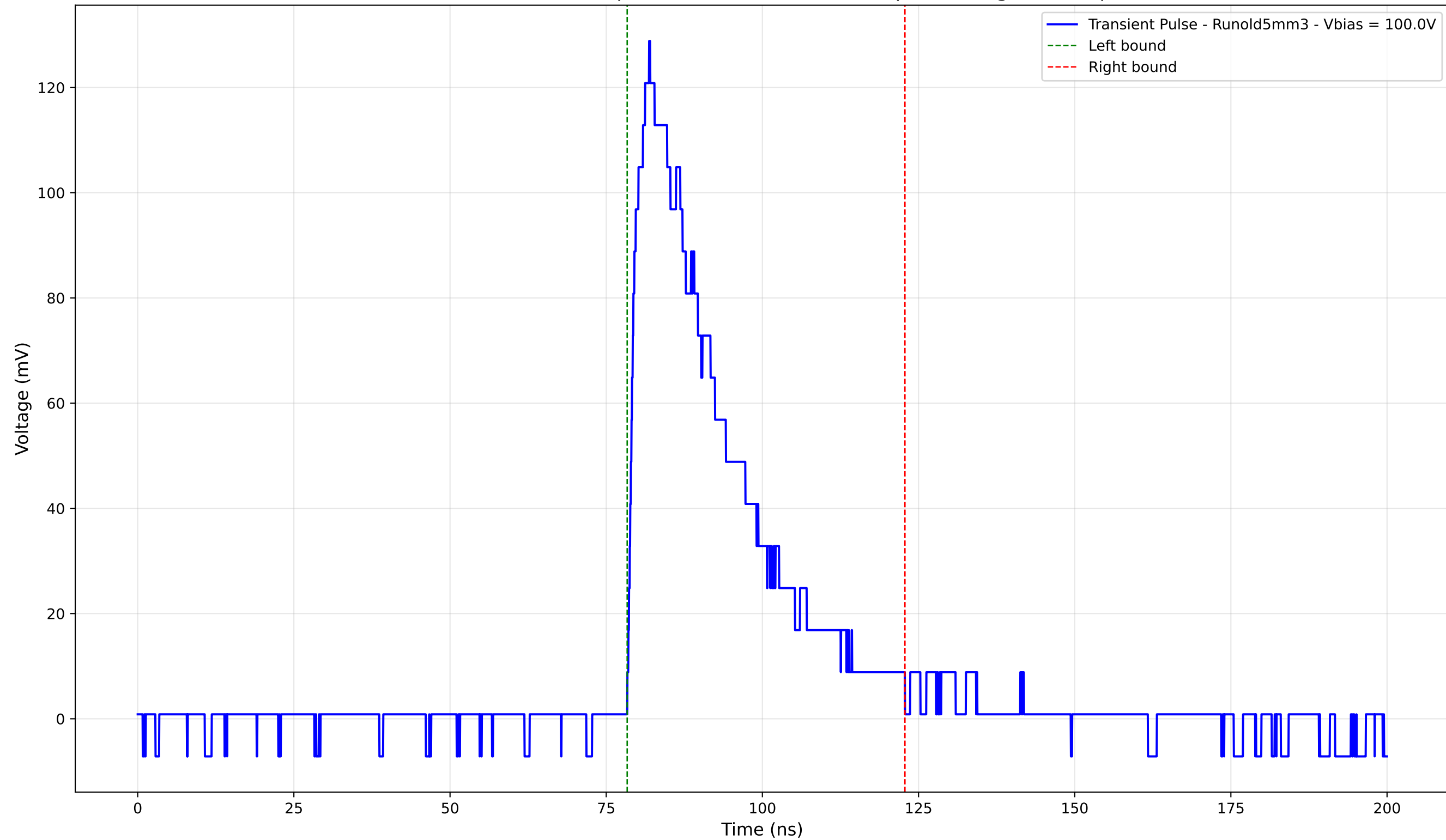
Transient Pulse - Sample: old5 - Position: 2735.0 \mu\text{m} - Charge: 40.42 pC
