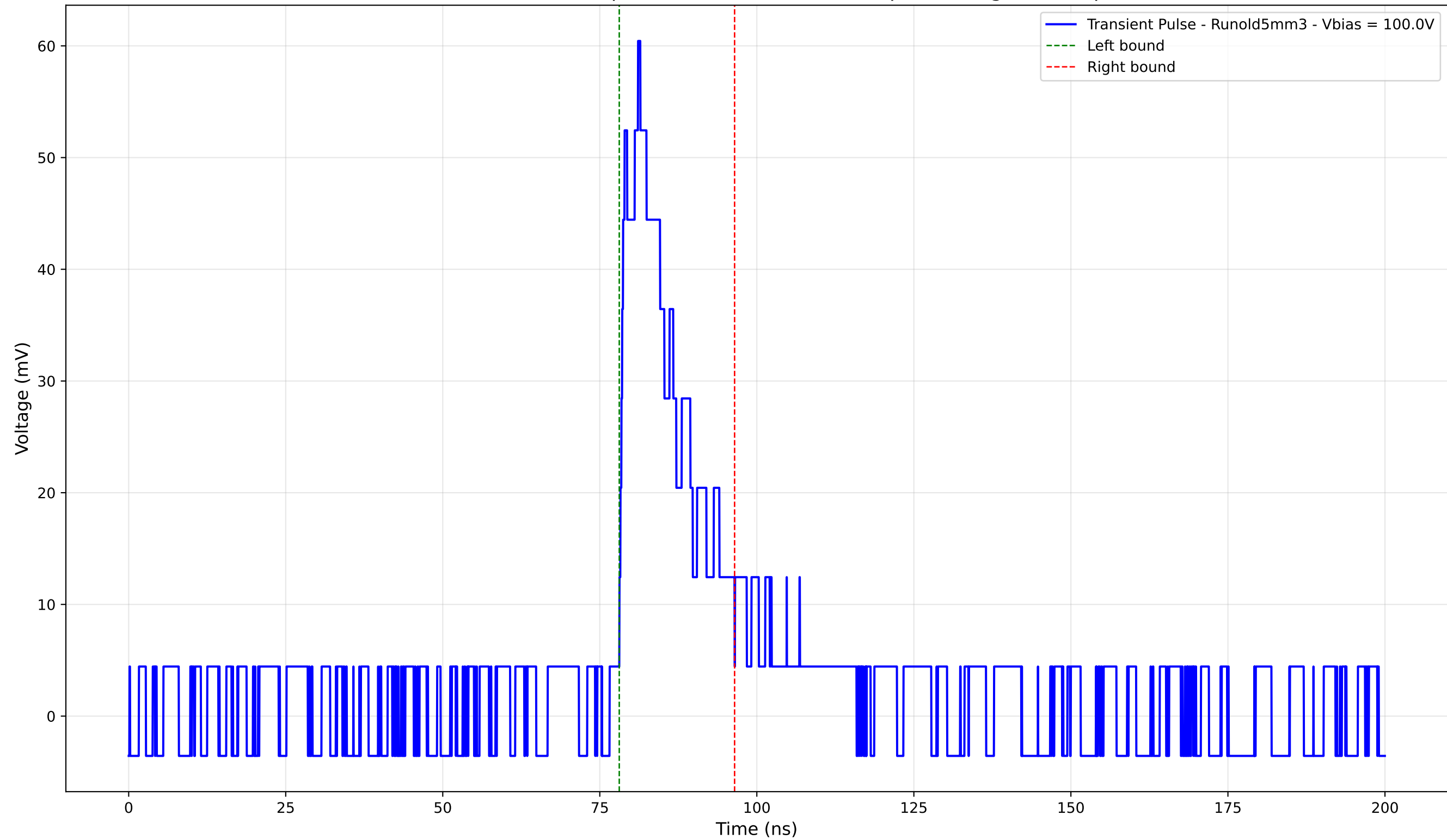
Transient Pulse - Sample: old5 - Position: 3915.0 \mu\text{m} - Charge: 10.95 pC
