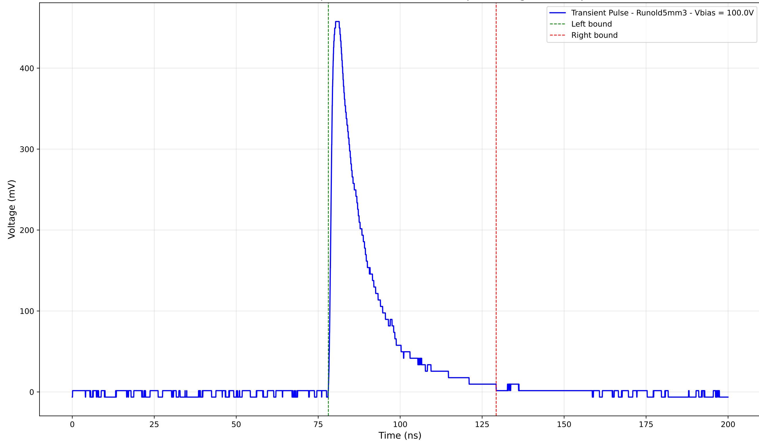
Transient Pulse - Sample: old5 - Position: 4290.0 \mu\text{m} - Charge: 105.01 pC
