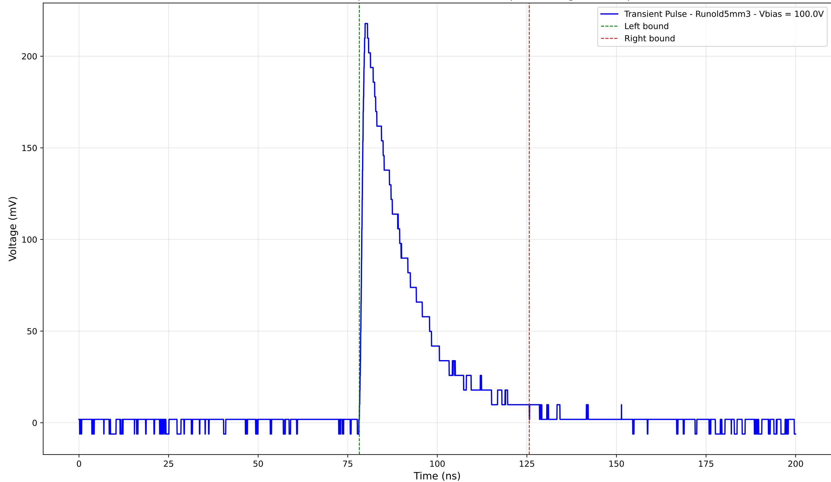
Transient Pulse - Sample: old5 - Position: 745.0 \mu\text{m} - Charge: 57.84 pC
