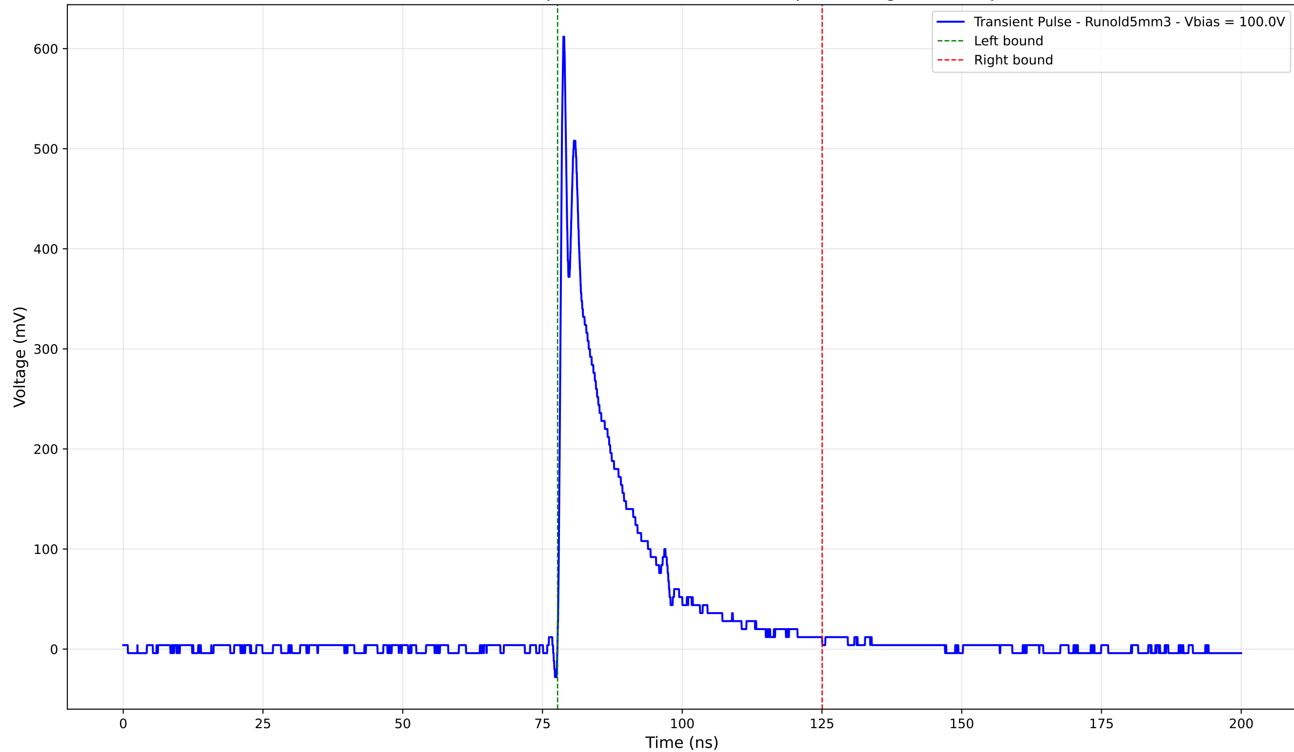
Transient Pulse - Sample: old5 - Position: 3400.0 \mu\text{m} - Charge: 105.20 pC
