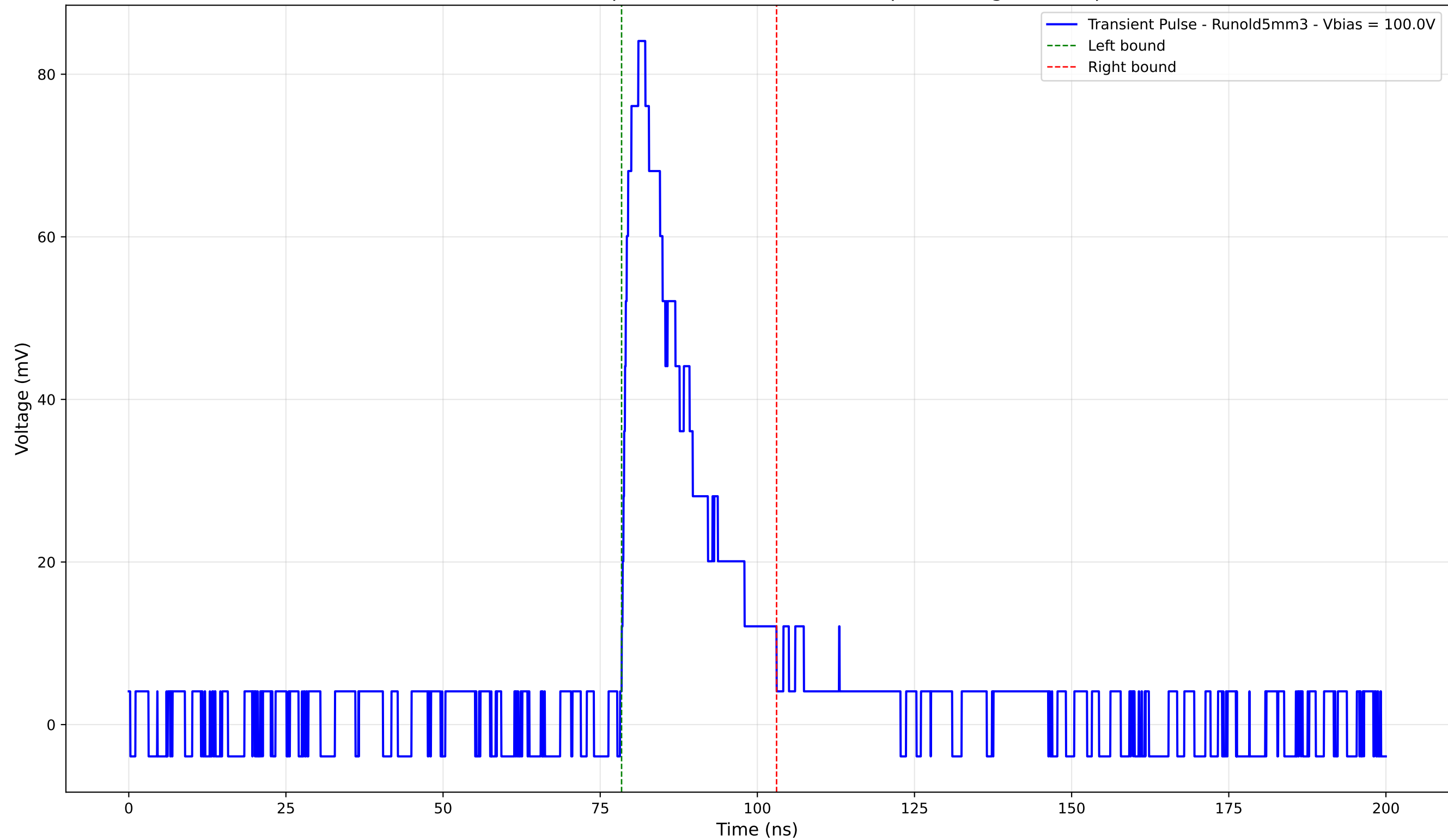
Transient Pulse - Sample: old5 - Position: 4220.0 \mu\text{m} - Charge: 18.20 pC
