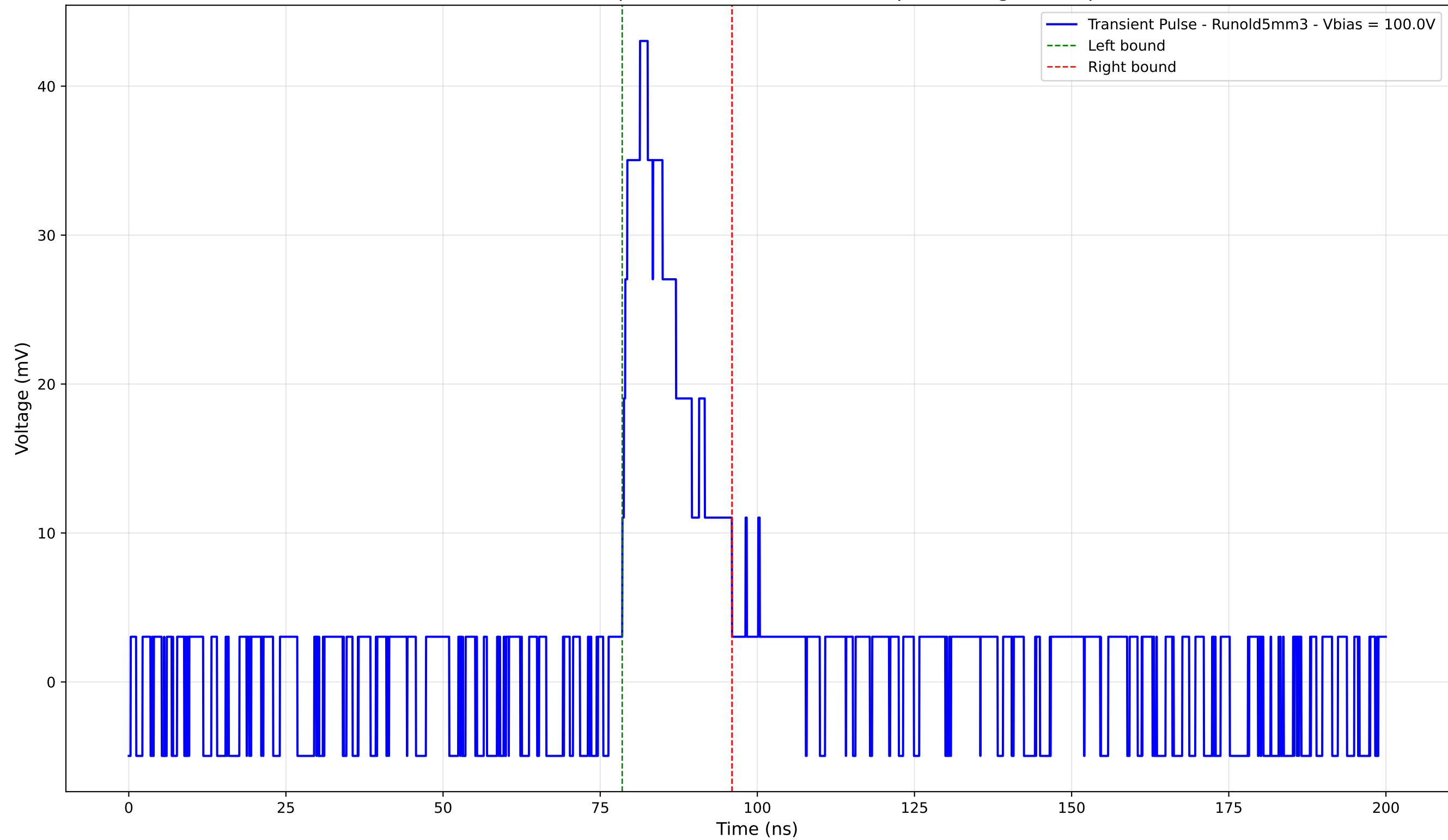
Transient Pulse - Sample: old5 - Position: 4510.0 \mu\text{m} - Charge: 8.11 pC
