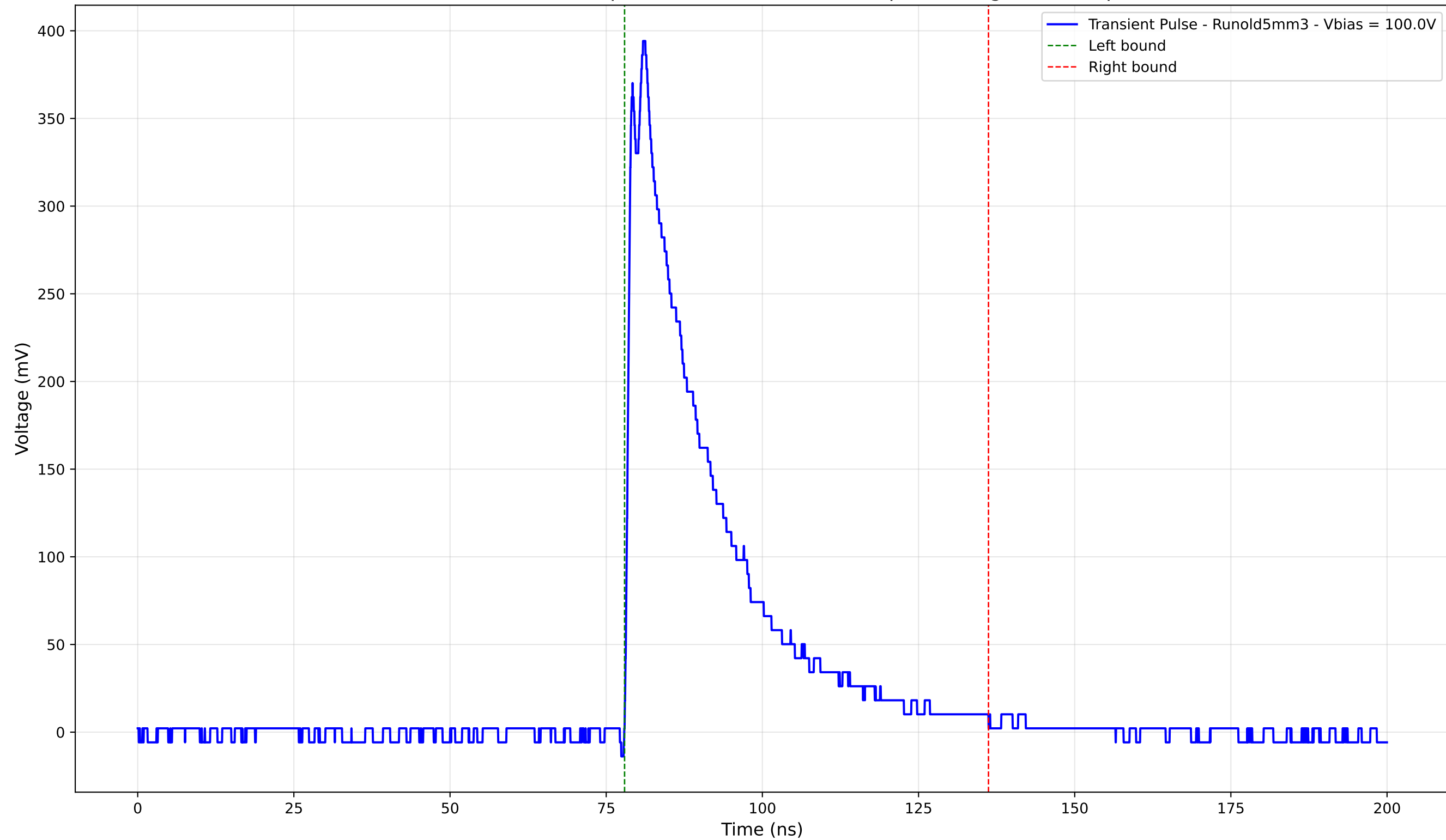
Transient Pulse - Sample: old5 - Position: 3115.0 \mu\text{m} - Charge: 106.55 pC
