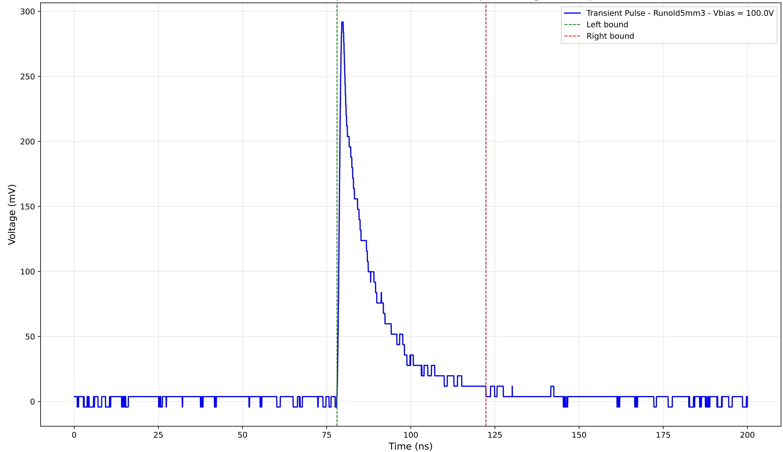
Transient Pulse - Sample: old5 - Position: 460.0 \mu\text{m} - Charge: 55.65 pC
