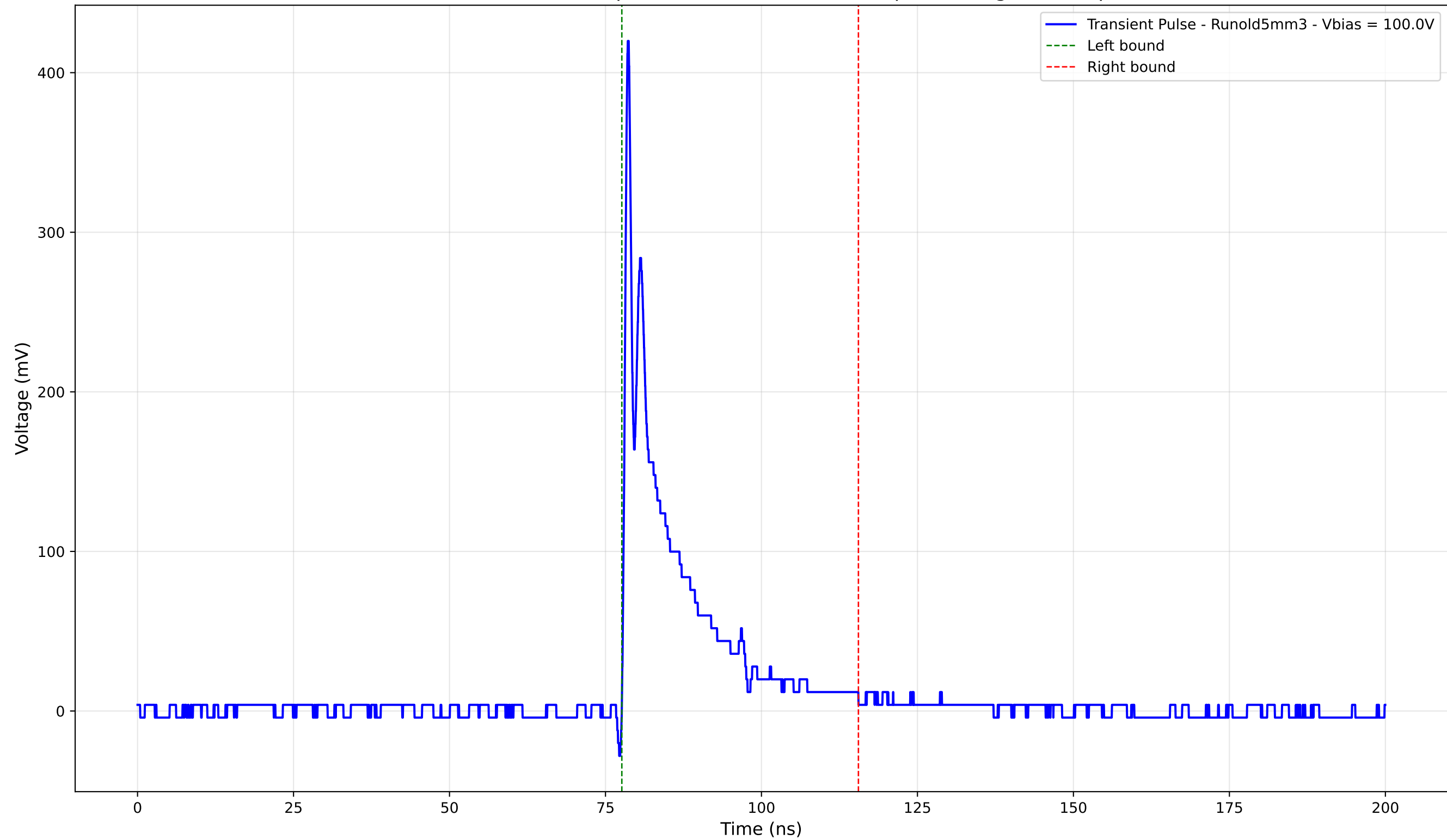
Transient Pulse - Sample: old5 - Position: 3515.0 \mu\text{m} - Charge: 50.40 pC
