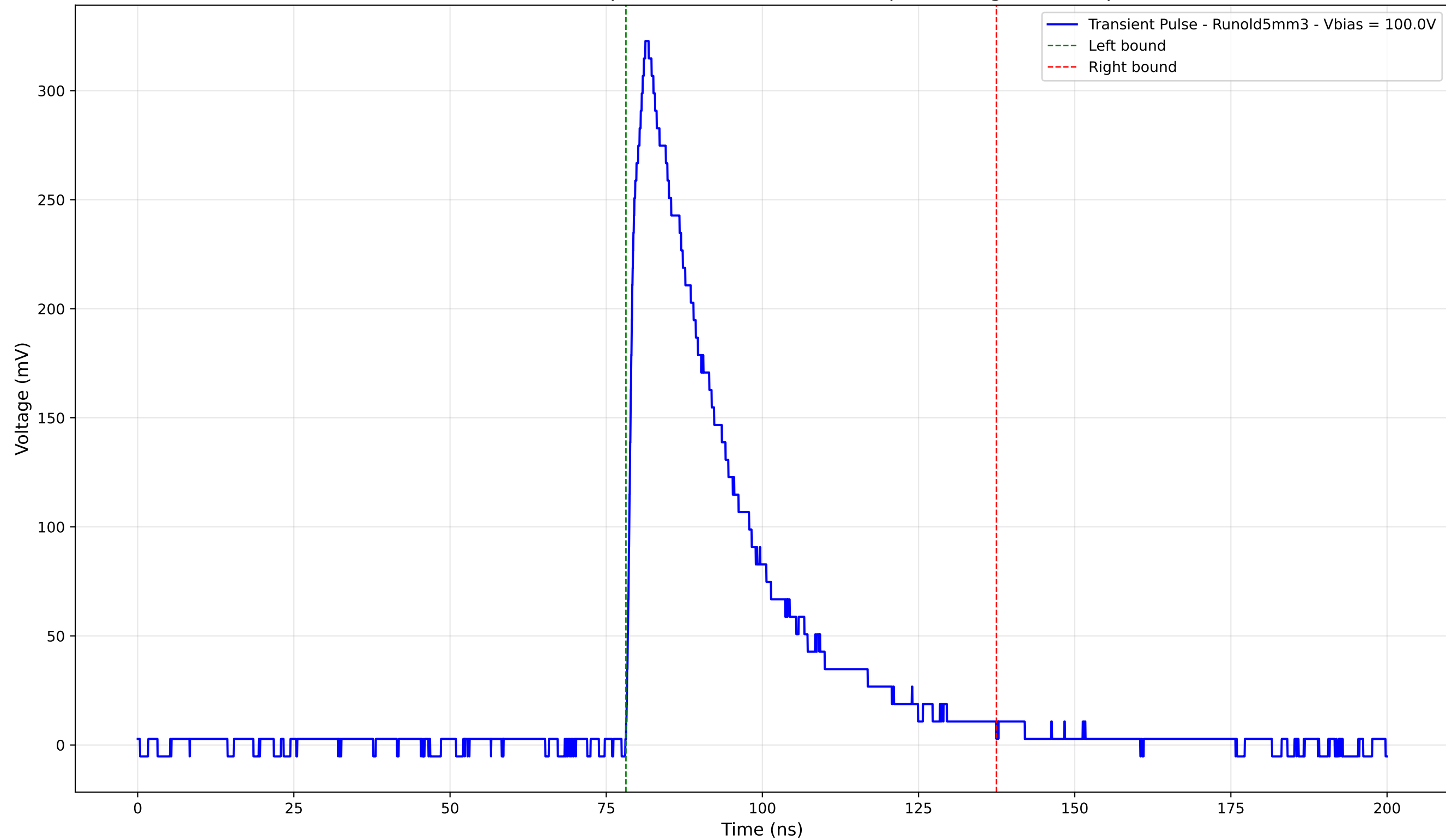
Transient Pulse - Sample: old5 - Position: 2840.0 \mu\text{m} - Charge: 105.94 pC
