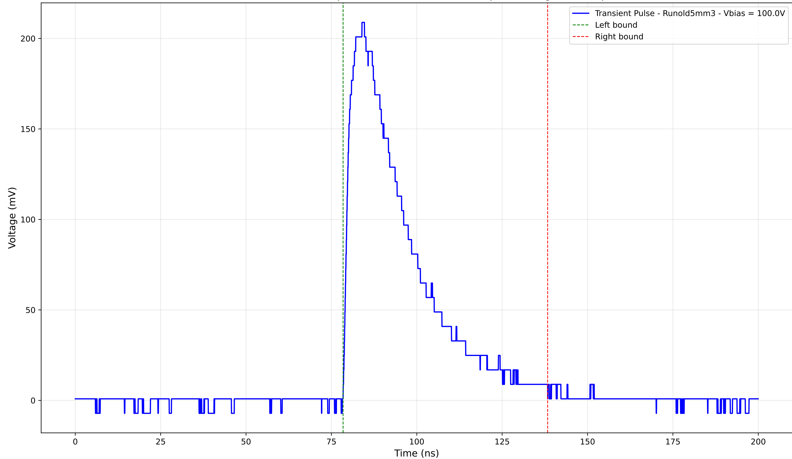
Transient Pulse - Sample: old5 - Position: 1675.0 \mu\text{m} - Charge: 82.91 pC
