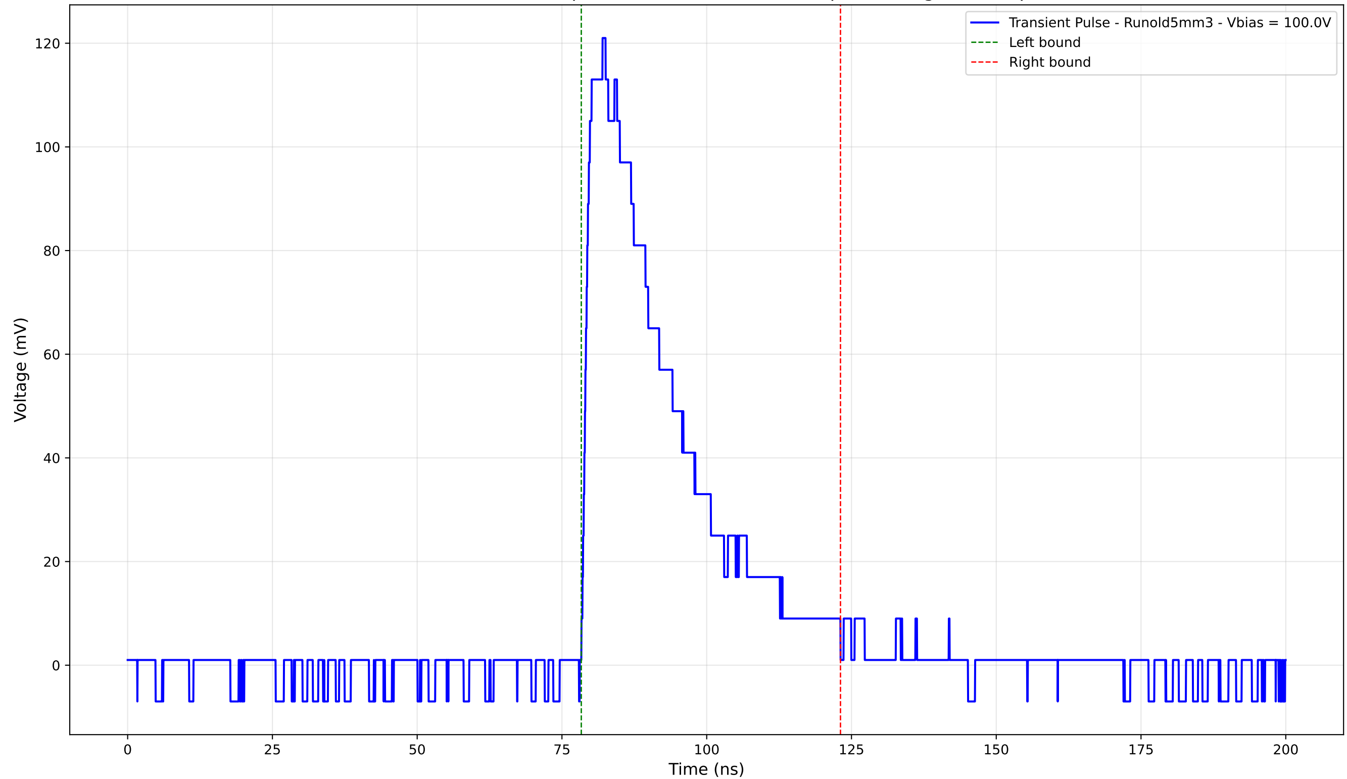
Transient Pulse - Sample: old5 - Position: 1005.0 \mu\text{m} - Charge: 38.81 pC
