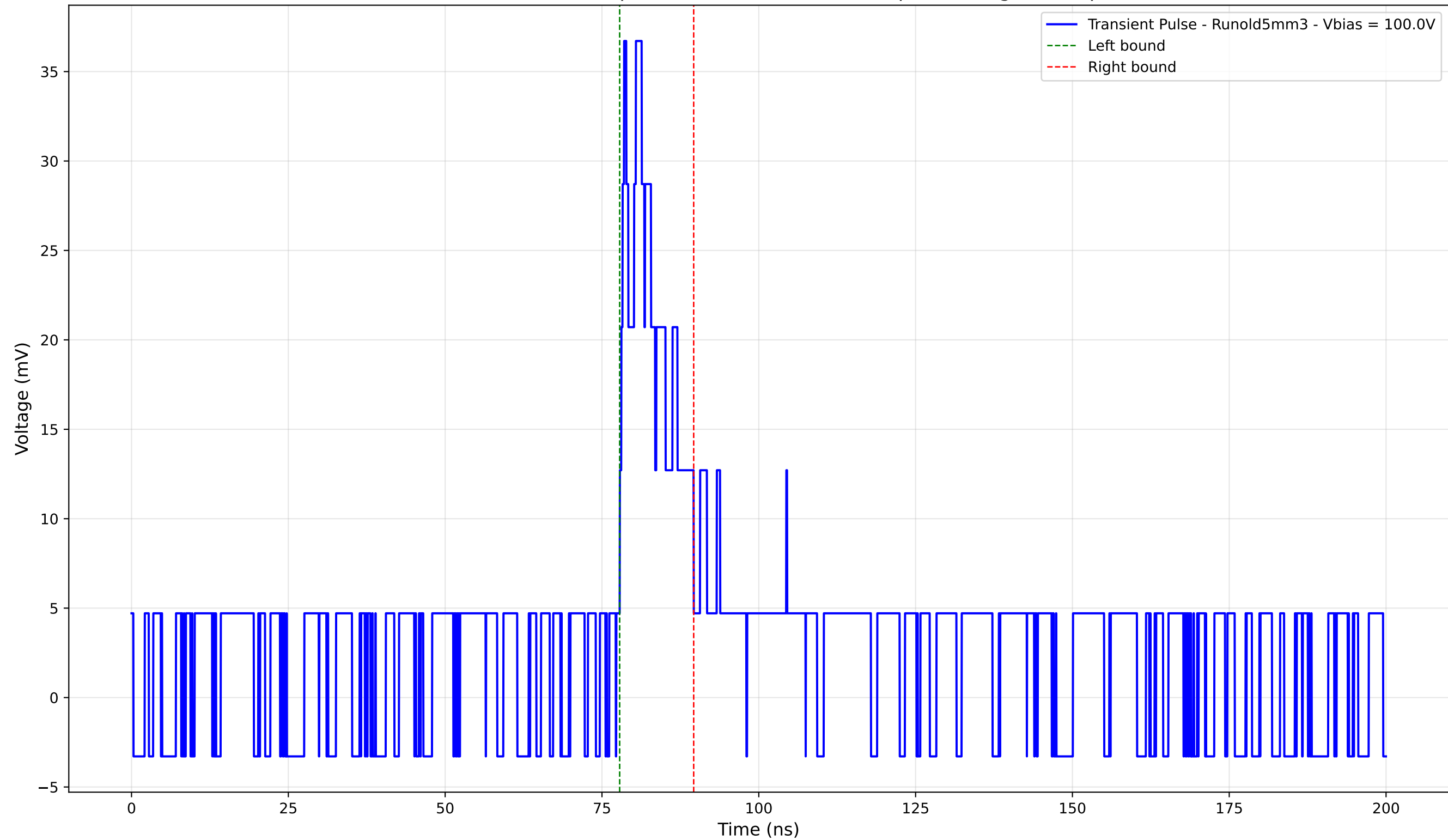
Transient Pulse - Sample: old5 - Position: 3590.0 \mu\text{m} - Charge: 5.00 pC
