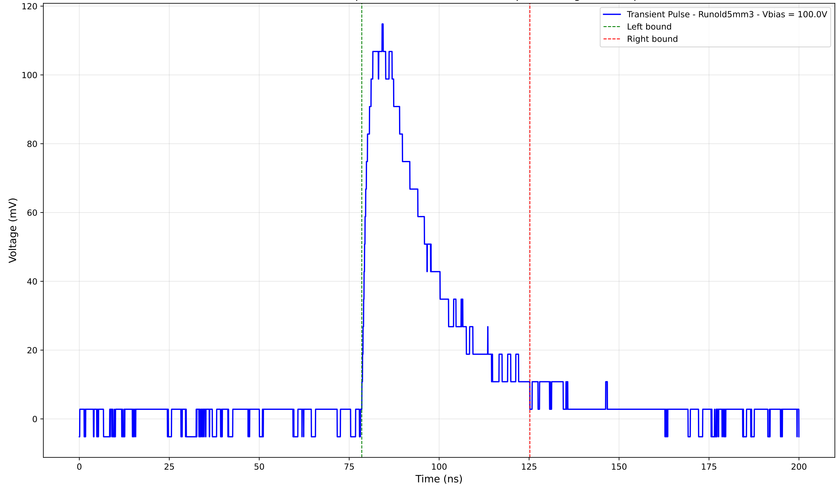
Transient Pulse - Sample: old5 - Position: 1540.0 \mu\text{m} - Charge: 42.79 pC
