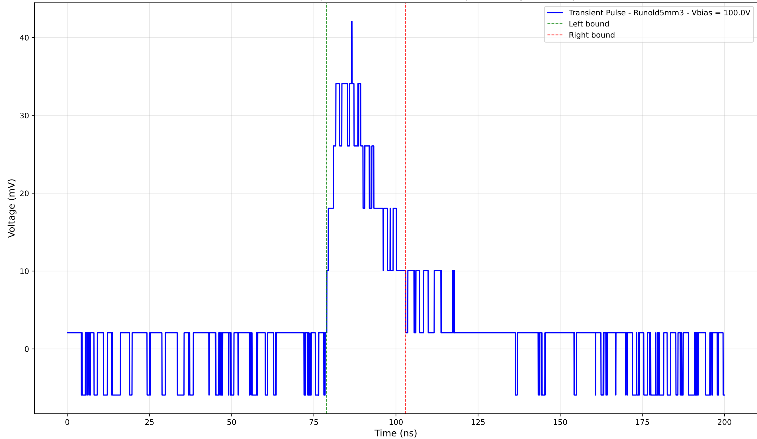
Transient Pulse - Sample: old5 - Position: 2195.0 \mu\text{m} - Charge: 10.48 pC
