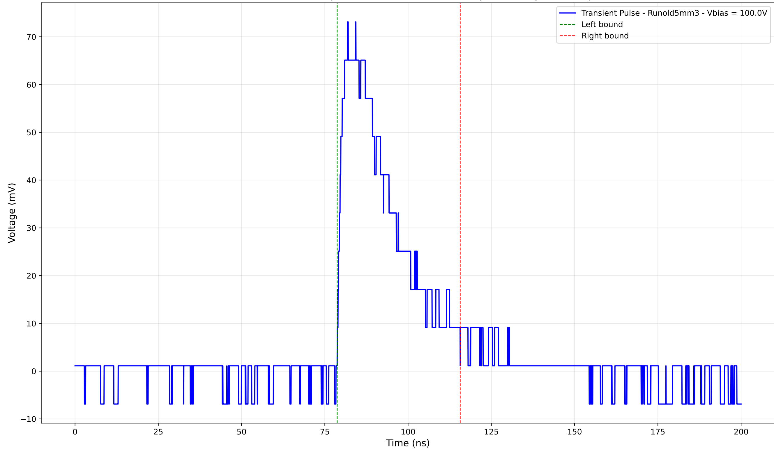
Transient Pulse - Sample: old5 - Position: 1355.0 \mu\text{m} - Charge: 24.38 pC
