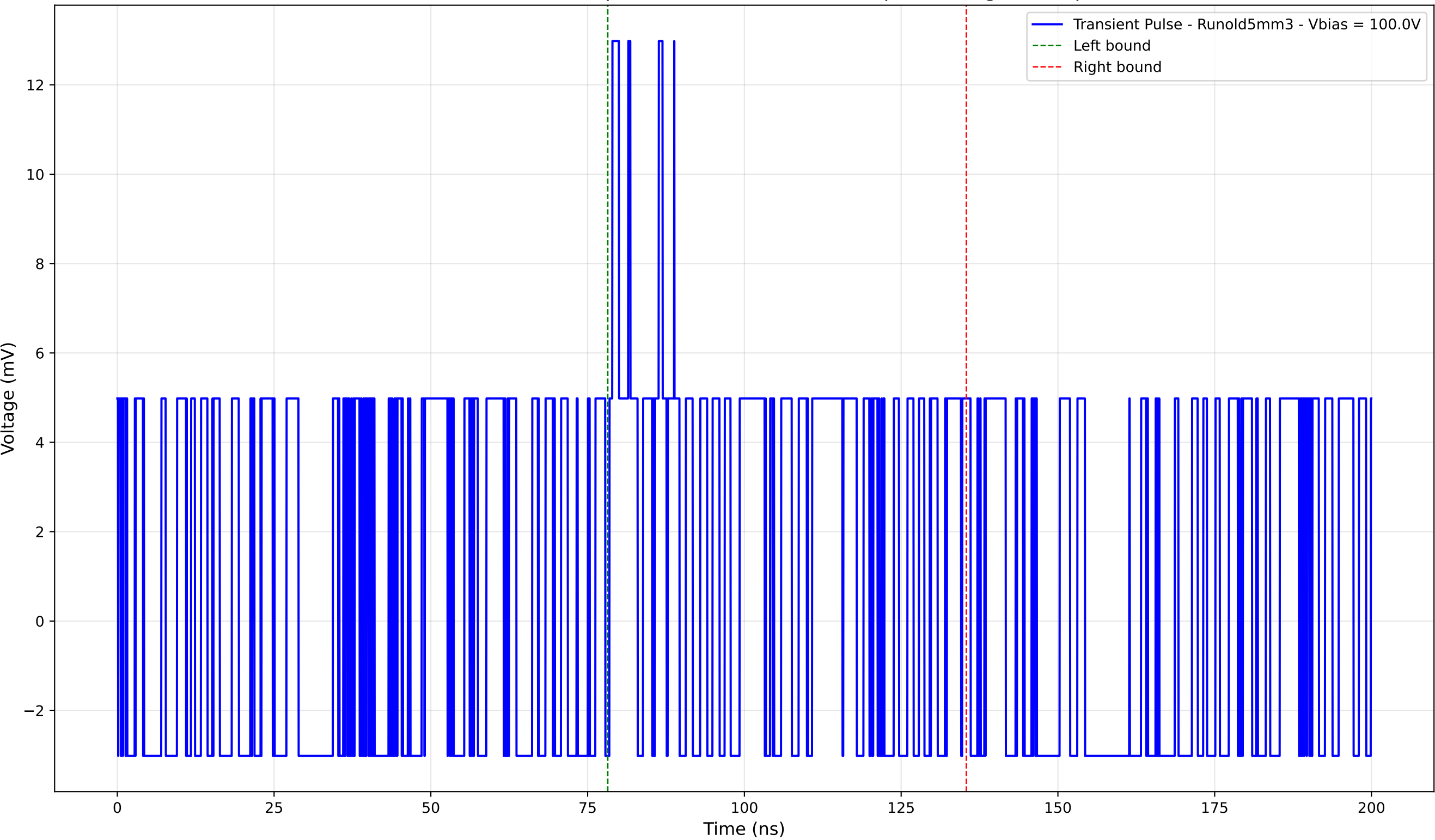
Transient Pulse - Sample: old5 - Position: 4995.0 \mu\text{m} - Charge: 2.95 pC
