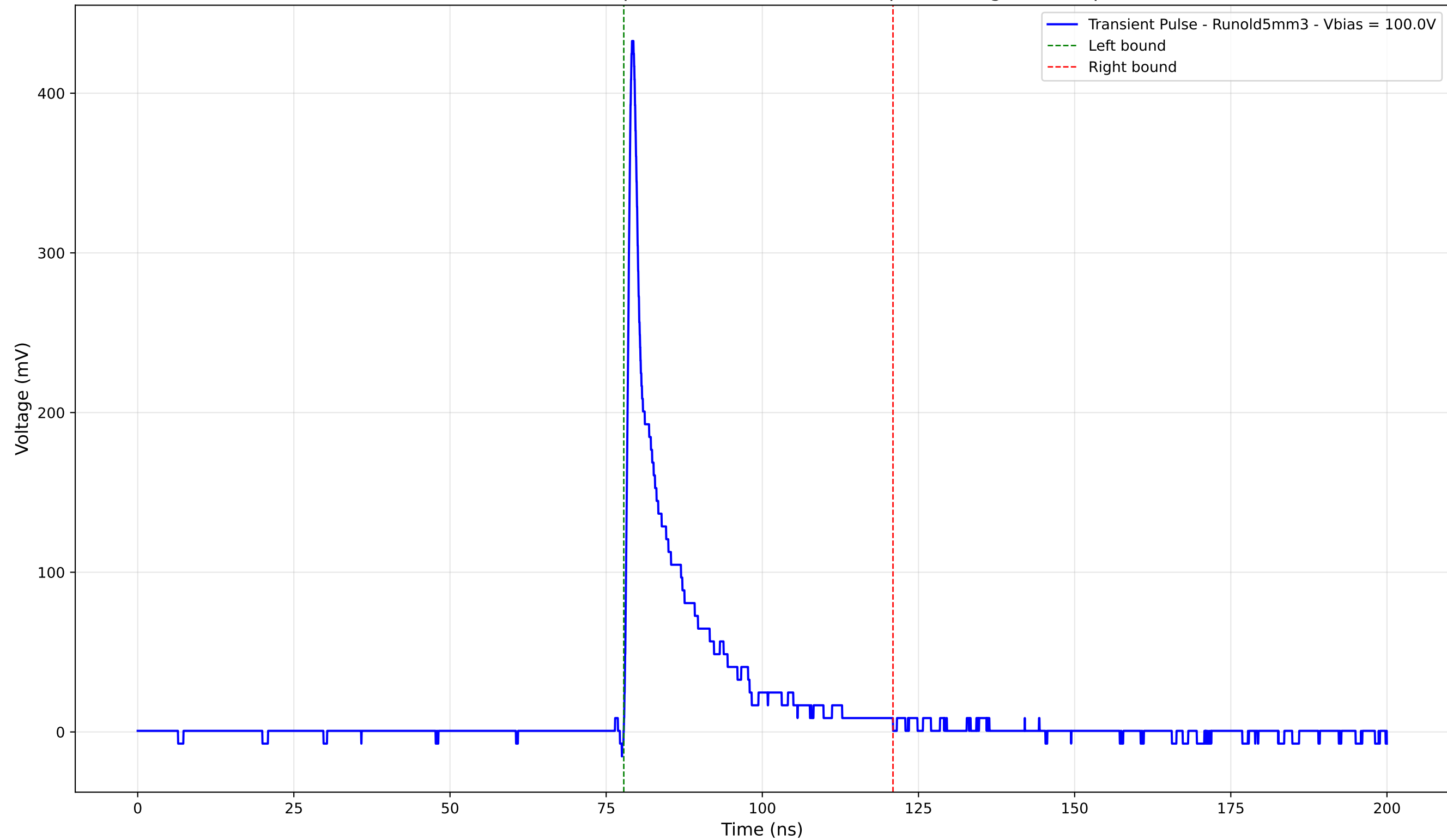
Transient Pulse - Sample: old5 - Position: 190.0 \mu\text{m} - Charge: 53.51 pC
