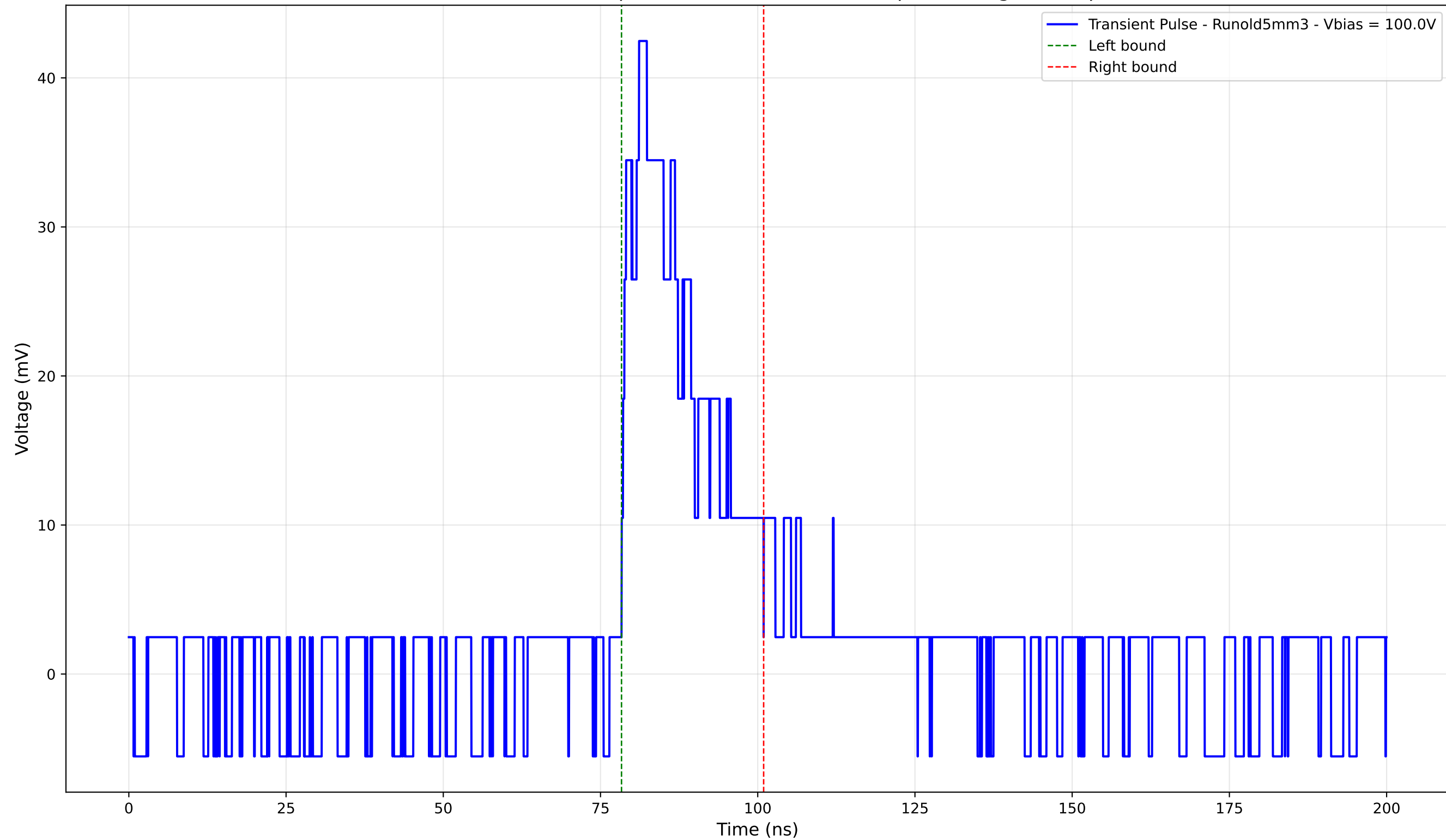
Transient Pulse - Sample: old5 - Position: 3005.0 \mu\text{m} - Charge: 9.89 pC
