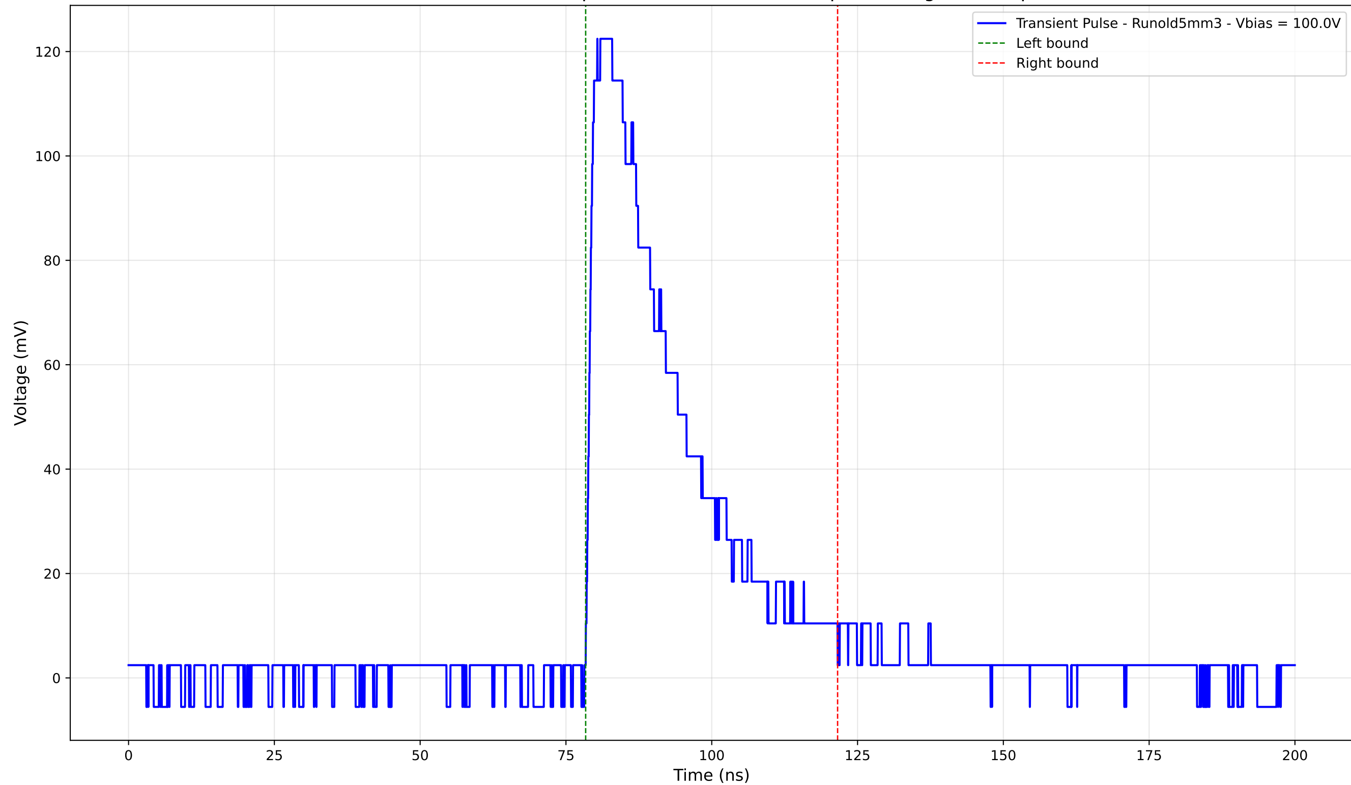
Transient Pulse - Sample: old5 - Position: 990.0 \mu\text{m} - Charge: 40.60 pC
