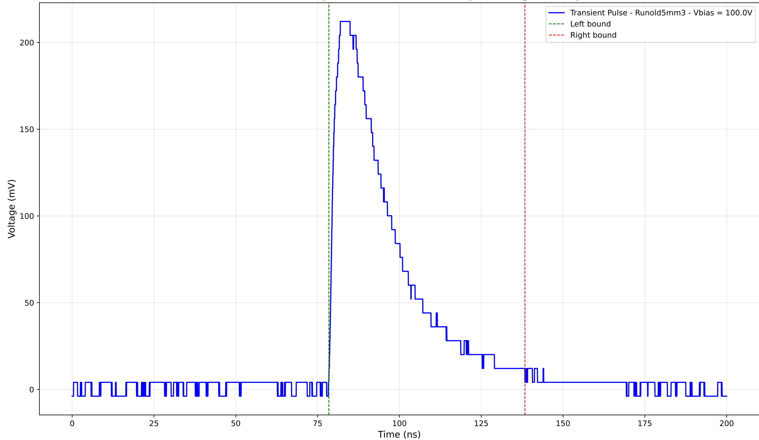
Transient Pulse - Sample: old5 - Position: 2110.0 \mu\text{m} - Charge: 87.93 pC
