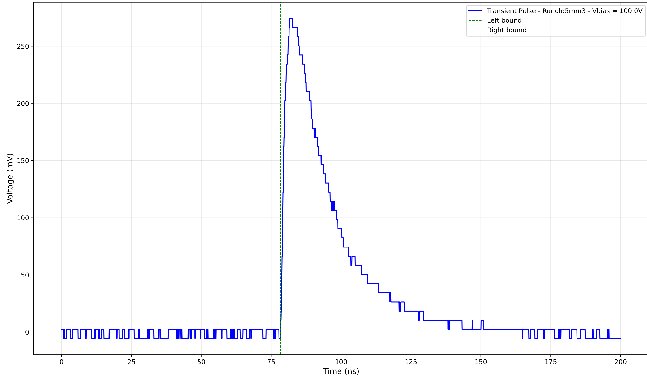
Transient Pulse - Sample: old5 - Position: 2530.0 \mu\text{m} - Charge: 102.35 pC
