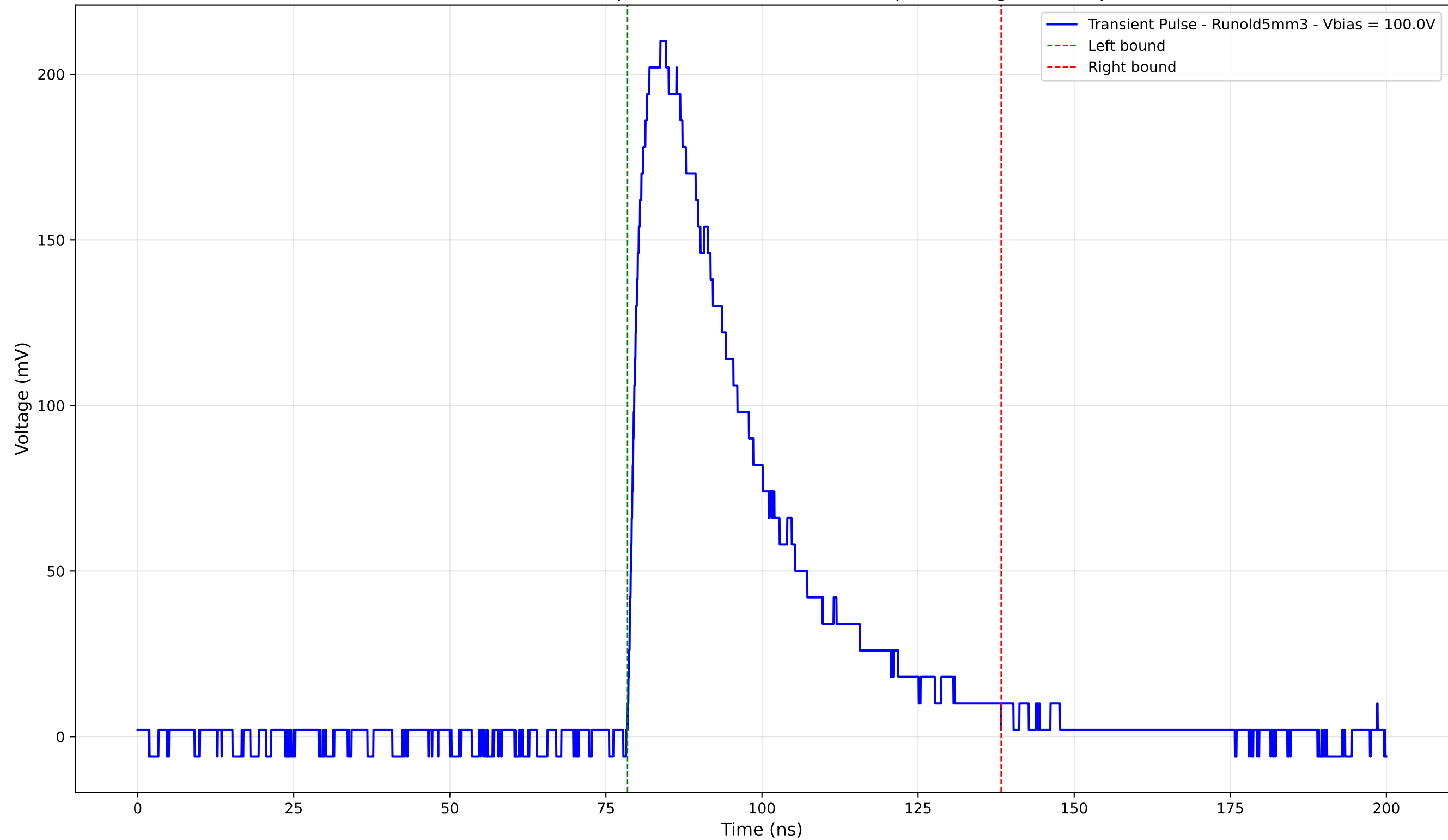
Transient Pulse - Sample: old5 - Position: 1875.0 \mu\text{m} - Charge: 85.11 pC
