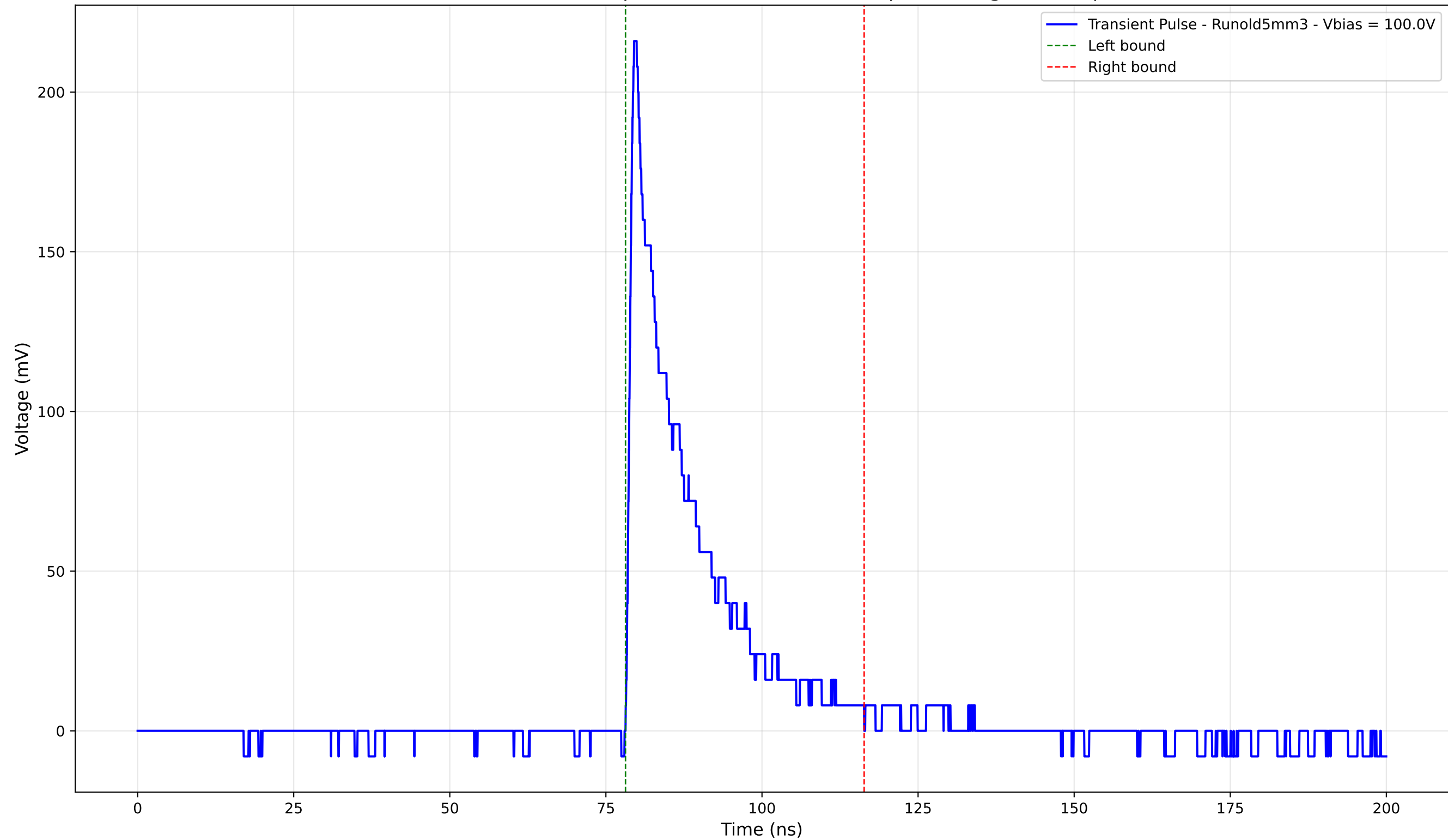
Transient Pulse - Sample: old5 - Position: 480.0 \mu\text{m} - Charge: 39.52 pC
