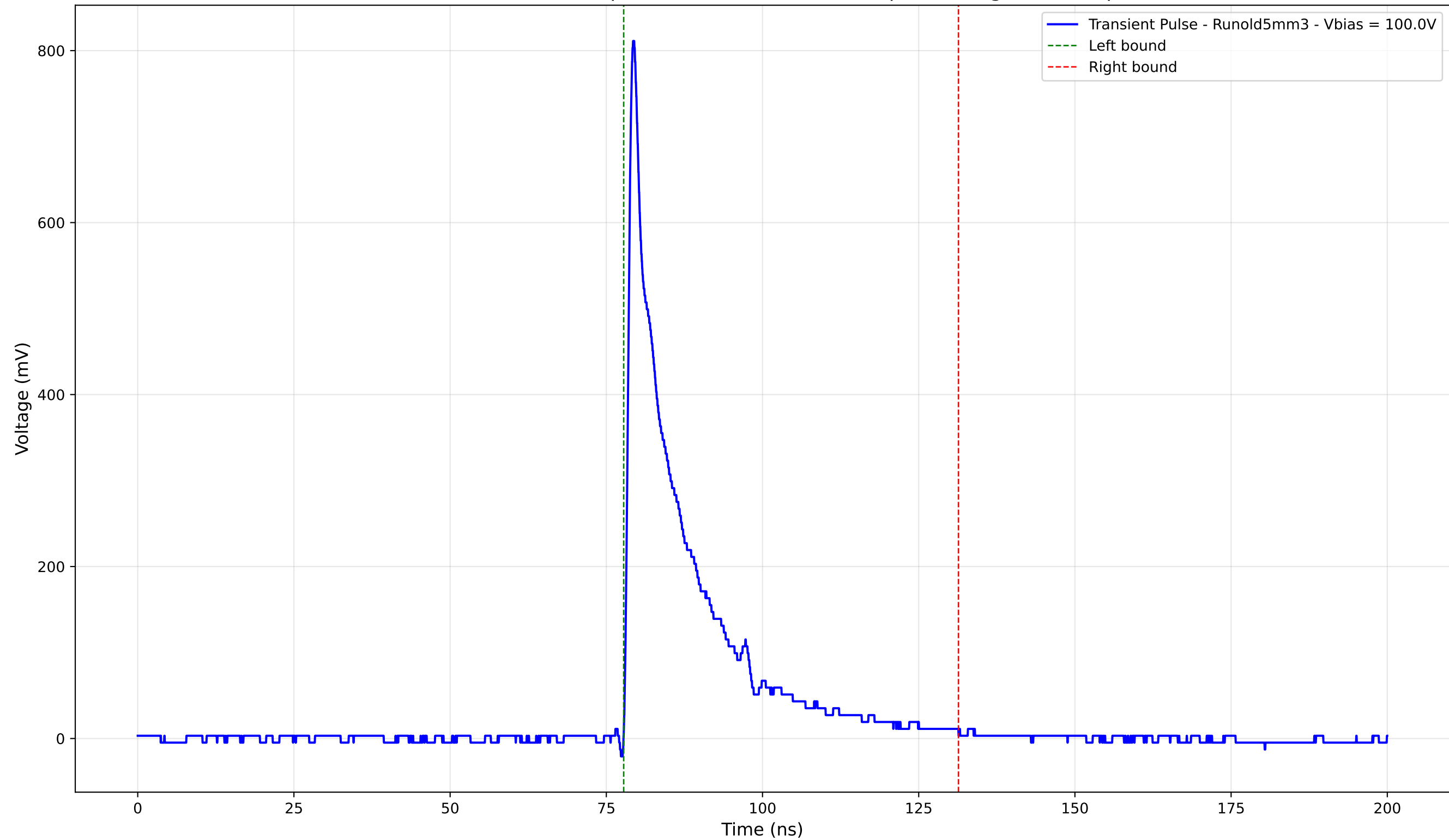
Transient Pulse - Sample: old5 - Position: 4785.0 \mu\text{m} - Charge: 133.50 pC
