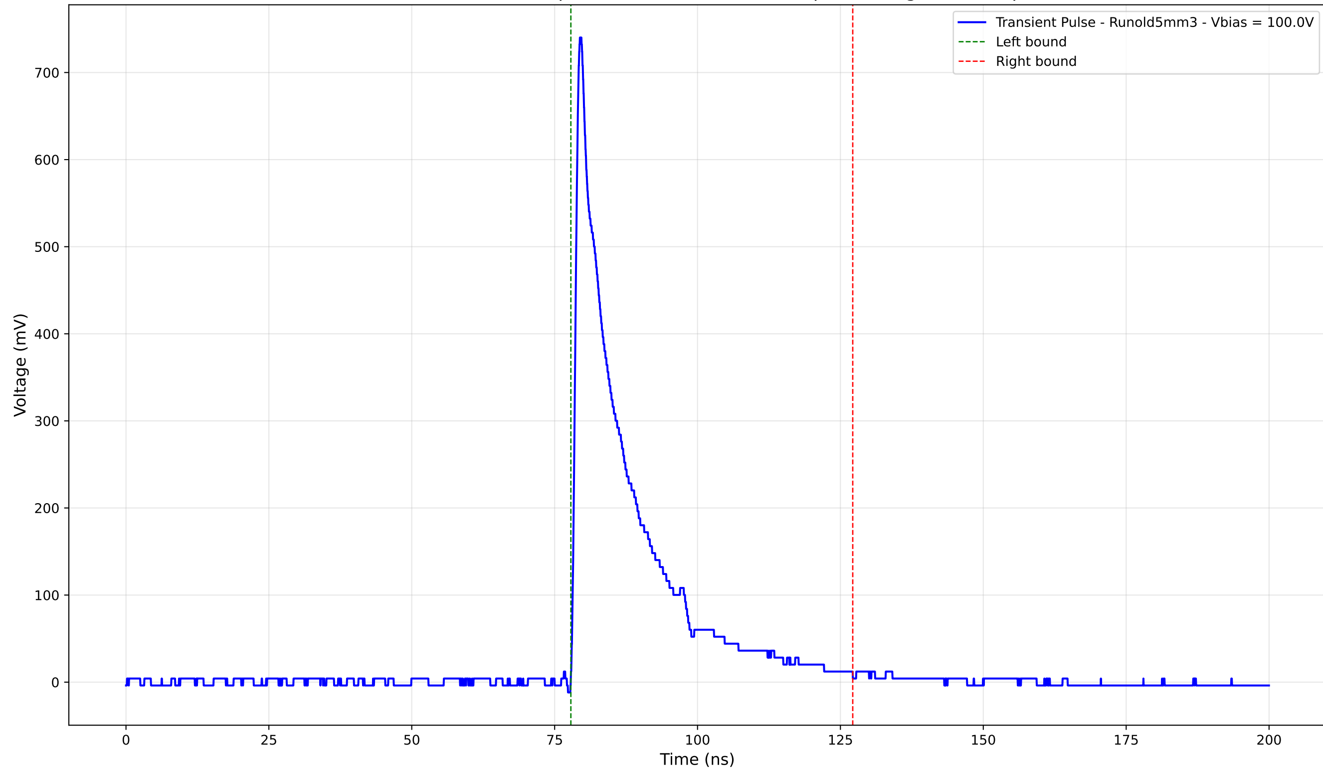
Transient Pulse - Sample: old5 - Position: 4720.0 \mu\text{m} - Charge: 133.06 pC
