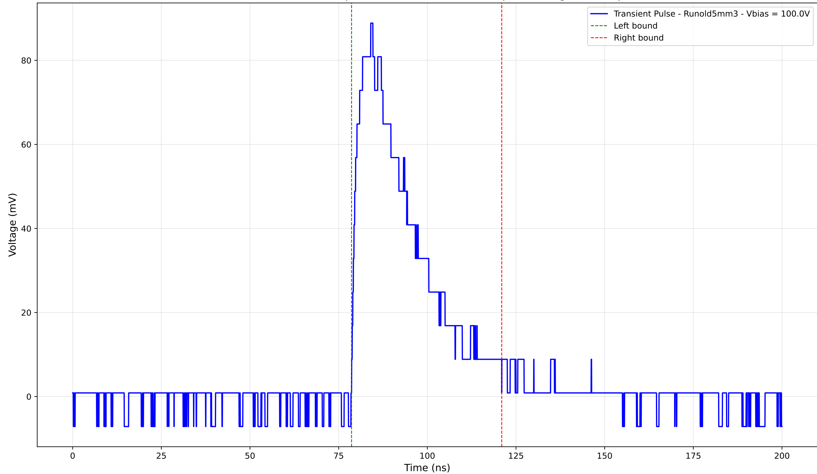
Transient Pulse - Sample: old5 - Position: 1420.0 \mu\text{m} - Charge: 30.73 pC
