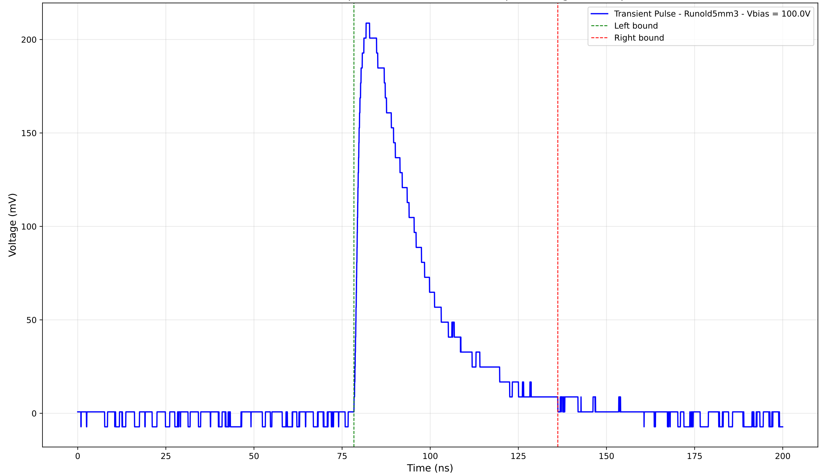
Transient Pulse - Sample: old5 - Position: 1270.0 \mu\text{m} - Charge: 78.57 pC
