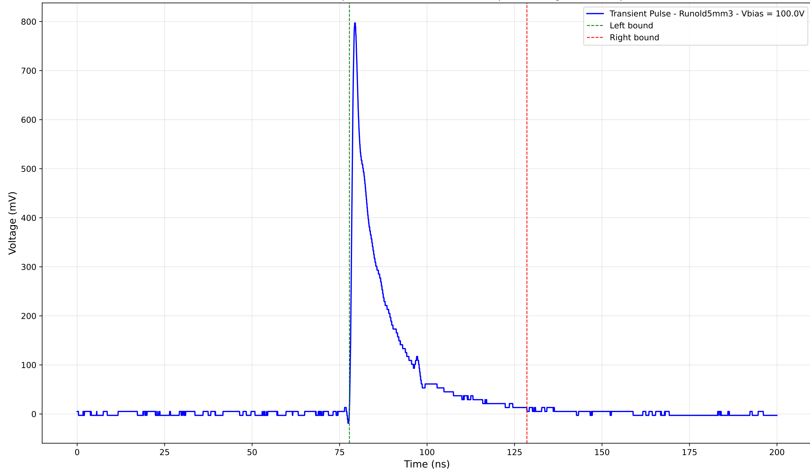
Transient Pulse - Sample: old5 - Position: 4770.0 \mu\text{m} - Charge: 135.16 pC
