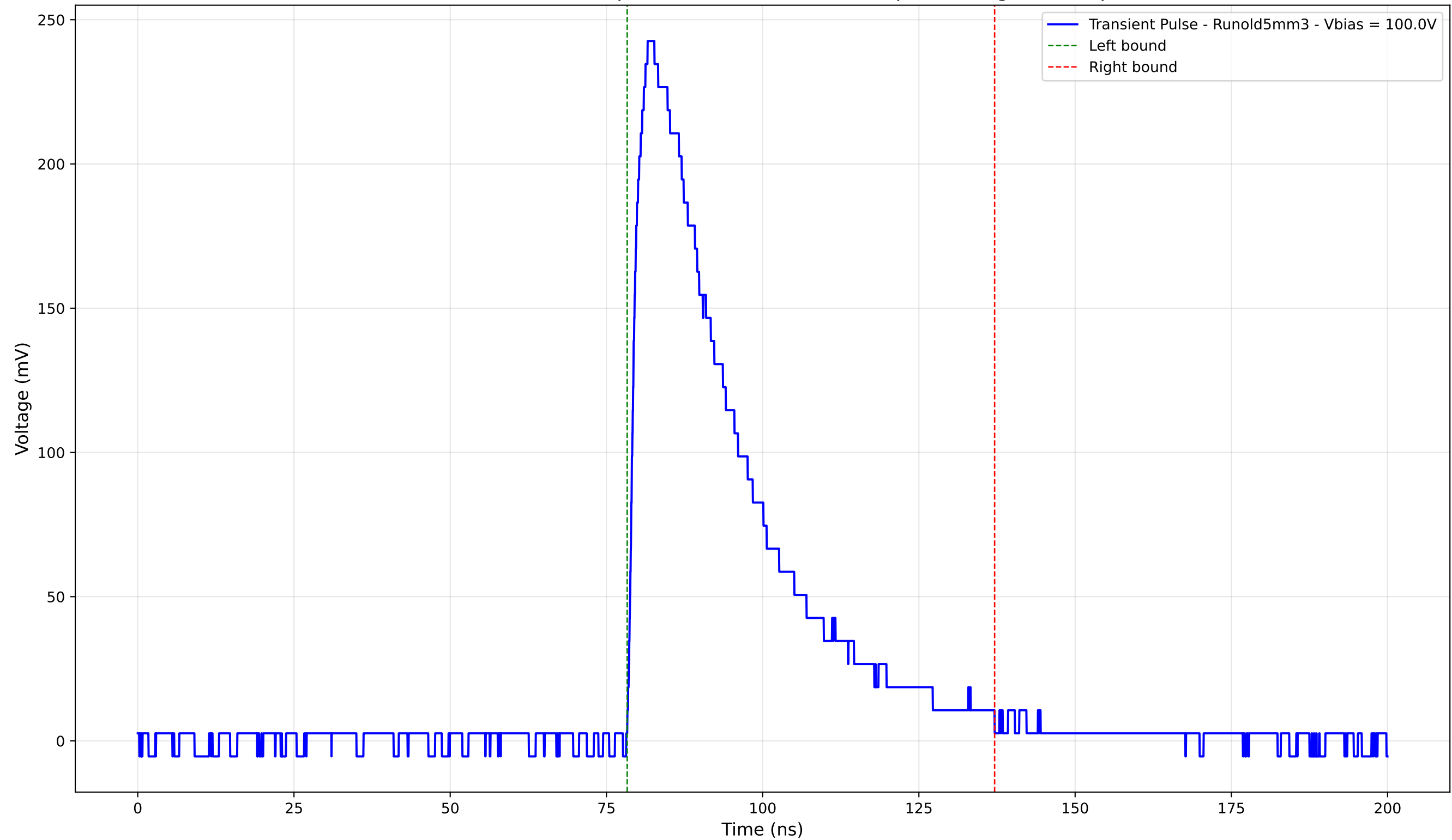
Transient Pulse - Sample: old5 - Position: 2570.0 \mu\text{m} - Charge: 89.97 pC
