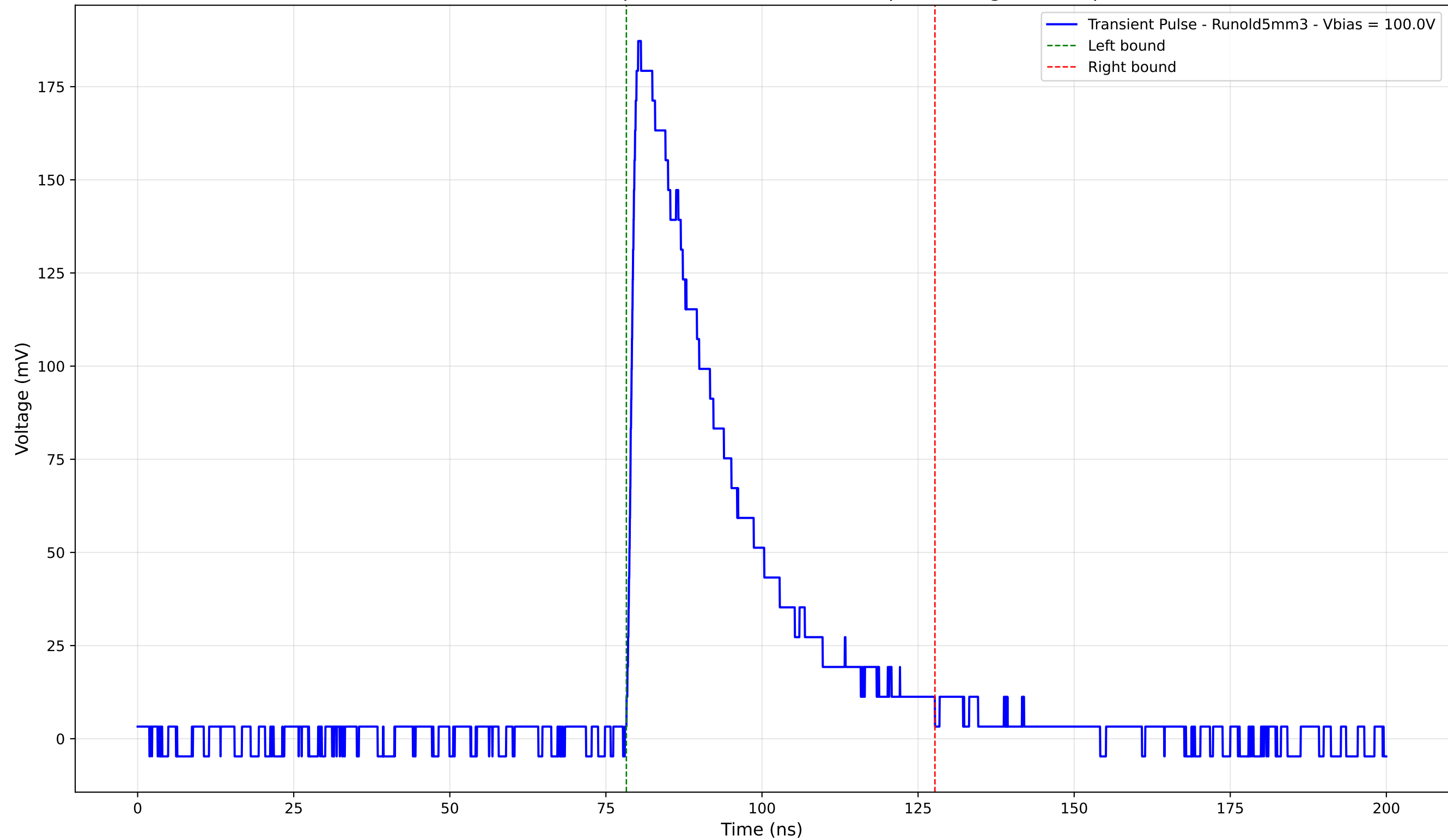
Transient Pulse - Sample: old5 - Position: 950.0 \mu\text{m} - Charge: 60.16 pC
