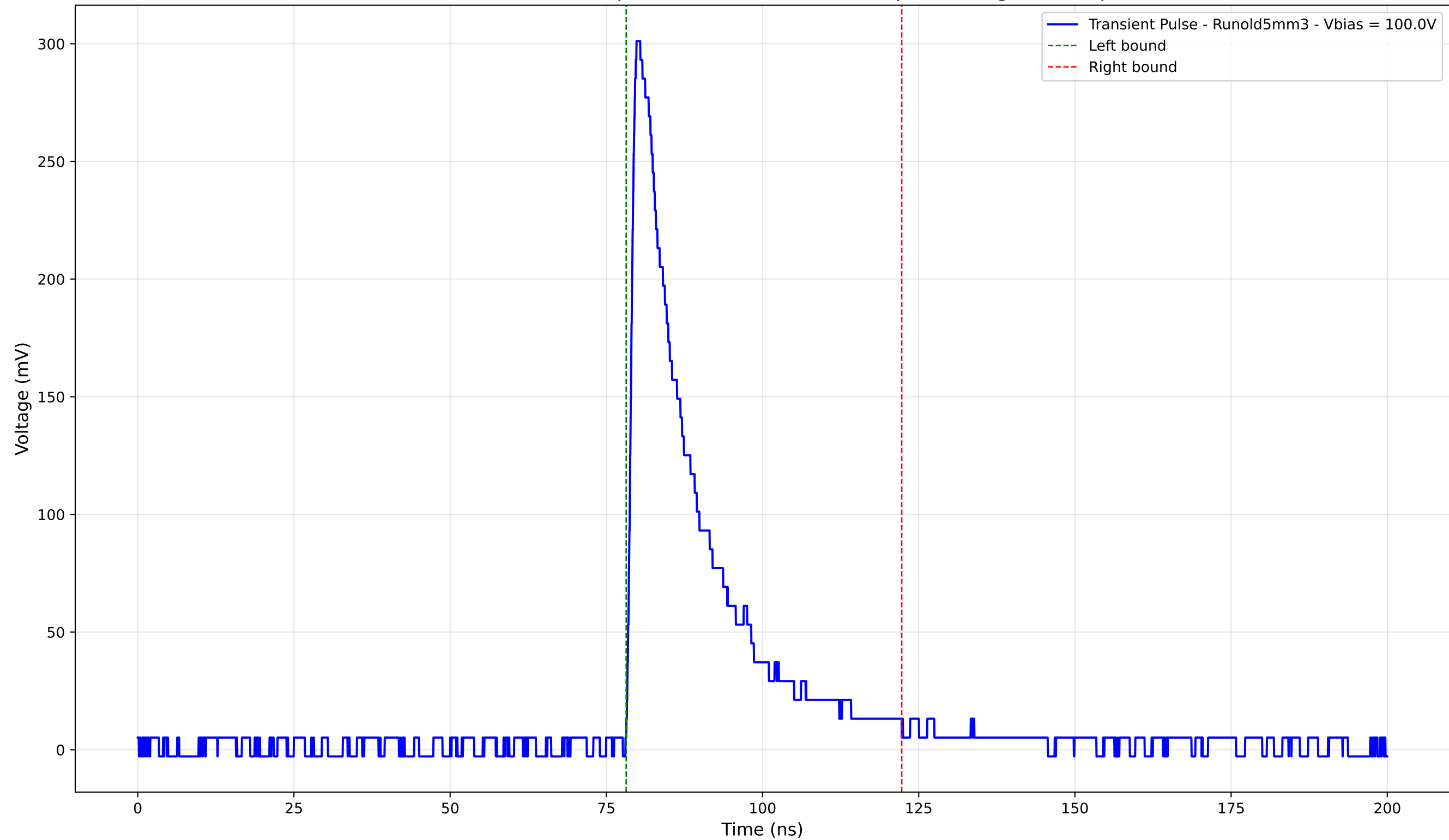
Transient Pulse - Sample: old5 - Position: 4420.0 \mu\text{m} - Charge: 66.32 pC
