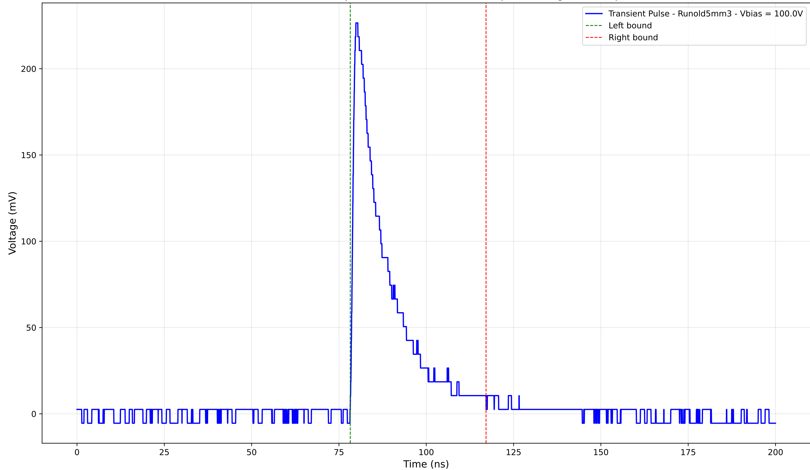
Transient Pulse - Sample: old5 - Position: 4430.0 \mu\text{m} - Charge: 46.91 pC
