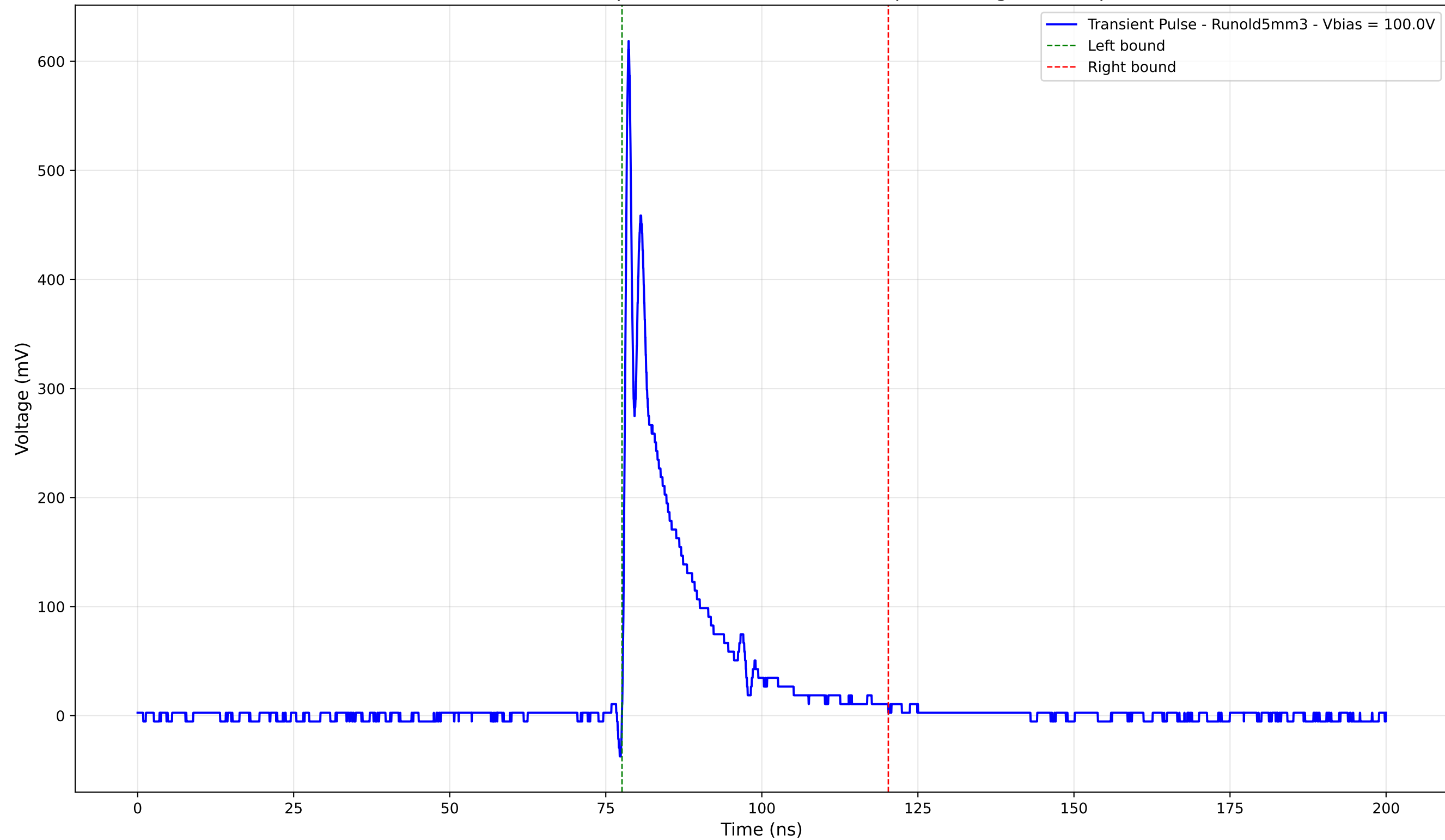
Transient Pulse - Sample: old5 - Position: 3670.0 \mu\text{m} - Charge: 81.21 pC
