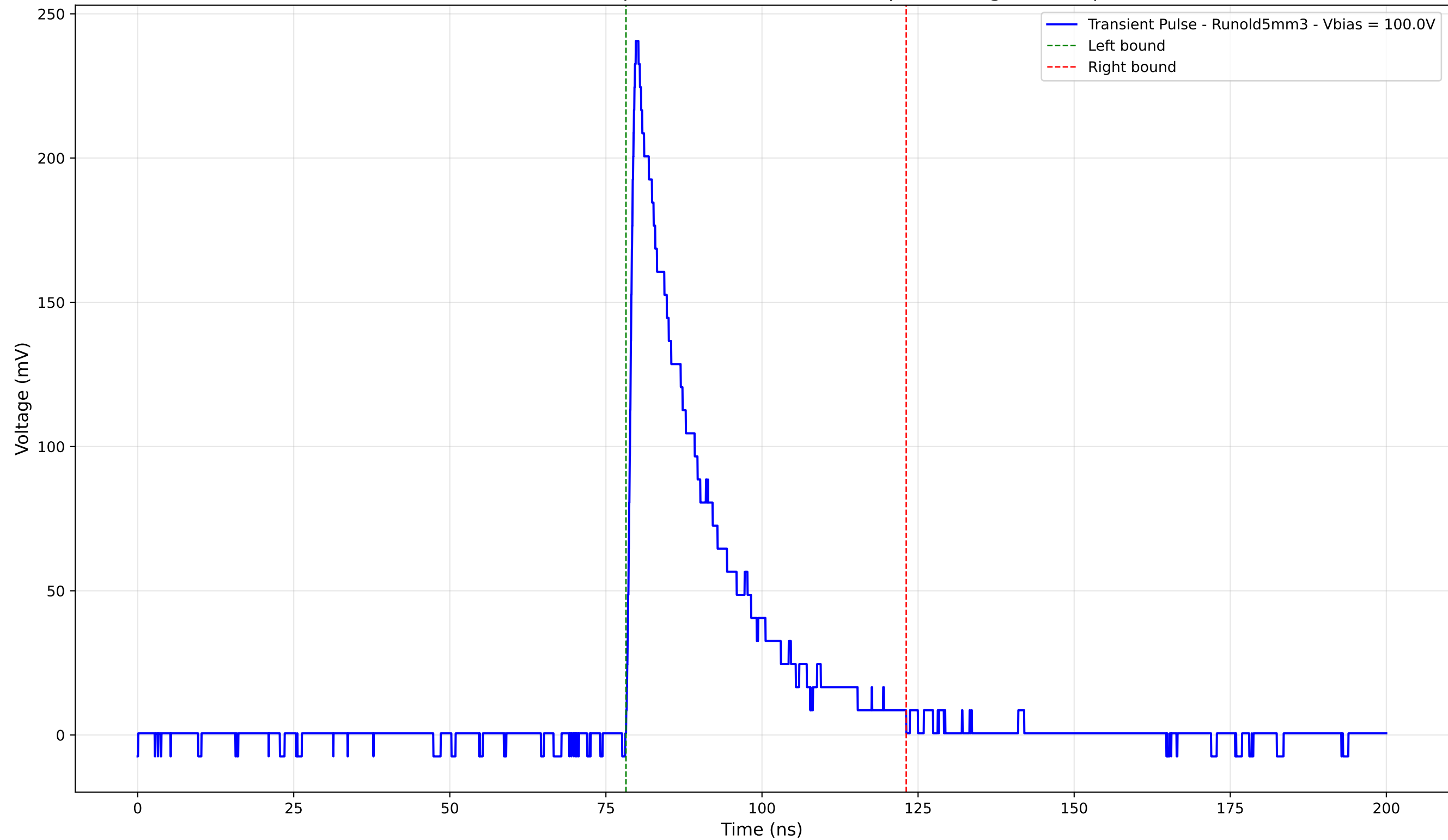
Transient Pulse - Sample: old5 - Position: 645.0 \mu\text{m} - Charge: 55.15 pC
