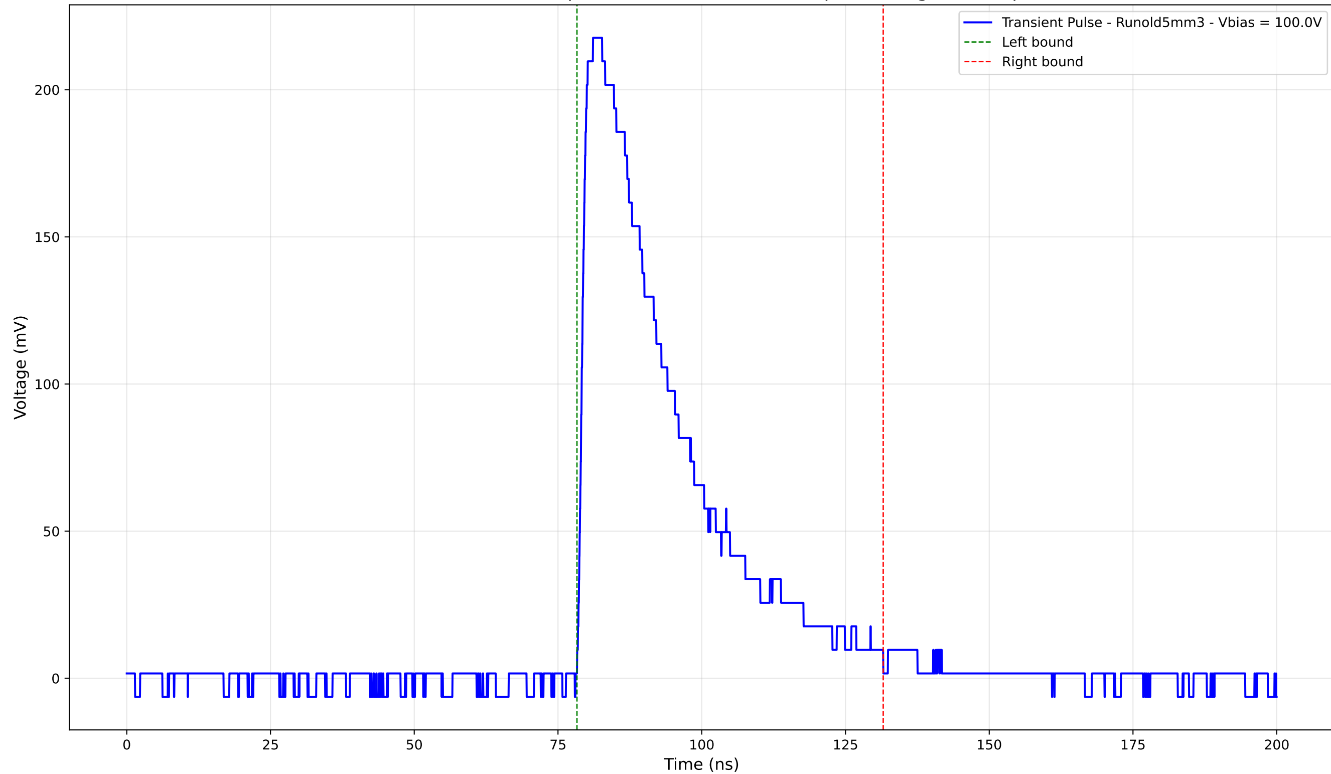
Transient Pulse - Sample: old5 - Position: 1055.0 \mu\text{m} - Charge: 77.57 pC
