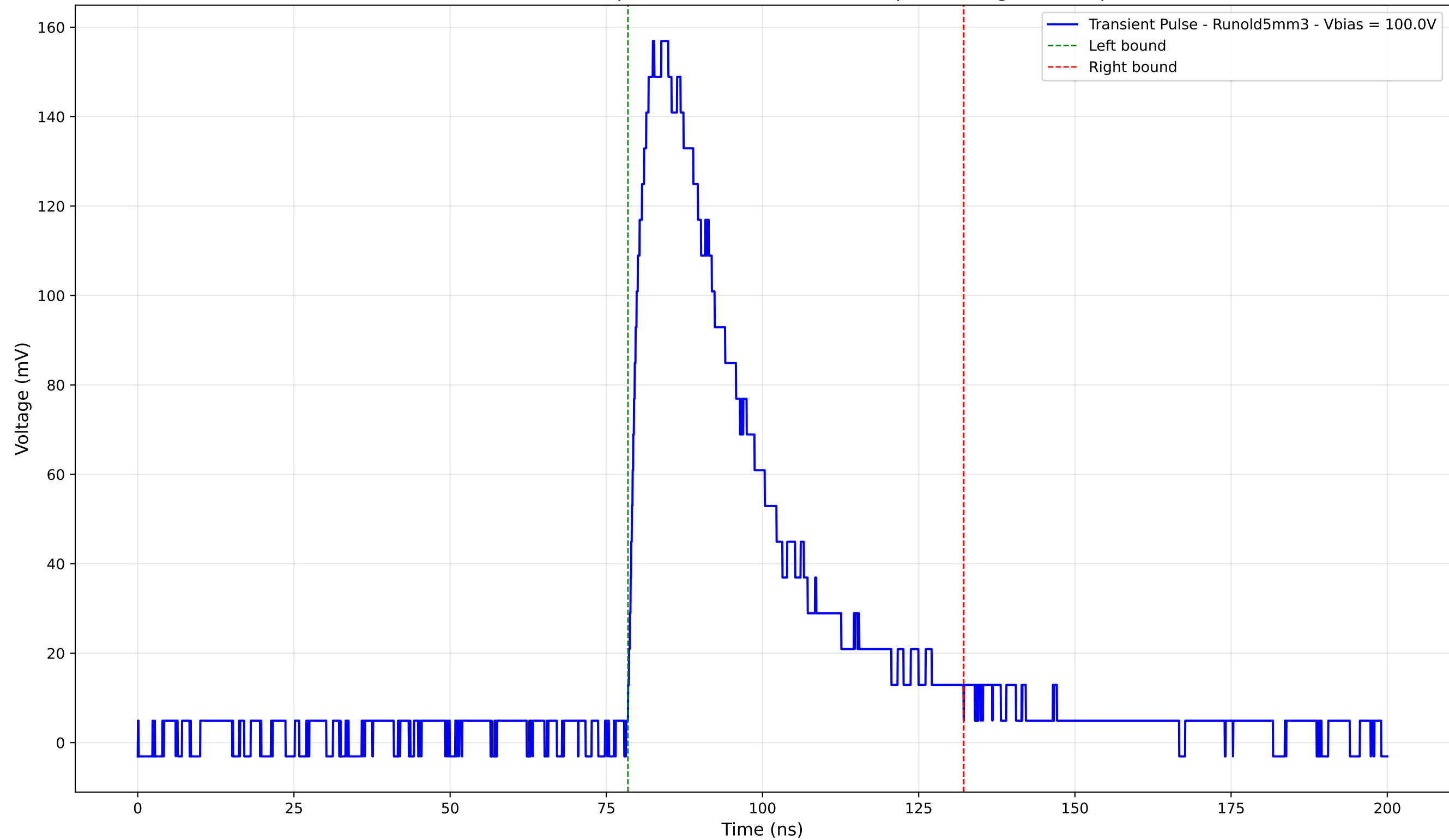
Transient Pulse - Sample: old5 - Position: 2045.0 \mu\text{m} - Charge: 63.36 pC
