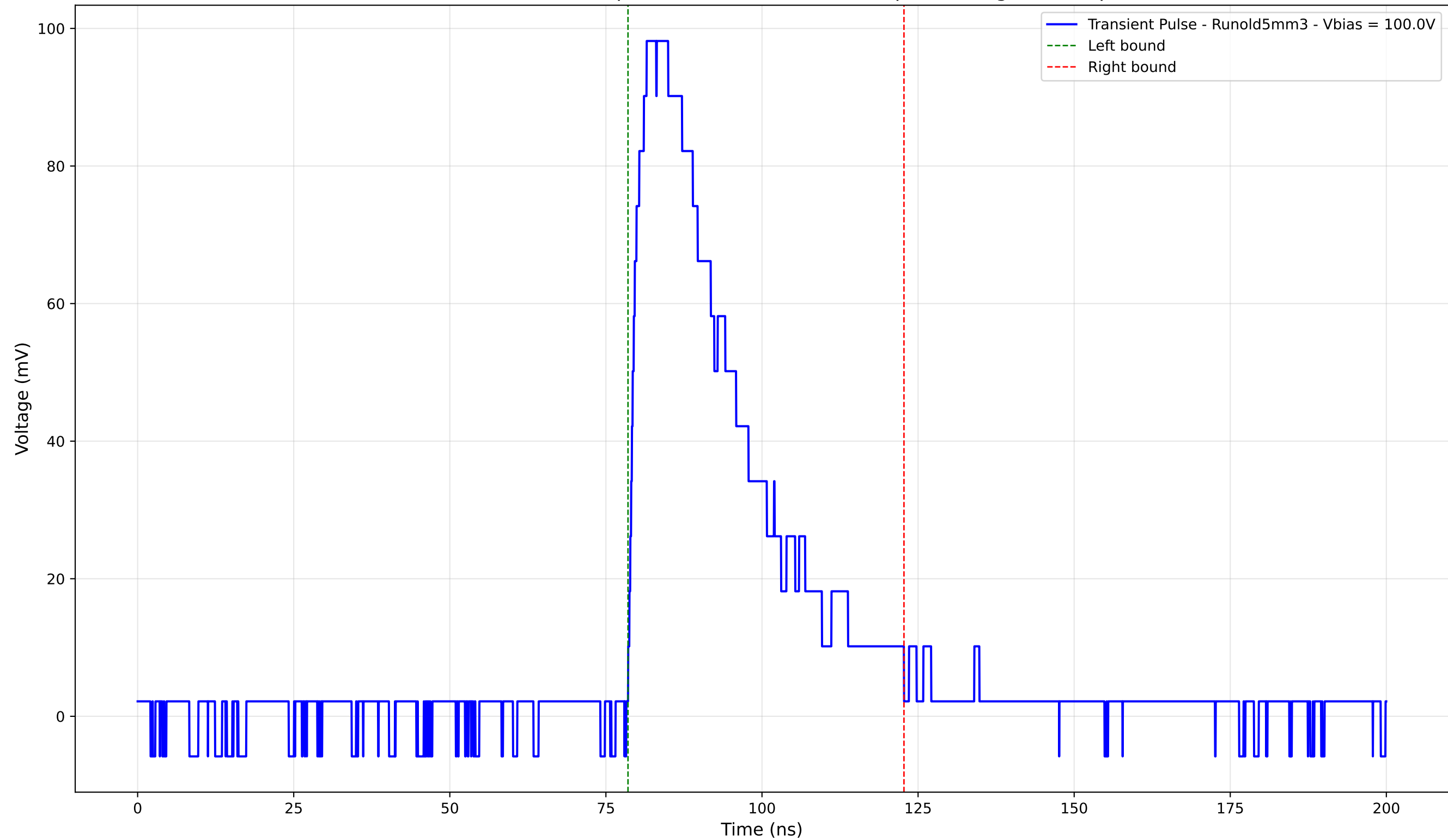
Transient Pulse - Sample: old5 - Position: 2430.0 \mu\text{m} - Charge: 36.40 pC
