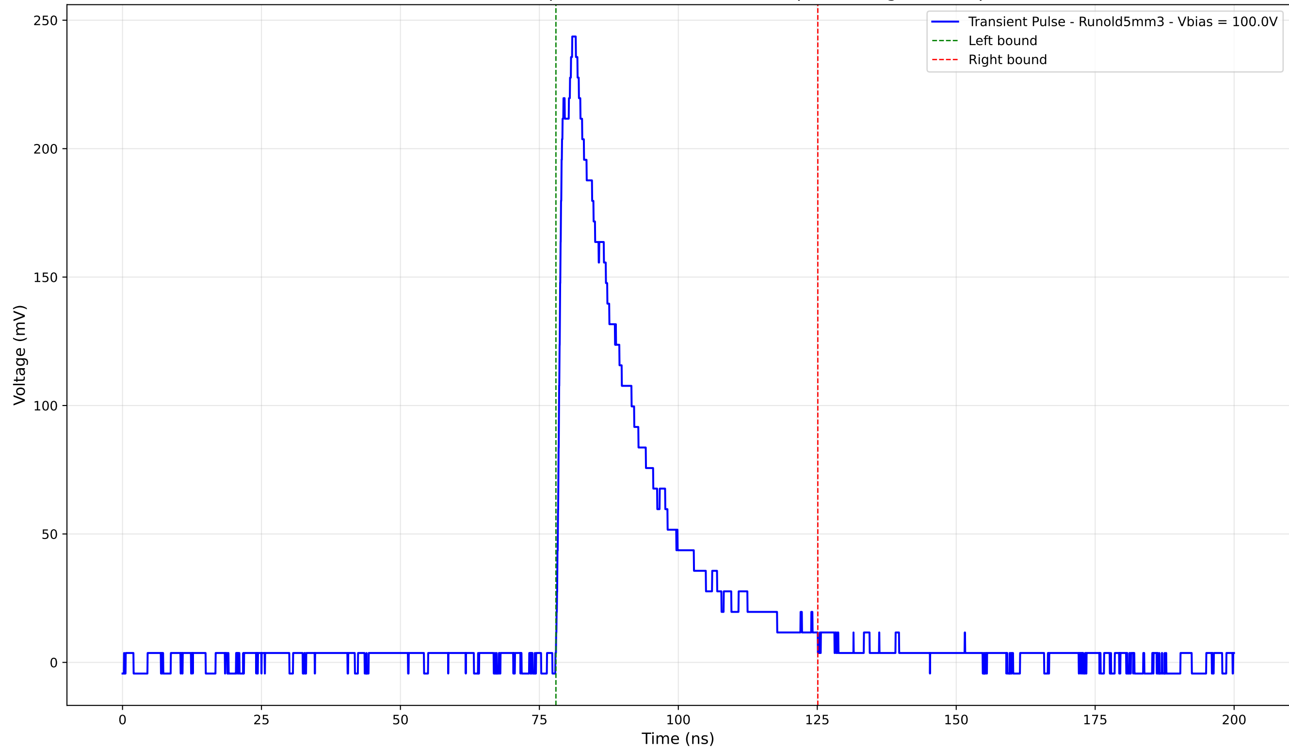
Transient Pulse - Sample: old5 - Position: 3055.0 \mu\text{m} - Charge: 68.42 pC
