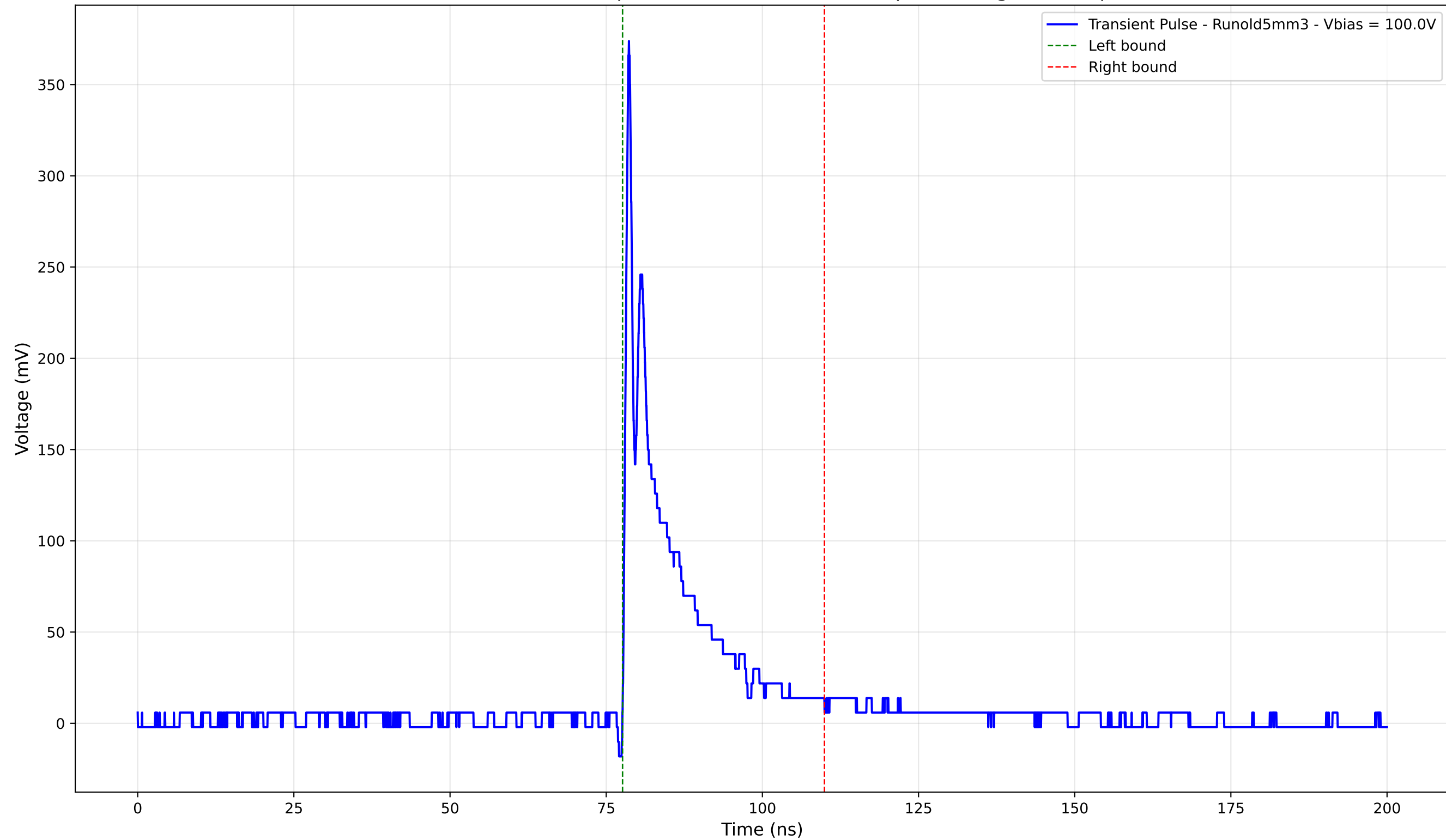
Transient Pulse - Sample: old5 - Position: 3520.0 \mu\text{m} - Charge: 43.88 pC
