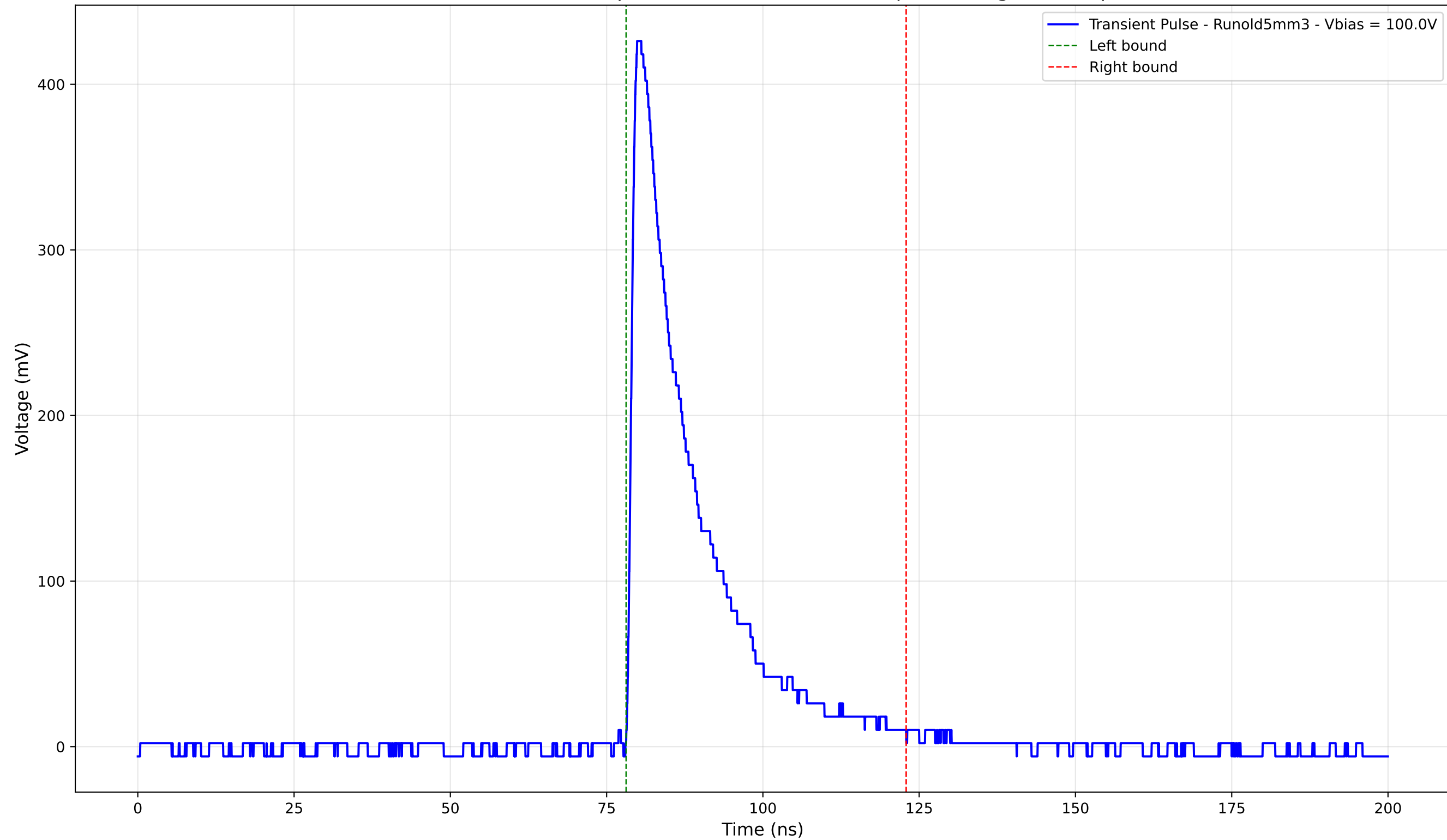
Transient Pulse - Sample: old5 - Position: 4400.0 \mu\text{m} - Charge: 91.77 pC
