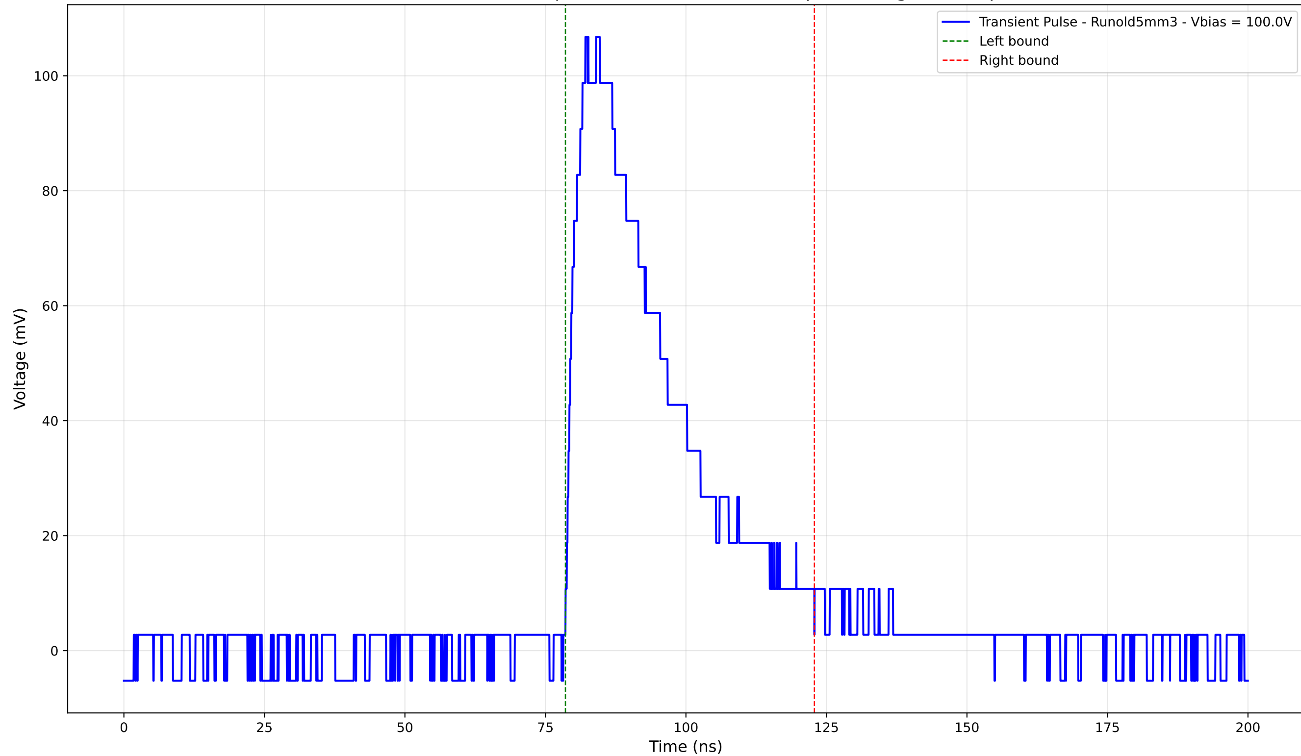
Transient Pulse - Sample: old5 - Position: 2230.0 \mu\text{m} - Charge: 39.68 pC
