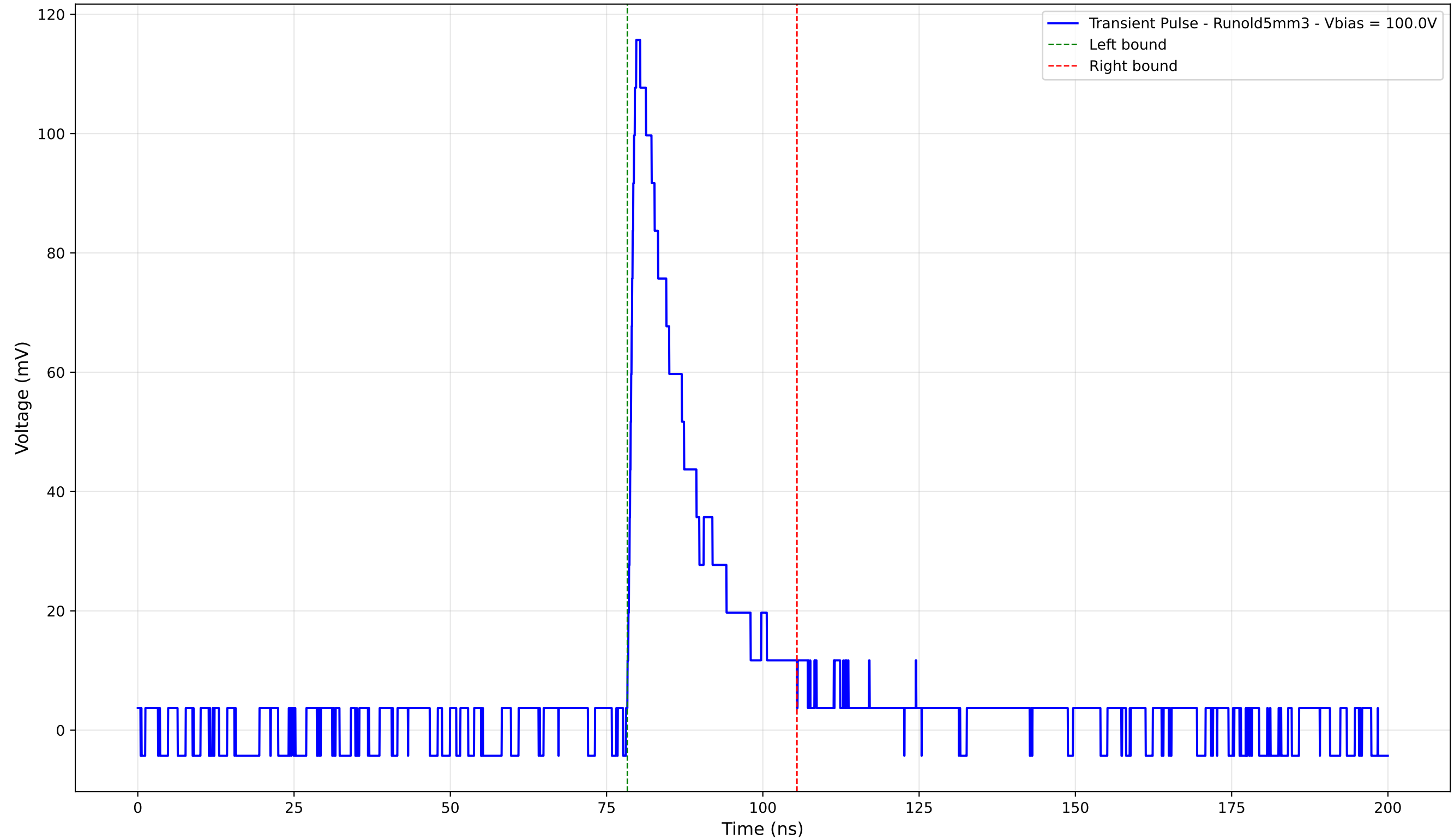
Transient Pulse - Sample: old5 - Position: 4450.0 \mu\text{m} - Charge: 22.38 pC
