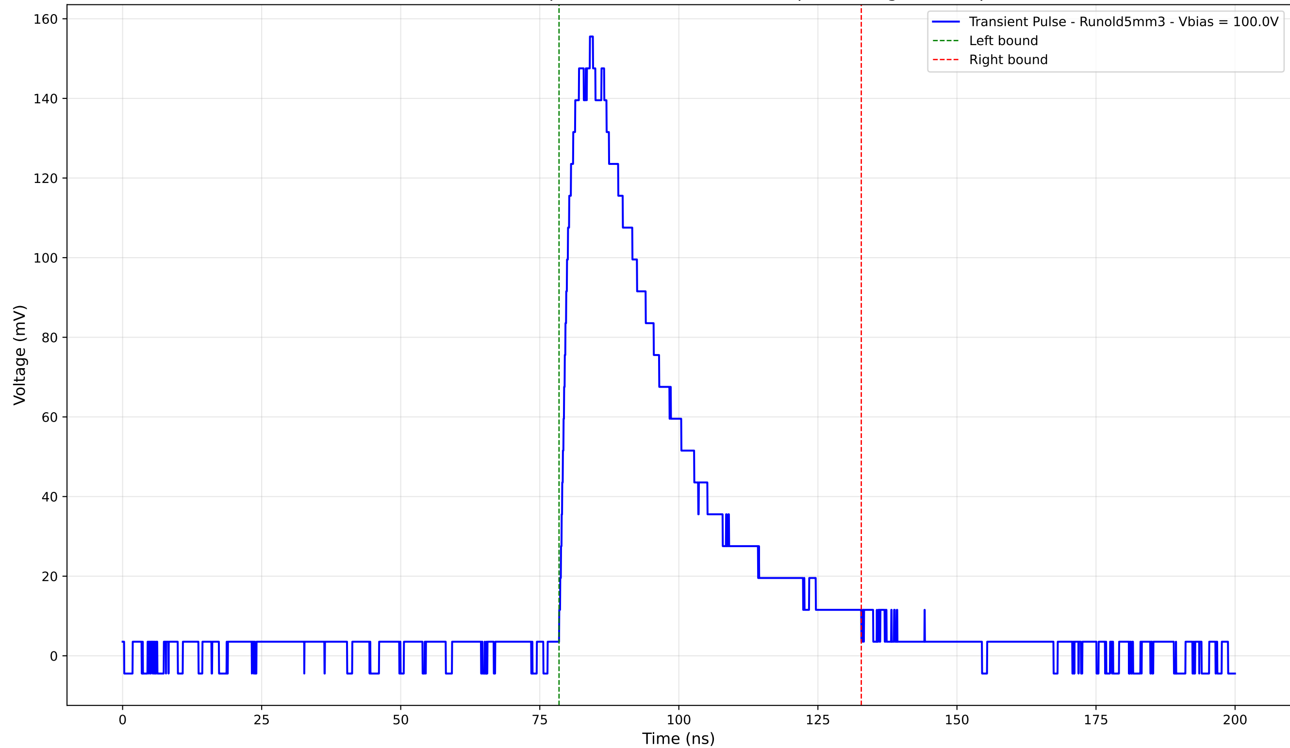
Transient Pulse - Sample: old5 - Position: 1730.0 \mu\text{m} - Charge: 61.31 pC
