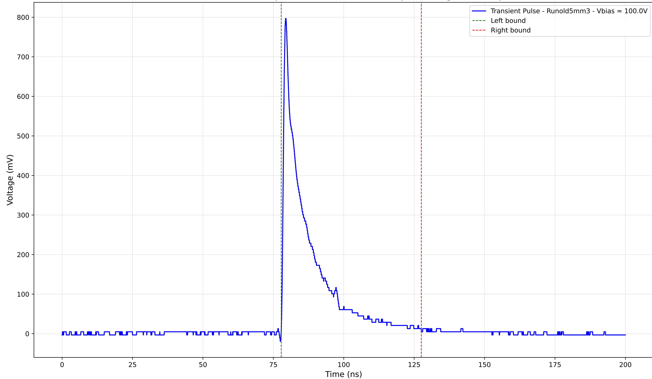
Transient Pulse - Sample: old5 - Position: 4765.0 \mu\text{m} - Charge: 135.79 pC
