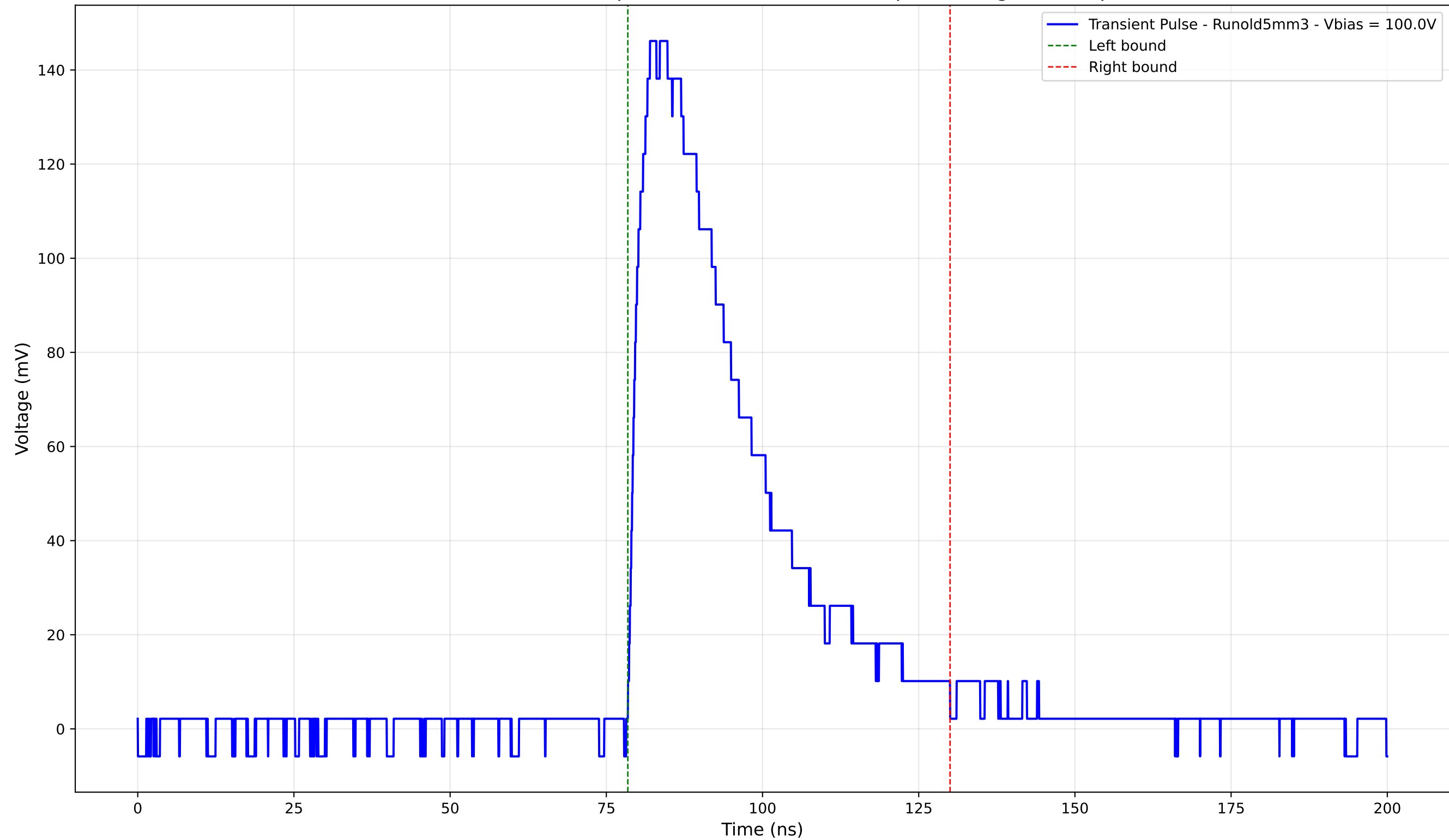
Transient Pulse - Sample: old5 - Position: 1935.0 \mu\text{m} - Charge: 57.99 pC
