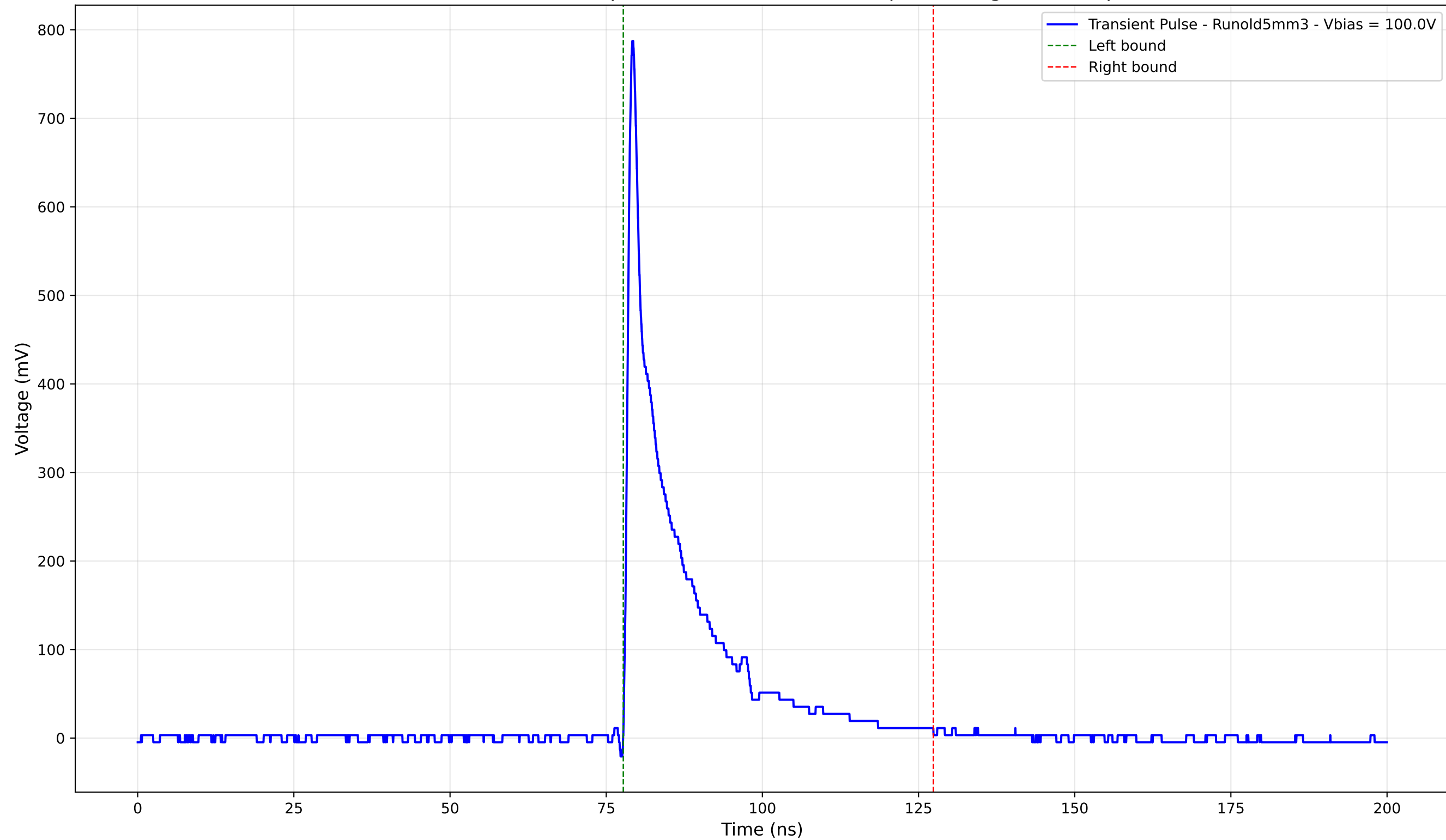
Transient Pulse - Sample: old5 - Position: 4845.0 \mu\text{m} - Charge: 113.14 pC
