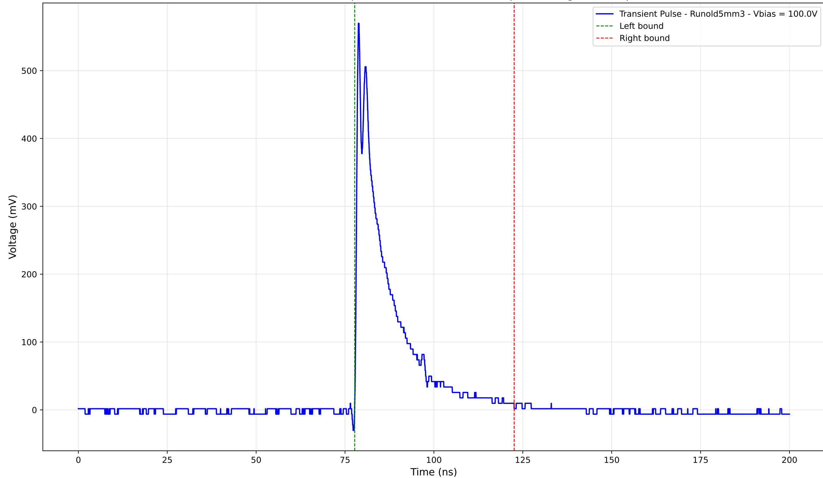
Transient Pulse - Sample: old5 - Position: 3780.0 \mu\text{m} - Charge: 97.73 pC
