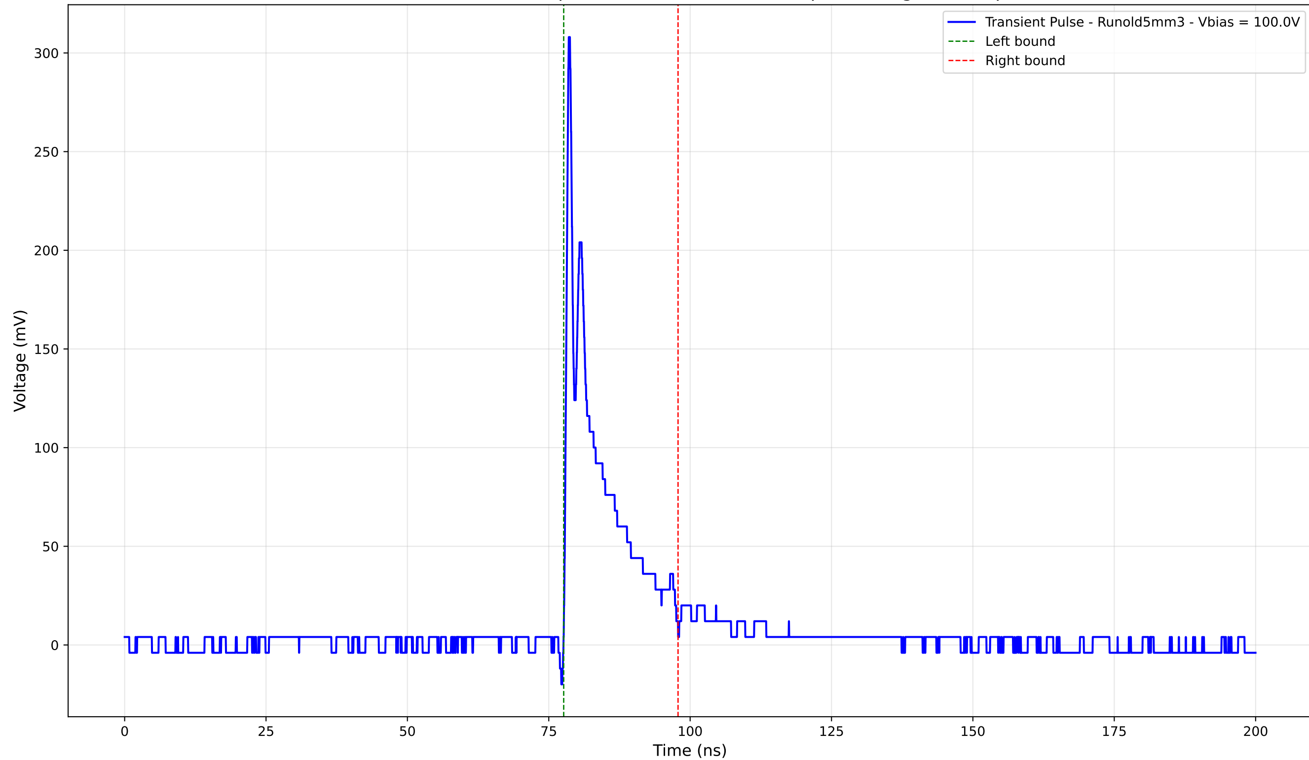
Transient Pulse - Sample: old5 - Position: 3525.0 \mu\text{m} - Charge: 32.50 pC
