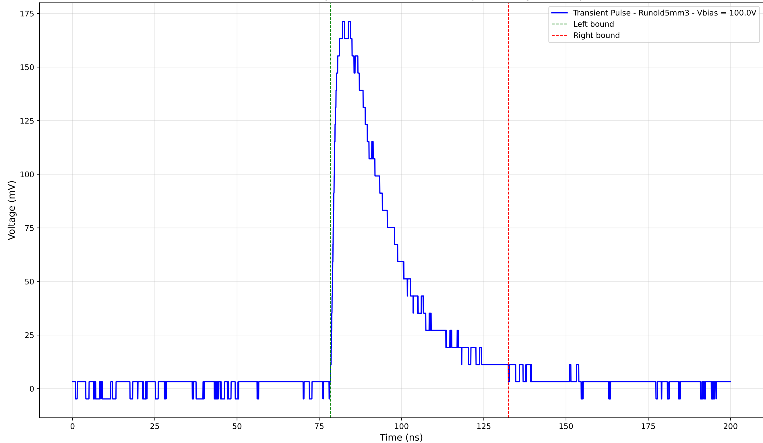
Transient Pulse - Sample: old5 - Position: 1320.0 \mu\text{m} - Charge: 65.19 pC
