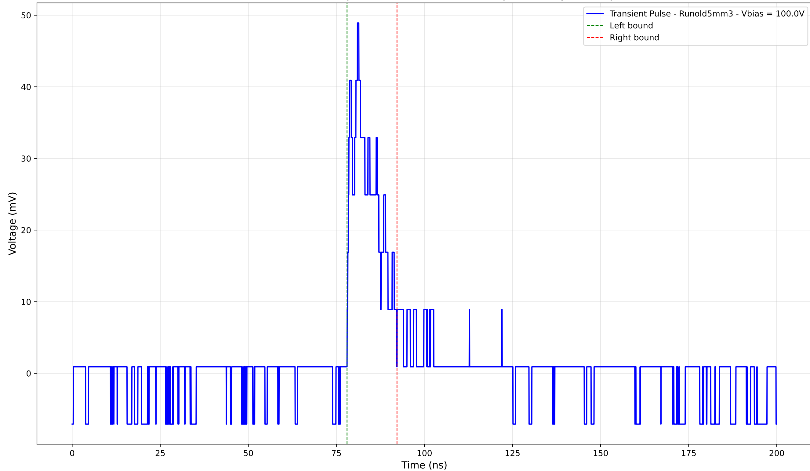
Transient Pulse - Sample: old5 - Position: 3305.0 \mu\text{m} - Charge: 7.00 pC
