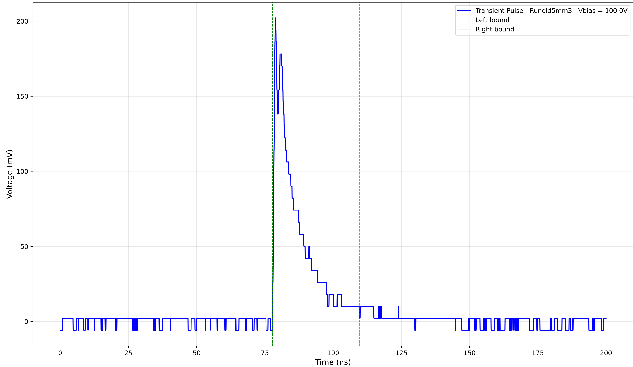
Transient Pulse - Sample: old5 - Position: 3830.0 \mu\text{m} - Charge: 33.42 pC
