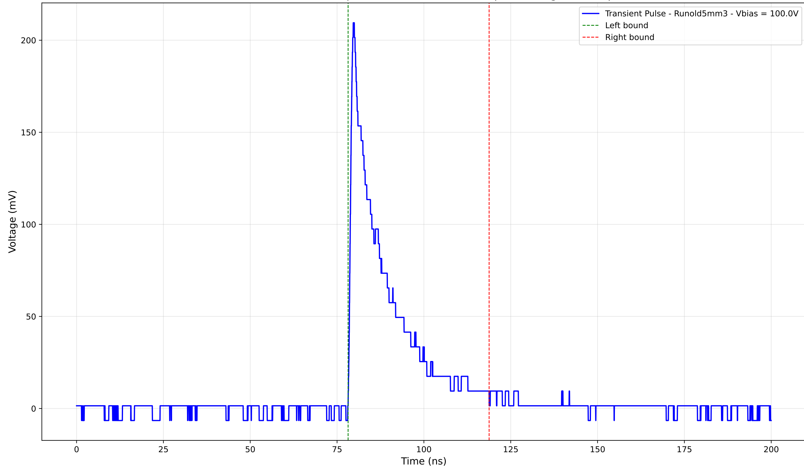
Transient Pulse - Sample: old5 - Position: 515.0 \mu\text{m} - Charge: 41.12 pC
