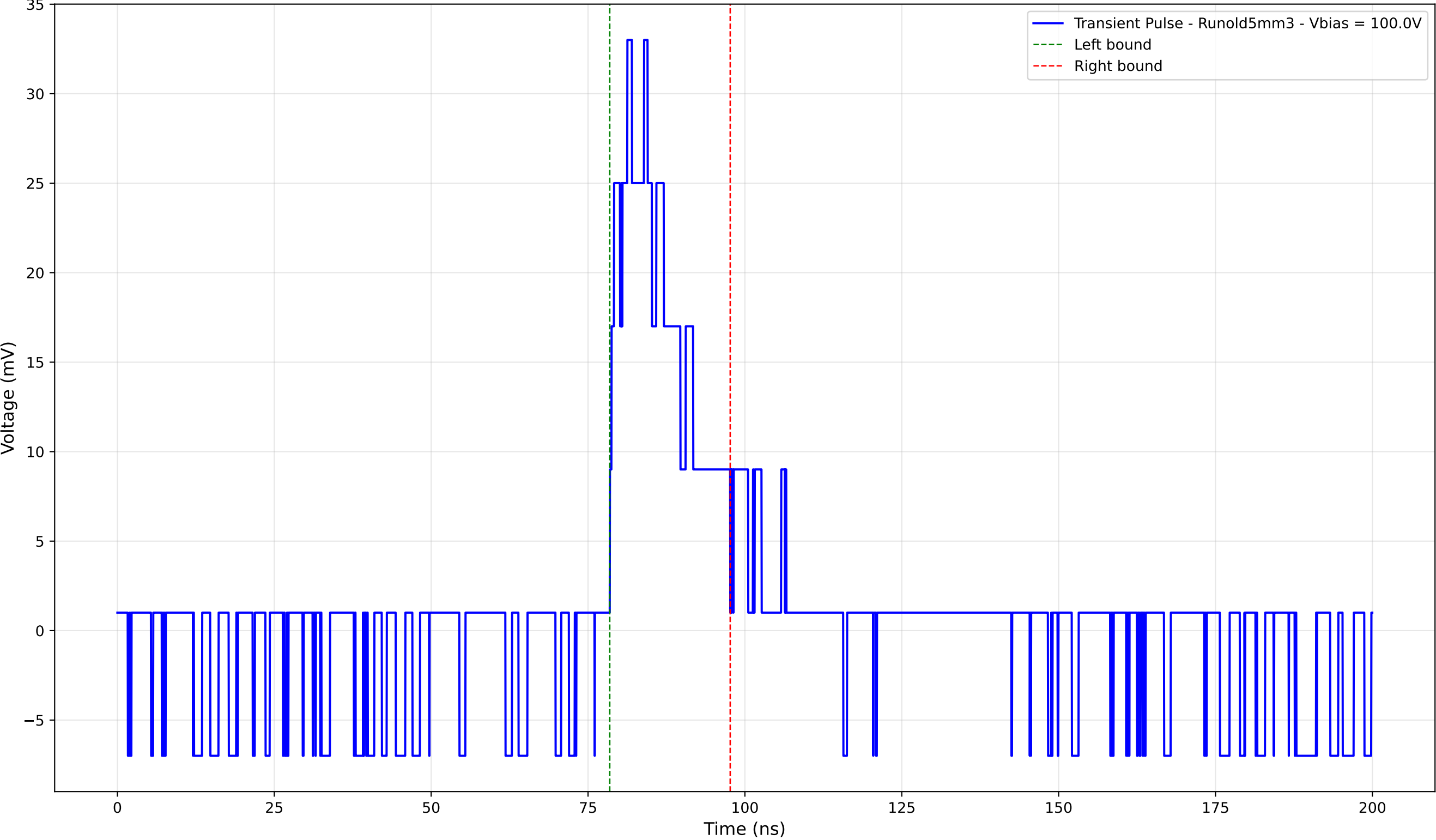
Transient Pulse - Sample: old5 - Position: 3000.0 \mu\text{m} - Charge: 6.73 pC
