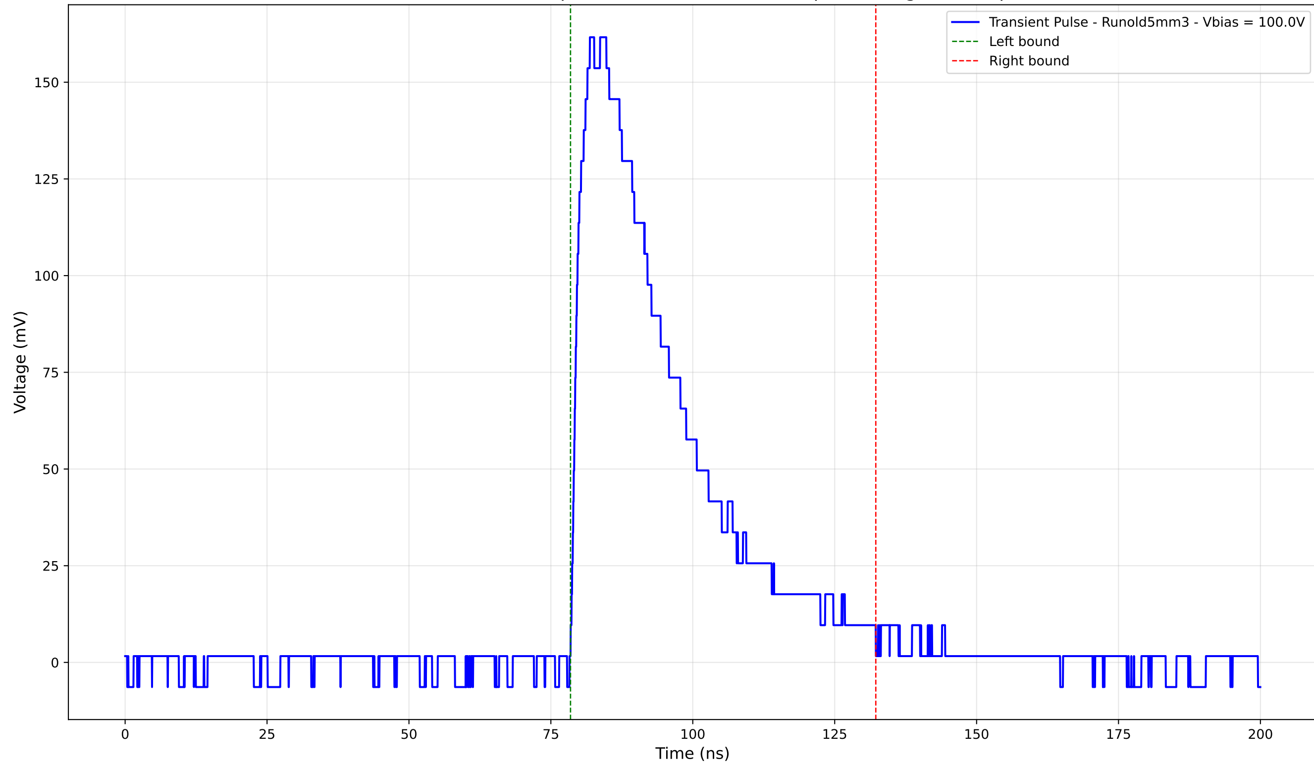
Transient Pulse - Sample: old5 - Position: 2340.0 \mu\text{m} - Charge: 62.62 pC
