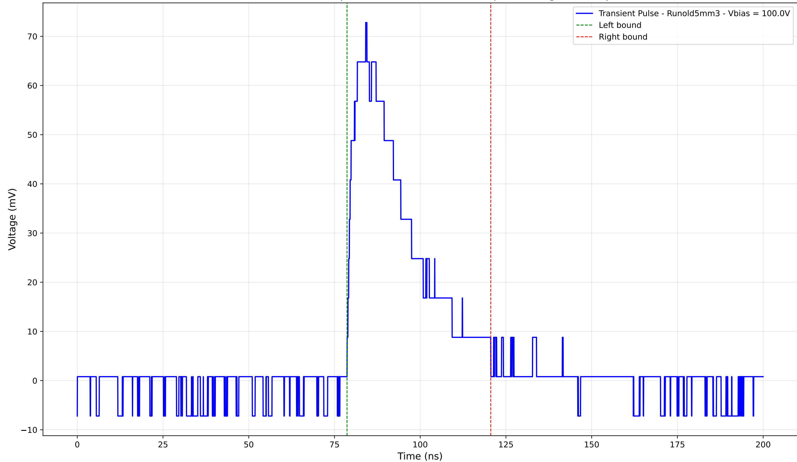
Transient Pulse - Sample: old5 - Position: 1760.0 \mu\text{m} - Charge: 25.34 pC
