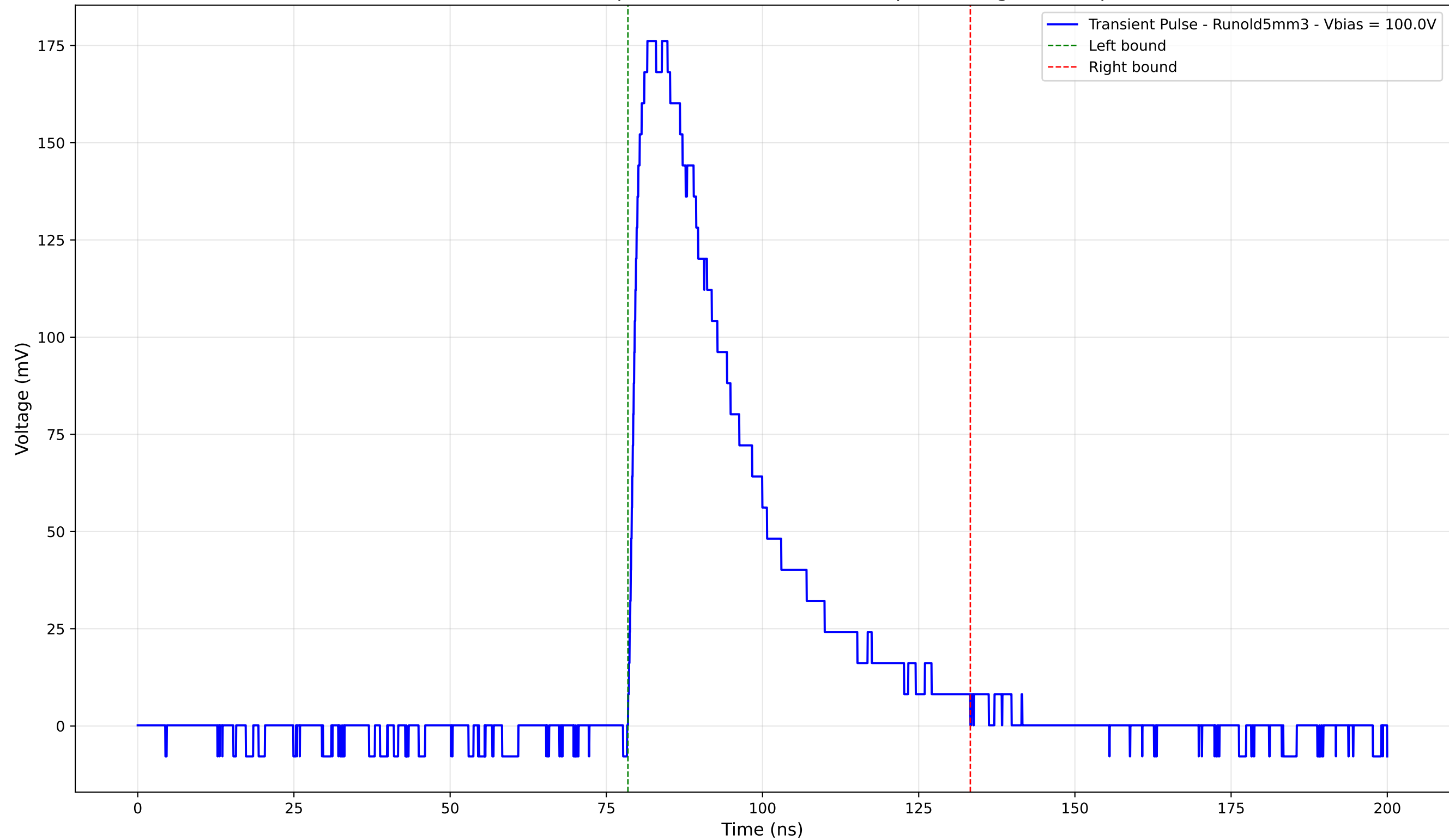
Transient Pulse - Sample: old5 - Position: 1315.0 \mu\text{m} - Charge: 66.53 pC
