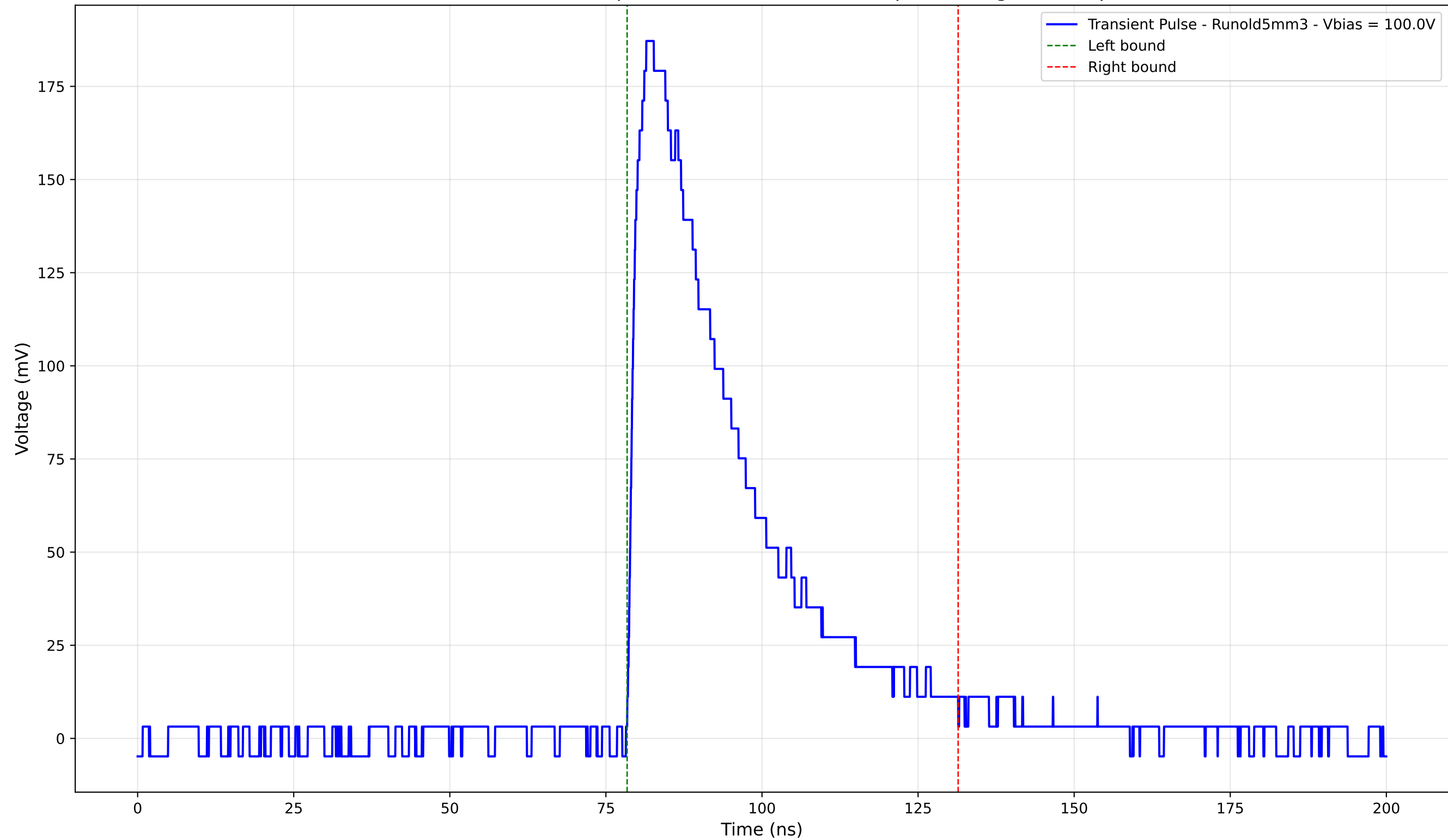
Transient Pulse - Sample: old5 - Position: 2590.0 \mu\text{m} - Charge: 68.78 pC
