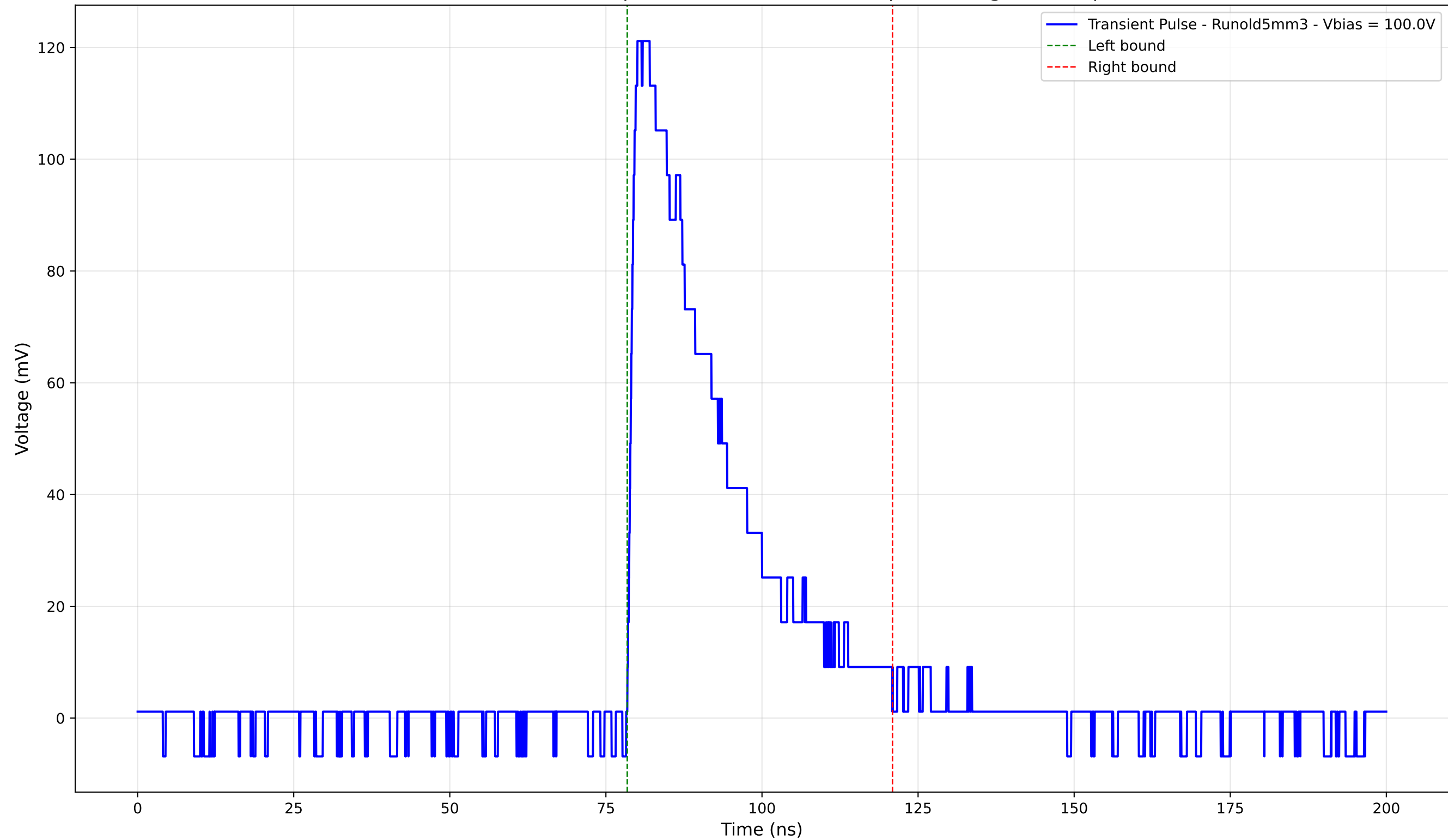
Transient Pulse - Sample: old5 - Position: 910.0 \mu\text{m} - Charge: 37.36 pC
