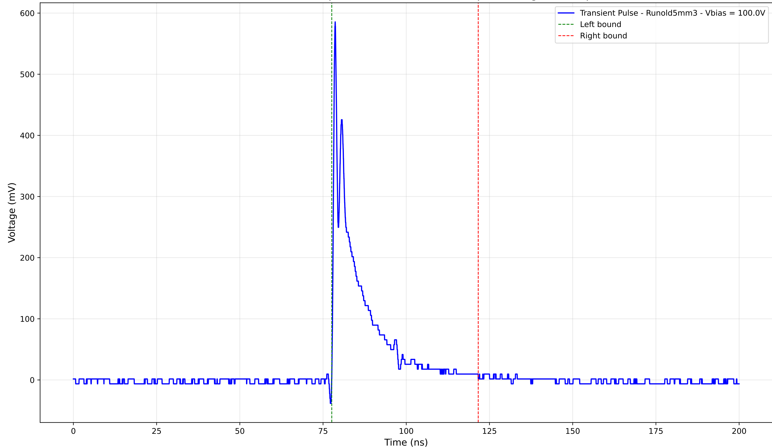
Transient Pulse - Sample: old5 - Position: 3665.0 \mu\text{m} - Charge: 74.94 pC
