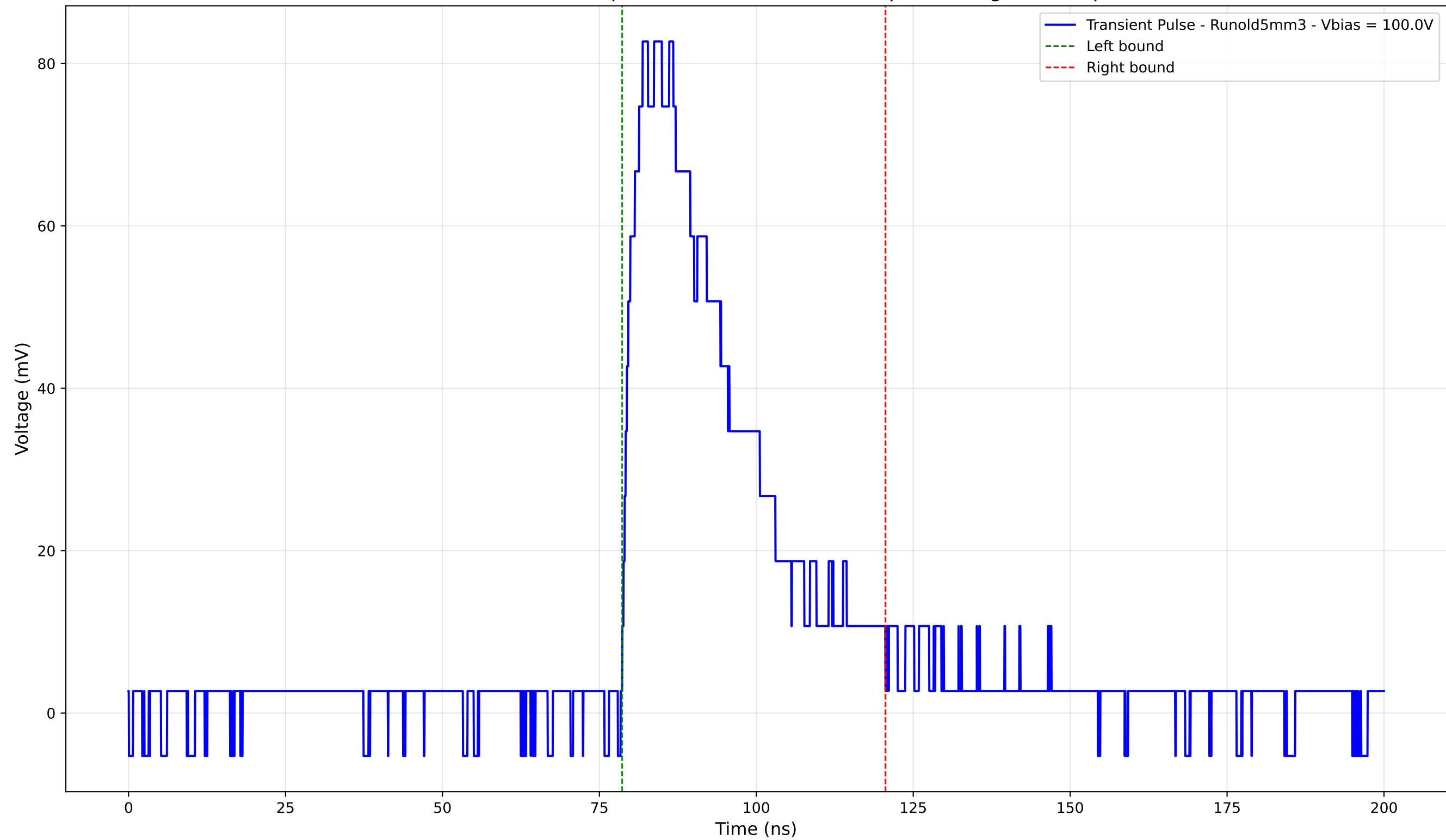
Transient Pulse - Sample: old5 - Position: 1550.0 \mu\text{m} - Charge: 30.82 pC
