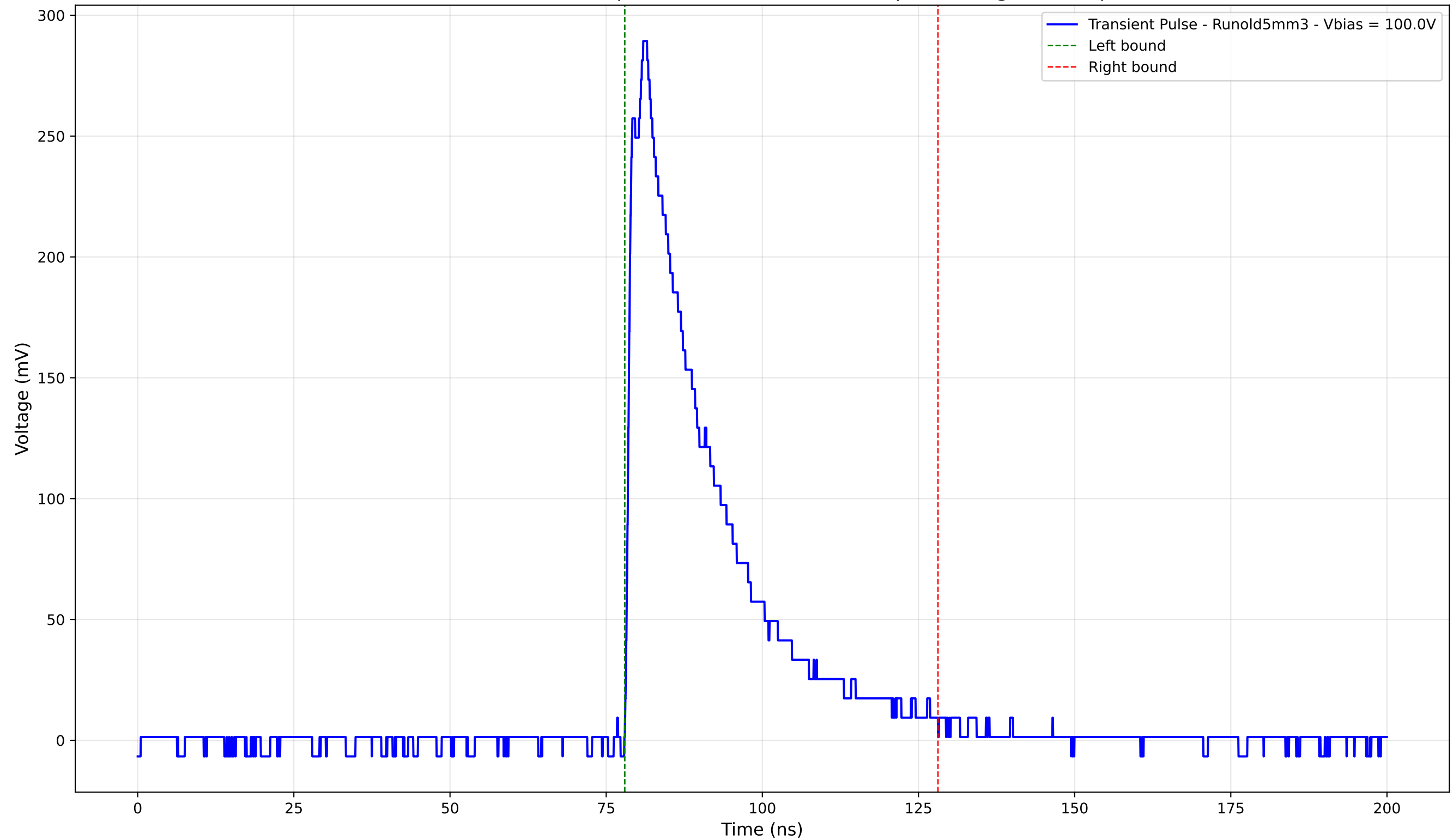
Transient Pulse - Sample: old5 - Position: 3065.0 \mu\text{m} - Charge: 79.73 pC
