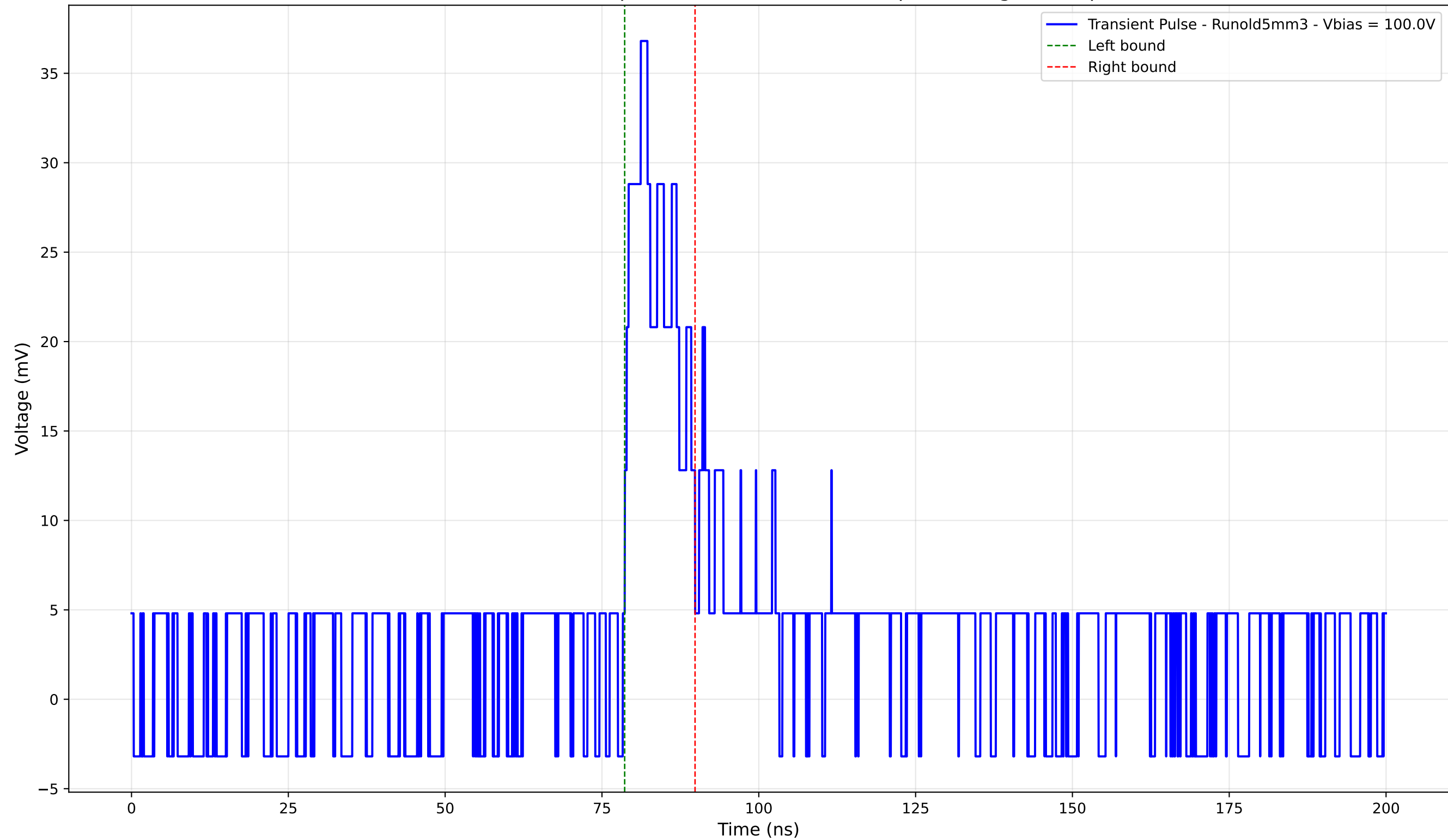
Transient Pulse - Sample: old5 - Position: 4485.0 \mu\text{m} - Charge: 5.36 pC
