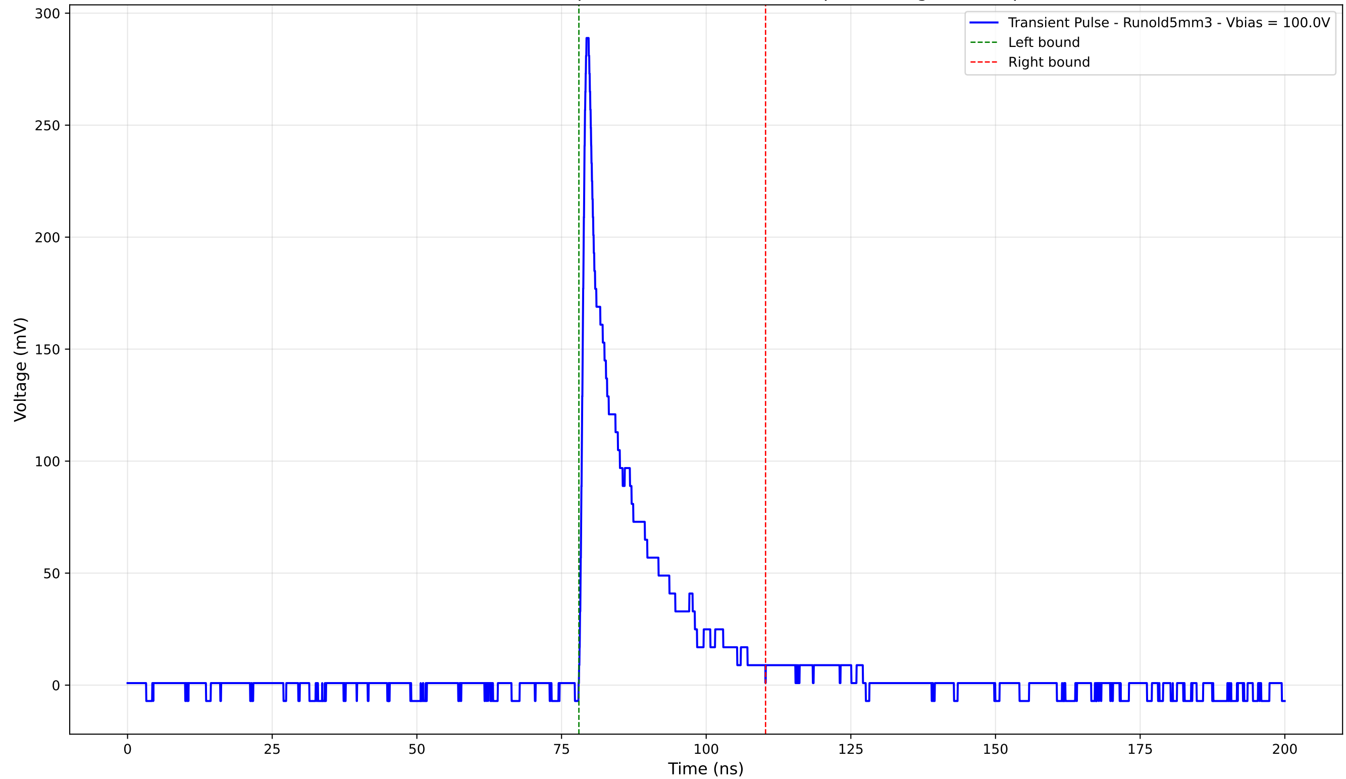
Transient Pulse - Sample: old5 - Position: 320.0 \mu\text{m} - Charge: 41.91 pC
