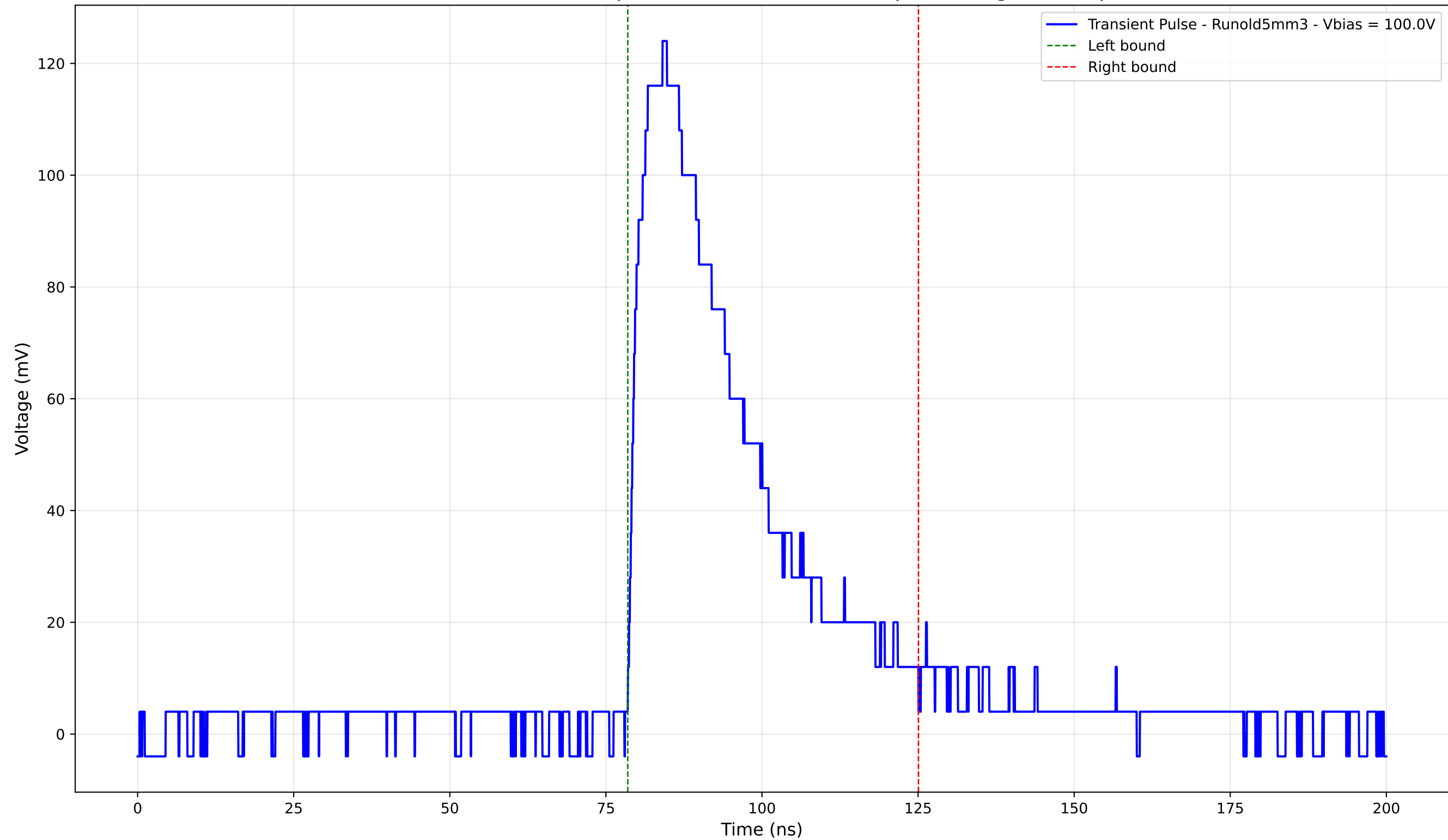
Transient Pulse - Sample: old5 - Position: 2035.0 \mu\text{m} - Charge: 47.91 pC
