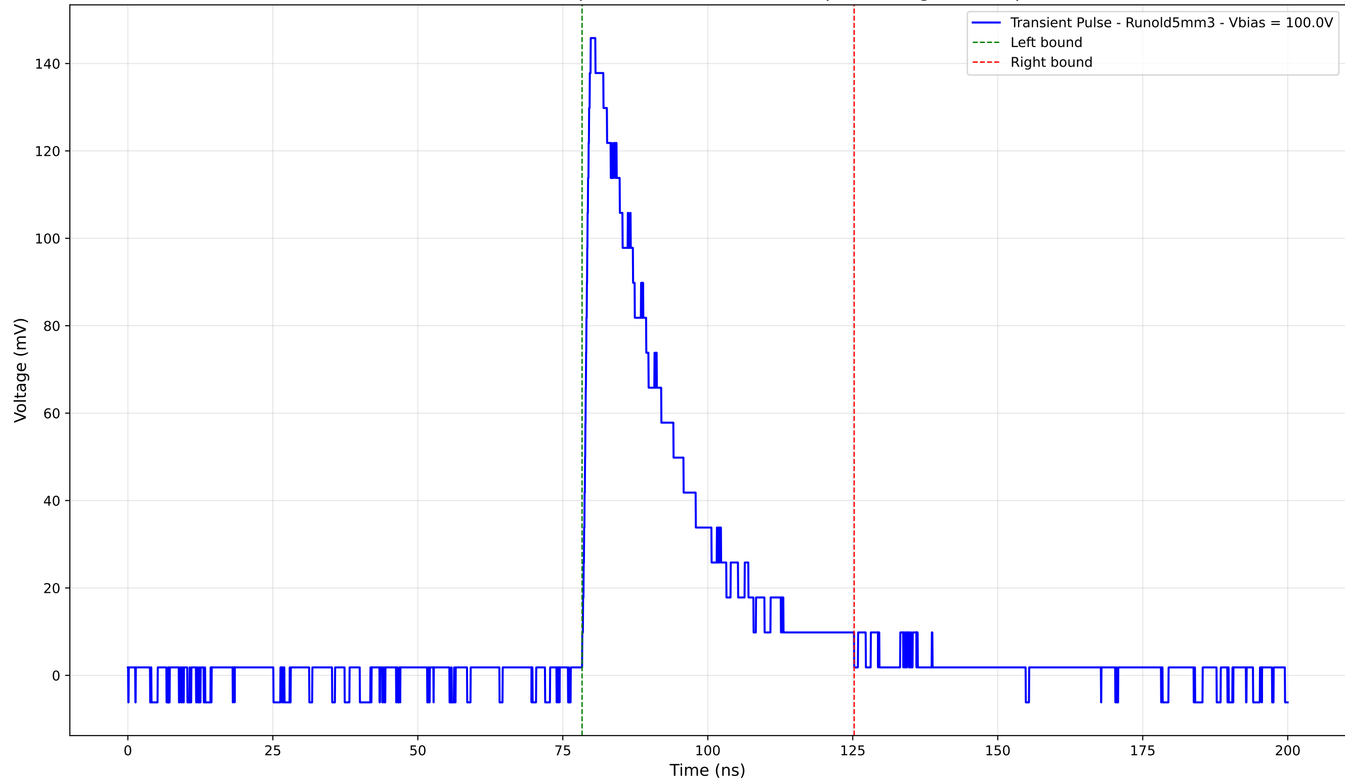
Transient Pulse - Sample: old5 - Position: 820.0 \mu\text{m} - Charge: 42.20 pC
