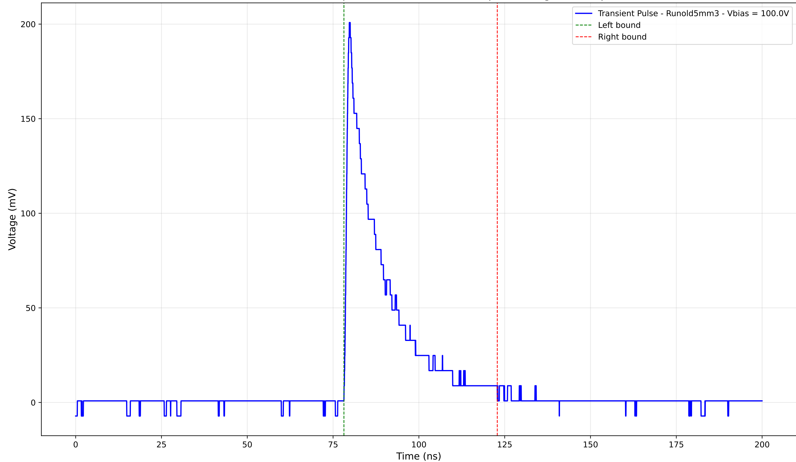
Transient Pulse - Sample: old5 - Position: 580.0 \mu\text{m} - Charge: 42.09 pC
