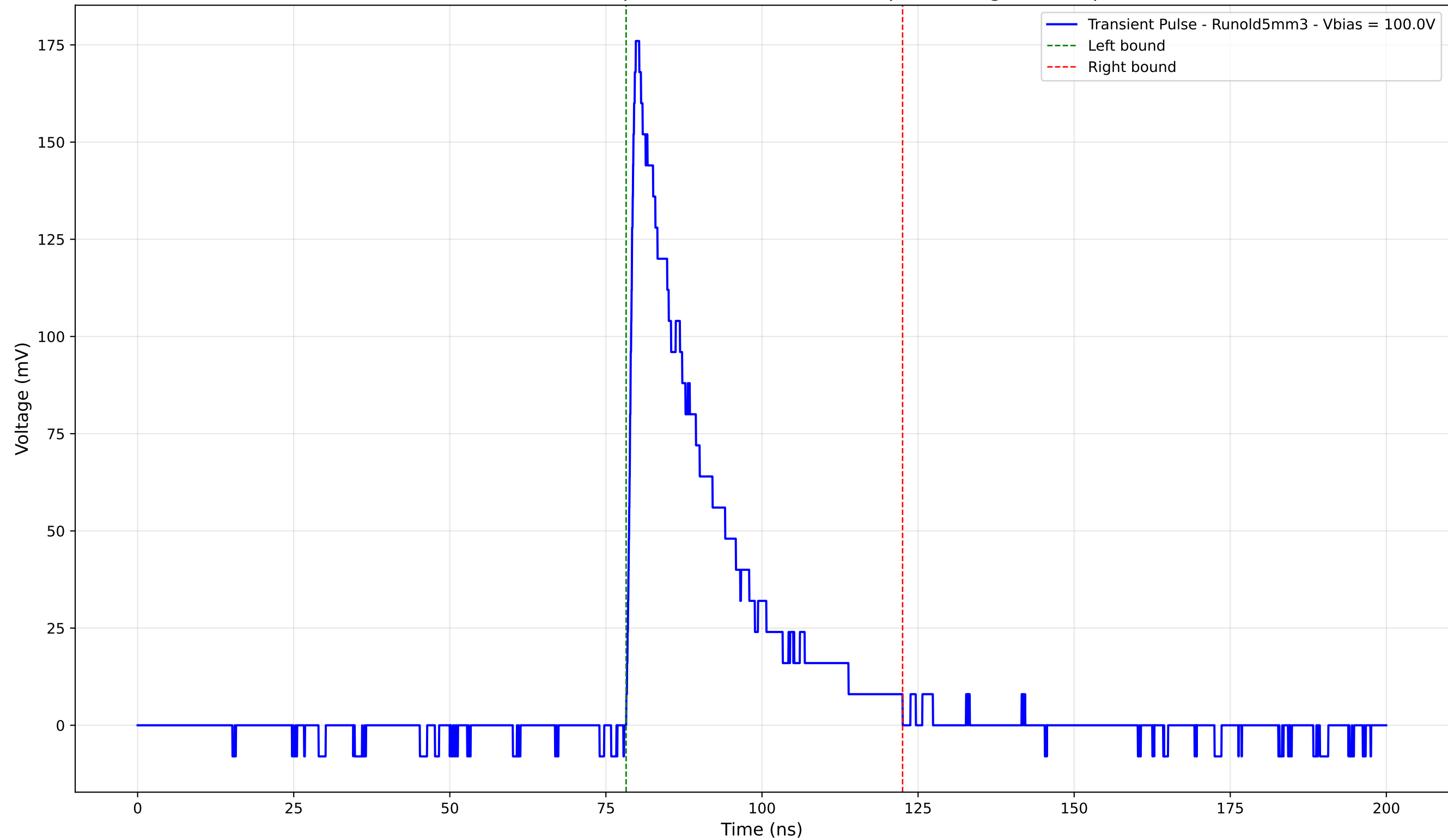
Transient Pulse - Sample: old5 - Position: 680.0 \mu\text{m} - Charge: 42.63 pC
