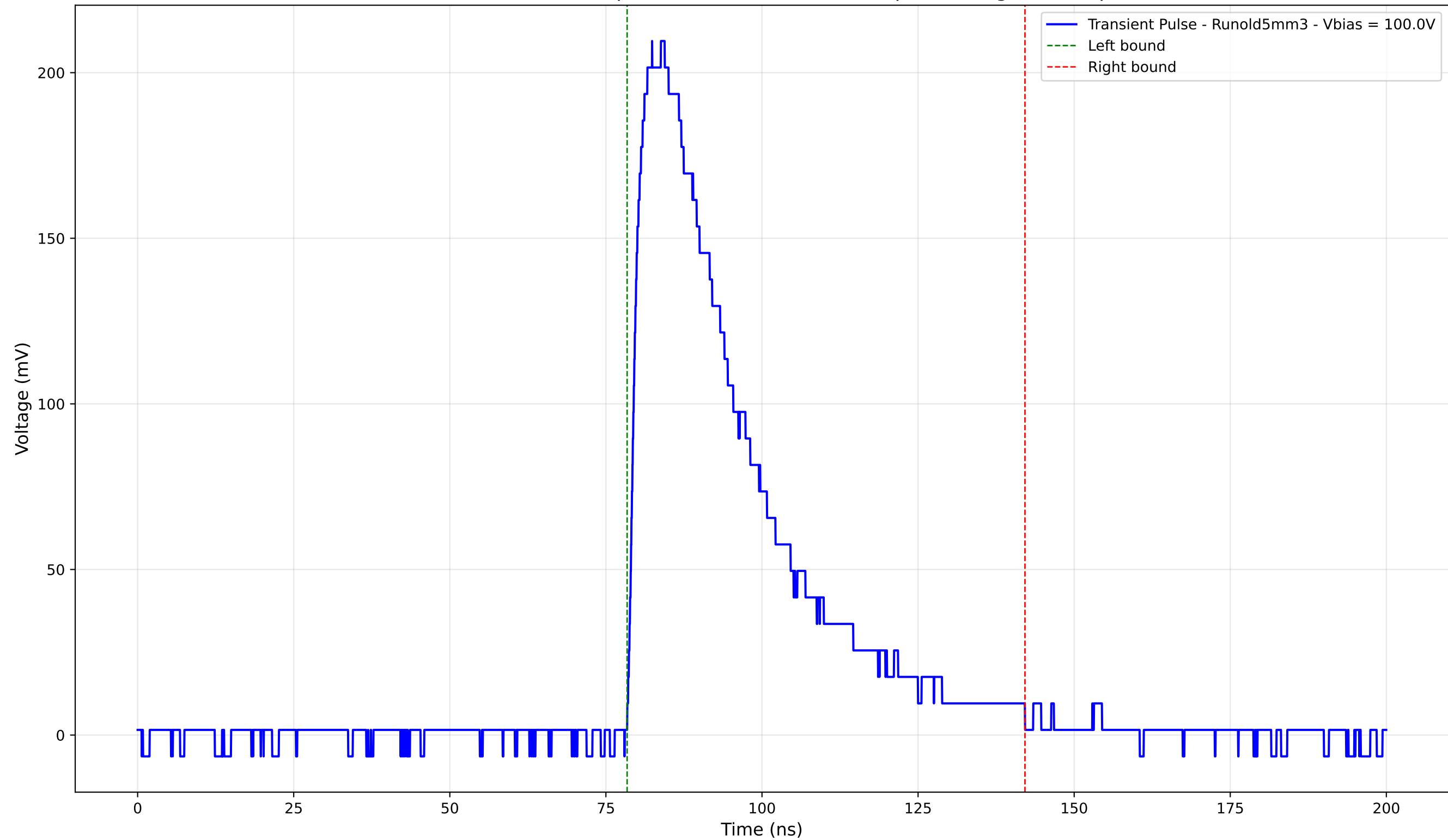
Transient Pulse - Sample: old5 - Position: 1495.0 \mu\text{m} - Charge: 83.60 pC
