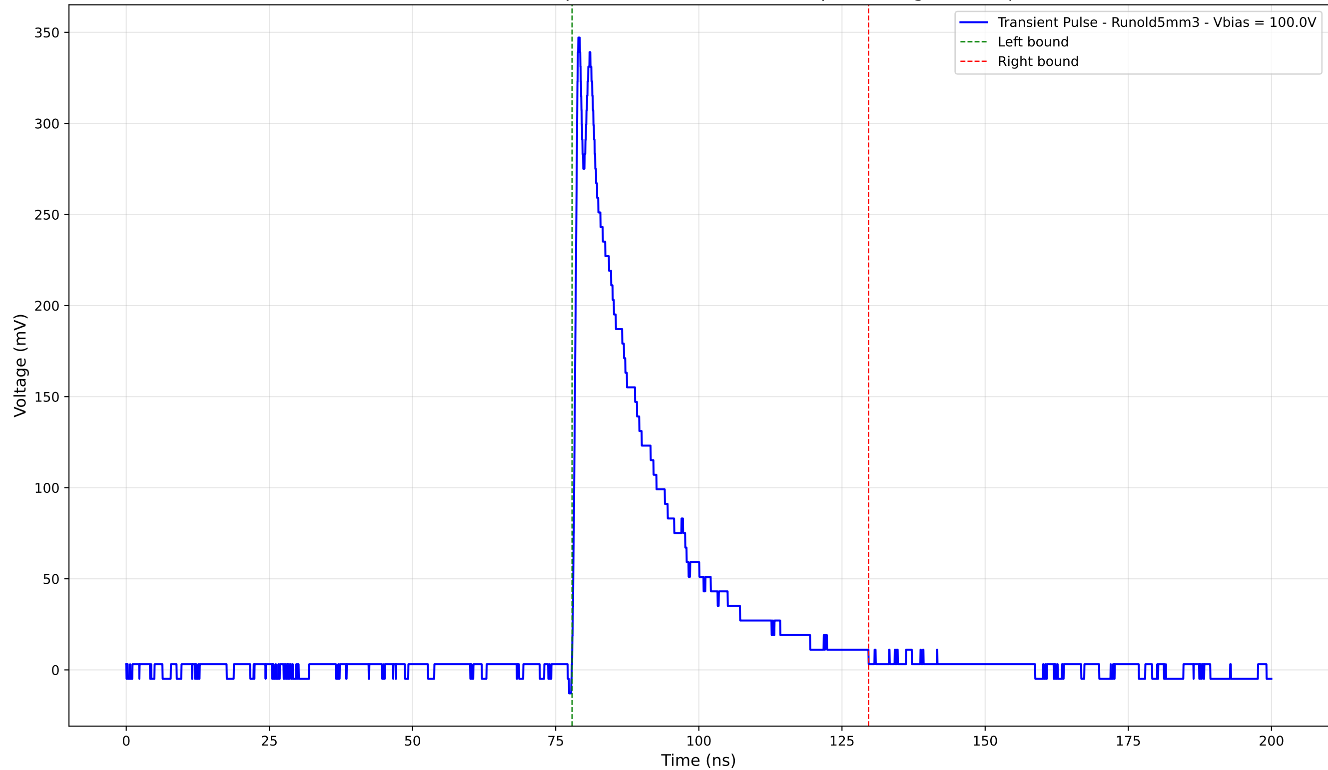
Transient Pulse - Sample: old5 - Position: 3185.0 \mu\text{m} - Charge: 85.26 pC
