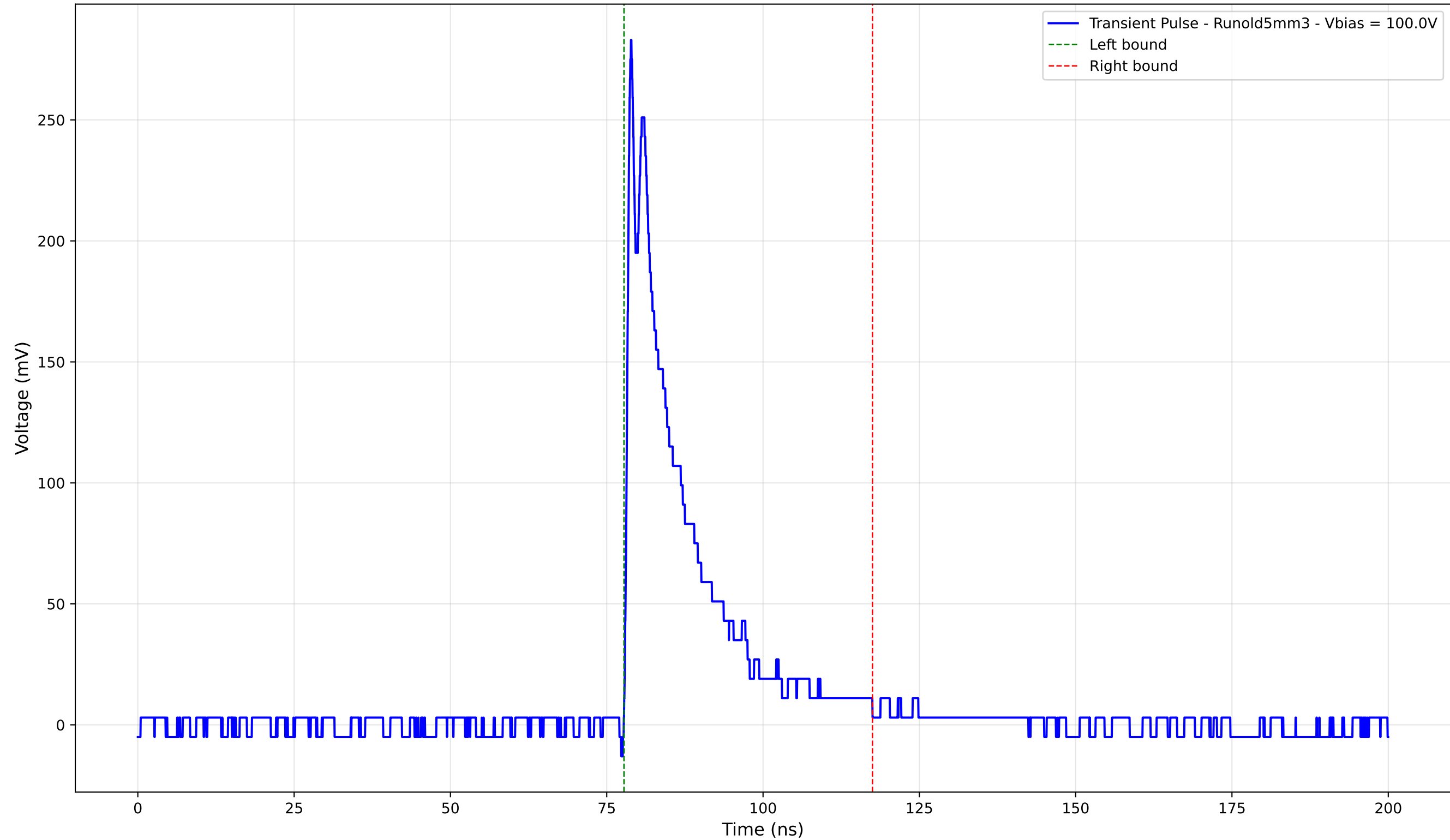
Transient Pulse - Sample: old5 - Position: 3820.0 \mu\text{m} - Charge: 48.86 pC
