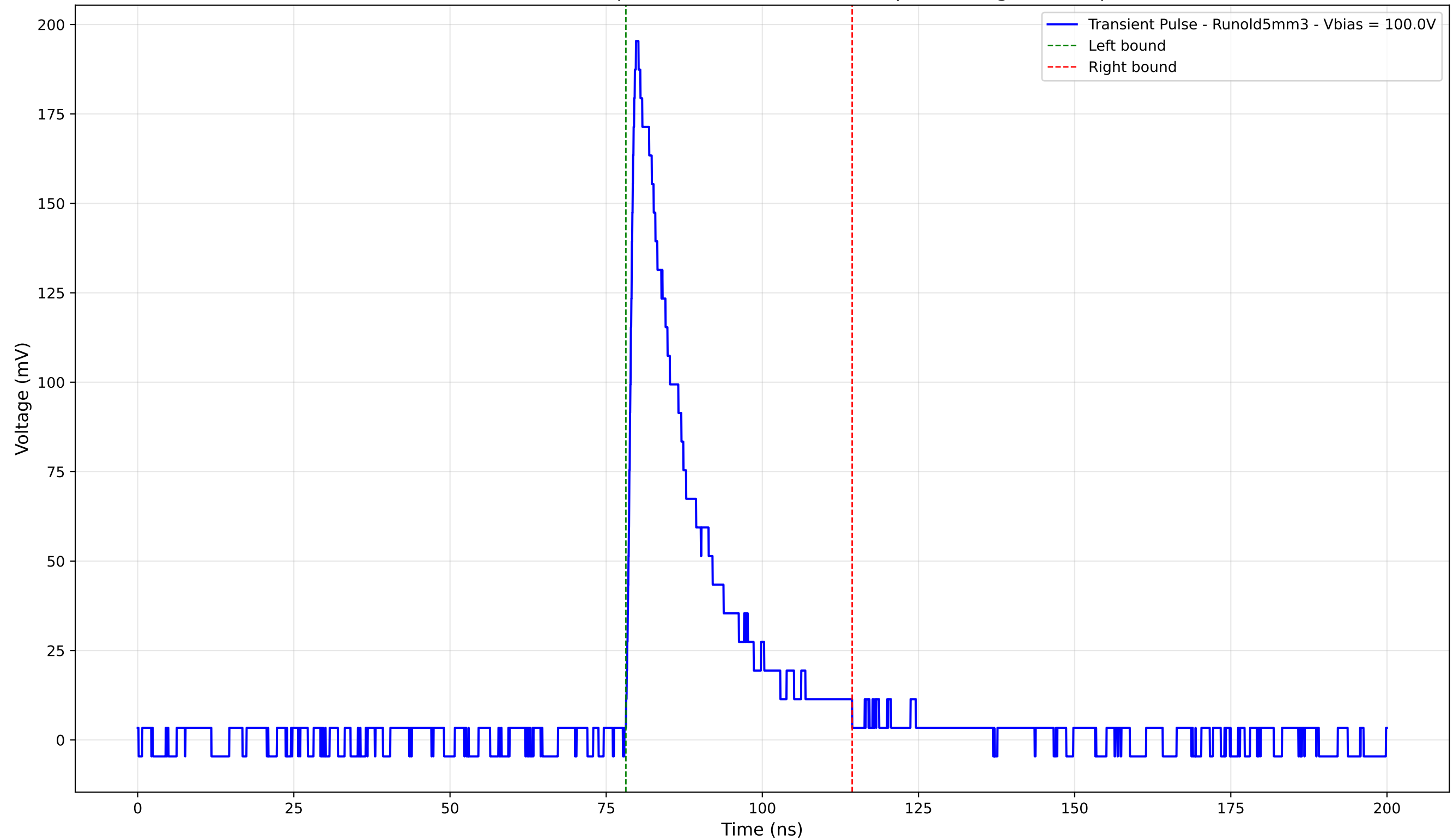
Transient Pulse - Sample: old5 - Position: 4545.0 \mu\text{m} - Charge: 39.13 pC
