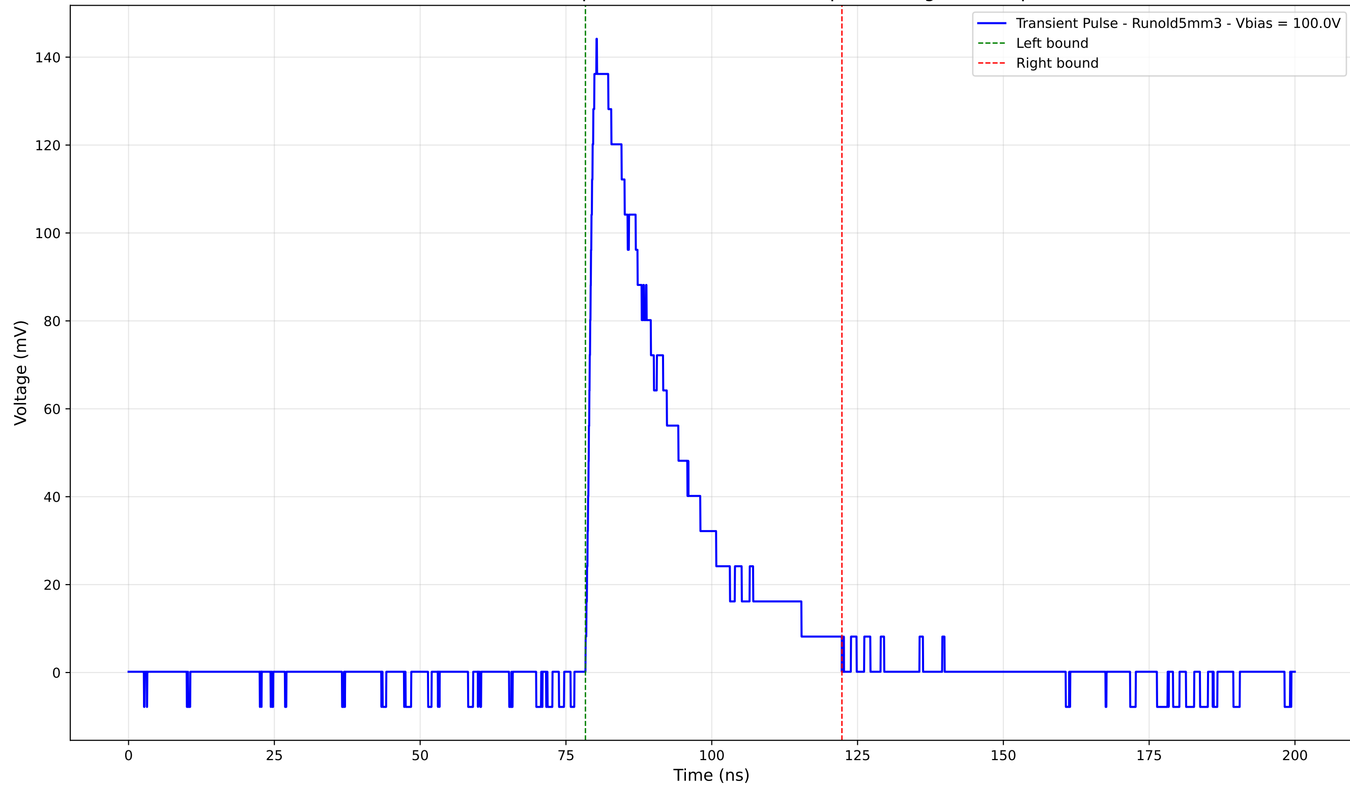
Transient Pulse - Sample: old5 - Position: 885.0 \mu\text{m} - Charge: 41.30 pC
