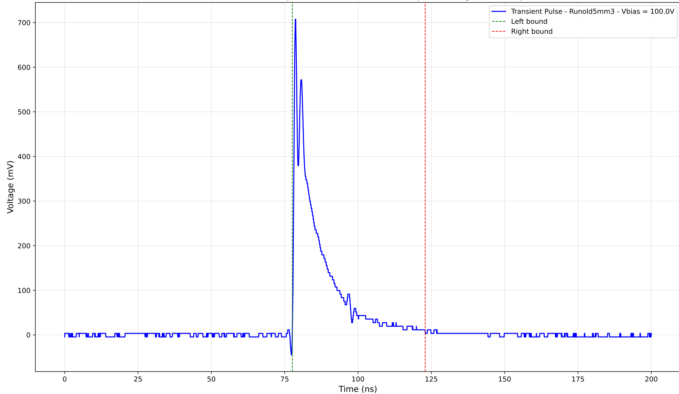
Transient Pulse - Sample: old5 - Position: 3705.0 \mu\text{m} - Charge: 106.21 pC
