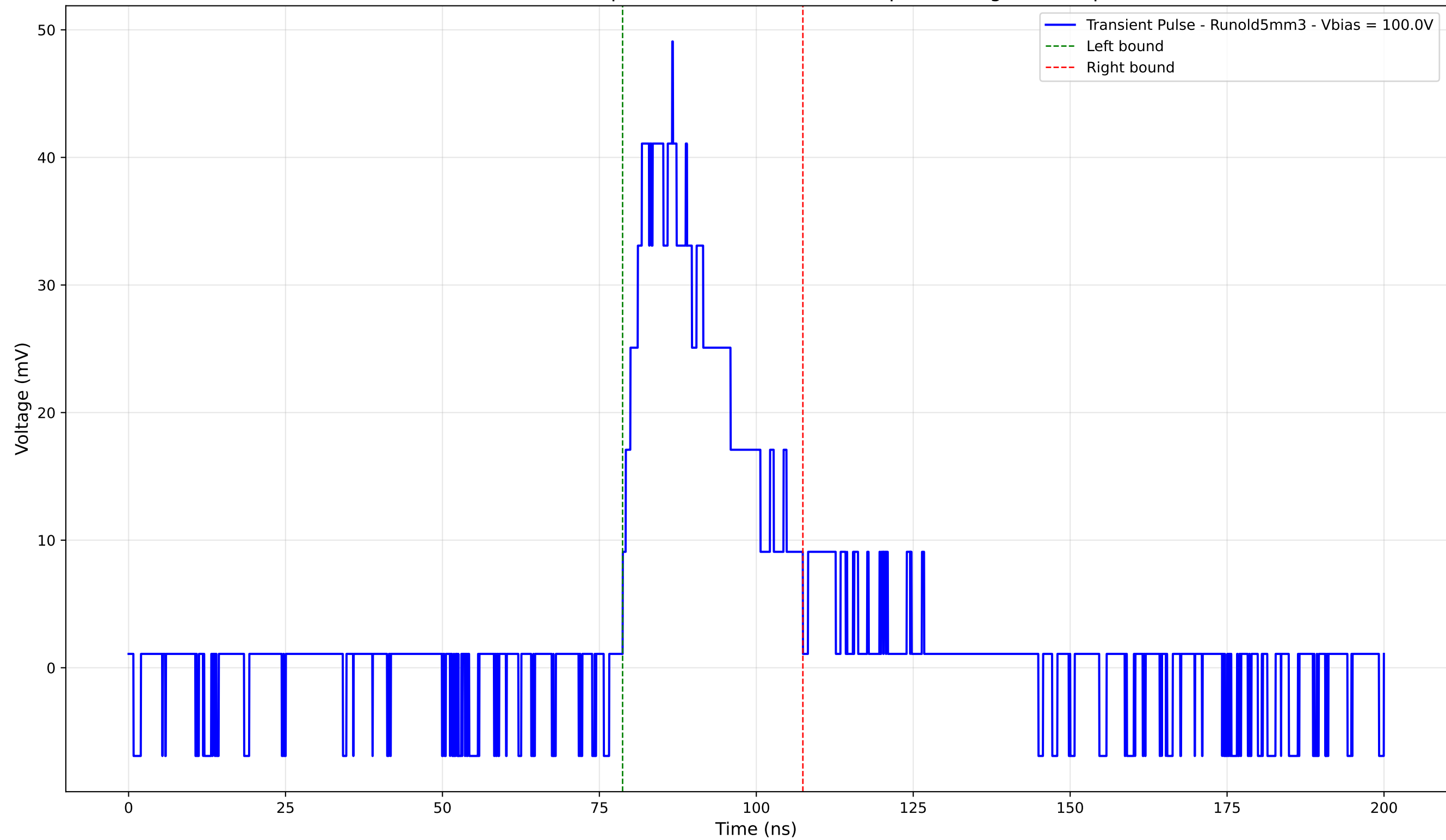
Transient Pulse - Sample: old5 - Position: 2005.0 \mu\text{m} - Charge: 13.71 pC
