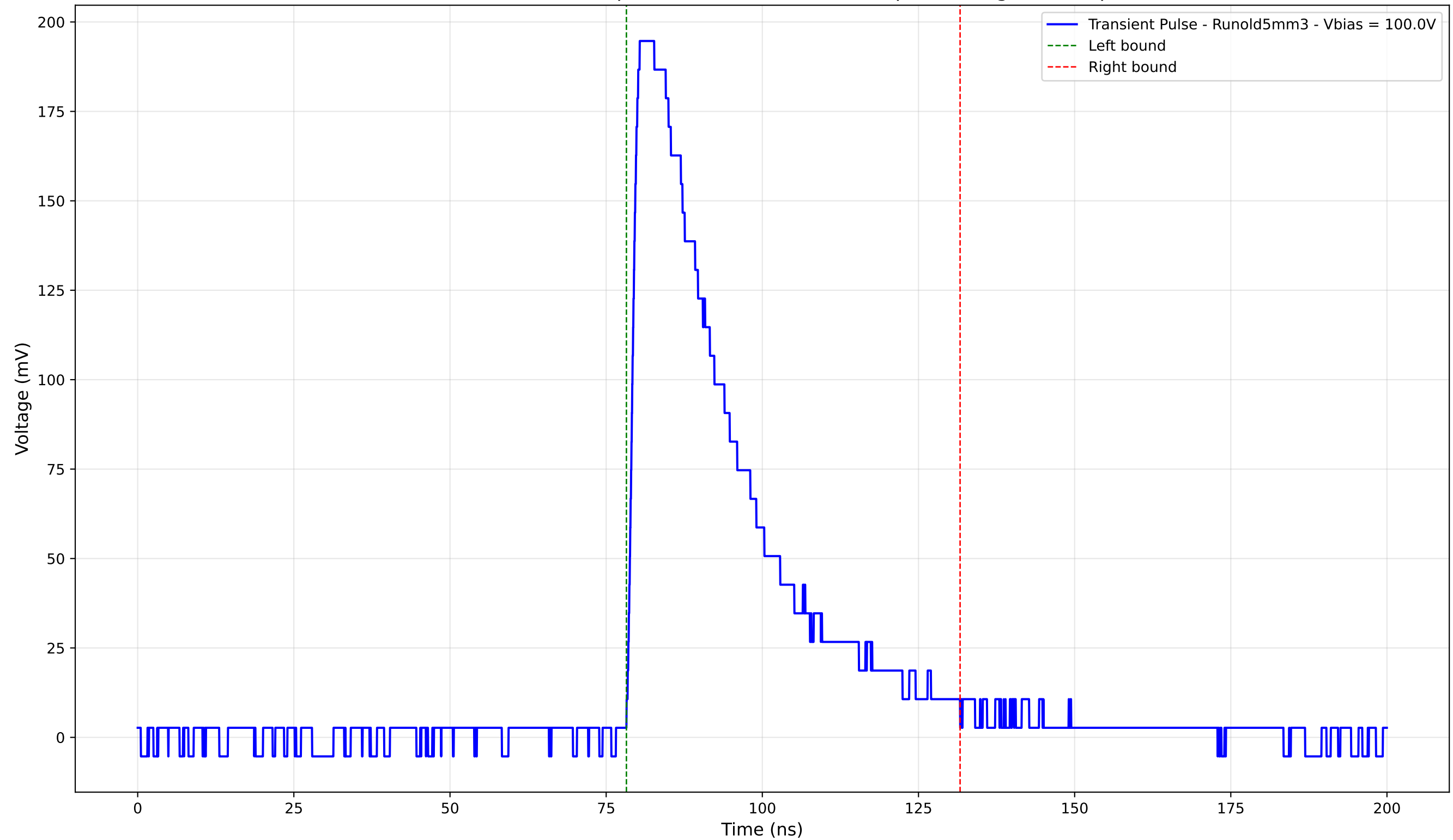
Transient Pulse - Sample: old5 - Position: 1045.0 \mu\text{m} - Charge: 70.52 pC
