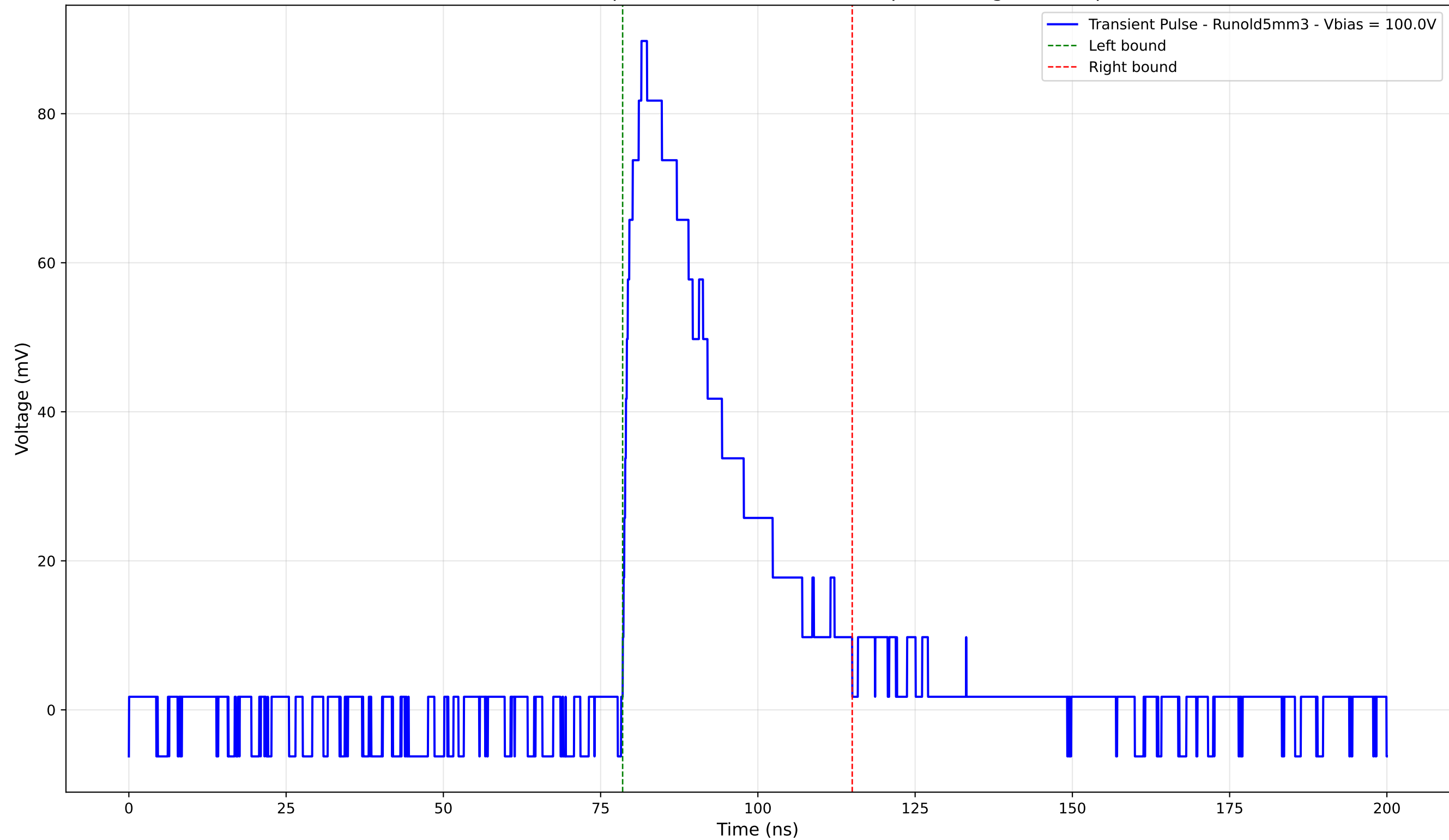
Transient Pulse - Sample: old5 - Position: 2725.0 \mu\text{m} - Charge: 28.22 pC
