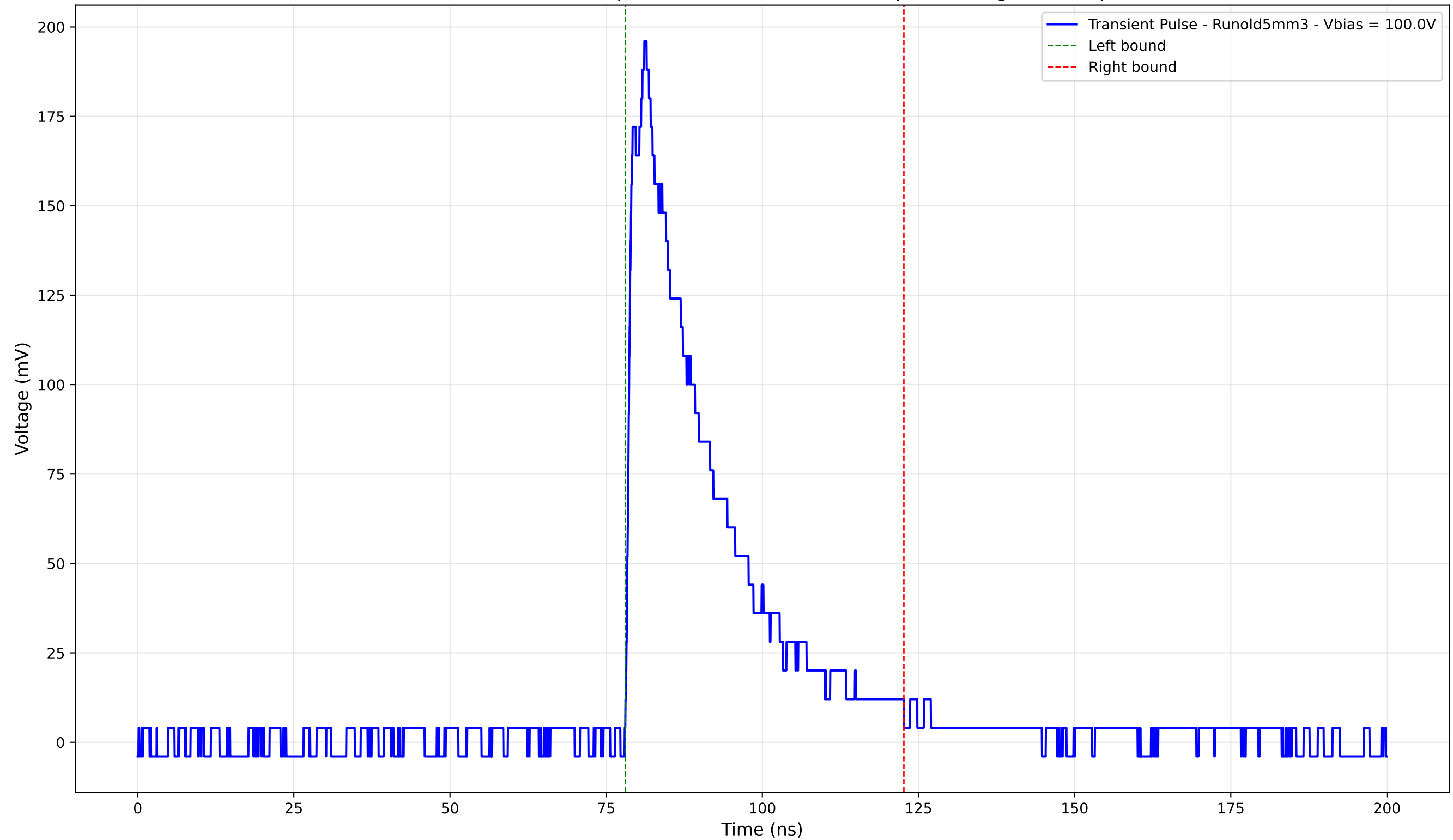
Transient Pulse - Sample: old5 - Position: 3045.0 \mu\text{m} - Charge: 53.44 pC
