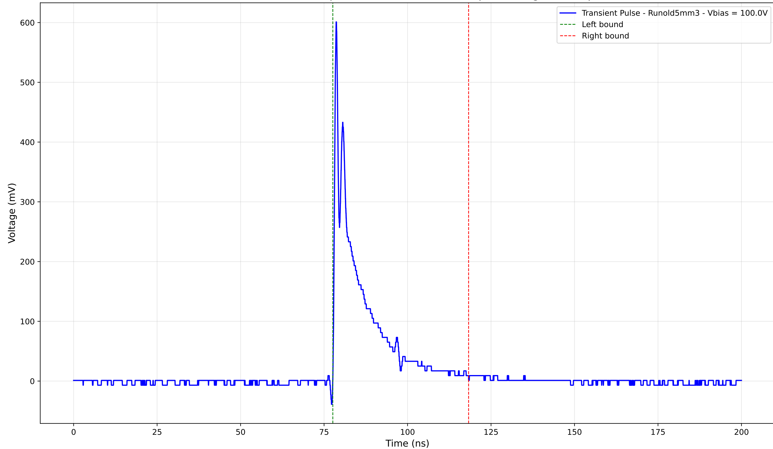
Transient Pulse - Sample: old5 - Position: 3495.0 \mu\text{m} - Charge: 76.57 pC
