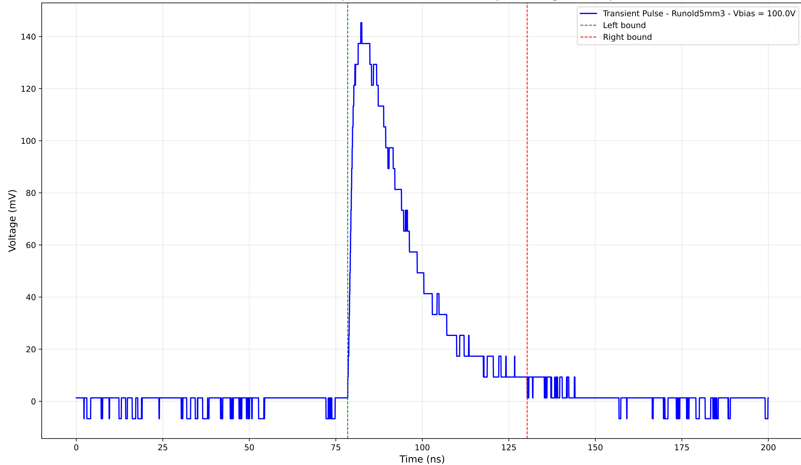
Transient Pulse - Sample: old5 - Position: 1330.0 \mu\text{m} - Charge: 53.44 pC
