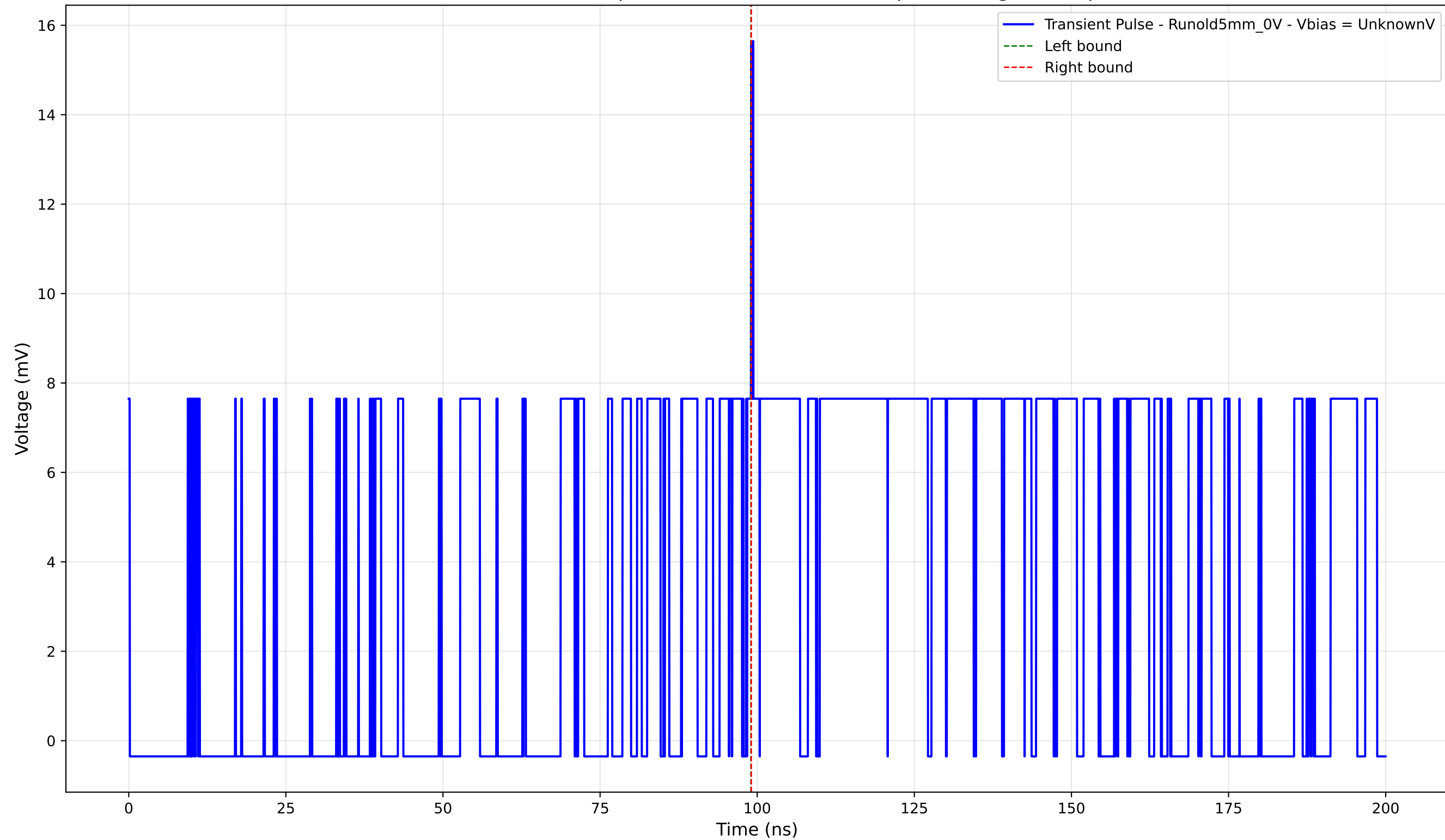
Transient Pulse - Sample: old5 - Position: 4505.0 \mu\text{m} - Charge: 0.02 pC
