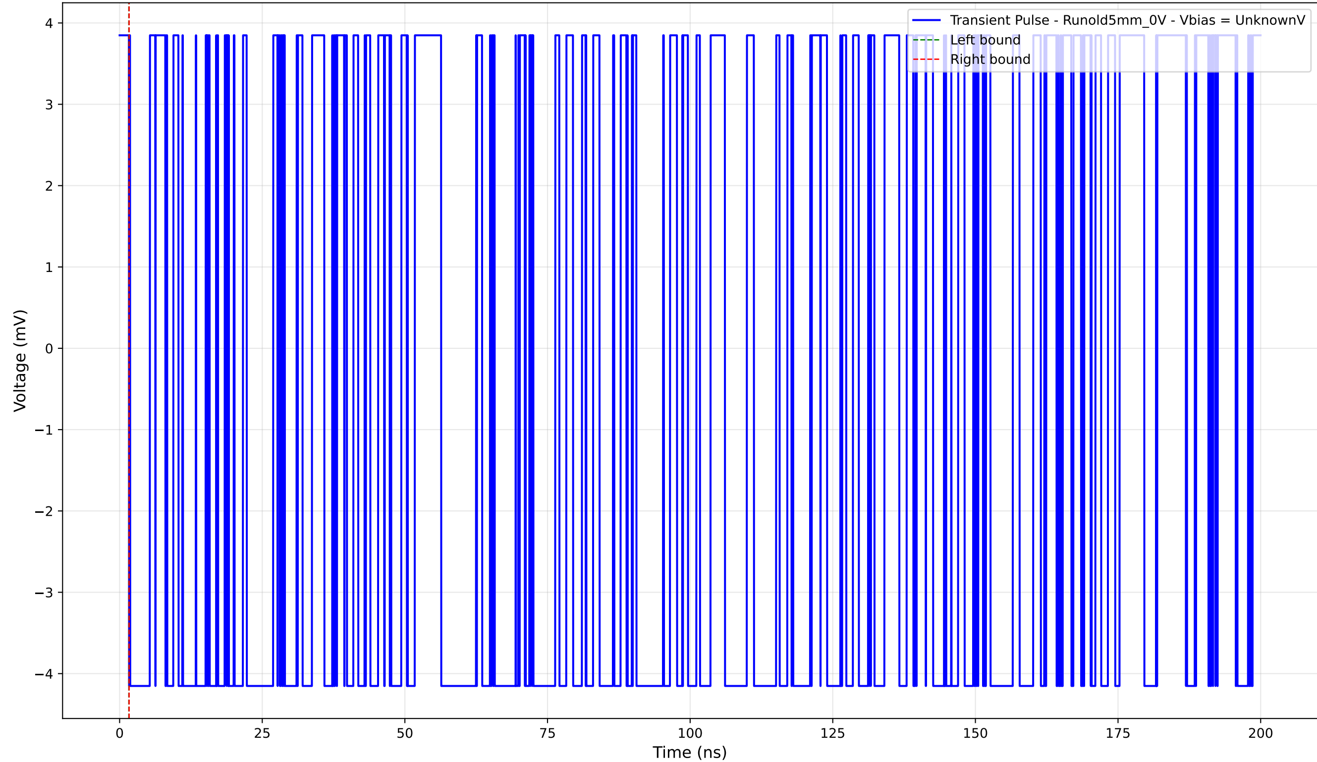
Transient Pulse - Sample: old5 - Position: 3270.0 \mu\text{m} - Charge: -0.00 pC
