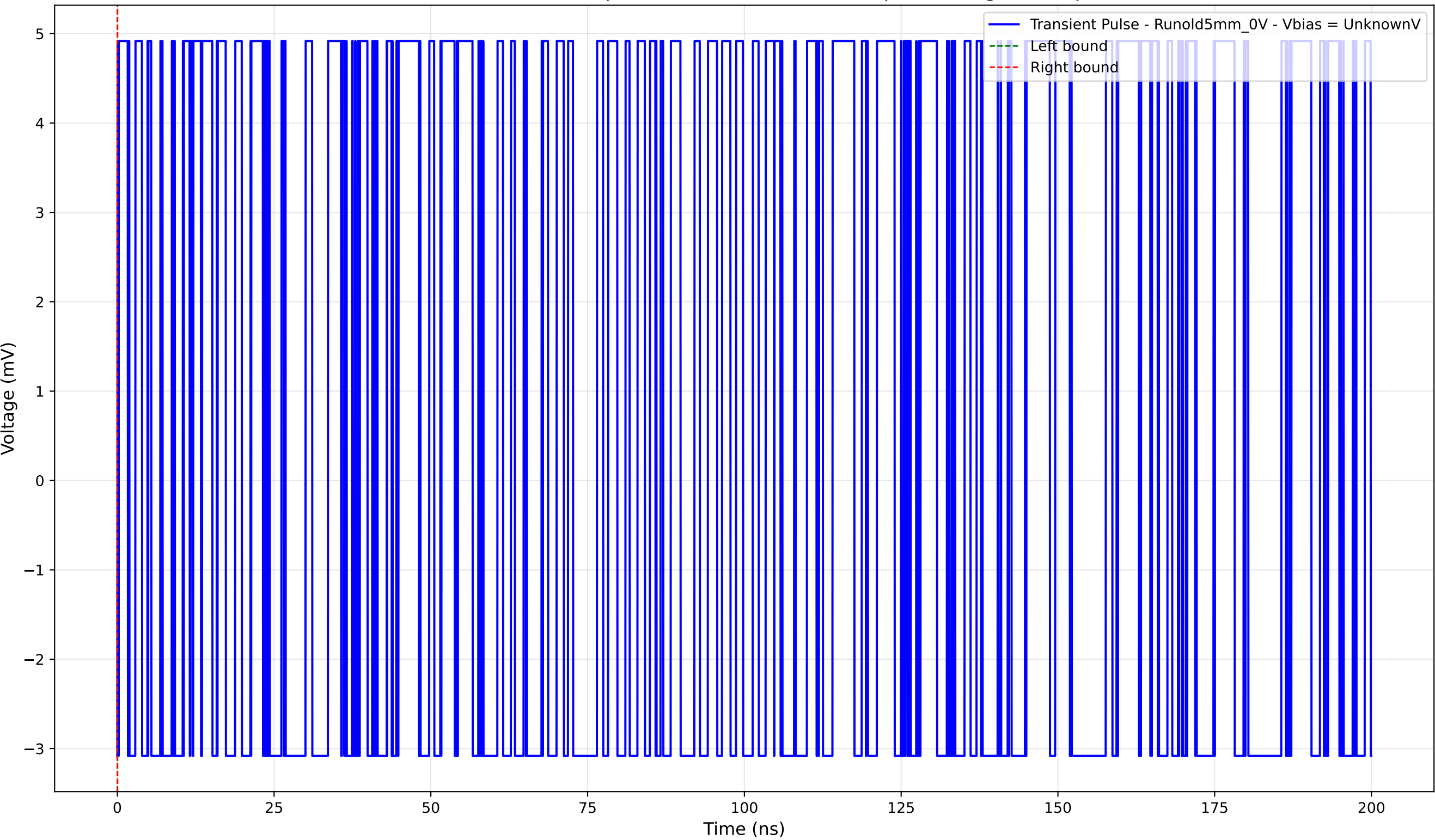
Transient Pulse - Sample: old5 - Position: 4275.0 \mu\text{m} - Charge: 0.00 pC
