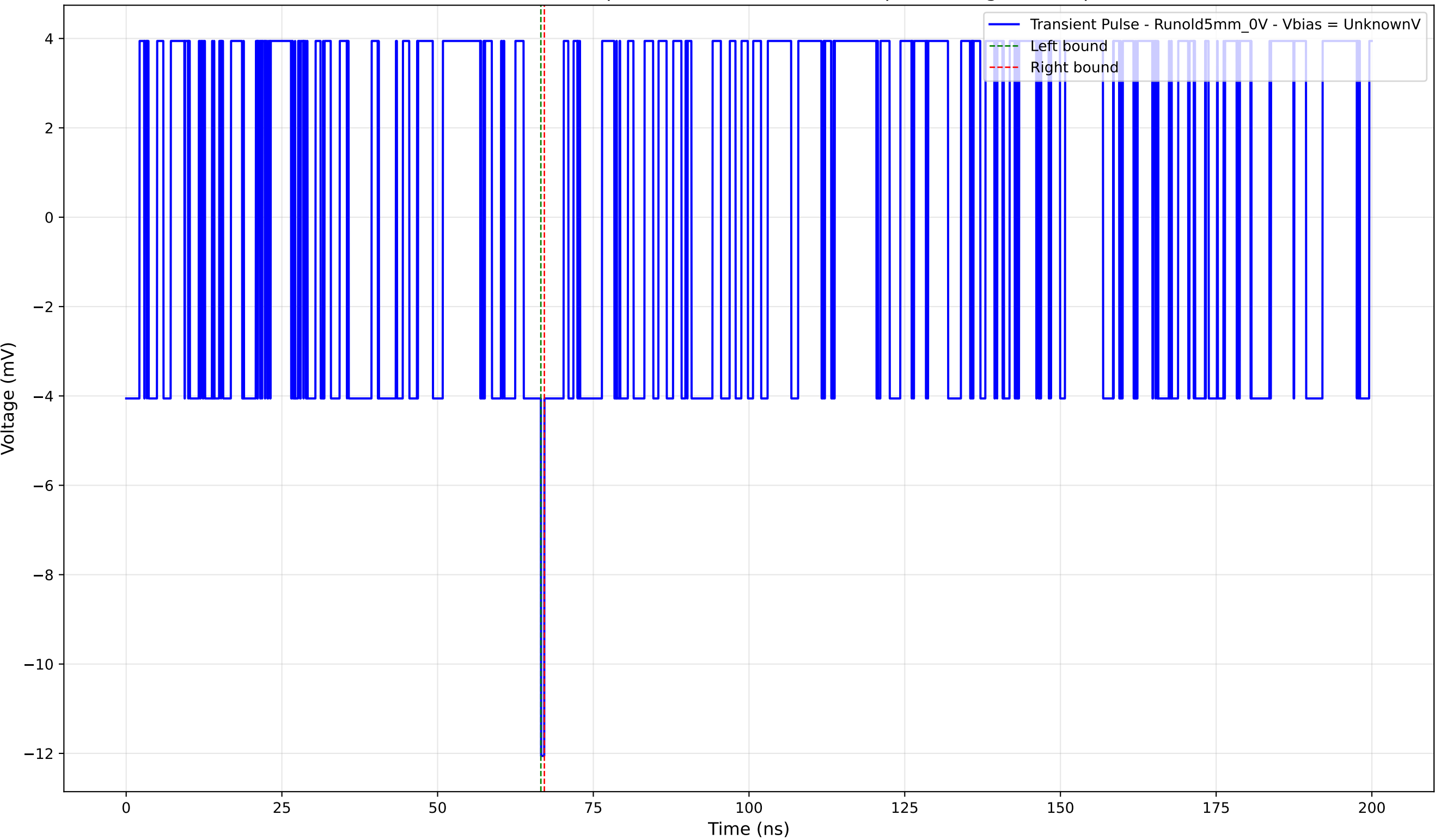
Transient Pulse - Sample: old5 - Position: 3925.0 \mu\text{m} - Charge: -0.13 pC
