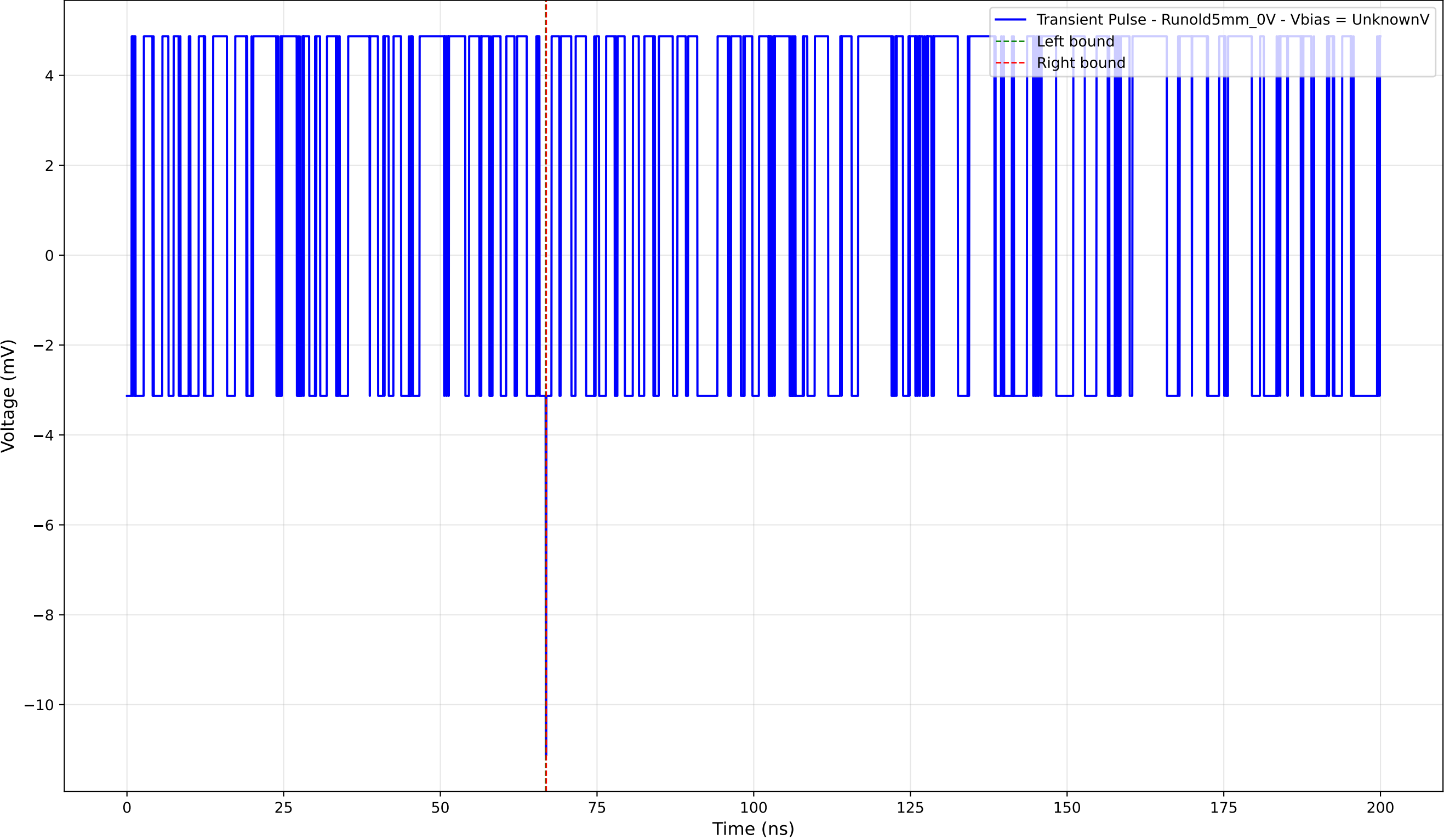
Transient Pulse - Sample: old5 - Position: 1840.0 \mu\text{m} - Charge: -0.02 pC
