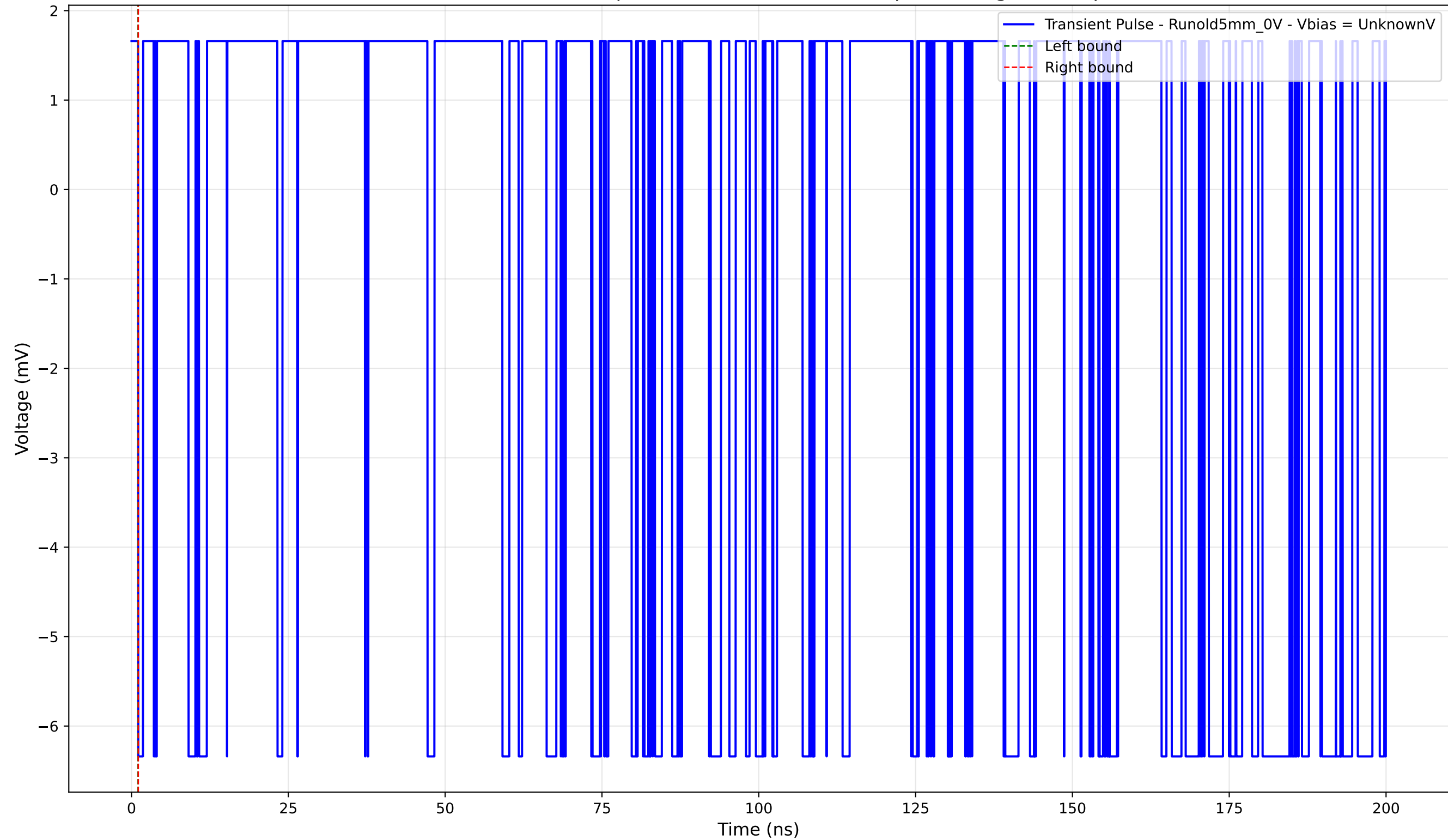
Transient Pulse - Sample: old5 - Position: 4060.0 \mu\text{m} - Charge: -0.00 pC
