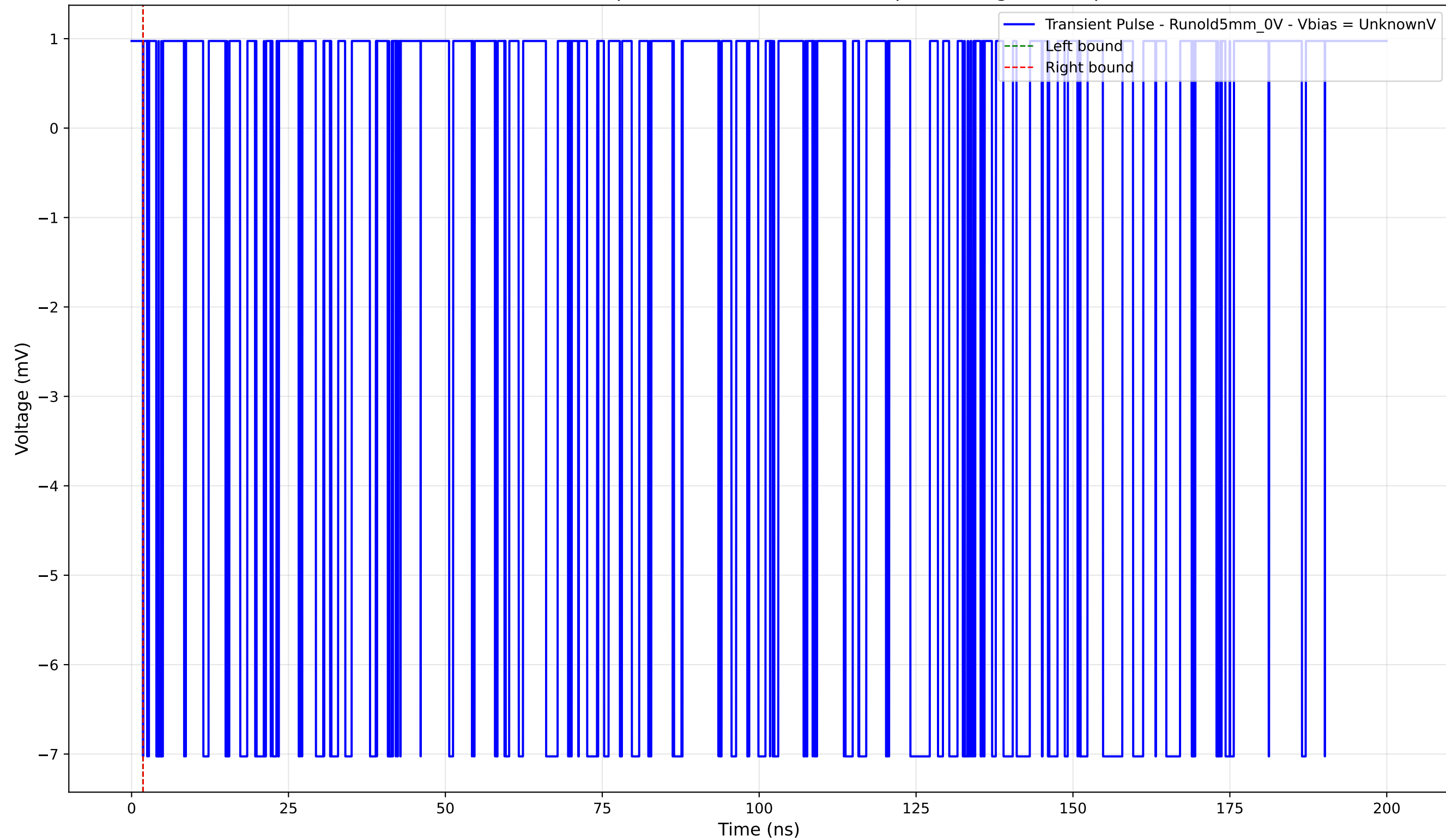
Transient Pulse - Sample: old5 - Position: 1310.0 \mu\text{m} - Charge: -0.00 pC
