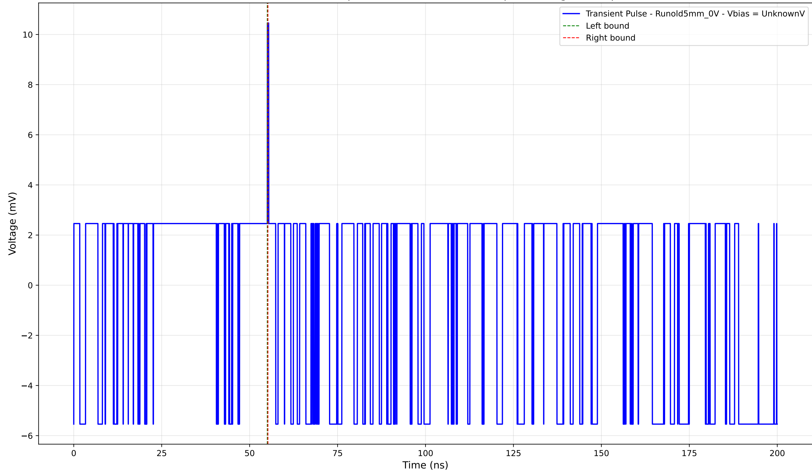
Transient Pulse - Sample: old5 - Position: 1445.0 \mu\text{m} - Charge: 0.03 pC
