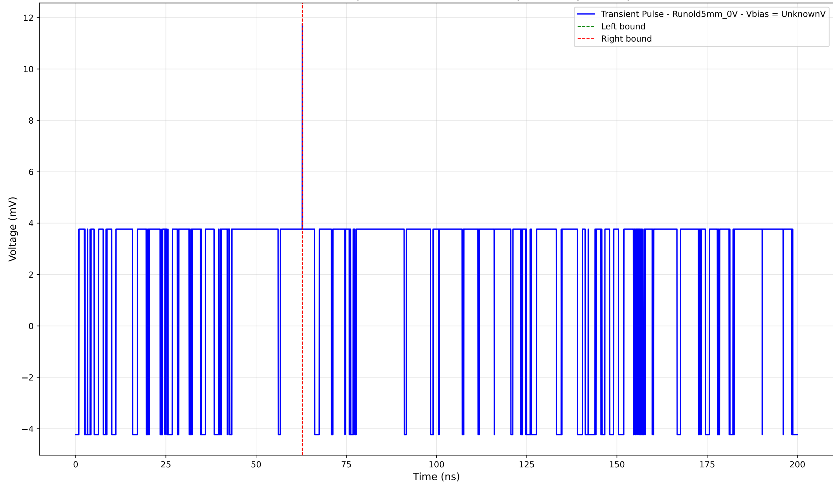
Transient Pulse - Sample: old5 - Position: 5000.0 \mu\text{m} - Charge: 0.02 pC
