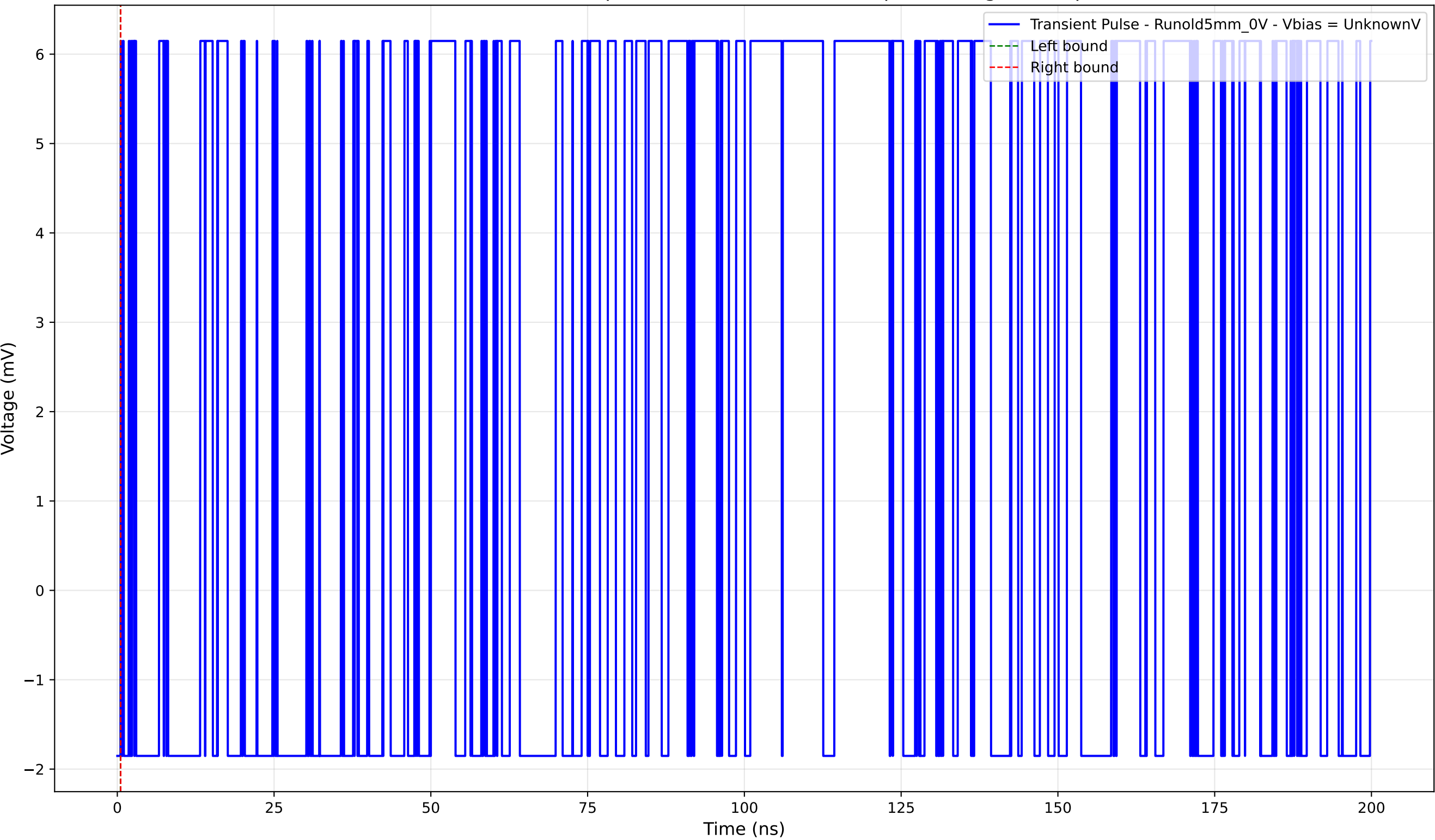
Transient Pulse - Sample: old5 - Position: 2005.0 \mu\text{m} - Charge: 0.00 pC
