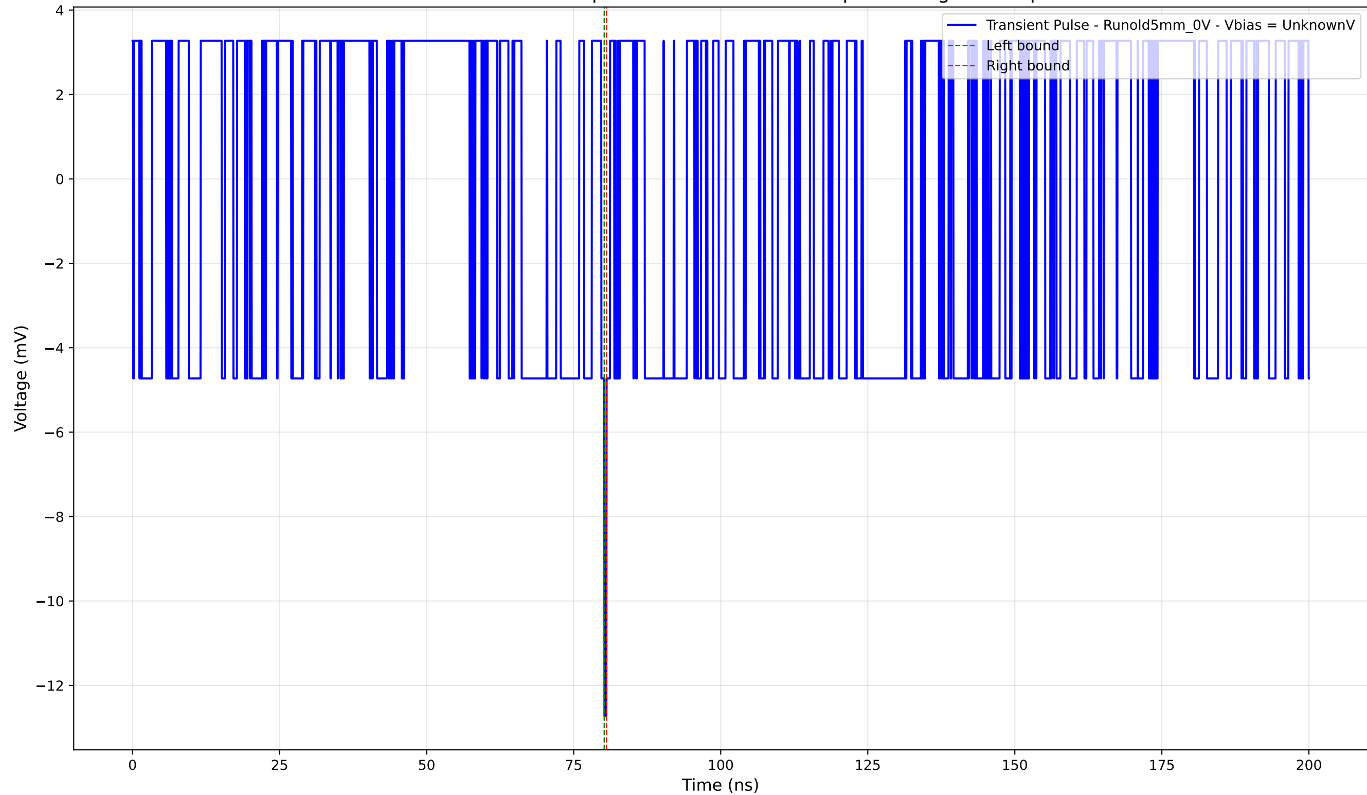
Transient Pulse - Sample: old5 - Position: 300.0 \mu\text{m} - Charge: -0.09 pC
