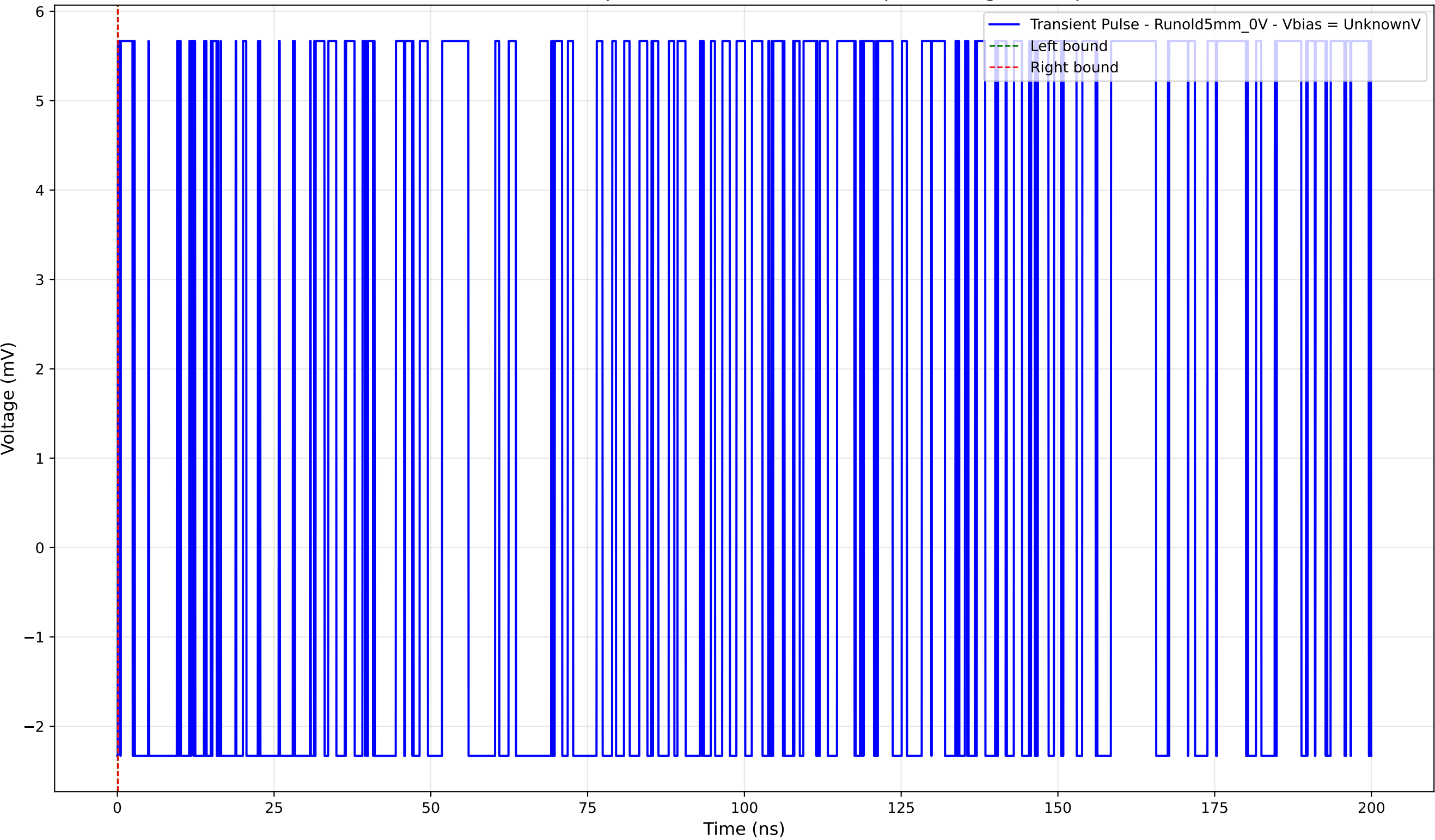
Transient Pulse - Sample: old5 - Position: 4725.0 \mu\text{m} - Charge: 0.00 pC
