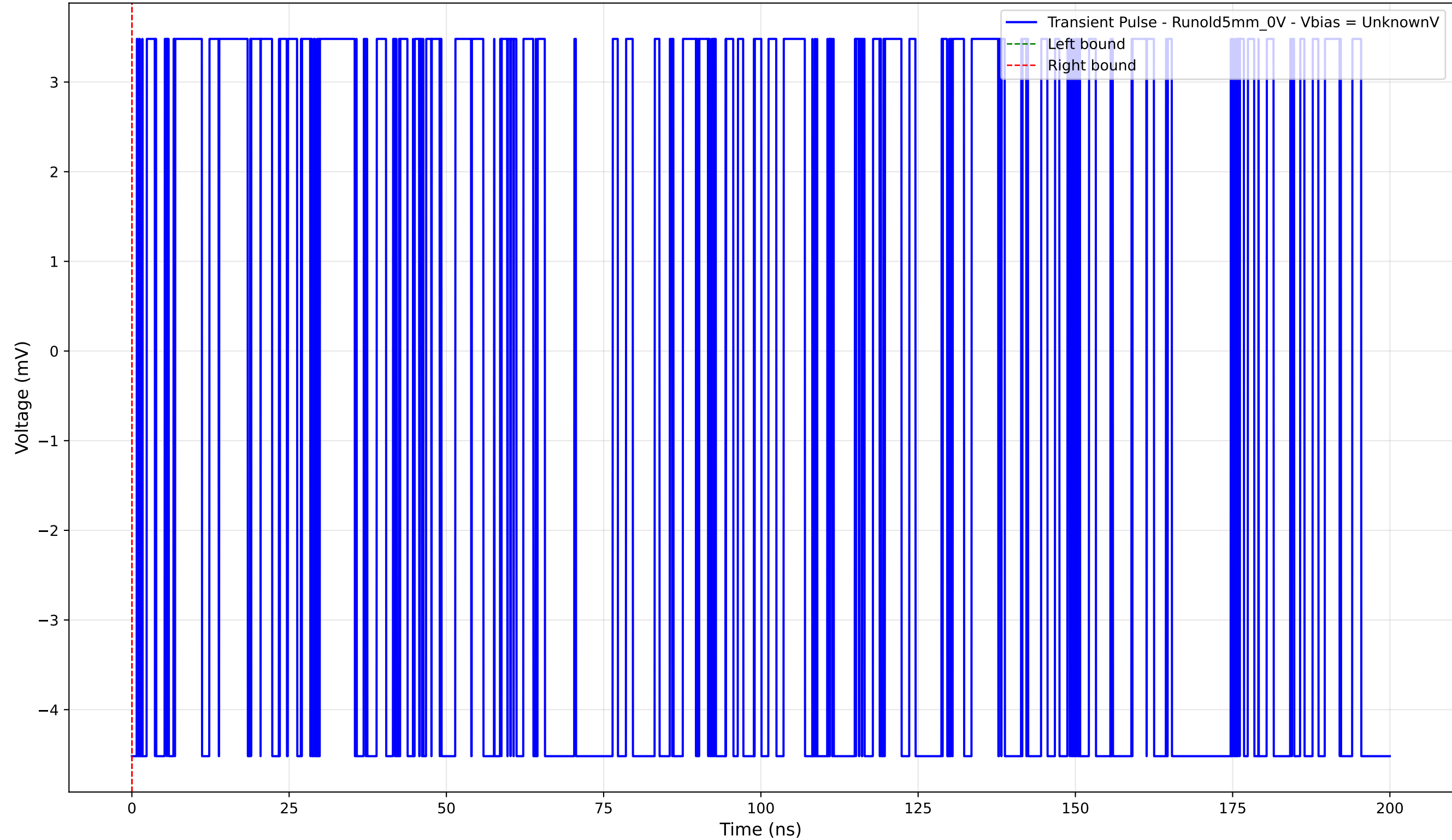
Transient Pulse - Sample: old5 - Position: 2605.0 \mu\text{m} - Charge: -0.00 pC
