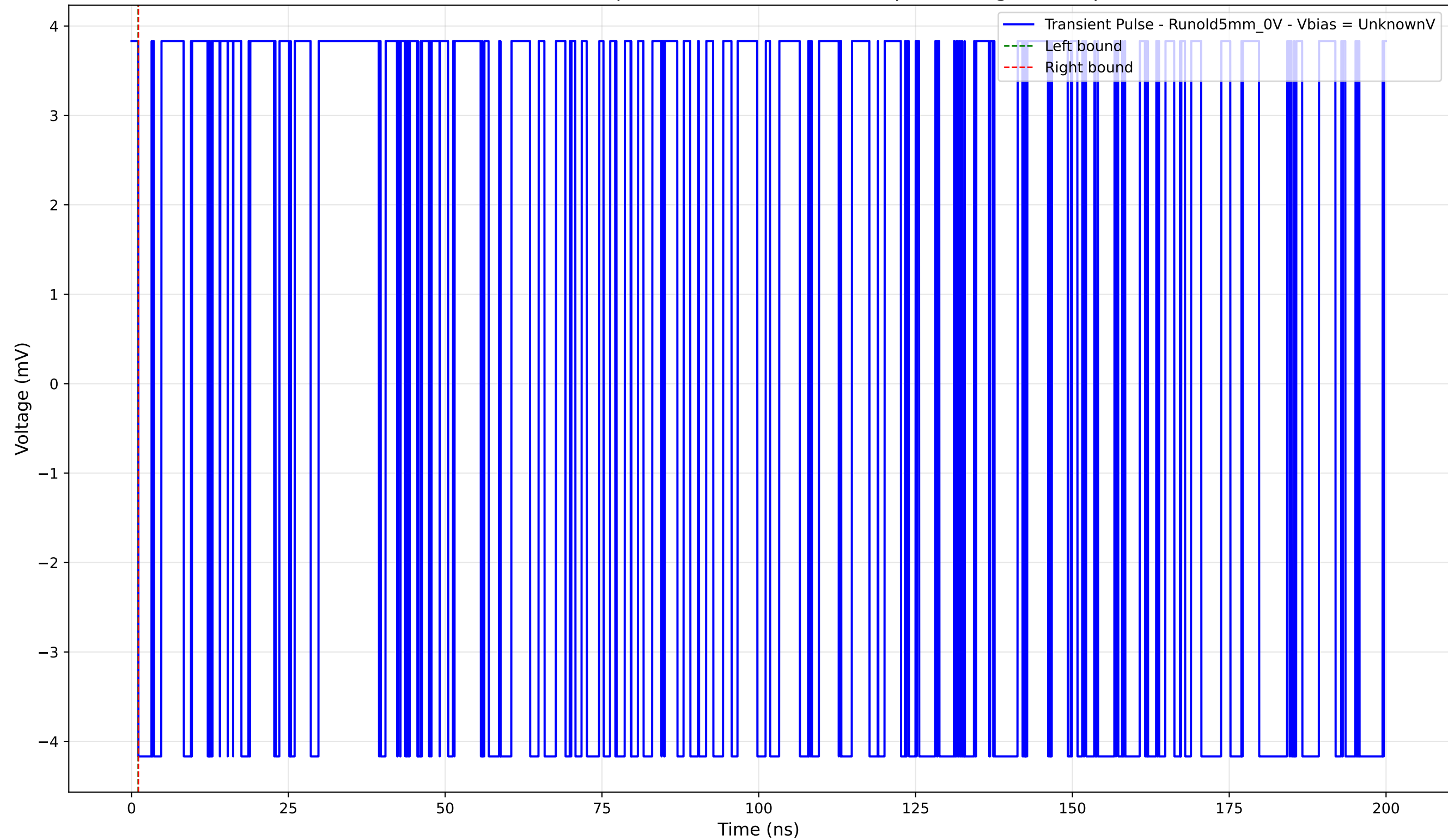
Transient Pulse - Sample: old5 - Position: 2060.0 \mu\text{m} - Charge: -0.00 pC
