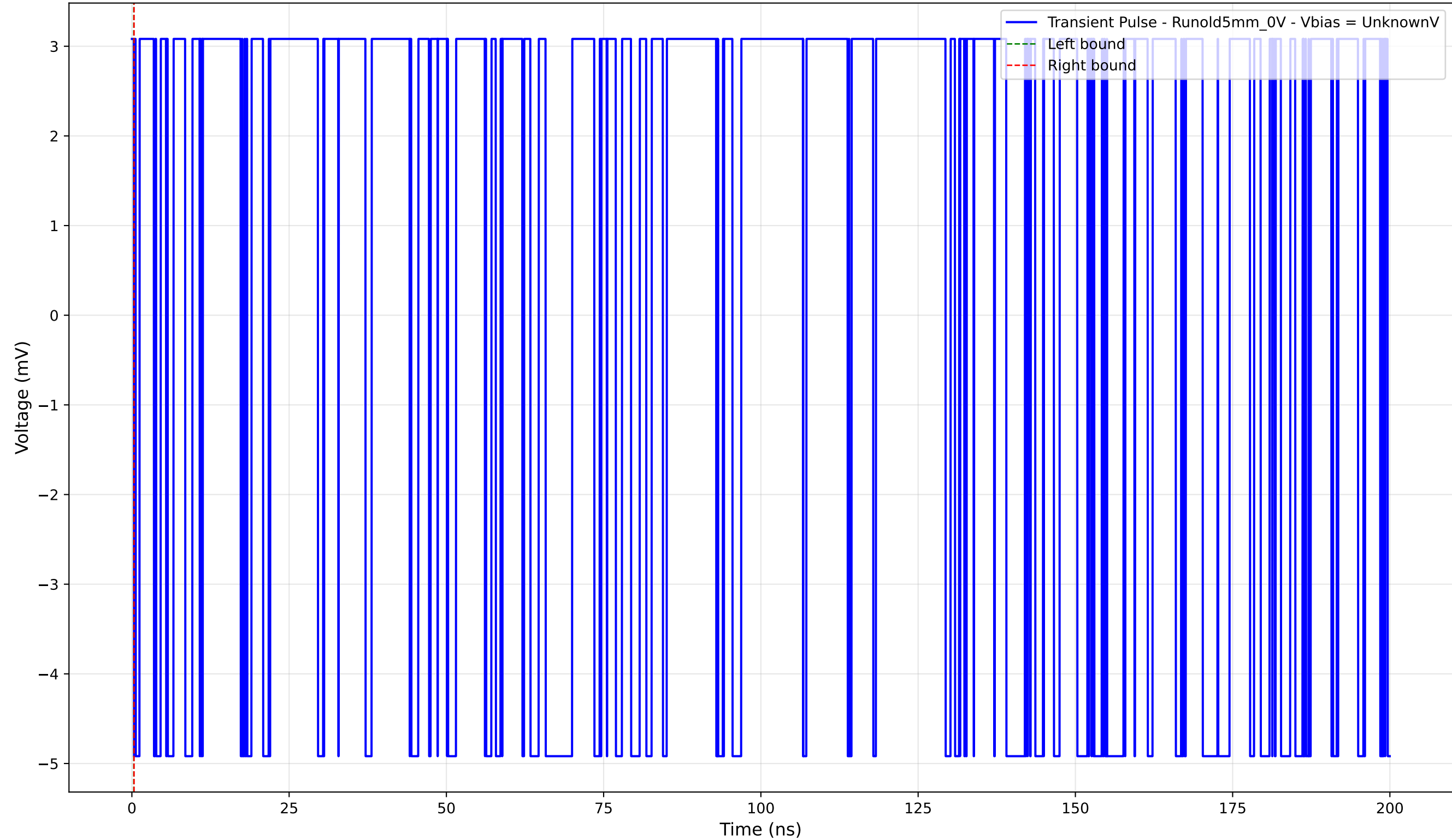
Transient Pulse - Sample: old5 - Position: 3790.0 \mu\text{m} - Charge: -0.00 pC
