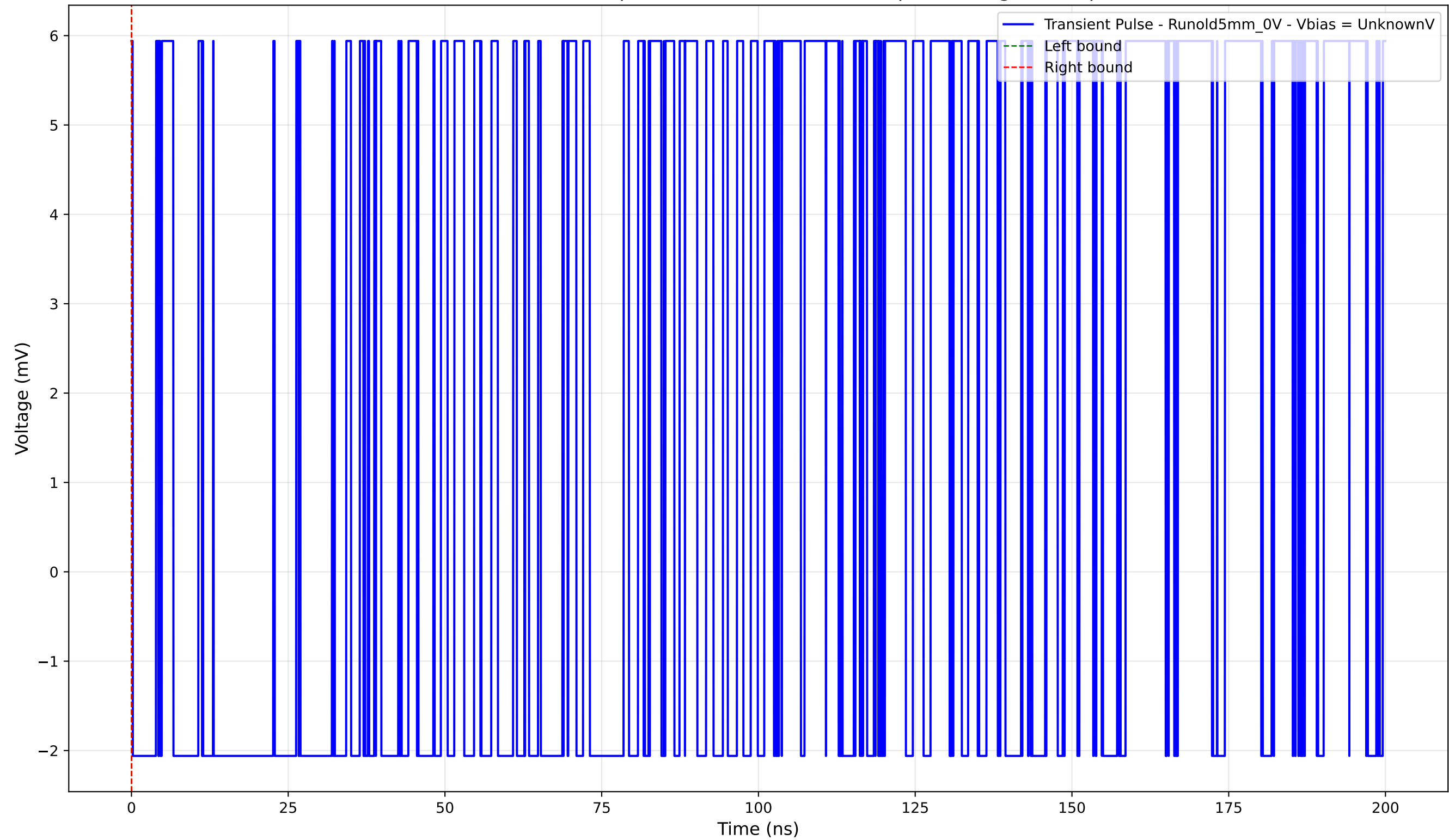
Transient Pulse - Sample: old5 - Position: 2695.0 \mu\text{m} - Charge: 0.00 pC
