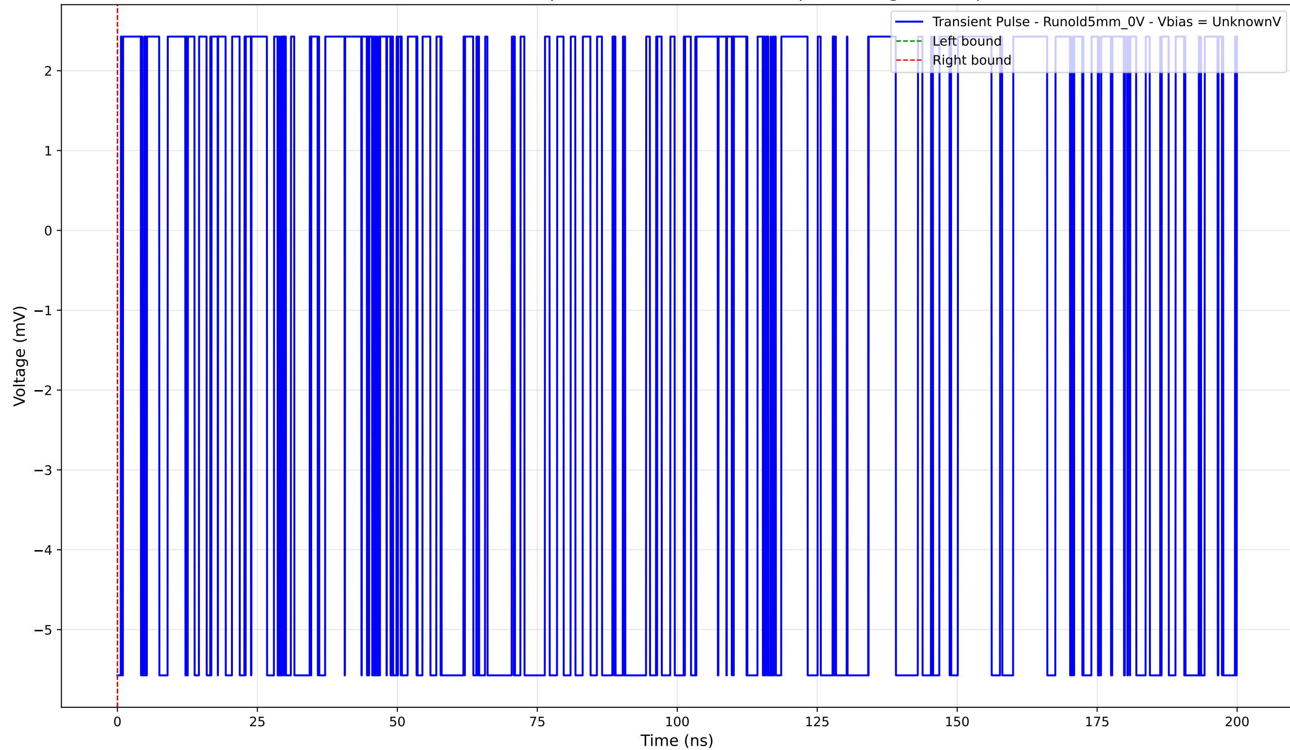
Transient Pulse - Sample: old5 - Position: 2325.0 \mu\text{m} - Charge: -0.00 pC
