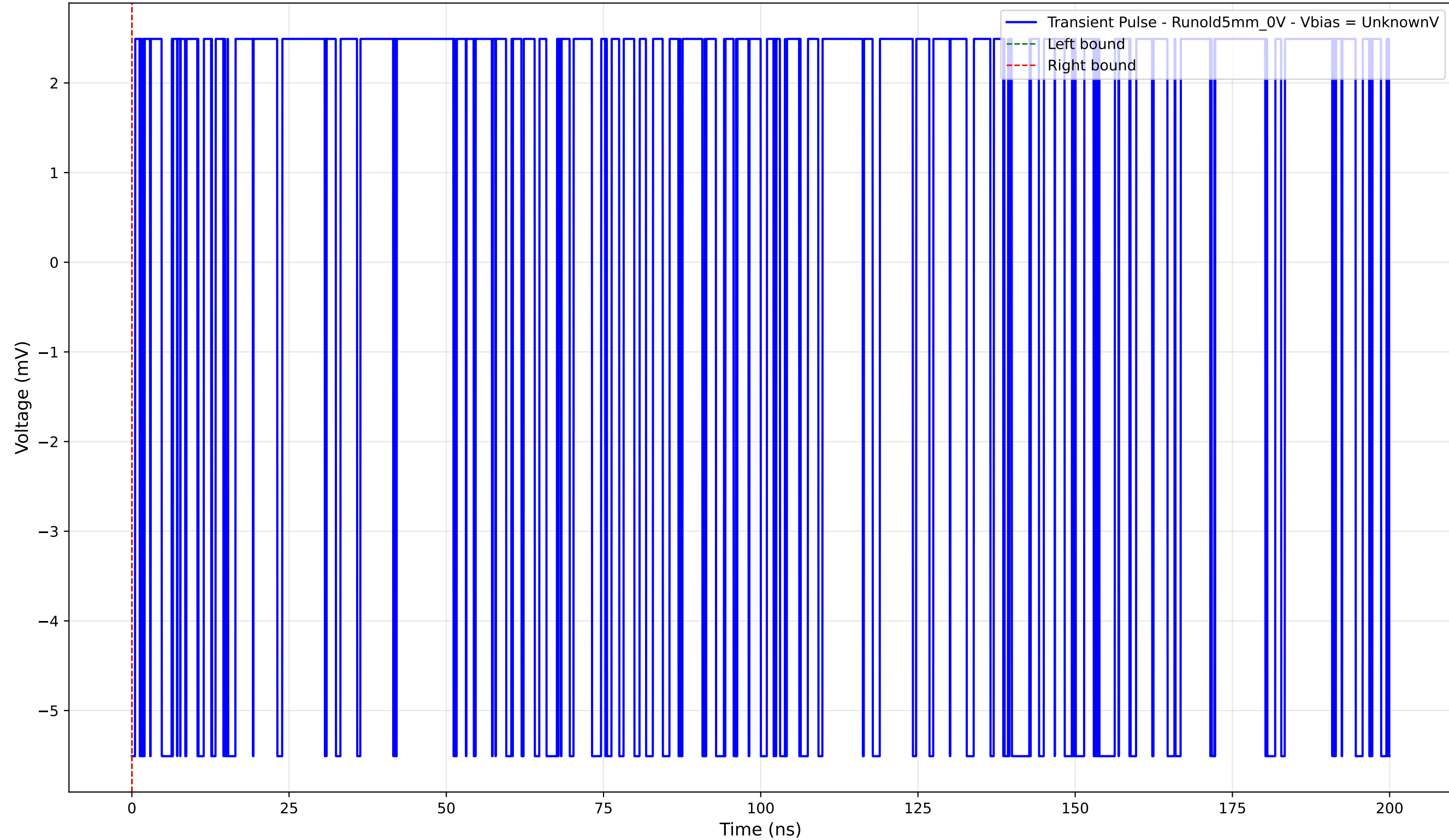
Transient Pulse - Sample: old5 - Position: 1085.0 \mu\text{m} - Charge: -0.00 pC
