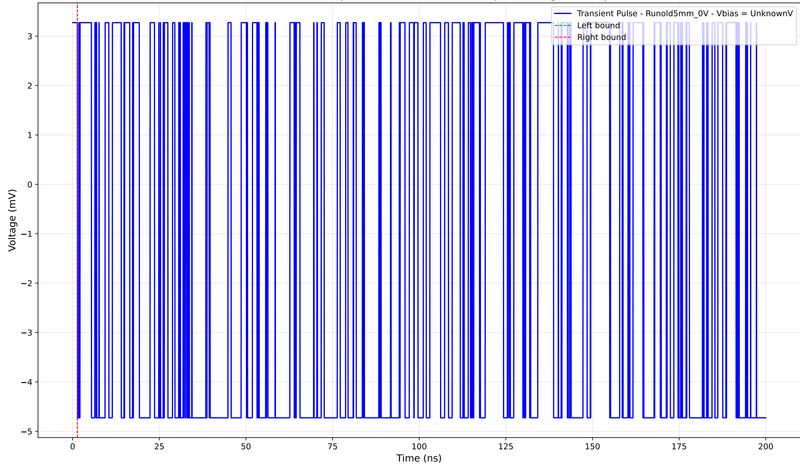
Transient Pulse - Sample: old5 - Position: 2715.0 \mu\text{m} - Charge: -0.00 pC
