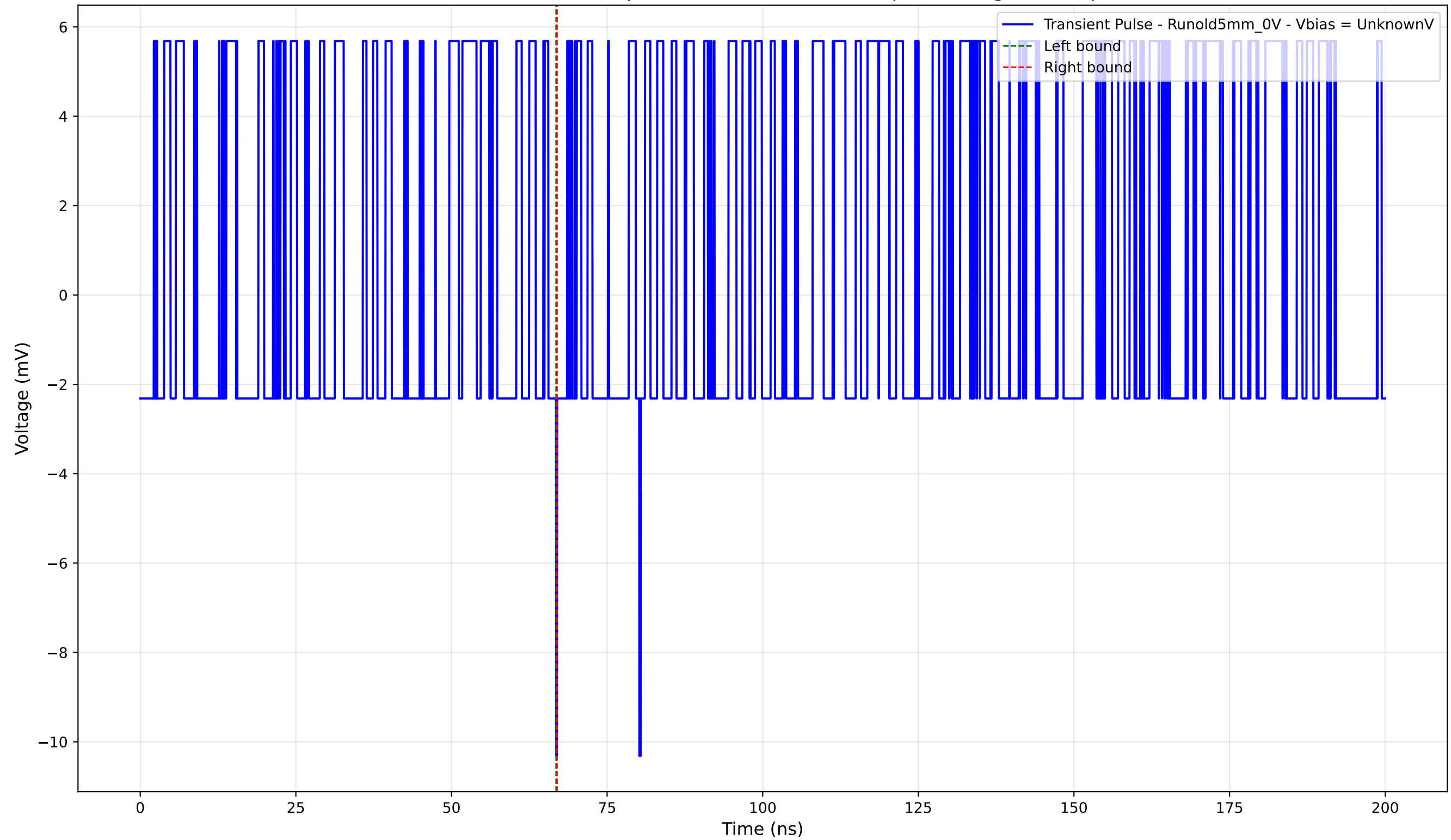
Transient Pulse - Sample: old5 - Position: 115.0 \mu\text{m} - Charge: -0.03 pC
