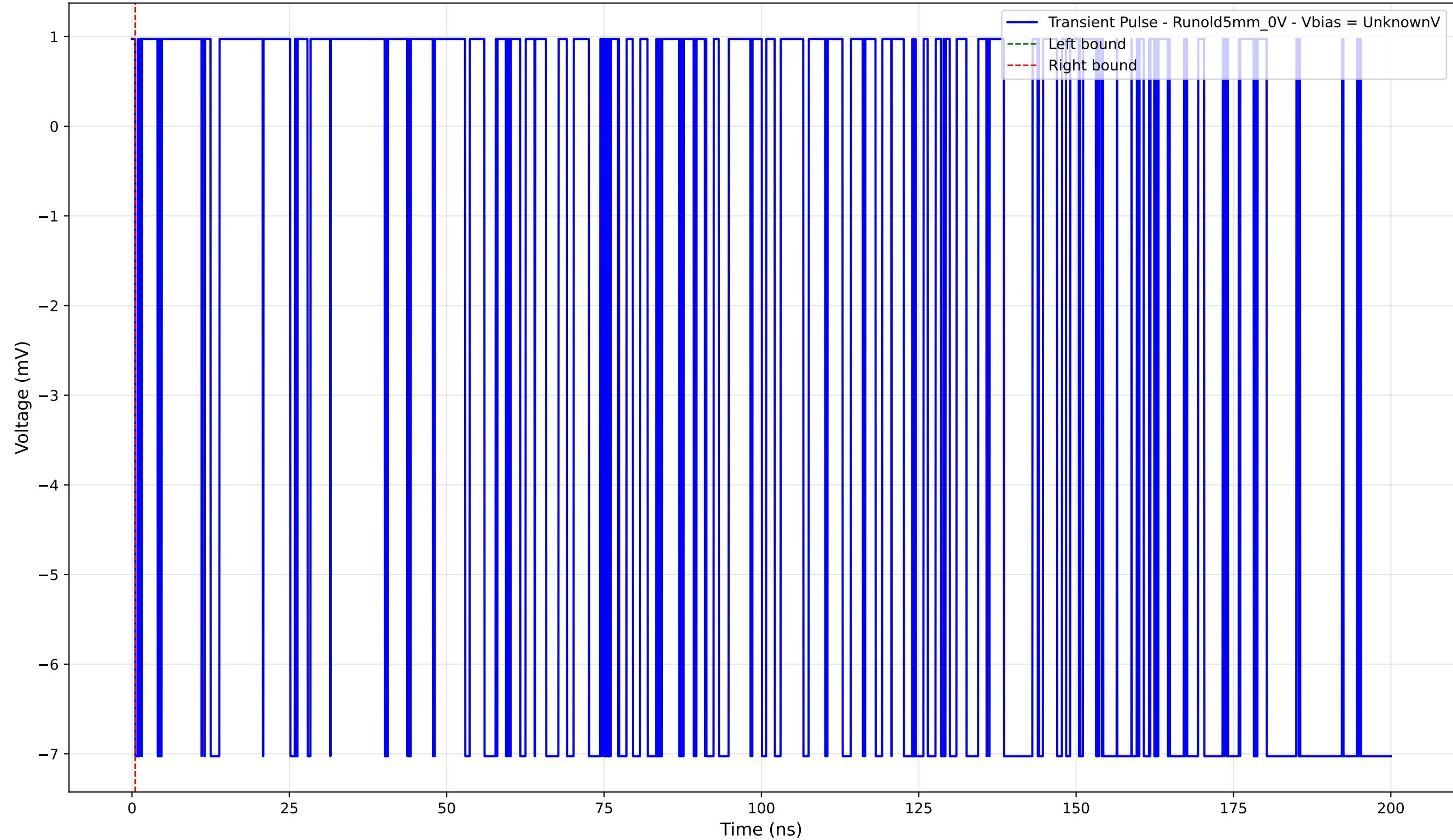
Transient Pulse - Sample: old5 - Position: 1855.0 \mu\text{m} - Charge: -0.00 pC
