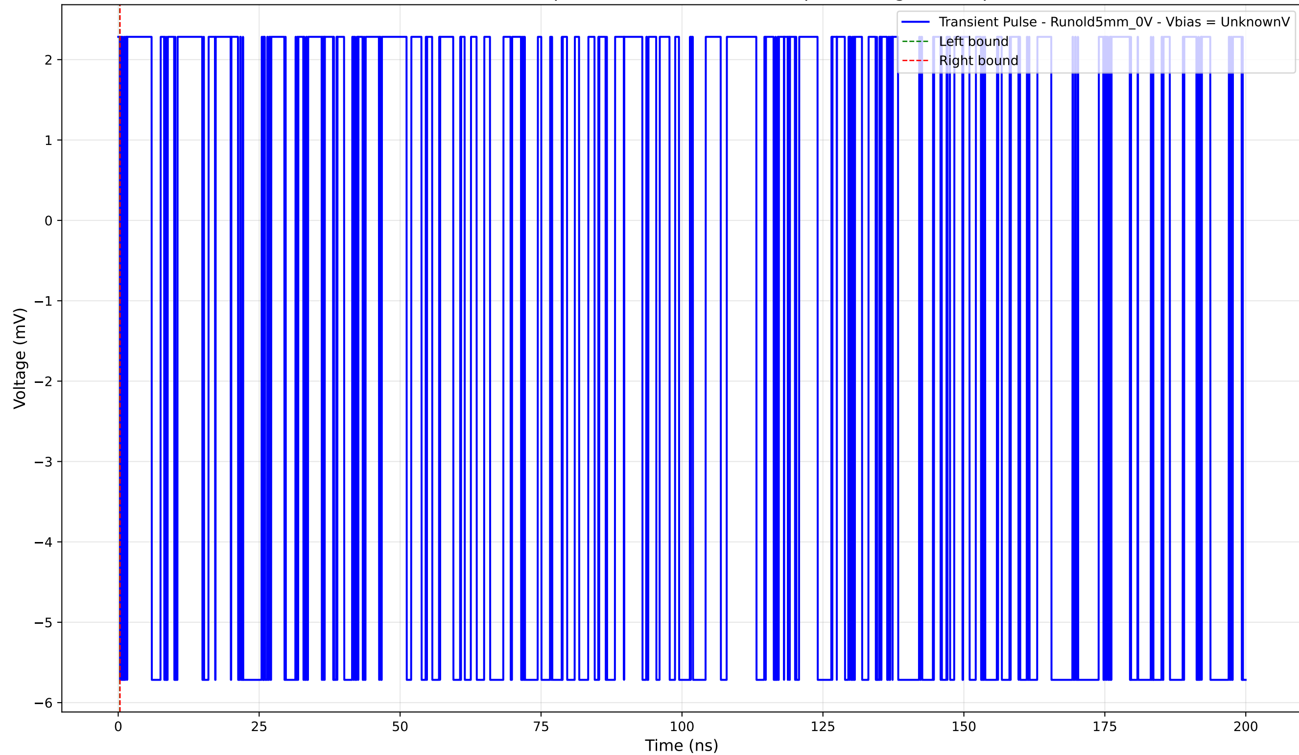
Transient Pulse - Sample: old5 - Position: 2860.0 \mu\text{m} - Charge: -0.00 pC
