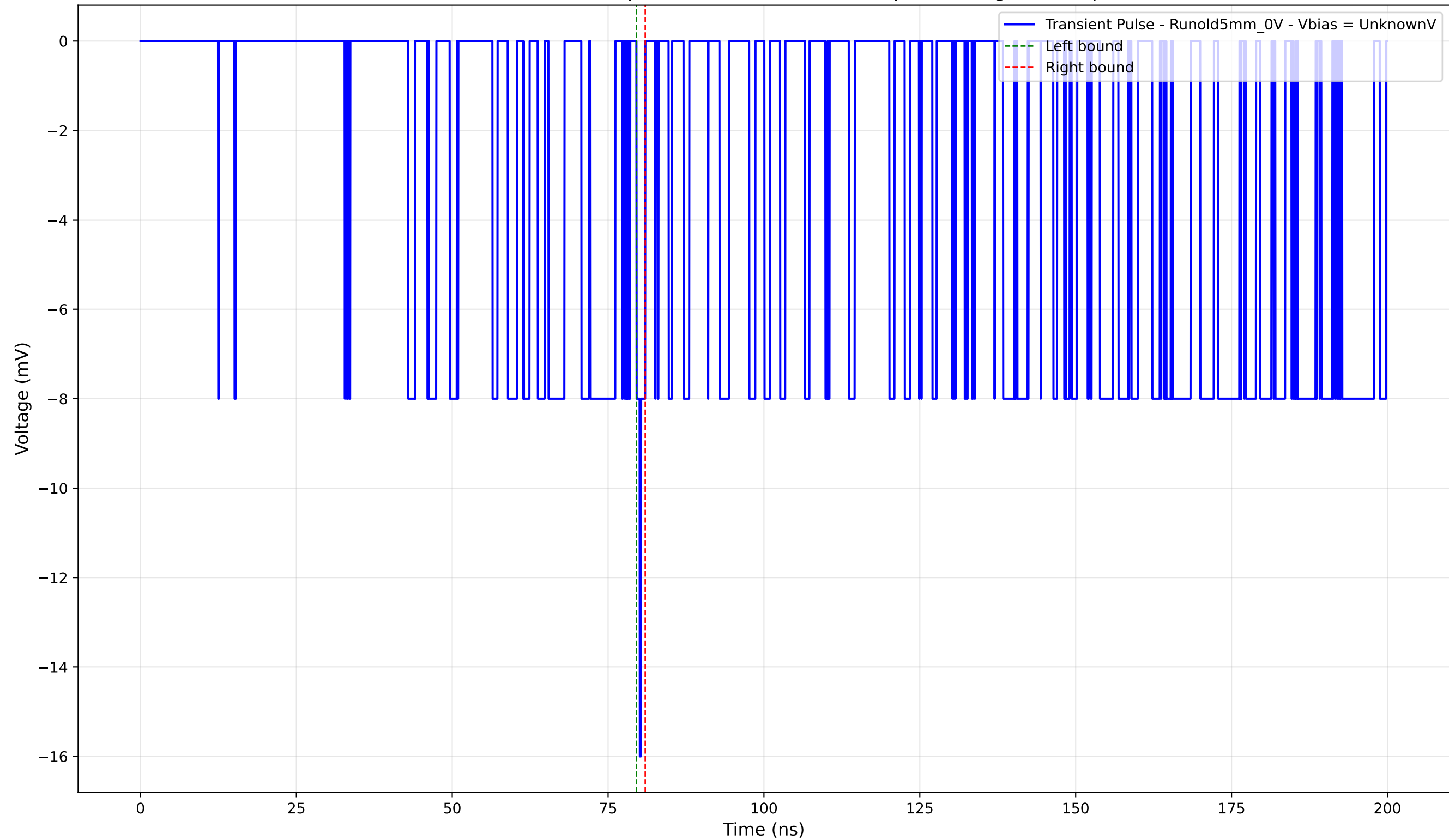
Transient Pulse - Sample: old5 - Position: 660.0 \mu\text{m} - Charge: -0.26 pC
