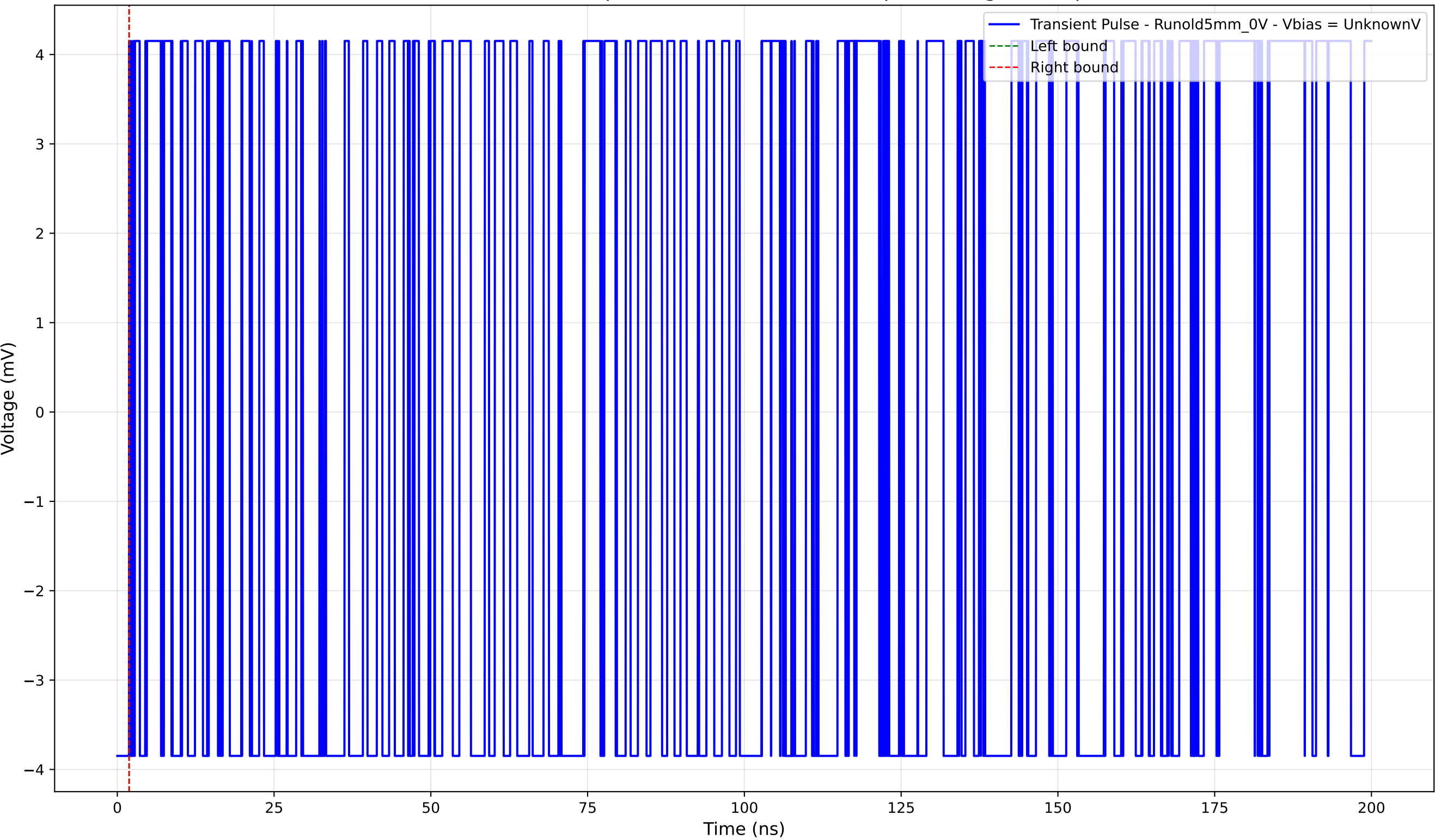
Transient Pulse - Sample: old5 - Position: 4535.0 \mu\text{m} - Charge: 0.00 pC
