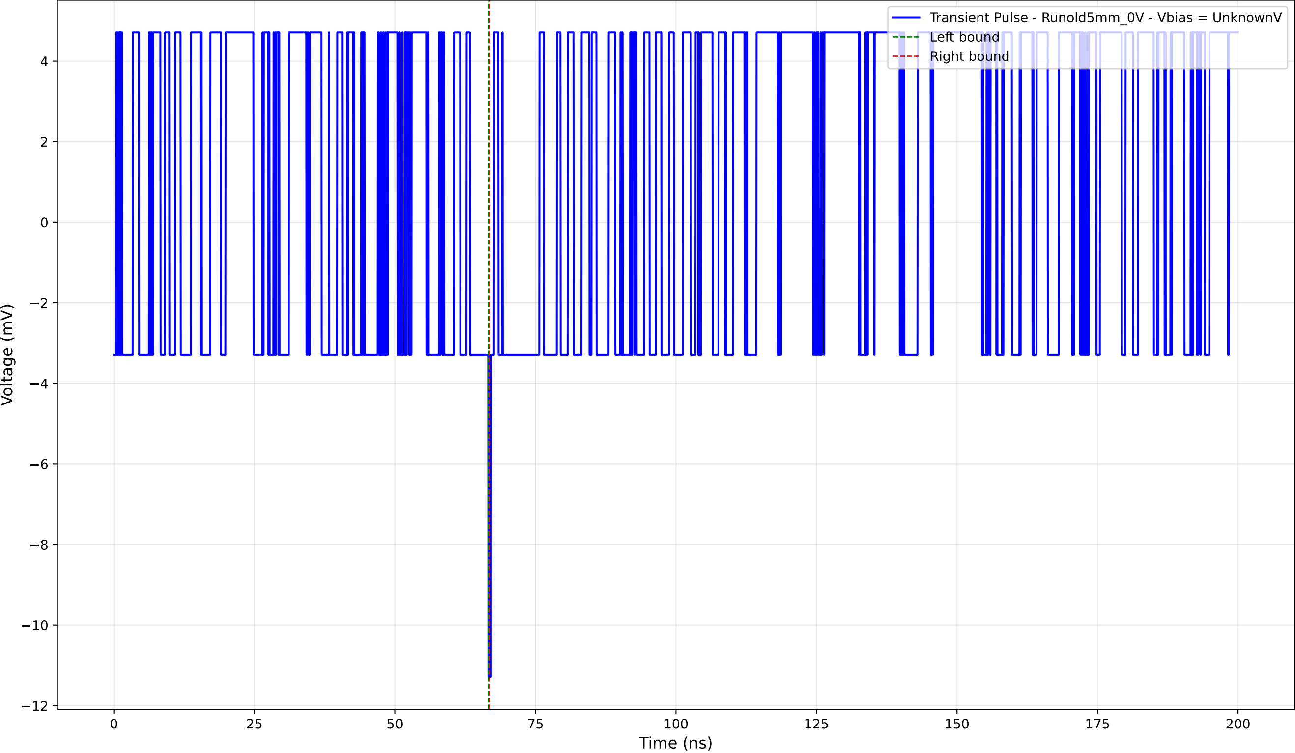
Transient Pulse - Sample: old5 - Position: 4530.0 \mu\text{m} - Charge: -0.06 pC
