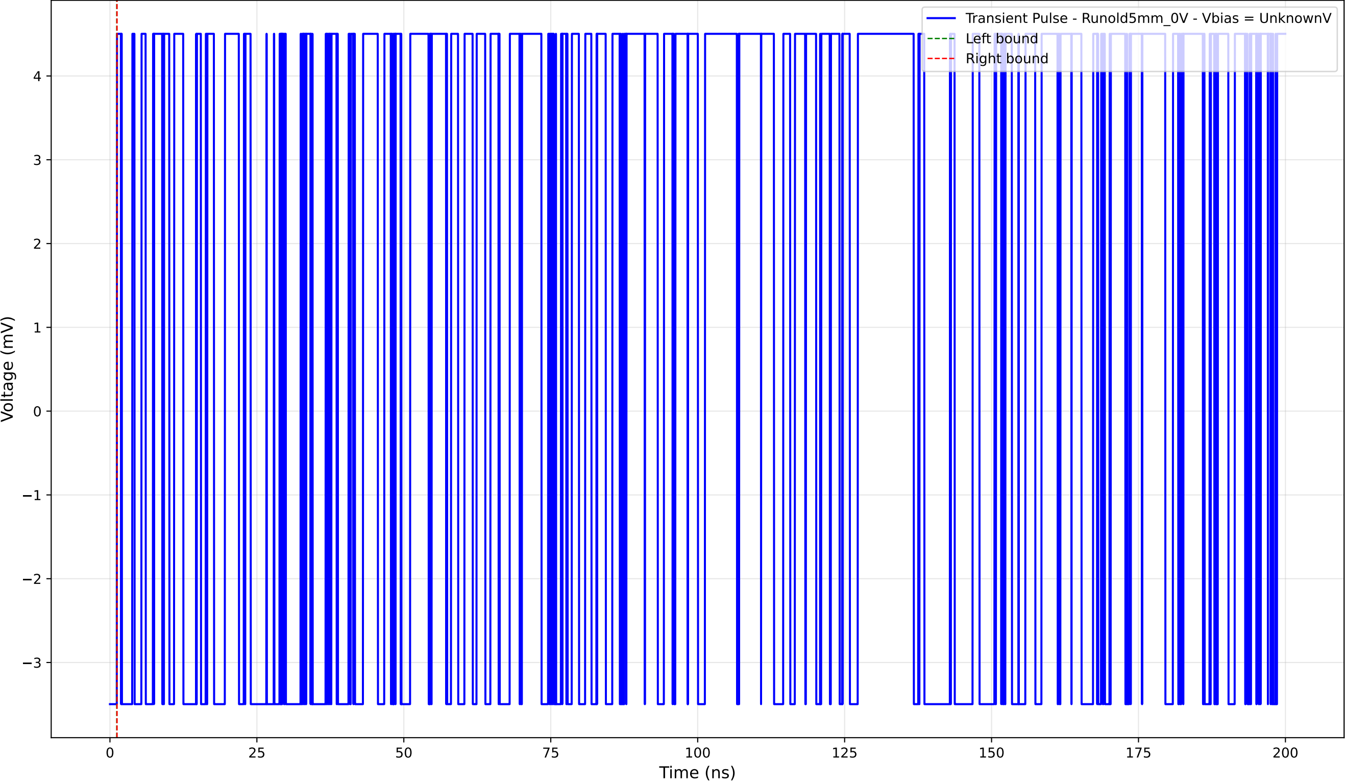
Transient Pulse - Sample: old5 - Position: 3525.0 \mu\text{m} - Charge: 0.00 pC
