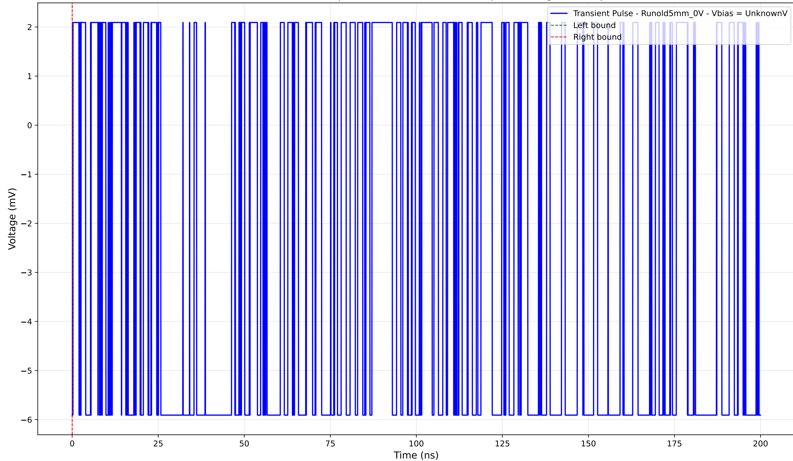
Transient Pulse - Sample: old5 - Position: 4625.0 \mu\text{m} - Charge: -0.00 pC
