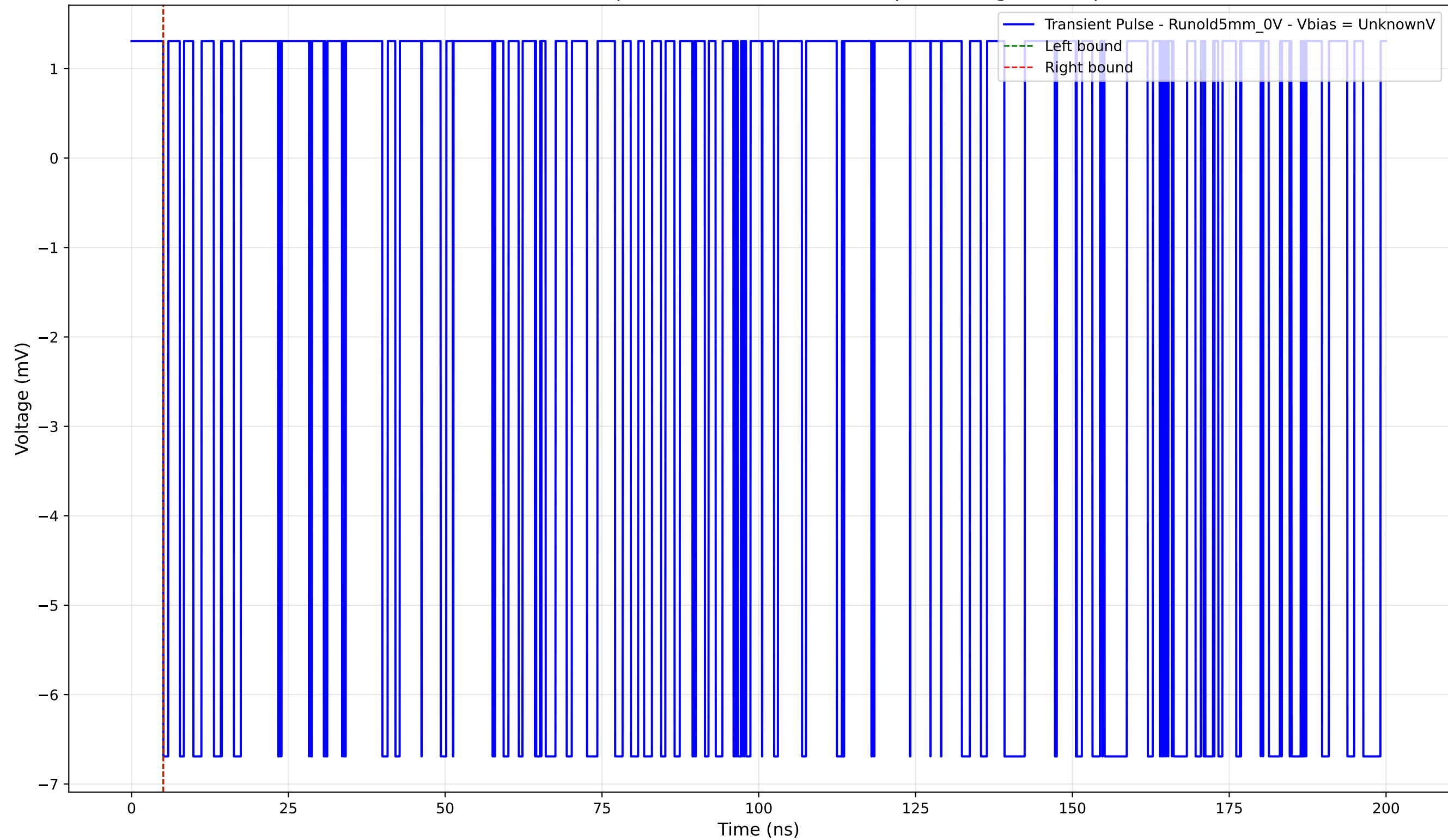
Transient Pulse - Sample: old5 - Position: 1100.0 \mu\text{m} - Charge: -0.00 pC
