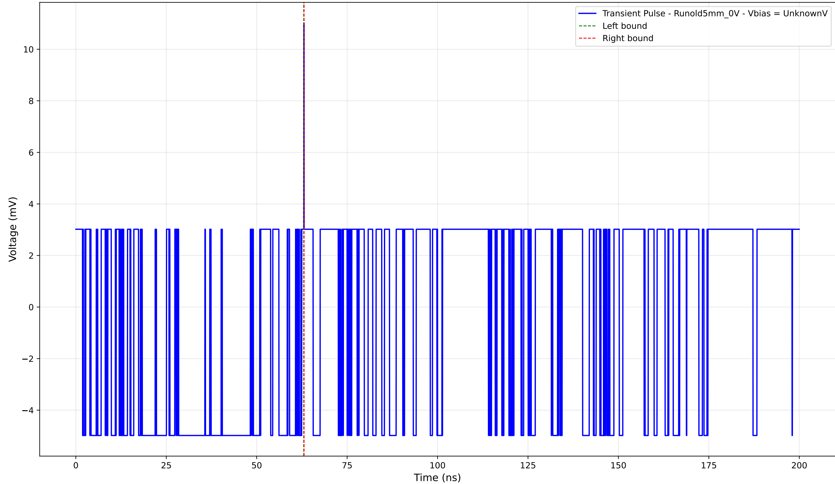
Transient Pulse - Sample: old5 - Position: 4855.0 \mu\text{m} - Charge: 0.02 pC
