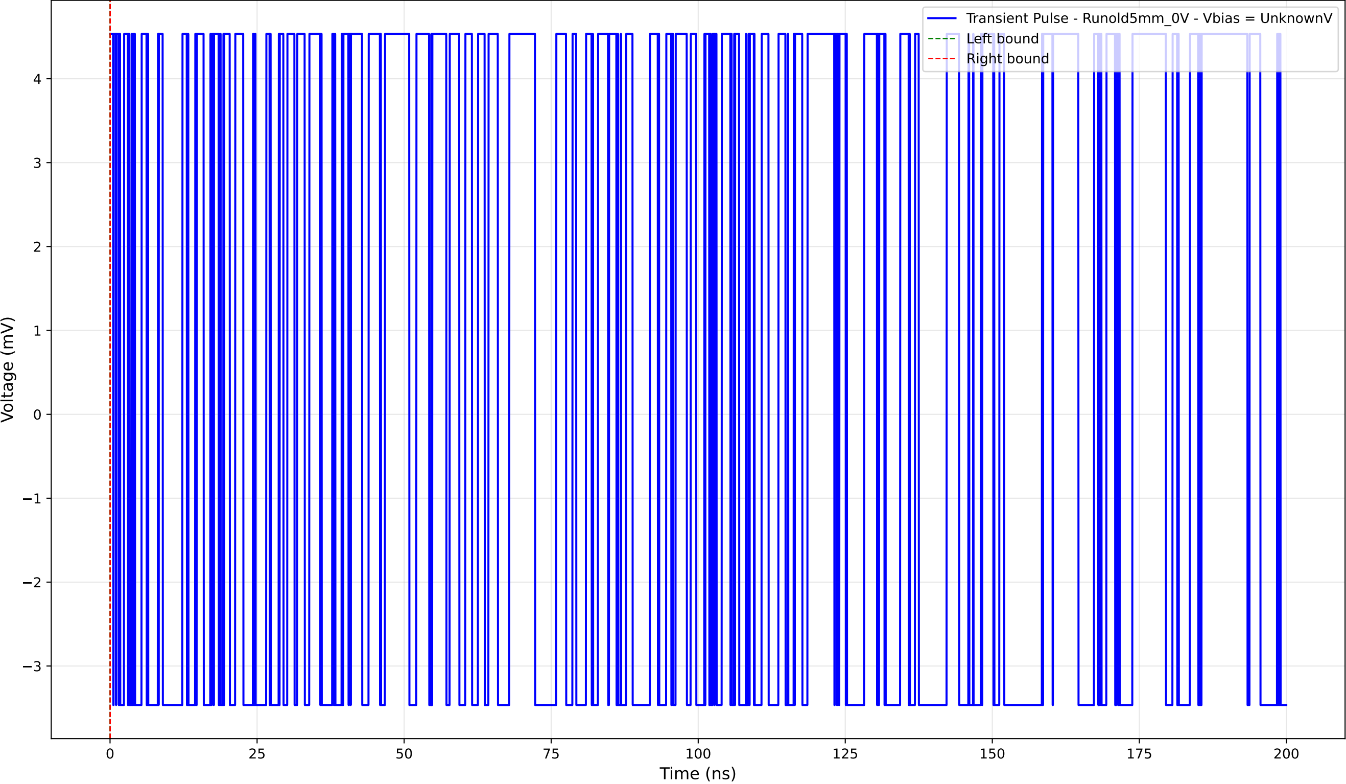
Transient Pulse - Sample: old5 - Position: 4710.0 \mu\text{m} - Charge: 0.00 pC
