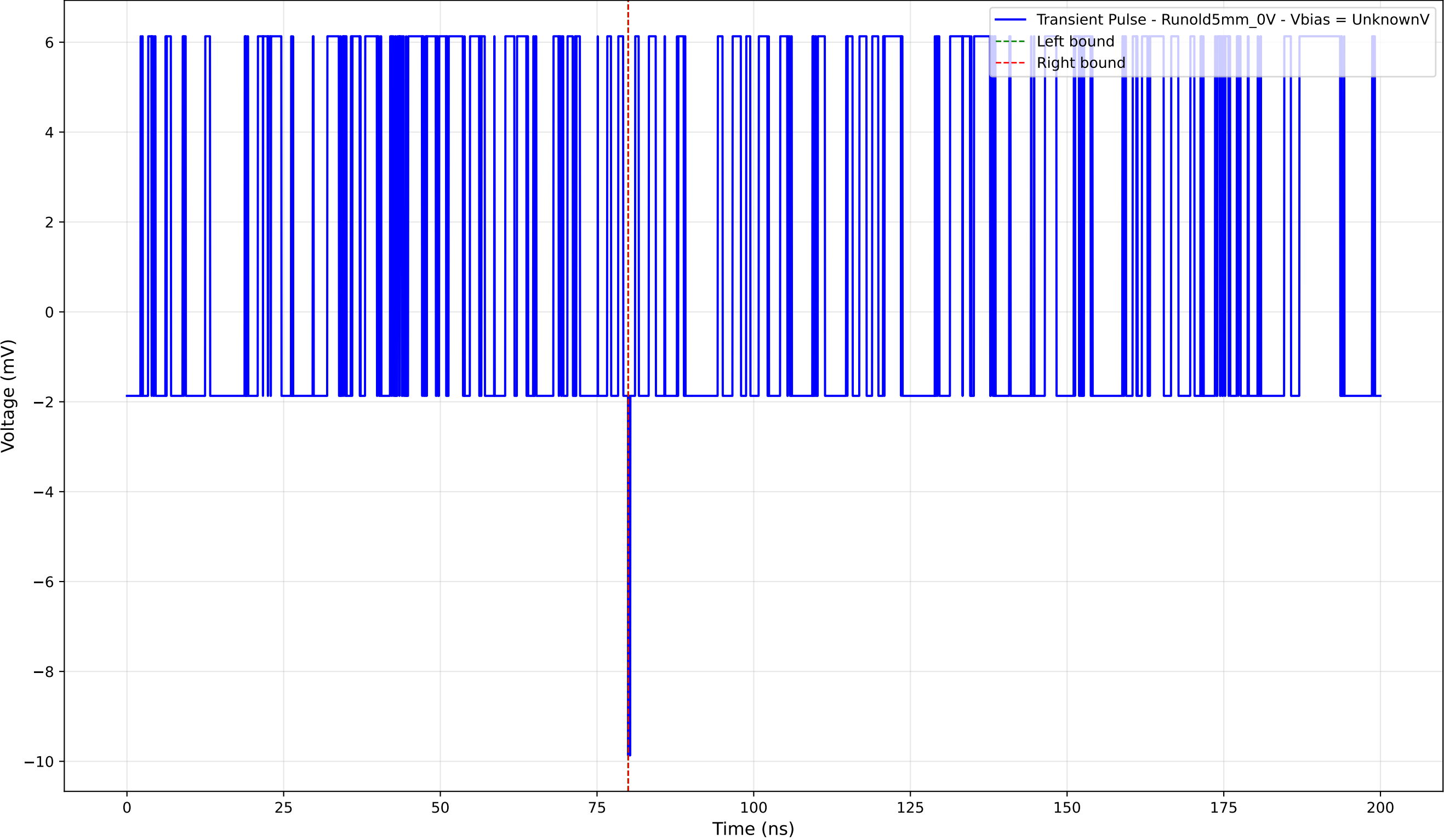
Transient Pulse - Sample: old5 - Position: 2265.0 \mu\text{m} - Charge: -0.01 pC
