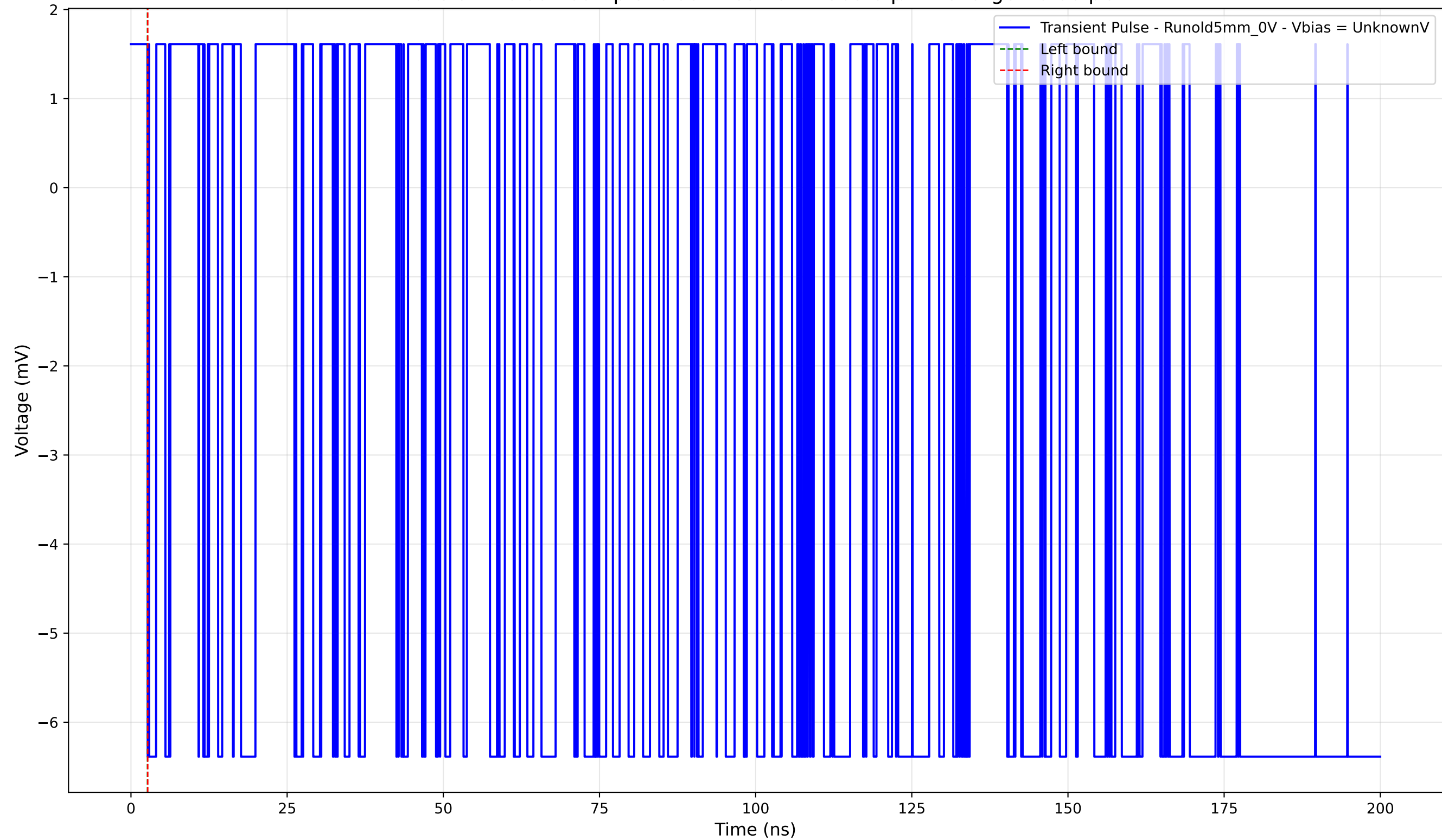
Transient Pulse - Sample: old5 - Position: 4305.0 \mu\text{m} - Charge: -0.00 pC
