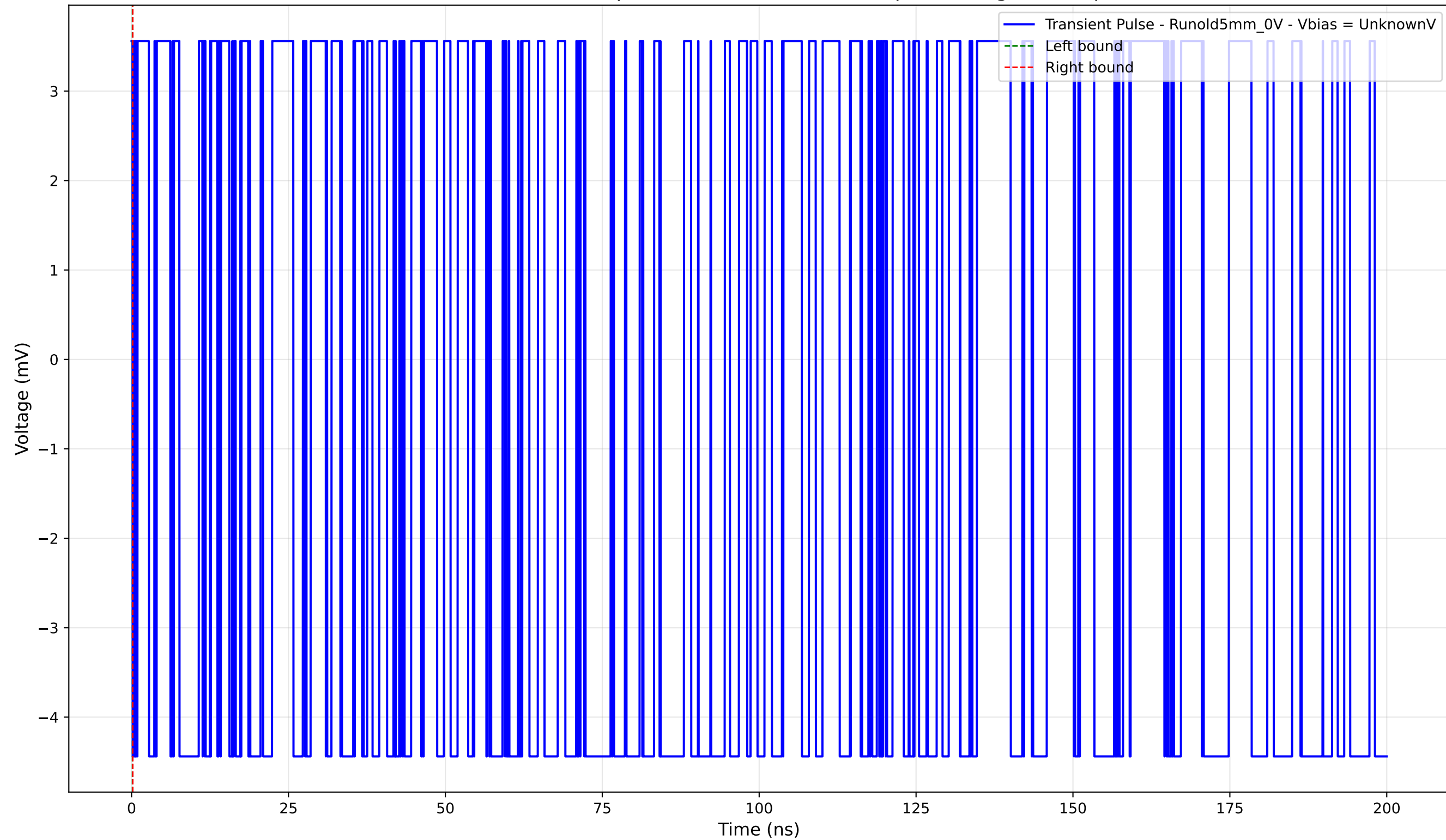
Transient Pulse - Sample: old5 - Position: 1745.0 \mu\text{m} - Charge: -0.00 pC
