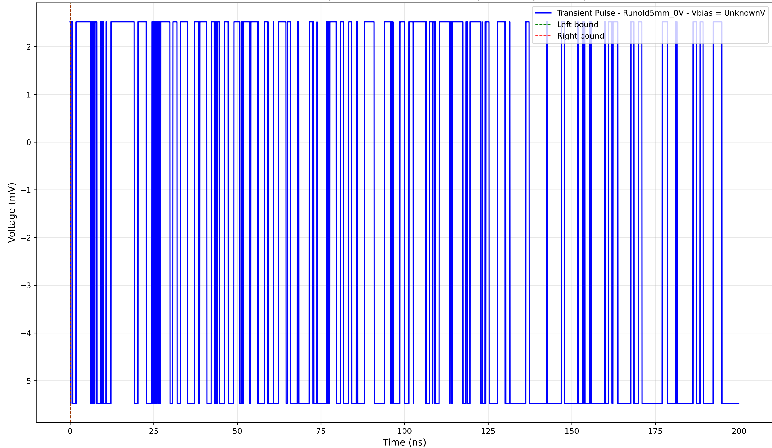
Transient Pulse - Sample: old5 - Position: 3215.0 \mu\text{m} - Charge: -0.00 pC
