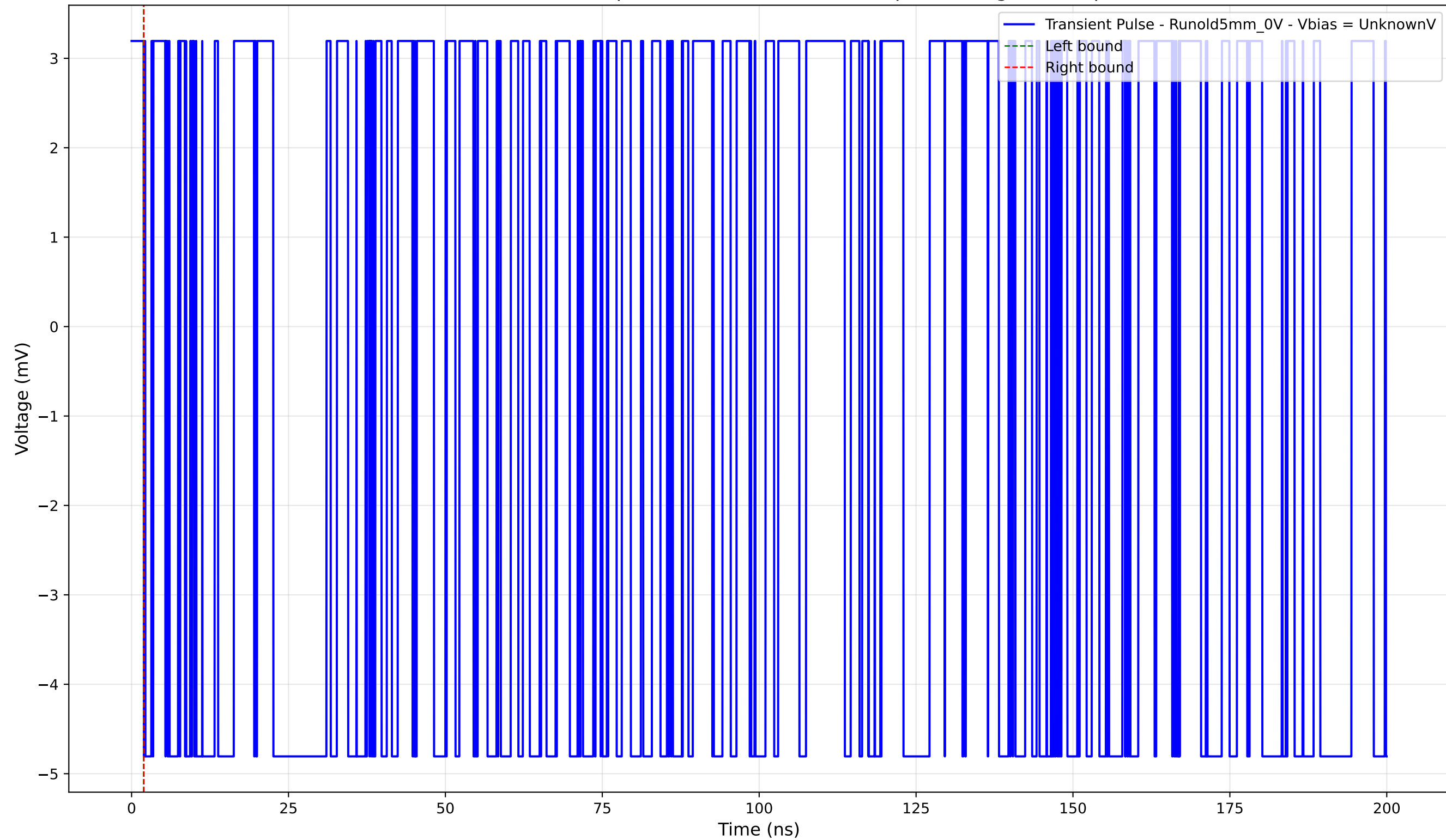
Transient Pulse - Sample: old5 - Position: 3155.0 \mu\text{m} - Charge: -0.00 pC
