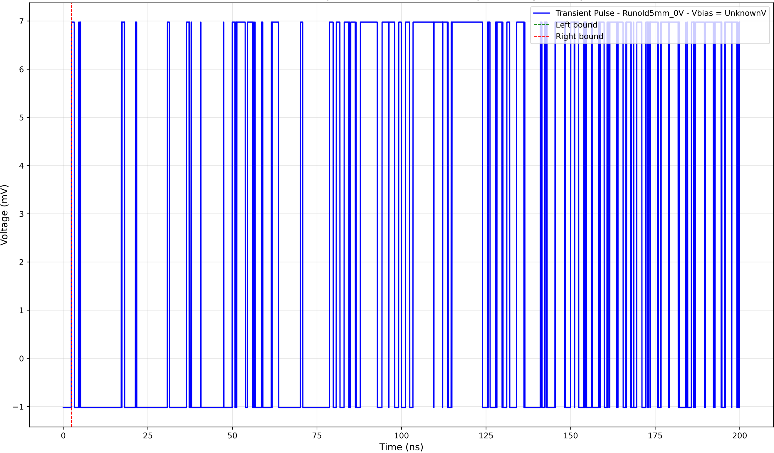
Transient Pulse - Sample: old5 - Position: 2035.0 \mu\text{m} - Charge: 0.00 pC
