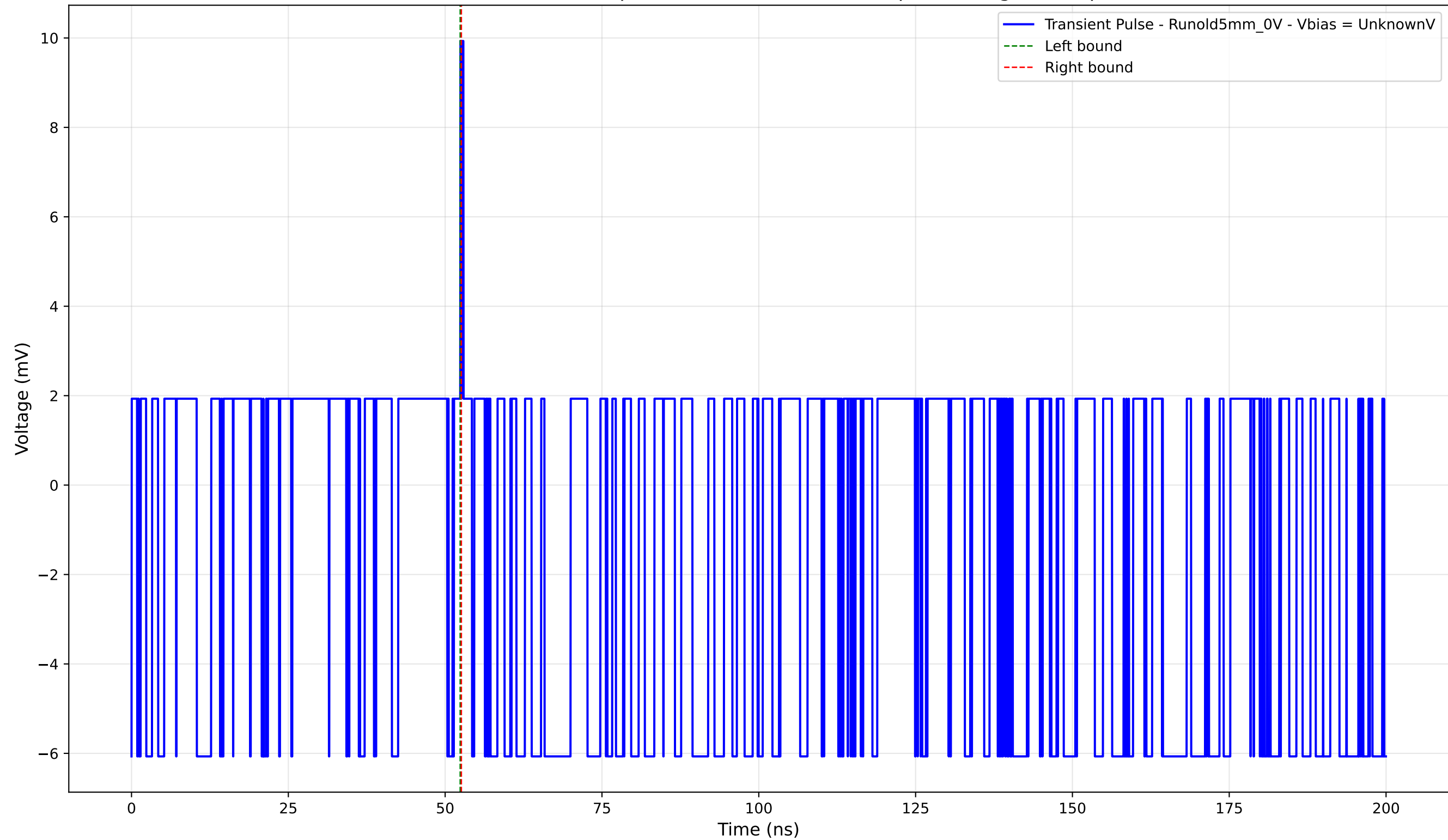
Transient Pulse - Sample: old5 - Position: 4340.0 \mu\text{m} - Charge: 0.03 pC
