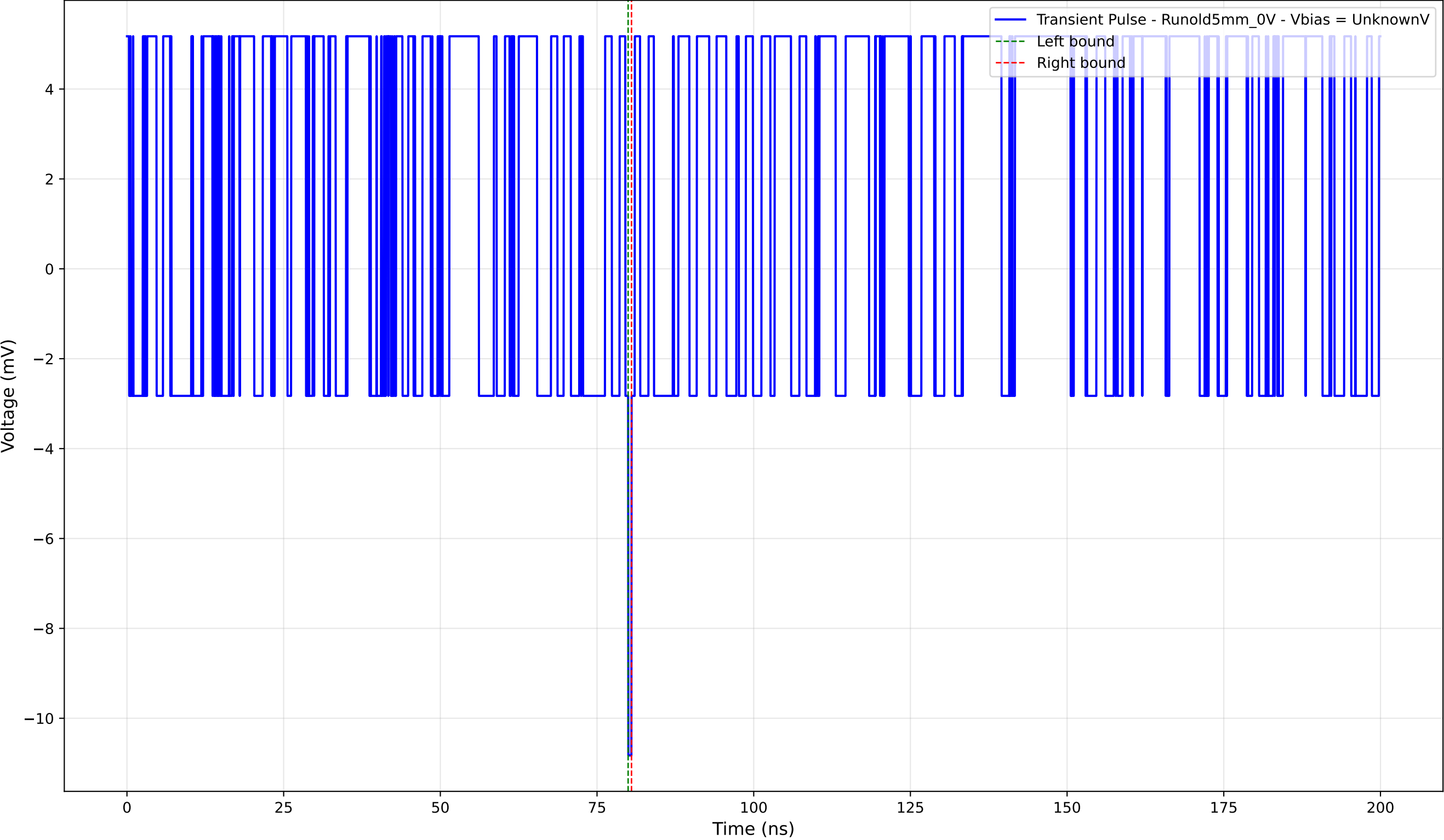
Transient Pulse - Sample: old5 - Position: 3895.0 \mu\text{m} - Charge: -0.11 pC
