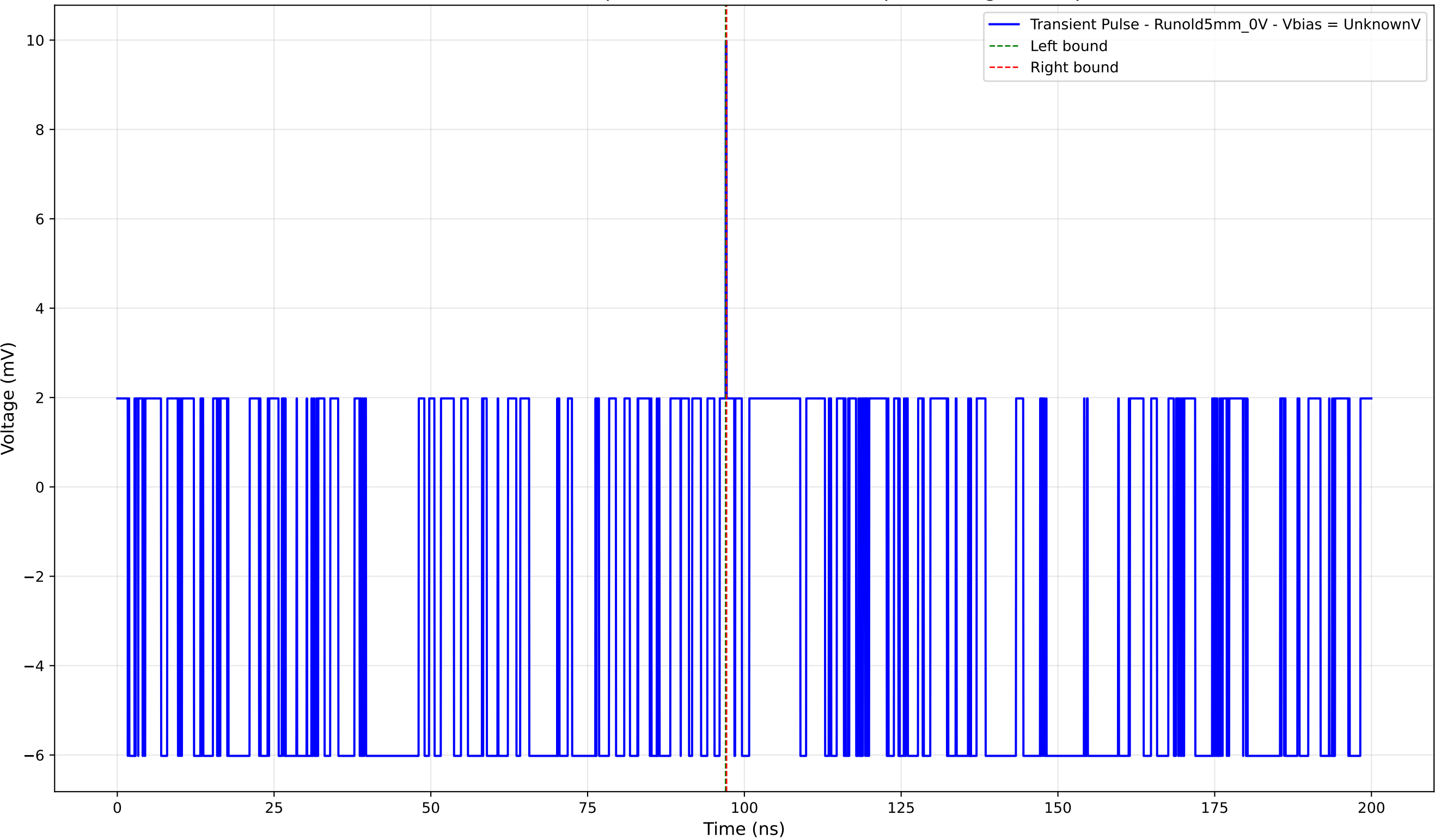
Transient Pulse - Sample: old5 - Position: 3275.0 \mu\text{m} - Charge: 0.03 pC
