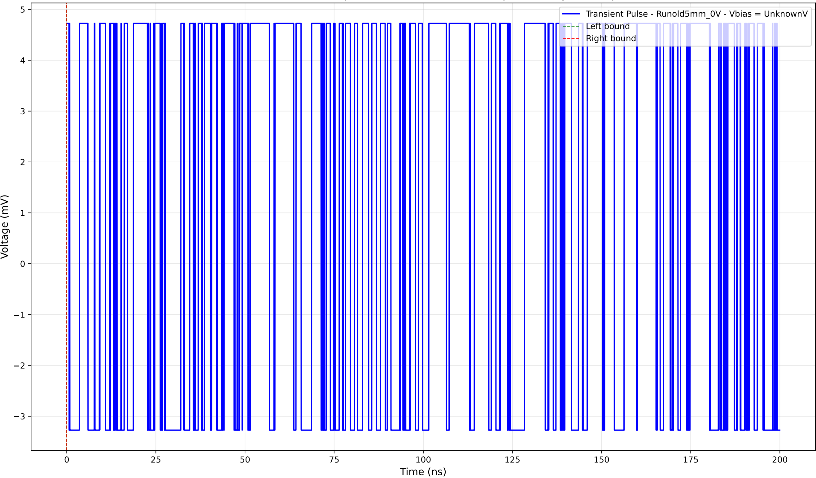
Transient Pulse - Sample: old5 - Position: 4030.0 \mu\text{m} - Charge: 0.00 pC
