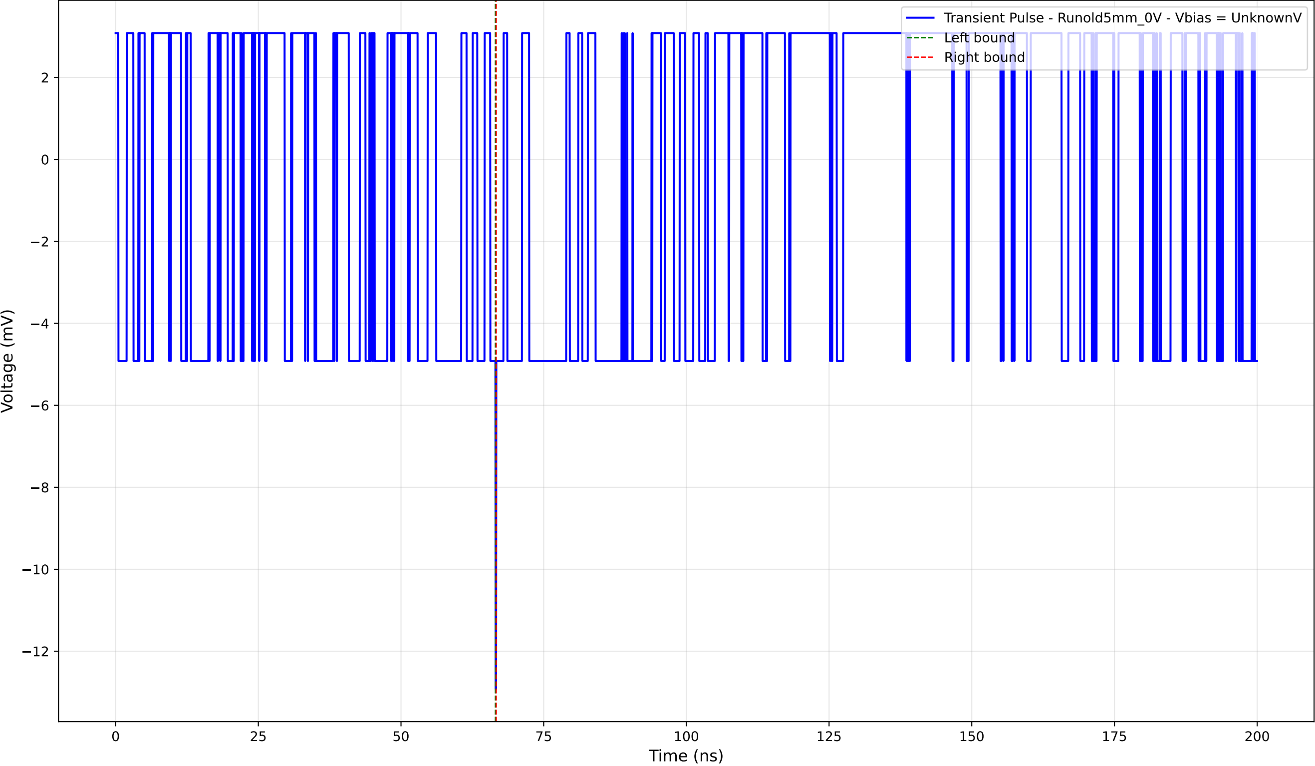
Transient Pulse - Sample: old5 - Position: 4965.0 \mu\text{m} - Charge: -0.03 pC
