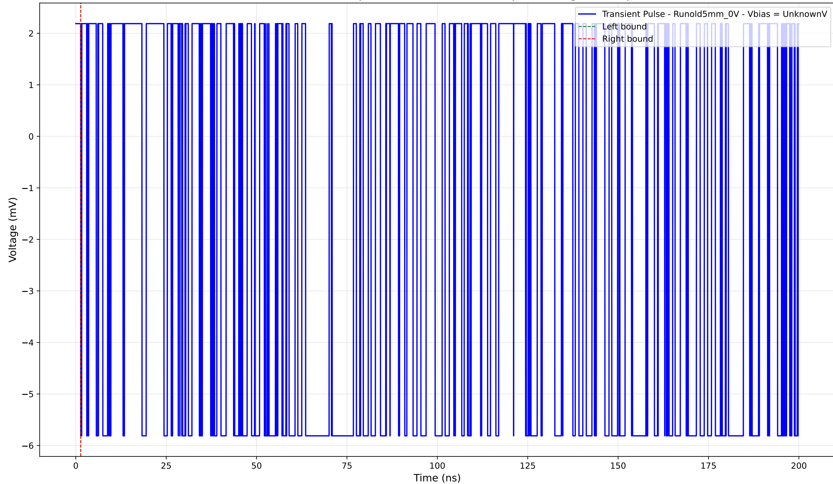
Transient Pulse - Sample: old5 - Position: 495.0 \mu\text{m} - Charge: -0.00 pC
