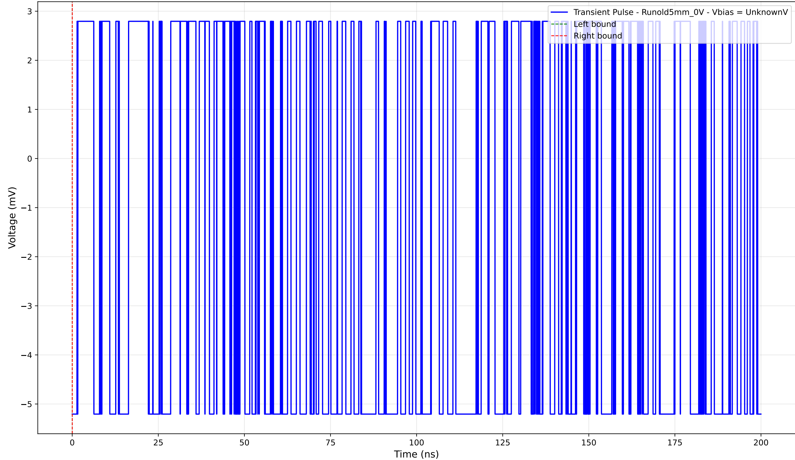
Transient Pulse - Sample: old5 - Position: 4765.0 \mu\text{m} - Charge: -0.00 pC
