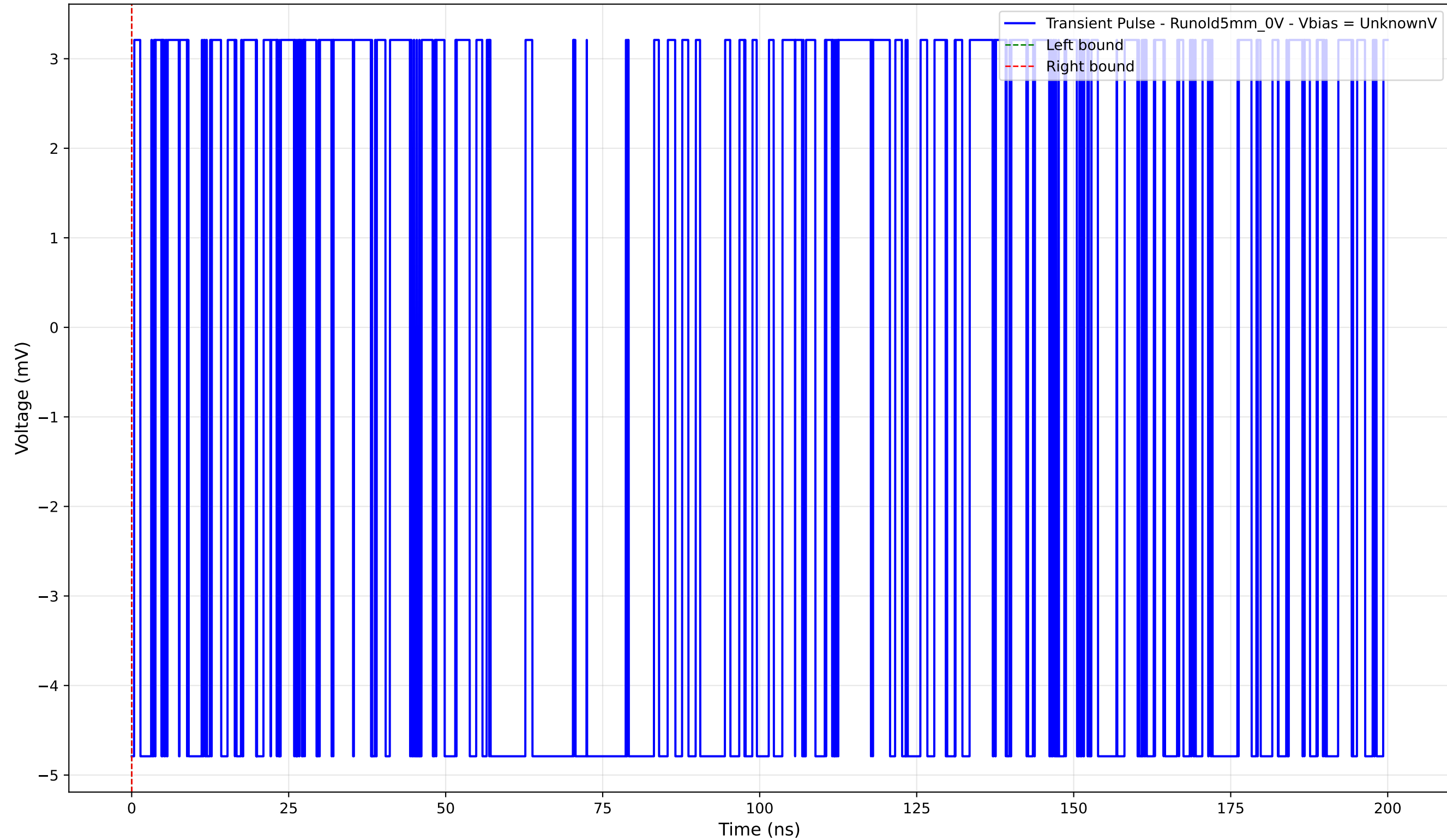
Transient Pulse - Sample: old5 - Position: 3630.0 \mu\text{m} - Charge: -0.00 pC
