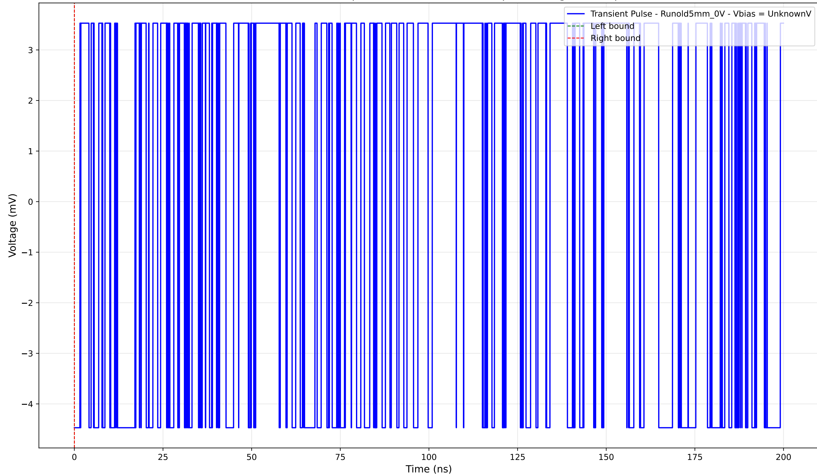
Transient Pulse - Sample: old5 - Position: 735.0 \mu\text{m} - Charge: -0.00 pC
