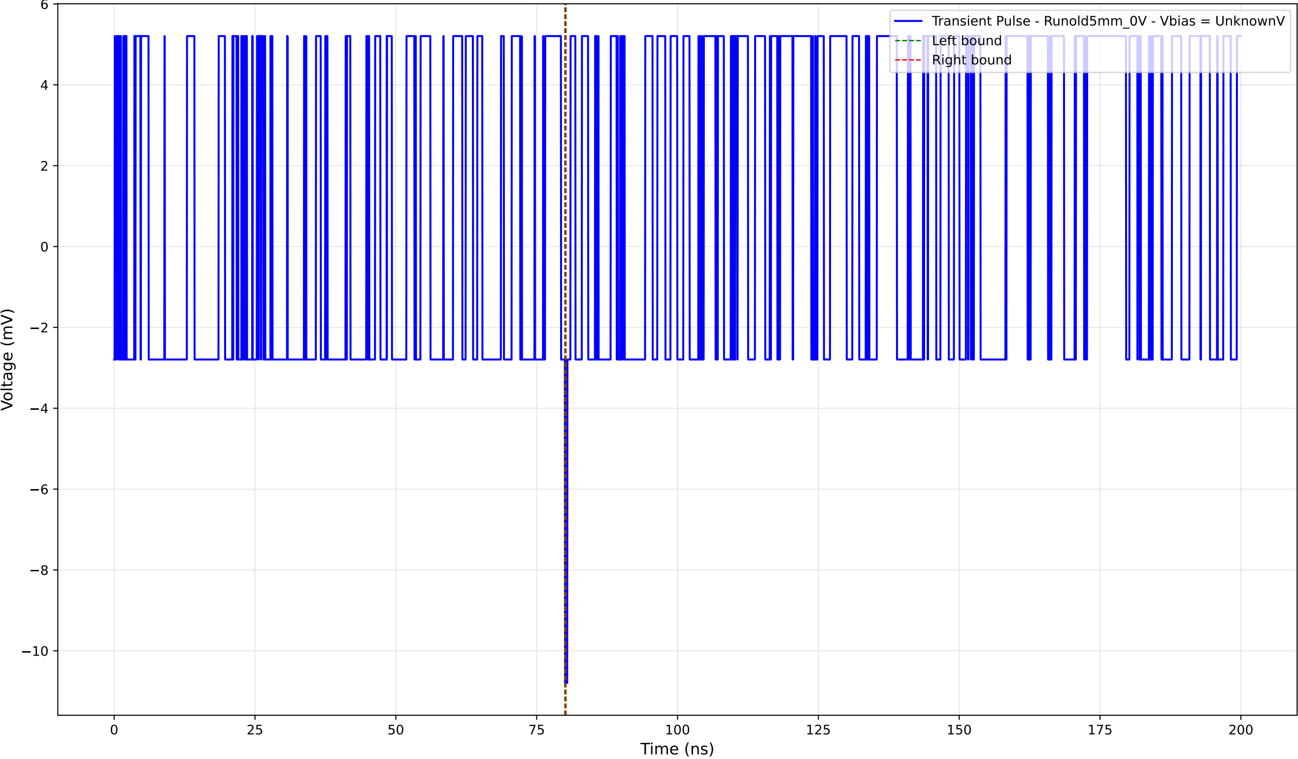
Transient Pulse - Sample: old5 - Position: 4190.0 \mu\text{m} - Charge: -0.04 pC
