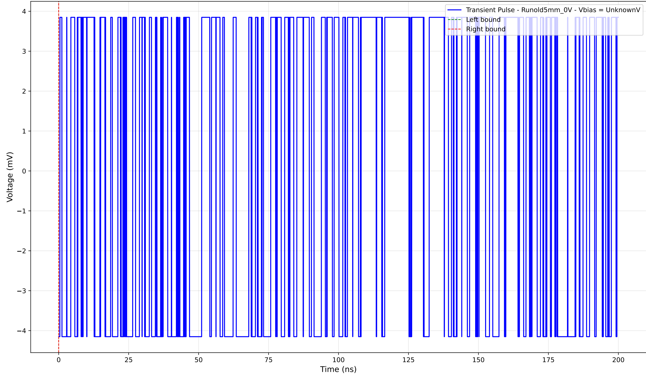
Transient Pulse - Sample: old5 - Position: 4680.0 \mu\text{m} - Charge: -0.00 pC
