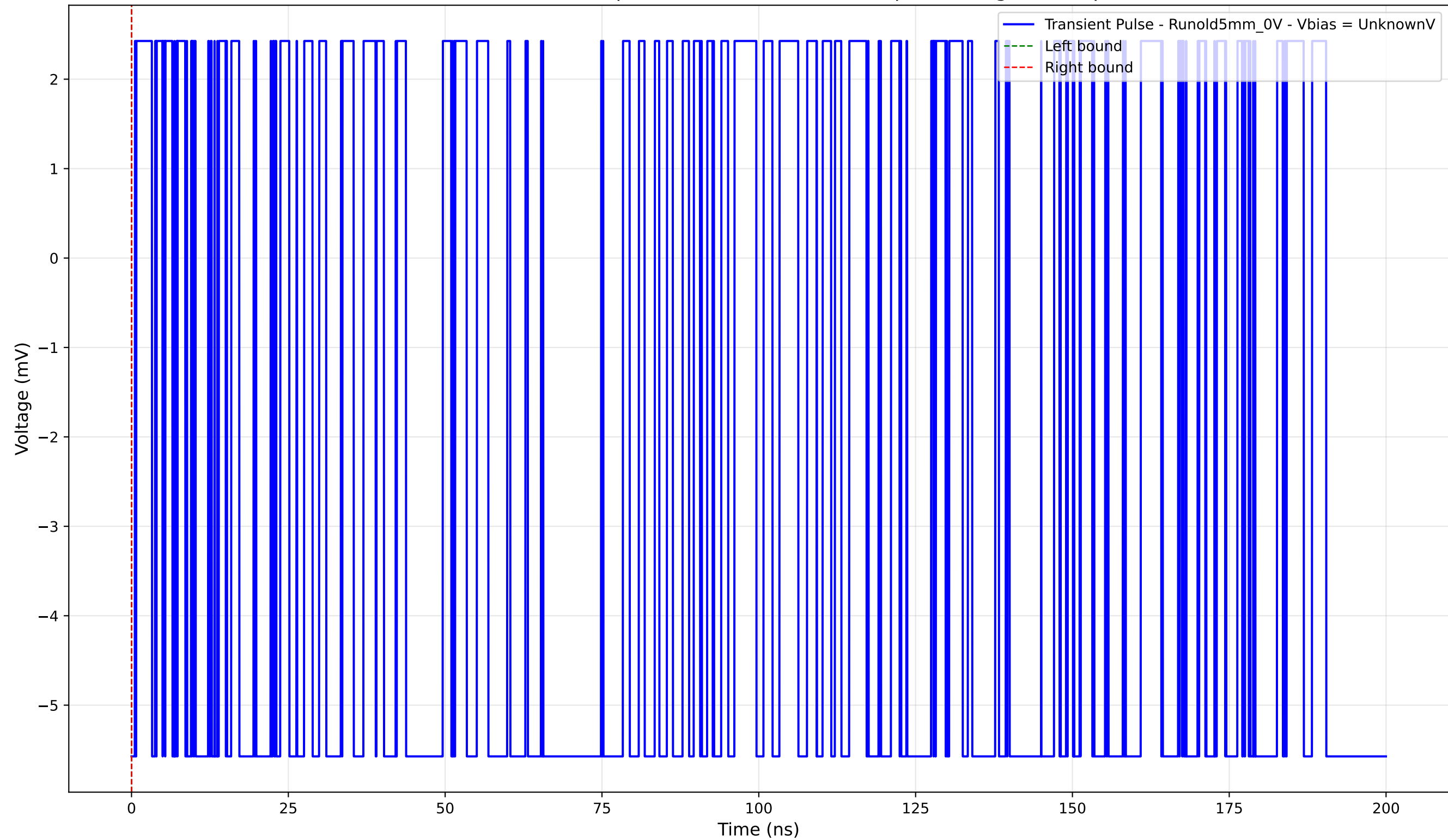
Transient Pulse - Sample: old5 - Position: 4100.0 \mu\text{m} - Charge: -0.00 pC
