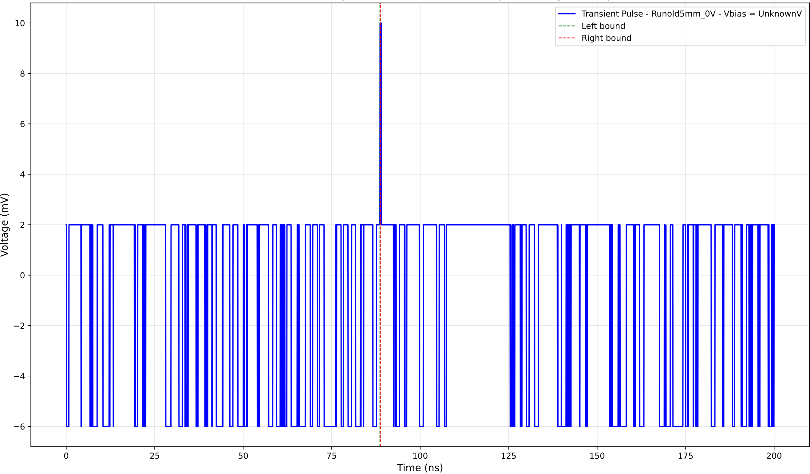
Transient Pulse - Sample: old5 - Position: 4440.0 \mu\text{m} - Charge: 0.04 pC
