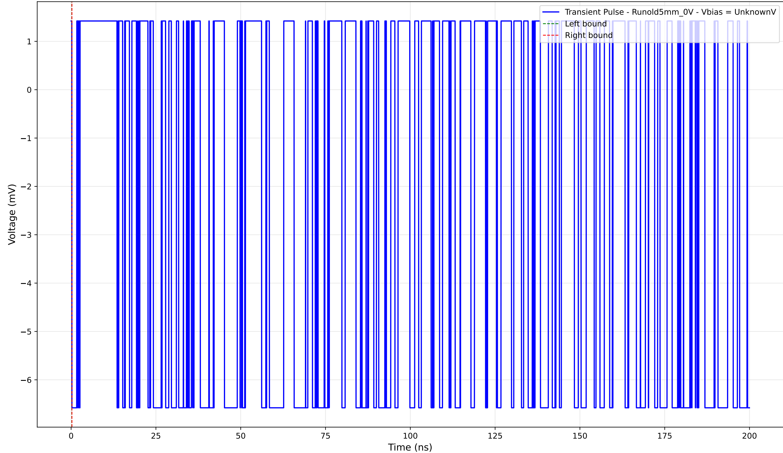
Transient Pulse - Sample: old5 - Position: 4795.0 \mu\text{m} - Charge: -0.00 pC
