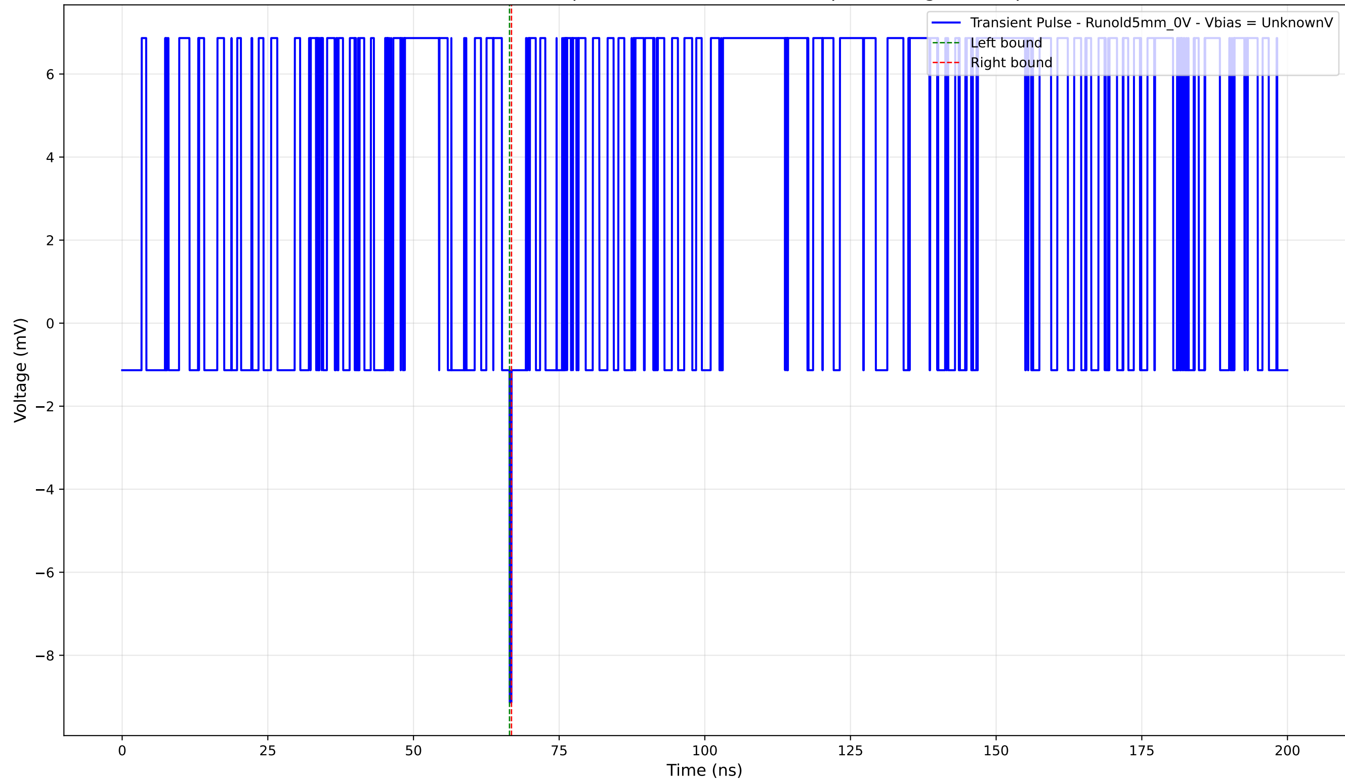
Transient Pulse - Sample: old5 - Position: 4295.0 \mu\text{m} - Charge: -0.06 pC
