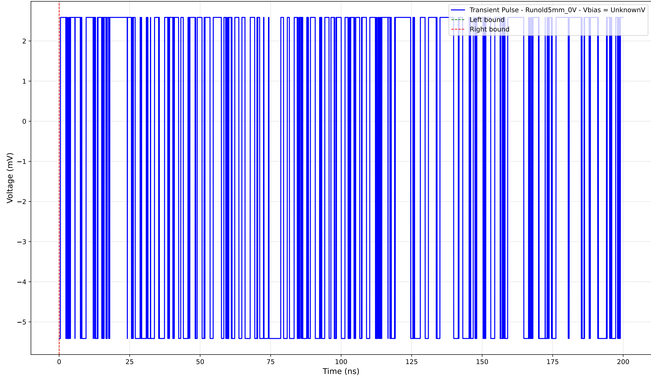
Transient Pulse - Sample: old5 - Position: 4945.0 \mu\text{m} - Charge: -0.00 pC
