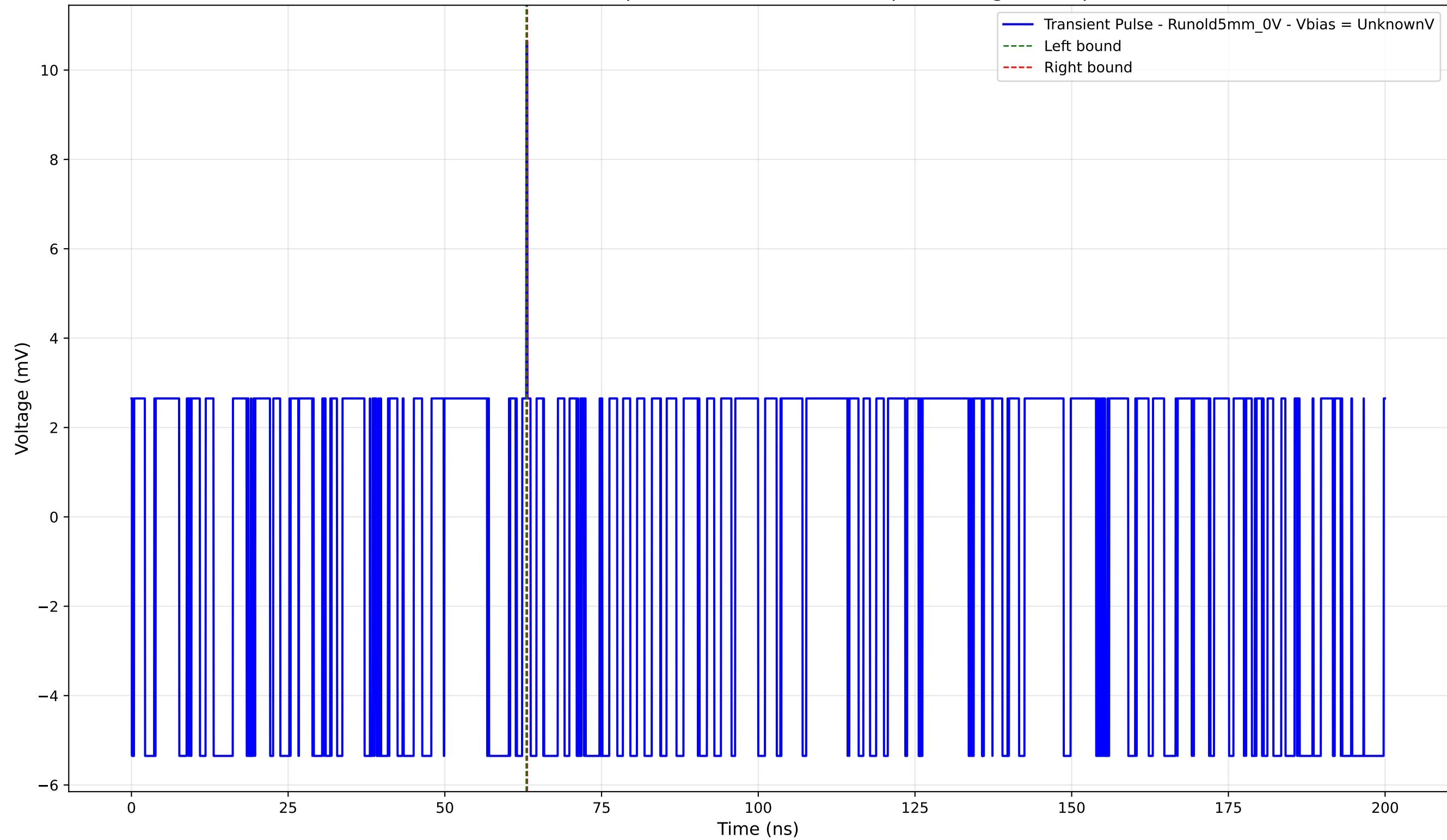
Transient Pulse - Sample: old5 - Position: 980.0 \mu\text{m} - Charge: 0.04 pC
