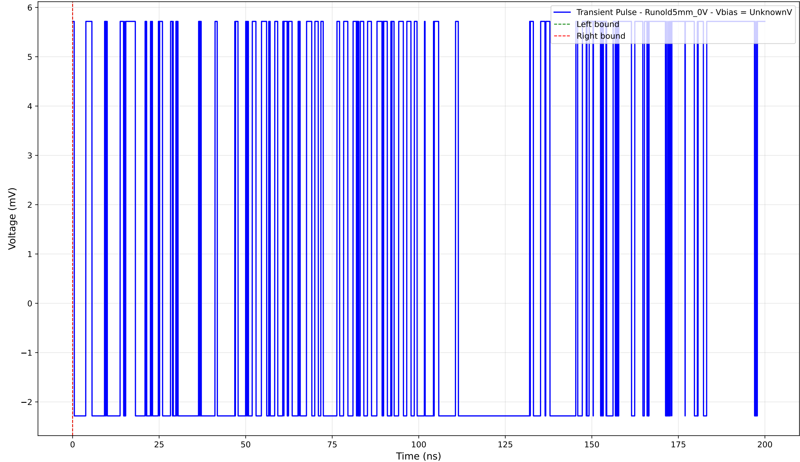
Transient Pulse - Sample: old5 - Position: 1770.0 \mu\text{m} - Charge: 0.00 pC
