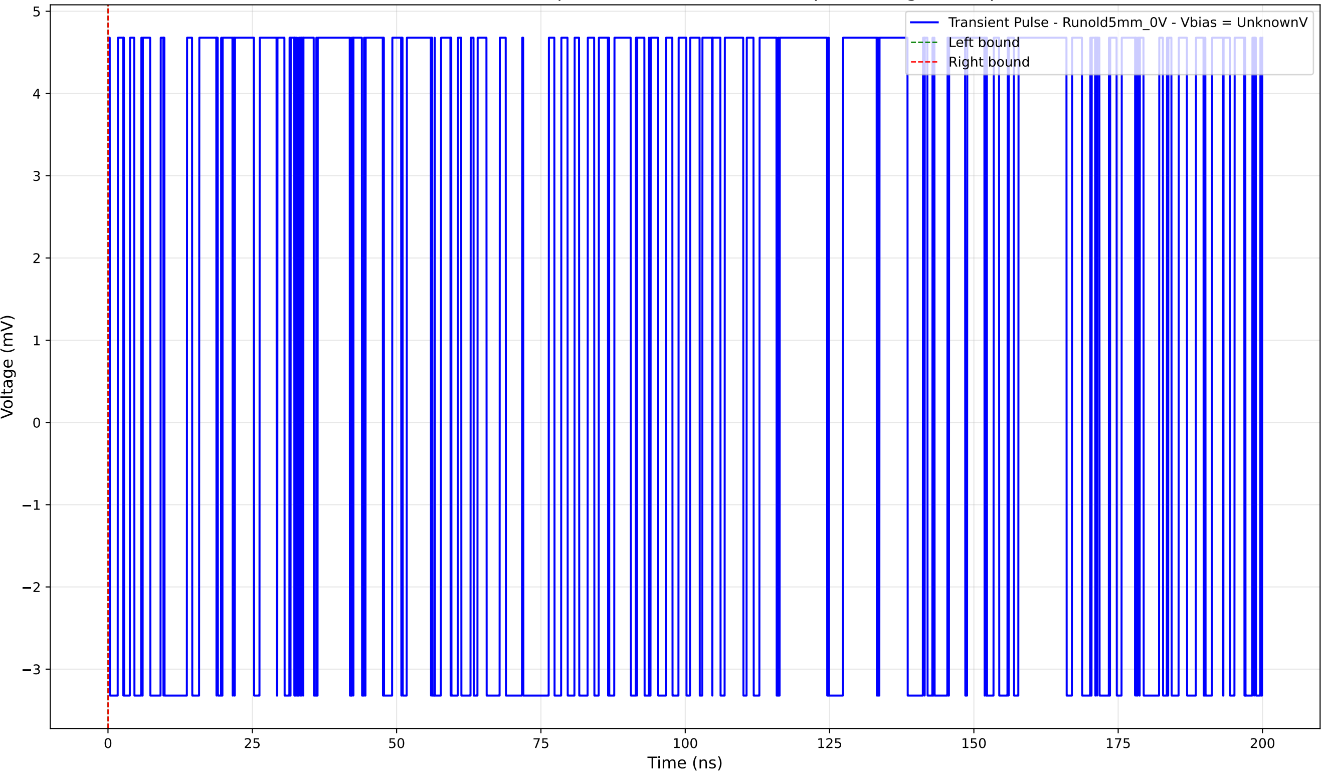
Transient Pulse - Sample: old5 - Position: 2030.0 \mu\text{m} - Charge: 0.00 pC
