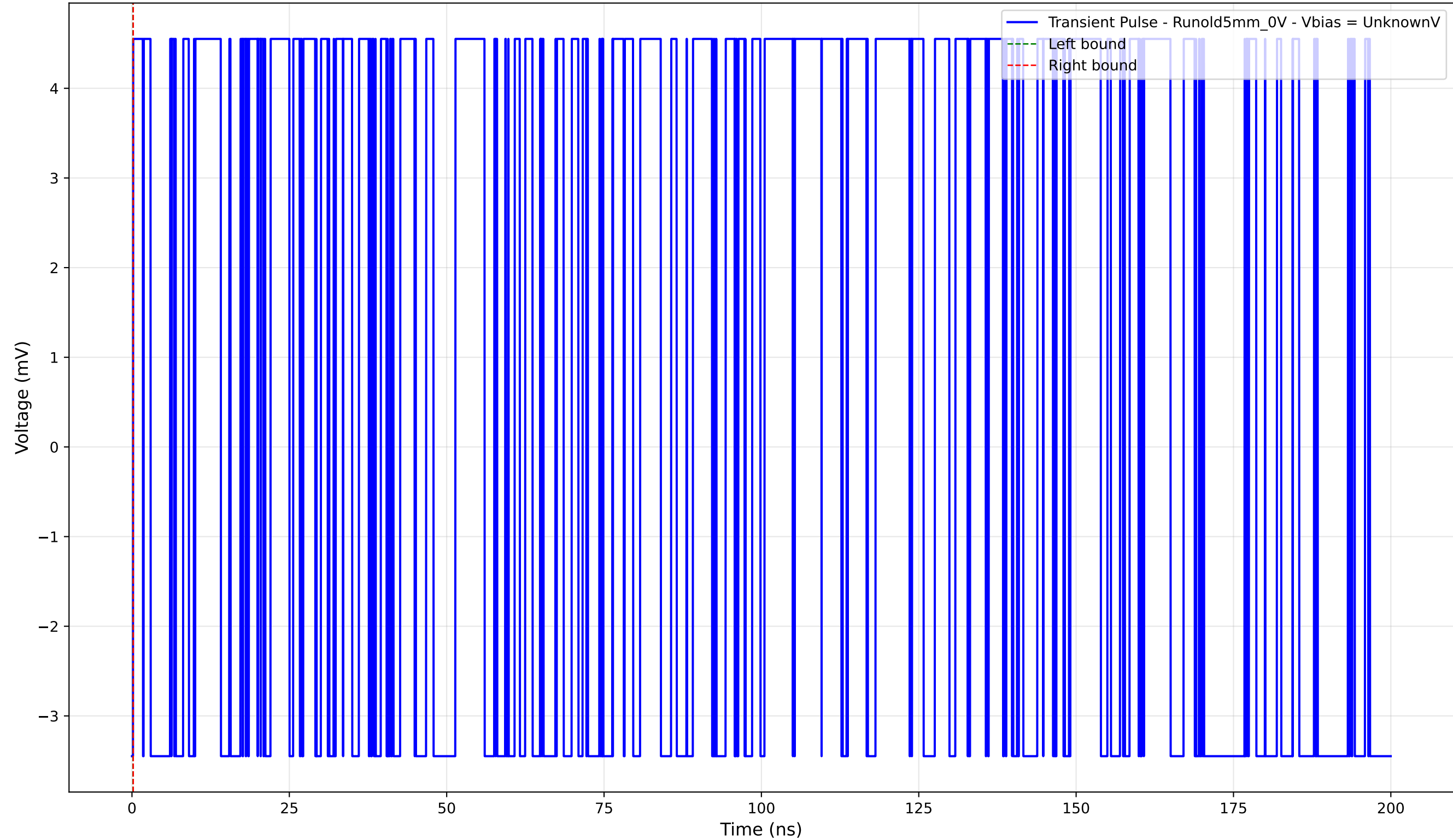
Transient Pulse - Sample: old5 - Position: 2155.0 \mu\text{m} - Charge: 0.00 pC
