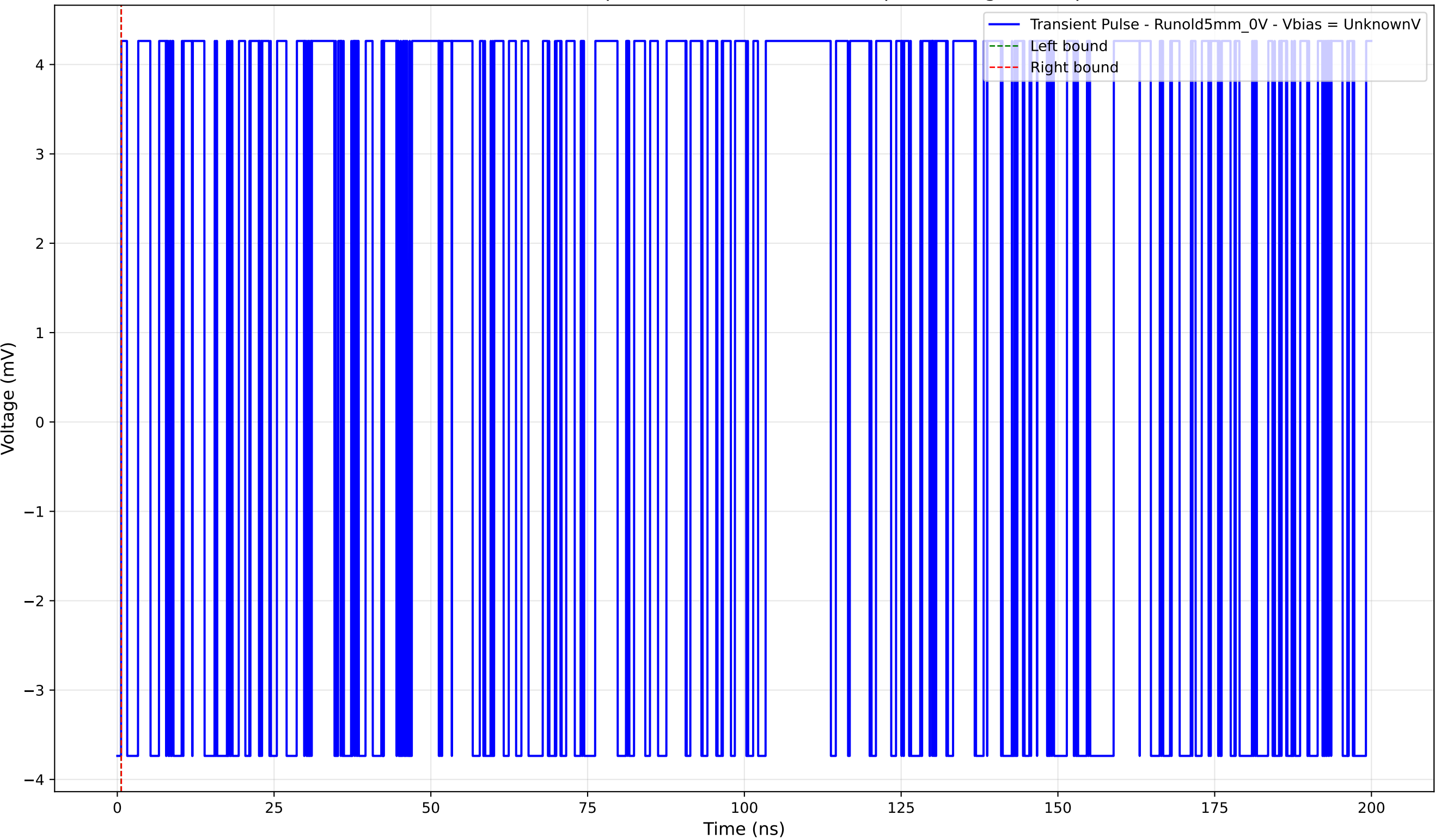
Transient Pulse - Sample: old5 - Position: 3135.0 \mu\text{m} - Charge: 0.00 pC
