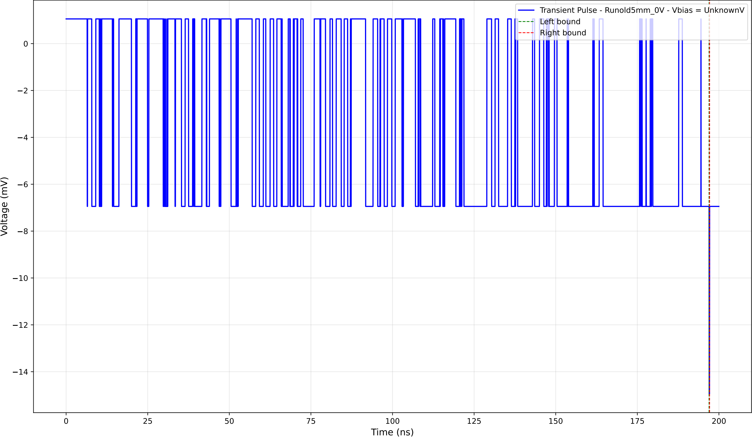
Transient Pulse - Sample: old5 - Position: 1300.0 \mu\text{m} - Charge: -0.04 pC
