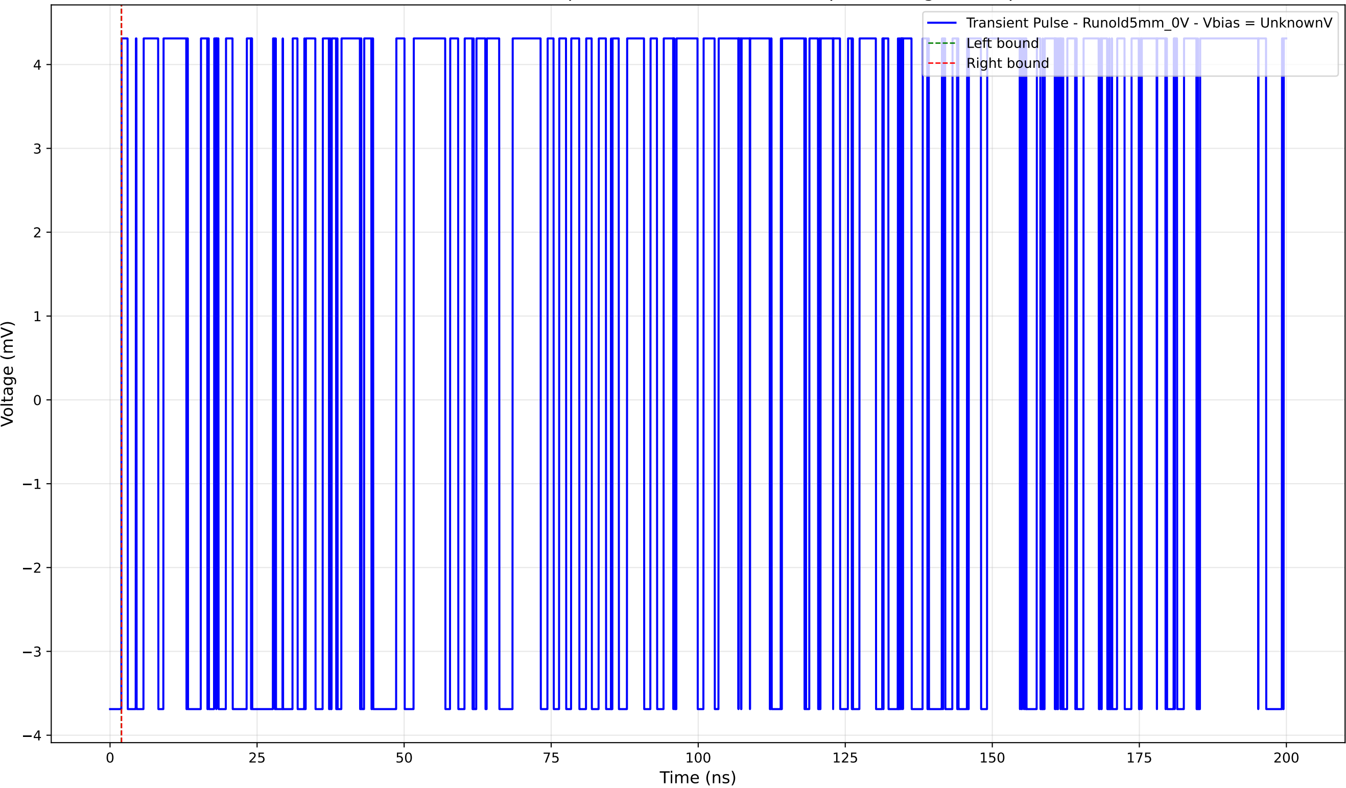
Transient Pulse - Sample: old5 - Position: 2015.0 \mu\text{m} - Charge: 0.00 pC
