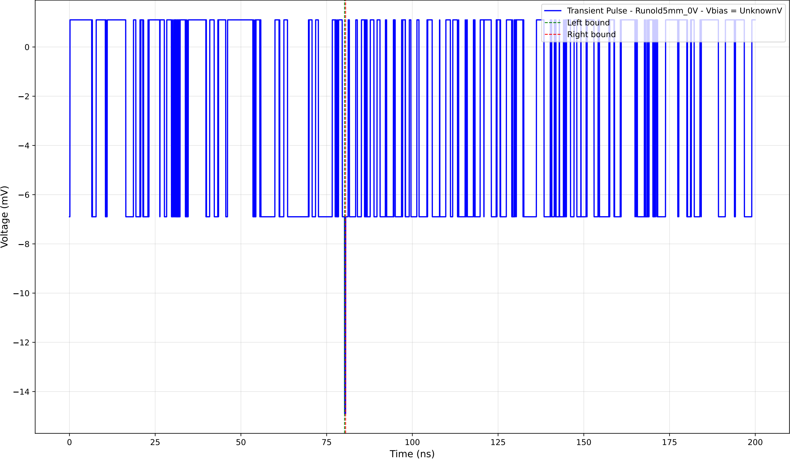
Transient Pulse - Sample: old5 - Position: 1560.0 \mu\text{m} - Charge: -0.09 pC
