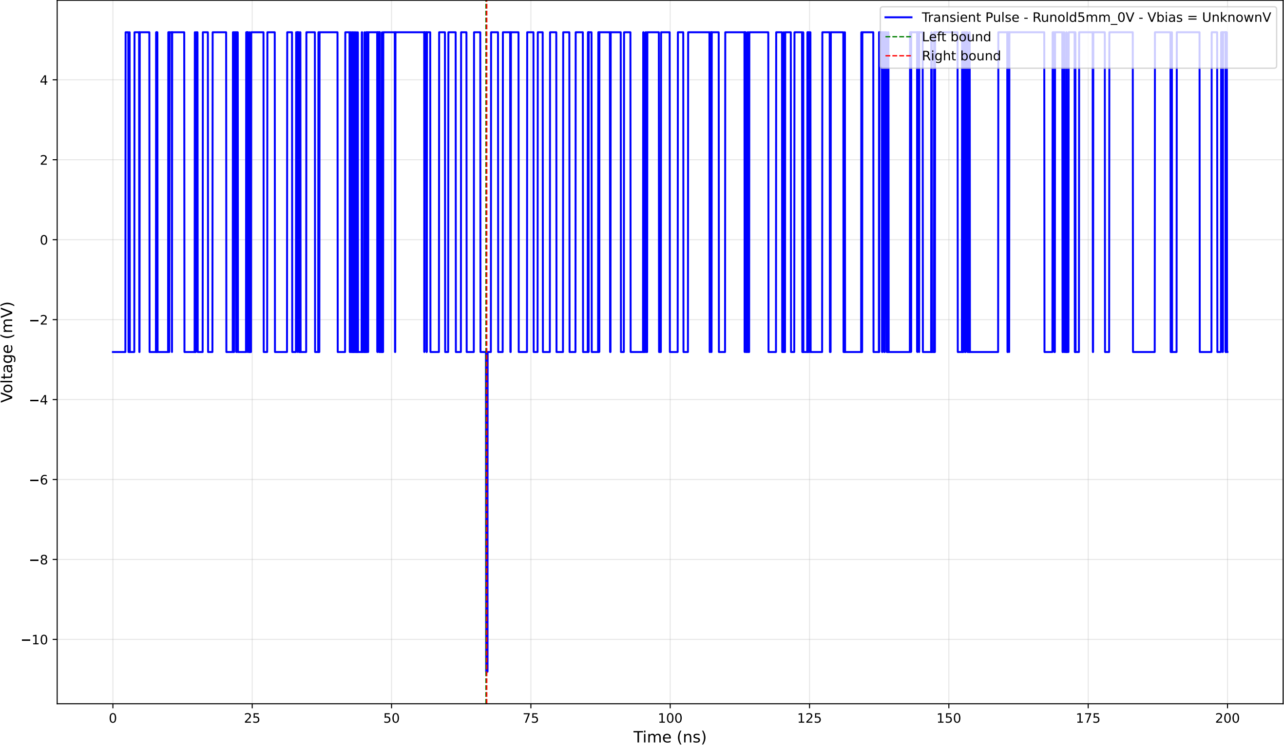
Transient Pulse - Sample: old5 - Position: 3965.0 \mu\text{m} - Charge: -0.03 pC
