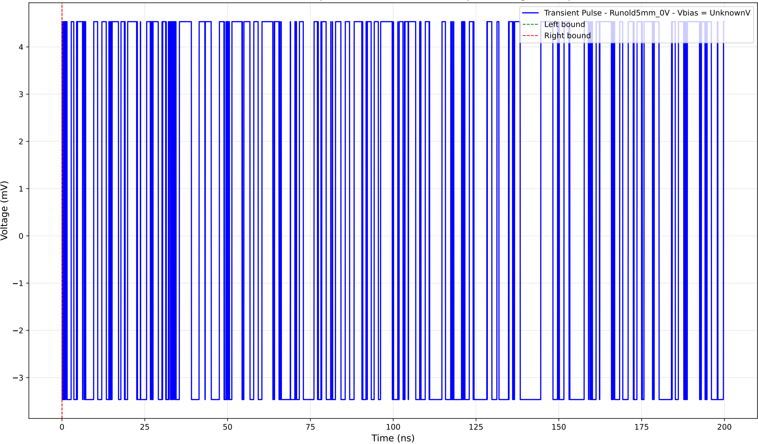
Transient Pulse - Sample: old5 - Position: 3070.0 \mu\text{m} - Charge: 0.00 pC
