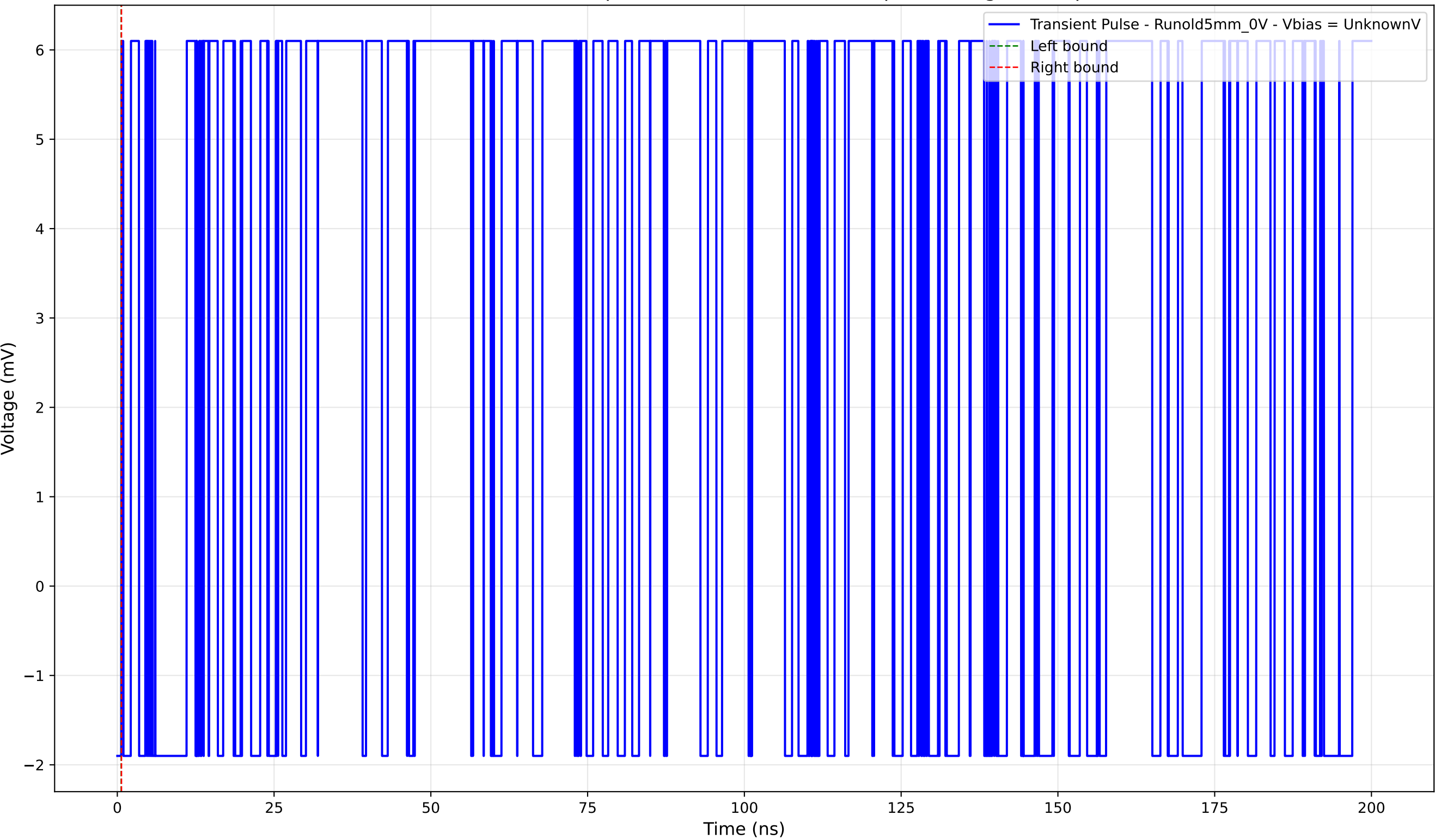
Transient Pulse - Sample: old5 - Position: 5185.0 \mu\text{m} - Charge: 0.00 pC
