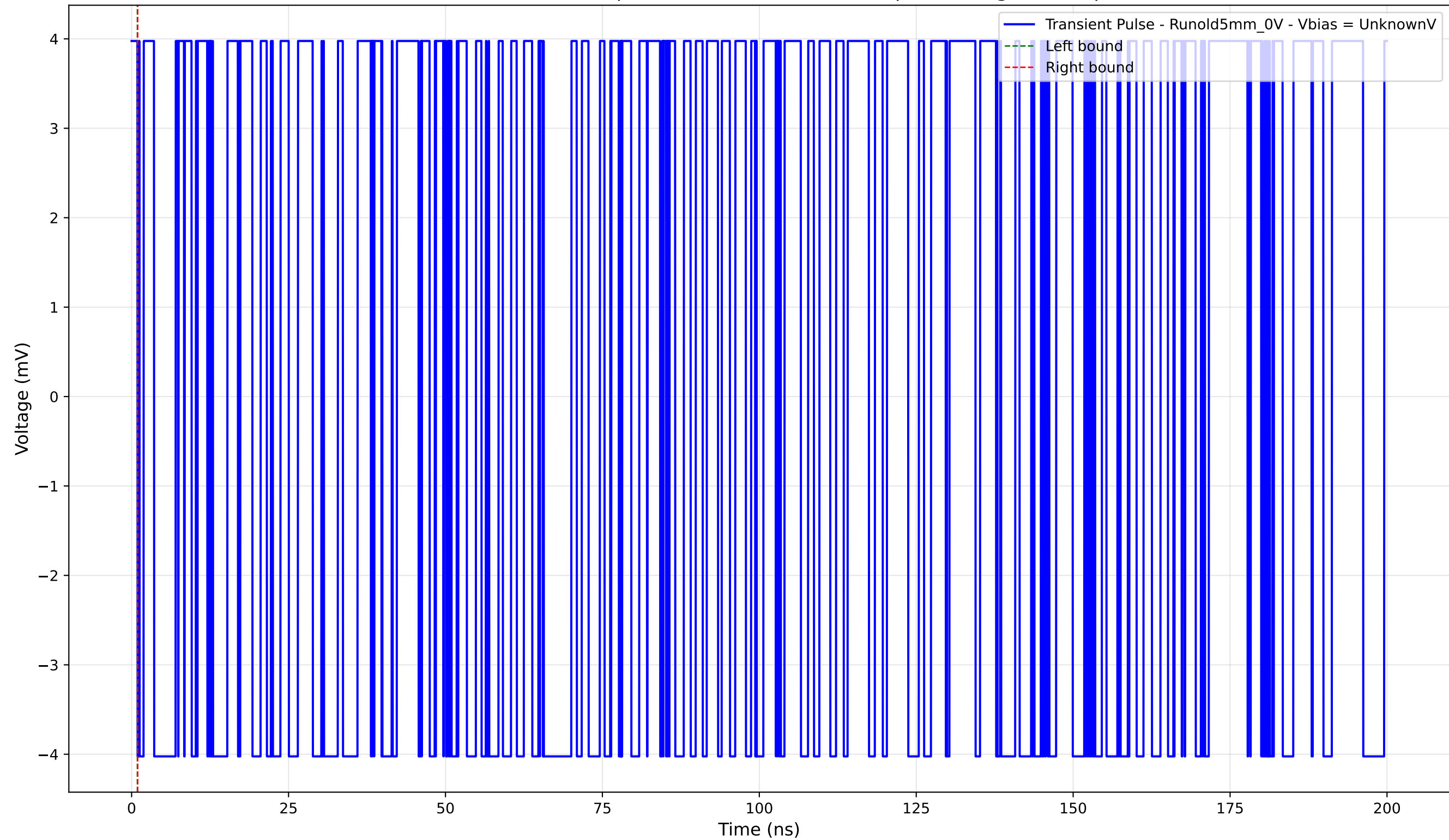
Transient Pulse - Sample: old5 - Position: 5160.0 \mu\text{m} - Charge: -0.00 pC
