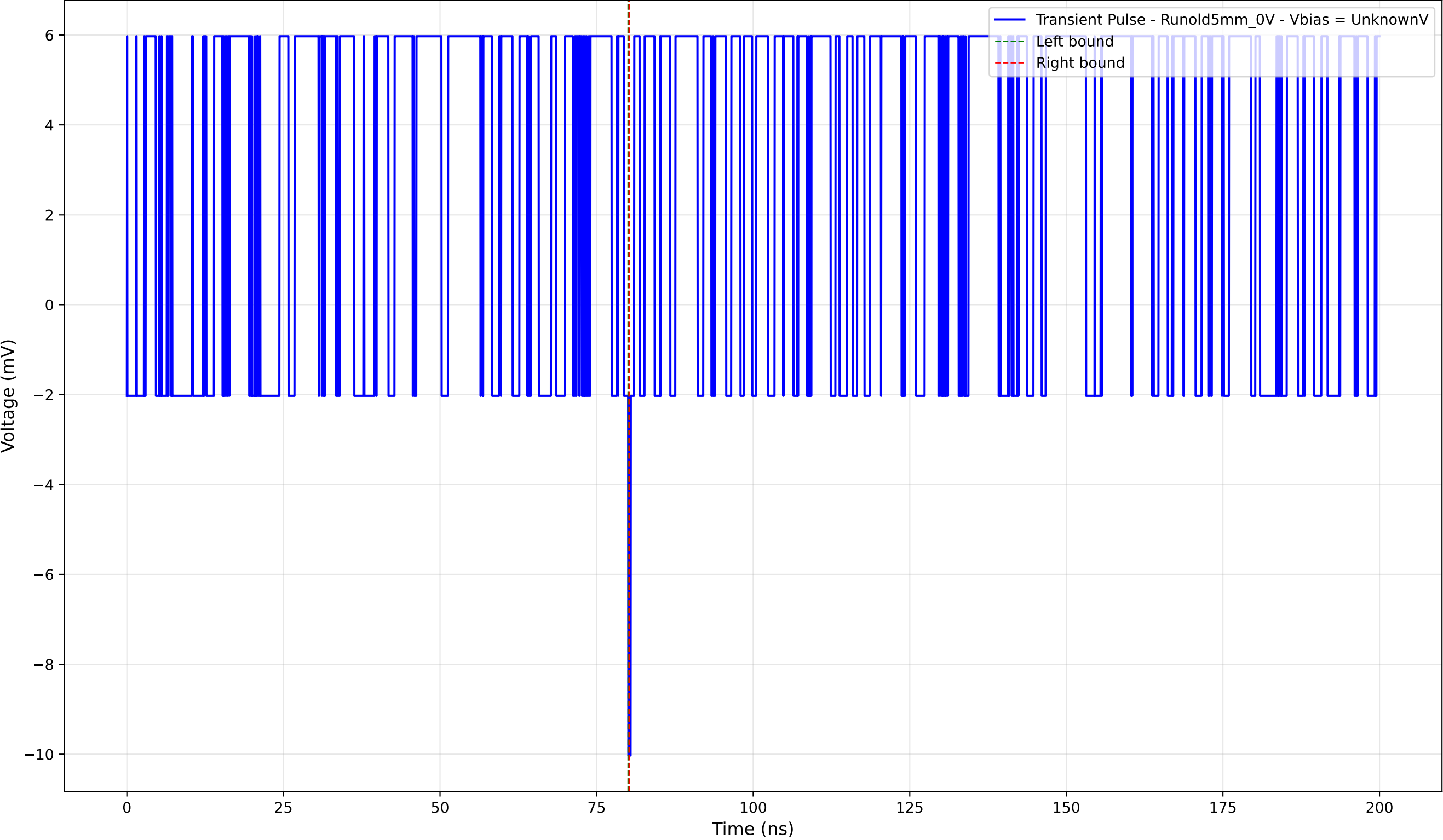
Transient Pulse - Sample: old5 - Position: 1470.0 \mu\text{m} - Charge: -0.03 pC
