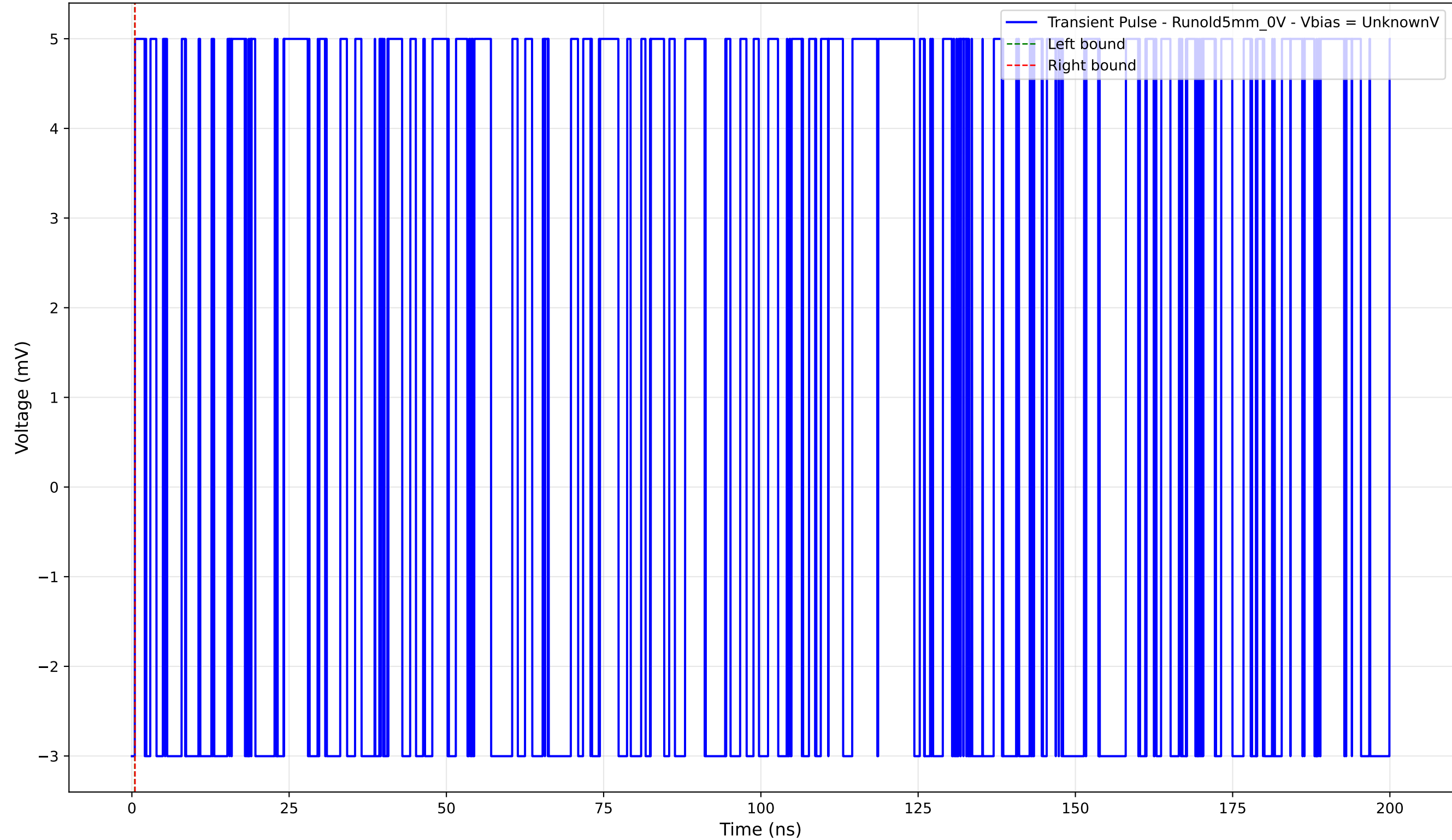
Transient Pulse - Sample: old5 - Position: 590.0 \mu\text{m} - Charge: 0.00 pC
