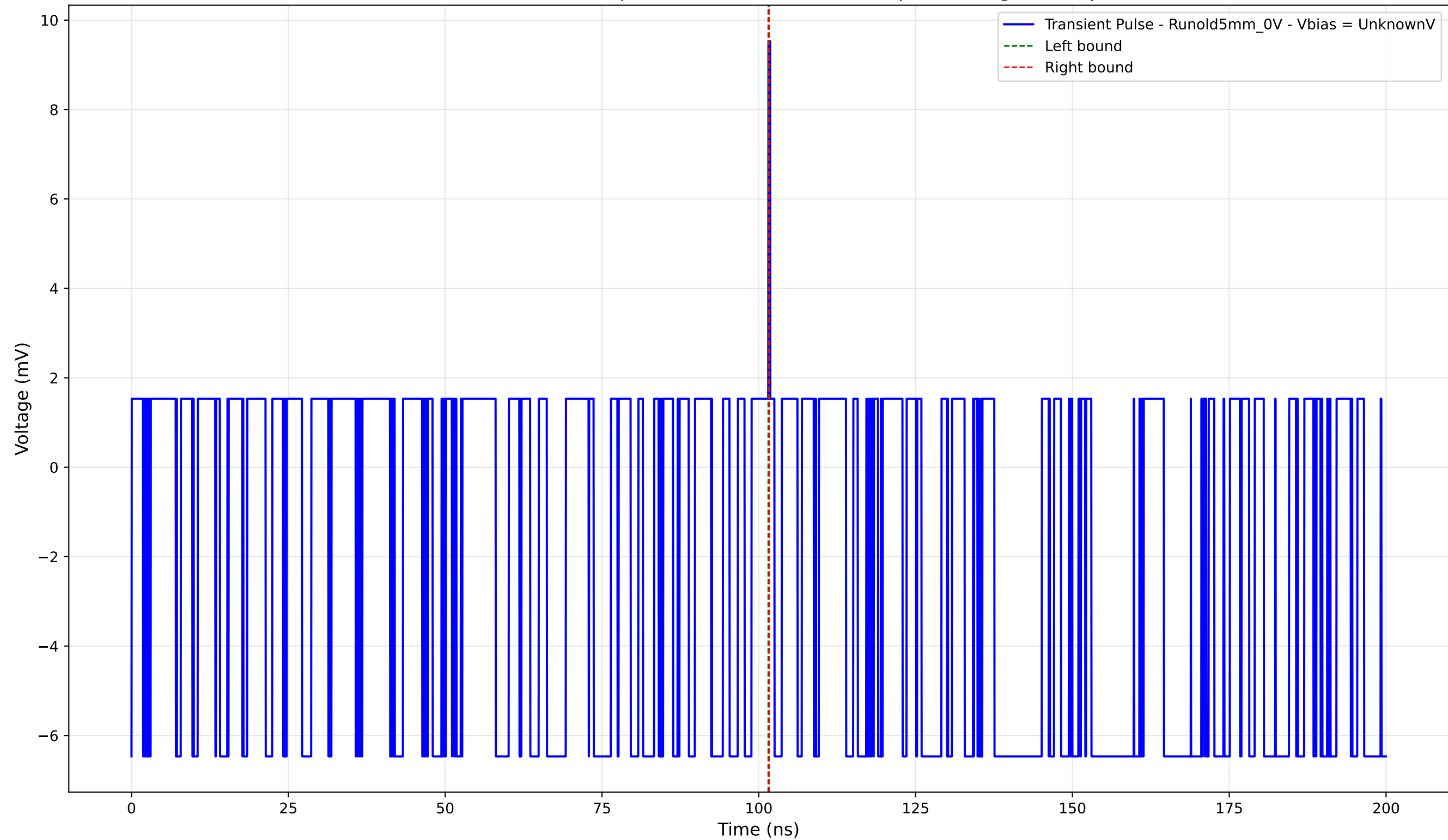
Transient Pulse - Sample: old5 - Position: 4770.0 \mu\text{m} - Charge: 0.02 pC
