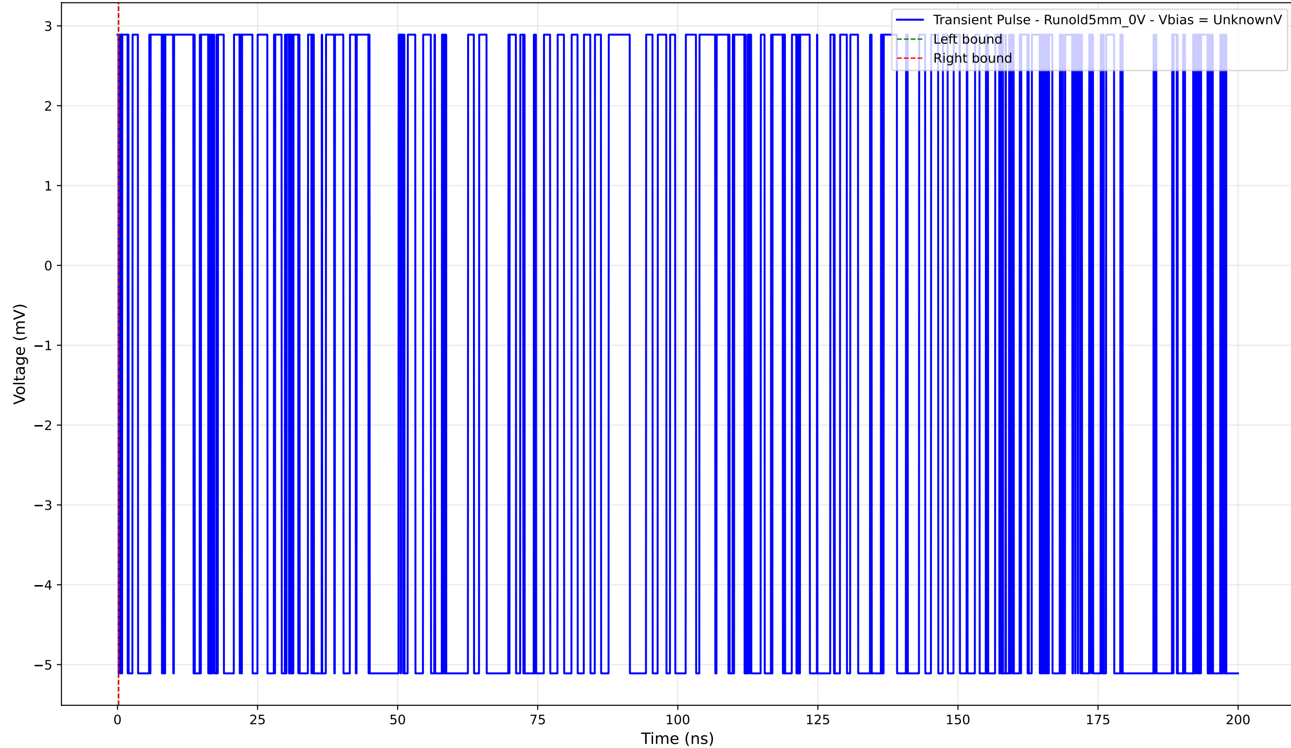
Transient Pulse - Sample: old5 - Position: 3190.0 \mu\text{m} - Charge: -0.00 pC
