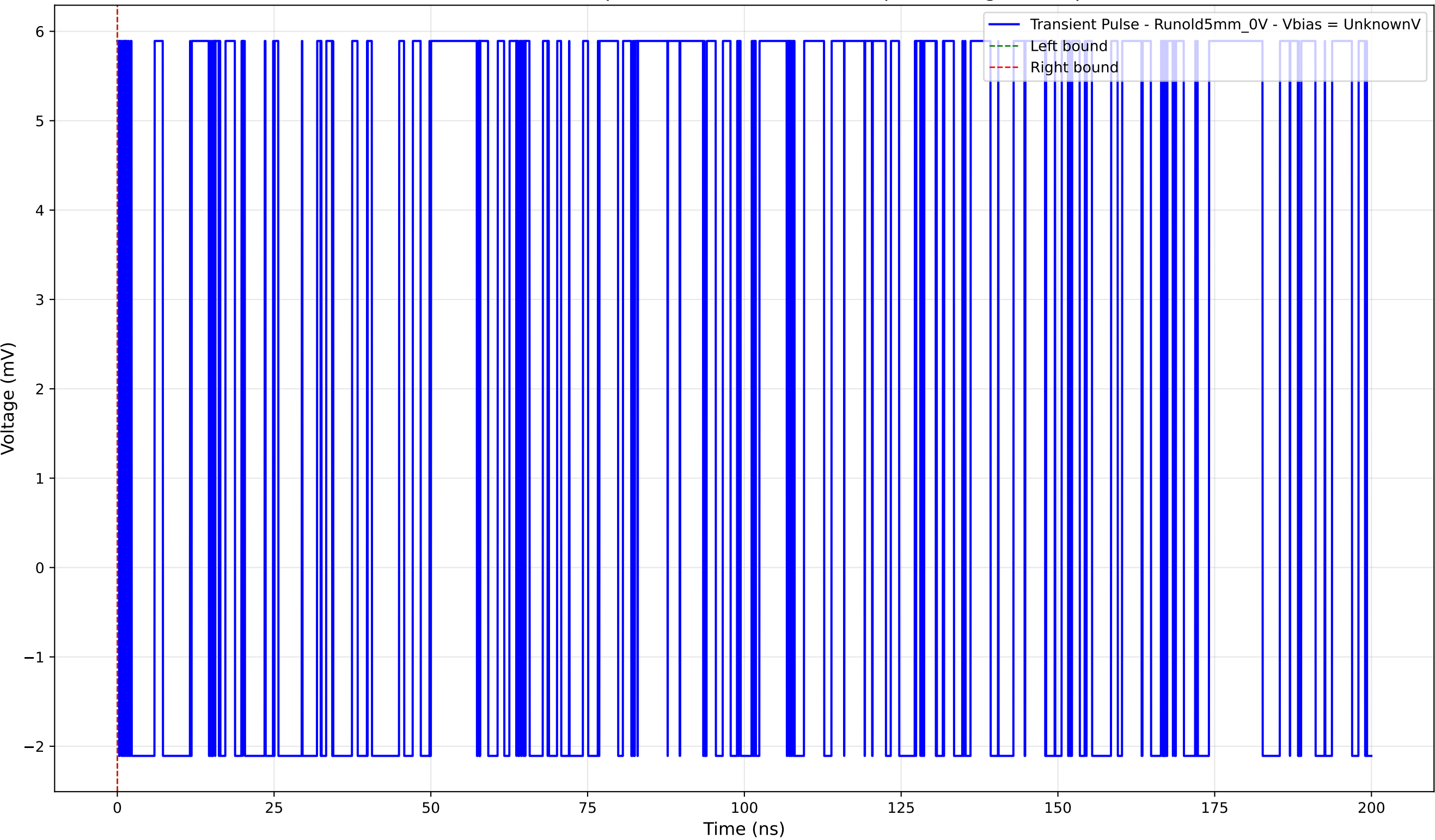
Transient Pulse - Sample: old5 - Position: 4240.0 \mu\text{m} - Charge: 0.00 pC
