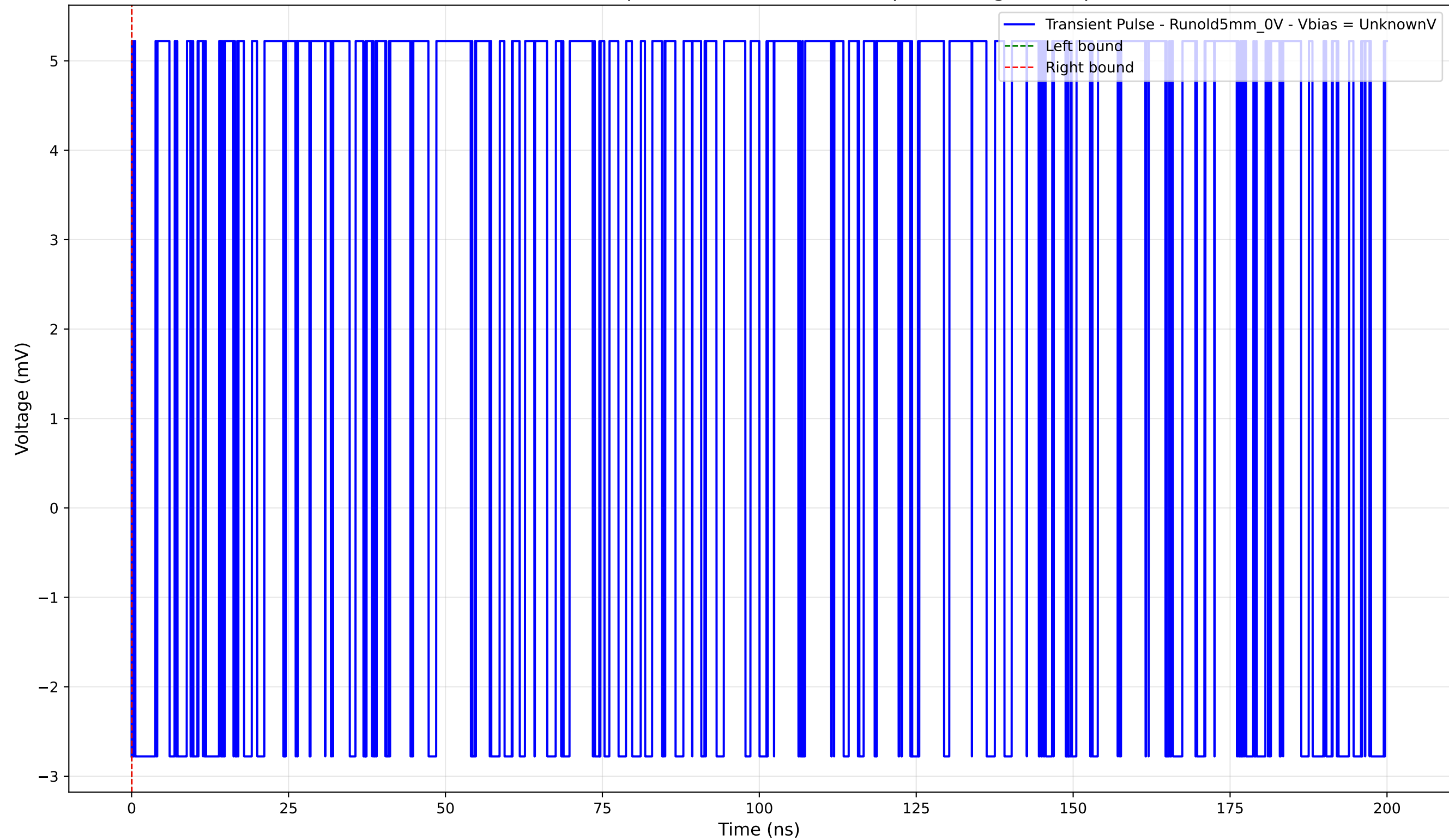
Transient Pulse - Sample: old5 - Position: 250.0 \mu\text{m} - Charge: 0.00 pC
