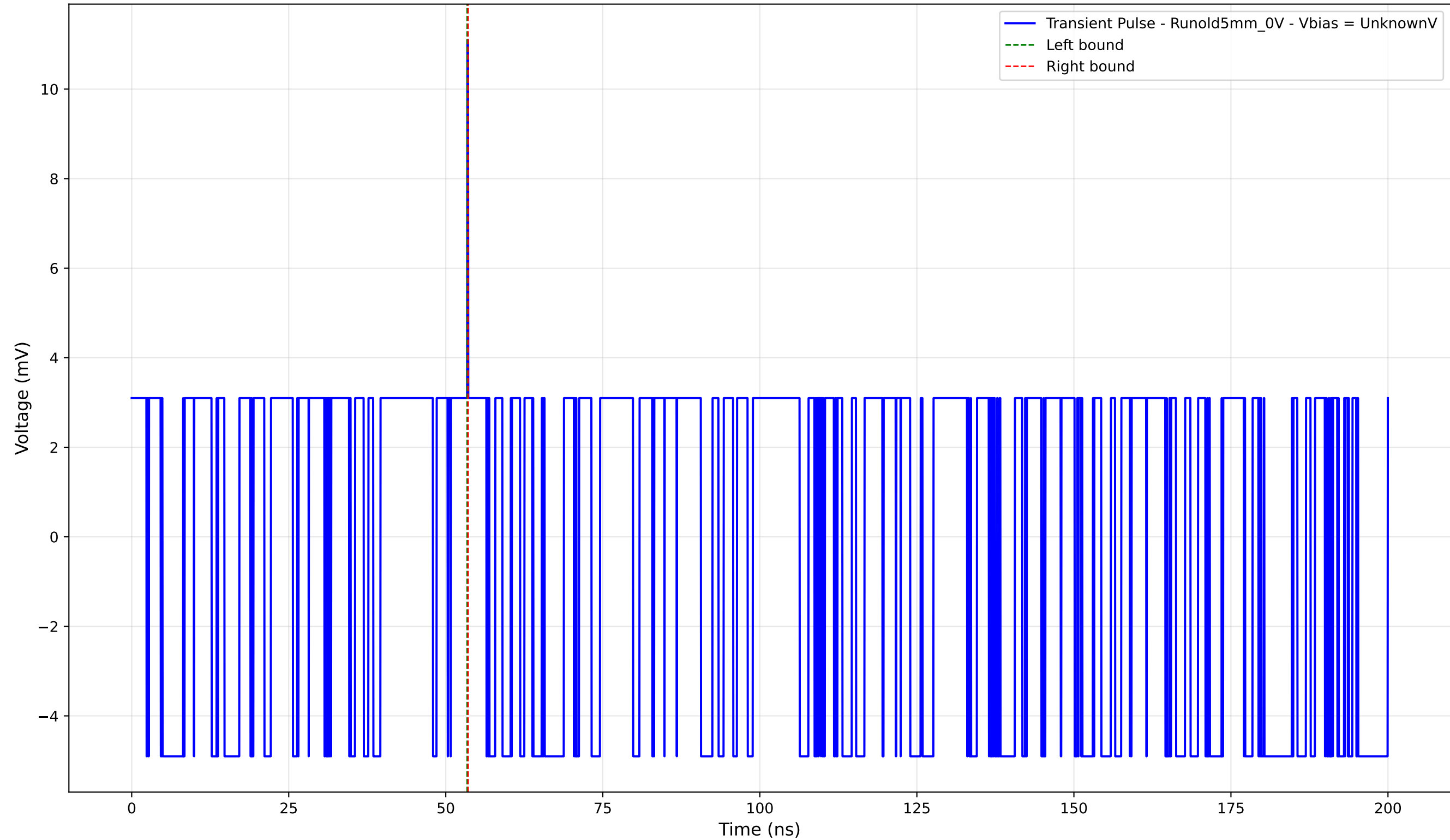
Transient Pulse - Sample: old5 - Position: 755.0 \mu\text{m} - Charge: 0.03 pC
