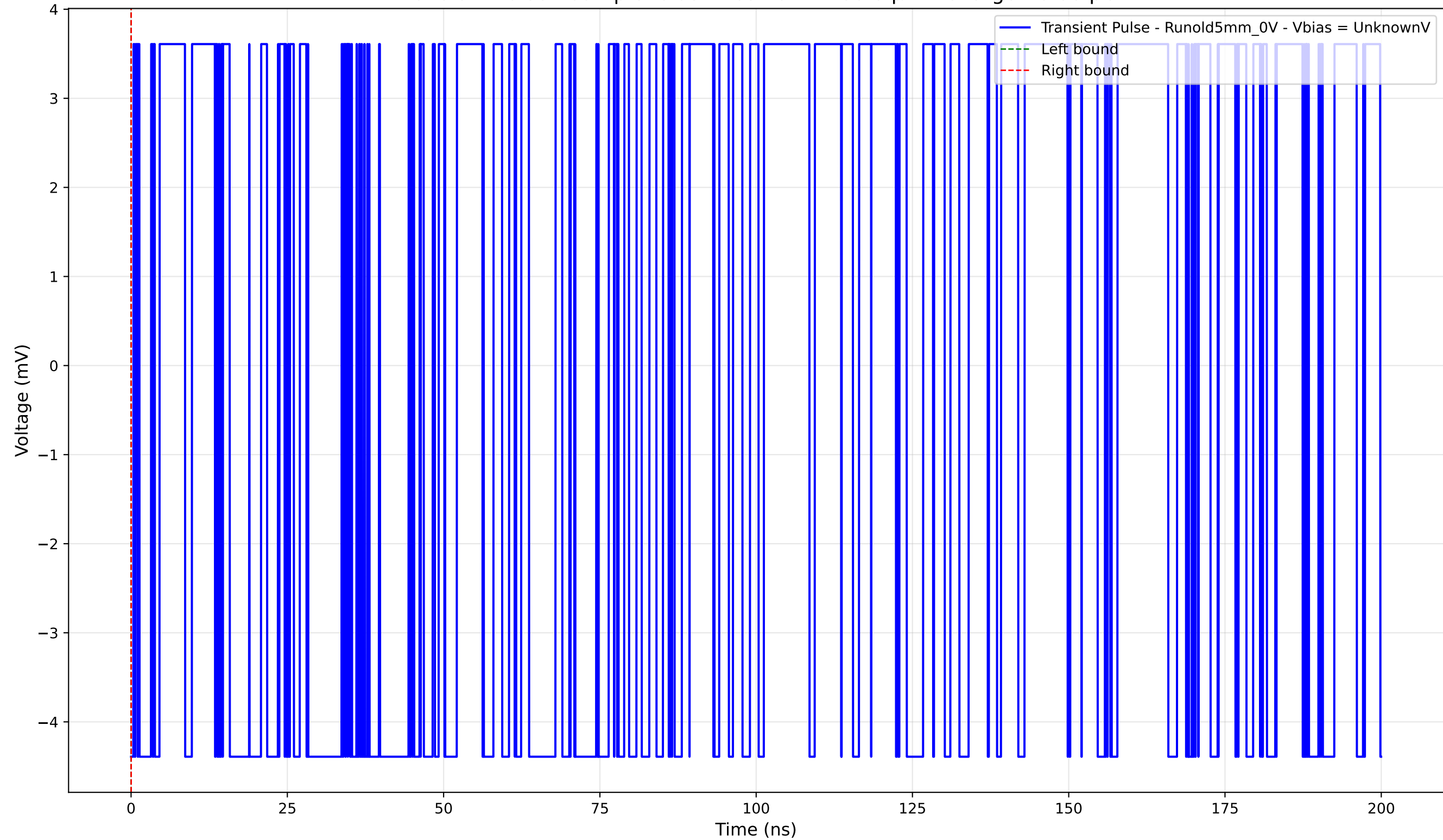
Transient Pulse - Sample: old5 - Position: 2780.0 \mu\text{m} - Charge: -0.00 pC
