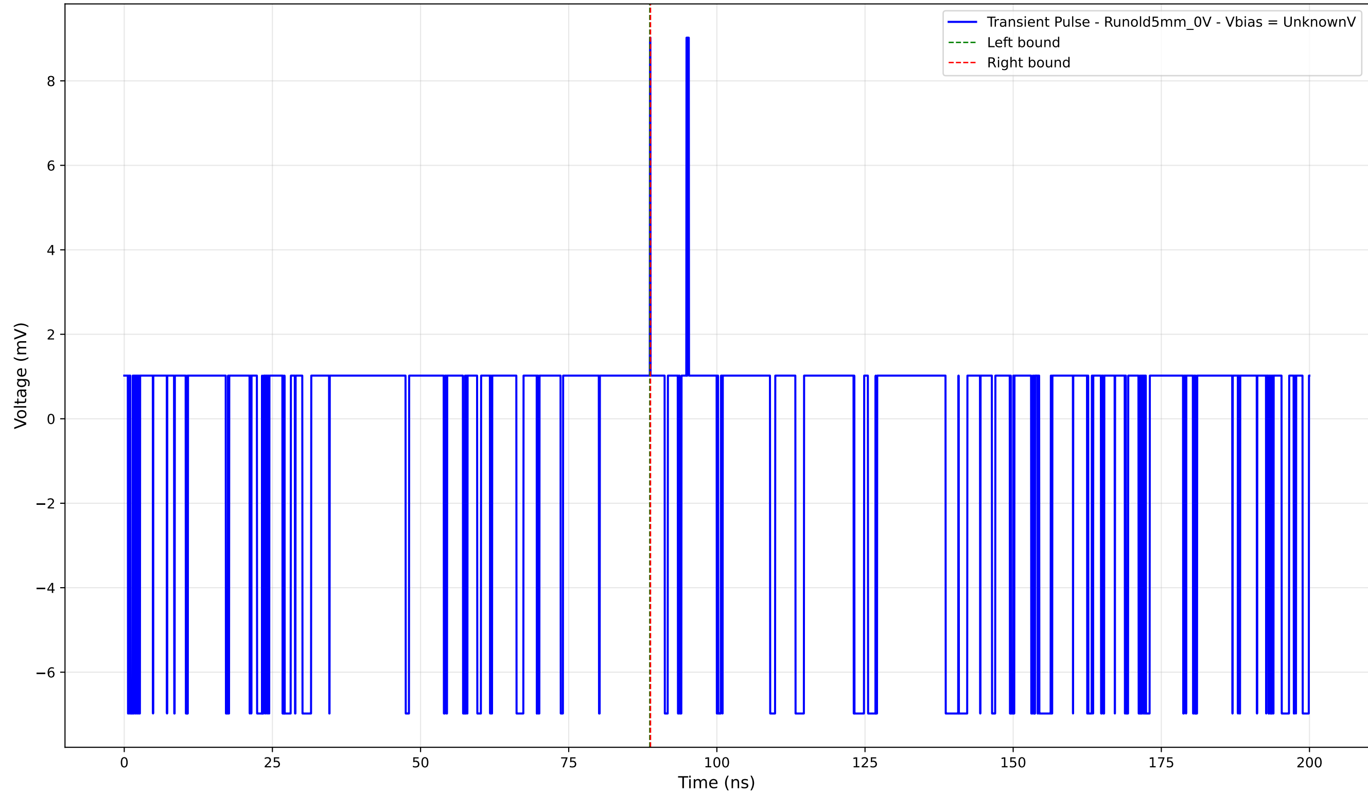
Transient Pulse - Sample: old5 - Position: 560.0 \mu\text{m} - Charge: 0.02 pC
