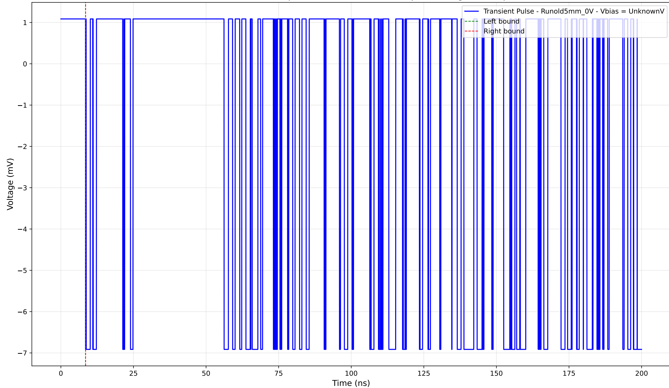
Transient Pulse - Sample: old5 - Position: 595.0 \mu\text{m} - Charge: -0.00 pC
