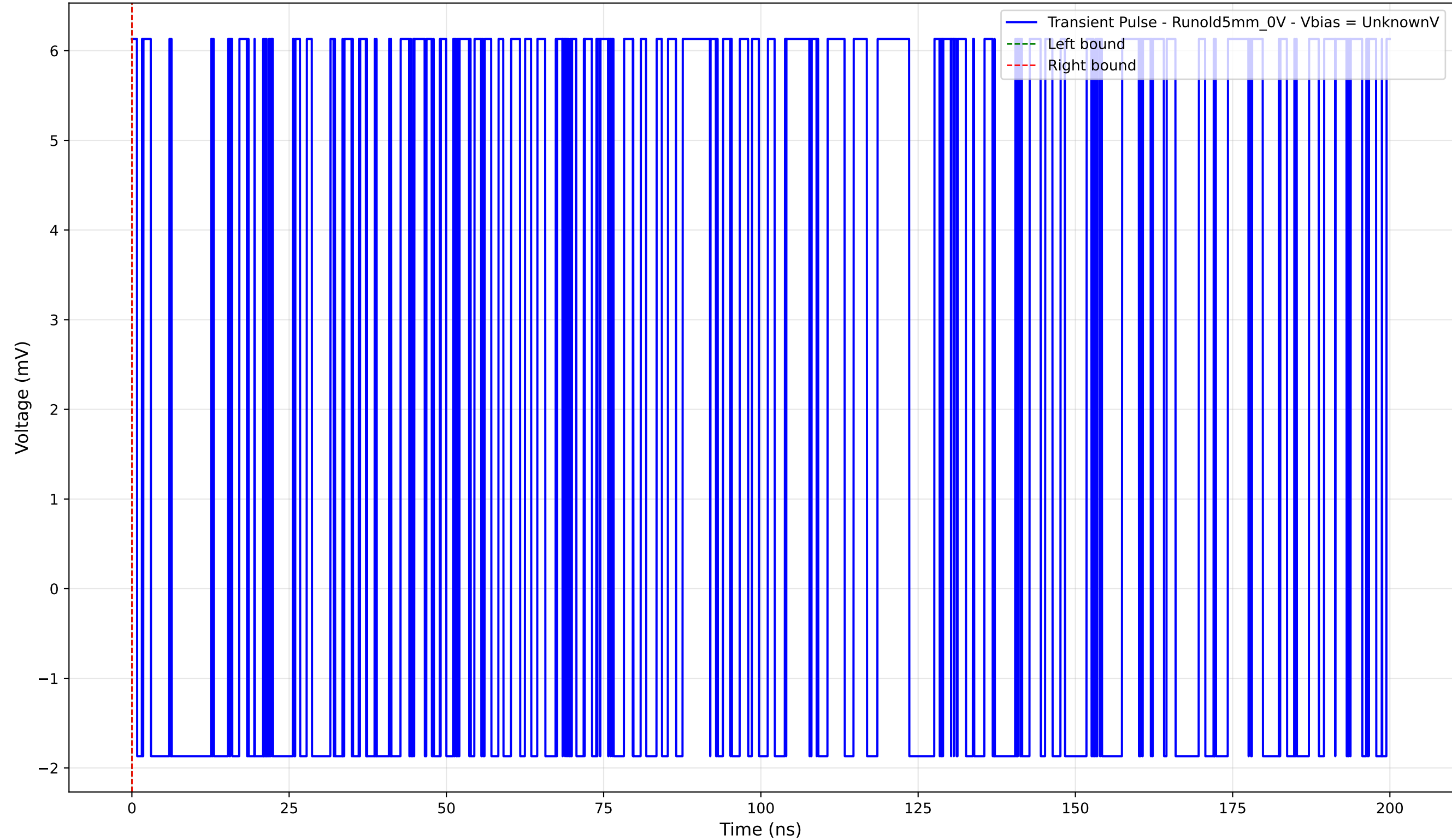
Transient Pulse - Sample: old5 - Position: 1665.0 \mu\text{m} - Charge: 0.00 pC
