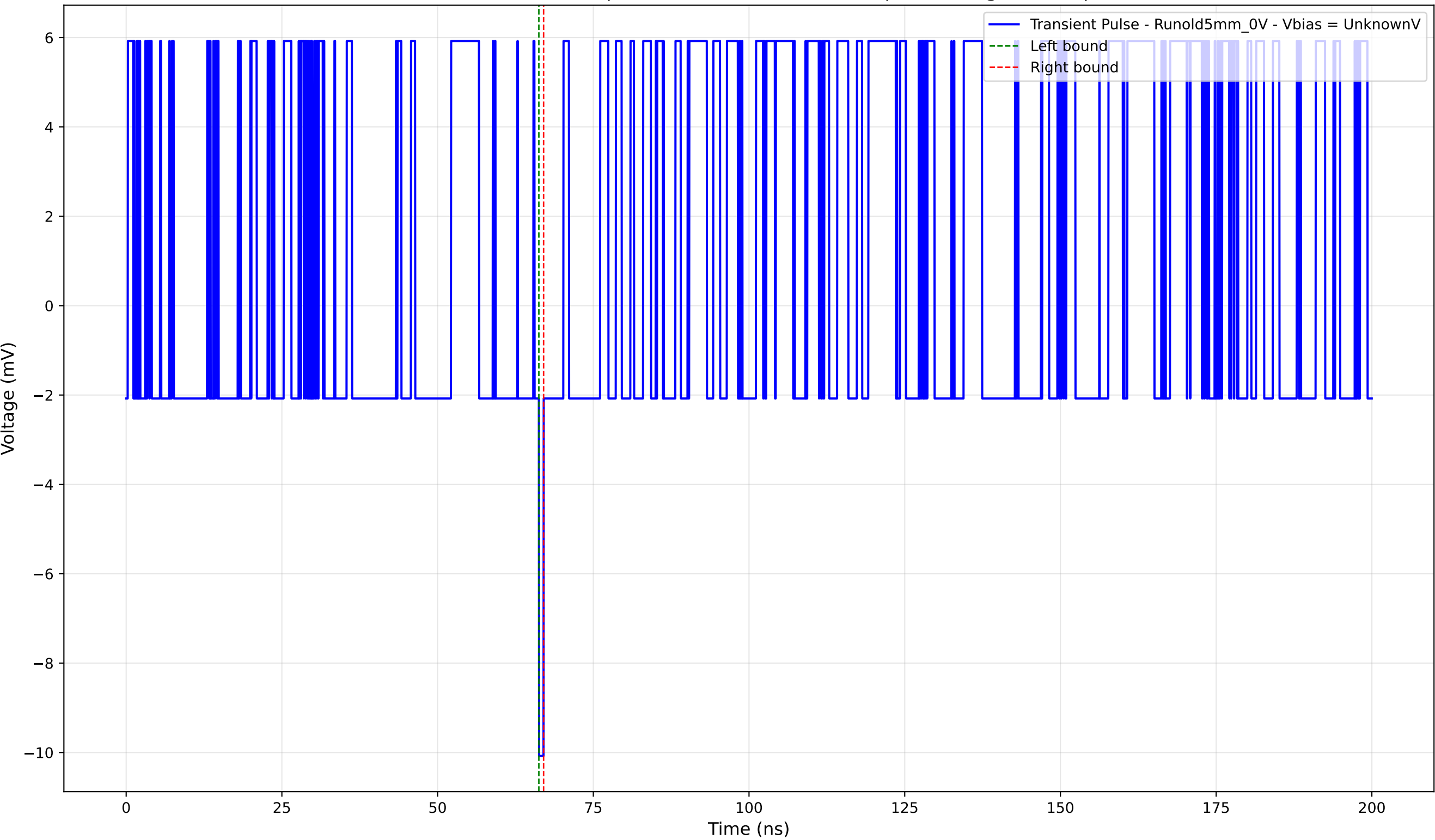
Transient Pulse - Sample: old5 - Position: 1765.0 \mu\text{m} - Charge: -0.15 pC
