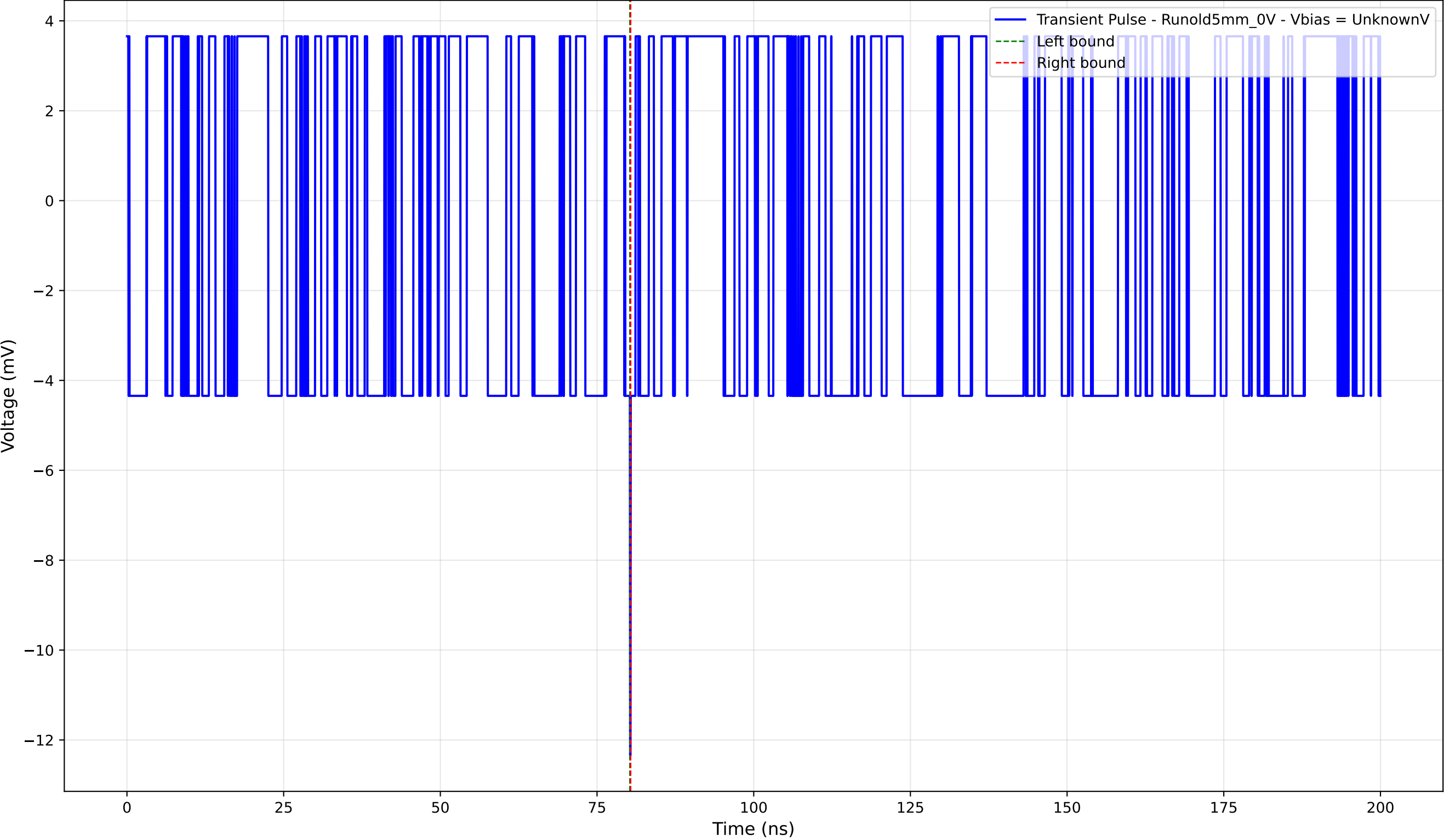
Transient Pulse - Sample: old5 - Position: 2160.0 \mu\text{m} - Charge: -0.03 pC
