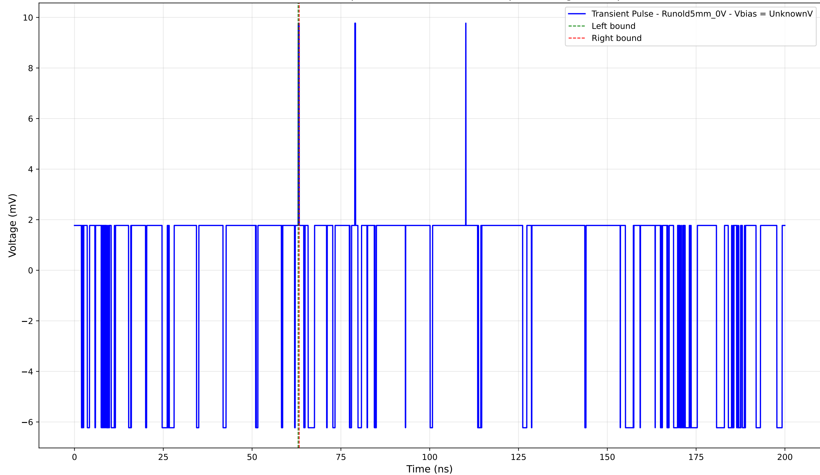
Transient Pulse - Sample: old5 - Position: 1030.0 \mu\text{m} - Charge: 0.06 pC
