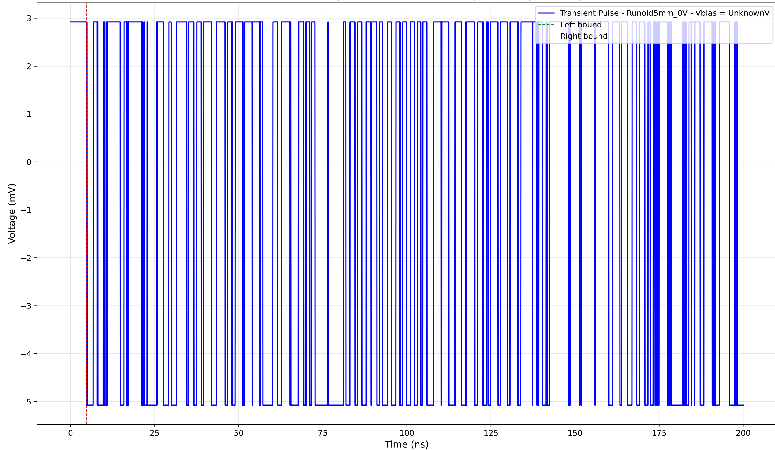
Transient Pulse - Sample: old5 - Position: 20.0 \mu\text{m} - Charge: -0.00 pC
