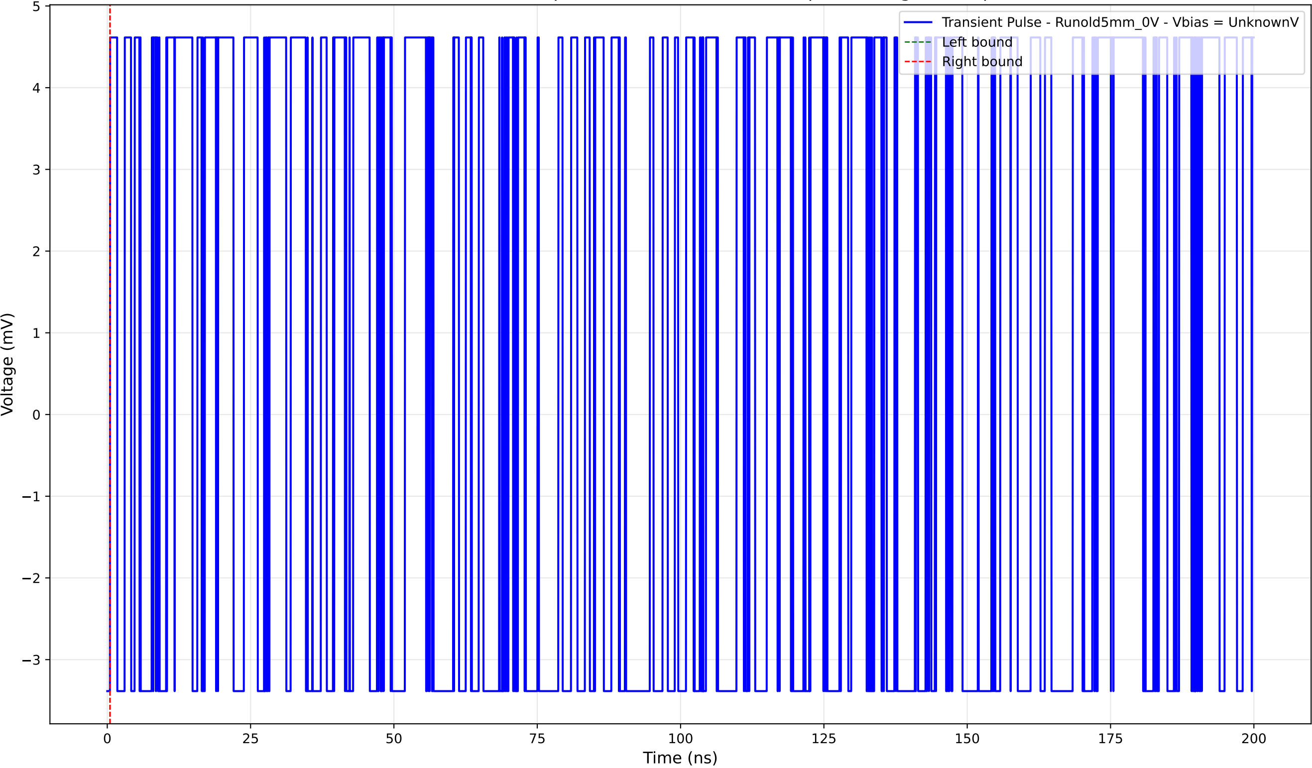
Transient Pulse - Sample: old5 - Position: 2500.0 \mu\text{m} - Charge: 0.00 pC
