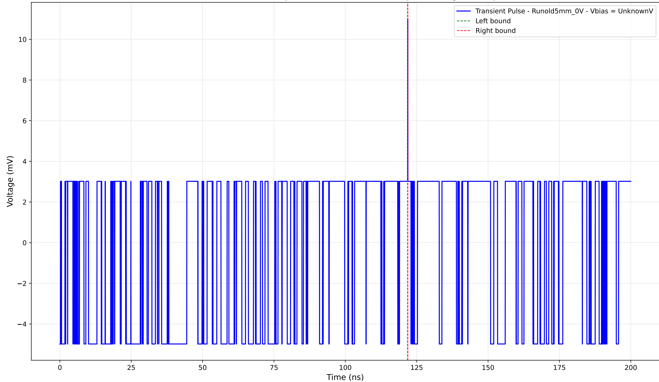
Transient Pulse - Sample: old5 - Position: 265.0 \mu\text{m} - Charge: 0.01 pC
