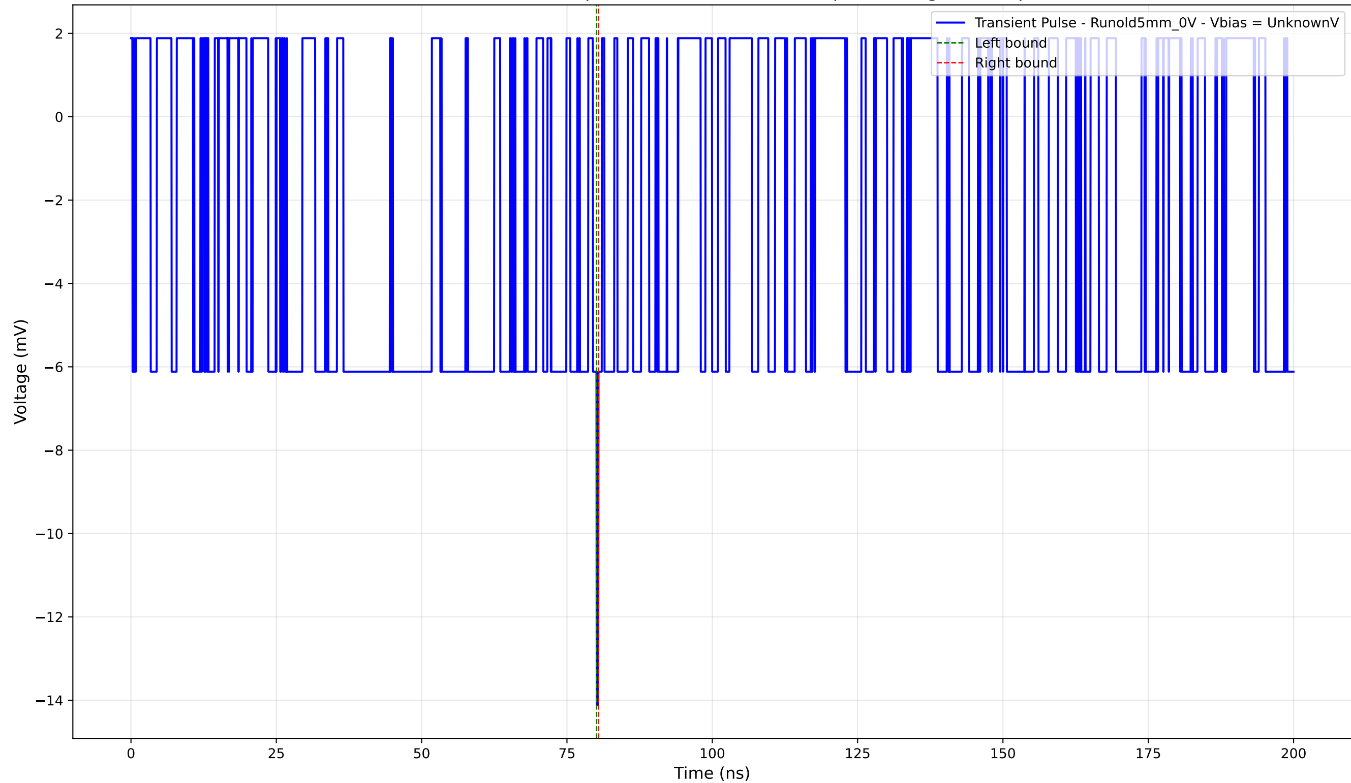
Transient Pulse - Sample: old5 - Position: 770.0 \mu\text{m} - Charge: -0.09 pC
