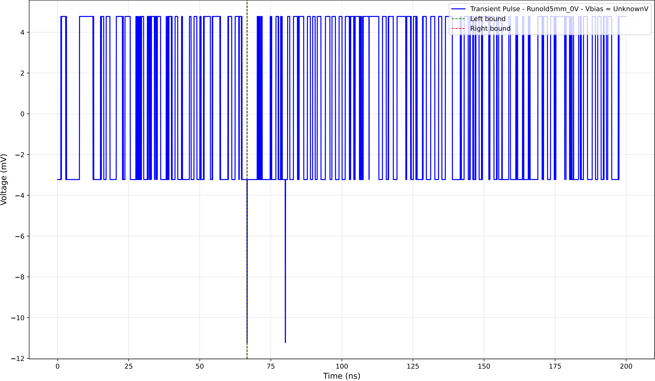
Transient Pulse - Sample: old5 - Position: 2255.0 \mu\text{m} - Charge: -0.03 pC
