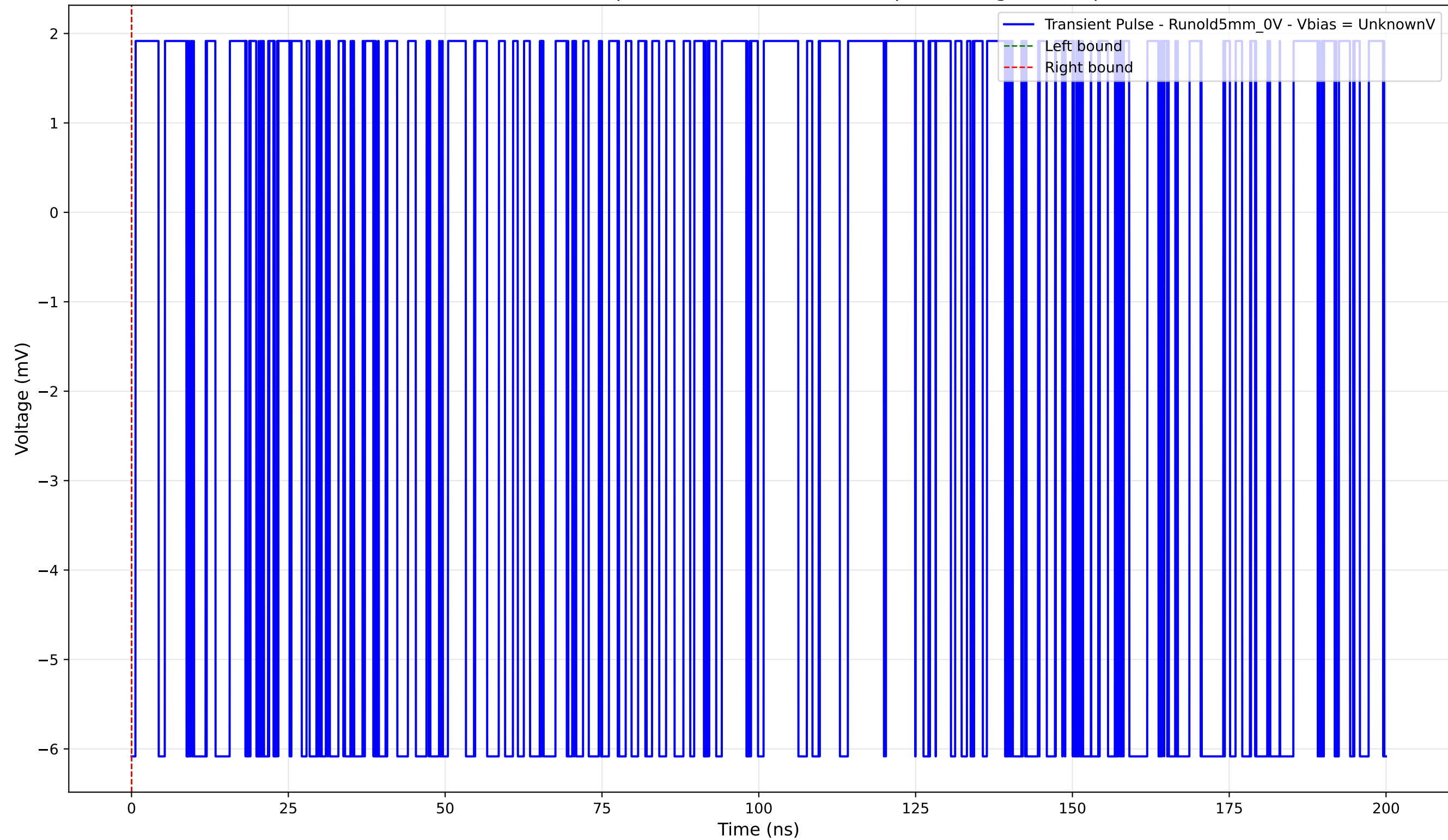
Transient Pulse - Sample: old5 - Position: 4705.0 \mu\text{m} - Charge: -0.00 pC
