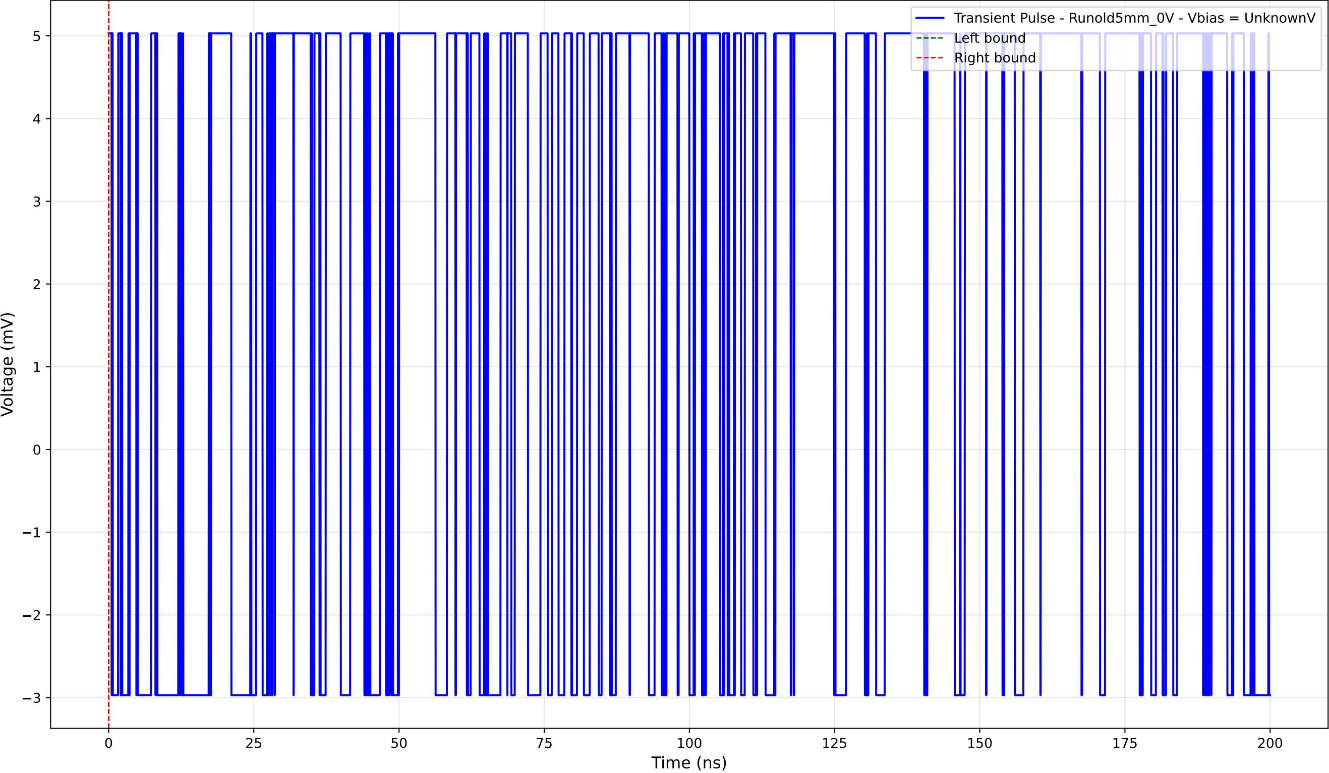
Transient Pulse - Sample: old5 - Position: 3930.0 \mu\text{m} - Charge: 0.00 pC
