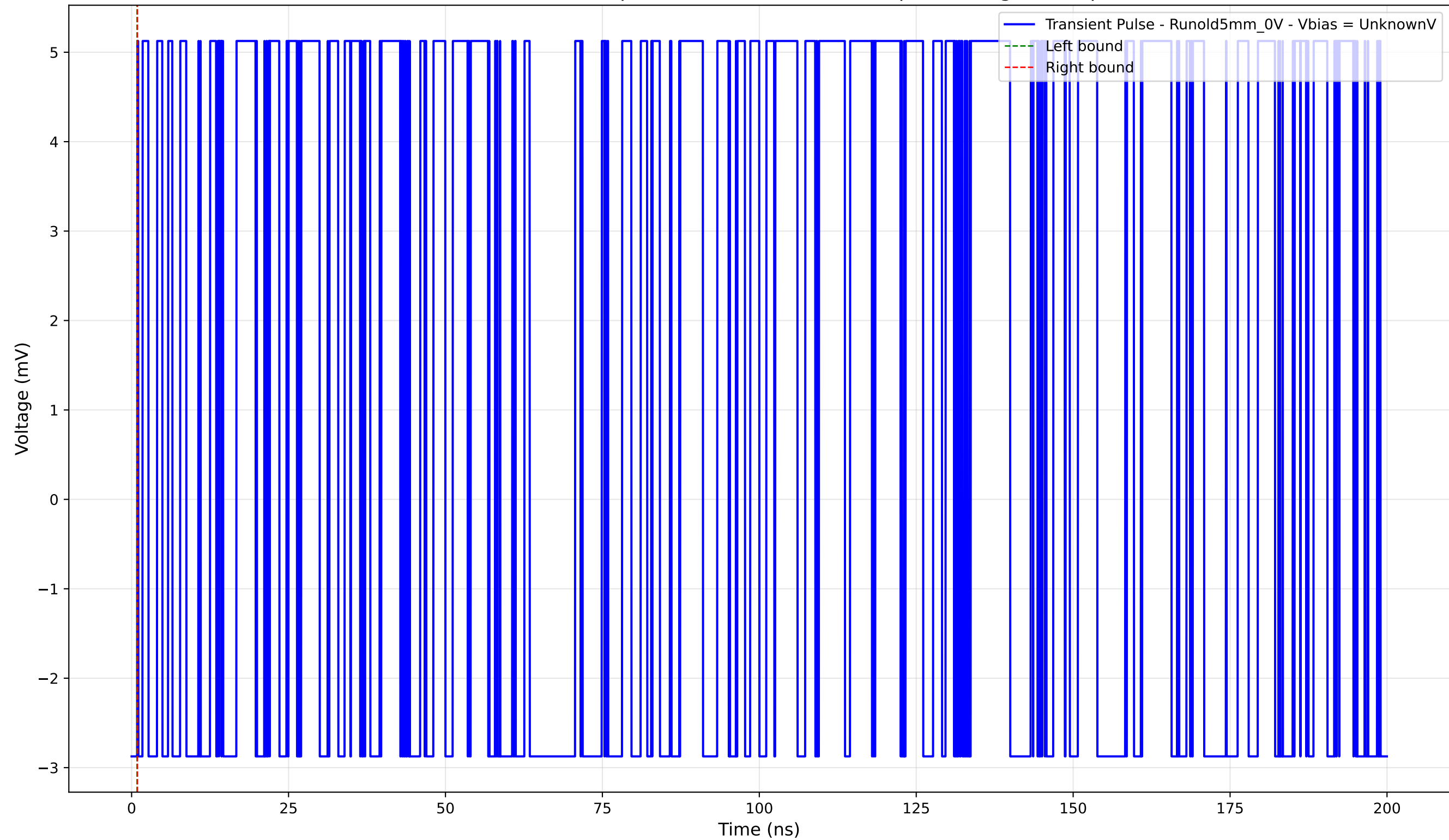
Transient Pulse - Sample: old5 - Position: 2615.0 \mu\text{m} - Charge: 0.00 pC
