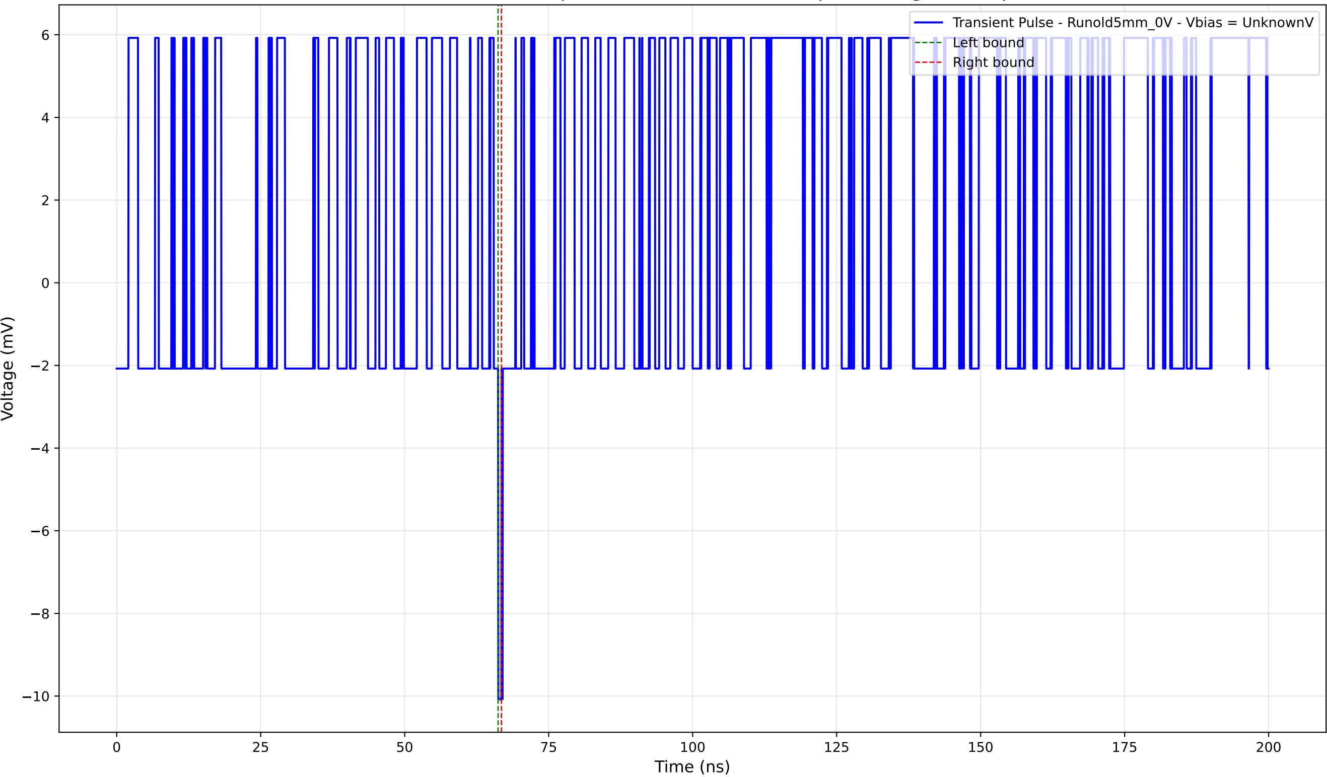
Transient Pulse - Sample: old5 - Position: 2065.0 \mu\text{m} - Charge: -0.11 pC
