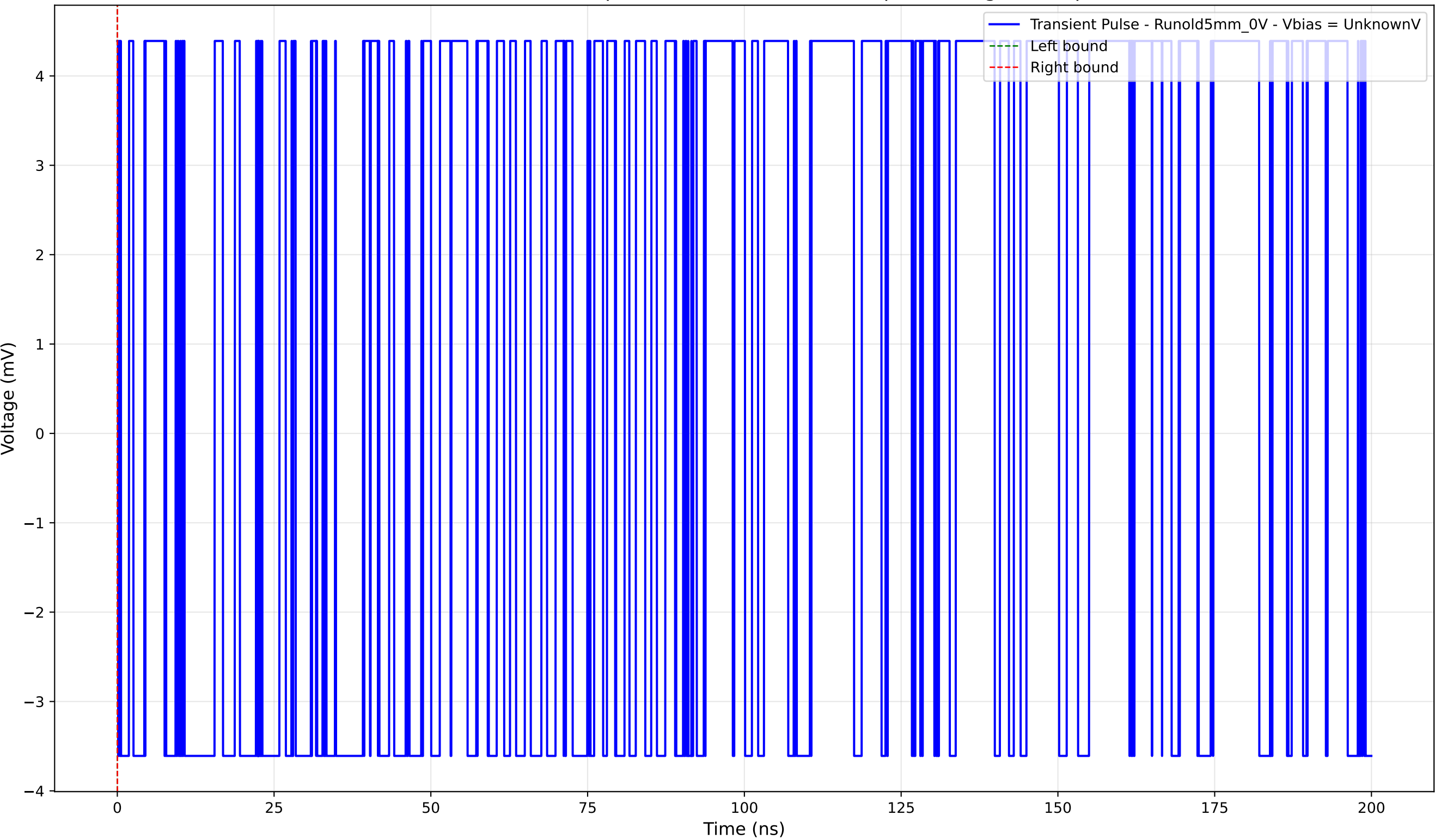
Transient Pulse - Sample: old5 - Position: 2250.0 \mu\text{m} - Charge: 0.00 pC
