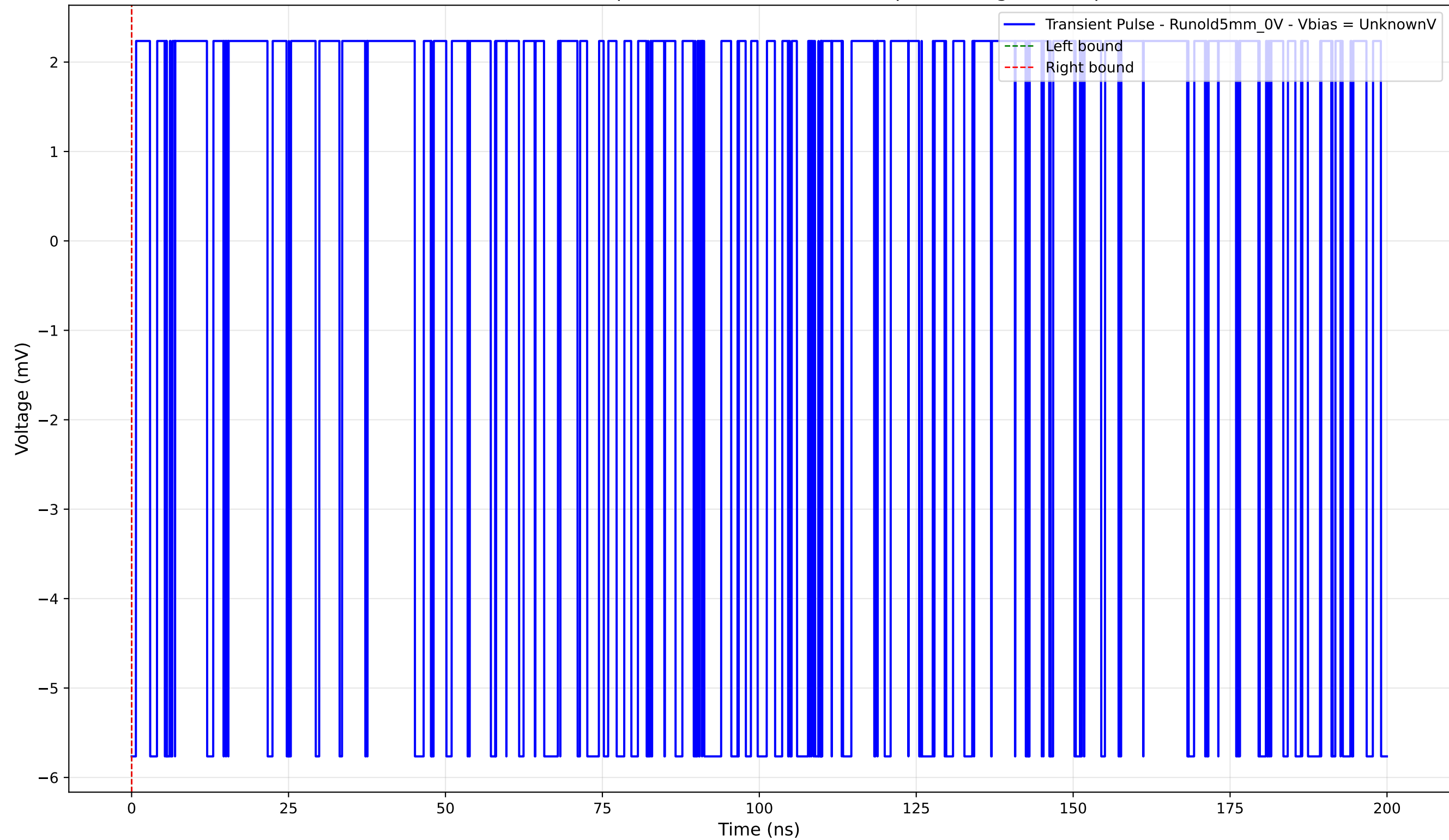
Transient Pulse - Sample: old5 - Position: 1670.0 \mu\text{m} - Charge: -0.00 pC
