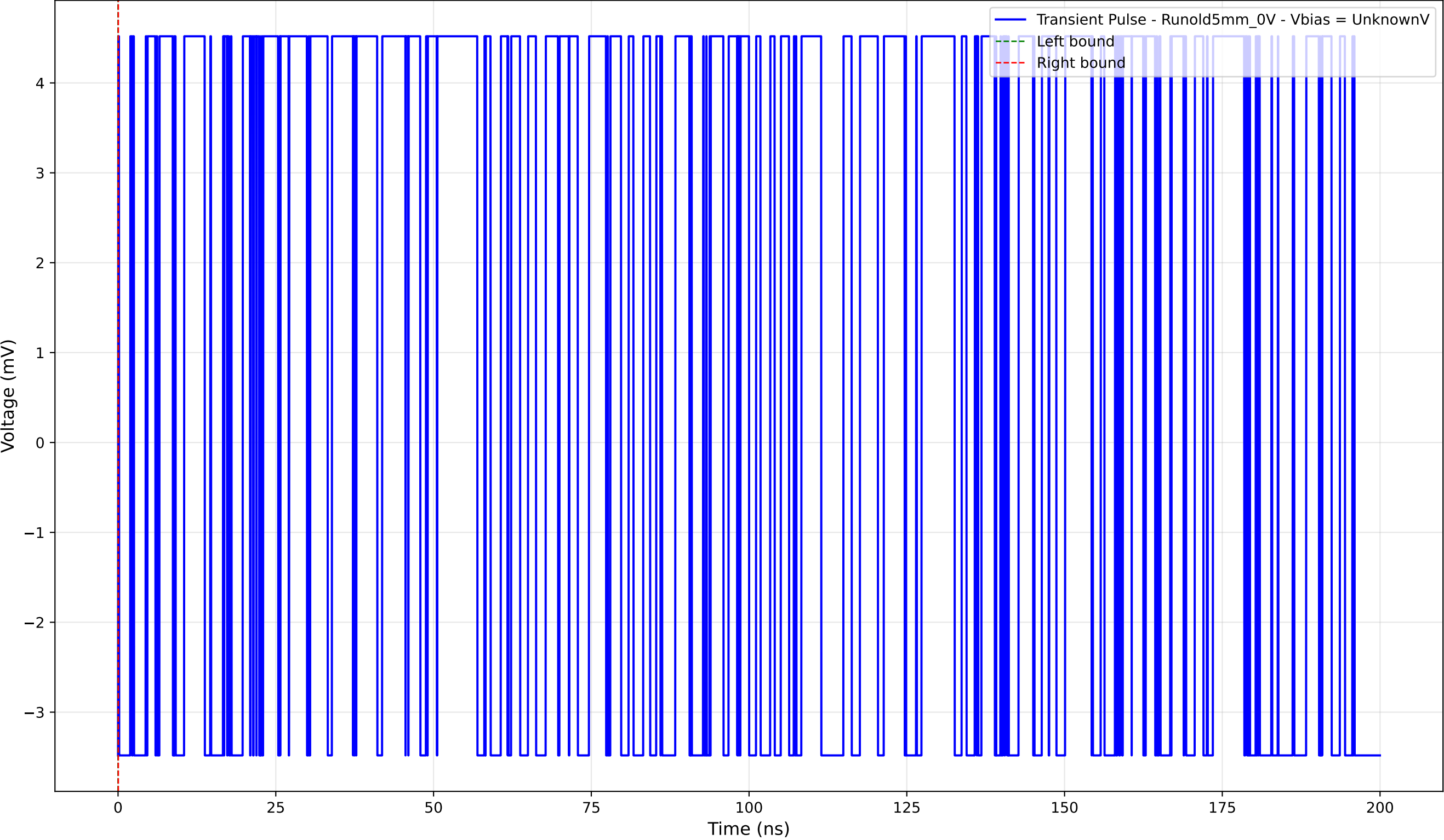
Transient Pulse - Sample: old5 - Position: 3305.0 \mu\text{m} - Charge: 0.00 pC
