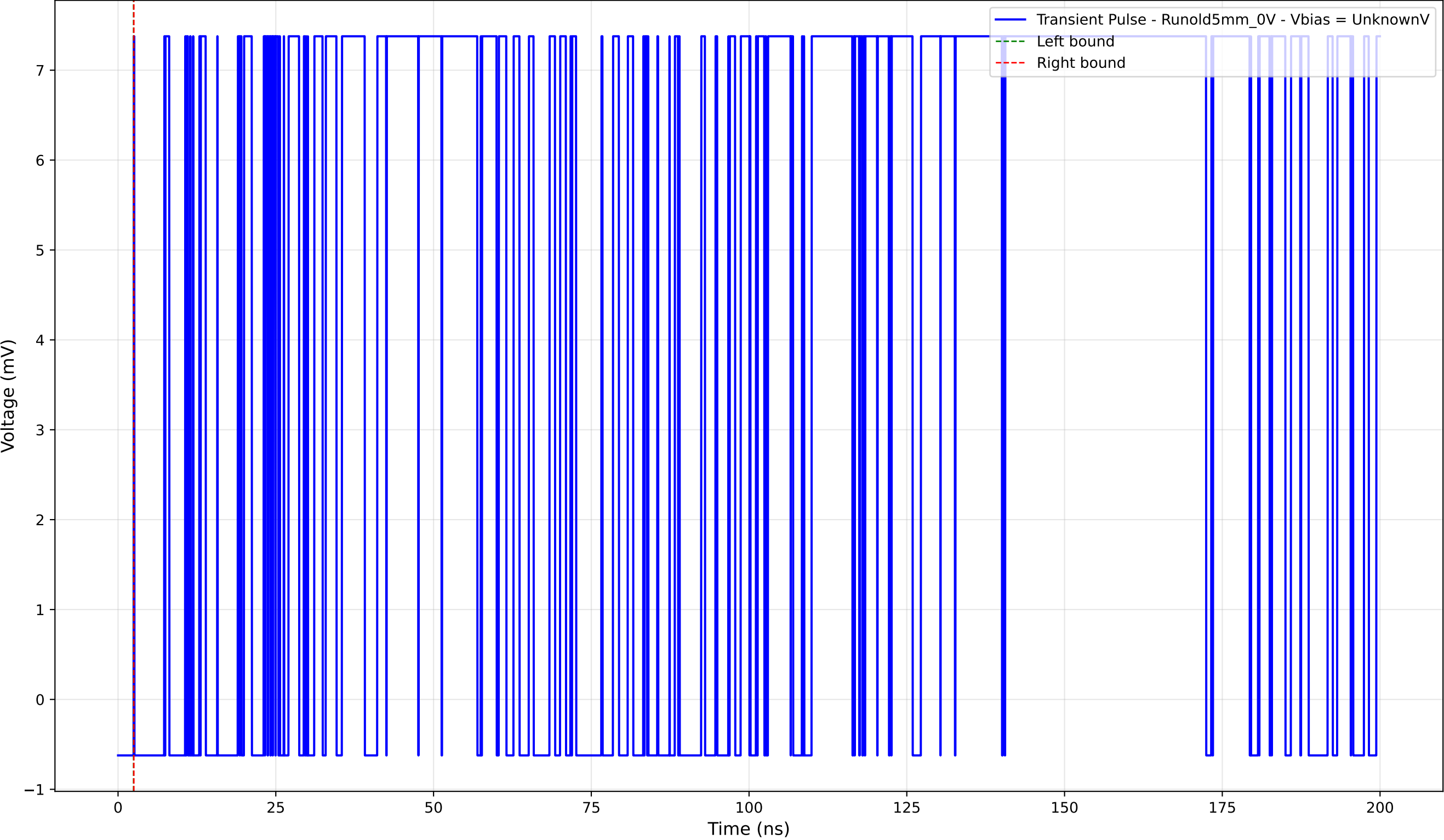
Transient Pulse - Sample: old5 - Position: 4835.0 \mu\text{m} - Charge: 0.00 pC
