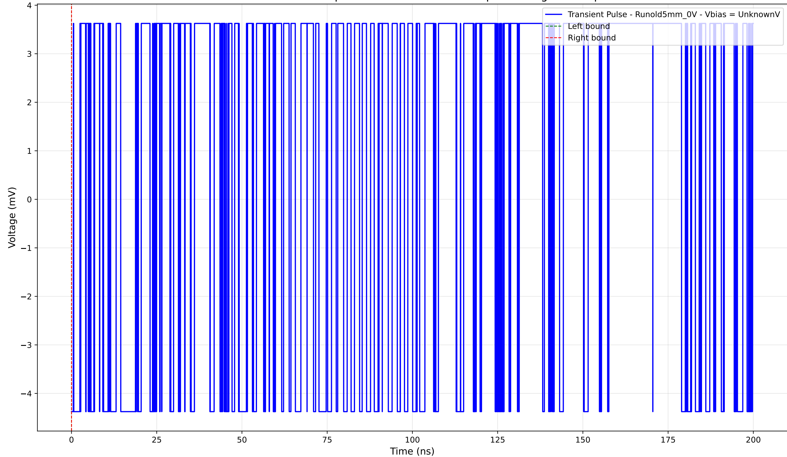
Transient Pulse - Sample: old5 - Position: 4755.0 \mu\text{m} - Charge: -0.00 pC
