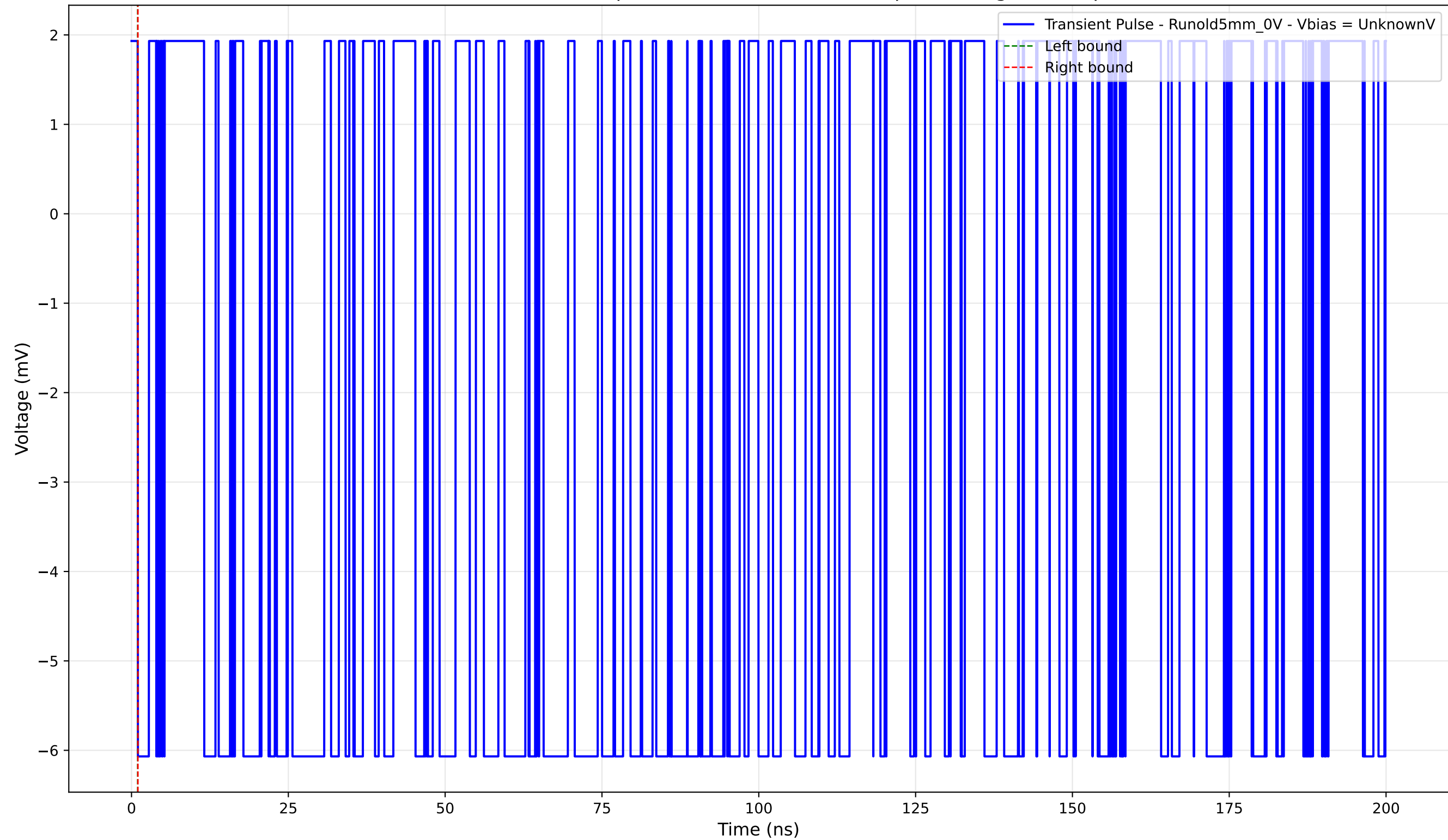
Transient Pulse - Sample: old5 - Position: 3705.0 \mu\text{m} - Charge: -0.00 pC
