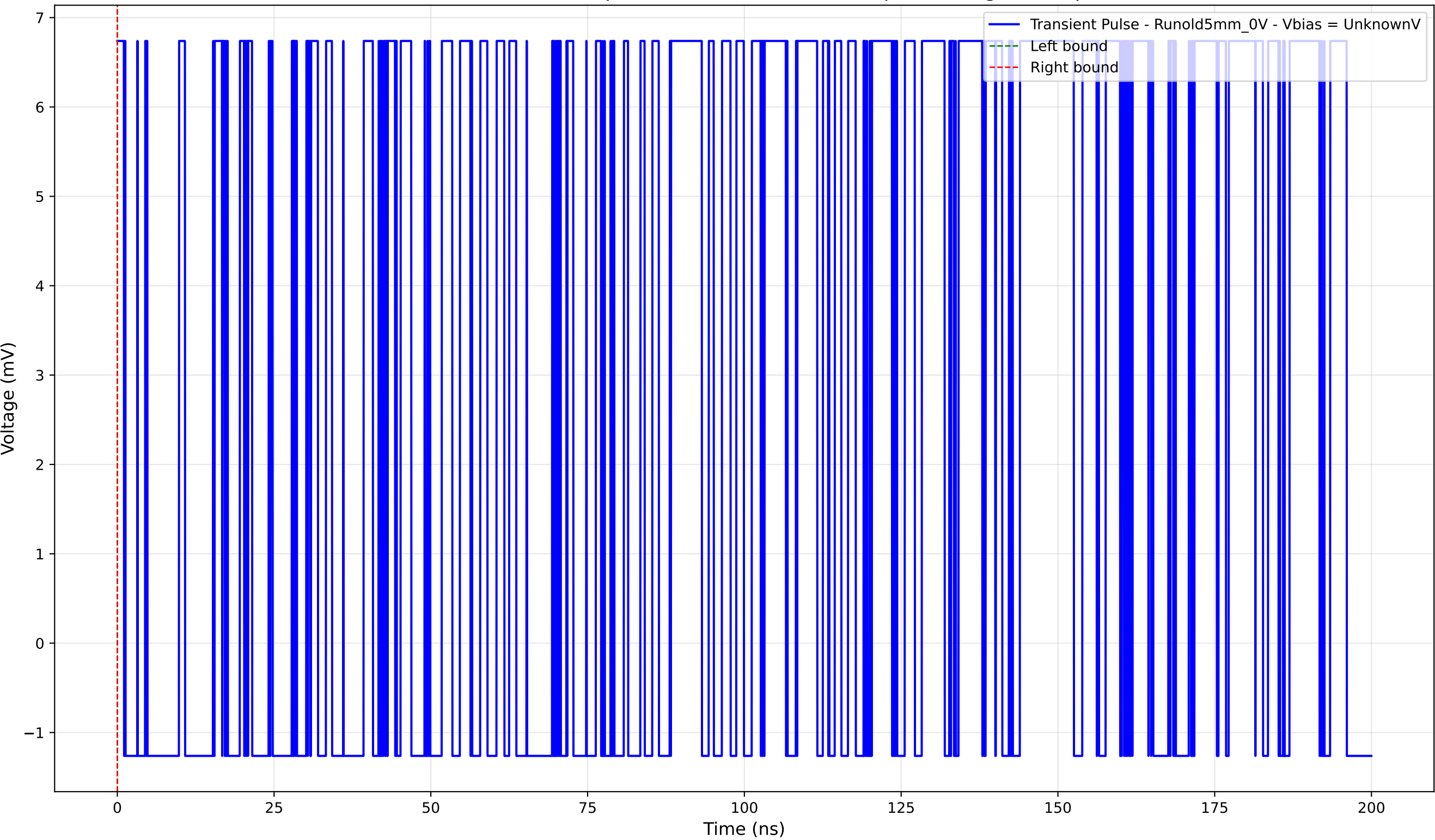
Transient Pulse - Sample: old5 - Position: 4875.0 \mu\text{m} - Charge: 0.00 pC
