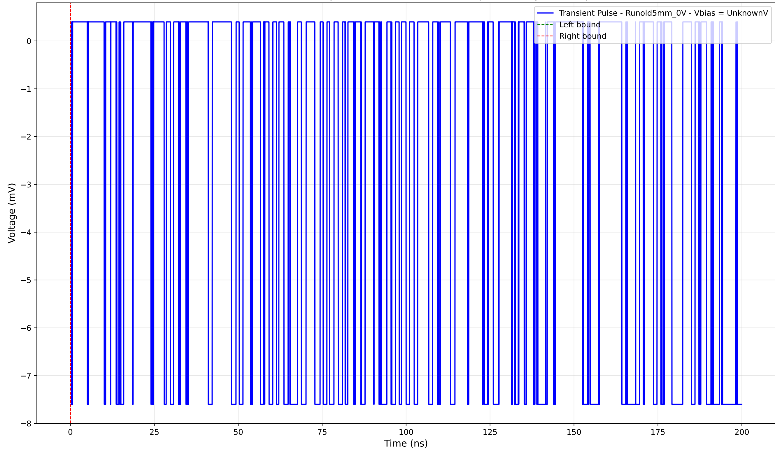
Transient Pulse - Sample: old5 - Position: 3465.0 \mu\text{m} - Charge: -0.00 pC
