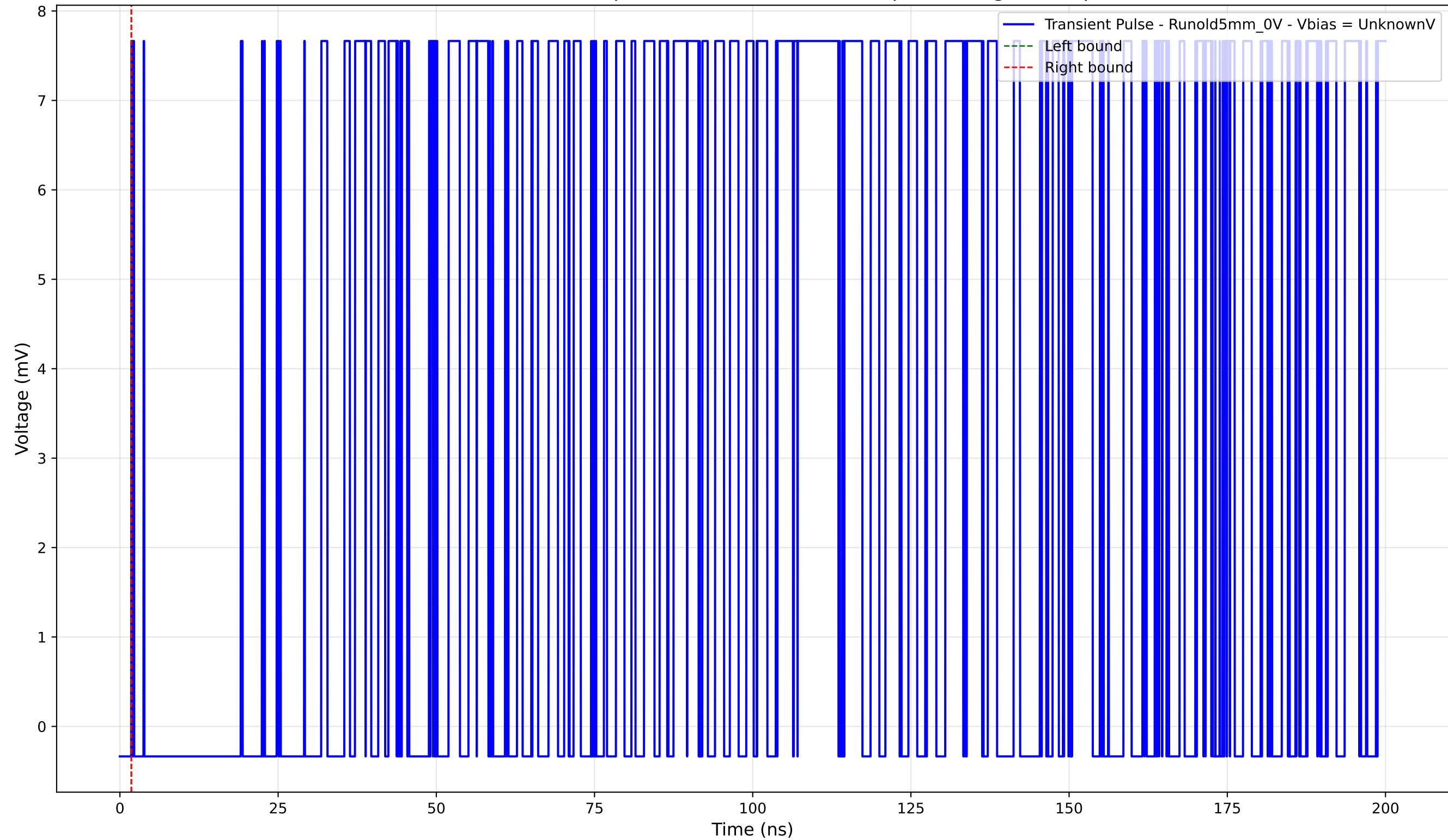
Transient Pulse - Sample: old5 - Position: 2530.0 \mu\text{m} - Charge: 0.00 pC
