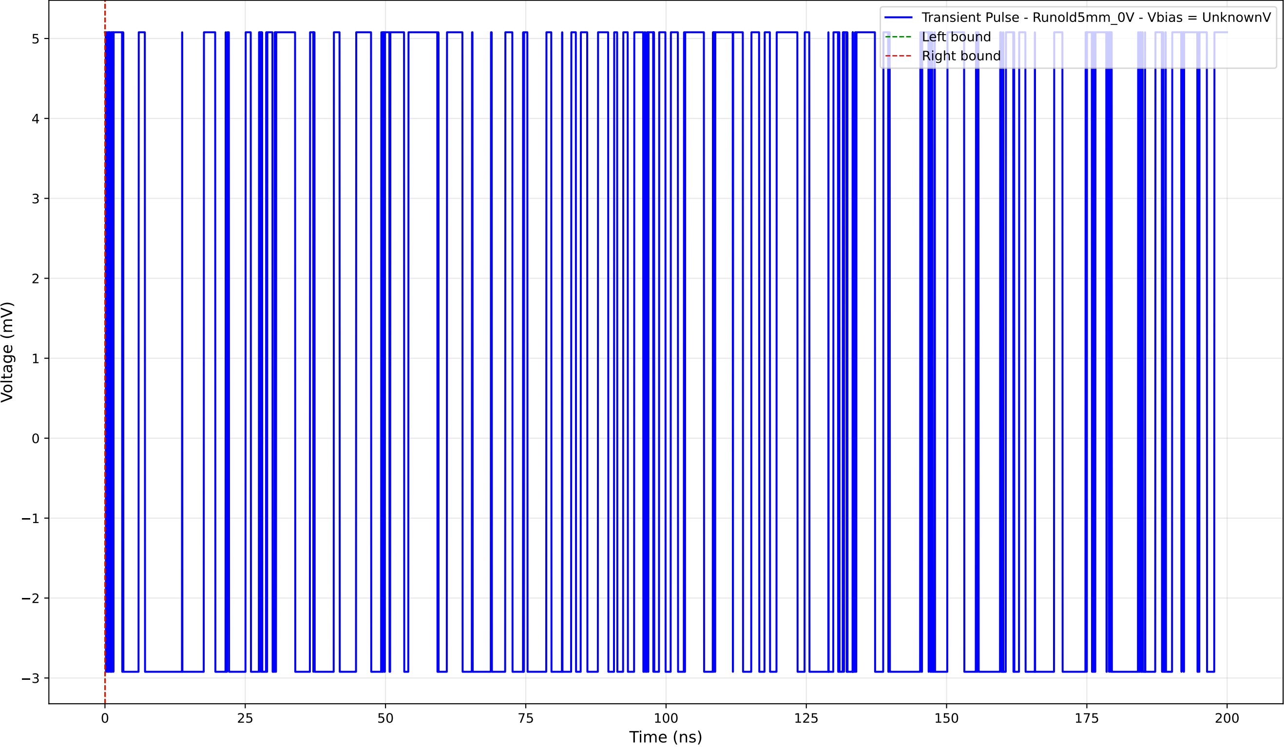
Transient Pulse - Sample: old5 - Position: 1295.0 \mu\text{m} - Charge: 0.00 pC
