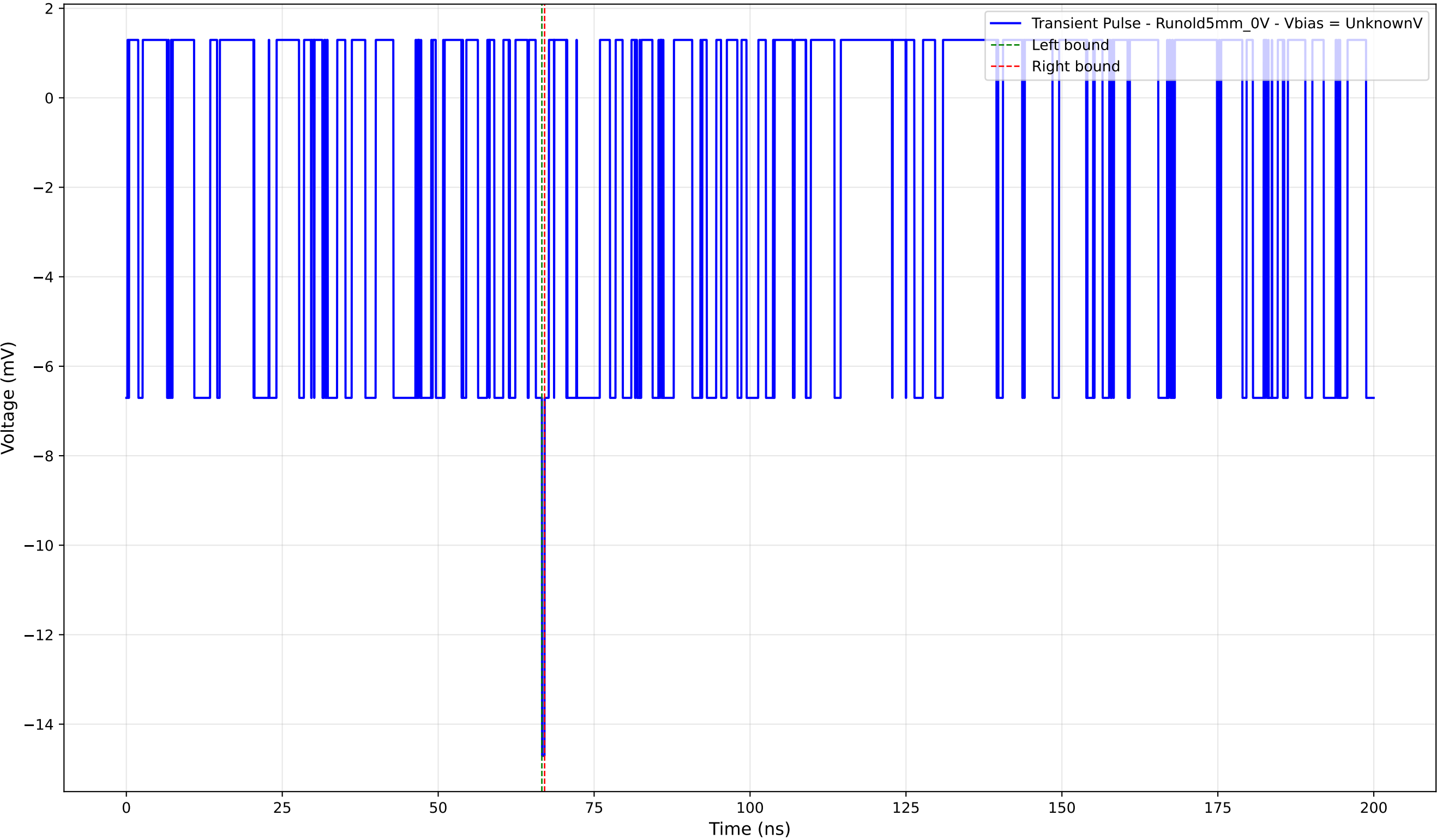
Transient Pulse - Sample: old5 - Position: 3545.0 \mu\text{m} - Charge: -0.13 pC
