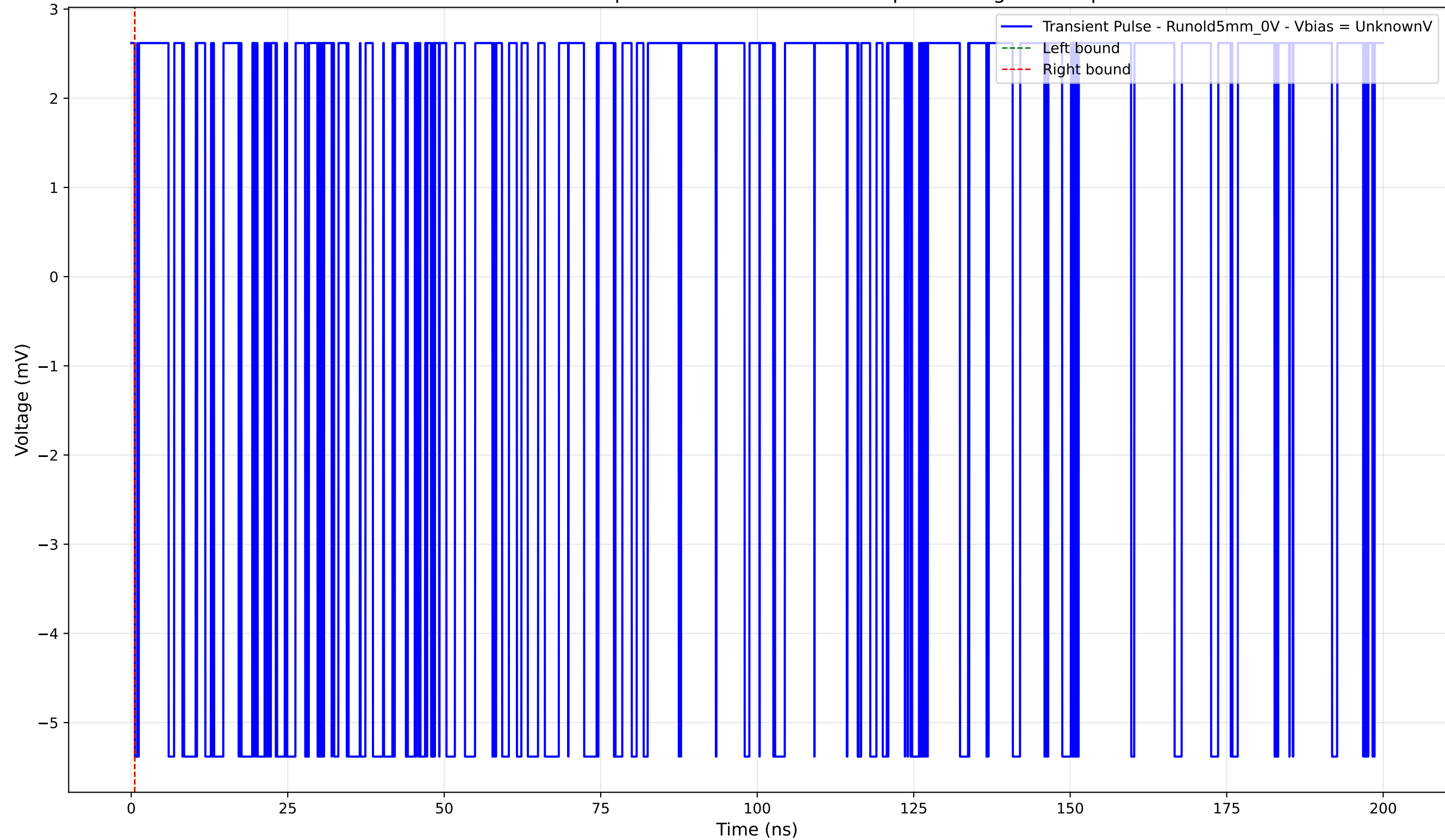
Transient Pulse - Sample: old5 - Position: 4620.0 \mu\text{m} - Charge: -0.00 pC
