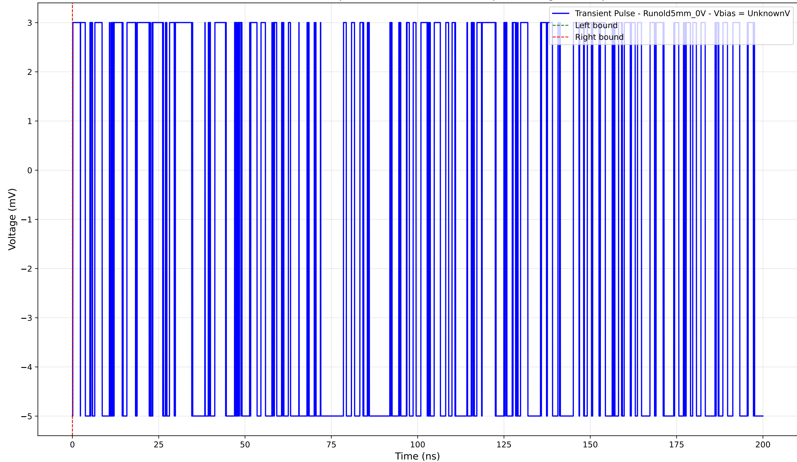
Transient Pulse - Sample: old5 - Position: 3035.0 \mu\text{m} - Charge: -0.00 pC
