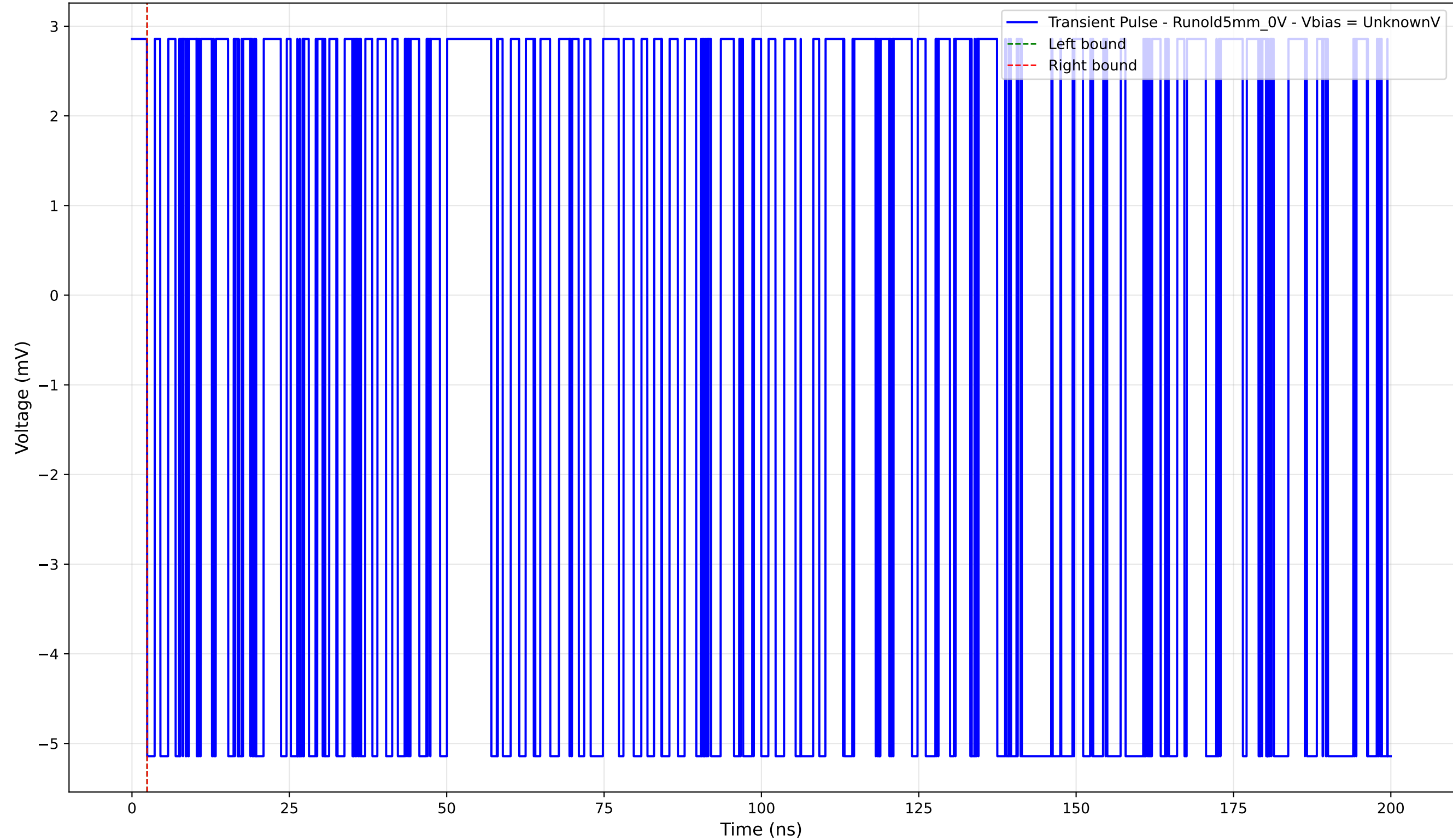
Transient Pulse - Sample: old5 - Position: 1000.0 \mu\text{m} - Charge: -0.00 pC
