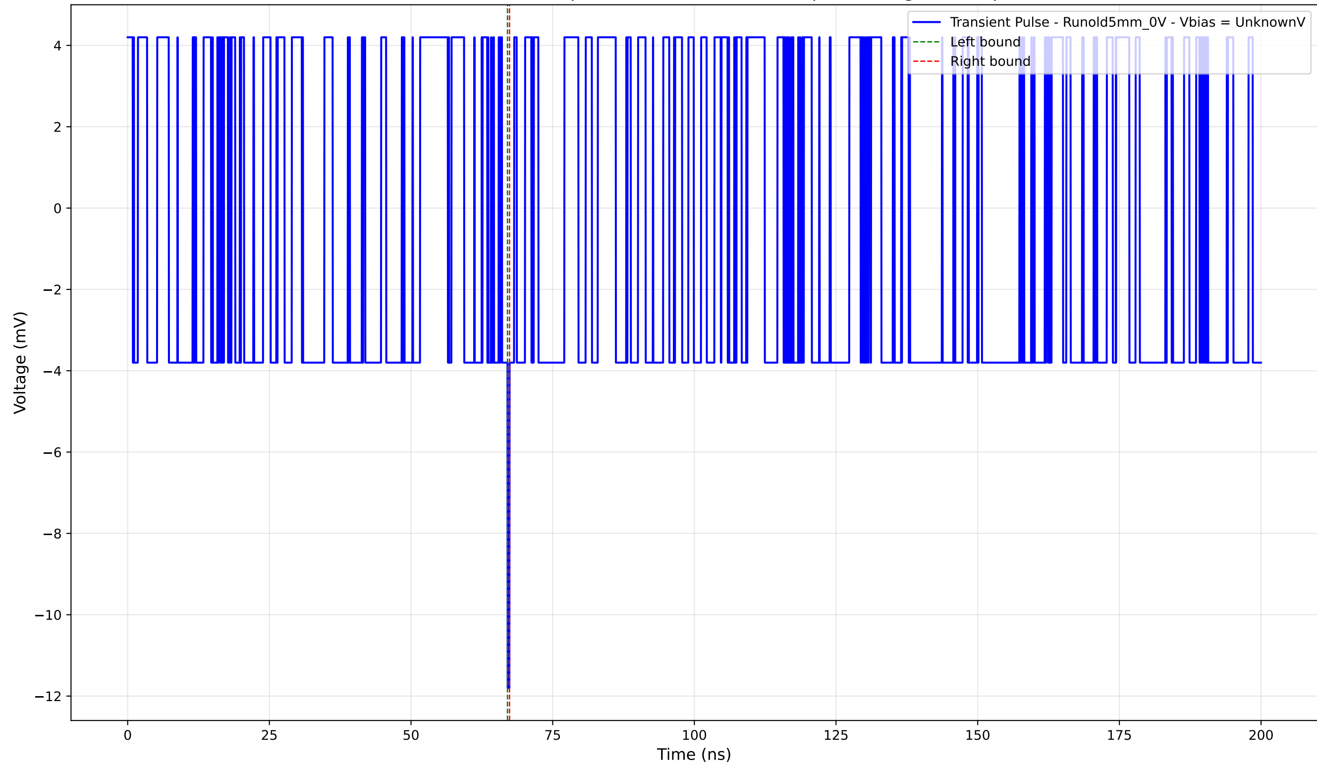
Transient Pulse - Sample: old5 - Position: 630.0 \mu\text{m} - Charge: -0.08 pC
