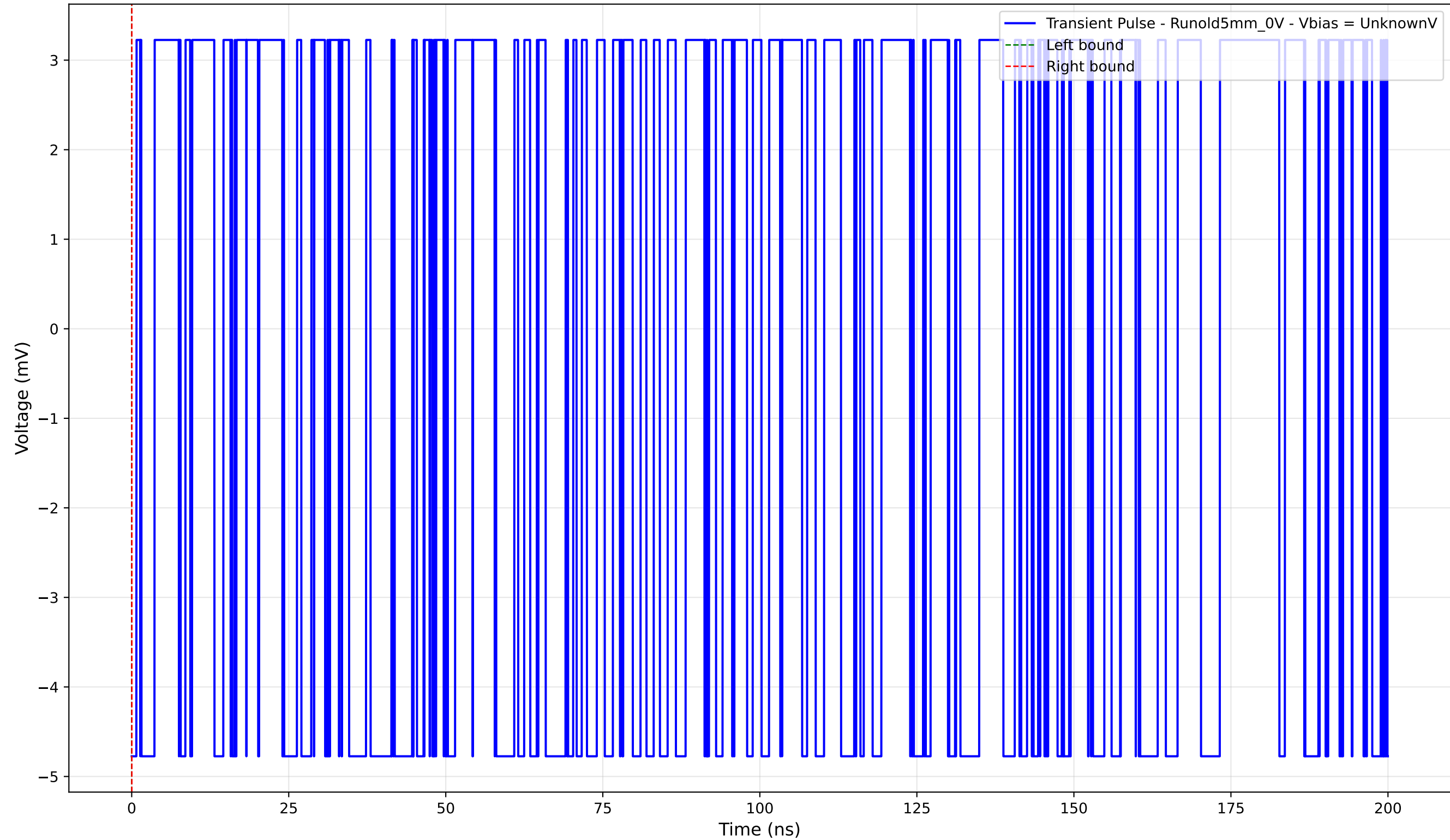
Transient Pulse - Sample: old5 - Position: 1125.0 \mu\text{m} - Charge: -0.00 pC
