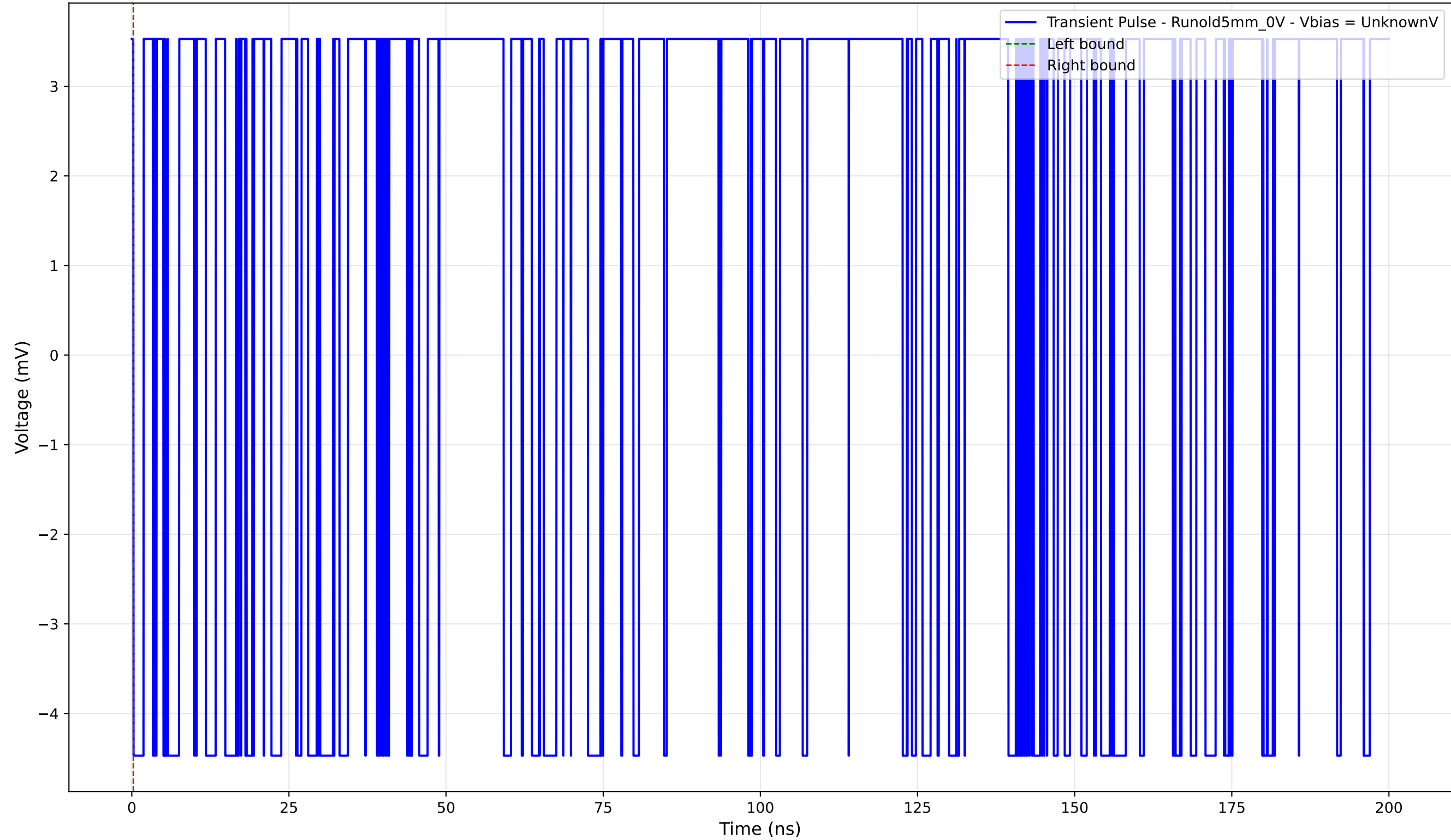
Transient Pulse - Sample: old5 - Position: 1135.0 \mu\text{m} - Charge: -0.00 pC
