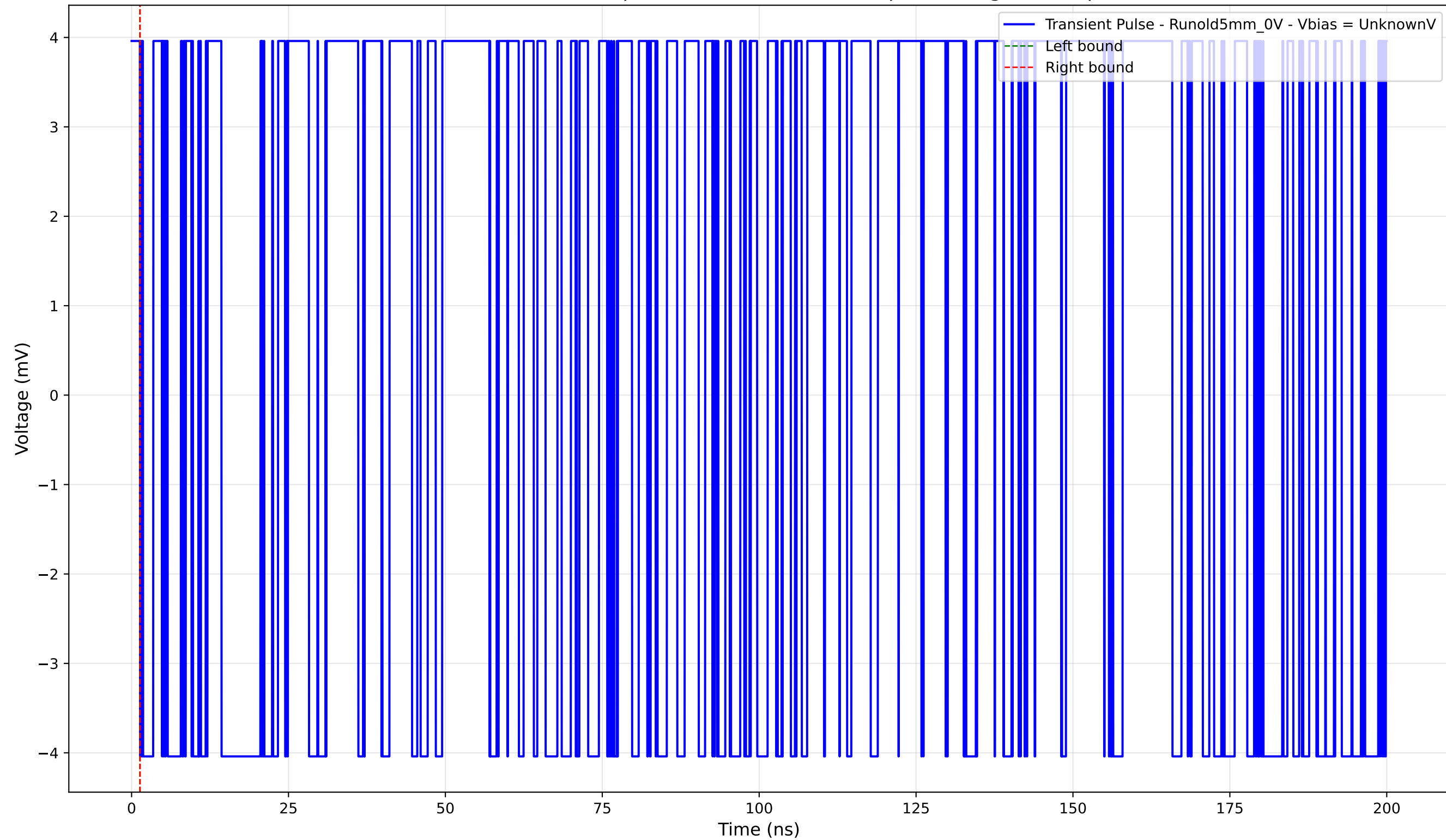
Transient Pulse - Sample: old5 - Position: 810.0 \mu\text{m} - Charge: -0.00 pC
