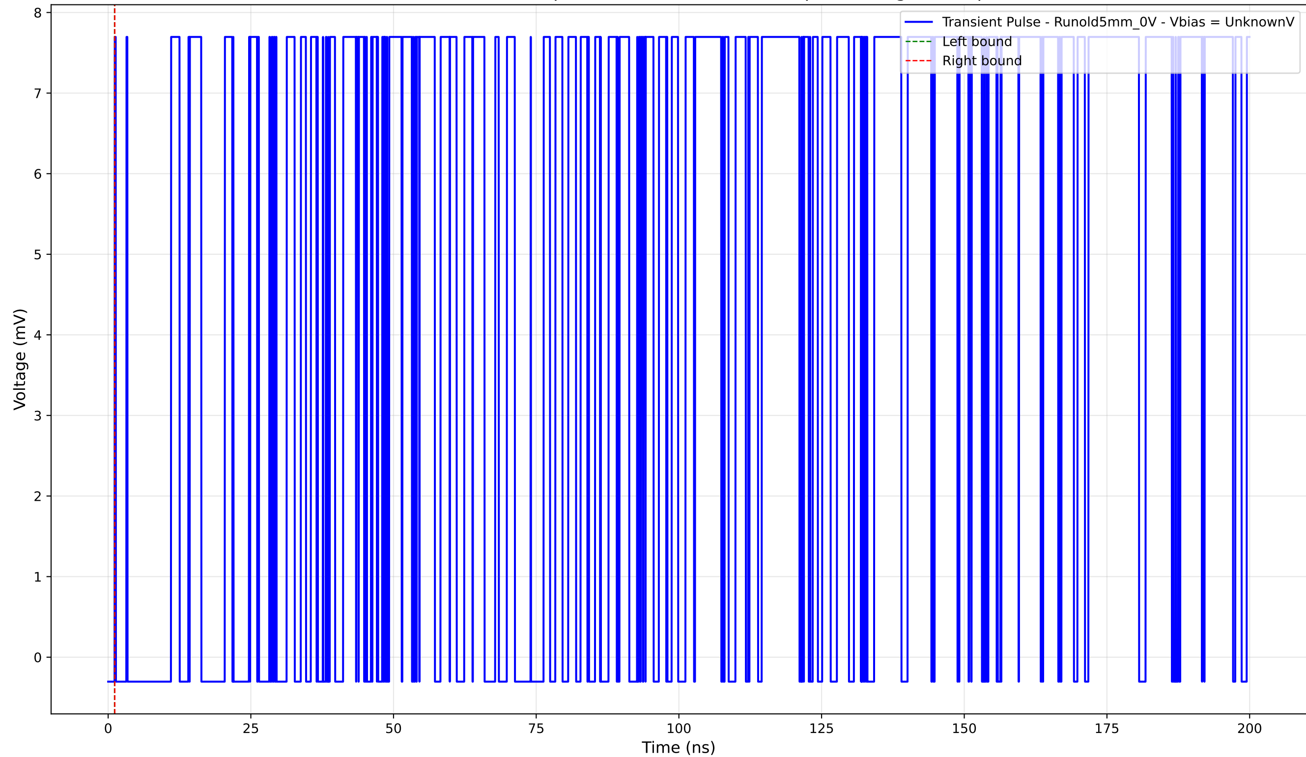
Transient Pulse - Sample: old5 - Position: 2915.0 \mu\text{m} - Charge: 0.00 pC
