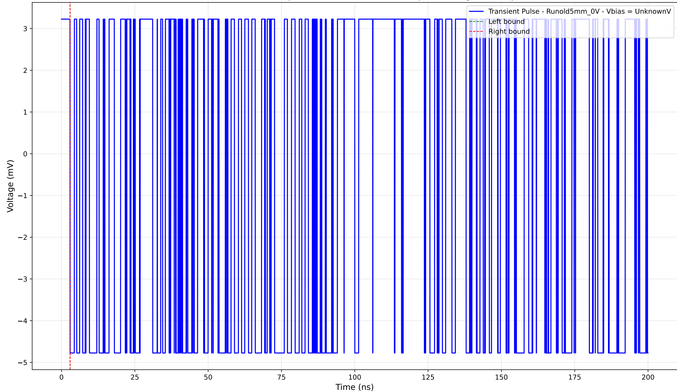
Transient Pulse - Sample: old5 - Position: 1495.0 \mu\text{m} - Charge: -0.00 pC
