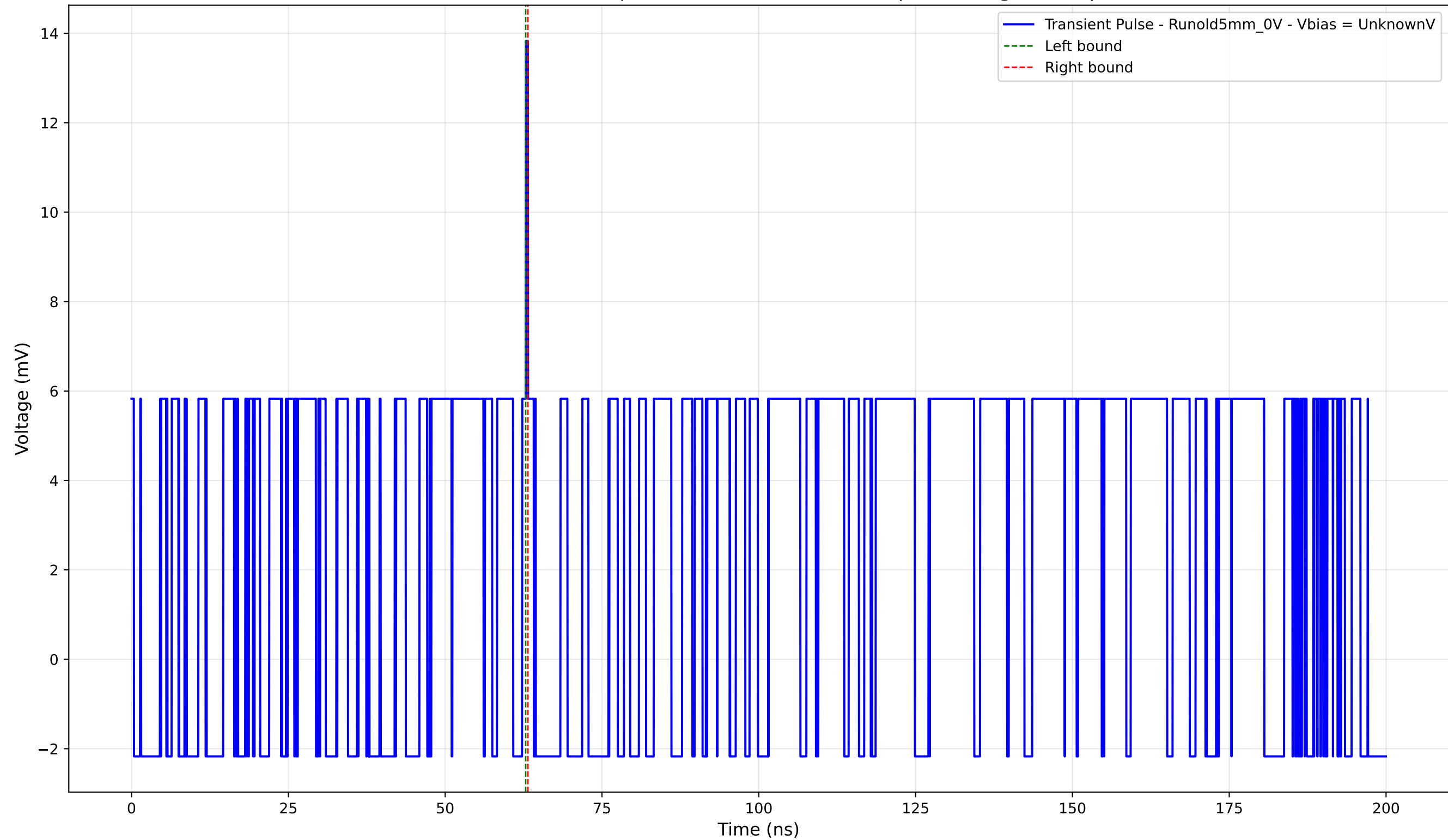
Transient Pulse - Sample: old5 - Position: 3640.0 \mu\text{m} - Charge: 0.10 pC
