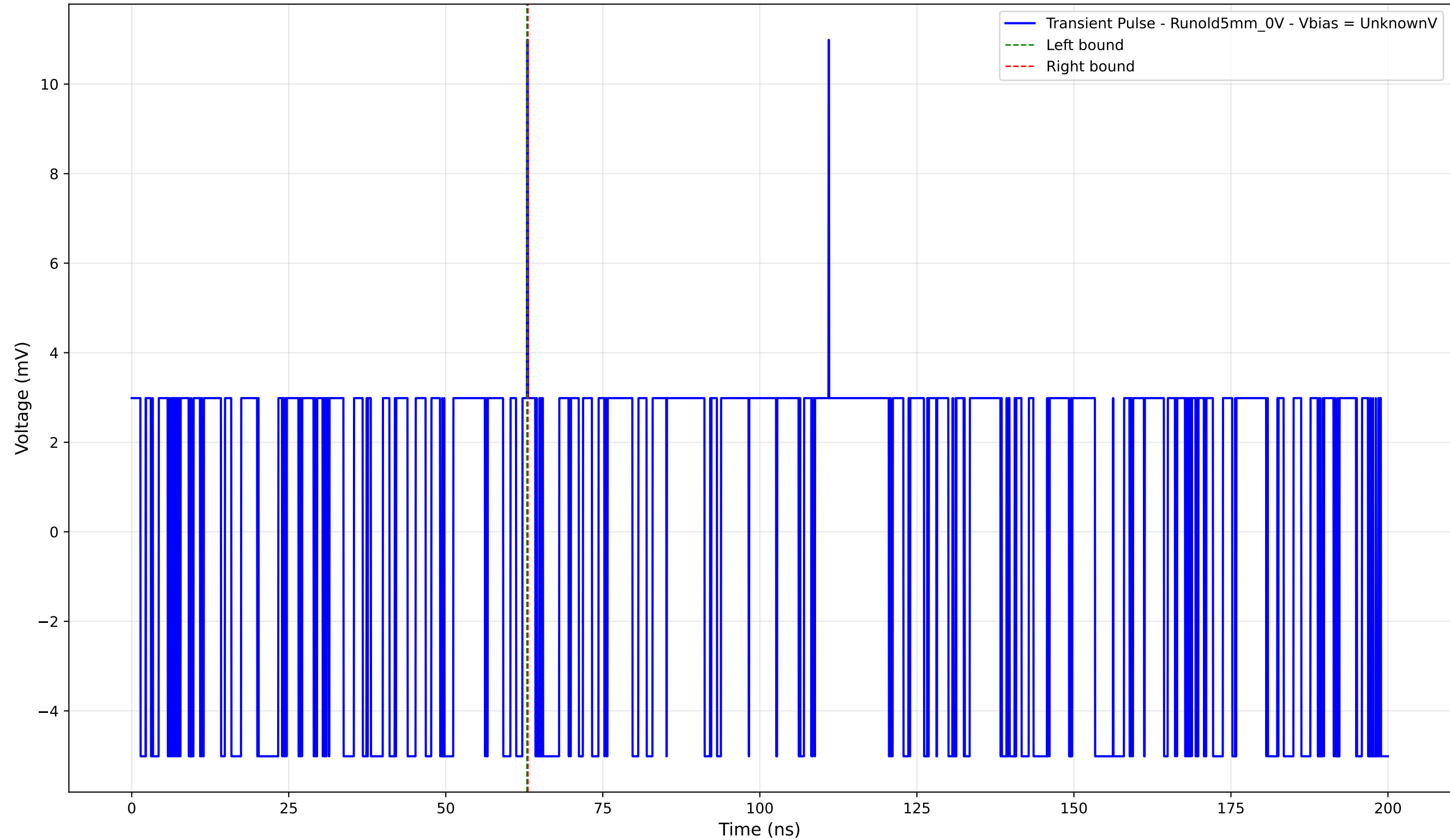
Transient Pulse - Sample: old5 - Position: 750.0 \mu\text{m} - Charge: 0.03 pC
