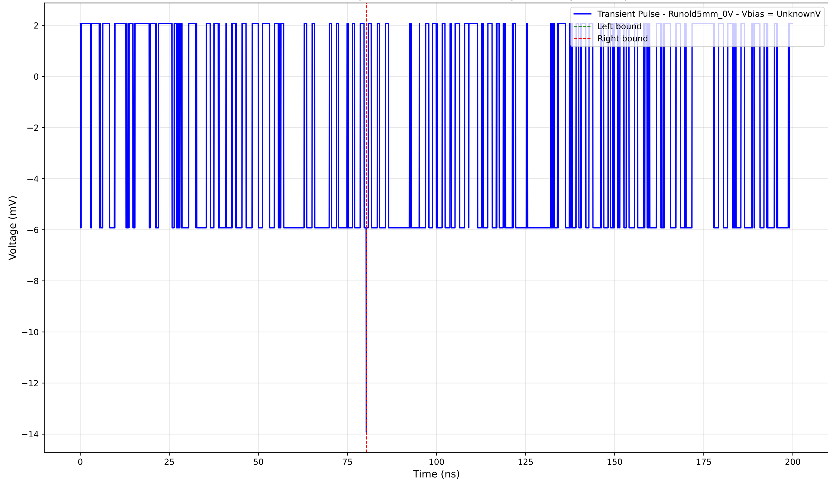
Transient Pulse - Sample: old5 - Position: 310.0 \mu\text{m} - Charge: -0.01 pC
