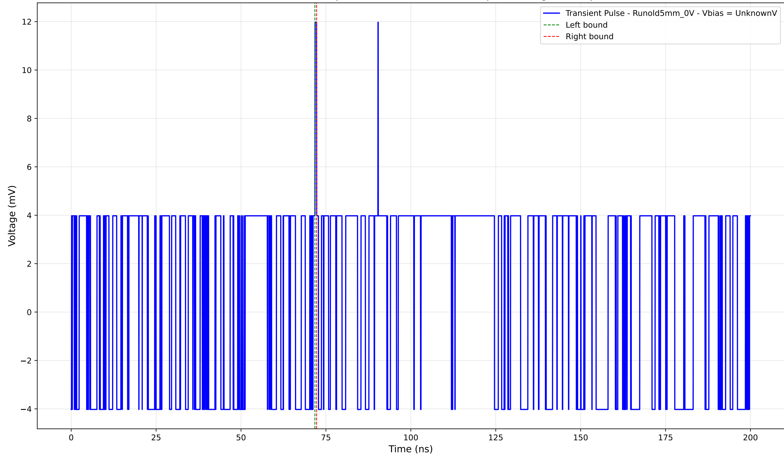
Transient Pulse - Sample: old5 - Position: 5095.0 \mu\text{m} - Charge: 0.12 pC
