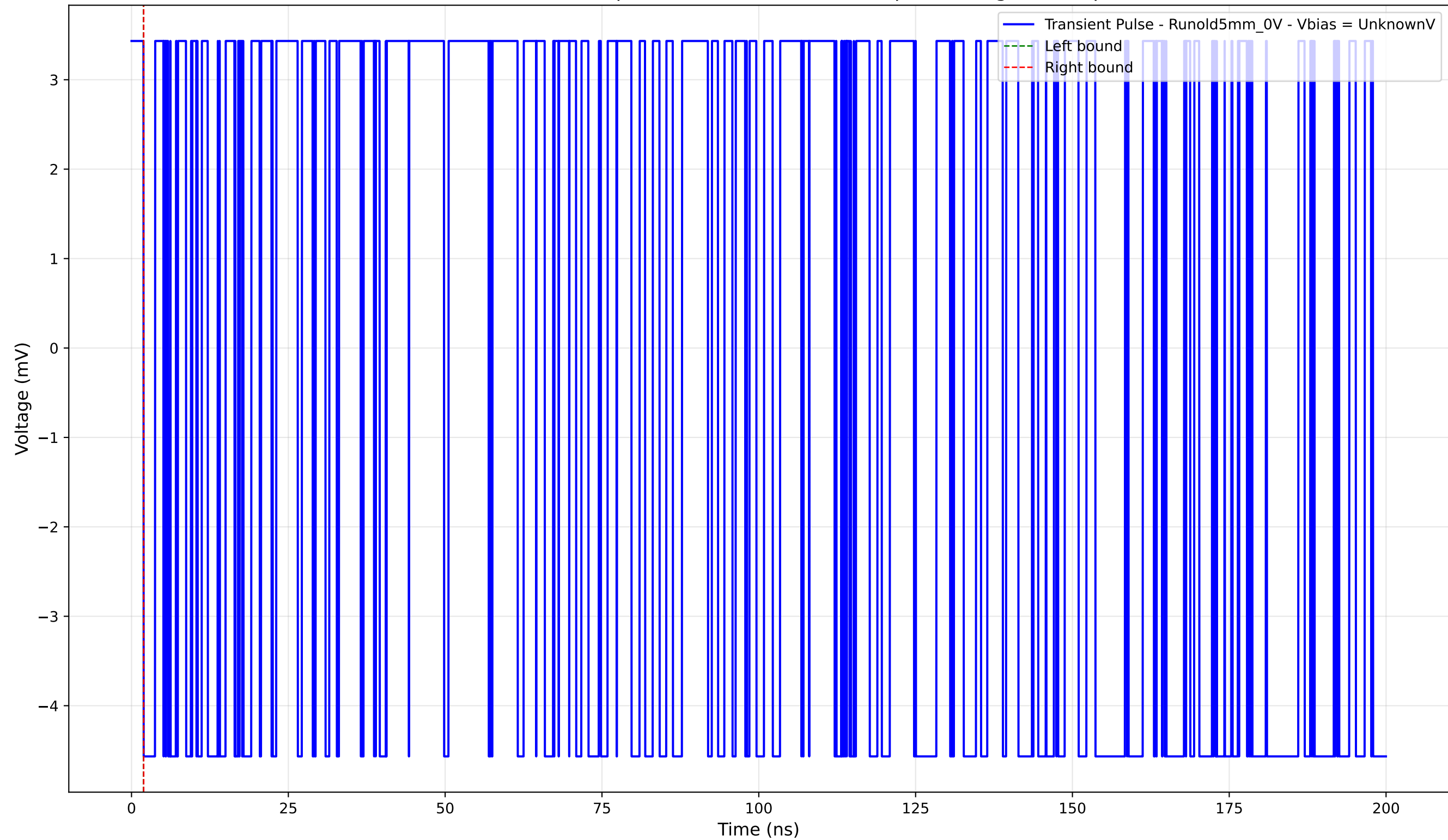
Transient Pulse - Sample: old5 - Position: 1335.0 \mu\text{m} - Charge: -0.00 pC
