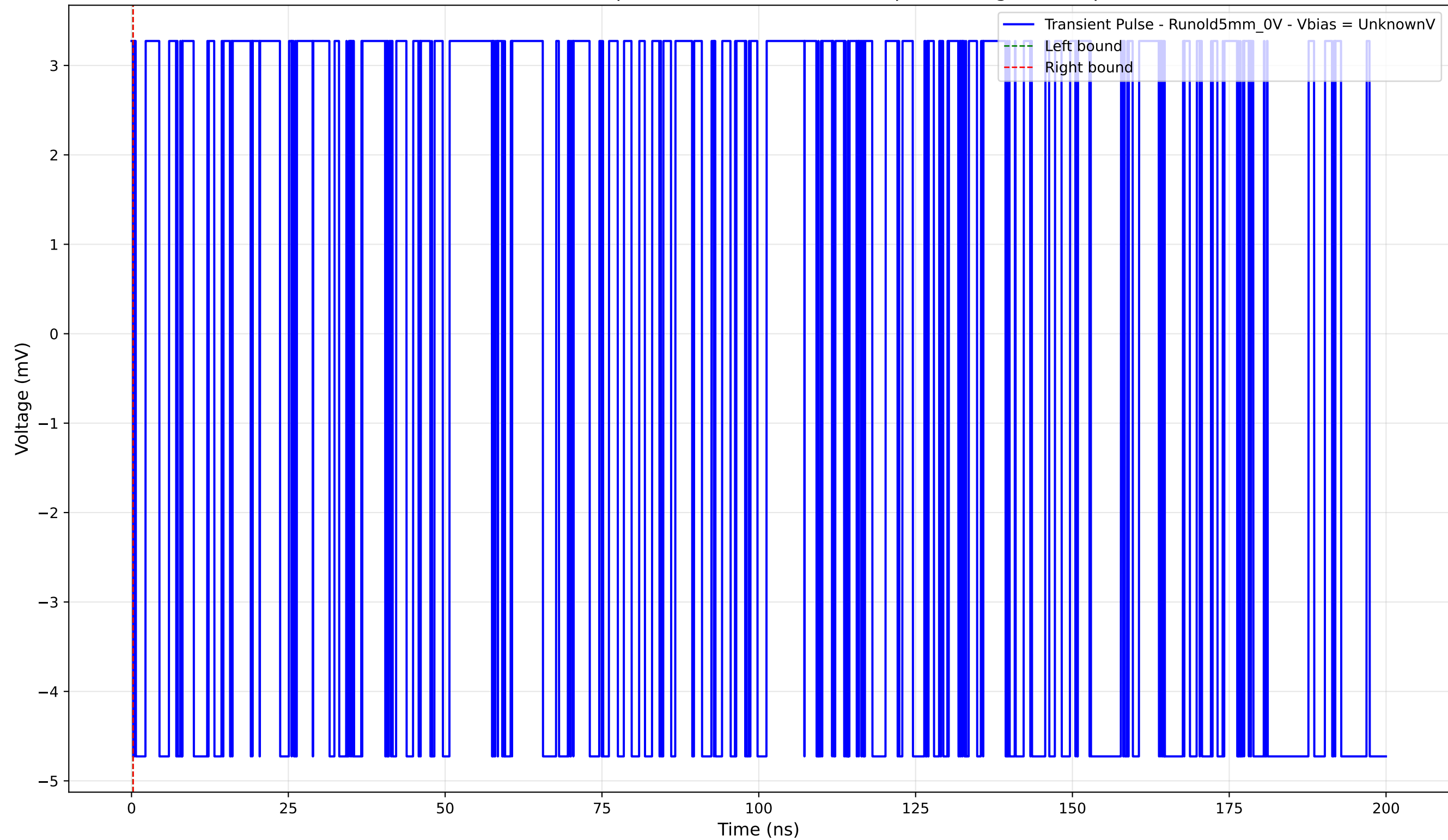
Transient Pulse - Sample: old5 - Position: 4950.0 \mu\text{m} - Charge: -0.00 pC
