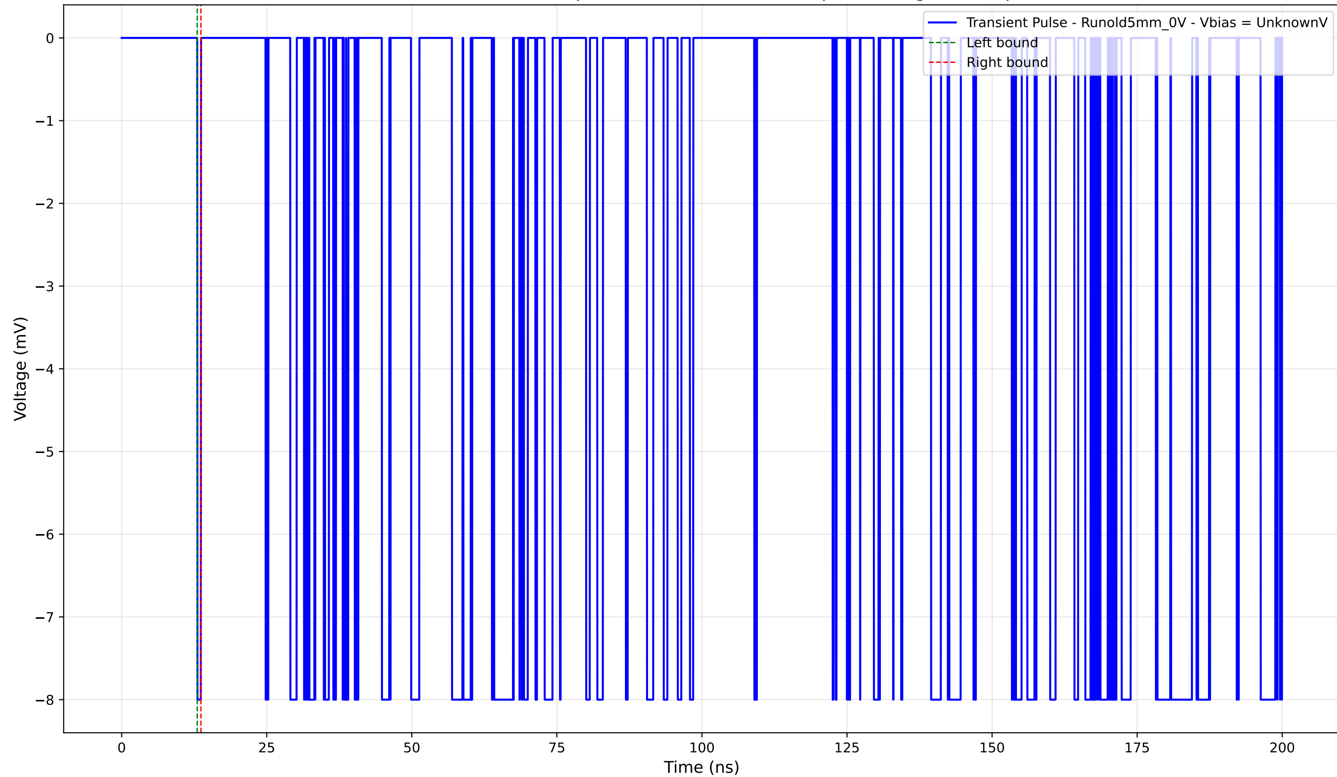
Transient Pulse - Sample: old5 - Position: 790.0 \mu\text{m} - Charge: -0.10 pC
