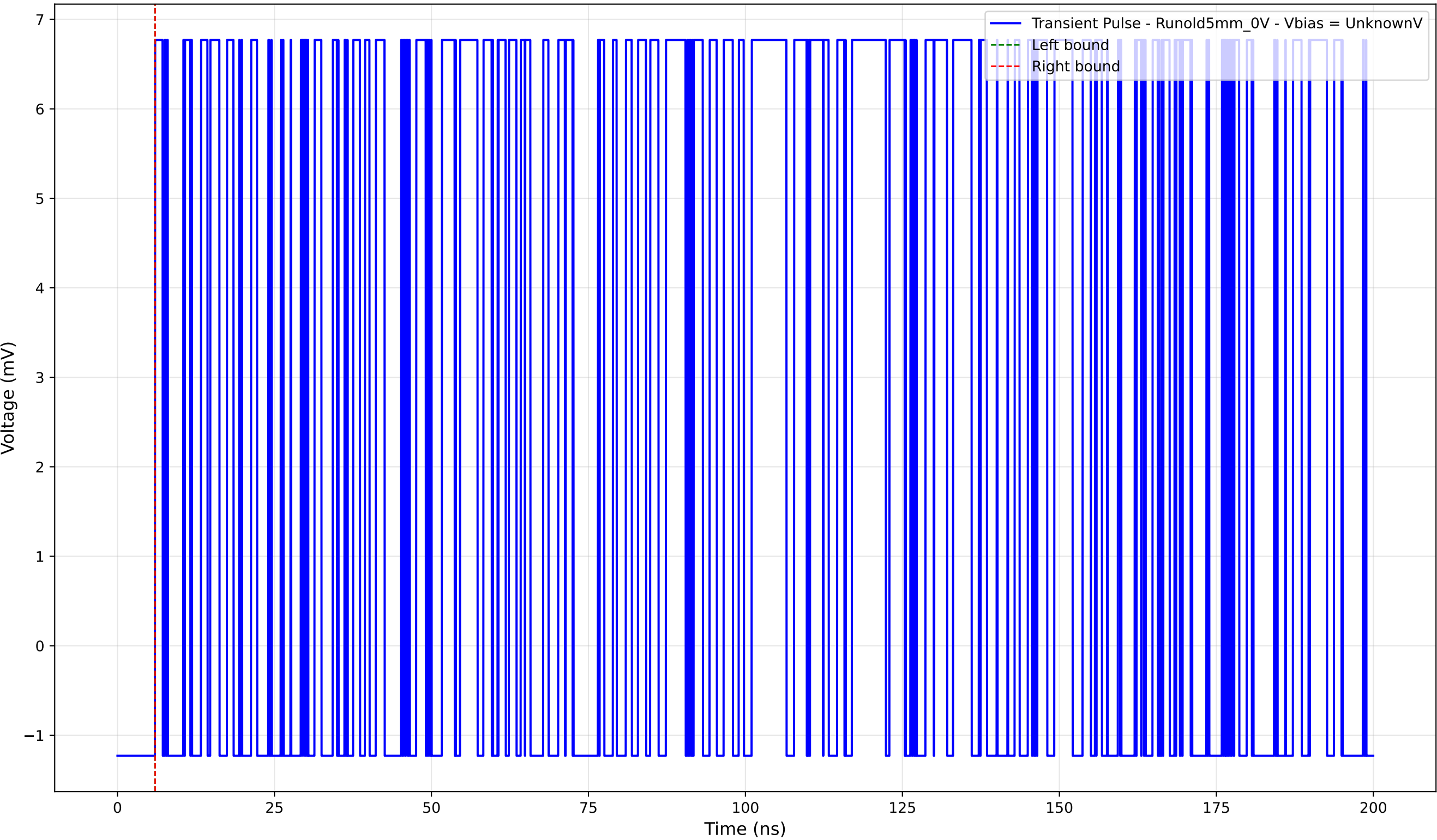
Transient Pulse - Sample: old5 - Position: 3935.0 \mu\text{m} - Charge: 0.00 pC
