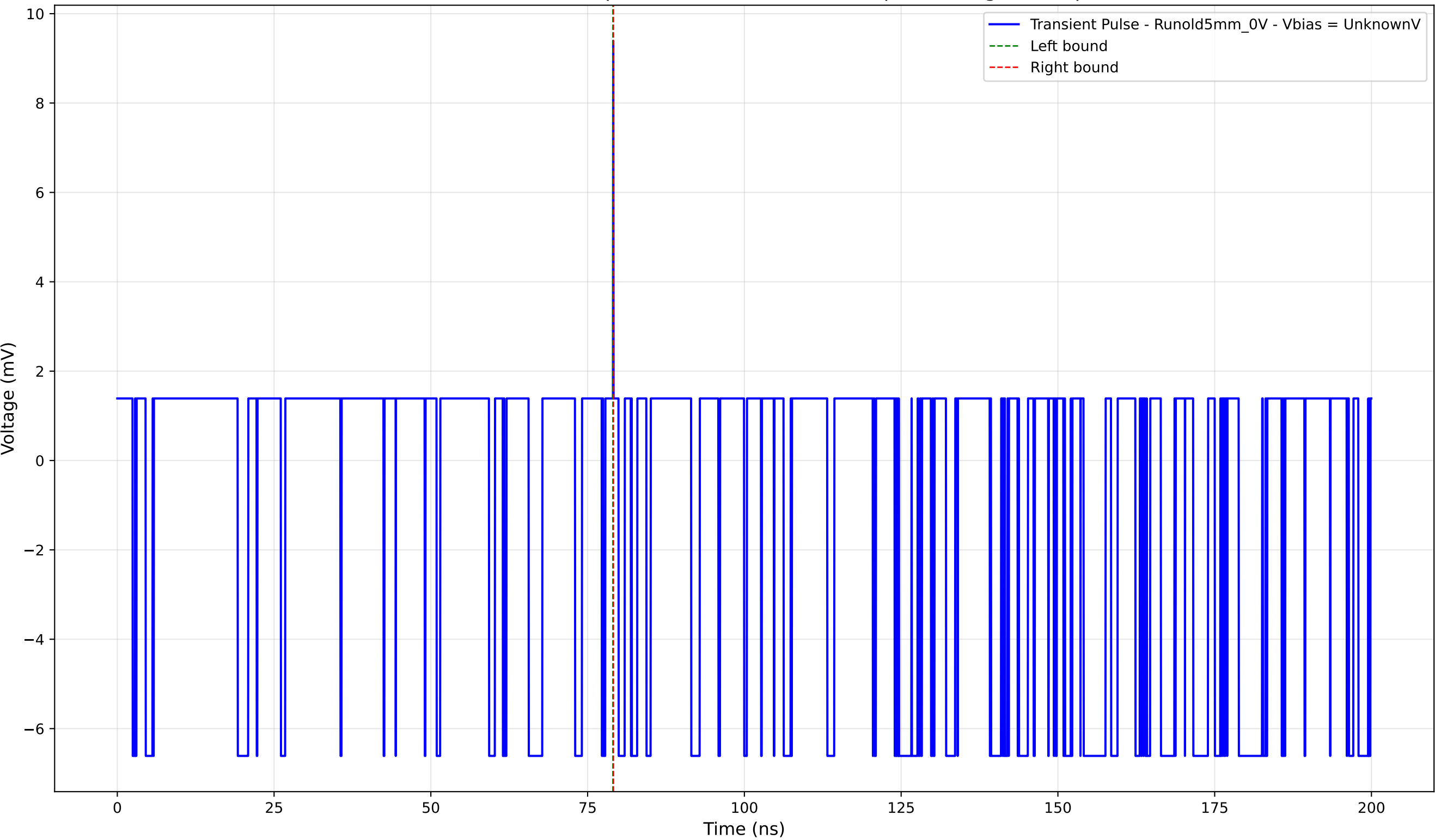
Transient Pulse - Sample: old5 - Position: 2140.0 \mu\text{m} - Charge: 0.01 pC
