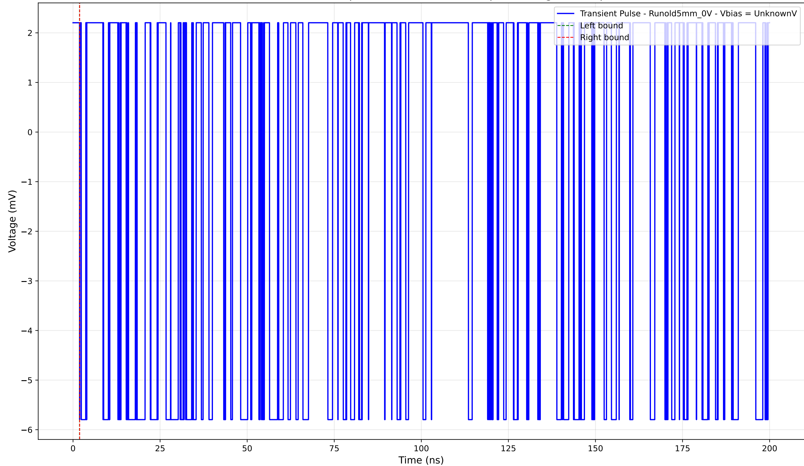
Transient Pulse - Sample: old5 - Position: 30.0 \mu\text{m} - Charge: -0.00 pC
