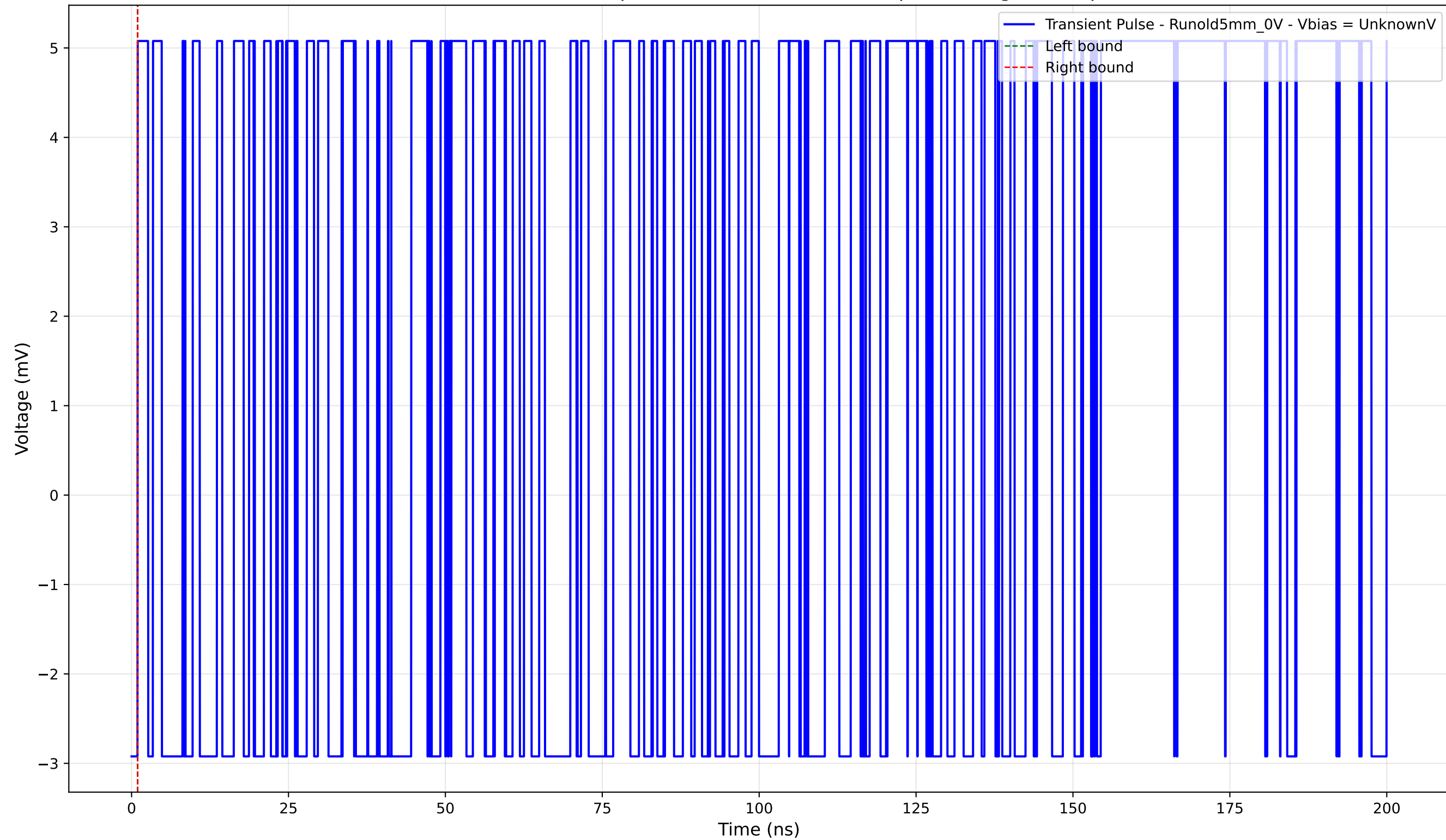
Transient Pulse - Sample: old5 - Position: 1660.0 \mu\text{m} - Charge: 0.00 pC
