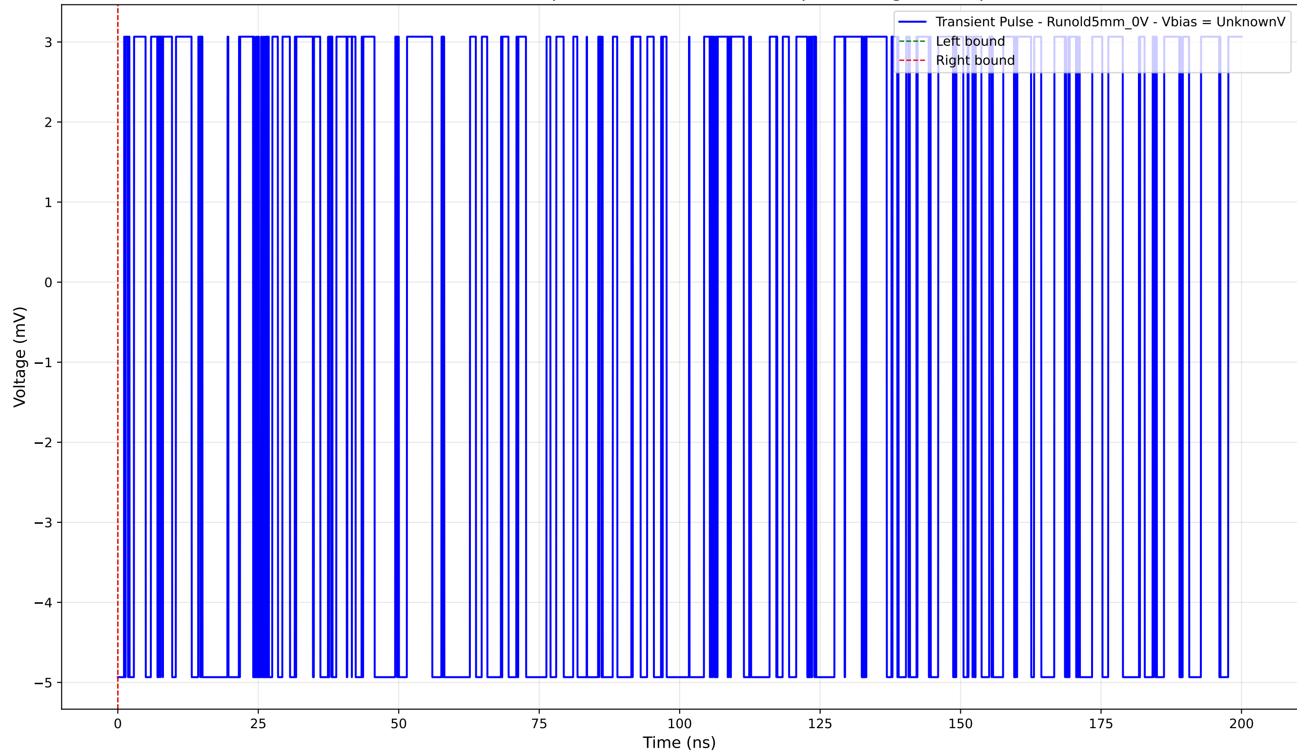
Transient Pulse - Sample: old5 - Position: 3045.0 \mu\text{m} - Charge: -0.00 pC
