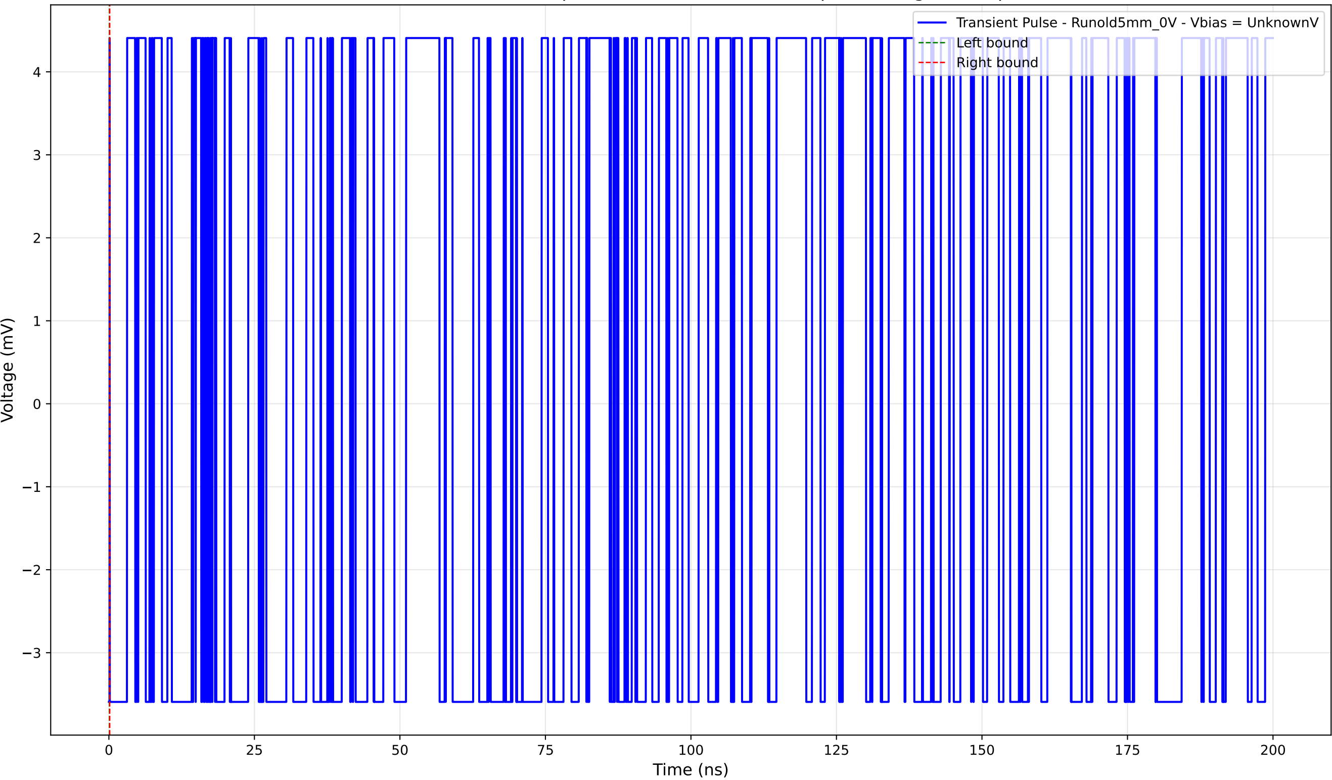
Transient Pulse - Sample: old5 - Position: 2845.0 \mu\text{m} - Charge: 0.00 pC
