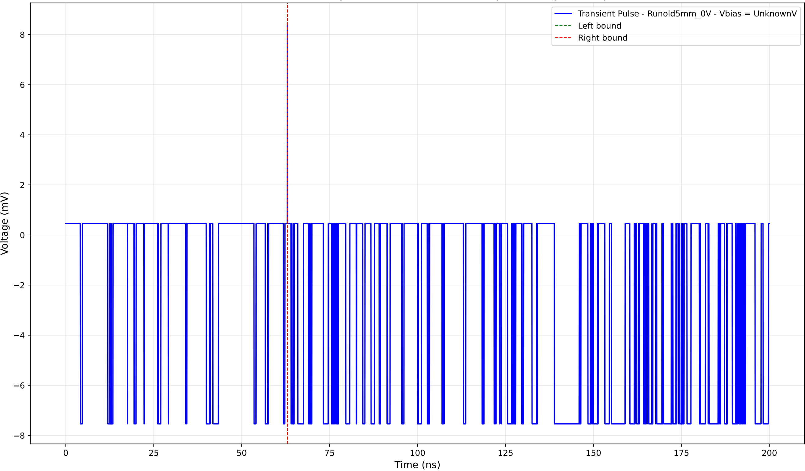
Transient Pulse - Sample: old5 - Position: 2670.0 \mu\text{m} - Charge: 0.01 pC
