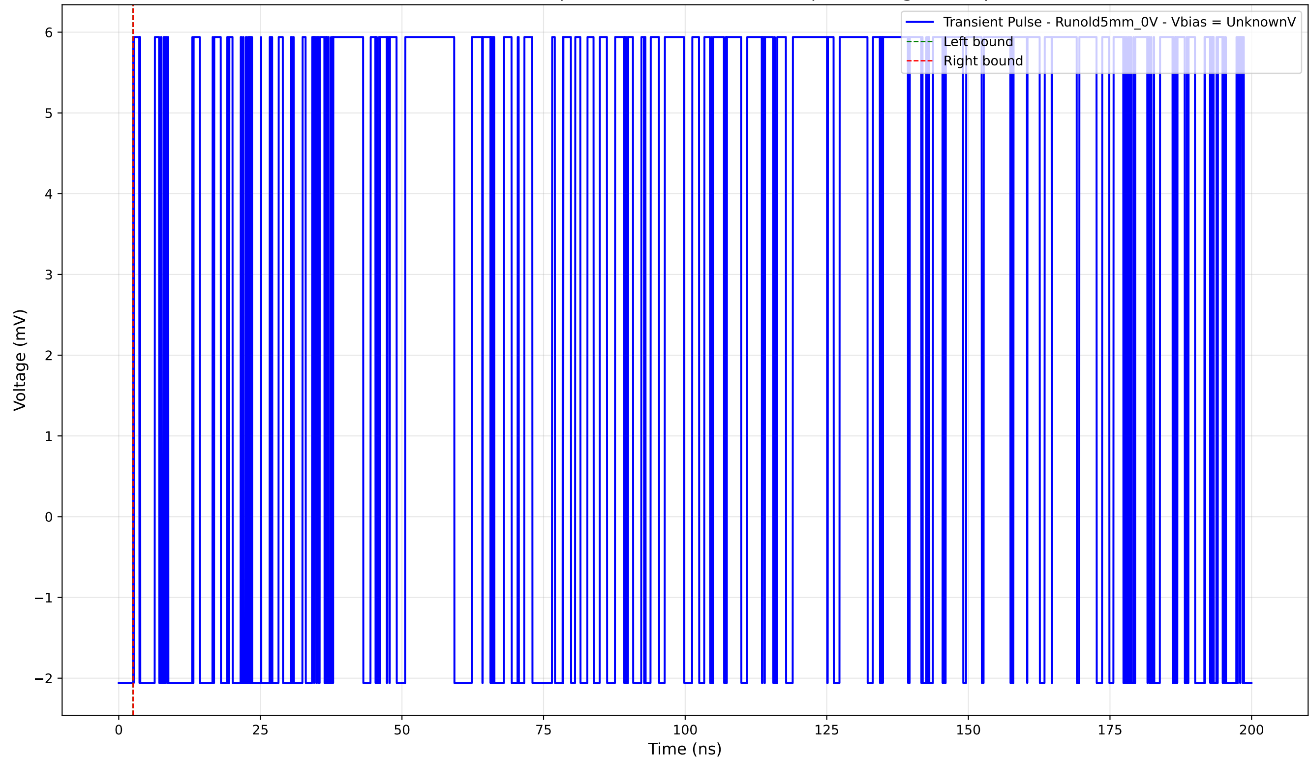
Transient Pulse - Sample: old5 - Position: 2205.0 \mu\text{m} - Charge: 0.00 pC
