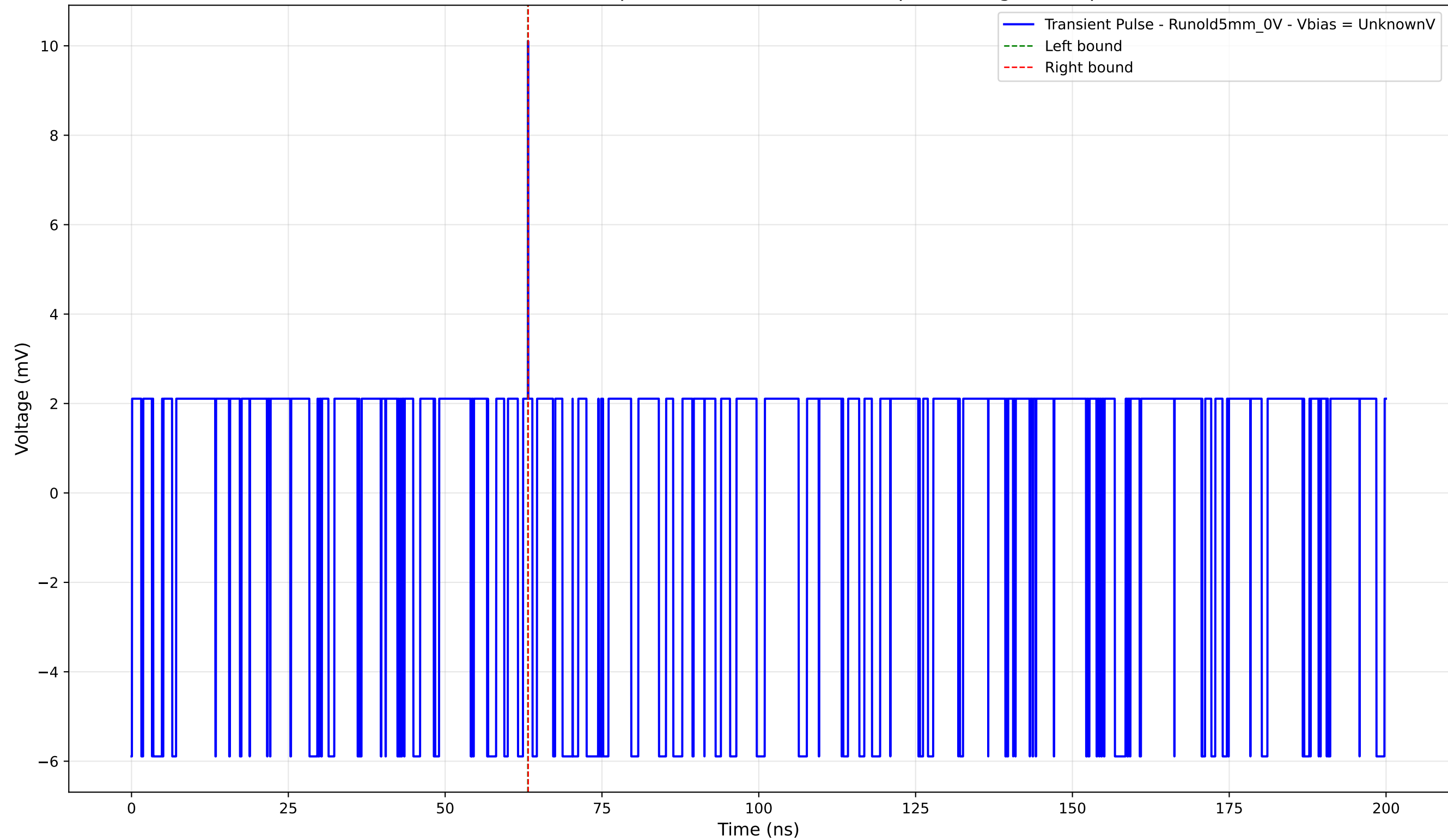
Transient Pulse - Sample: old5 - Position: 5115.0 \mu\text{m} - Charge: 0.01 pC
