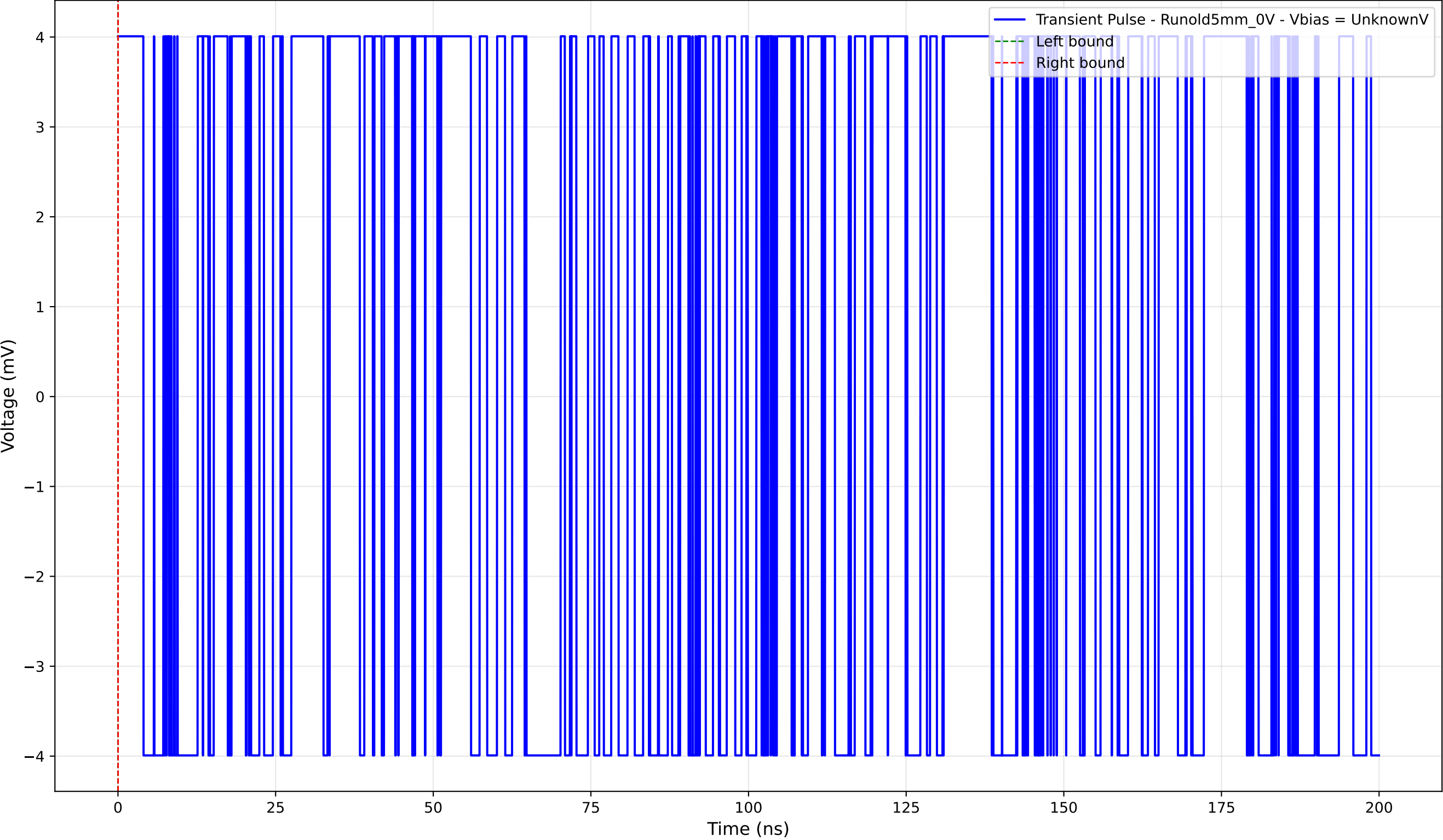
Transient Pulse - Sample: old5 - Position: 3600.0 \mu\text{m} - Charge: 0.00 pC
