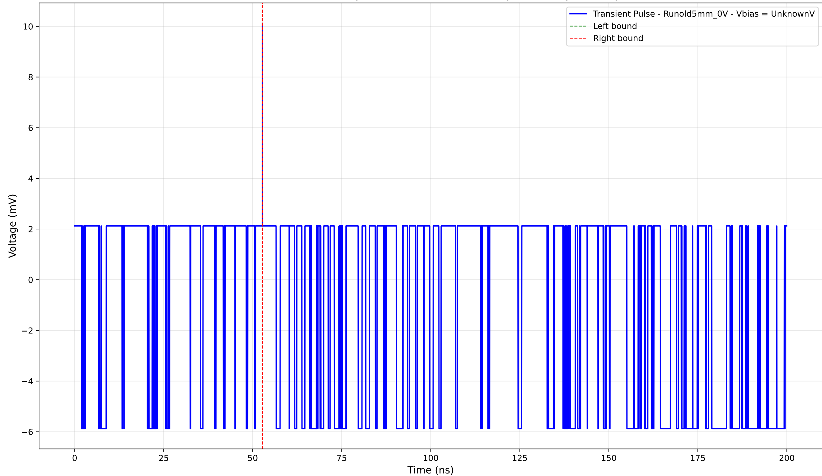
Transient Pulse - Sample: old5 - Position: 545.0 \mu\text{m} - Charge: 0.01 pC
