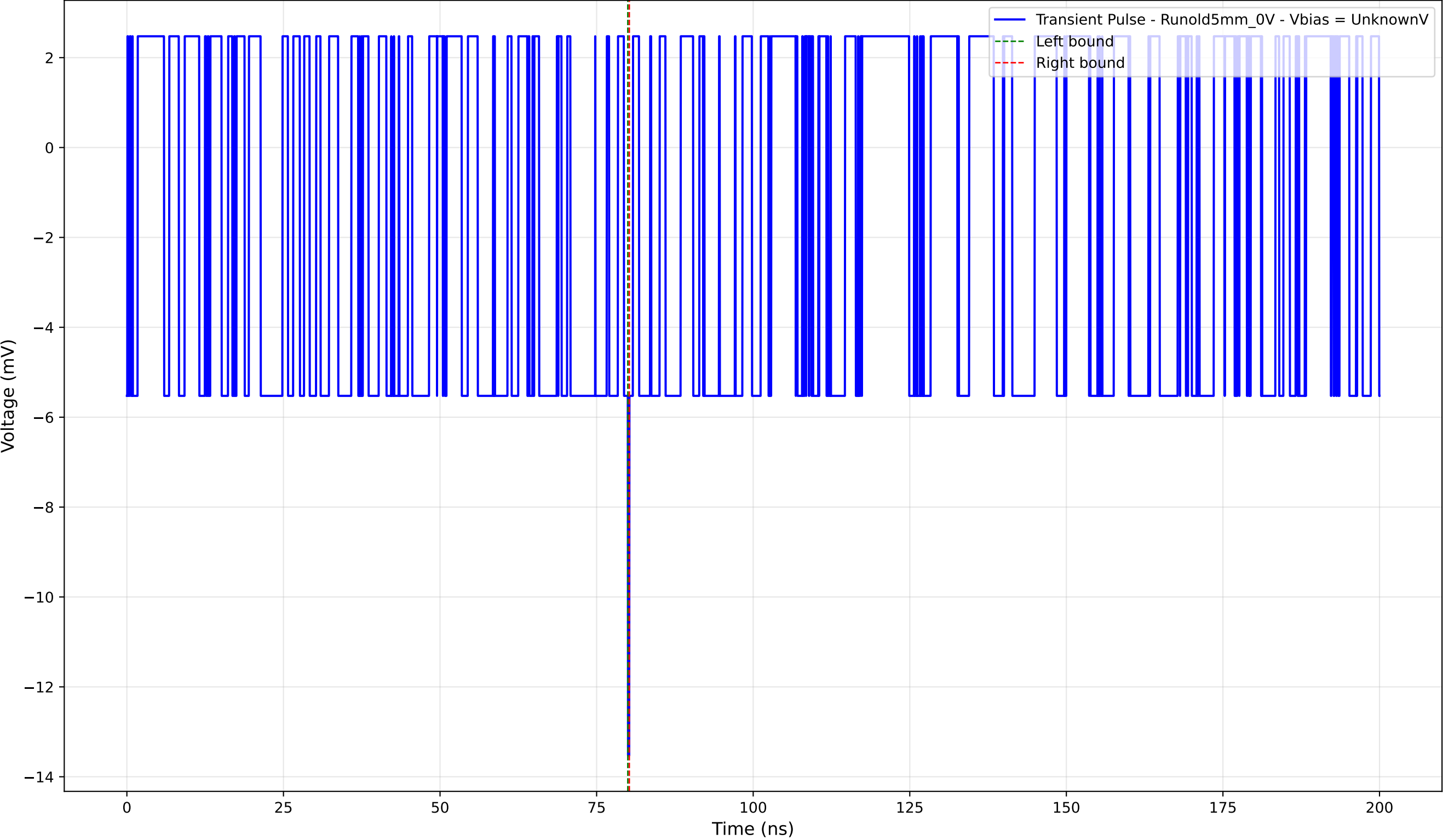
Transient Pulse - Sample: old5 - Position: 2430.0 \mu\text{m} - Charge: -0.06 pC
