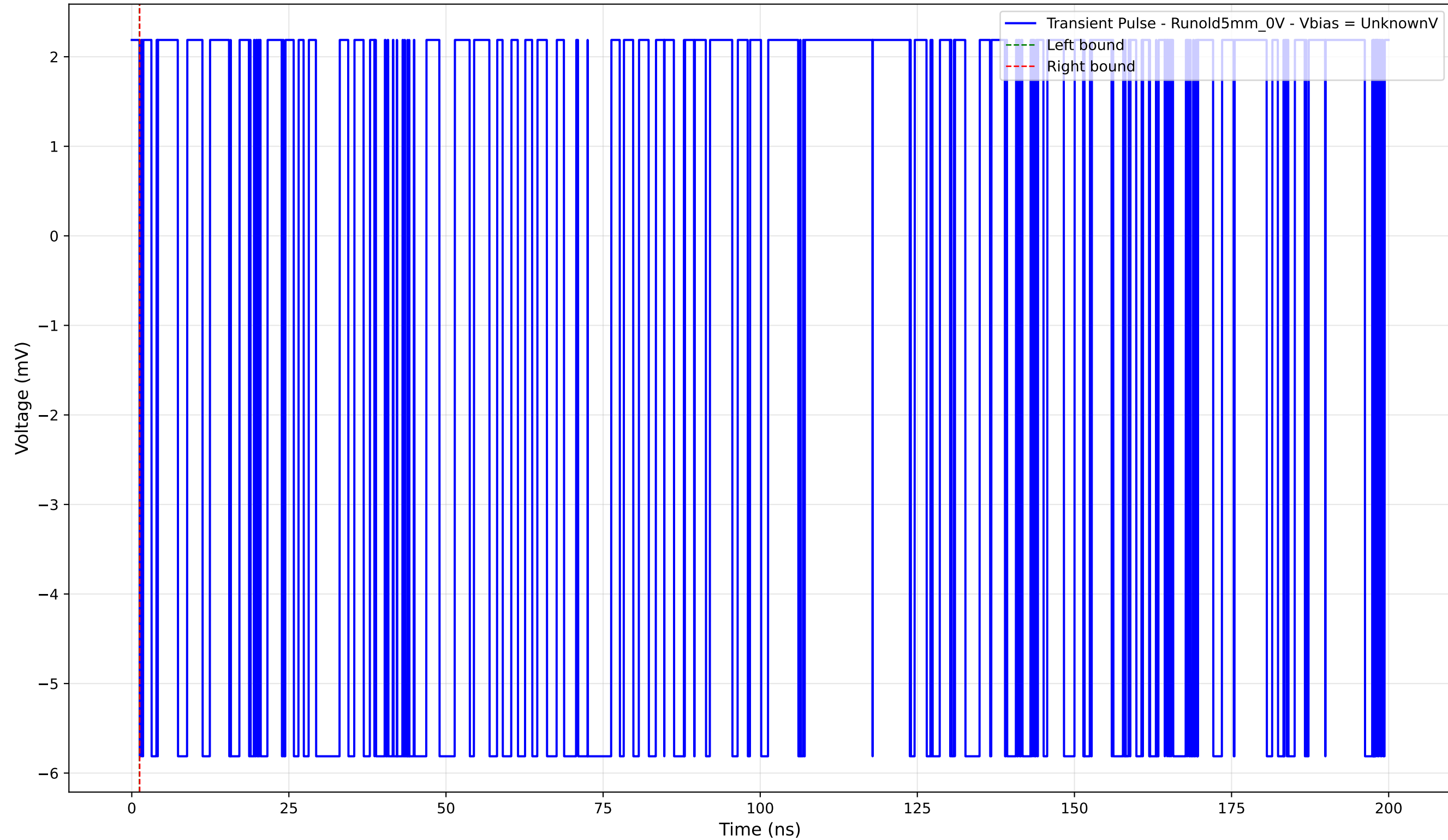
Transient Pulse - Sample: old5 - Position: 1020.0 \mu\text{m} - Charge: -0.00 pC
