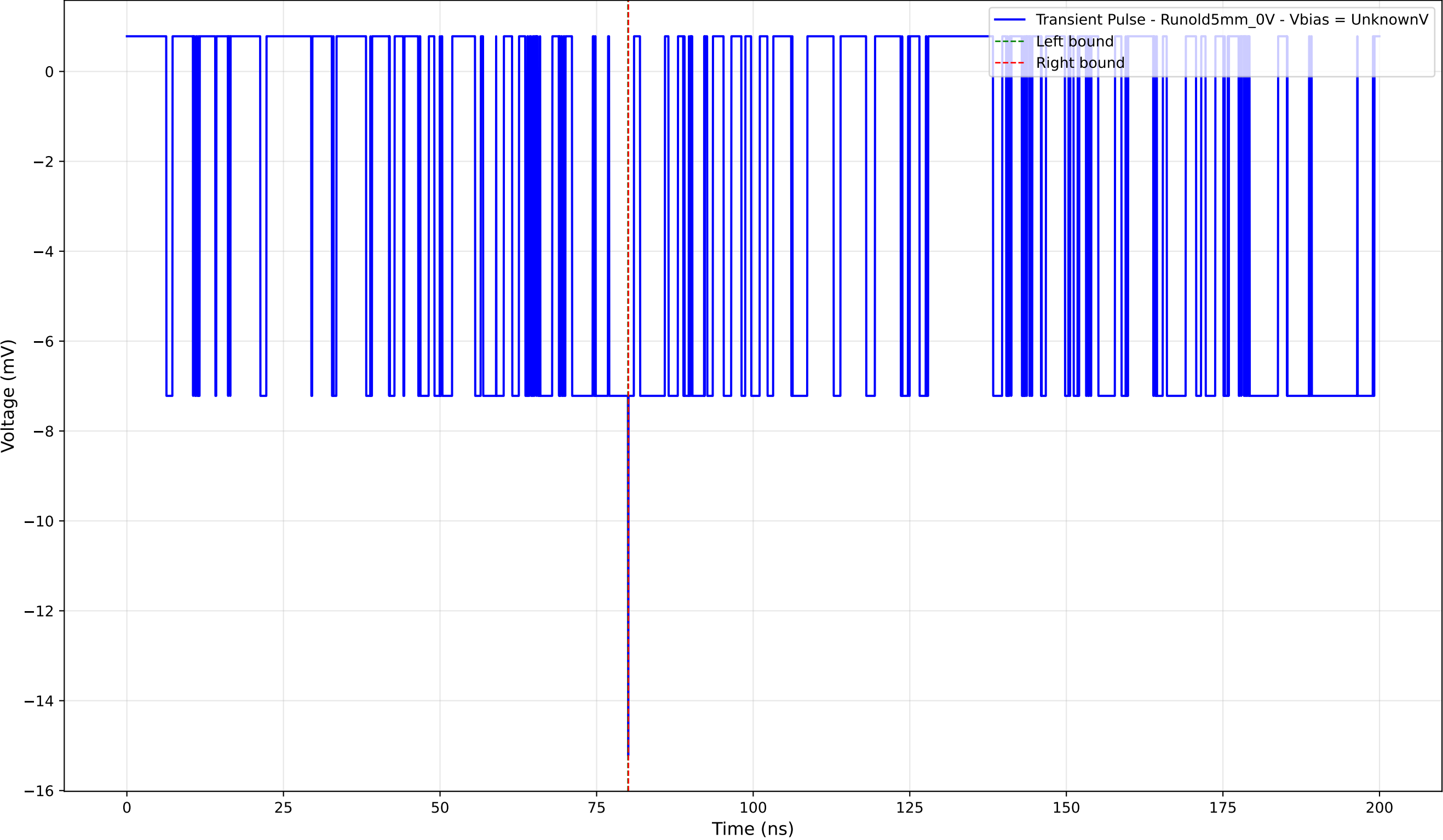
Transient Pulse - Sample: old5 - Position: 2200.0 \mu\text{m} - Charge: -0.02 pC
