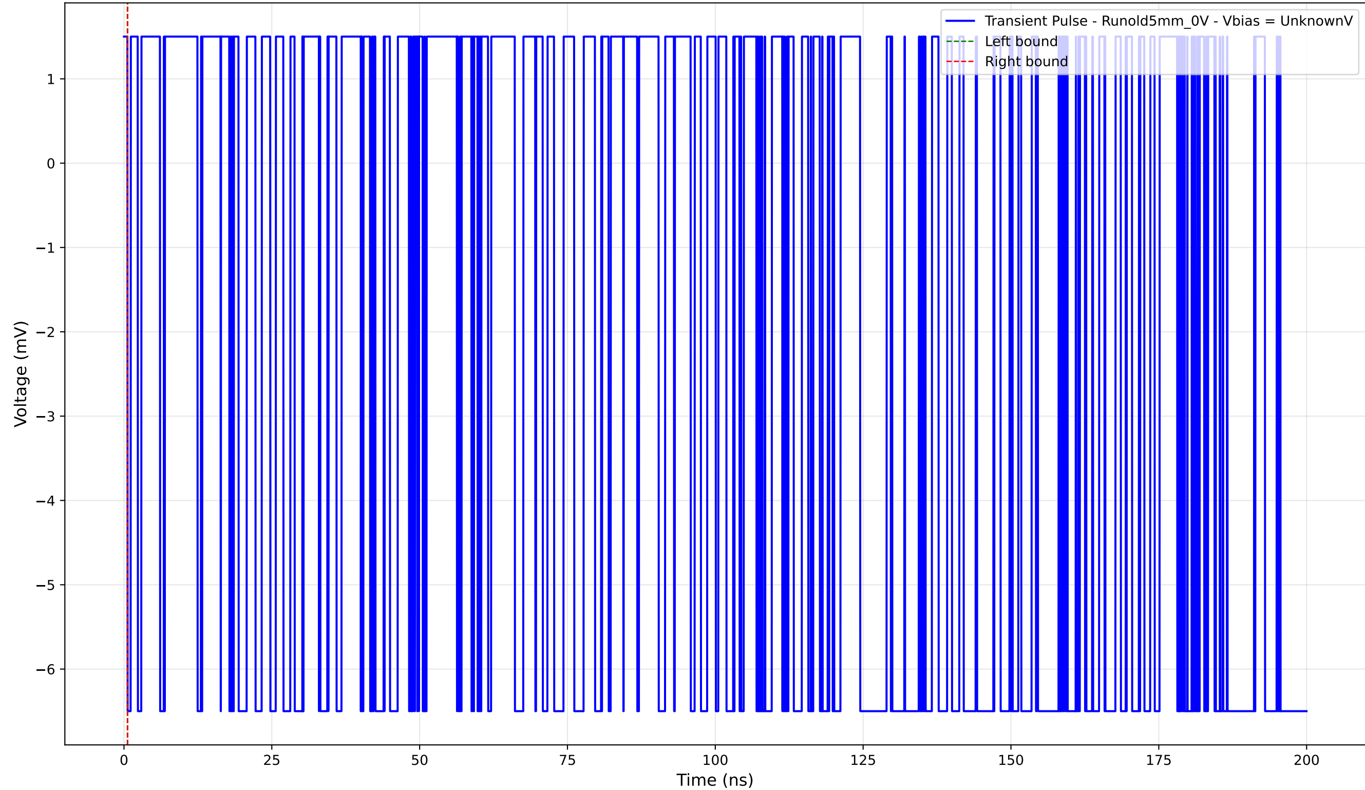
Transient Pulse - Sample: old5 - Position: 3140.0 \mu\text{m} - Charge: -0.00 pC
