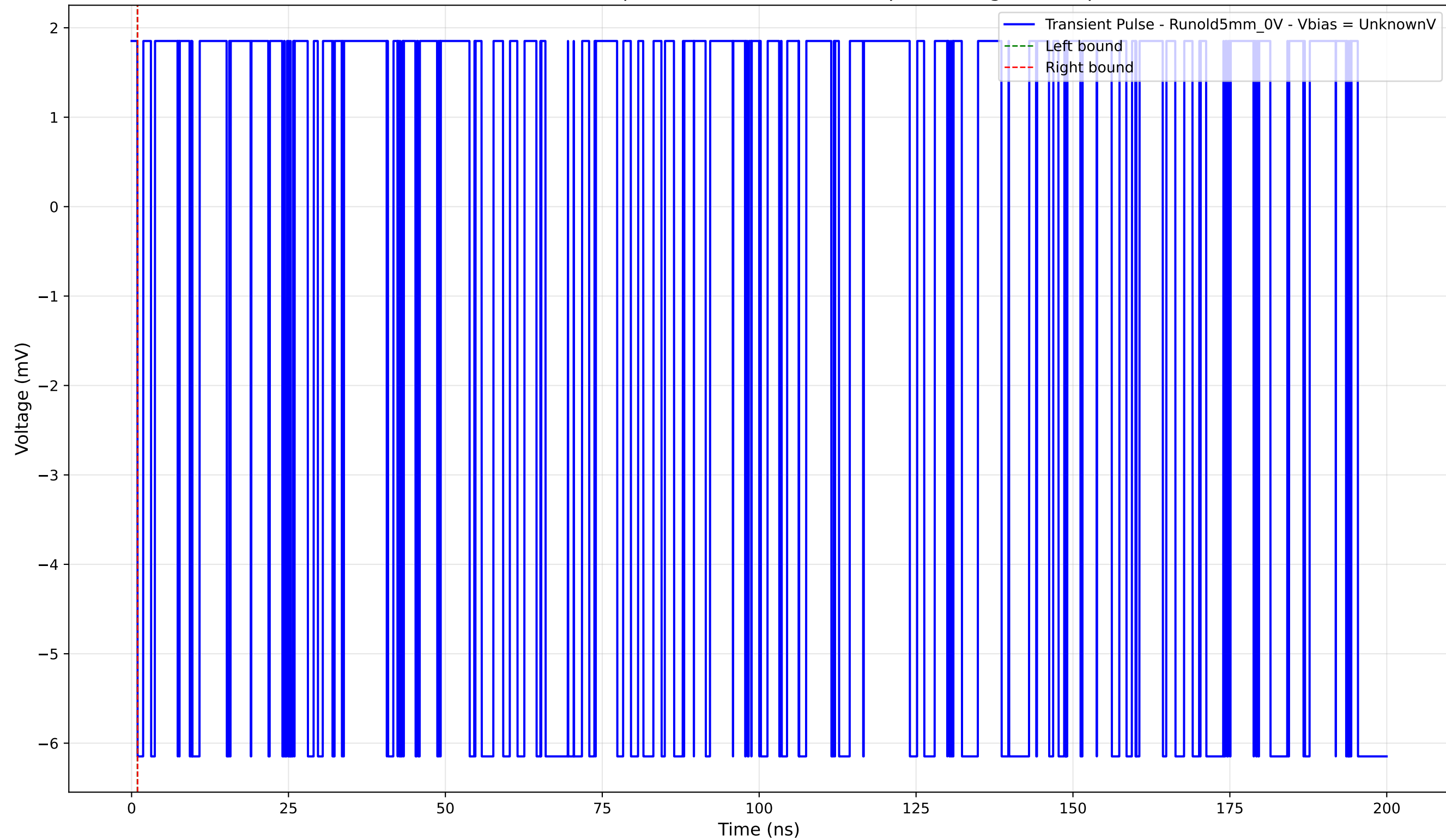
Transient Pulse - Sample: old5 - Position: 780.0 \mu\text{m} - Charge: -0.00 pC
