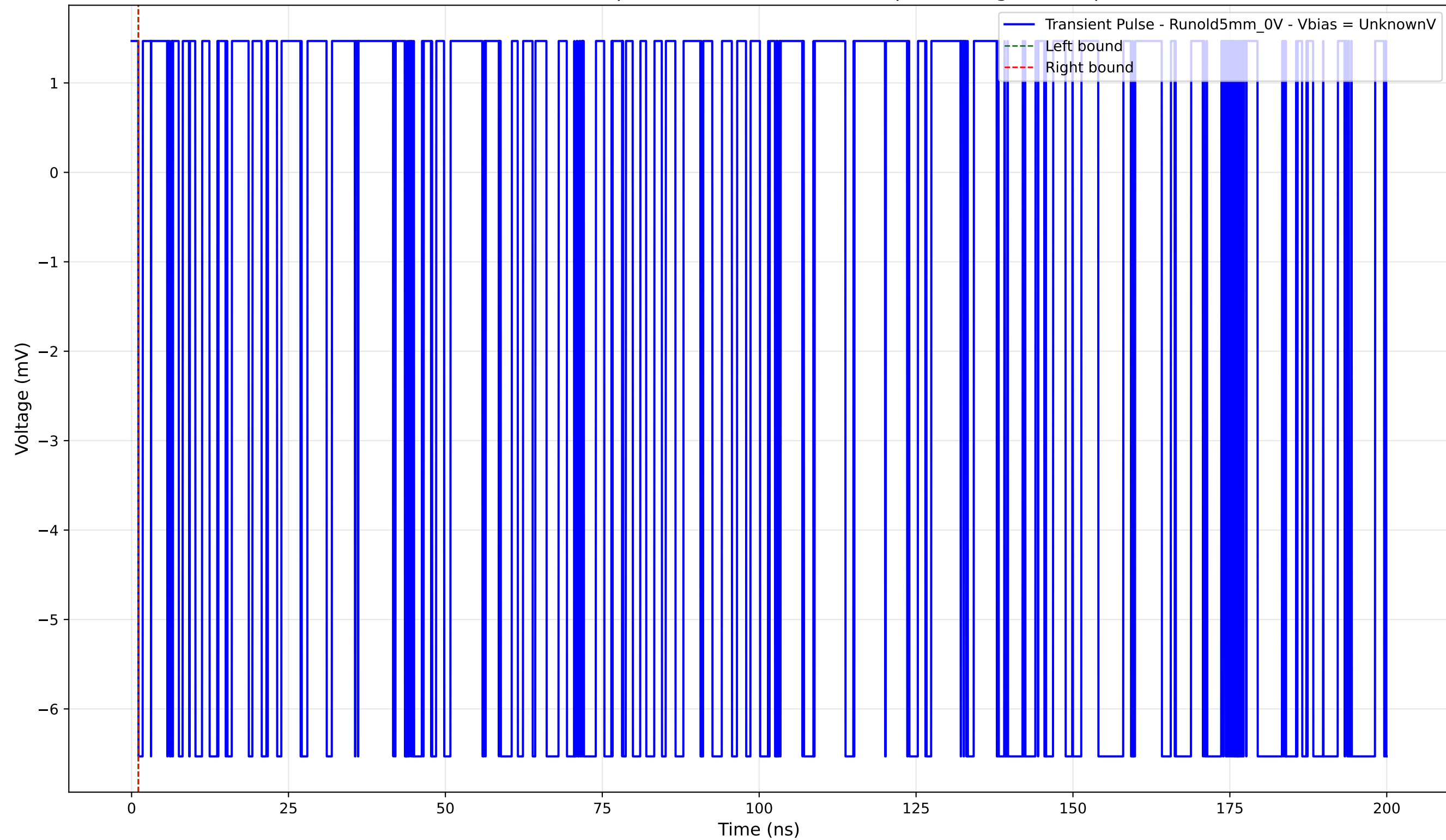
Transient Pulse - Sample: old5 - Position: 1825.0 \mu\text{m} - Charge: -0.00 pC
