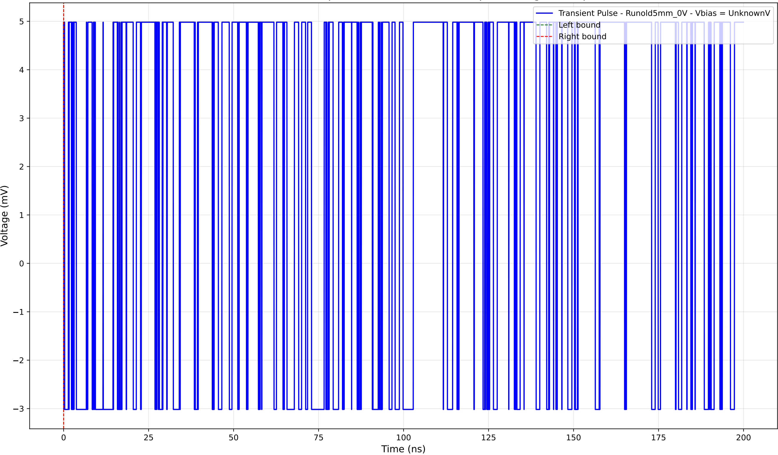
Transient Pulse - Sample: old5 - Position: 3355.0 \mu\text{m} - Charge: 0.00 pC
