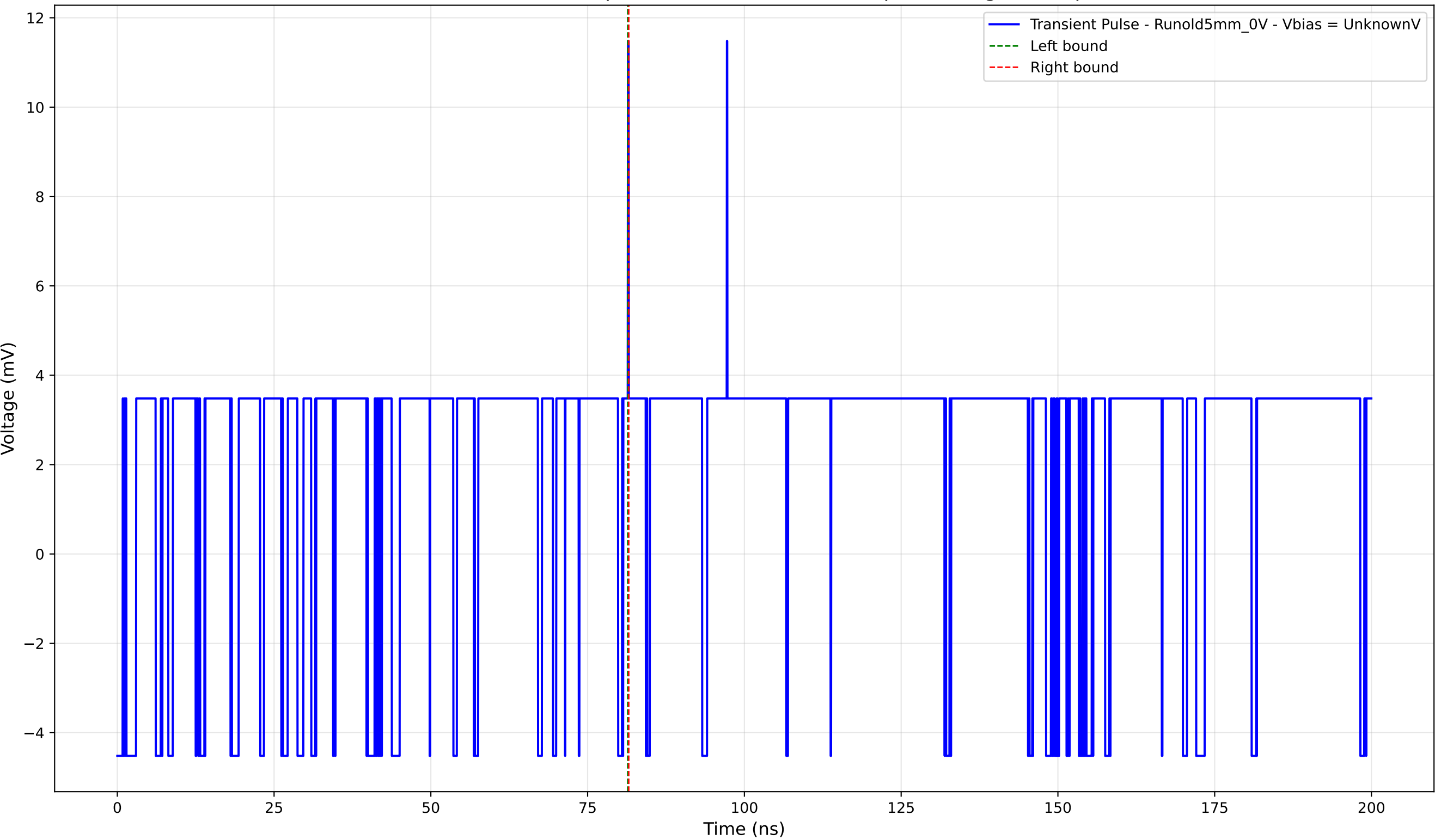
Transient Pulse - Sample: old5 - Position: 5065.0 \mu\text{m} - Charge: 0.03 pC
