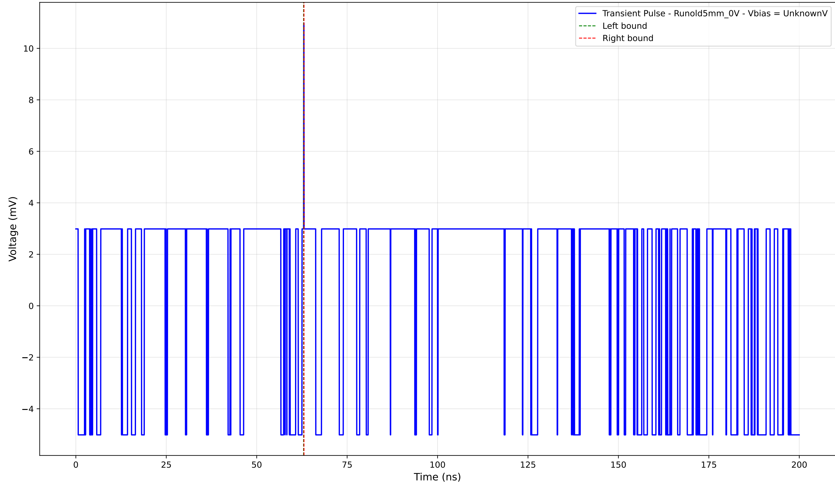
Transient Pulse - Sample: old5 - Position: 255.0 \mu\text{m} - Charge: 0.02 pC
