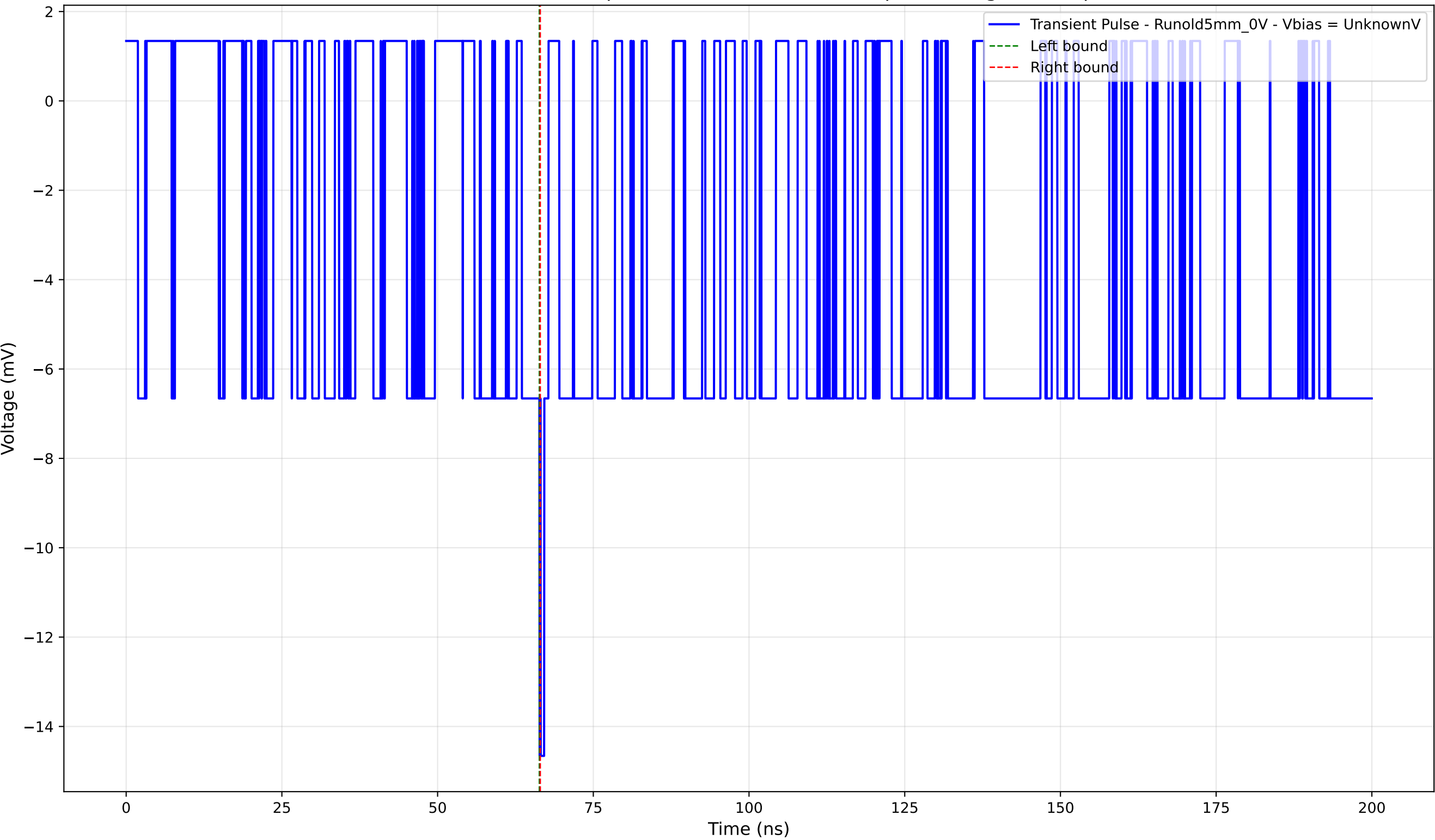
Transient Pulse - Sample: old5 - Position: 3520.0 \mu\text{m} - Charge: -0.04 pC
