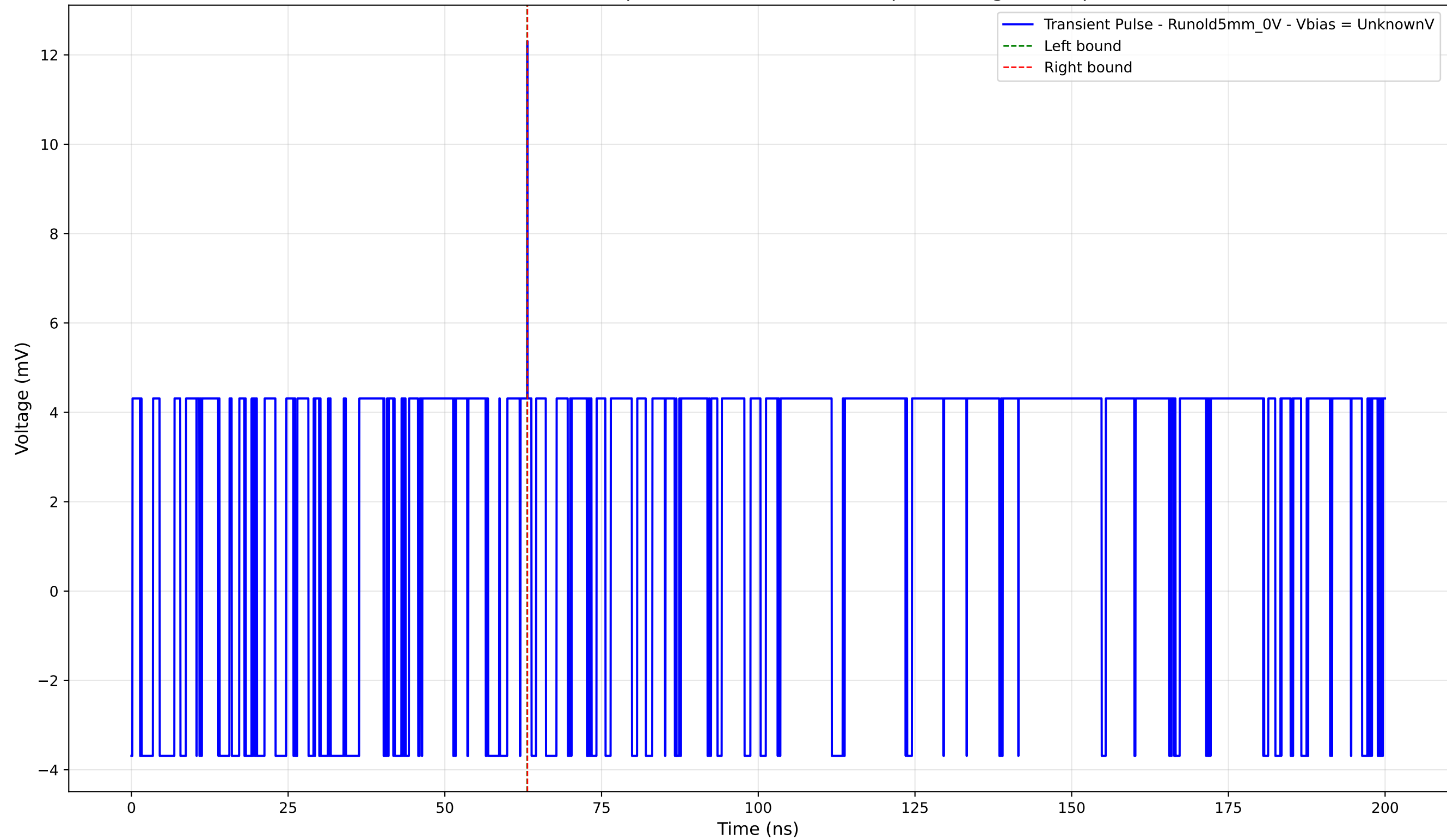
Transient Pulse - Sample: old5 - Position: 510.0 \mu\text{m} - Charge: 0.01 pC
