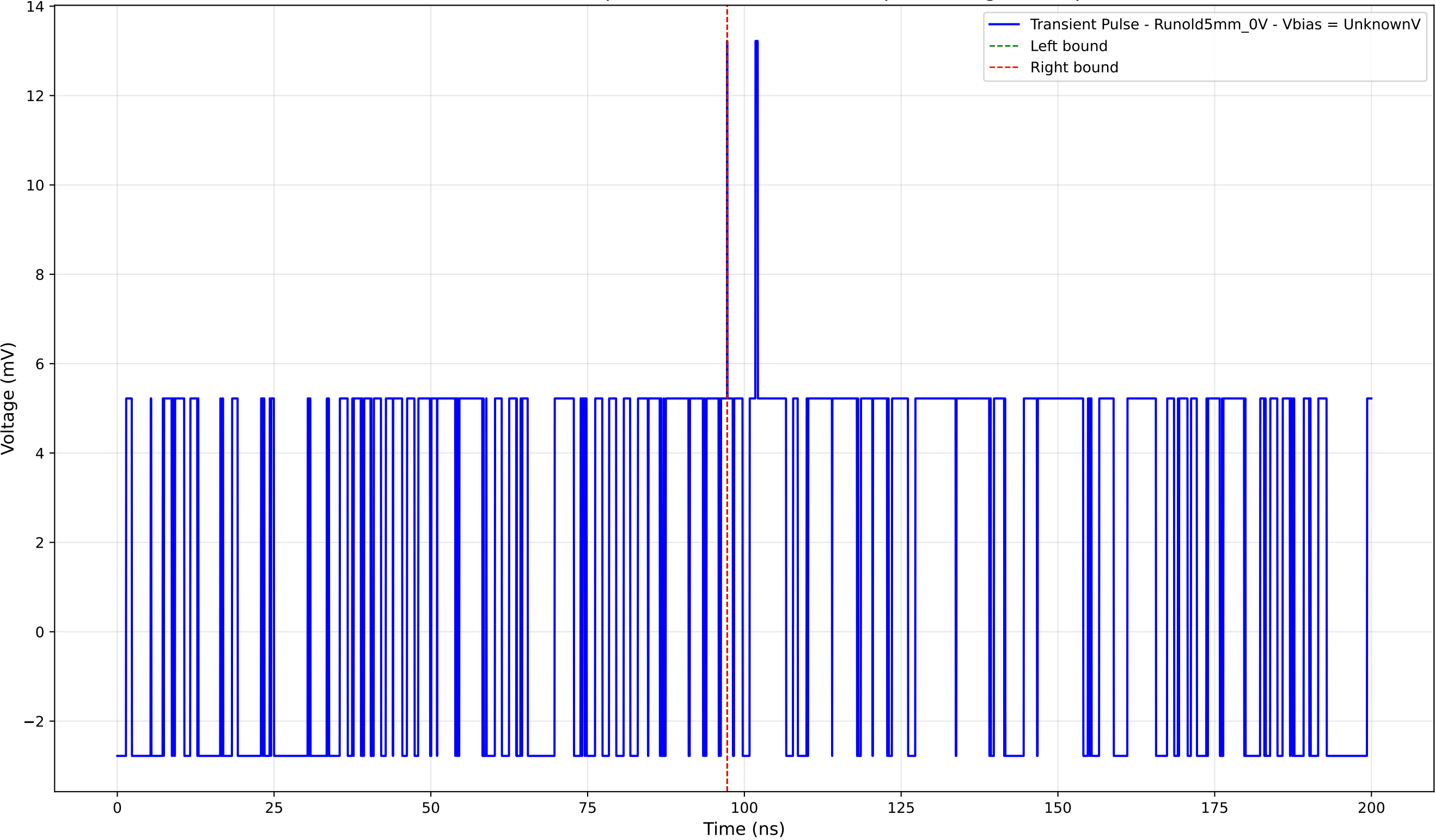
Transient Pulse - Sample: old5 - Position: 1520.0 \mu\text{m} - Charge: 0.01 pC
