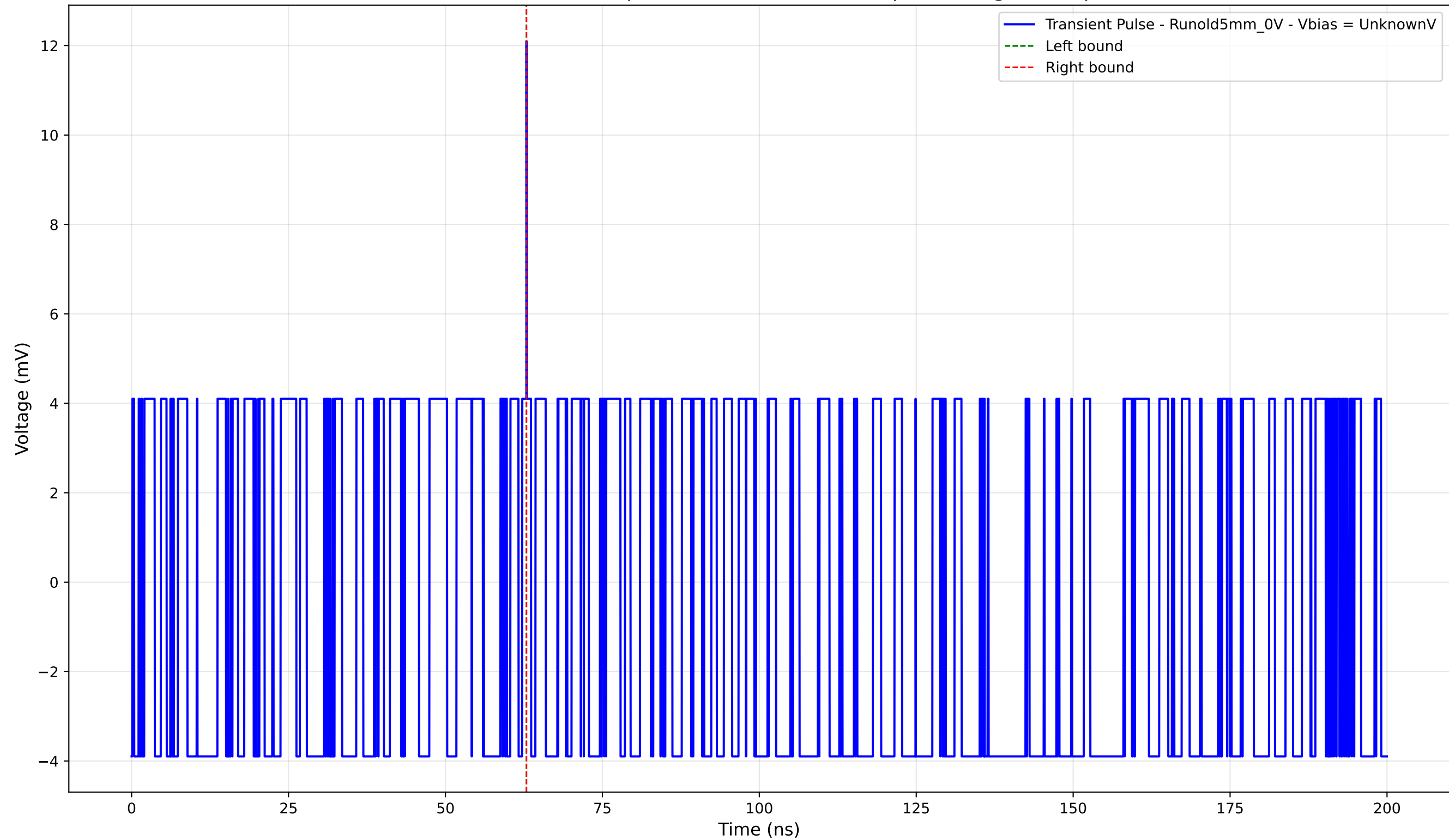
Transient Pulse - Sample: old5 - Position: 200.0 \mu\text{m} - Charge: 0.01 pC
