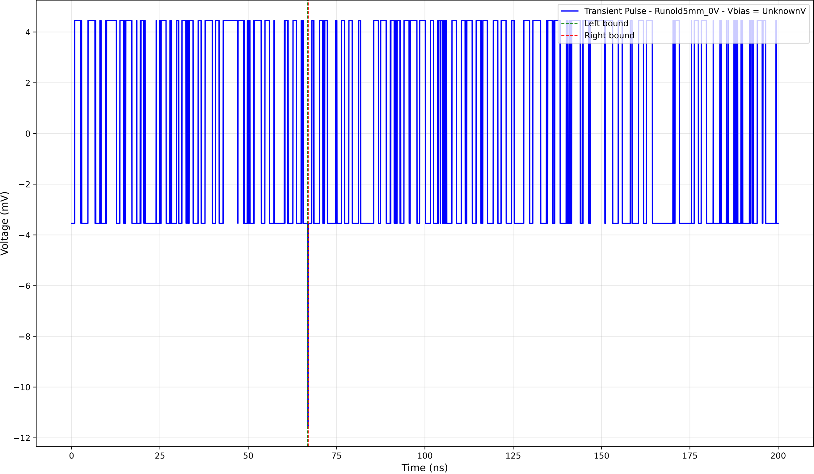
Transient Pulse - Sample: old5 - Position: 4235.0 \mu\text{m} - Charge: -0.03 pC
