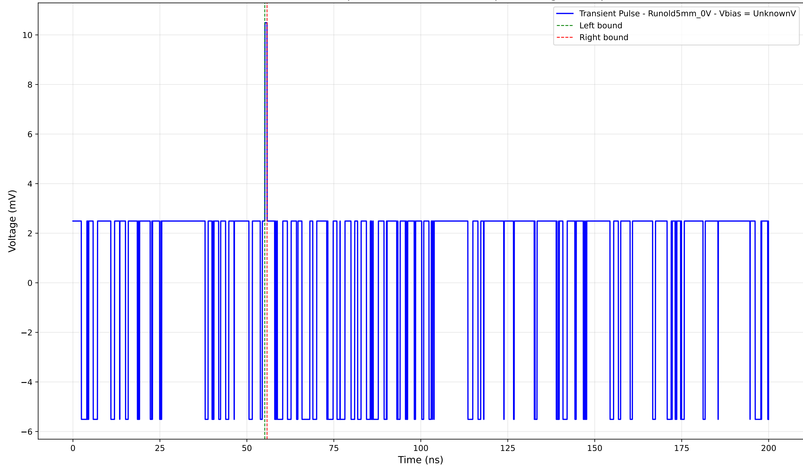
Transient Pulse - Sample: old5 - Position: 745.0 \mu\text{m} - Charge: 0.13 pC
