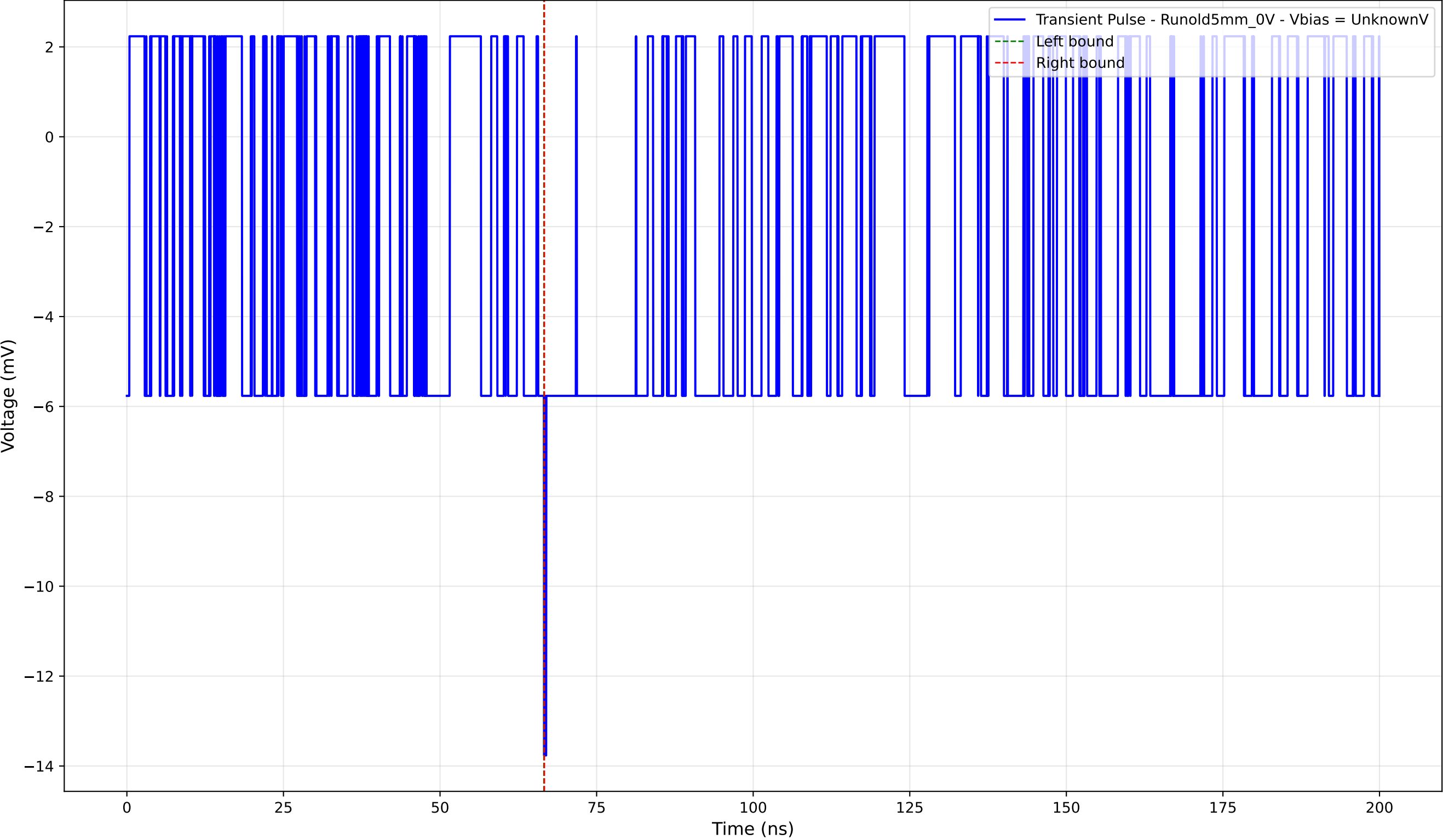
Transient Pulse - Sample: old5 - Position: 4540.0 \mu\text{m} - Charge: -0.02 pC
