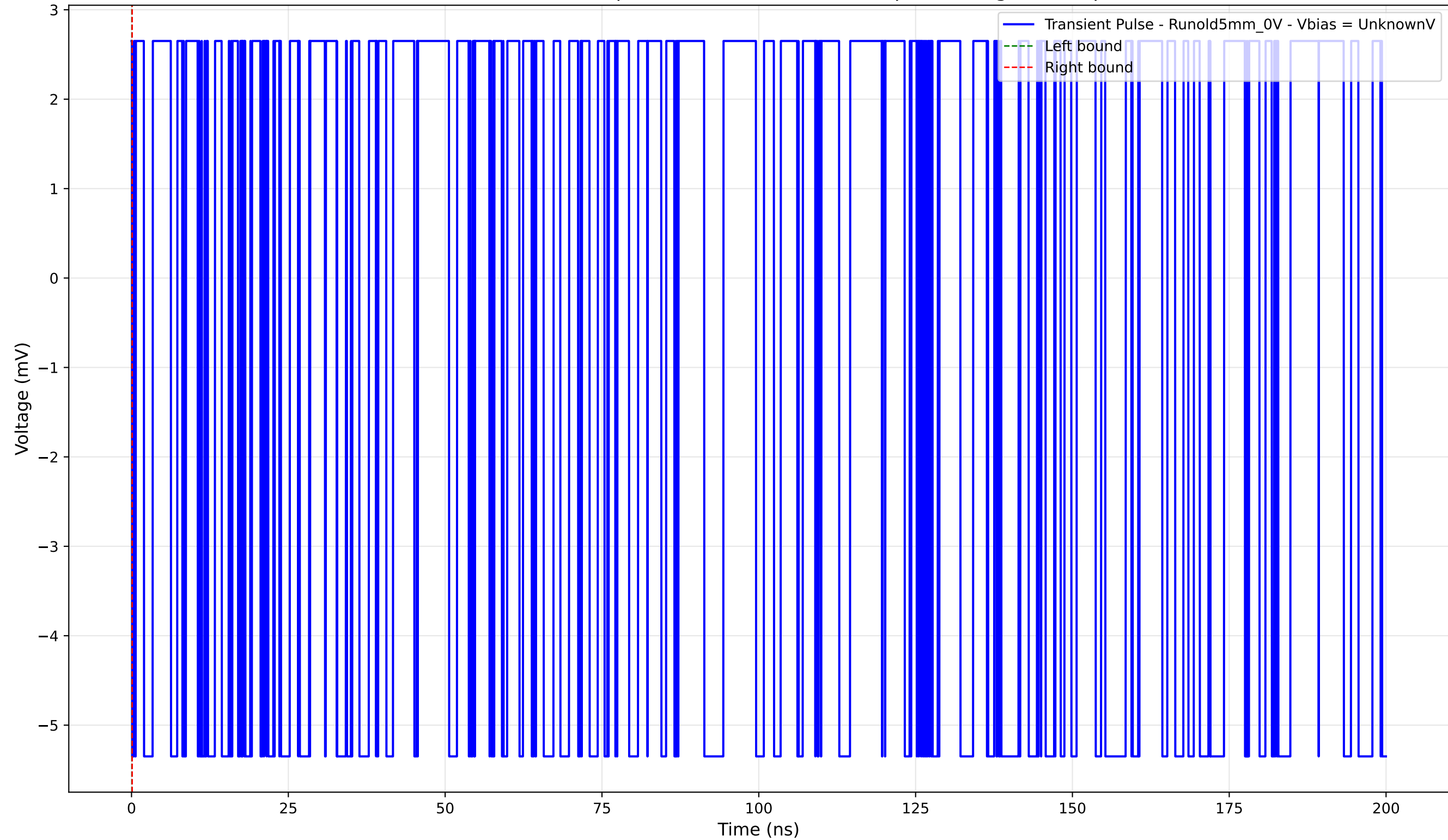
Transient Pulse - Sample: old5 - Position: 2515.0 \mu\text{m} - Charge: -0.00 pC
