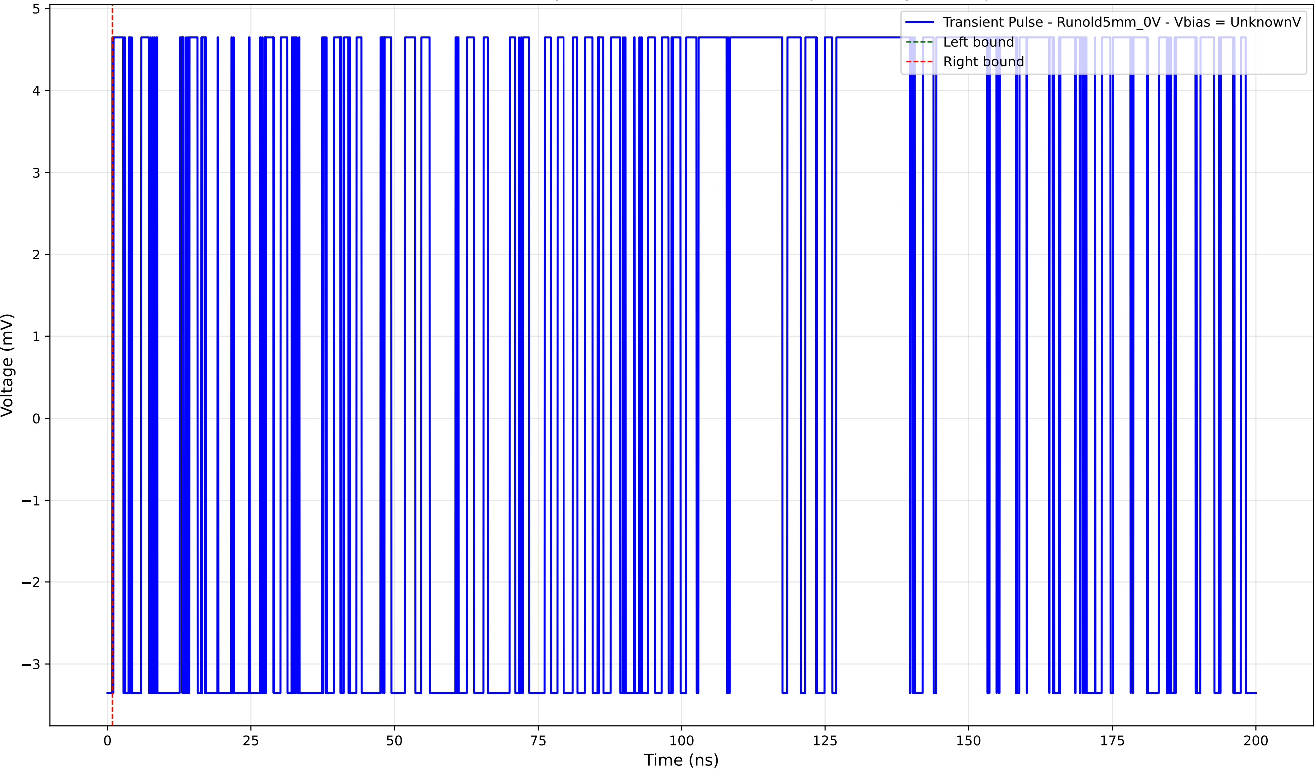
Transient Pulse - Sample: old5 - Position: 1850.0 \mu\text{m} - Charge: 0.00 pC
