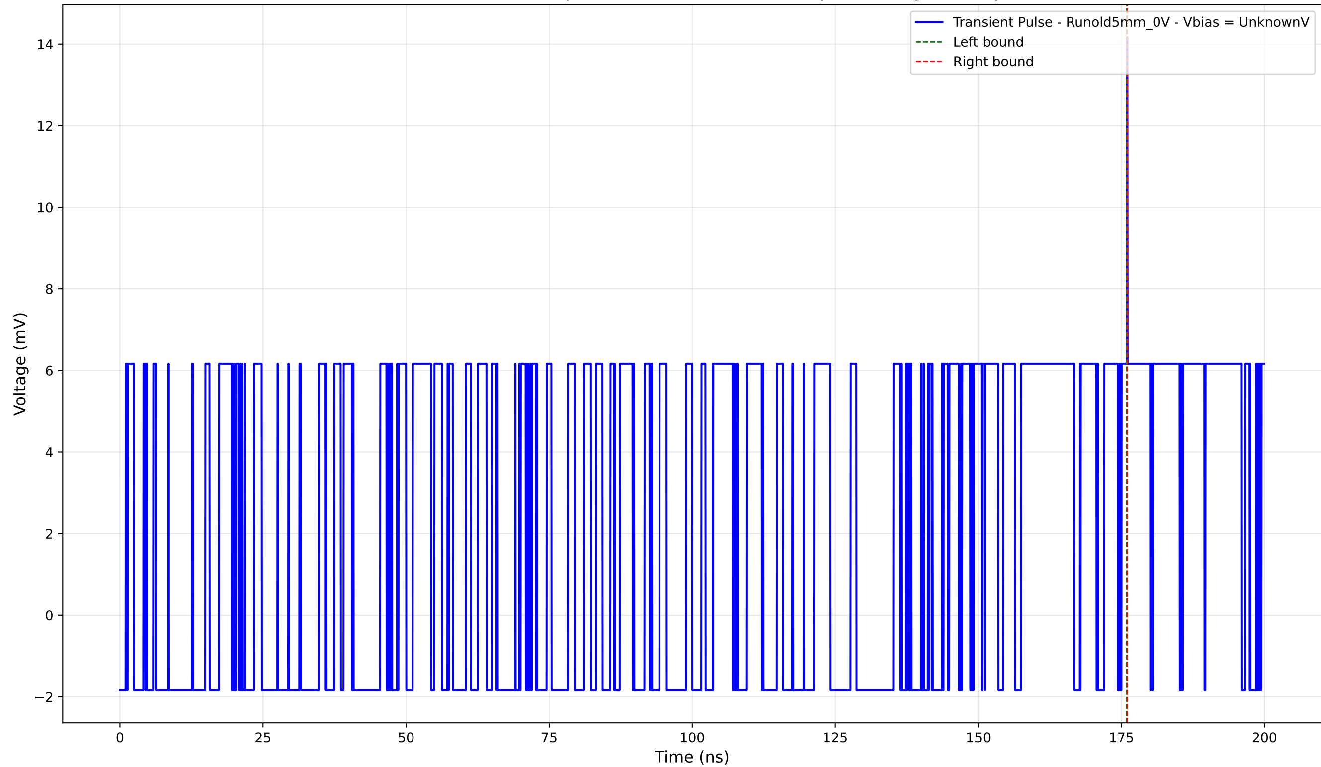
Transient Pulse - Sample: old5 - Position: 4840.0 \mu\text{m} - Charge: 0.03 pC
