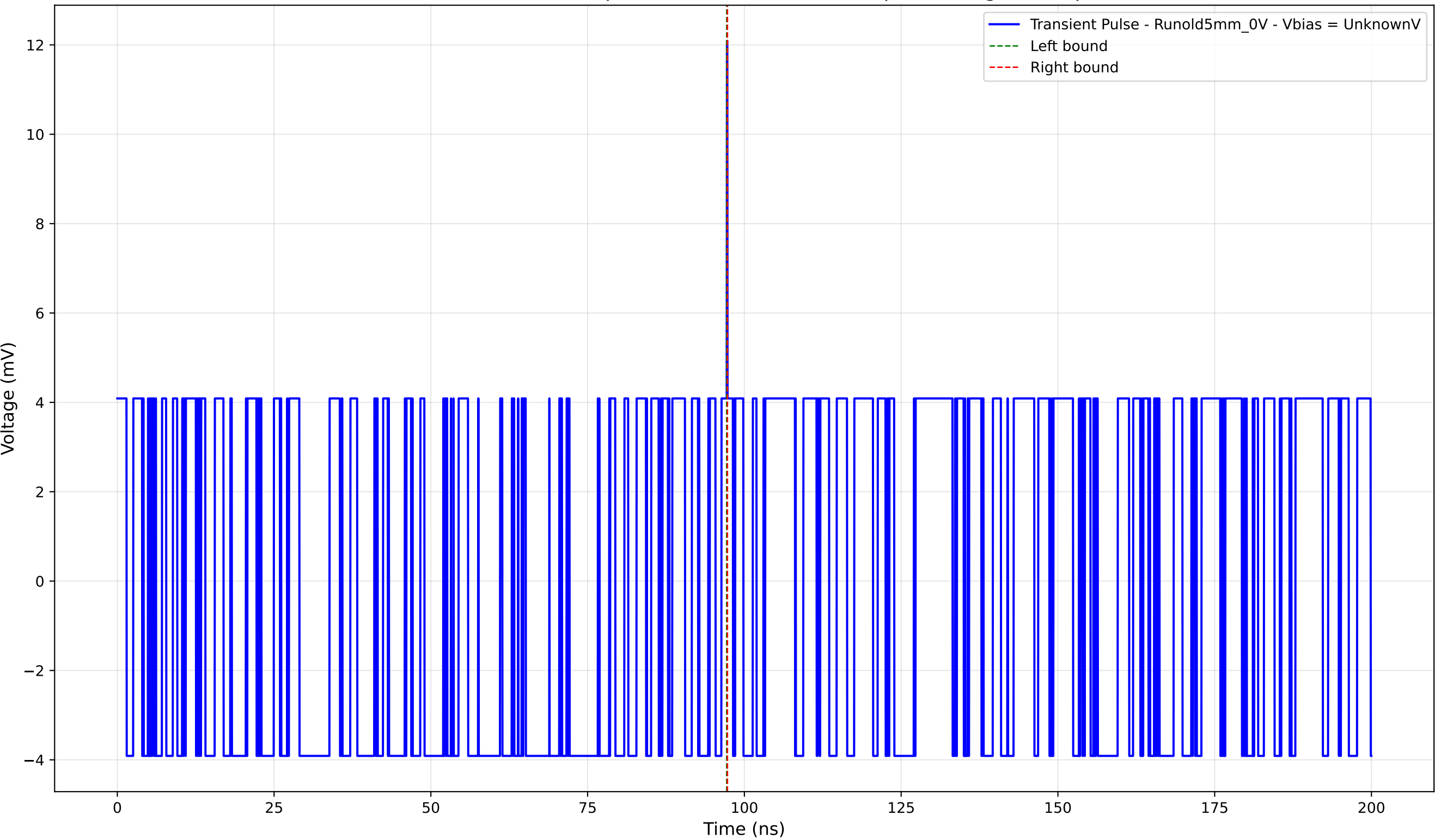
Transient Pulse - Sample: old5 - Position: 2470.0 \mu\text{m} - Charge: 0.03 pC
