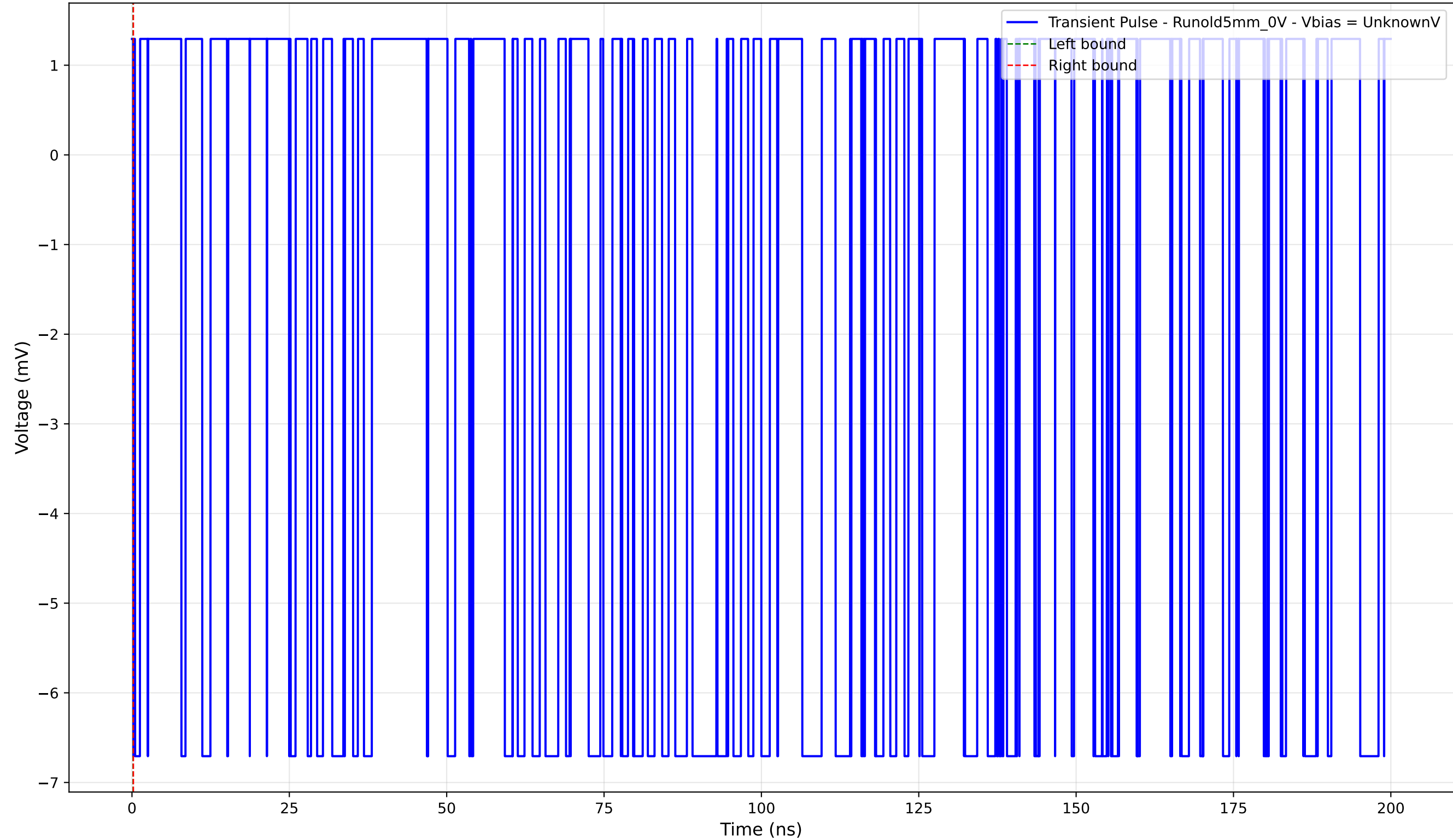
Transient Pulse - Sample: old5 - Position: 1145.0 \mu\text{m} - Charge: -0.00 pC
