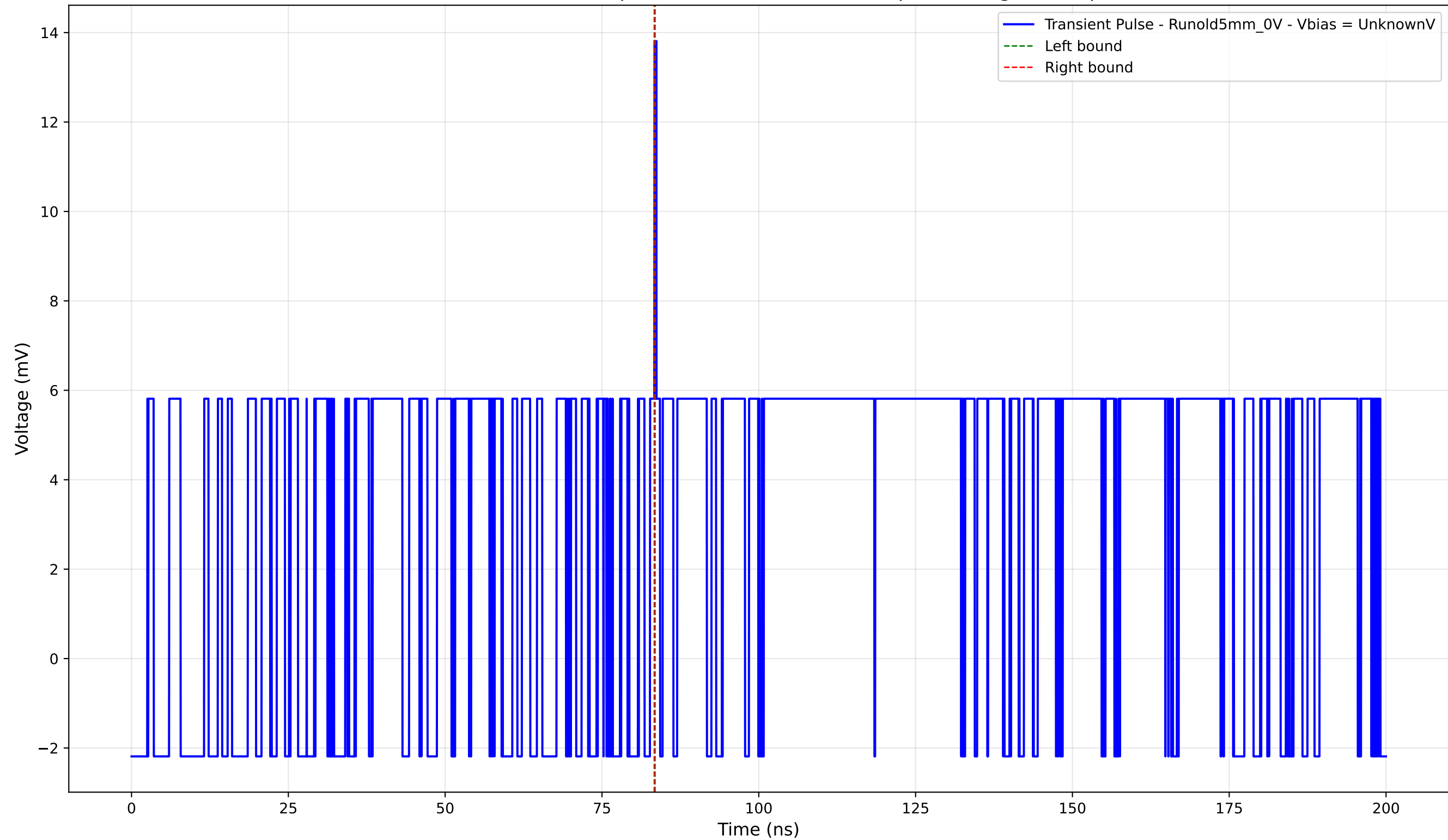
Transient Pulse - Sample: old5 - Position: 3985.0 \mu\text{m} - Charge: 0.03 pC
