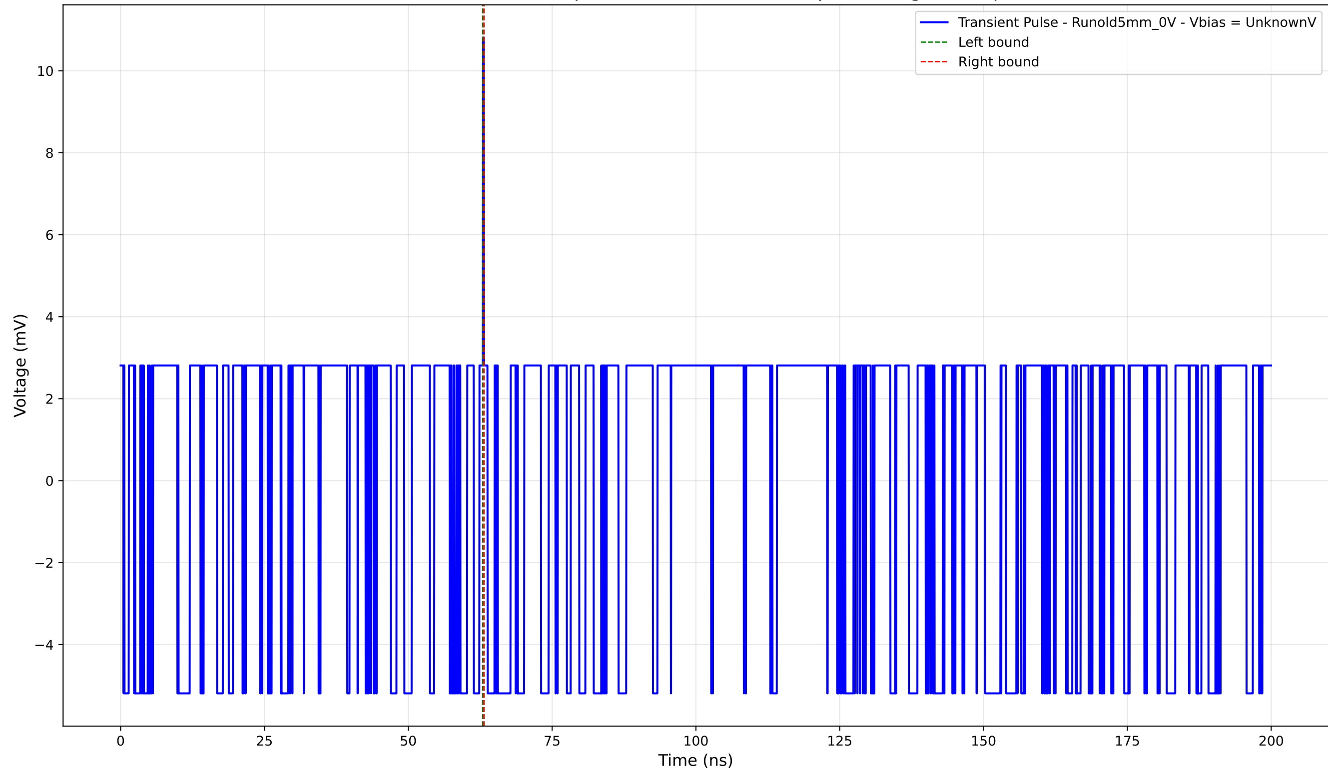
Transient Pulse - Sample: old5 - Position: 395.0 \mu\text{m} - Charge: 0.04 pC
