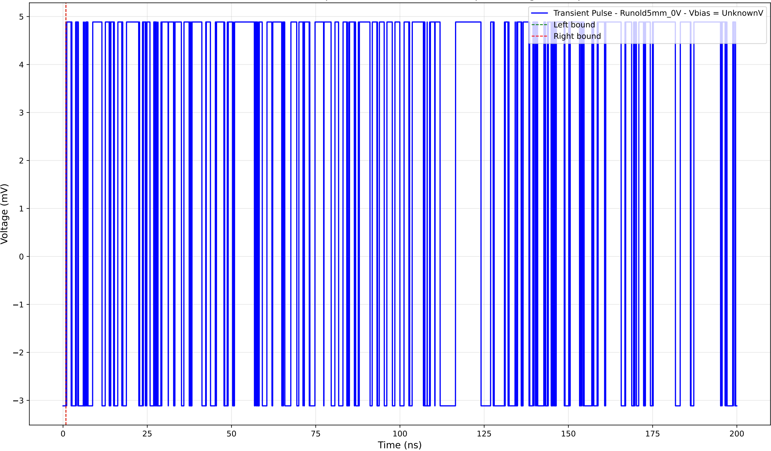
Transient Pulse - Sample: old5 - Position: 1305.0 \mu\text{m} - Charge: 0.00 pC
