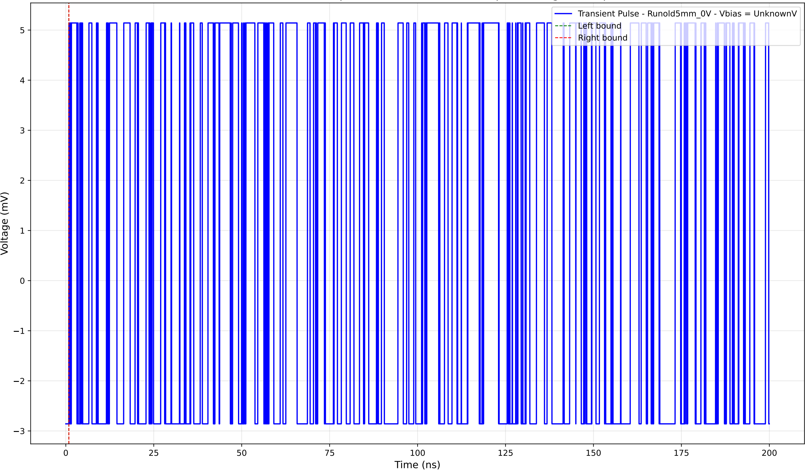
Transient Pulse - Sample: old5 - Position: 4300.0 \mu\text{m} - Charge: 0.00 pC
