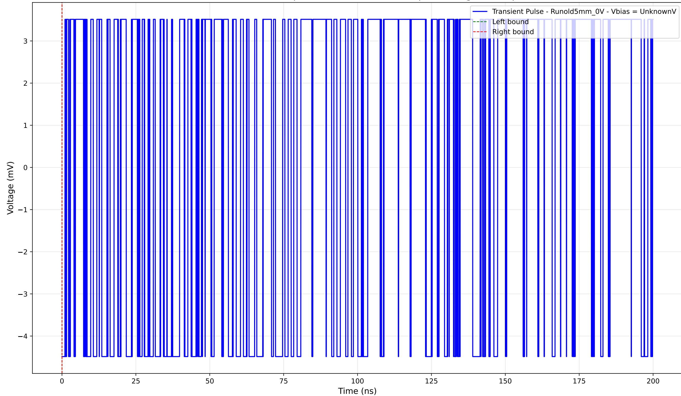
Transient Pulse - Sample: old5 - Position: 710.0 \mu\text{m} - Charge: -0.00 pC
