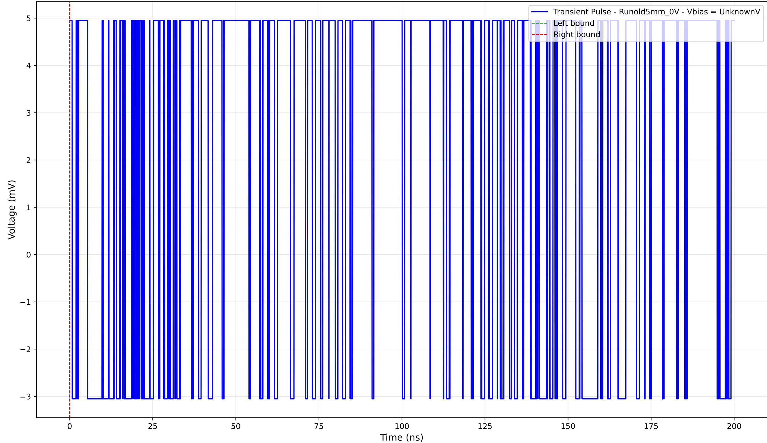
Transient Pulse - Sample: old5 - Position: 410.0 \mu\text{m} - Charge: 0.00 pC
