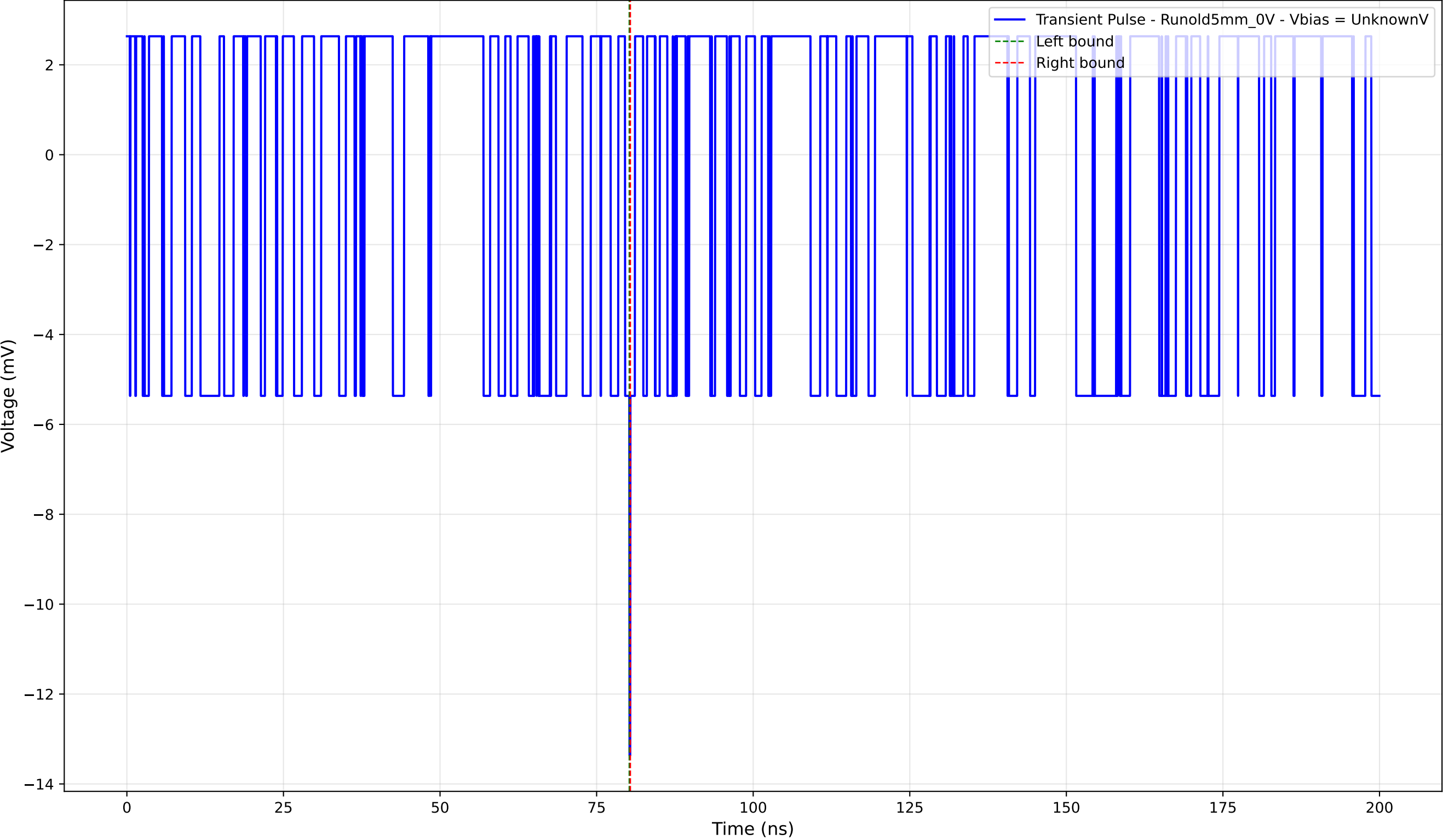
Transient Pulse - Sample: old5 - Position: 3670.0 \mu\text{m} - Charge: -0.04 pC
