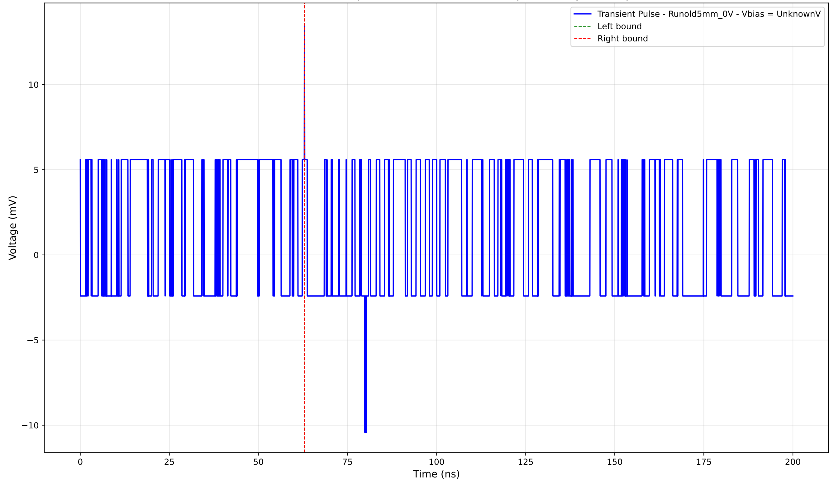
Transient Pulse - Sample: old5 - Position: 3085.0 \mu\text{m} - Charge: 0.03 pC
