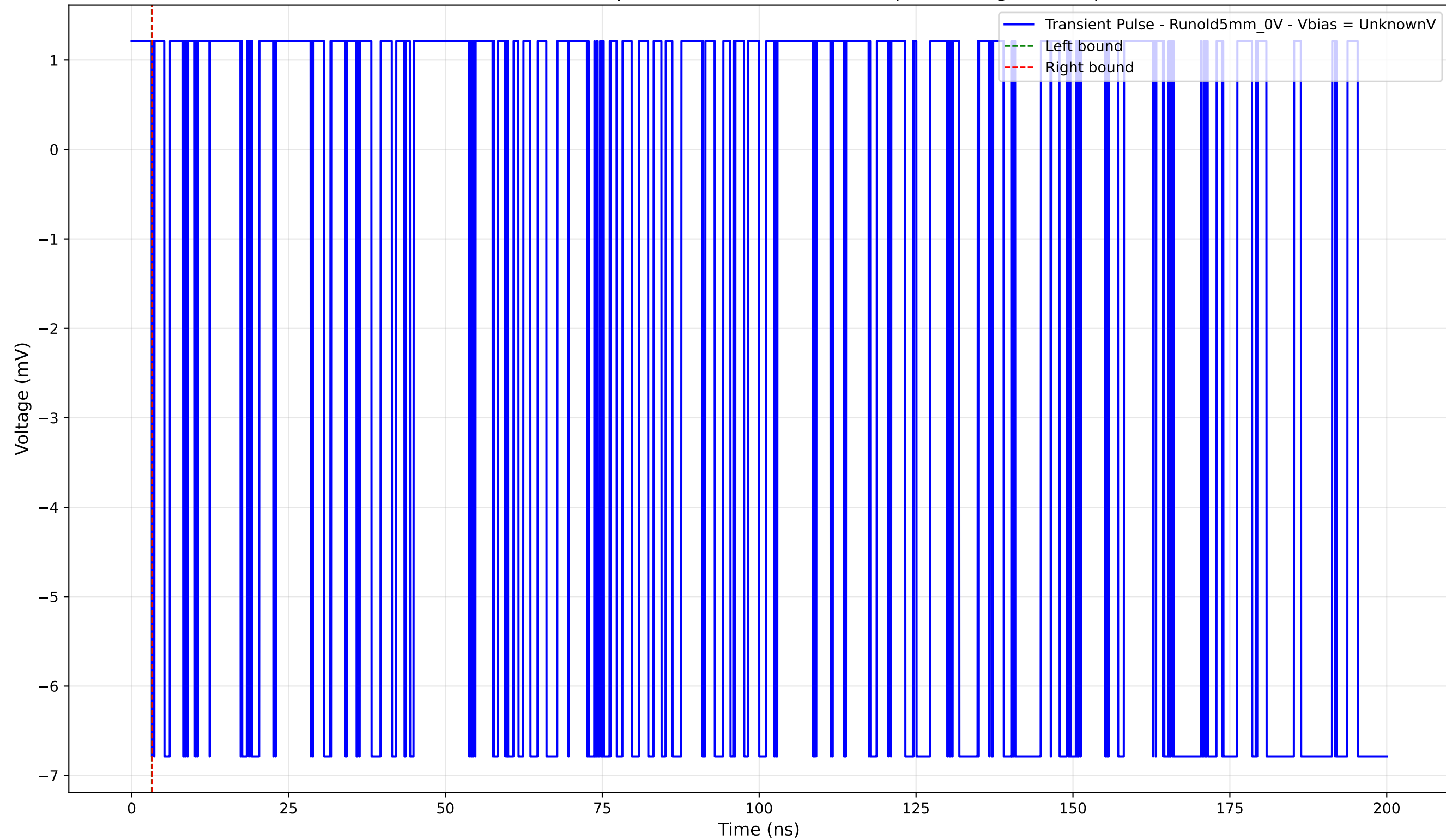
Transient Pulse - Sample: old5 - Position: 3555.0 \mu\text{m} - Charge: -0.00 pC
