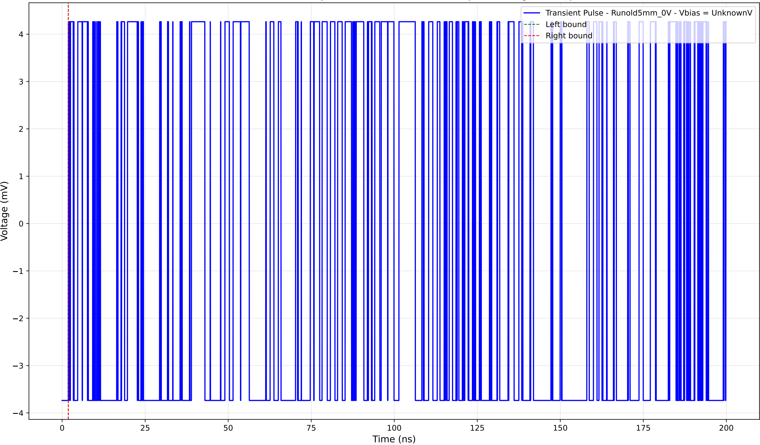
Transient Pulse - Sample: old5 - Position: 2285.0 \mu\text{m} - Charge: 0.00 pC
