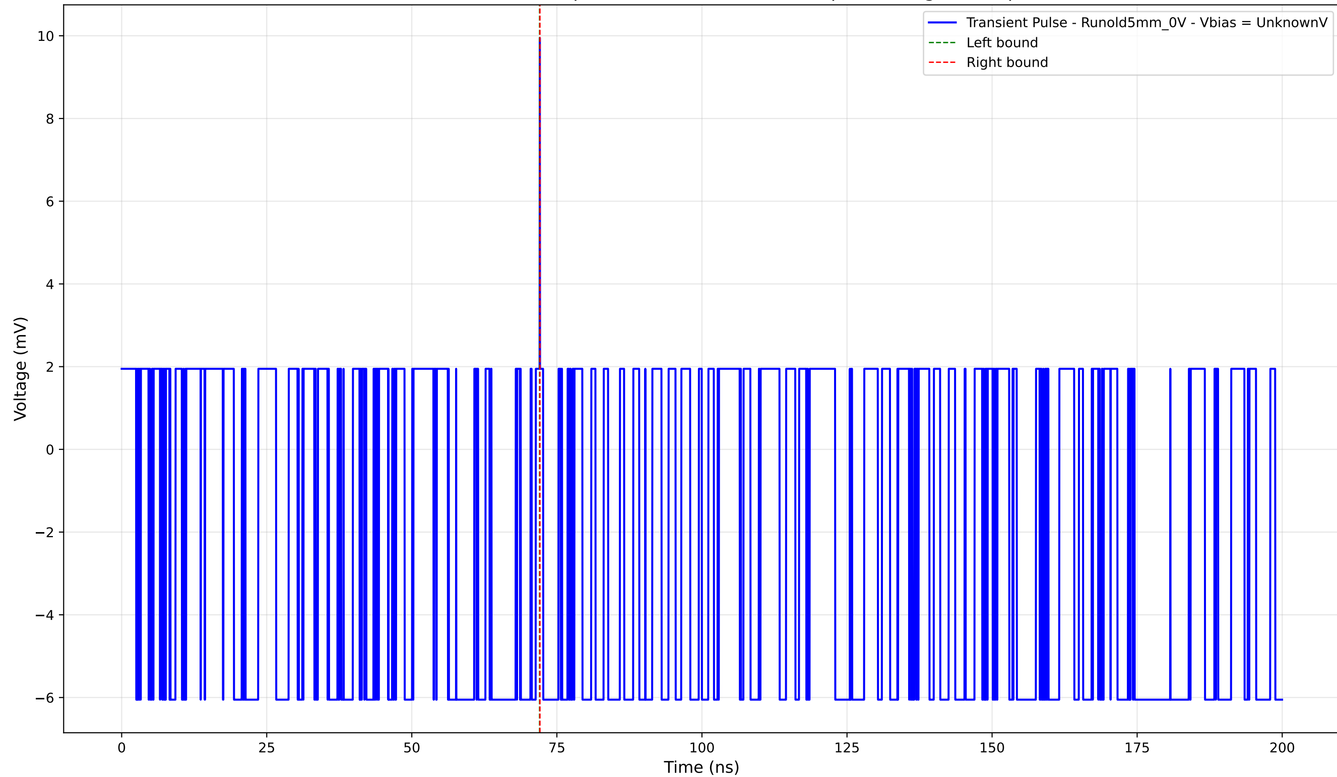
Transient Pulse - Sample: old5 - Position: 5090.0 \mu\text{m} - Charge: 0.01 pC
