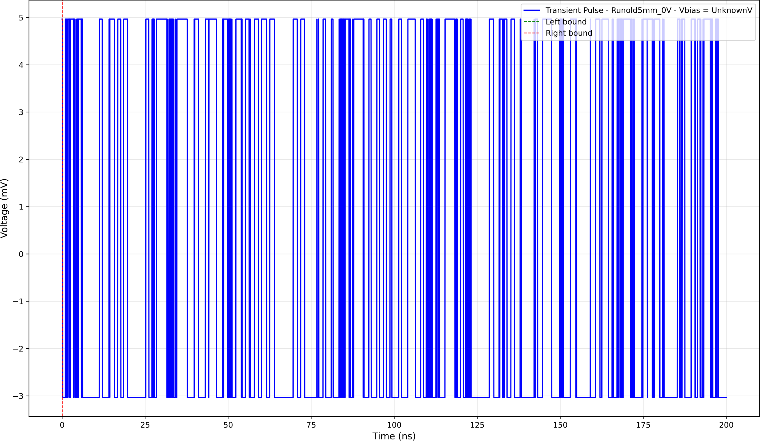
Transient Pulse - Sample: old5 - Position: 3420.0 \mu\text{m} - Charge: 0.00 pC
