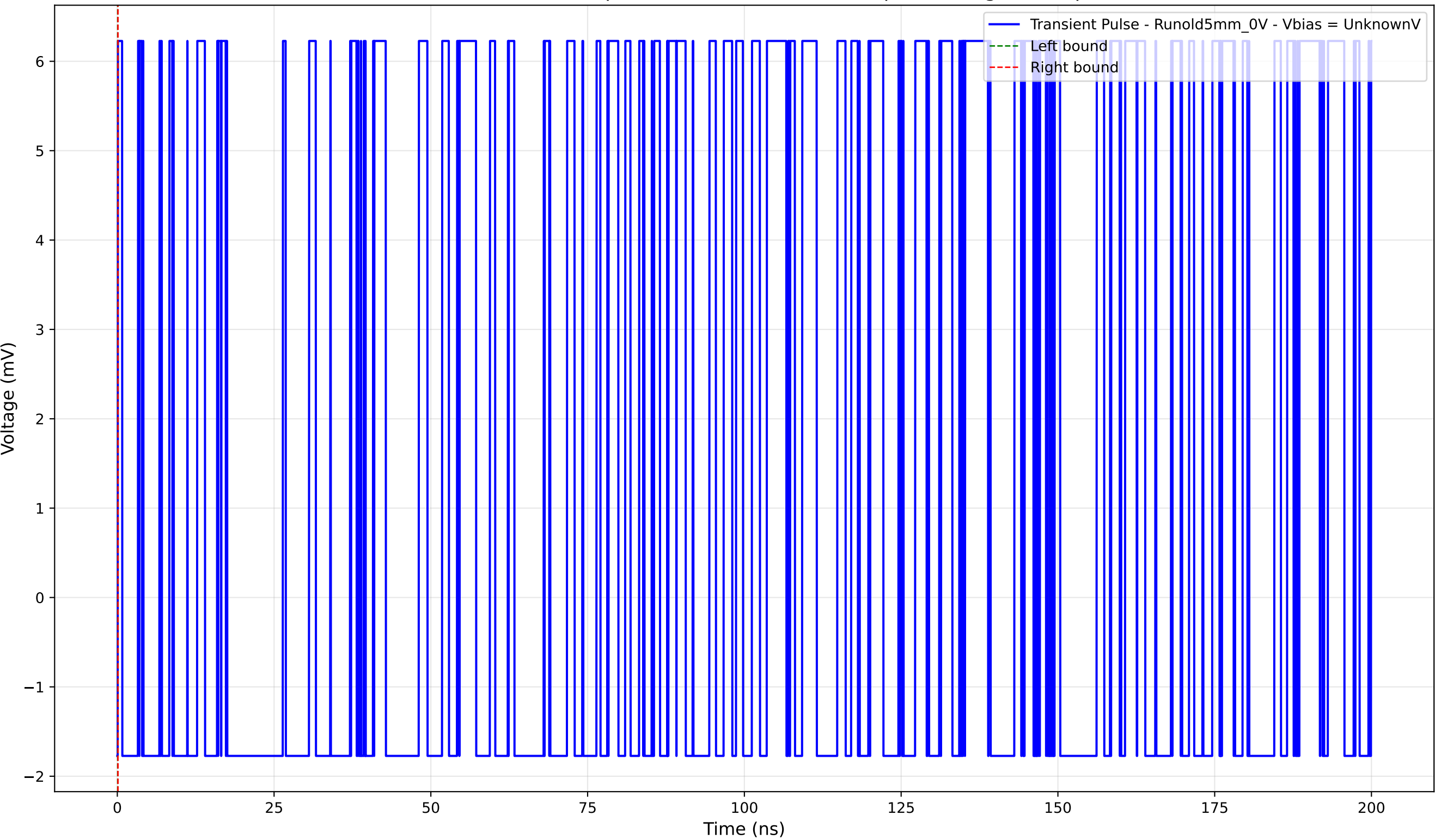
Transient Pulse - Sample: old5 - Position: 3040.0 \mu\text{m} - Charge: 0.00 pC
