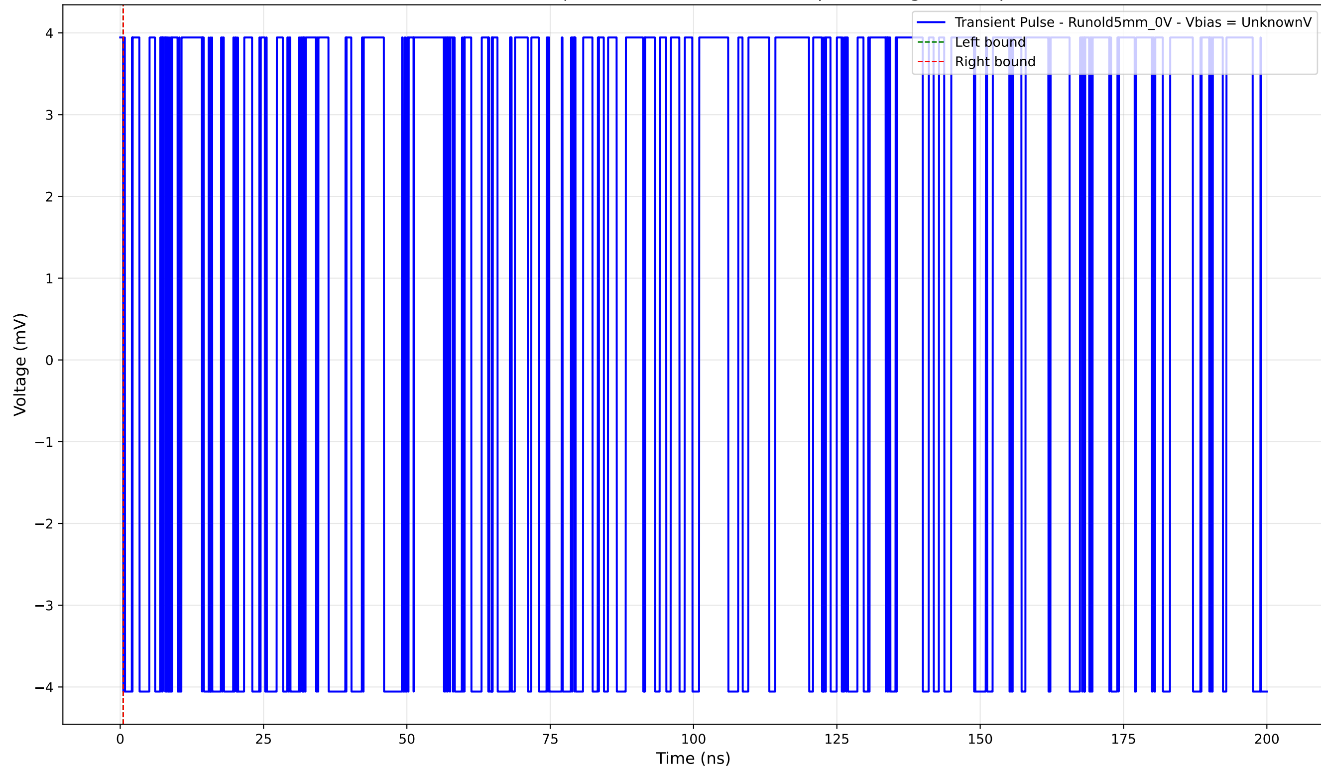
Transient Pulse - Sample: old5 - Position: 4790.0 \mu\text{m} - Charge: -0.00 pC
