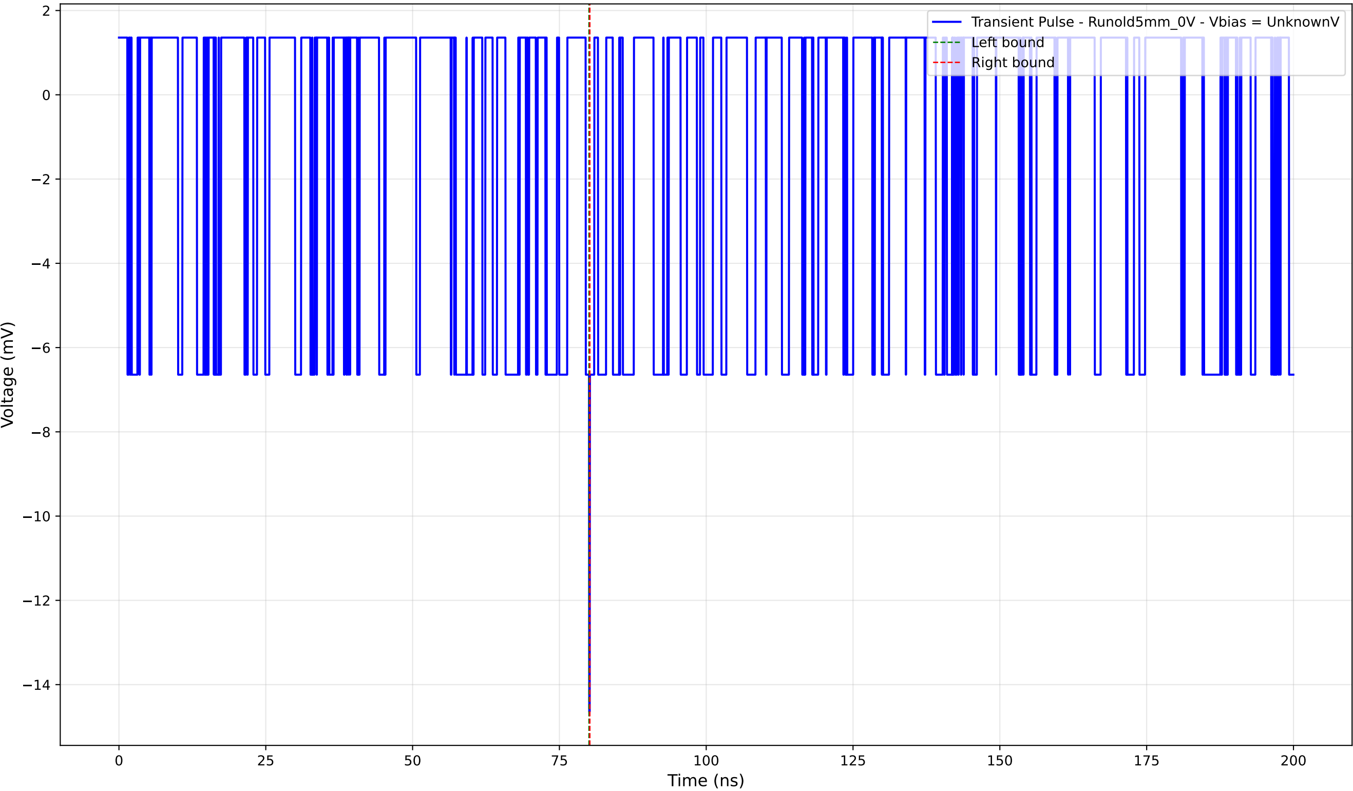
Transient Pulse - Sample: old5 - Position: 2385.0 \mu\text{m} - Charge: -0.04 pC
