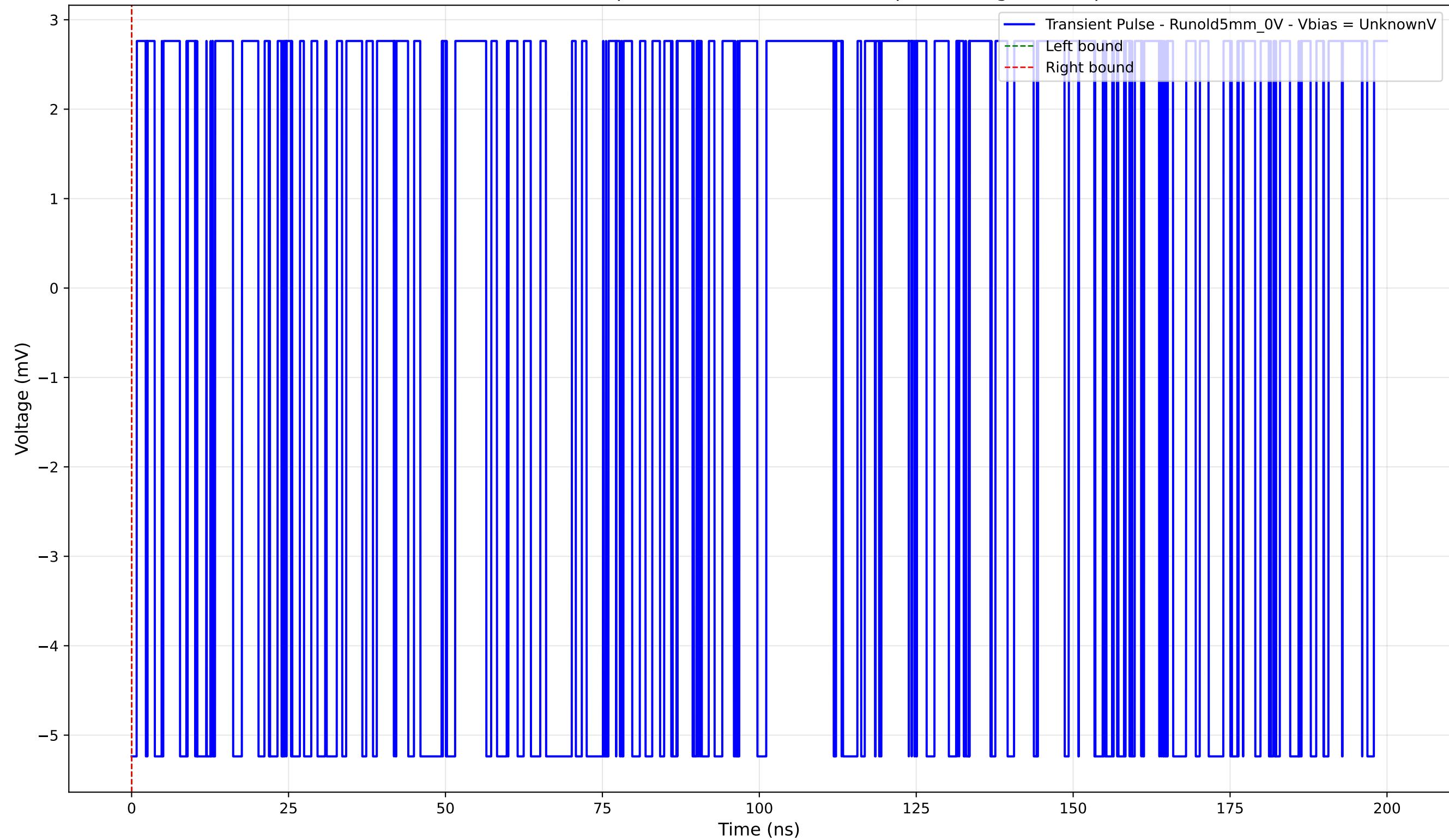
Transient Pulse - Sample: old5 - Position: 1280.0 \mu\text{m} - Charge: -0.00 pC
