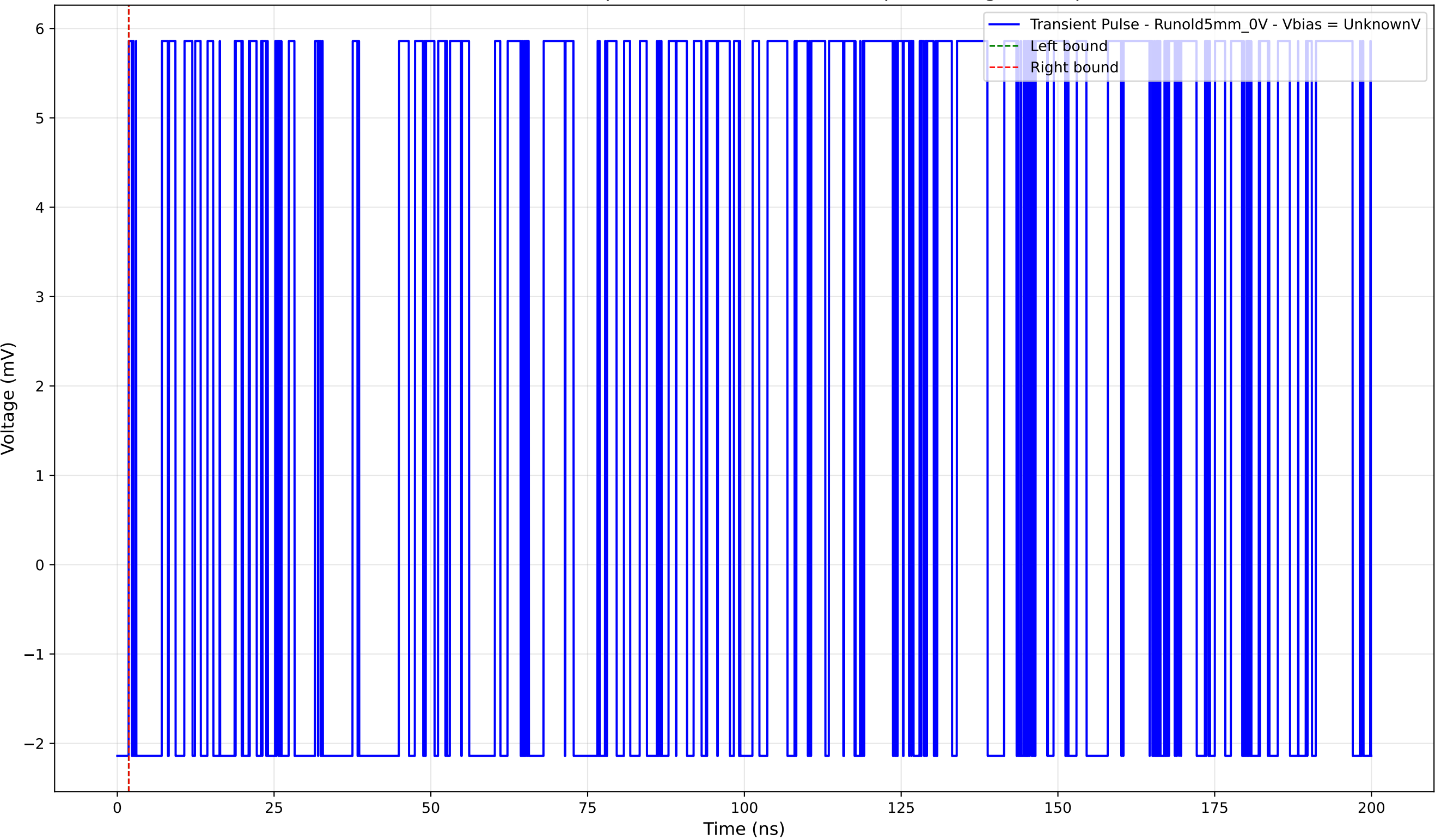
Transient Pulse - Sample: old5 - Position: 4785.0 \mu\text{m} - Charge: 0.00 pC
