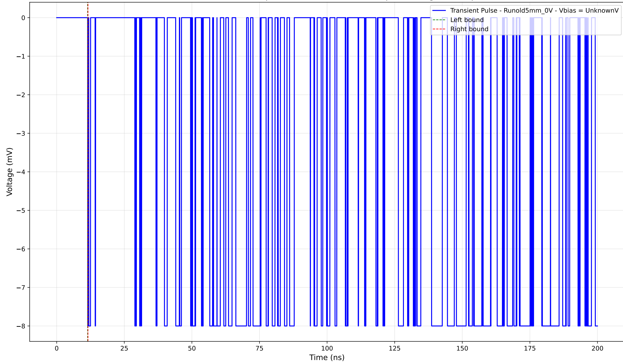
Transient Pulse - Sample: old5 - Position: 2400.0 \mu\text{m} - Charge: -0.02 pC
