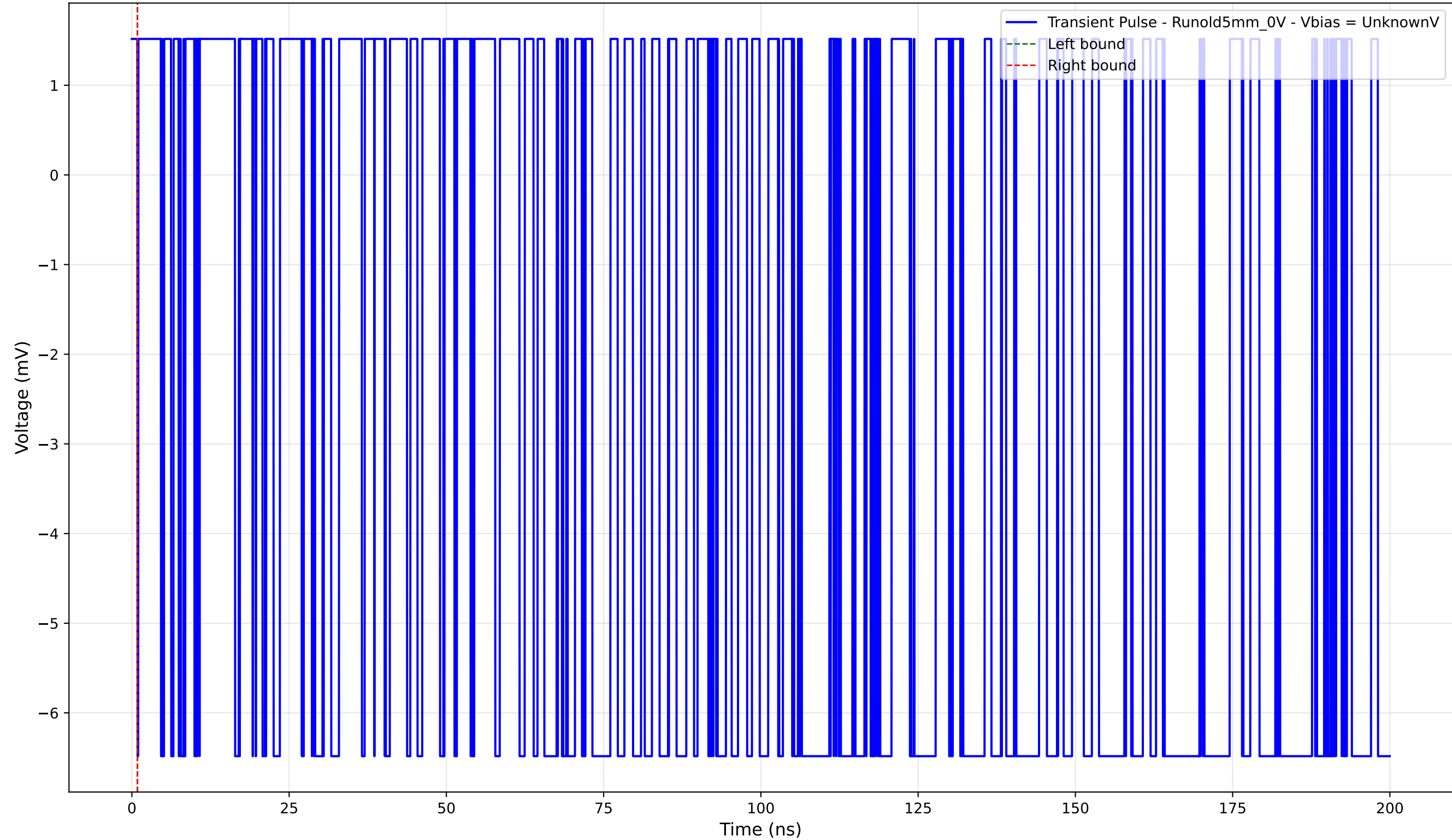
Transient Pulse - Sample: old5 - Position: 1330.0 \mu\text{m} - Charge: -0.00 pC
