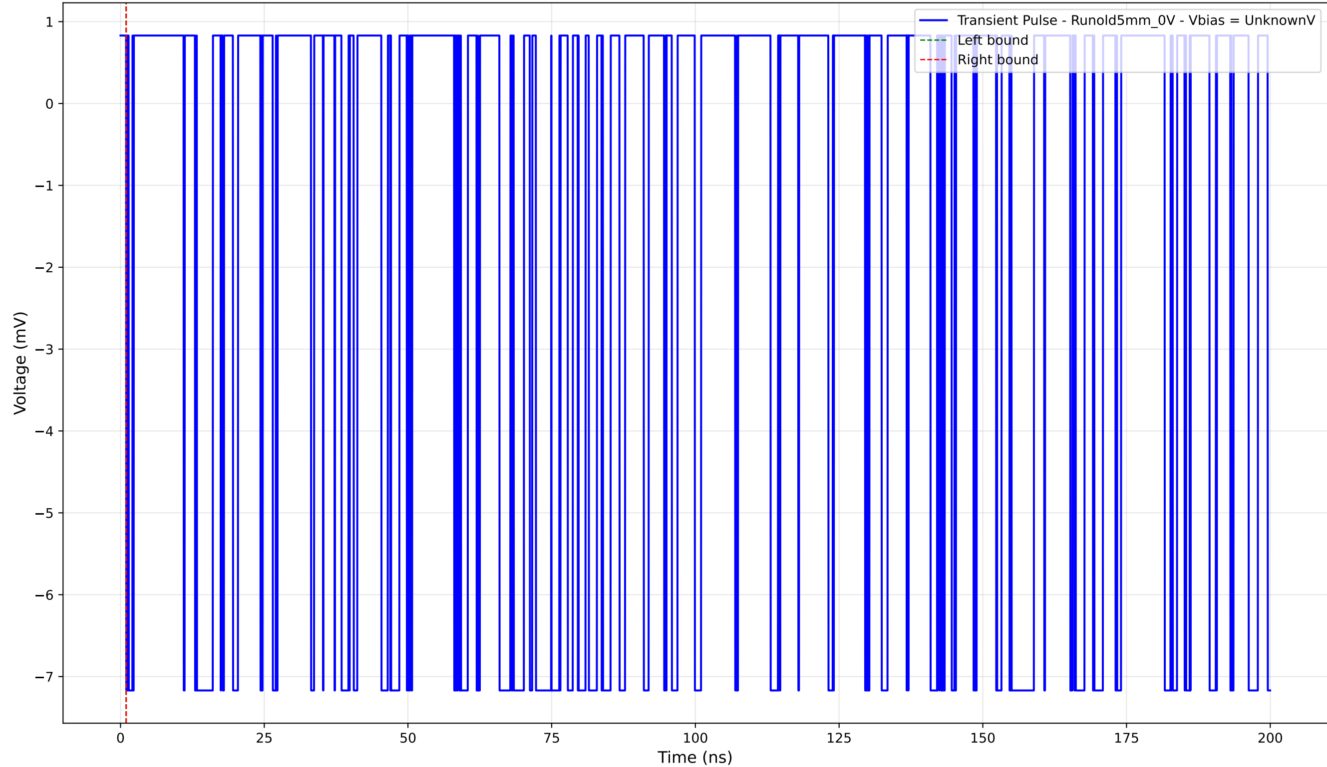
Transient Pulse - Sample: old5 - Position: 2075.0 \mu\text{m} - Charge: -0.00 pC
