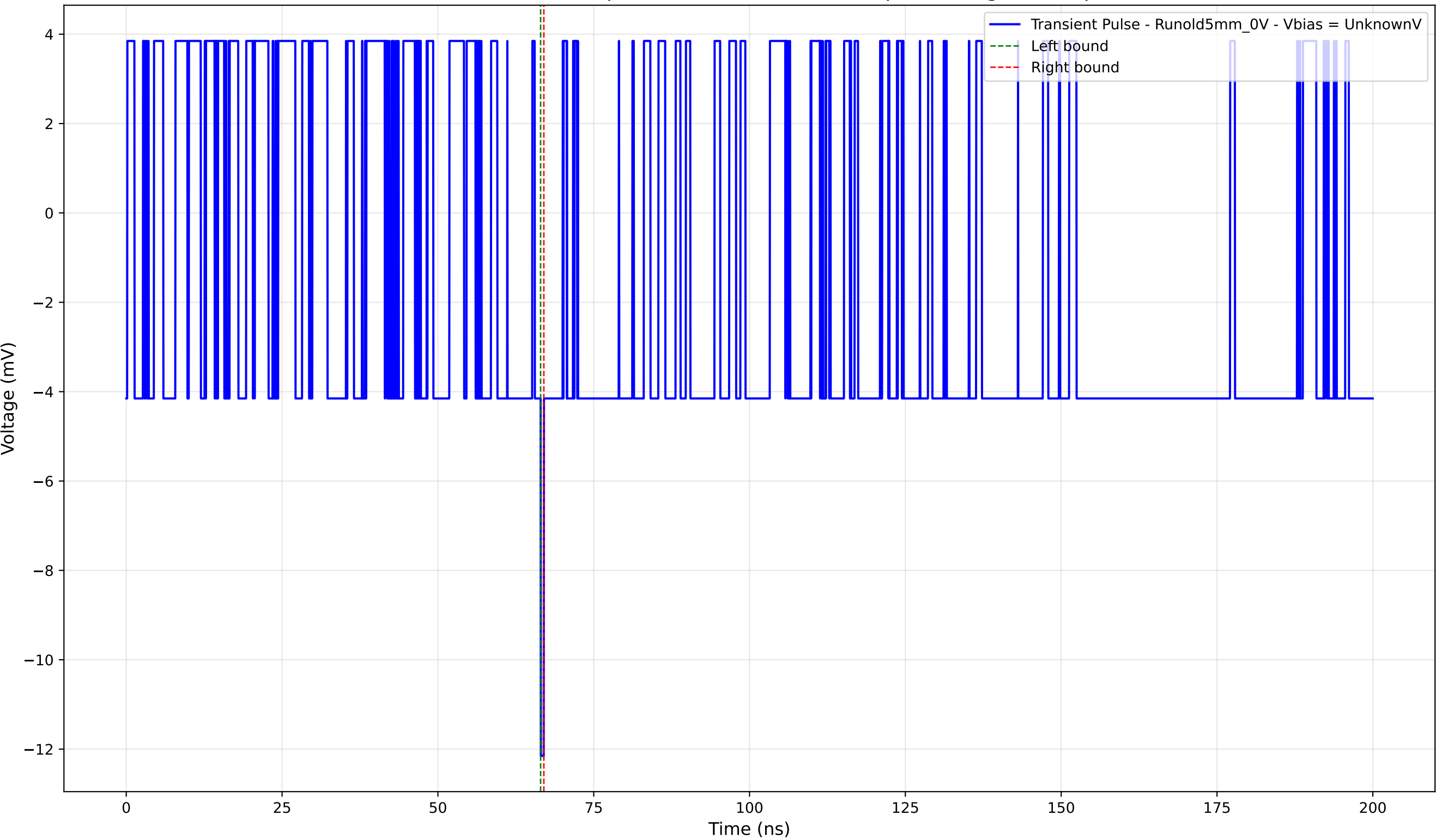
Transient Pulse - Sample: old5 - Position: 1885.0 \mu\text{m} - Charge: -0.12 pC
