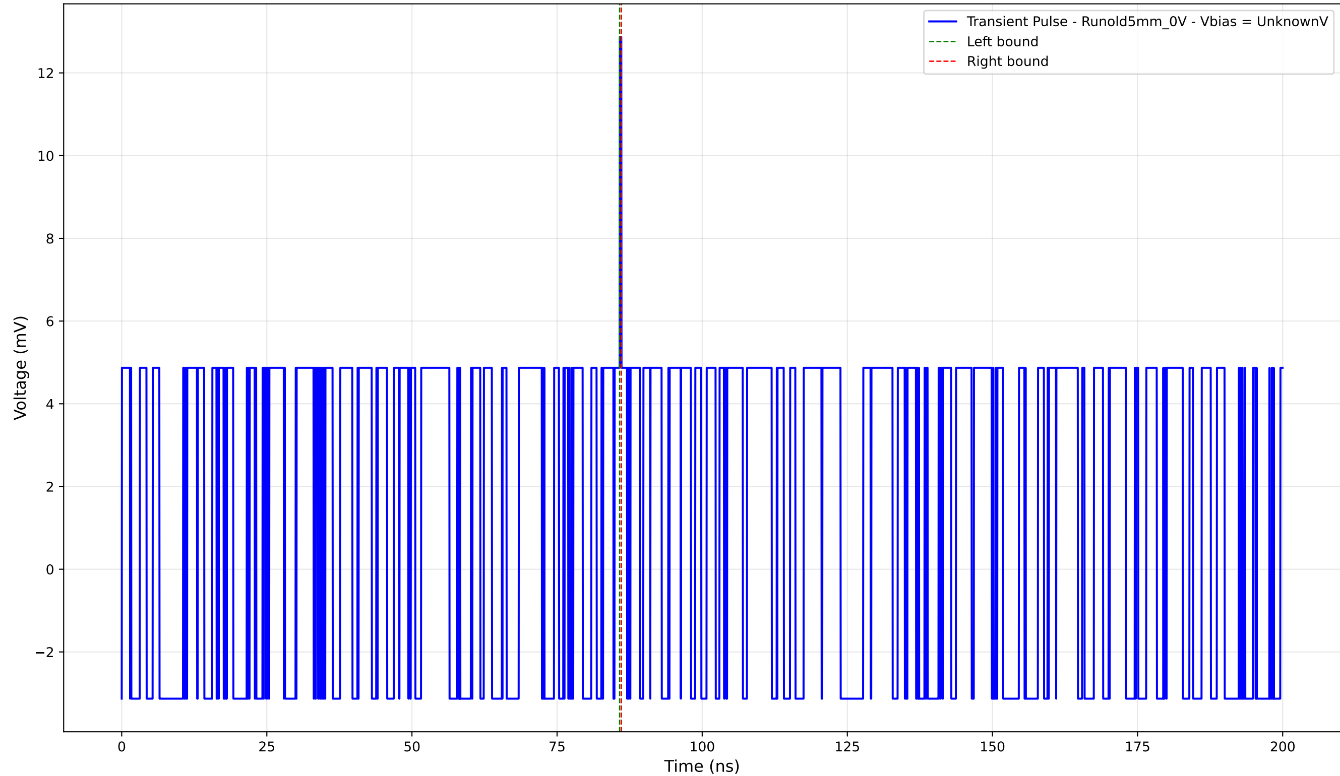
Transient Pulse - Sample: old5 - Position: 155.0 \mu\text{m} - Charge: 0.07 pC
