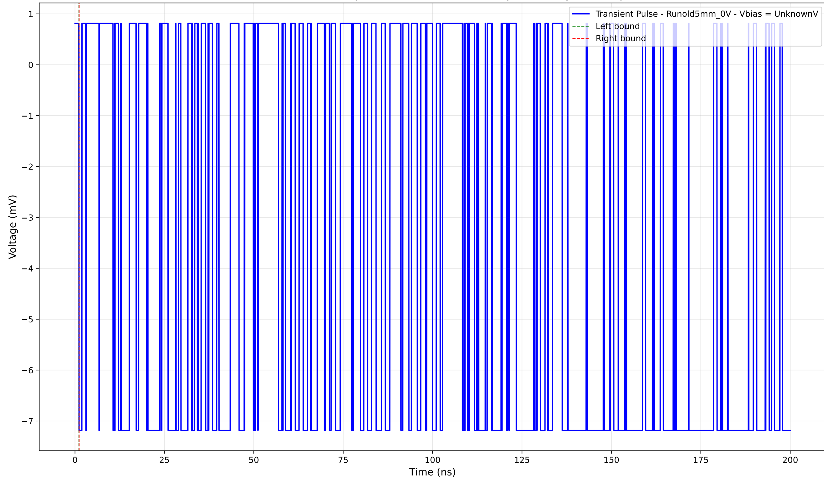
Transient Pulse - Sample: old5 - Position: 230.0 \mu\text{m} - Charge: -0.00 pC
