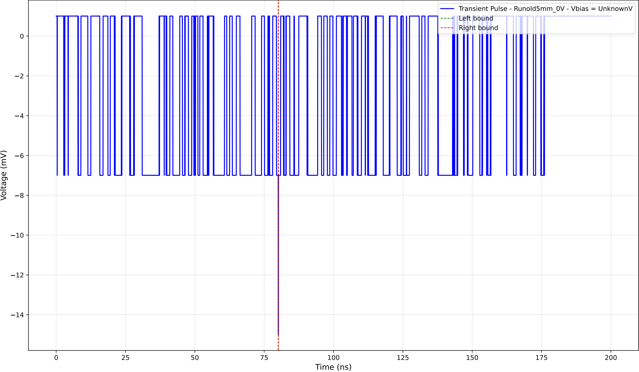
Transient Pulse - Sample: old5 - Position: 2210.0 \mu\text{m} - Charge: -0.02 pC
