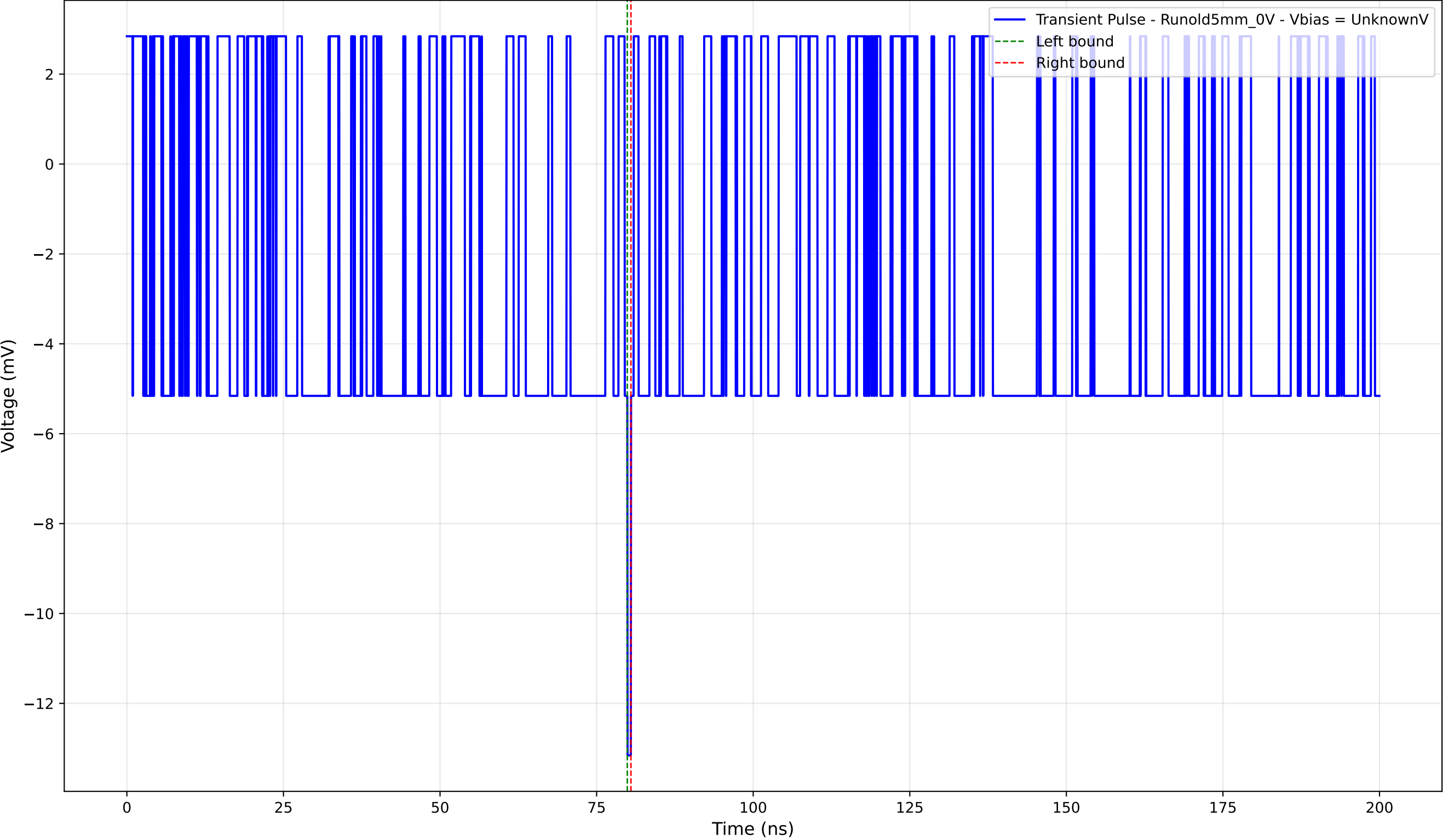
Transient Pulse - Sample: old5 - Position: 2960.0 \mu\text{m} - Charge: -0.15 pC
