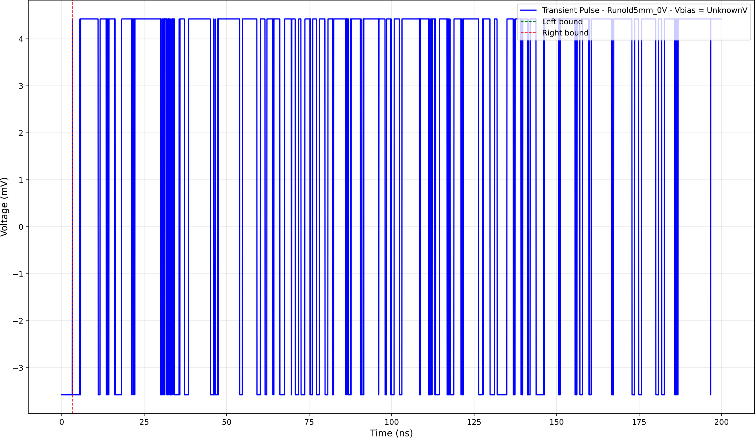
Transient Pulse - Sample: old5 - Position: 2295.0 \mu\text{m} - Charge: 0.00 pC
