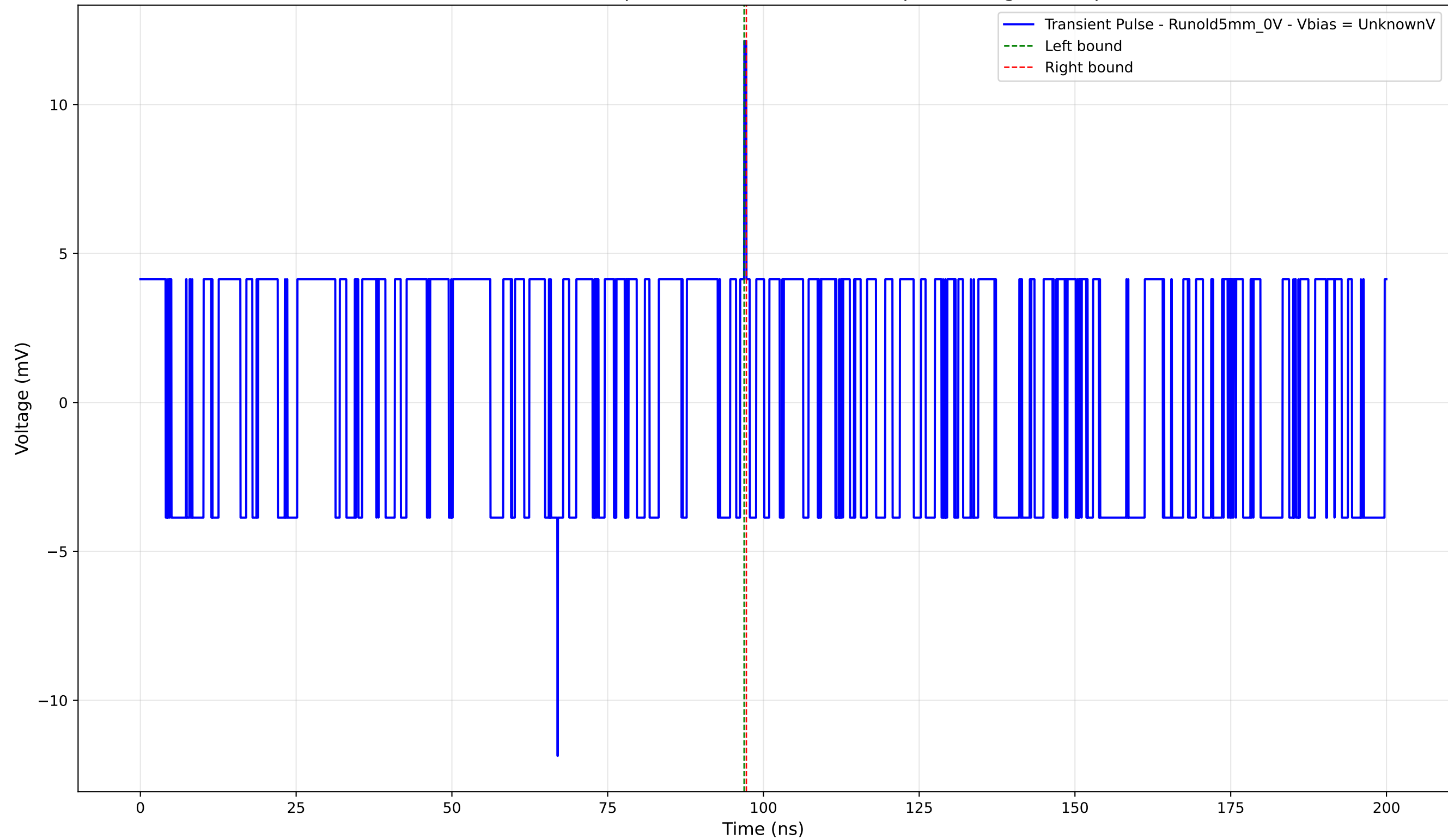
Transient Pulse - Sample: old5 - Position: 2595.0 \mu\text{m} - Charge: 0.08 pC
