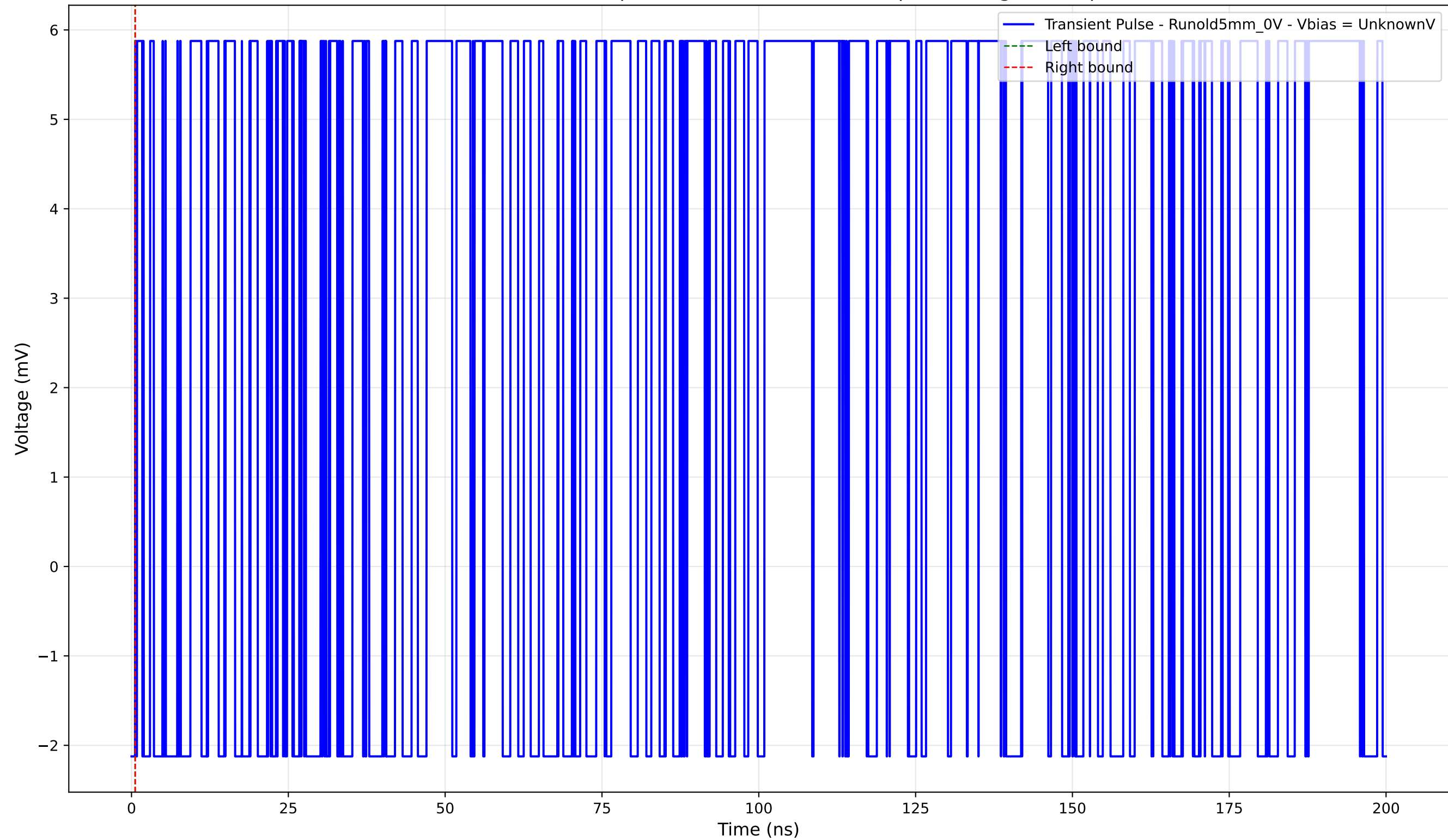
Transient Pulse - Sample: old5 - Position: 2820.0 \mu\text{m} - Charge: 0.00 pC
