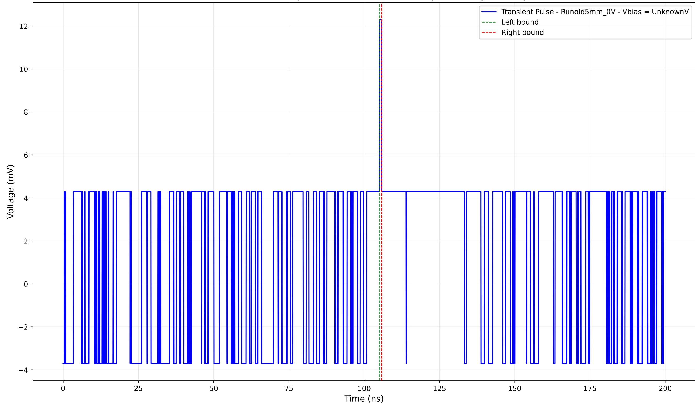
Transient Pulse - Sample: old5 - Position: 3760.0 \mu\text{m} - Charge: 0.19 pC
