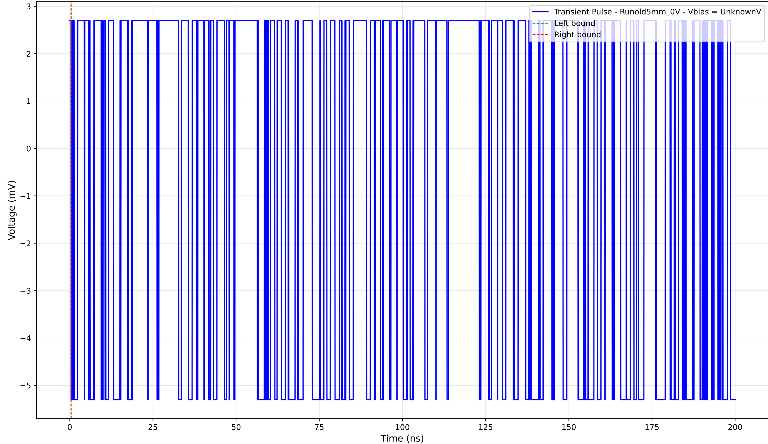
Transient Pulse - Sample: old5 - Position: 1215.0 \mu\text{m} - Charge: -0.00 pC
