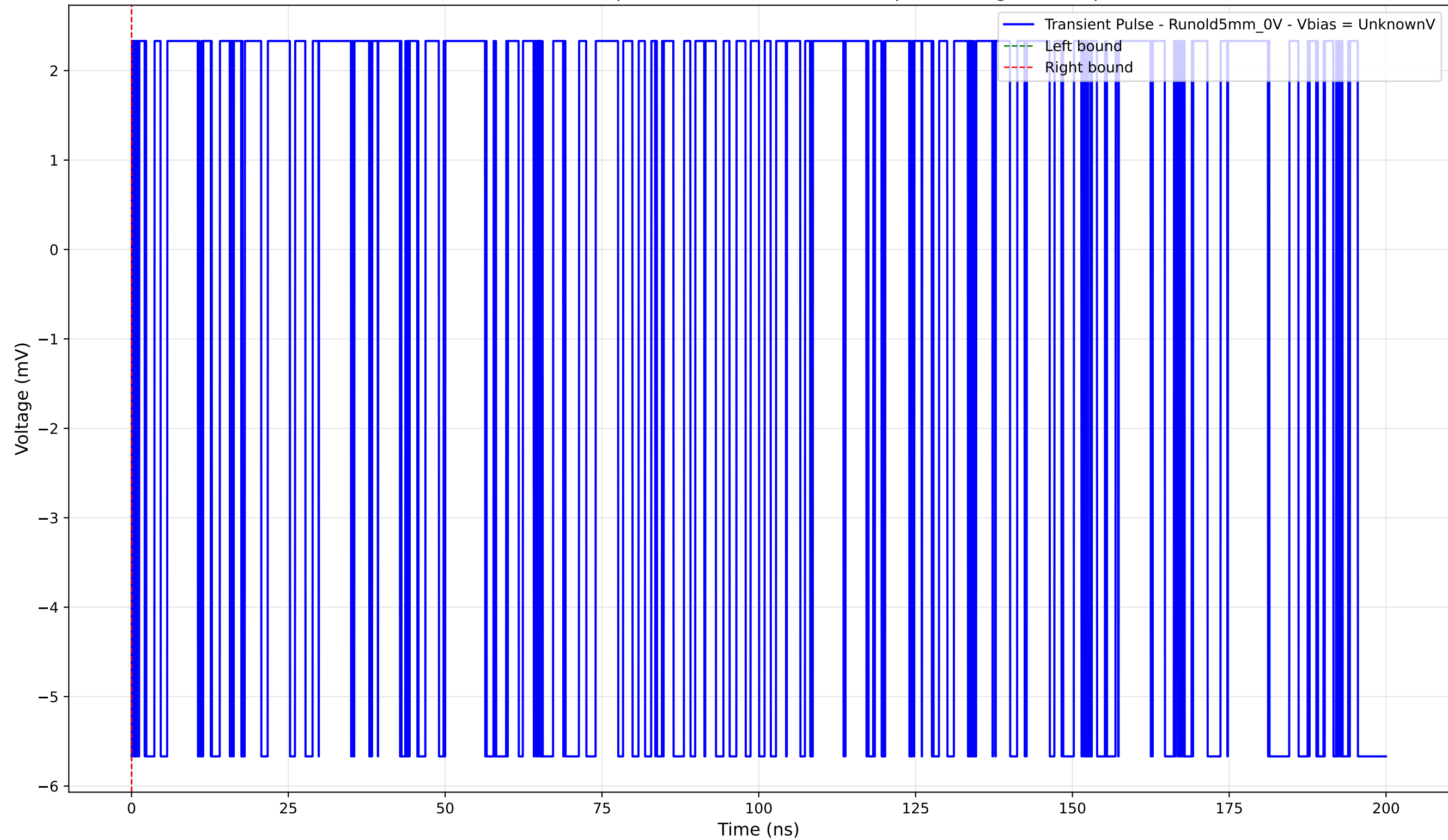
Transient Pulse - Sample: old5 - Position: 2350.0 \mu\text{m} - Charge: -0.00 pC
