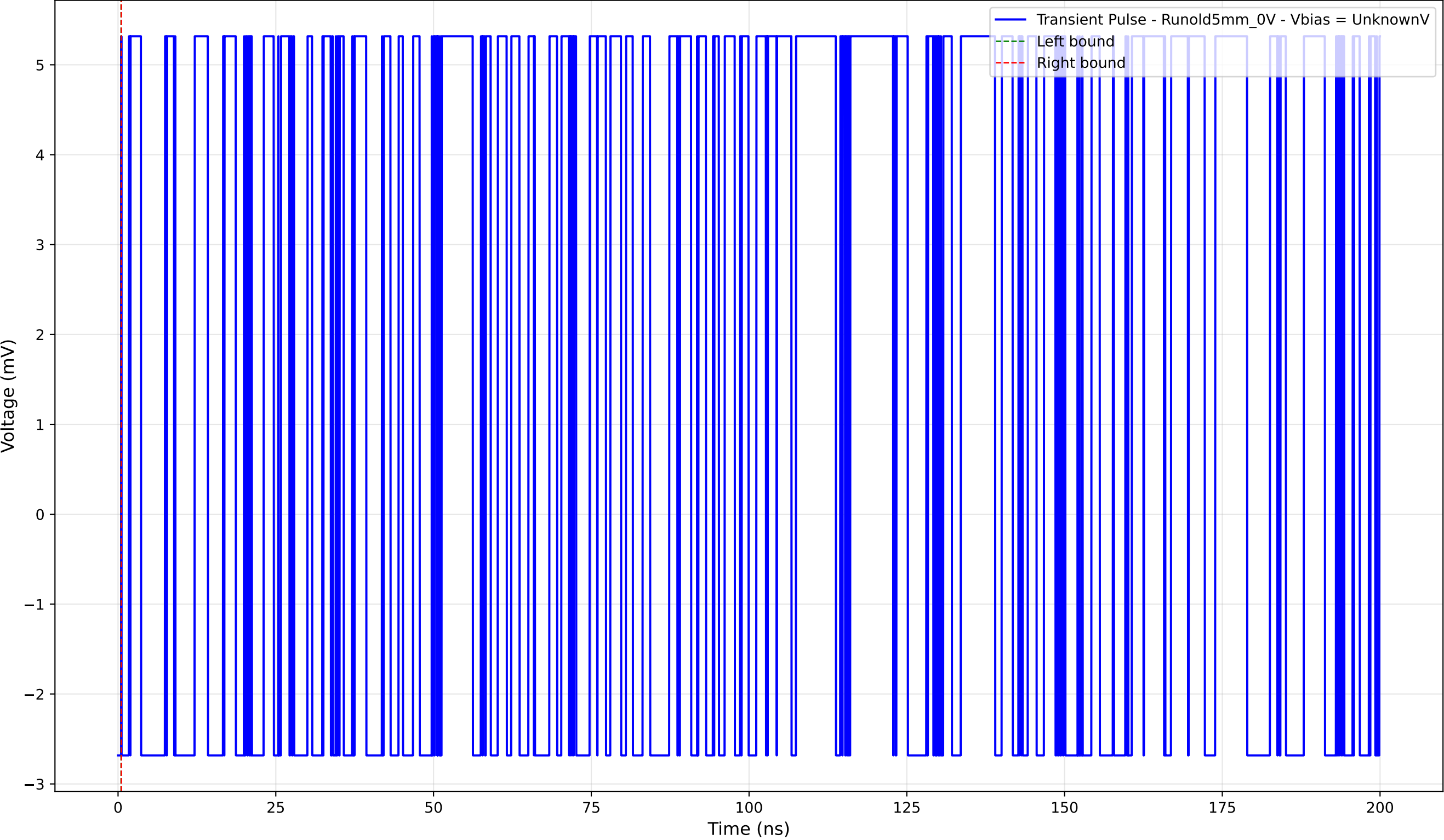
Transient Pulse - Sample: old5 - Position: 1810.0 \mu\text{m} - Charge: 0.00 pC
