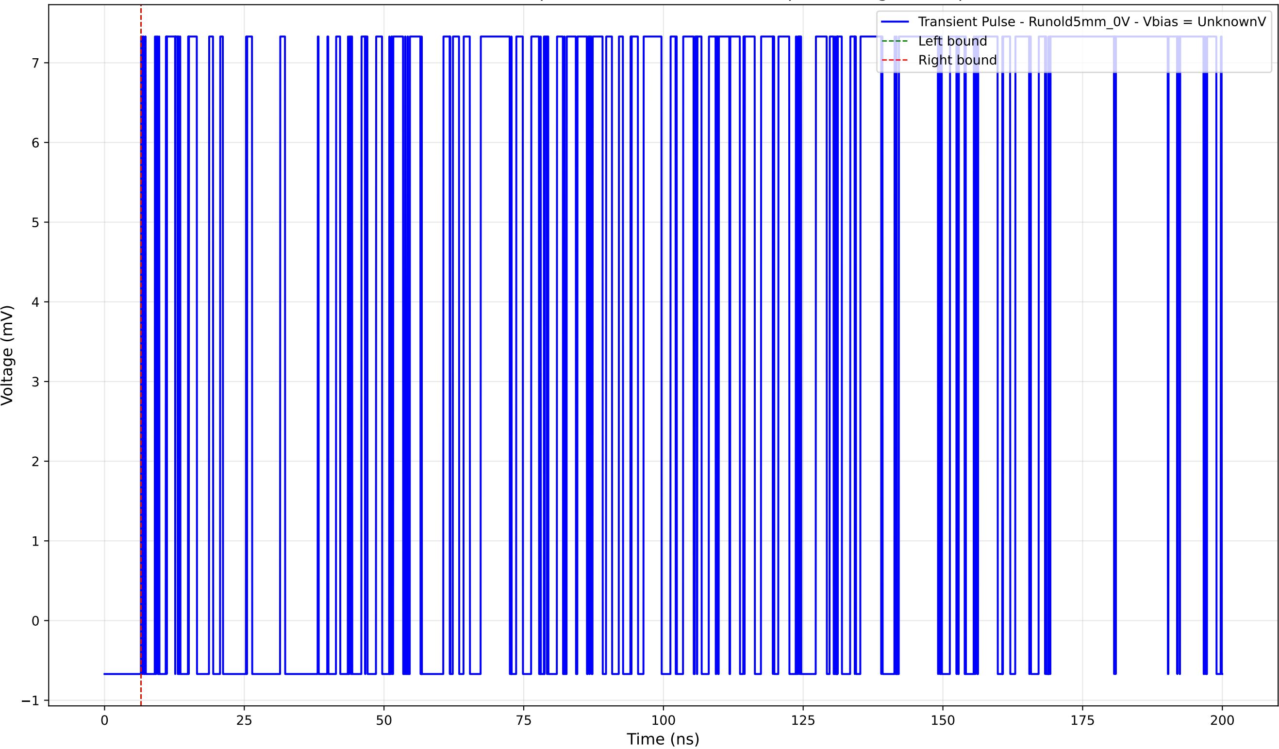
Transient Pulse - Sample: old5 - Position: 4495.0 \mu\text{m} - Charge: 0.00 pC
