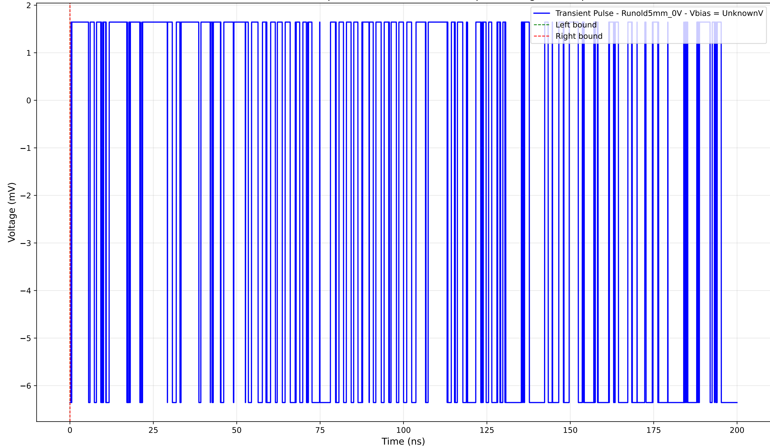
Transient Pulse - Sample: old5 - Position: 3980.0 \mu\text{m} - Charge: -0.00 pC
