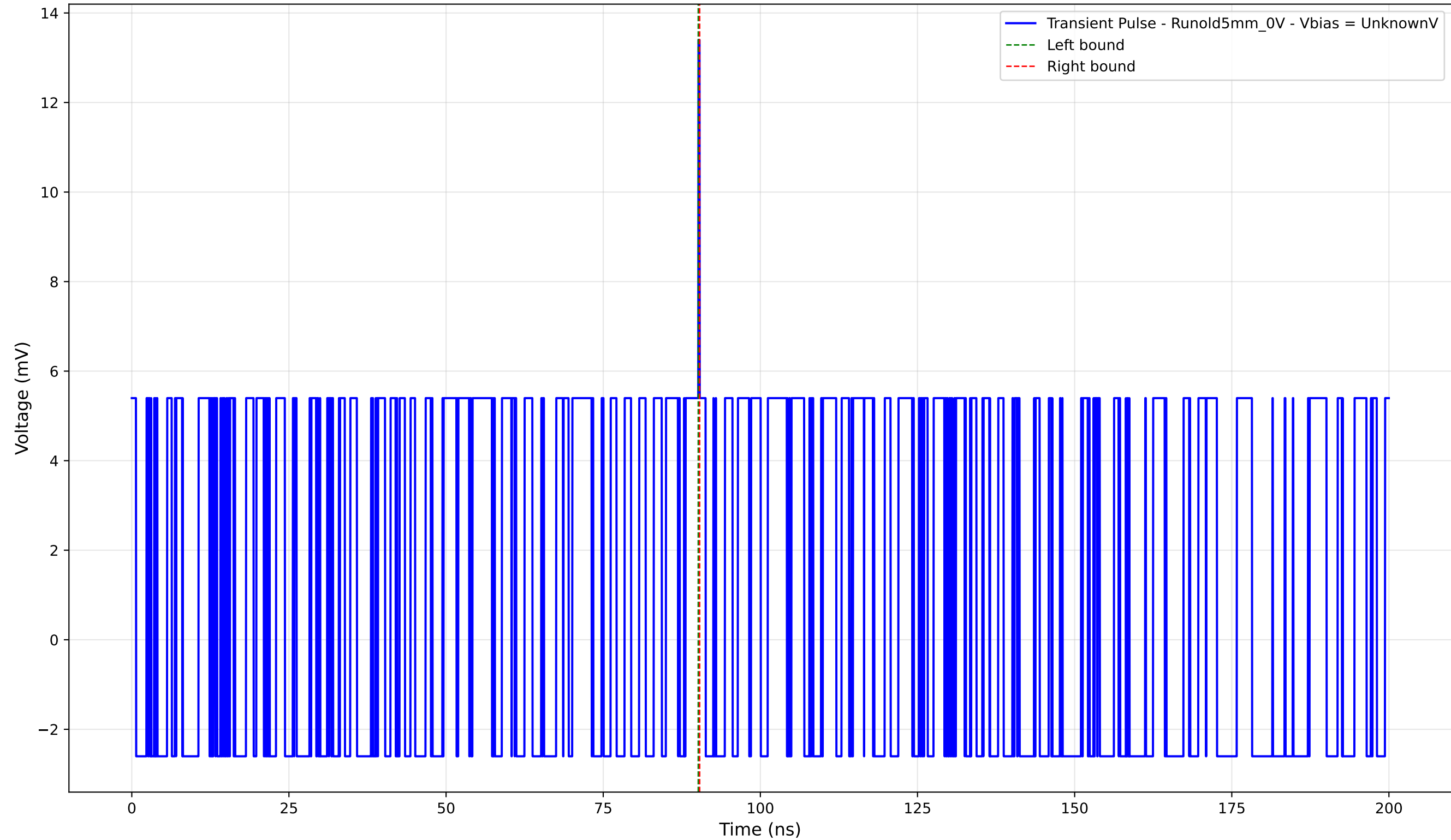
Transient Pulse - Sample: old5 - Position: 3185.0 \mu\text{m} - Charge: 0.06 pC
