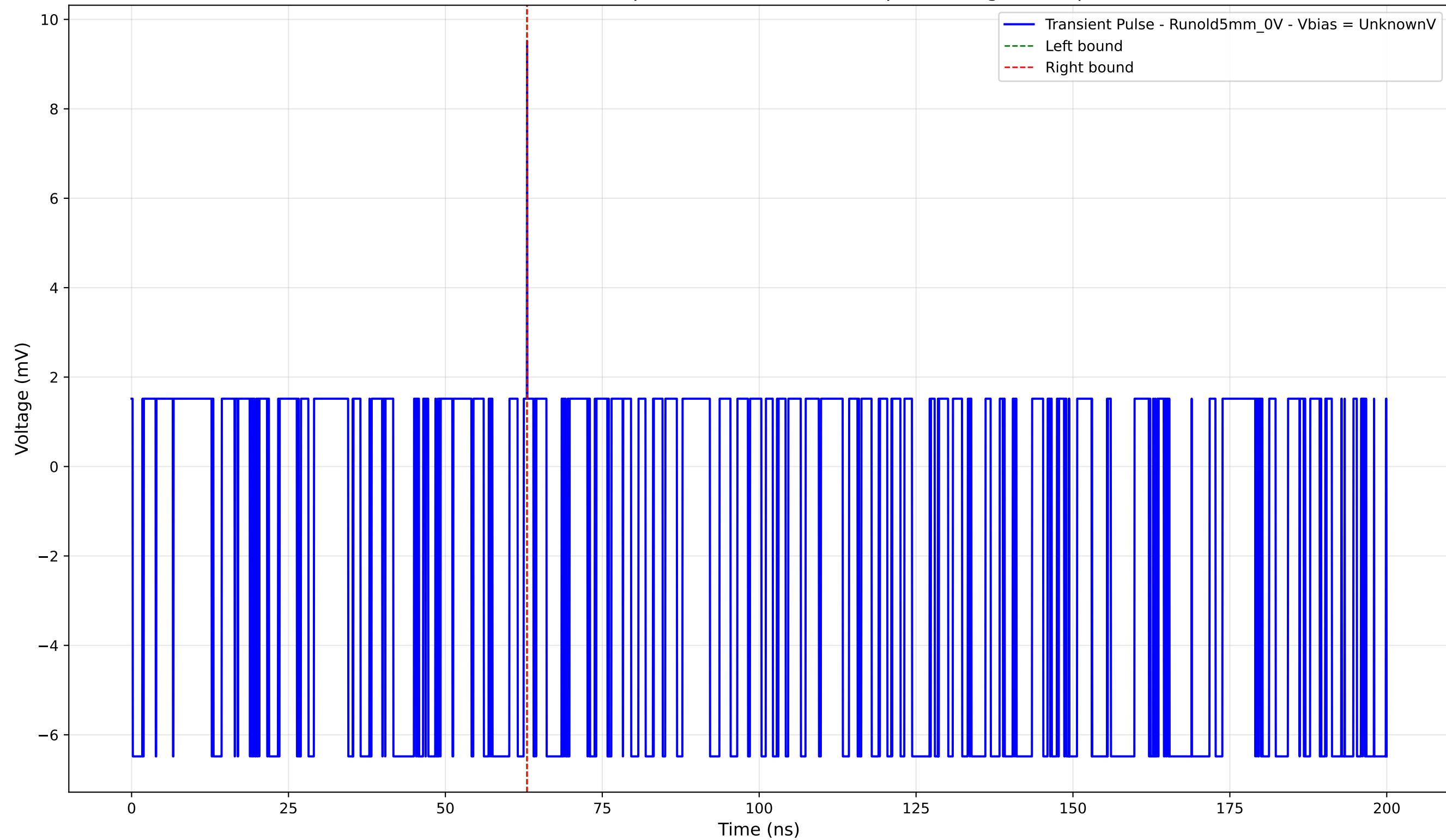
Transient Pulse - Sample: old5 - Position: 10.0 \mu\text{m} - Charge: 0.01 pC
