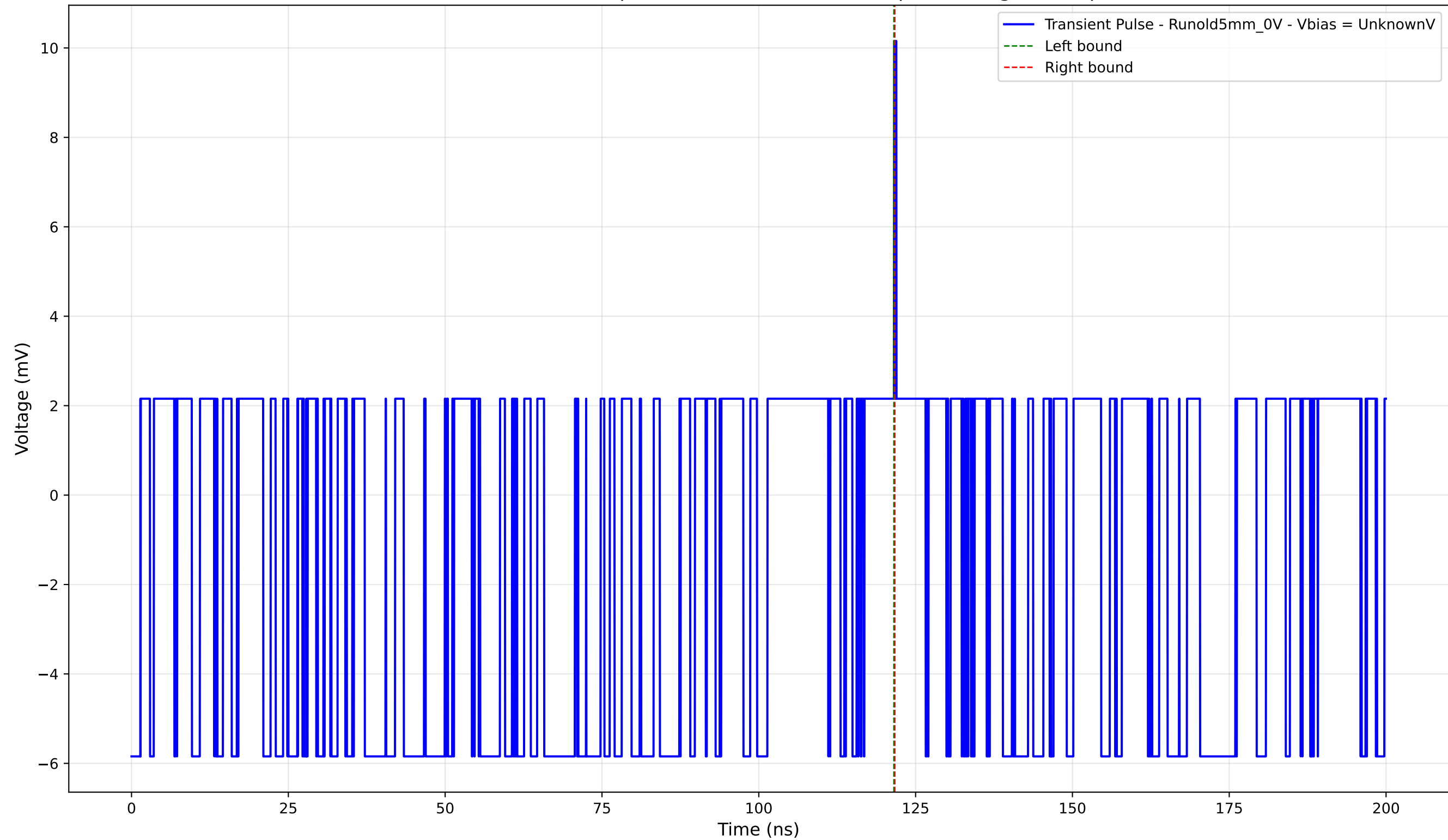
Transient Pulse - Sample: old5 - Position: 2765.0 \mu\text{m} - Charge: 0.03 pC
