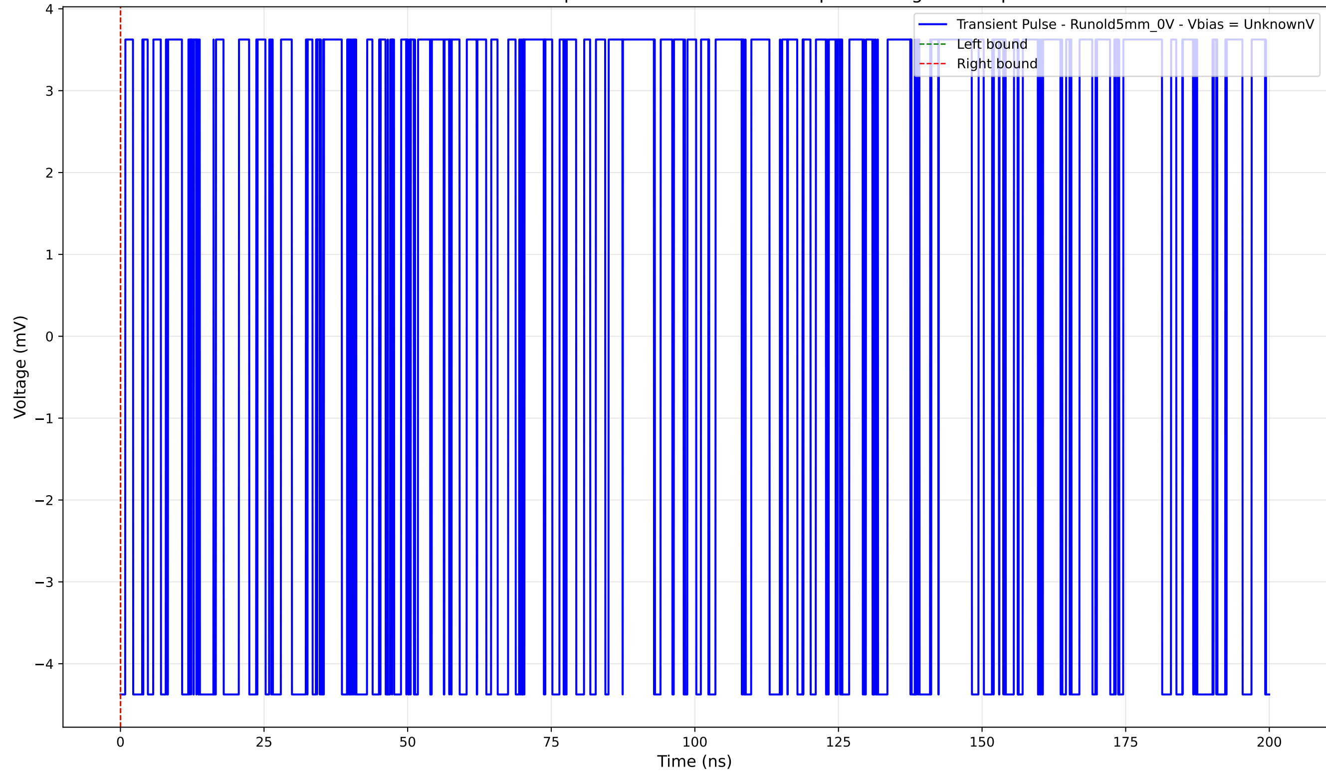
Transient Pulse - Sample: old5 - Position: 2425.0 \mu\text{m} - Charge: -0.00 pC
