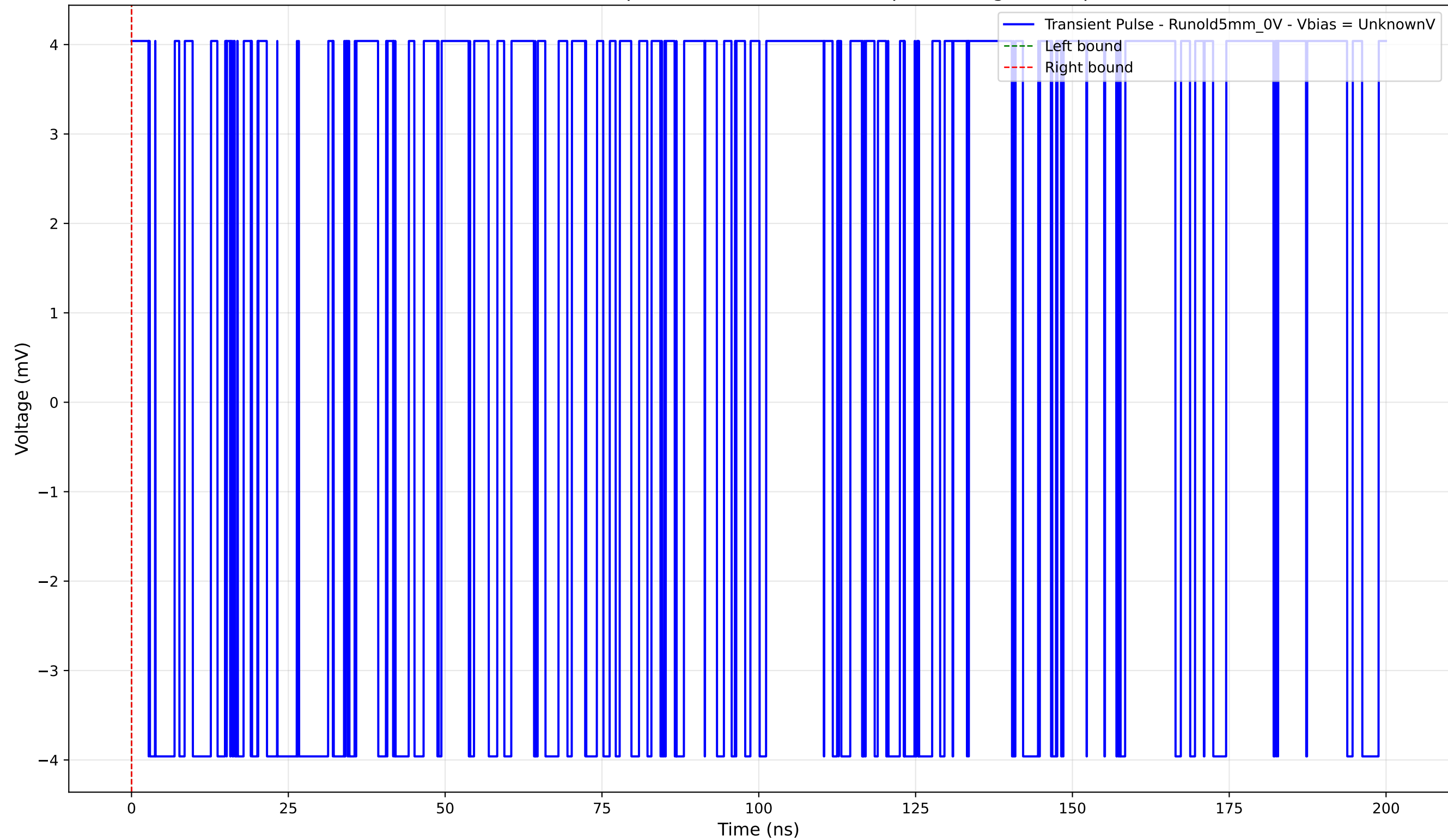
Transient Pulse - Sample: old5 - Position: 205.0 \mu\text{m} - Charge: 0.00 pC
