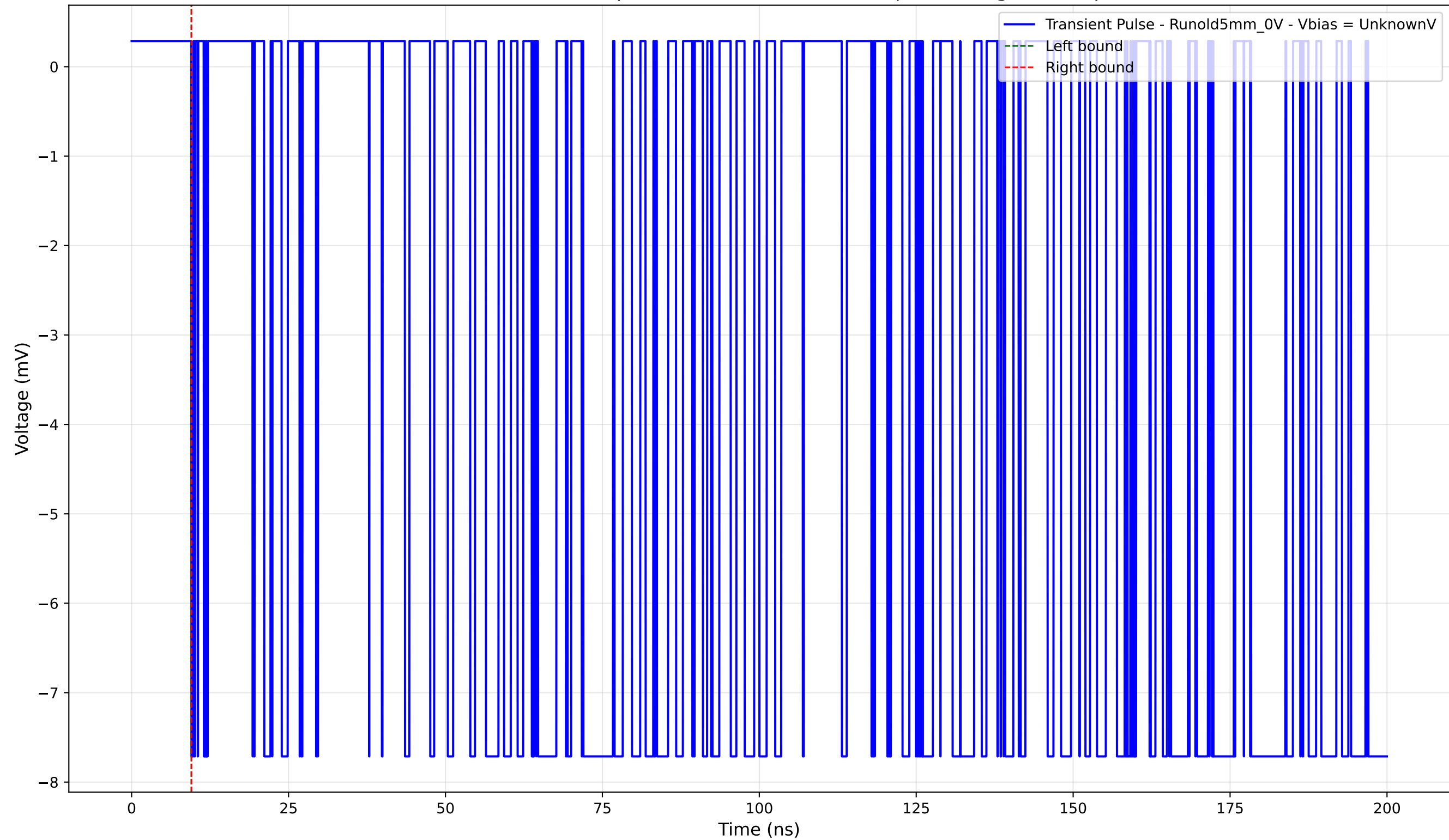
Transient Pulse - Sample: old5 - Position: 2655.0 \mu\text{m} - Charge: -0.00 pC
