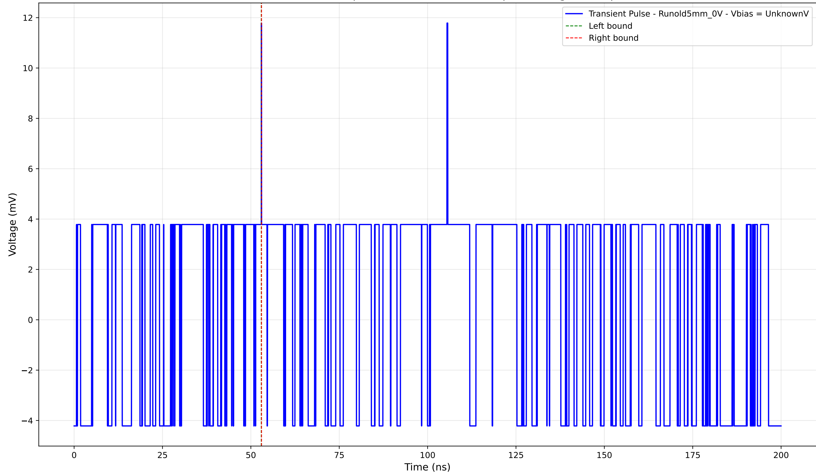
Transient Pulse - Sample: old5 - Position: 775.0 \mu\text{m} - Charge: 0.02 pC
