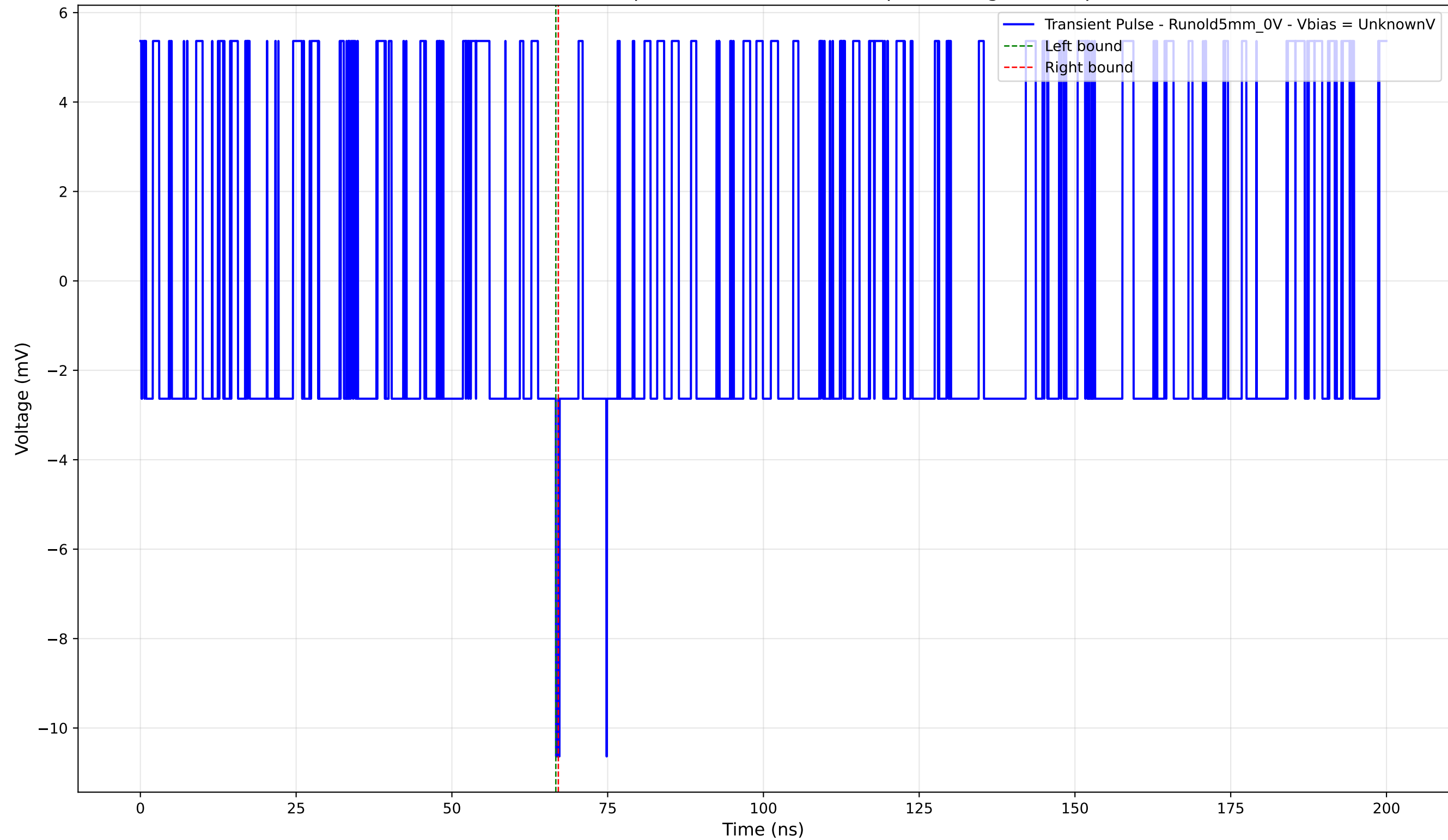
Transient Pulse - Sample: old5 - Position: 90.0 \mu\text{m} - Charge: -0.08 pC
