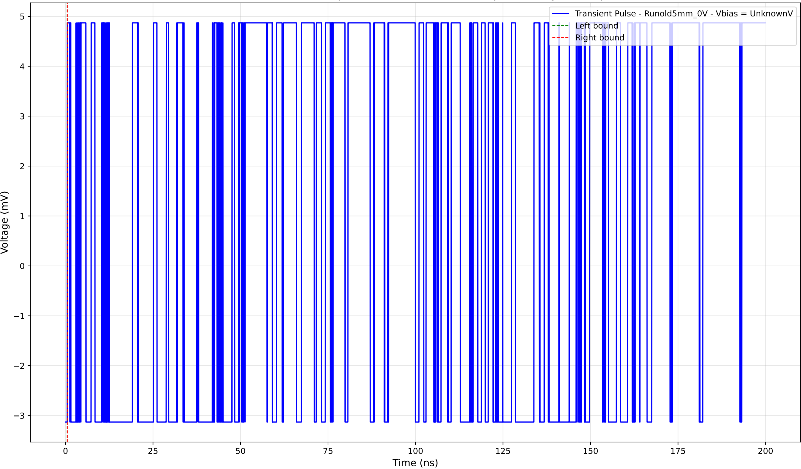
Transient Pulse - Sample: old5 - Position: 1510.0 \mu\text{m} - Charge: 0.00 pC
