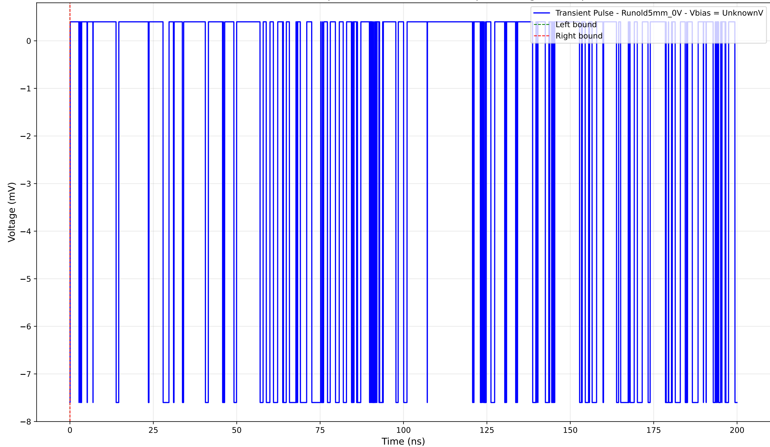
Transient Pulse - Sample: old5 - Position: 1705.0 \mu\text{m} - Charge: -0.00 pC
