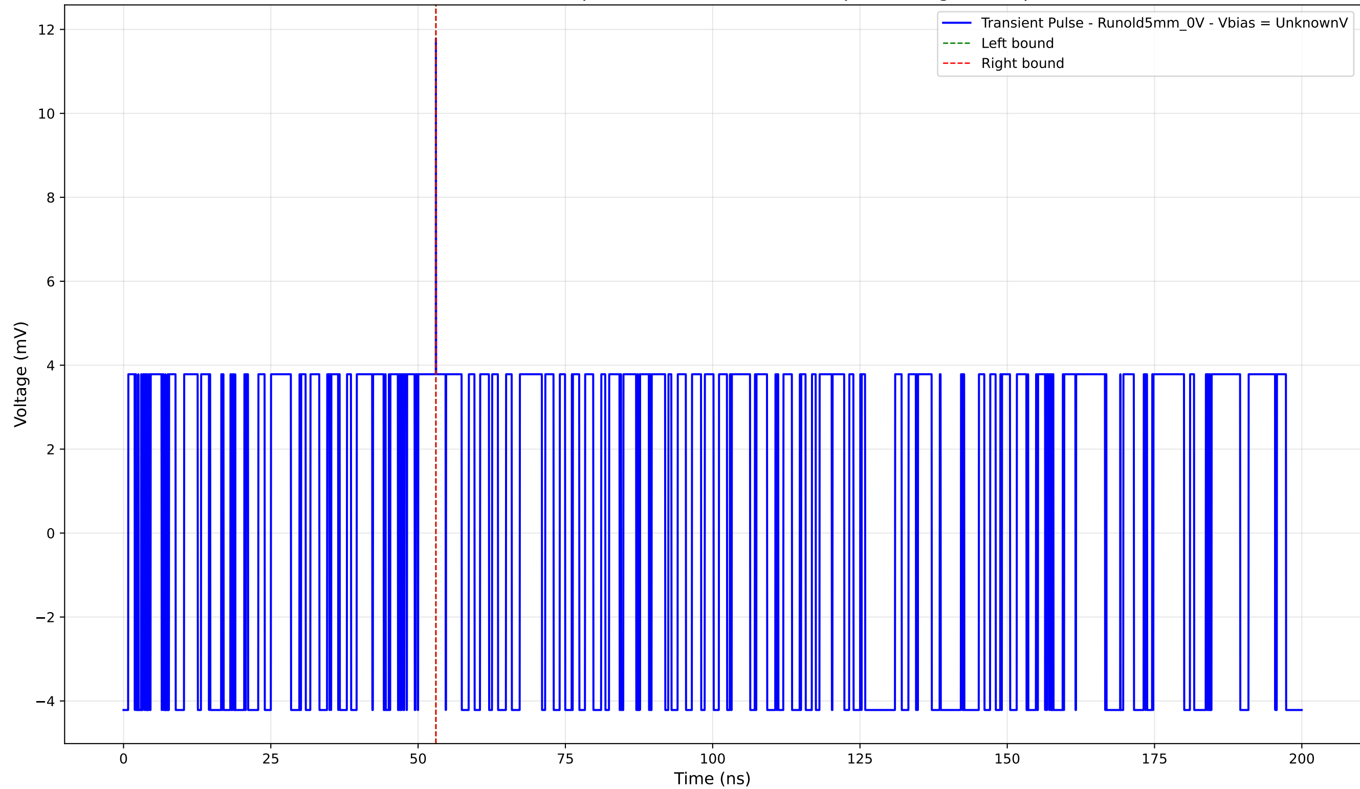
Transient Pulse - Sample: old5 - Position: 3835.0 \mu\text{m} - Charge: 0.01 pC
