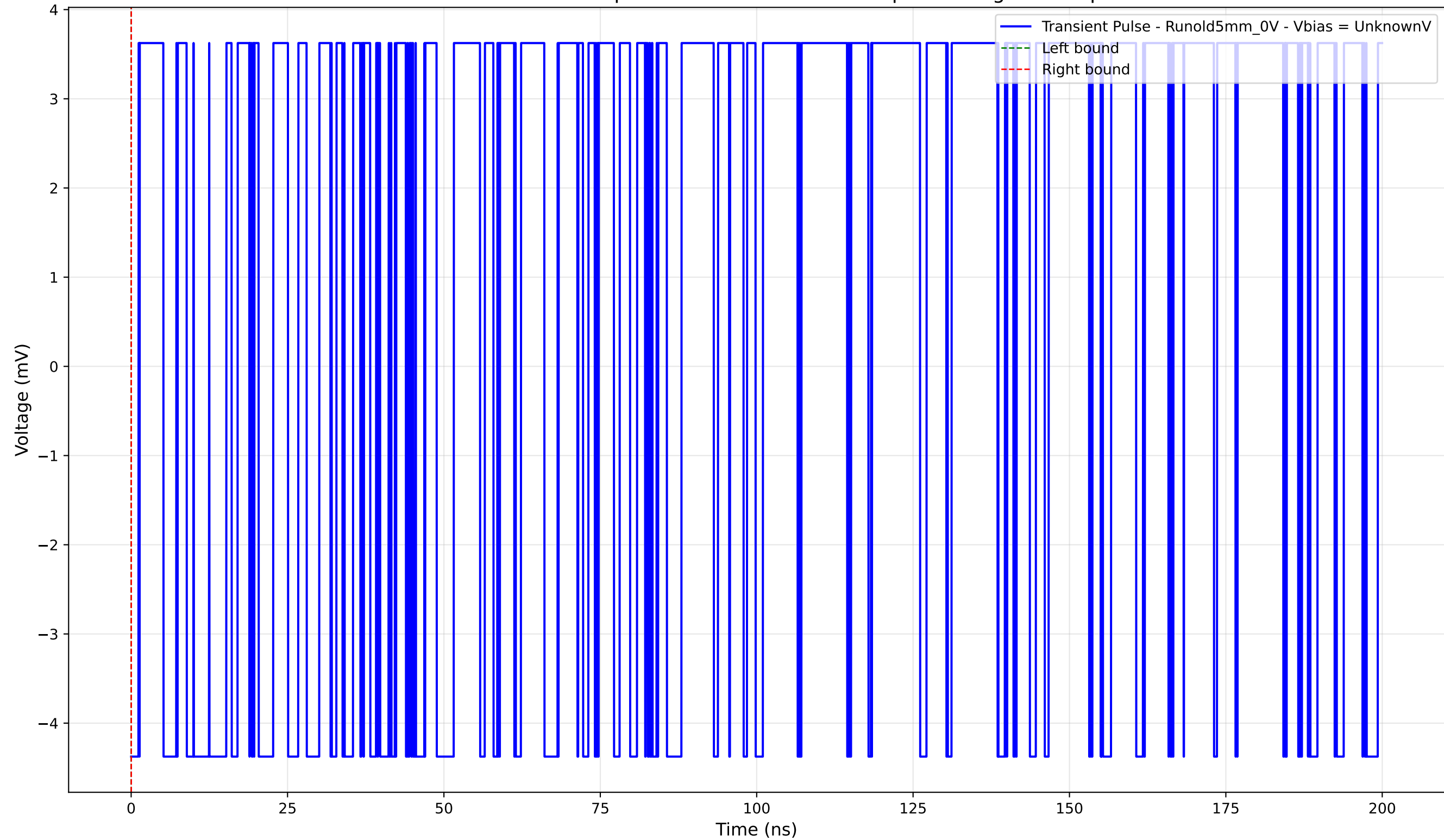
Transient Pulse - Sample: old5 - Position: 4645.0 \mu\text{m} - Charge: -0.00 pC
