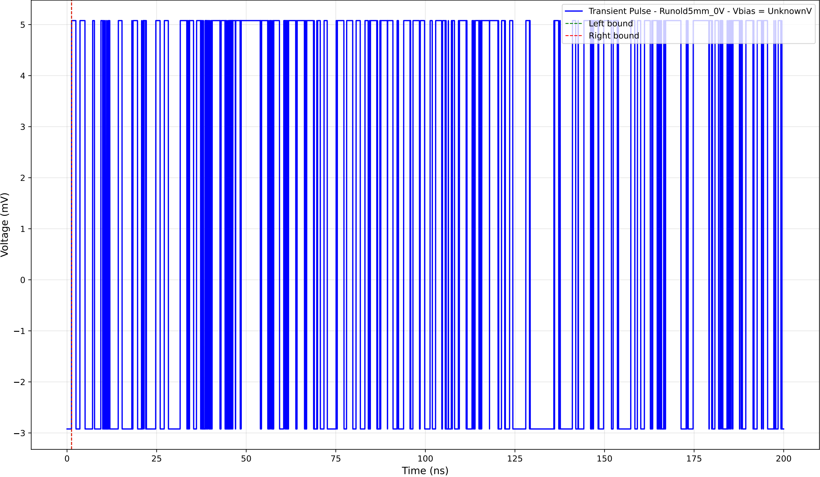
Transient Pulse - Sample: old5 - Position: 1385.0 \mu\text{m} - Charge: 0.00 pC
