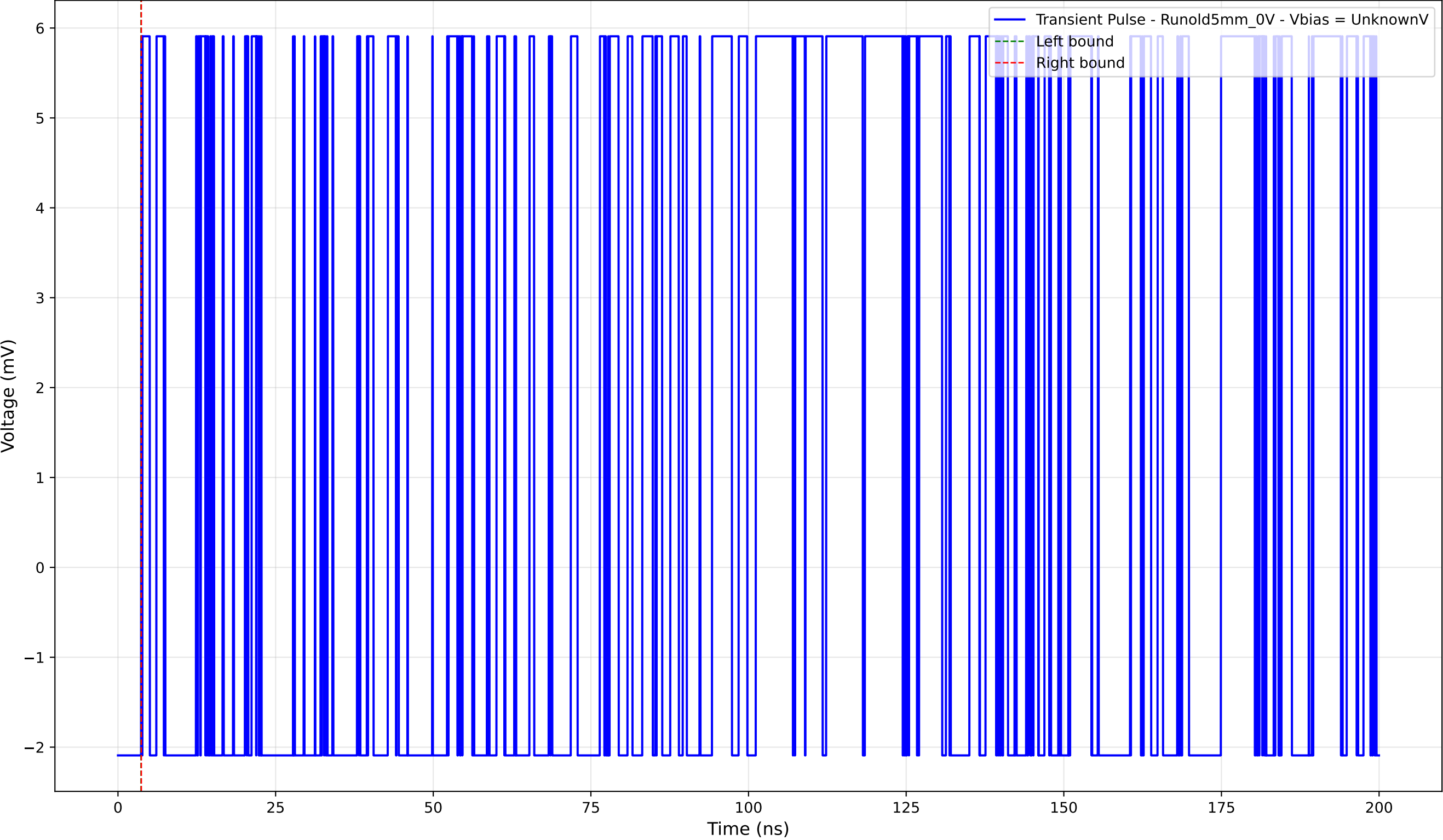
Transient Pulse - Sample: old5 - Position: 2435.0 \mu\text{m} - Charge: 0.00 pC
