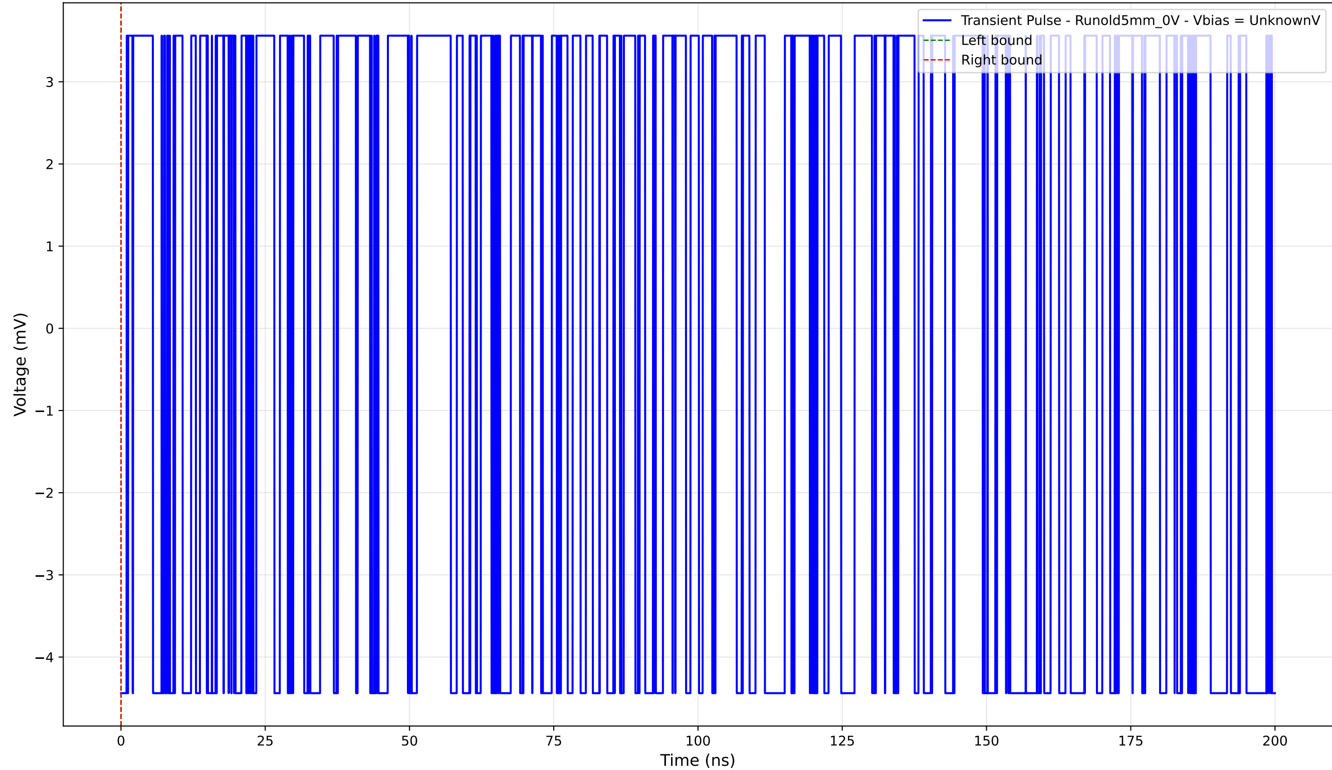
Transient Pulse - Sample: old5 - Position: 4845.0 \mu\text{m} - Charge: -0.00 pC
