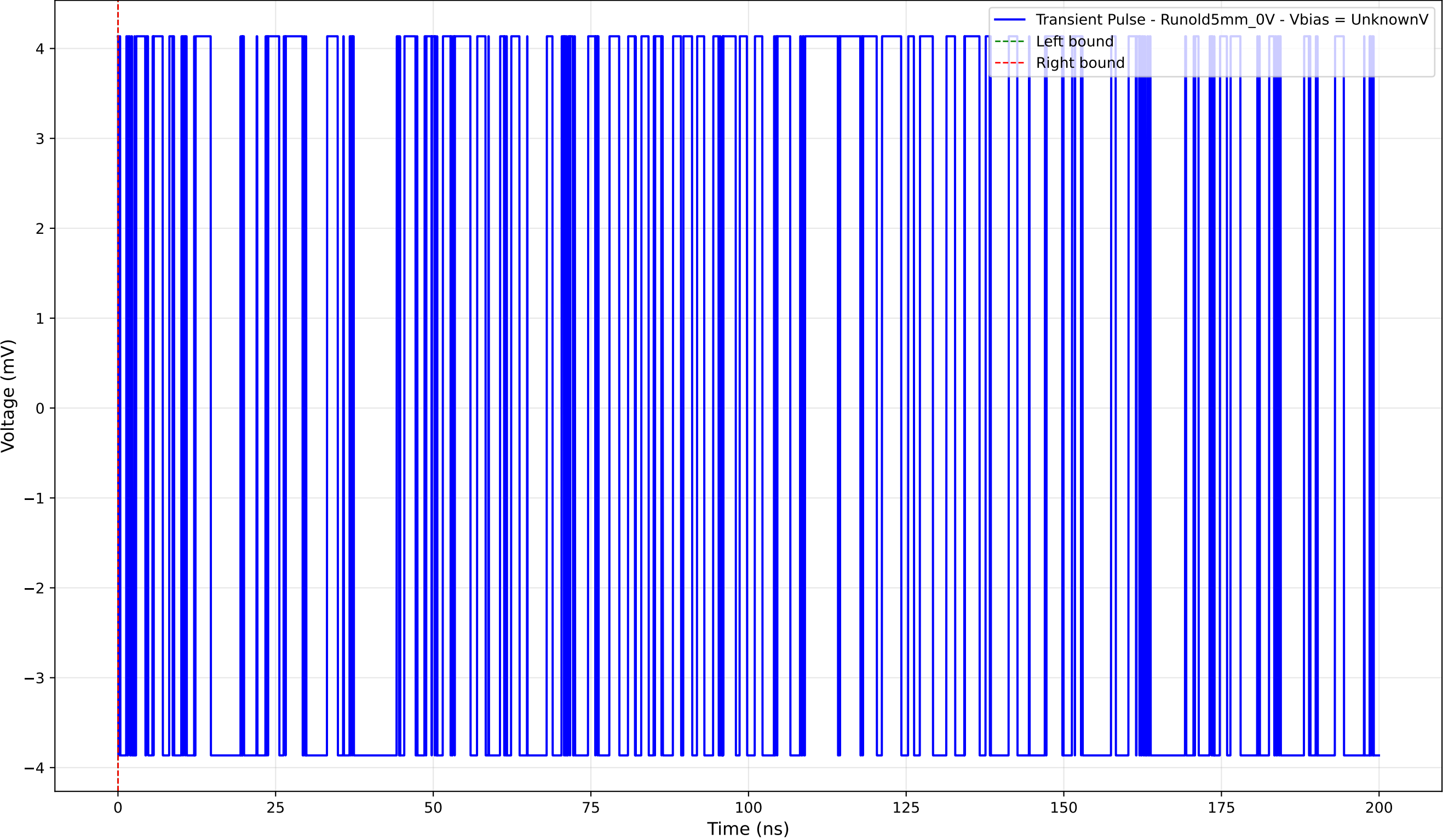
Transient Pulse - Sample: old5 - Position: 4820.0 \mu\text{m} - Charge: 0.00 pC
