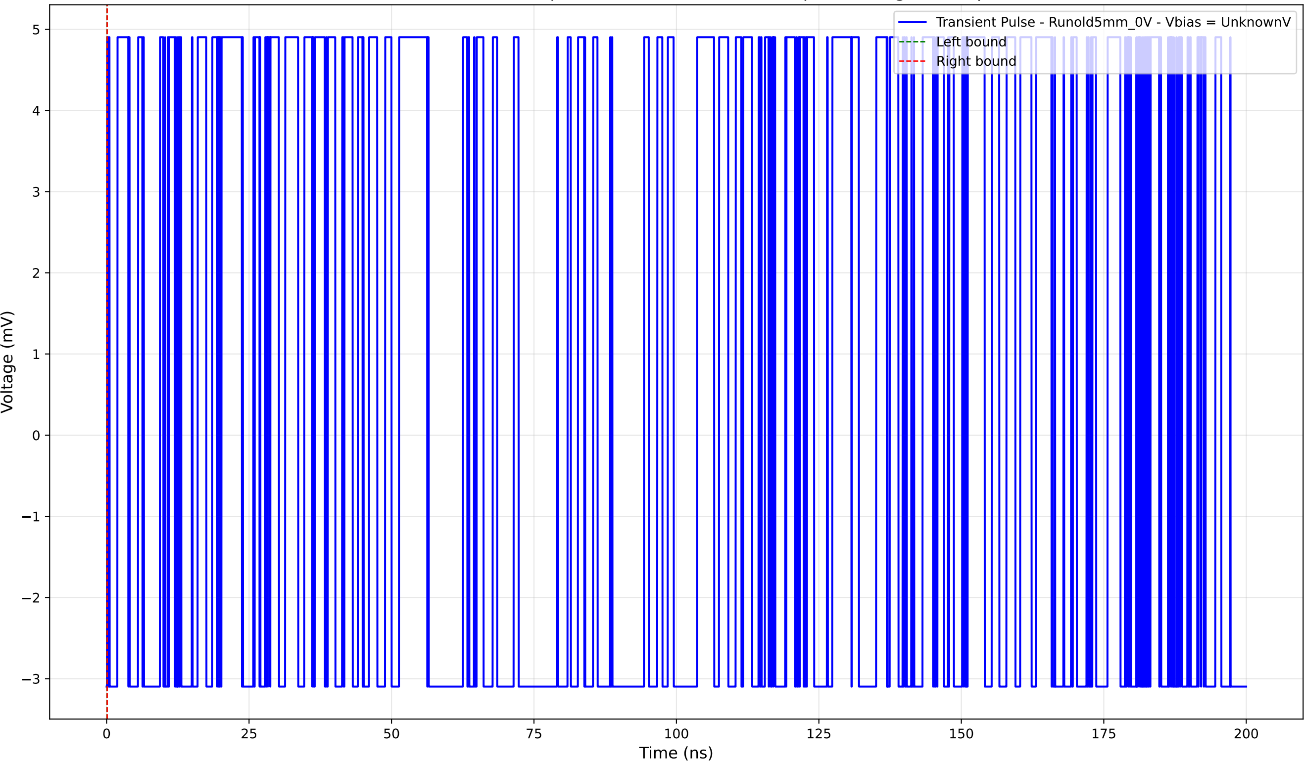
Transient Pulse - Sample: old5 - Position: 4265.0 \mu\text{m} - Charge: 0.00 pC
