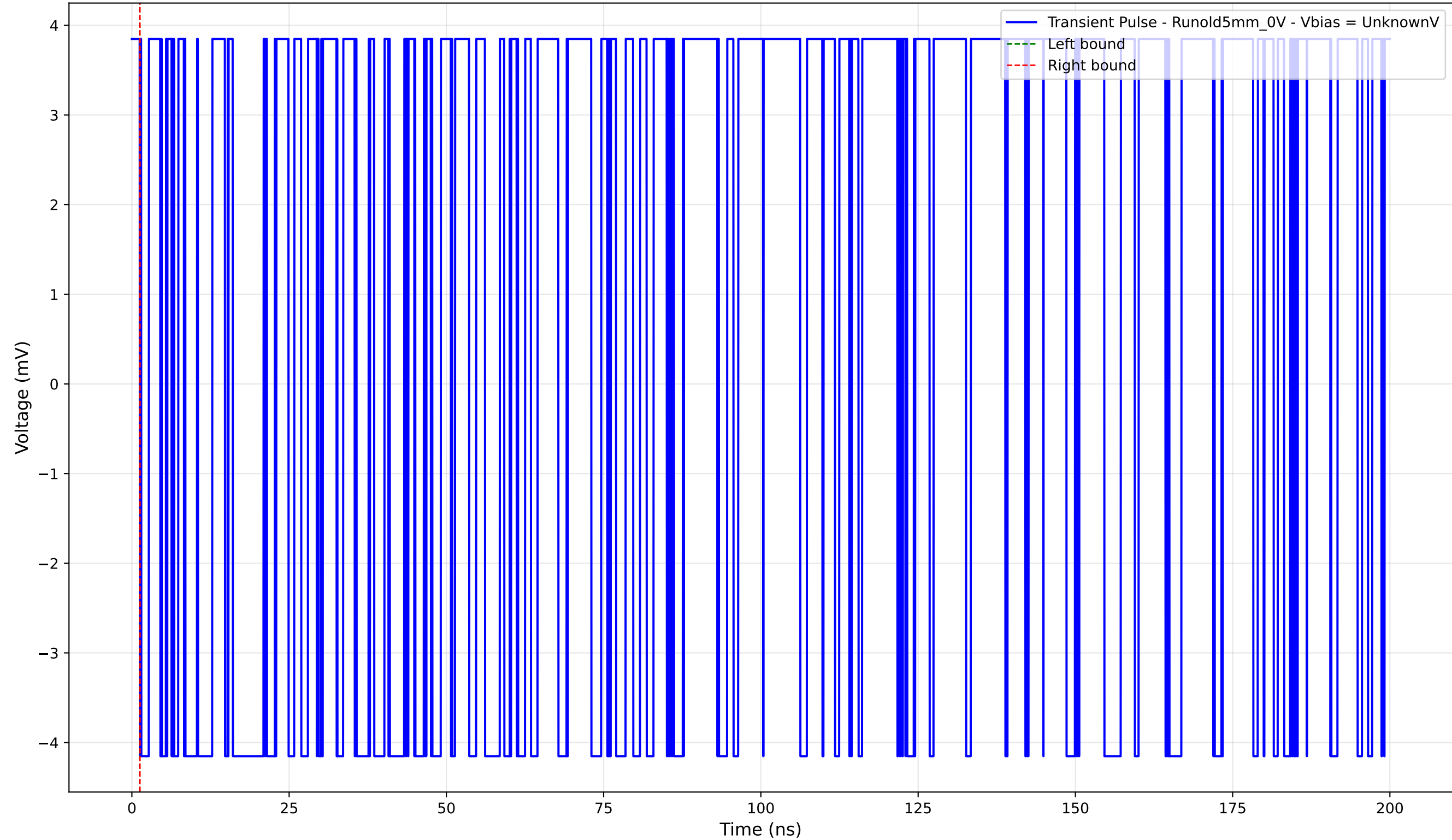
Transient Pulse - Sample: old5 - Position: 3900.0 \mu\text{m} - Charge: -0.00 pC
