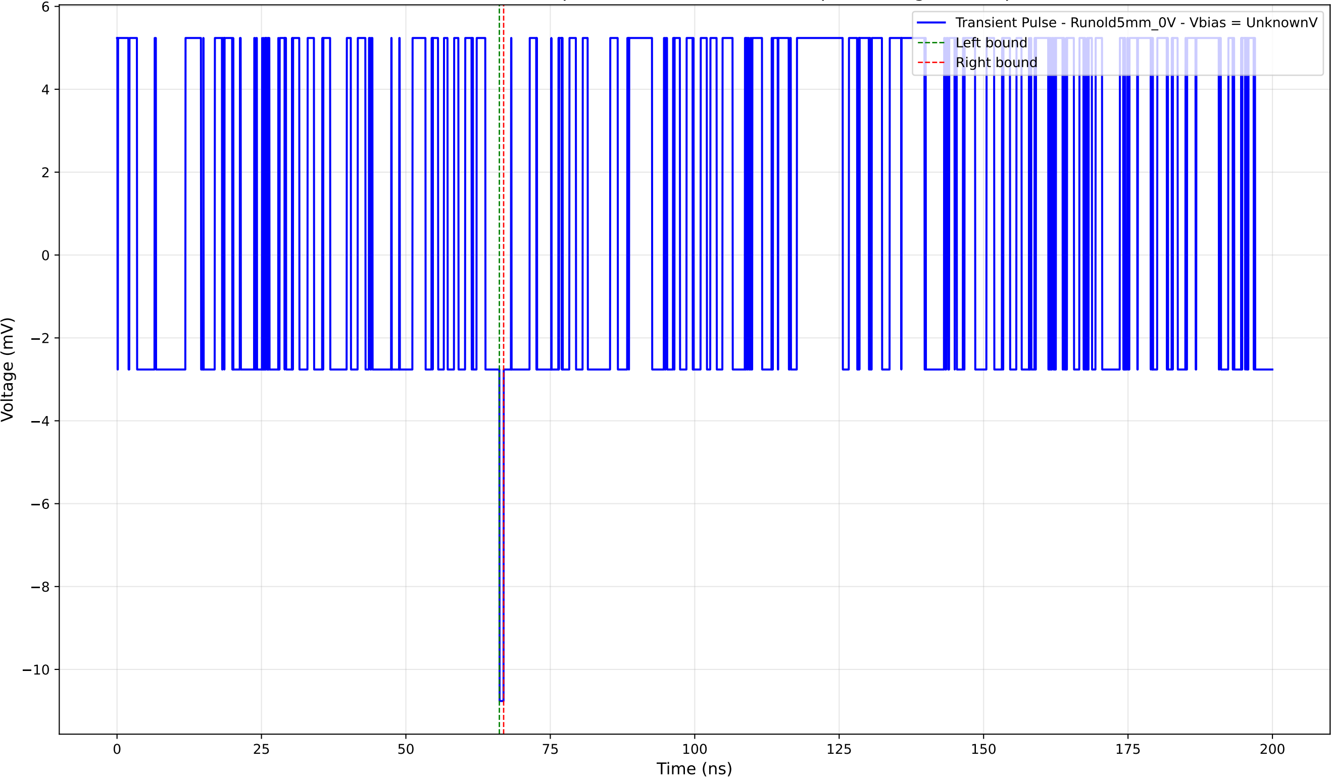
Transient Pulse - Sample: old5 - Position: 4565.0 \mu\text{m} - Charge: -0.16 pC
