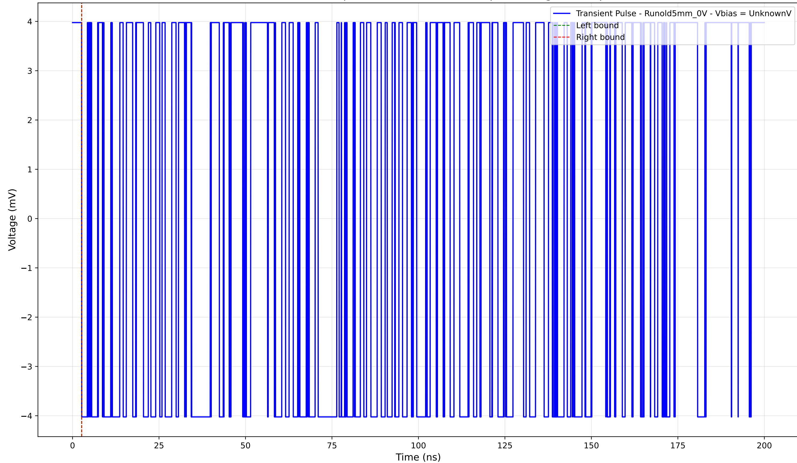
Transient Pulse - Sample: old5 - Position: 515.0 \mu\text{m} - Charge: -0.00 pC
