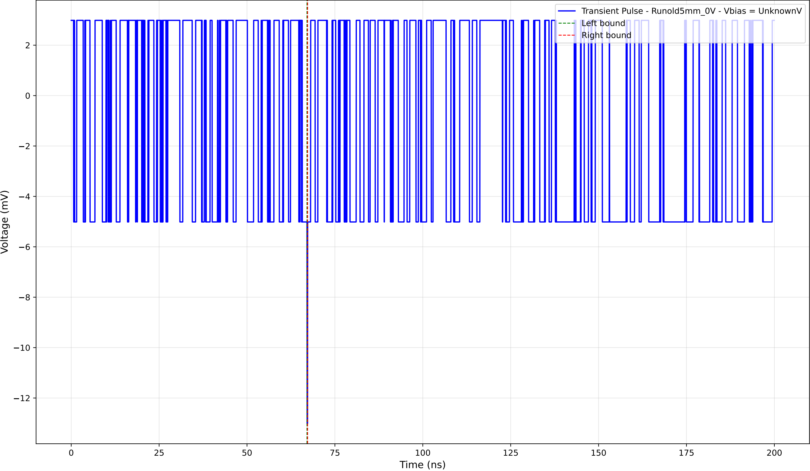
Transient Pulse - Sample: old5 - Position: 4975.0 \mu\text{m} - Charge: -0.04 pC
