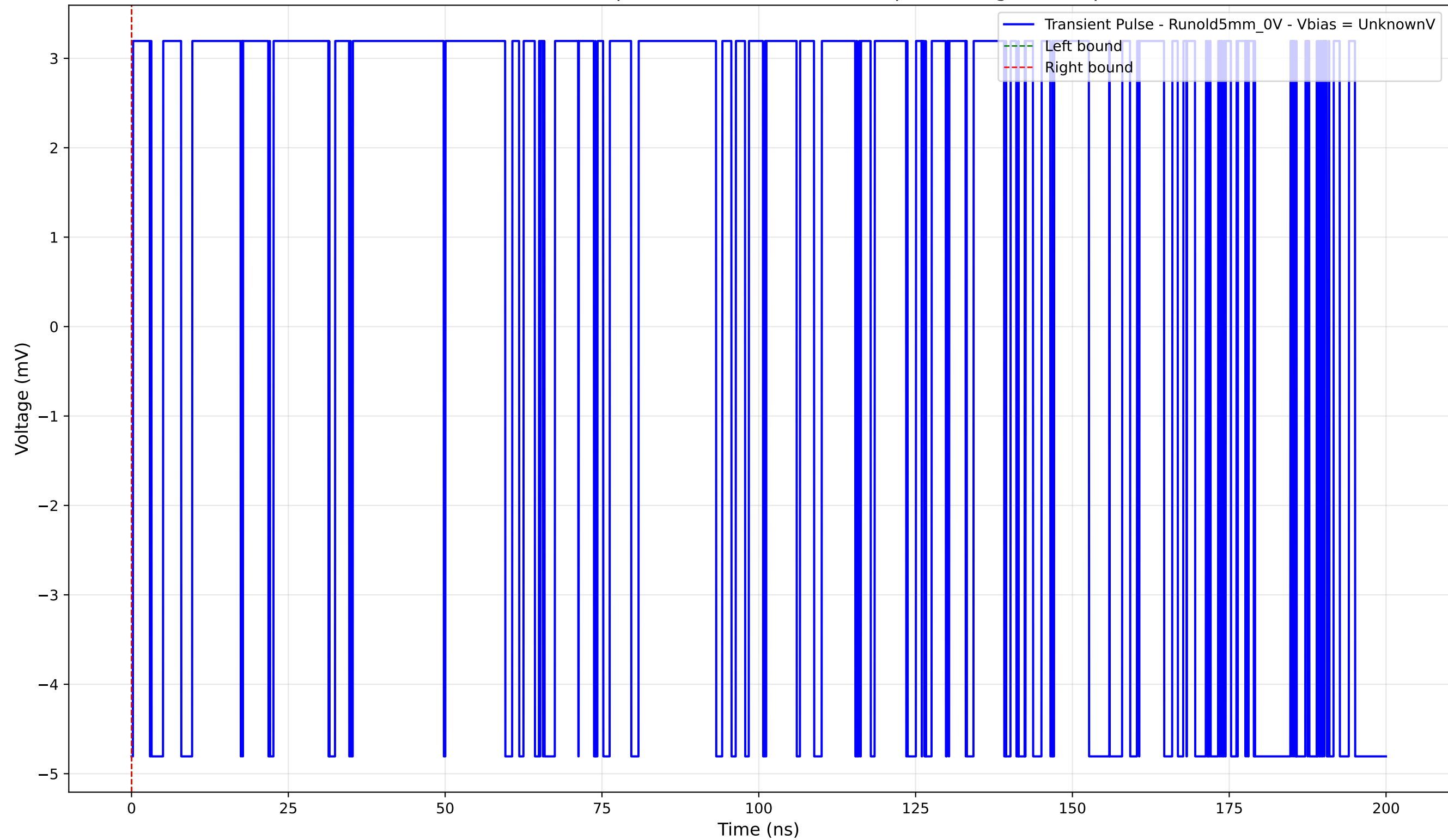
Transient Pulse - Sample: old5 - Position: 3195.0 \mu\text{m} - Charge: -0.00 pC
