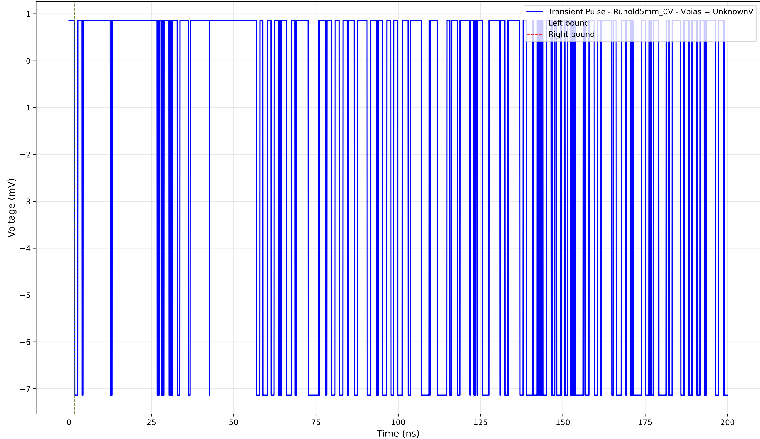
Transient Pulse - Sample: old5 - Position: 1435.0 \mu\text{m} - Charge: -0.00 pC
