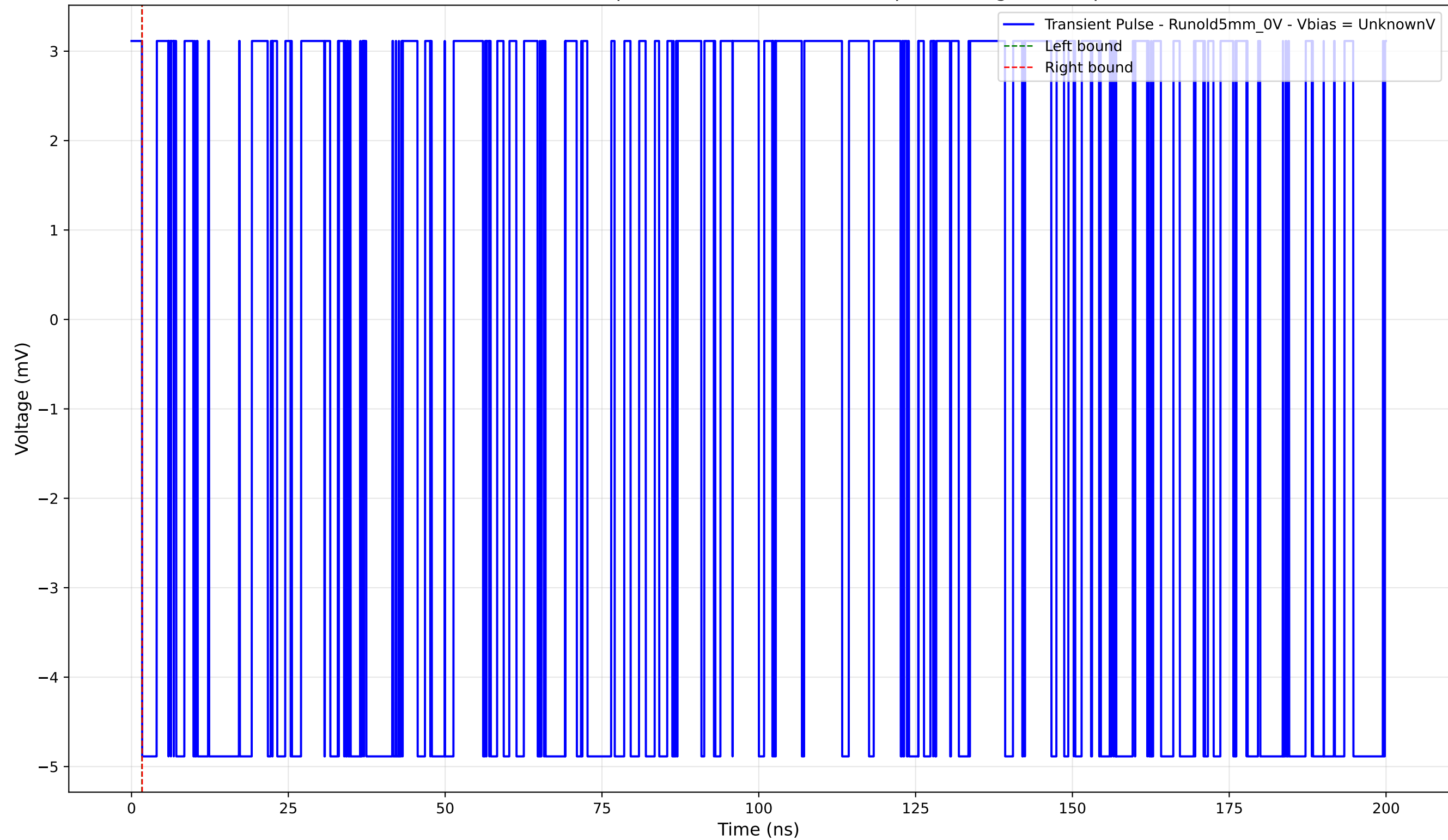
Transient Pulse - Sample: old5 - Position: 4500.0 \mu\text{m} - Charge: -0.00 pC
