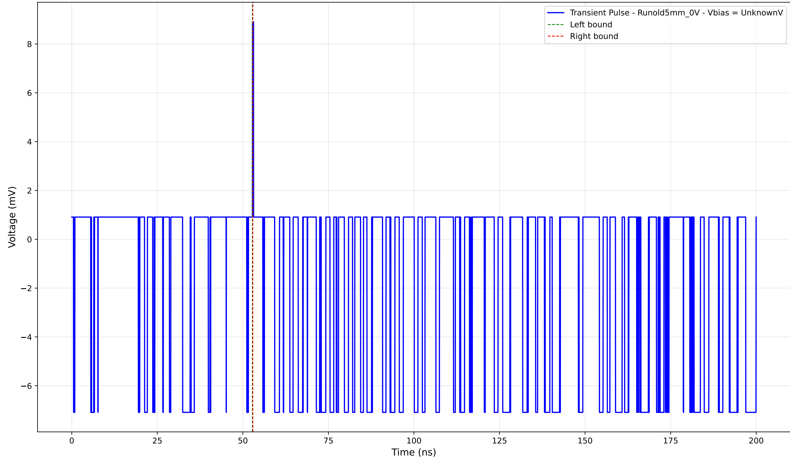
Transient Pulse - Sample: old5 - Position: 650.0 \mu\text{m} - Charge: 0.02 pC
