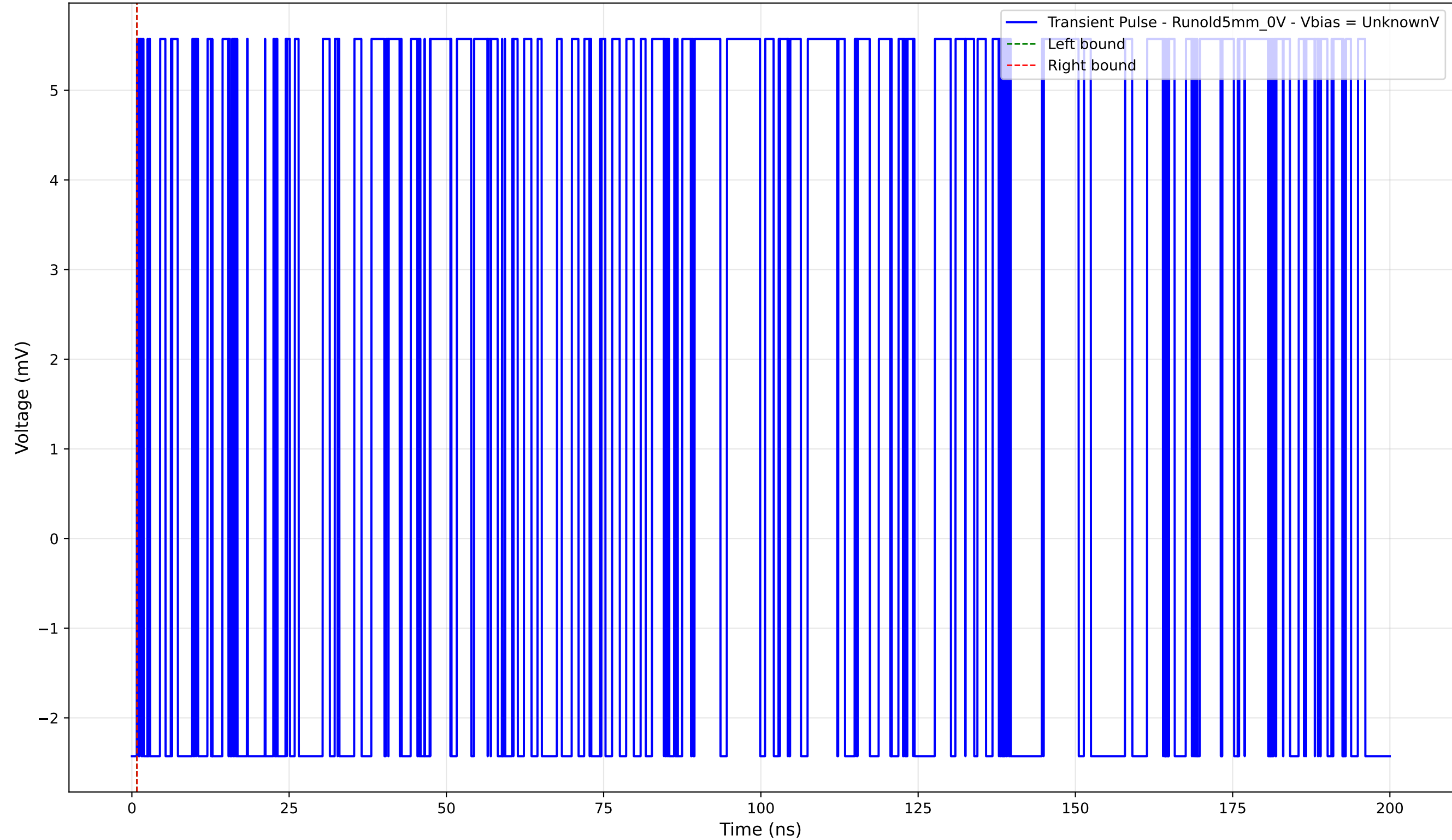
Transient Pulse - Sample: old5 - Position: 145.0 \mu\text{m} - Charge: 0.00 pC
