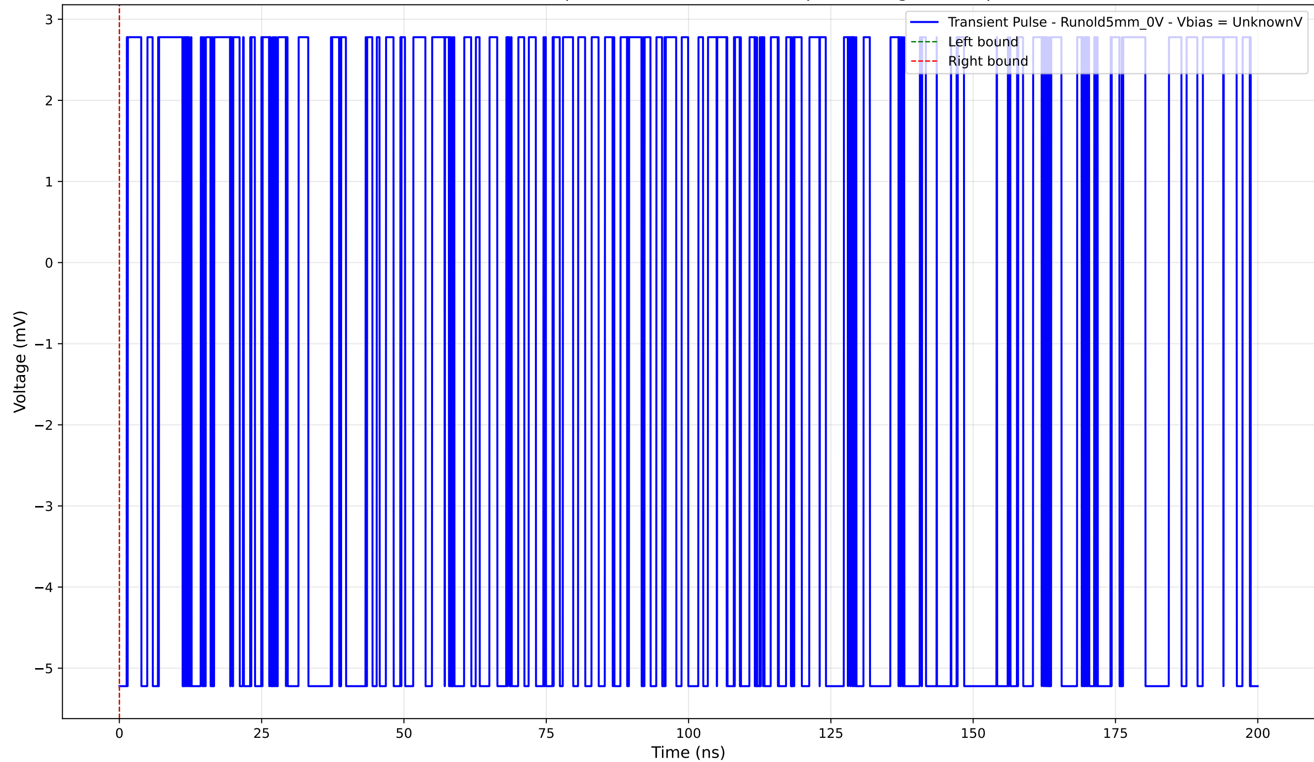
Transient Pulse - Sample: old5 - Position: 420.0 \mu\text{m} - Charge: -0.00 pC
