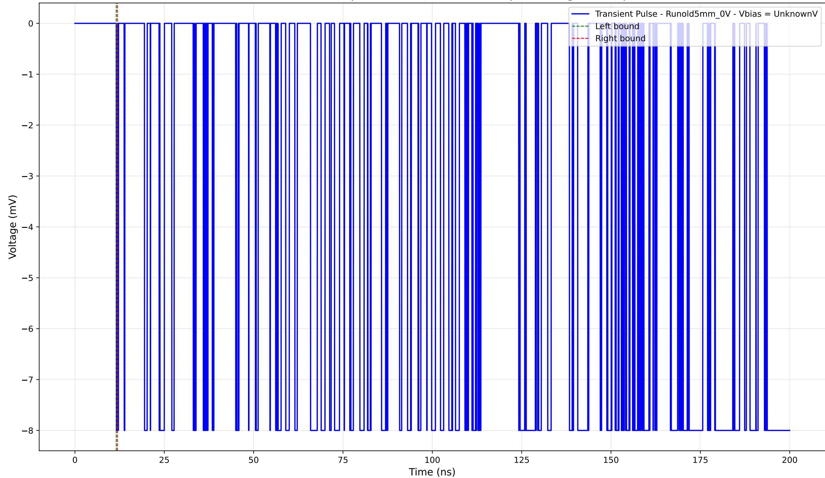
Transient Pulse - Sample: old5 - Position: 4635.0 \mu\text{m} - Charge: -0.05 pC
