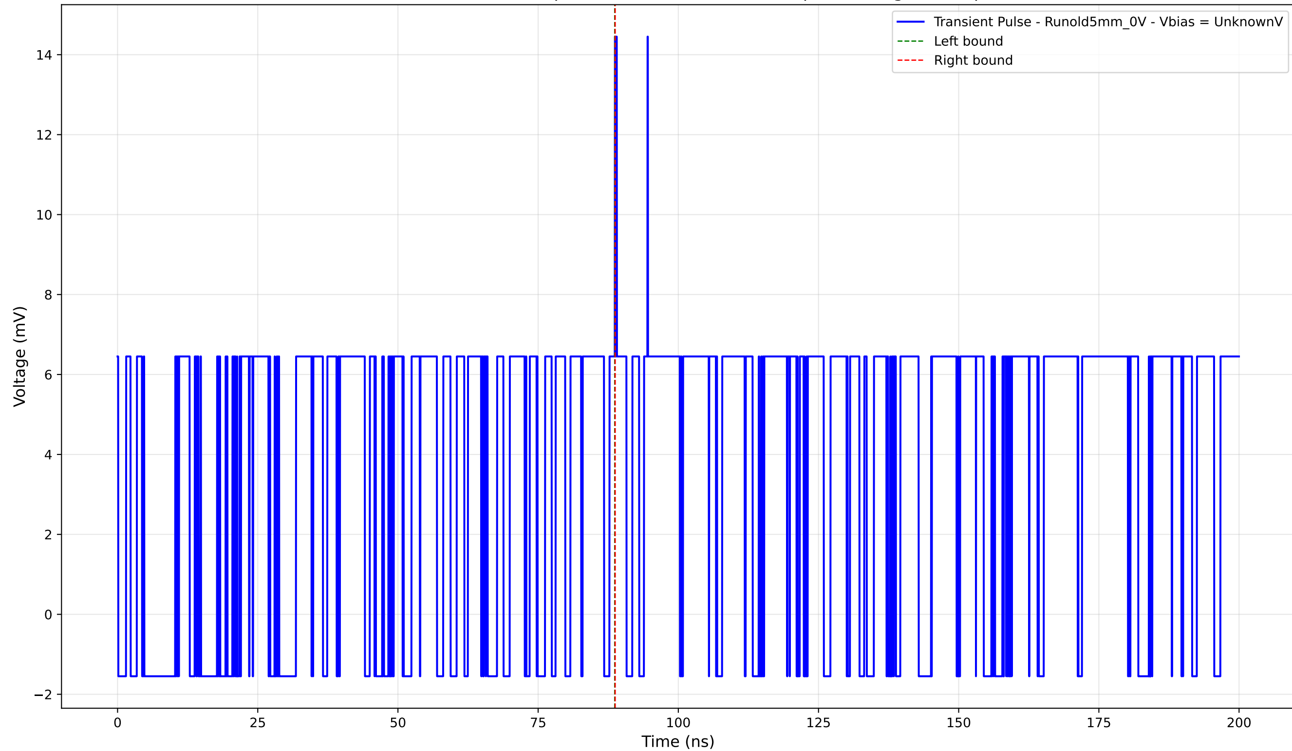
Transient Pulse - Sample: old5 - Position: 3645.0 \mu\text{m} - Charge: 0.02 pC
