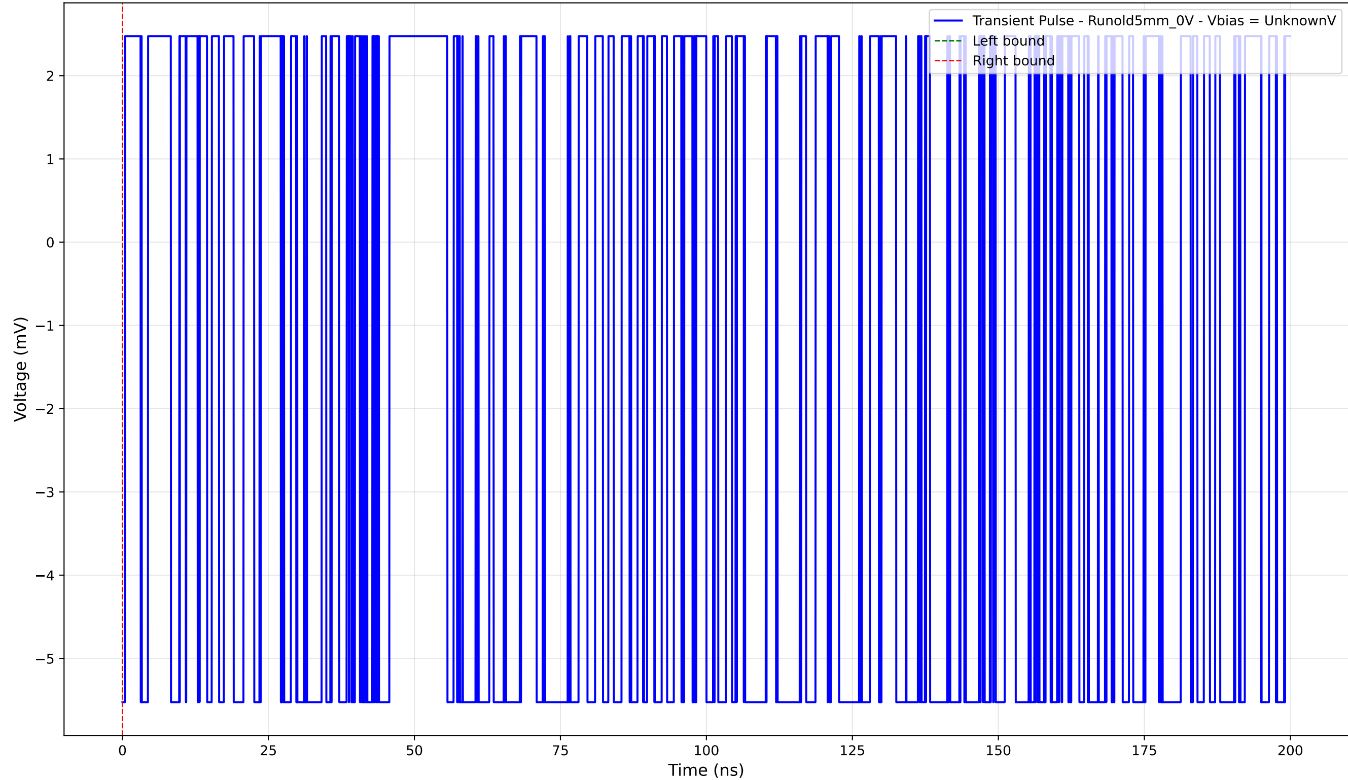
Transient Pulse - Sample: old5 - Position: 2020.0 \mu\text{m} - Charge: -0.00 pC
