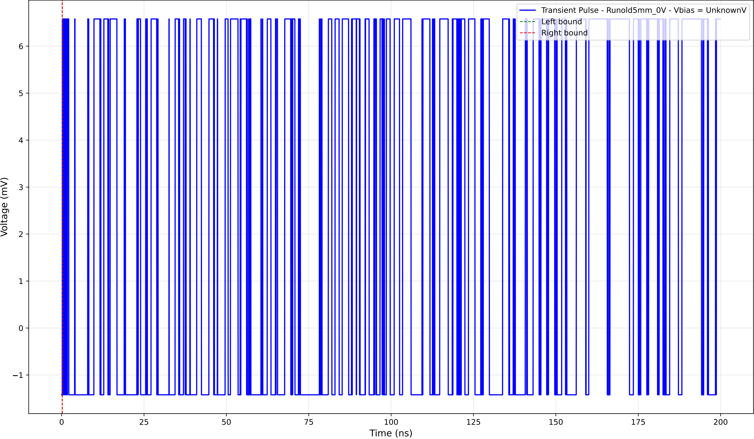
Transient Pulse - Sample: old5 - Position: 2130.0 \mu\text{m} - Charge: 0.00 pC
