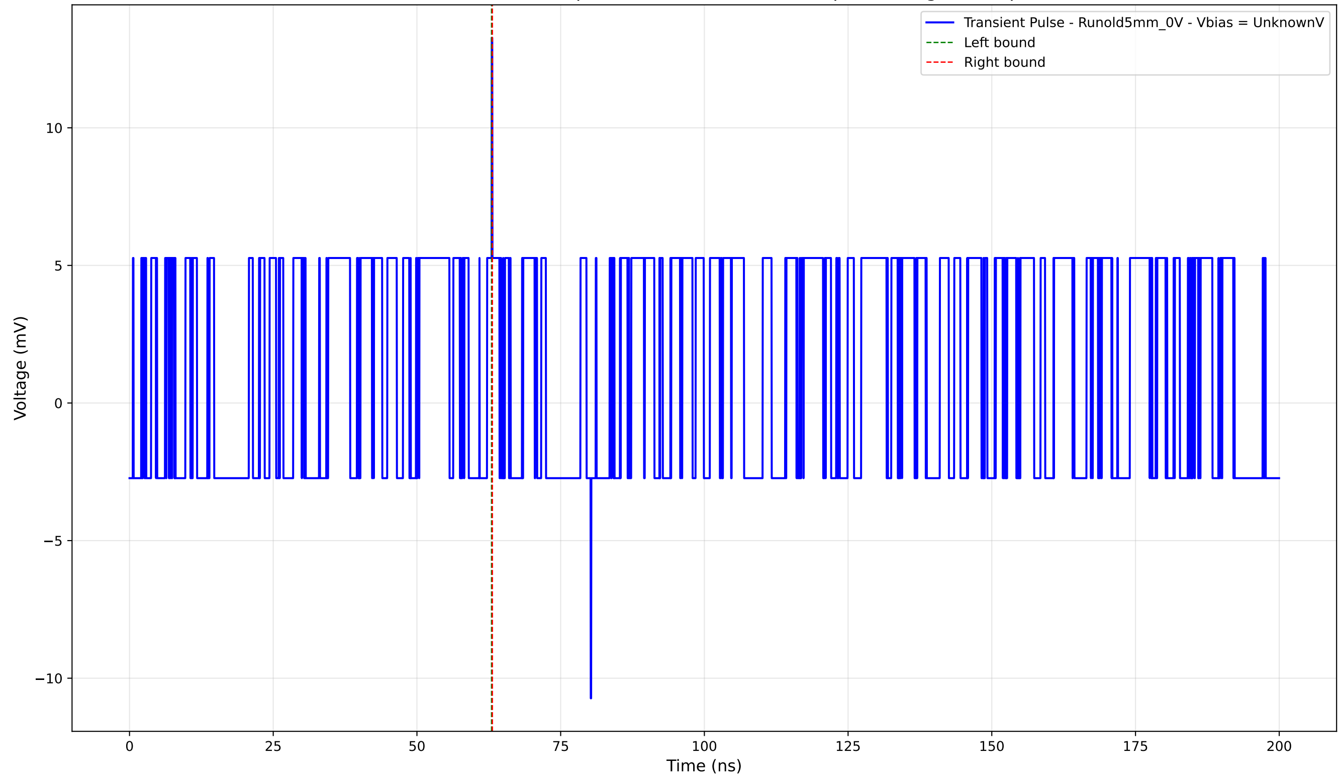
Transient Pulse - Sample: old5 - Position: 3115.0 \mu\text{m} - Charge: 0.03 pC
