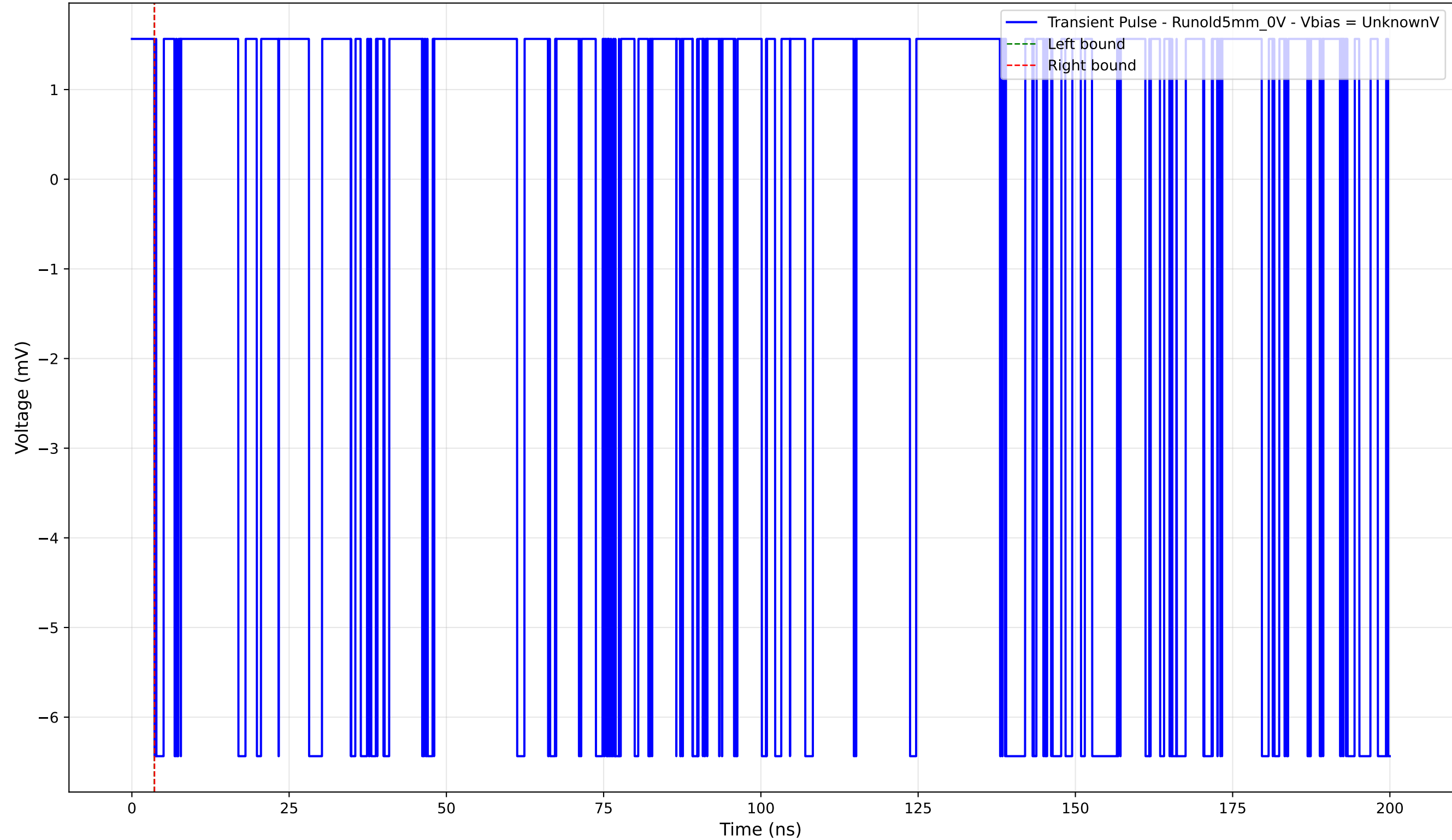
Transient Pulse - Sample: old5 - Position: 1600.0 \mu\text{m} - Charge: -0.00 pC
