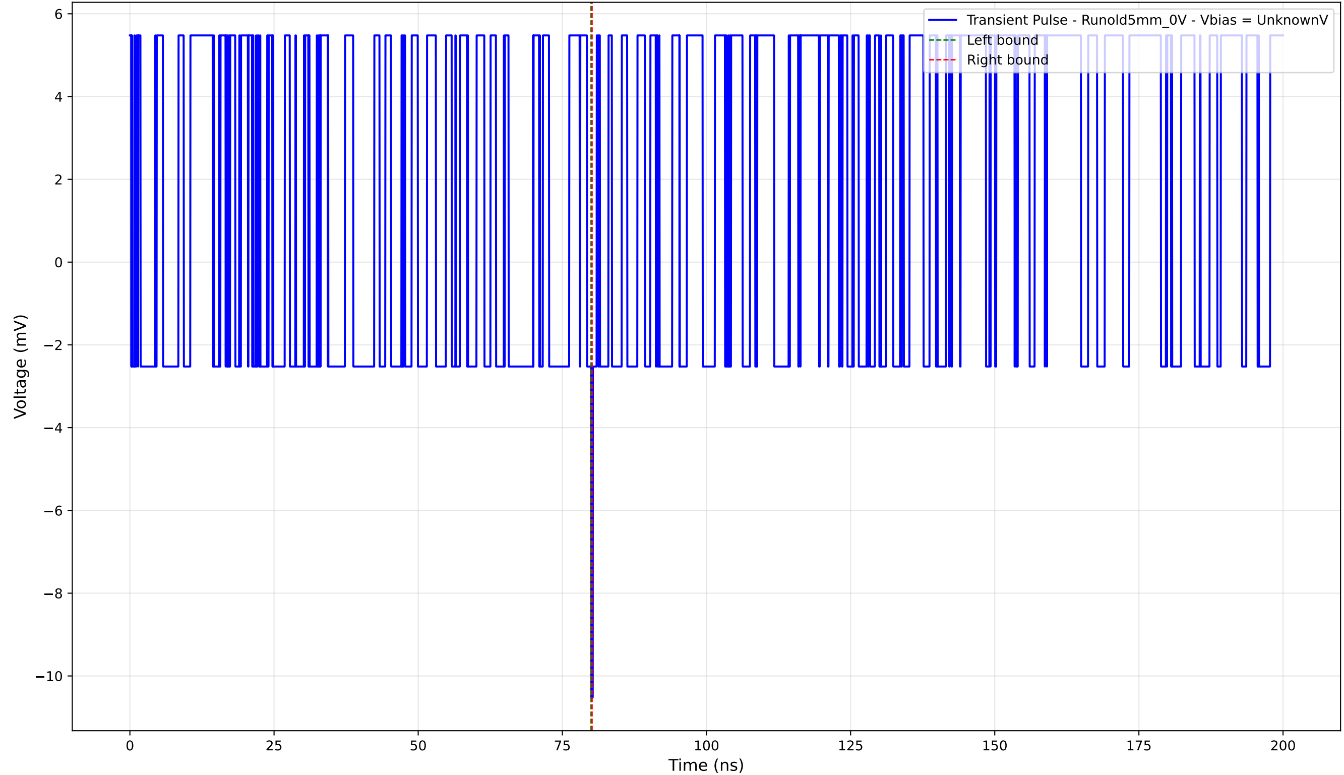
Transient Pulse - Sample: old5 - Position: 890.0 \mu\text{m} - Charge: -0.03 pC
