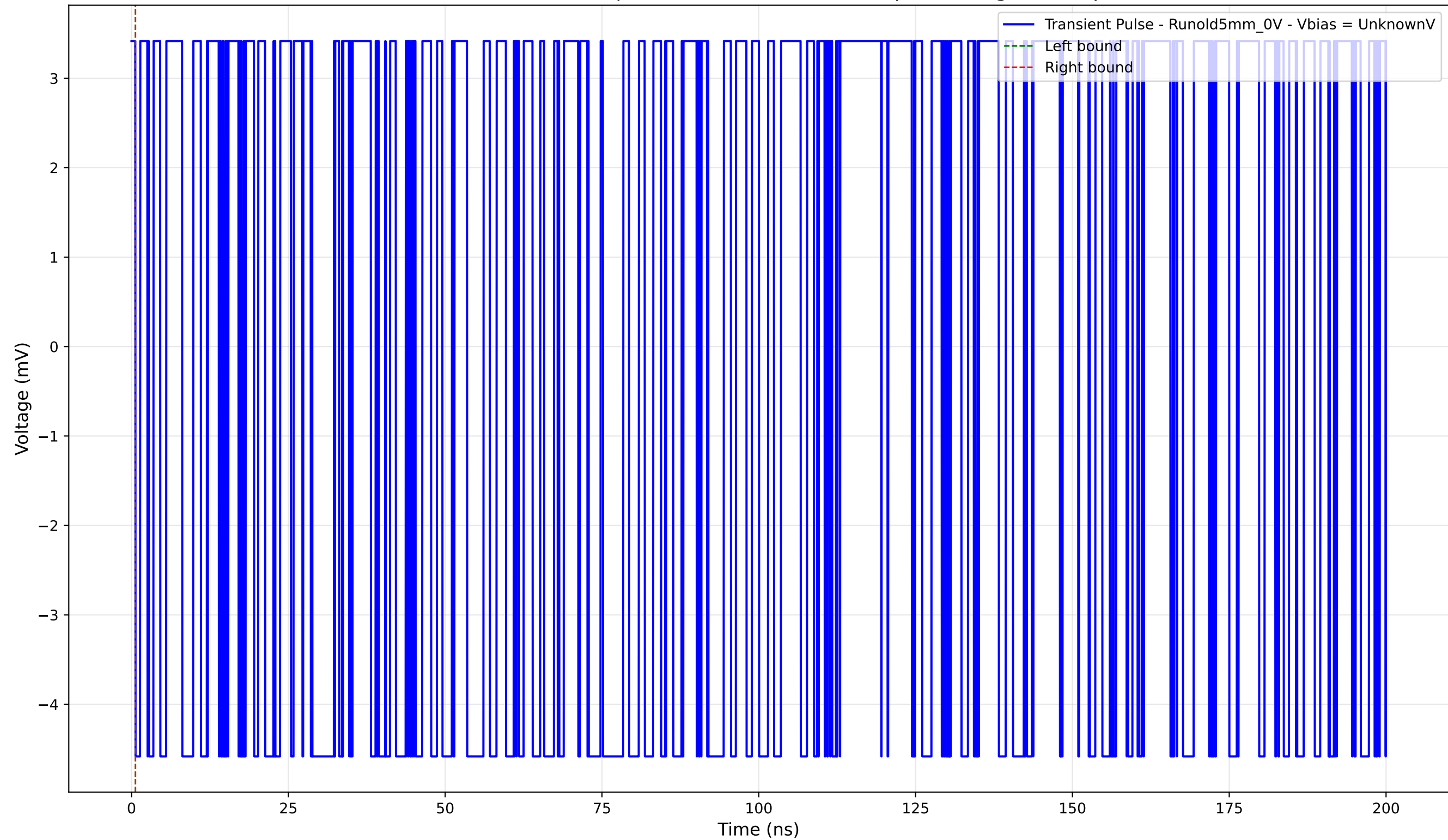
Transient Pulse - Sample: old5 - Position: 4830.0 \mu\text{m} - Charge: -0.00 pC
