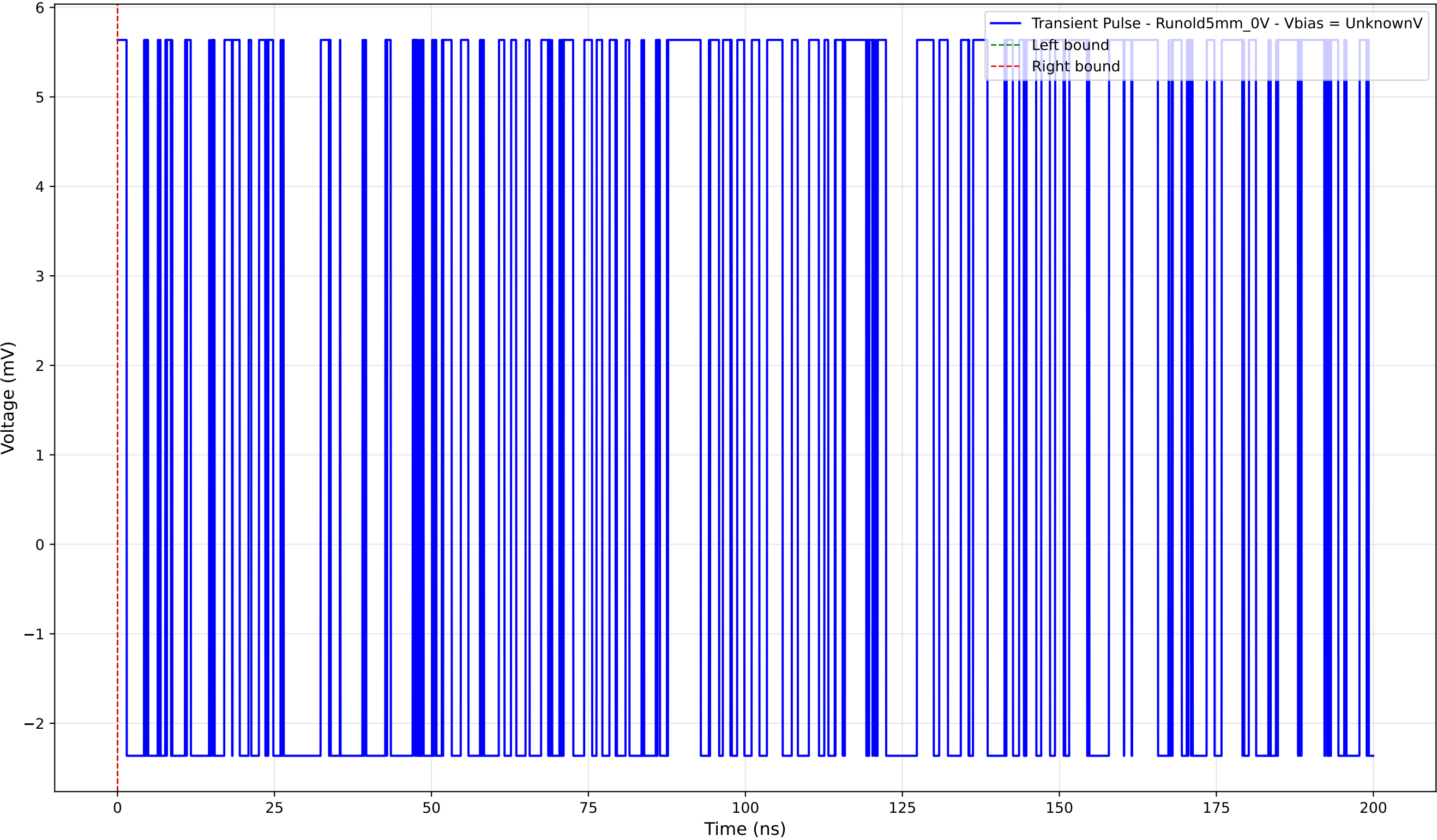
Transient Pulse - Sample: old5 - Position: 2360.0 \mu\text{m} - Charge: 0.00 pC
