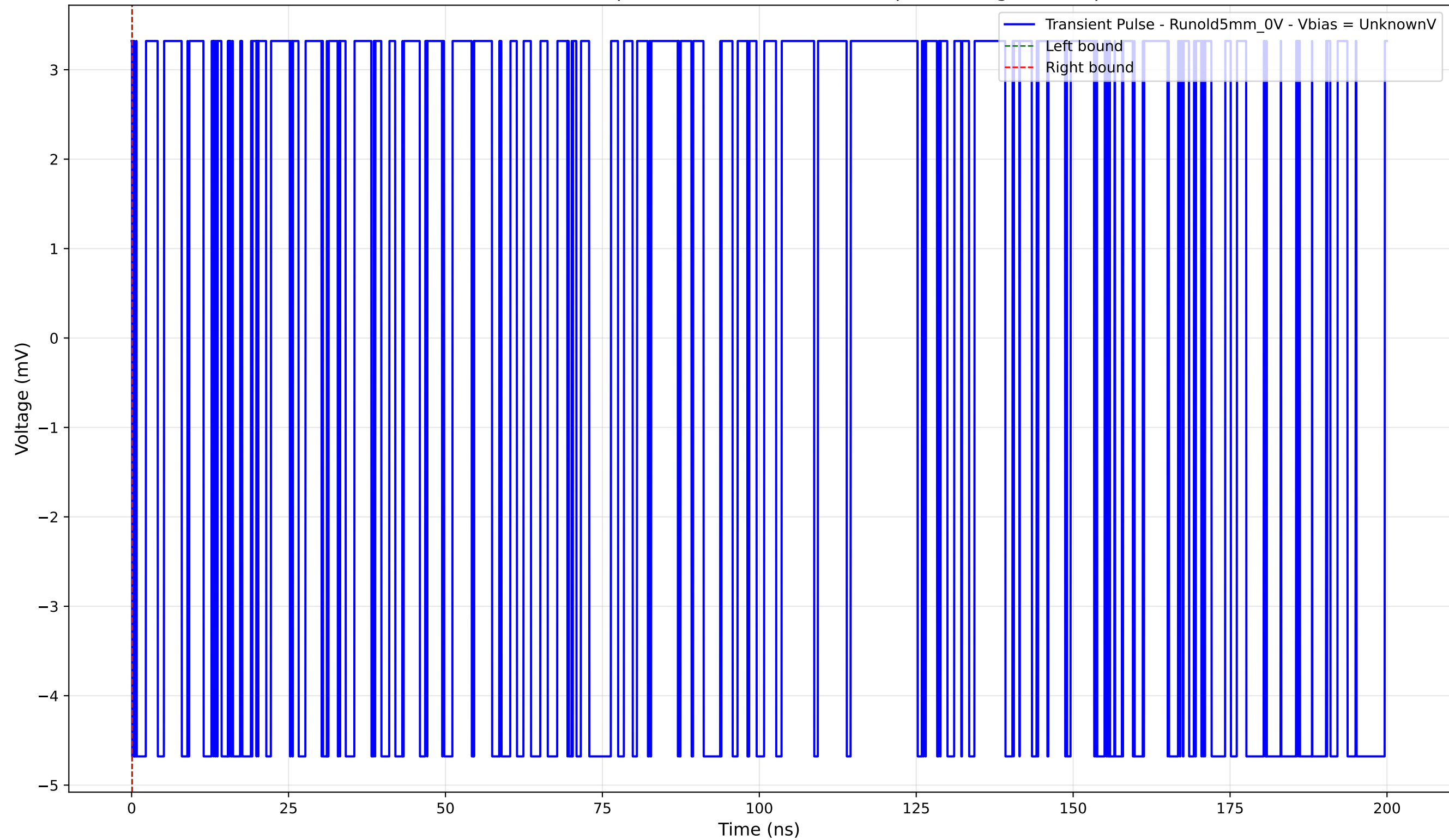
Transient Pulse - Sample: old5 - Position: 1045.0 \mu\text{m} - Charge: -0.00 pC
