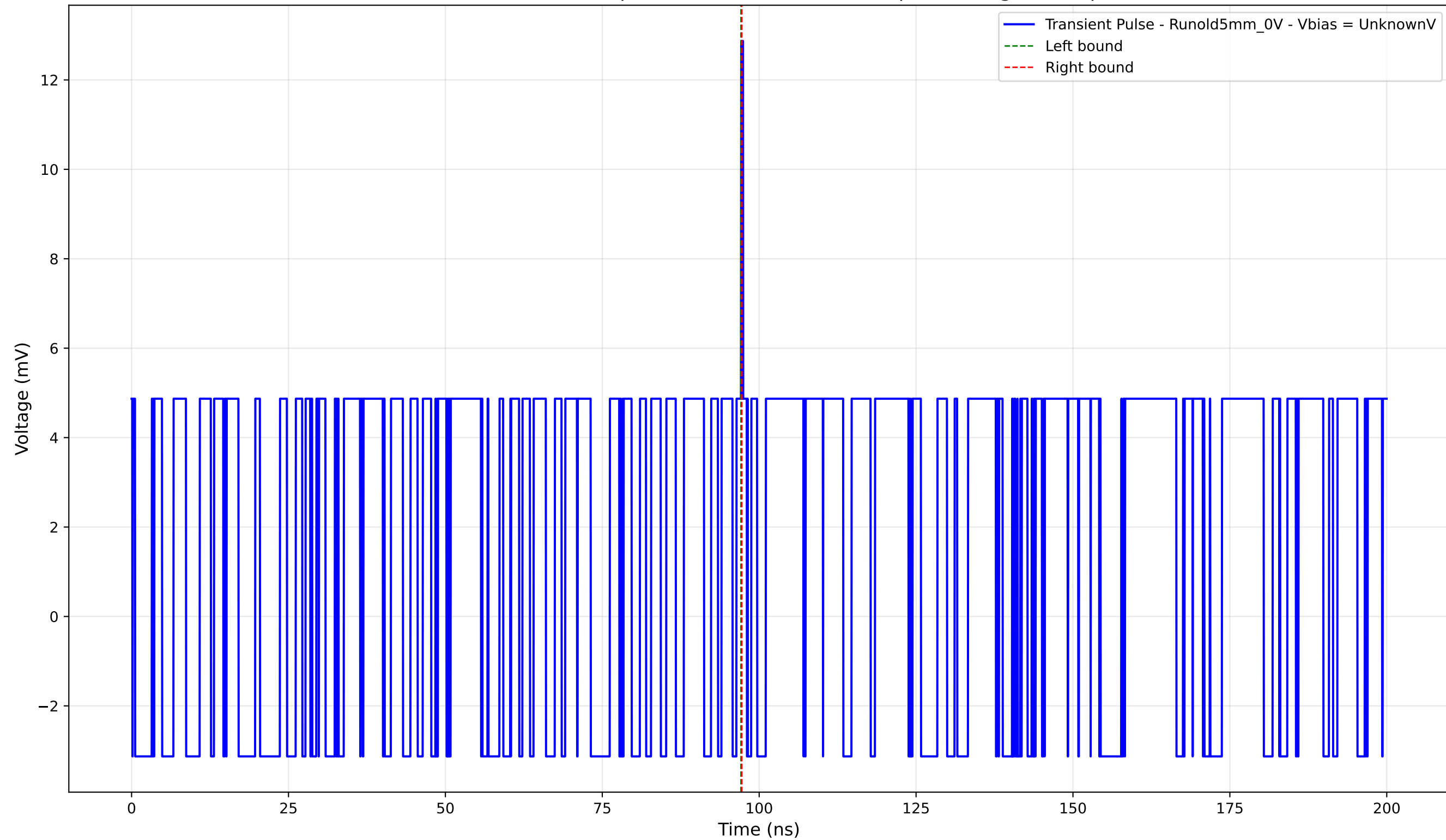
Transient Pulse - Sample: old5 - Position: 3090.0 \mu\text{m} - Charge: 0.03 pC
