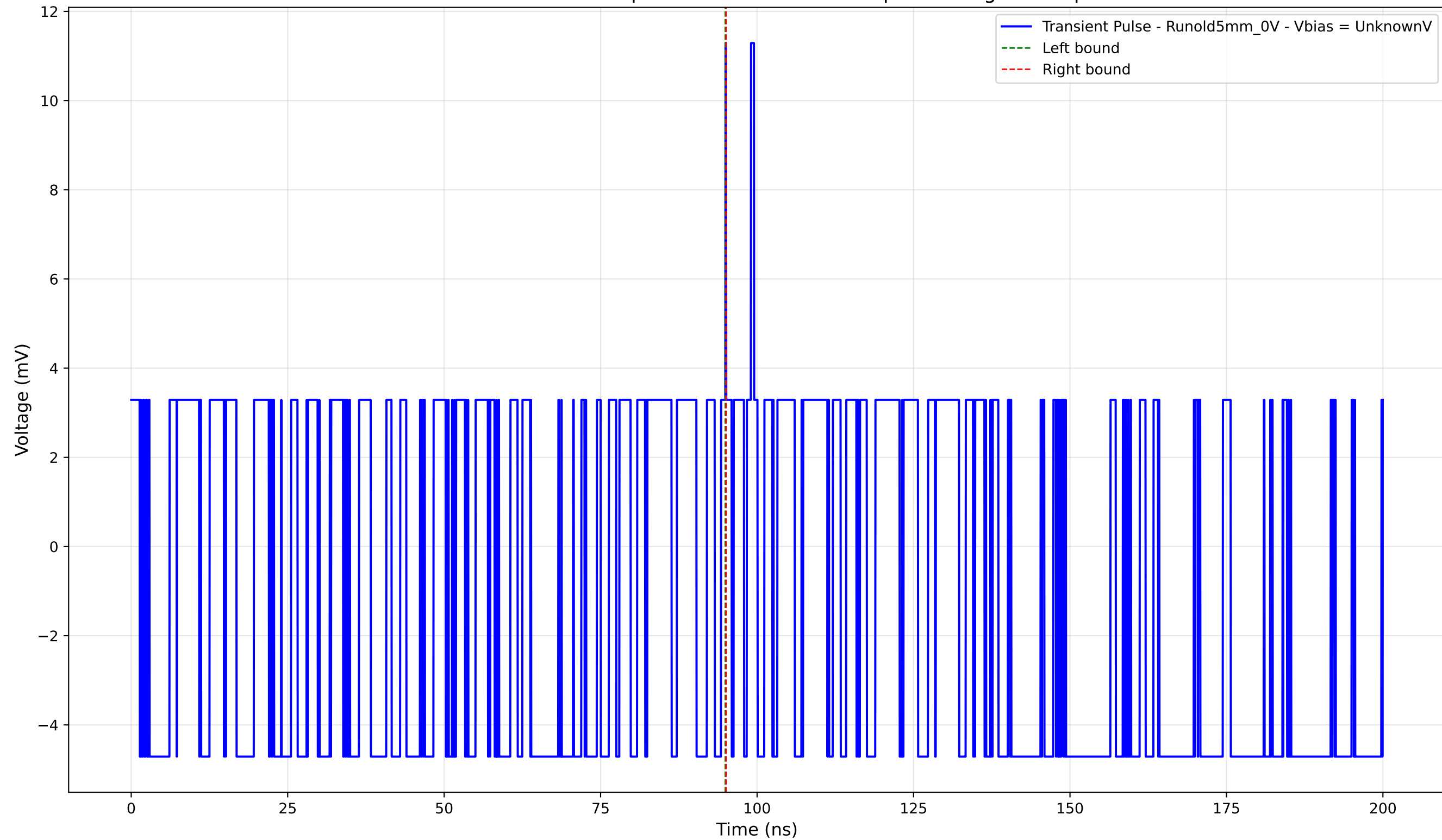
Transient Pulse - Sample: old5 - Position: 35.0 \mu\text{m} - Charge: 0.03 pC
