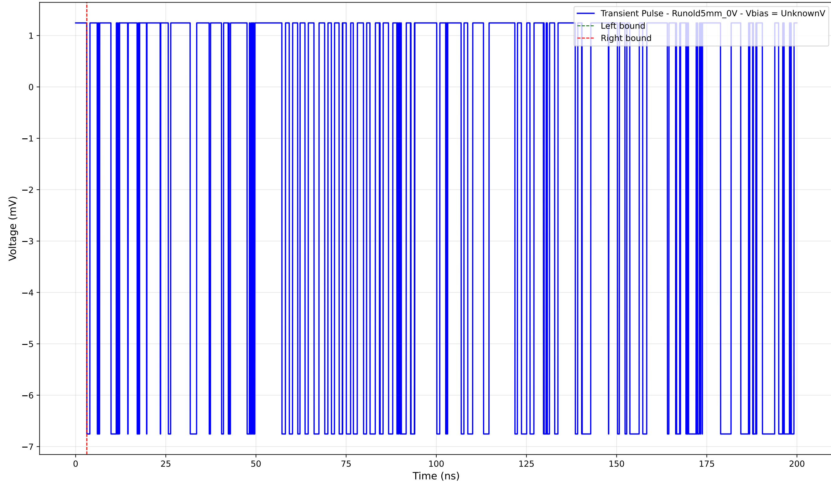
Transient Pulse - Sample: old5 - Position: 1750.0 \mu\text{m} - Charge: -0.00 pC
