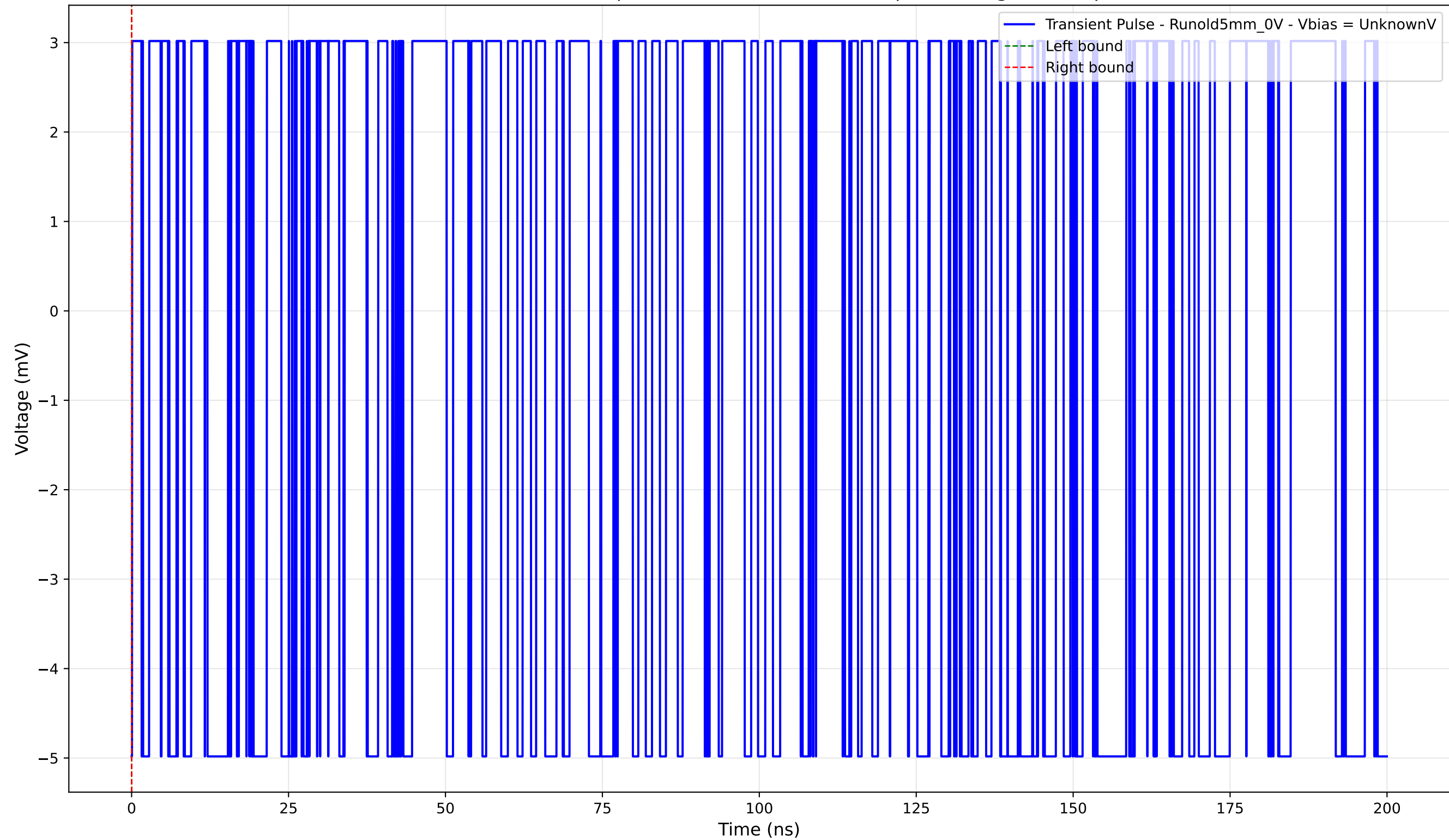
Transient Pulse - Sample: old5 - Position: 4260.0 \mu\text{m} - Charge: -0.00 pC
