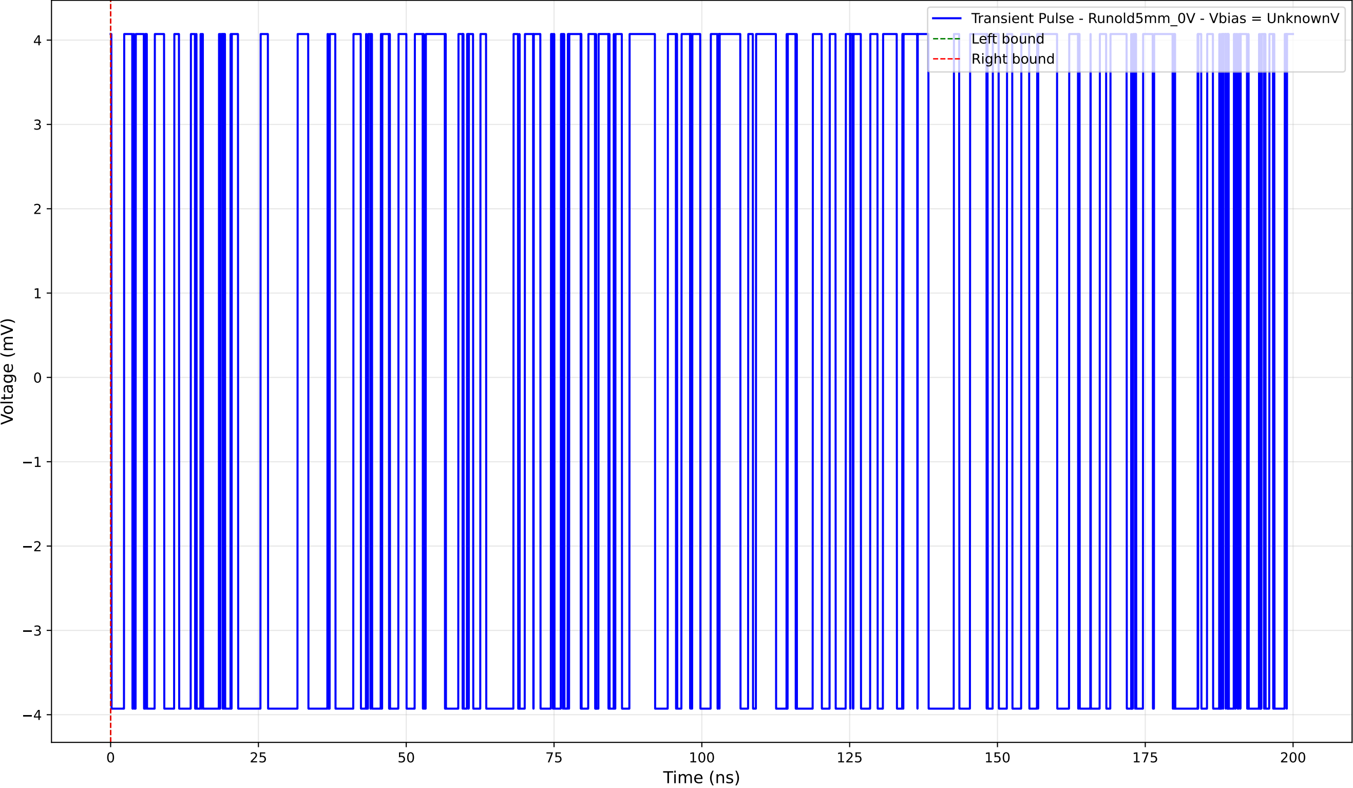
Transient Pulse - Sample: old5 - Position: 5035.0 \mu\text{m} - Charge: 0.00 pC
