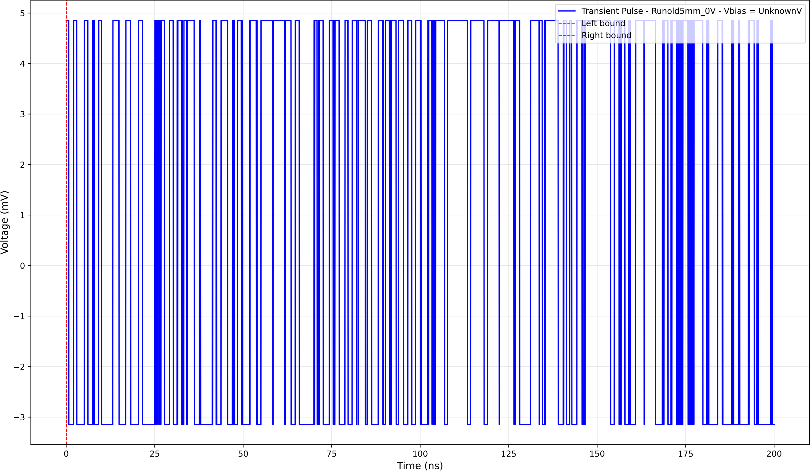
Transient Pulse - Sample: old5 - Position: 2690.0 \mu\text{m} - Charge: 0.00 pC
