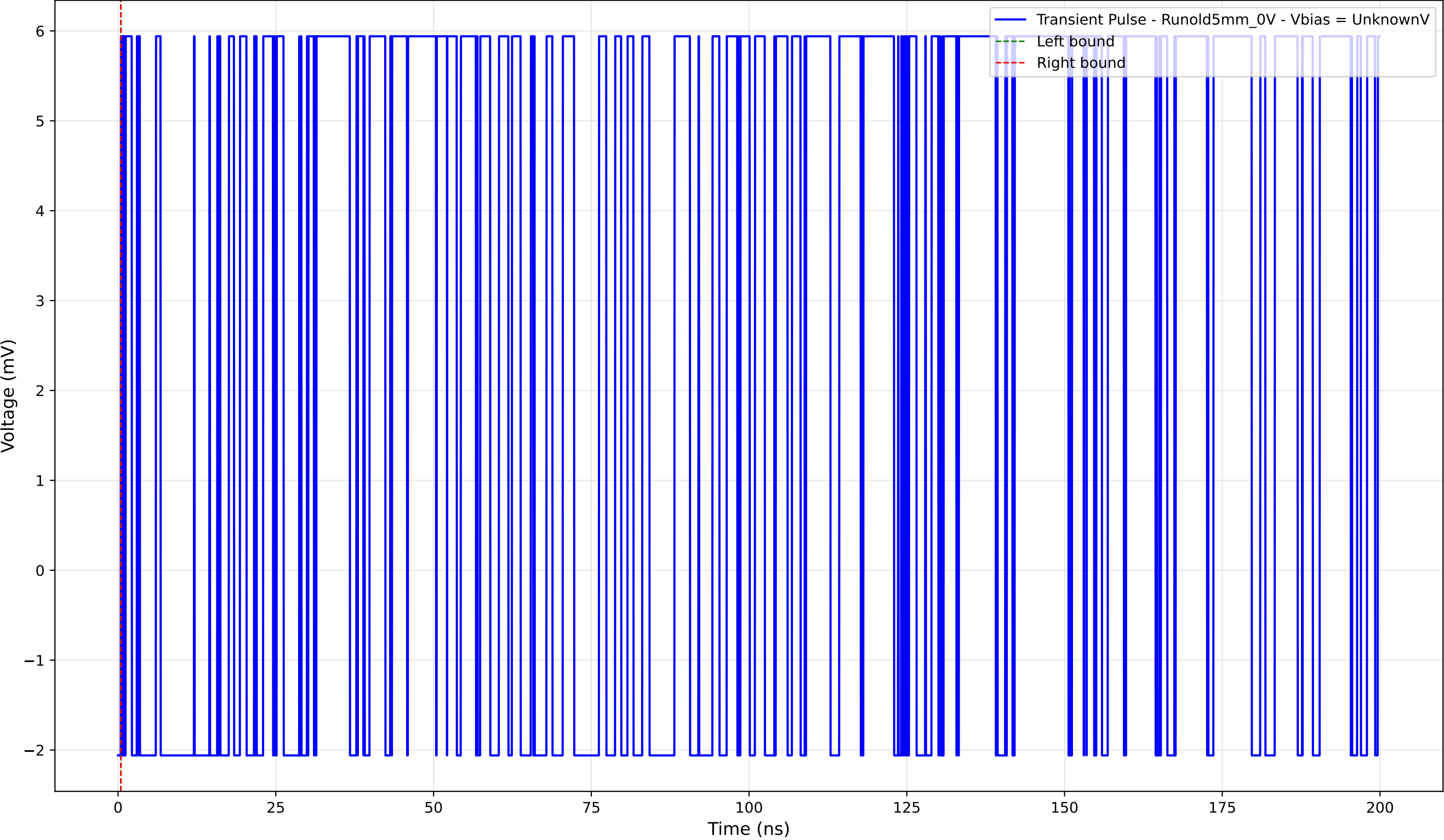
Transient Pulse - Sample: old5 - Position: 1130.0 \mu\text{m} - Charge: 0.00 pC
