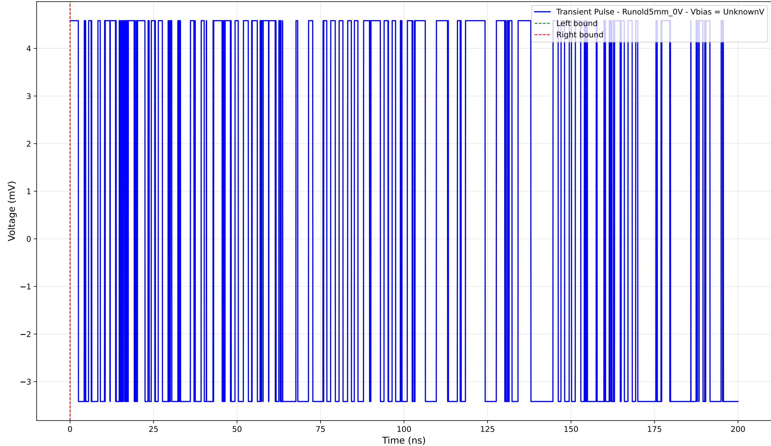
Transient Pulse - Sample: old5 - Position: 3005.0 \mu\text{m} - Charge: 0.00 pC
