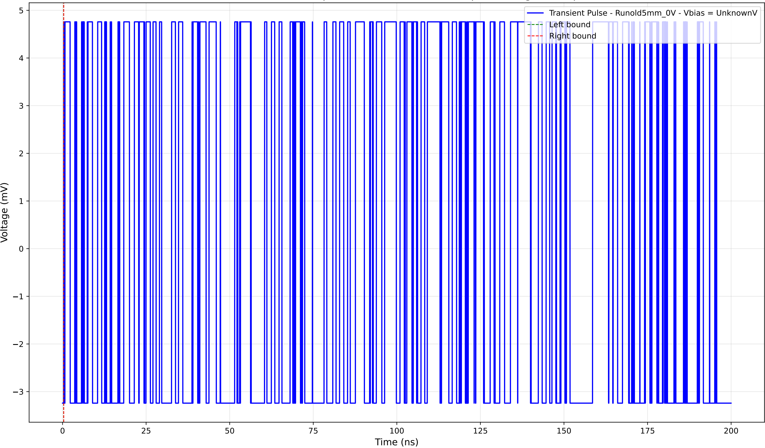
Transient Pulse - Sample: old5 - Position: 4380.0 \mu\text{m} - Charge: 0.00 pC
