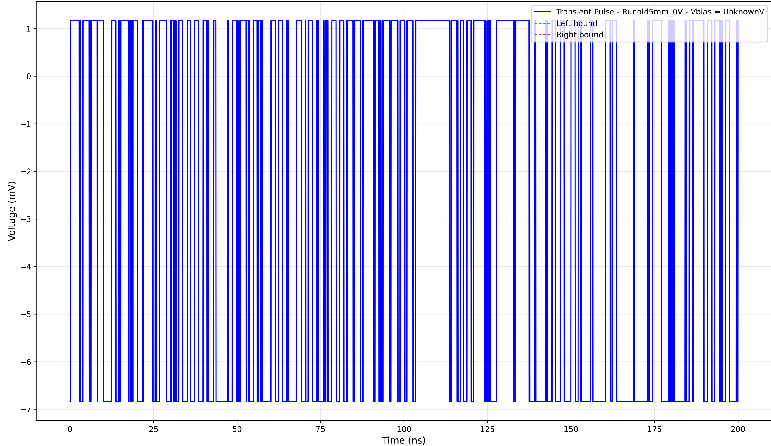
Transient Pulse - Sample: old5 - Position: 4435.0 \mu\text{m} - Charge: -0.00 pC
