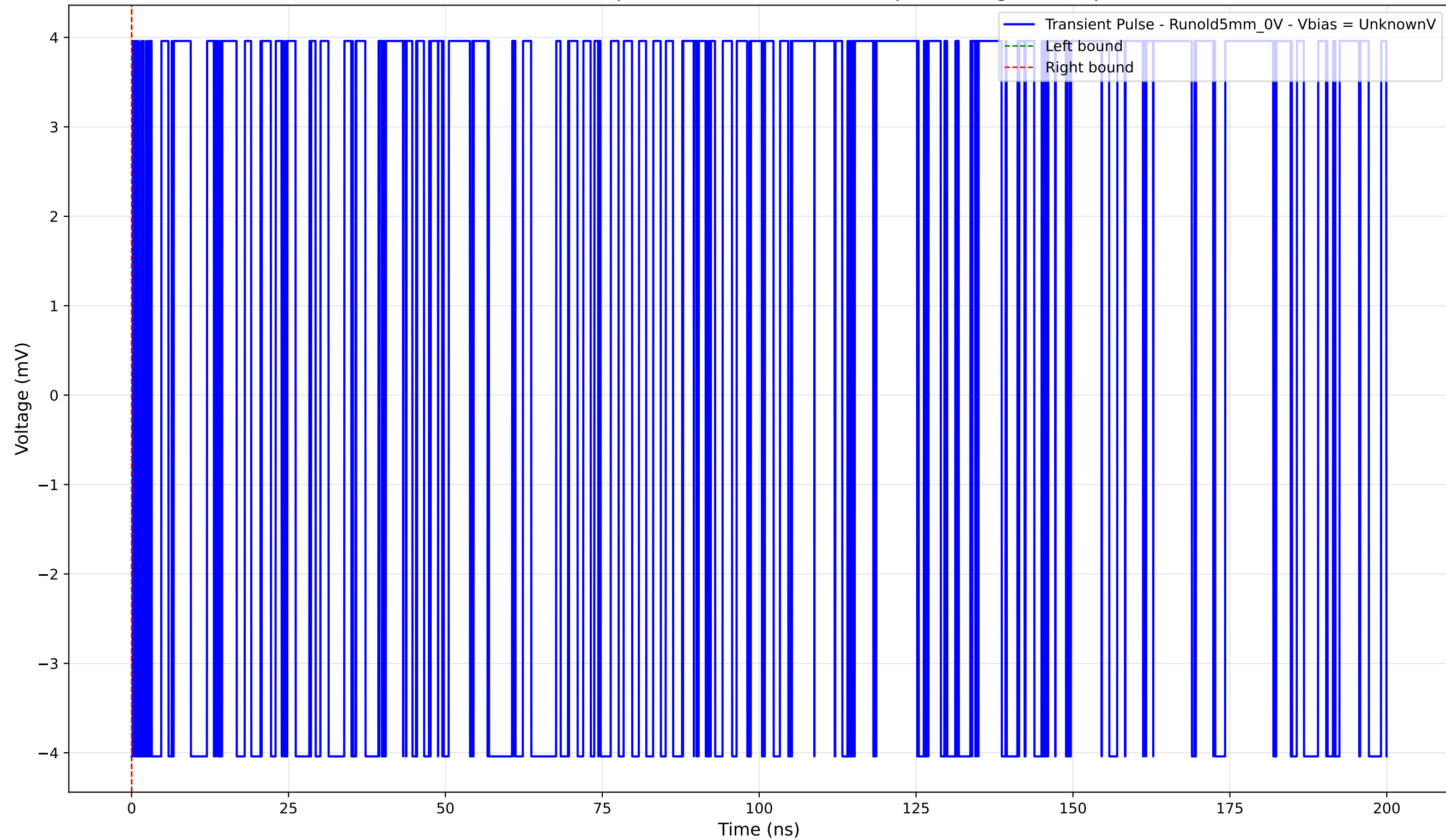
Transient Pulse - Sample: old5 - Position: 4025.0 \mu\text{m} - Charge: -0.00 pC
