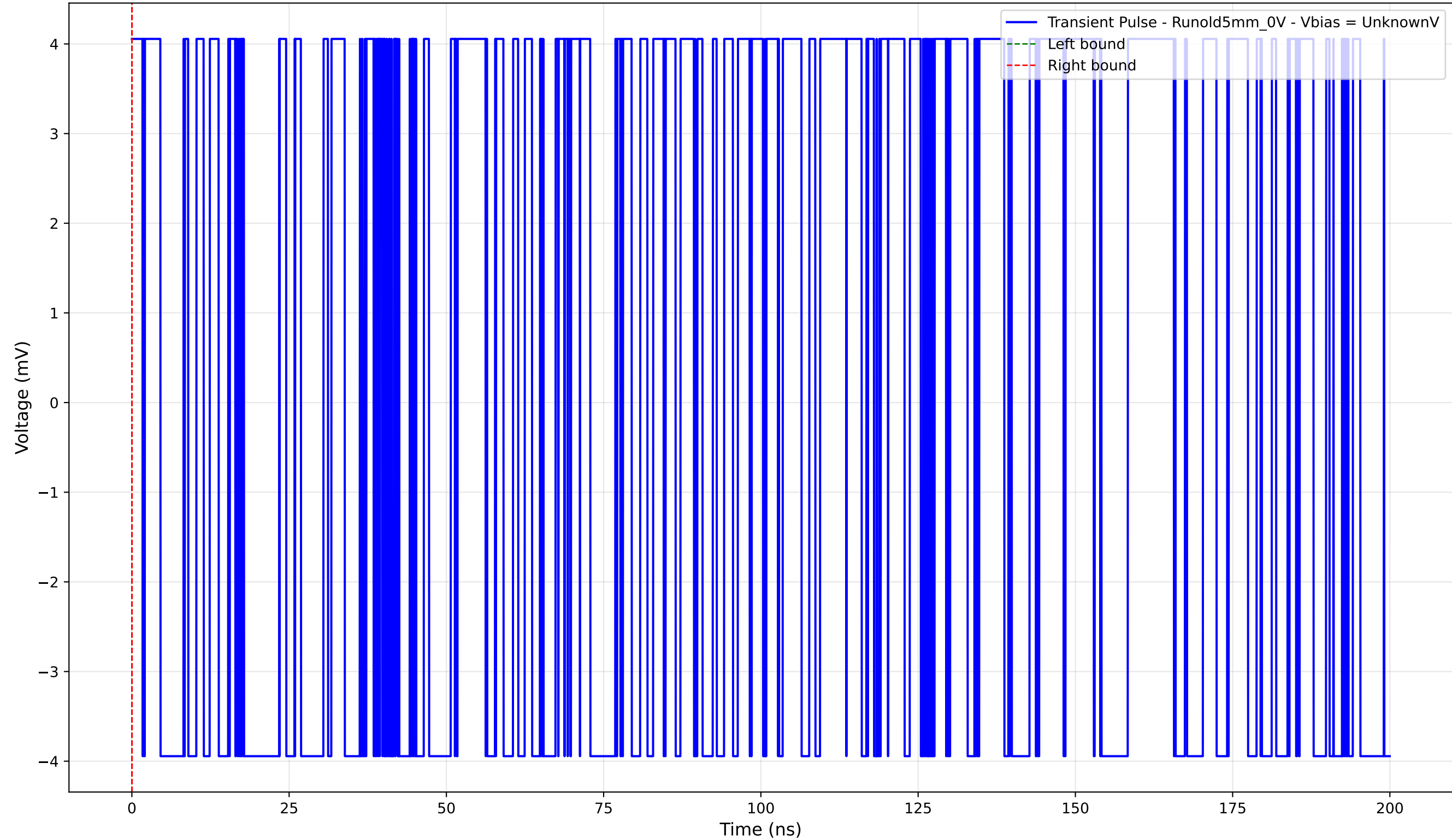
Transient Pulse - Sample: old5 - Position: 3510.0 \mu\text{m} - Charge: 0.00 pC
