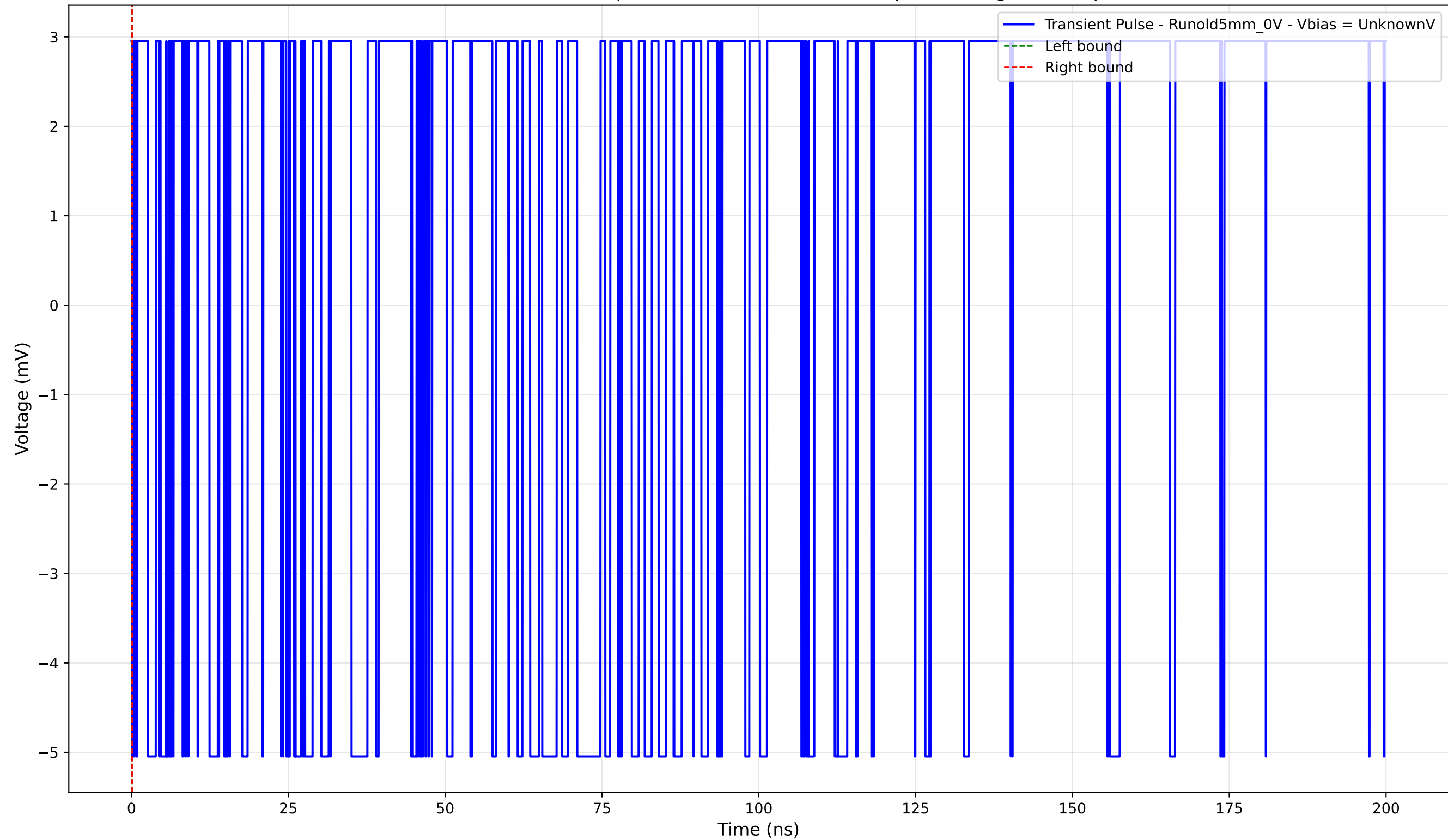
Transient Pulse - Sample: old5 - Position: 1115.0 \mu\text{m} - Charge: -0.00 pC
