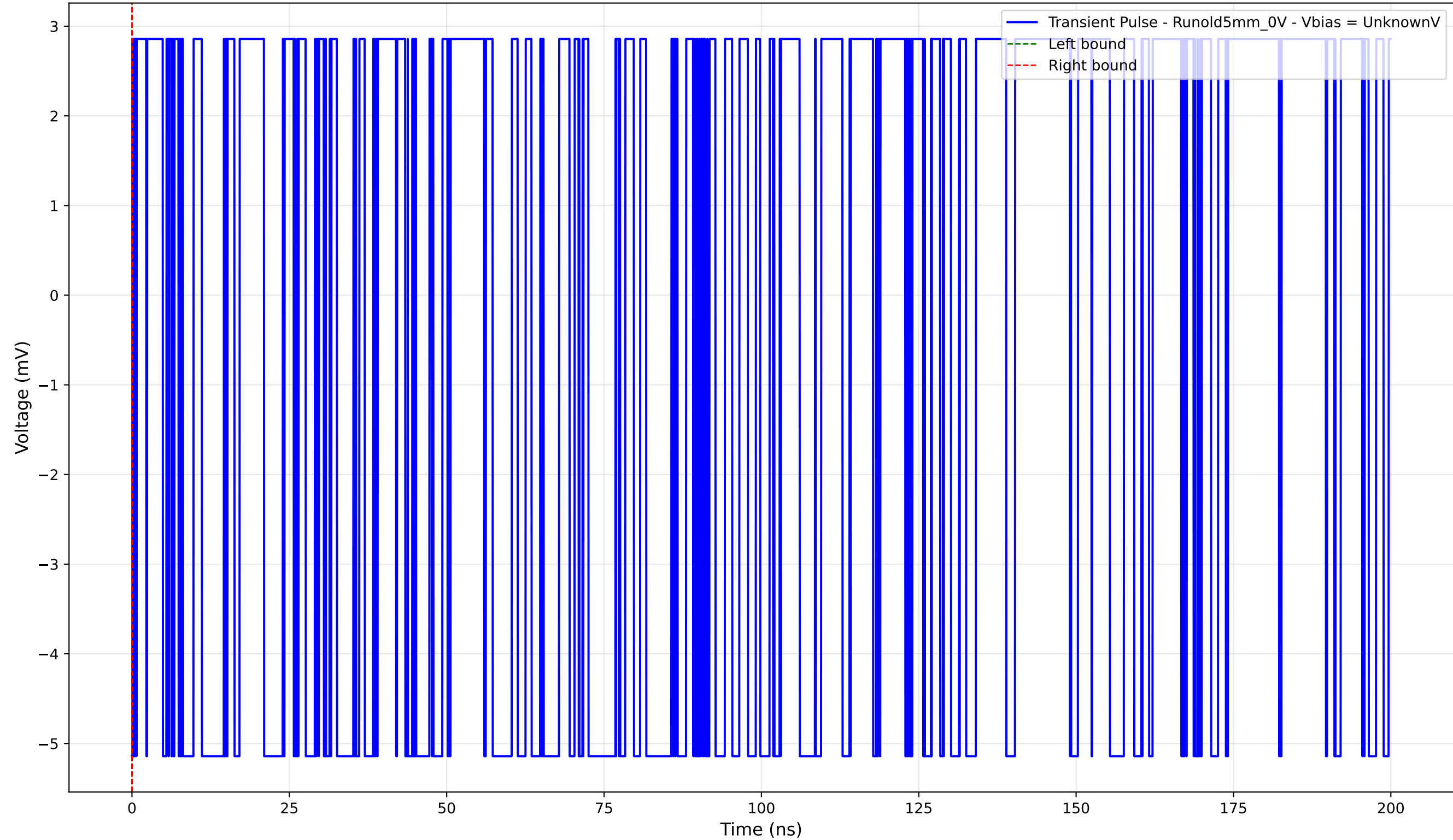
Transient Pulse - Sample: old5 - Position: 1930.0 \mu\text{m} - Charge: -0.00 pC
