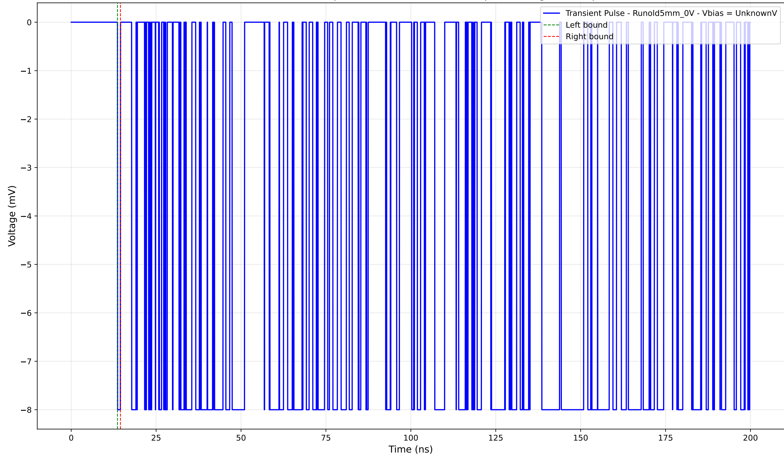
Transient Pulse - Sample: old5 - Position: 1610.0 \mu\text{m} - Charge: -0.14 pC
