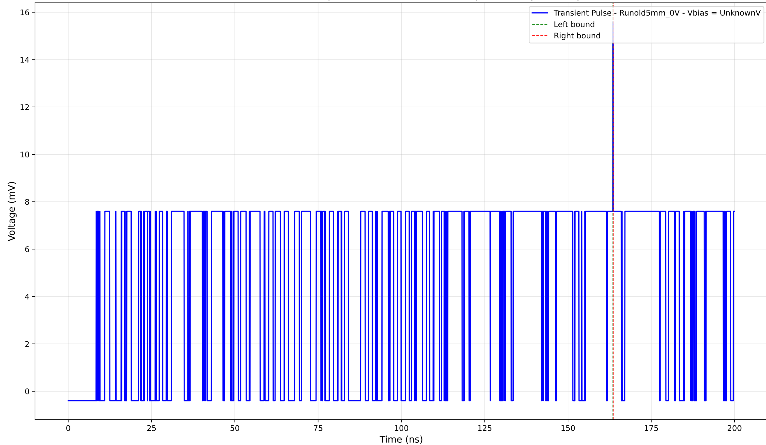
Transient Pulse - Sample: old5 - Position: 4640.0 \mu\text{m} - Charge: 0.02 pC
