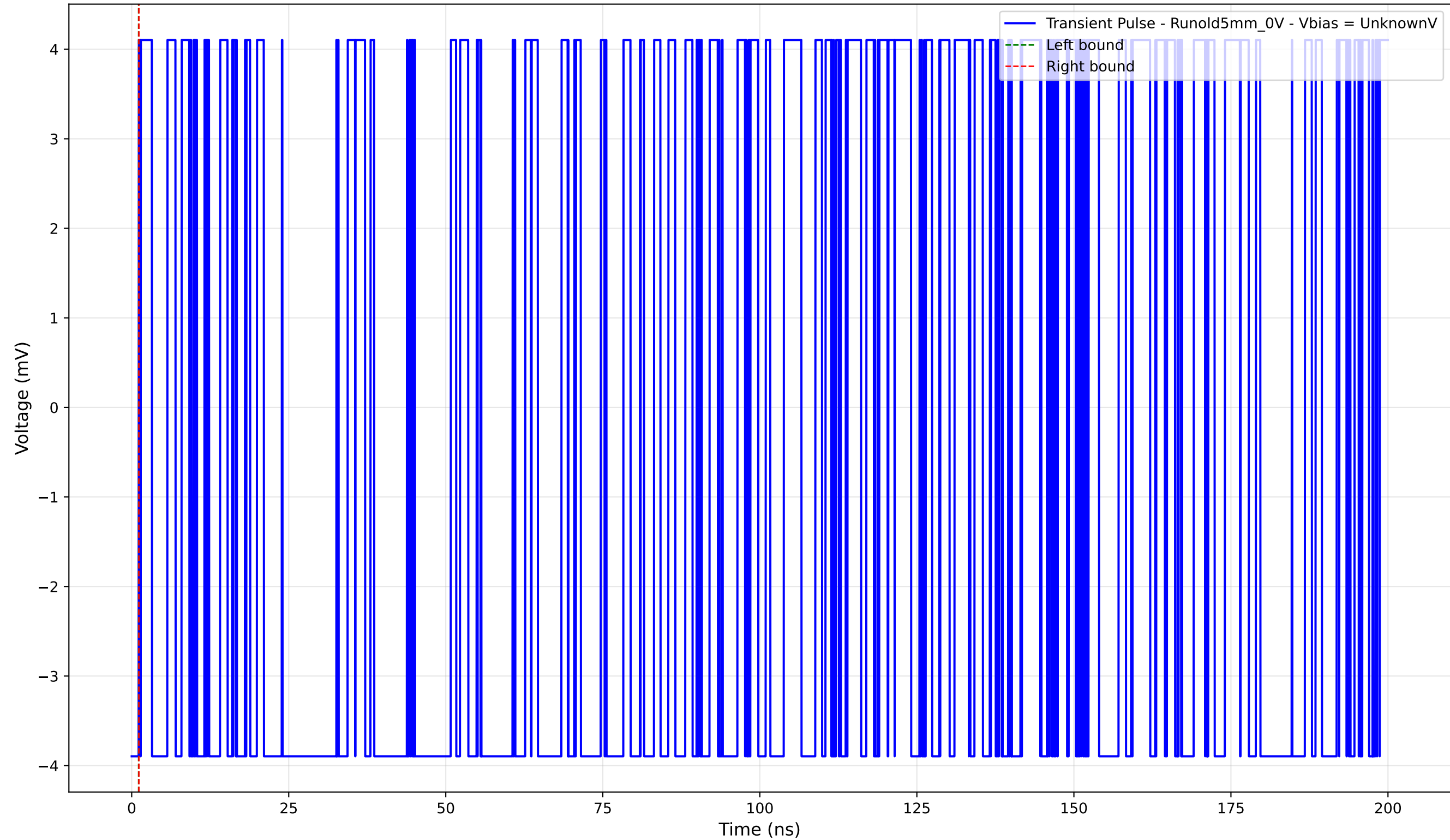
Transient Pulse - Sample: old5 - Position: 655.0 \mu\text{m} - Charge: 0.00 pC
