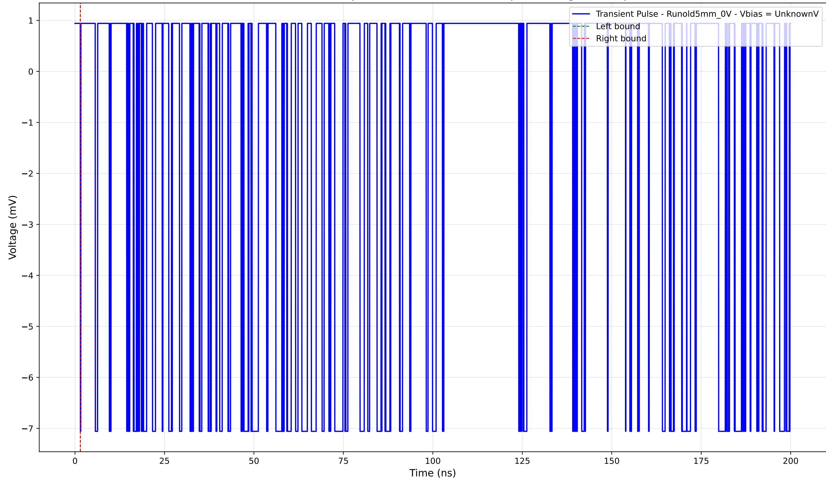
Transient Pulse - Sample: old5 - Position: 1340.0 \mu\text{m} - Charge: -0.00 pC
