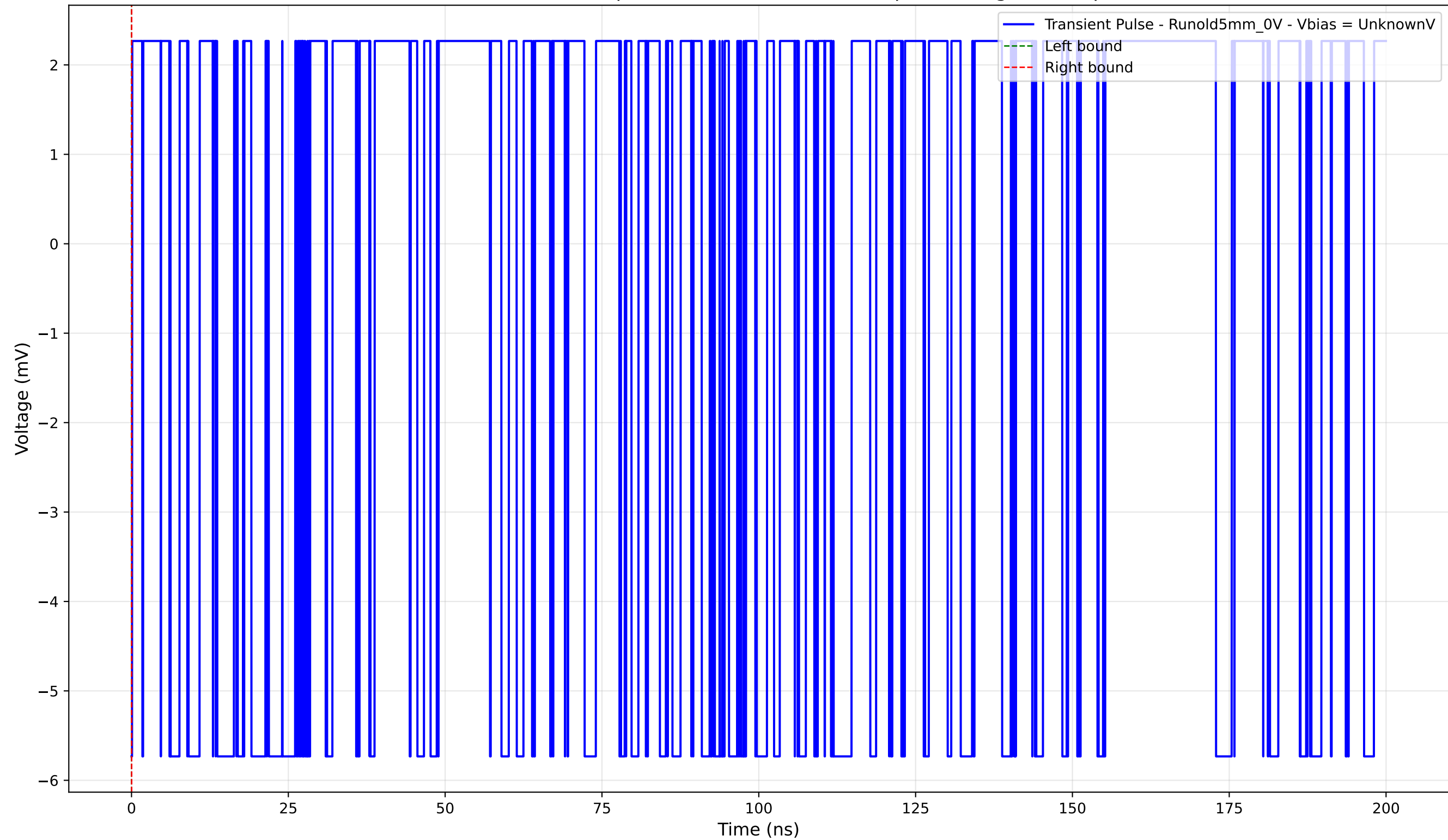
Transient Pulse - Sample: old5 - Position: 3685.0 \mu\text{m} - Charge: -0.00 pC
