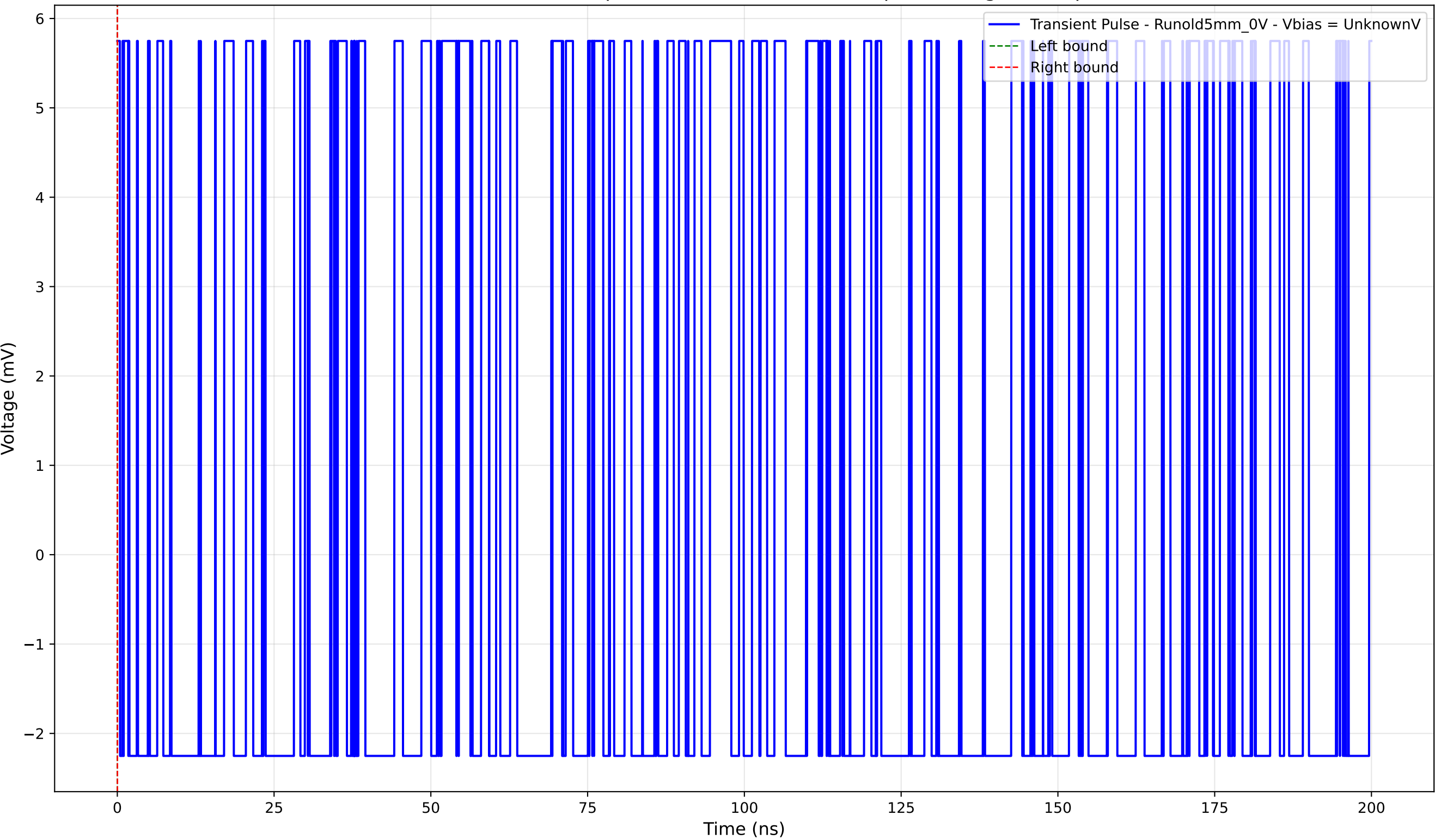
Transient Pulse - Sample: old5 - Position: 1475.0 \mu\text{m} - Charge: 0.00 pC
