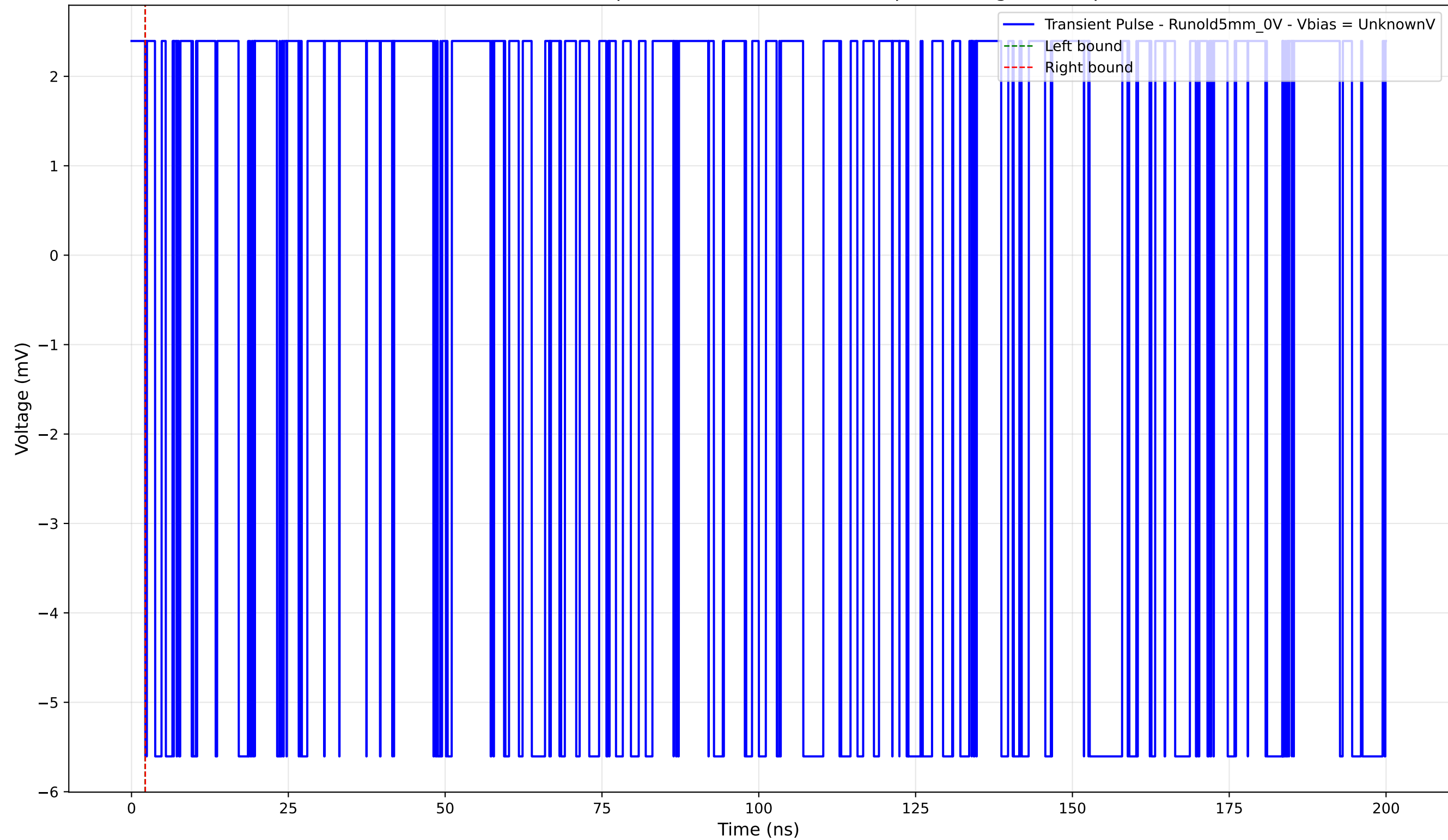
Transient Pulse - Sample: old5 - Position: 1440.0 \mu\text{m} - Charge: -0.00 pC
