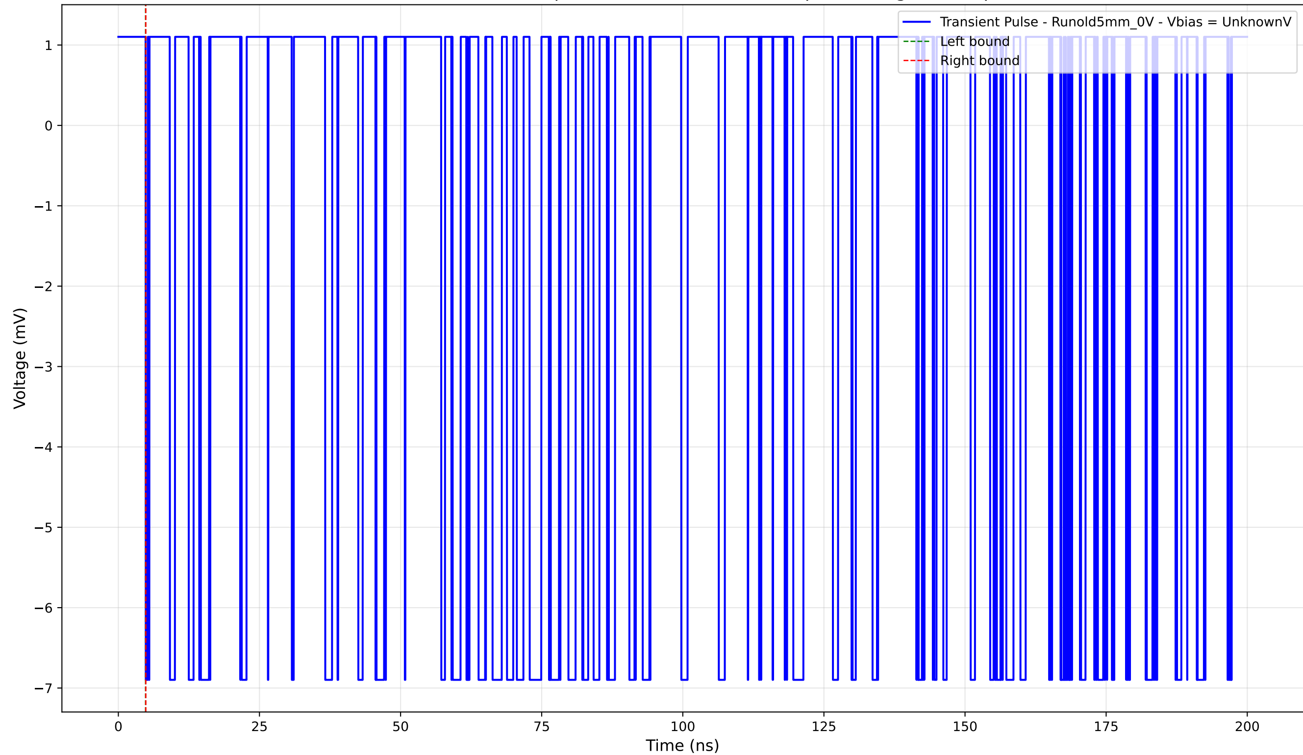
Transient Pulse - Sample: old5 - Position: 1350.0 \mu\text{m} - Charge: -0.00 pC
