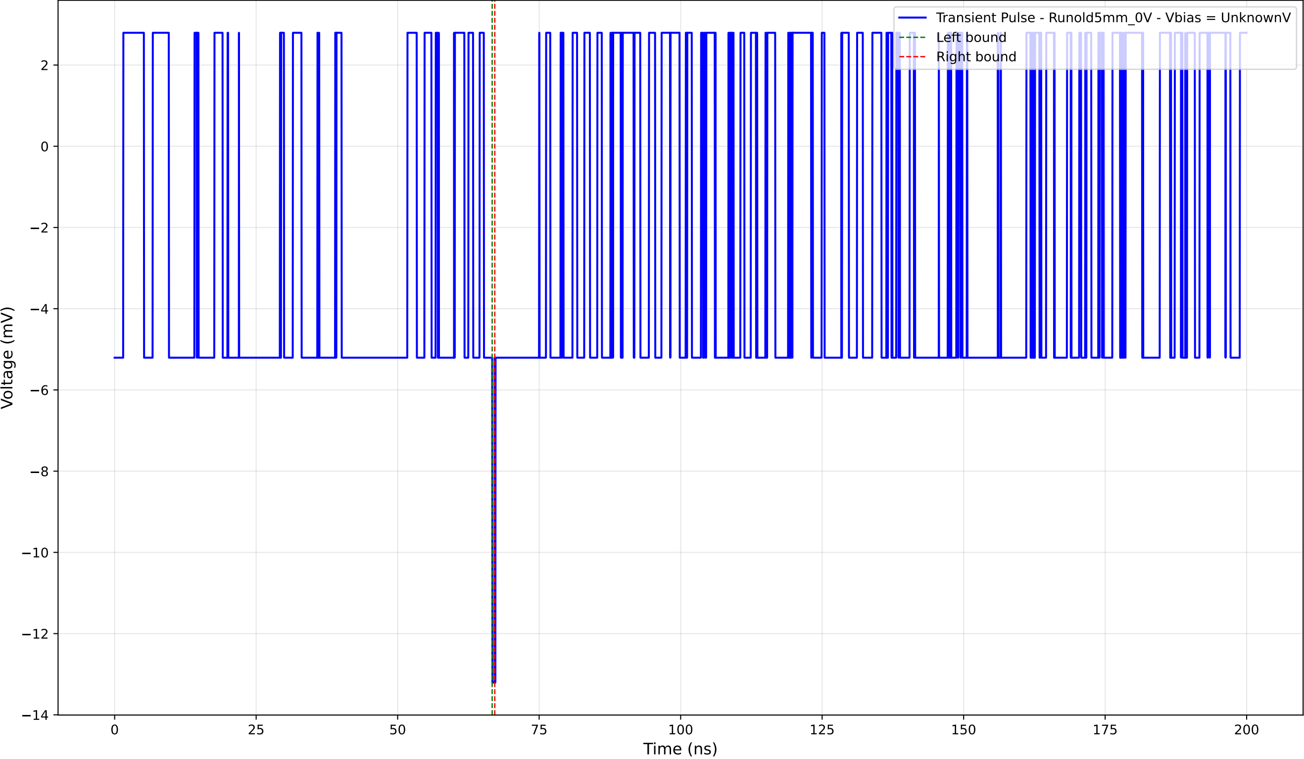
Transient Pulse - Sample: old5 - Position: 5195.0 \mu\text{m} - Charge: -0.12 pC
