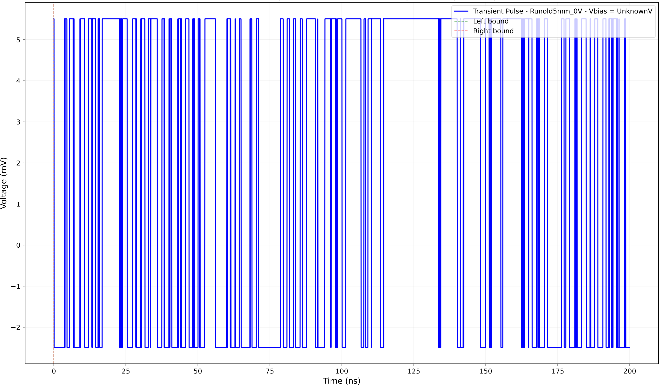
Transient Pulse - Sample: old5 - Position: 1990.0 \mu\text{m} - Charge: 0.00 pC
