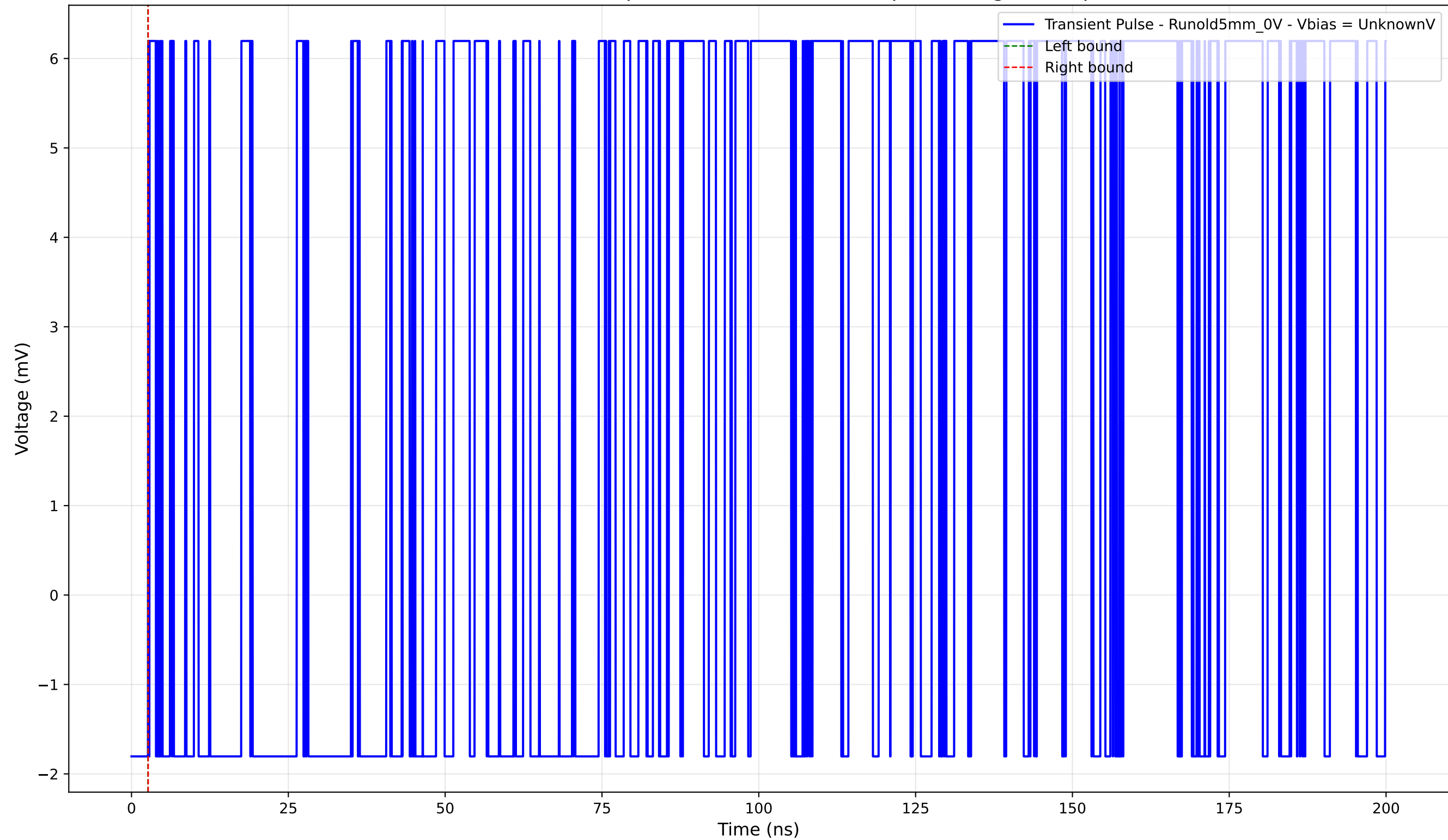
Transient Pulse - Sample: old5 - Position: 165.0 \mu\text{m} - Charge: 0.00 pC
