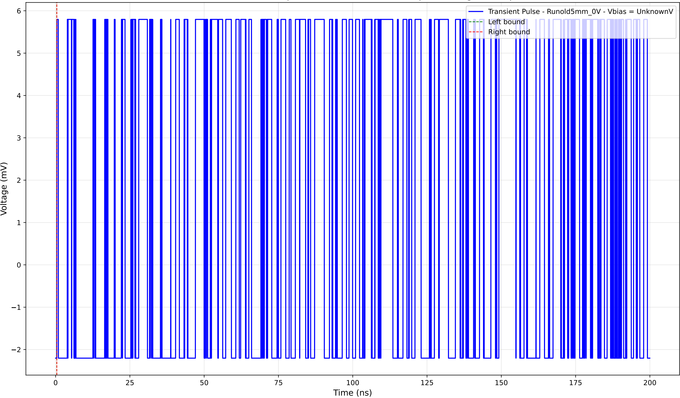
Transient Pulse - Sample: old5 - Position: 2920.0 \mu\text{m} - Charge: 0.00 pC
