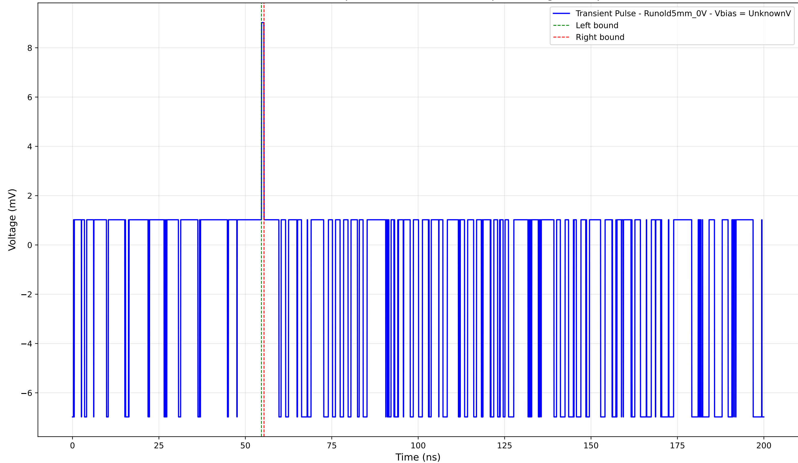
Transient Pulse - Sample: old5 - Position: 875.0 \mu\text{m} - Charge: 0.13 pC
