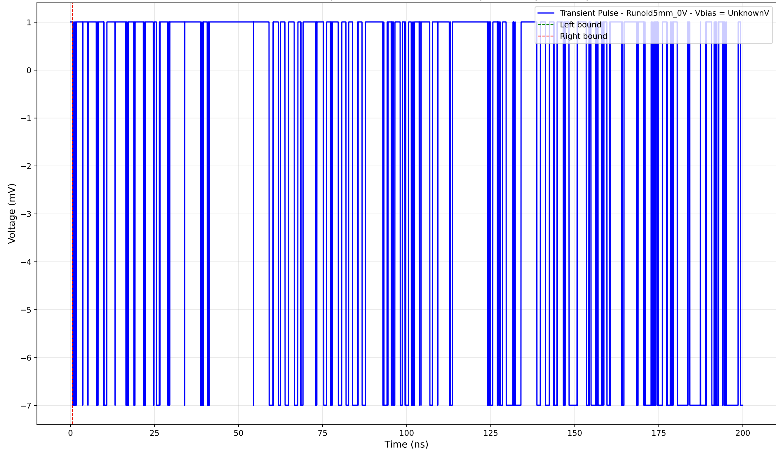
Transient Pulse - Sample: old5 - Position: 2220.0 \mu\text{m} - Charge: -0.00 pC
