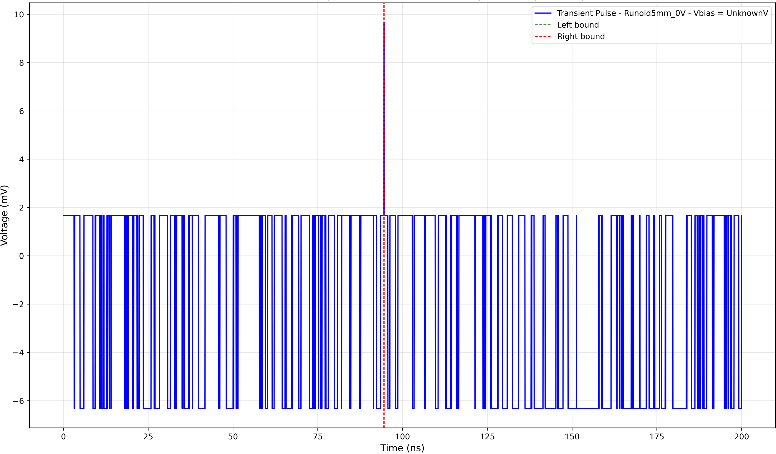
Transient Pulse - Sample: old5 - Position: 2745.0 \mu\text{m} - Charge: 0.02 pC
