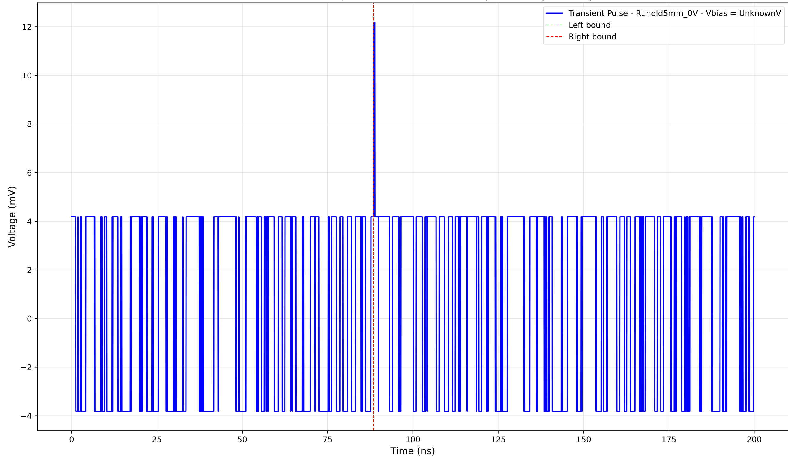
Transient Pulse - Sample: old5 - Position: 470.0 \mu\text{m} - Charge: 0.01 pC
