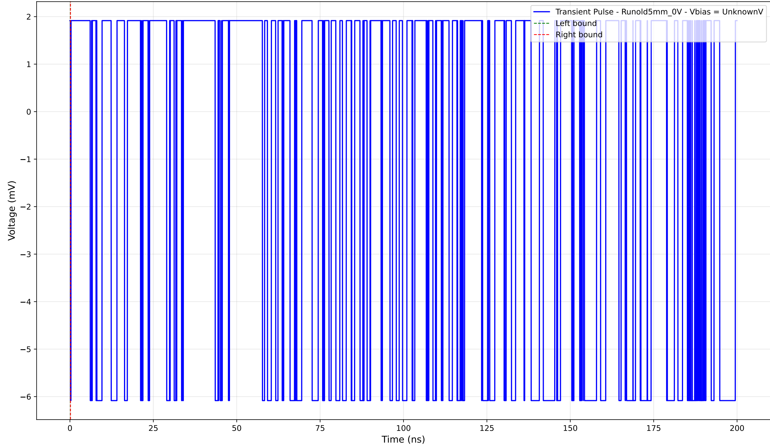
Transient Pulse - Sample: old5 - Position: 1865.0 \mu\text{m} - Charge: -0.00 pC
