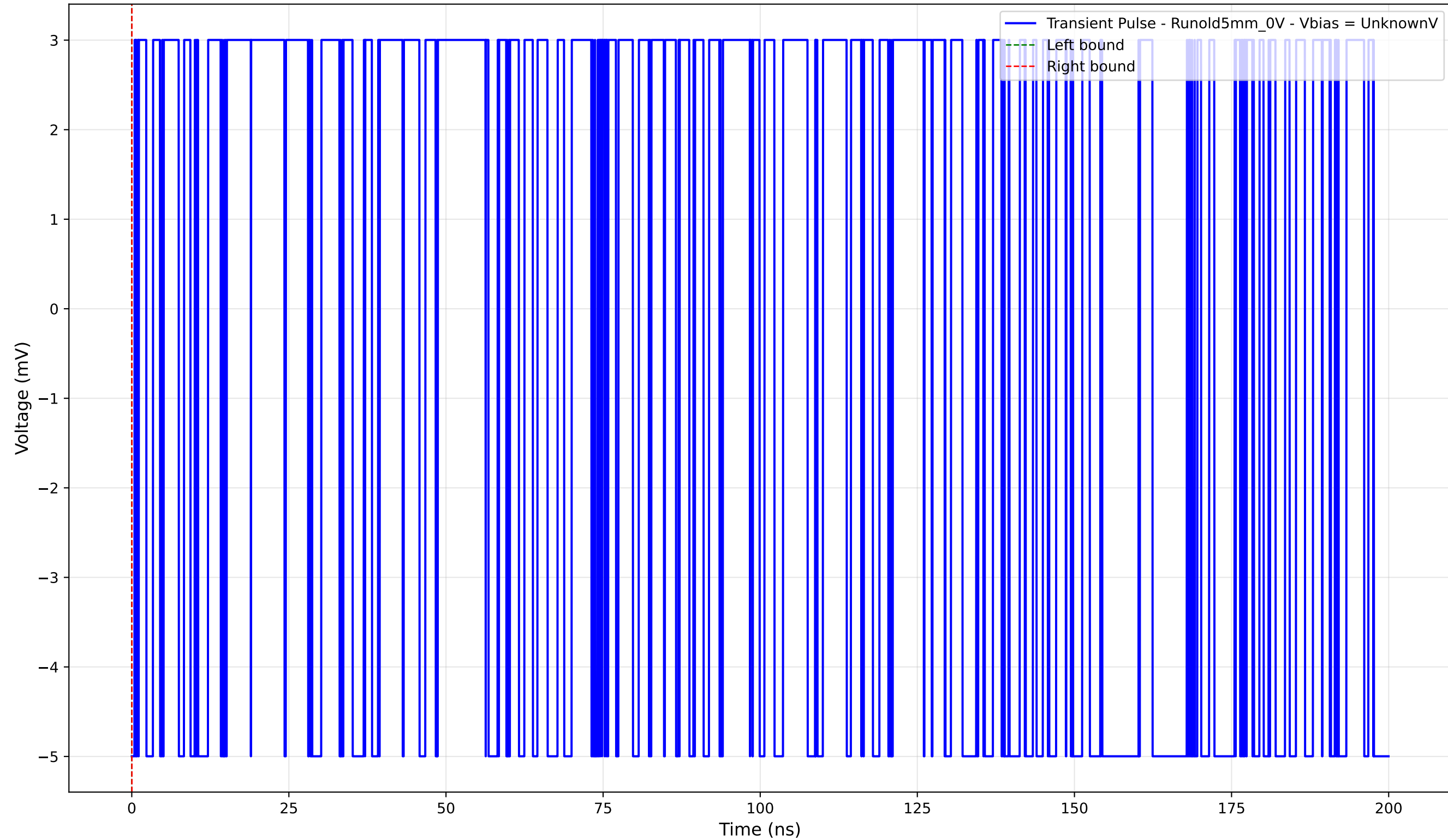
Transient Pulse - Sample: old5 - Position: 3715.0 \mu\text{m} - Charge: -0.00 pC
