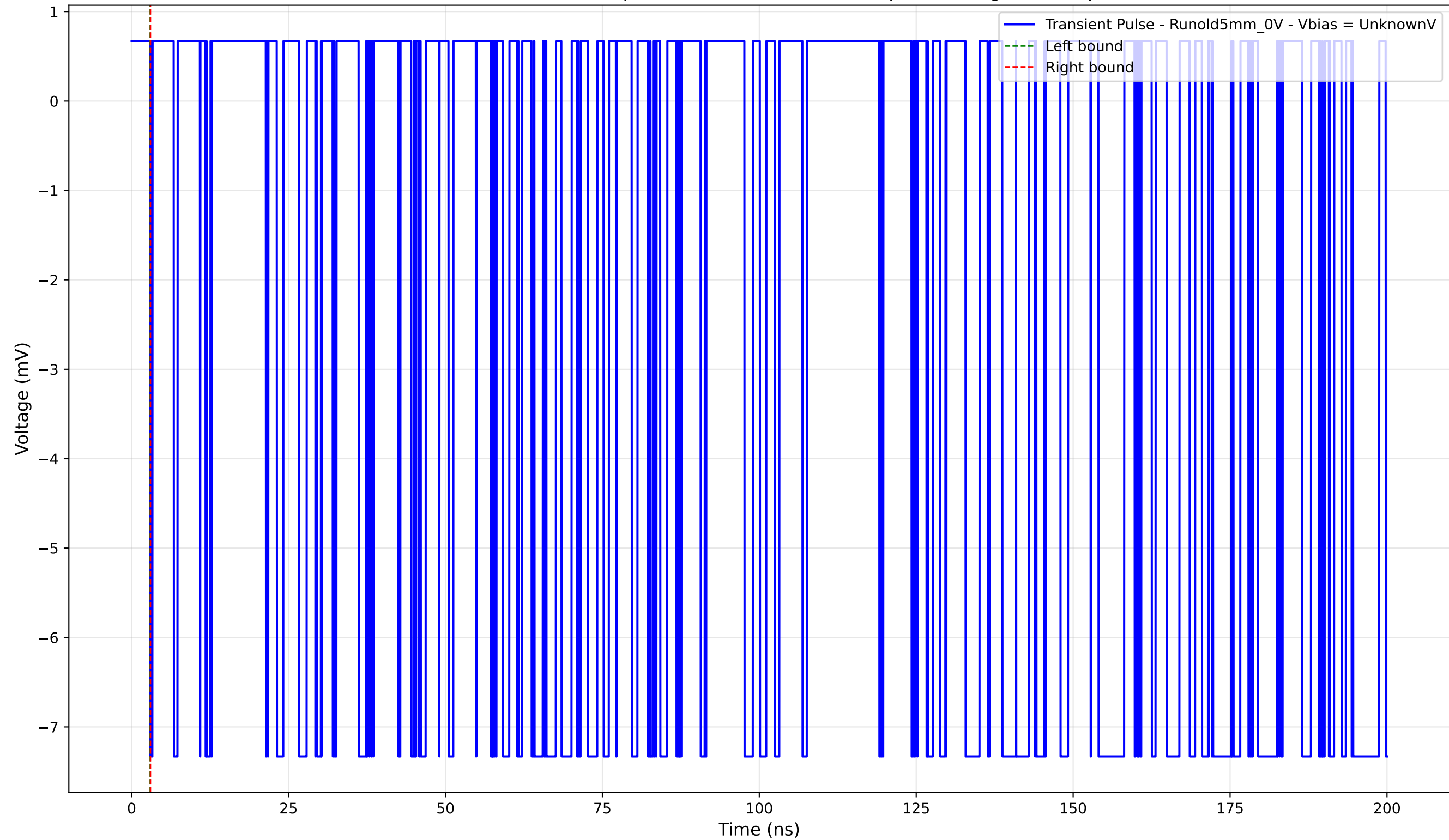
Transient Pulse - Sample: old5 - Position: 600.0 \mu\text{m} - Charge: -0.00 pC
