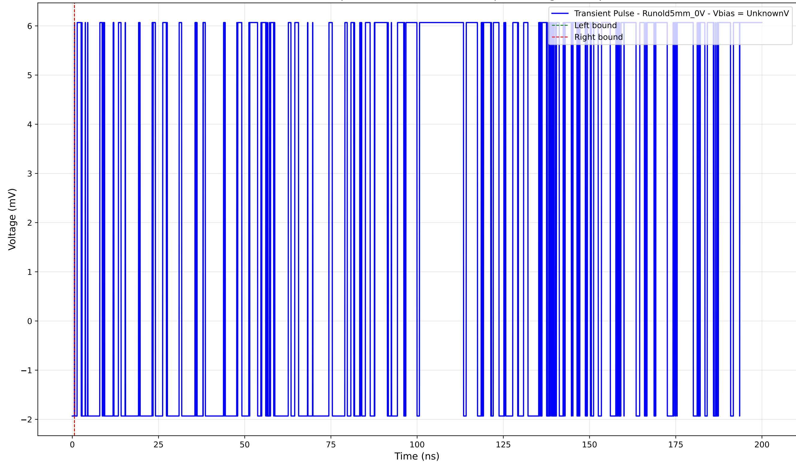
Transient Pulse - Sample: old5 - Position: 1800.0 \mu\text{m} - Charge: 0.00 pC
