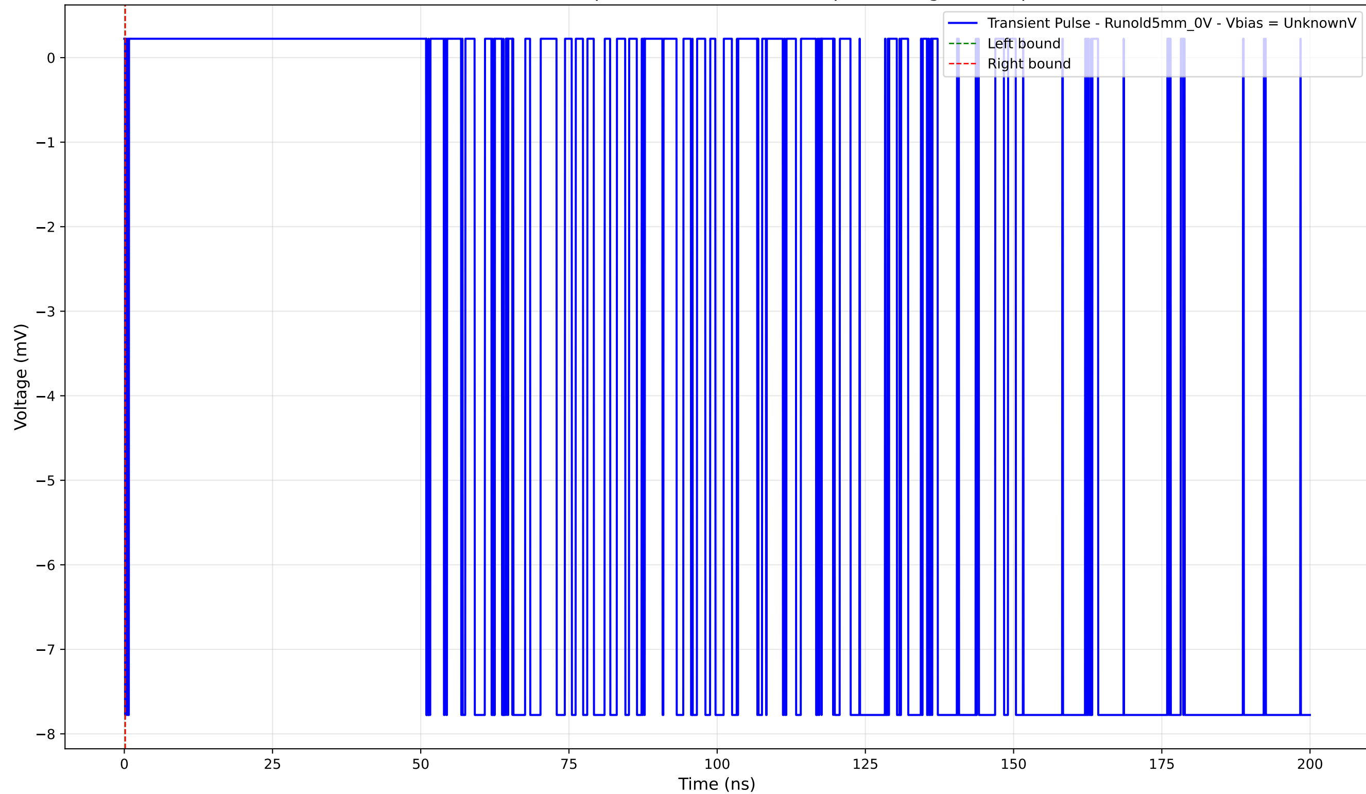
Transient Pulse - Sample: old5 - Position: 45.0 \mu\text{m} - Charge: -0.00 pC
