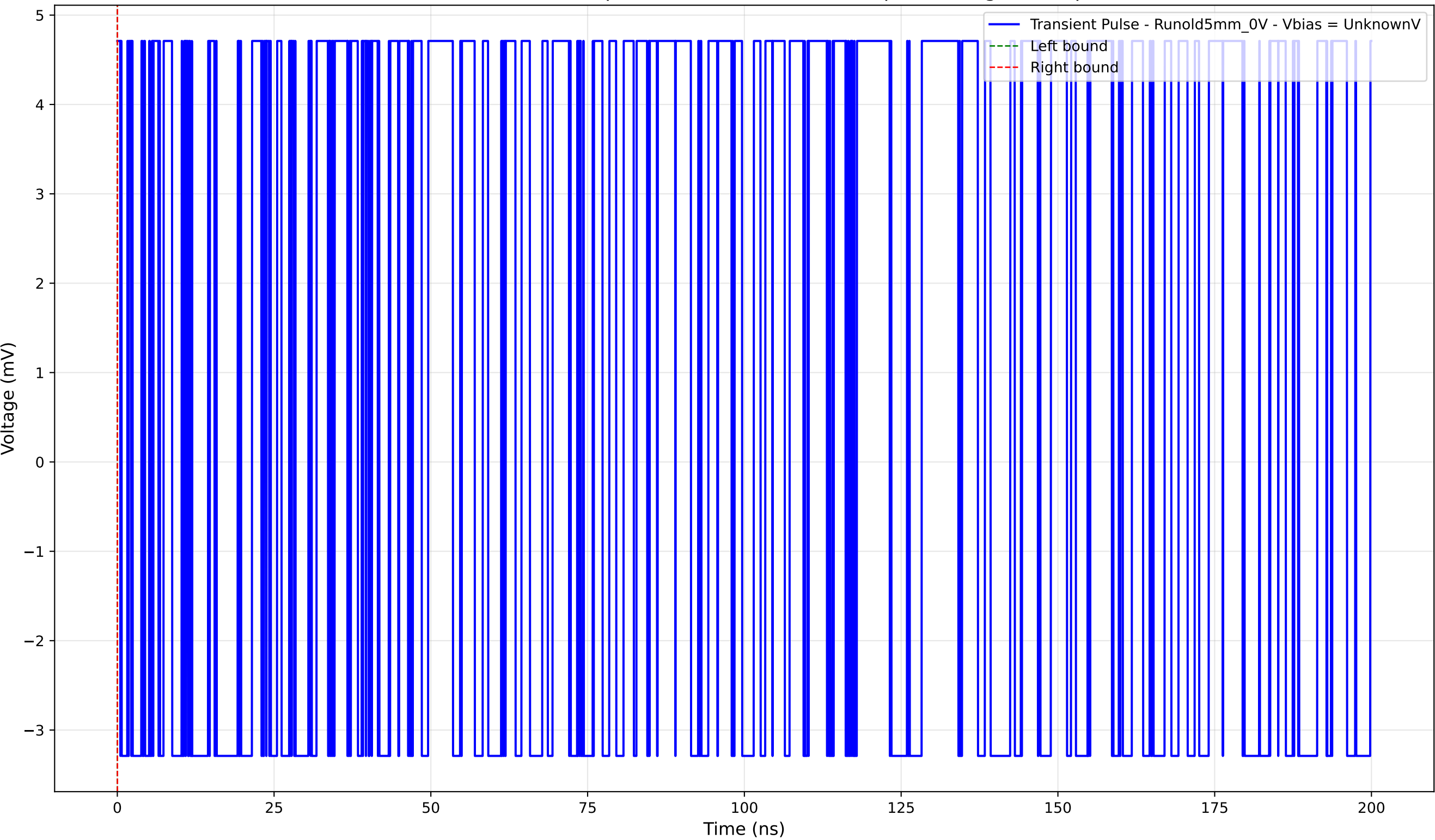
Transient Pulse - Sample: old5 - Position: 3785.0 \mu\text{m} - Charge: 0.00 pC
