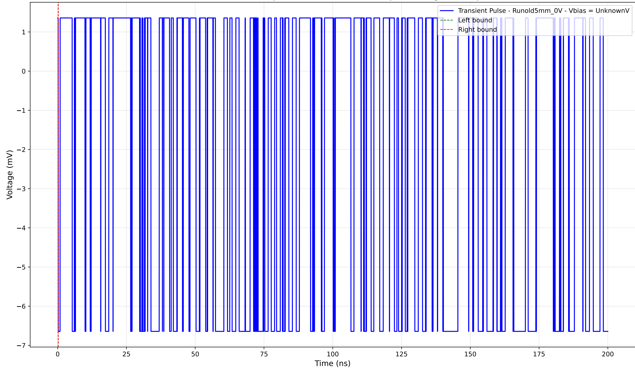
Transient Pulse - Sample: old5 - Position: 520.0 \mu\text{m} - Charge: -0.00 pC
