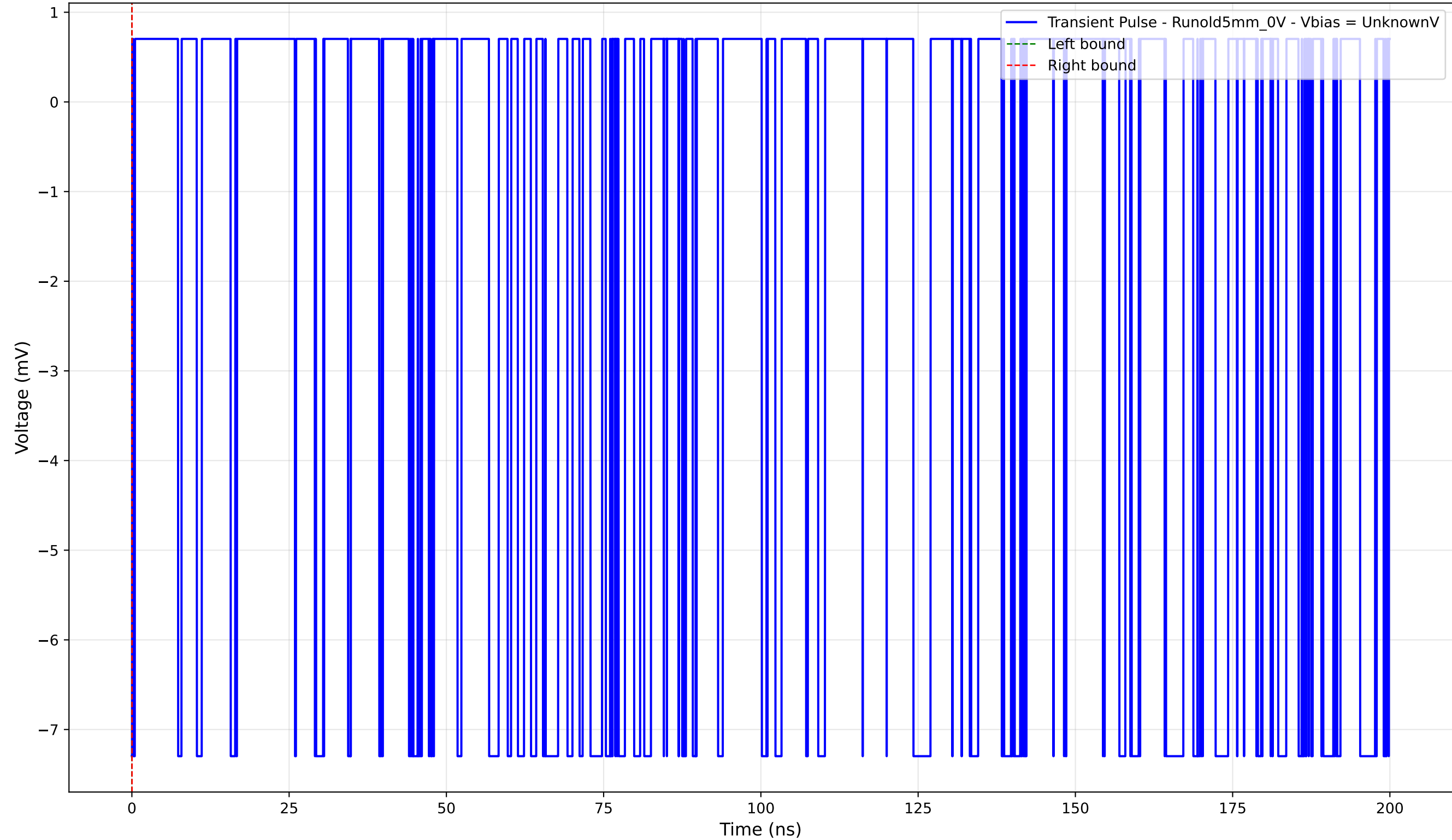
Transient Pulse - Sample: old5 - Position: 1325.0 \mu\text{m} - Charge: -0.00 pC
