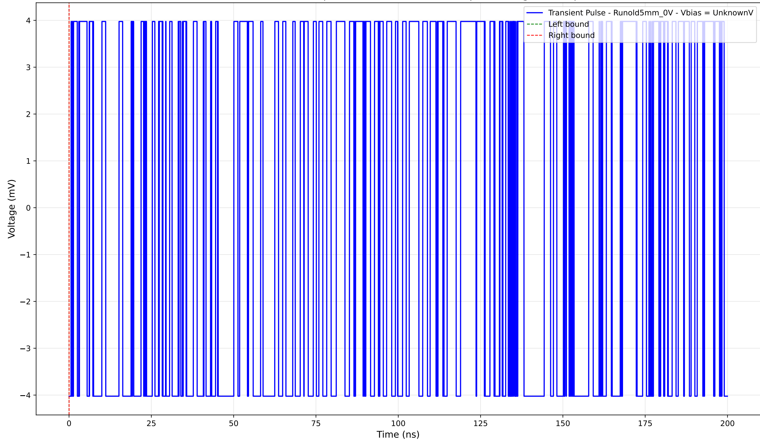
Transient Pulse - Sample: old5 - Position: 4355.0 \mu\text{m} - Charge: -0.00 pC
