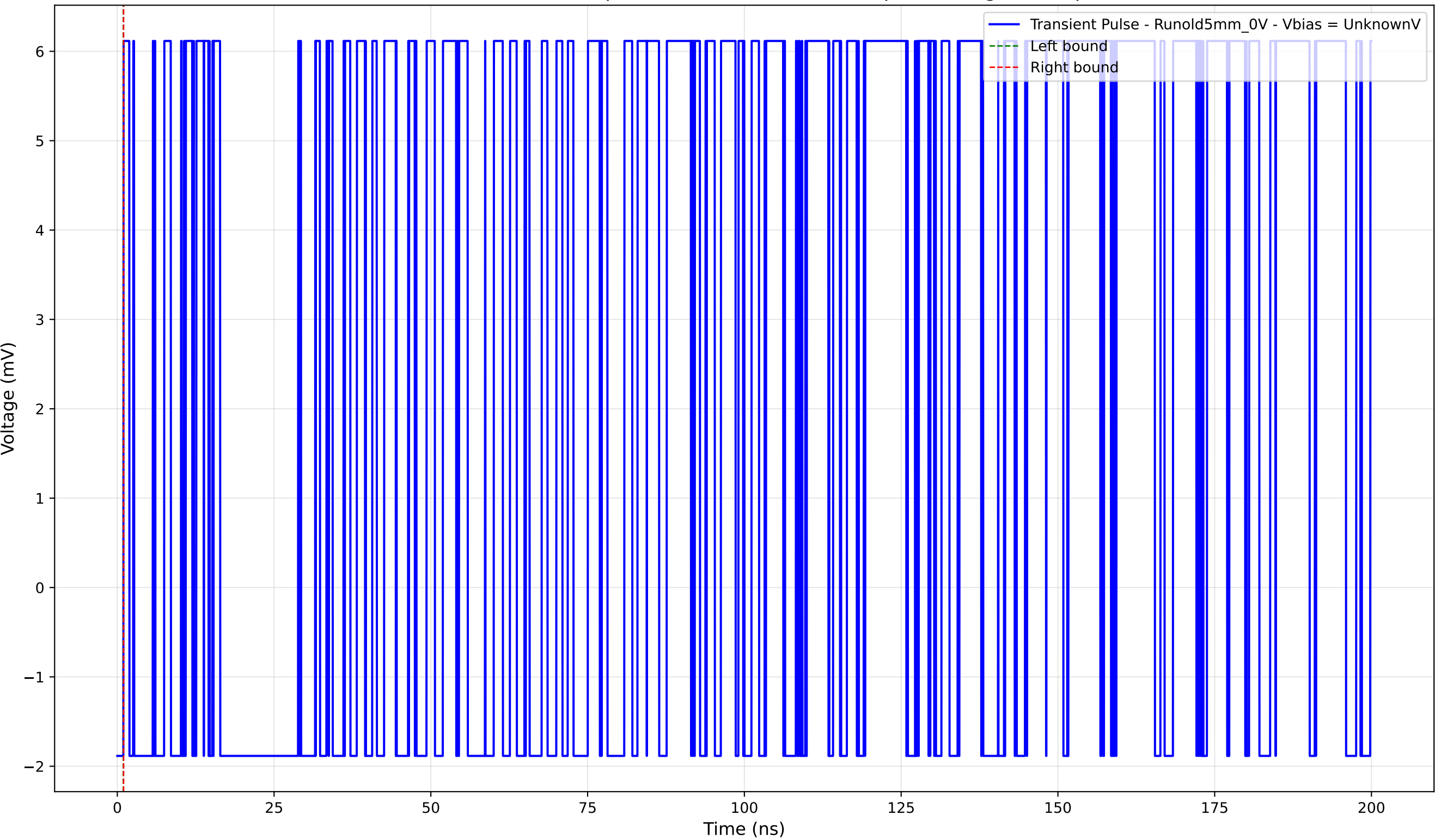
Transient Pulse - Sample: old5 - Position: 3580.0 \mu\text{m} - Charge: 0.00 pC
