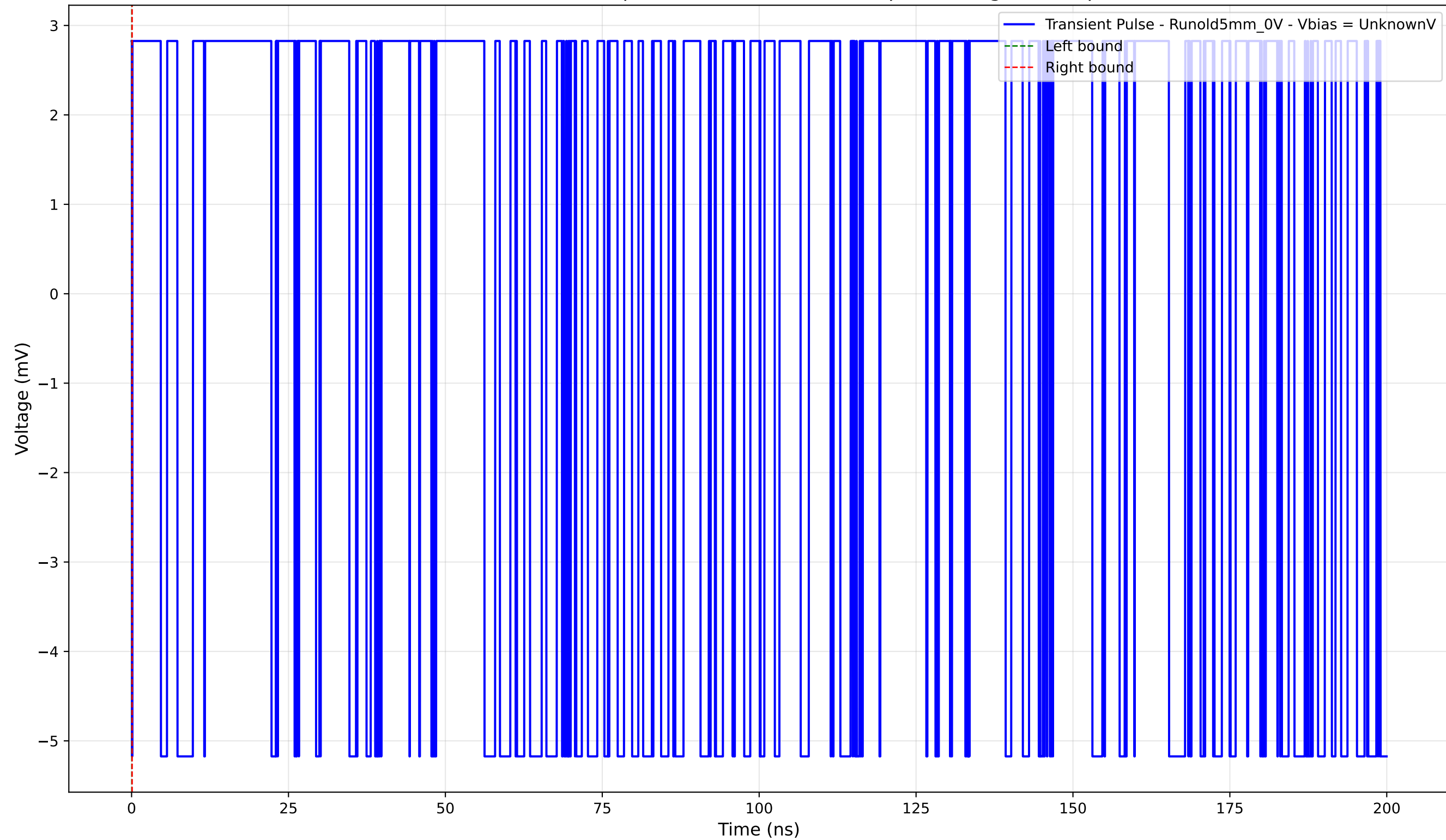
Transient Pulse - Sample: old5 - Position: 290.0 \mu\text{m} - Charge: -0.00 pC
