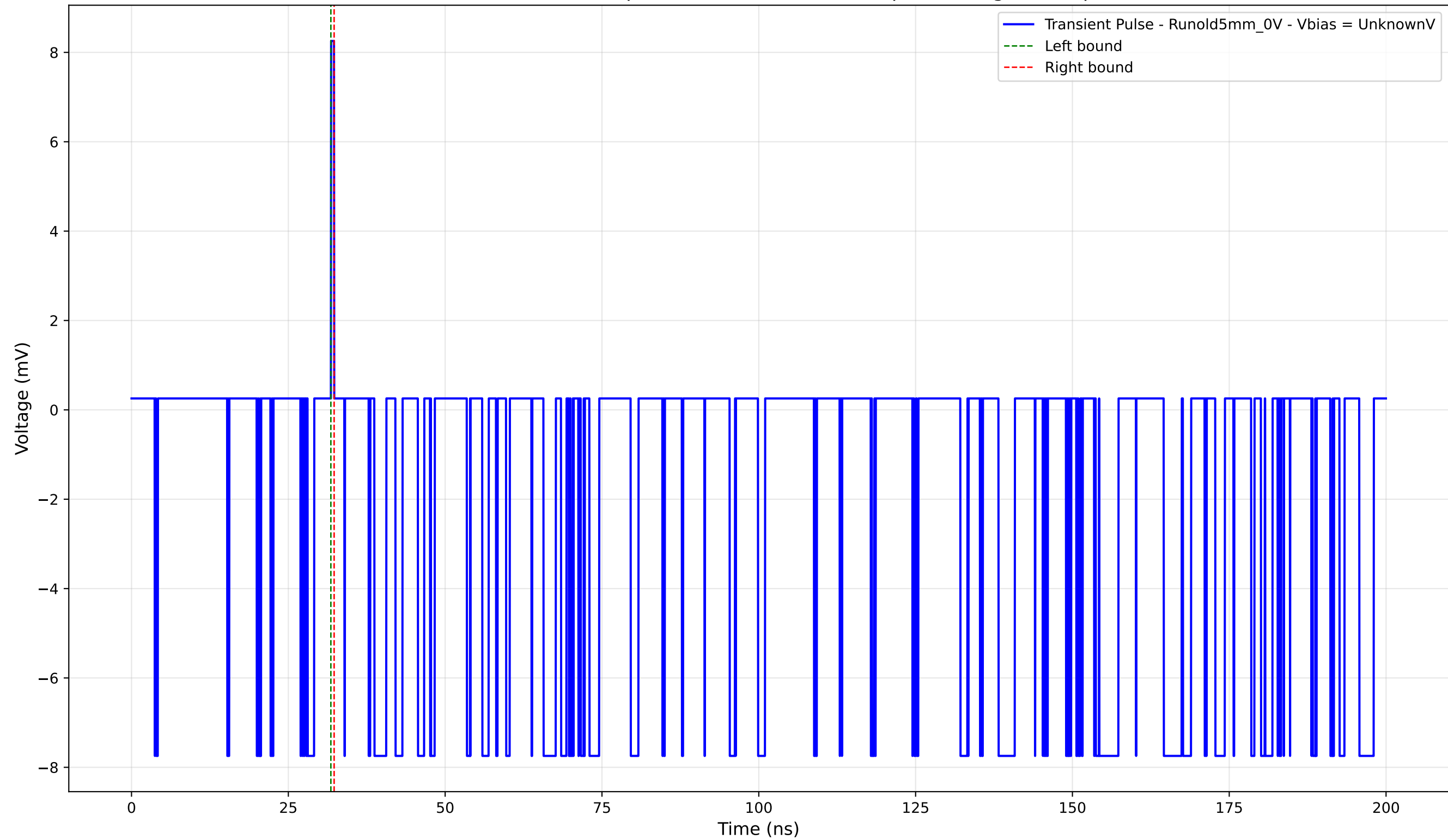
Transient Pulse - Sample: old5 - Position: 855.0 \mu\text{m} - Charge: 0.08 pC
