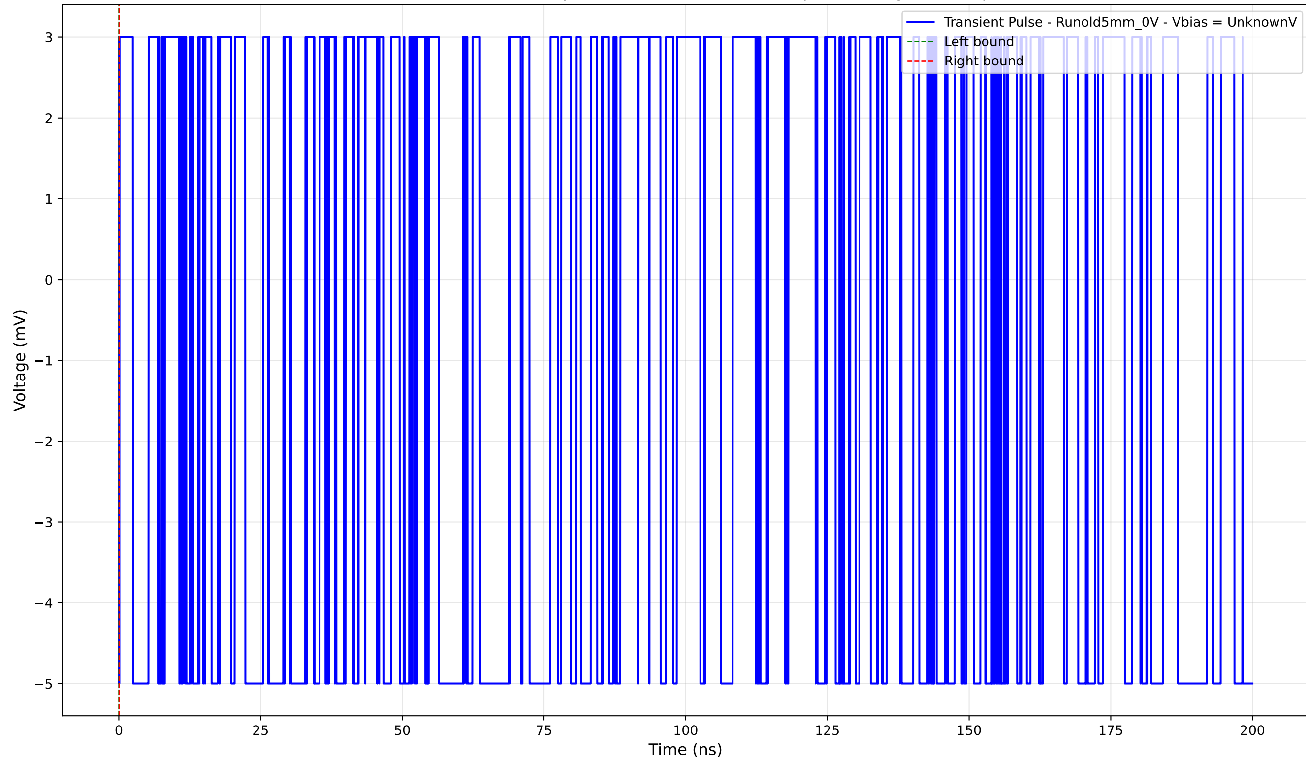
Transient Pulse - Sample: old5 - Position: 330.0 \mu\text{m} - Charge: -0.00 pC
