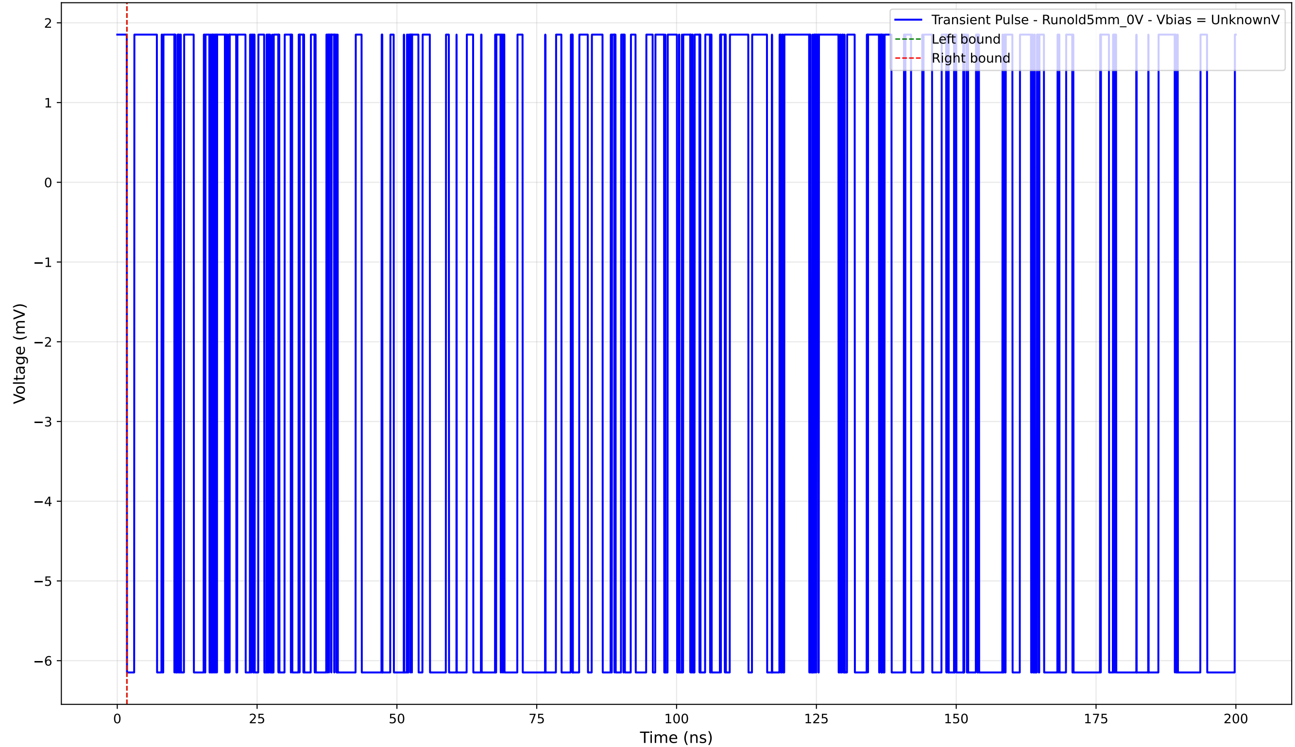
Transient Pulse - Sample: old5 - Position: 4250.0 \mu\text{m} - Charge: -0.00 pC
