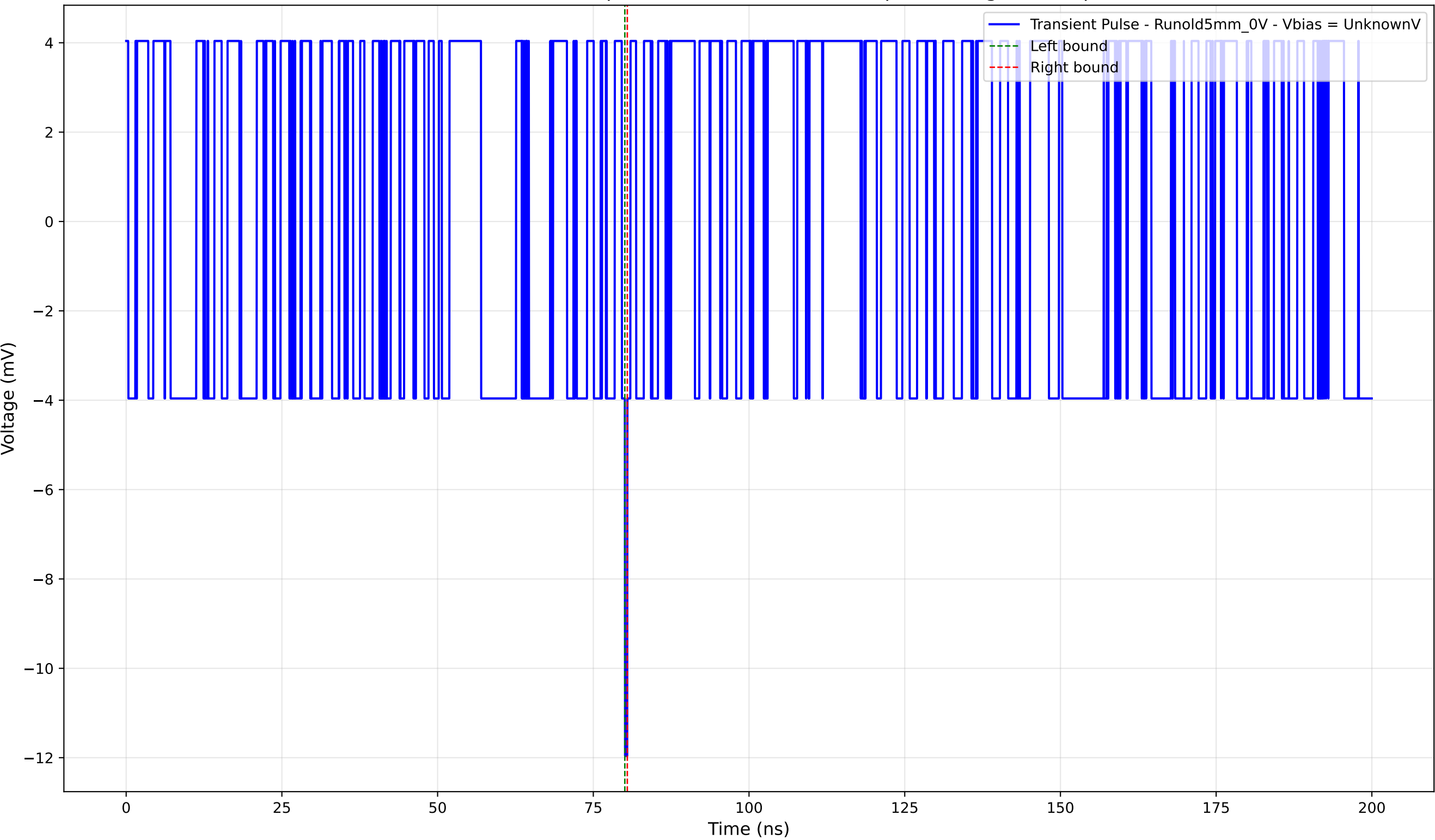
Transient Pulse - Sample: old5 - Position: 1950.0 \mu\text{m} - Charge: -0.09 pC
