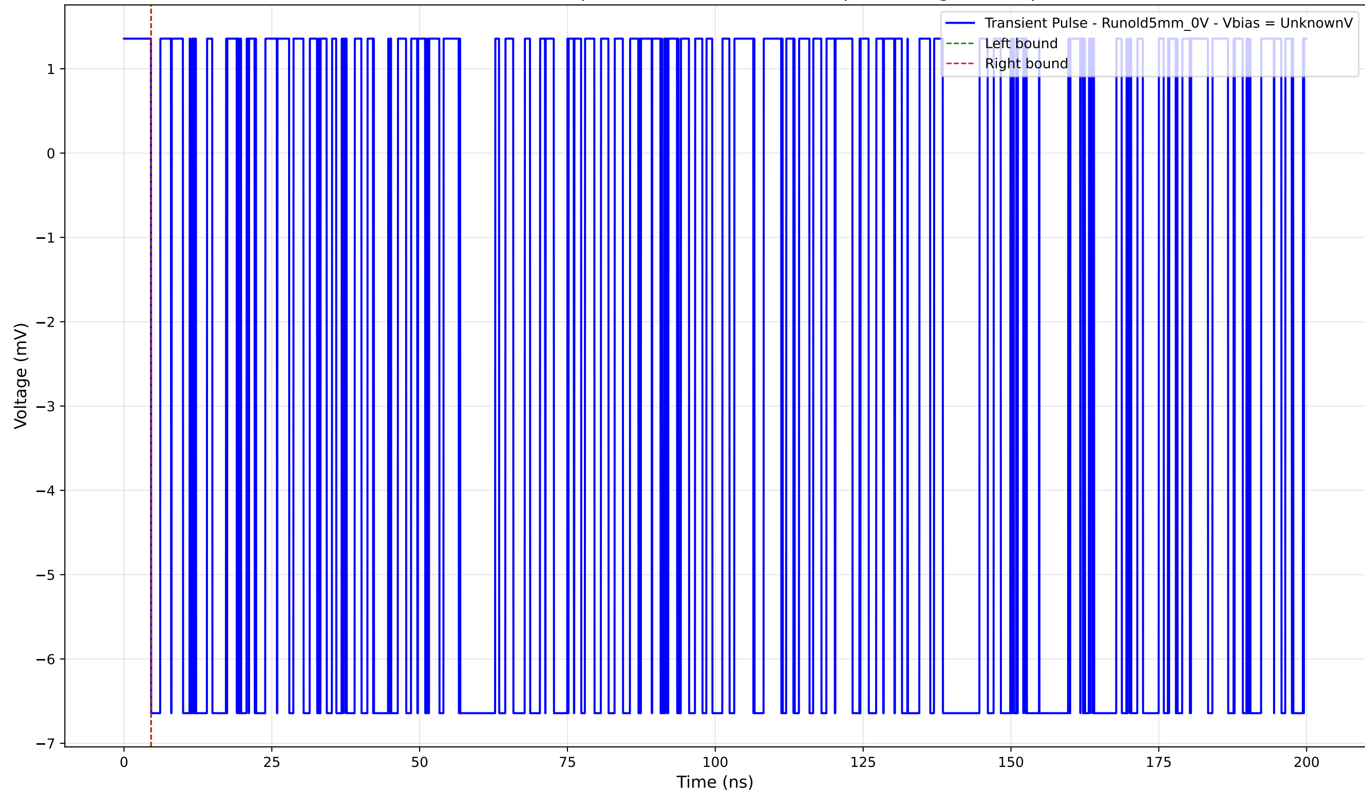
Transient Pulse - Sample: old5 - Position: 2460.0 \mu\text{m} - Charge: -0.00 pC
