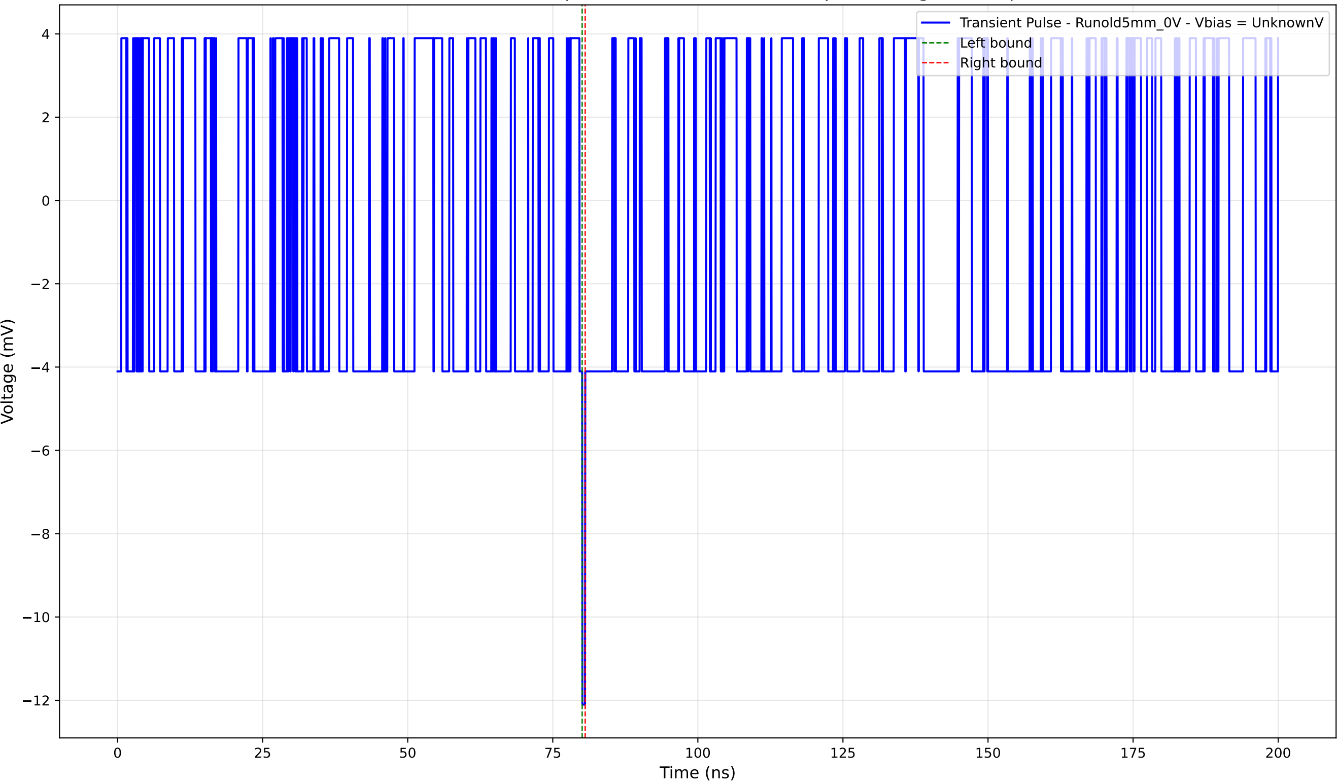
Transient Pulse - Sample: old5 - Position: 4205.0 \mu\text{m} - Charge: -0.12 pC
