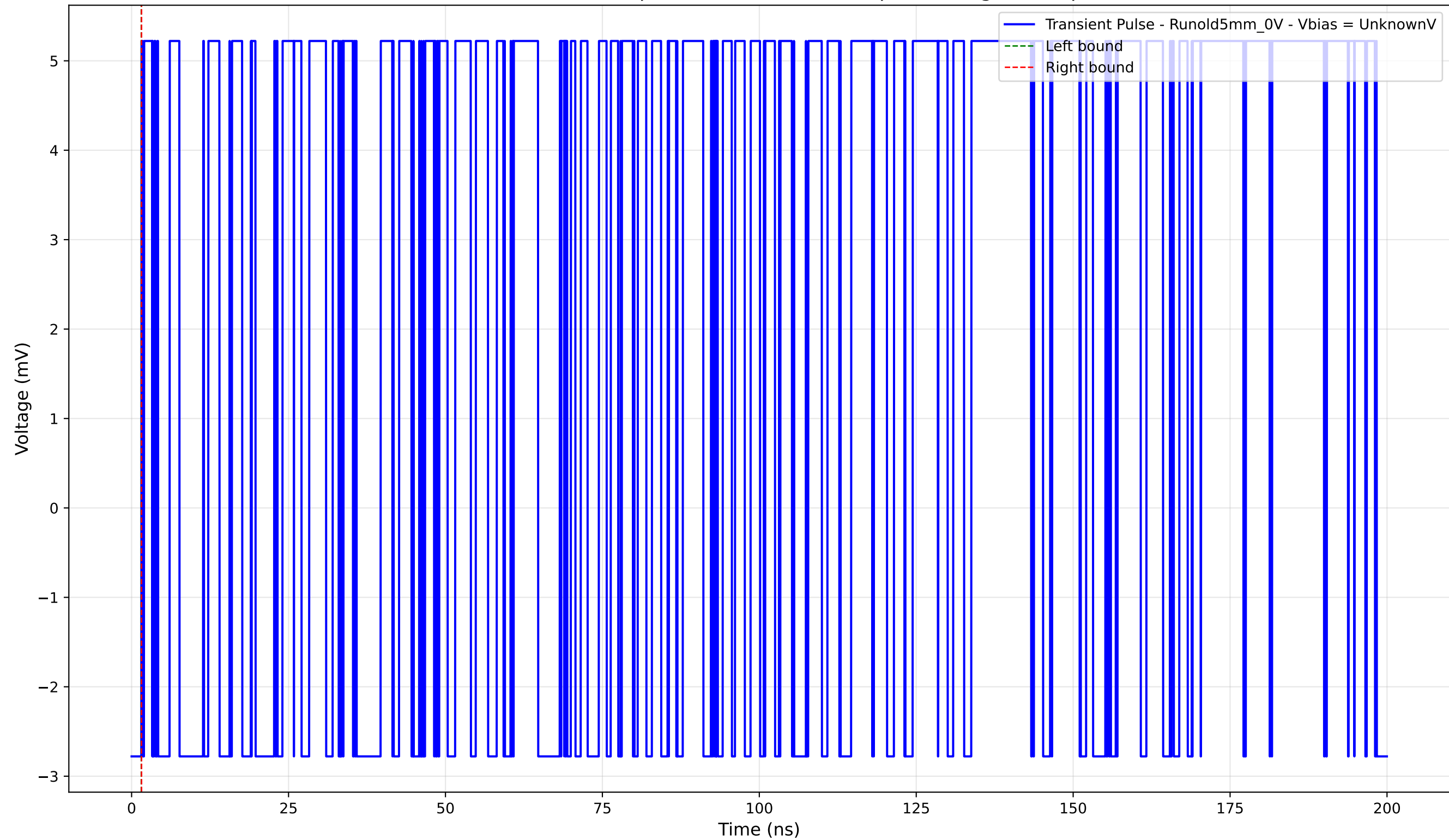
Transient Pulse - Sample: old5 - Position: 0.0 \mu\text{m} - Charge: 0.00 pC
