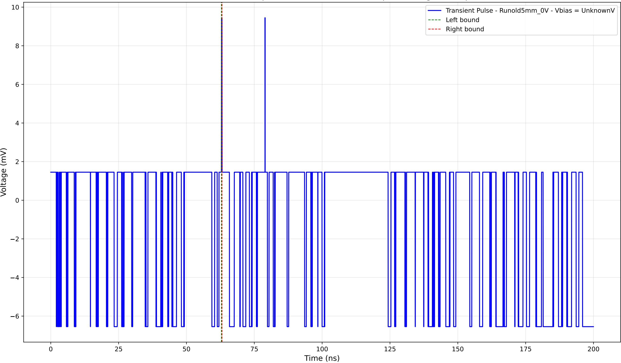
Transient Pulse - Sample: old5 - Position: 4740.0 \mu\text{m} - Charge: 0.04 pC
