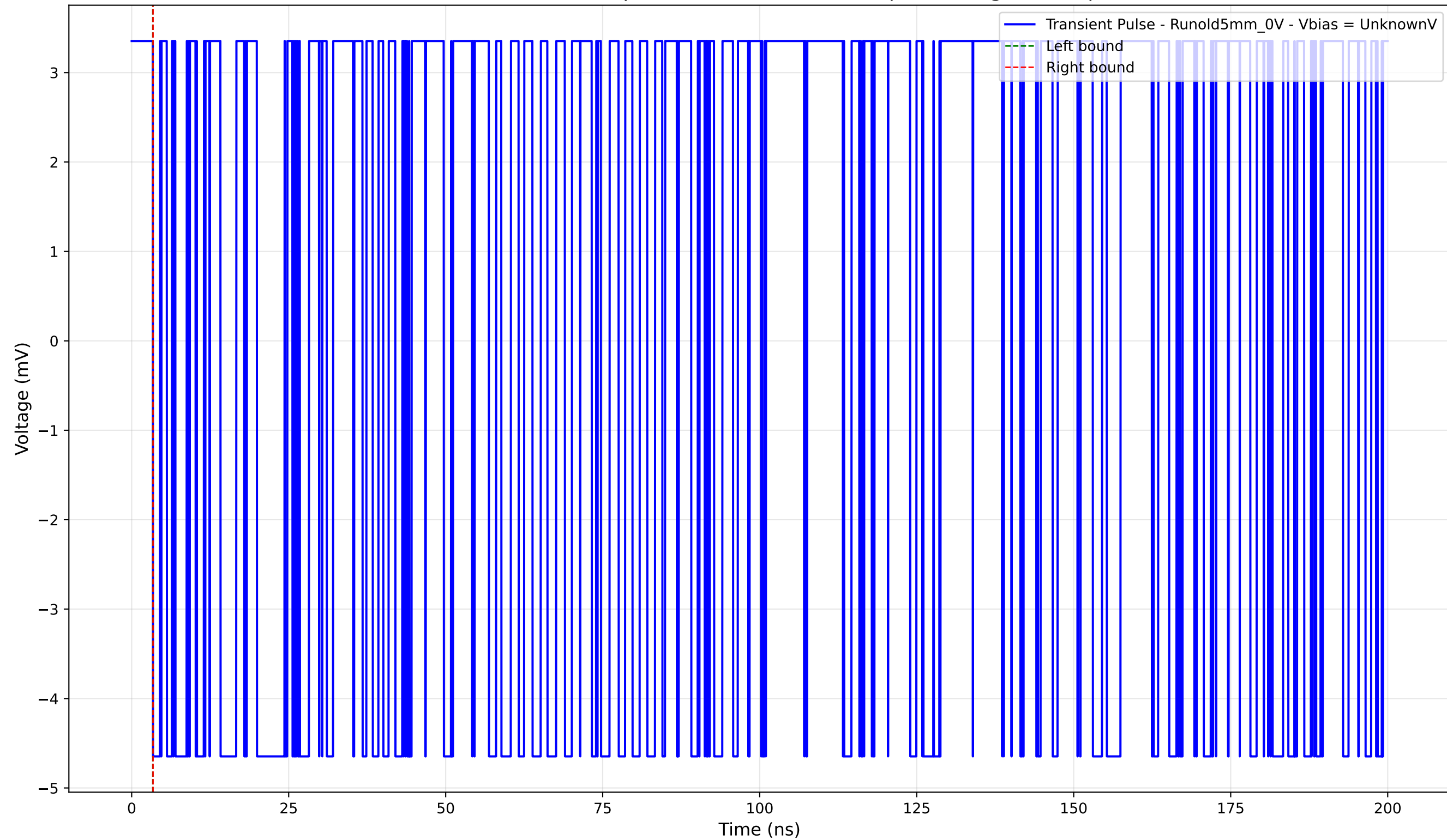
Transient Pulse - Sample: old5 - Position: 315.0 \mu\text{m} - Charge: -0.00 pC
