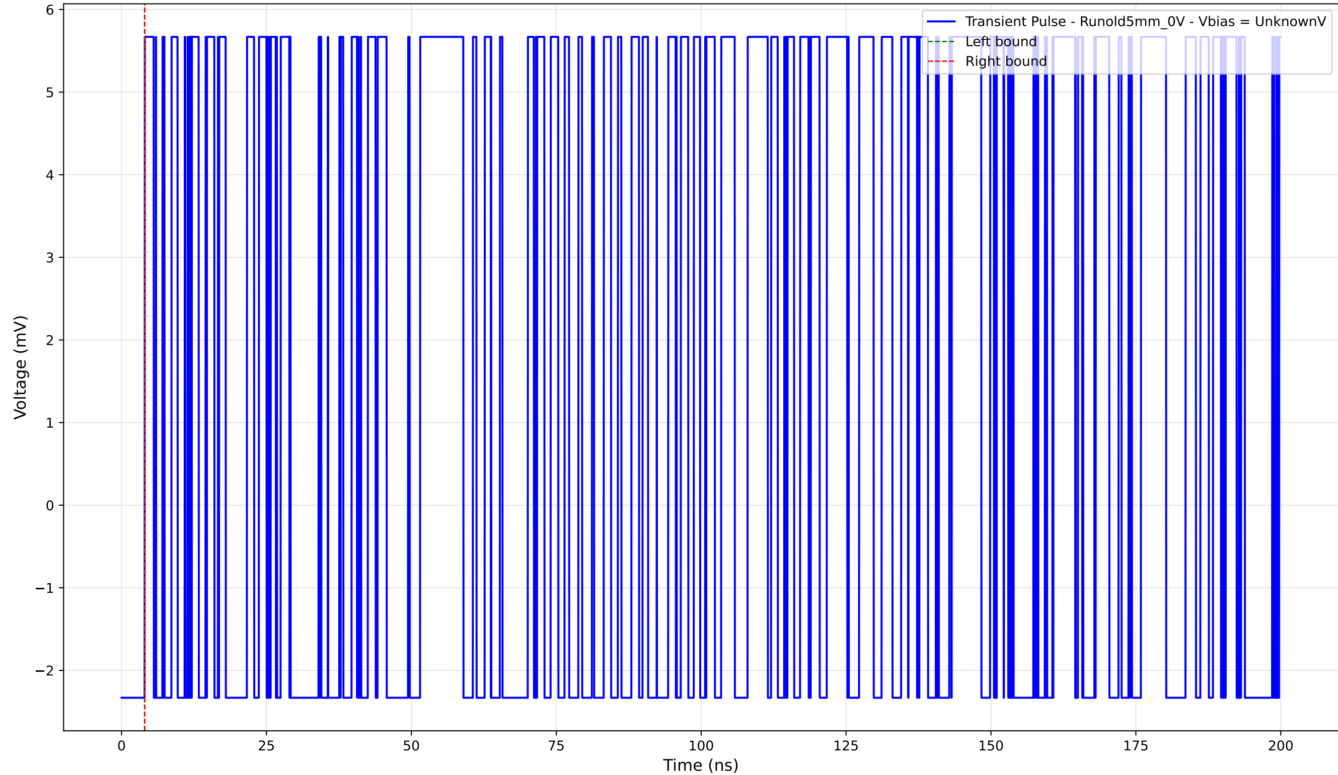
Transient Pulse - Sample: old5 - Position: 1185.0 \mu\text{m} - Charge: 0.00 pC
