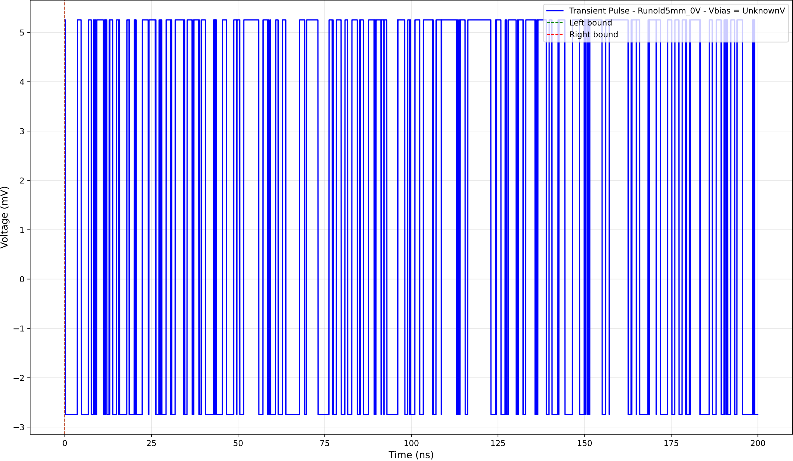
Transient Pulse - Sample: old5 - Position: 2145.0 \mu\text{m} - Charge: 0.00 pC
