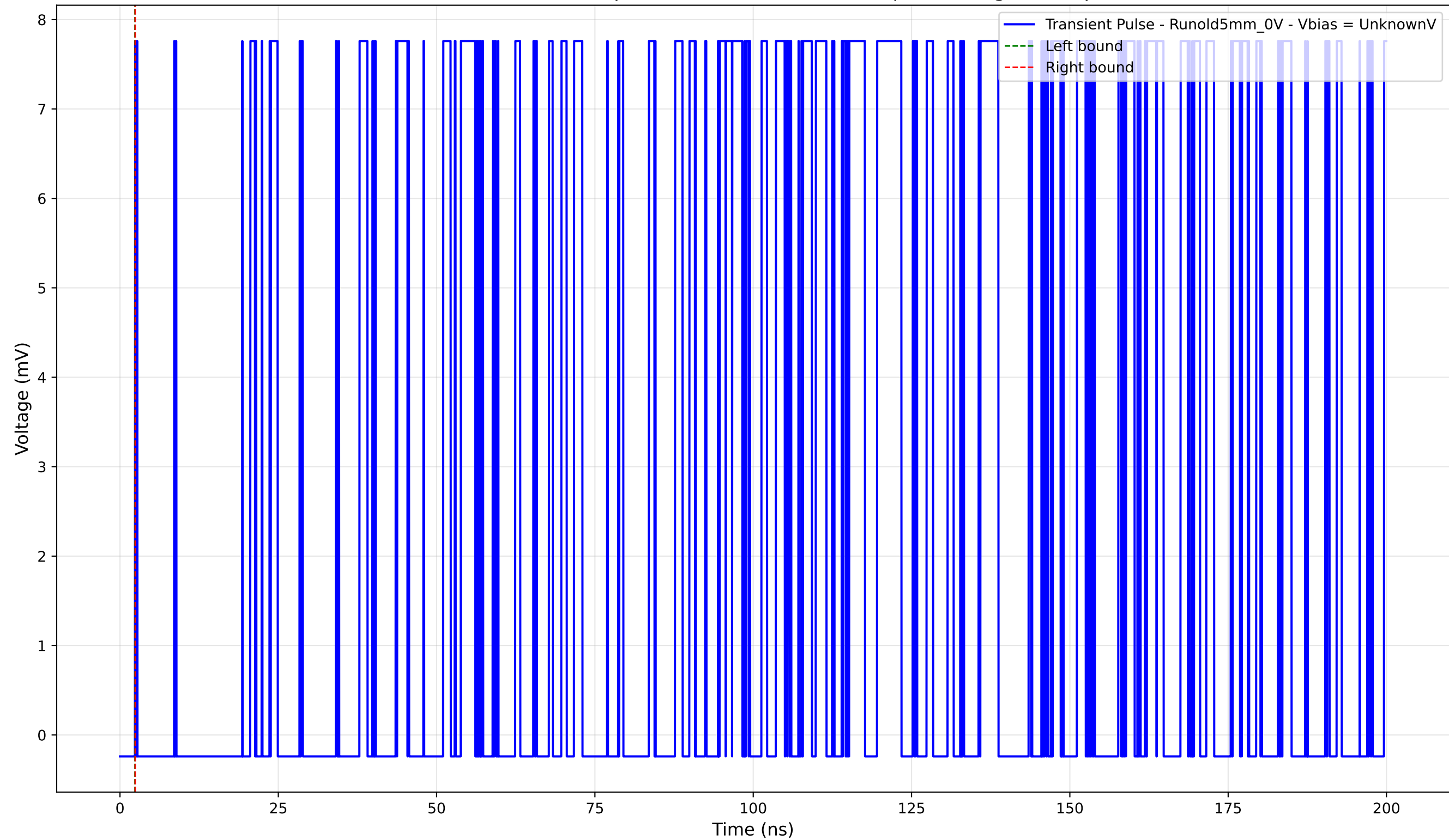
Transient Pulse - Sample: old5 - Position: 5130.0 \mu\text{m} - Charge: 0.00 pC
