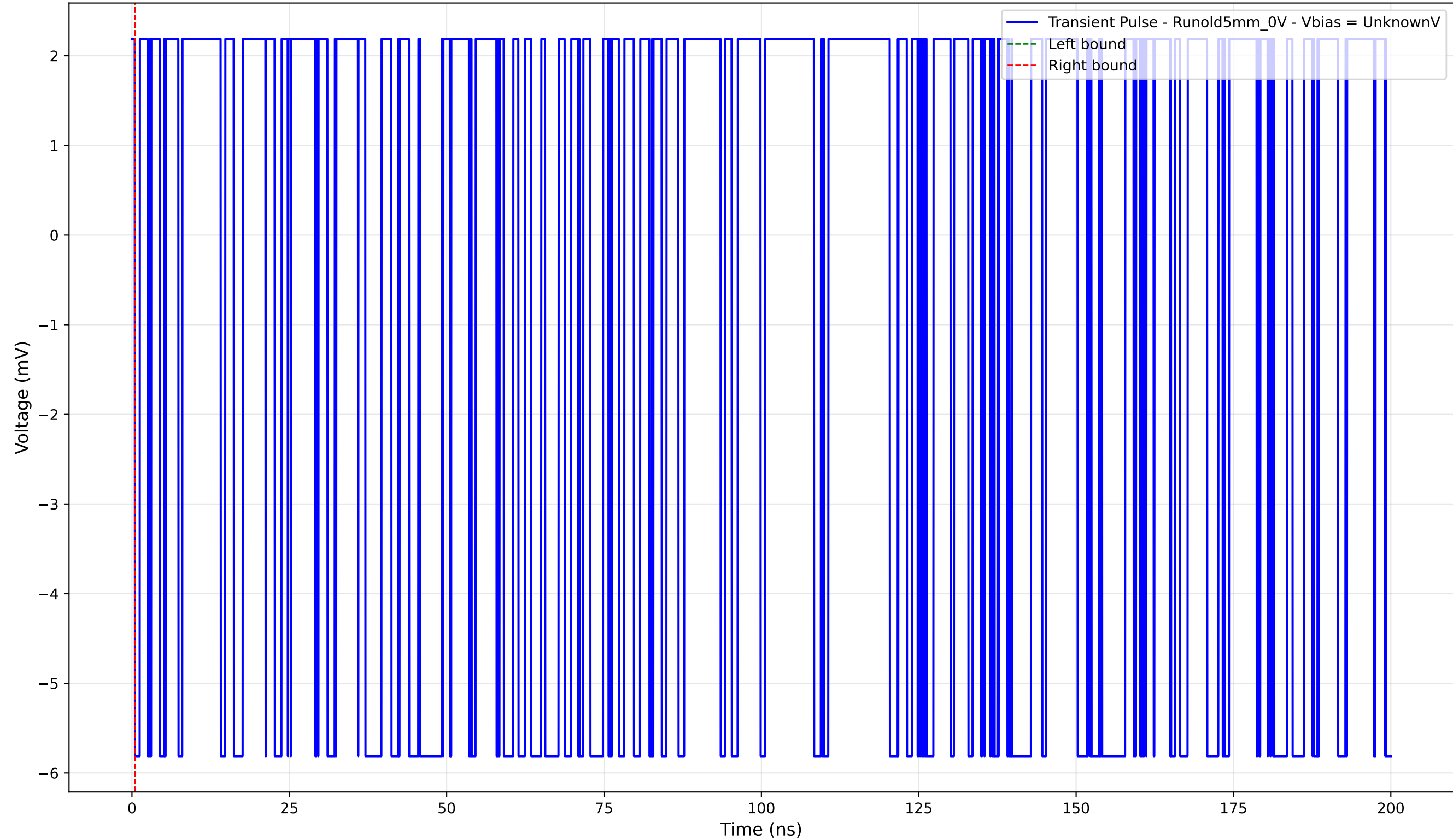
Transient Pulse - Sample: old5 - Position: 1485.0 \mu\text{m} - Charge: -0.00 pC
