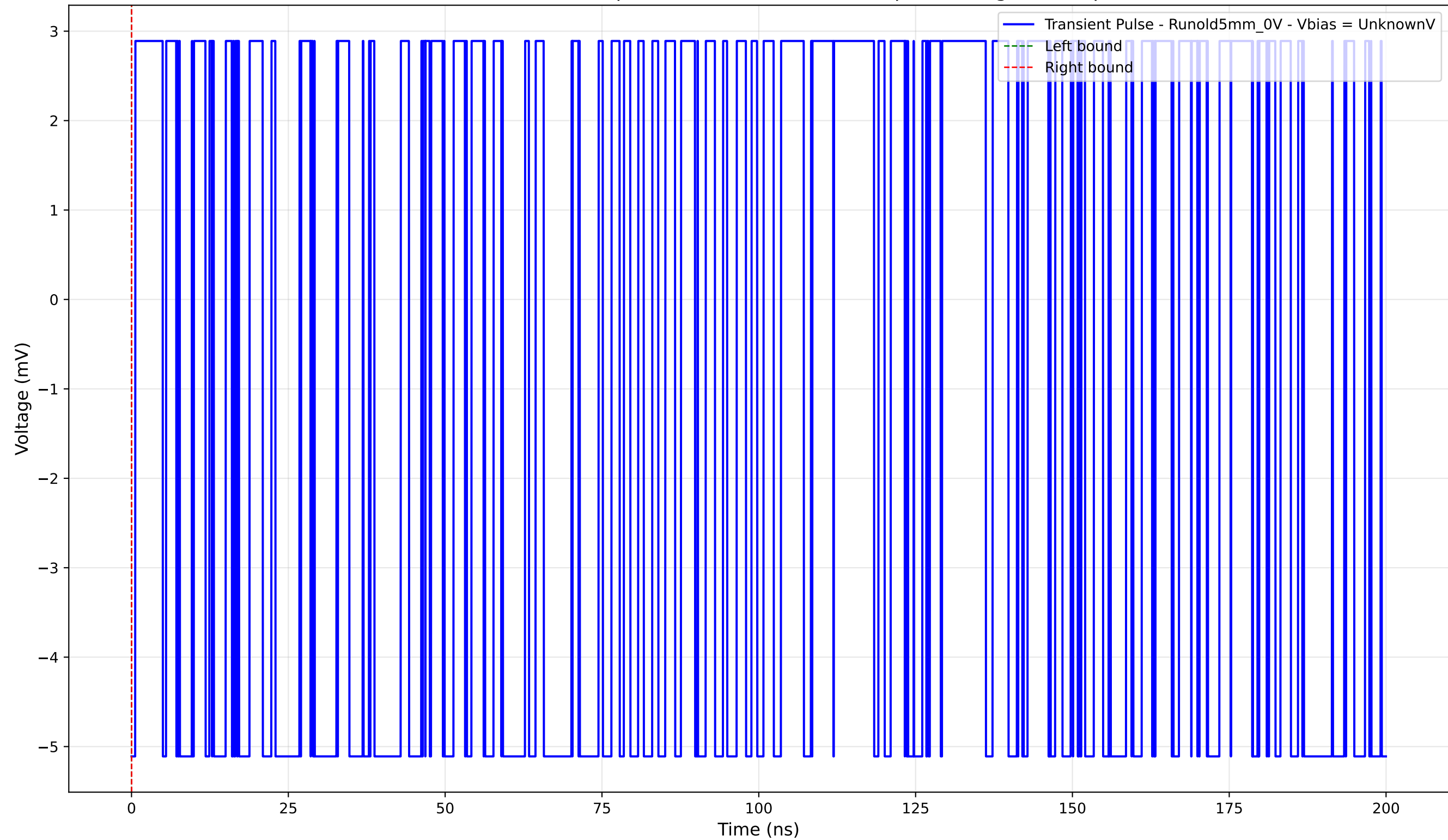
Transient Pulse - Sample: old5 - Position: 3765.0 \mu\text{m} - Charge: -0.00 pC
