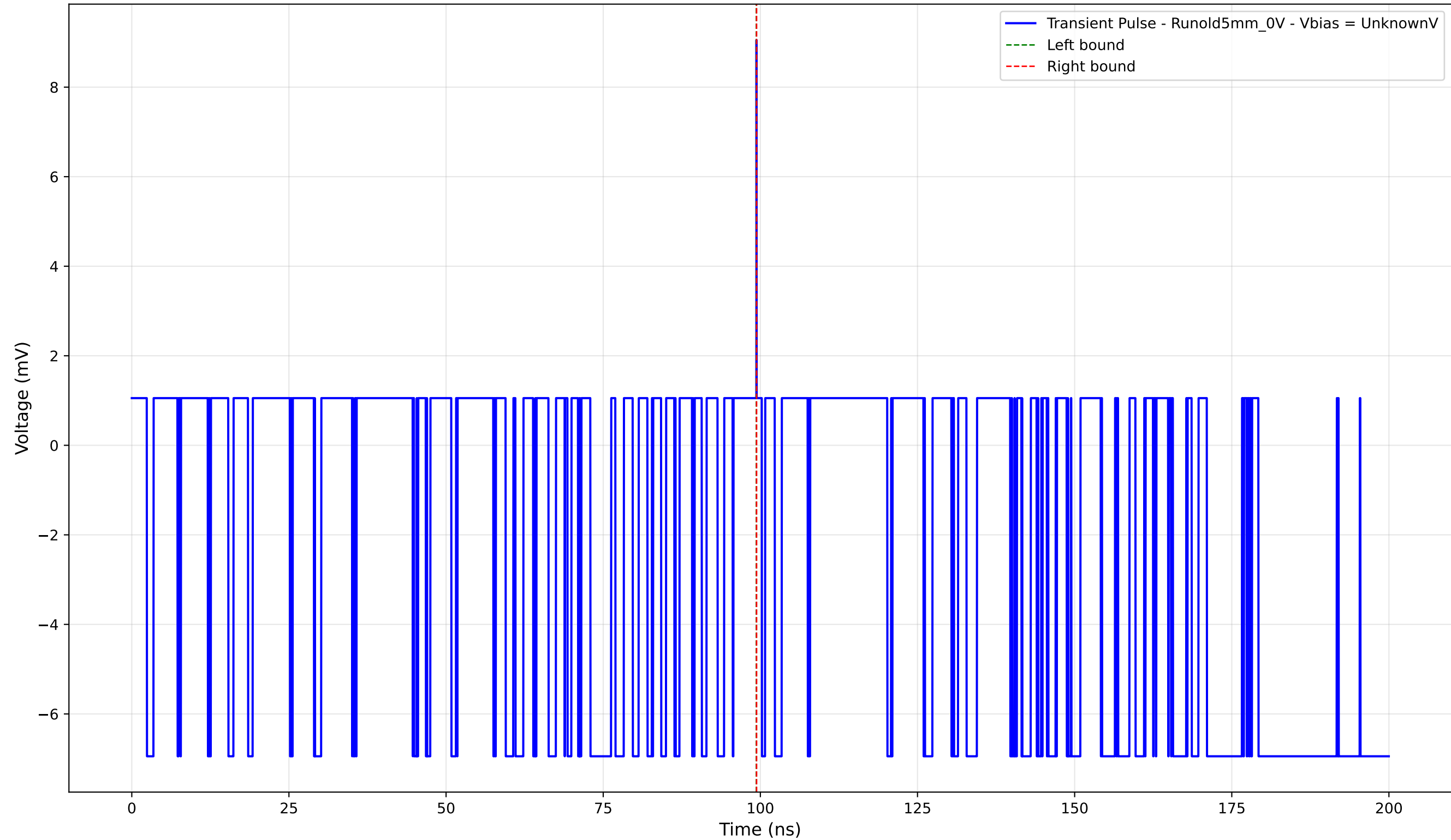
Transient Pulse - Sample: old5 - Position: 625.0 \mu\text{m} - Charge: 0.00 pC
