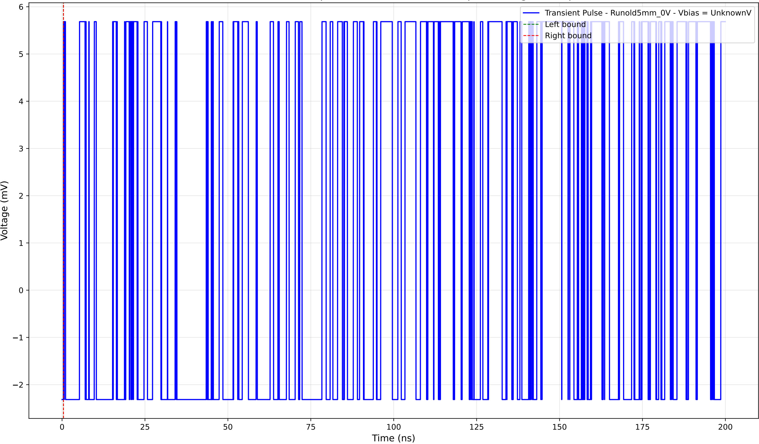
Transient Pulse - Sample: old5 - Position: 3050.0 \mu\text{m} - Charge: 0.00 pC
