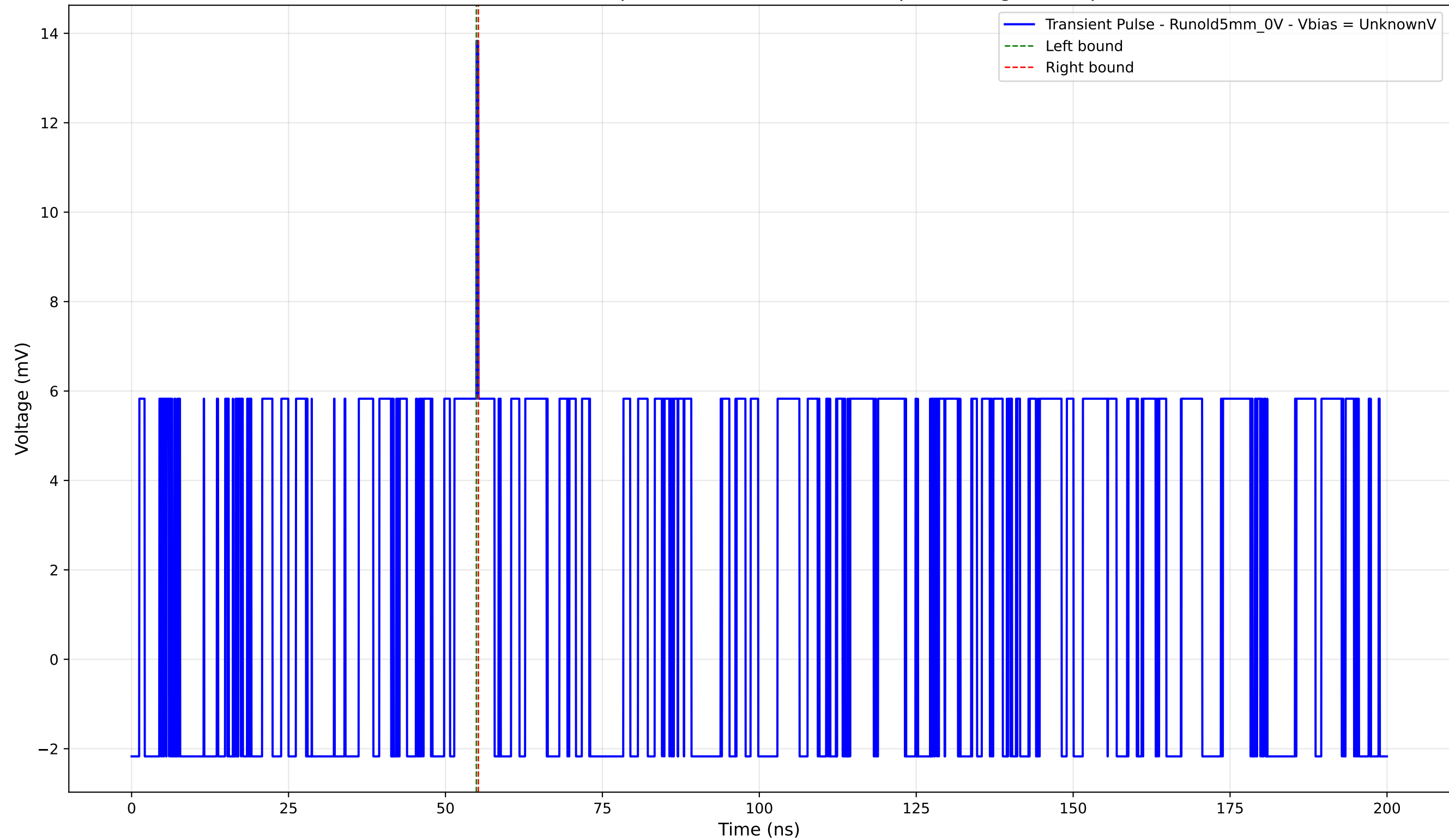
Transient Pulse - Sample: old5 - Position: 2840.0 \mu\text{m} - Charge: 0.09 pC
