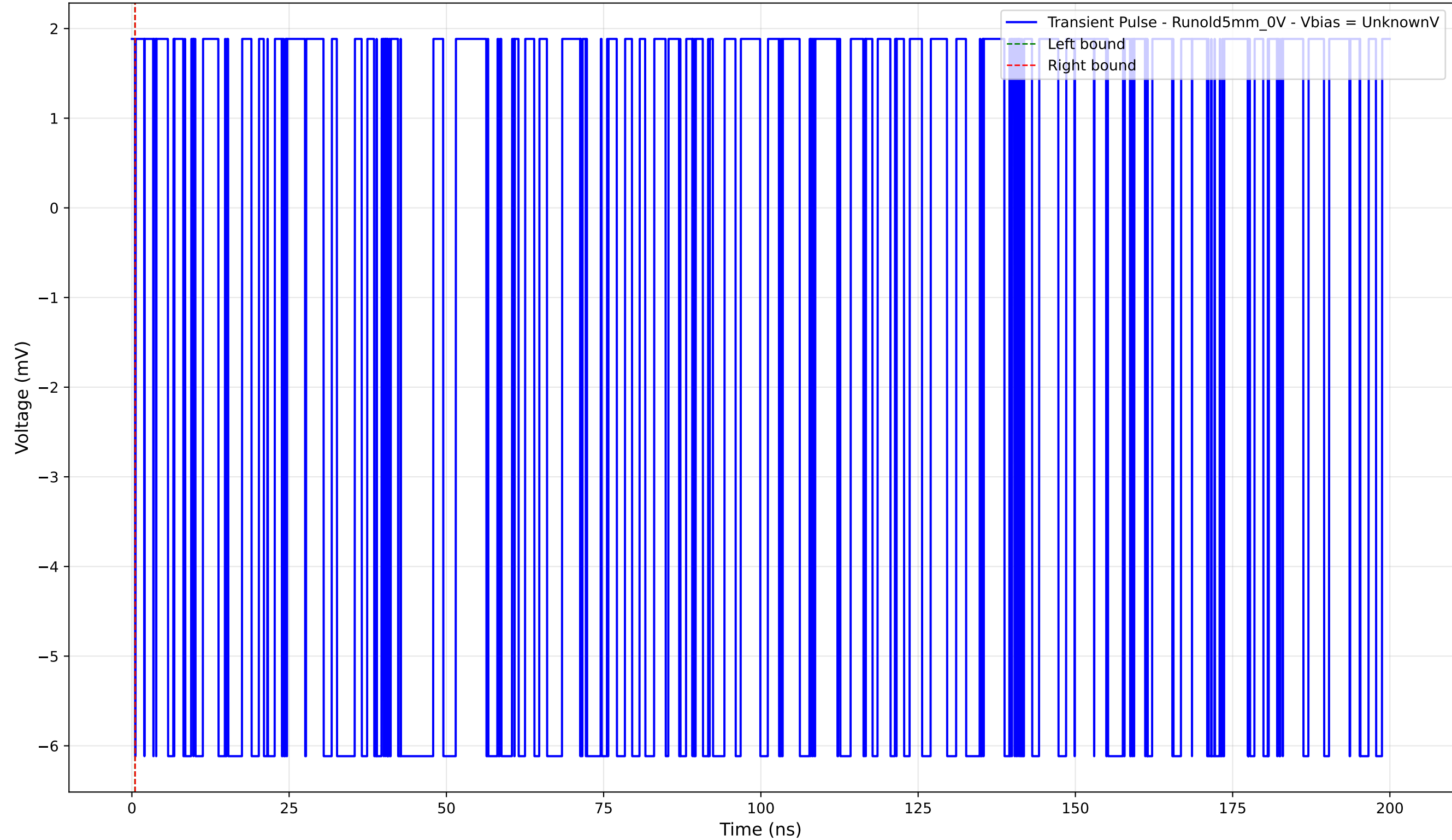
Transient Pulse - Sample: old5 - Position: 3235.0 \mu\text{m} - Charge: -0.00 pC
