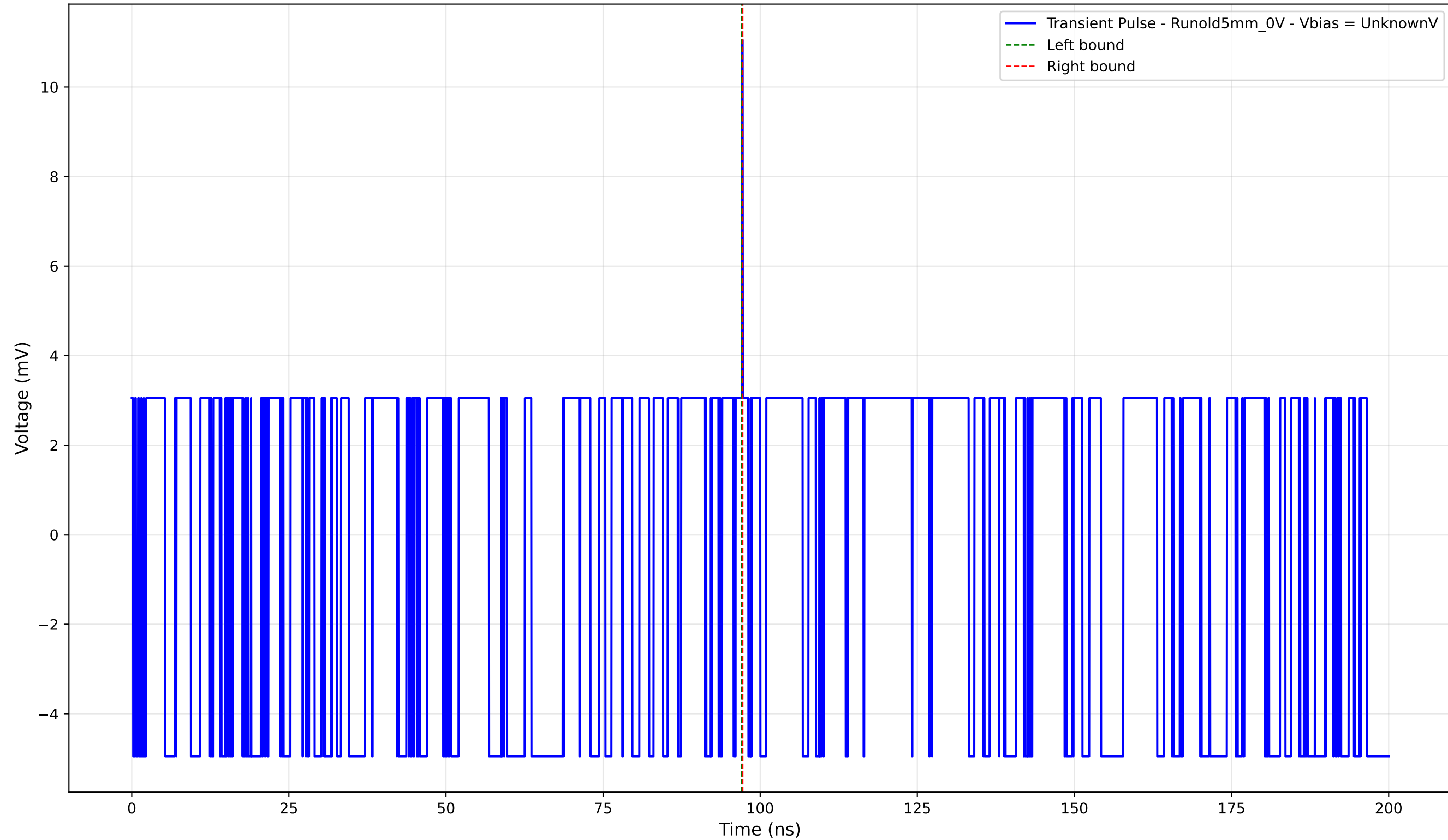
Transient Pulse - Sample: old5 - Position: 50.0 \mu\text{m} - Charge: 0.03 pC
