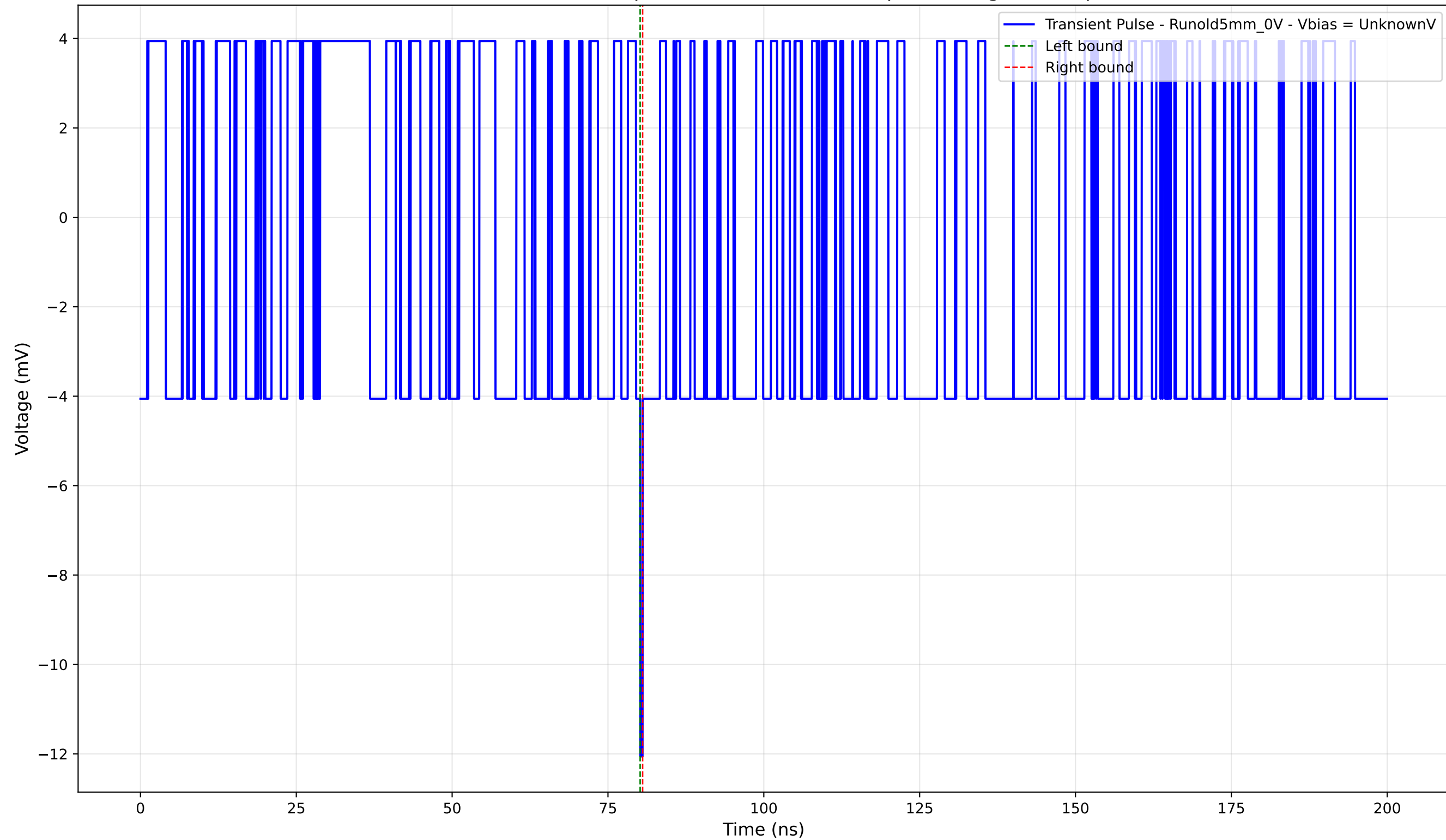
Transient Pulse - Sample: old5 - Position: 70.0 \mu\text{m} - Charge: -0.09 pC
