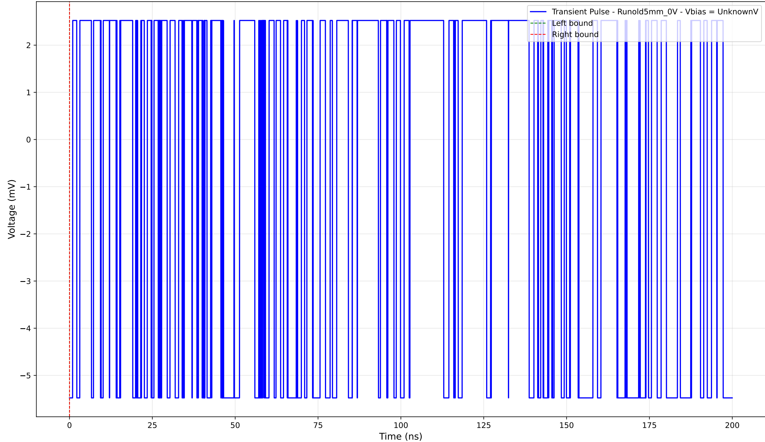
Transient Pulse - Sample: old5 - Position: 4480.0 \mu\text{m} - Charge: -0.00 pC
