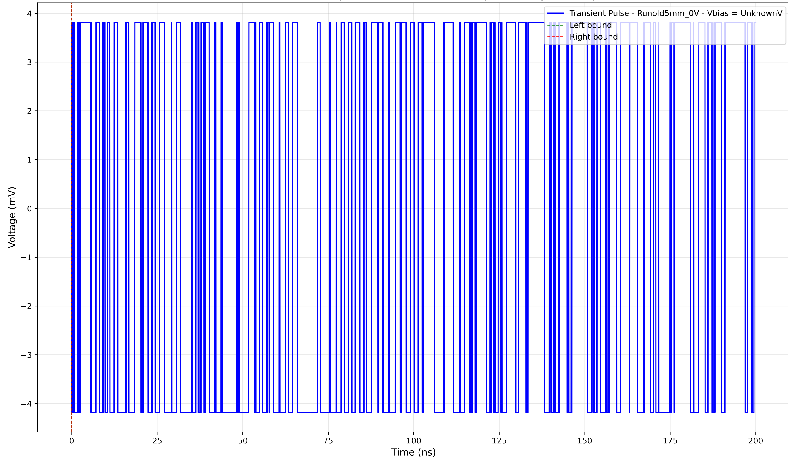
Transient Pulse - Sample: old5 - Position: 785.0 \mu\text{m} - Charge: -0.00 pC
