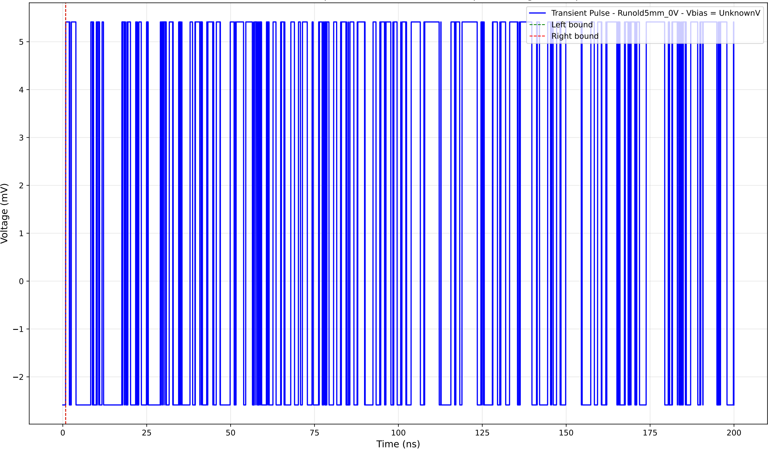
Transient Pulse - Sample: old5 - Position: 2110.0 \mu\text{m} - Charge: 0.00 pC
