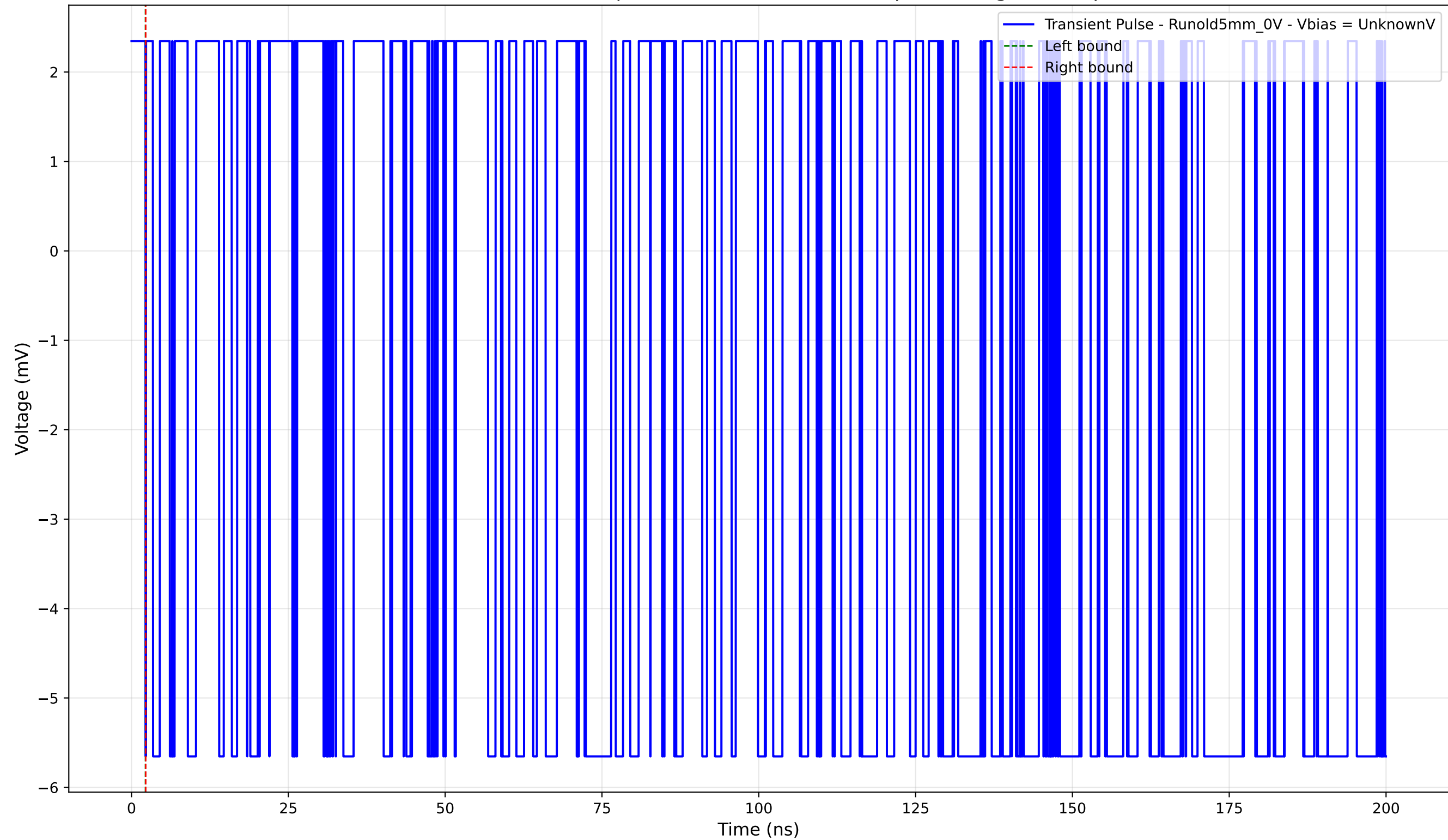
Transient Pulse - Sample: old5 - Position: 2775.0 \mu\text{m} - Charge: -0.00 pC
