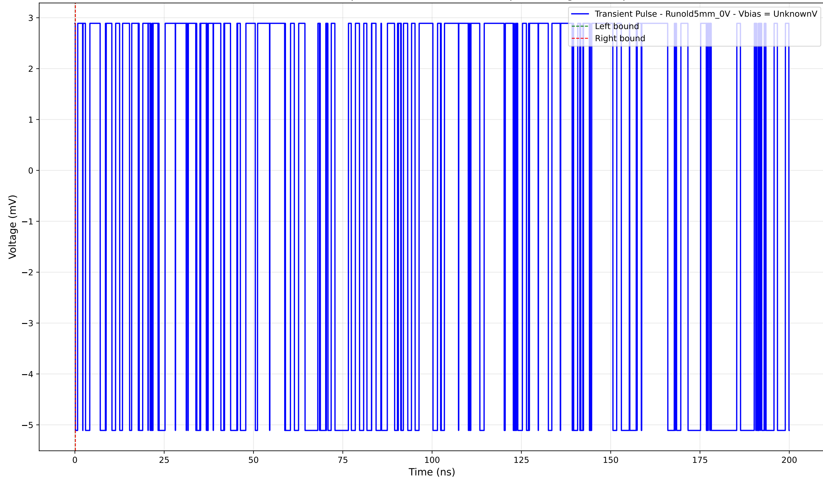
Transient Pulse - Sample: old5 - Position: 3360.0 \mu\text{m} - Charge: -0.00 pC
