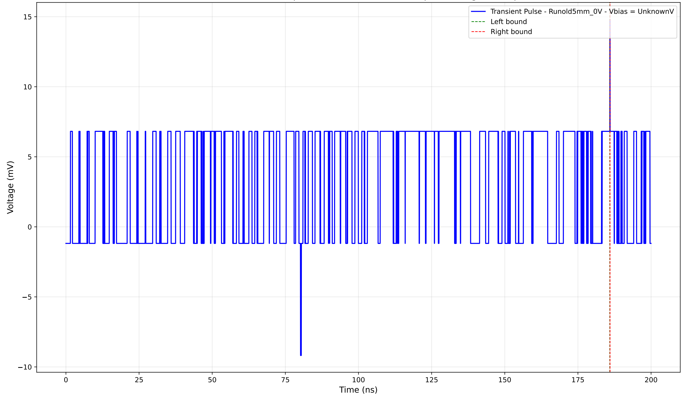
Transient Pulse - Sample: old5 - Position: 3540.0 \mu\text{m} - Charge: 0.02 pC
