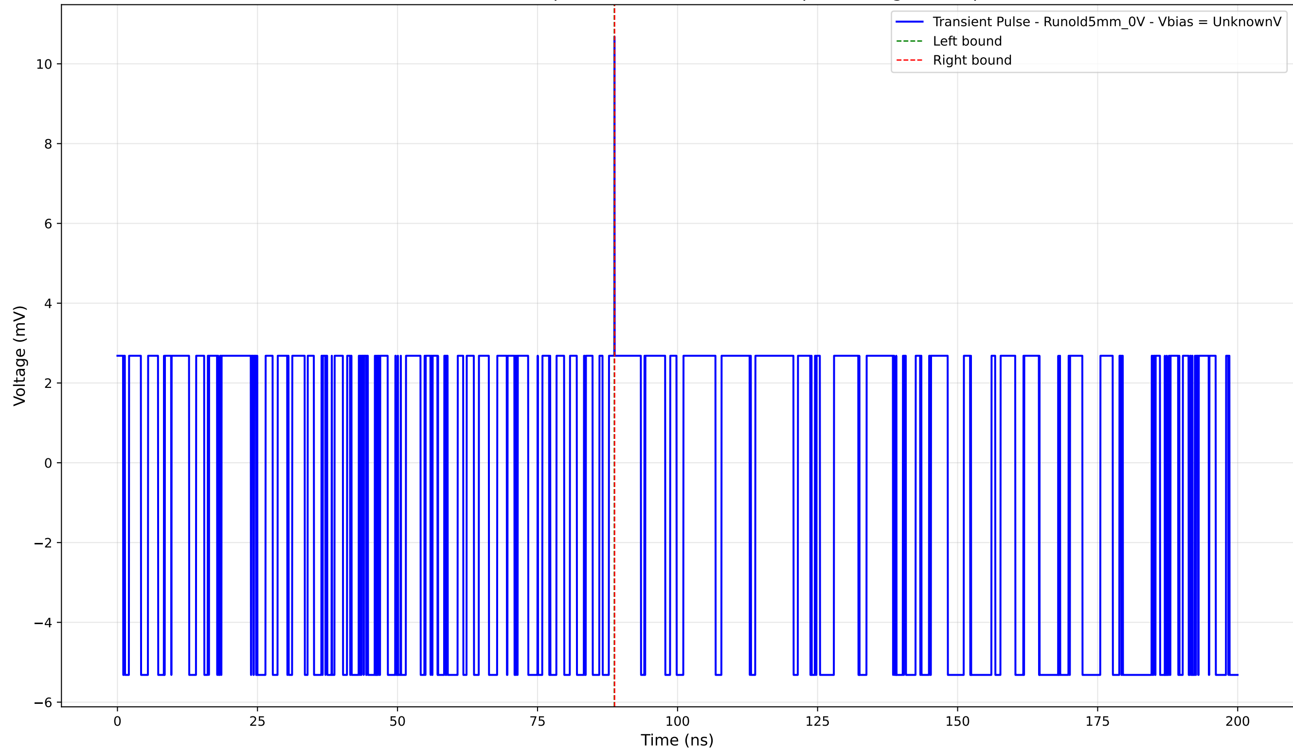
Transient Pulse - Sample: old5 - Position: 3725.0 \mu\text{m} - Charge: 0.01 pC
