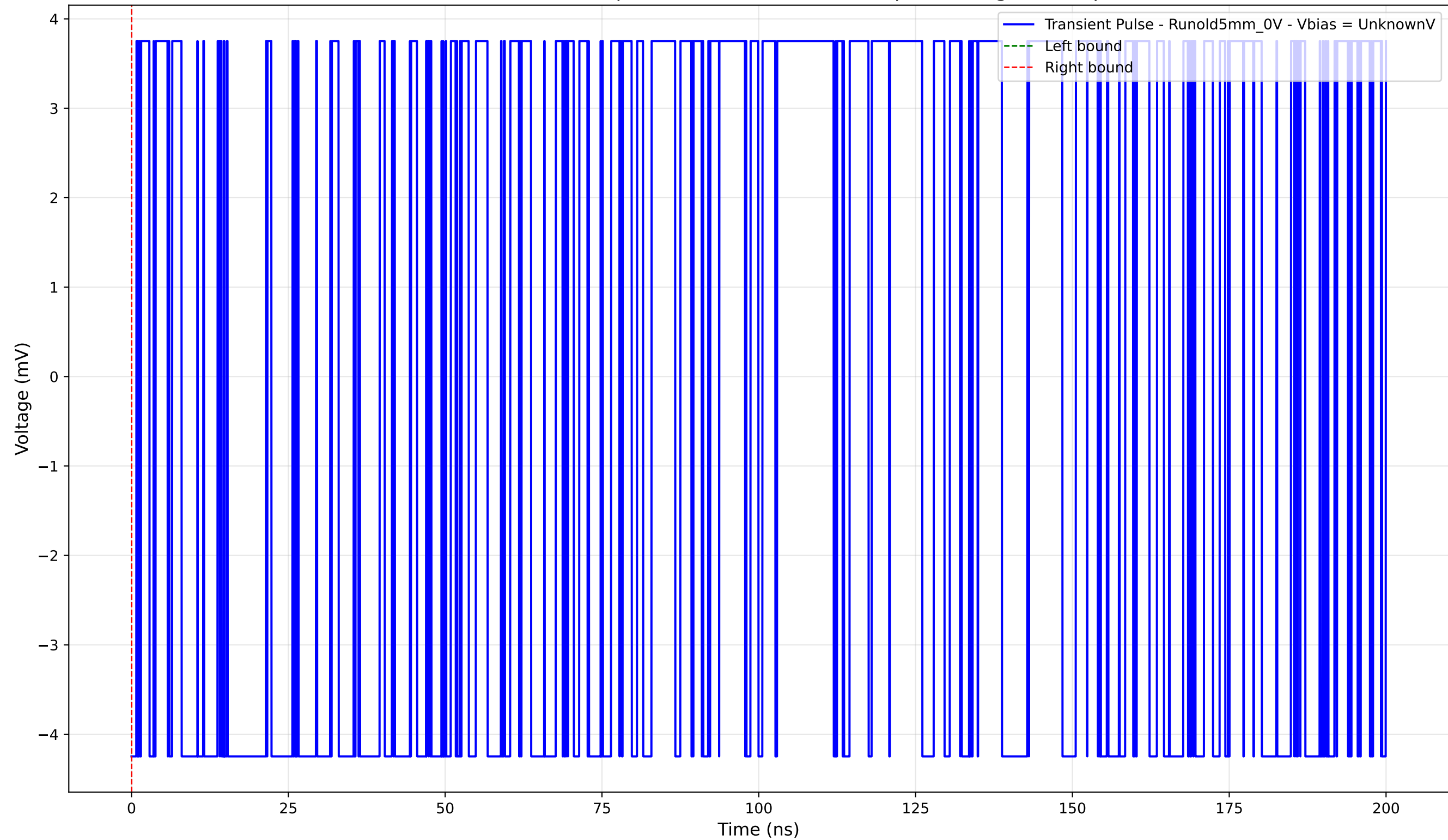
Transient Pulse - Sample: old5 - Position: 1955.0 \mu\text{m} - Charge: -0.00 pC
