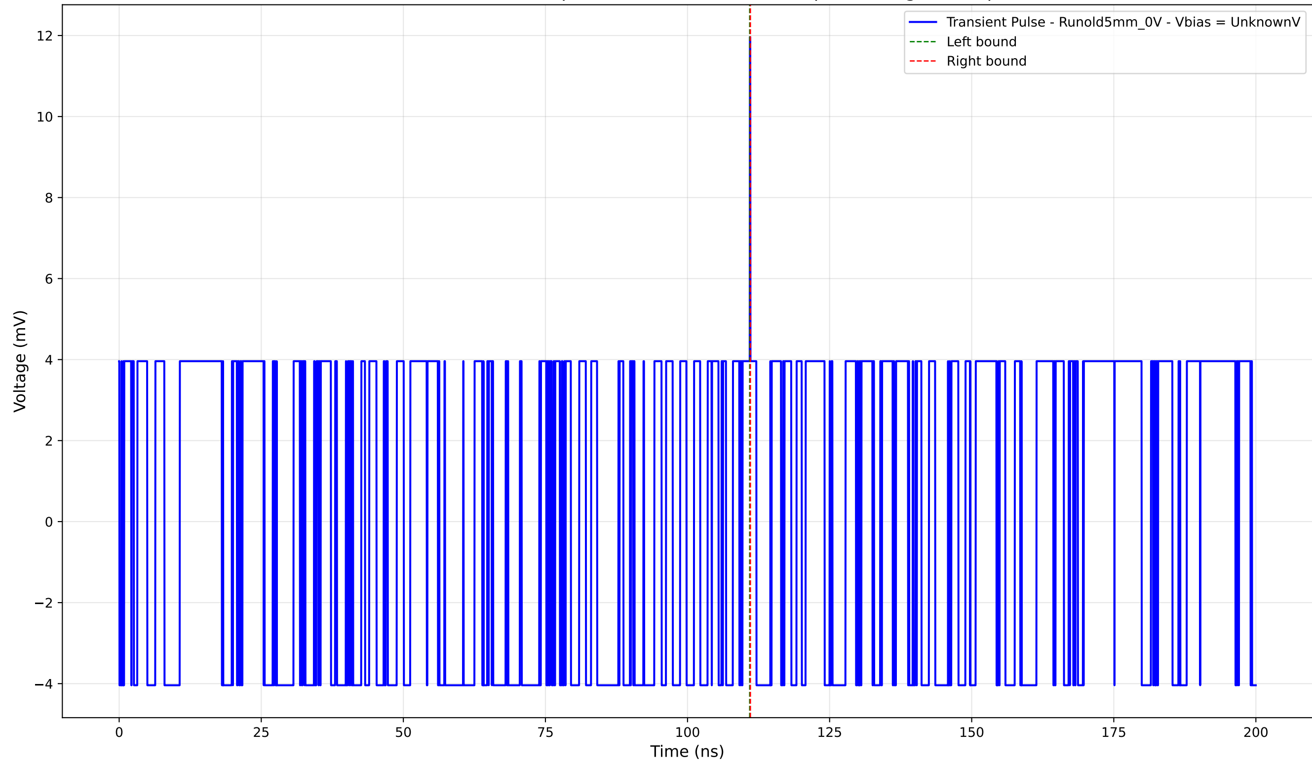
Transient Pulse - Sample: old5 - Position: 1945.0 \mu\text{m} - Charge: 0.03 pC
