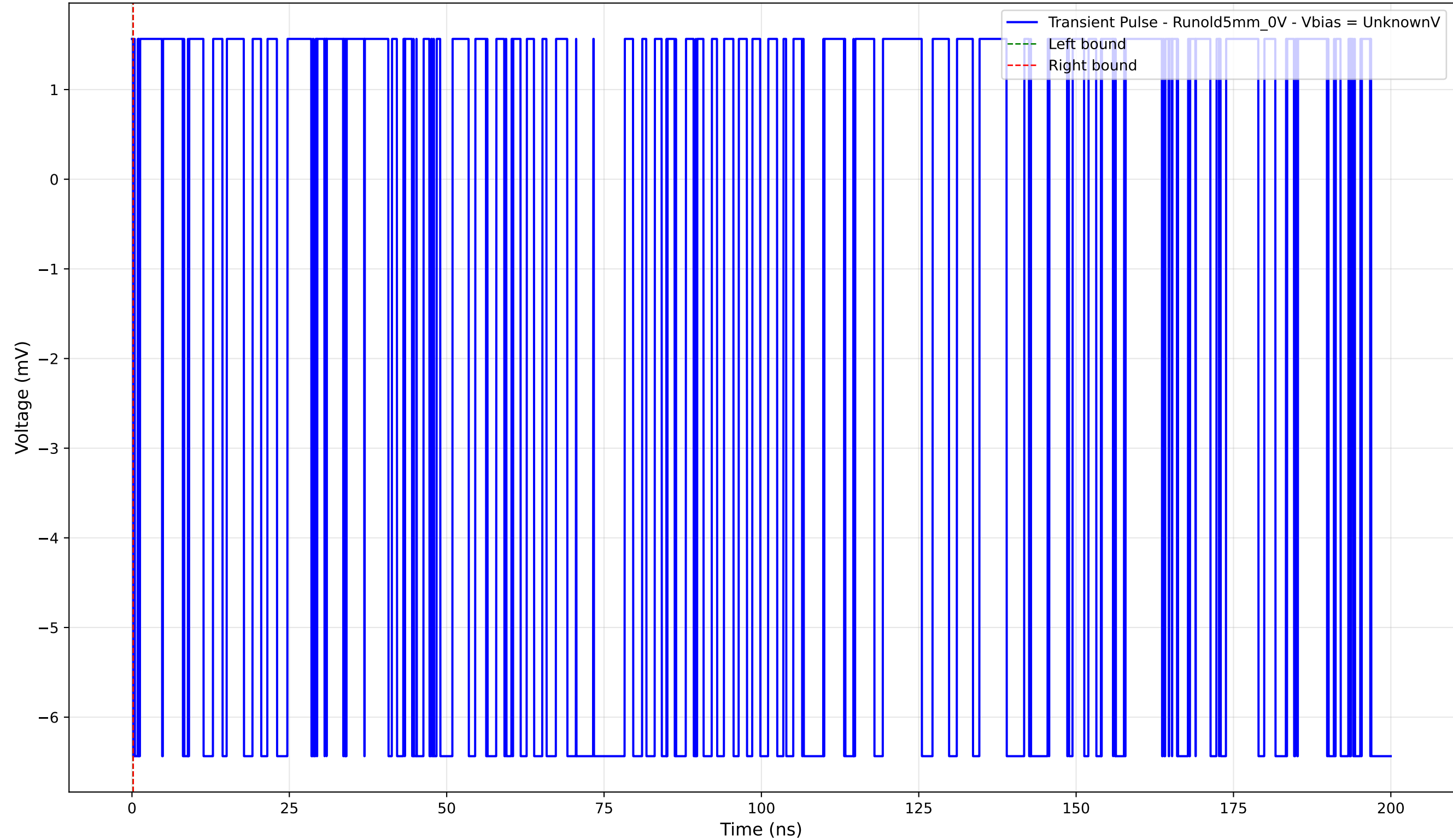
Transient Pulse - Sample: old5 - Position: 1695.0 \mu\text{m} - Charge: -0.00 pC
