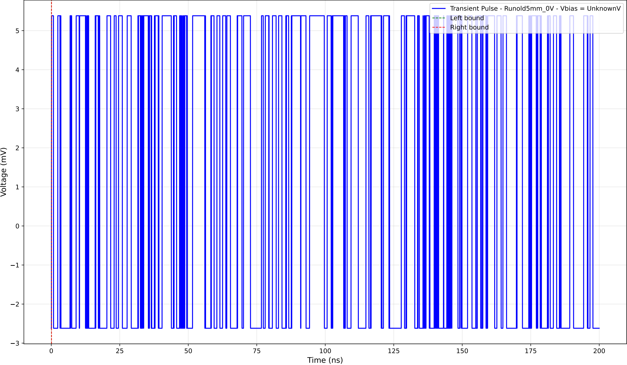
Transient Pulse - Sample: old5 - Position: 3865.0 \mu\text{m} - Charge: 0.00 pC
