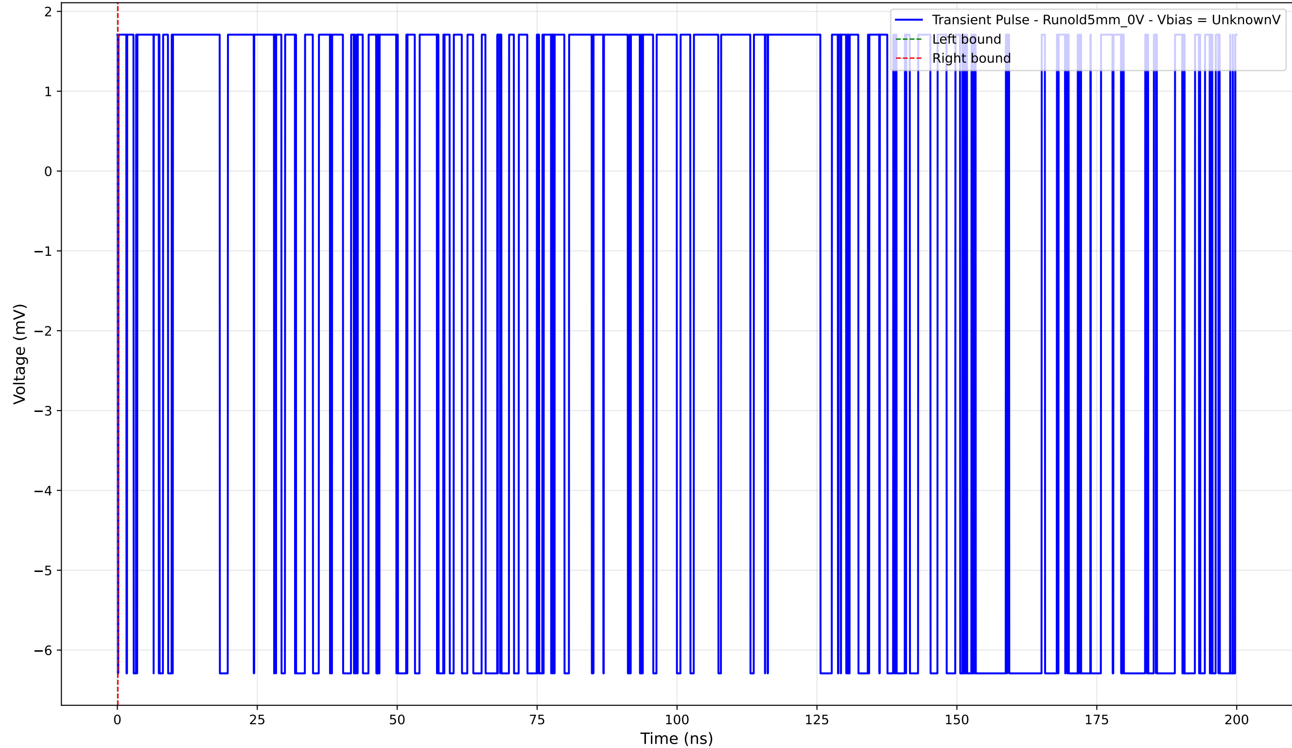
Transient Pulse - Sample: old5 - Position: 2215.0 \mu\text{m} - Charge: -0.00 pC
