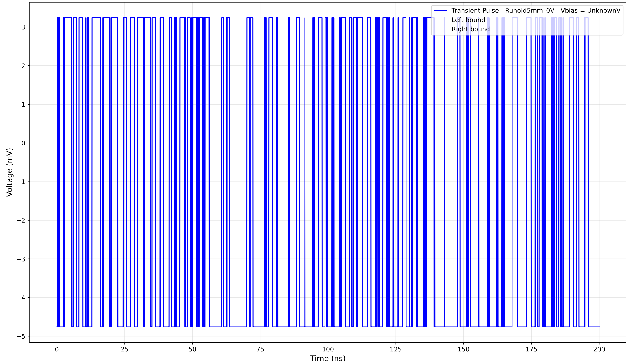
Transient Pulse - Sample: old5 - Position: 3350.0 \mu\text{m} - Charge: -0.00 pC
