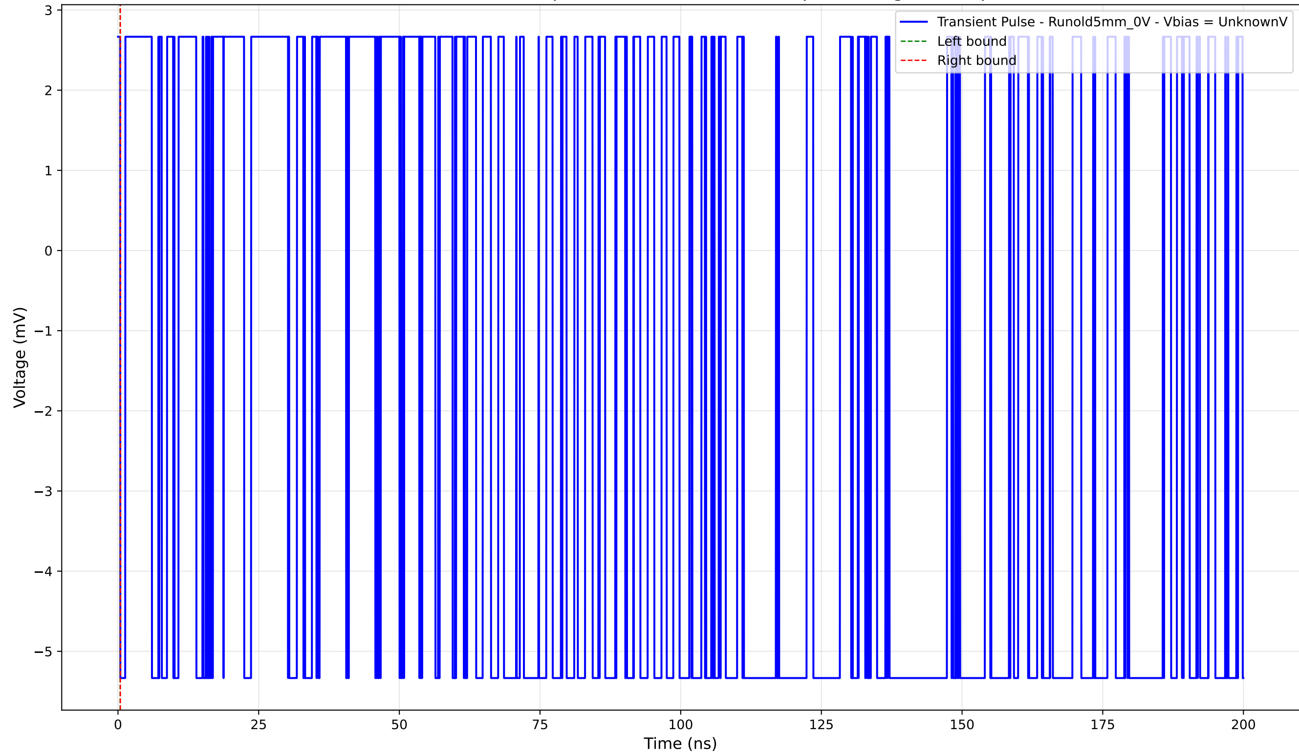
Transient Pulse - Sample: old5 - Position: 2760.0 \mu\text{m} - Charge: -0.00 pC
