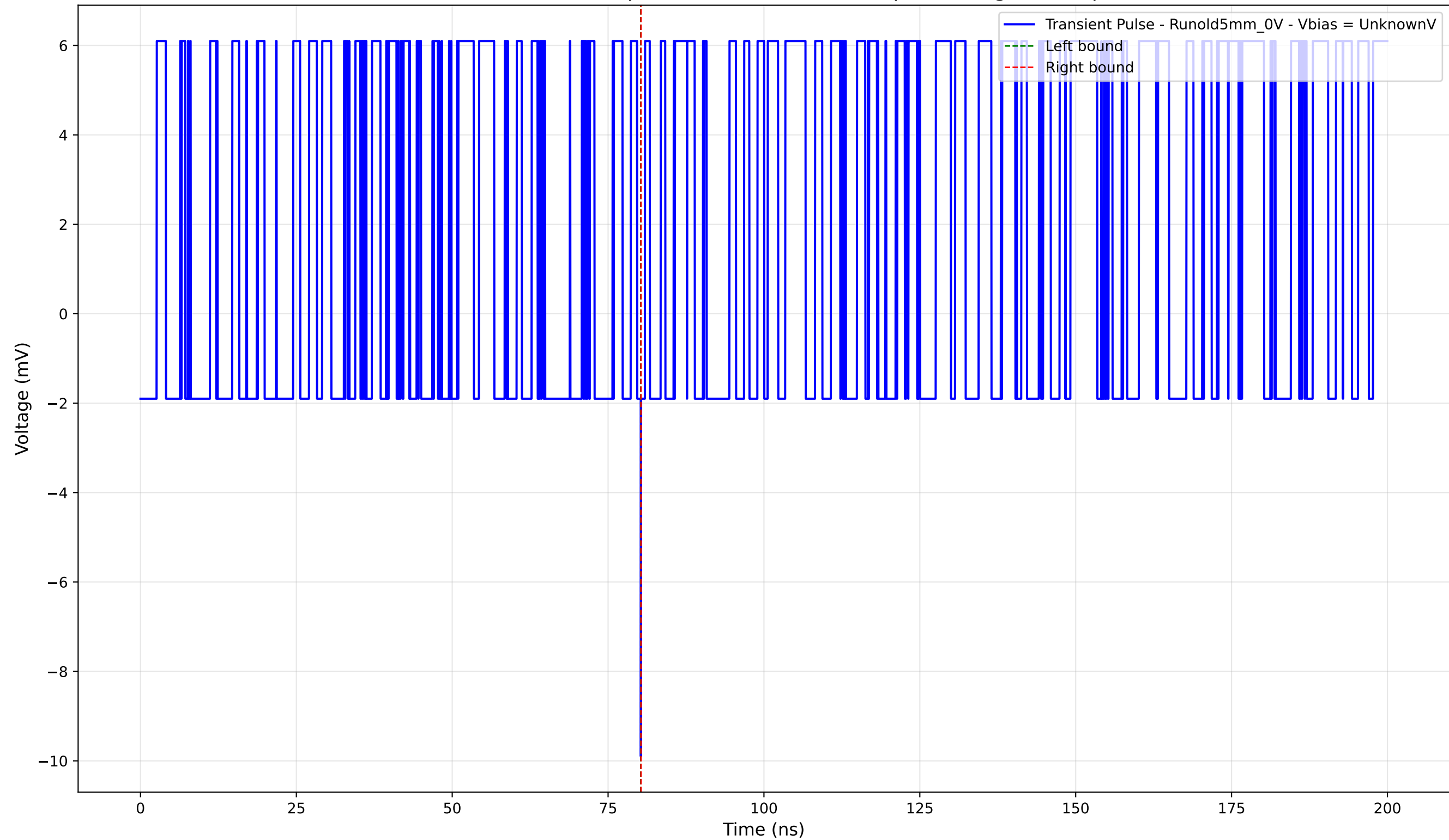
Transient Pulse - Sample: old5 - Position: 130.0 \mu\text{m} - Charge: -0.00 pC
