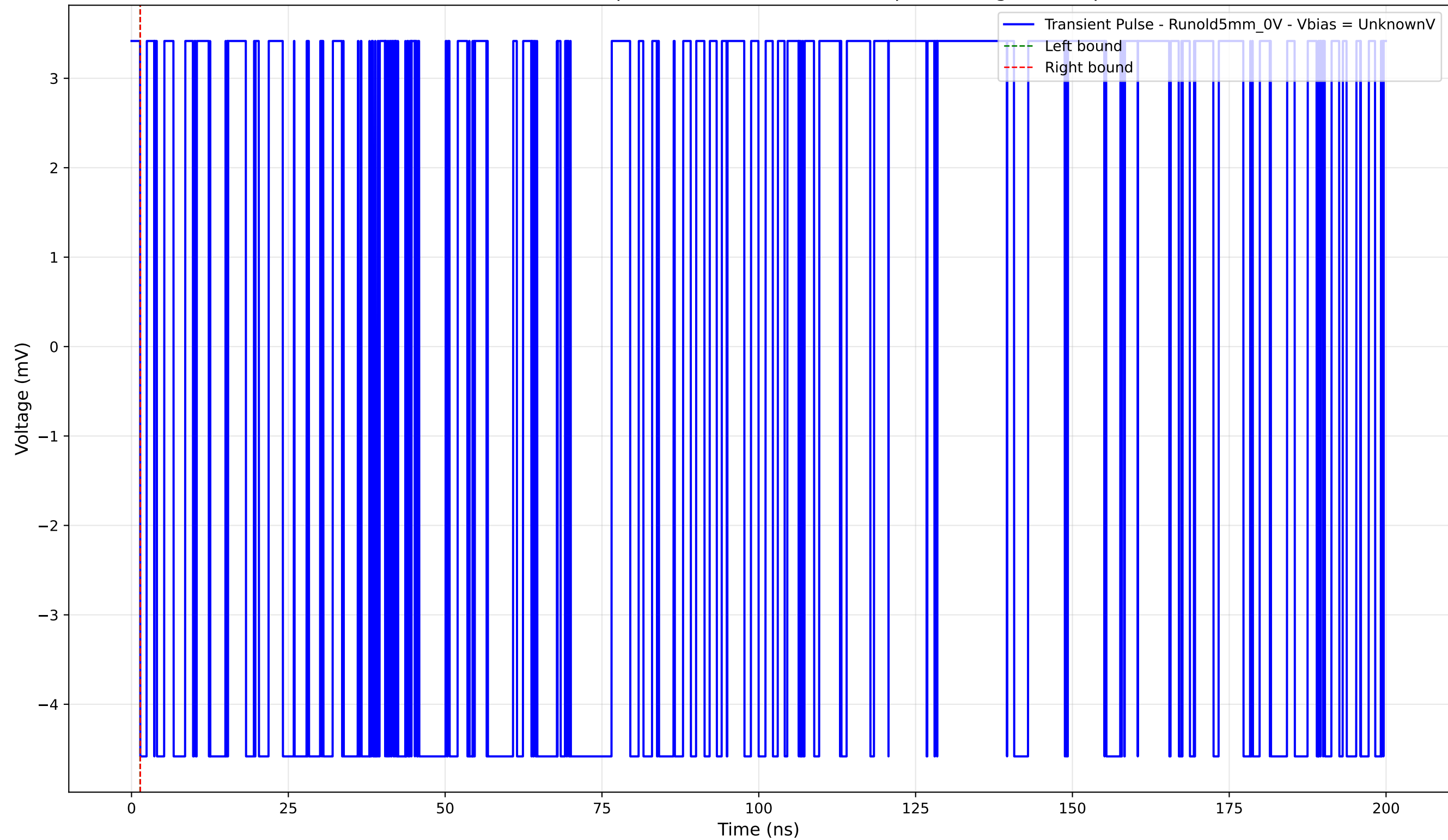
Transient Pulse - Sample: old5 - Position: 2505.0 \mu\text{m} - Charge: -0.00 pC
