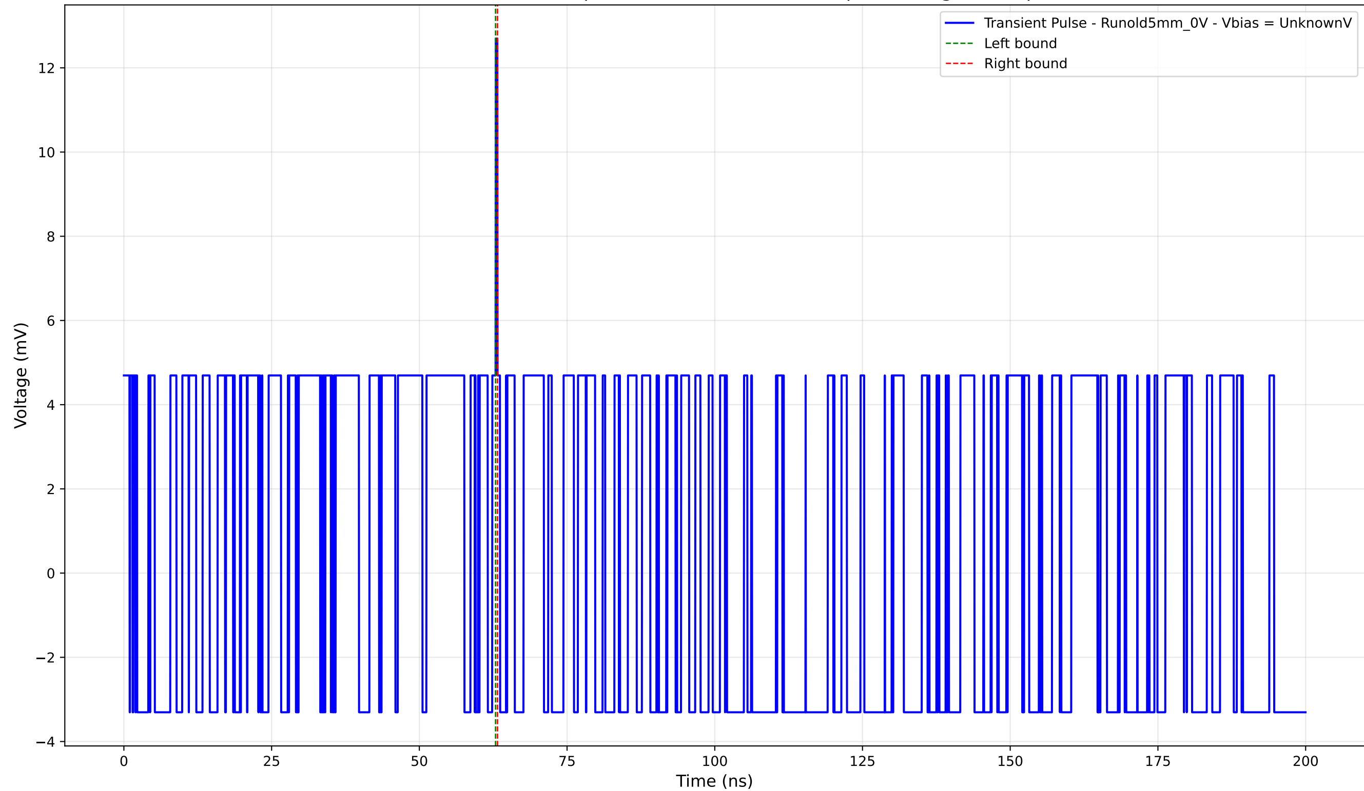
Transient Pulse - Sample: old5 - Position: 1835.0 \mu\text{m} - Charge: 0.08 pC
