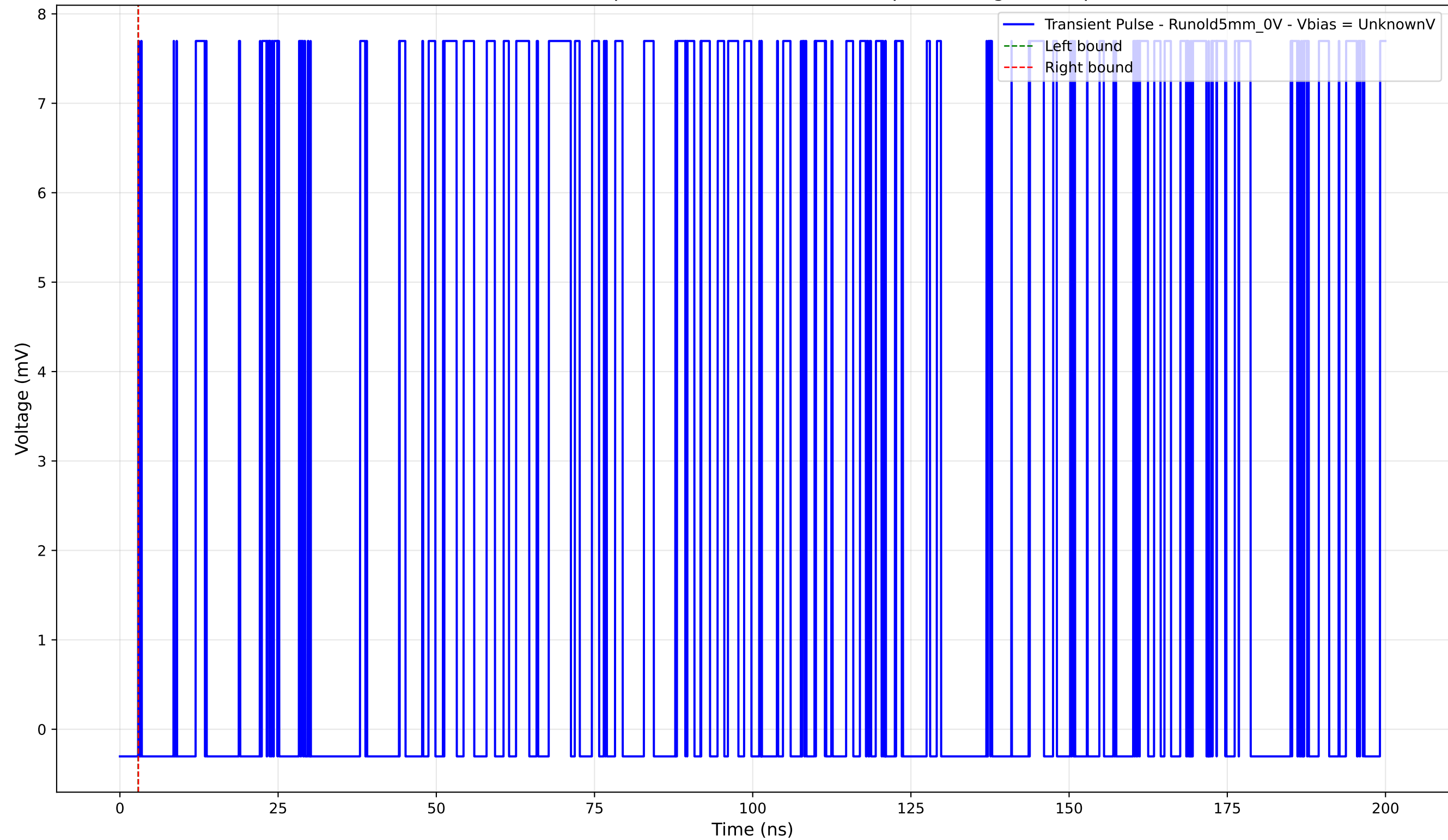
Transient Pulse - Sample: old5 - Position: 3160.0 \mu\text{m} - Charge: 0.00 pC
