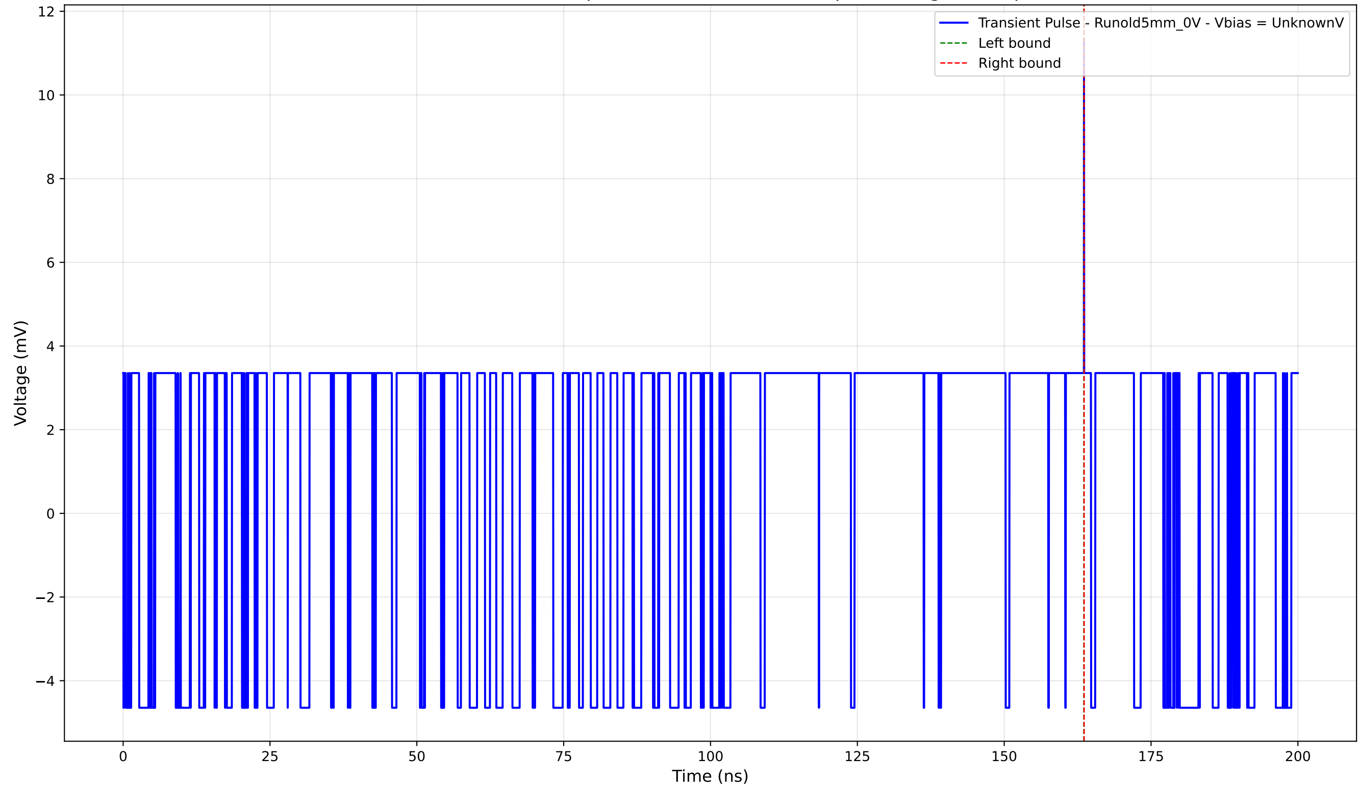
Transient Pulse - Sample: old5 - Position: 380.0 \mu\text{m} - Charge: 0.01 pC
