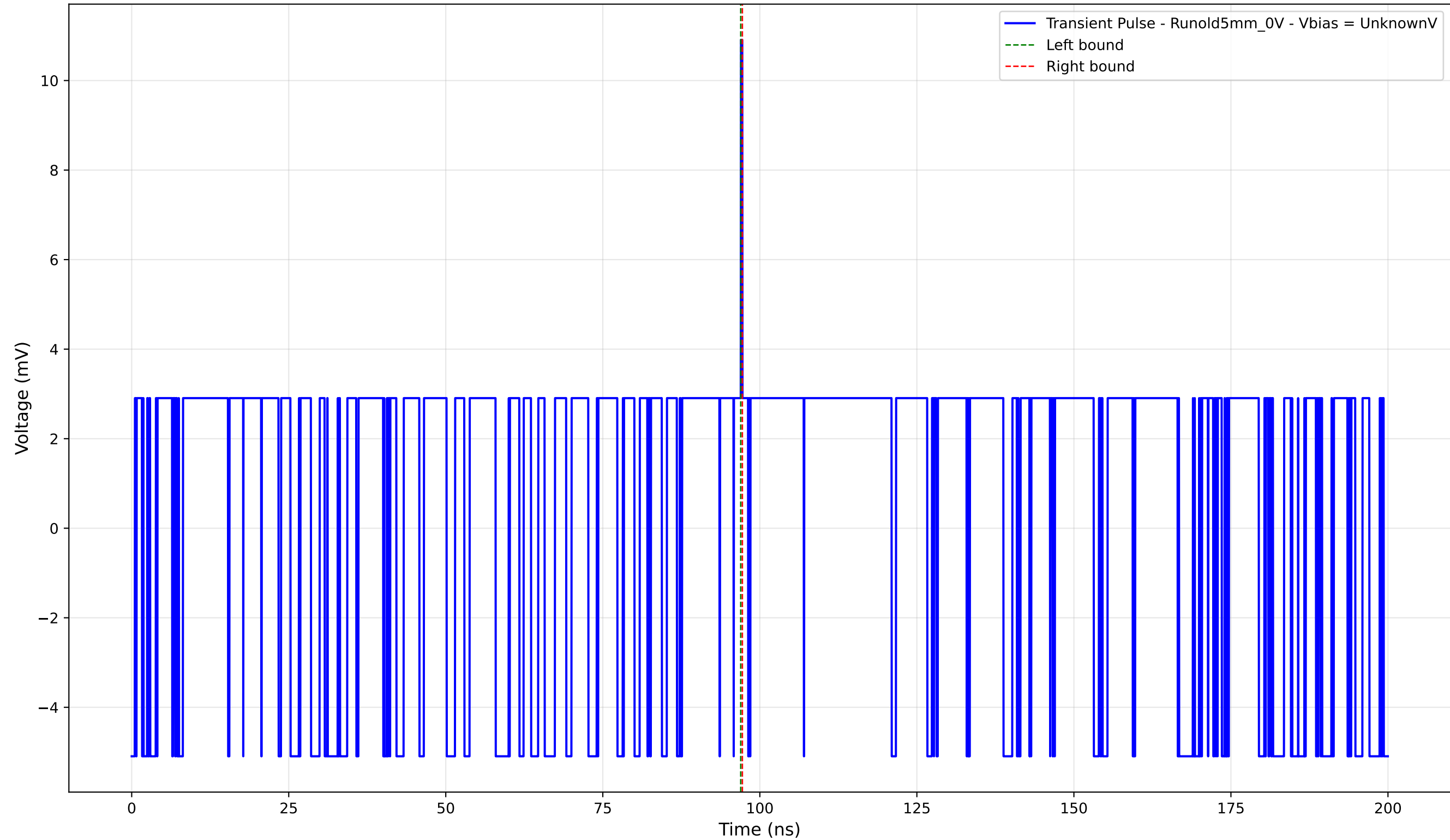
Transient Pulse - Sample: old5 - Position: 225.0 \mu\text{m} - Charge: 0.05 pC
