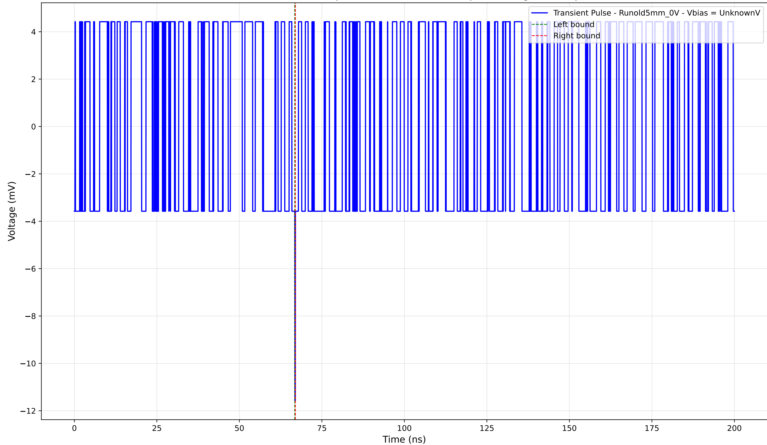
Transient Pulse - Sample: old5 - Position: 55.0 \mu\text{m} - Charge: -0.04 pC
