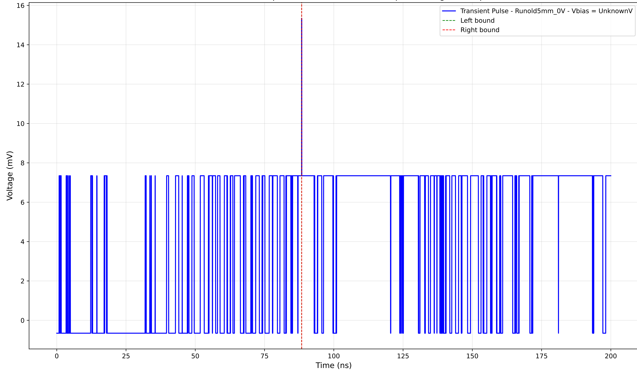
Transient Pulse - Sample: old5 - Position: 2940.0 \mu\text{m} - Charge: 0.01 pC
