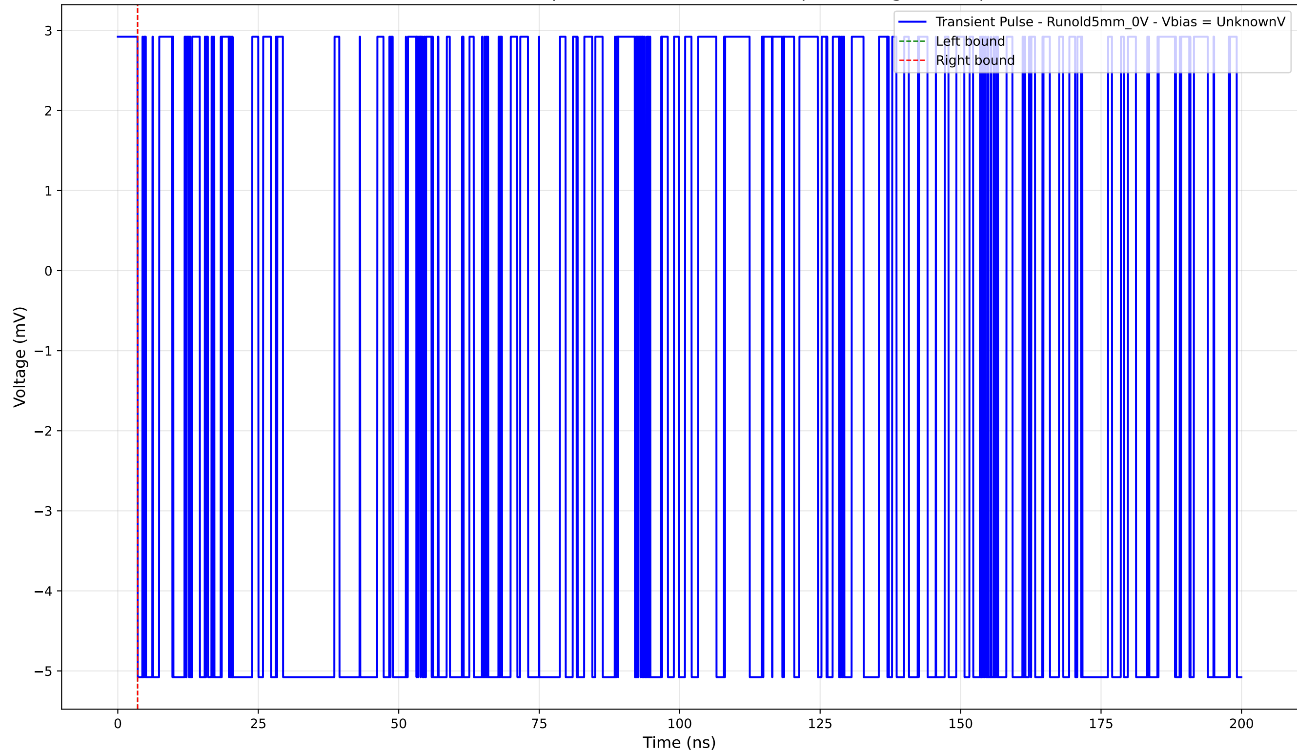
Transient Pulse - Sample: old5 - Position: 4720.0 \mu\text{m} - Charge: -0.00 pC
