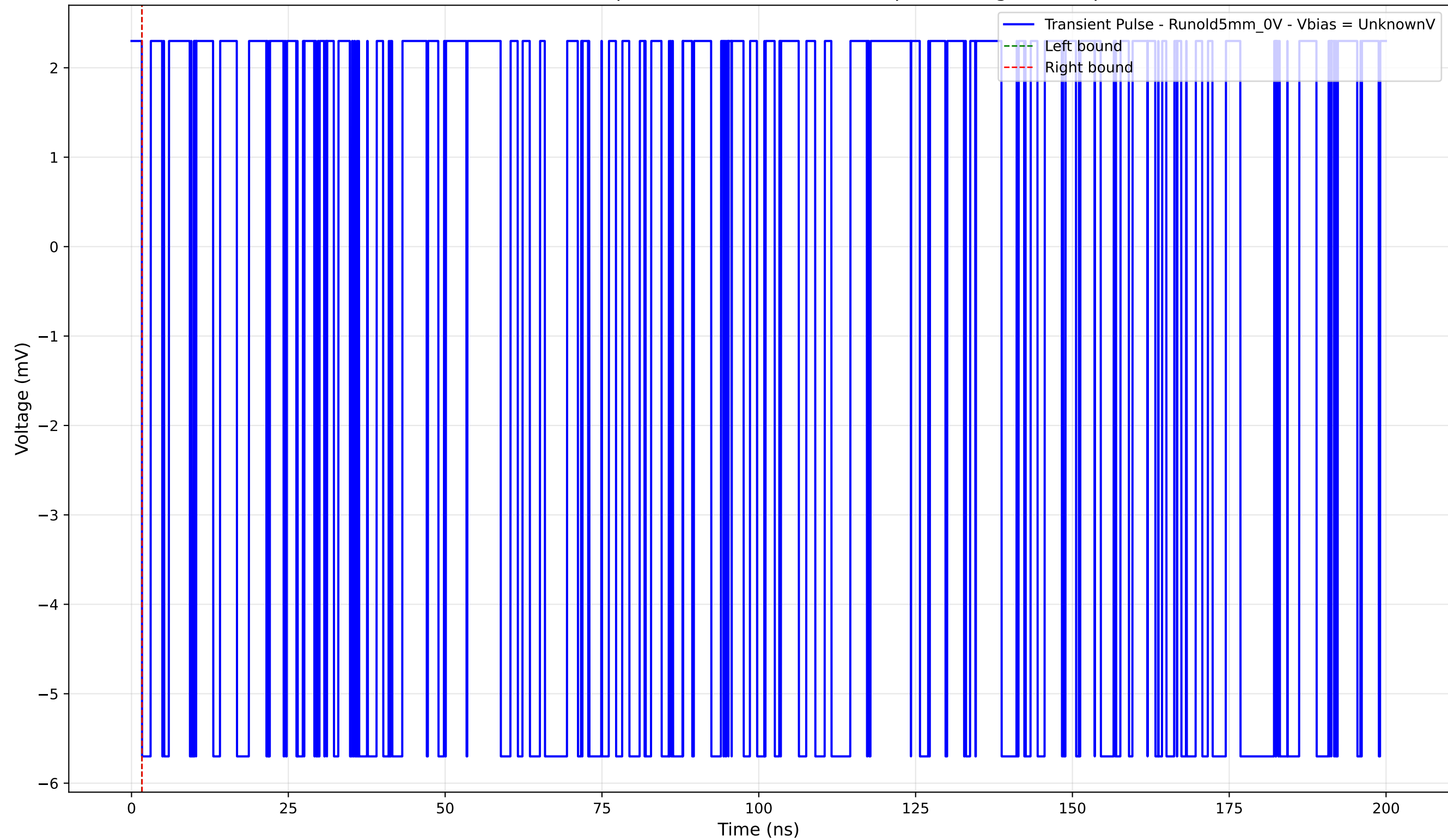
Transient Pulse - Sample: old5 - Position: 1390.0 \mu\text{m} - Charge: -0.00 pC
