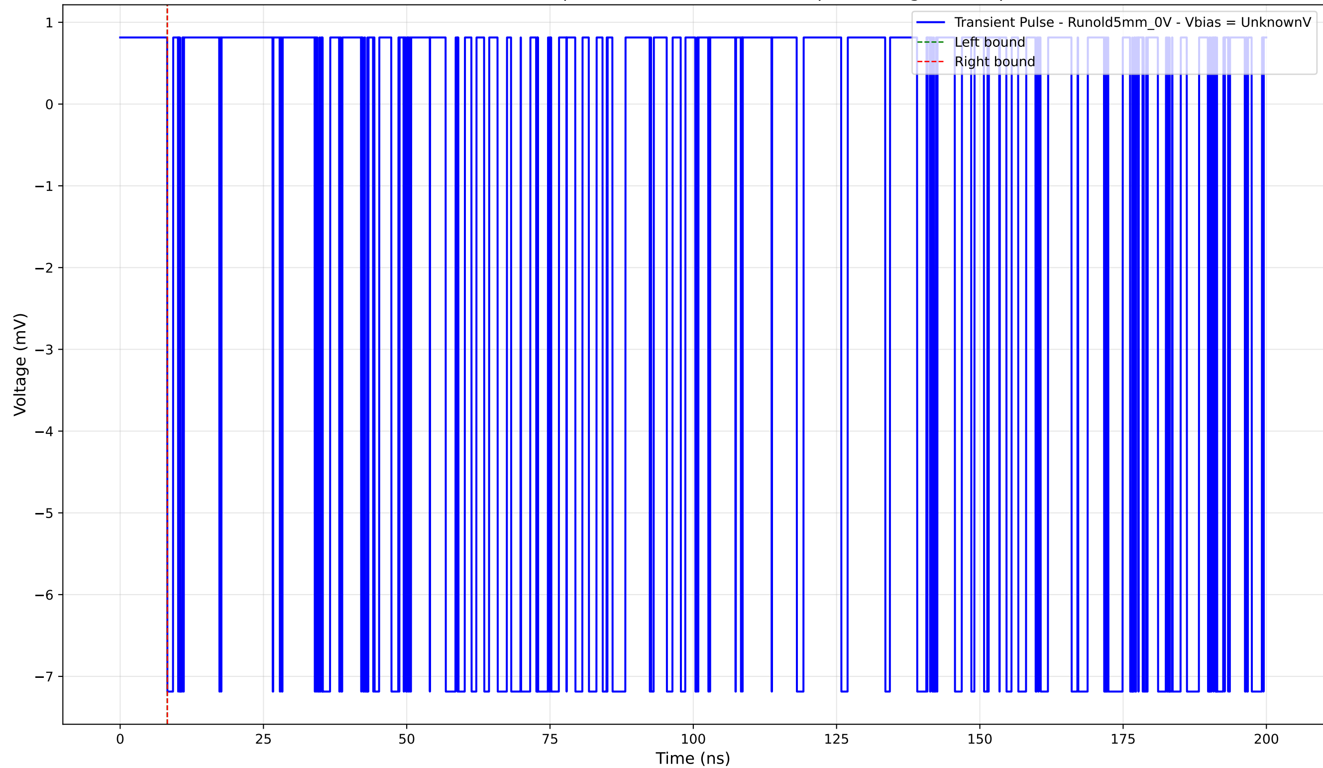
Transient Pulse - Sample: old5 - Position: 3485.0 \mu\text{m} - Charge: -0.00 pC
