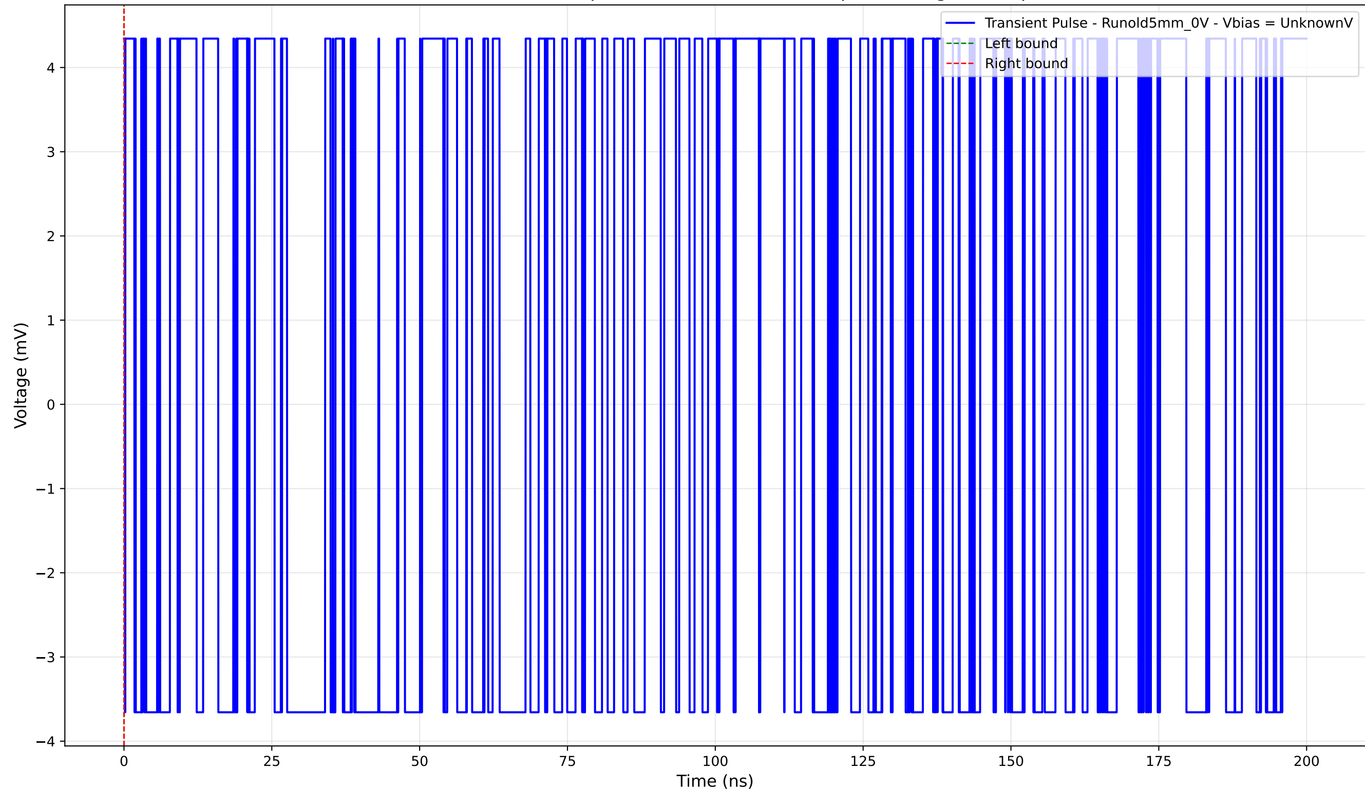
Transient Pulse - Sample: old5 - Position: 475.0 \mu\text{m} - Charge: 0.00 pC
