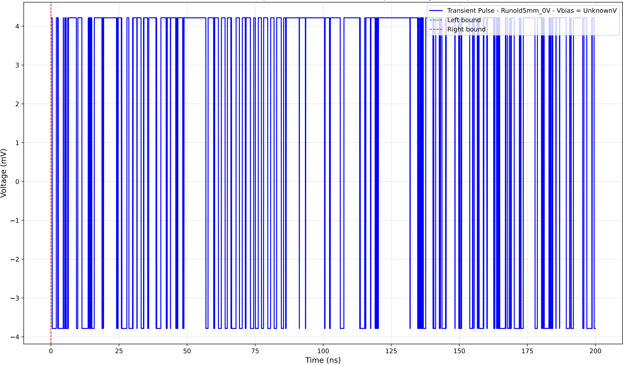
Transient Pulse - Sample: old5 - Position: 5165.0 \mu\text{m} - Charge: 0.00 pC
