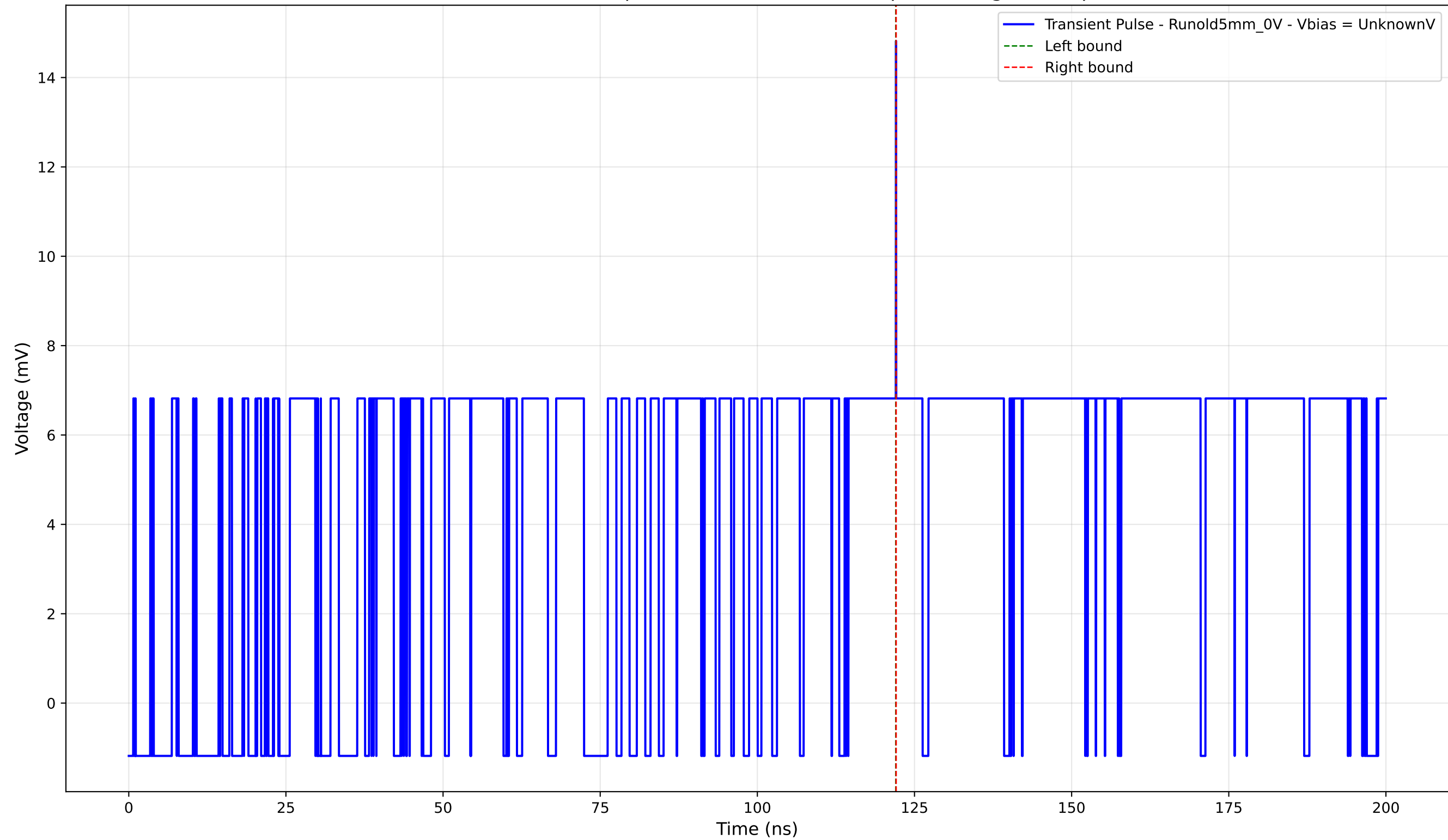
Transient Pulse - Sample: old5 - Position: 620.0 \mu\text{m} - Charge: 0.01 pC
