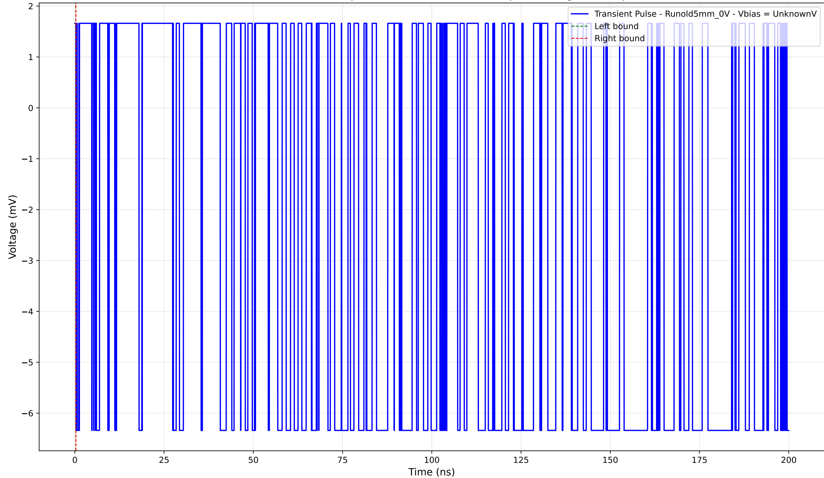
Transient Pulse - Sample: old5 - Position: 1225.0 \mu\text{m} - Charge: -0.00 pC
