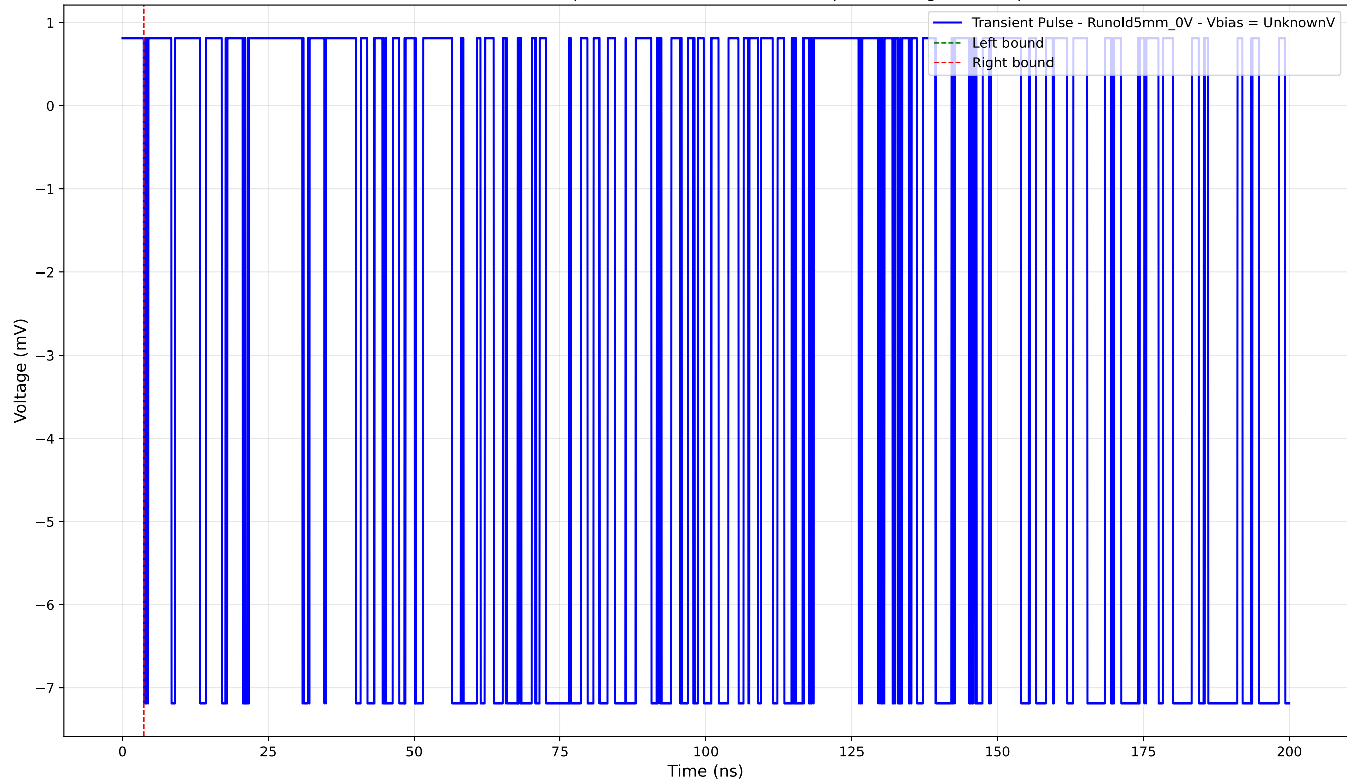
Transient Pulse - Sample: old5 - Position: 1070.0 \mu\text{m} - Charge: -0.00 pC
