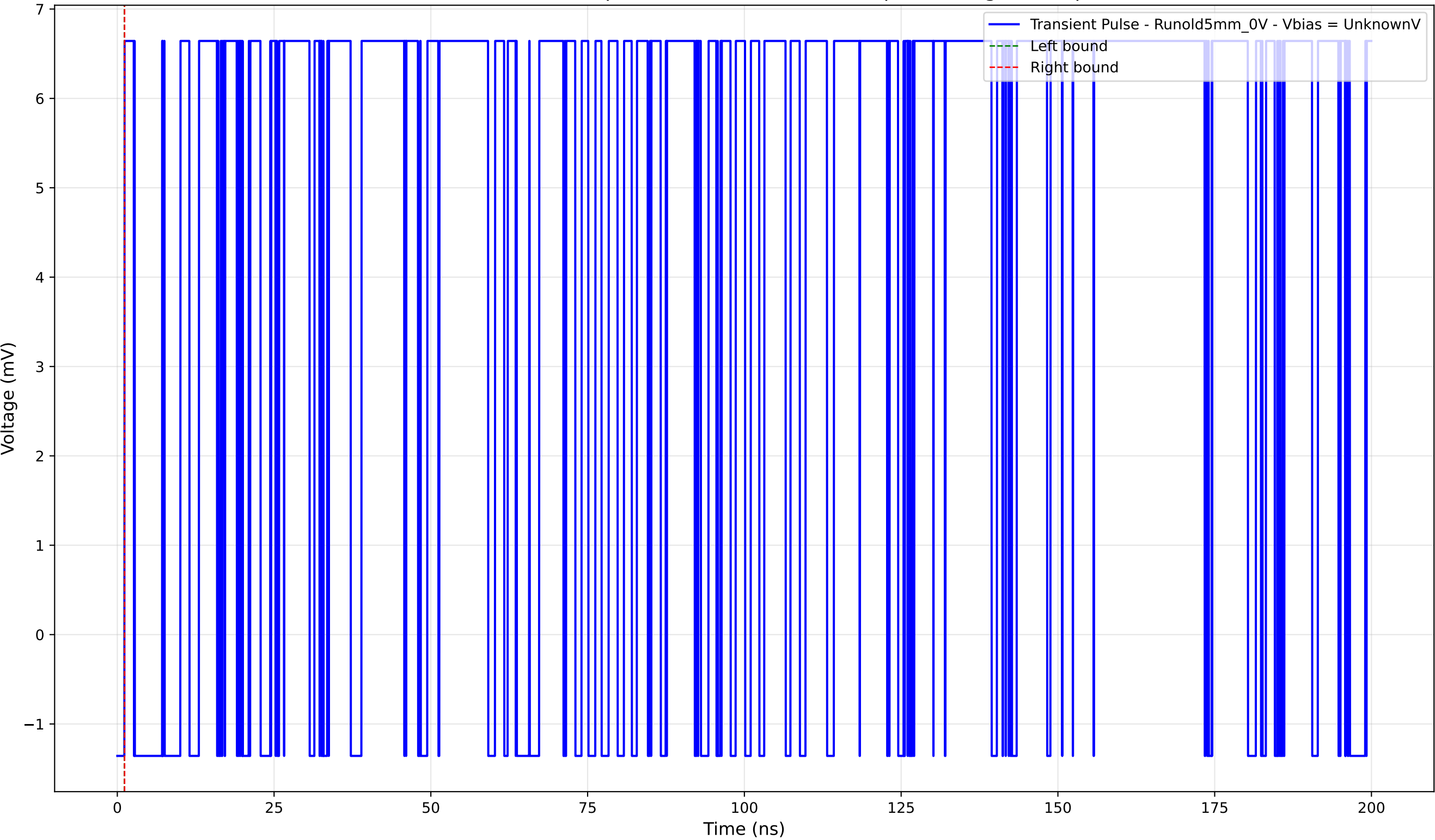
Transient Pulse - Sample: old5 - Position: 1530.0 \mu\text{m} - Charge: 0.00 pC
