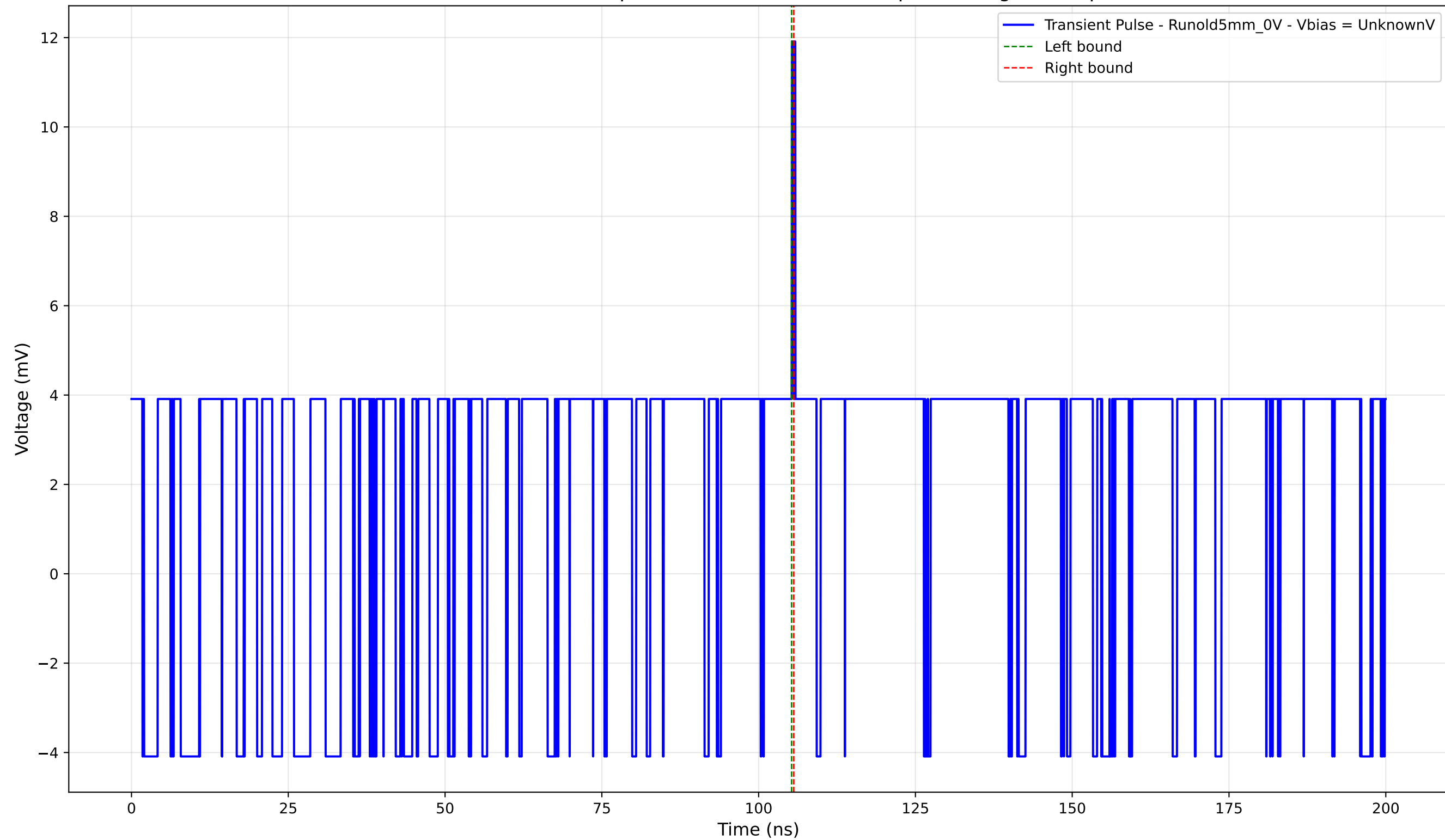
Transient Pulse - Sample: old5 - Position: 1375.0 \mu\text{m} - Charge: 0.08 pC
