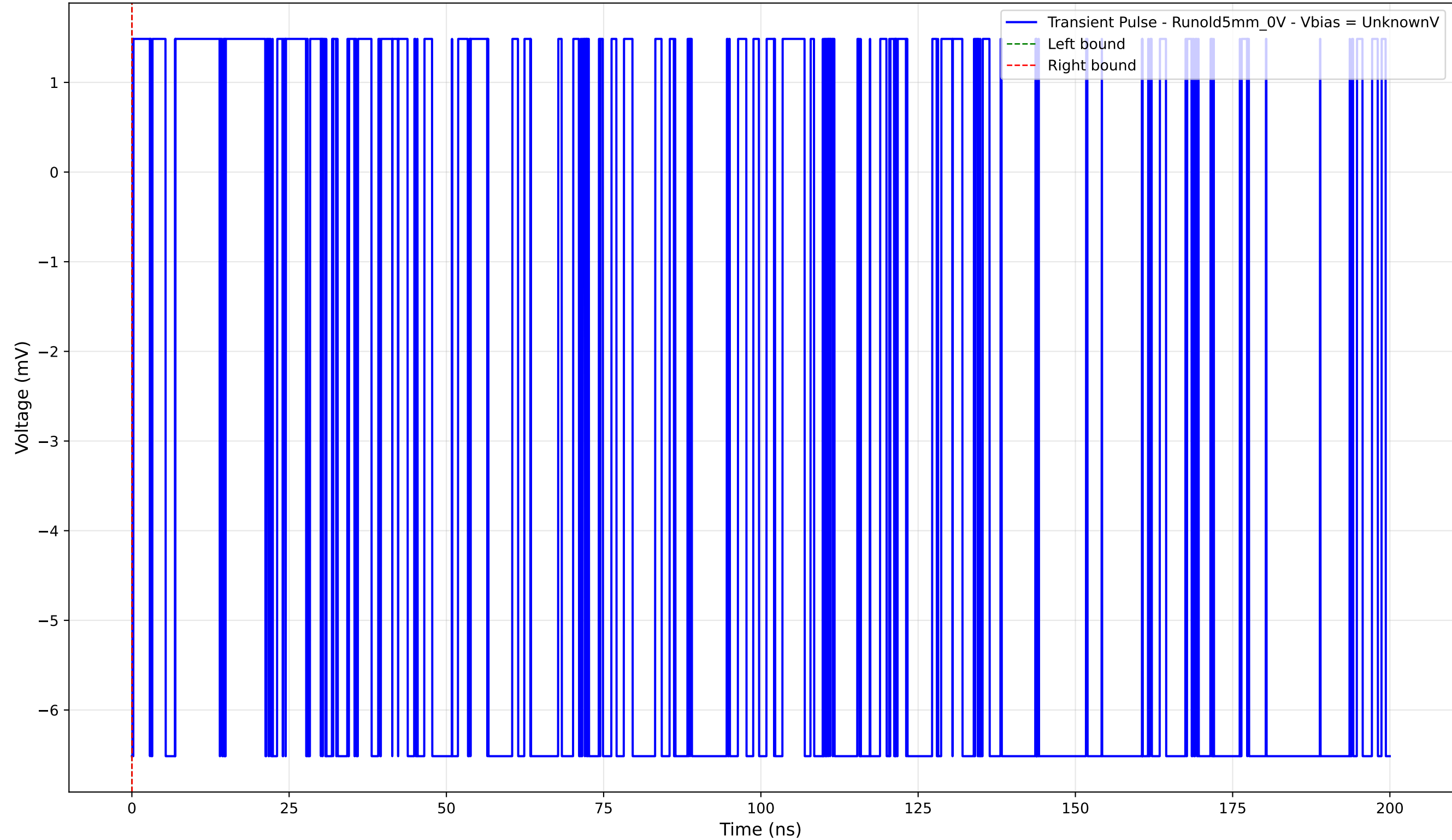
Transient Pulse - Sample: old5 - Position: 3870.0 \mu\text{m} - Charge: -0.00 pC
