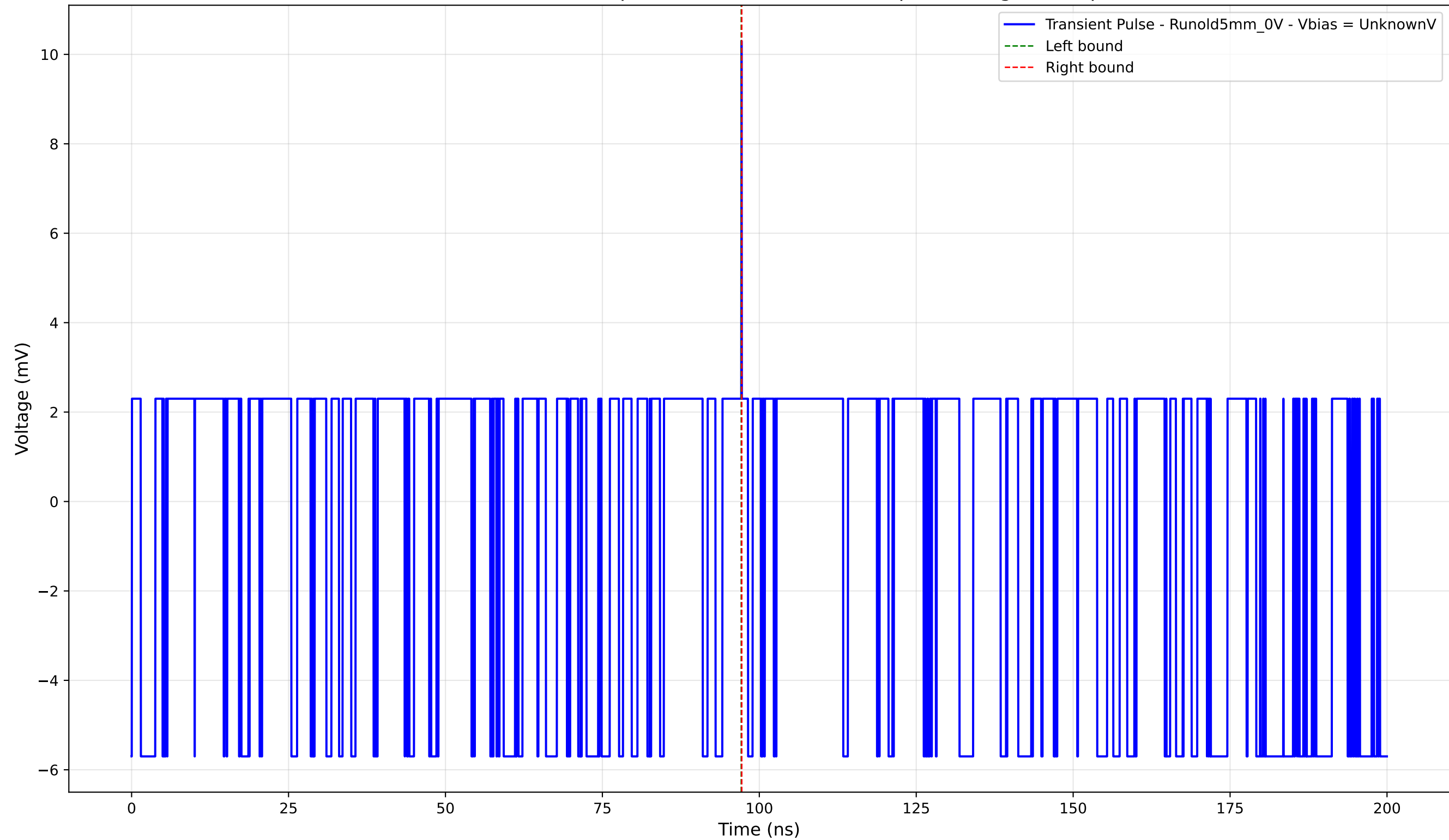
Transient Pulse - Sample: old5 - Position: 4490.0 \mu\text{m} - Charge: 0.01 pC
