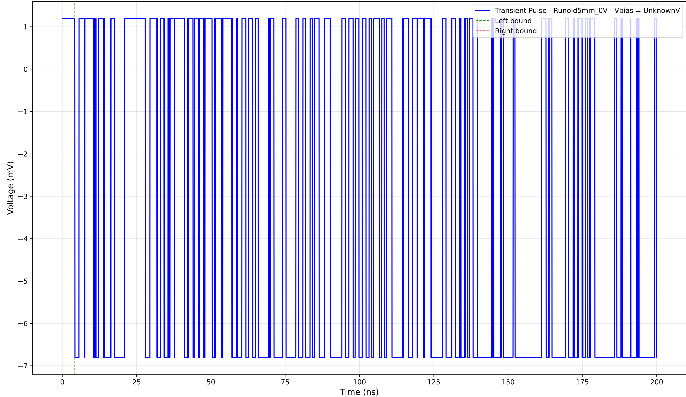
Transient Pulse - Sample: old5 - Position: 5040.0 \mu\text{m} - Charge: -0.00 pC
