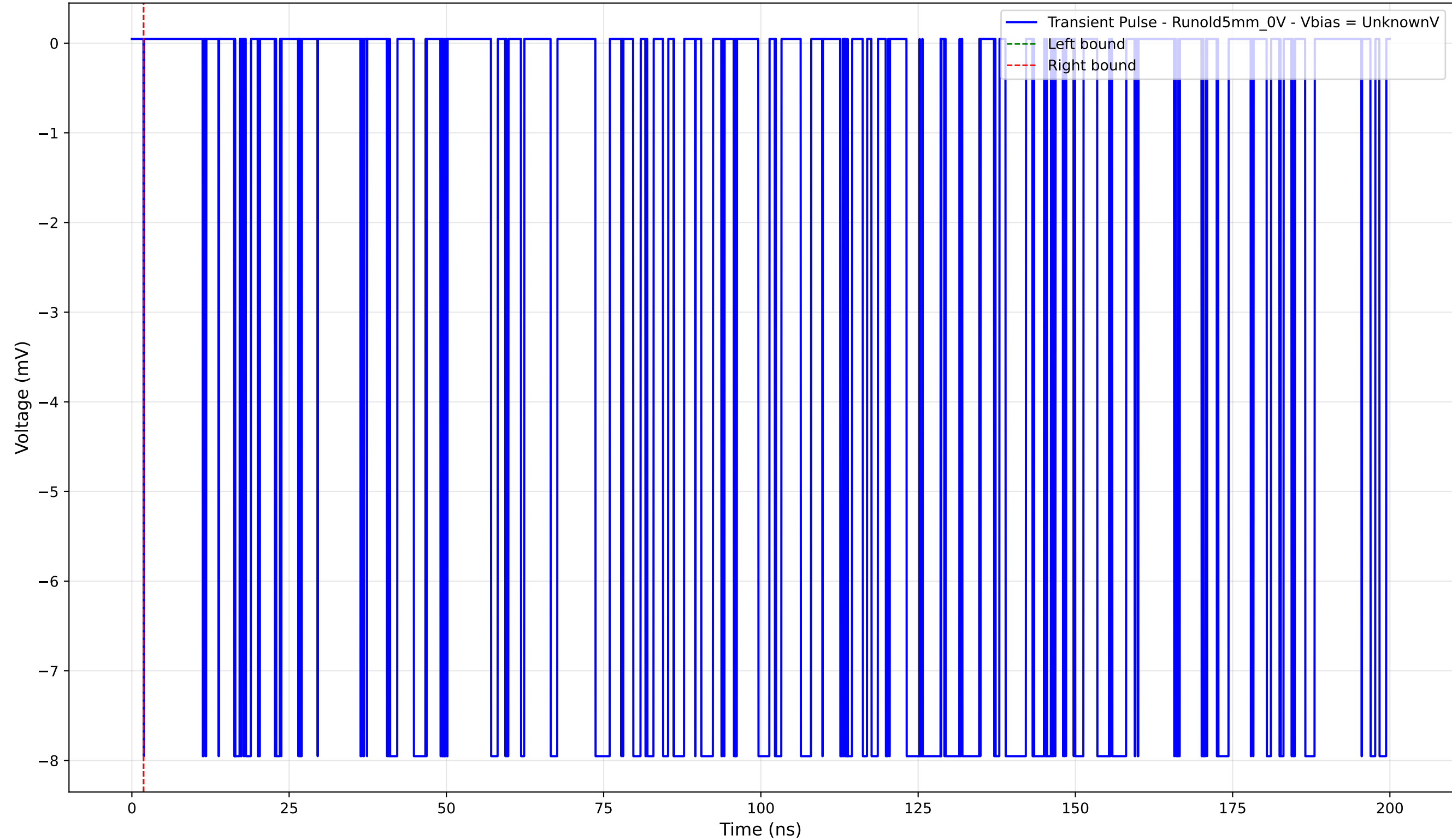
Transient Pulse - Sample: old5 - Position: 1155.0 \mu\text{m} - Charge: -0.00 pC
