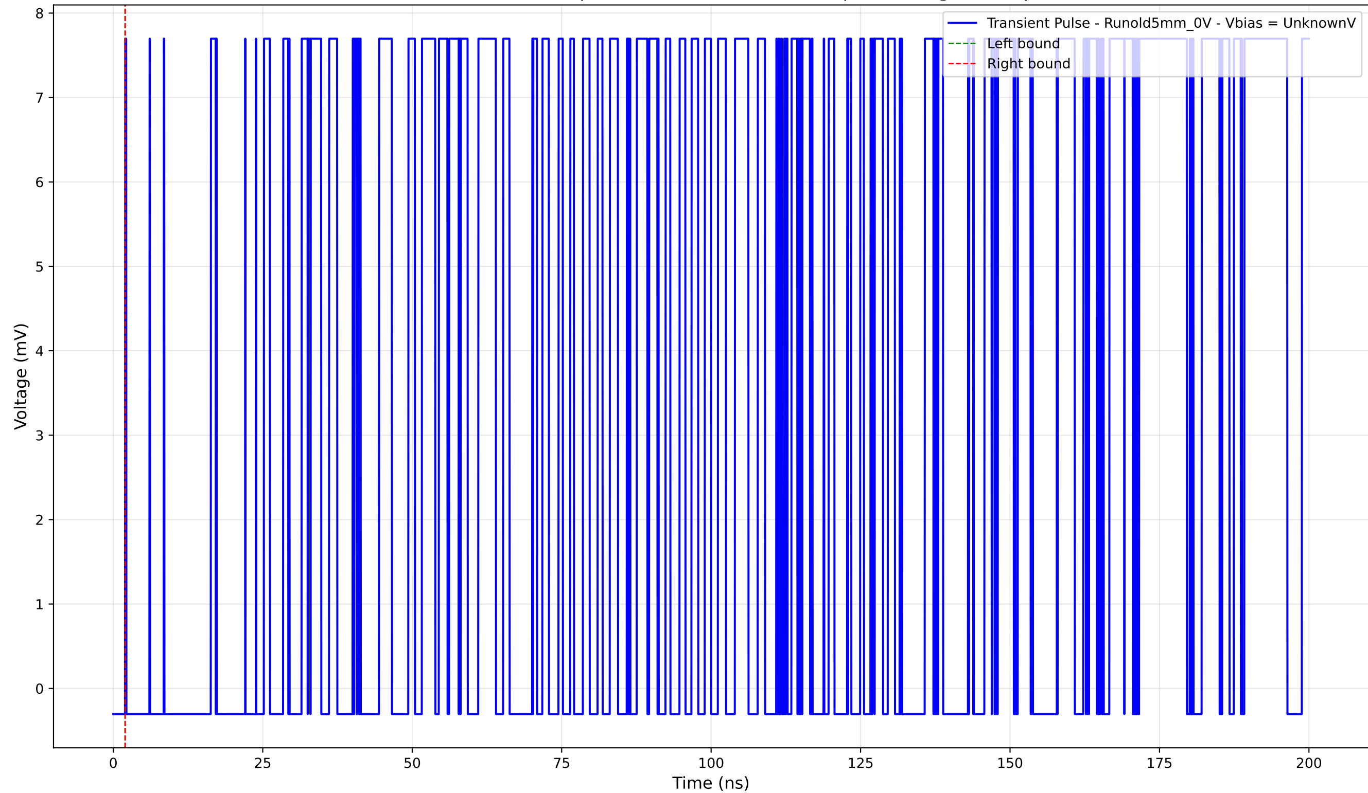
Transient Pulse - Sample: old5 - Position: 1105.0 \mu\text{m} - Charge: 0.00 pC
