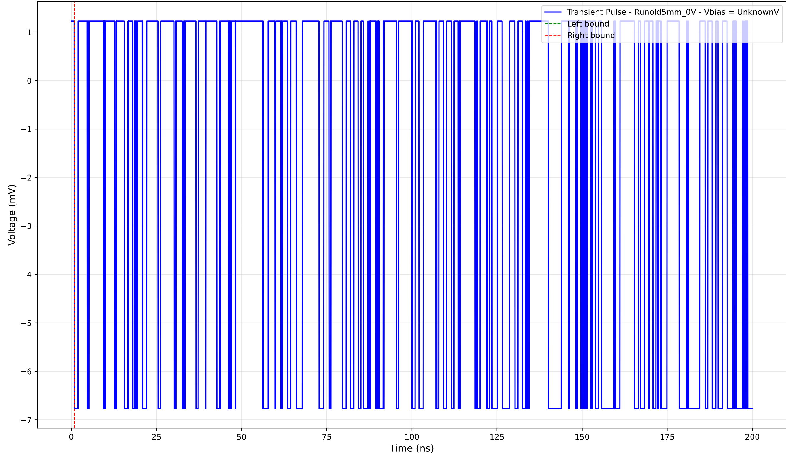
Transient Pulse - Sample: old5 - Position: 1270.0 \mu\text{m} - Charge: -0.00 pC
