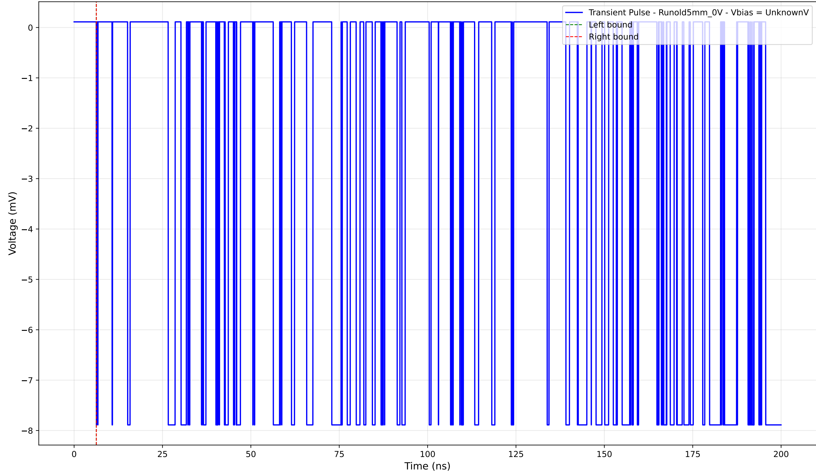
Transient Pulse - Sample: old5 - Position: 4065.0 \mu\text{m} - Charge: -0.00 pC
