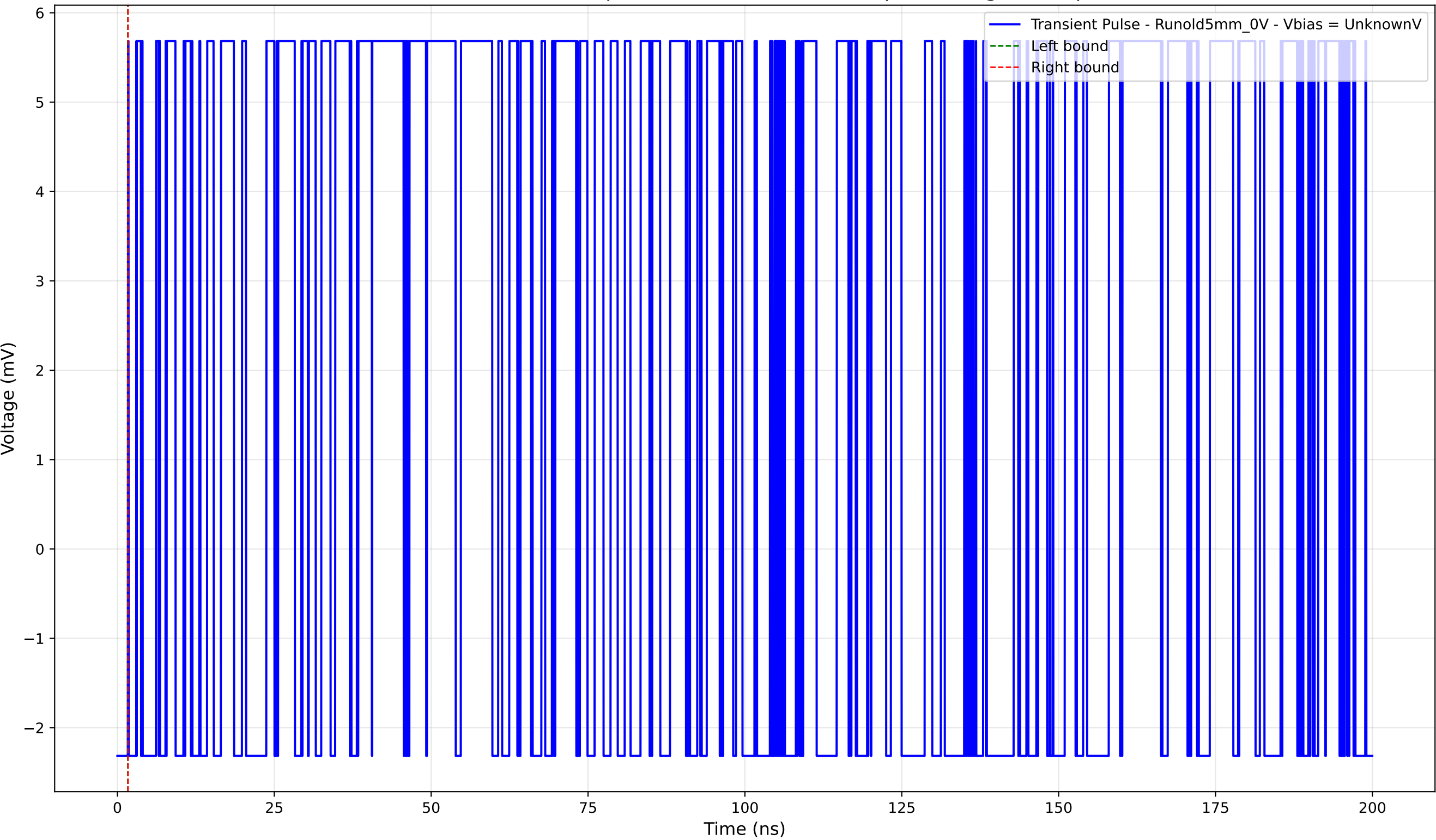
Transient Pulse - Sample: old5 - Position: 3310.0 \mu\text{m} - Charge: 0.00 pC
