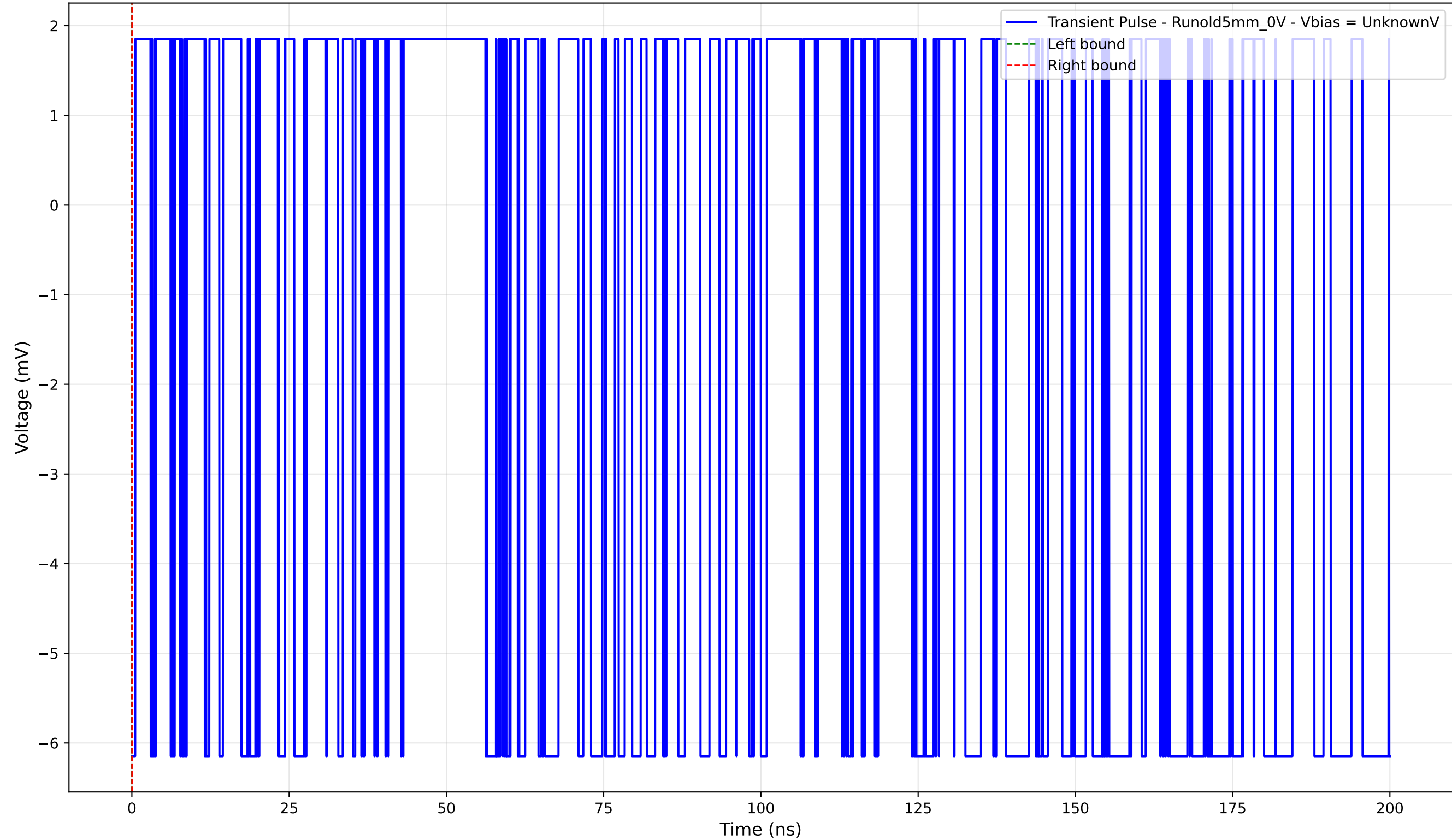
Transient Pulse - Sample: old5 - Position: 2675.0 \mu\text{m} - Charge: -0.00 pC
