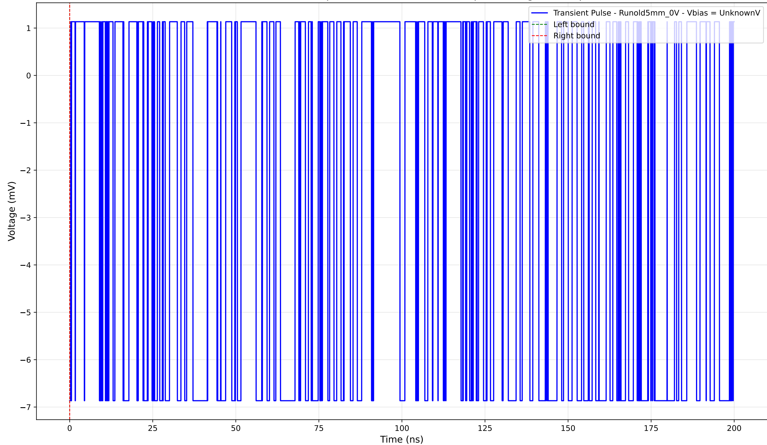
Transient Pulse - Sample: old5 - Position: 1730.0 \mu\text{m} - Charge: -0.00 pC
