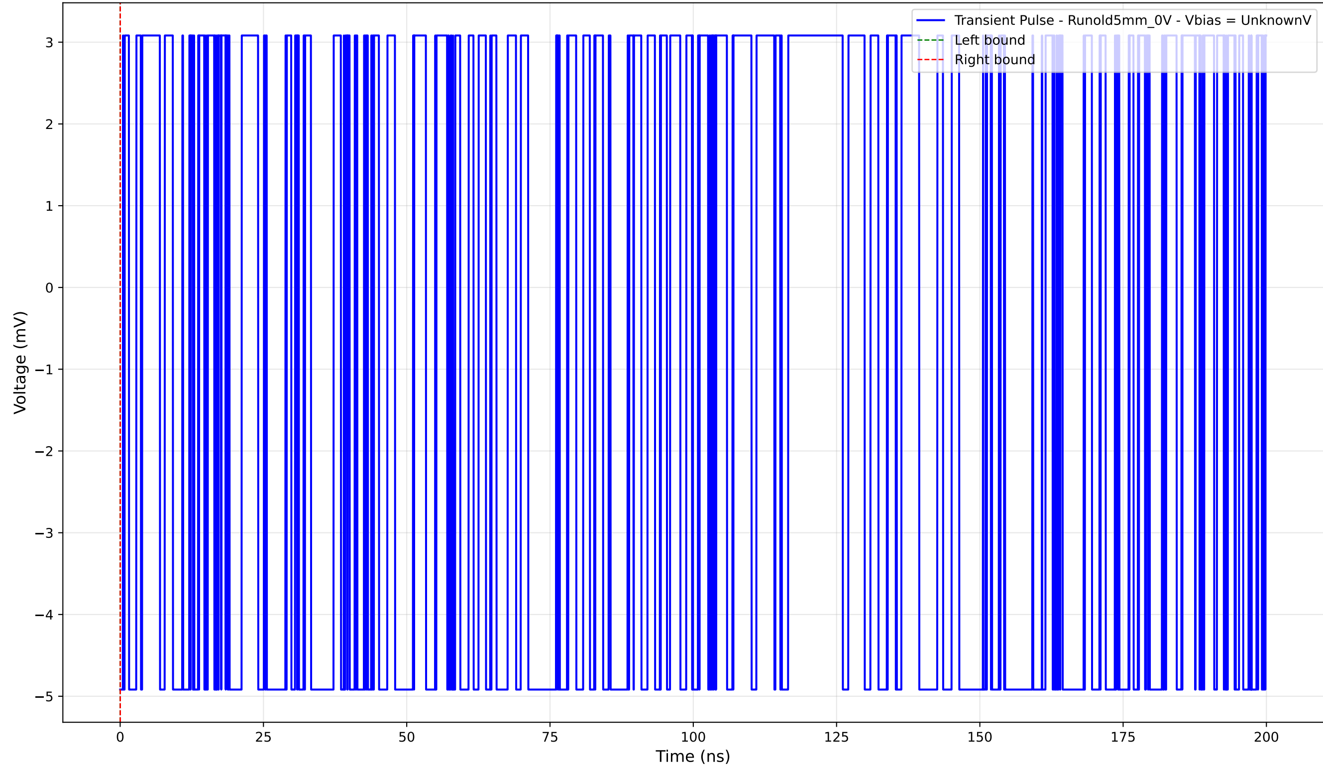
Transient Pulse - Sample: old5 - Position: 3625.0 \mu\text{m} - Charge: -0.00 pC
