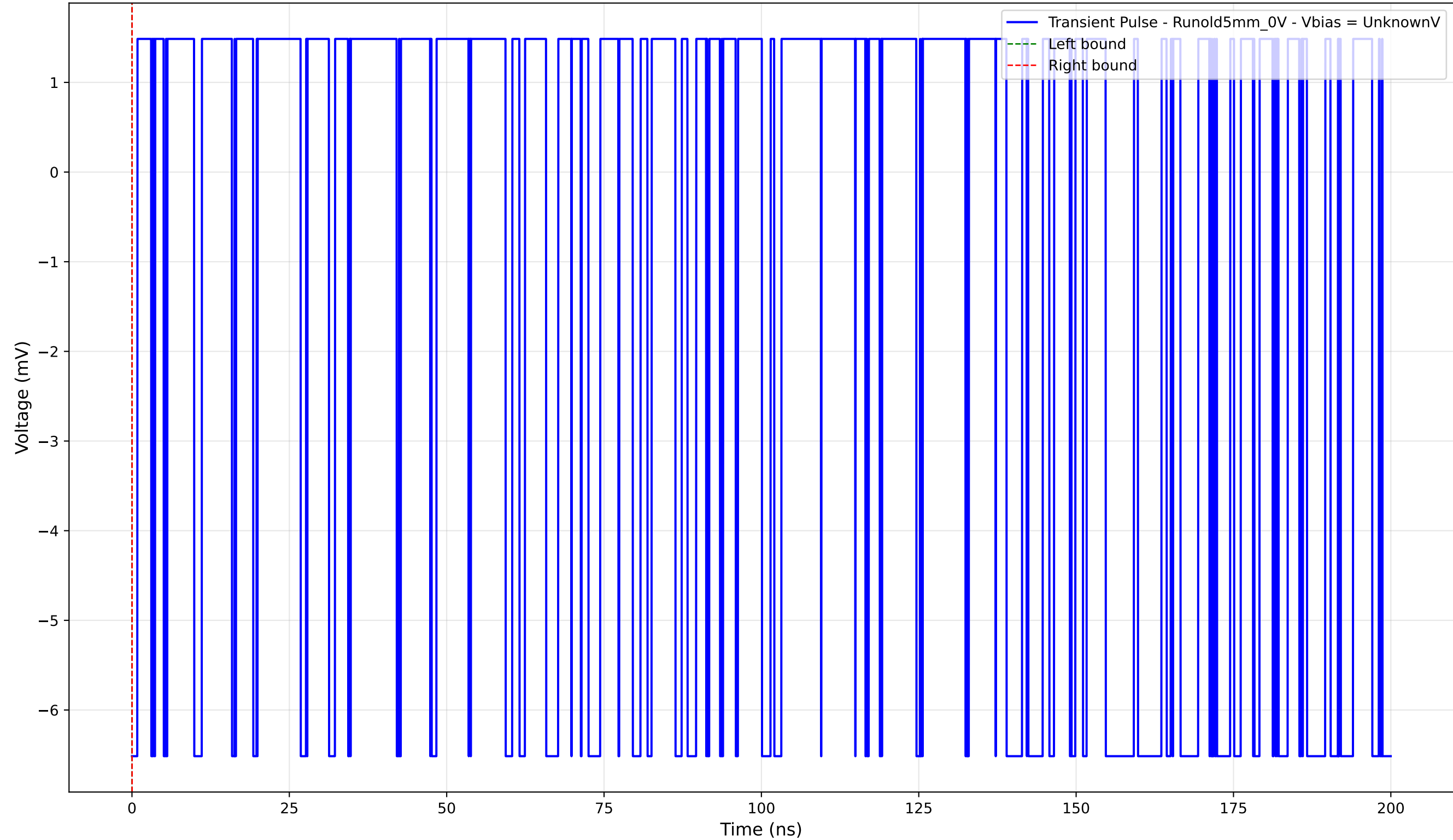
Transient Pulse - Sample: old5 - Position: 3330.0 \mu\text{m} - Charge: -0.00 pC
