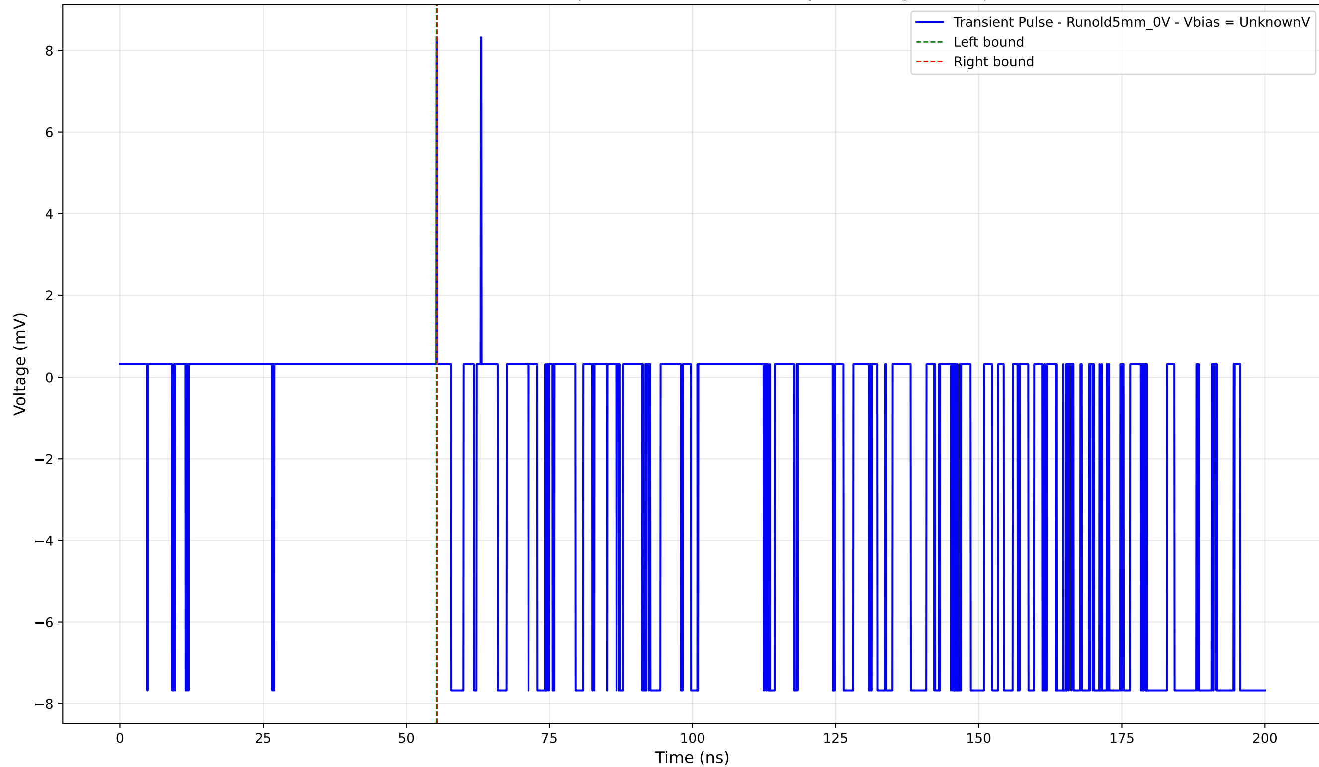
Transient Pulse - Sample: old5 - Position: 25.0 \mu\text{m} - Charge: 0.02 pC
