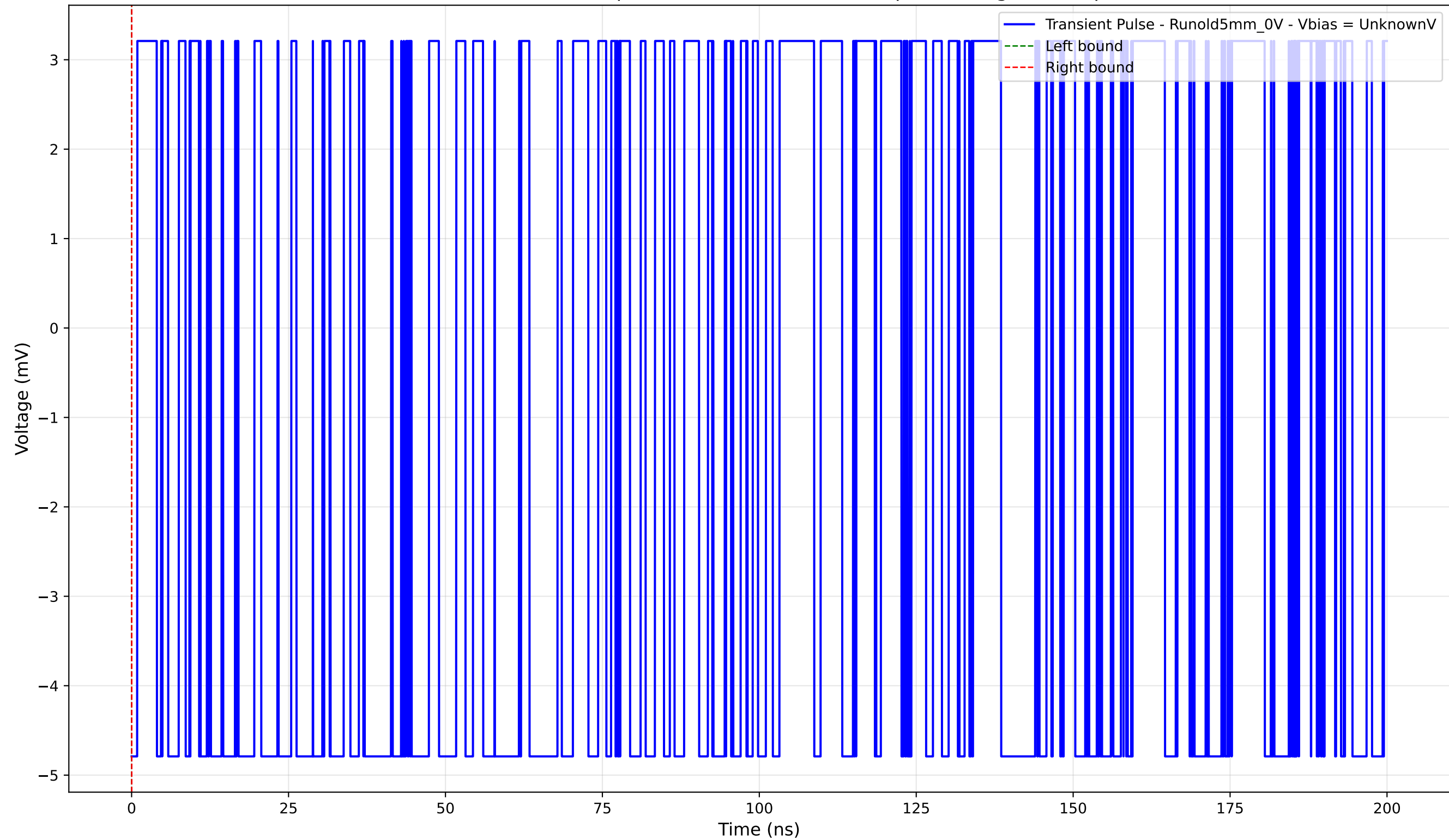
Transient Pulse - Sample: old5 - Position: 2865.0 \mu\text{m} - Charge: -0.00 pC
