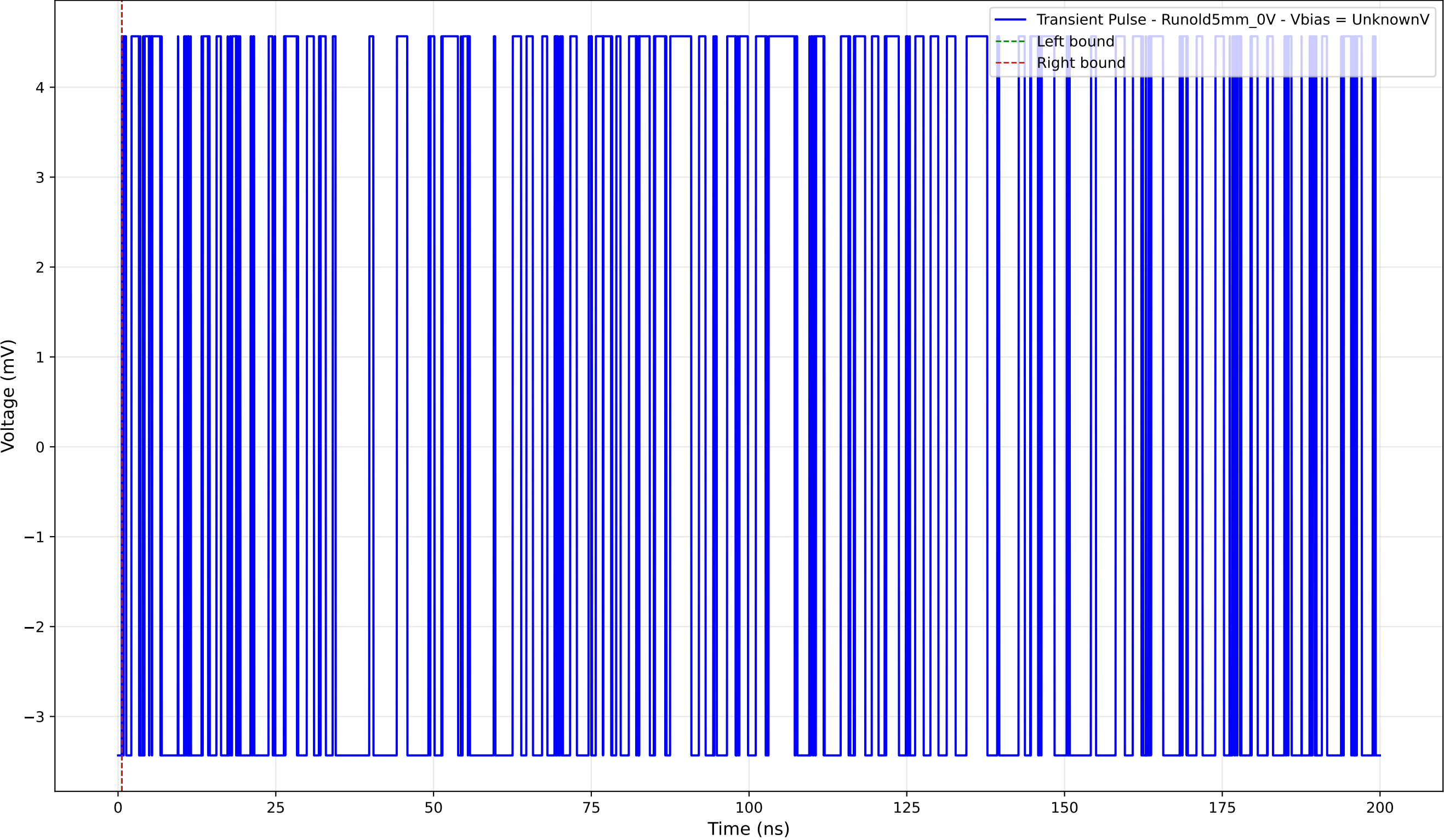
Transient Pulse - Sample: old5 - Position: 2315.0 \mu\text{m} - Charge: 0.00 pC
