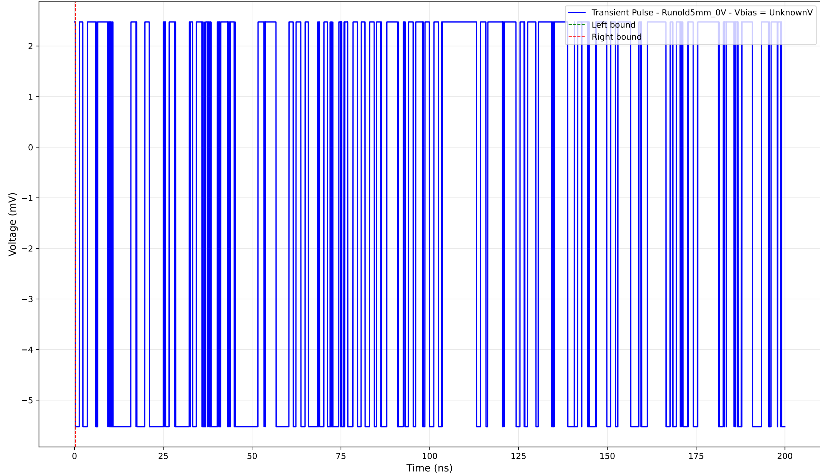
Transient Pulse - Sample: old5 - Position: 5045.0 \mu\text{m} - Charge: -0.00 pC
