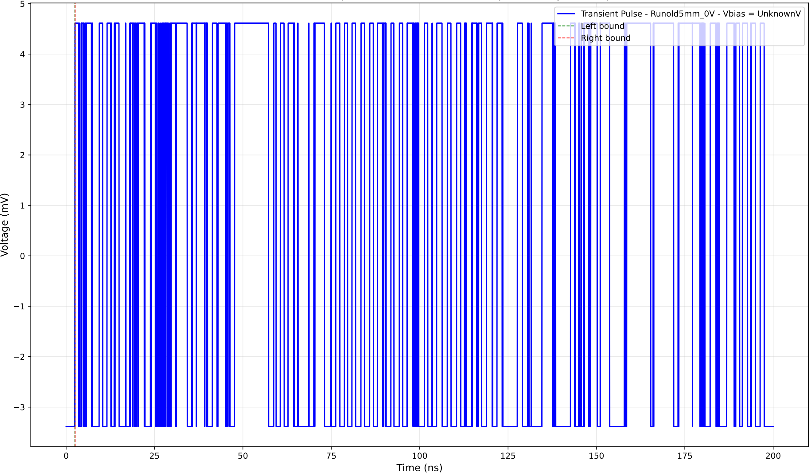
Transient Pulse - Sample: old5 - Position: 3700.0 \mu\text{m} - Charge: 0.00 pC
