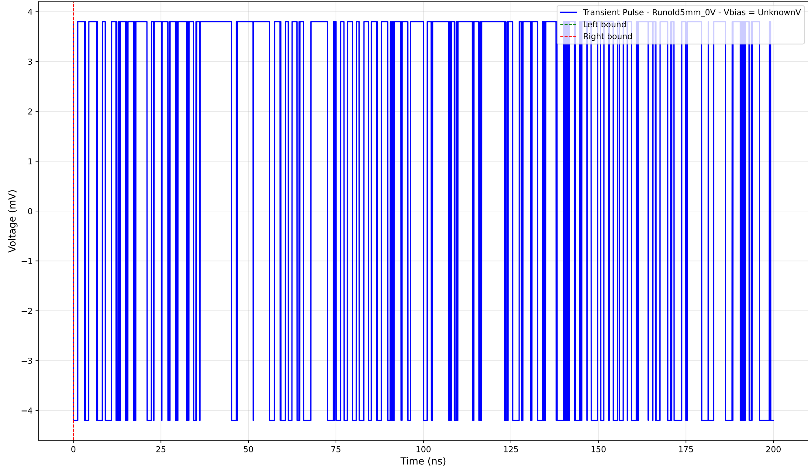
Transient Pulse - Sample: old5 - Position: 1260.0 \mu\text{m} - Charge: -0.00 pC
