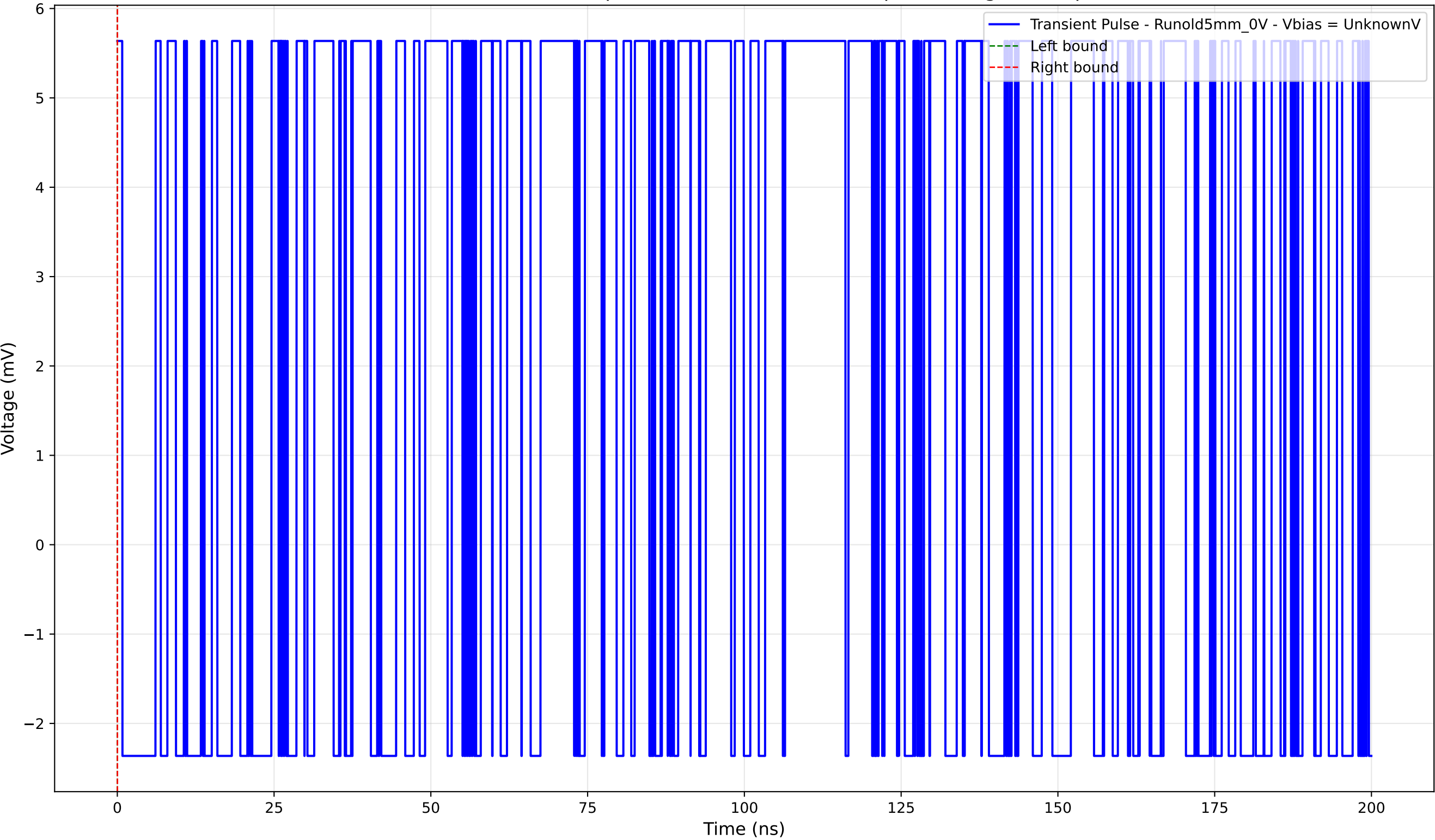
Transient Pulse - Sample: old5 - Position: 3850.0 \mu\text{m} - Charge: 0.00 pC
