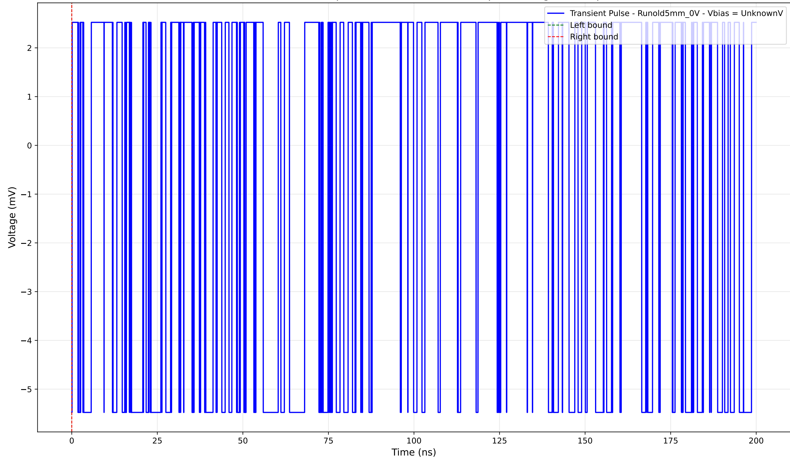
Transient Pulse - Sample: old5 - Position: 4460.0 \mu\text{m} - Charge: -0.00 pC
