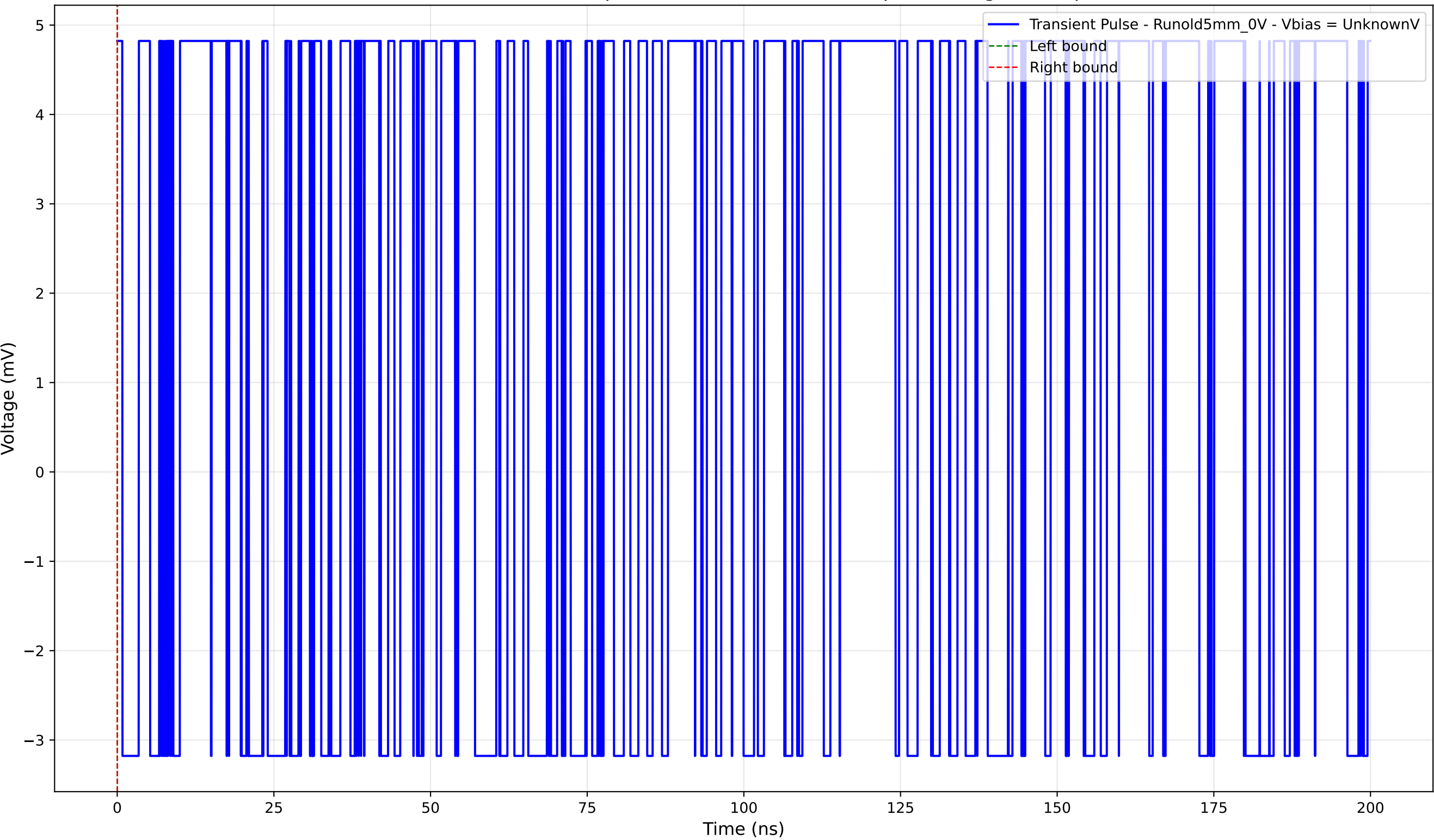
Transient Pulse - Sample: old5 - Position: 1405.0 \mu\text{m} - Charge: 0.00 pC
