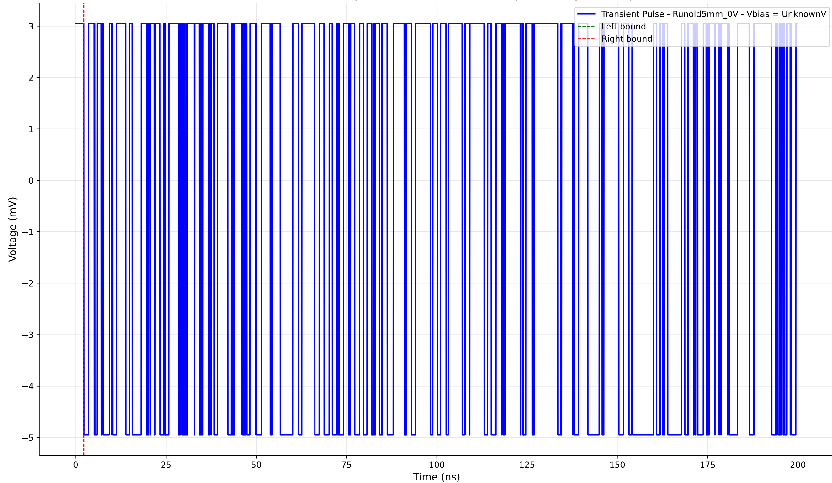
Transient Pulse - Sample: old5 - Position: 4860.0 \mu\text{m} - Charge: -0.00 pC
