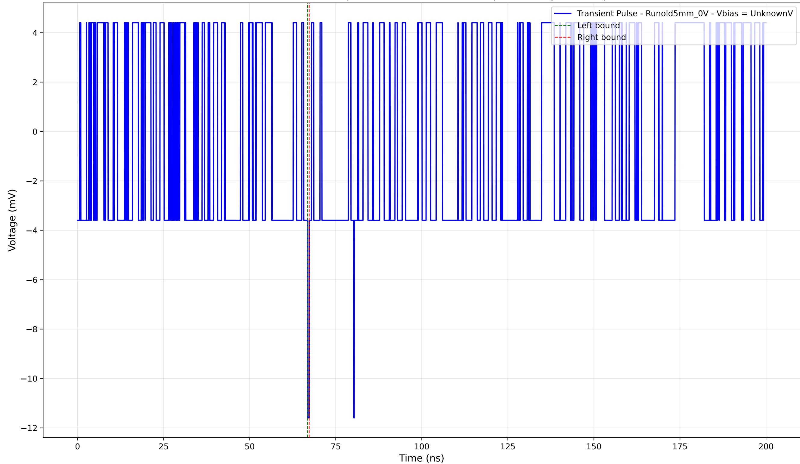
Transient Pulse - Sample: old5 - Position: 435.0 \mu\text{m} - Charge: -0.10 pC
