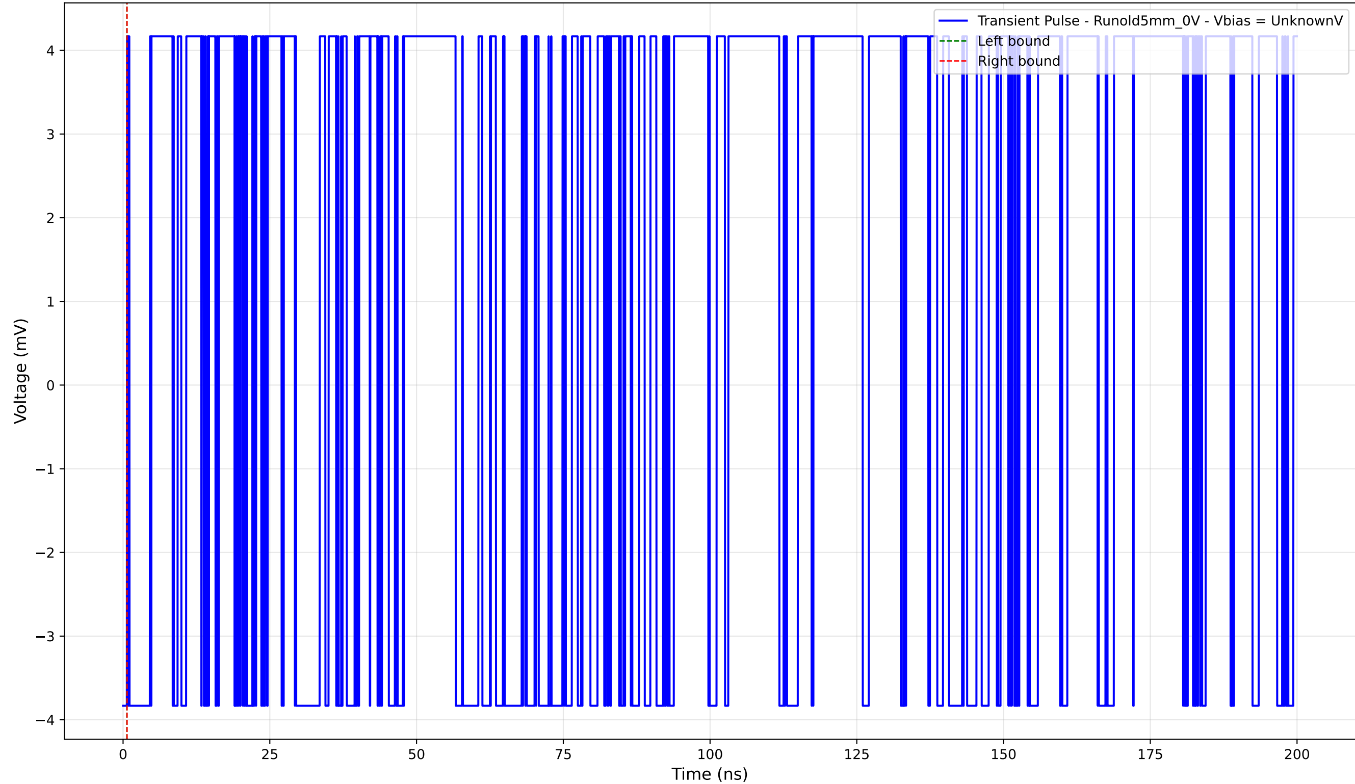
Transient Pulse - Sample: old5 - Position: 645.0 \mu\text{m} - Charge: 0.00 pC
