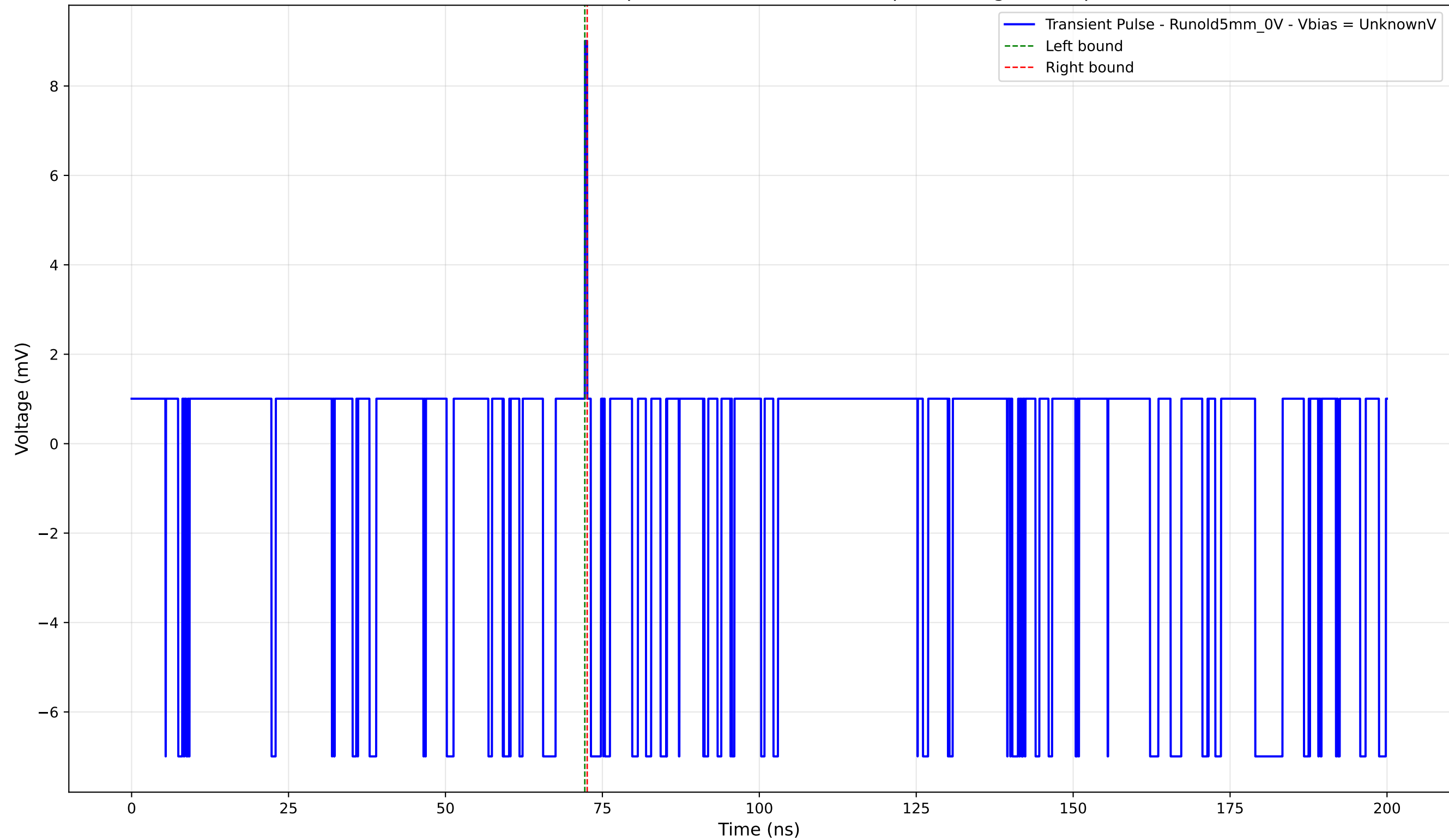
Transient Pulse - Sample: old5 - Position: 935.0 \mu\text{m} - Charge: 0.07 pC
