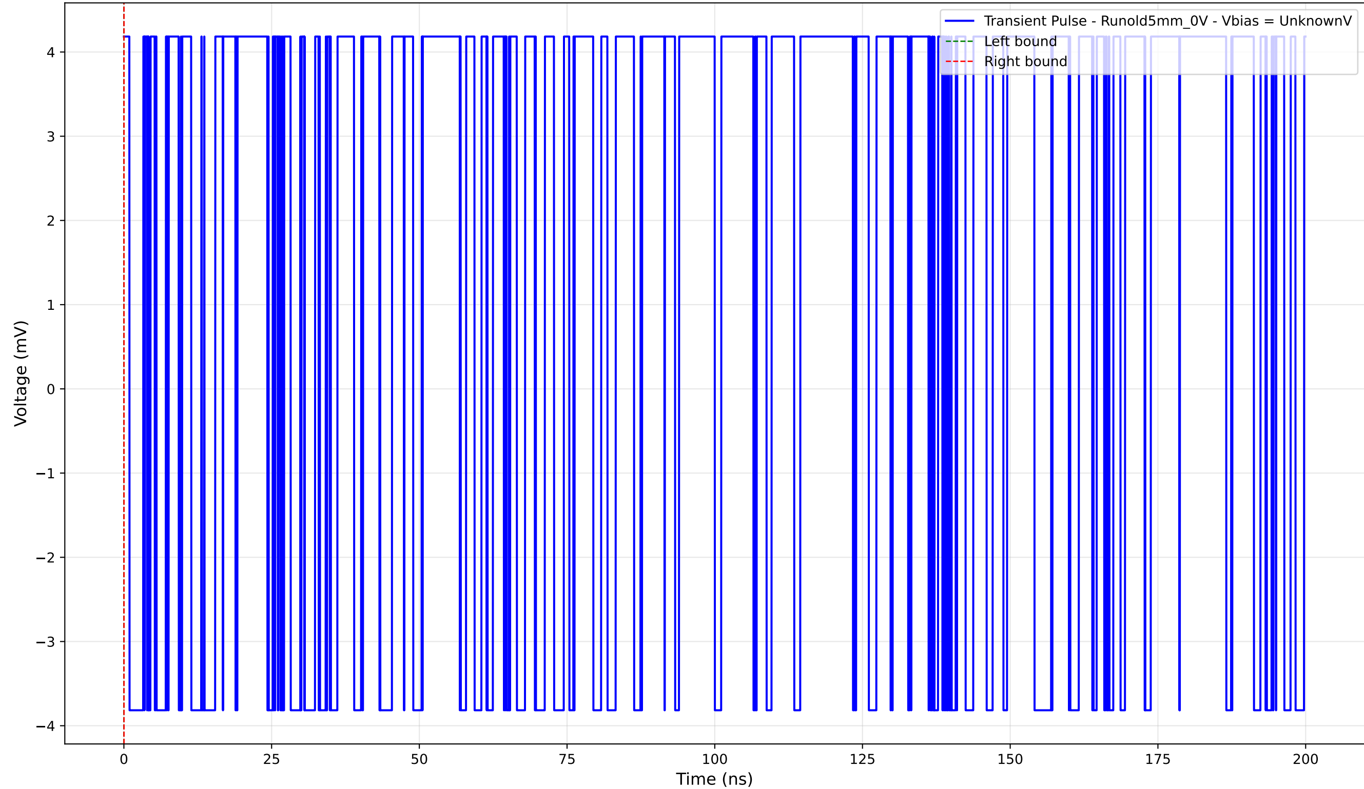
Transient Pulse - Sample: old5 - Position: 955.0 \mu\text{m} - Charge: 0.00 pC
