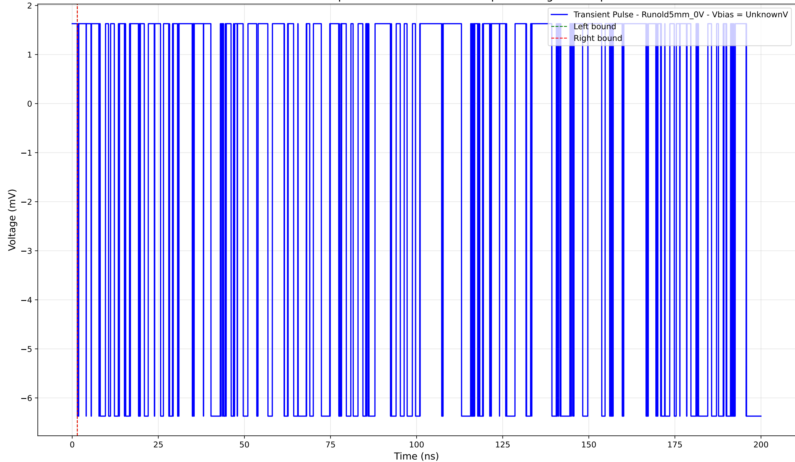
Transient Pulse - Sample: old5 - Position: 2410.0 \mu\text{m} - Charge: -0.00 pC
