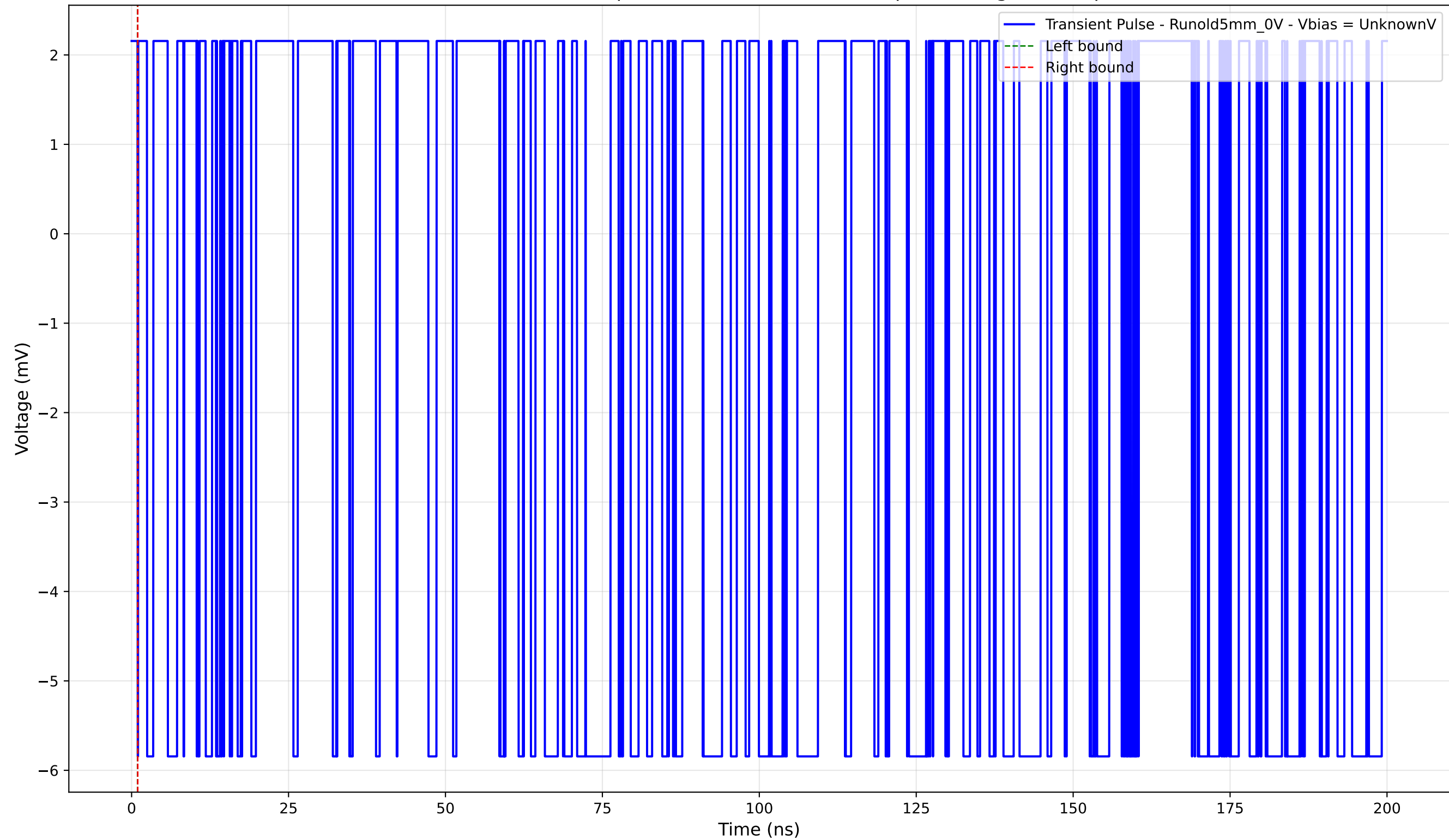
Transient Pulse - Sample: old5 - Position: 2700.0 \mu\text{m} - Charge: -0.00 pC
