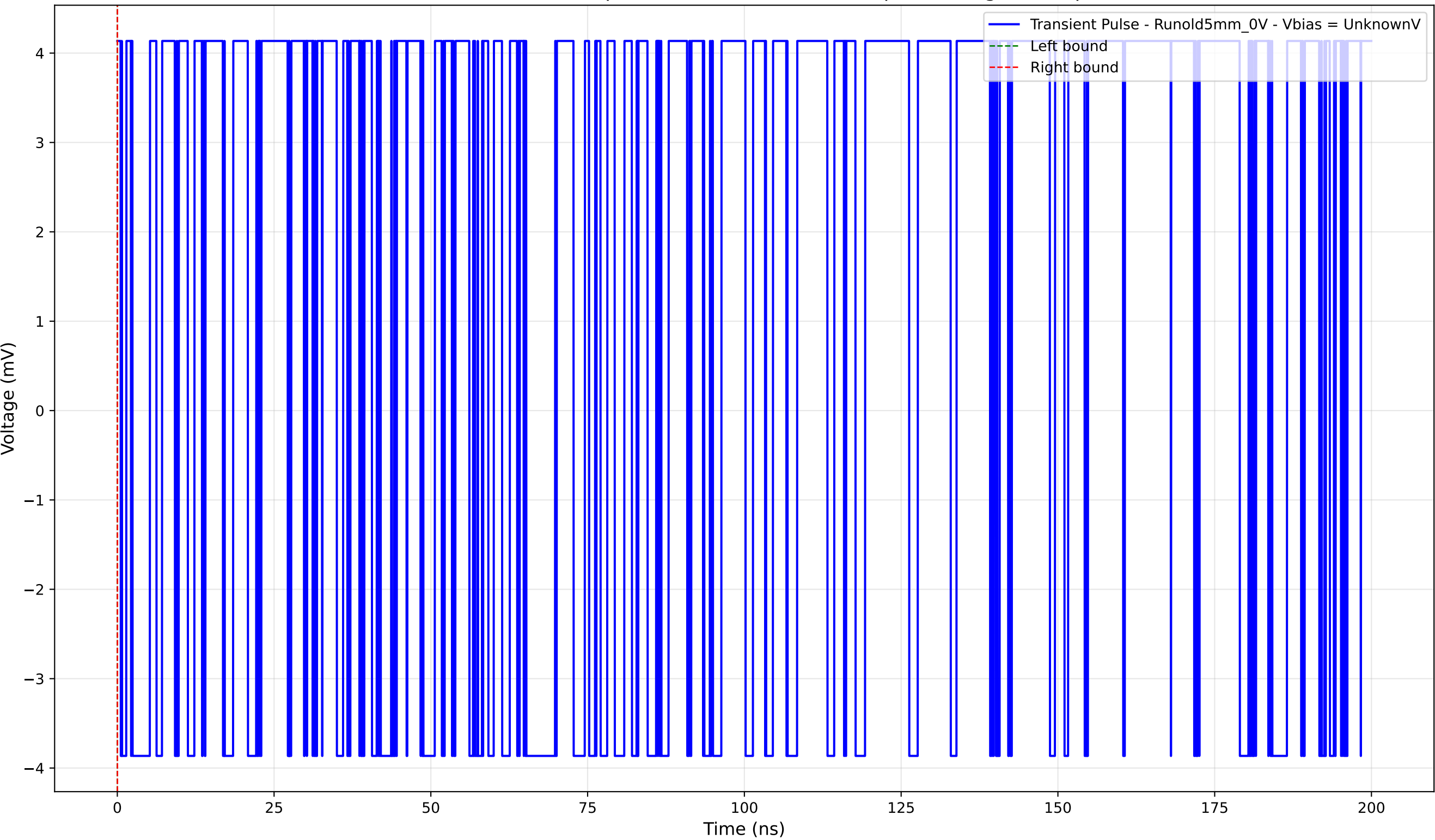
Transient Pulse - Sample: old5 - Position: 5060.0 \mu\text{m} - Charge: 0.00 pC
