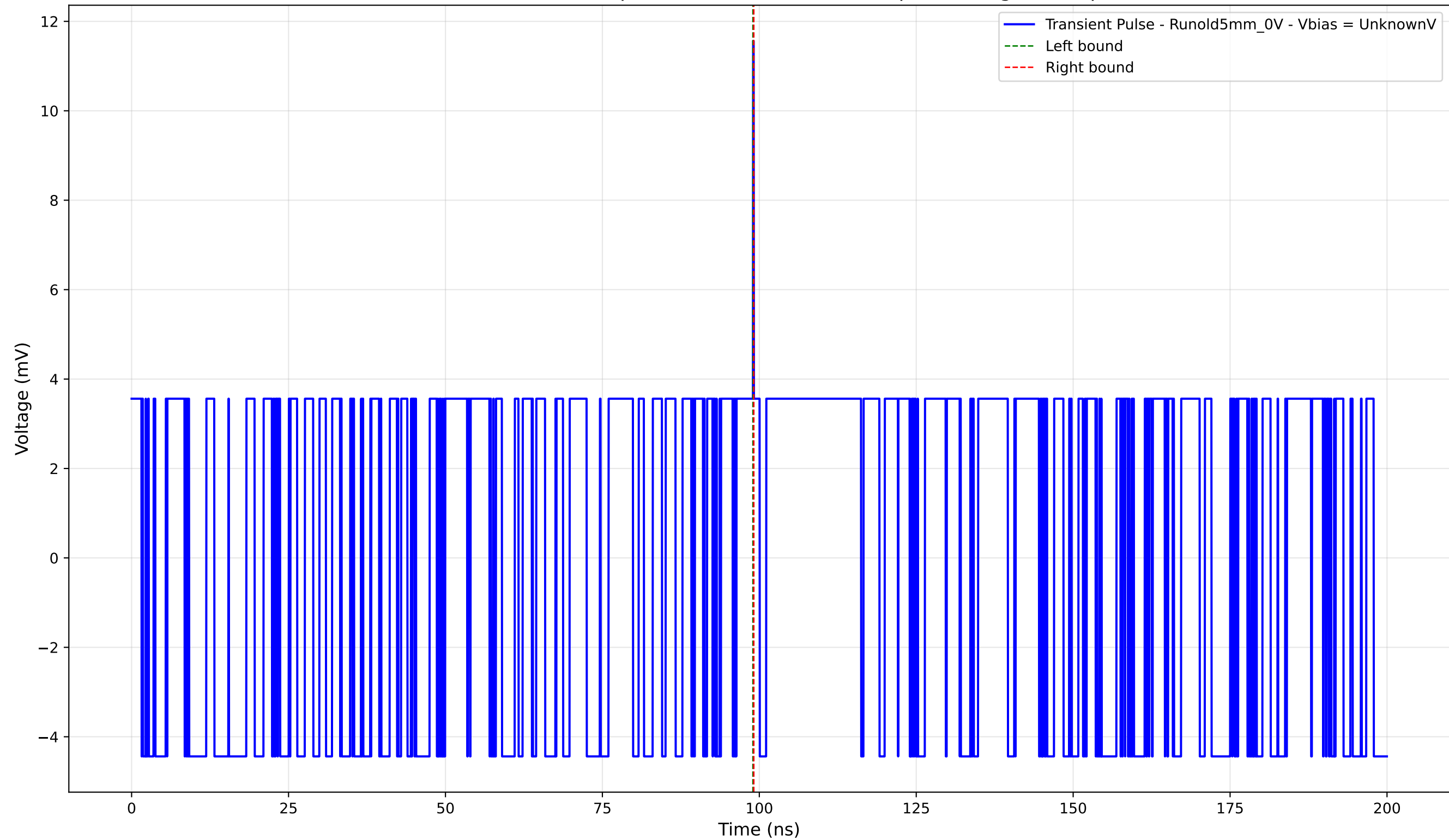
Transient Pulse - Sample: old5 - Position: 2185.0 \mu\text{m} - Charge: 0.03 pC
