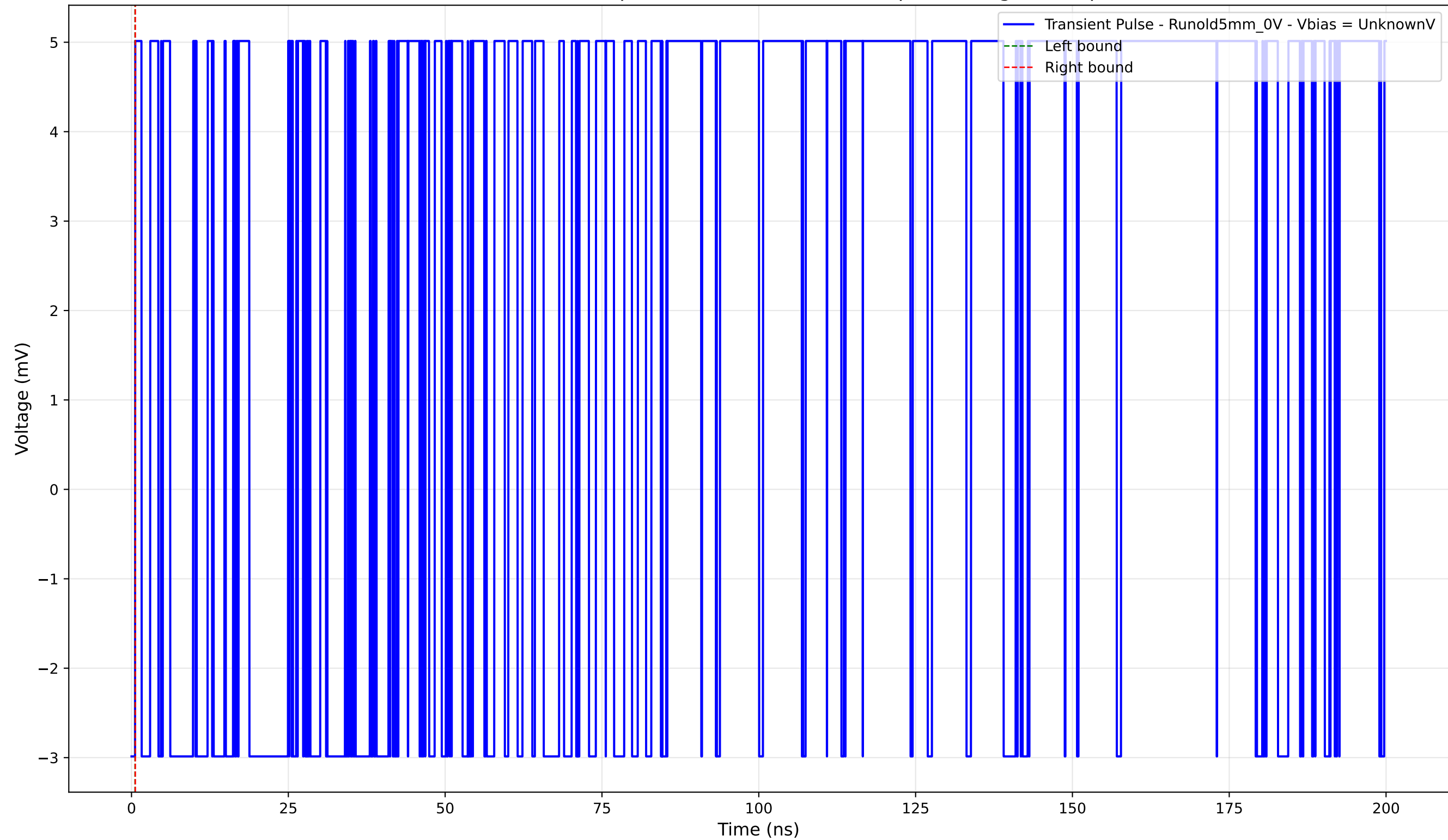
Transient Pulse - Sample: old5 - Position: 2050.0 \mu\text{m} - Charge: 0.00 pC
