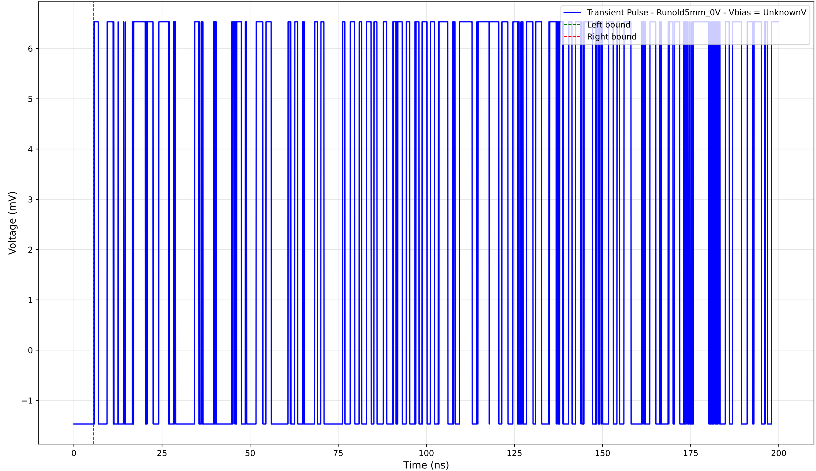
Transient Pulse - Sample: old5 - Position: 105.0 \mu\text{m} - Charge: 0.00 pC
