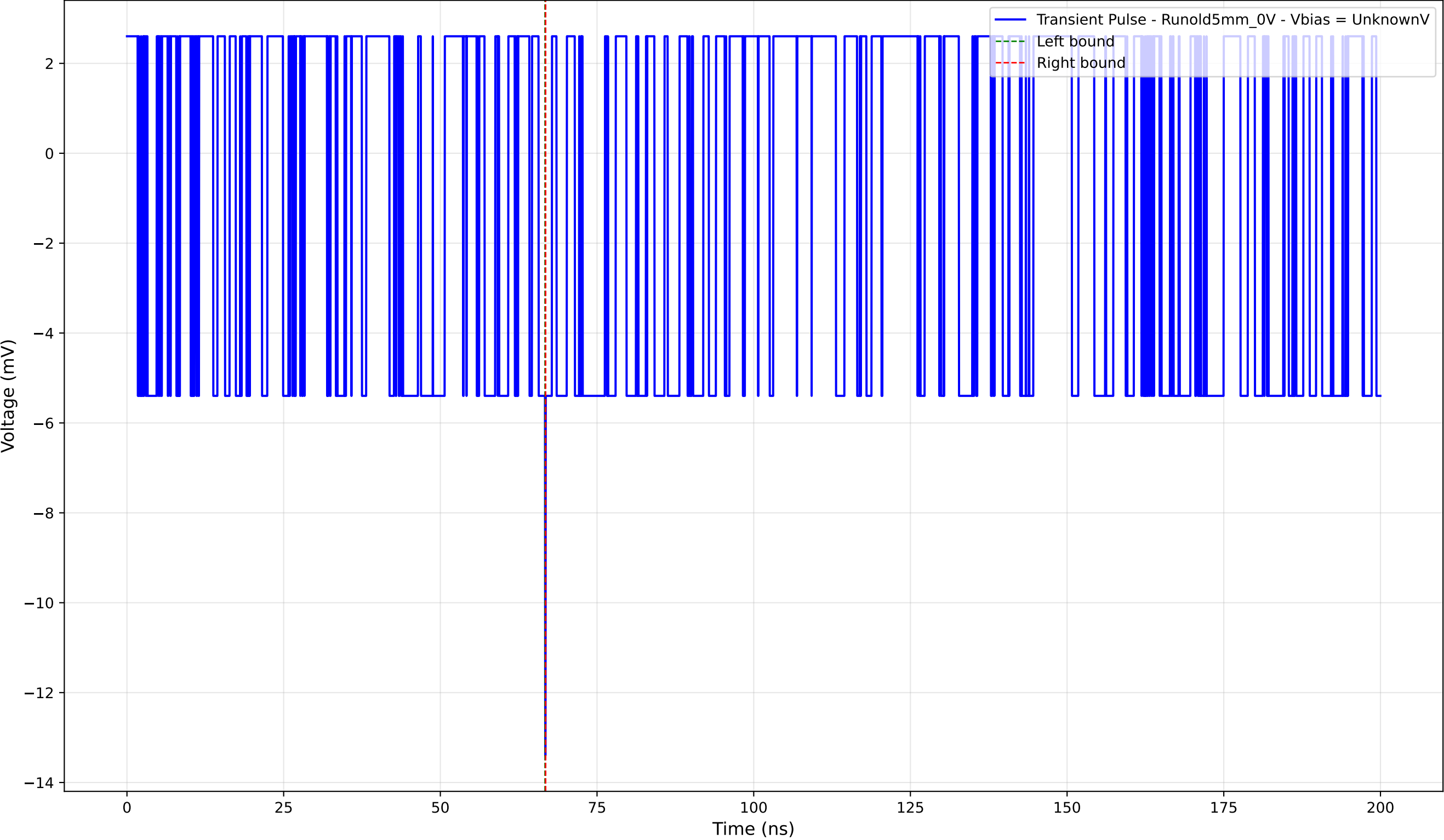
Transient Pulse - Sample: old5 - Position: 4675.0 \mu\text{m} - Charge: -0.02 pC
