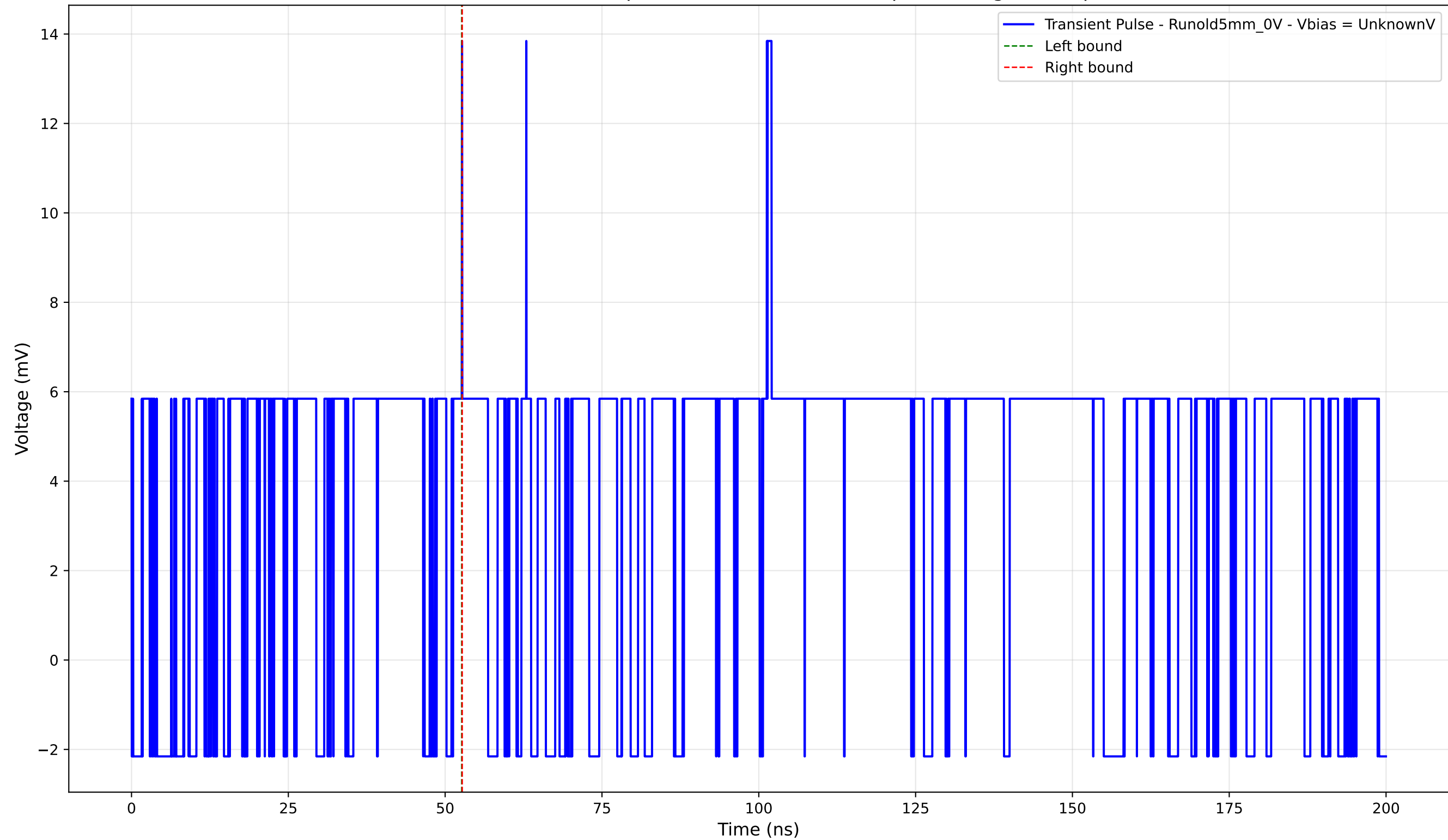
Transient Pulse - Sample: old5 - Position: 285.0 \mu\text{m} - Charge: 0.02 pC
