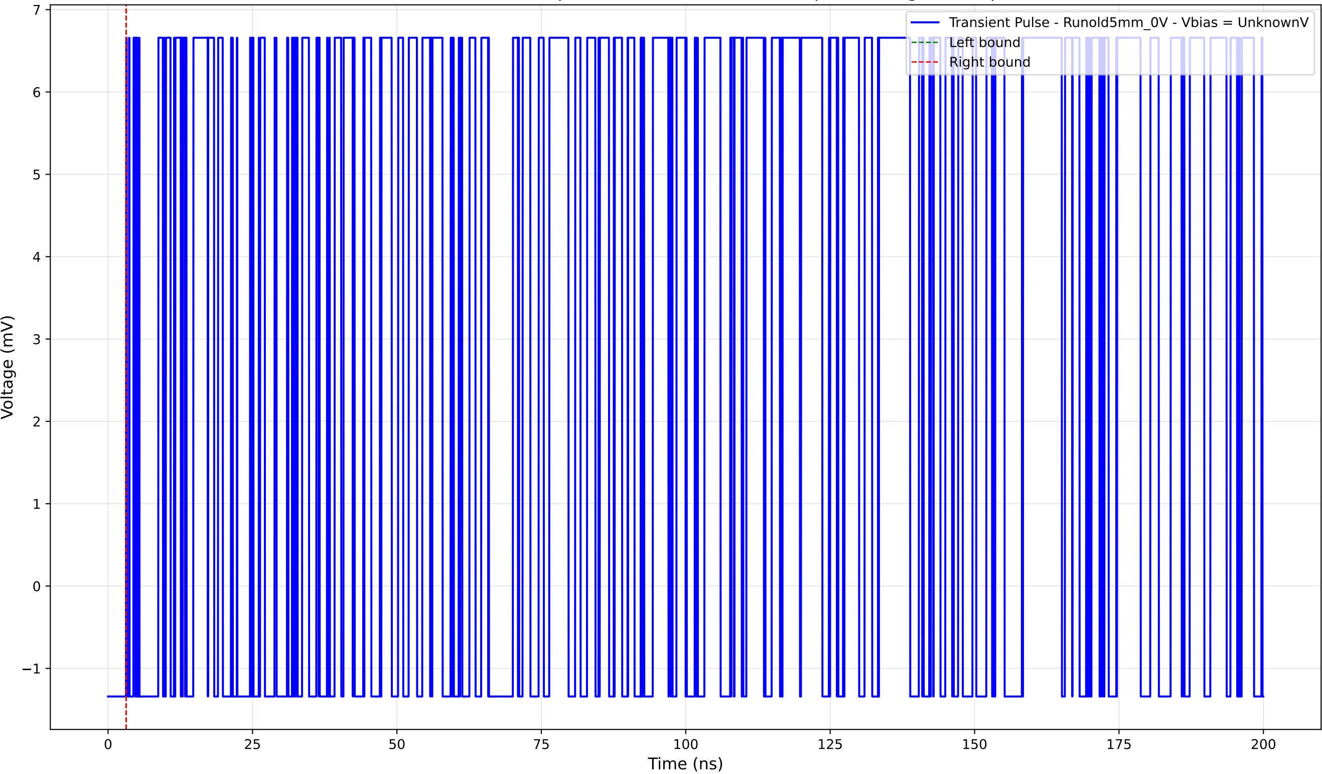
Transient Pulse - Sample: old5 - Position: 3415.0 \mu\text{m} - Charge: 0.00 pC
