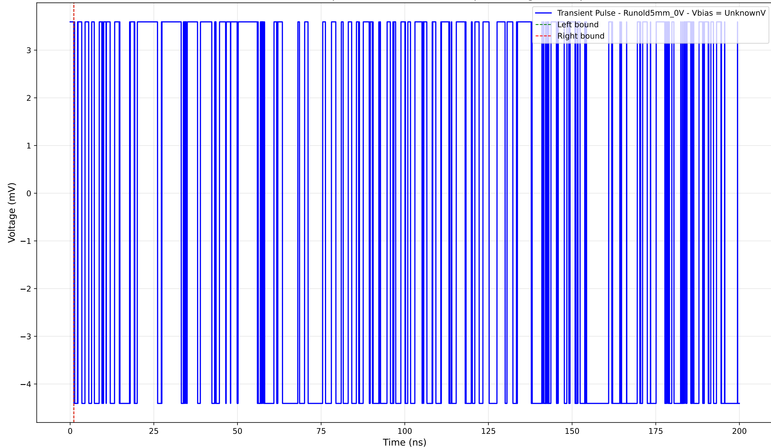
Transient Pulse - Sample: old5 - Position: 805.0 \mu\text{m} - Charge: -0.00 pC
