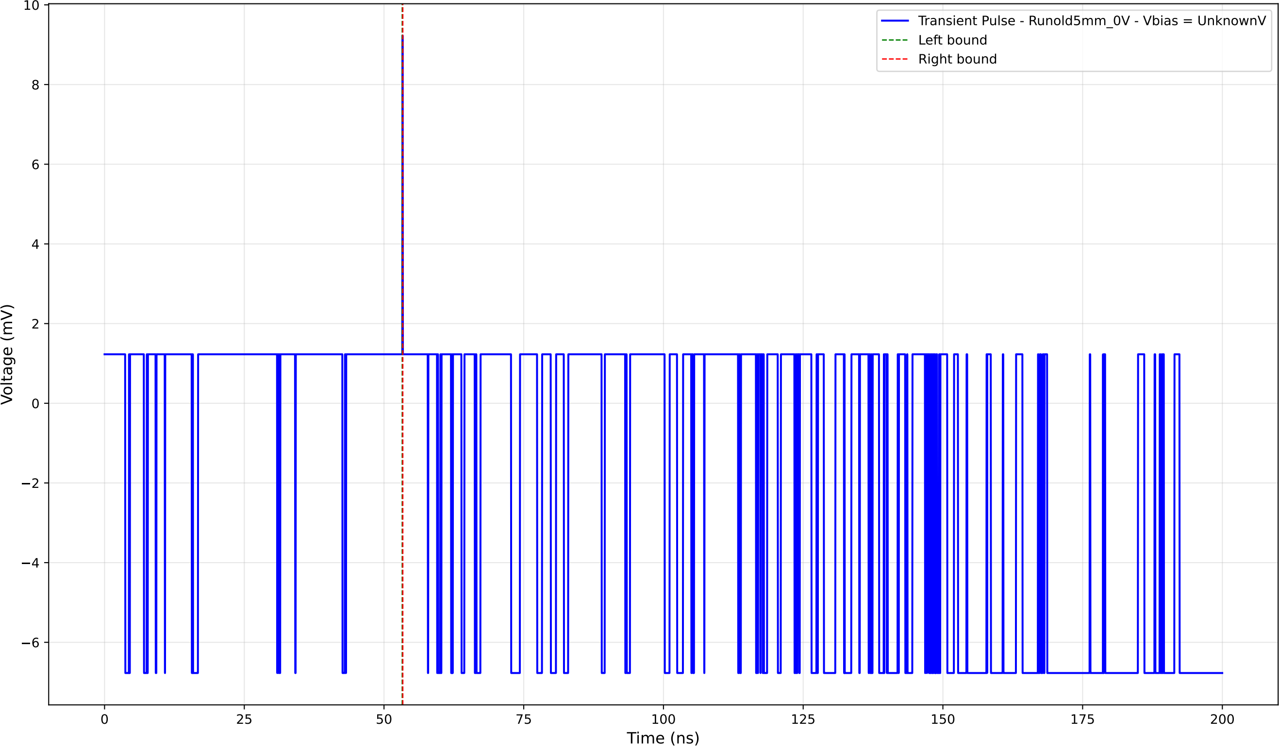
Transient Pulse - Sample: old5 - Position: 2165.0 \mu\text{m} - Charge: 0.02 pC
