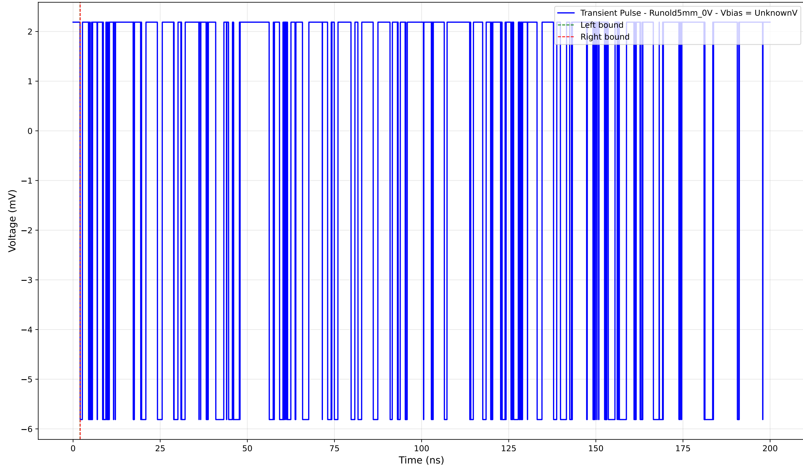
Transient Pulse - Sample: old5 - Position: 1720.0 \mu\text{m} - Charge: -0.00 pC
