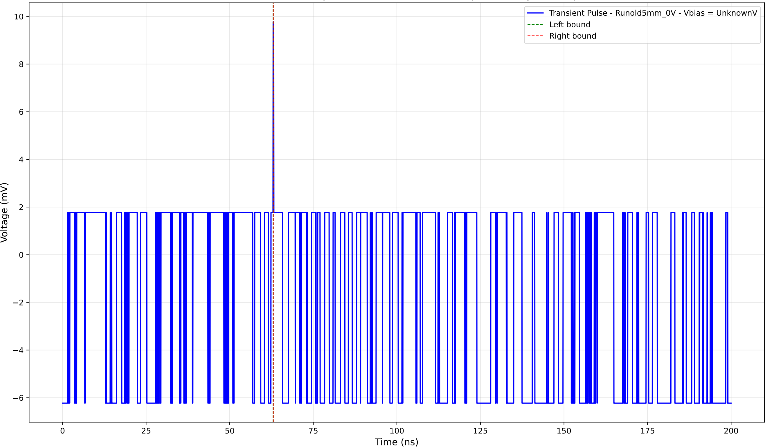
Transient Pulse - Sample: old5 - Position: 1565.0 \mu\text{m} - Charge: 0.04 pC
