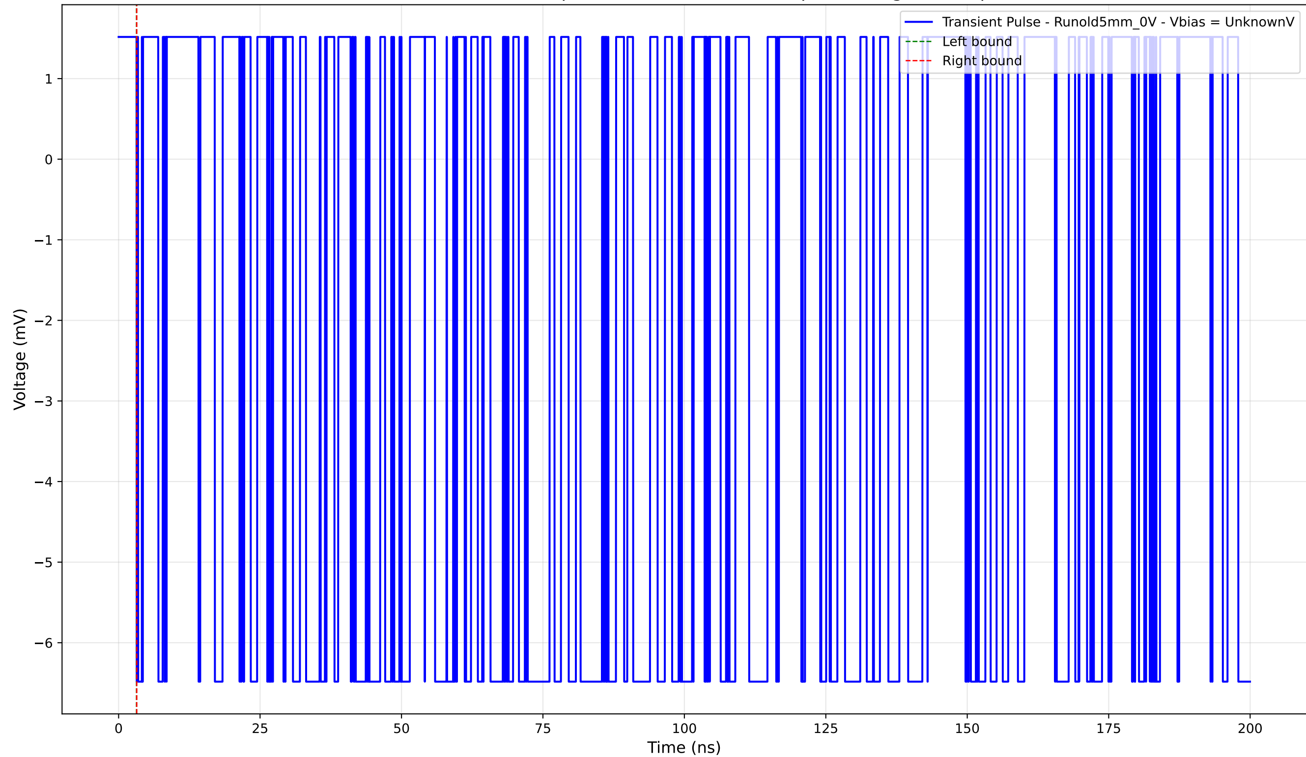
Transient Pulse - Sample: old5 - Position: 950.0 \mu\text{m} - Charge: -0.00 pC
