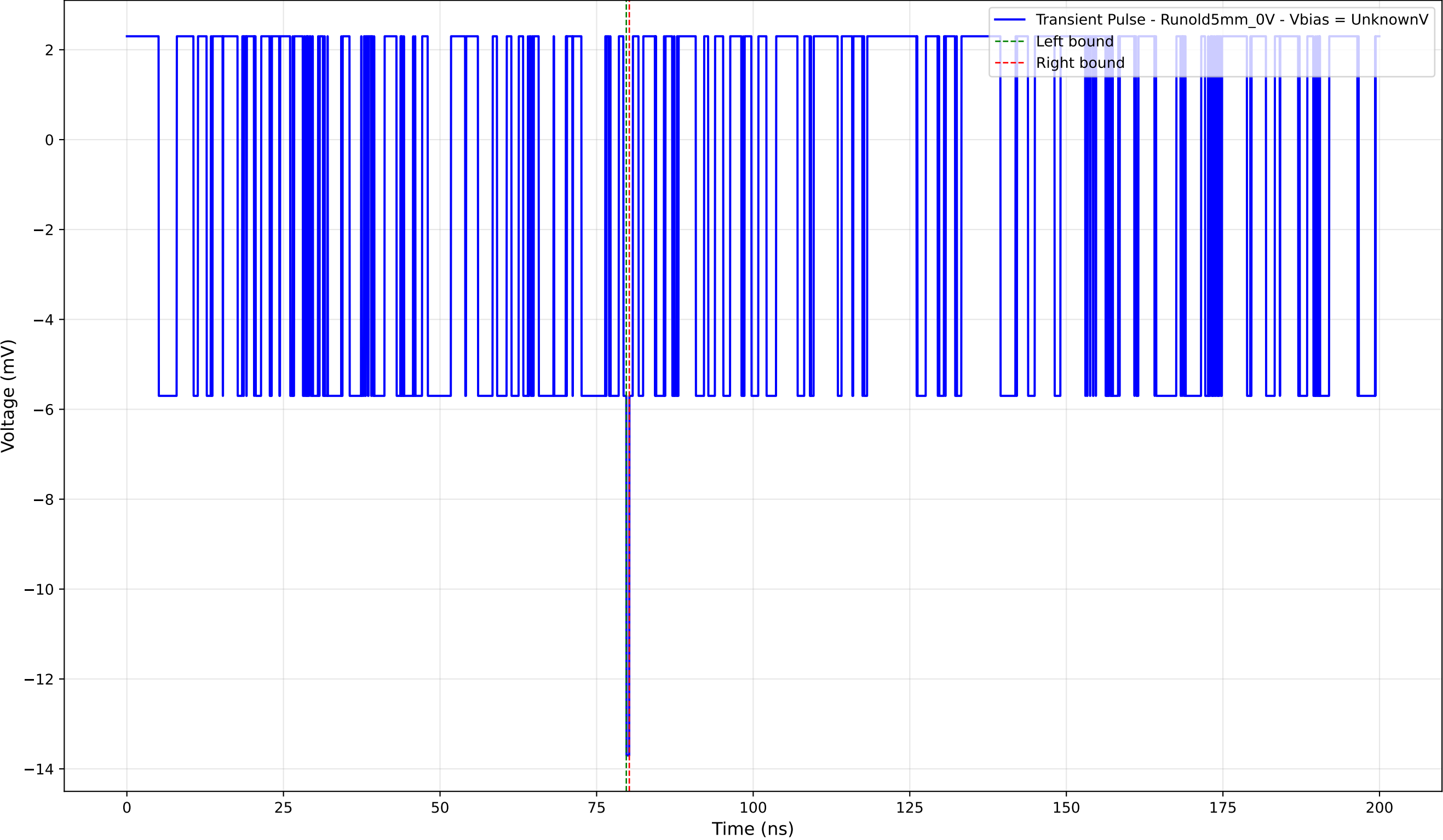
Transient Pulse - Sample: old5 - Position: 2475.0 \mu\text{m} - Charge: -0.13 pC
