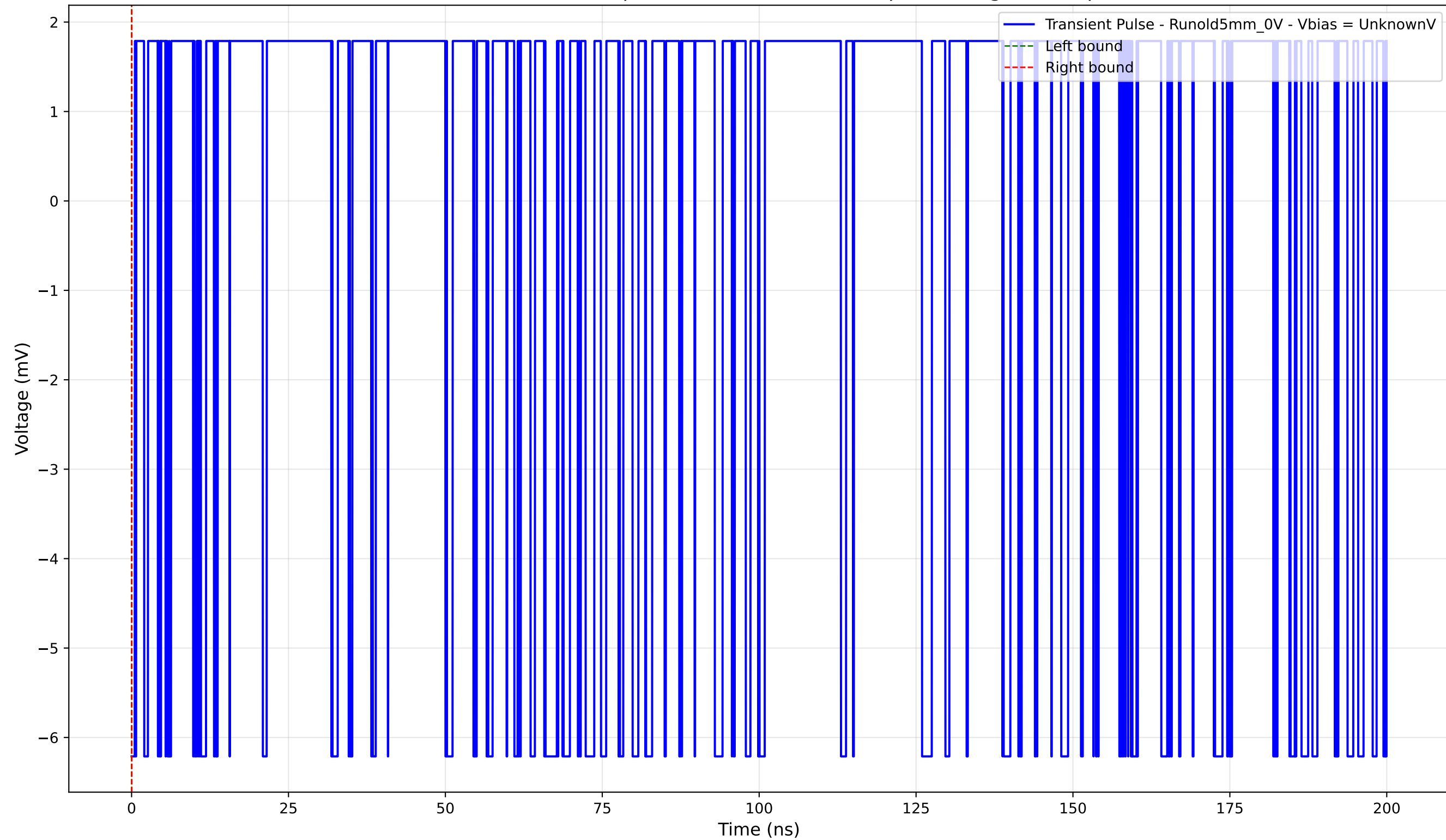
Transient Pulse - Sample: old5 - Position: 550.0 \mu\text{m} - Charge: -0.00 pC
