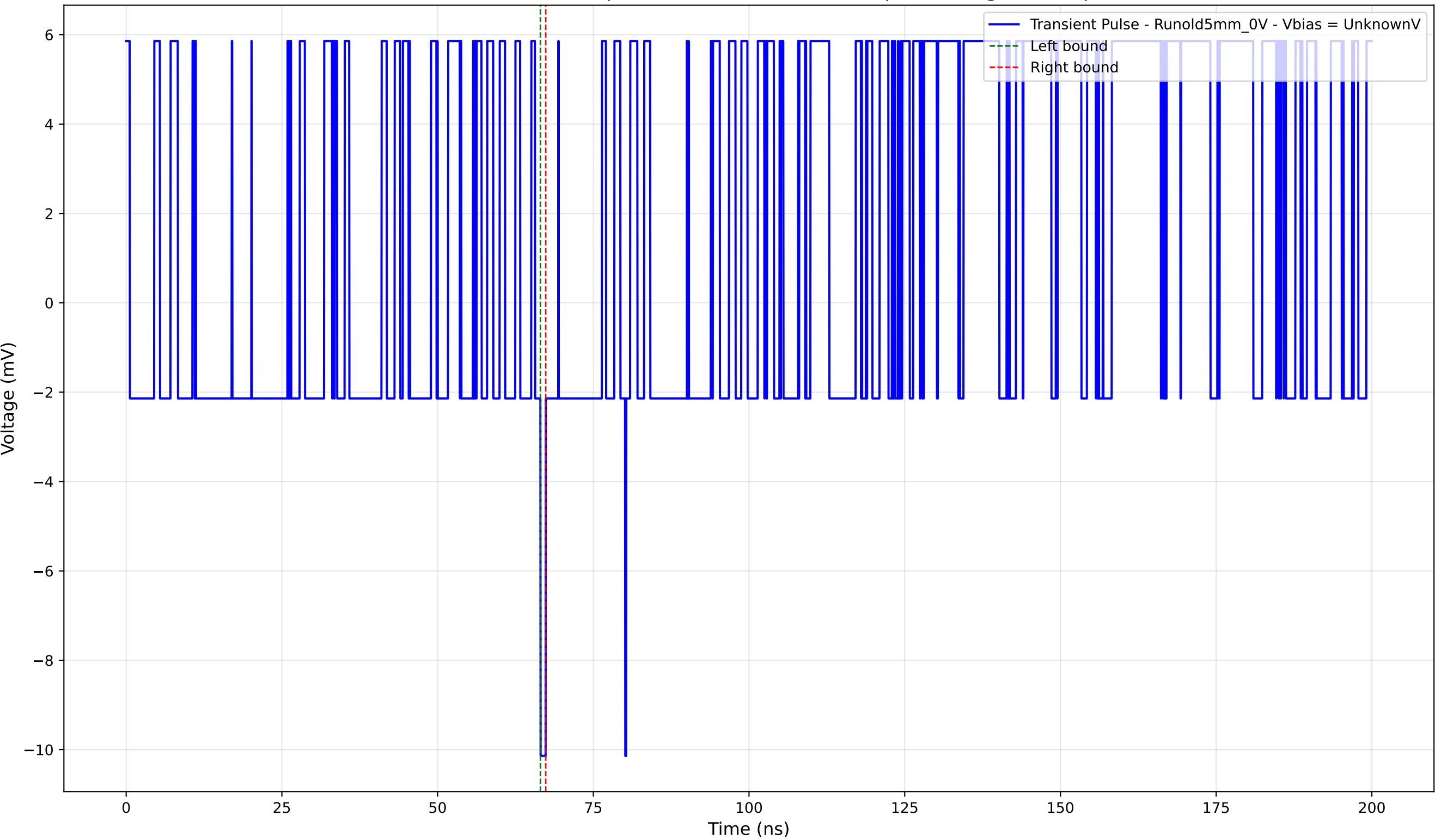
Transient Pulse - Sample: old5 - Position: 1780.0 \mu\text{m} - Charge: -0.17 pC
