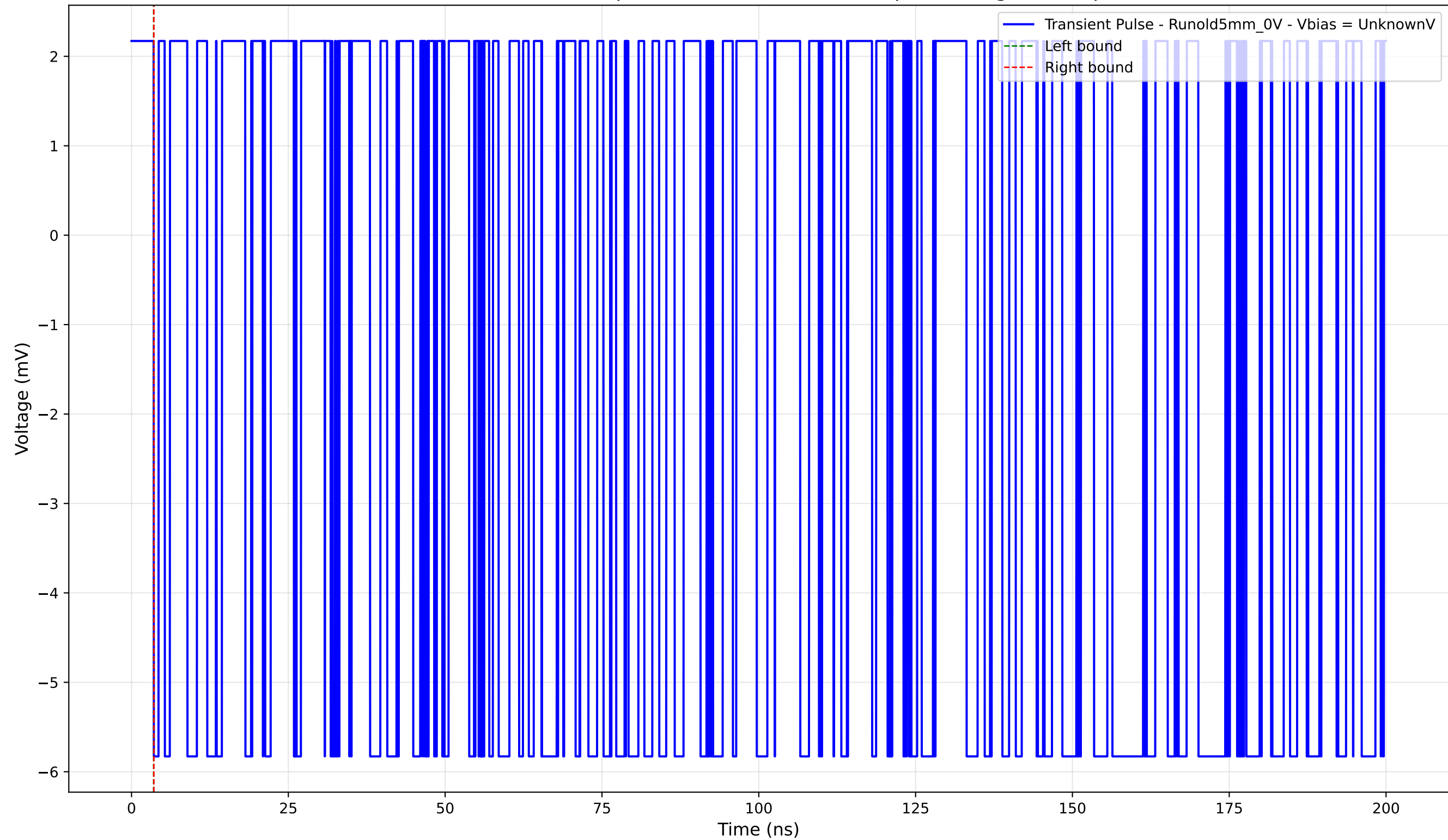
Transient Pulse - Sample: old5 - Position: 1860.0 \mu\text{m} - Charge: -0.00 pC
