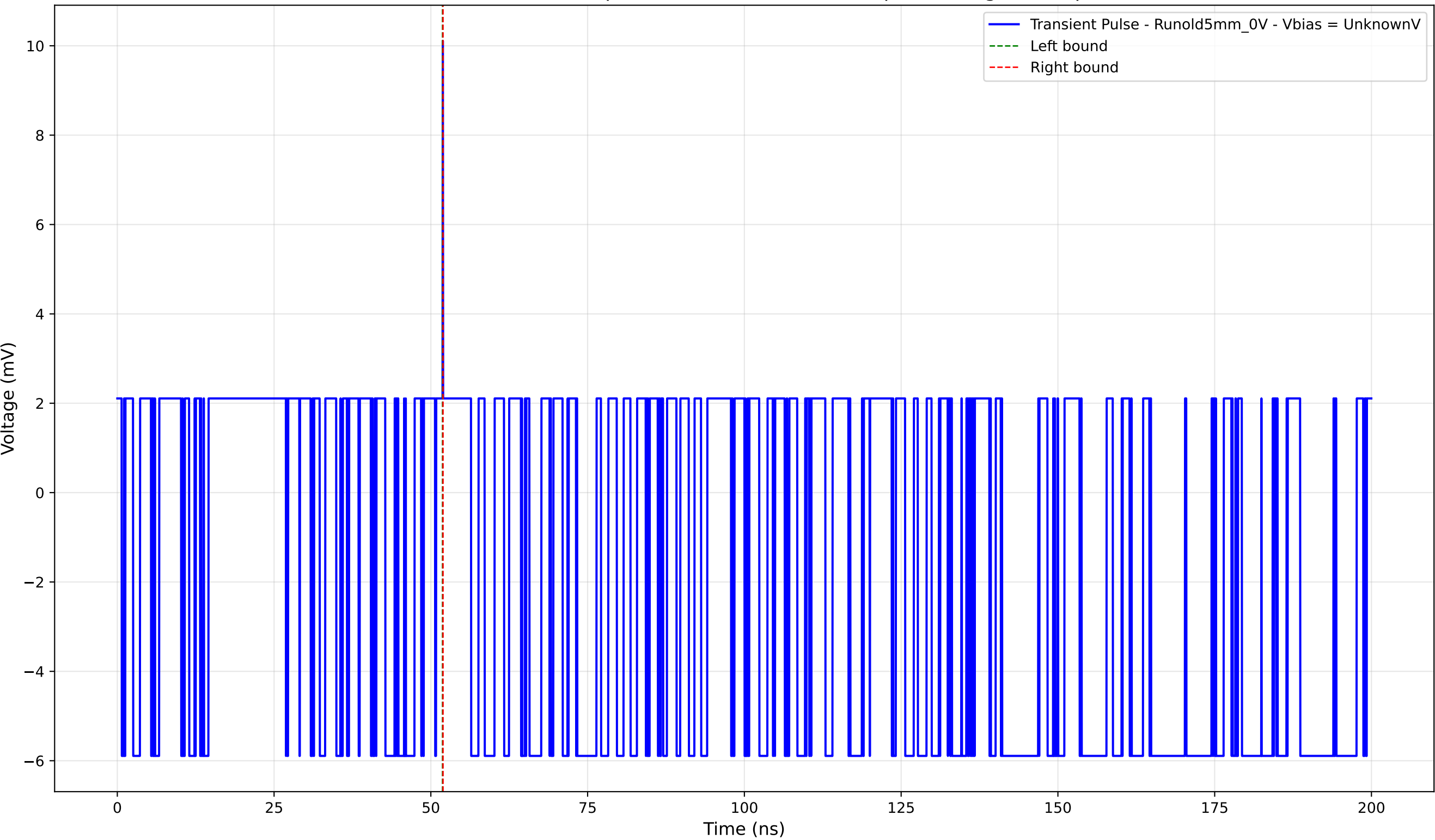
Transient Pulse - Sample: old5 - Position: 4255.0 \mu\text{m} - Charge: 0.01 pC
