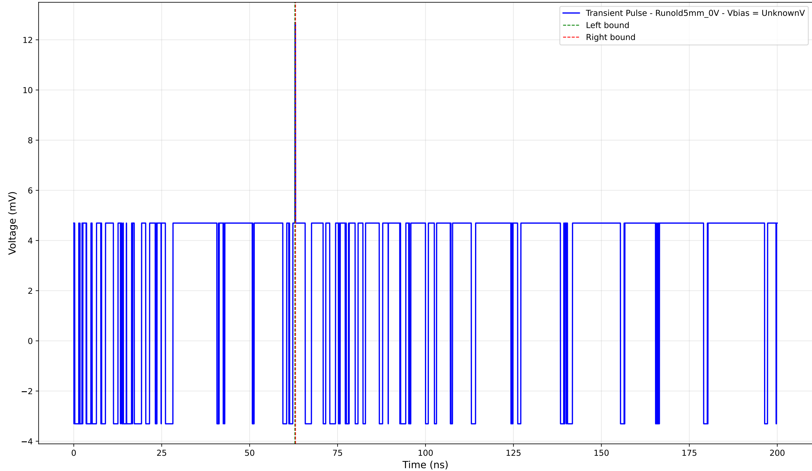
Transient Pulse - Sample: old5 - Position: 840.0 \mu\text{m} - Charge: 0.04 pC
