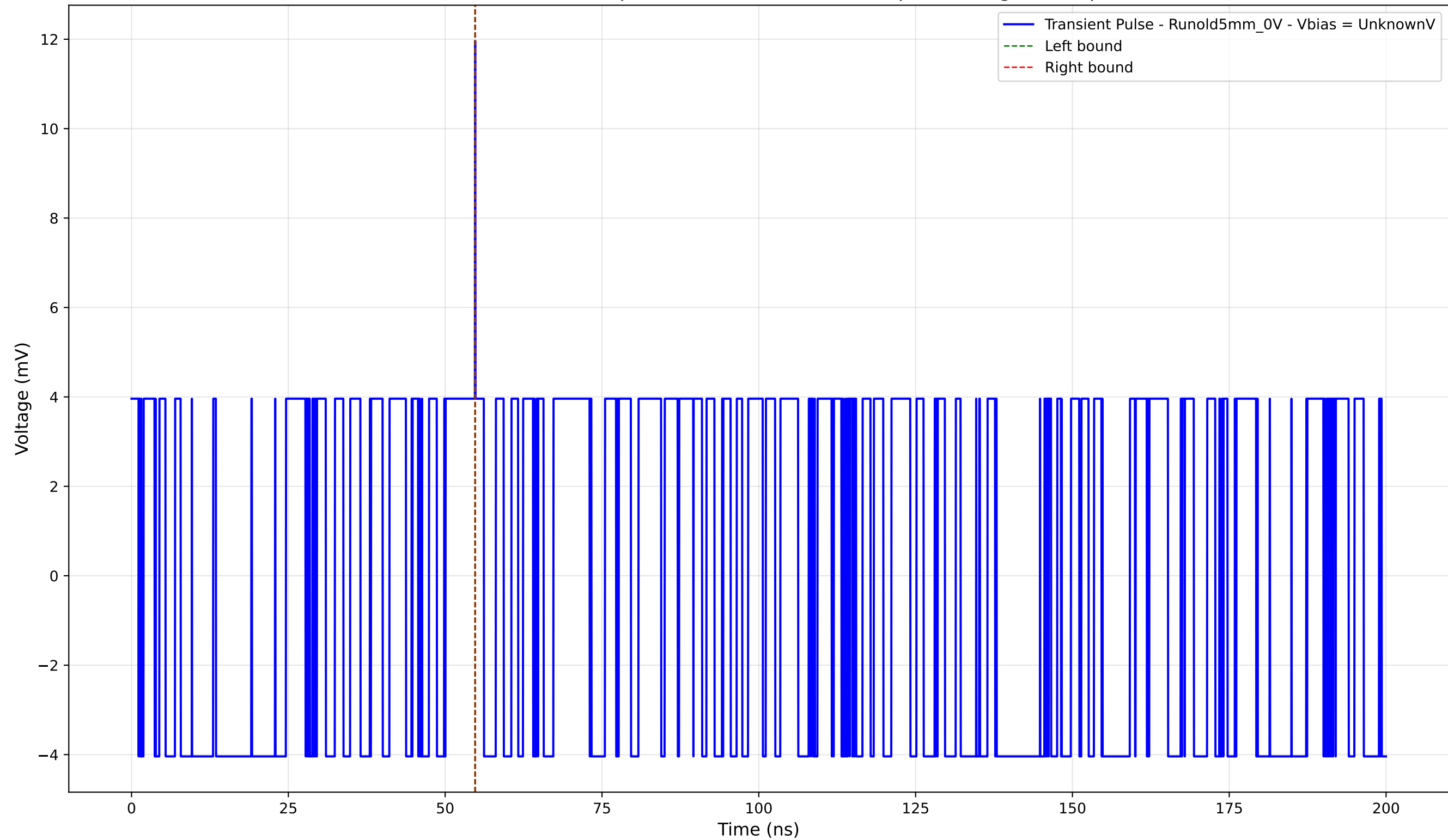
Transient Pulse - Sample: old5 - Position: 4910.0 \mu\text{m} - Charge: 0.02 pC
