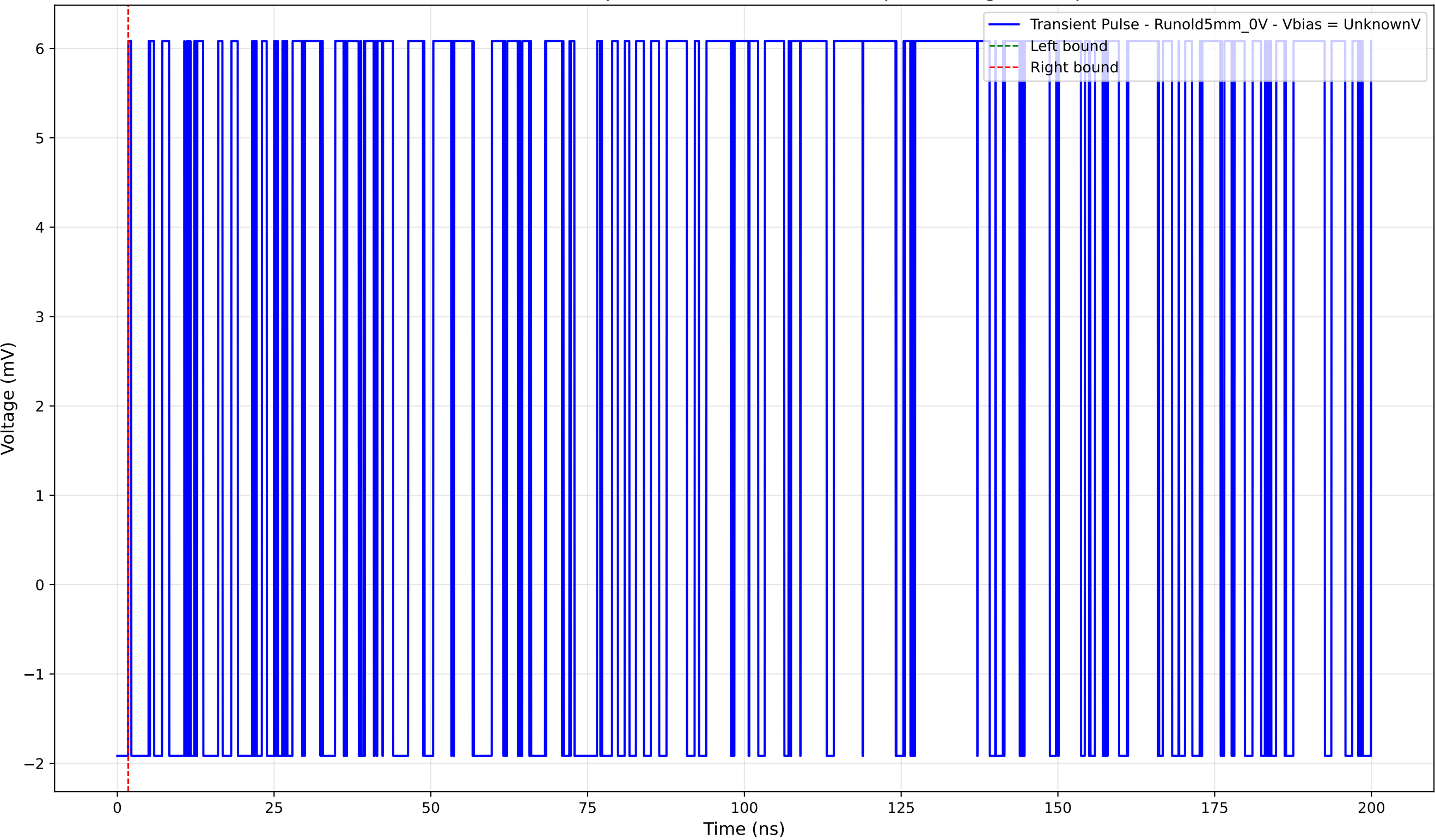
Transient Pulse - Sample: old5 - Position: 2055.0 \mu\text{m} - Charge: 0.00 pC
