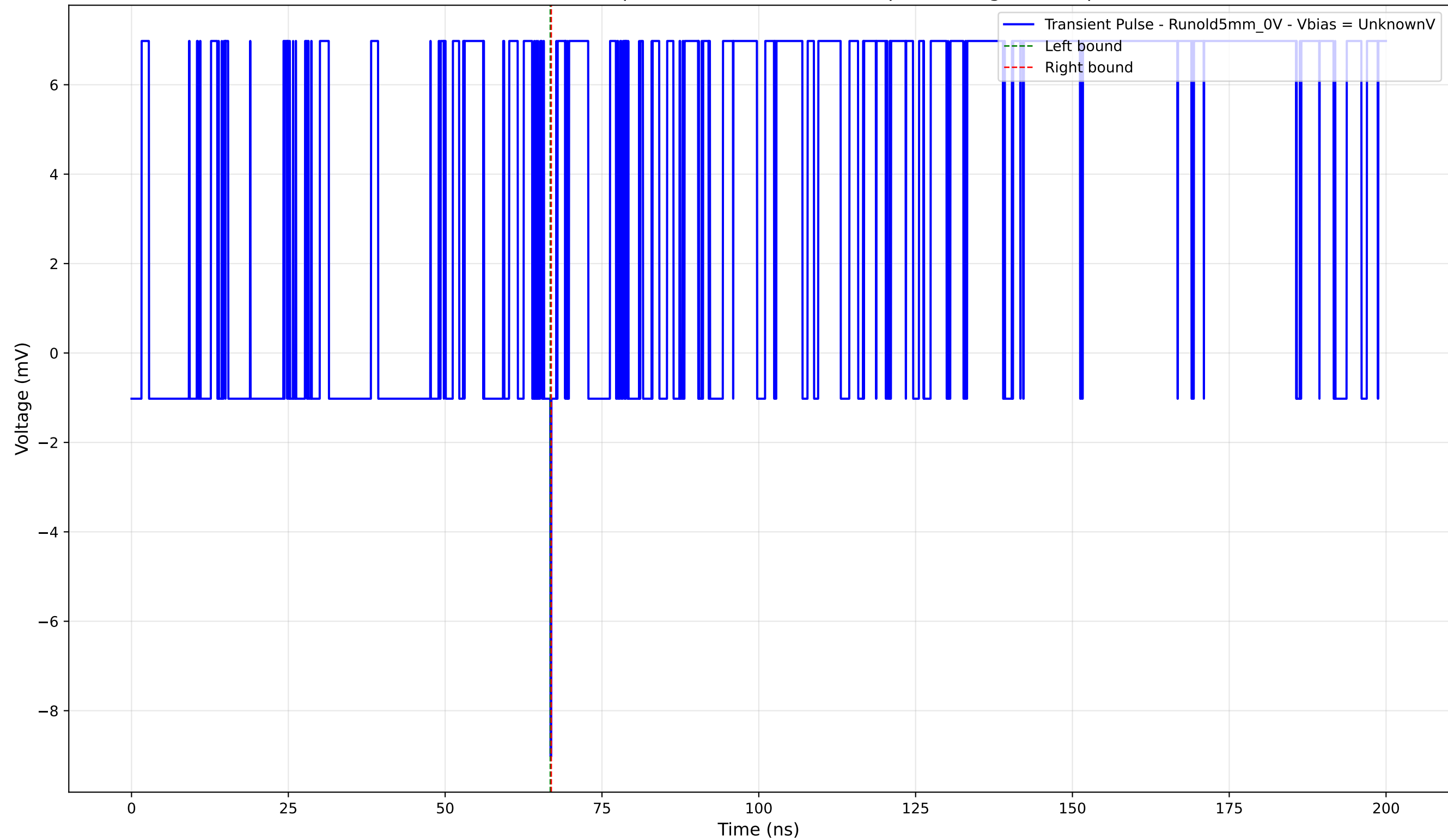
Transient Pulse - Sample: old5 - Position: 530.0 \mu\text{m} - Charge: -0.03 pC
