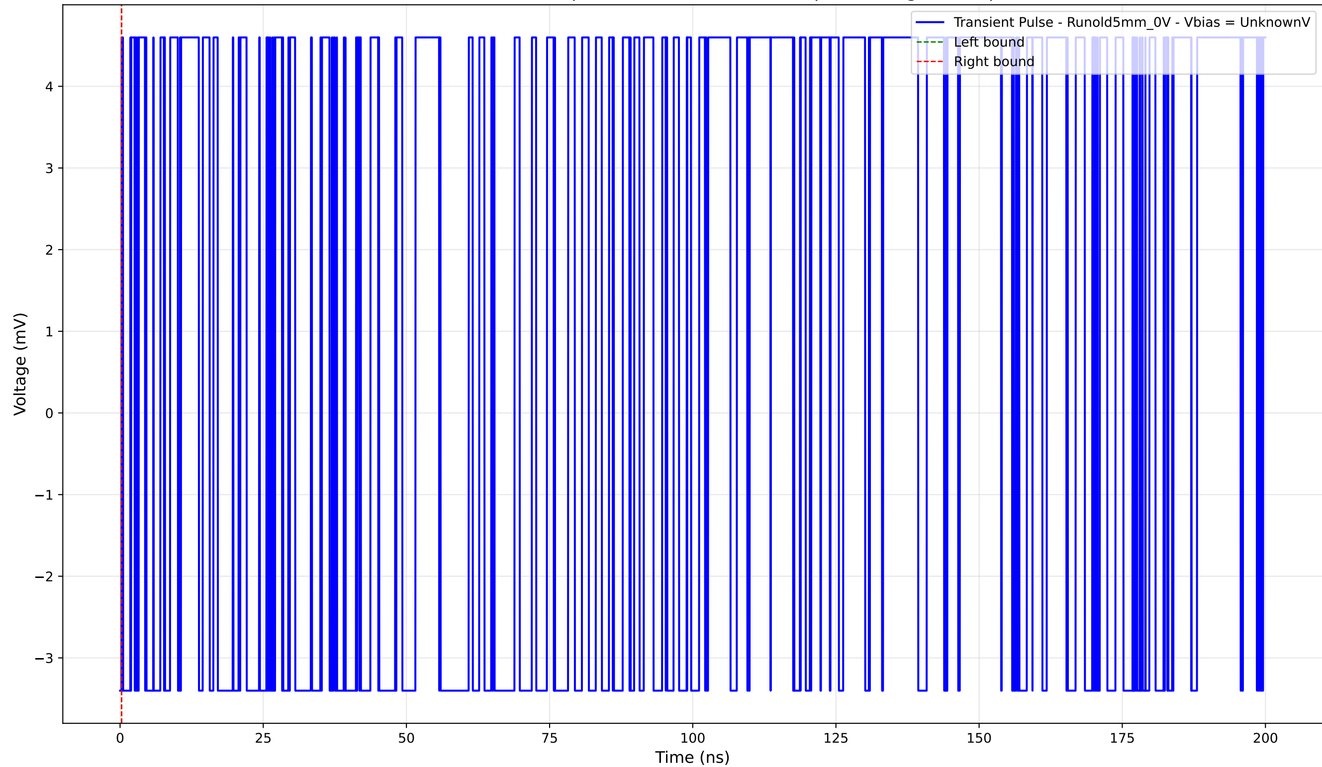
Transient Pulse - Sample: old5 - Position: 675.0 \mu\text{m} - Charge: 0.00 pC
