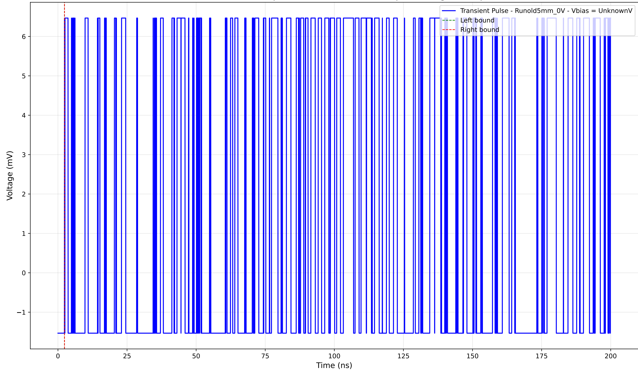
Transient Pulse - Sample: old5 - Position: 5110.0 \mu\text{m} - Charge: 0.00 pC
