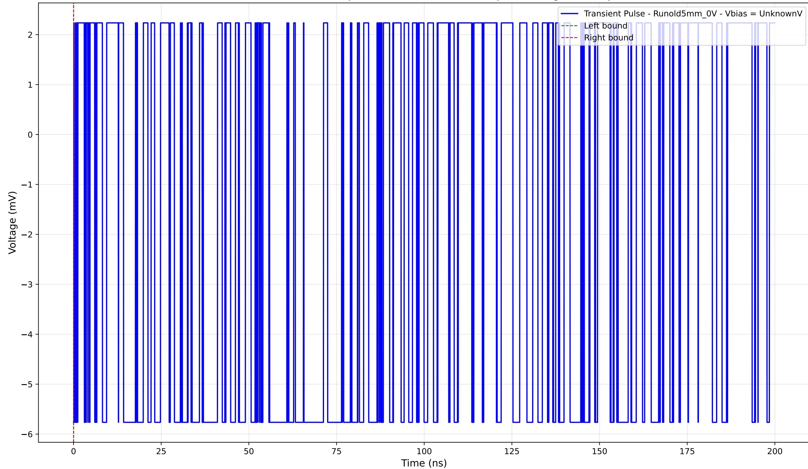
Transient Pulse - Sample: old5 - Position: 575.0 \mu\text{m} - Charge: -0.00 pC
