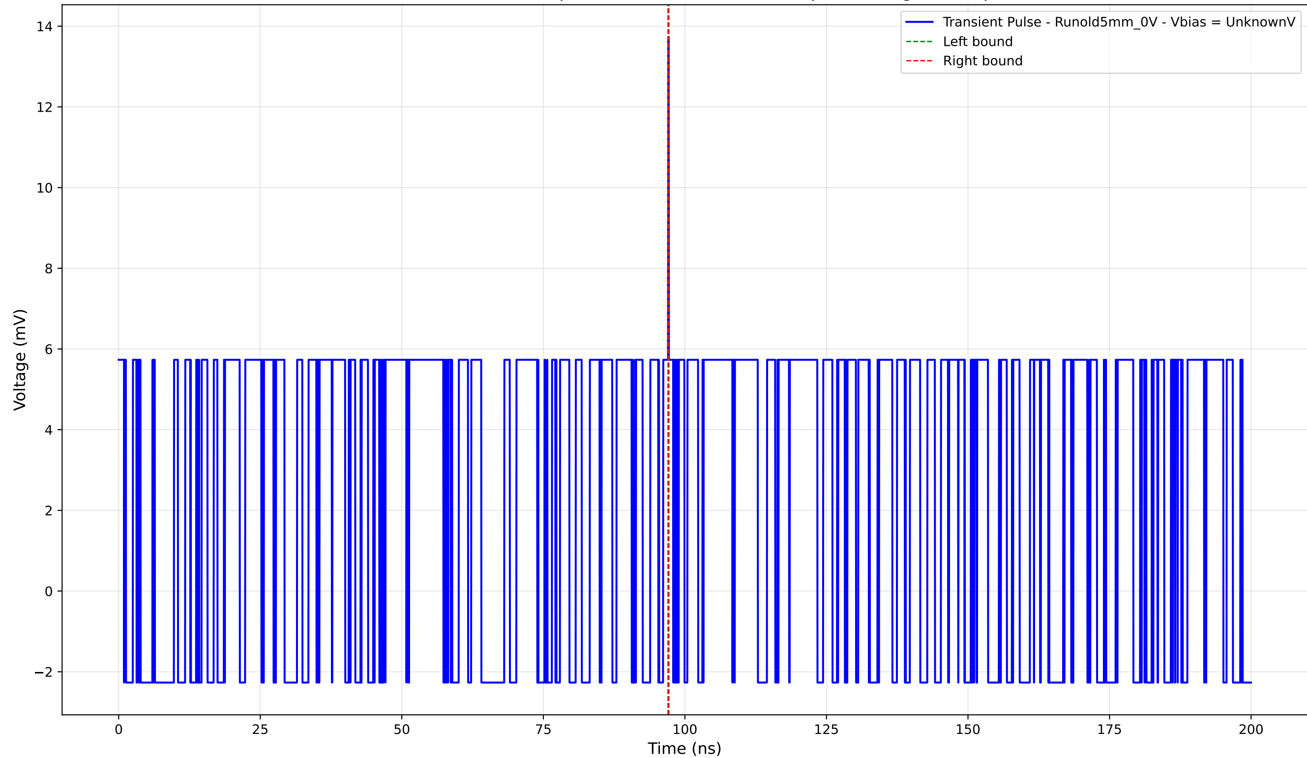
Transient Pulse - Sample: old5 - Position: 2640.0 \mu\text{m} - Charge: 0.04 pC
