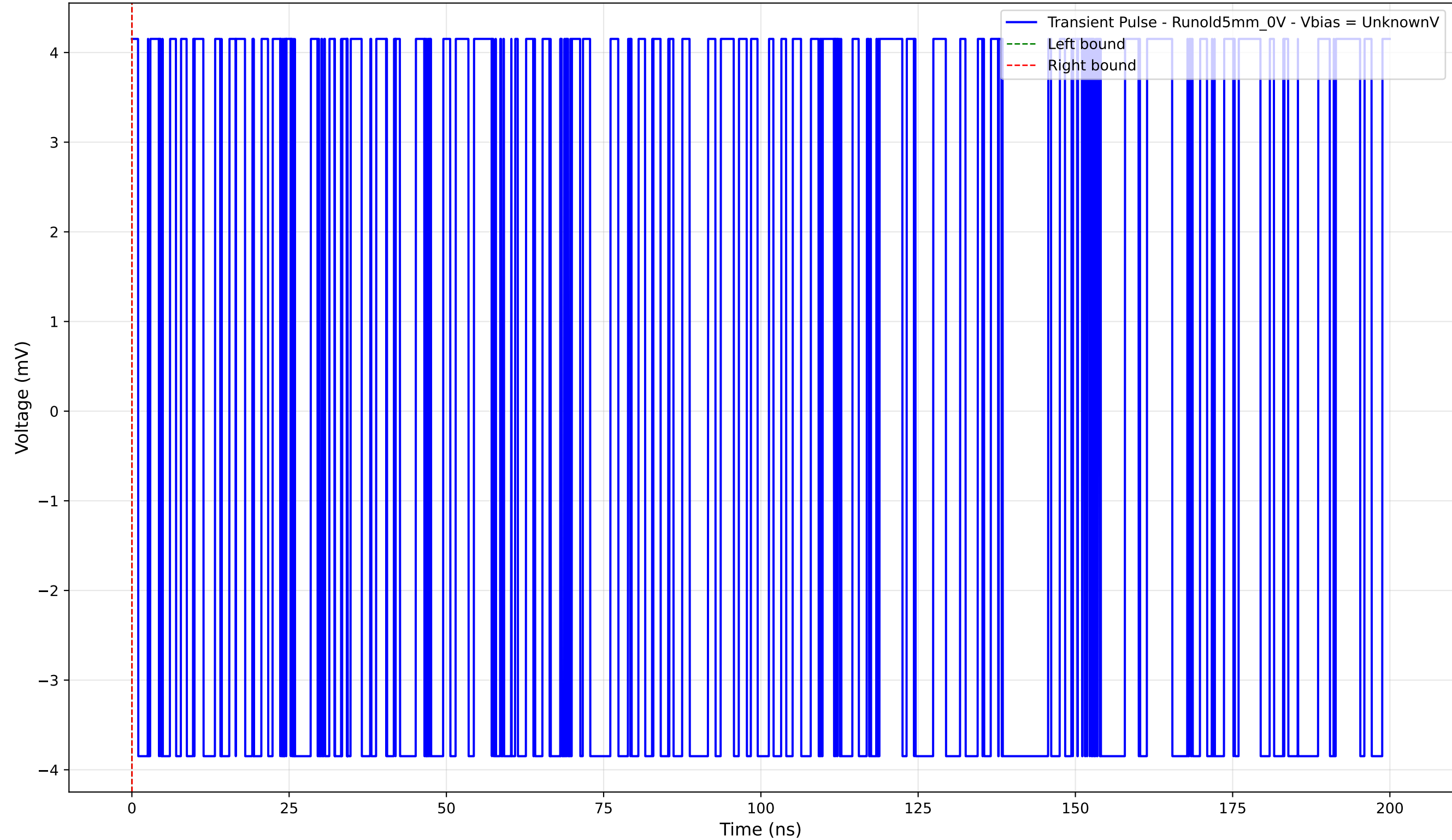
Transient Pulse - Sample: old5 - Position: 4210.0 \mu\text{m} - Charge: 0.00 pC
