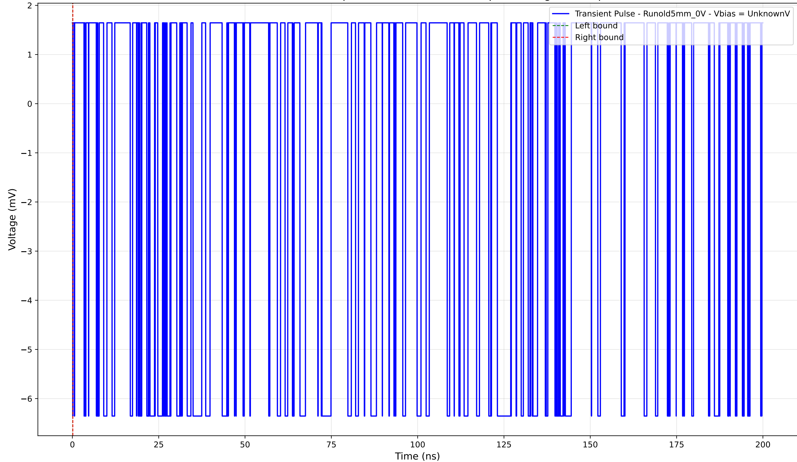
Transient Pulse - Sample: old5 - Position: 580.0 \mu\text{m} - Charge: -0.00 pC
