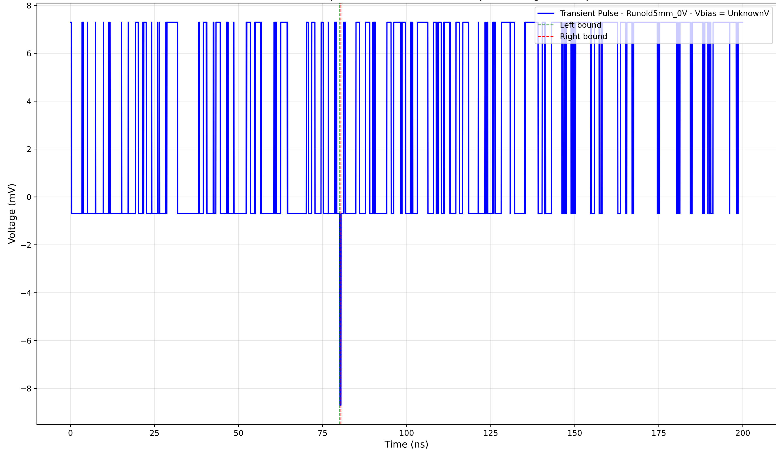
Transient Pulse - Sample: old5 - Position: 4760.0 \mu\text{m} - Charge: -0.06 pC
