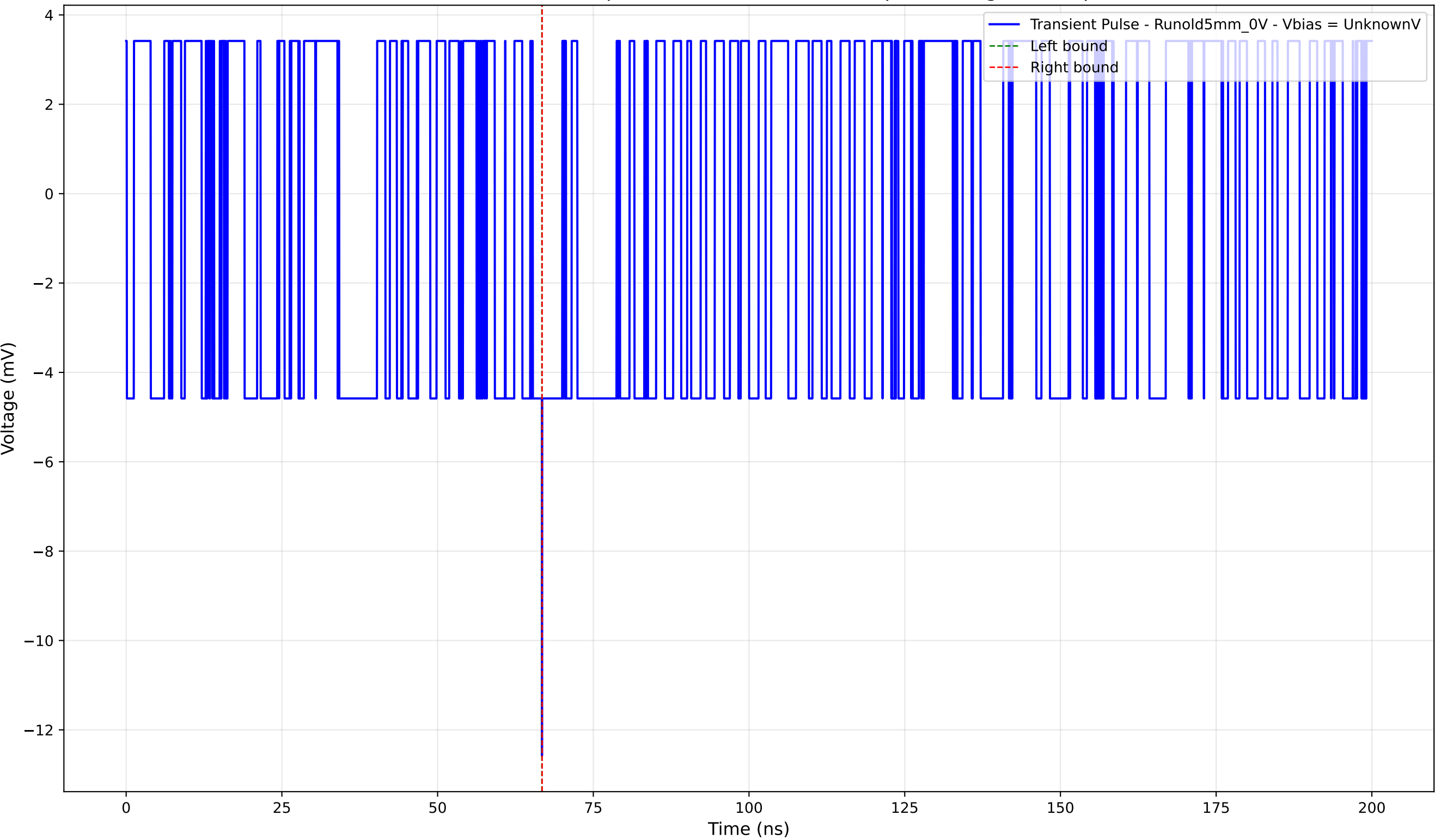
Transient Pulse - Sample: old5 - Position: 3615.0 \mu\text{m} - Charge: -0.01 pC
