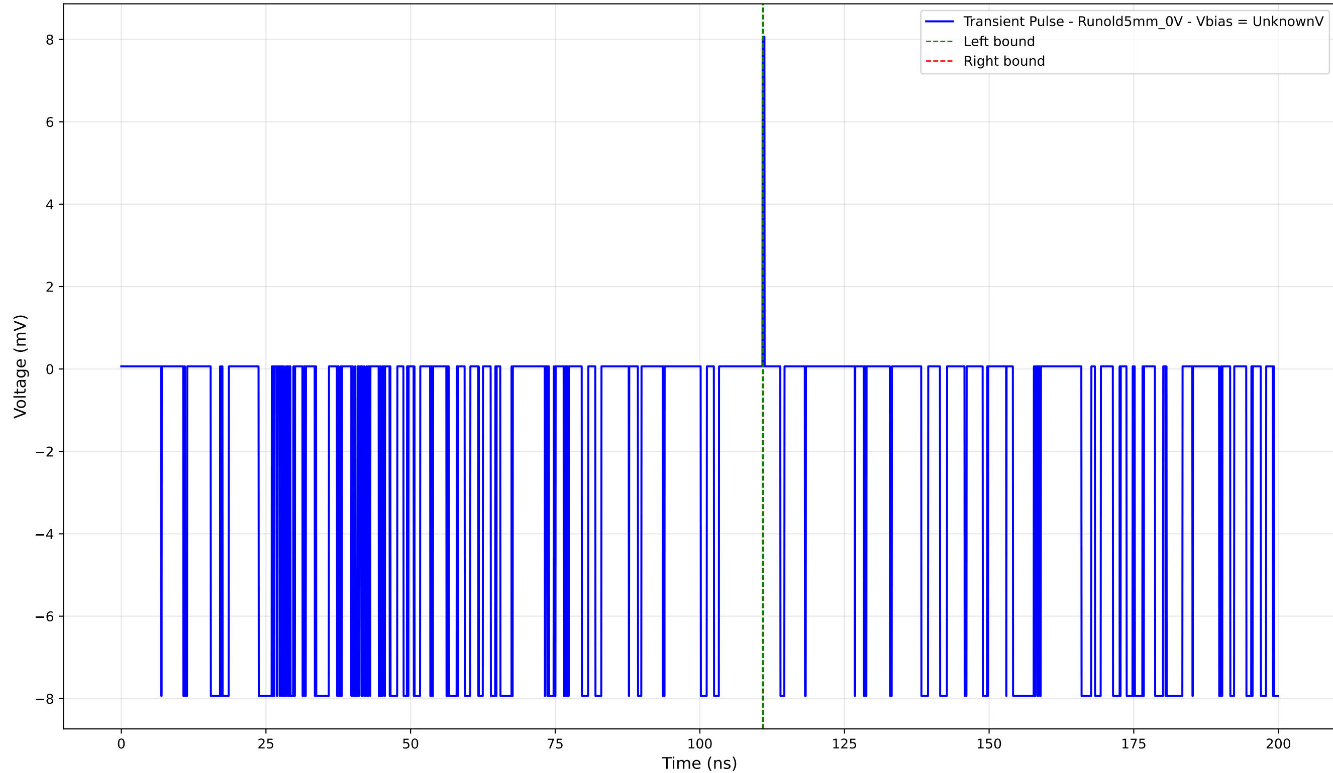
Transient Pulse - Sample: old5 - Position: 3100.0 \mu\text{m} - Charge: 0.03 pC
