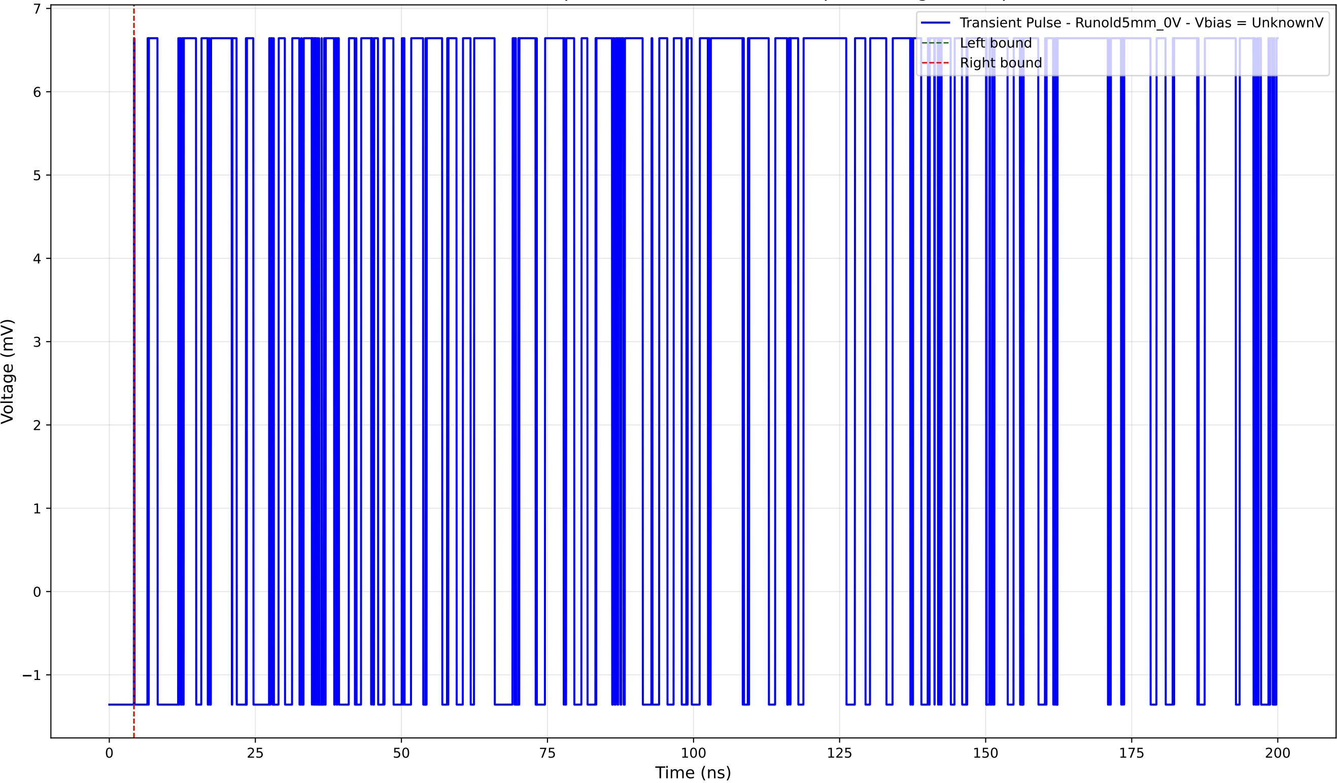
Transient Pulse - Sample: old5 - Position: 2000.0 \mu\text{m} - Charge: 0.00 pC
