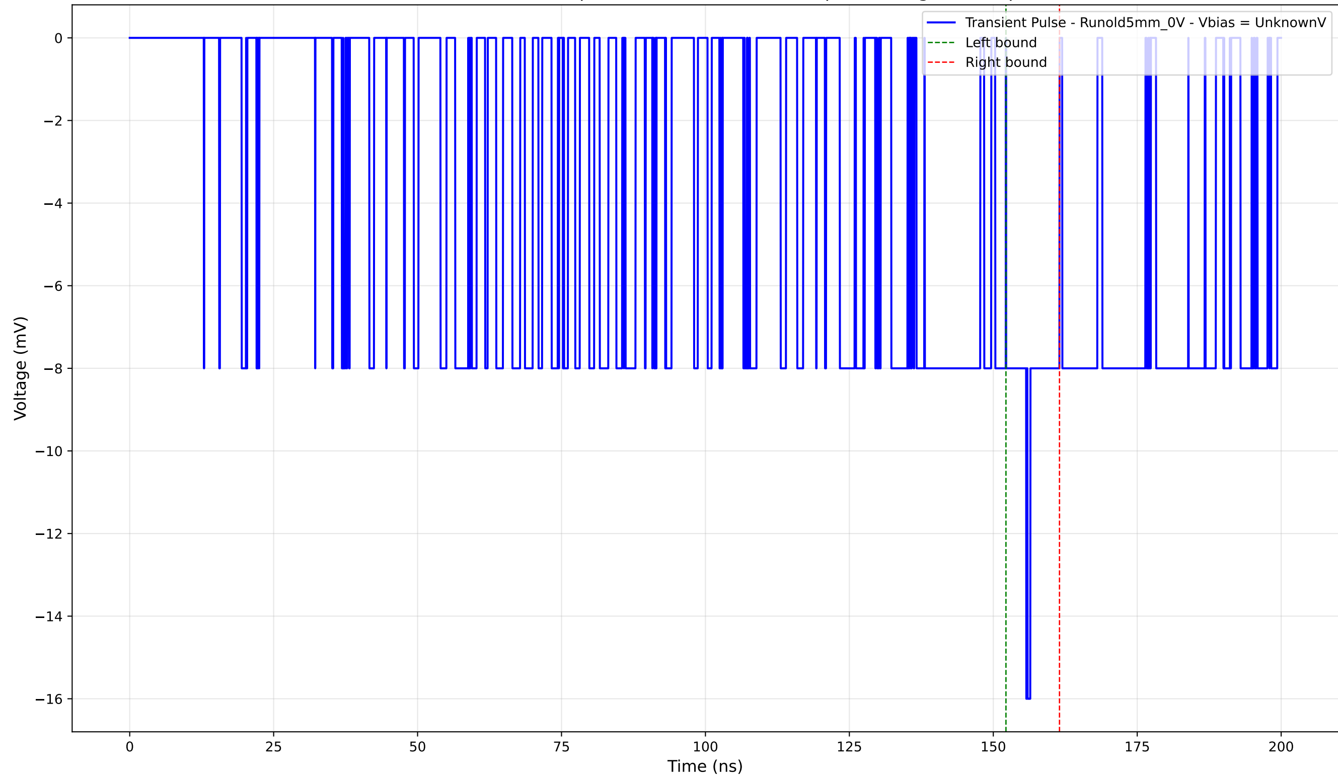
Transient Pulse - Sample: old5 - Position: 465.0 \mu\text{m} - Charge: -1.58 pC
