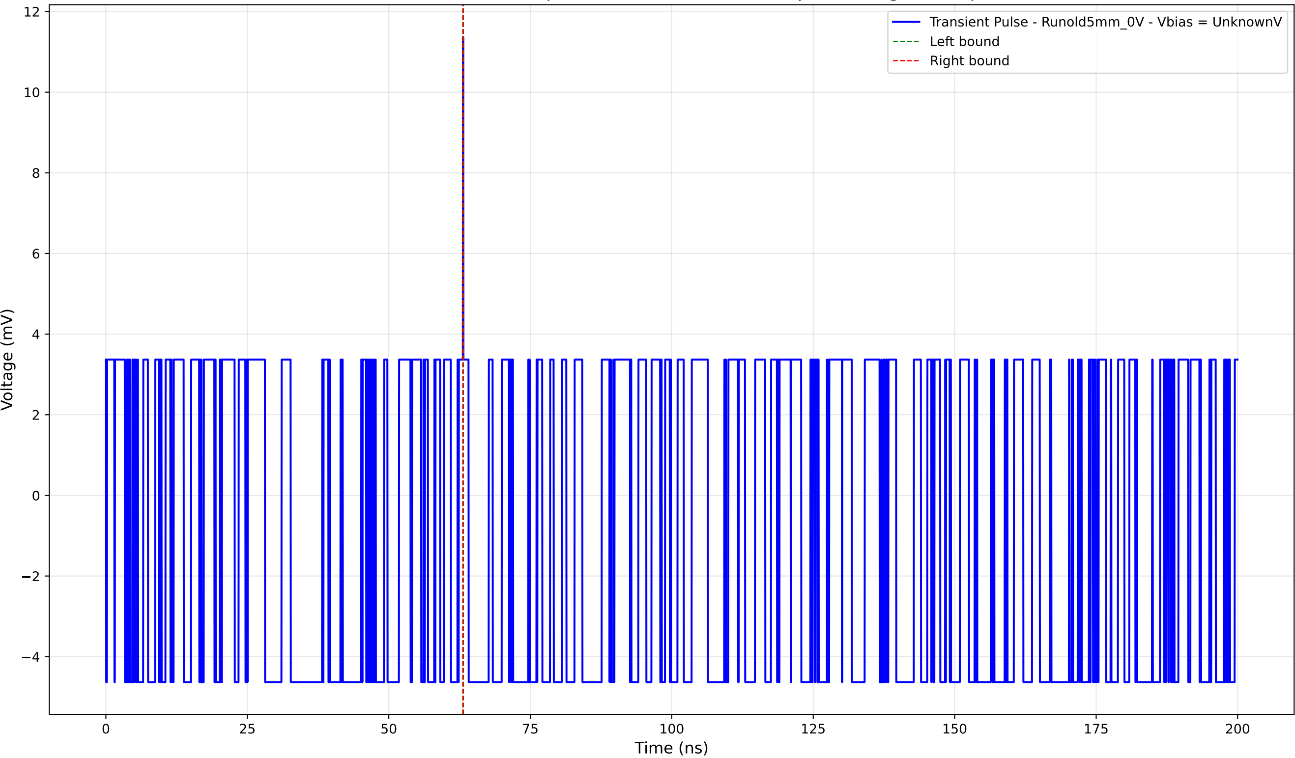
Transient Pulse - Sample: old5 - Position: 3445.0 \mu\text{m} - Charge: 0.01 pC
