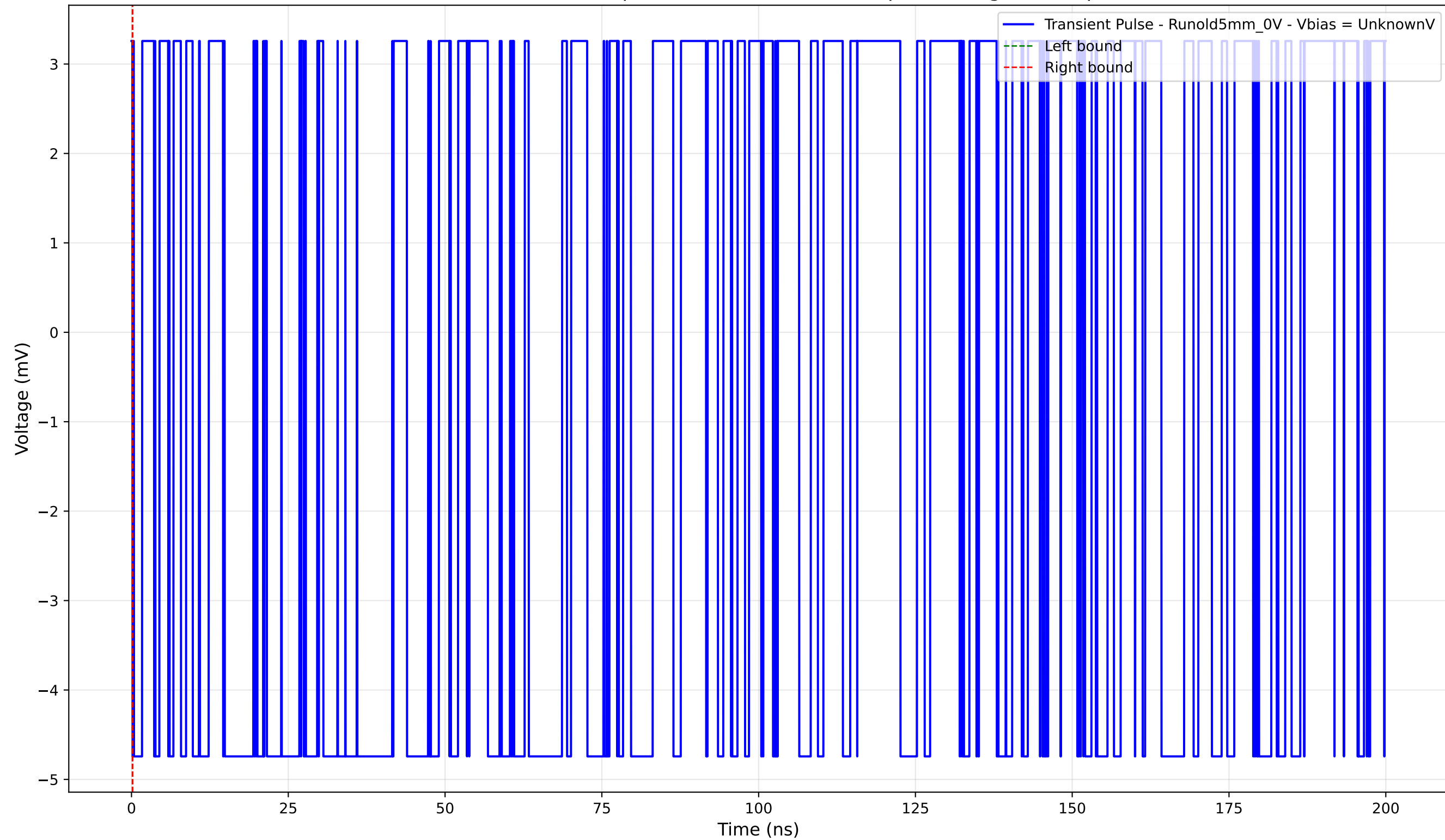
Transient Pulse - Sample: old5 - Position: 670.0 \mu\text{m} - Charge: -0.00 pC
