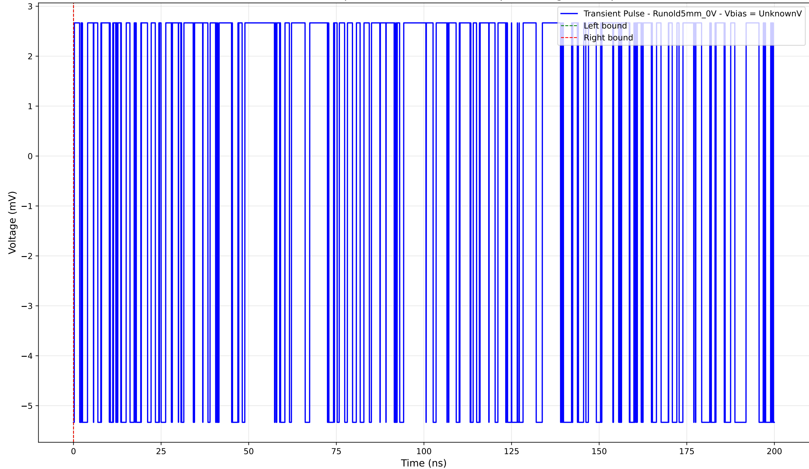
Transient Pulse - Sample: old5 - Position: 4900.0 \mu\text{m} - Charge: -0.00 pC
