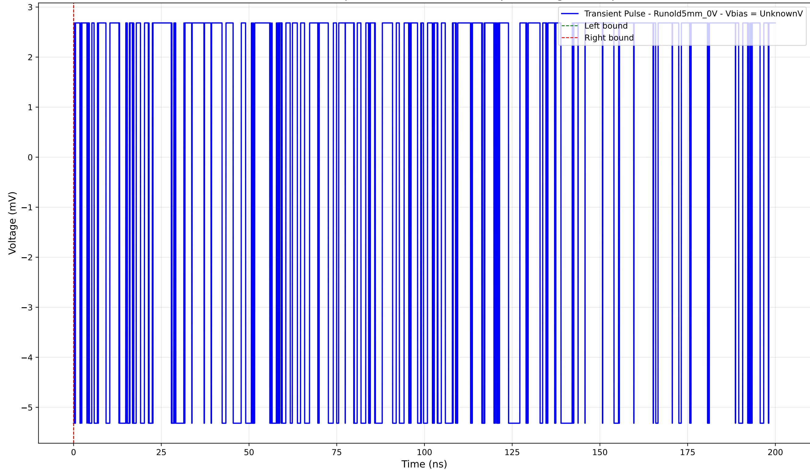
Transient Pulse - Sample: old5 - Position: 4045.0 \mu\text{m} - Charge: -0.00 pC
