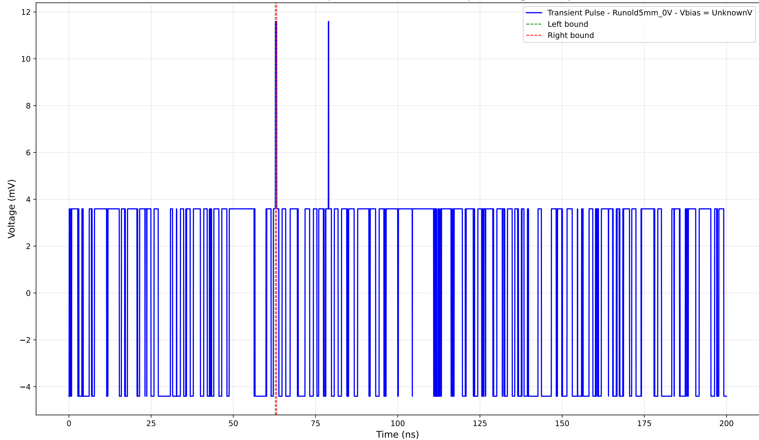
Transient Pulse - Sample: old5 - Position: 640.0 \mu\text{m} - Charge: 0.09 pC
