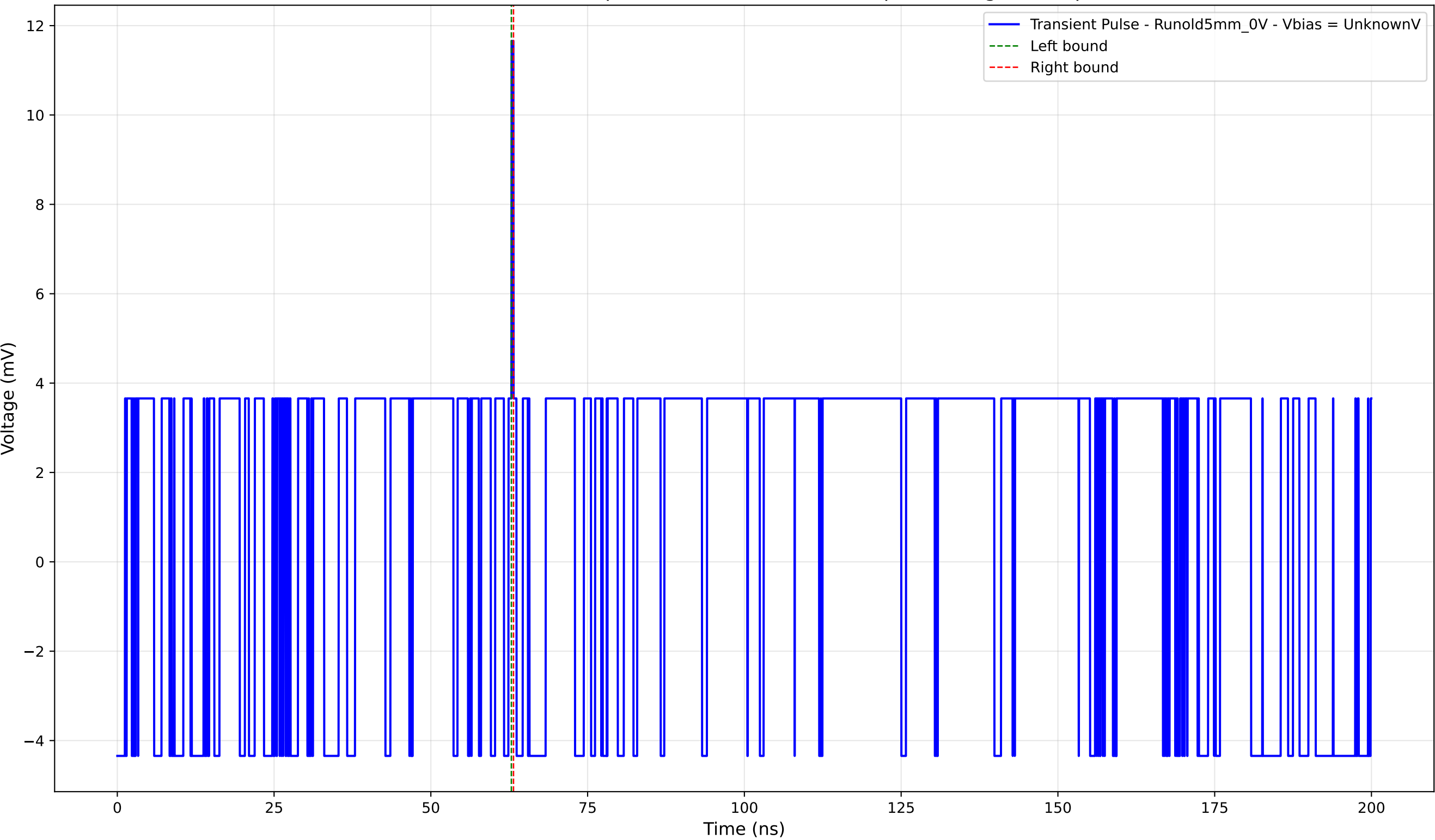
Transient Pulse - Sample: old5 - Position: 1785.0 \mu\text{m} - Charge: 0.08 pC
