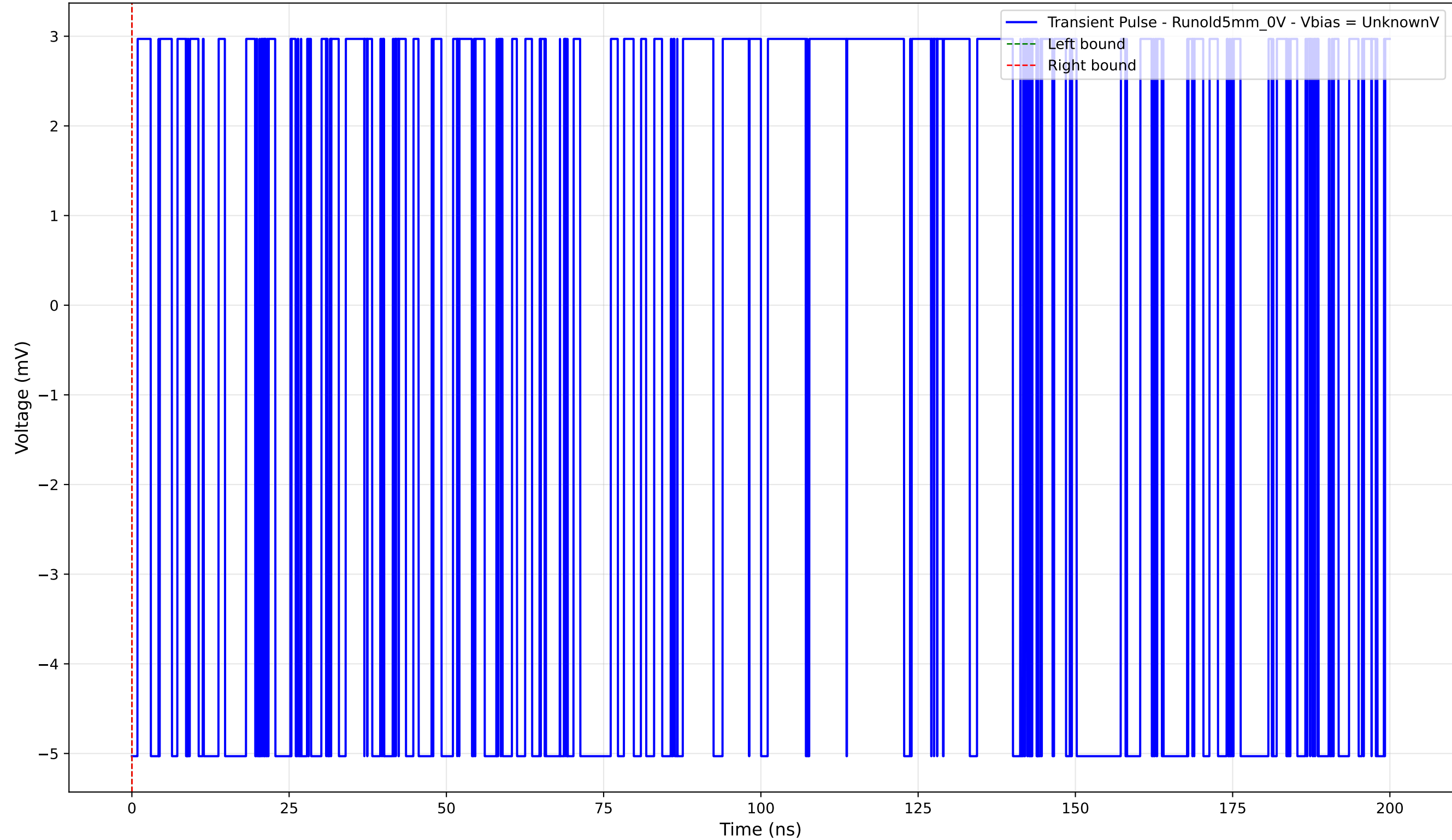
Transient Pulse - Sample: old5 - Position: 2950.0 \mu\text{m} - Charge: -0.00 pC
