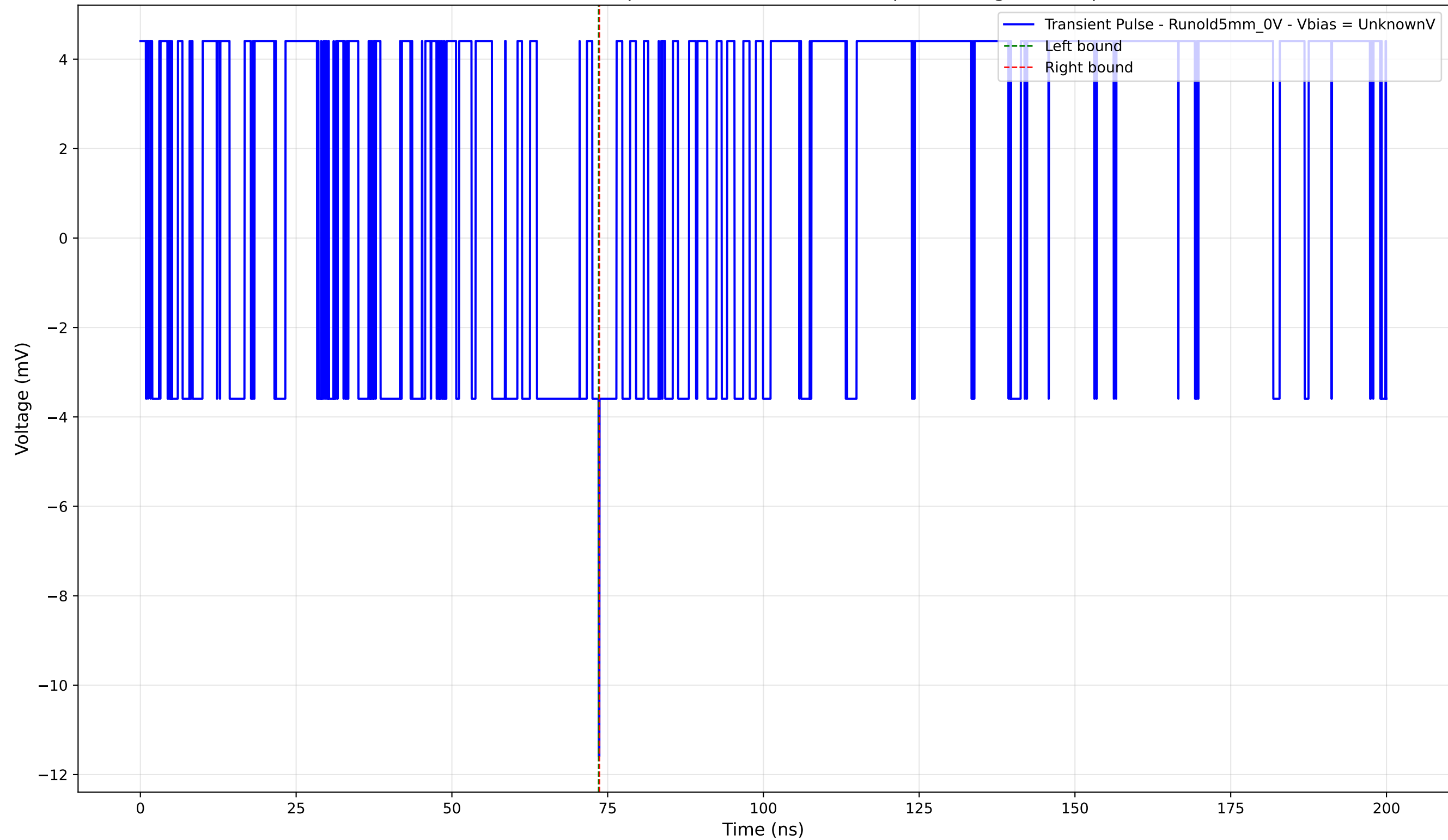
Transient Pulse - Sample: old5 - Position: 850.0 \mu\text{m} - Charge: -0.03 pC
