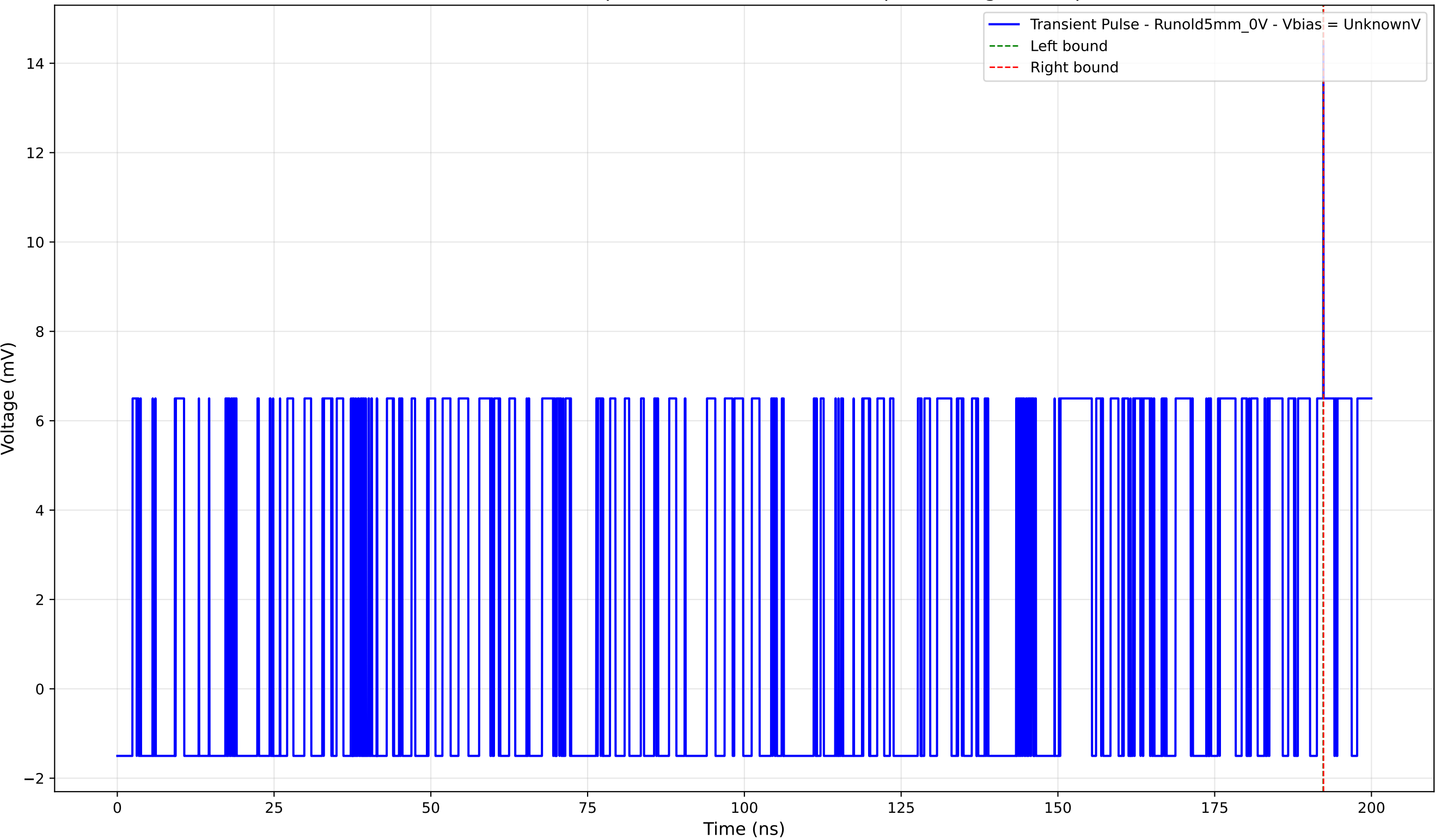
Transient Pulse - Sample: old5 - Position: 4345.0 \mu\text{m} - Charge: 0.01 pC
