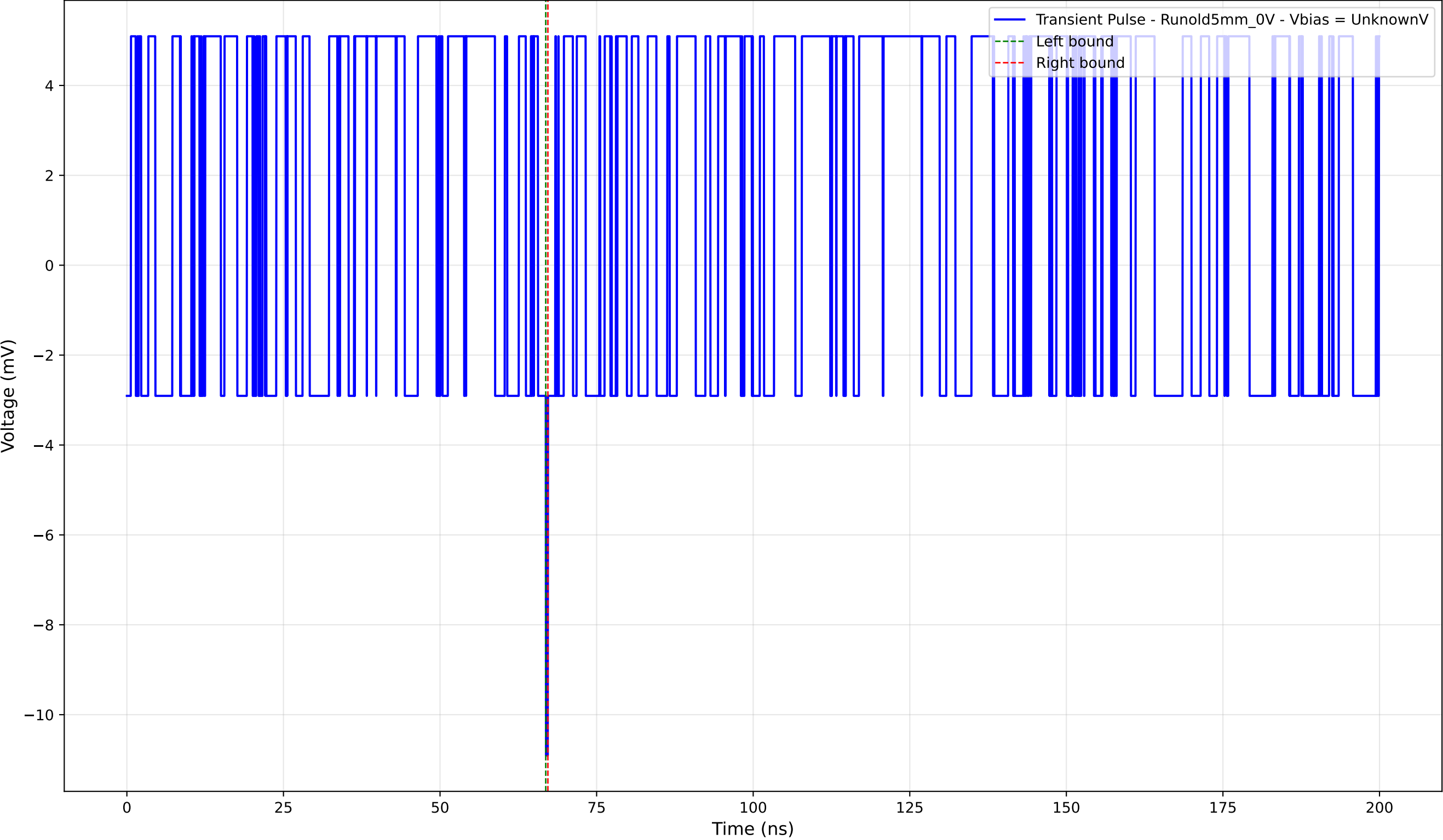
Transient Pulse - Sample: old5 - Position: 1890.0 \mu\text{m} - Charge: -0.07 pC
