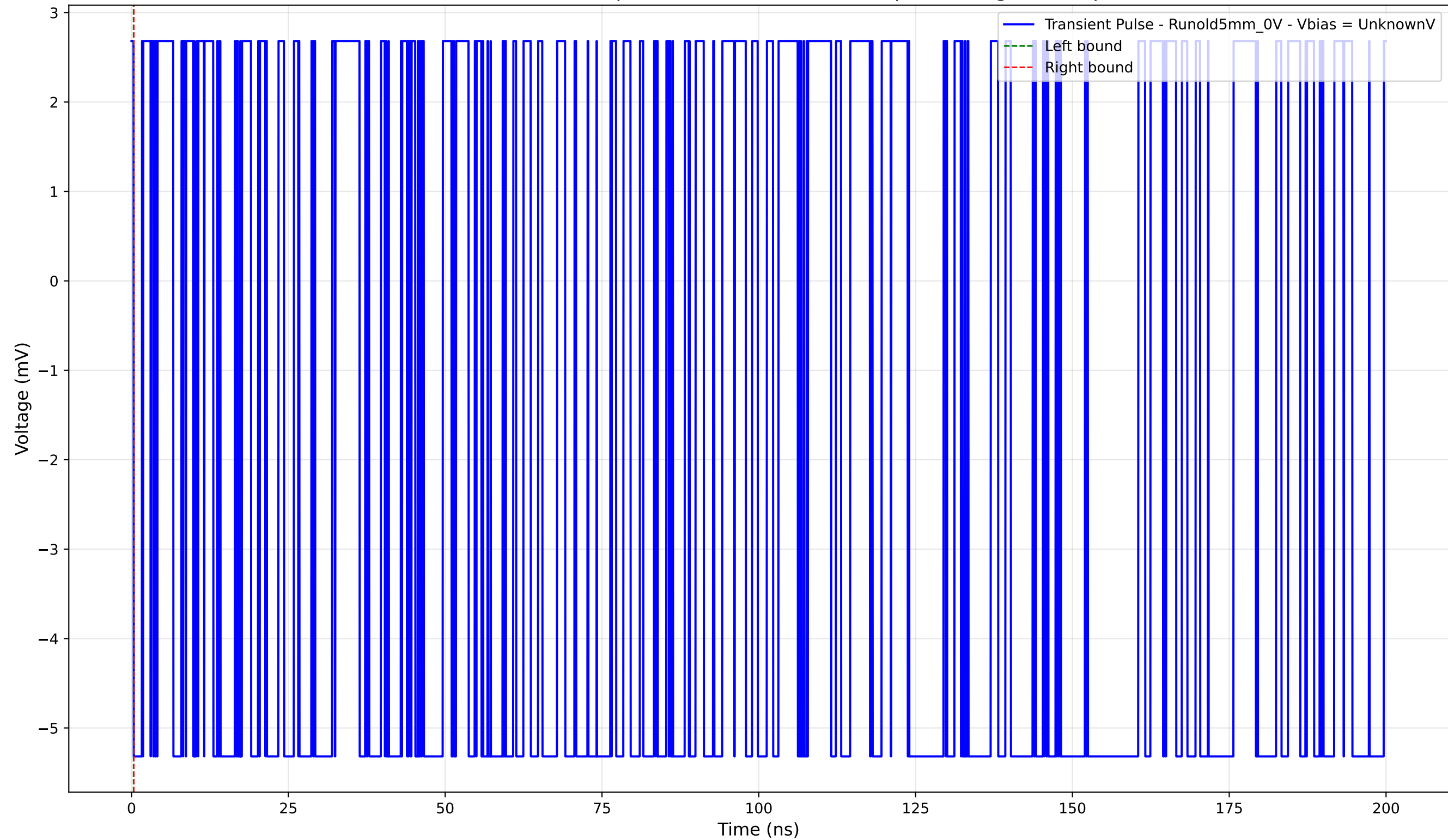
Transient Pulse - Sample: old5 - Position: 5150.0 \mu\text{m} - Charge: -0.00 pC
