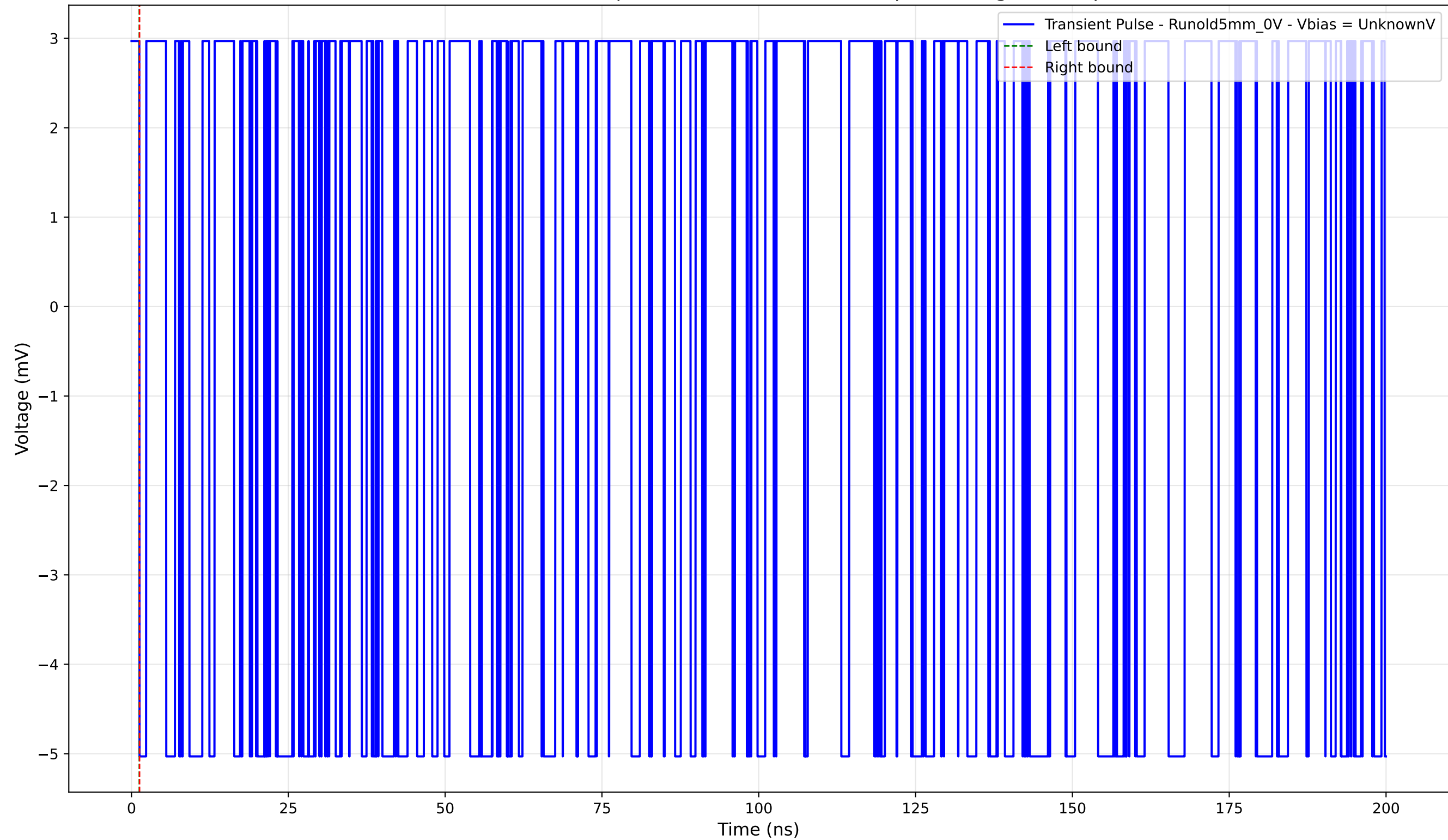
Transient Pulse - Sample: old5 - Position: 4335.0 \mu\text{m} - Charge: -0.00 pC
