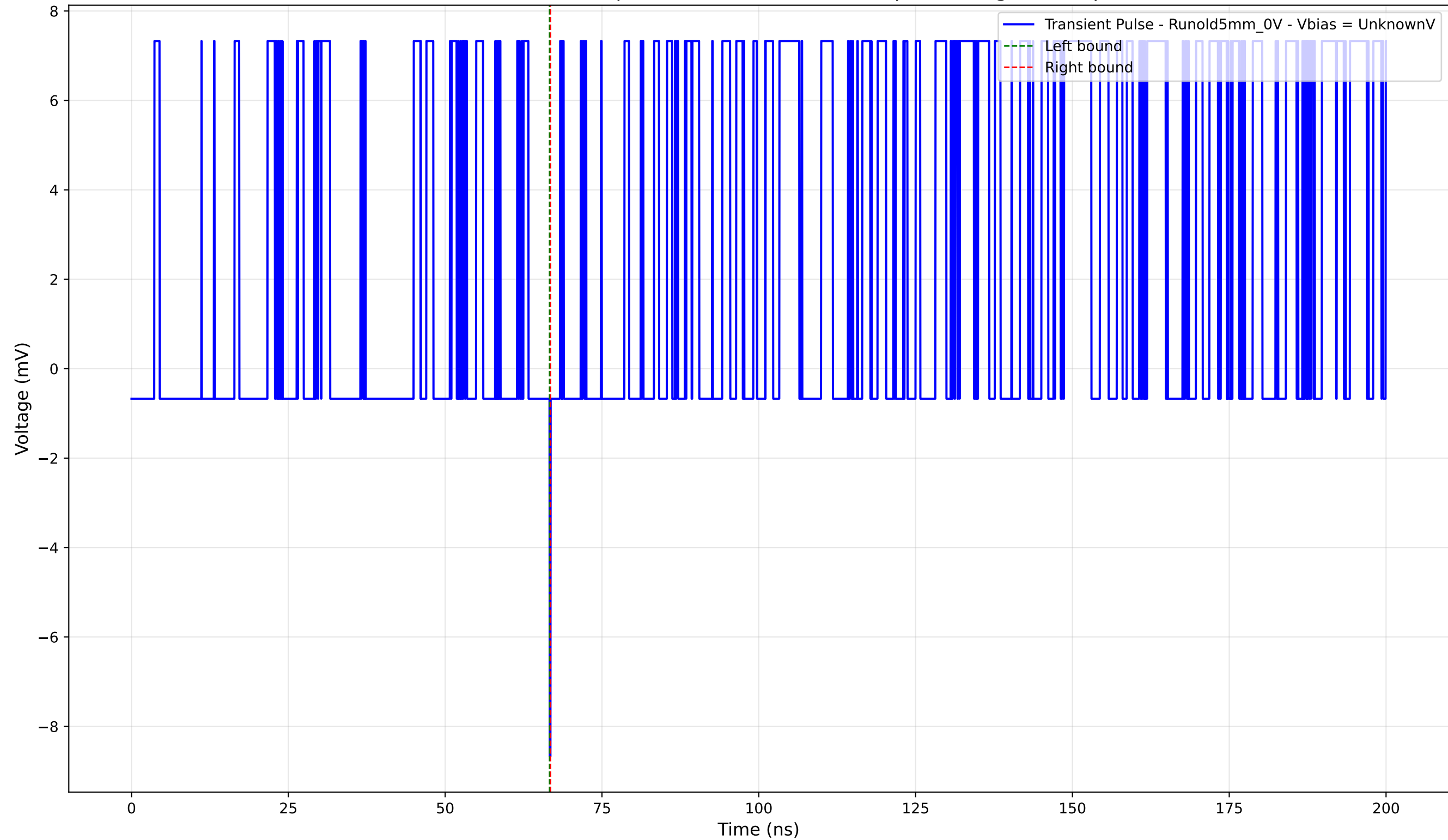
Transient Pulse - Sample: old5 - Position: 4325.0 \mu\text{m} - Charge: -0.02 pC
