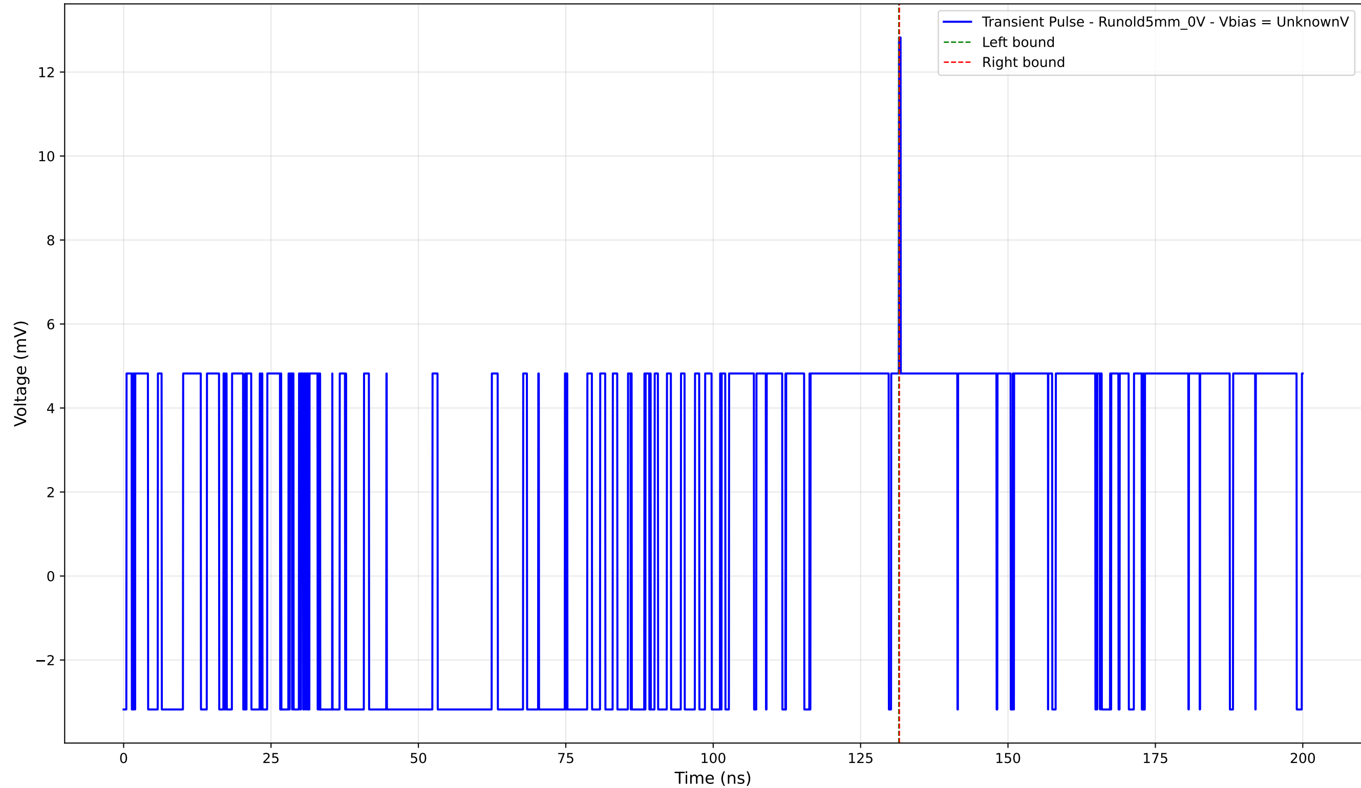
Transient Pulse - Sample: old5 - Position: 4035.0 \mu\text{m} - Charge: 0.02 pC
