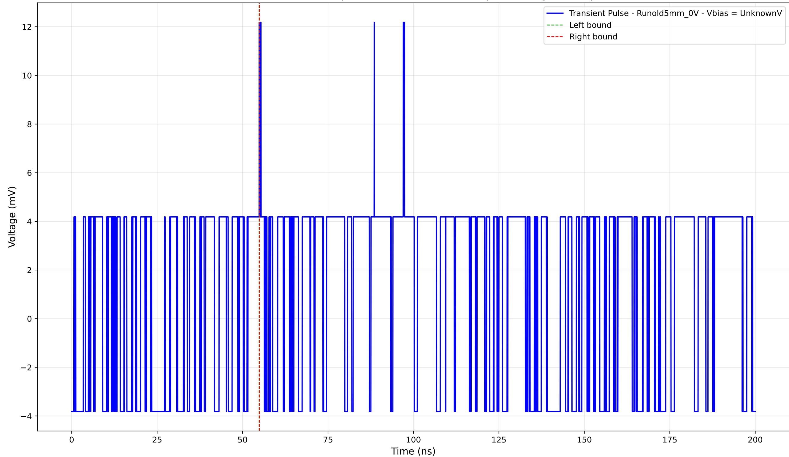
Transient Pulse - Sample: old5 - Position: 440.0 \mu\text{m} - Charge: 0.02 pC
