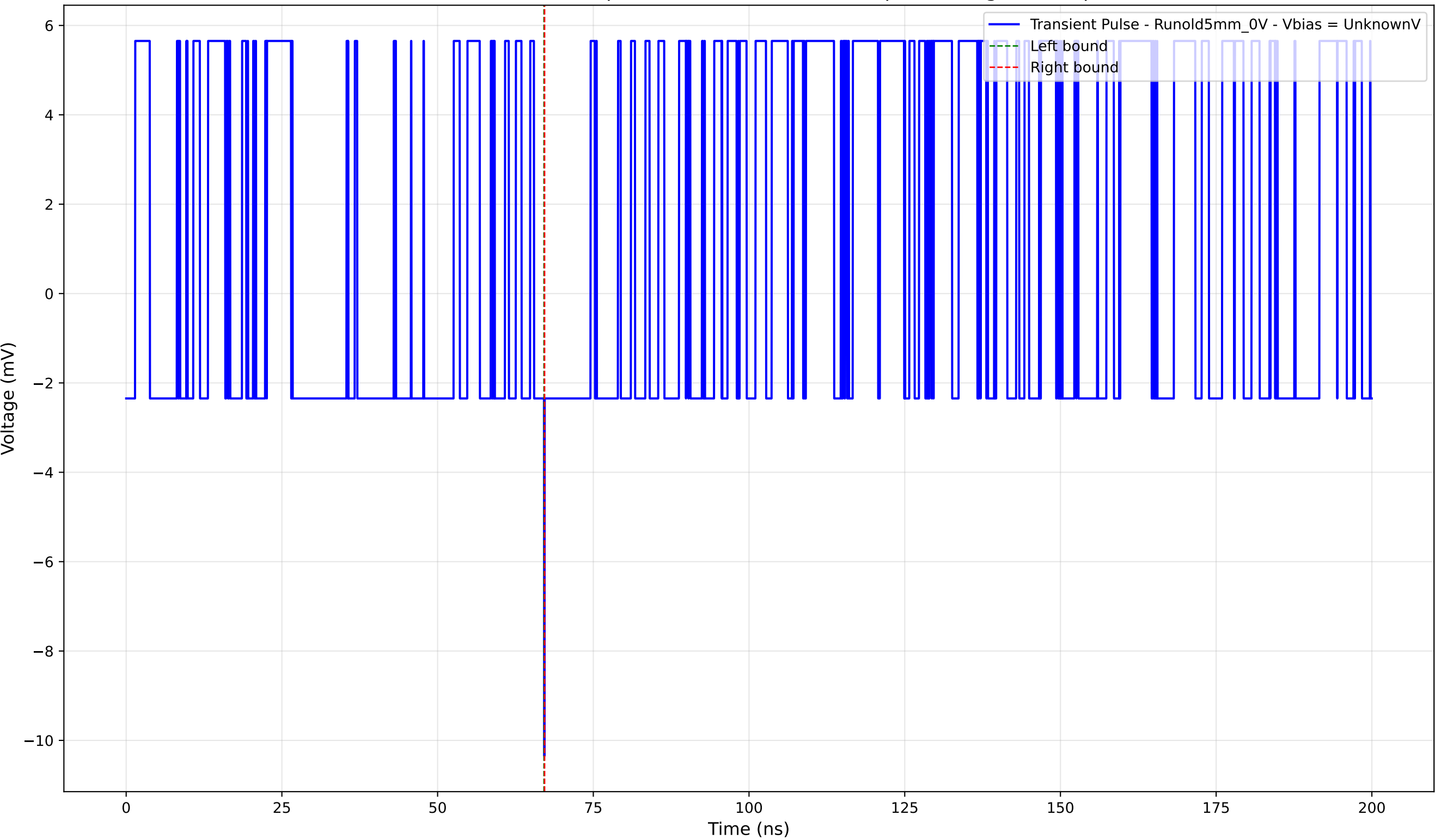
Transient Pulse - Sample: old5 - Position: 1685.0 \mu\text{m} - Charge: -0.02 pC
