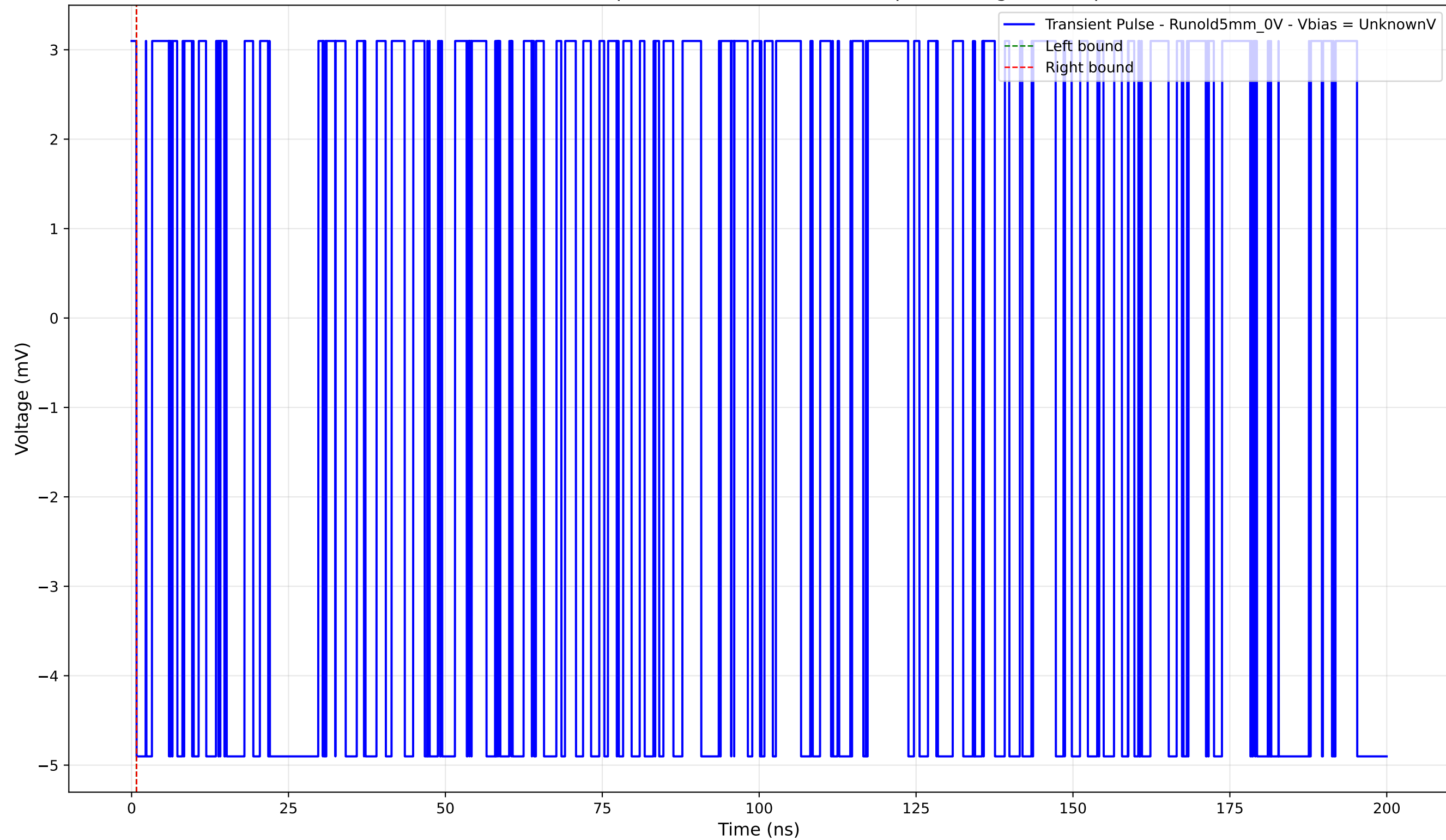
Transient Pulse - Sample: old5 - Position: 5135.0 \mu\text{m} - Charge: -0.00 pC
