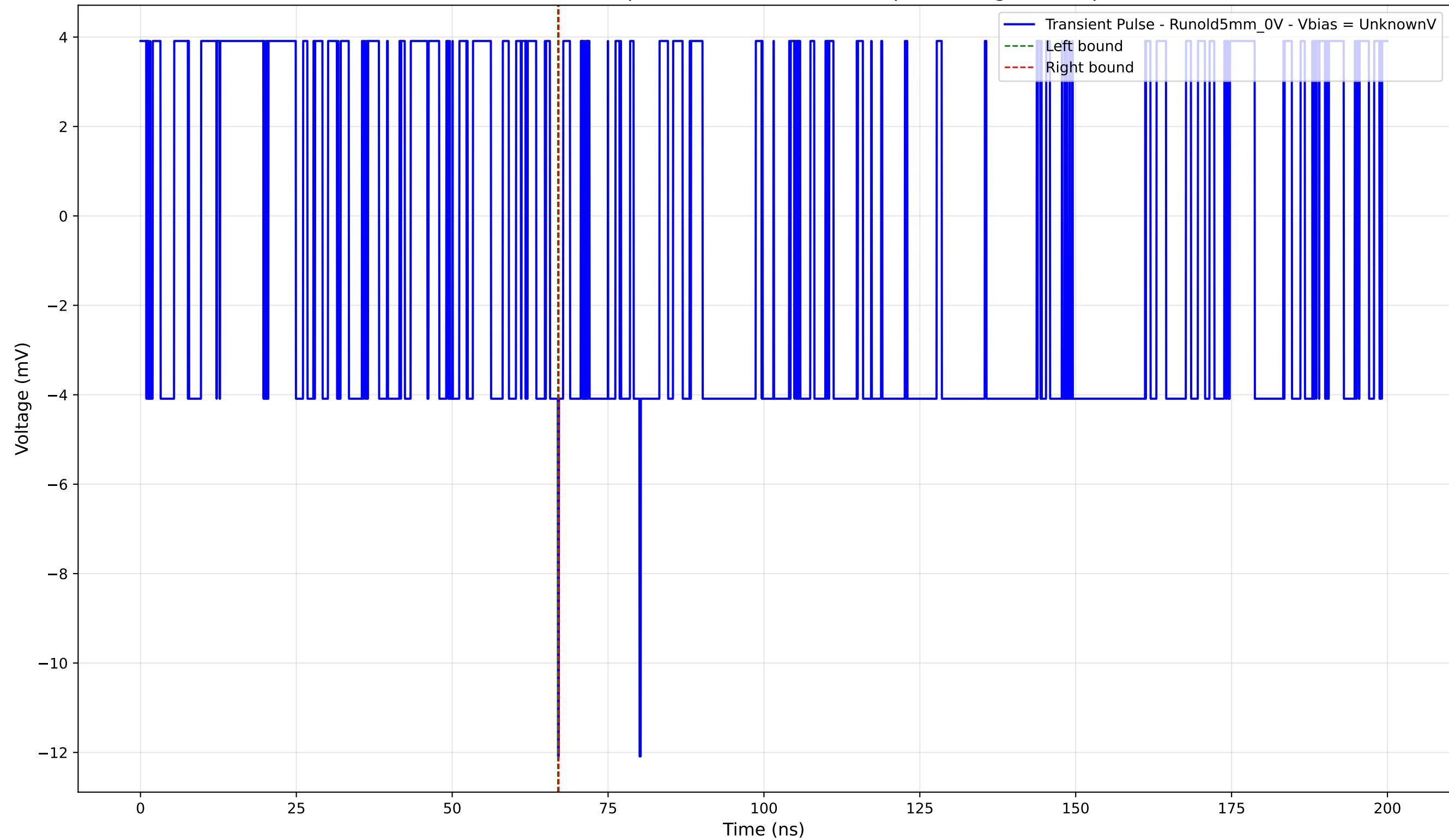
Transient Pulse - Sample: old5 - Position: 695.0 \mu\text{m} - Charge: -0.04 pC
