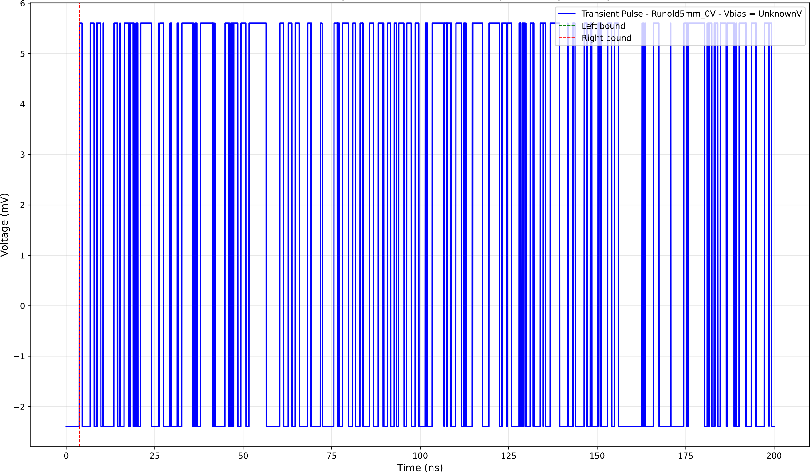
Transient Pulse - Sample: old5 - Position: 4095.0 \mu\text{m} - Charge: 0.00 pC
