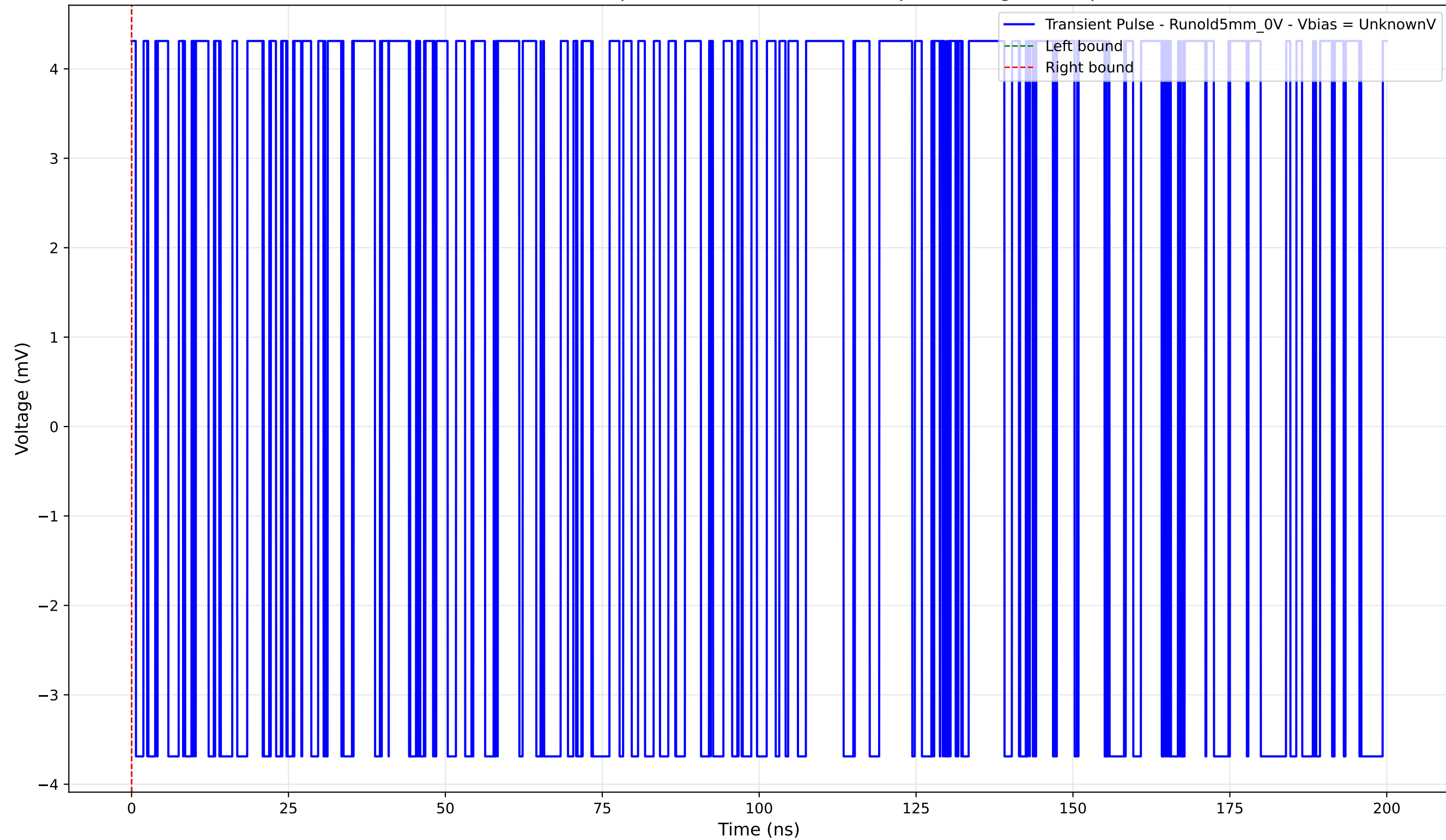
Transient Pulse - Sample: old5 - Position: 2680.0 \mu\text{m} - Charge: 0.00 pC
