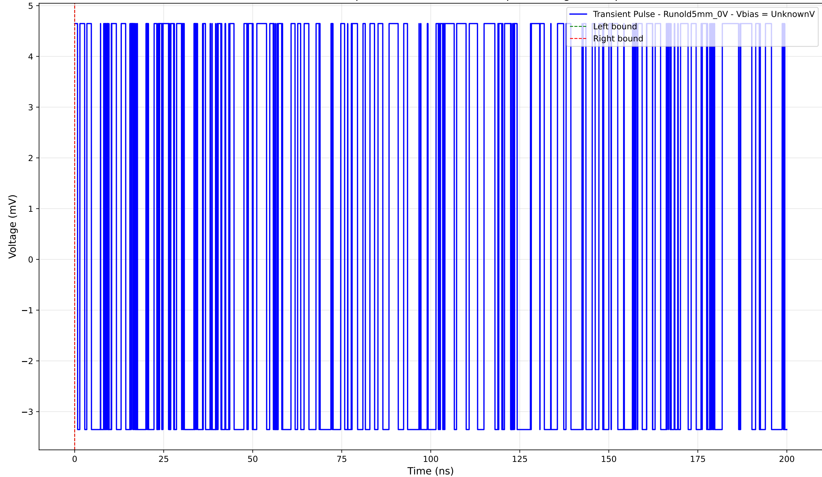
Transient Pulse - Sample: old5 - Position: 450.0 \mu\text{m} - Charge: 0.00 pC
