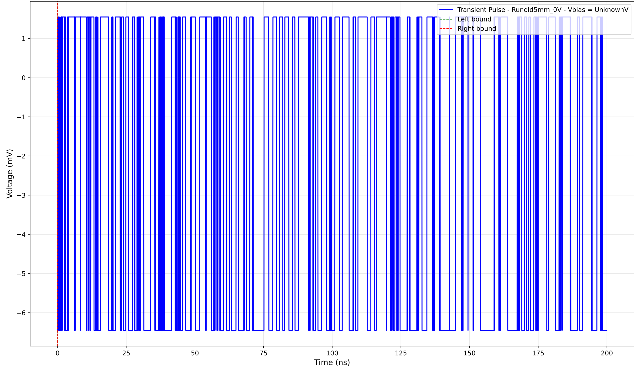
Transient Pulse - Sample: old5 - Position: 3200.0 \mu\text{m} - Charge: -0.00 pC
