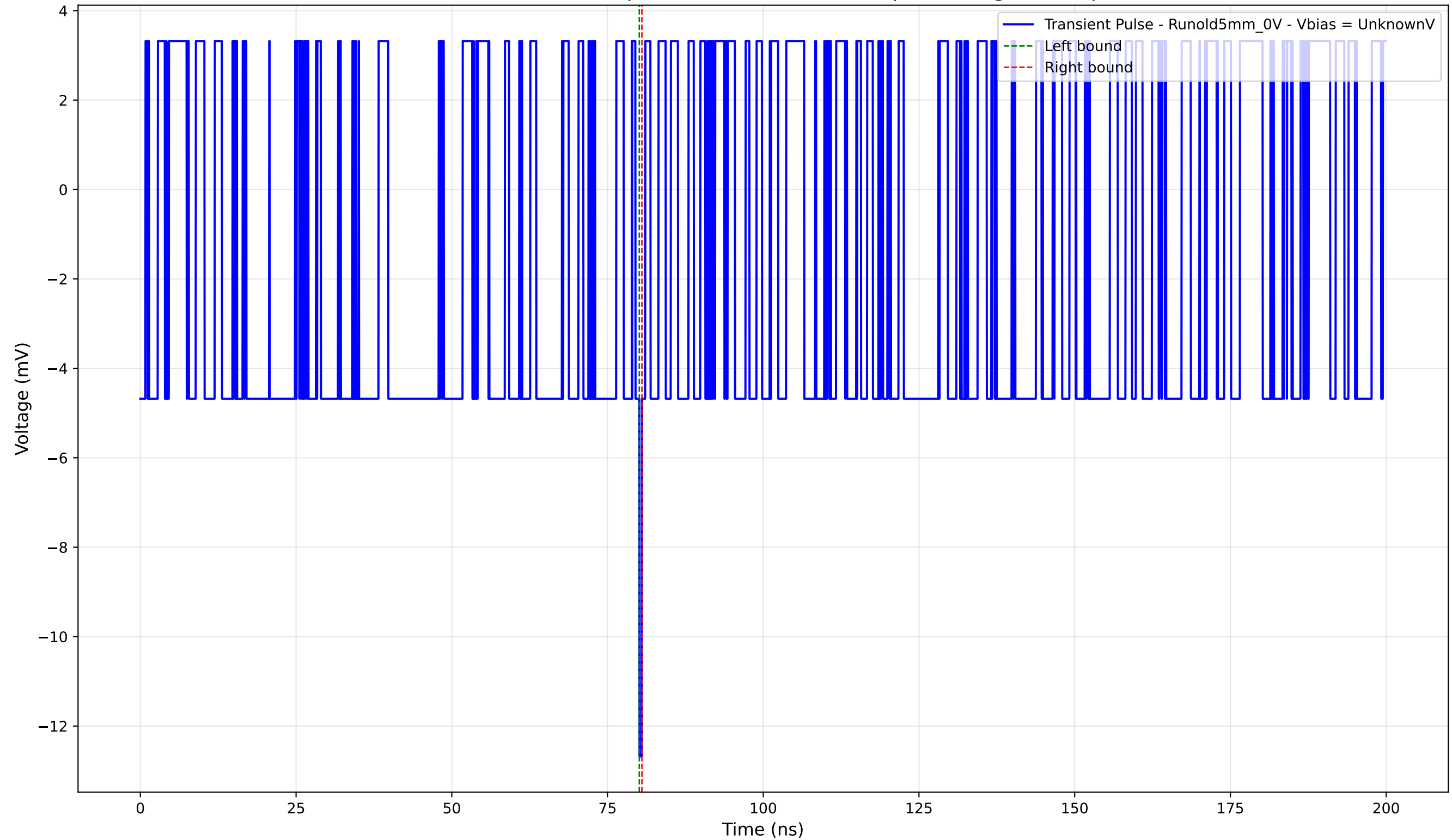
Transient Pulse - Sample: old5 - Position: 210.0 \mu\text{m} - Charge: -0.10 pC
