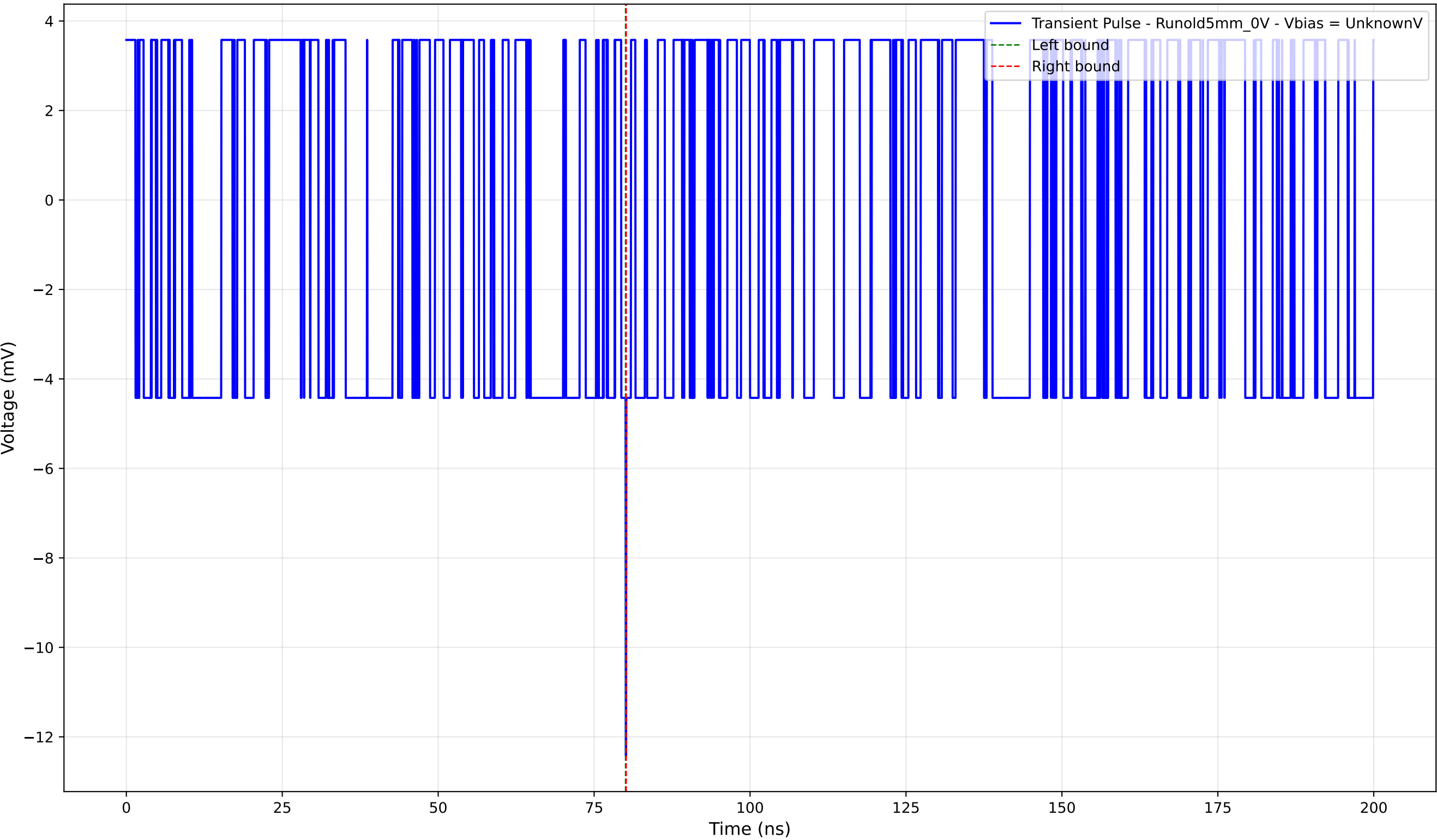
Transient Pulse - Sample: old5 - Position: 2365.0 \mu\text{m} - Charge: -0.02 pC
