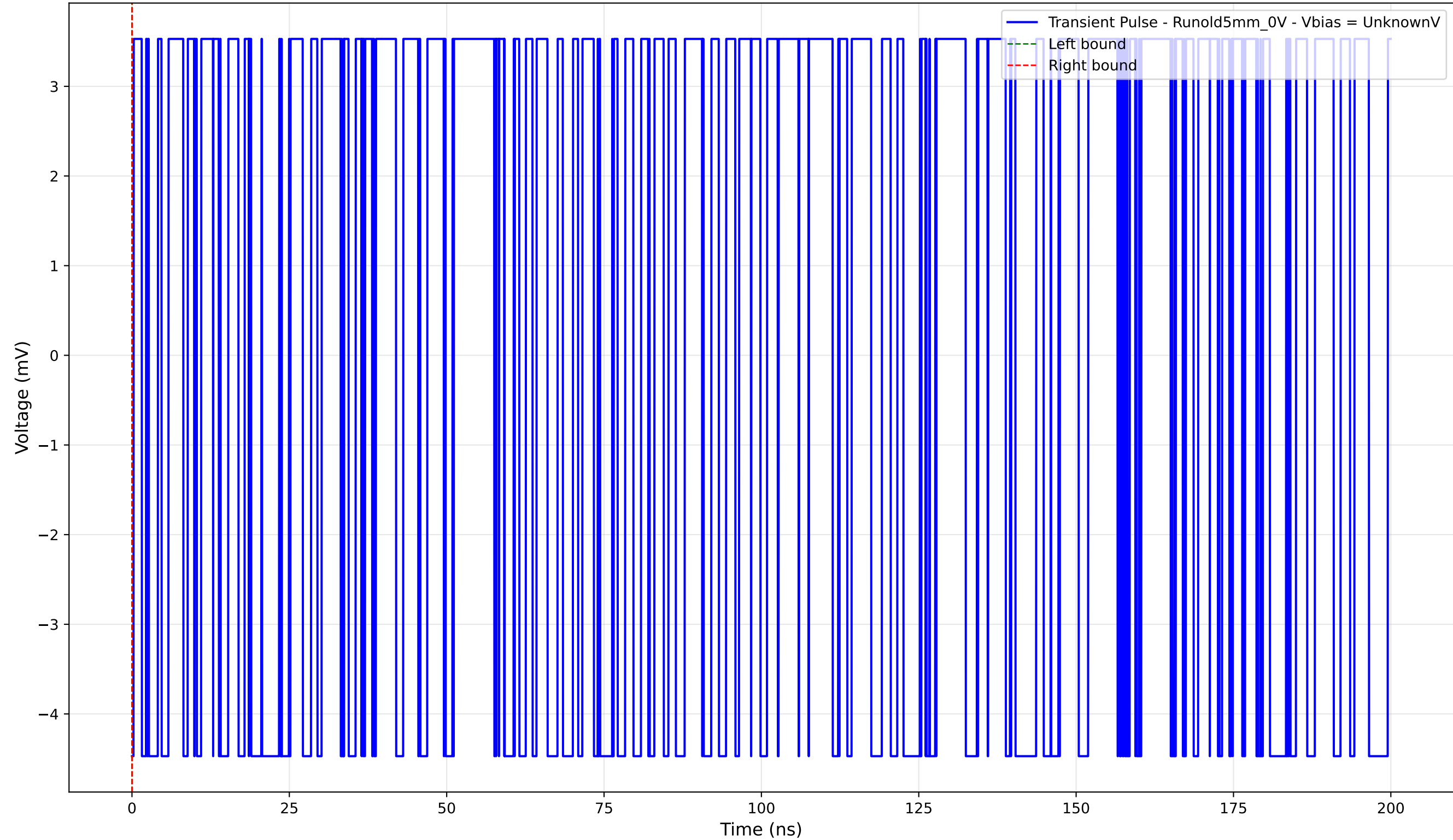
Transient Pulse - Sample: old5 - Position: 2770.0 \mu\text{m} - Charge: -0.00 pC
