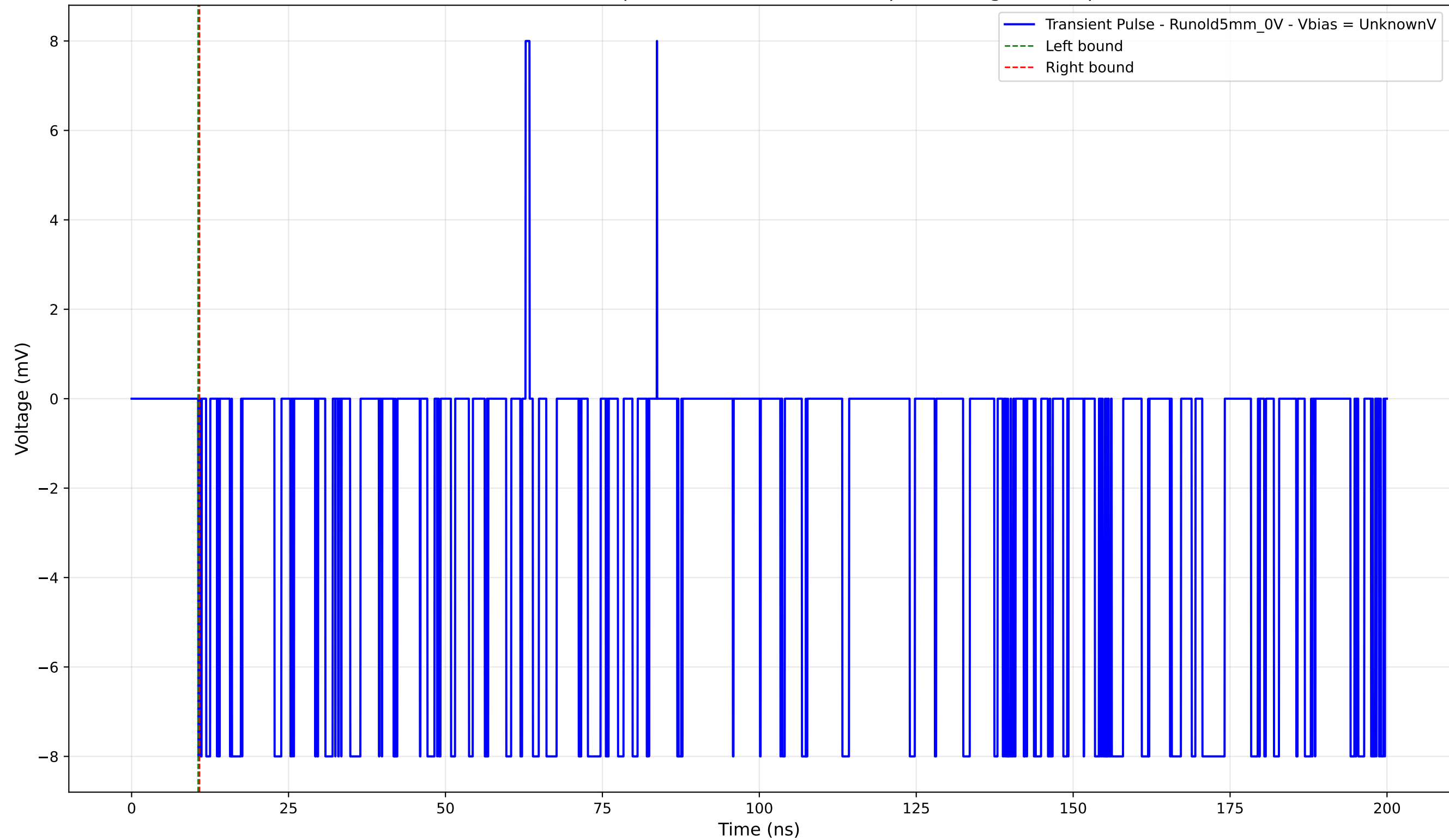
Transient Pulse - Sample: old5 - Position: 295.0 \mu\text{m} - Charge: -0.03 pC
