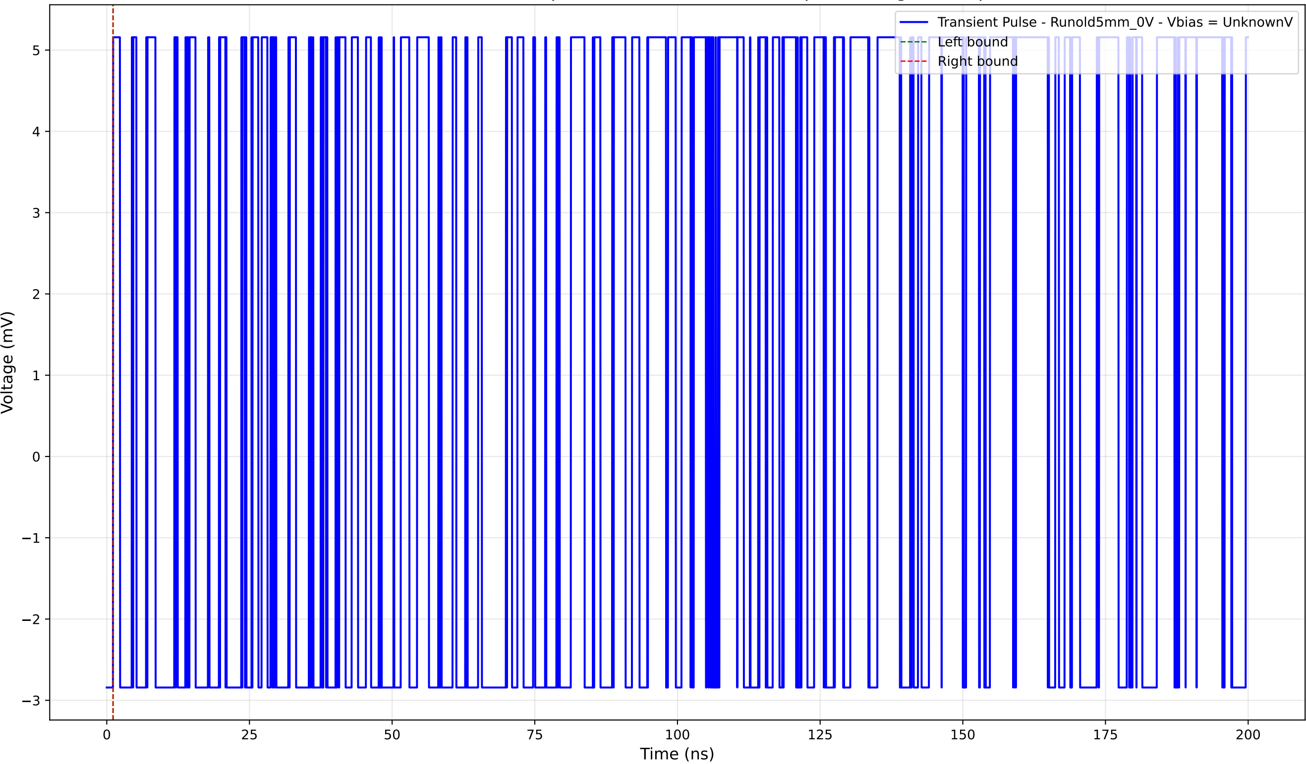
Transient Pulse - Sample: old5 - Position: 2520.0 \mu\text{m} - Charge: 0.00 pC
