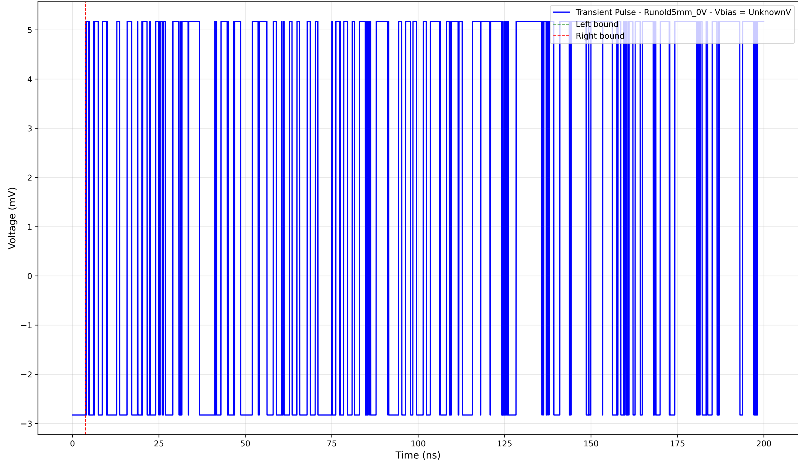
Transient Pulse - Sample: old5 - Position: 835.0 \mu\text{m} - Charge: 0.00 pC
