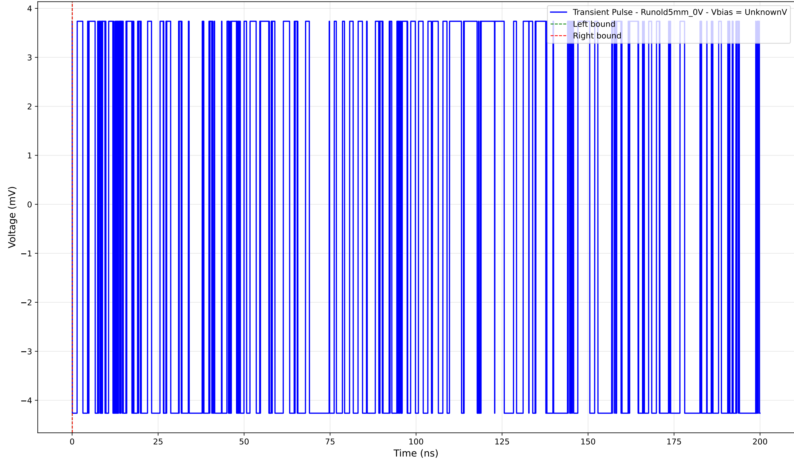
Transient Pulse - Sample: old5 - Position: 4990.0 \mu\text{m} - Charge: -0.00 pC
