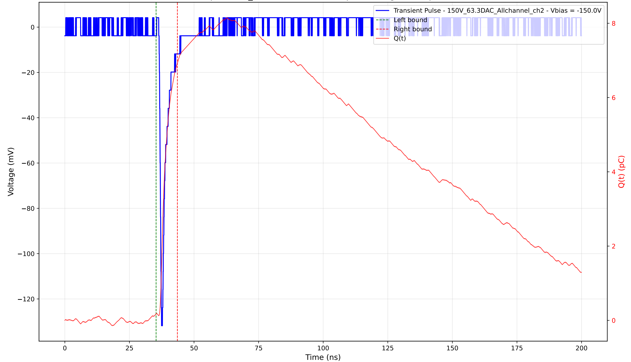
Transient Pulse - Sample: 1cm_42 - Position: 2240.0 \mu\text{m} - Charge: 6.75 pC - Rise Time: 0.75 ns
