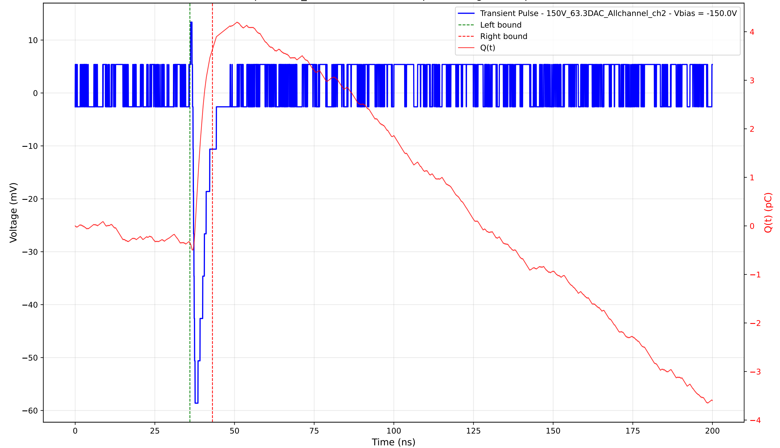
Transient Pulse - Sample: 1cm_42 - Position: 4085.0 \mu\text{m} - Charge: 3.99 pC - Rise Time: 0.66 ns
