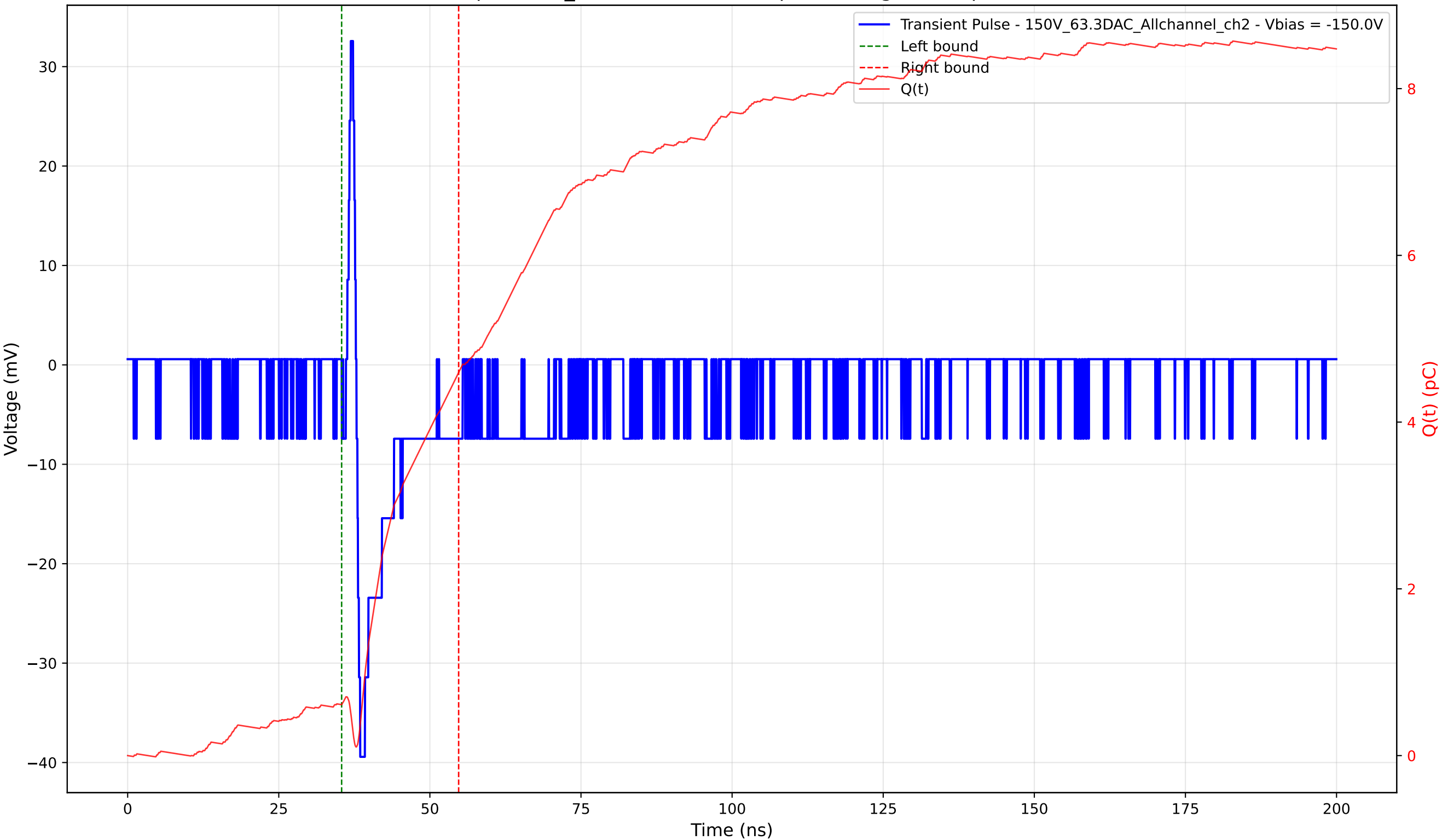
Transient Pulse - Sample: 1cm_42 - Position: 925.0 \mu\text{m} - Charge: 3.99 pC - Rise Time: 0.62 ns
