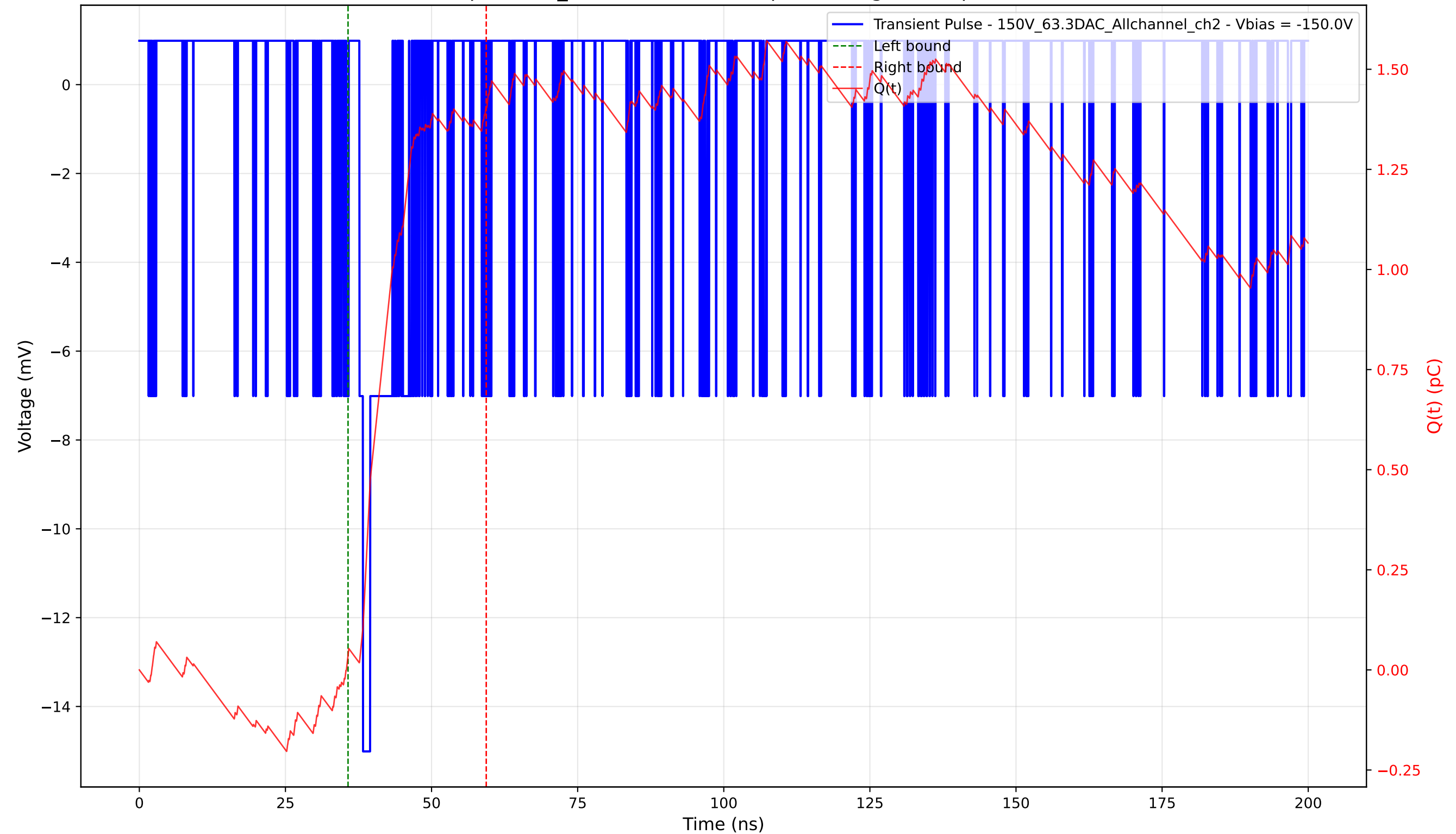
Transient Pulse - Sample: 1cm_42 - Position: 145.0 \mu\text{m} - Charge: 1.37 pC - Rise Time: 0.64 ns
