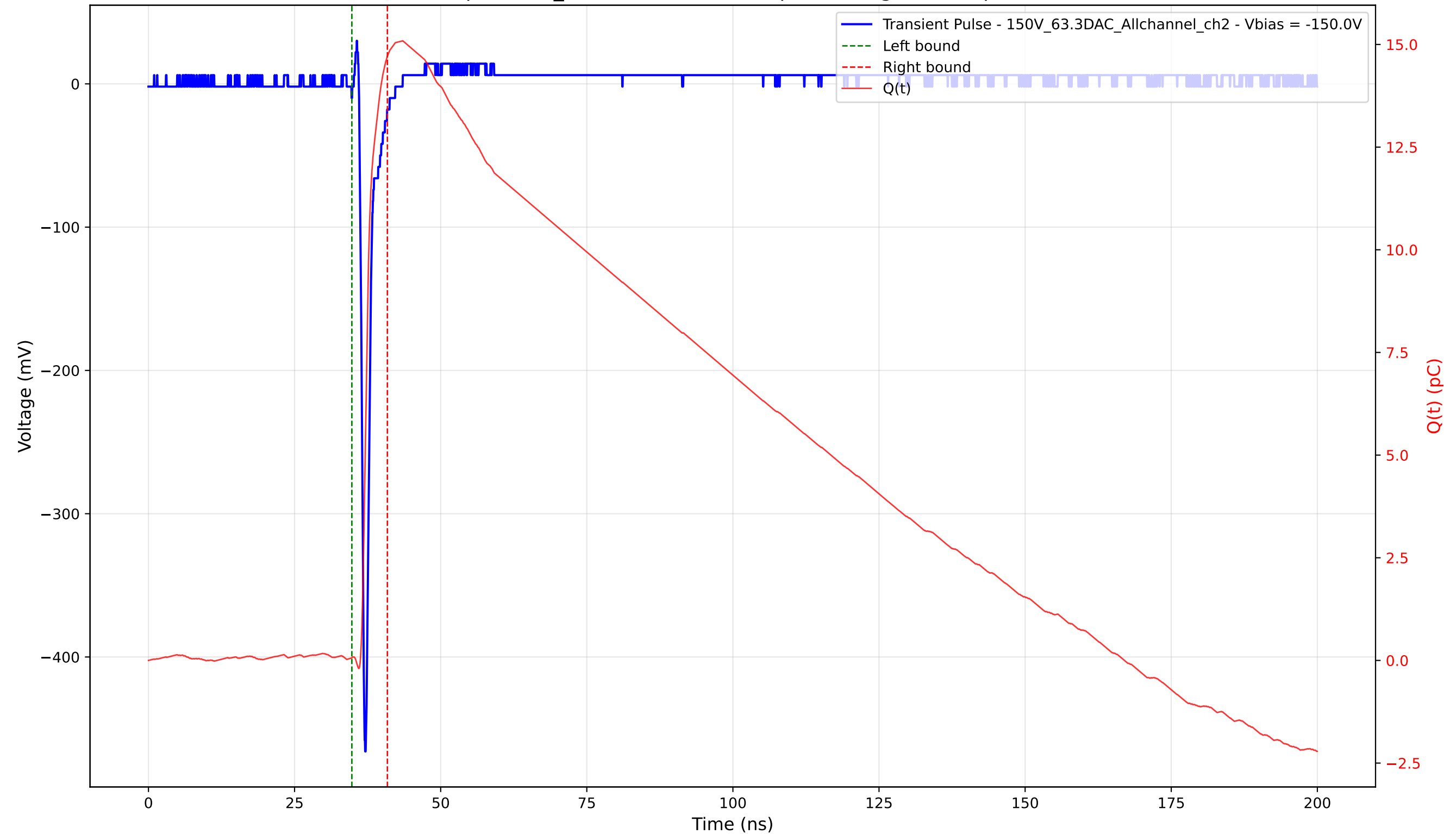
Transient Pulse - Sample: 1cm_42 - Position: 3170.0 \mu\text{m} - Charge: 14.65 pC - Rise Time: 0.70 ns
