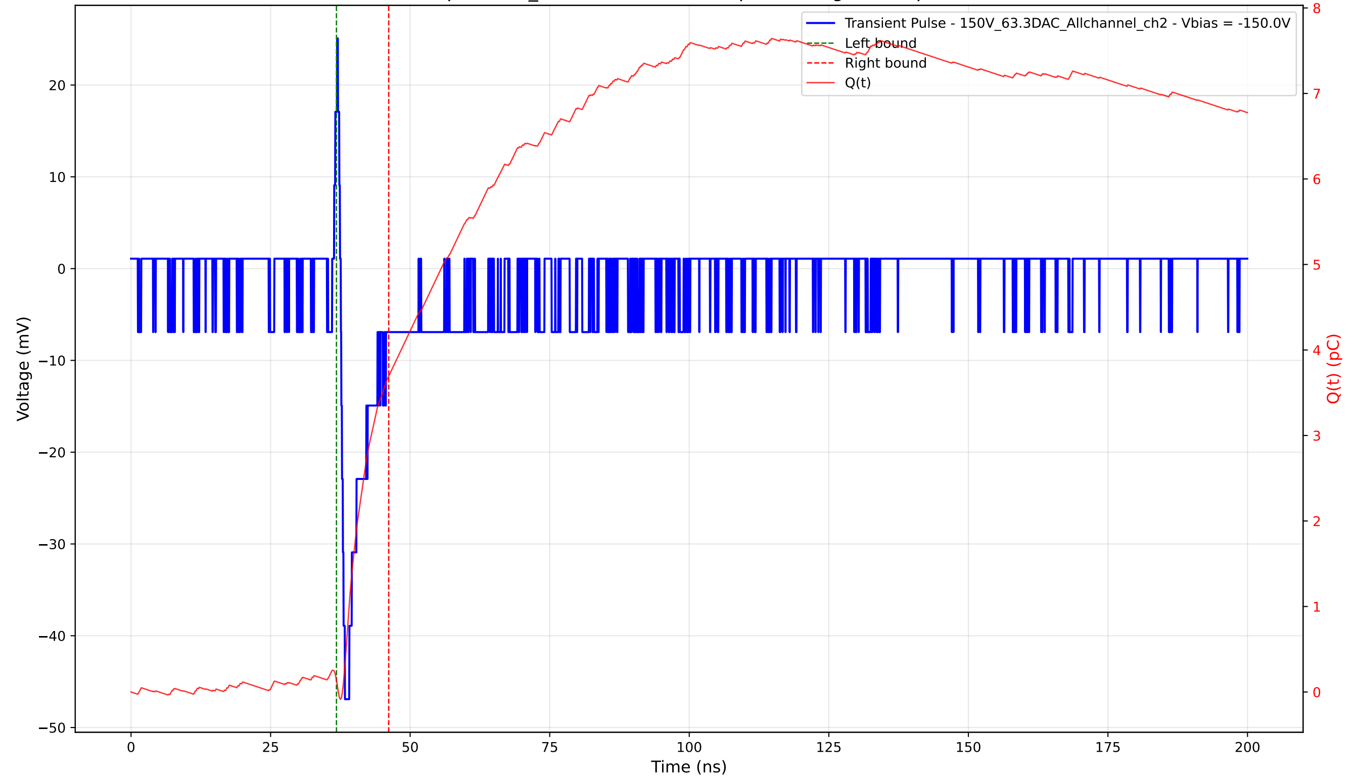
Transient Pulse - Sample: 1cm_42 - Position: 1525.0 \mu\text{m} - Charge: 3.56 pC - Rise Time: 0.74 ns
