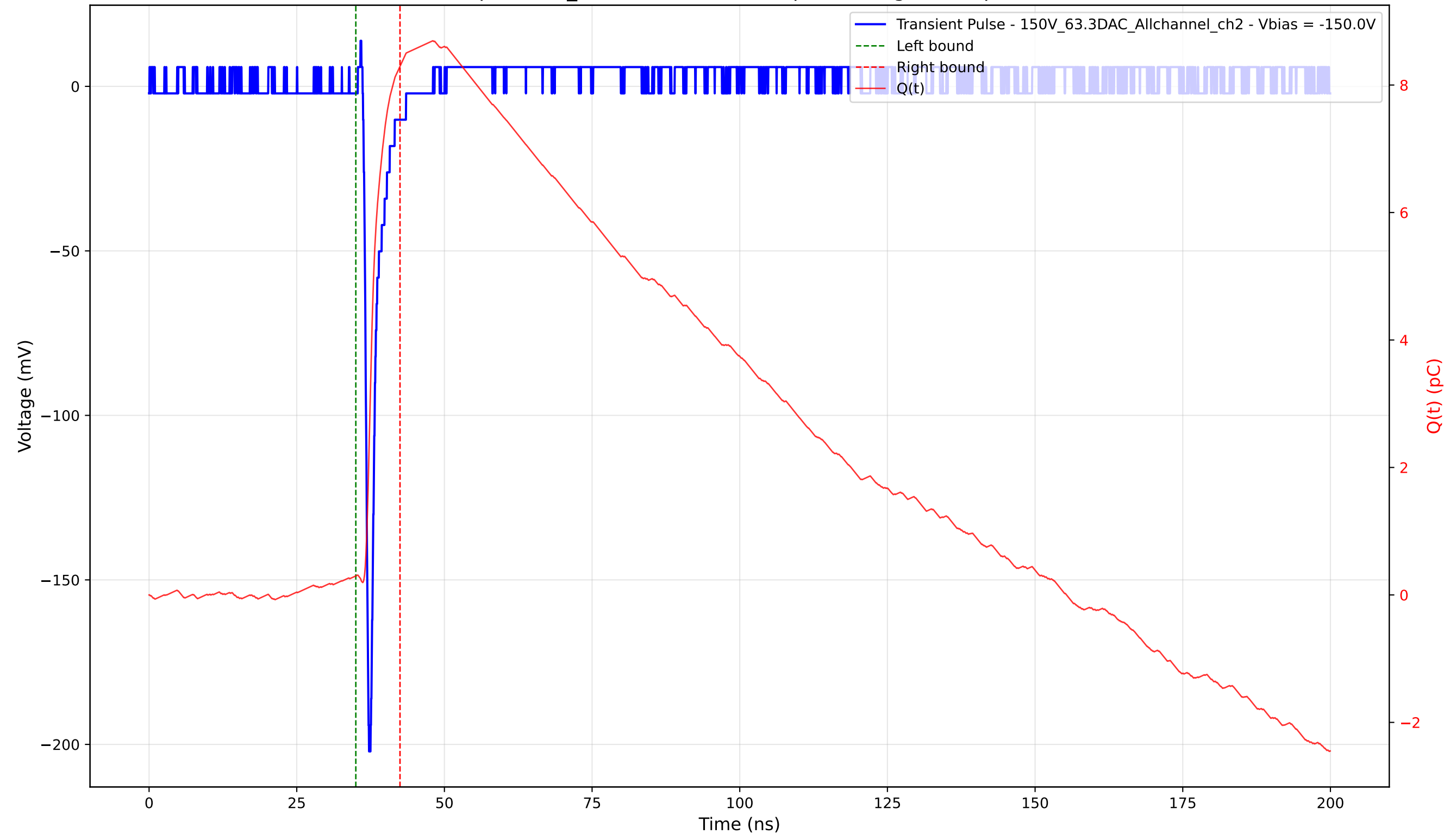
Transient Pulse - Sample: 1cm_42 - Position: 2505.0 \mu\text{m} - Charge: 8.00 pC - Rise Time: 0.77 ns
