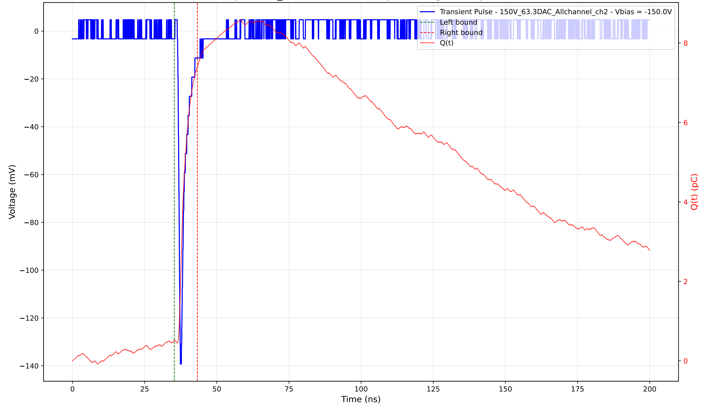
Transient Pulse - Sample: 1cm_42 - Position: 2300.0 \mu\text{m} - Charge: 6.90 pC - Rise Time: 0.79 ns
