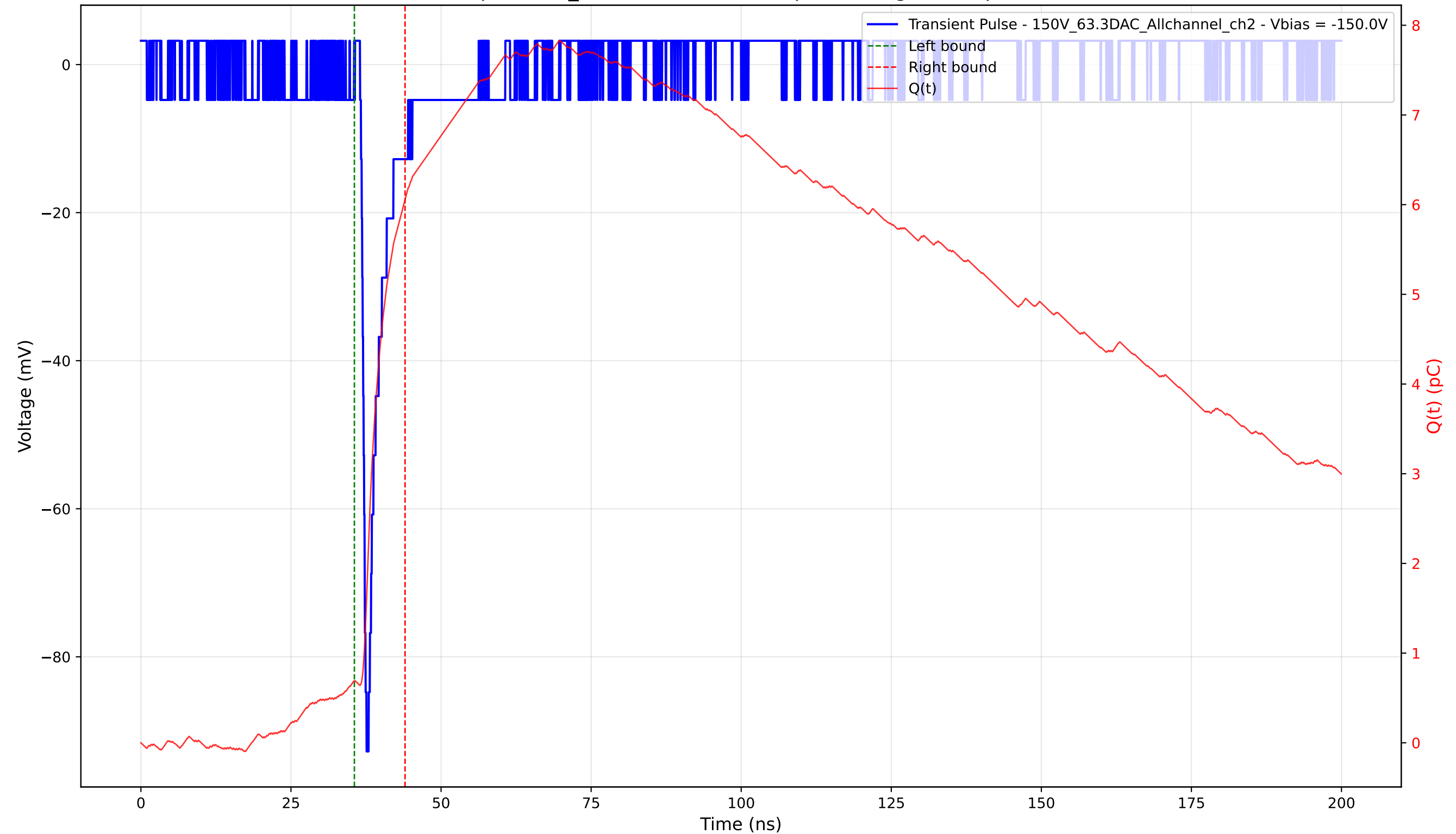
Transient Pulse - Sample: 1cm_42 - Position: 2100.0 \mu\text{m} - Charge: 5.37 pC - Rise Time: 0.78 ns
