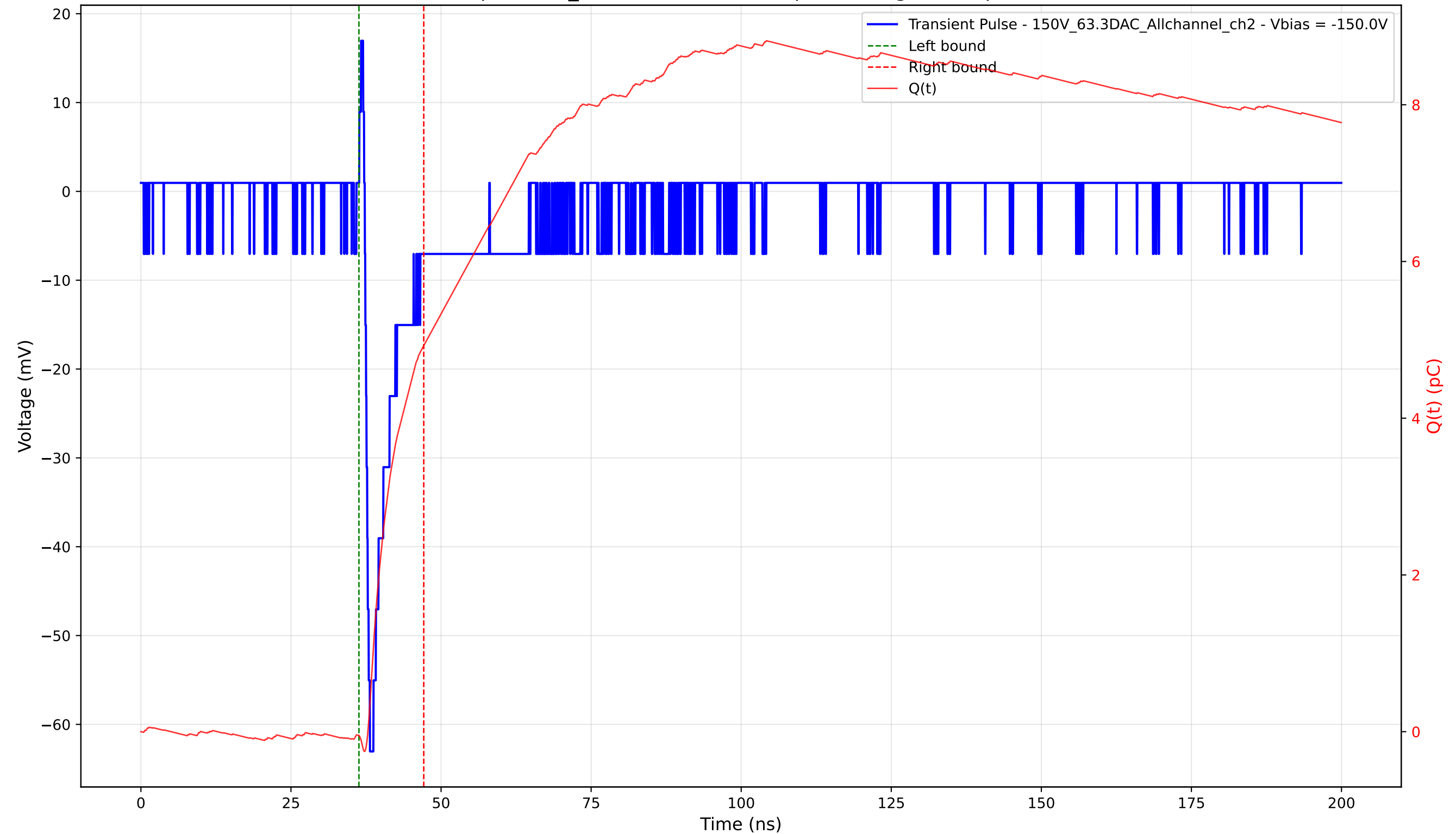
Transient Pulse - Sample: 1cm_42 - Position: 1715.0 \mu\text{m} - Charge: 4.97 pC - Rise Time: 0.84 ns
