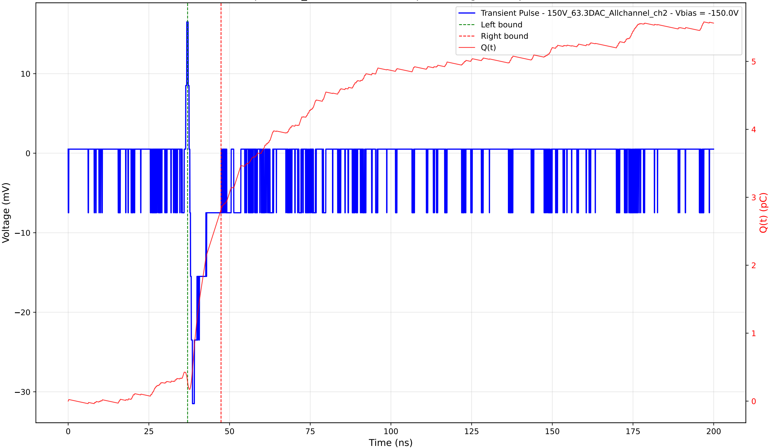
Transient Pulse - Sample: 1cm_42 - Position: 385.0 \mu\text{m} - Charge: 2.54 pC - Rise Time: 0.82 ns
