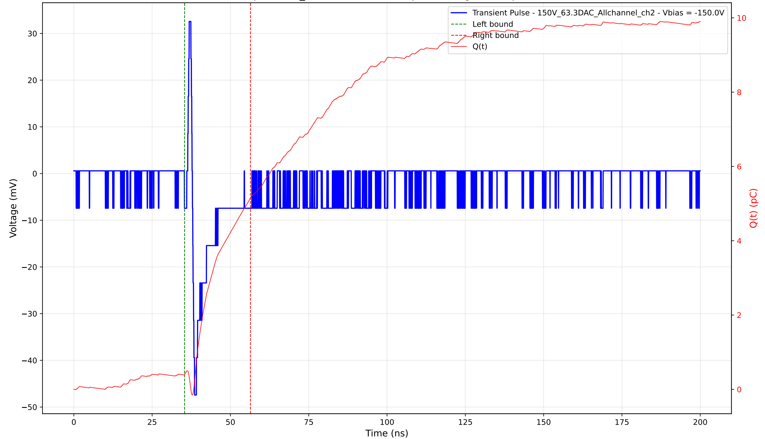
Transient Pulse - Sample: 1cm_42 - Position: 740.0 \mu\text{m} - Charge: 4.76 pC - Rise Time: 0.70 ns
