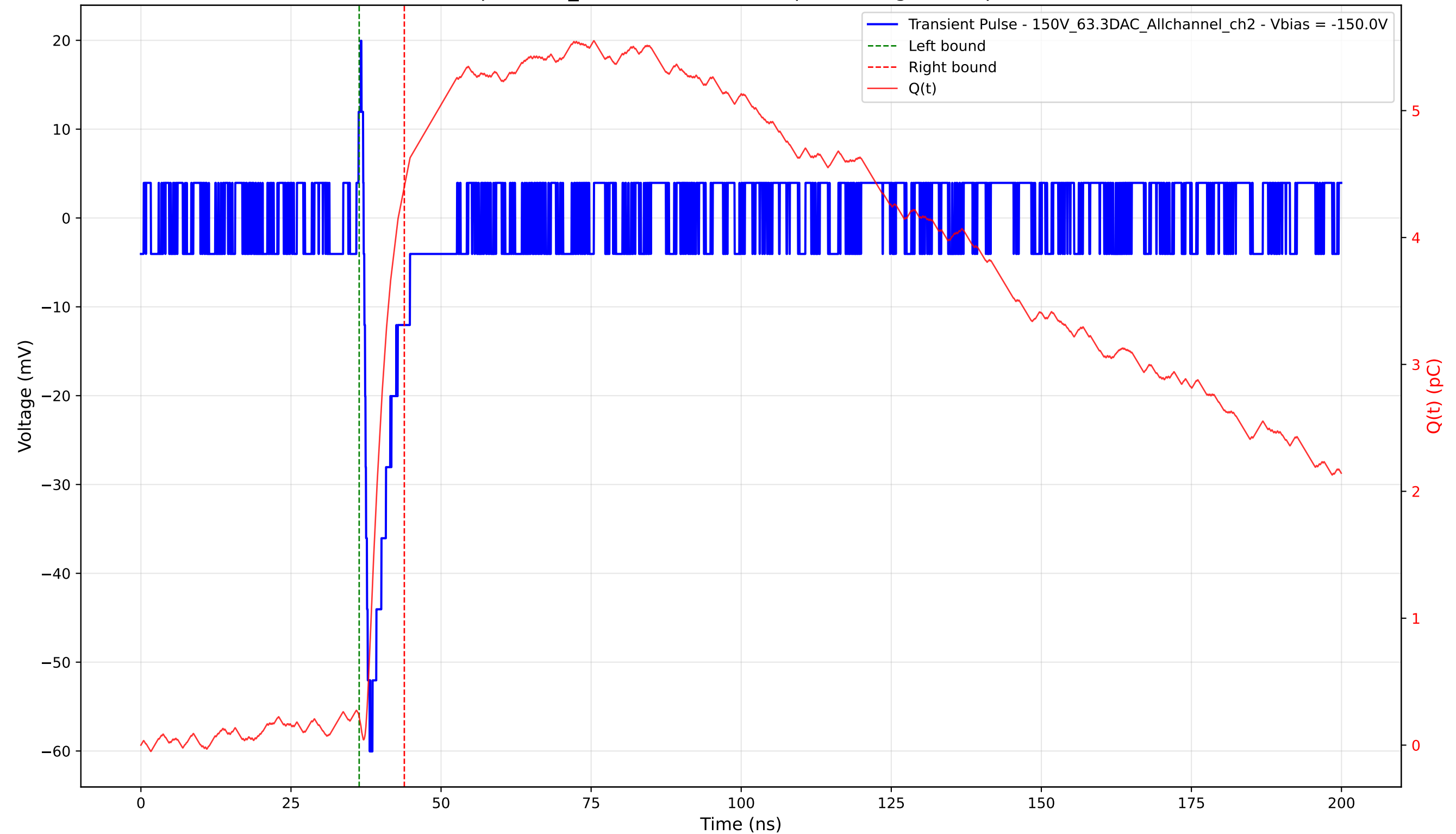
Transient Pulse - Sample: 1cm_42 - Position: 4265.0 \mu\text{m} - Charge: 4.18 pC - Rise Time: 0.91 ns
