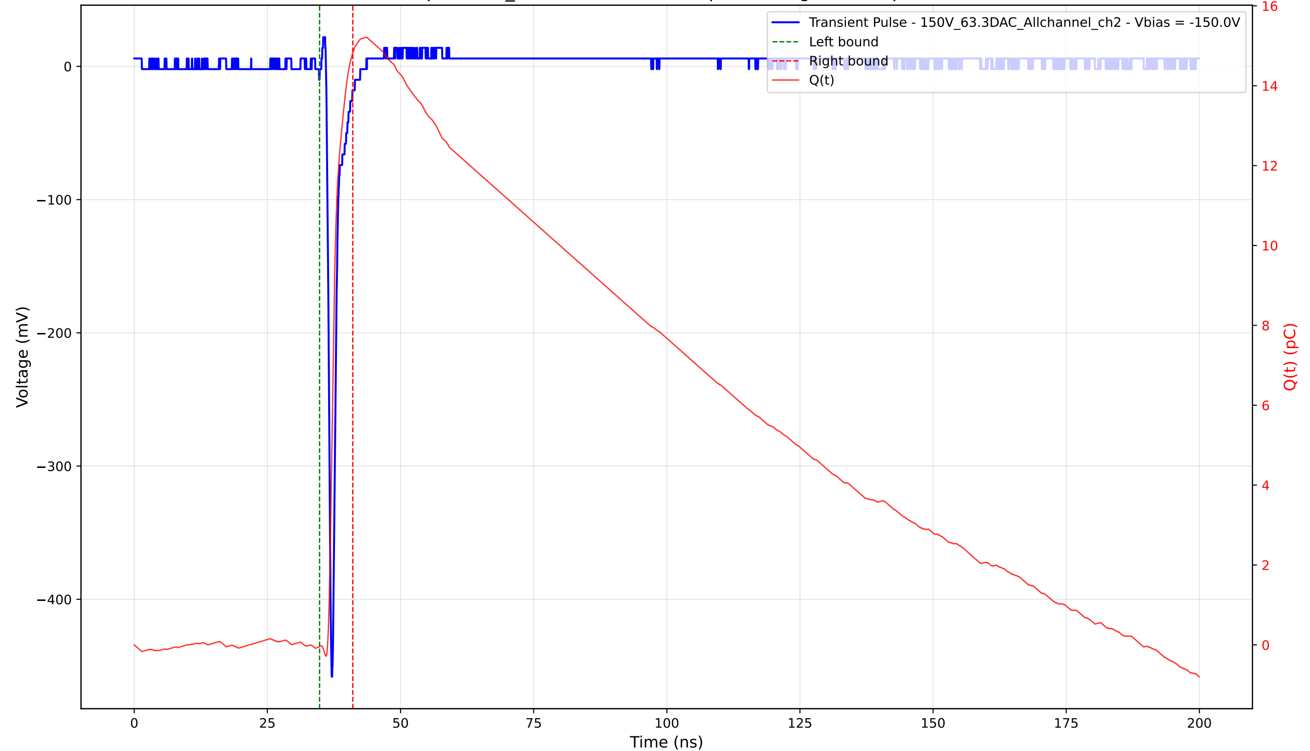
Transient Pulse - Sample: 1cm_42 - Position: 3215.0 \mu\text{m} - Charge: 14.87 pC - Rise Time: 0.68 ns
