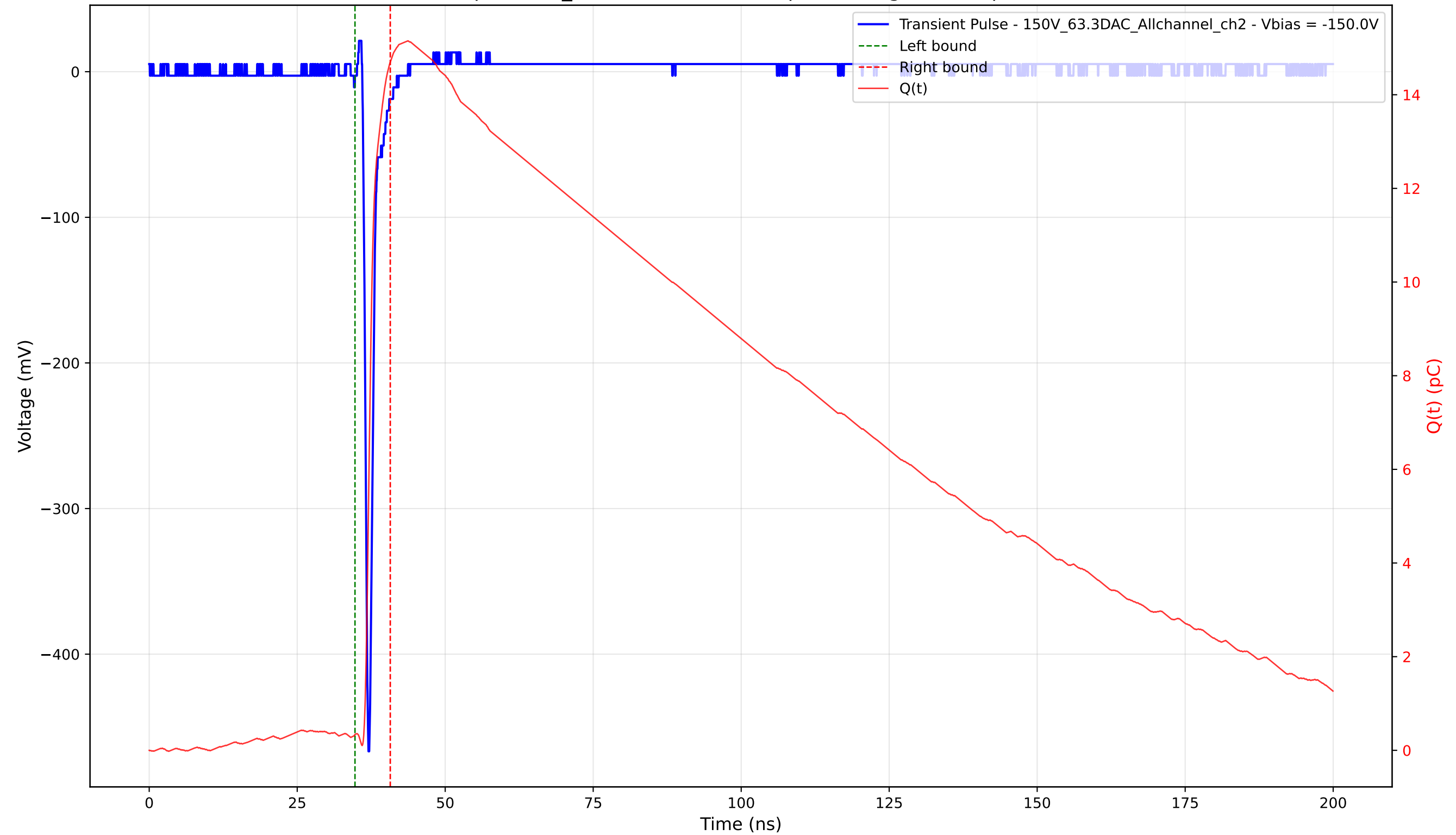
Transient Pulse - Sample: 1cm_42 - Position: 2930.0 \mu\text{m} - Charge: 14.36 pC - Rise Time: 0.73 ns
