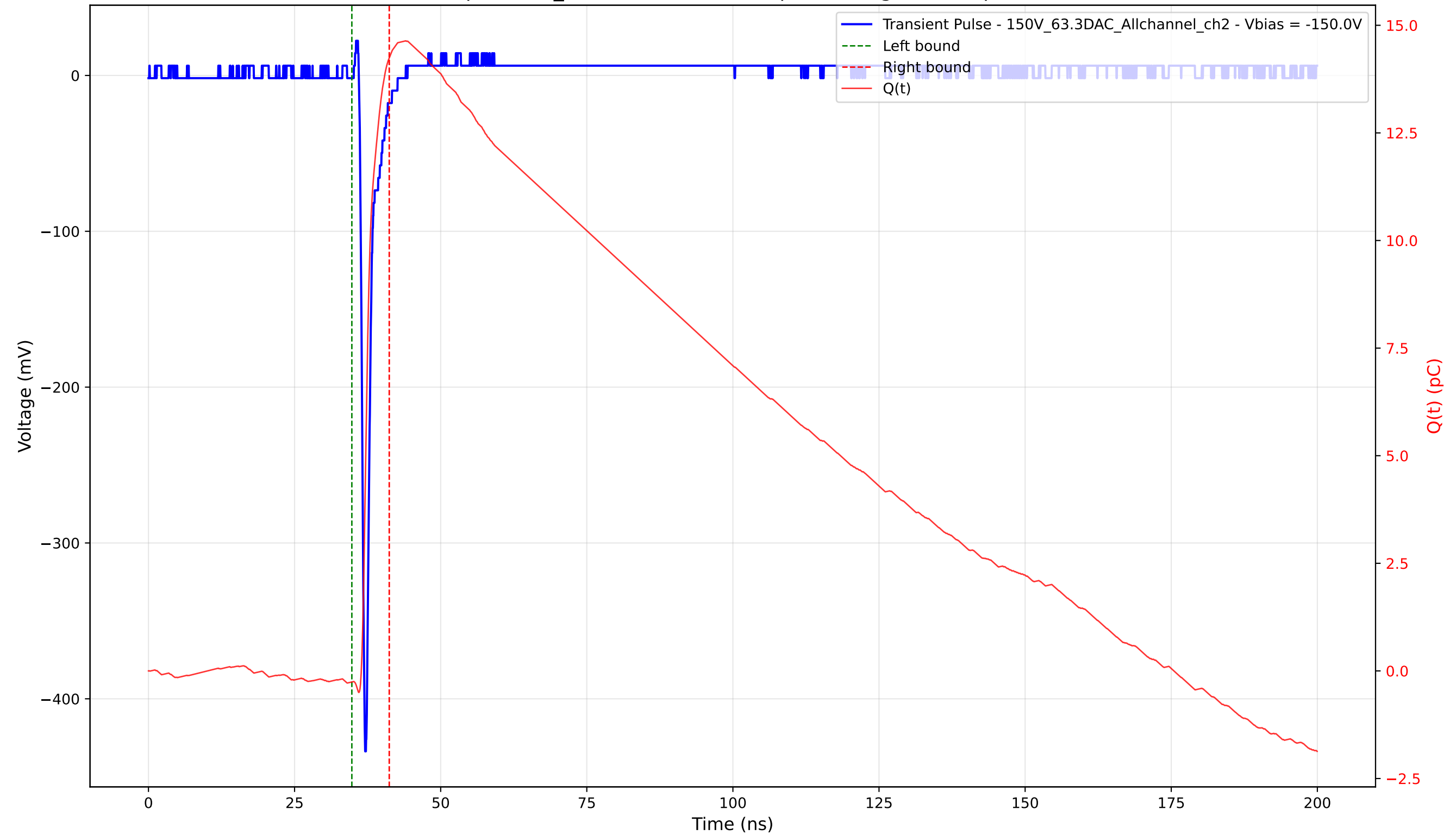
Transient Pulse - Sample: 1cm_42 - Position: 3280.0 \mu\text{m} - Charge: 14.50 pC - Rise Time: 0.73 ns
