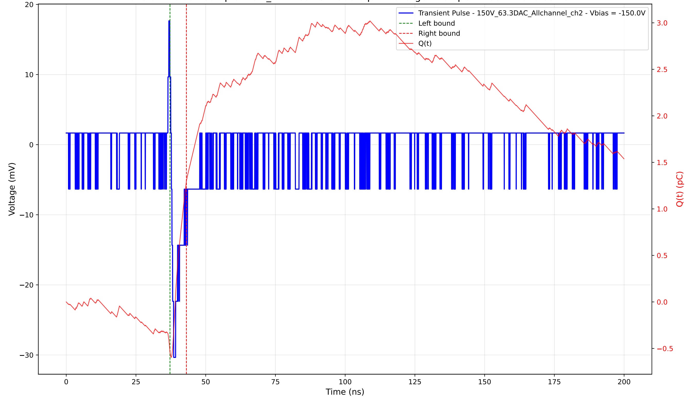
Transient Pulse - Sample: 1cm_42 - Position: 380.0 \mu\text{m} - Charge: 1.84 pC - Rise Time: 0.83 ns
