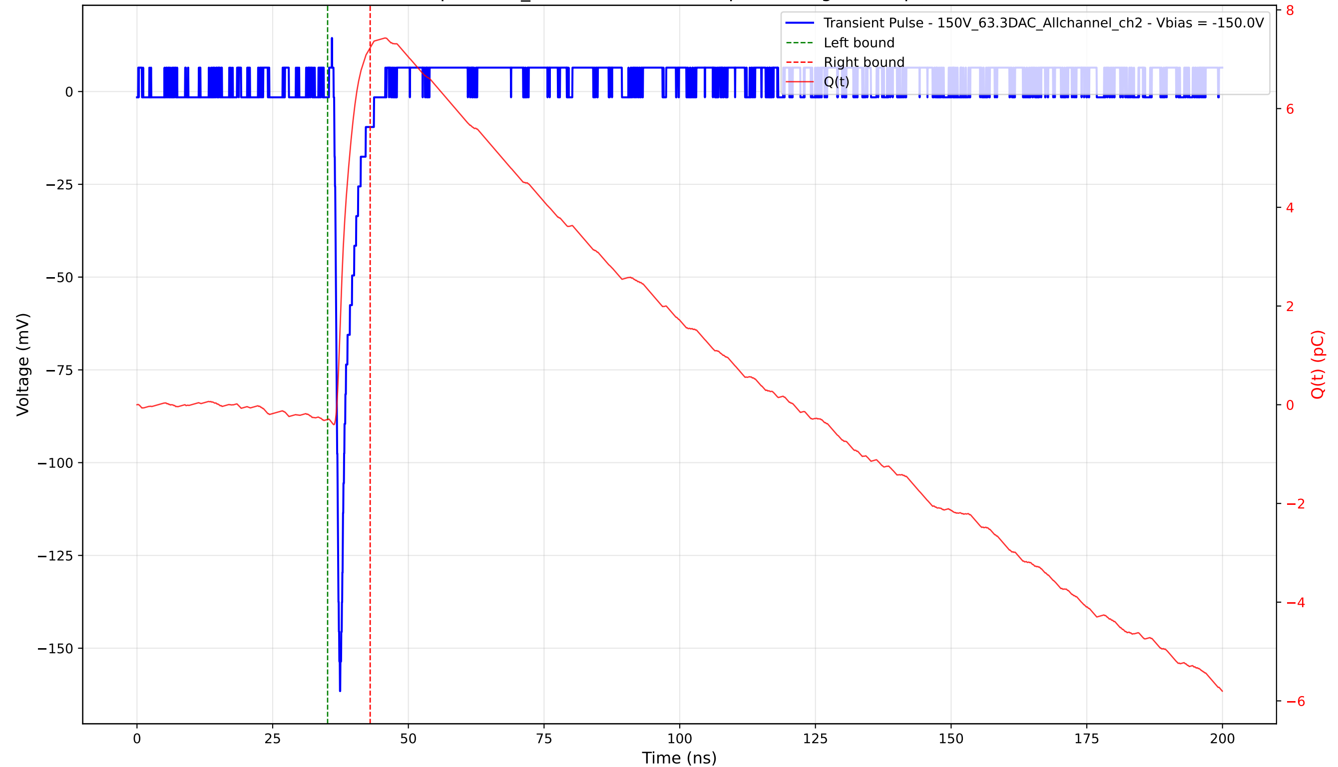
Transient Pulse - Sample: 1cm_42 - Position: 3630.0 \mu\text{m} - Charge: 7.53 pC - Rise Time: 0.81 ns
