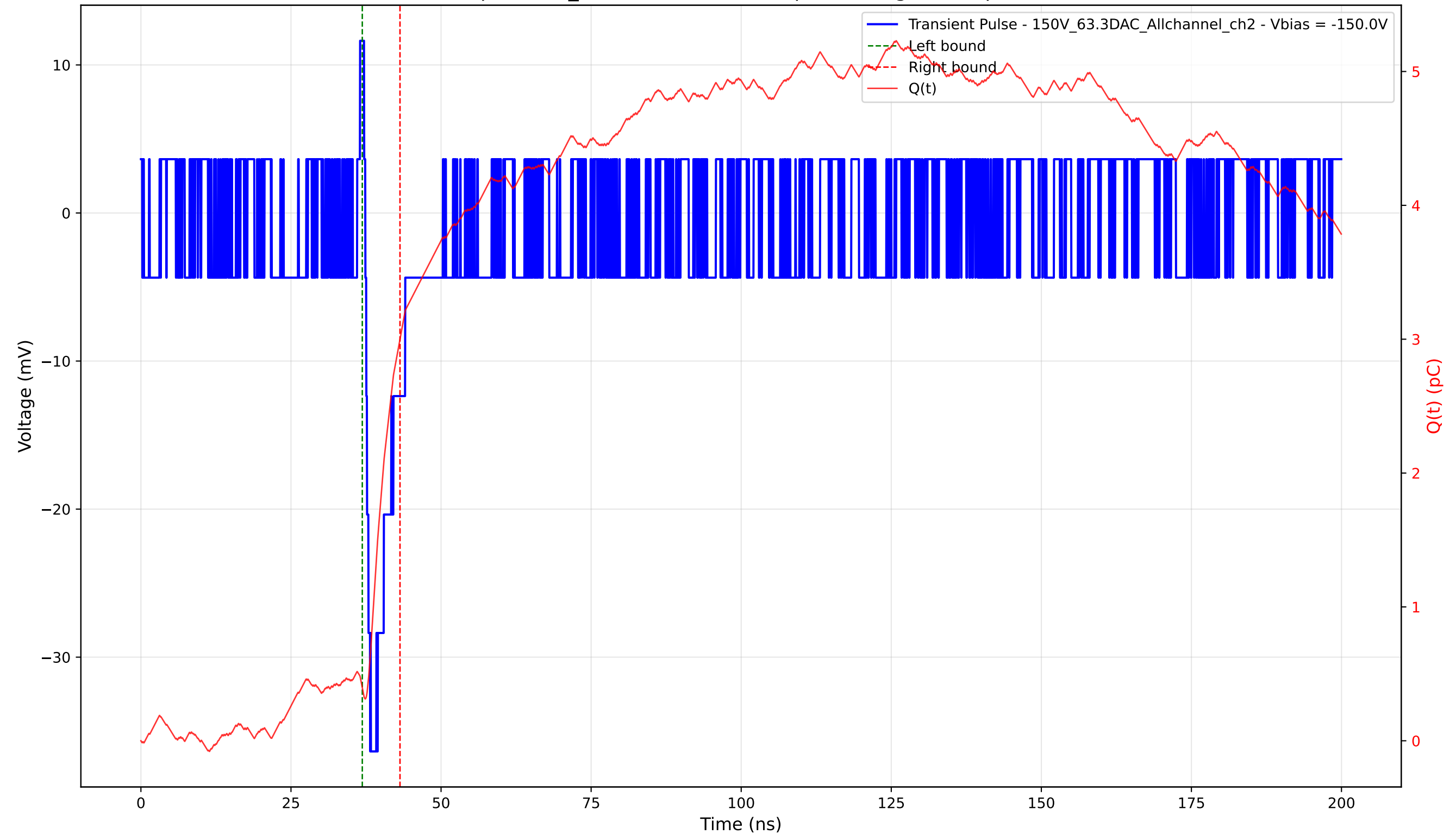
Transient Pulse - Sample: 1cm_42 - Position: 4640.0 \mu\text{m} - Charge: 2.61 pC - Rise Time: 0.84 ns
