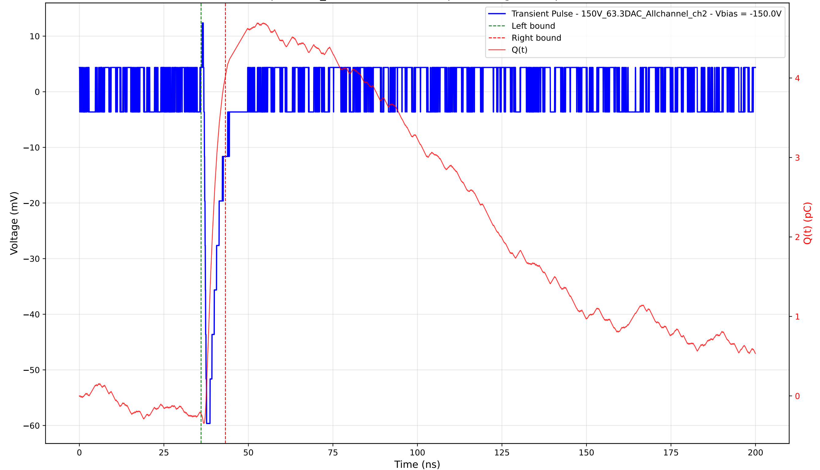
Transient Pulse - Sample: 1cm_42 - Position: 4090.0 \mu\text{m} - Charge: 4.25 pC - Rise Time: 0.67 ns
