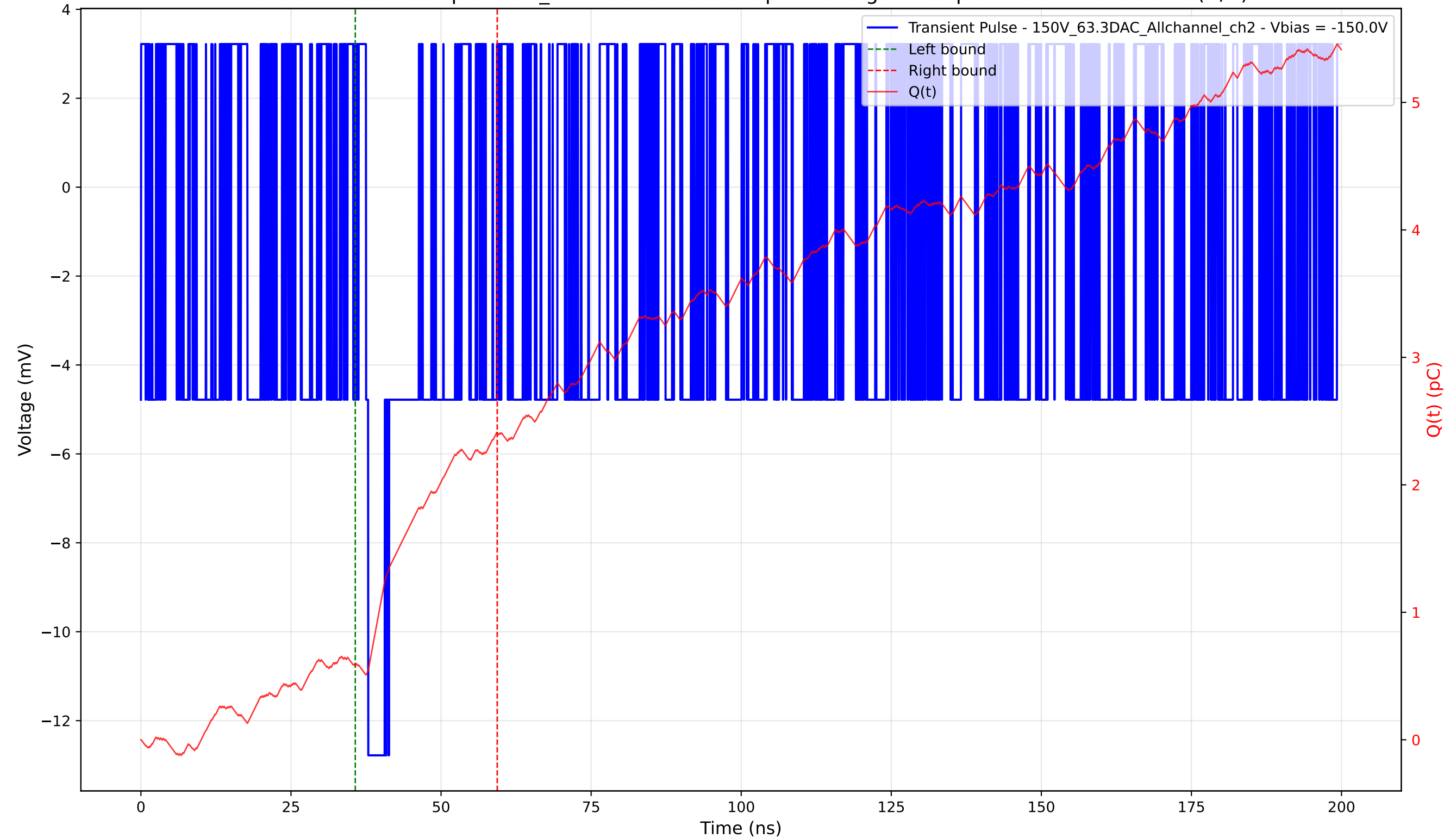
Transient Pulse - Sample: 1cm_42 - Position: 5050.0 \mu\text{m} - Charge: 1.83 pC - Rise Time: 0.00 ns (N/A)
