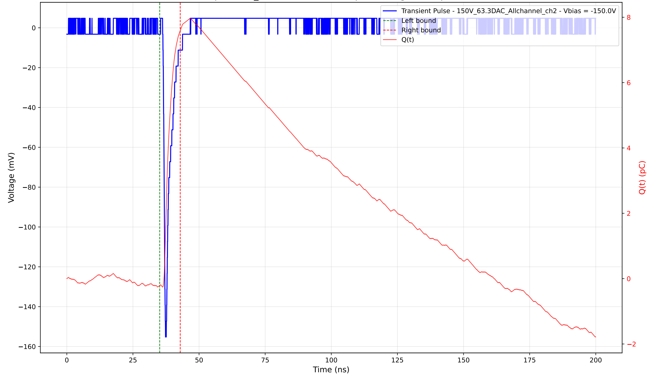
Transient Pulse - Sample: 1cm_42 - Position: 3645.0 \mu\text{m} - Charge: 7.80 pC - Rise Time: 0.82 ns
