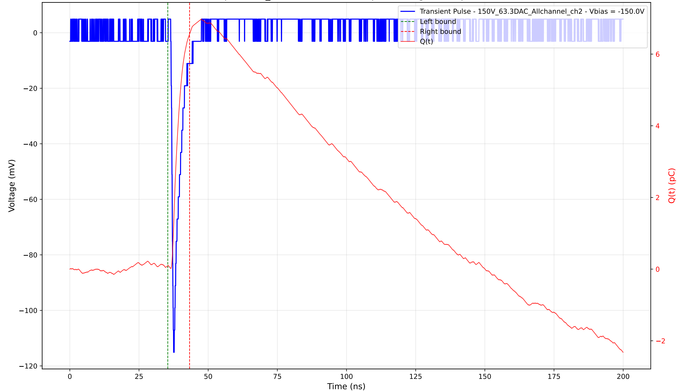
Transient Pulse - Sample: 1cm_42 - Position: 3860.0 \mu\text{m} - Charge: 6.46 pC - Rise Time: 0.80 ns
