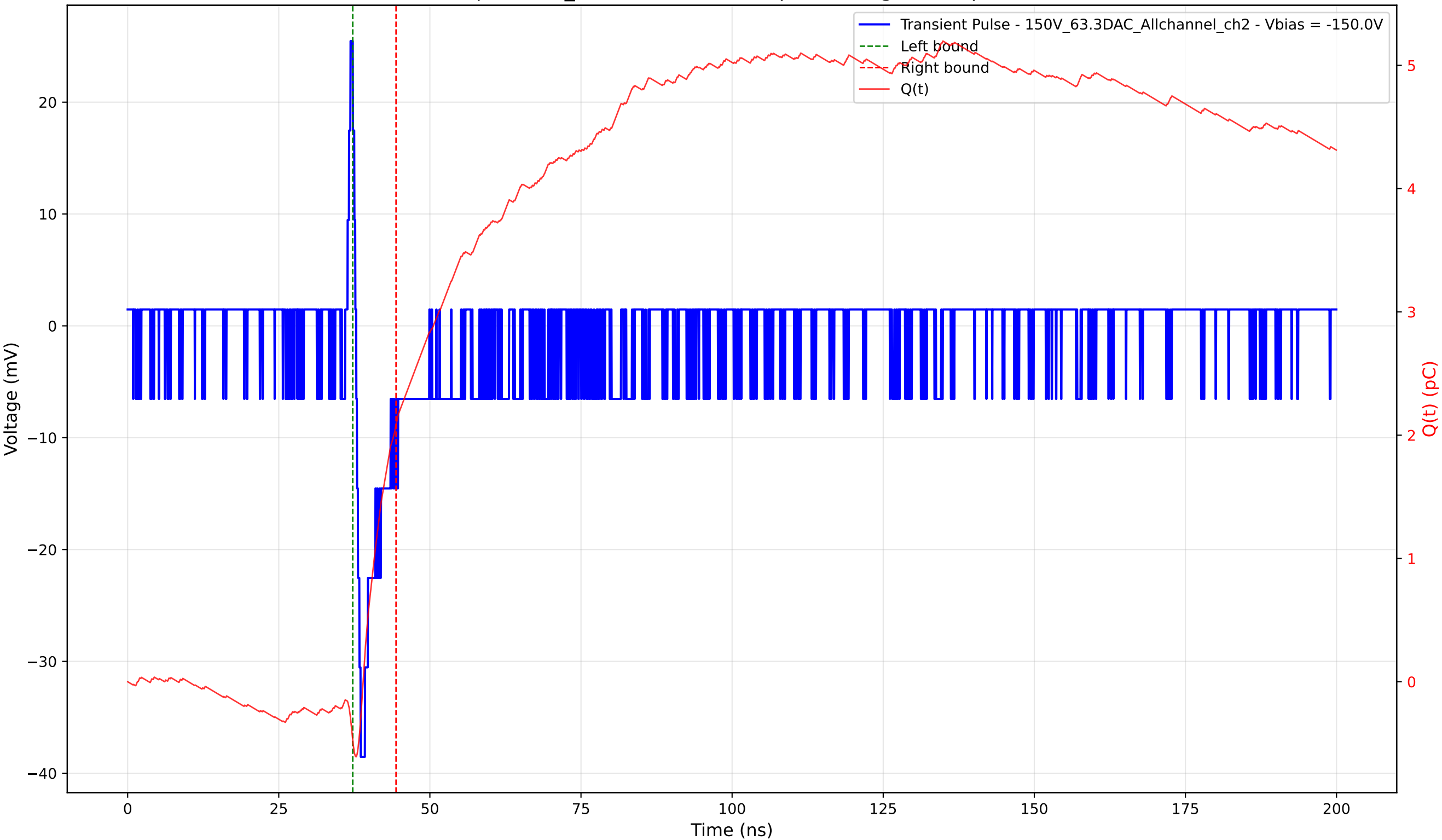
Transient Pulse - Sample: 1cm_42 - Position: 550.0 \mu\text{m} - Charge: 2.57 pC - Rise Time: 0.74 ns
