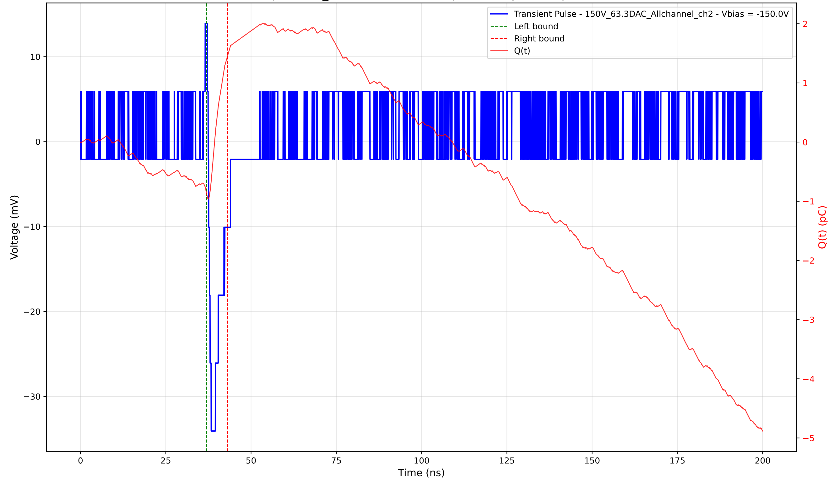
Transient Pulse - Sample: 1cm_42 - Position: 4790.0 \mu\text{m} - Charge: 2.33 pC - Rise Time: 0.75 ns
