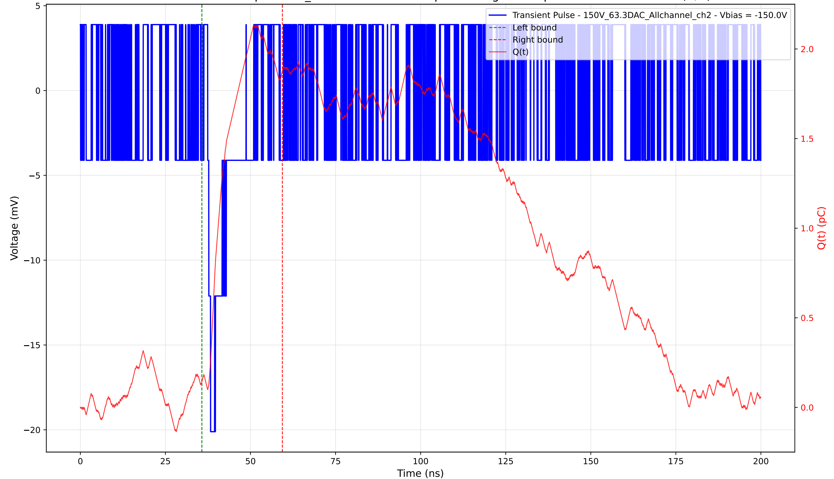
Transient Pulse - Sample: 1cm_42 - Position: 5005.0 \mu\text{m} - Charge: 1.73 pC - Rise Time: 0.00 ns (N/A)
