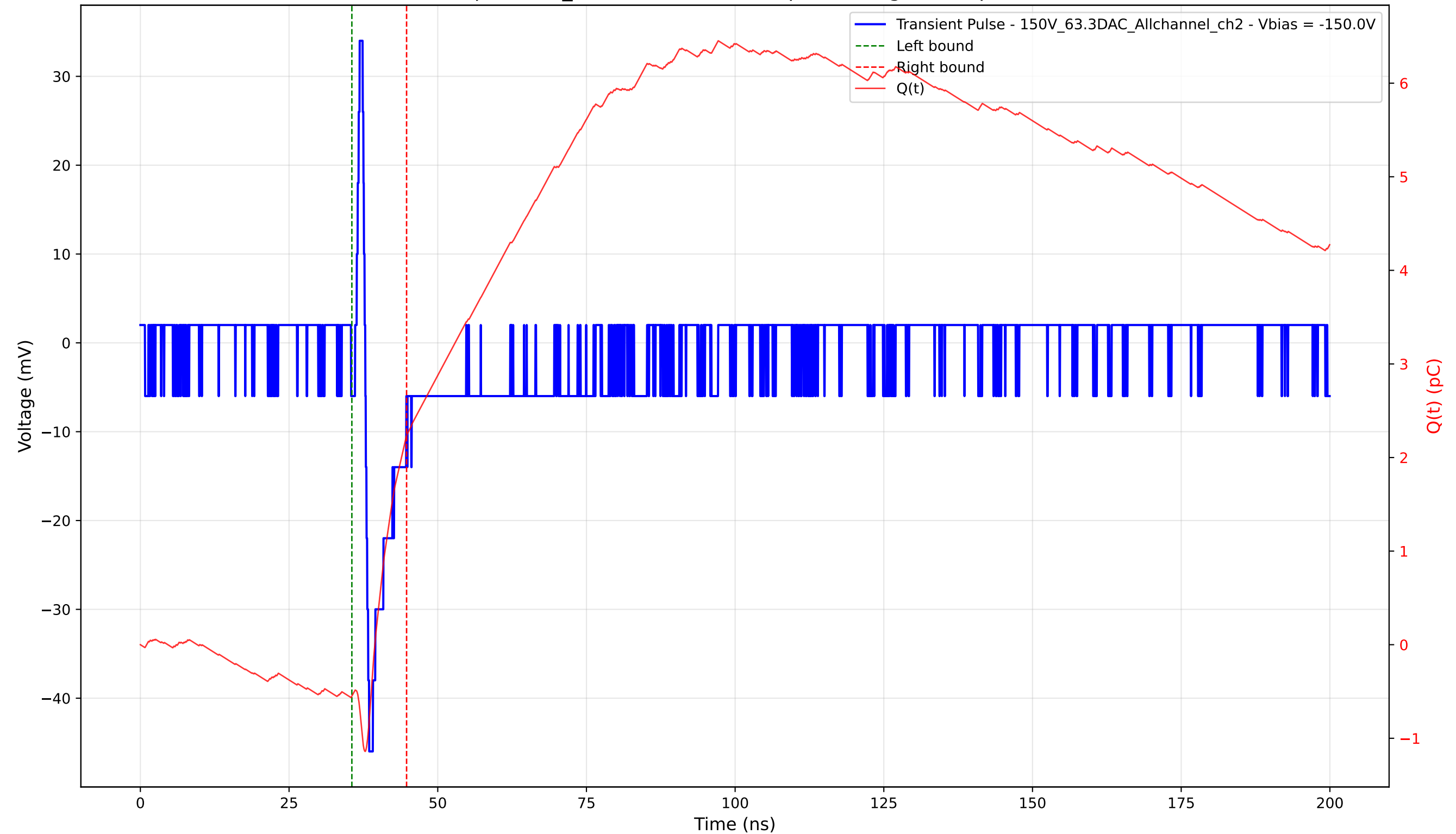
Transient Pulse - Sample: 1cm_42 - Position: 1170.0 \mu\text{m} - Charge: 2.78 pC - Rise Time: 0.65 ns
