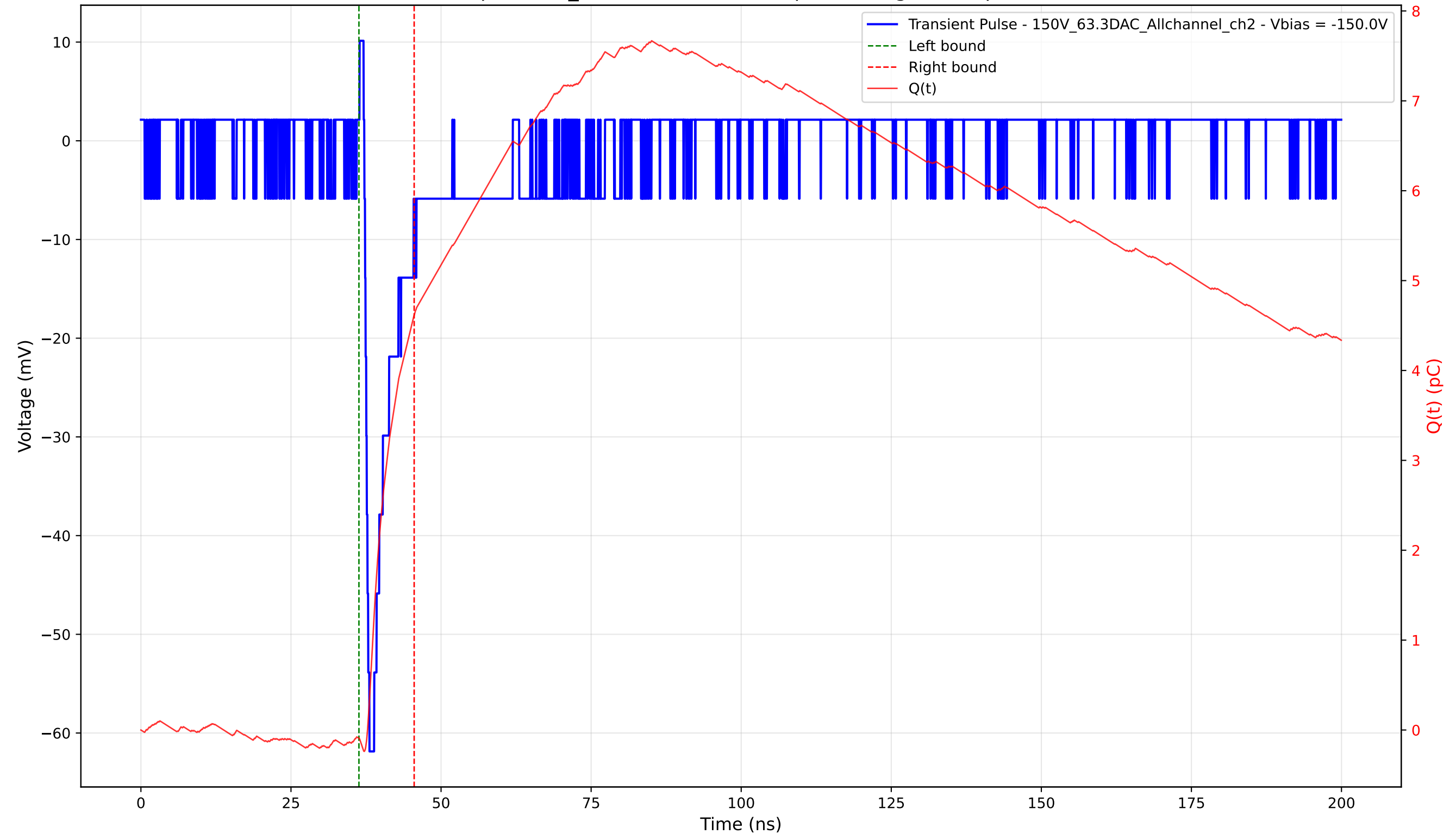
Transient Pulse - Sample: 1cm_42 - Position: 1790.0 \mu\text{m} - Charge: 4.70 pC - Rise Time: 0.76 ns
