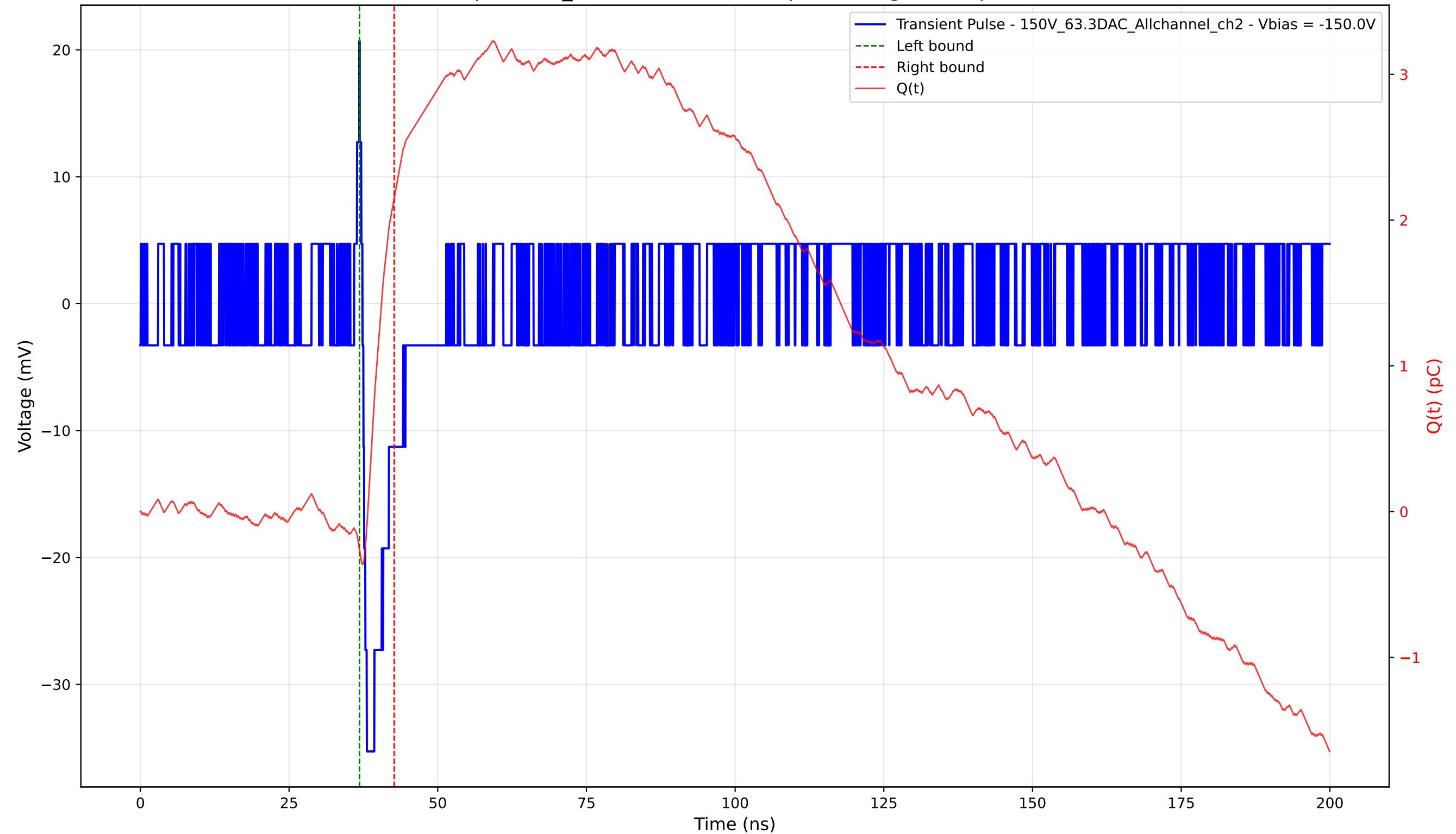
Transient Pulse - Sample: 1cm_42 - Position: 4540.0 \mu\text{m} - Charge: 2.42 pC - Rise Time: 0.60 ns
