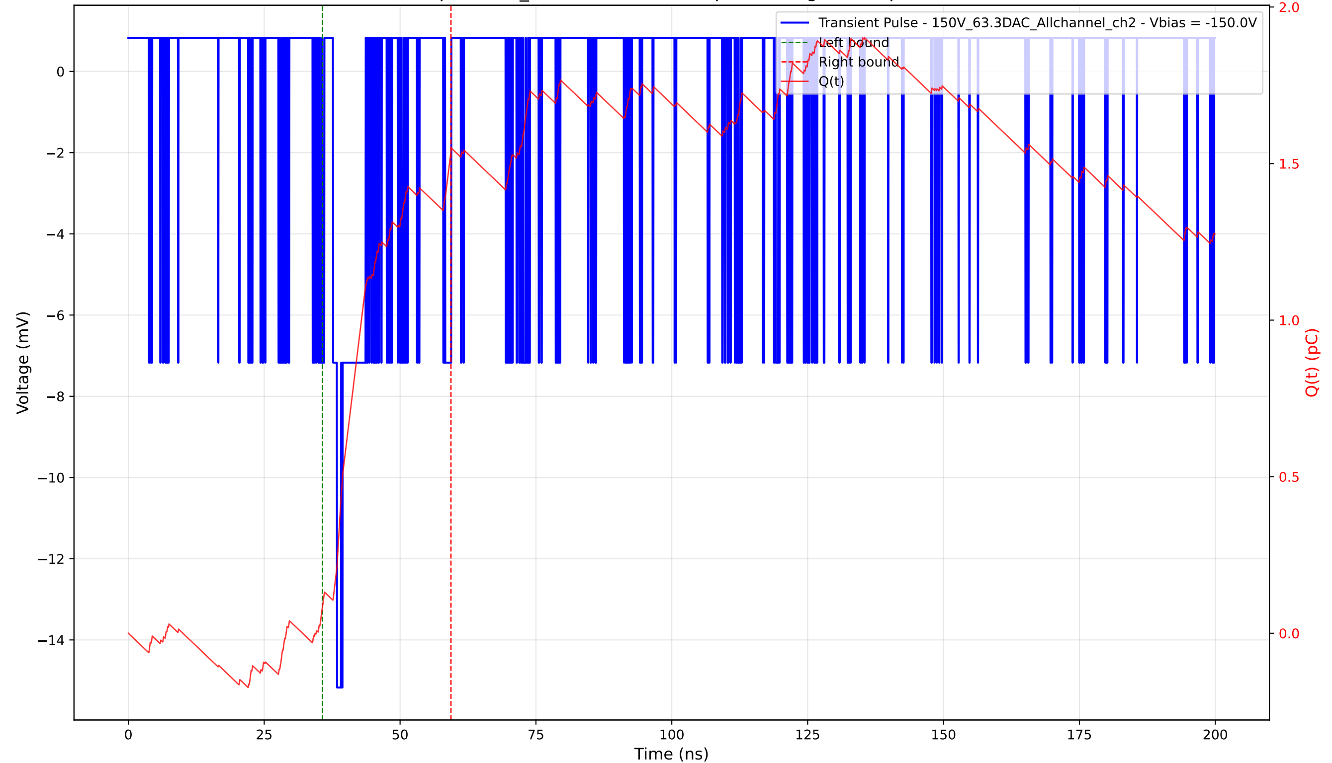
Transient Pulse - Sample: 1cm_42 - Position: 125.0 \mu\text{m} - Charge: 1.45 pC - Rise Time: 0.76 ns
