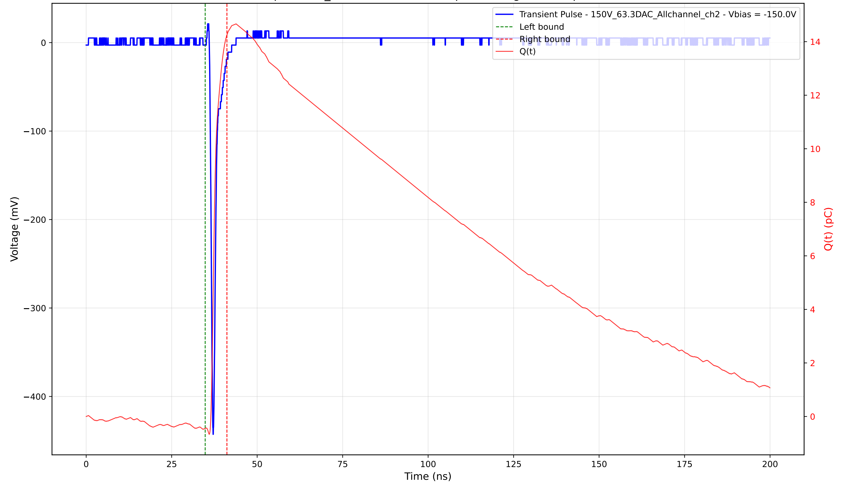
Transient Pulse - Sample: 1cm_42 - Position: 3265.0 \mu\text{m} - Charge: 14.70 pC - Rise Time: 0.73 ns
