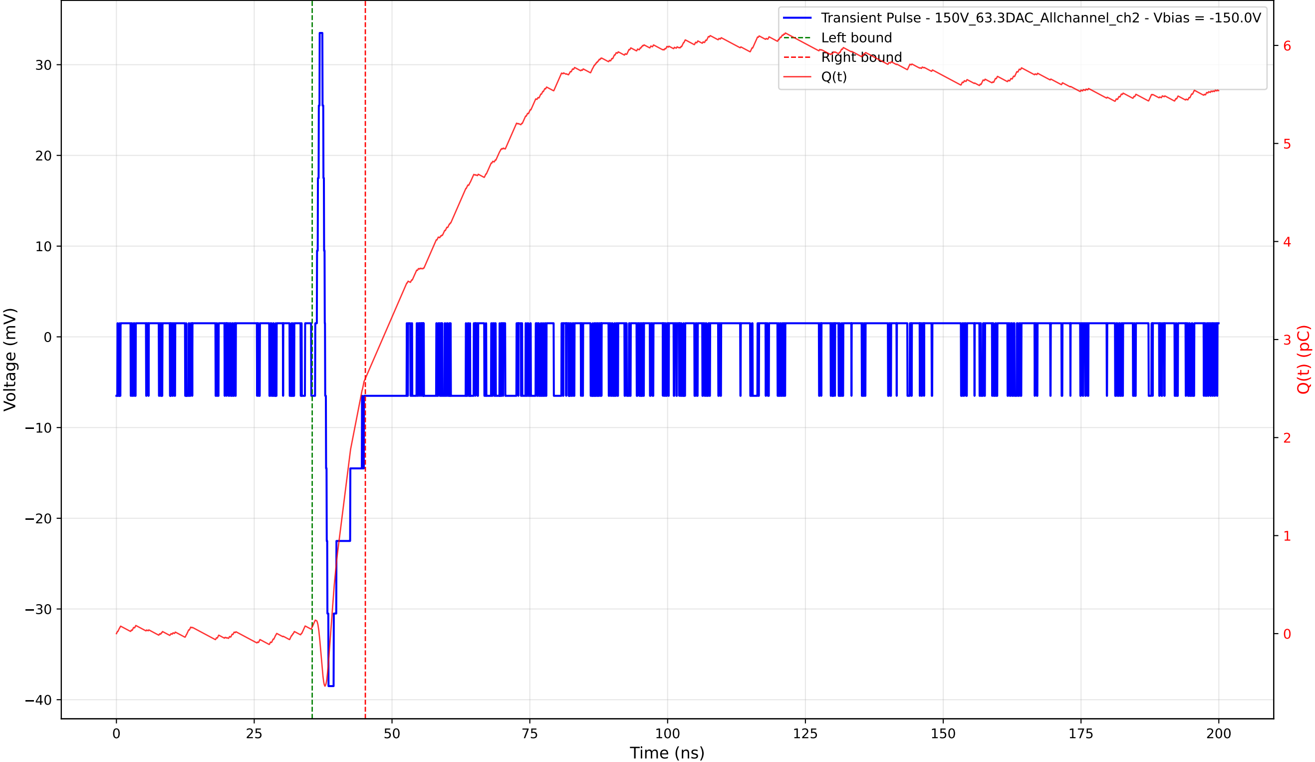
Transient Pulse - Sample: 1cm_42 - Position: 845.0 \mu\text{m} - Charge: 2.53 pC - Rise Time: 0.62 ns
