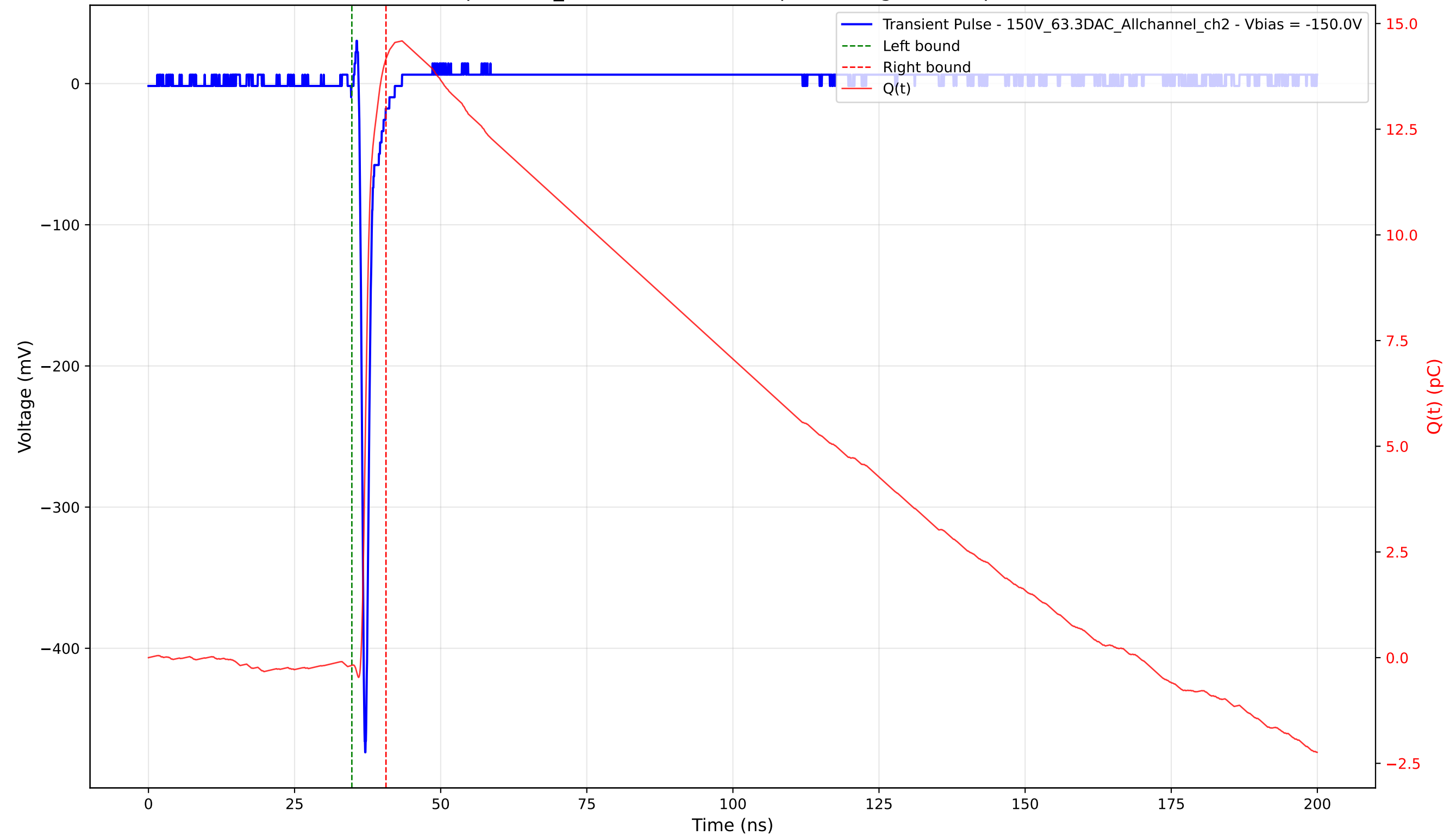
Transient Pulse - Sample: 1cm_42 - Position: 2915.0 \mu\text{m} - Charge: 14.35 pC - Rise Time: 0.71 ns
