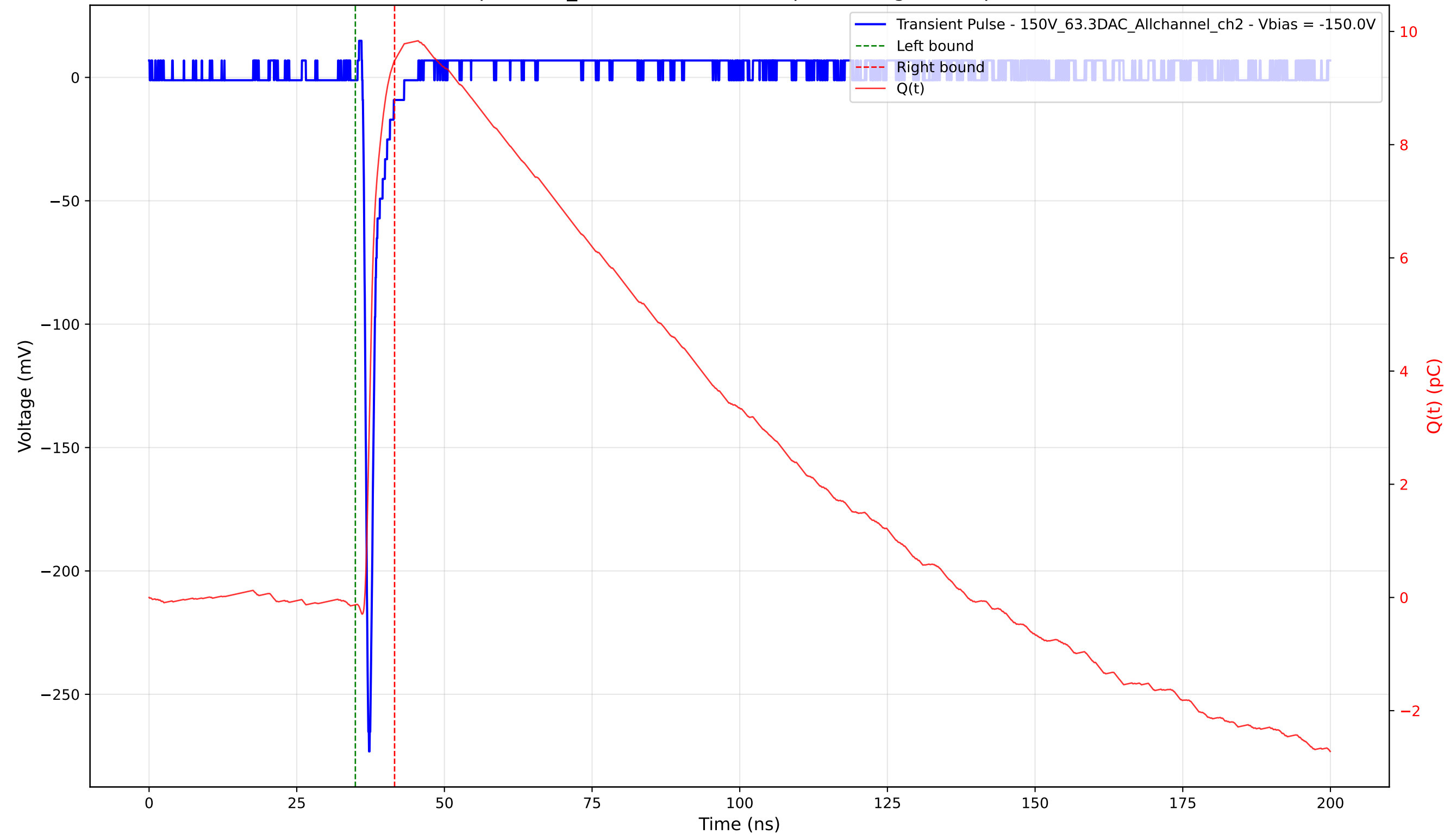
Transient Pulse - Sample: 1cm_42 - Position: 2595.0 \mu\text{m} - Charge: 9.61 pC - Rise Time: 0.73 ns
