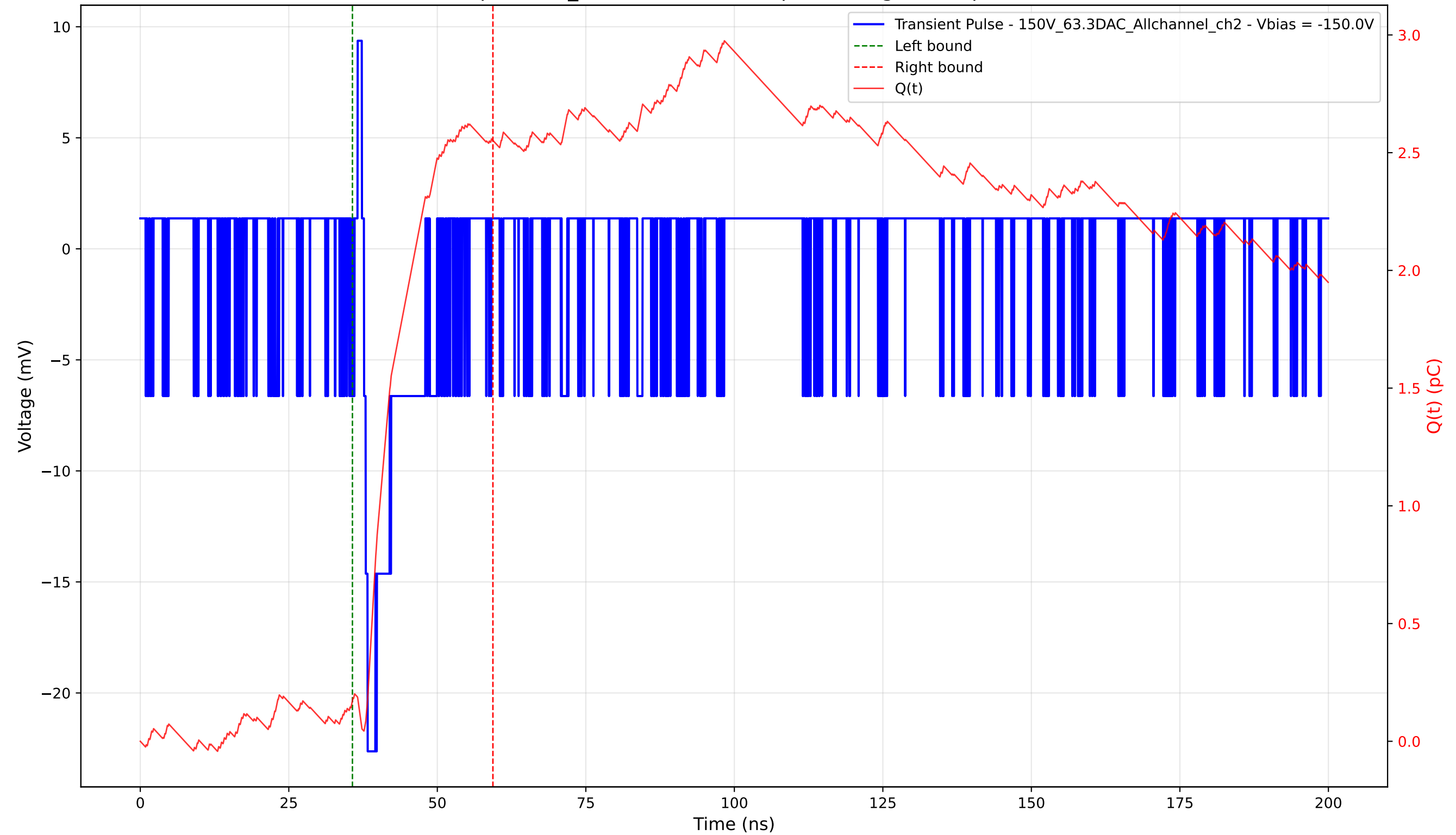
Transient Pulse - Sample: 1cm_42 - Position: 270.0 \mu\text{m} - Charge: 2.38 pC - Rise Time: 0.63 ns
