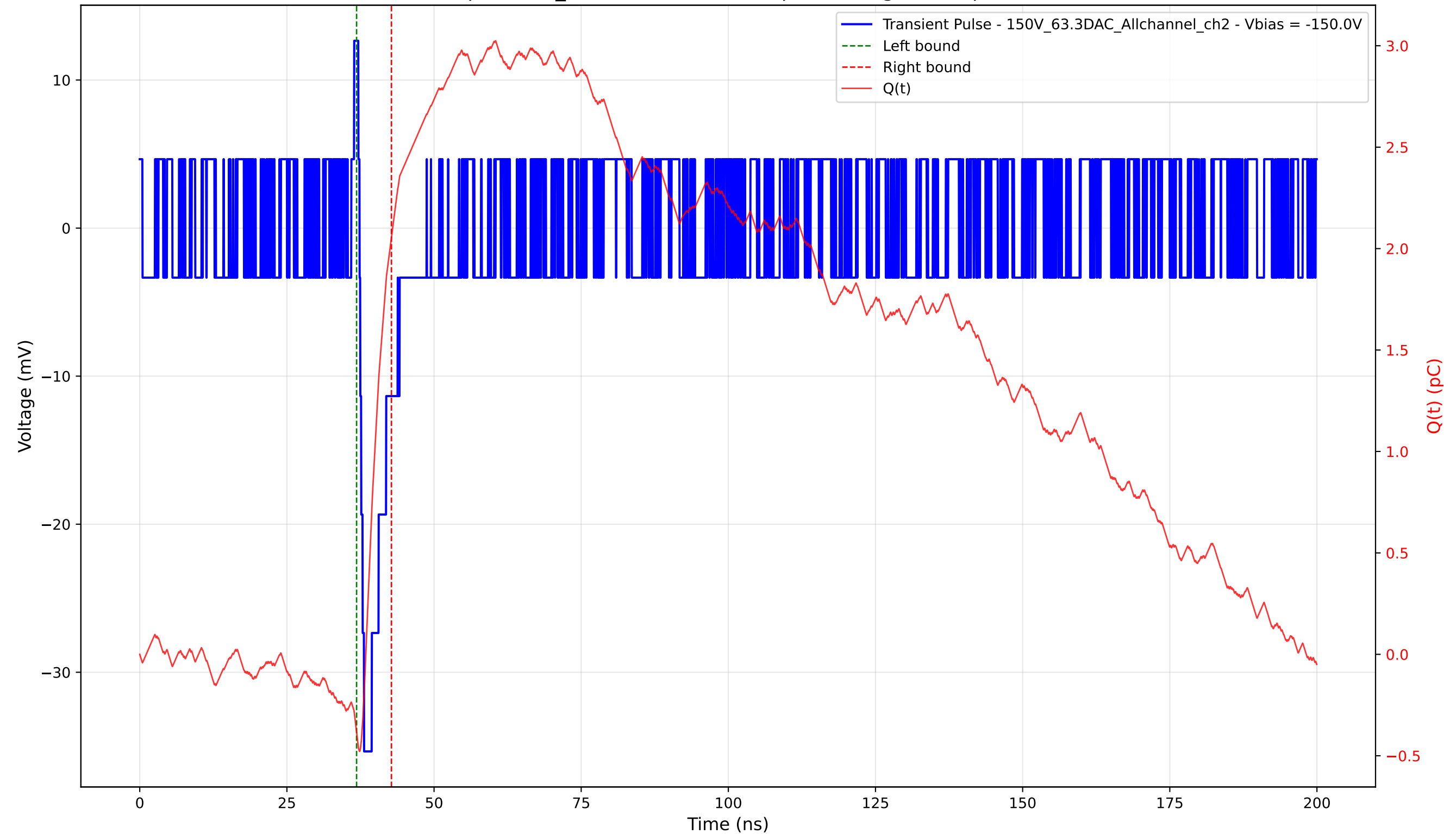
Transient Pulse - Sample: 1cm_42 - Position: 4525.0 \mu\text{m} - Charge: 2.44 pC - Rise Time: 0.68 ns
