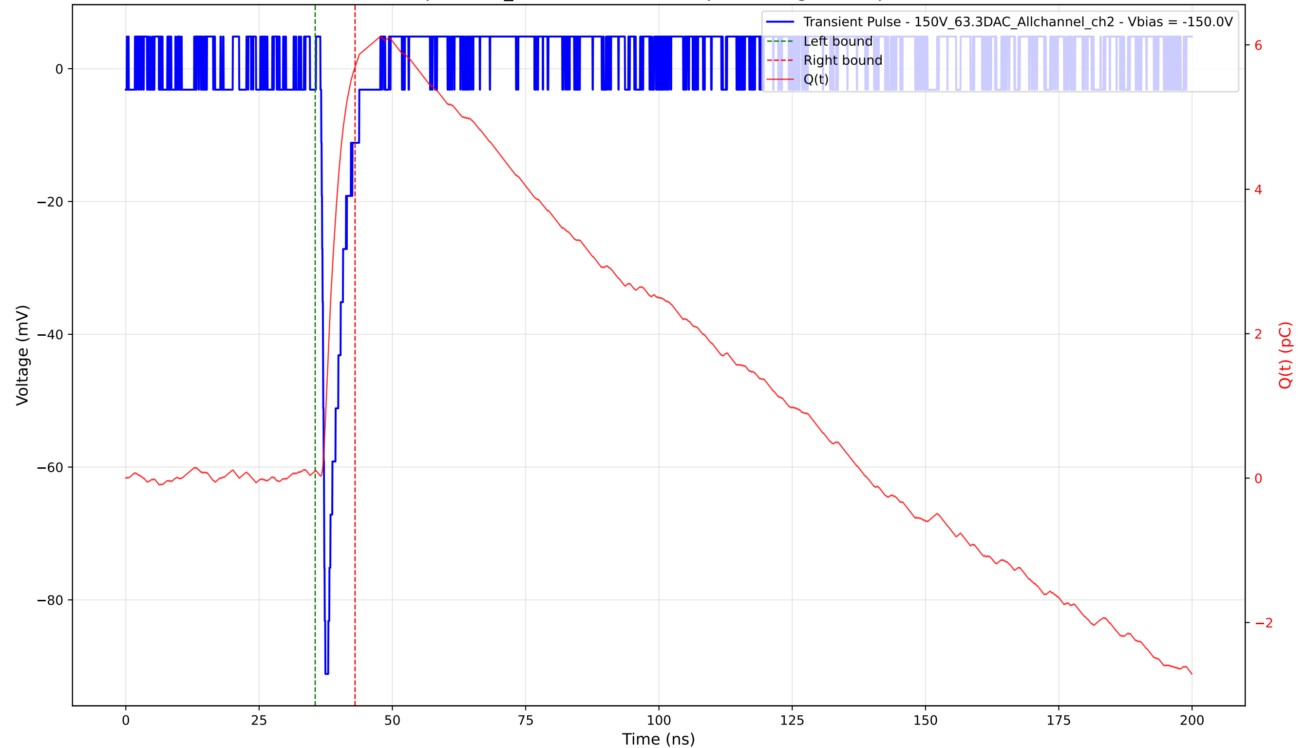
Transient Pulse - Sample: 1cm_42 - Position: 3920.0 \mu\text{m} - Charge: 5.60 pC - Rise Time: 0.65 ns
