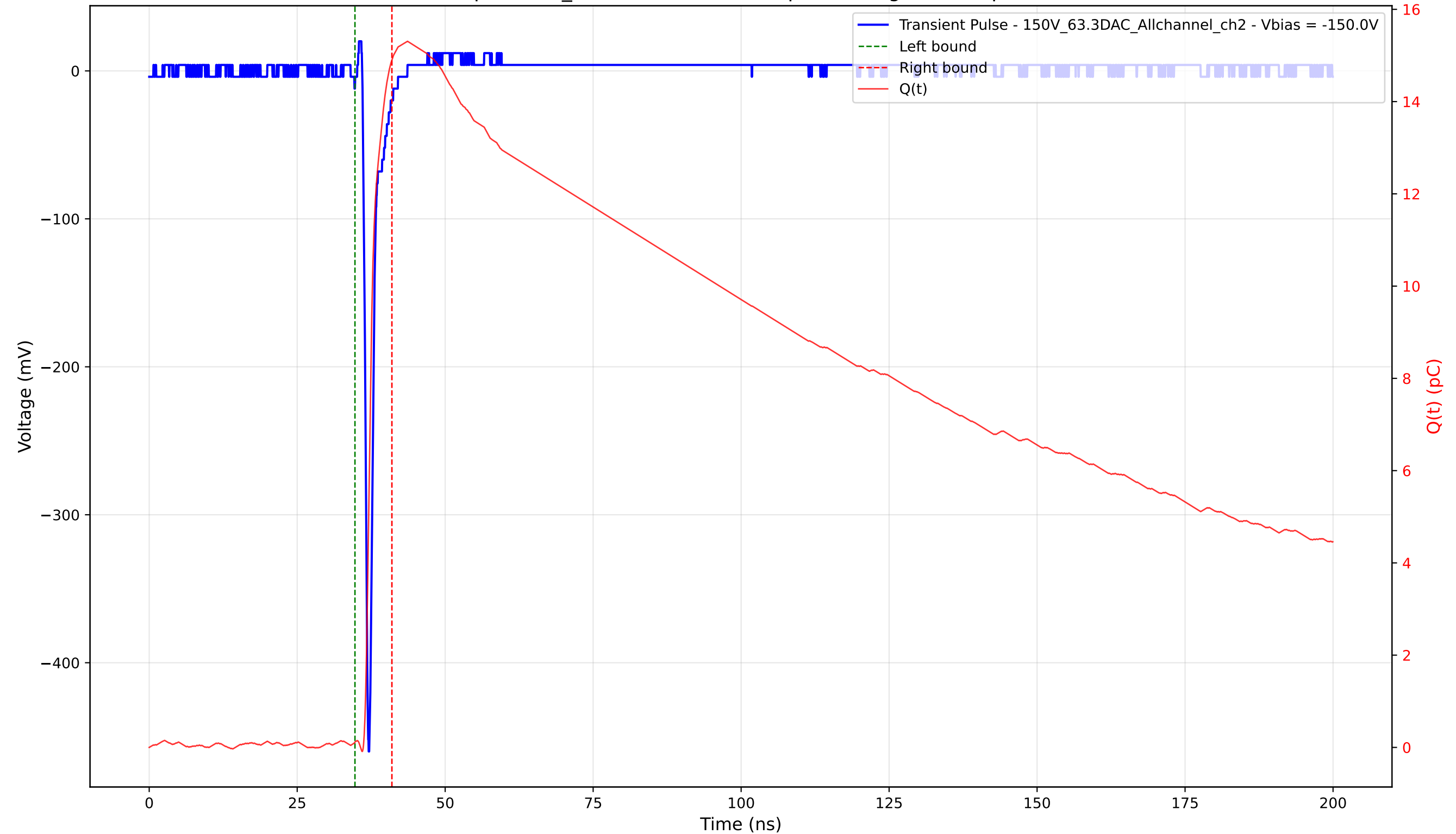
Transient Pulse - Sample: 1cm_42 - Position: 3180.0 \mu\text{m} - Charge: 14.79 pC - Rise Time: 0.70 ns
