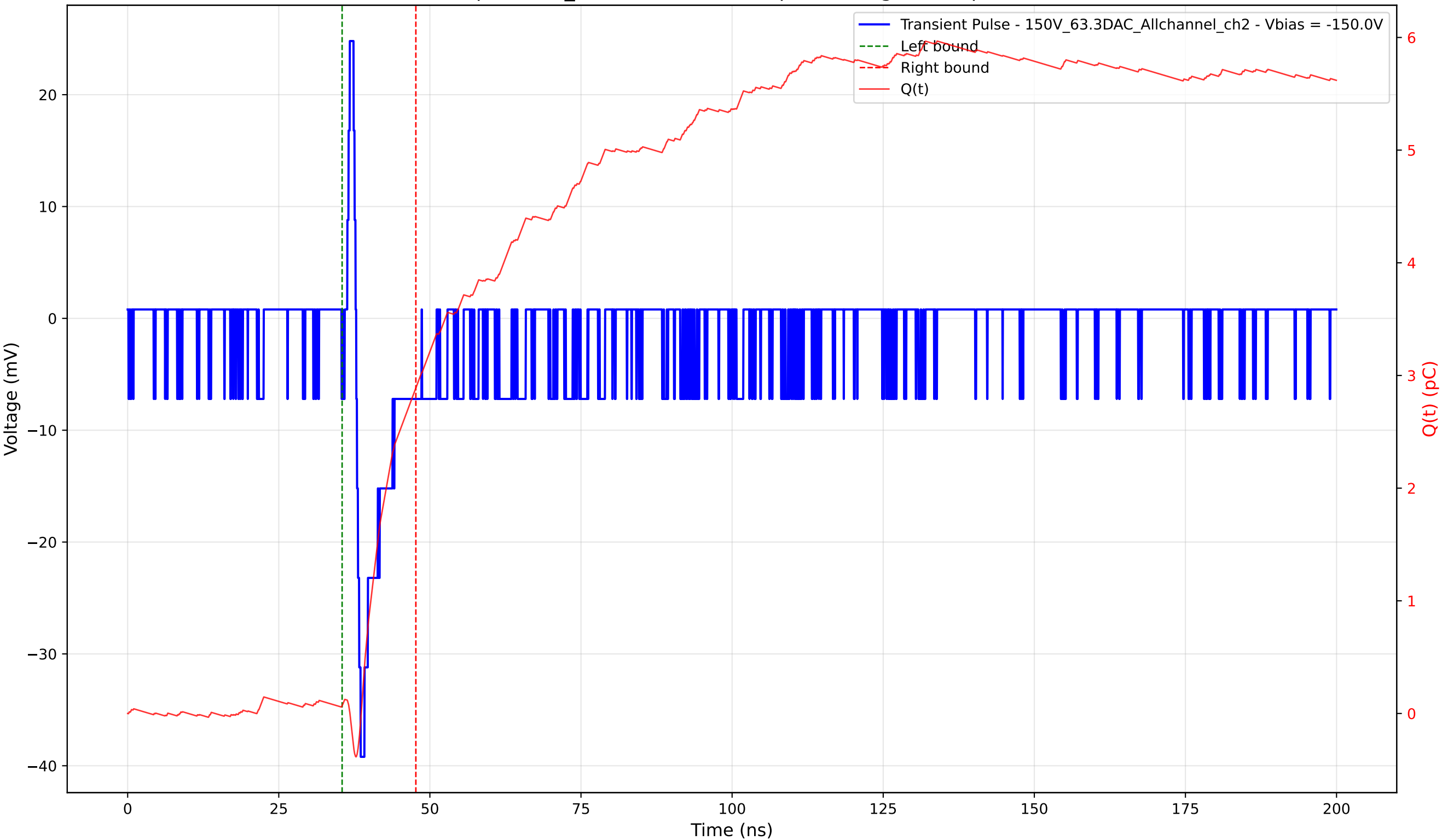
Transient Pulse - Sample: 1cm_42 - Position: 570.0 \mu\text{m} - Charge: 2.82 pC - Rise Time: 0.74 ns
