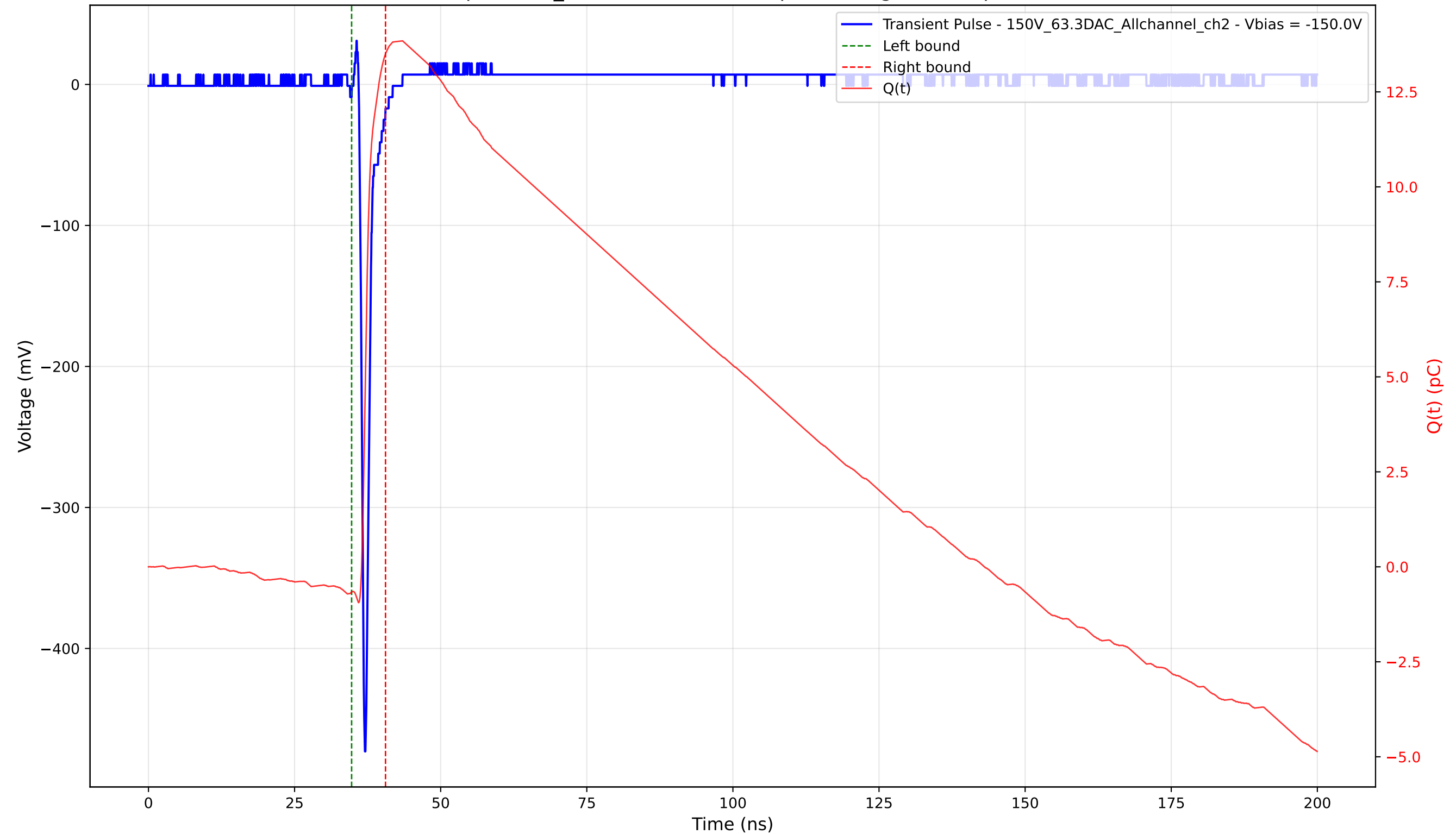
Transient Pulse - Sample: 1cm_42 - Position: 2980.0 \mu\text{m} - Charge: 14.16 pC - Rise Time: 0.67 ns
