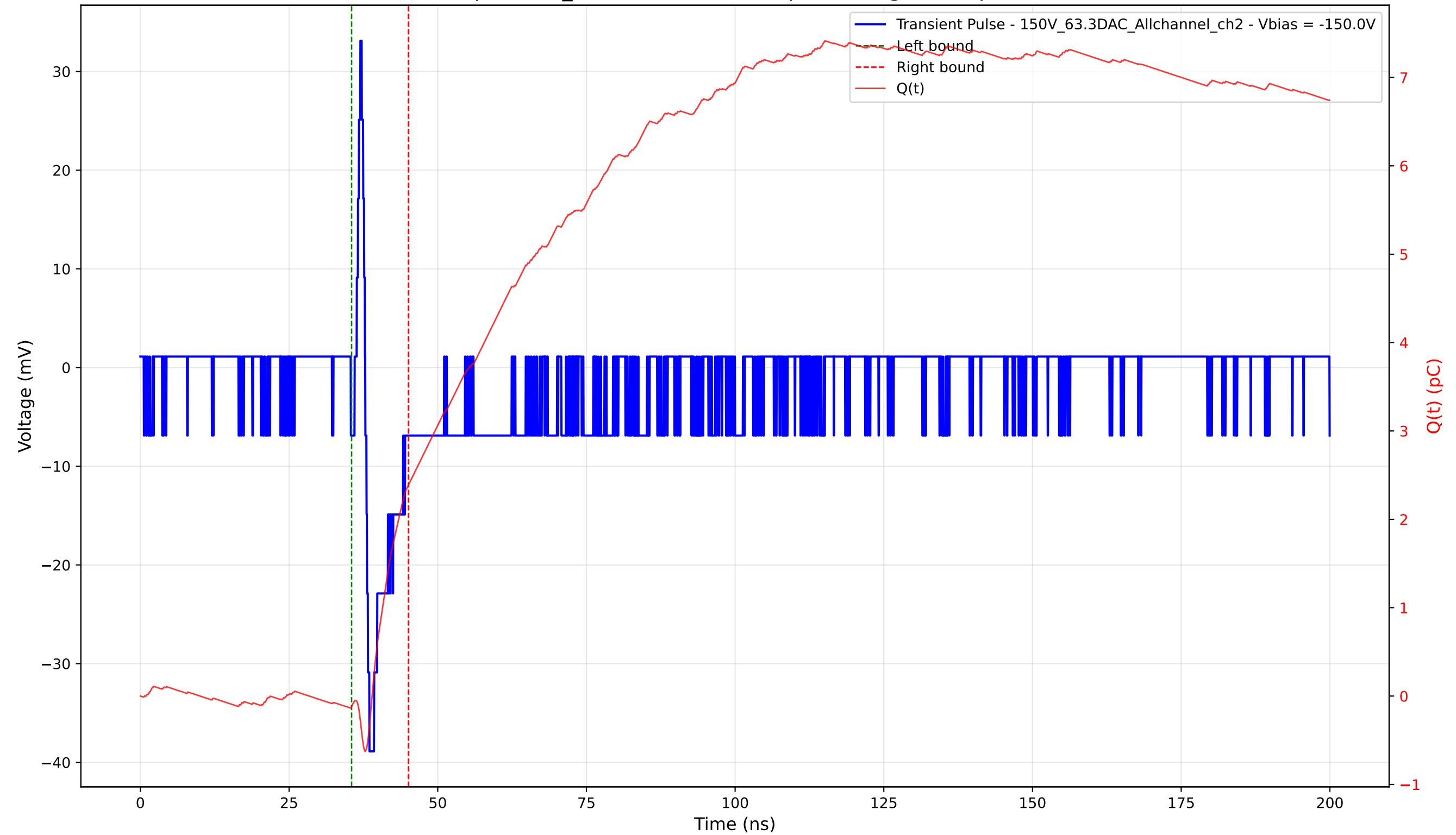
Transient Pulse - Sample: 1cm_42 - Position: 1005.0 \mu\text{m} - Charge: 2.51 pC - Rise Time: 0.70 ns
