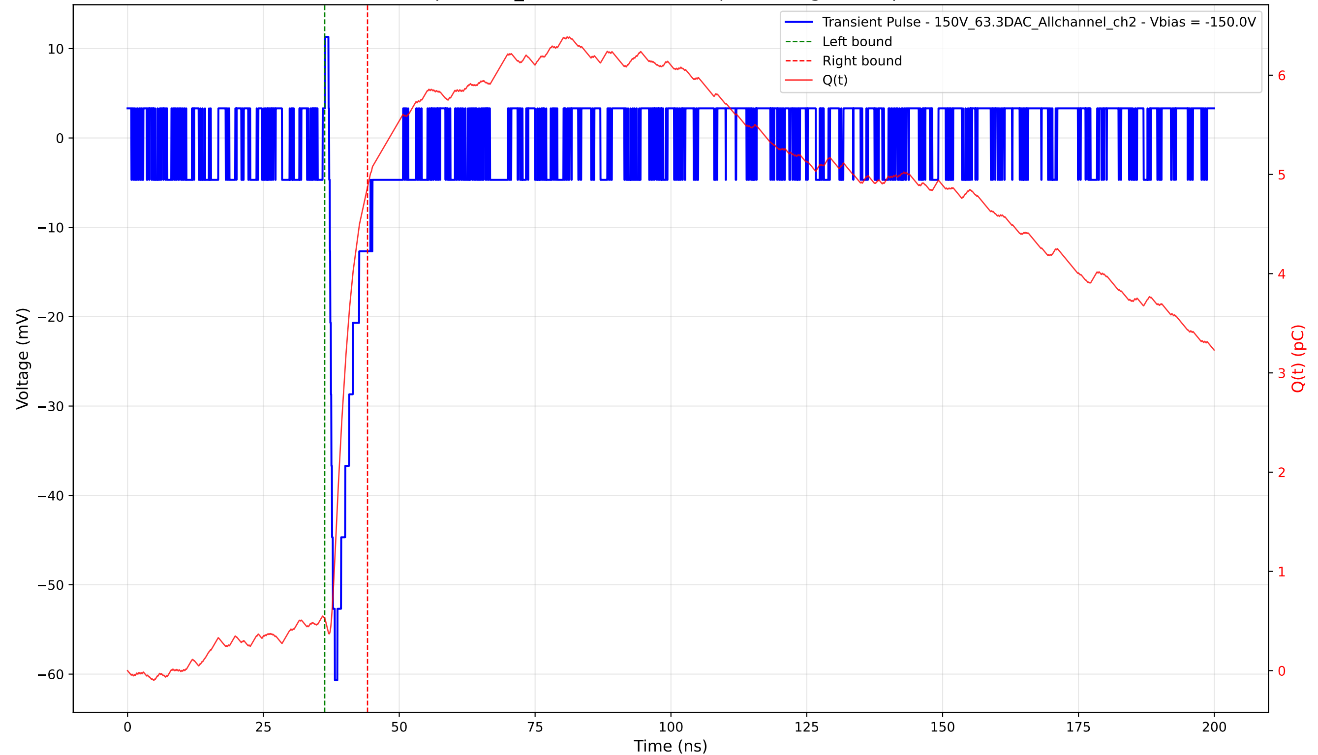
Transient Pulse - Sample: 1cm_42 - Position: 4260.0 \mu\text{m} - Charge: 4.35 pC - Rise Time: 0.95 ns
