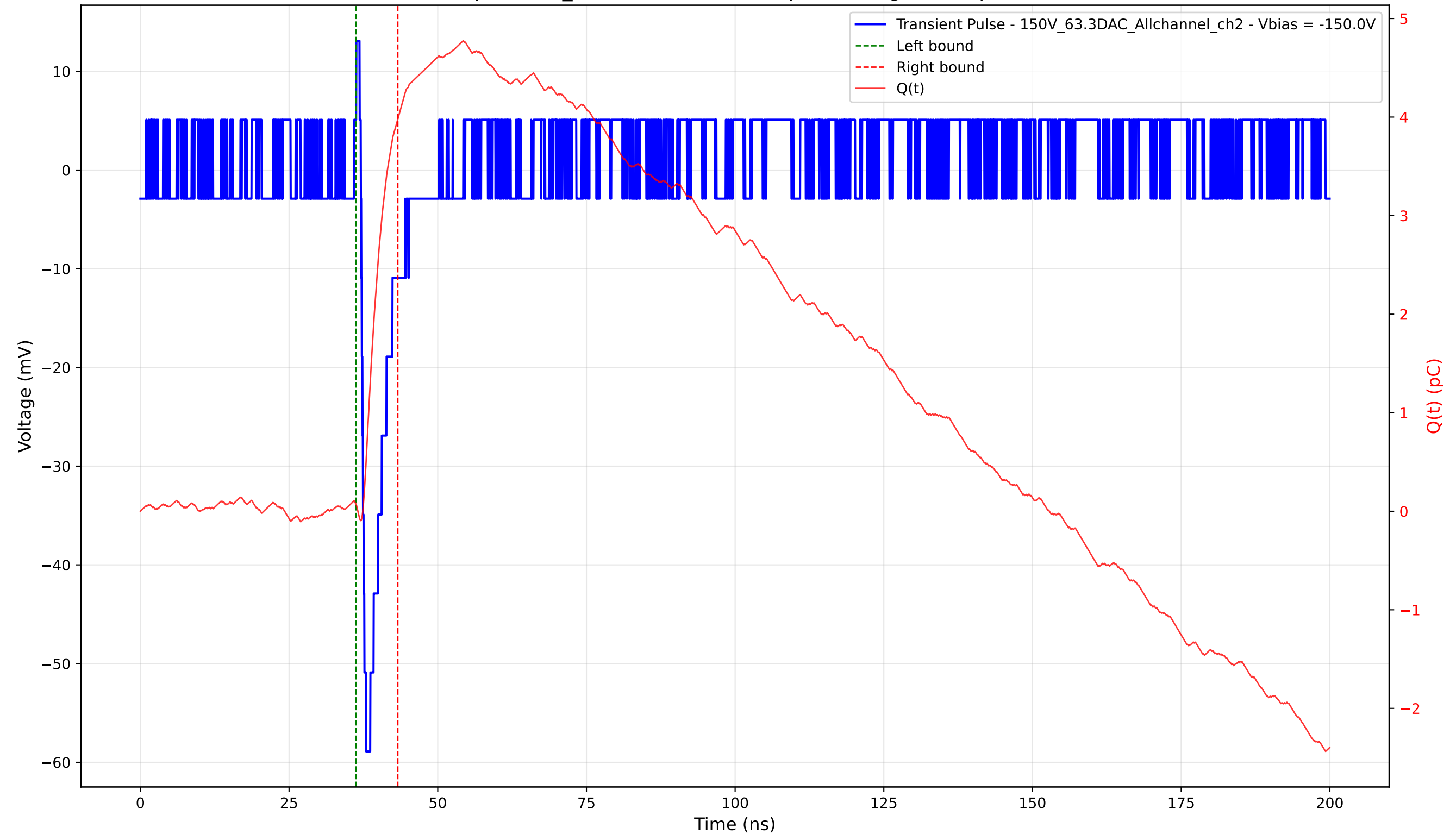
Transient Pulse - Sample: 1cm_42 - Position: 4180.0 \mu\text{m} - Charge: 3.90 pC - Rise Time: 0.83 ns
