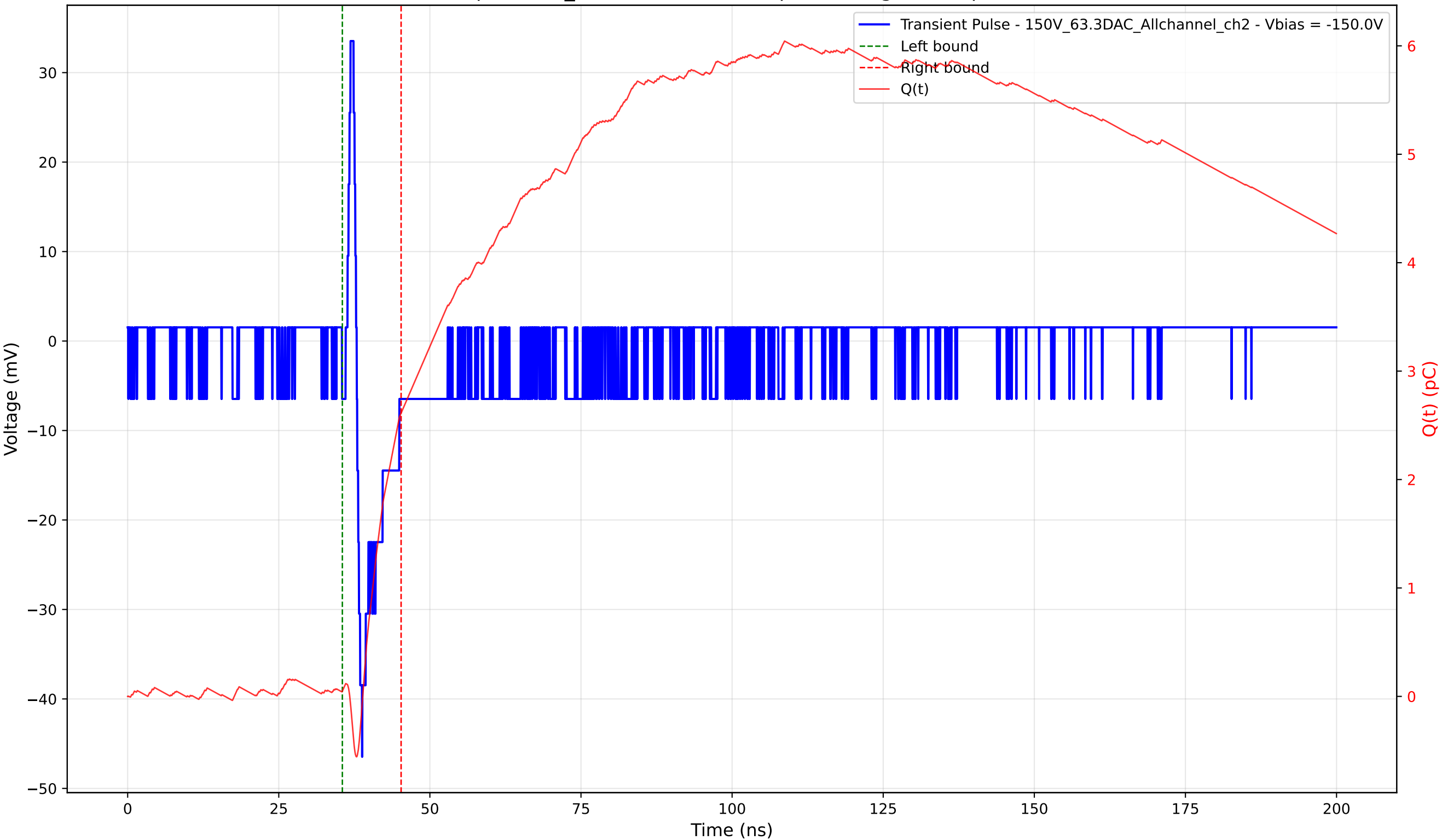
Transient Pulse - Sample: 1cm_42 - Position: 835.0 \mu\text{m} - Charge: 2.56 pC - Rise Time: 0.89 ns
