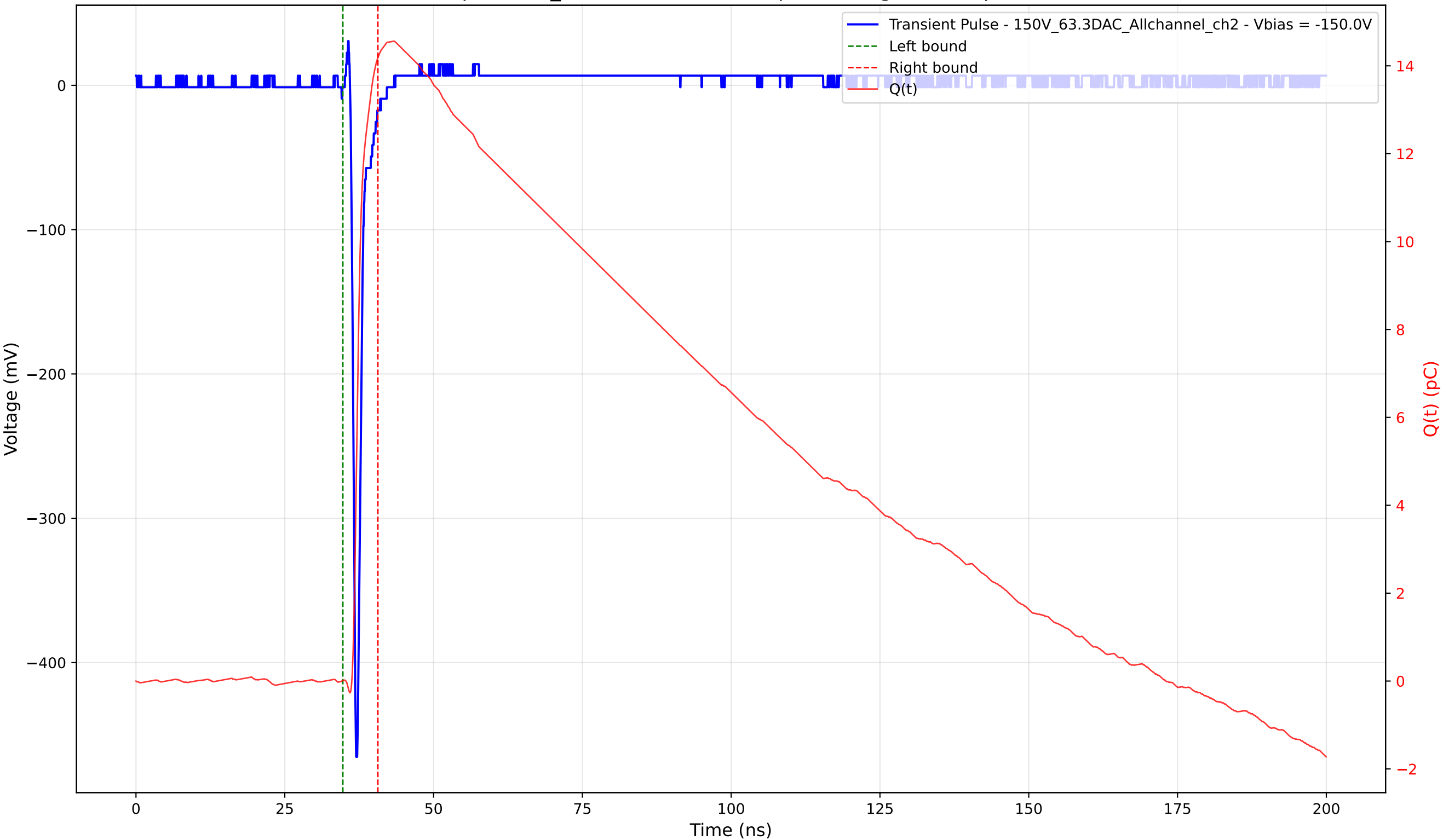
Transient Pulse - Sample: 1cm_42 - Position: 3075.0 \mu\text{m} - Charge: 14.17 pC - Rise Time: 0.67 ns
