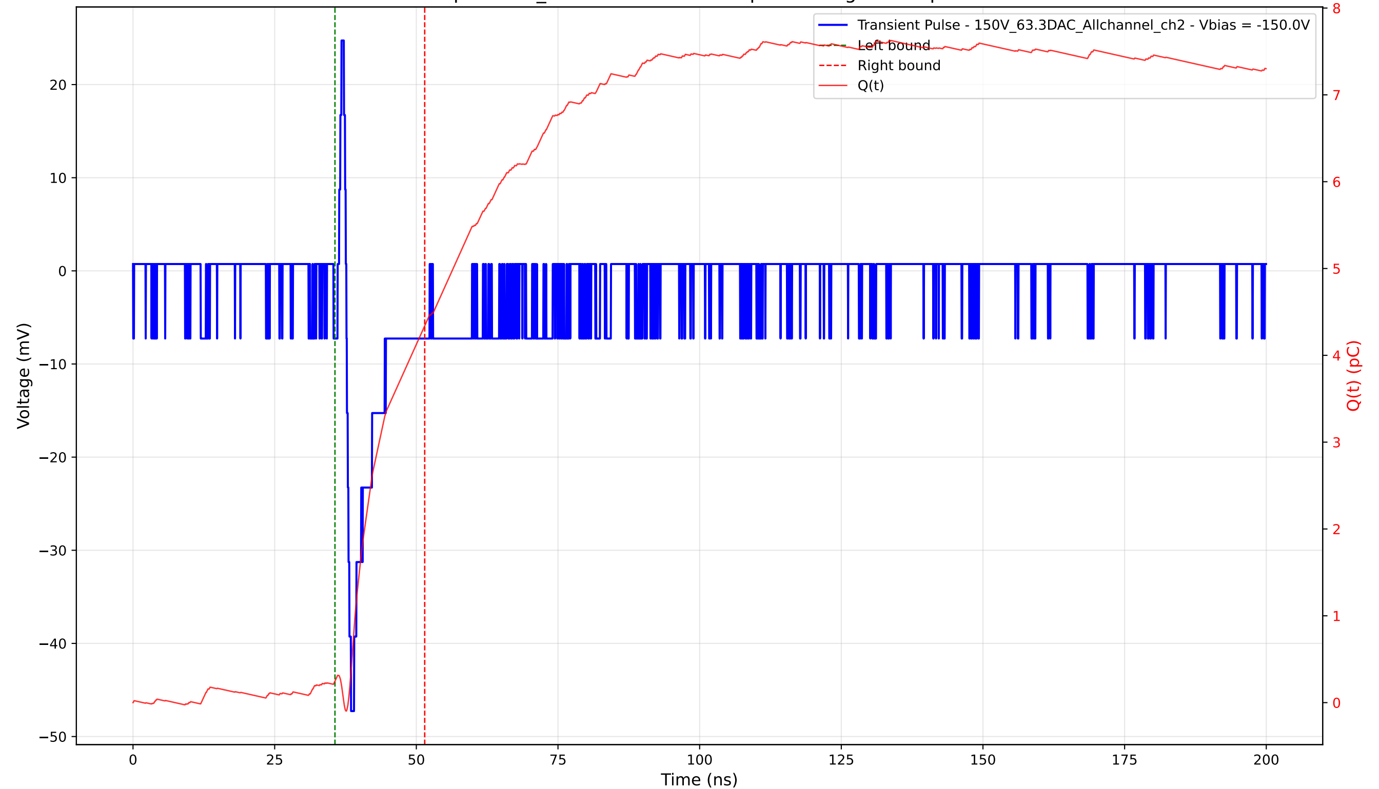
Transient Pulse - Sample: 1cm_42 - Position: 1465.0 \mu\text{m} - Charge: 4.09 pC - Rise Time: 0.82 ns
