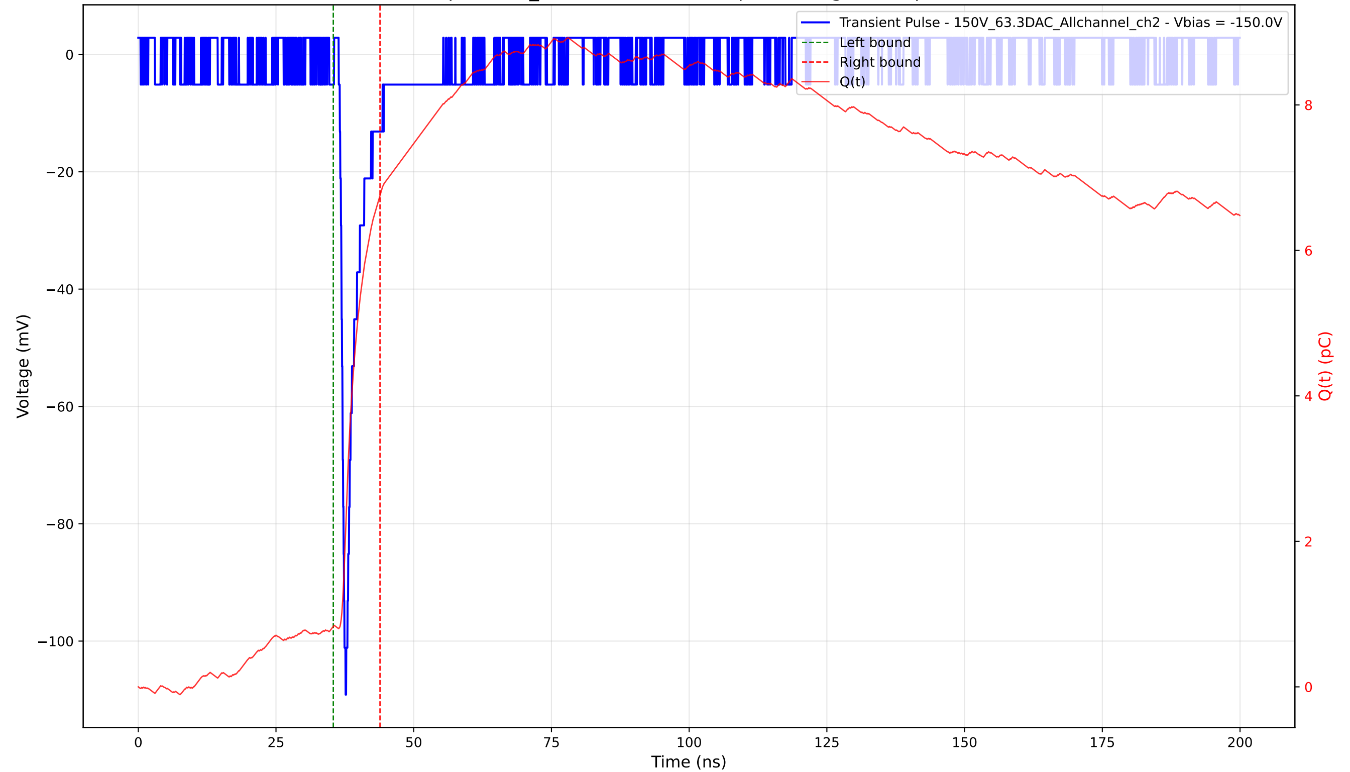
Transient Pulse - Sample: 1cm_42 - Position: 2150.0 \mu\text{m} - Charge: 5.92 pC - Rise Time: 0.85 ns
