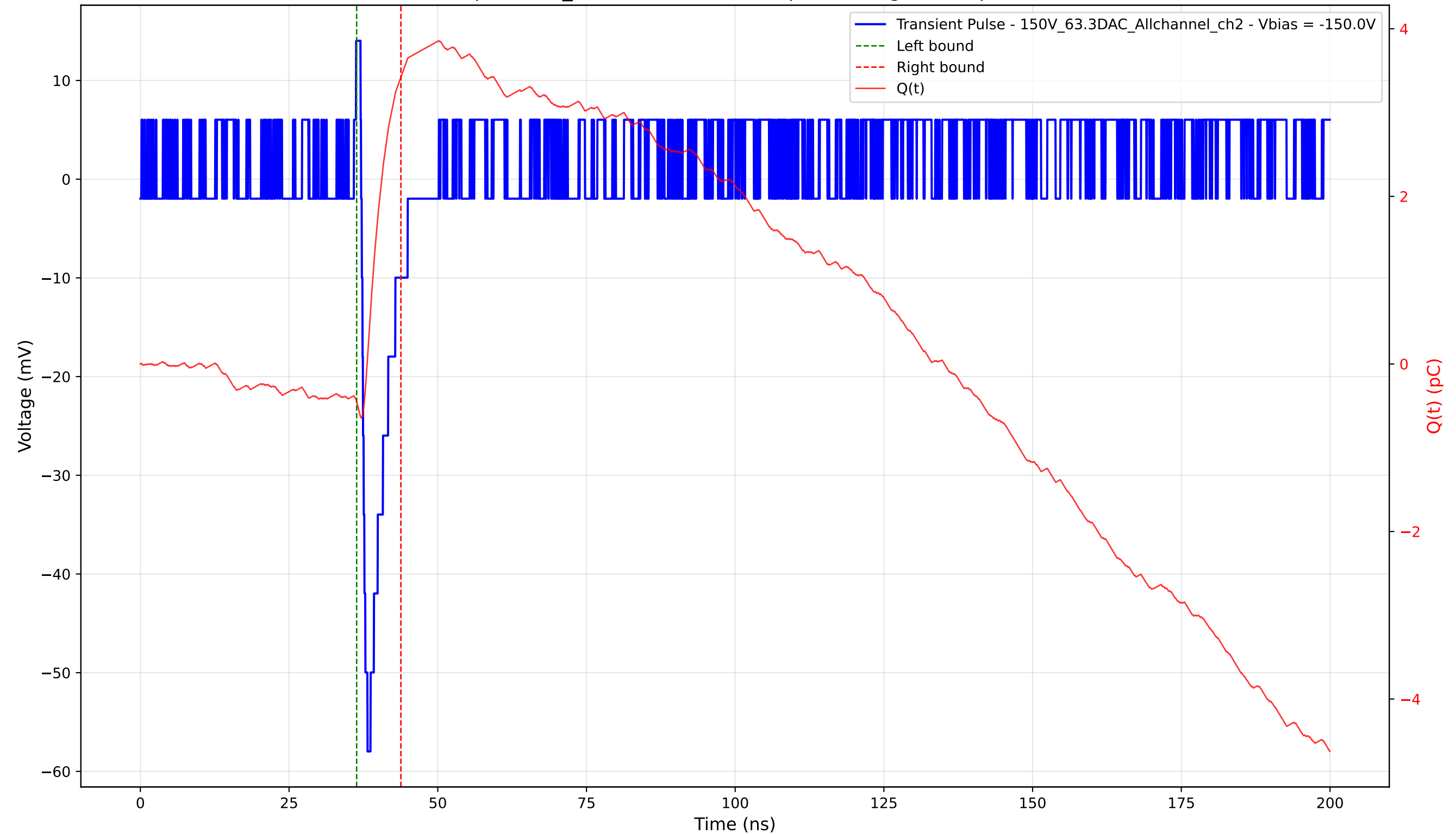
Transient Pulse - Sample: 1cm_42 - Position: 4290.0 \mu\text{m} - Charge: 3.87 pC - Rise Time: 0.98 ns
