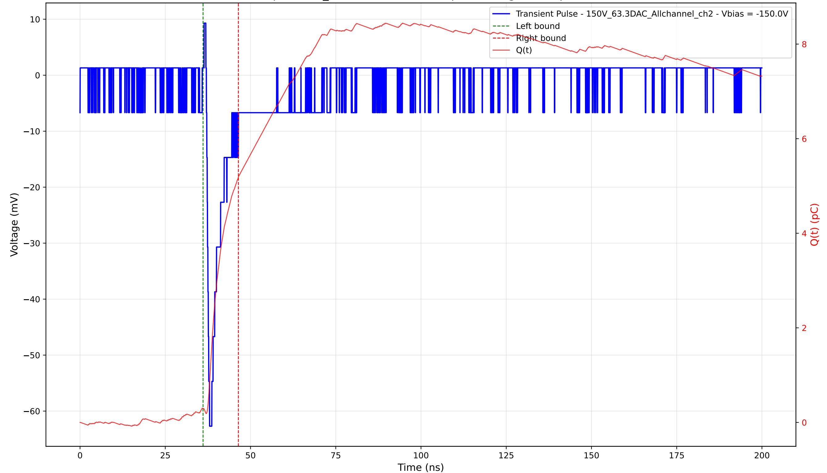
Transient Pulse - Sample: 1cm_42 - Position: 1880.0 \mu\text{m} - Charge: 4.89 pC - Rise Time: 0.92 ns
