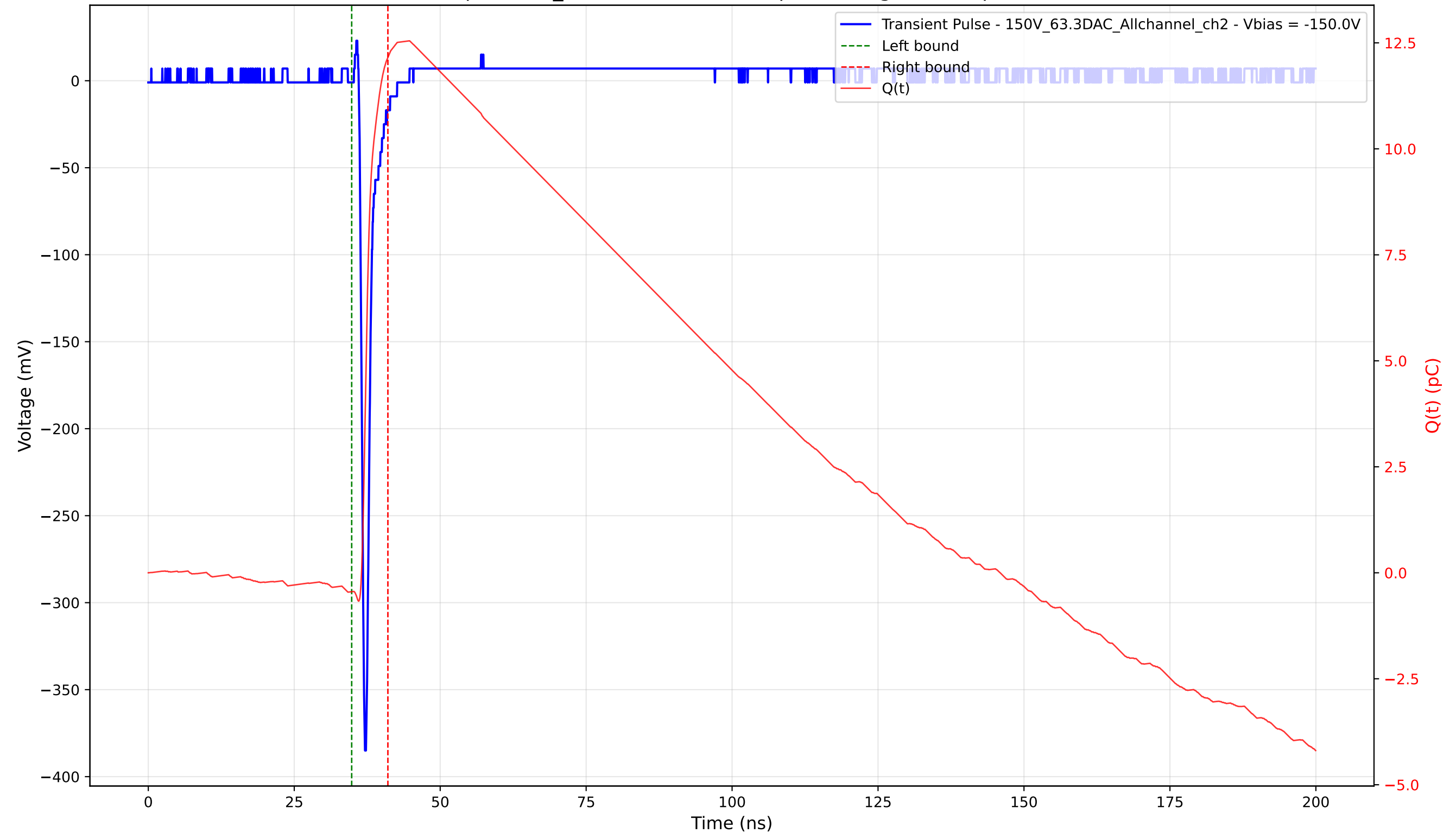
Transient Pulse - Sample: 1cm_42 - Position: 2700.0 \mu\text{m} - Charge: 12.61 pC - Rise Time: 0.71 ns
