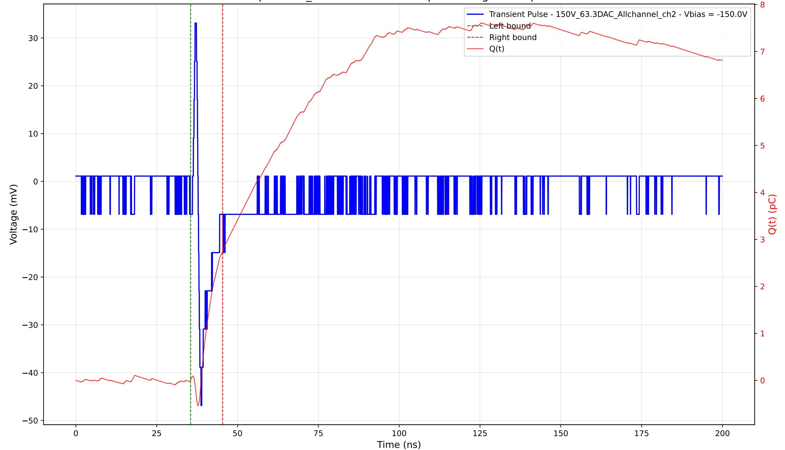
Transient Pulse - Sample: 1cm_42 - Position: 1115.0 \mu\text{m} - Charge: 2.73 pC - Rise Time: 0.90 ns
