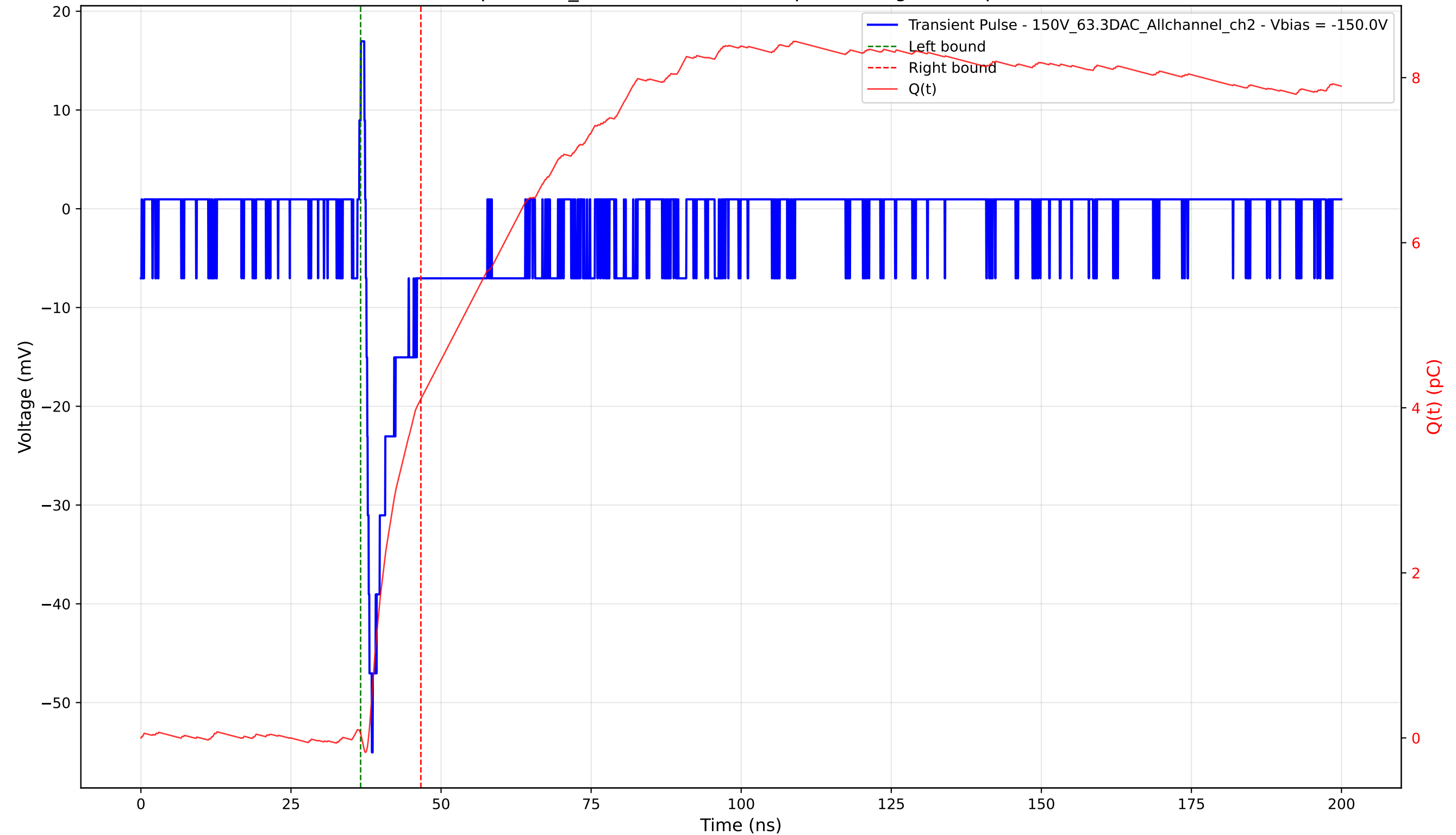
Transient Pulse - Sample: 1cm_42 - Position: 1590.0 \mu\text{m} - Charge: 4.05 pC - Rise Time: 1.01 ns
