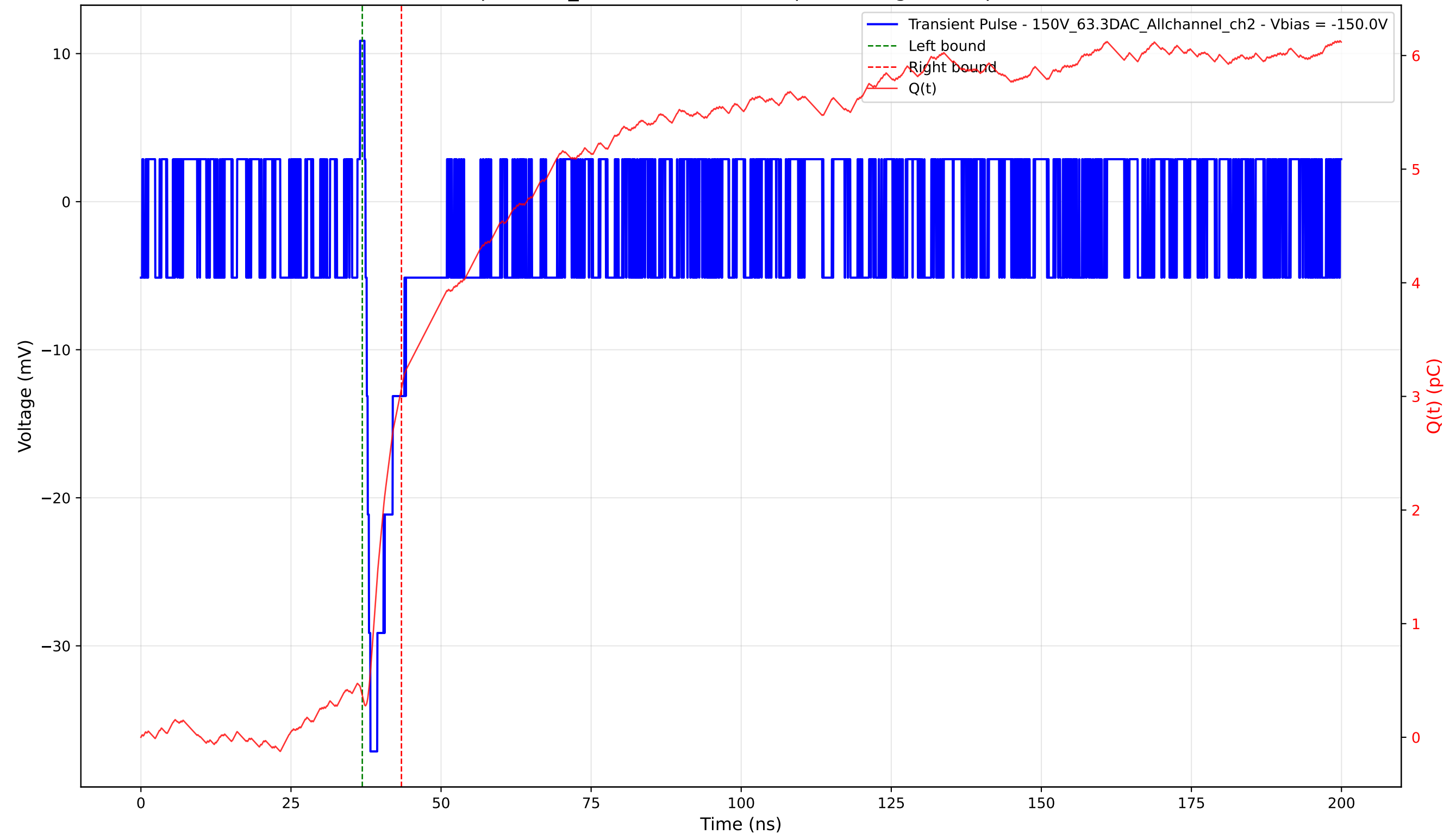
Transient Pulse - Sample: 1cm_42 - Position: 4715.0 \mu\text{m} - Charge: 2.70 pC - Rise Time: 0.83 ns
