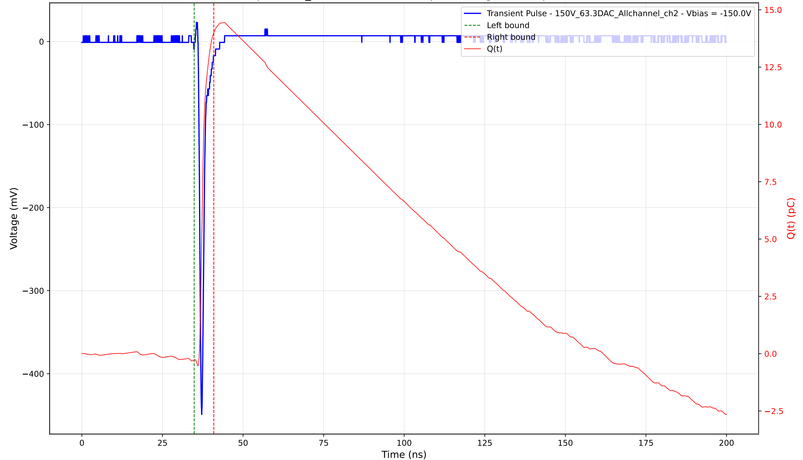
Transient Pulse - Sample: 1cm_42 - Position: 2760.0 \mu\text{m} - Charge: 14.28 pC - Rise Time: 0.71 ns
