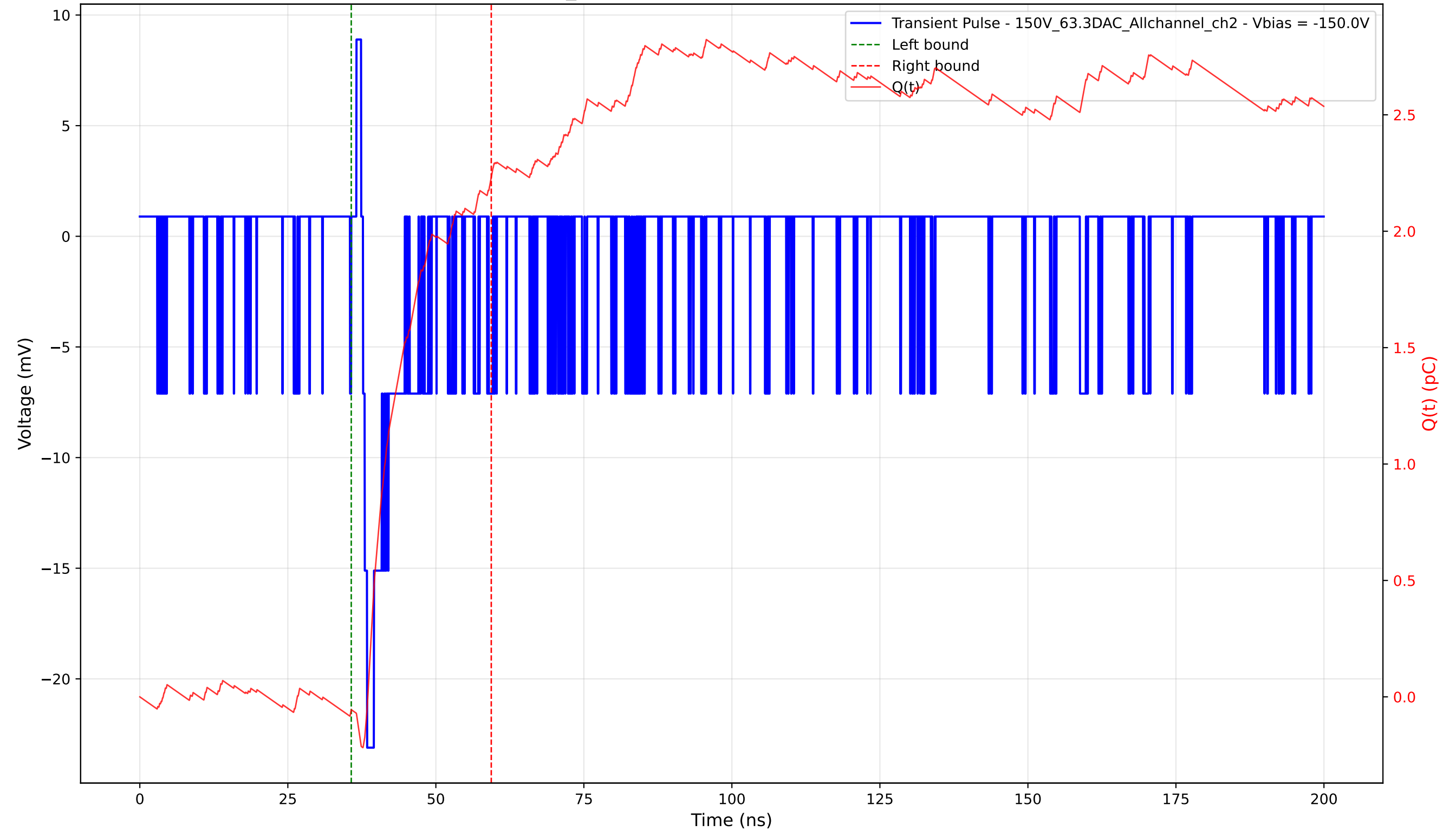
Transient Pulse - Sample: 1cm_42 - Position: 245.0 \mu\text{m} - Charge: 2.28 pC - Rise Time: 0.71 ns
