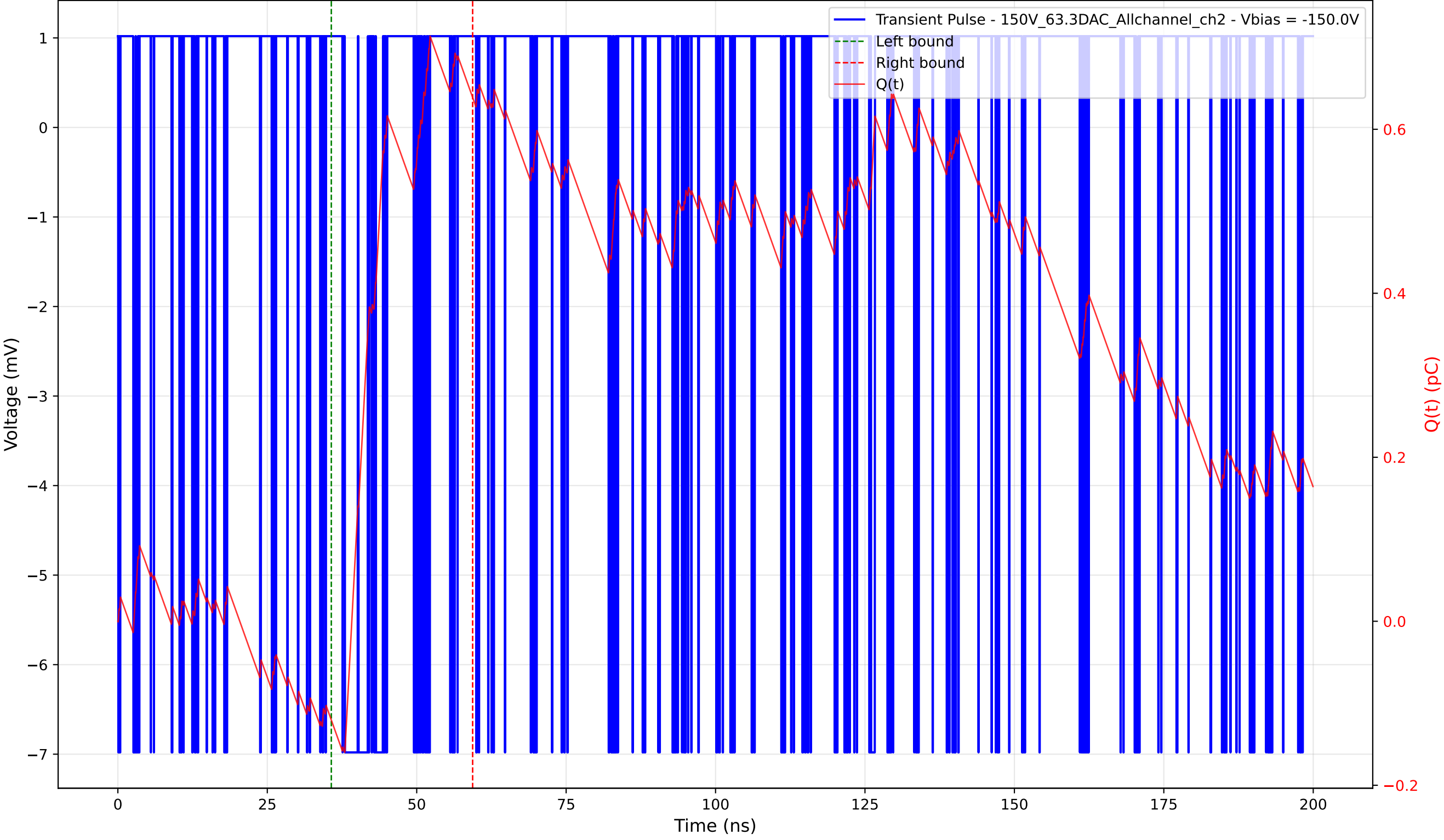
Transient Pulse - Sample: 1cm_42 - Position: 60.0 \mu\text{m} - Charge: 0.76 pC - Rise Time: 0.00 ns (N/A)
