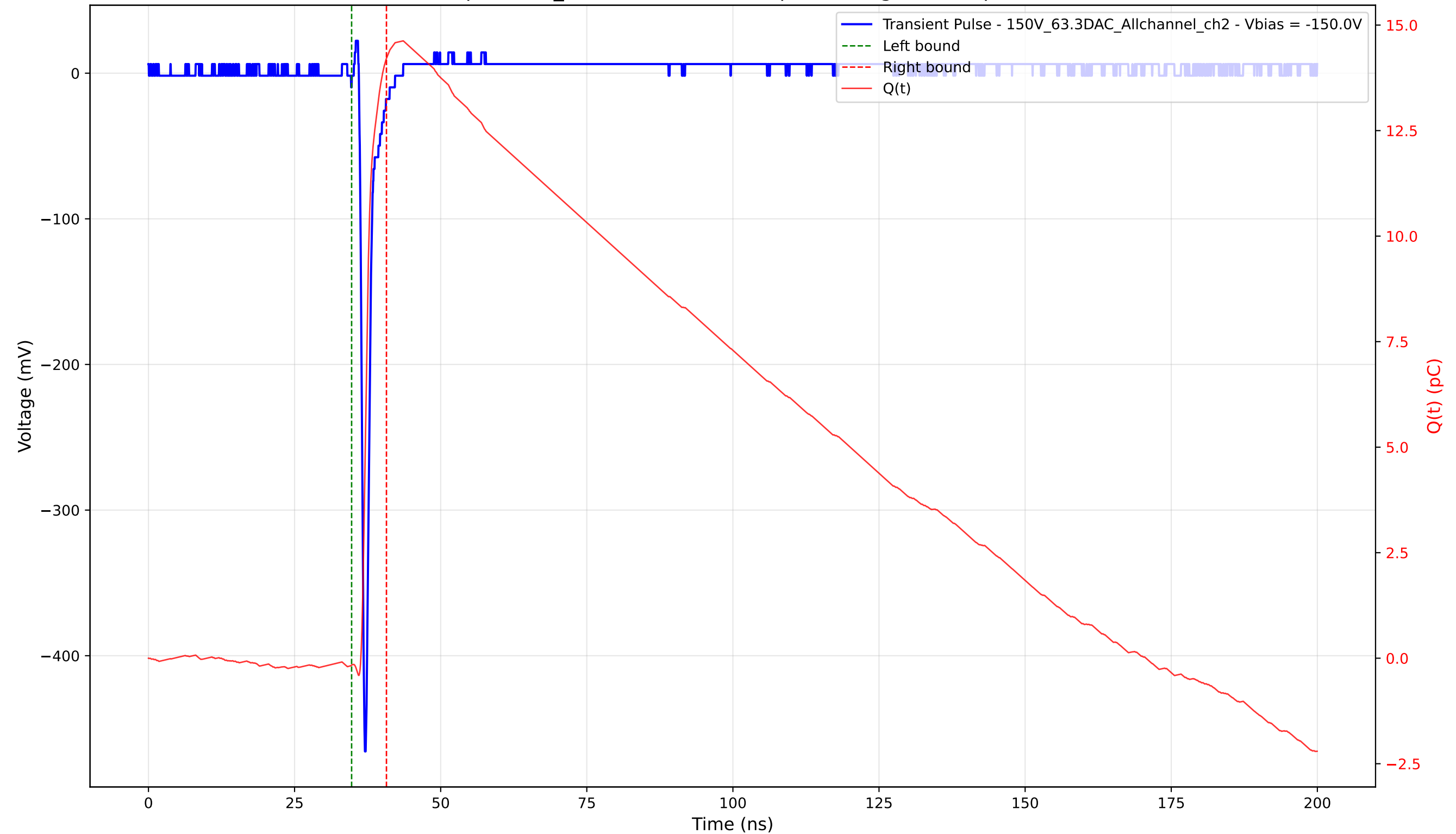
Transient Pulse - Sample: 1cm_42 - Position: 2905.0 \mu\text{m} - Charge: 14.37 pC - Rise Time: 0.72 ns
