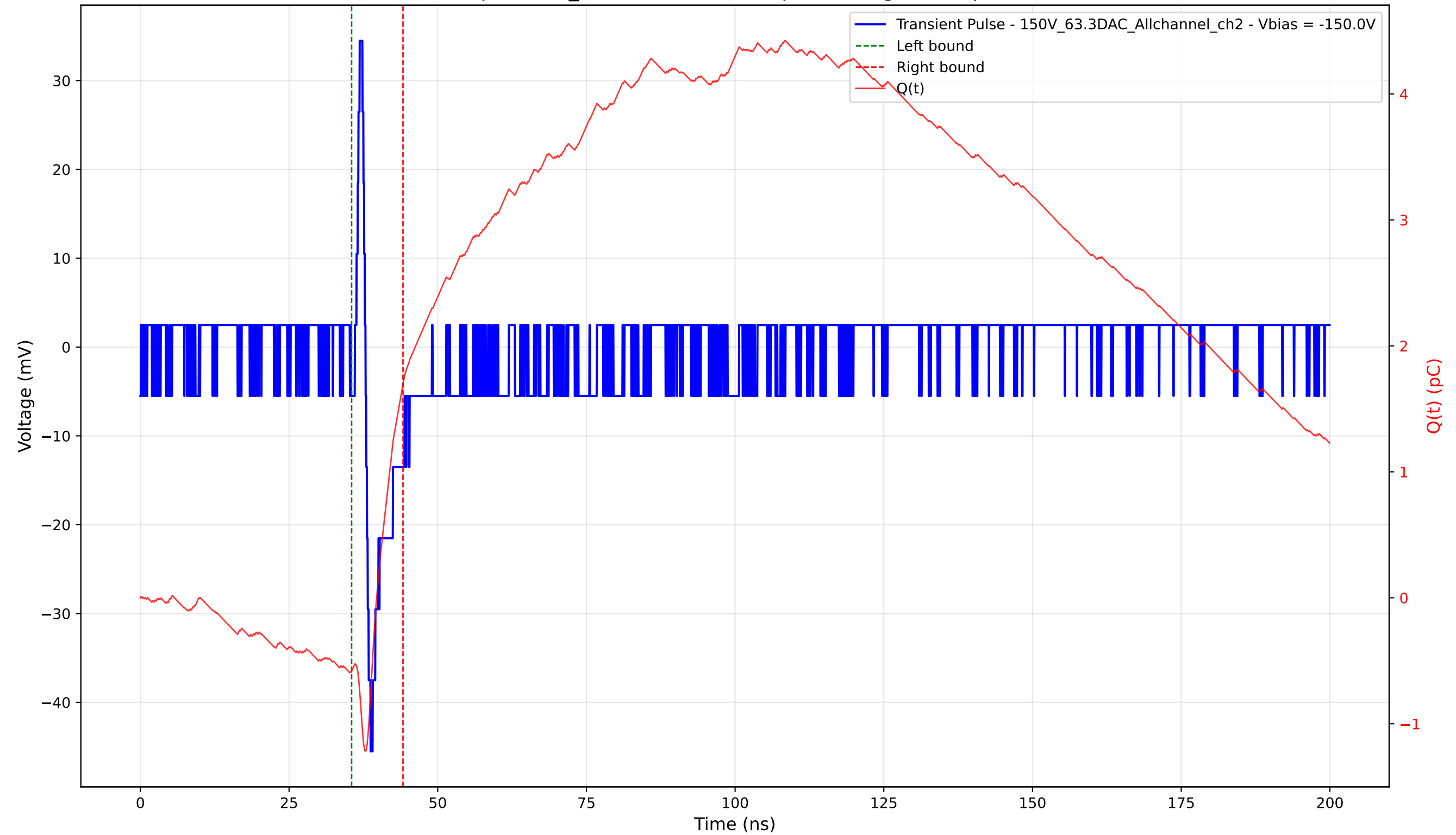
Transient Pulse - Sample: 1cm_42 - Position: 695.0 \mu\text{m} - Charge: 2.28 pC - Rise Time: 0.85 ns
