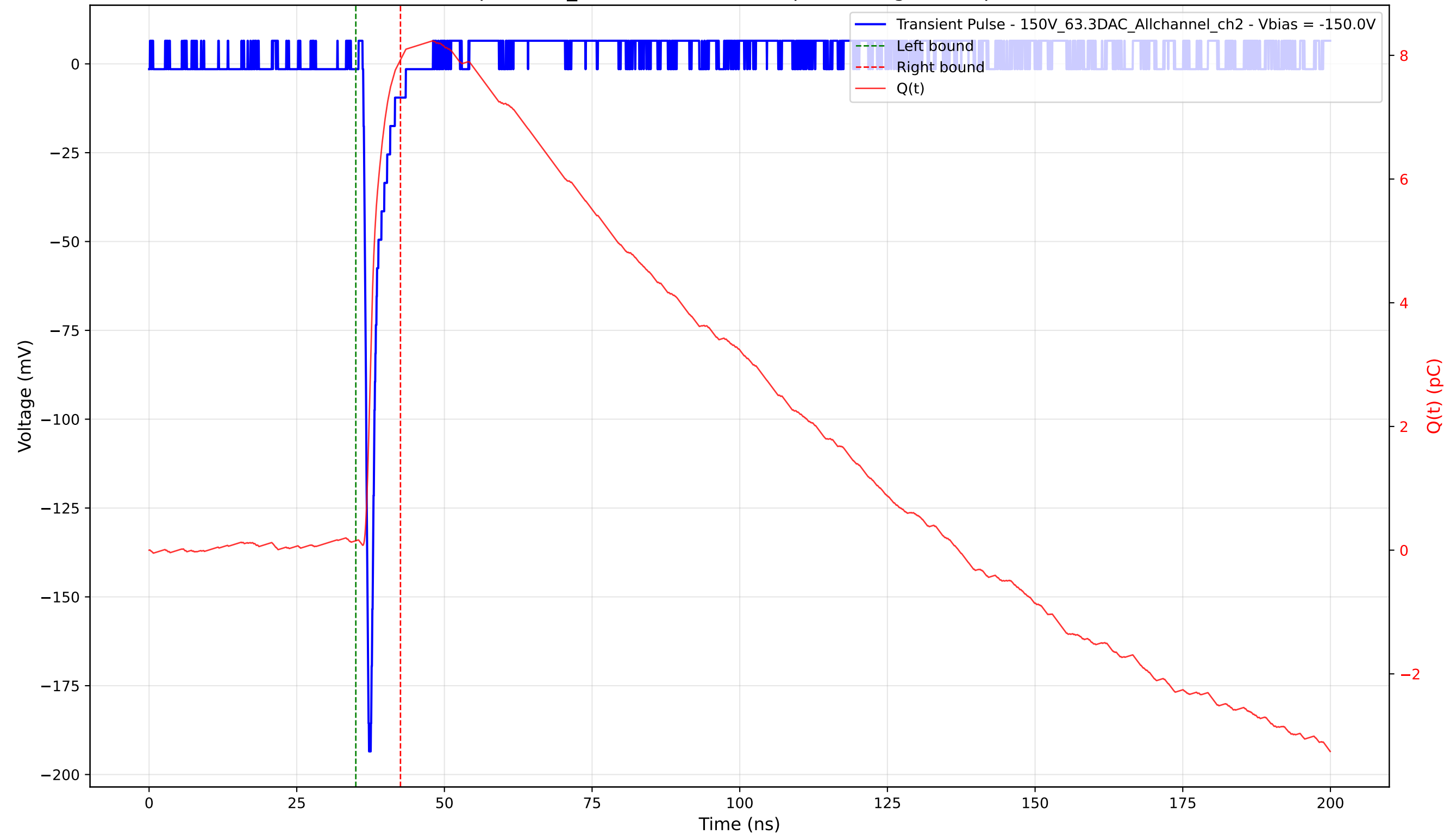
Transient Pulse - Sample: 1cm_42 - Position: 2500.0 \mu\text{m} - Charge: 7.78 pC - Rise Time: 0.73 ns
