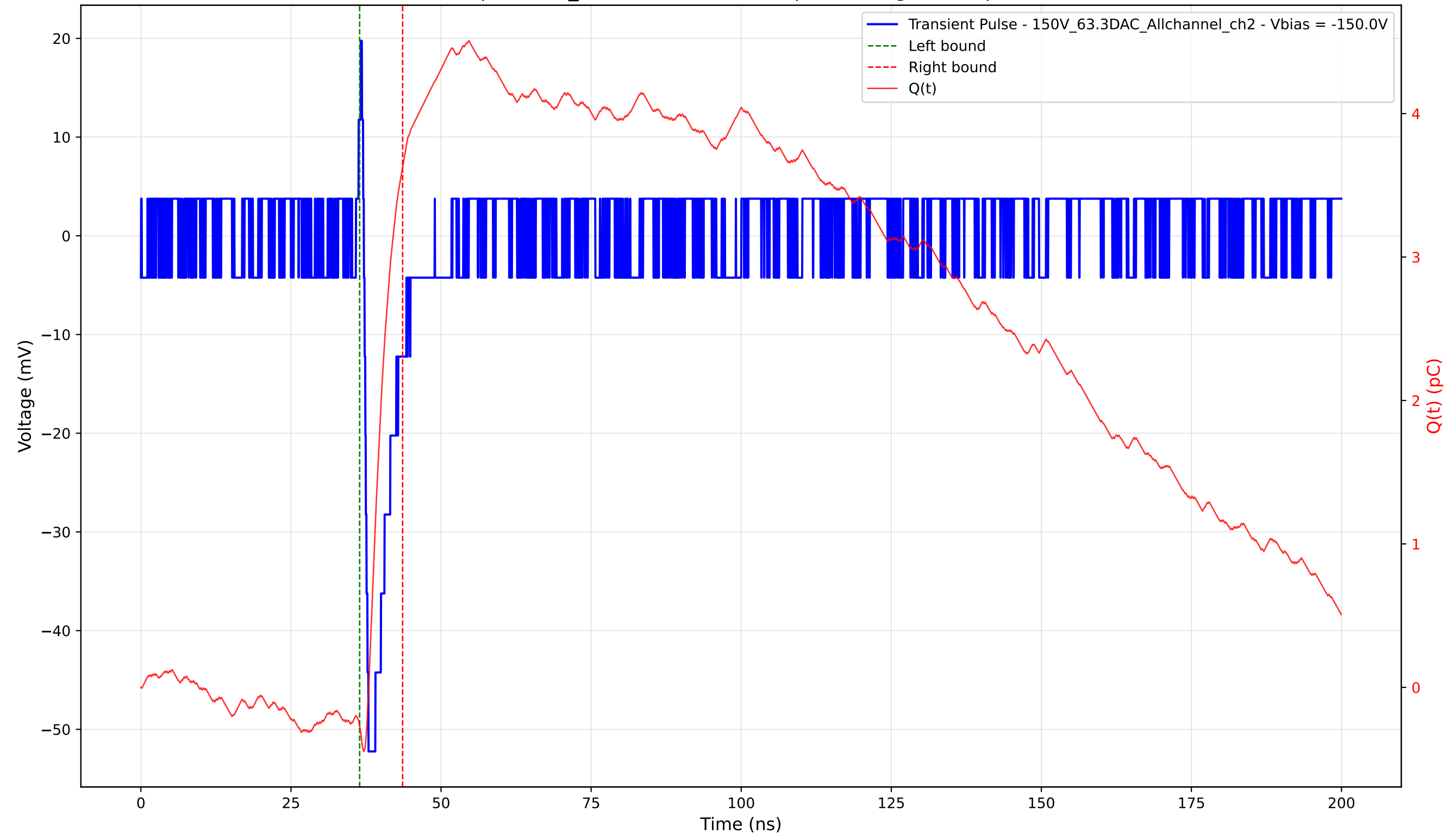
Transient Pulse - Sample: 1cm_42 - Position: 4345.0 \mu\text{m} - Charge: 3.90 pC - Rise Time: 0.68 ns
