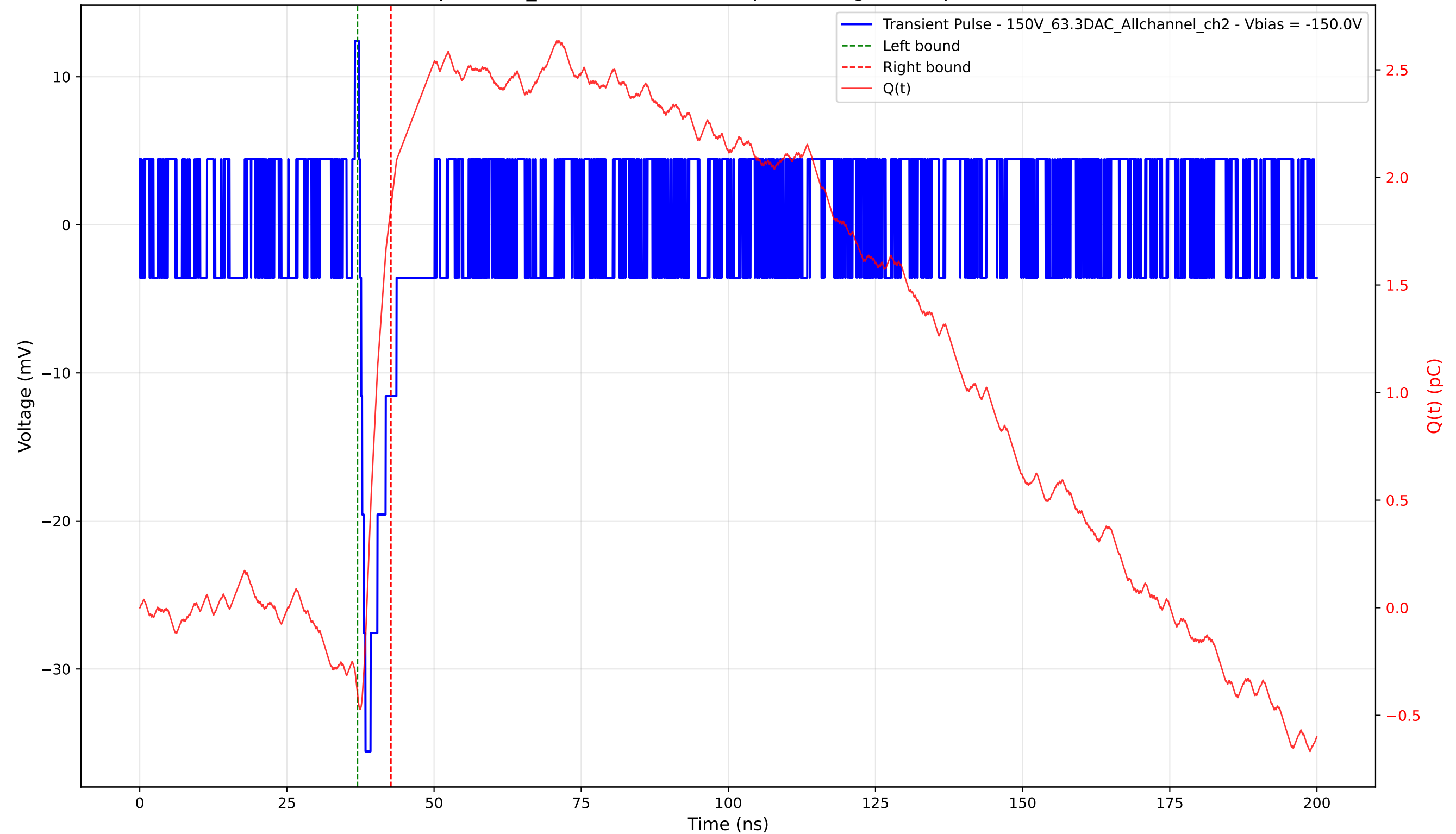
Transient Pulse - Sample: 1cm_42 - Position: 4835.0 \mu\text{m} - Charge: 2.26 pC - Rise Time: 0.00 ns (N/A)
