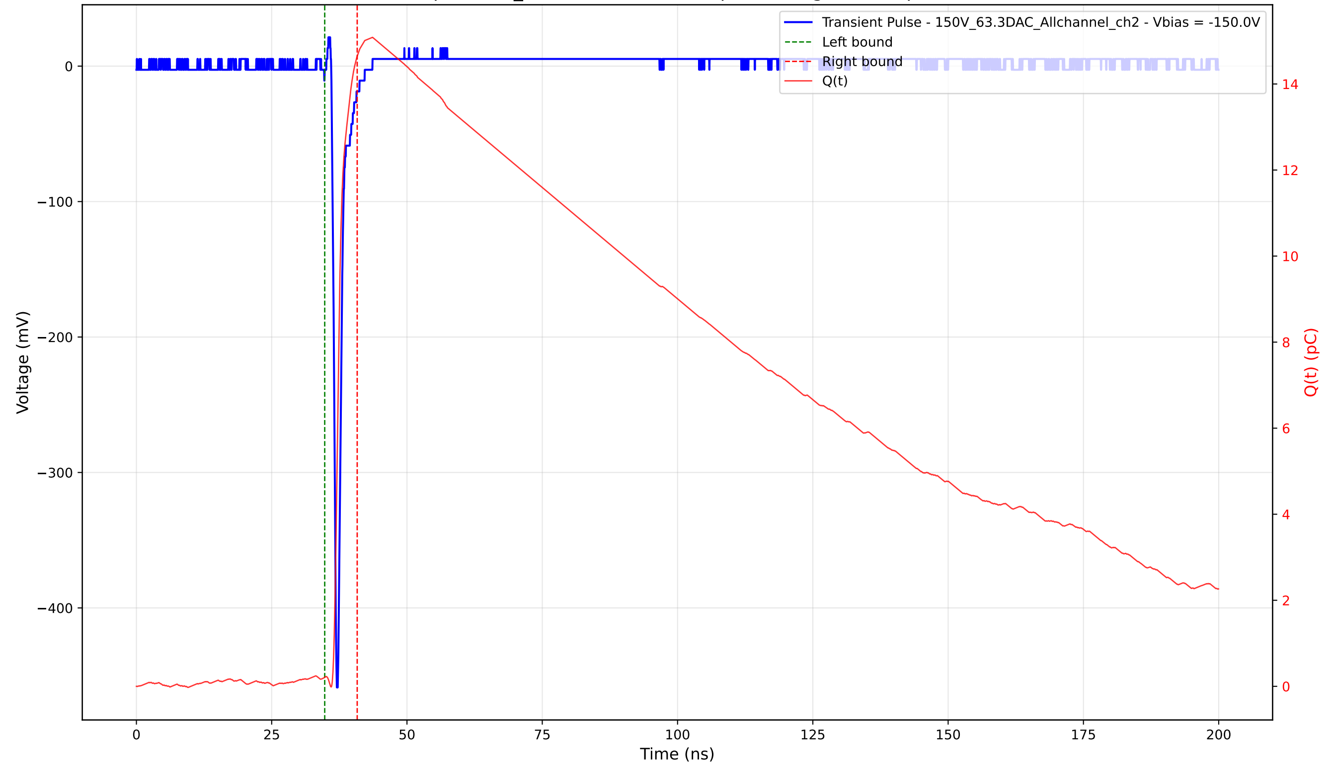
Transient Pulse - Sample: 1cm_42 - Position: 2875.0 \mu\text{m} - Charge: 14.43 pC - Rise Time: 0.70 ns
