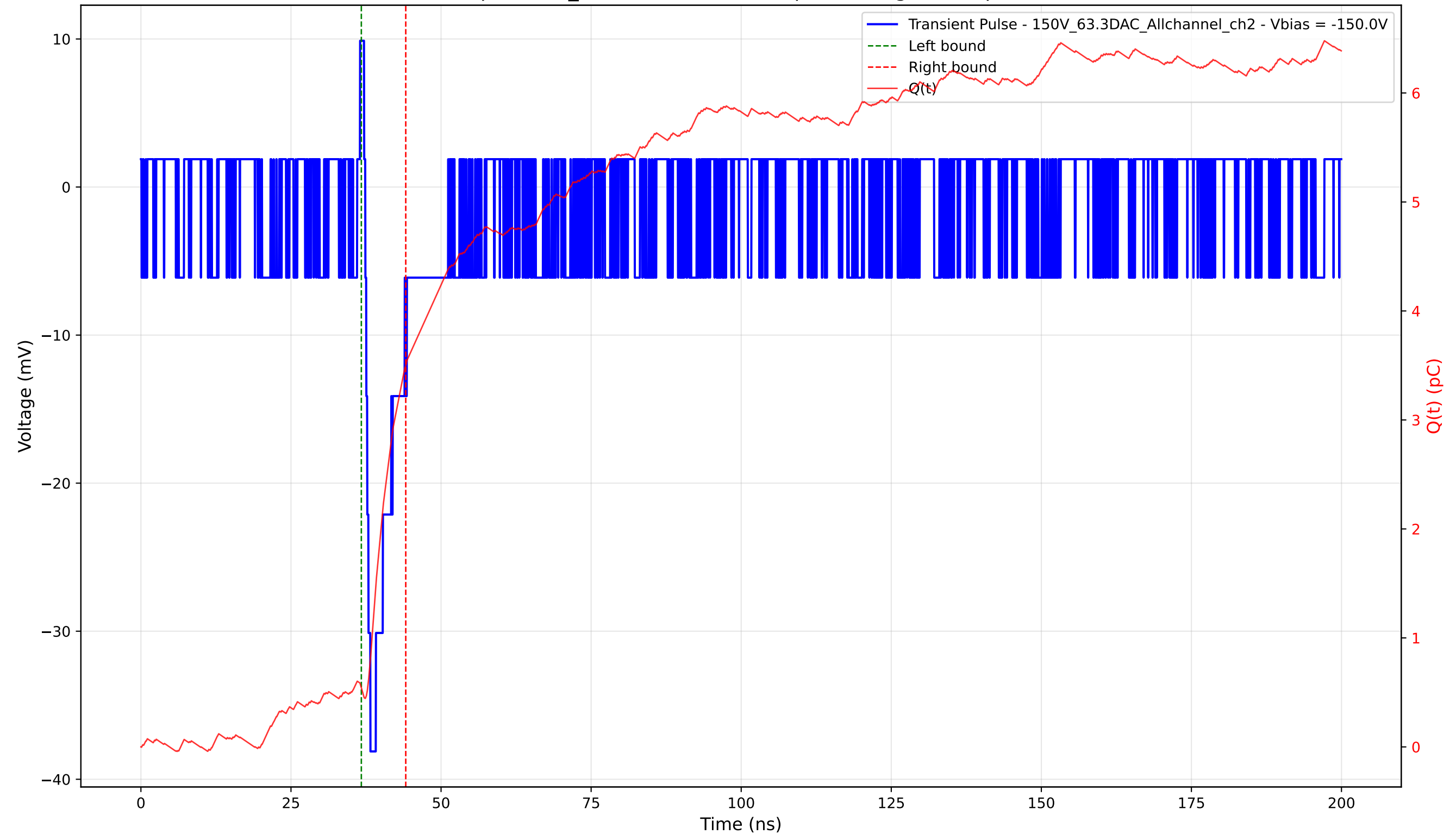
Transient Pulse - Sample: 1cm_42 - Position: 4605.0 \mu\text{m} - Charge: 2.95 pC - Rise Time: 0.86 ns
