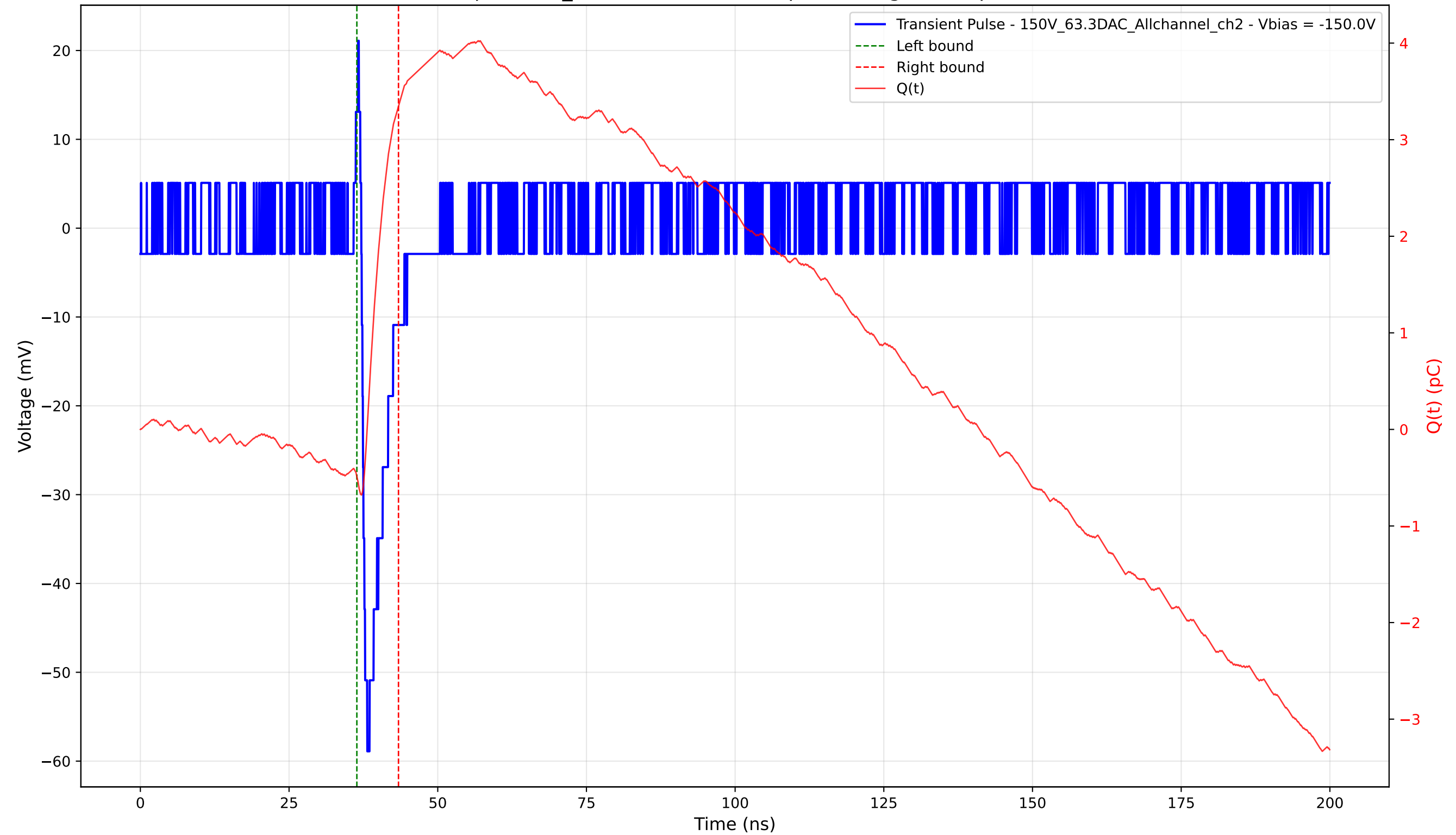
Transient Pulse - Sample: 1cm_42 - Position: 4255.0 \mu\text{m} - Charge: 3.83 pC - Rise Time: 0.95 ns
