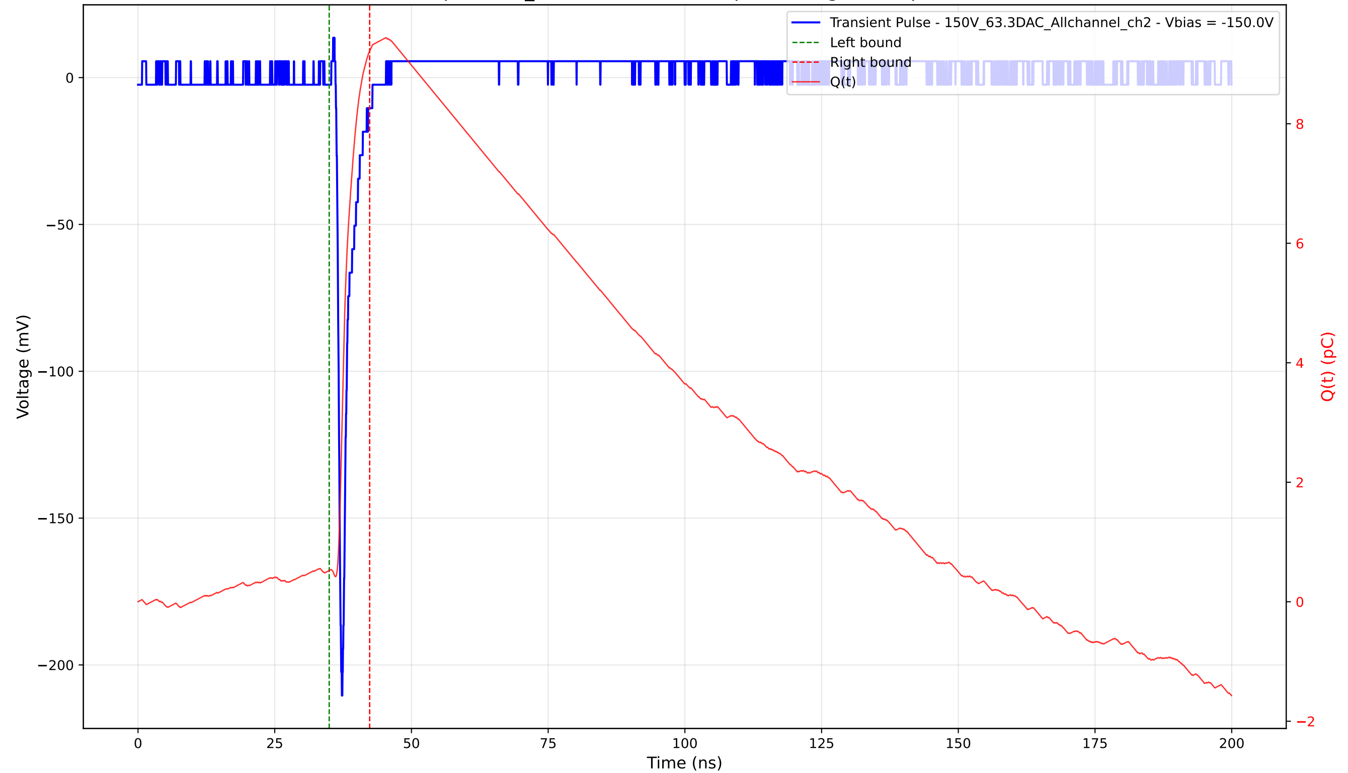
Transient Pulse - Sample: 1cm_42 - Position: 3525.0 \mu\text{m} - Charge: 8.69 pC - Rise Time: 0.80 ns
