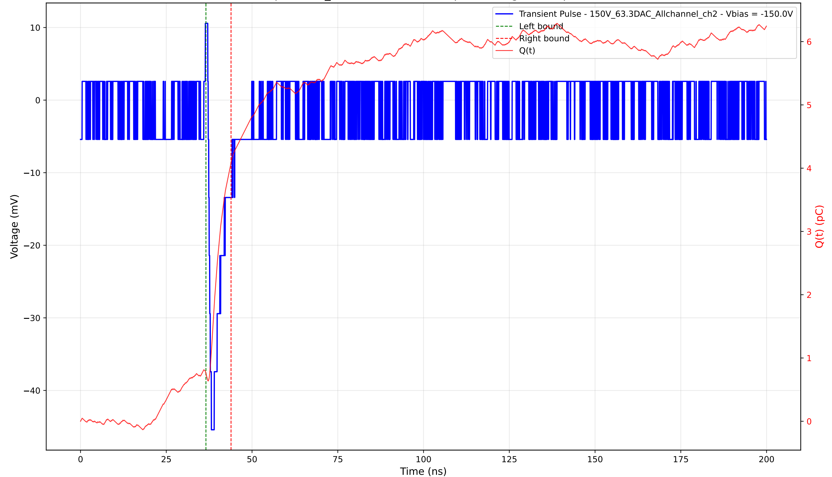
Transient Pulse - Sample: 1cm_42 - Position: 4455.0 \mu\text{m} - Charge: 3.33 pC - Rise Time: 0.93 ns
