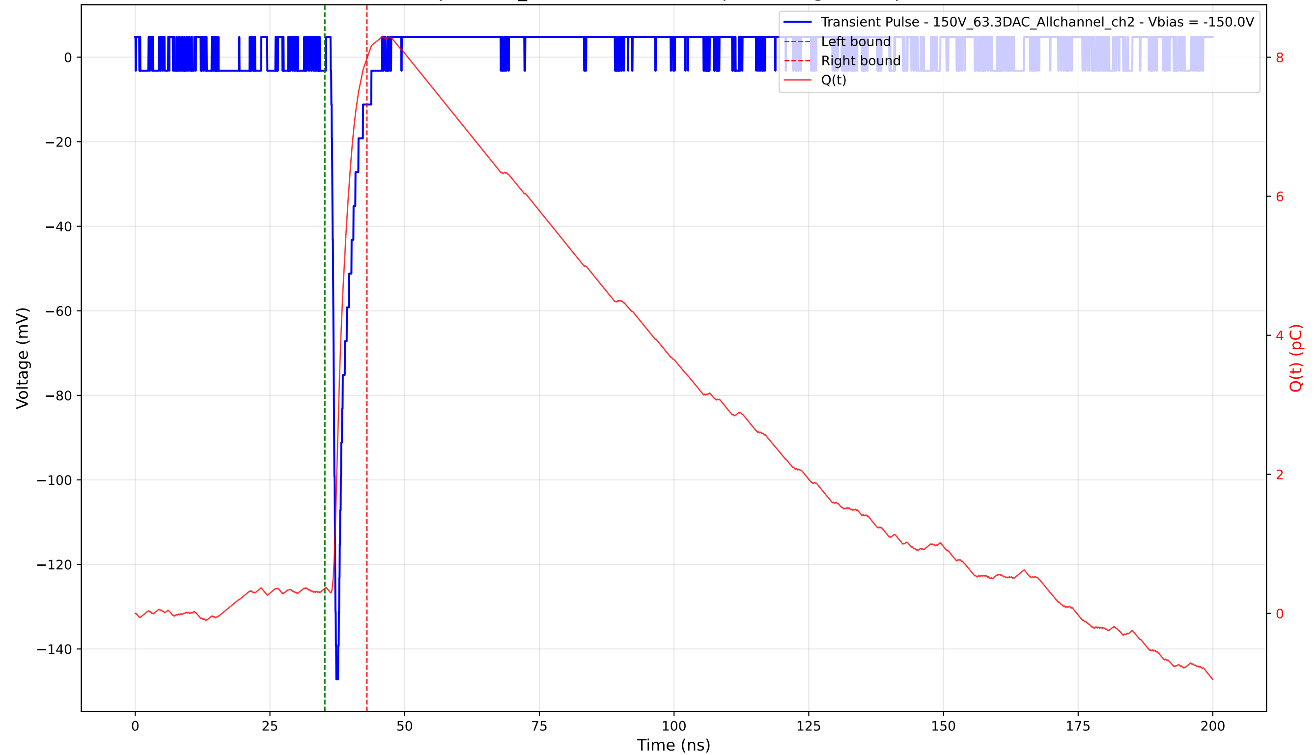
Transient Pulse - Sample: 1cm_42 - Position: 3670.0 \mu\text{m} - Charge: 7.62 pC - Rise Time: 0.78 ns
