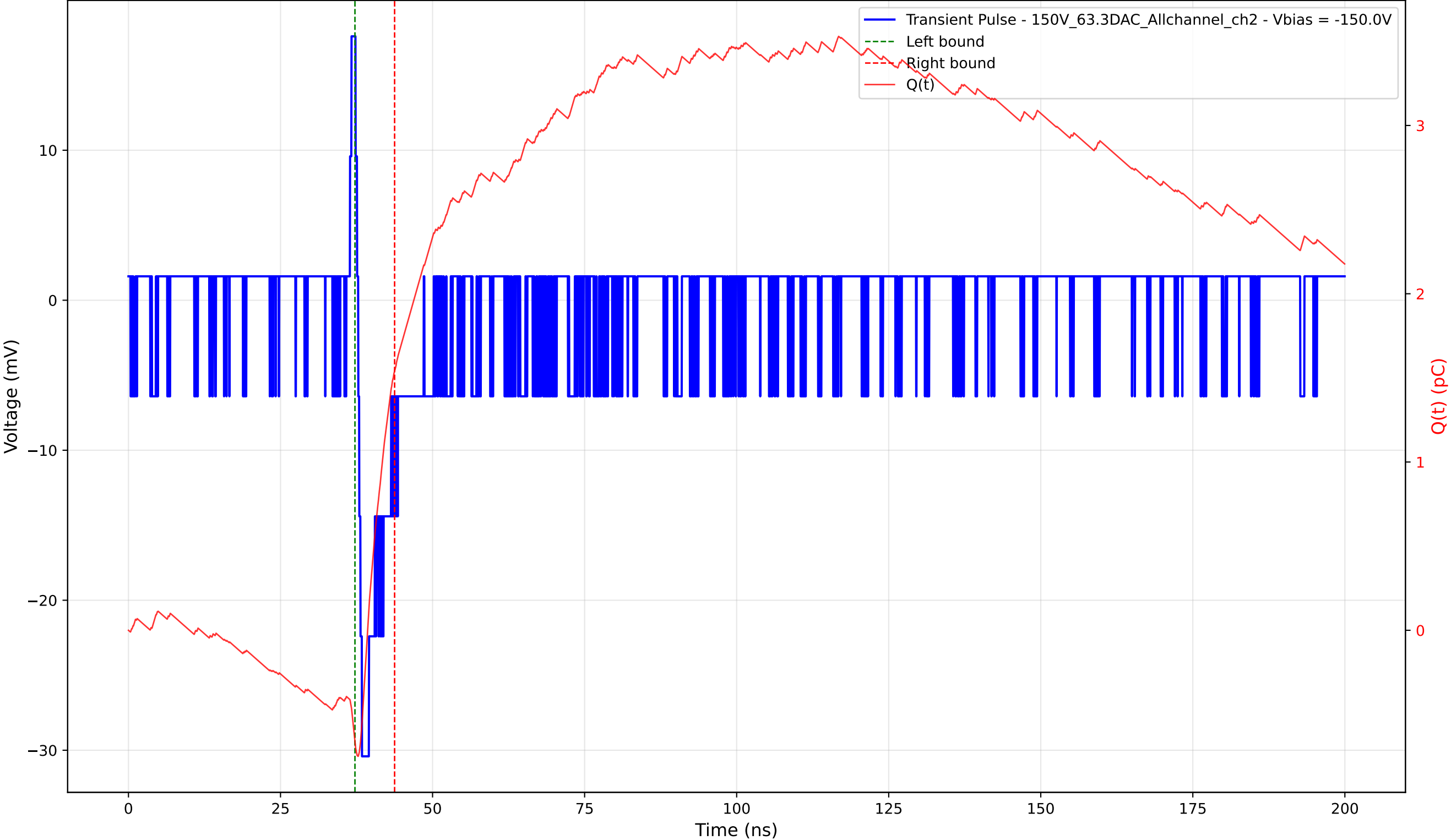
Transient Pulse - Sample: 1cm_42 - Position: 480.0 \mu\text{m} - Charge: 2.20 pC - Rise Time: 0.63 ns
