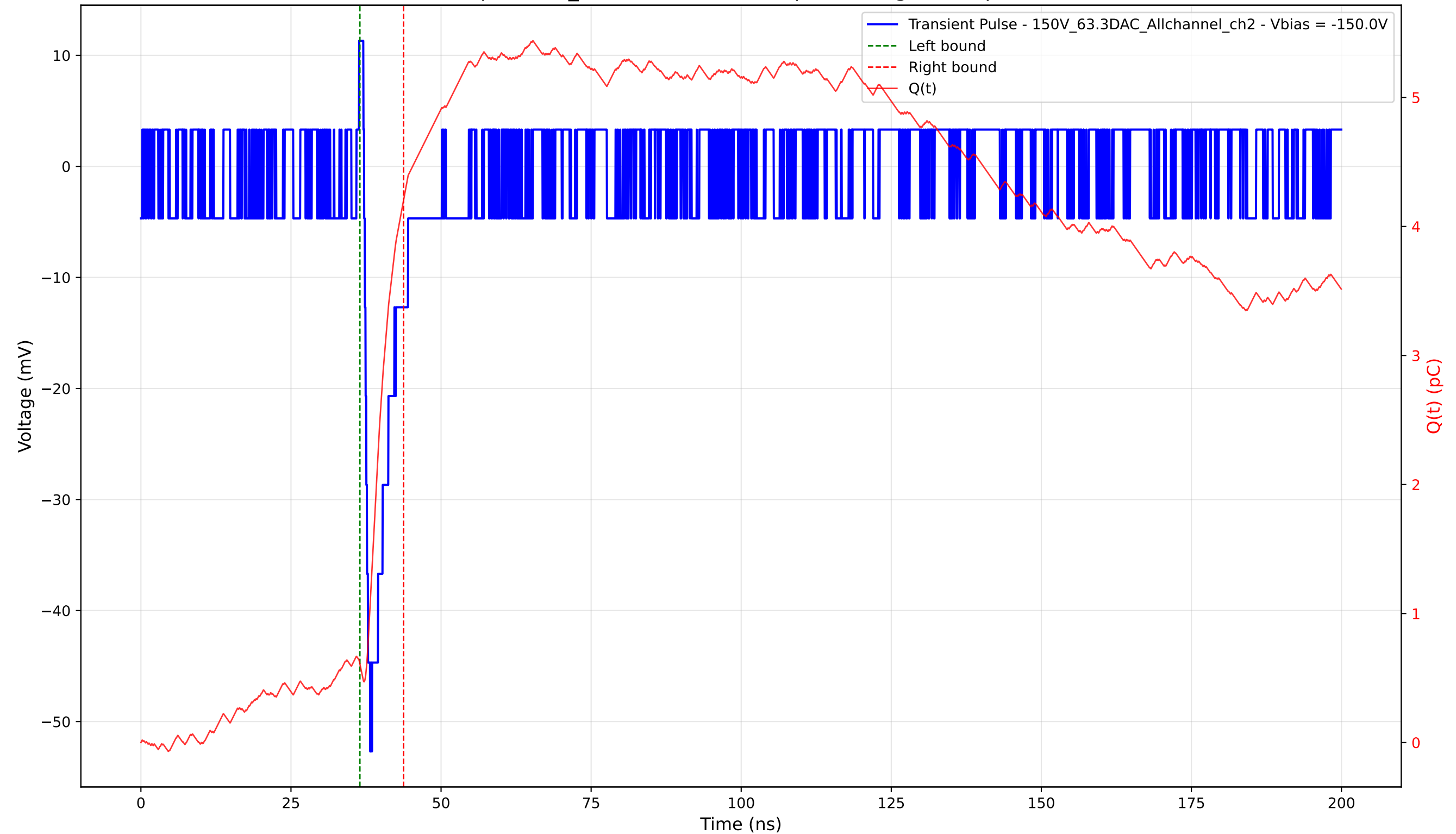
Transient Pulse - Sample: 1cm_42 - Position: 4390.0 \mu\text{m} - Charge: 3.60 pC - Rise Time: 0.92 ns
