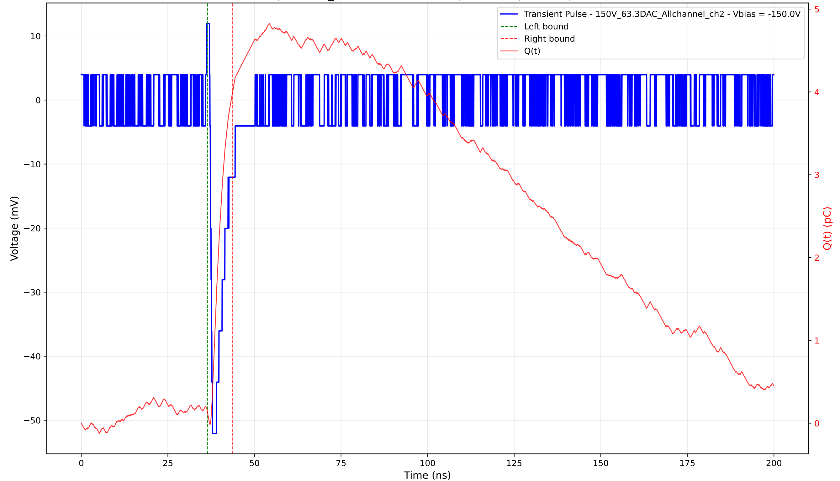
Transient Pulse - Sample: 1cm_42 - Position: 4350.0 \mu\text{m} - Charge: 3.83 pC - Rise Time: 0.67 ns
