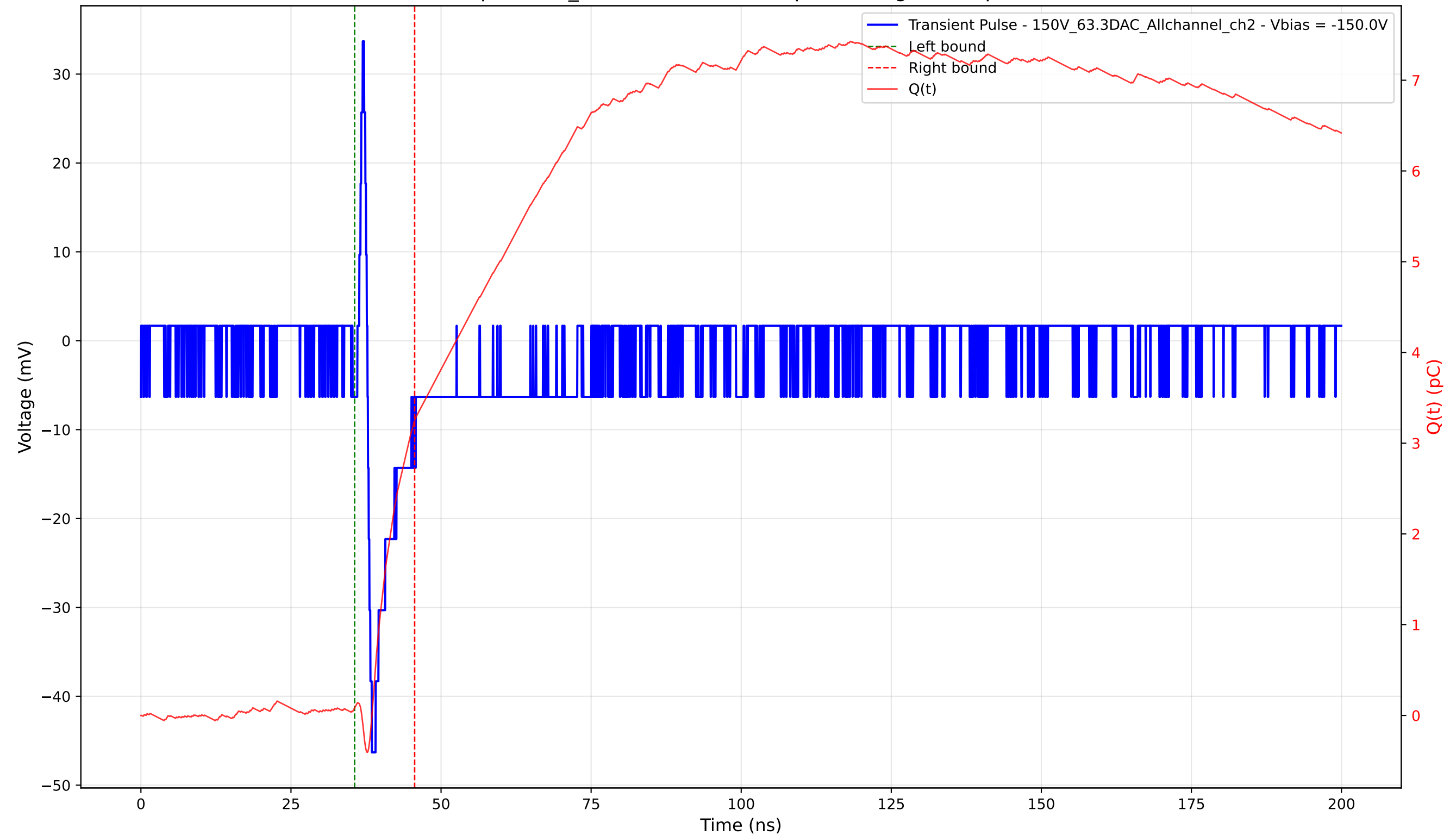
Transient Pulse - Sample: 1cm_42 - Position: 1385.0 \mu\text{m} - Charge: 3.16 pC - Rise Time: 0.73 ns
