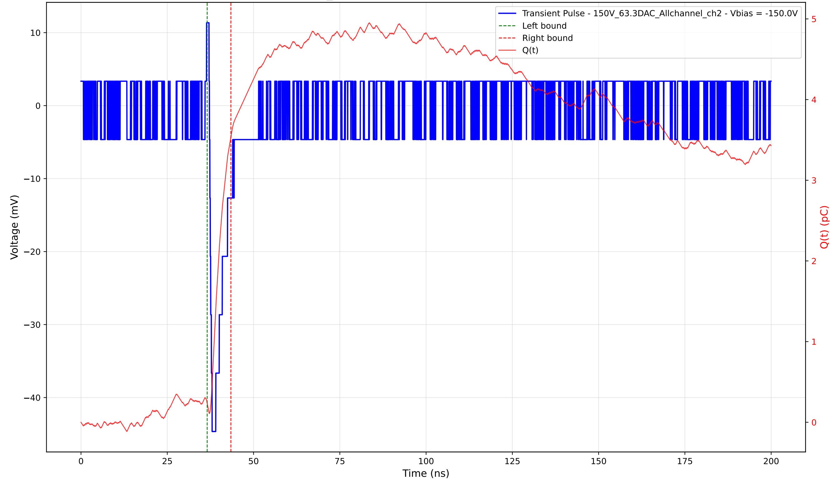
Transient Pulse - Sample: 1cm_42 - Position: 4430.0 \mu\text{m} - Charge: 3.30 pC - Rise Time: 0.77 ns
