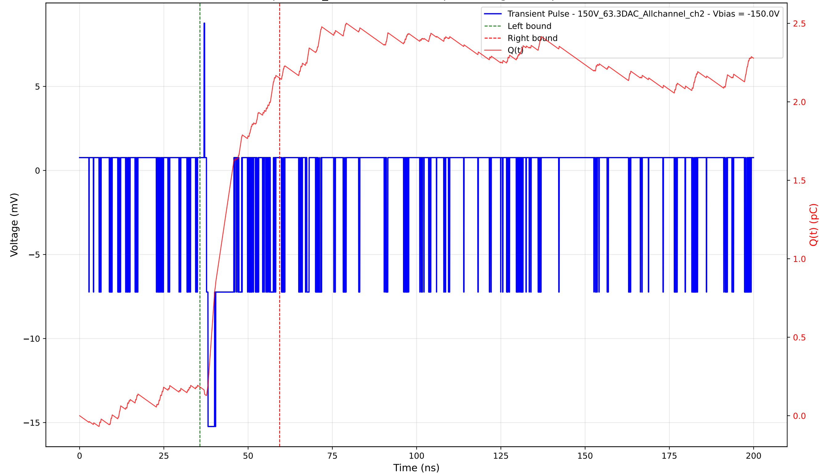
Transient Pulse - Sample: 1cm_42 - Position: 175.0 \mu\text{m} - Charge: 1.97 pC - Rise Time: 0.48 ns
