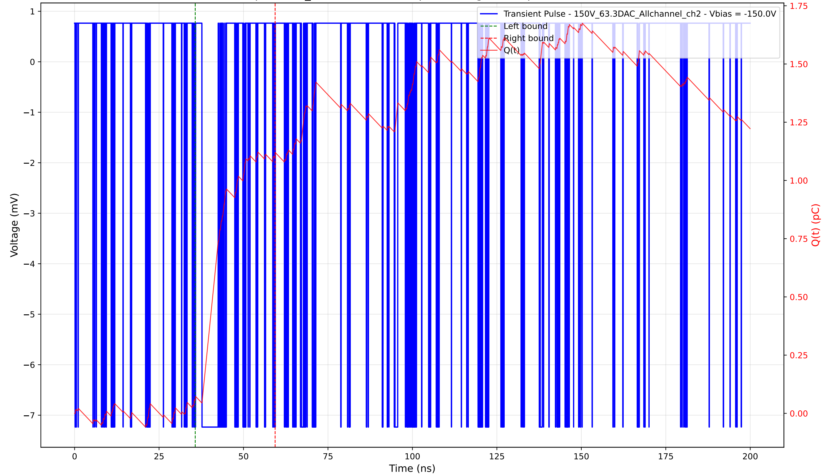
Transient Pulse - Sample: 1cm_42 - Position: 80.0 \mu\text{m} - Charge: 1.05 pC - Rise Time: 0.00 ns (N/A)
