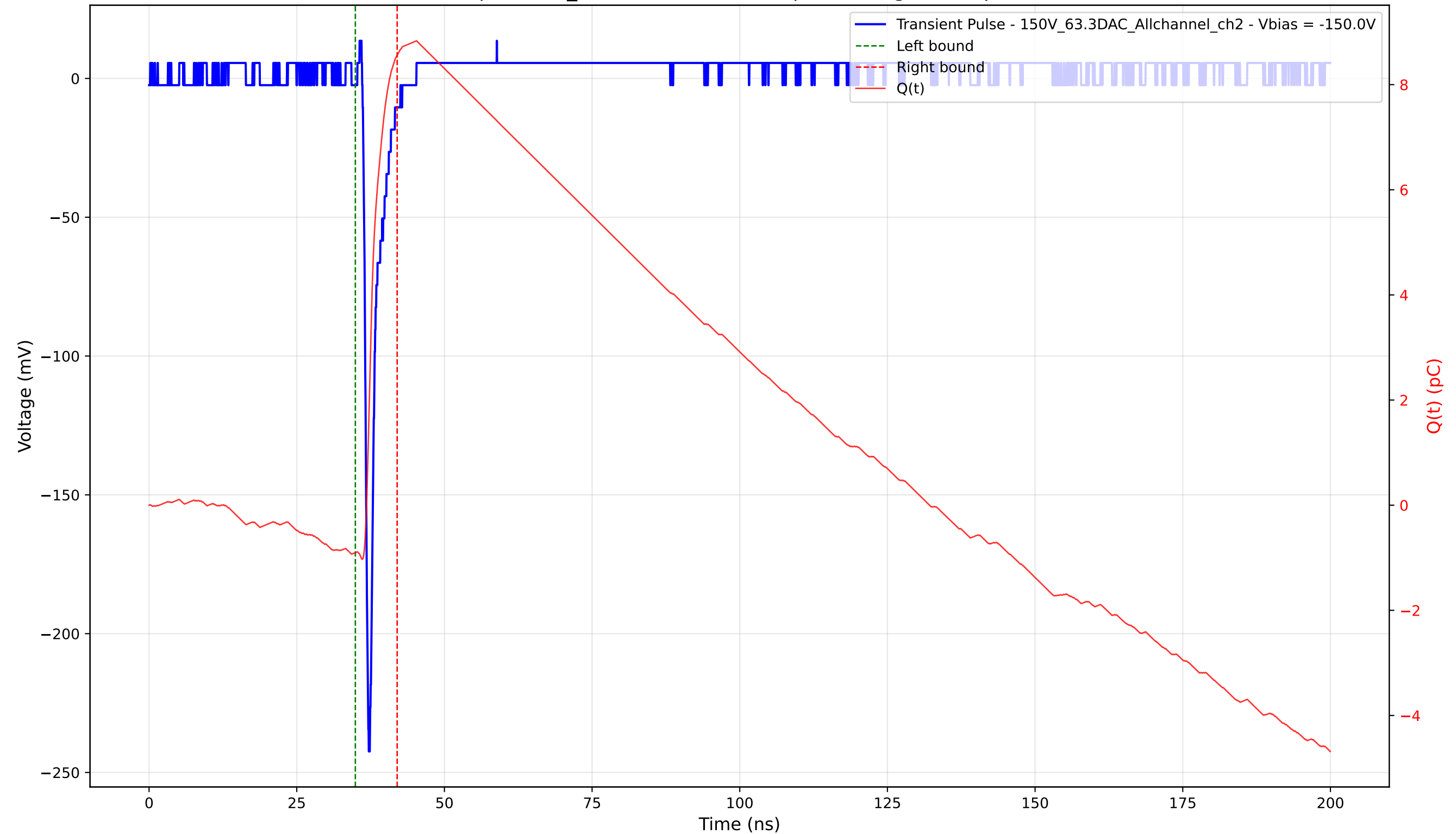
Transient Pulse - Sample: 1cm_42 - Position: 3480.0 \mu\text{m} - Charge: 9.46 pC - Rise Time: 0.77 ns
