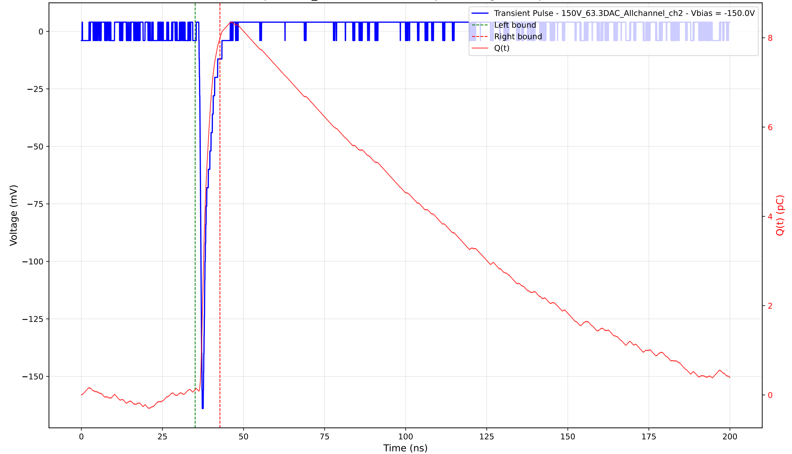
Transient Pulse - Sample: 1cm_42 - Position: 3615.0 \mu\text{m} - Charge: 7.87 pC - Rise Time: 0.78 ns
