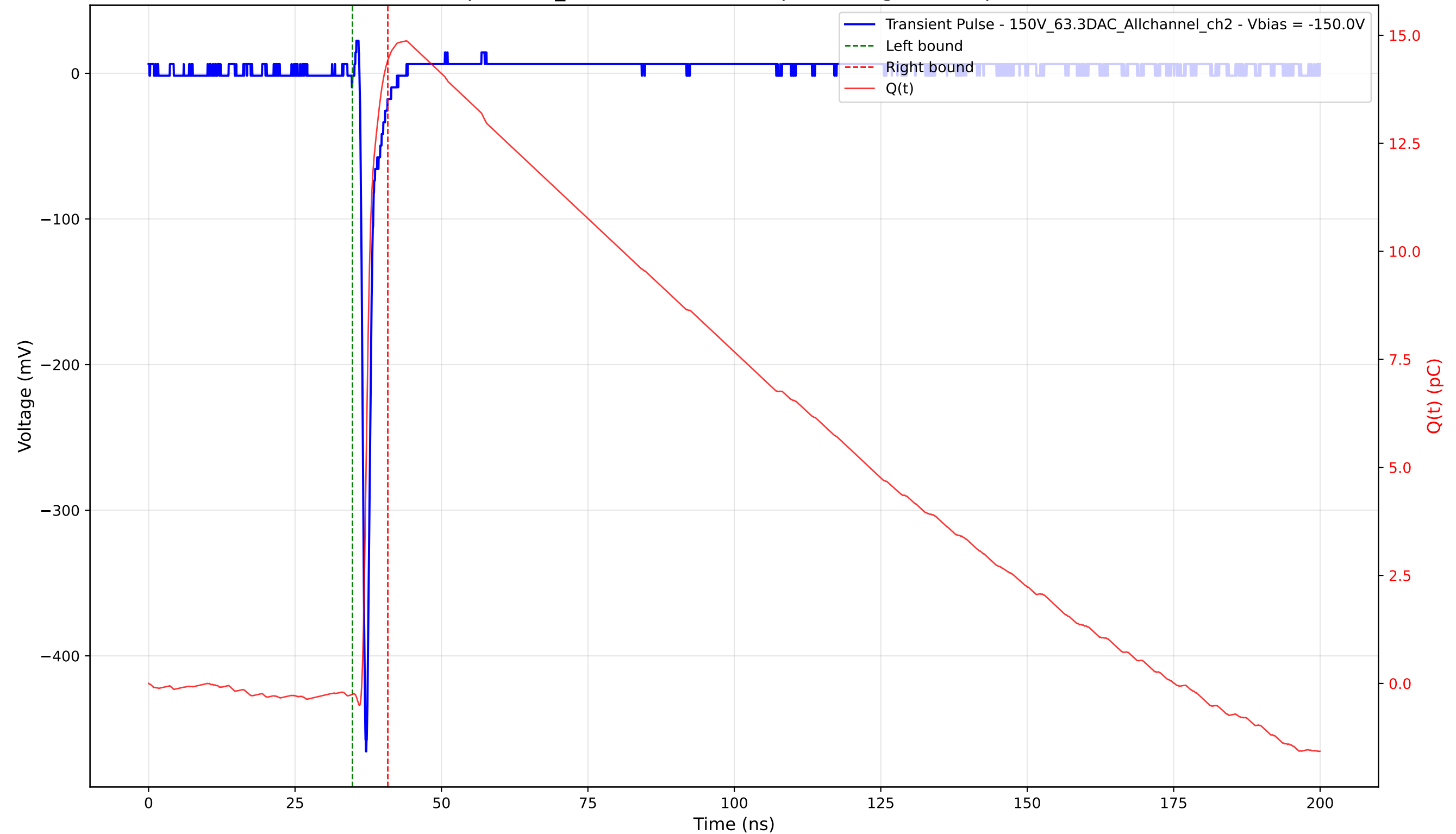
Transient Pulse - Sample: 1cm_42 - Position: 2820.0 \mu\text{m} - Charge: 14.67 pC - Rise Time: 0.73 ns
