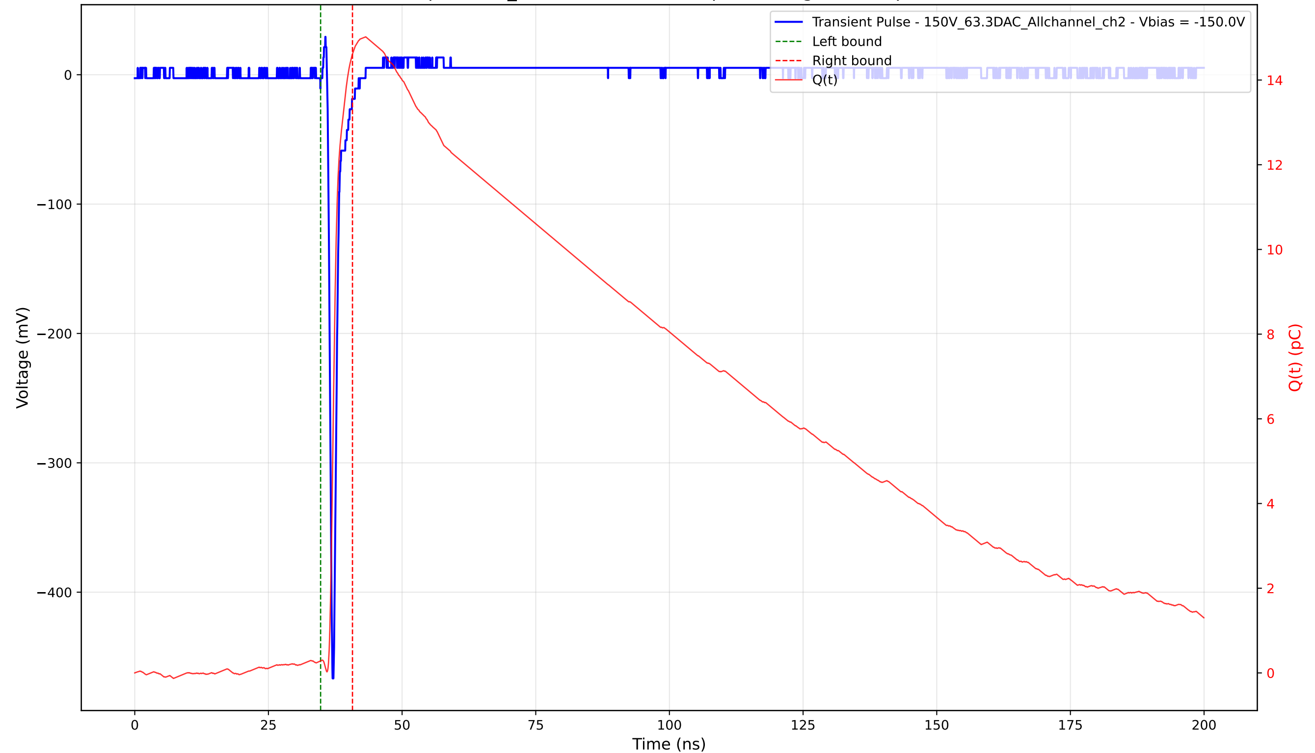
Transient Pulse - Sample: 1cm_42 - Position: 3070.0 \mu\text{m} - Charge: 14.33 pC - Rise Time: 0.71 ns
