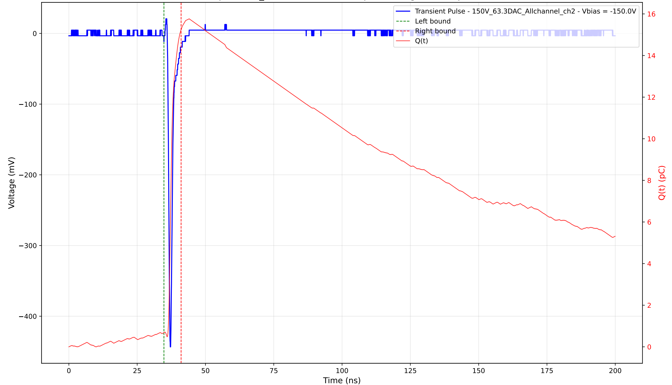
Transient Pulse - Sample: 1cm_42 - Position: 2755.0 \mu\text{m} - Charge: 14.56 pC - Rise Time: 0.72 ns
