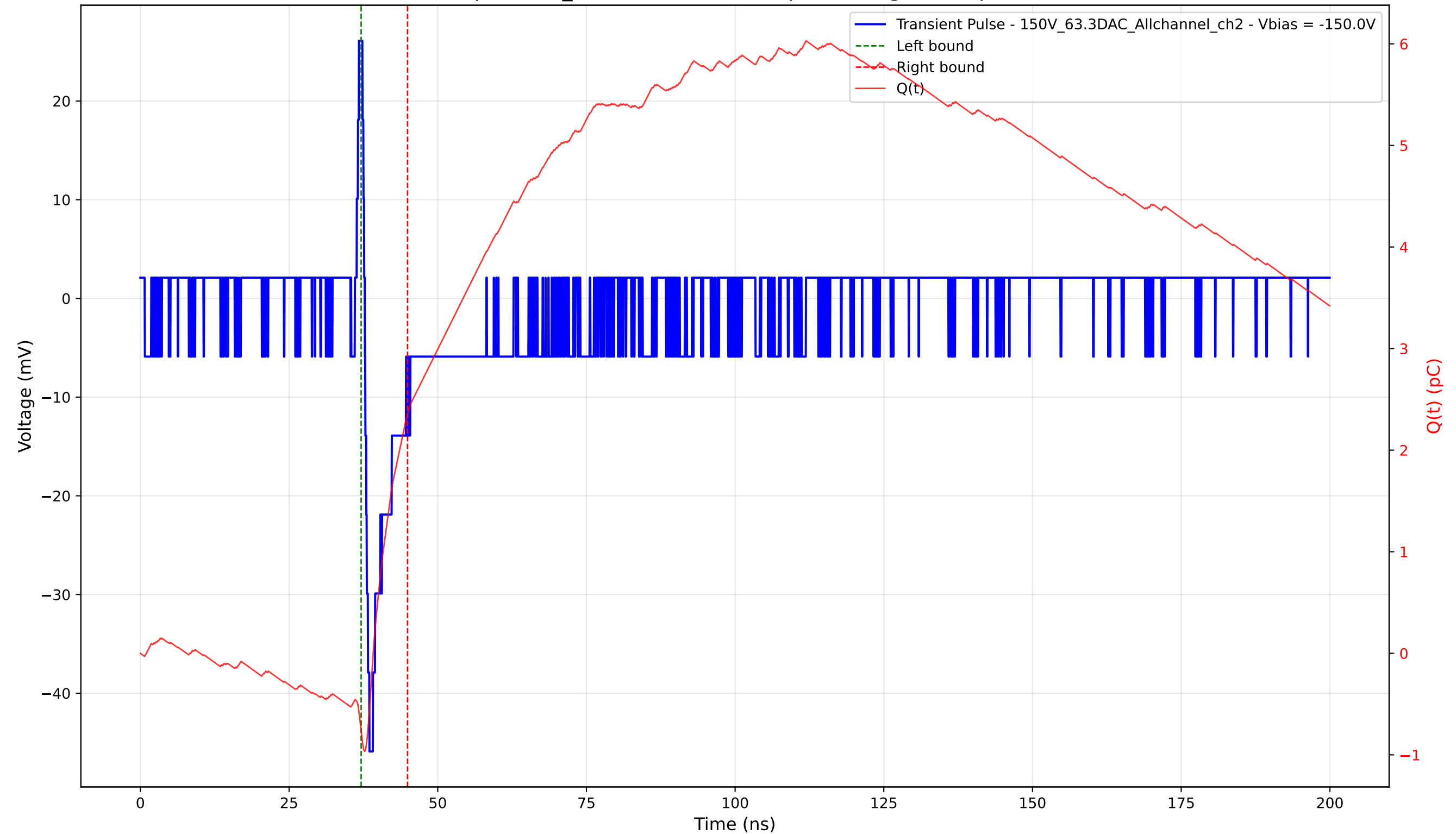
Transient Pulse - Sample: 1cm_42 - Position: 1395.0 \mu\text{m} - Charge: 3.12 pC - Rise Time: 0.77 ns
