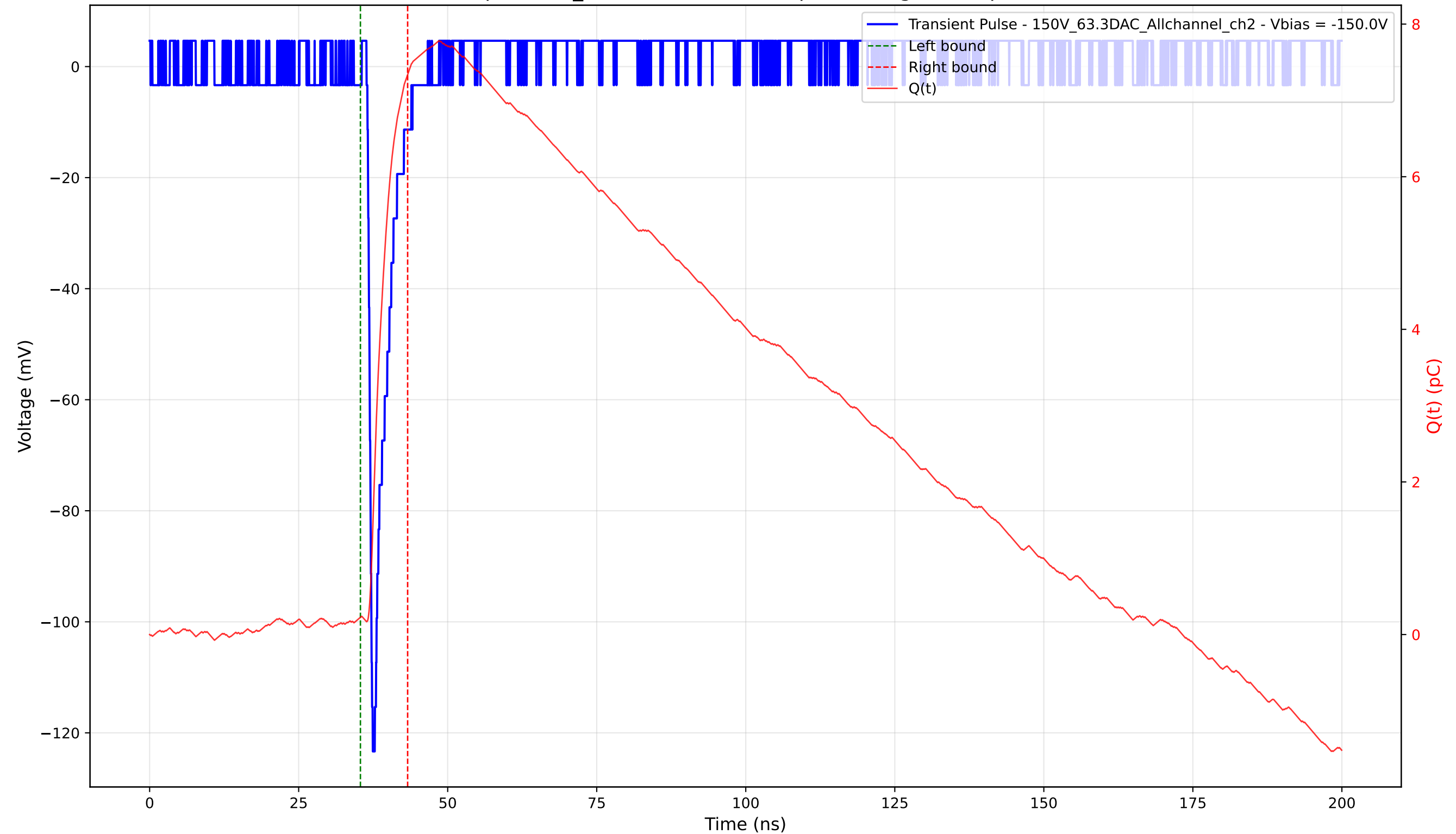
Transient Pulse - Sample: 1cm_42 - Position: 3815.0 \mu\text{m} - Charge: 7.11 pC - Rise Time: 0.72 ns
