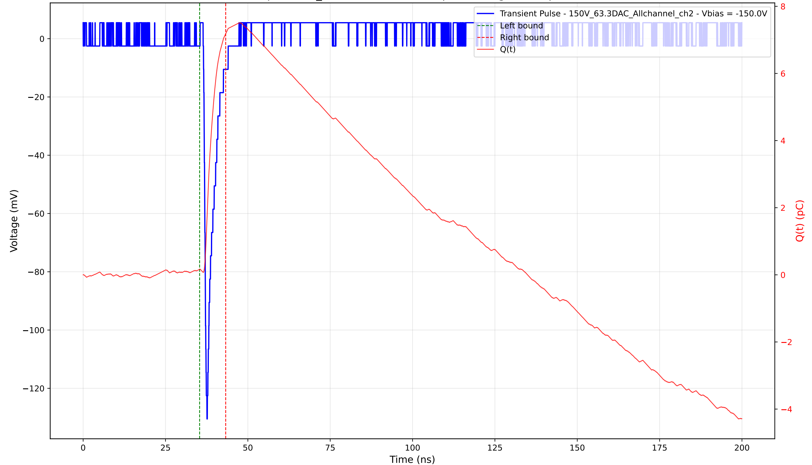
Transient Pulse - Sample: 1cm_42 - Position: 3805.0 \mu\text{m} - Charge: 7.02 pC - Rise Time: 0.79 ns
