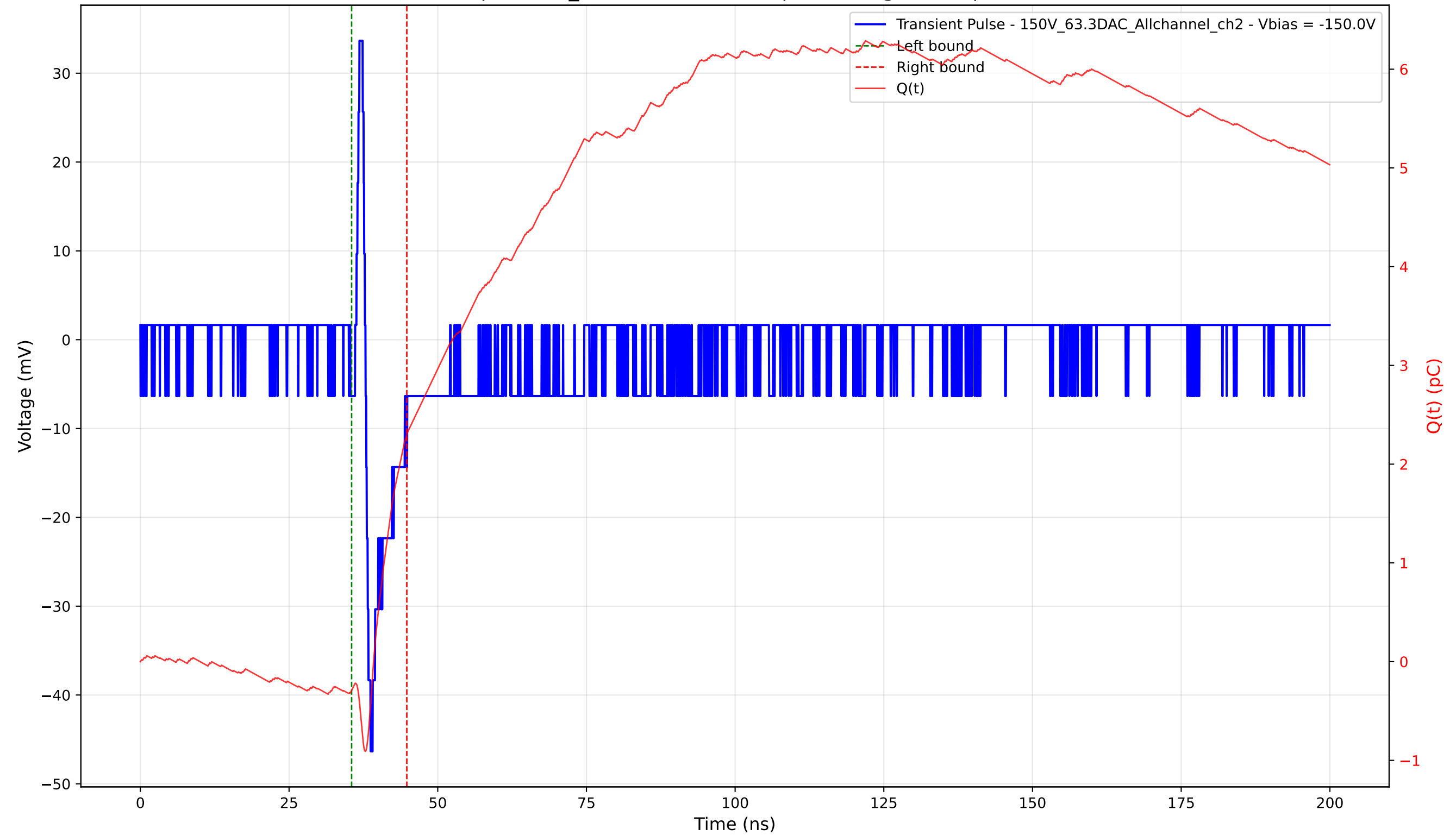
Transient Pulse - Sample: 1cm_42 - Position: 780.0 \mu\text{m} - Charge: 2.59 pC - Rise Time: 0.85 ns
