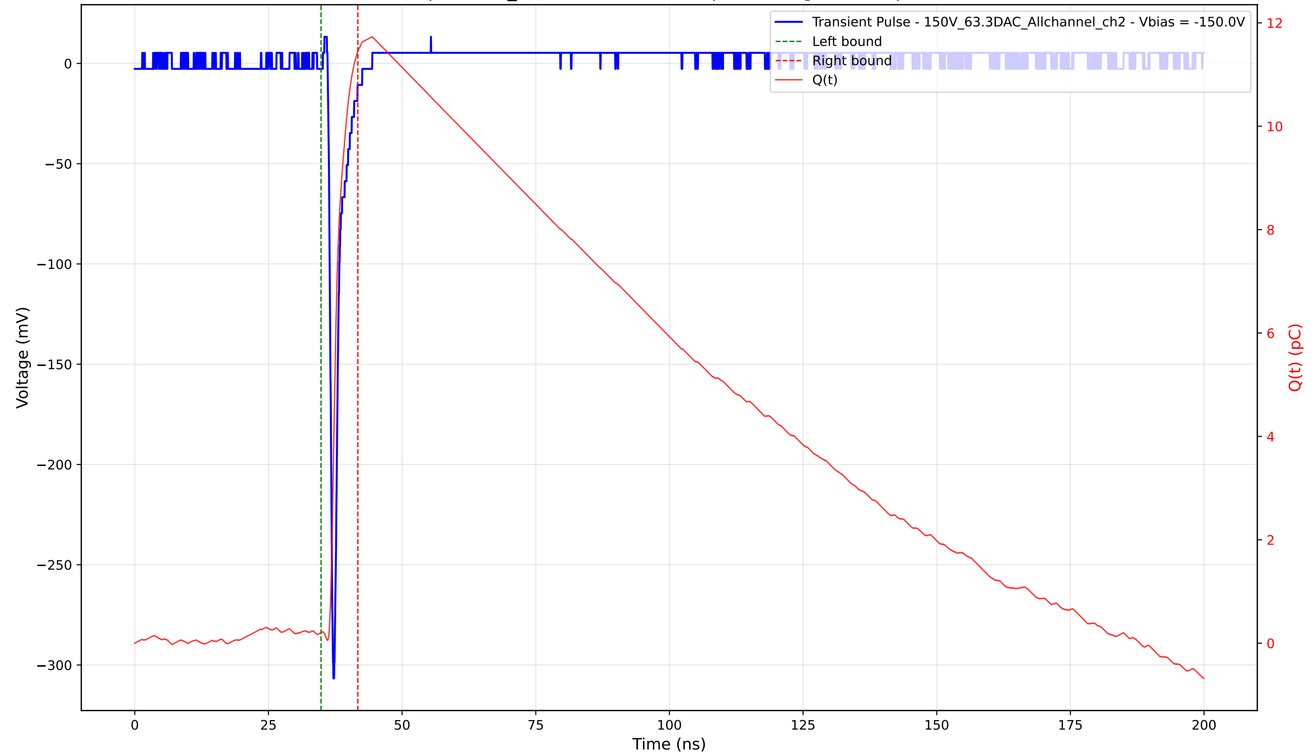
Transient Pulse - Sample: 1cm_42 - Position: 3415.0 \mu\text{m} - Charge: 11.25 pC - Rise Time: 0.75 ns
