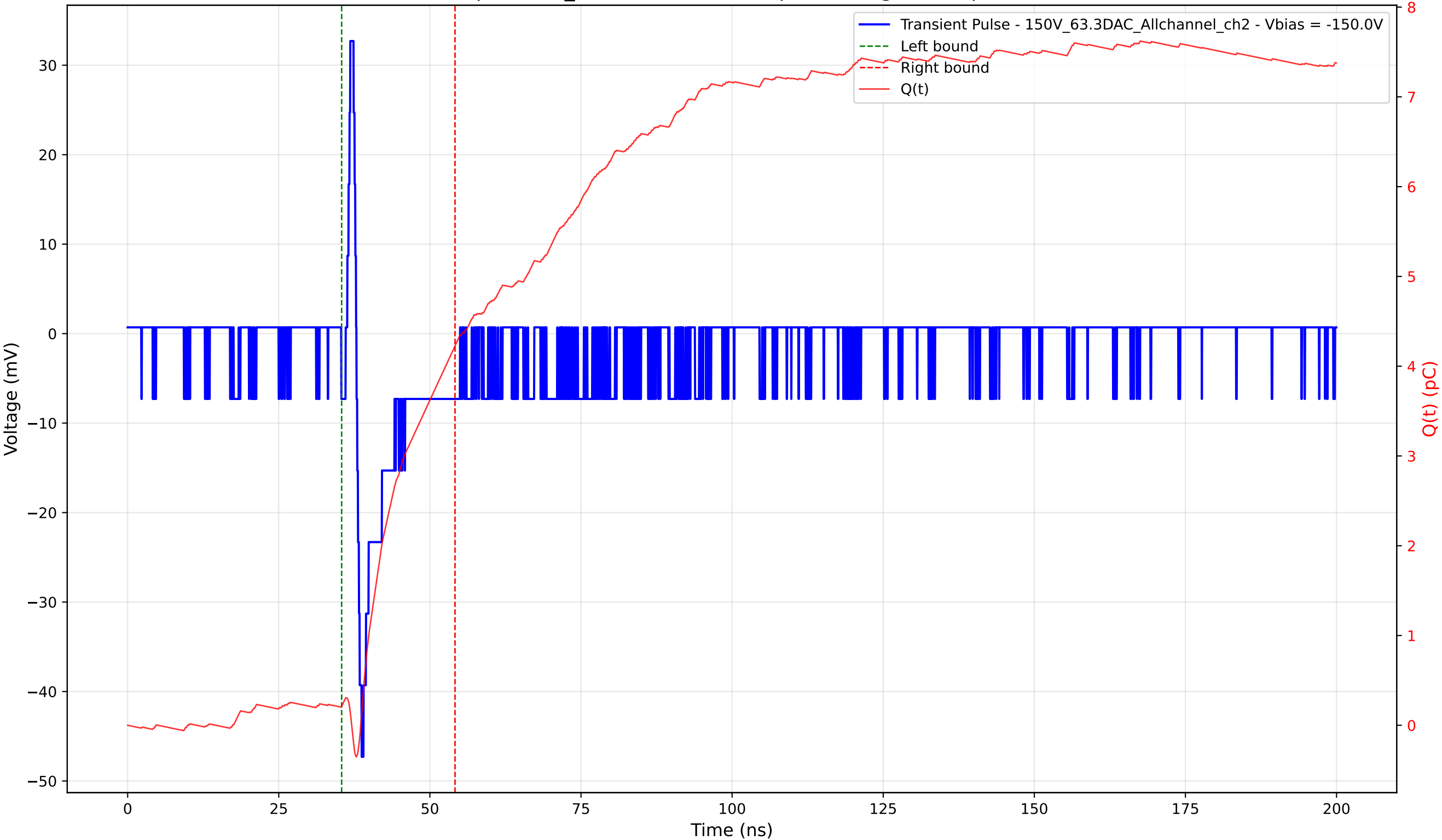
Transient Pulse - Sample: 1cm_42 - Position: 830.0 \mu\text{m} - Charge: 4.02 pC - Rise Time: 0.86 ns
