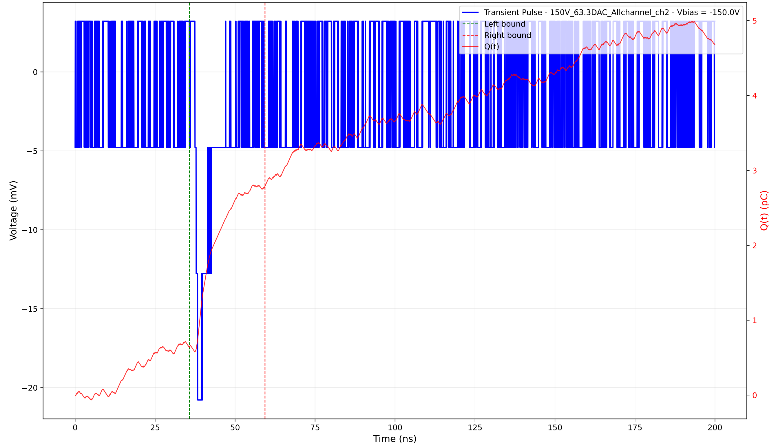
Transient Pulse - Sample: 1cm_42 - Position: 5010.0 \mu\text{m} - Charge: 2.15 pC - Rise Time: 0.00 ns (N/A)
