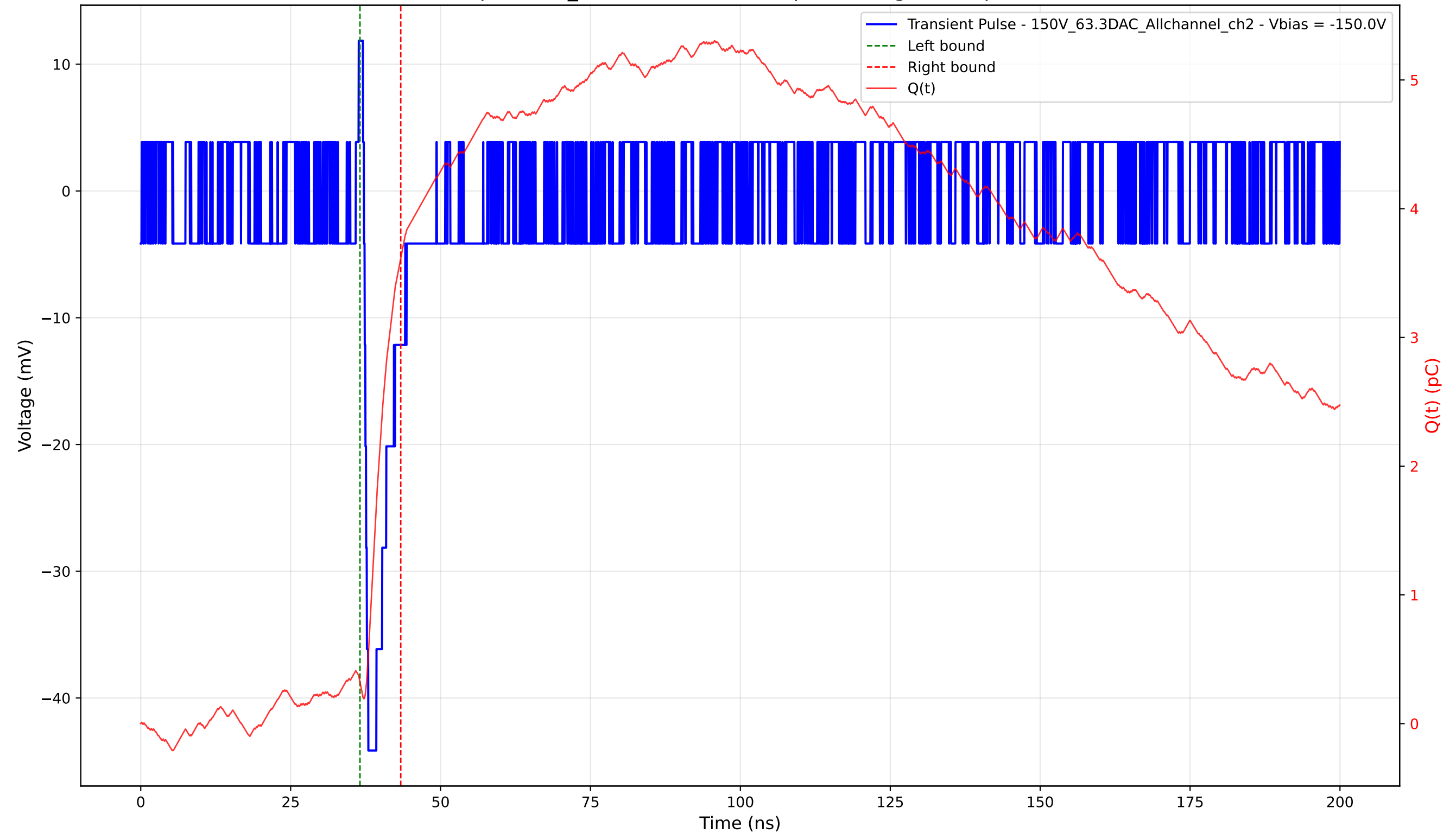
Transient Pulse - Sample: 1cm_42 - Position: 4415.0 \mu\text{m} - Charge: 3.29 pC - Rise Time: 0.64 ns
