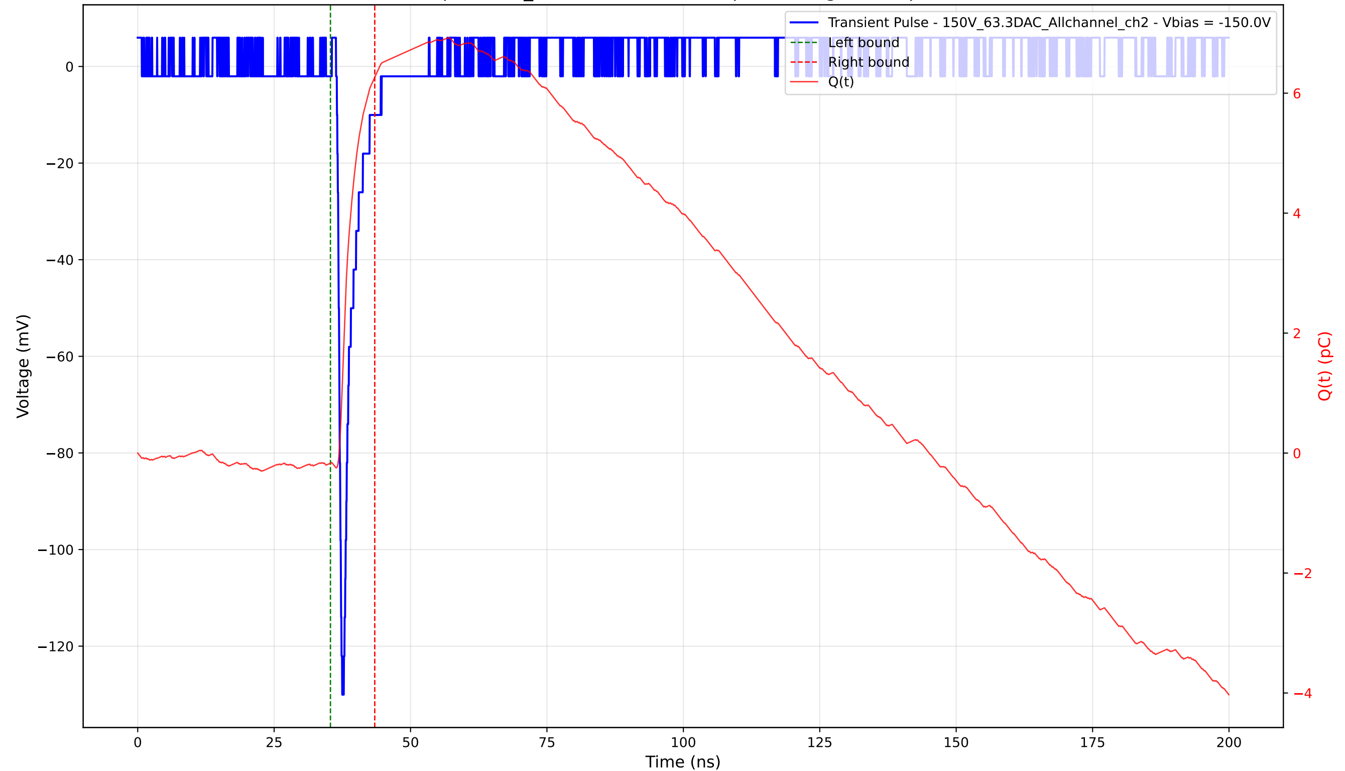
Transient Pulse - Sample: 1cm_42 - Position: 2235.0 \mu\text{m} - Charge: 6.43 pC - Rise Time: 0.79 ns
