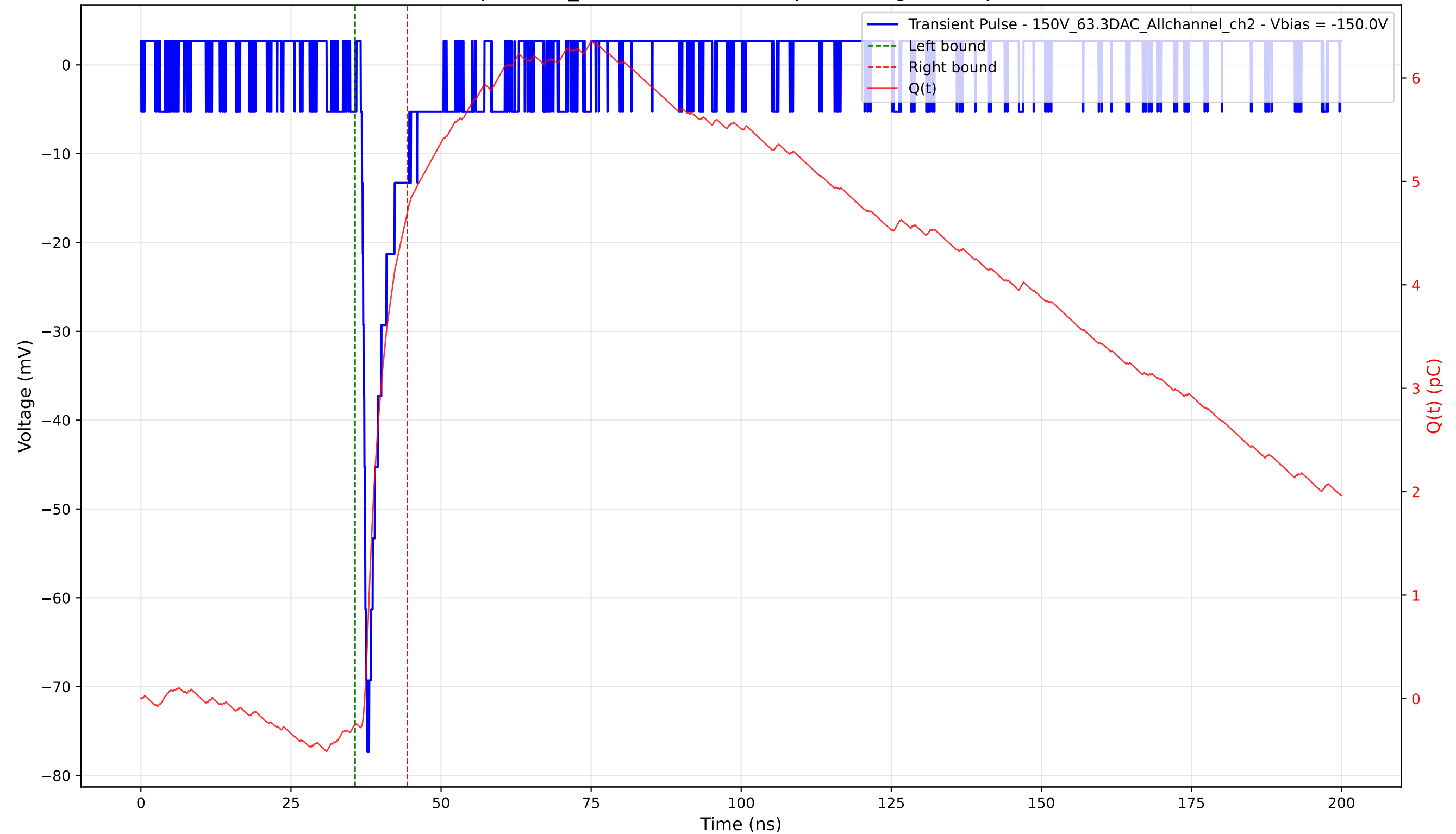
Transient Pulse - Sample: 1cm_42 - Position: 2030.0 \mu\text{m} - Charge: 4.95 pC - Rise Time: 0.91 ns
