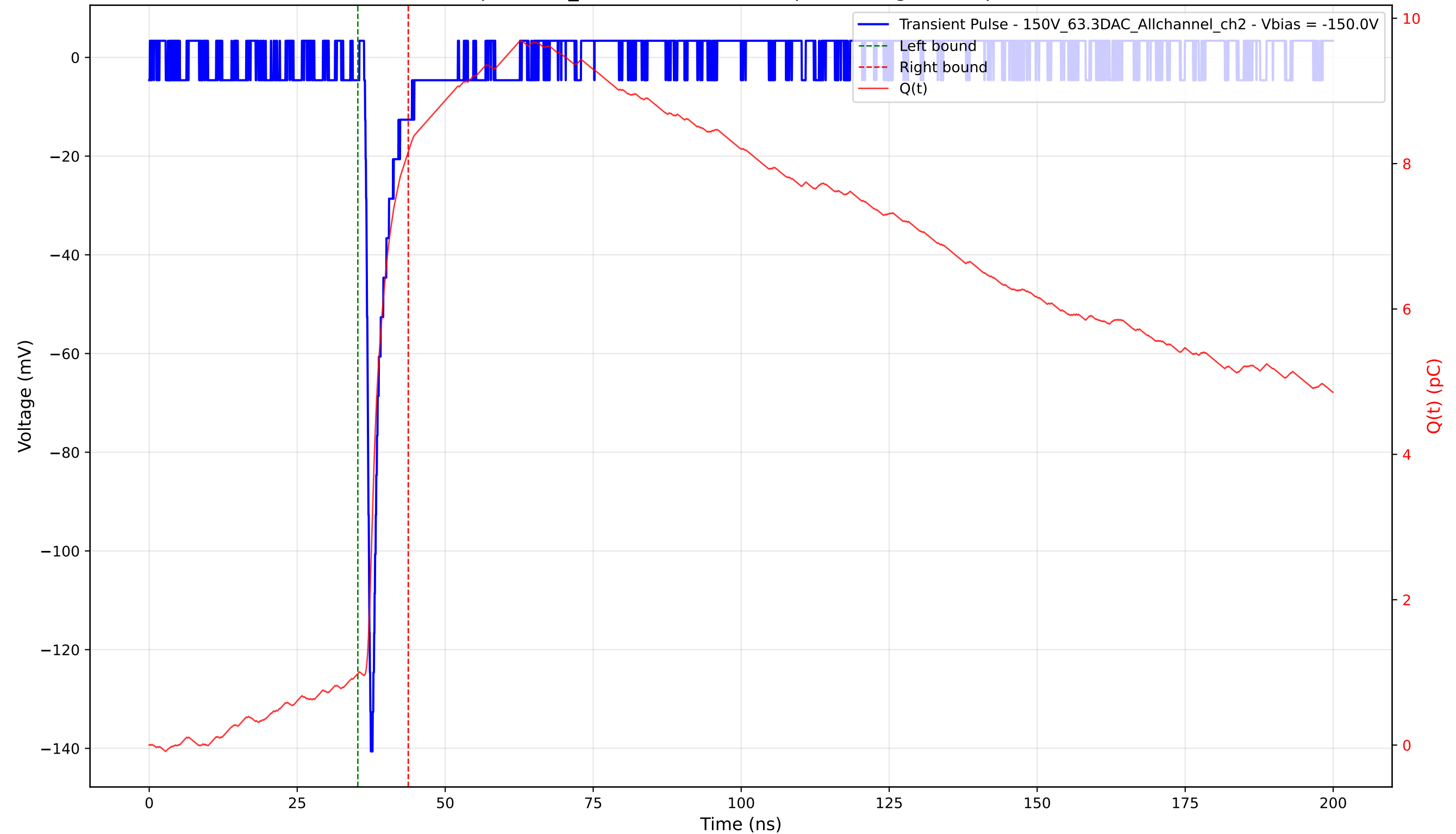
Transient Pulse - Sample: 1cm_42 - Position: 2275.0 \mu\text{m} - Charge: 7.18 pC - Rise Time: 0.83 ns
