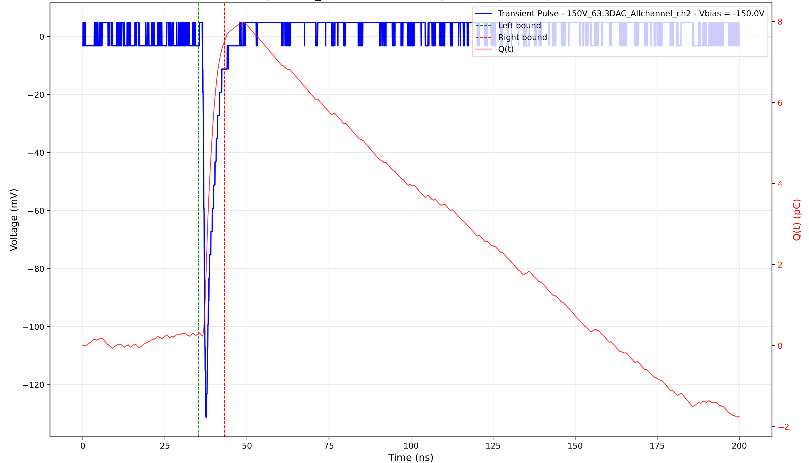
Transient Pulse - Sample: 1cm_42 - Position: 3785.0 \mu\text{m} - Charge: 7.19 pC - Rise Time: 0.79 ns
