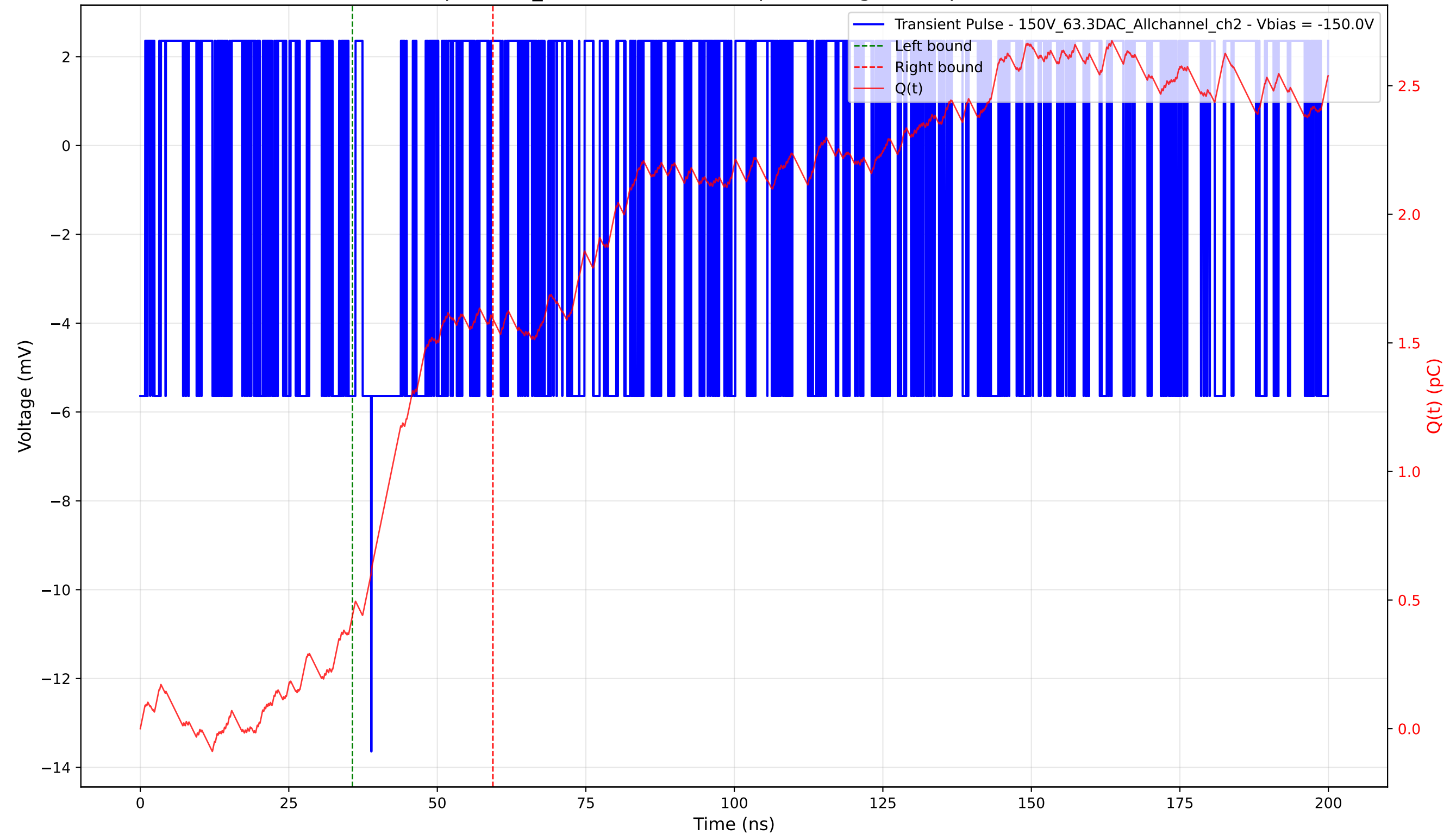
Transient Pulse - Sample: 1cm_42 - Position: 5135.0 \mu\text{m} - Charge: 1.16 pC - Rise Time: 0.00 ns (N/A)
