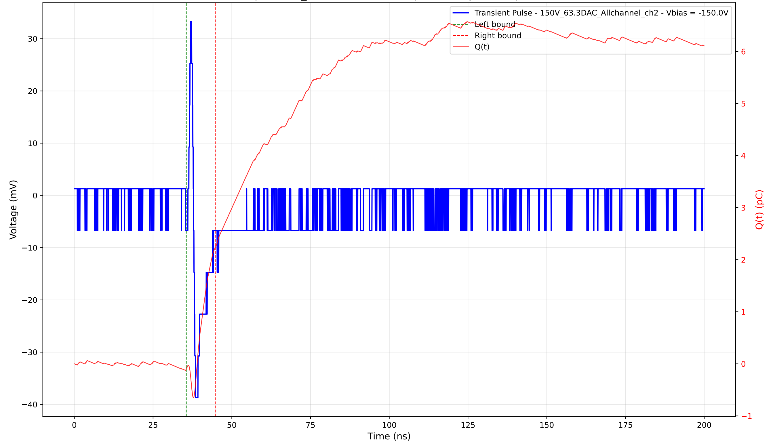
Transient Pulse - Sample: 1cm_42 - Position: 960.0 \mu\text{m} - Charge: 2.33 pC - Rise Time: 0.66 ns
