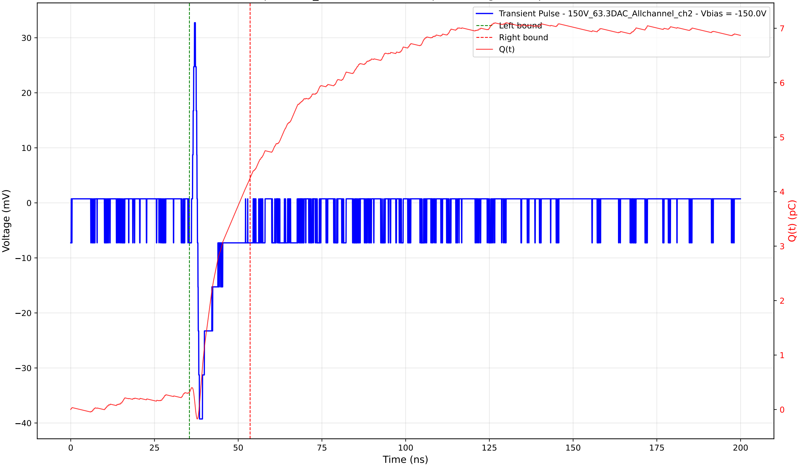
Transient Pulse - Sample: 1cm_42 - Position: 640.0 \mu\text{m} - Charge: 3.94 pC - Rise Time: 0.62 ns
