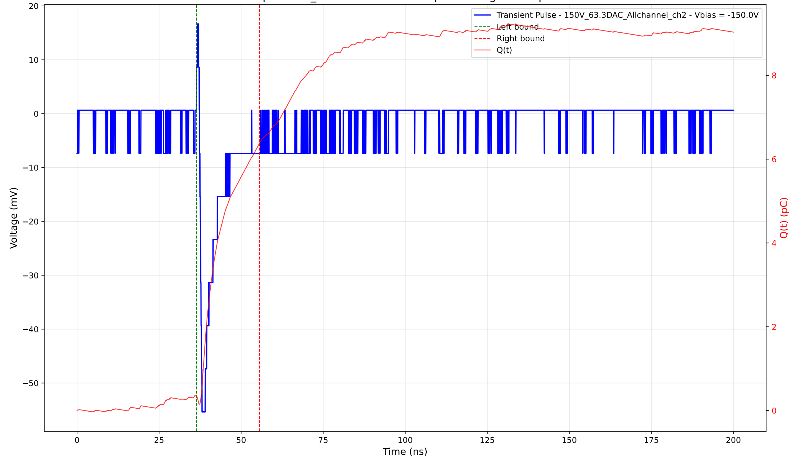
Transient Pulse - Sample: 1cm_42 - Position: 1675.0 \mu\text{m} - Charge: 6.02 pC - Rise Time: 0.73 ns
