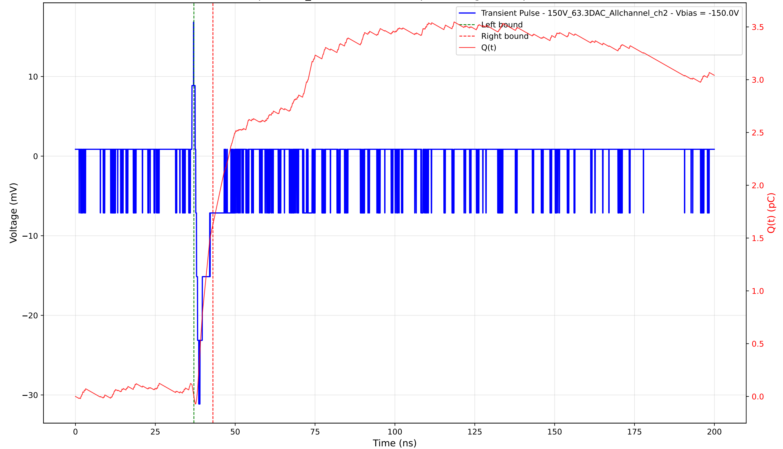
Transient Pulse - Sample: 1cm_42 - Position: 330.0 \mu\text{m} - Charge: 1.63 pC - Rise Time: 0.99 ns
