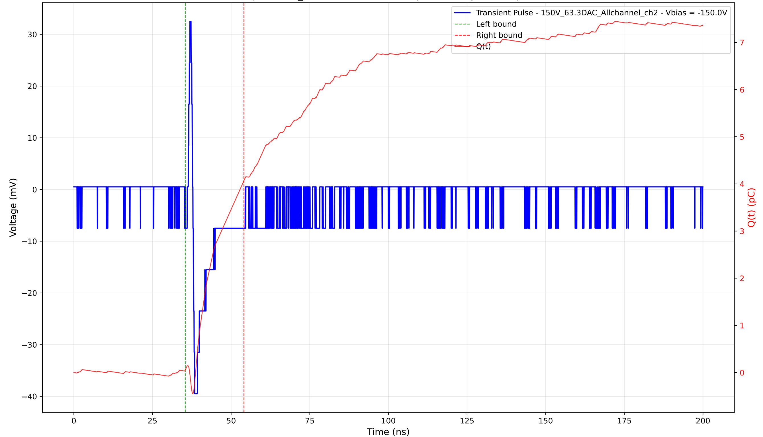
Transient Pulse - Sample: 1cm_42 - Position: 1065.0 \mu\text{m} - Charge: 4.02 pC - Rise Time: 0.58 ns
