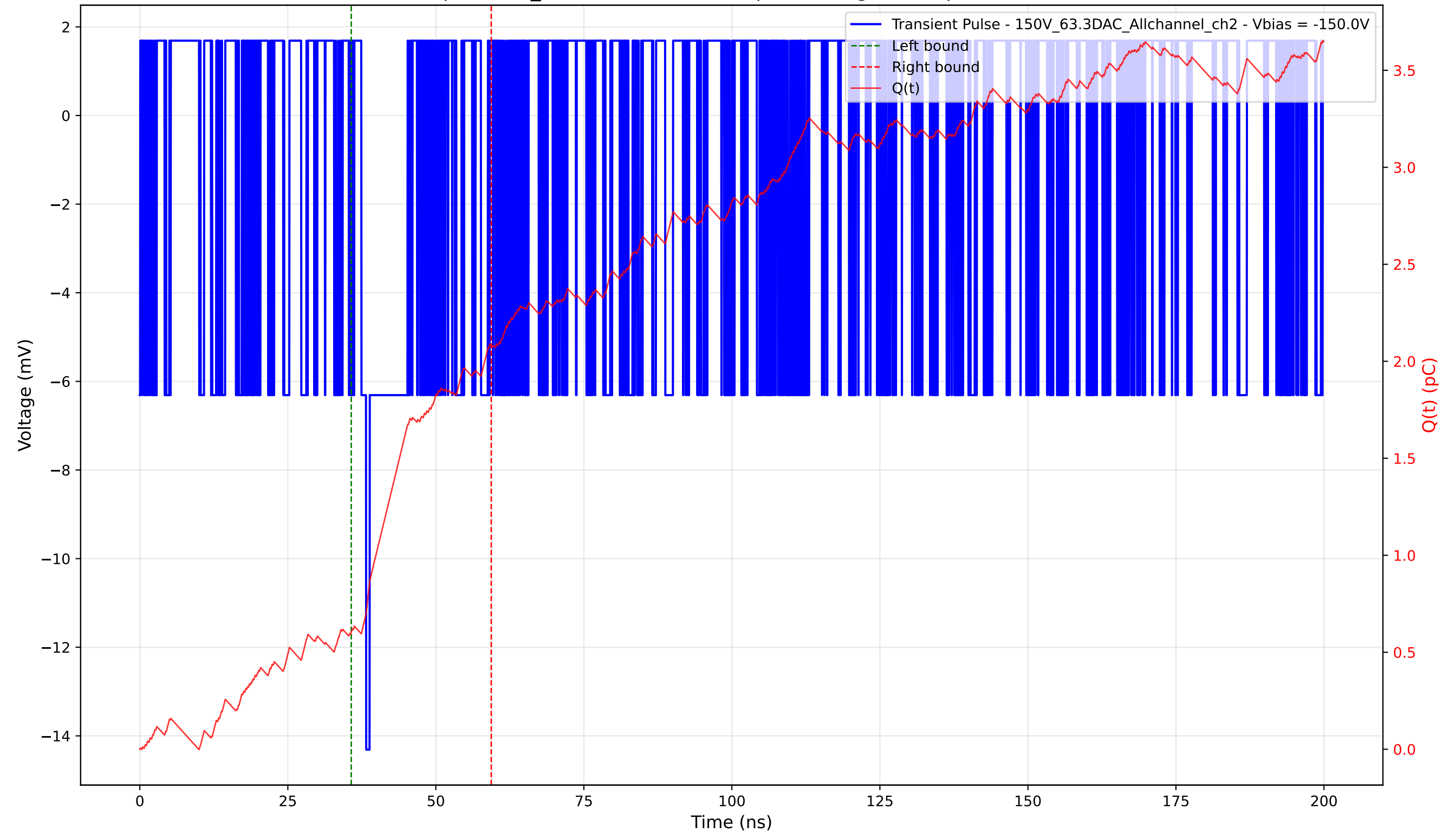
Transient Pulse - Sample: 1cm_42 - Position: 5120.0 \mu\text{m} - Charge: 1.48 pC - Rise Time: 0.00 ns (N/A)
