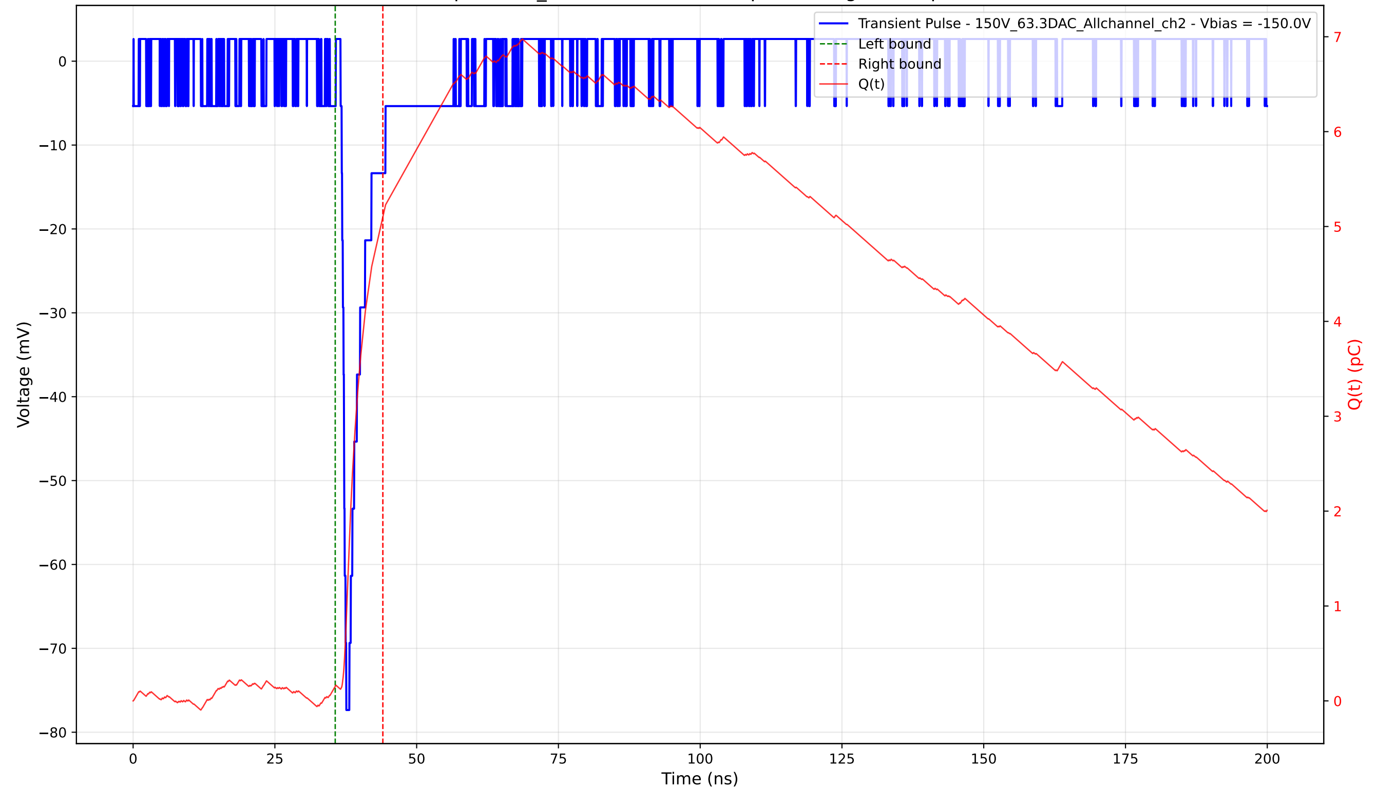
Transient Pulse - Sample: 1cm_42 - Position: 2050.0 \mu\text{m} - Charge: 4.95 pC - Rise Time: 0.83 ns
