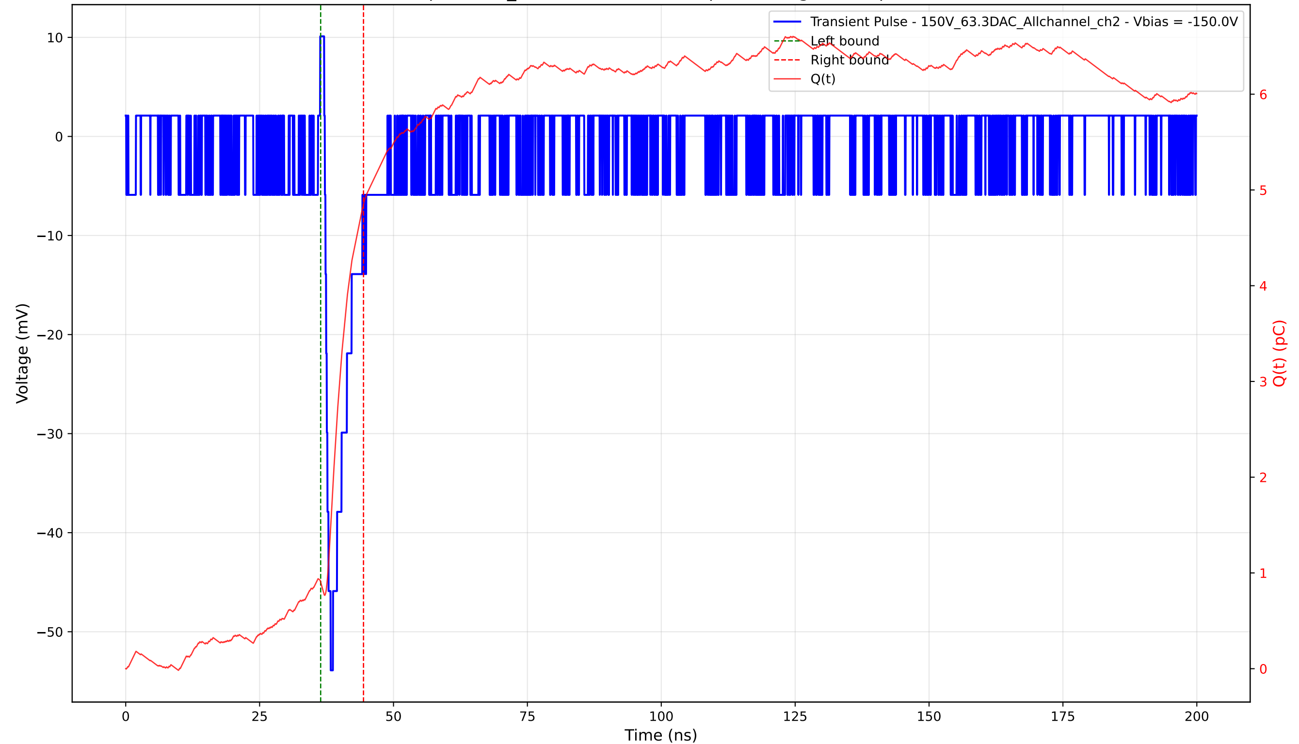
Transient Pulse - Sample: 1cm_42 - Position: 4380.0 \mu\text{m} - Charge: 3.94 pC - Rise Time: 1.09 ns
