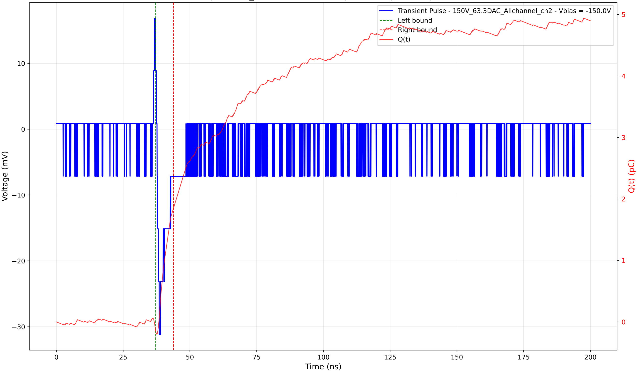
Transient Pulse - Sample: 1cm_42 - Position: 375.0 \mu\text{m} - Charge: 1.96 pC - Rise Time: 0.83 ns
