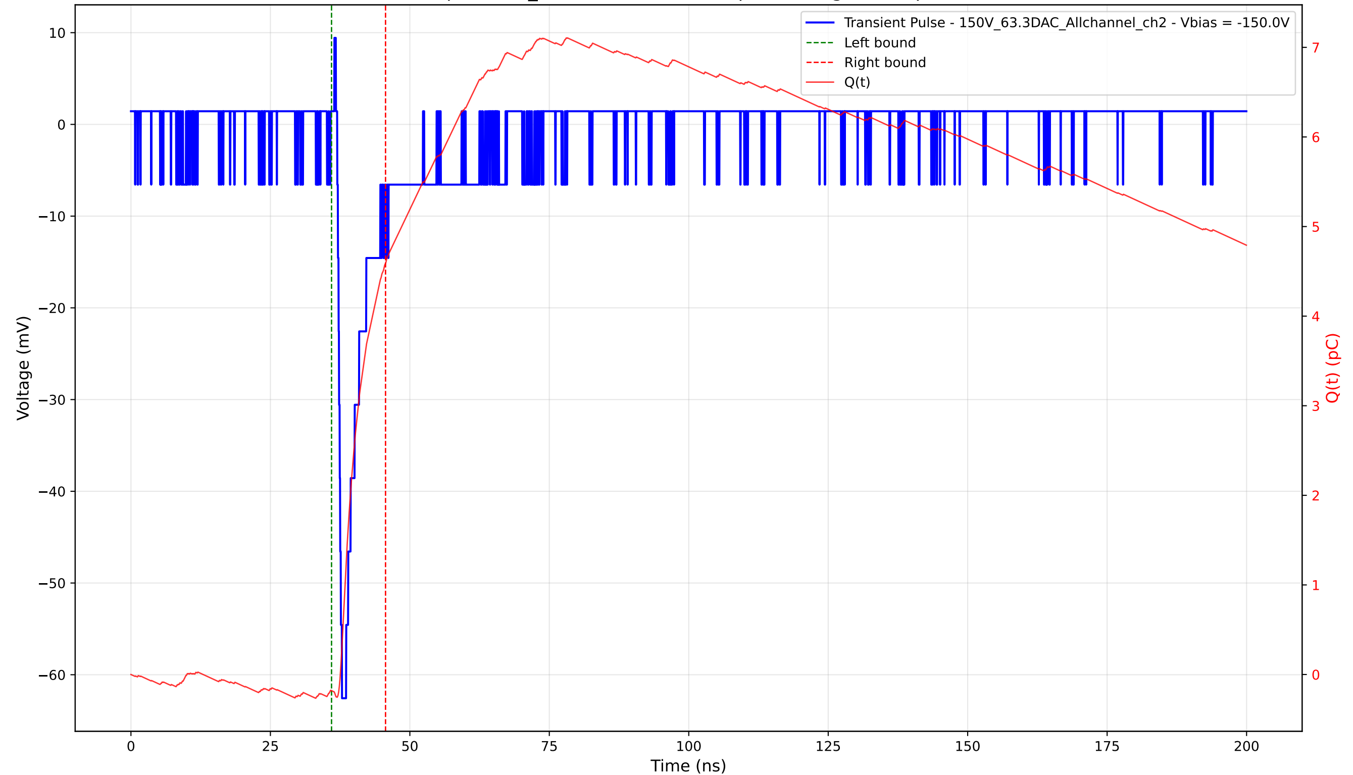
Transient Pulse - Sample: 1cm_42 - Position: 1925.0 \mu\text{m} - Charge: 4.77 pC - Rise Time: 0.84 ns
