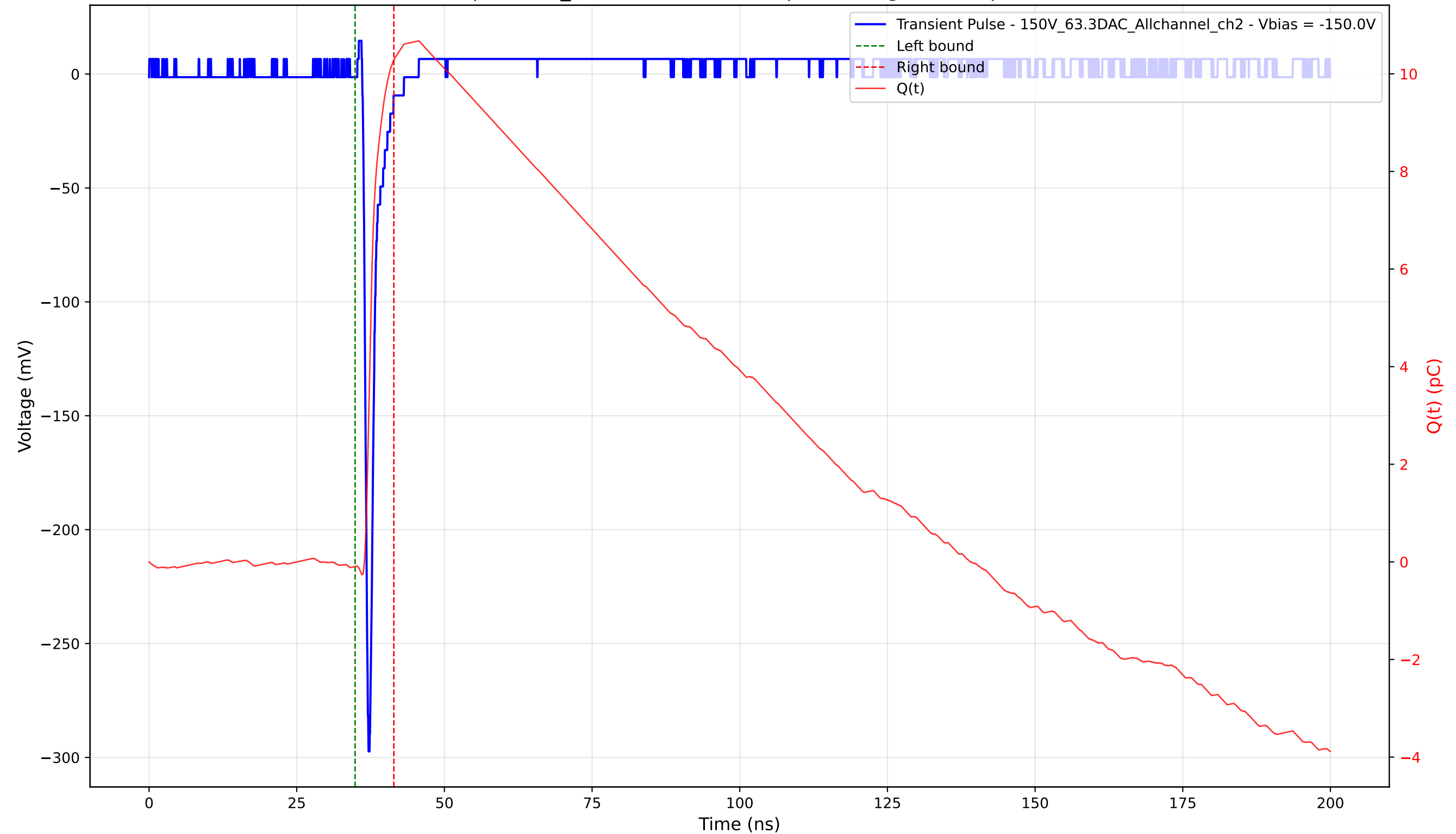
Transient Pulse - Sample: 1cm_42 - Position: 2620.0 \mu\text{m} - Charge: 10.38 pC - Rise Time: 0.78 ns
