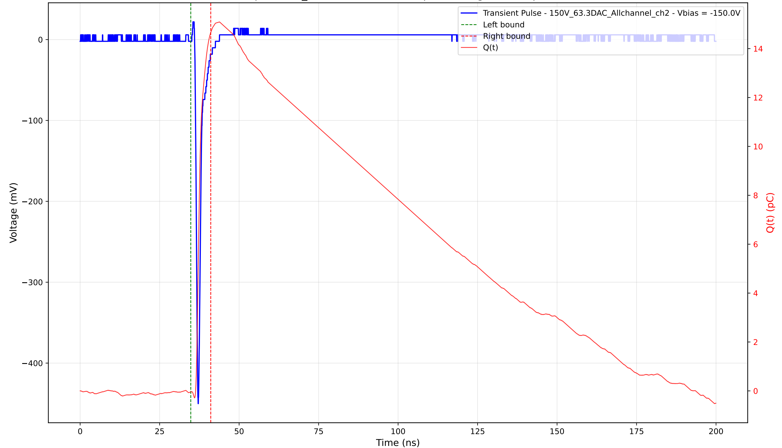
Transient Pulse - Sample: 1cm_42 - Position: 3245.0 \mu\text{m} - Charge: 14.71 pC - Rise Time: 0.74 ns
