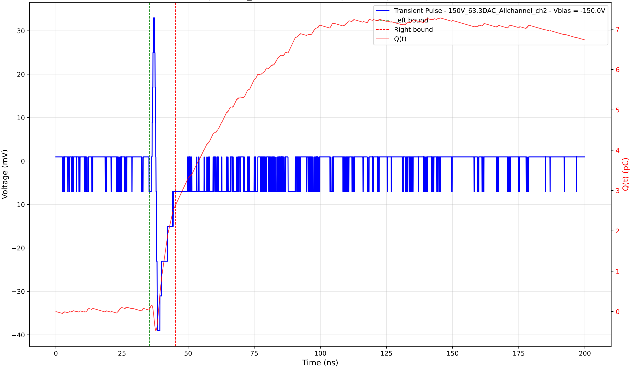
Transient Pulse - Sample: 1cm_42 - Position: 915.0 \mu\text{m} - Charge: 2.56 pC - Rise Time: 0.66 ns
