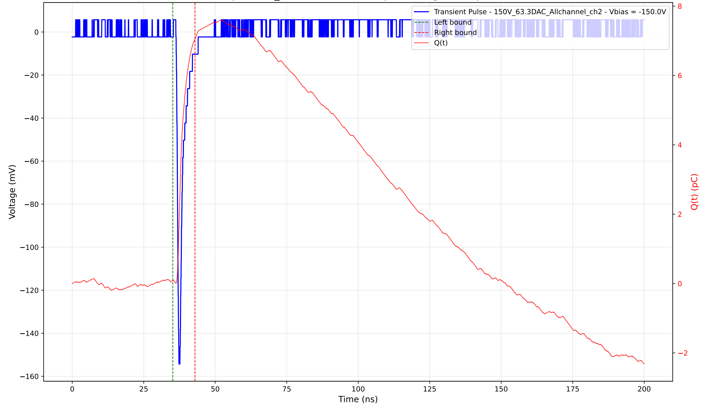
Transient Pulse - Sample: 1cm_42 - Position: 2410.0 \mu\text{m} - Charge: 6.96 pC - Rise Time: 0.81 ns
