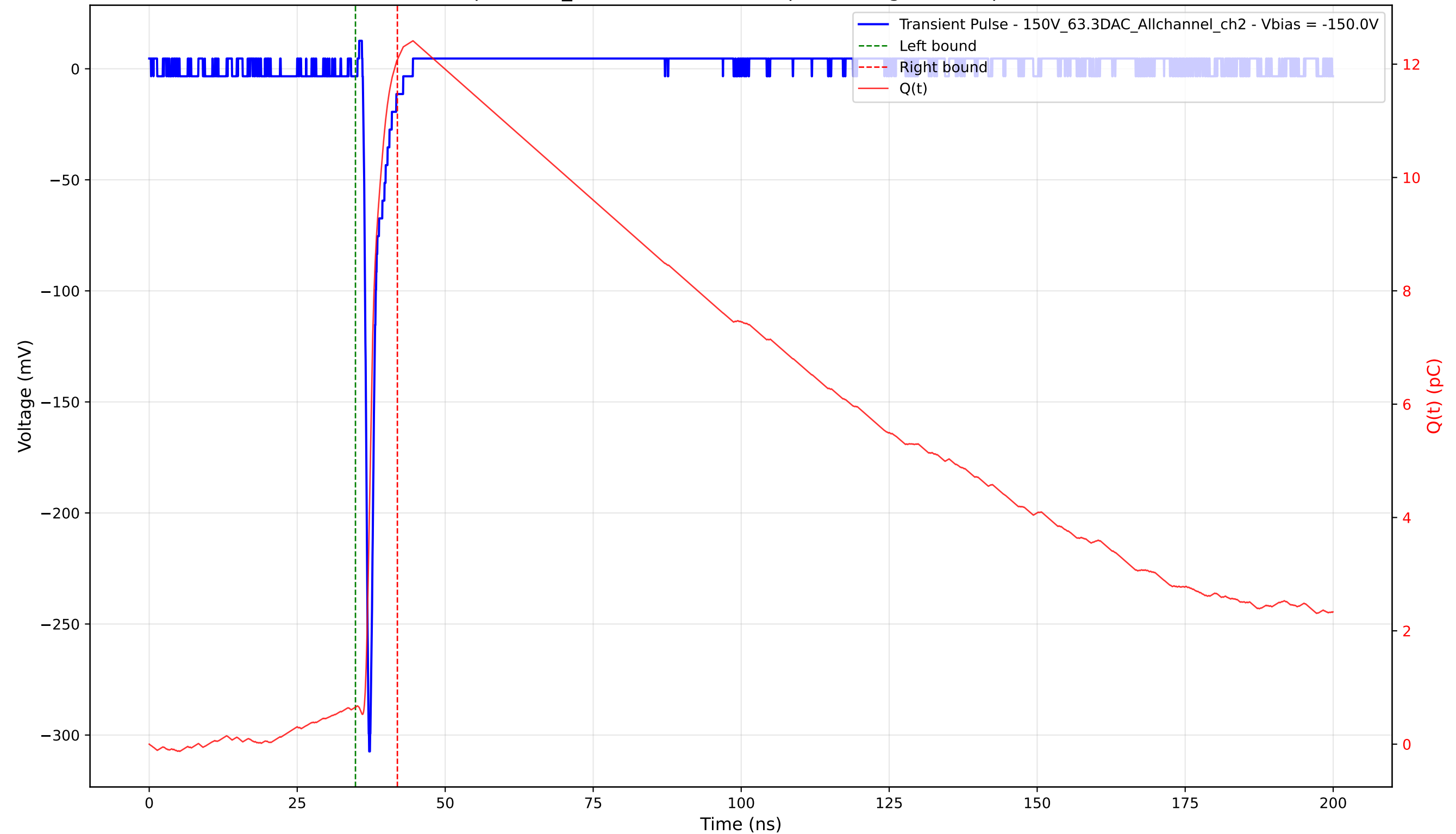
Transient Pulse - Sample: 1cm_42 - Position: 3420.0 \mu\text{m} - Charge: 11.43 pC - Rise Time: 0.75 ns
