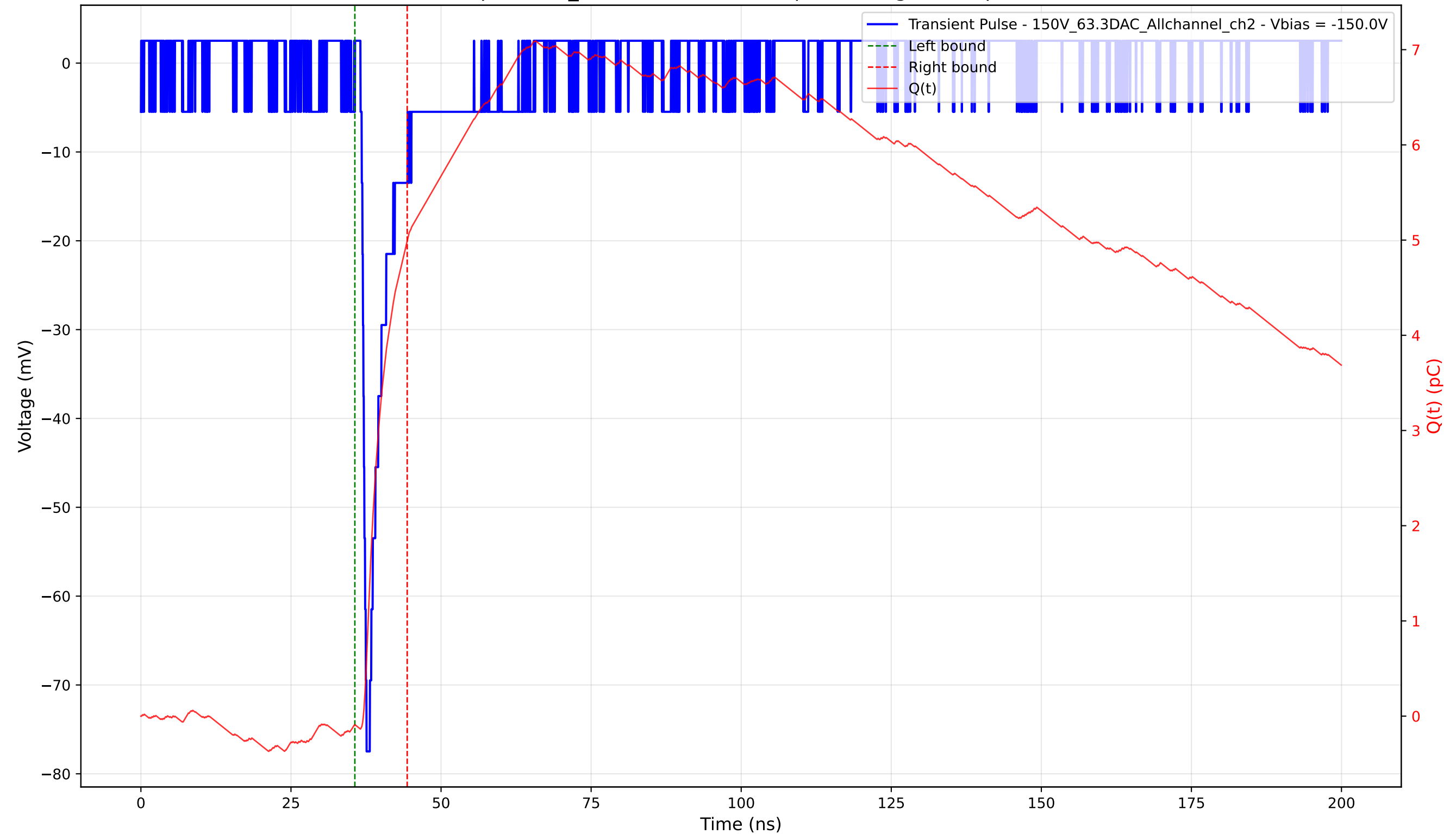
Transient Pulse - Sample: 1cm_42 - Position: 2040.0 \mu\text{m} - Charge: 5.09 pC - Rise Time: 0.83 ns
