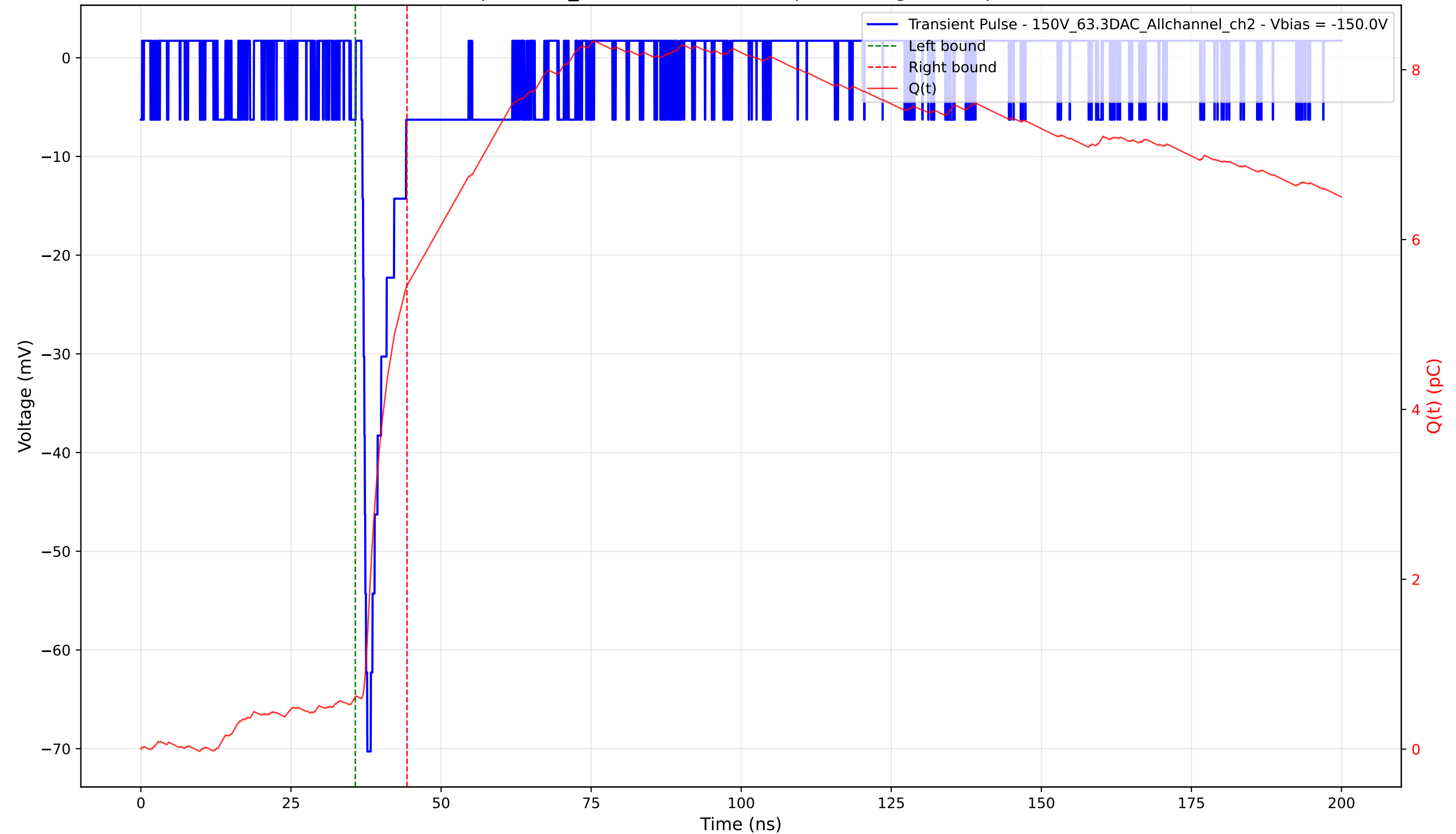
Transient Pulse - Sample: 1cm_42 - Position: 2000.0 \mu\text{m} - Charge: 4.84 pC - Rise Time: 0.84 ns
