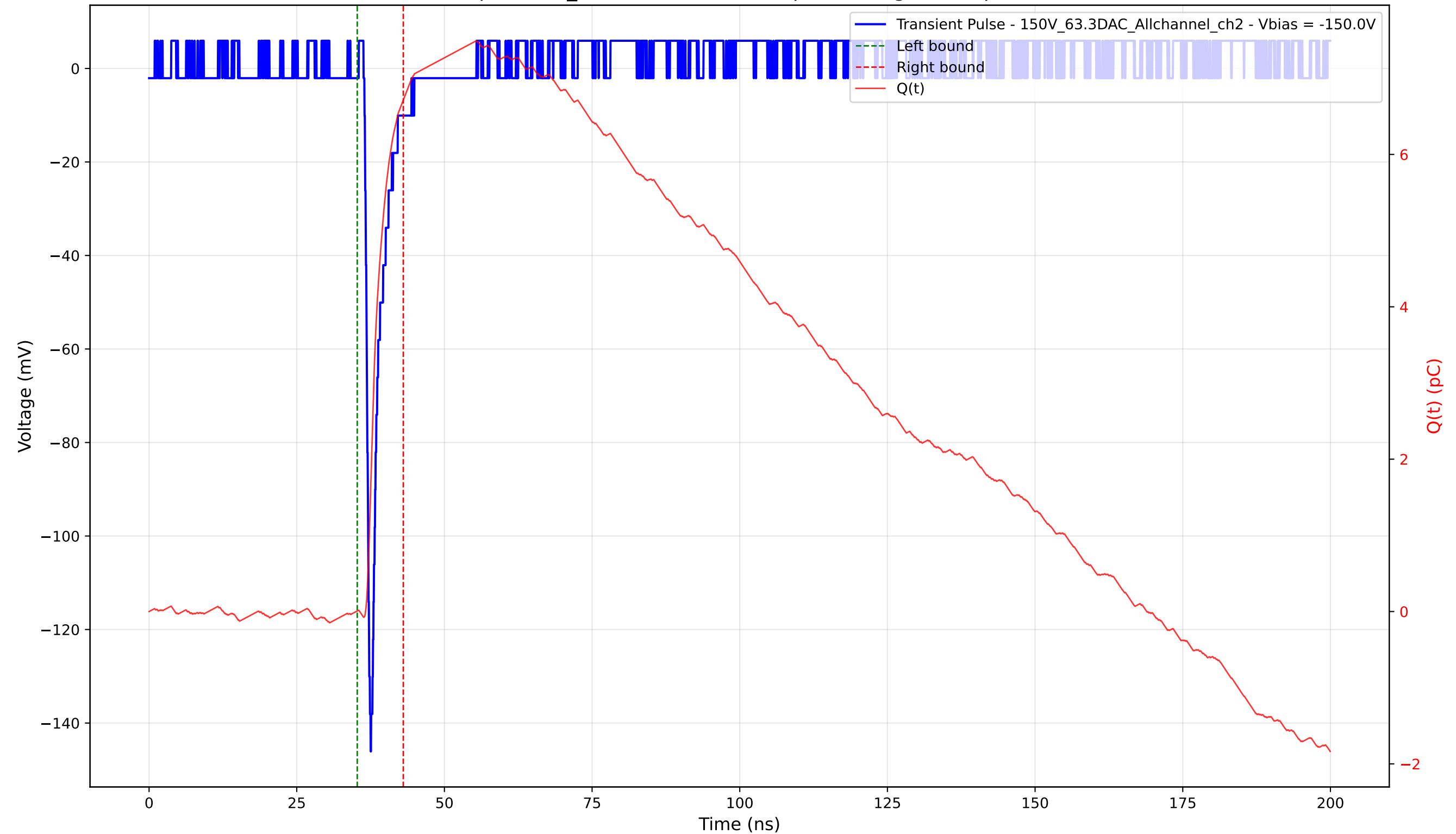
Transient Pulse - Sample: 1cm_42 - Position: 2315.0 \mu\text{m} - Charge: 6.71 pC - Rise Time: 0.86 ns
