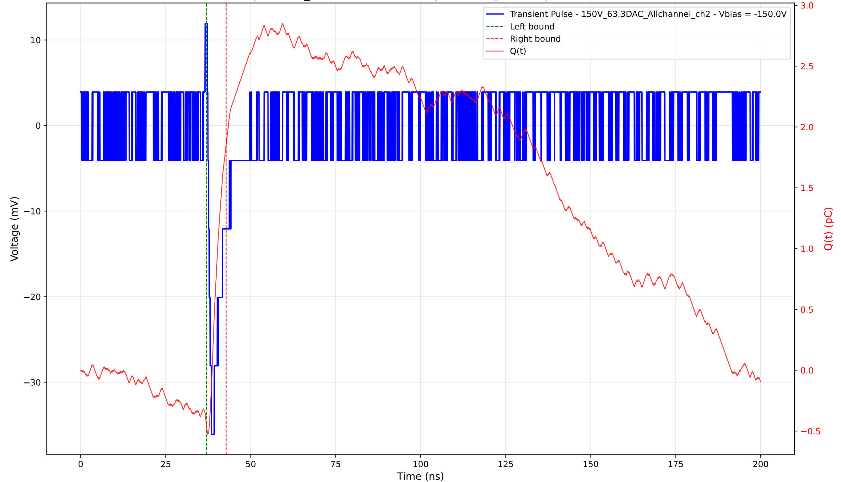
Transient Pulse - Sample: 1cm_42 - Position: 4855.0 \mu\text{m} - Charge: 2.30 pC - Rise Time: 0.00 ns (N/A)
