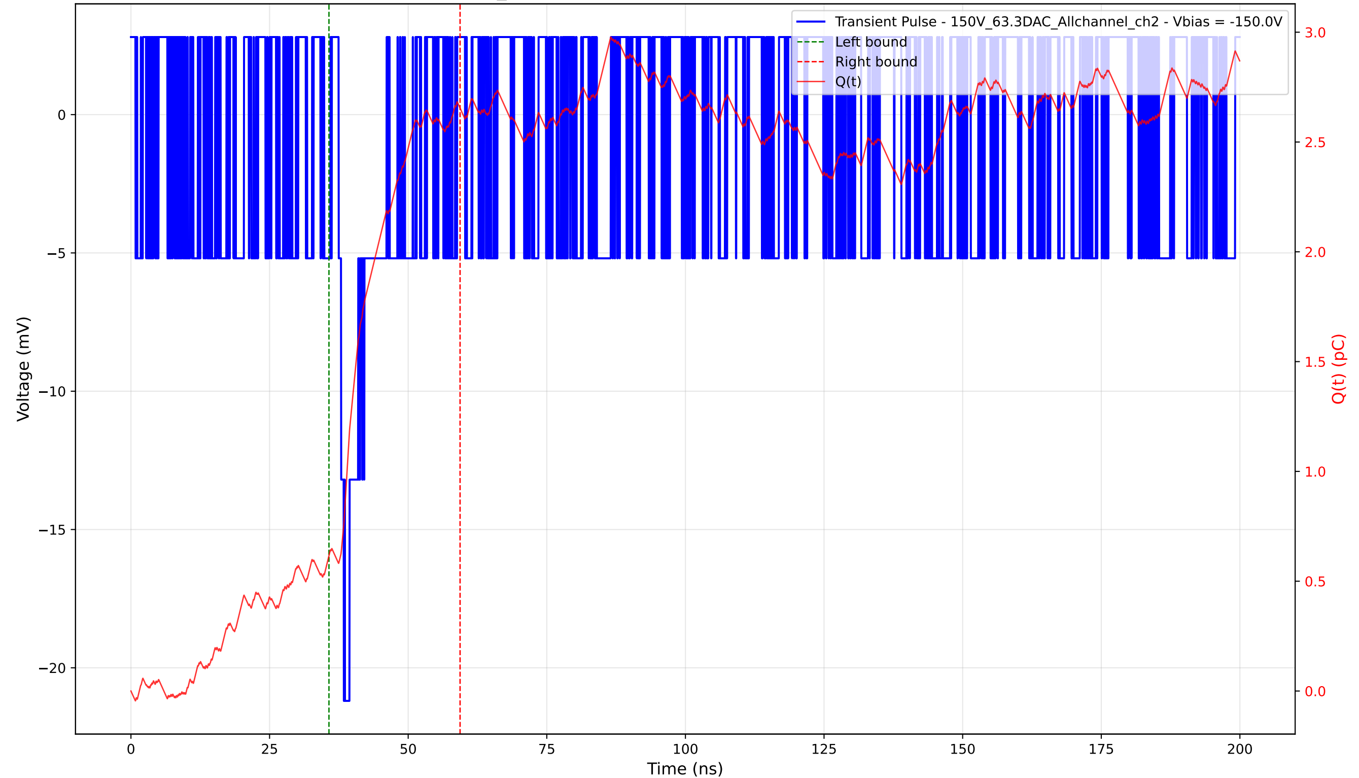
Transient Pulse - Sample: 1cm_42 - Position: 5020.0 \mu\text{m} - Charge: 2.04 pC - Rise Time: 0.00 ns (N/A)
