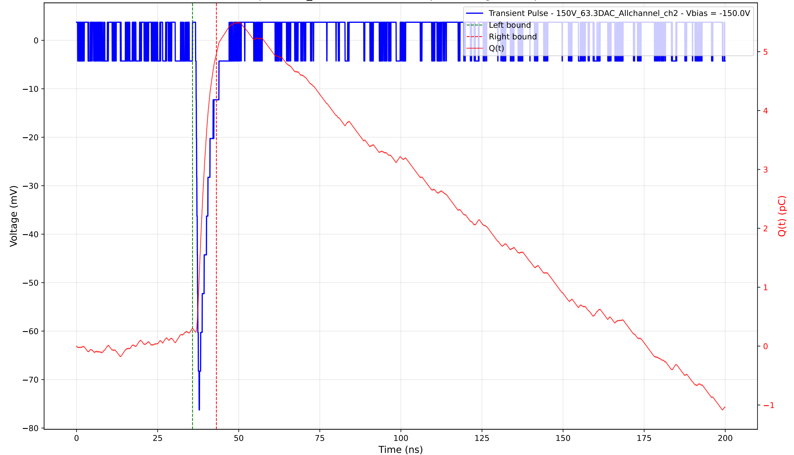
Transient Pulse - Sample: 1cm_42 - Position: 4015.0 \mu\text{m} - Charge: 4.66 pC - Rise Time: 0.94 ns
