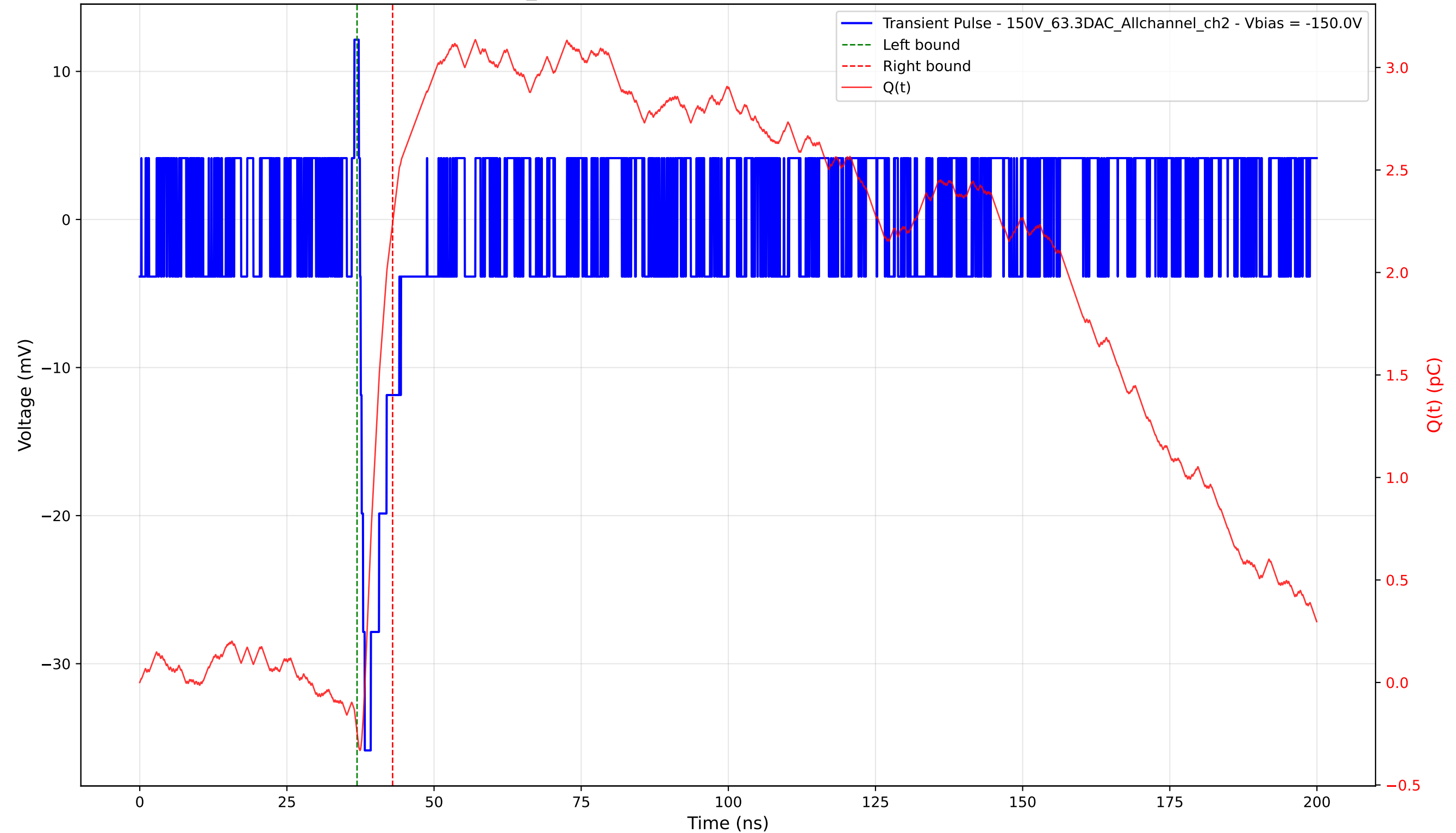
Transient Pulse - Sample: 1cm_42 - Position: 4645.0 \mu\text{m} - Charge: 2.49 pC - Rise Time: 0.00 ns (N/A)
