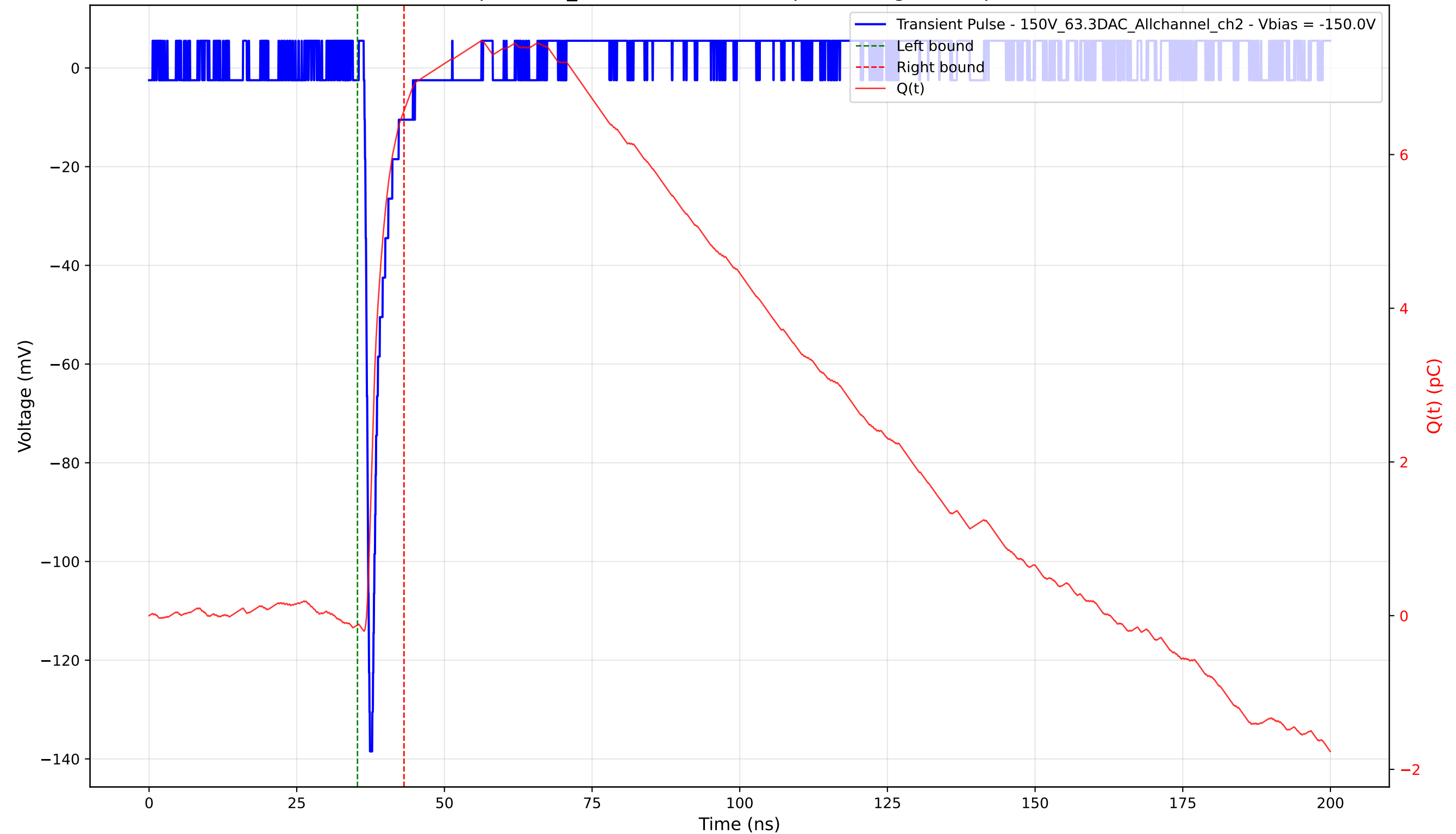
Transient Pulse - Sample: 1cm_42 - Position: 2310.0 \mu\text{m} - Charge: 6.69 pC - Rise Time: 0.78 ns
