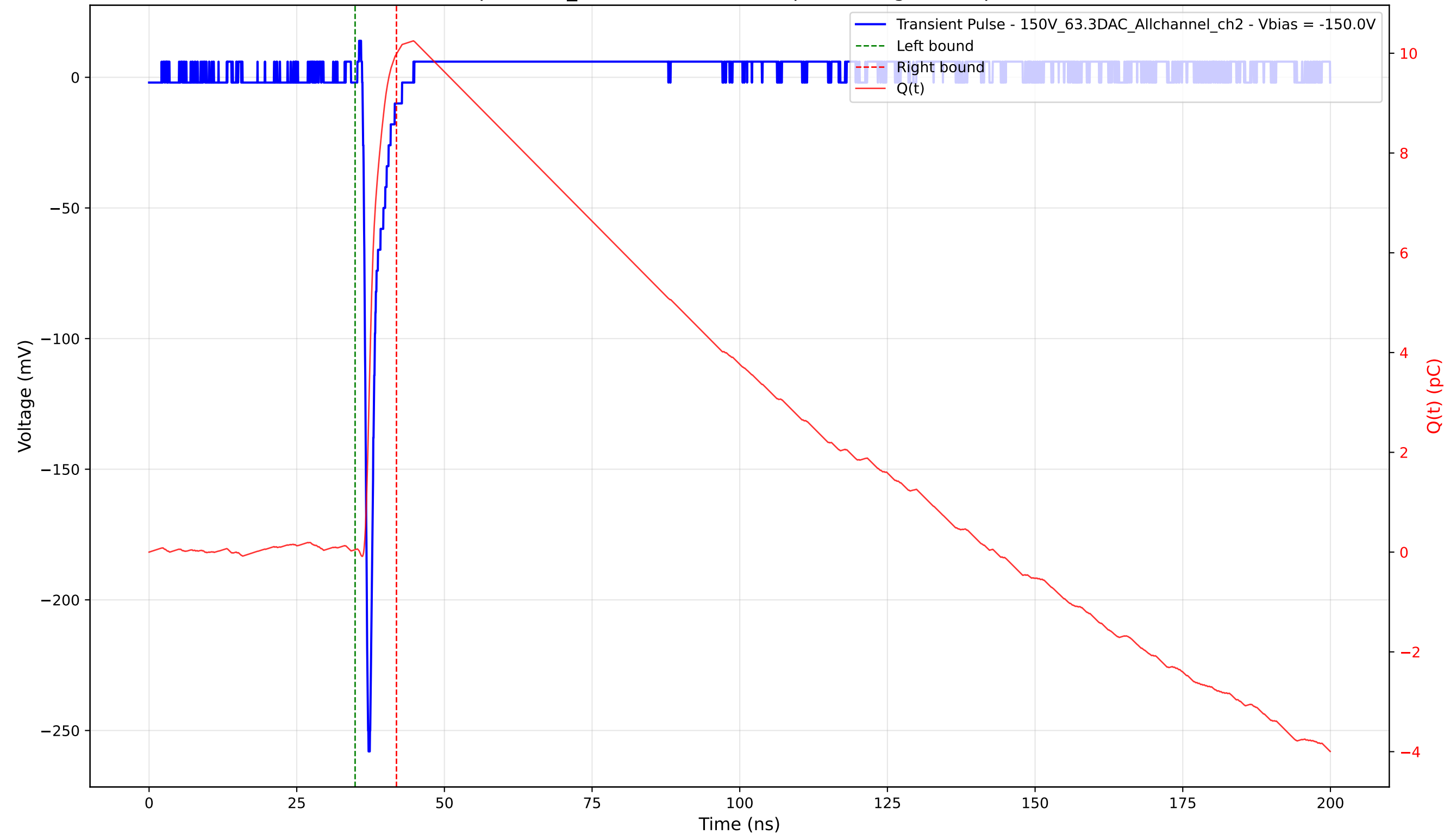
Transient Pulse - Sample: 1cm_42 - Position: 3460.0 \mu\text{m} - Charge: 9.94 pC - Rise Time: 0.75 ns
