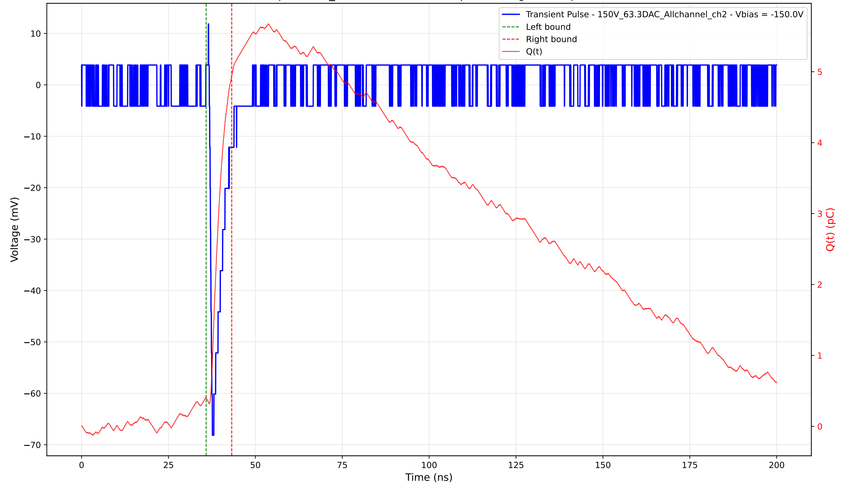
Transient Pulse - Sample: 1cm_42 - Position: 4035.0 \mu\text{m} - Charge: 4.55 pC - Rise Time: 0.79 ns
