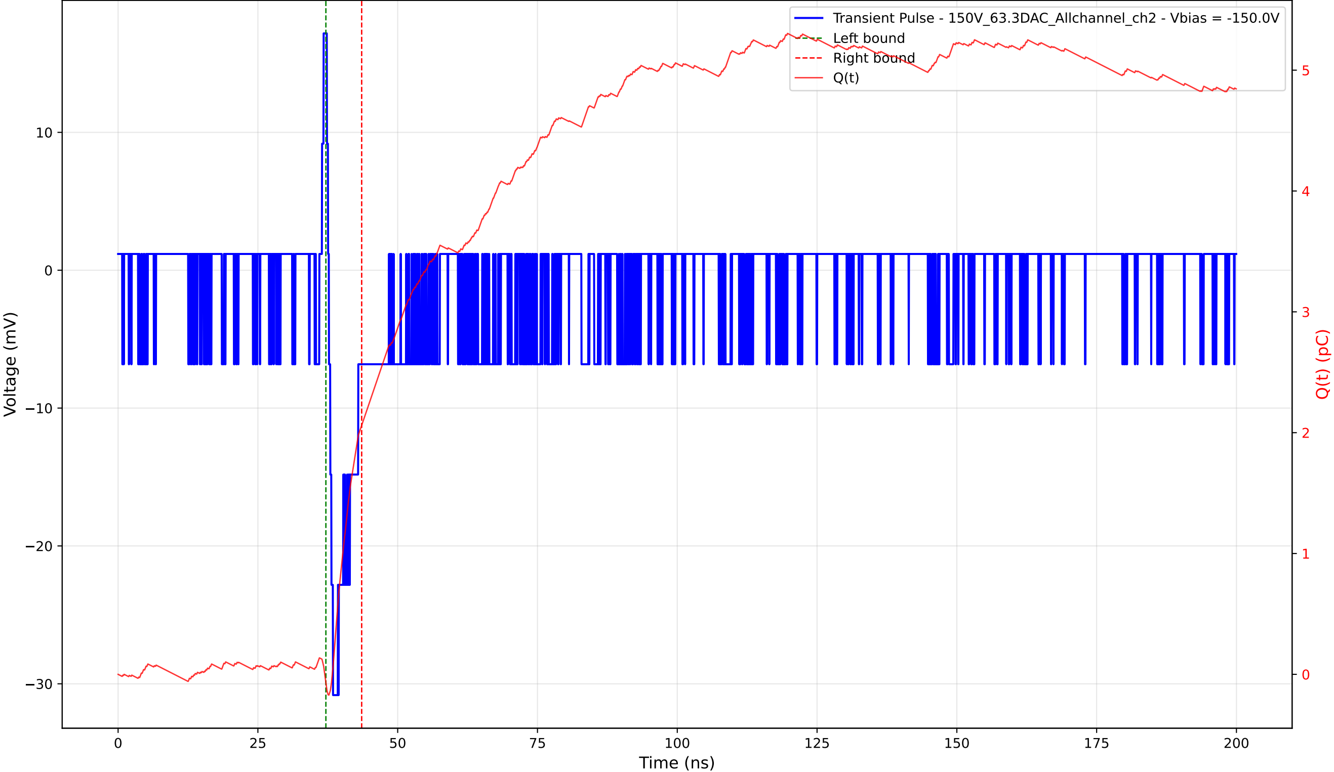
Transient Pulse - Sample: 1cm_42 - Position: 430.0 \mu\text{m} - Charge: 2.13 pC - Rise Time: 0.75 ns
