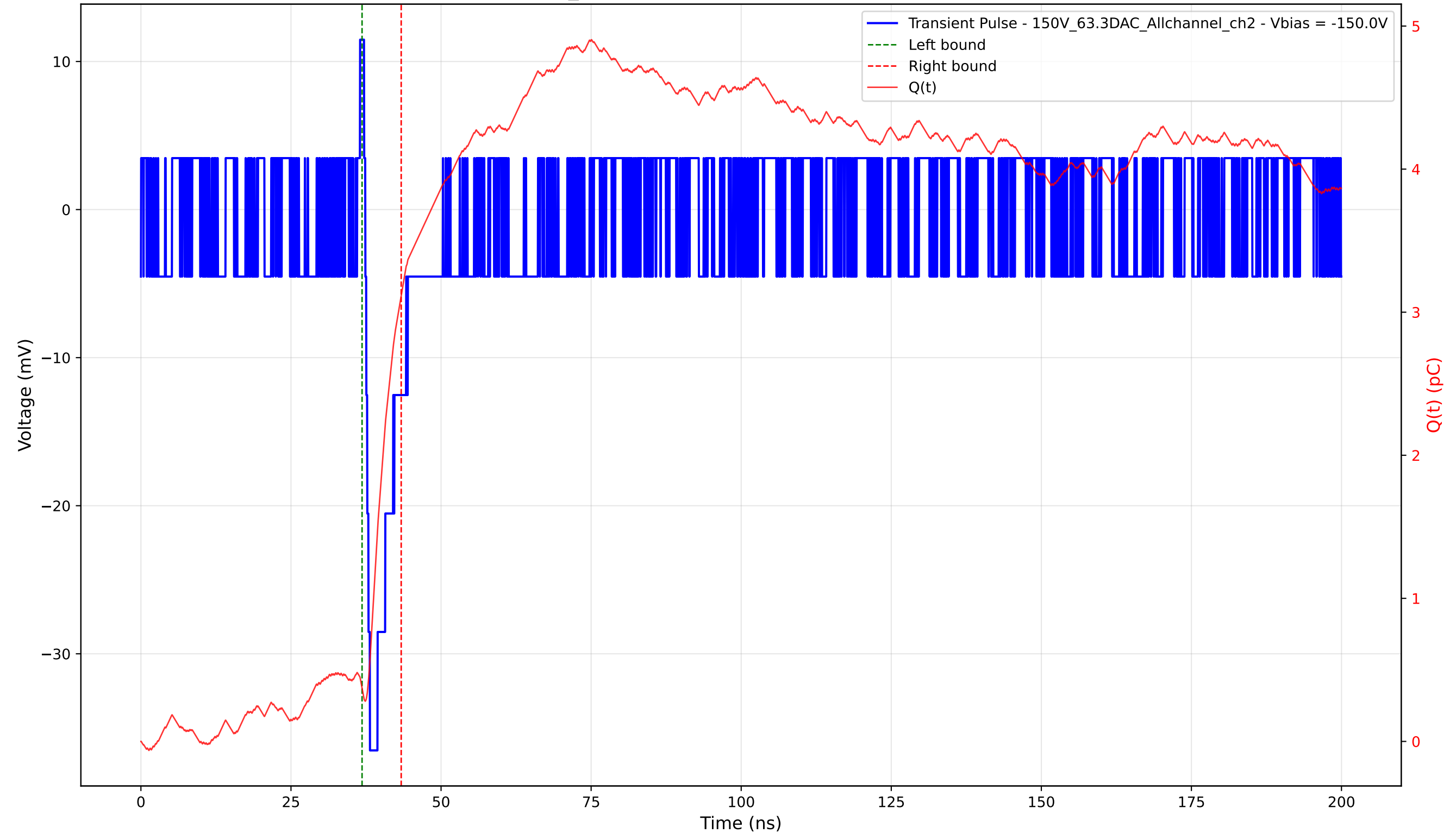
Transient Pulse - Sample: 1cm_42 - Position: 4670.0 \mu\text{m} - Charge: 2.74 pC - Rise Time: 0.79 ns
