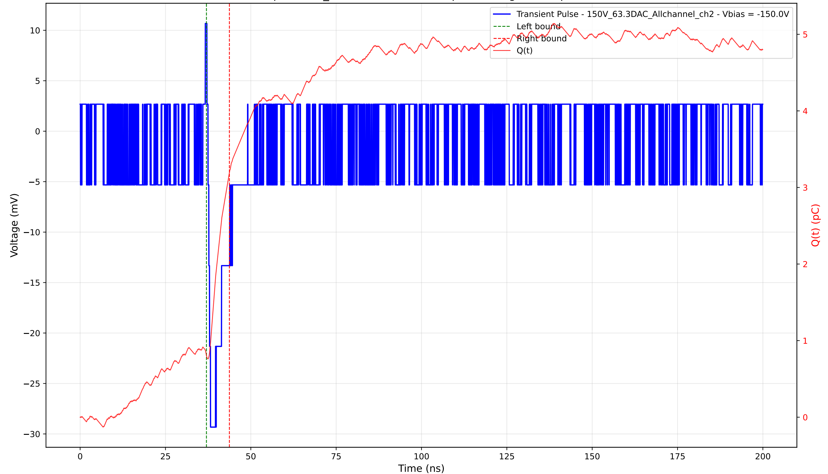
Transient Pulse - Sample: 1cm_42 - Position: 4900.0 \mu\text{m} - Charge: 2.39 pC - Rise Time: 0.76 ns
