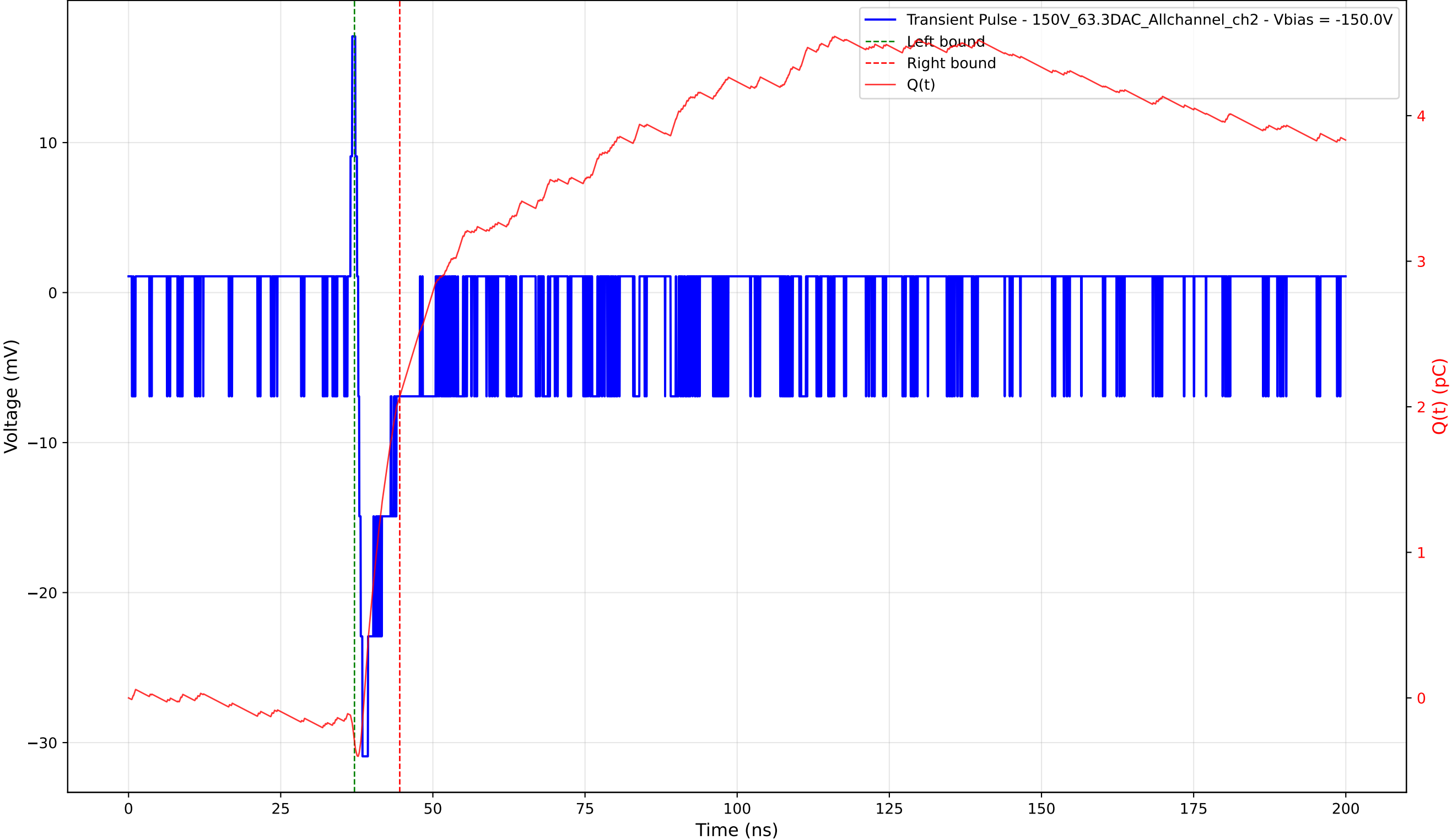
Transient Pulse - Sample: 1cm_42 - Position: 435.0 \mu\text{m} - Charge: 2.37 pC - Rise Time: 0.71 ns
