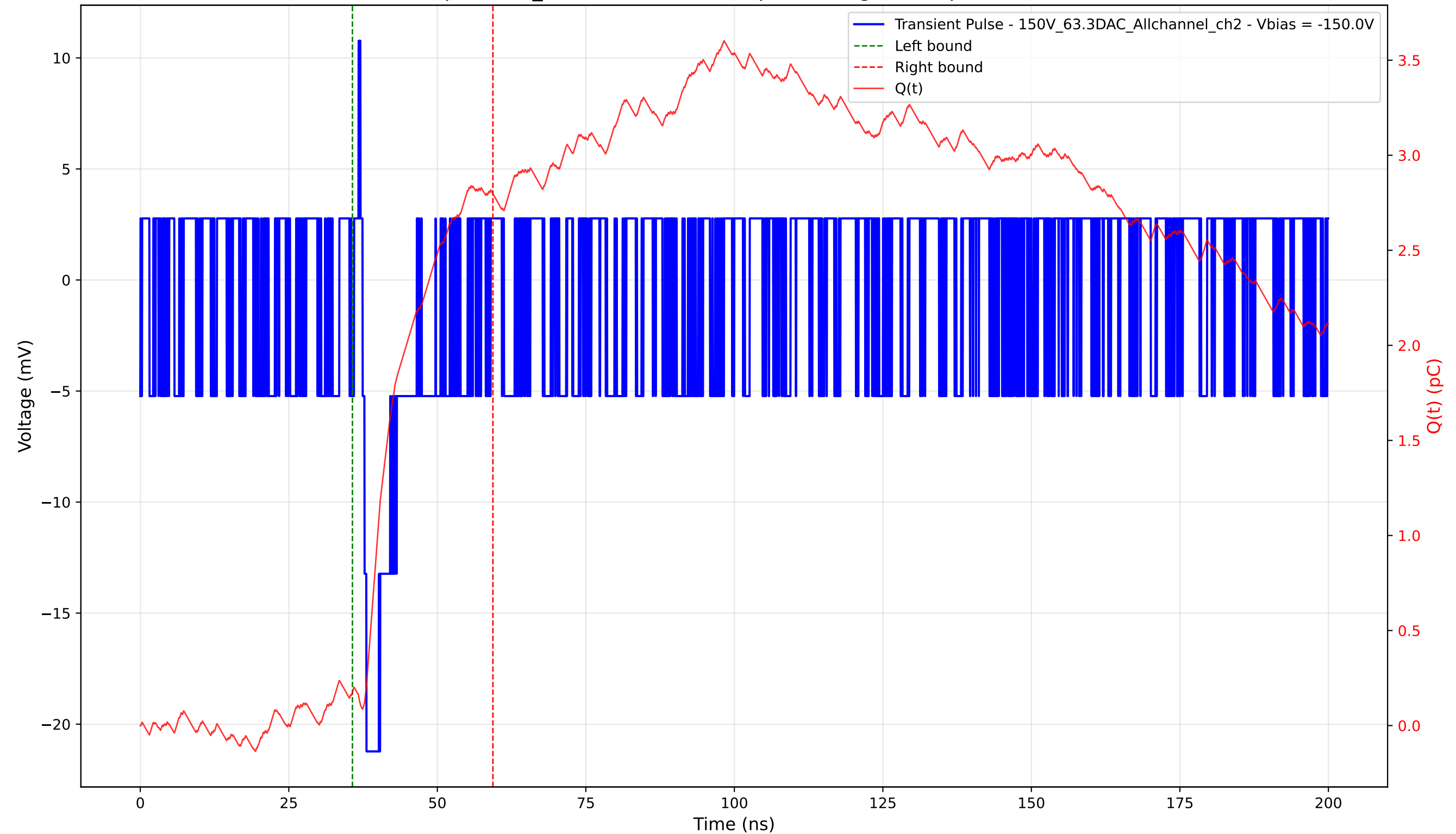
Transient Pulse - Sample: 1cm_42 - Position: 4980.0 \mu\text{m} - Charge: 2.62 pC - Rise Time: 0.00 ns (N/A)
