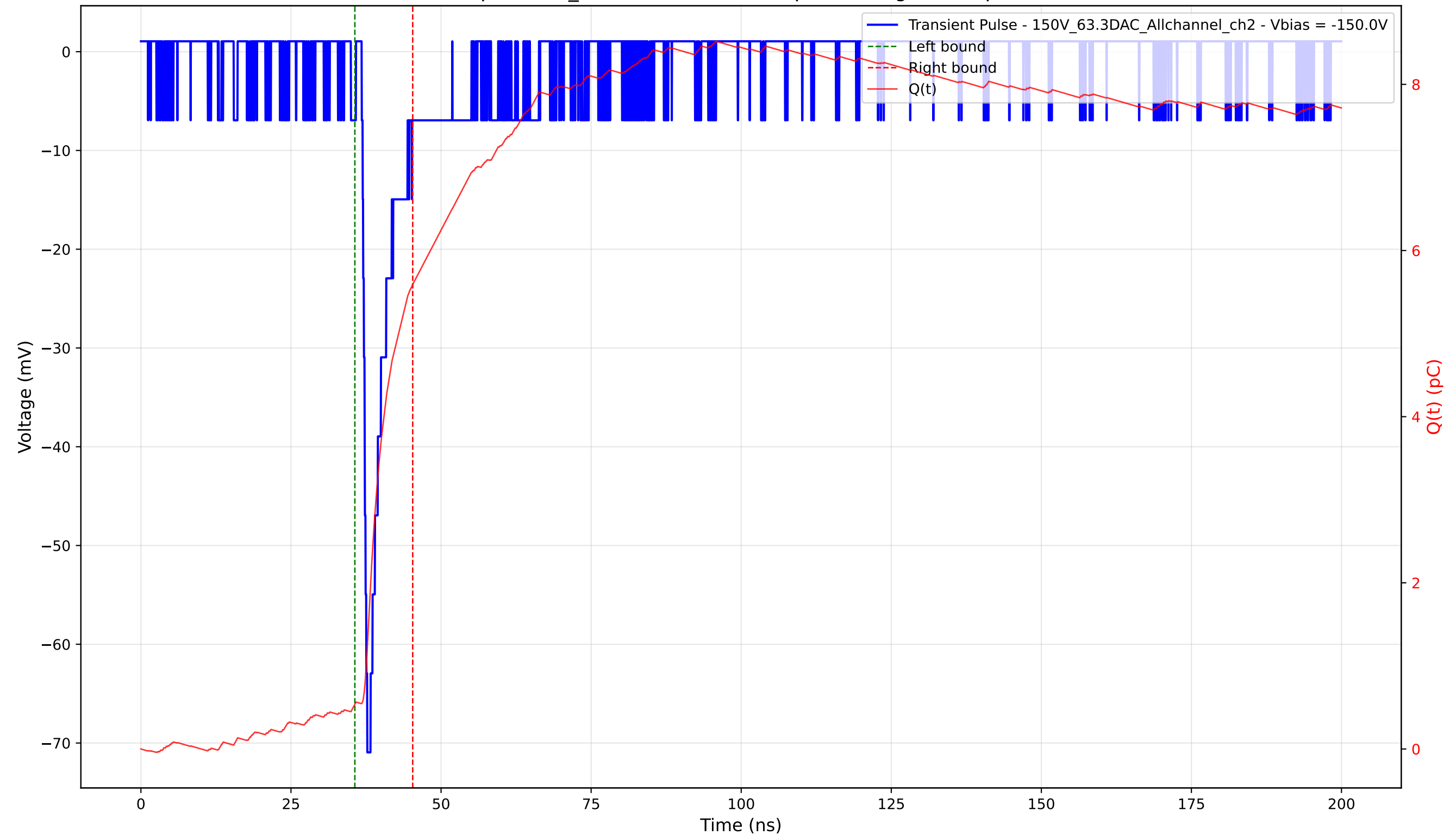
Transient Pulse - Sample: 1cm_42 - Position: 1995.0 \mu\text{m} - Charge: 5.05 pC - Rise Time: 0.80 ns
