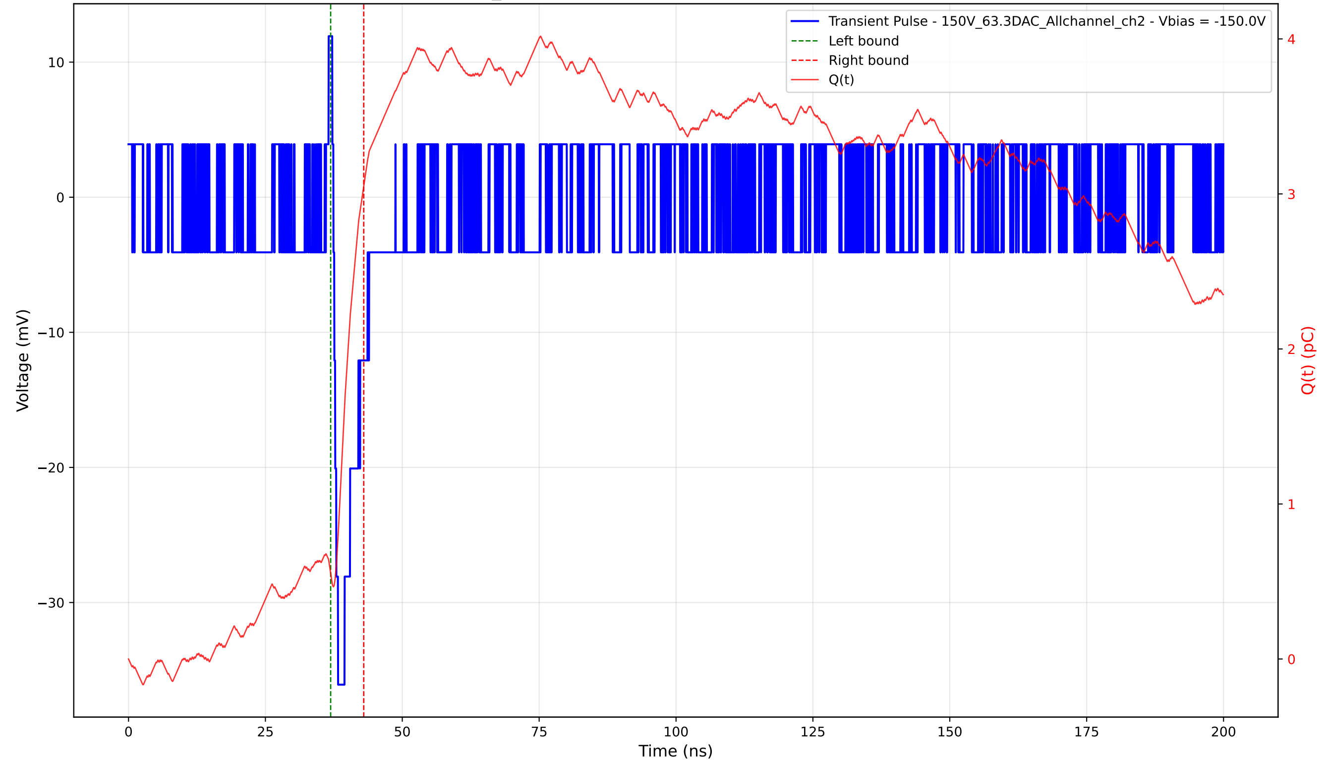
Transient Pulse - Sample: 1cm_42 - Position: 4665.0 \mu\text{m} - Charge: 2.51 pC - Rise Time: 0.00 ns (N/A)
