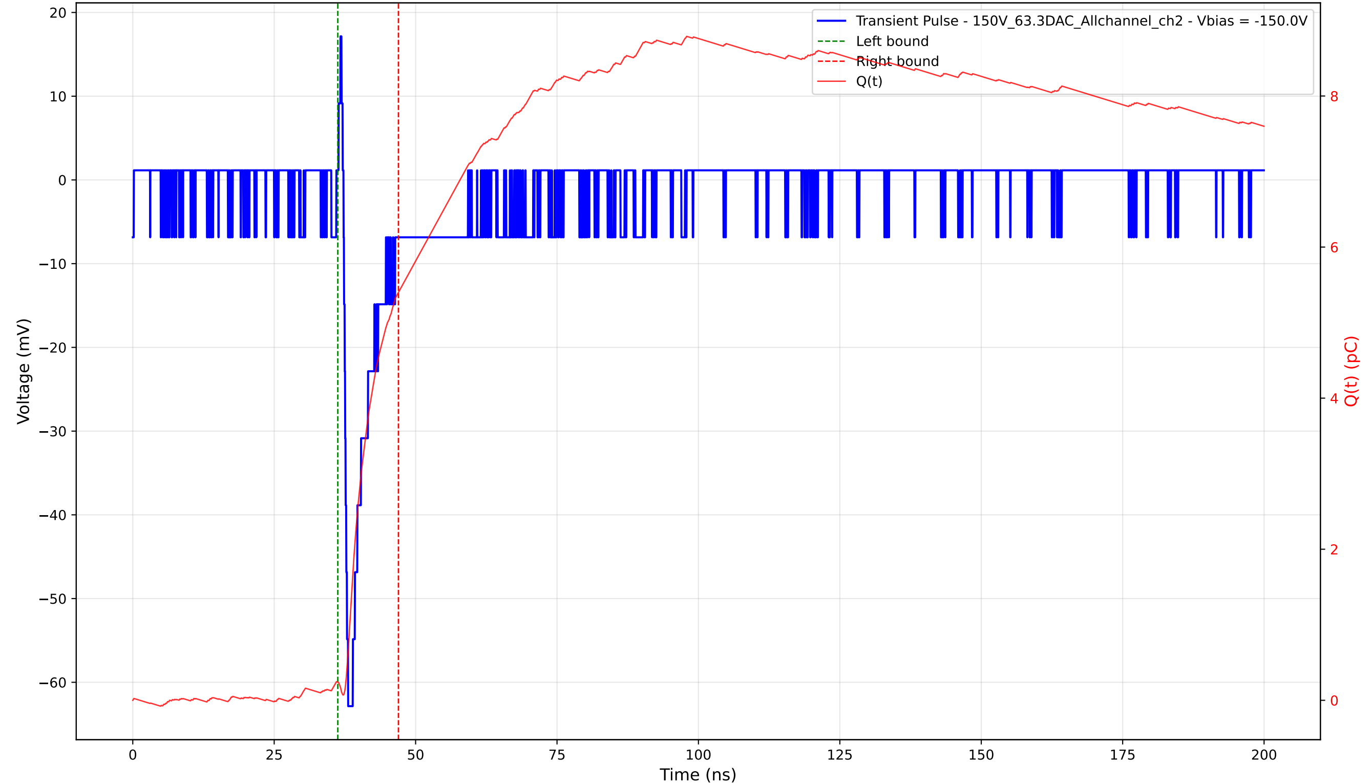
Transient Pulse - Sample: 1cm_42 - Position: 1755.0 \mu\text{m} - Charge: 5.16 pC - Rise Time: 0.80 ns
