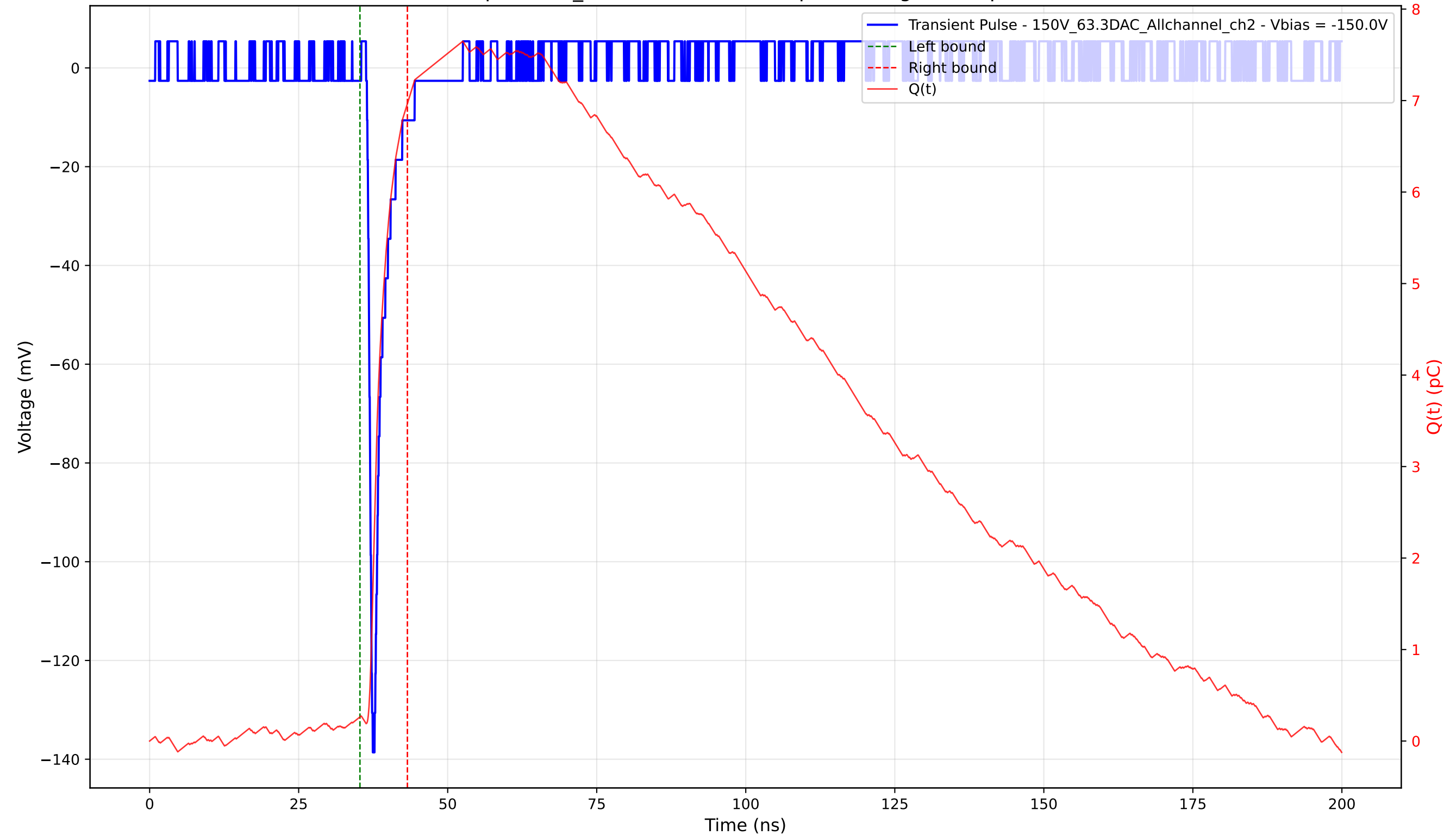
Transient Pulse - Sample: 1cm_42 - Position: 2305.0 \mu\text{m} - Charge: 6.70 pC - Rise Time: 0.78 ns
