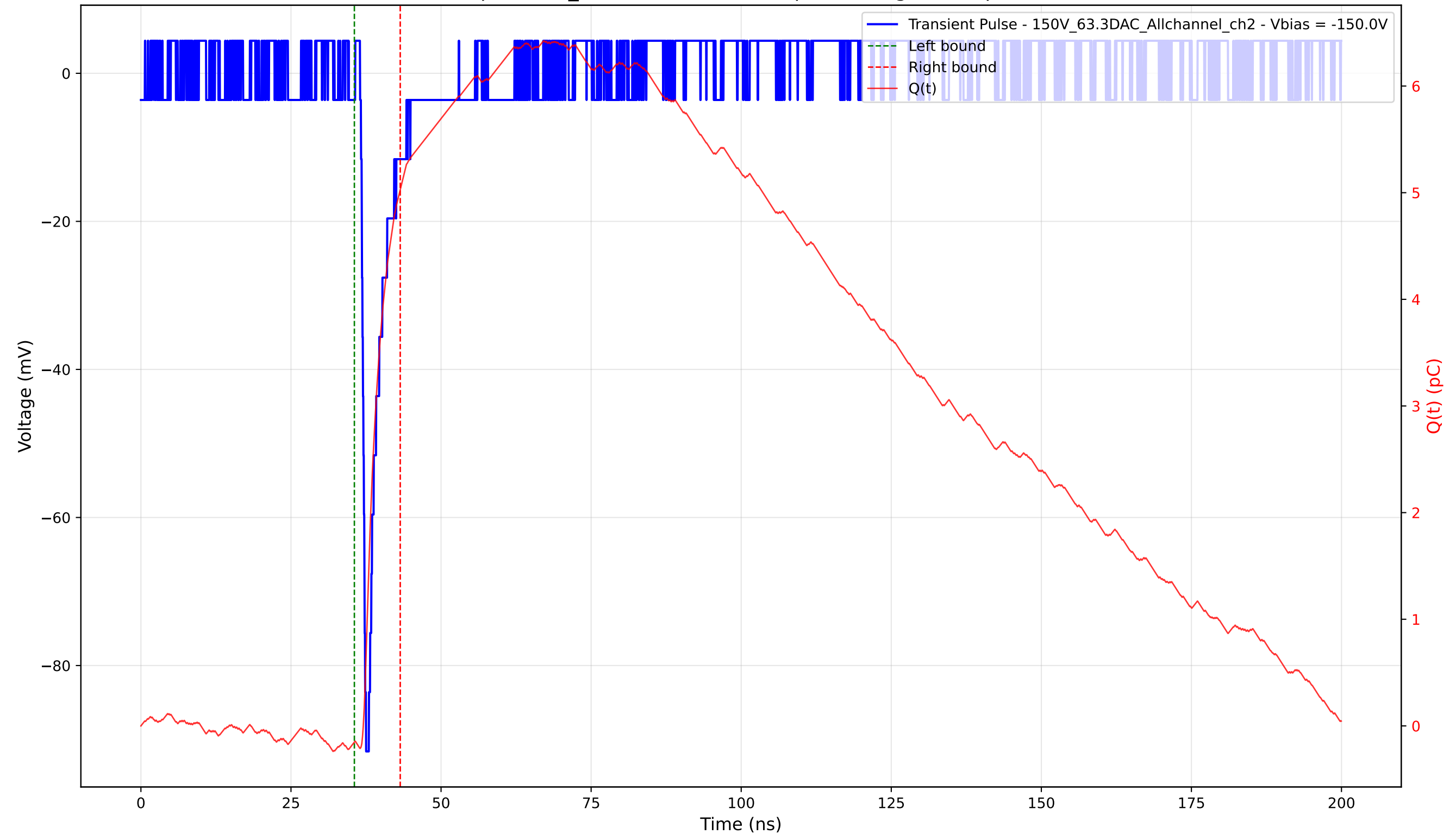
Transient Pulse - Sample: 1cm_42 - Position: 2110.0 \mu\text{m} - Charge: 5.18 pC - Rise Time: 0.69 ns
