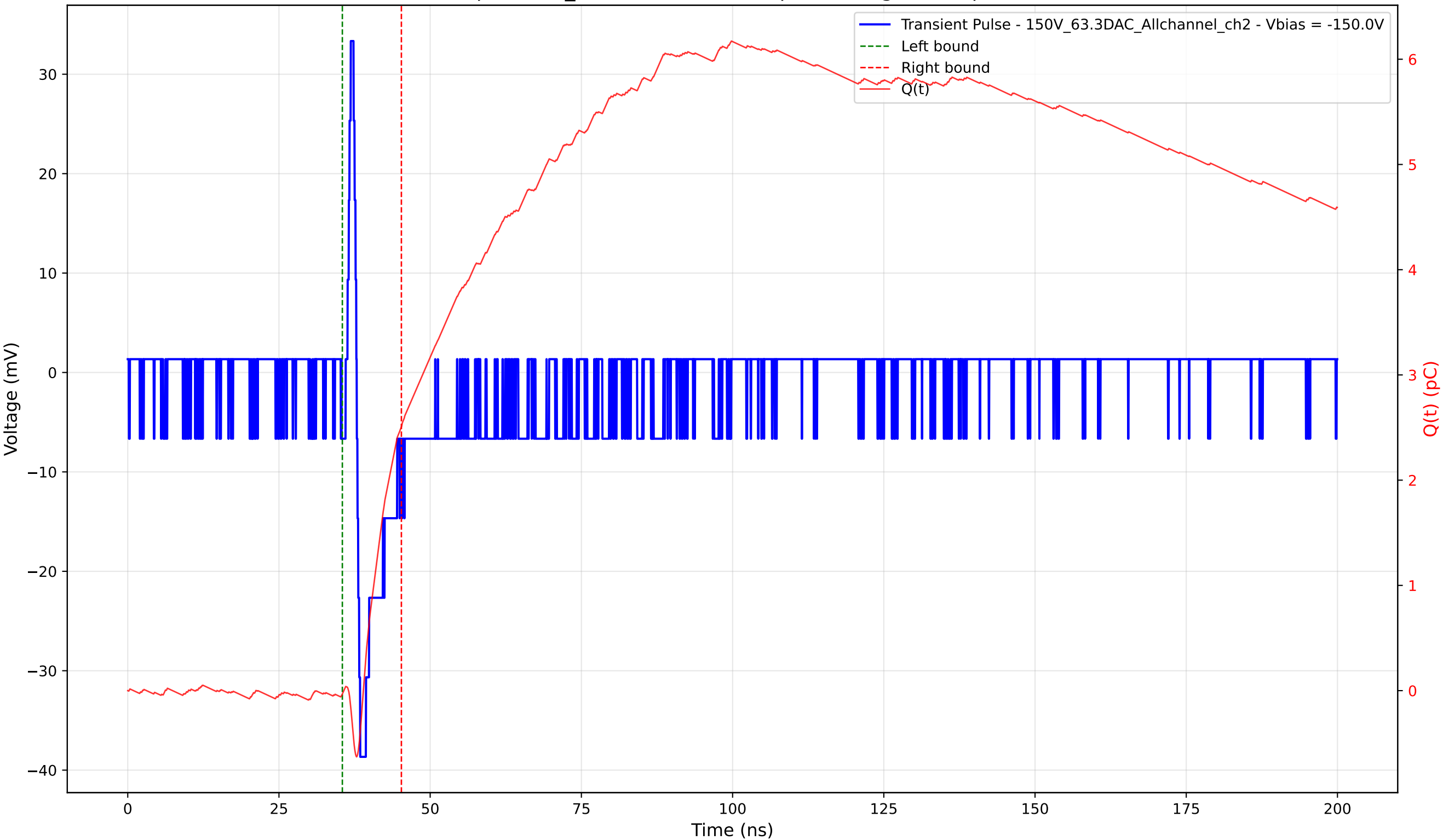
Transient Pulse - Sample: 1cm_42 - Position: 860.0 \mu\text{m} - Charge: 2.54 pC - Rise Time: 0.58 ns
