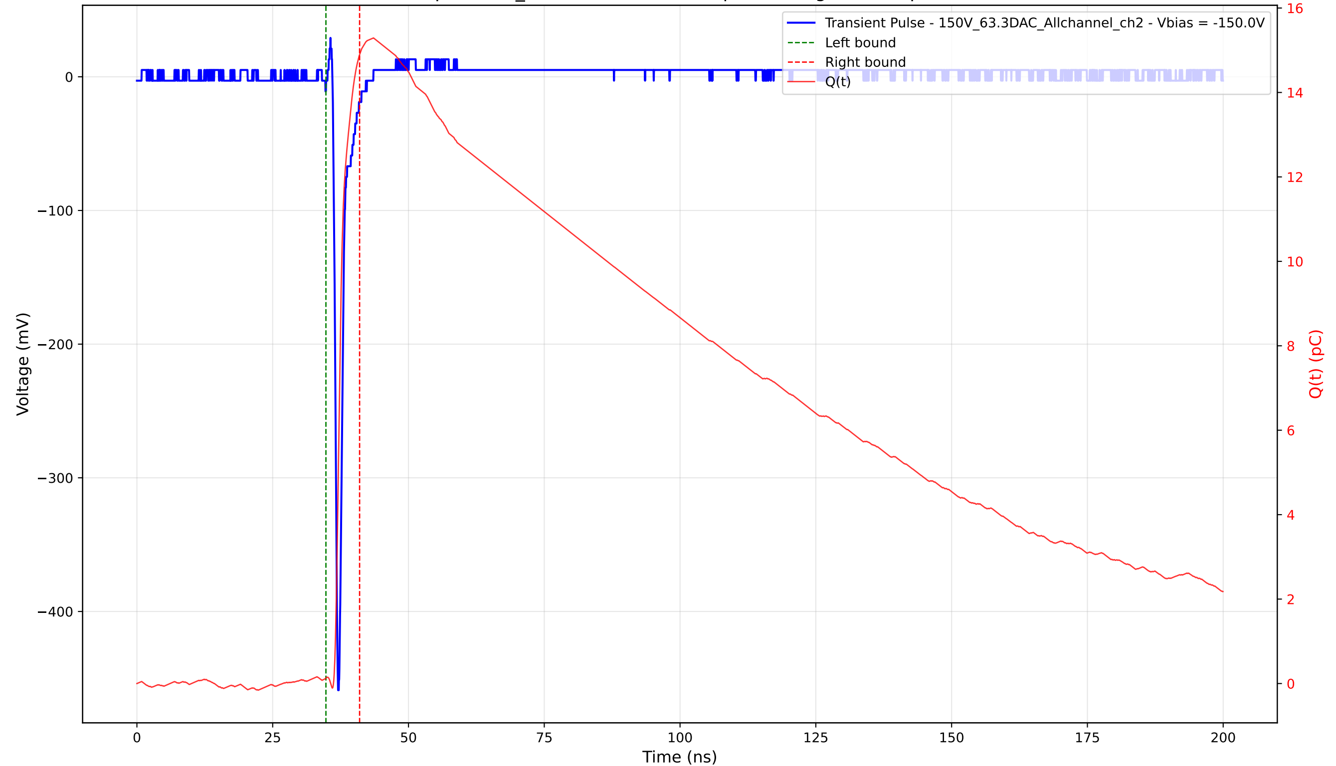
Transient Pulse - Sample: 1cm_42 - Position: 3195.0 \mu\text{m} - Charge: 14.76 pC - Rise Time: 0.70 ns
