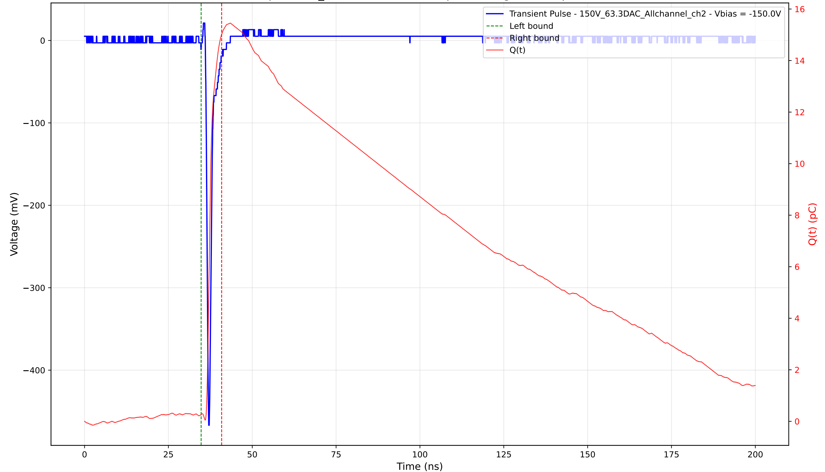
Transient Pulse - Sample: 1cm_42 - Position: 3155.0 \mu\text{m} - Charge: 14.75 pC - Rise Time: 0.72 ns
