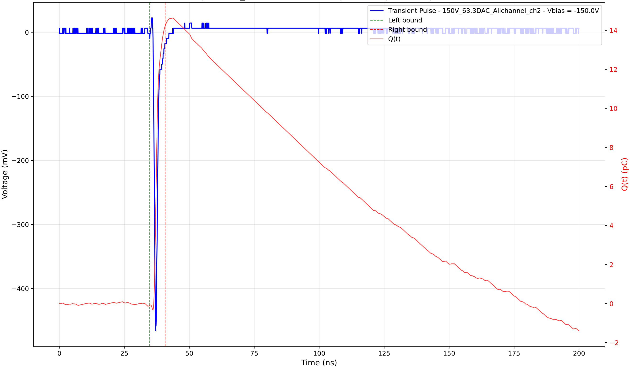
Transient Pulse - Sample: 1cm_42 - Position: 2885.0 \mu\text{m} - Charge: 14.30 pC - Rise Time: 0.69 ns
