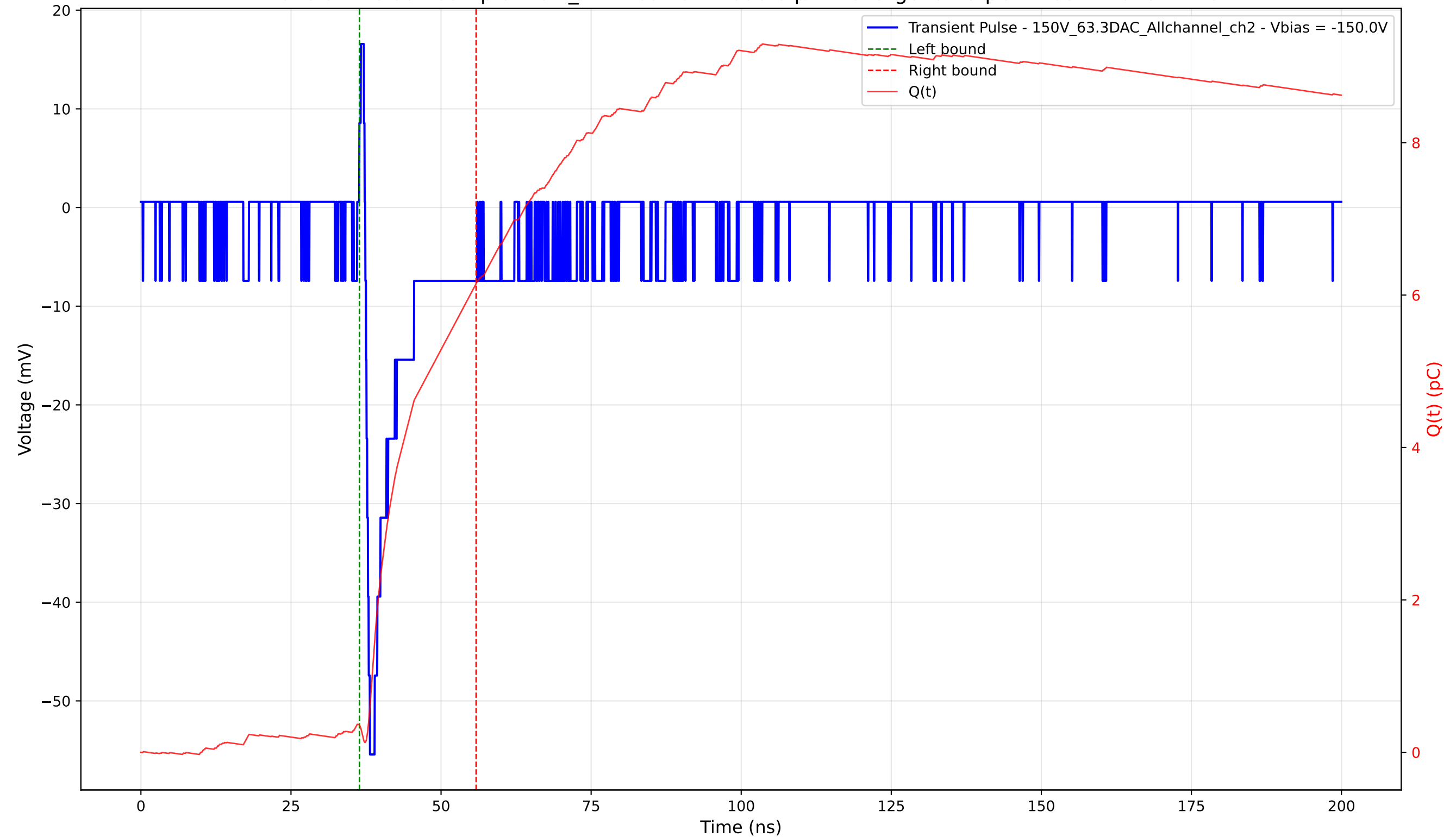
Transient Pulse - Sample: 1cm_42 - Position: 1650.0 \mu\text{m} - Charge: 5.79 pC - Rise Time: 0.77 ns
