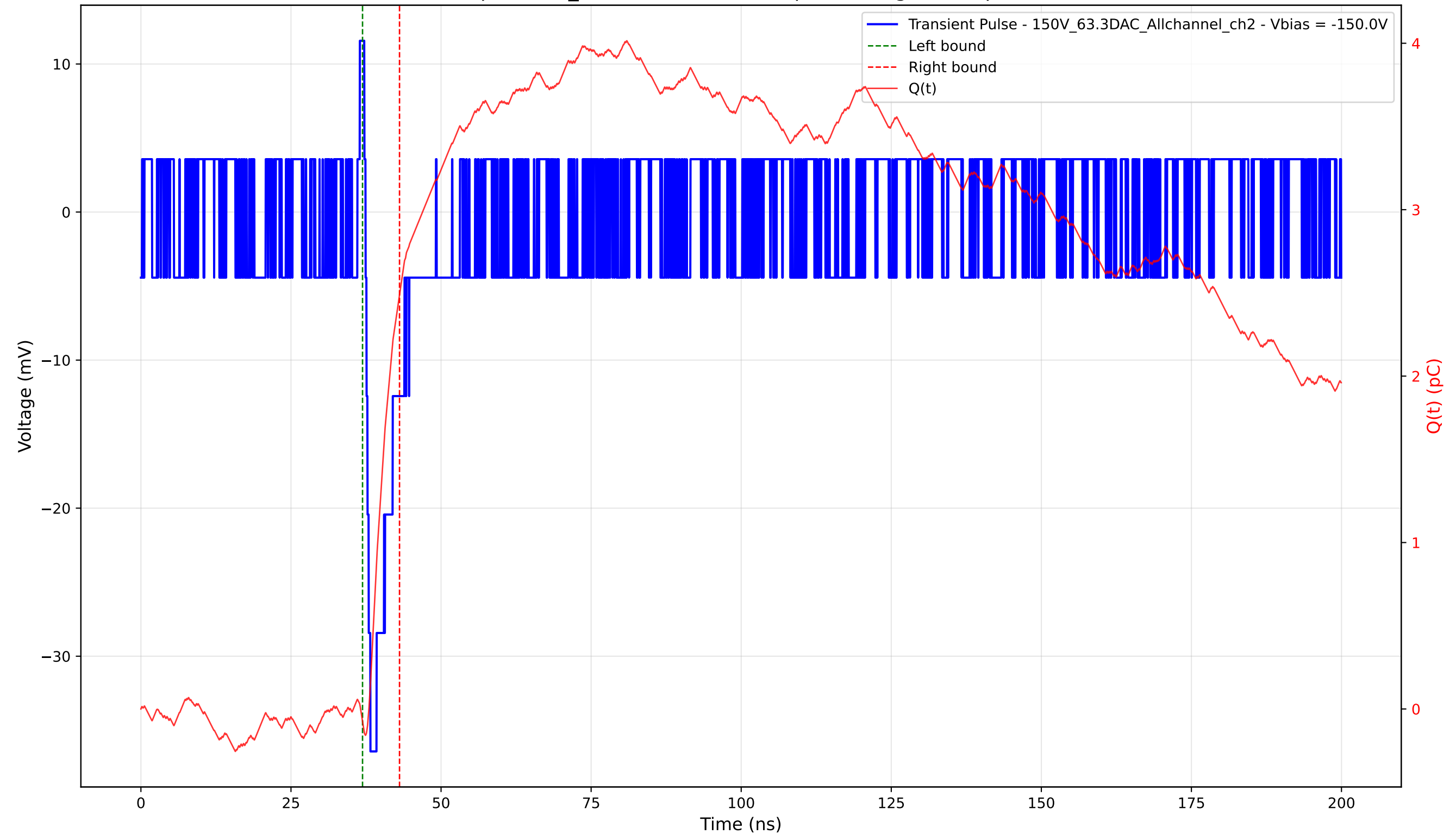
Transient Pulse - Sample: 1cm_42 - Position: 4690.0 \mu\text{m} - Charge: 2.57 pC - Rise Time: 0.84 ns
