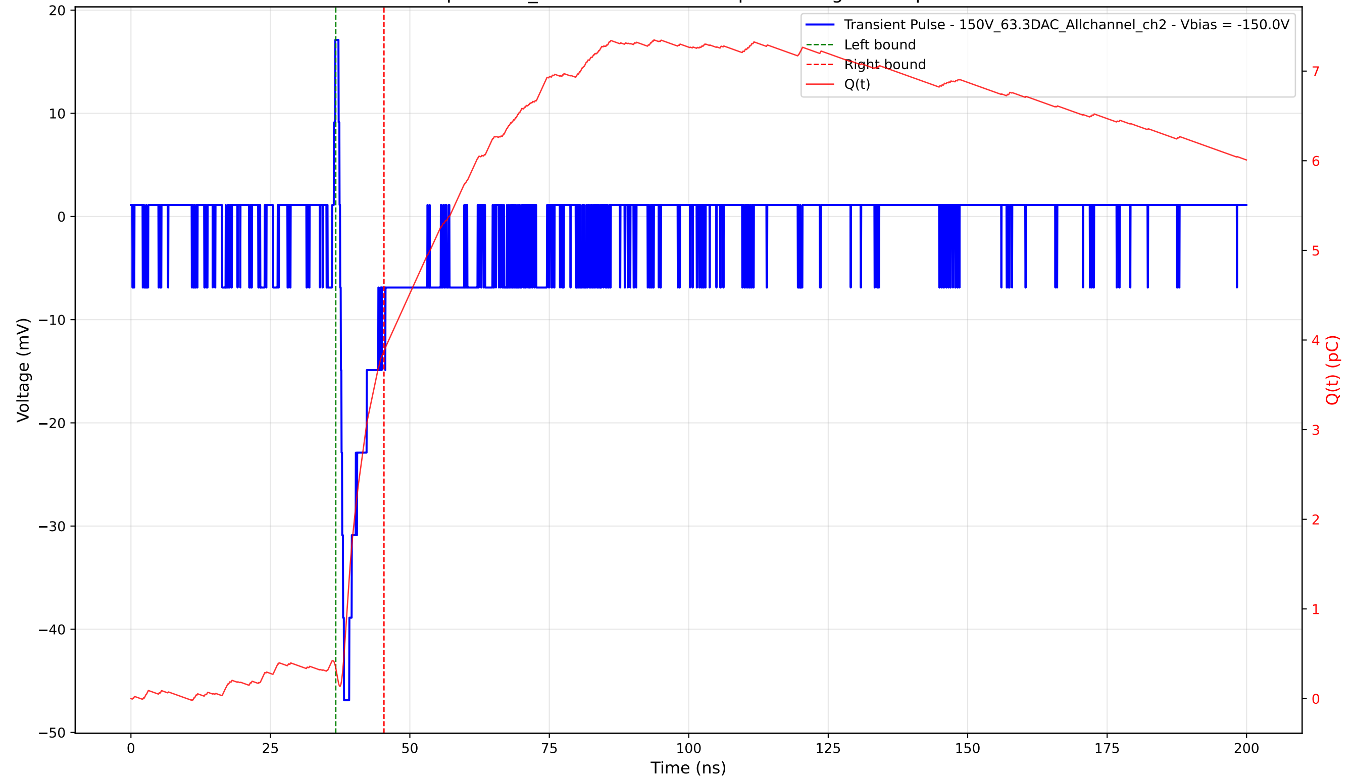
Transient Pulse - Sample: 1cm_42 - Position: 1560.0 \mu\text{m} - Charge: 3.54 pC - Rise Time: 0.70 ns
