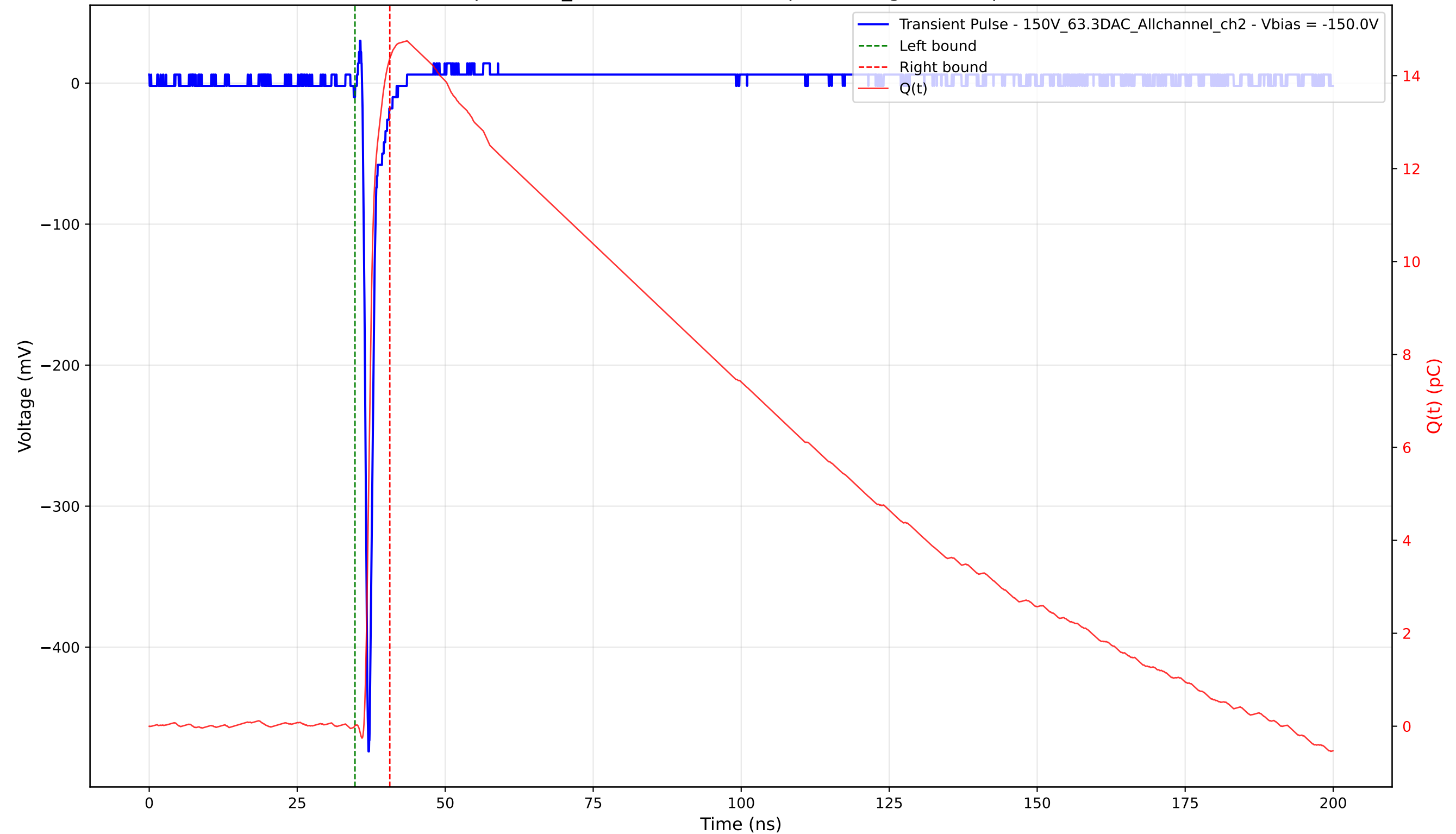
Transient Pulse - Sample: 1cm_42 - Position: 2965.0 \mu\text{m} - Charge: 14.36 pC - Rise Time: 0.67 ns
