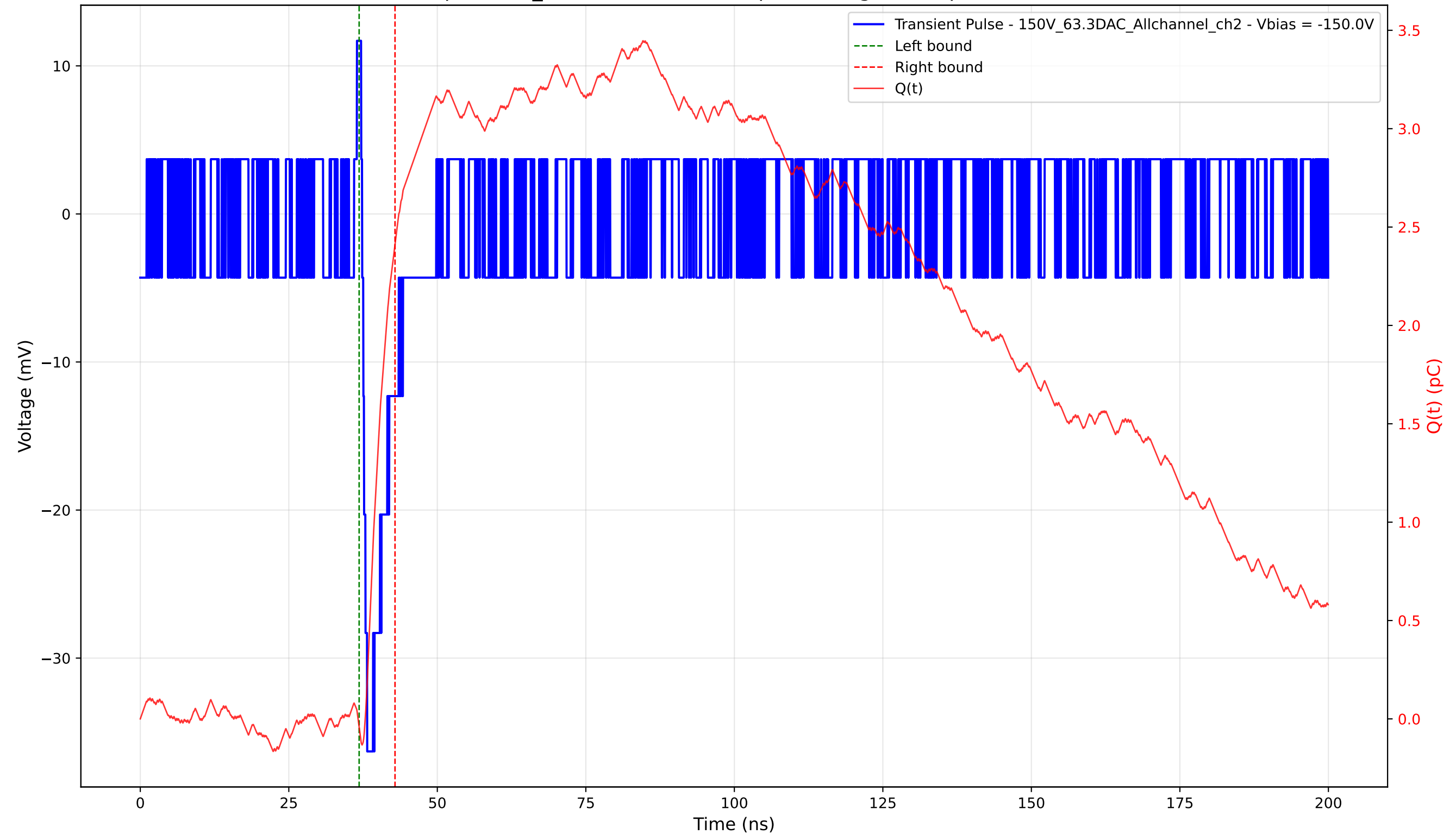
Transient Pulse - Sample: 1cm_42 - Position: 4620.0 \mu\text{m} - Charge: 2.46 pC - Rise Time: 0.00 ns (N/A)
