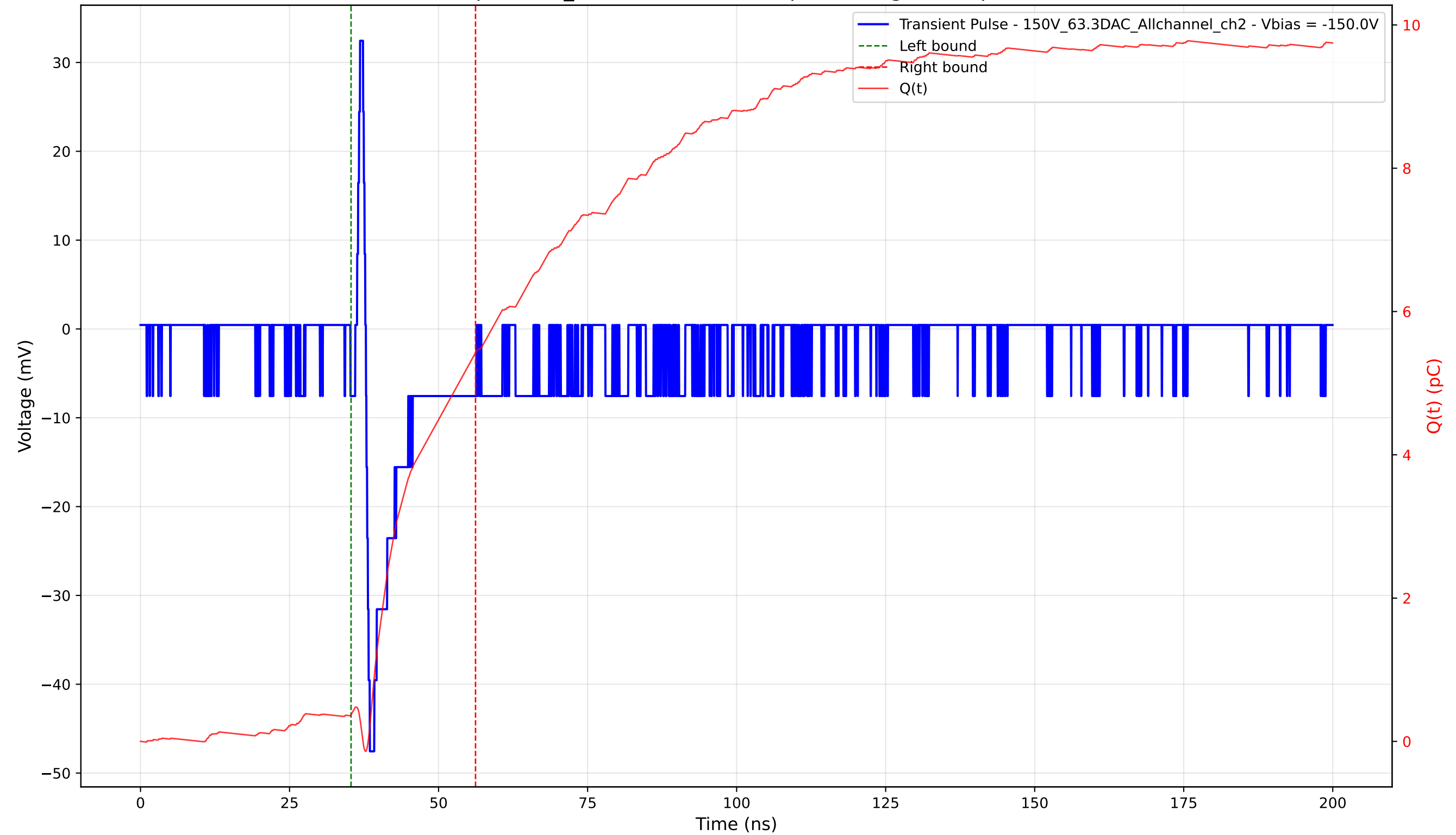
Transient Pulse - Sample: 1cm_42 - Position: 1205.0 \mu\text{m} - Charge: 5.06 pC - Rise Time: 0.66 ns
