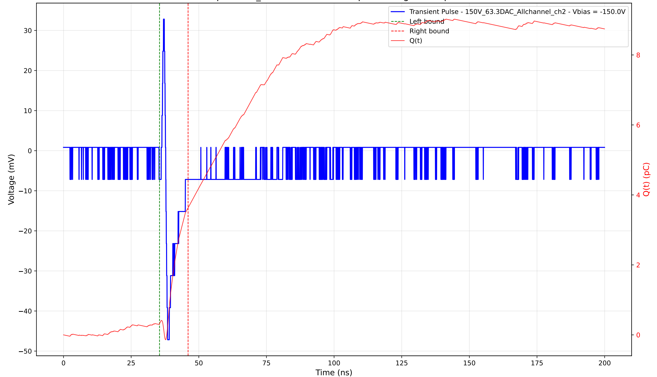
Transient Pulse - Sample: 1cm_42 - Position: 1360.0 \mu\text{m} - Charge: 3.31 pC - Rise Time: 0.70 ns
