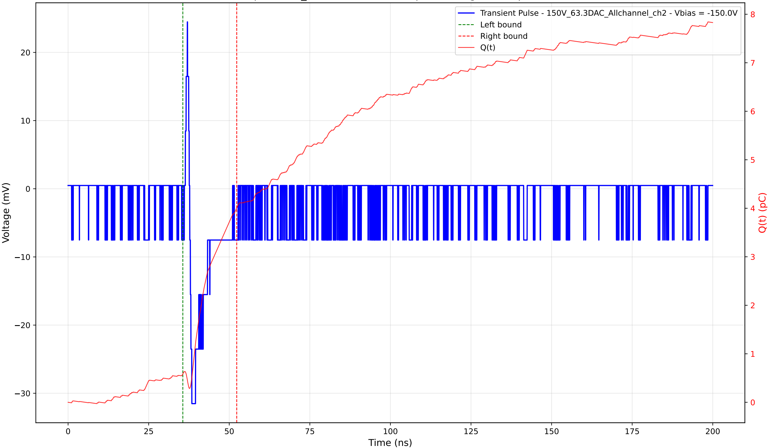
Transient Pulse - Sample: 1cm_42 - Position: 500.0 \mu\text{m} - Charge: 3.42 pC - Rise Time: 0.66 ns
