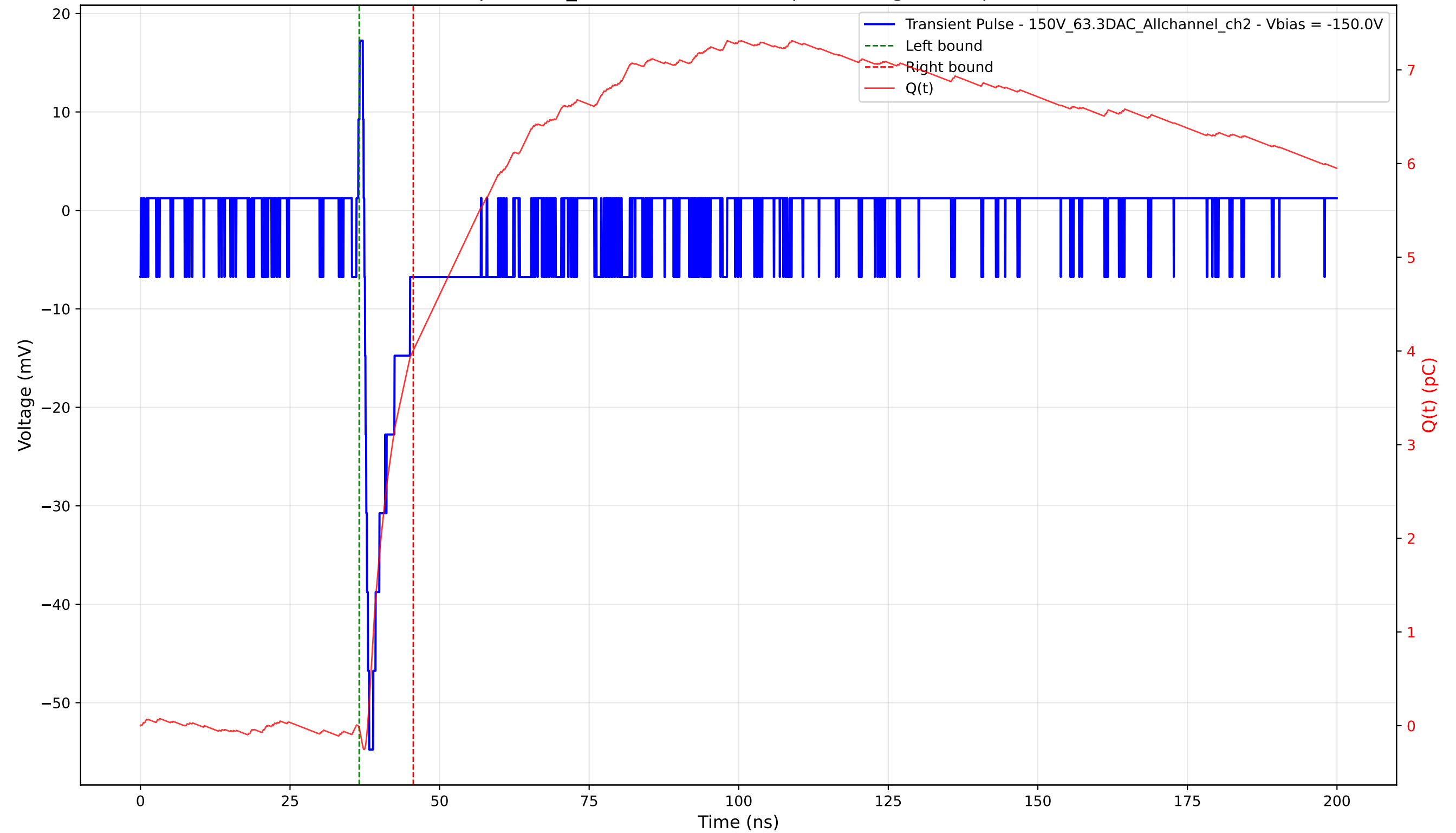
Transient Pulse - Sample: 1cm_42 - Position: 1630.0 \mu\text{m} - Charge: 4.03 pC - Rise Time: 0.81 ns
