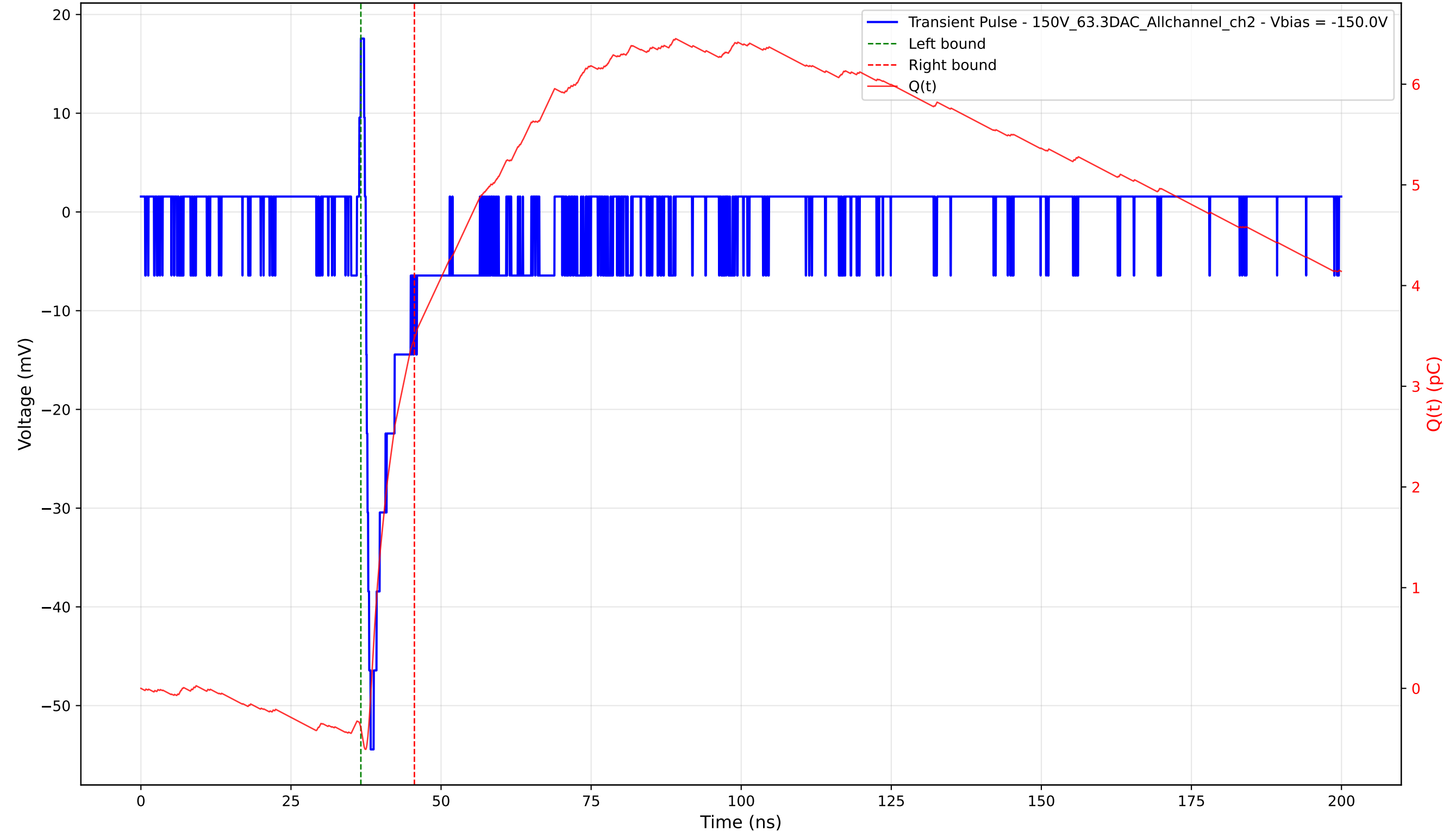
Transient Pulse - Sample: 1cm_42 - Position: 1615.0 \mu\text{m} - Charge: 3.87 pC - Rise Time: 0.81 ns
