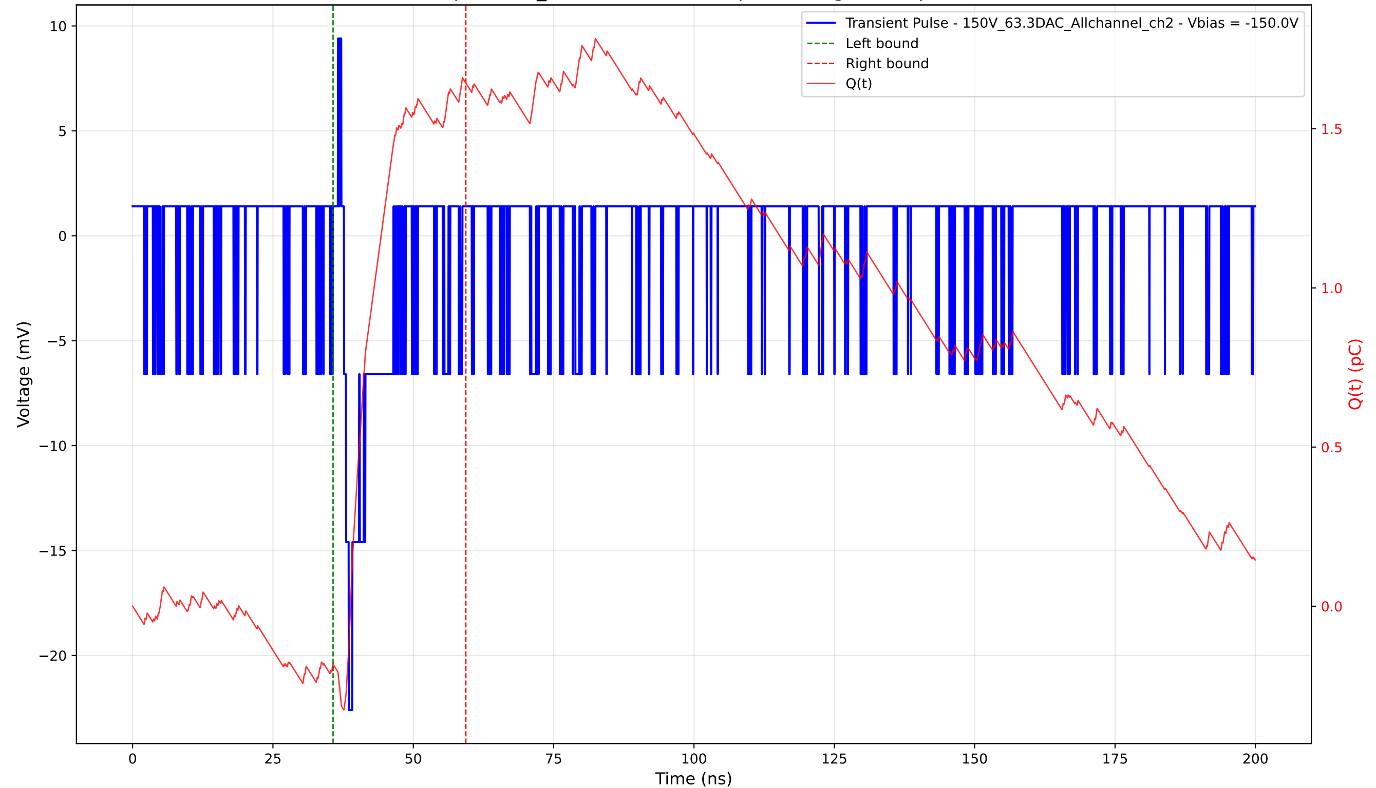
Transient Pulse - Sample: 1cm_42 - Position: 200.0 \mu\text{m} - Charge: 1.83 pC - Rise Time: 0.87 ns
