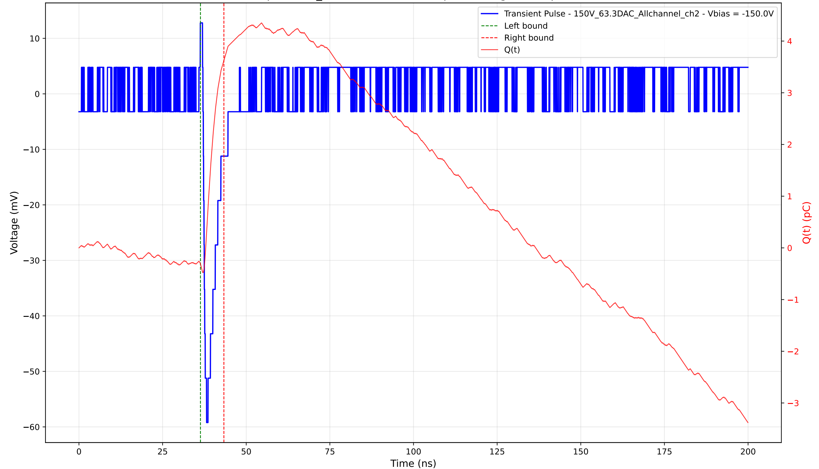
Transient Pulse - Sample: 1cm_42 - Position: 4205.0 \mu\text{m} - Charge: 3.94 pC - Rise Time: 0.99 ns
