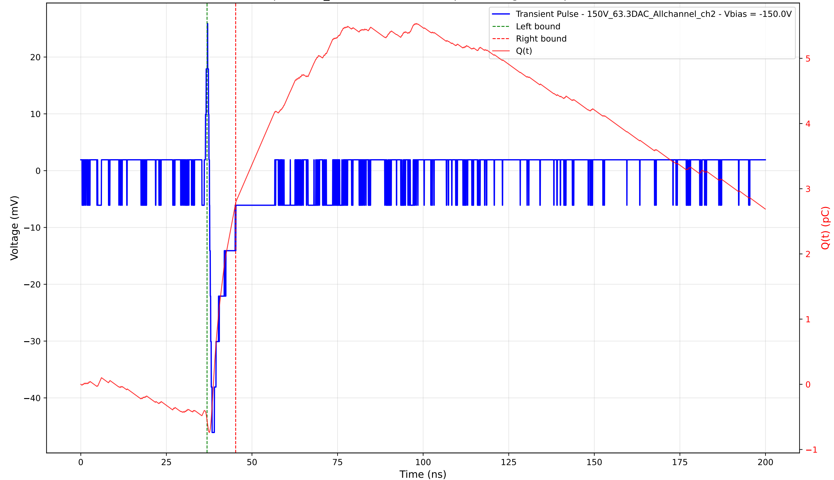
Transient Pulse - Sample: 1cm_42 - Position: 1515.0 \mu\text{m} - Charge: 3.33 pC - Rise Time: 0.77 ns
