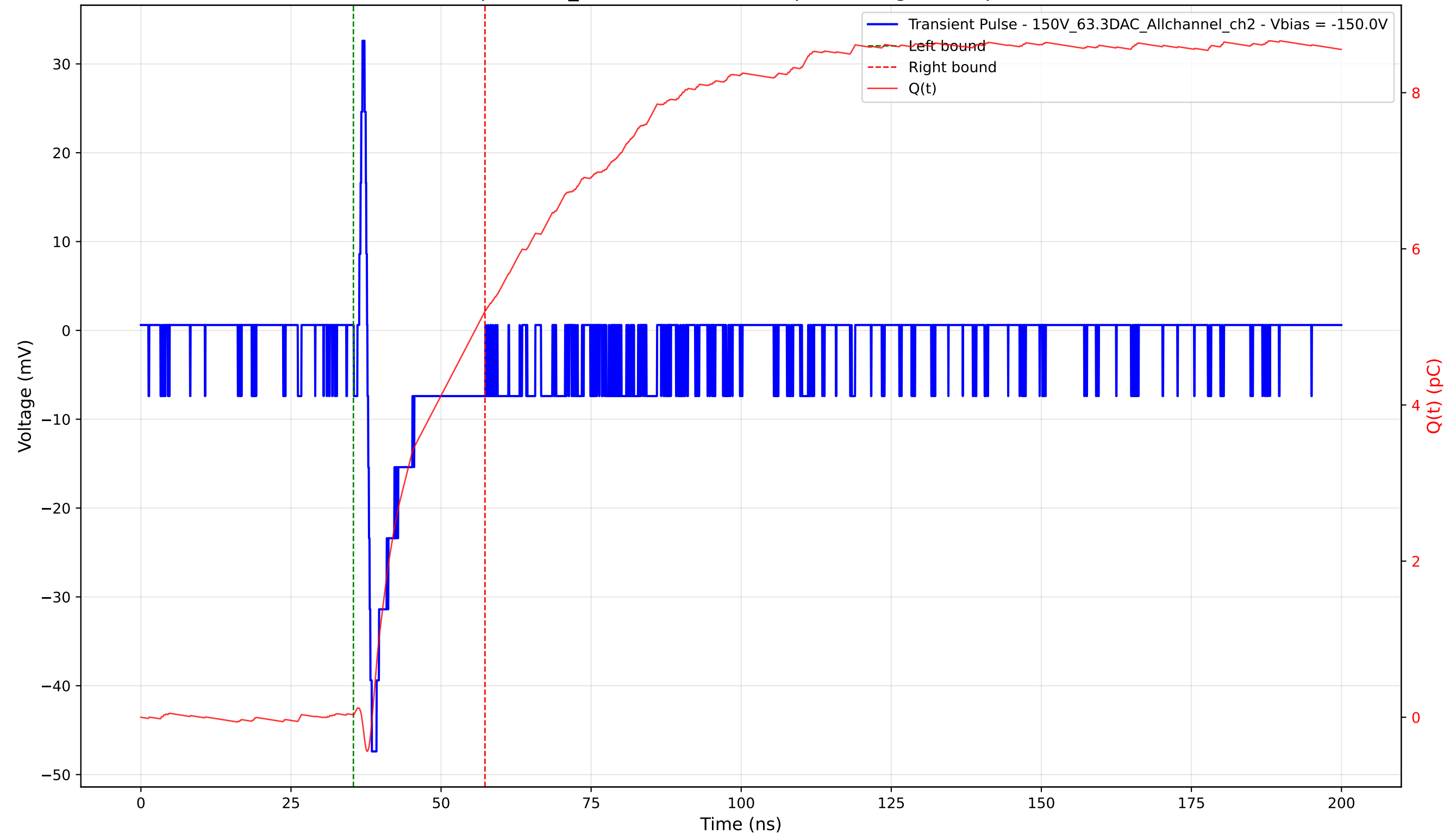
Transient Pulse - Sample: 1cm_42 - Position: 1335.0 \mu\text{m} - Charge: 5.17 pC - Rise Time: 0.74 ns
