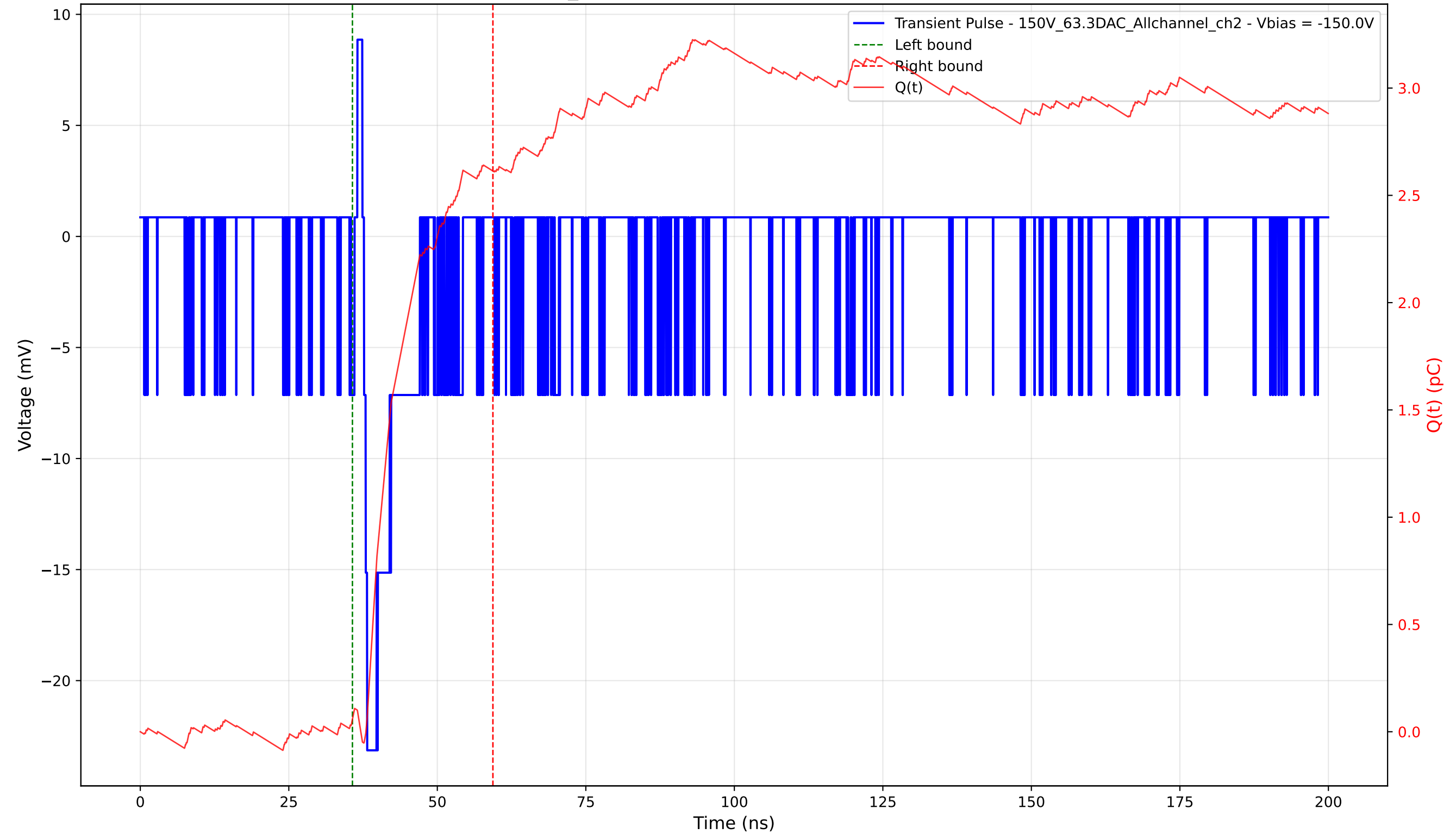
Transient Pulse - Sample: 1cm_42 - Position: 315.0 \mu\text{m} - Charge: 2.55 pC - Rise Time: 0.55 ns
