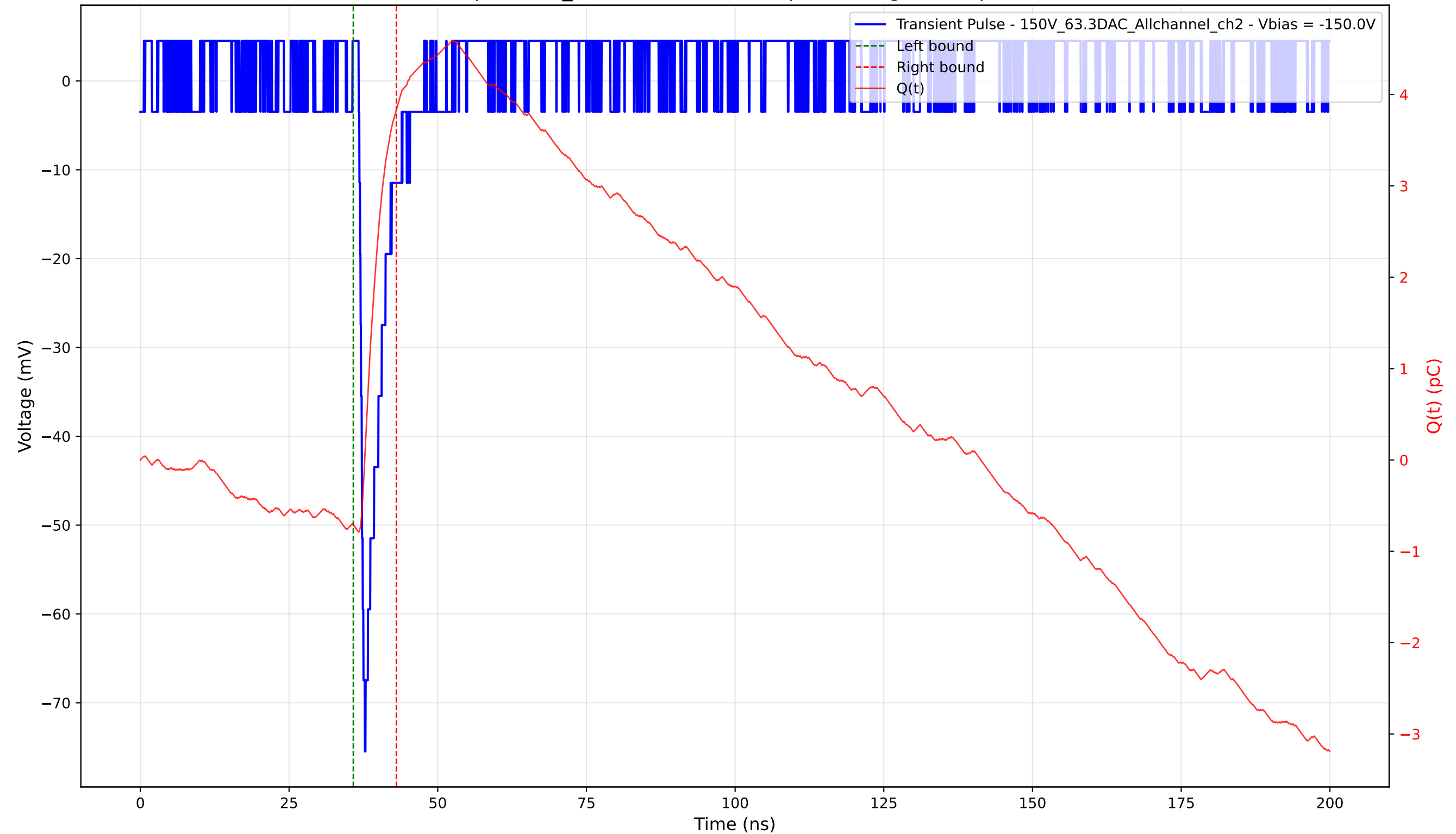
Transient Pulse - Sample: 1cm_42 - Position: 4010.0 \mu\text{m} - Charge: 4.54 pC - Rise Time: 0.94 ns
