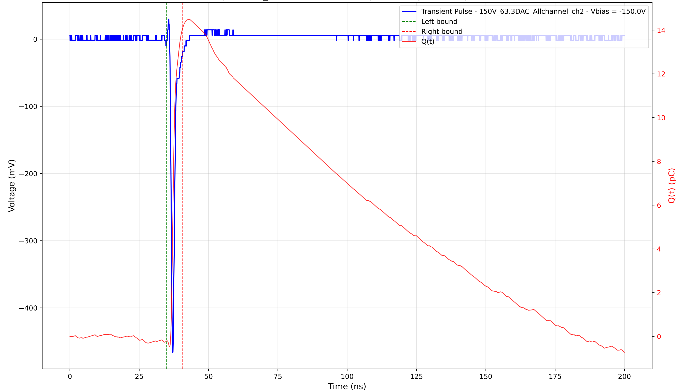
Transient Pulse - Sample: 1cm_42 - Position: 3085.0 \mu\text{m} - Charge: 14.33 pC - Rise Time: 0.68 ns
