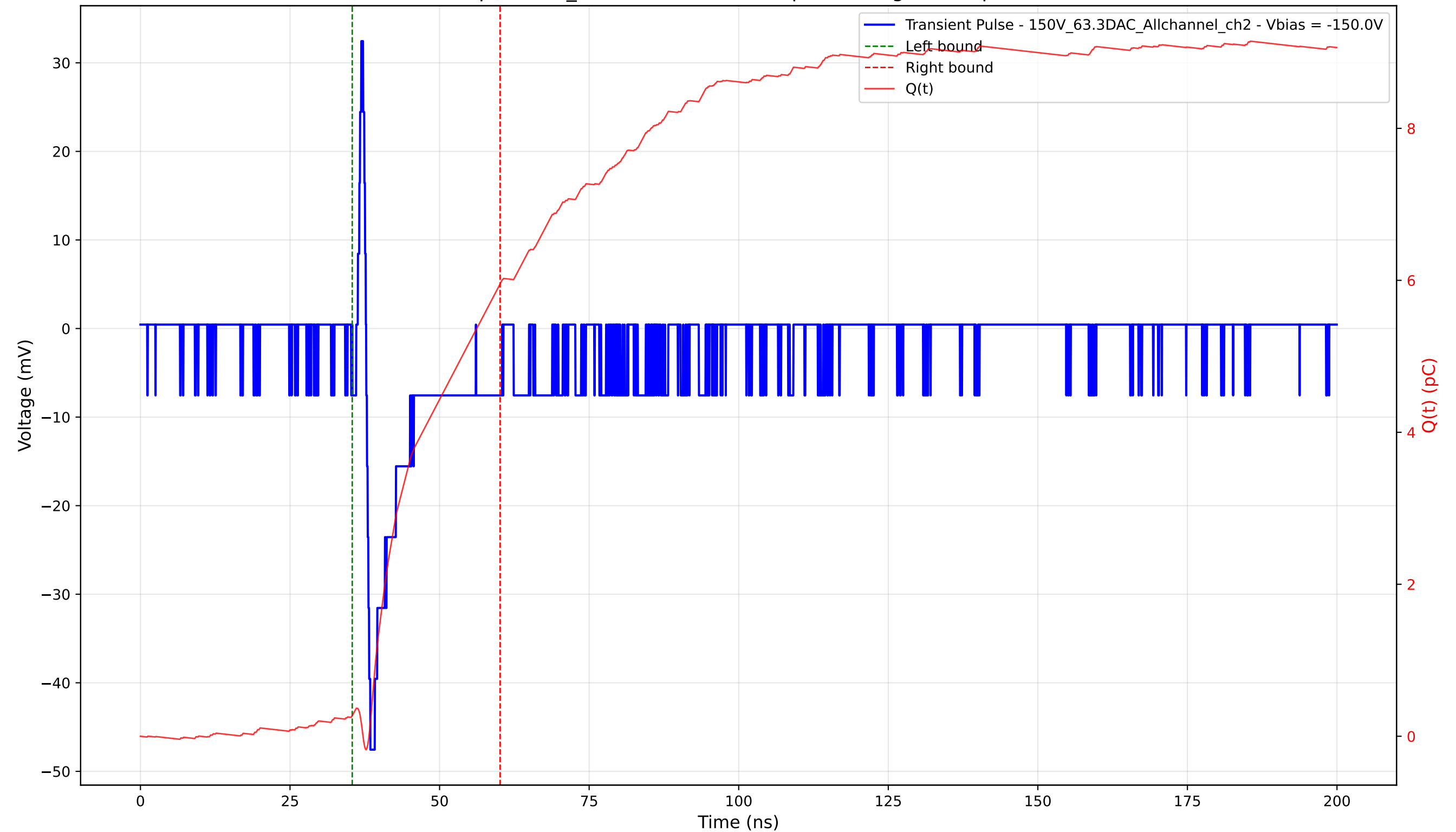
Transient Pulse - Sample: 1cm_42 - Position: 1340.0 \mu\text{m} - Charge: 5.68 pC - Rise Time: 0.70 ns
