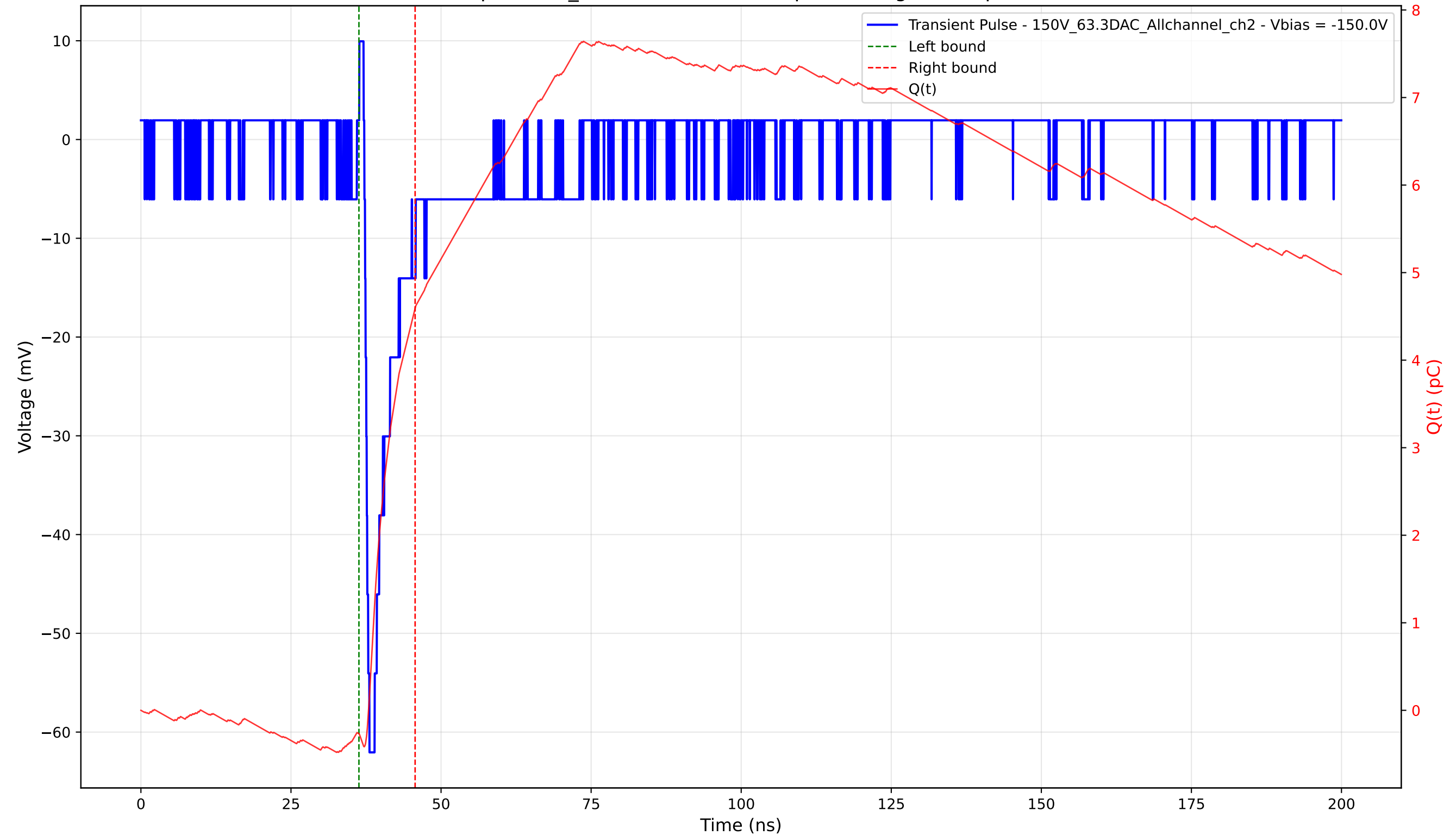
Transient Pulse - Sample: 1cm_42 - Position: 1785.0 \mu\text{m} - Charge: 4.86 pC - Rise Time: 0.76 ns
