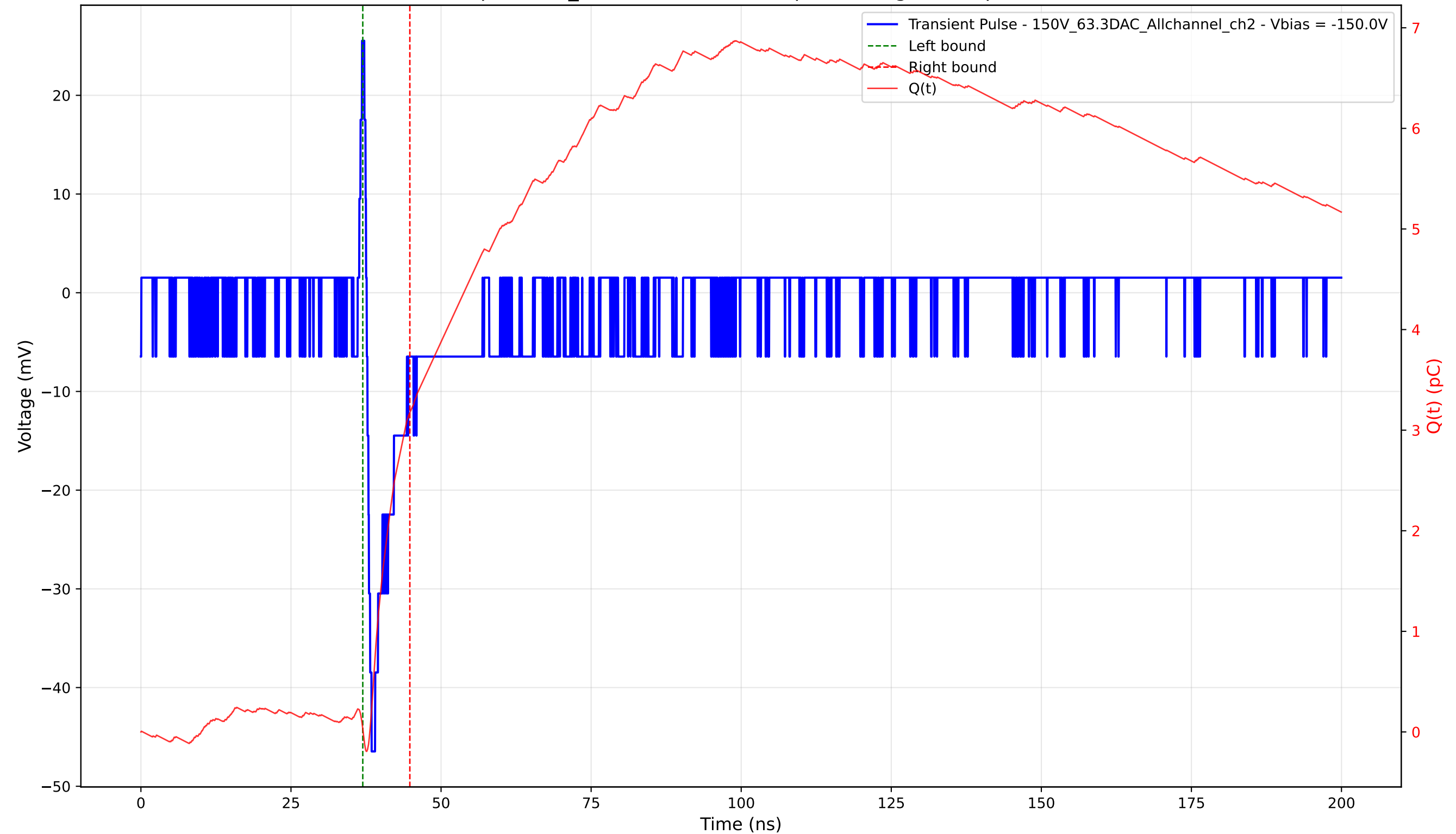
Transient Pulse - Sample: 1cm_42 - Position: 1470.0 \mu\text{m} - Charge: 3.15 pC - Rise Time: 0.81 ns
