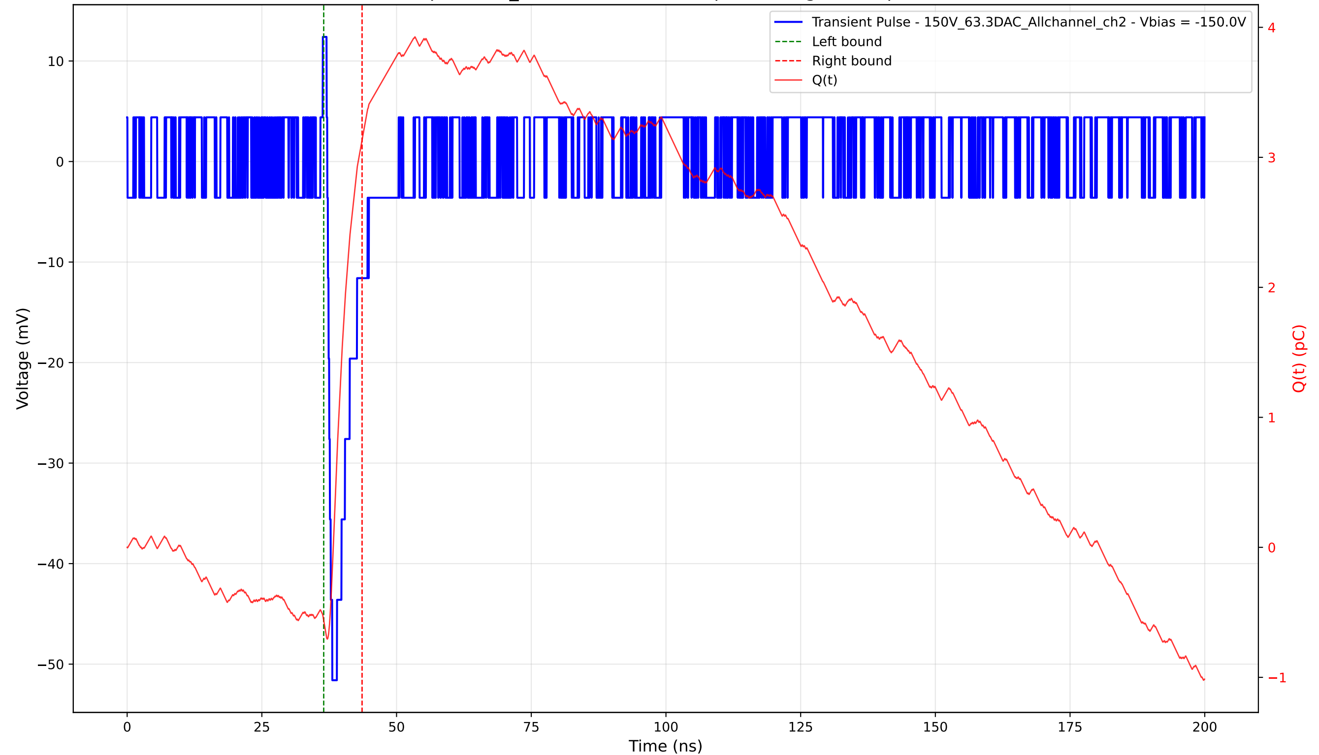
Transient Pulse - Sample: 1cm_42 - Position: 4365.0 \mu\text{m} - Charge: 3.70 pC - Rise Time: 0.83 ns
