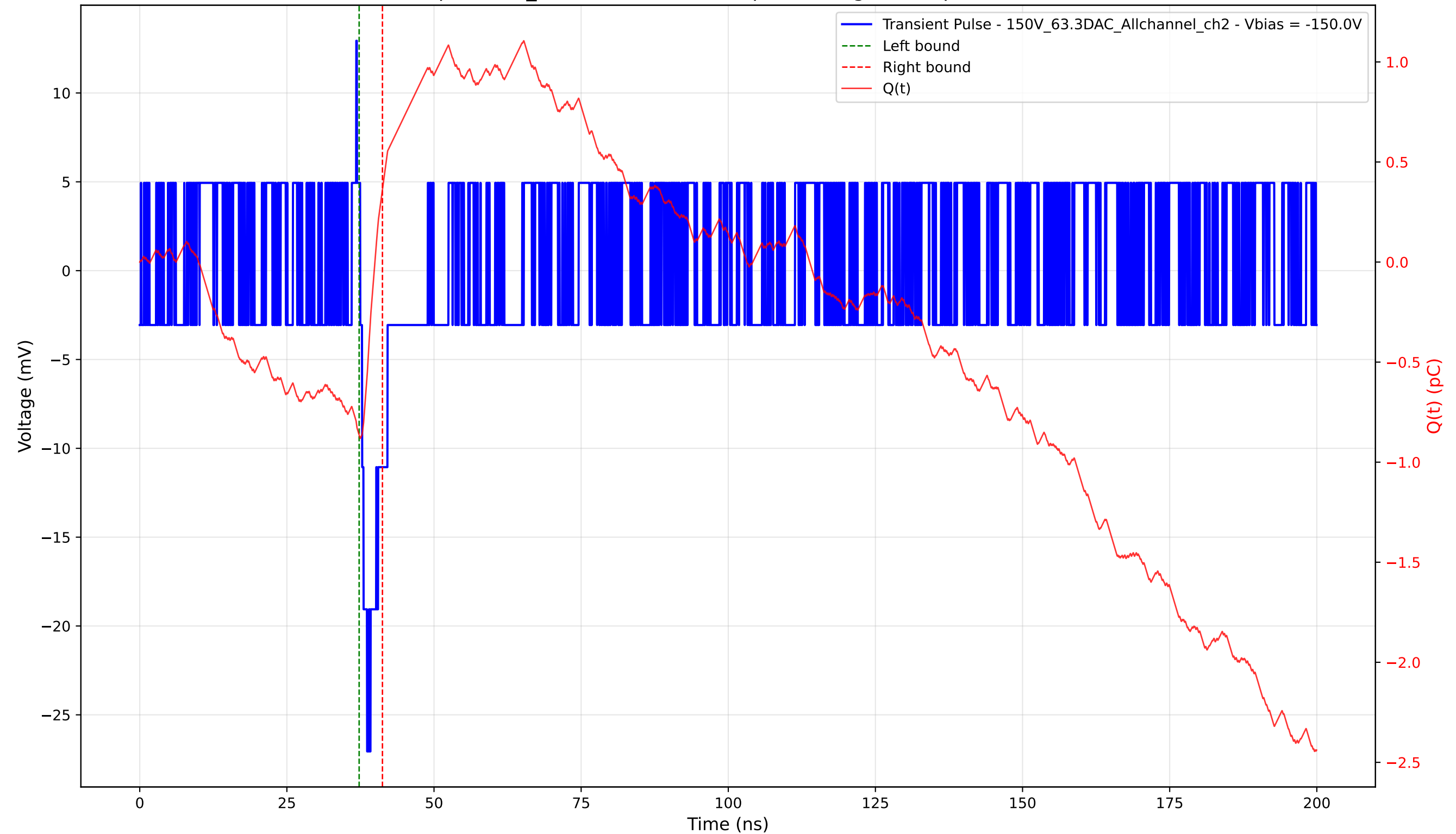
Transient Pulse - Sample: 1cm_42 - Position: 4970.0 \mu\text{m} - Charge: 1.23 pC - Rise Time: 0.00 ns (N/A)
