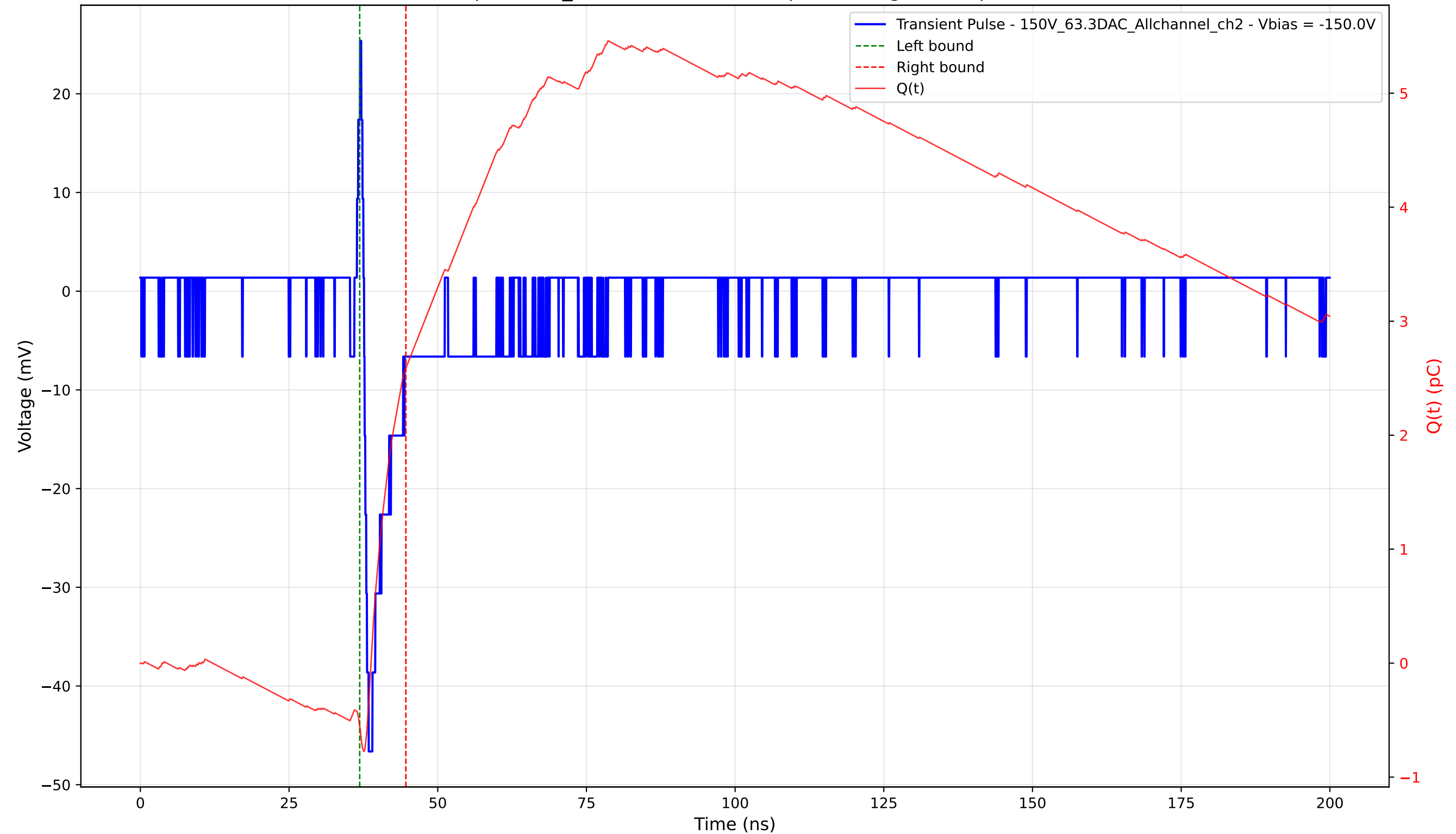
Transient Pulse - Sample: 1cm_42 - Position: 1505.0 \mu\text{m} - Charge: 3.14 pC - Rise Time: 0.77 ns
