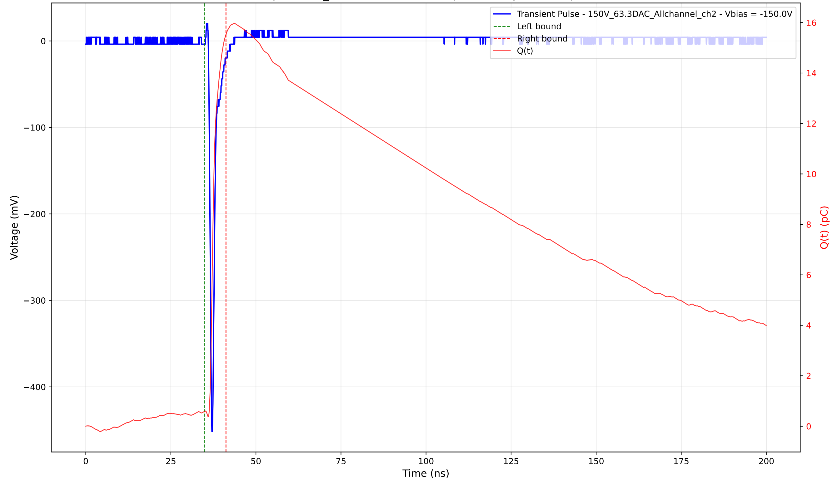
Transient Pulse - Sample: 1cm_42 - Position: 3225.0 \mu\text{m} - Charge: 14.94 pC - Rise Time: 0.69 ns
