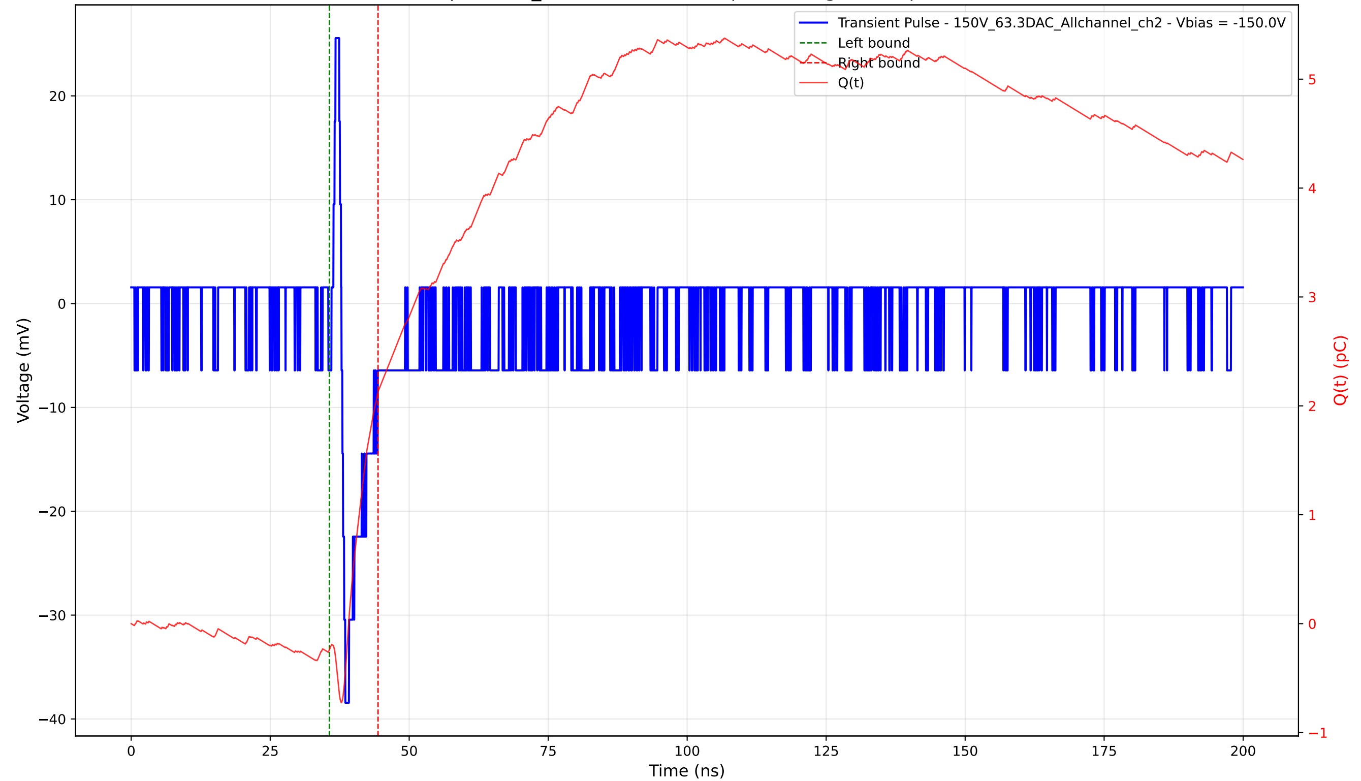
Transient Pulse - Sample: 1cm_42 - Position: 610.0 \mu\text{m} - Charge: 2.37 pC - Rise Time: 0.70 ns
