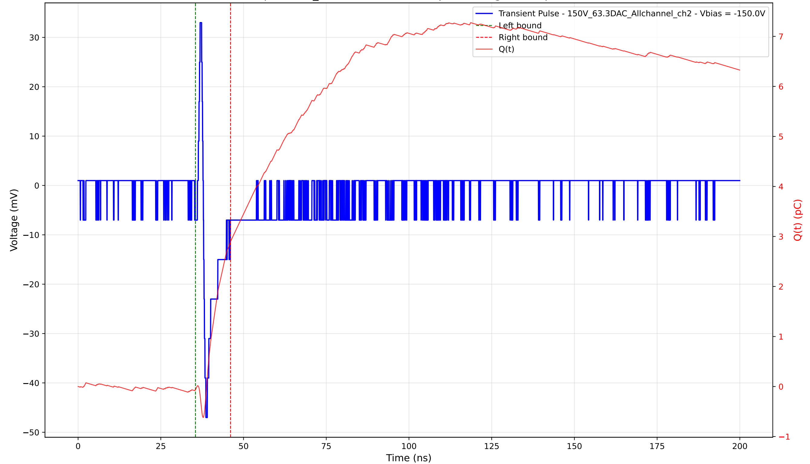
Transient Pulse - Sample: 1cm_42 - Position: 1125.0 \mu\text{m} - Charge: 2.96 pC - Rise Time: 0.78 ns
