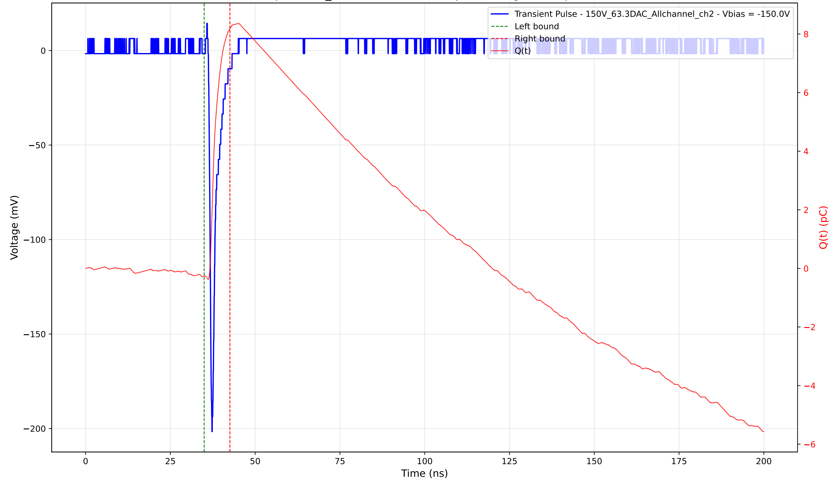
Transient Pulse - Sample: 1cm_42 - Position: 3535.0 \mu\text{m} - Charge: 8.45 pC - Rise Time: 0.79 ns
