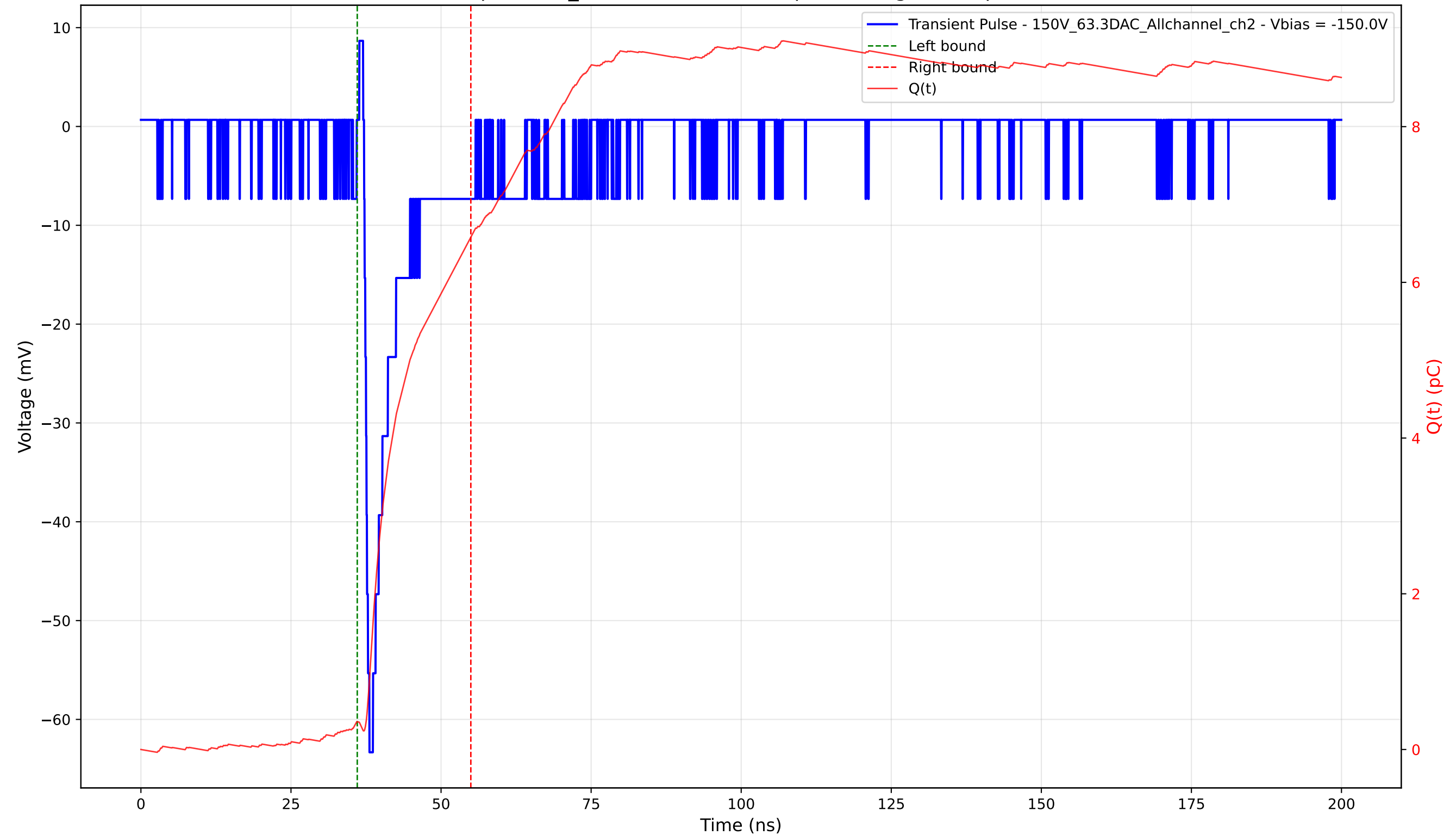
Transient Pulse - Sample: 1cm_42 - Position: 1840.0 \mu\text{m} - Charge: 6.23 pC - Rise Time: 0.89 ns
