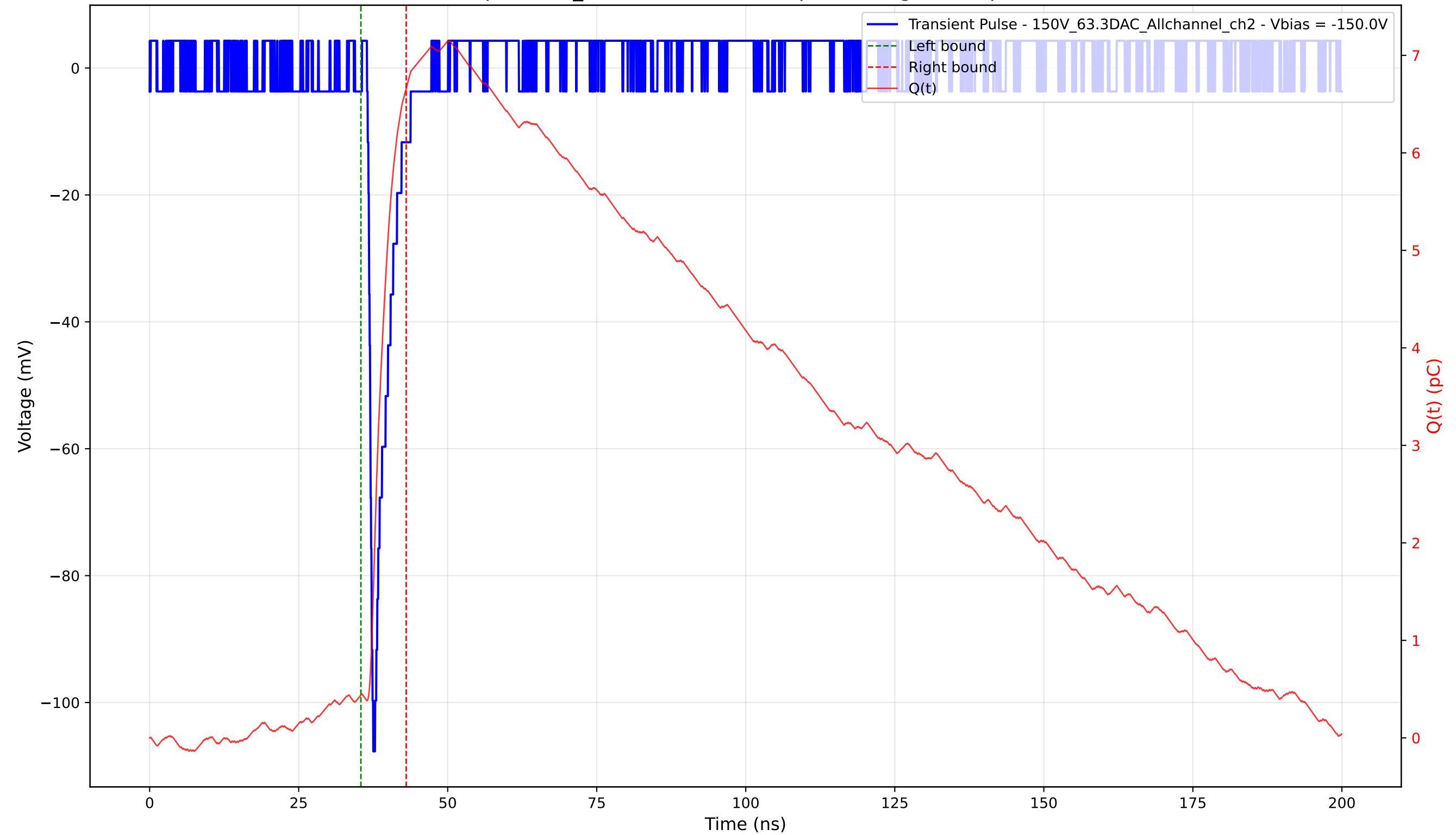
Transient Pulse - Sample: 1cm_42 - Position: 3885.0 \mu\text{m} - Charge: 6.22 pC - Rise Time: 0.80 ns
