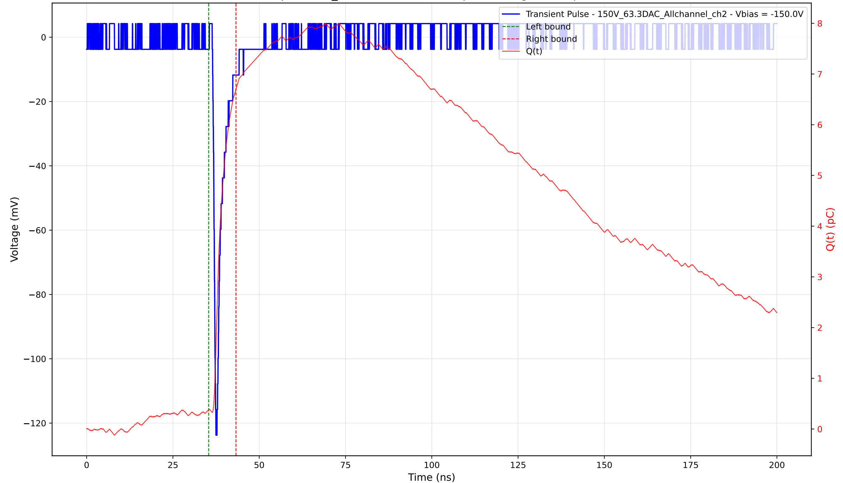
Transient Pulse - Sample: 1cm_42 - Position: 2210.0 \mu\text{m} - Charge: 6.32 pC - Rise Time: 0.80 ns
