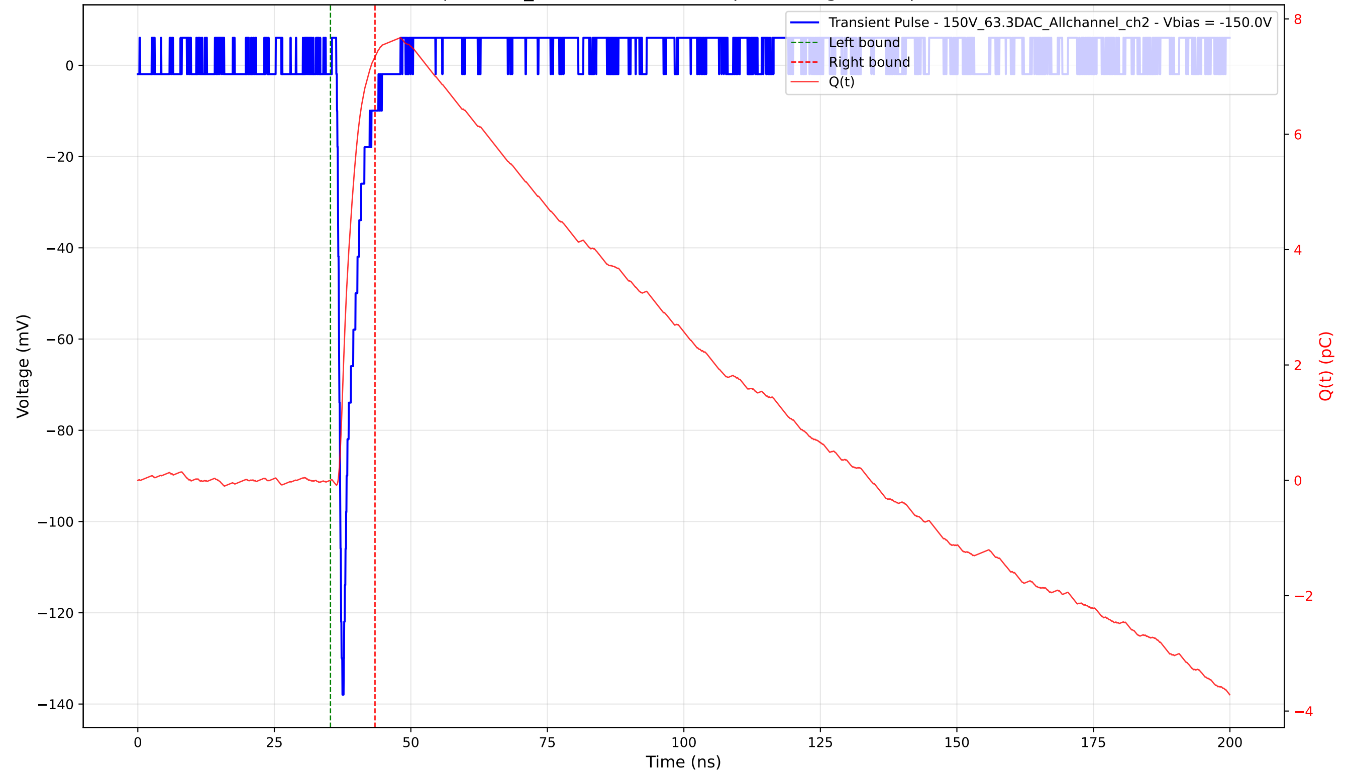
Transient Pulse - Sample: 1cm_42 - Position: 3730.0 \mu\text{m} - Charge: 7.34 pC - Rise Time: 0.78 ns
