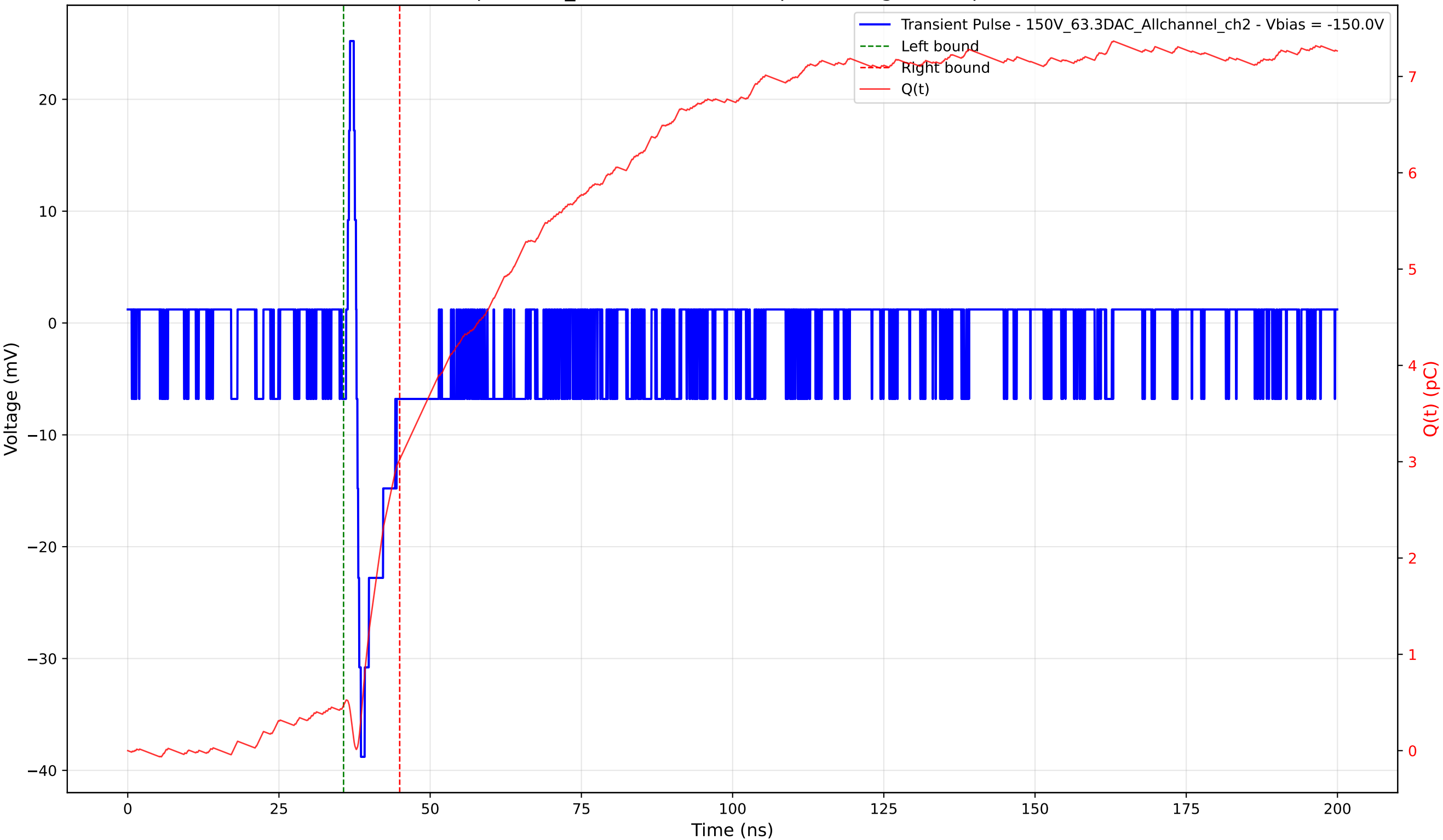
Transient Pulse - Sample: 1cm_42 - Position: 605.0 \mu\text{m} - Charge: 2.55 pC - Rise Time: 0.74 ns
