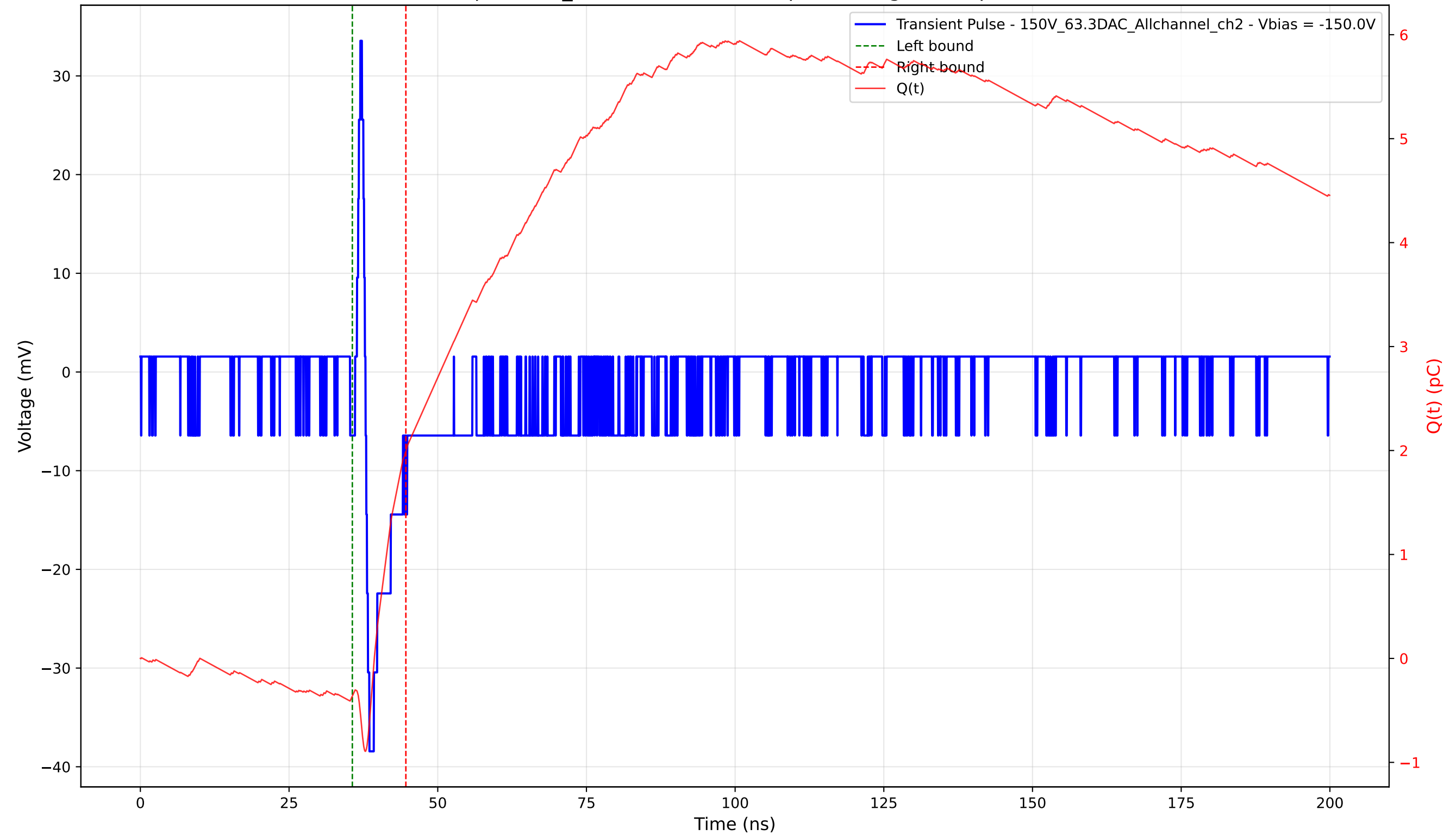
Transient Pulse - Sample: 1cm_42 - Position: 1015.0 \mu\text{m} - Charge: 2.35 pC - Rise Time: 0.66 ns
