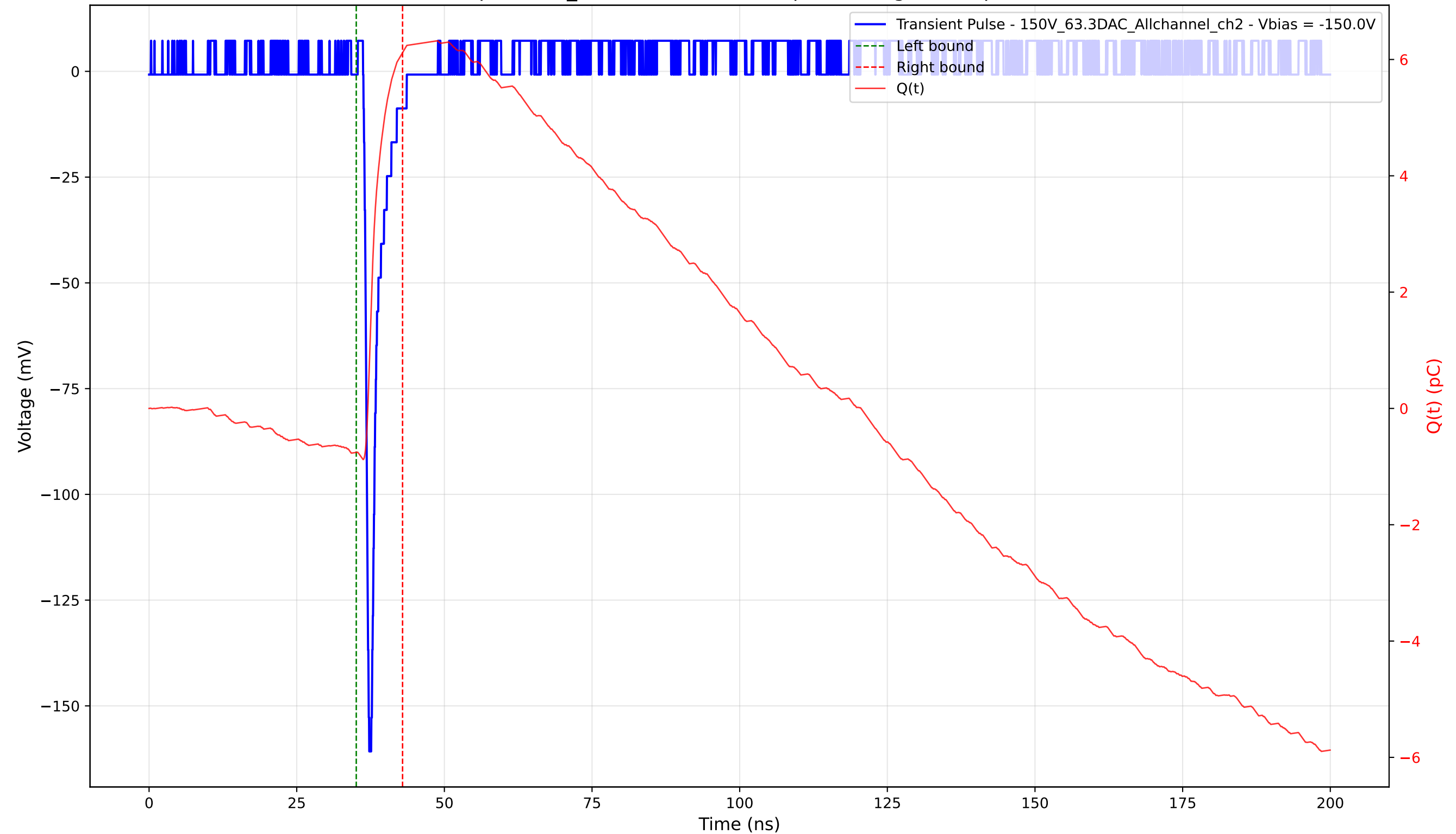
Transient Pulse - Sample: 1cm_42 - Position: 2435.0 \mu\text{m} - Charge: 6.88 pC - Rise Time: 0.76 ns
