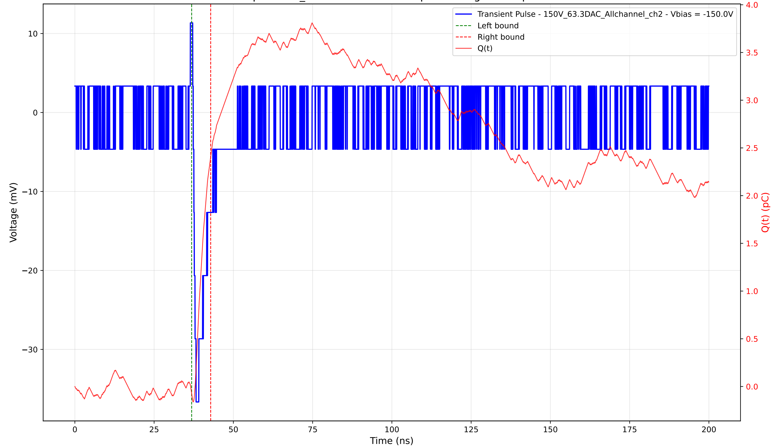
Transient Pulse - Sample: 1cm_42 - Position: 4625.0 \mu\text{m} - Charge: 2.48 pC - Rise Time: 0.91 ns
