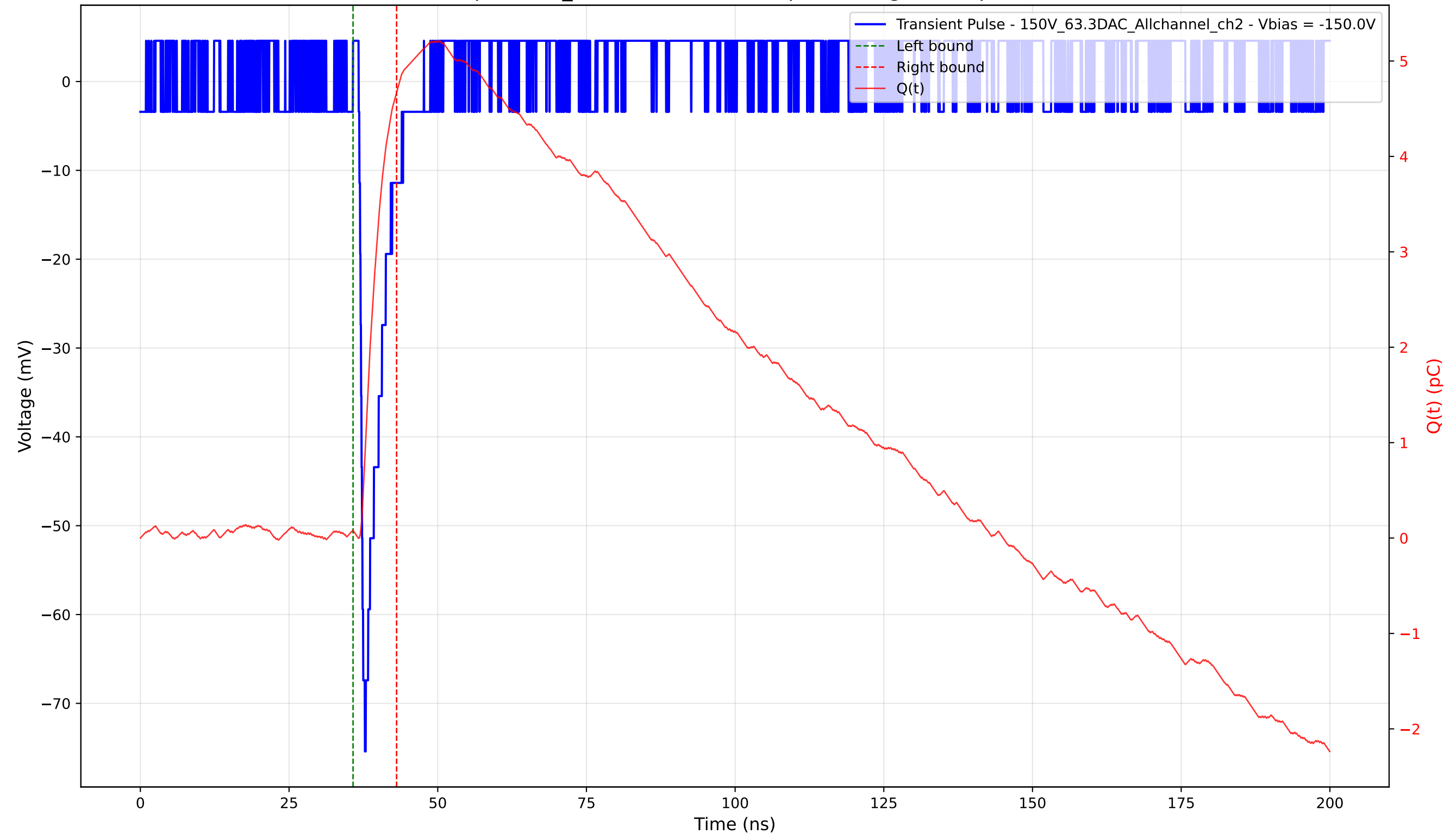
Transient Pulse - Sample: 1cm_42 - Position: 4005.0 \mu\text{m} - Charge: 4.59 pC - Rise Time: 0.94 ns
