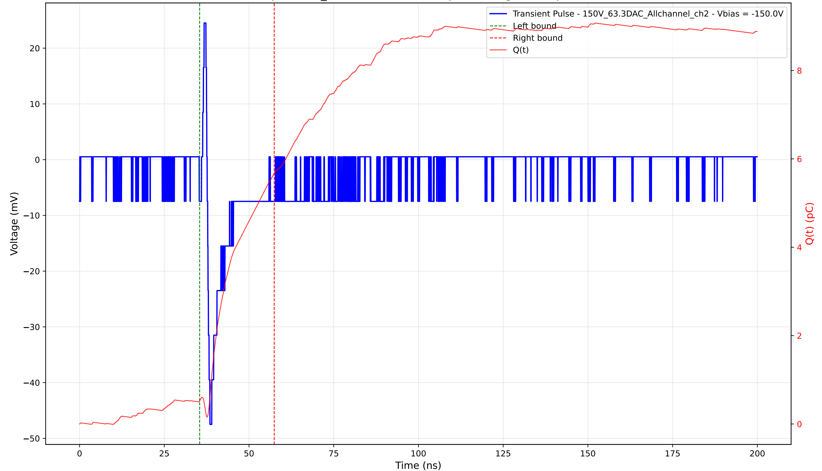
Transient Pulse - Sample: 1cm_42 - Position: 1450.0 \mu\text{m} - Charge: 5.16 pC - Rise Time: 0.82 ns
