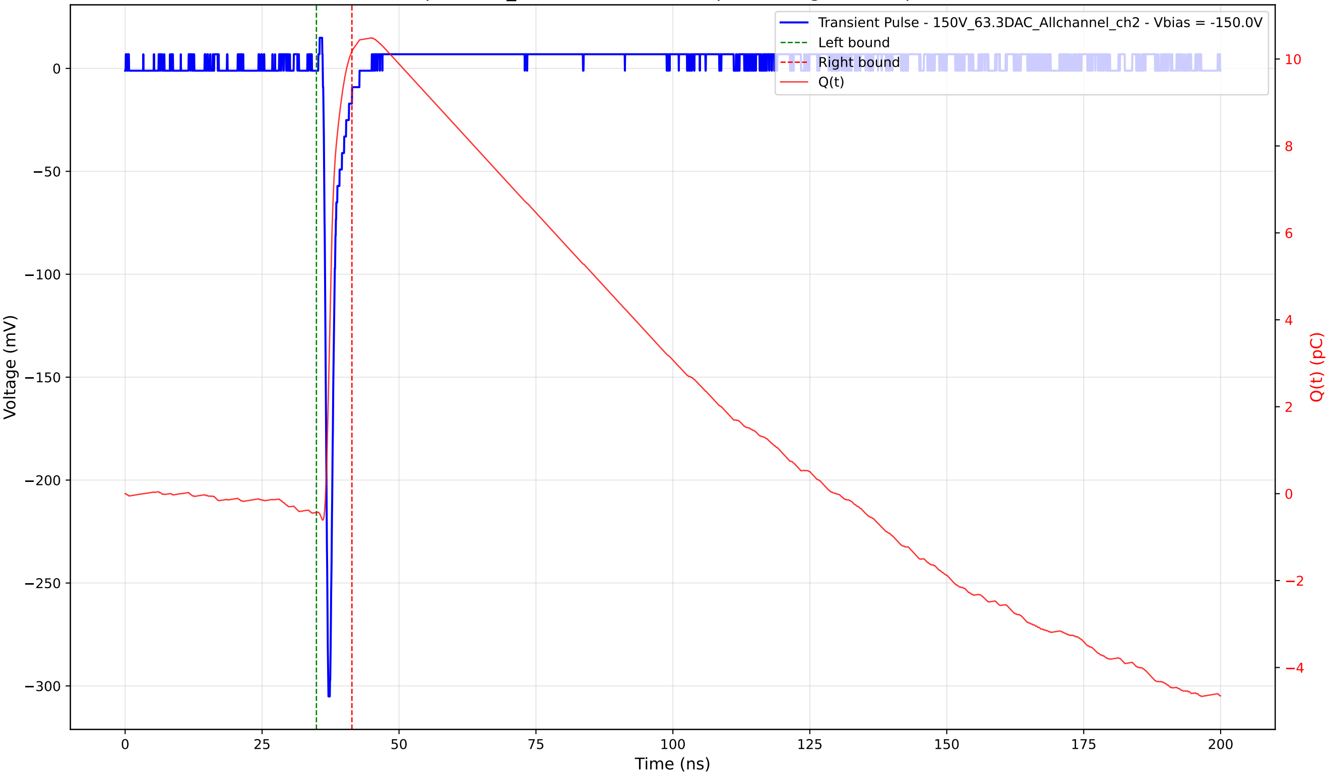
Transient Pulse - Sample: 1cm_42 - Position: 2630.0 \mu\text{m} - Charge: 10.61 pC - Rise Time: 0.70 ns
