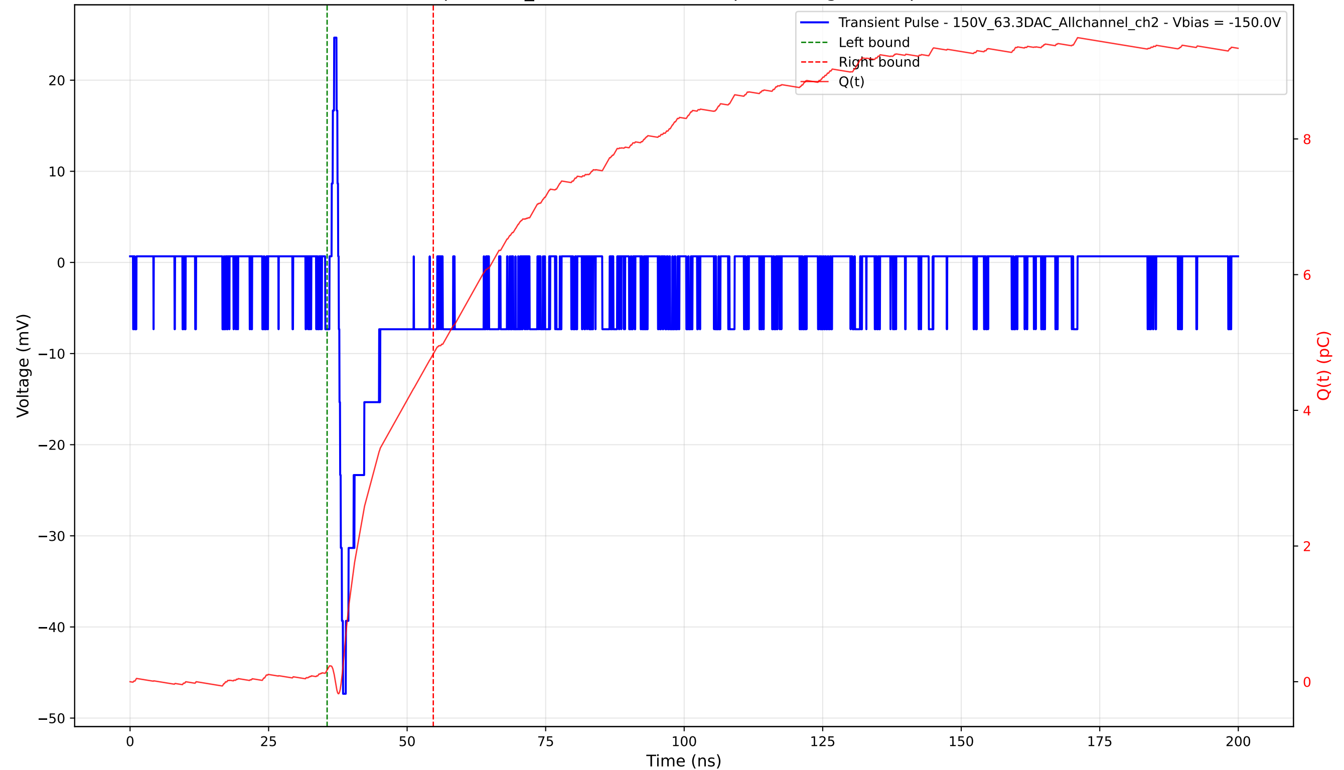
Transient Pulse - Sample: 1cm_42 - Position: 1445.0 \mu\text{m} - Charge: 4.66 pC - Rise Time: 0.78 ns
