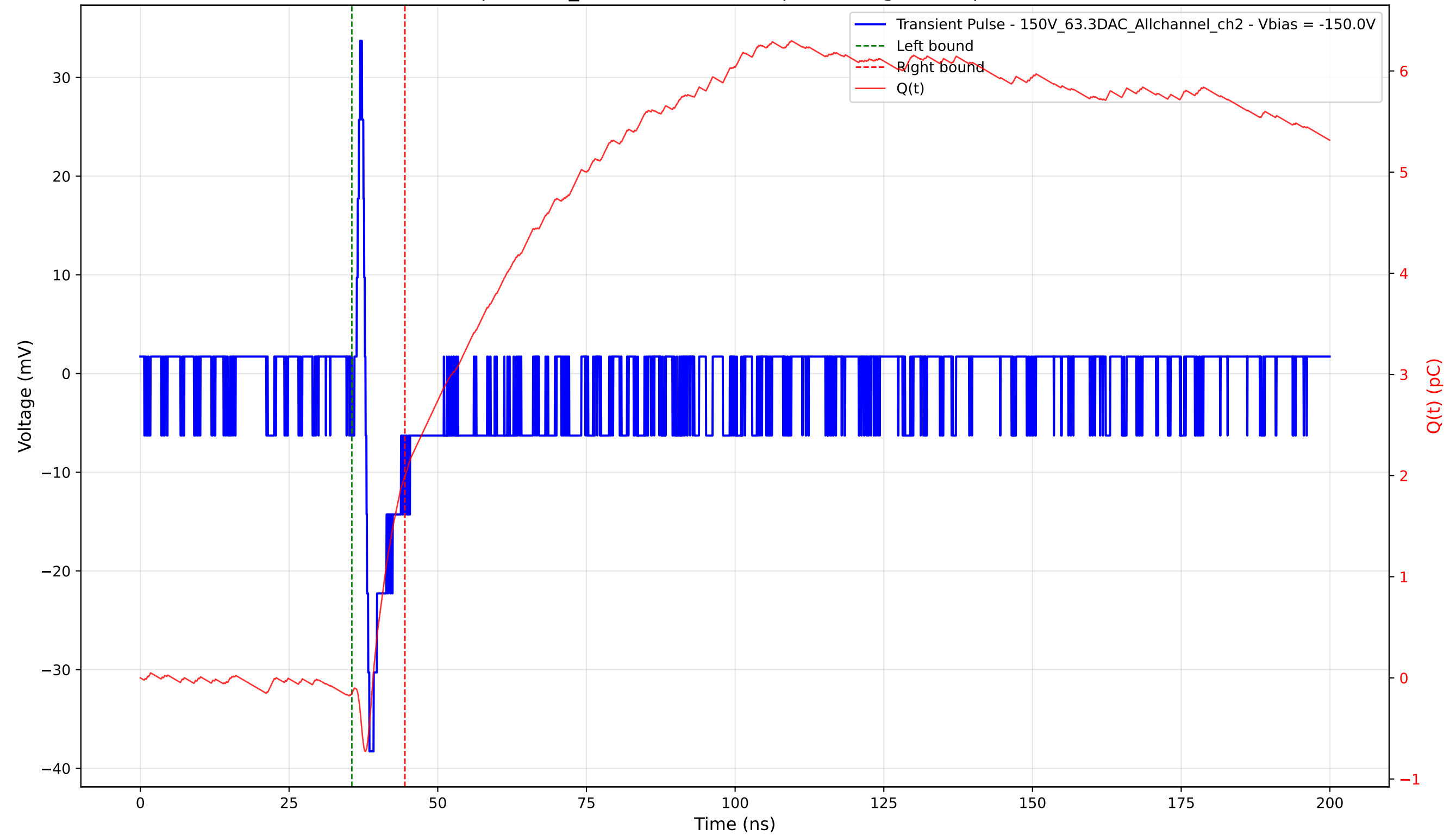
Transient Pulse - Sample: 1cm_42 - Position: 965.0 \mu\text{m} - Charge: 2.14 pC - Rise Time: 0.66 ns
