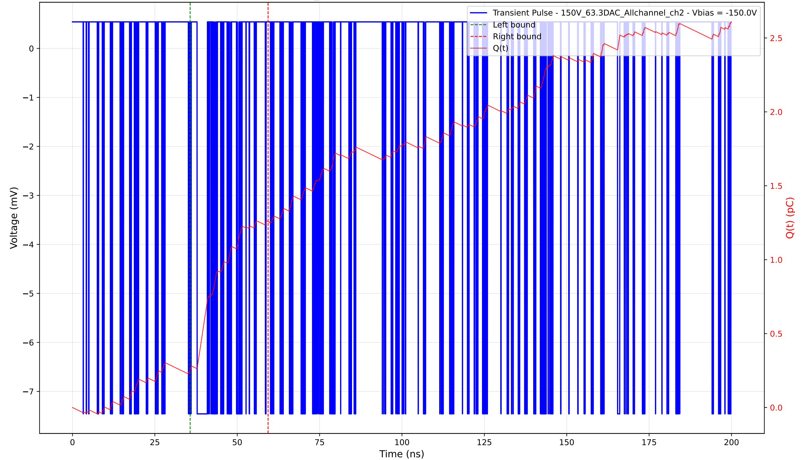
Transient Pulse - Sample: 1cm_42 - Position: 65.0 \mu\text{m} - Charge: 1.00 pC - Rise Time: 0.04 ns
