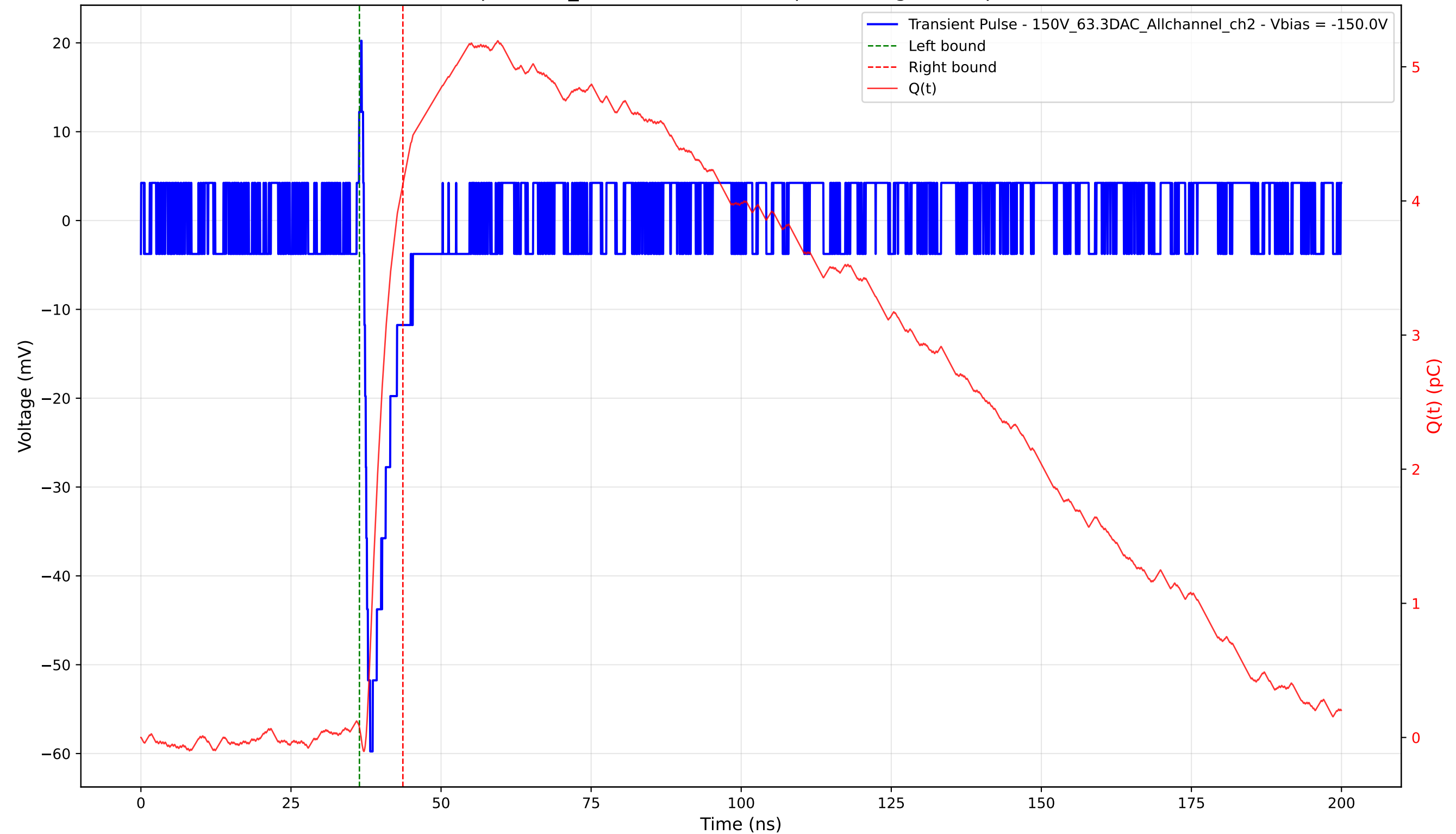
Transient Pulse - Sample: 1cm_42 - Position: 4295.0 \mu\text{m} - Charge: 4.05 pC - Rise Time: 0.99 ns
