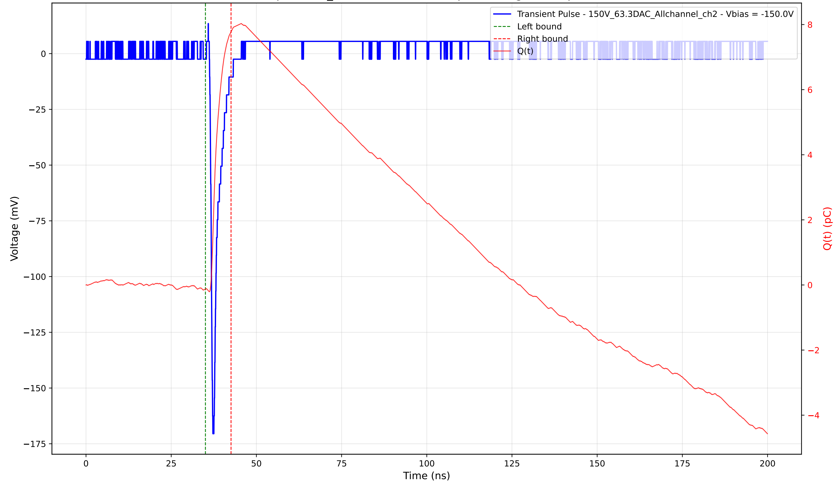
Transient Pulse - Sample: 1cm_42 - Position: 3585.0 \mu\text{m} - Charge: 7.90 pC - Rise Time: 0.76 ns
