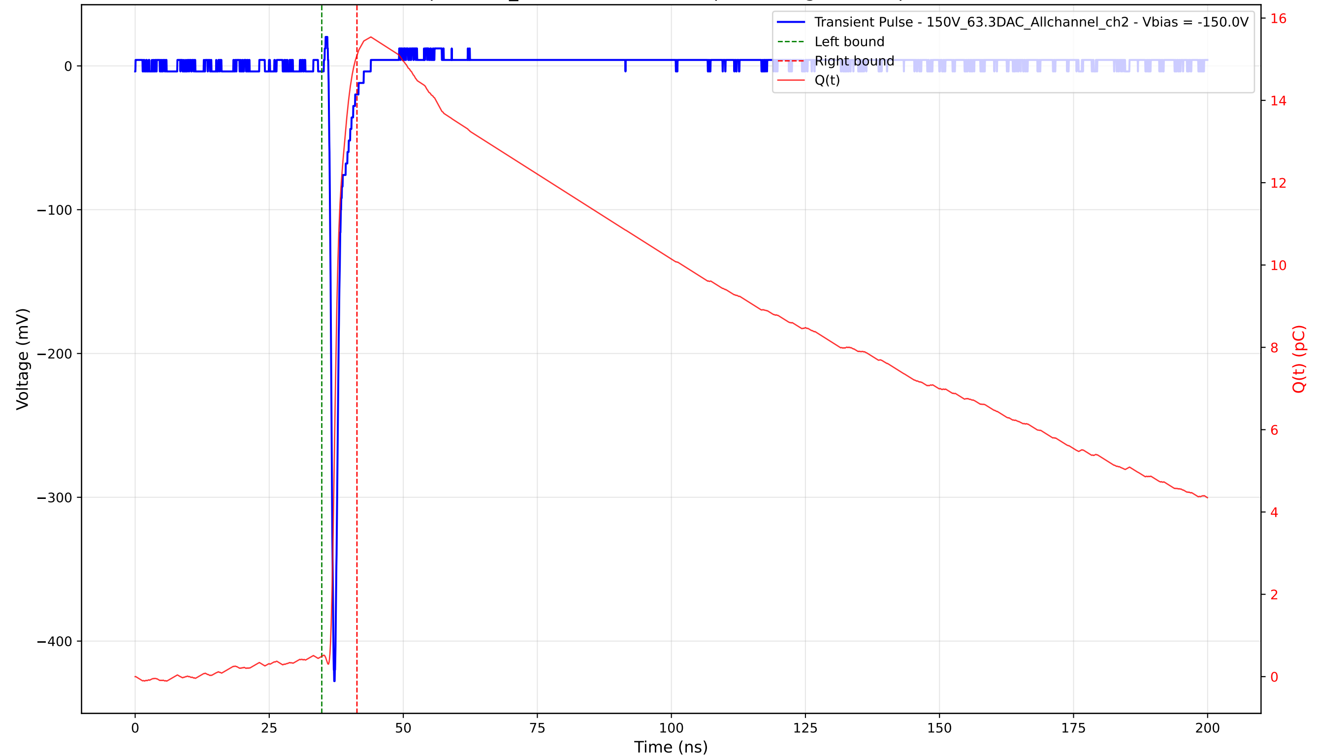
Transient Pulse - Sample: 1cm_42 - Position: 3300.0 \mu\text{m} - Charge: 14.60 pC - Rise Time: 0.73 ns
