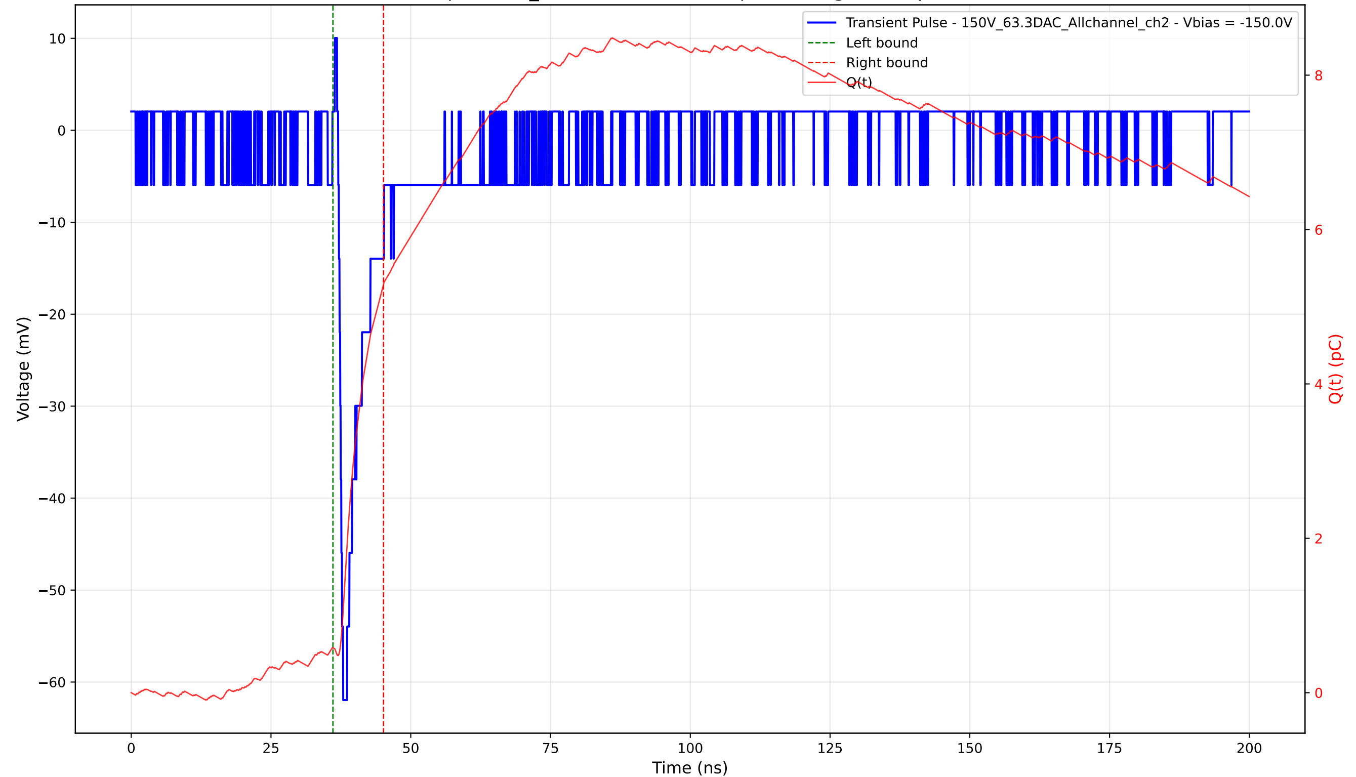
Transient Pulse - Sample: 1cm_42 - Position: 1900.0 \mu\text{m} - Charge: 4.71 pC - Rise Time: 0.80 ns
