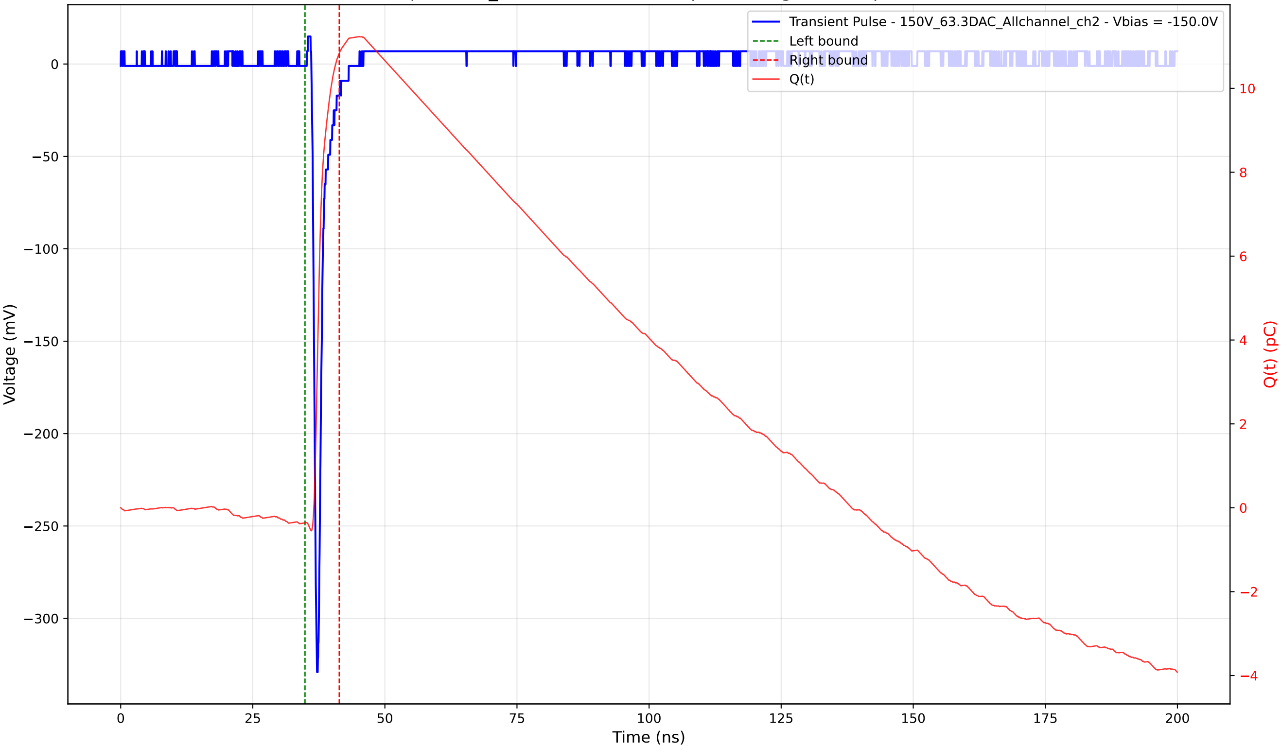
Transient Pulse - Sample: 1cm_42 - Position: 2650.0 \mu\text{m} - Charge: 11.20 pC - Rise Time: 0.76 ns
