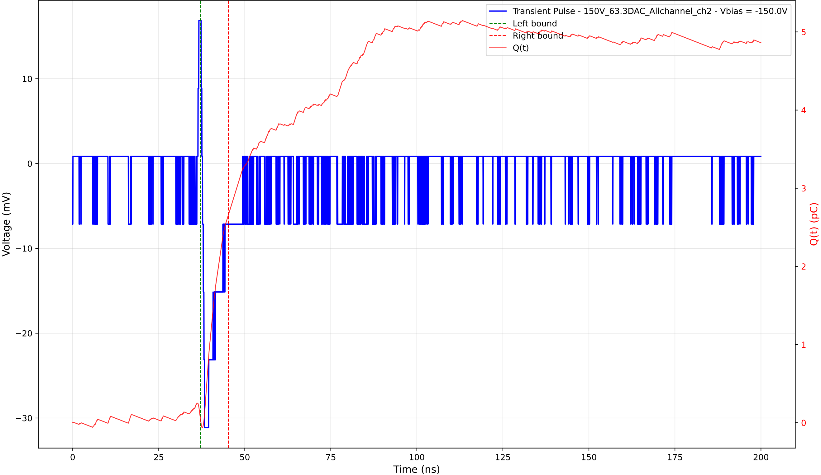
Transient Pulse - Sample: 1cm_42 - Position: 475.0 \mu\text{m} - Charge: 2.60 pC - Rise Time: 0.59 ns
