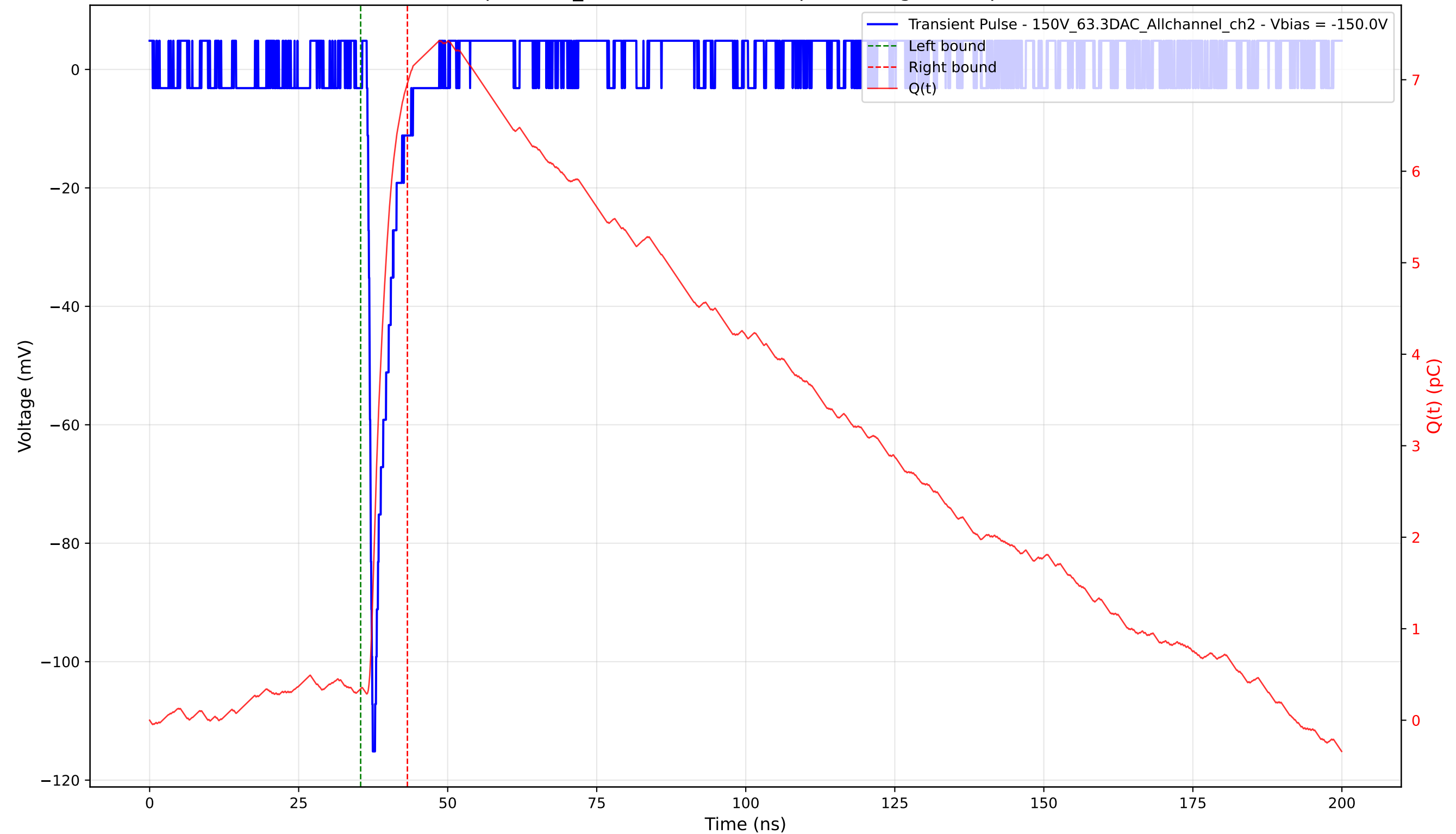
Transient Pulse - Sample: 1cm_42 - Position: 3855.0 \mu\text{m} - Charge: 6.62 pC - Rise Time: 0.72 ns
