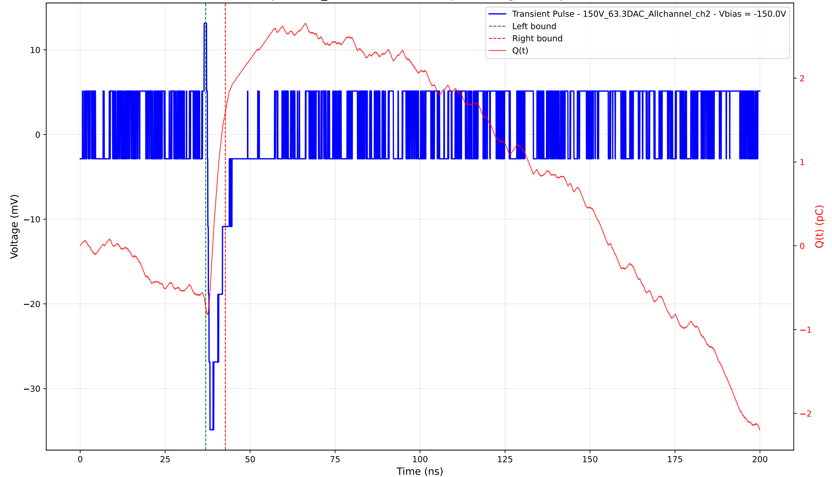
Transient Pulse - Sample: 1cm_42 - Position: 4630.0 \mu\text{m} - Charge: 2.33 pC - Rise Time: 0.68 ns
