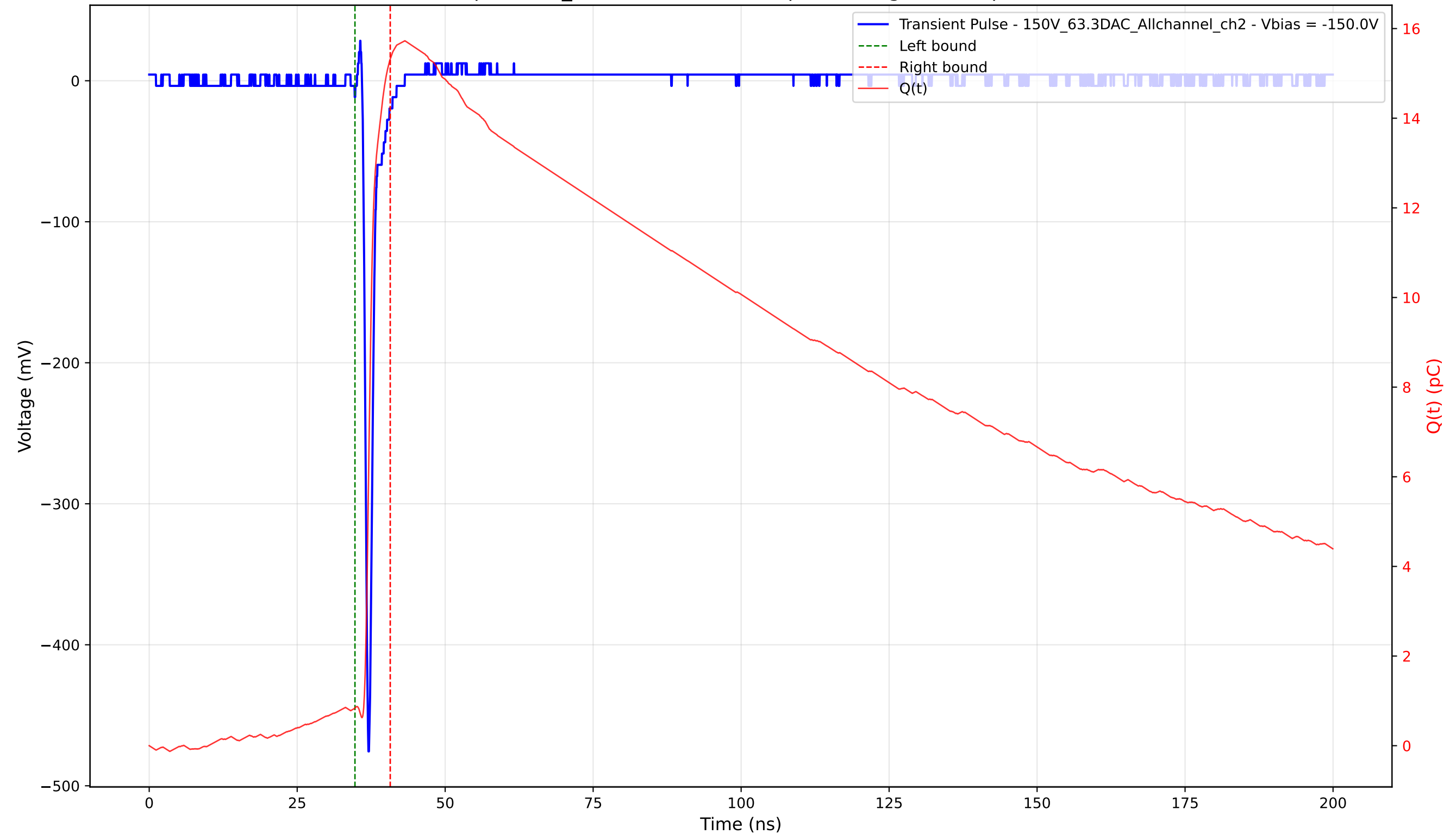
Transient Pulse - Sample: 1cm_42 - Position: 2990.0 \mu\text{m} - Charge: 14.48 pC - Rise Time: 0.73 ns
