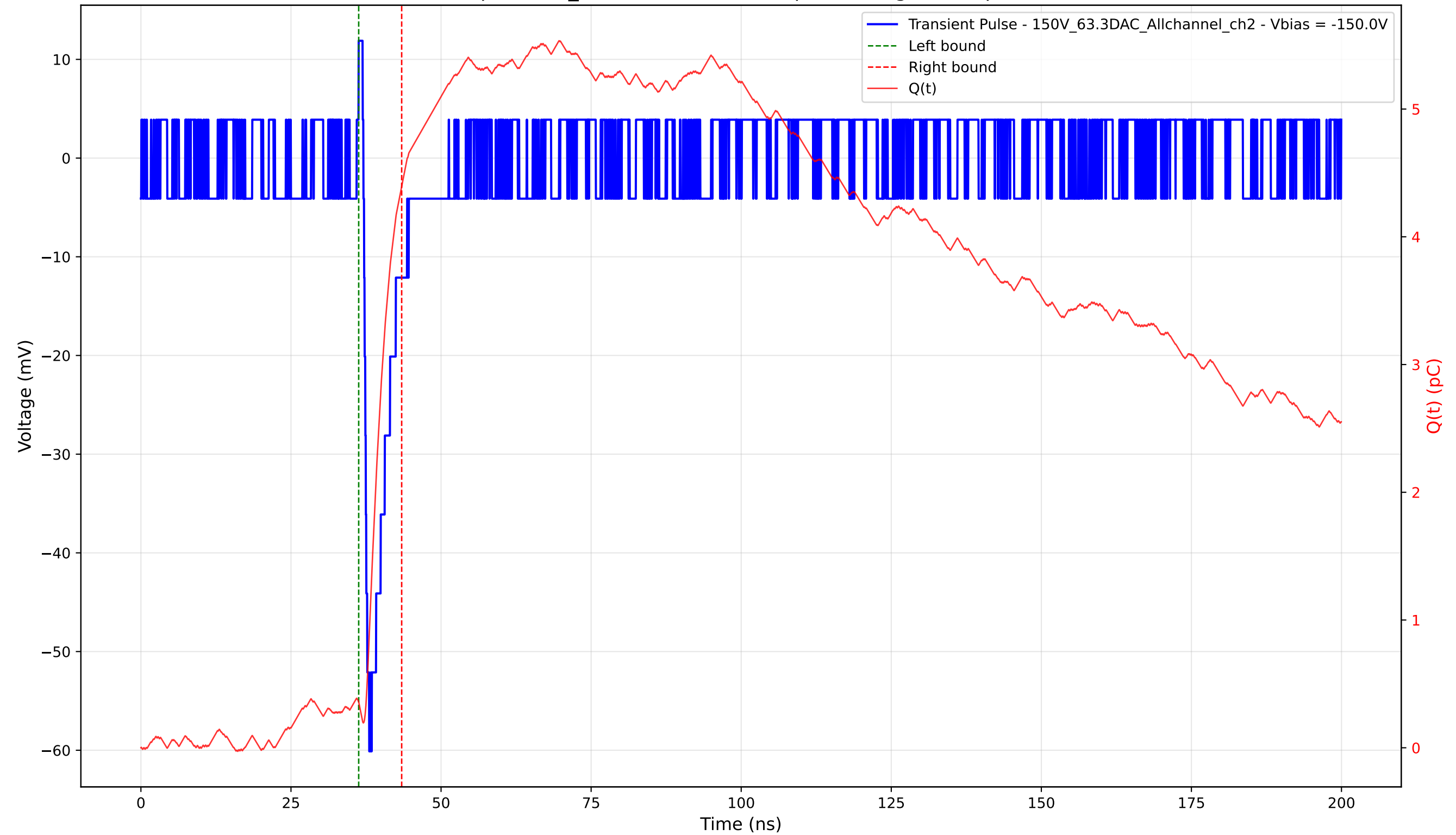
Transient Pulse - Sample: 1cm_42 - Position: 4195.0 \mu\text{m} - Charge: 4.04 pC - Rise Time: 0.87 ns
