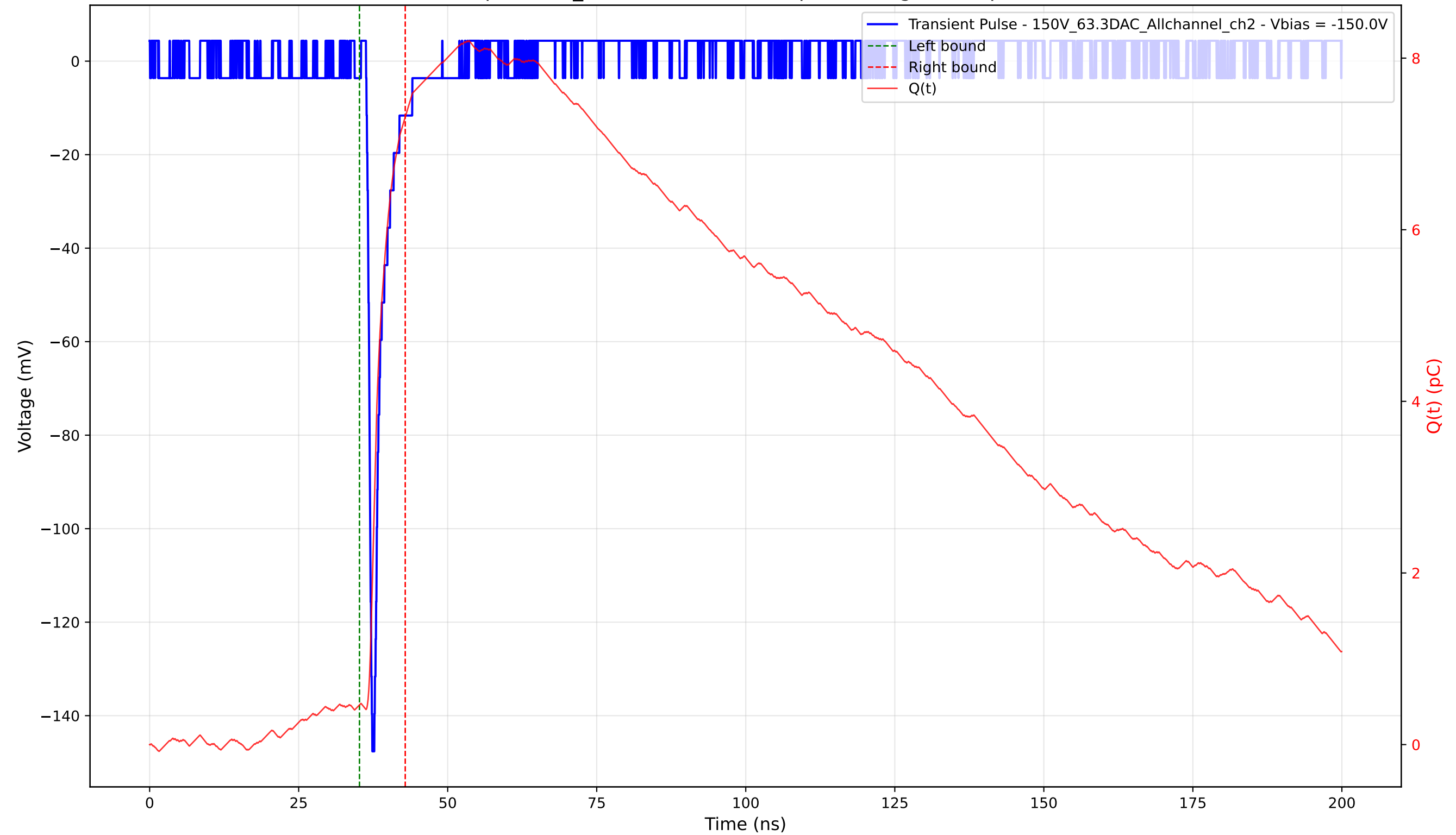
Transient Pulse - Sample: 1cm_42 - Position: 2375.0 \mu\text{m} - Charge: 6.85 pC - Rise Time: 0.82 ns
