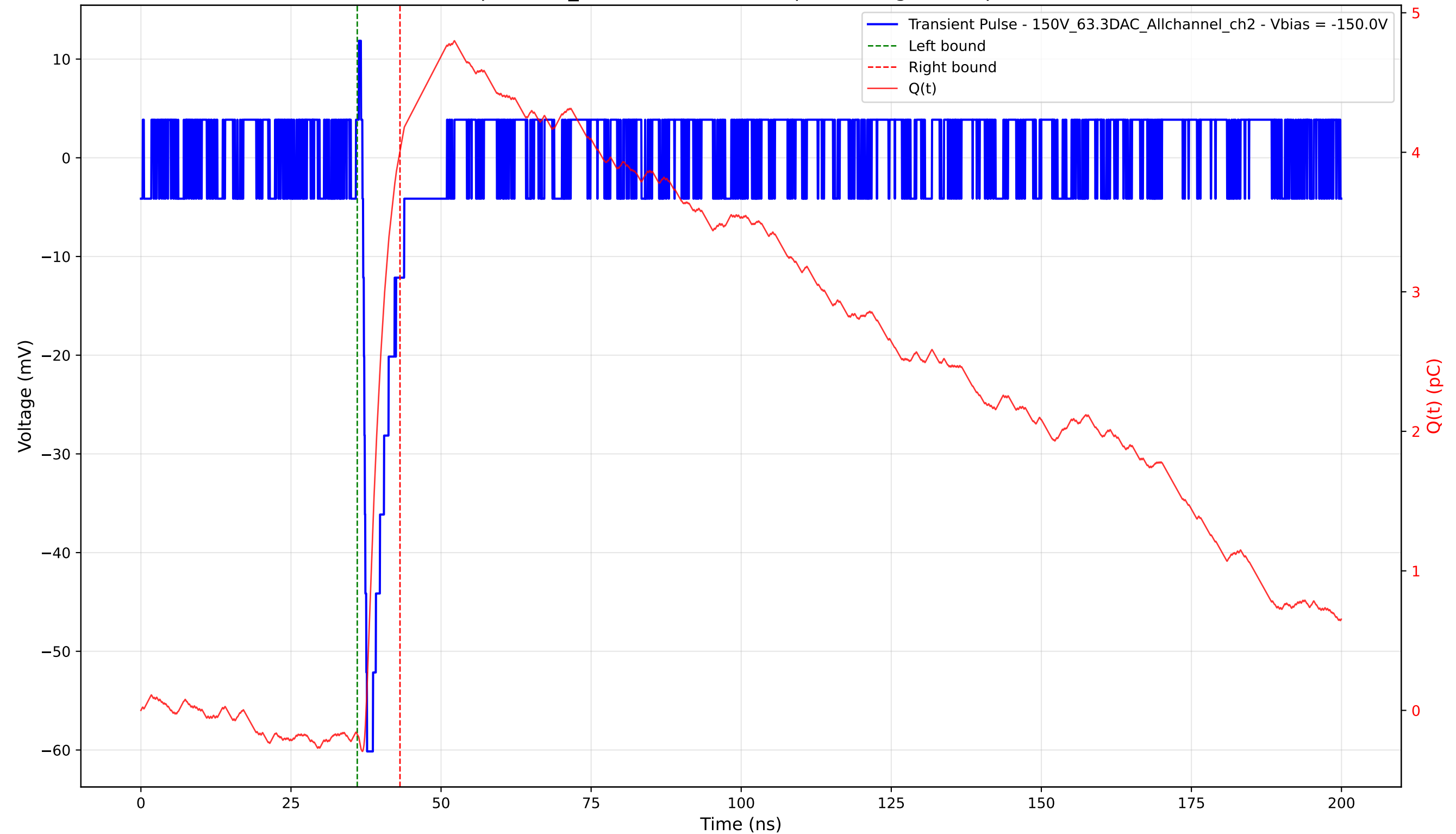
Transient Pulse - Sample: 1cm_42 - Position: 4100.0 \mu\text{m} - Charge: 4.18 pC - Rise Time: 0.67 ns
