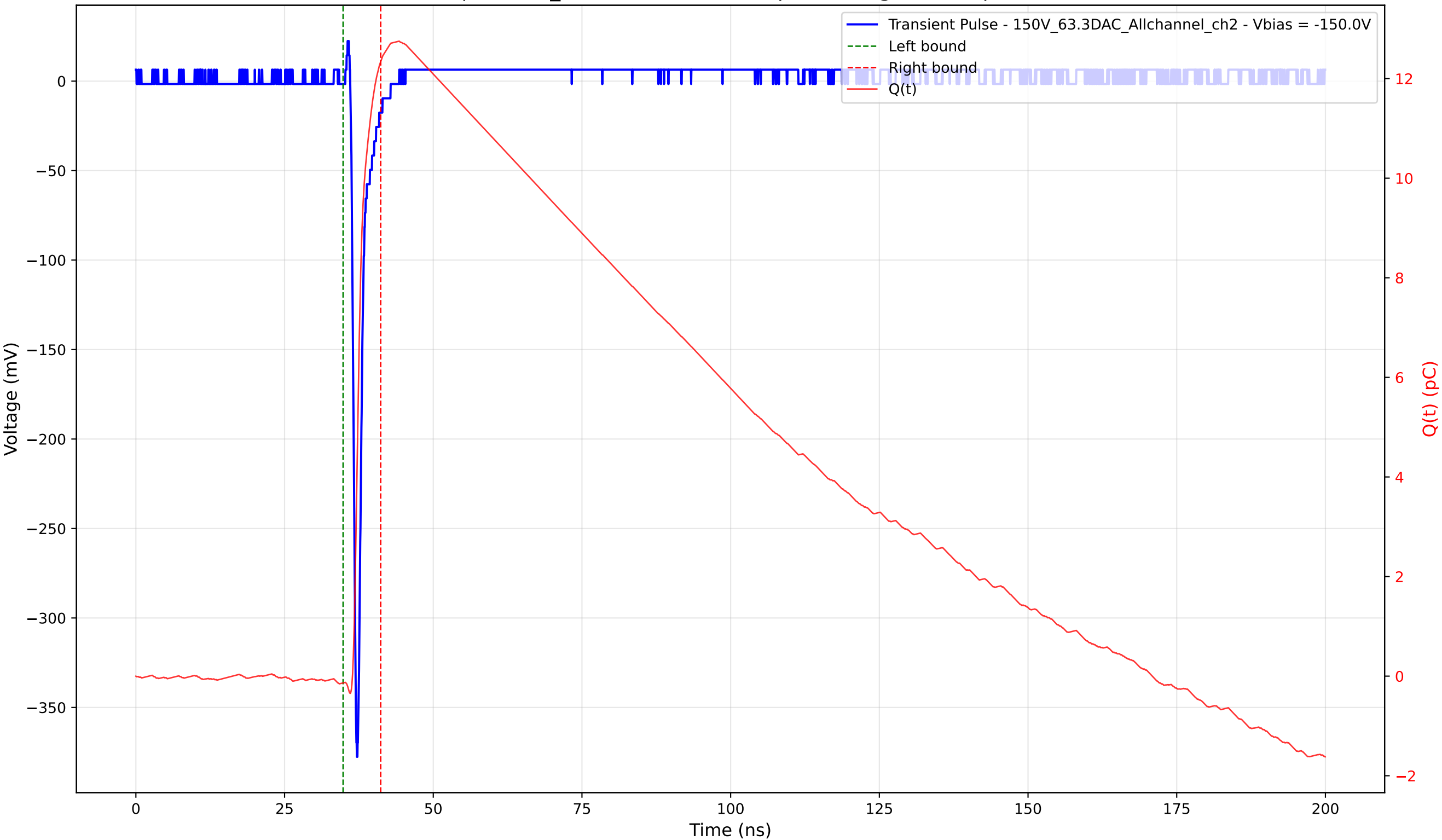
Transient Pulse - Sample: 1cm_42 - Position: 2690.0 \mu\text{m} - Charge: 12.48 pC - Rise Time: 0.71 ns
