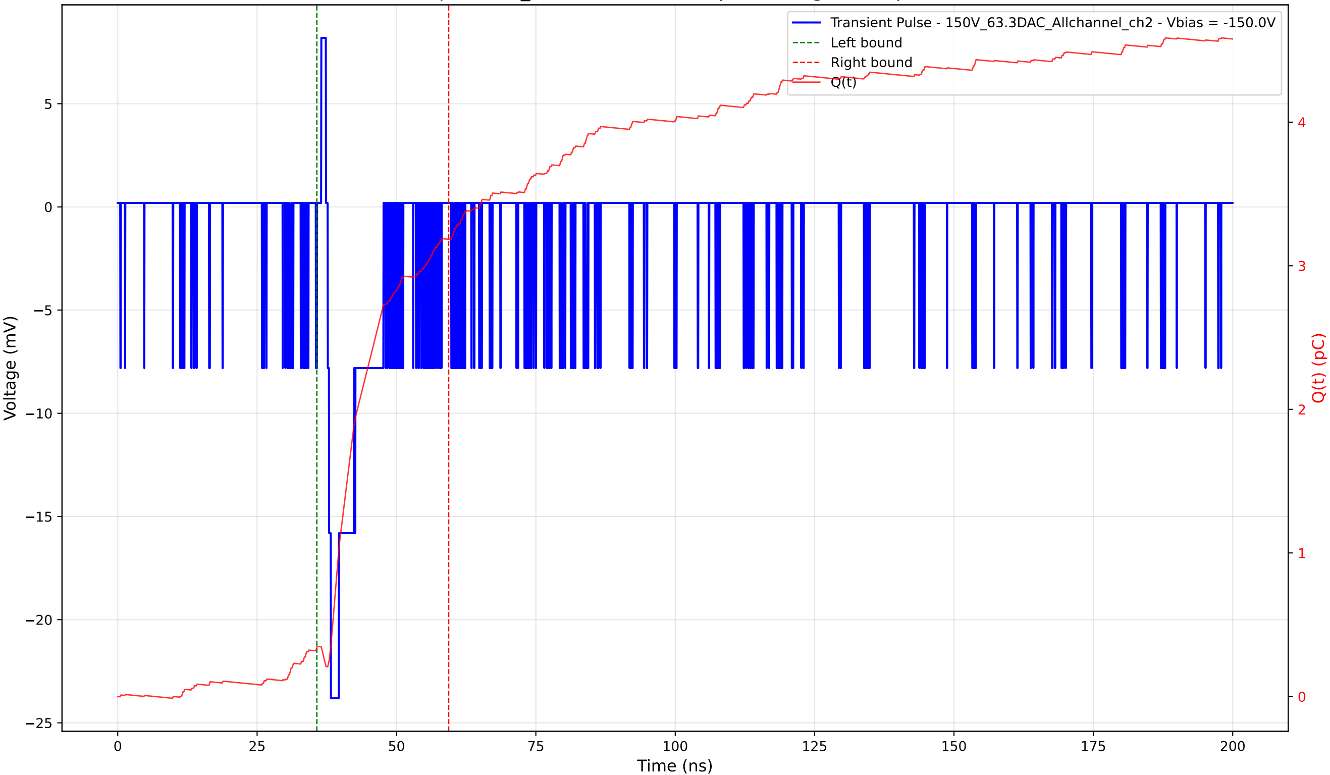
Transient Pulse - Sample: 1cm_42 - Position: 295.0 \mu\text{m} - Charge: 2.84 pC - Rise Time: 0.59 ns
