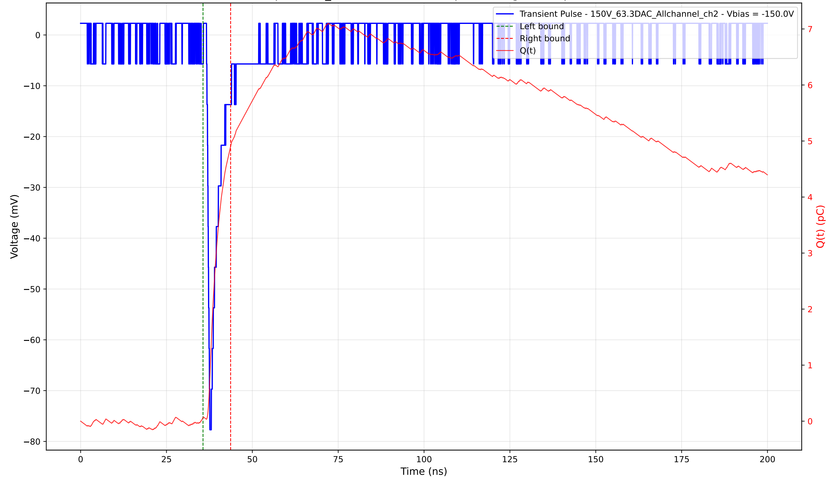
Transient Pulse - Sample: 1cm_42 - Position: 2035.0 \mu\text{m} - Charge: 4.84 pC - Rise Time: 0.87 ns
