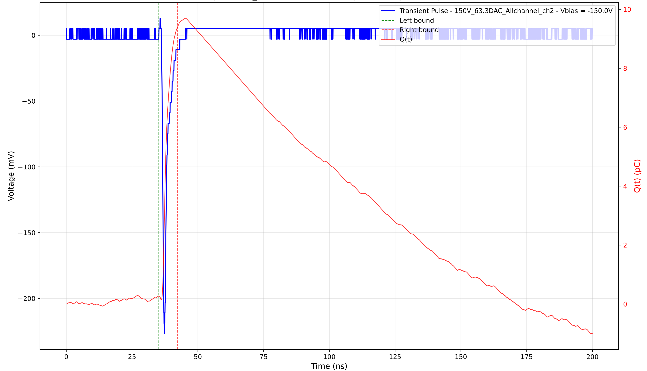
Transient Pulse - Sample: 1cm_42 - Position: 3500.0 \mu\text{m} - Charge: 9.15 pC - Rise Time: 0.78 ns
