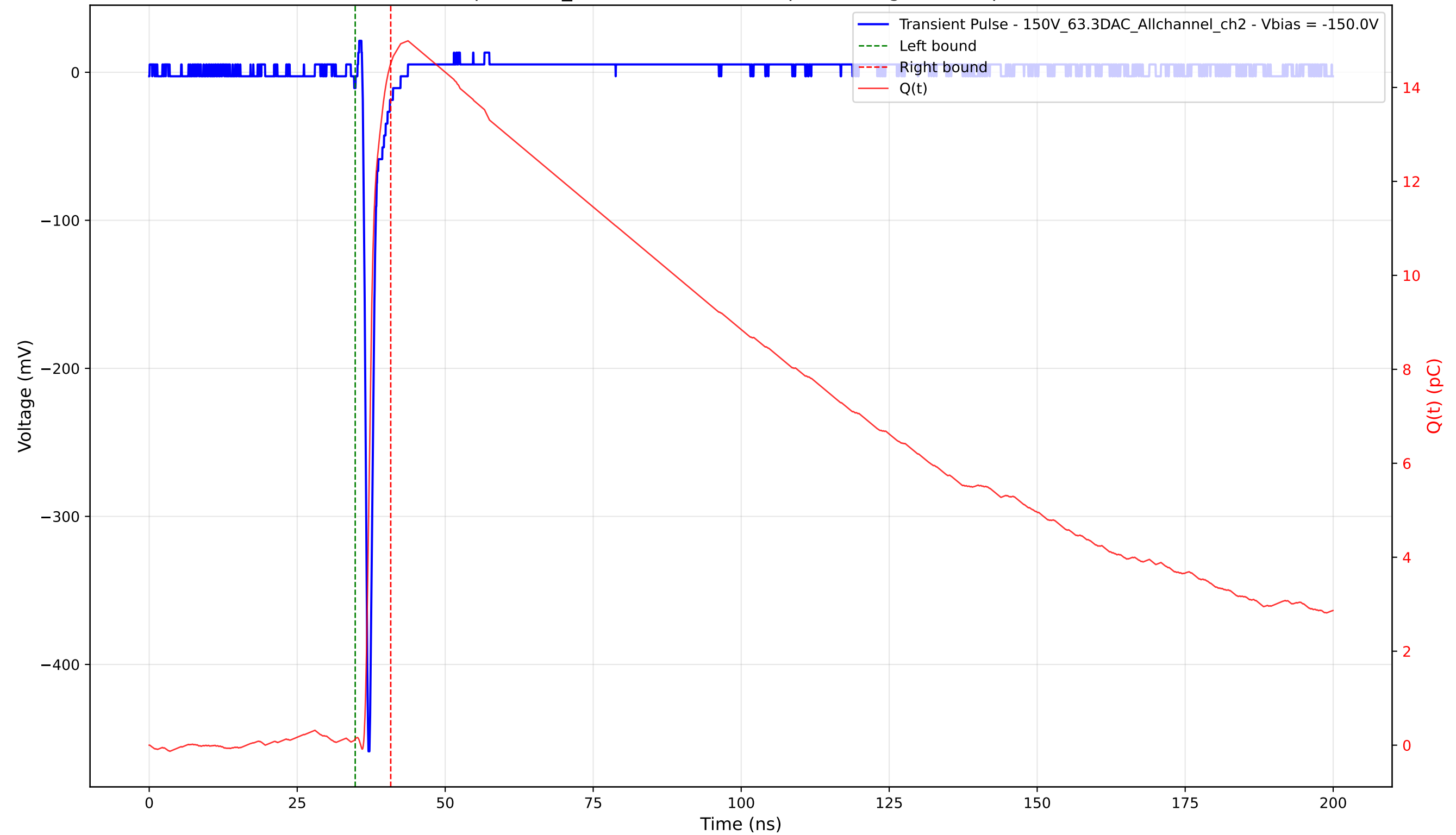
Transient Pulse - Sample: 1cm_42 - Position: 2880.0 \mu\text{m} - Charge: 14.38 pC - Rise Time: 0.70 ns
