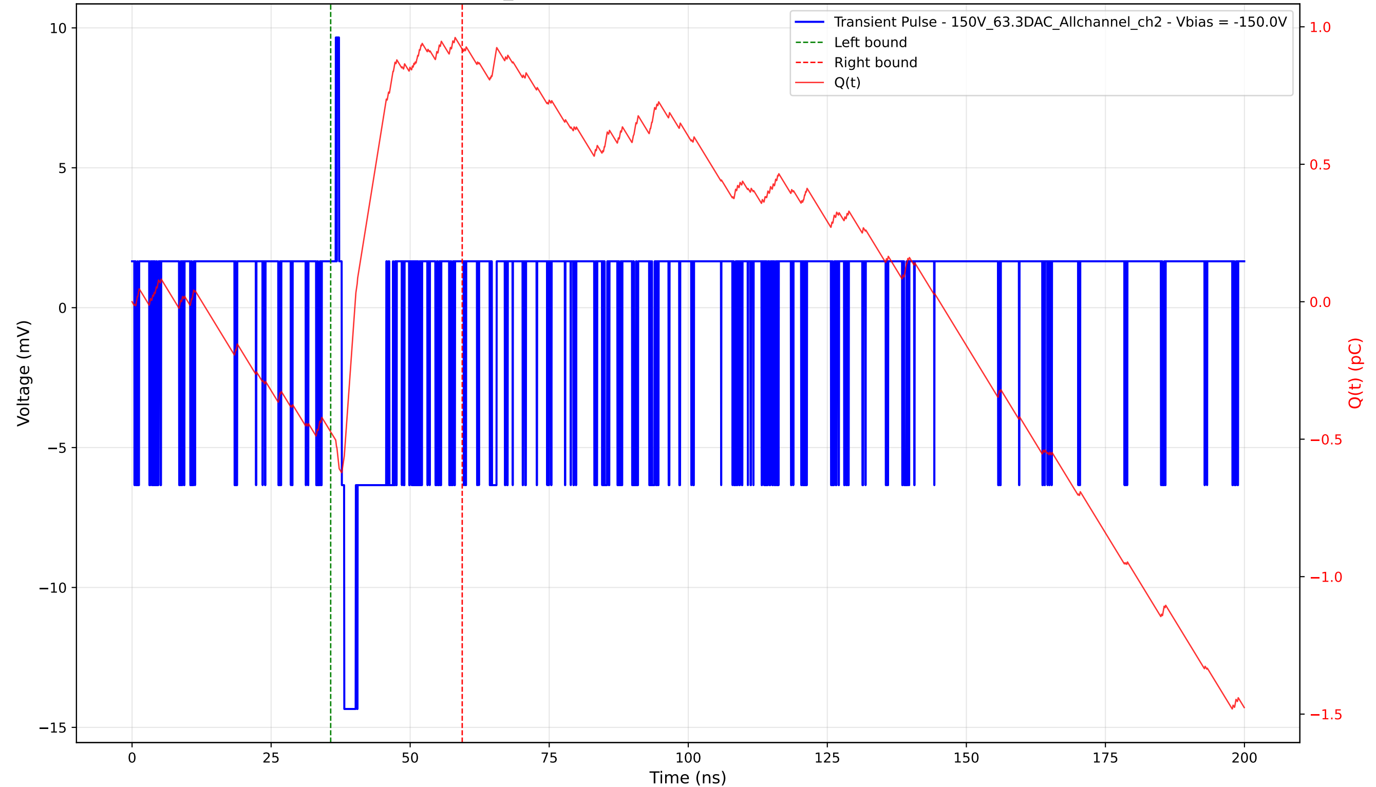
Transient Pulse - Sample: 1cm_42 - Position: 180.0 \mu\text{m} - Charge: 1.39 pC - Rise Time: 0.00 ns (N/A)
