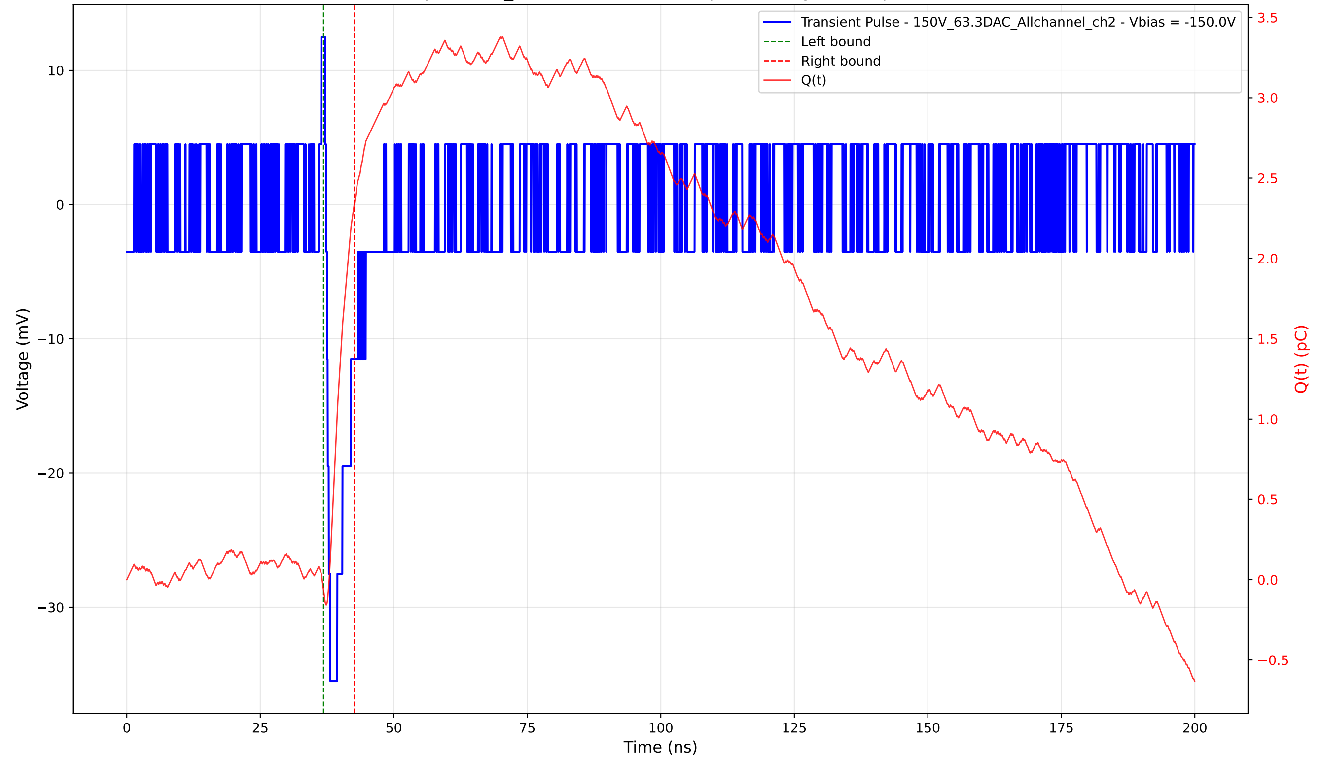
Transient Pulse - Sample: 1cm_42 - Position: 4560.0 \mu\text{m} - Charge: 2.40 pC - Rise Time: 0.64 ns
