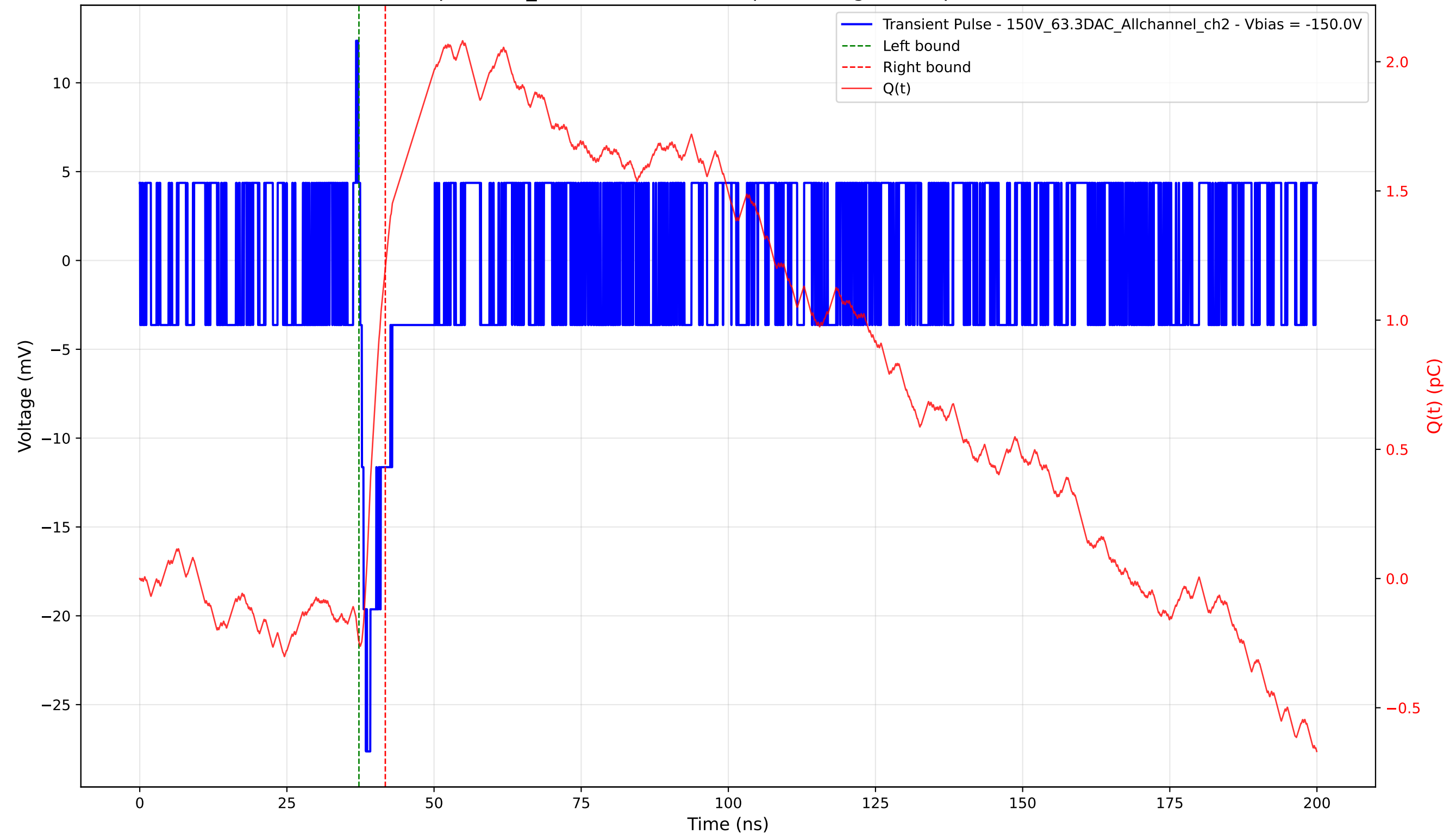
Transient Pulse - Sample: 1cm_42 - Position: 4960.0 \mu\text{m} - Charge: 1.45 pC - Rise Time: 0.00 ns (N/A)
