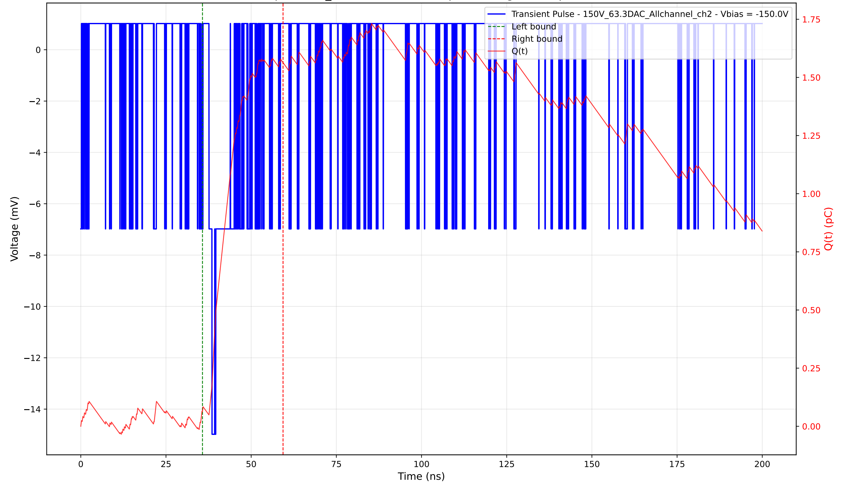
Transient Pulse - Sample: 1cm_42 - Position: 130.0 \mu\text{m} - Charge: 1.50 pC - Rise Time: 0.92 ns
