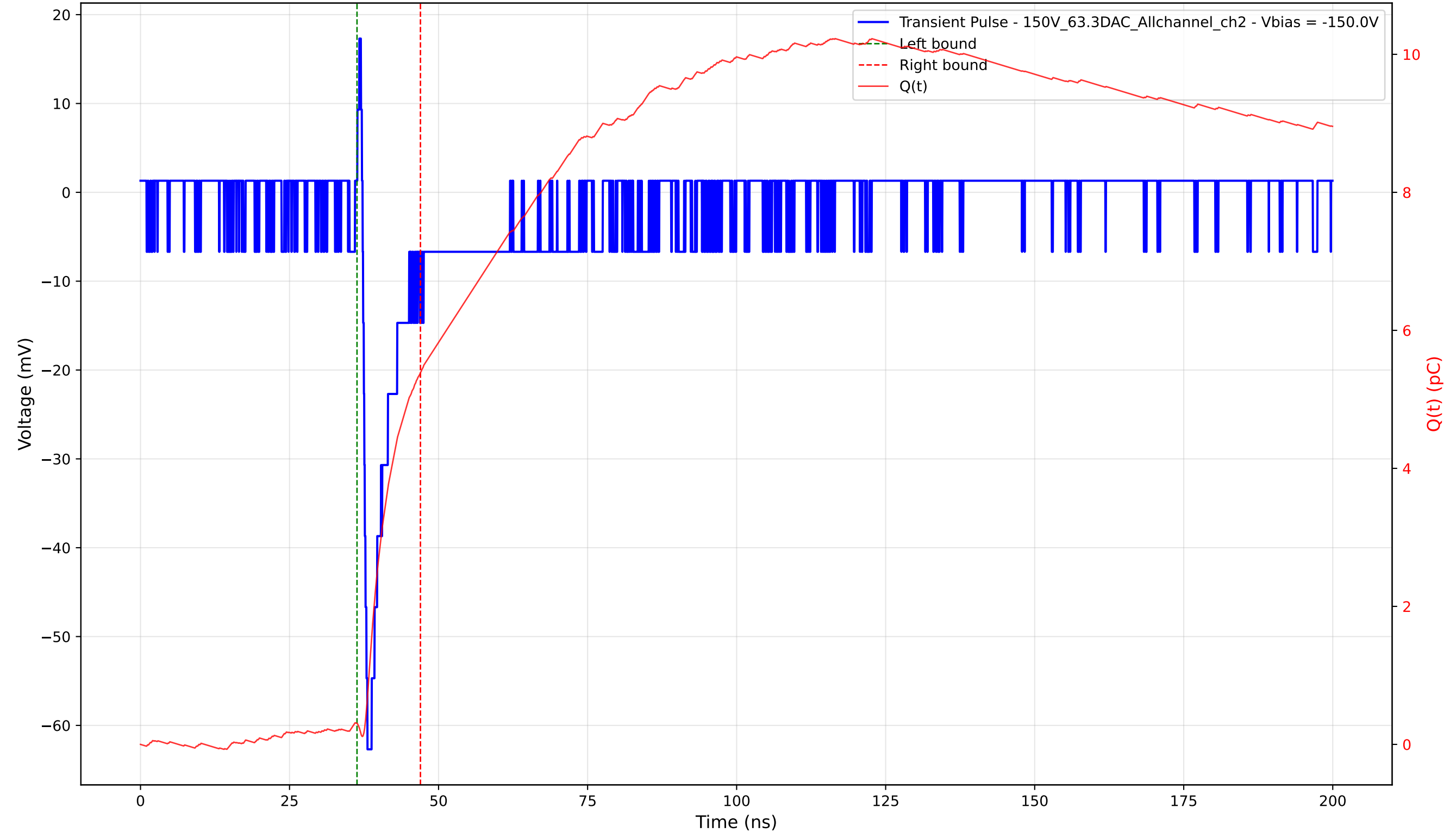
Transient Pulse - Sample: 1cm_42 - Position: 1730.0 \mu\text{m} - Charge: 5.08 pC - Rise Time: 0.80 ns
