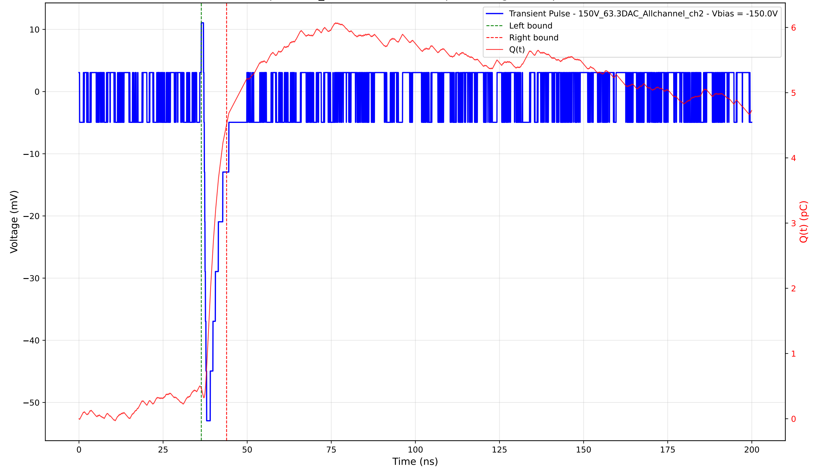
Transient Pulse - Sample: 1cm_42 - Position: 4355.0 \mu\text{m} - Charge: 4.04 pC - Rise Time: 0.72 ns
