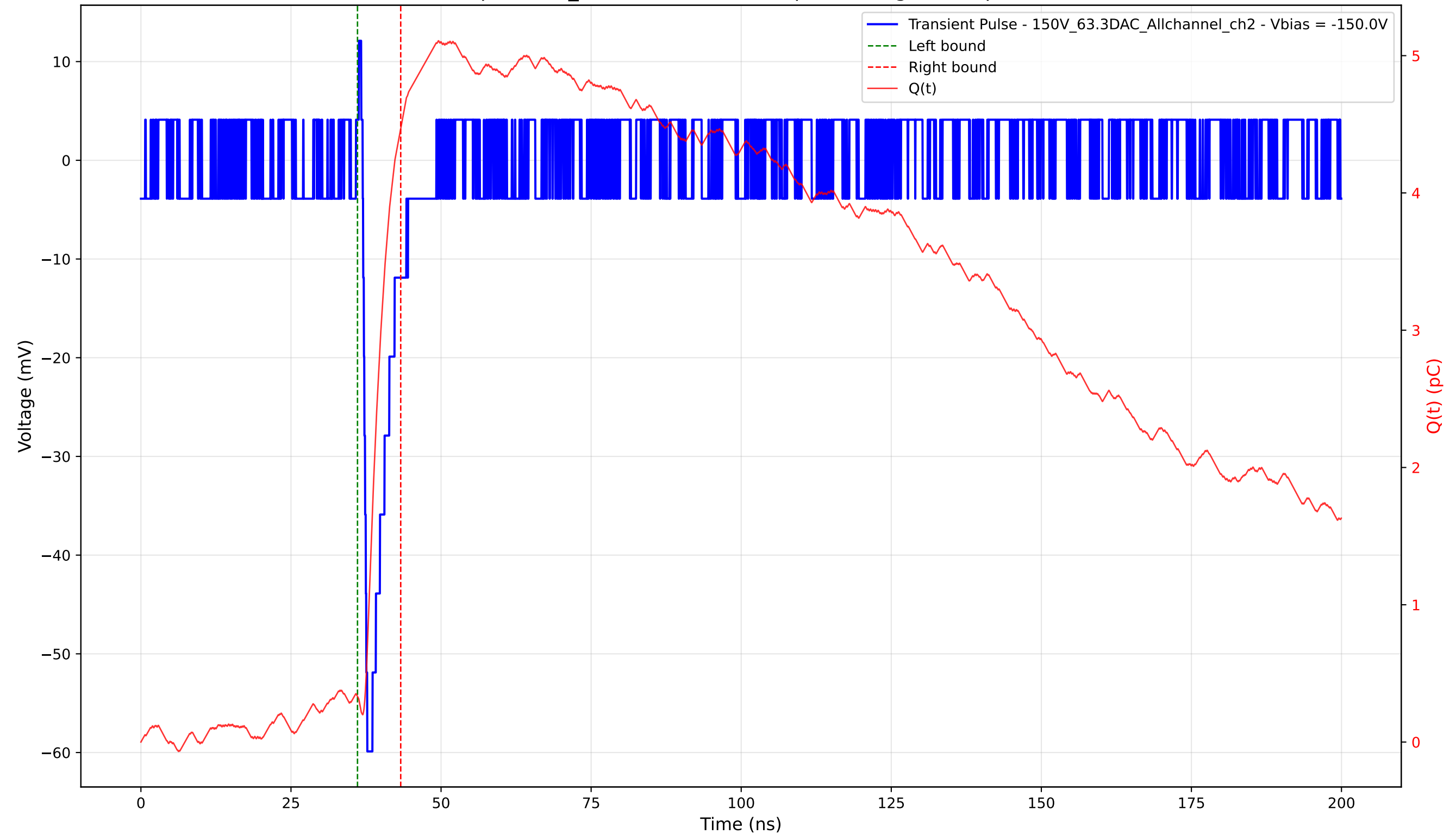
Transient Pulse - Sample: 1cm_42 - Position: 4115.0 \mu\text{m} - Charge: 4.14 pC - Rise Time: 0.71 ns
