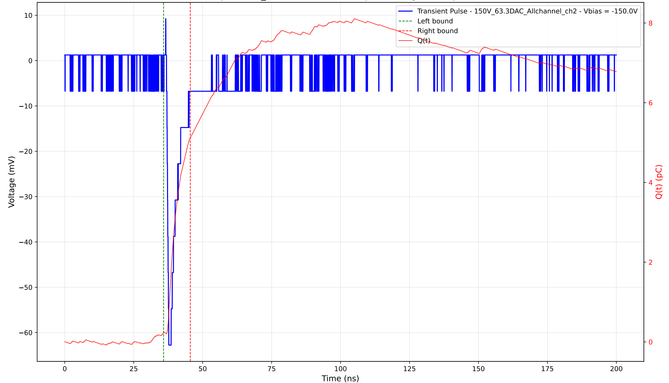
Transient Pulse - Sample: 1cm_42 - Position: 1950.0 \mu\text{m} - Charge: 4.88 pC - Rise Time: 0.80 ns
