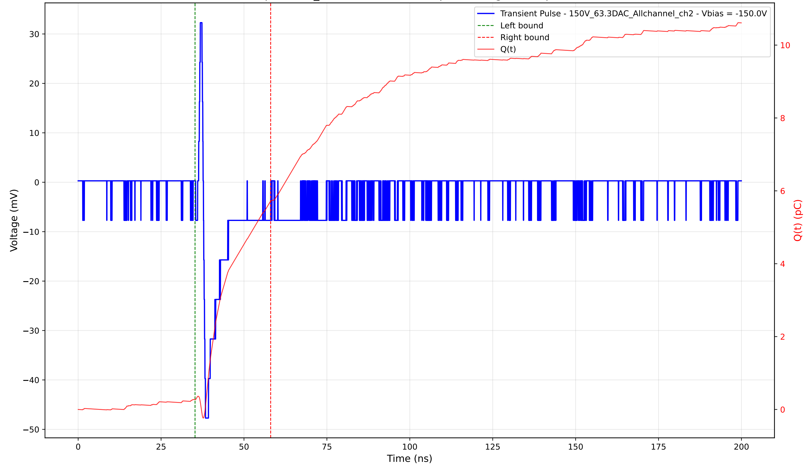
Transient Pulse - Sample: 1cm_42 - Position: 1290.0 \mu\text{m} - Charge: 5.45 pC - Rise Time: 0.62 ns
