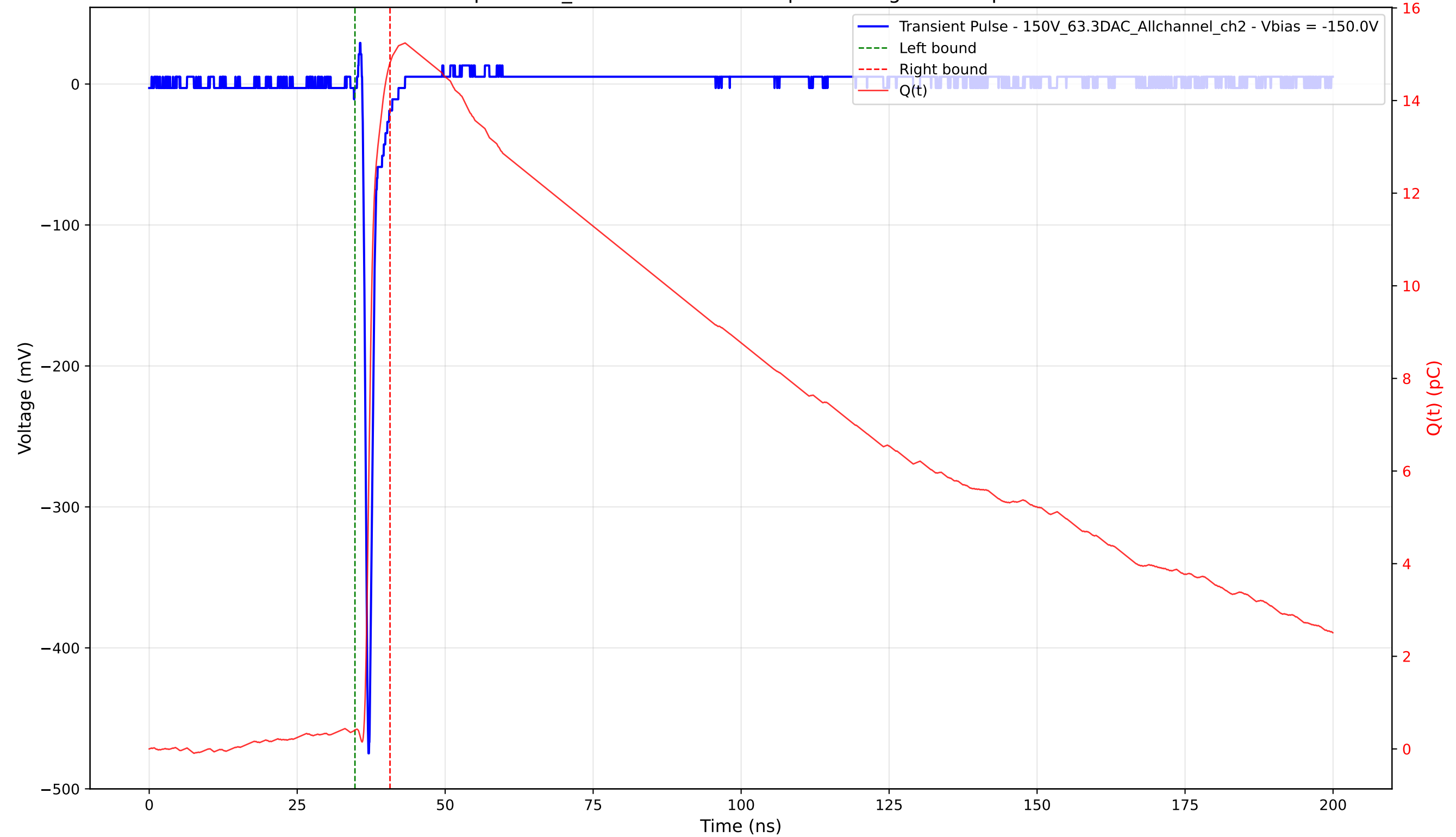
Transient Pulse - Sample: 1cm_42 - Position: 2975.0 \mu\text{m} - Charge: 14.40 pC - Rise Time: 0.73 ns
