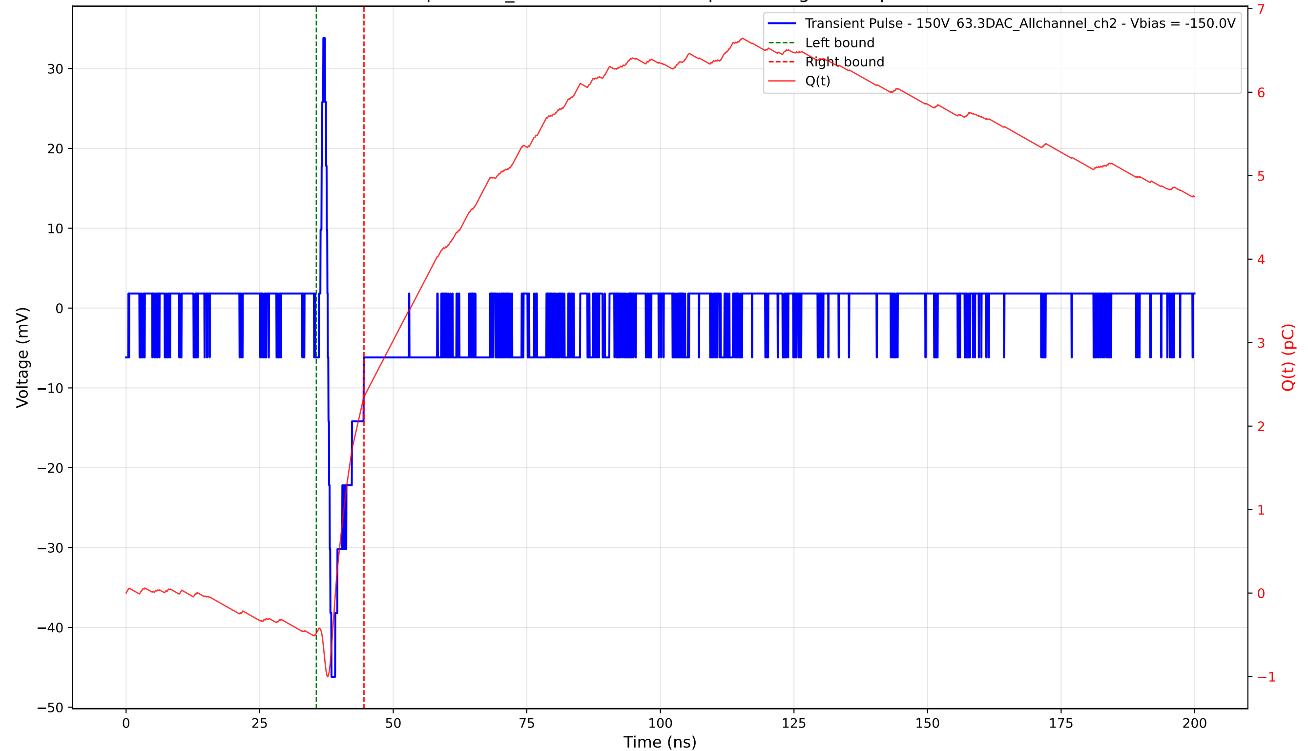
Transient Pulse - Sample: 1cm_42 - Position: 1365.0 \mu\text{m} - Charge: 2.83 pC - Rise Time: 0.69 ns
