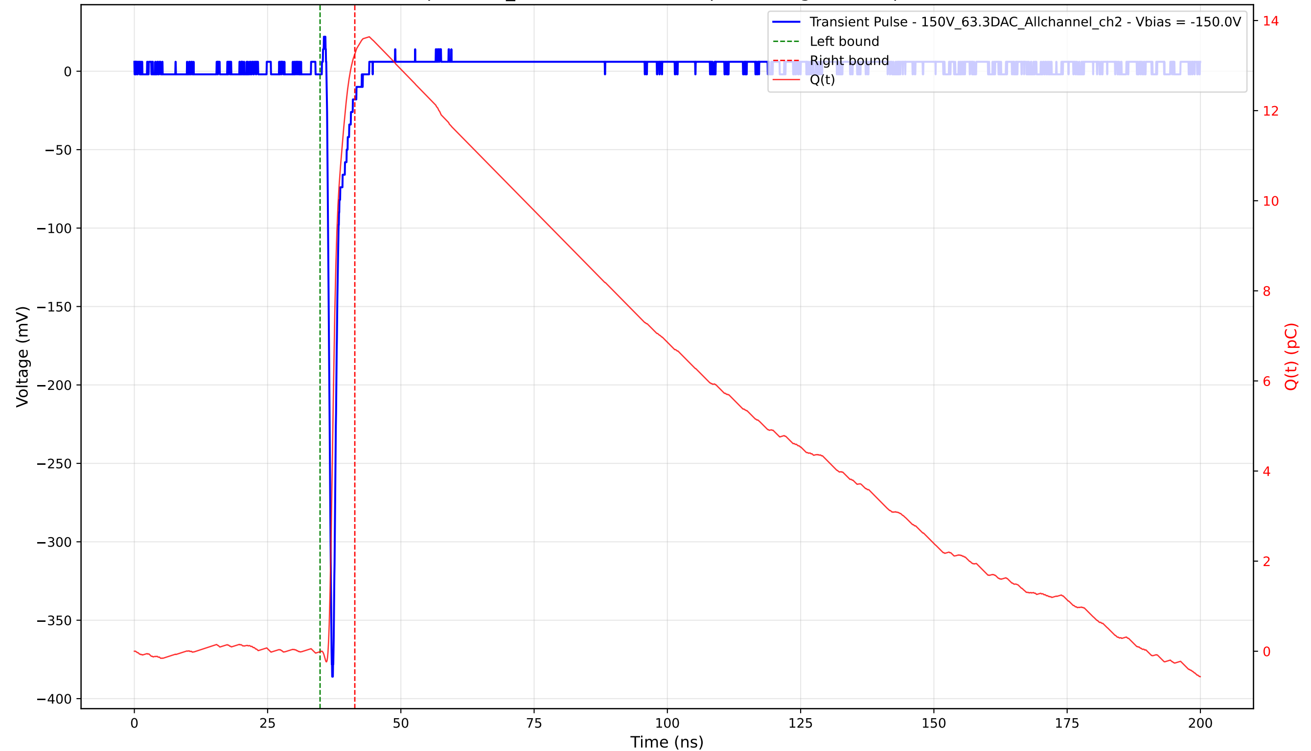
Transient Pulse - Sample: 1cm_42 - Position: 3345.0 \mu\text{m} - Charge: 13.27 pC - Rise Time: 0.70 ns
