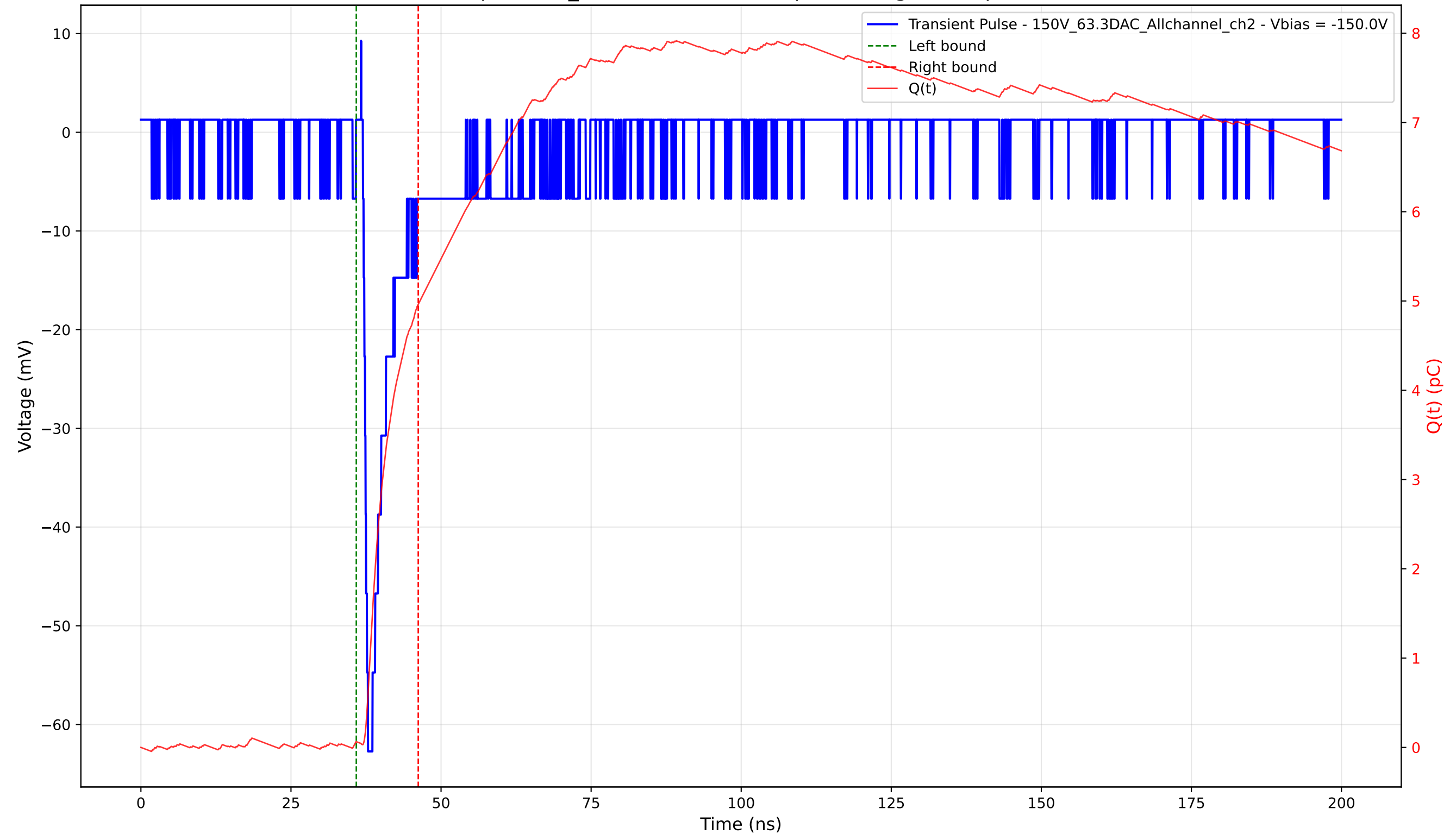
Transient Pulse - Sample: 1cm_42 - Position: 1930.0 \mu\text{m} - Charge: 4.90 pC - Rise Time: 0.84 ns
