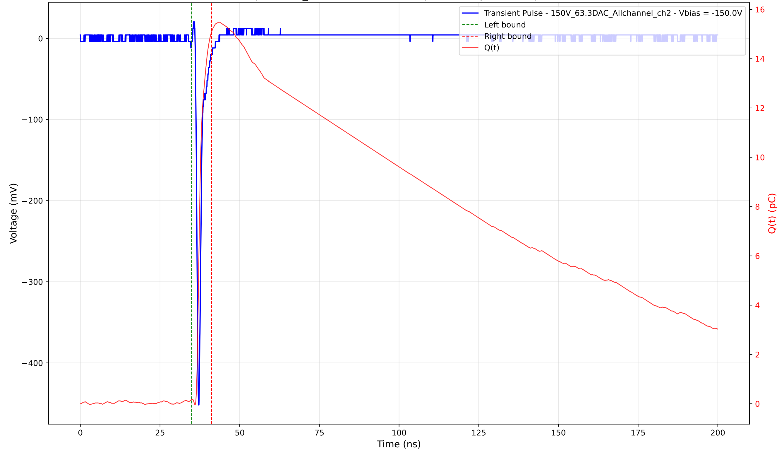
Transient Pulse - Sample: 1cm_42 - Position: 3230.0 \mu\text{m} - Charge: 14.92 pC - Rise Time: 0.69 ns
