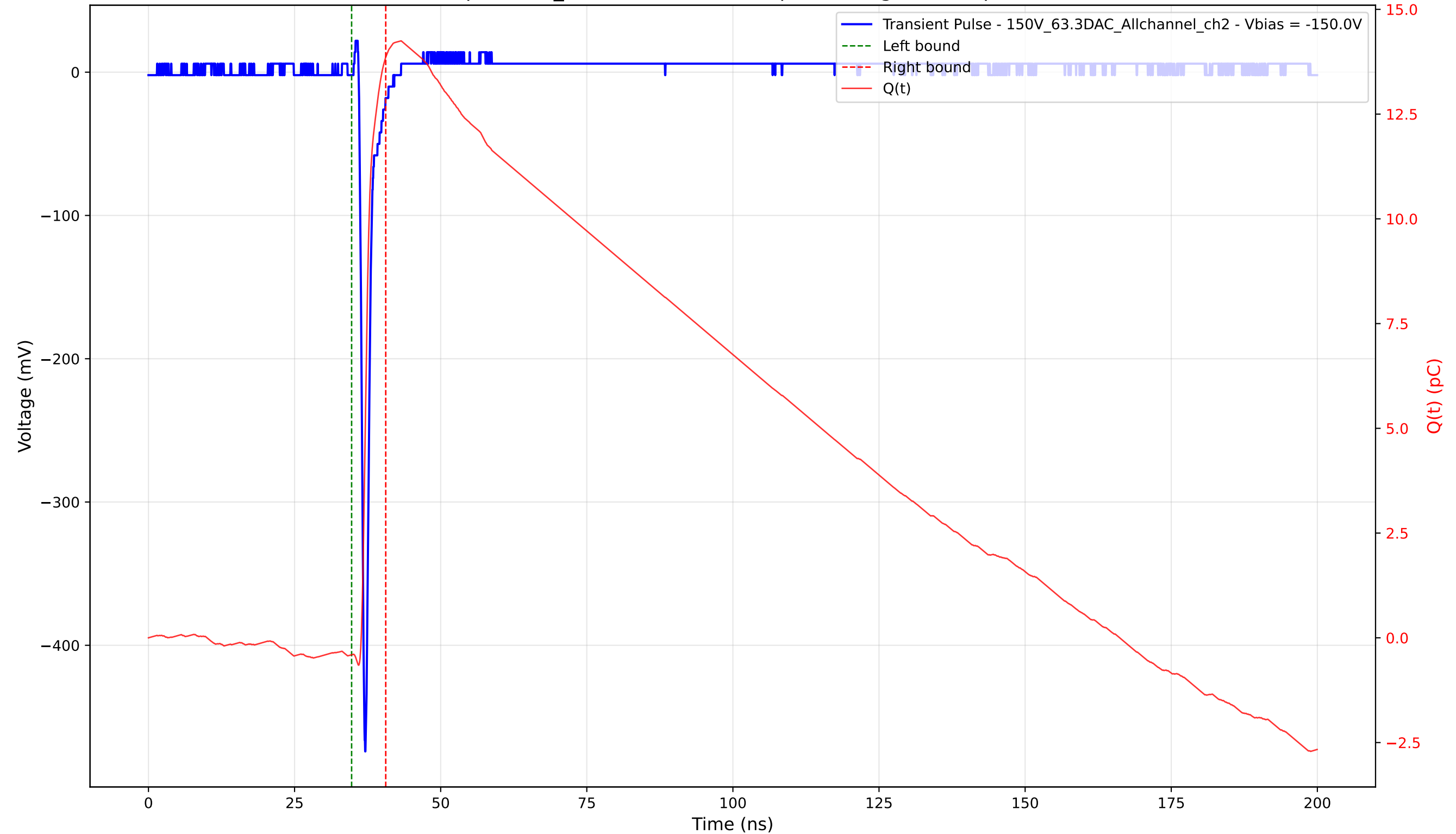
Transient Pulse - Sample: 1cm_42 - Position: 2955.0 \mu\text{m} - Charge: 14.26 pC - Rise Time: 0.73 ns
