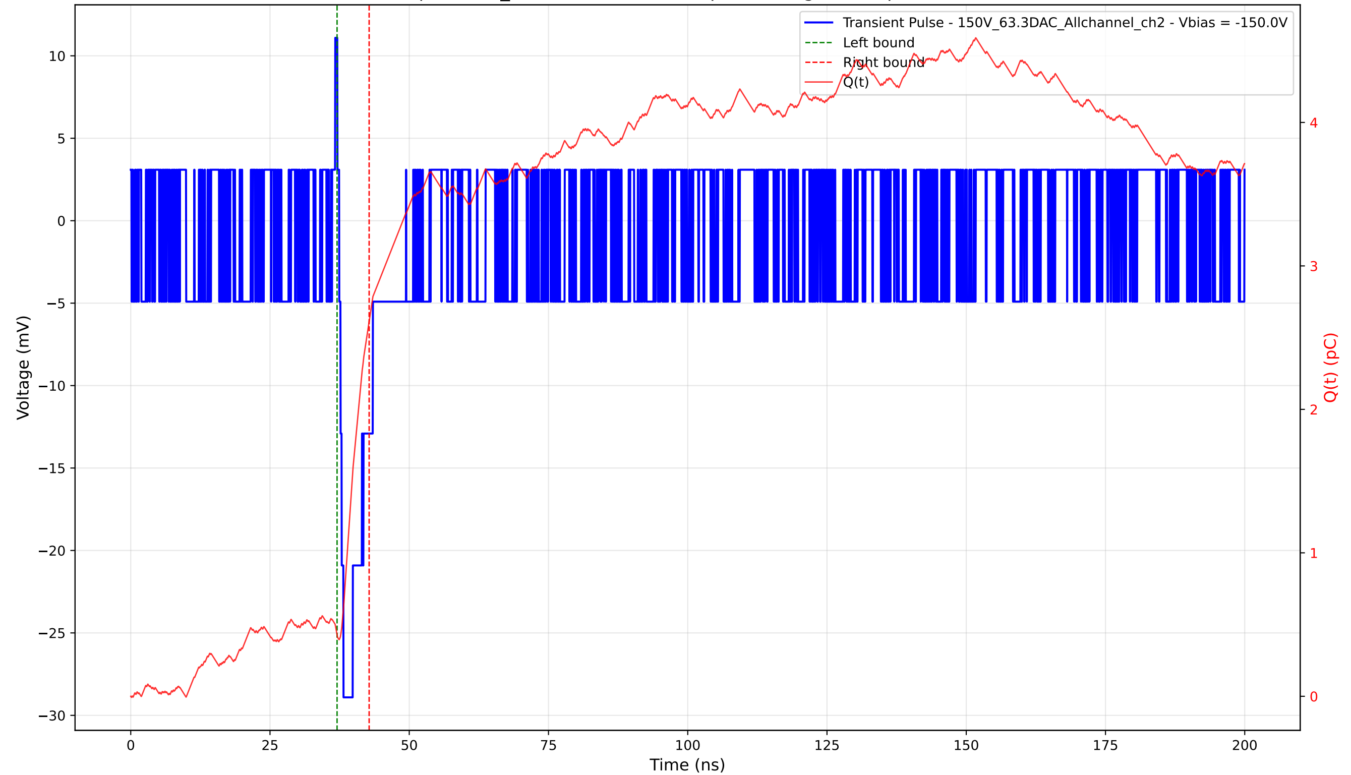
Transient Pulse - Sample: 1cm_42 - Position: 4895.0 \mu\text{m} - Charge: 2.19 pC - Rise Time: 0.00 ns (N/A)
