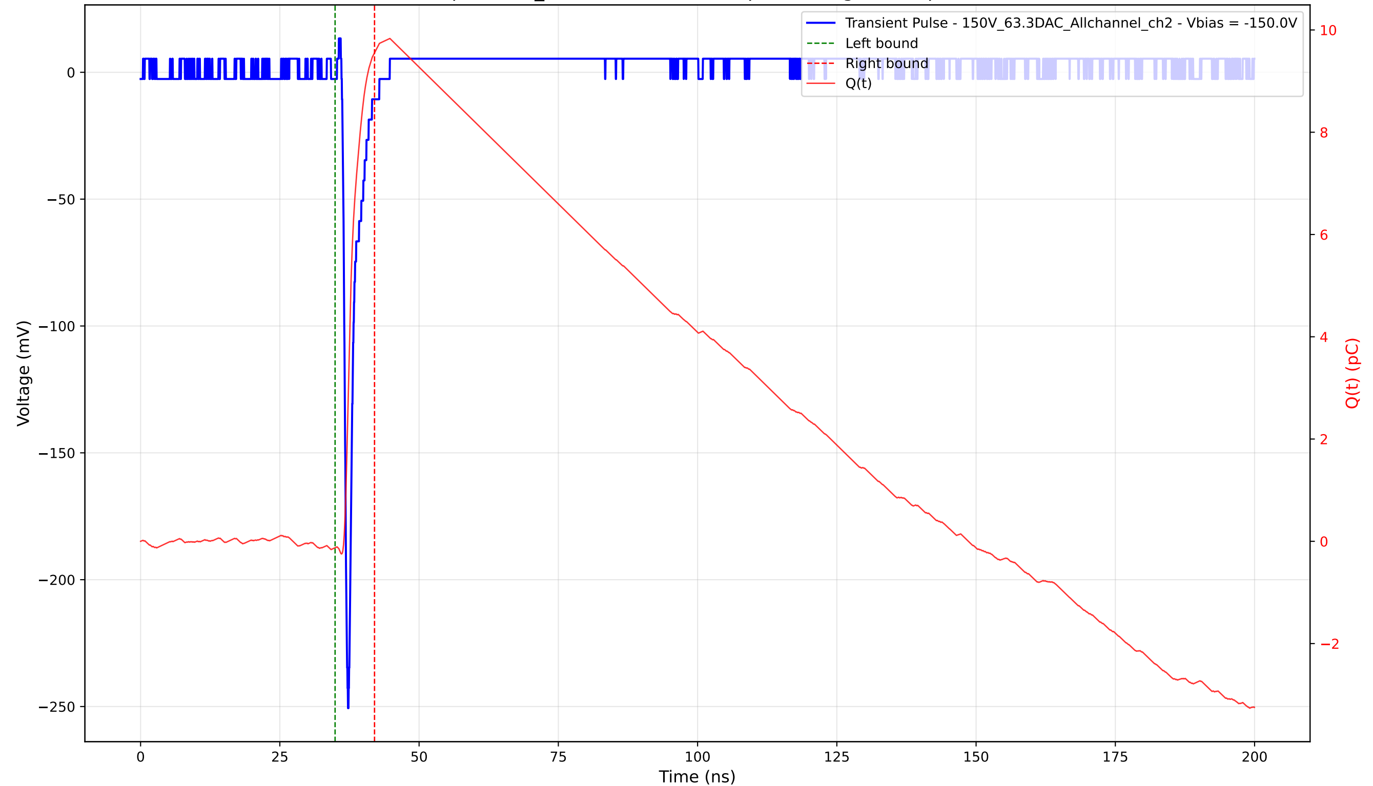
Transient Pulse - Sample: 1cm_42 - Position: 3475.0 \mu\text{m} - Charge: 9.68 pC - Rise Time: 0.76 ns
