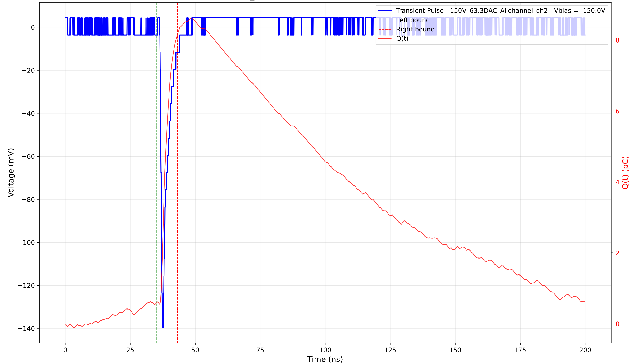
Transient Pulse - Sample: 1cm_42 - Position: 3705.0 \mu\text{m} - Charge: 7.57 pC - Rise Time: 0.79 ns
