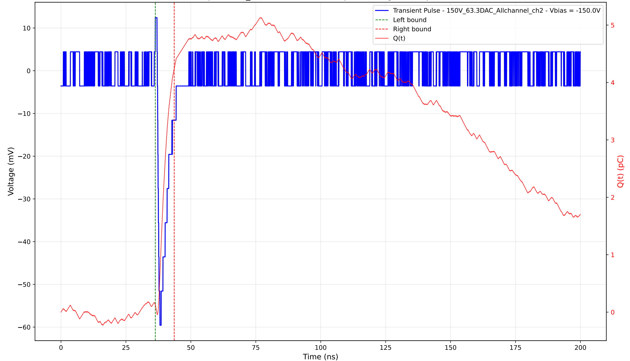
Transient Pulse - Sample: 1cm_42 - Position: 4245.0 \mu\text{m} - Charge: 4.11 pC - Rise Time: 0.91 ns
