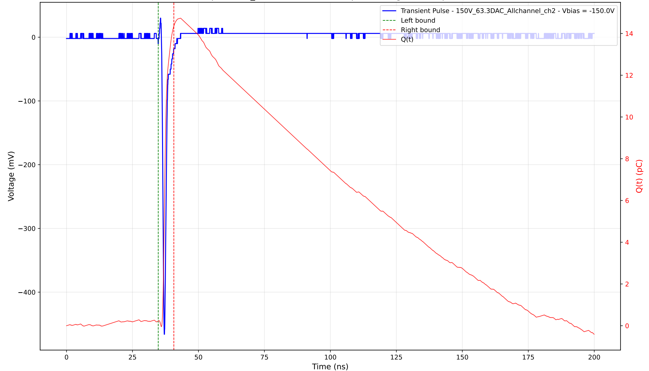
Transient Pulse - Sample: 1cm_42 - Position: 3040.0 \mu\text{m} - Charge: 14.14 pC - Rise Time: 0.68 ns
