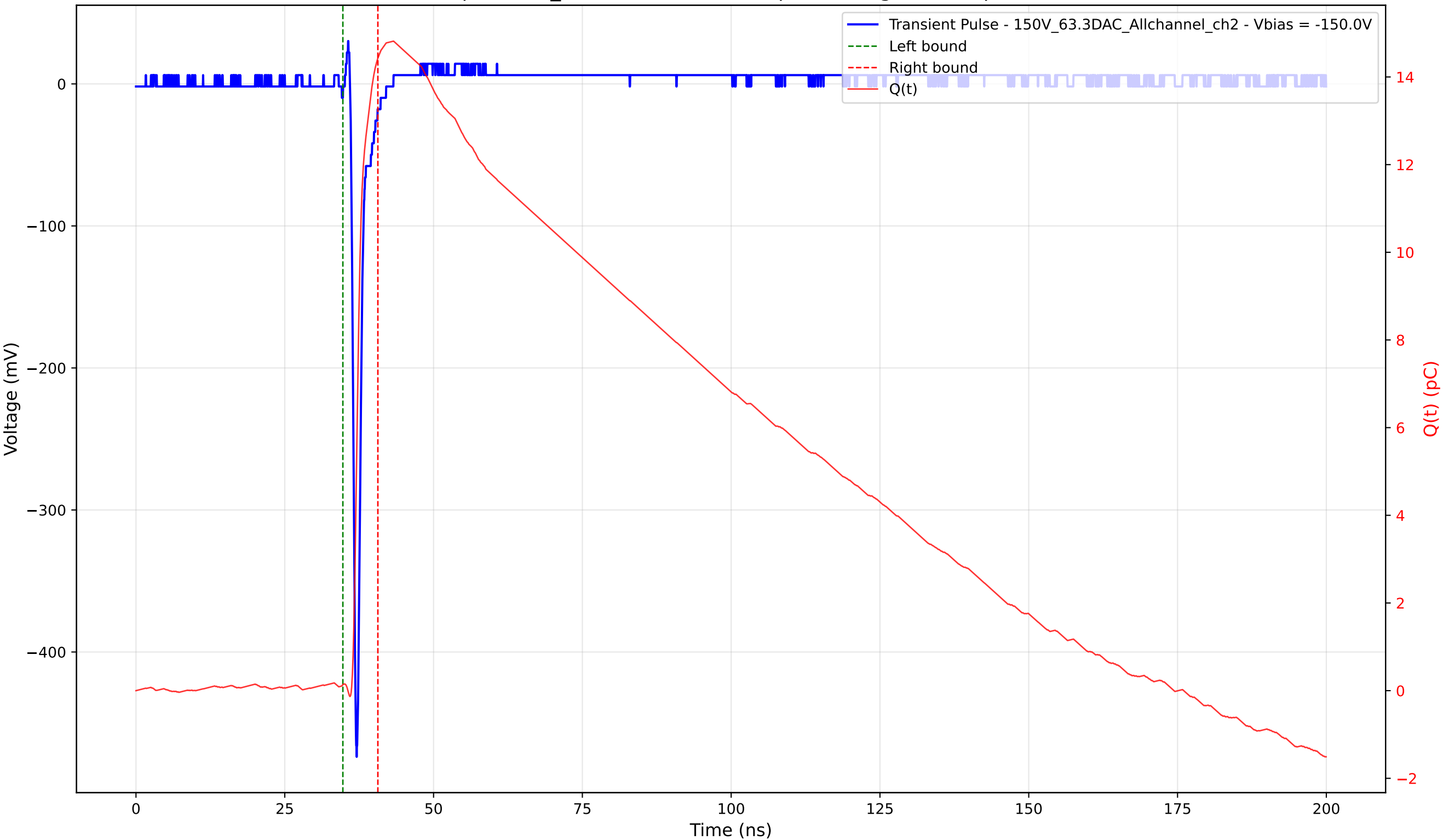
Transient Pulse - Sample: 1cm_42 - Position: 3080.0 \mu\text{m} - Charge: 14.29 pC - Rise Time: 0.71 ns
