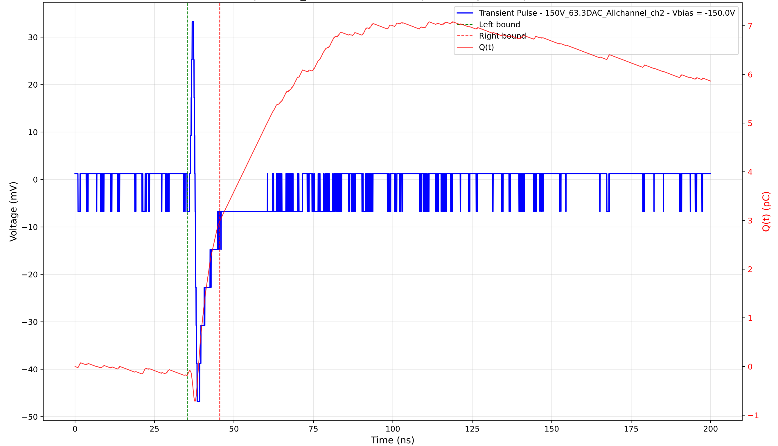
Transient Pulse - Sample: 1cm_42 - Position: 1310.0 \mu\text{m} - Charge: 3.14 pC - Rise Time: 0.66 ns
