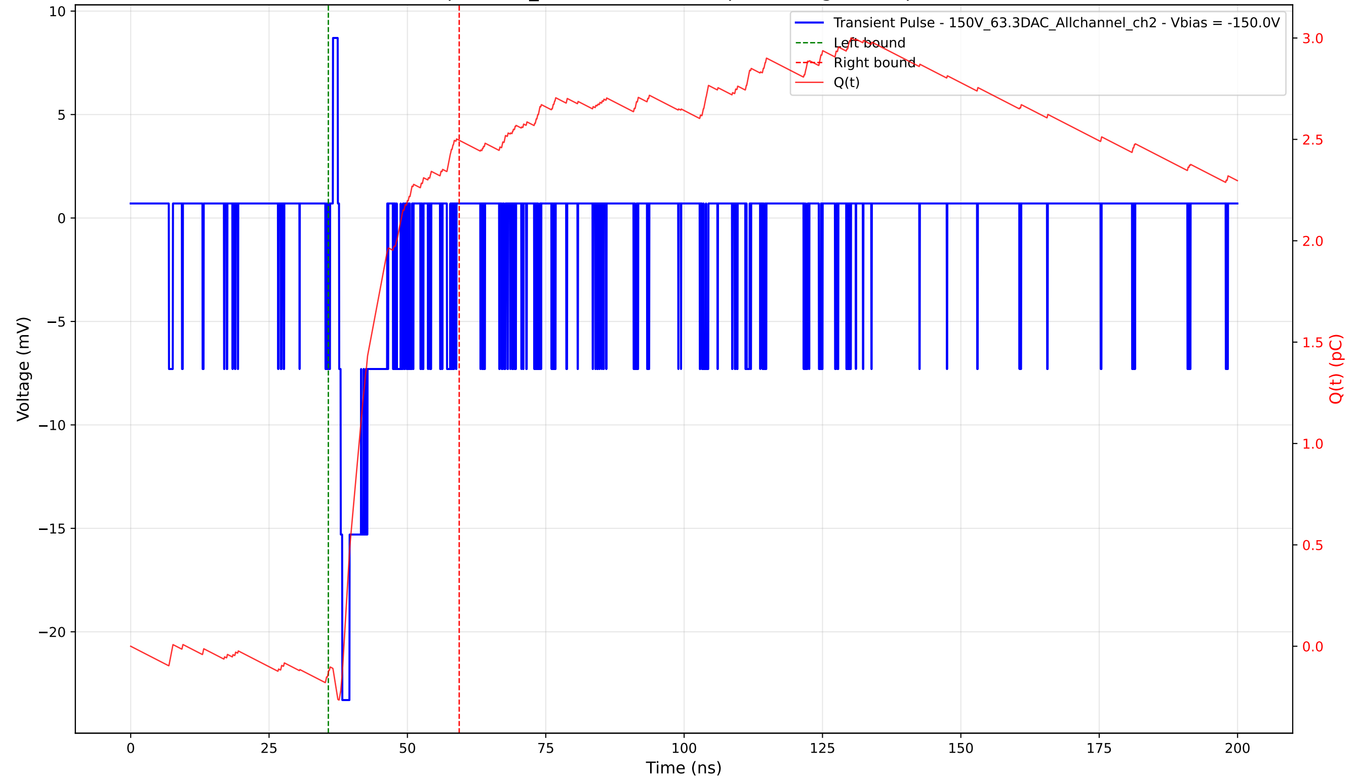
Transient Pulse - Sample: 1cm_42 - Position: 300.0 \mu\text{m} - Charge: 2.62 pC - Rise Time: 0.59 ns
