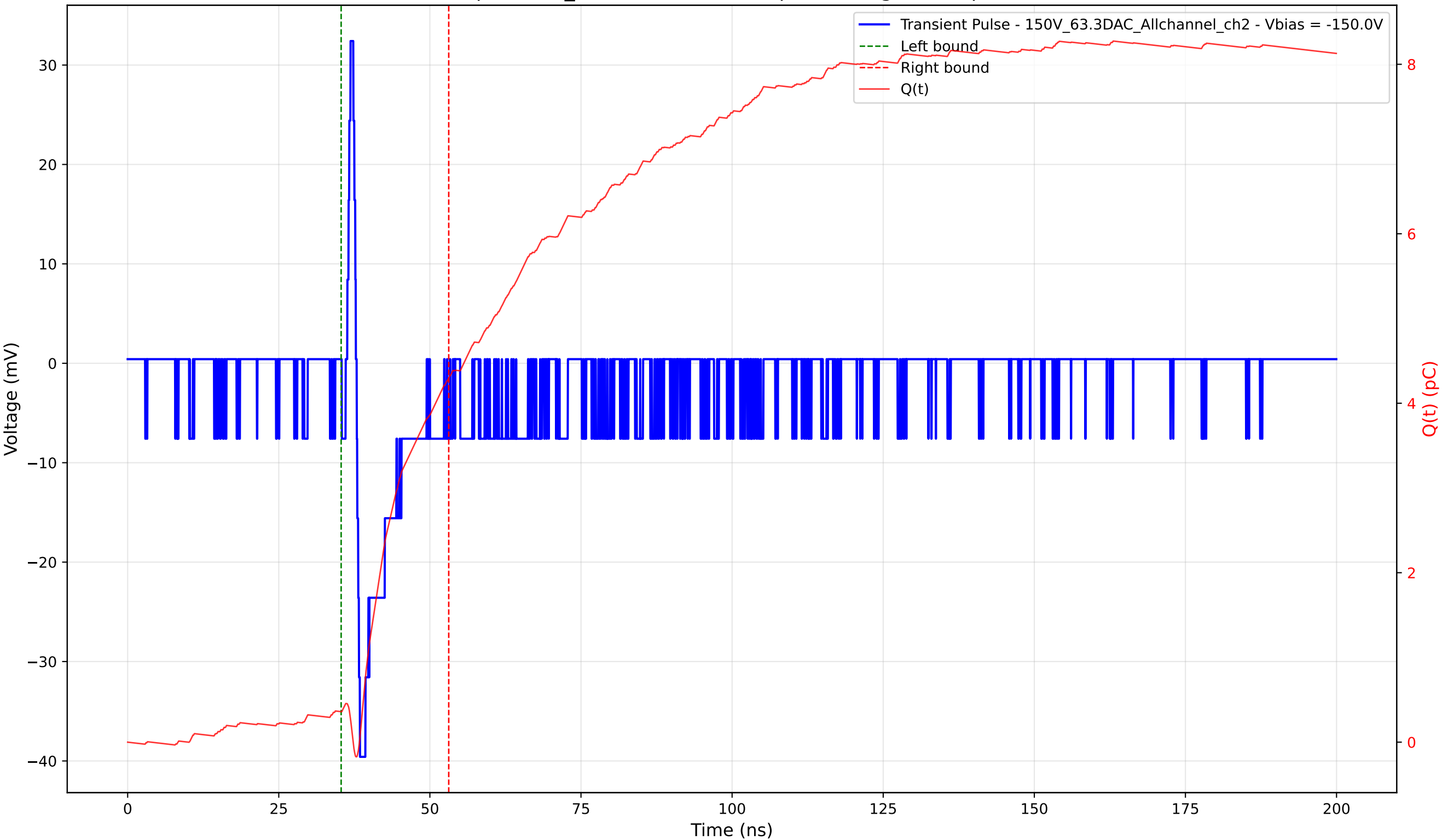
Transient Pulse - Sample: 1cm_42 - Position: 875.0 \mu\text{m} - Charge: 3.94 pC - Rise Time: 0.54 ns
