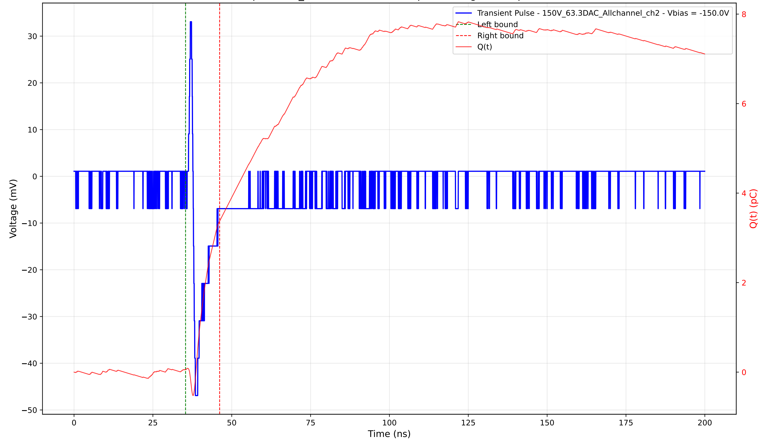
Transient Pulse - Sample: 1cm_42 - Position: 1320.0 \mu\text{m} - Charge: 3.32 pC - Rise Time: 0.70 ns
