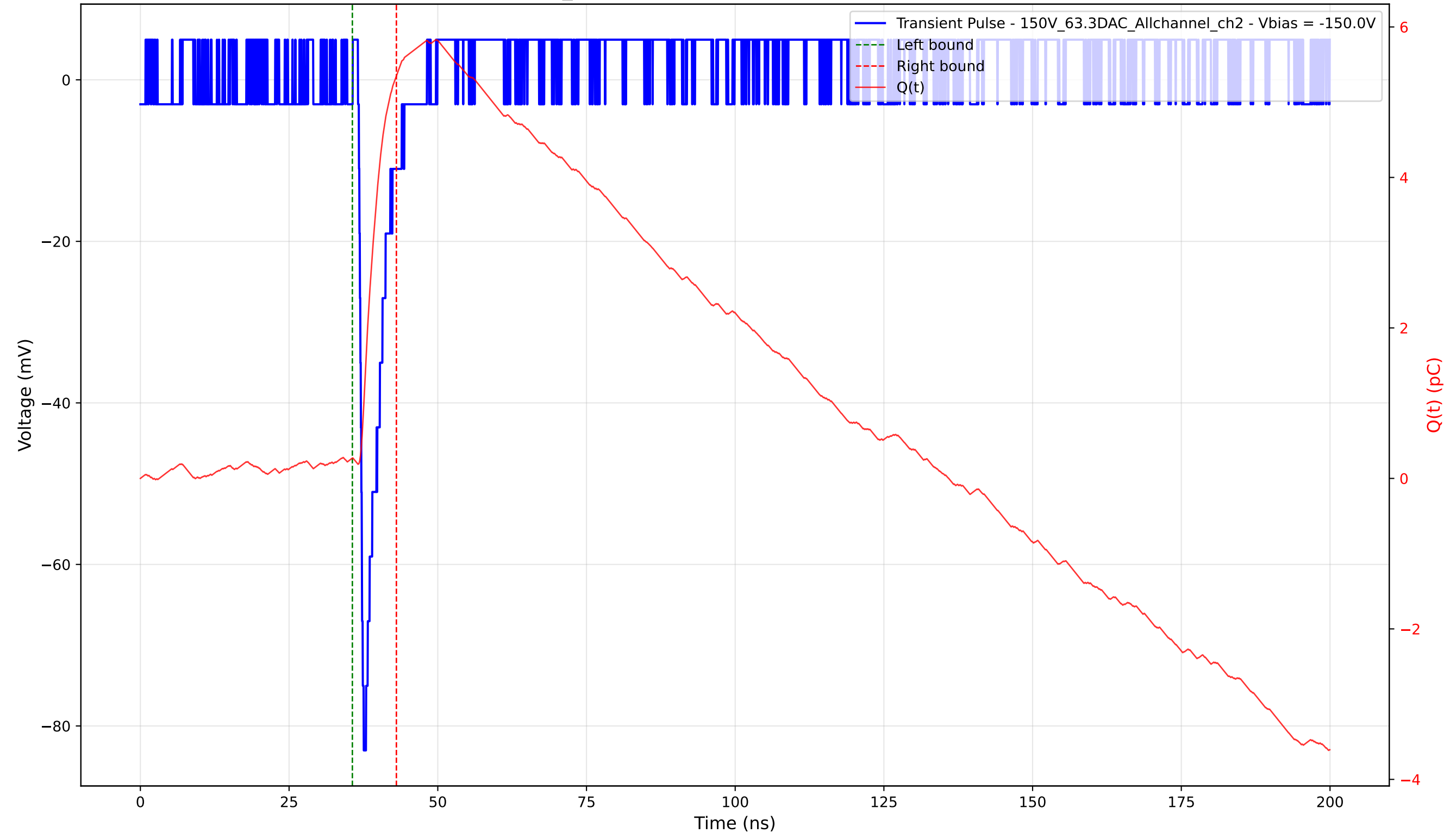
Transient Pulse - Sample: 1cm_42 - Position: 3955.0 \mu\text{m} - Charge: 5.08 pC - Rise Time: 0.65 ns
