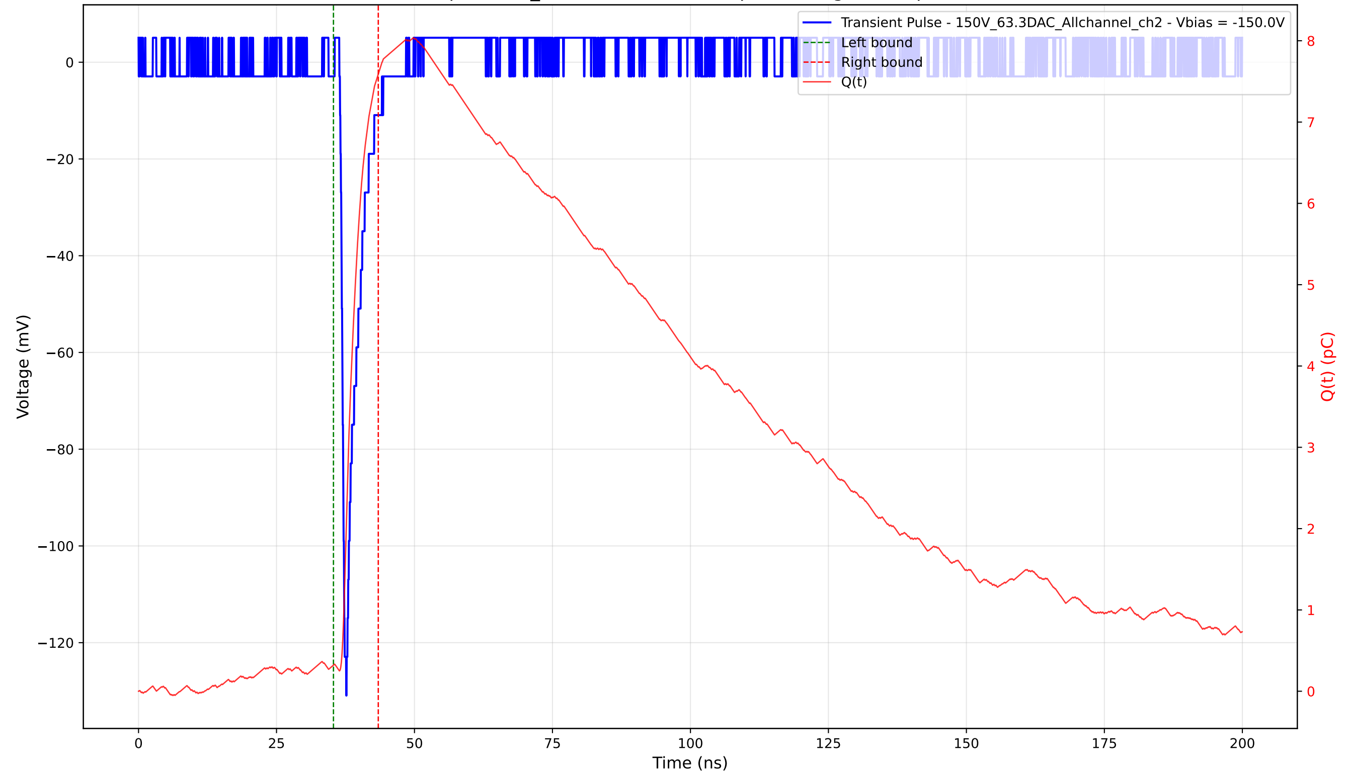
Transient Pulse - Sample: 1cm_42 - Position: 3810.0 \mu\text{m} - Charge: 7.27 pC - Rise Time: 0.79 ns
