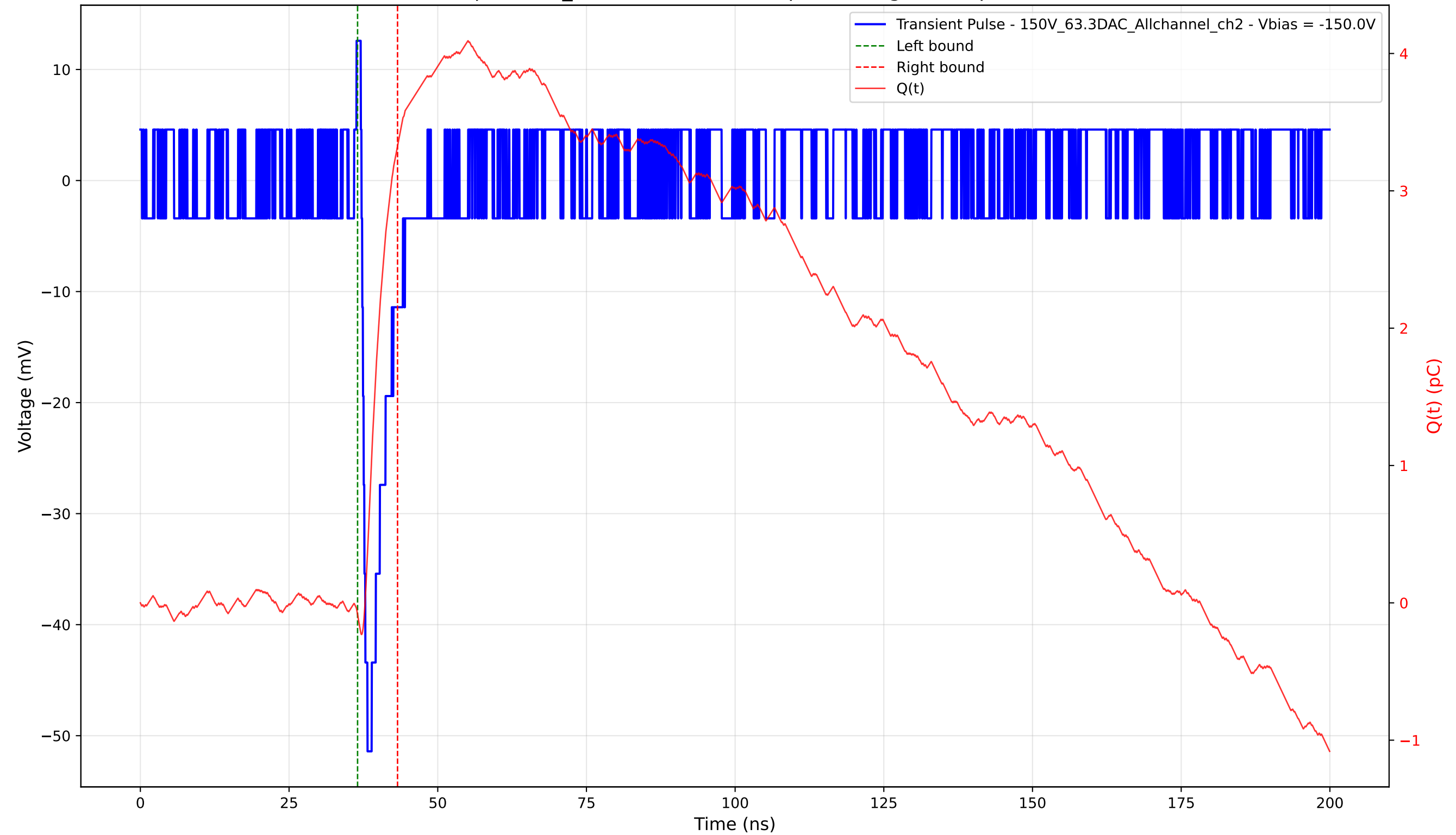
Transient Pulse - Sample: 1cm_42 - Position: 4385.0 \mu\text{m} - Charge: 3.41 pC - Rise Time: 0.91 ns
