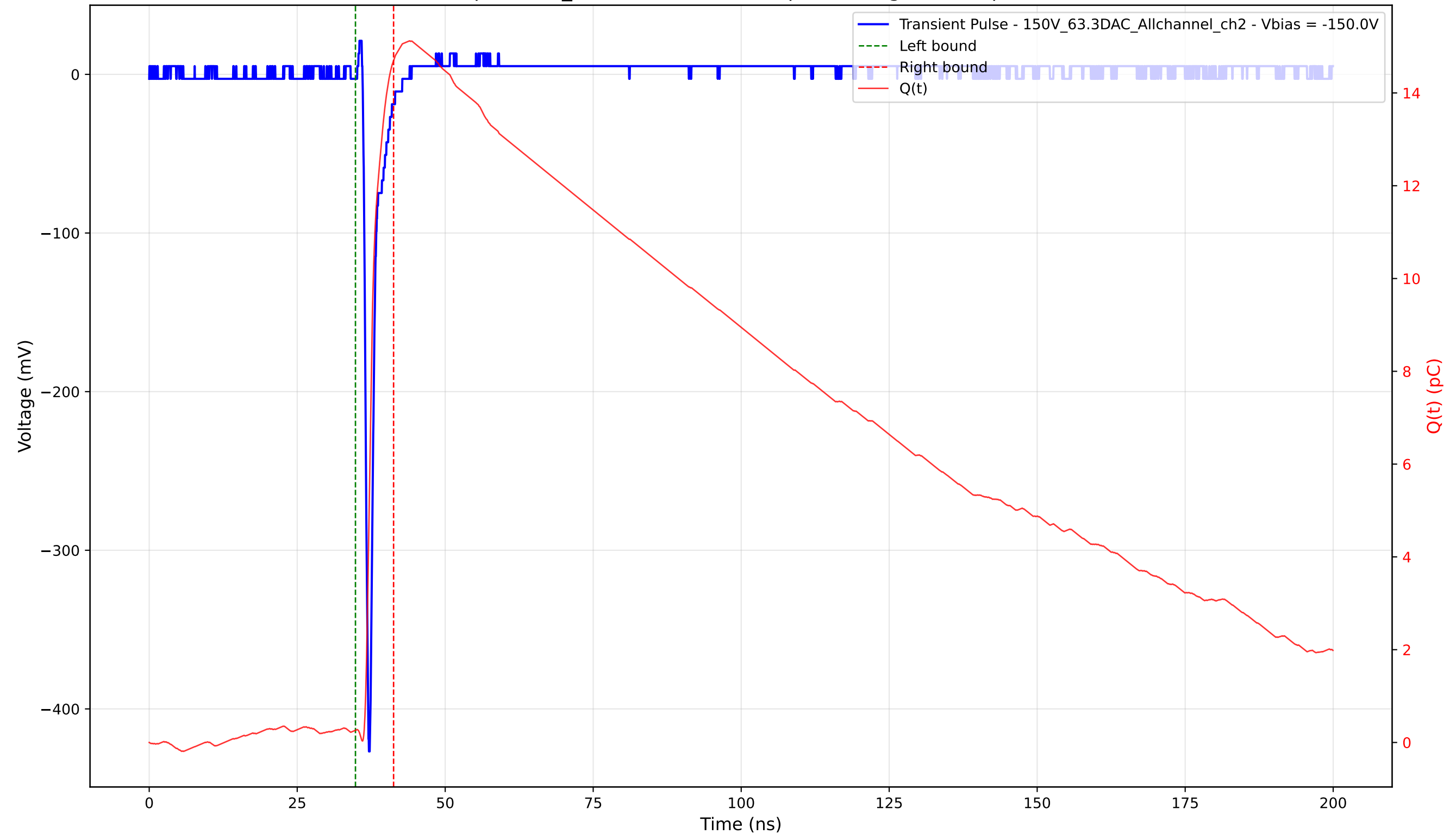
Transient Pulse - Sample: 1cm_42 - Position: 3295.0 \mu\text{m} - Charge: 14.43 pC - Rise Time: 0.73 ns
