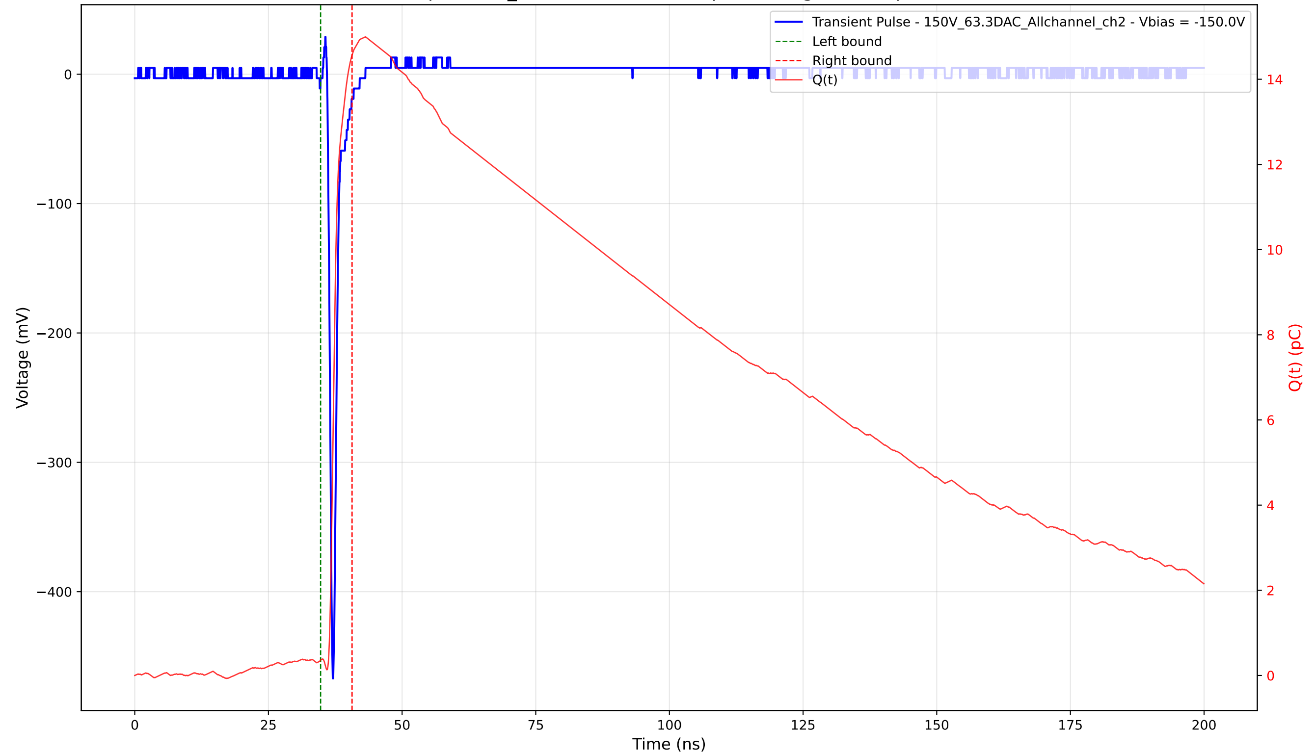
Transient Pulse - Sample: 1cm_42 - Position: 3020.0 \mu\text{m} - Charge: 14.20 pC - Rise Time: 0.68 ns
