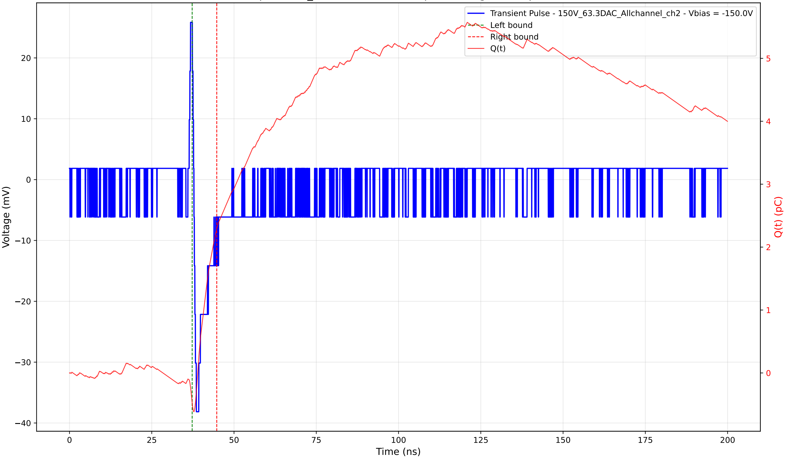
Transient Pulse - Sample: 1cm_42 - Position: 590.0 \mu\text{m} - Charge: 2.78 pC - Rise Time: 0.74 ns
