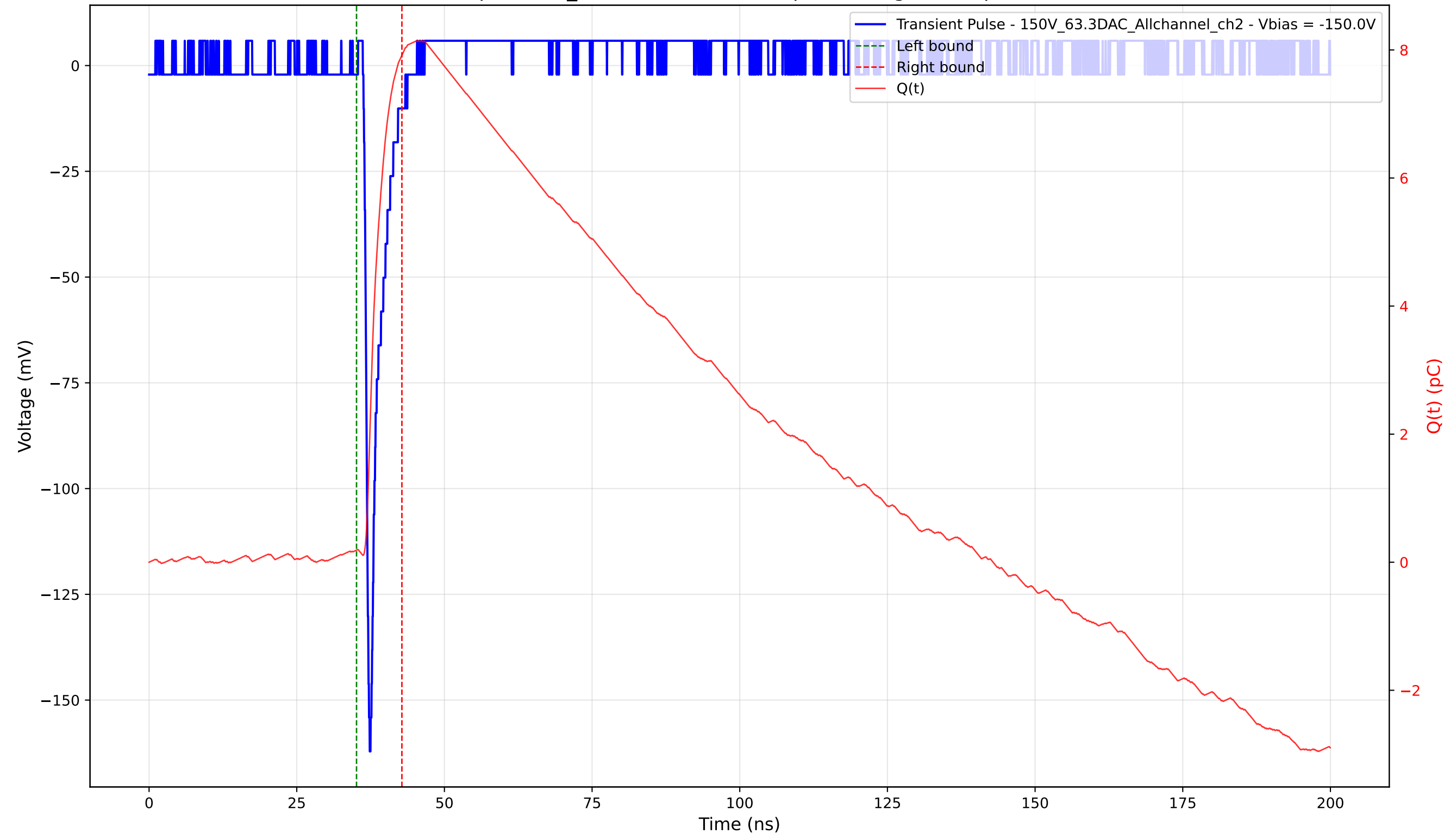
Transient Pulse - Sample: 1cm_42 - Position: 3625.0 \mu\text{m} - Charge: 7.73 pC - Rise Time: 0.77 ns
