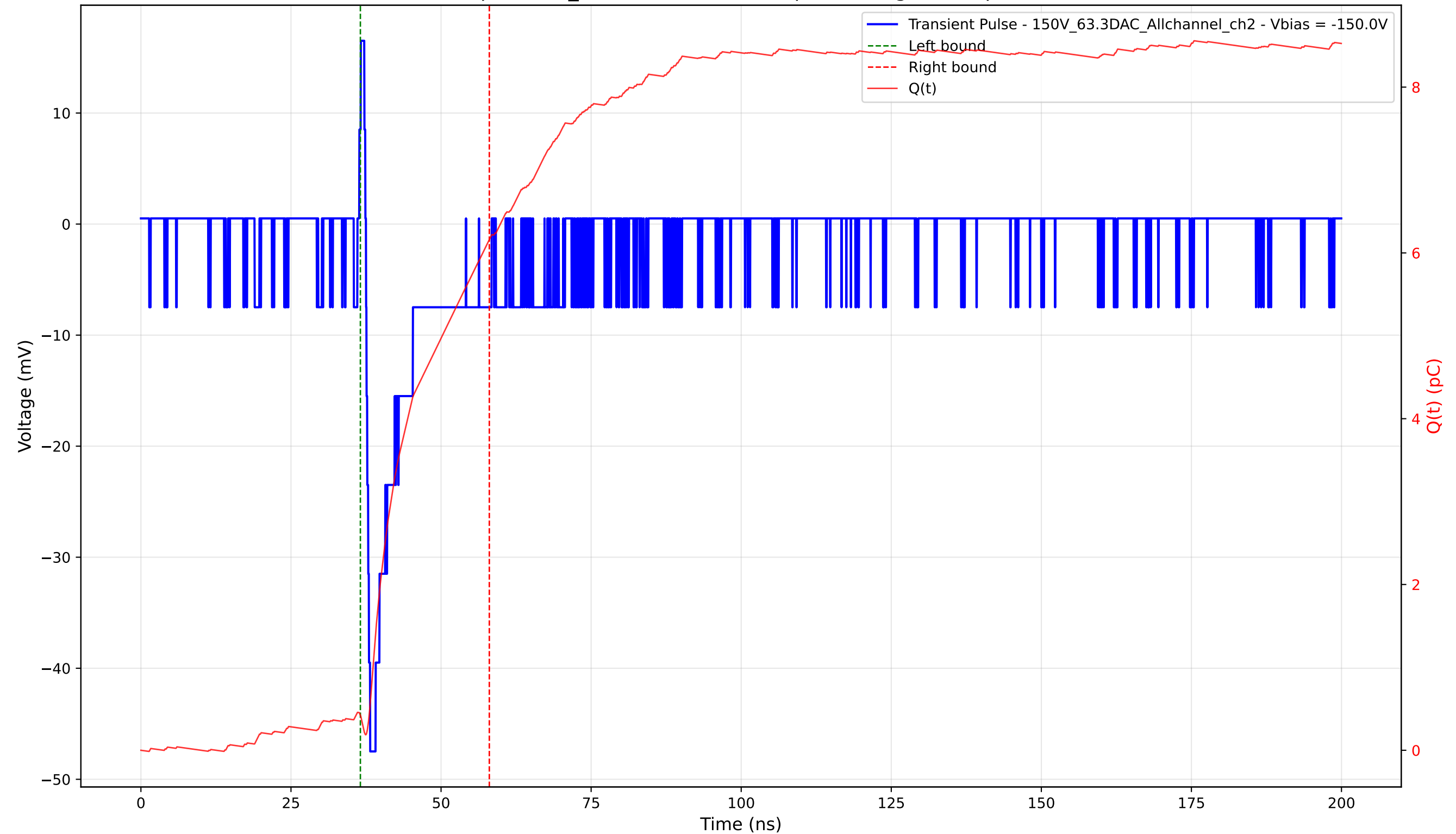
Transient Pulse - Sample: 1cm_42 - Position: 1570.0 \mu\text{m} - Charge: 5.74 pC - Rise Time: 0.70 ns
