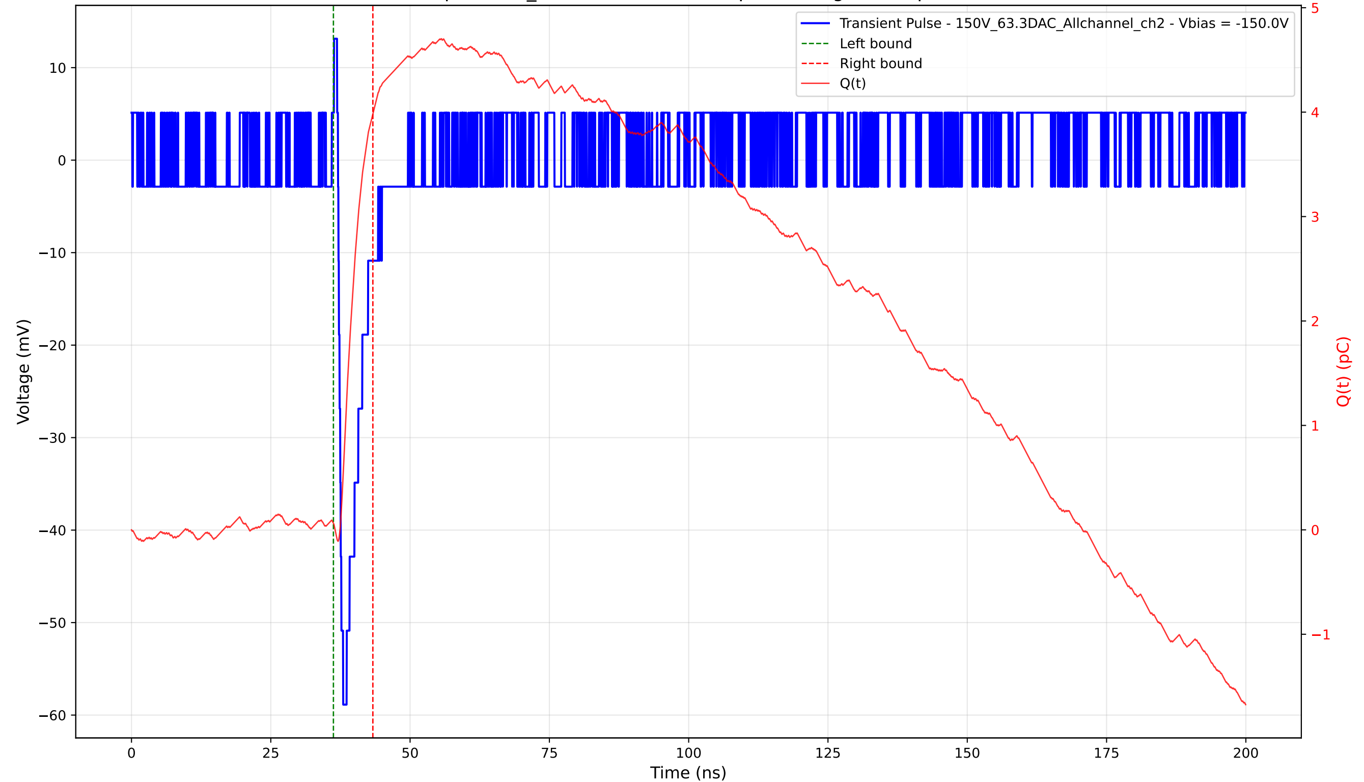
Transient Pulse - Sample: 1cm_42 - Position: 4190.0 \mu\text{m} - Charge: 3.92 pC - Rise Time: 0.86 ns
