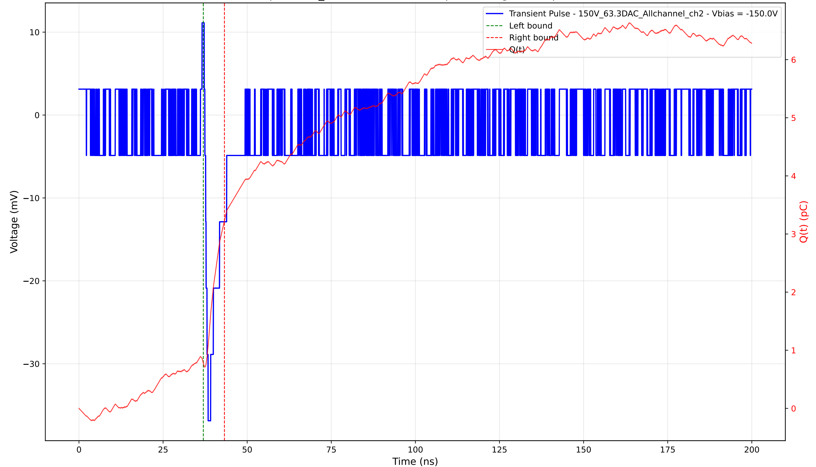
Transient Pulse - Sample: 1cm_42 - Position: 4875.0 \mu\text{m} - Charge: 2.45 pC - Rise Time: 0.99 ns
