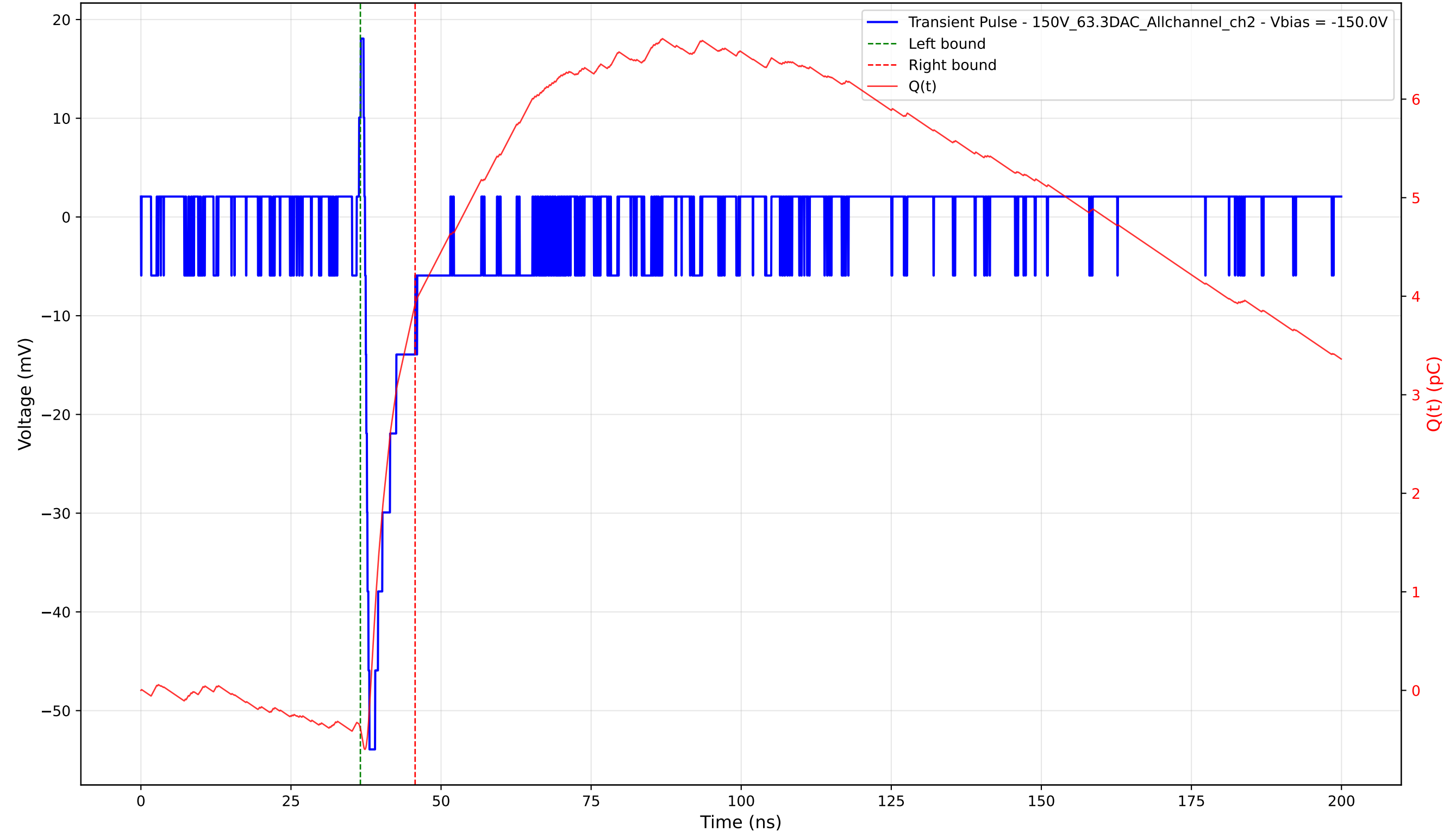
Transient Pulse - Sample: 1cm_42 - Position: 1680.0 \mu\text{m} - Charge: 4.31 pC - Rise Time: 0.73 ns
