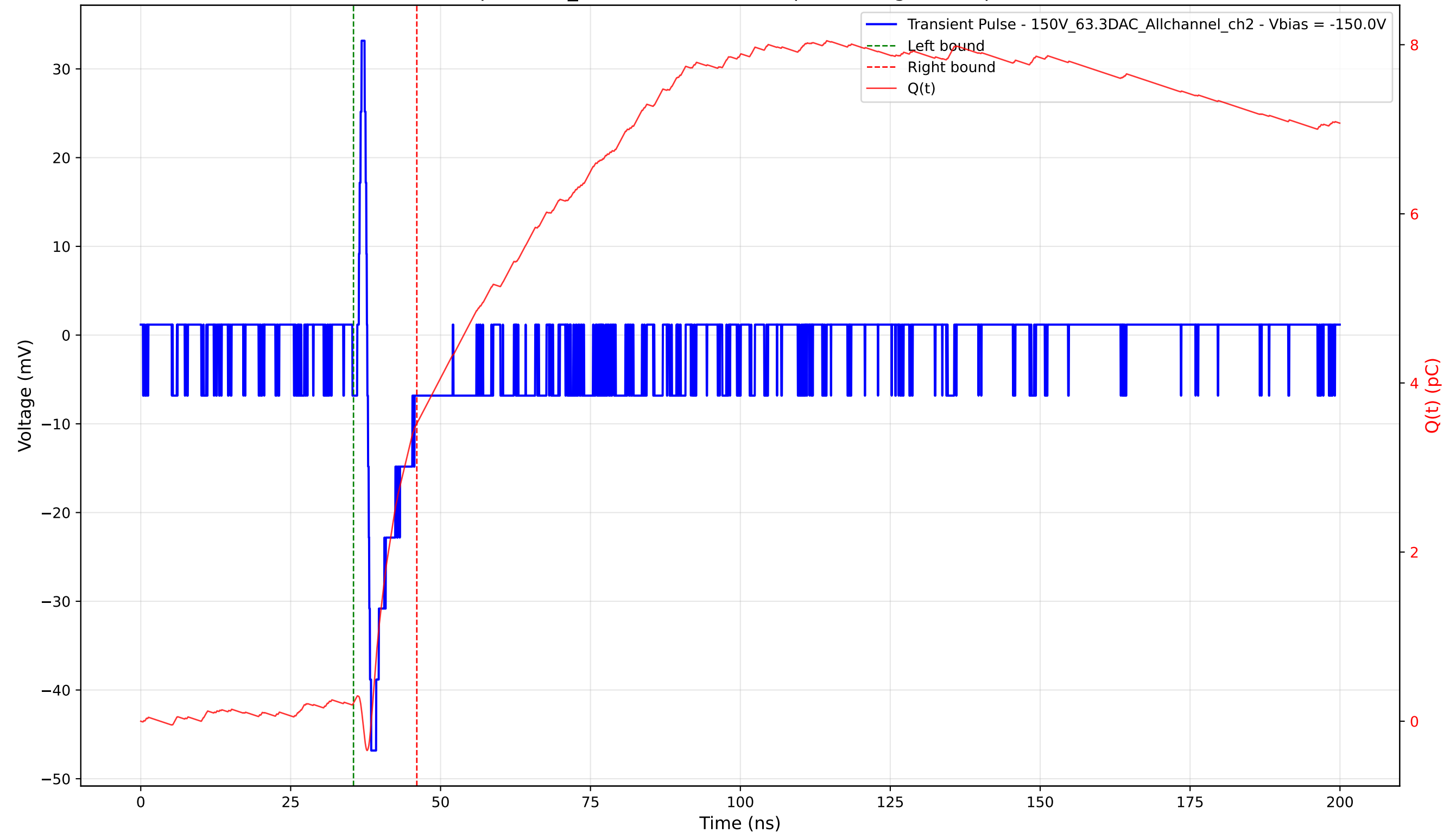
Transient Pulse - Sample: 1cm_42 - Position: 1215.0 \mu\text{m} - Charge: 3.30 pC - Rise Time: 0.66 ns
