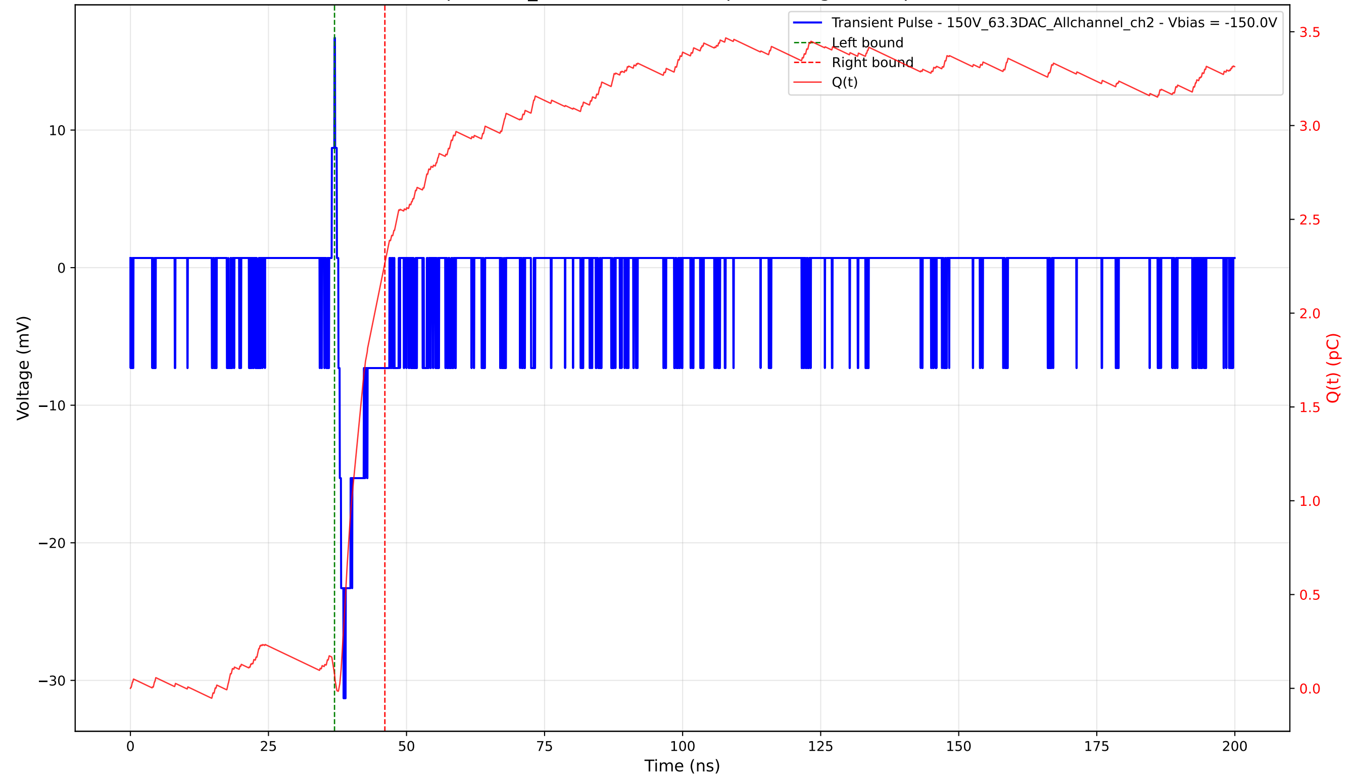
Transient Pulse - Sample: 1cm_42 - Position: 365.0 \mu\text{m} - Charge: 2.19 pC - Rise Time: 0.95 ns
