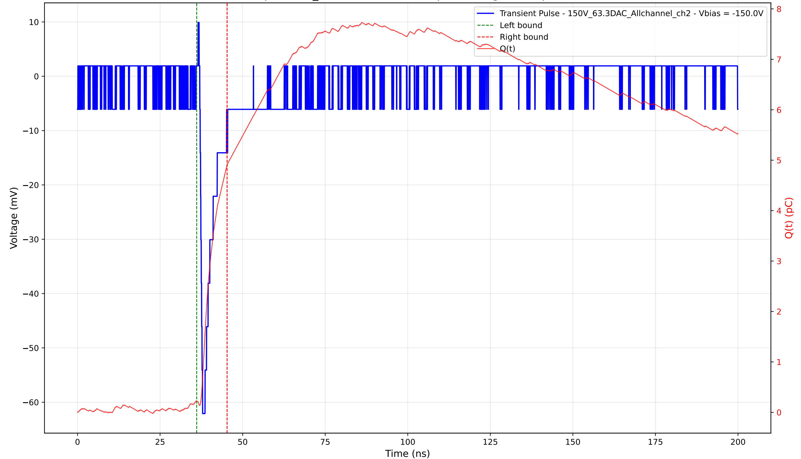
Transient Pulse - Sample: 1cm_42 - Position: 1905.0 \mu\text{m} - Charge: 4.67 pC - Rise Time: 0.76 ns
