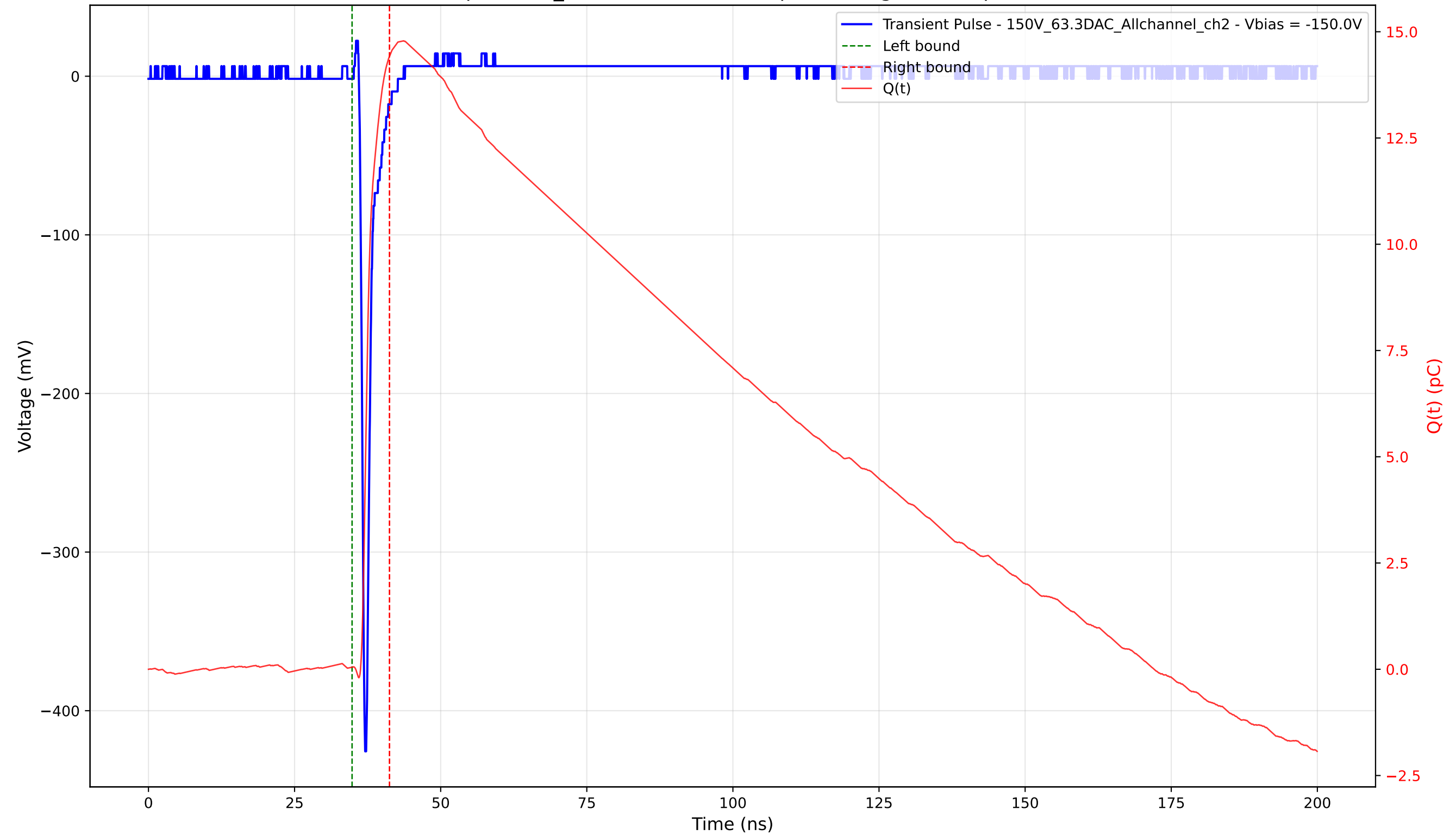
Transient Pulse - Sample: 1cm_42 - Position: 3290.0 \mu\text{m} - Charge: 14.37 pC - Rise Time: 0.68 ns
