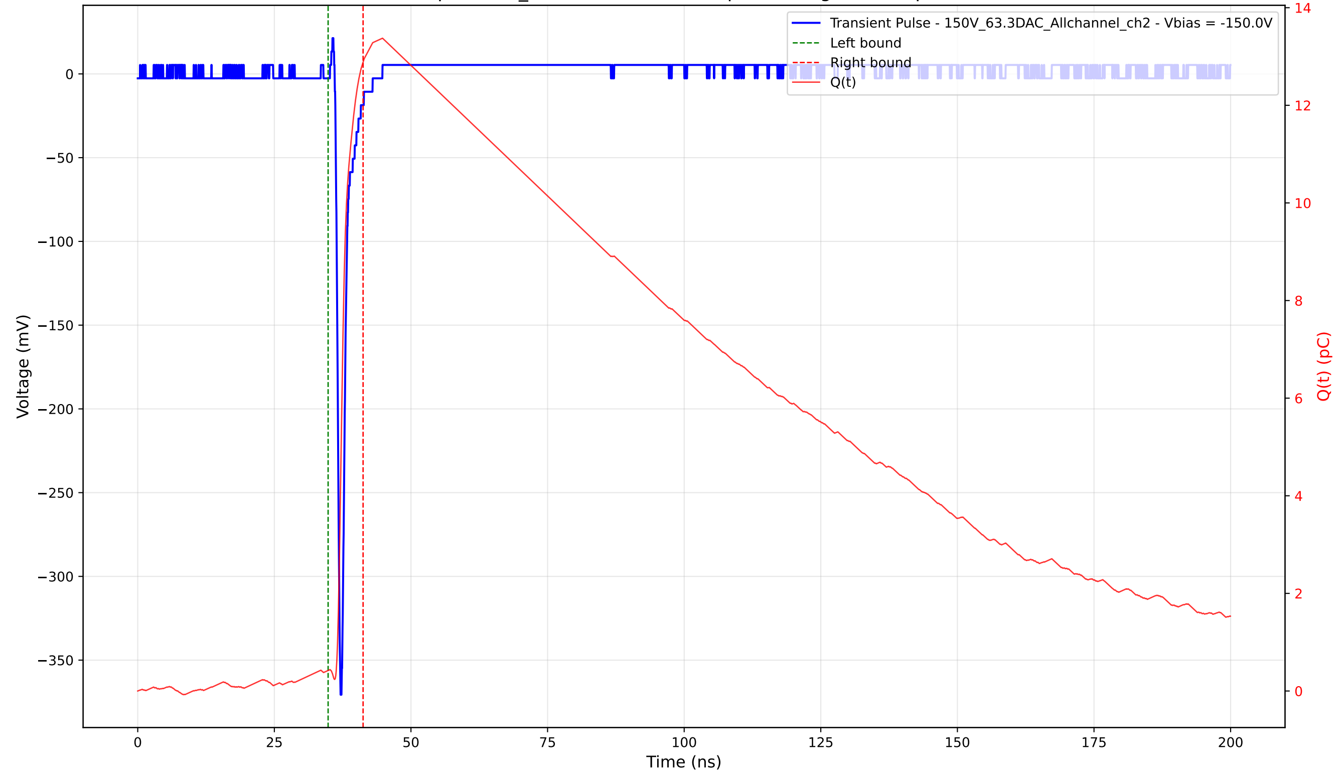
Transient Pulse - Sample: 1cm_42 - Position: 2685.0 \mu\text{m} - Charge: 12.47 pC - Rise Time: 0.72 ns
