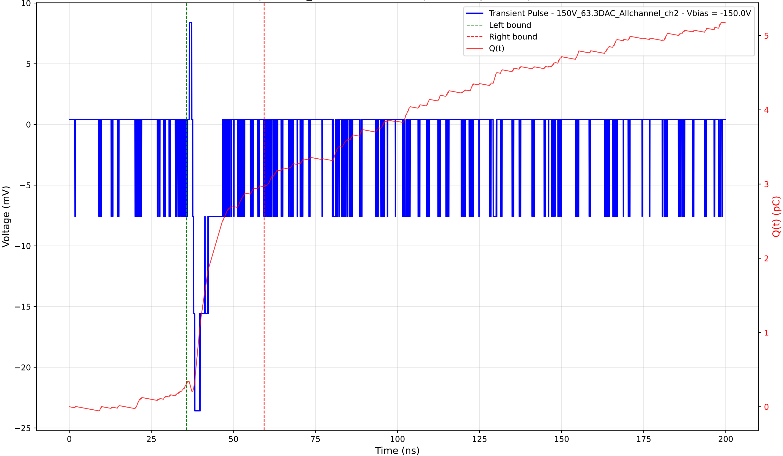
Transient Pulse - Sample: 1cm_42 - Position: 250.0 \mu\text{m} - Charge: 2.65 pC - Rise Time: 0.63 ns
