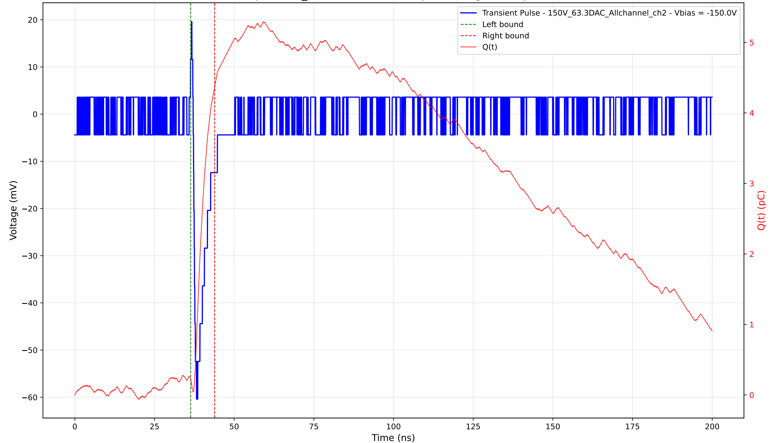
Transient Pulse - Sample: 1cm_42 - Position: 4300.0 \mu\text{m} - Charge: 4.15 pC - Rise Time: 0.95 ns
