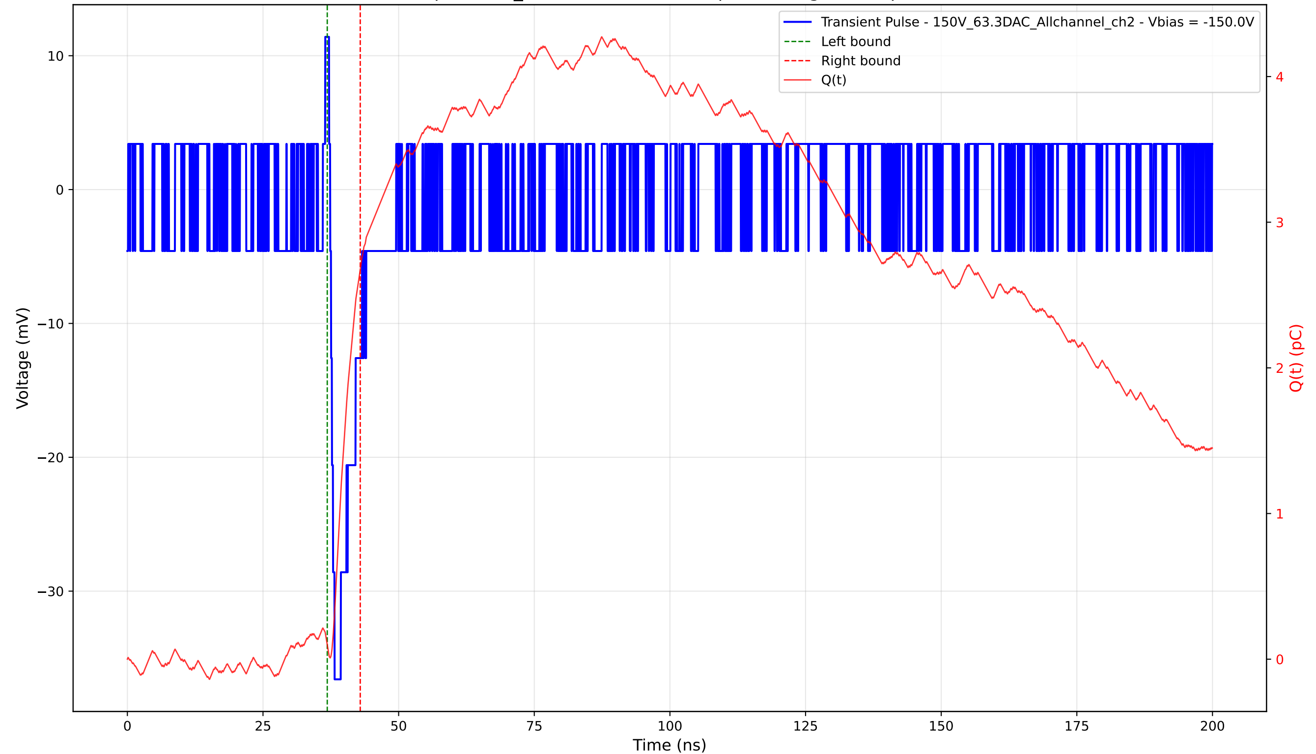
Transient Pulse - Sample: 1cm_42 - Position: 4615.0 \mu\text{m} - Charge: 2.58 pC - Rise Time: 0.83 ns
