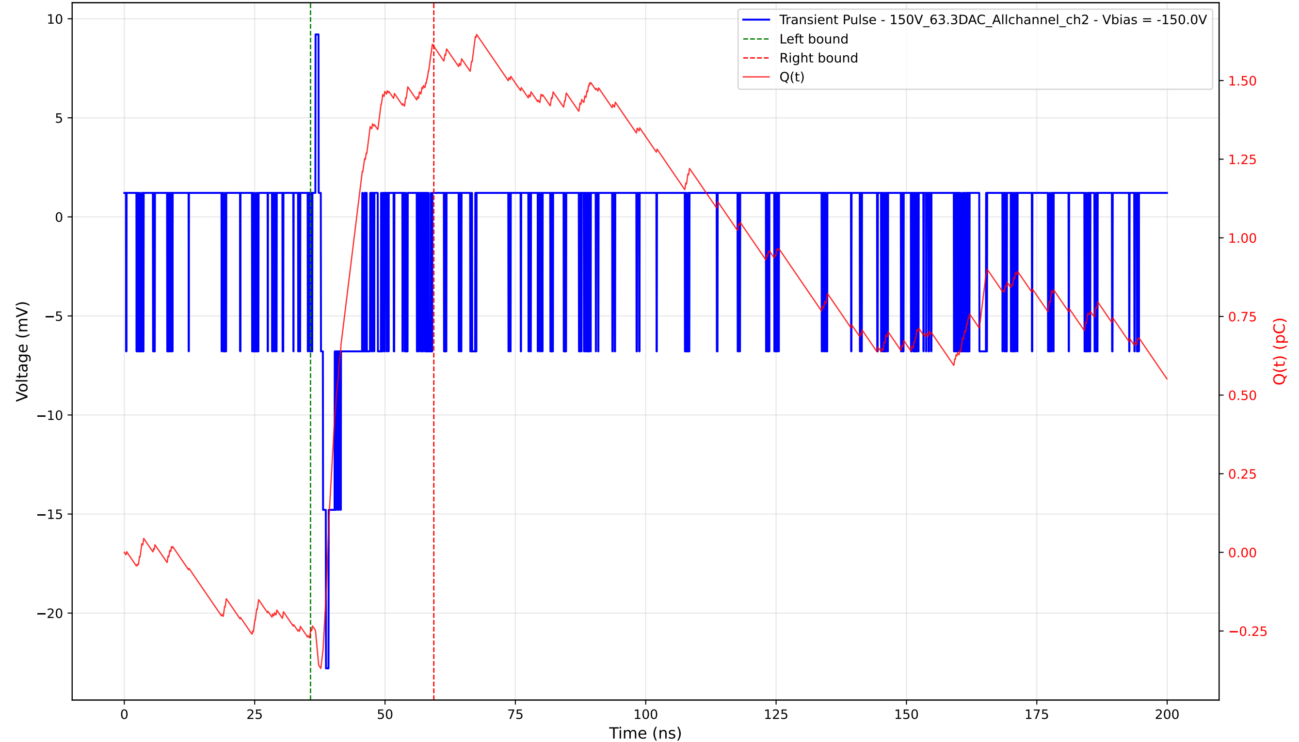
Transient Pulse - Sample: 1cm_42 - Position: 195.0 \mu\text{m} - Charge: 1.86 pC - Rise Time: 0.99 ns
