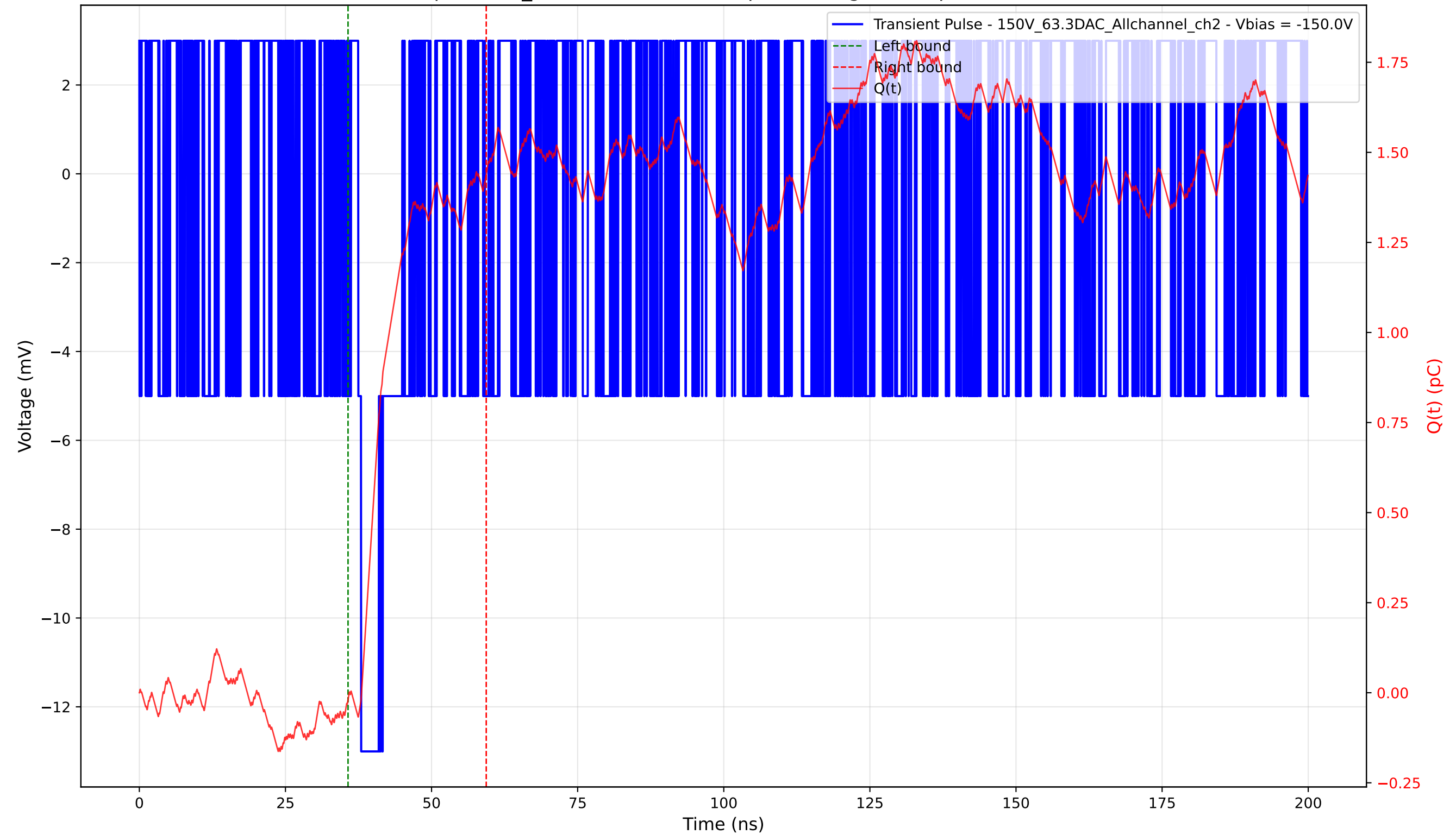
Transient Pulse - Sample: 1cm_42 - Position: 5055.0 \mu\text{m} - Charge: 1.45 pC - Rise Time: 0.00 ns (N/A)
