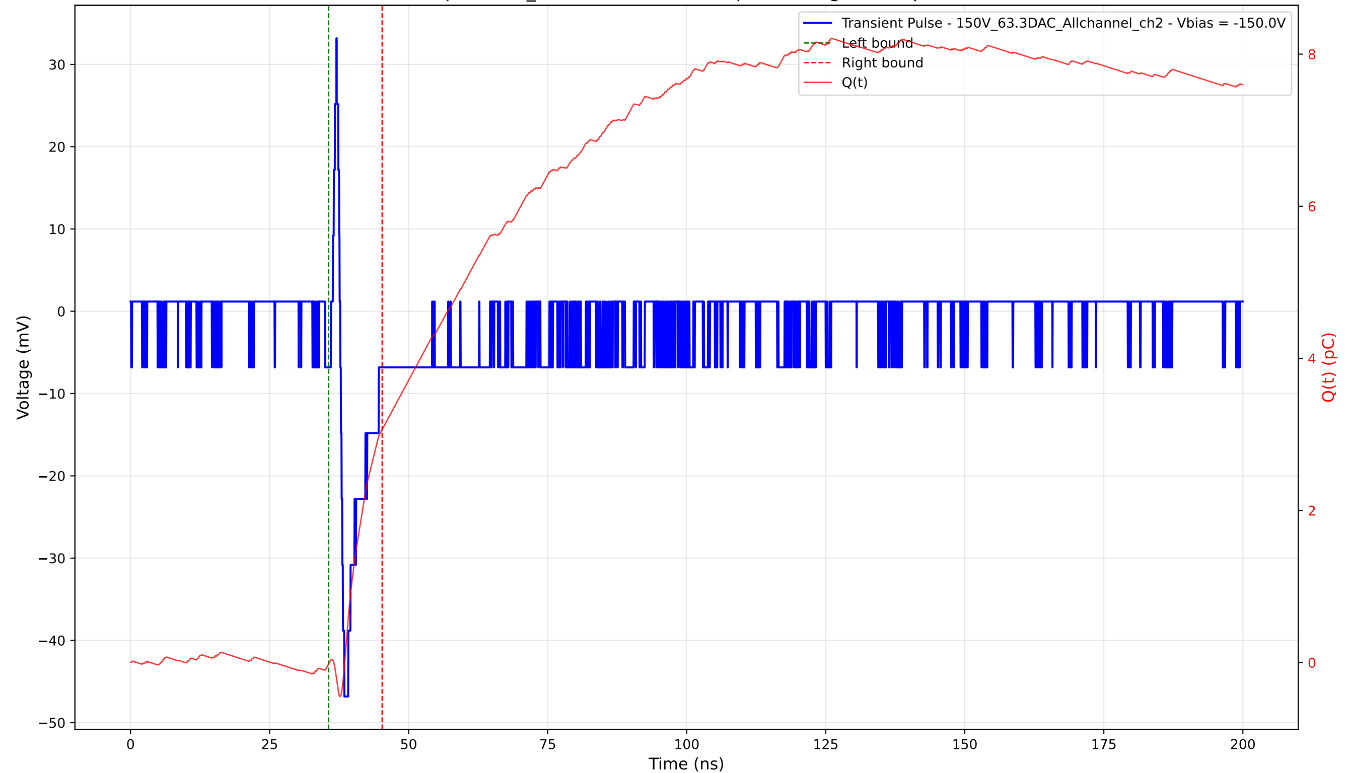
Transient Pulse - Sample: 1cm_42 - Position: 1410.0 \mu\text{m} - Charge: 3.08 pC - Rise Time: 0.74 ns
