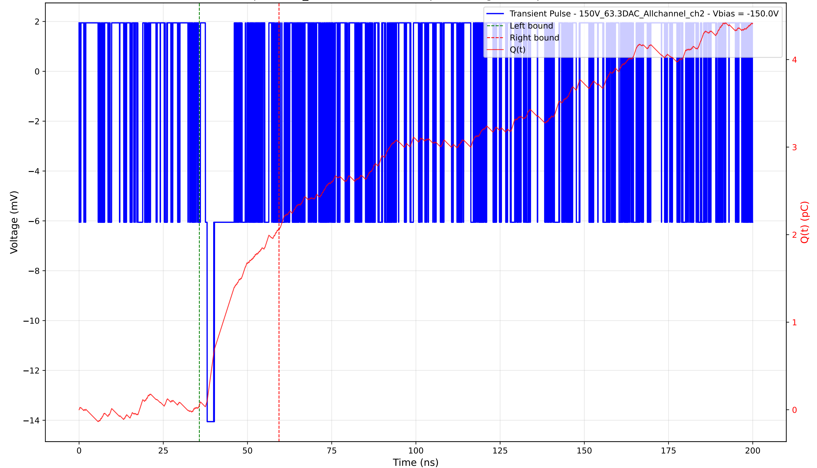
Transient Pulse - Sample: 1cm_42 - Position: 5065.0 \mu\text{m} - Charge: 2.01 pC - Rise Time: 0.00 ns (N/A)
