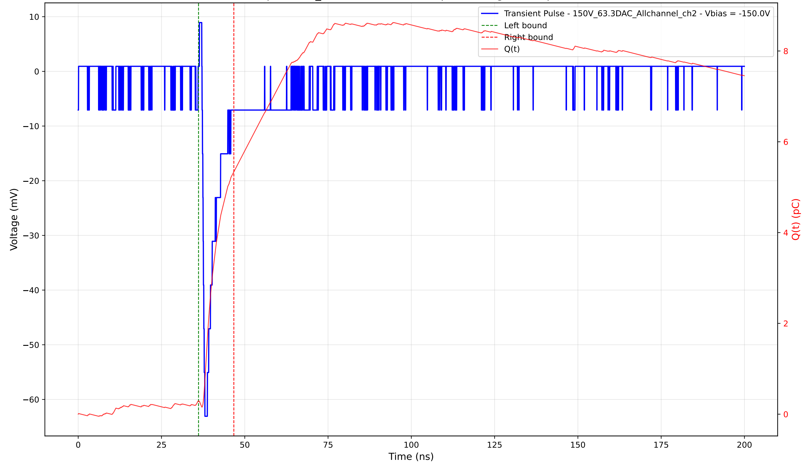
Transient Pulse - Sample: 1cm_42 - Position: 1815.0 \mu\text{m} - Charge: 5.05 pC - Rise Time: 0.84 ns
