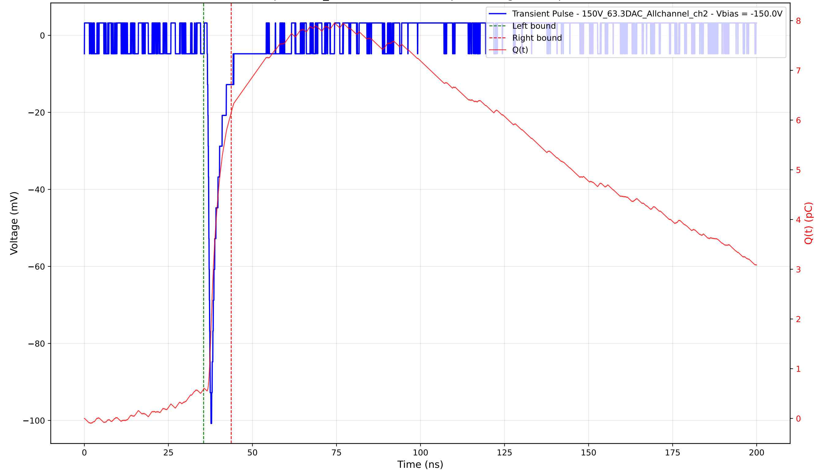
Transient Pulse - Sample: 1cm_42 - Position: 2125.0 \mu\text{m} - Charge: 5.56 pC - Rise Time: 0.81 ns
