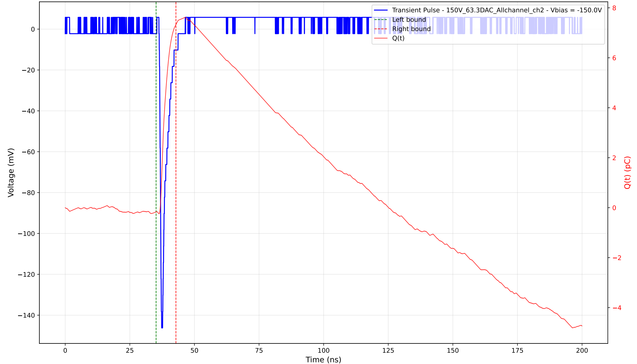
Transient Pulse - Sample: 1cm_42 - Position: 3665.0 \mu\text{m} - Charge: 7.49 pC - Rise Time: 0.74 ns
