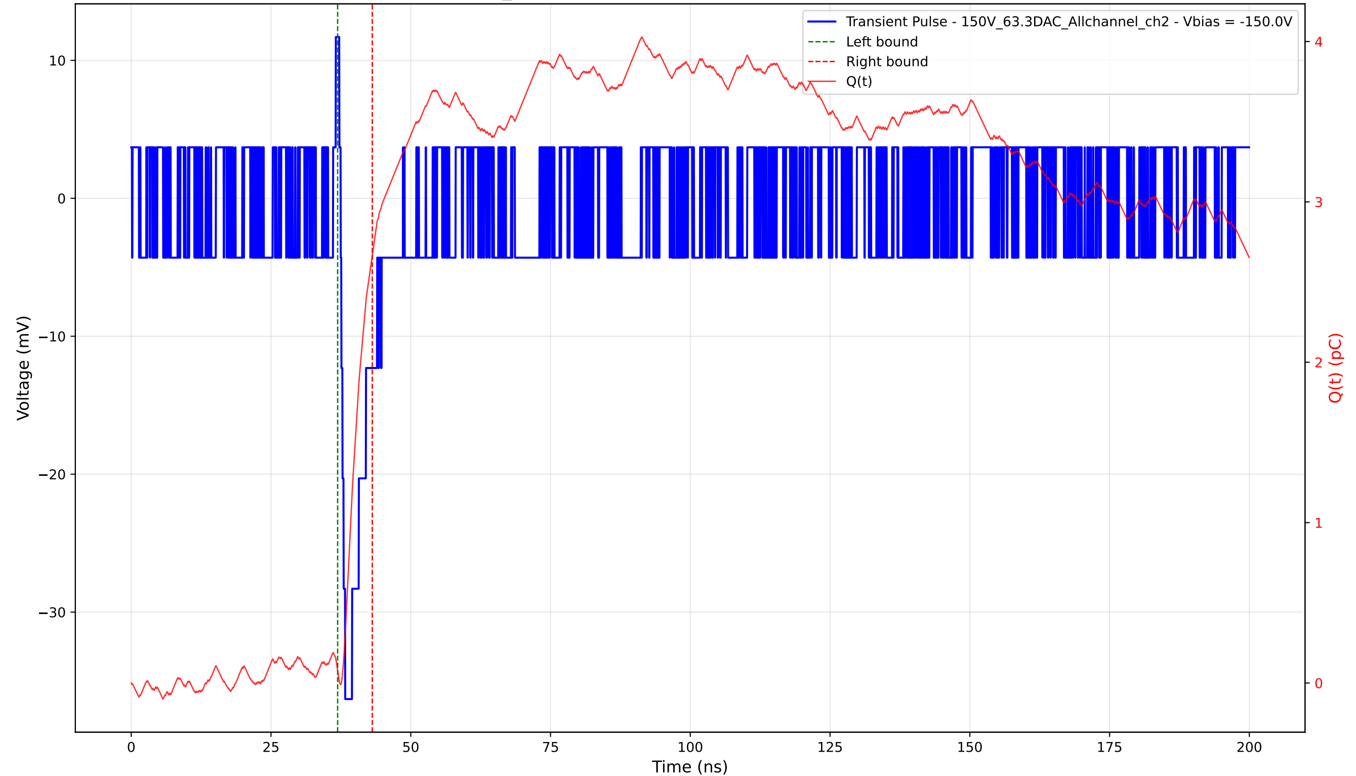
Transient Pulse - Sample: 1cm_42 - Position: 4800.0 \mu\text{m} - Charge: 2.59 pC - Rise Time: 0.00 ns (N/A)
