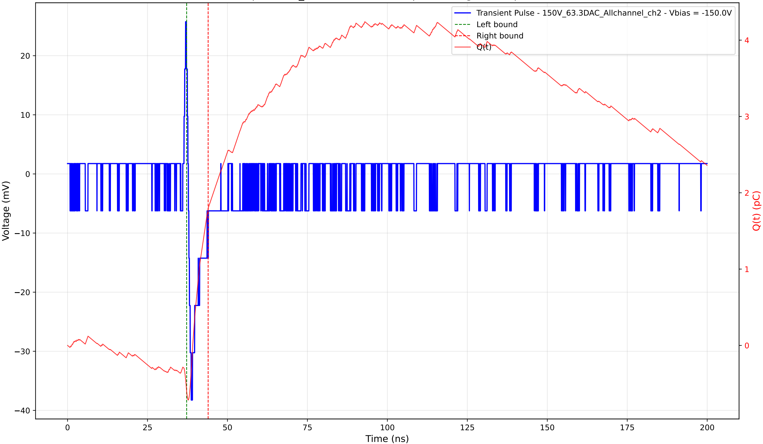
Transient Pulse - Sample: 1cm_42 - Position: 520.0 \mu\text{m} - Charge: 2.39 pC - Rise Time: 0.90 ns
