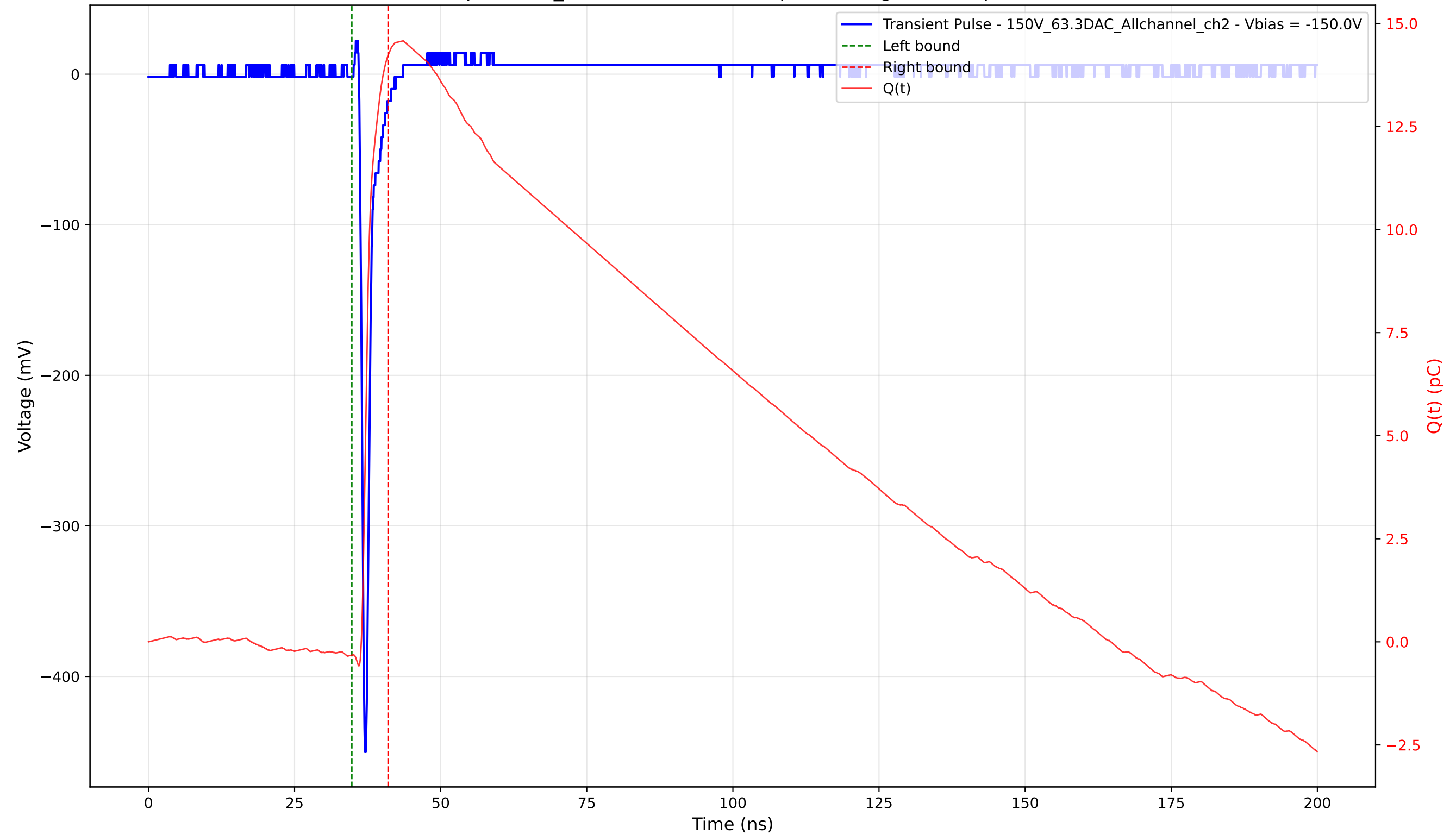
Transient Pulse - Sample: 1cm_42 - Position: 3205.0 \mu\text{m} - Charge: 14.54 pC - Rise Time: 0.70 ns
