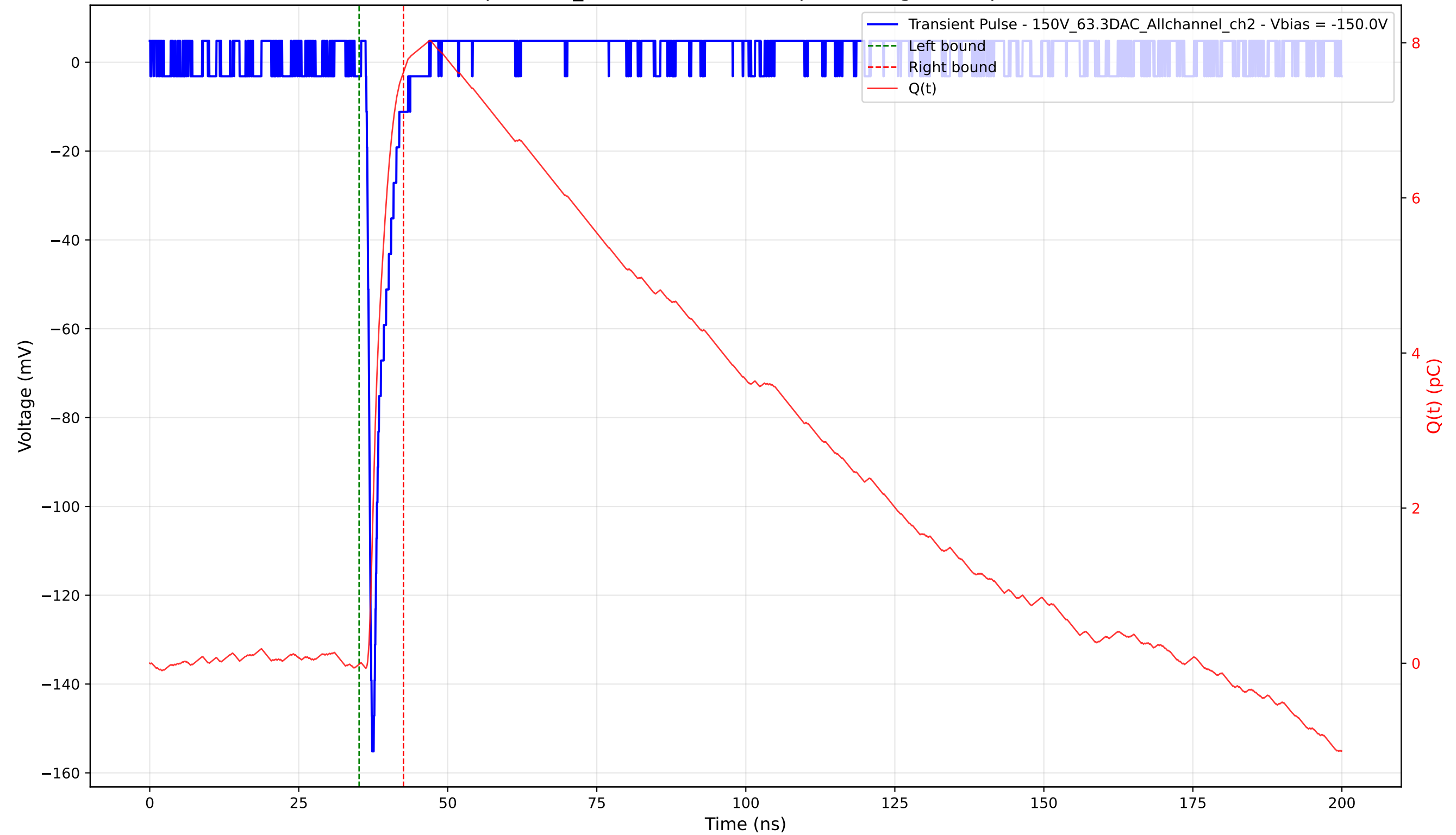
Transient Pulse - Sample: 1cm_42 - Position: 3640.0 \mu\text{m} - Charge: 7.63 pC - Rise Time: 0.82 ns
