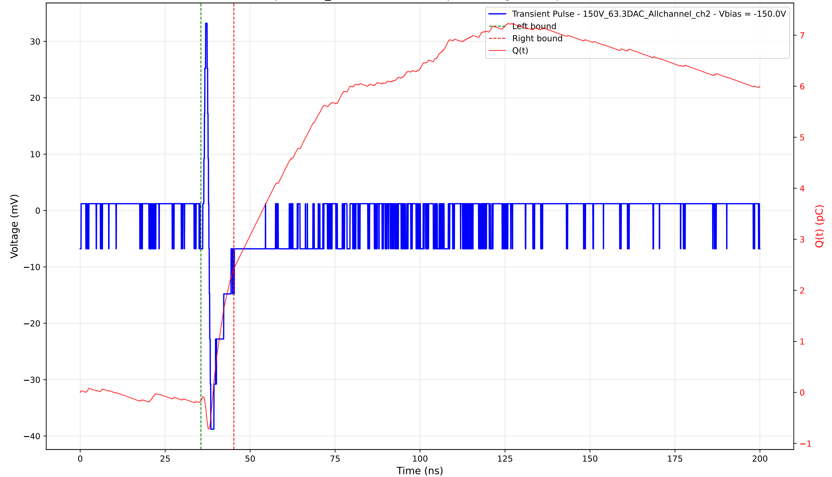
Transient Pulse - Sample: 1cm_42 - Position: 865.0 \mu\text{m} - Charge: 2.56 pC - Rise Time: 0.58 ns
