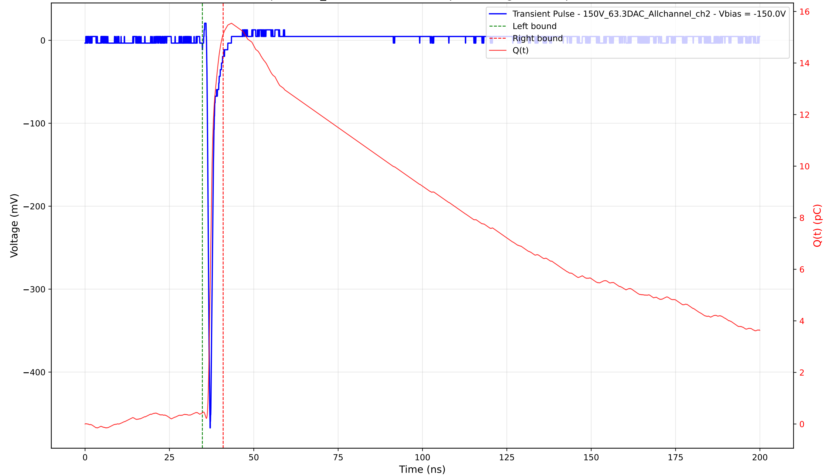
Transient Pulse - Sample: 1cm_42 - Position: 3165.0 \mu\text{m} - Charge: 14.68 pC - Rise Time: 0.70 ns
