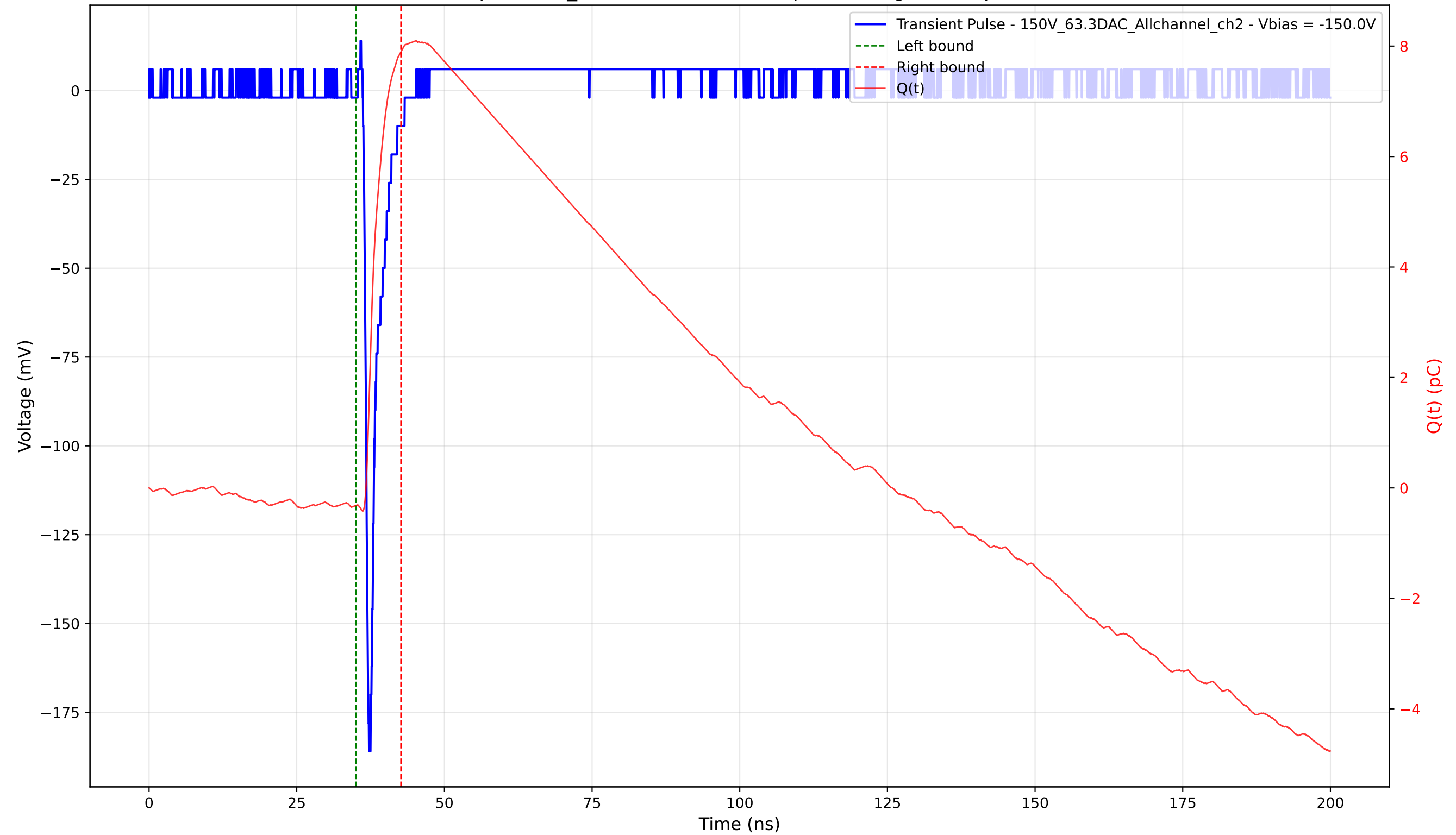
Transient Pulse - Sample: 1cm_42 - Position: 3555.0 \mu\text{m} - Charge: 8.22 pC - Rise Time: 0.72 ns
