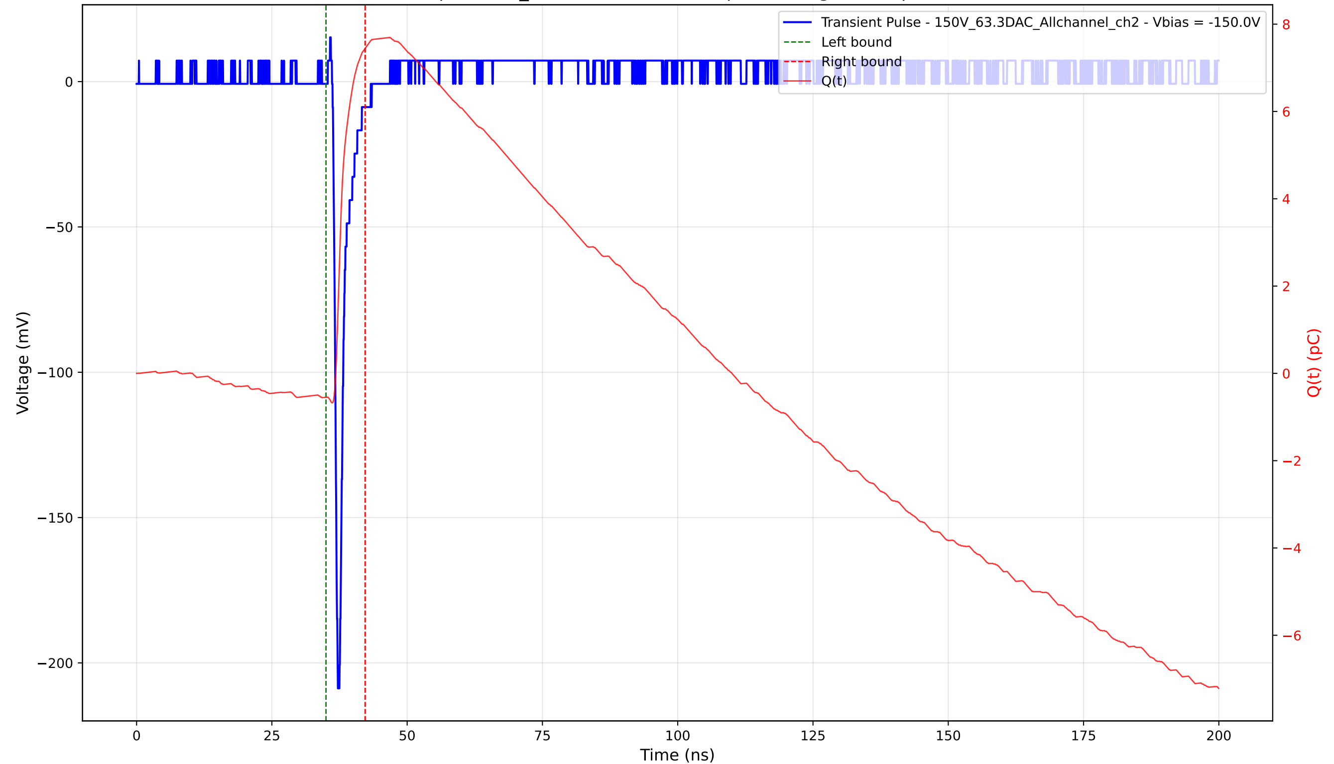
Transient Pulse - Sample: 1cm_42 - Position: 2525.0 \mu\text{m} - Charge: 7.99 pC - Rise Time: 0.76 ns
