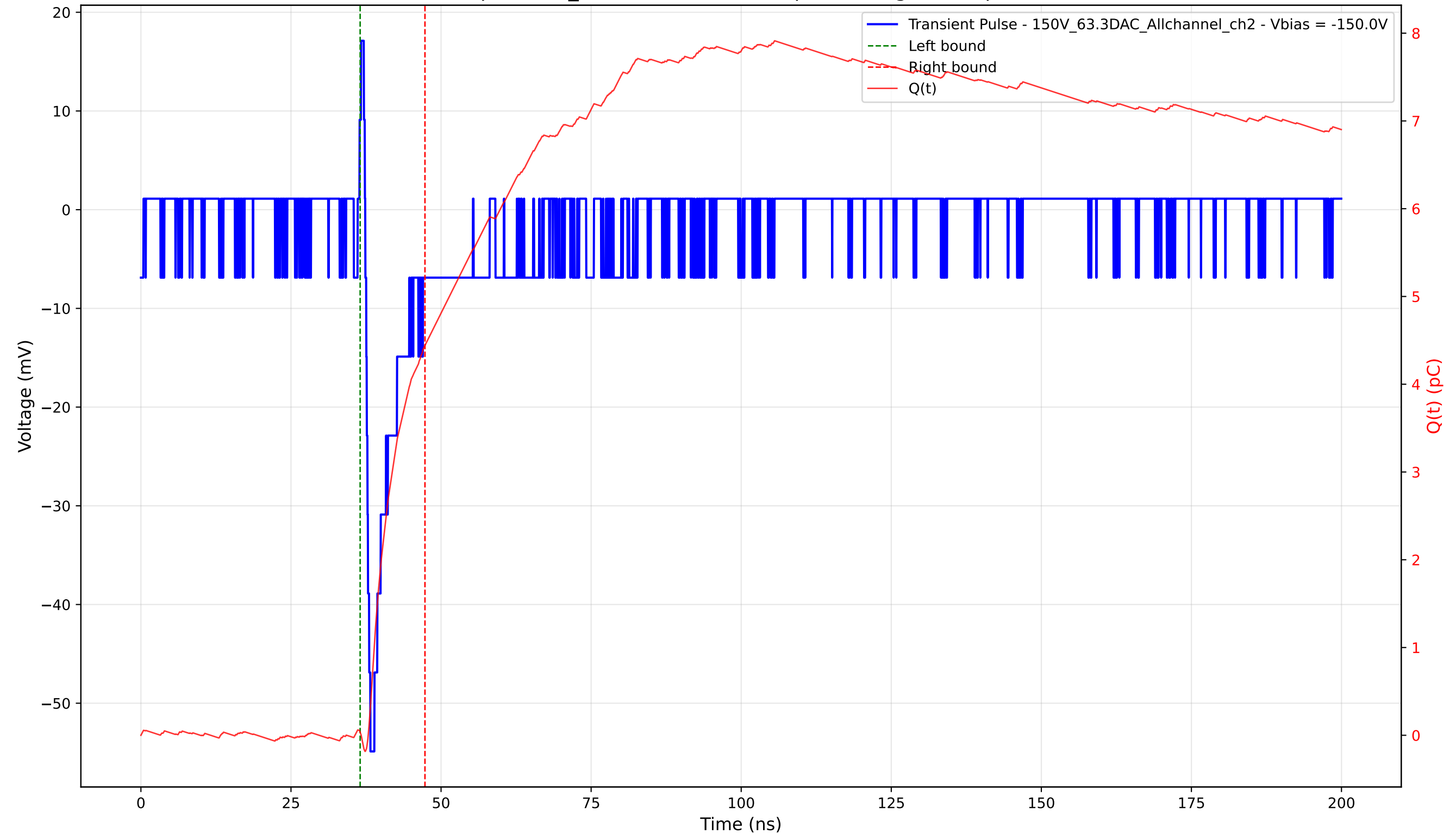
Transient Pulse - Sample: 1cm_42 - Position: 1635.0 \mu\text{m} - Charge: 4.41 pC - Rise Time: 0.85 ns
