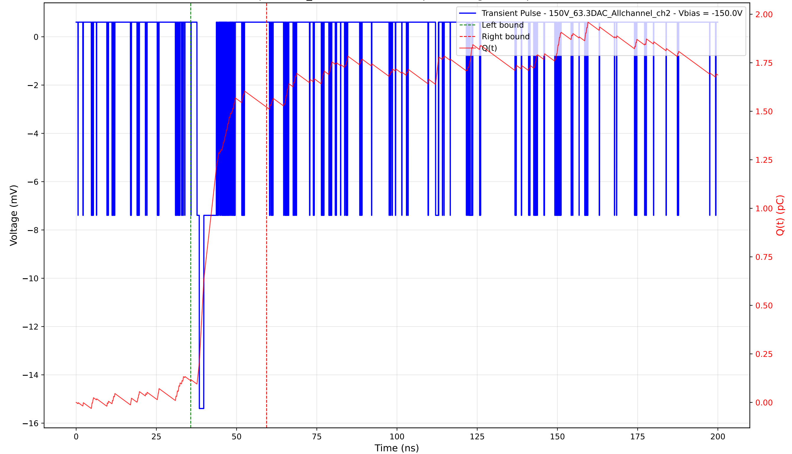
Transient Pulse - Sample: 1cm_42 - Position: 150.0 \mu\text{m} - Charge: 1.41 pC - Rise Time: 0.75 ns
