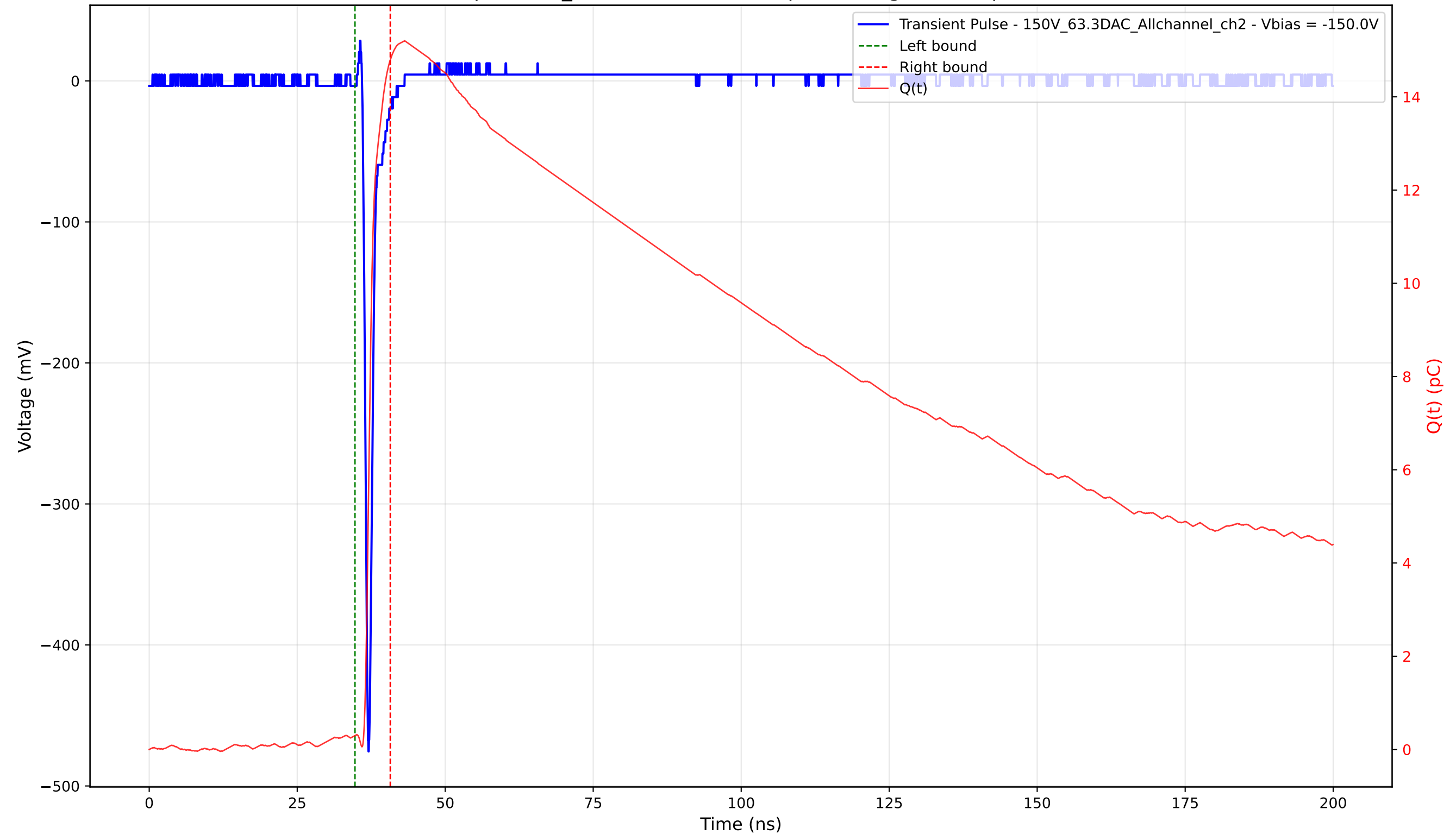
Transient Pulse - Sample: 1cm_42 - Position: 3025.0 \mu\text{m} - Charge: 14.49 pC - Rise Time: 0.69 ns
