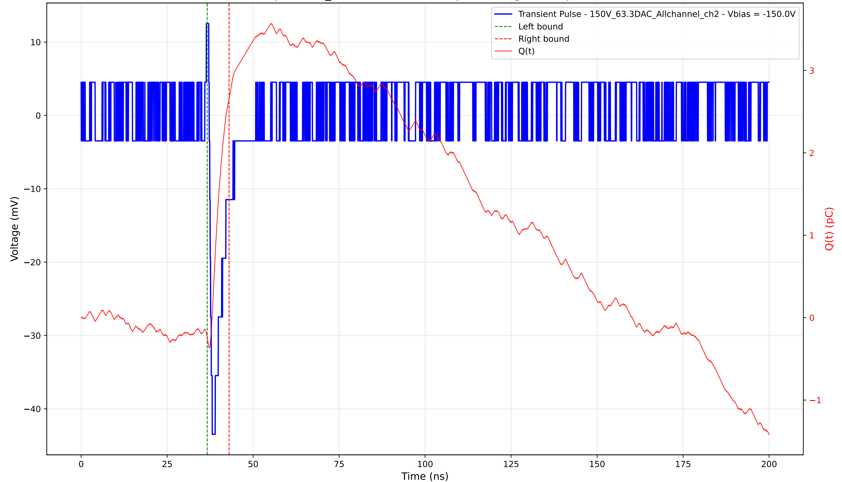
Transient Pulse - Sample: 1cm_42 - Position: 4465.0 \mu\text{m} - Charge: 2.90 pC - Rise Time: 0.76 ns
