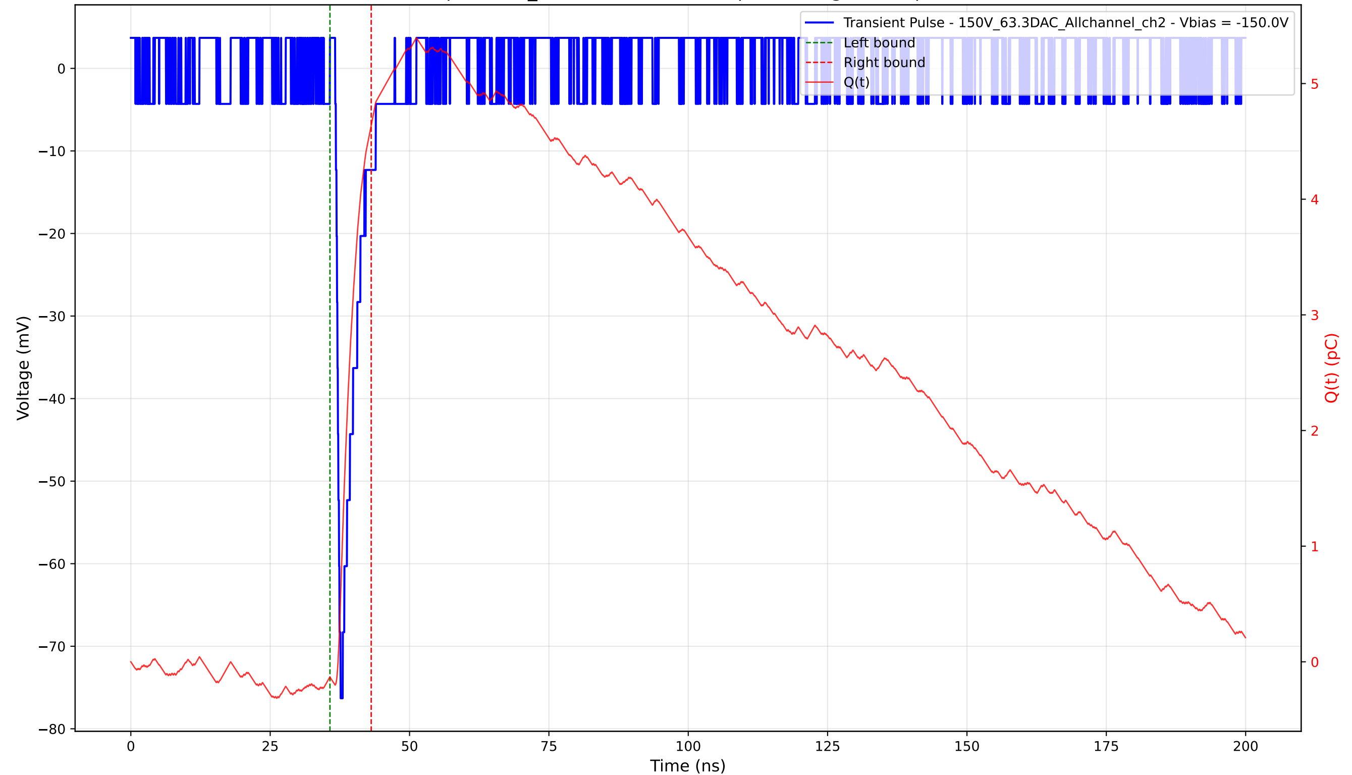
Transient Pulse - Sample: 1cm_42 - Position: 4000.0 \mu\text{m} - Charge: 4.77 pC - Rise Time: 0.86 ns
