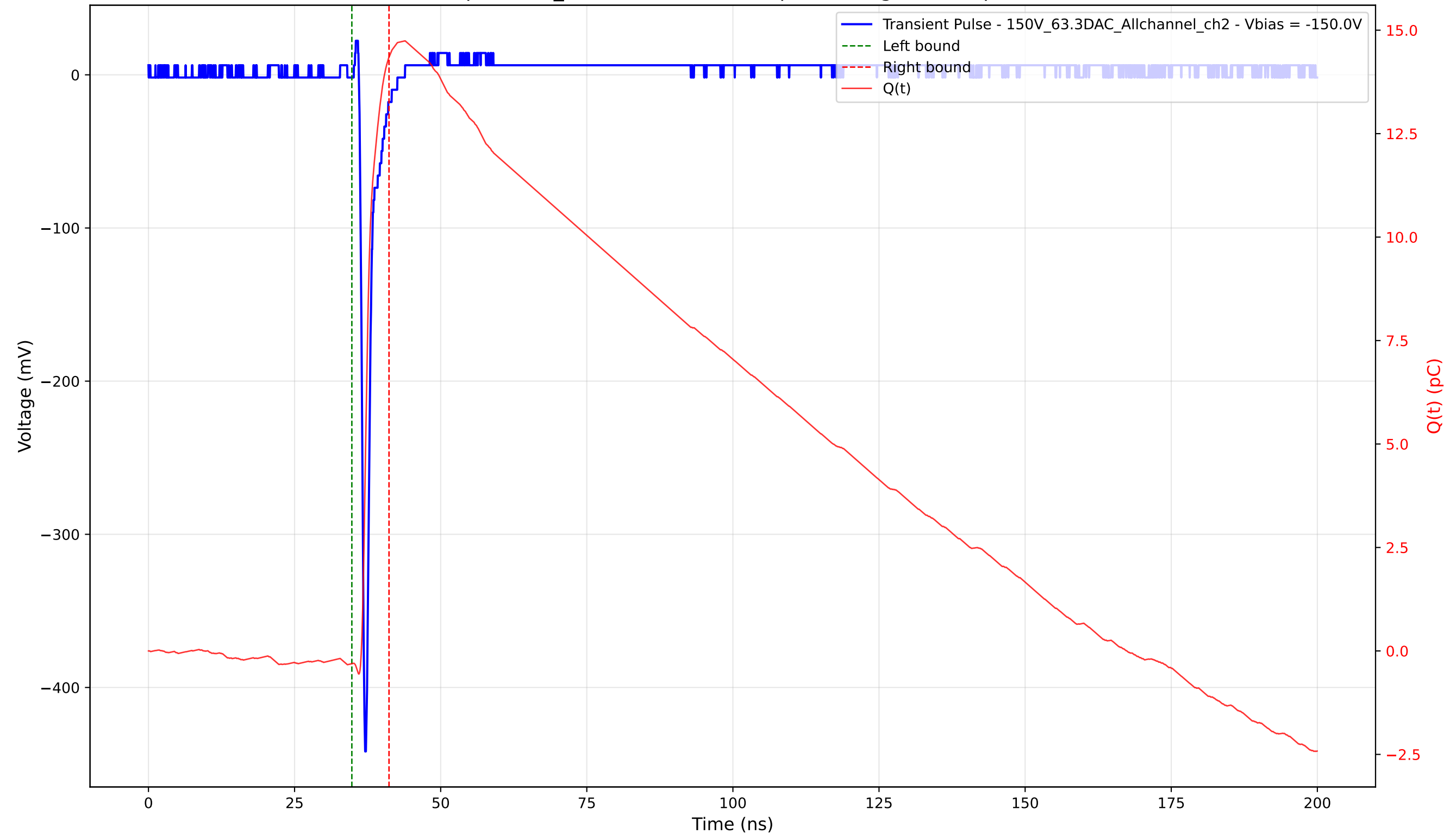
Transient Pulse - Sample: 1cm_42 - Position: 3260.0 \mu\text{m} - Charge: 14.65 pC - Rise Time: 0.69 ns
