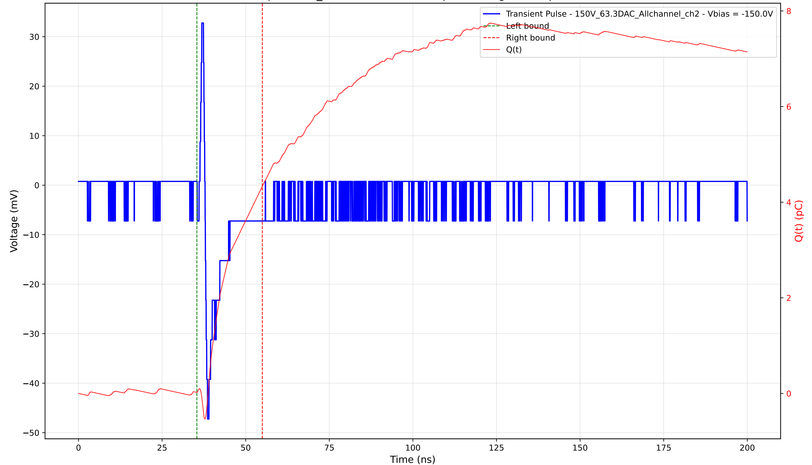
Transient Pulse - Sample: 1cm_42 - Position: 1150.0 \mu\text{m} - Charge: 4.31 pC - Rise Time: 0.74 ns
