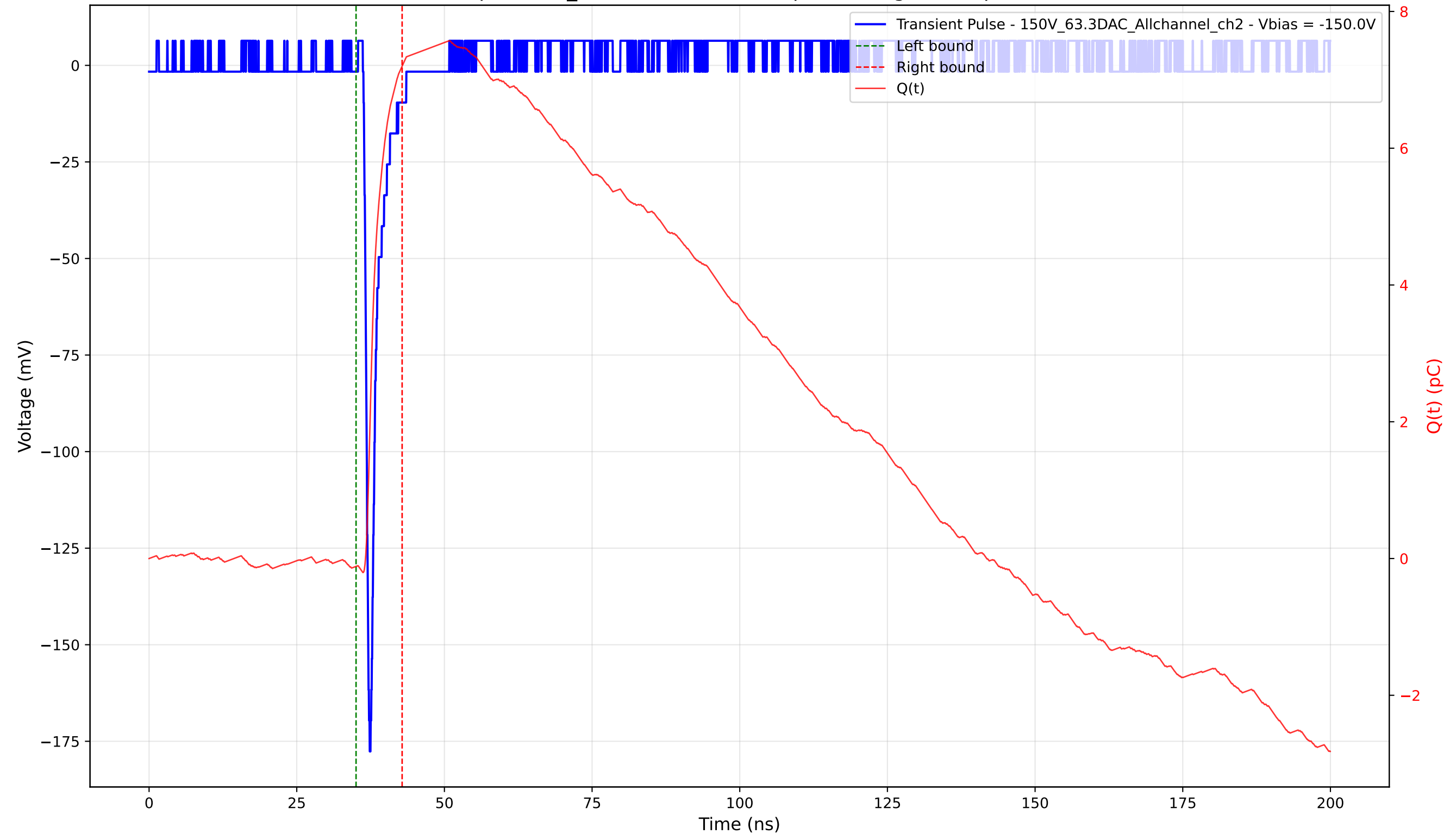
Transient Pulse - Sample: 1cm_42 - Position: 2455.0 \mu\text{m} - Charge: 7.32 pC - Rise Time: 0.76 ns
