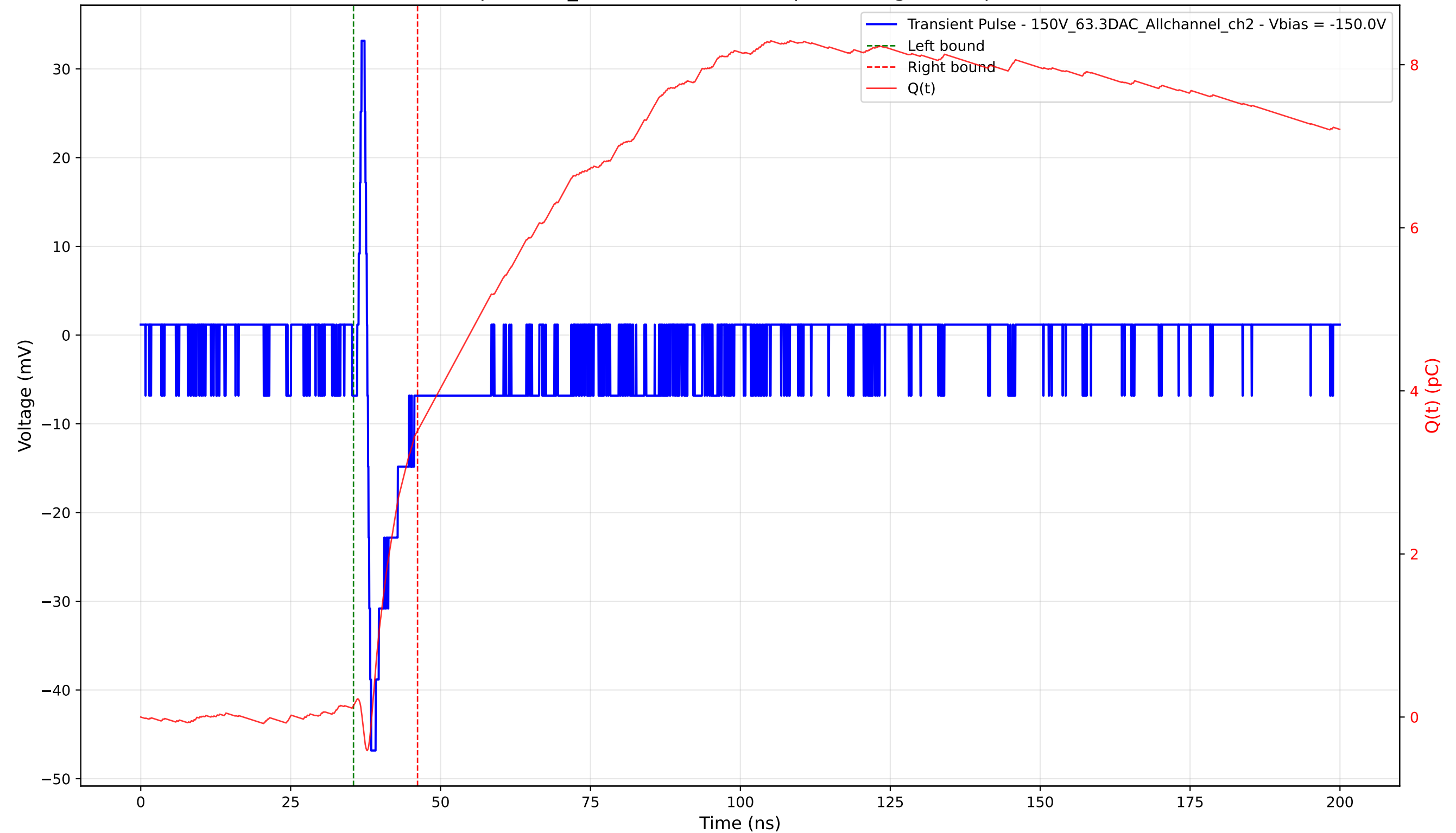
Transient Pulse - Sample: 1cm_42 - Position: 1200.0 \mu\text{m} - Charge: 3.37 pC - Rise Time: 0.66 ns
