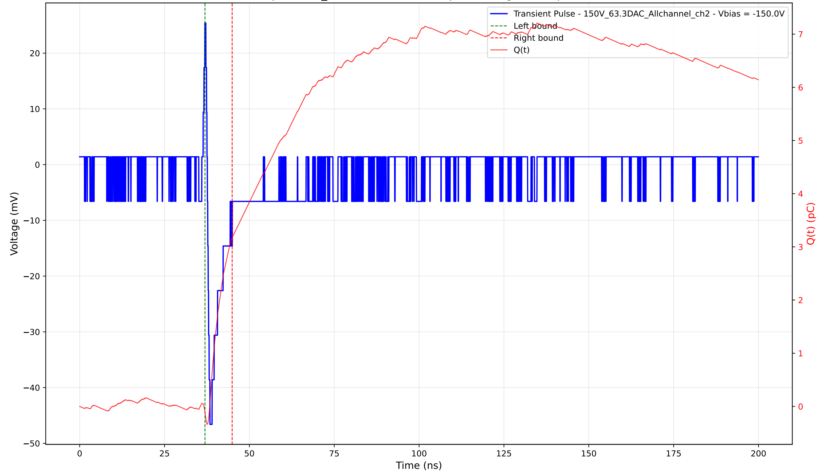
Transient Pulse - Sample: 1cm_42 - Position: 1490.0 \mu\text{m} - Charge: 3.27 pC - Rise Time: 0.77 ns
