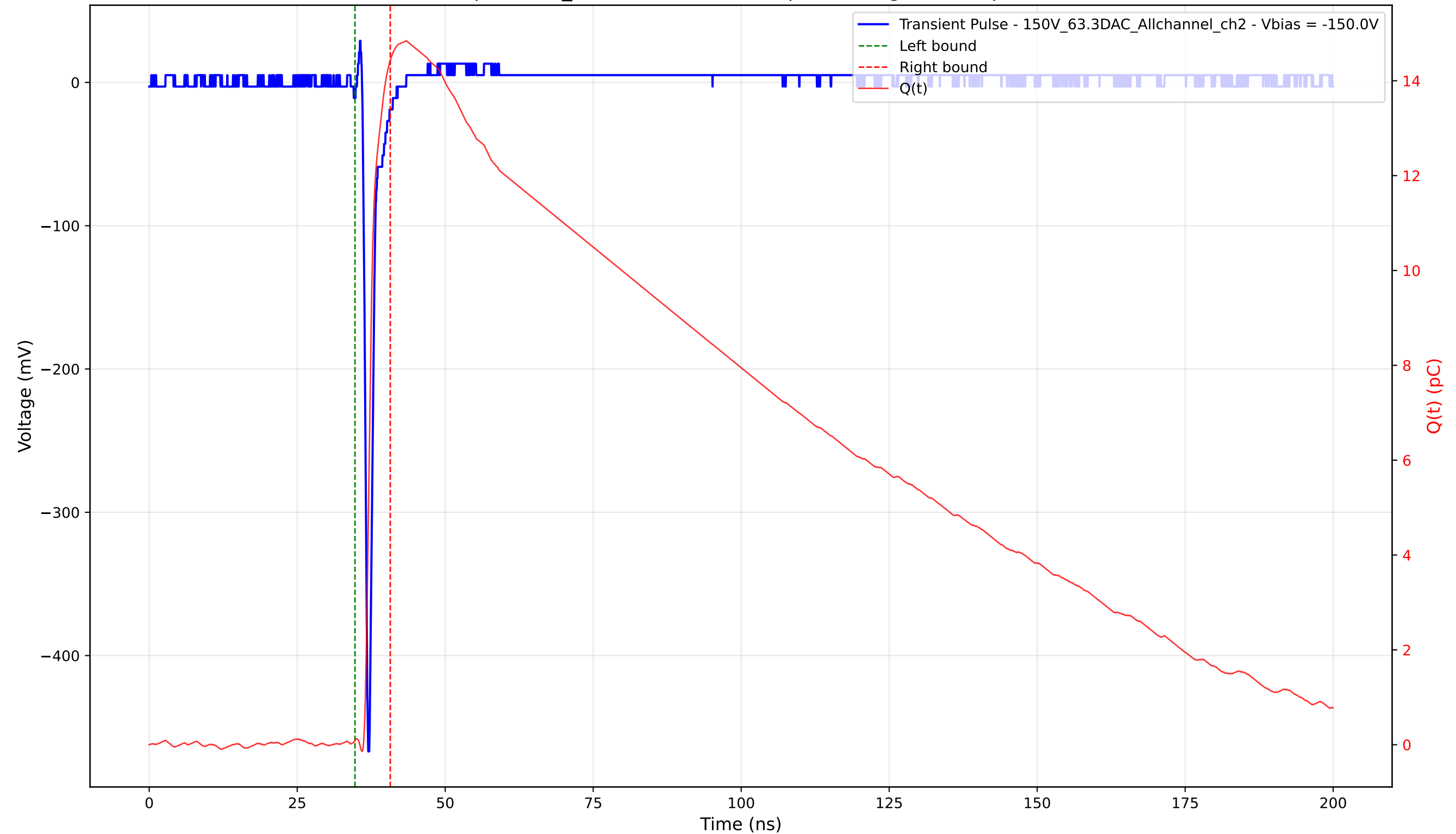
Transient Pulse - Sample: 1cm_42 - Position: 3055.0 \mu\text{m} - Charge: 14.34 pC - Rise Time: 0.68 ns
