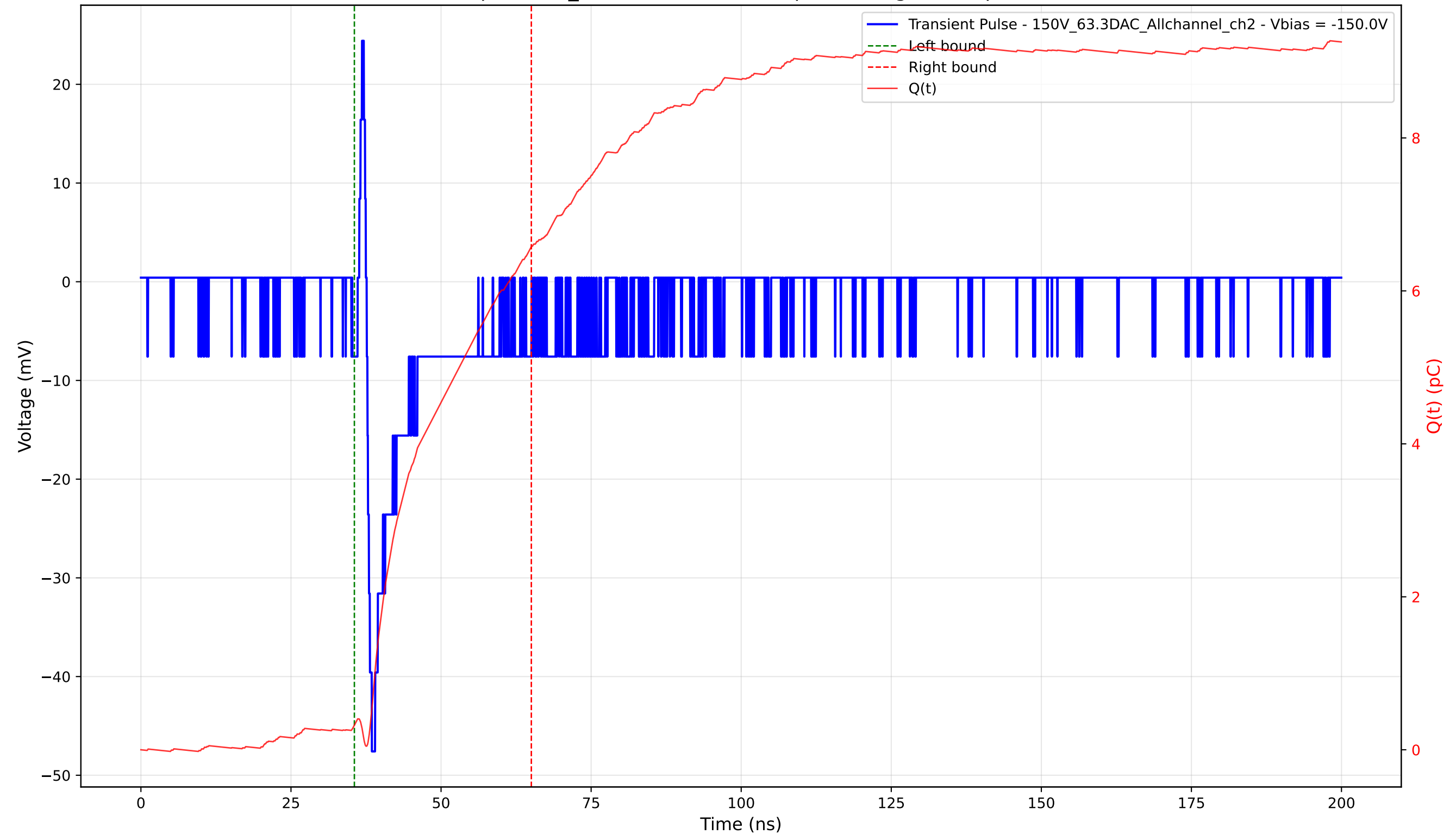
Transient Pulse - Sample: 1cm_42 - Position: 1500.0 \mu\text{m} - Charge: 6.26 pC - Rise Time: 0.86 ns
