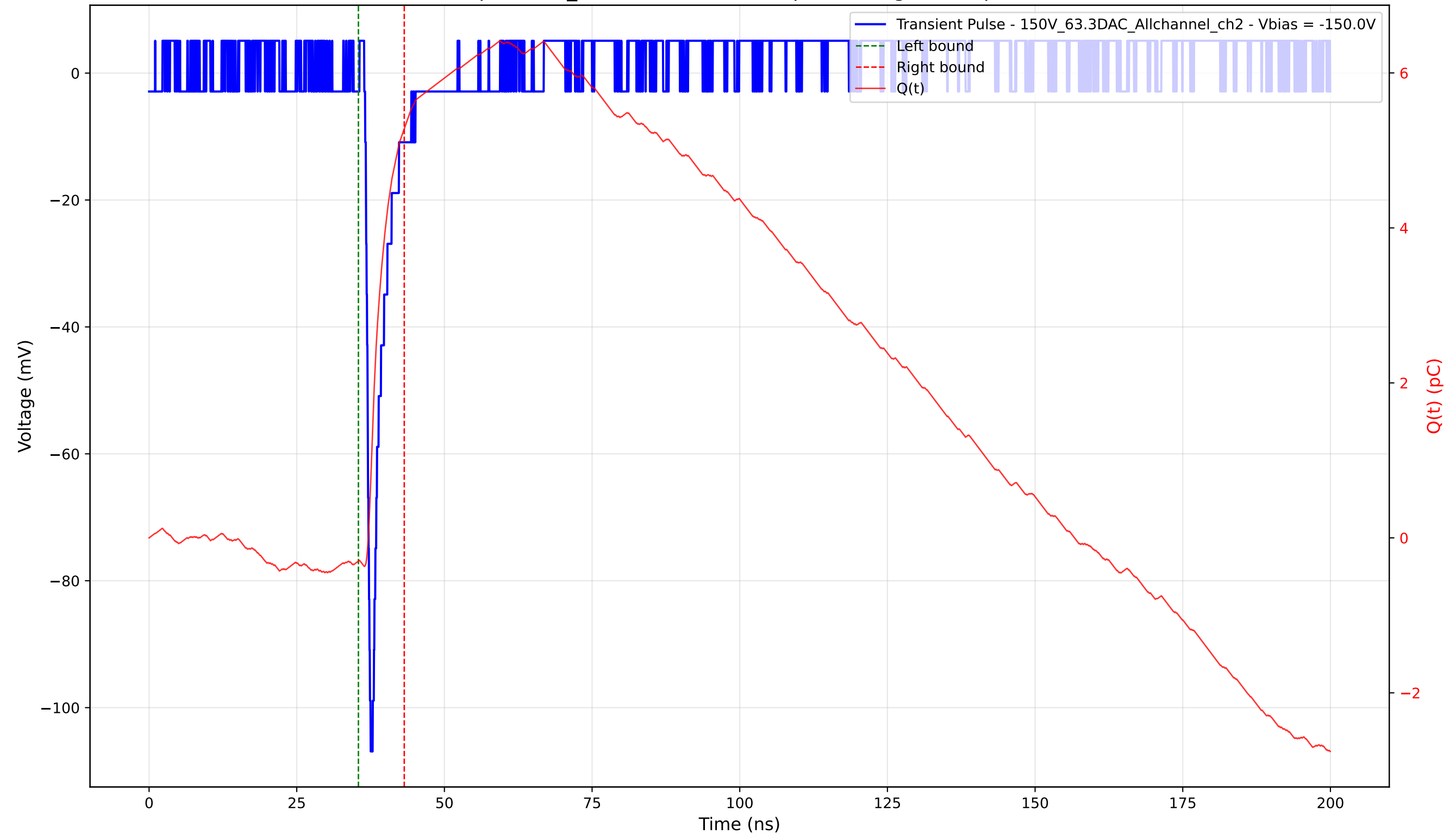
Transient Pulse - Sample: 1cm_42 - Position: 2165.0 \mu\text{m} - Charge: 5.58 pC - Rise Time: 0.80 ns
