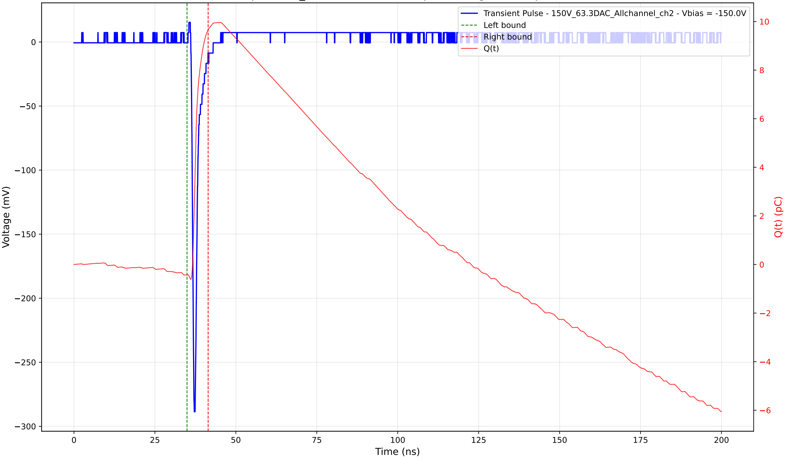
Transient Pulse - Sample: 1cm_42 - Position: 2615.0 \mu\text{m} - Charge: 10.08 pC - Rise Time: 0.71 ns
