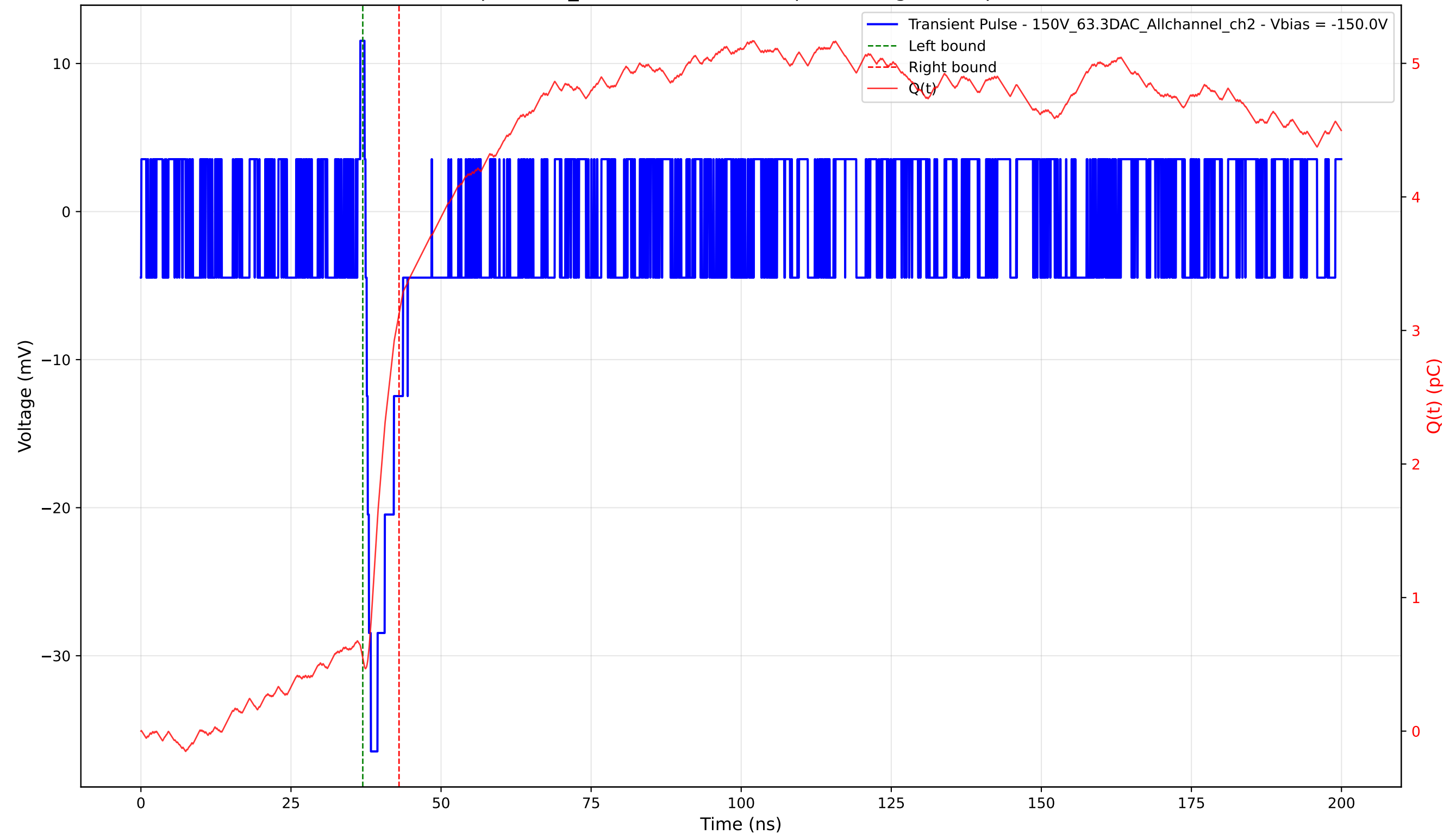
Transient Pulse - Sample: 1cm_42 - Position: 4760.0 \mu\text{m} - Charge: 2.58 pC - Rise Time: 0.92 ns
