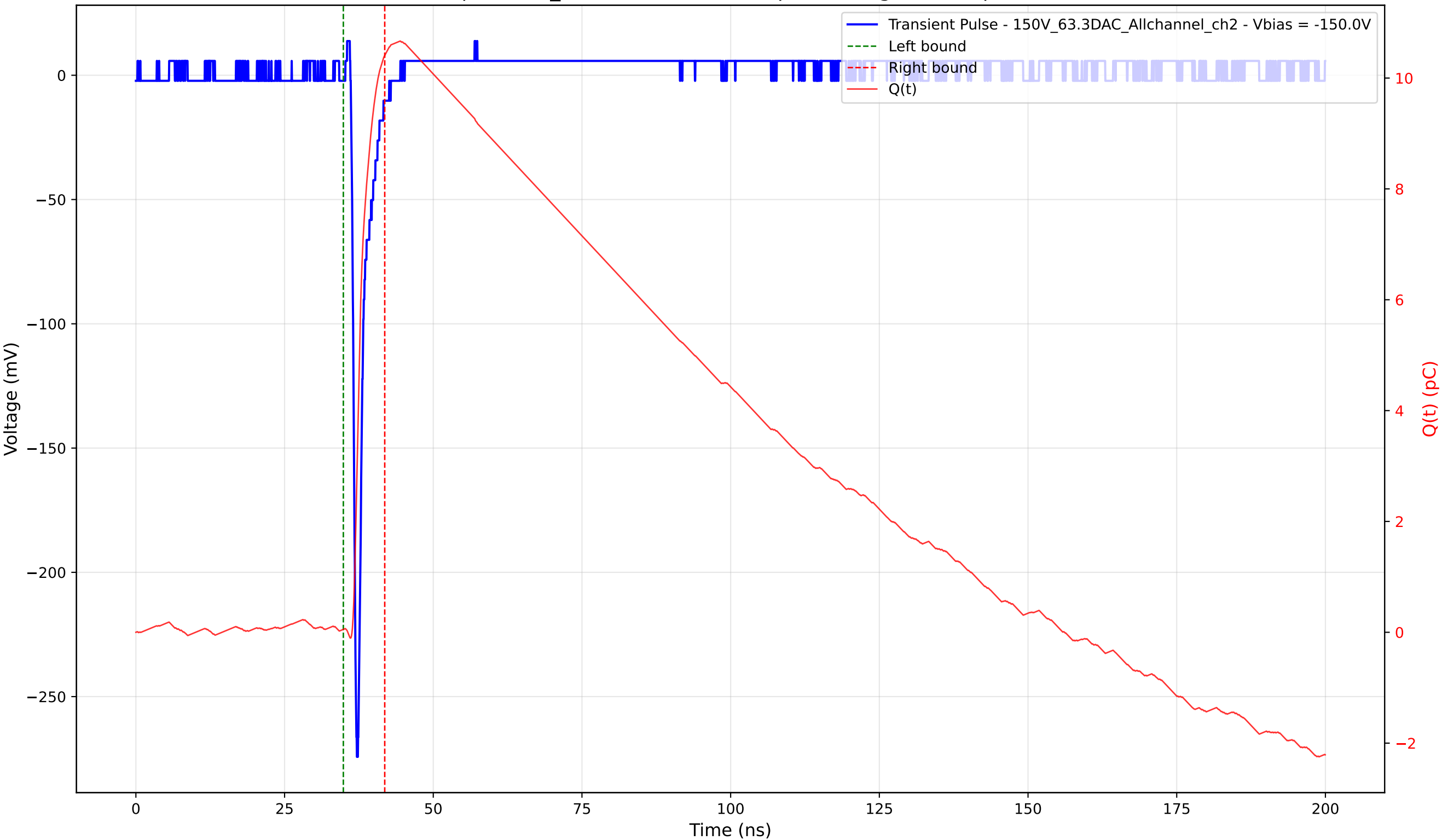
Transient Pulse - Sample: 1cm_42 - Position: 3445.0 \mu\text{m} - Charge: 10.36 pC - Rise Time: 0.74 ns
