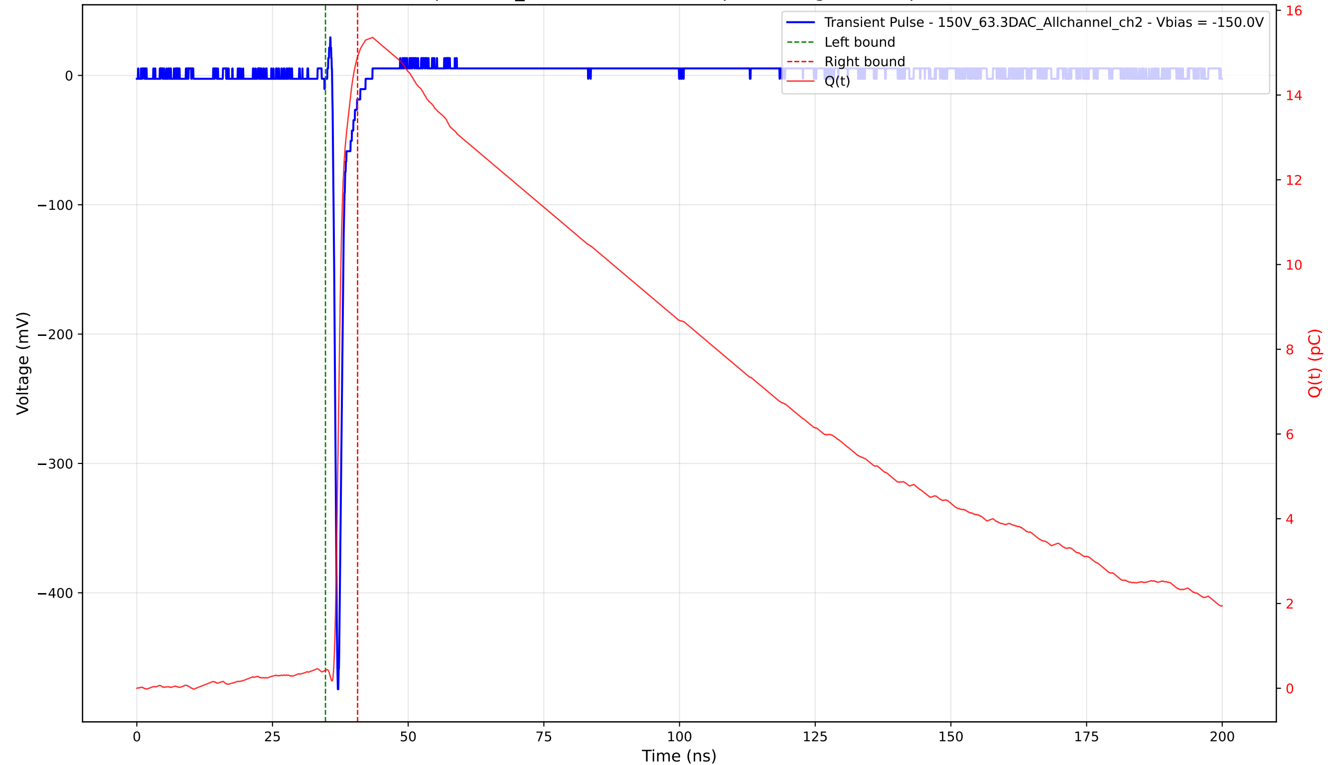
Transient Pulse - Sample: 1cm_42 - Position: 2935.0 \mu\text{m} - Charge: 14.48 pC - Rise Time: 0.73 ns
