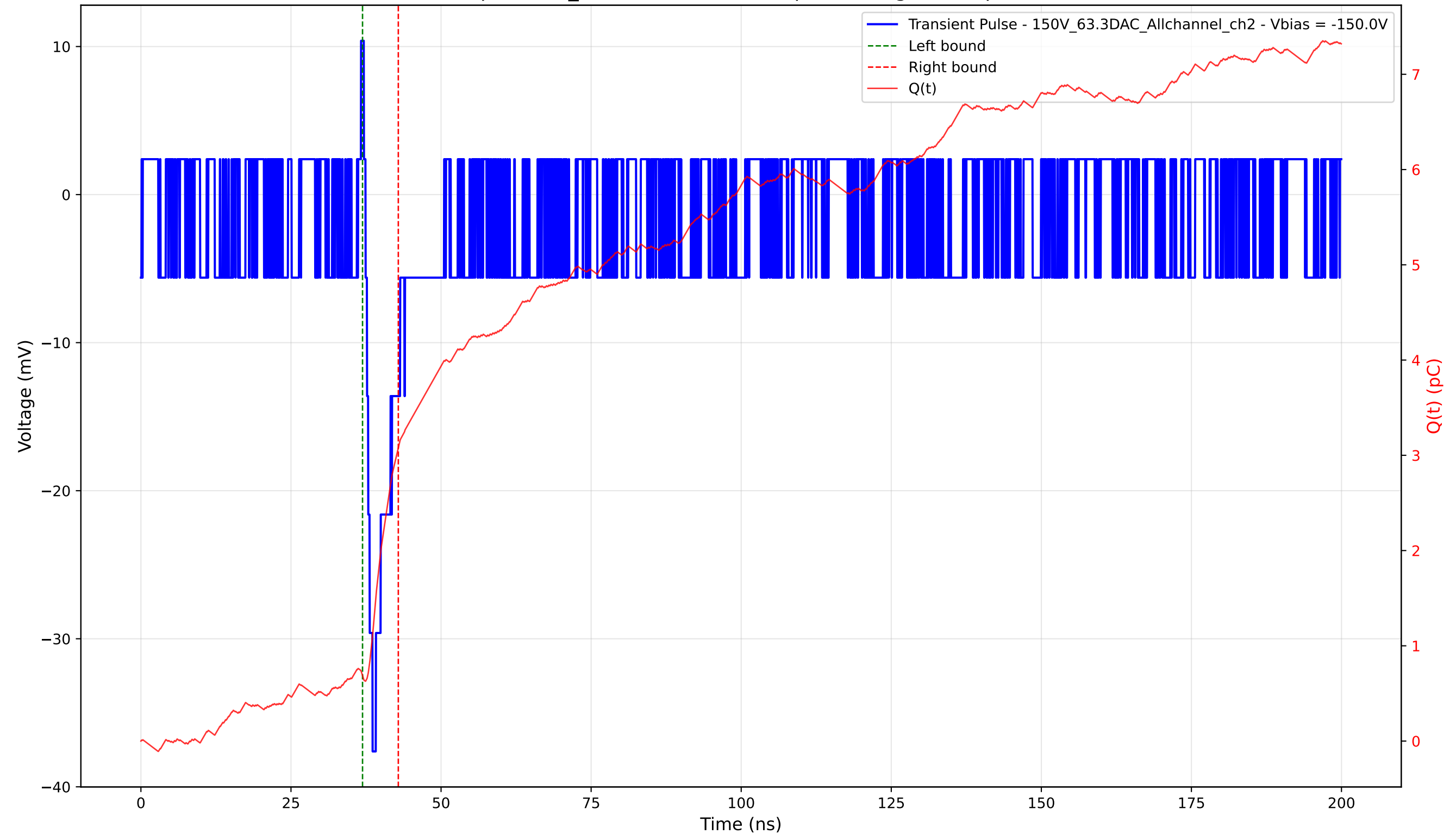
Transient Pulse - Sample: 1cm_42 - Position: 4885.0 \mu\text{m} - Charge: 2.39 pC - Rise Time: 1.18 ns
