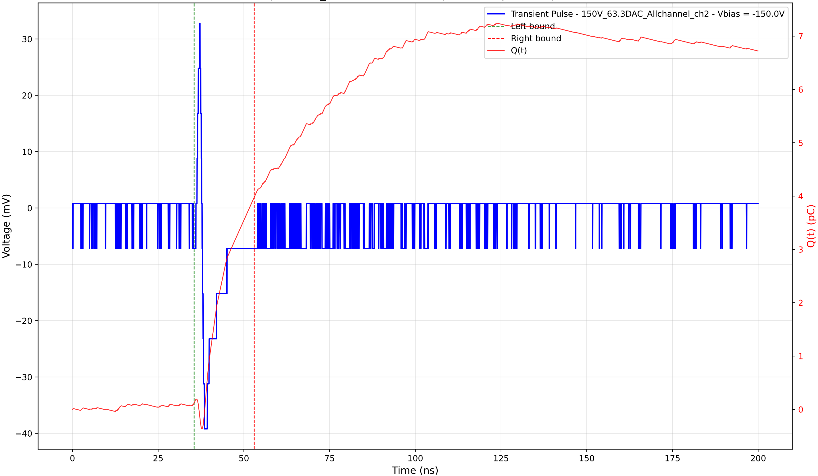
Transient Pulse - Sample: 1cm_42 - Position: 635.0 \mu\text{m} - Charge: 3.86 pC - Rise Time: 0.66 ns
