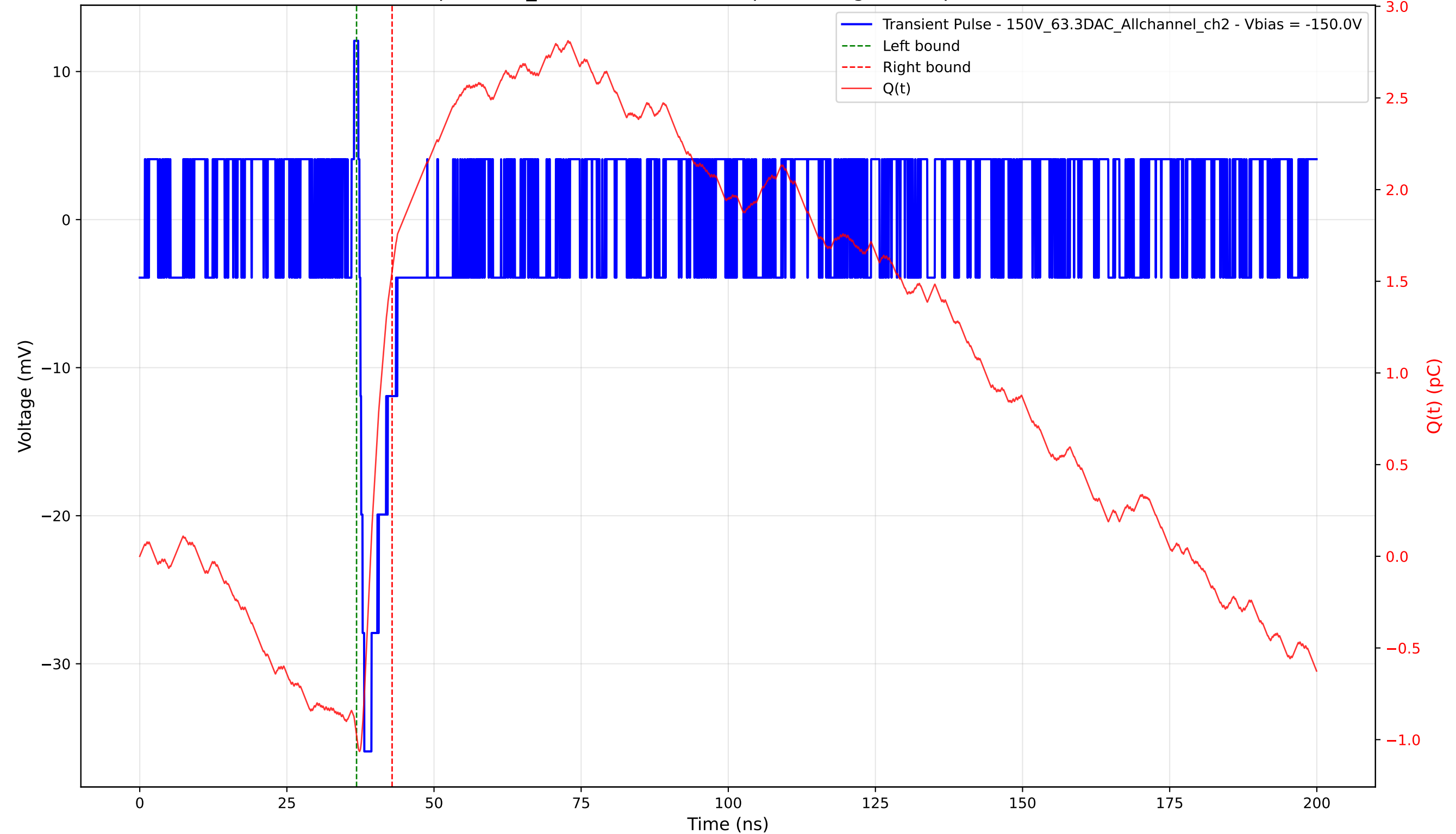
Transient Pulse - Sample: 1cm_42 - Position: 4570.0 \mu\text{m} - Charge: 2.53 pC - Rise Time: 0.00 ns (N/A)
