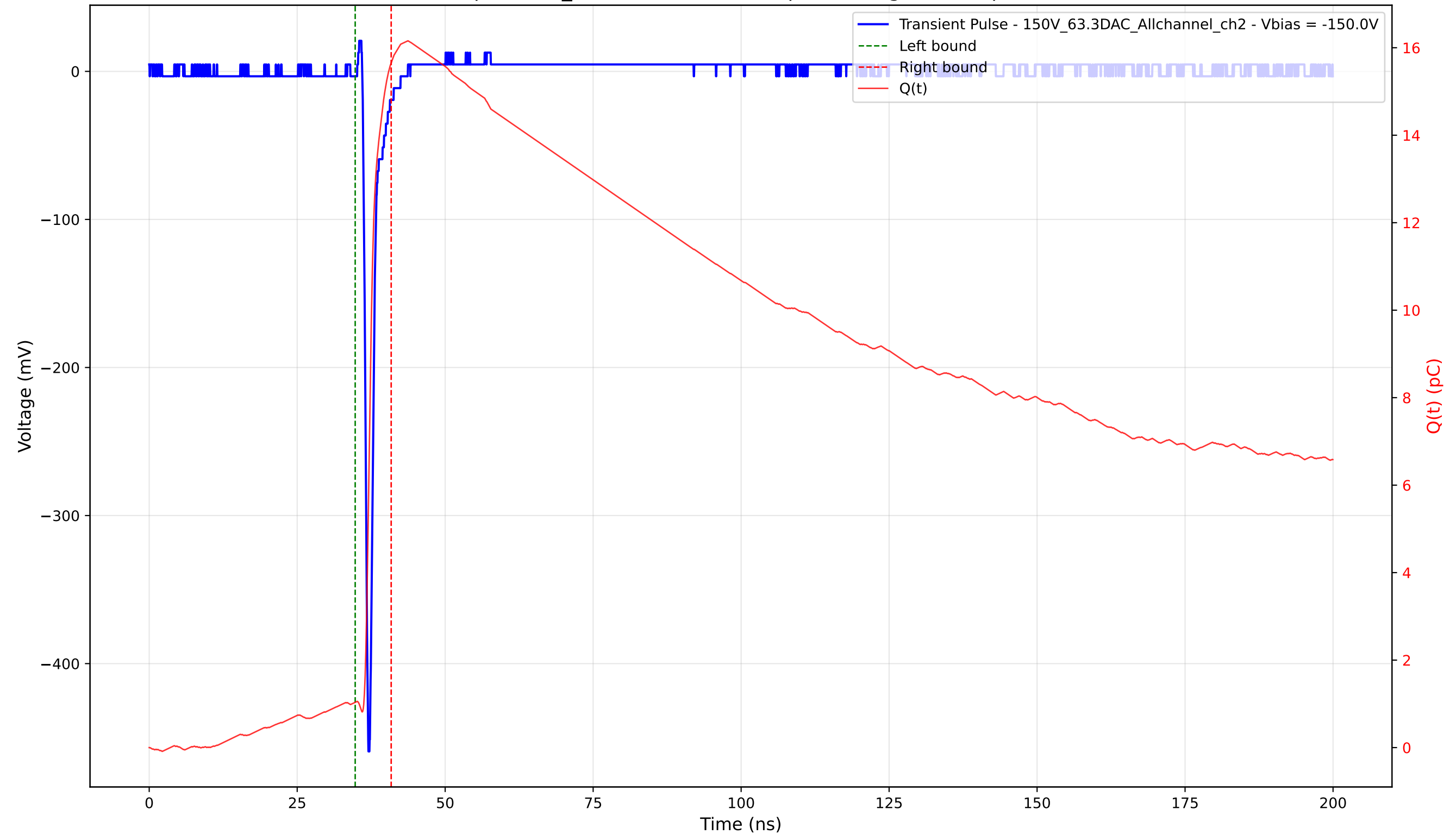
Transient Pulse - Sample: 1cm_42 - Position: 2870.0 \mu\text{m} - Charge: 14.62 pC - Rise Time: 0.72 ns
