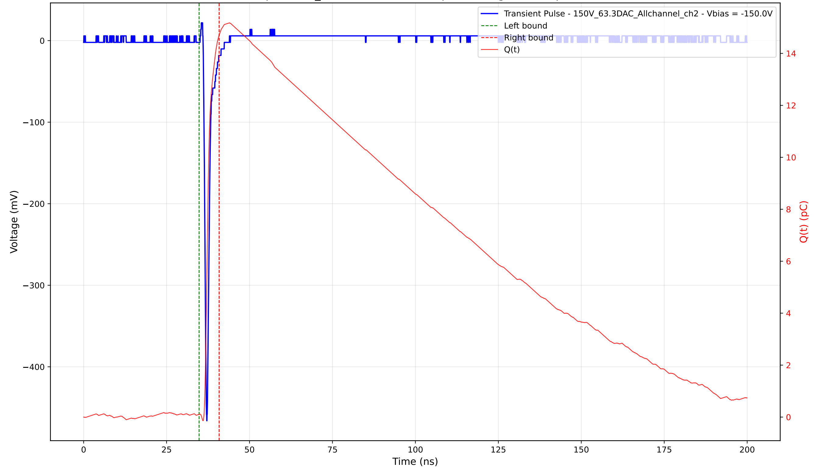
Transient Pulse - Sample: 1cm_42 - Position: 2840.0 \mu\text{m} - Charge: 14.60 pC - Rise Time: 0.75 ns
