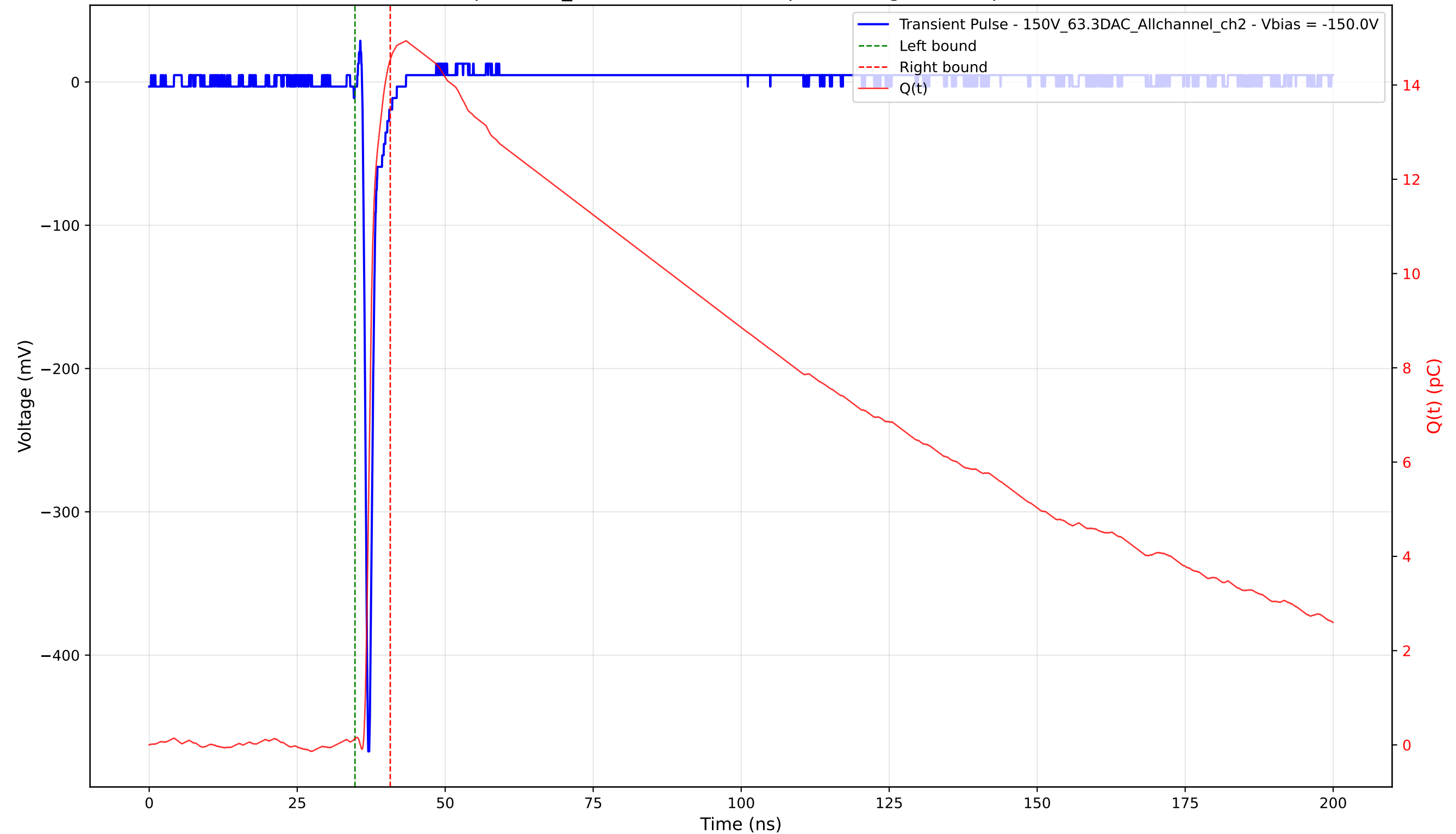
Transient Pulse - Sample: 1cm_42 - Position: 2985.0 \mu\text{m} - Charge: 14.40 pC - Rise Time: 0.71 ns
