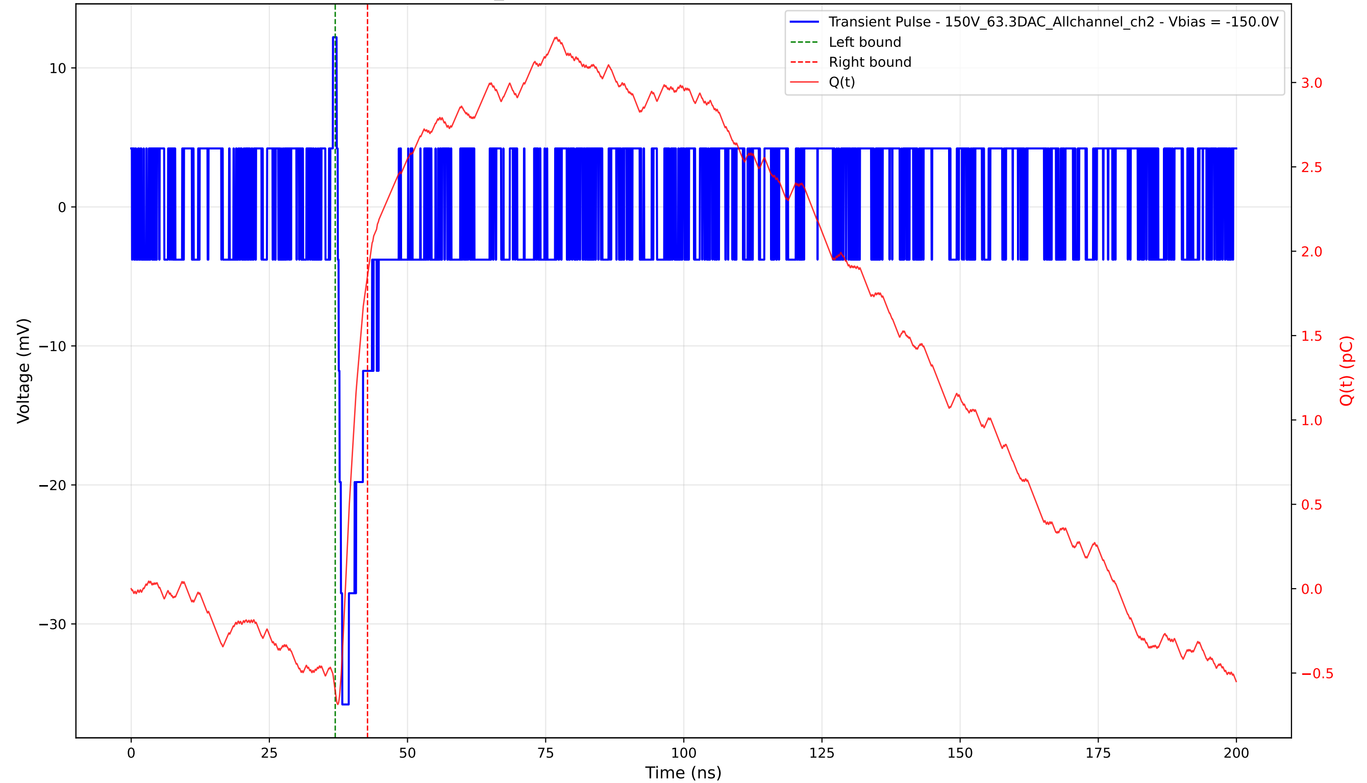
Transient Pulse - Sample: 1cm_42 - Position: 4680.0 \mu\text{m} - Charge: 2.46 pC - Rise Time: 0.00 ns (N/A)
