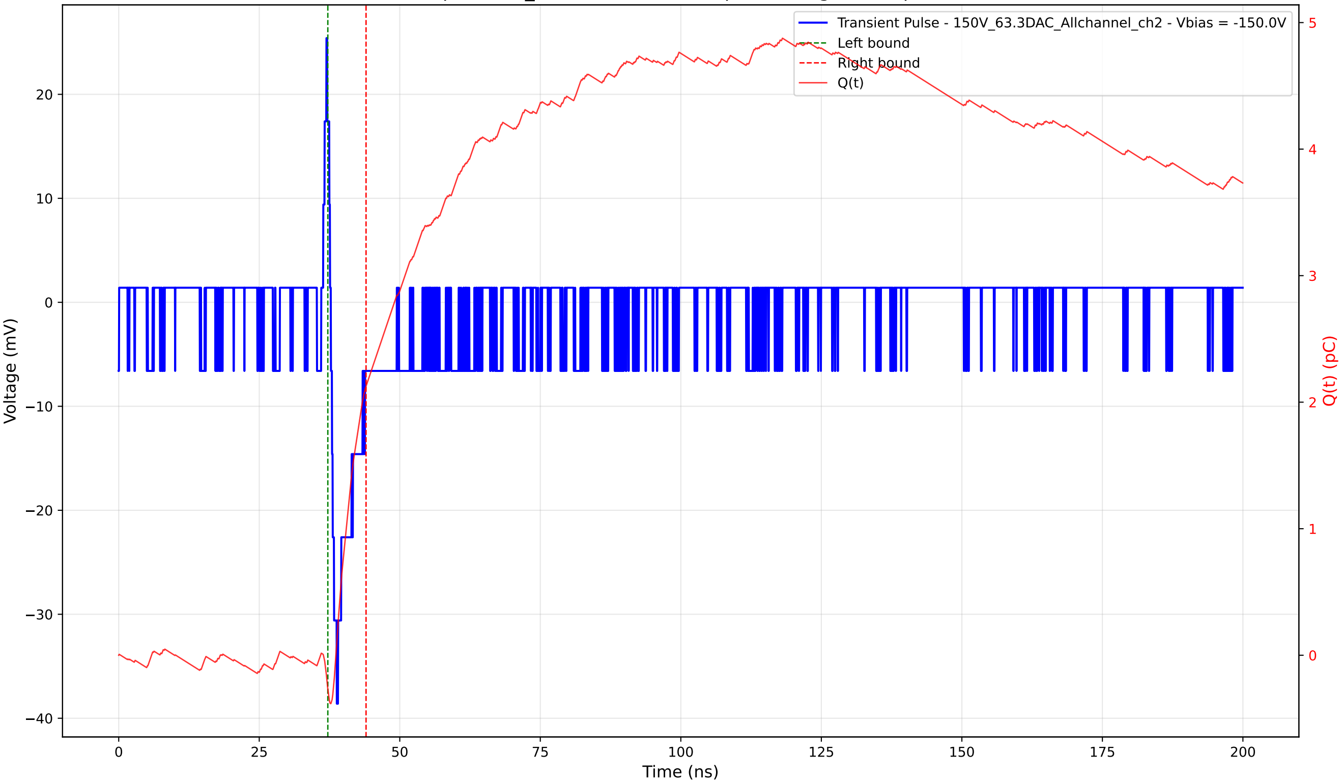
Transient Pulse - Sample: 1cm_42 - Position: 505.0 \mu\text{m} - Charge: 2.39 pC - Rise Time: 1.06 ns
