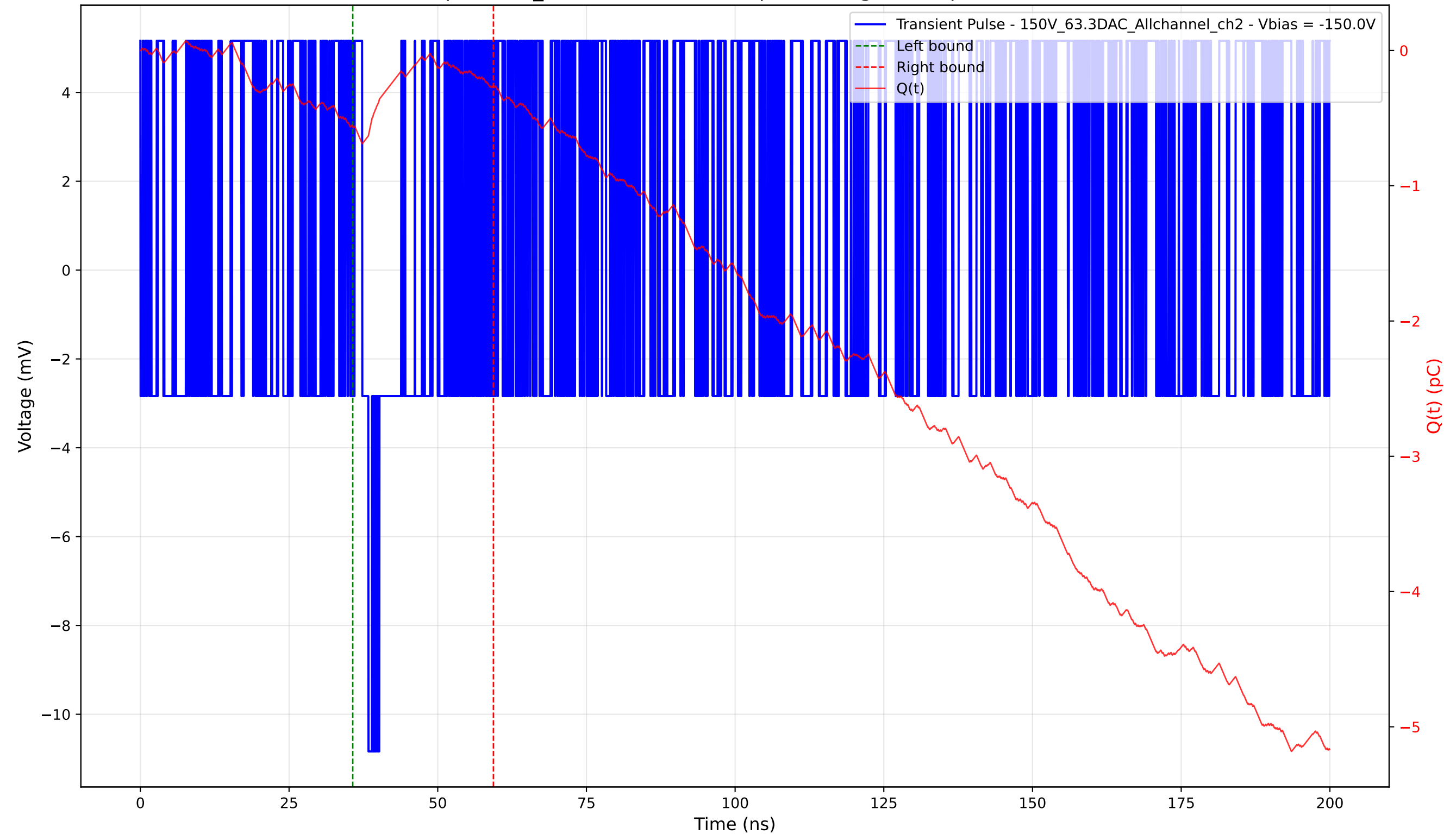
Transient Pulse - Sample: 1cm_42 - Position: 5110.0 \mu\text{m} - Charge: 0.31 pC - Rise Time: 0.00 ns (N/A)
