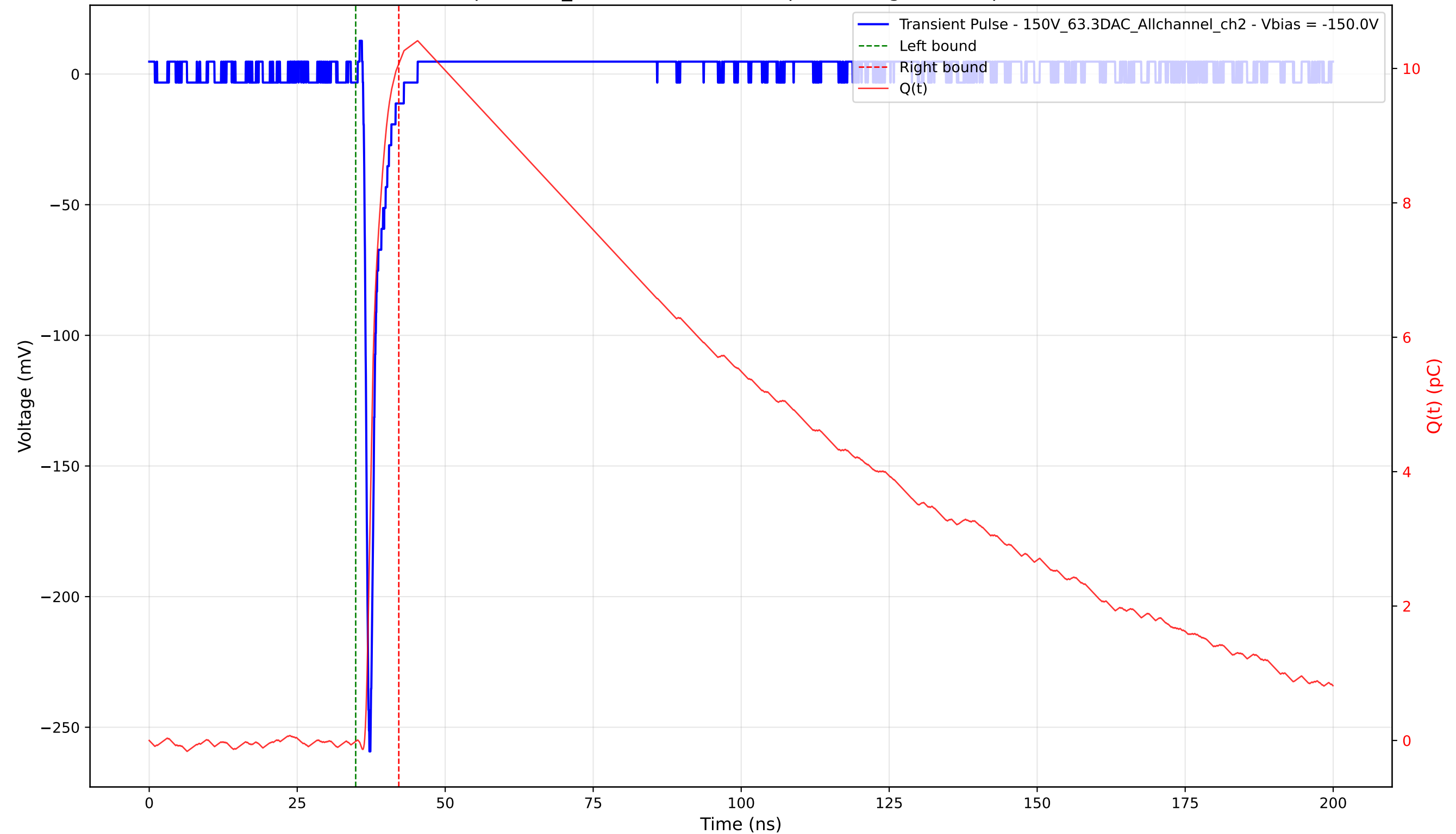
Transient Pulse - Sample: 1cm_42 - Position: 3465.0 \mu\text{m} - Charge: 10.08 pC - Rise Time: 0.72 ns
