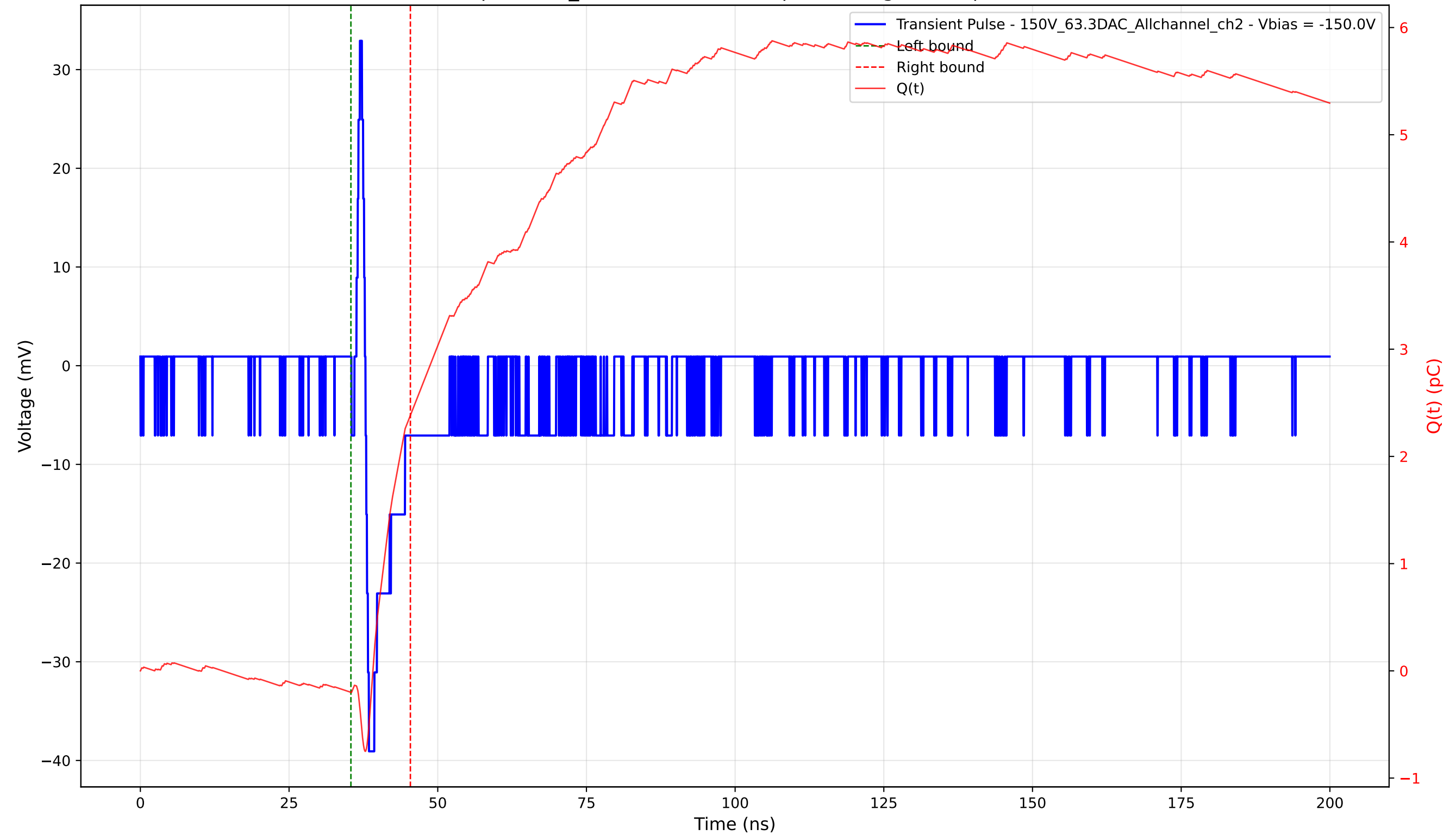
Transient Pulse - Sample: 1cm_42 - Position: 660.0 \mu\text{m} - Charge: 2.58 pC - Rise Time: 0.58 ns
