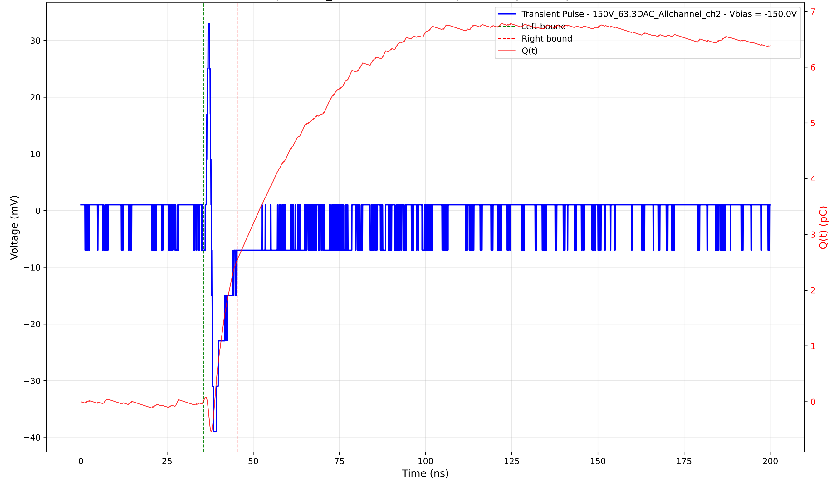
Transient Pulse - Sample: 1cm_42 - Position: 1070.0 \mu\text{m} - Charge: 2.53 pC - Rise Time: 0.58 ns
