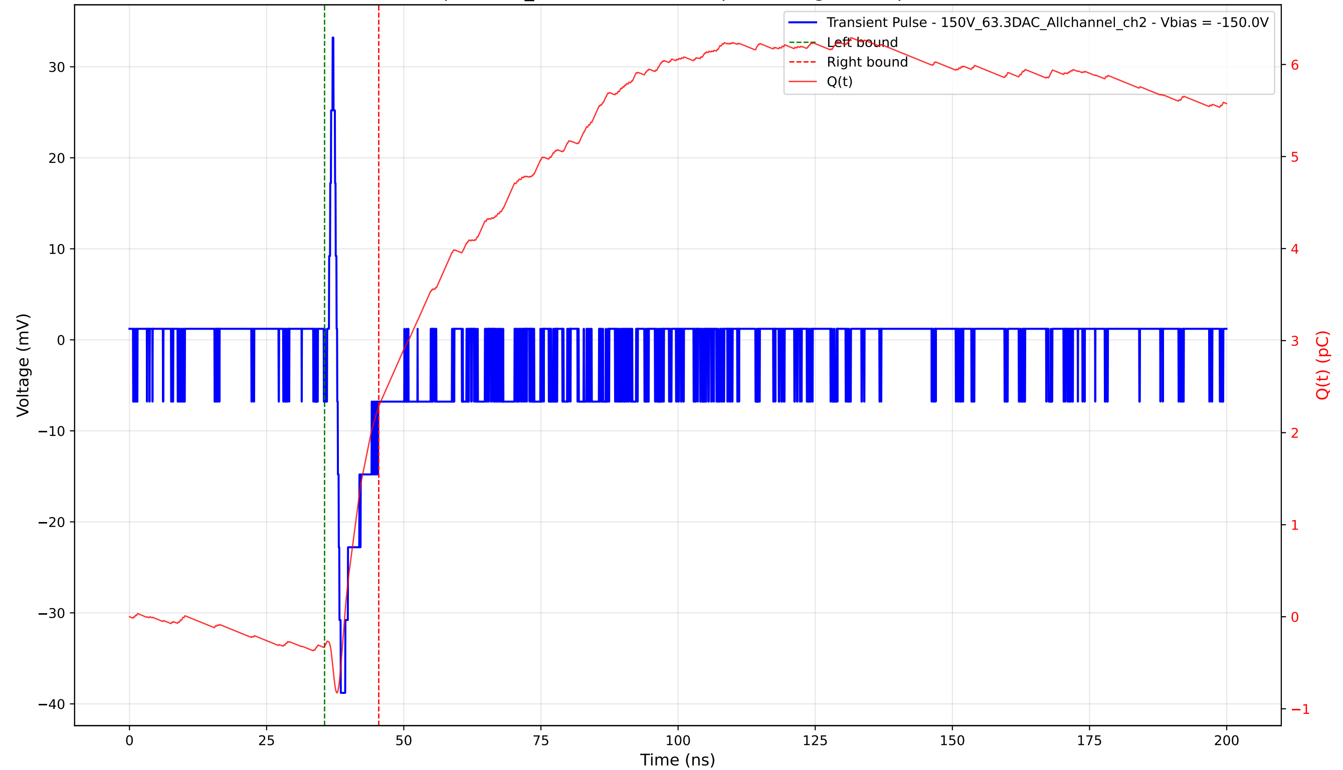
Transient Pulse - Sample: 1cm_42 - Position: 625.0 \mu\text{m} - Charge: 2.60 pC - Rise Time: 0.66 ns
