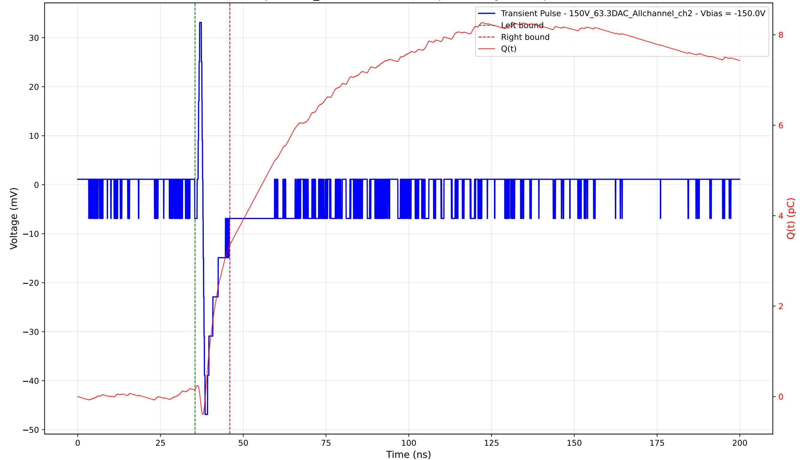
Transient Pulse - Sample: 1cm_42 - Position: 1195.0 \mu\text{m} - Charge: 3.20 pC - Rise Time: 0.66 ns
