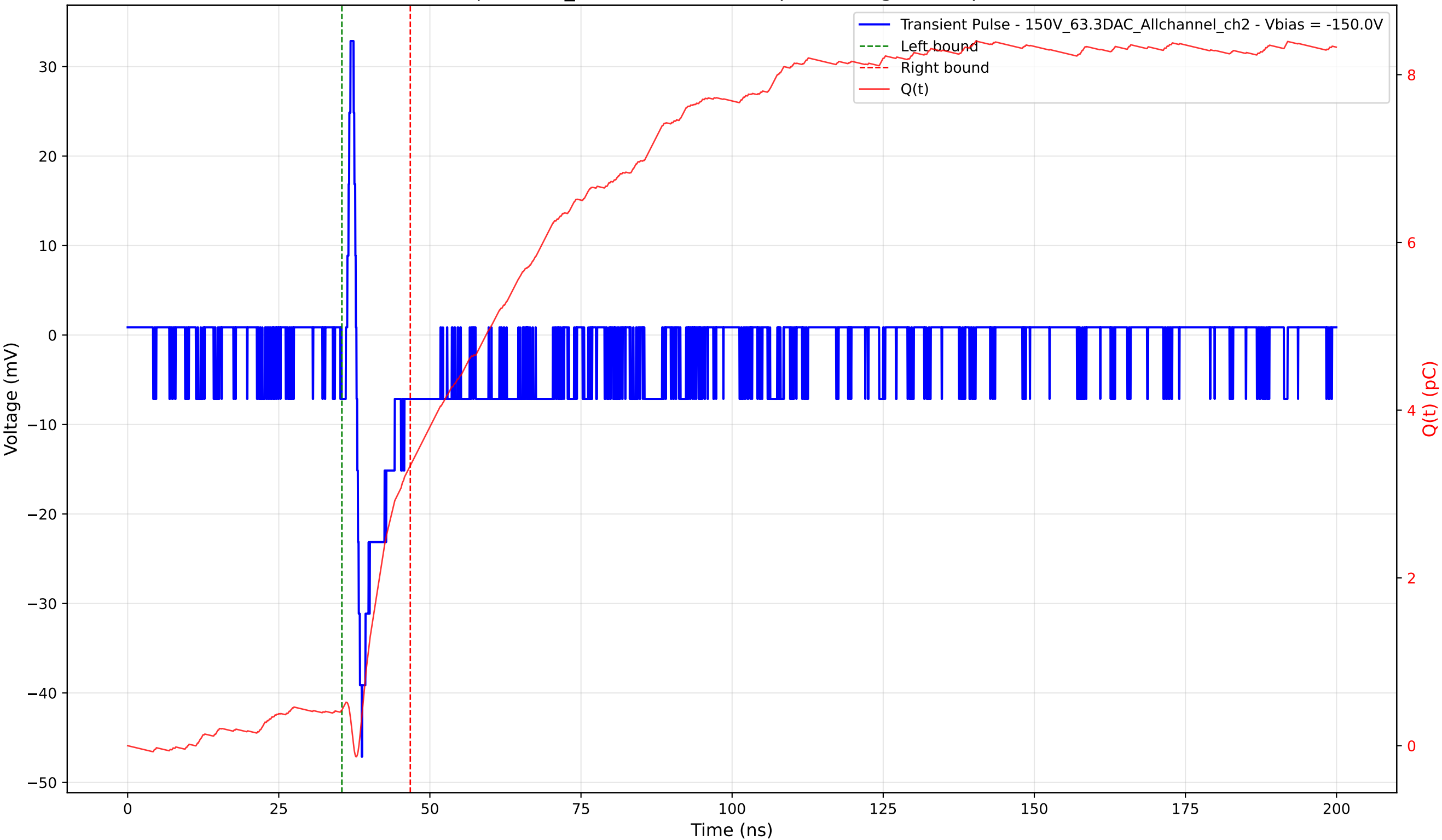
Transient Pulse - Sample: 1cm_42 - Position: 840.0 \mu\text{m} - Charge: 2.92 pC - Rise Time: 0.90 ns
