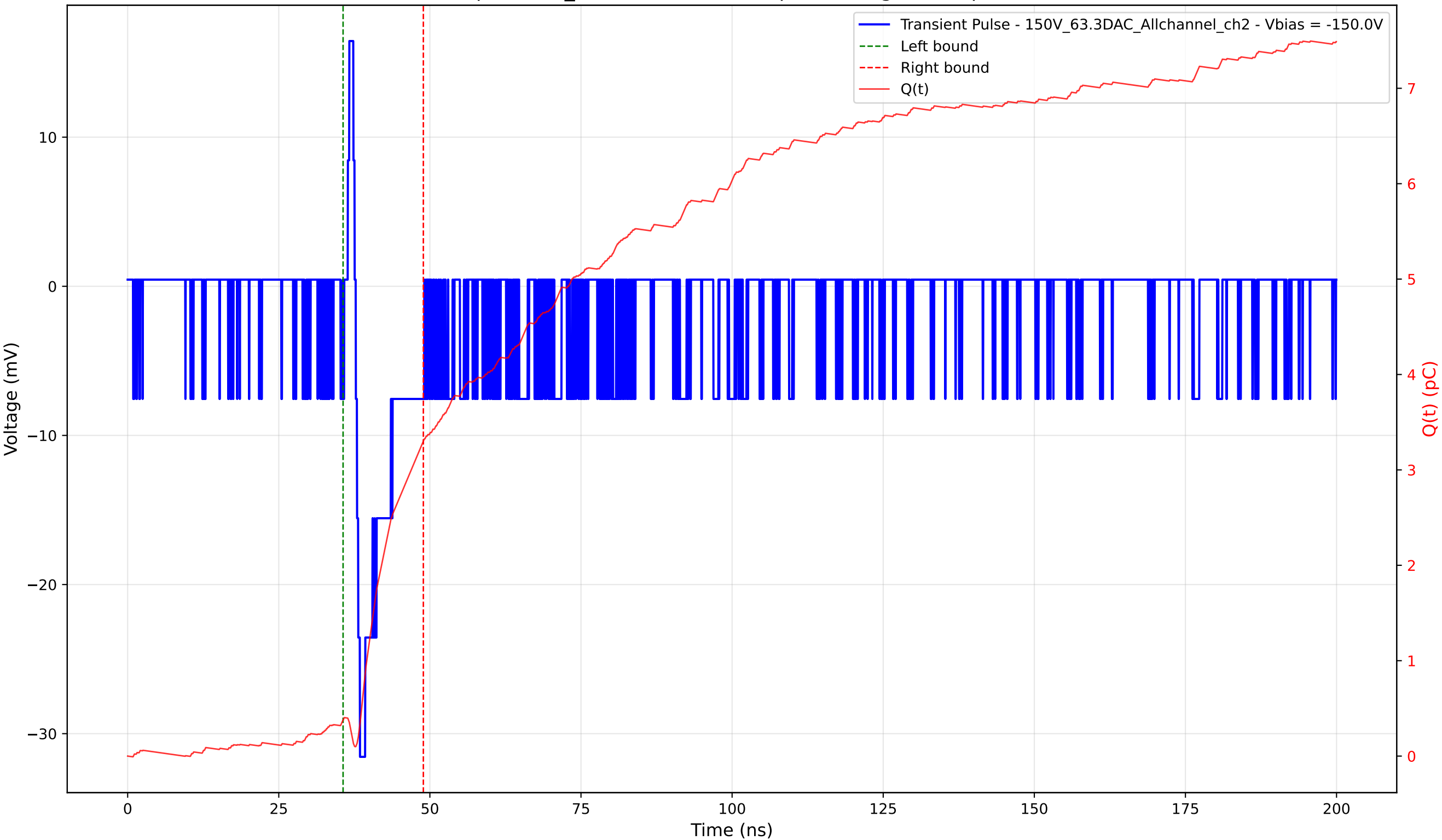
Transient Pulse - Sample: 1cm_42 - Position: 445.0 \mu\text{m} - Charge: 2.93 pC - Rise Time: 0.70 ns
