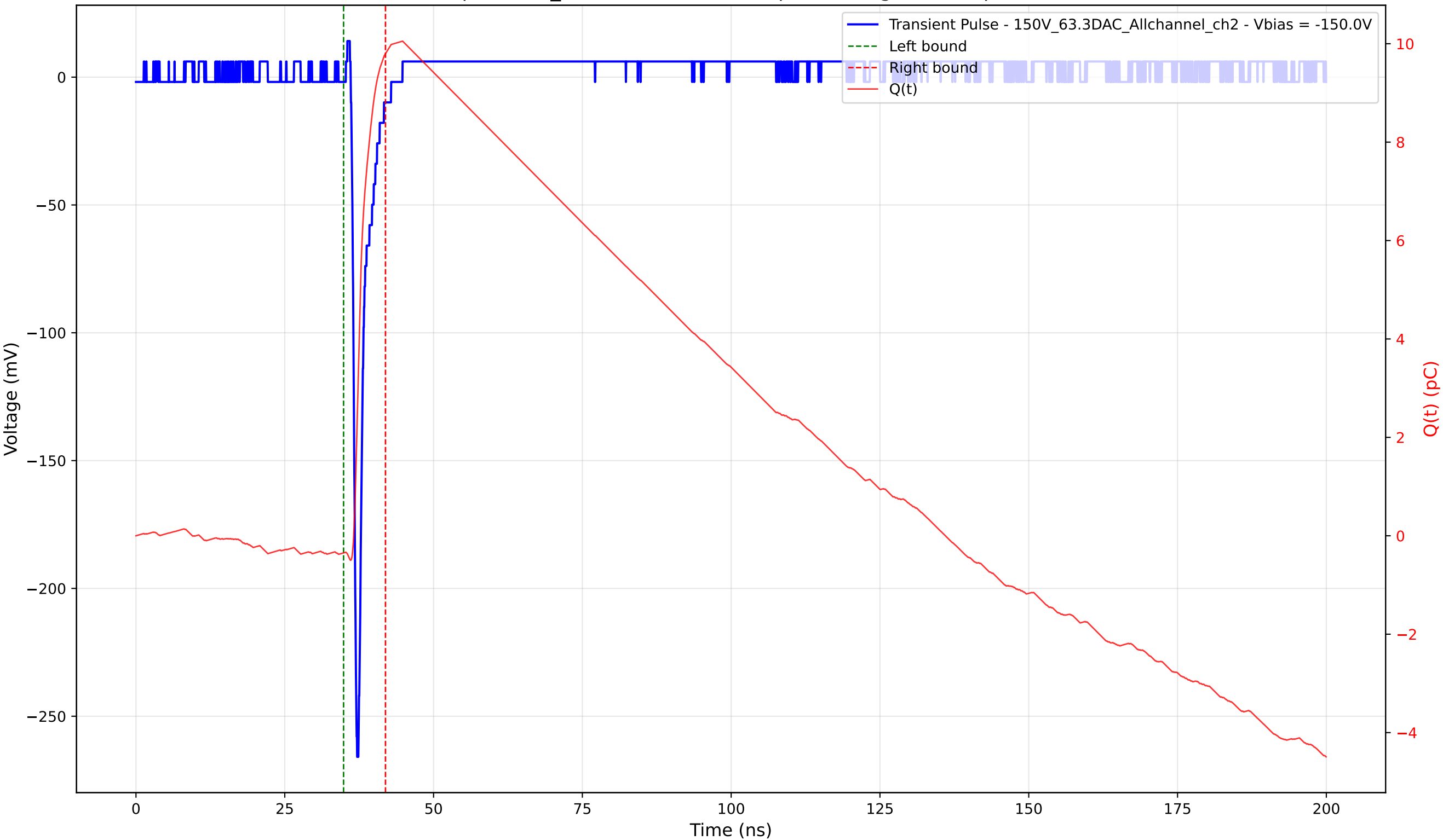
Transient Pulse - Sample: 1cm_42 - Position: 3455.0 \mu\text{m} - Charge: 10.14 pC - Rise Time: 0.74 ns
