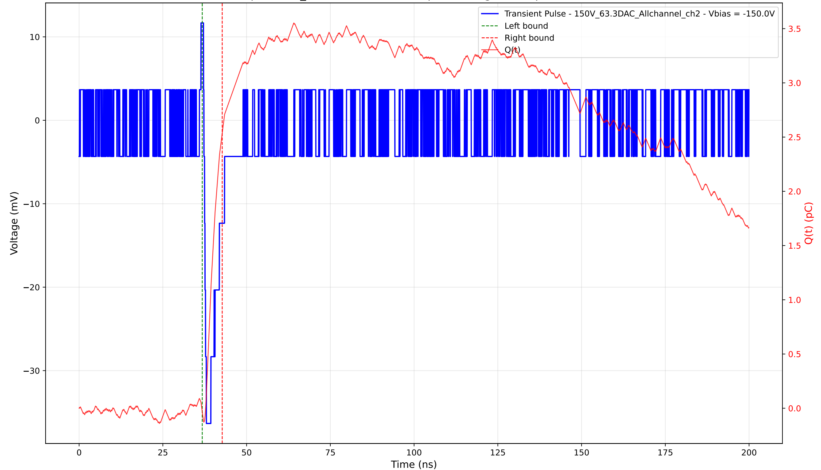
Transient Pulse - Sample: 1cm_42 - Position: 4535.0 \mu\text{m} - Charge: 2.57 pC - Rise Time: 0.00 ns (N/A)
