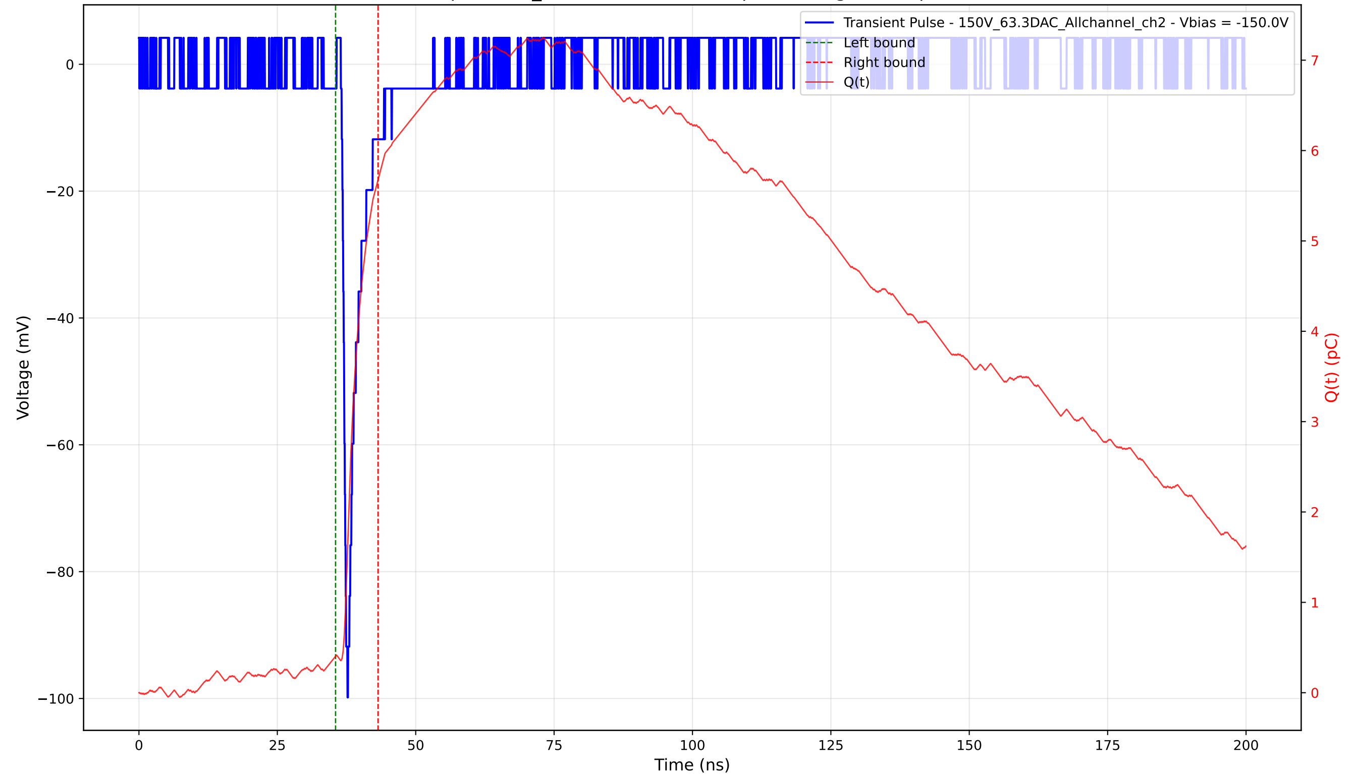
Transient Pulse - Sample: 1cm_42 - Position: 2120.0 \mu\text{m} - Charge: 5.28 pC - Rise Time: 0.81 ns
