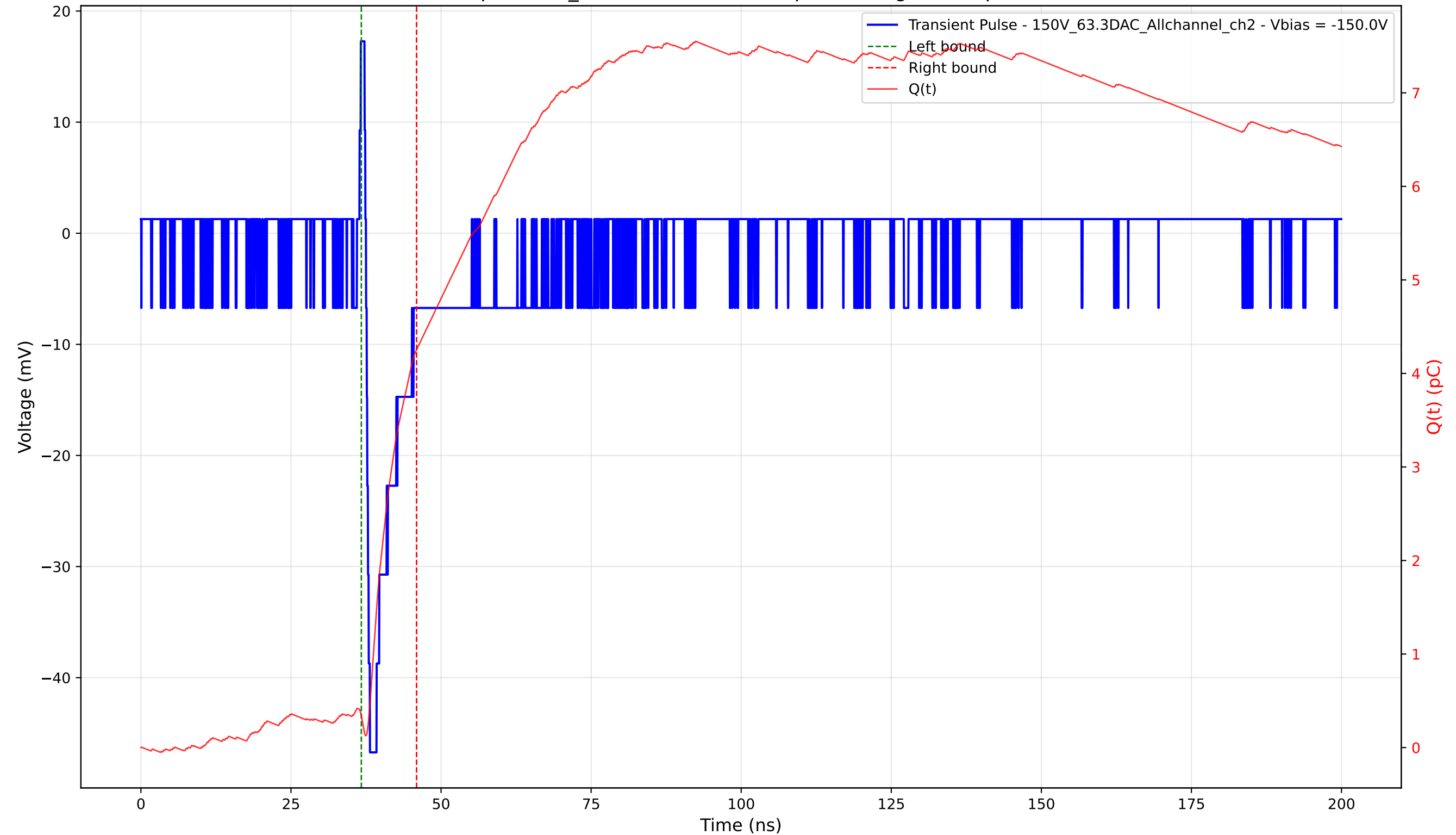
Transient Pulse - Sample: 1cm_42 - Position: 1580.0 \mu\text{m} - Charge: 3.92 pC - Rise Time: 0.66 ns
