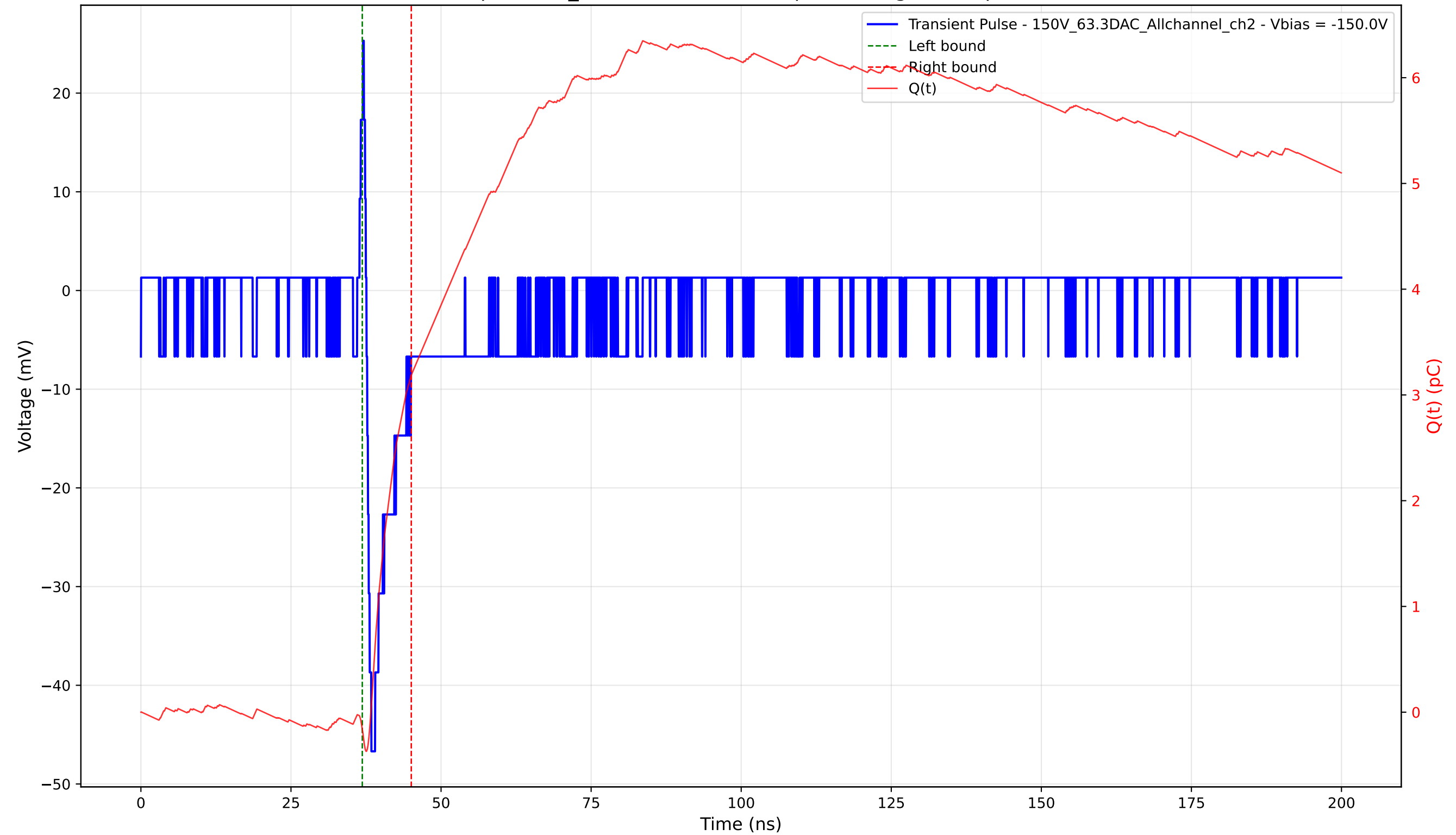
Transient Pulse - Sample: 1cm_42 - Position: 1510.0 \mu\text{m} - Charge: 3.35 pC - Rise Time: 0.82 ns
