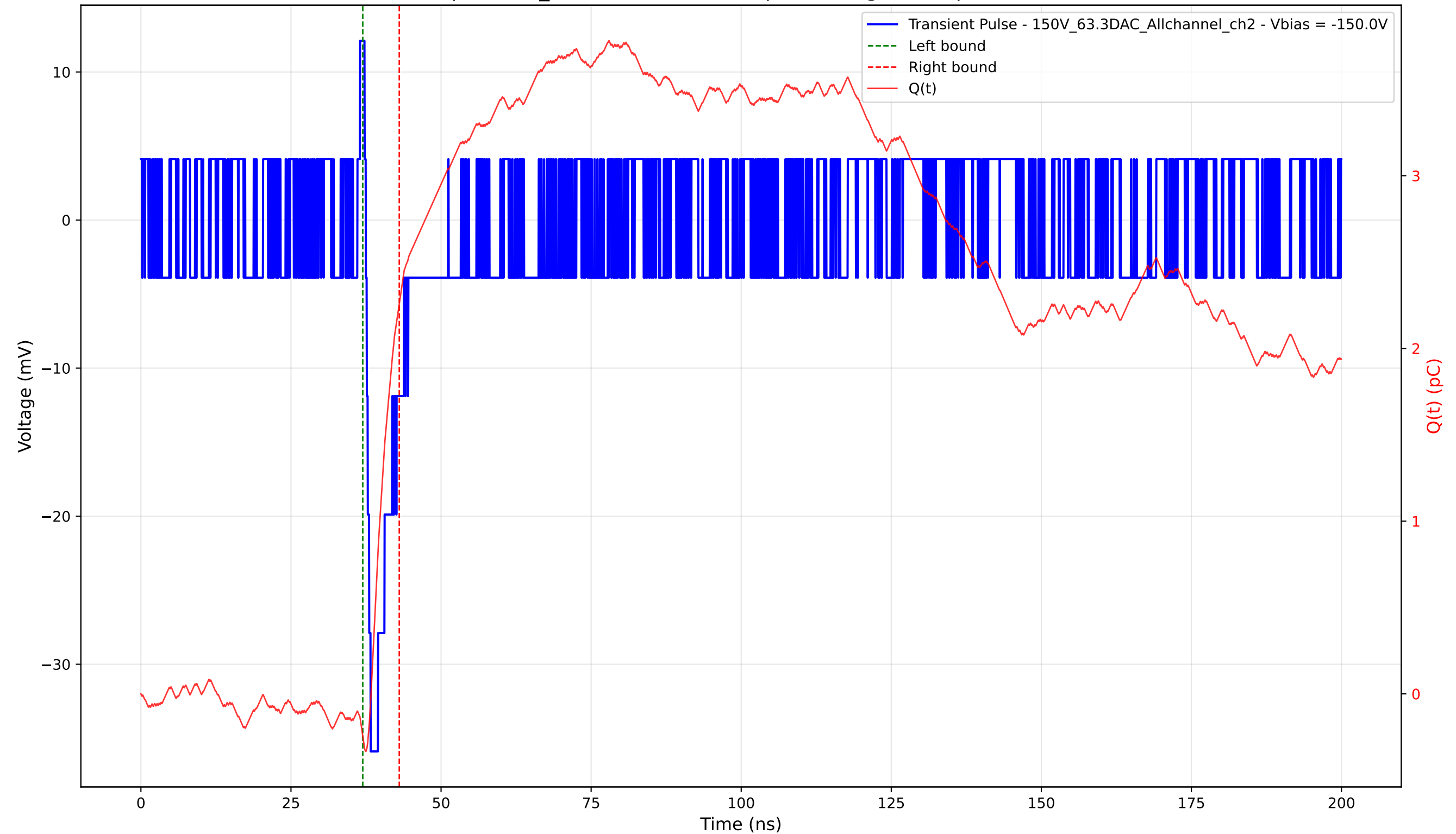
Transient Pulse - Sample: 1cm_42 - Position: 4805.0 \mu\text{m} - Charge: 2.51 pC - Rise Time: 0.00 ns (N/A)
