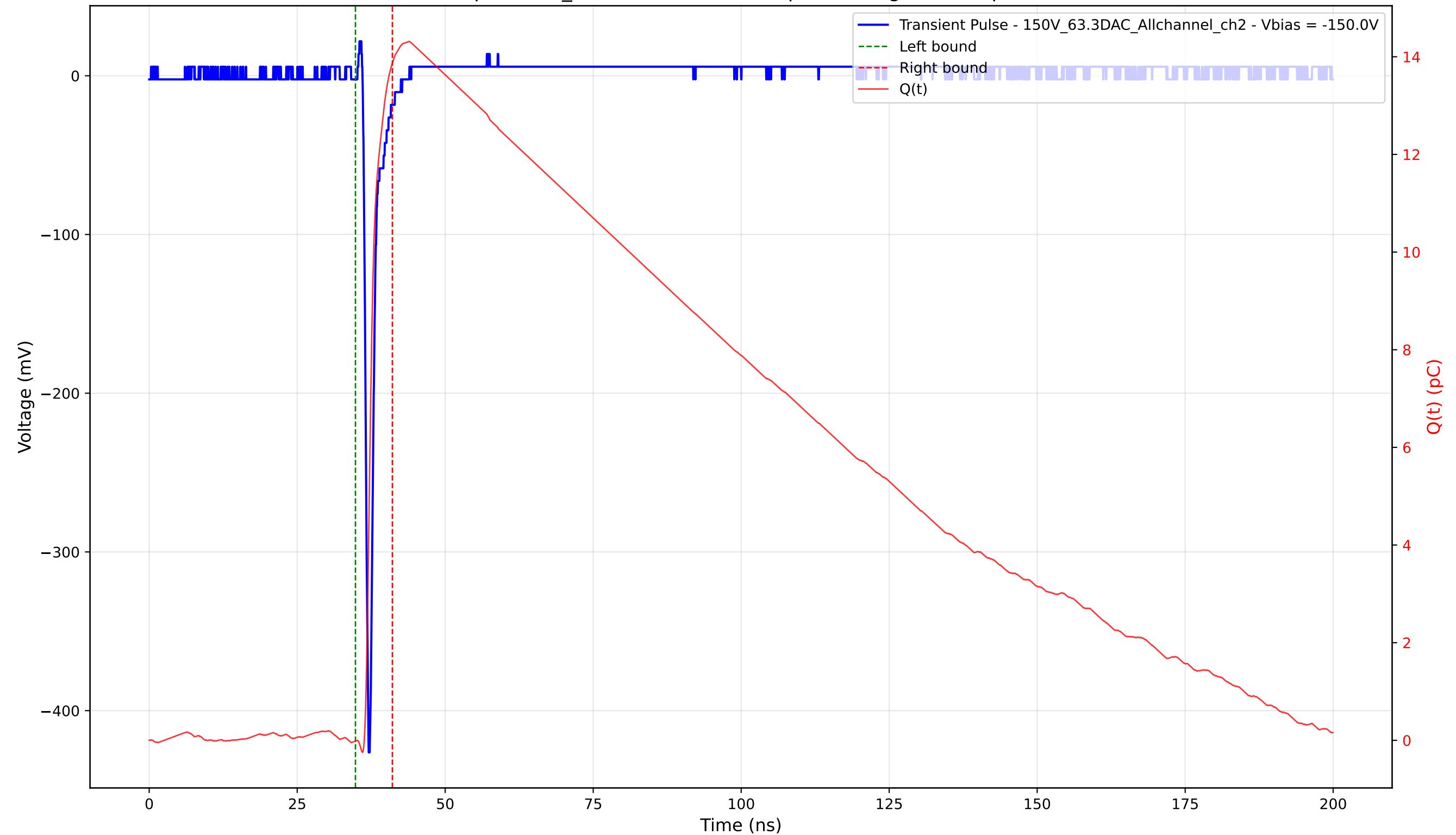
Transient Pulse - Sample: 1cm_42 - Position: 2740.0 \mu\text{m} - Charge: 13.89 pC - Rise Time: 0.71 ns
