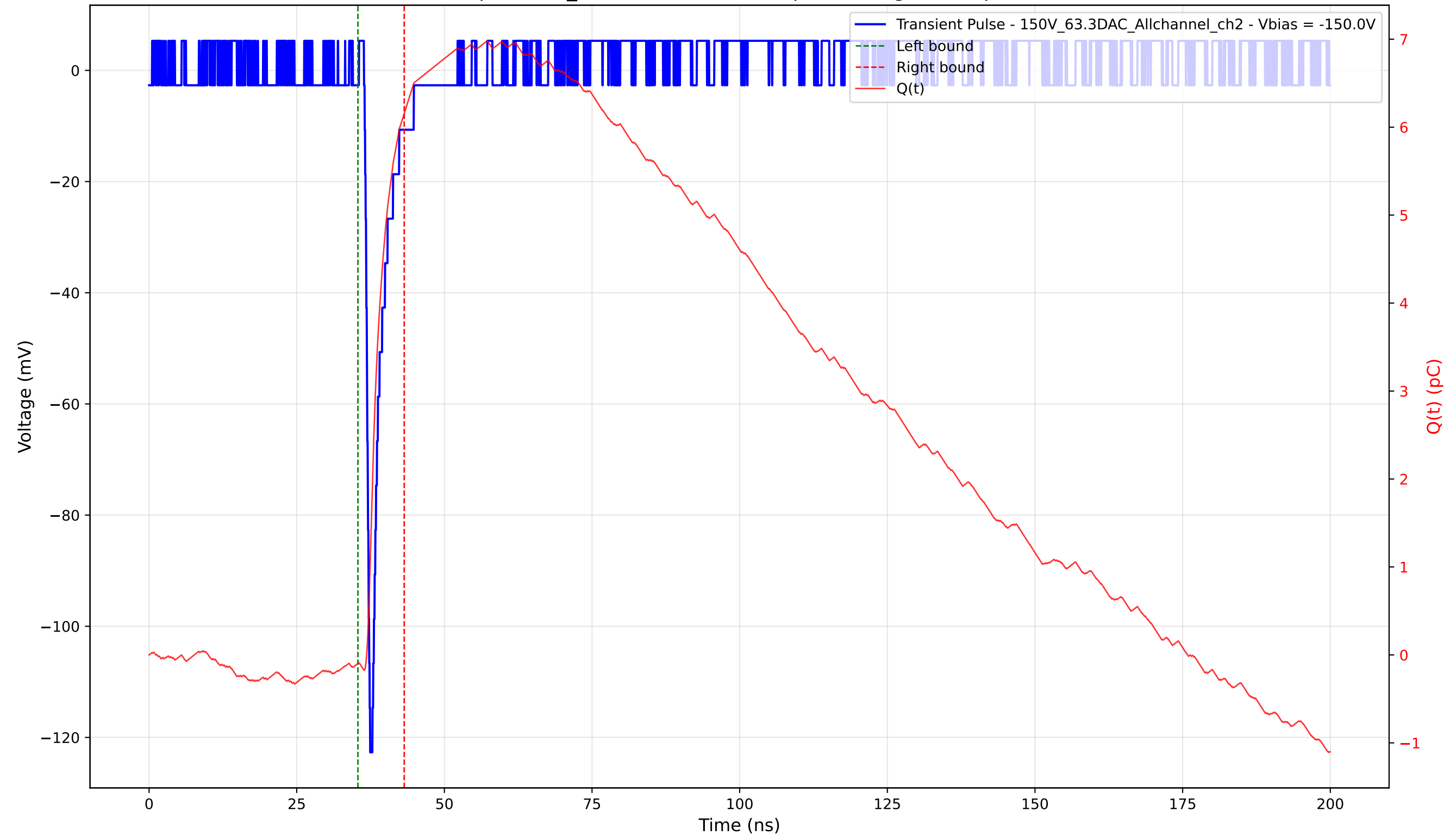
Transient Pulse - Sample: 1cm_42 - Position: 2215.0 \mu\text{m} - Charge: 6.25 pC - Rise Time: 0.79 ns
