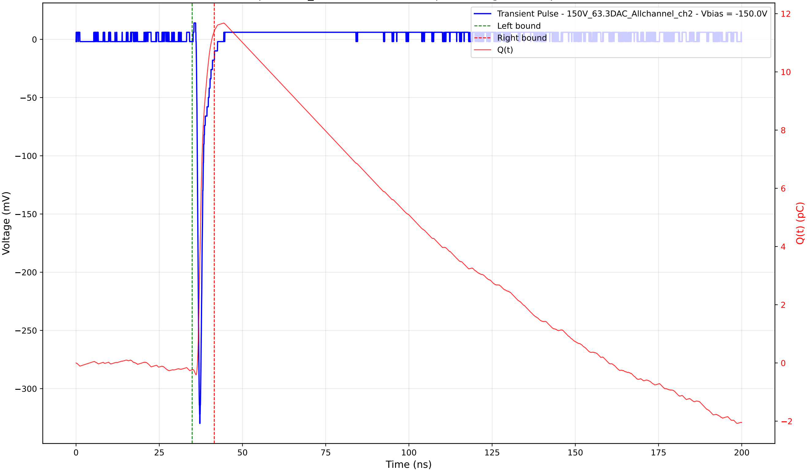
Transient Pulse - Sample: 1cm_42 - Position: 3400.0 \mu\text{m} - Charge: 11.64 pC - Rise Time: 0.74 ns
