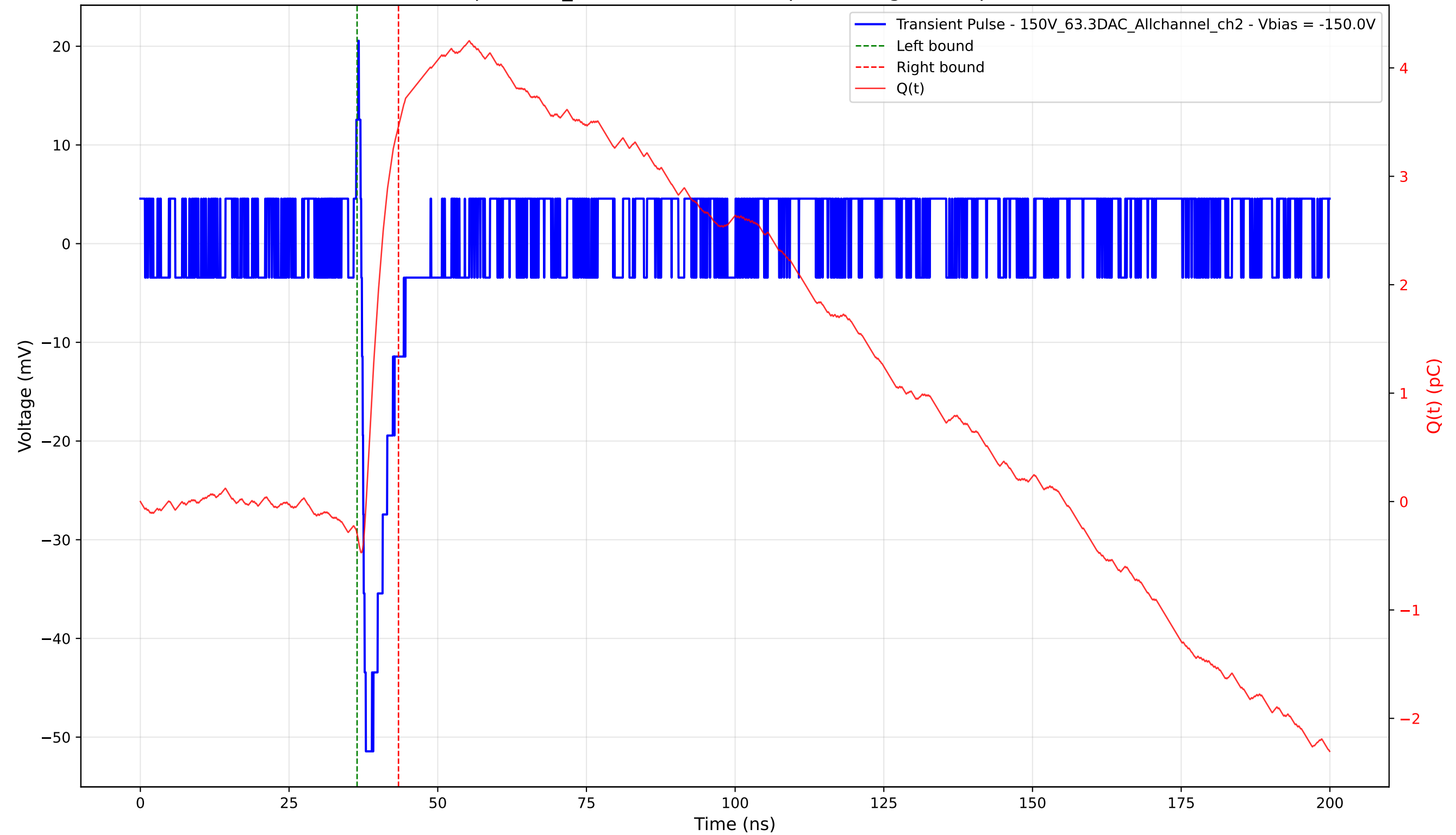
Transient Pulse - Sample: 1cm_42 - Position: 4340.0 \mu\text{m} - Charge: 3.76 pC - Rise Time: 0.67 ns
