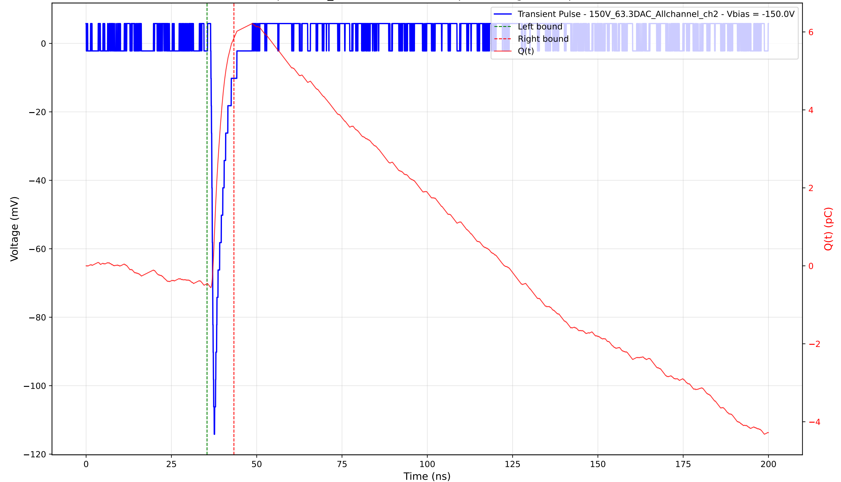
Transient Pulse - Sample: 1cm_42 - Position: 3870.0 \mu\text{m} - Charge: 6.30 pC - Rise Time: 0.75 ns
