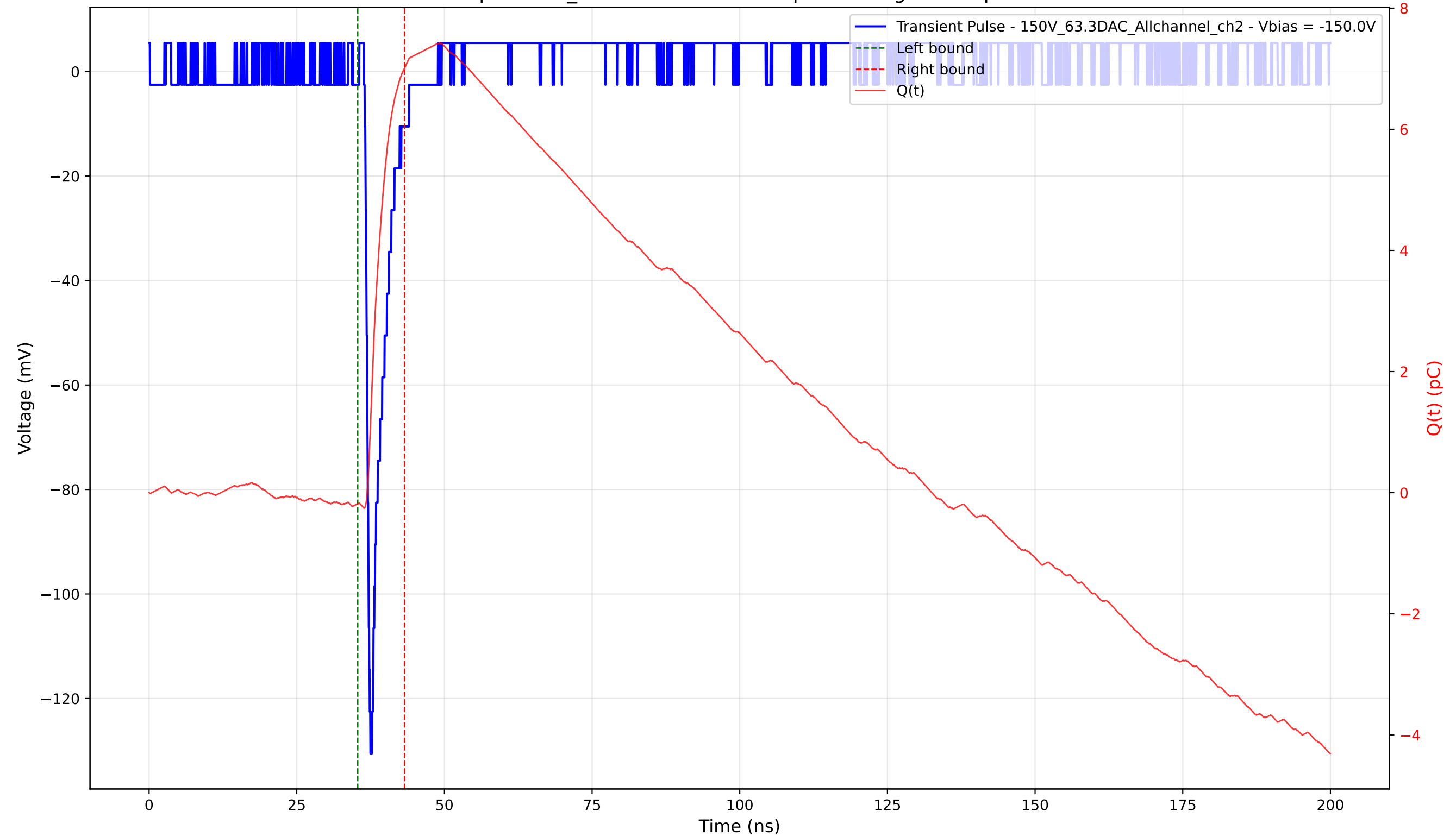
Transient Pulse - Sample: 1cm_42 - Position: 3790.0 \mu\text{m} - Charge: 7.19 pC - Rise Time: 0.75 ns
