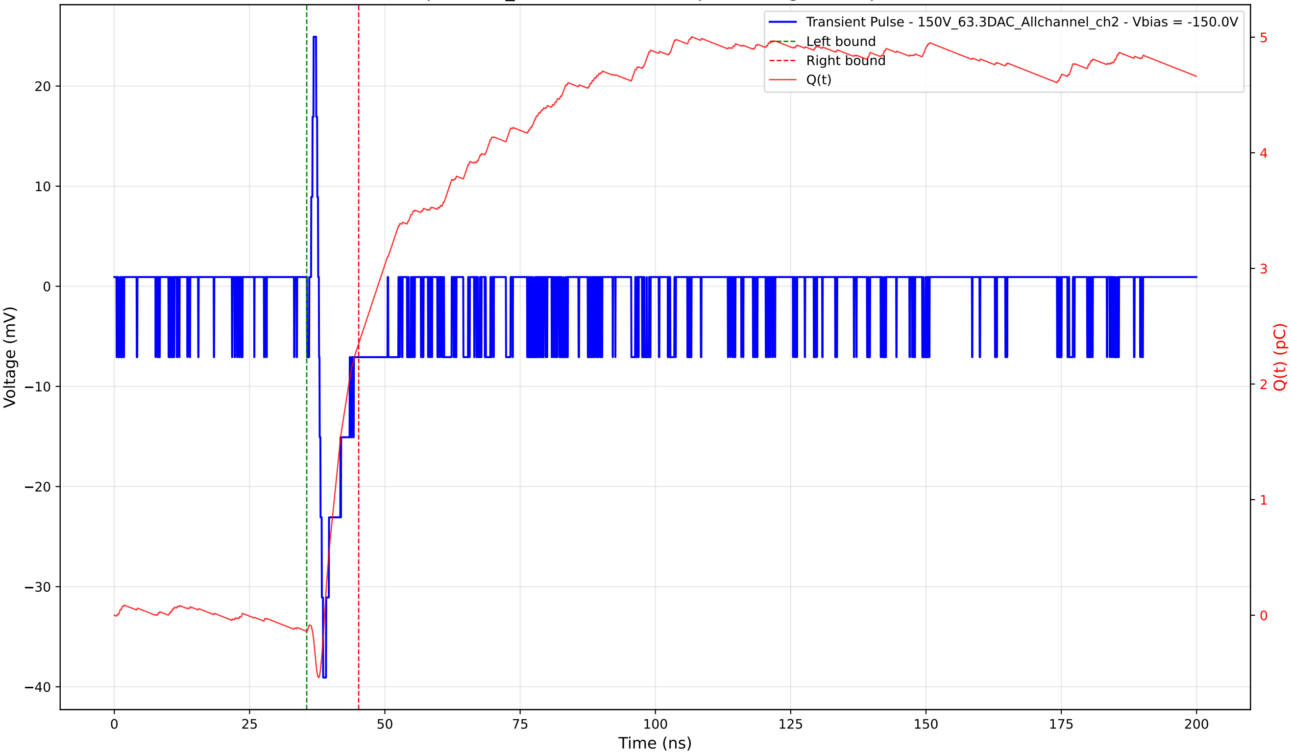
Transient Pulse - Sample: 1cm_42 - Position: 560.0 \mu\text{m} - Charge: 2.49 pC - Rise Time: 0.78 ns
