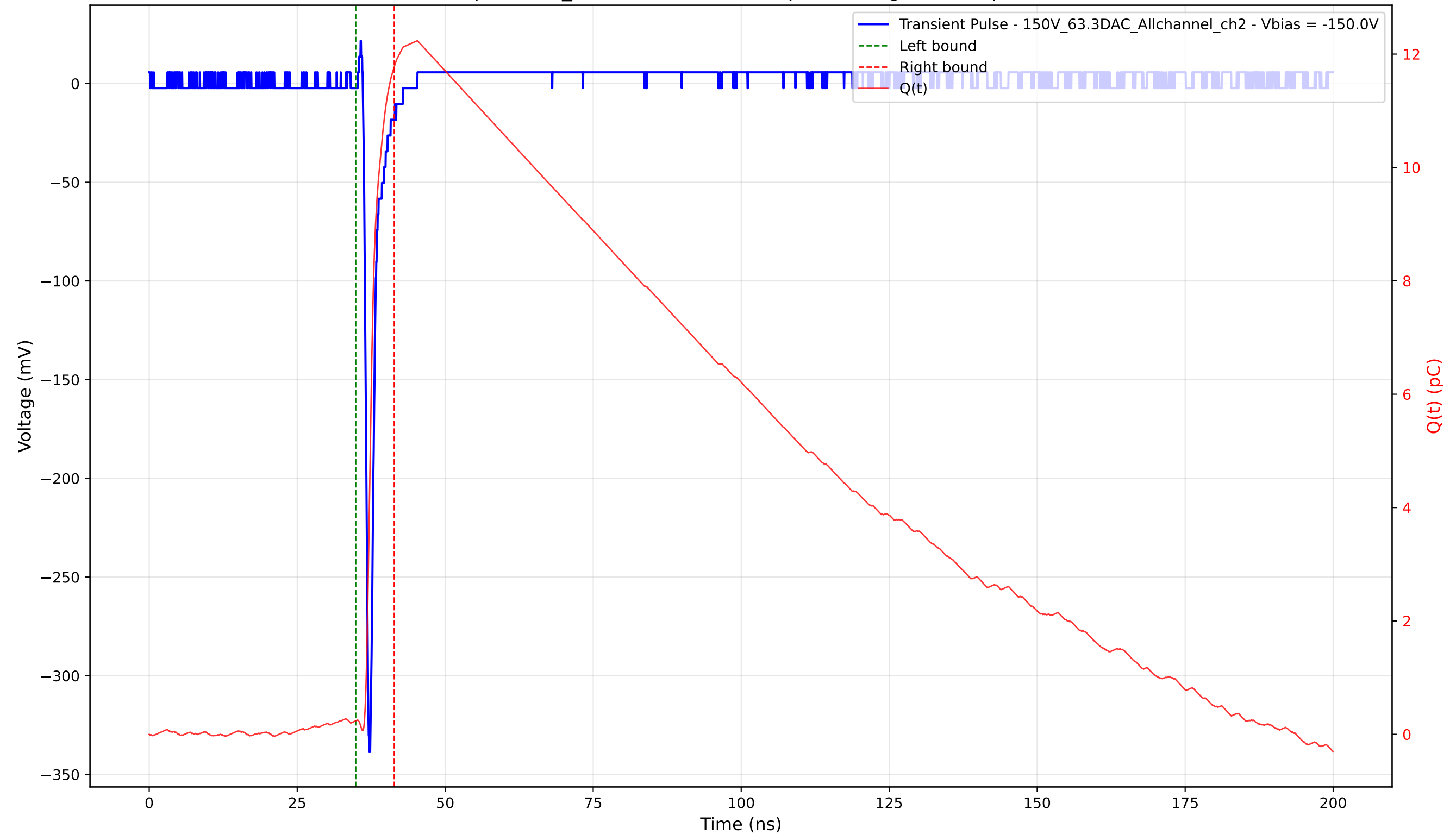
Transient Pulse - Sample: 1cm_42 - Position: 2660.0 \mu\text{m} - Charge: 11.55 pC - Rise Time: 0.71 ns
