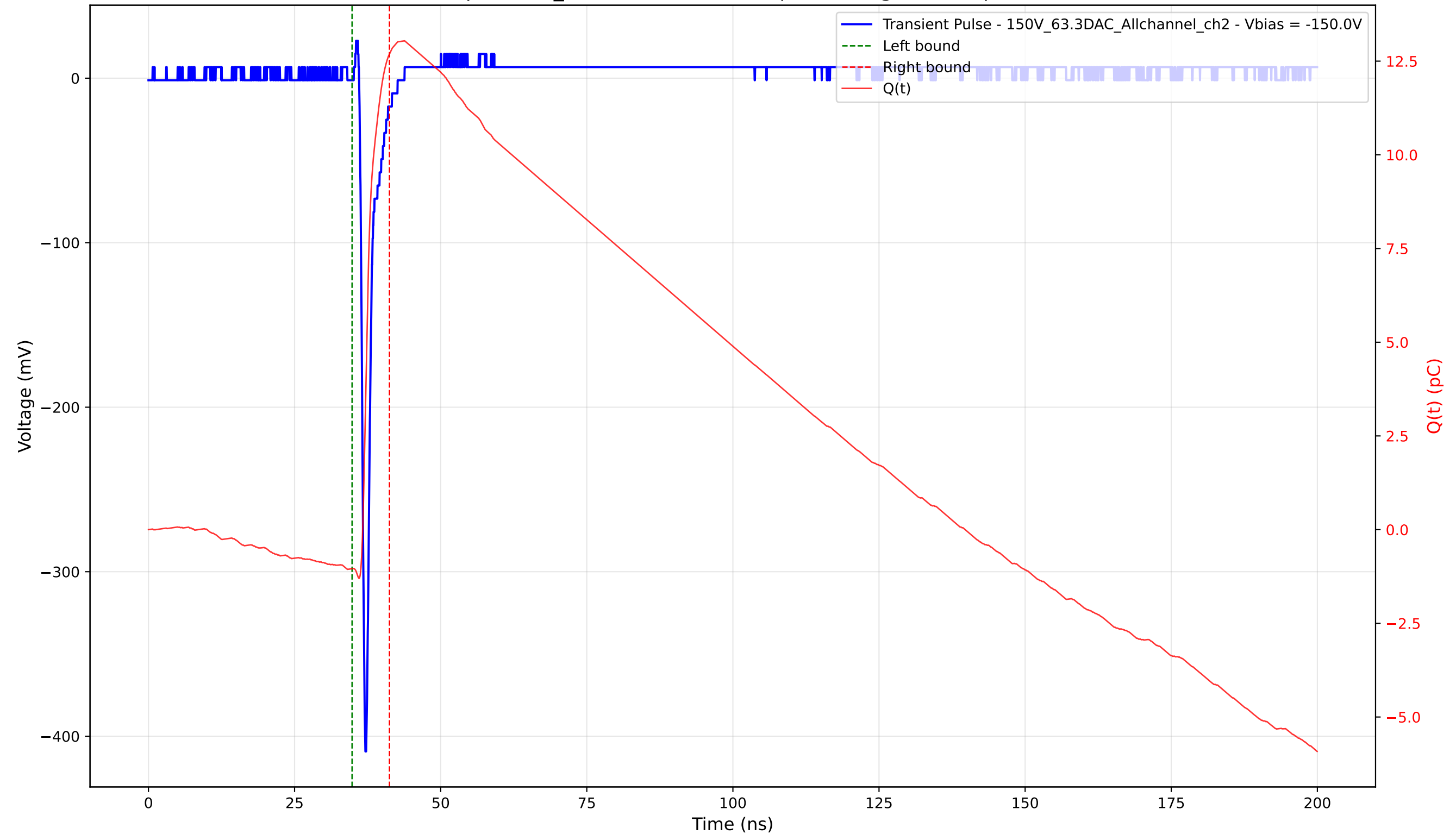
Transient Pulse - Sample: 1cm_42 - Position: 3325.0 \mu\text{m} - Charge: 13.73 pC - Rise Time: 0.72 ns
