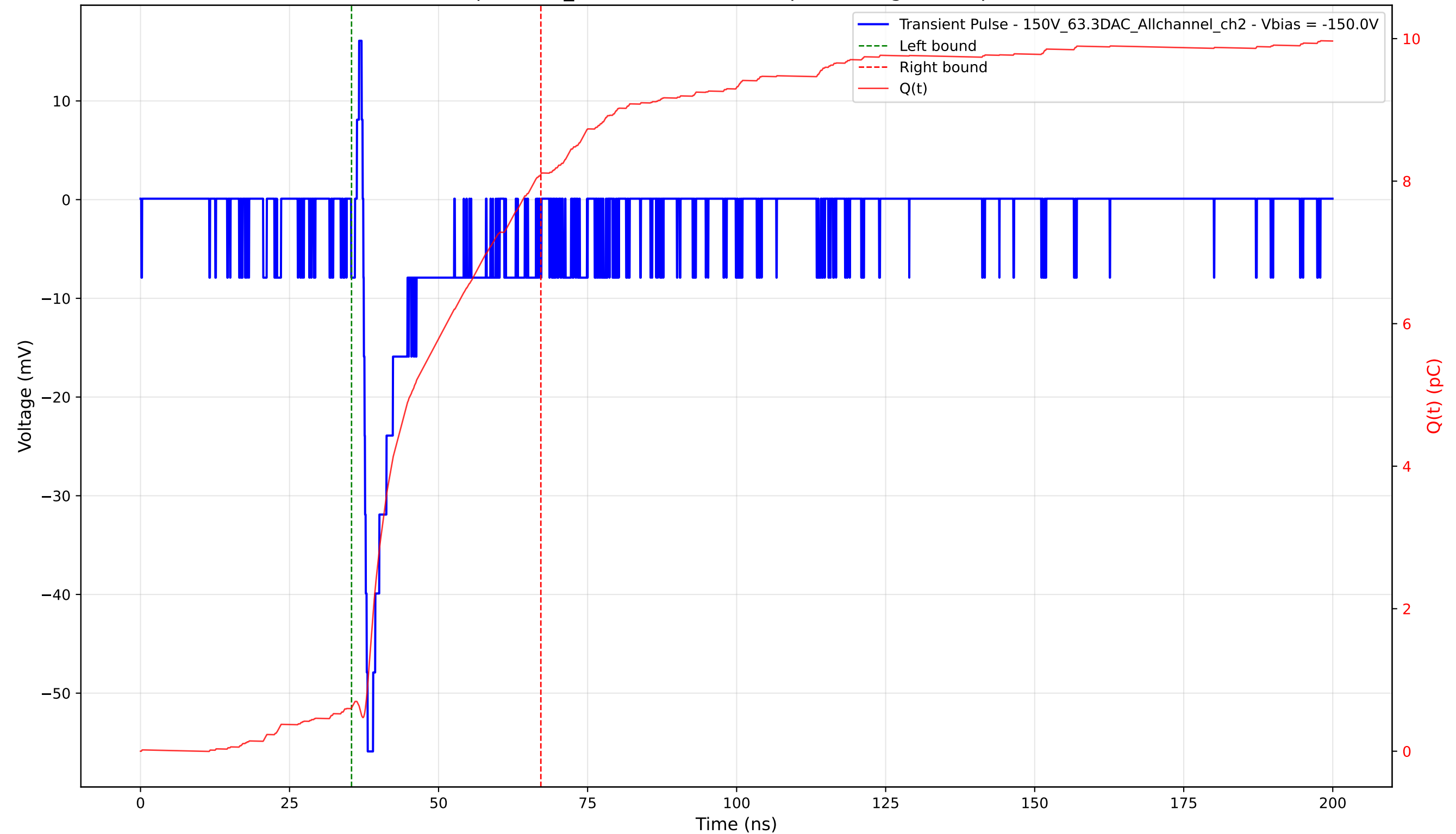
Transient Pulse - Sample: 1cm_42 - Position: 1665.0 \mu\text{m} - Charge: 7.49 pC - Rise Time: 0.73 ns
