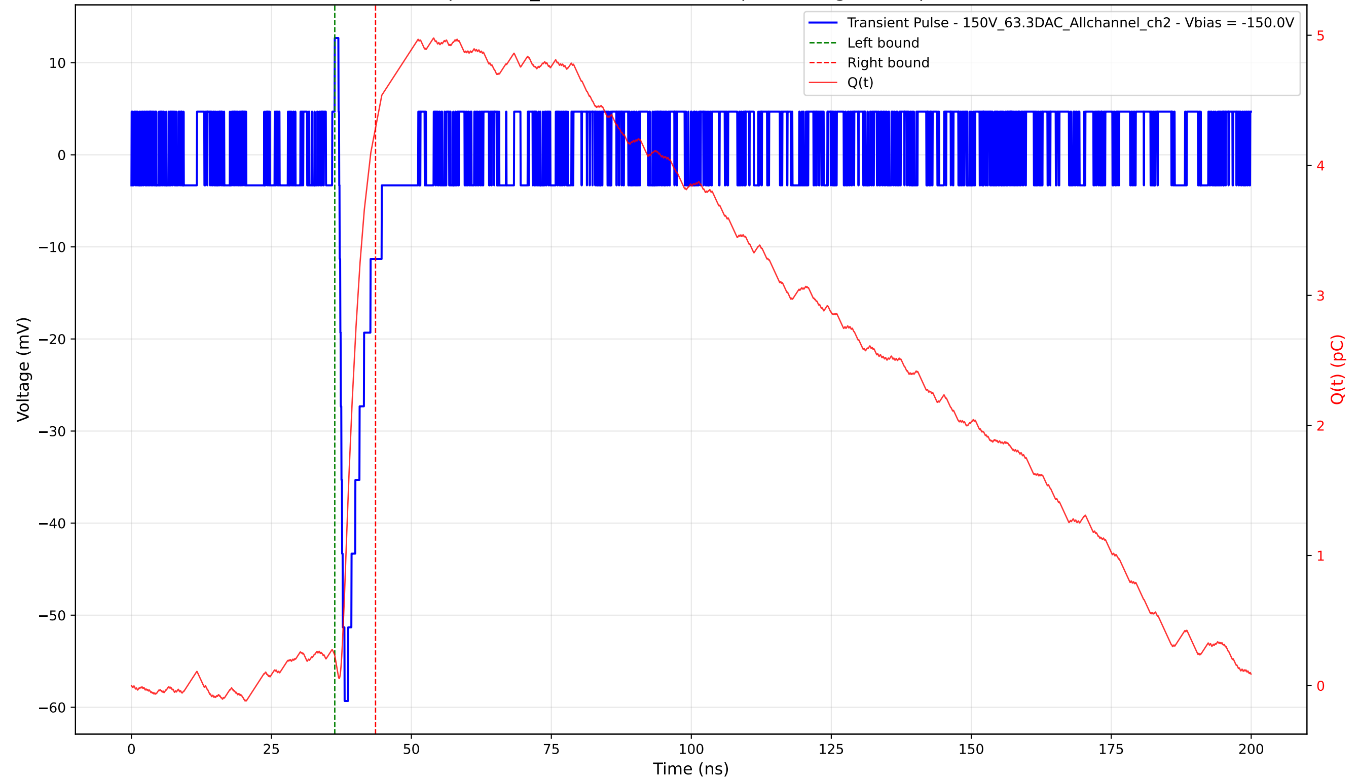
Transient Pulse - Sample: 1cm_42 - Position: 4240.0 \mu\text{m} - Charge: 4.06 pC - Rise Time: 0.91 ns
