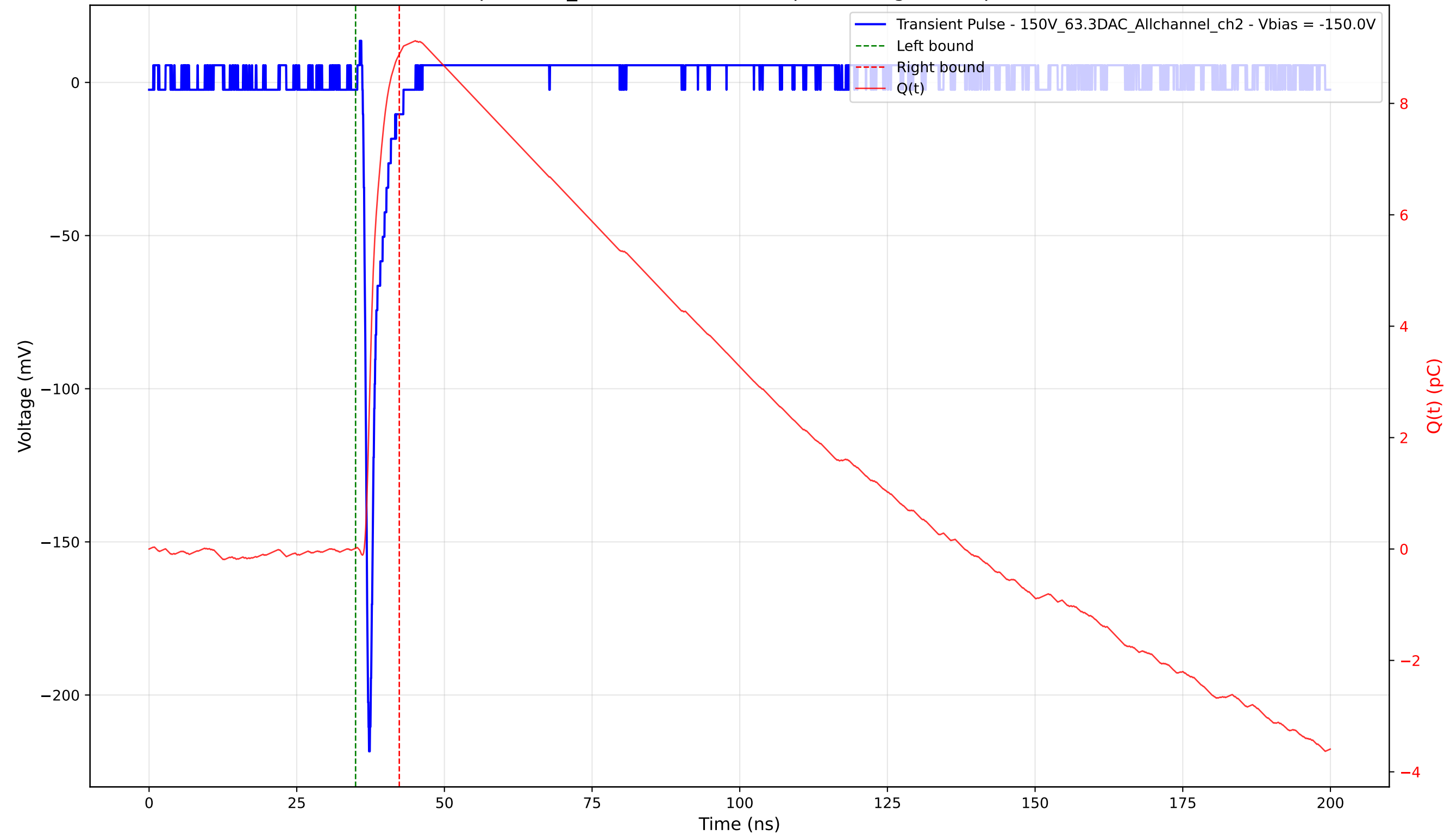
Transient Pulse - Sample: 1cm_42 - Position: 3510.0 \mu\text{m} - Charge: 8.87 pC - Rise Time: 0.78 ns
