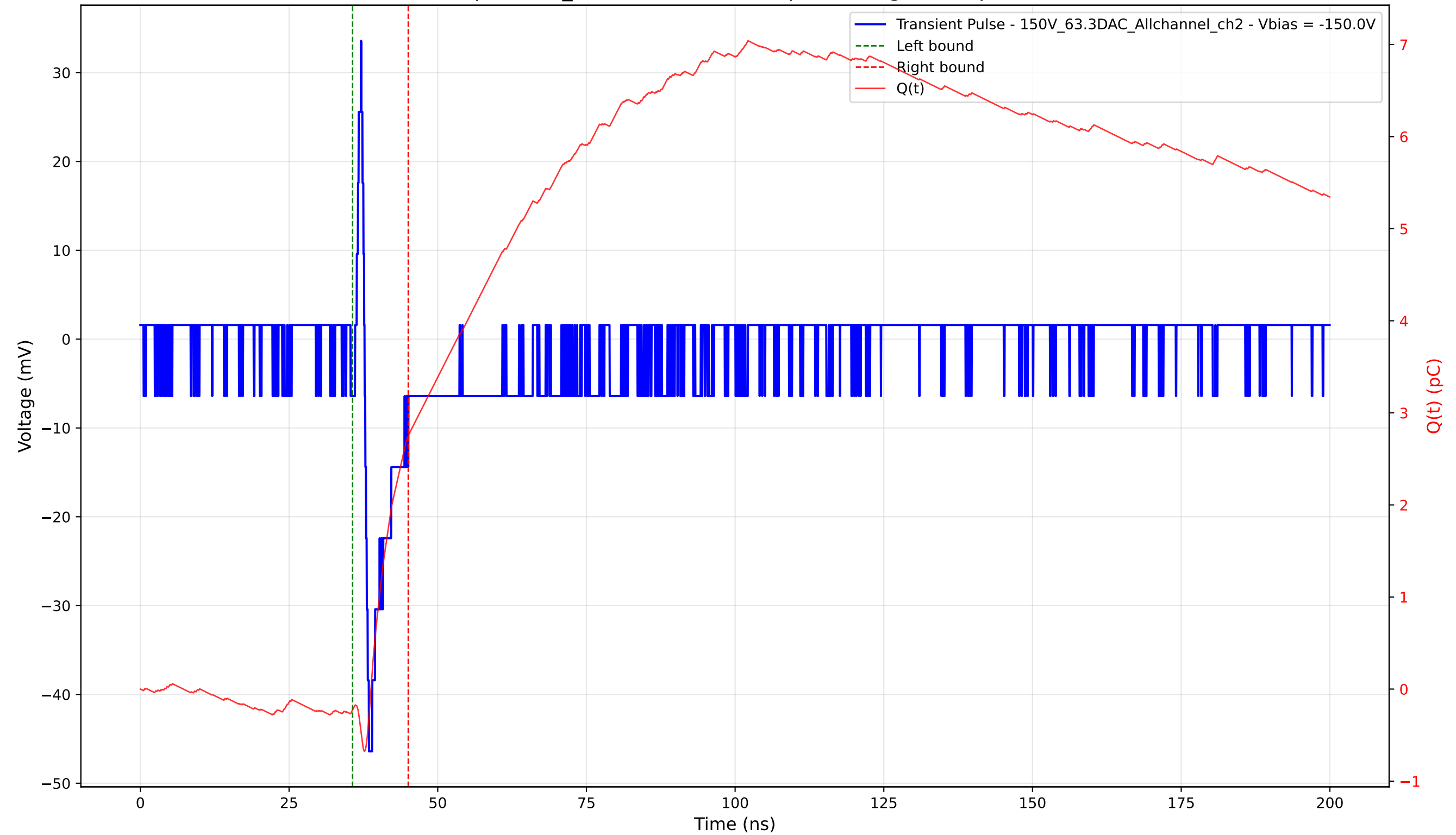
Transient Pulse - Sample: 1cm_42 - Position: 1415.0 \mu\text{m} - Charge: 2.98 pC - Rise Time: 0.73 ns
