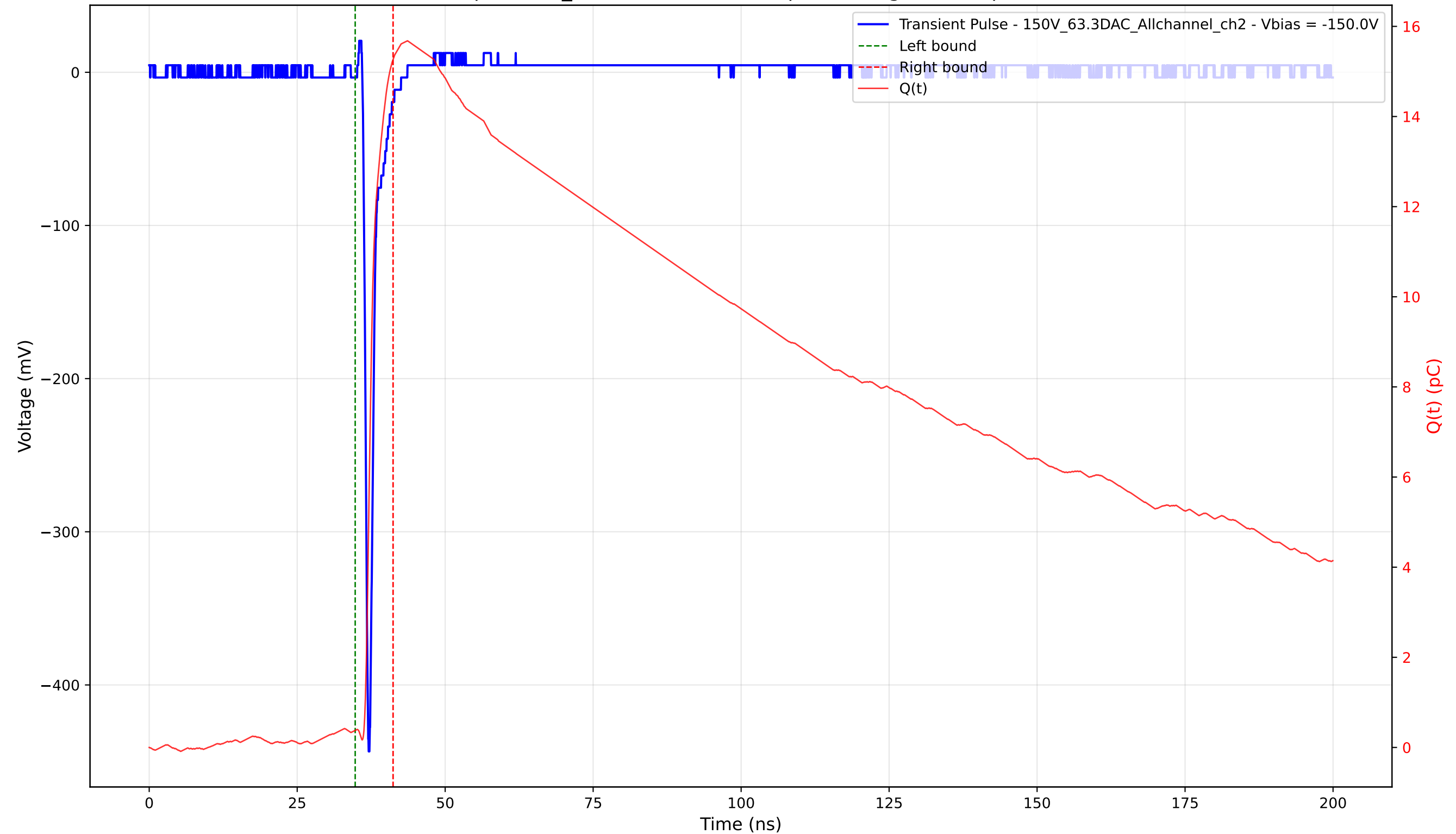
Transient Pulse - Sample: 1cm_42 - Position: 3255.0 \mu\text{m} - Charge: 14.89 pC - Rise Time: 0.69 ns
