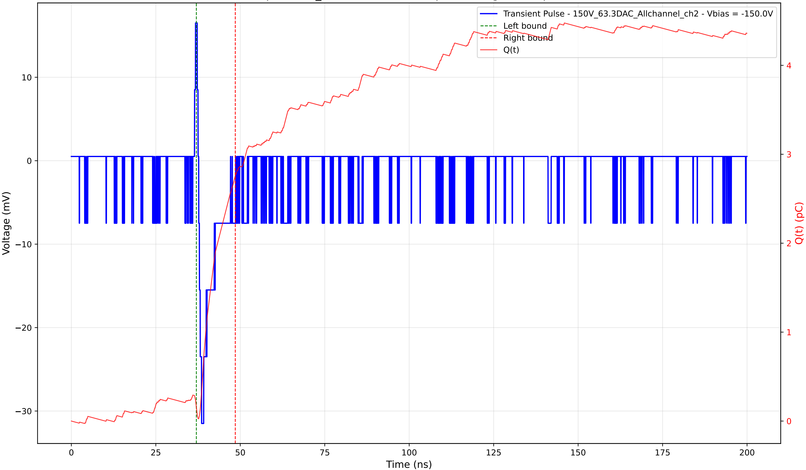
Transient Pulse - Sample: 1cm_42 - Position: 400.0 \mu\text{m} - Charge: 2.61 pC - Rise Time: 0.86 ns
