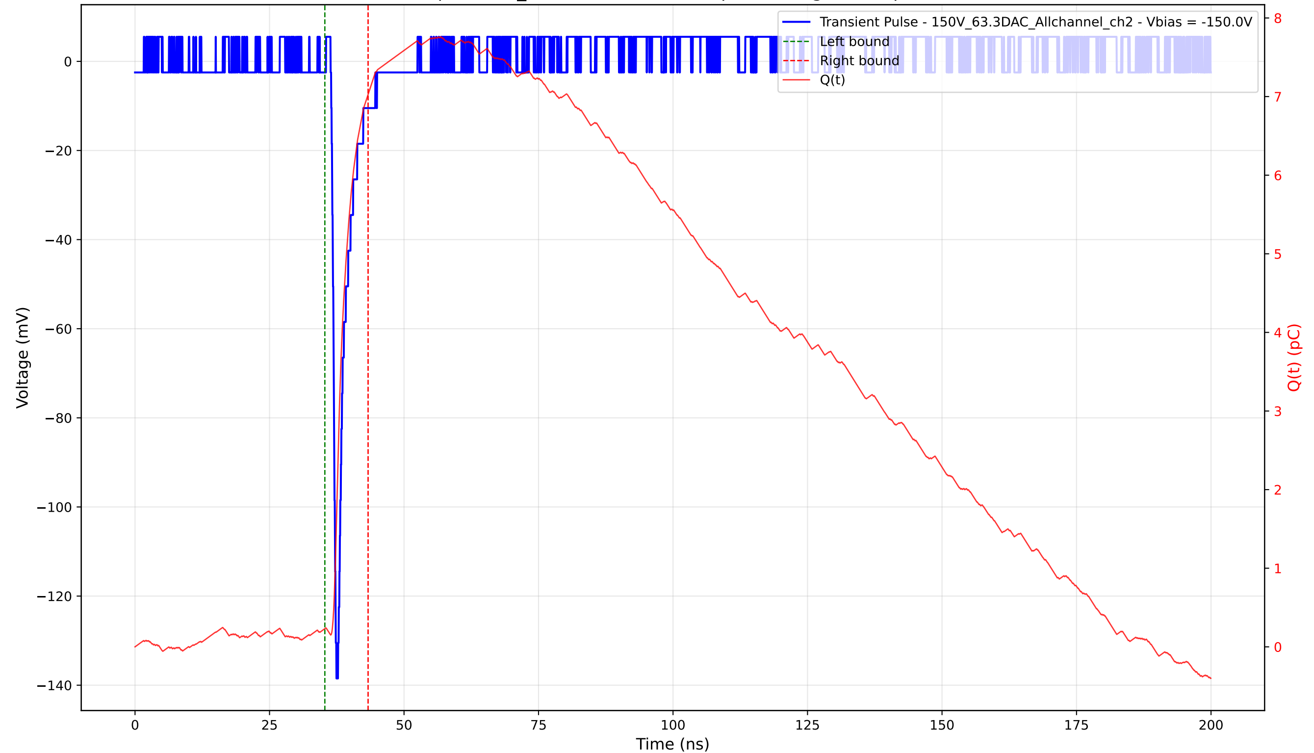
Transient Pulse - Sample: 1cm_42 - Position: 2280.0 \mu\text{m} - Charge: 6.80 pC - Rise Time: 0.78 ns
