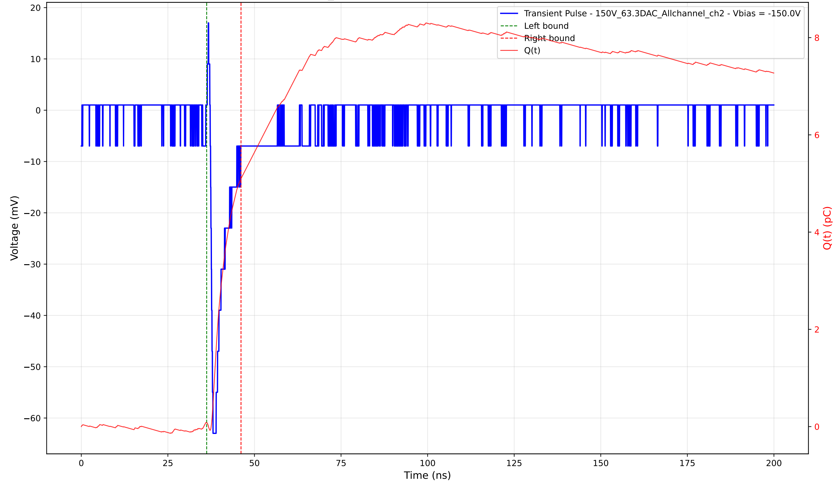
Transient Pulse - Sample: 1cm_42 - Position: 1770.0 \mu\text{m} - Charge: 5.02 pC - Rise Time: 0.80 ns
