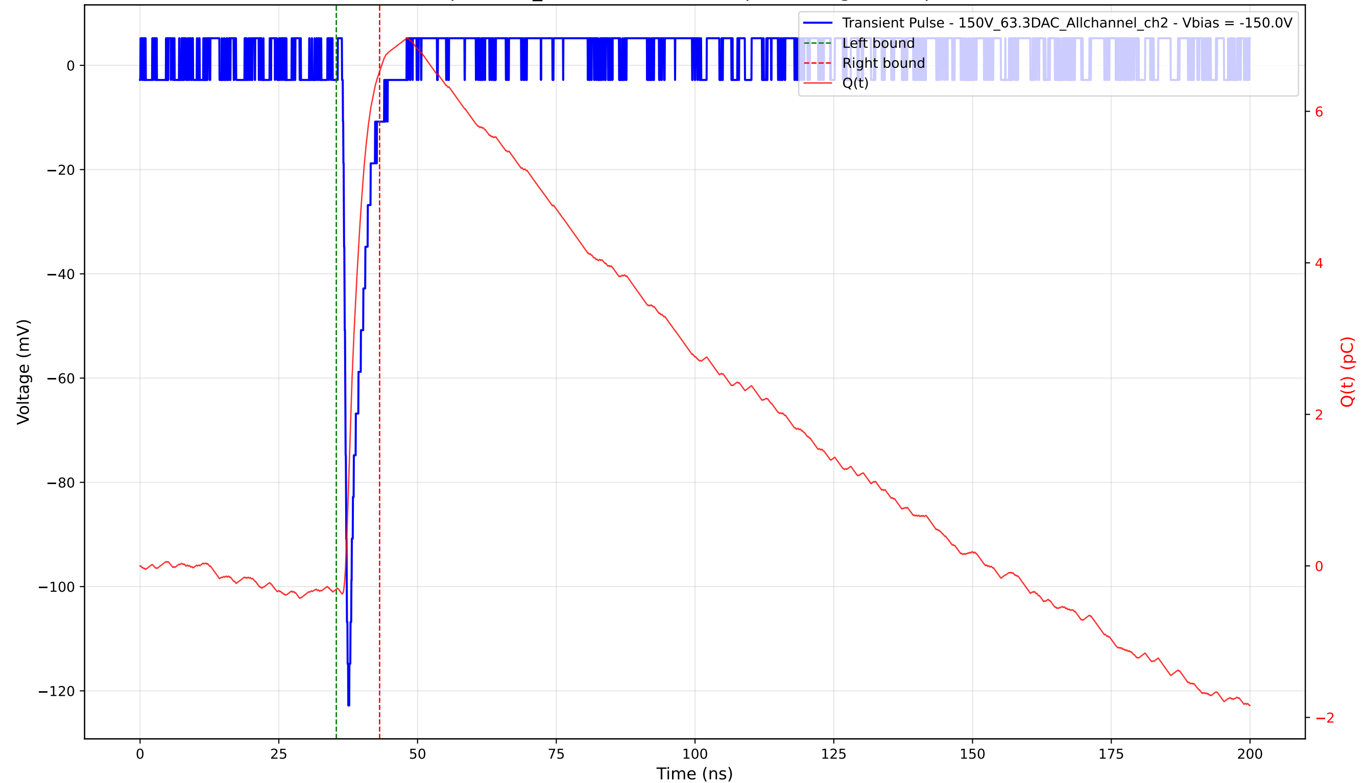
Transient Pulse - Sample: 1cm_42 - Position: 3840.0 \mu\text{m} - Charge: 6.83 pC - Rise Time: 0.79 ns
