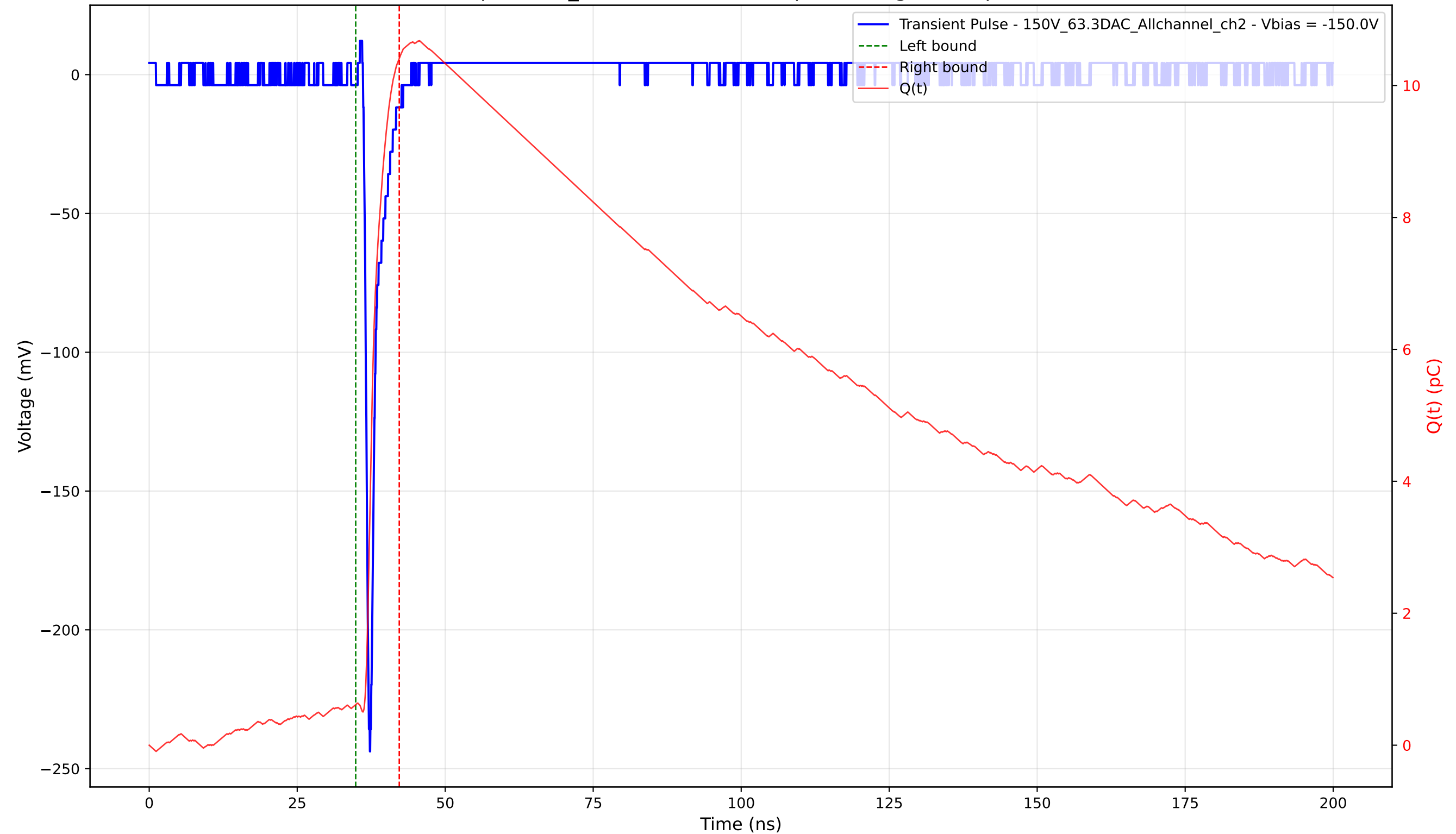
Transient Pulse - Sample: 1cm_42 - Position: 3485.0 \mu\text{m} - Charge: 9.80 pC - Rise Time: 0.78 ns
