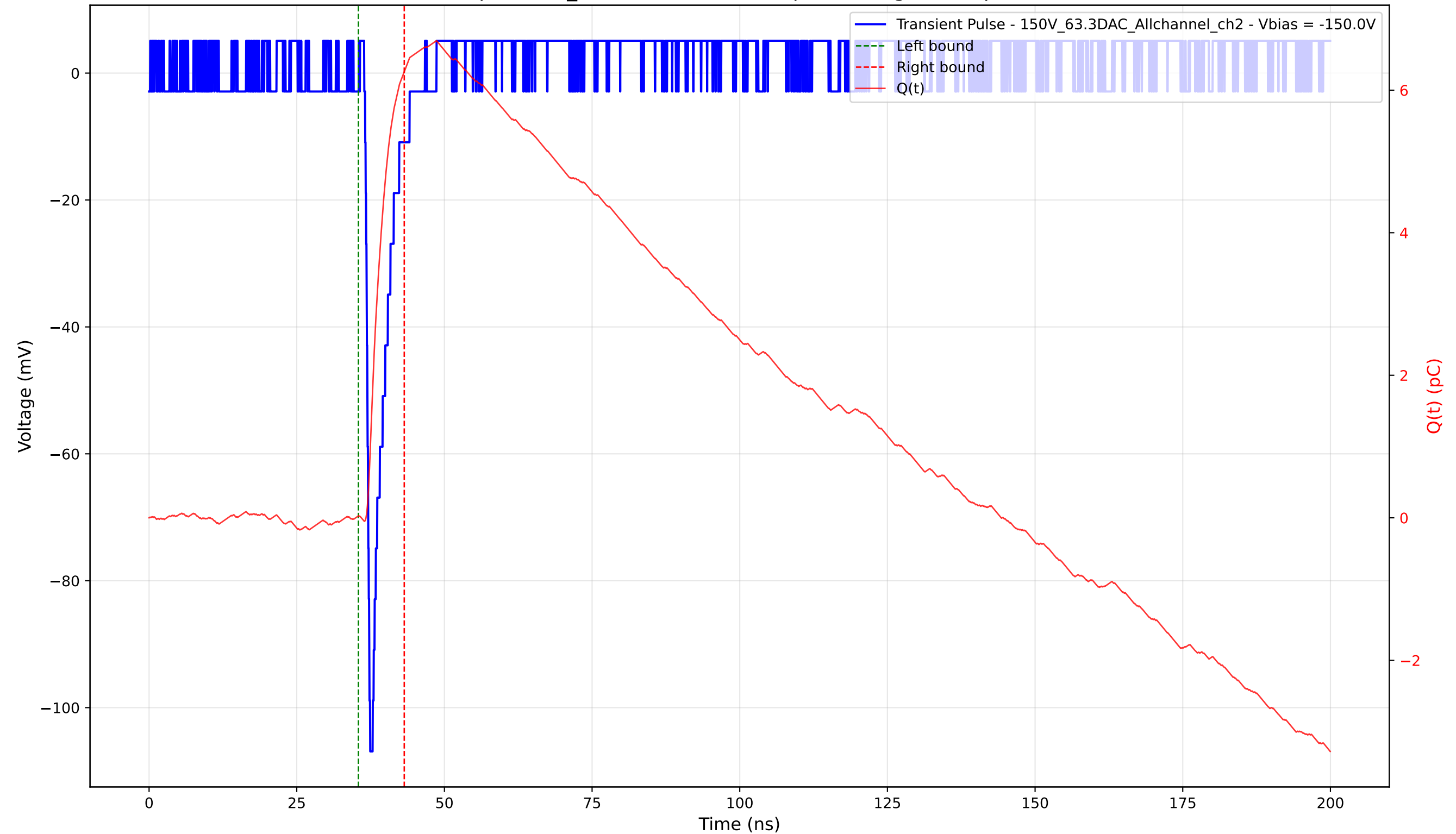
Transient Pulse - Sample: 1cm_42 - Position: 3875.0 \mu\text{m} - Charge: 6.23 pC - Rise Time: 0.72 ns
