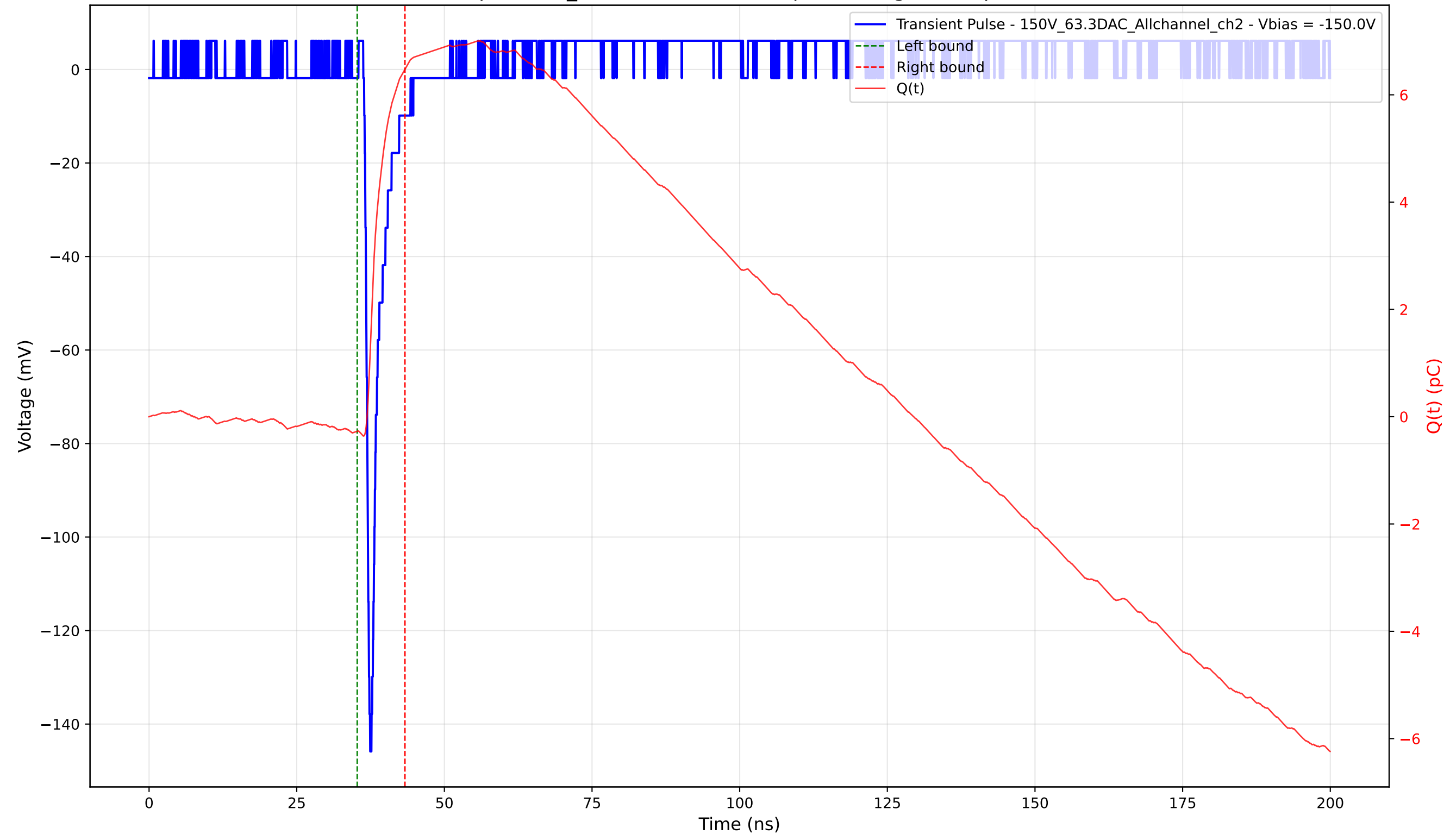
Transient Pulse - Sample: 1cm_42 - Position: 2350.0 \mu\text{m} - Charge: 6.75 pC - Rise Time: 0.82 ns
