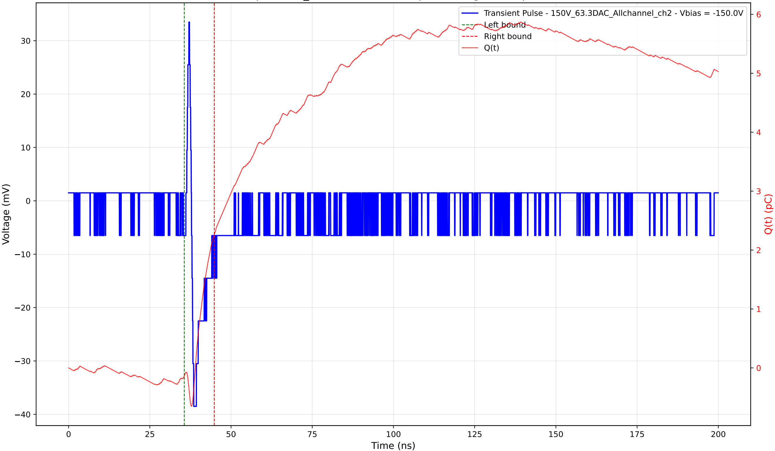
Transient Pulse - Sample: 1cm_42 - Position: 630.0 \mu\text{m} - Charge: 2.40 pC - Rise Time: 0.70 ns
