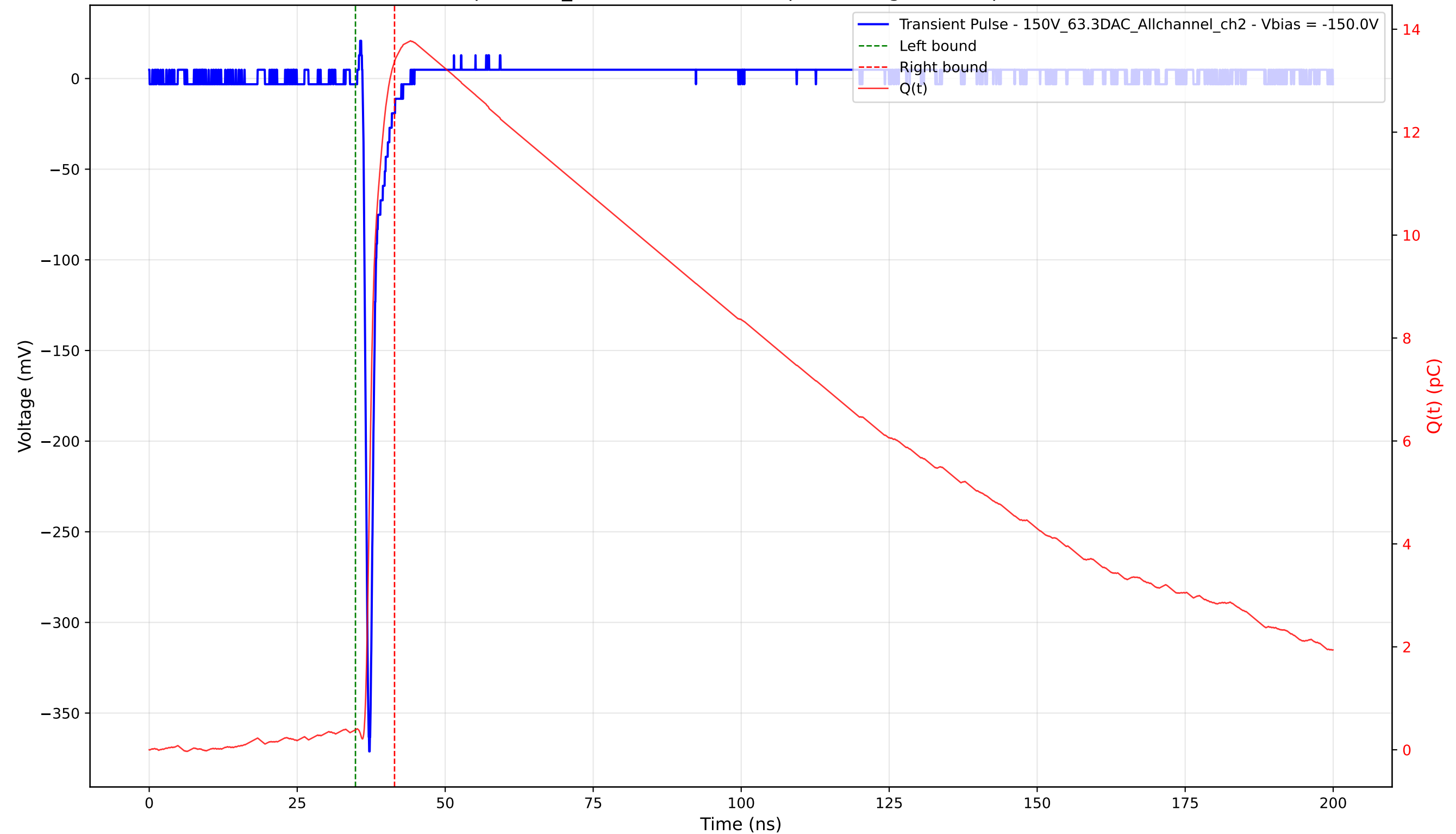
Transient Pulse - Sample: 1cm_42 - Position: 3360.0 \mu\text{m} - Charge: 12.99 pC - Rise Time: 0.73 ns
