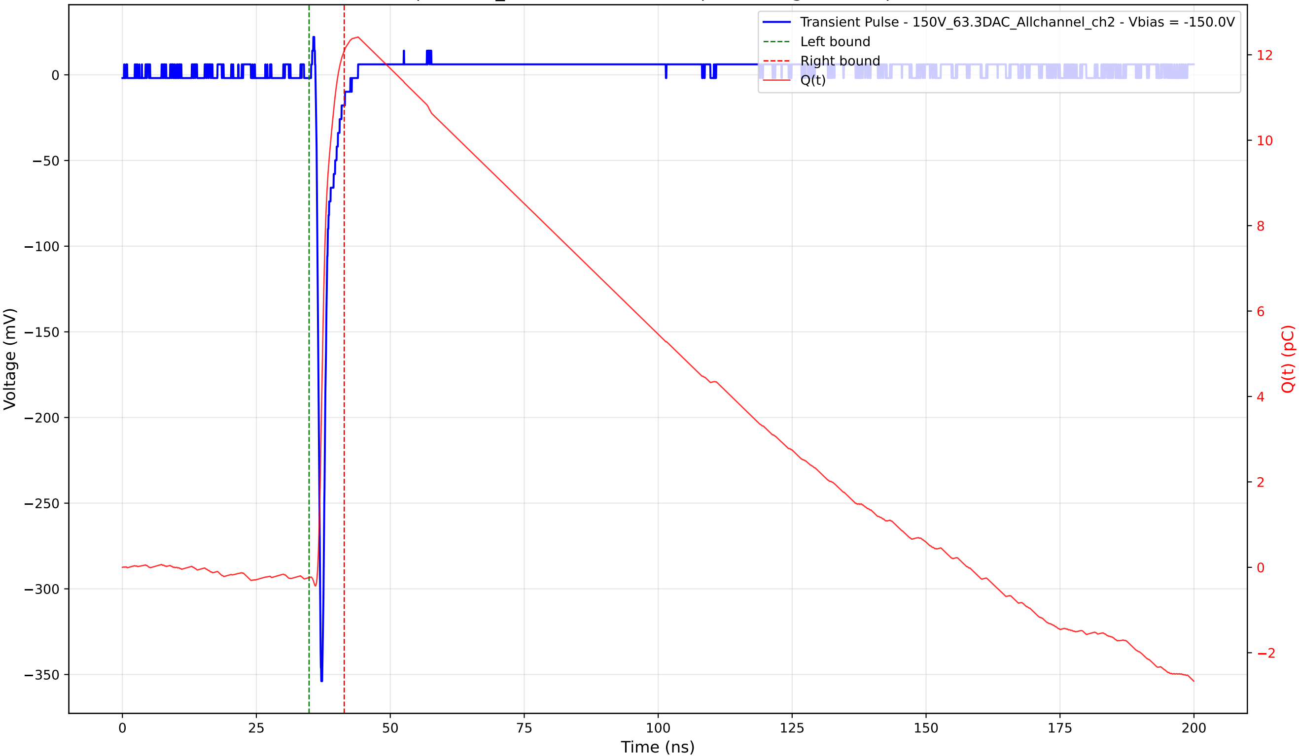
Transient Pulse - Sample: 1cm_42 - Position: 3370.0 \mu\text{m} - Charge: 12.34 pC - Rise Time: 0.74 ns
