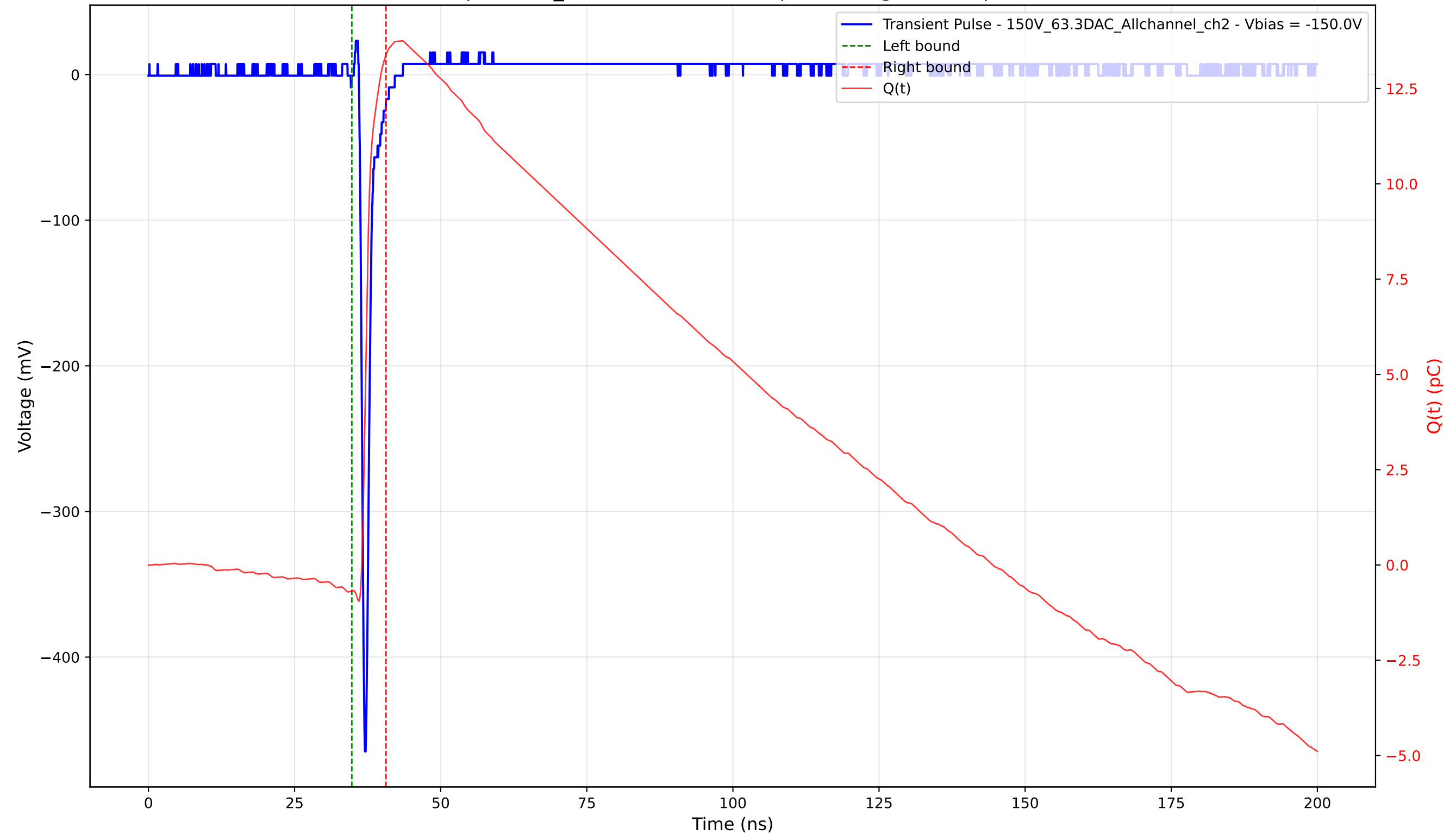
Transient Pulse - Sample: 1cm_42 - Position: 2910.0 \mu\text{m} - Charge: 14.07 pC - Rise Time: 0.70 ns
