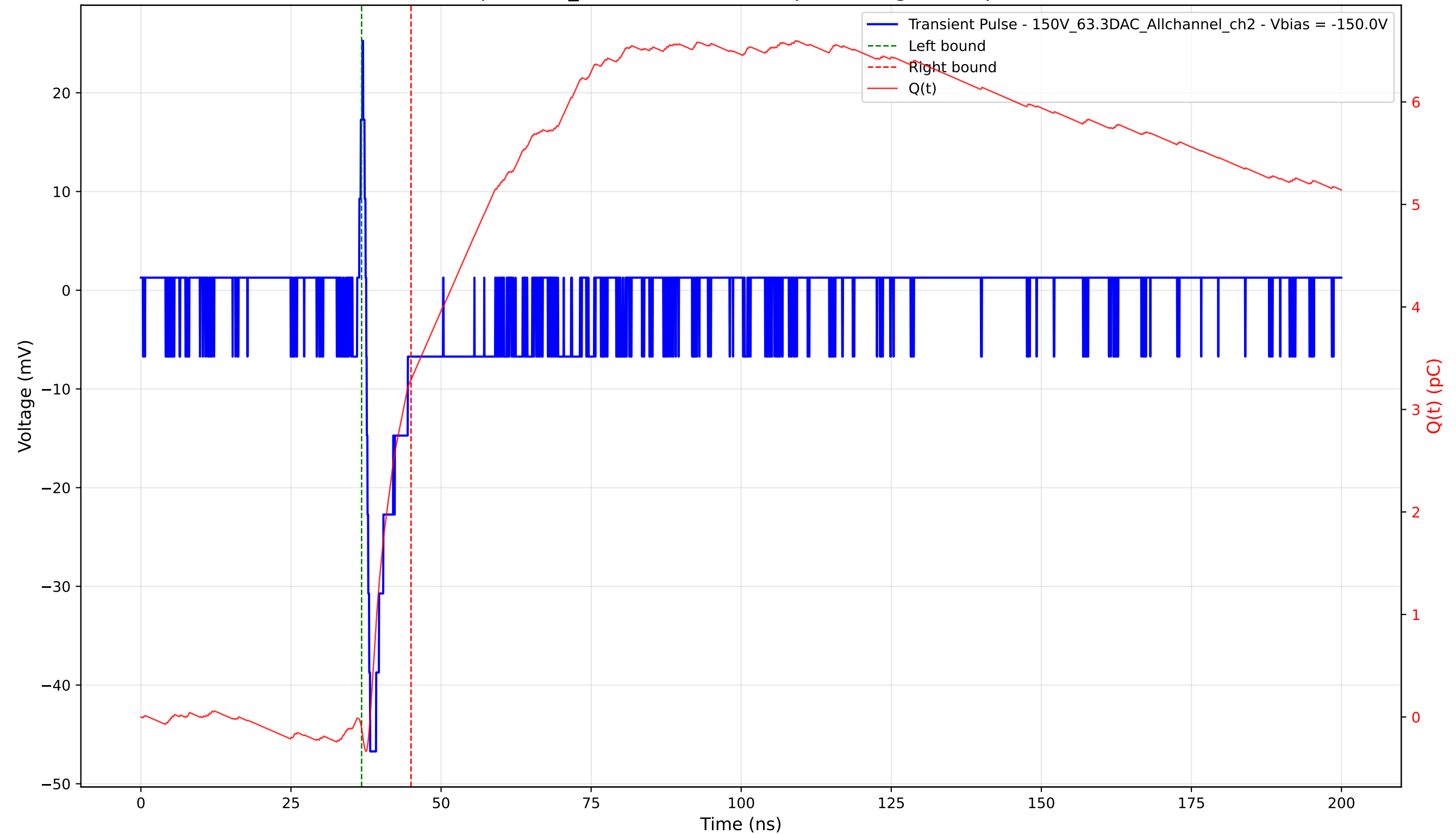
Transient Pulse - Sample: 1cm_42 - Position: 1550.0 \mu\text{m} - Charge: 3.40 pC - Rise Time: 0.66 ns
