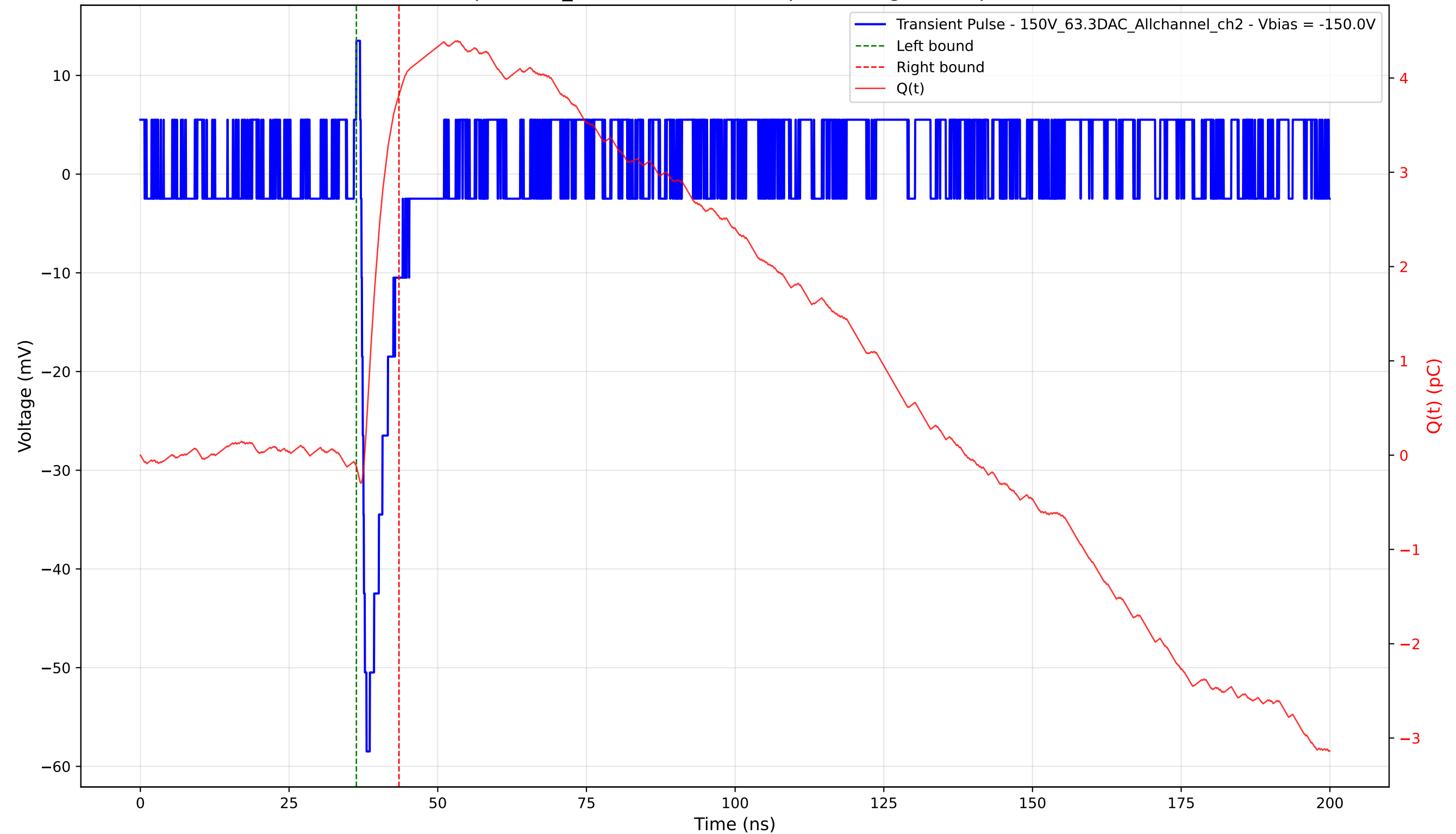
Transient Pulse - Sample: 1cm_42 - Position: 4225.0 \mu\text{m} - Charge: 3.94 pC - Rise Time: 0.86 ns
