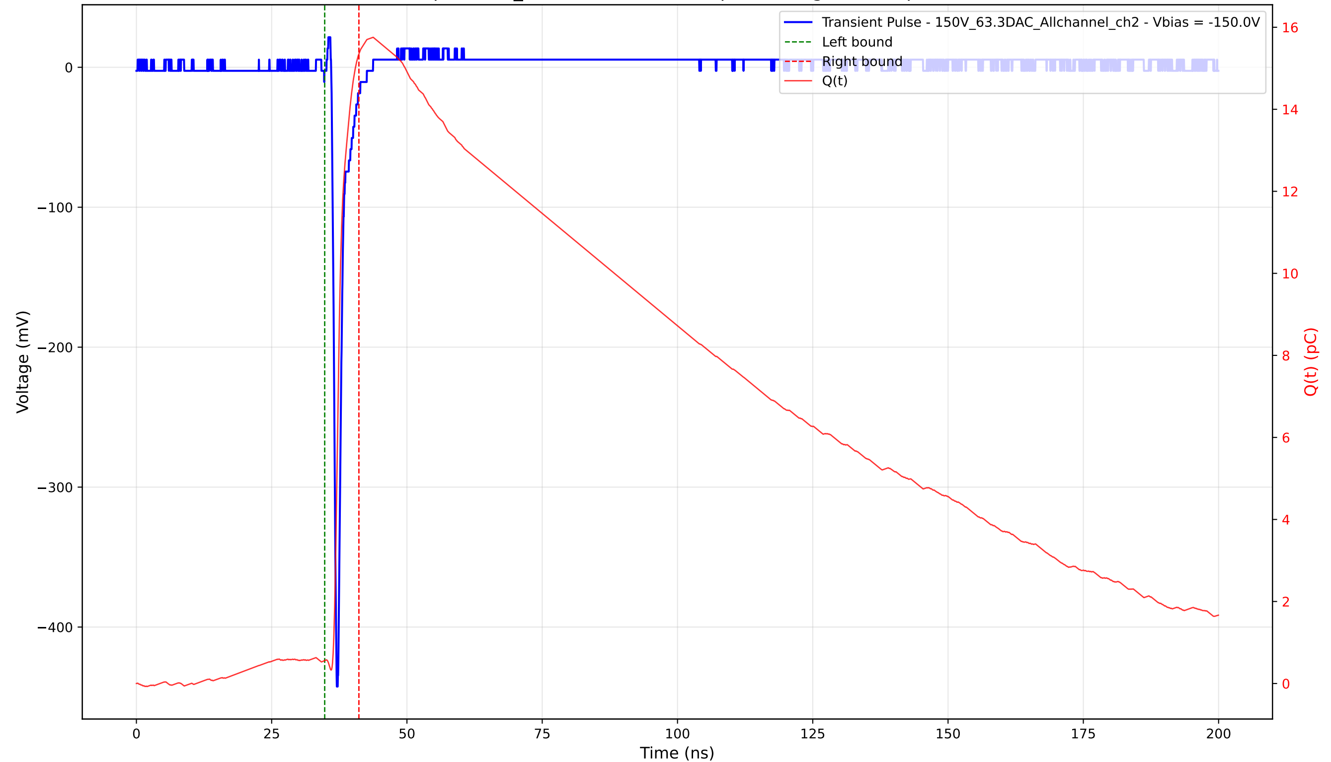
Transient Pulse - Sample: 1cm_42 - Position: 3250.0 \mu\text{m} - Charge: 14.79 pC - Rise Time: 0.69 ns
