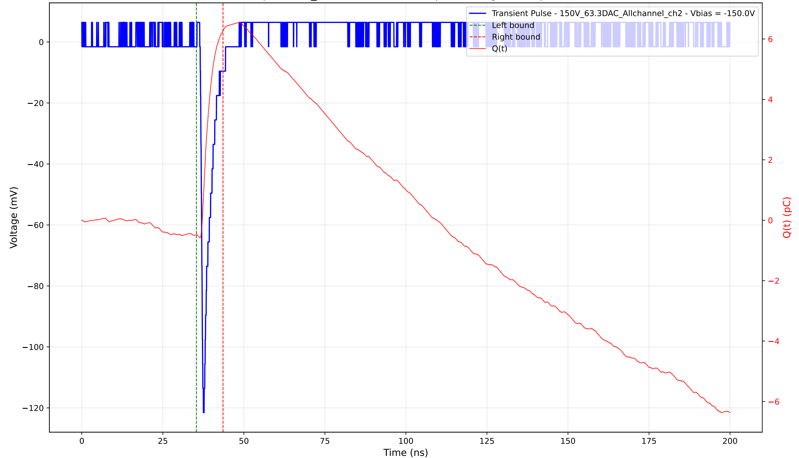
Transient Pulse - Sample: 1cm_42 - Position: 3835.0 \mu\text{m} - Charge: 6.75 pC - Rise Time: 0.75 ns
