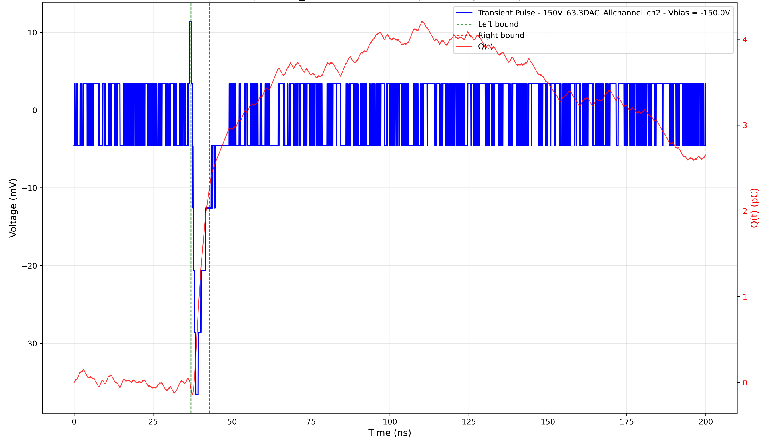
Transient Pulse - Sample: 1cm_42 - Position: 4870.0 \mu\text{m} - Charge: 2.32 pC - Rise Time: 0.99 ns
