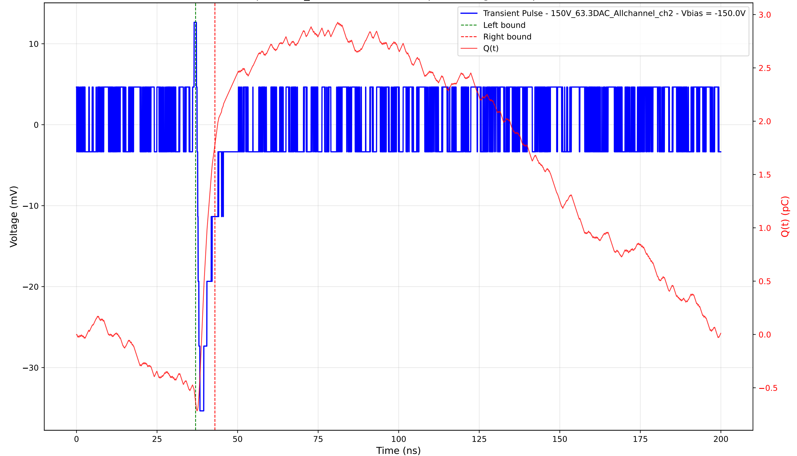
Transient Pulse - Sample: 1cm_42 - Position: 4730.0 \mu\text{m} - Charge: 2.41 pC - Rise Time: 0.72 ns
