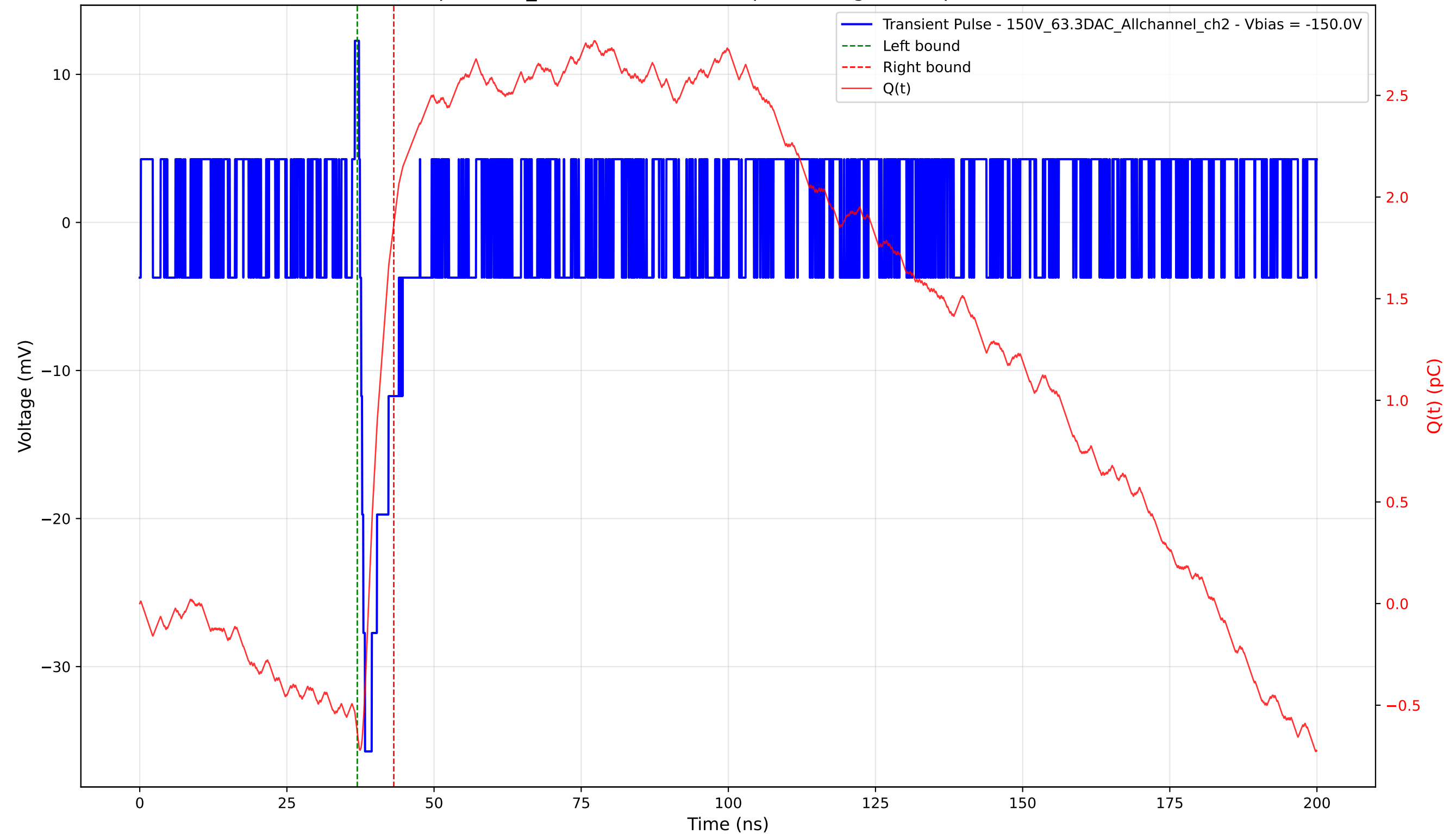
Transient Pulse - Sample: 1cm_42 - Position: 4825.0 \mu\text{m} - Charge: 2.50 pC - Rise Time: 0.00 ns (N/A)
