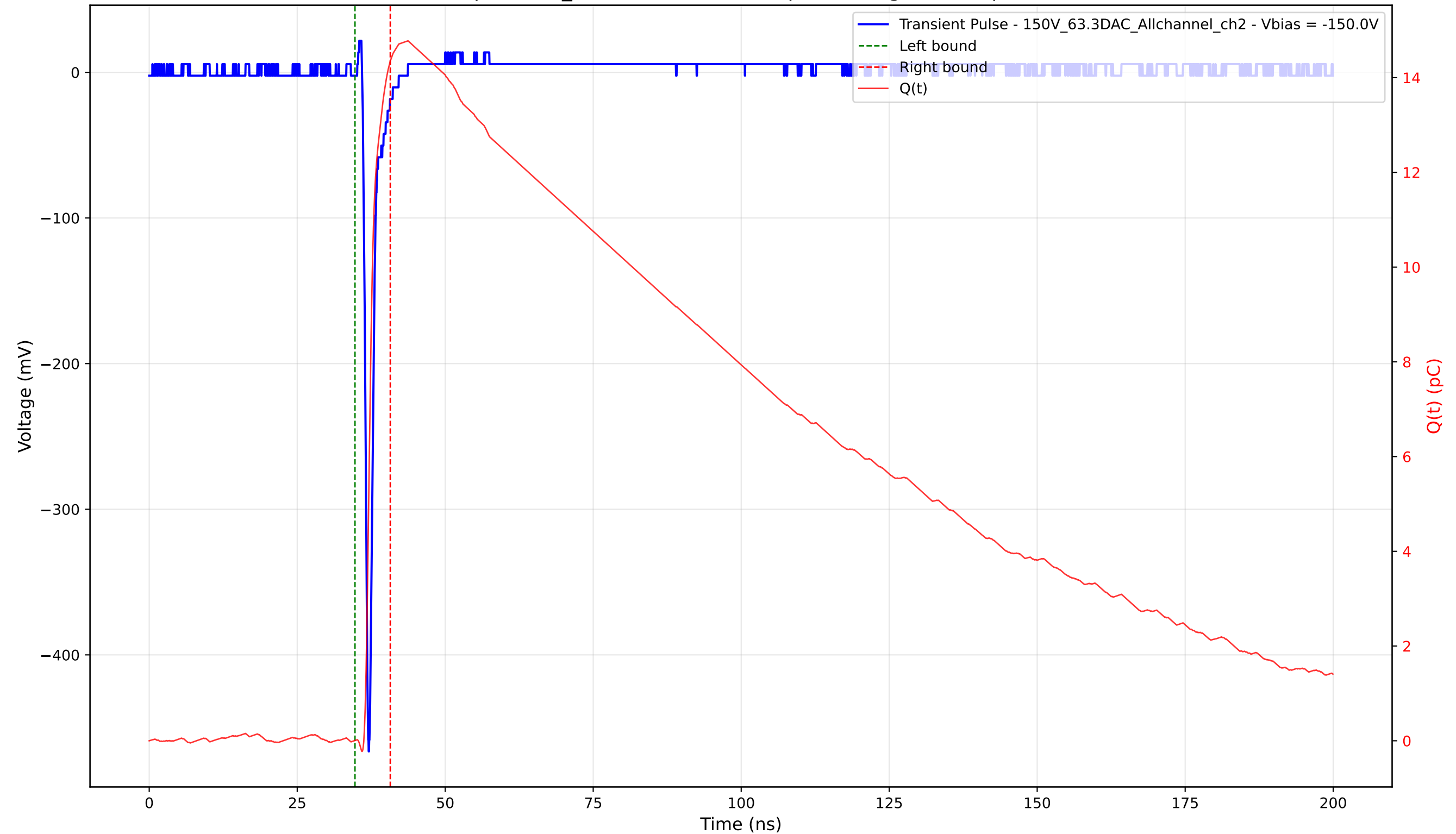
Transient Pulse - Sample: 1cm_42 - Position: 2900.0 \mu\text{m} - Charge: 14.34 pC - Rise Time: 0.71 ns
