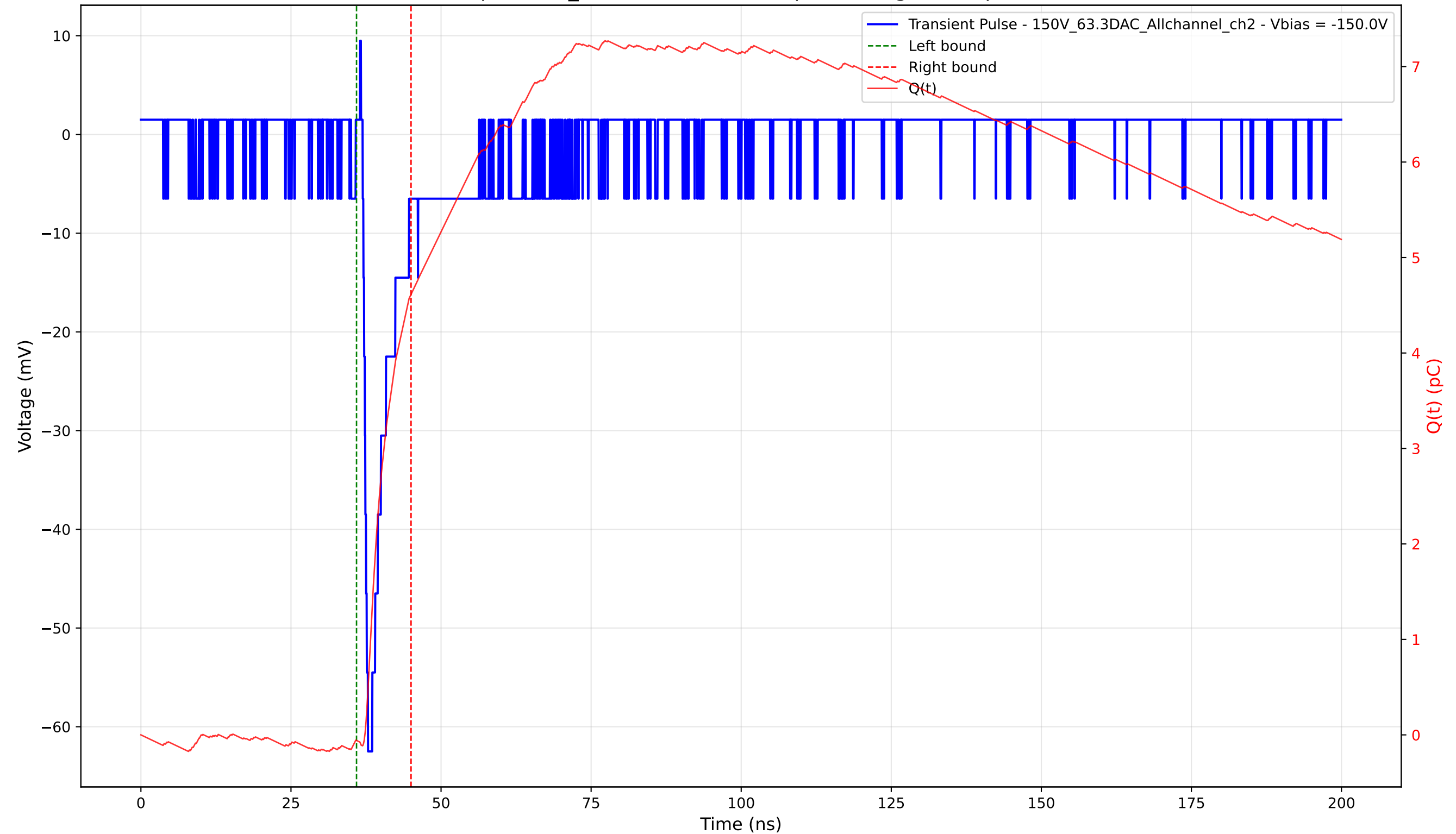
Transient Pulse - Sample: 1cm_42 - Position: 1935.0 \mu\text{m} - Charge: 4.67 pC - Rise Time: 0.88 ns
