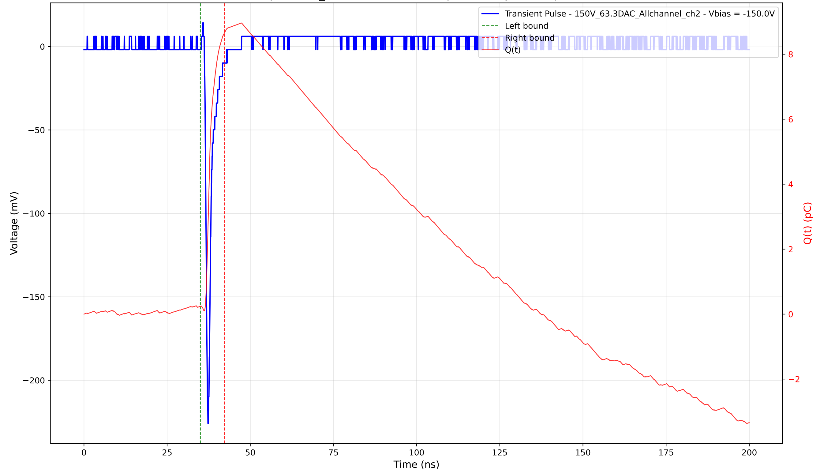
Transient Pulse - Sample: 1cm_42 - Position: 2540.0 \mu\text{m} - Charge: 8.40 pC - Rise Time: 0.74 ns
