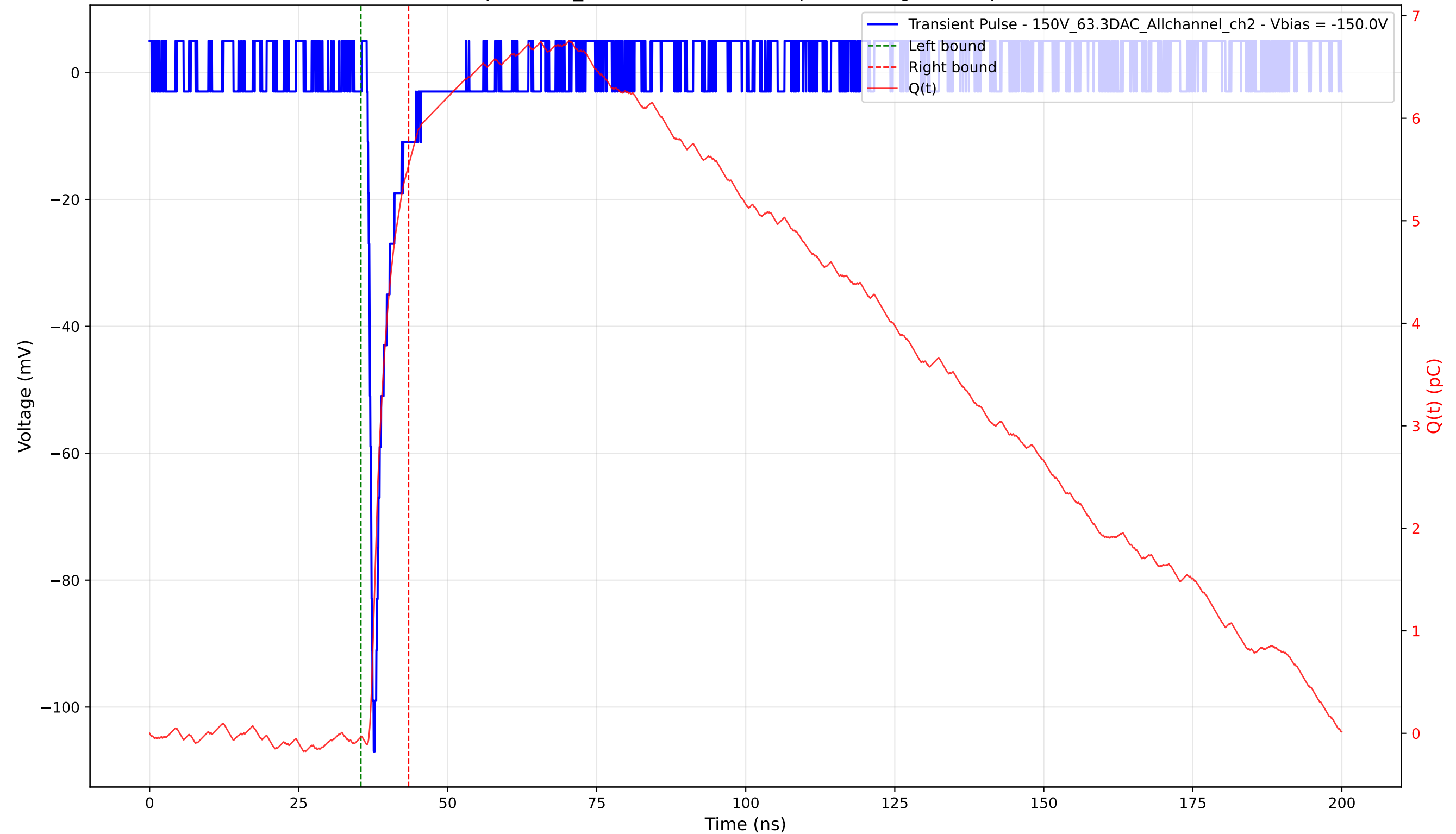
Transient Pulse - Sample: 1cm_42 - Position: 2155.0 \mu\text{m} - Charge: 5.58 pC - Rise Time: 0.80 ns
