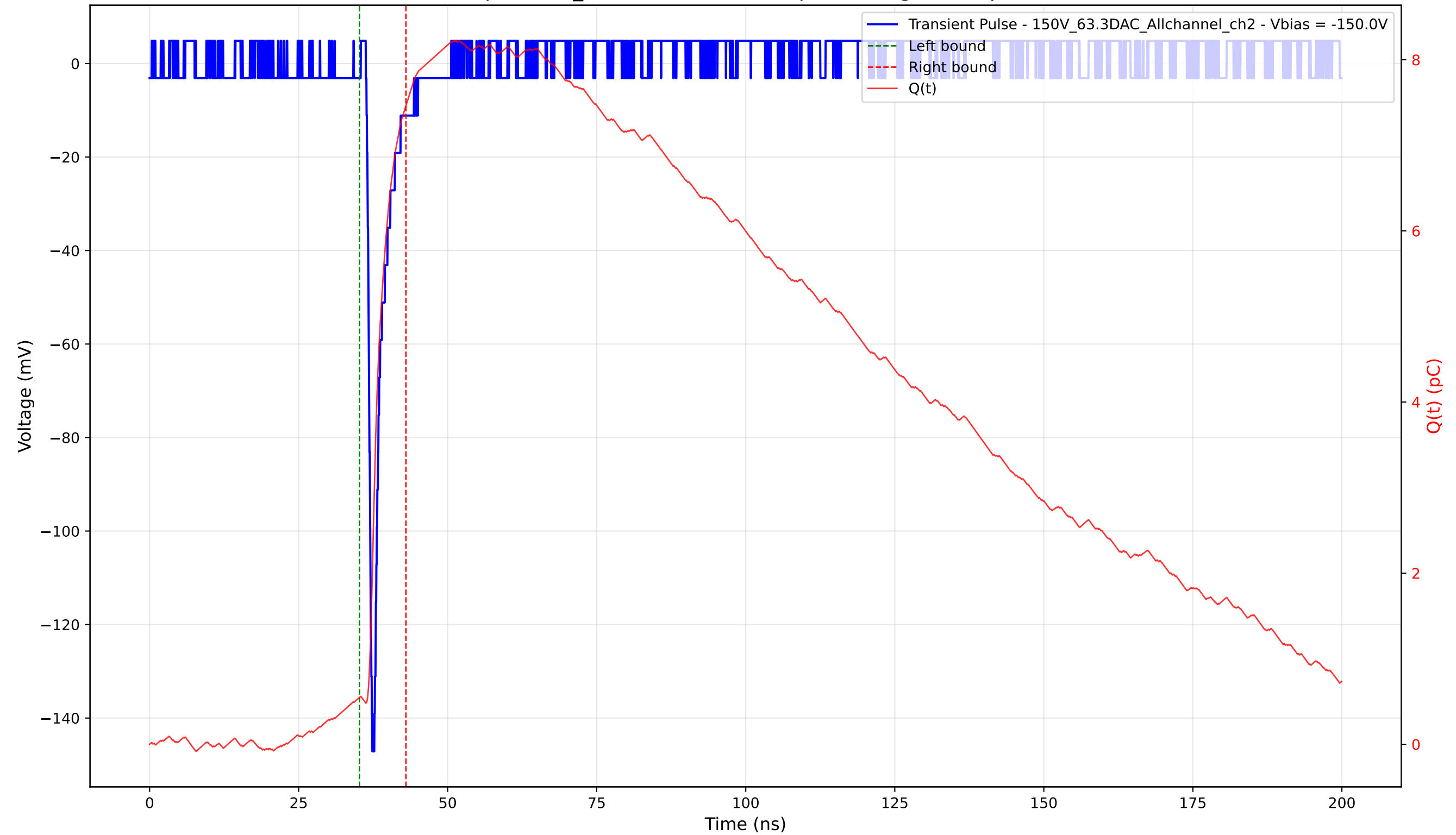
Transient Pulse - Sample: 1cm_42 - Position: 2380.0 \mu\text{m} - Charge: 6.92 pC - Rise Time: 0.82 ns
