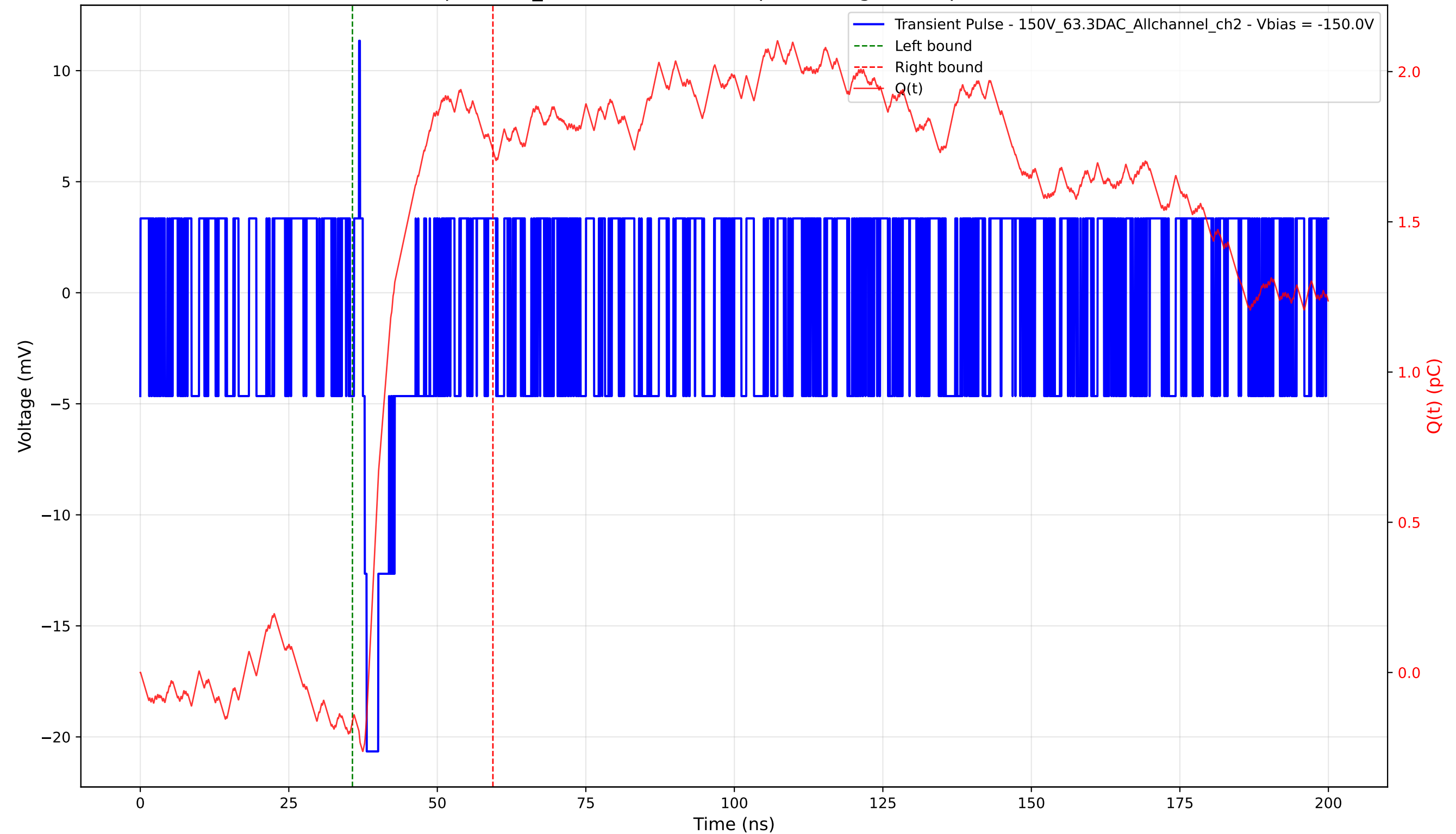
Transient Pulse - Sample: 1cm_42 - Position: 4985.0 \mu\text{m} - Charge: 1.91 pC - Rise Time: 0.00 ns (N/A)
