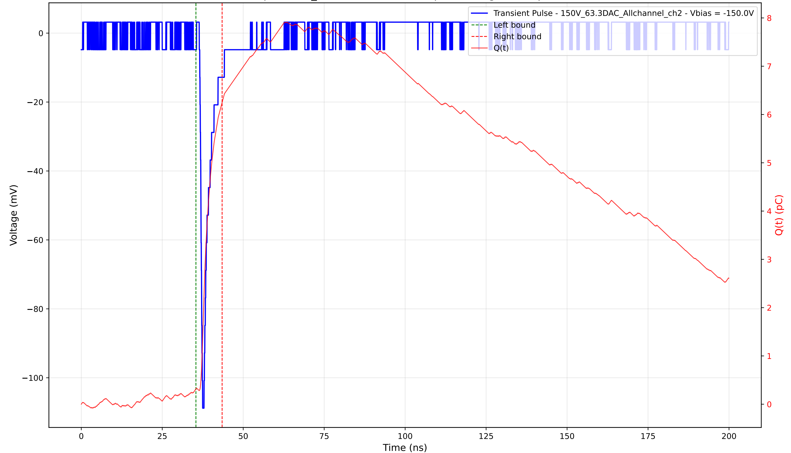
Transient Pulse - Sample: 1cm_42 - Position: 2170.0 \mu\text{m} - Charge: 5.93 pC - Rise Time: 0.77 ns
