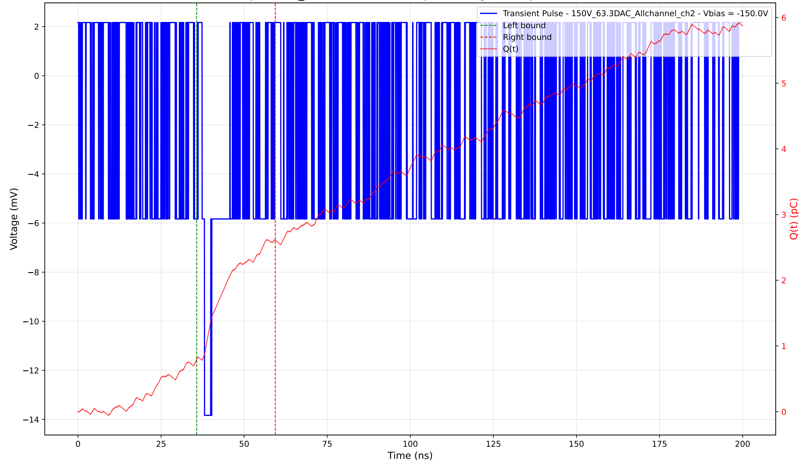
Transient Pulse - Sample: 1cm_42 - Position: 5080.0 \mu\text{m} - Charge: 1.82 pC - Rise Time: 0.00 ns (N/A)
