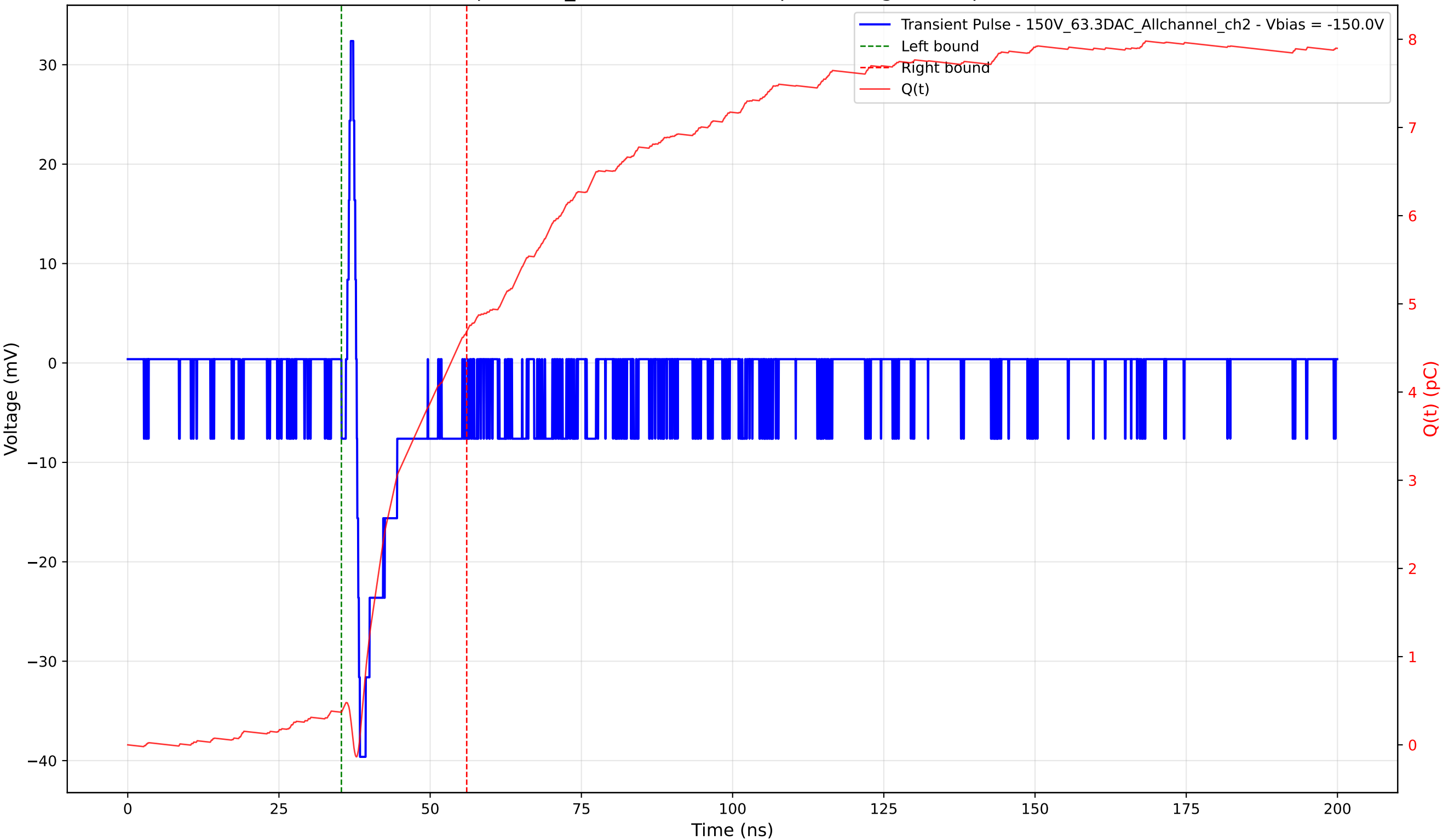
Transient Pulse - Sample: 1cm_42 - Position: 665.0 \mu\text{m} - Charge: 4.32 pC - Rise Time: 0.54 ns
