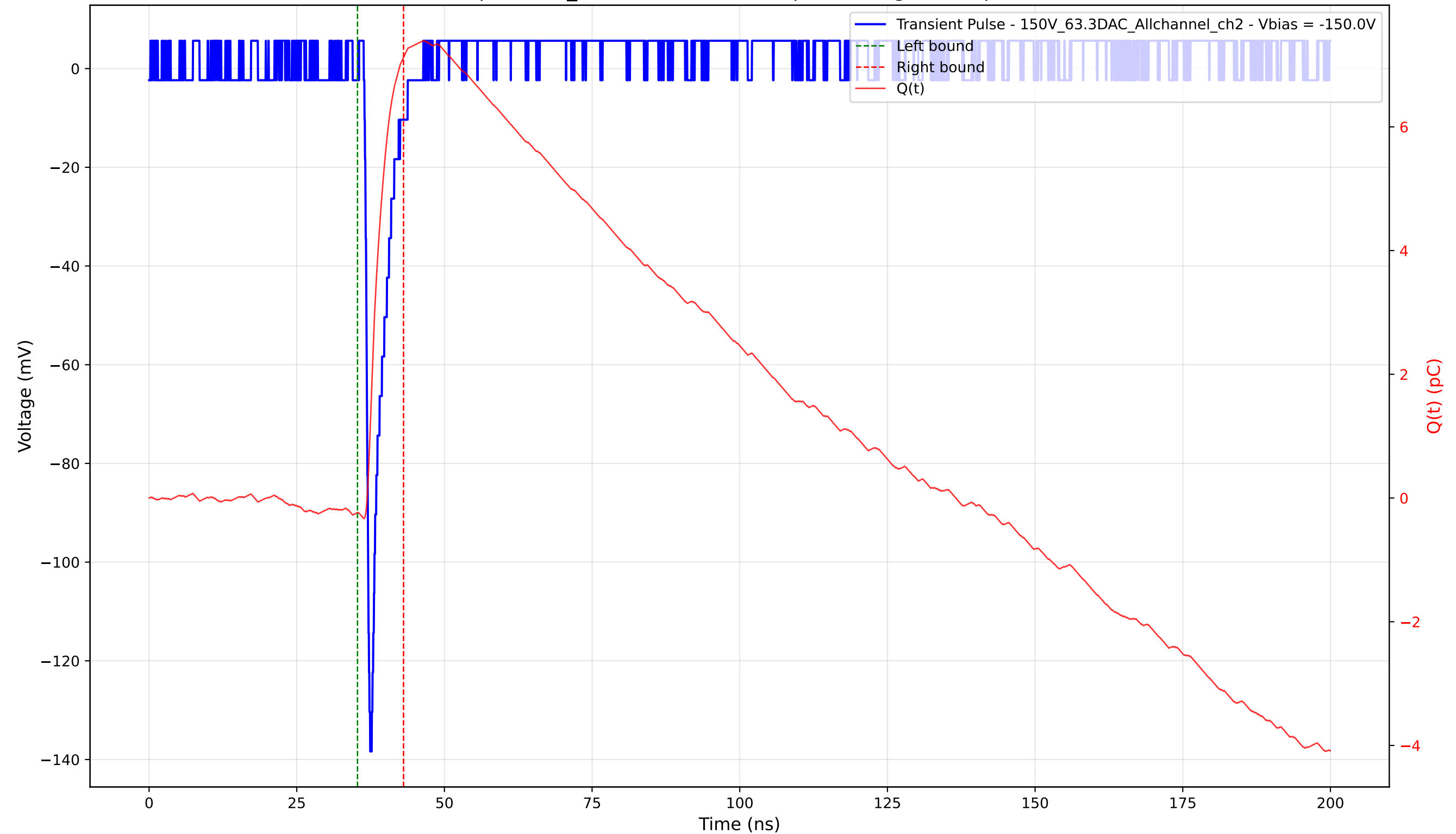
Transient Pulse - Sample: 1cm_42 - Position: 3725.0 \mu\text{m} - Charge: 7.36 pC - Rise Time: 0.78 ns
