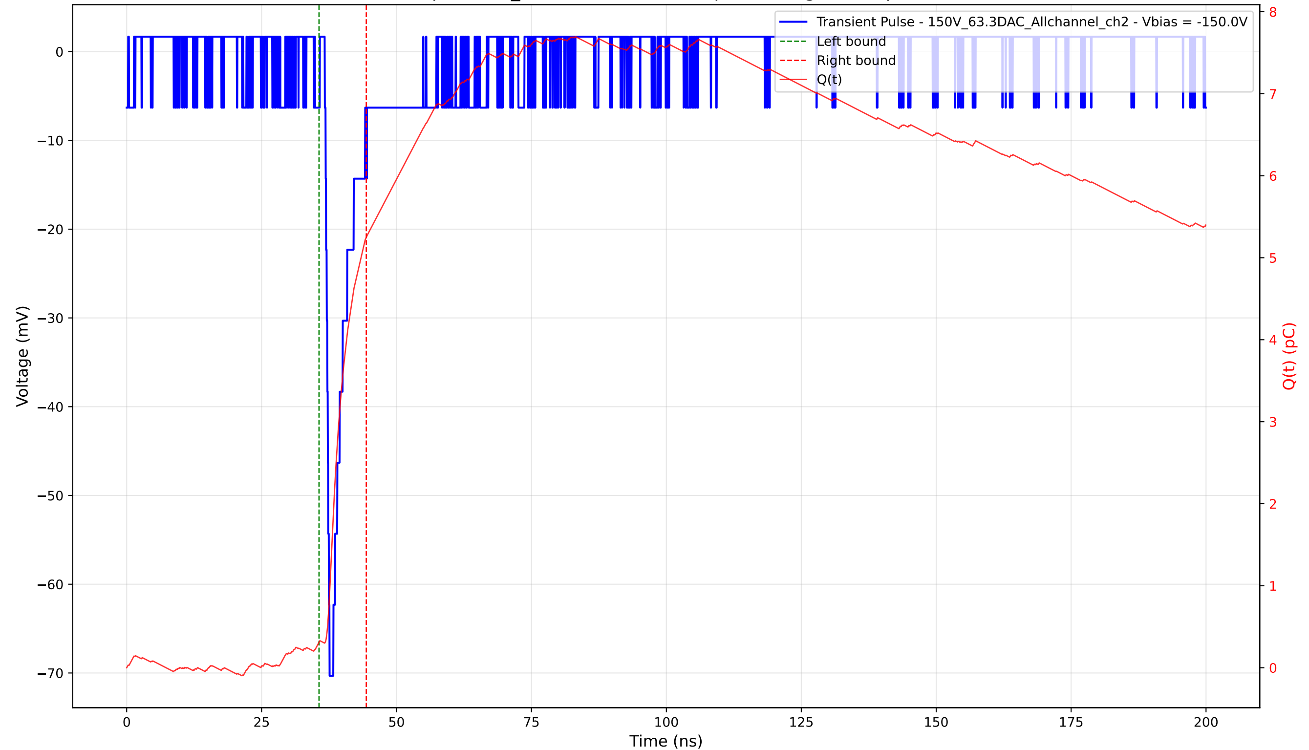
Transient Pulse - Sample: 1cm_42 - Position: 2015.0 \mu\text{m} - Charge: 4.93 pC - Rise Time: 0.76 ns
