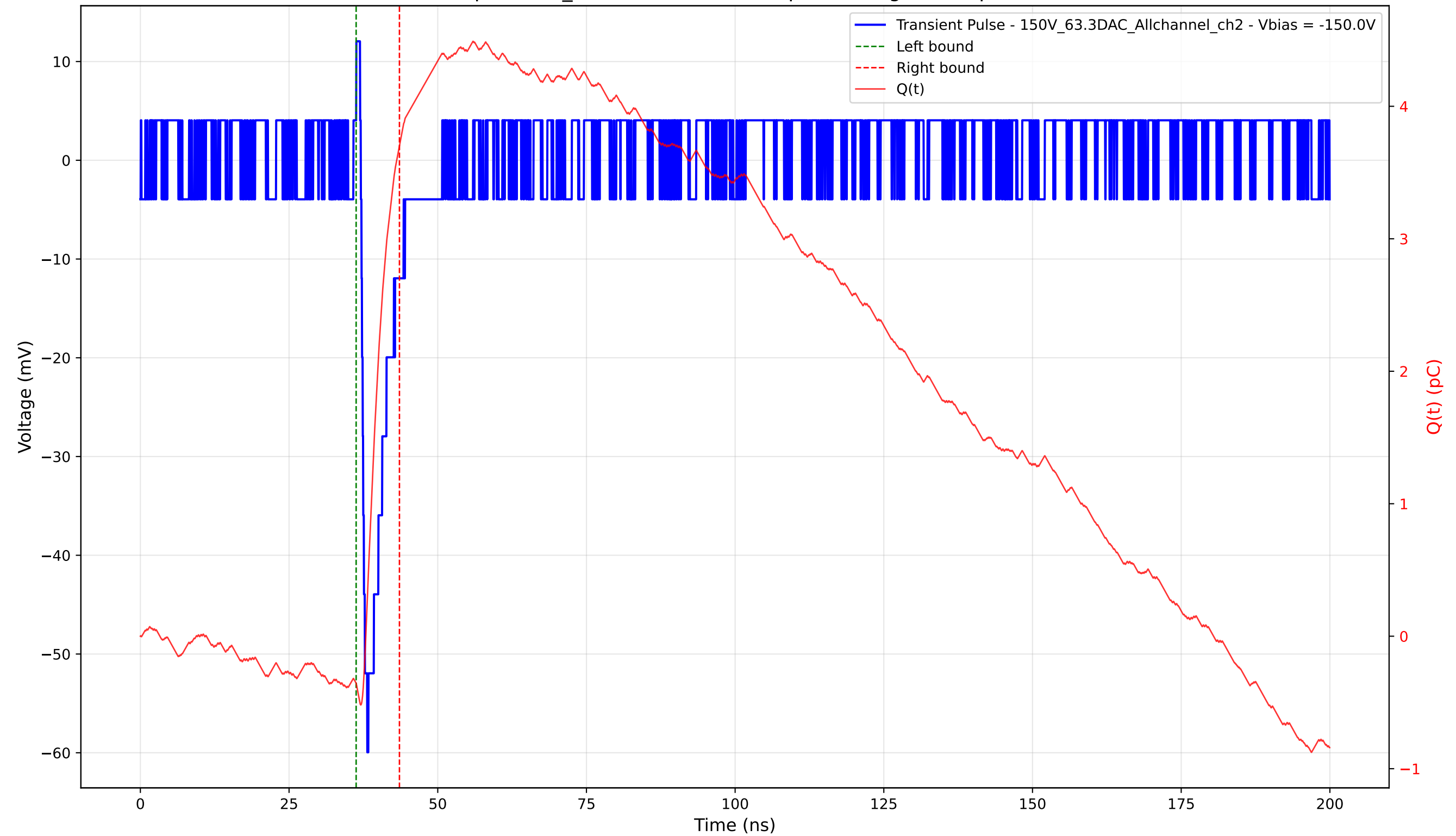
Transient Pulse - Sample: 1cm_42 - Position: 4210.0 \mu\text{m} - Charge: 4.06 pC - Rise Time: 0.99 ns
