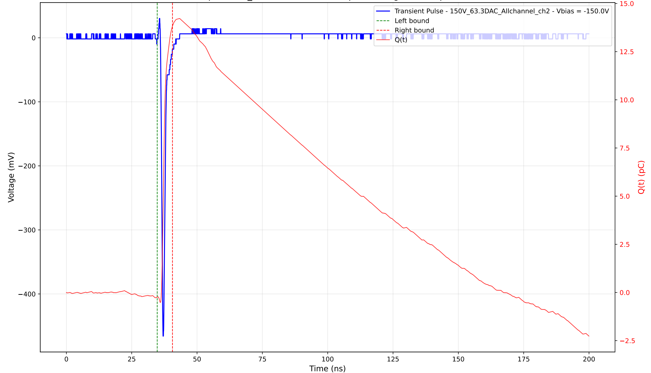
Transient Pulse - Sample: 1cm_42 - Position: 3030.0 \mu\text{m} - Charge: 14.07 pC - Rise Time: 0.68 ns
