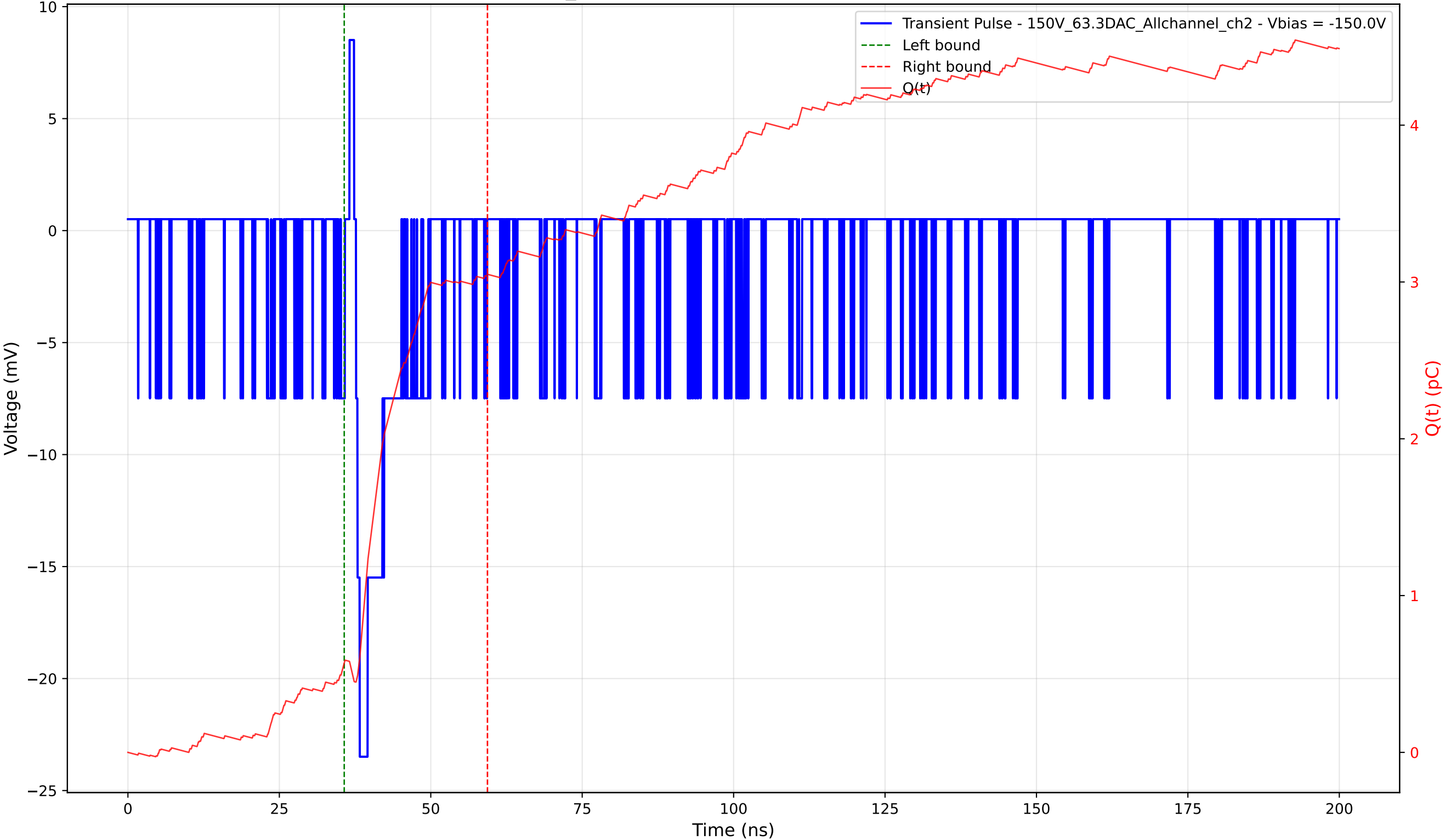
Transient Pulse - Sample: 1cm_42 - Position: 255.0 \mu\text{m} - Charge: 2.48 pC - Rise Time: 0.63 ns
