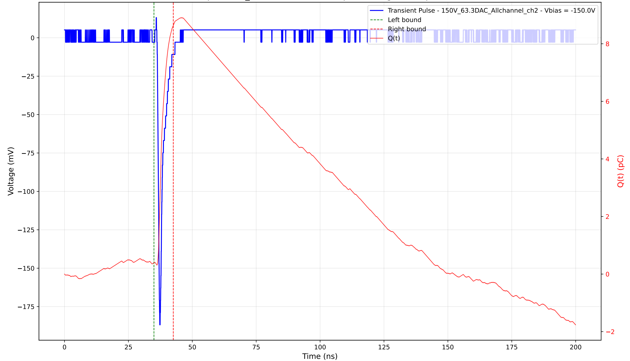
Transient Pulse - Sample: 1cm_42 - Position: 3565.0 \mu\text{m} - Charge: 8.24 pC - Rise Time: 0.76 ns
