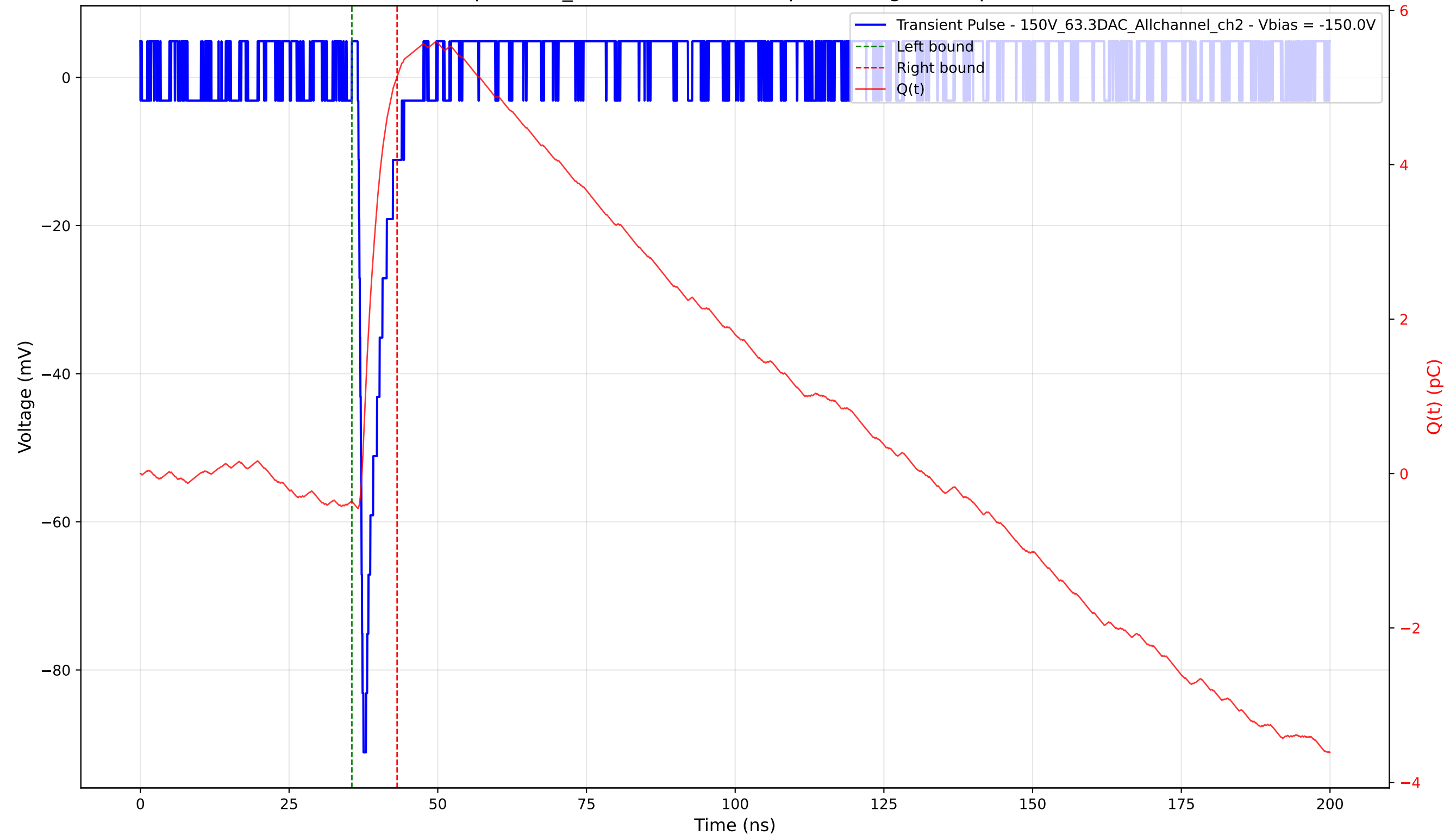
Transient Pulse - Sample: 1cm_42 - Position: 3930.0 \mu\text{m} - Charge: 5.50 pC - Rise Time: 0.69 ns
