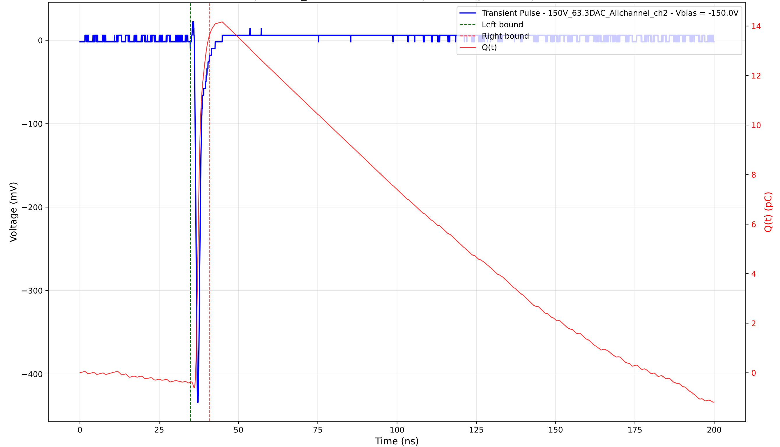
Transient Pulse - Sample: 1cm_42 - Position: 2745.0 \mu\text{m} - Charge: 14.06 pC - Rise Time: 0.70 ns
