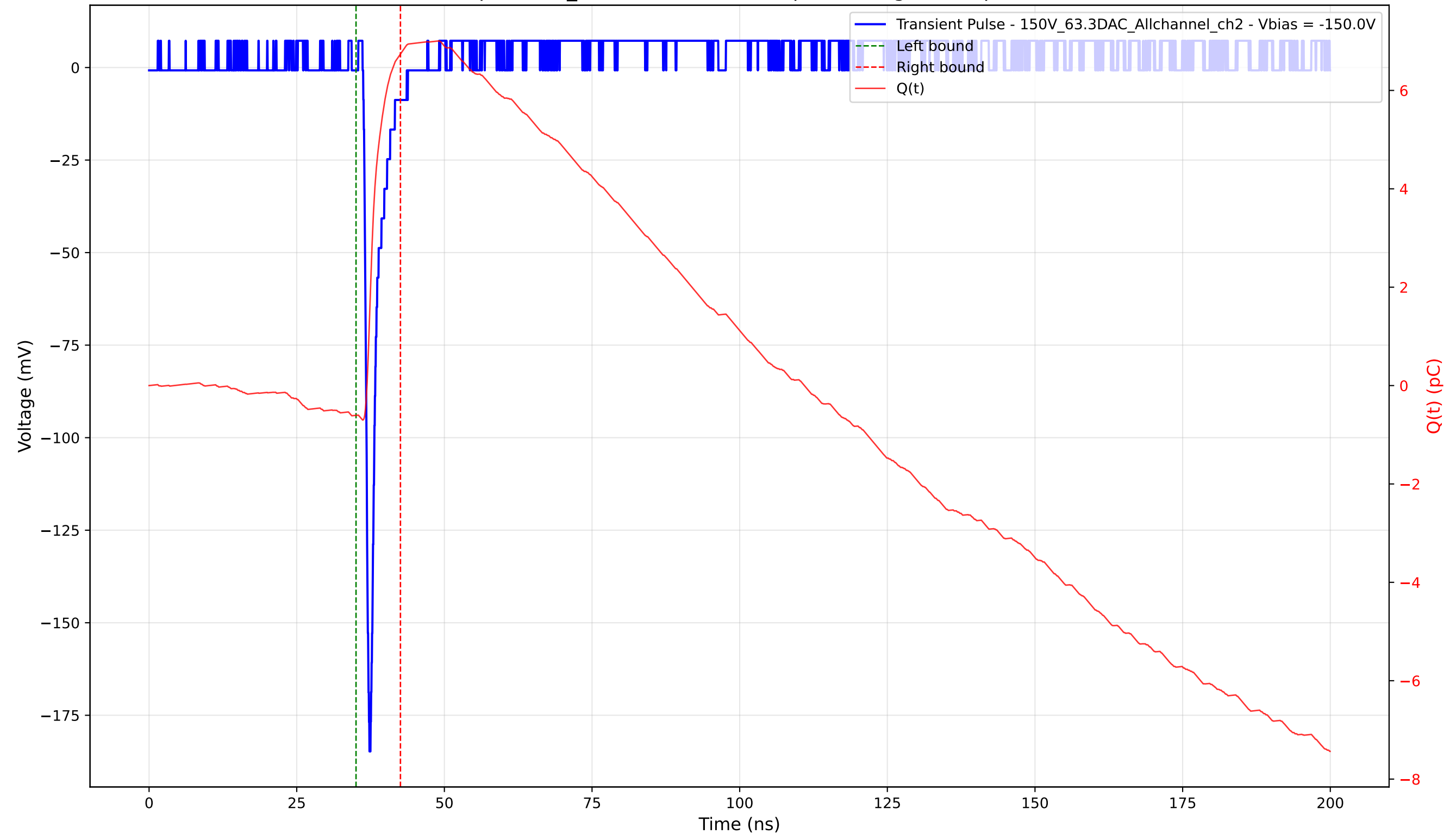
Transient Pulse - Sample: 1cm_42 - Position: 2475.0 \mu\text{m} - Charge: 7.34 pC - Rise Time: 0.75 ns
