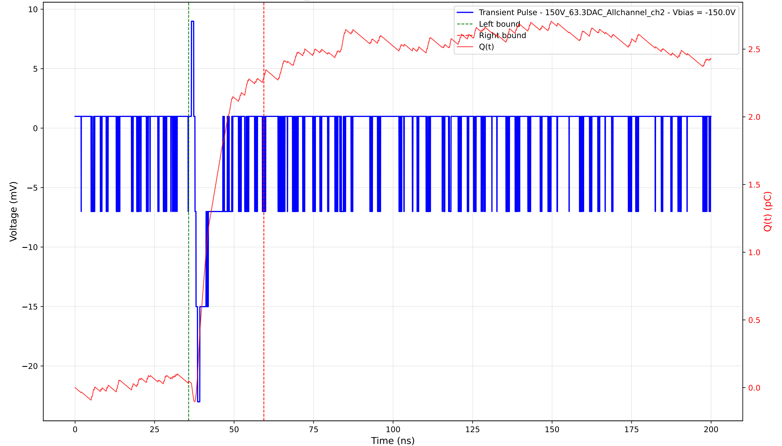
Transient Pulse - Sample: 1cm_42 - Position: 220.0 \mu\text{m} - Charge: 2.24 pC - Rise Time: 0.83 ns
