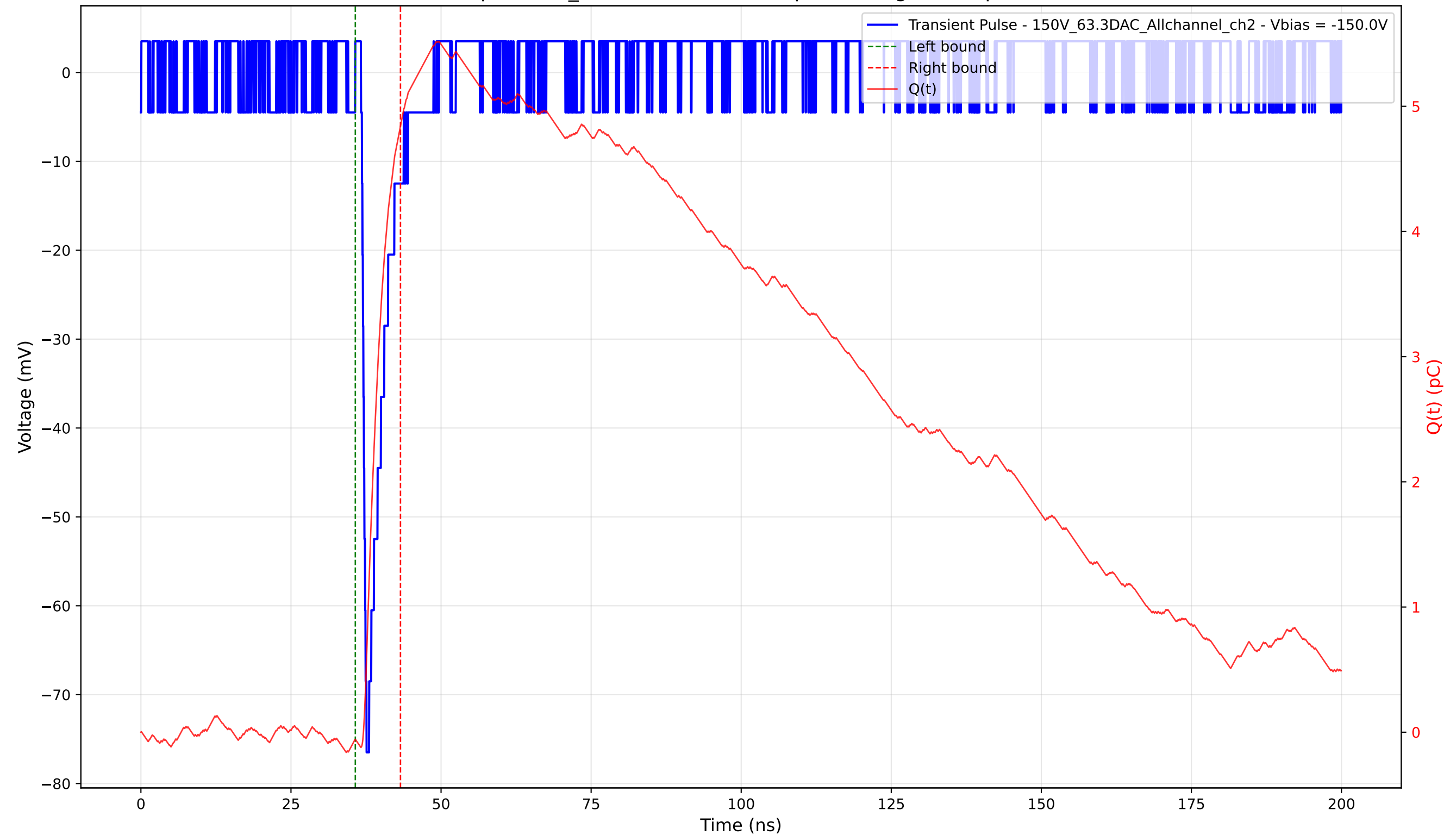
Transient Pulse - Sample: 1cm_42 - Position: 3995.0 \mu\text{m} - Charge: 4.90 pC - Rise Time: 0.78 ns
