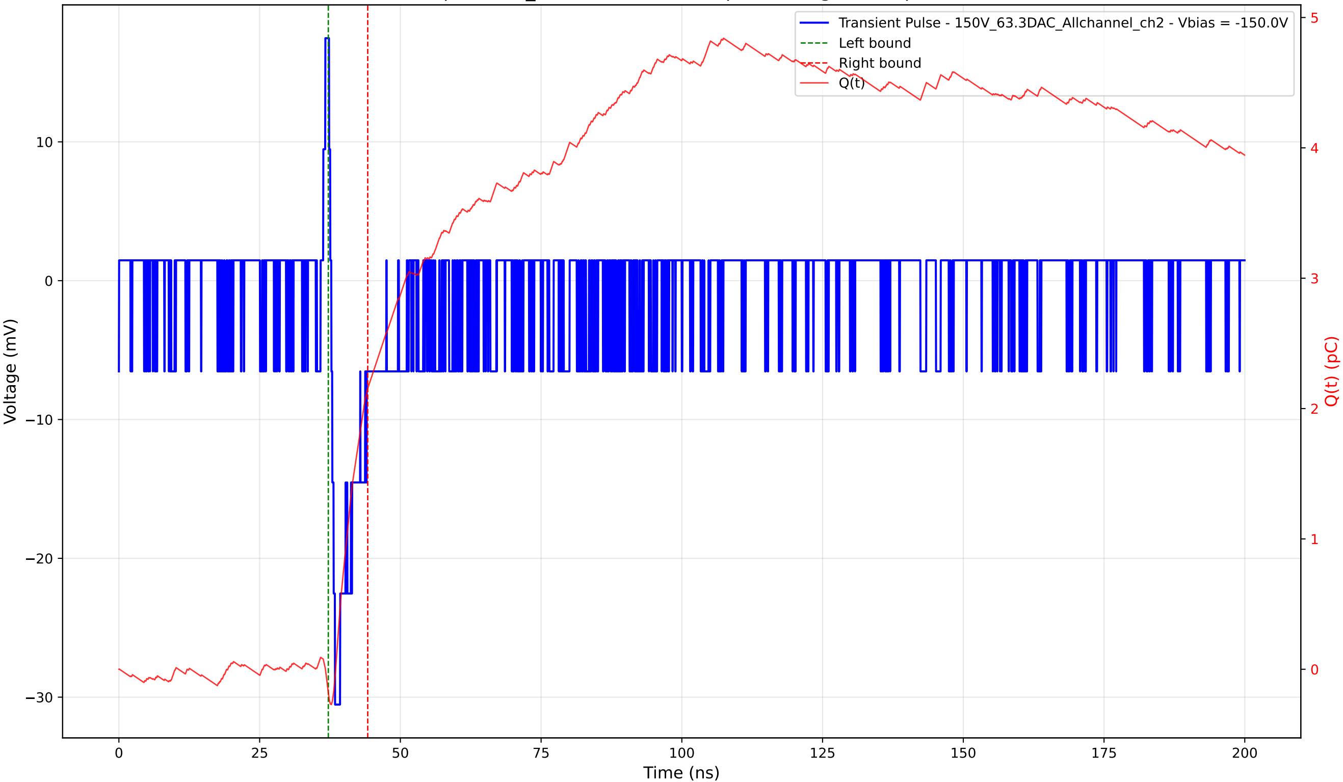
Transient Pulse - Sample: 1cm_42 - Position: 440.0 \mu\text{m} - Charge: 2.33 pC - Rise Time: 0.67 ns
