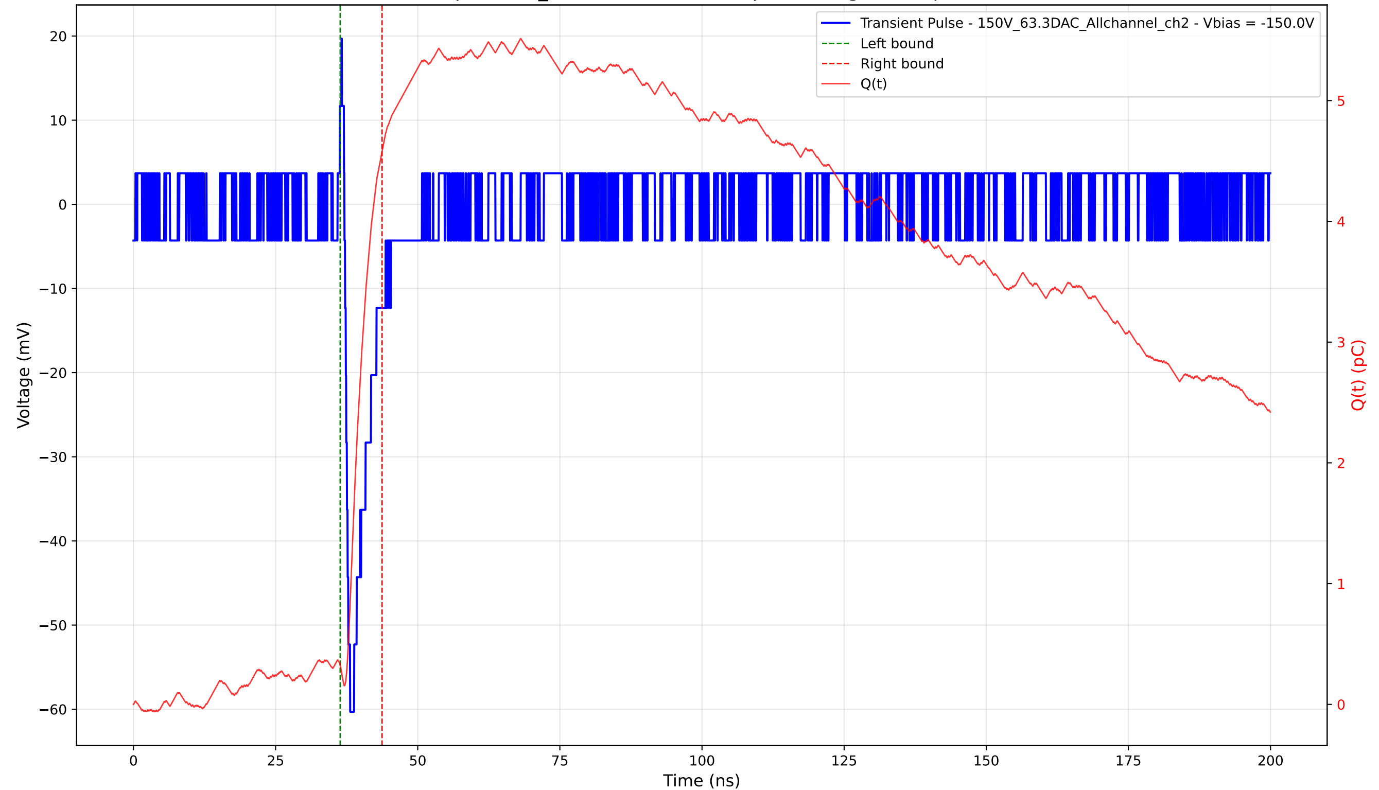
Transient Pulse - Sample: 1cm_42 - Position: 4270.0 \mu\text{m} - Charge: 4.25 pC - Rise Time: 0.91 ns
