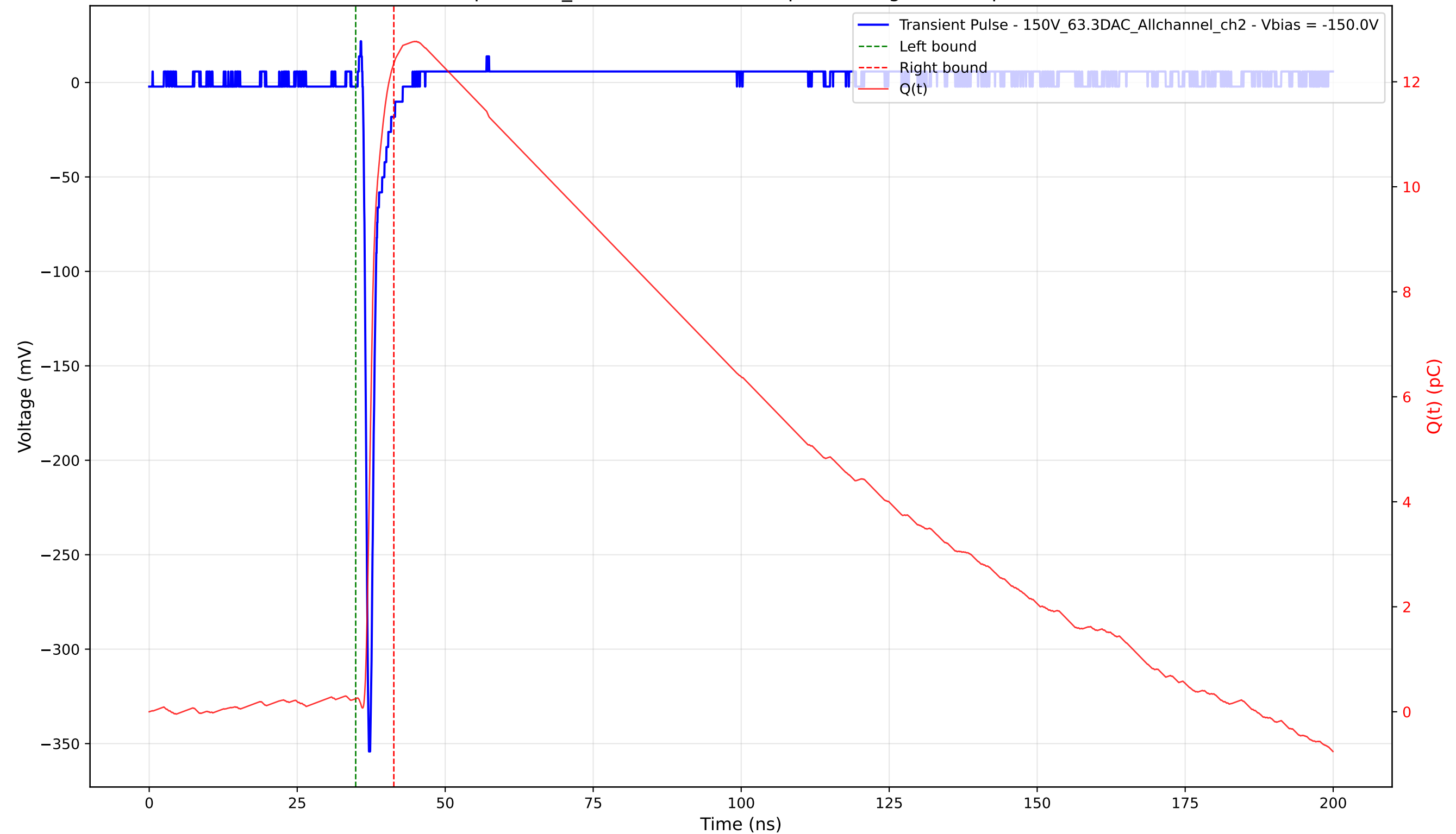
Transient Pulse - Sample: 1cm_42 - Position: 2675.0 \mu\text{m} - Charge: 12.10 pC - Rise Time: 0.72 ns
