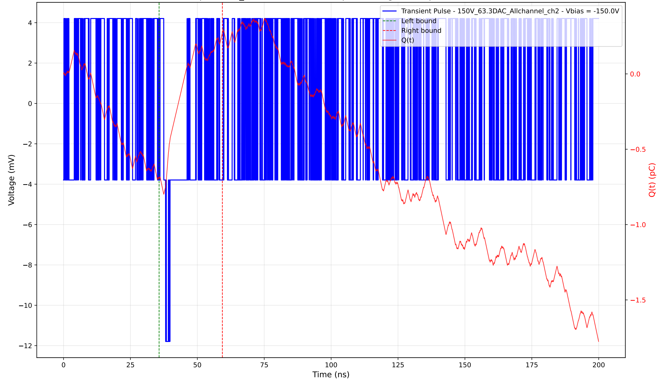
Transient Pulse - Sample: 1cm_42 - Position: 5100.0 \mu\text{m} - Charge: 0.95 pC - Rise Time: 0.00 ns (N/A)
