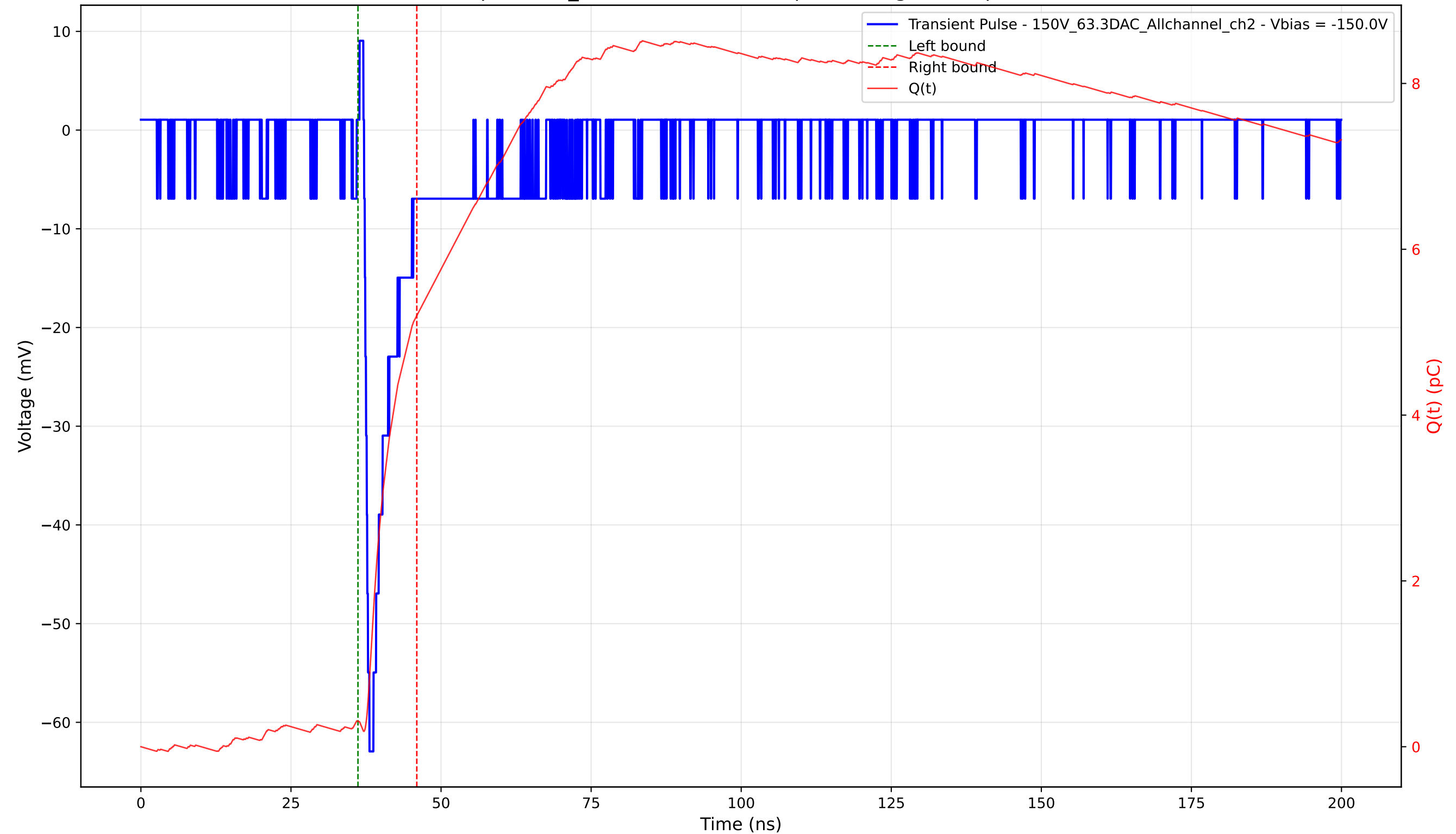
Transient Pulse - Sample: 1cm_42 - Position: 1830.0 \mu\text{m} - Charge: 4.89 pC - Rise Time: 0.88 ns
