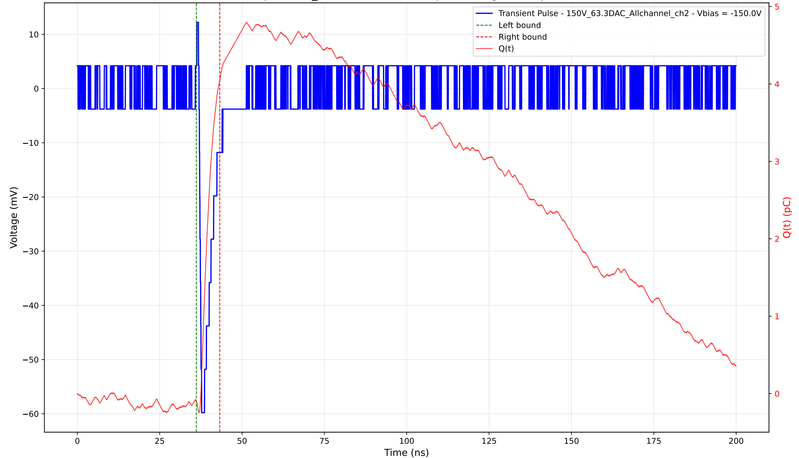
Transient Pulse - Sample: 1cm_42 - Position: 4125.0 \mu\text{m} - Charge: 4.16 pC - Rise Time: 0.71 ns
