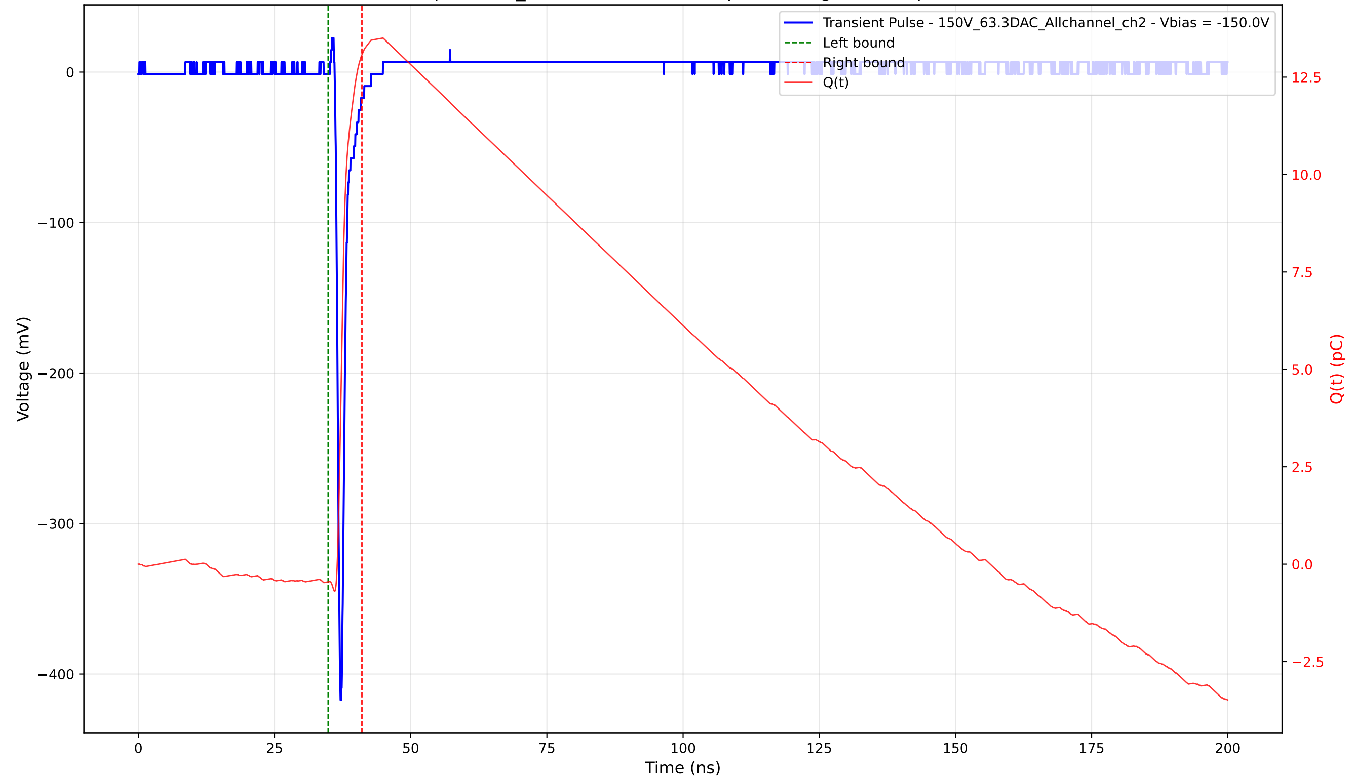
Transient Pulse - Sample: 1cm_42 - Position: 2725.0 \mu\text{m} - Charge: 13.53 pC - Rise Time: 0.71 ns
