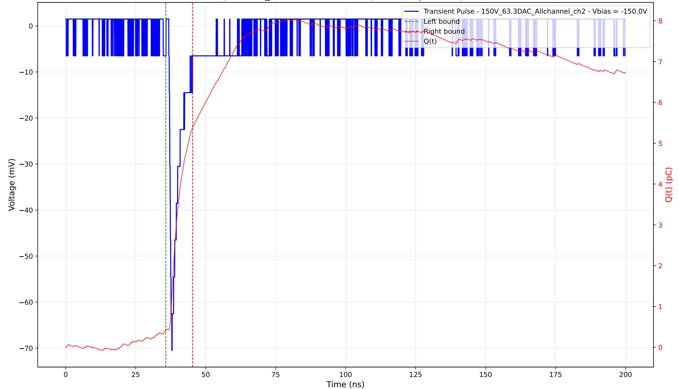
Transient Pulse - Sample: 1cm_42 - Position: 1970.0 \mu\text{m} - Charge: 4.96 pC - Rise Time: 0.96 ns
