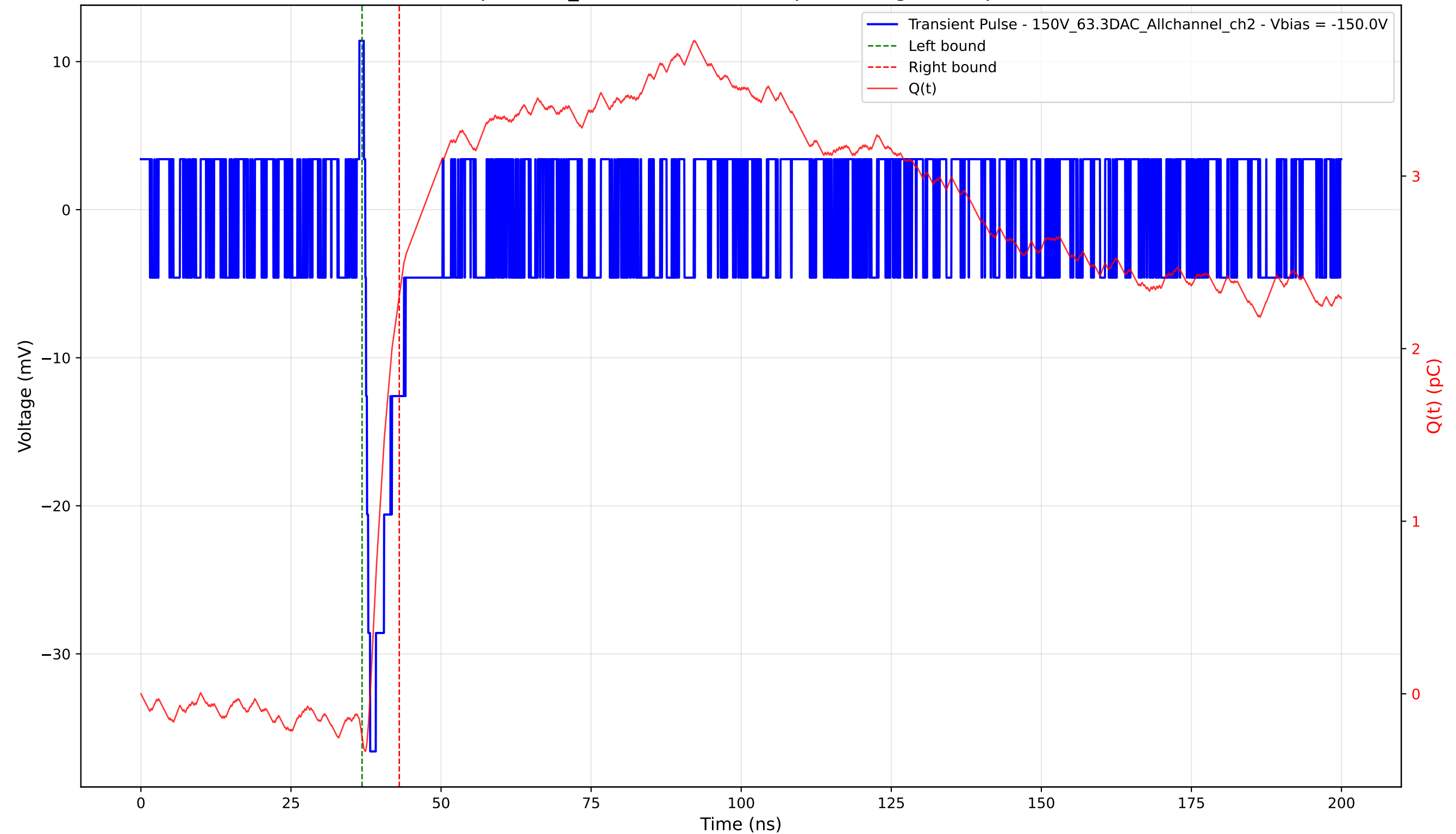
Transient Pulse - Sample: 1cm_42 - Position: 4565.0 \mu\text{m} - Charge: 2.56 pC - Rise Time: 0.83 ns
