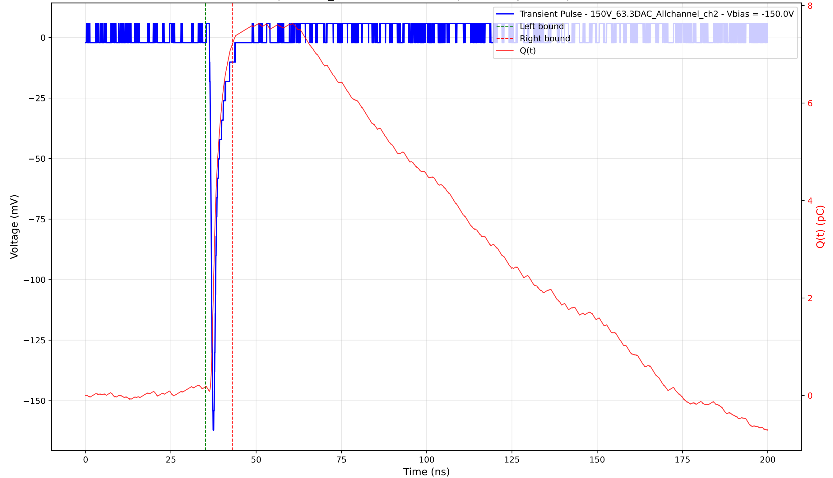
Transient Pulse - Sample: 1cm_42 - Position: 2415.0 \mu\text{m} - Charge: 7.03 pC - Rise Time: 0.77 ns
