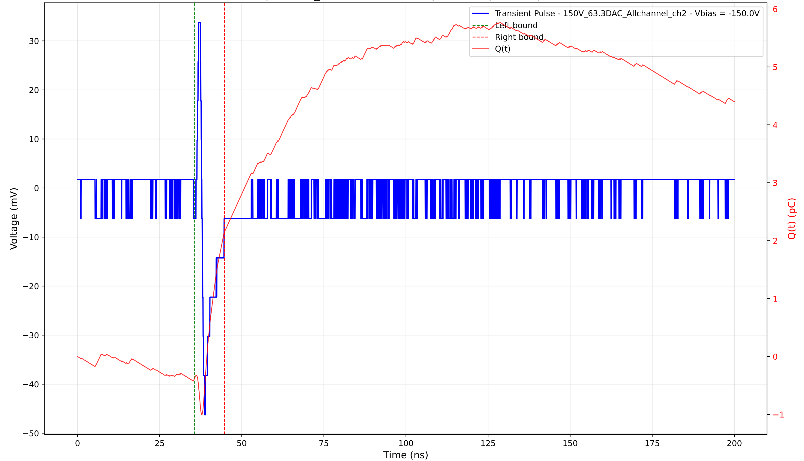
Transient Pulse - Sample: 1cm_42 - Position: 820.0 \mu\text{m} - Charge: 2.53 pC - Rise Time: 0.85 ns
