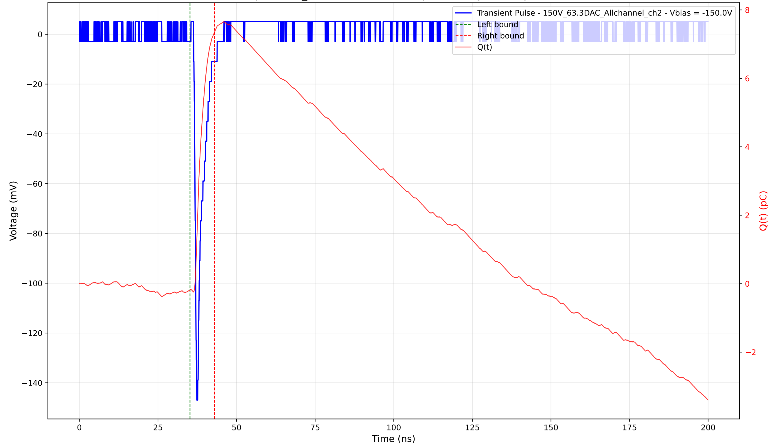
Transient Pulse - Sample: 1cm_42 - Position: 3680.0 \mu\text{m} - Charge: 7.52 pC - Rise Time: 0.82 ns
