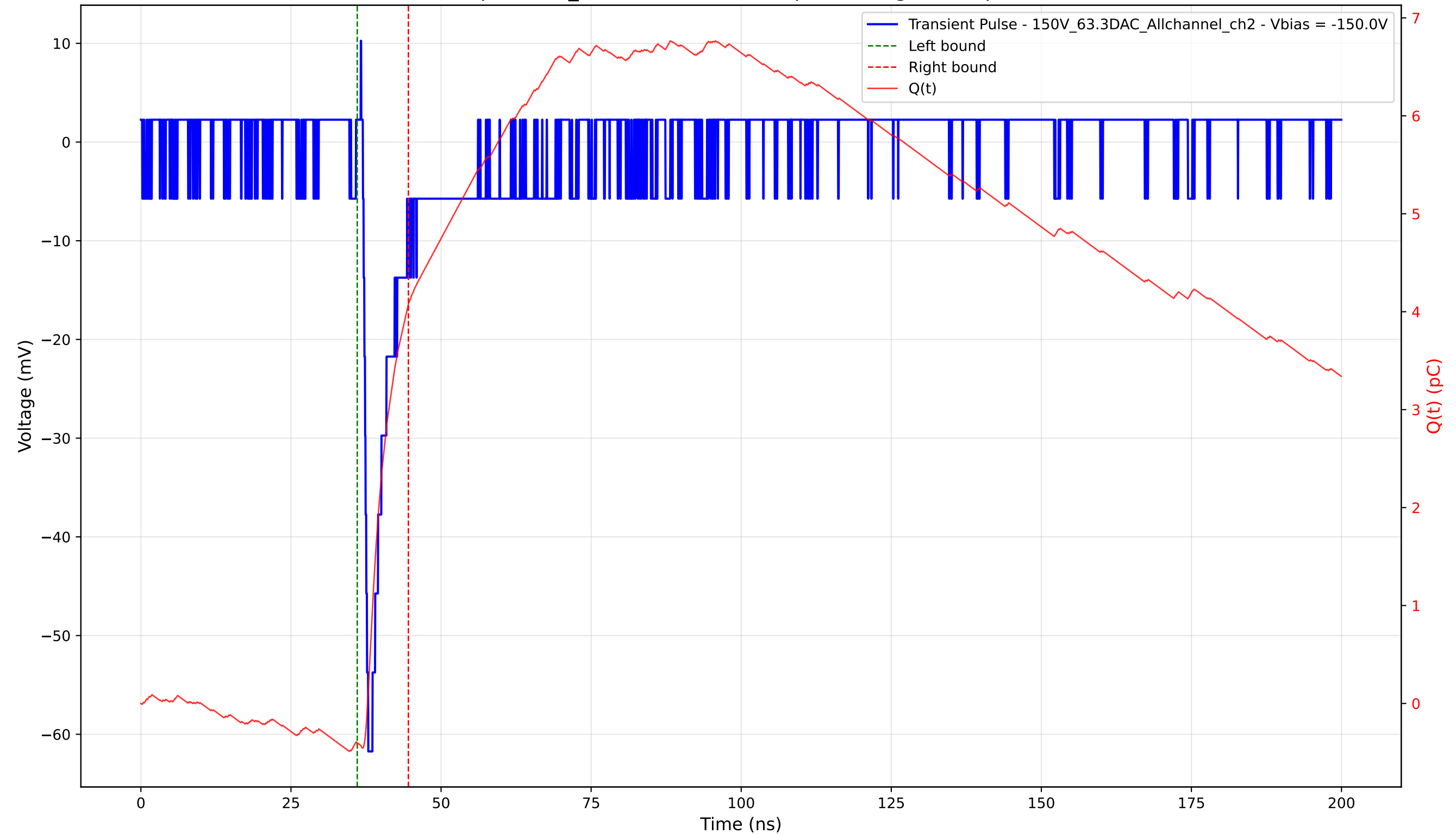
Transient Pulse - Sample: 1cm_42 - Position: 1920.0 \mu\text{m} - Charge: 4.48 pC - Rise Time: 0.80 ns
