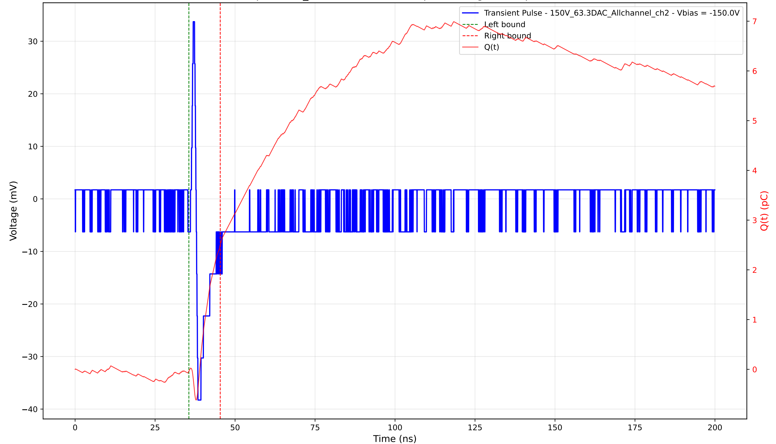
Transient Pulse - Sample: 1cm_42 - Position: 1075.0 \mu\text{m} - Charge: 2.53 pC - Rise Time: 0.54 ns
