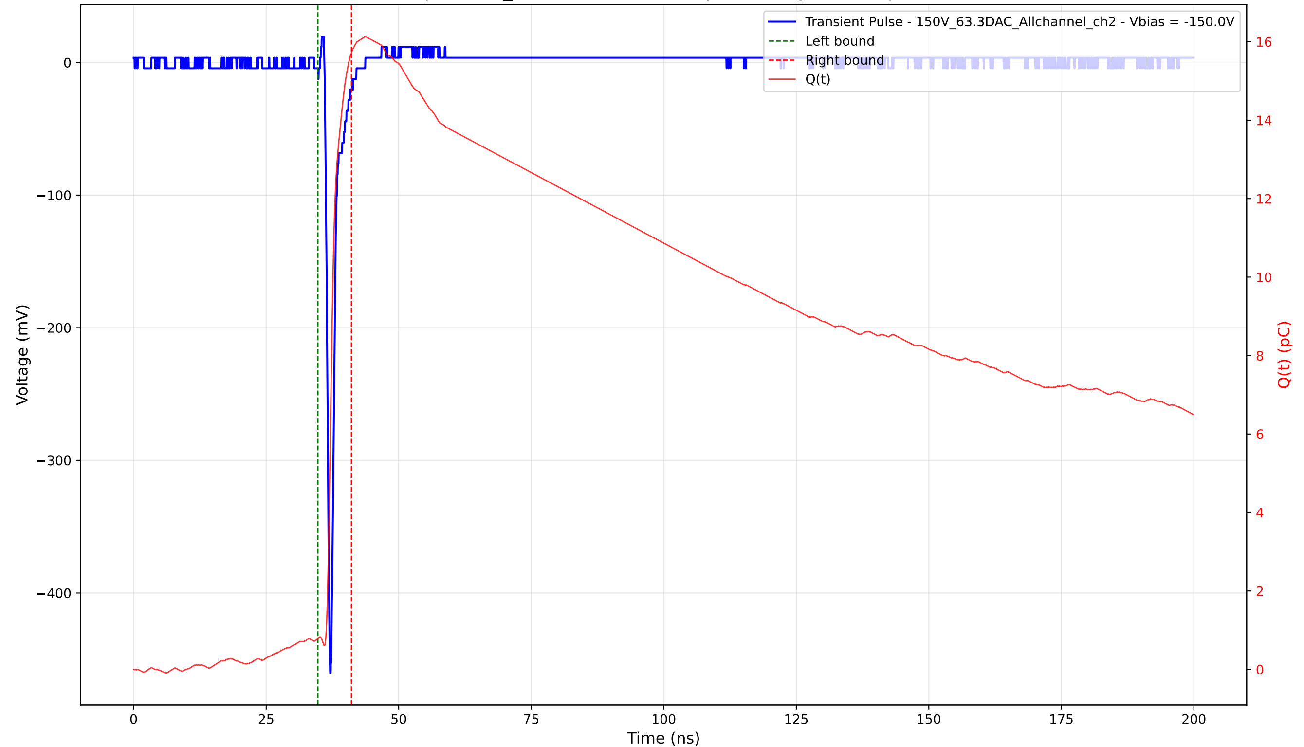
Transient Pulse - Sample: 1cm_42 - Position: 3190.0 \mu\text{m} - Charge: 14.94 pC - Rise Time: 0.71 ns
