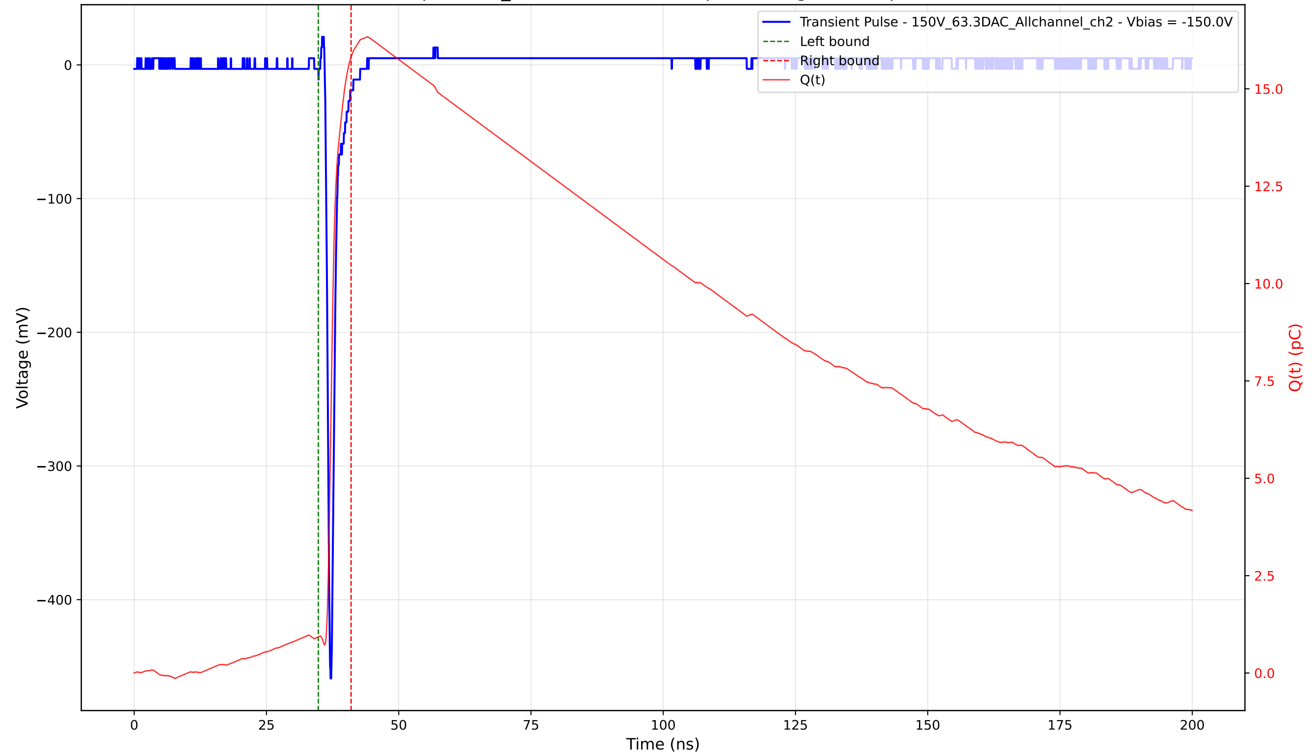
Transient Pulse - Sample: 1cm_42 - Position: 2780.0 \mu\text{m} - Charge: 14.90 pC - Rise Time: 0.72 ns
