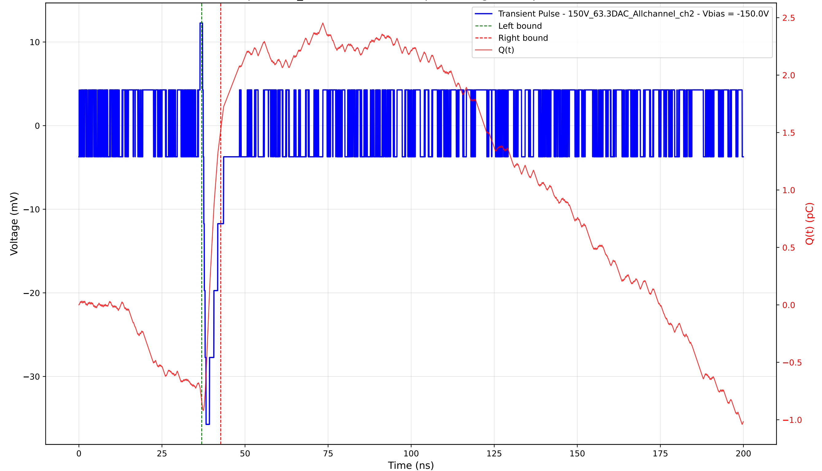
Transient Pulse - Sample: 1cm_42 - Position: 4695.0 \mu\text{m} - Charge: 2.36 pC - Rise Time: 0.00 ns (N/A)
