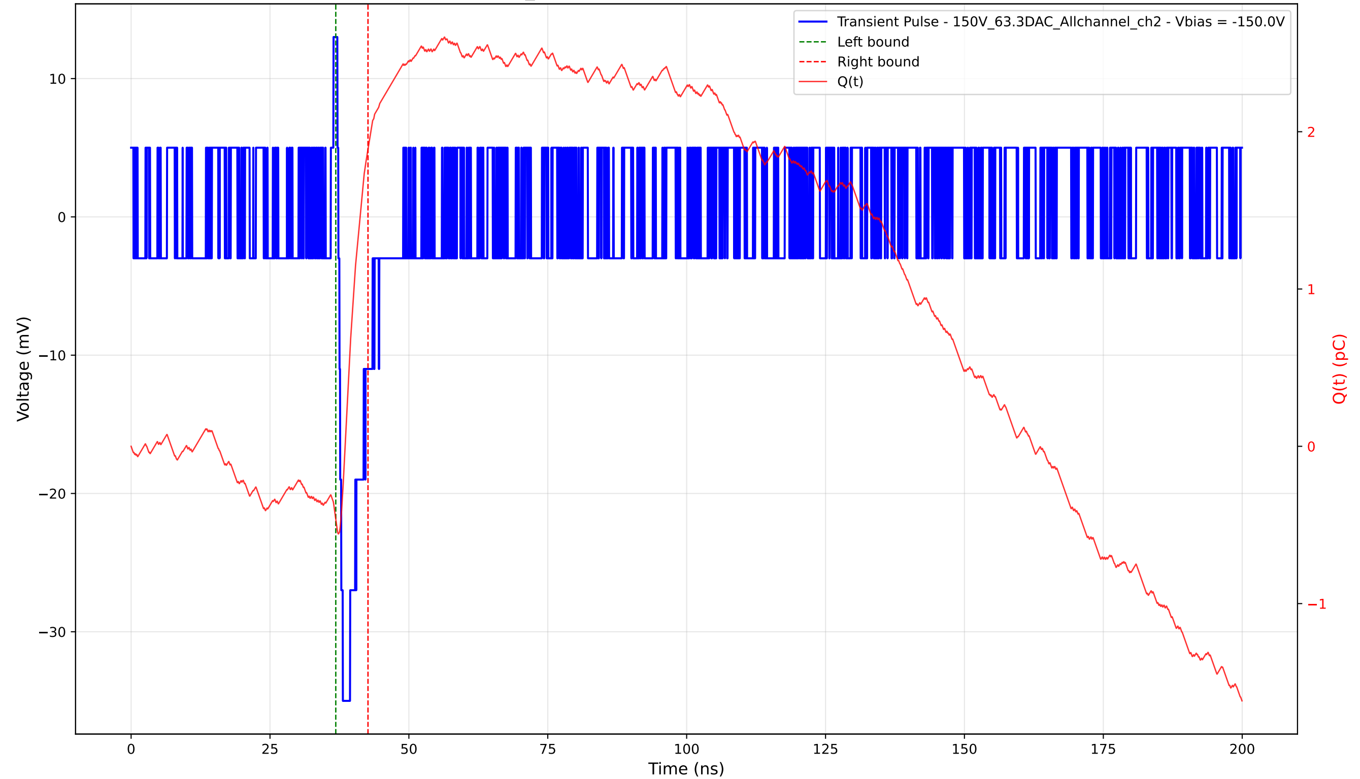
Transient Pulse - Sample: 1cm_42 - Position: 4550.0 \mu\text{m} - Charge: 2.35 pC - Rise Time: 0.64 ns
