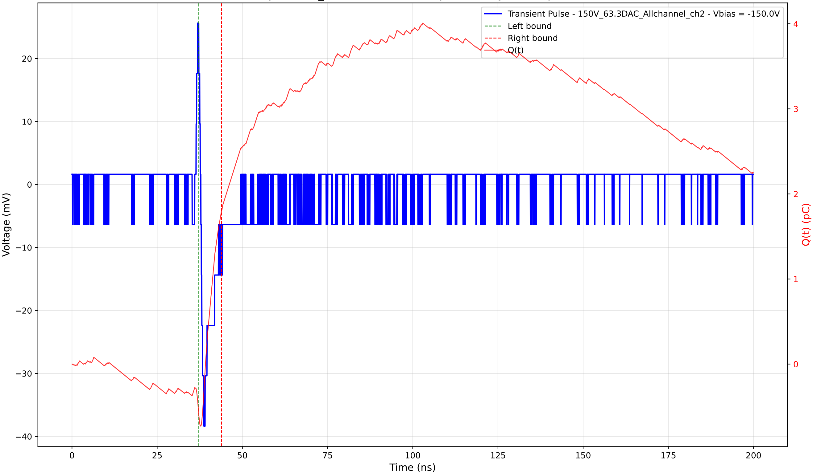
Transient Pulse - Sample: 1cm_42 - Position: 530.0 \mu\text{m} - Charge: 2.40 pC - Rise Time: 0.90 ns
