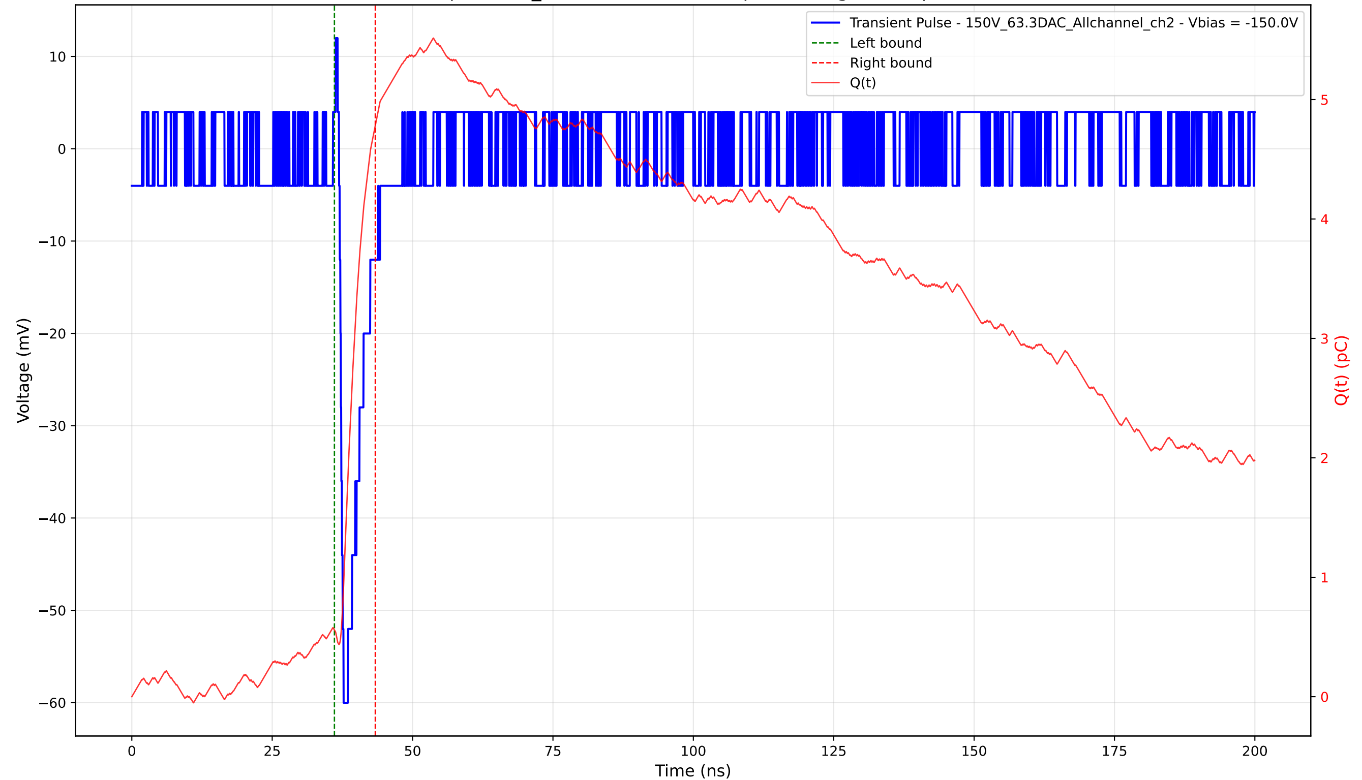
Transient Pulse - Sample: 1cm_42 - Position: 4120.0 \mu\text{m} - Charge: 4.23 pC - Rise Time: 0.71 ns
