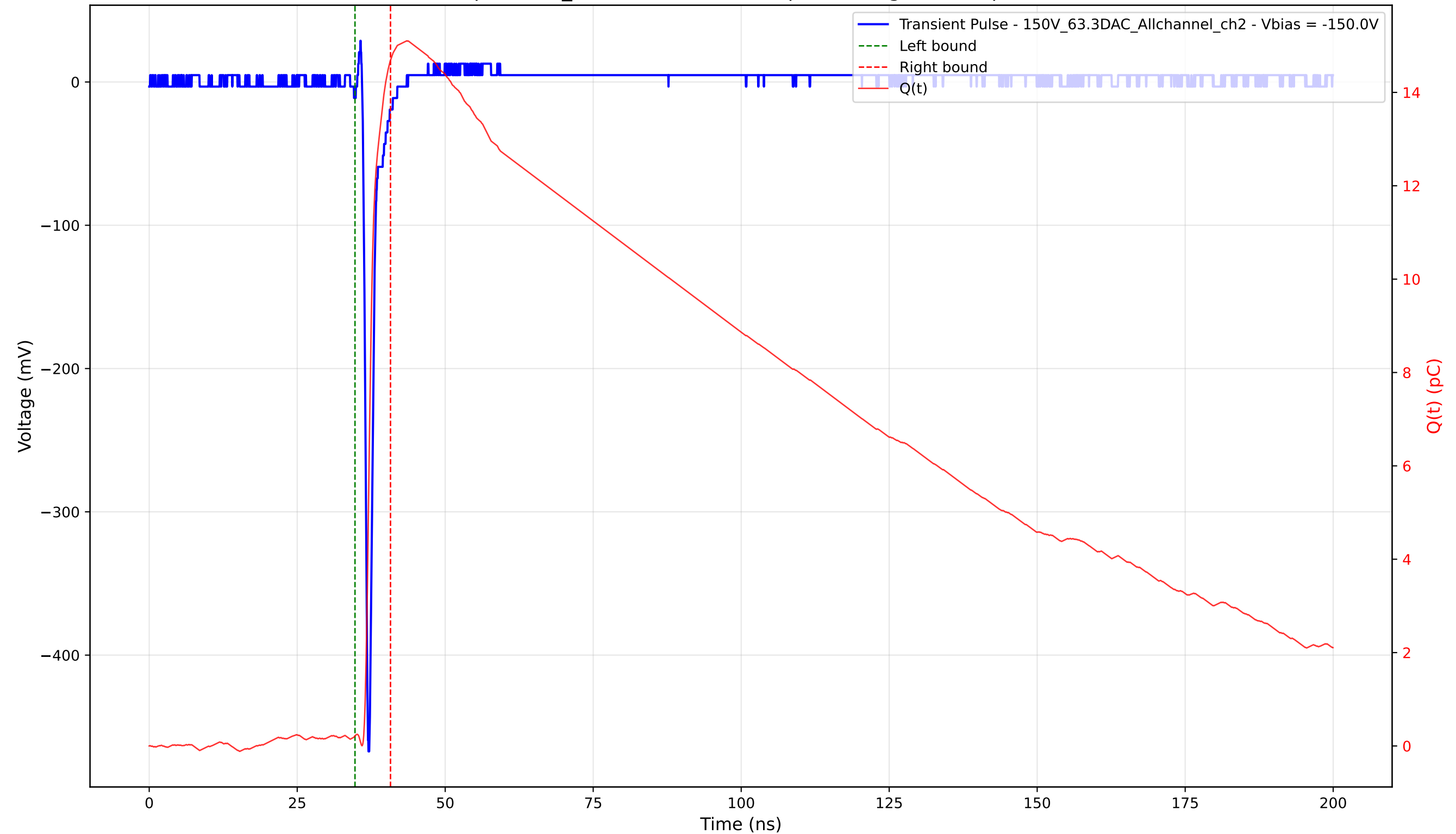
Transient Pulse - Sample: 1cm_42 - Position: 3090.0 \mu\text{m} - Charge: 14.47 pC - Rise Time: 0.68 ns
