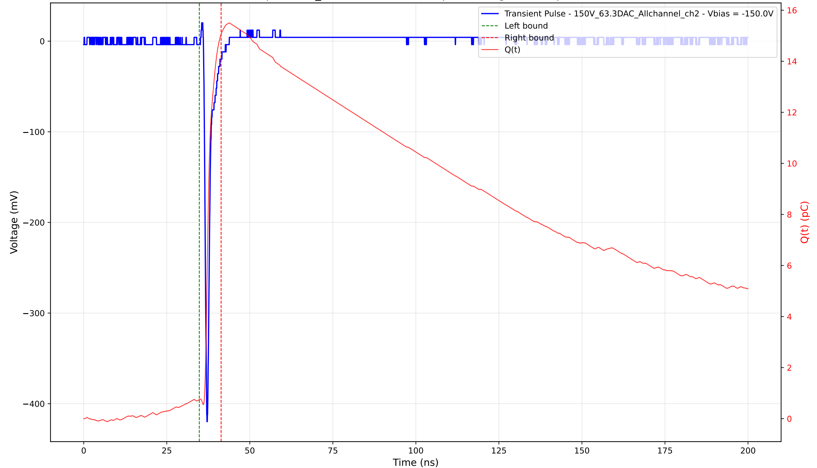
Transient Pulse - Sample: 1cm_42 - Position: 3305.0 \mu\text{m} - Charge: 14.31 pC - Rise Time: 0.72 ns
