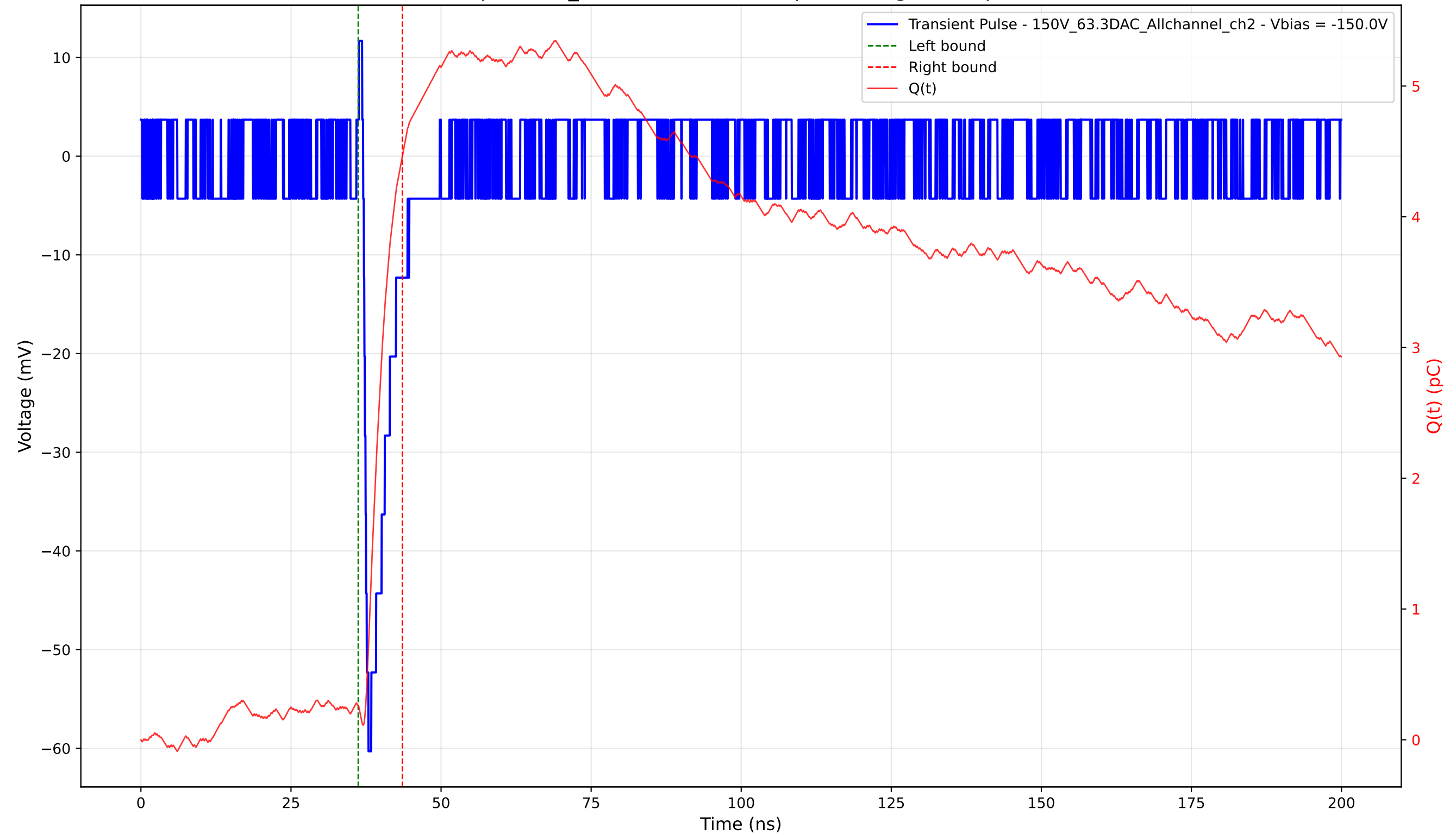
Transient Pulse - Sample: 1cm_42 - Position: 4170.0 \mu\text{m} - Charge: 4.20 pC - Rise Time: 0.79 ns
