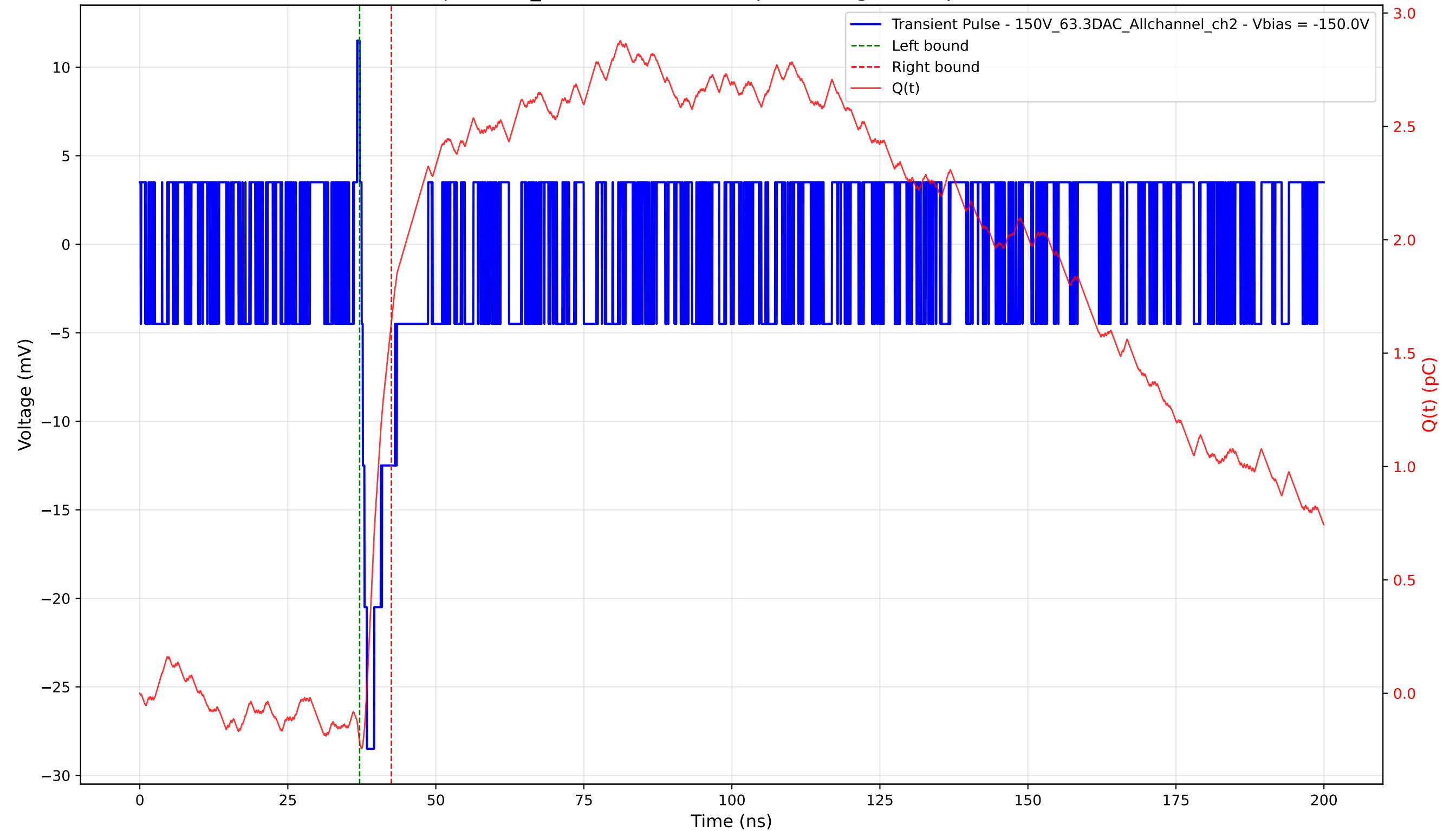
Transient Pulse - Sample: 1cm_42 - Position: 4925.0 \mu\text{m} - Charge: 1.85 pC - Rise Time: 0.00 ns (N/A)
