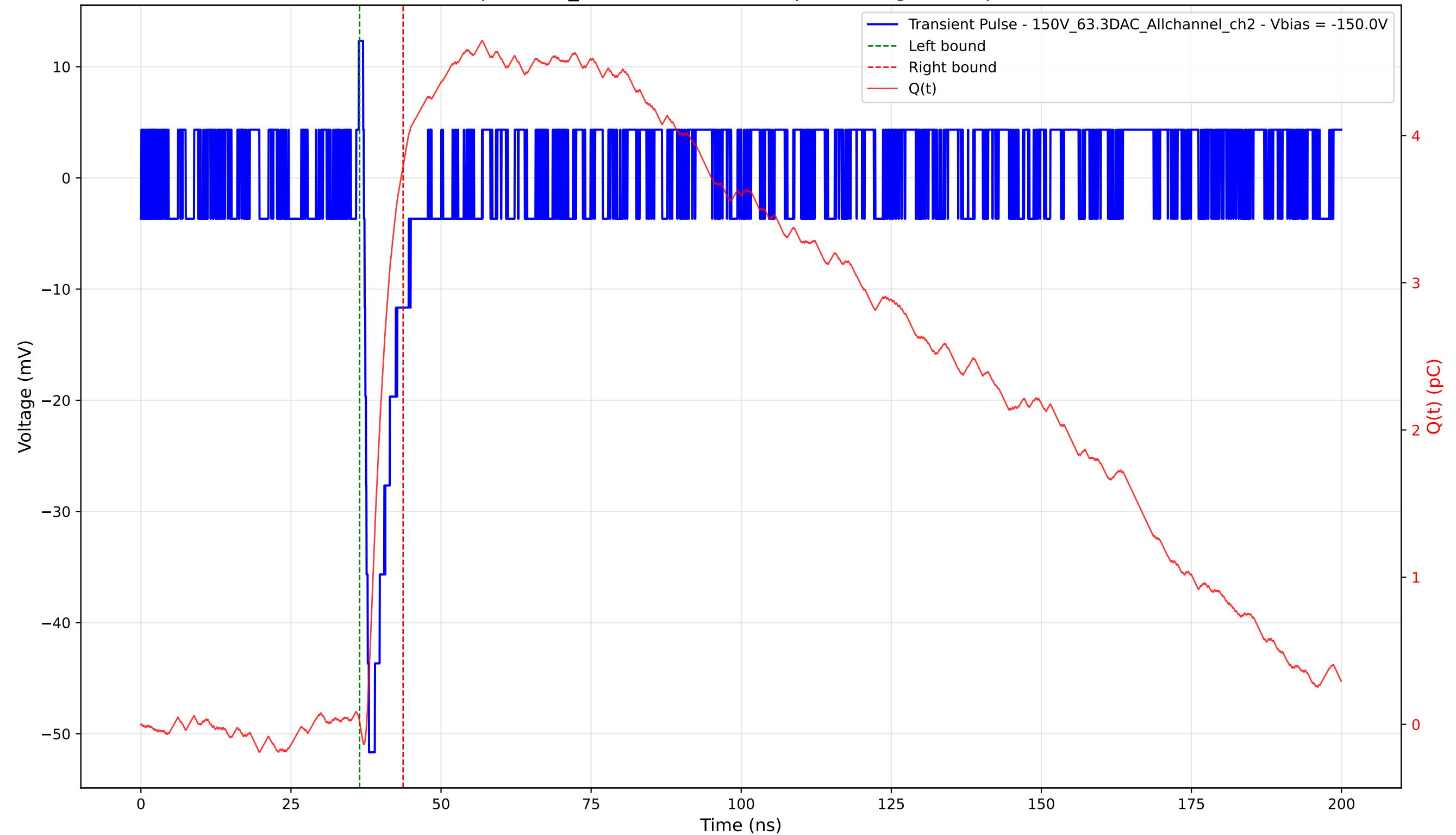
Transient Pulse - Sample: 1cm_42 - Position: 4360.0 \mu\text{m} - Charge: 3.78 pC - Rise Time: 0.75 ns
