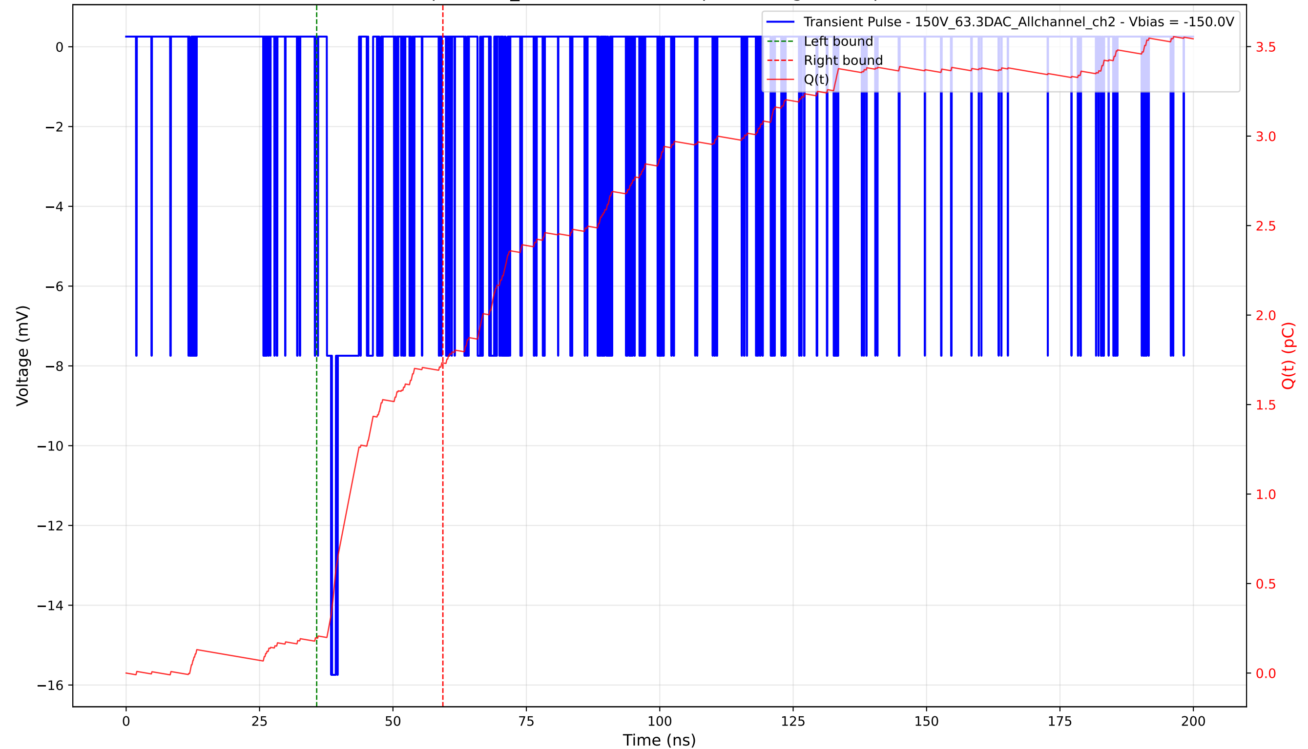
Transient Pulse - Sample: 1cm_42 - Position: 120.0 \mu\text{m} - Charge: 1.54 pC - Rise Time: 0.83 ns
