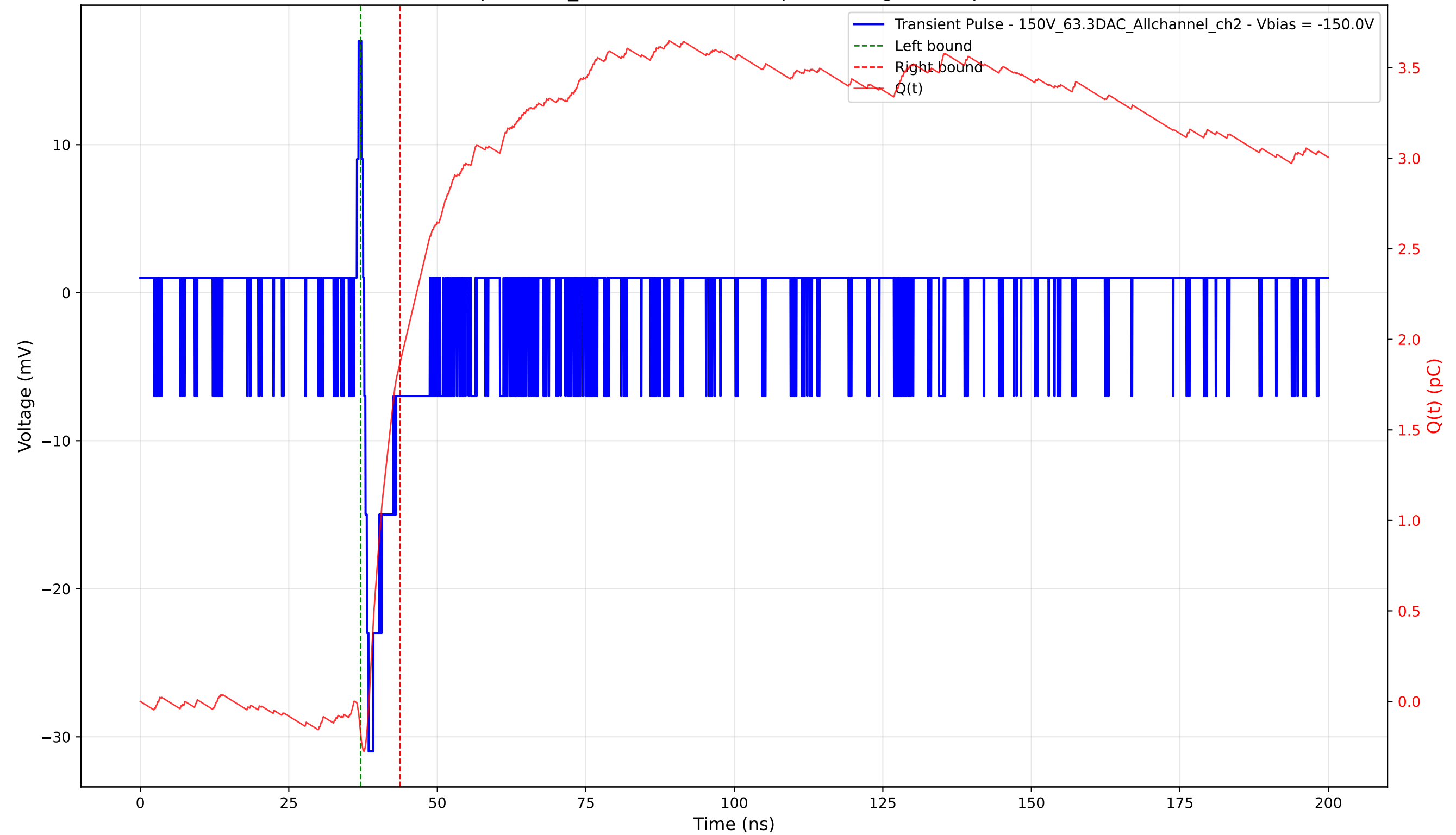
Transient Pulse - Sample: 1cm_42 - Position: 410.0 \mu\text{m} - Charge: 2.04 pC - Rise Time: 0.75 ns
