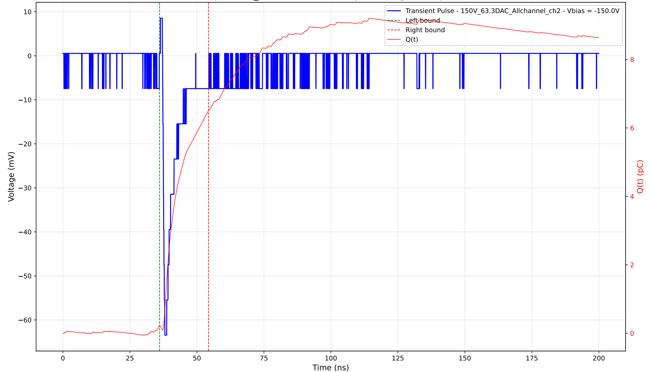
Transient Pulse - Sample: 1cm_42 - Position: 1805.0 \mu\text{m} - Charge: 6.30 pC - Rise Time: 0.81 ns
