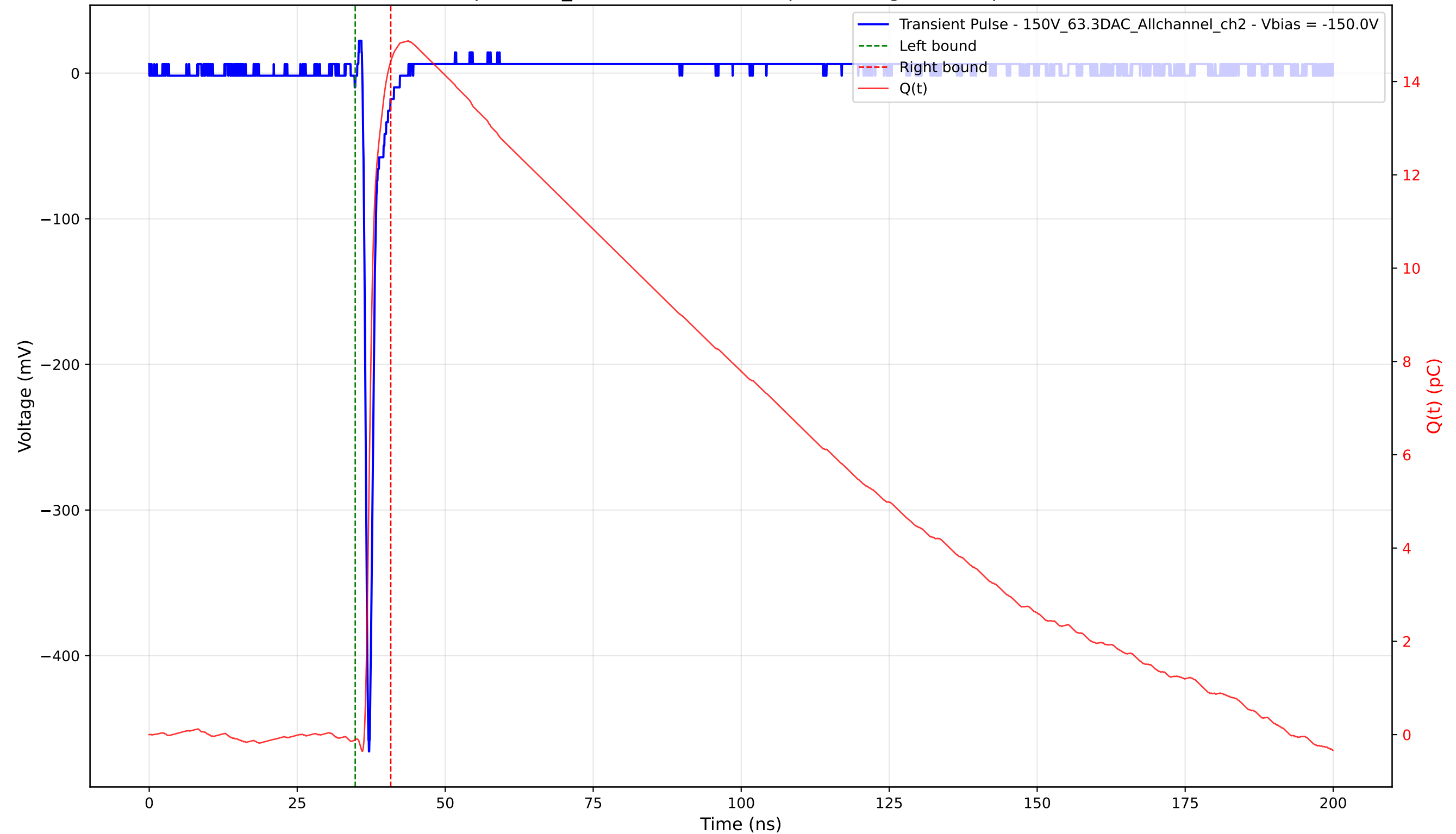
Transient Pulse - Sample: 1cm_42 - Position: 2850.0 \mu\text{m} - Charge: 14.54 pC - Rise Time: 0.75 ns
