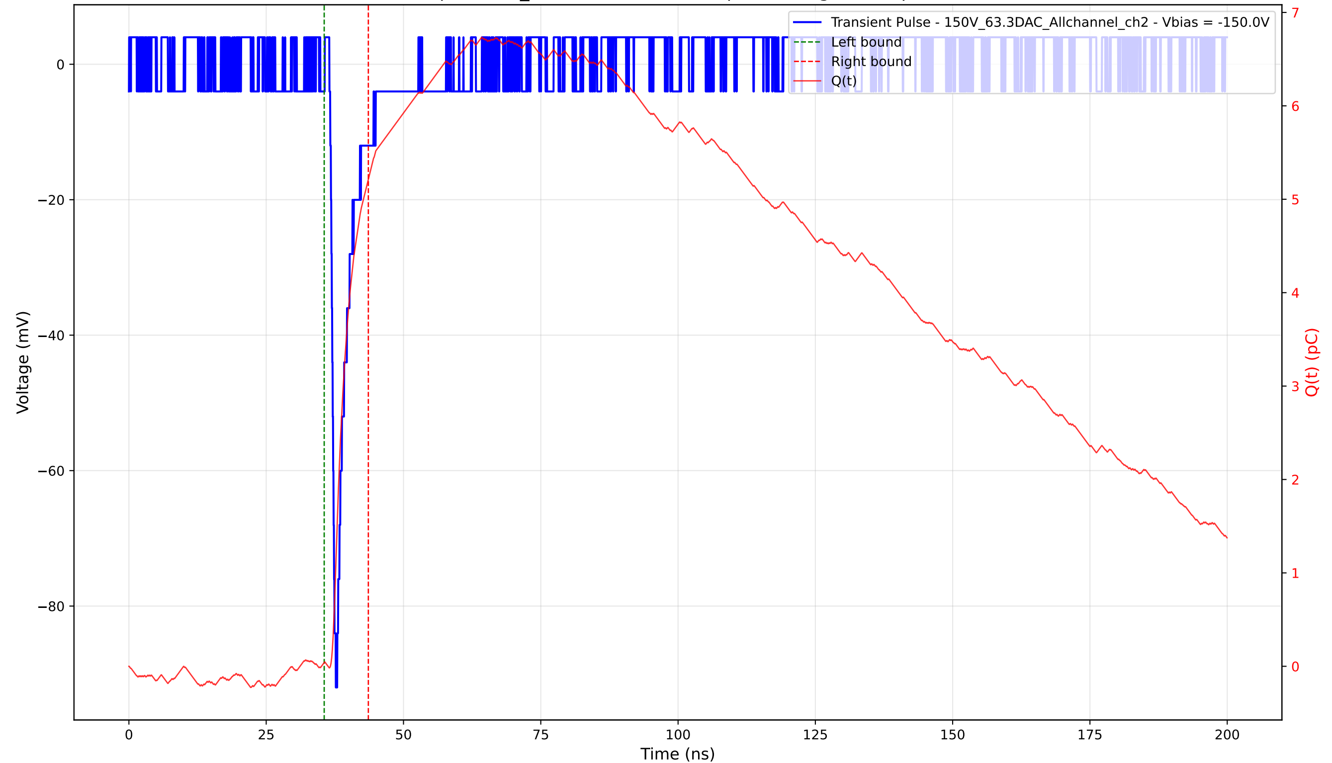
Transient Pulse - Sample: 1cm_42 - Position: 2095.0 \mu\text{m} - Charge: 5.17 pC - Rise Time: 0.77 ns
