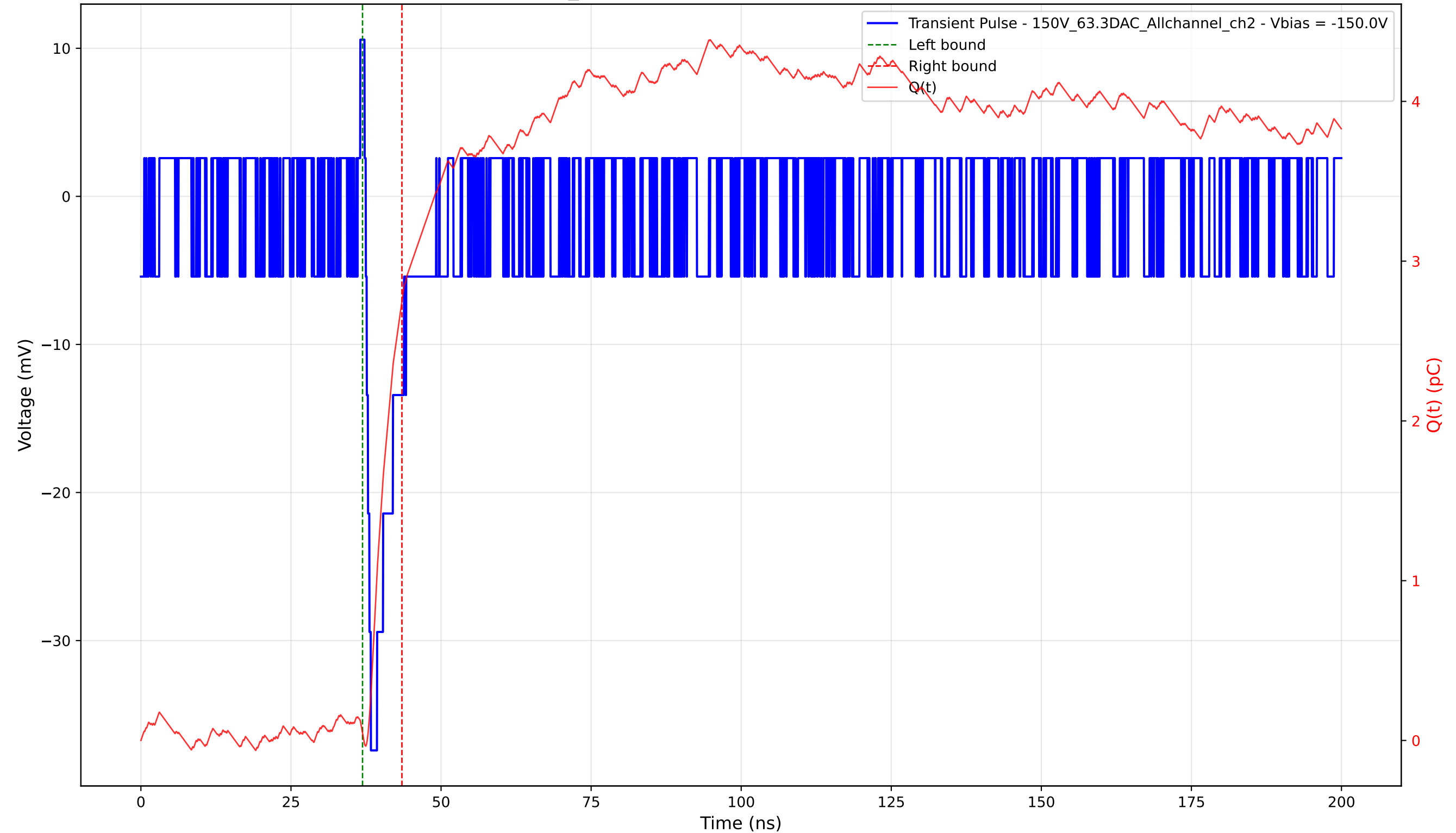
Transient Pulse - Sample: 1cm_42 - Position: 4830.0 \mu\text{m} - Charge: 2.70 pC - Rise Time: 0.86 ns
