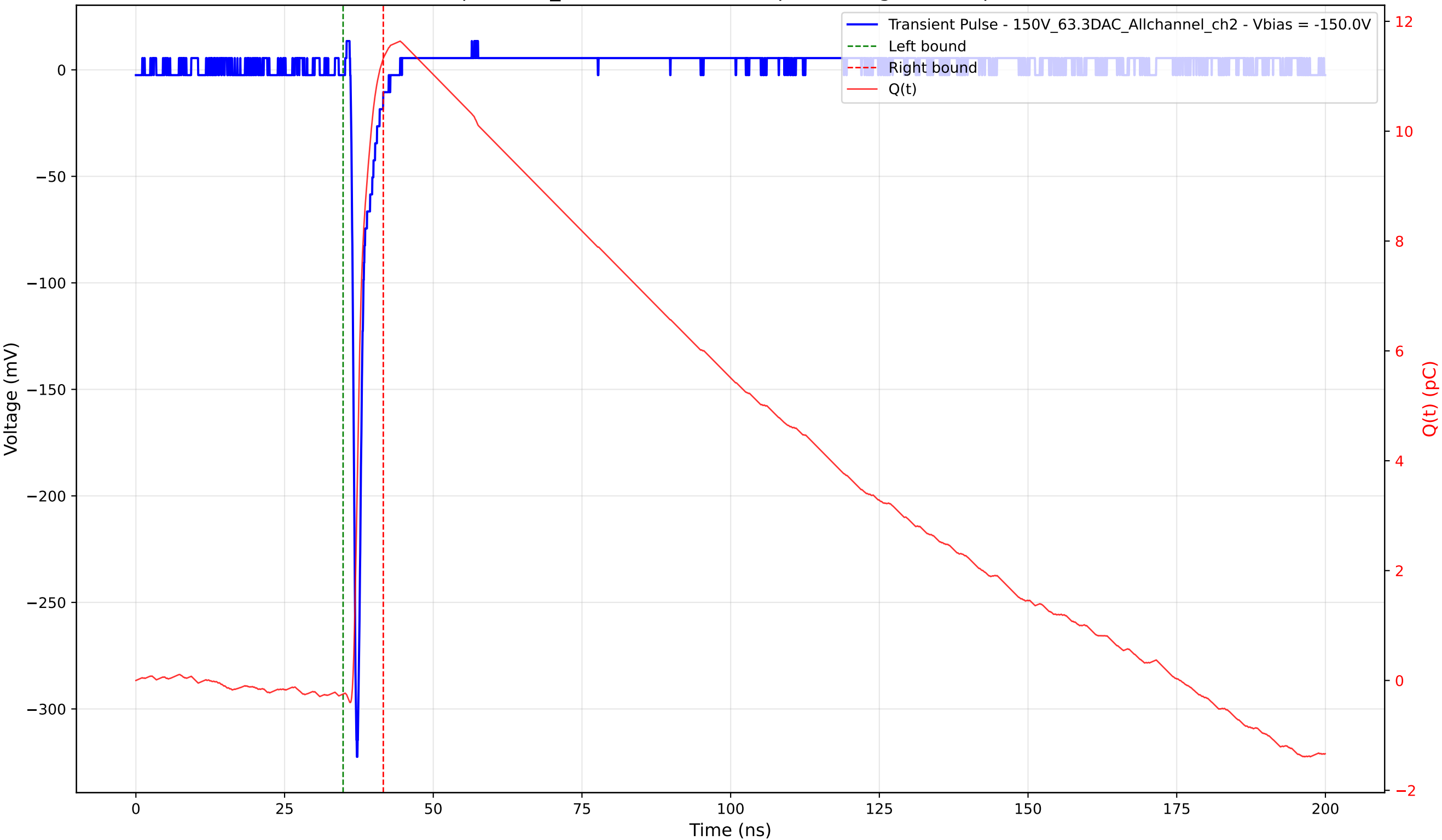
Transient Pulse - Sample: 1cm_42 - Position: 3405.0 \mu\text{m} - Charge: 11.58 pC - Rise Time: 0.73 ns
