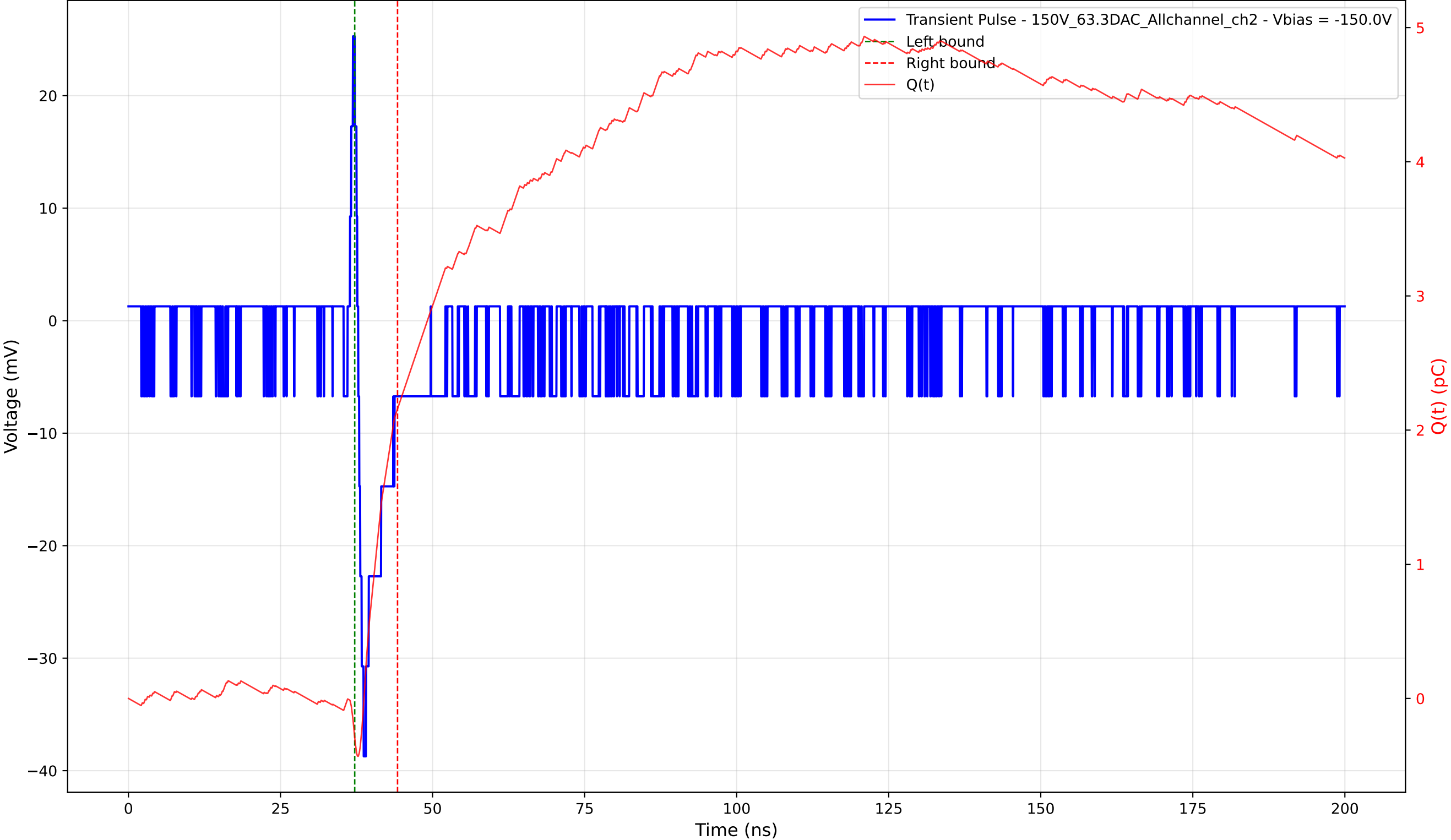
Transient Pulse - Sample: 1cm_42 - Position: 510.0 \mu\text{m} - Charge: 2.46 pC - Rise Time: 0.90 ns
