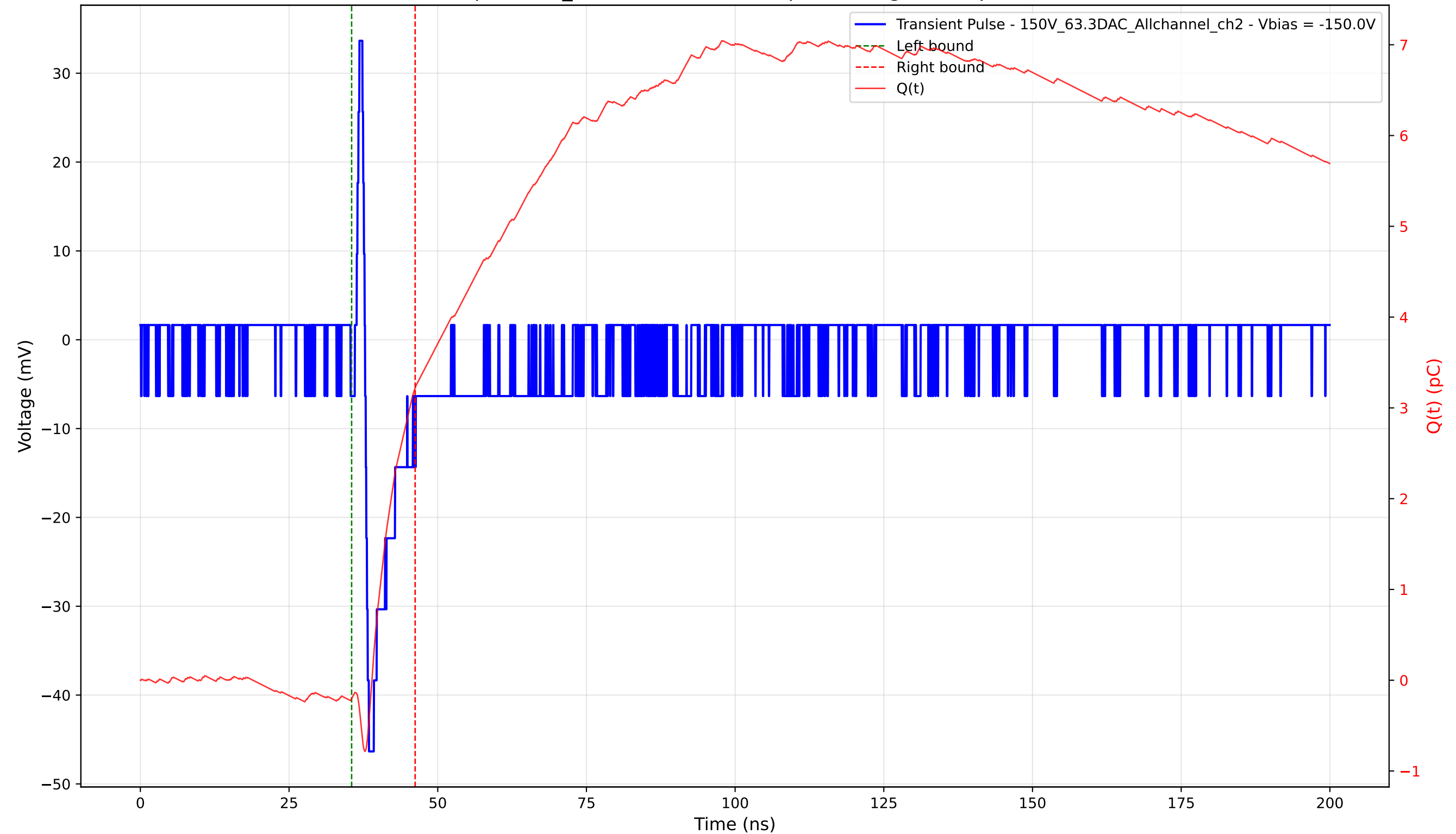
Transient Pulse - Sample: 1cm_42 - Position: 1275.0 \mu\text{m} - Charge: 3.42 pC - Rise Time: 0.65 ns
