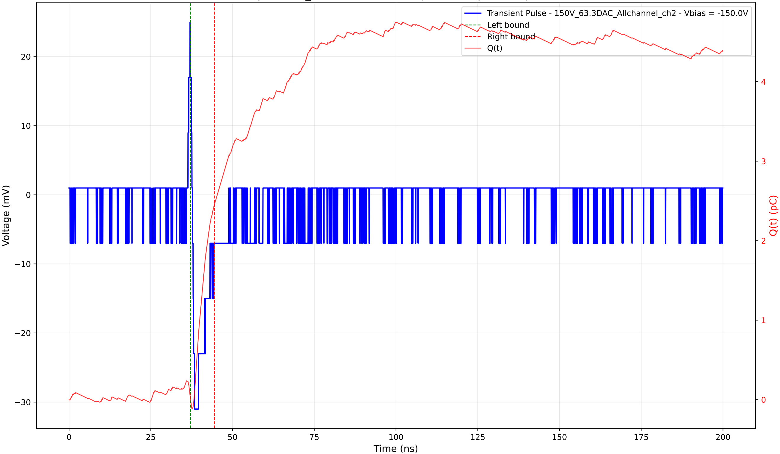
Transient Pulse - Sample: 1cm_42 - Position: 490.0 \mu\text{m} - Charge: 2.44 pC - Rise Time: 0.67 ns
