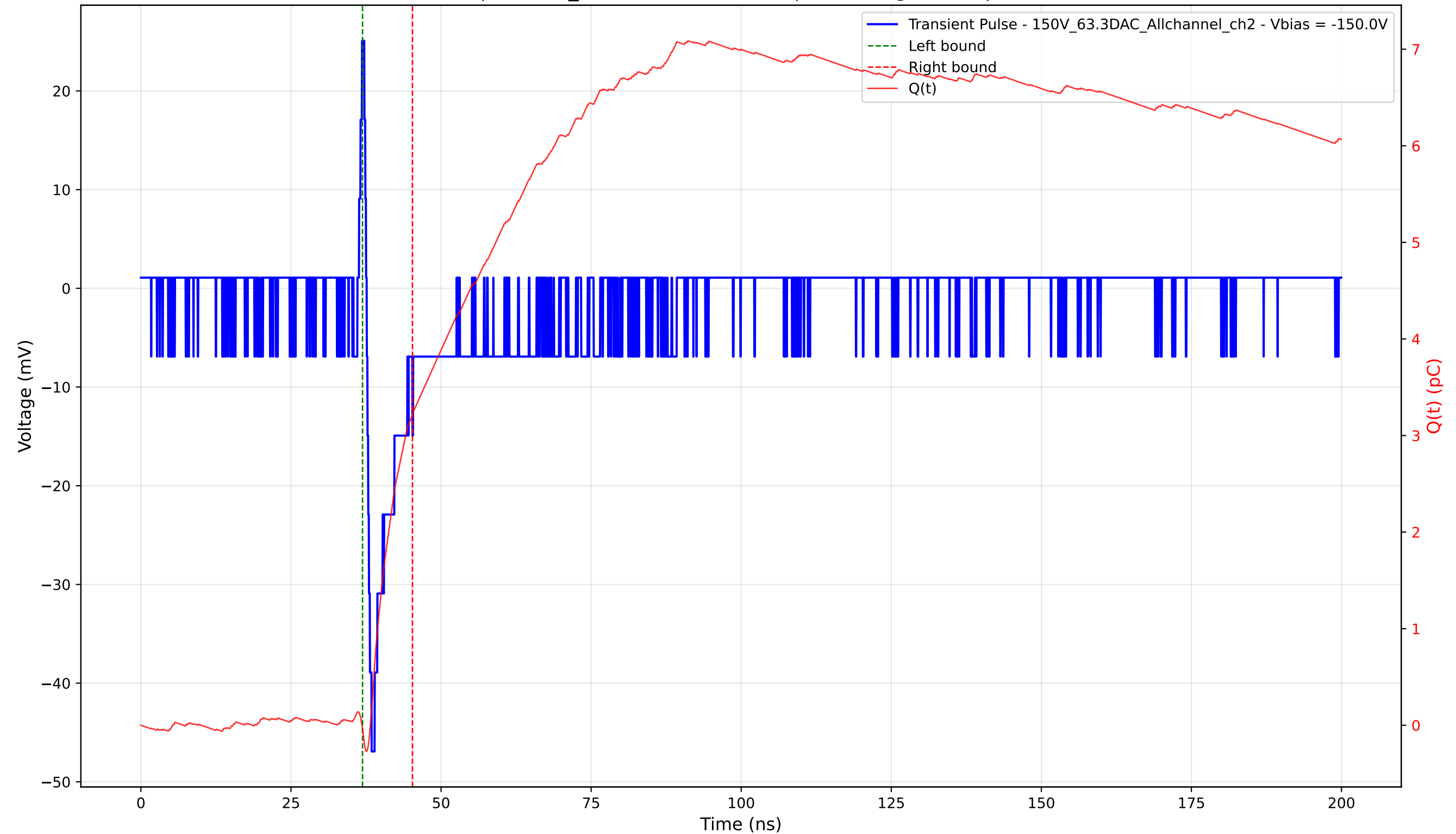
Transient Pulse - Sample: 1cm_42 - Position: 1485.0 \mu\text{m} - Charge: 3.25 pC - Rise Time: 0.82 ns
