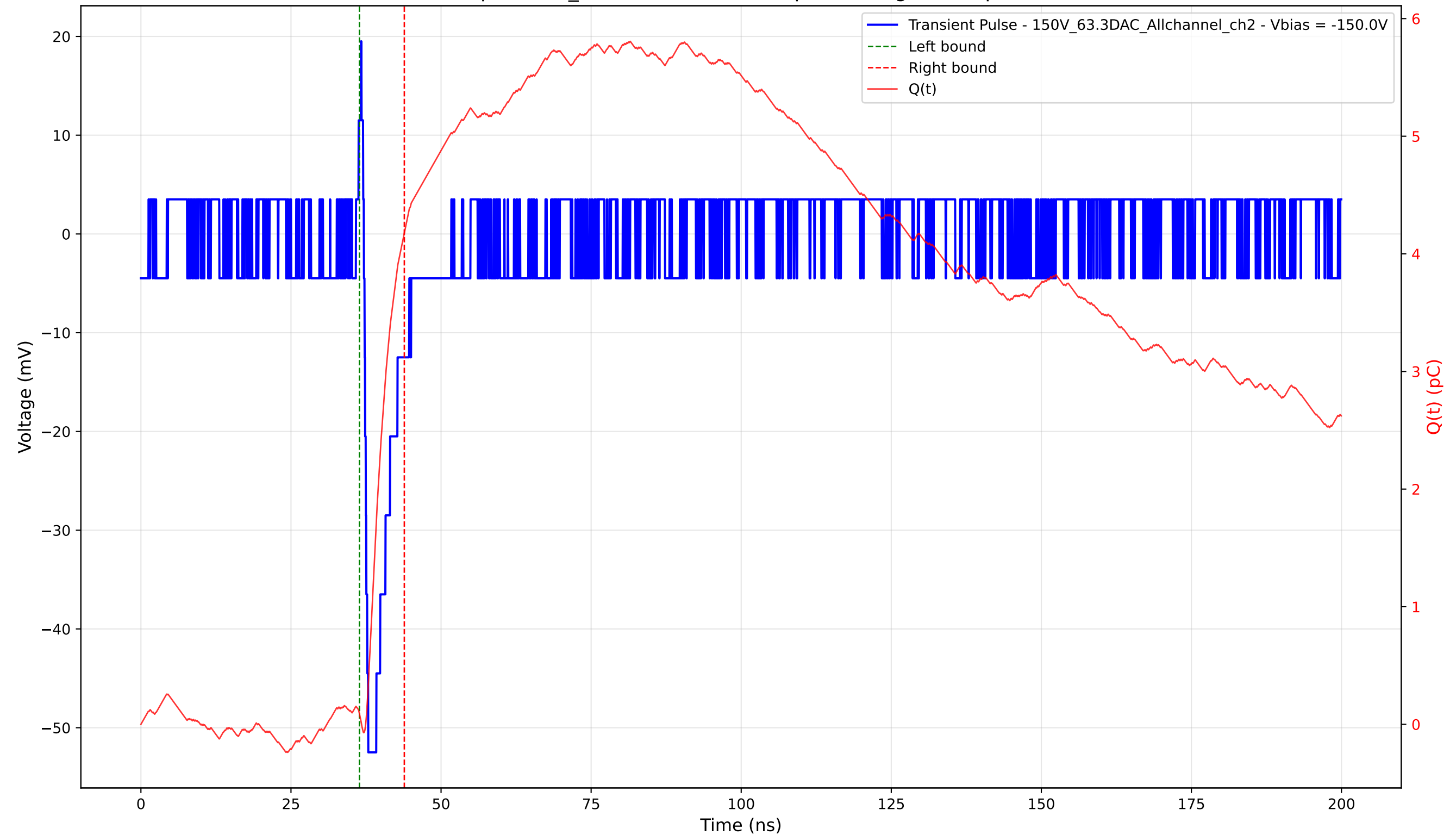
Transient Pulse - Sample: 1cm_42 - Position: 4325.0 \mu\text{m} - Charge: 4.09 pC - Rise Time: 0.64 ns
