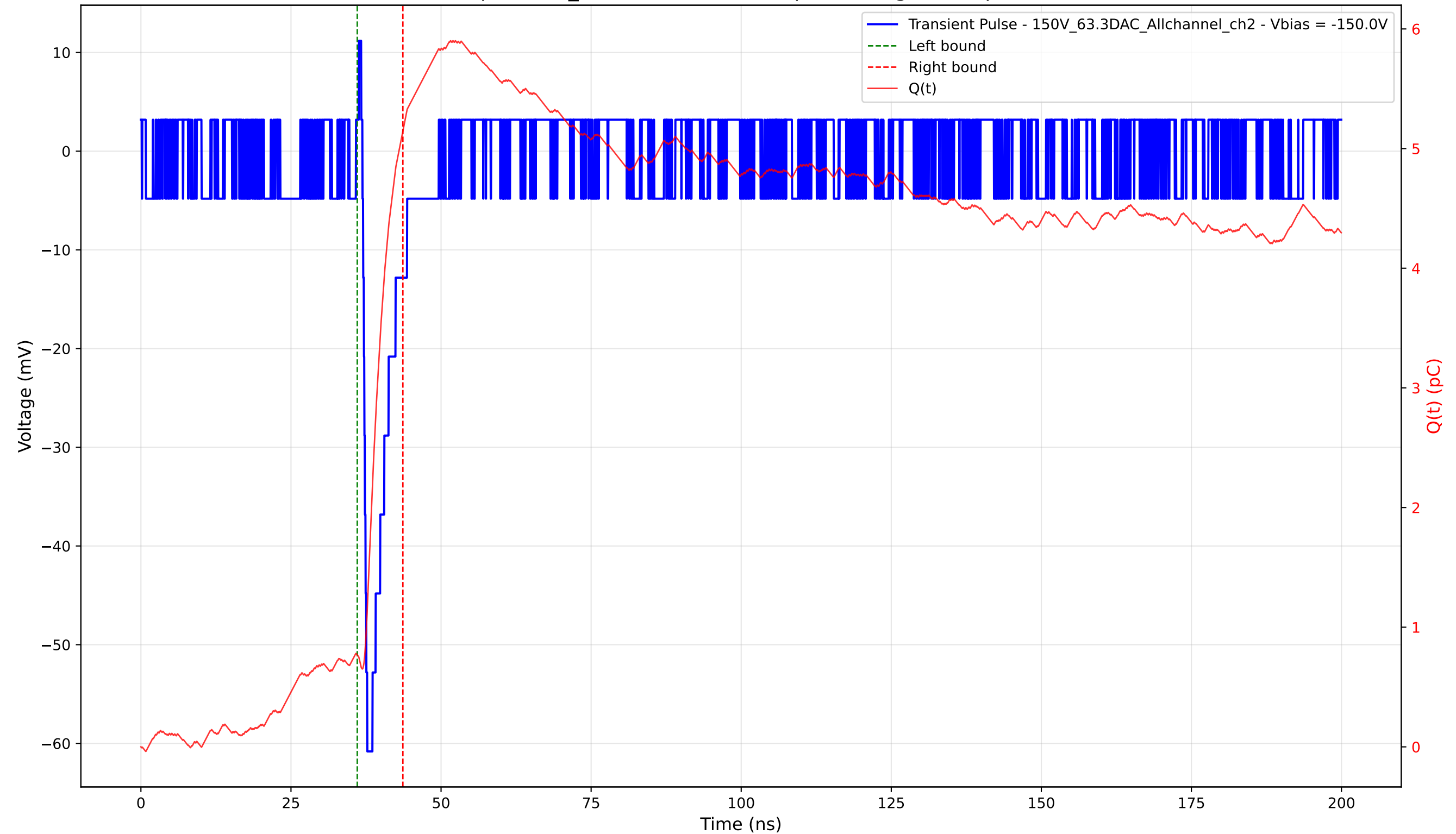
Transient Pulse - Sample: 1cm_42 - Position: 4105.0 \mu\text{m} - Charge: 4.38 pC - Rise Time: 0.71 ns
