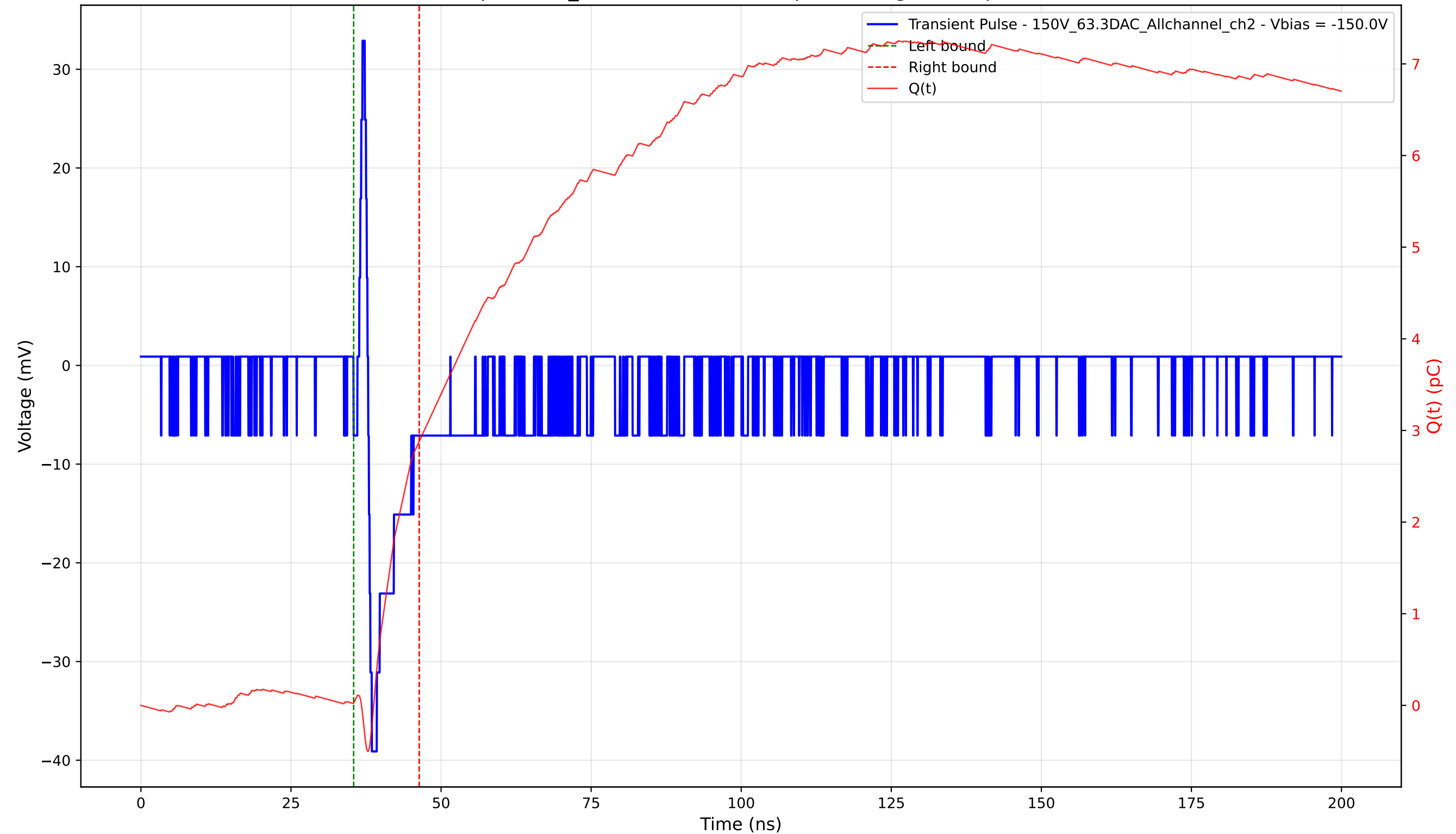
Transient Pulse - Sample: 1cm_42 - Position: 1050.0 \mu\text{m} - Charge: 2.86 pC - Rise Time: 0.62 ns
