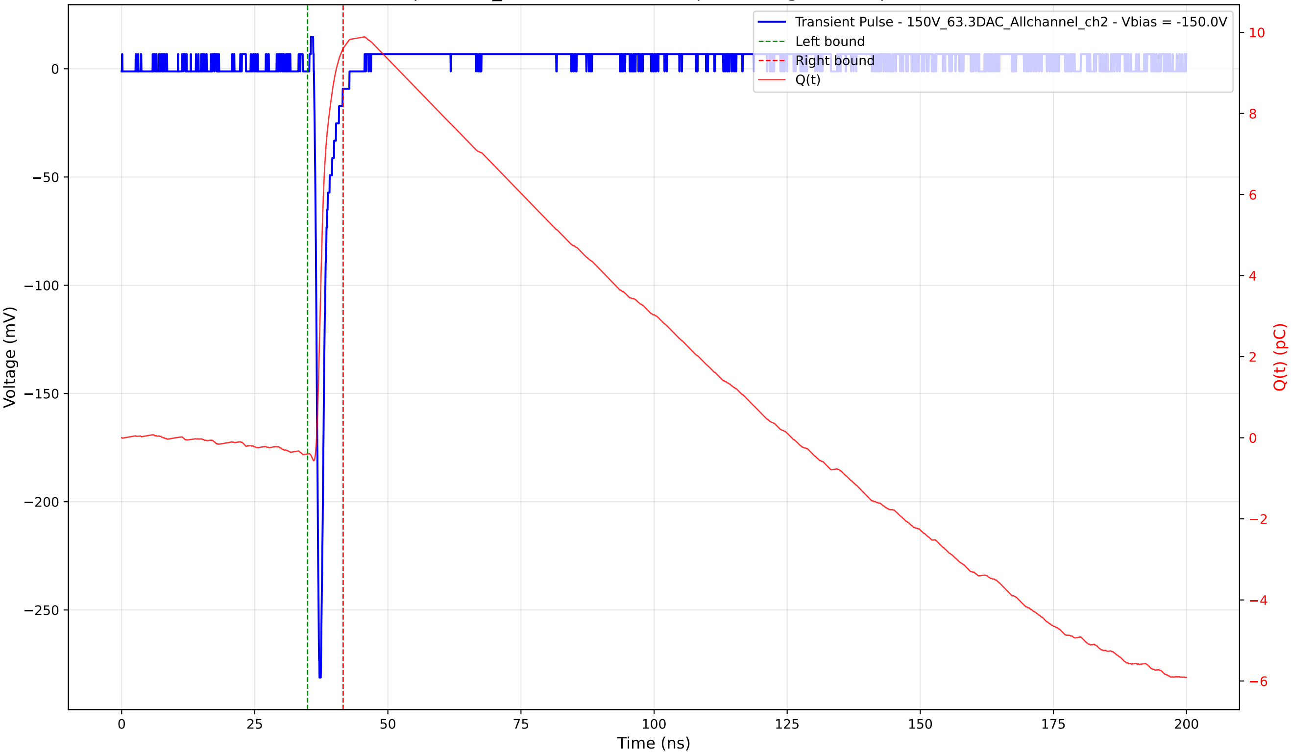
Transient Pulse - Sample: 1cm_42 - Position: 2605.0 \mu\text{m} - Charge: 10.00 pC - Rise Time: 0.72 ns
