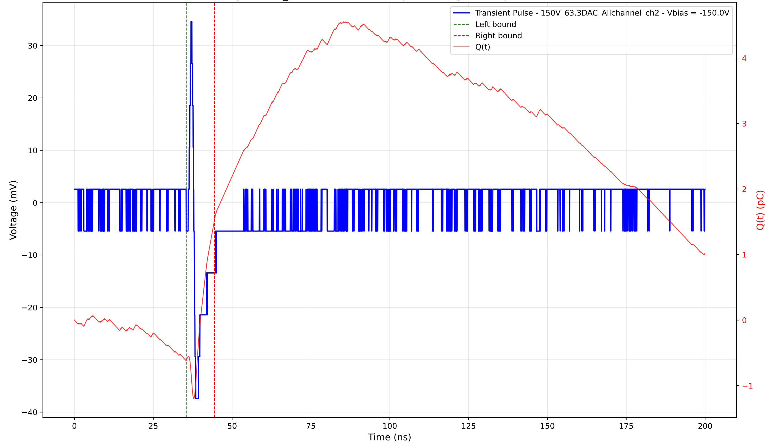
Transient Pulse - Sample: 1cm_42 - Position: 1000.0 \mu\text{m} - Charge: 2.11 pC - Rise Time: 0.00 ns (N/A)
