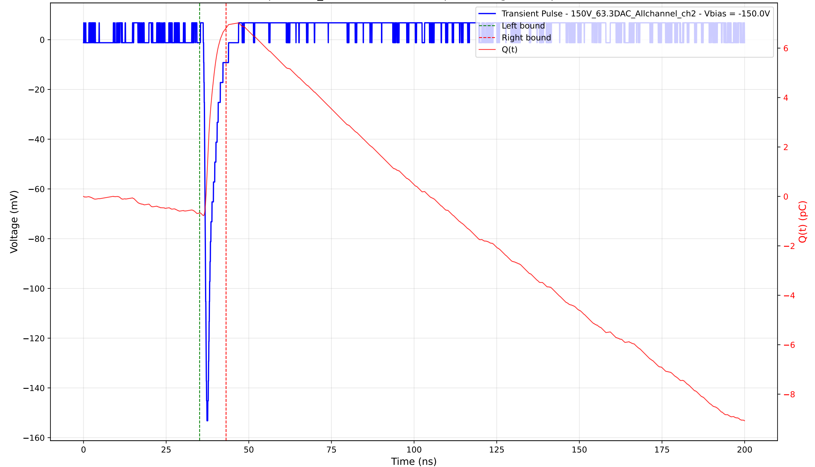
Transient Pulse - Sample: 1cm_42 - Position: 3650.0 \mu\text{m} - Charge: 7.49 pC - Rise Time: 0.81 ns
