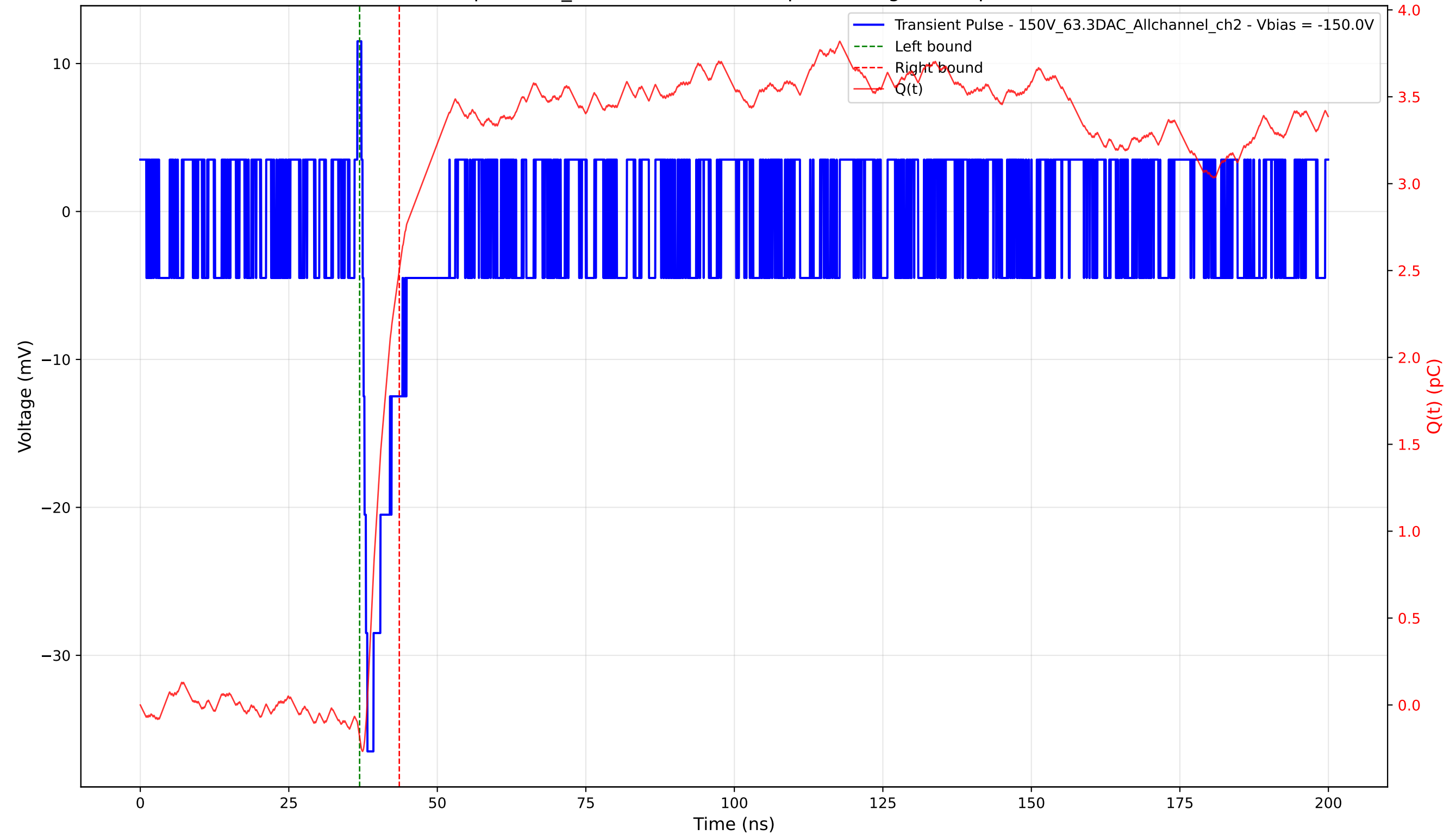
Transient Pulse - Sample: 1cm_42 - Position: 4725.0 \mu\text{m} - Charge: 2.69 pC - Rise Time: 0.83 ns
