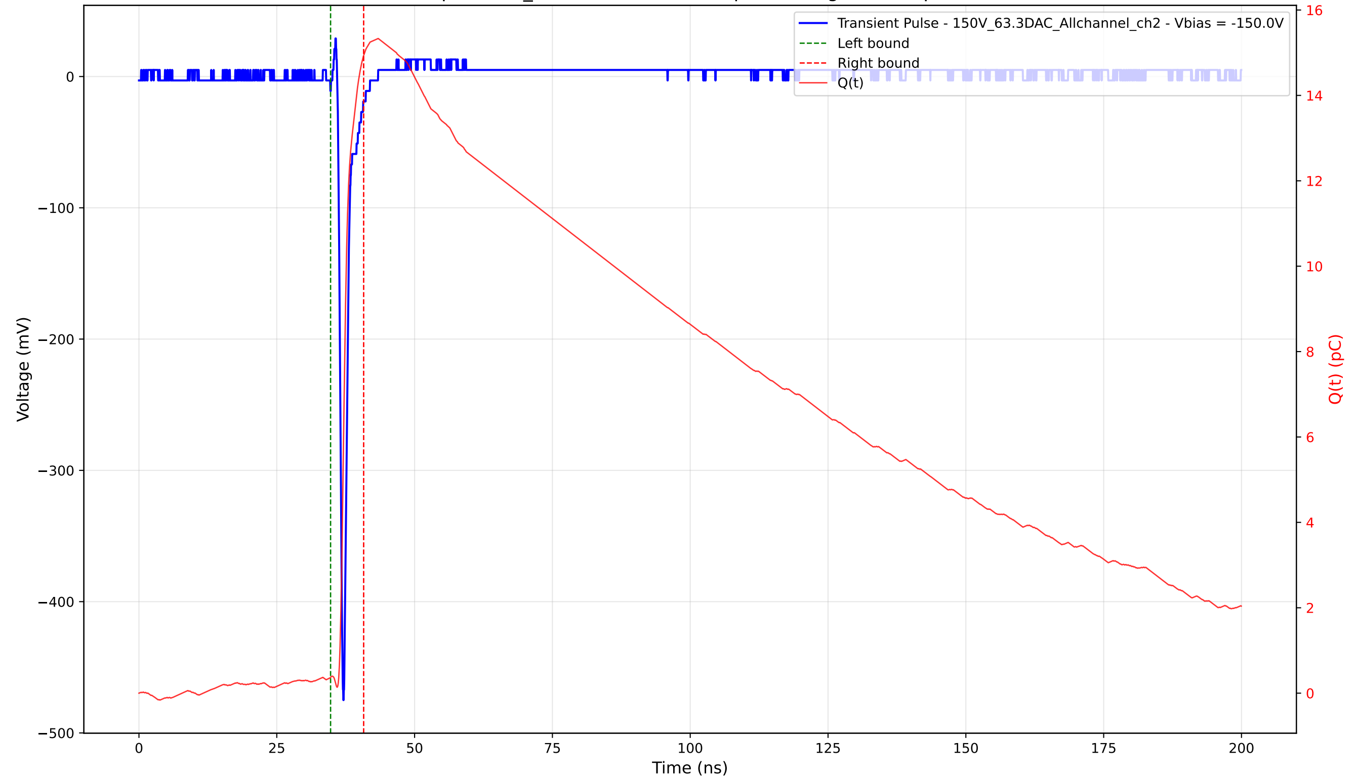
Transient Pulse - Sample: 1cm_42 - Position: 3110.0 \mu\text{m} - Charge: 14.56 pC - Rise Time: 0.71 ns
