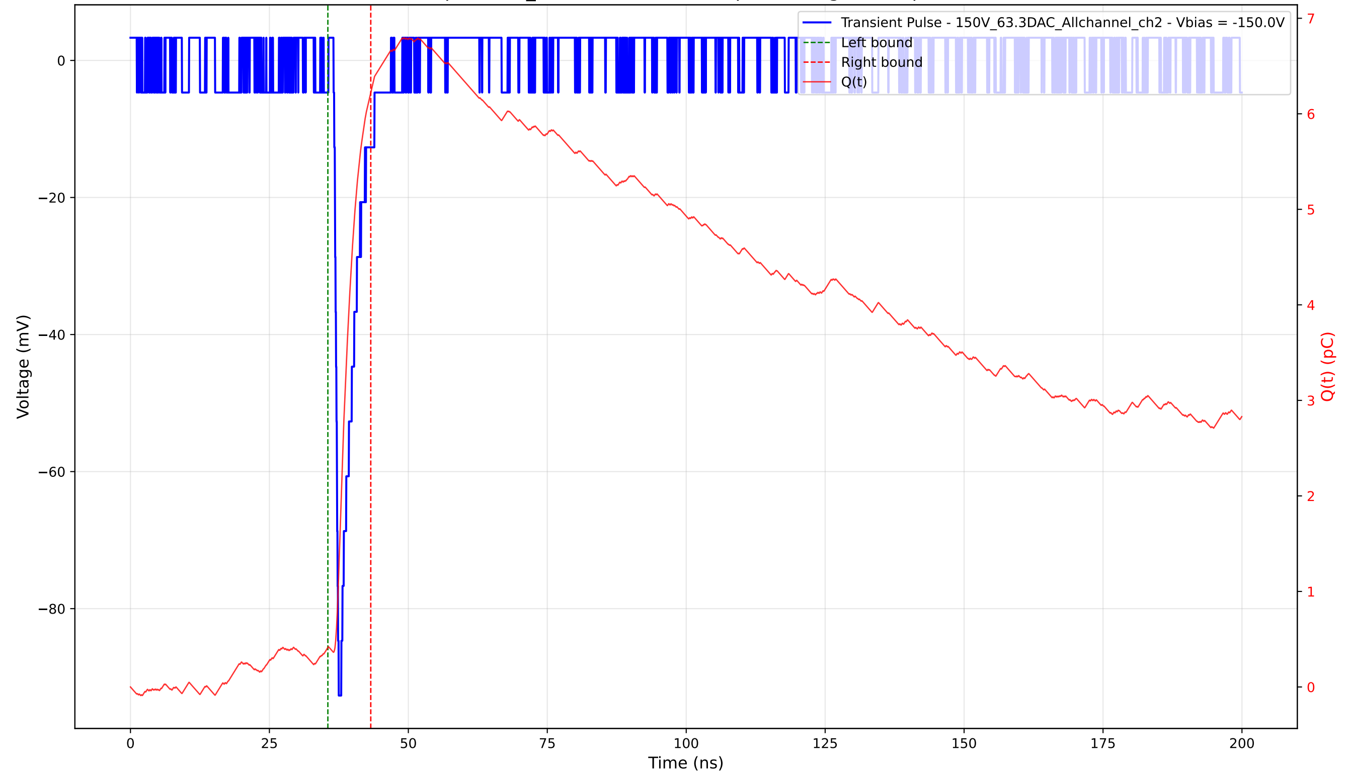
Transient Pulse - Sample: 1cm_42 - Position: 3925.0 \mu\text{m} - Charge: 5.81 pC - Rise Time: 0.70 ns
