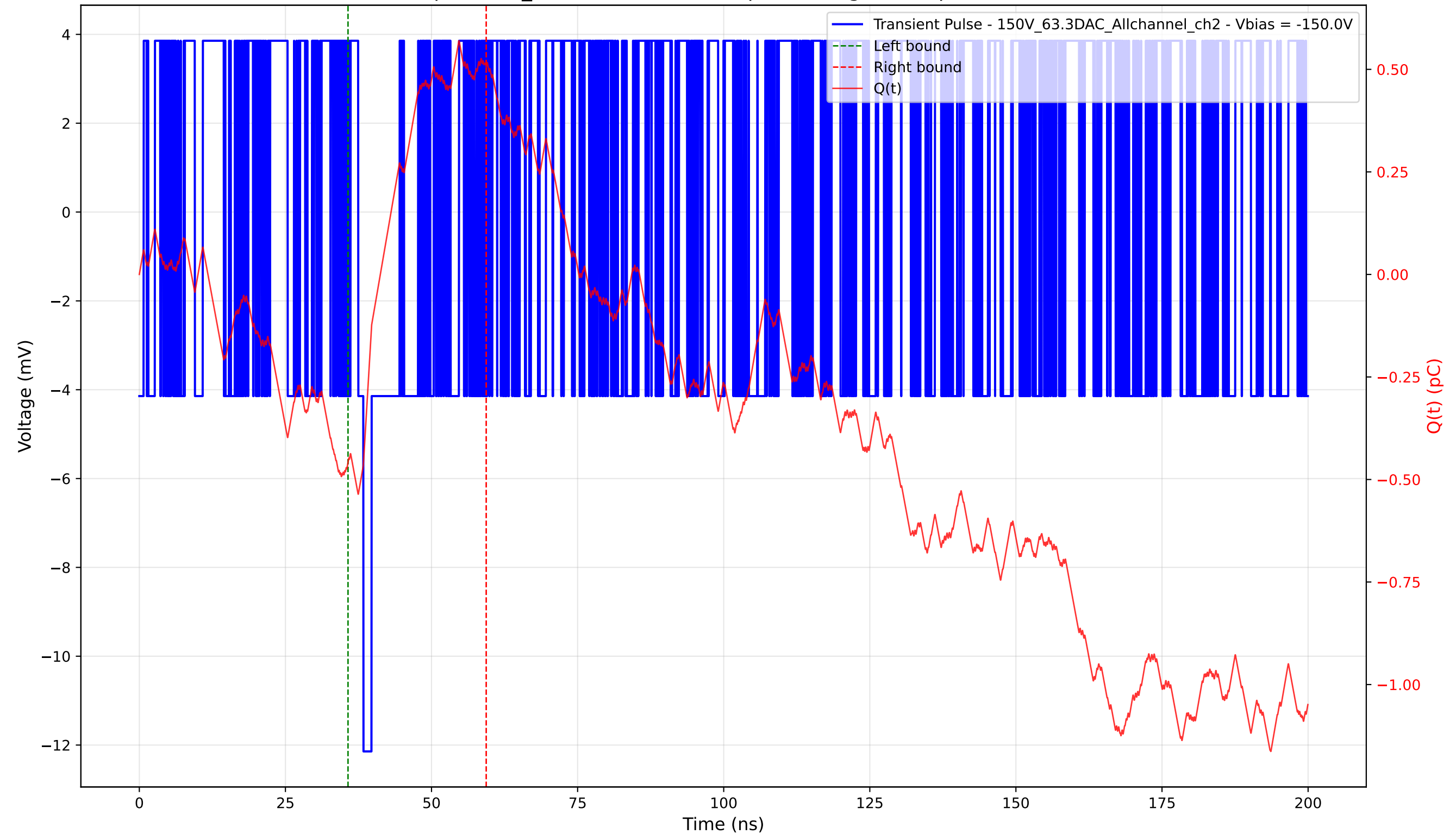
Transient Pulse - Sample: 1cm_42 - Position: 5105.0 \mu\text{m} - Charge: 0.97 pC - Rise Time: 0.00 ns (N/A)
