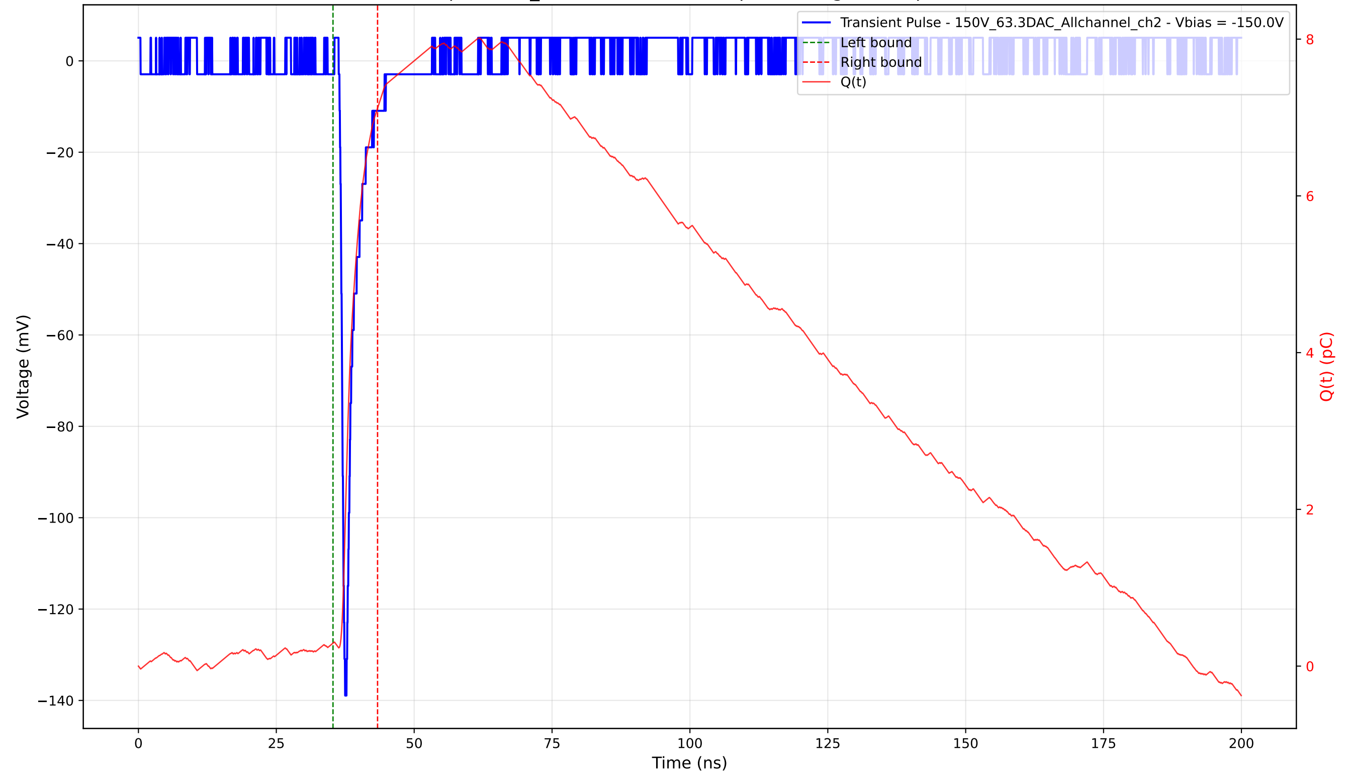
Transient Pulse - Sample: 1cm_42 - Position: 2260.0 \mu\text{m} - Charge: 6.83 pC - Rise Time: 0.83 ns
