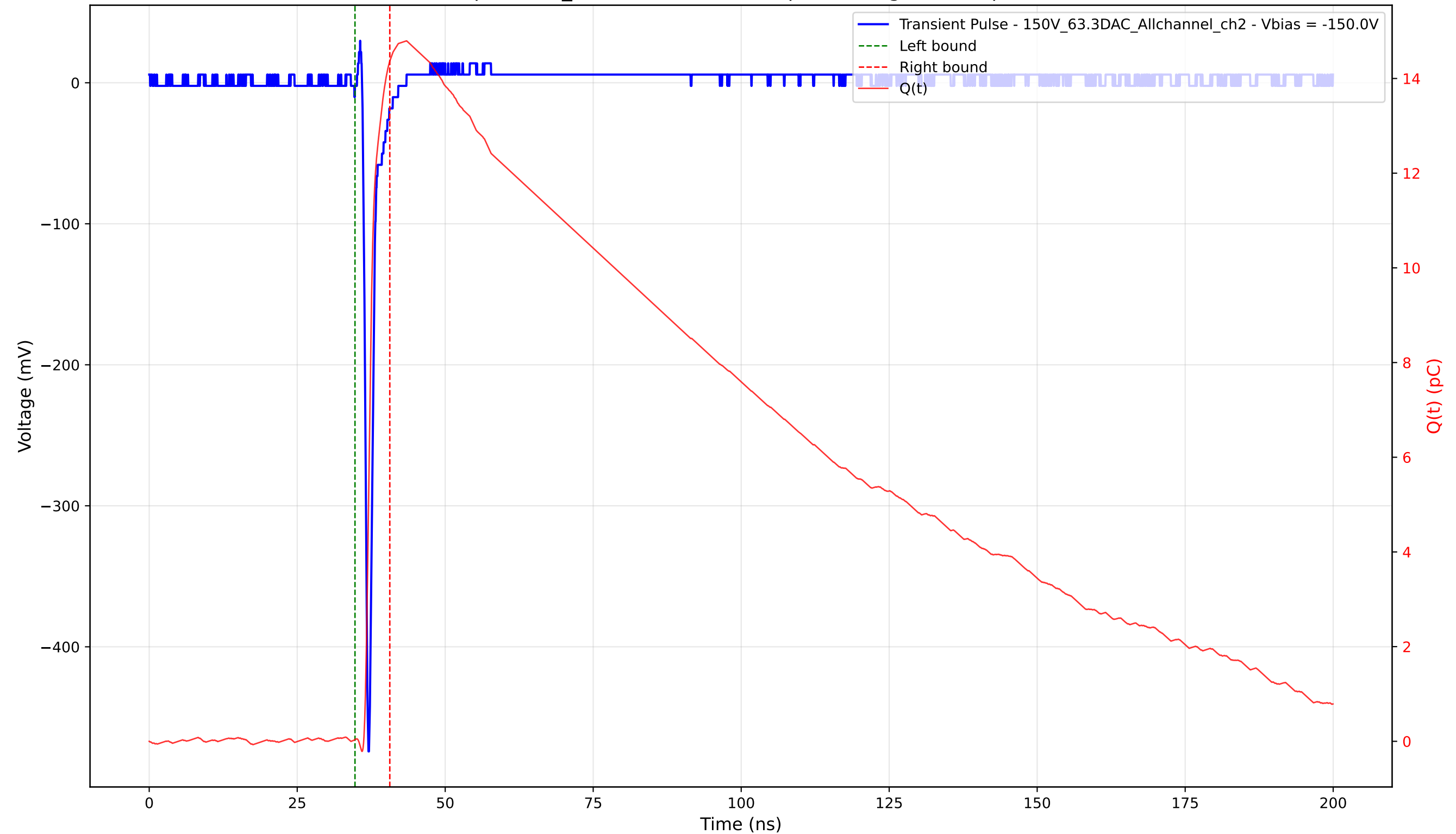
Transient Pulse - Sample: 1cm_42 - Position: 3000.0 \mu\text{m} - Charge: 14.33 pC - Rise Time: 0.67 ns
