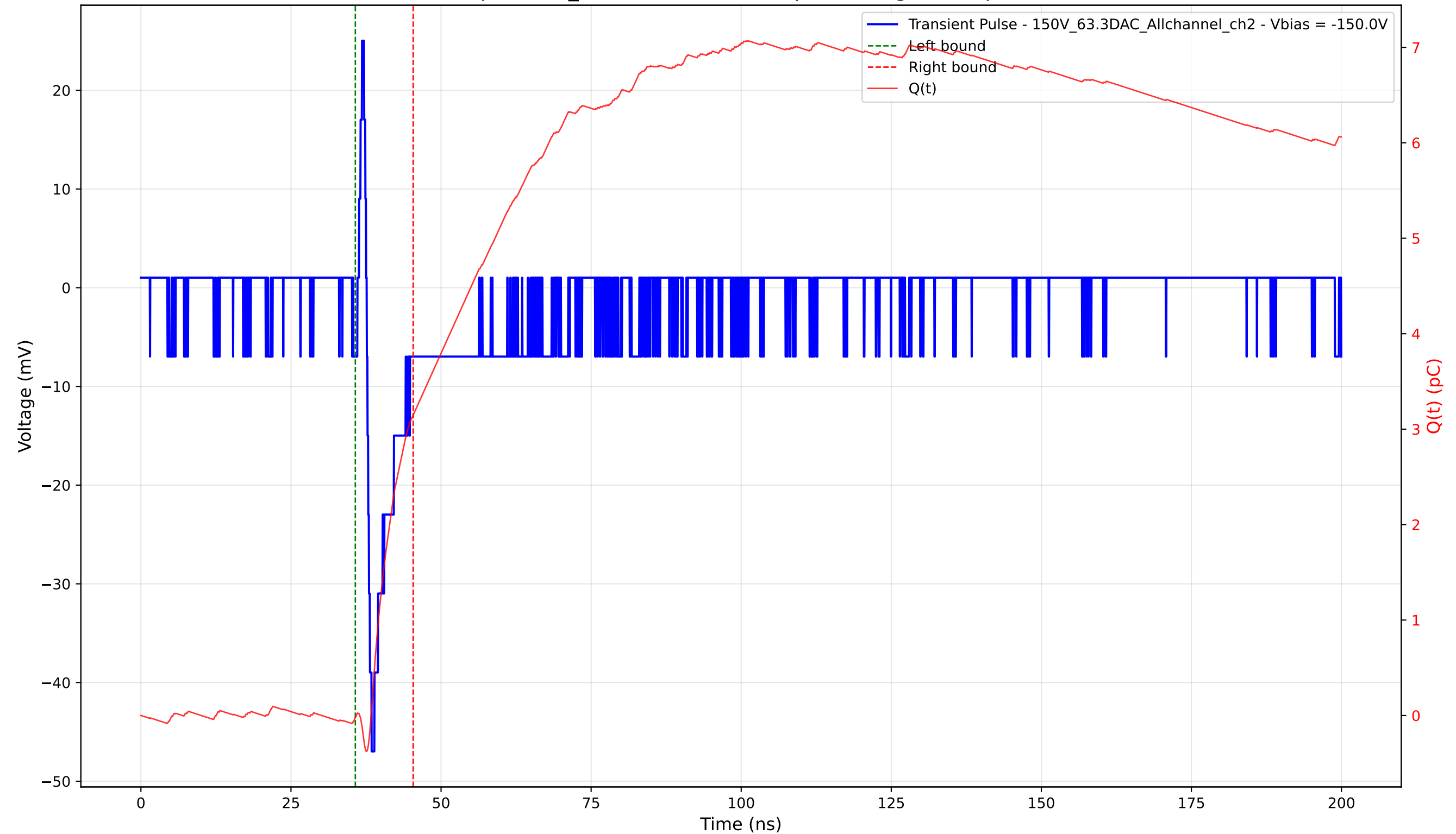
Transient Pulse - Sample: 1cm_42 - Position: 1495.0 \mu\text{m} - Charge: 3.17 pC - Rise Time: 0.82 ns
