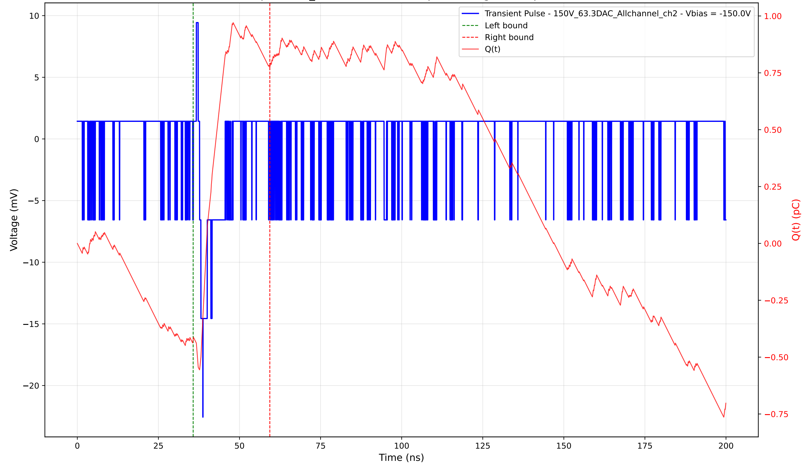
Transient Pulse - Sample: 1cm_42 - Position: 185.0 \mu\text{m} - Charge: 1.20 pC - Rise Time: 1.03 ns
