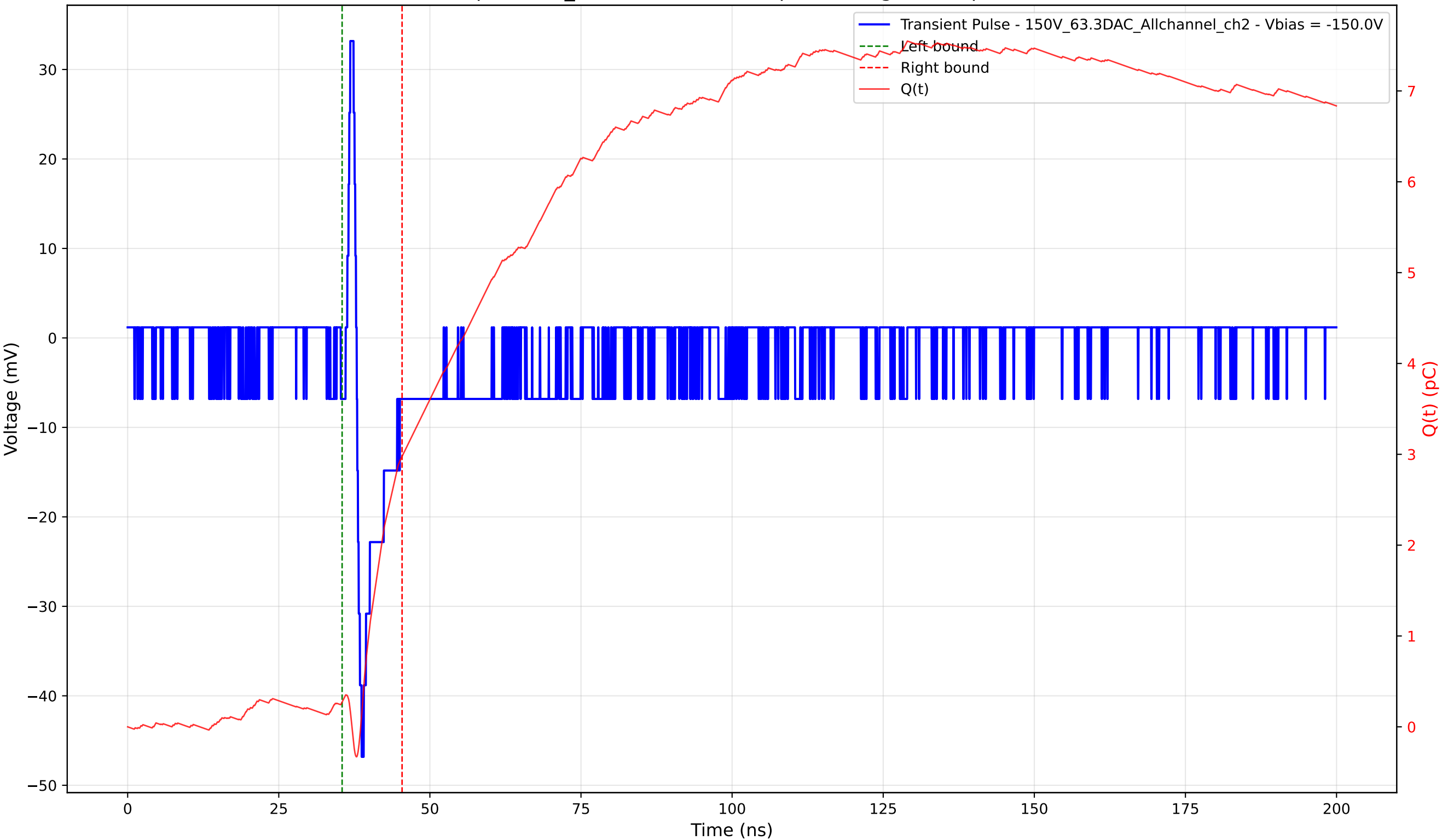
Transient Pulse - Sample: 1cm_42 - Position: 810.0 \mu\text{m} - Charge: 2.70 pC - Rise Time: 0.82 ns
