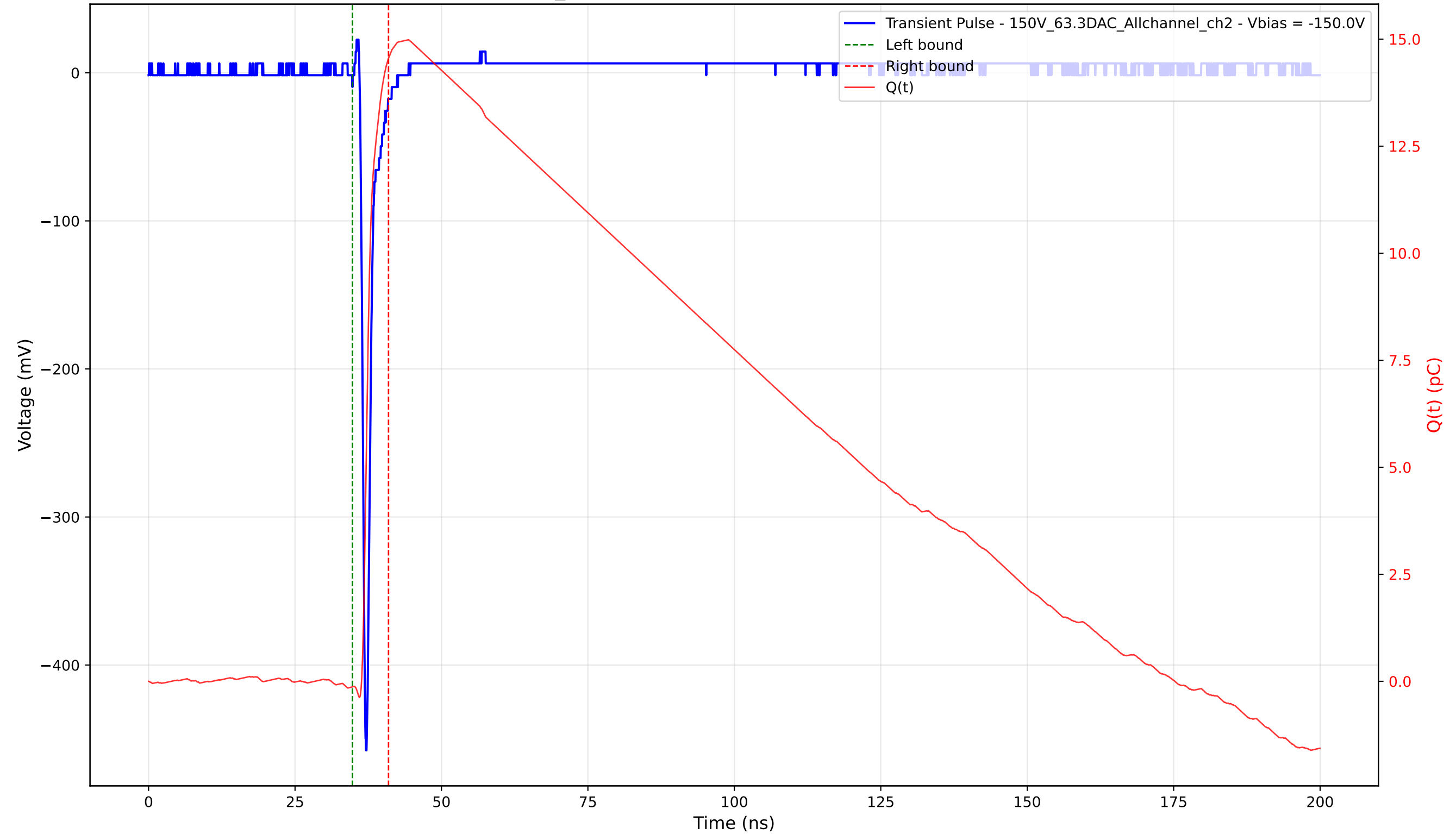
Transient Pulse - Sample: 1cm_42 - Position: 2765.0 \mu\text{m} - Charge: 14.68 pC - Rise Time: 0.72 ns
