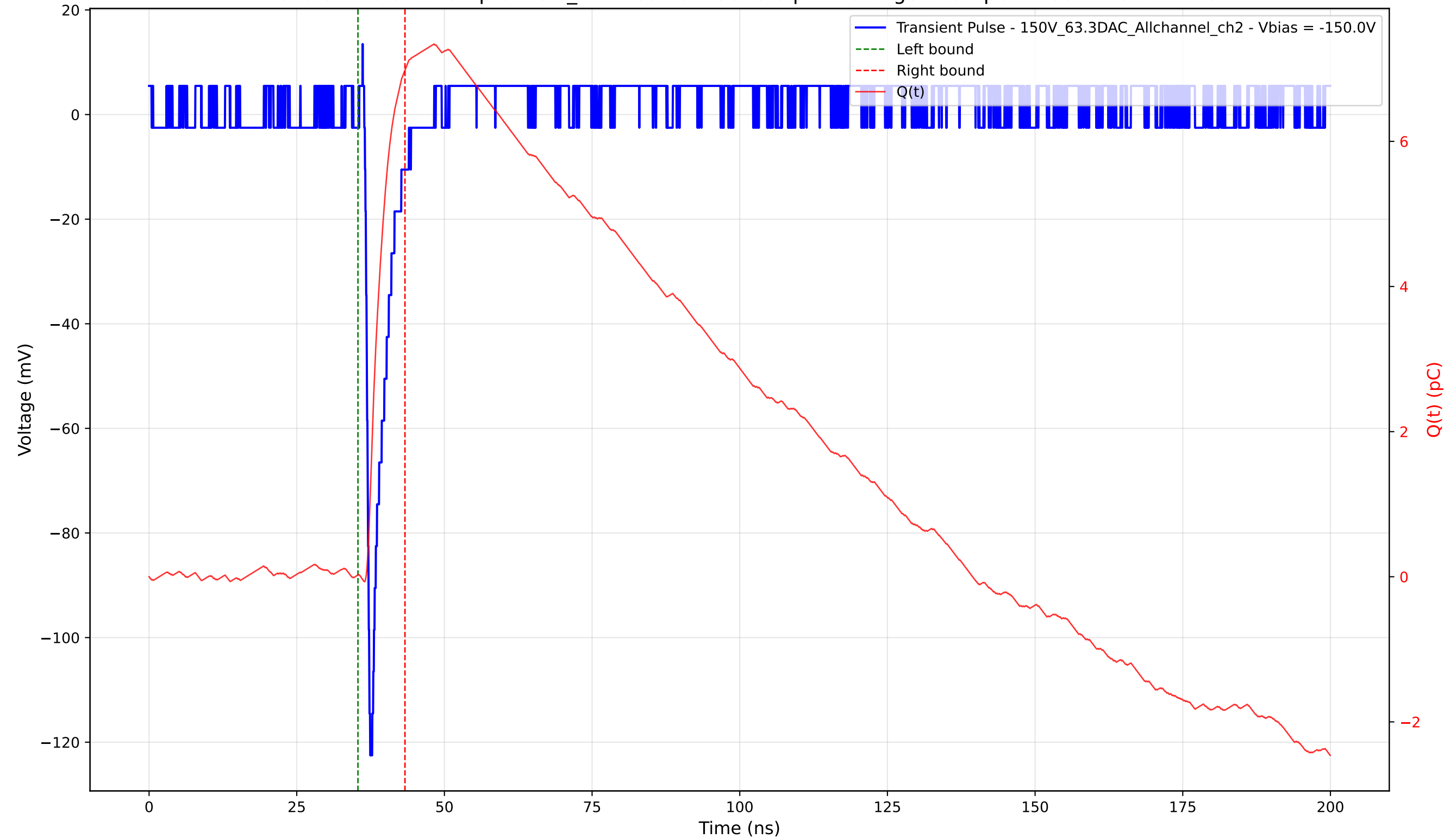
Transient Pulse - Sample: 1cm_42 - Position: 3830.0 \mu\text{m} - Charge: 6.96 pC - Rise Time: 0.71 ns
