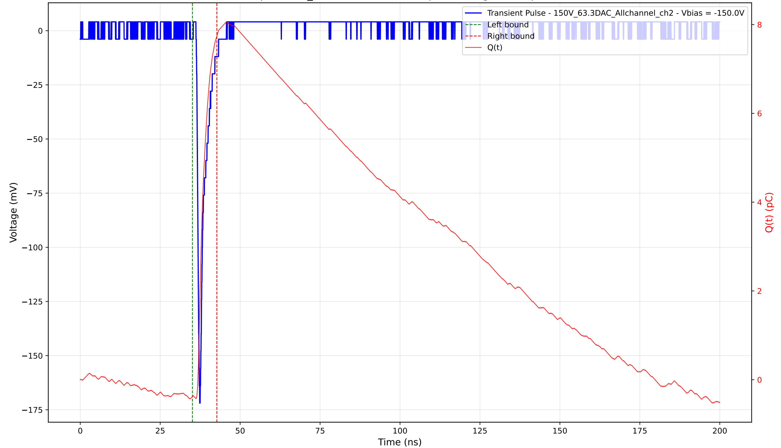
Transient Pulse - Sample: 1cm_42 - Position: 3610.0 \mu\text{m} - Charge: 8.12 pC - Rise Time: 0.77 ns
