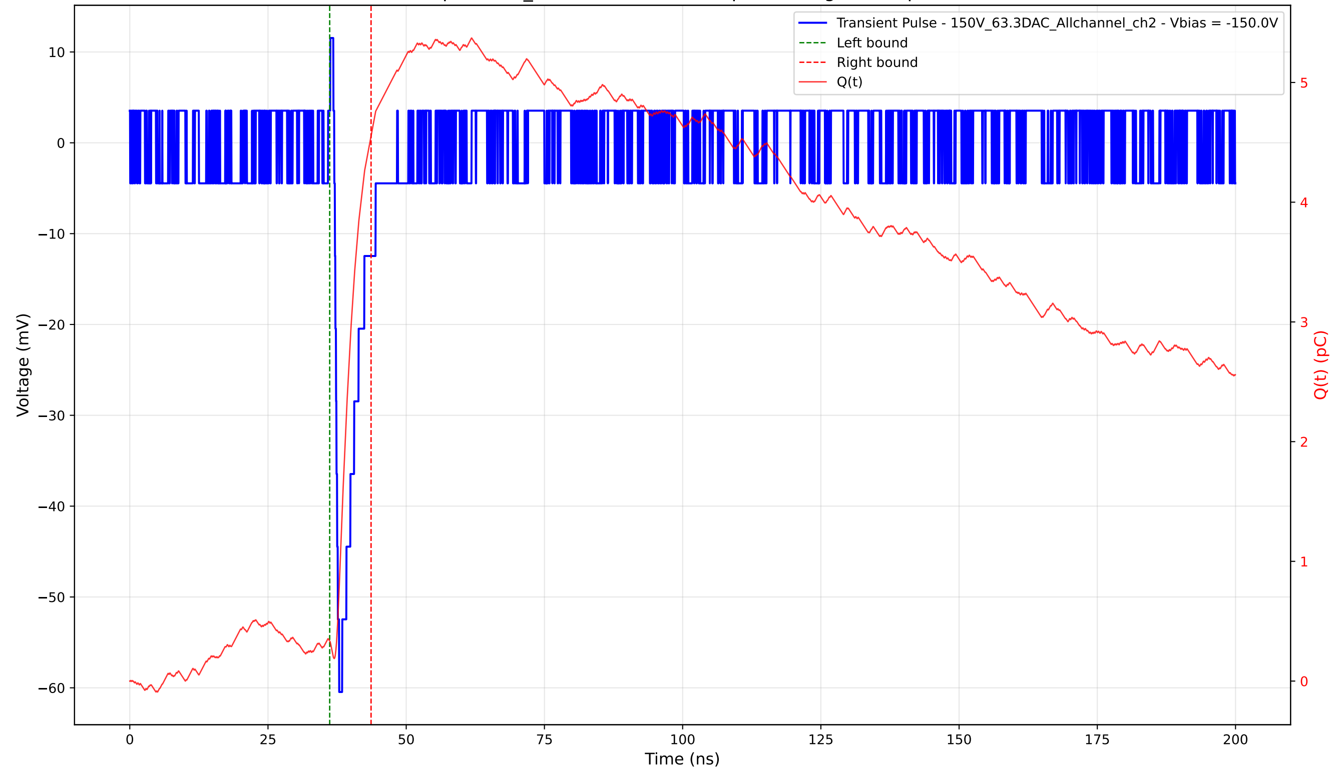
Transient Pulse - Sample: 1cm_42 - Position: 4155.0 \mu\text{m} - Charge: 4.22 pC - Rise Time: 0.79 ns
