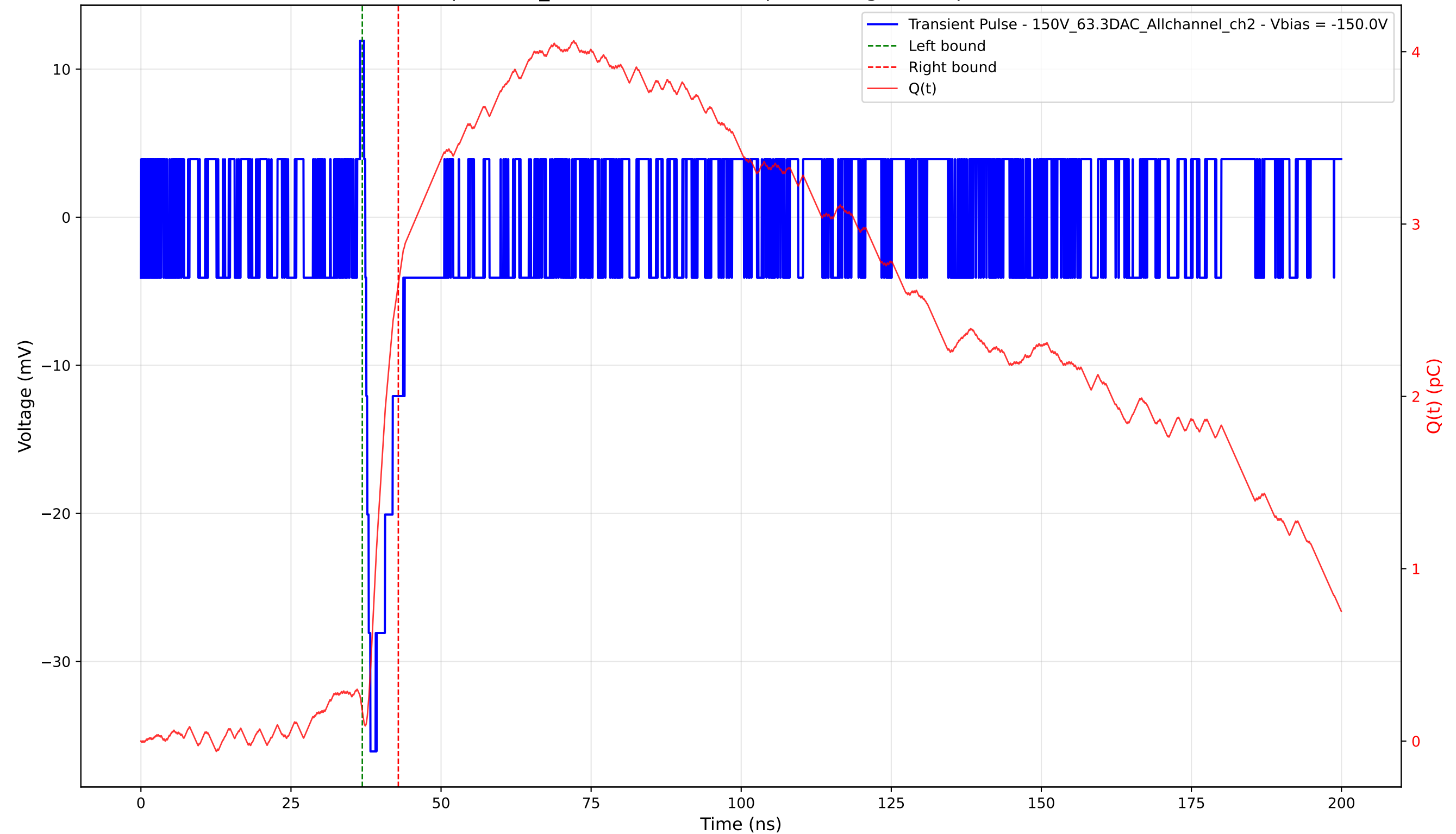
Transient Pulse - Sample: 1cm_42 - Position: 4650.0 \mu\text{m} - Charge: 2.48 pC - Rise Time: 0.00 ns (N/A)
