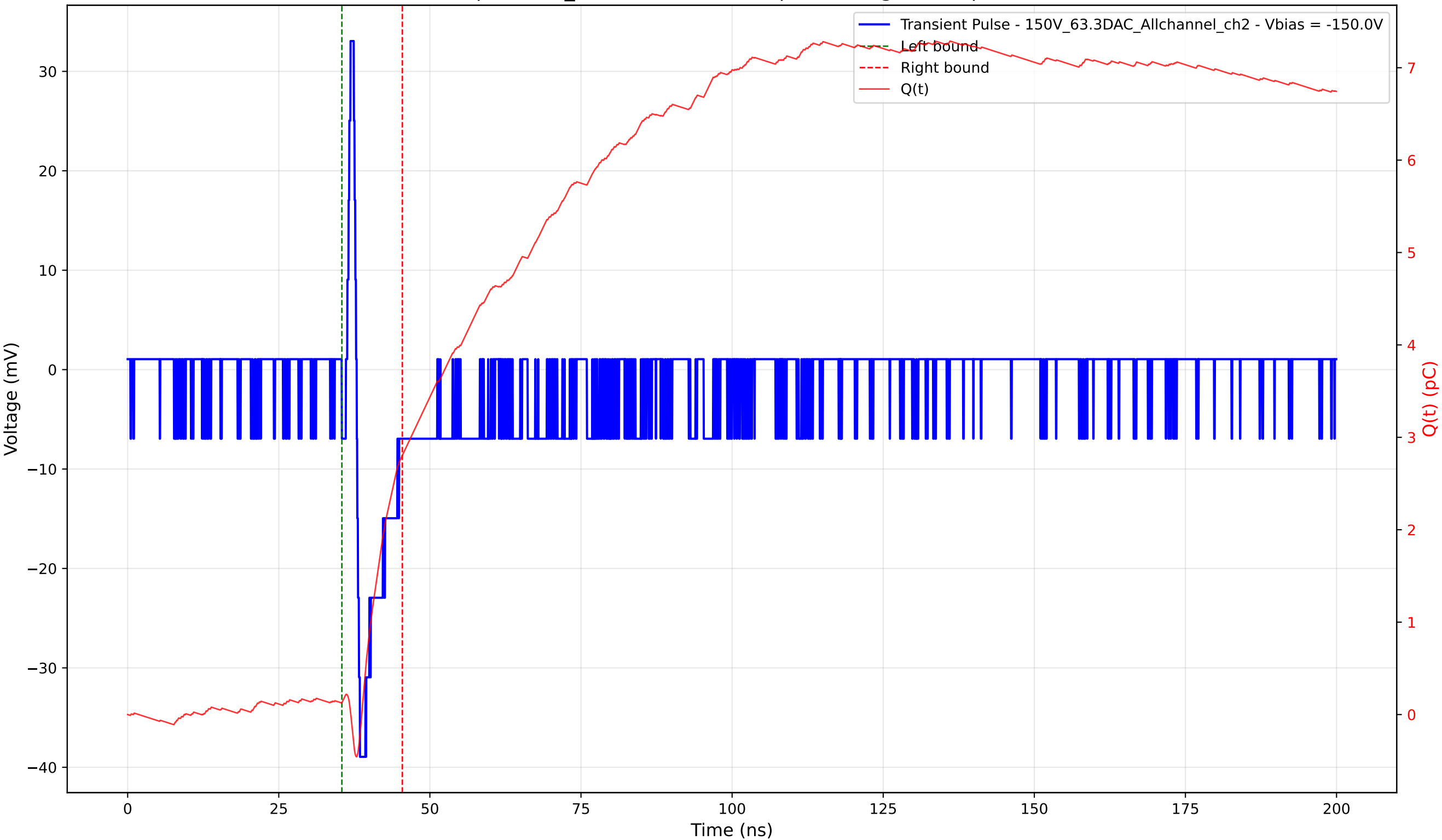
Transient Pulse - Sample: 1cm_42 - Position: 825.0 \mu\text{m} - Charge: 2.68 pC - Rise Time: 0.54 ns
