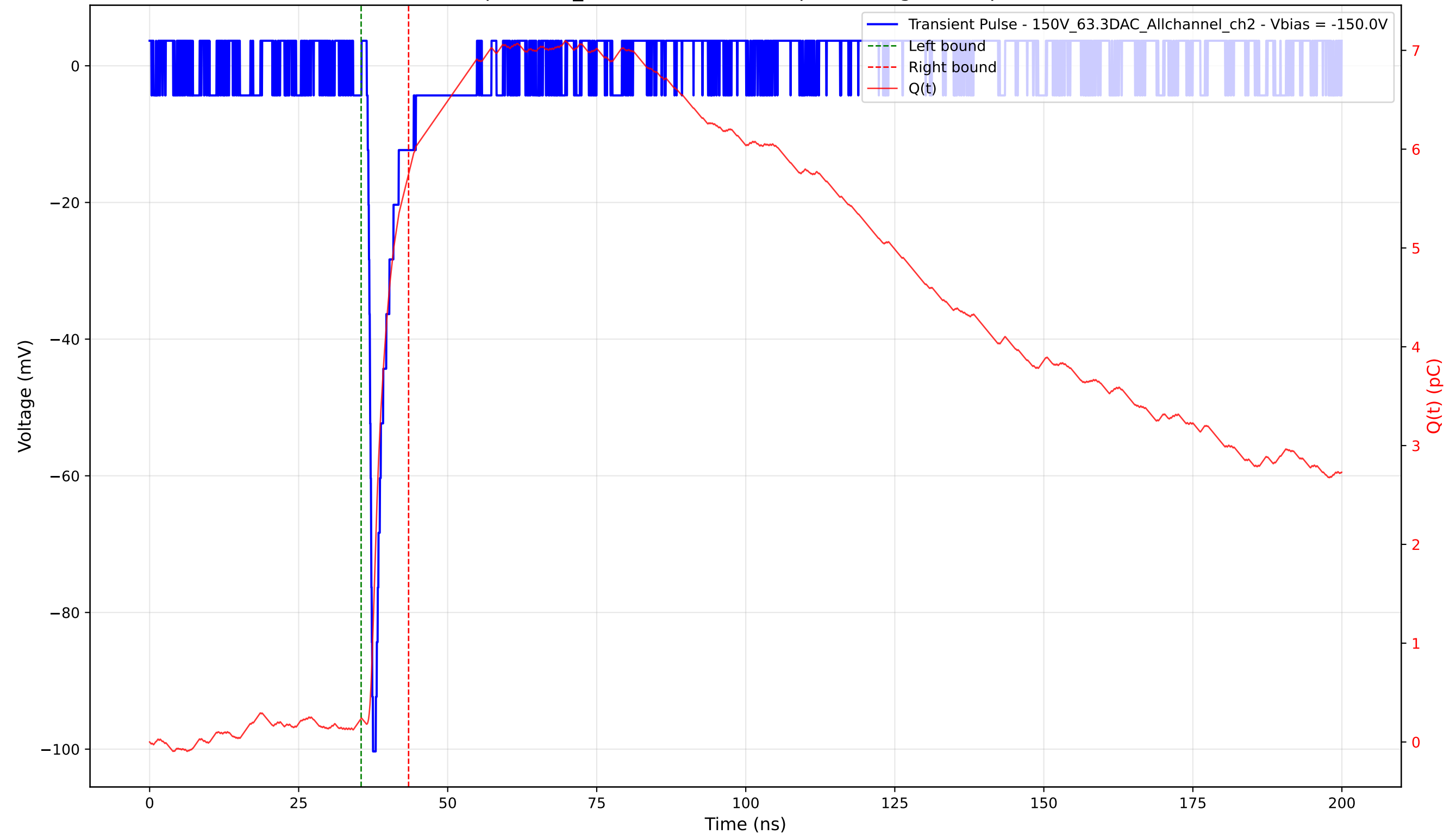
Transient Pulse - Sample: 1cm_42 - Position: 2145.0 \mu\text{m} - Charge: 5.51 pC - Rise Time: 0.77 ns
