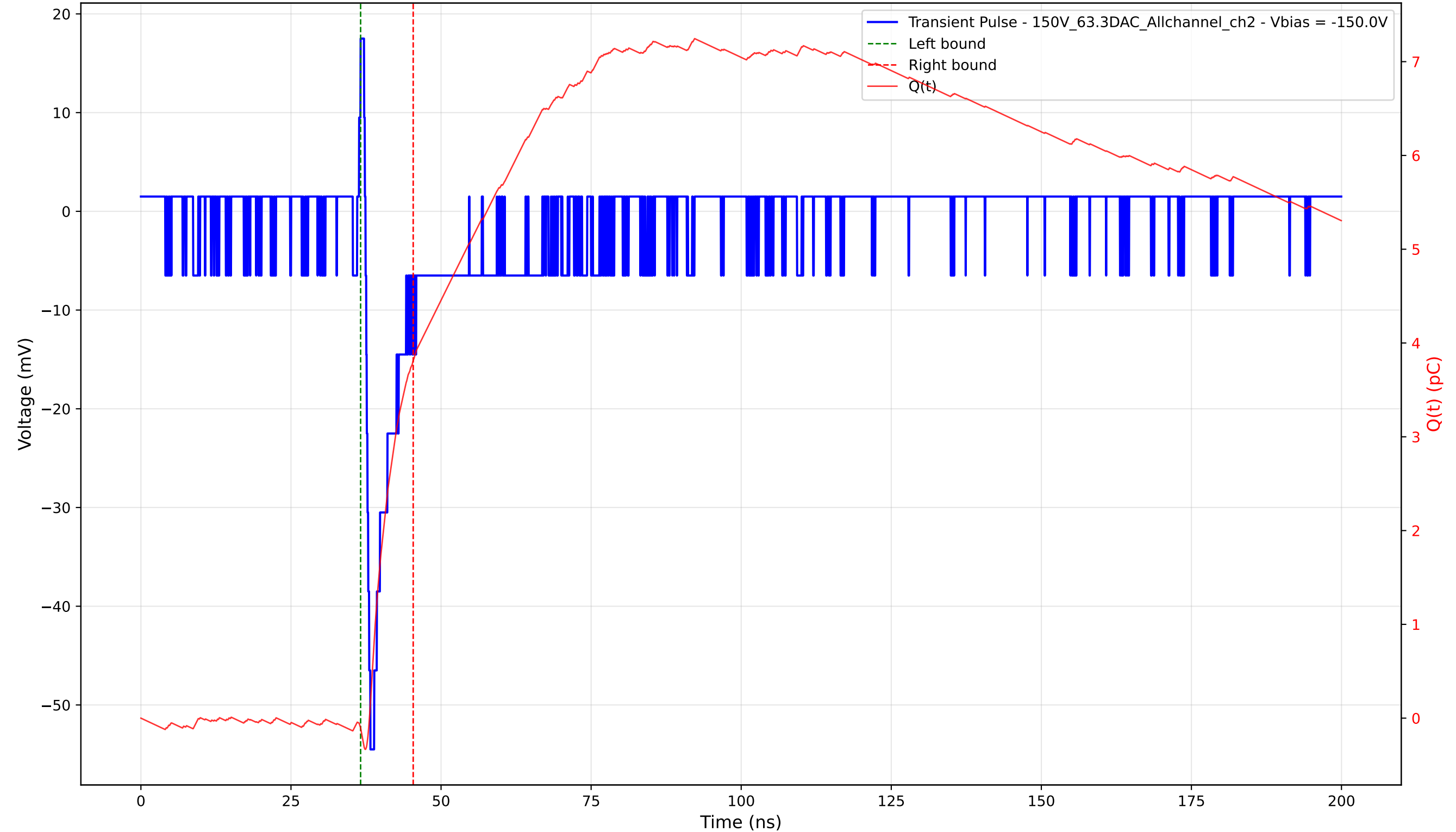
Transient Pulse - Sample: 1cm_42 - Position: 1620.0 \mu\text{m} - Charge: 3.92 pC - Rise Time: 0.81 ns
