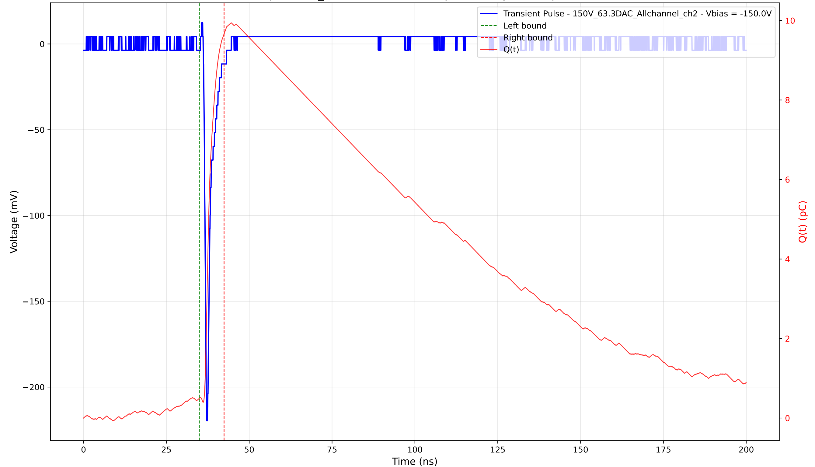
Transient Pulse - Sample: 1cm_42 - Position: 3505.0 \mu\text{m} - Charge: 9.17 pC - Rise Time: 0.75 ns
