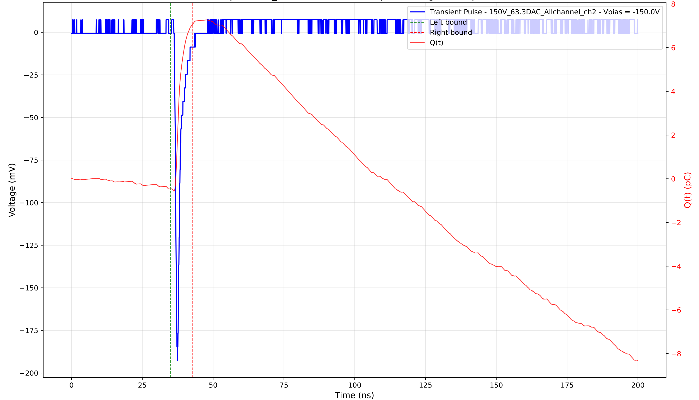
Transient Pulse - Sample: 1cm_42 - Position: 2490.0 \mu\text{m} - Charge: 7.50 pC - Rise Time: 0.79 ns
