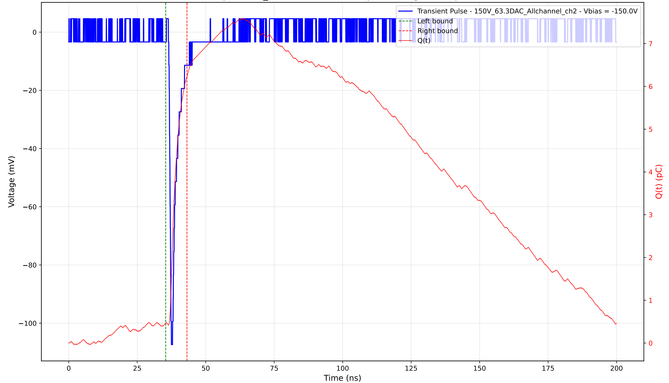
Transient Pulse - Sample: 1cm_42 - Position: 2175.0 \mu\text{m} - Charge: 5.77 pC - Rise Time: 0.76 ns
