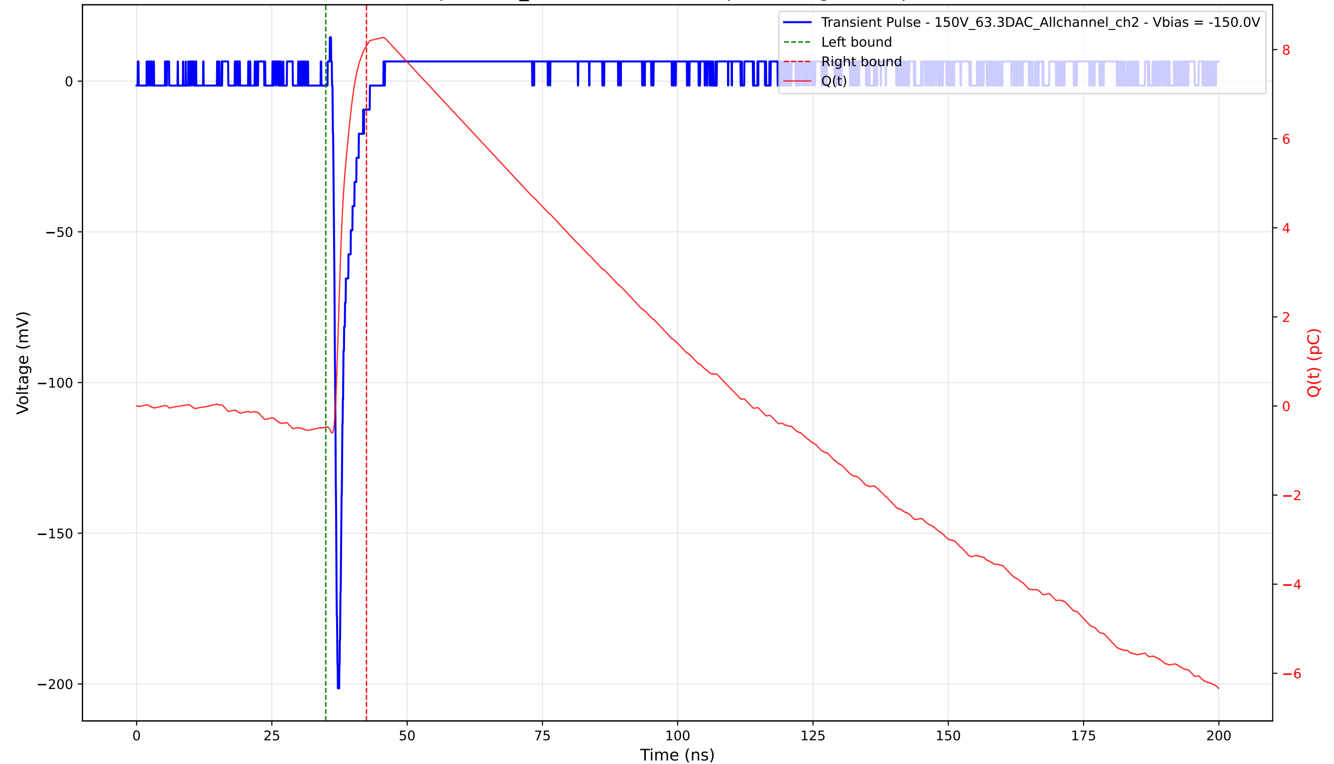
Transient Pulse - Sample: 1cm_42 - Position: 3530.0 \mu\text{m} - Charge: 8.56 pC - Rise Time: 0.73 ns
