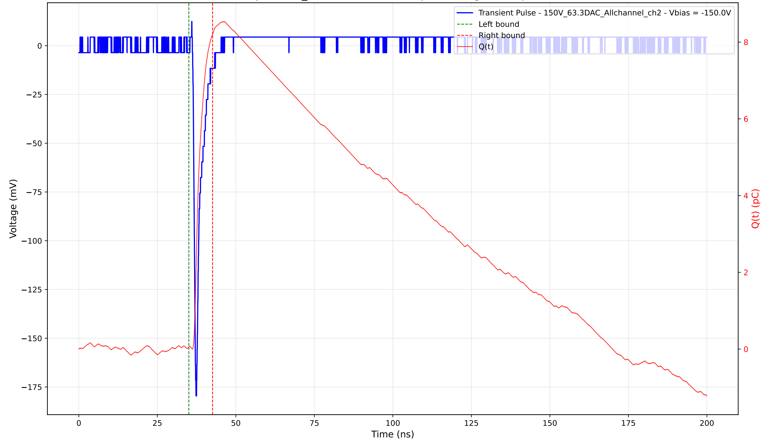
Transient Pulse - Sample: 1cm_42 - Position: 3575.0 \mu\text{m} - Charge: 8.16 pC - Rise Time: 0.77 ns
