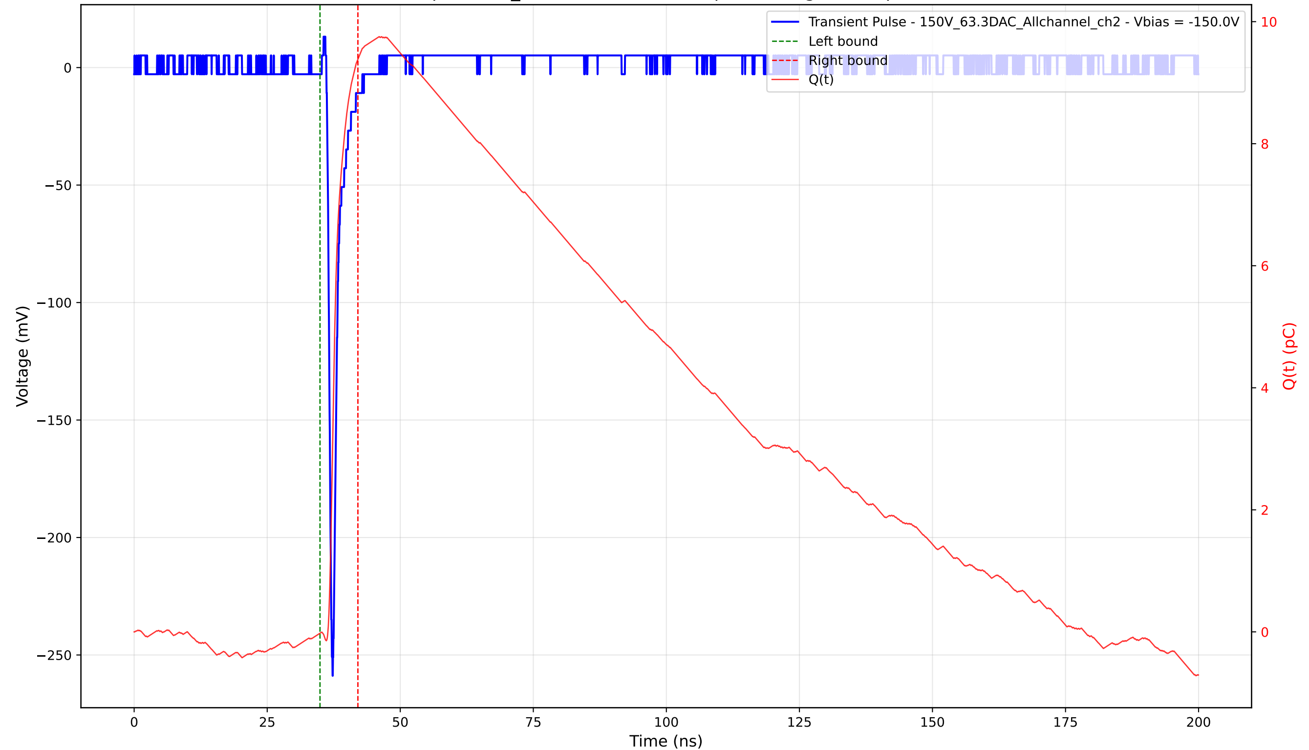
Transient Pulse - Sample: 1cm_42 - Position: 2575.0 \mu\text{m} - Charge: 9.41 pC - Rise Time: 0.76 ns
