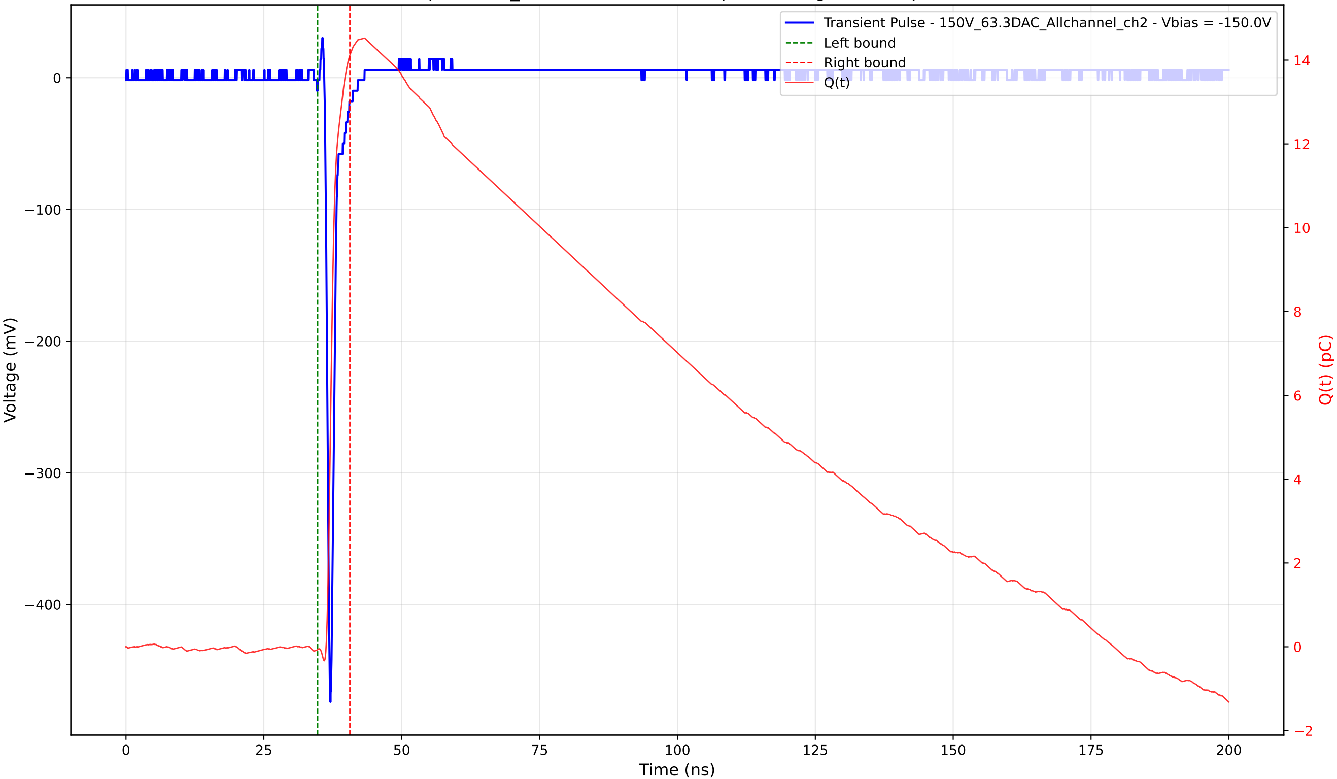
Transient Pulse - Sample: 1cm_42 - Position: 2995.0 \mu\text{m} - Charge: 14.18 pC - Rise Time: 0.73 ns
