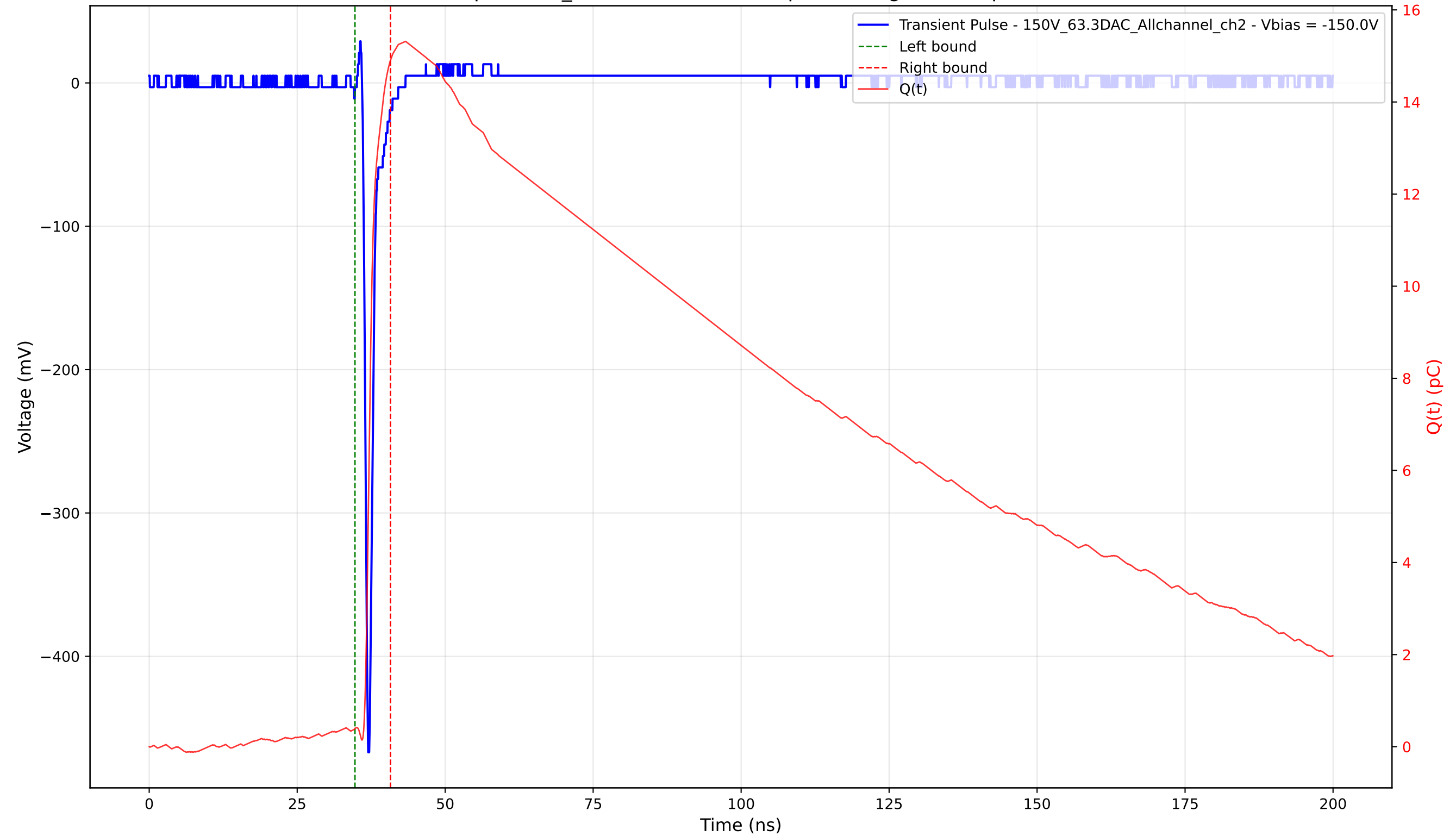
Transient Pulse - Sample: 1cm_42 - Position: 3115.0 \mu\text{m} - Charge: 14.51 pC - Rise Time: 0.68 ns
