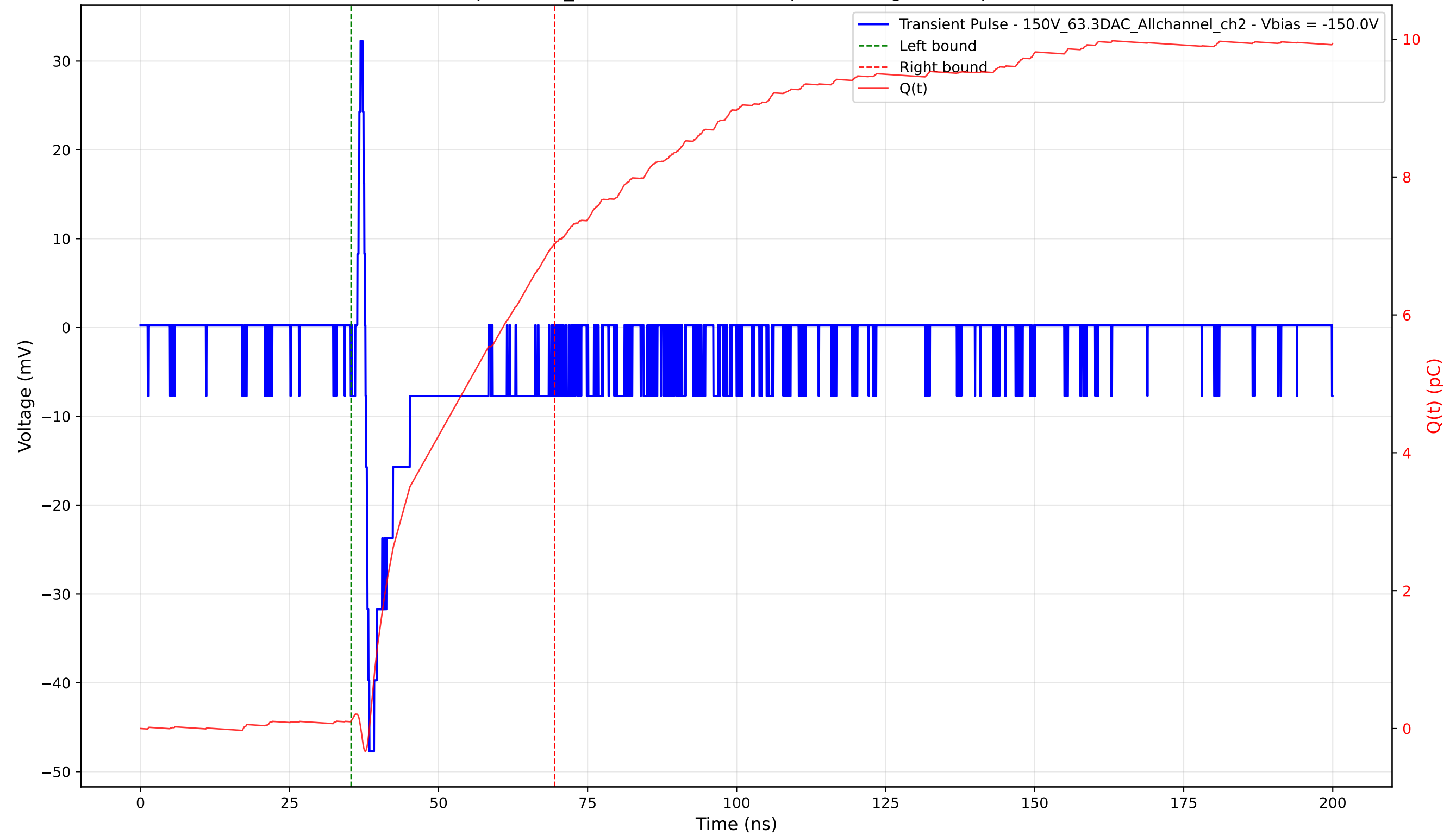
Transient Pulse - Sample: 1cm_42 - Position: 1345.0 \mu\text{m} - Charge: 6.92 pC - Rise Time: 0.66 ns
