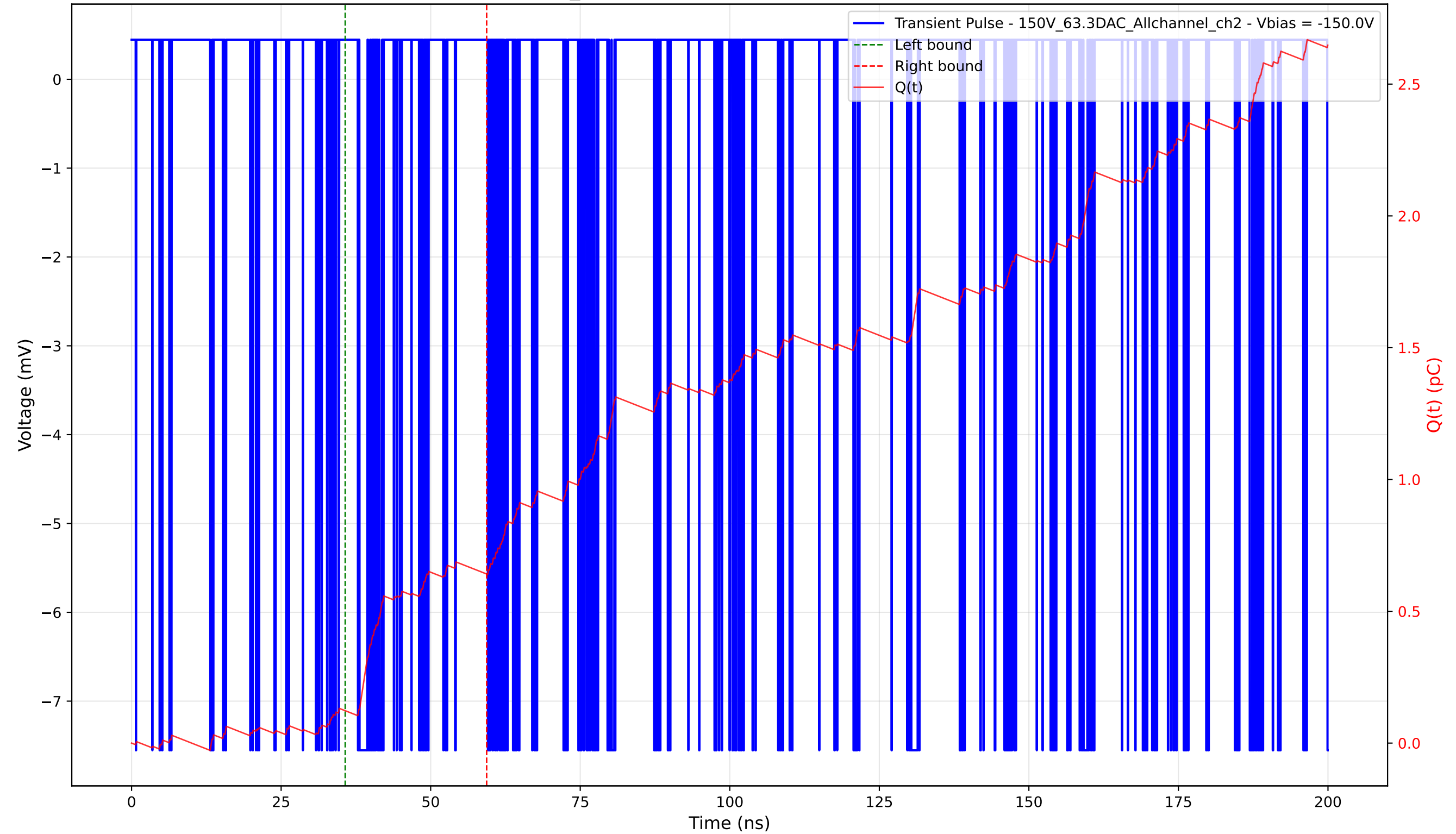
Transient Pulse - Sample: 1cm_42 - Position: 15.0 \mu\text{m} - Charge: 0.52 pC - Rise Time: 0.04 ns
