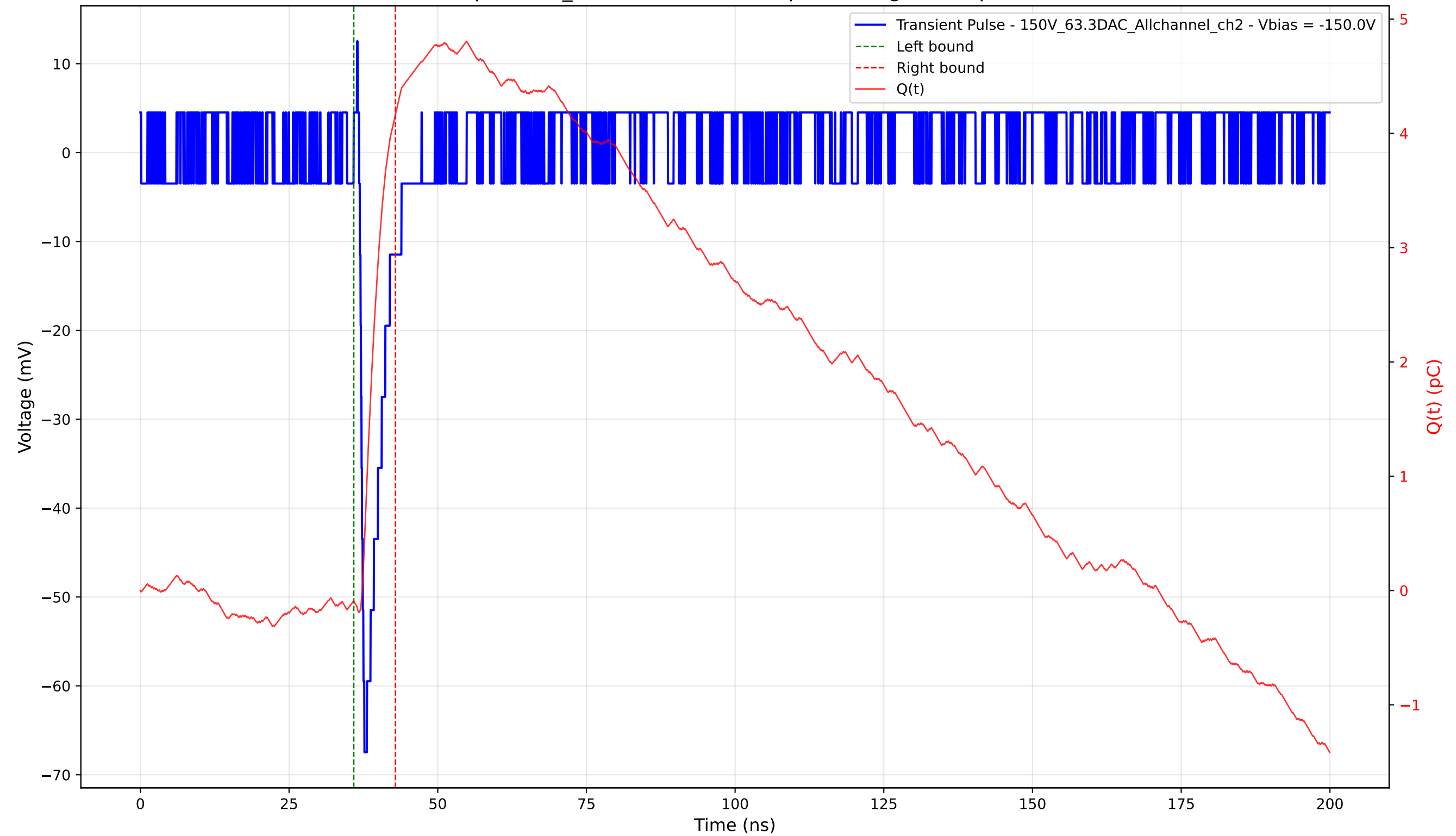
Transient Pulse - Sample: 1cm_42 - Position: 4045.0 \mu\text{m} - Charge: 4.26 pC - Rise Time: 0.78 ns
