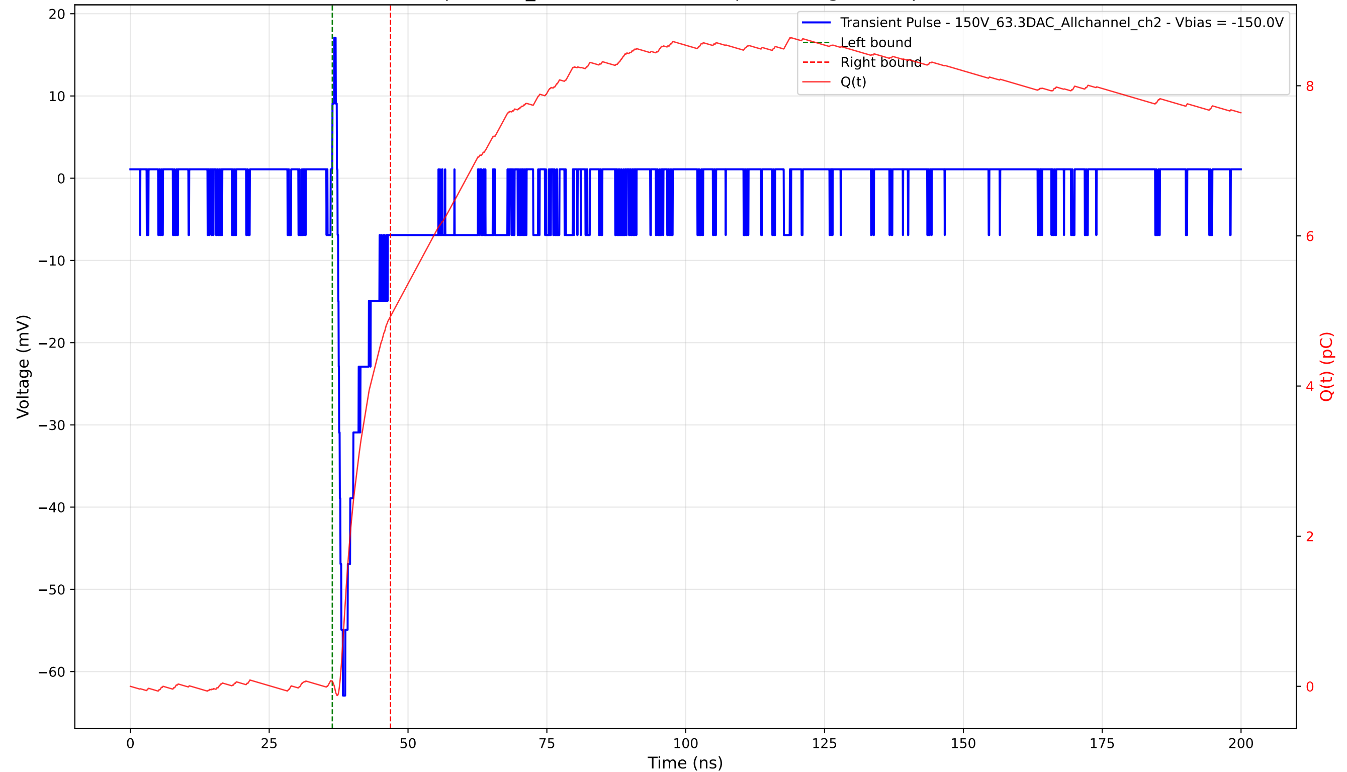
Transient Pulse - Sample: 1cm_42 - Position: 1700.0 \mu\text{m} - Charge: 4.86 pC - Rise Time: 0.96 ns
