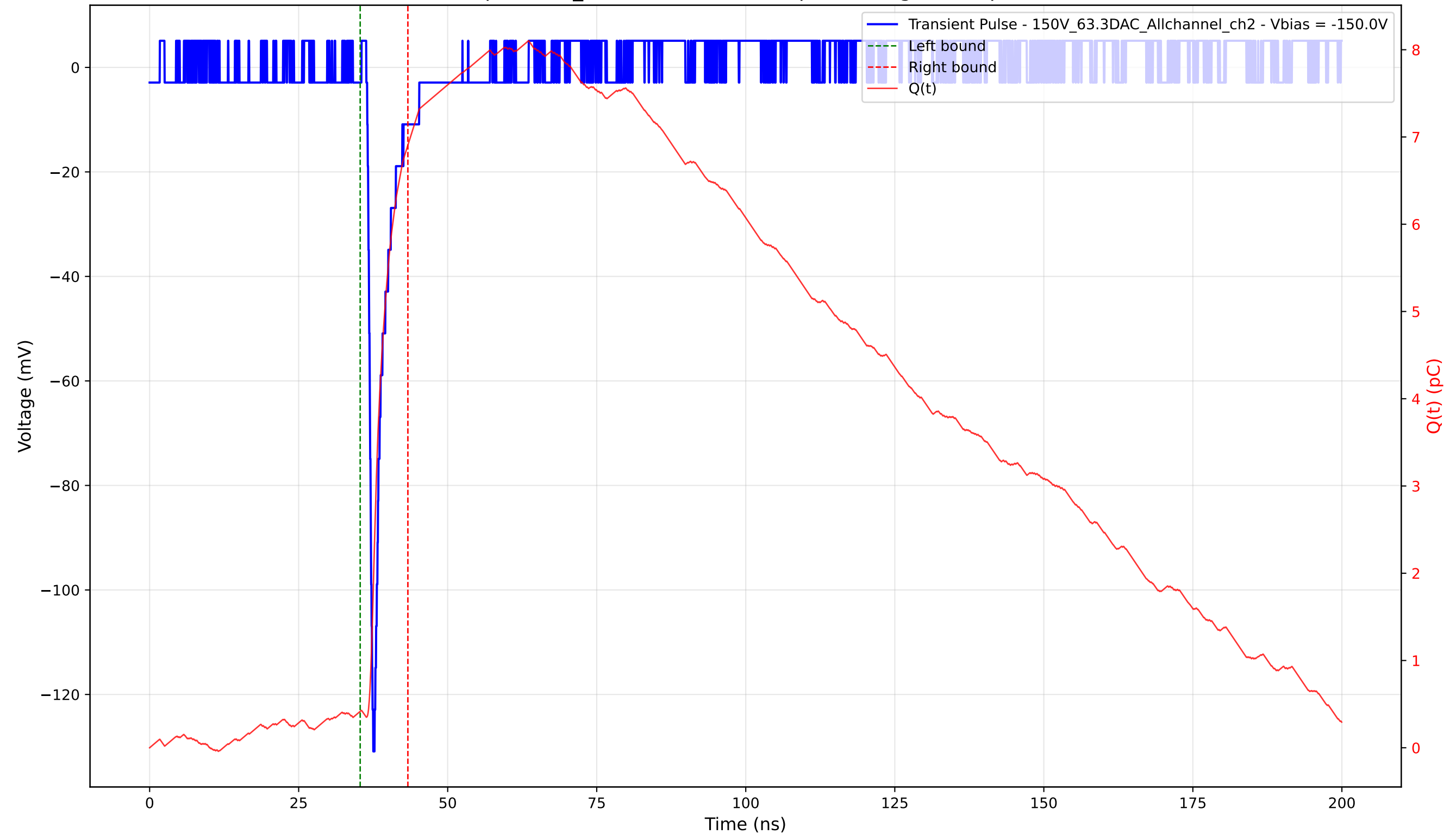
Transient Pulse - Sample: 1cm_42 - Position: 2225.0 \mu\text{m} - Charge: 6.49 pC - Rise Time: 0.83 ns
