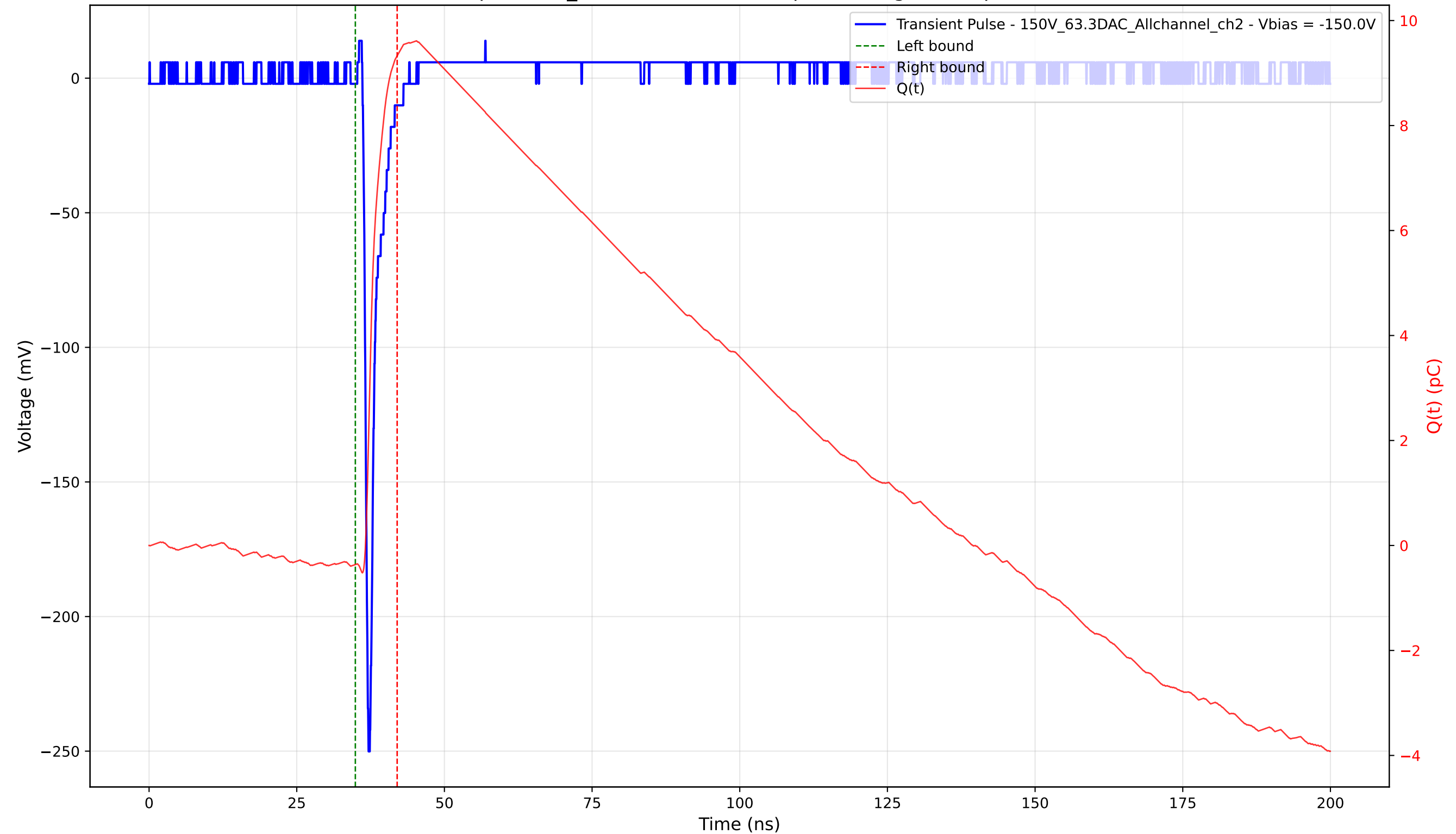
Transient Pulse - Sample: 1cm_42 - Position: 3470.0 \mu\text{m} - Charge: 9.69 pC - Rise Time: 0.72 ns
