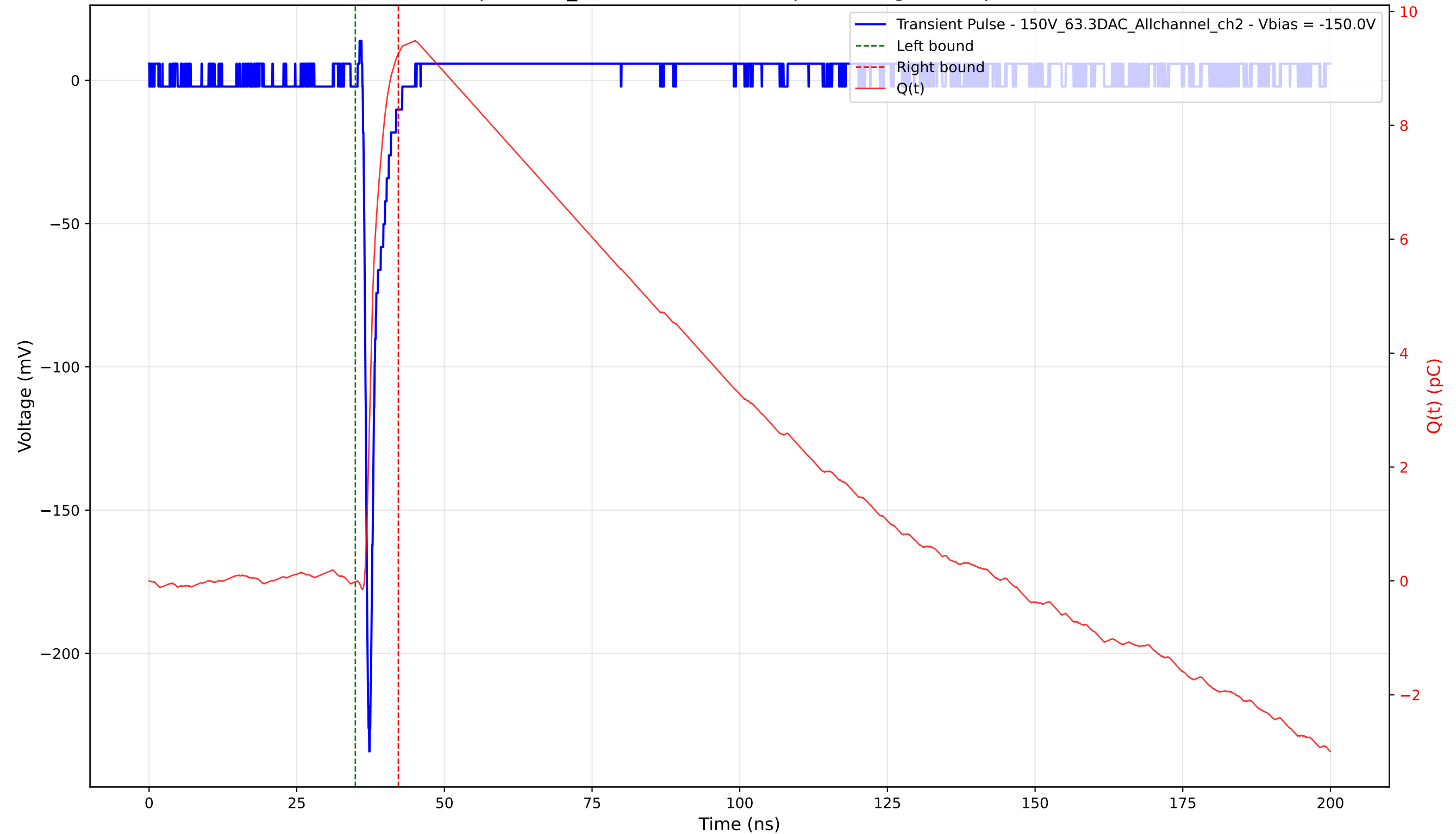
Transient Pulse - Sample: 1cm_42 - Position: 3495.0 \mu\text{m} - Charge: 9.27 pC - Rise Time: 0.77 ns
