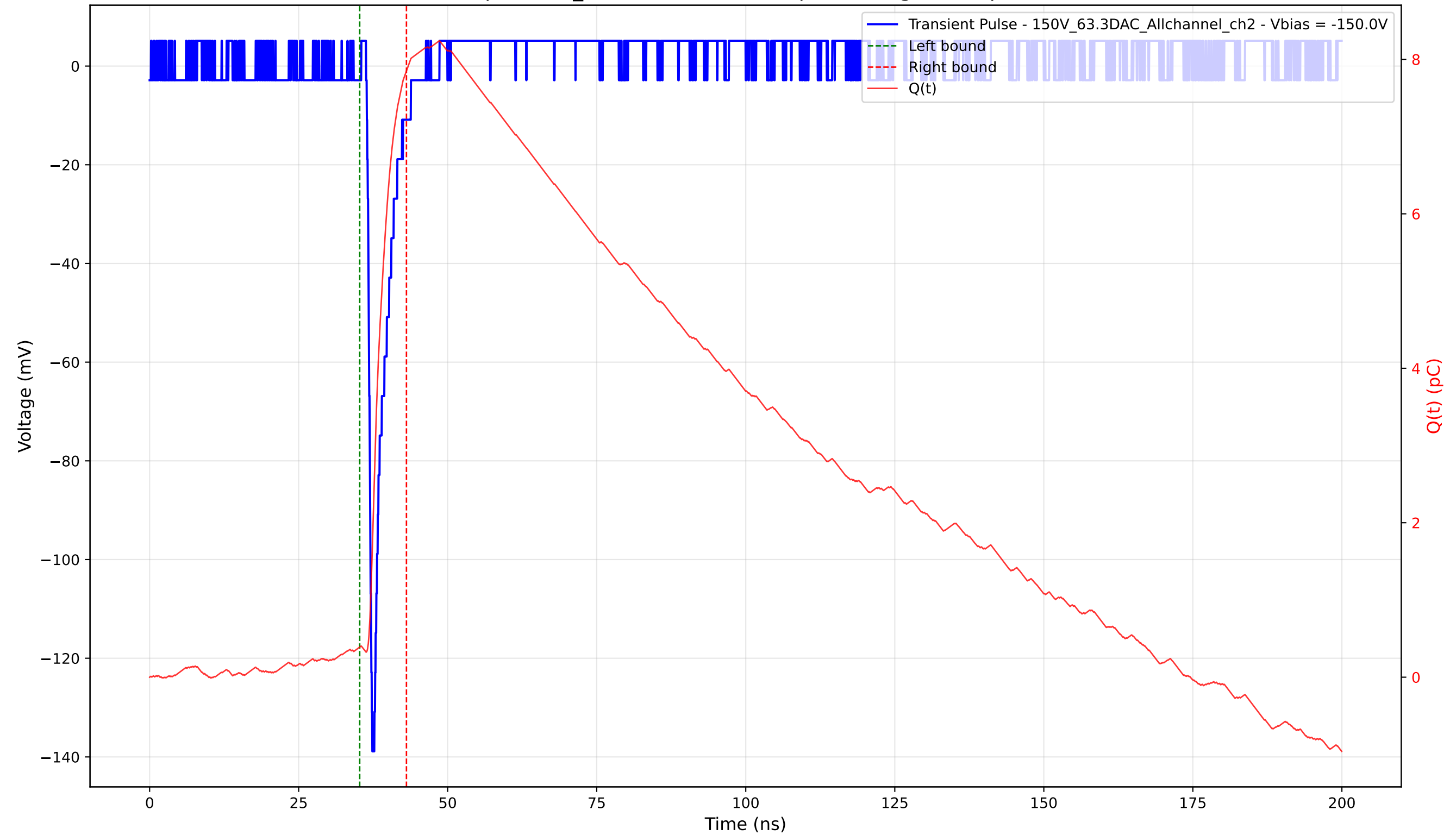
Transient Pulse - Sample: 1cm_42 - Position: 3715.0 \mu\text{m} - Charge: 7.46 pC - Rise Time: 0.78 ns
