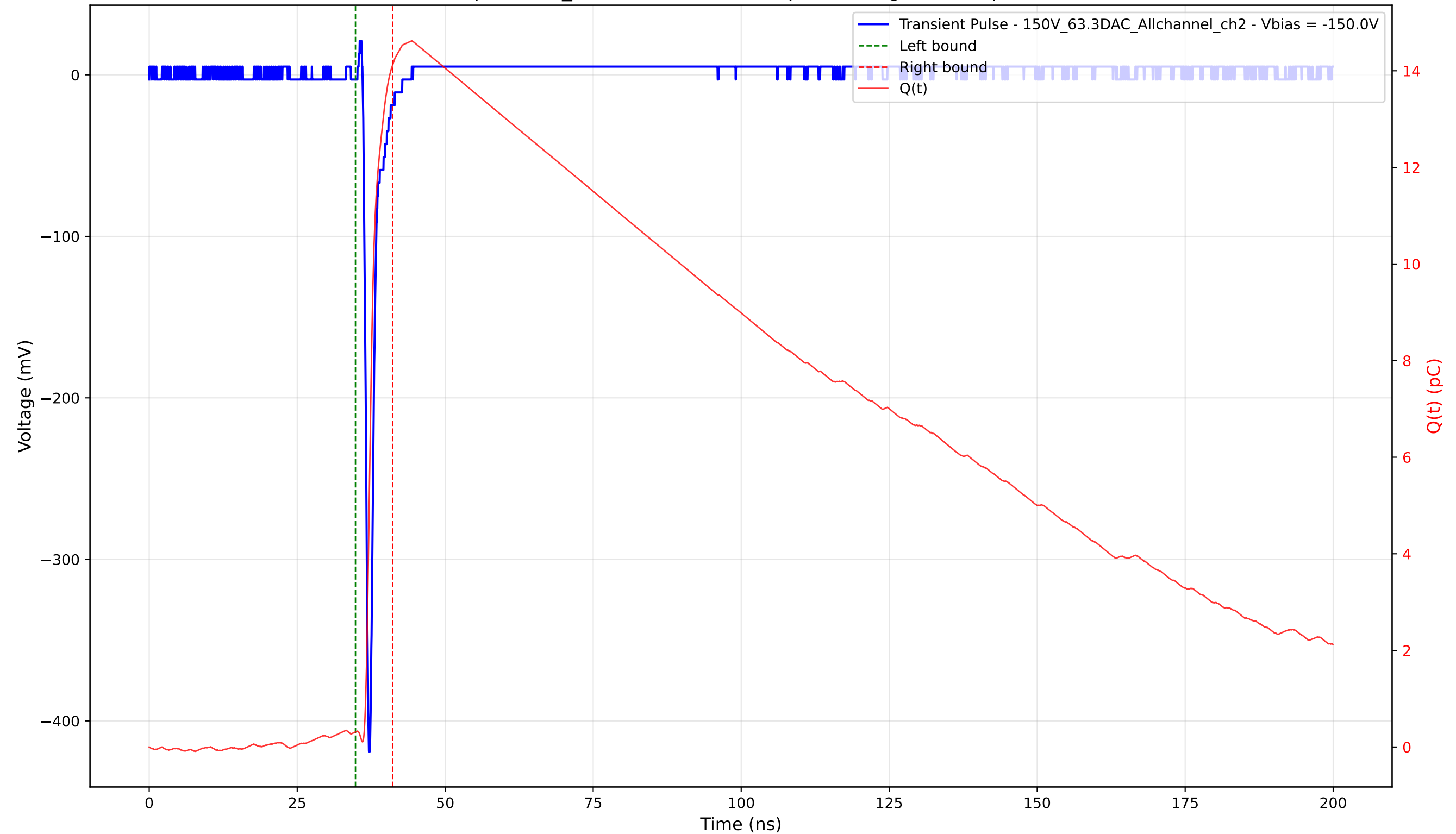
Transient Pulse - Sample: 1cm_42 - Position: 2730.0 \mu\text{m} - Charge: 13.81 pC - Rise Time: 0.71 ns
