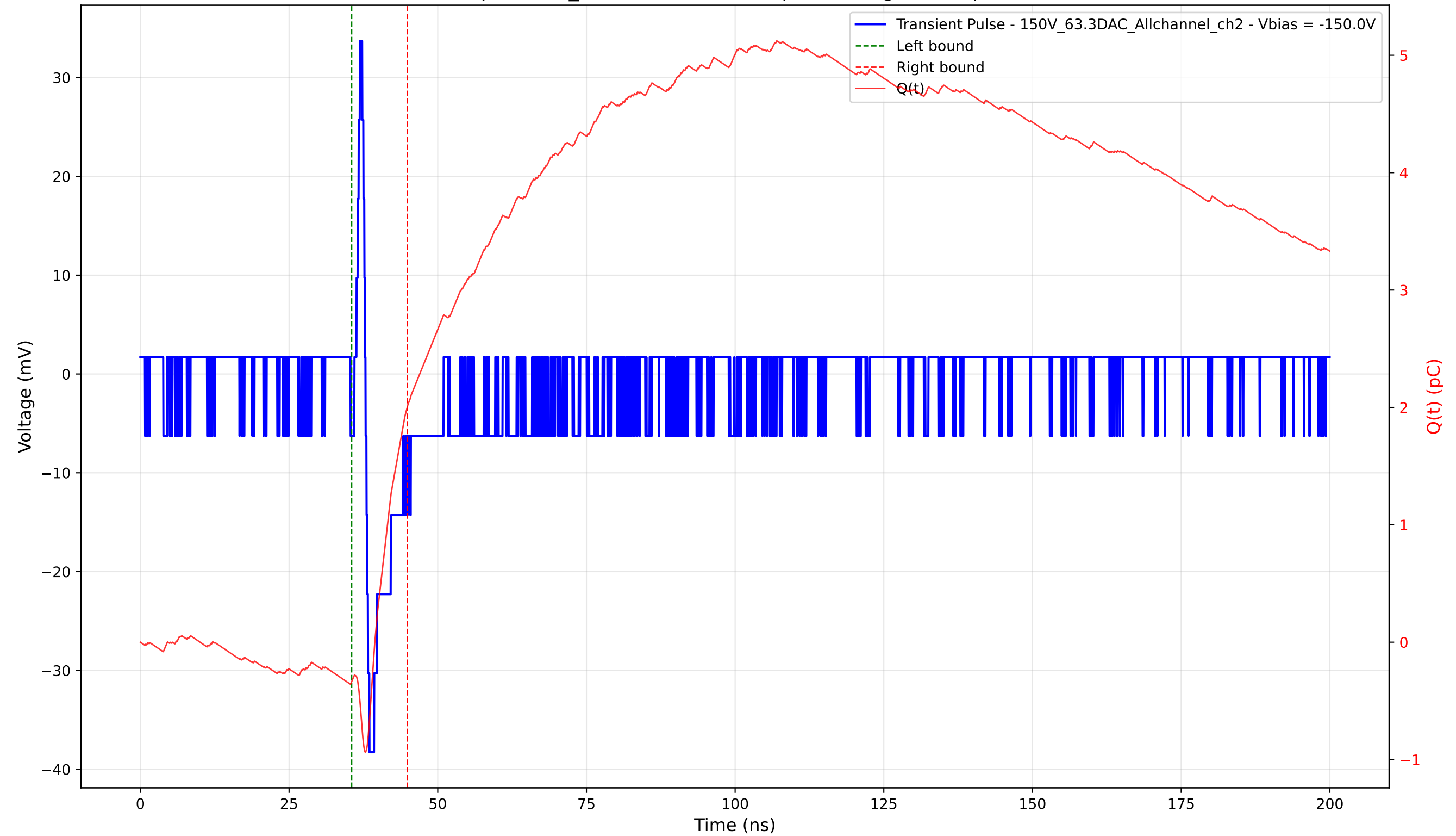
Transient Pulse - Sample: 1cm_42 - Position: 905.0 \mu\text{m} - Charge: 2.34 pC - Rise Time: 0.66 ns
