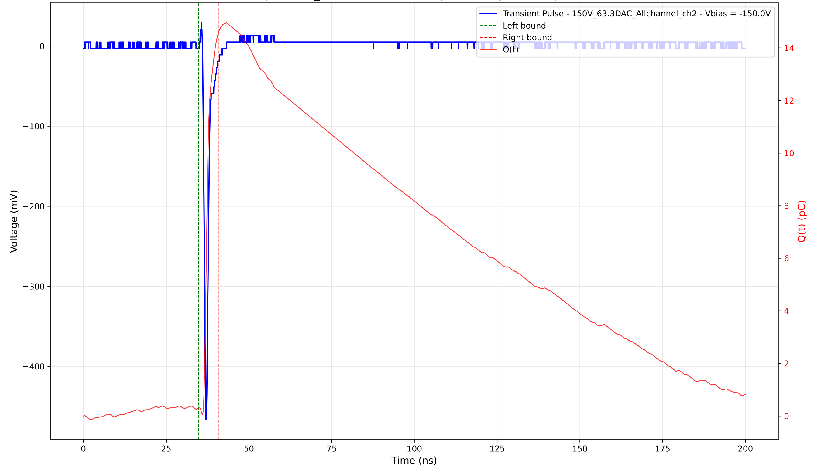
Transient Pulse - Sample: 1cm_42 - Position: 3050.0 \mu\text{m} - Charge: 14.25 pC - Rise Time: 0.71 ns
