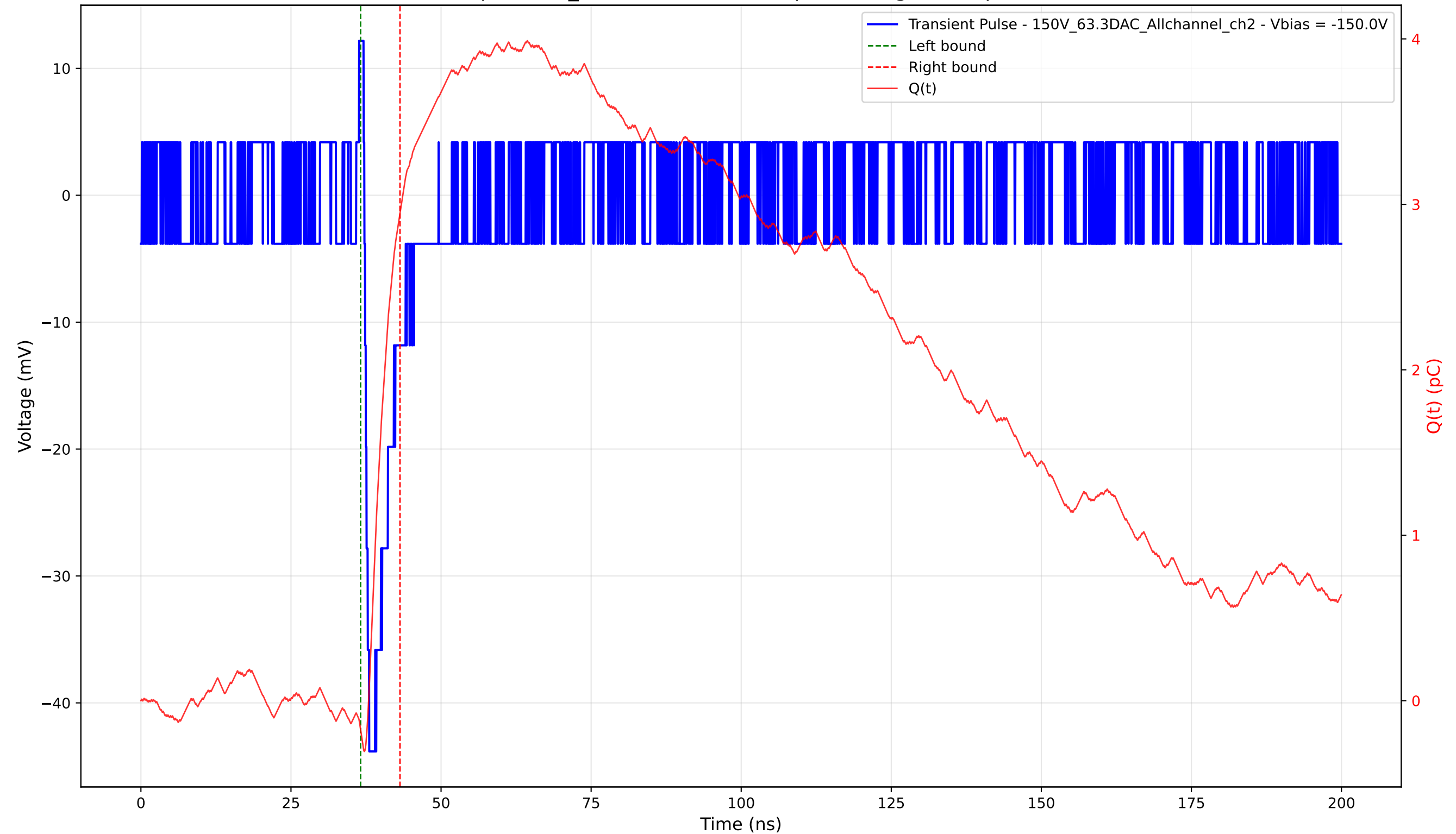
Transient Pulse - Sample: 1cm_42 - Position: 4435.0 \mu\text{m} - Charge: 3.12 pC - Rise Time: 0.72 ns
