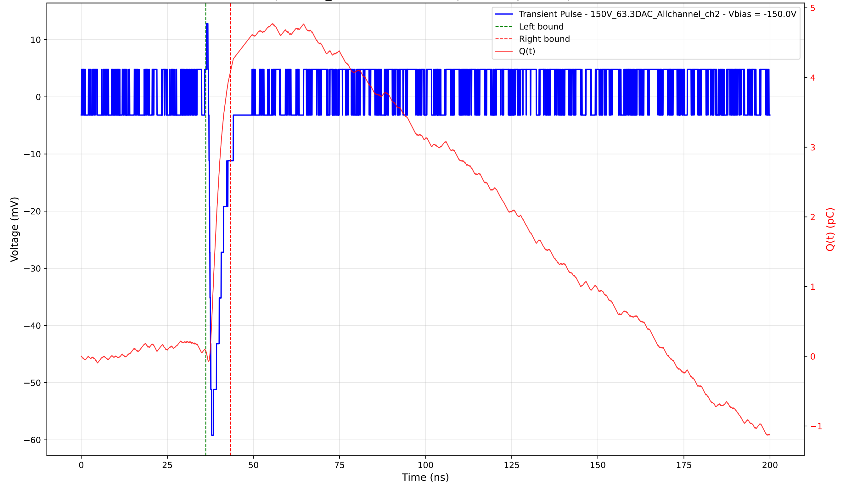
Transient Pulse - Sample: 1cm_42 - Position: 4150.0 \mu\text{m} - Charge: 4.00 pC - Rise Time: 0.79 ns
