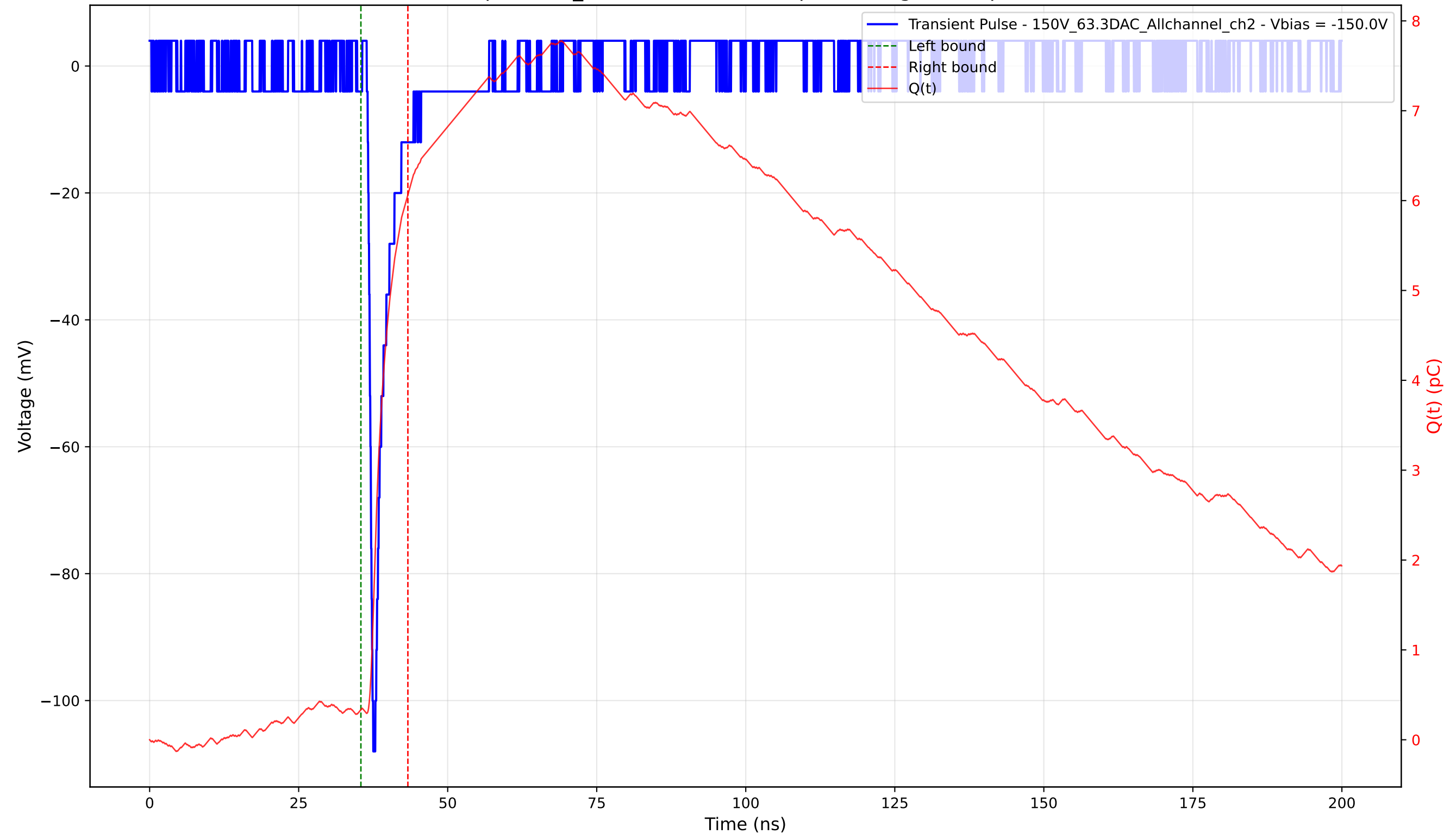
Transient Pulse - Sample: 1cm_42 - Position: 2160.0 \mu\text{m} - Charge: 5.73 pC - Rise Time: 0.81 ns
