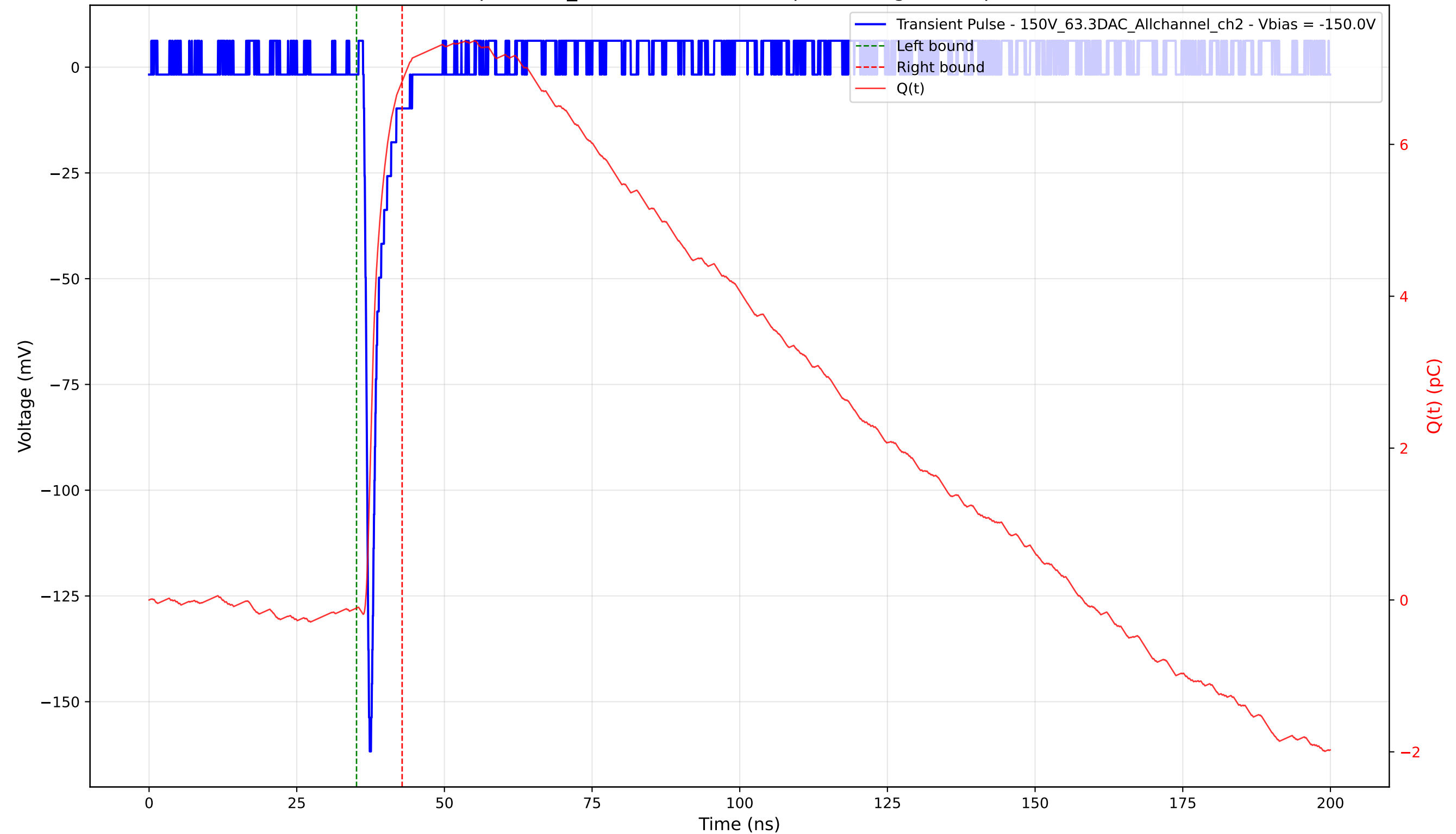
Transient Pulse - Sample: 1cm_42 - Position: 2425.0 \mu\text{m} - Charge: 6.94 pC - Rise Time: 0.77 ns
