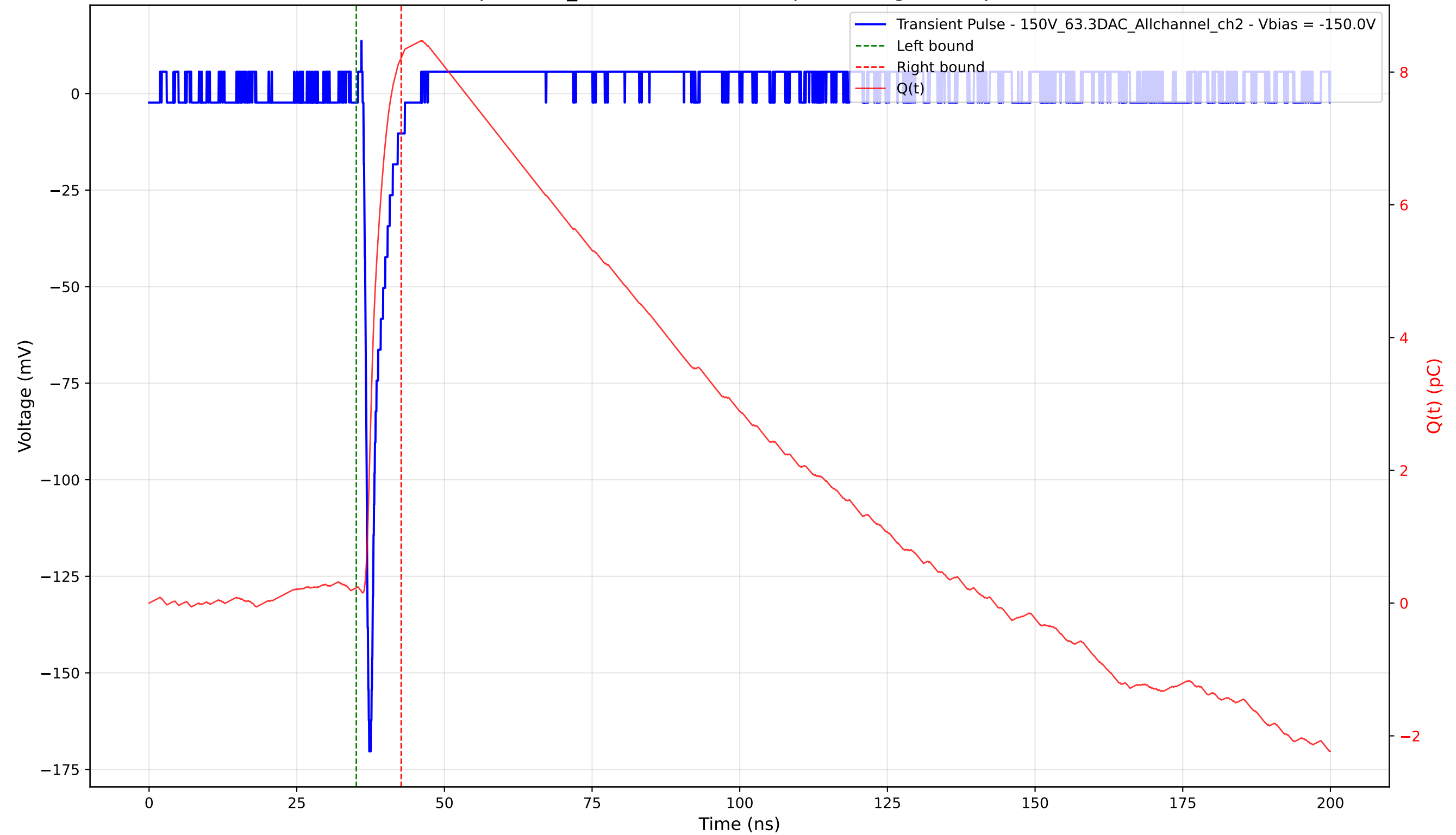
Transient Pulse - Sample: 1cm_42 - Position: 3590.0 \mu\text{m} - Charge: 7.99 pC - Rise Time: 0.77 ns
