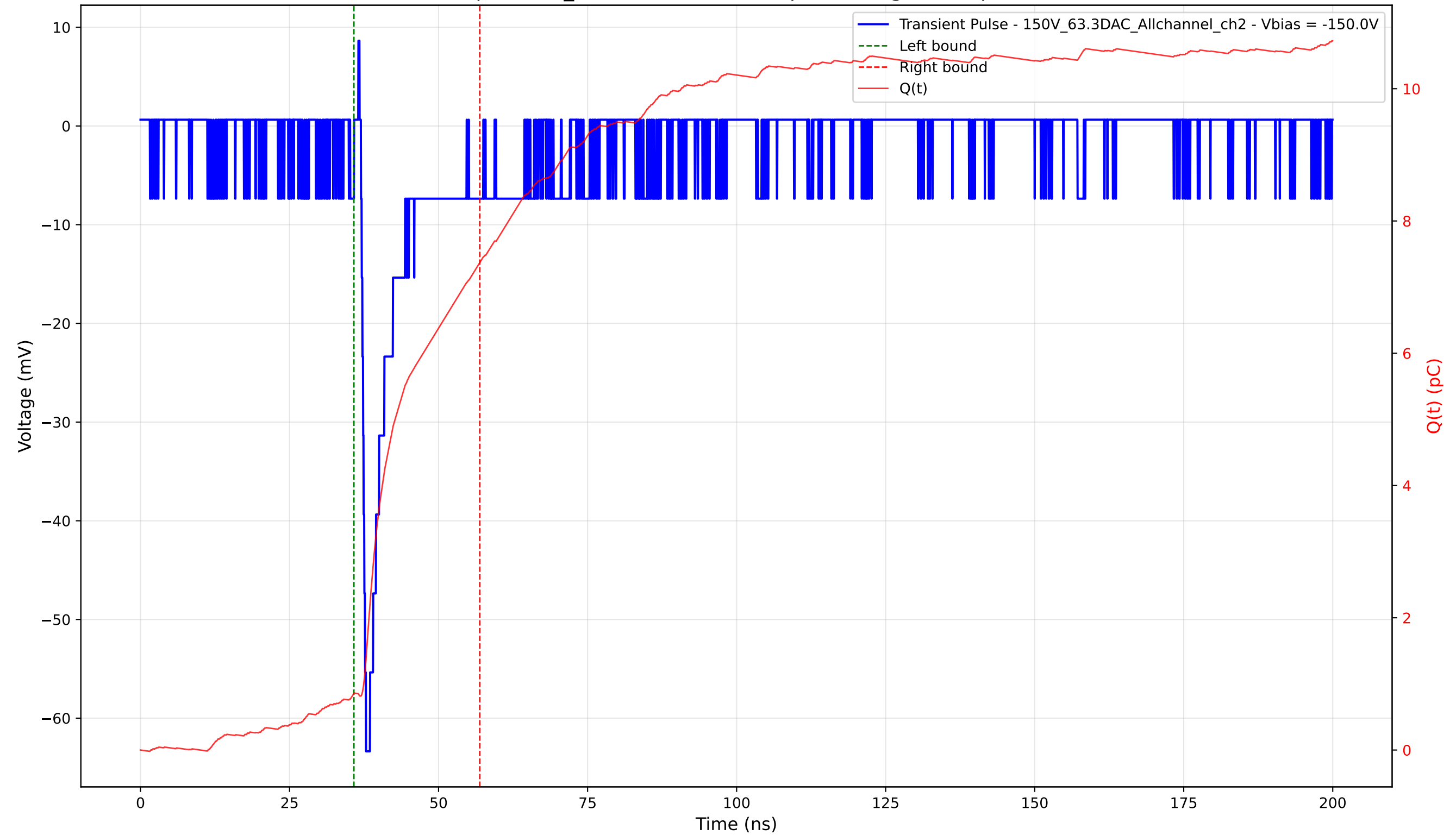
Transient Pulse - Sample: 1cm_42 - Position: 1915.0 \mu\text{m} - Charge: 6.51 pC - Rise Time: 0.85 ns
