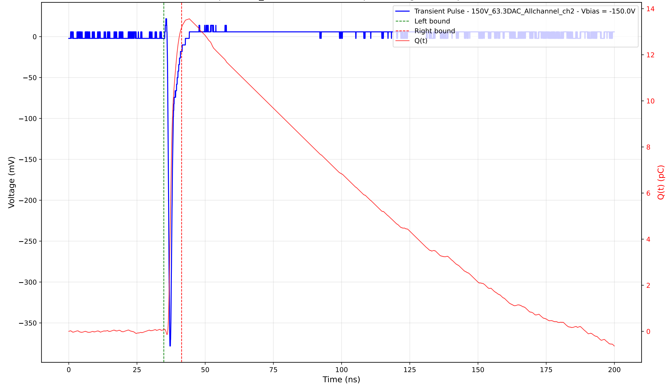
Transient Pulse - Sample: 1cm_42 - Position: 3350.0 \mu\text{m} - Charge: 13.11 pC - Rise Time: 0.68 ns
