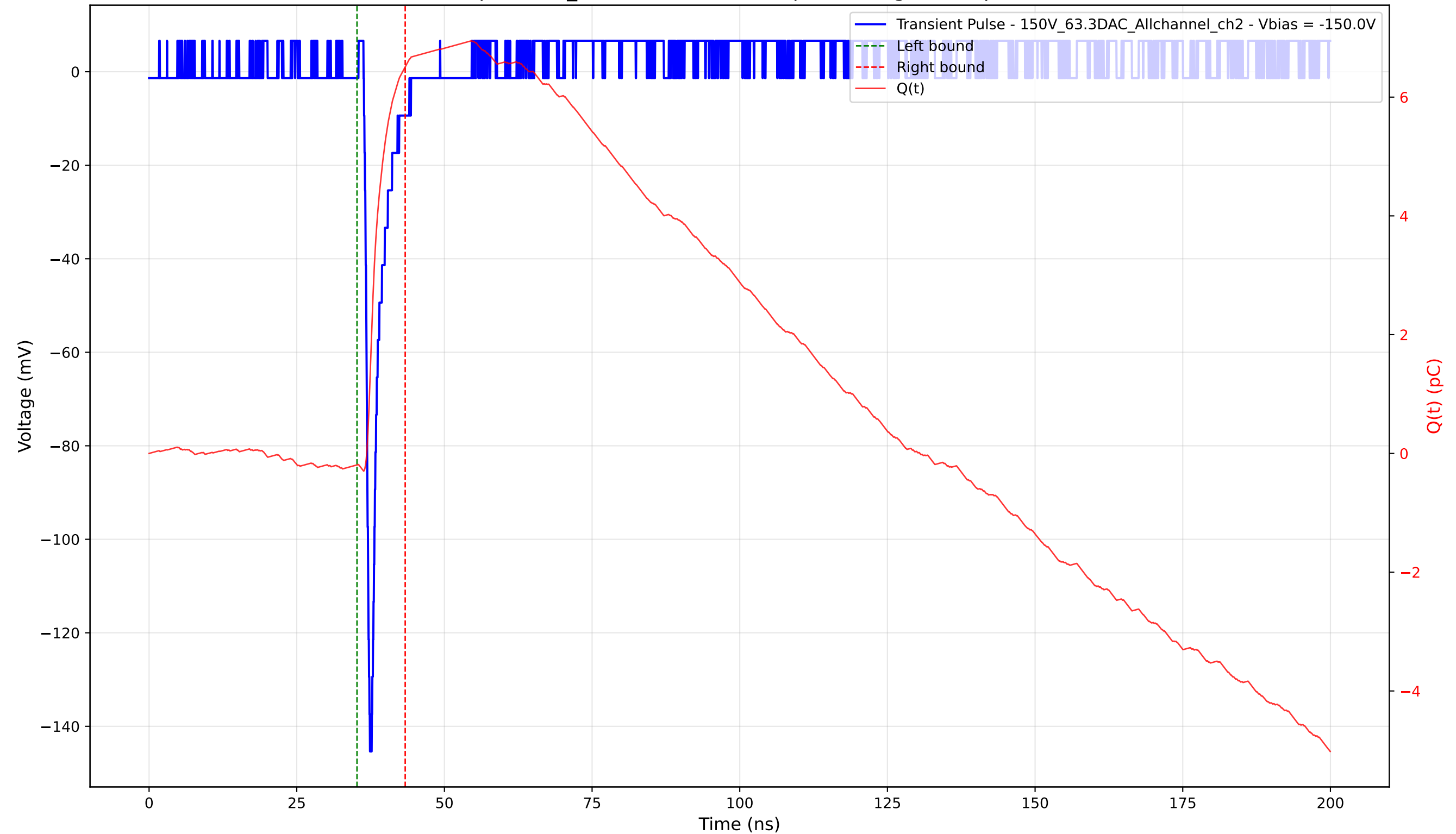
Transient Pulse - Sample: 1cm_42 - Position: 2360.0 \mu\text{m} - Charge: 6.70 pC - Rise Time: 0.85 ns
