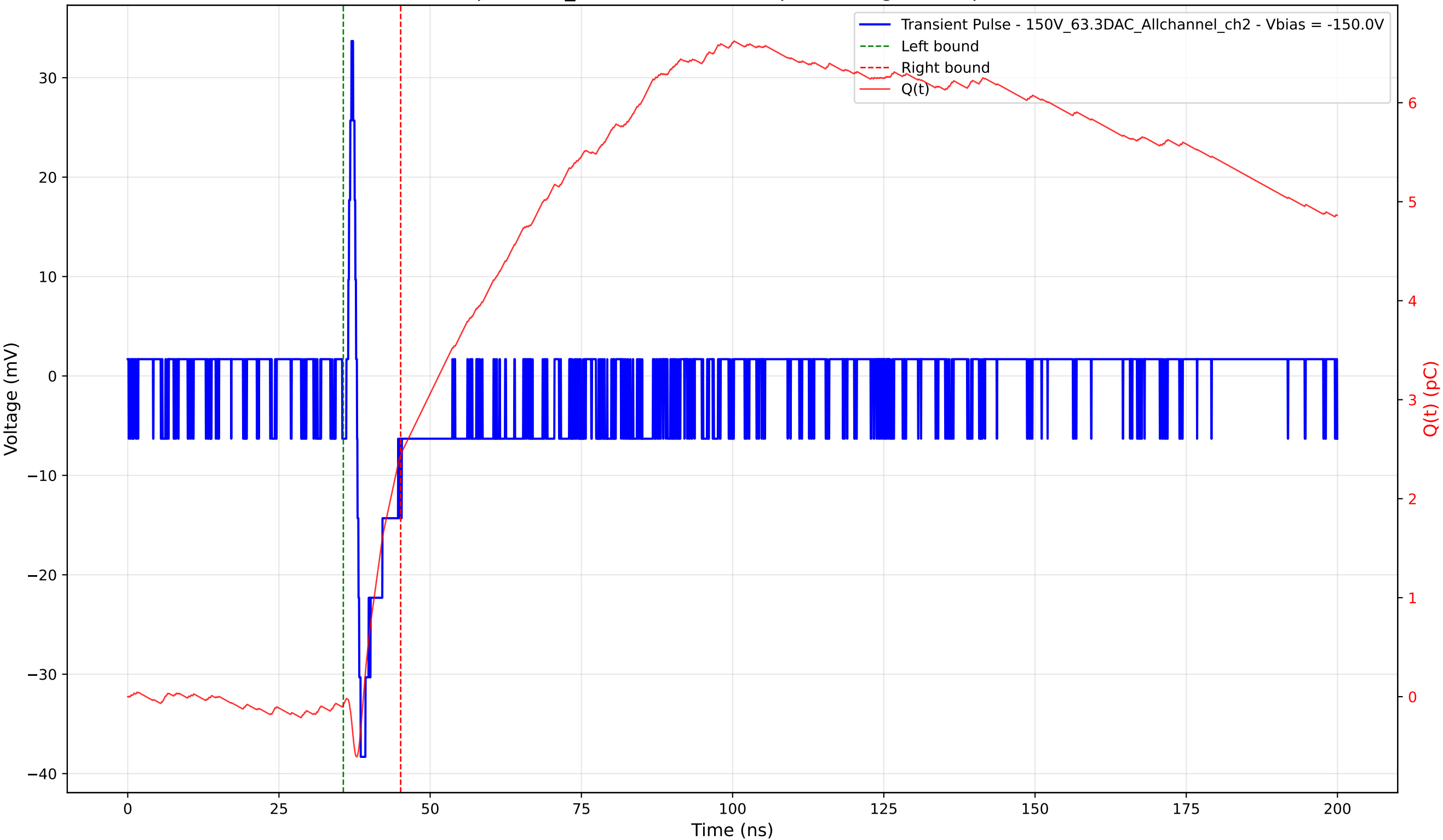
Transient Pulse - Sample: 1cm_42 - Position: 995.0 \mu\text{m} - Charge: 2.51 pC - Rise Time: 0.62 ns
