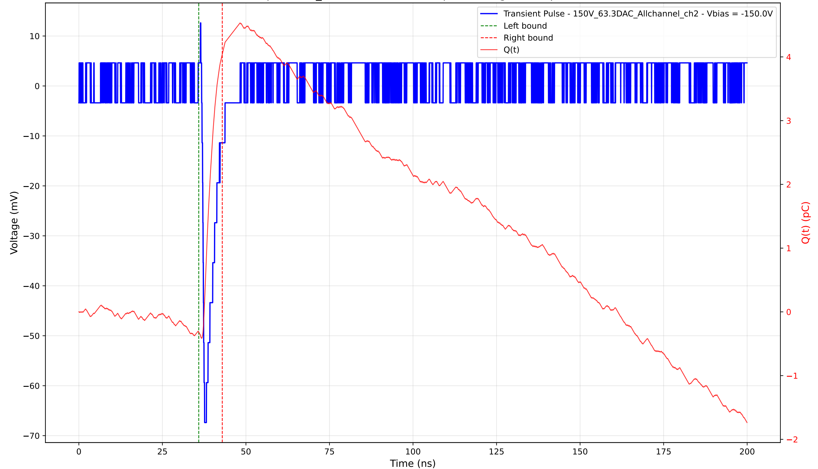
Transient Pulse - Sample: 1cm_42 - Position: 4040.0 \mu\text{m} - Charge: 4.36 pC - Rise Time: 0.78 ns
