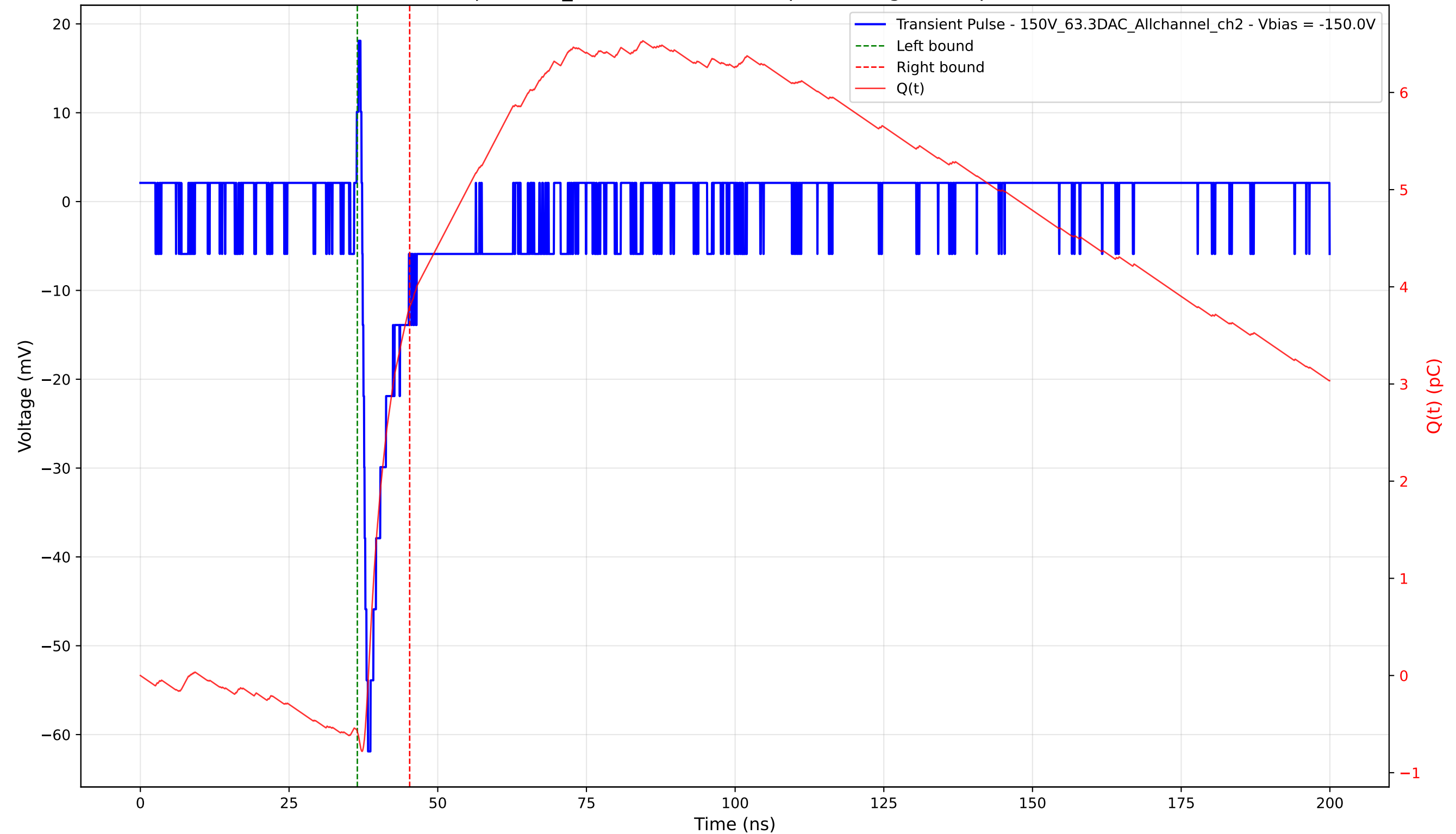
Transient Pulse - Sample: 1cm_42 - Position: 1695.0 \mu\text{m} - Charge: 4.37 pC - Rise Time: 0.92 ns
