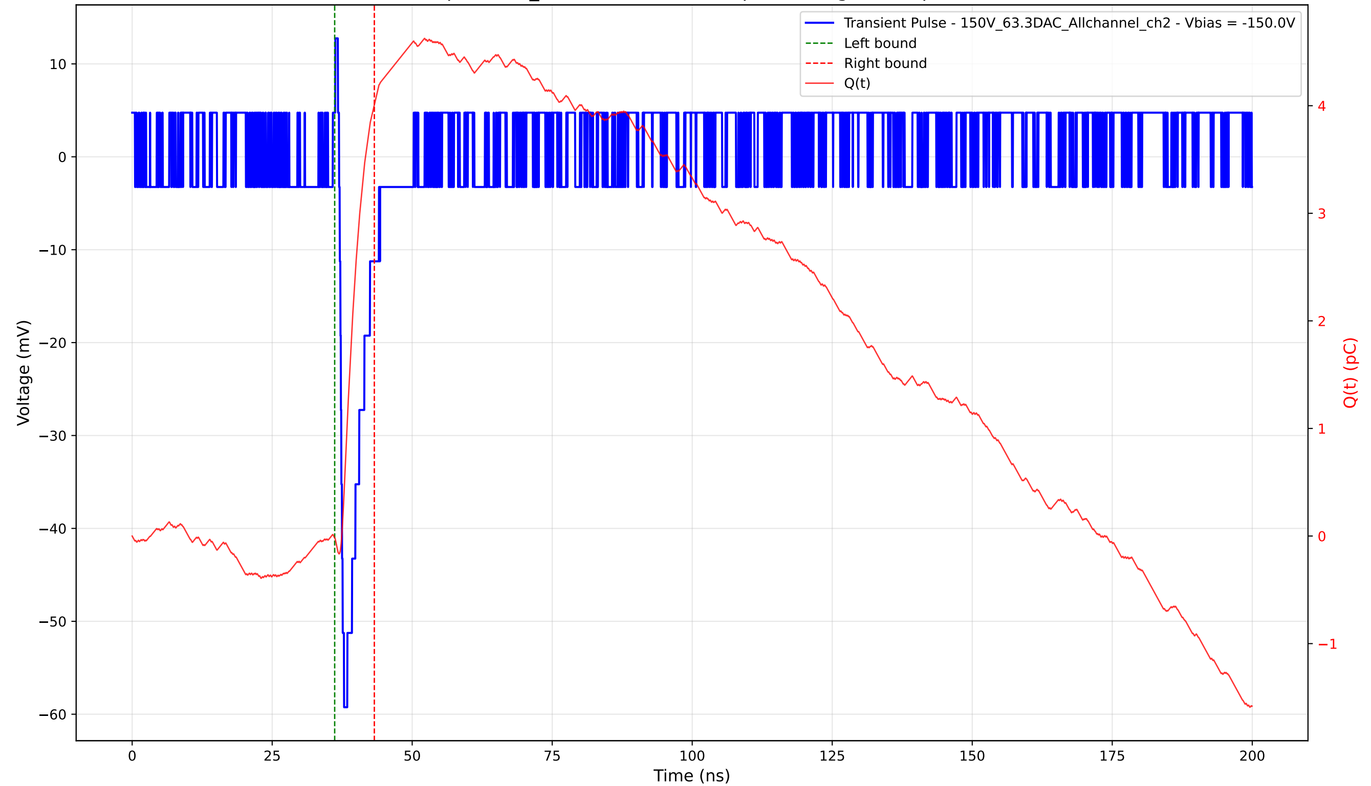
Transient Pulse - Sample: 1cm_42 - Position: 4135.0 \mu\text{m} - Charge: 4.03 pC - Rise Time: 0.79 ns
