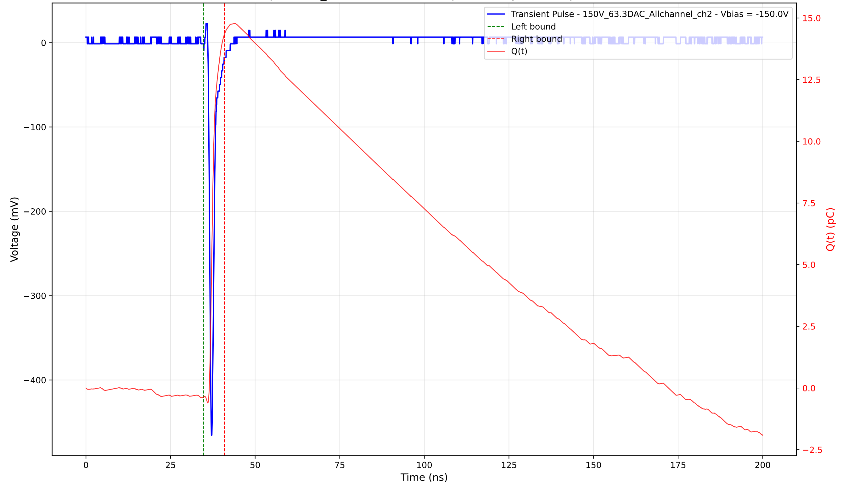
Transient Pulse - Sample: 1cm_42 - Position: 2810.0 \mu\text{m} - Charge: 14.68 pC - Rise Time: 0.73 ns
