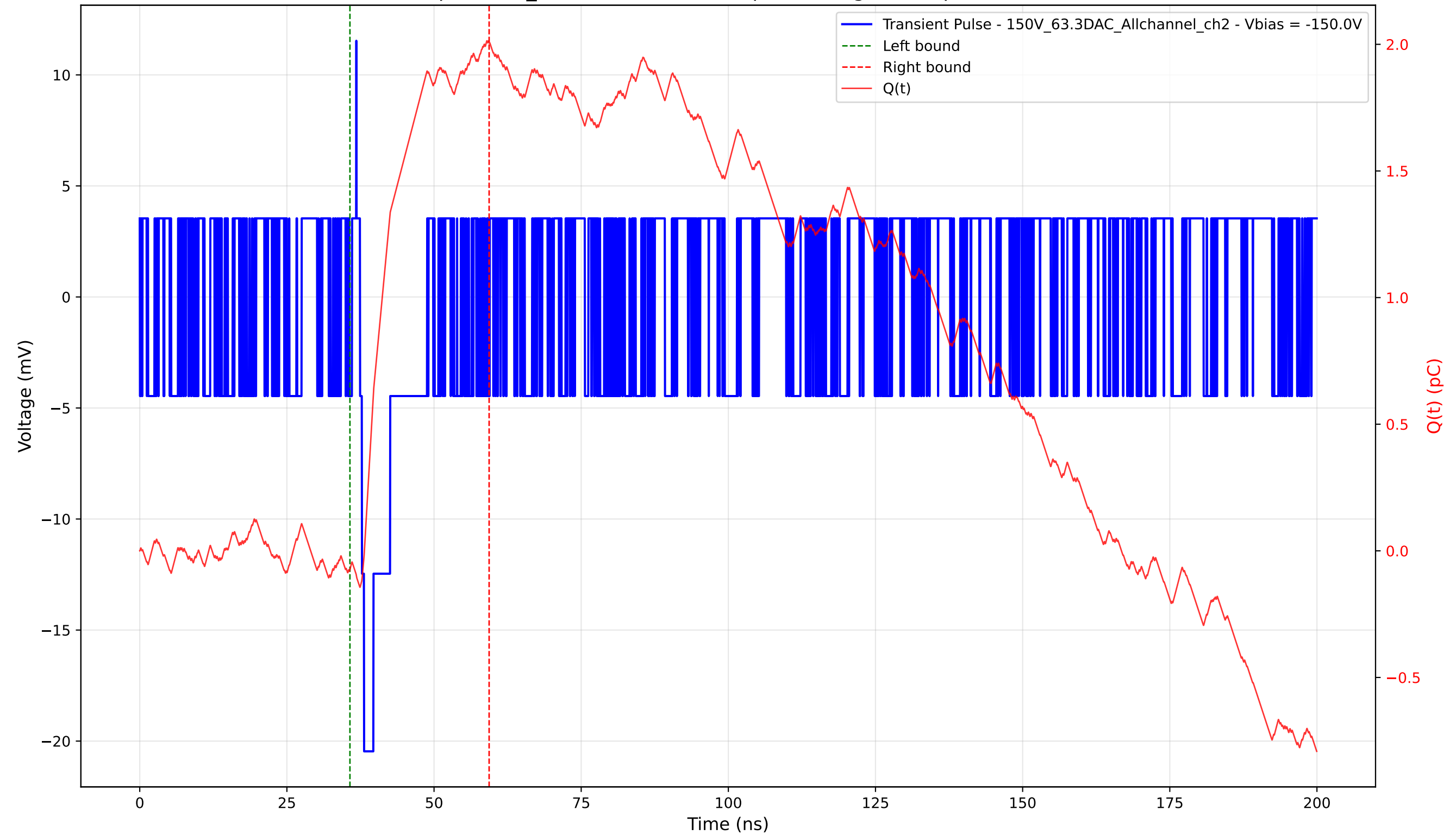
Transient Pulse - Sample: 1cm_42 - Position: 4990.0 \mu\text{m} - Charge: 2.08 pC - Rise Time: 0.00 ns (N/A)
