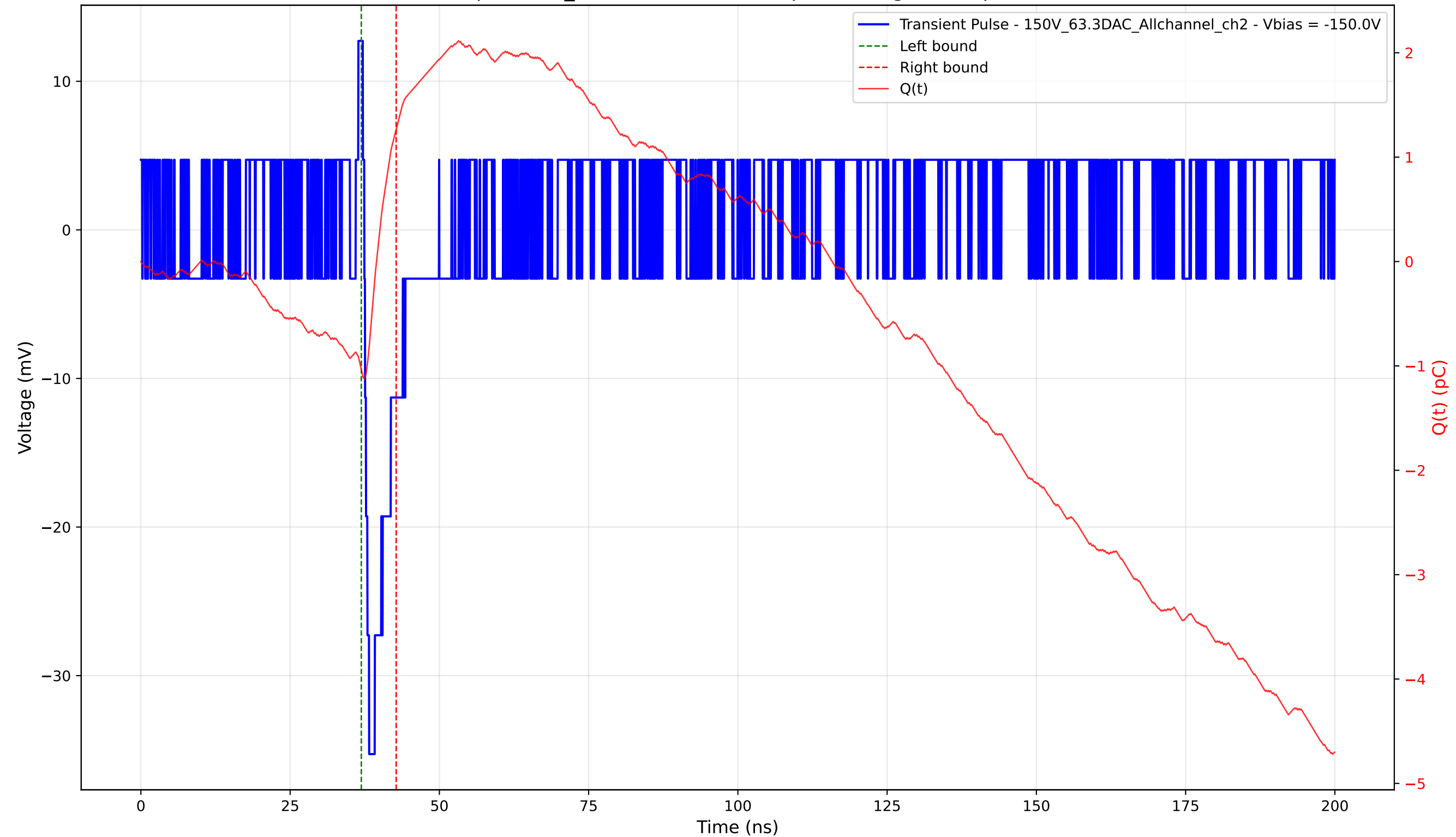
Transient Pulse - Sample: 1cm_42 - Position: 4610.0 \mu\text{m} - Charge: 2.30 pC - Rise Time: 0.72 ns
