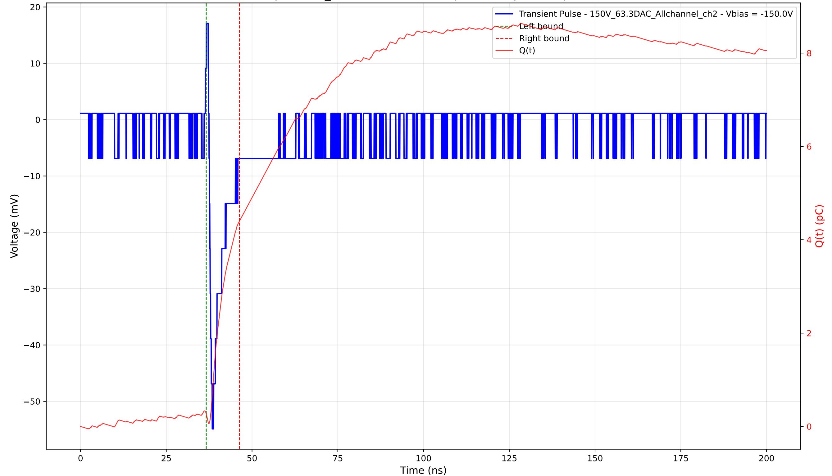
Transient Pulse - Sample: 1cm_42 - Position: 1600.0 \mu\text{m} - Charge: 4.12 pC - Rise Time: 0.93 ns
