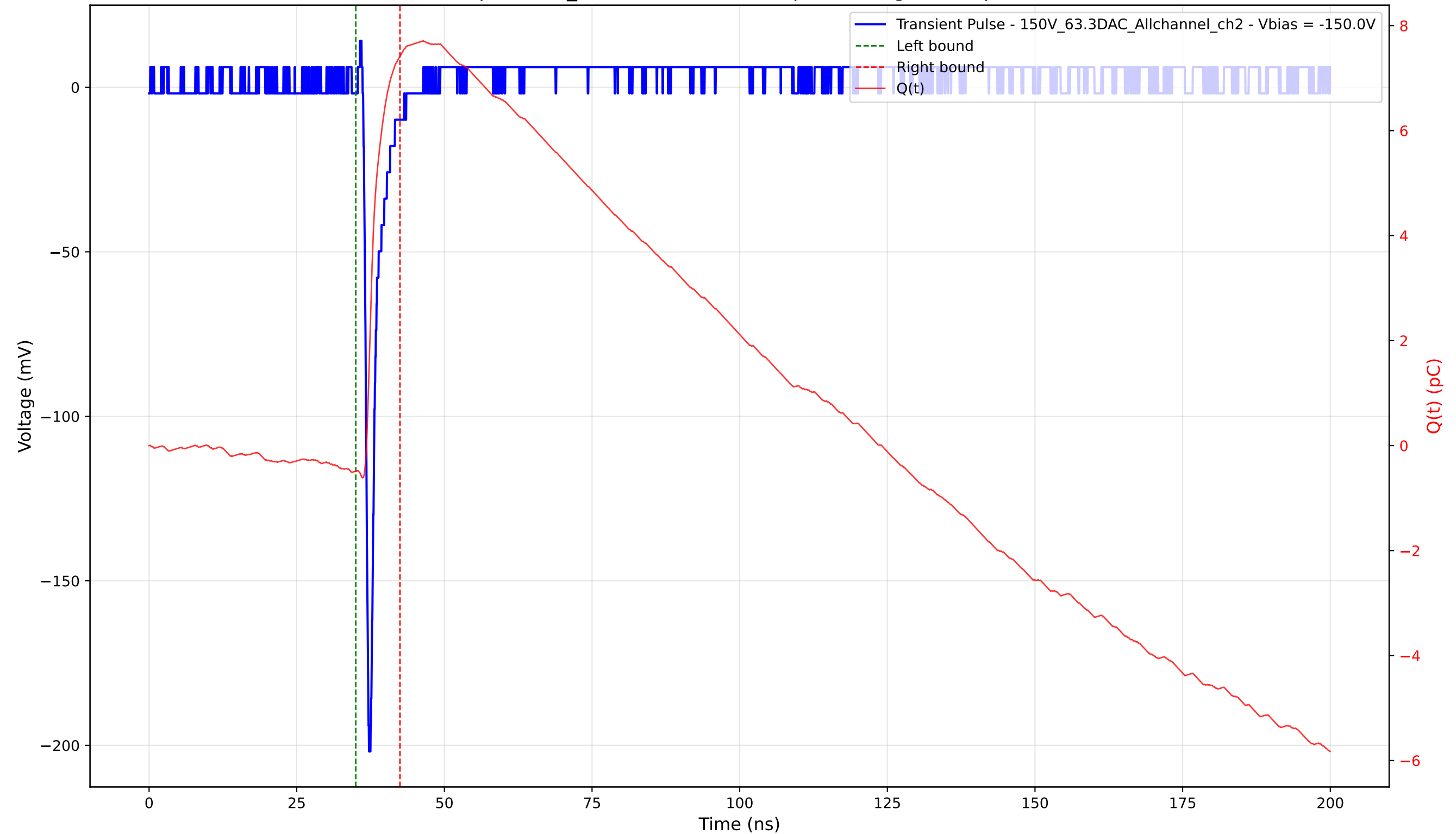
Transient Pulse - Sample: 1cm_42 - Position: 2510.0 \mu\text{m} - Charge: 7.90 pC - Rise Time: 0.73 ns
