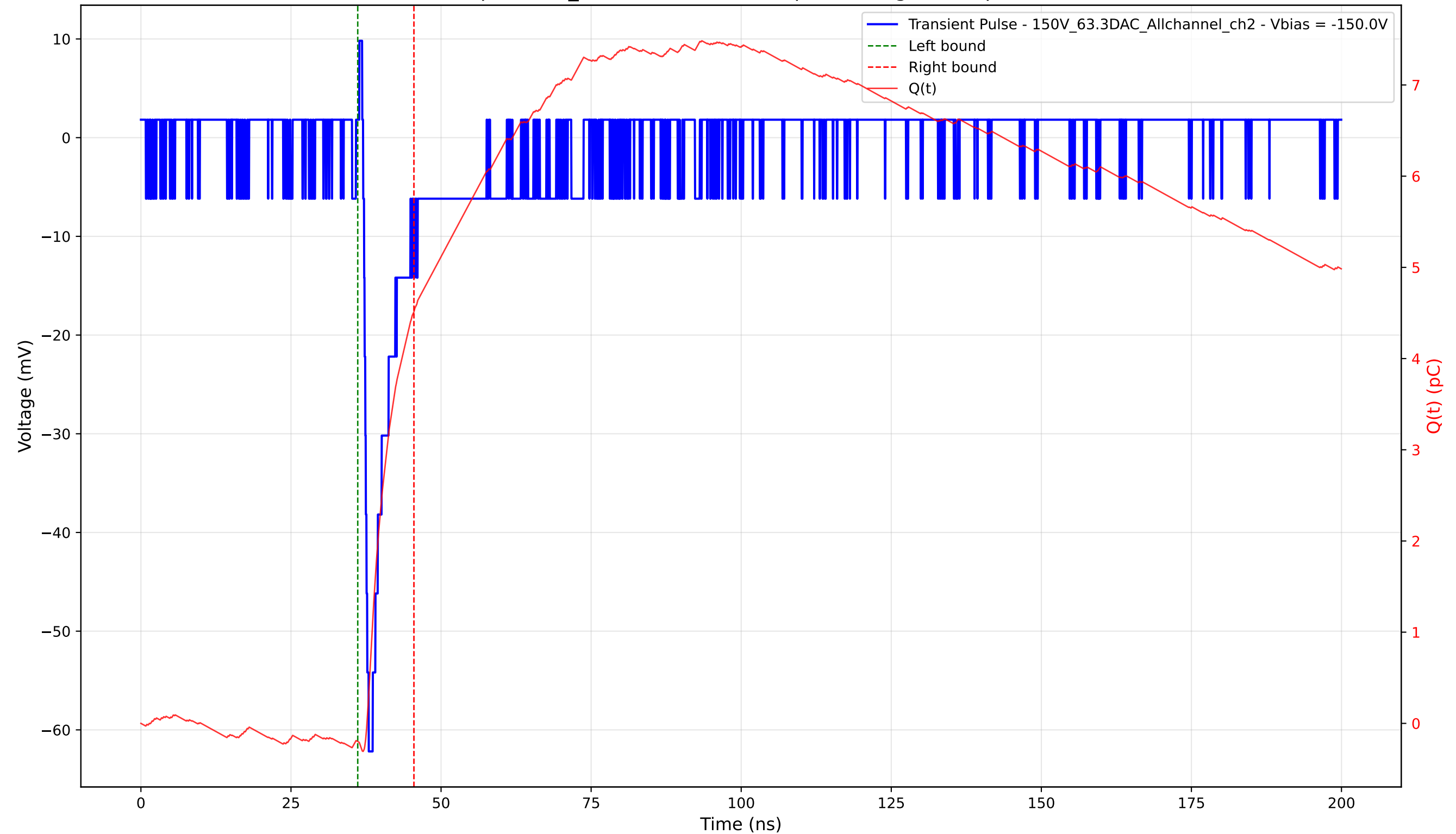
Transient Pulse - Sample: 1cm_42 - Position: 1895.0 \mu\text{m} - Charge: 4.71 pC - Rise Time: 0.80 ns
