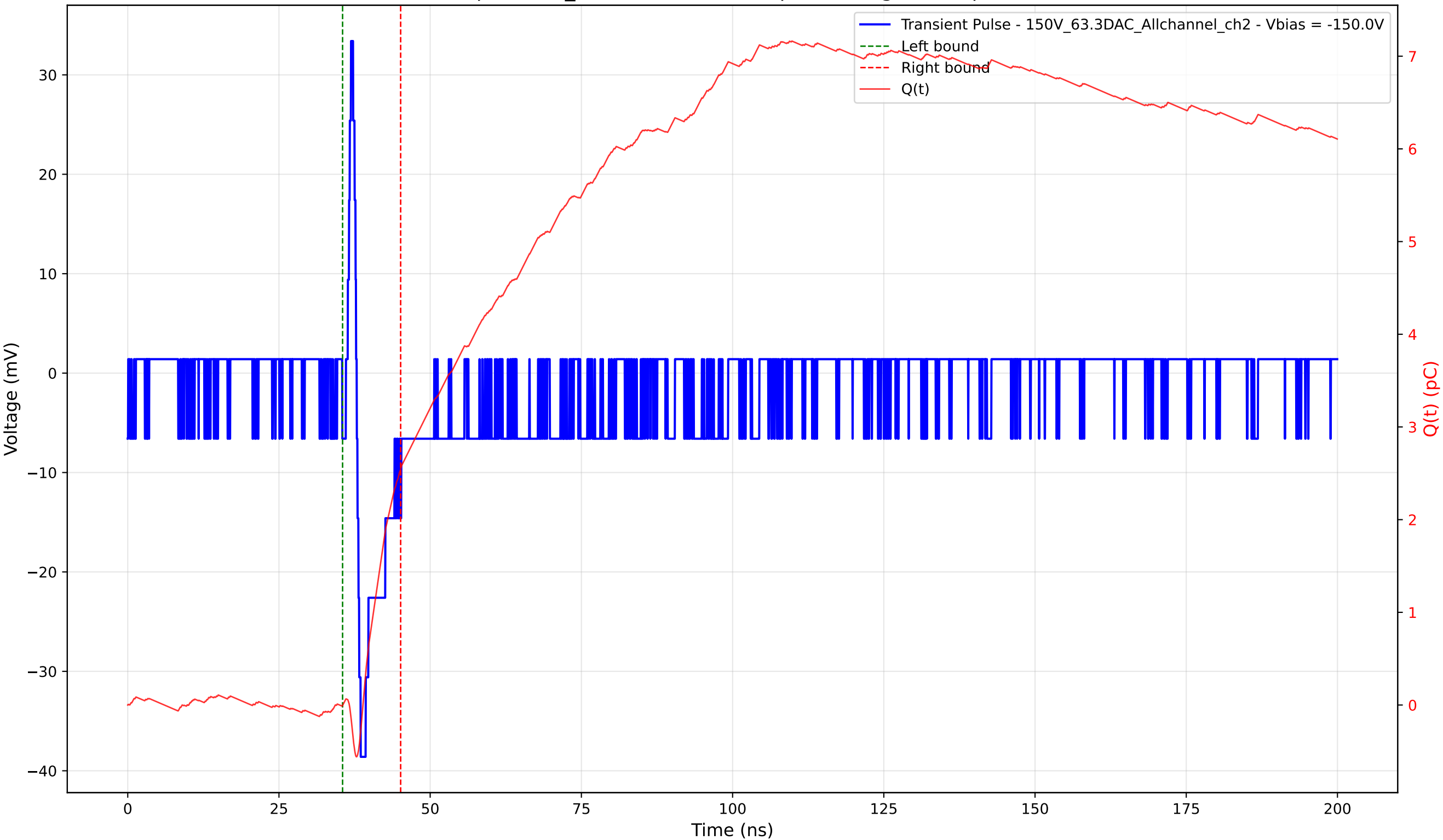
Transient Pulse - Sample: 1cm_42 - Position: 930.0 \mu\text{m} - Charge: 2.55 pC - Rise Time: 0.66 ns
