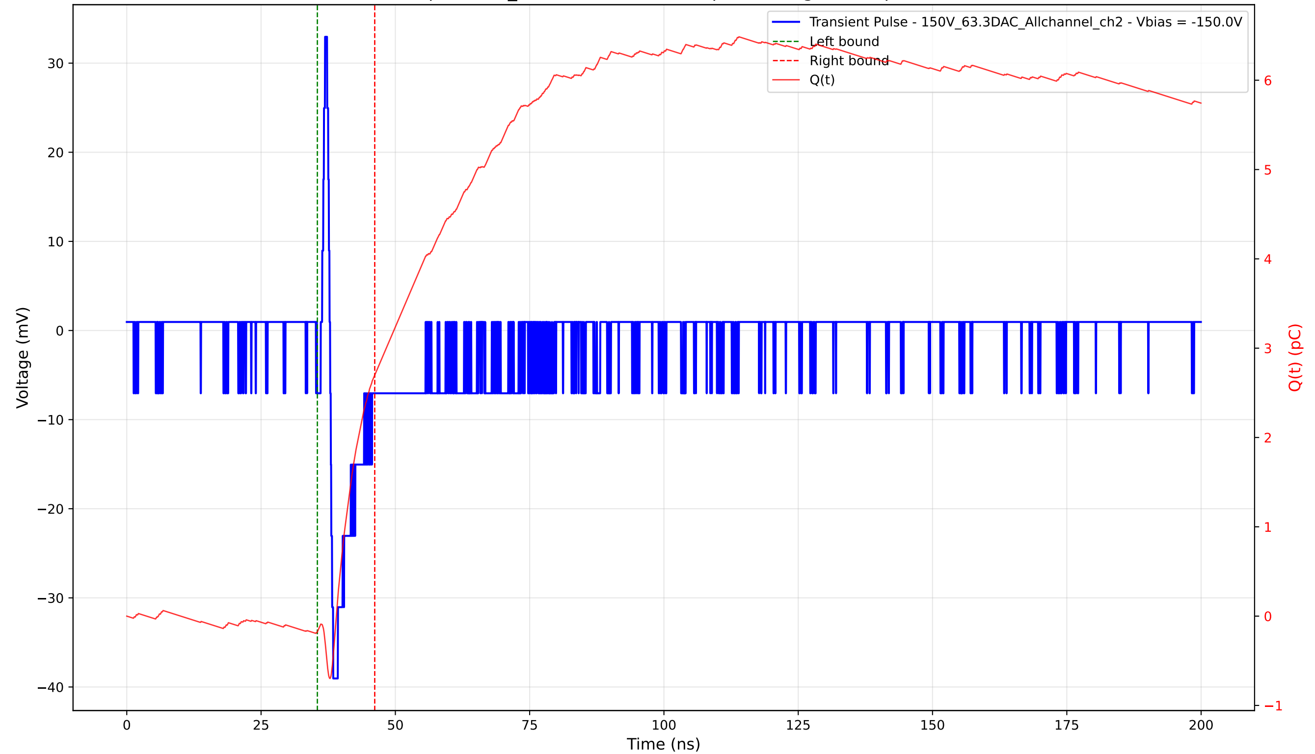
Transient Pulse - Sample: 1cm_42 - Position: 1090.0 \mu\text{m} - Charge: 2.87 pC - Rise Time: 0.58 ns
