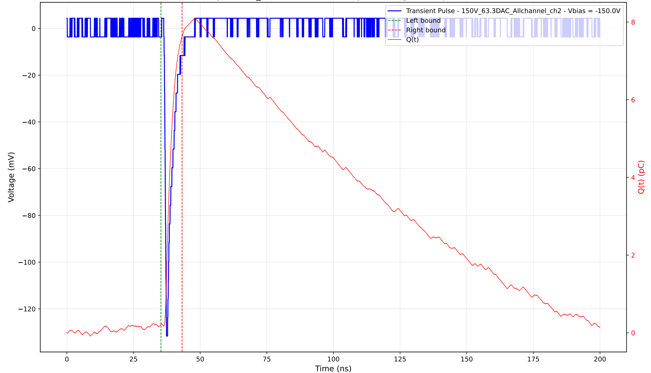
Transient Pulse - Sample: 1cm_42 - Position: 3750.0 \mu\text{m} - Charge: 7.41 pC - Rise Time: 0.71 ns
