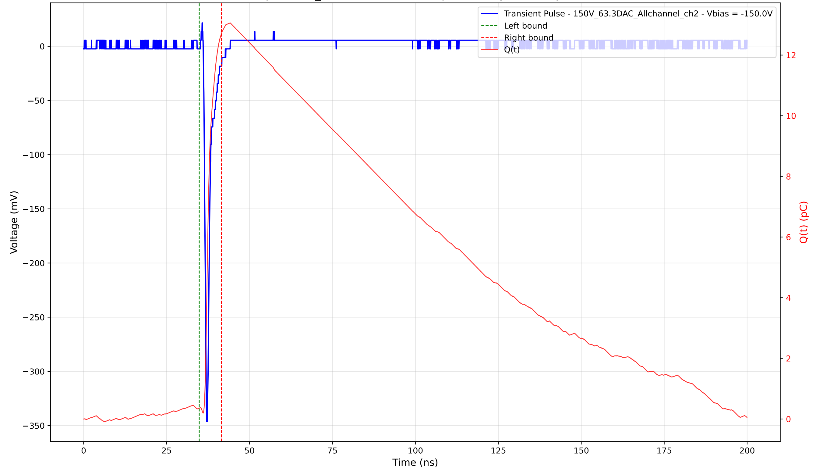
Transient Pulse - Sample: 1cm_42 - Position: 3380.0 \mu\text{m} - Charge: 12.34 pC - Rise Time: 0.71 ns
