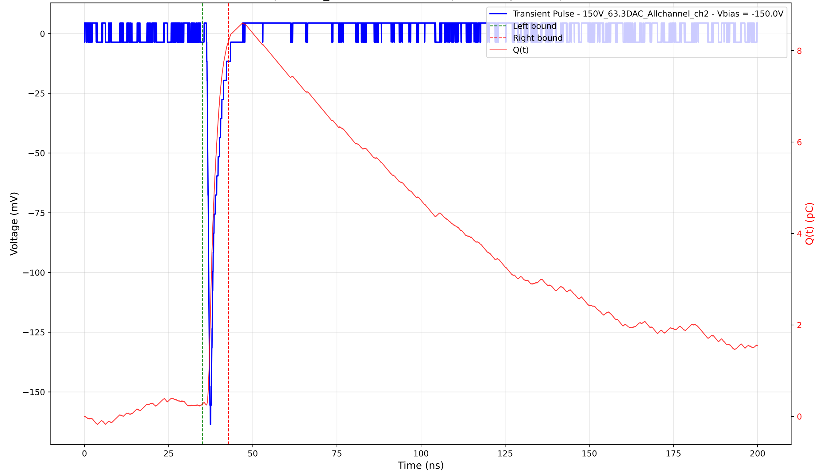
Transient Pulse - Sample: 1cm_42 - Position: 3635.0 \mu\text{m} - Charge: 7.93 pC - Rise Time: 0.78 ns
