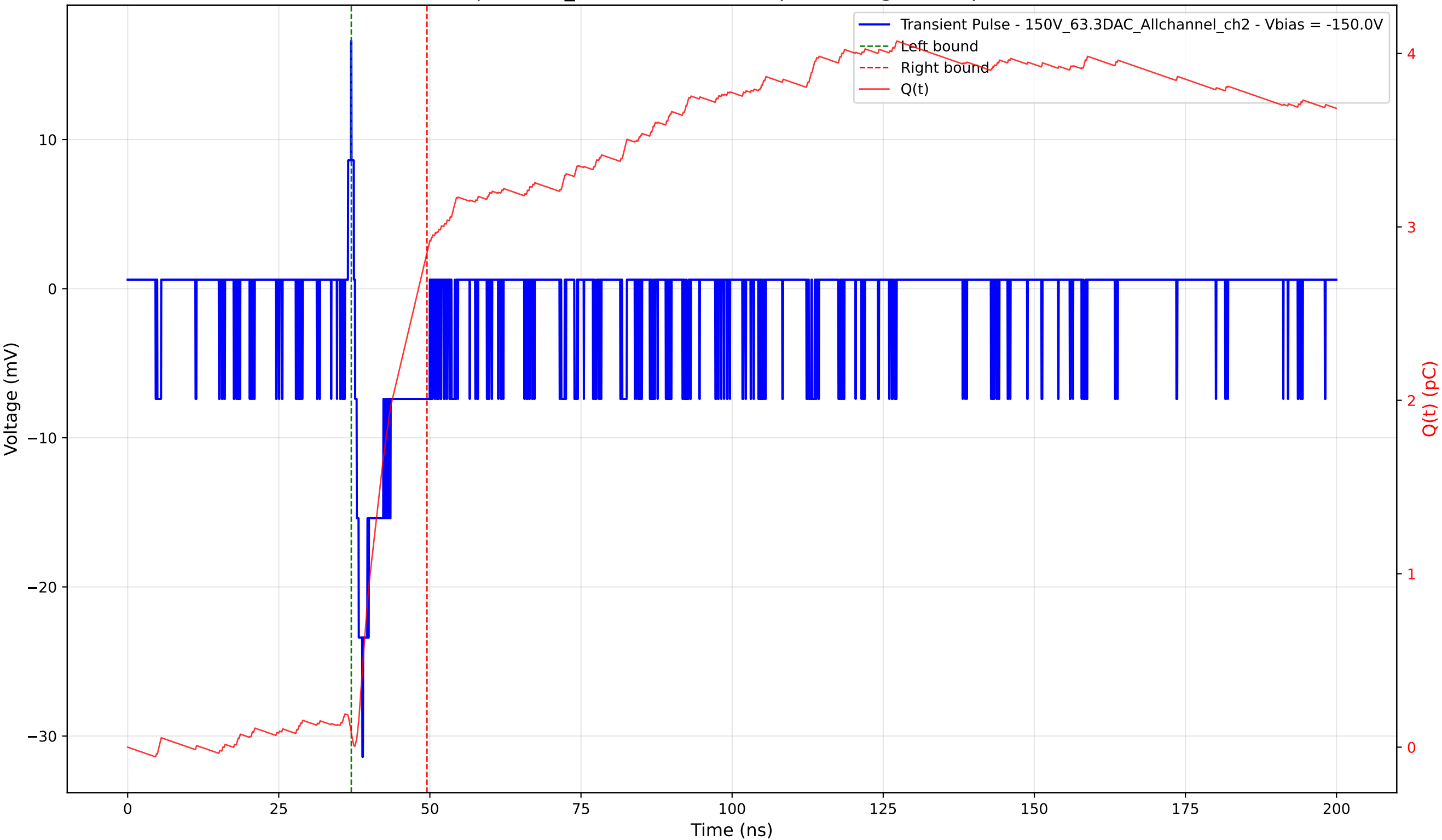
Transient Pulse - Sample: 1cm_42 - Position: 345.0 \mu\text{m} - Charge: 2.77 pC - Rise Time: 1.23 ns
