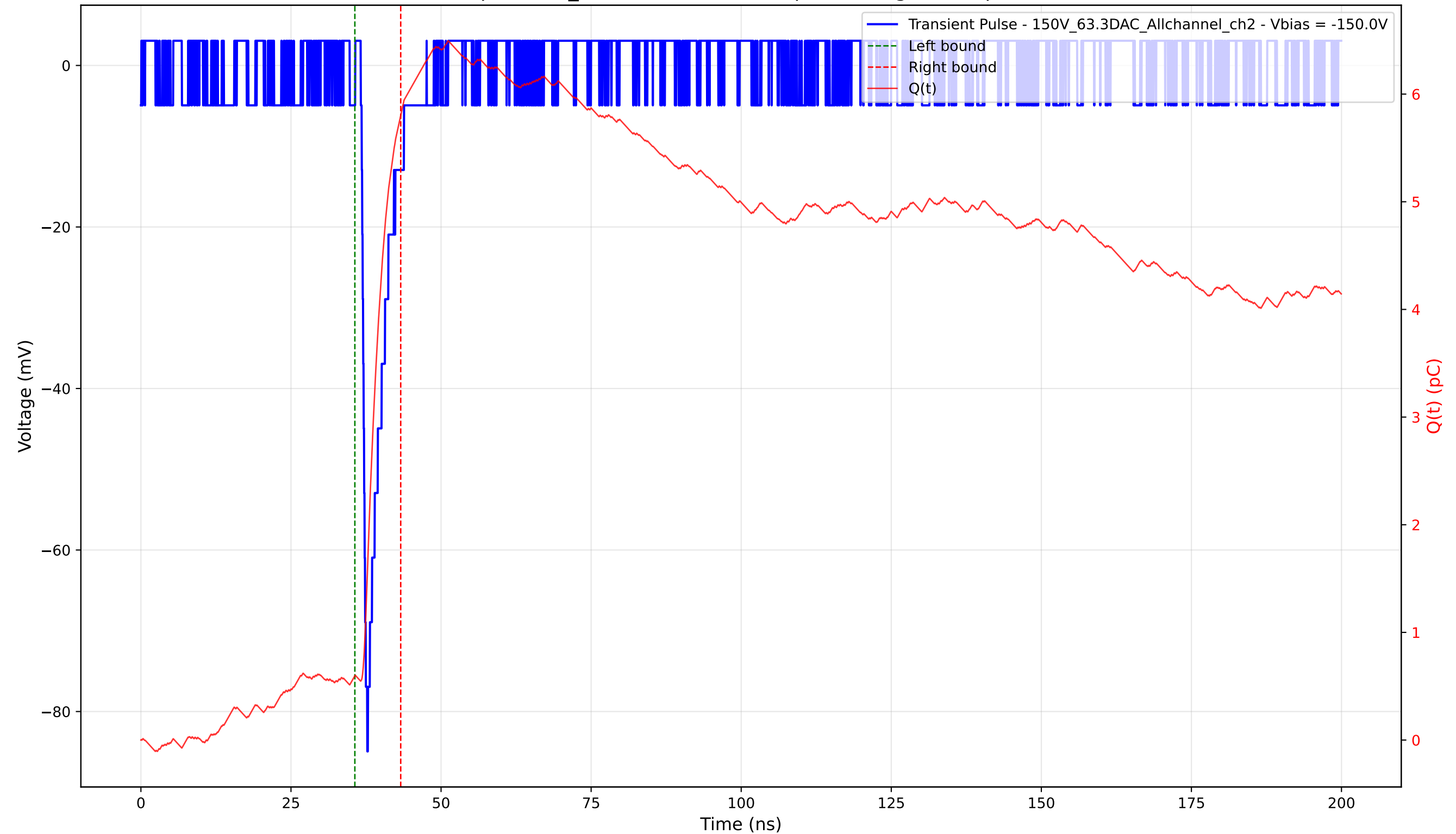
Transient Pulse - Sample: 1cm_42 - Position: 3975.0 \mu\text{m} - Charge: 5.21 pC - Rise Time: 0.70 ns
