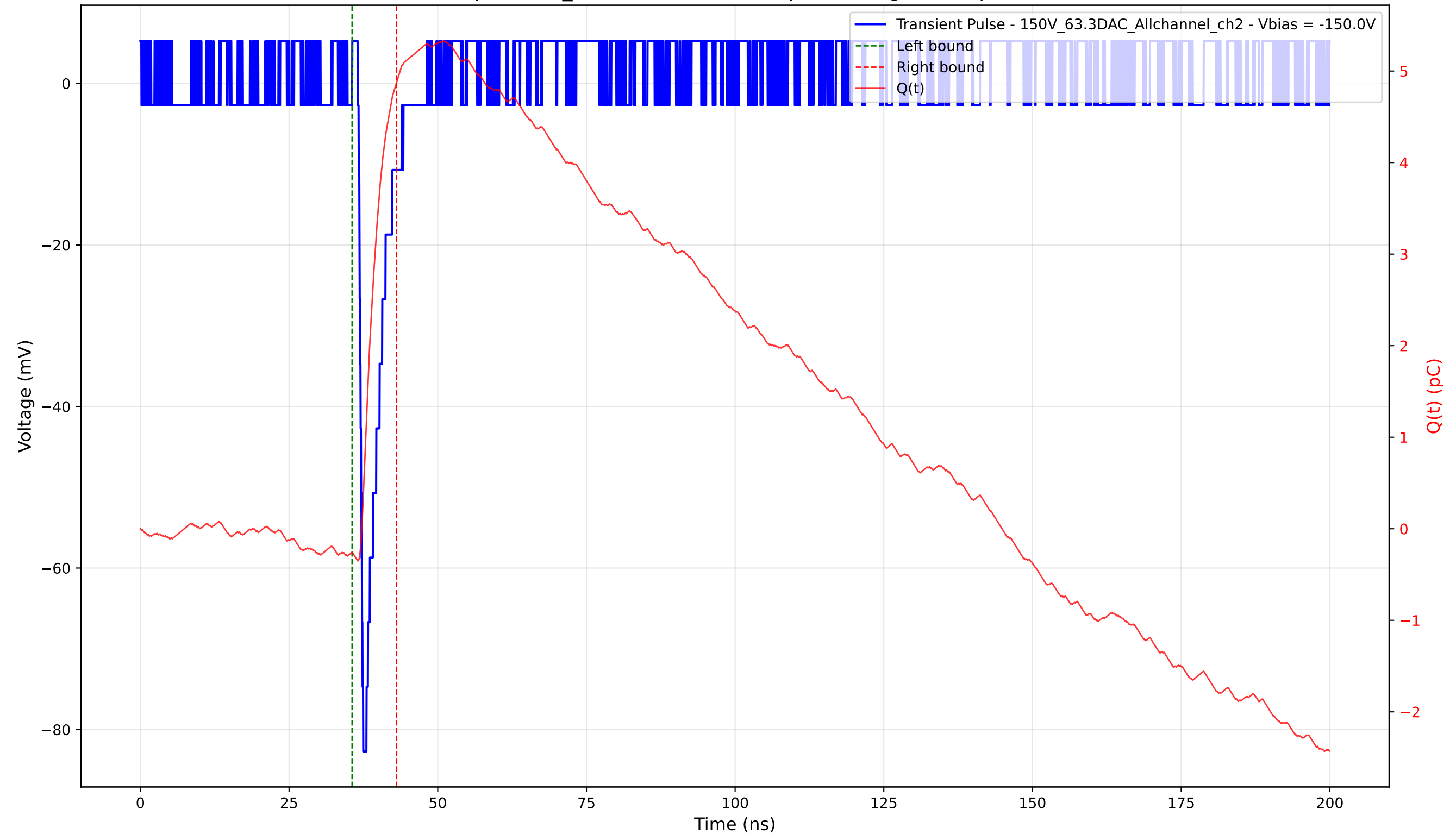
Transient Pulse - Sample: 1cm_42 - Position: 3950.0 \mu\text{m} - Charge: 5.13 pC - Rise Time: 0.65 ns
