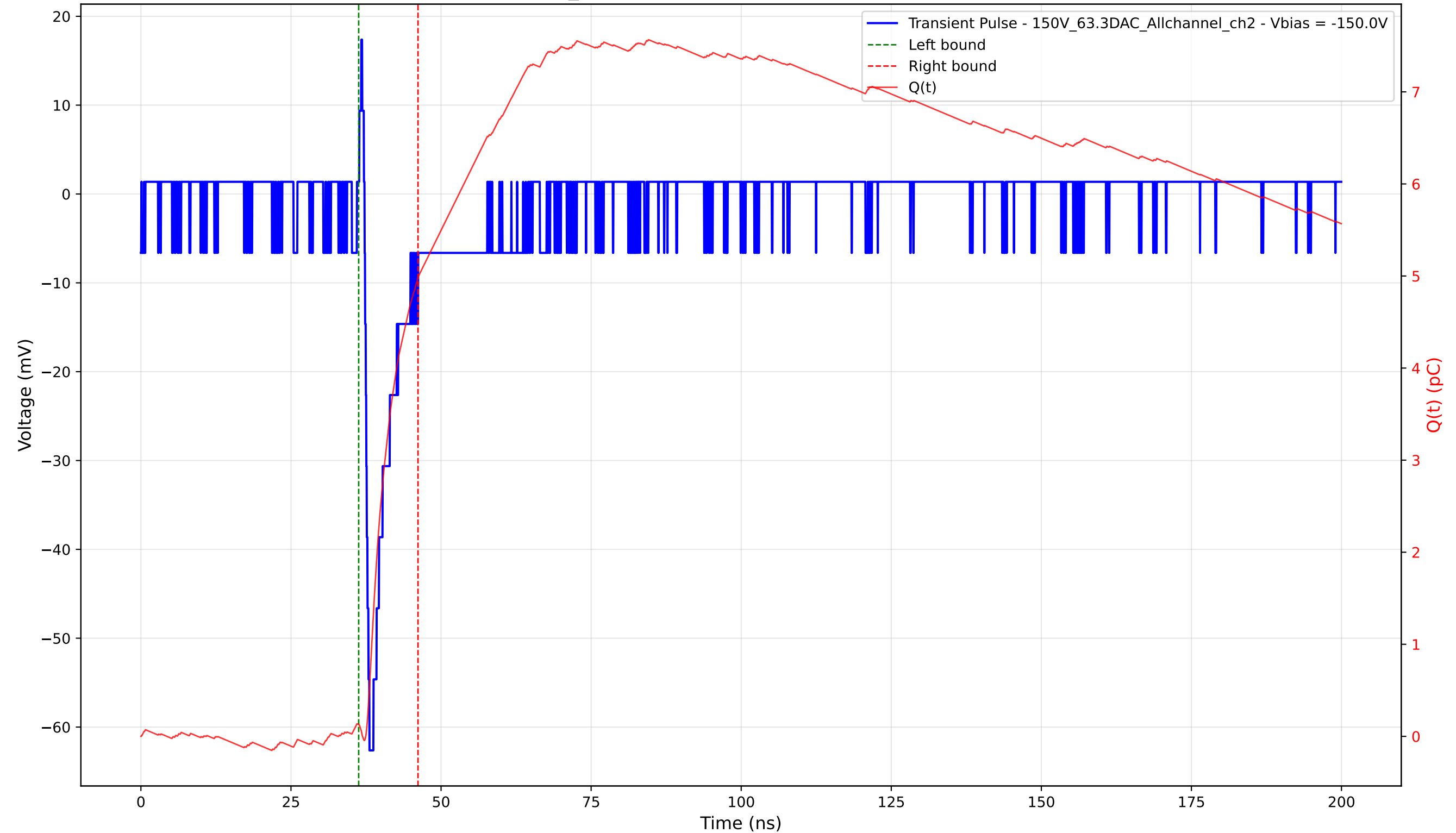
Transient Pulse - Sample: 1cm_42 - Position: 1740.0 \mu\text{m} - Charge: 4.86 pC - Rise Time: 0.80 ns
