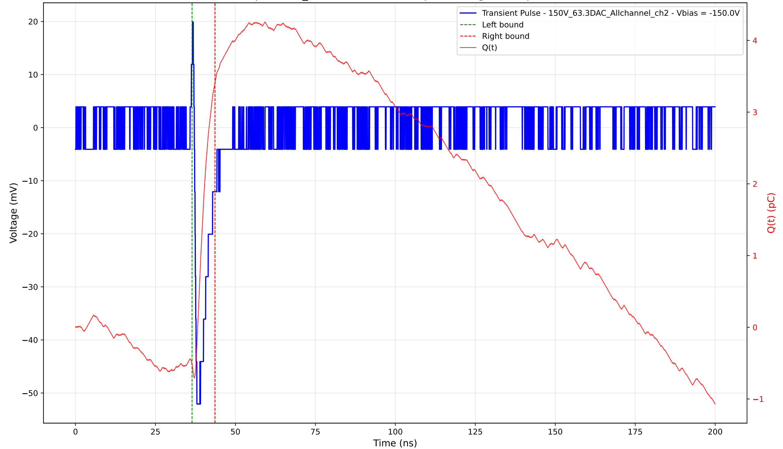
Transient Pulse - Sample: 1cm_42 - Position: 4335.0 \mu\text{m} - Charge: 3.93 pC - Rise Time: 0.71 ns
