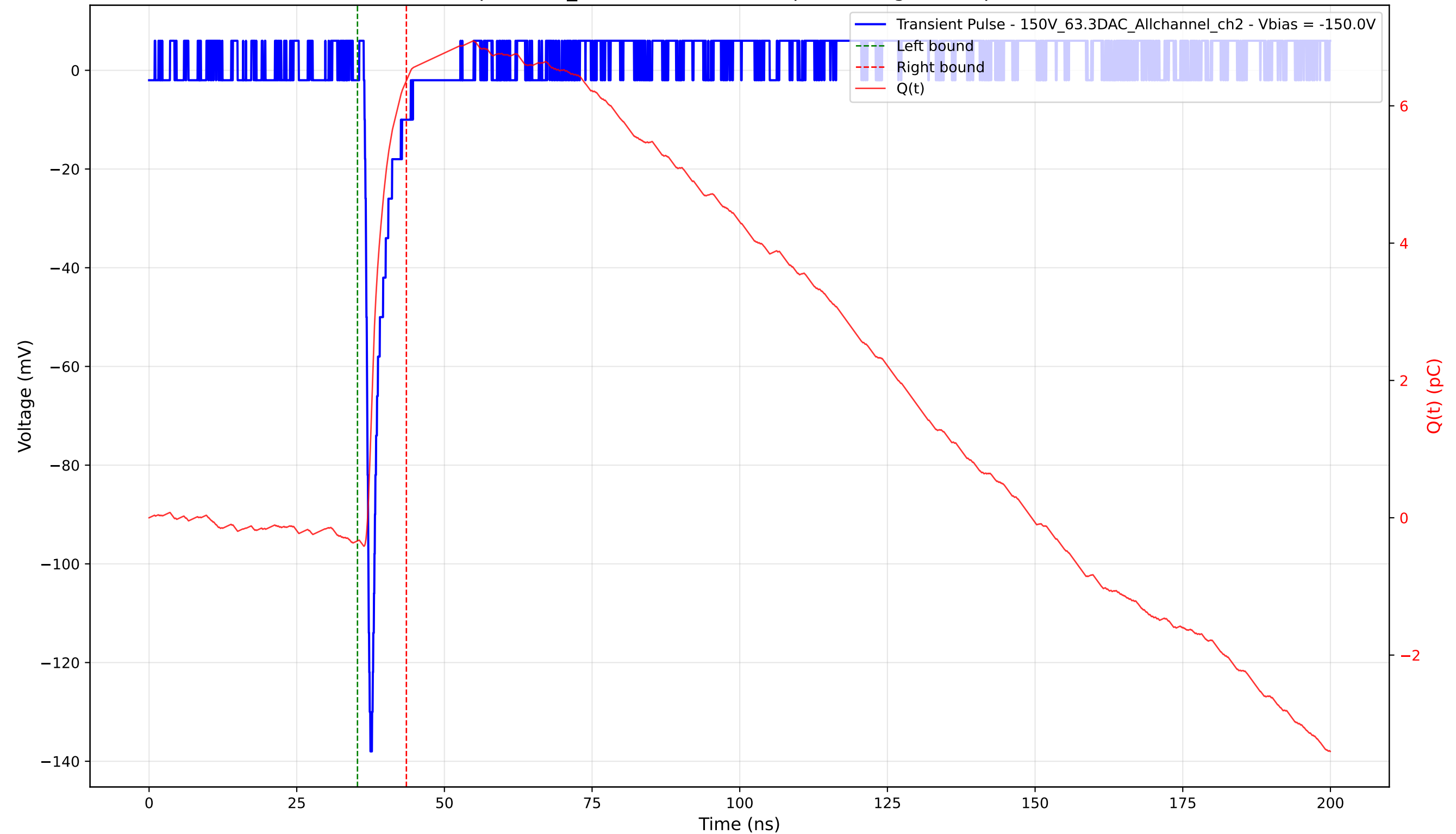
Transient Pulse - Sample: 1cm_42 - Position: 2270.0 \mu\text{m} - Charge: 6.70 pC - Rise Time: 0.82 ns
