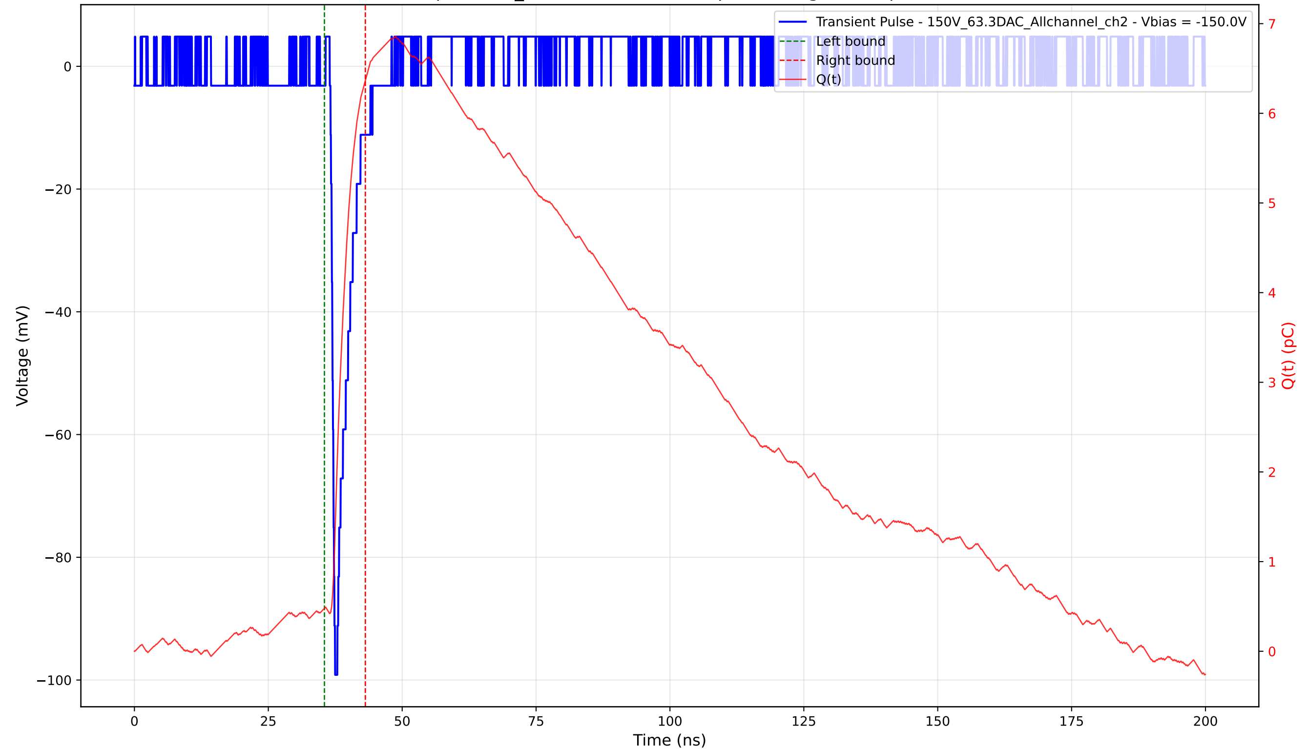
Transient Pulse - Sample: 1cm_42 - Position: 3905.0 \mu\text{m} - Charge: 5.89 pC - Rise Time: 0.73 ns
