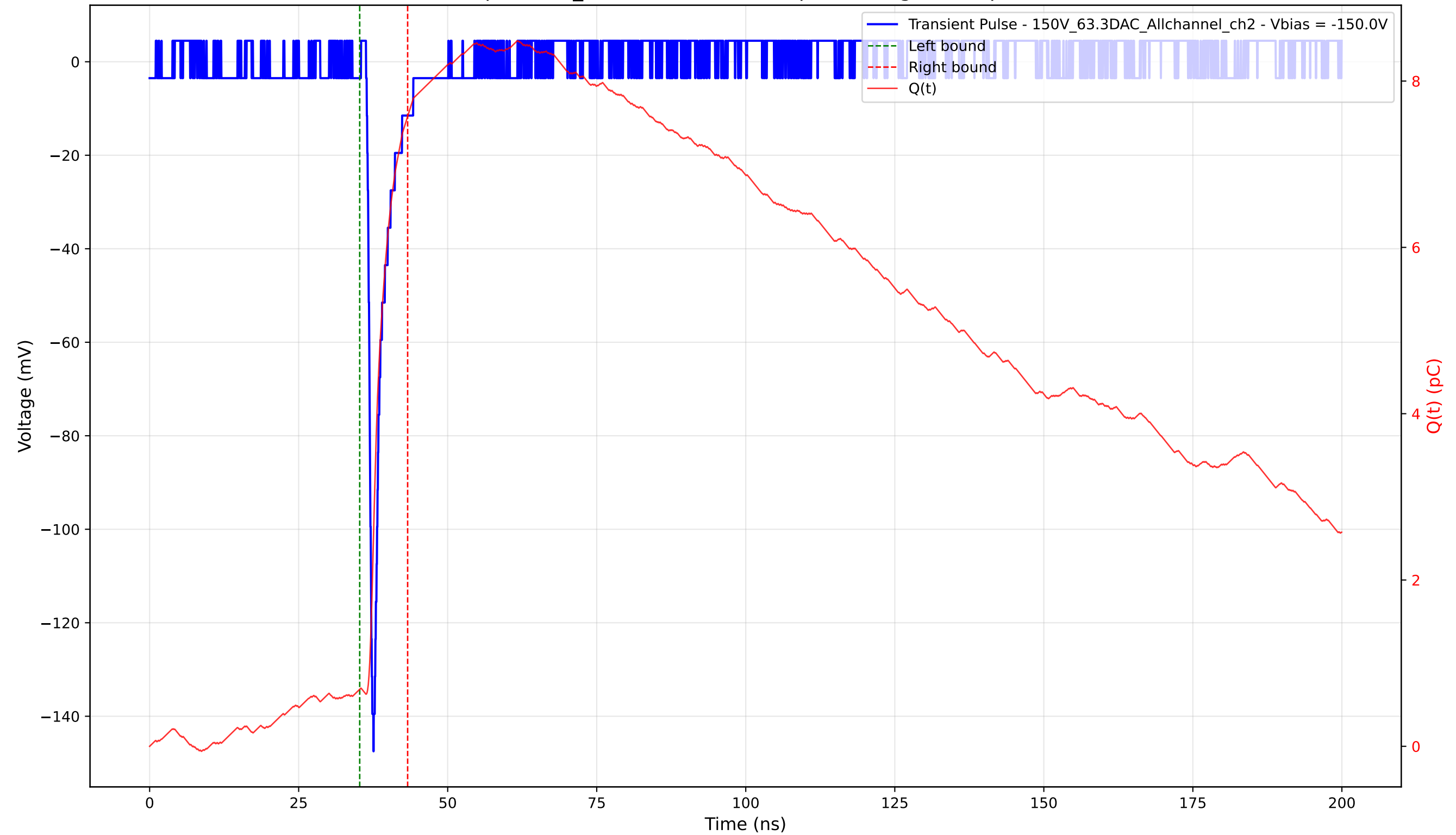
Transient Pulse - Sample: 1cm_42 - Position: 2335.0 \mu\text{m} - Charge: 6.89 pC - Rise Time: 0.86 ns
