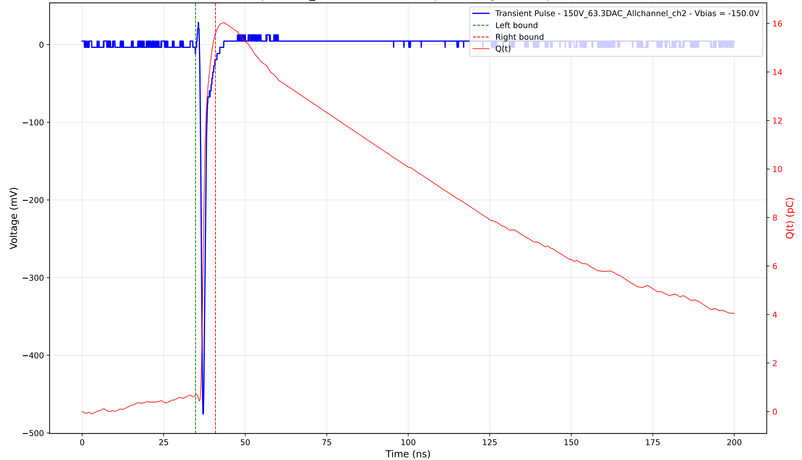
Transient Pulse - Sample: 1cm_42 - Position: 3130.0 \mu\text{m} - Charge: 14.90 pC - Rise Time: 0.73 ns
