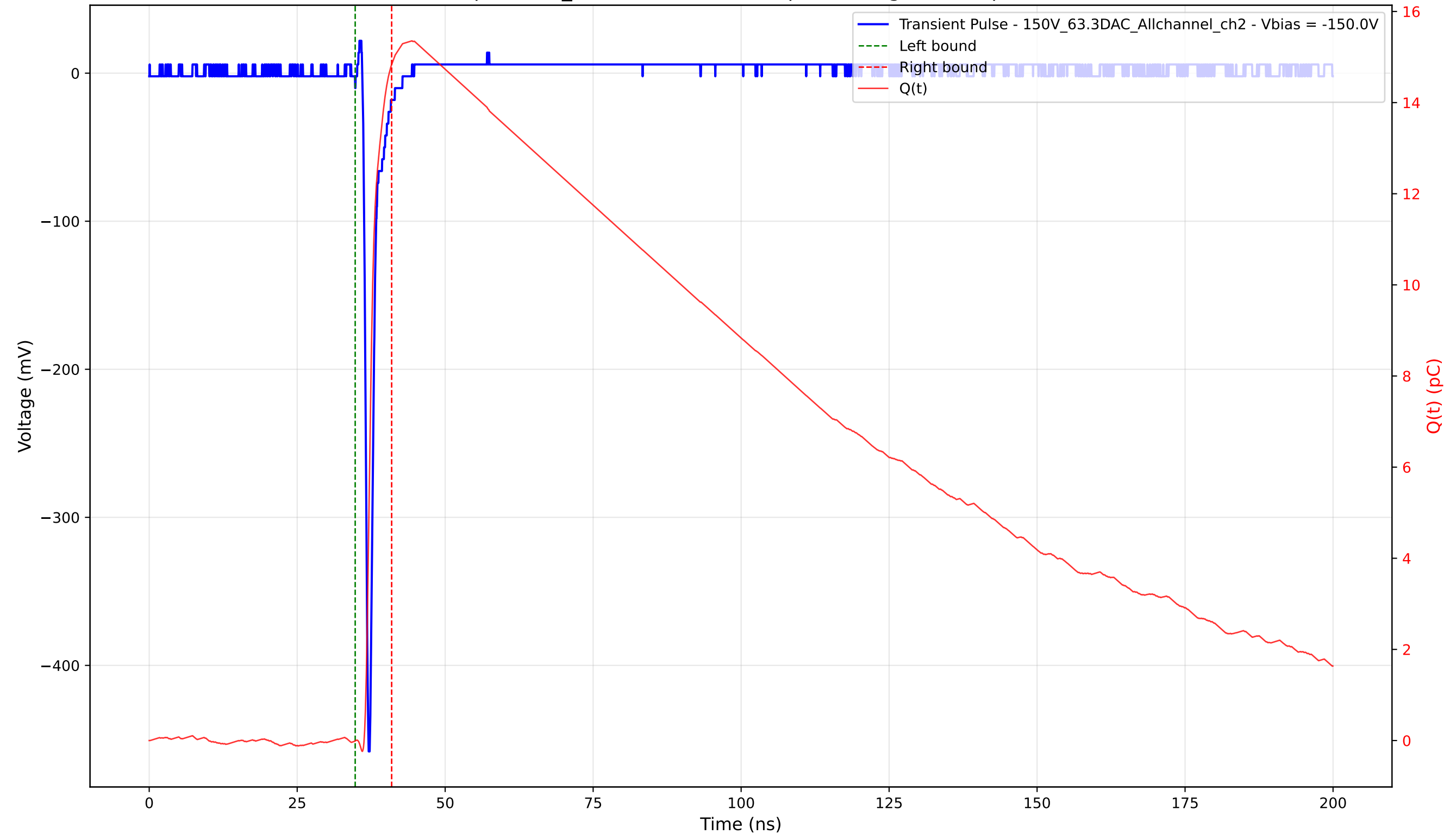
Transient Pulse - Sample: 1cm_42 - Position: 2775.0 \mu\text{m} - Charge: 14.85 pC - Rise Time: 0.72 ns
