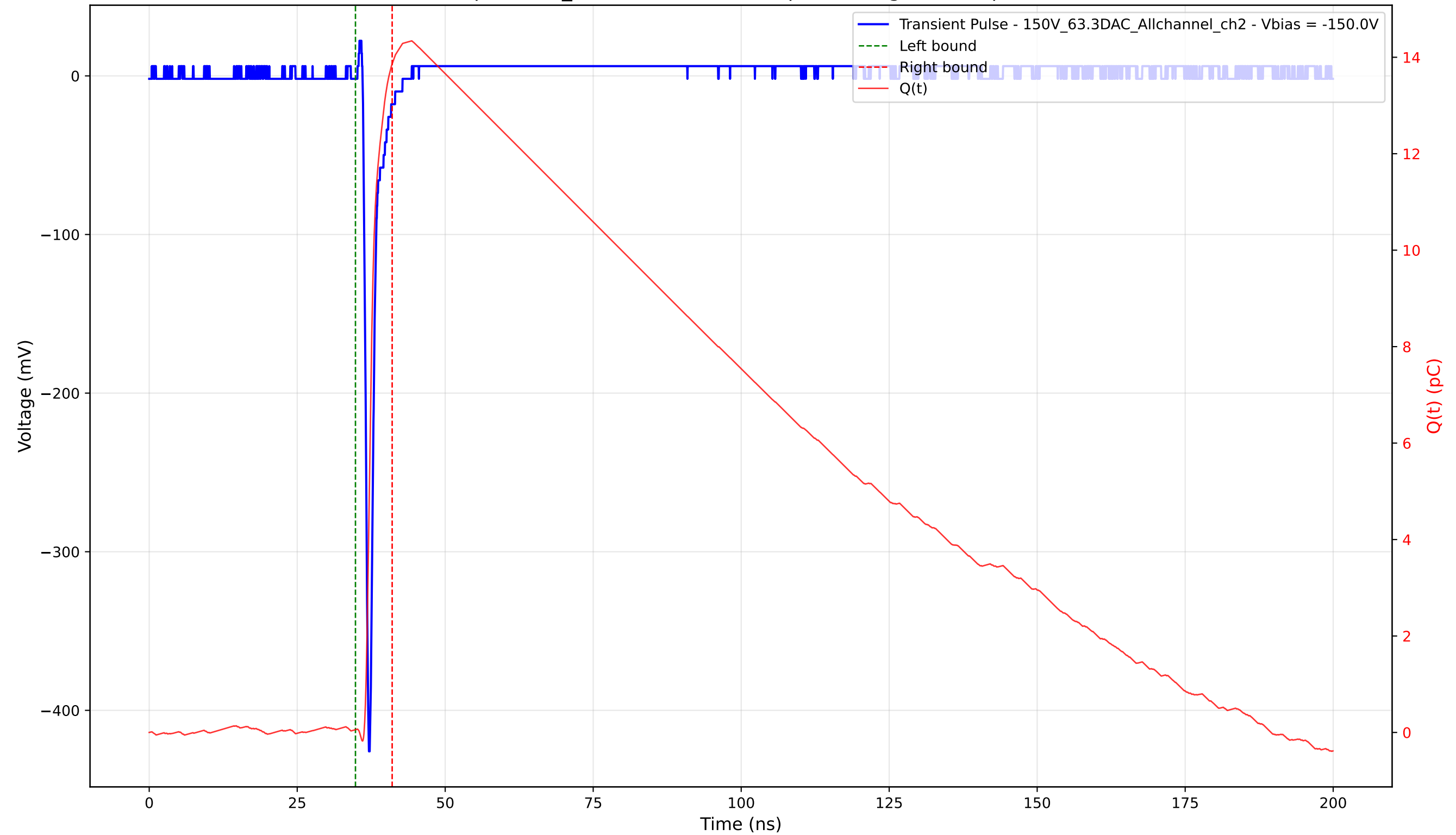
Transient Pulse - Sample: 1cm_42 - Position: 2735.0 \mu\text{m} - Charge: 13.80 pC - Rise Time: 0.71 ns
