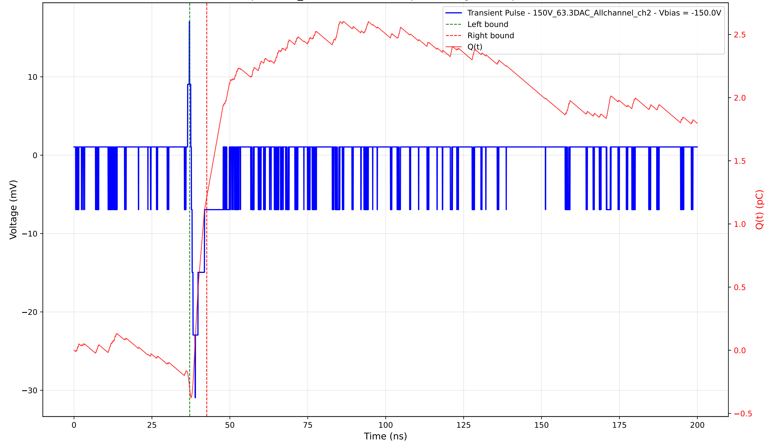
Transient Pulse - Sample: 1cm_42 - Position: 340.0 \mu\text{m} - Charge: 1.52 pC - Rise Time: 1.23 ns
