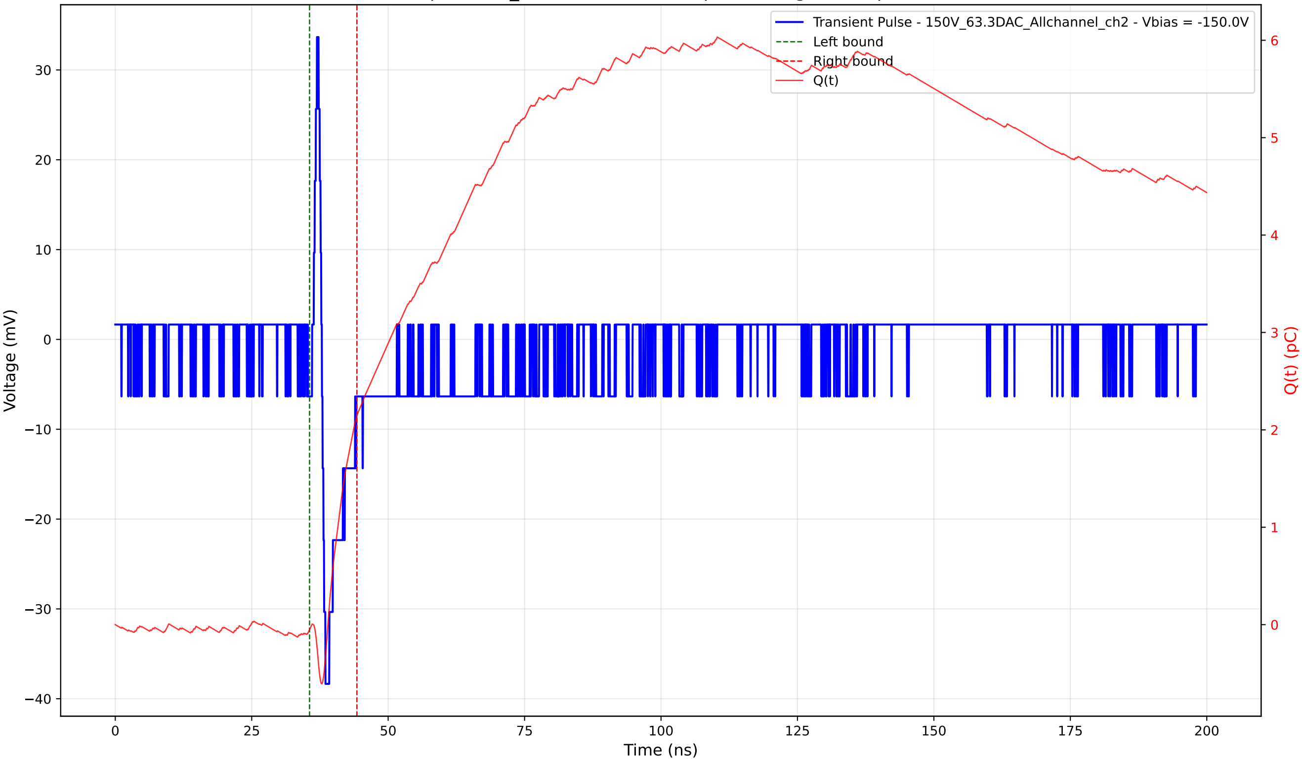
Transient Pulse - Sample: 1cm_42 - Position: 980.0 \mu\text{m} - Charge: 2.20 pC - Rise Time: 0.66 ns
