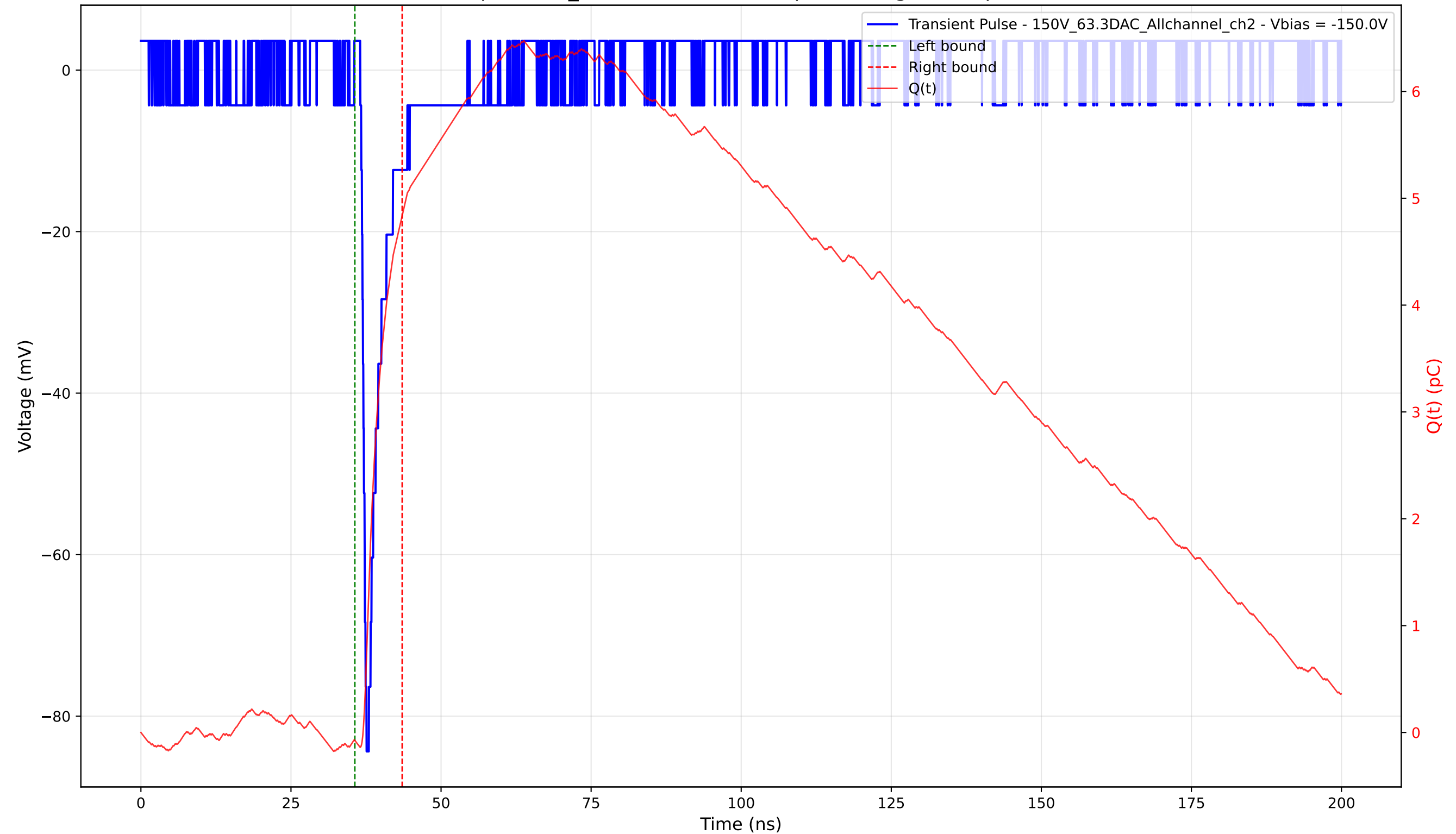
Transient Pulse - Sample: 1cm_42 - Position: 2075.0 \mu\text{m} - Charge: 4.91 pC - Rise Time: 0.74 ns
