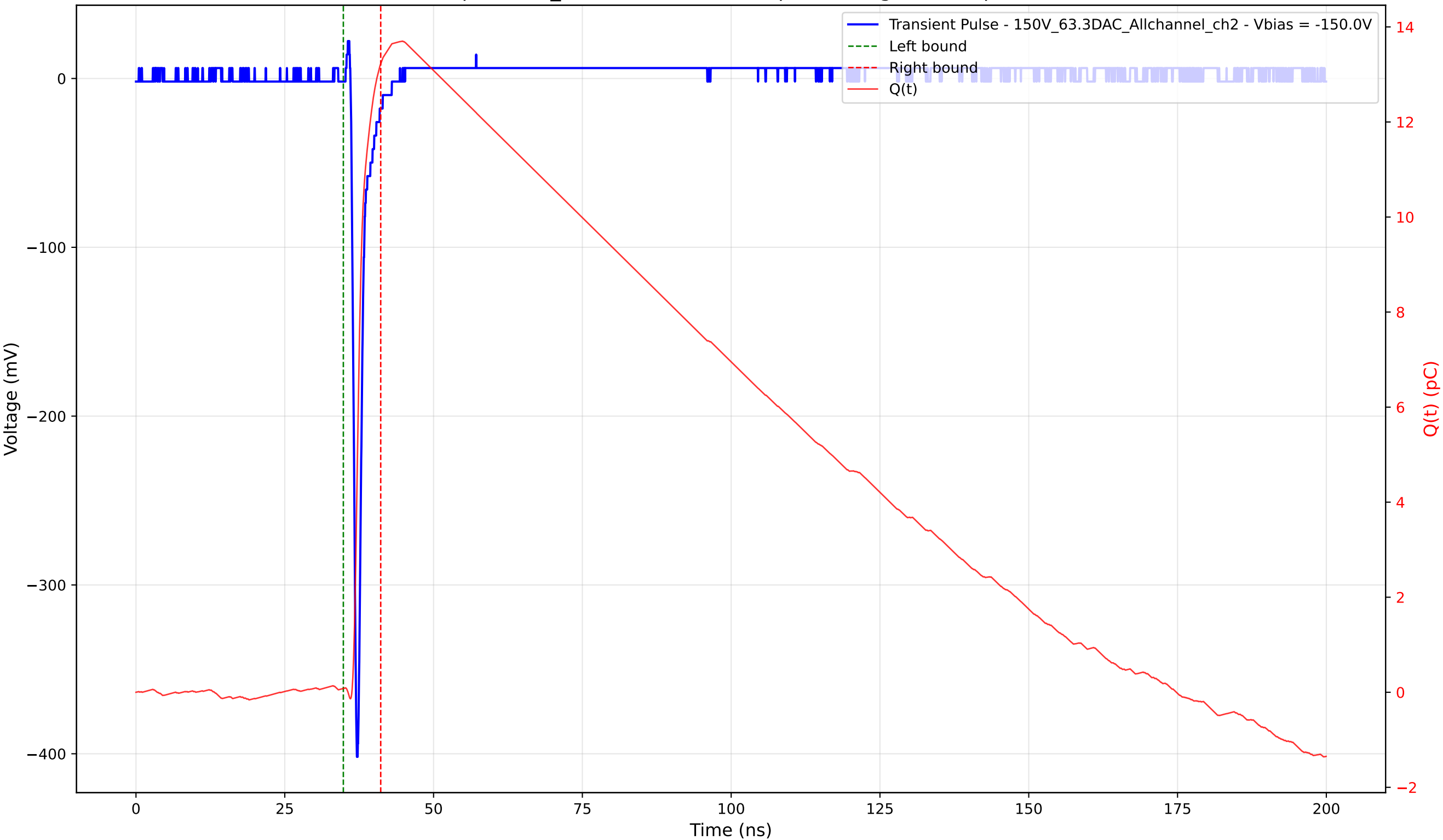
Transient Pulse - Sample: 1cm_42 - Position: 2710.0 \mu\text{m} - Charge: 13.14 pC - Rise Time: 0.72 ns
