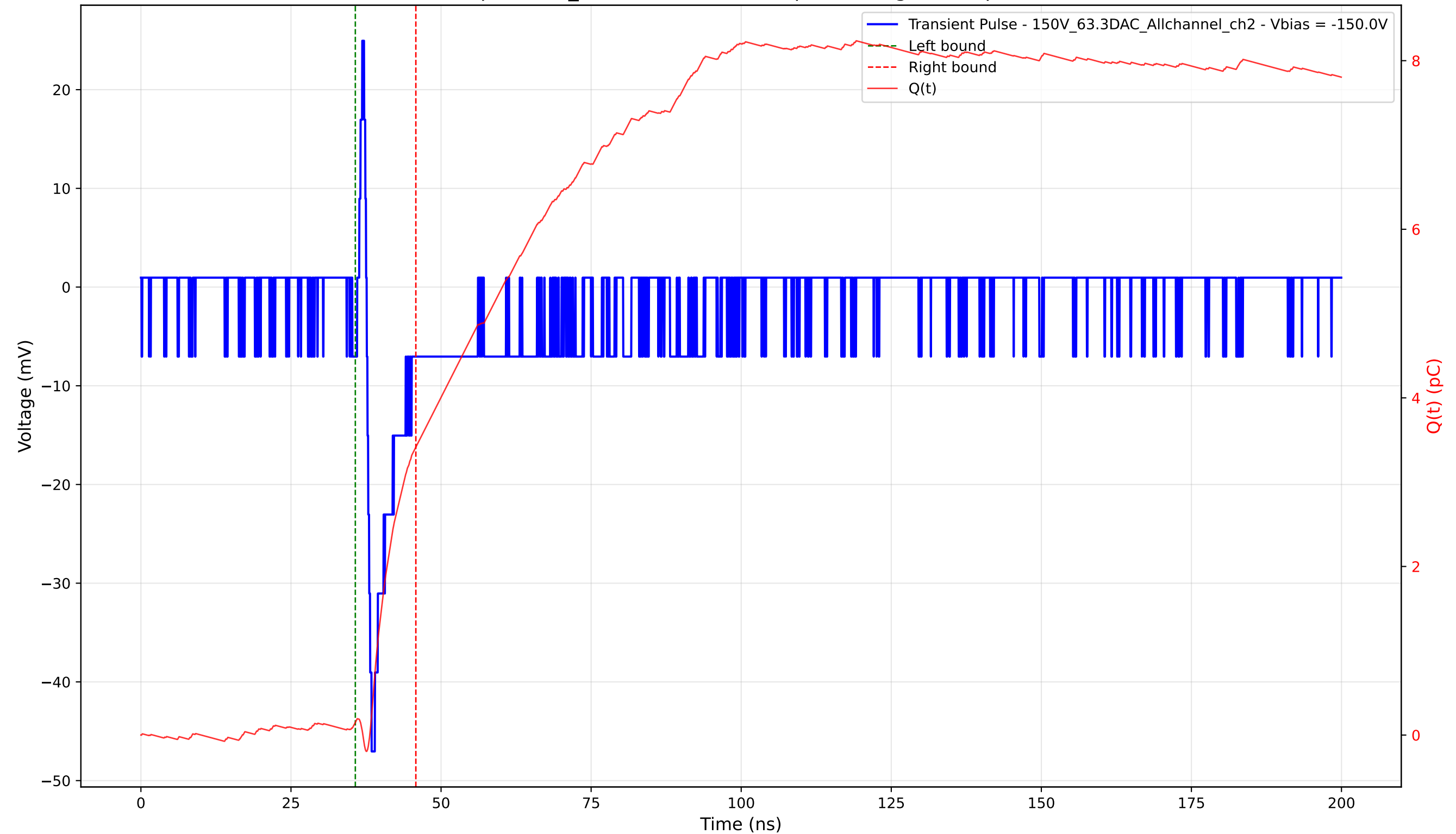
Transient Pulse - Sample: 1cm_42 - Position: 1480.0 \mu\text{m} - Charge: 3.26 pC - Rise Time: 0.82 ns
