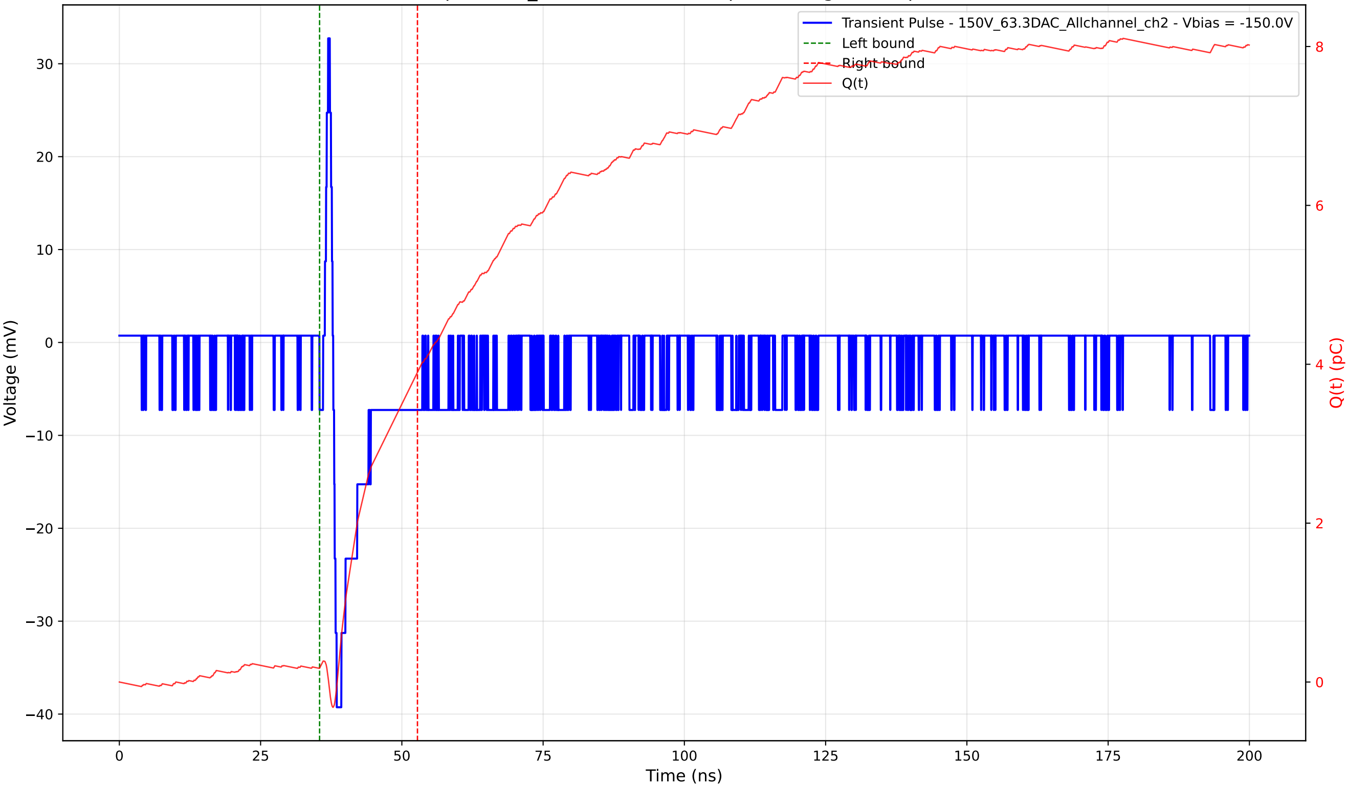
Transient Pulse - Sample: 1cm_42 - Position: 900.0 \mu\text{m} - Charge: 3.73 pC - Rise Time: 0.62 ns
