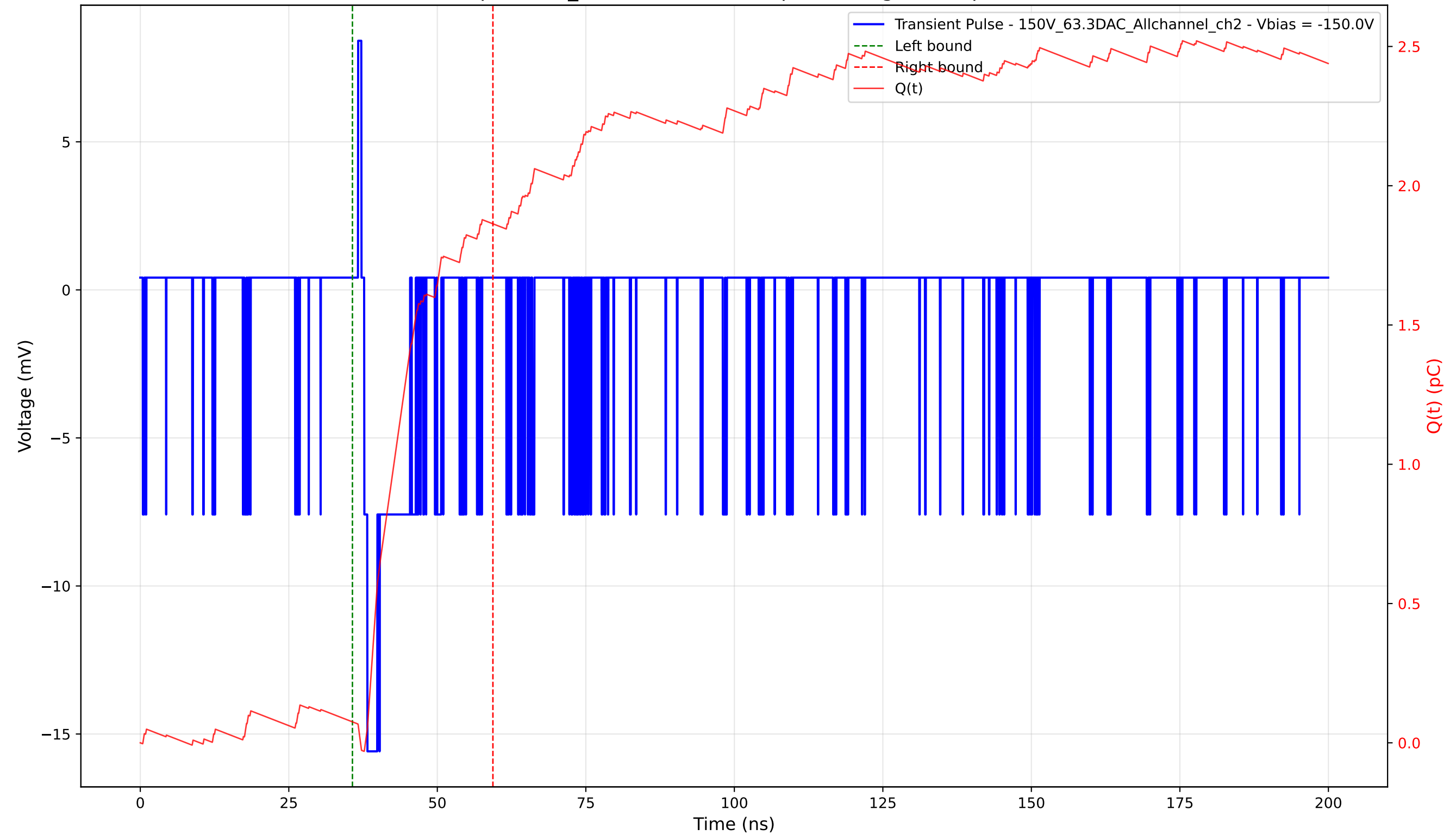
Transient Pulse - Sample: 1cm_42 - Position: 170.0 \mu\text{m} - Charge: 1.79 pC - Rise Time: 0.55 ns
