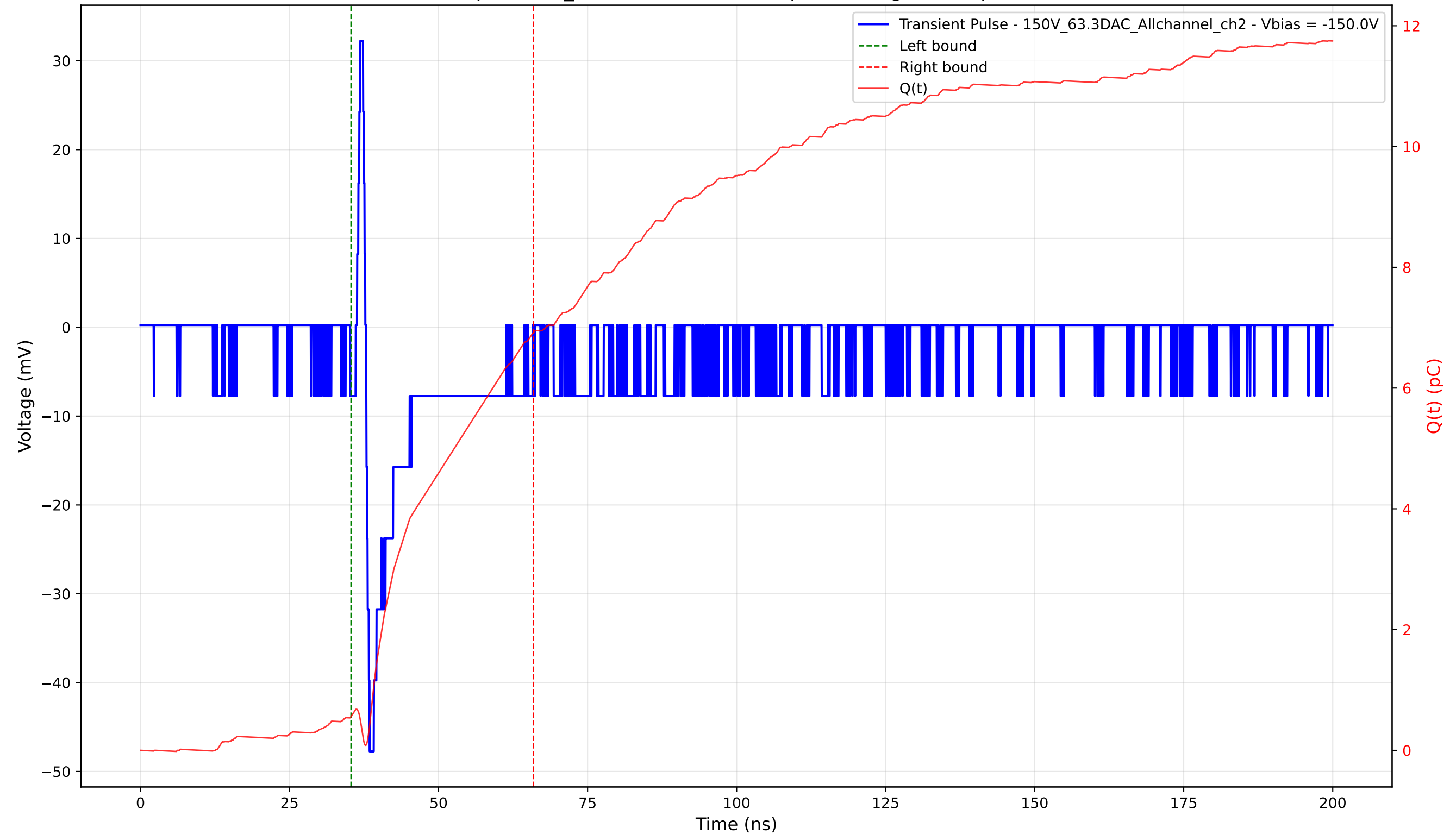
Transient Pulse - Sample: 1cm_42 - Position: 1185.0 \mu\text{m} - Charge: 6.36 pC - Rise Time: 0.62 ns
