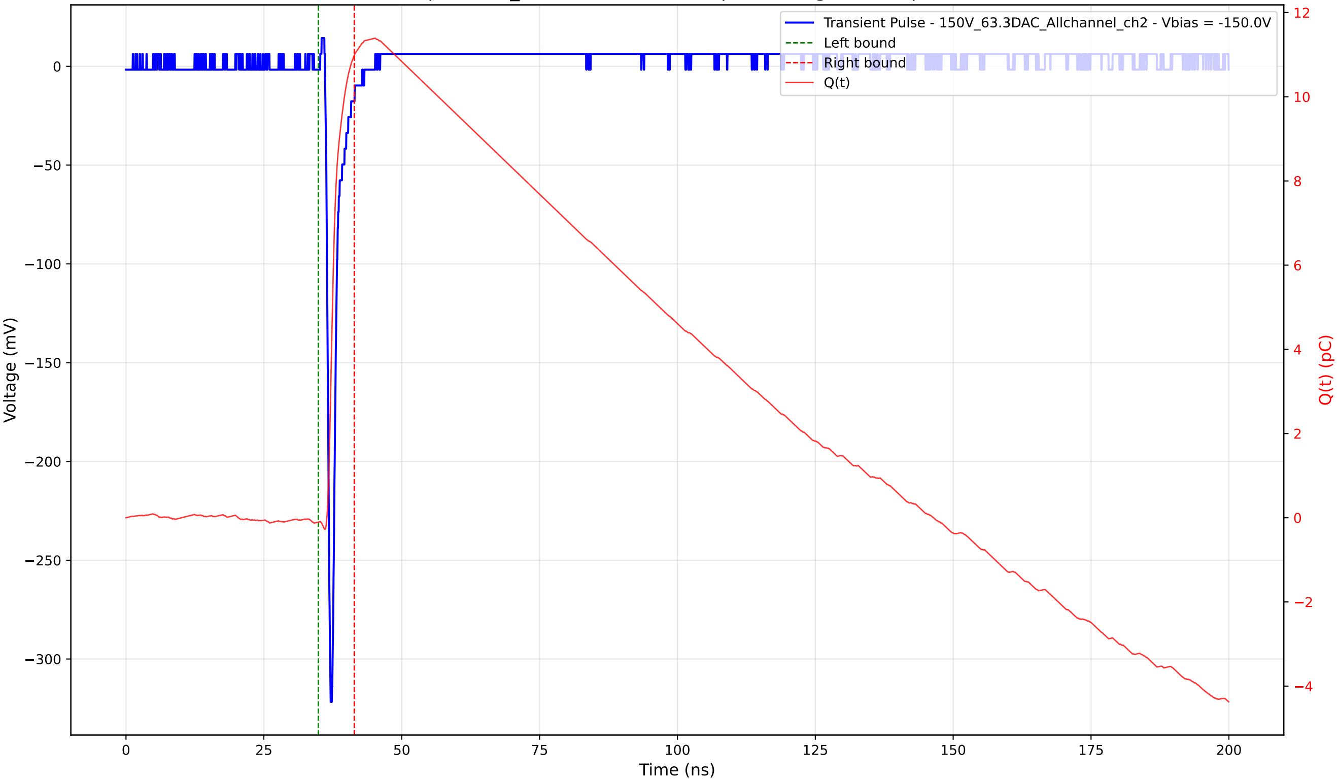
Transient Pulse - Sample: 1cm_42 - Position: 2645.0 \mu\text{m} - Charge: 11.09 pC - Rise Time: 0.73 ns
