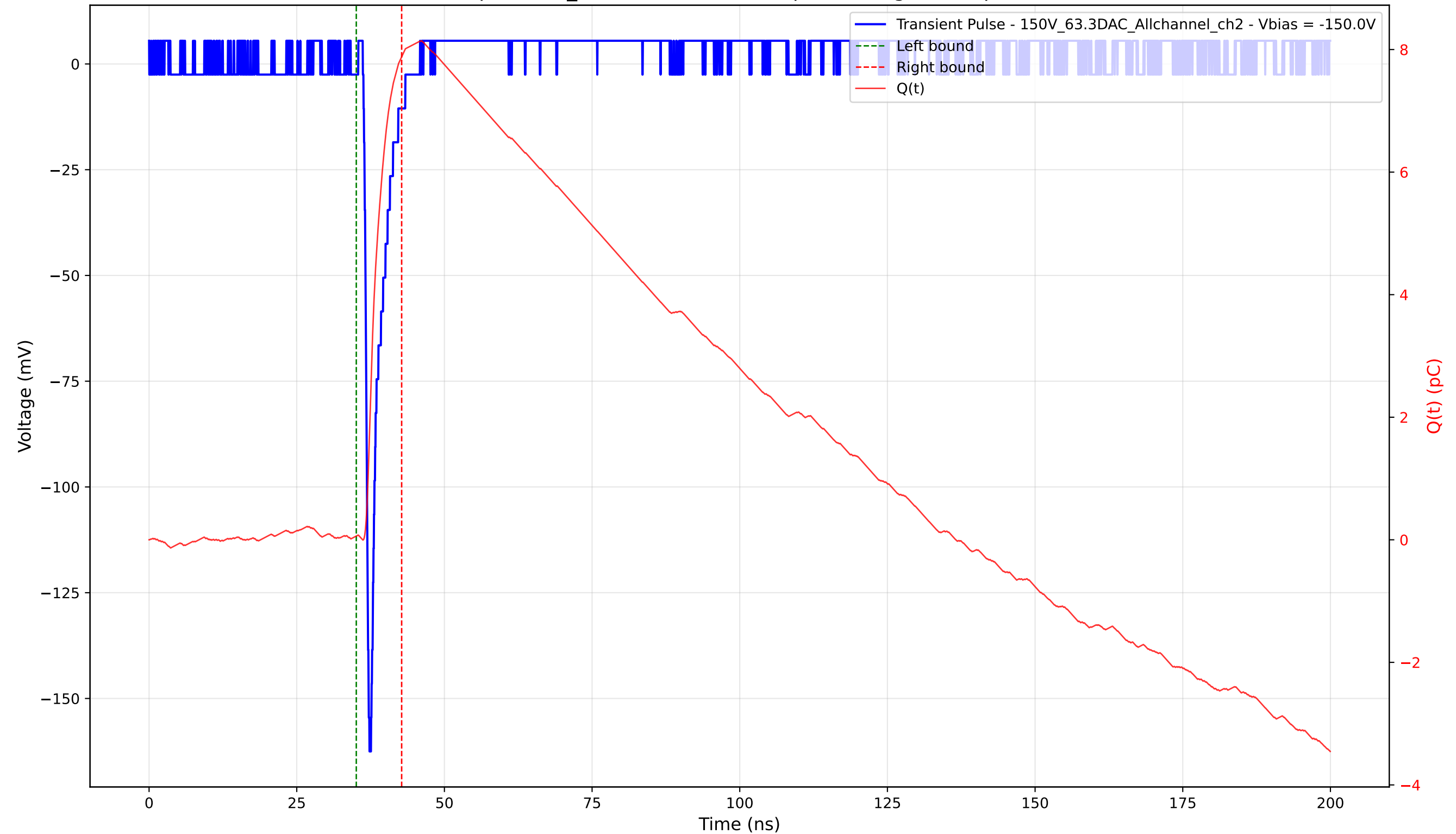
Transient Pulse - Sample: 1cm_42 - Position: 3620.0 \mu\text{m} - Charge: 7.82 pC - Rise Time: 0.77 ns
