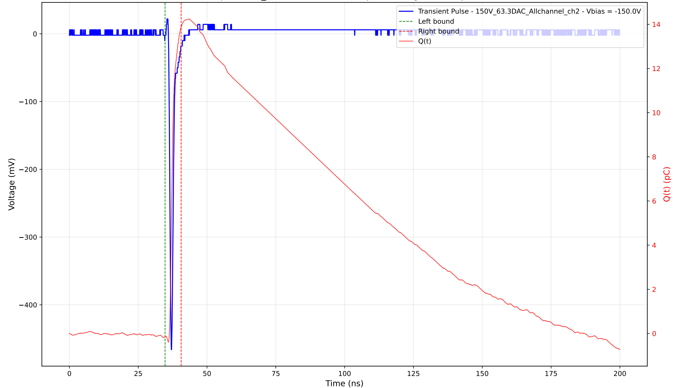
Transient Pulse - Sample: 1cm_42 - Position: 3010.0 \mu\text{m} - Charge: 14.01 pC - Rise Time: 0.68 ns
