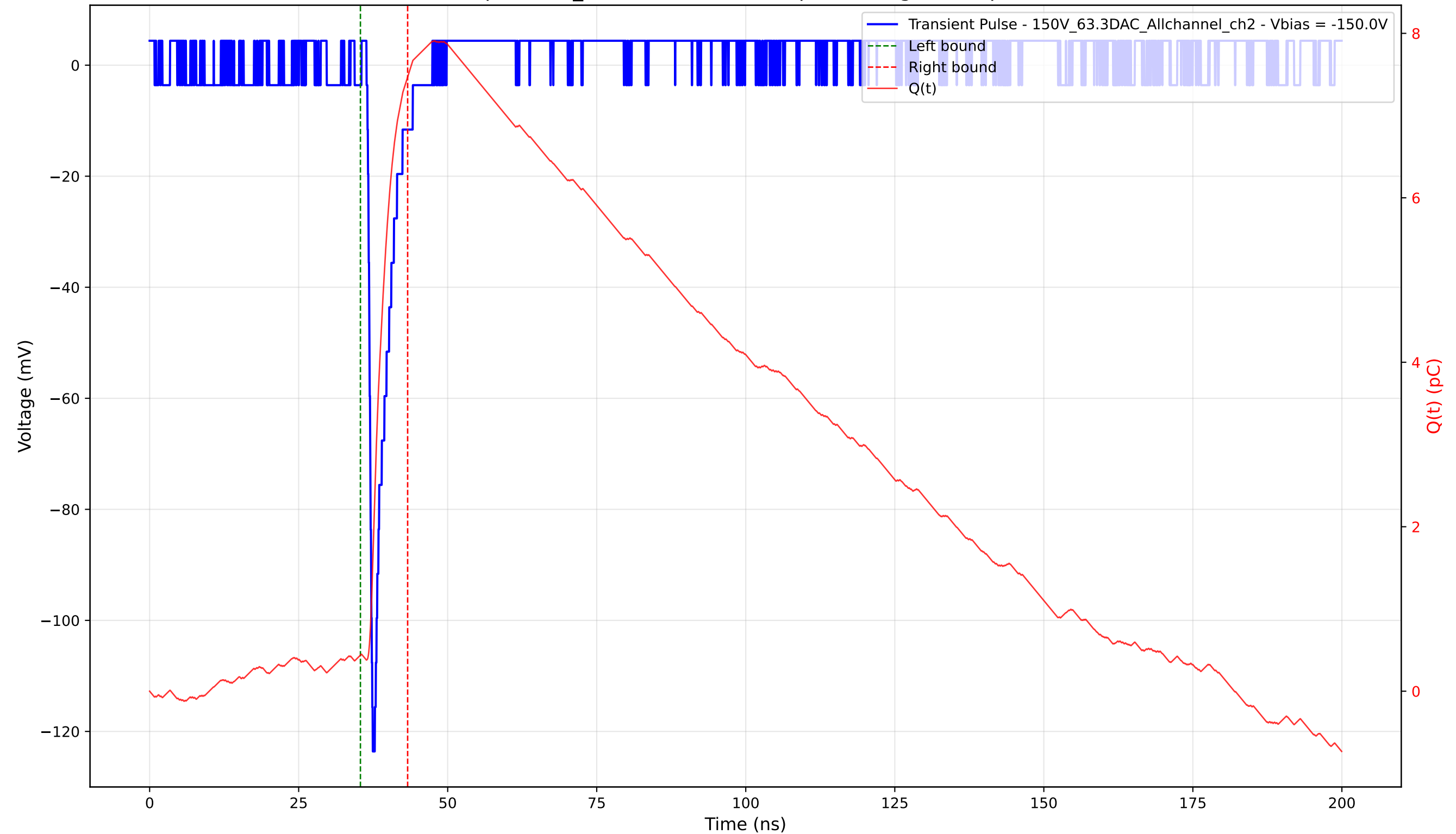
Transient Pulse - Sample: 1cm_42 - Position: 3825.0 \mu\text{m} - Charge: 7.03 pC - Rise Time: 0.76 ns
