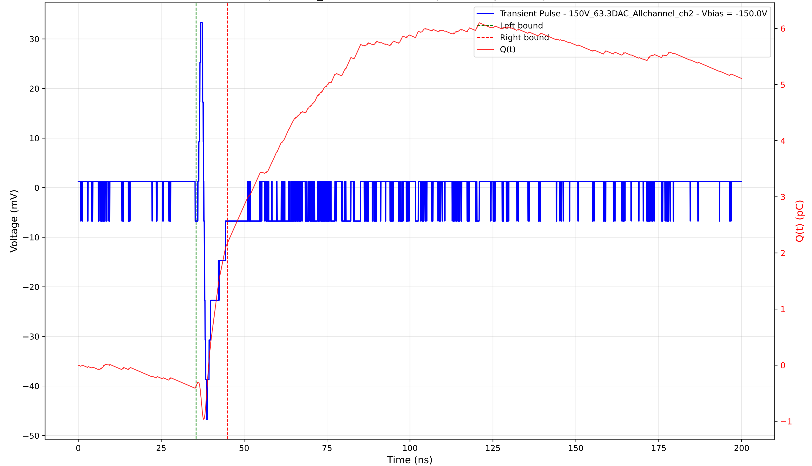
Transient Pulse - Sample: 1cm_42 - Position: 725.0 \mu\text{m} - Charge: 2.54 pC - Rise Time: 0.82 ns
