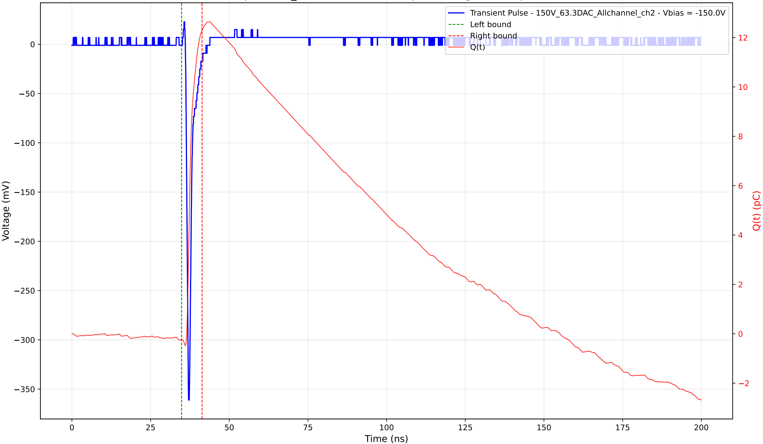
Transient Pulse - Sample: 1cm_42 - Position: 3365.0 \mu\text{m} - Charge: 12.54 pC - Rise Time: 0.69 ns
