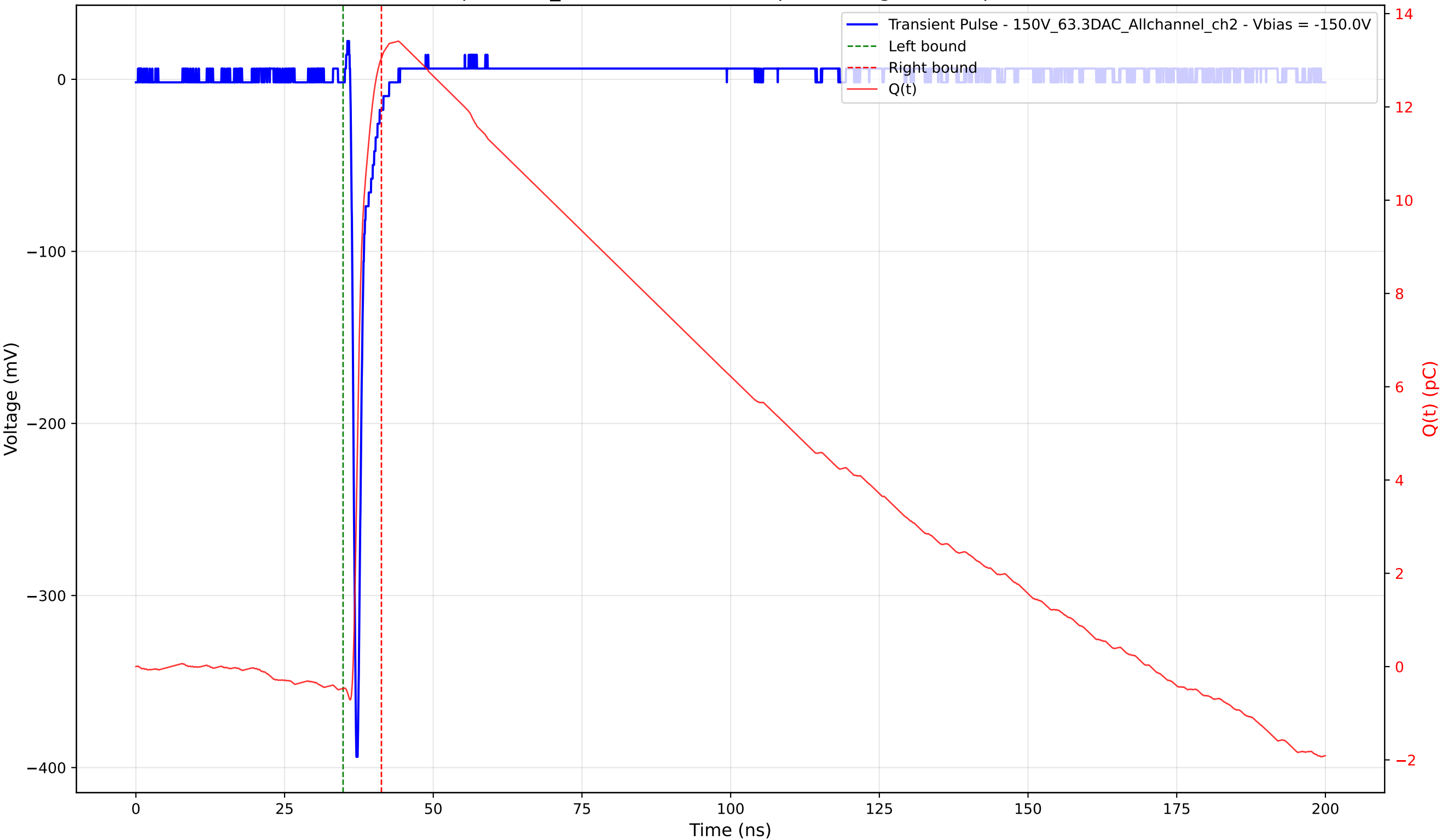
Transient Pulse - Sample: 1cm_42 - Position: 3335.0 \mu\text{m} - Charge: 13.52 pC - Rise Time: 0.70 ns
