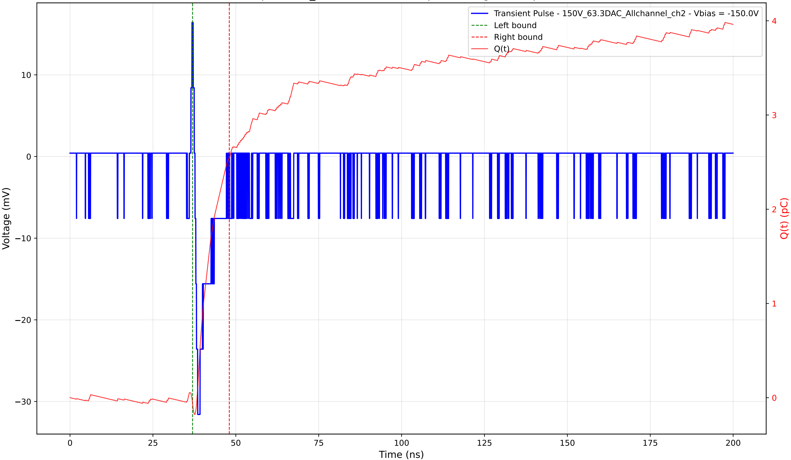
Transient Pulse - Sample: 1cm_42 - Position: 390.0 \mu\text{m} - Charge: 2.61 pC - Rise Time: 0.82 ns
