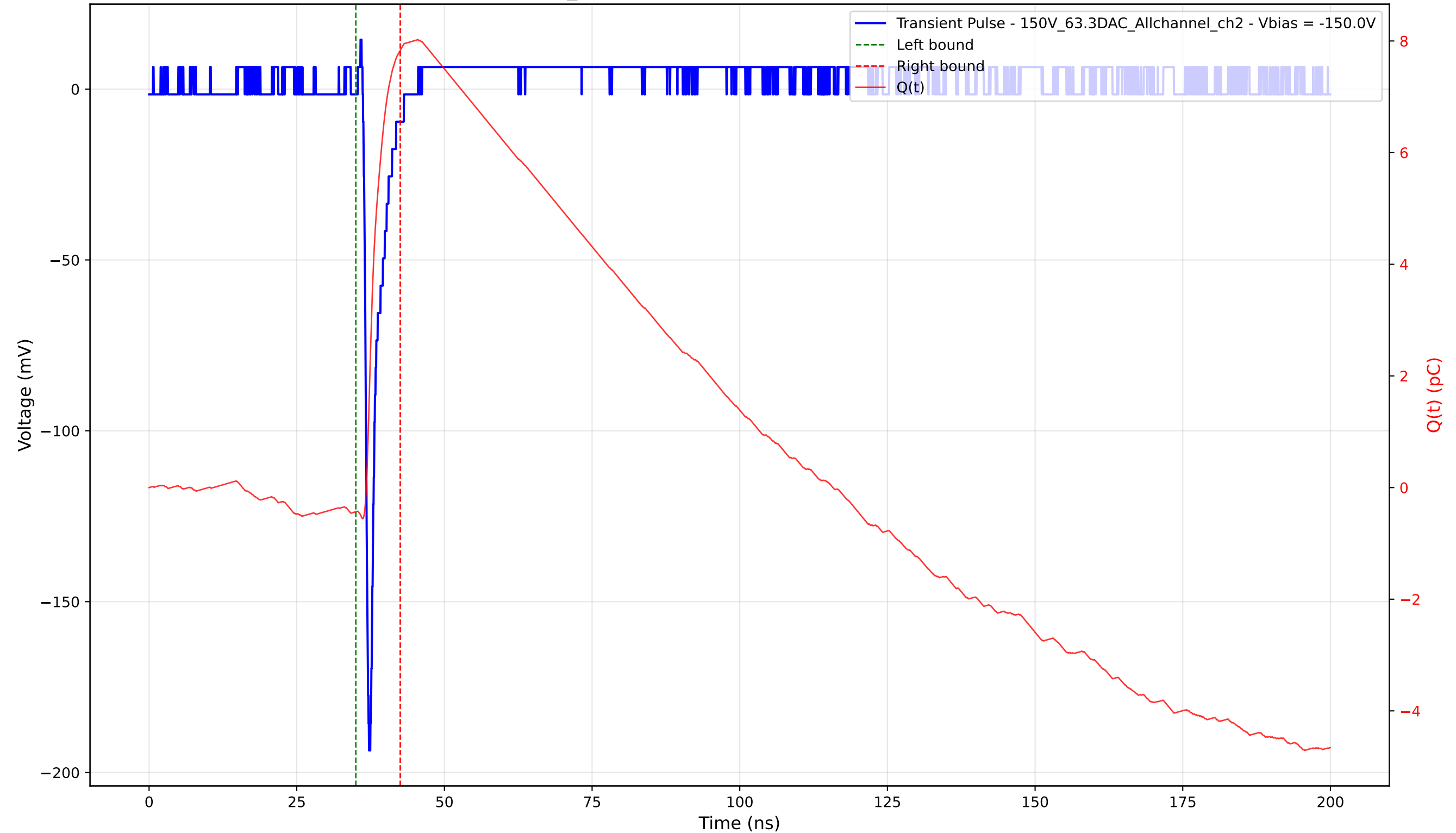
Transient Pulse - Sample: 1cm_42 - Position: 3545.0 \mu\text{m} - Charge: 8.27 pC - Rise Time: 0.75 ns
