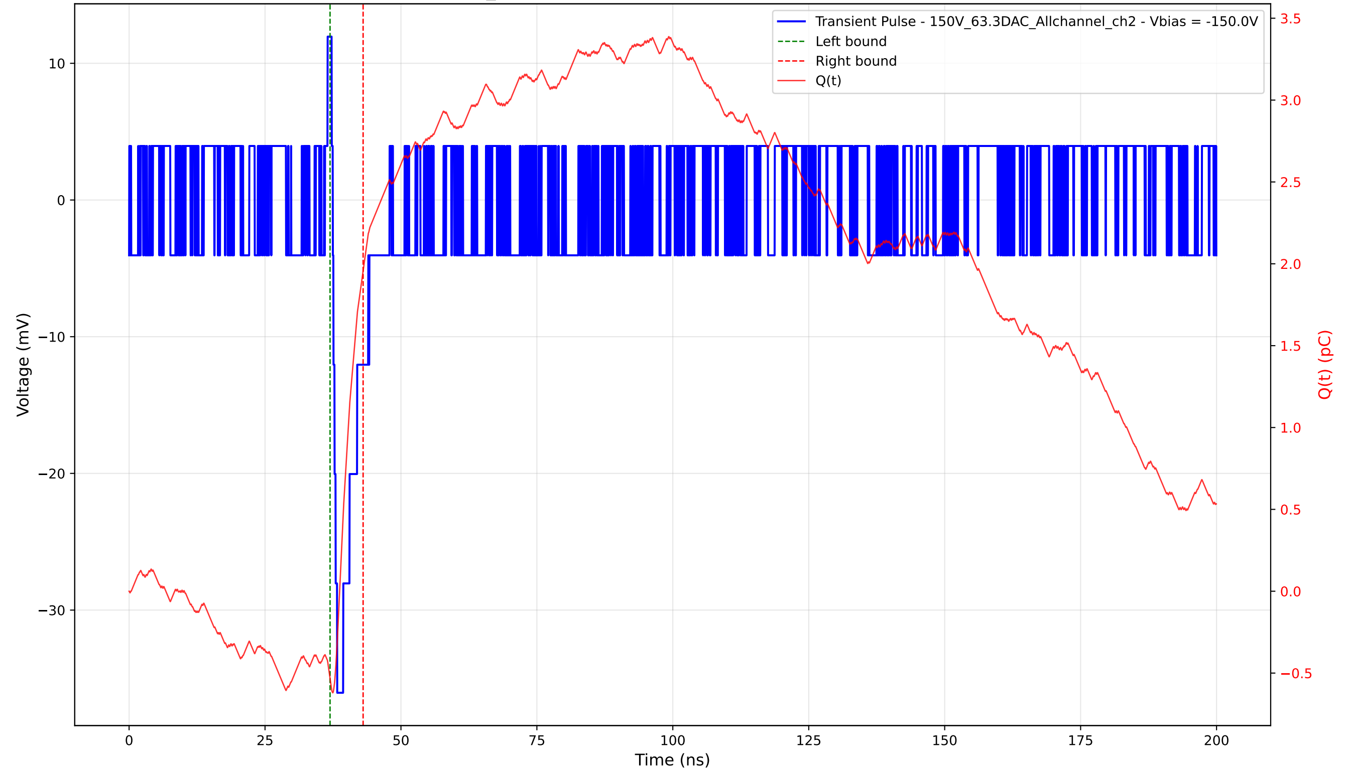
Transient Pulse - Sample: 1cm_42 - Position: 4720.0 \mu\text{m} - Charge: 2.49 pC - Rise Time: 0.00 ns (N/A)
