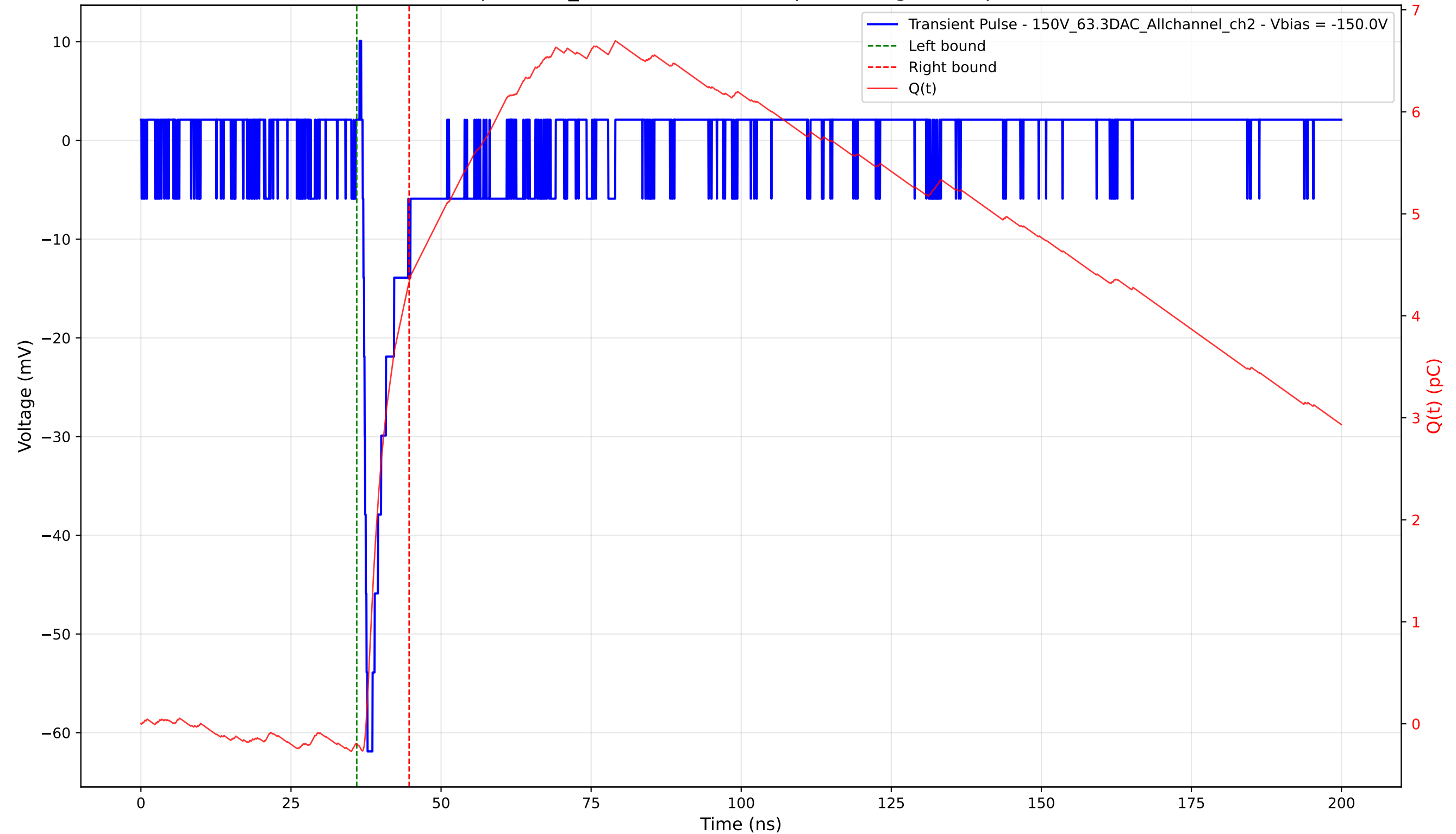
Transient Pulse - Sample: 1cm_42 - Position: 1940.0 \mu\text{m} - Charge: 4.53 pC - Rise Time: 0.72 ns
