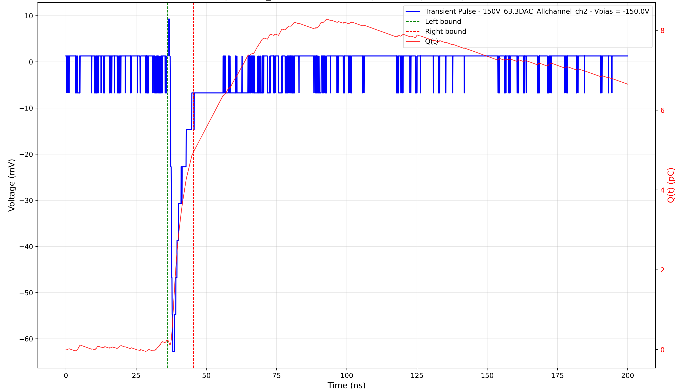
Transient Pulse - Sample: 1cm_42 - Position: 1865.0 \mu\text{m} - Charge: 4.71 pC - Rise Time: 0.92 ns
