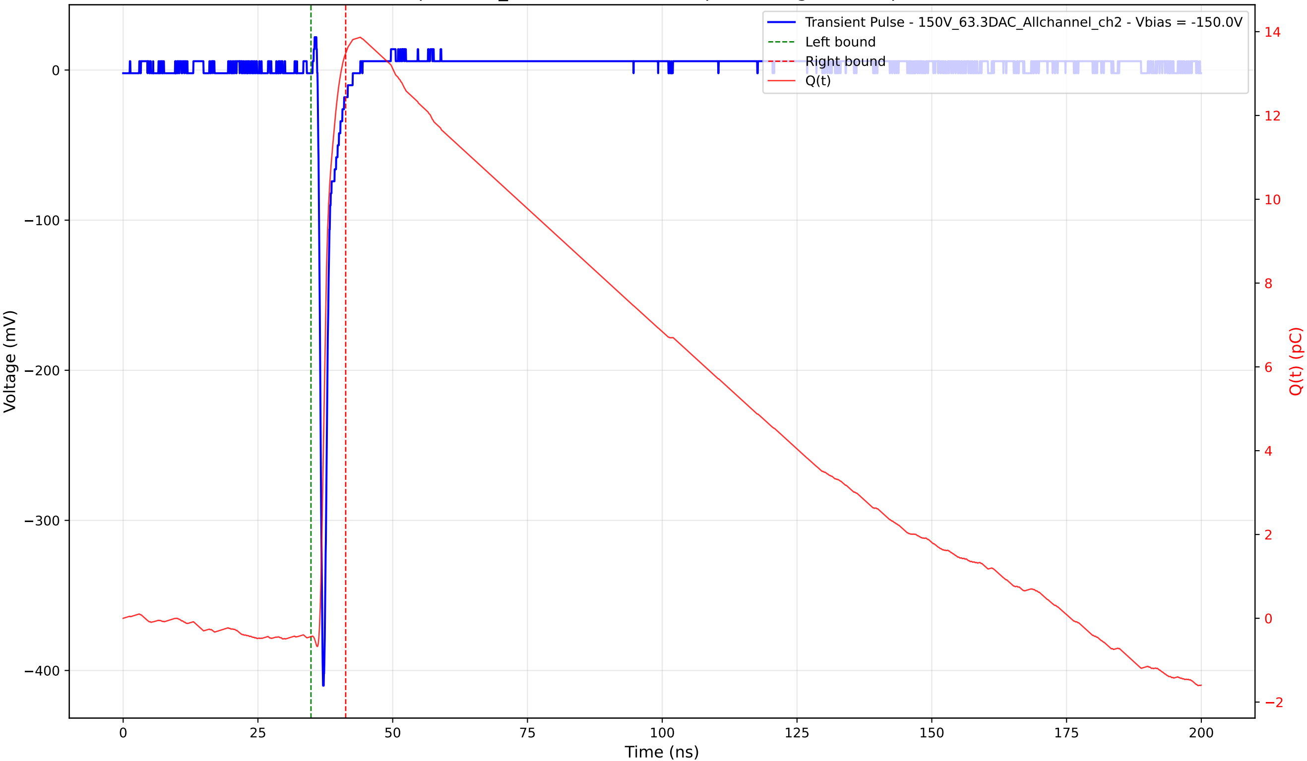
Transient Pulse - Sample: 1cm_42 - Position: 3320.0 \mu\text{m} - Charge: 13.92 pC - Rise Time: 0.74 ns
