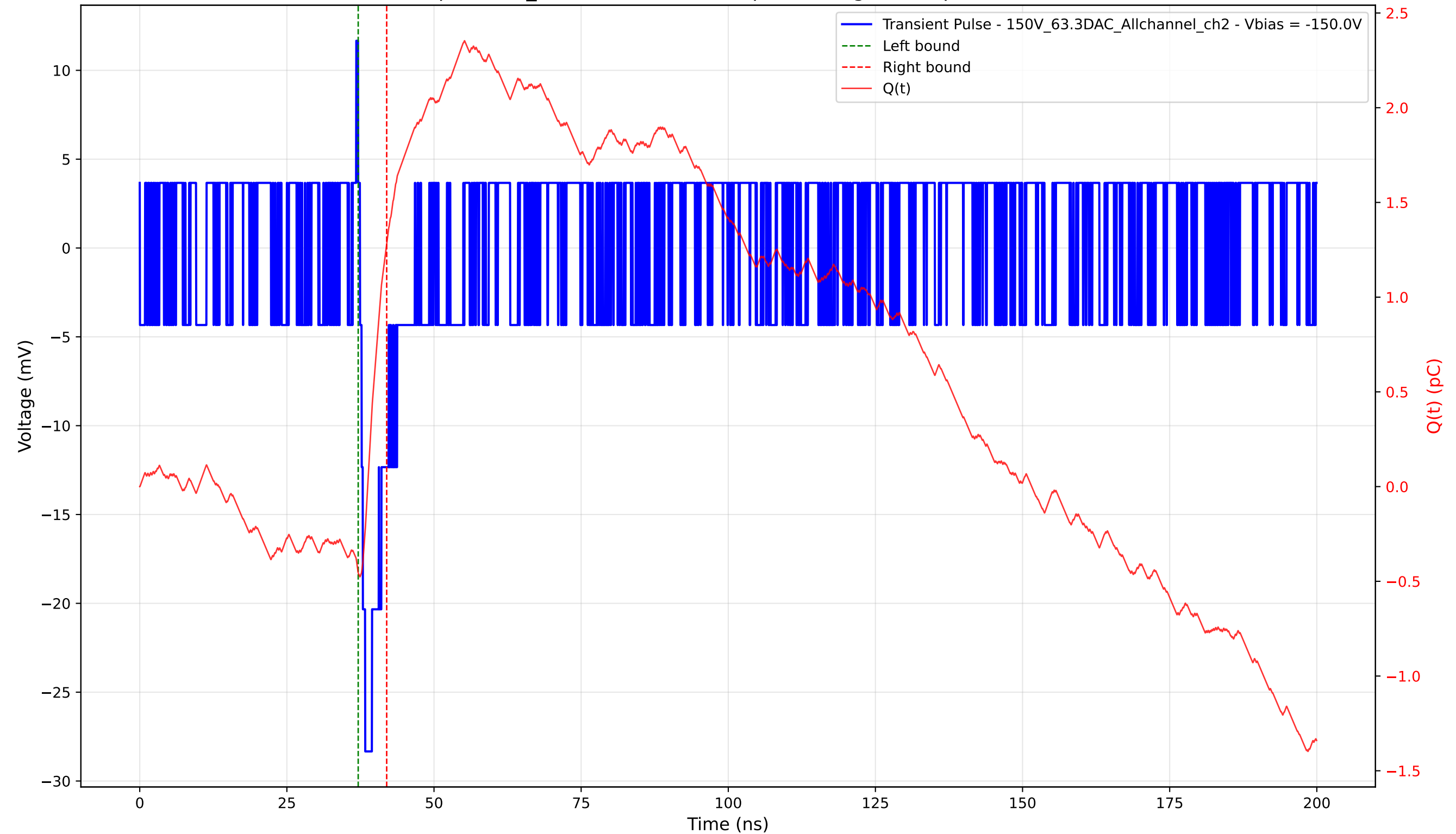
Transient Pulse - Sample: 1cm_42 - Position: 4935.0 \mu\text{m} - Charge: 1.74 pC - Rise Time: 0.00 ns (N/A)
