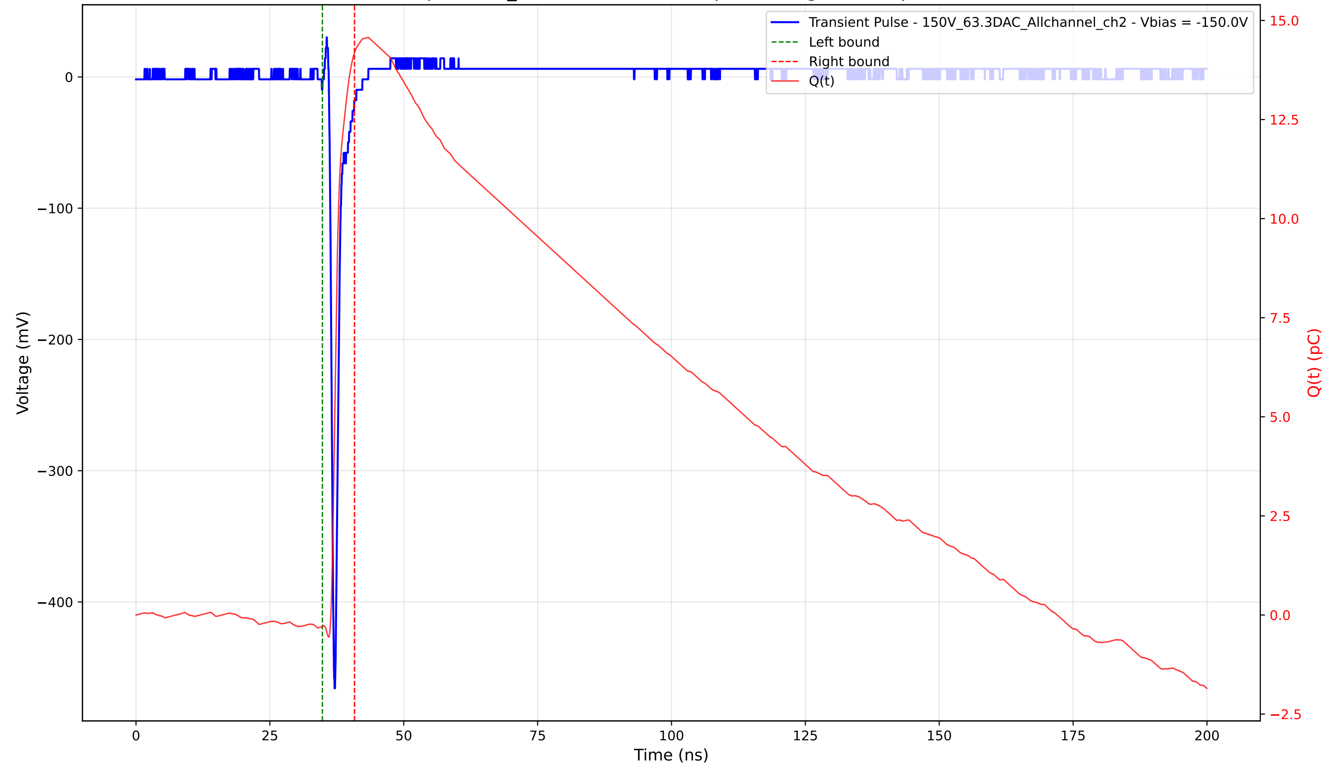
Transient Pulse - Sample: 1cm_42 - Position: 3145.0 \mu\text{m} - Charge: 14.47 pC - Rise Time: 0.72 ns
