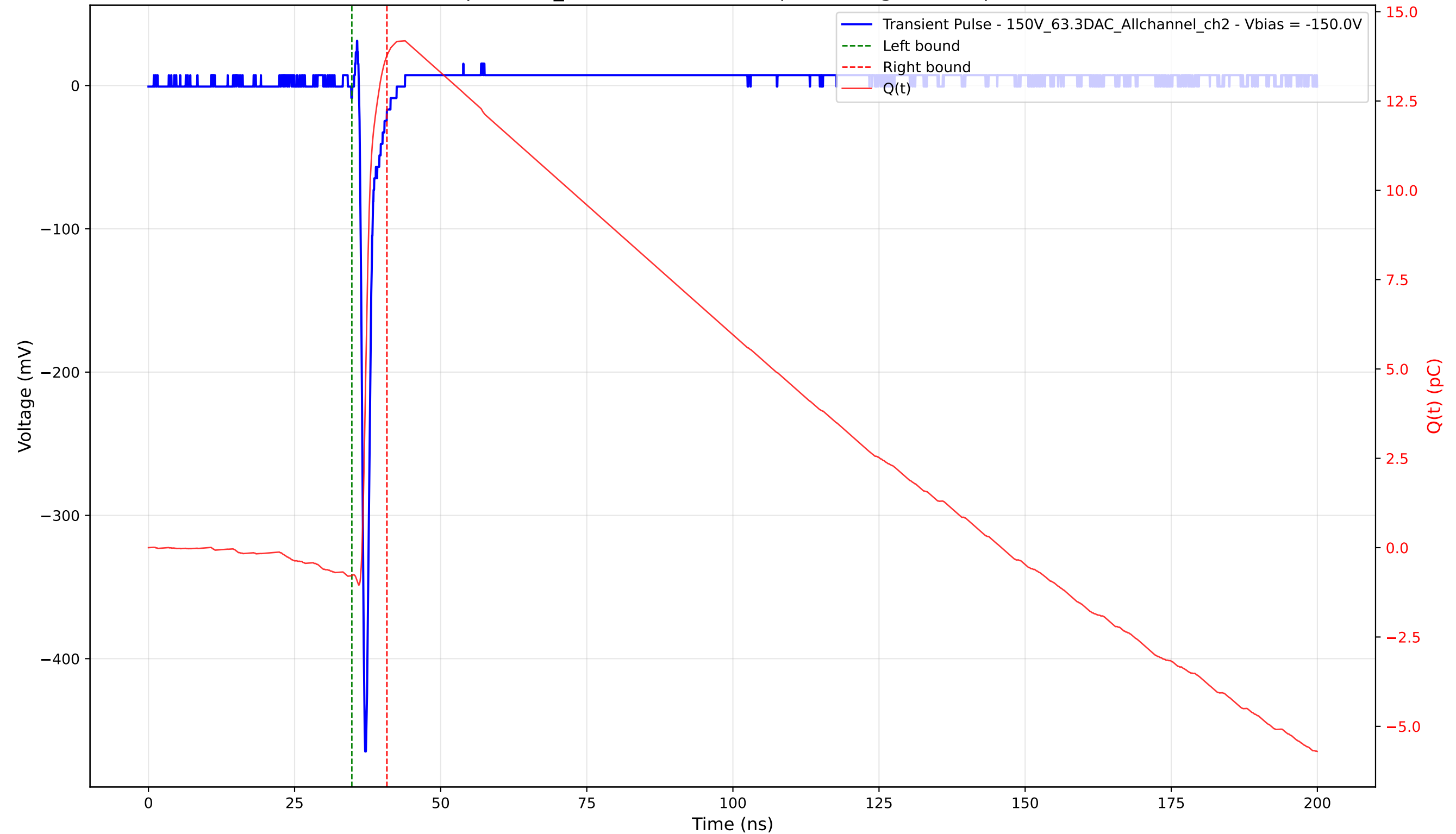
Transient Pulse - Sample: 1cm_42 - Position: 2830.0 \mu\text{m} - Charge: 14.55 pC - Rise Time: 0.73 ns
