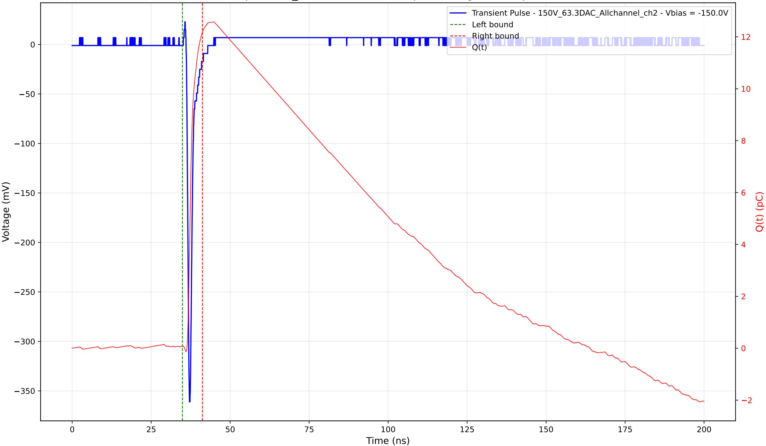
Transient Pulse - Sample: 1cm_42 - Position: 2680.0 \mu\text{m} - Charge: 12.11 pC - Rise Time: 0.72 ns
