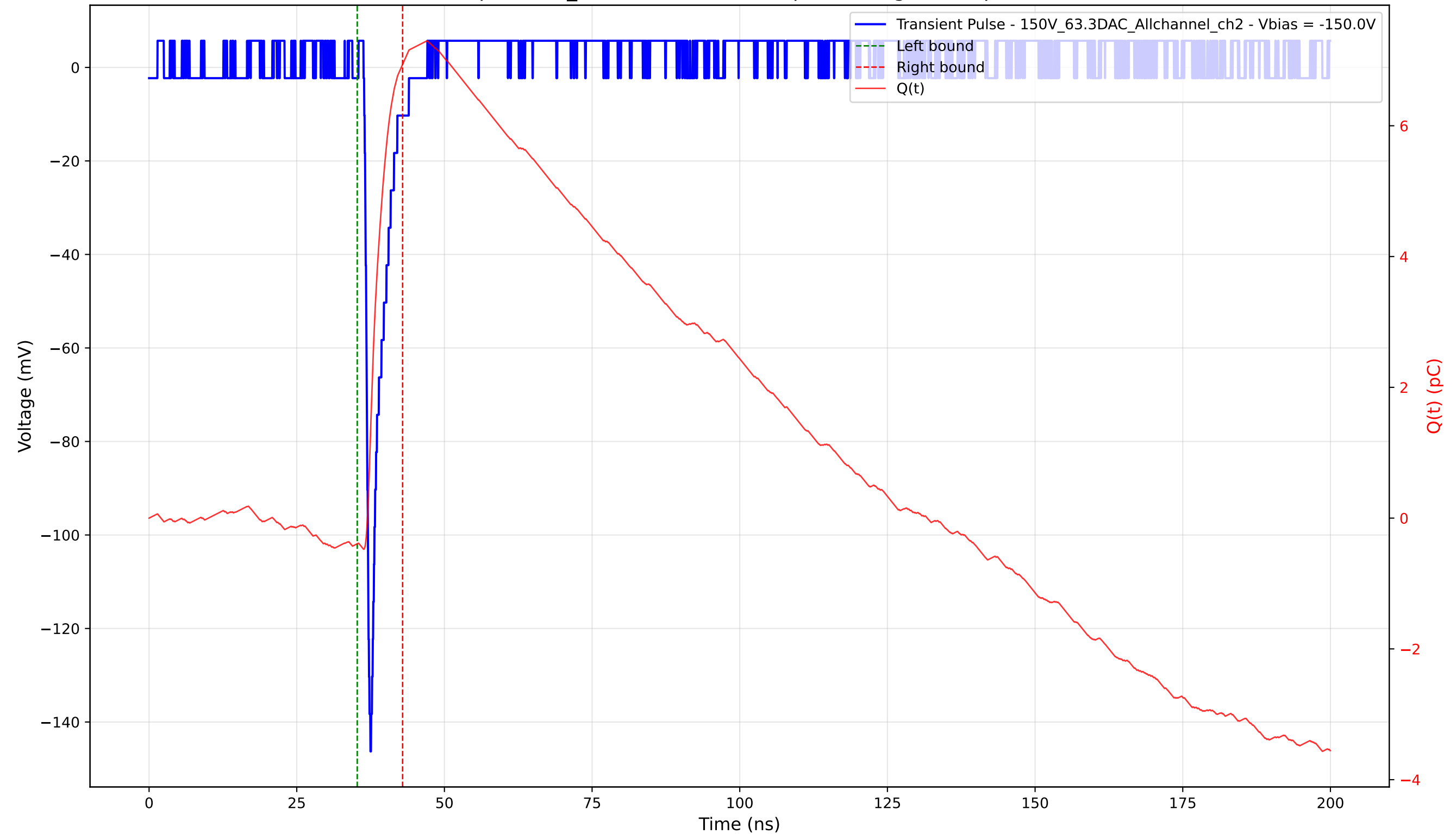
Transient Pulse - Sample: 1cm_42 - Position: 3695.0 \mu\text{m} - Charge: 7.33 pC - Rise Time: 0.82 ns
