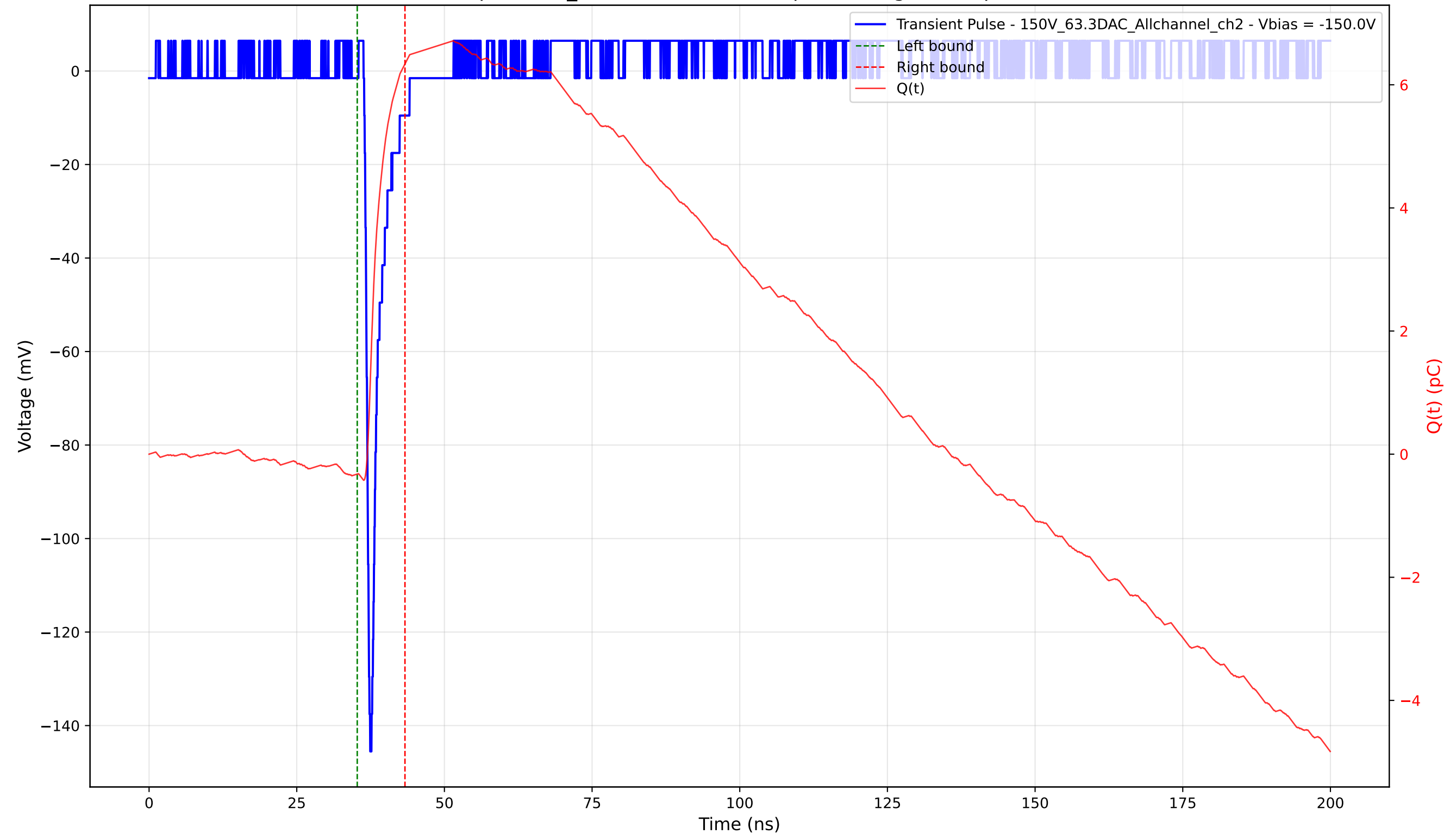
Transient Pulse - Sample: 1cm_42 - Position: 2345.0 \mu\text{m} - Charge: 6.66 pC - Rise Time: 0.81 ns
