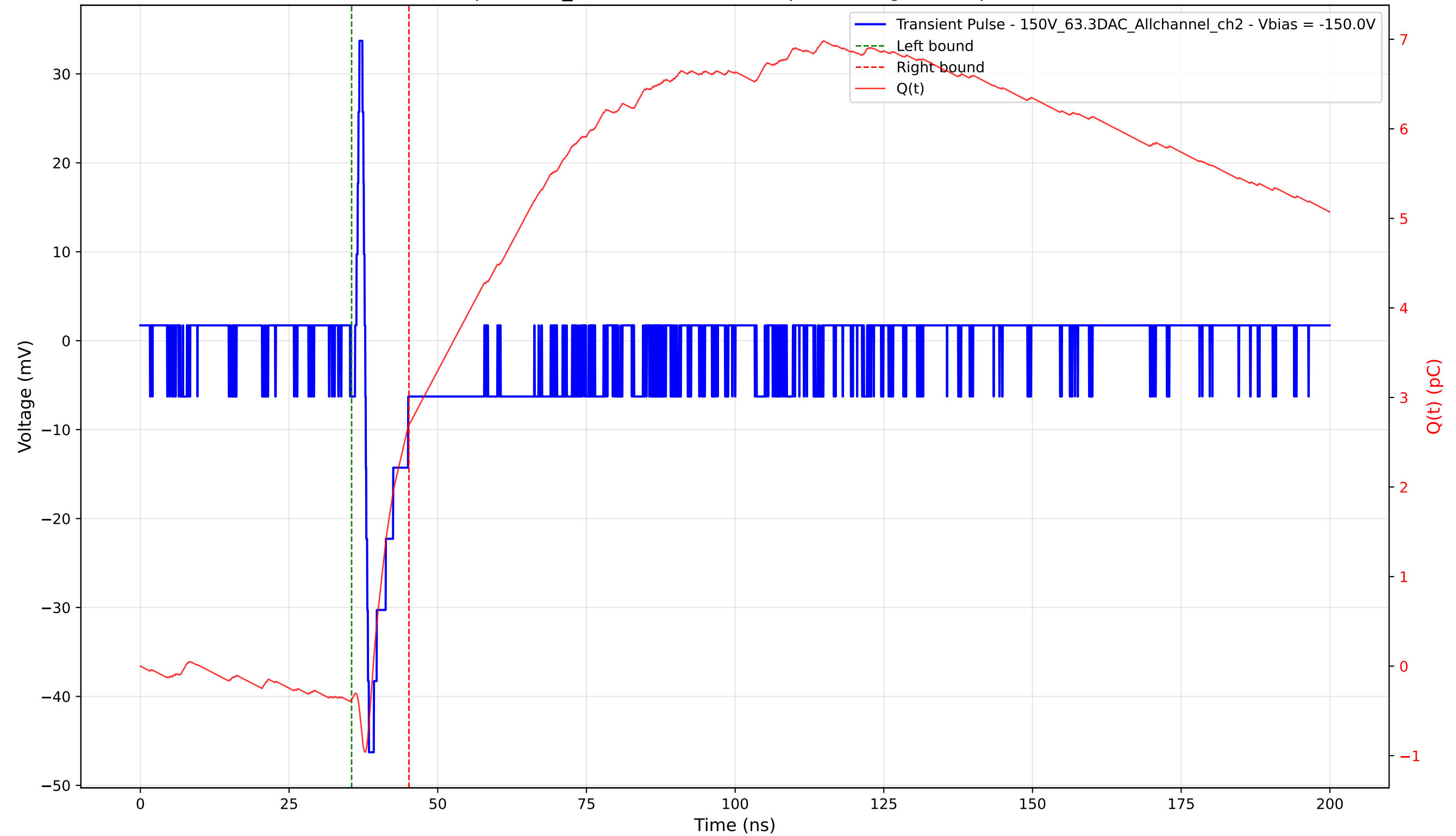
Transient Pulse - Sample: 1cm_42 - Position: 1210.0 \mu\text{m} - Charge: 3.07 pC - Rise Time: 0.61 ns
