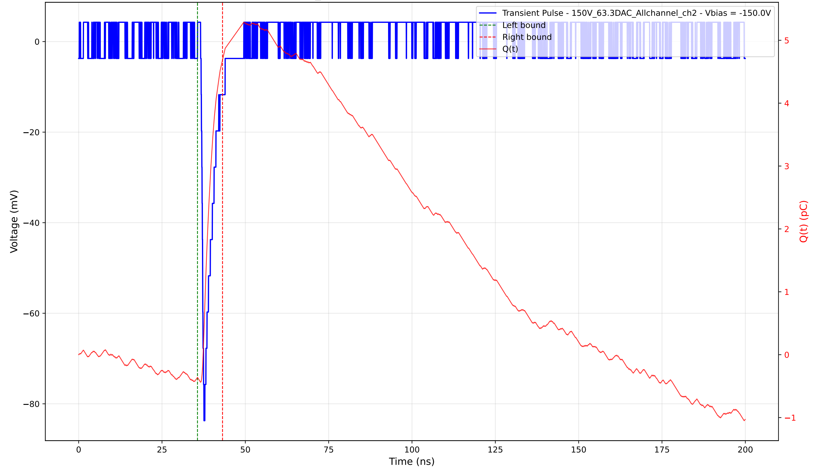
Transient Pulse - Sample: 1cm_42 - Position: 3970.0 \mu\text{m} - Charge: 5.05 pC - Rise Time: 0.74 ns
