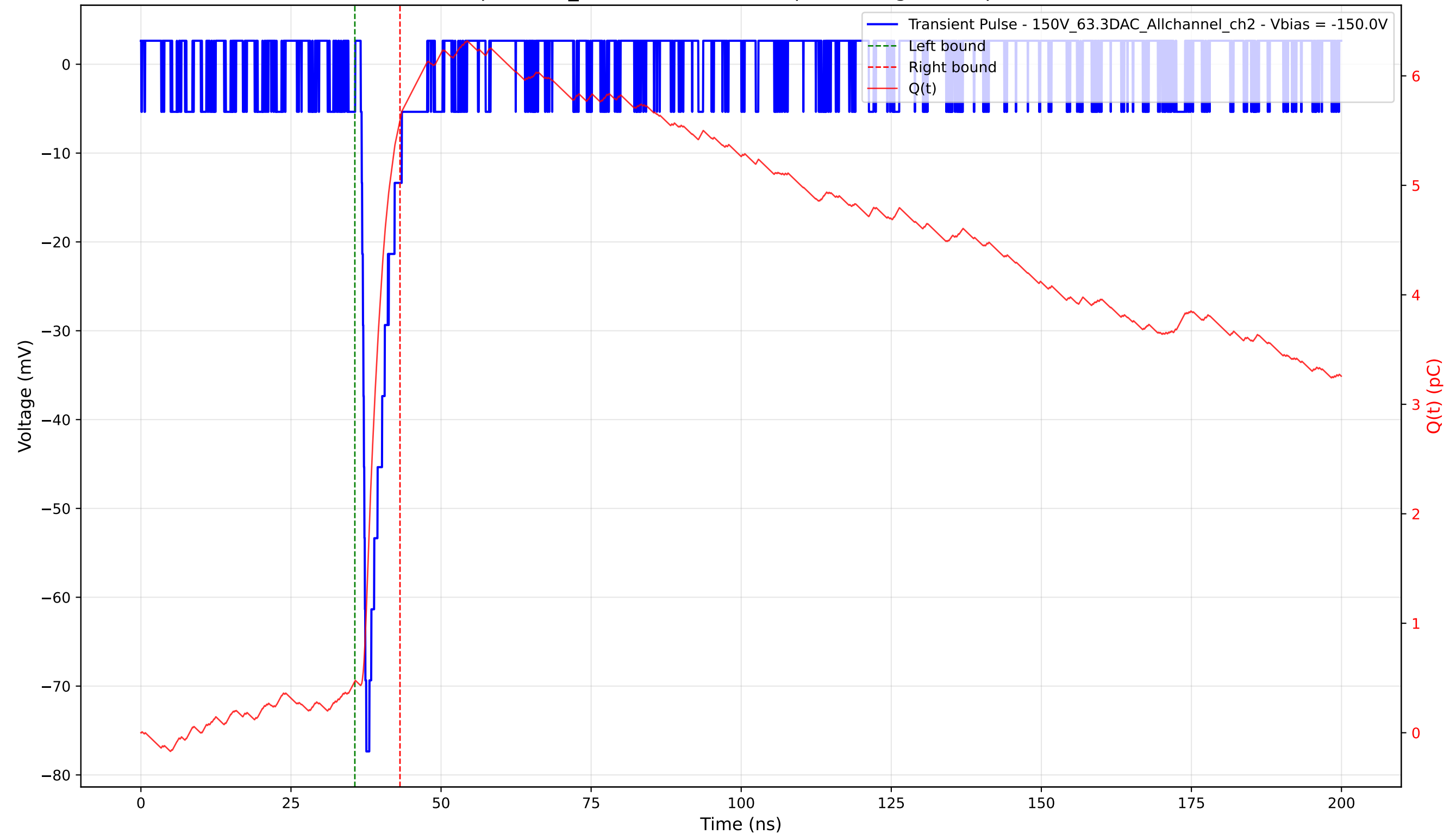
Transient Pulse - Sample: 1cm_42 - Position: 3990.0 \mu\text{m} - Charge: 5.12 pC - Rise Time: 0.79 ns
