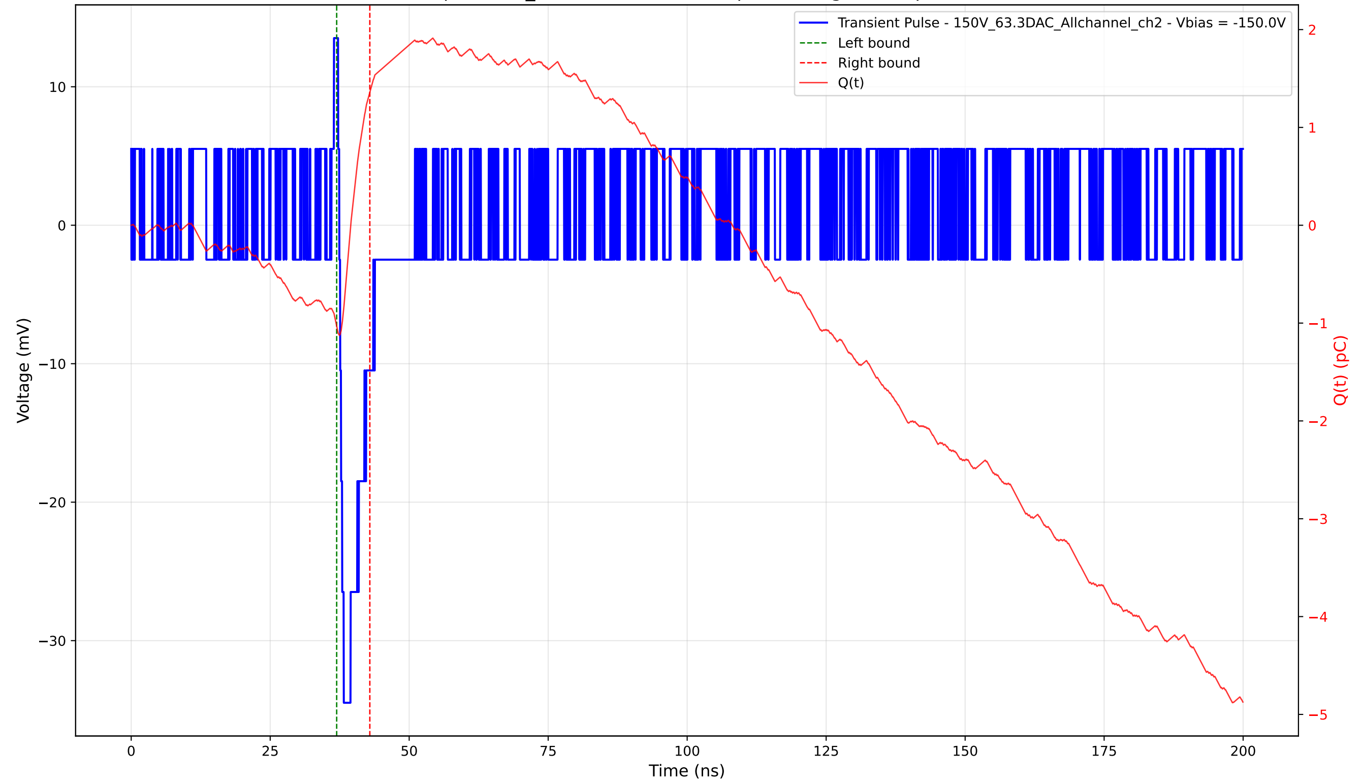
Transient Pulse - Sample: 1cm_42 - Position: 4740.0 \mu\text{m} - Charge: 2.39 pC - Rise Time: 0.68 ns
