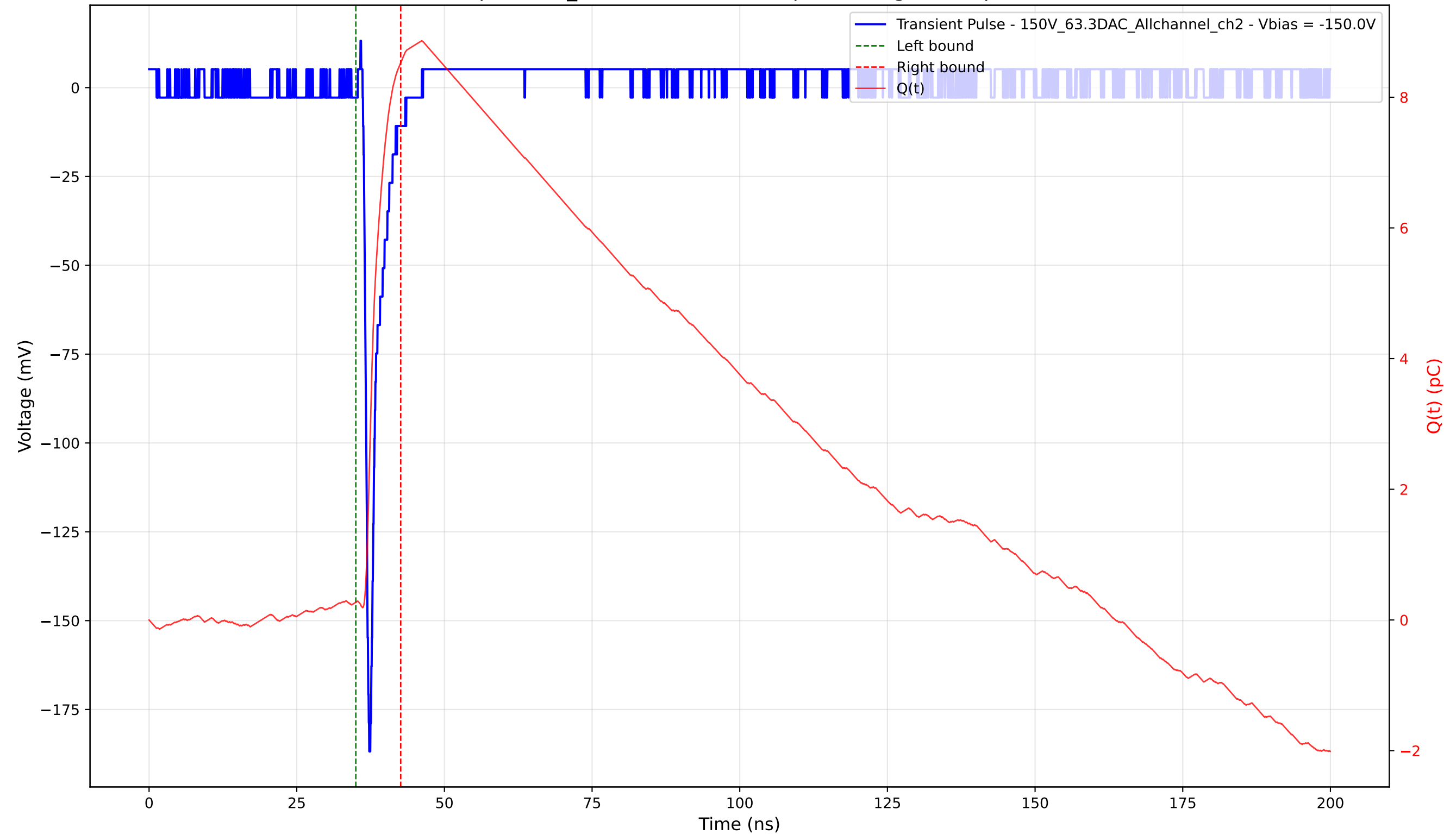
Transient Pulse - Sample: 1cm_42 - Position: 3560.0 \mu\text{m} - Charge: 8.26 pC - Rise Time: 0.80 ns
