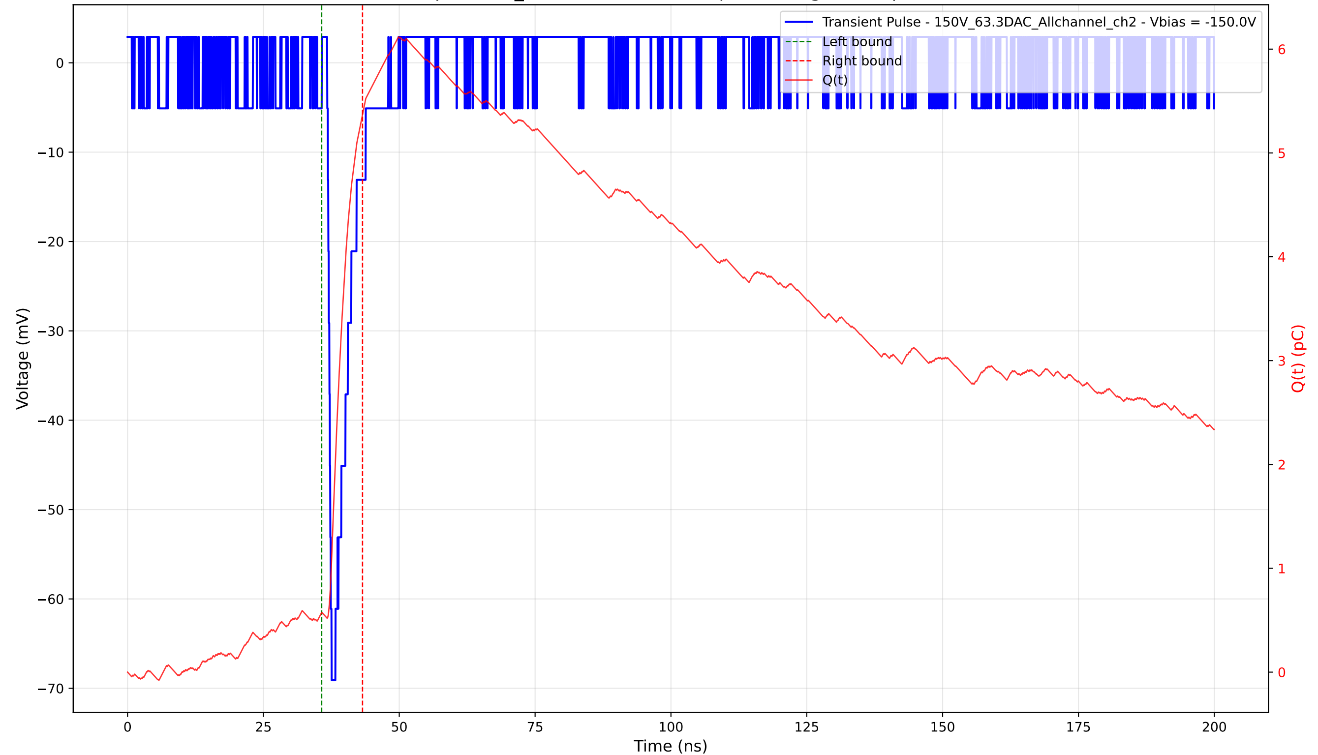
Transient Pulse - Sample: 1cm_42 - Position: 4020.0 \mu\text{m} - Charge: 4.80 pC - Rise Time: 0.71 ns
