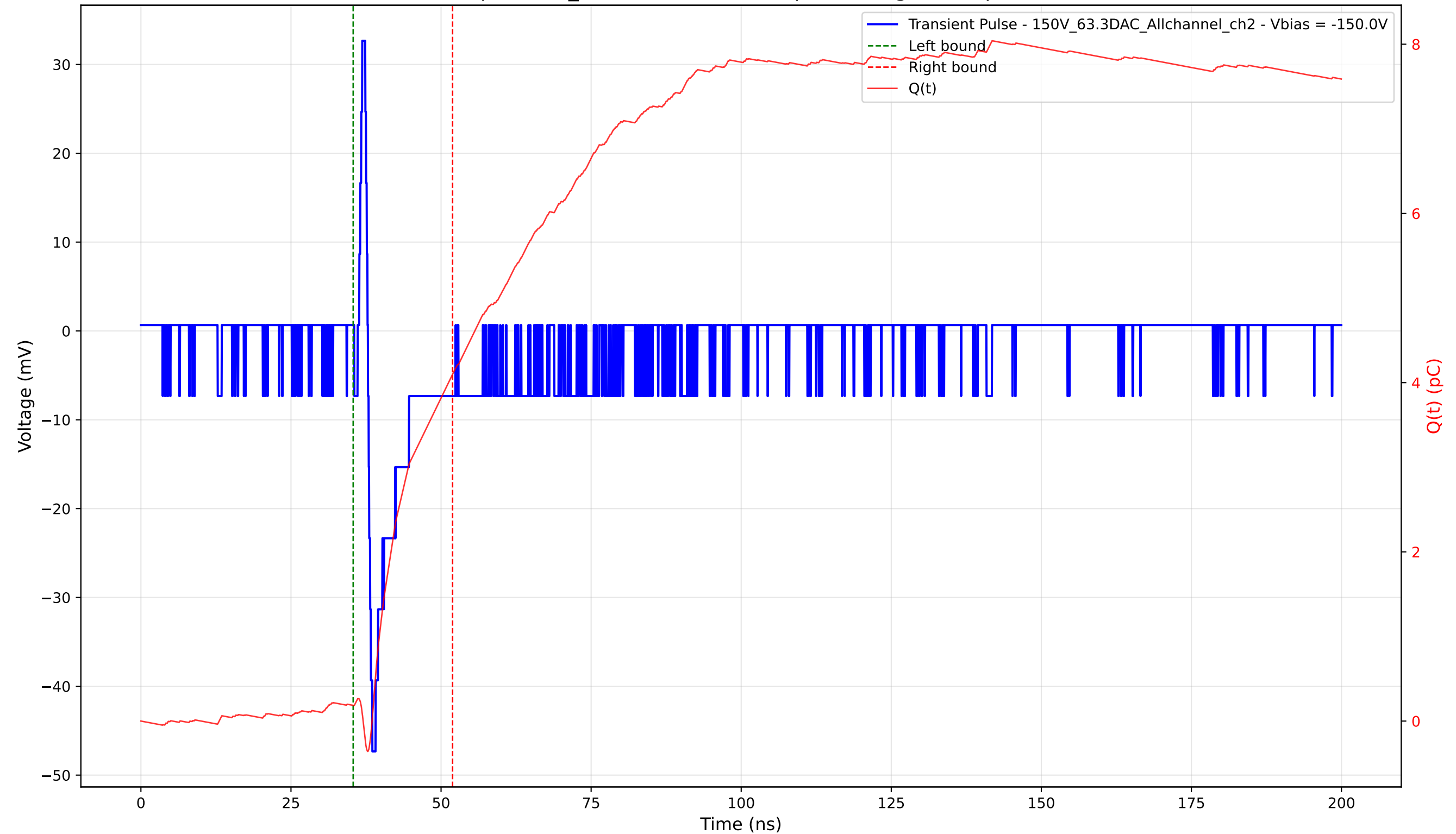
Transient Pulse - Sample: 1cm_42 - Position: 1140.0 \mu\text{m} - Charge: 3.92 pC - Rise Time: 0.74 ns
