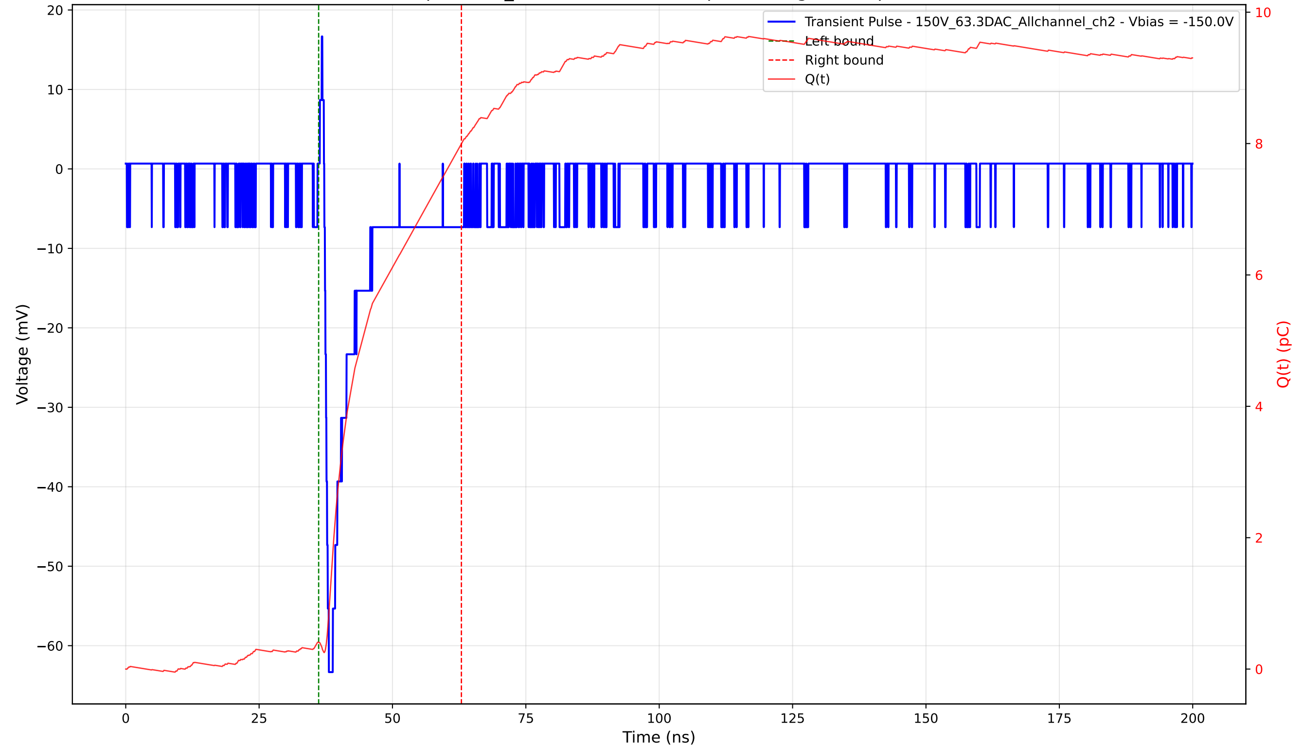
Transient Pulse - Sample: 1cm_42 - Position: 1745.0 \mu\text{m} - Charge: 7.59 pC - Rise Time: 0.85 ns
