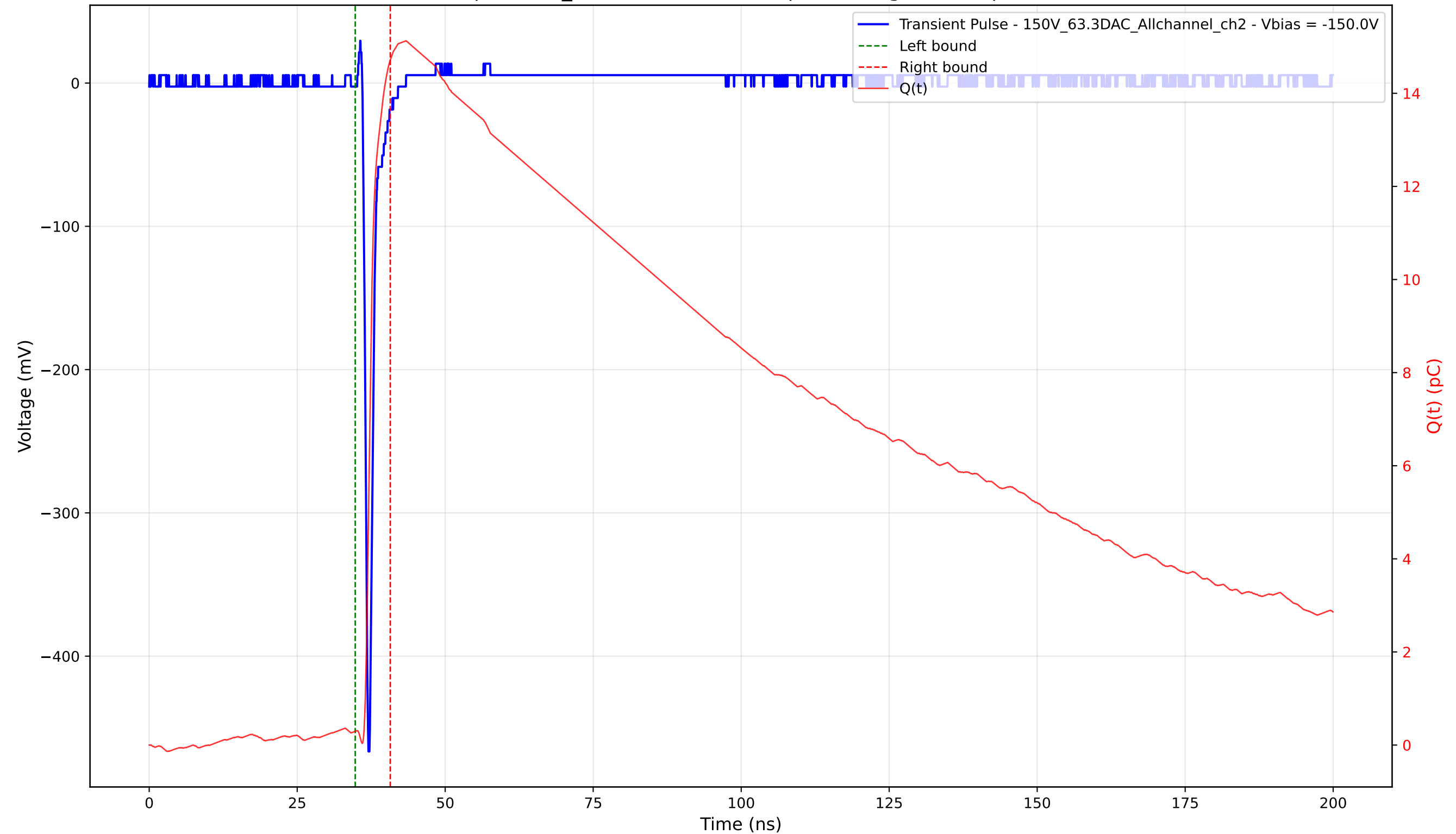
Transient Pulse - Sample: 1cm_42 - Position: 2920.0 \mu\text{m} - Charge: 14.42 pC - Rise Time: 0.71 ns
