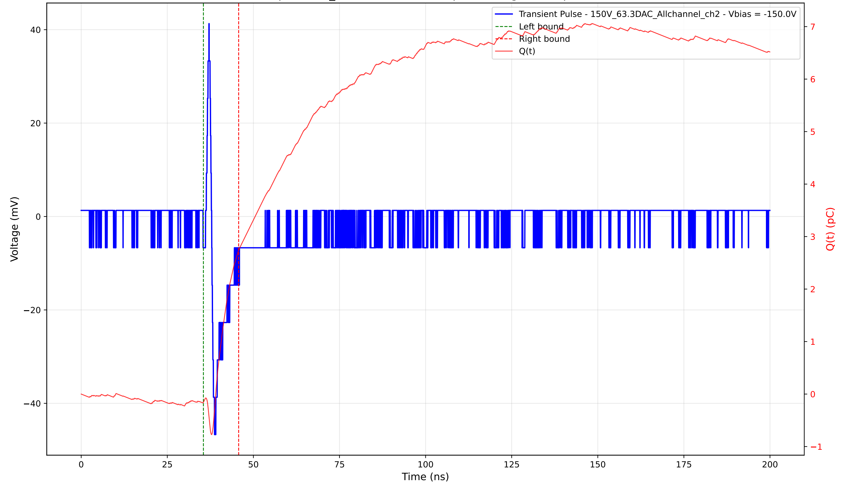
Transient Pulse - Sample: 1cm_42 - Position: 750.0 \mu\text{m} - Charge: 2.89 pC - Rise Time: 0.82 ns
