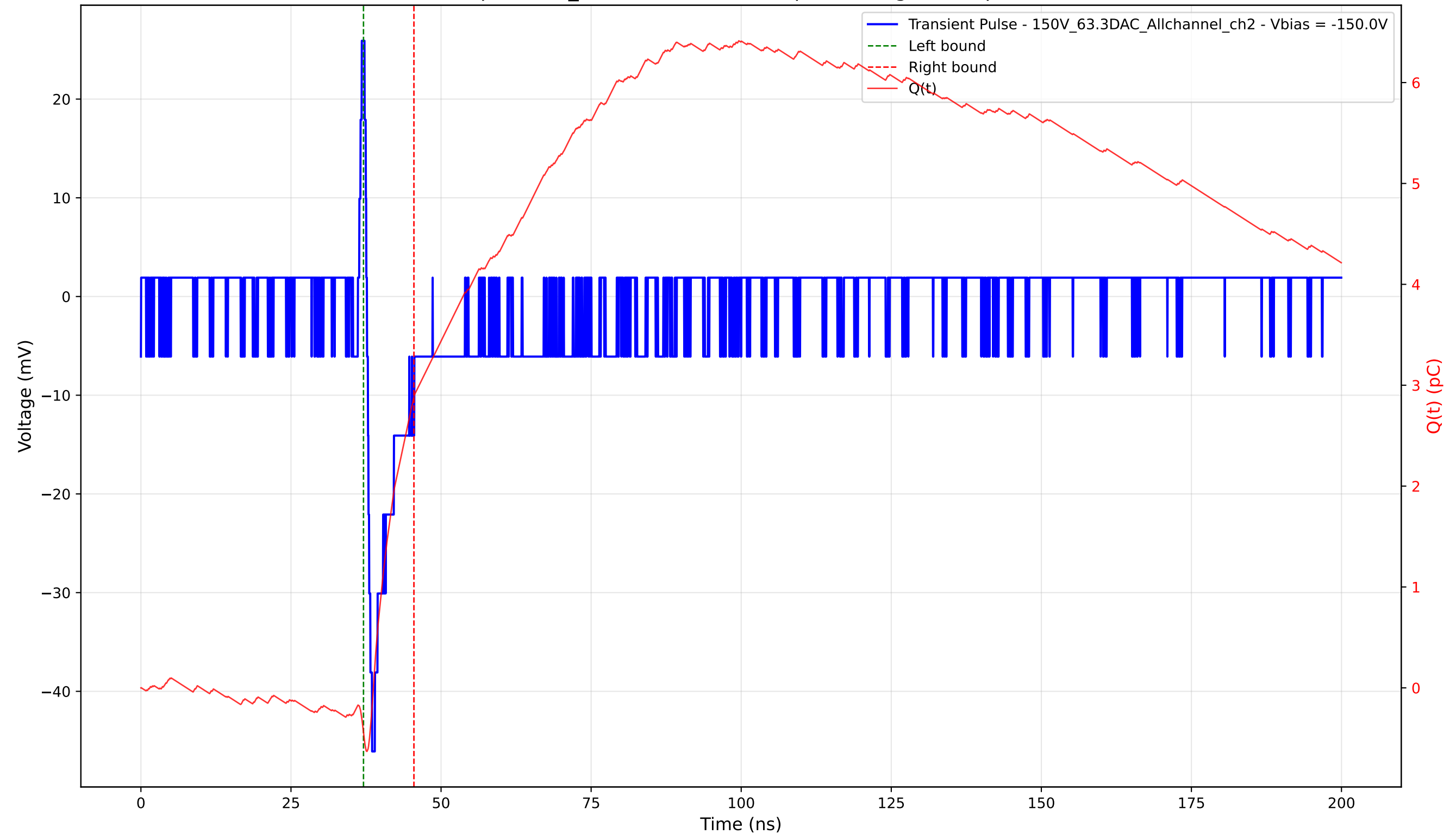
Transient Pulse - Sample: 1cm_42 - Position: 1435.0 \mu\text{m} - Charge: 3.33 pC - Rise Time: 0.85 ns
