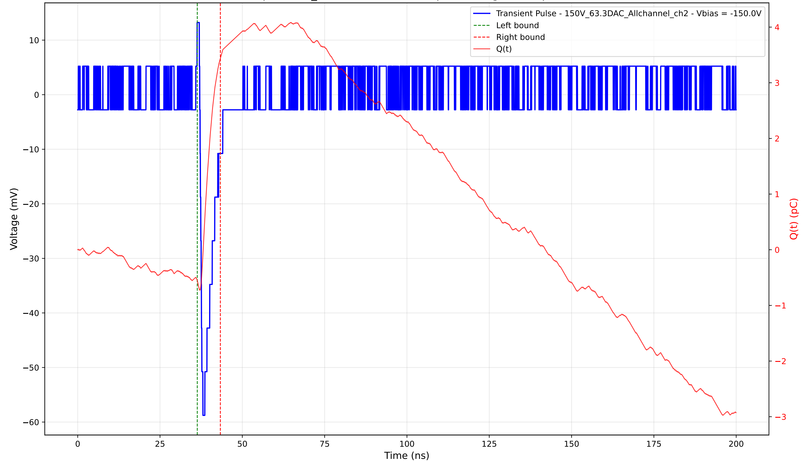
Transient Pulse - Sample: 1cm_42 - Position: 4220.0 \mu\text{m} - Charge: 3.99 pC - Rise Time: 0.86 ns
