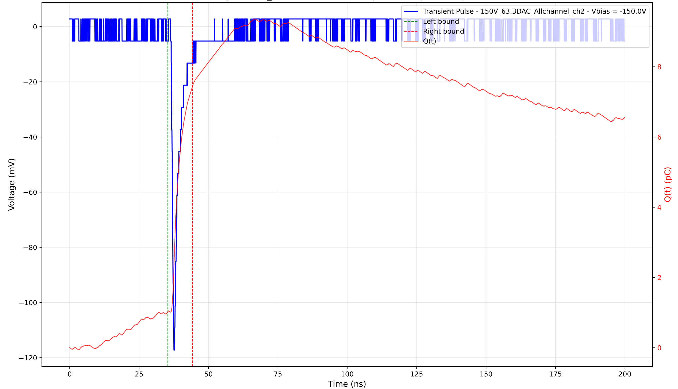
Transient Pulse - Sample: 1cm_42 - Position: 2180.0 \mu\text{m} - Charge: 6.41 pC - Rise Time: 0.85 ns
