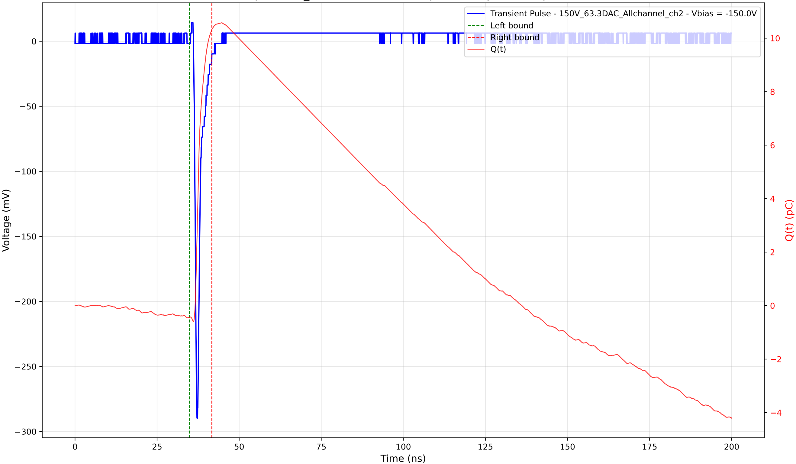
Transient Pulse - Sample: 1cm_42 - Position: 3430.0 \mu\text{m} - Charge: 10.76 pC - Rise Time: 0.76 ns
