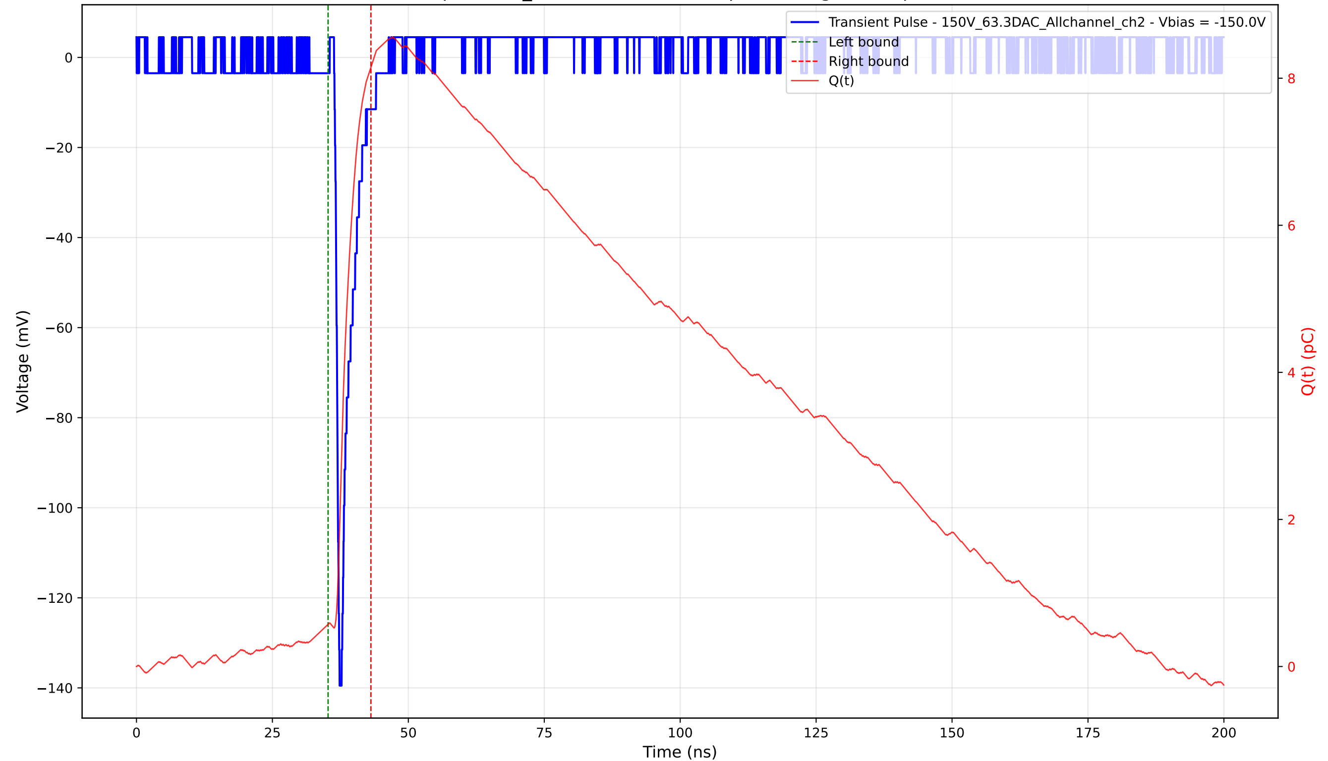
Transient Pulse - Sample: 1cm_42 - Position: 3710.0 \mu\text{m} - Charge: 7.58 pC - Rise Time: 0.79 ns
