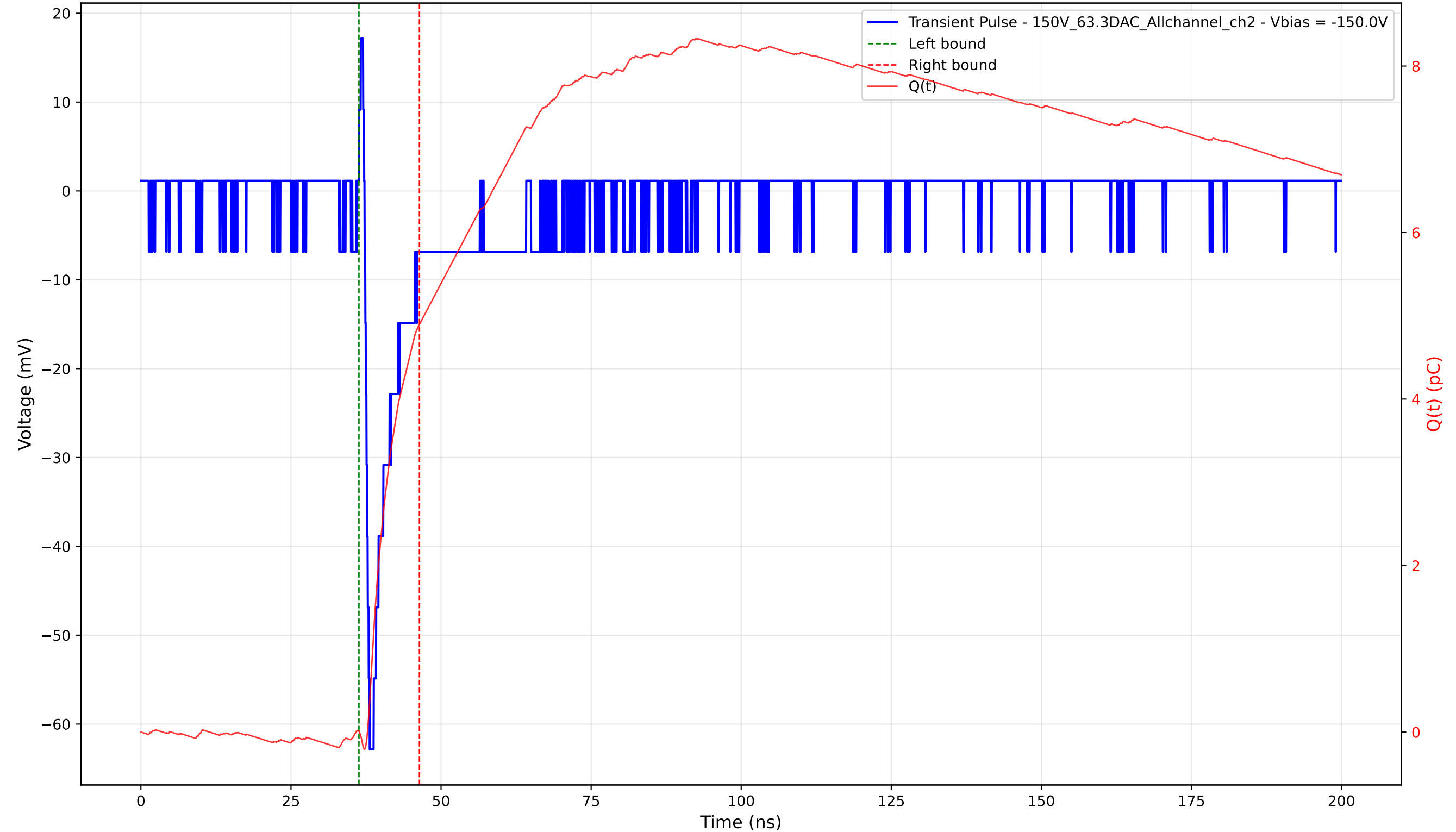
Transient Pulse - Sample: 1cm_42 - Position: 1720.0 \mu\text{m} - Charge: 4.89 pC - Rise Time: 0.84 ns
