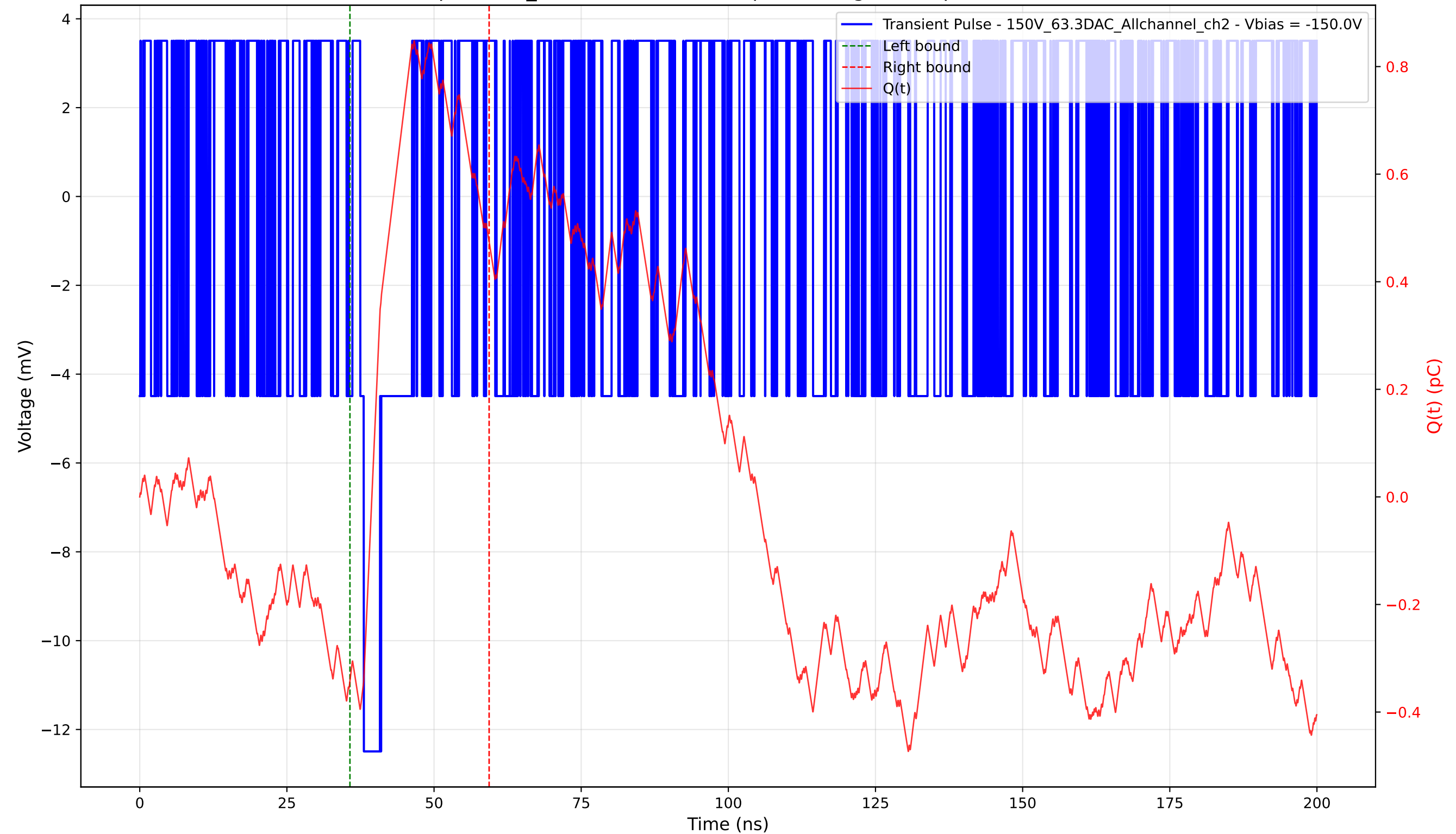
Transient Pulse - Sample: 1cm_42 - Position: 5070.0 \mu\text{m} - Charge: 0.82 pC - Rise Time: 0.00 ns (N/A)
