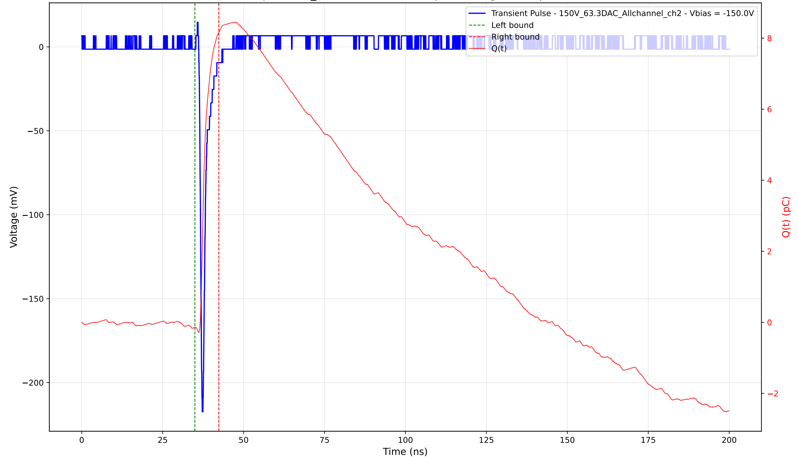
Transient Pulse - Sample: 1cm_42 - Position: 2530.0 \mu\text{m} - Charge: 8.31 pC - Rise Time: 0.75 ns
