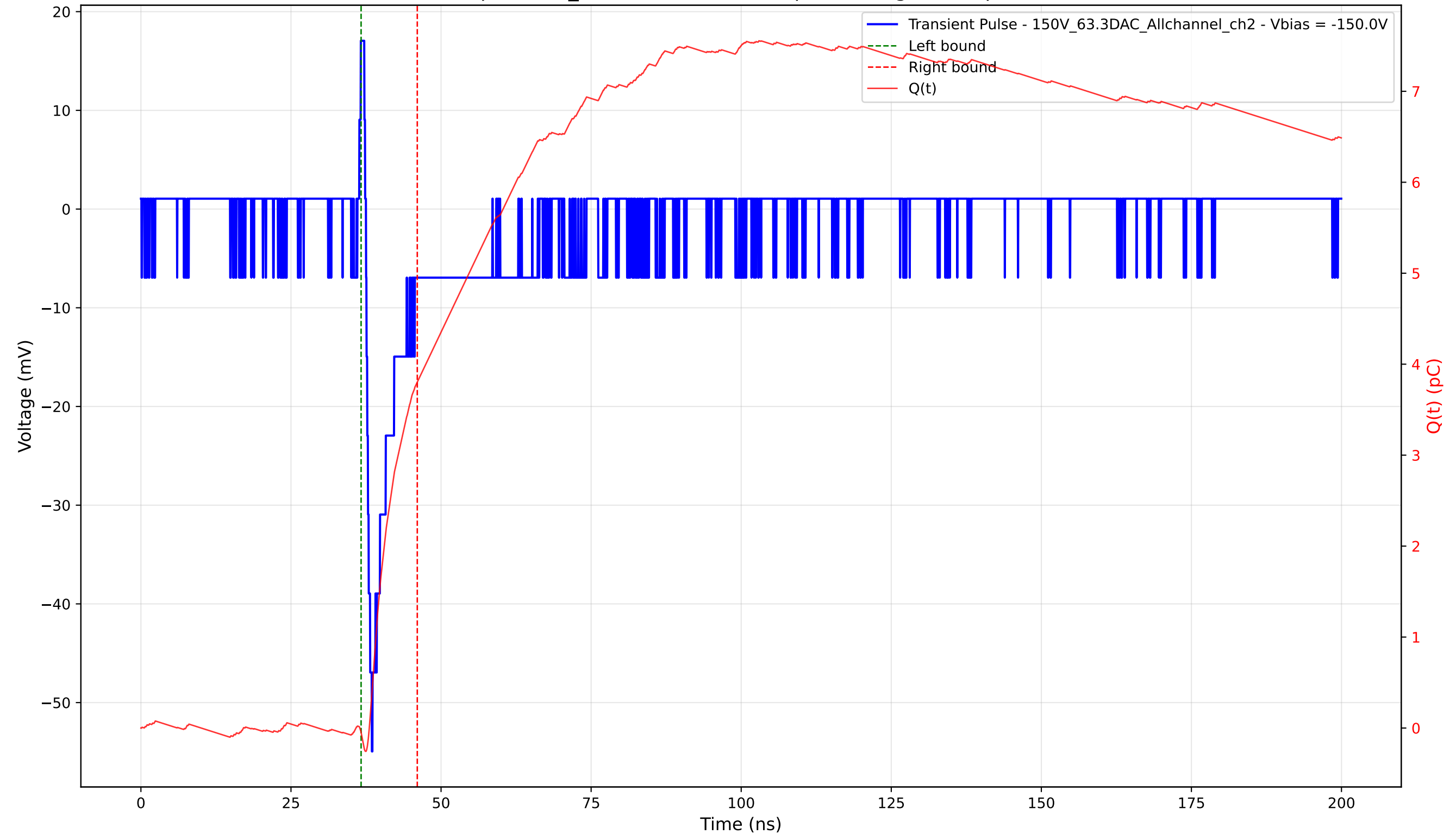
Transient Pulse - Sample: 1cm_42 - Position: 1575.0 \mu\text{m} - Charge: 3.85 pC - Rise Time: 0.97 ns
