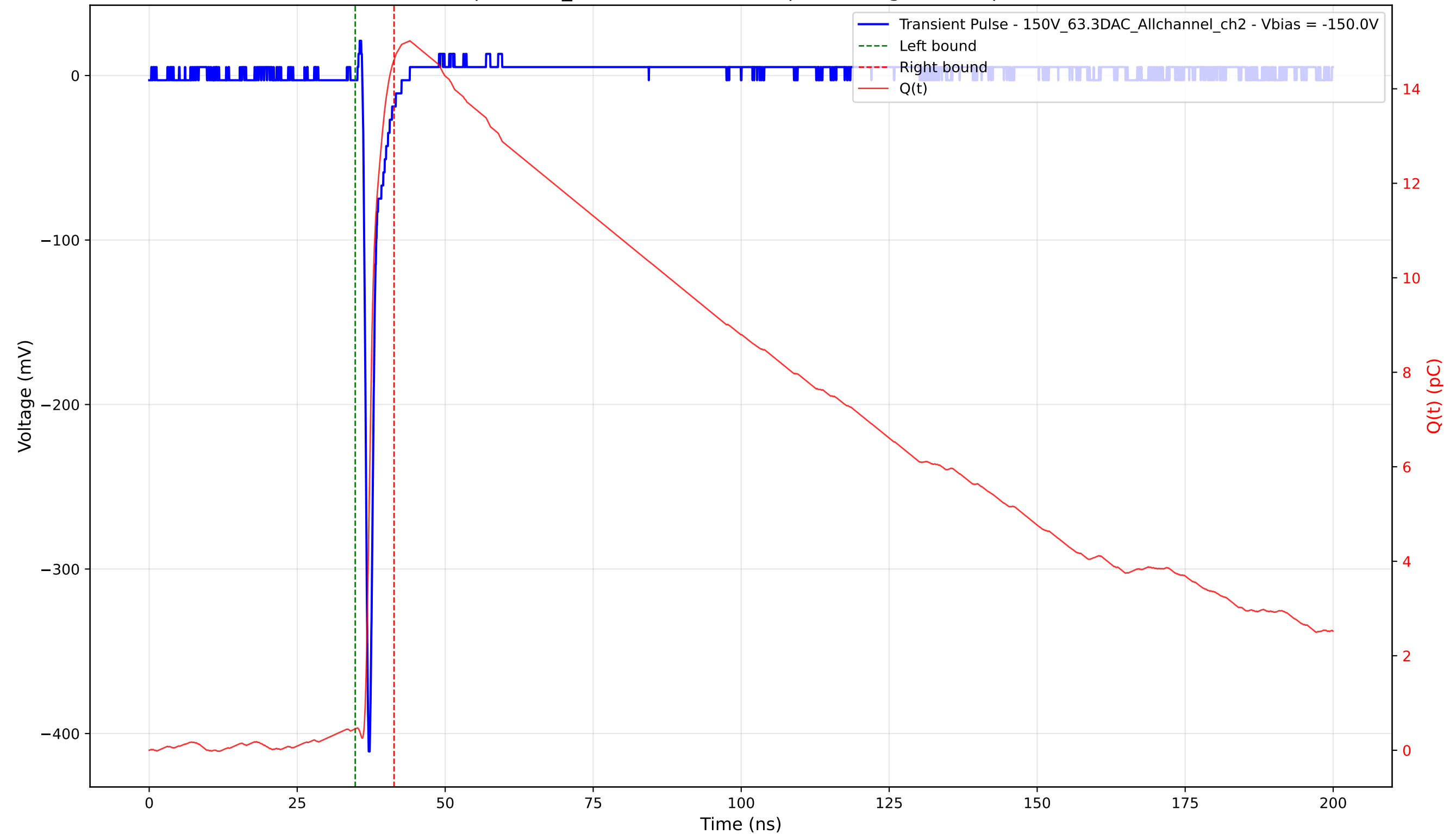
Transient Pulse - Sample: 1cm_42 - Position: 3315.0 \mu\text{m} - Charge: 14.16 pC - Rise Time: 0.70 ns
