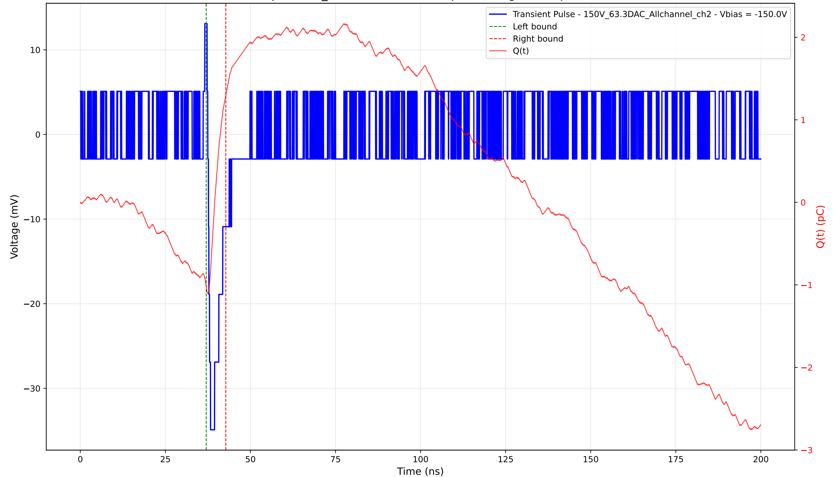
Transient Pulse - Sample: 1cm_42 - Position: 4810.0 \mu\text{m} - Charge: 2.31 pC - Rise Time: 0.64 ns
