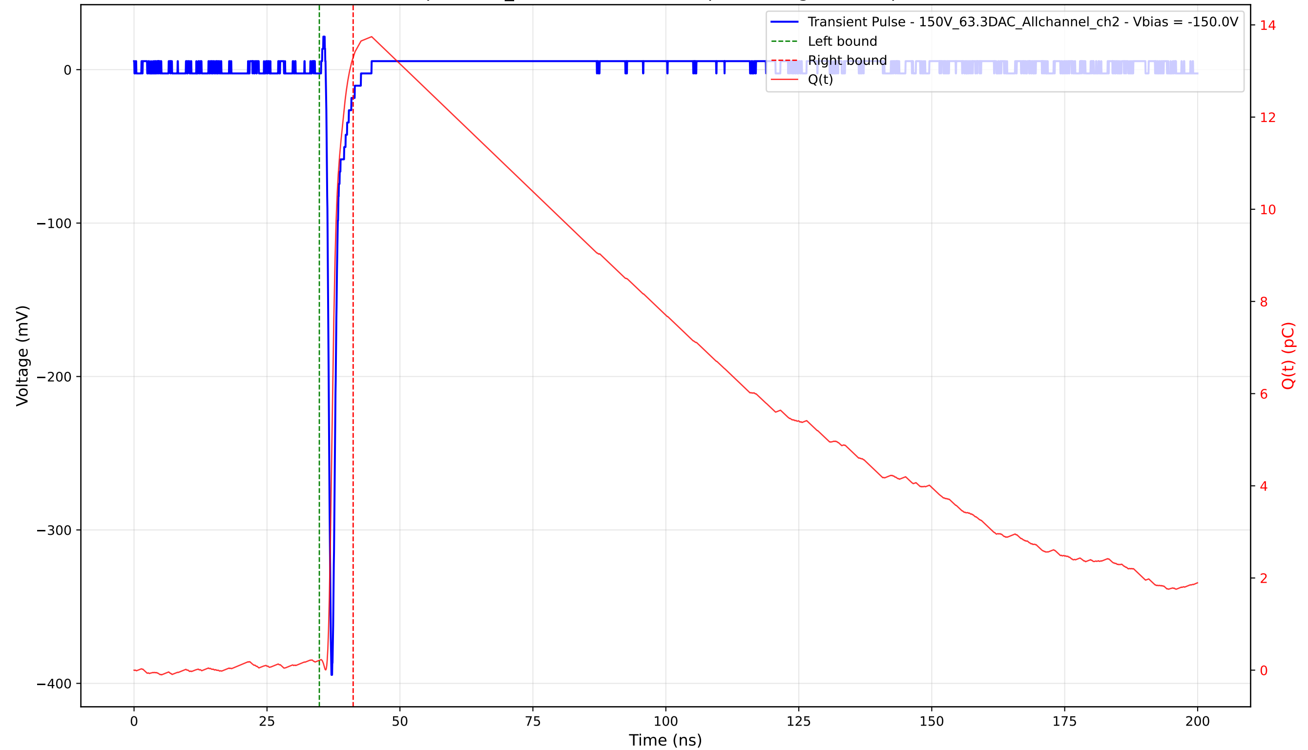
Transient Pulse - Sample: 1cm_42 - Position: 2705.0 \mu\text{m} - Charge: 13.08 pC - Rise Time: 0.73 ns
