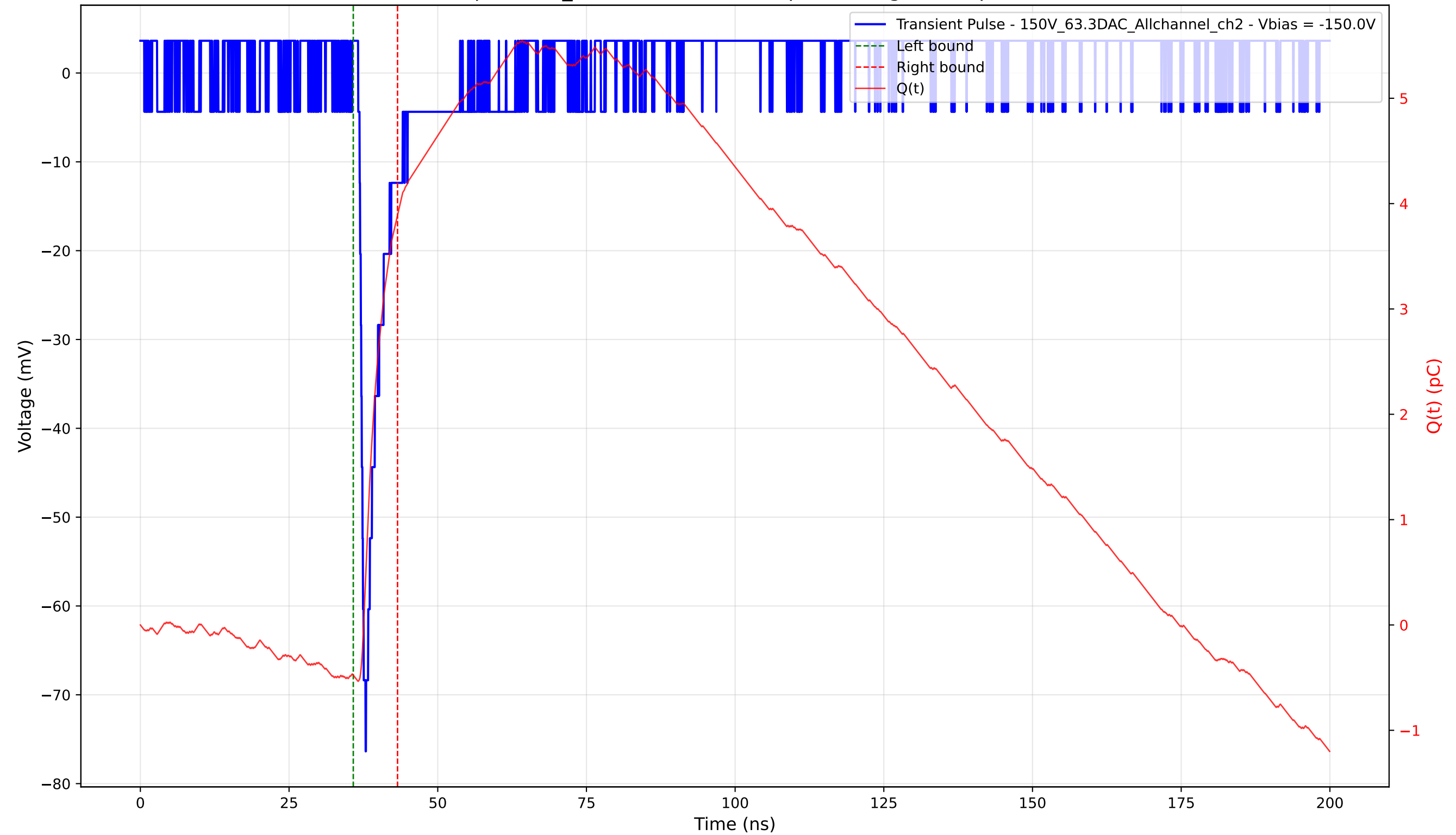
Transient Pulse - Sample: 1cm_42 - Position: 2020.0 \mu\text{m} - Charge: 4.37 pC - Rise Time: 1.02 ns
