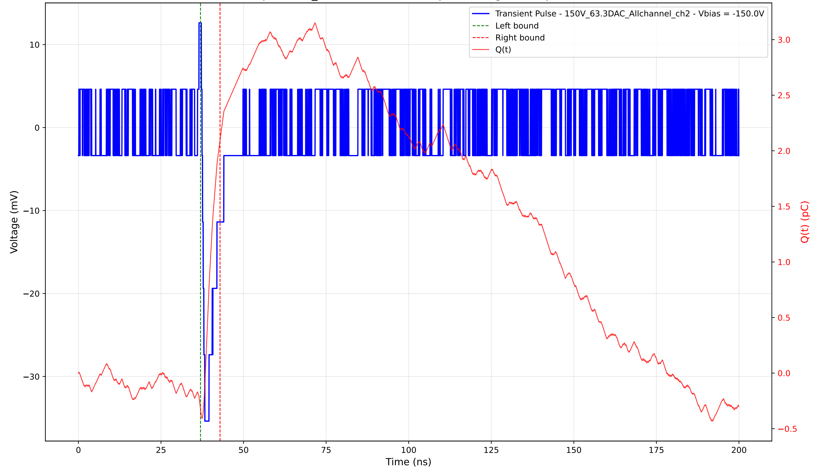
Transient Pulse - Sample: 1cm_42 - Position: 4755.0 \mu\text{m} - Charge: 2.42 pC - Rise Time: 0.72 ns
