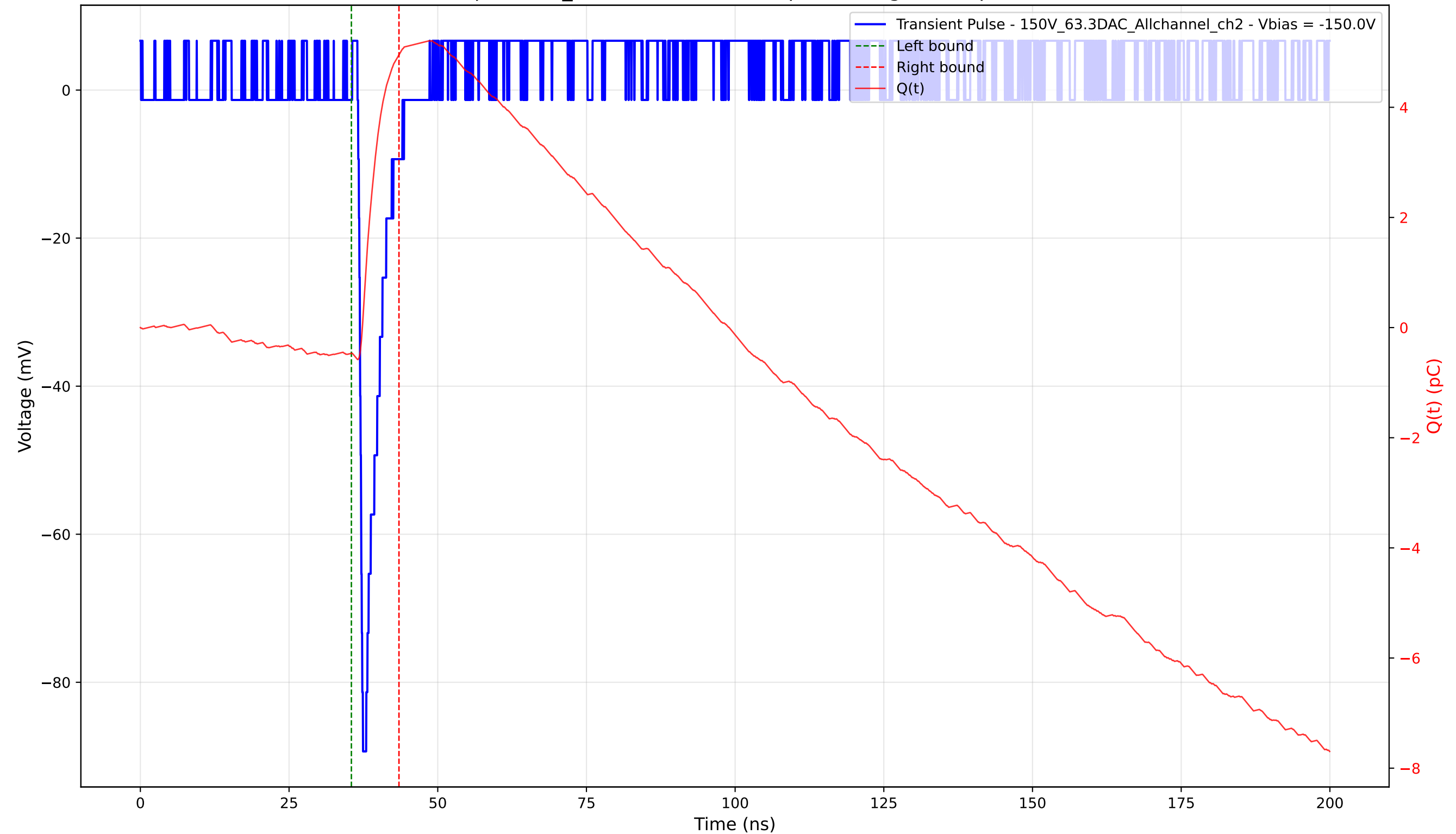
Transient Pulse - Sample: 1cm_42 - Position: 3915.0 \mu\text{m} - Charge: 5.42 pC - Rise Time: 0.68 ns
