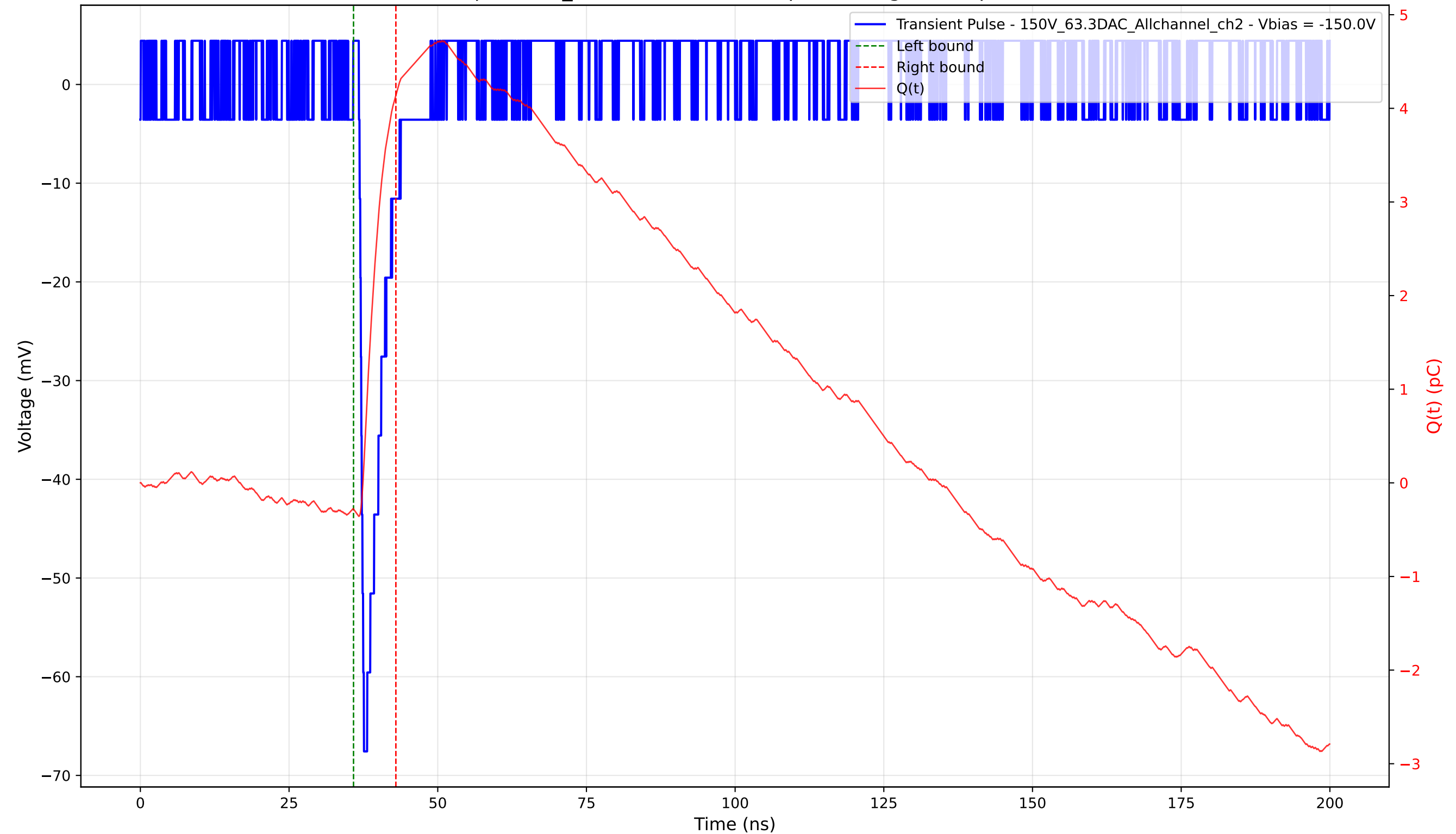
Transient Pulse - Sample: 1cm_42 - Position: 4030.0 \mu\text{m} - Charge: 4.42 pC - Rise Time: 0.74 ns
