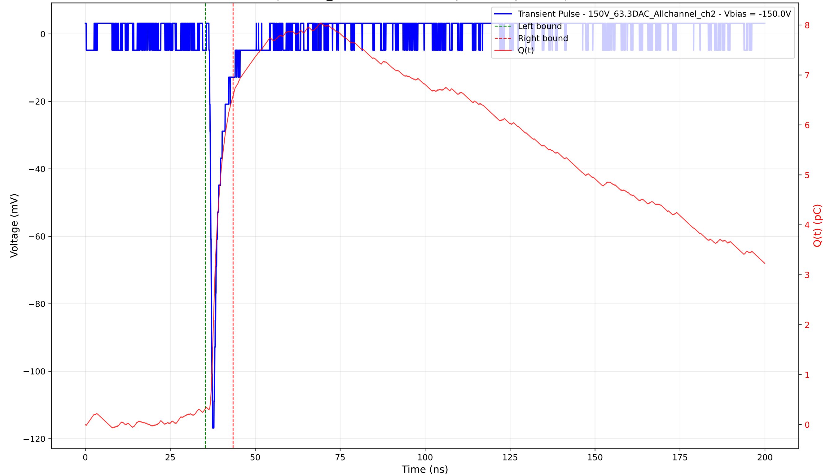
Transient Pulse - Sample: 1cm_42 - Position: 2190.0 \mu\text{m} - Charge: 6.27 pC - Rise Time: 0.81 ns
