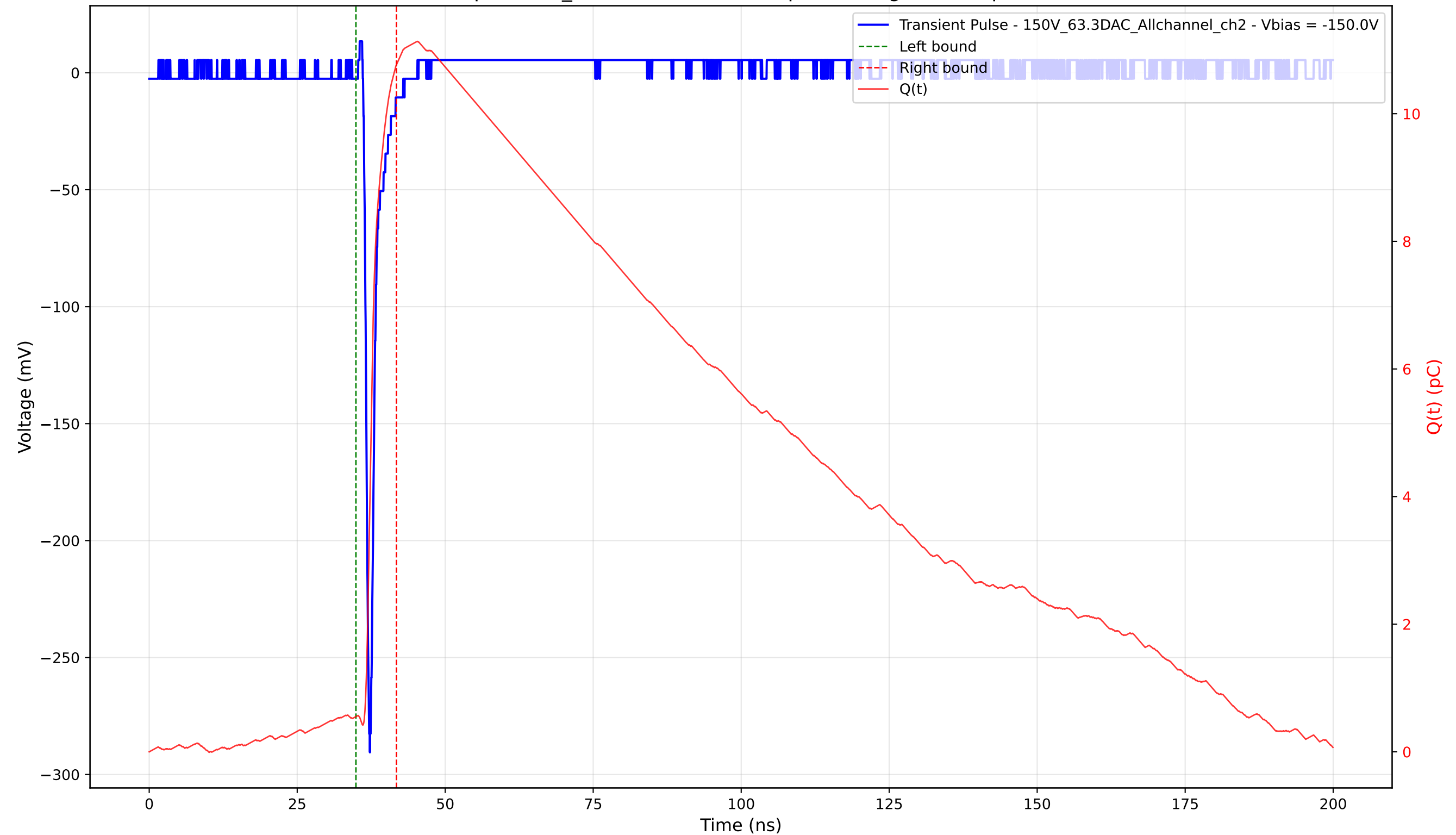
Transient Pulse - Sample: 1cm_42 - Position: 2610.0 \mu\text{m} - Charge: 10.21 pC - Rise Time: 0.79 ns
