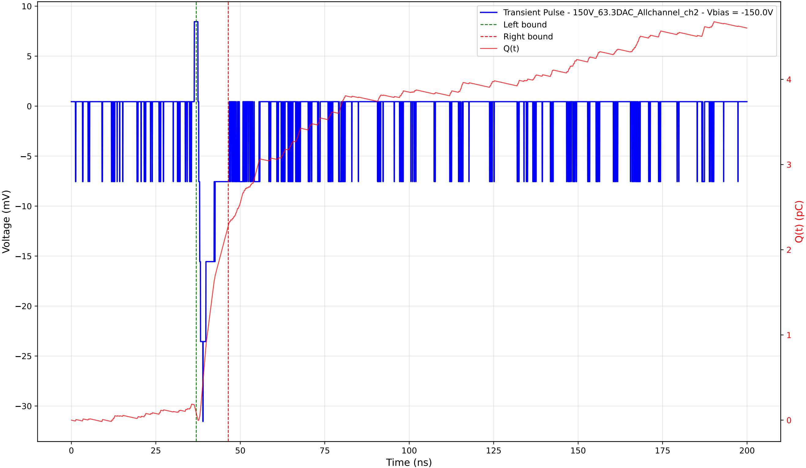
Transient Pulse - Sample: 1cm_42 - Position: 335.0 \mu\text{m} - Charge: 2.20 pC - Rise Time: 1.26 ns
