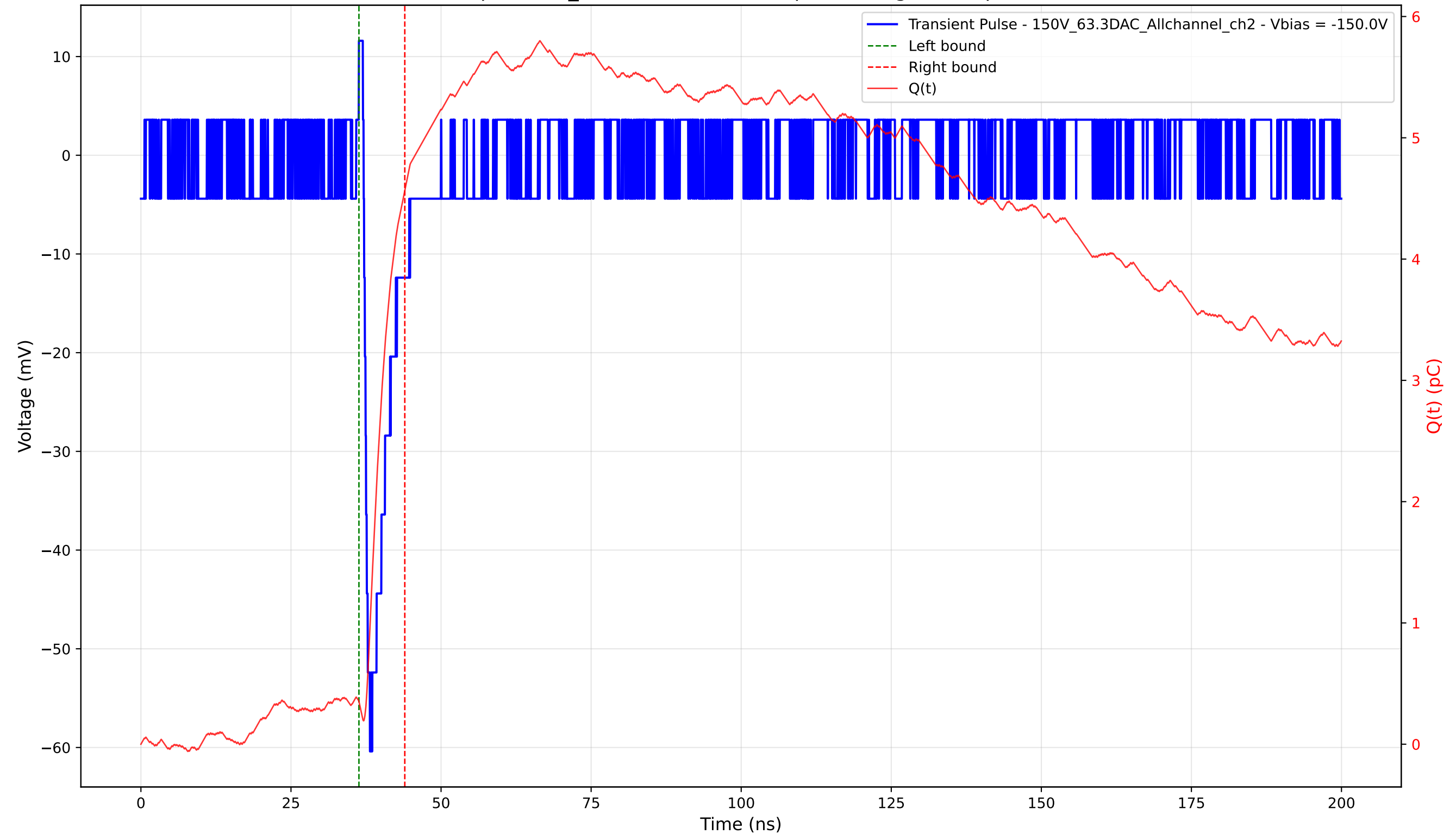
Transient Pulse - Sample: 1cm_42 - Position: 4250.0 \mu\text{m} - Charge: 4.21 pC - Rise Time: 0.99 ns
