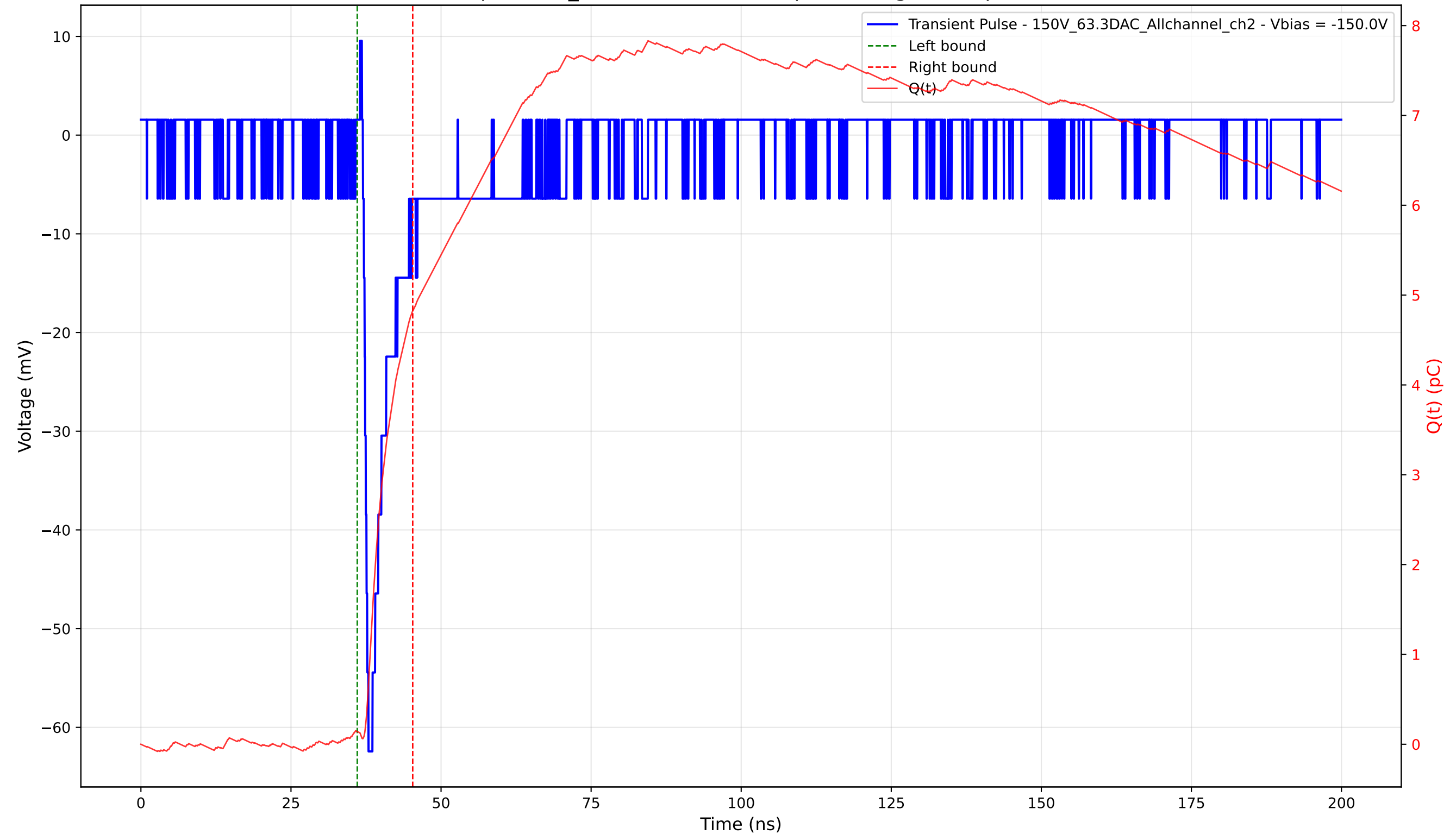
Transient Pulse - Sample: 1cm_42 - Position: 1910.0 \mu\text{m} - Charge: 4.68 pC - Rise Time: 0.92 ns
