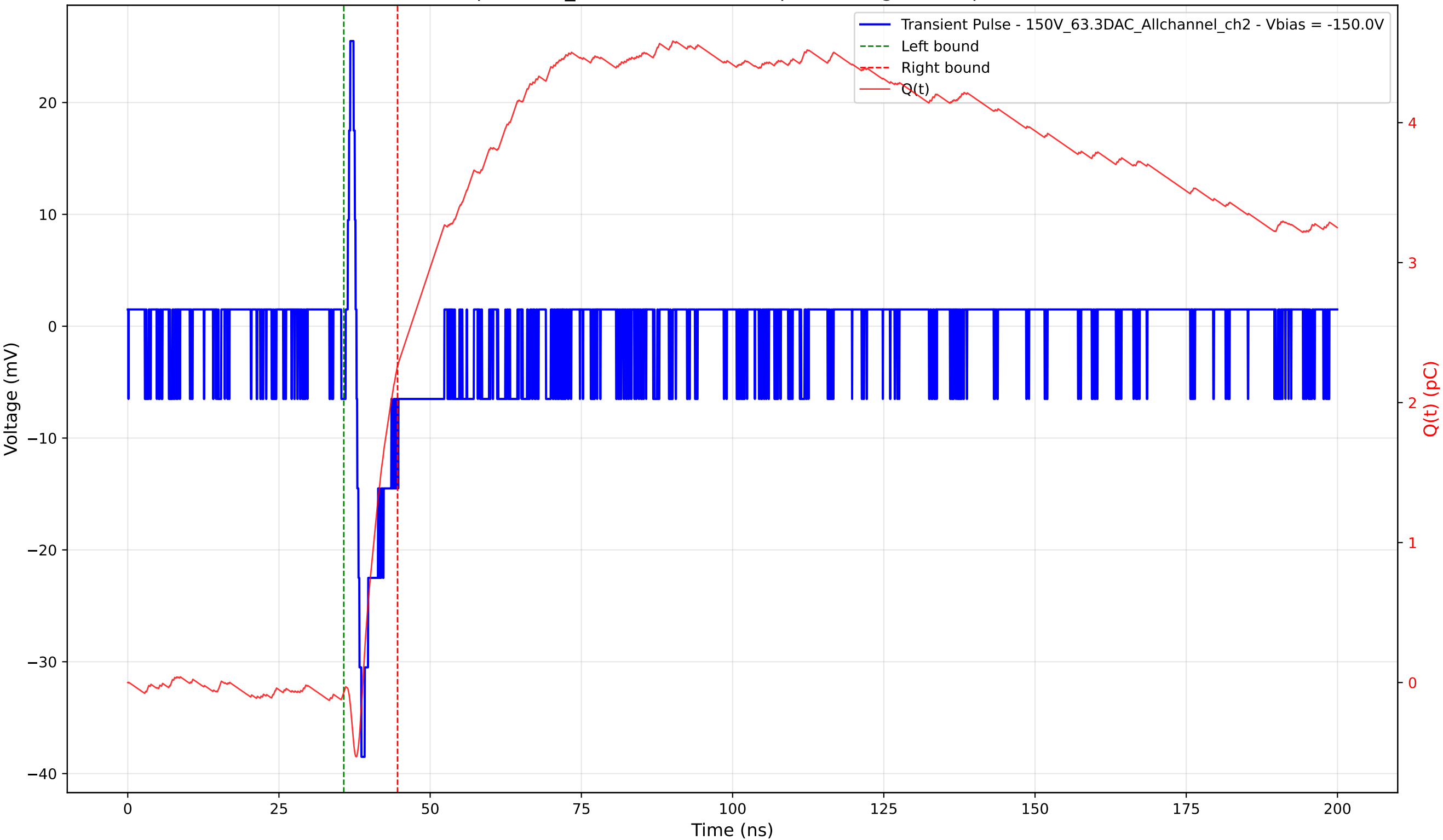
Transient Pulse - Sample: 1cm_42 - Position: 565.0 \mu\text{m} - Charge: 2.33 pC - Rise Time: 0.82 ns
