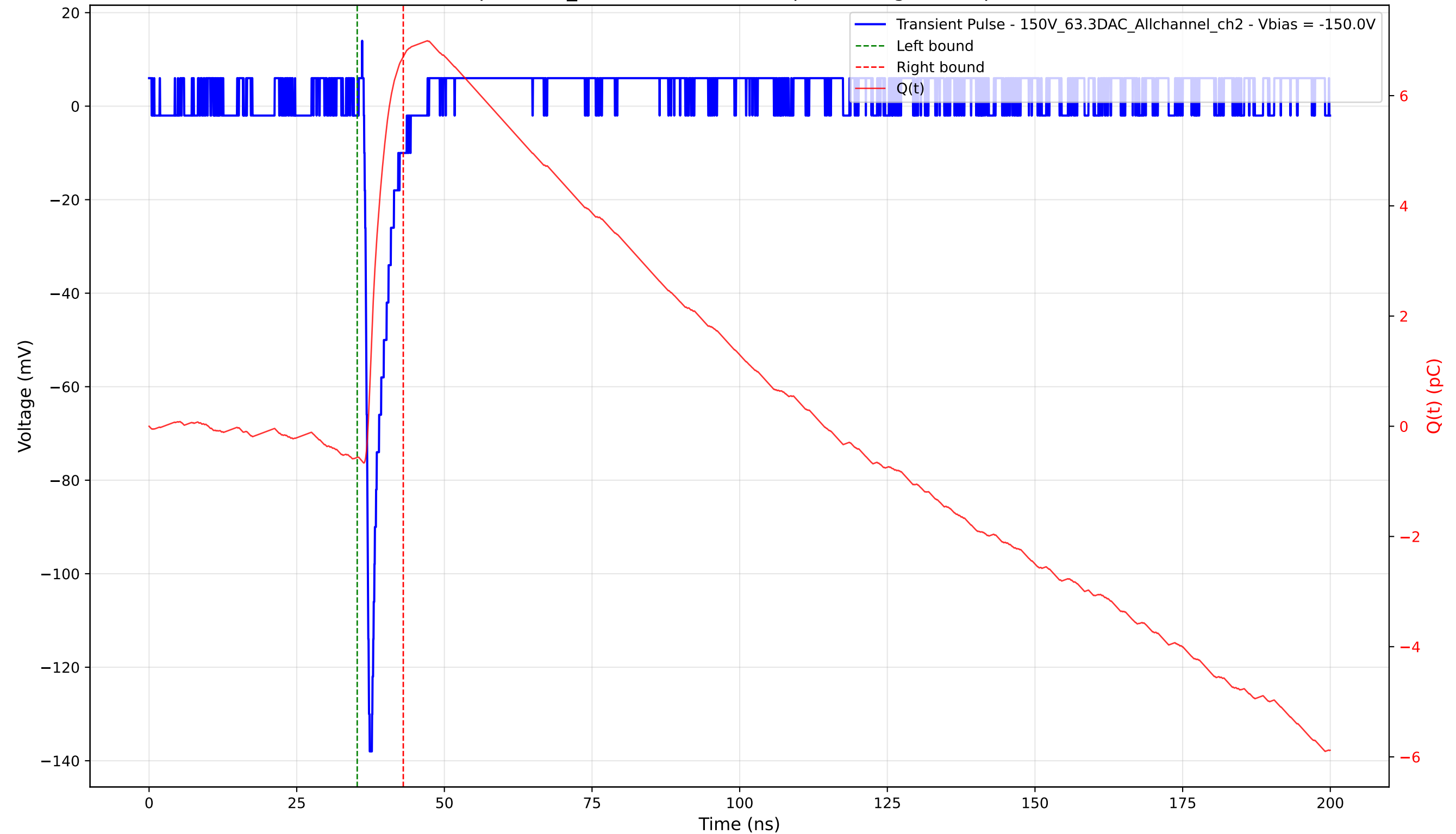
Transient Pulse - Sample: 1cm_42 - Position: 3700.0 \mu\text{m} - Charge: 7.27 pC - Rise Time: 0.74 ns
