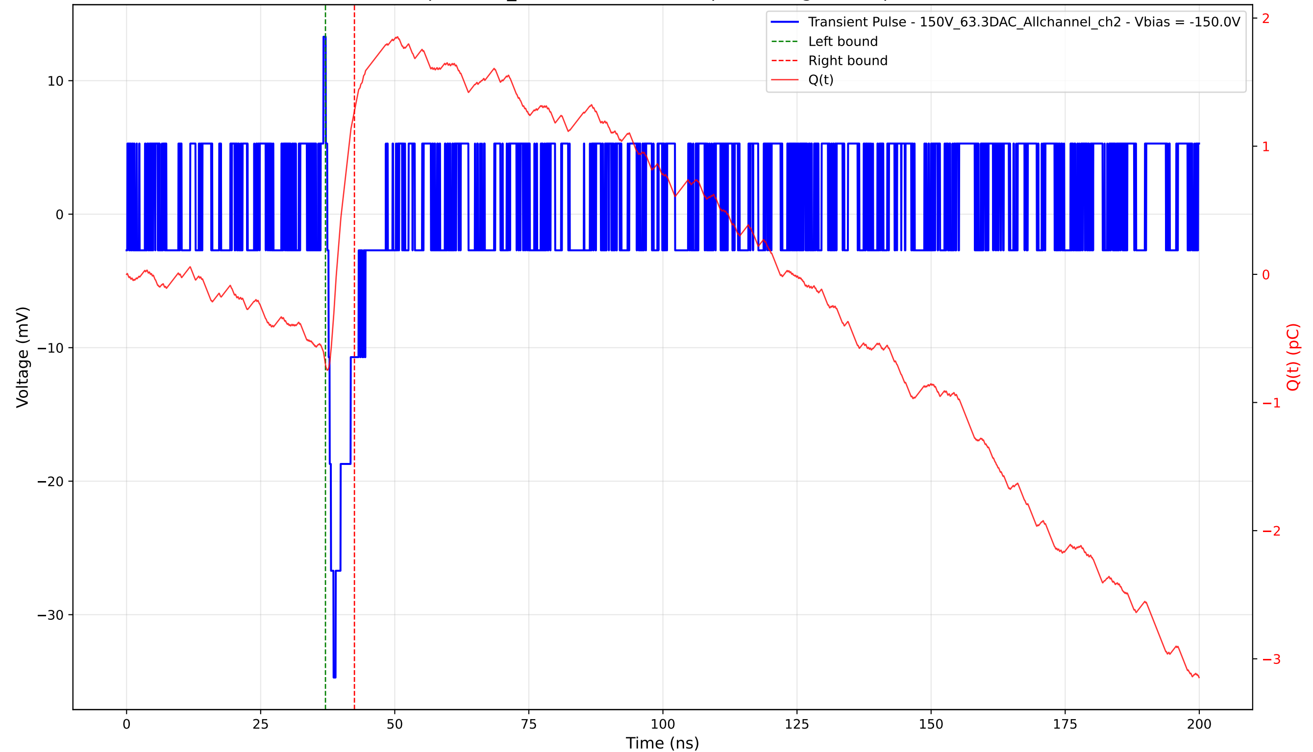
Transient Pulse - Sample: 1cm_42 - Position: 4890.0 \mu\text{m} - Charge: 1.98 pC - Rise Time: 0.96 ns
