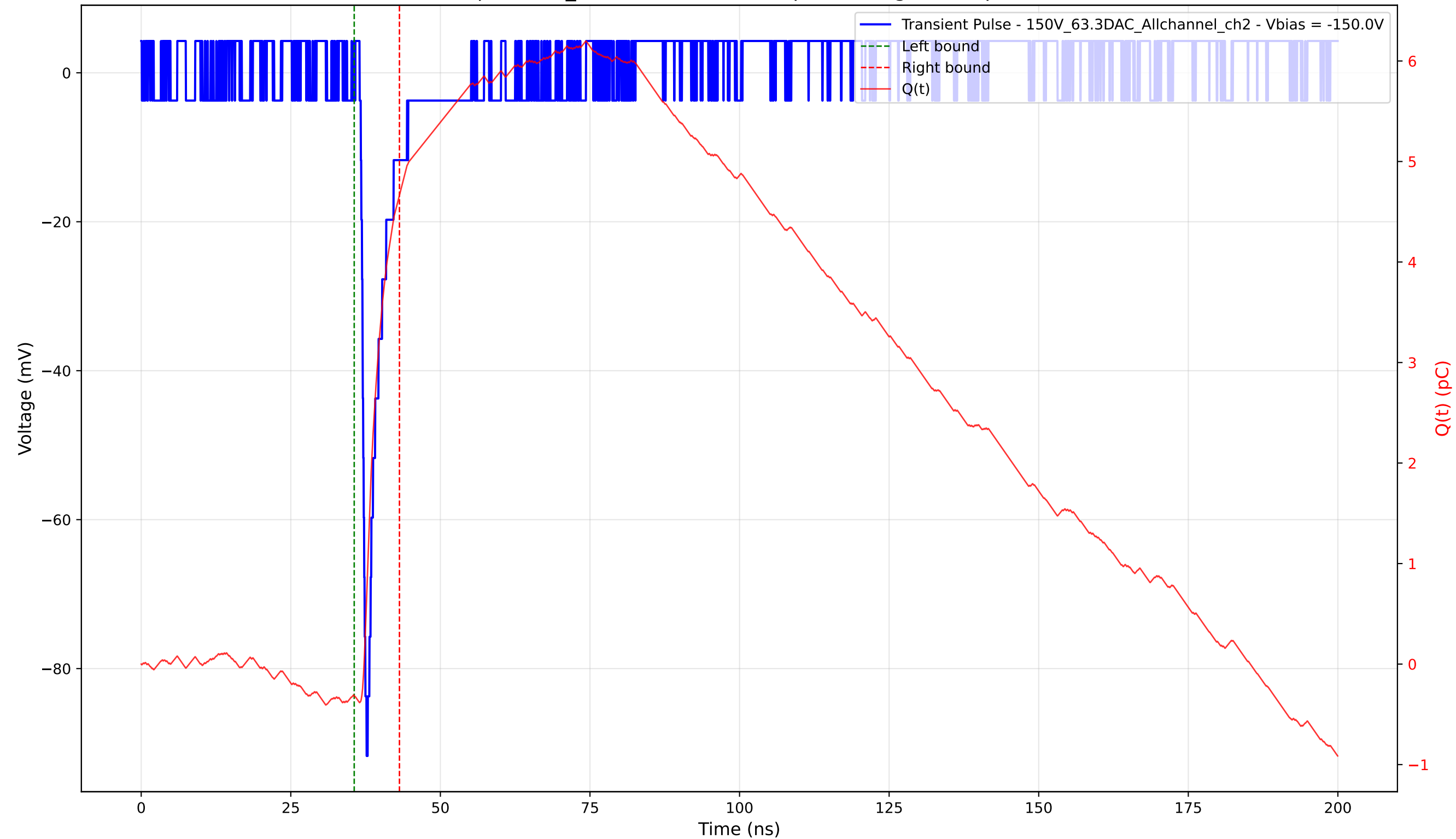
Transient Pulse - Sample: 1cm_42 - Position: 2090.0 \mu\text{m} - Charge: 4.98 pC - Rise Time: 0.77 ns
