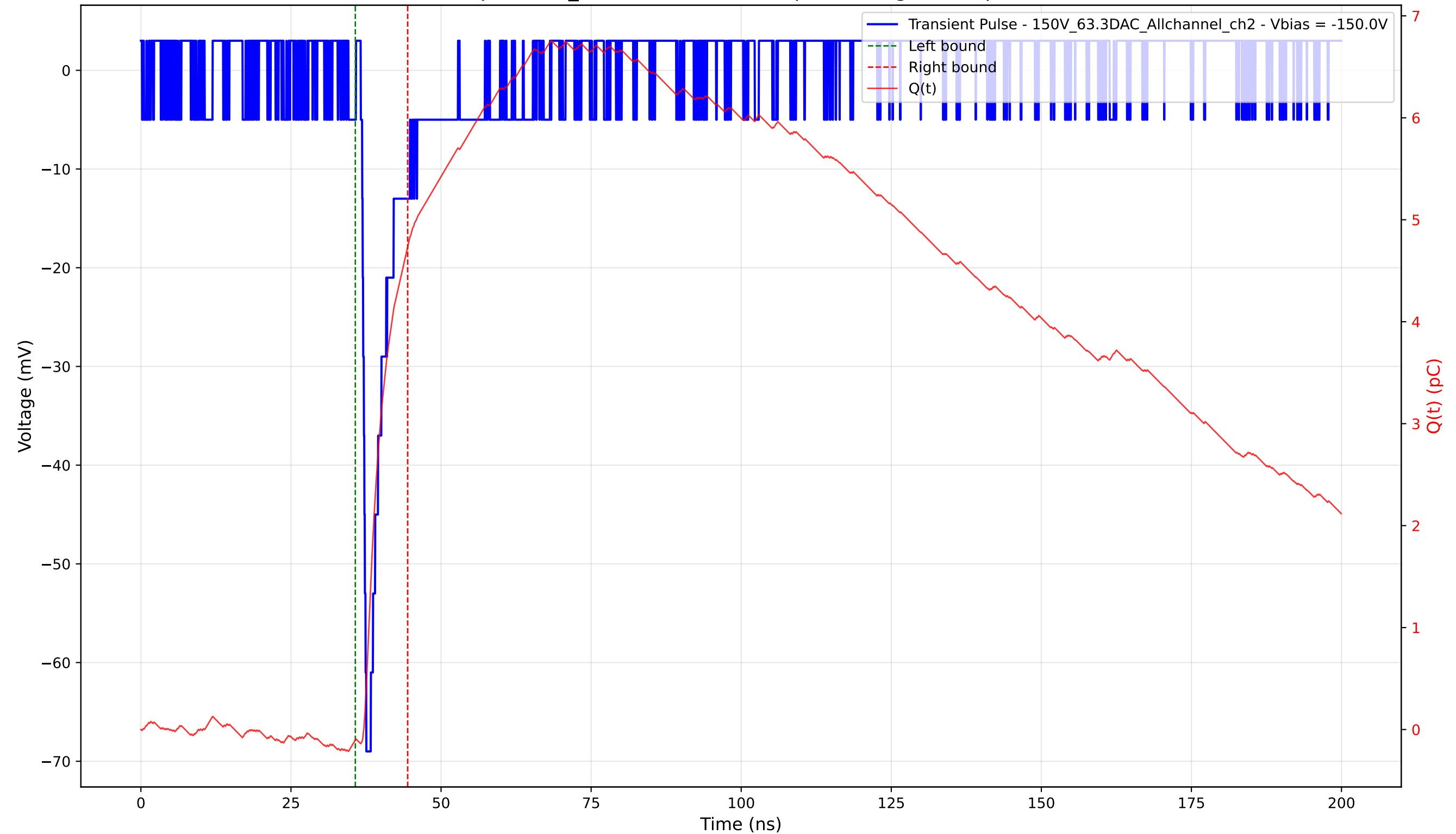
Transient Pulse - Sample: 1cm_42 - Position: 2025.0 \mu\text{m} - Charge: 4.84 pC - Rise Time: 0.71 ns
