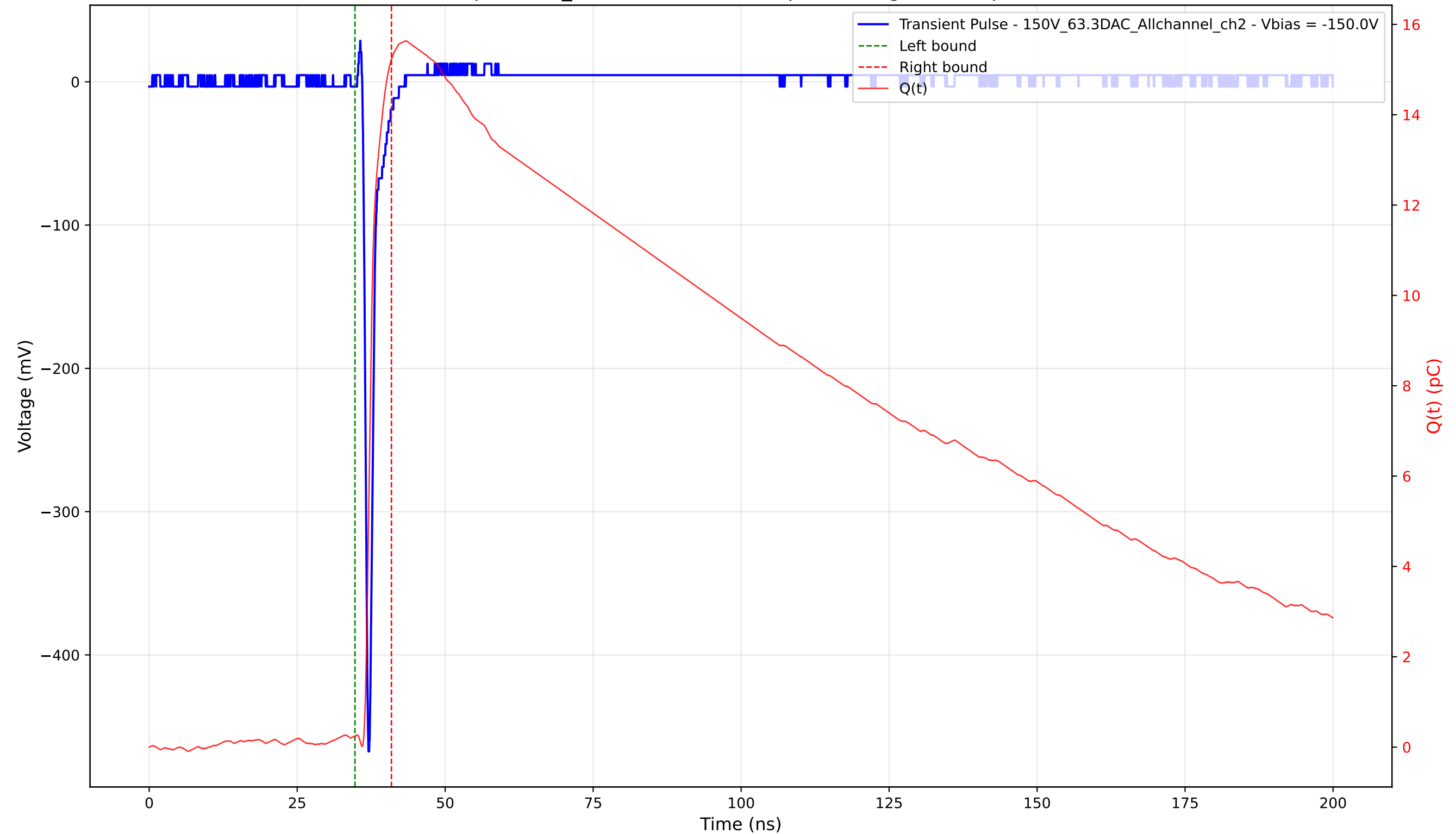
Transient Pulse - Sample: 1cm_42 - Position: 3175.0 \mu\text{m} - Charge: 14.98 pC - Rise Time: 0.71 ns
