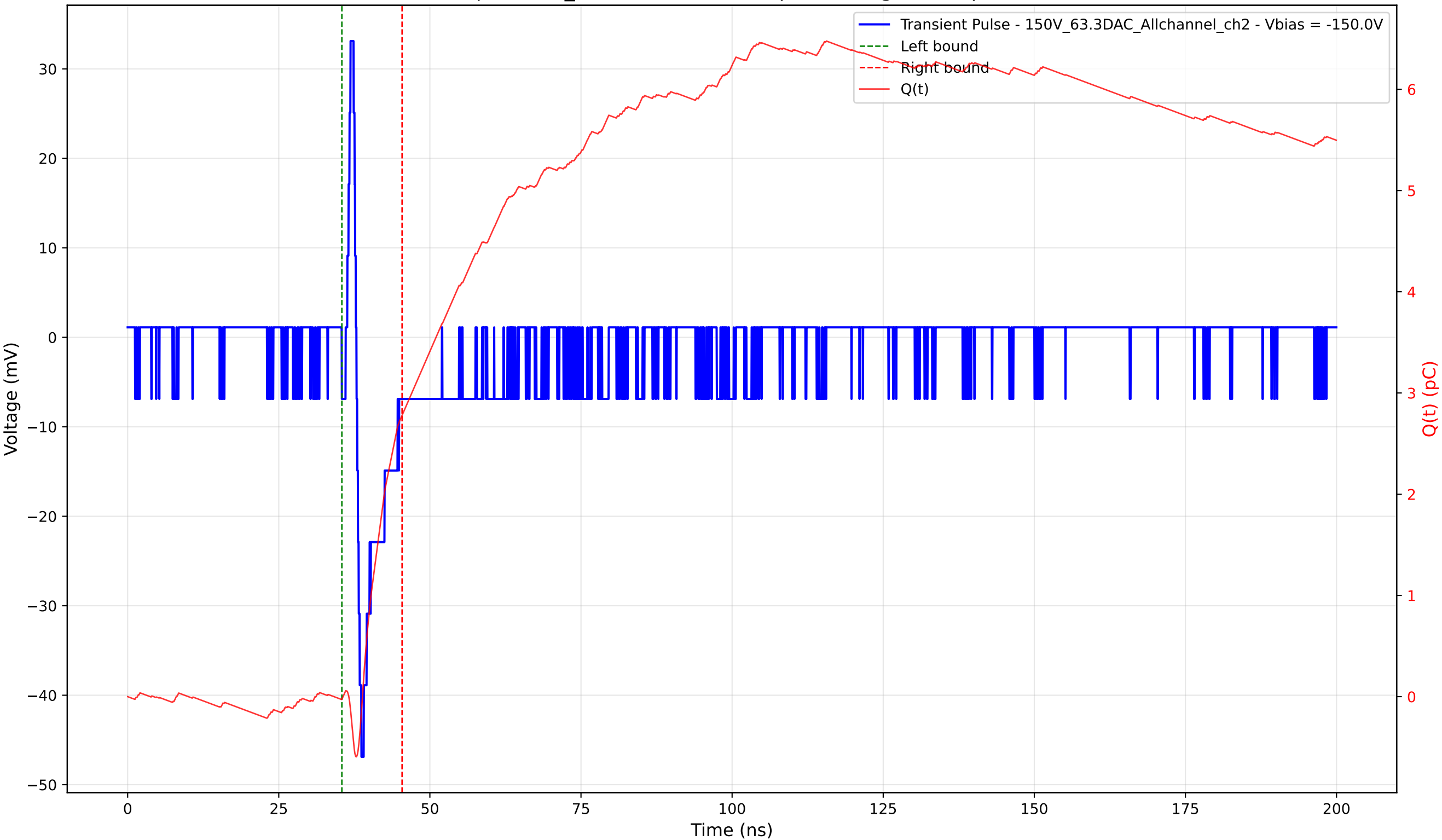
Transient Pulse - Sample: 1cm_42 - Position: 710.0 \mu\text{m} - Charge: 2.80 pC - Rise Time: 0.82 ns
