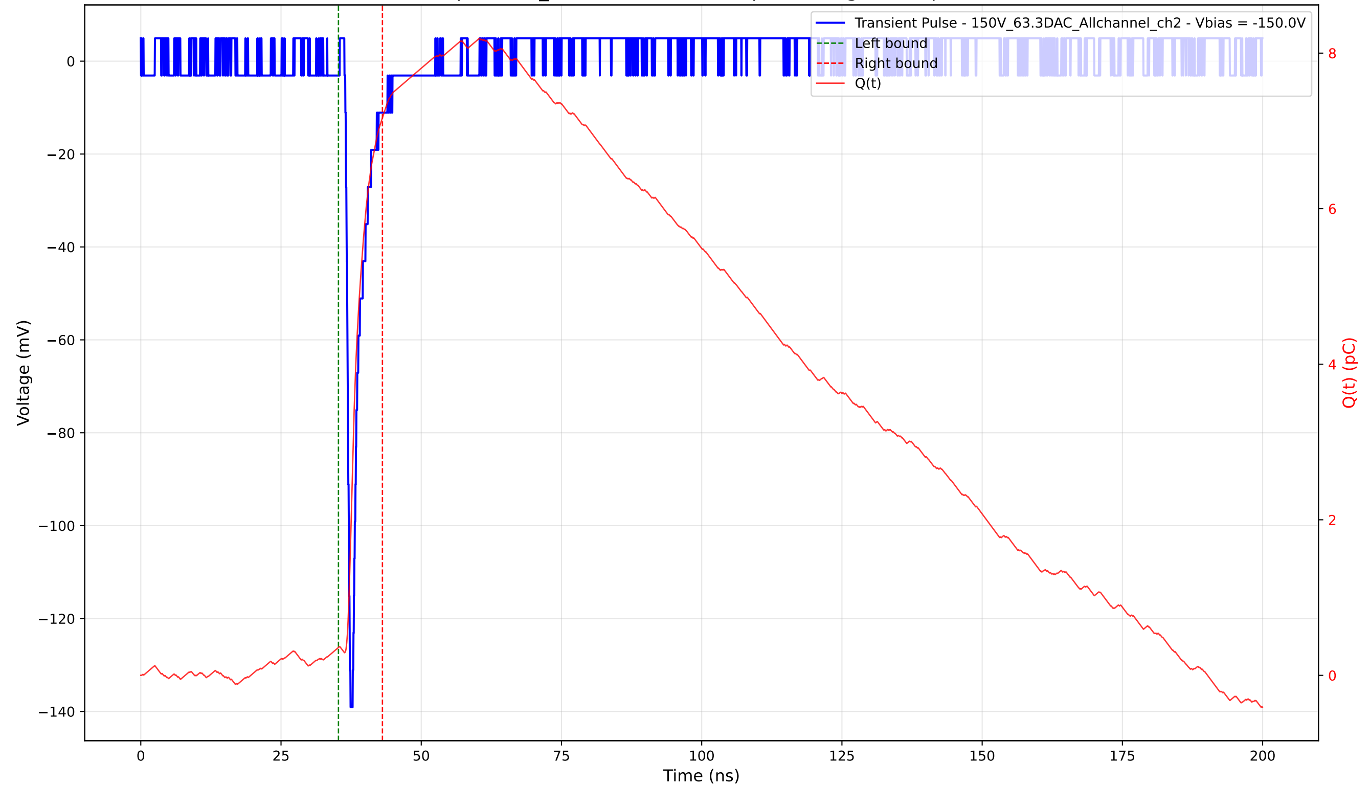
Transient Pulse - Sample: 1cm_42 - Position: 2320.0 \mu\text{m} - Charge: 6.81 pC - Rise Time: 0.75 ns
