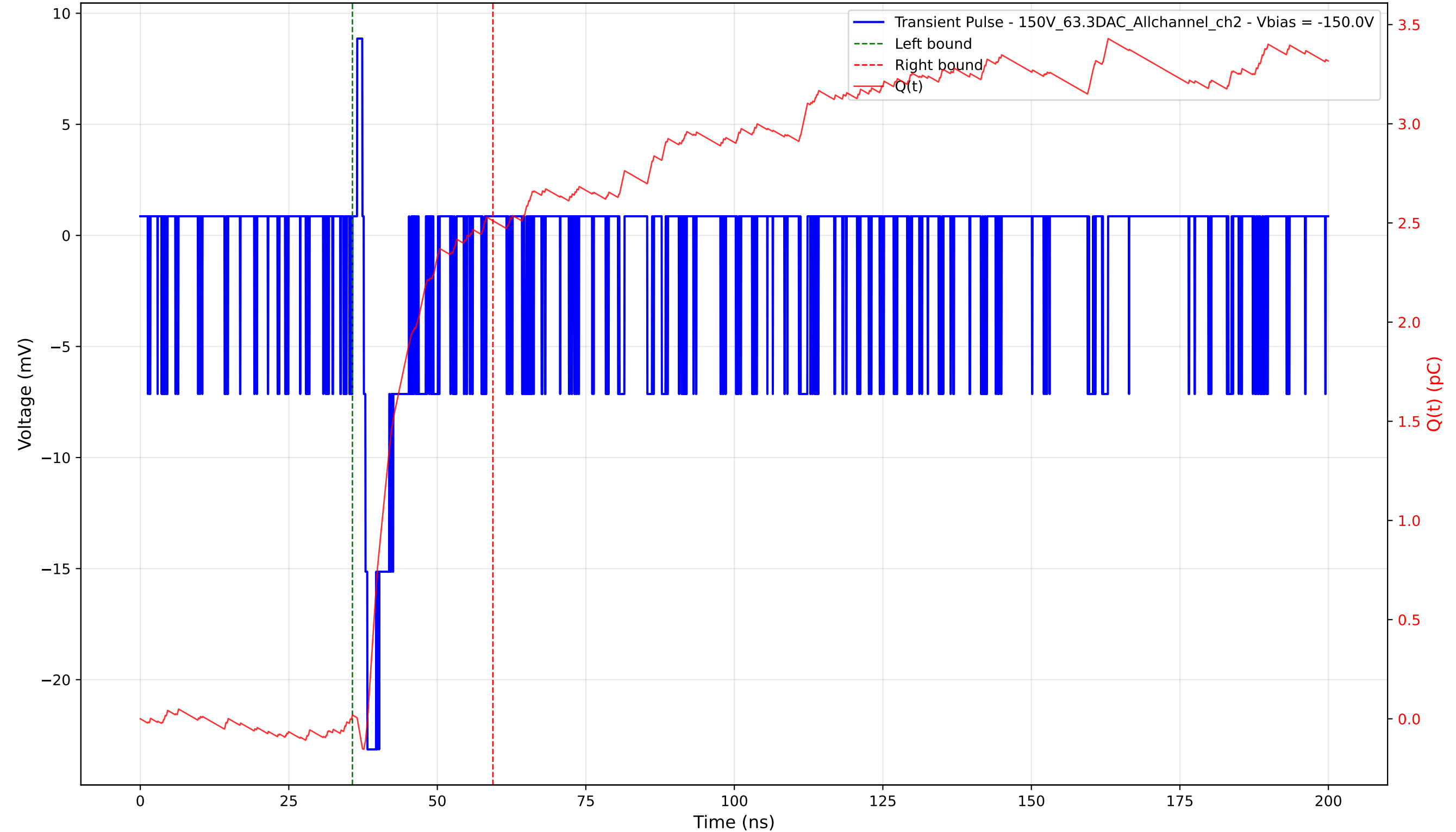
Transient Pulse - Sample: 1cm_42 - Position: 325.0 \mu\text{m} - Charge: 2.49 pC - Rise Time: 0.63 ns
