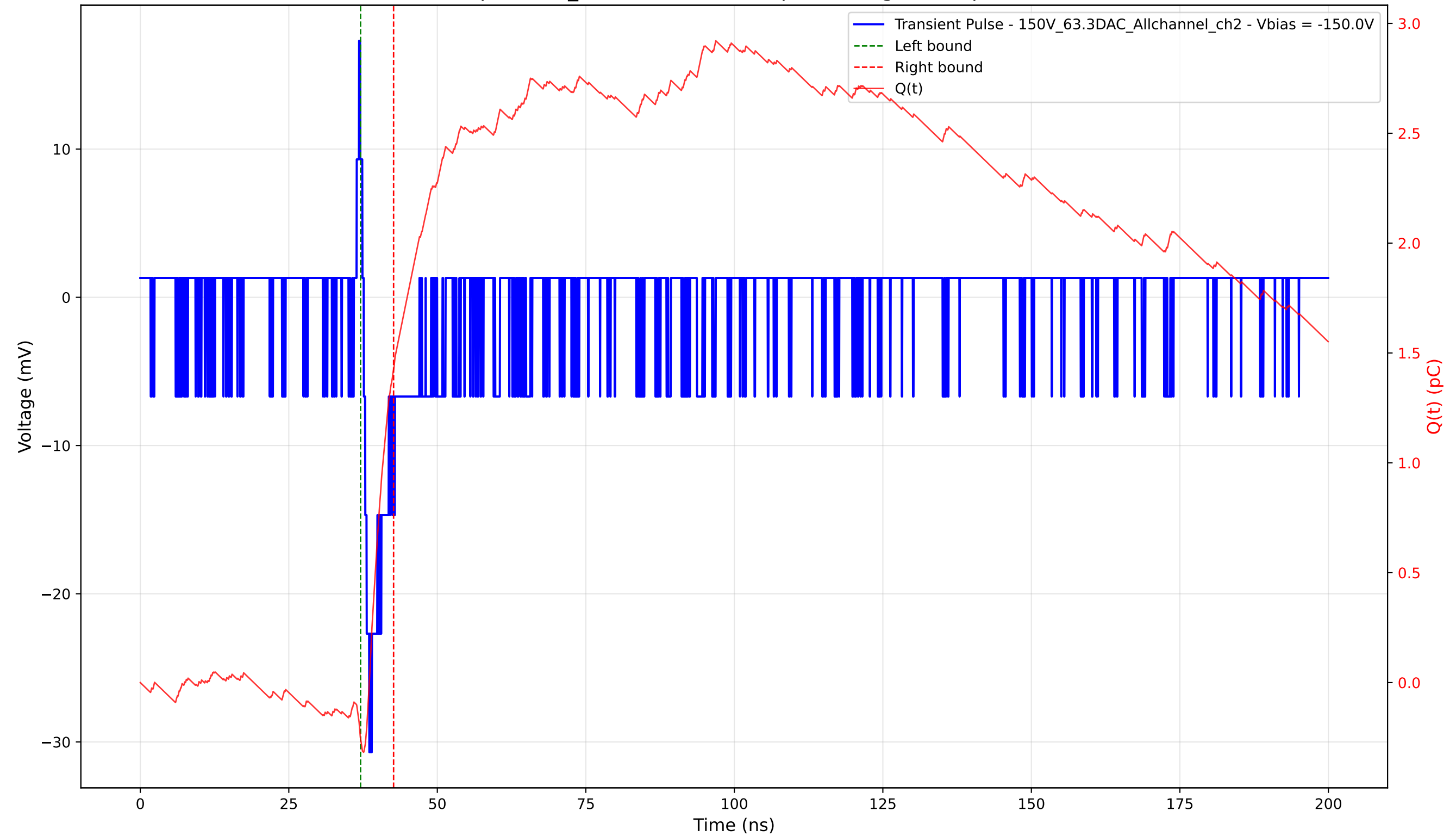
Transient Pulse - Sample: 1cm_42 - Position: 355.0 \mu\text{m} - Charge: 1.68 pC - Rise Time: 0.95 ns
