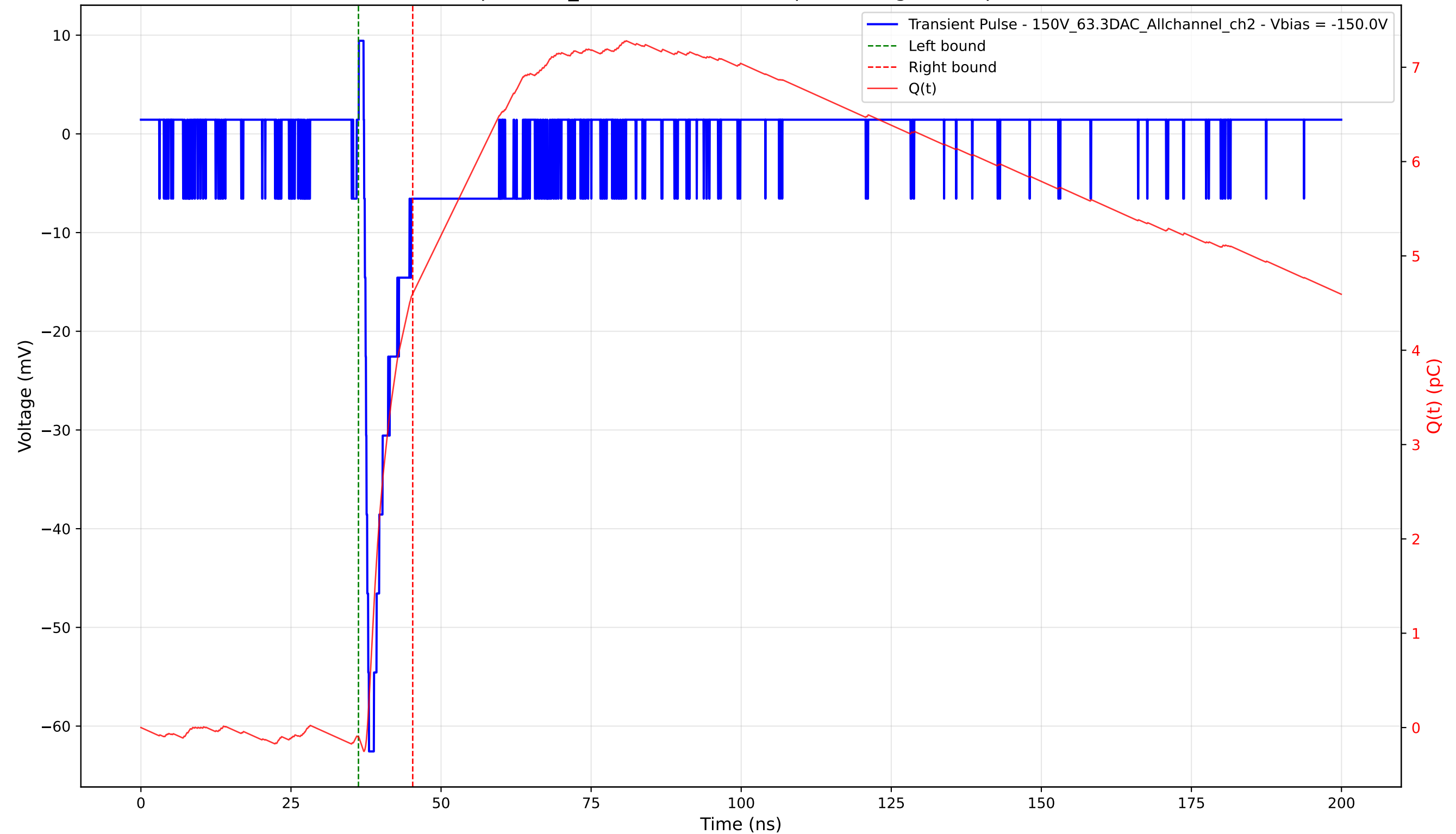
Transient Pulse - Sample: 1cm_42 - Position: 1810.0 \mu\text{m} - Charge: 4.70 pC - Rise Time: 0.80 ns
