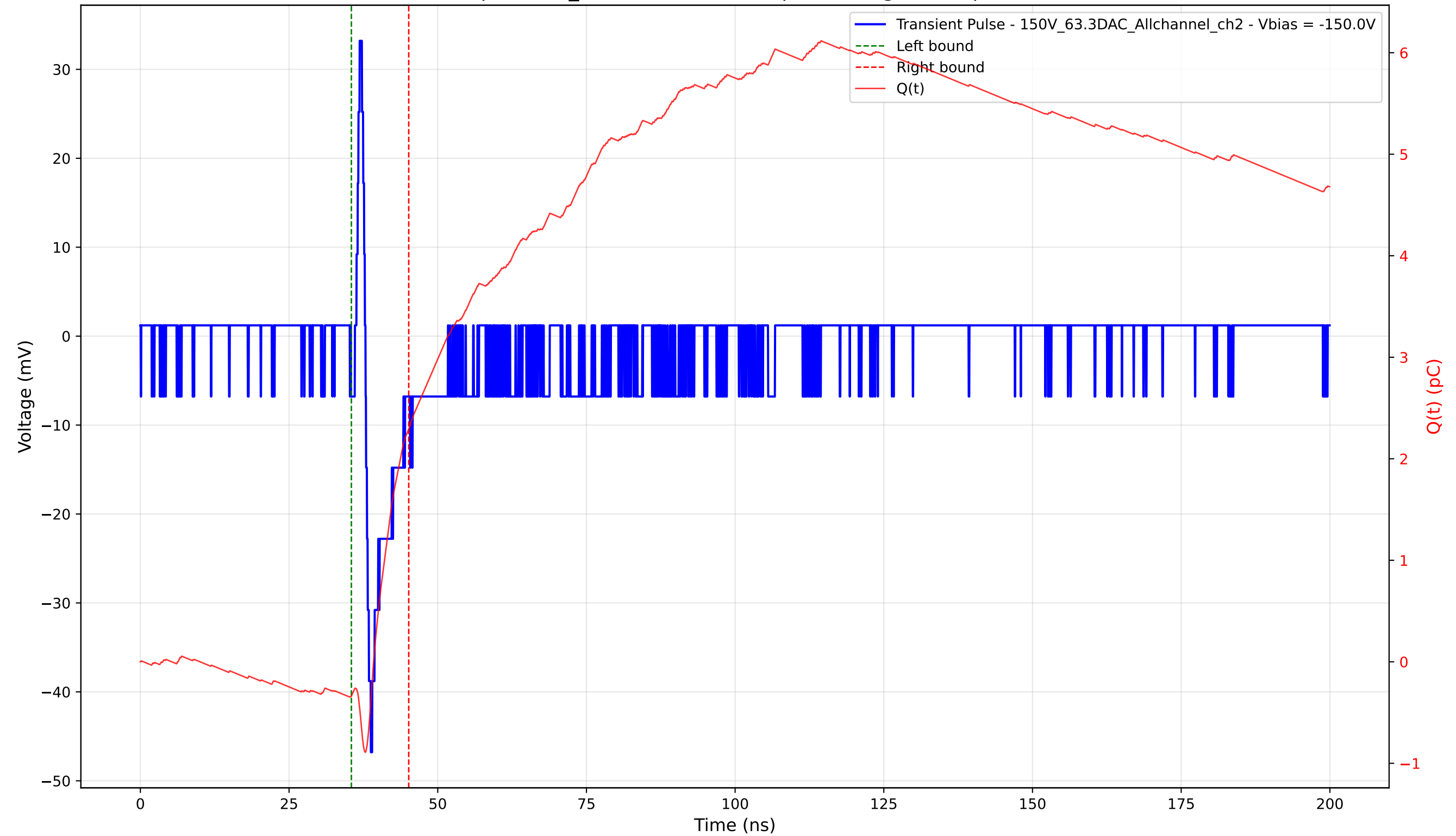
Transient Pulse - Sample: 1cm_42 - Position: 690.0 \mu\text{m} - Charge: 2.63 pC - Rise Time: 0.90 ns
