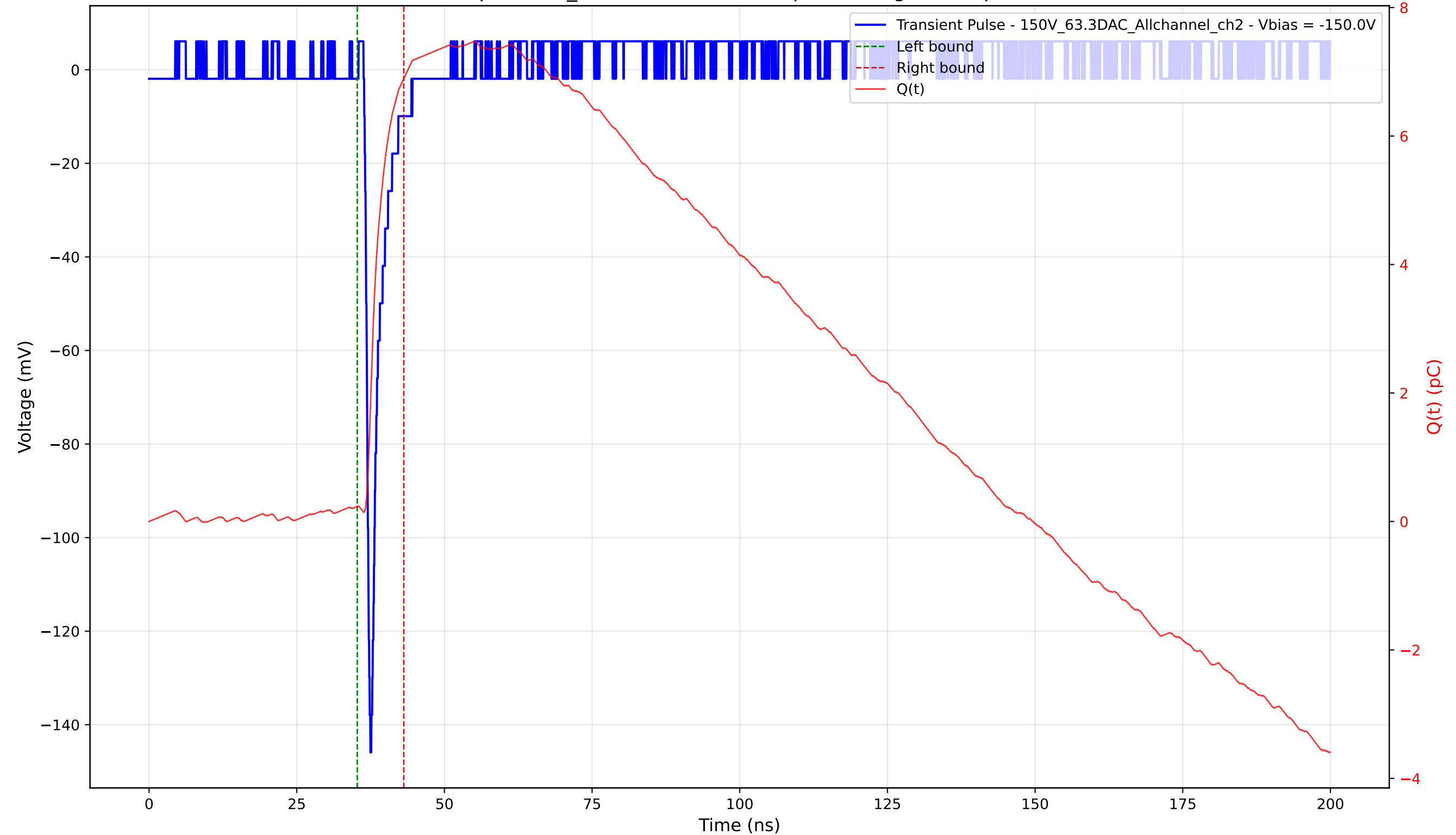
Transient Pulse - Sample: 1cm_42 - Position: 2330.0 \mu\text{m} - Charge: 6.66 pC - Rise Time: 0.86 ns
