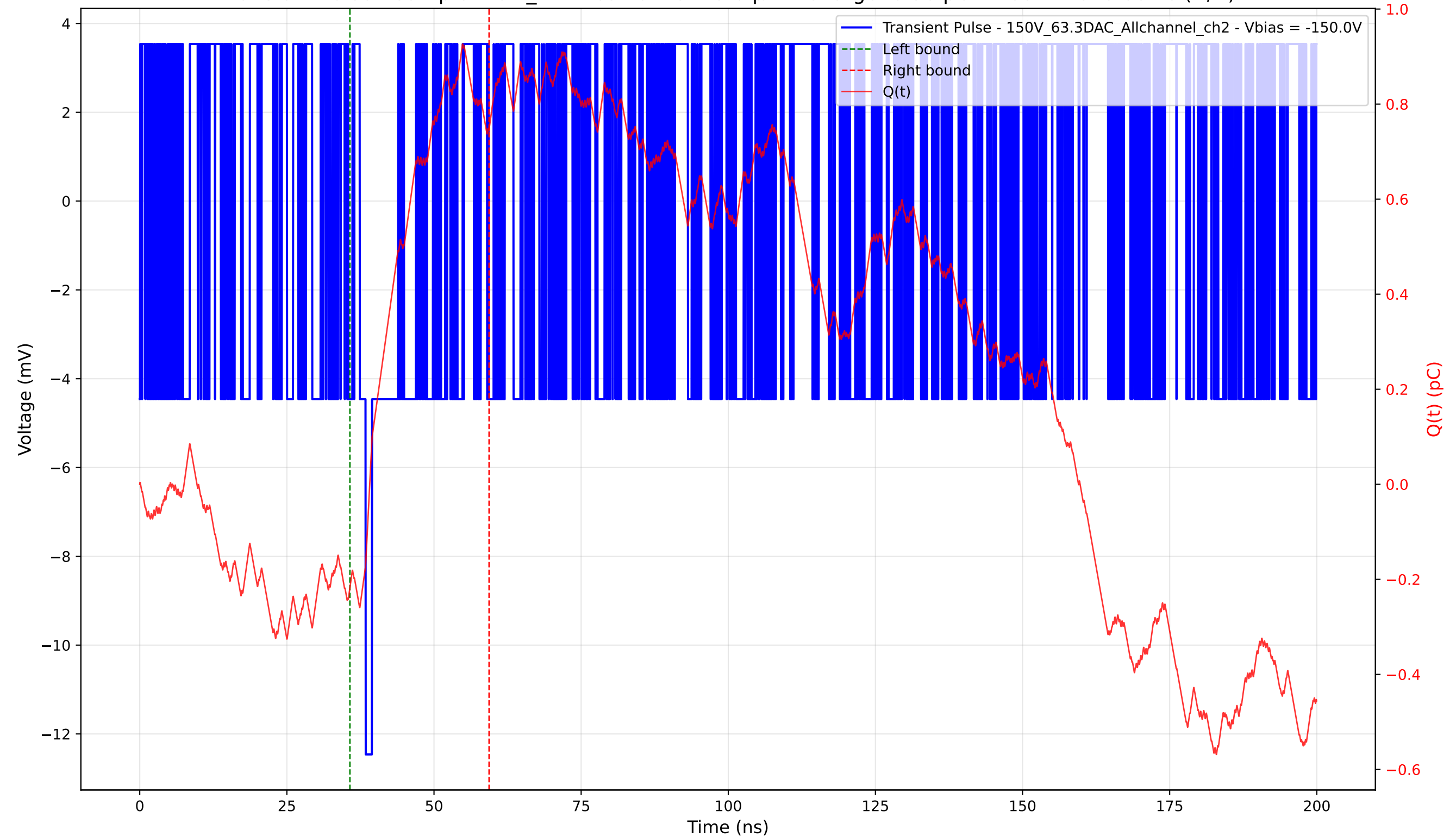
Transient Pulse - Sample: 1cm_42 - Position: 5115.0 \mu\text{m} - Charge: 0.96 pC - Rise Time: 0.00 ns (N/A)
