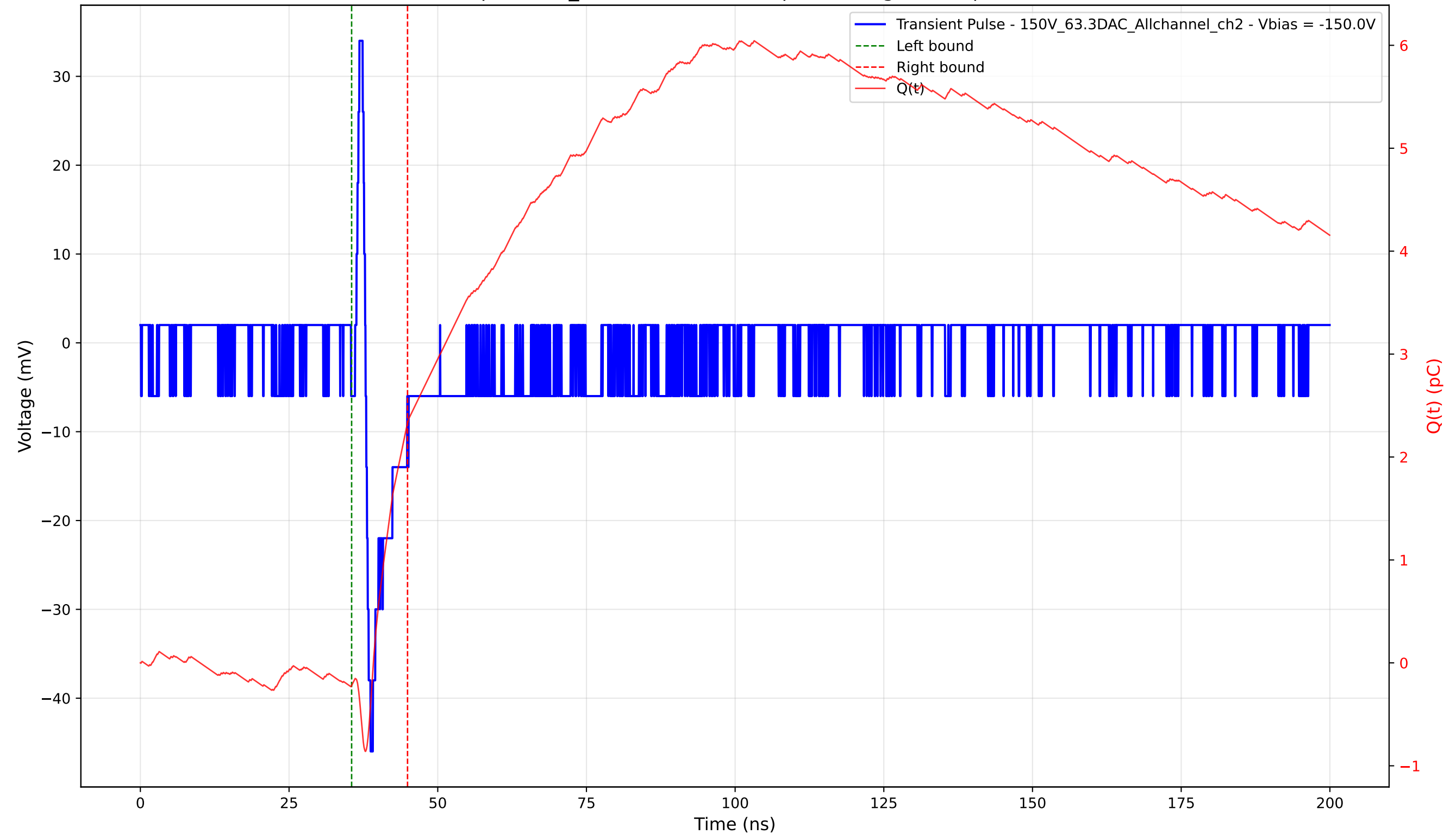
Transient Pulse - Sample: 1cm_42 - Position: 760.0 \mu\text{m} - Charge: 2.55 pC - Rise Time: 0.85 ns
