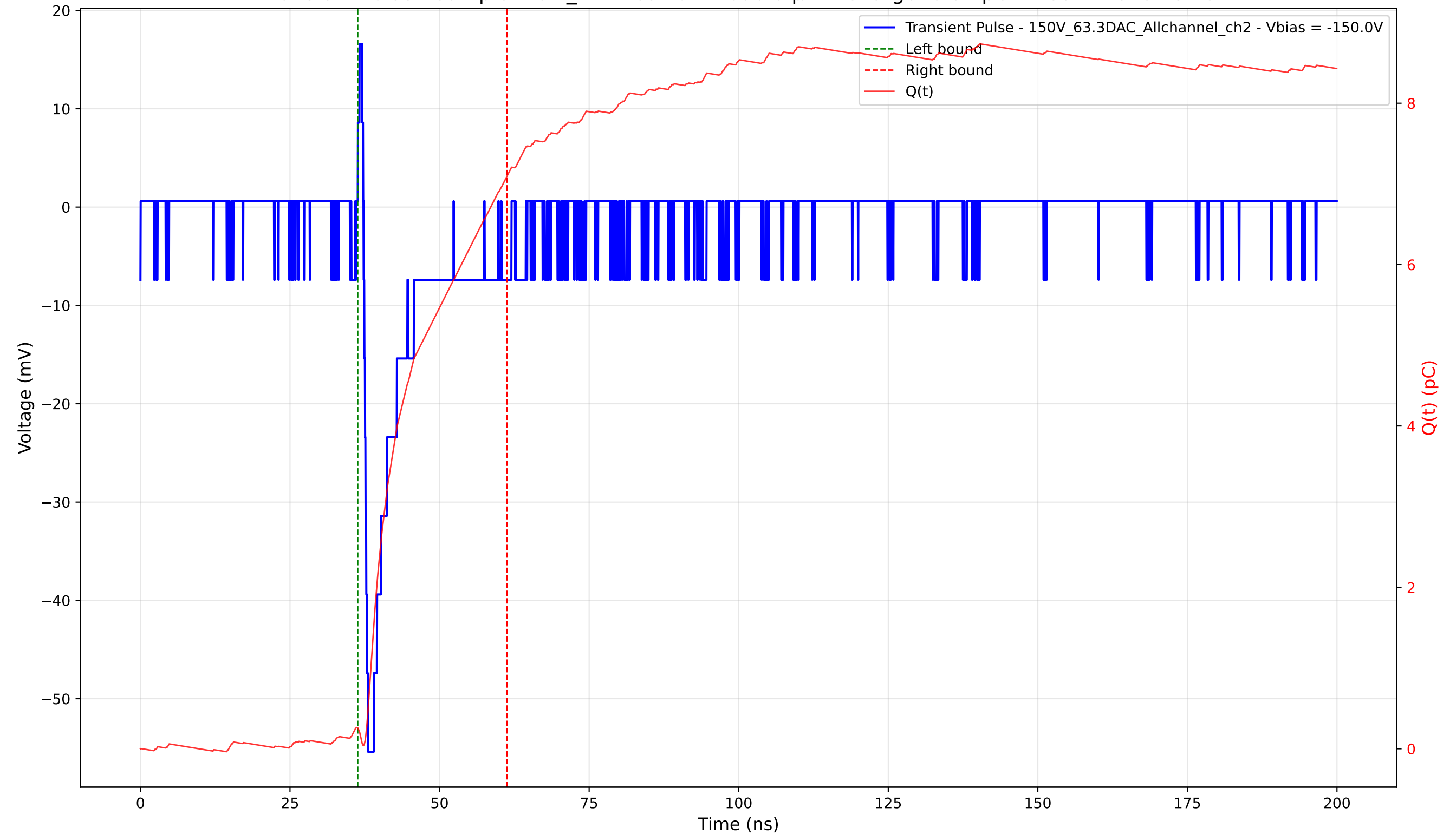
Transient Pulse - Sample: 1cm_42 - Position: 1690.0 \mu\text{m} - Charge: 6.84 pC - Rise Time: 0.73 ns
