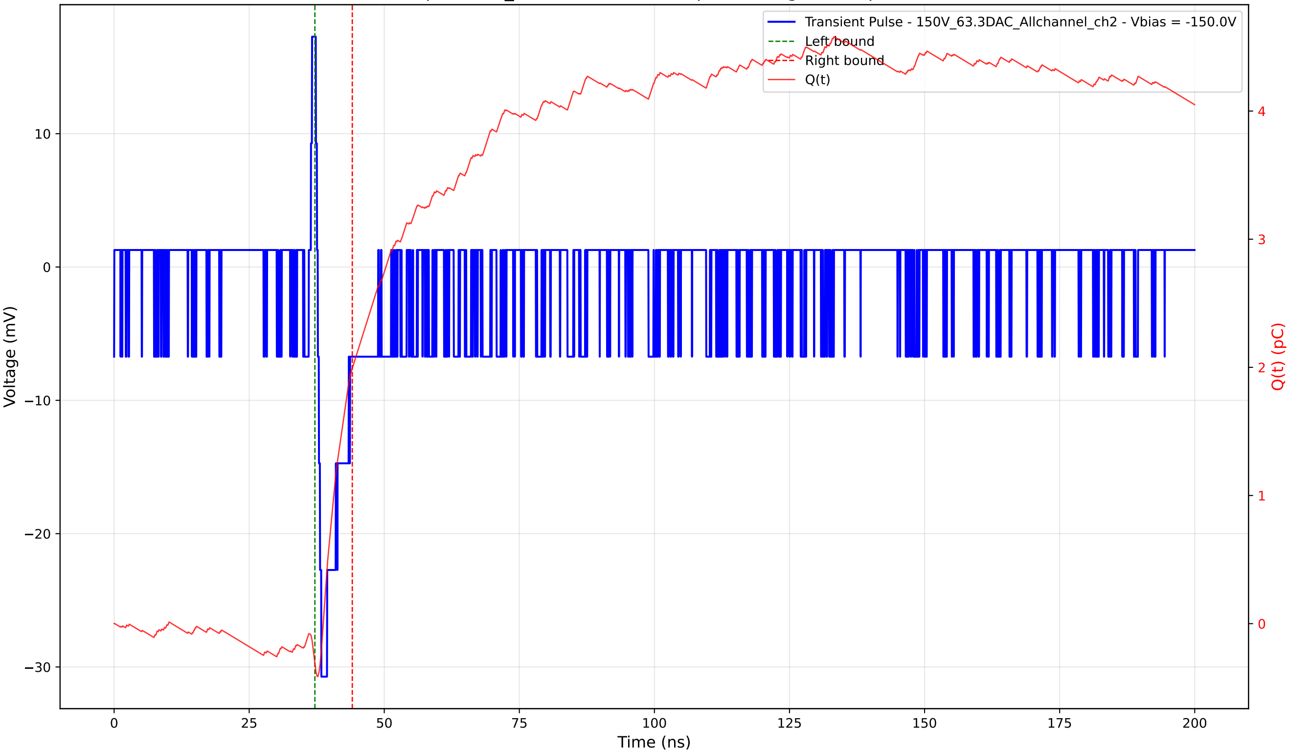
Transient Pulse - Sample: 1cm_42 - Position: 450.0 \mu\text{m} - Charge: 2.30 pC - Rise Time: 0.67 ns
