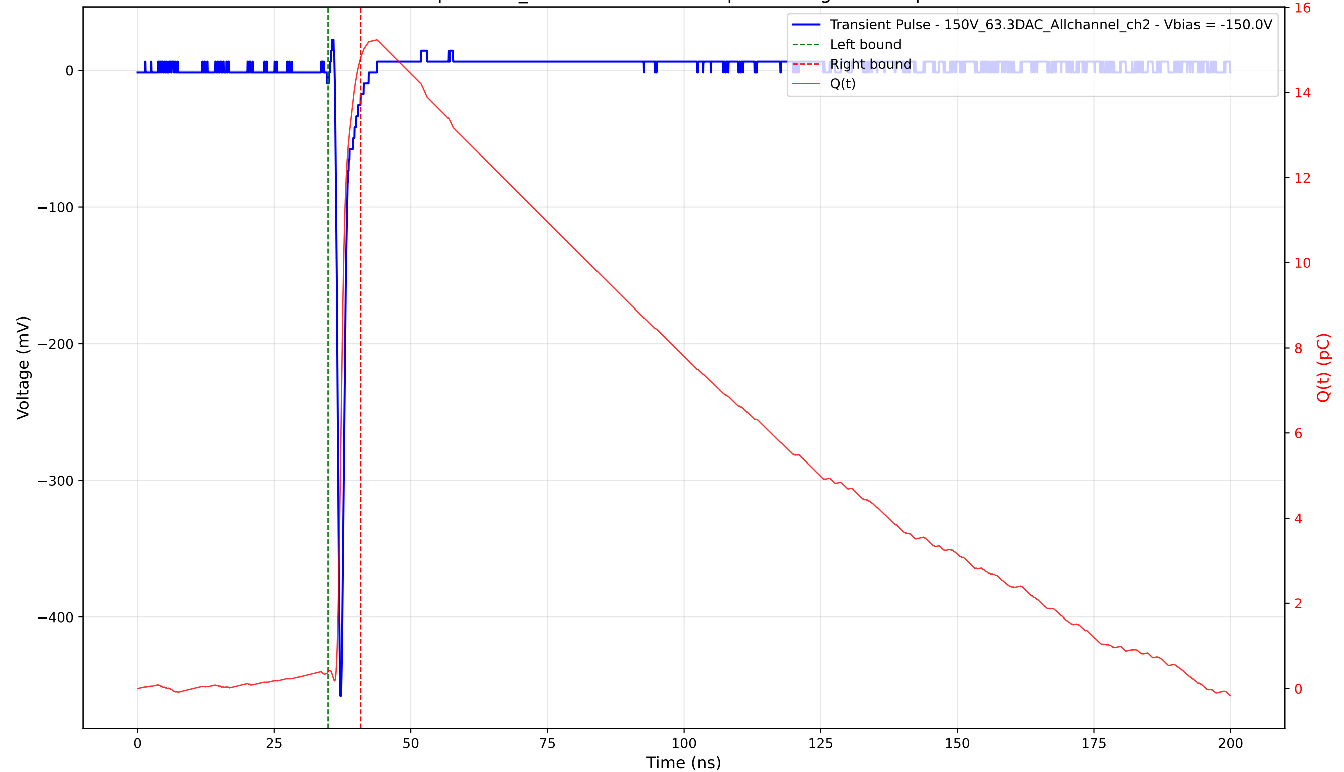
Transient Pulse - Sample: 1cm_42 - Position: 2865.0 \mu\text{m} - Charge: 14.43 pC - Rise Time: 0.74 ns
