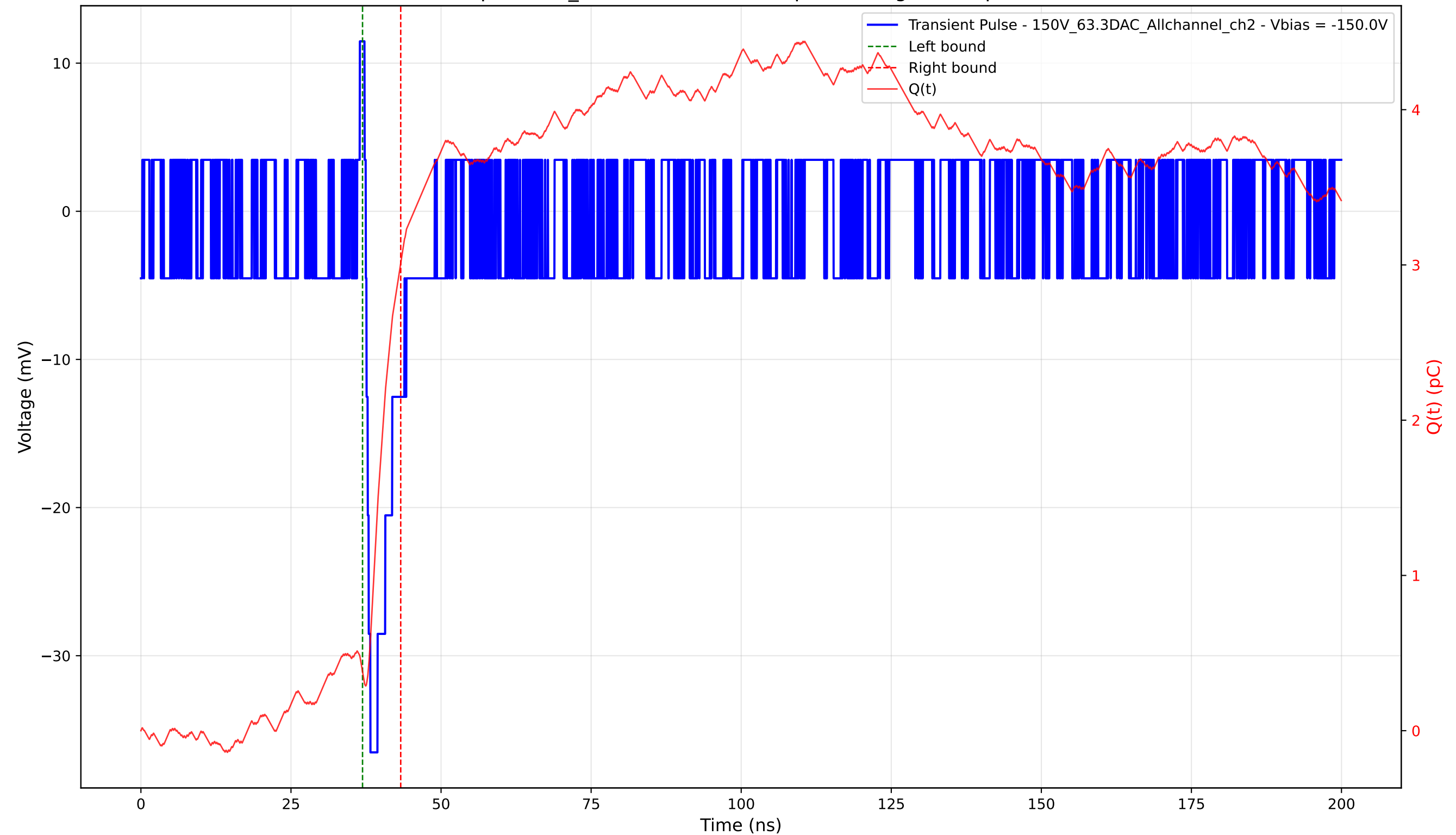
Transient Pulse - Sample: 1cm_42 - Position: 4750.0 \mu\text{m} - Charge: 2.63 pC - Rise Time: 0.79 ns
