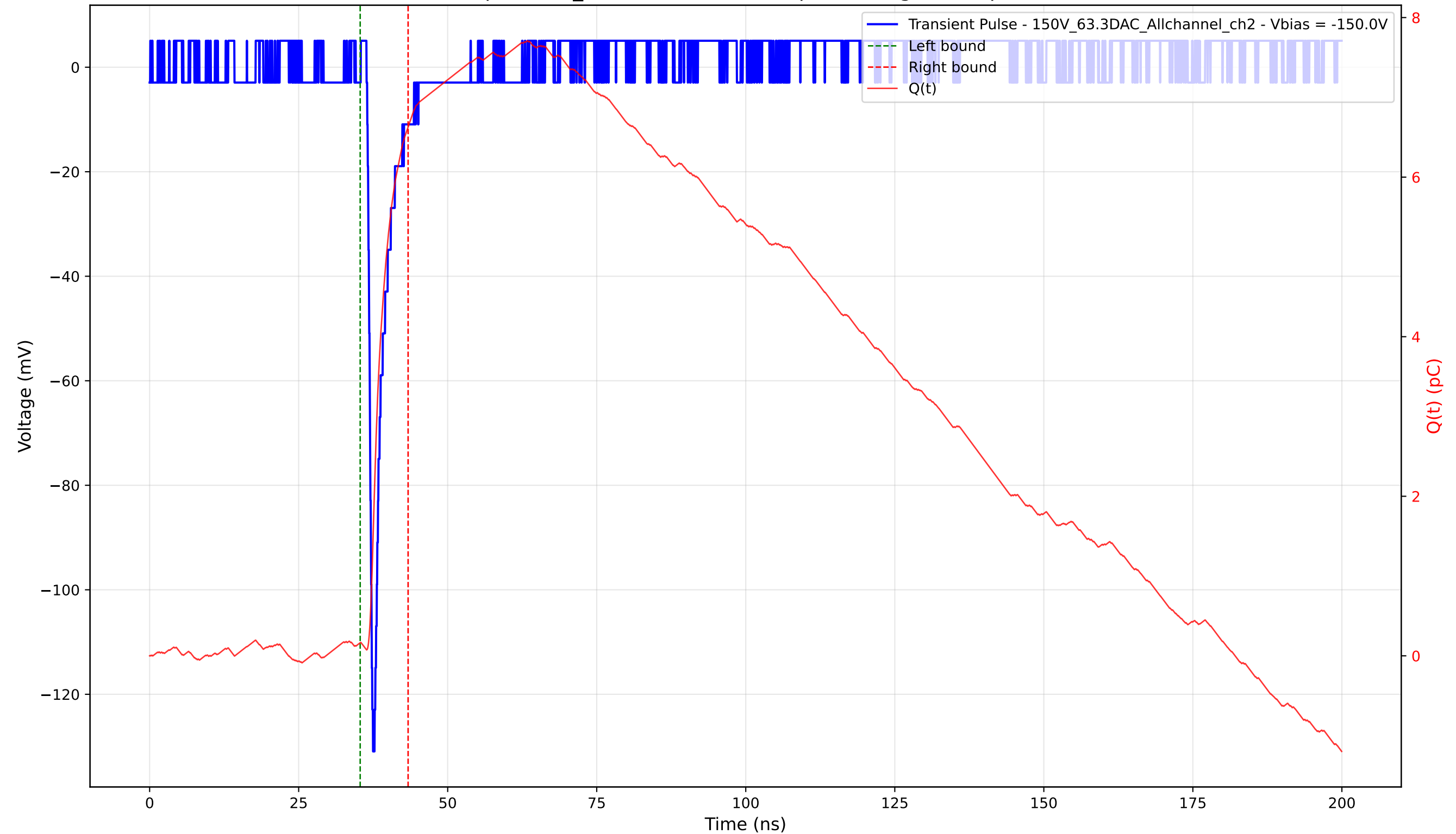
Transient Pulse - Sample: 1cm_42 - Position: 2230.0 \mu\text{m} - Charge: 6.47 pC - Rise Time: 0.79 ns
