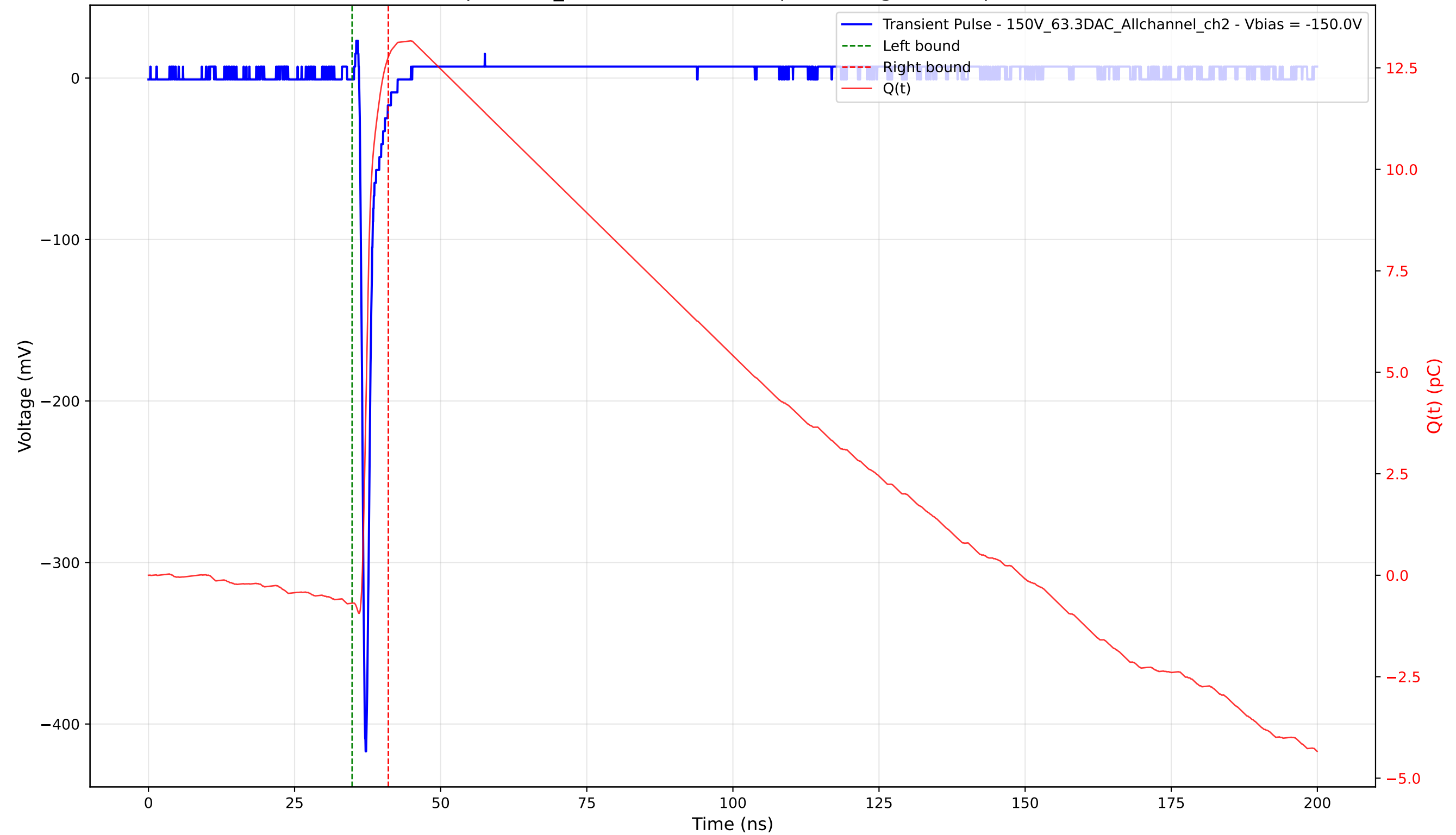
Transient Pulse - Sample: 1cm_42 - Position: 2720.0 \mu\text{m} - Charge: 13.46 pC - Rise Time: 0.75 ns
