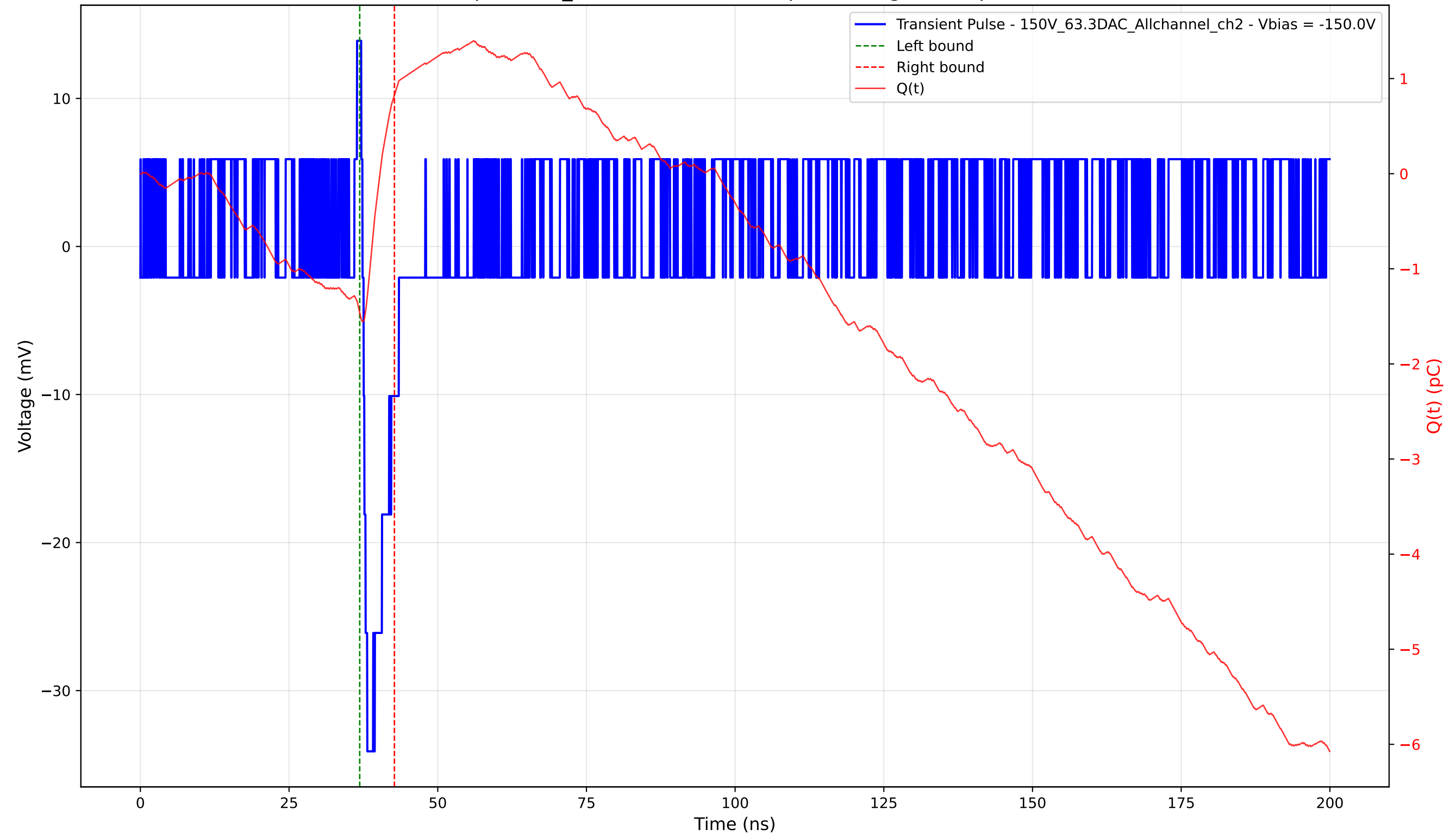
Transient Pulse - Sample: 1cm_42 - Position: 4585.0 \mu\text{m} - Charge: 2.29 pC - Rise Time: 0.63 ns
