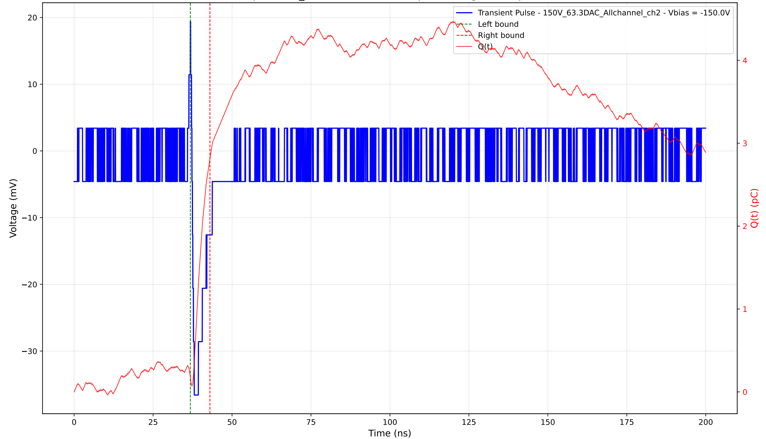
Transient Pulse - Sample: 1cm_42 - Position: 4530.0 \mu\text{m} - Charge: 2.64 pC - Rise Time: 0.75 ns
