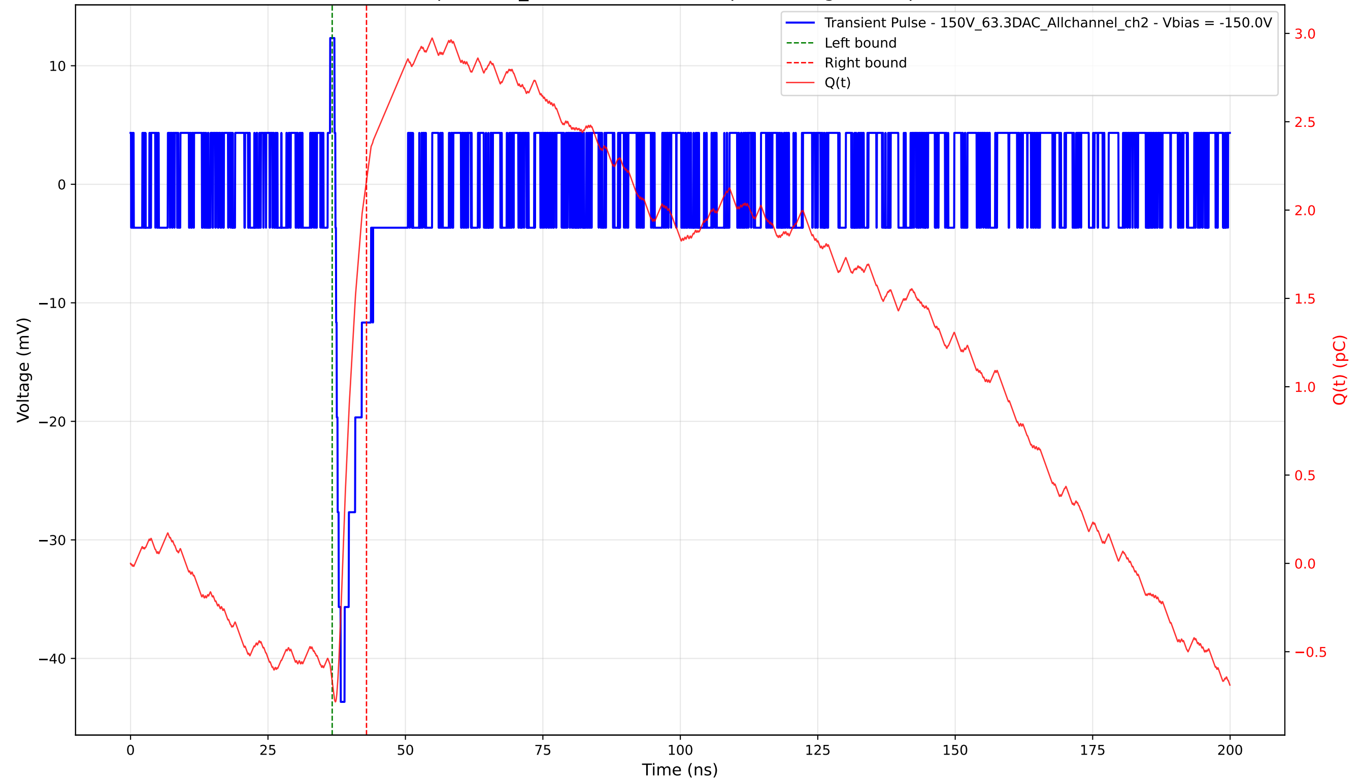
Transient Pulse - Sample: 1cm_42 - Position: 4470.0 \mu\text{m} - Charge: 2.84 pC - Rise Time: 0.88 ns
