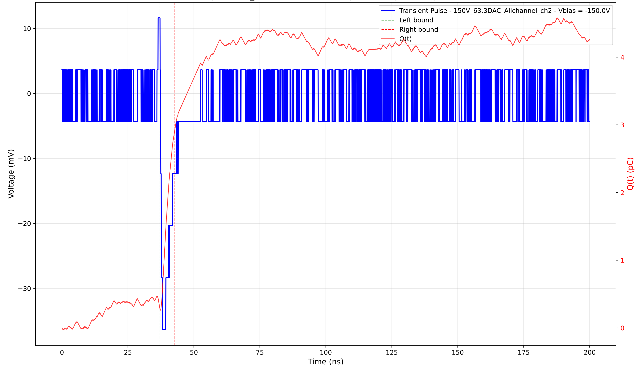
Transient Pulse - Sample: 1cm_42 - Position: 4520.0 \mu\text{m} - Charge: 2.58 pC - Rise Time: 0.80 ns
