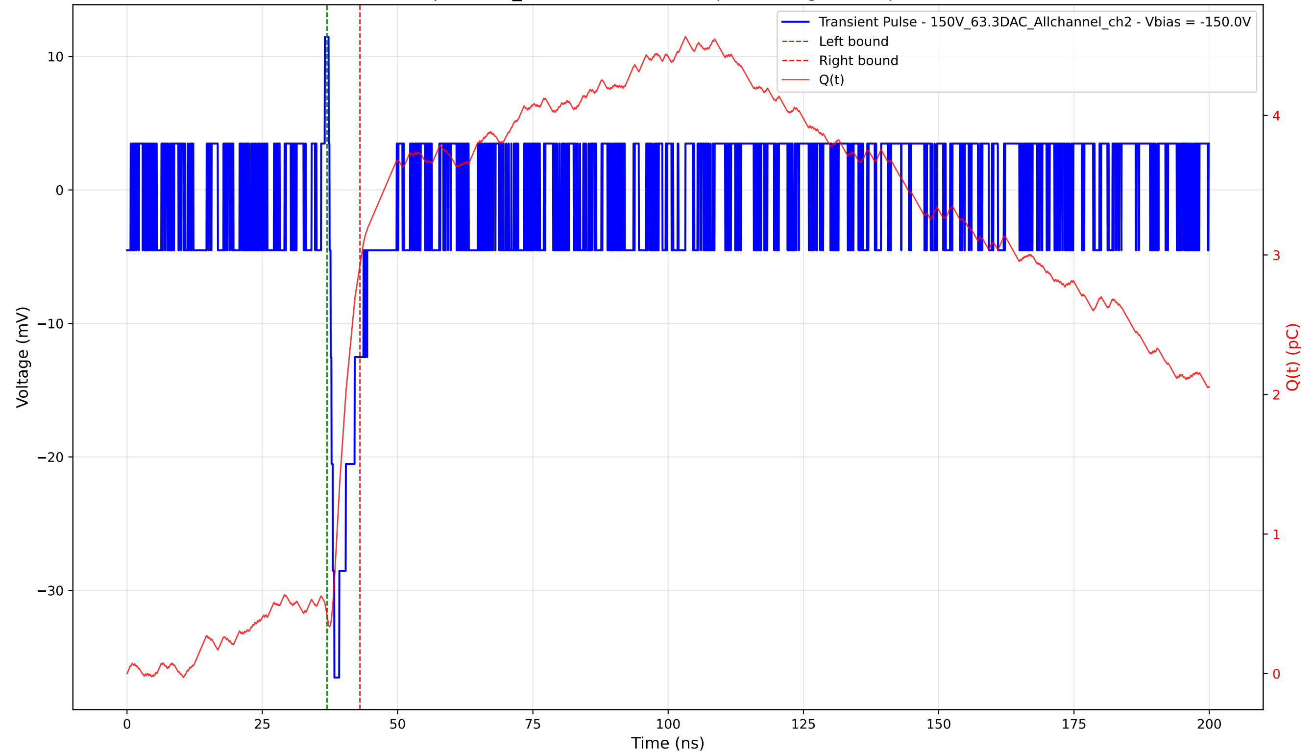
Transient Pulse - Sample: 1cm_42 - Position: 4840.0 \mu\text{m} - Charge: 2.51 pC - Rise Time: 0.91 ns
