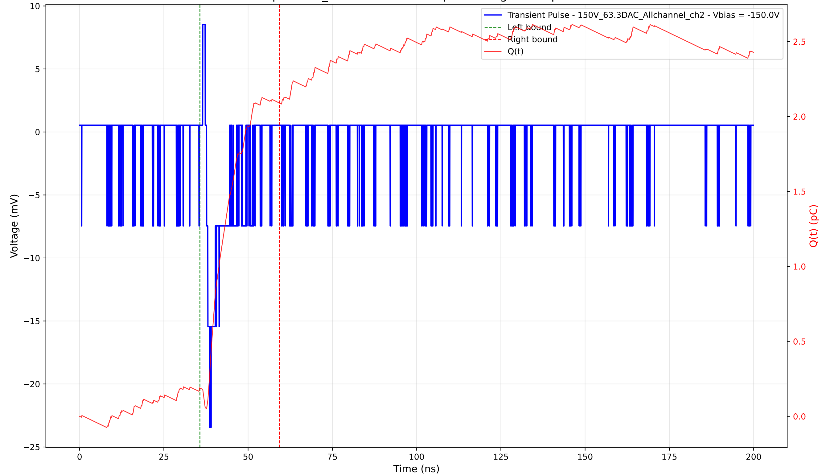
Transient Pulse - Sample: 1cm_42 - Position: 205.0 \mu\text{m} - Charge: 1.90 pC - Rise Time: 0.91 ns
