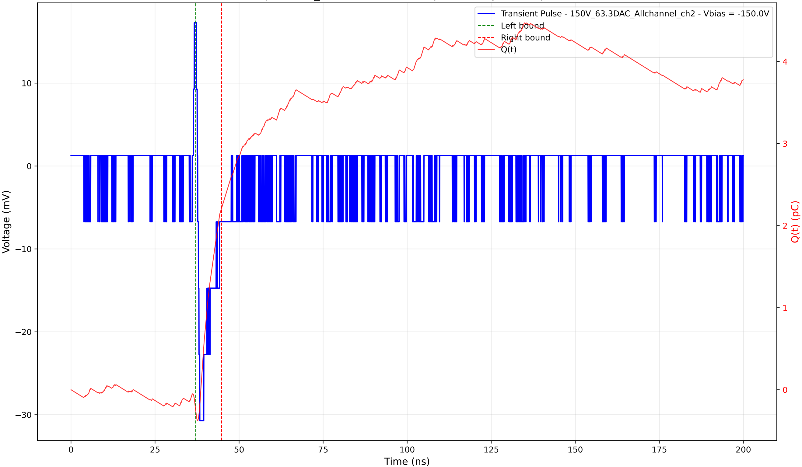
Transient Pulse - Sample: 1cm_42 - Position: 470.0 \mu\text{m} - Charge: 2.47 pC - Rise Time: 0.63 ns
