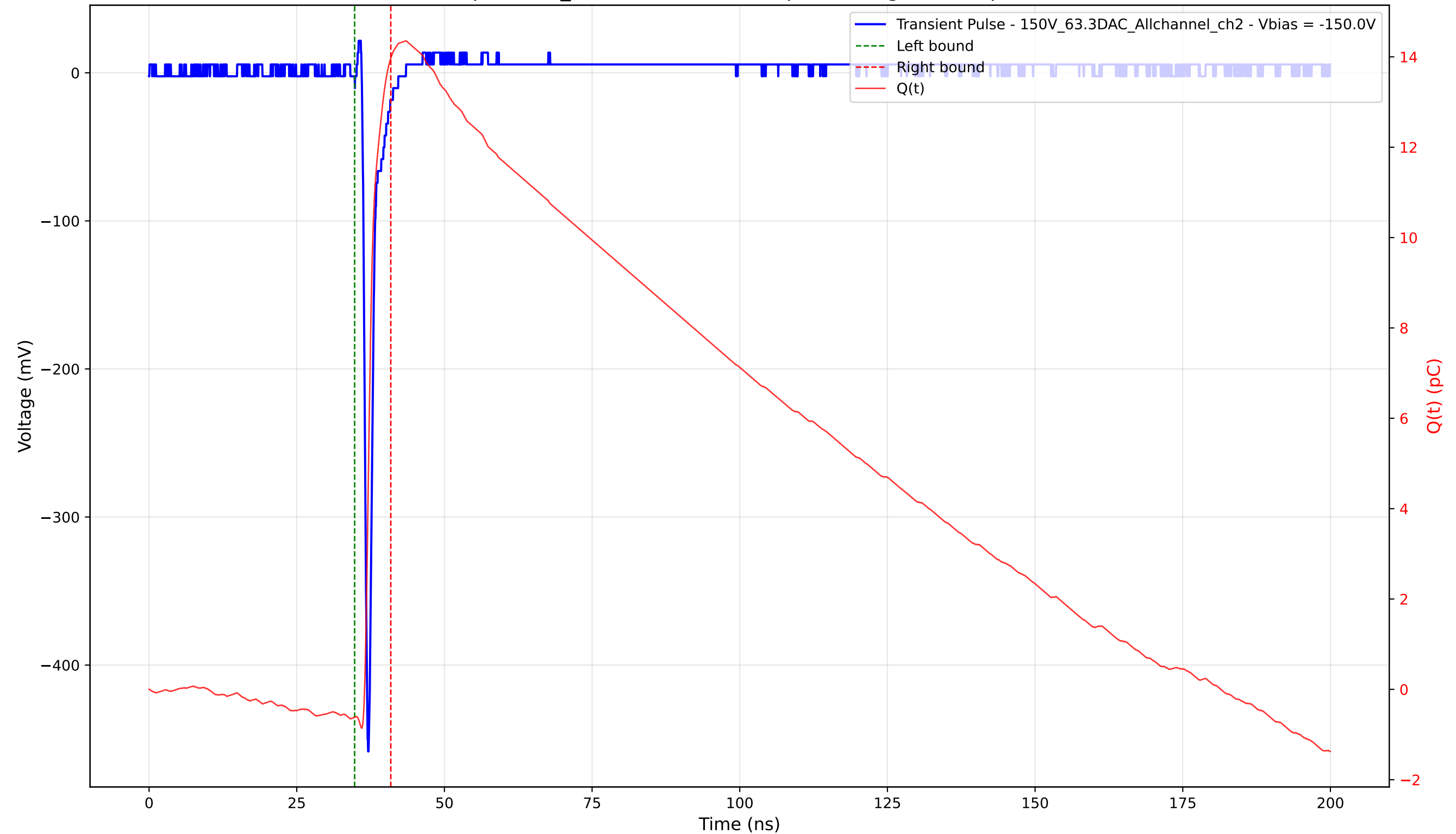
Transient Pulse - Sample: 1cm_42 - Position: 3185.0 \mu\text{m} - Charge: 14.60 pC - Rise Time: 0.74 ns
