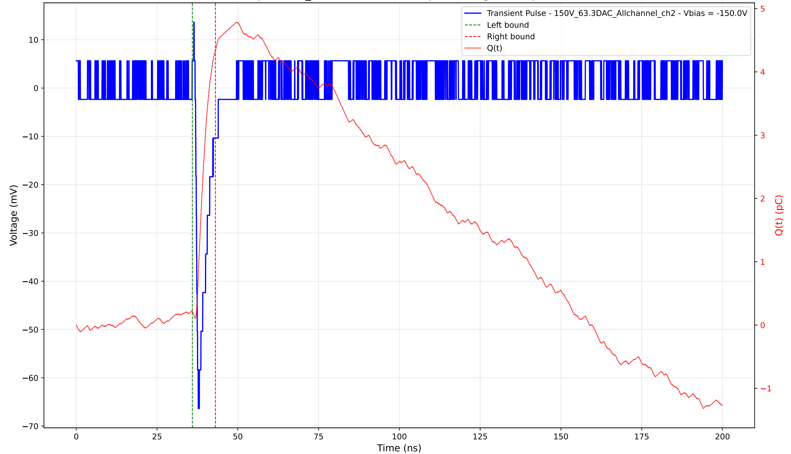
Transient Pulse - Sample: 1cm_42 - Position: 4060.0 \mu\text{m} - Charge: 4.12 pC - Rise Time: 0.82 ns
