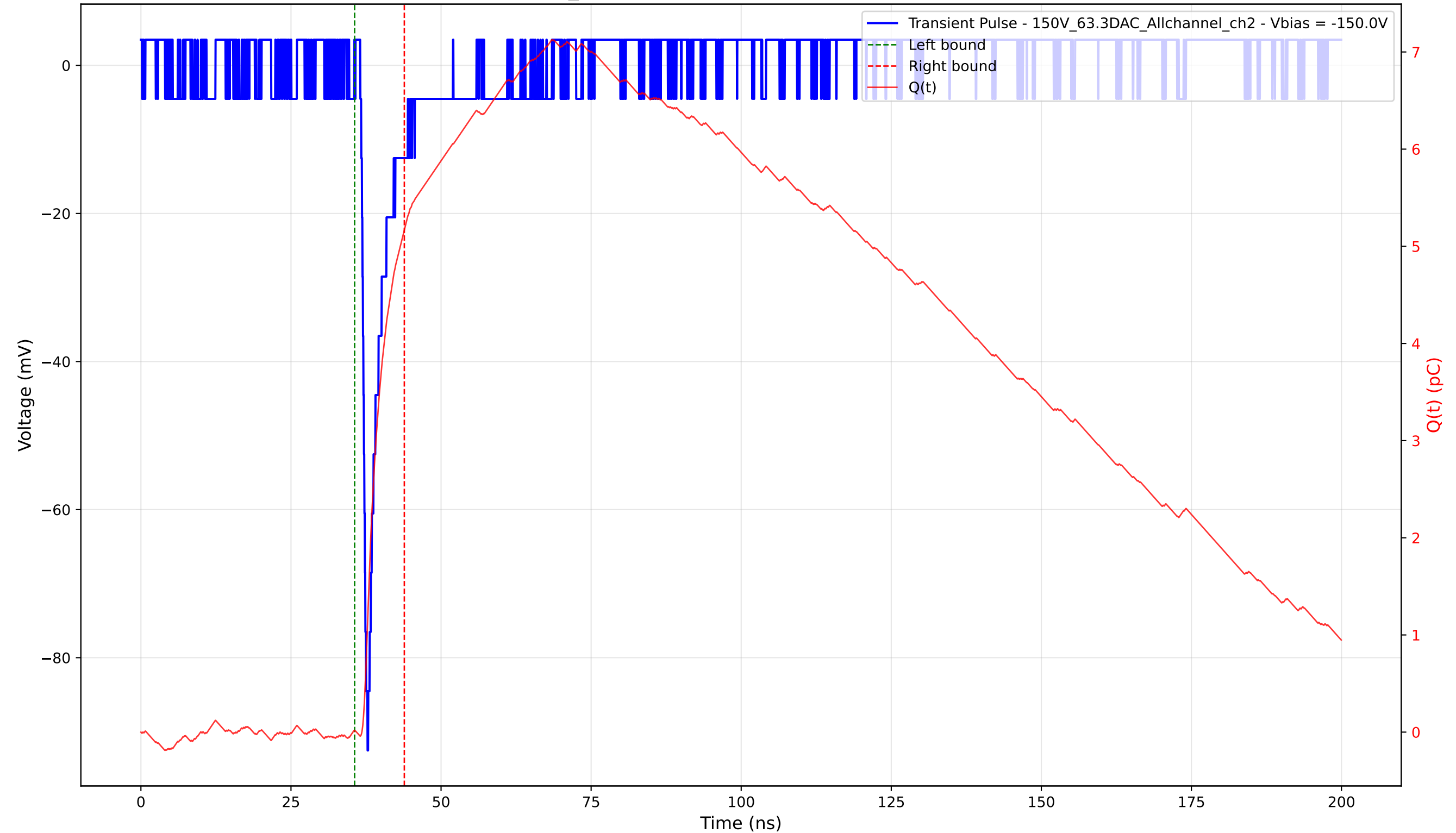
Transient Pulse - Sample: 1cm_42 - Position: 2080.0 \mu\text{m} - Charge: 5.15 pC - Rise Time: 0.82 ns
