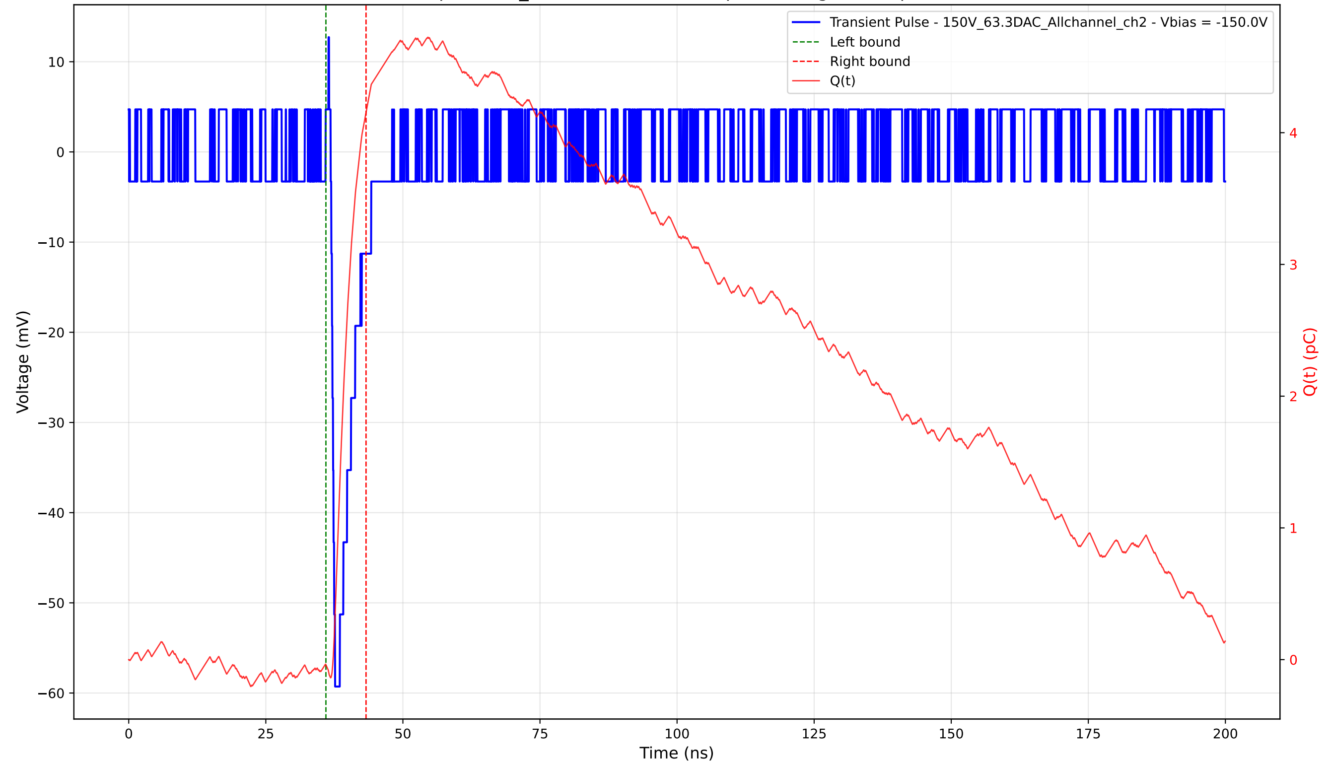
Transient Pulse - Sample: 1cm_42 - Position: 4080.0 \mu\text{m} - Charge: 4.19 pC - Rise Time: 0.71 ns
