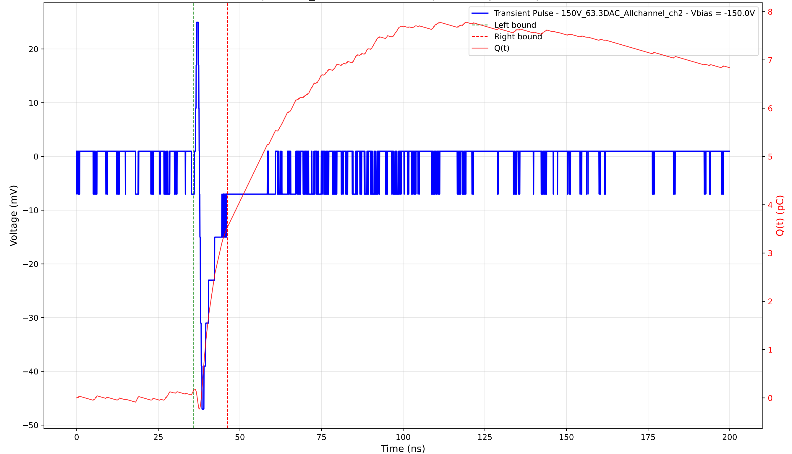
Transient Pulse - Sample: 1cm_42 - Position: 1455.0 \mu\text{m} - Charge: 3.41 pC - Rise Time: 0.78 ns
