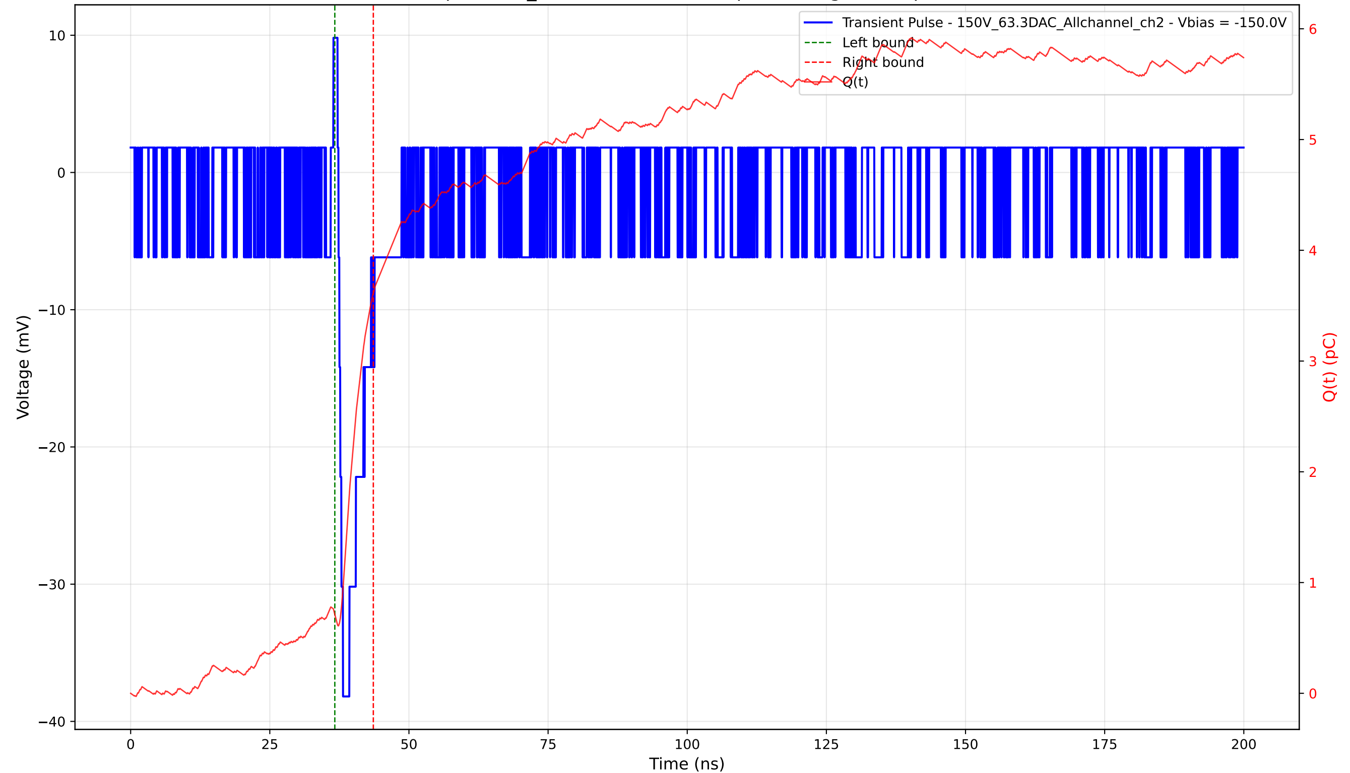
Transient Pulse - Sample: 1cm_42 - Position: 4590.0 \mu\text{m} - Charge: 2.90 pC - Rise Time: 0.82 ns
