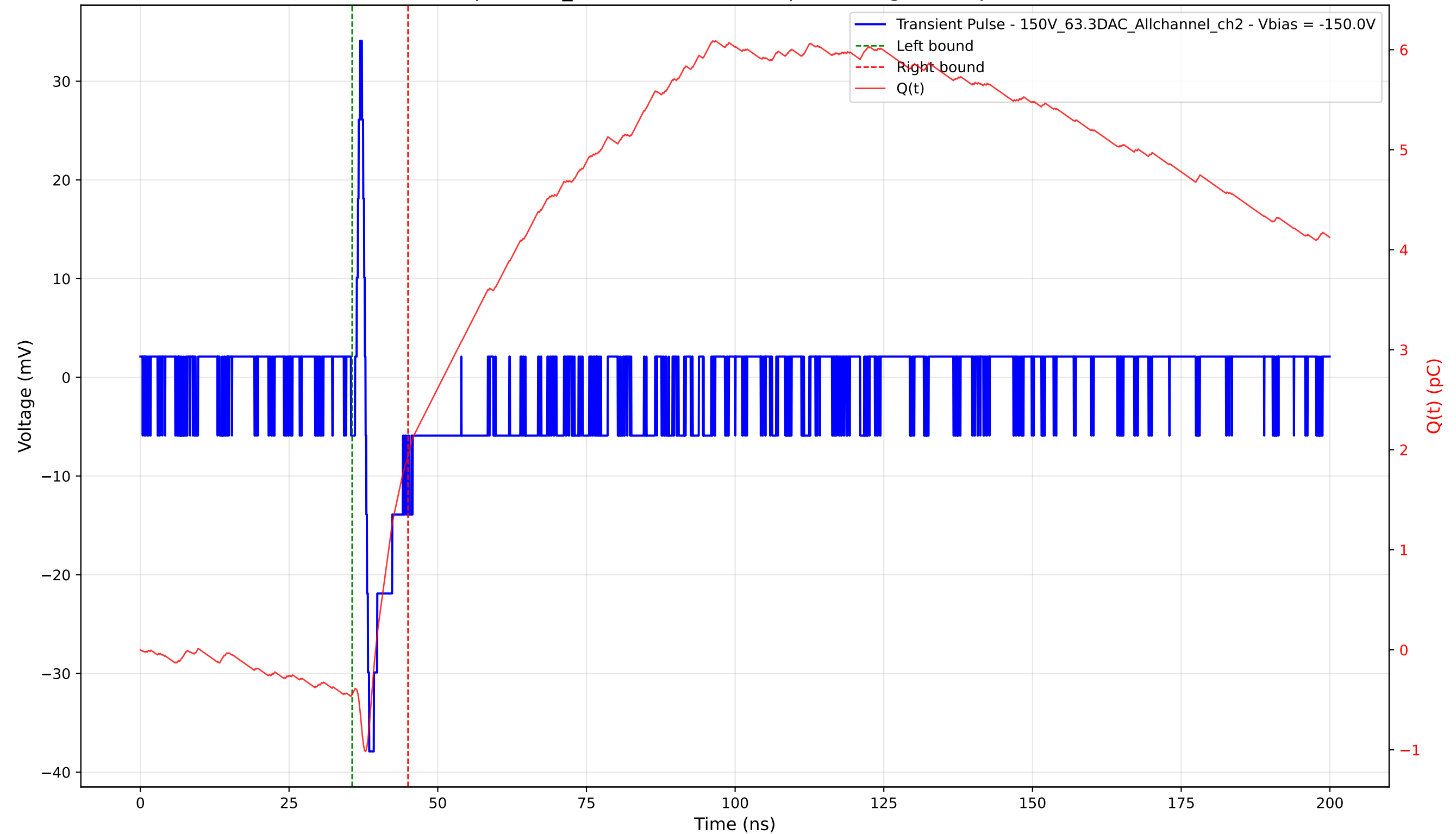
Transient Pulse - Sample: 1cm_42 - Position: 1035.0 \mu\text{m} - Charge: 2.39 pC - Rise Time: 0.62 ns
