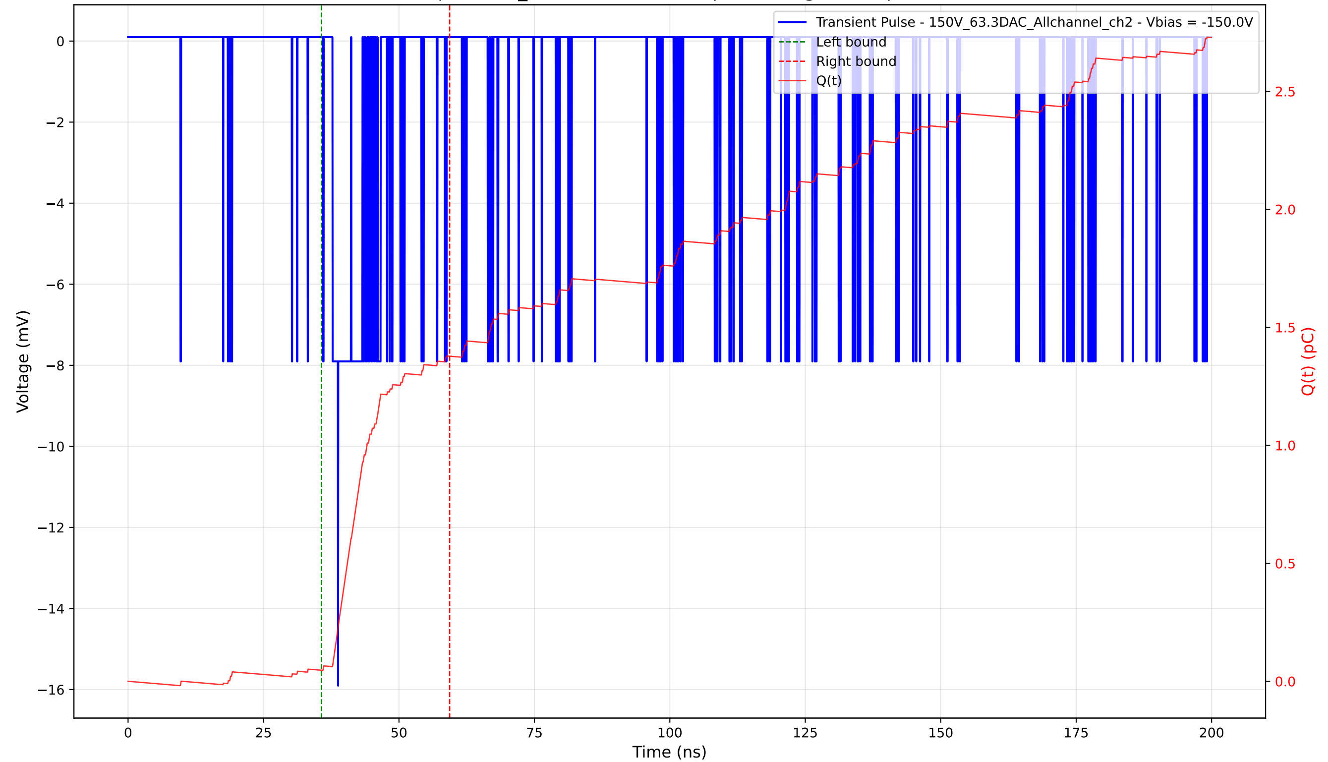
Transient Pulse - Sample: 1cm_42 - Position: 100.0 \mu\text{m} - Charge: 1.33 pC - Rise Time: 1.03 ns
