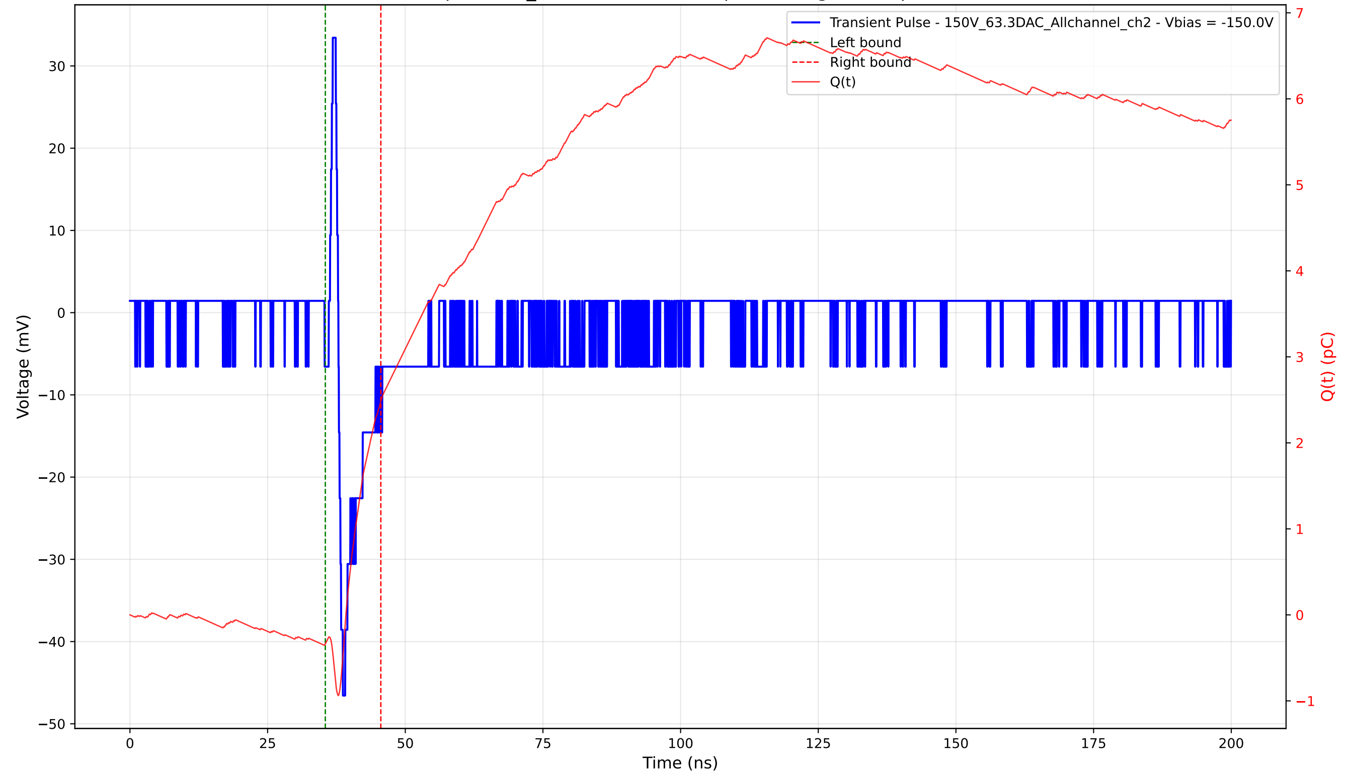
Transient Pulse - Sample: 1cm_42 - Position: 745.0 \mu\text{m} - Charge: 2.83 pC - Rise Time: 0.81 ns
