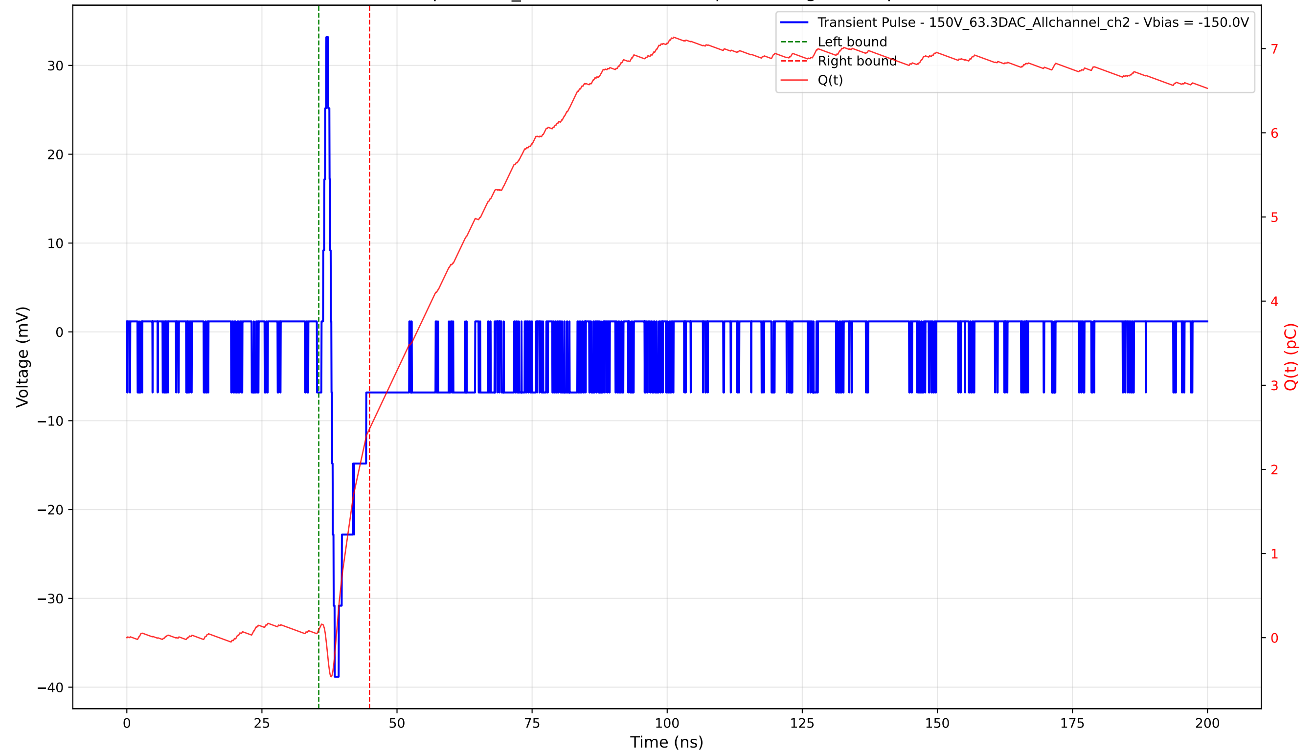
Transient Pulse - Sample: 1cm_42 - Position: 1020.0 \mu\text{m} - Charge: 2.39 pC - Rise Time: 0.62 ns
