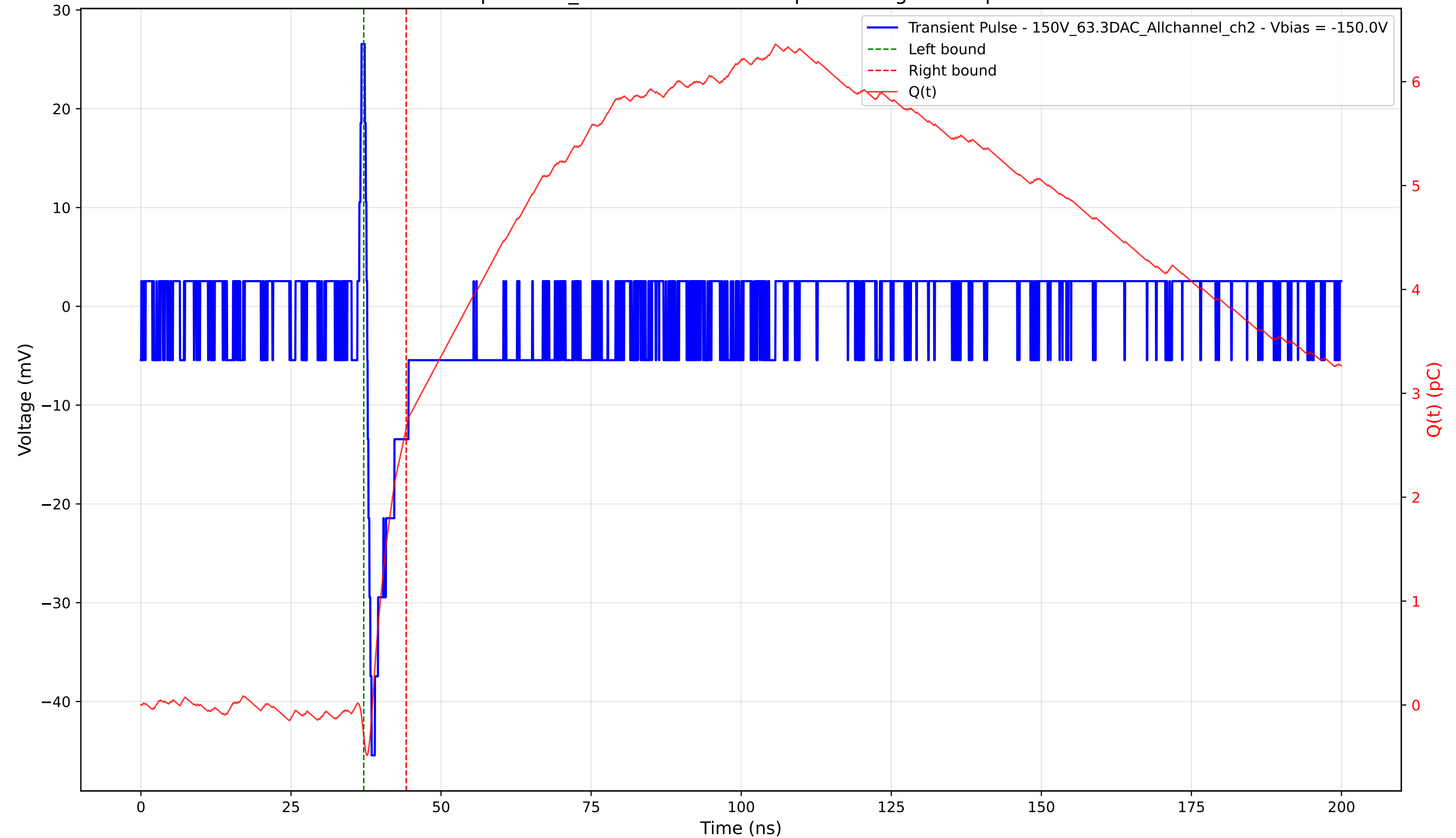
Transient Pulse - Sample: 1cm_42 - Position: 1425.0 \mu\text{m} - Charge: 2.96 pC - Rise Time: 0.73 ns
