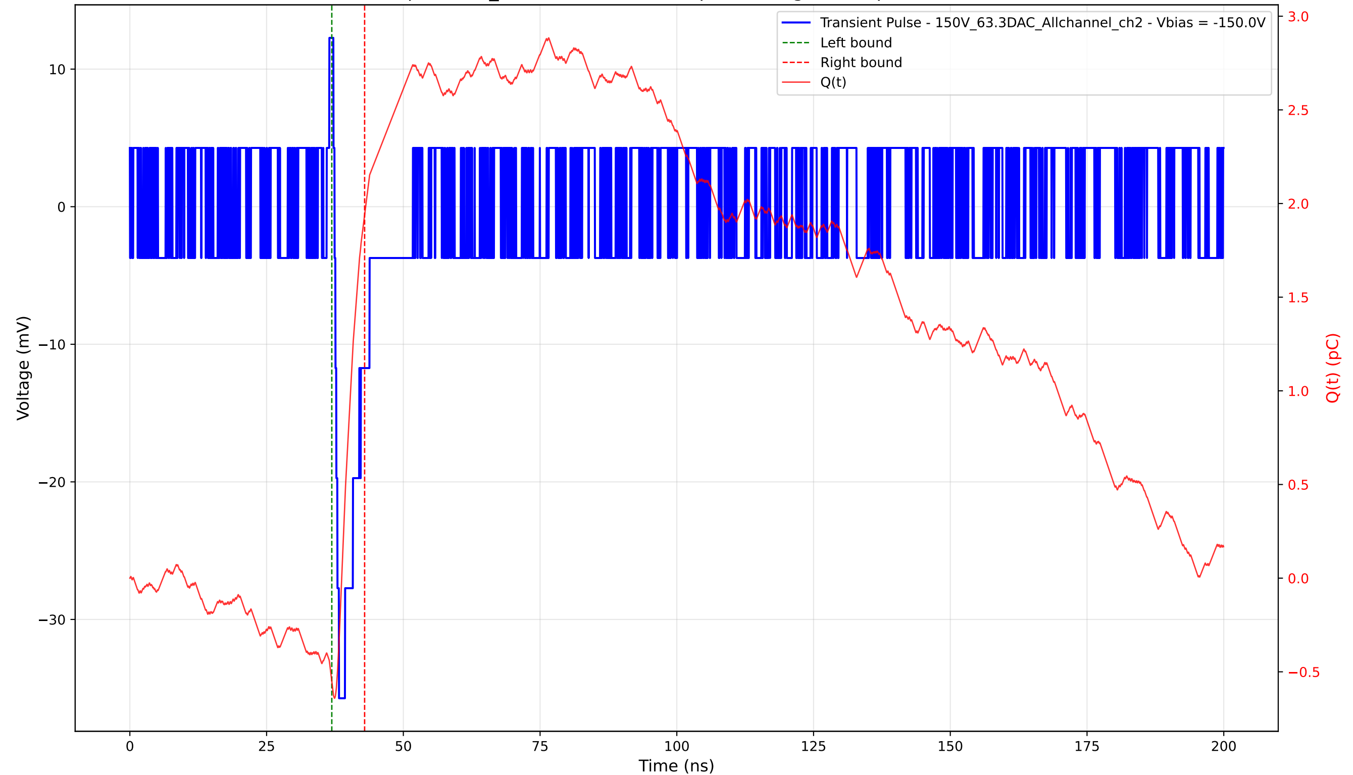
Transient Pulse - Sample: 1cm_42 - Position: 4685.0 \mu\text{m} - Charge: 2.49 pC - Rise Time: 0.00 ns (N/A)
