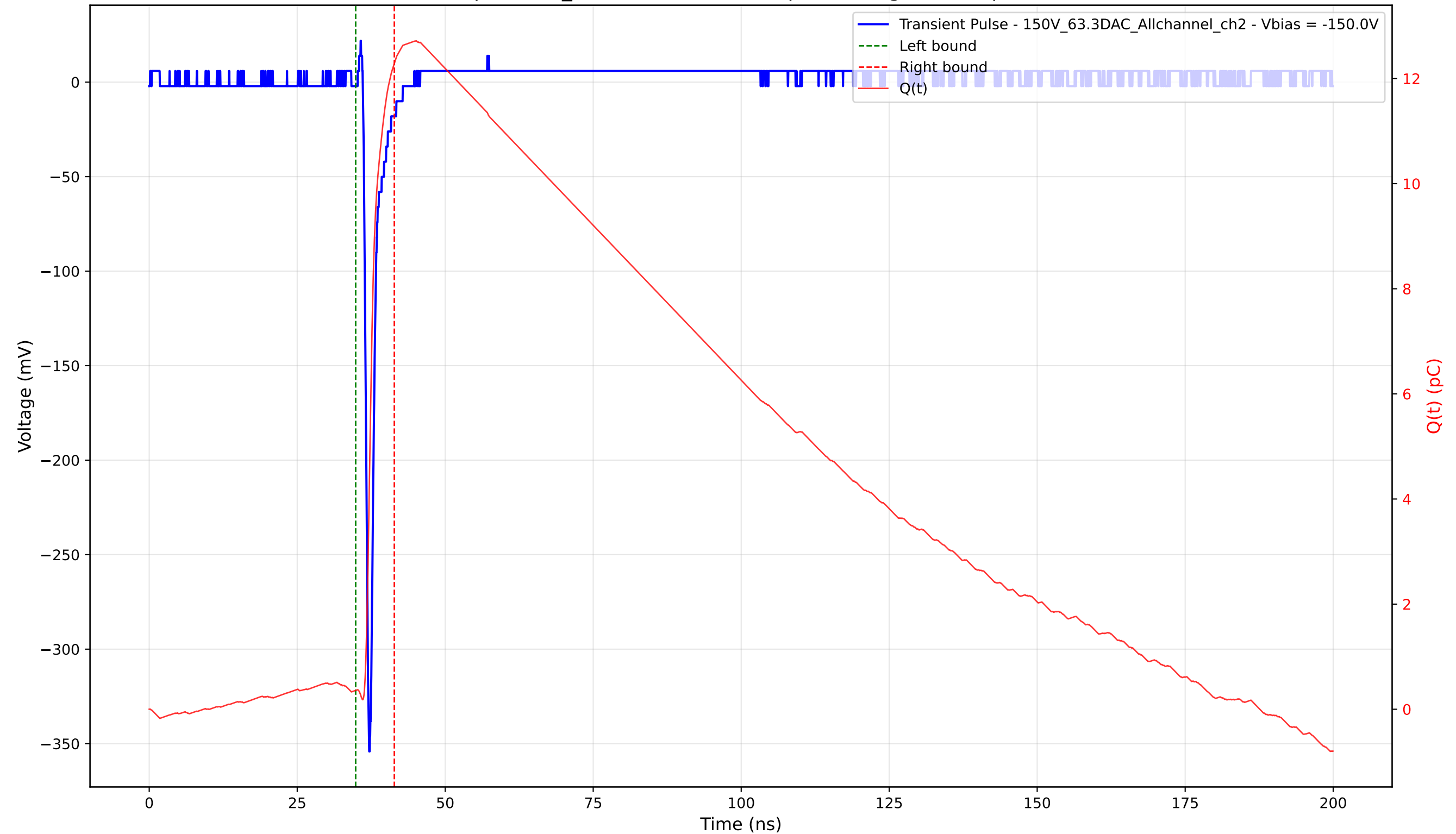
Transient Pulse - Sample: 1cm_42 - Position: 2670.0 \mu\text{m} - Charge: 11.93 pC - Rise Time: 0.74 ns
