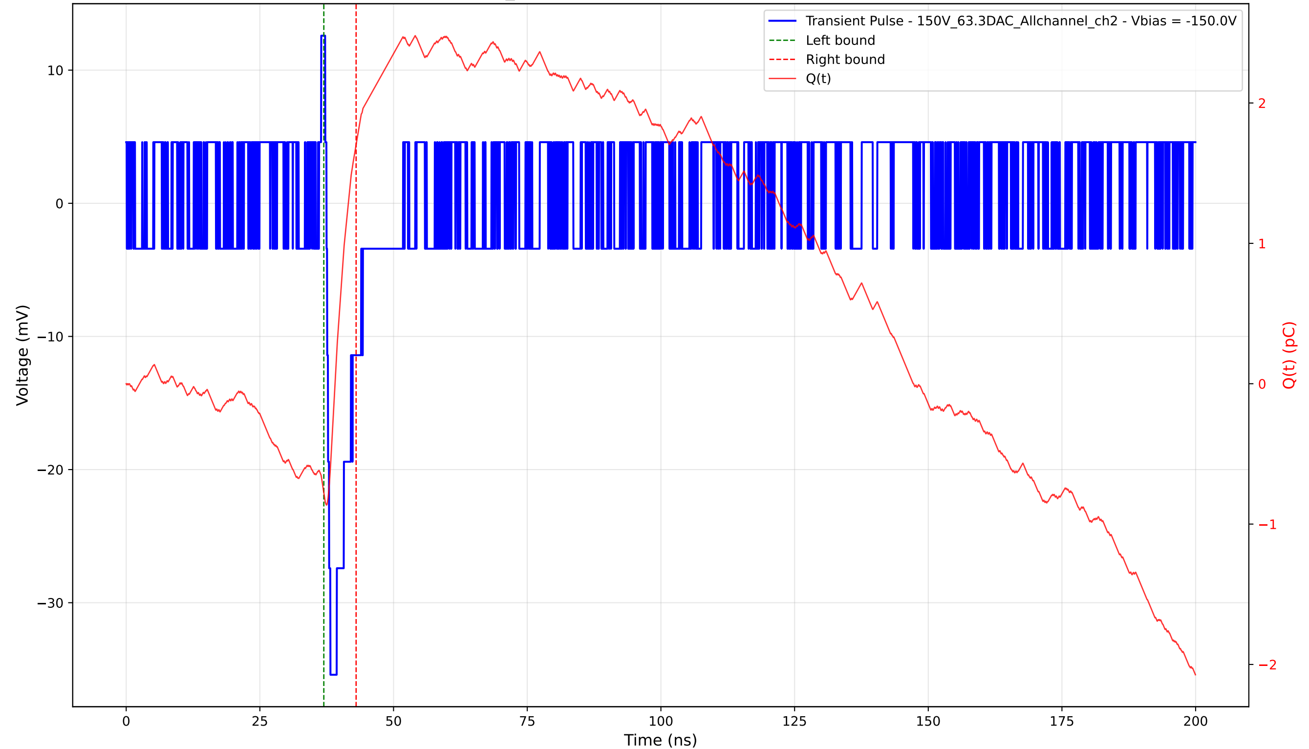
Transient Pulse - Sample: 1cm_42 - Position: 4775.0 \mu\text{m} - Charge: 2.48 pC - Rise Time: 0.64 ns
