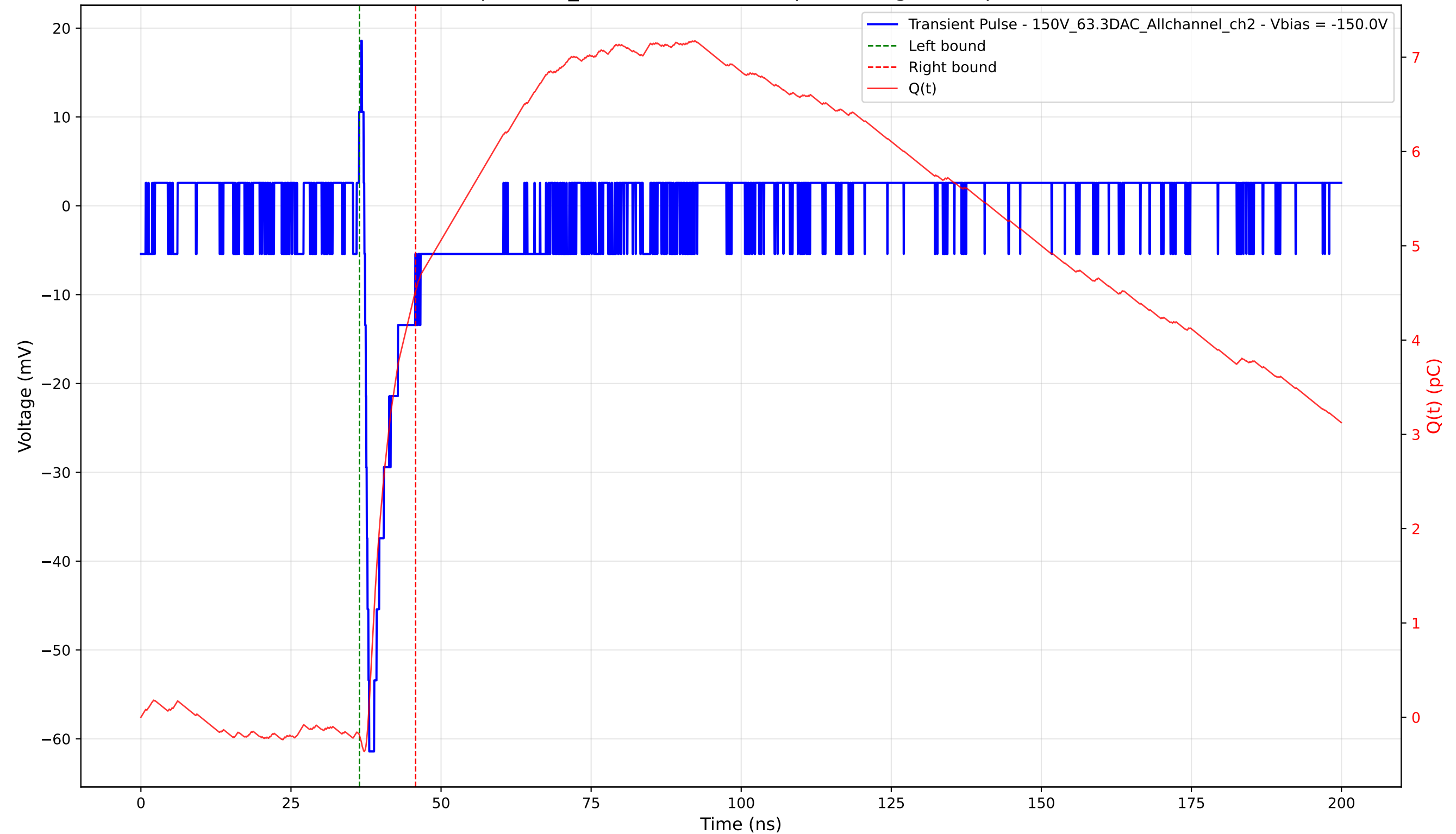
Transient Pulse - Sample: 1cm_42 - Position: 1750.0 \mu\text{m} - Charge: 4.71 pC - Rise Time: 0.72 ns
