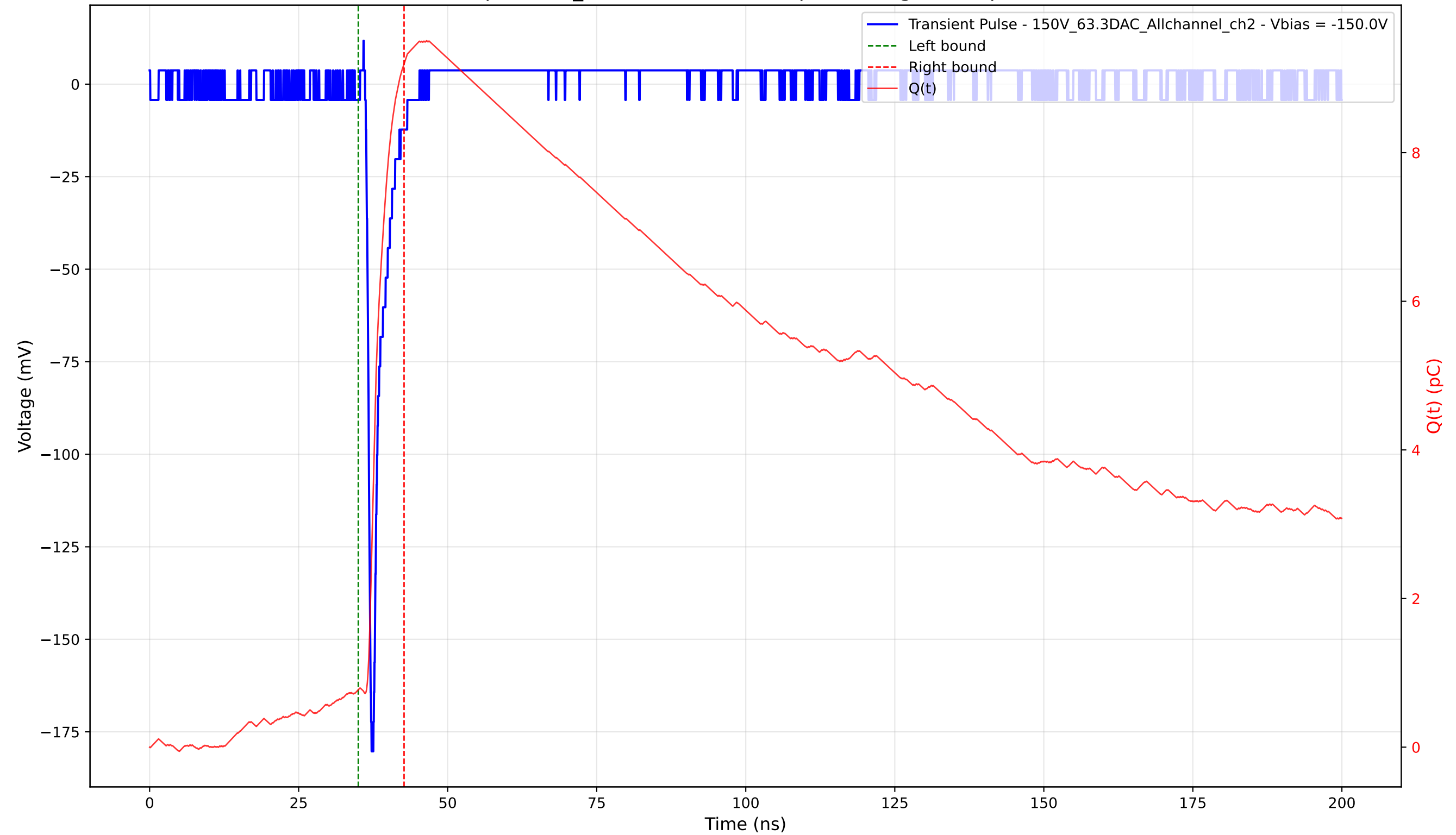
Transient Pulse - Sample: 1cm_42 - Position: 3570.0 \mu\text{m} - Charge: 8.42 pC - Rise Time: 0.73 ns
