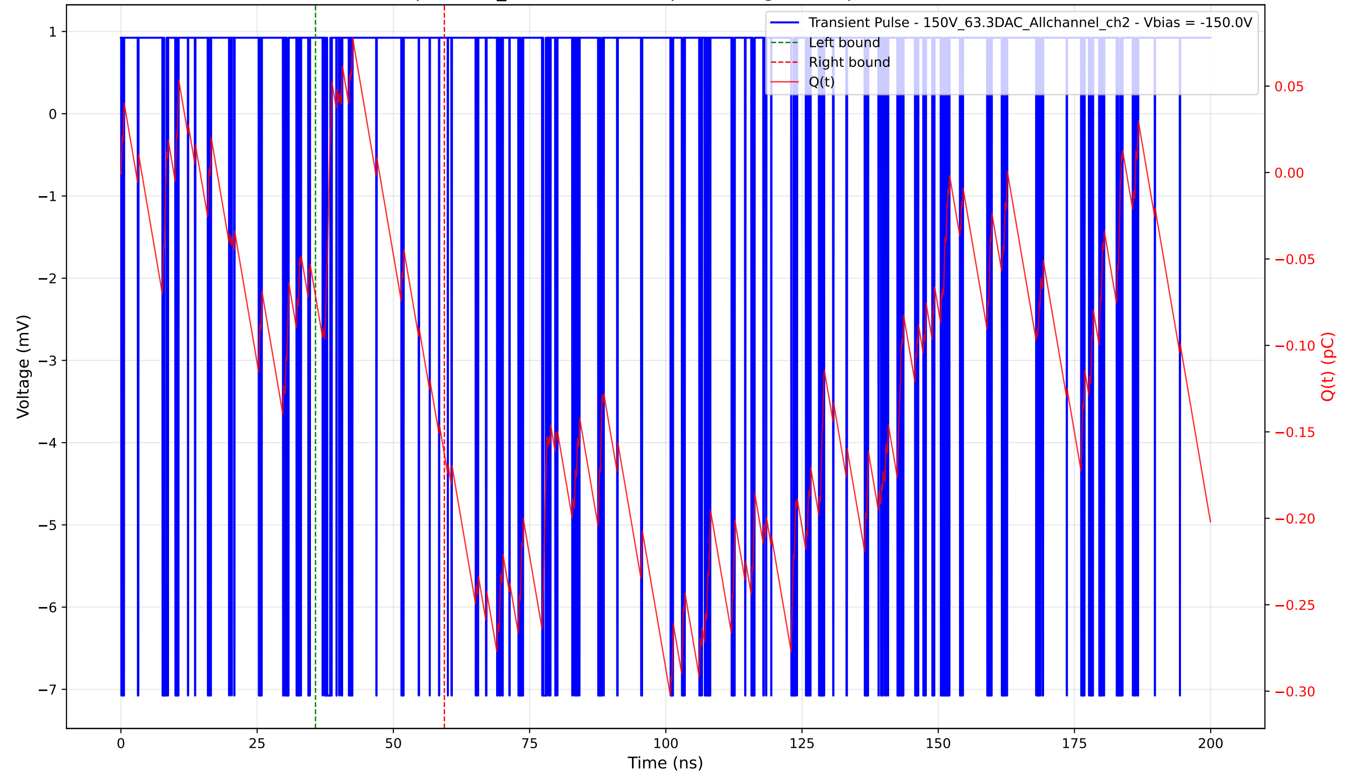
Transient Pulse - Sample: 1cm_42 - Position: 0.0 \mu\text{m} - Charge: 0.09 pC - Rise Time: 0.00 ns (N/A)
