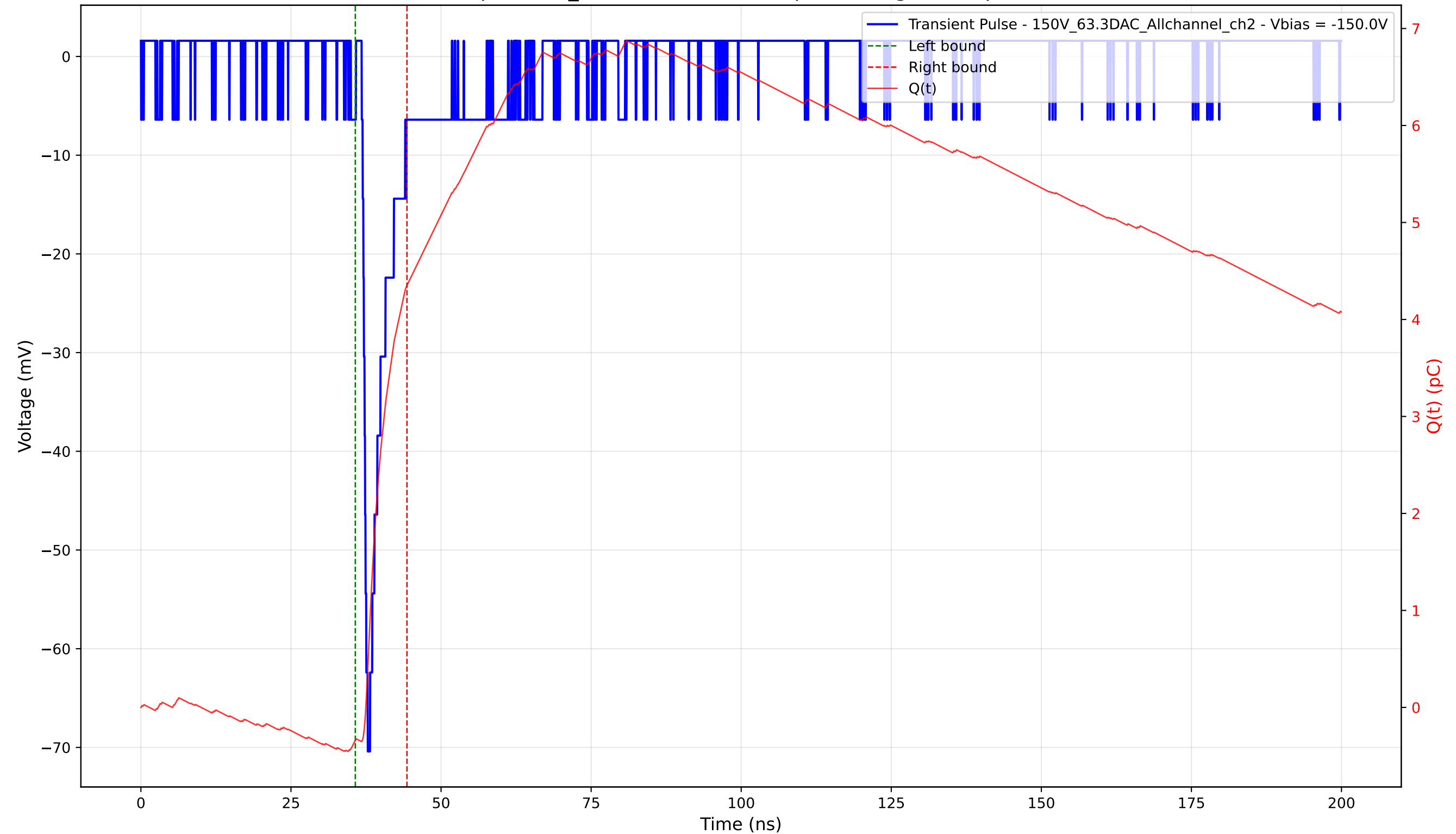
Transient Pulse - Sample: 1cm_42 - Position: 1990.0 \mu\text{m} - Charge: 4.69 pC - Rise Time: 0.88 ns
