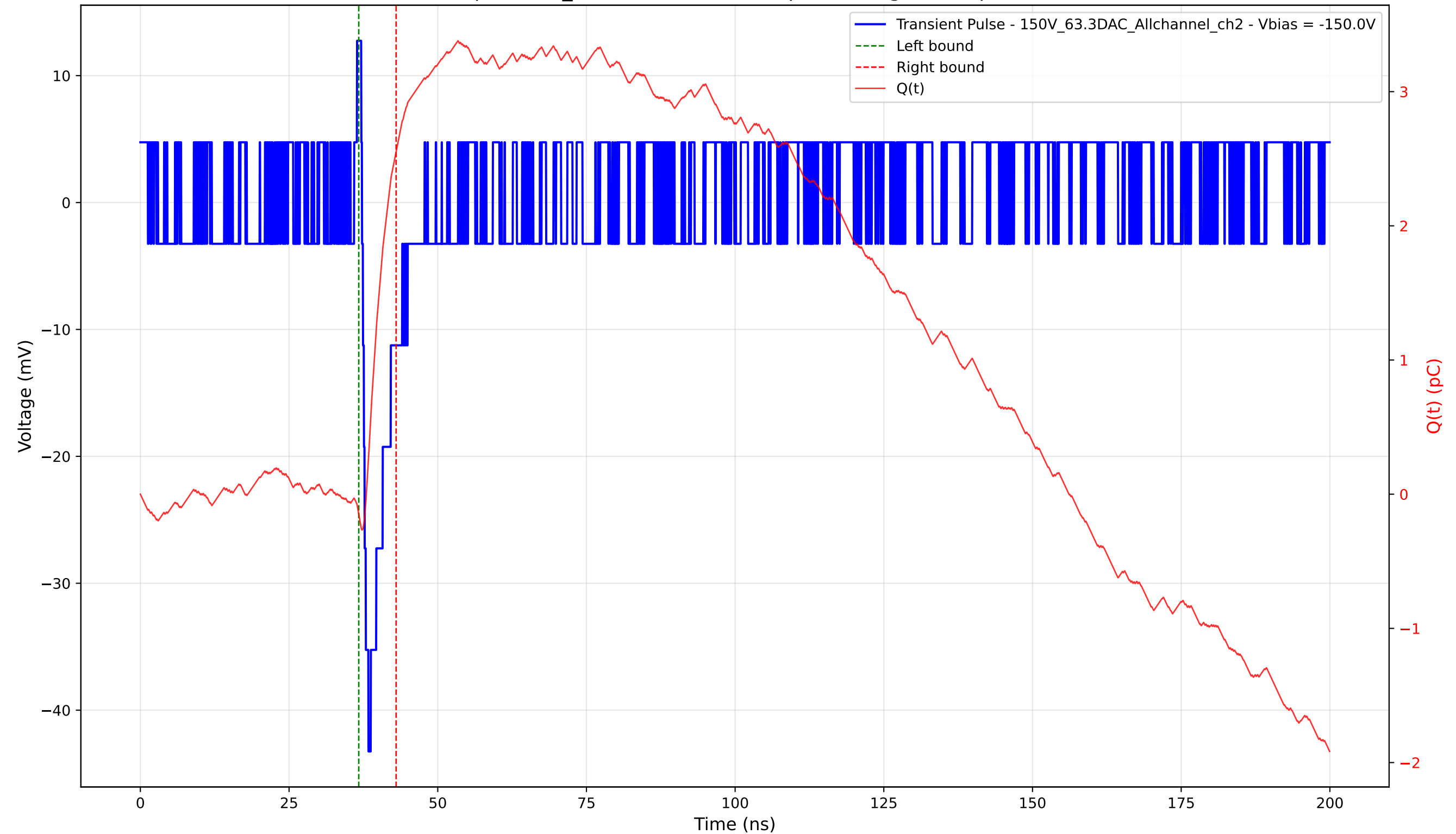
Transient Pulse - Sample: 1cm_42 - Position: 4490.0 \mu\text{m} - Charge: 2.70 pC - Rise Time: 0.95 ns
