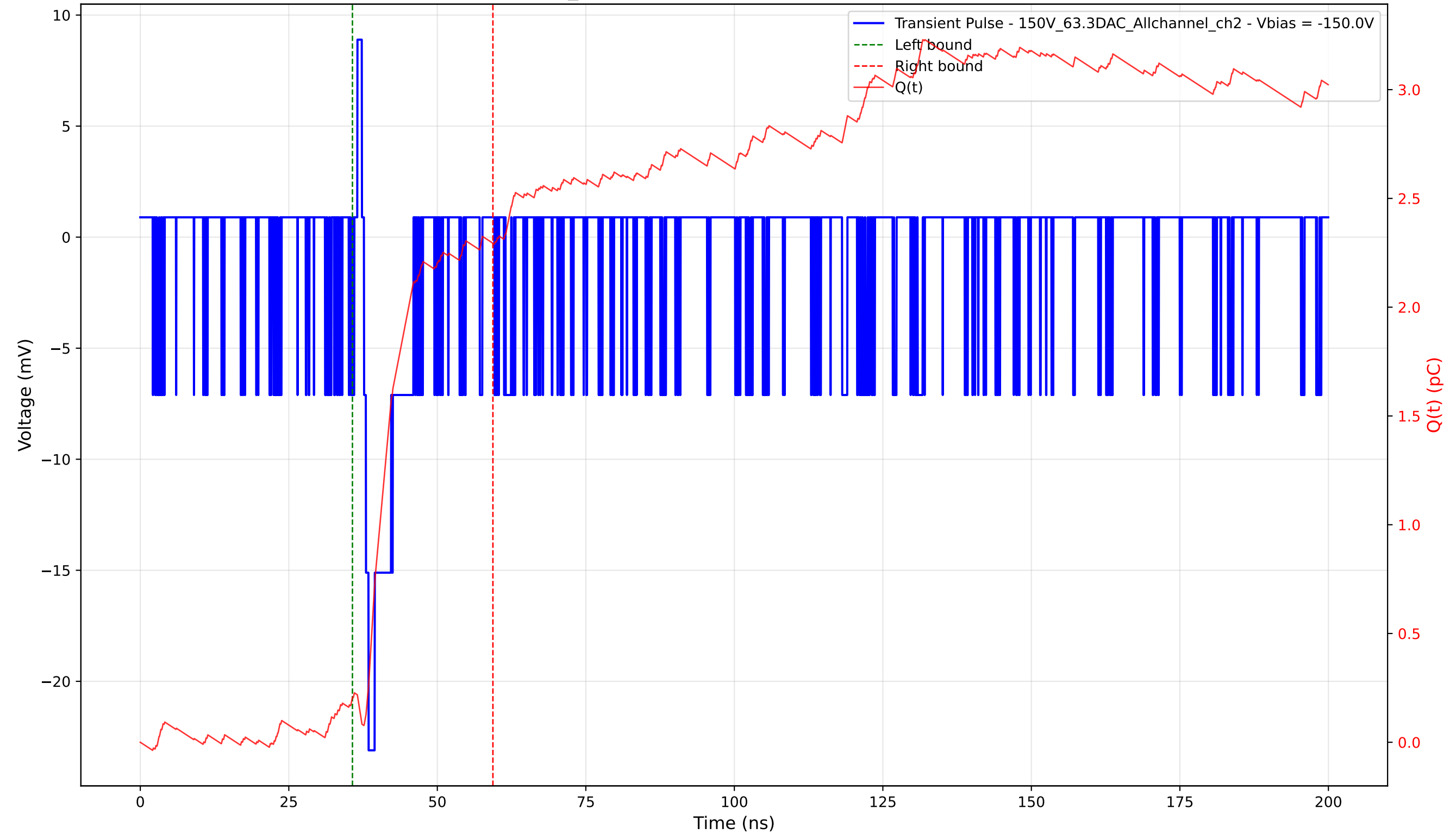
Transient Pulse - Sample: 1cm_42 - Position: 240.0 \mu\text{m} - Charge: 2.09 pC - Rise Time: 0.79 ns
