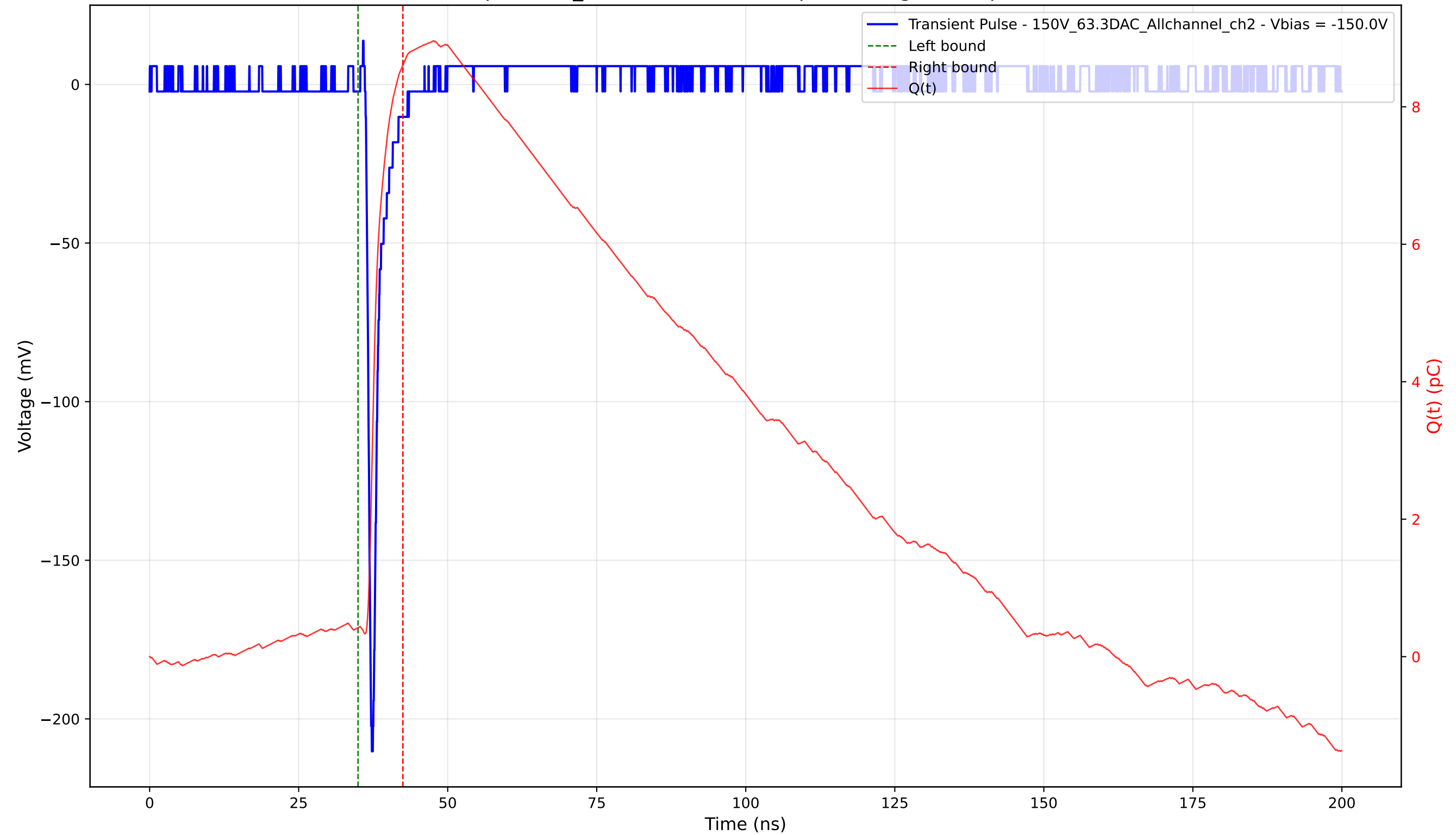
Transient Pulse - Sample: 1cm_42 - Position: 2520.0 \mu\text{m} - Charge: 8.19 pC - Rise Time: 0.76 ns
