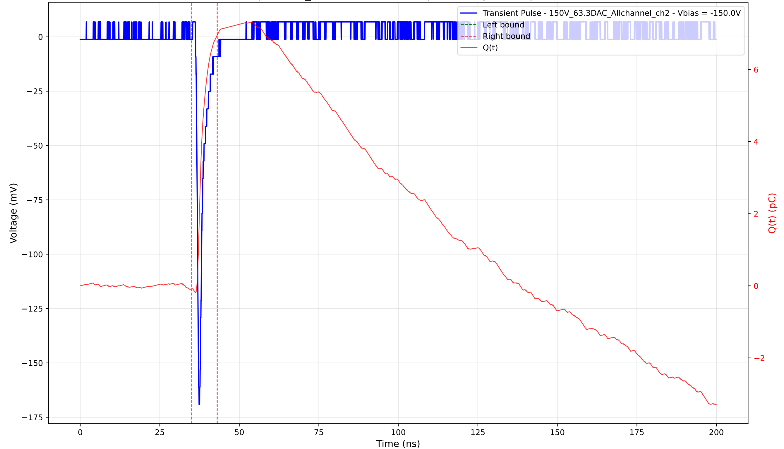
Transient Pulse - Sample: 1cm_42 - Position: 2440.0 \mu\text{m} - Charge: 7.03 pC - Rise Time: 0.80 ns
