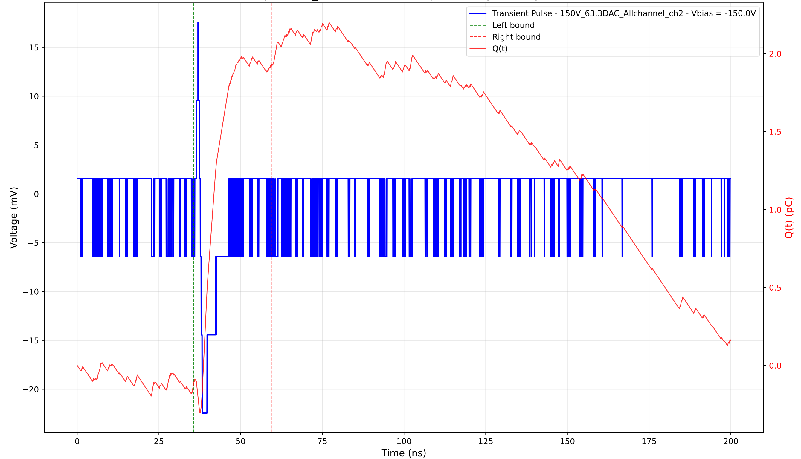
Transient Pulse - Sample: 1cm_42 - Position: 320.0 \mu\text{m} - Charge: 2.02 pC - Rise Time: 0.59 ns
