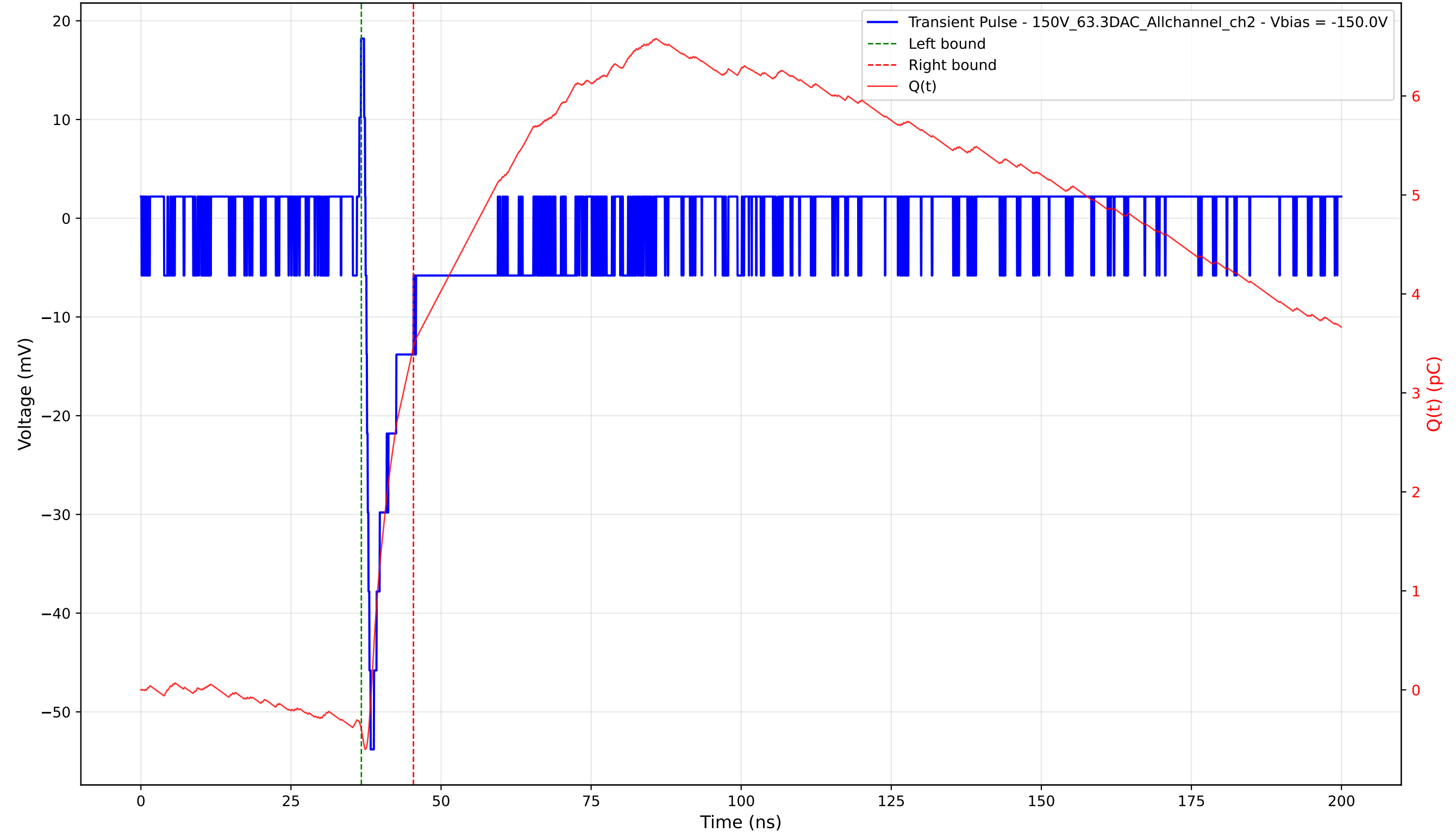
Transient Pulse - Sample: 1cm_42 - Position: 1610.0 \mu\text{m} - Charge: 3.87 pC - Rise Time: 0.84 ns
