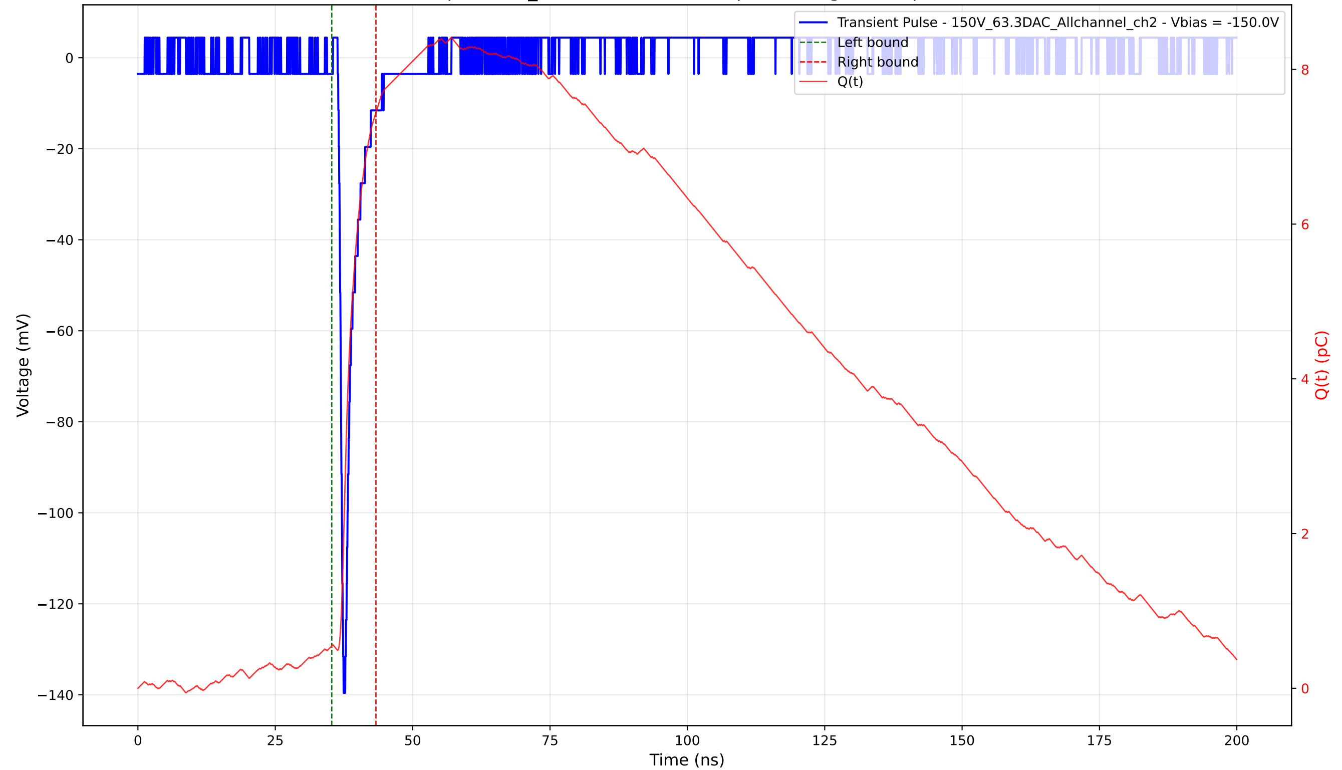
Transient Pulse - Sample: 1cm_42 - Position: 2265.0 \mu\text{m} - Charge: 6.89 pC - Rise Time: 0.83 ns
