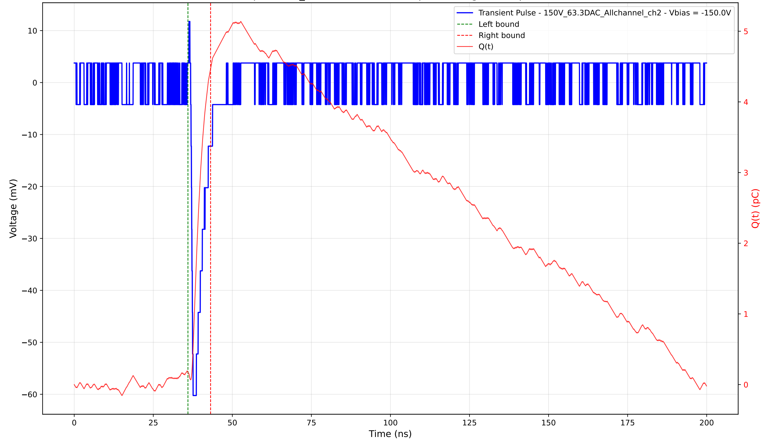
Transient Pulse - Sample: 1cm_42 - Position: 4070.0 \mu\text{m} - Charge: 4.29 pC - Rise Time: 0.67 ns
