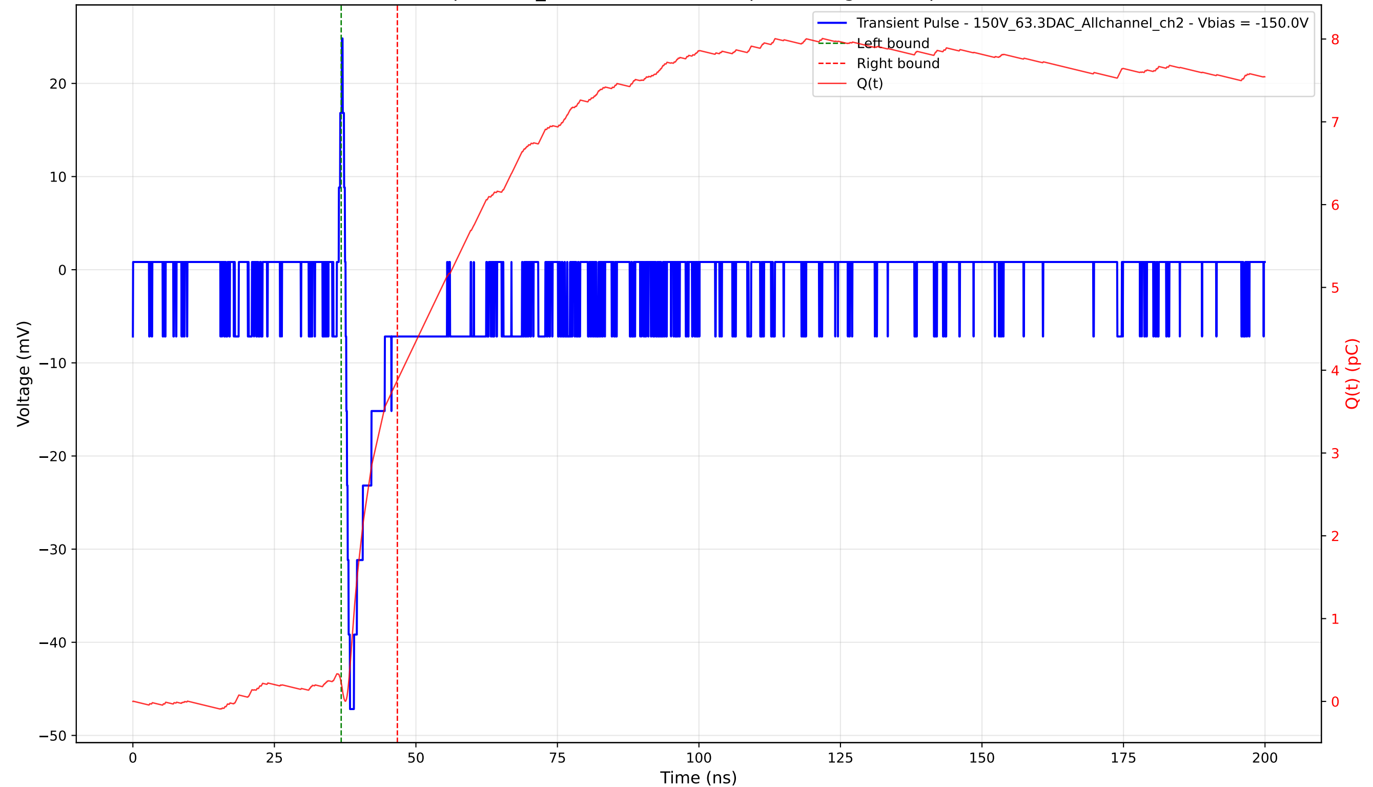
Transient Pulse - Sample: 1cm_42 - Position: 1520.0 \mu\text{m} - Charge: 3.65 pC - Rise Time: 0.78 ns
