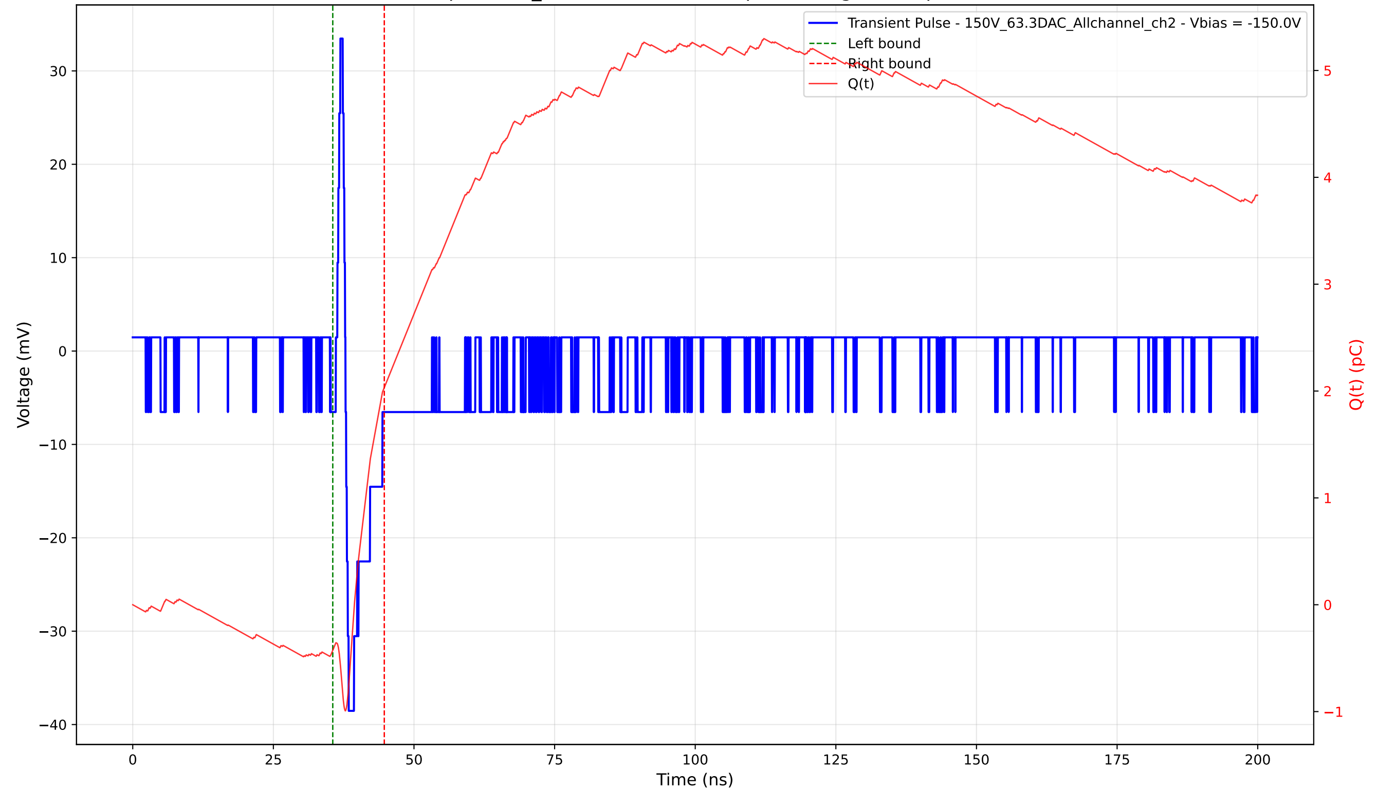
Transient Pulse - Sample: 1cm_42 - Position: 1095.0 \mu\text{m} - Charge: 2.46 pC - Rise Time: 0.58 ns
