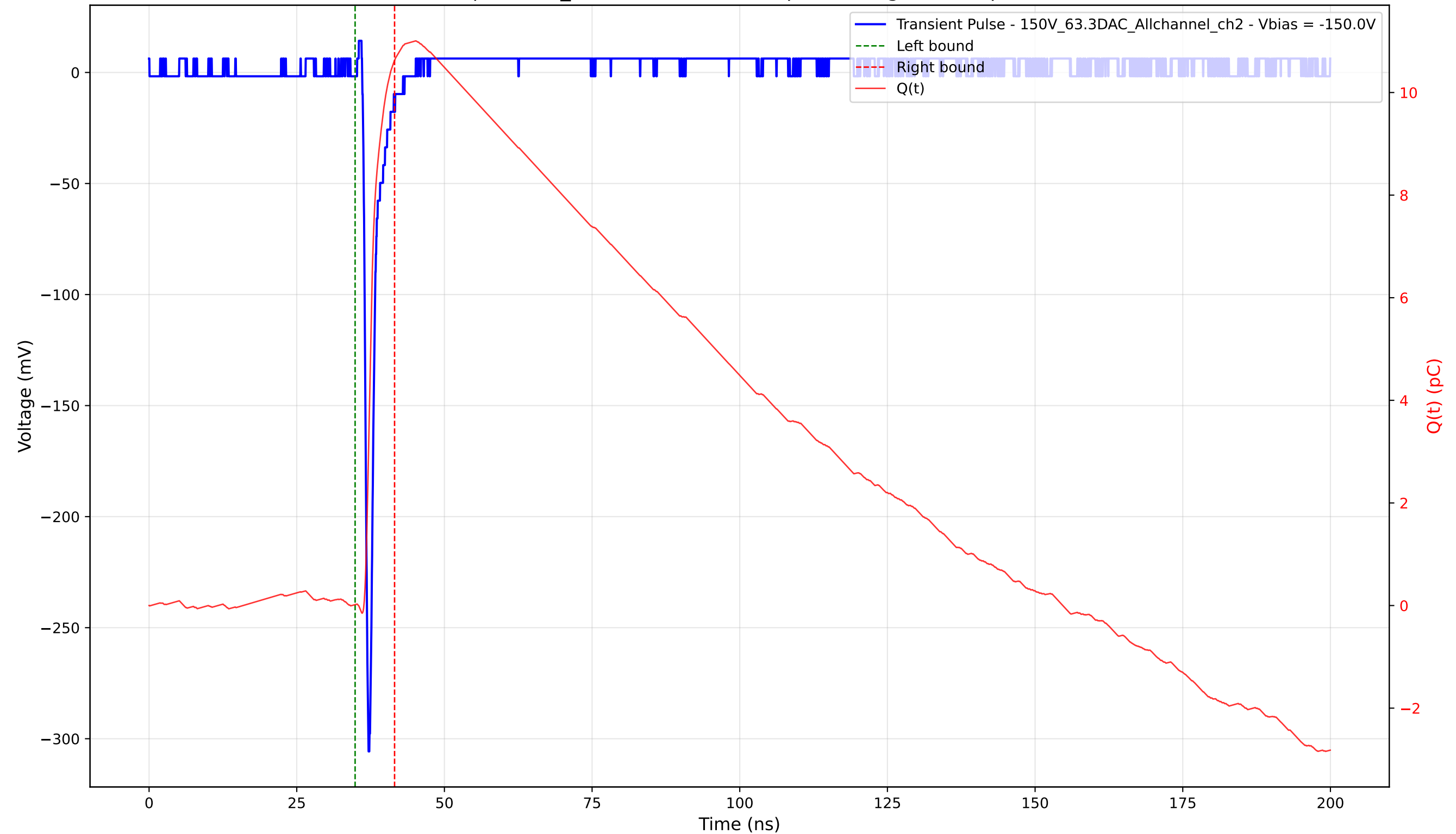
Transient Pulse - Sample: 1cm_42 - Position: 2625.0 \mu\text{m} - Charge: 10.60 pC - Rise Time: 0.74 ns
