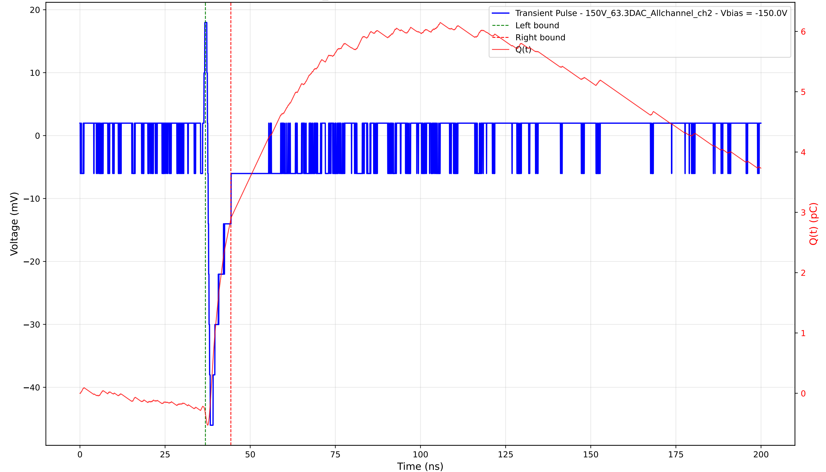
Transient Pulse - Sample: 1cm_42 - Position: 1540.0 \mu\text{m} - Charge: 3.24 pC - Rise Time: 0.73 ns
