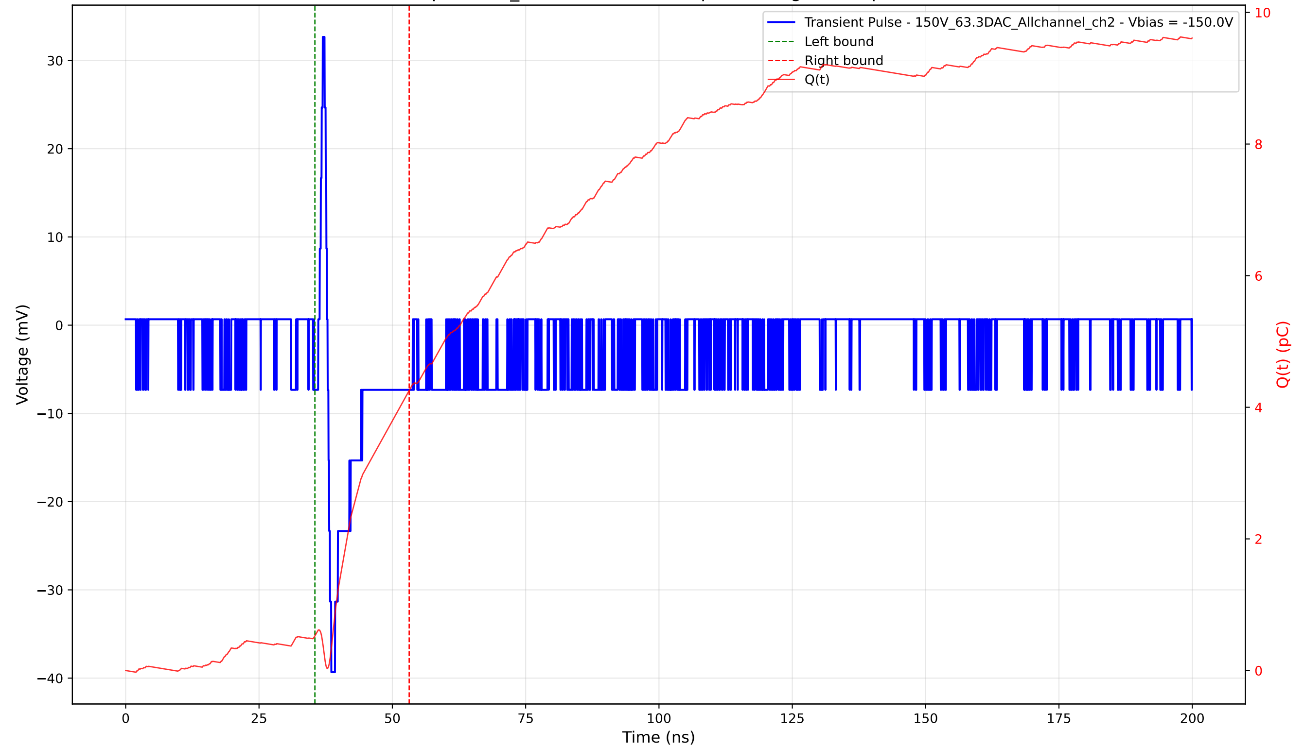
Transient Pulse - Sample: 1cm_42 - Position: 935.0 \mu\text{m} - Charge: 3.73 pC - Rise Time: 0.70 ns
