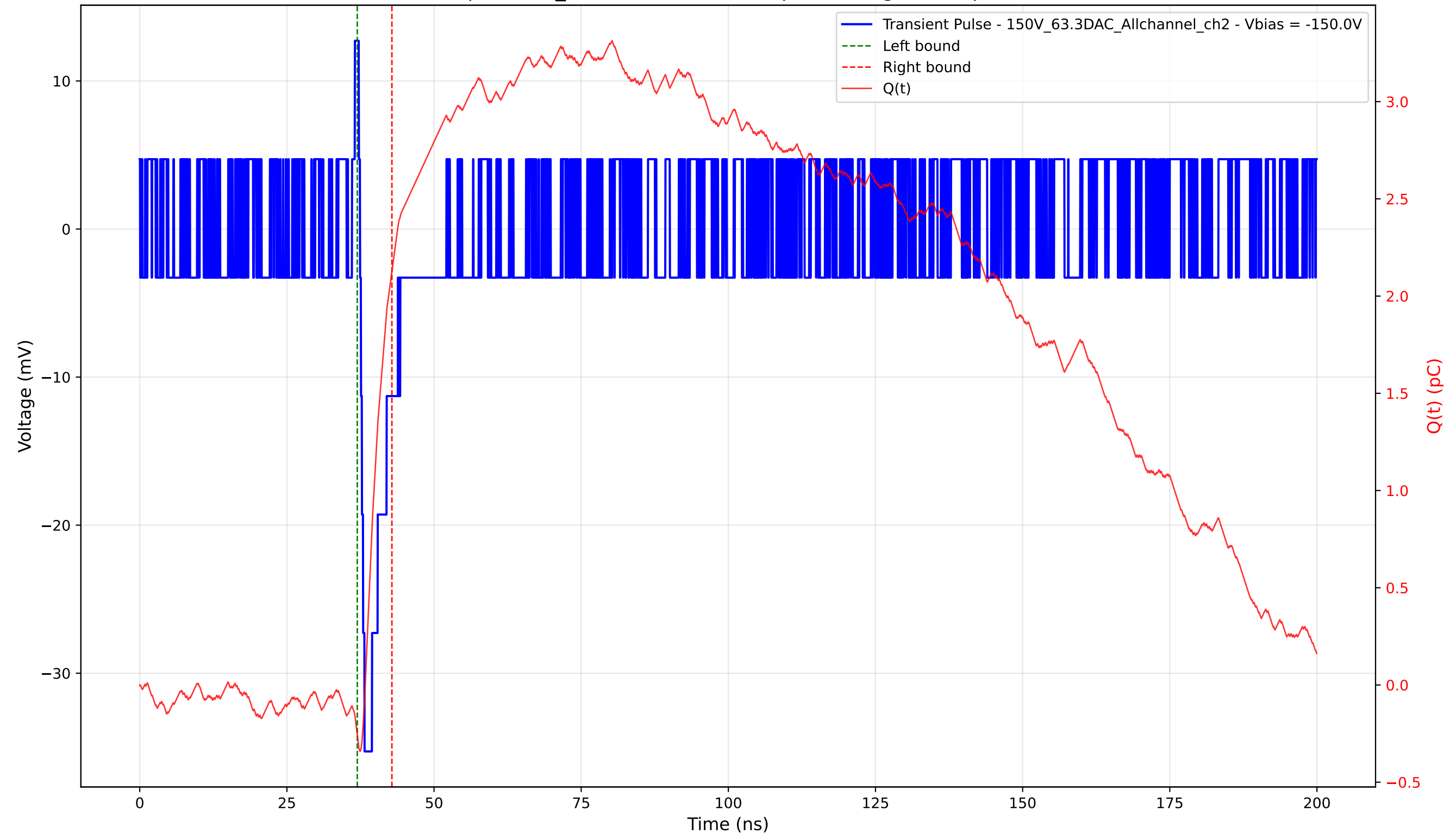
Transient Pulse - Sample: 1cm_42 - Position: 4765.0 \mu\text{m} - Charge: 2.39 pC - Rise Time: 0.64 ns
