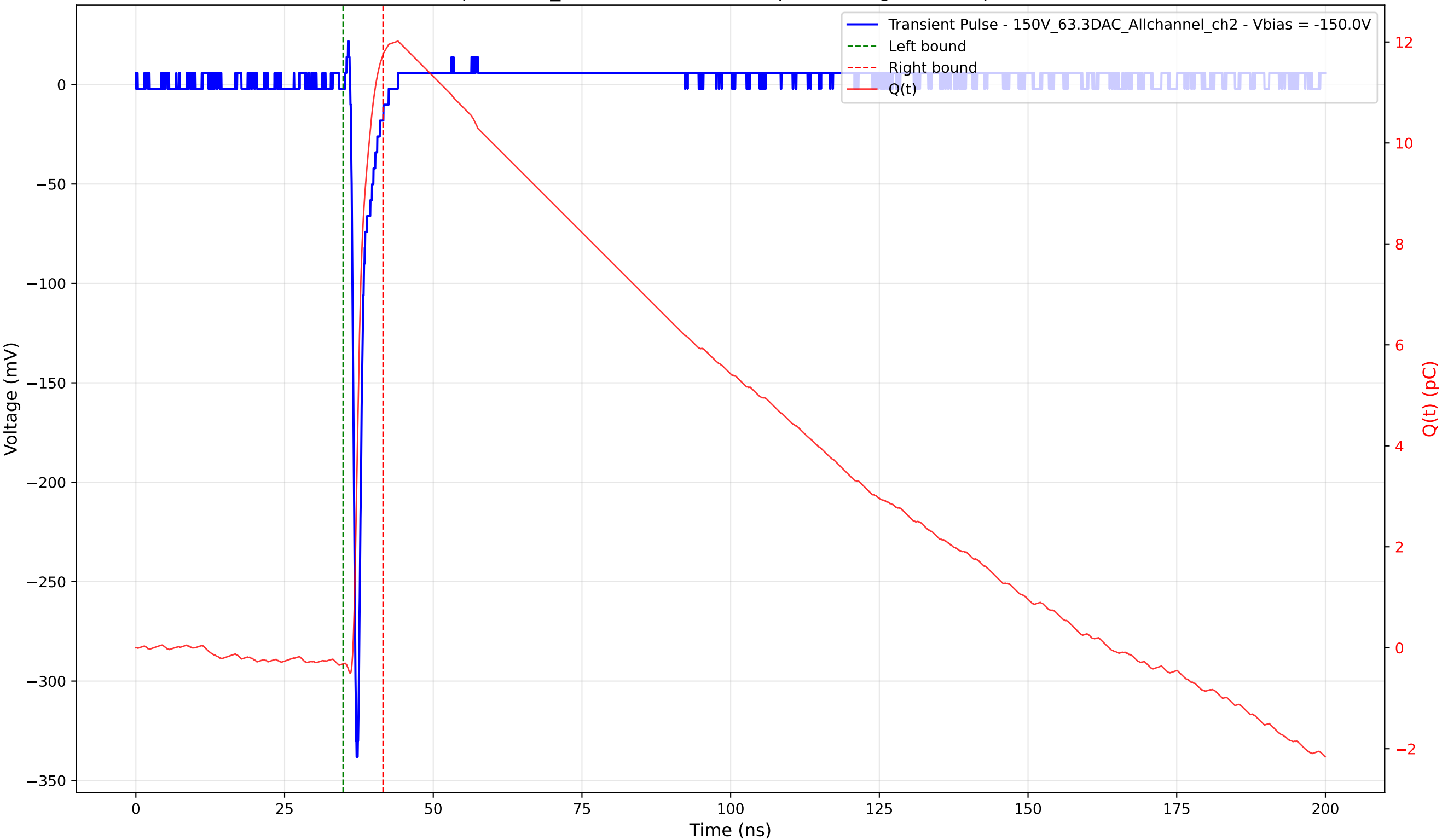
Transient Pulse - Sample: 1cm_42 - Position: 3385.0 \mu\text{m} - Charge: 12.07 pC - Rise Time: 0.76 ns
