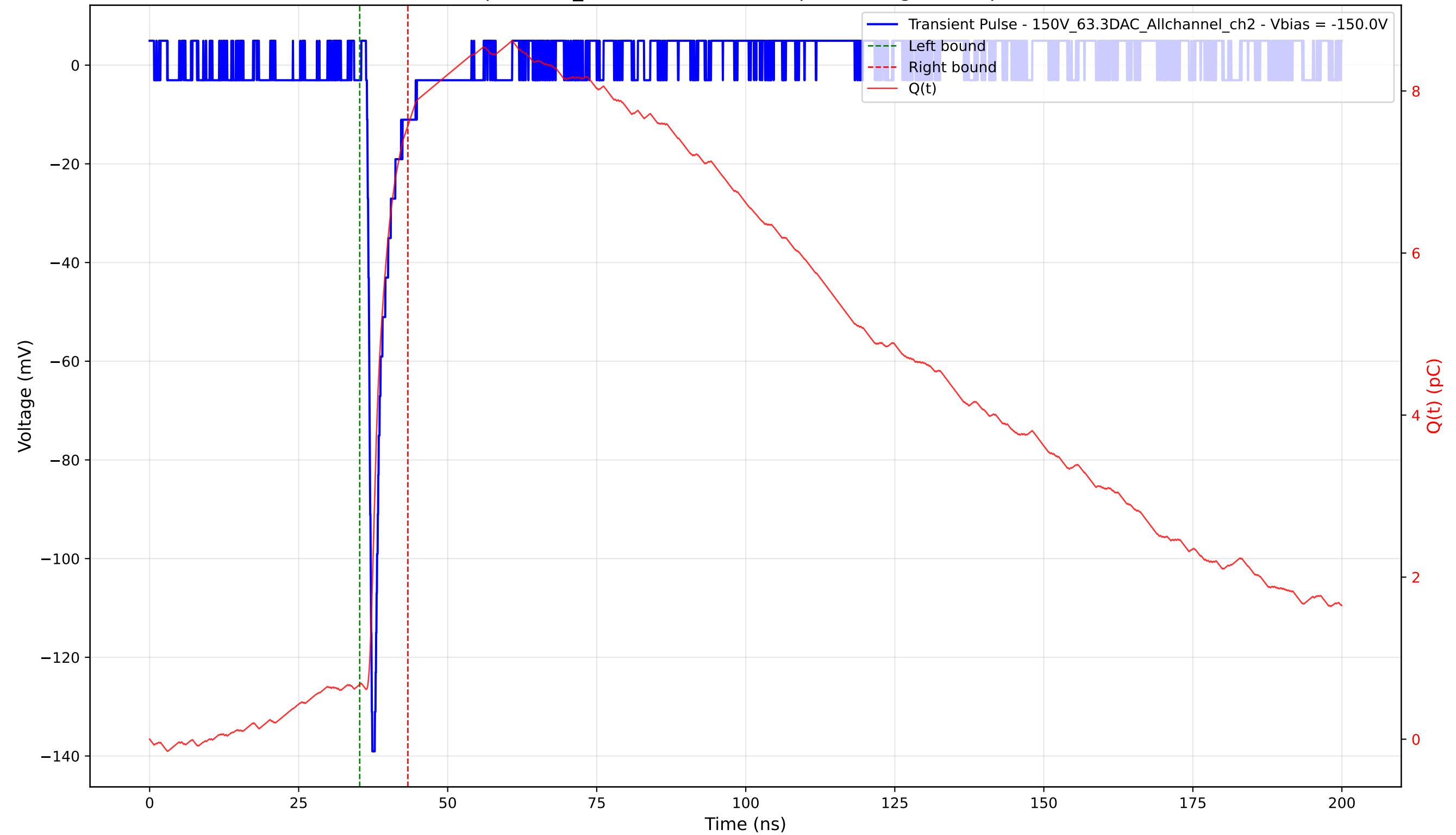
Transient Pulse - Sample: 1cm_42 - Position: 2325.0 \mu\text{m} - Charge: 6.90 pC - Rise Time: 0.75 ns
