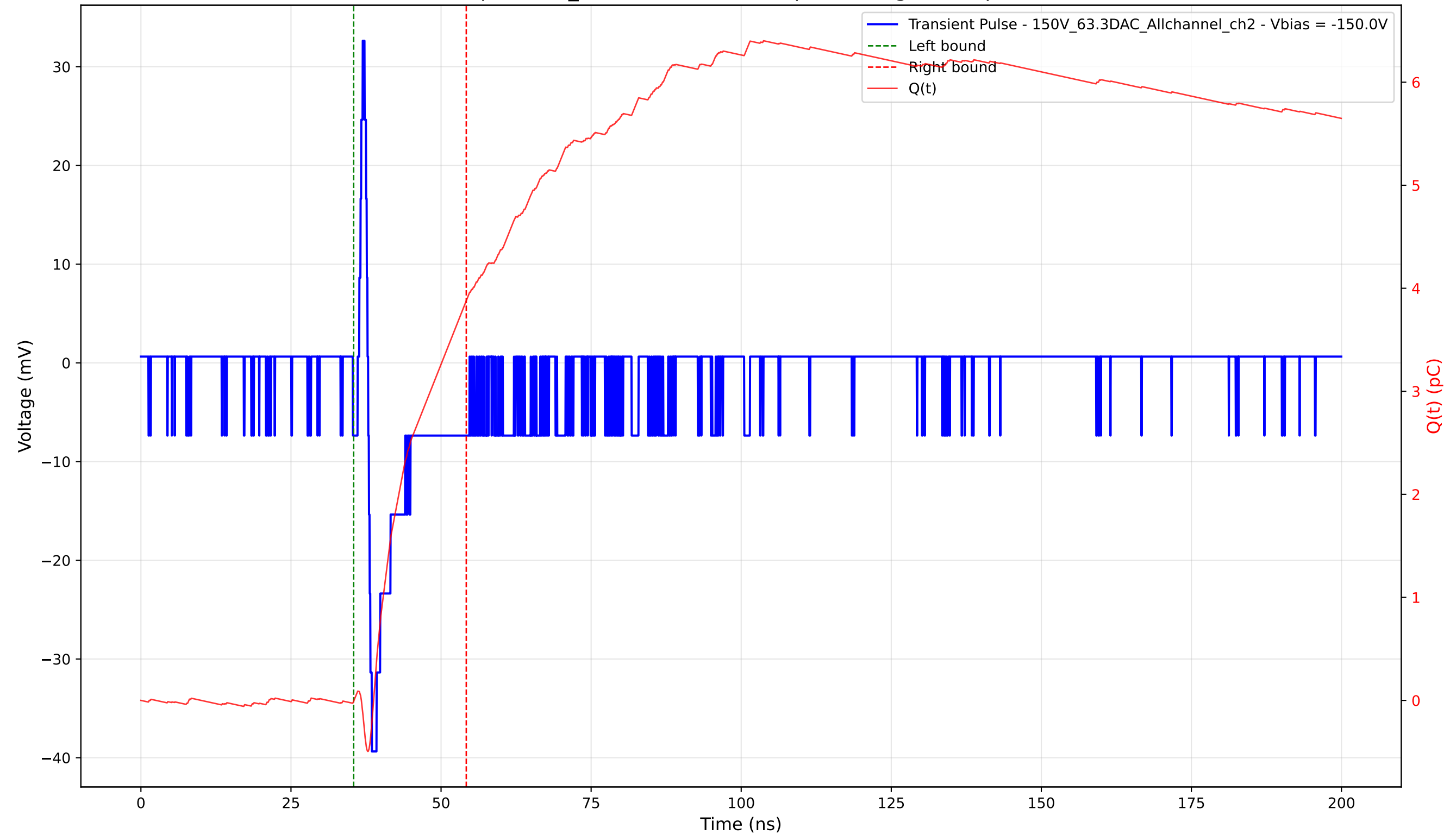
Transient Pulse - Sample: 1cm_42 - Position: 1060.0 \mu\text{m} - Charge: 3.89 pC - Rise Time: 0.62 ns
