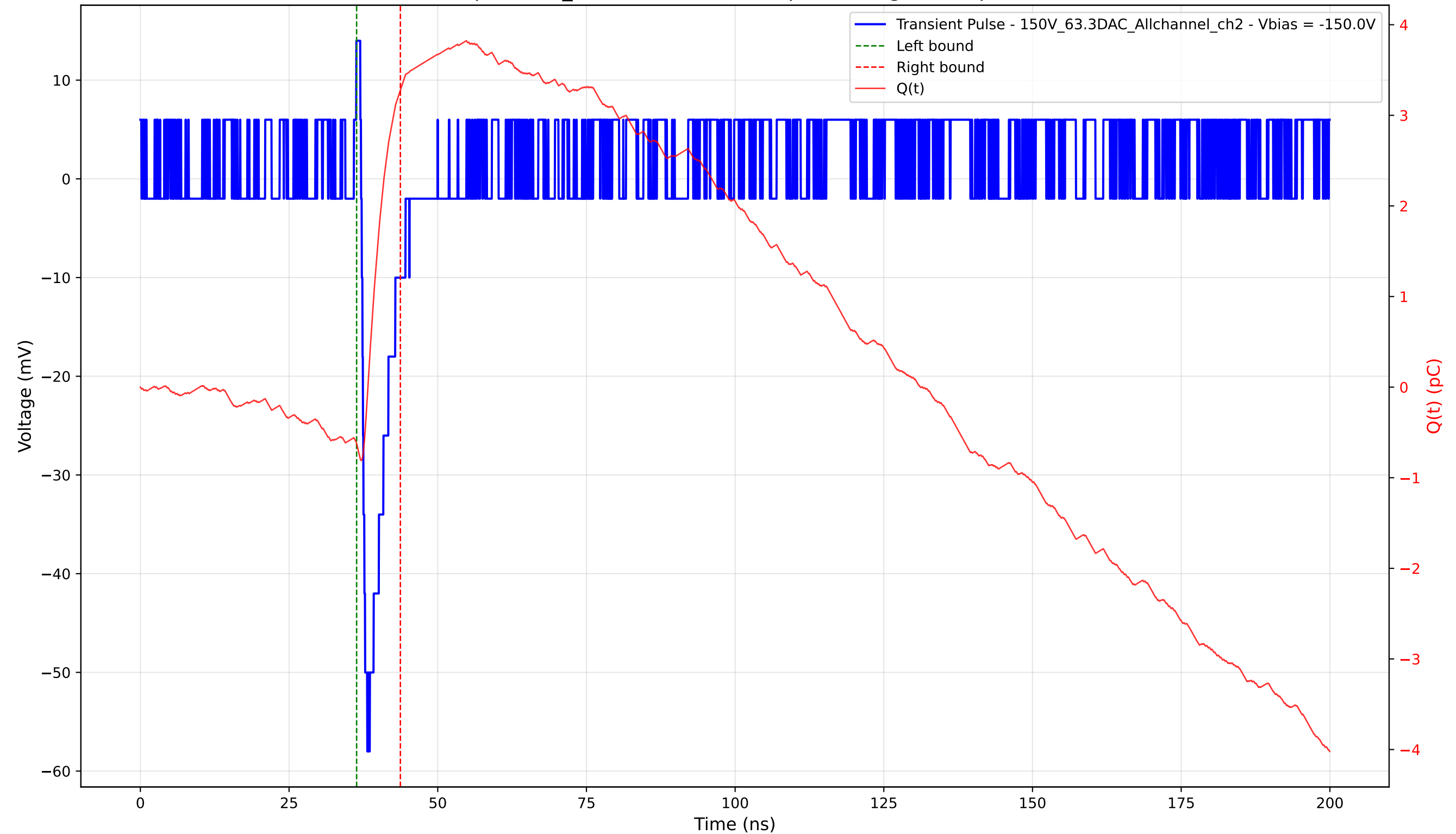
Transient Pulse - Sample: 1cm_42 - Position: 4285.0 \mu\text{m} - Charge: 3.90 pC - Rise Time: 0.94 ns
