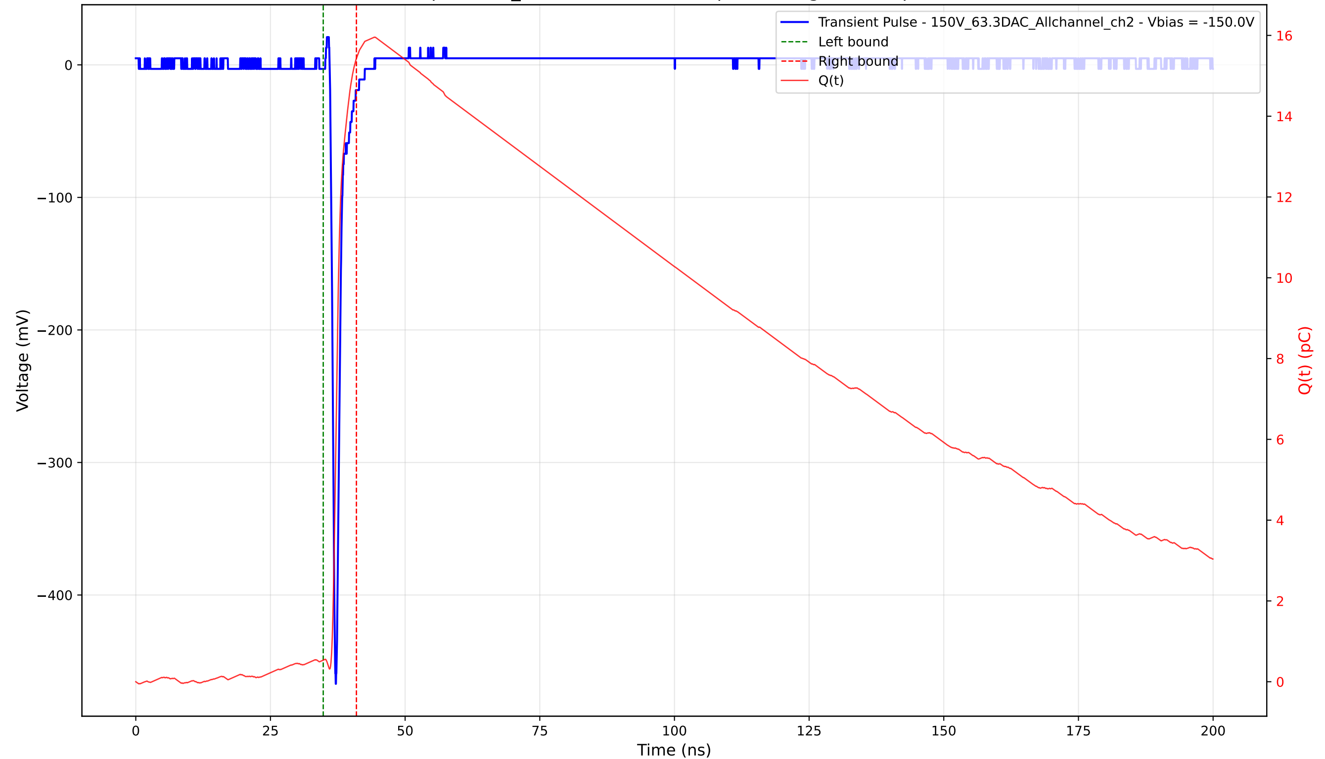
Transient Pulse - Sample: 1cm_42 - Position: 2825.0 \mu\text{m} - Charge: 14.89 pC - Rise Time: 0.73 ns
