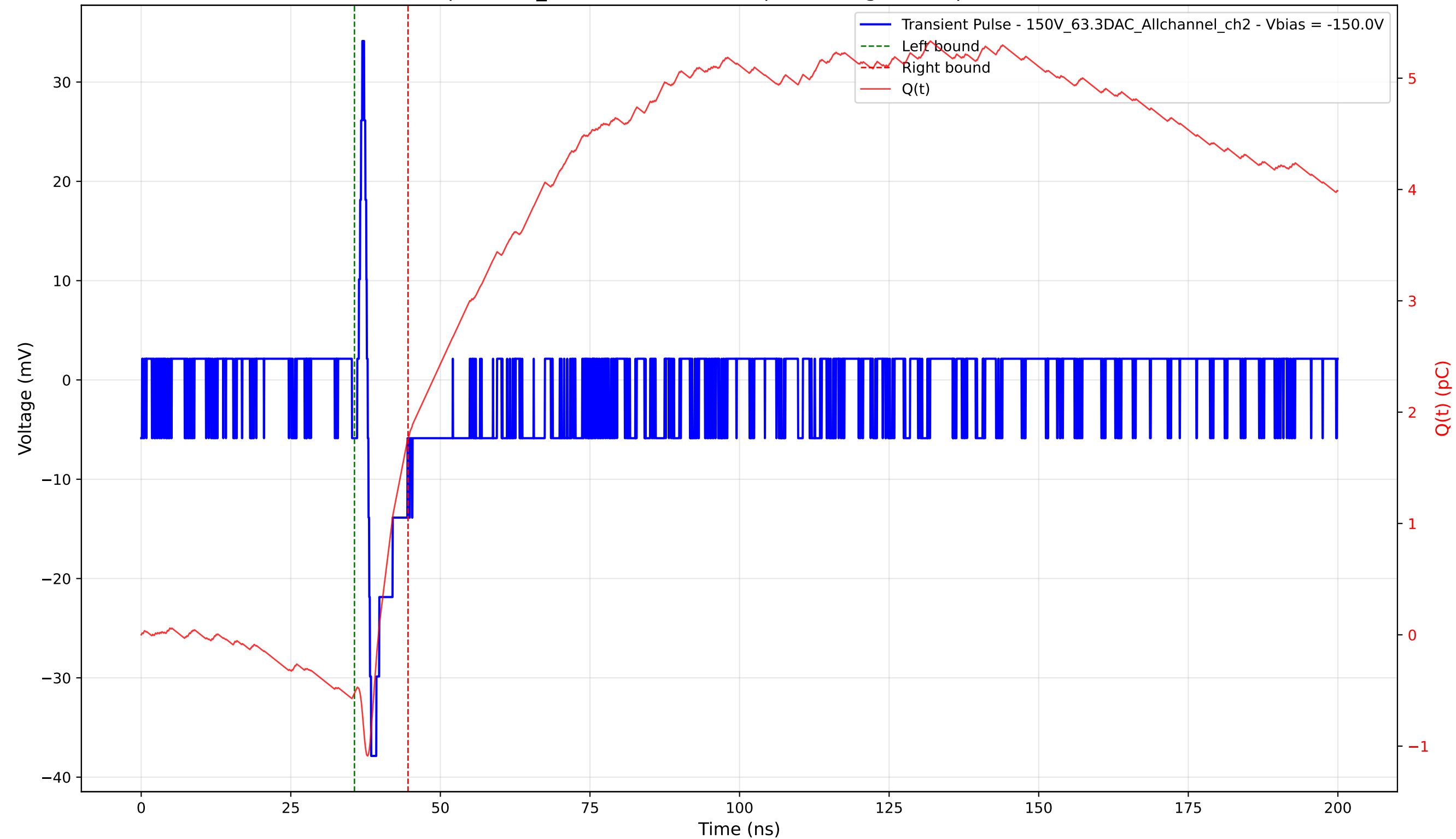
Transient Pulse - Sample: 1cm_42 - Position: 1030.0 \mu\text{m} - Charge: 2.29 pC - Rise Time: 0.00 ns (N/A)
