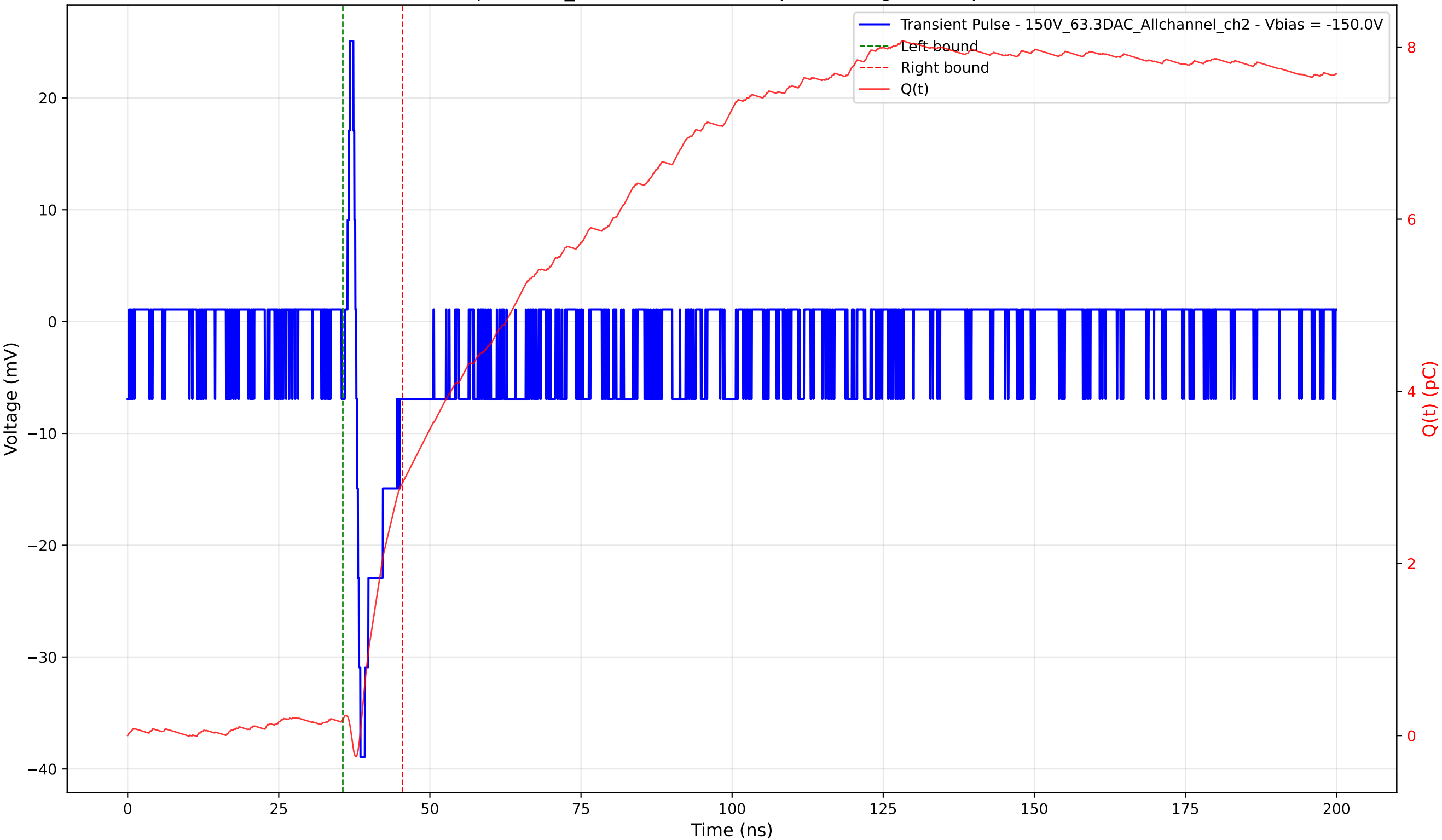
Transient Pulse - Sample: 1cm_42 - Position: 580.0 \mu\text{m} - Charge: 2.75 pC - Rise Time: 0.70 ns
