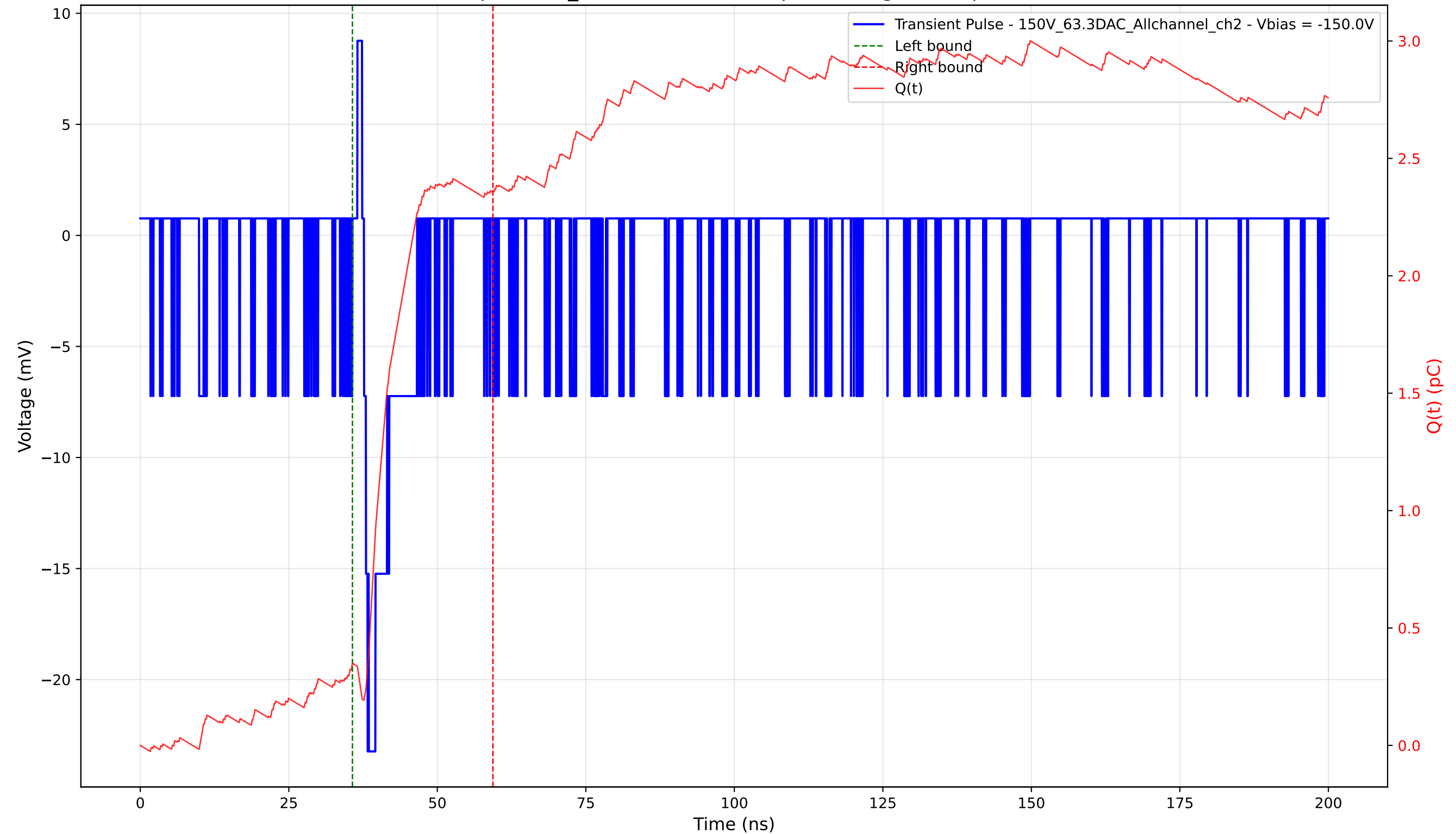
Transient Pulse - Sample: 1cm_42 - Position: 265.0 \mu\text{m} - Charge: 2.01 pC - Rise Time: 0.63 ns
