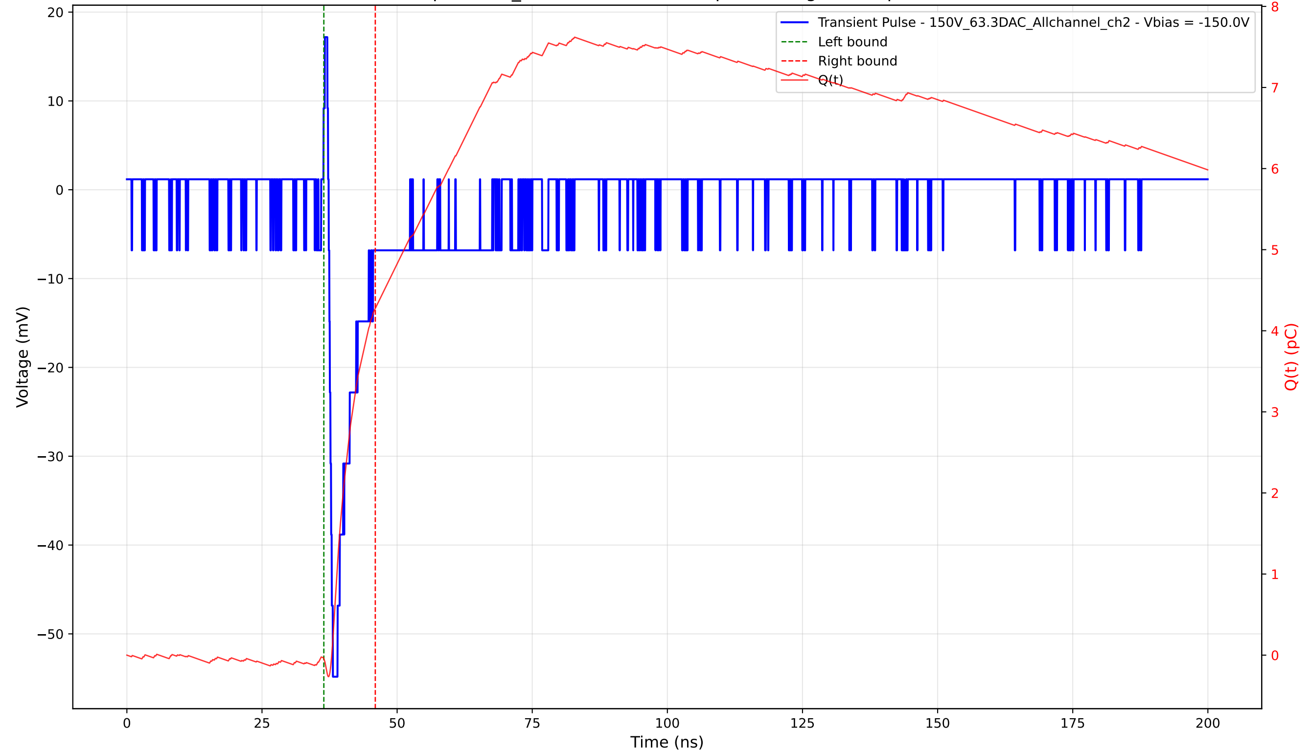
Transient Pulse - Sample: 1cm_42 - Position: 1670.0 \mu\text{m} - Charge: 4.32 pC - Rise Time: 0.77 ns
