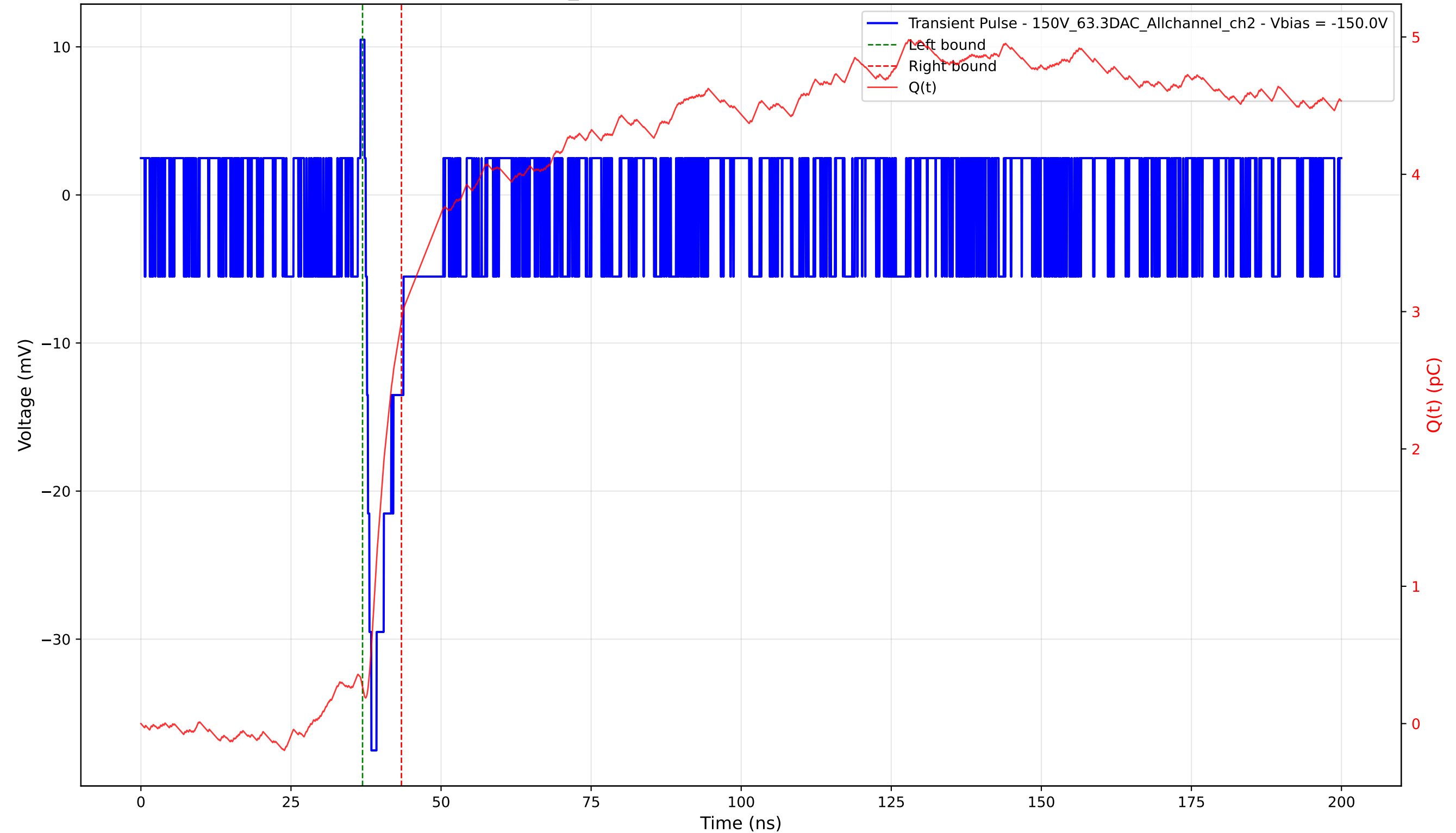
Transient Pulse - Sample: 1cm_42 - Position: 4850.0 \mu\text{m} - Charge: 2.66 pC - Rise Time: 0.94 ns
