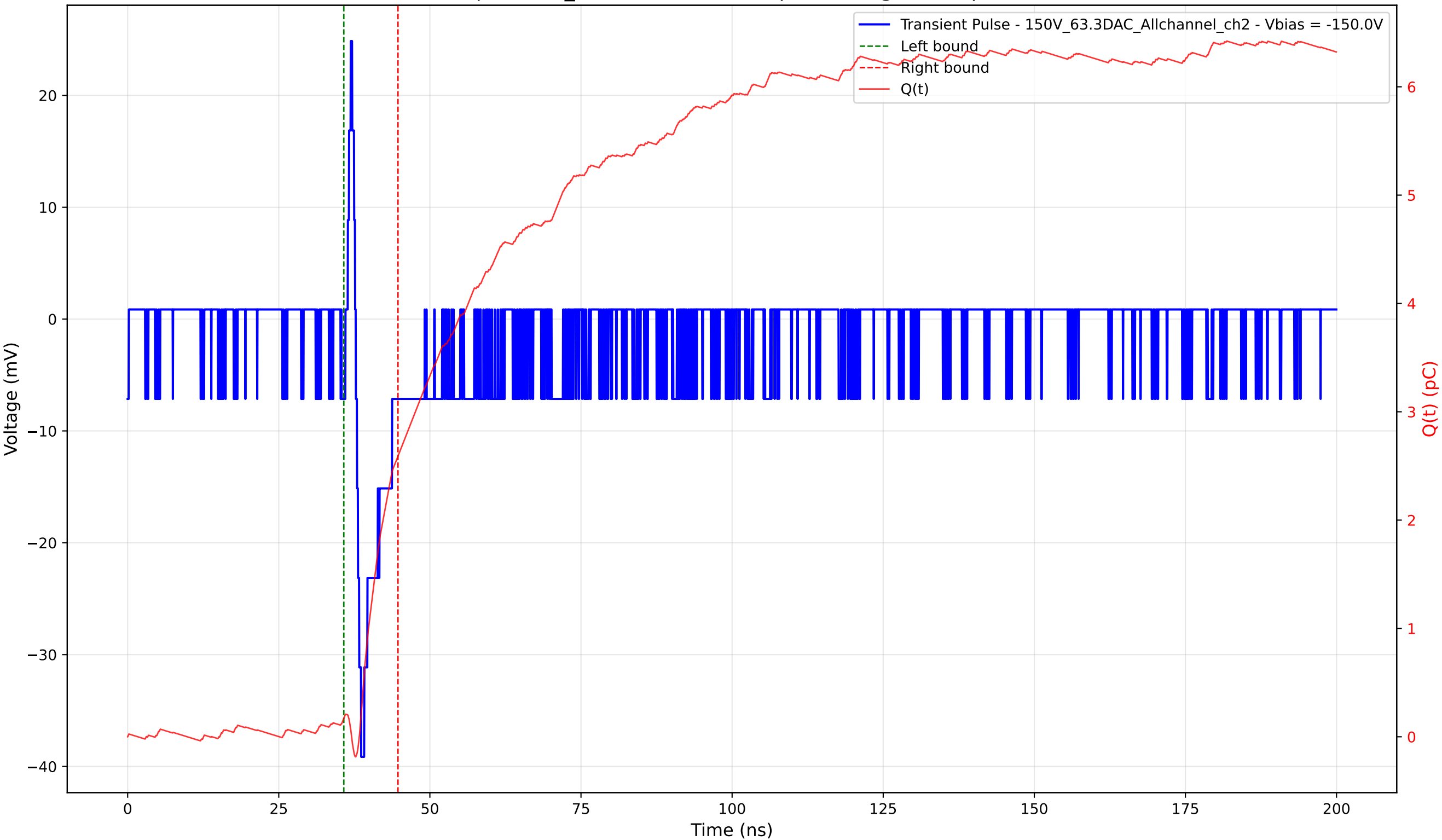
Transient Pulse - Sample: 1cm_42 - Position: 525.0 \mu\text{m} - Charge: 2.42 pC - Rise Time: 0.90 ns
