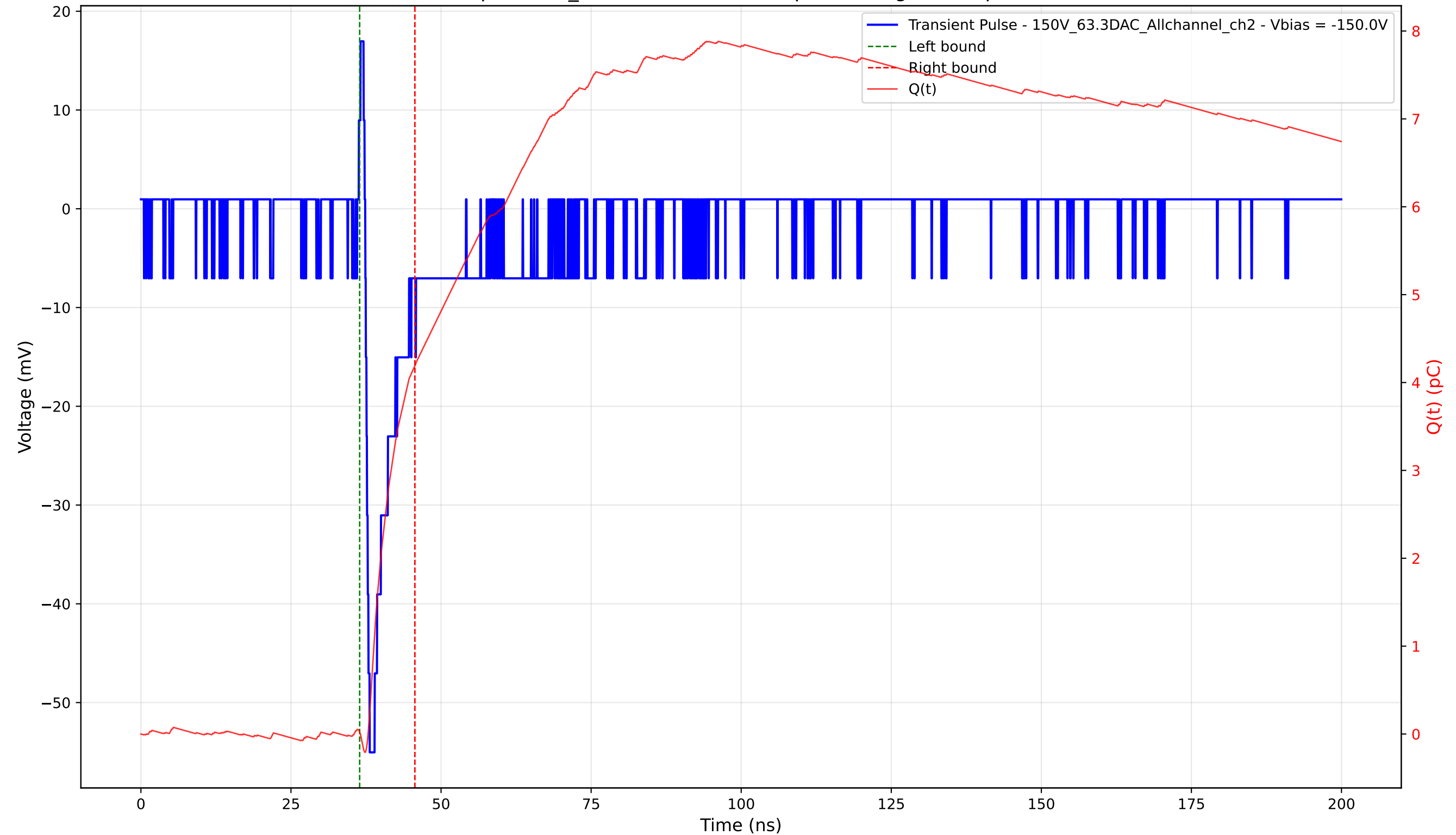
Transient Pulse - Sample: 1cm_42 - Position: 1655.0 \mu\text{m} - Charge: 4.16 pC - Rise Time: 0.73 ns
