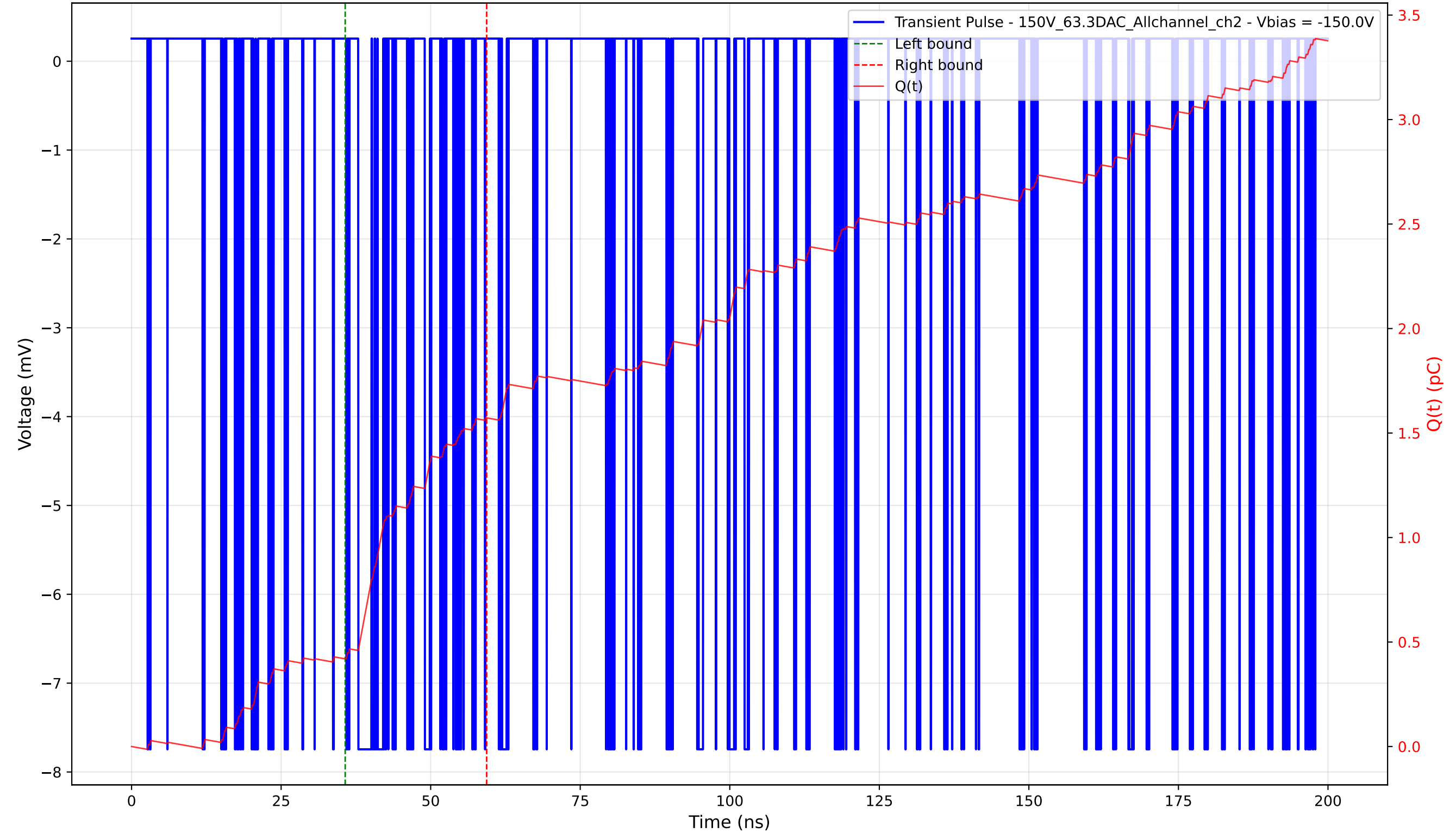
Transient Pulse - Sample: 1cm_42 - Position: 50.0 \mu\text{m} - Charge: 1.15 pC - Rise Time: 0.04 ns
