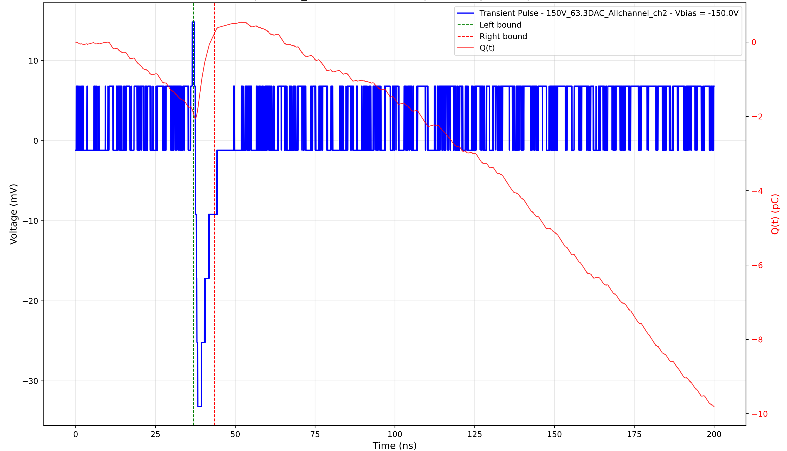
Transient Pulse - Sample: 1cm_42 - Position: 4770.0 \mu\text{m} - Charge: 2.17 pC - Rise Time: 0.71 ns
