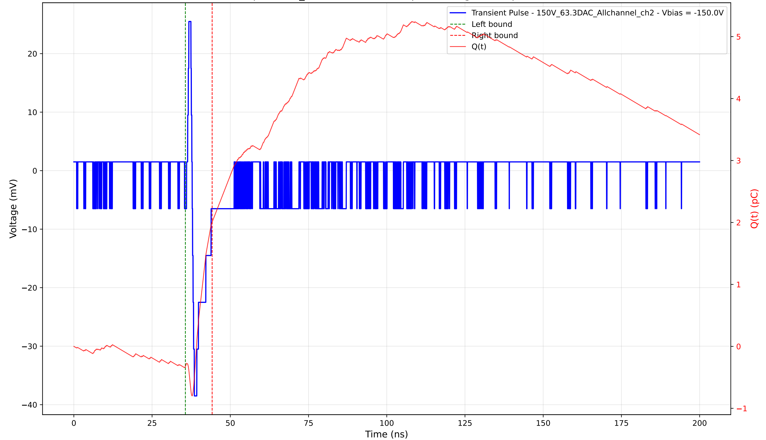
Transient Pulse - Sample: 1cm_42 - Position: 600.0 \mu\text{m} - Charge: 2.33 pC - Rise Time: 0.70 ns
