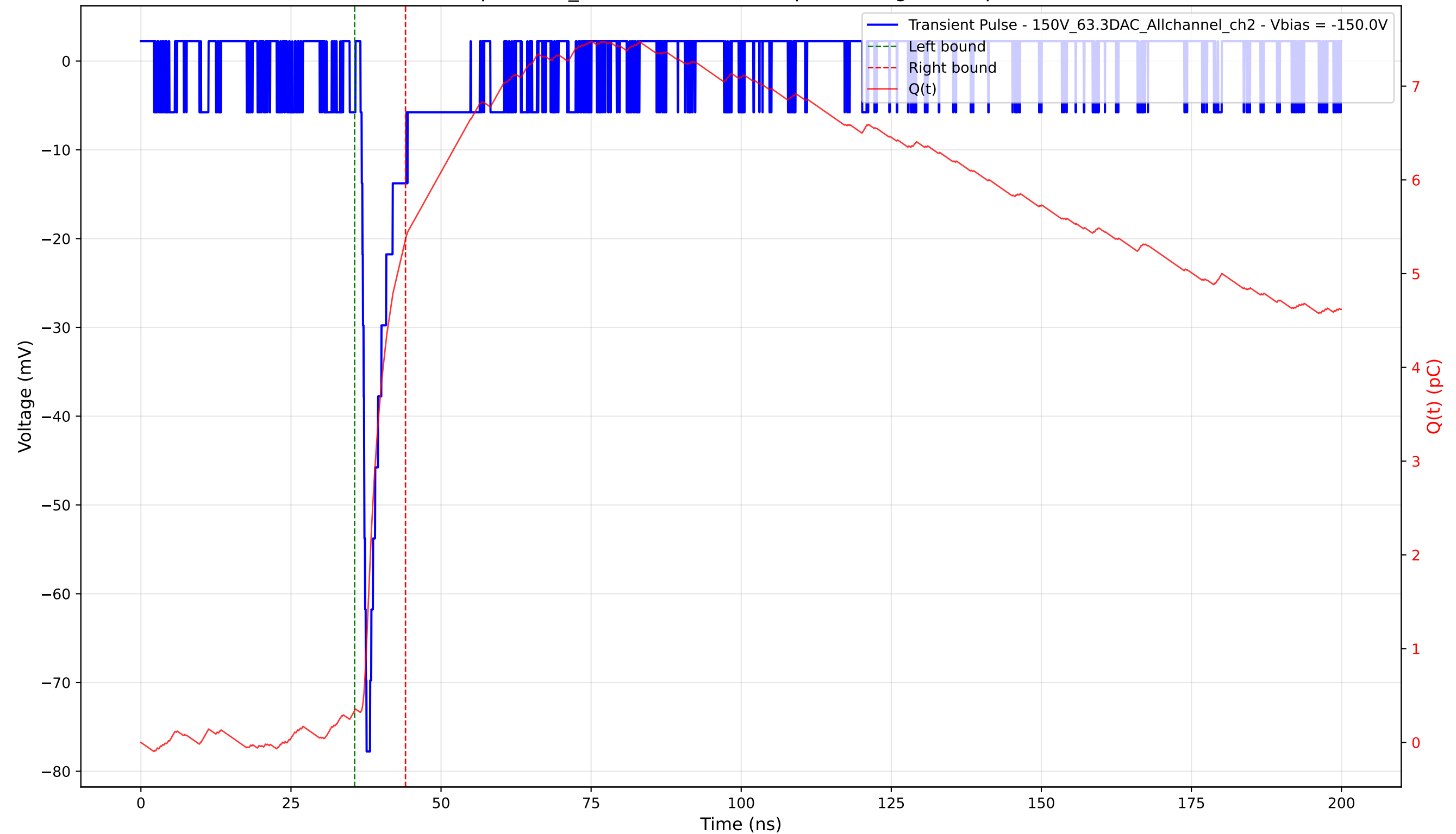
Transient Pulse - Sample: 1cm_42 - Position: 2045.0 \mu\text{m} - Charge: 5.03 pC - Rise Time: 0.83 ns
