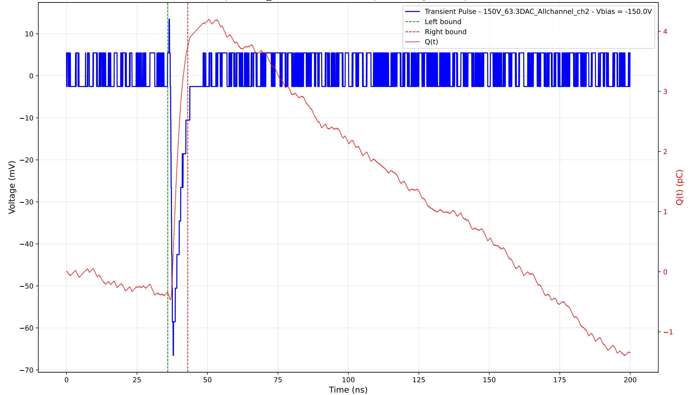
Transient Pulse - Sample: 1cm_42 - Position: 4065.0 \mu\text{m} - Charge: 4.09 pC - Rise Time: 0.90 ns
