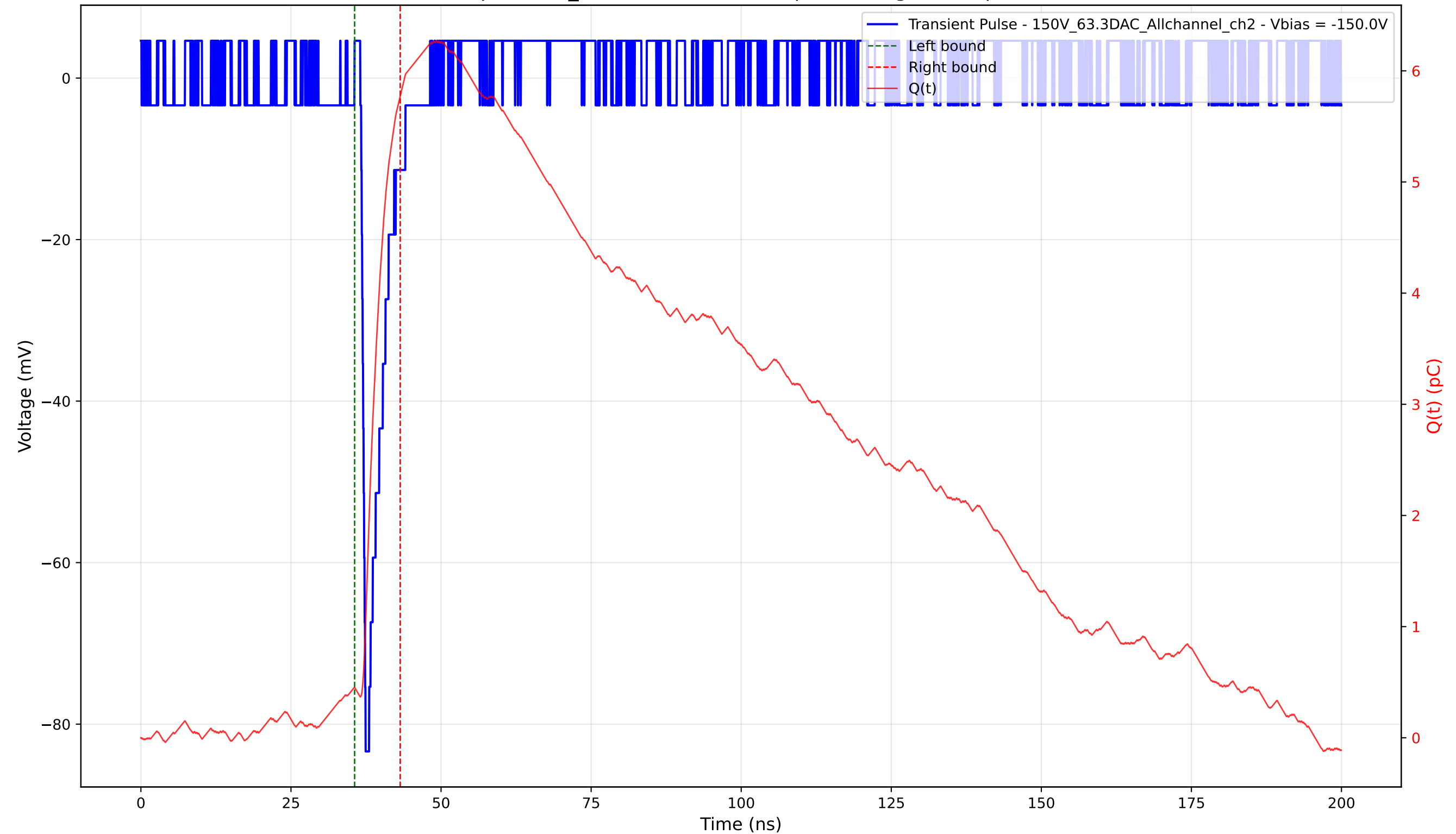
Transient Pulse - Sample: 1cm_42 - Position: 3945.0 \mu\text{m} - Charge: 5.32 pC - Rise Time: 0.66 ns
