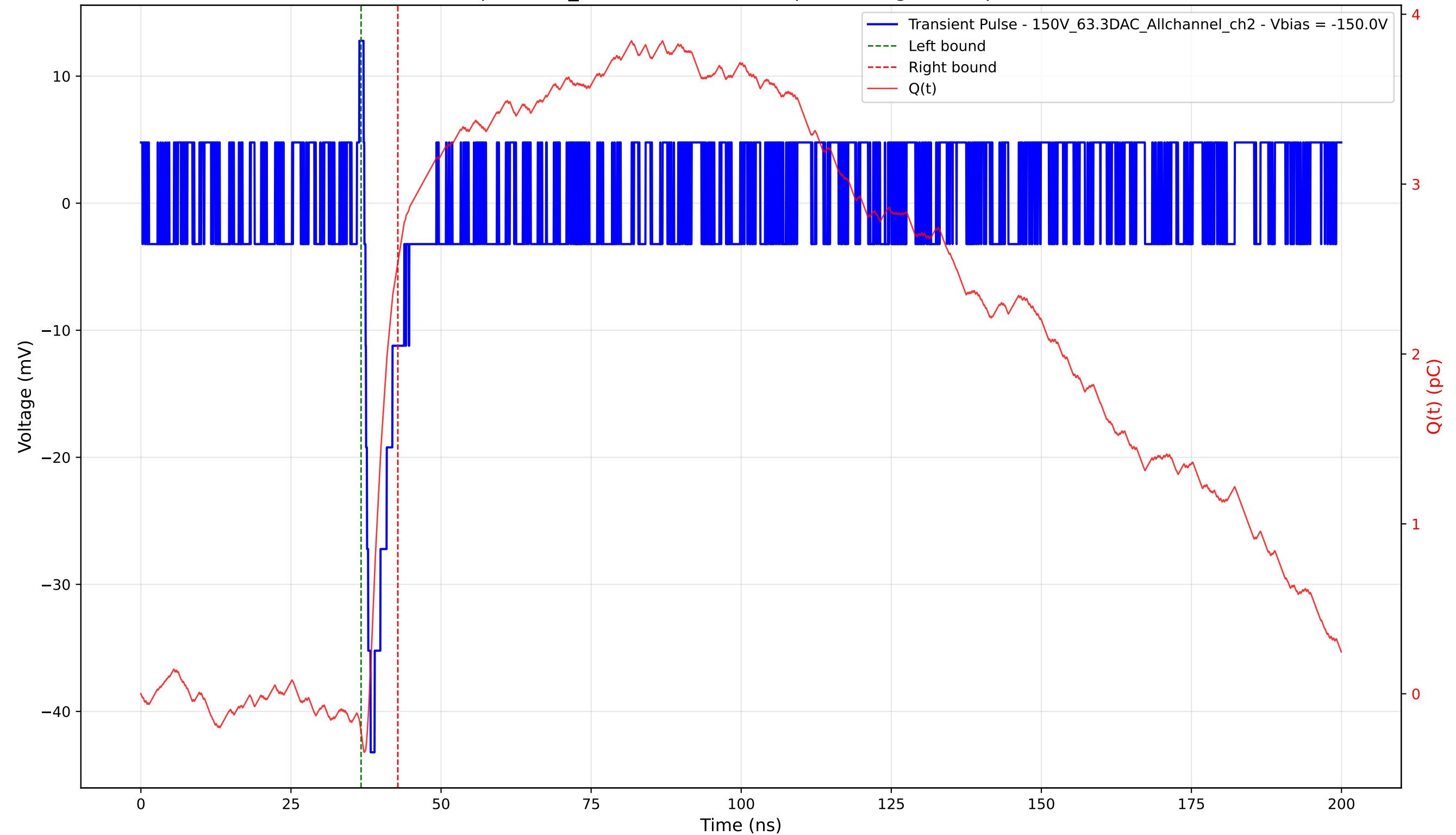
Transient Pulse - Sample: 1cm_42 - Position: 4480.0 \mu\text{m} - Charge: 2.77 pC - Rise Time: 0.87 ns
