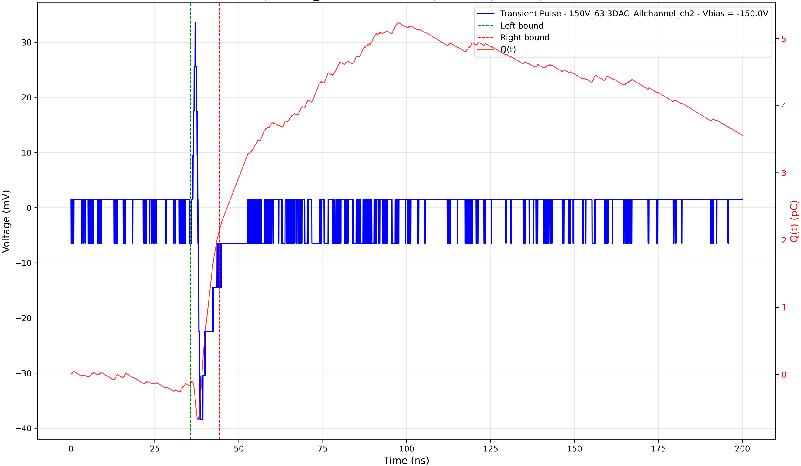
Transient Pulse - Sample: 1cm_42 - Position: 620.0 \mu\text{m} - Charge: 2.31 pC - Rise Time: 0.66 ns
