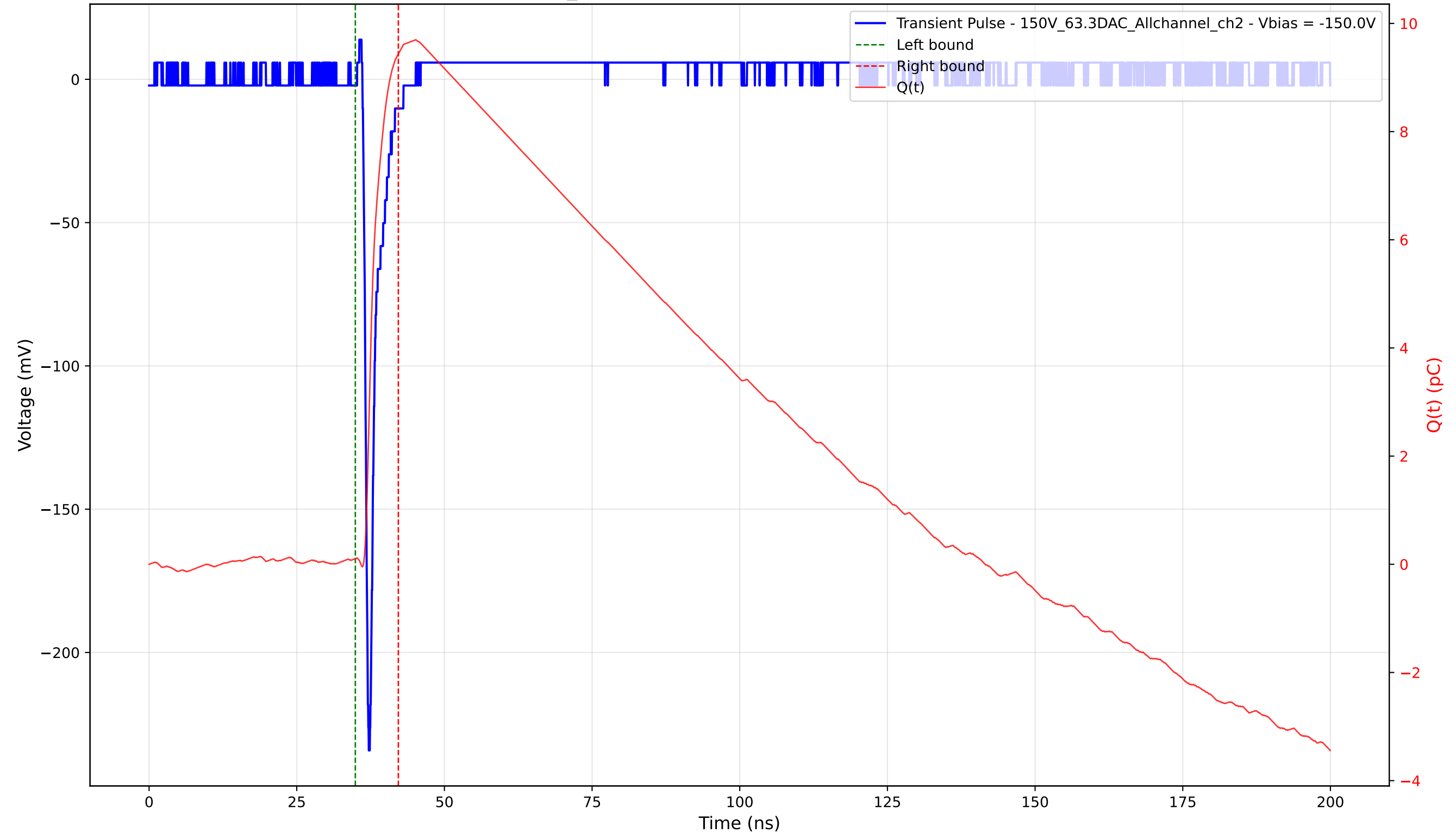
Transient Pulse - Sample: 1cm_42 - Position: 3490.0 \mu\text{m} - Charge: 9.33 pC - Rise Time: 0.77 ns
