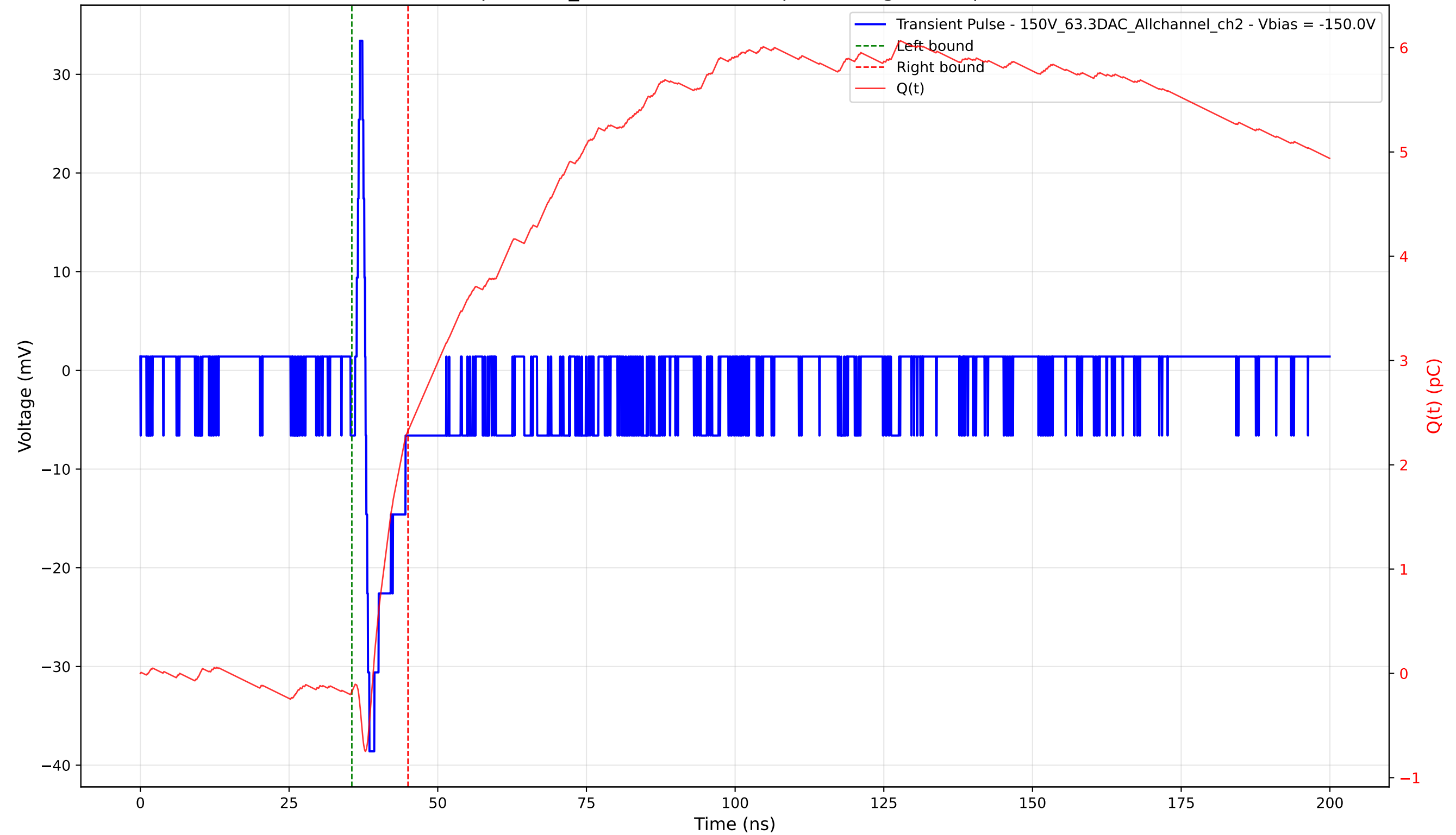
Transient Pulse - Sample: 1cm_42 - Position: 895.0 \mu\text{m} - Charge: 2.50 pC - Rise Time: 0.66 ns
