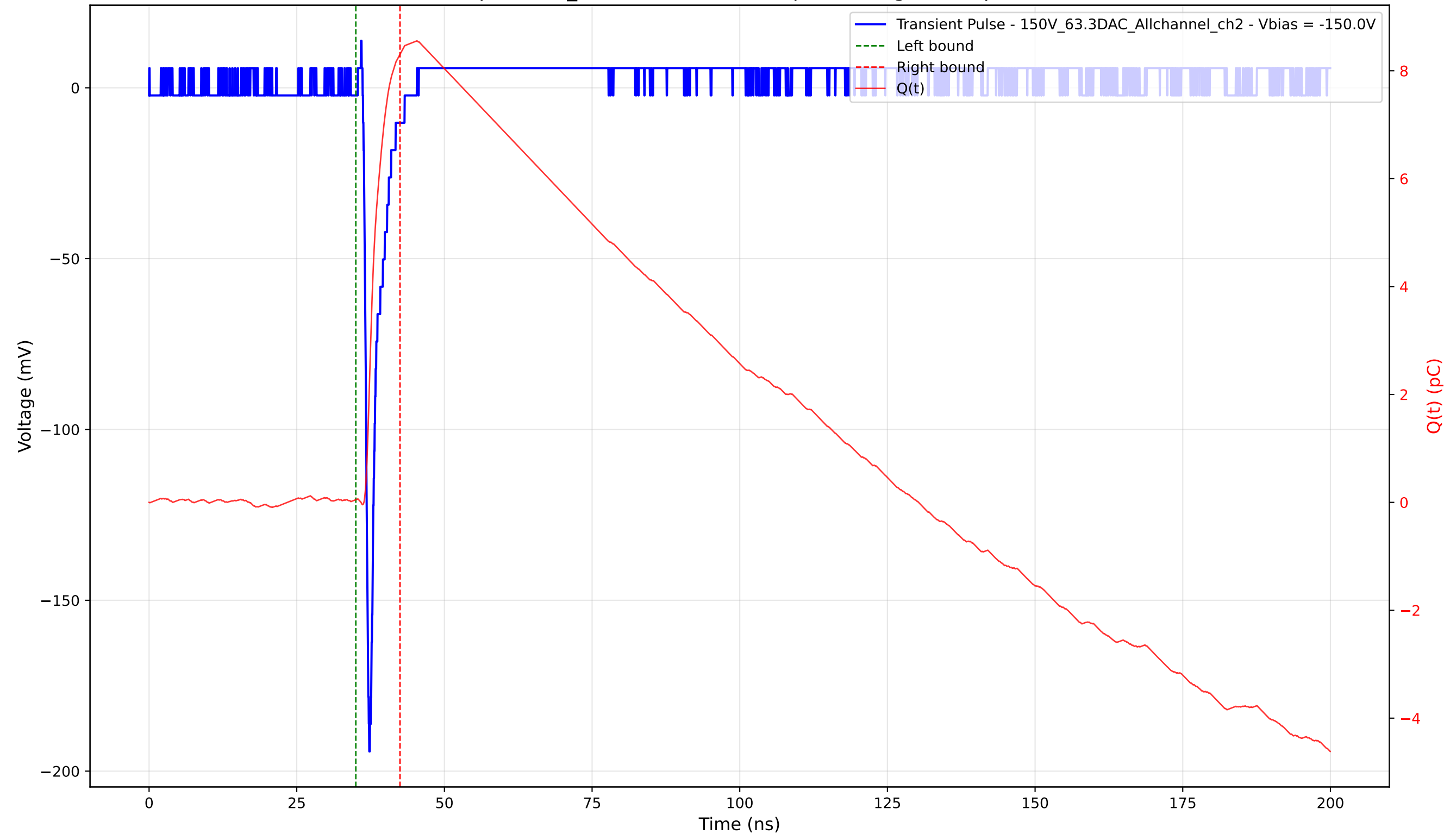
Transient Pulse - Sample: 1cm_42 - Position: 3550.0 \mu\text{m} - Charge: 8.25 pC - Rise Time: 0.75 ns
