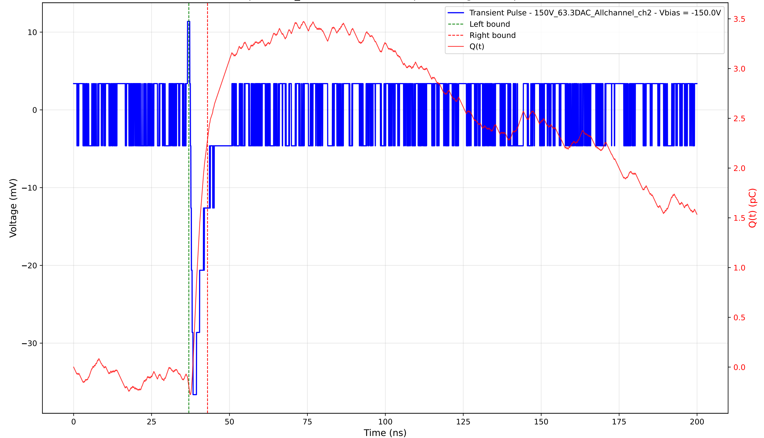
Transient Pulse - Sample: 1cm_42 - Position: 4815.0 \mu\text{m} - Charge: 2.48 pC - Rise Time: 0.87 ns
