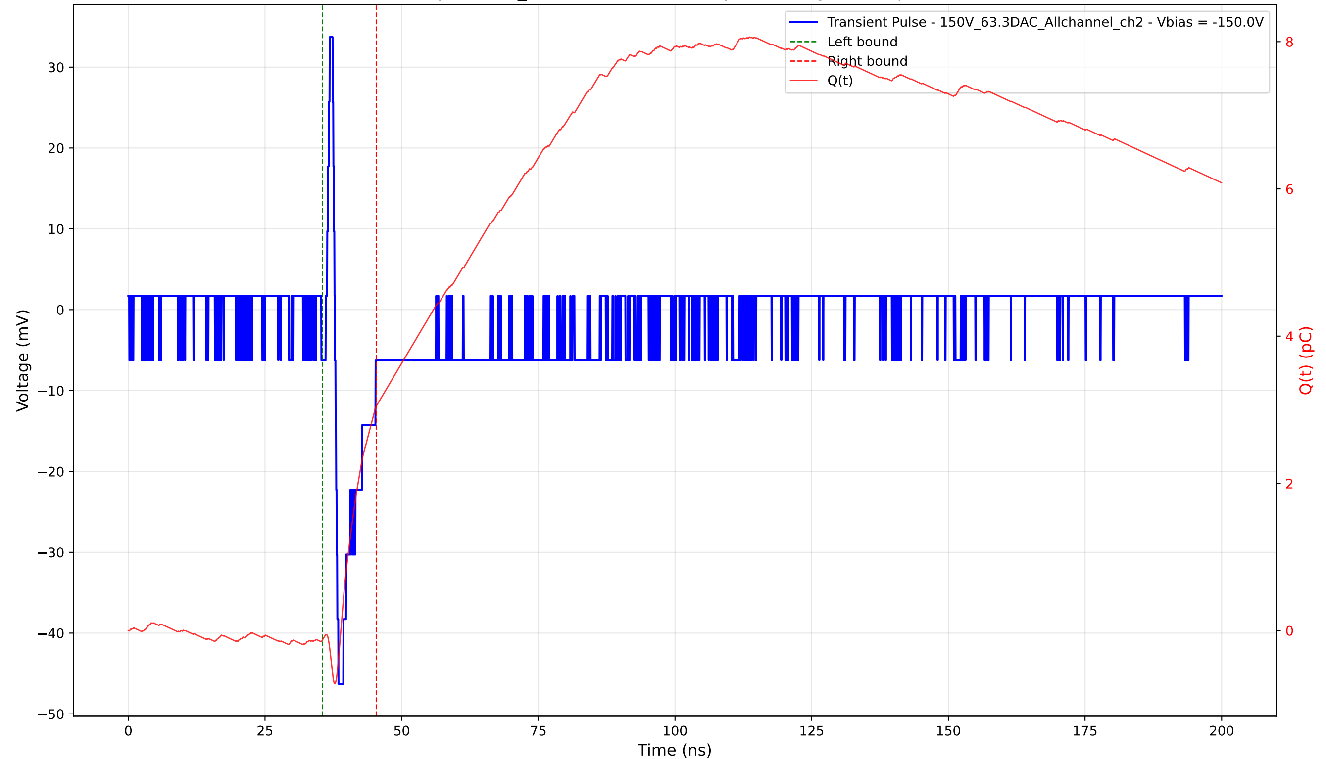
Transient Pulse - Sample: 1cm_42 - Position: 1230.0 \mu\text{m} - Charge: 3.17 pC - Rise Time: 0.65 ns
