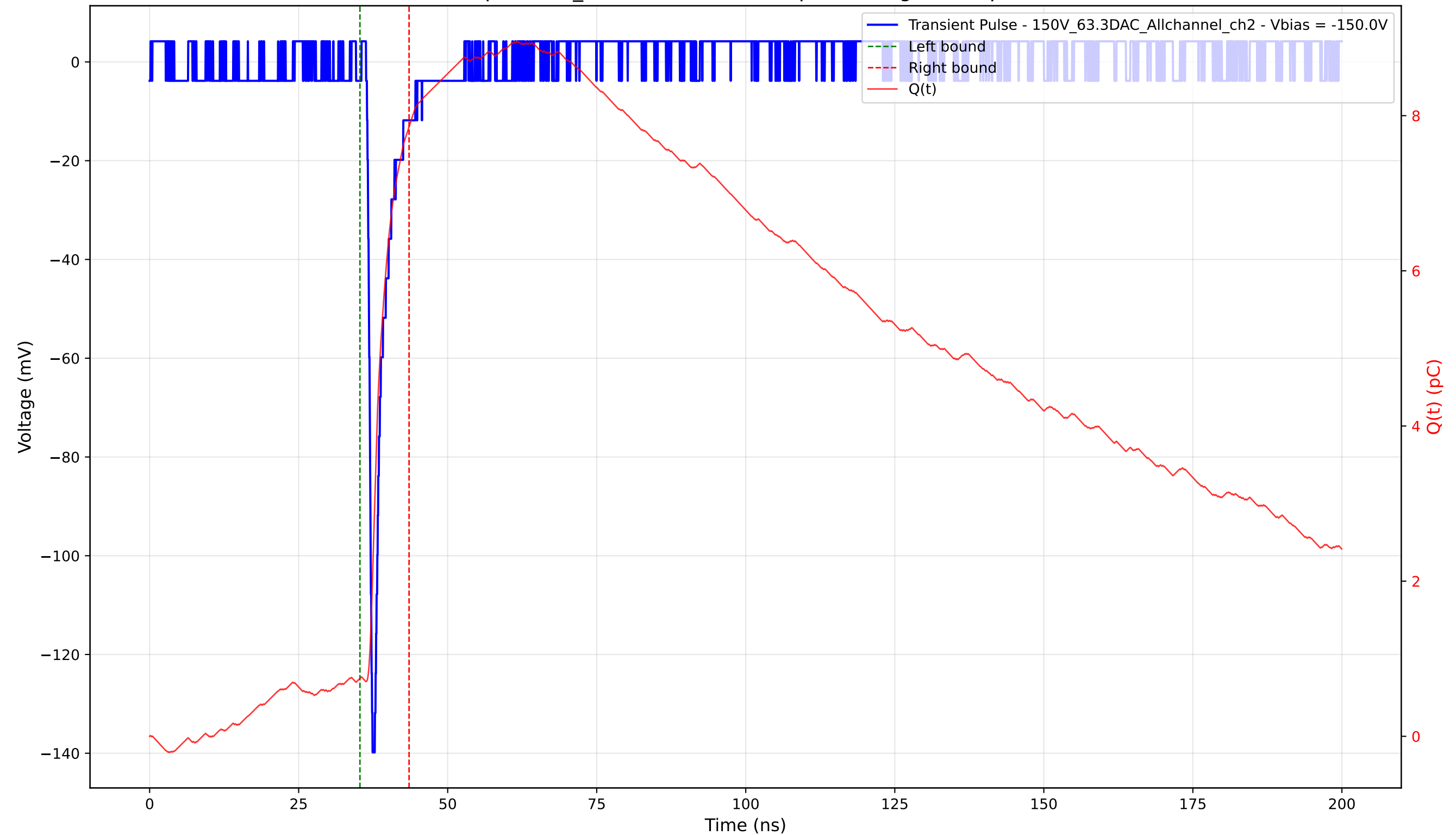
Transient Pulse - Sample: 1cm_42 - Position: 2290.0 \mu\text{m} - Charge: 7.11 pC - Rise Time: 0.79 ns
