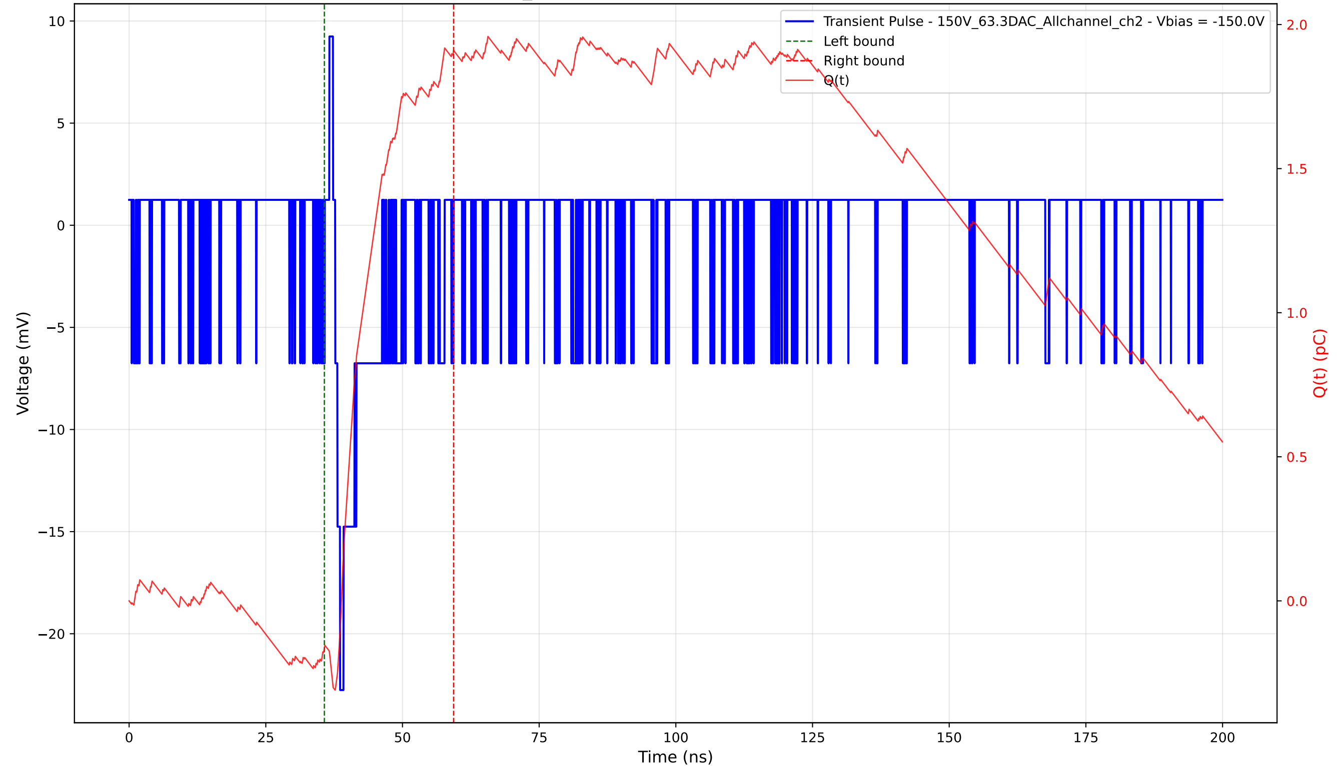
Transient Pulse - Sample: 1cm_42 - Position: 215.0 \mu\text{m} - Charge: 2.07 pC - Rise Time: 0.91 ns
