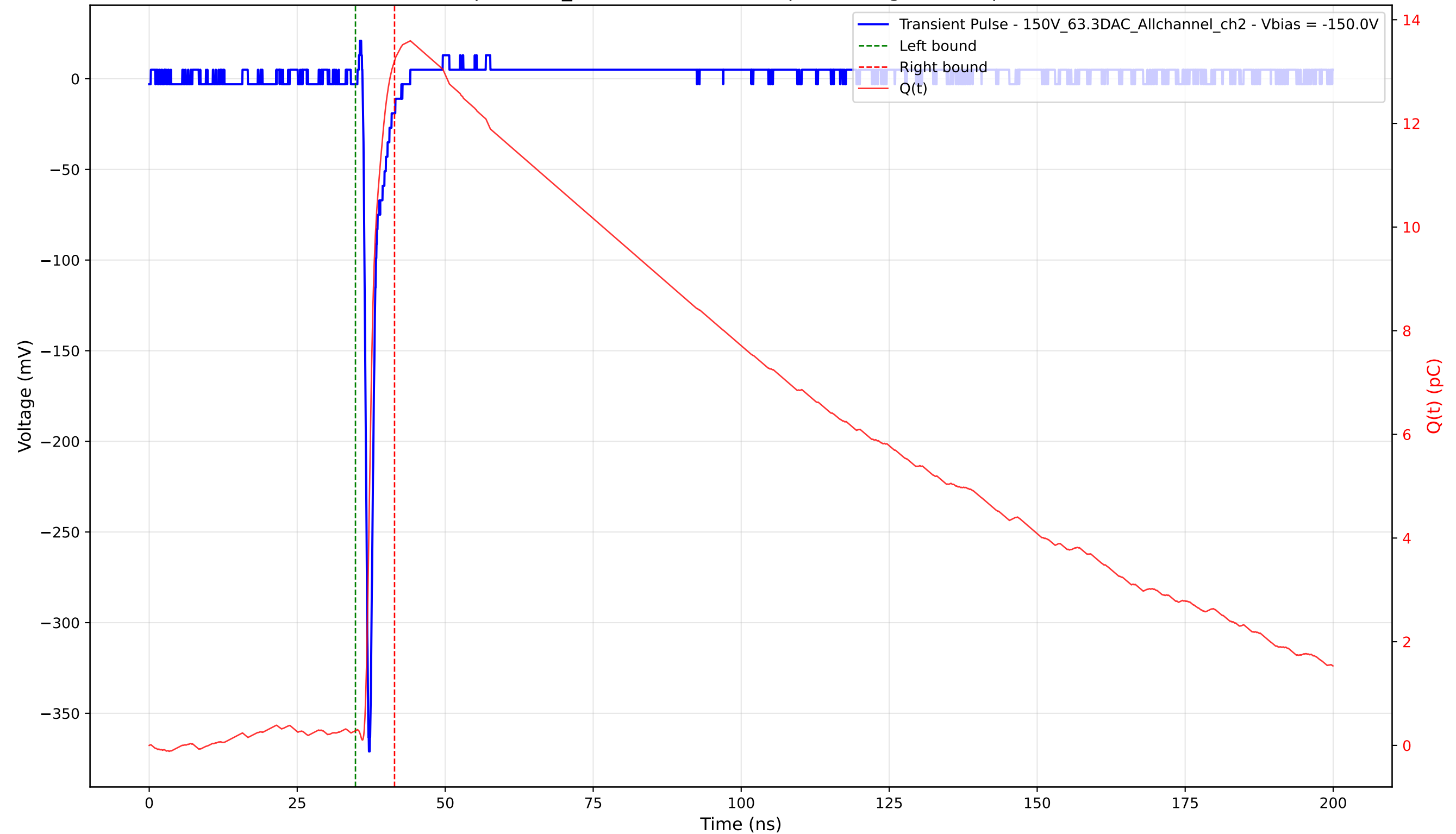
Transient Pulse - Sample: 1cm_42 - Position: 3355.0 \mu\text{m} - Charge: 12.92 pC - Rise Time: 0.74 ns
