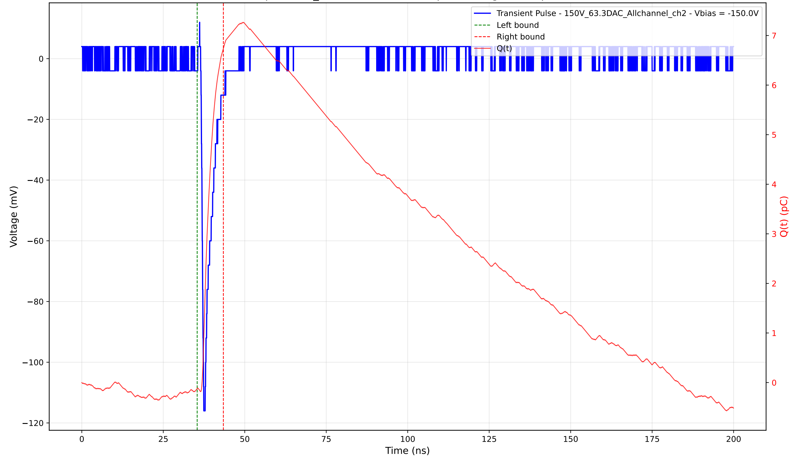
Transient Pulse - Sample: 1cm_42 - Position: 3850.0 \mu\text{m} - Charge: 6.86 pC - Rise Time: 0.76 ns
