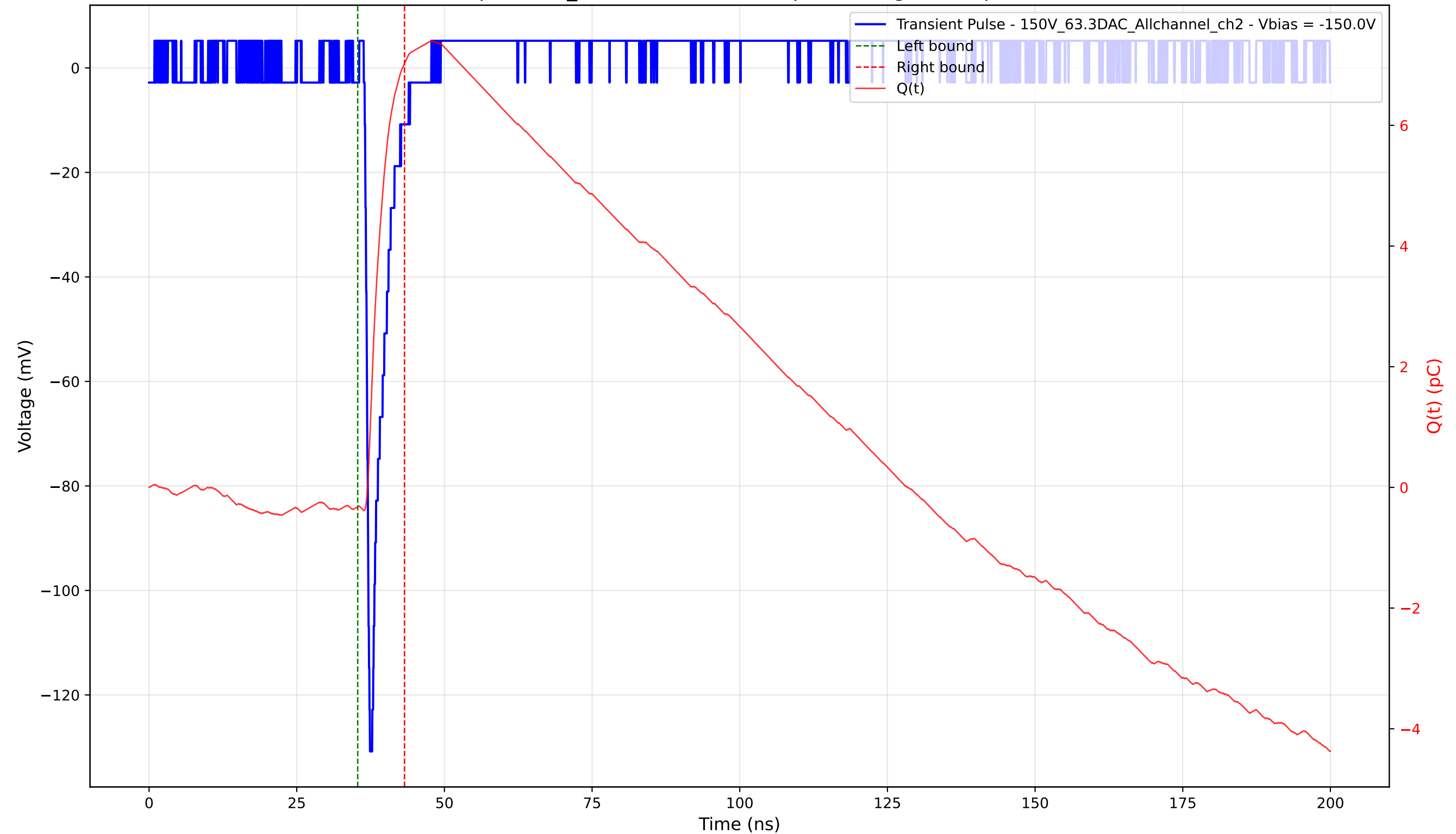
Transient Pulse - Sample: 1cm_42 - Position: 3760.0 \mu\text{m} - Charge: 7.35 pC - Rise Time: 0.75 ns
