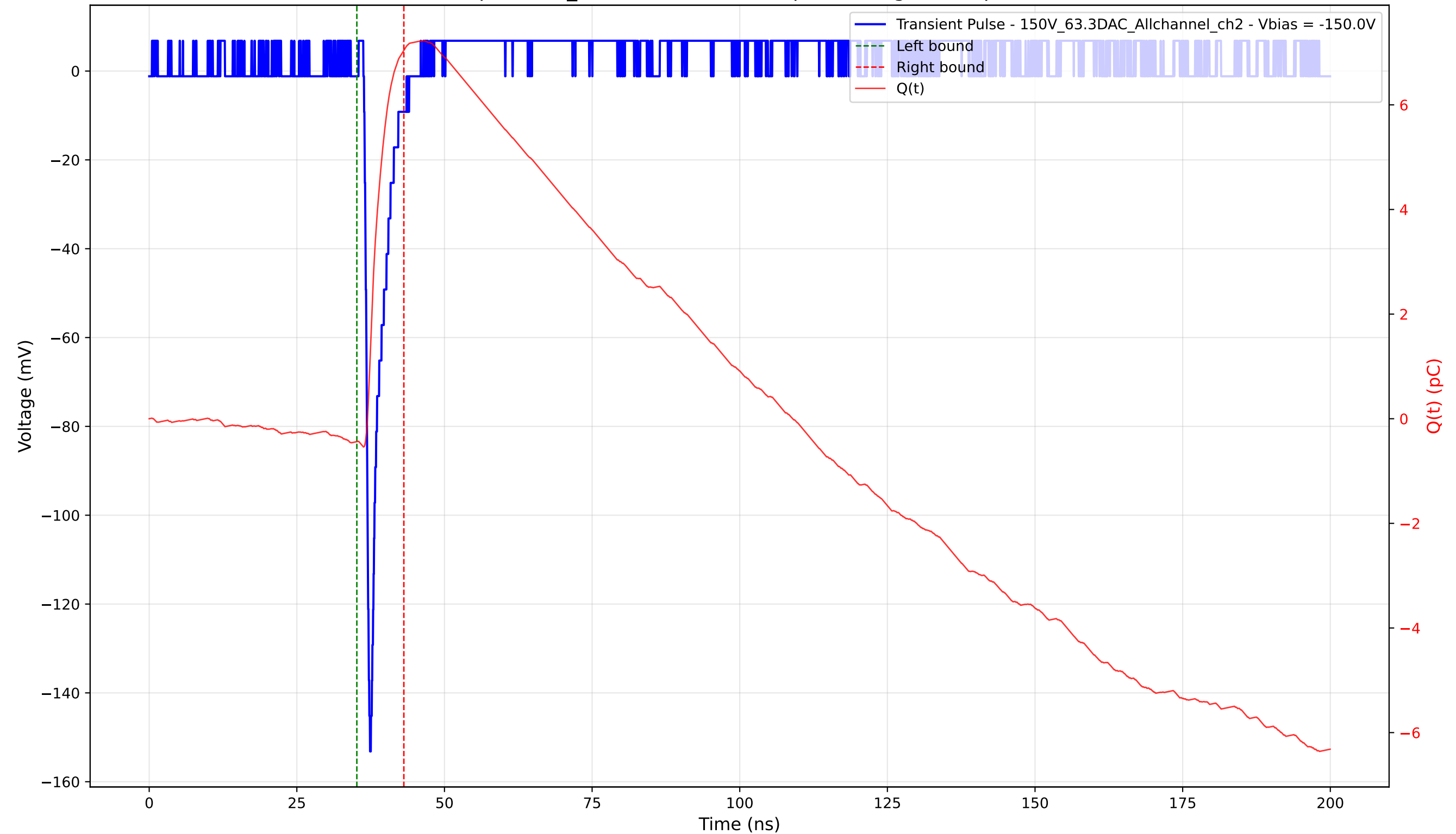
Transient Pulse - Sample: 1cm_42 - Position: 3660.0 \mu\text{m} - Charge: 7.48 pC - Rise Time: 0.81 ns
