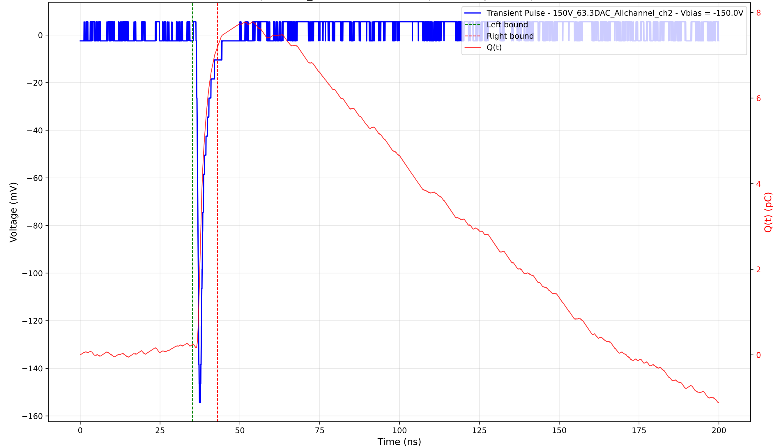
Transient Pulse - Sample: 1cm_42 - Position: 2405.0 \mu\text{m} - Charge: 6.95 pC - Rise Time: 0.78 ns
