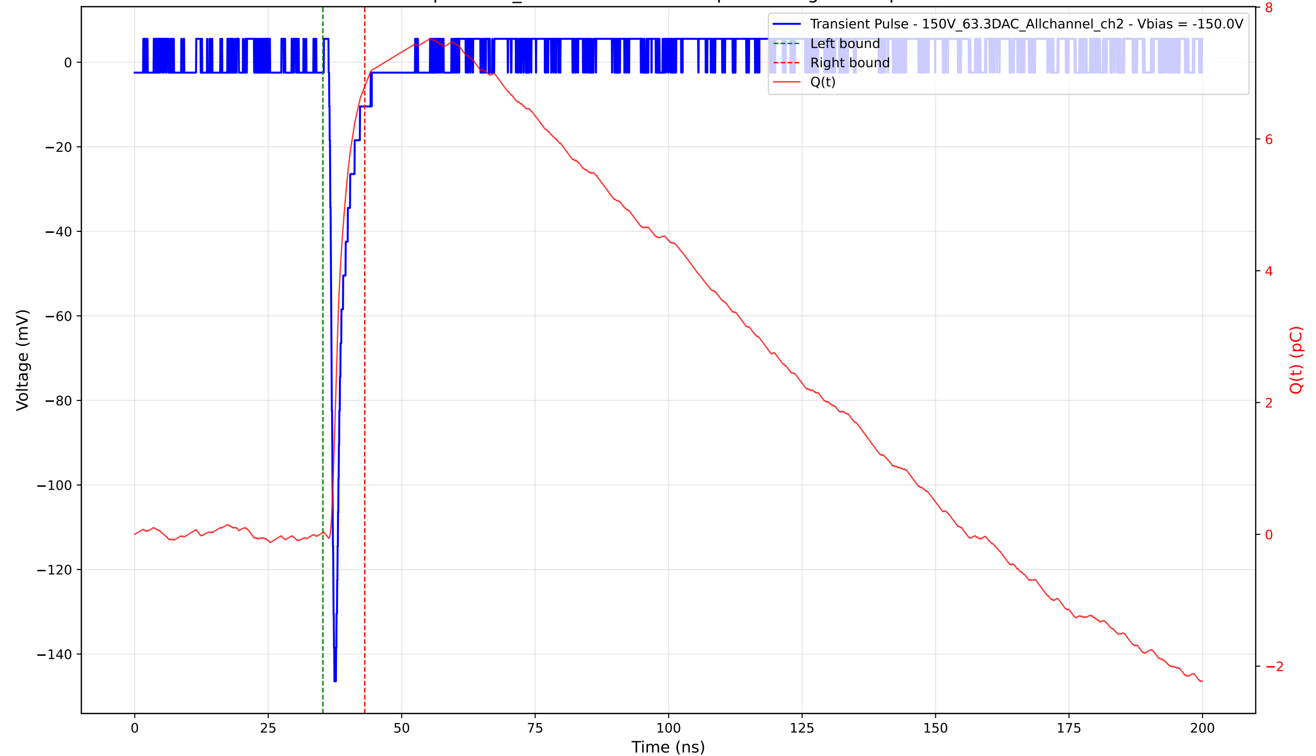
Transient Pulse - Sample: 1cm_42 - Position: 2355.0 \mu\text{m} - Charge: 6.77 pC - Rise Time: 0.82 ns
