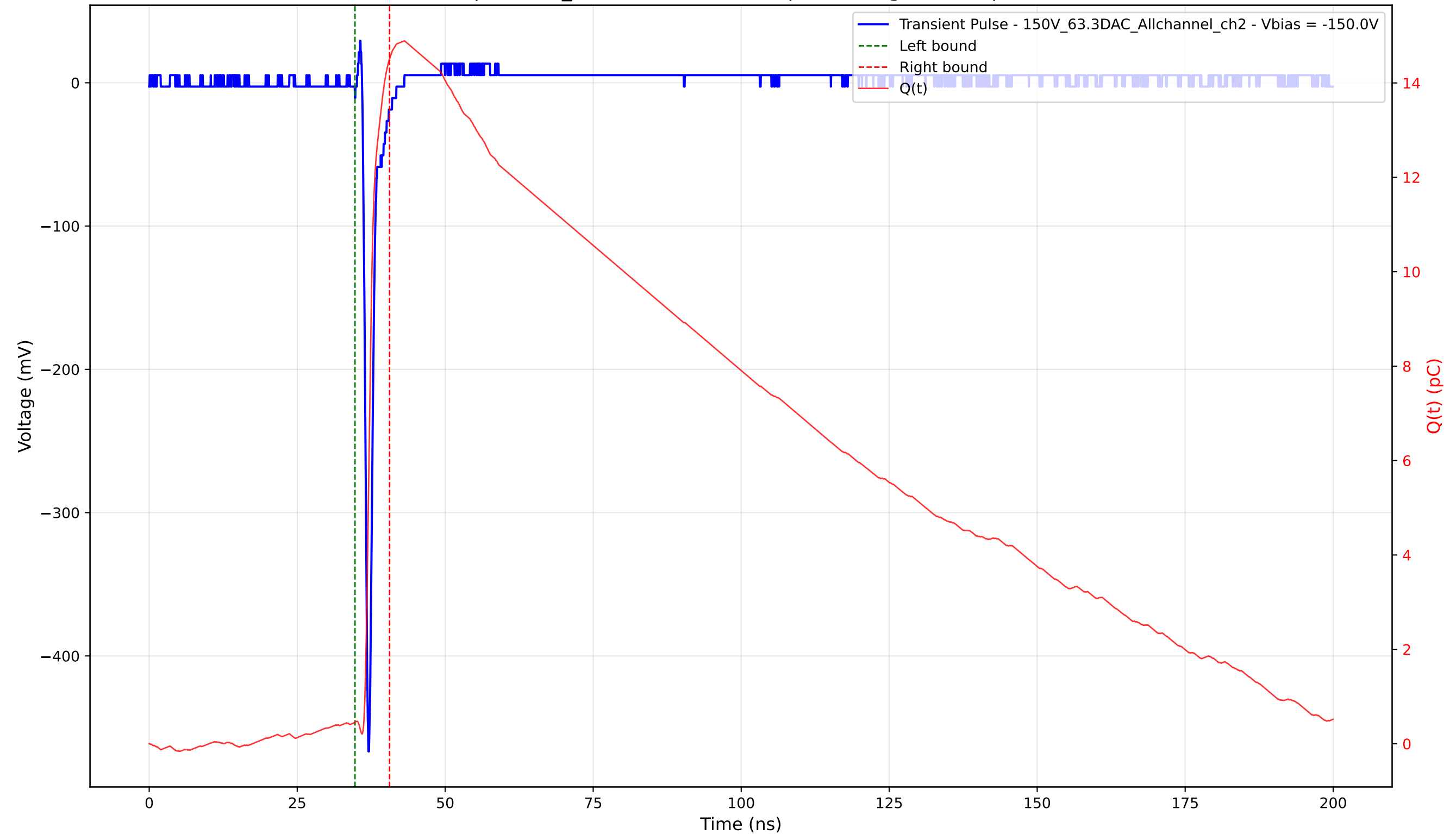
Transient Pulse - Sample: 1cm_42 - Position: 3015.0 \mu\text{m} - Charge: 14.06 pC - Rise Time: 0.68 ns
