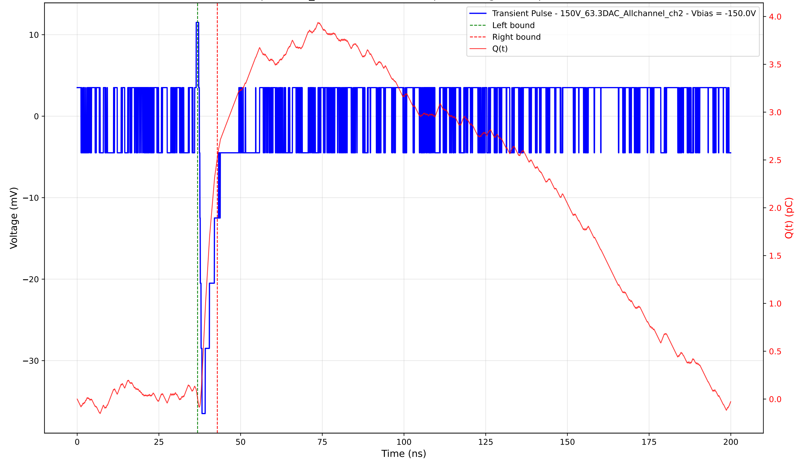
Transient Pulse - Sample: 1cm_42 - Position: 4580.0 \mu\text{m} - Charge: 2.52 pC - Rise Time: 0.83 ns
