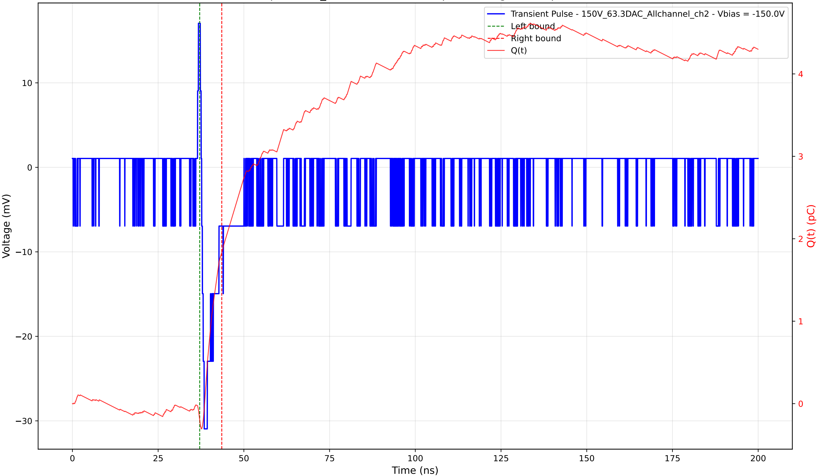
Transient Pulse - Sample: 1cm_42 - Position: 425.0 \mu\text{m} - Charge: 2.03 pC - Rise Time: 0.75 ns
