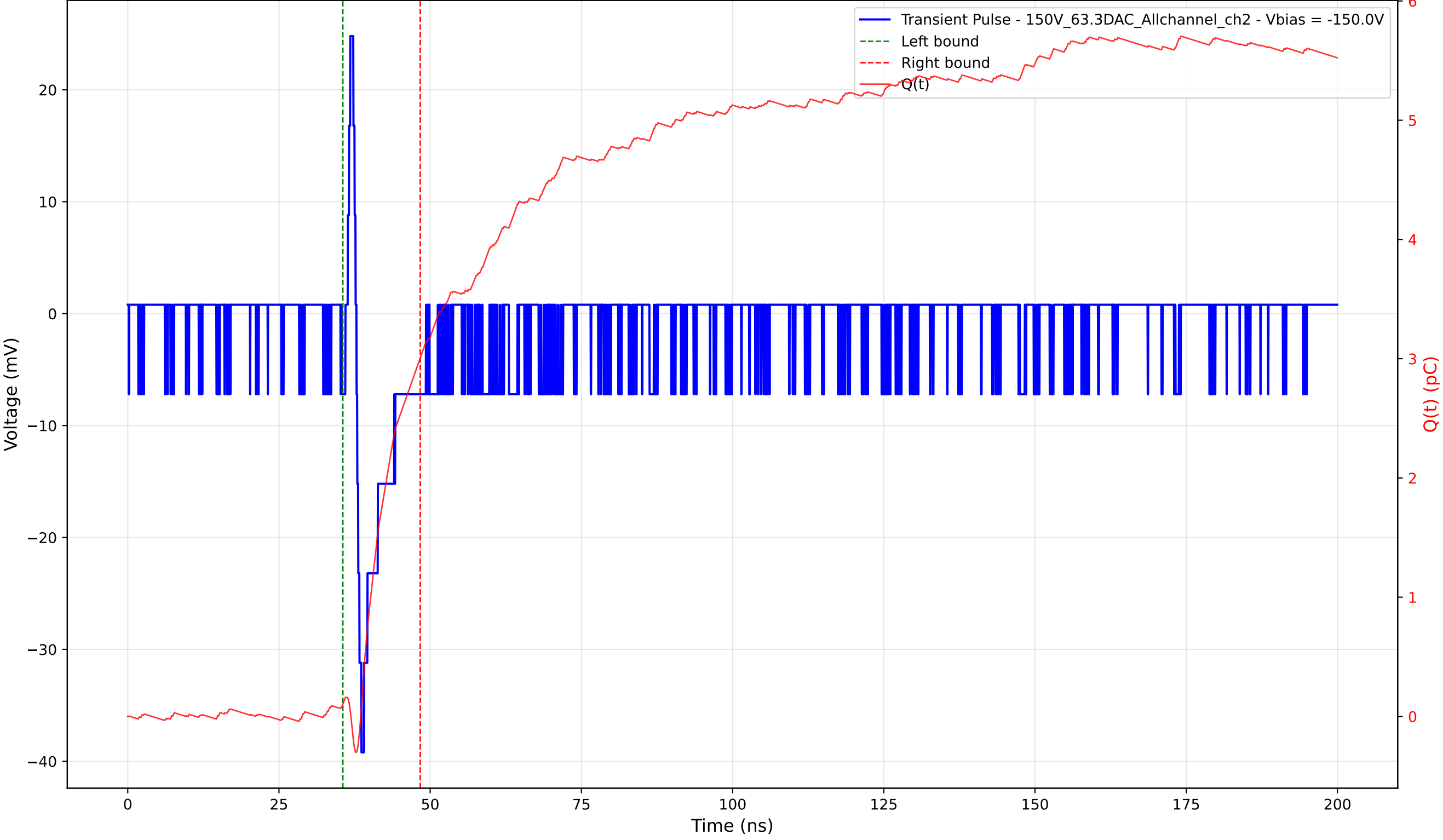
Transient Pulse - Sample: 1cm_42 - Position: 555.0 \mu\text{m} - Charge: 2.91 pC - Rise Time: 0.82 ns
