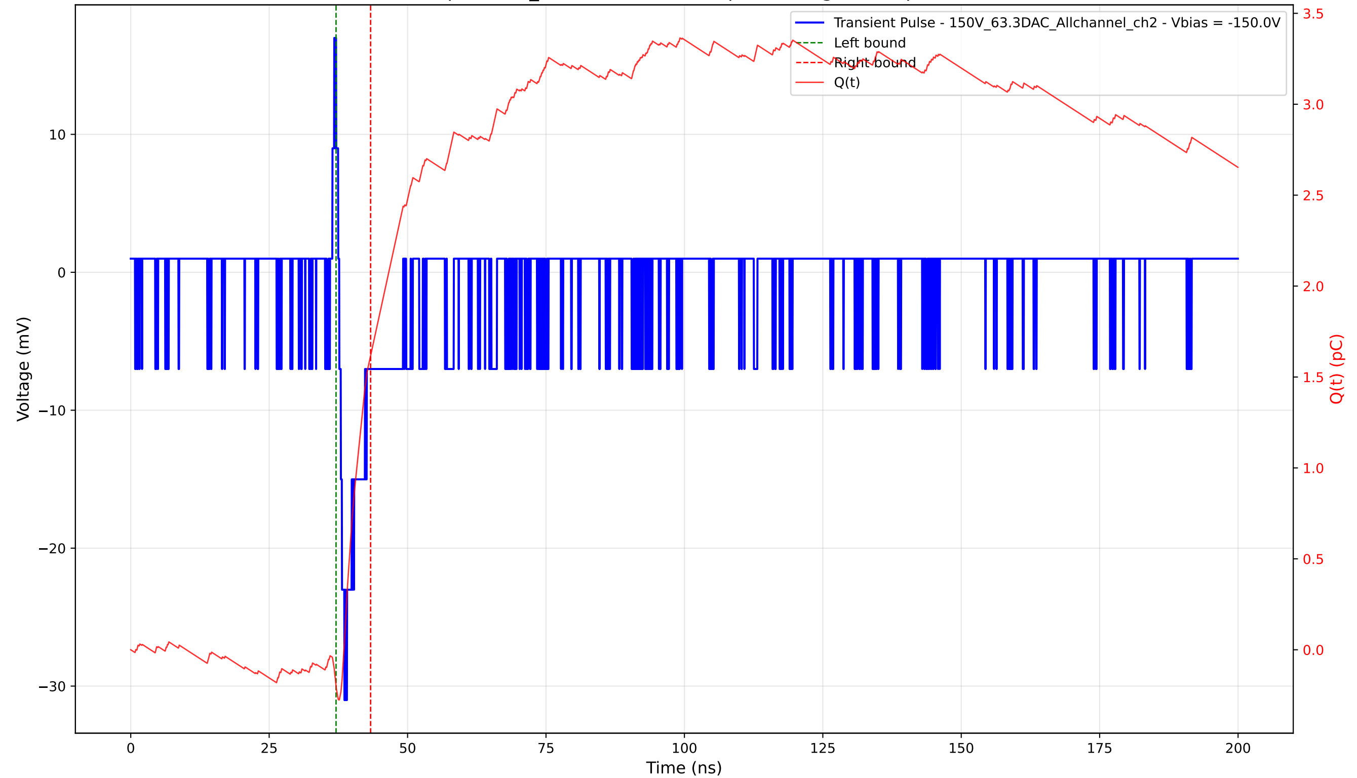
Transient Pulse - Sample: 1cm_42 - Position: 370.0 \mu\text{m} - Charge: 1.82 pC - Rise Time: 0.95 ns
