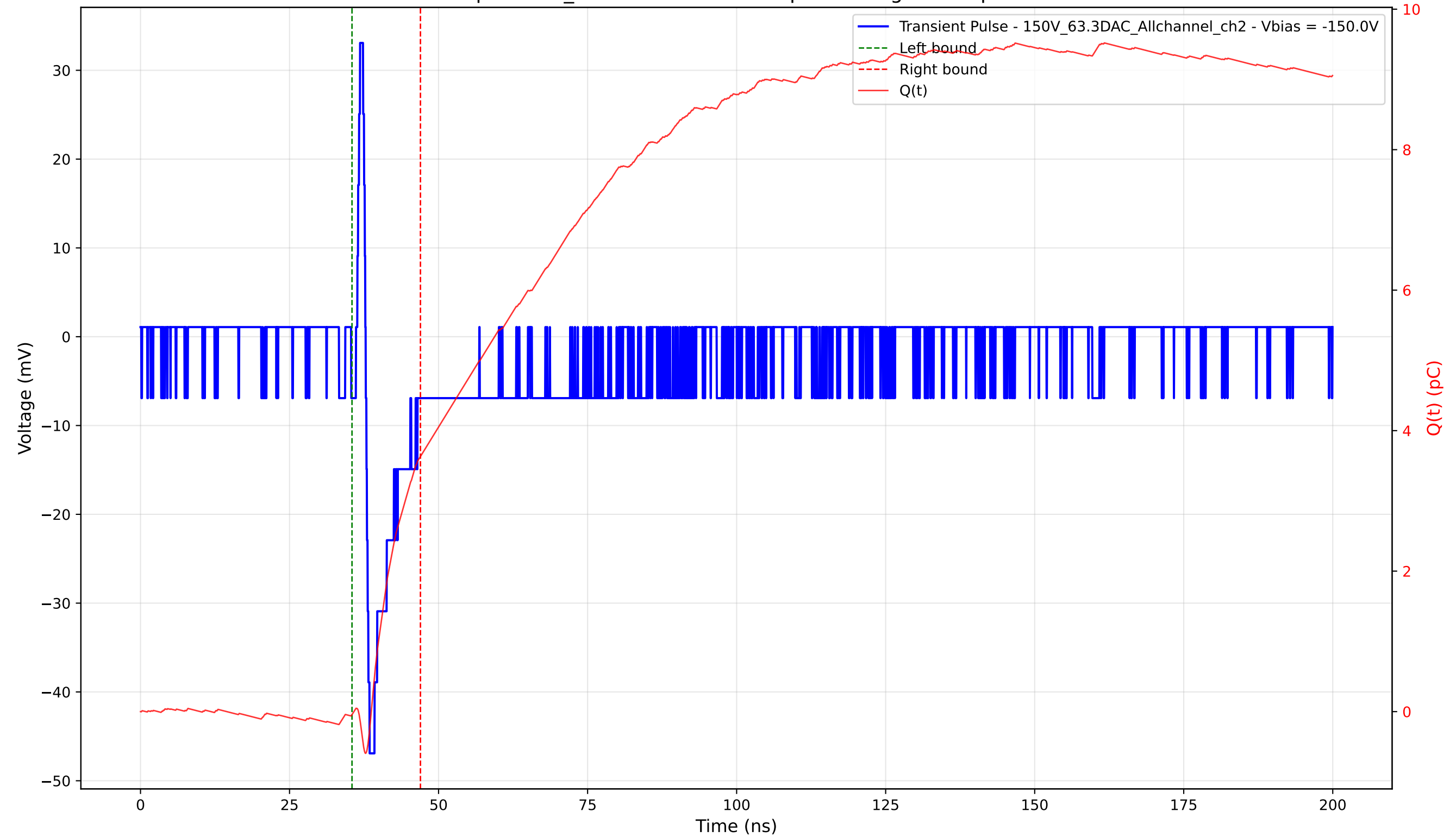
Transient Pulse - Sample: 1cm_42 - Position: 1240.0 \mu\text{m} - Charge: 3.67 pC - Rise Time: 0.66 ns
