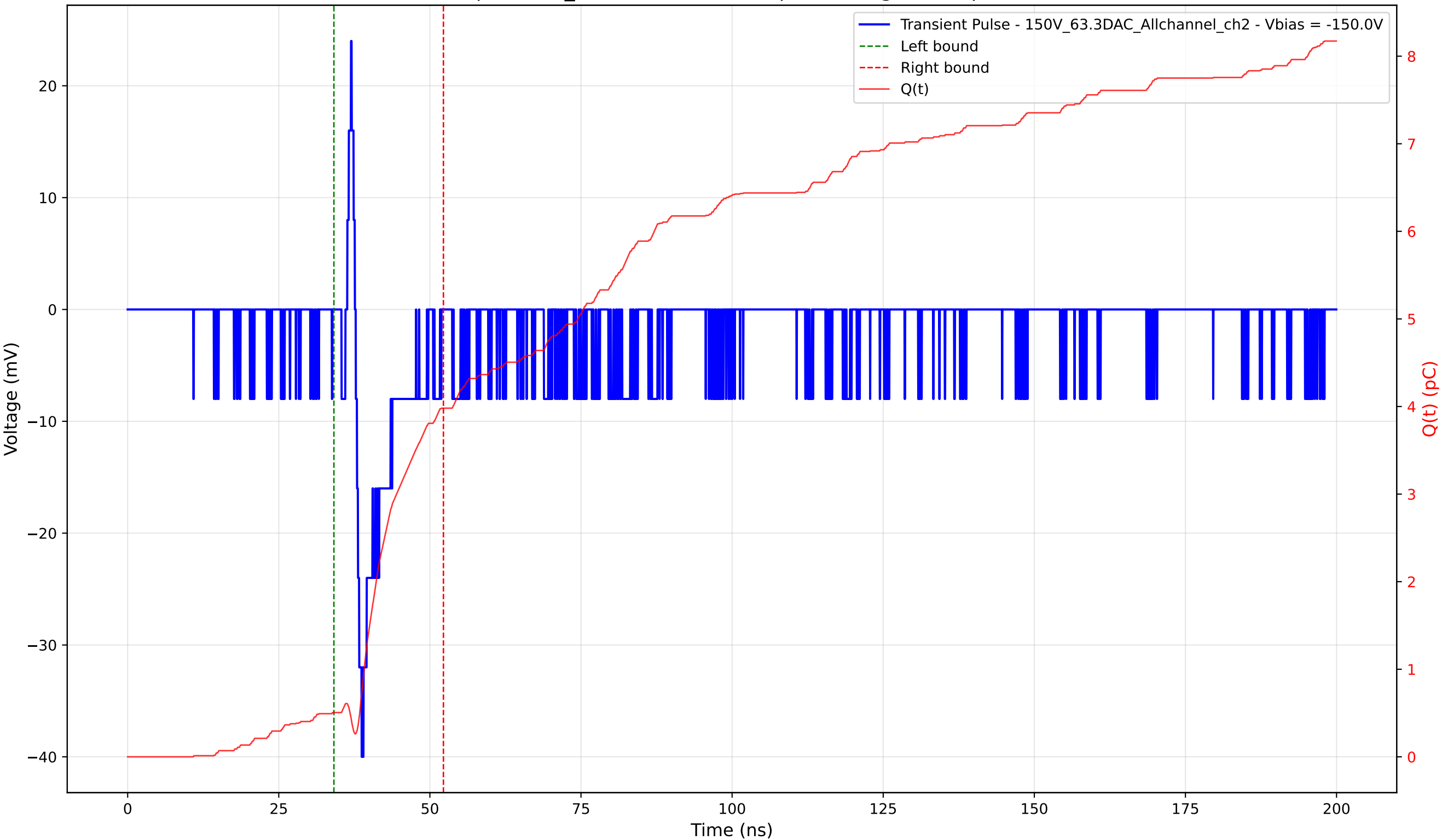
Transient Pulse - Sample: 1cm_42 - Position: 485.0 \mu\text{m} - Charge: 3.48 pC - Rise Time: 0.98 ns
