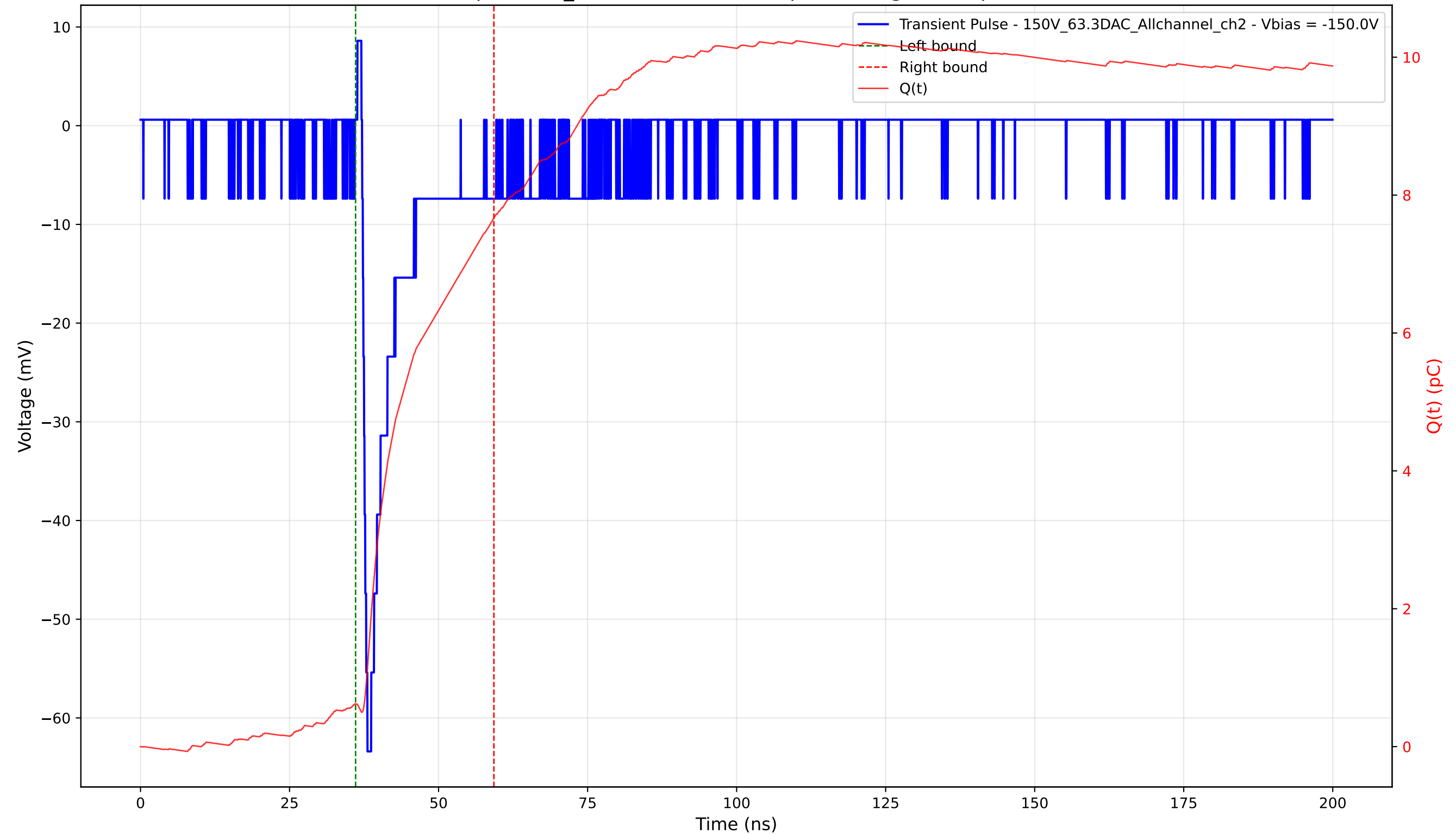
Transient Pulse - Sample: 1cm_42 - Position: 1825.0 \mu\text{m} - Charge: 7.05 pC - Rise Time: 0.89 ns
