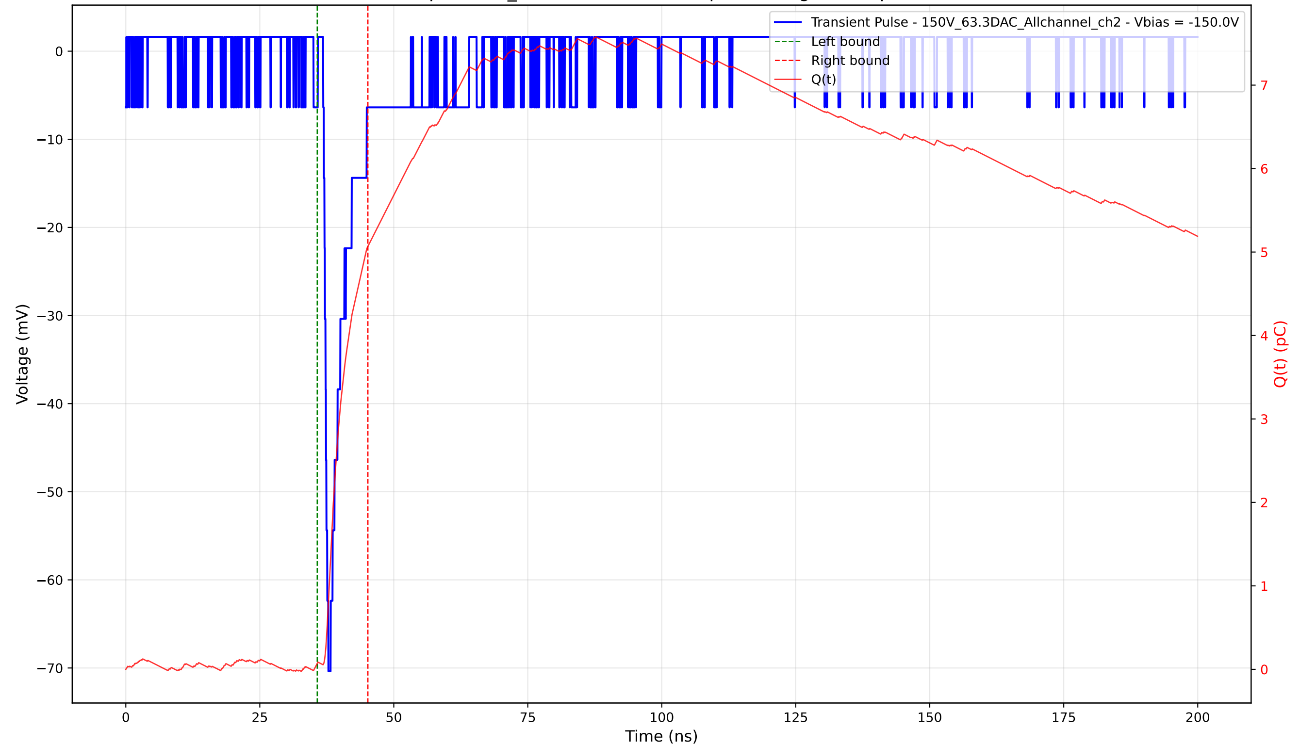
Transient Pulse - Sample: 1cm_42 - Position: 1985.0 \mu\text{m} - Charge: 4.99 pC - Rise Time: 0.88 ns
