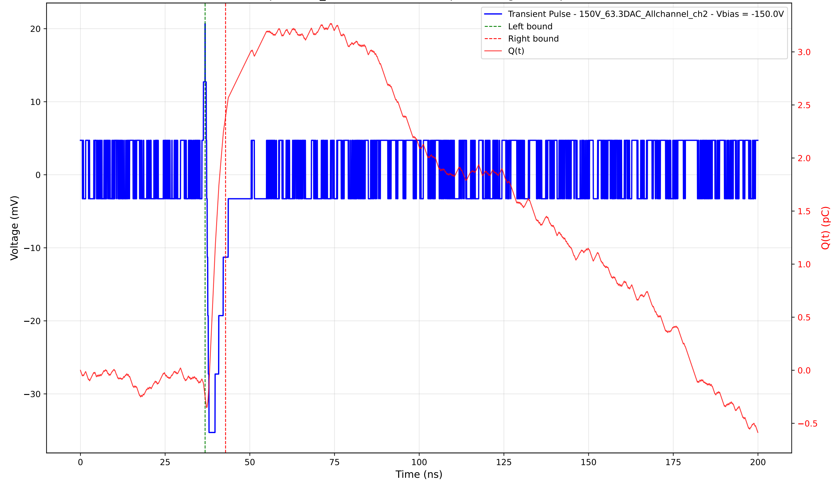
Transient Pulse - Sample: 1cm_42 - Position: 4505.0 \mu\text{m} - Charge: 2.64 pC - Rise Time: 0.56 ns
