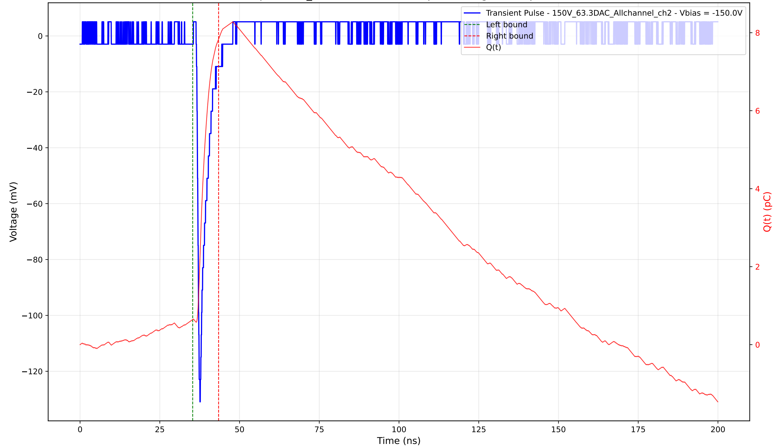
Transient Pulse - Sample: 1cm_42 - Position: 3800.0 \mu\text{m} - Charge: 7.19 pC - Rise Time: 0.75 ns
