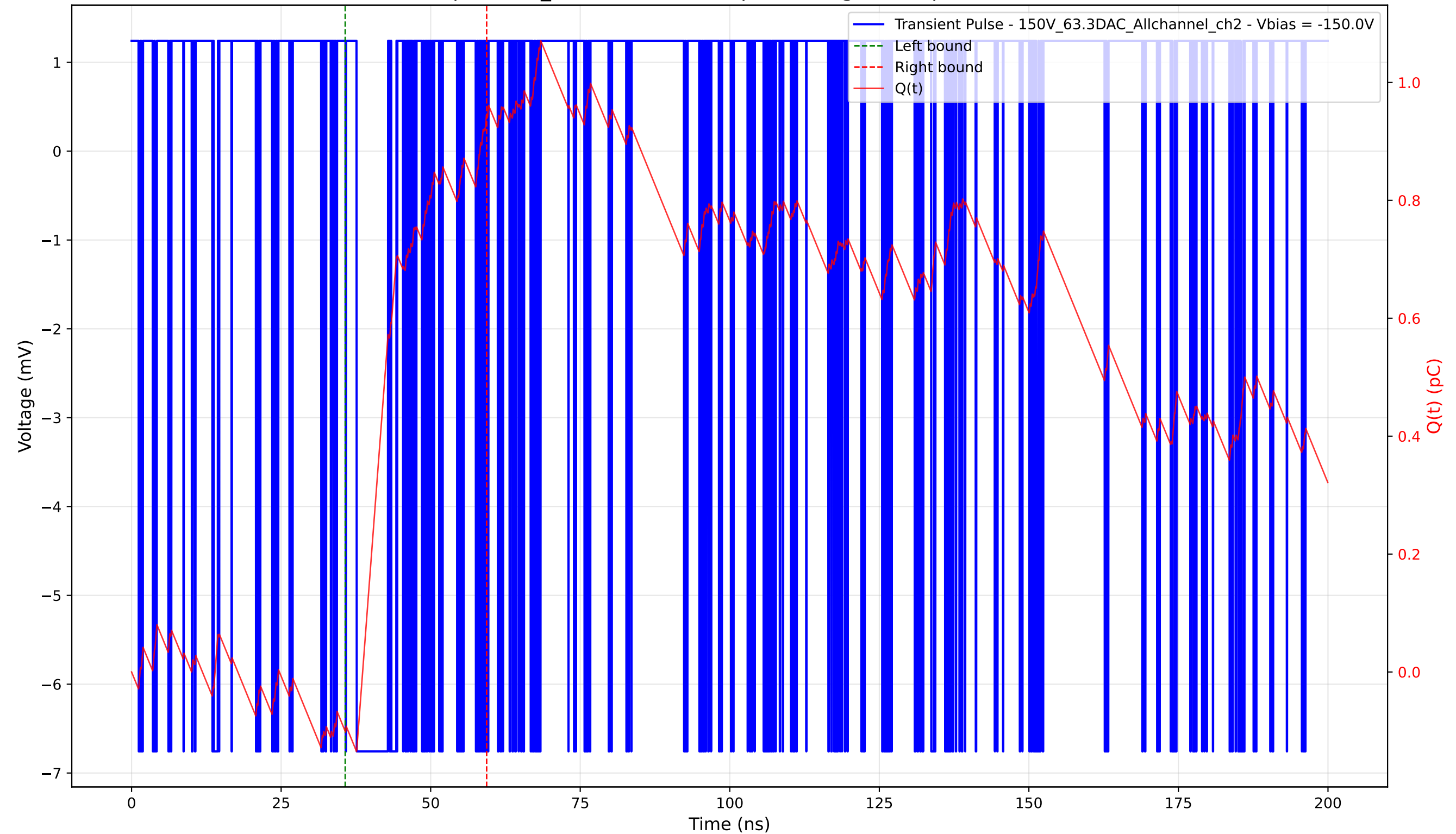
Transient Pulse - Sample: 1cm_42 - Position: 75.0 \mu\text{m} - Charge: 1.05 pC - Rise Time: 0.00 ns (N/A)
