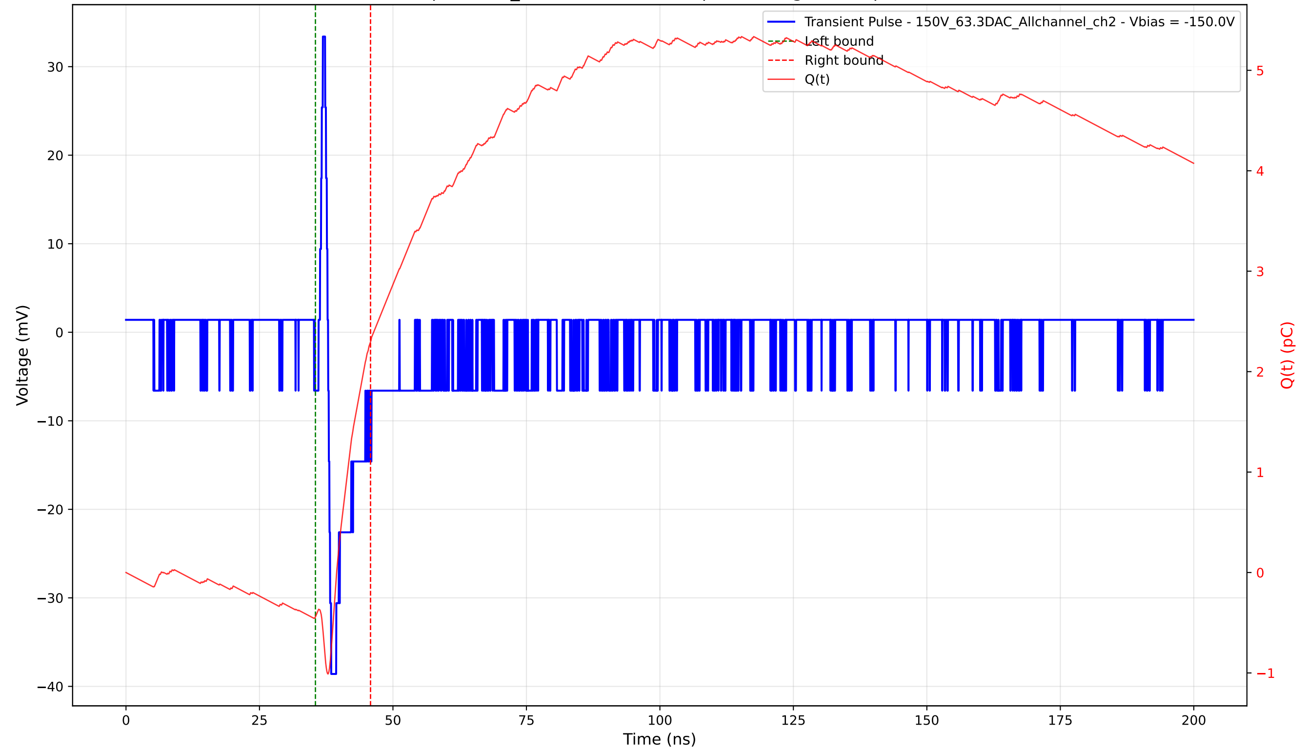
Transient Pulse - Sample: 1cm_42 - Position: 675.0 \mu\text{m} - Charge: 2.74 pC - Rise Time: 0.58 ns
