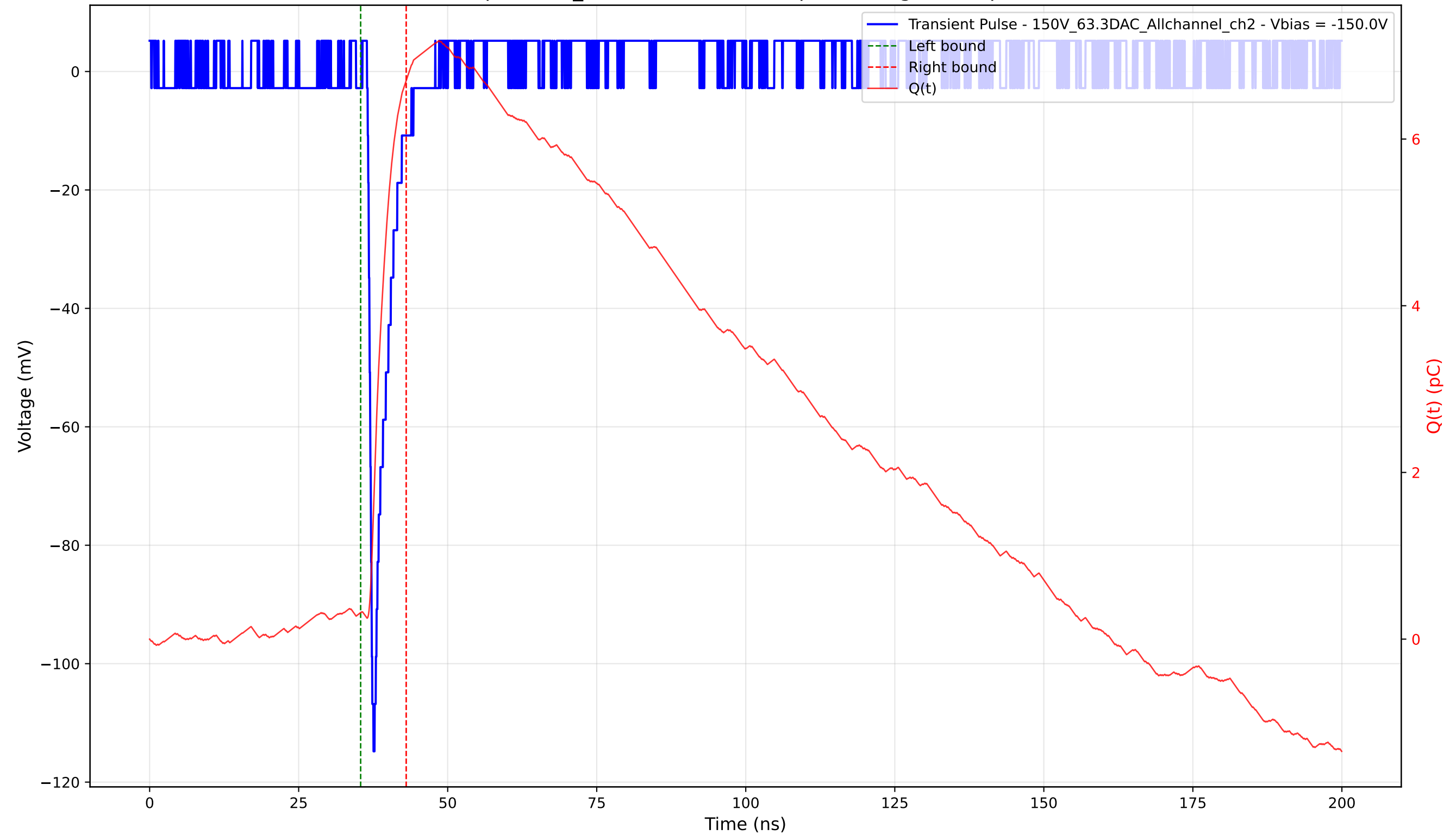
Transient Pulse - Sample: 1cm_42 - Position: 3865.0 \mu\text{m} - Charge: 6.38 pC - Rise Time: 0.72 ns
