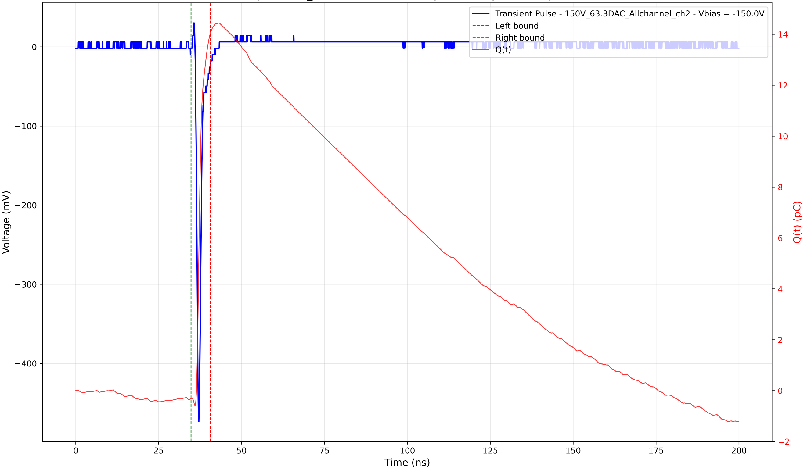
Transient Pulse - Sample: 1cm_42 - Position: 2940.0 \mu\text{m} - Charge: 14.38 pC - Rise Time: 0.73 ns
