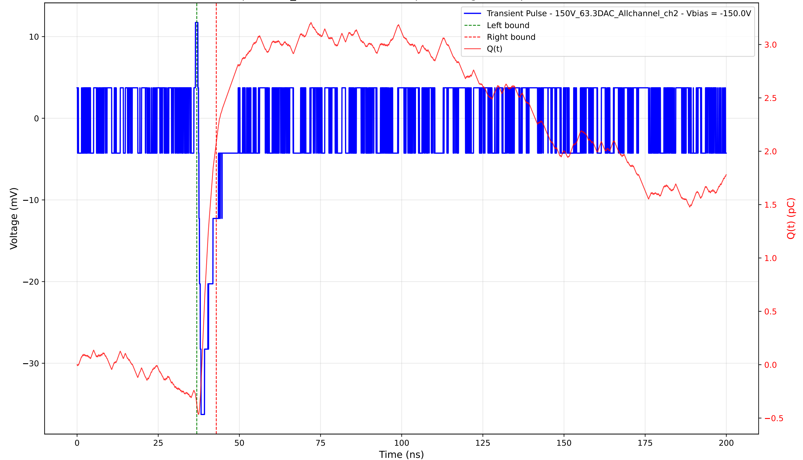
Transient Pulse - Sample: 1cm_42 - Position: 4635.0 \mu\text{m} - Charge: 2.45 pC - Rise Time: 0.00 ns (N/A)
