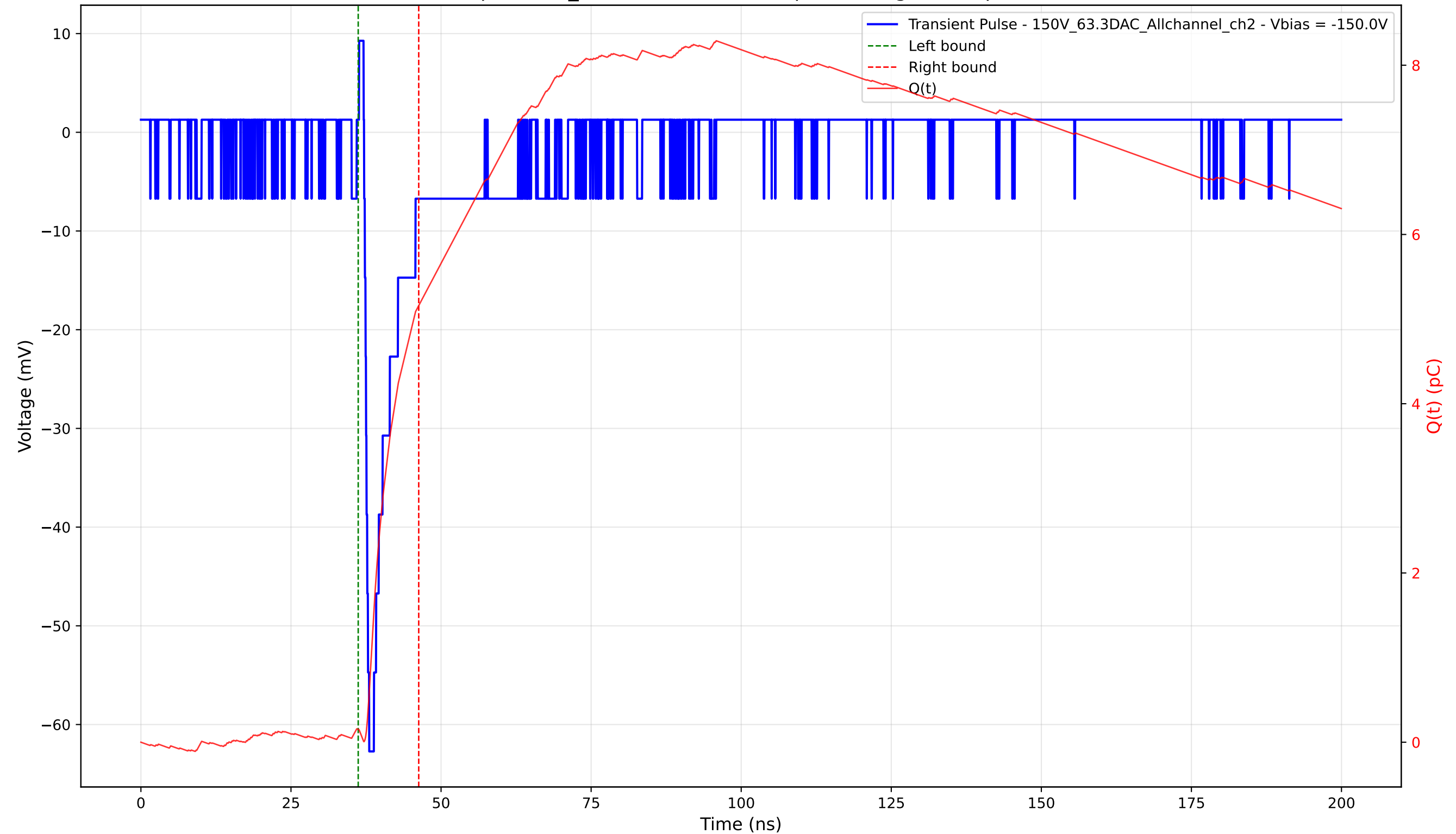
Transient Pulse - Sample: 1cm_42 - Position: 1820.0 \mu\text{m} - Charge: 5.01 pC - Rise Time: 0.84 ns
