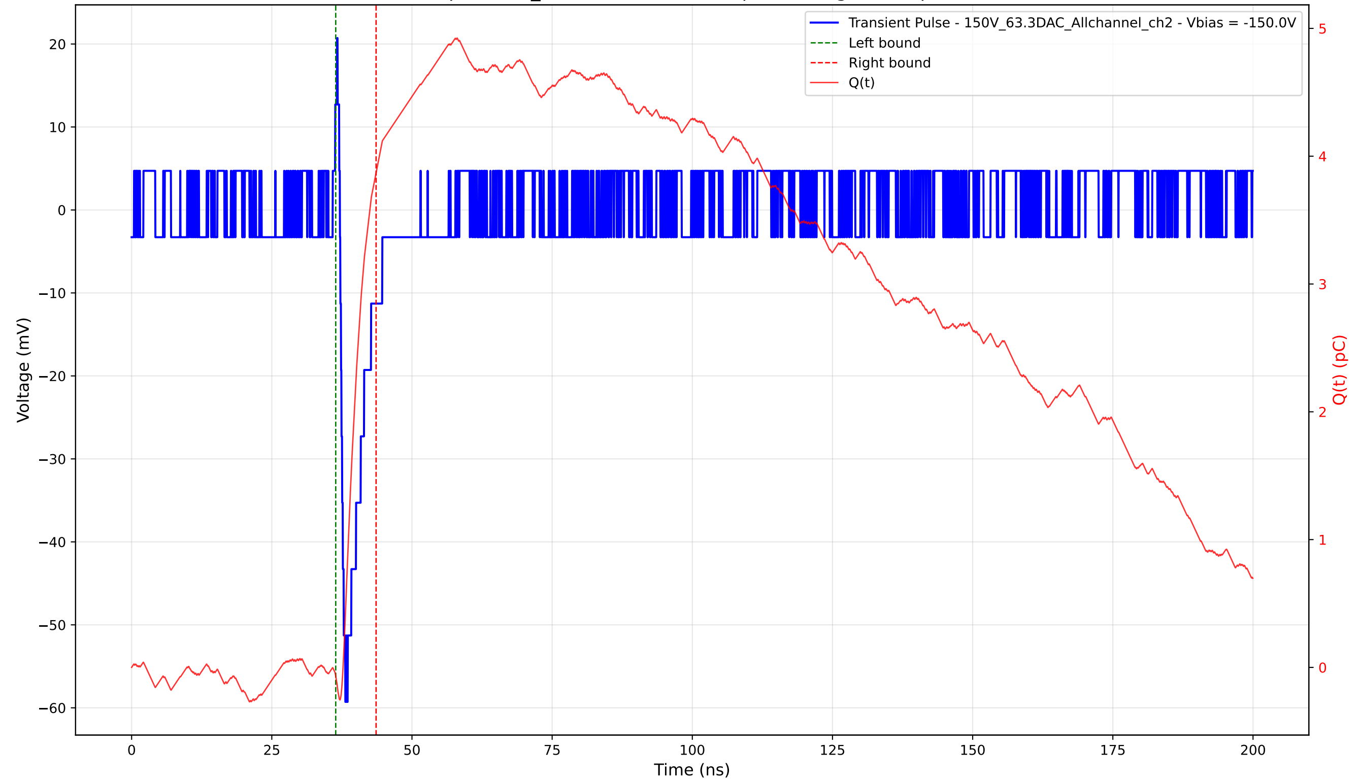
Transient Pulse - Sample: 1cm_42 - Position: 4310.0 \mu\text{m} - Charge: 3.94 pC - Rise Time: 0.91 ns
