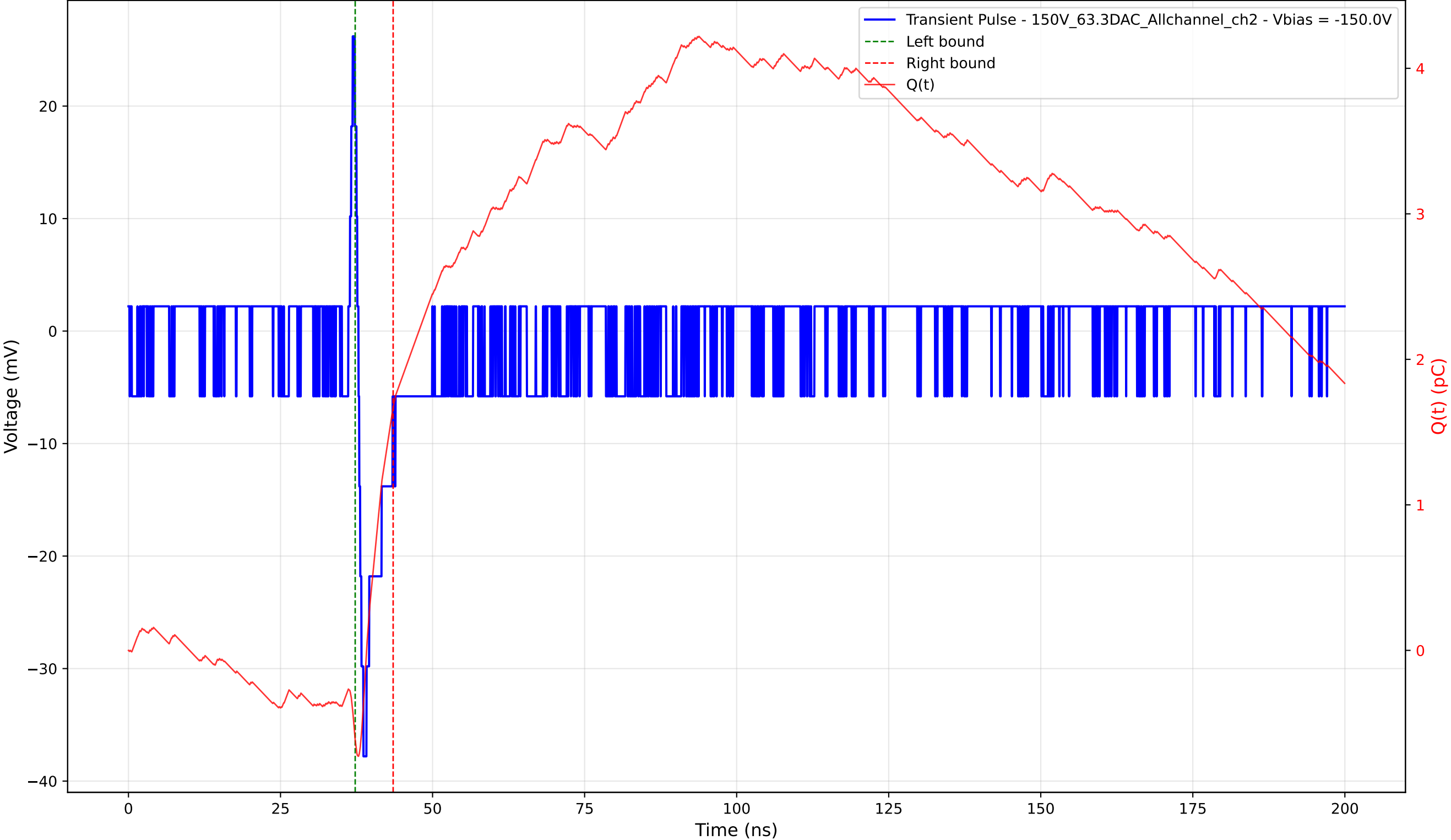
Transient Pulse - Sample: 1cm_42 - Position: 545.0 \mu\text{m} - Charge: 2.28 pC - Rise Time: 0.82 ns
