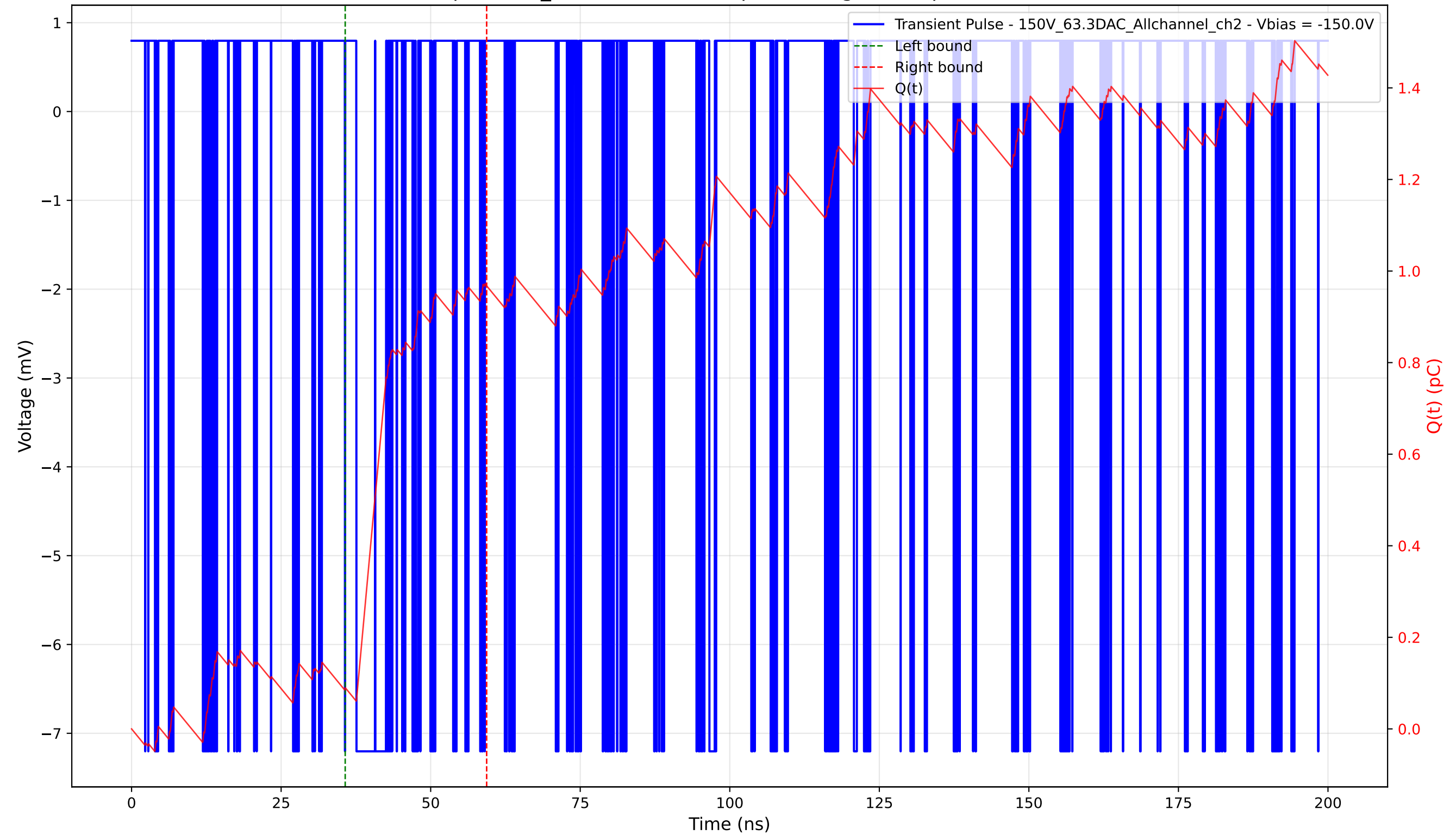
Transient Pulse - Sample: 1cm_42 - Position: 55.0 \mu\text{m} - Charge: 0.88 pC - Rise Time: 0.00 ns (N/A)
