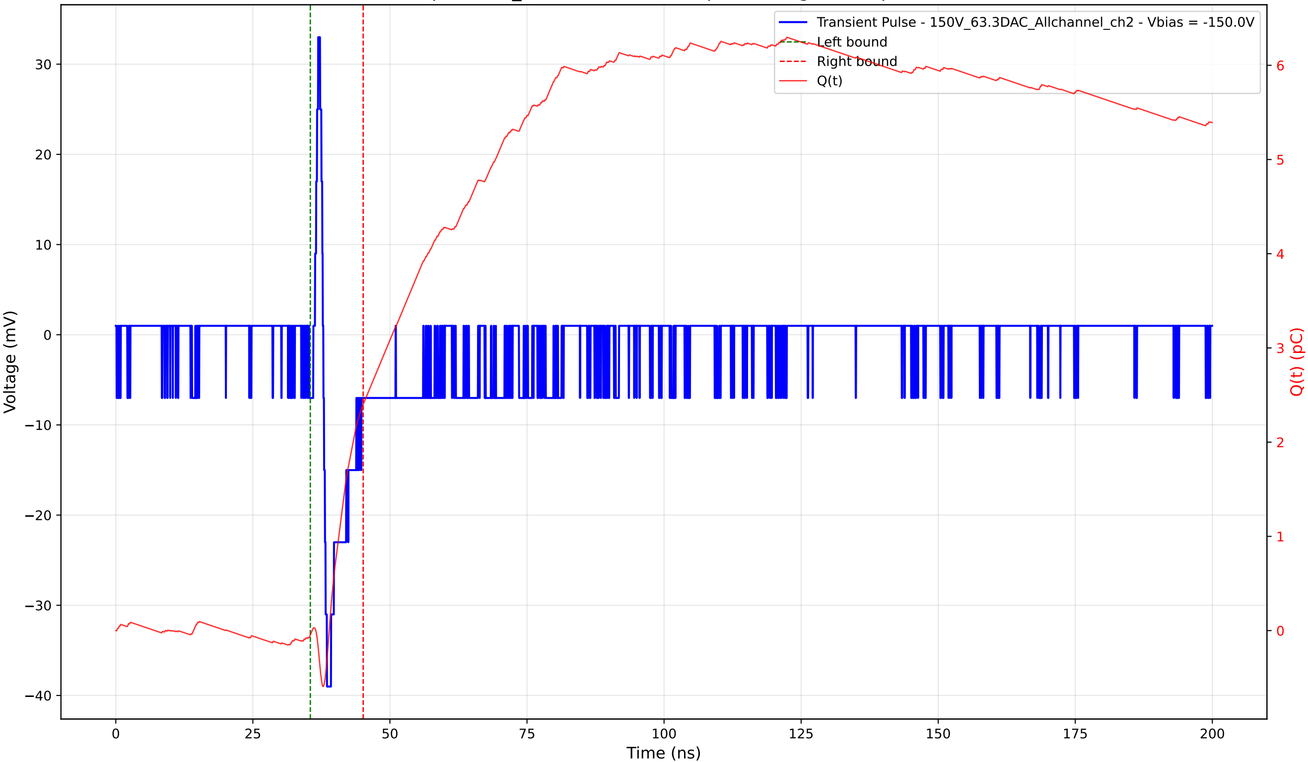
Transient Pulse - Sample: 1cm_42 - Position: 955.0 \mu\text{m} - Charge: 2.45 pC - Rise Time: 0.66 ns
