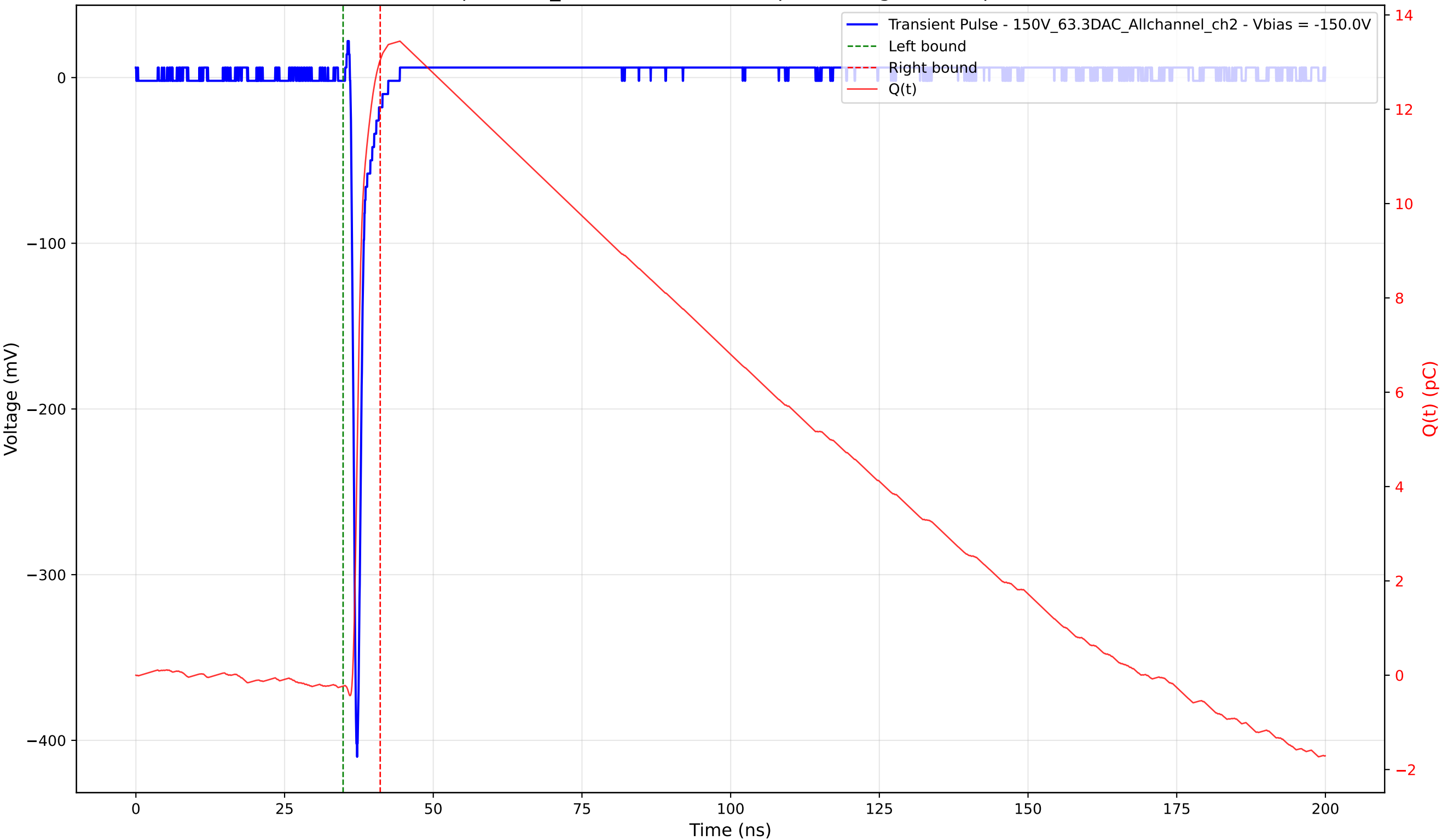
Transient Pulse - Sample: 1cm_42 - Position: 2715.0 \mu\text{m} - Charge: 13.27 pC - Rise Time: 0.76 ns
