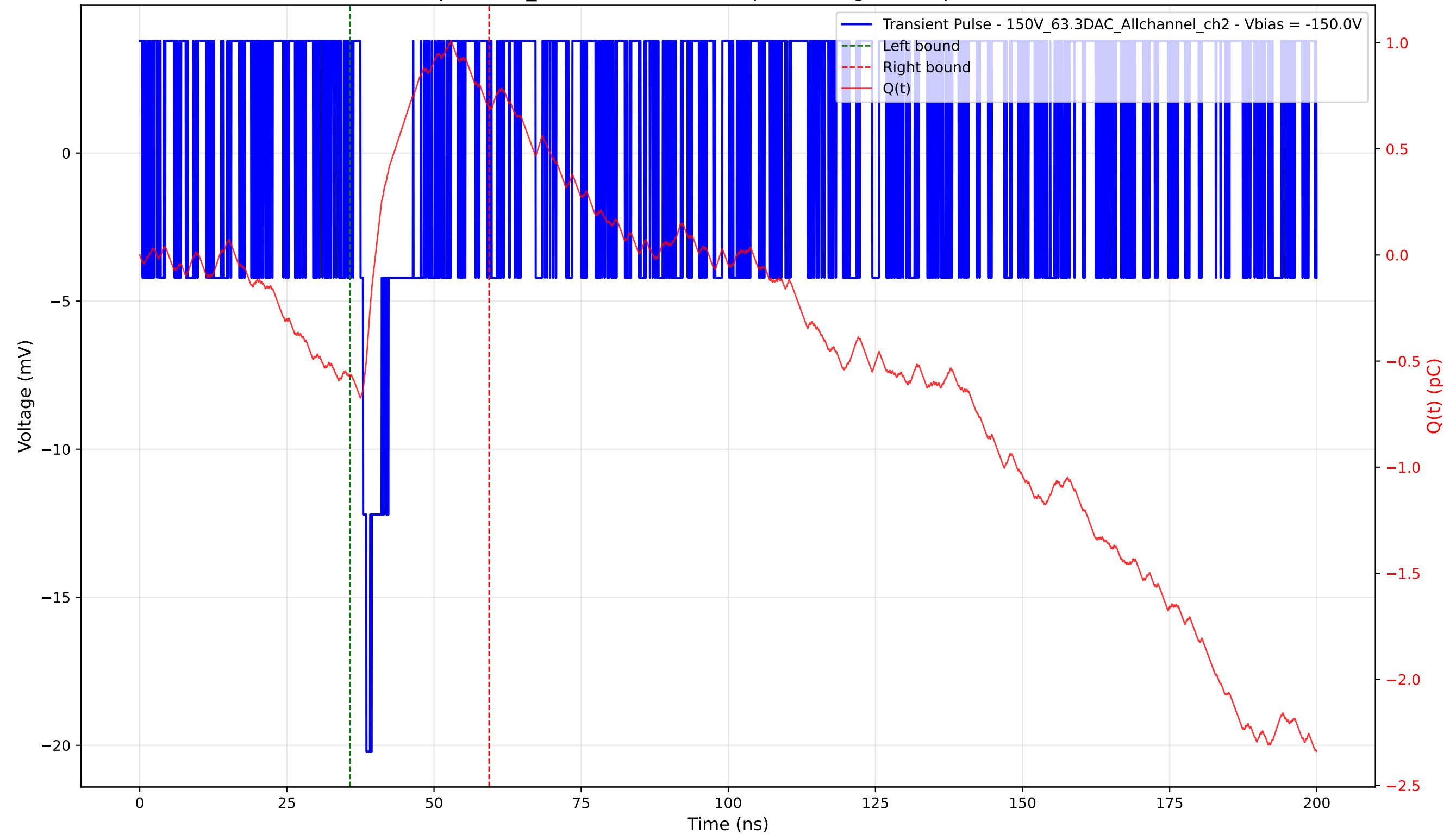
Transient Pulse - Sample: 1cm_42 - Position: 5025.0 \mu\text{m} - Charge: 1.27 pC - Rise Time: 0.00 ns (N/A)
