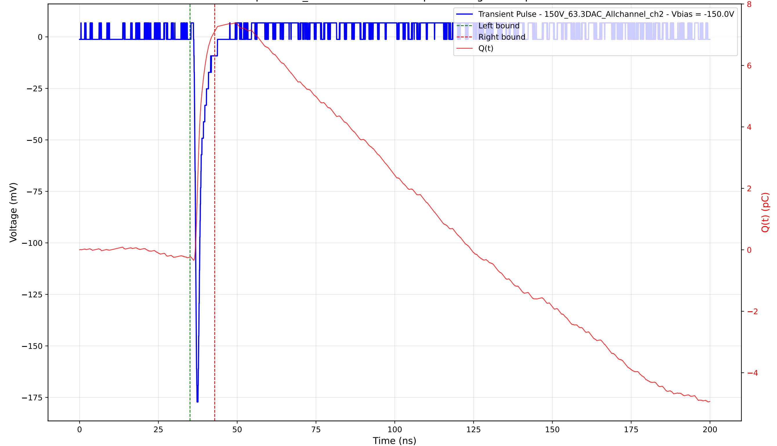
Transient Pulse - Sample: 1cm_42 - Position: 2470.0 \mu\text{m} - Charge: 7.35 pC - Rise Time: 0.72 ns
