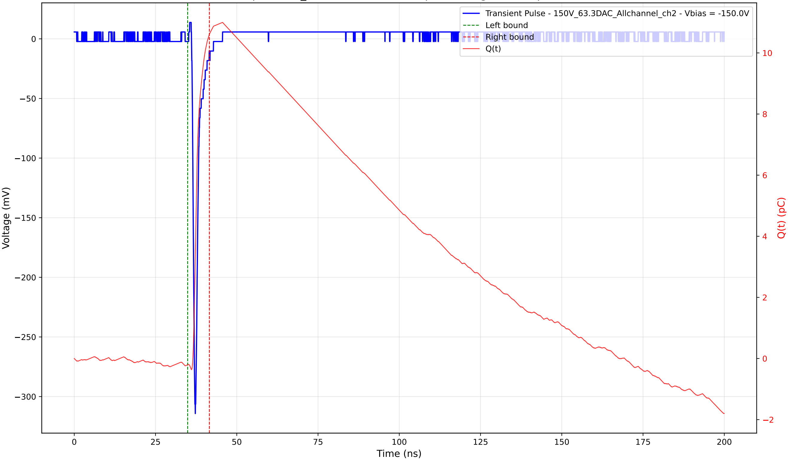
Transient Pulse - Sample: 1cm_42 - Position: 2635.0 \mu\text{m} - Charge: 10.82 pC - Rise Time: 0.75 ns
