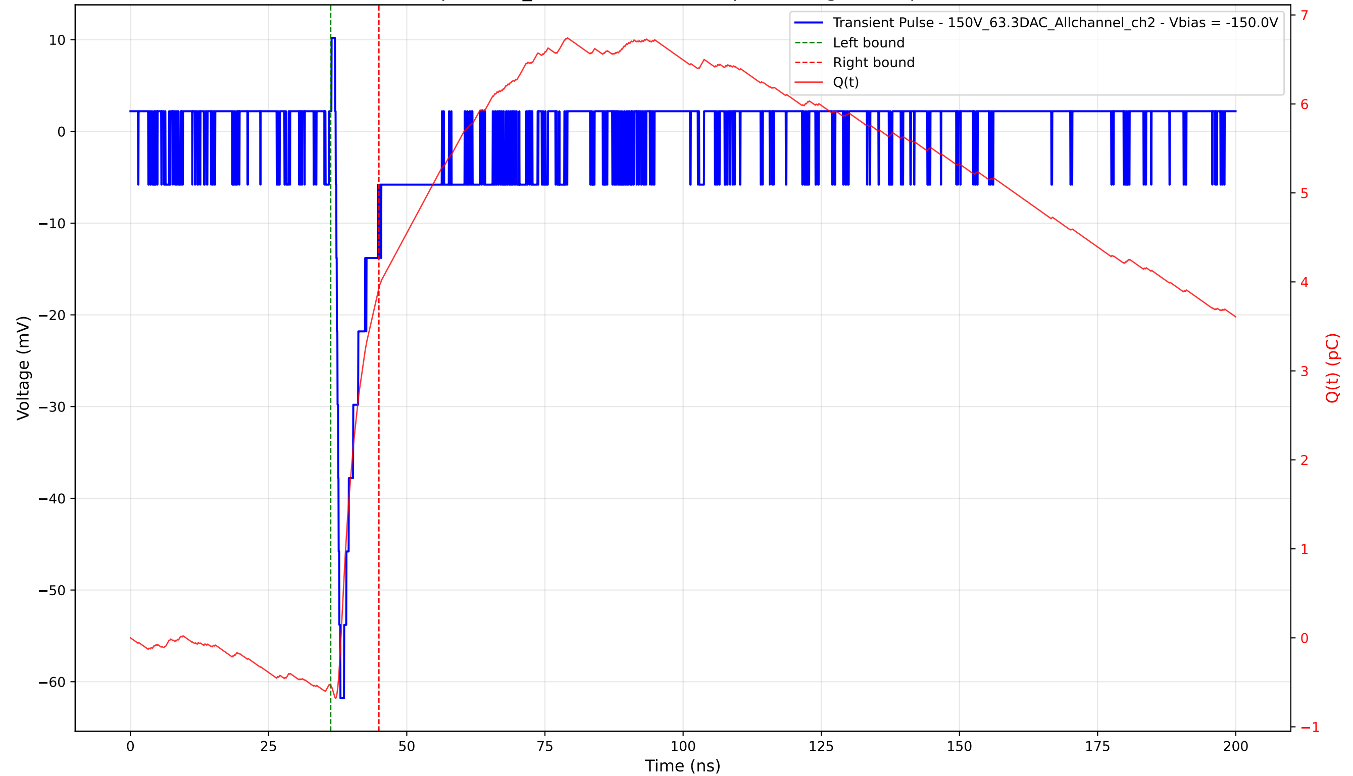
Transient Pulse - Sample: 1cm_42 - Position: 1855.0 \mu\text{m} - Charge: 4.47 pC - Rise Time: 0.76 ns
