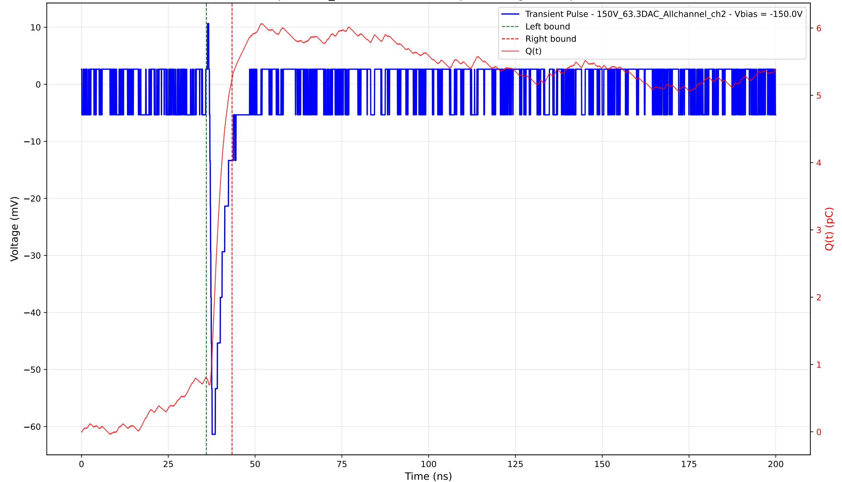
Transient Pulse - Sample: 1cm_42 - Position: 4095.0 \mu\text{m} - Charge: 4.45 pC - Rise Time: 0.68 ns
