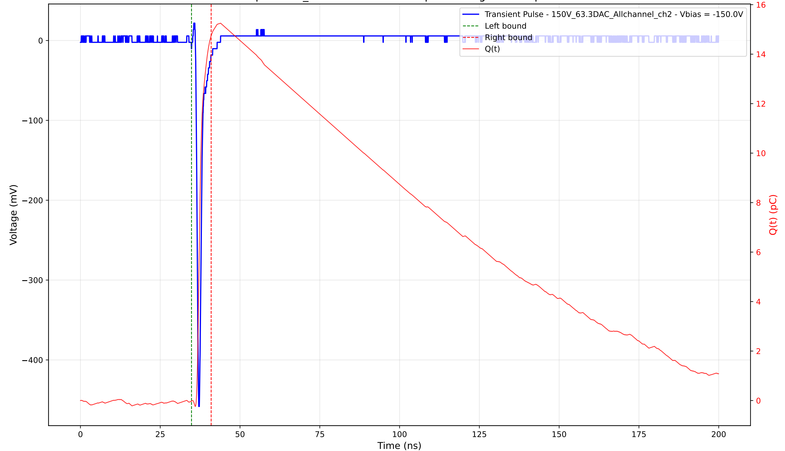
Transient Pulse - Sample: 1cm_42 - Position: 2795.0 \mu\text{m} - Charge: 14.77 pC - Rise Time: 0.74 ns
