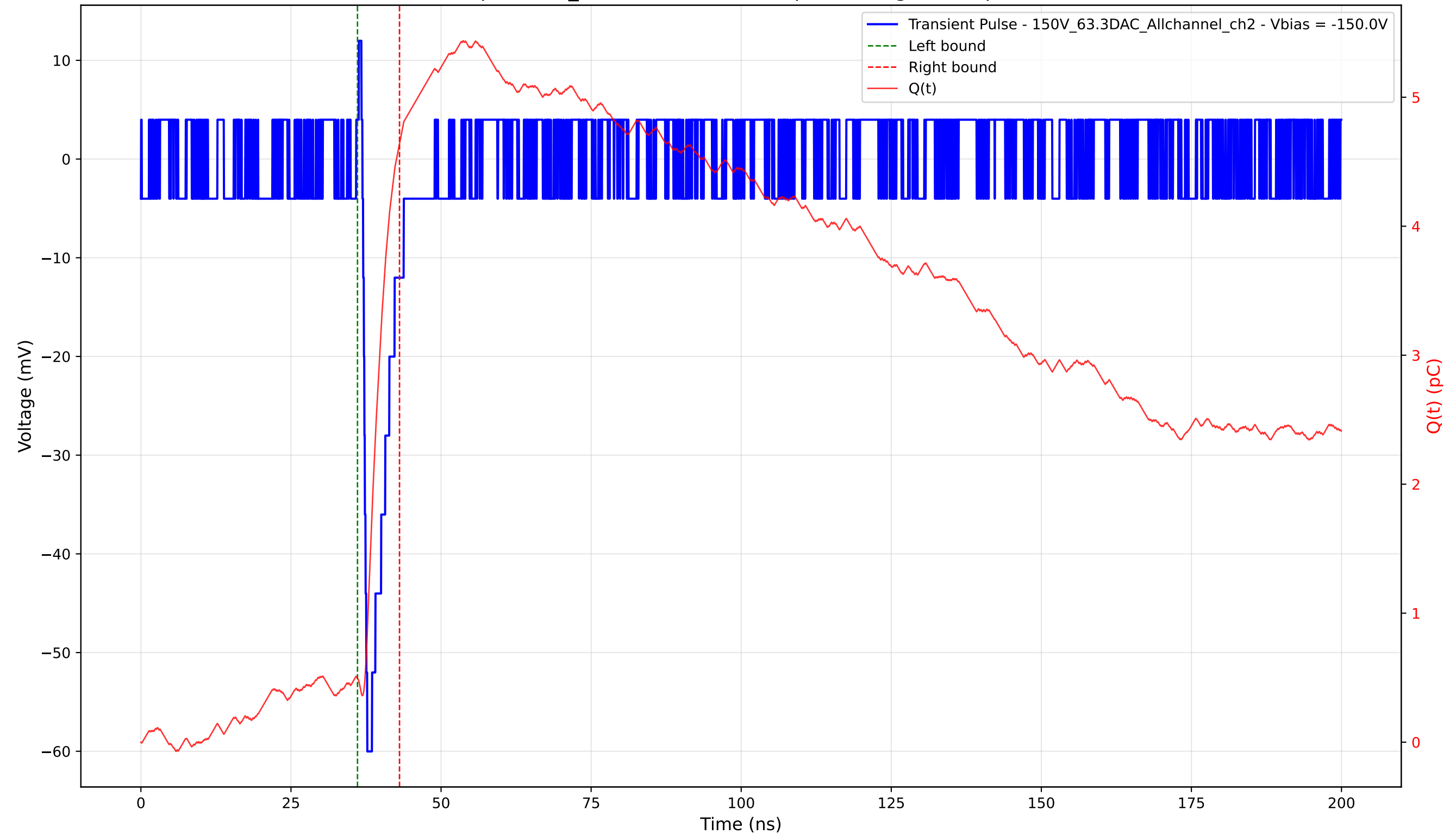
Transient Pulse - Sample: 1cm_42 - Position: 4110.0 \mu\text{m} - Charge: 4.15 pC - Rise Time: 0.71 ns
