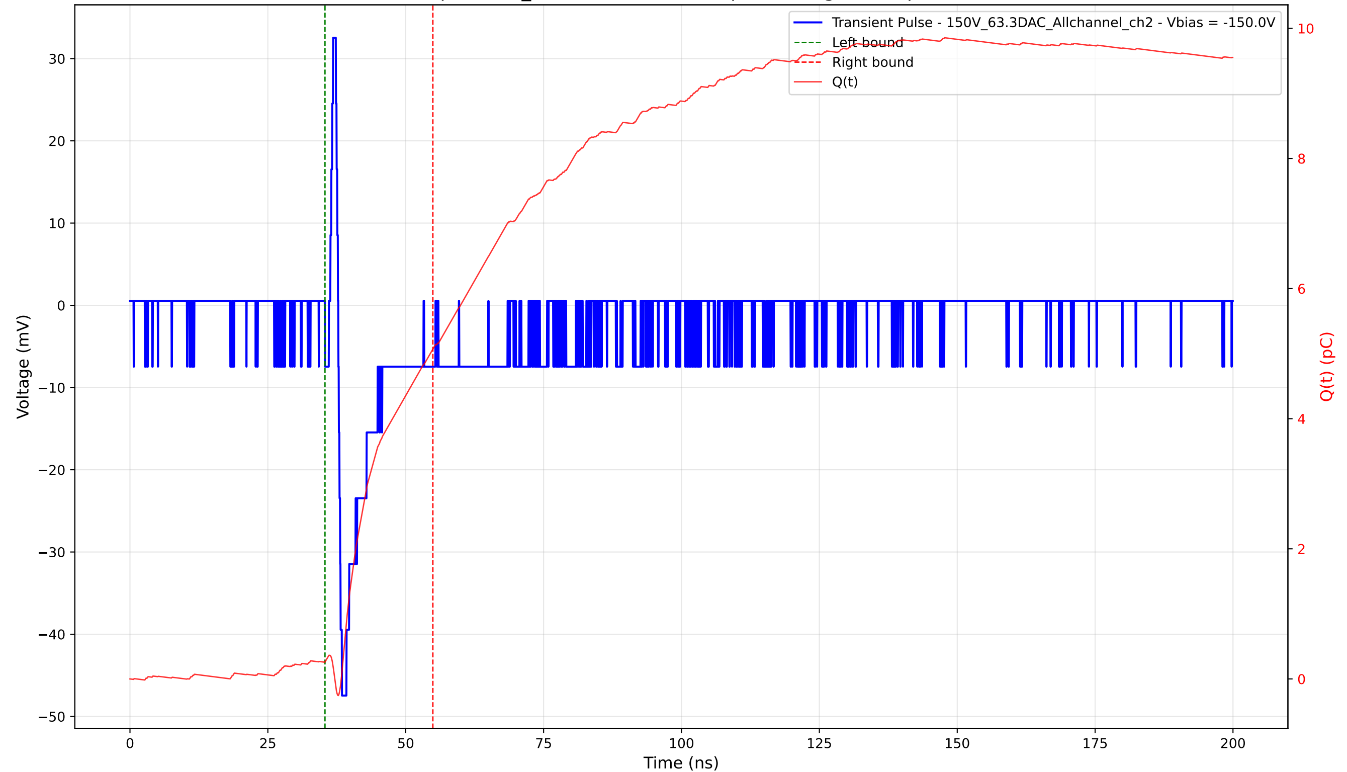
Transient Pulse - Sample: 1cm_42 - Position: 1260.0 \mu\text{m} - Charge: 4.81 pC - Rise Time: 0.66 ns
