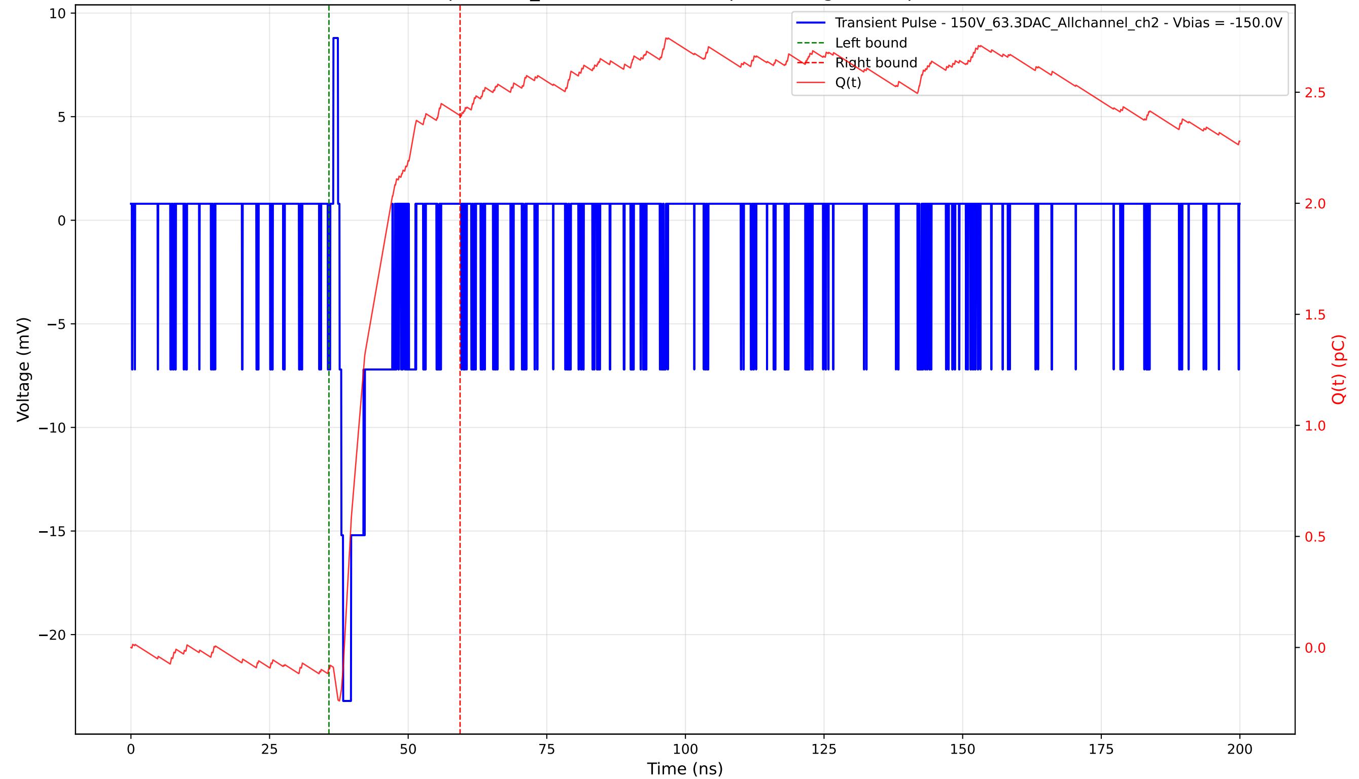
Transient Pulse - Sample: 1cm_42 - Position: 290.0 \mu\text{m} - Charge: 2.49 pC - Rise Time: 0.67 ns
