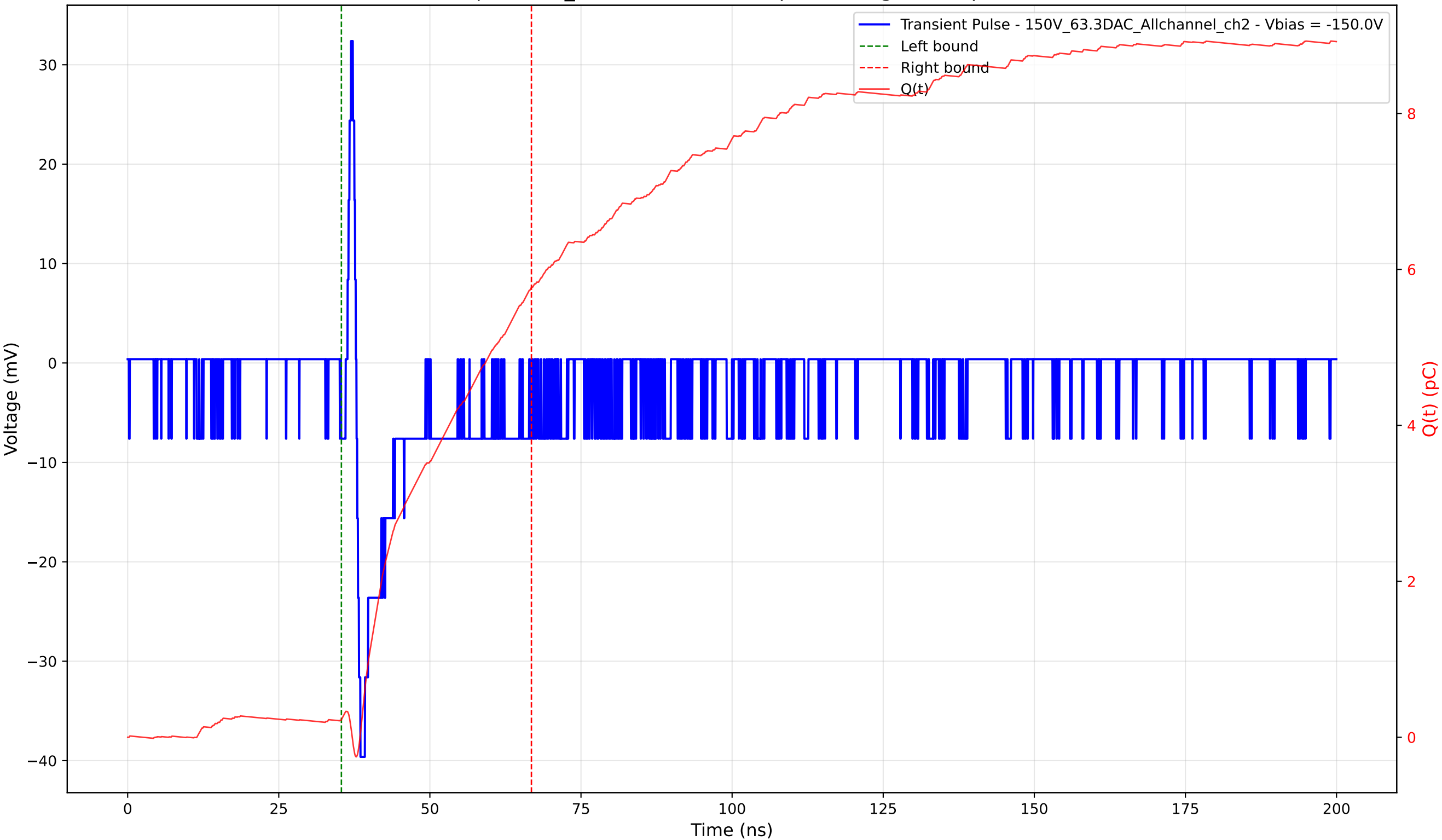
Transient Pulse - Sample: 1cm_42 - Position: 975.0 \mu\text{m} - Charge: 5.55 pC - Rise Time: 0.66 ns
