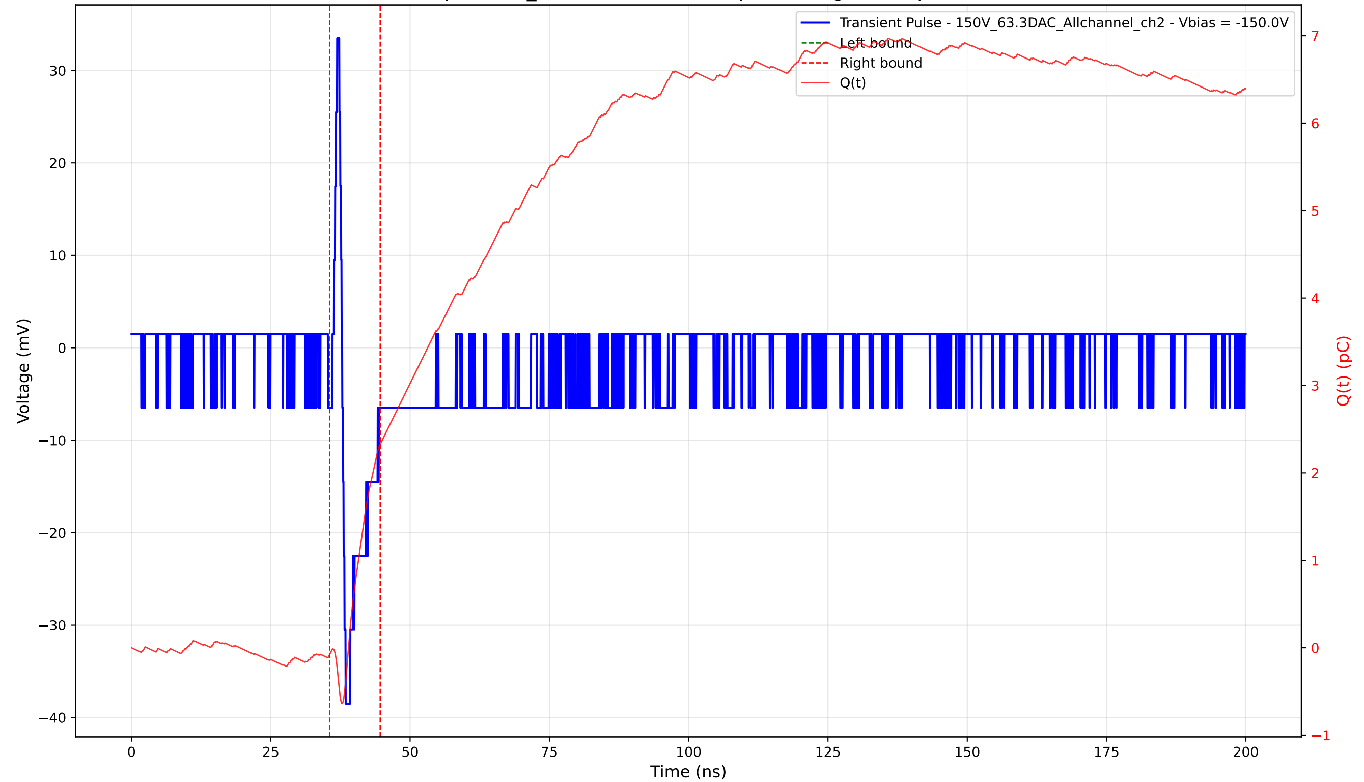
Transient Pulse - Sample: 1cm_42 - Position: 1025.0 \mu\text{m} - Charge: 2.40 pC - Rise Time: 0.62 ns
