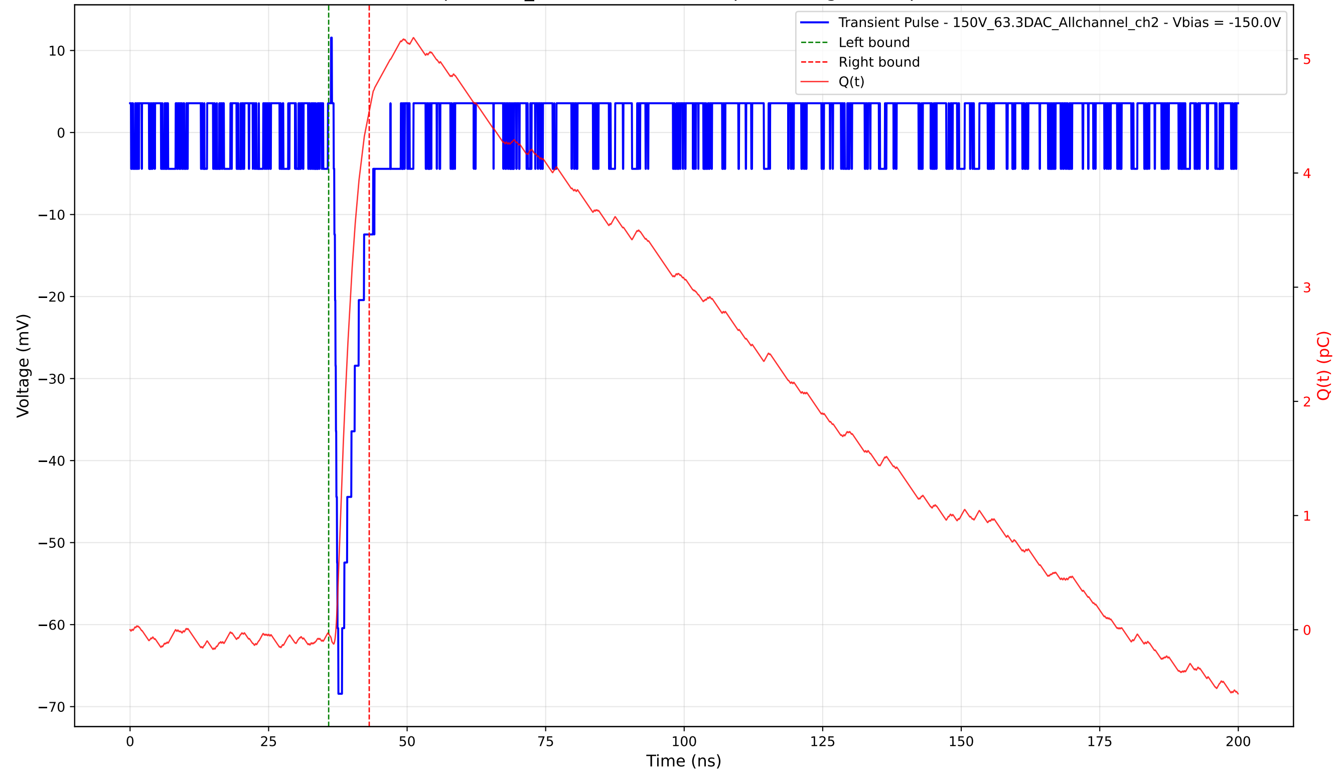
Transient Pulse - Sample: 1cm_42 - Position: 4025.0 \mu\text{m} - Charge: 4.58 pC - Rise Time: 0.75 ns
