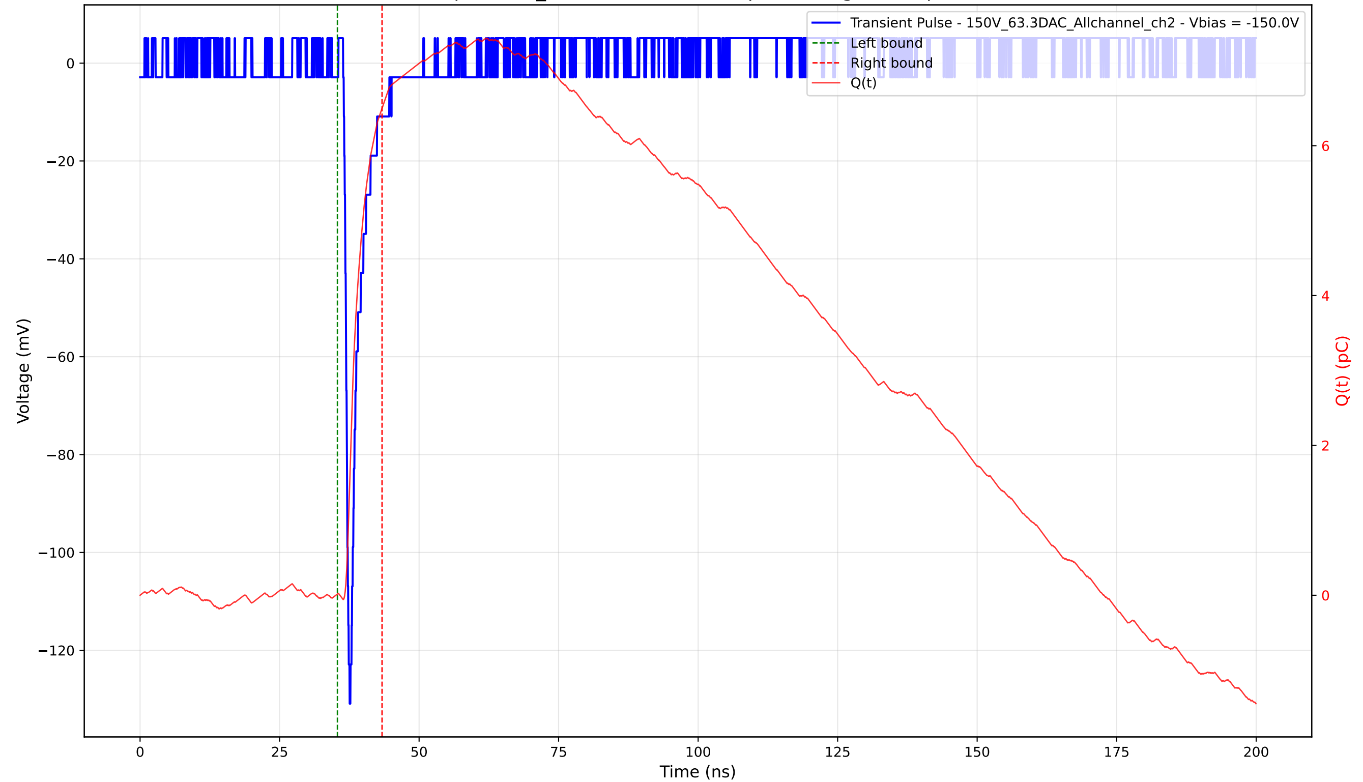
Transient Pulse - Sample: 1cm_42 - Position: 2220.0 \mu\text{m} - Charge: 6.48 pC - Rise Time: 0.83 ns
