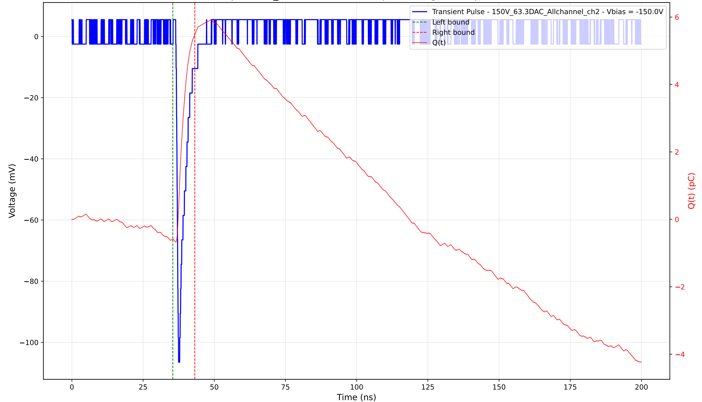
Transient Pulse - Sample: 1cm_42 - Position: 3880.0 \mu\text{m} - Charge: 6.06 pC - Rise Time: 0.68 ns
