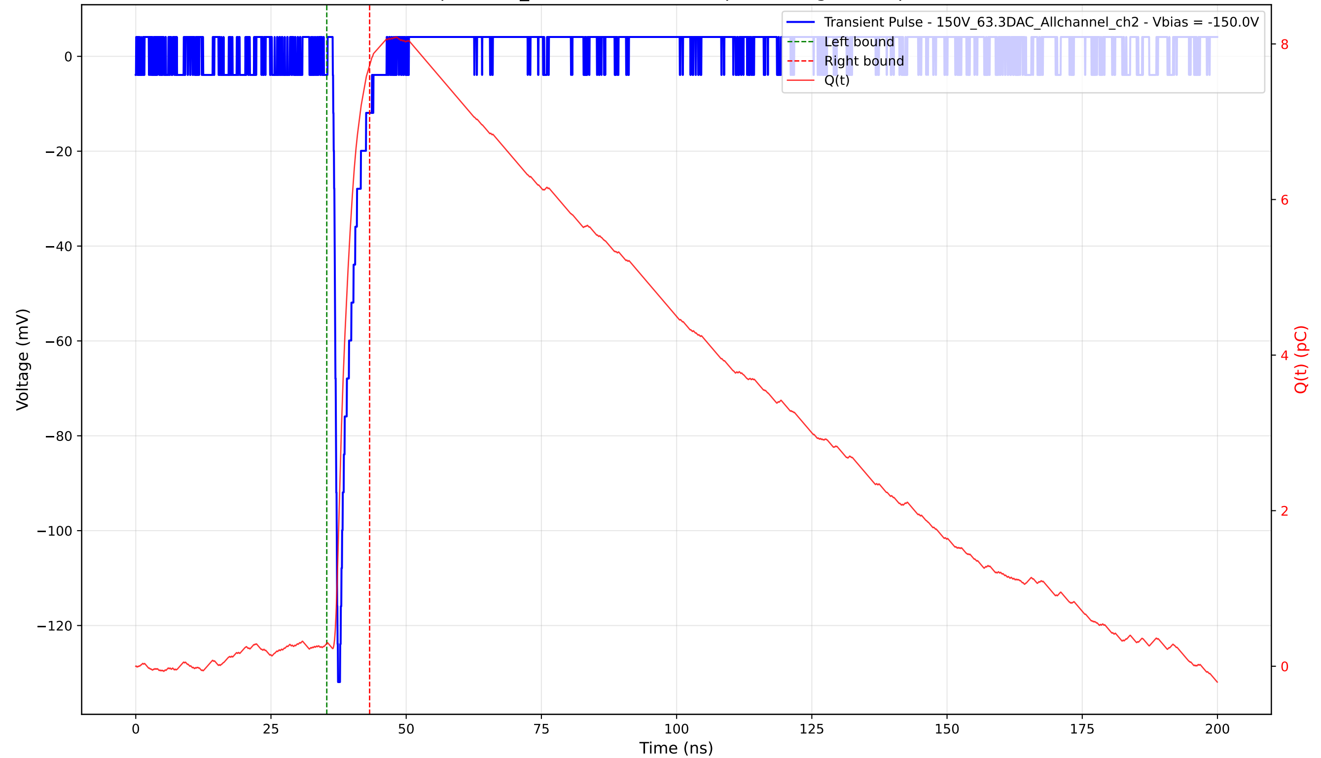
Transient Pulse - Sample: 1cm_42 - Position: 3775.0 \mu\text{m} - Charge: 7.43 pC - Rise Time: 0.75 ns
