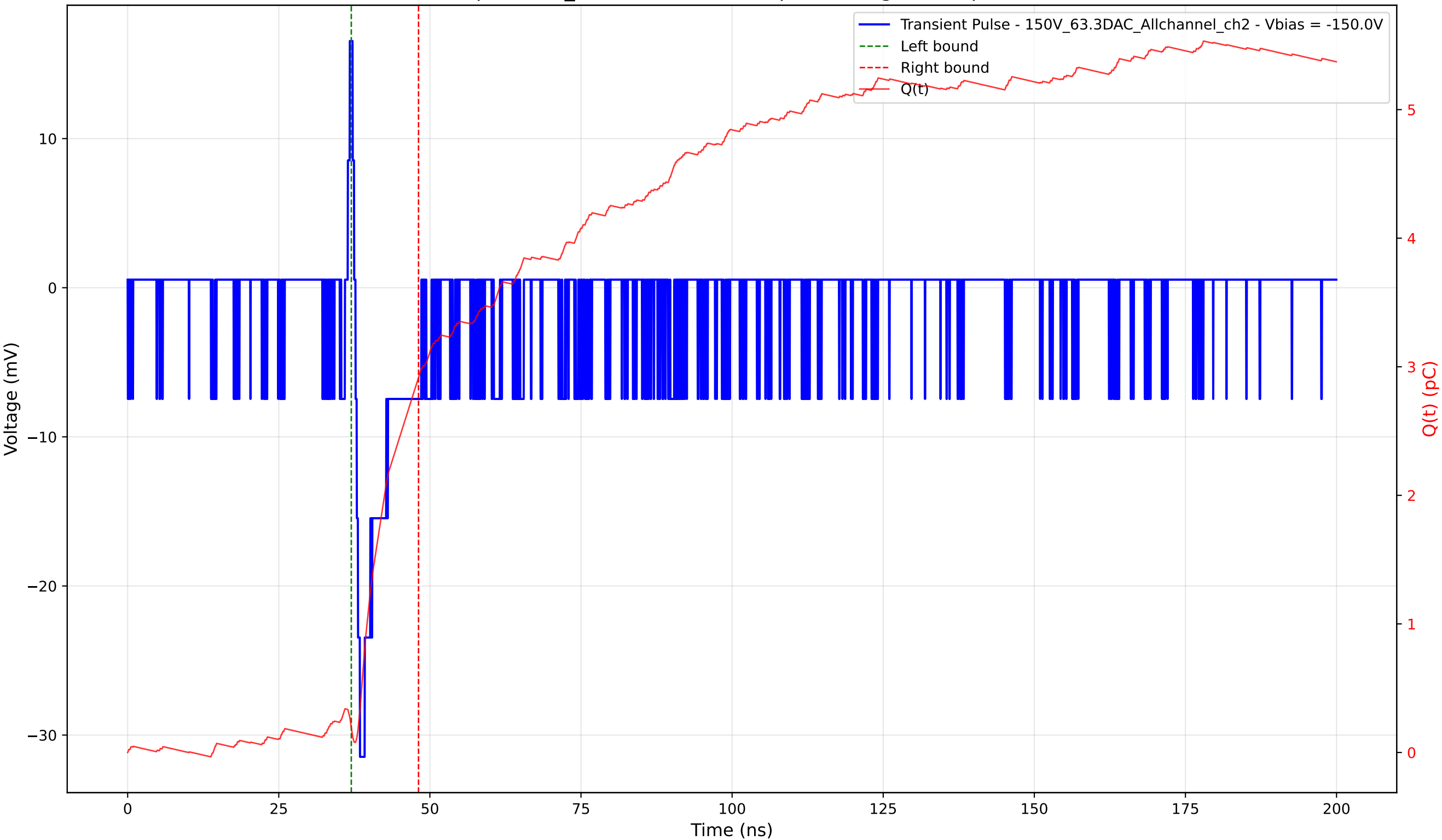
Transient Pulse - Sample: 1cm_42 - Position: 405.0 \mu\text{m} - Charge: 2.72 pC - Rise Time: 0.74 ns
