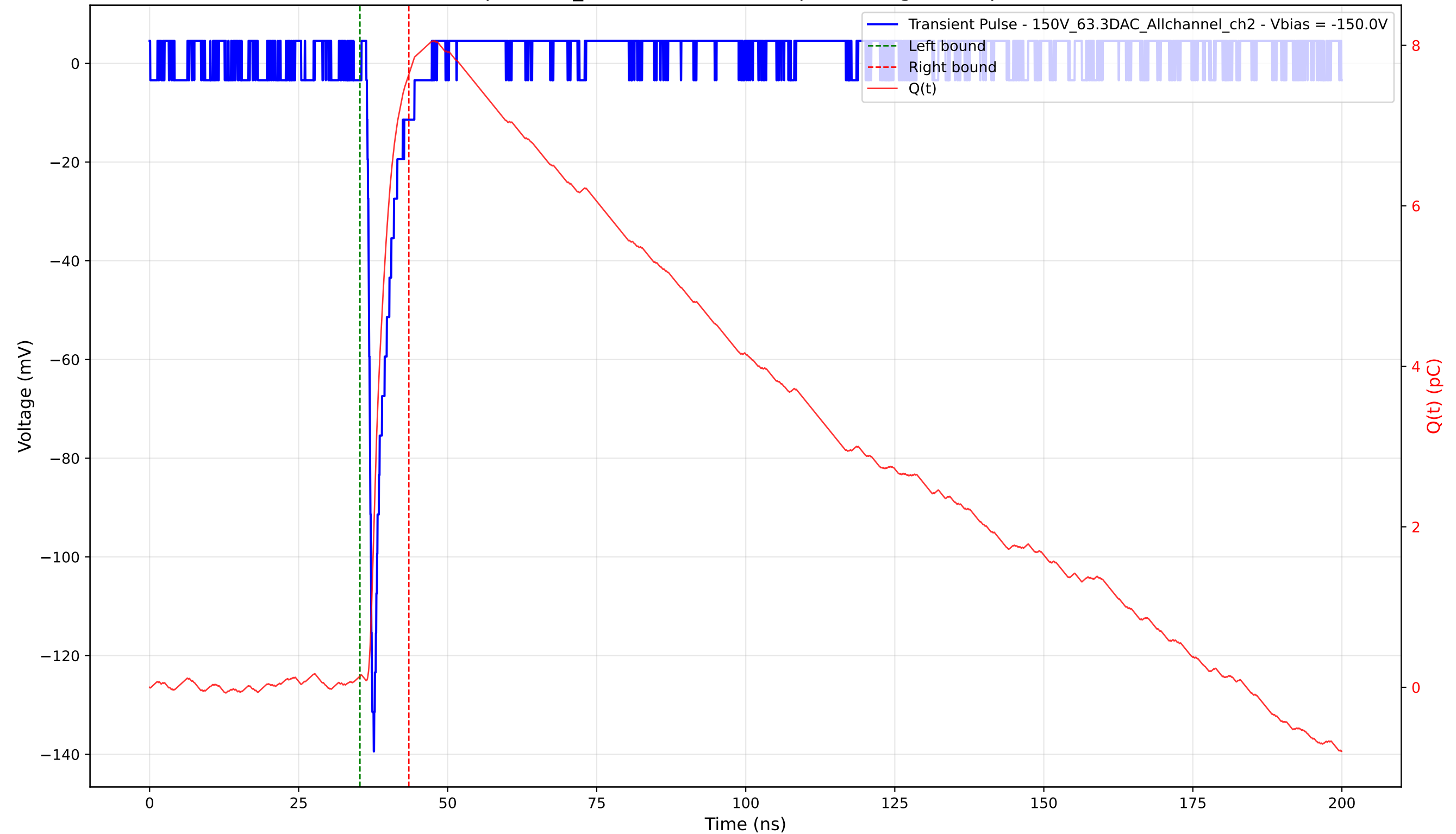
Transient Pulse - Sample: 1cm_42 - Position: 3740.0 \mu\text{m} - Charge: 7.50 pC - Rise Time: 0.83 ns
