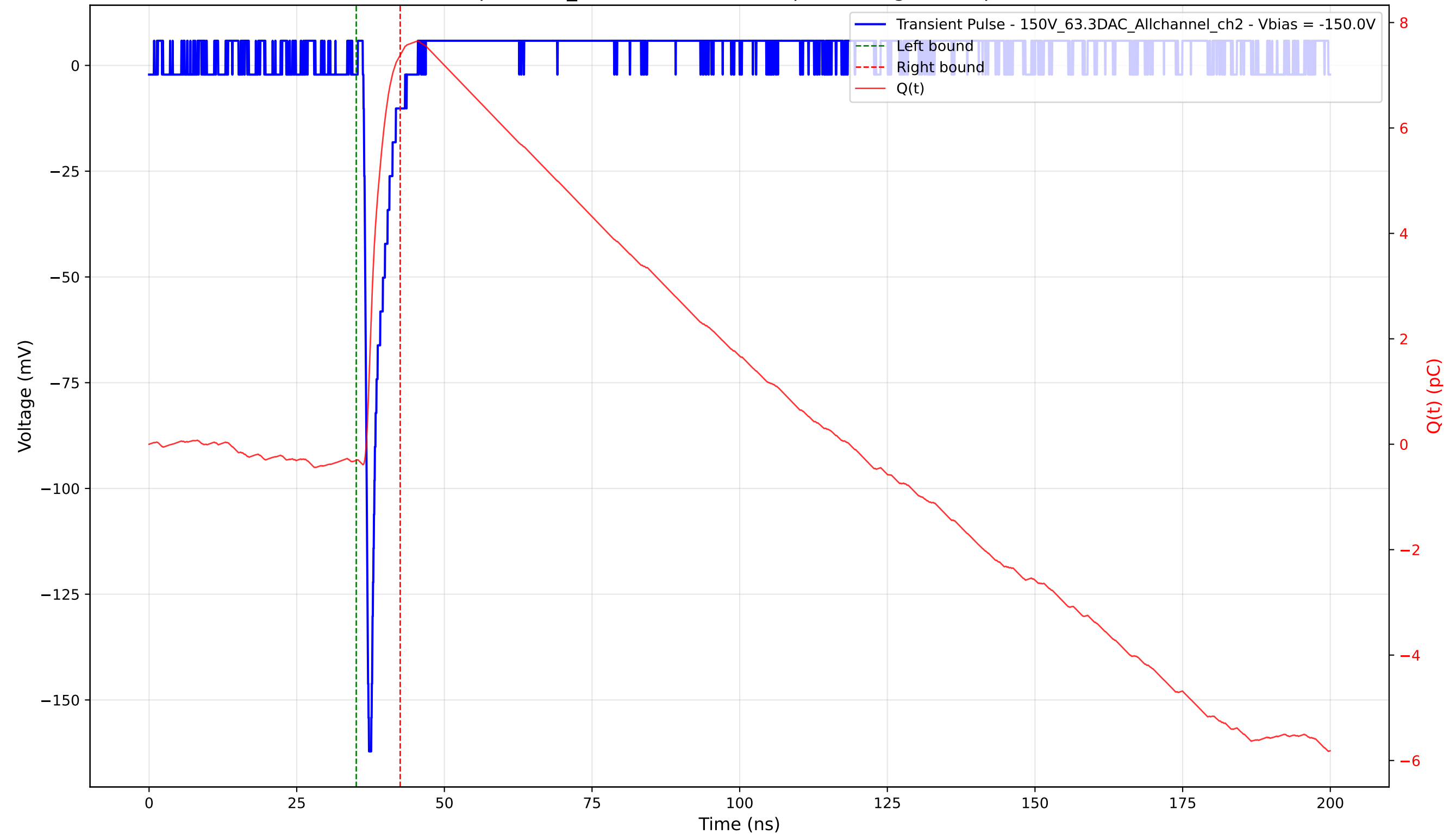
Transient Pulse - Sample: 1cm_42 - Position: 3600.0 \mu\text{m} - Charge: 7.69 pC - Rise Time: 0.69 ns
