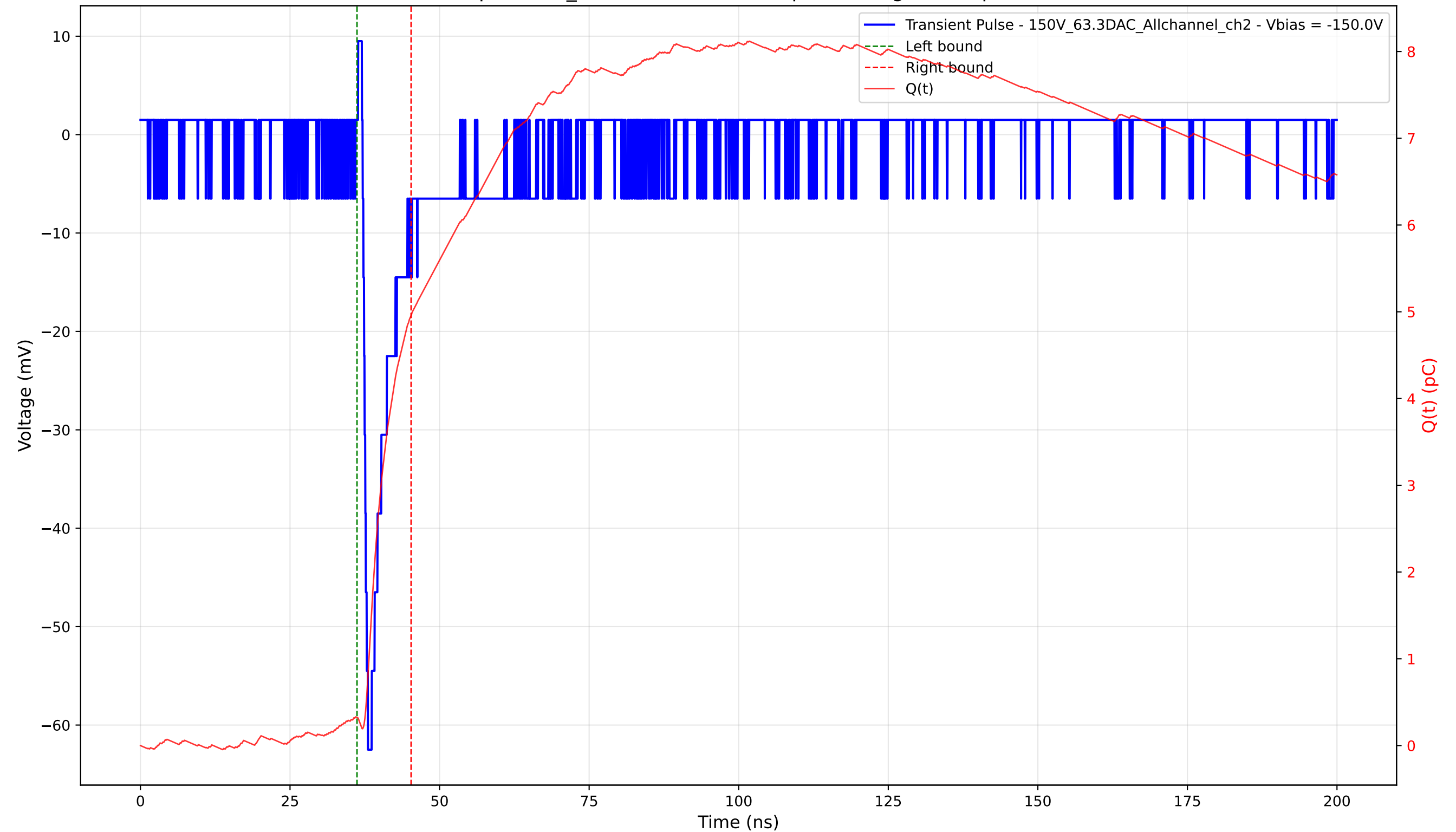
Transient Pulse - Sample: 1cm_42 - Position: 1850.0 \mu\text{m} - Charge: 4.63 pC - Rise Time: 0.88 ns
