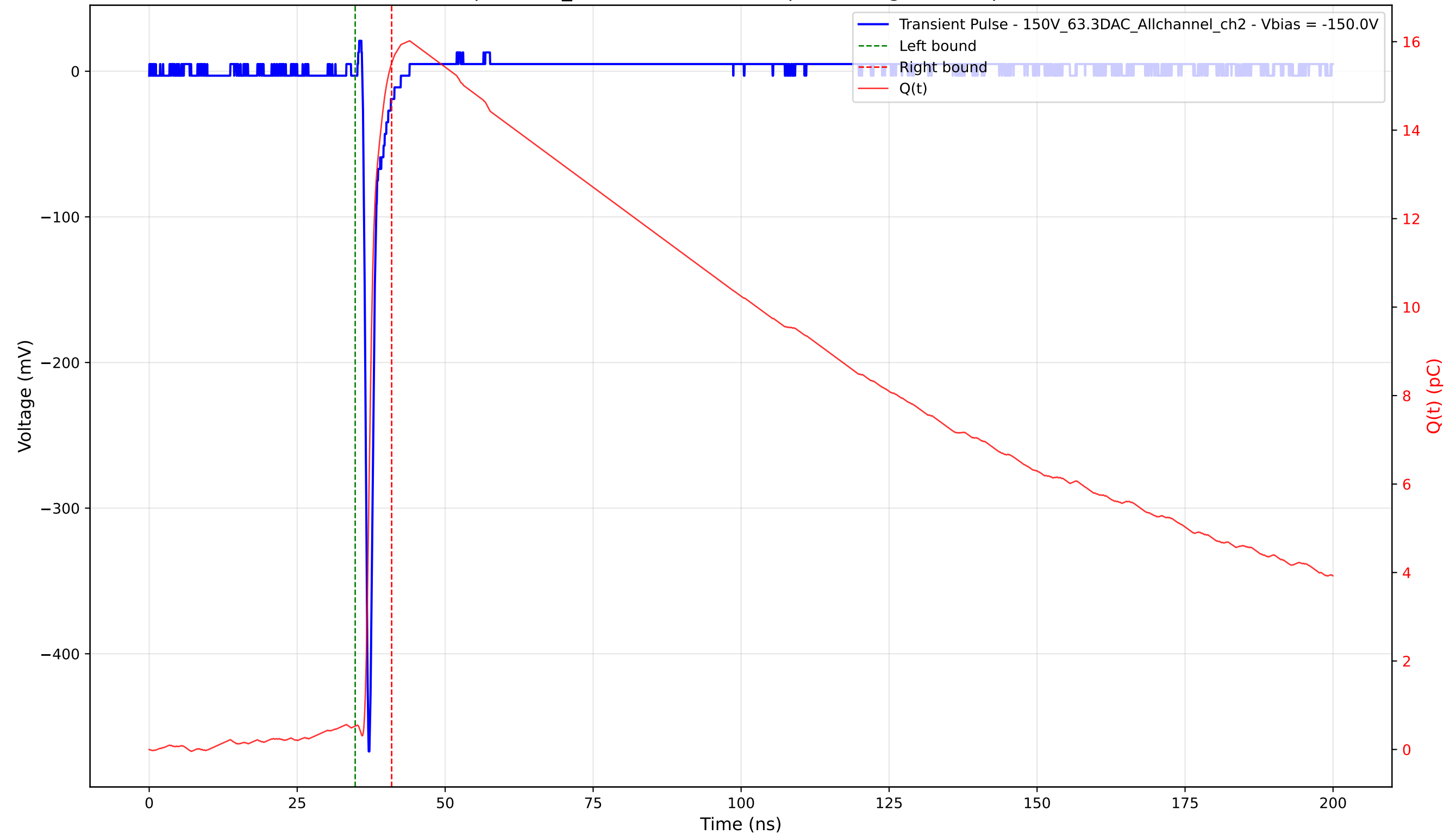
Transient Pulse - Sample: 1cm_42 - Position: 2815.0 \mu\text{m} - Charge: 14.99 pC - Rise Time: 0.73 ns
