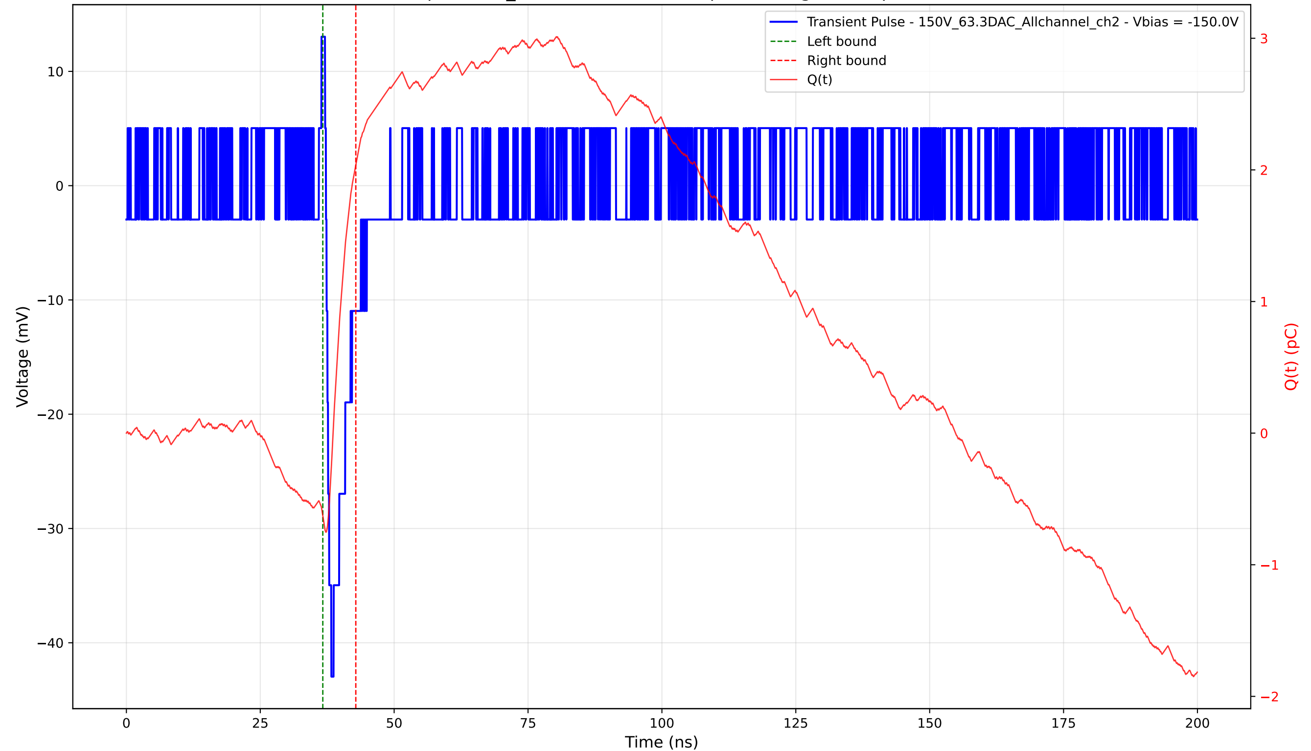
Transient Pulse - Sample: 1cm_42 - Position: 4485.0 \mu\text{m} - Charge: 2.67 pC - Rise Time: 0.91 ns
