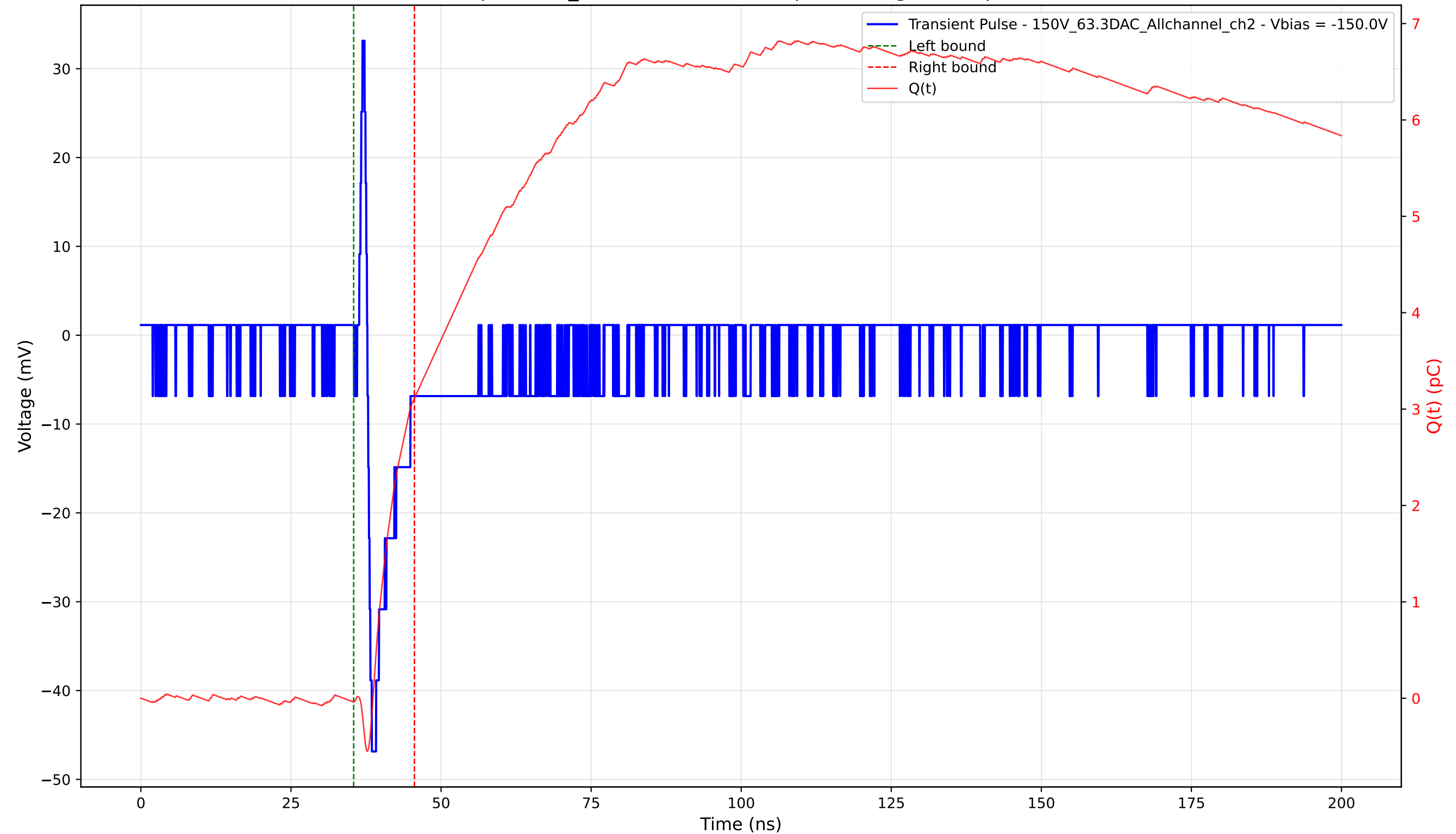
Transient Pulse - Sample: 1cm_42 - Position: 1355.0 \mu\text{m} - Charge: 3.15 pC - Rise Time: 0.74 ns
