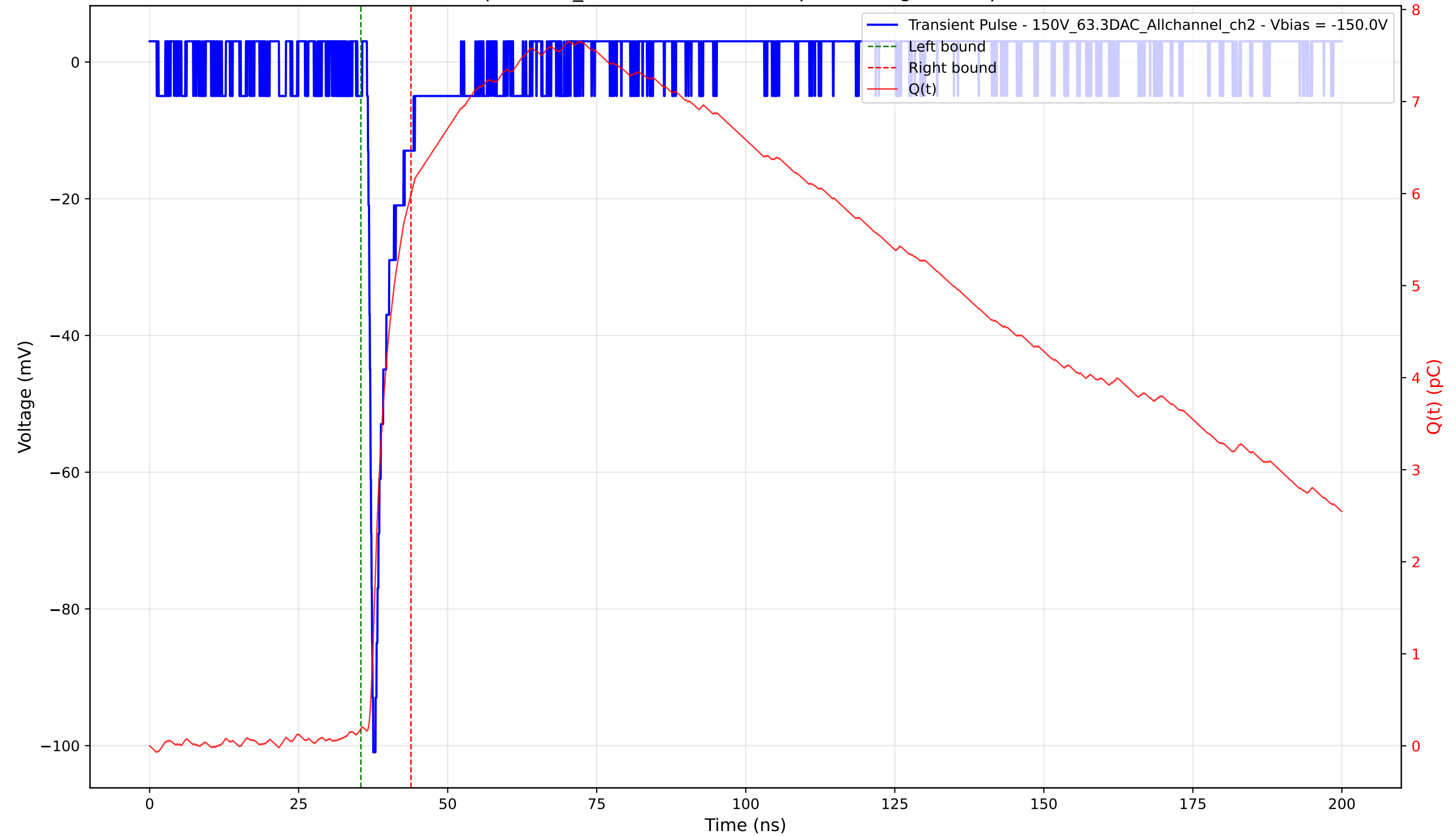
Transient Pulse - Sample: 1cm_42 - Position: 2135.0 \mu\text{m} - Charge: 5.81 pC - Rise Time: 0.77 ns
