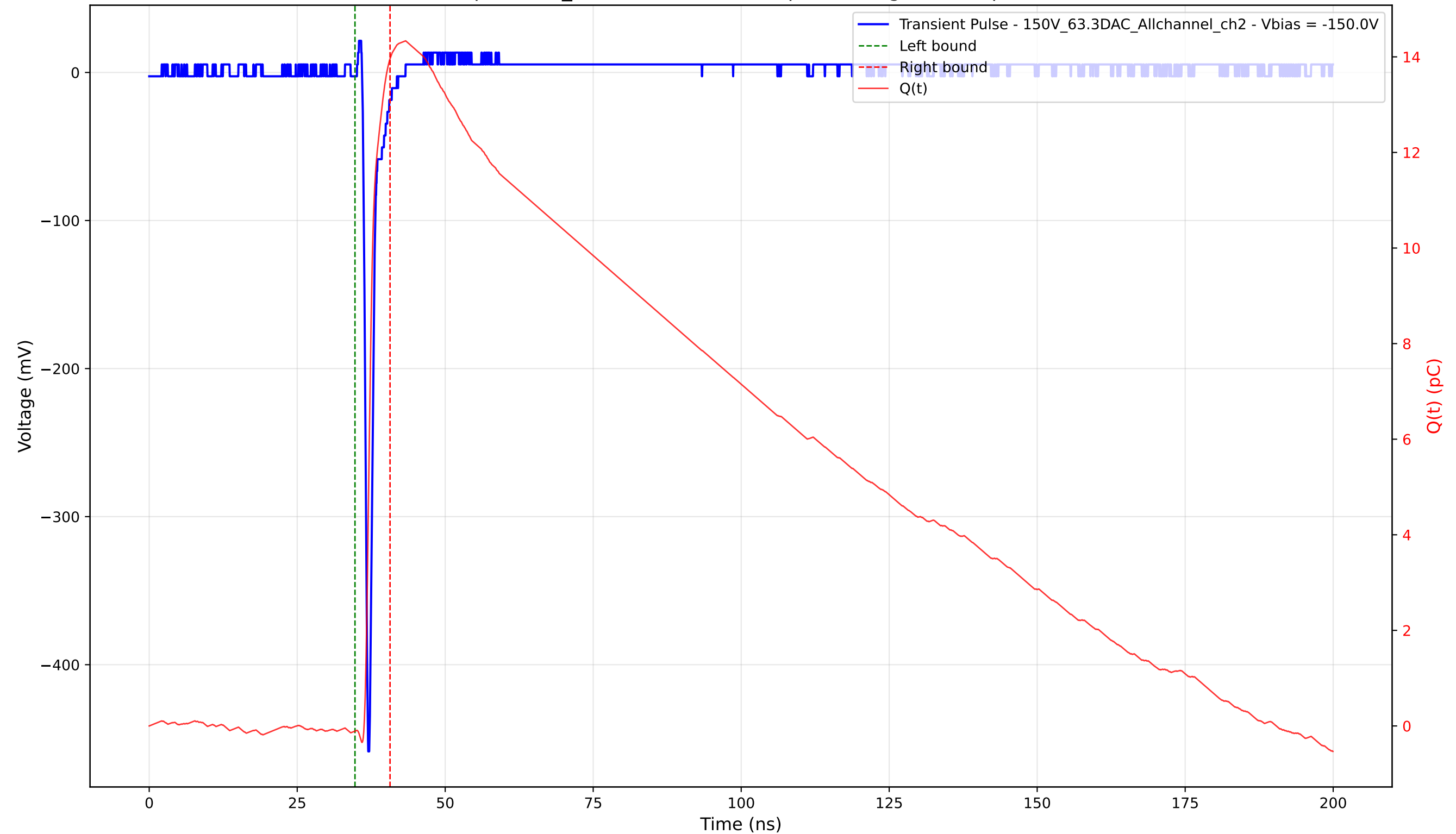
Transient Pulse - Sample: 1cm_42 - Position: 3060.0 \mu\text{m} - Charge: 14.07 pC - Rise Time: 0.72 ns
