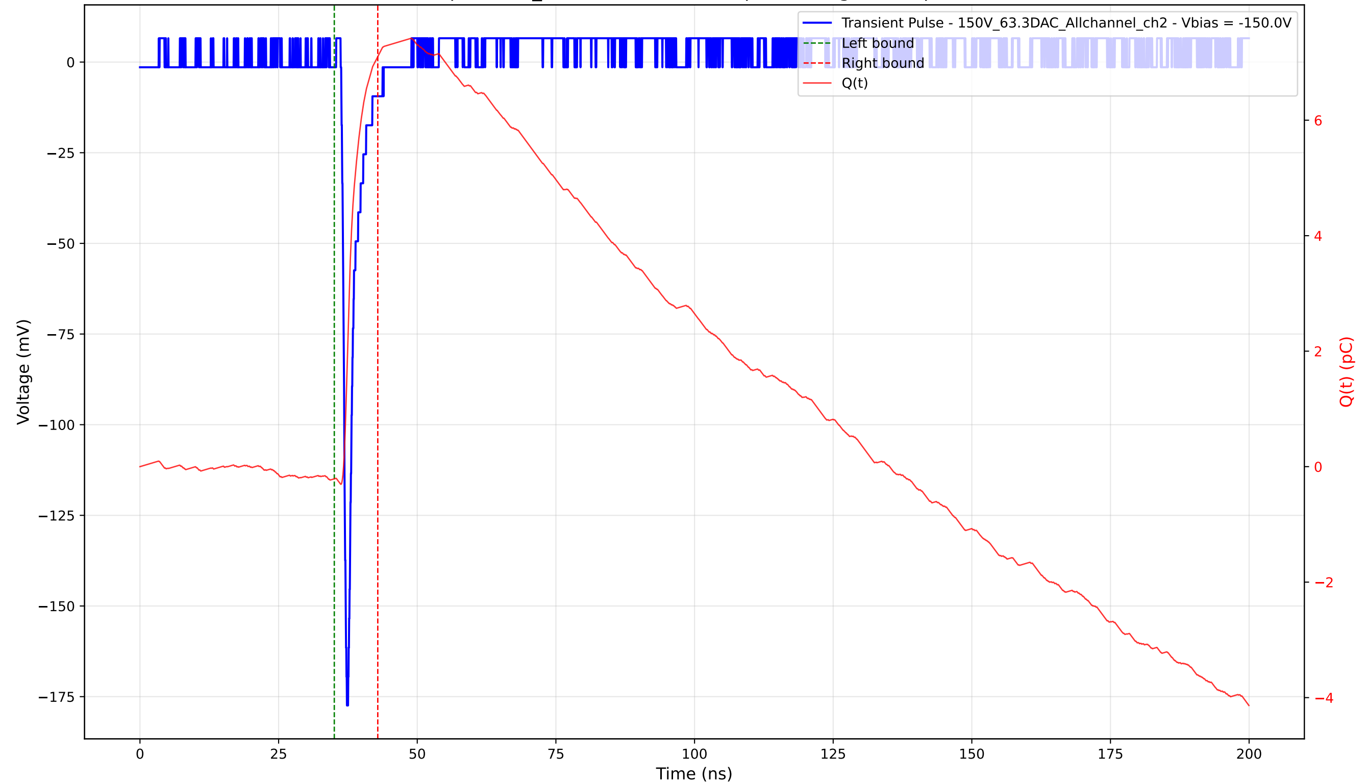
Transient Pulse - Sample: 1cm_42 - Position: 2460.0 \mu\text{m} - Charge: 7.31 pC - Rise Time: 0.76 ns
