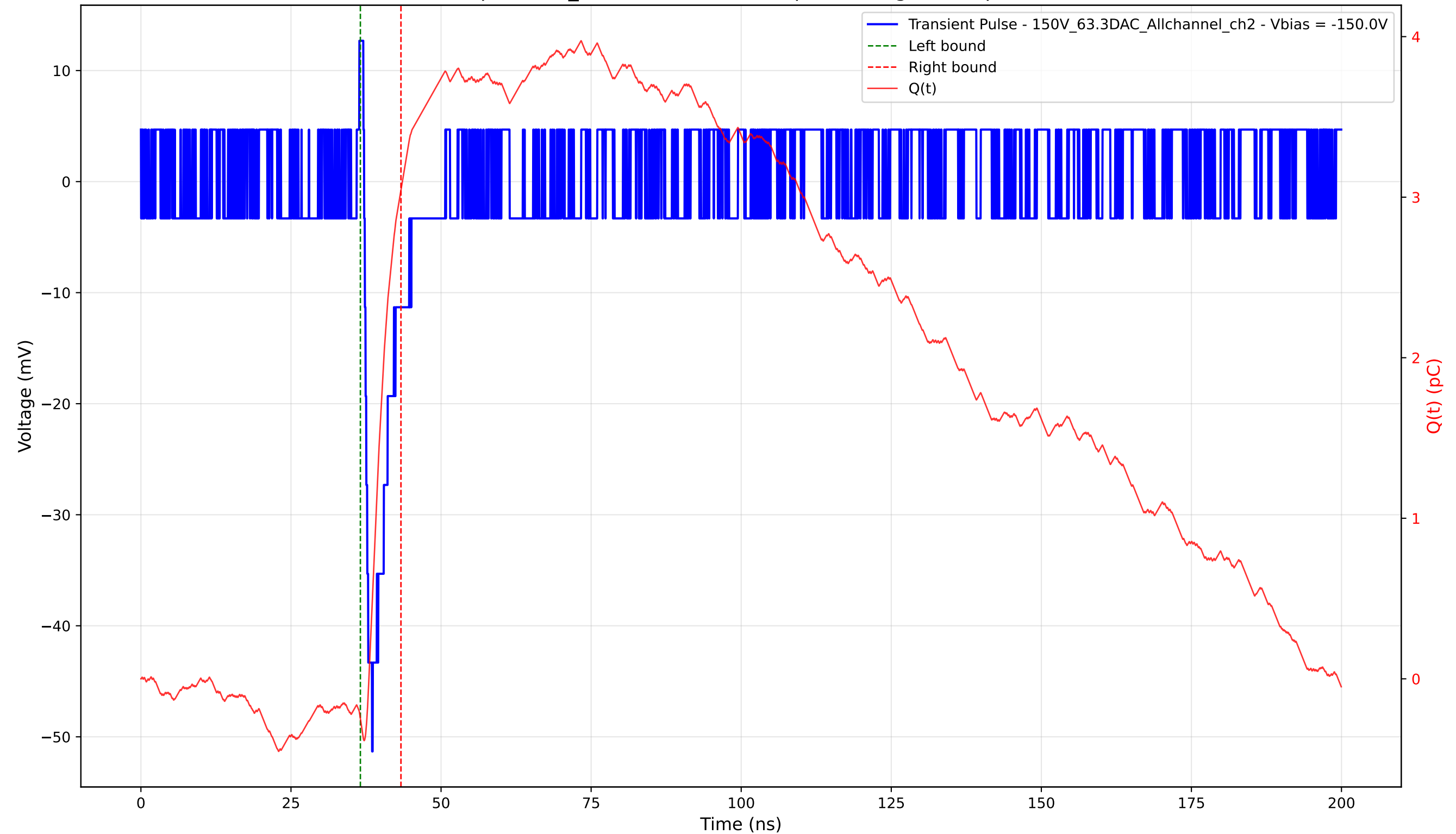
Transient Pulse - Sample: 1cm_42 - Position: 4400.0 \mu\text{m} - Charge: 3.29 pC - Rise Time: 1.23 ns
