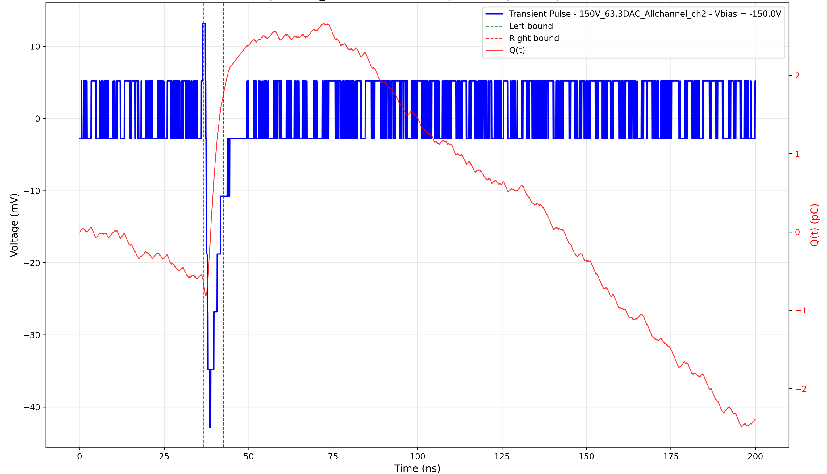
Transient Pulse - Sample: 1cm_42 - Position: 4500.0 \mu\text{m} - Charge: 2.46 pC - Rise Time: 0.99 ns
