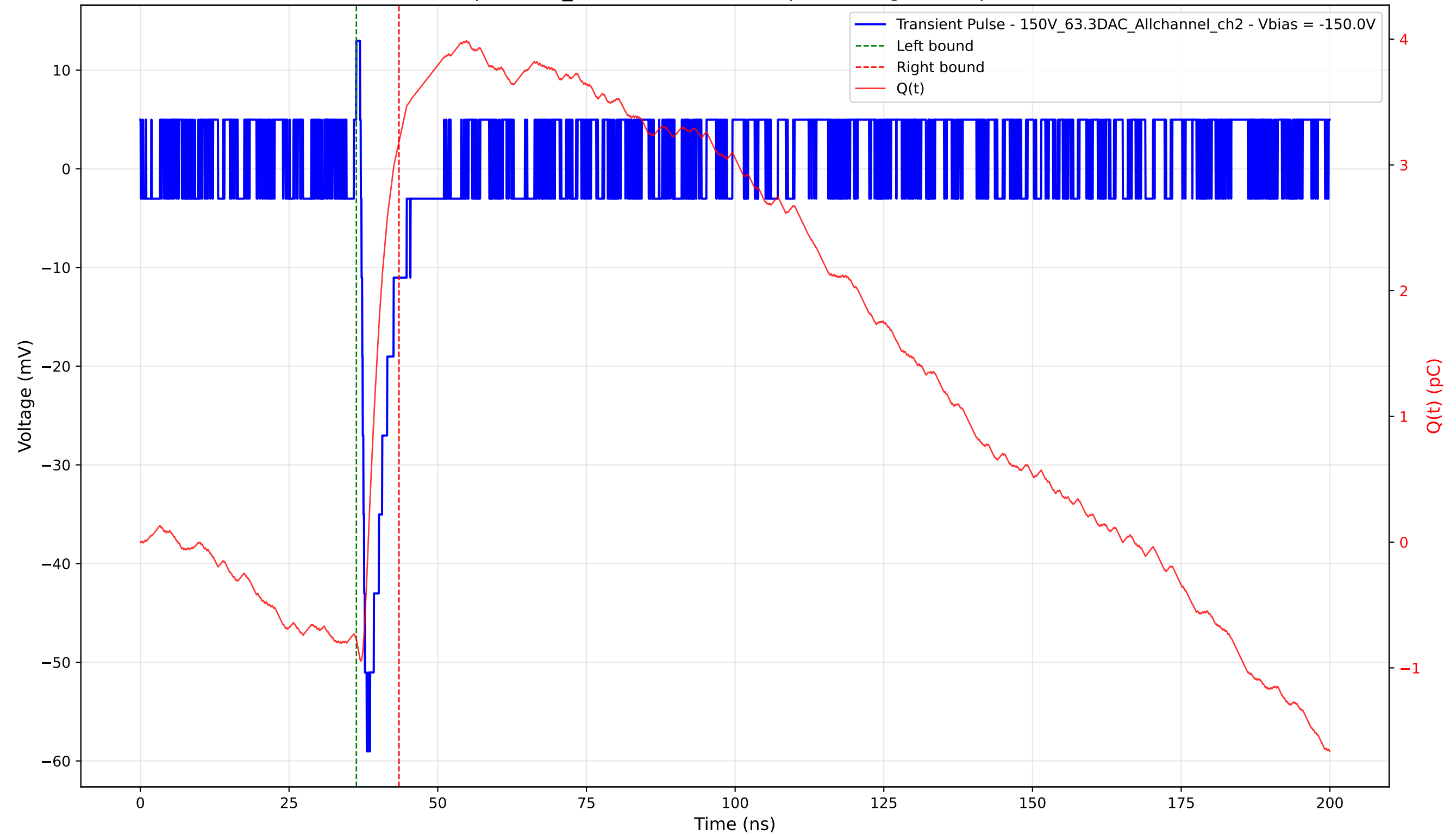
Transient Pulse - Sample: 1cm_42 - Position: 4230.0 \mu\text{m} - Charge: 3.96 pC - Rise Time: 0.91 ns
