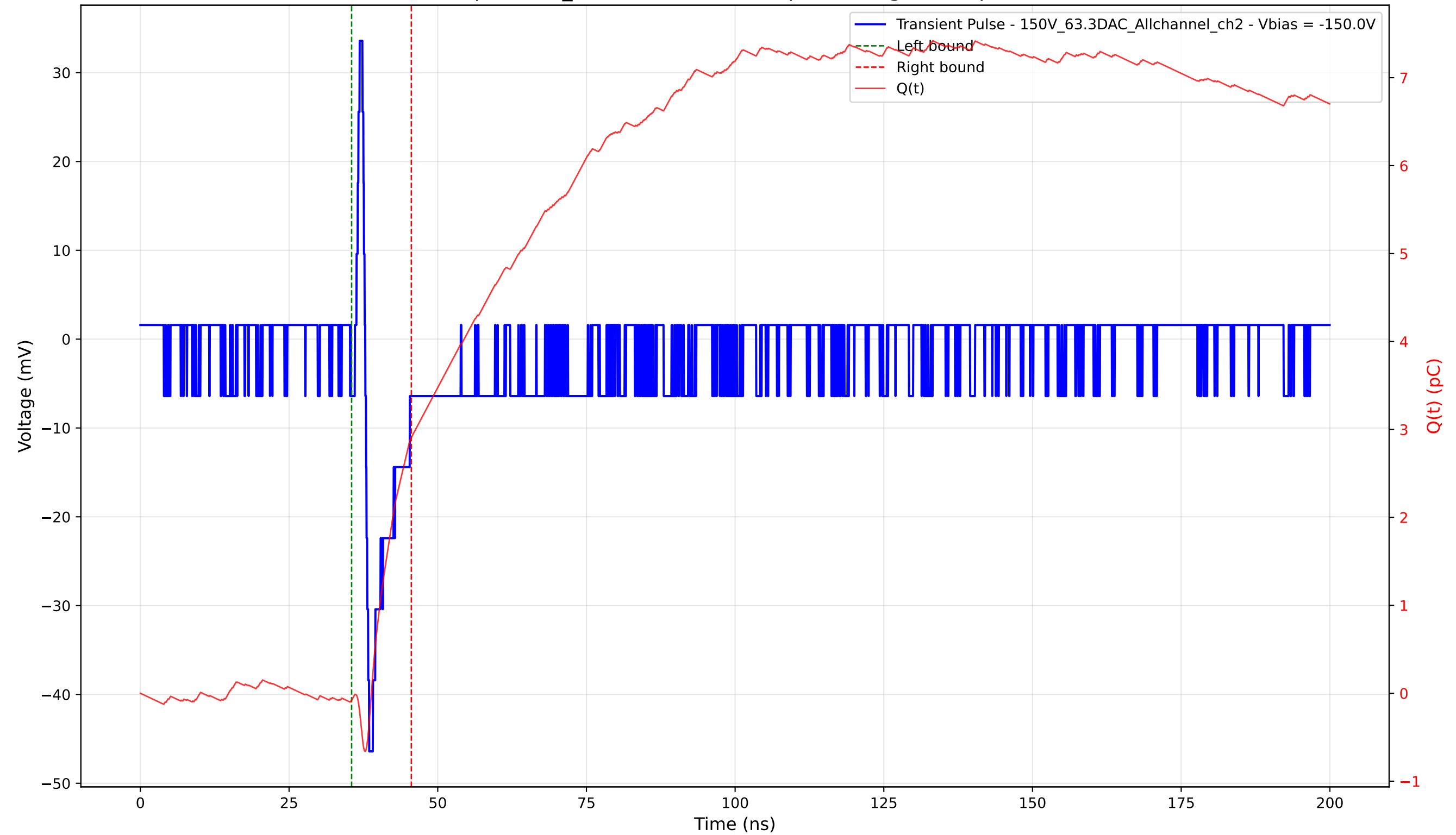
Transient Pulse - Sample: 1cm_42 - Position: 1160.0 \mu\text{m} - Charge: 2.99 pC - Rise Time: 0.65 ns
