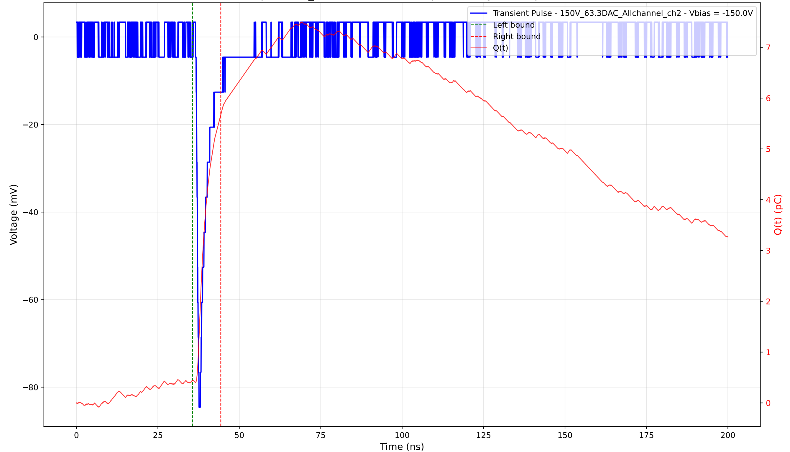
Transient Pulse - Sample: 1cm_42 - Position: 2065.0 \mu\text{m} - Charge: 5.23 pC - Rise Time: 0.74 ns
