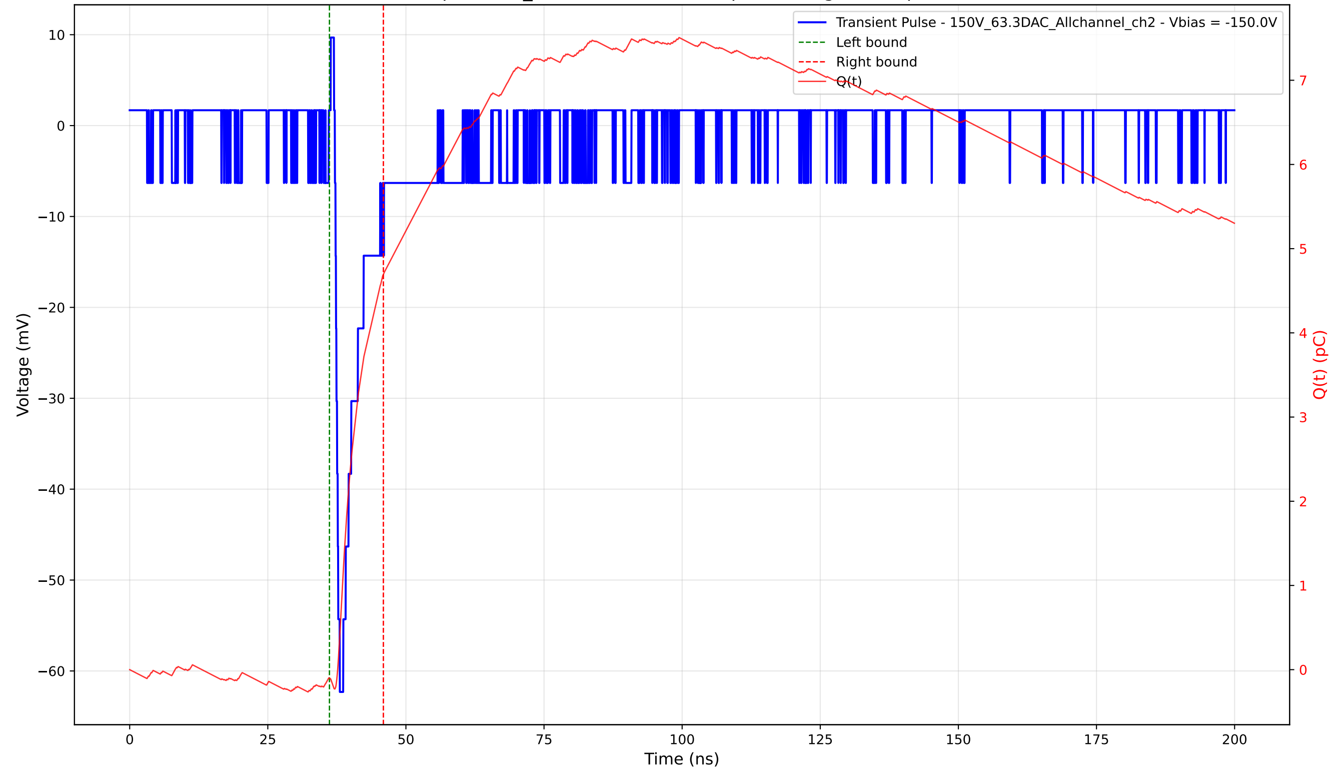
Transient Pulse - Sample: 1cm_42 - Position: 1860.0 \mu\text{m} - Charge: 4.79 pC - Rise Time: 0.88 ns
