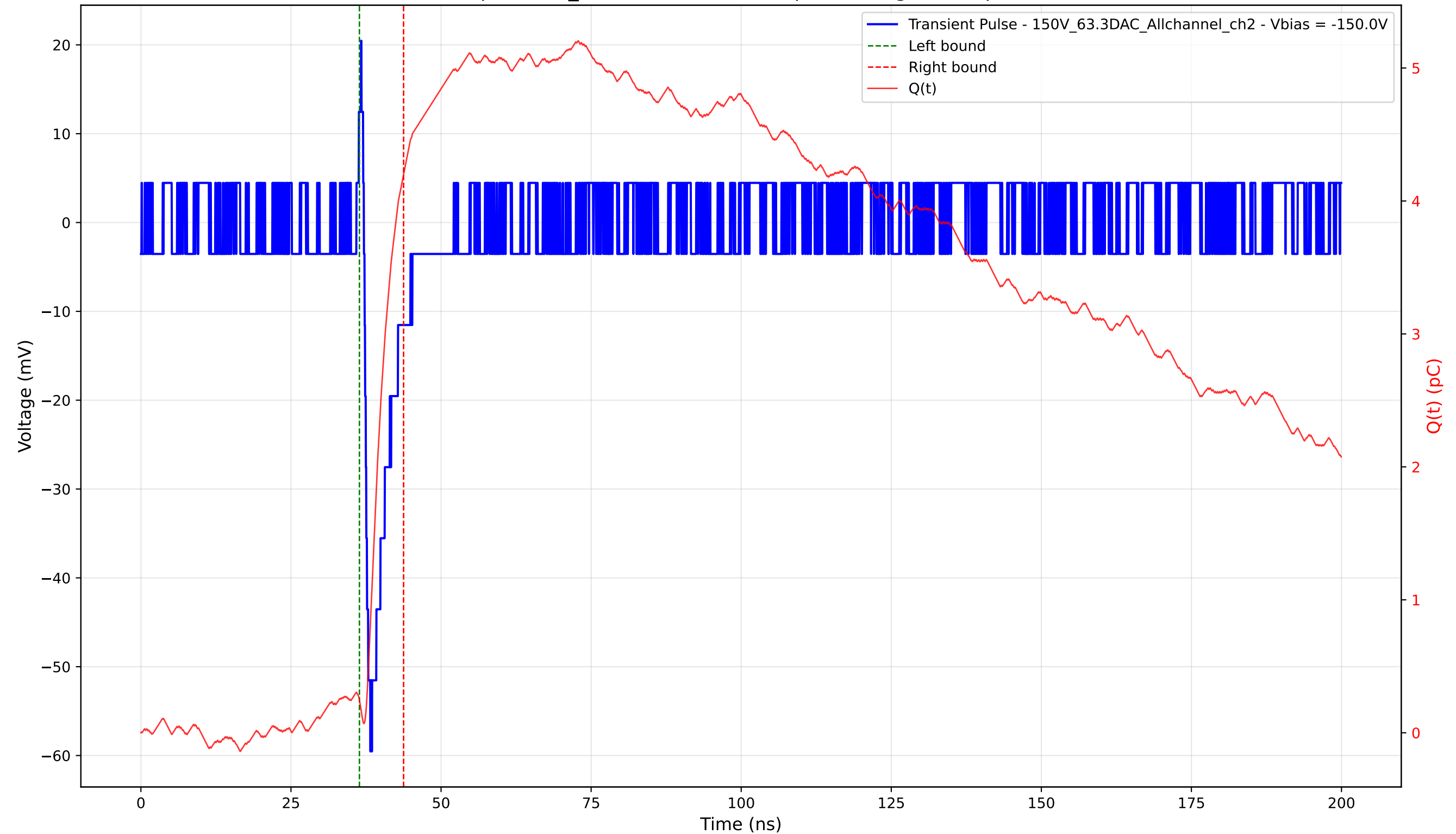
Transient Pulse - Sample: 1cm_42 - Position: 4315.0 \mu\text{m} - Charge: 3.95 pC - Rise Time: 0.99 ns
