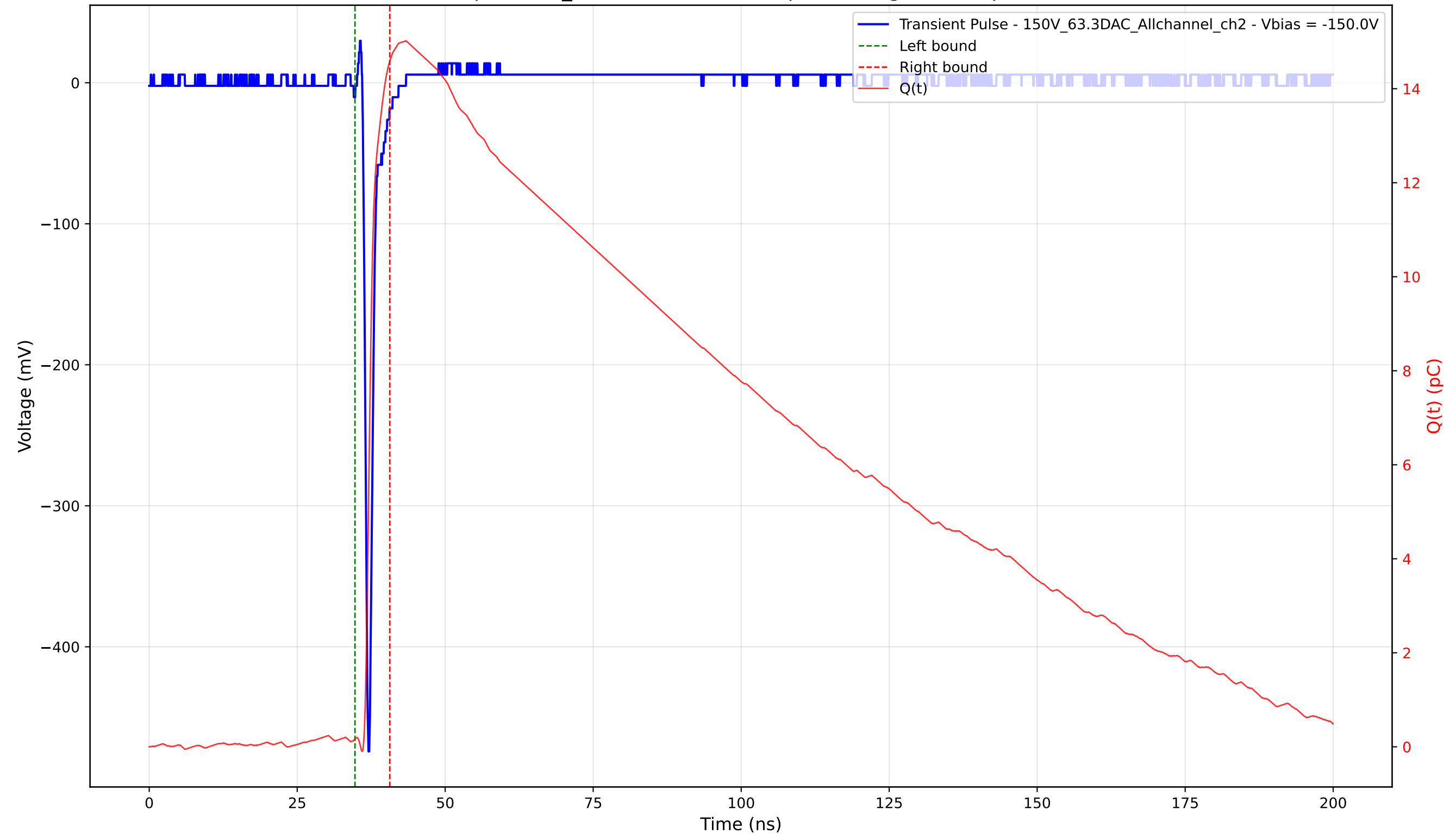
Transient Pulse - Sample: 1cm_42 - Position: 2960.0 \mu\text{m} - Charge: 14.42 pC - Rise Time: 0.67 ns
