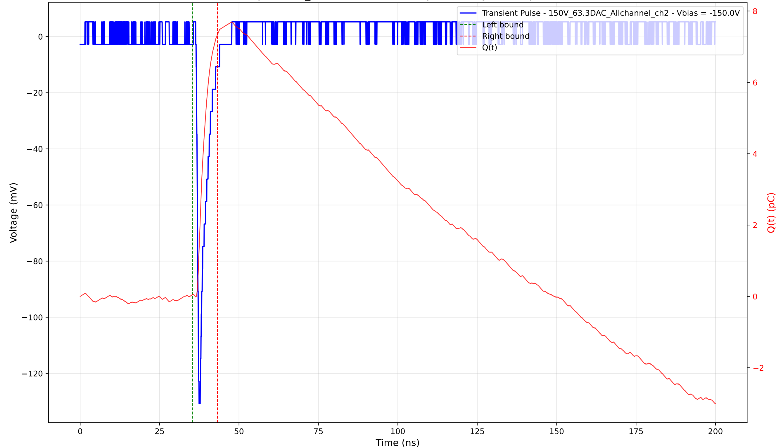
Transient Pulse - Sample: 1cm_42 - Position: 3765.0 \mu\text{m} - Charge: 7.30 pC - Rise Time: 0.75 ns
