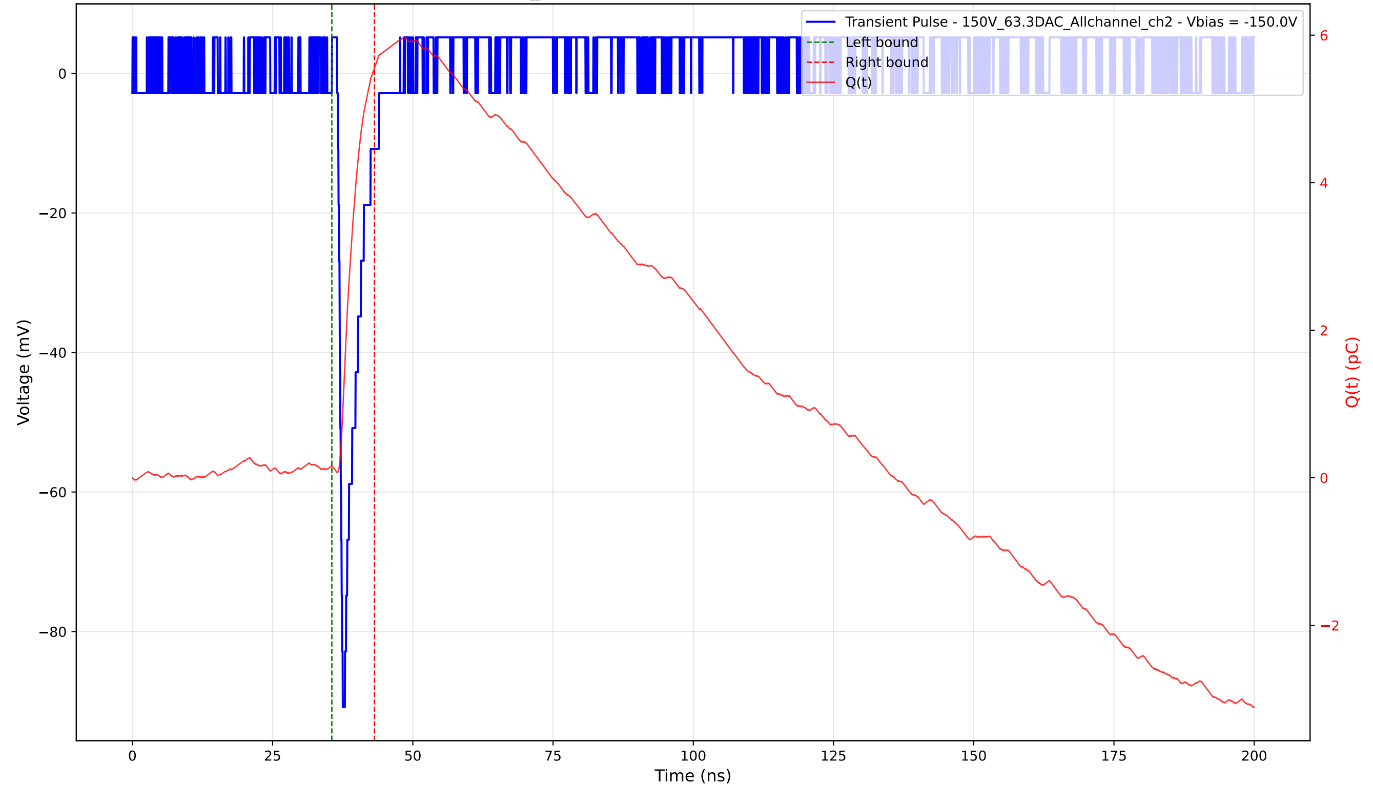
Transient Pulse - Sample: 1cm_42 - Position: 3935.0 \mu\text{m} - Charge: 5.39 pC - Rise Time: 0.73 ns
