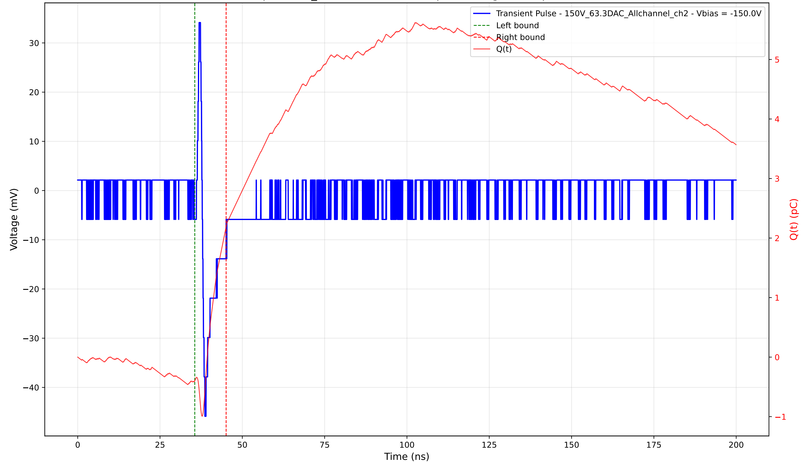
Transient Pulse - Sample: 1cm_42 - Position: 1120.0 \mu\text{m} - Charge: 2.60 pC - Rise Time: 0.81 ns
