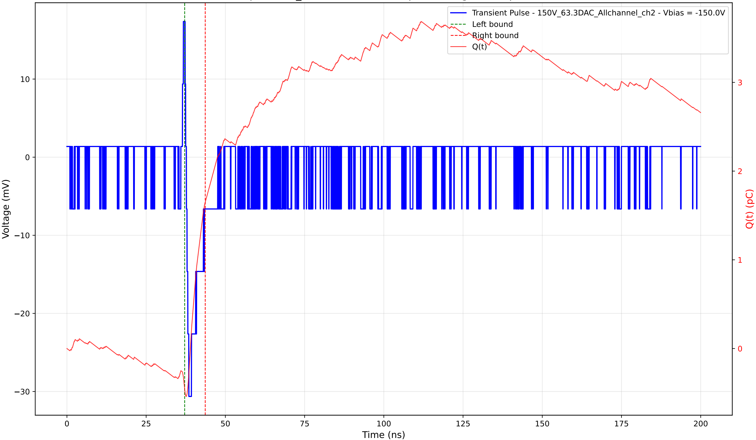
Transient Pulse - Sample: 1cm_42 - Position: 415.0 \mu\text{m} - Charge: 2.11 pC - Rise Time: 0.79 ns
