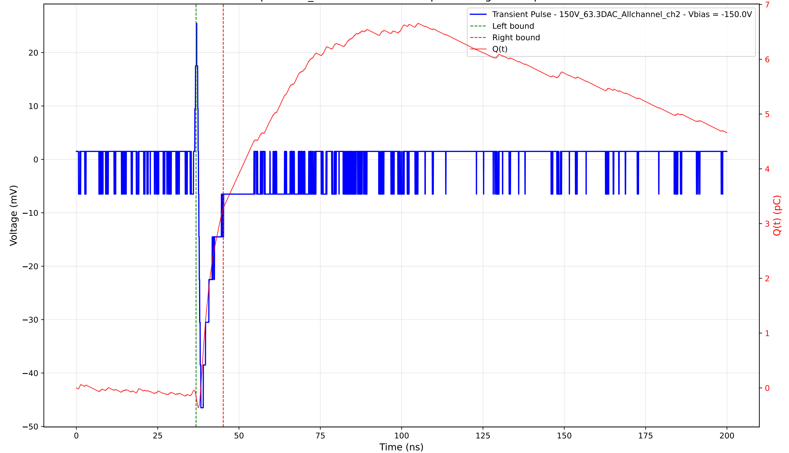
Transient Pulse - Sample: 1cm_42 - Position: 1535.0 \mu\text{m} - Charge: 3.43 pC - Rise Time: 0.73 ns
