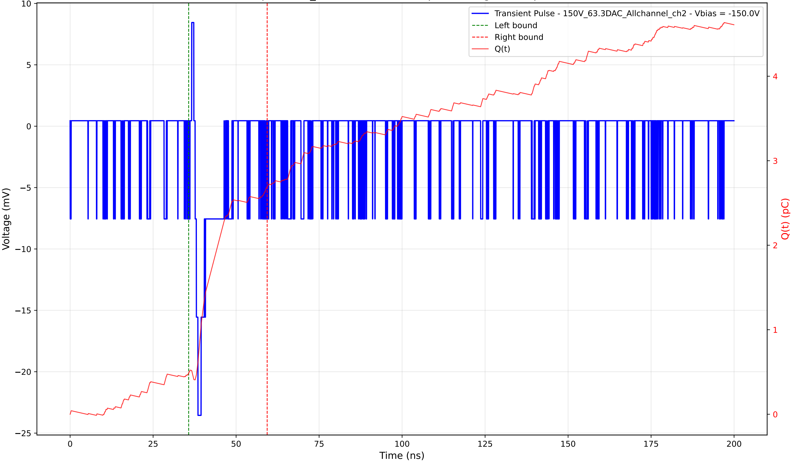
Transient Pulse - Sample: 1cm_42 - Position: 210.0 \mu\text{m} - Charge: 2.20 pC - Rise Time: 0.87 ns
