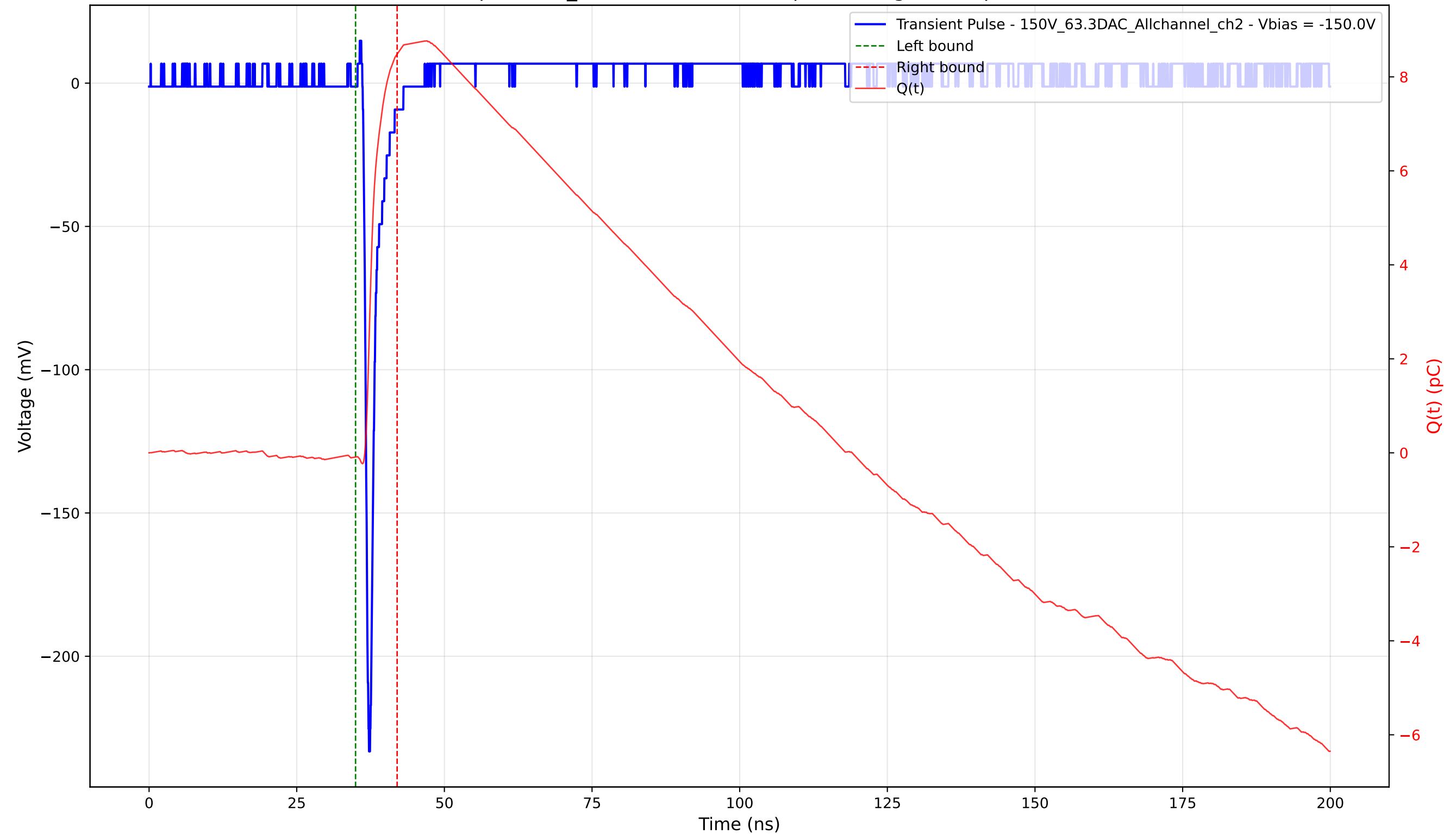
Transient Pulse - Sample: 1cm_42 - Position: 2550.0 \mu\text{m} - Charge: 8.57 pC - Rise Time: 0.77 ns
