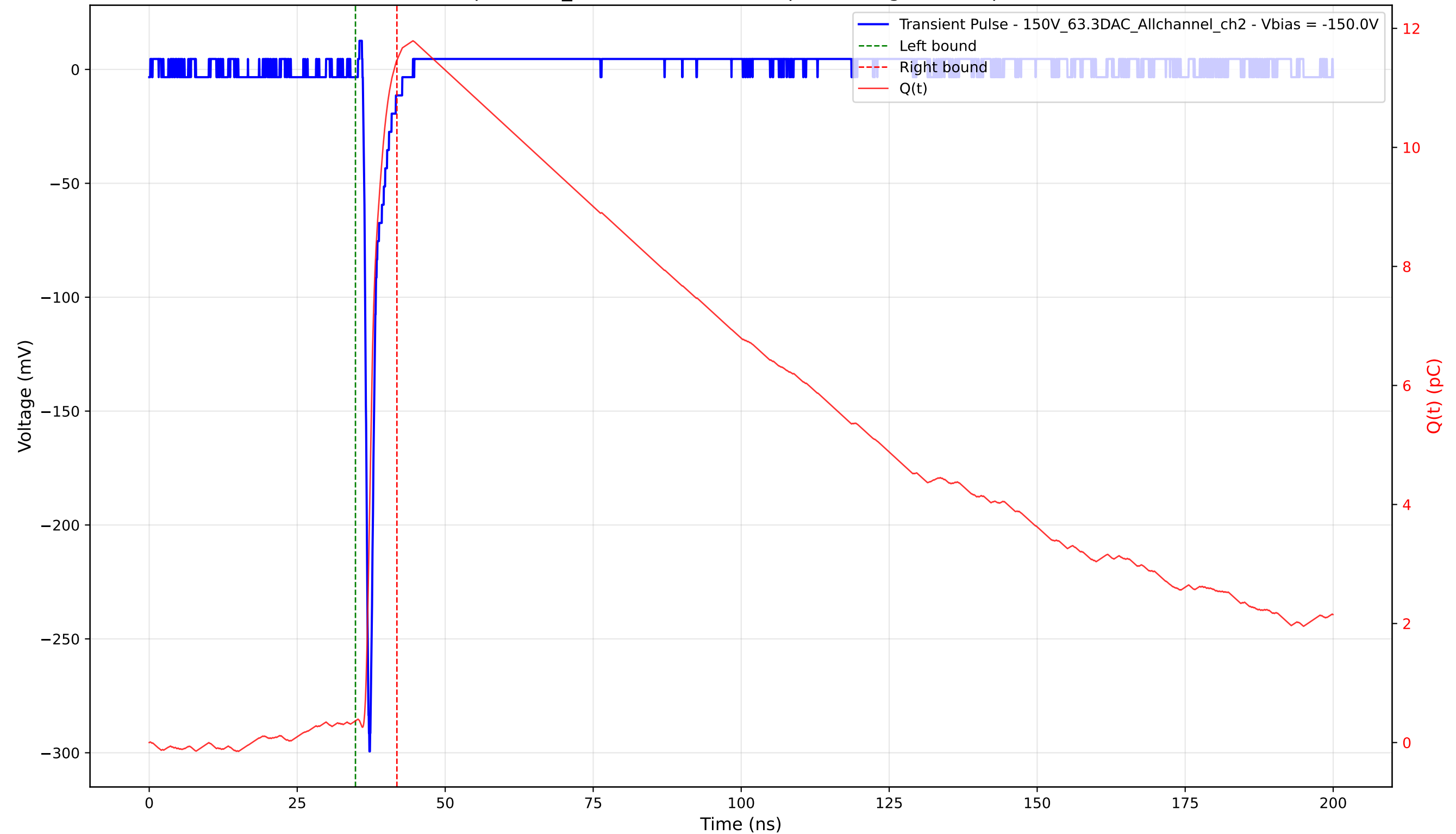
Transient Pulse - Sample: 1cm_42 - Position: 3425.0 \mu\text{m} - Charge: 11.10 pC - Rise Time: 0.76 ns
