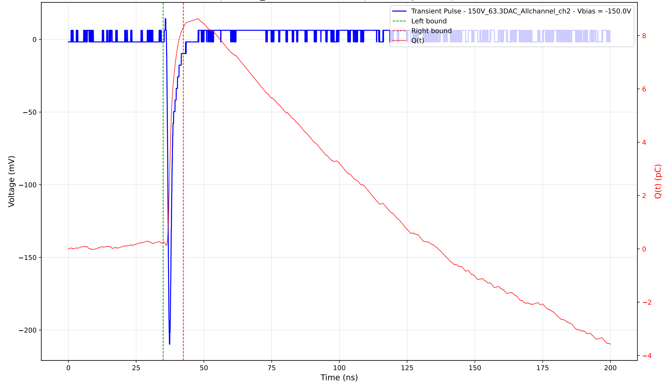
Transient Pulse - Sample: 1cm_42 - Position: 2515.0 \mu\text{m} - Charge: 8.06 pC - Rise Time: 0.78 ns
