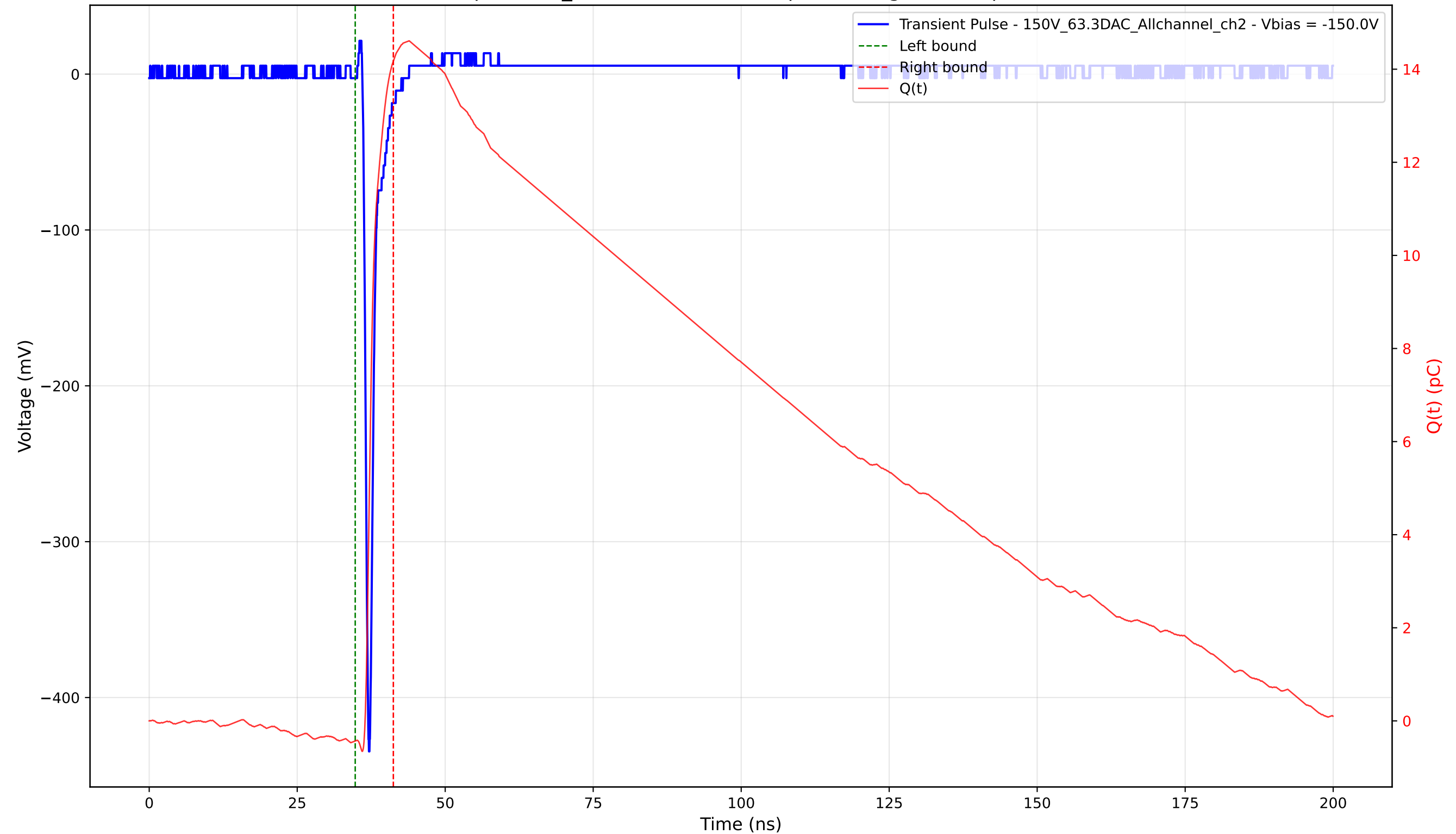
Transient Pulse - Sample: 1cm_42 - Position: 3275.0 \mu\text{m} - Charge: 14.60 pC - Rise Time: 0.73 ns
