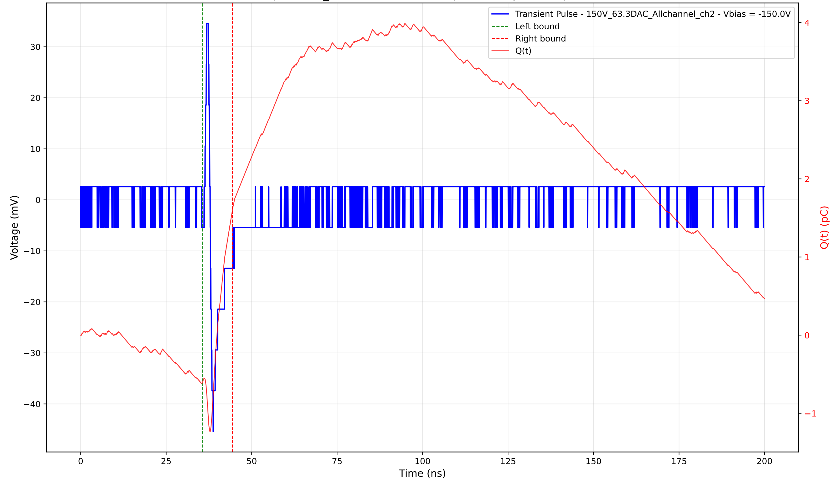
Transient Pulse - Sample: 1cm_42 - Position: 1100.0 \mu\text{m} - Charge: 2.22 pC - Rise Time: 0.89 ns
