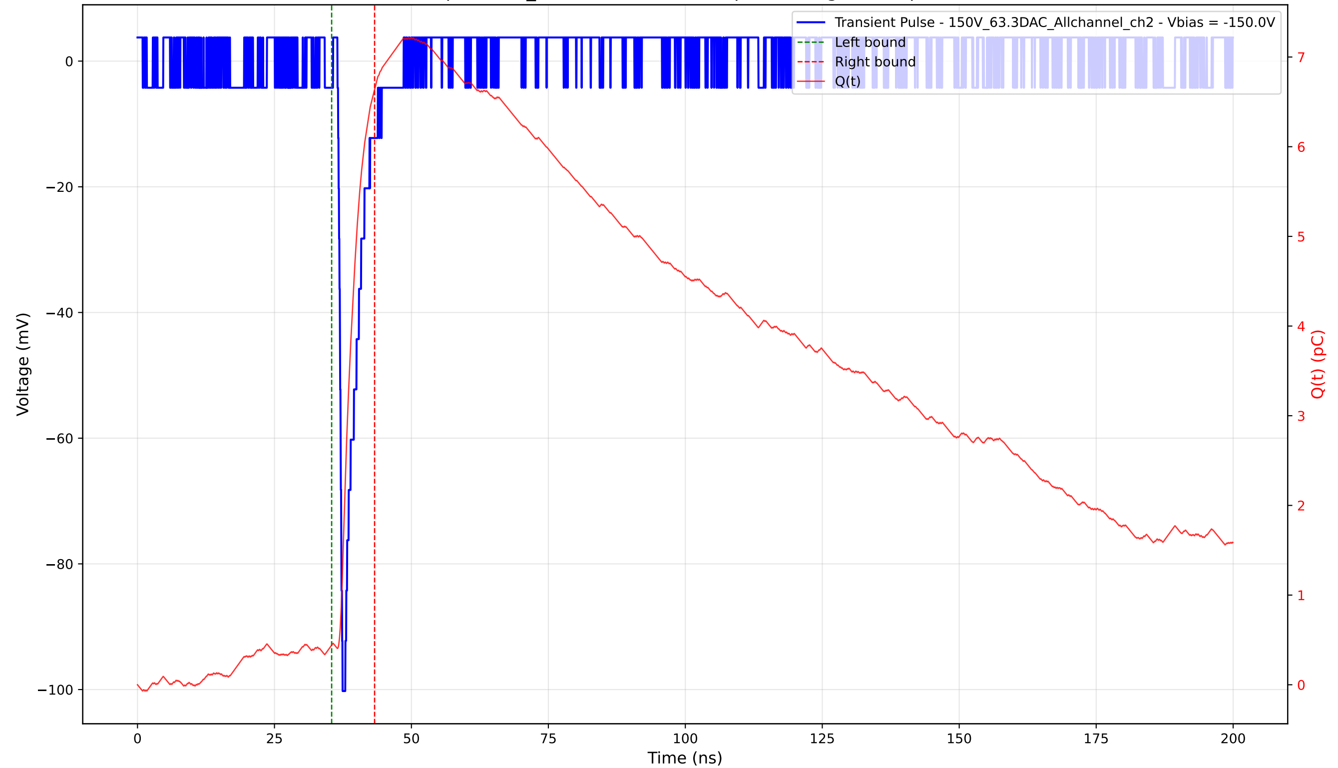
Transient Pulse - Sample: 1cm_42 - Position: 3900.0 \mu\text{m} - Charge: 6.20 pC - Rise Time: 0.73 ns
