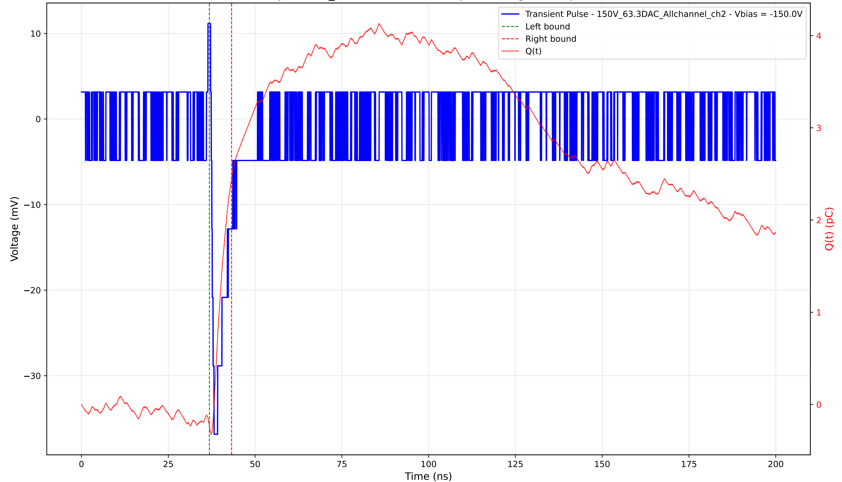
Transient Pulse - Sample: 1cm_42 - Position: 4600.0 \mu\text{m} - Charge: 2.68 pC - Rise Time: 0.83 ns
