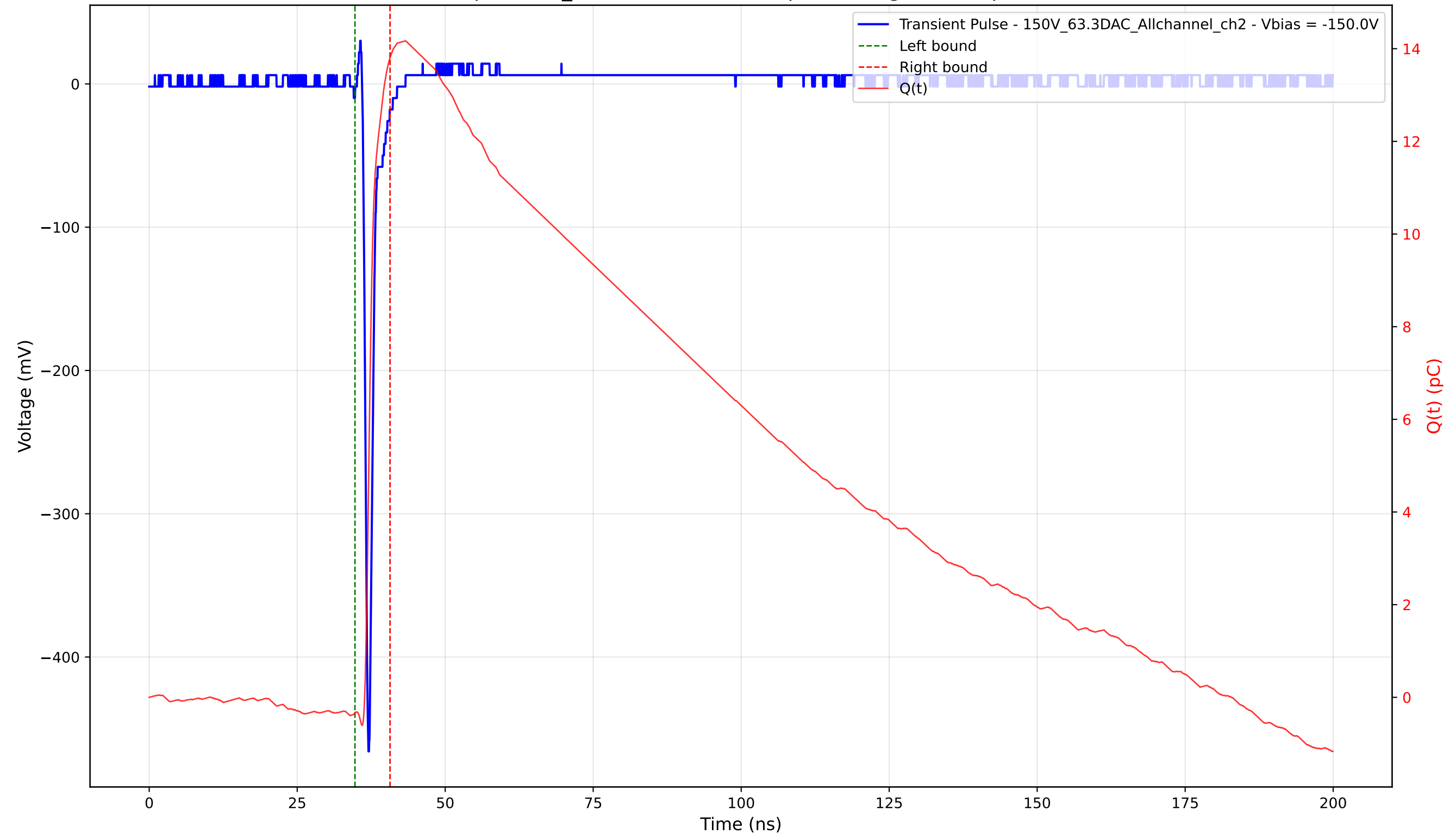
Transient Pulse - Sample: 1cm_42 - Position: 3065.0 \mu\text{m} - Charge: 14.14 pC - Rise Time: 0.68 ns
