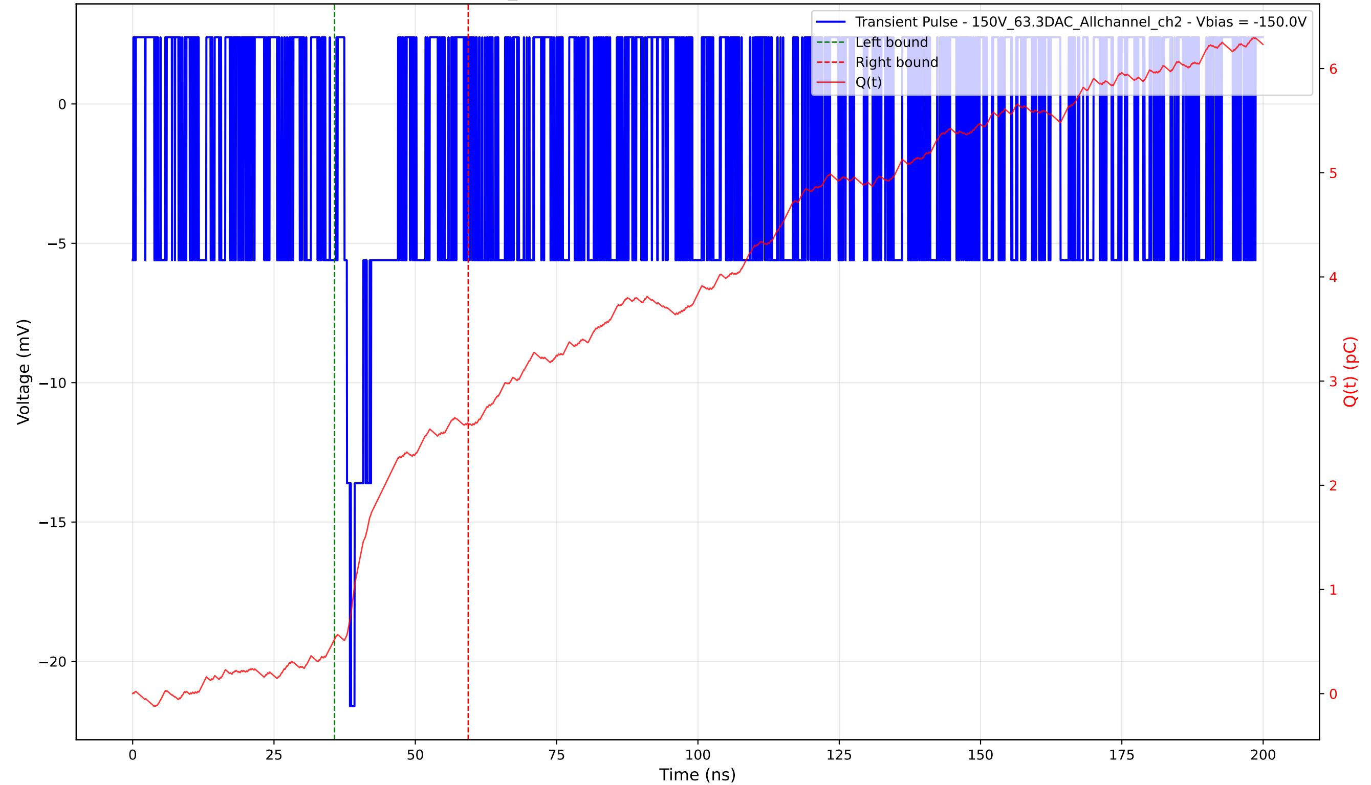
Transient Pulse - Sample: 1cm_42 - Position: 5035.0 \mu\text{m} - Charge: 2.07 pC - Rise Time: 0.00 ns (N/A)
