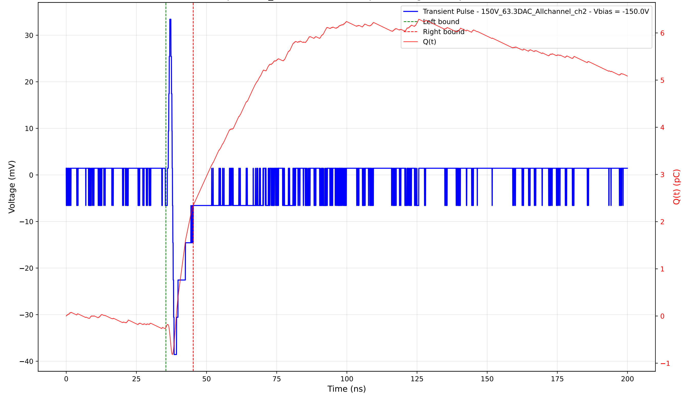
Transient Pulse - Sample: 1cm_42 - Position: 885.0 \mu\text{m} - Charge: 2.58 pC - Rise Time: 0.58 ns
