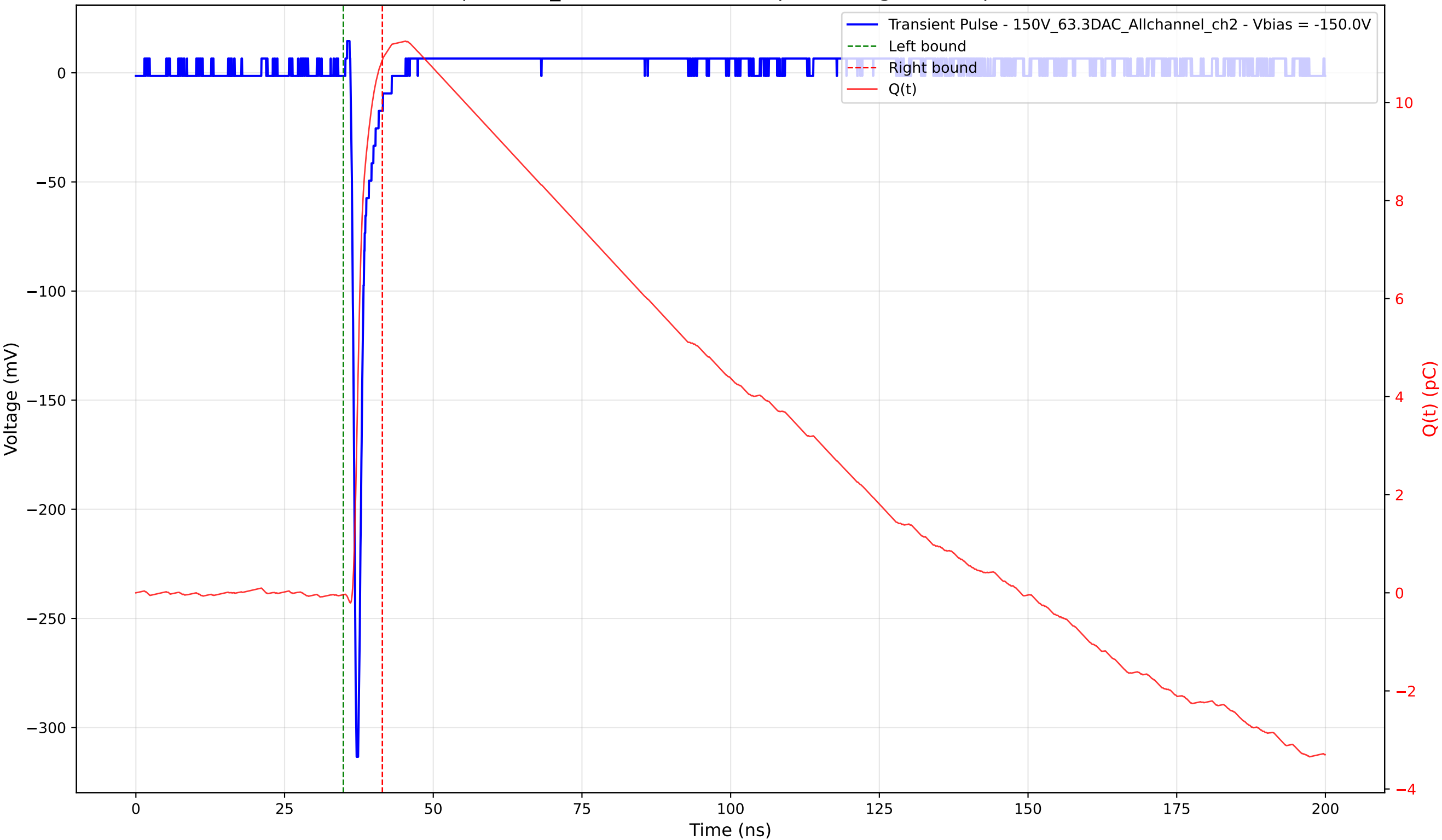
Transient Pulse - Sample: 1cm_42 - Position: 2640.0 \mu\text{m} - Charge: 10.91 pC - Rise Time: 0.73 ns
