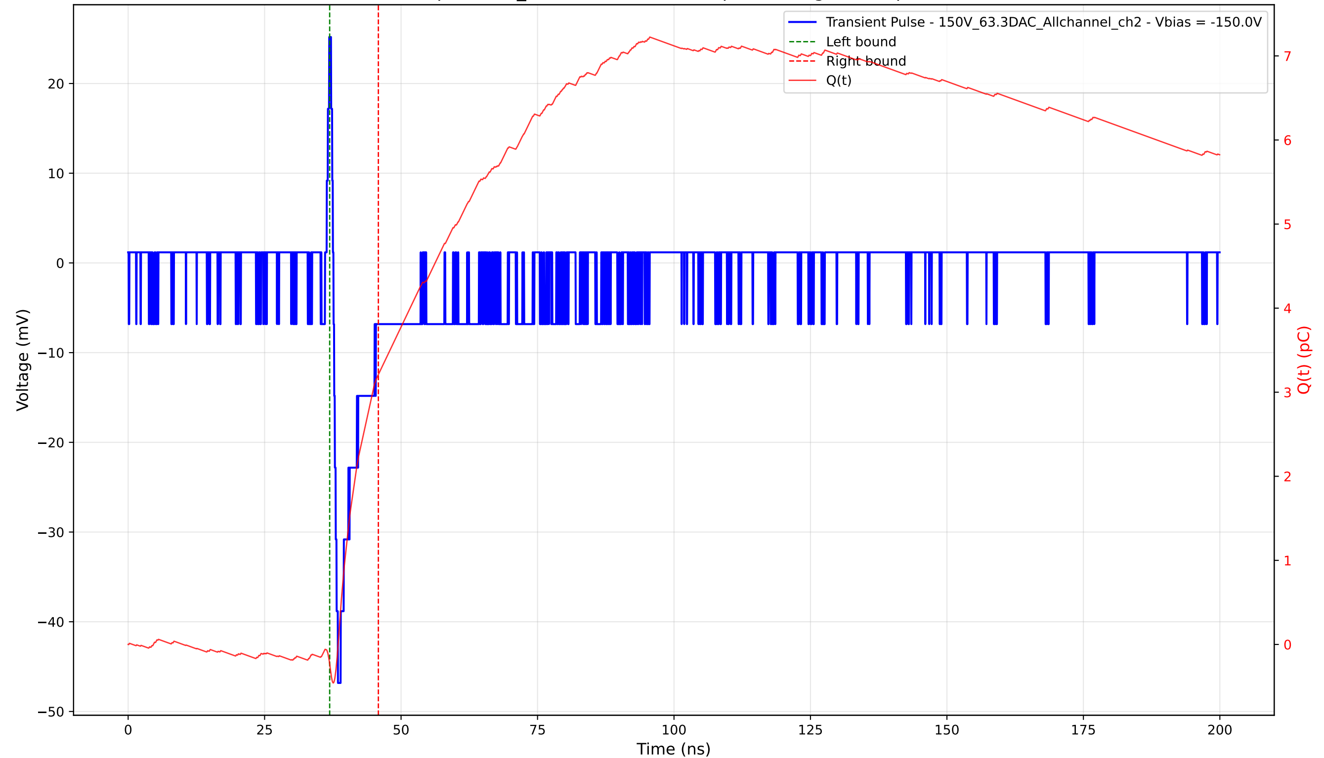
Transient Pulse - Sample: 1cm_42 - Position: 1475.0 \mu\text{m} - Charge: 3.44 pC - Rise Time: 0.82 ns
