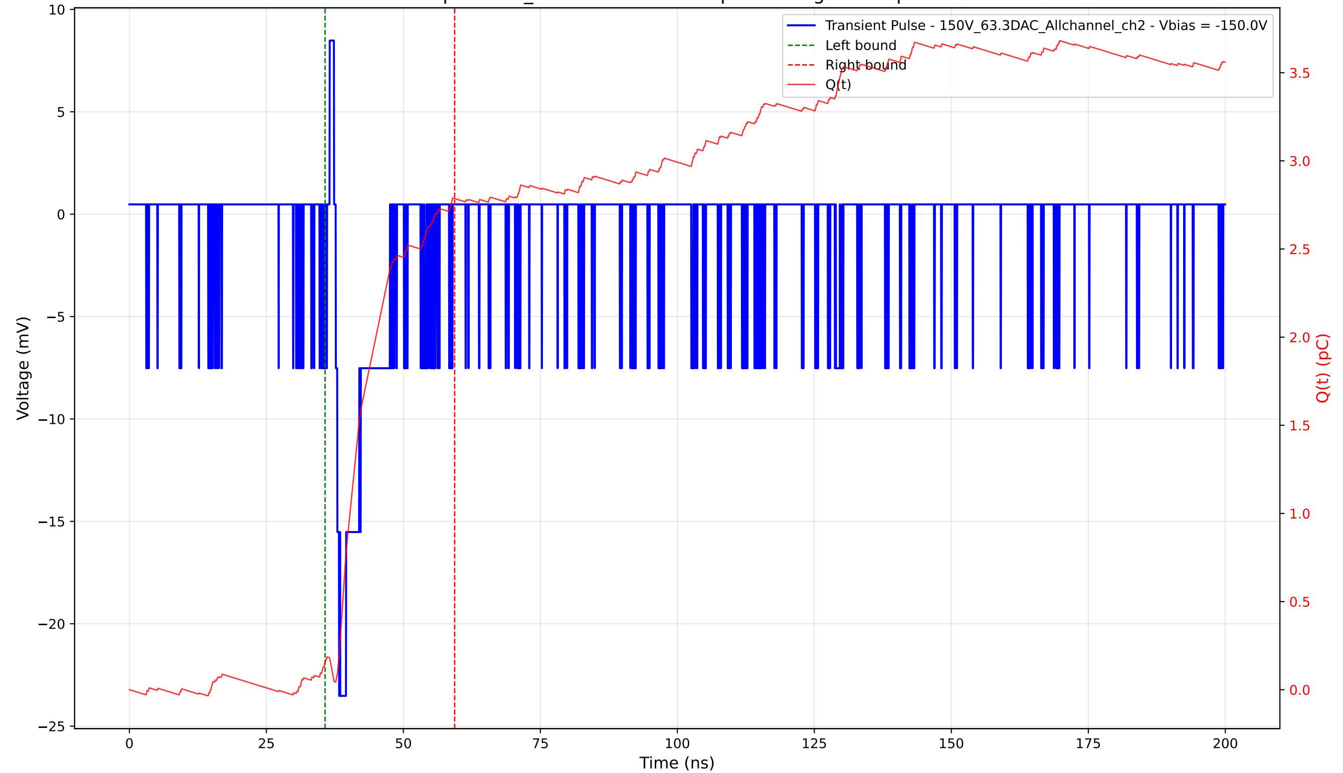
Transient Pulse - Sample: 1cm_42 - Position: 260.0 \mu\text{m} - Charge: 2.63 pC - Rise Time: 0.63 ns
