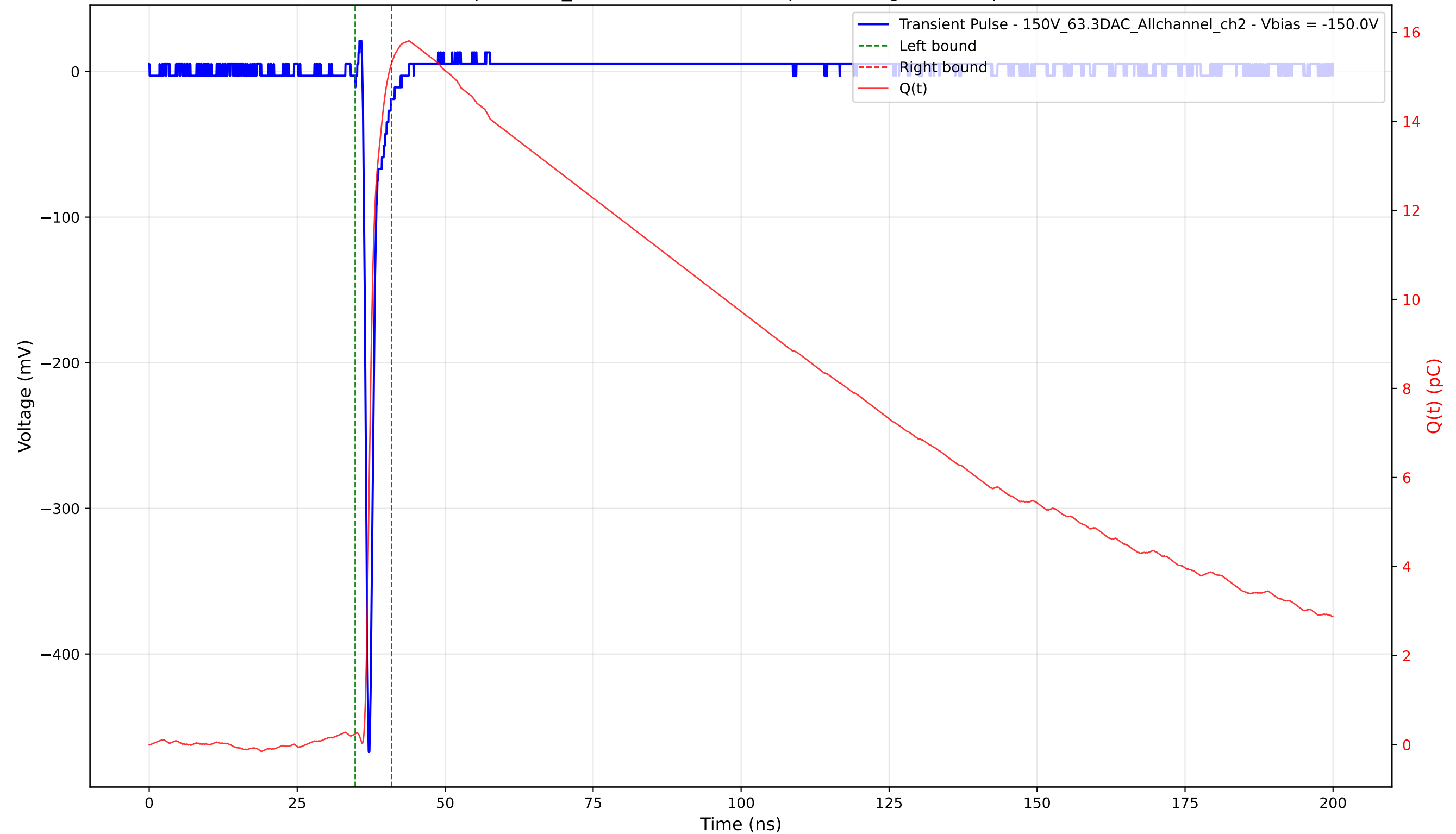
Transient Pulse - Sample: 1cm_42 - Position: 2805.0 \mu\text{m} - Charge: 15.07 pC - Rise Time: 0.73 ns
