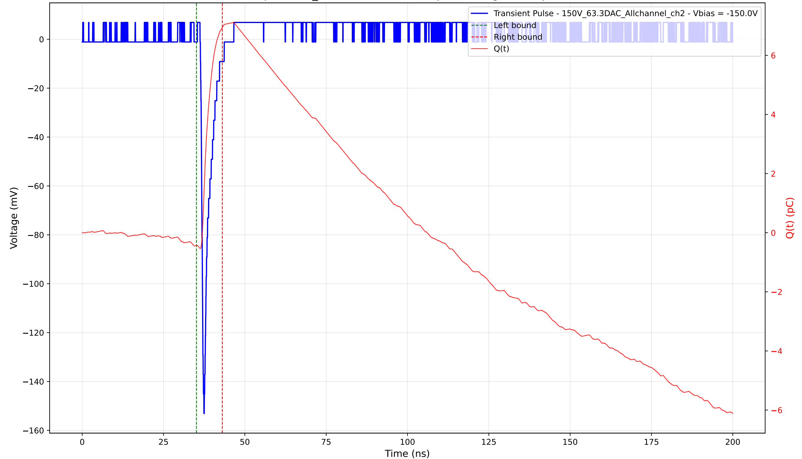
Transient Pulse - Sample: 1cm_42 - Position: 3655.0 \mu\text{m} - Charge: 7.37 pC - Rise Time: 0.85 ns
