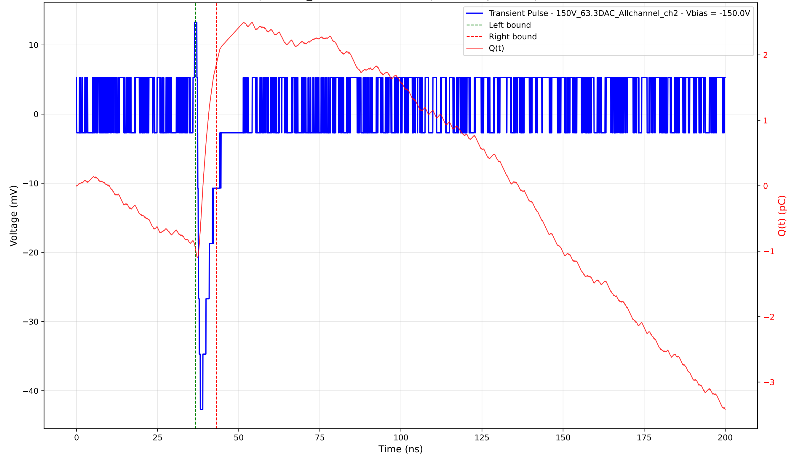
Transient Pulse - Sample: 1cm_42 - Position: 4450.0 \mu\text{m} - Charge: 2.83 pC - Rise Time: 0.79 ns
