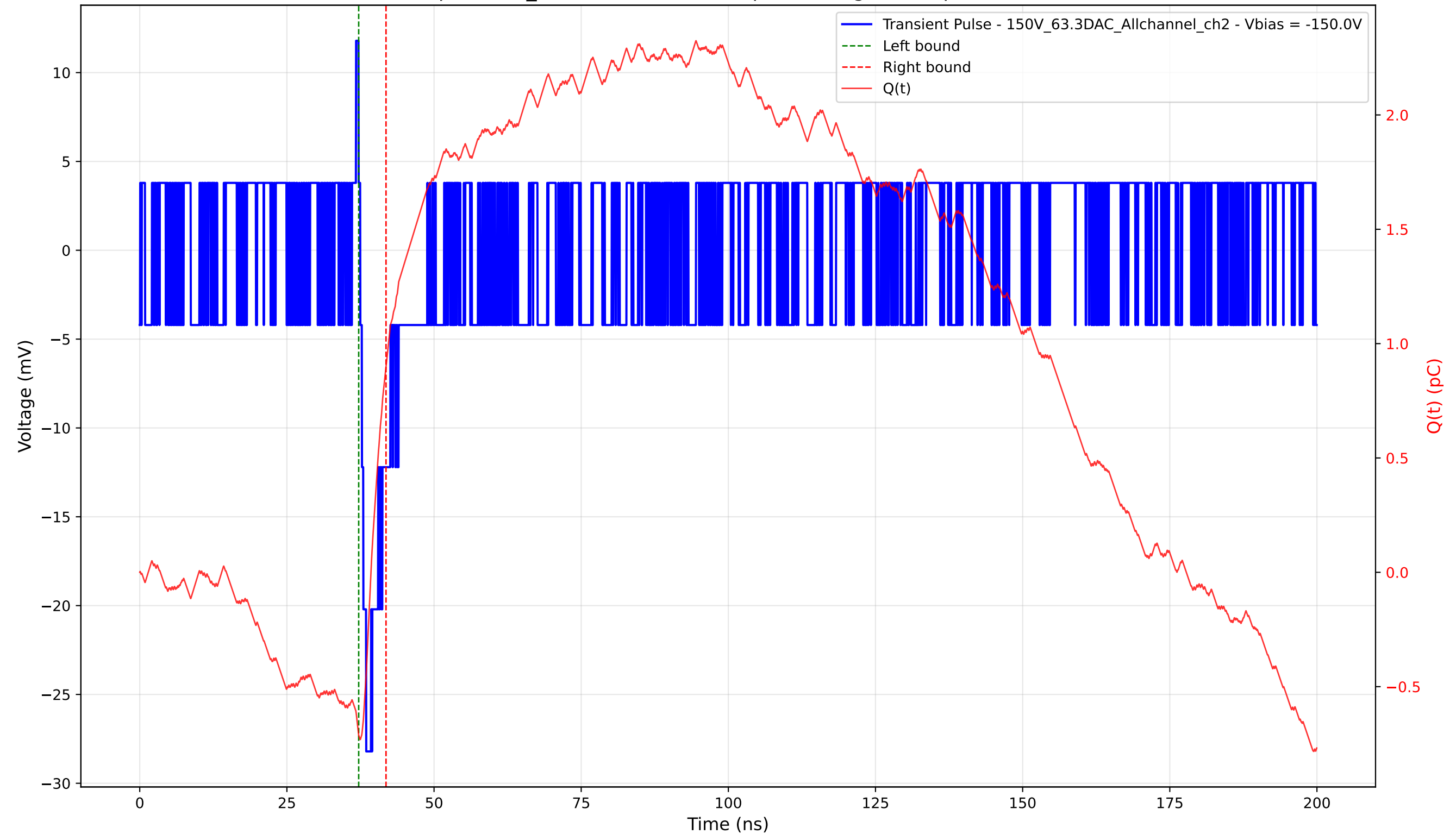
Transient Pulse - Sample: 1cm_42 - Position: 4940.0 \mu\text{m} - Charge: 1.61 pC - Rise Time: 0.00 ns (N/A)
