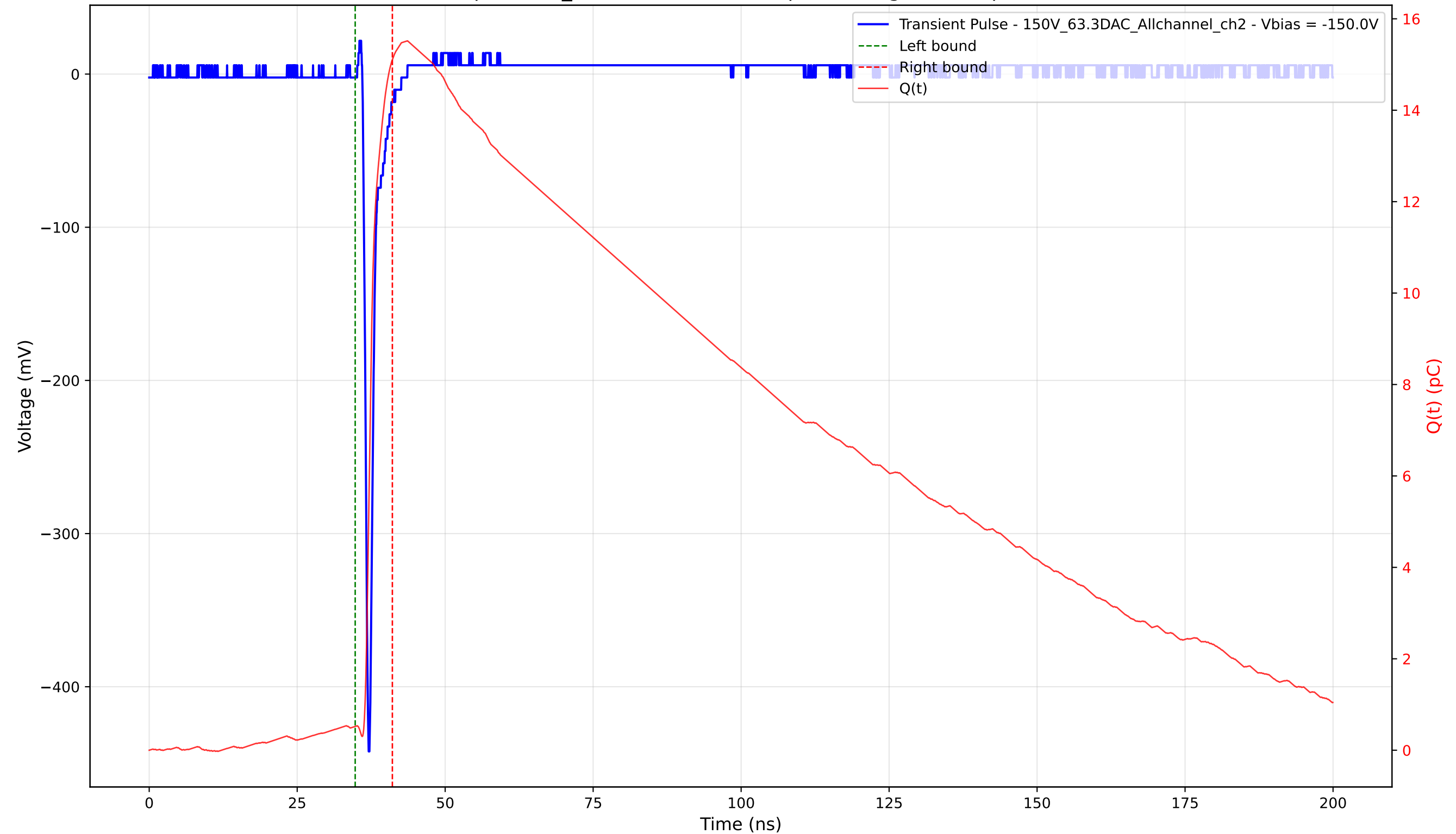
Transient Pulse - Sample: 1cm_42 - Position: 3240.0 \mu\text{m} - Charge: 14.58 pC - Rise Time: 0.69 ns
