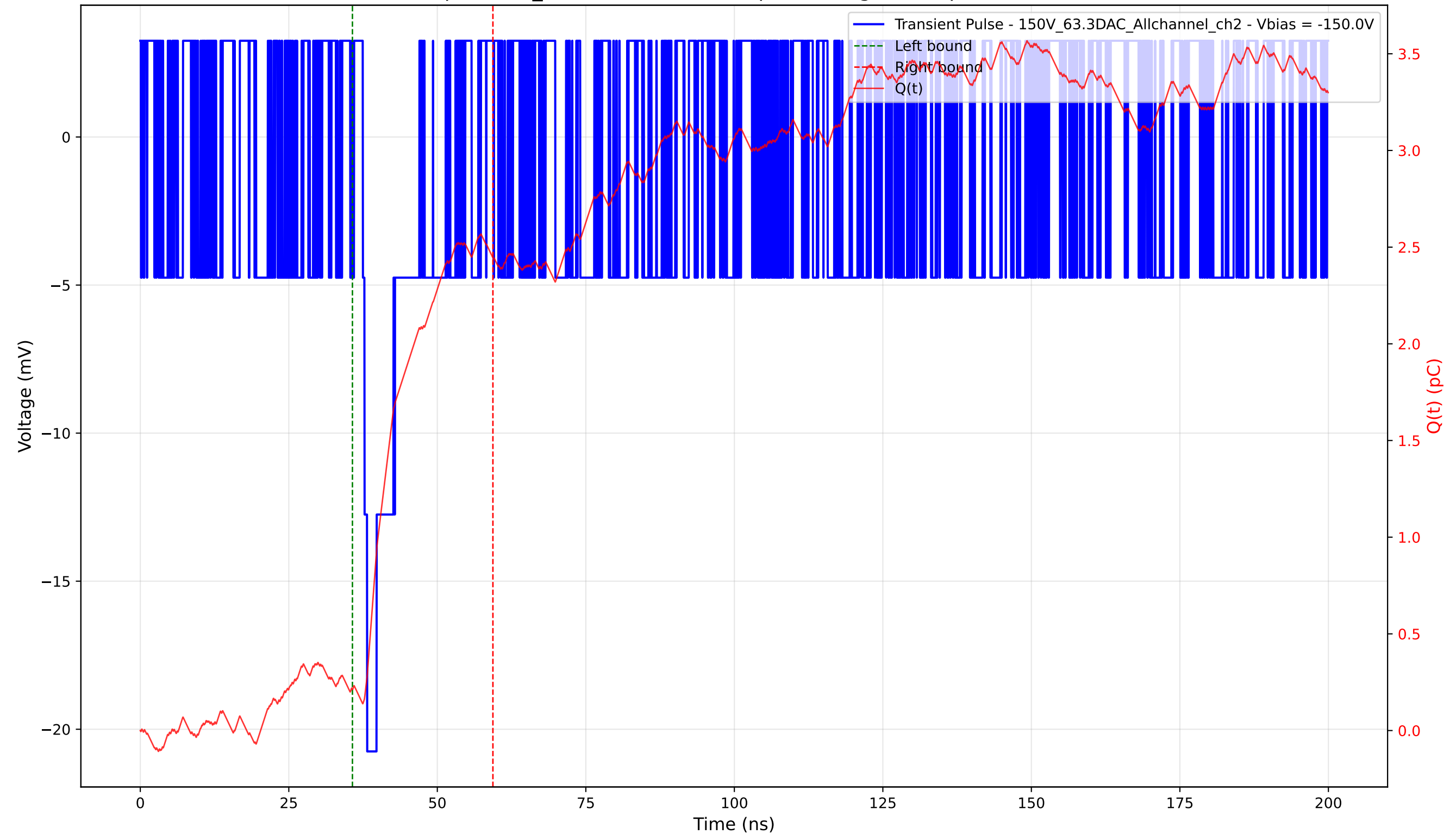
Transient Pulse - Sample: 1cm_42 - Position: 4995.0 \mu\text{m} - Charge: 2.24 pC - Rise Time: 0.00 ns (N/A)
