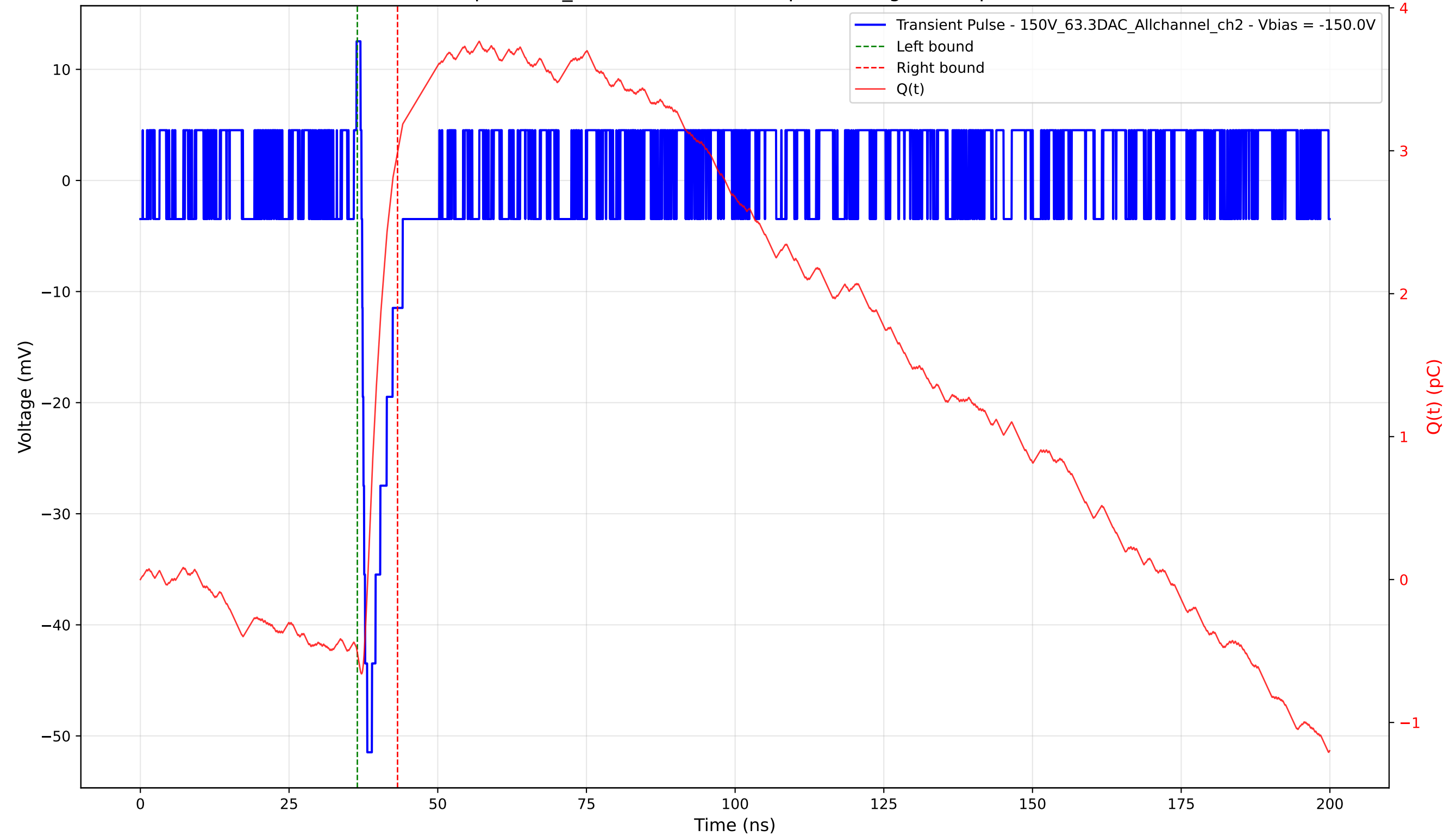
Transient Pulse - Sample: 1cm_42 - Position: 4375.0 \mu\text{m} - Charge: 3.50 pC - Rise Time: 0.87 ns
