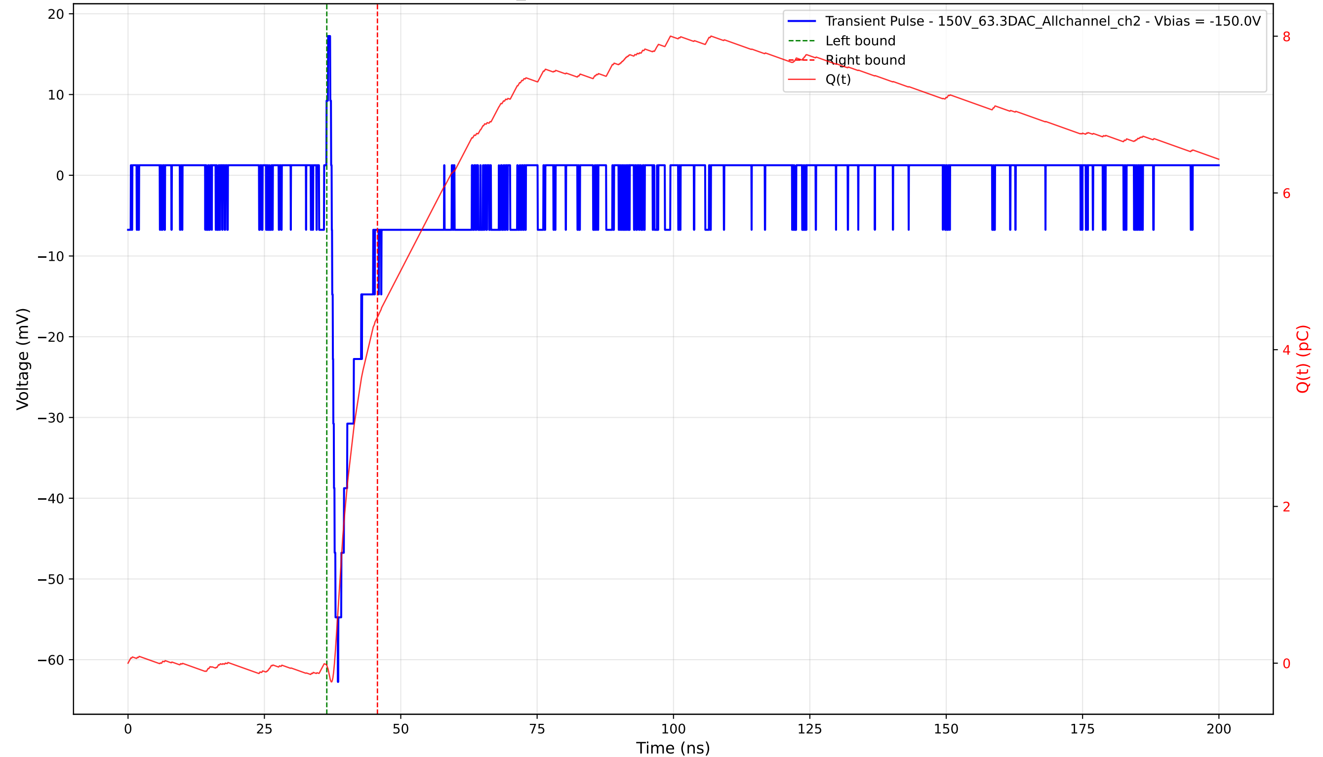
Transient Pulse - Sample: 1cm_42 - Position: 1685.0 \mu\text{m} - Charge: 4.44 pC - Rise Time: 1.12 ns
