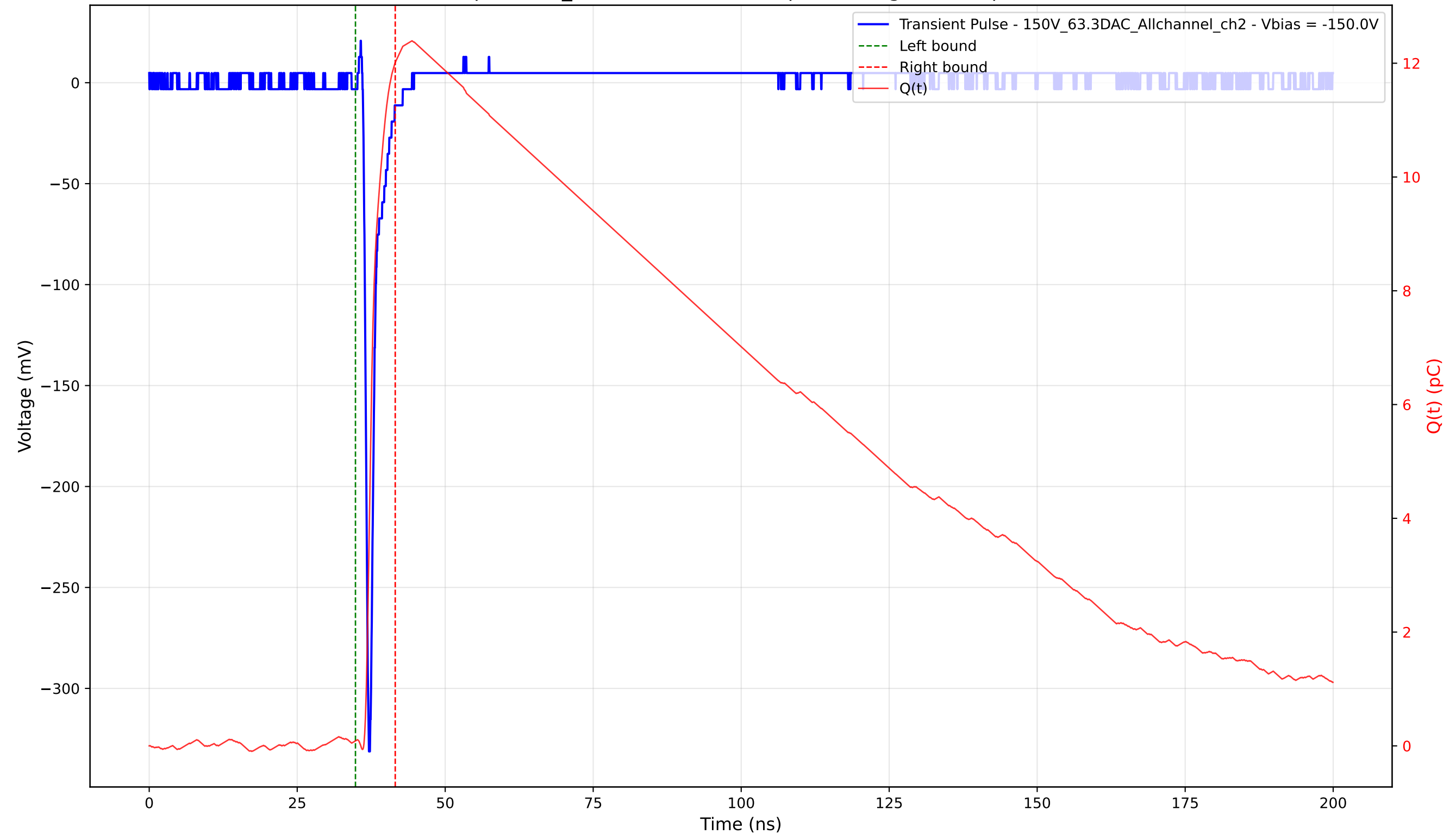
Transient Pulse - Sample: 1cm_42 - Position: 3390.0 \mu\text{m} - Charge: 11.92 pC - Rise Time: 0.74 ns
