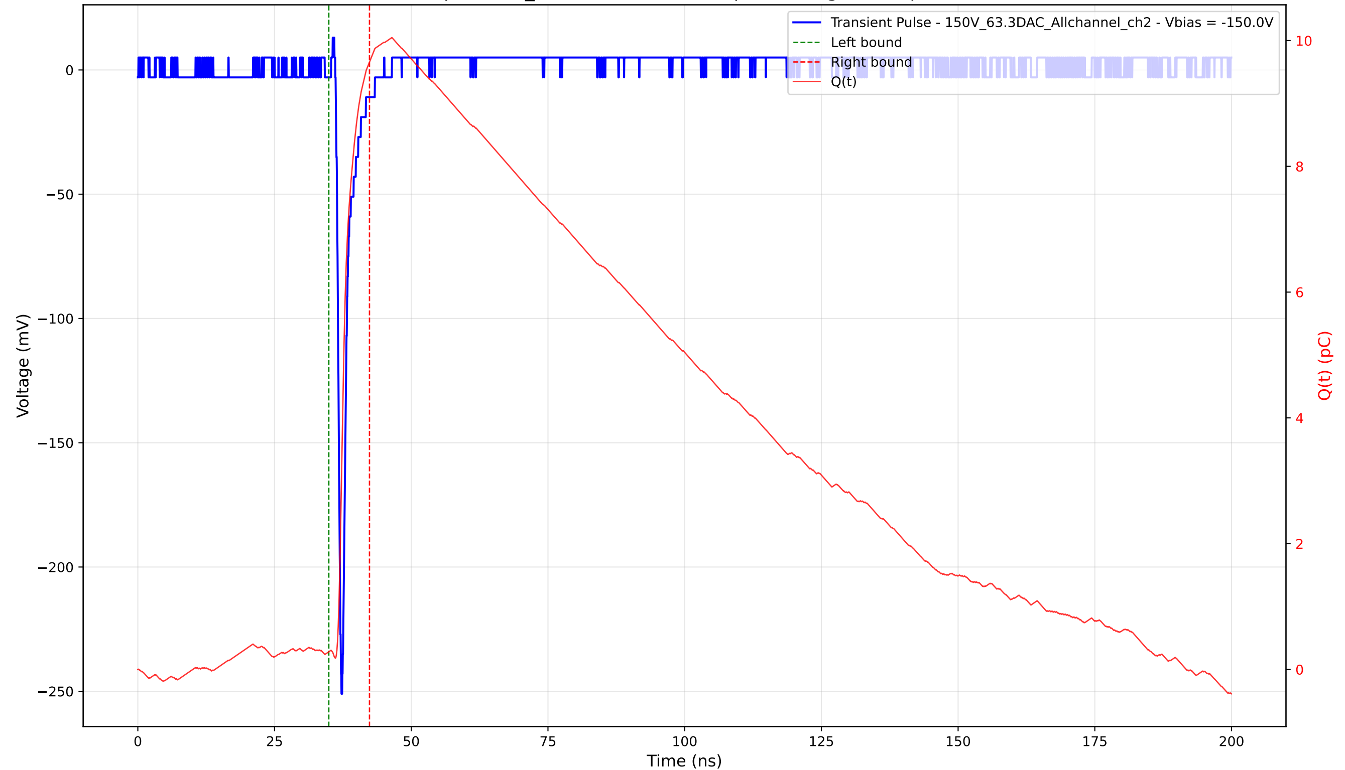
Transient Pulse - Sample: 1cm_42 - Position: 2570.0 \mu\text{m} - Charge: 9.38 pC - Rise Time: 0.77 ns
