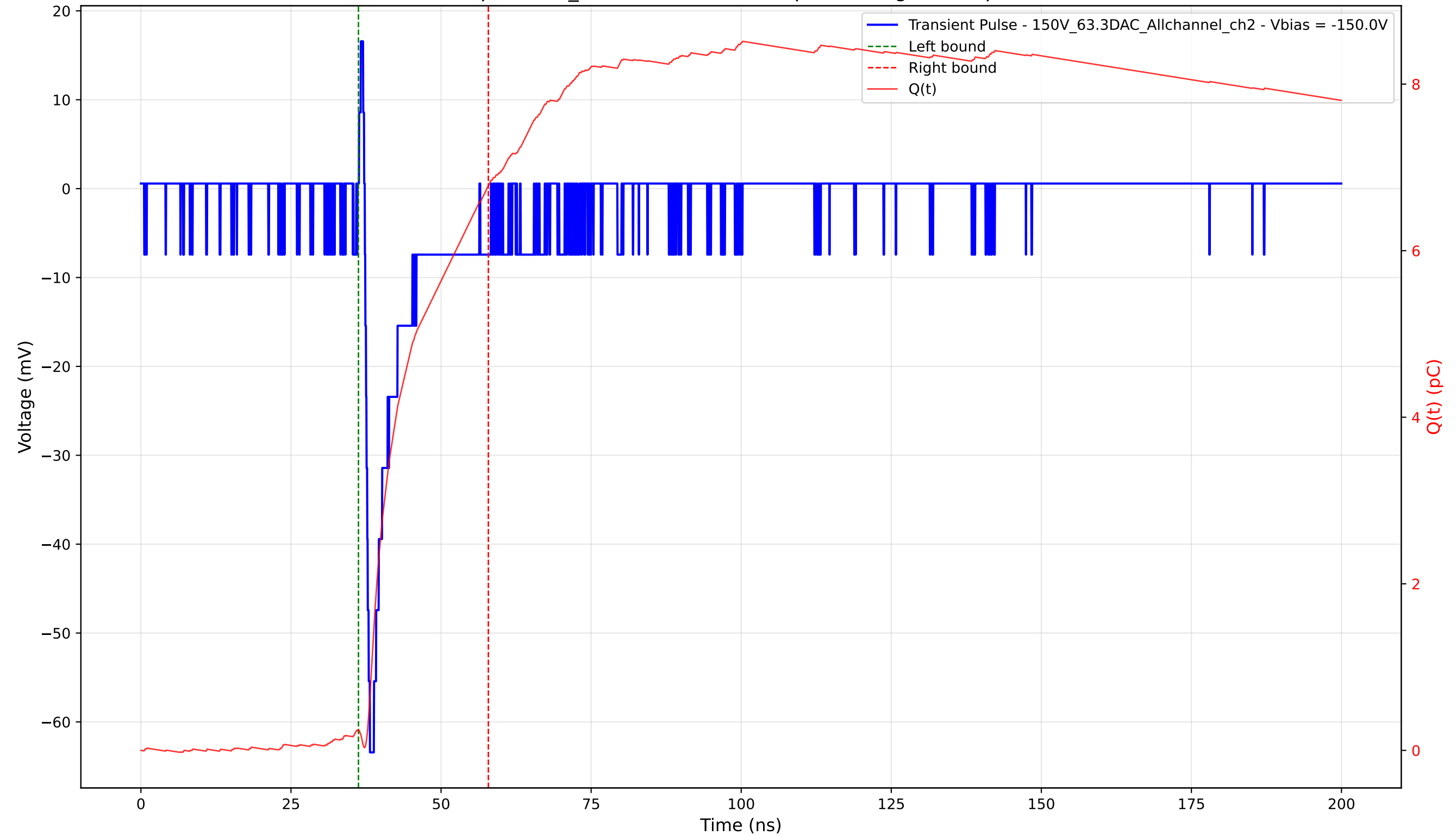
Transient Pulse - Sample: 1cm_42 - Position: 1705.0 \mu\text{m} - Charge: 6.54 pC - Rise Time: 0.85 ns
