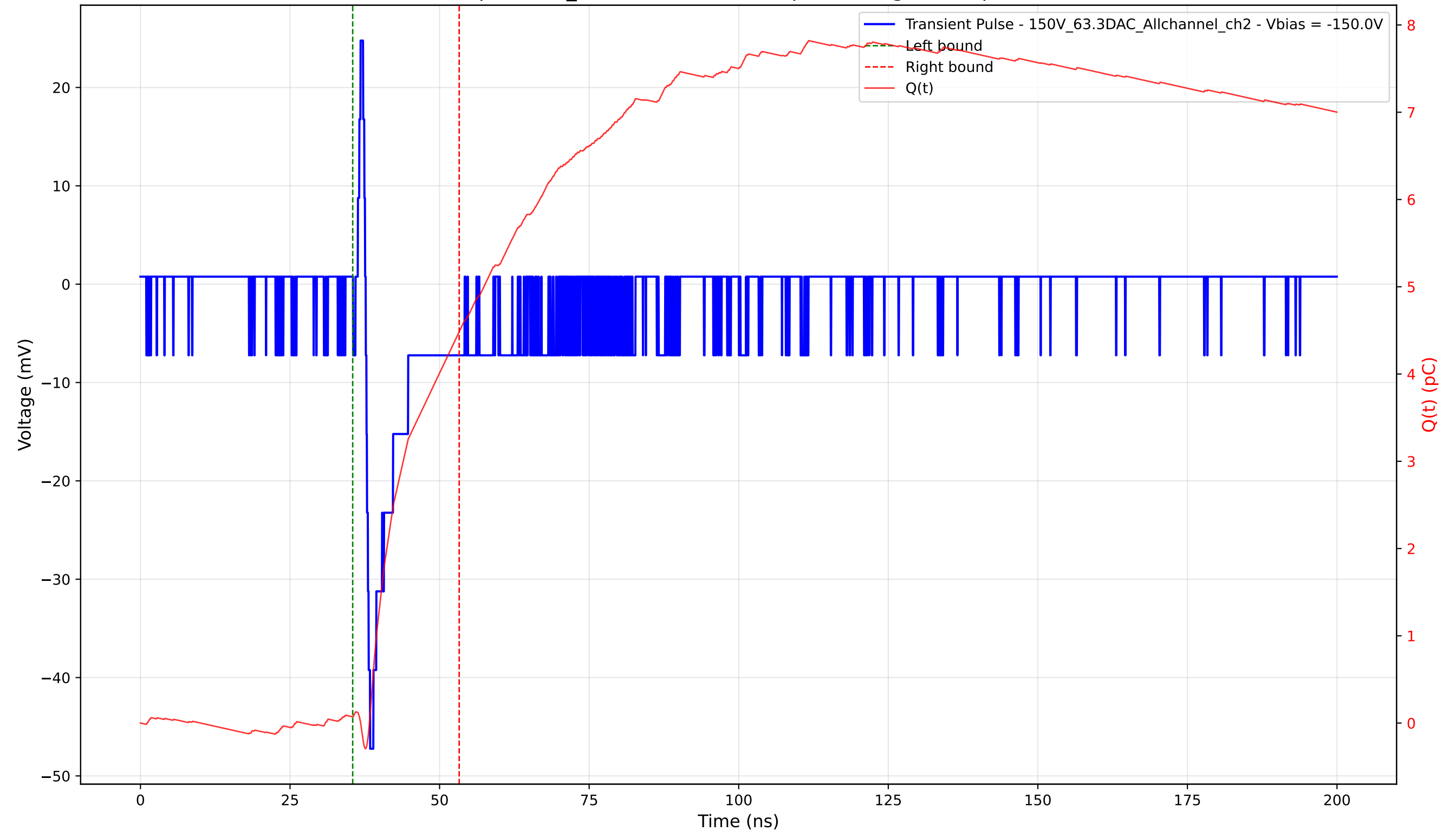
Transient Pulse - Sample: 1cm_42 - Position: 1460.0 \mu\text{m} - Charge: 4.42 pC - Rise Time: 0.74 ns
