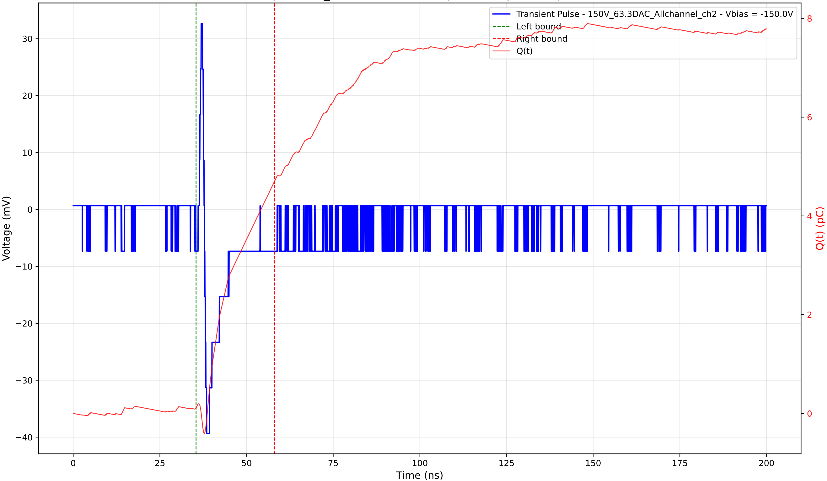
Transient Pulse - Sample: 1cm_42 - Position: 910.0 \mu\text{m} - Charge: 4.59 pC - Rise Time: 0.66 ns
