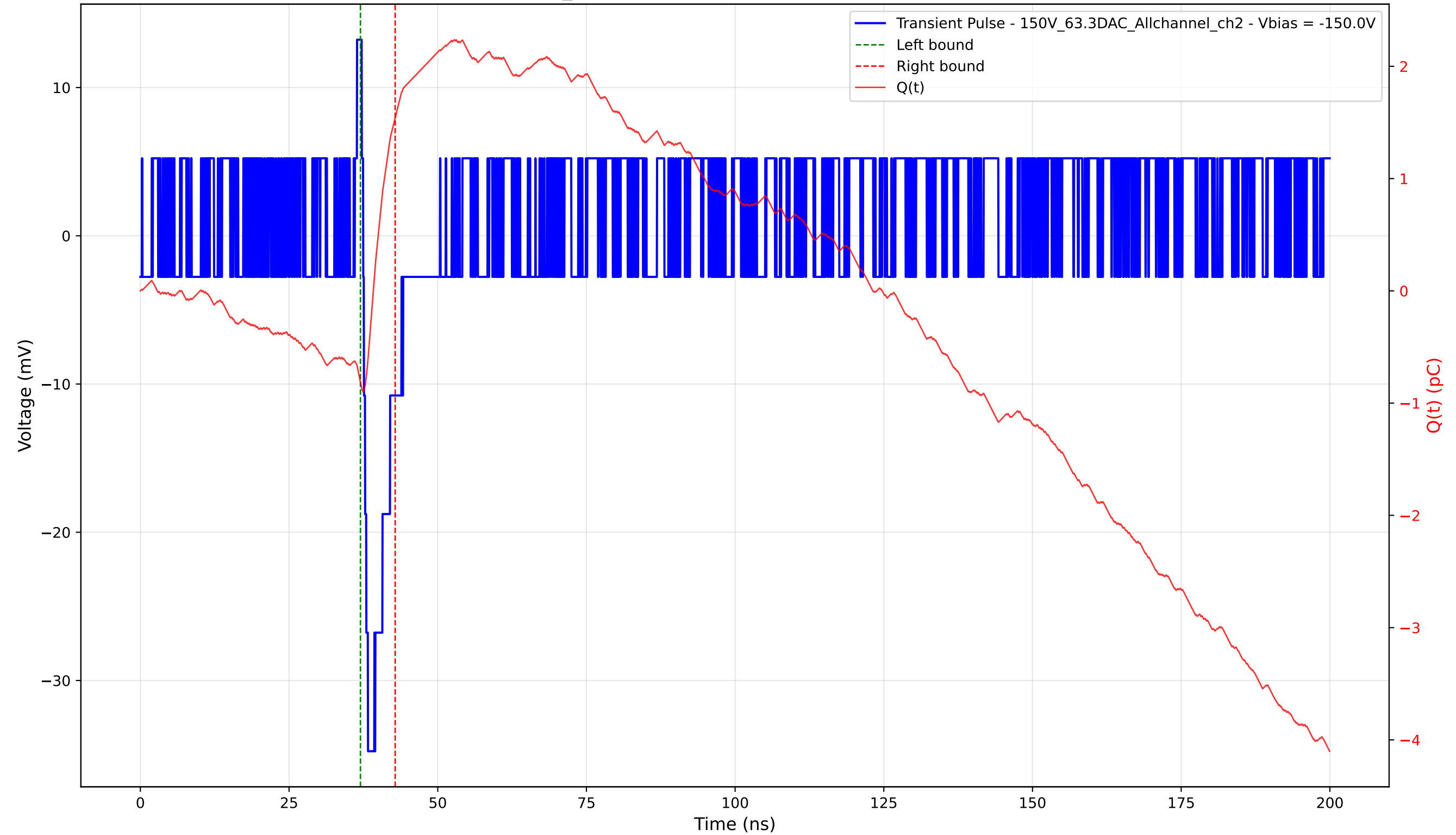
Transient Pulse - Sample: 1cm_42 - Position: 4735.0 \mu\text{m} - Charge: 2.36 pC - Rise Time: 0.72 ns
