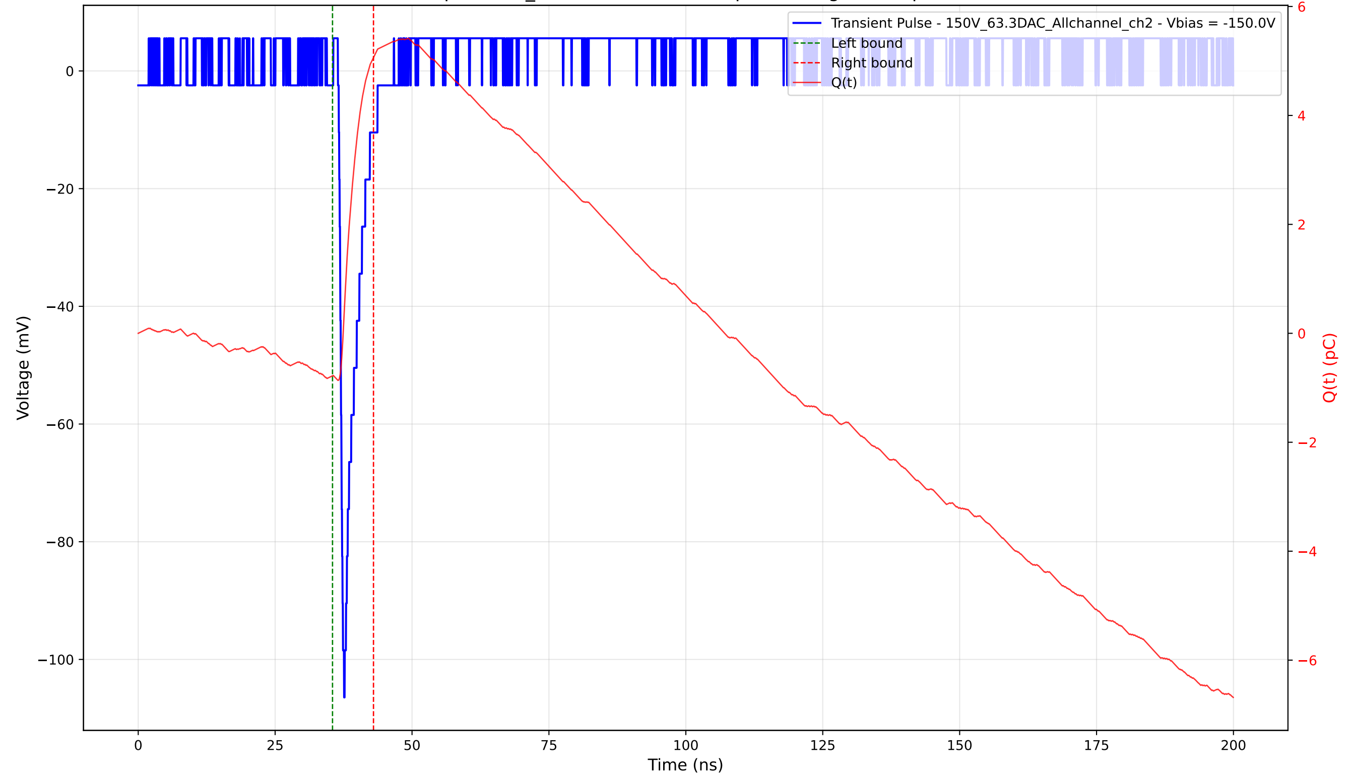
Transient Pulse - Sample: 1cm_42 - Position: 3890.0 \mu\text{m} - Charge: 5.84 pC - Rise Time: 0.72 ns
