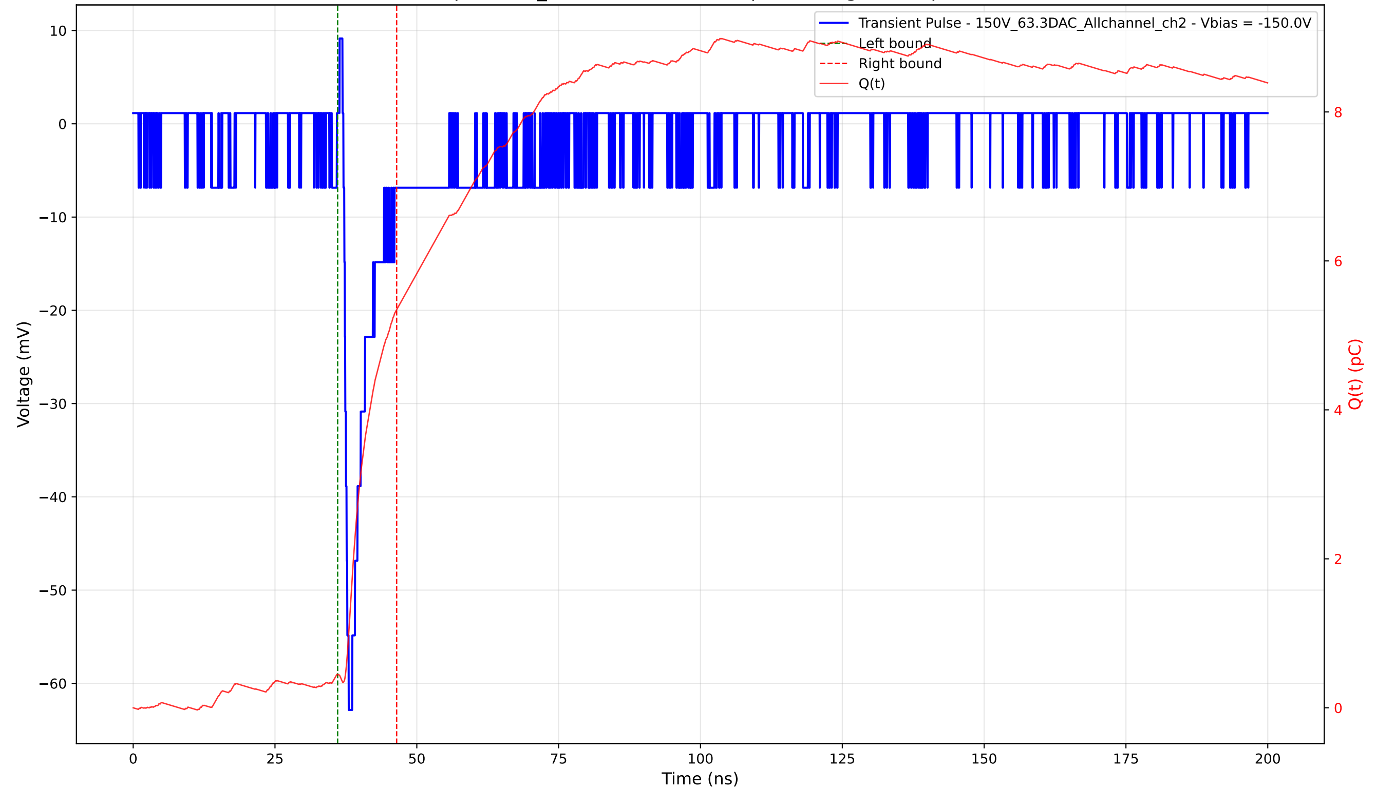
Transient Pulse - Sample: 1cm_42 - Position: 1885.0 \mu\text{m} - Charge: 4.90 pC - Rise Time: 0.92 ns
