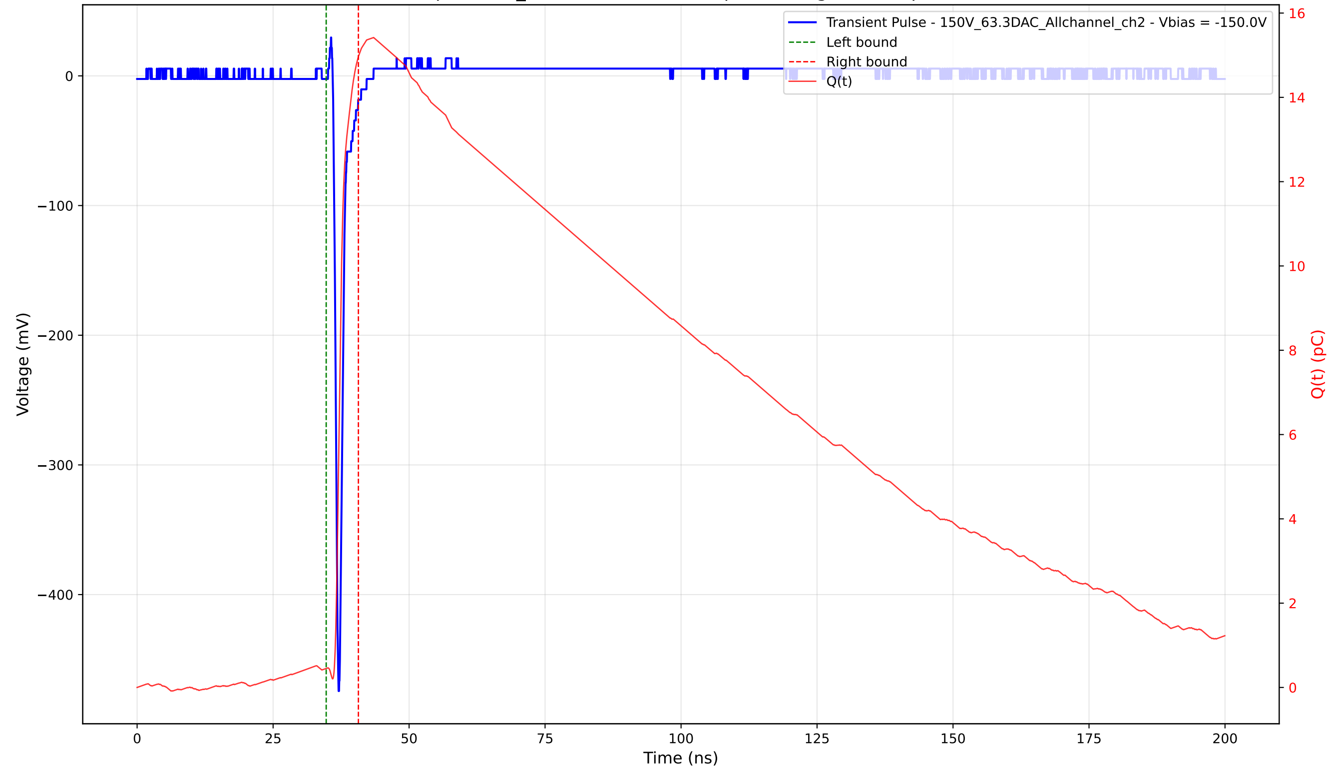
Transient Pulse - Sample: 1cm_42 - Position: 2945.0 \mu\text{m} - Charge: 14.52 pC - Rise Time: 0.73 ns
