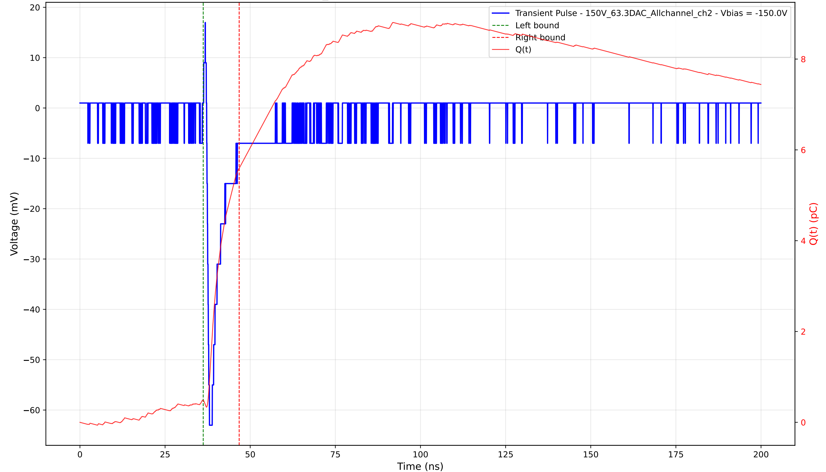
Transient Pulse - Sample: 1cm_42 - Position: 1795.0 \mu\text{m} - Charge: 5.11 pC - Rise Time: 0.80 ns
