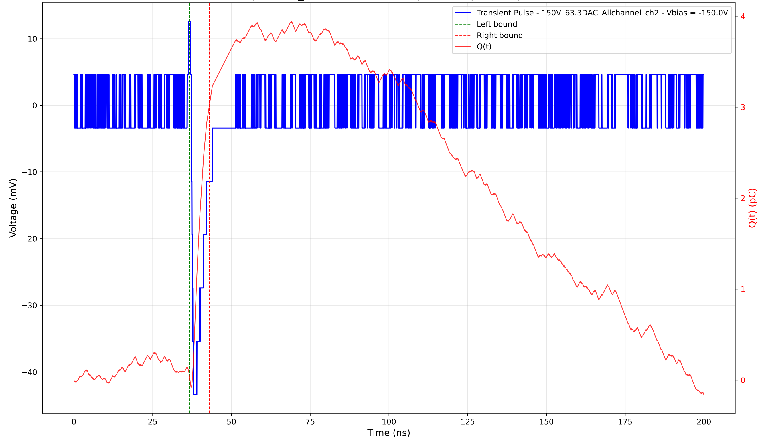
Transient Pulse - Sample: 1cm_42 - Position: 4445.0 \mu\text{m} - Charge: 2.98 pC - Rise Time: 0.68 ns
