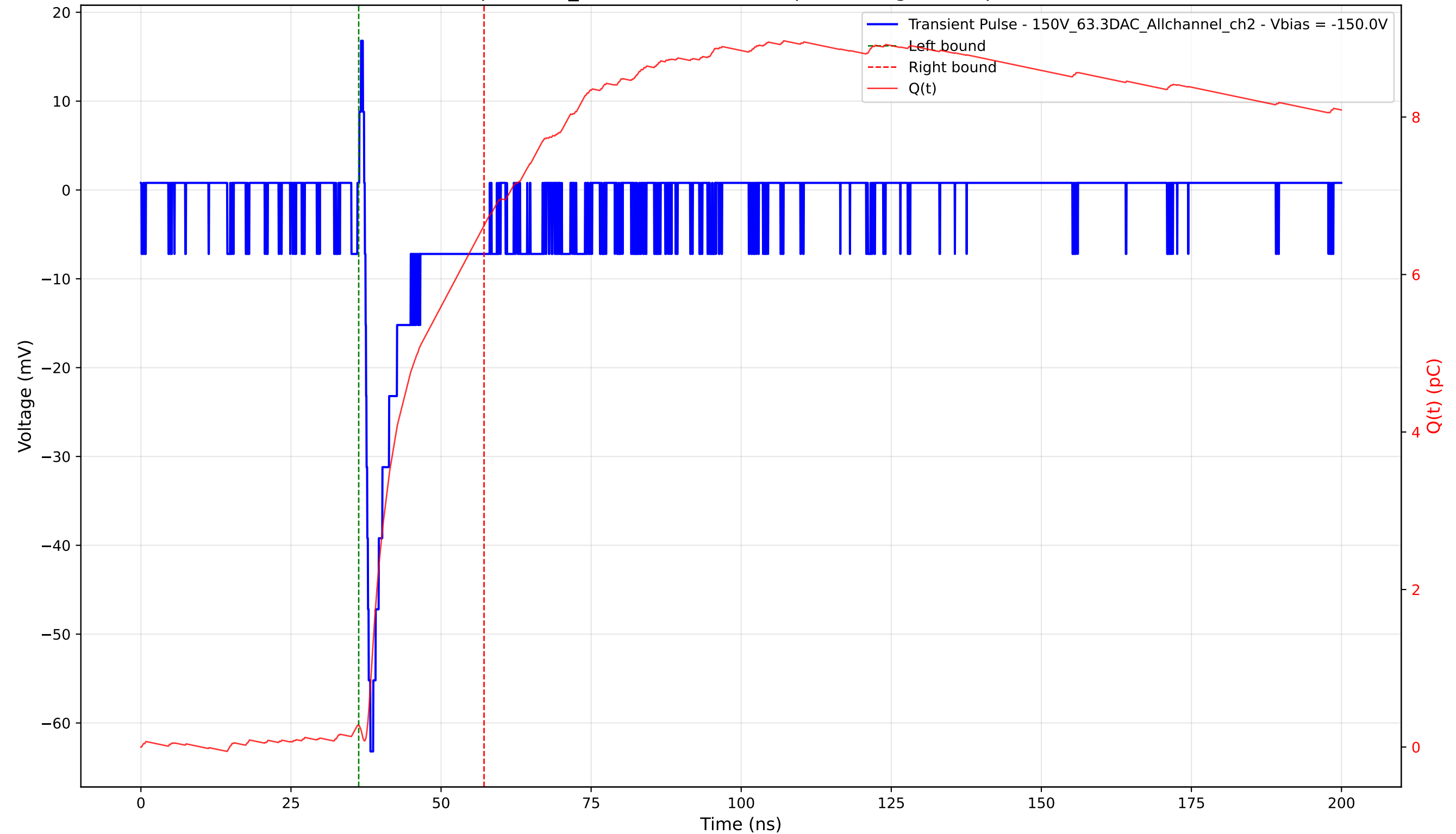
Transient Pulse - Sample: 1cm_42 - Position: 1710.0 \mu\text{m} - Charge: 6.35 pC - Rise Time: 0.93 ns
