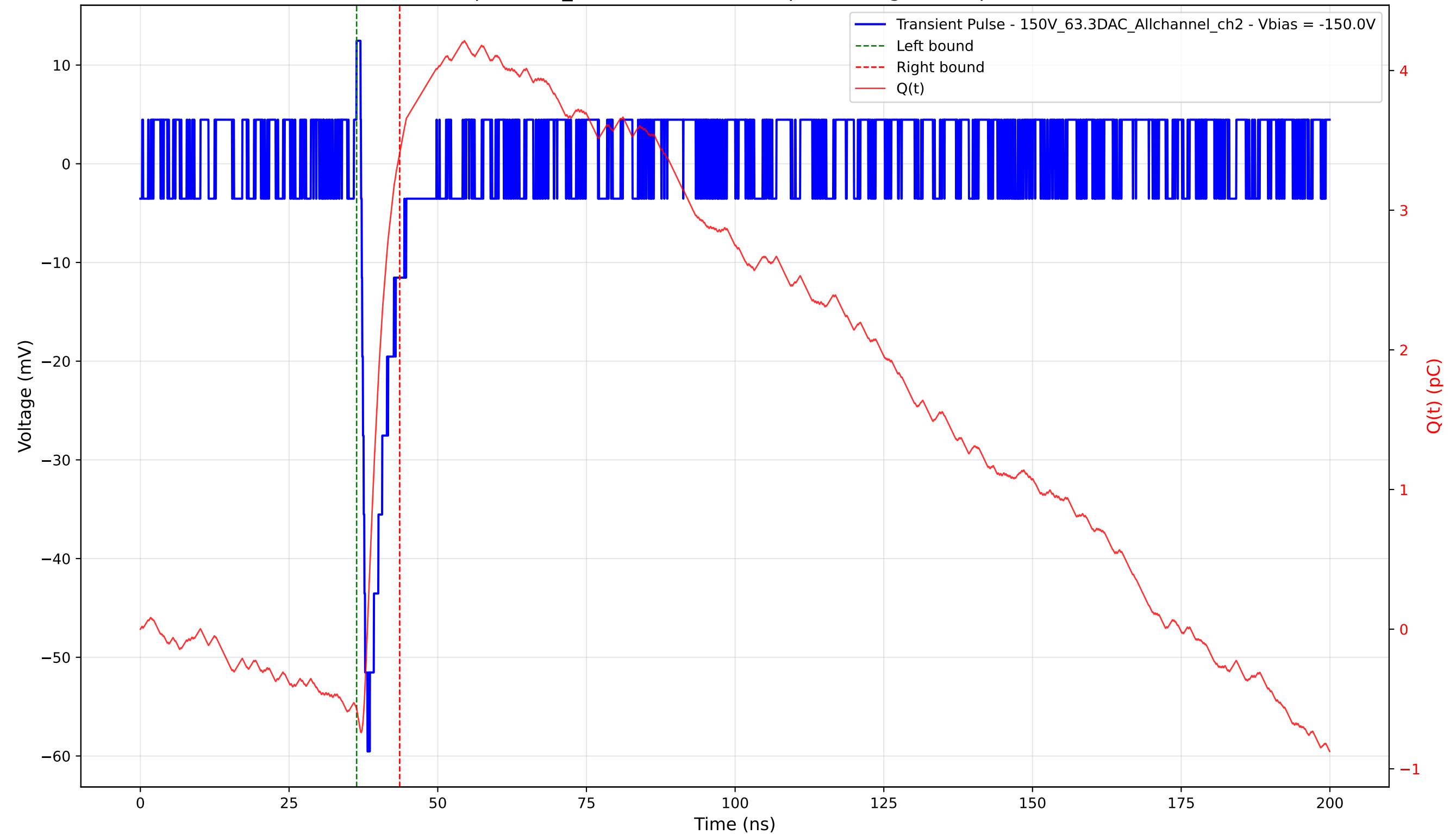
Transient Pulse - Sample: 1cm_42 - Position: 4280.0 \mu\text{m} - Charge: 3.98 pC - Rise Time: 0.99 ns
