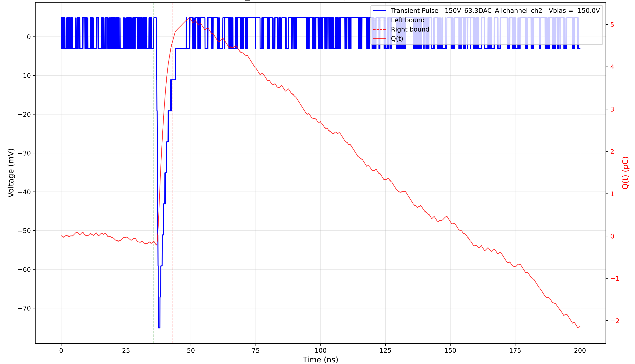
Transient Pulse - Sample: 1cm_42 - Position: 3985.0 \mu\text{m} - Charge: 4.76 pC - Rise Time: 0.74 ns
