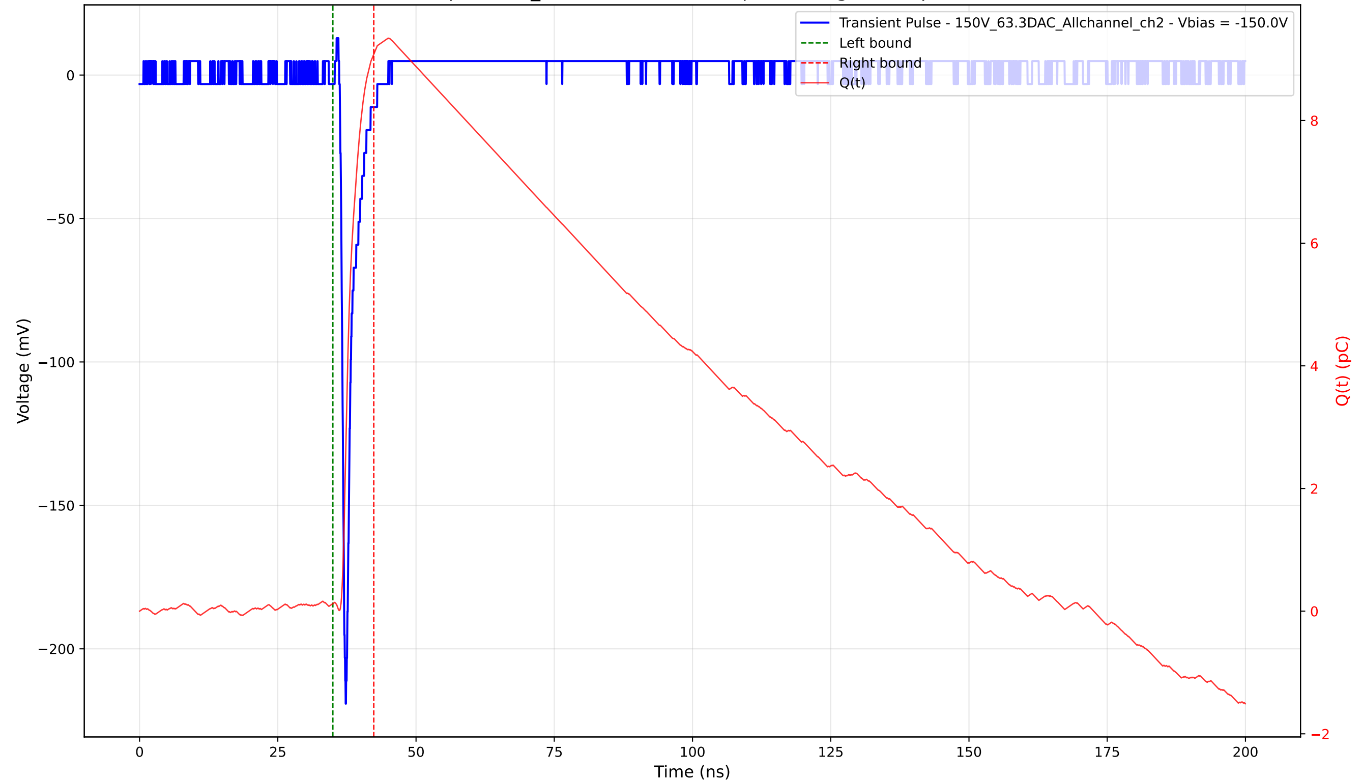
Transient Pulse - Sample: 1cm_42 - Position: 3515.0 \mu\text{m} - Charge: 8.96 pC - Rise Time: 0.83 ns
