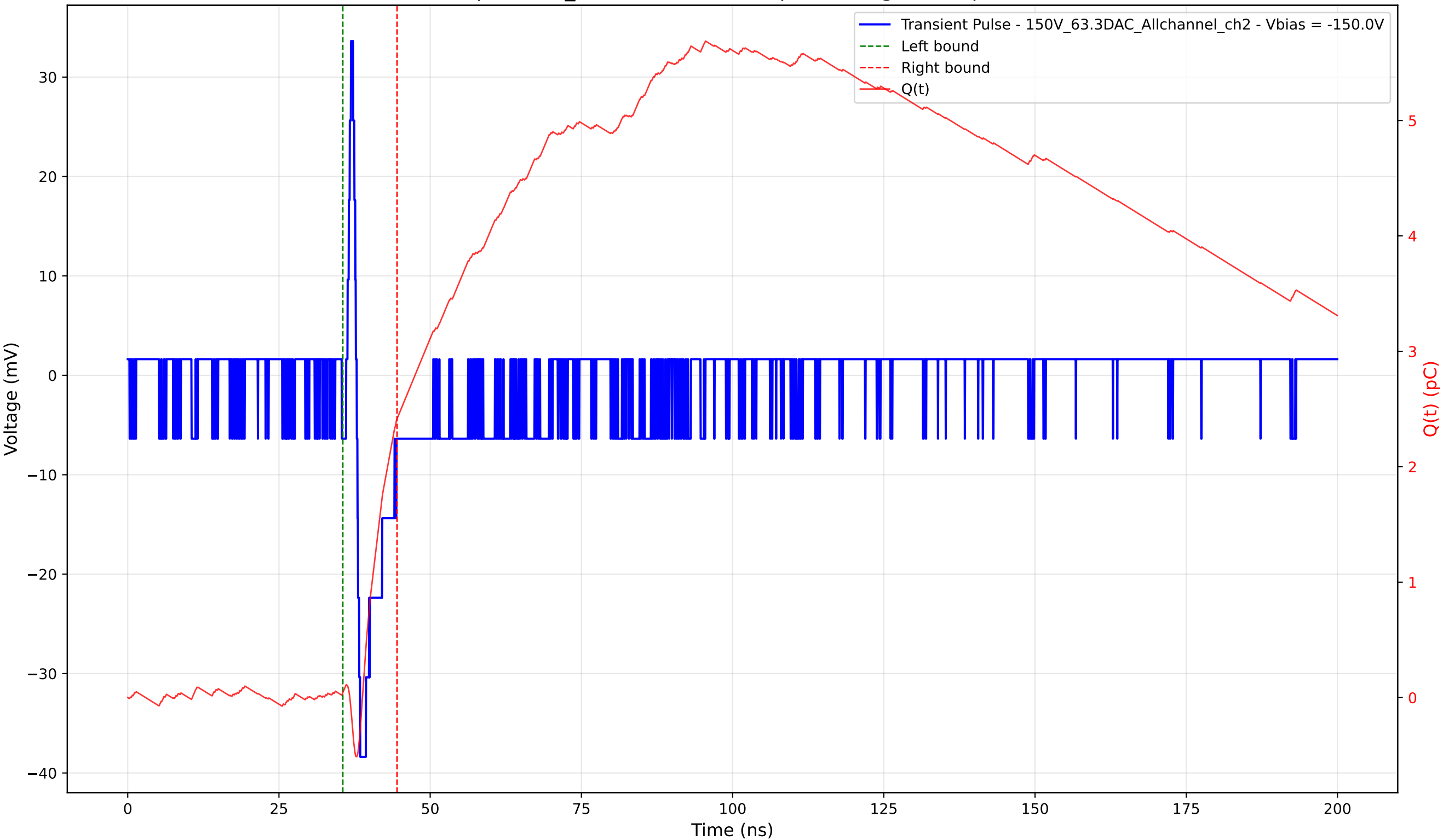
Transient Pulse - Sample: 1cm_42 - Position: 655.0 \mu\text{m} - Charge: 2.37 pC - Rise Time: 0.58 ns
