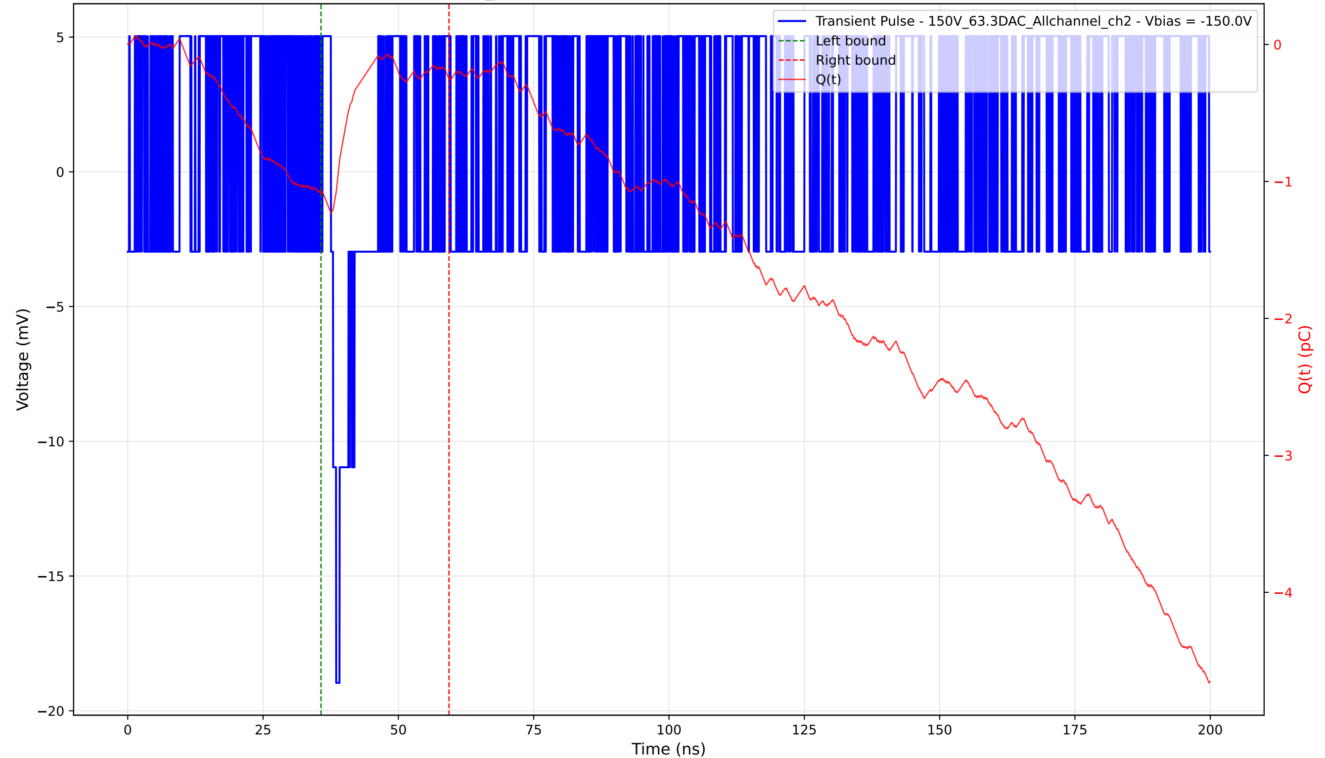
Transient Pulse - Sample: 1cm_42 - Position: 5040.0 \mu\text{m} - Charge: 0.84 pC - Rise Time: 0.00 ns (N/A)
