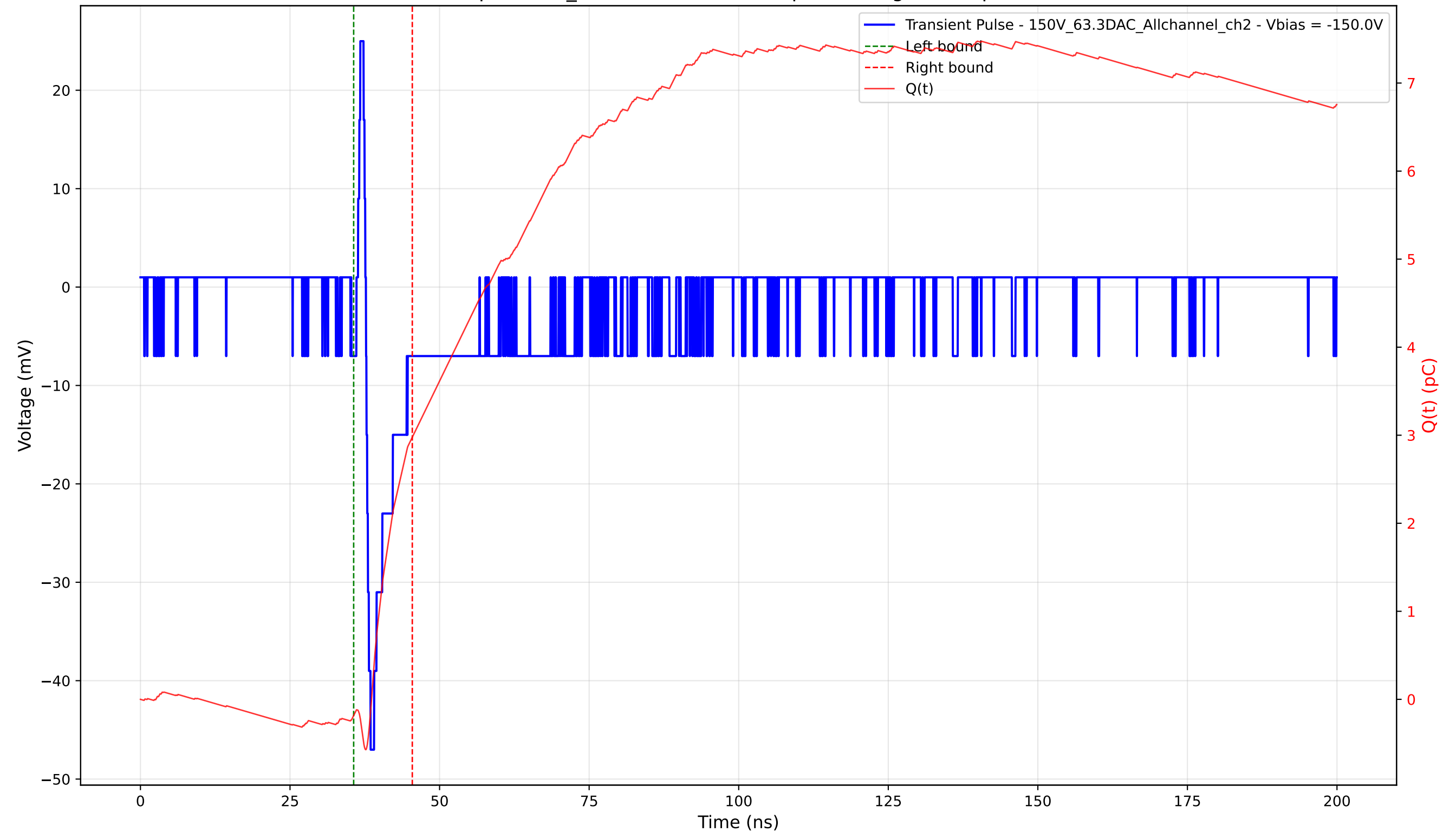
Transient Pulse - Sample: 1cm_42 - Position: 1440.0 \mu\text{m} - Charge: 3.16 pC - Rise Time: 0.78 ns
