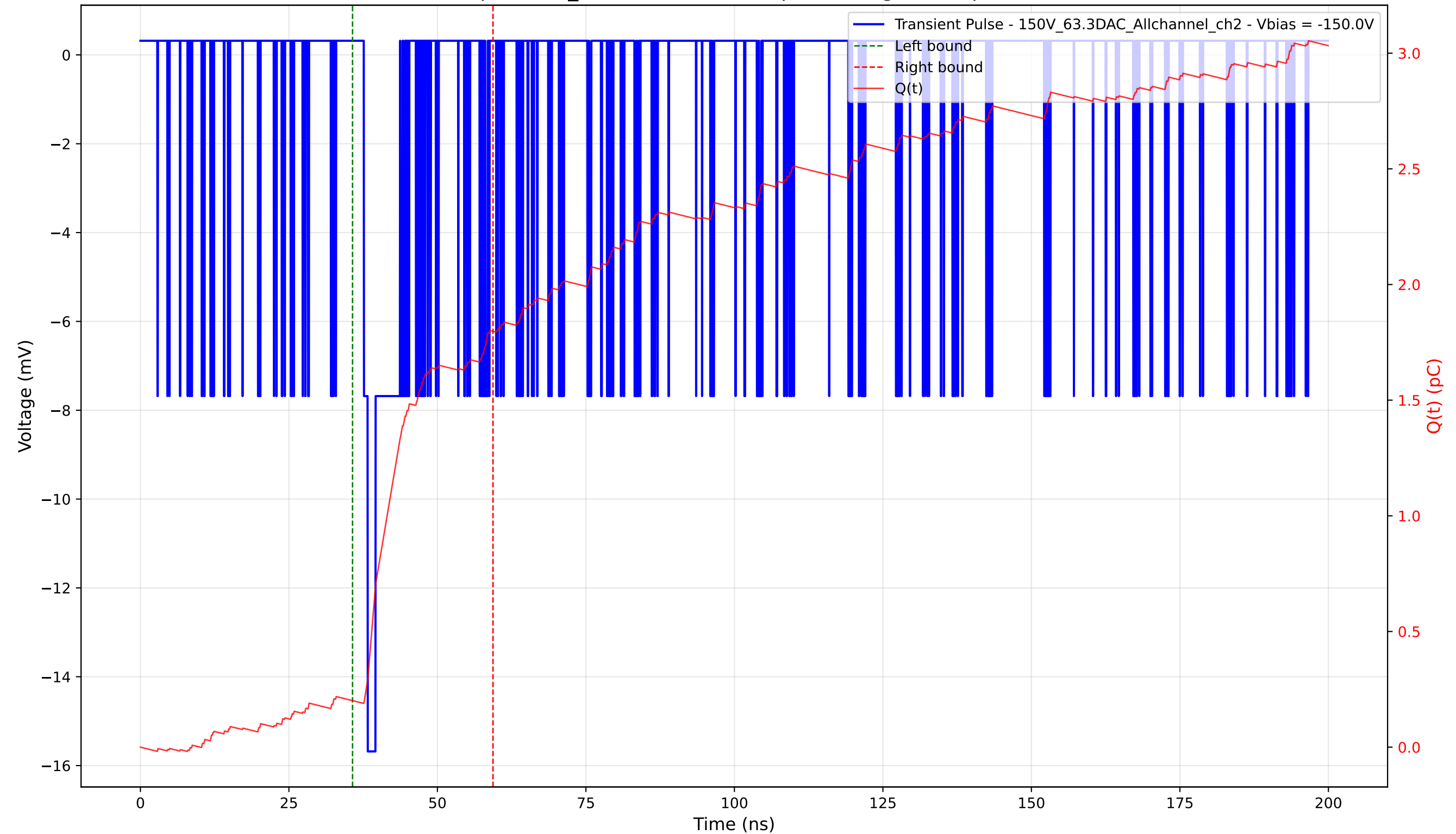
Transient Pulse - Sample: 1cm_42 - Position: 140.0 \mu\text{m} - Charge: 1.60 pC - Rise Time: 0.67 ns
