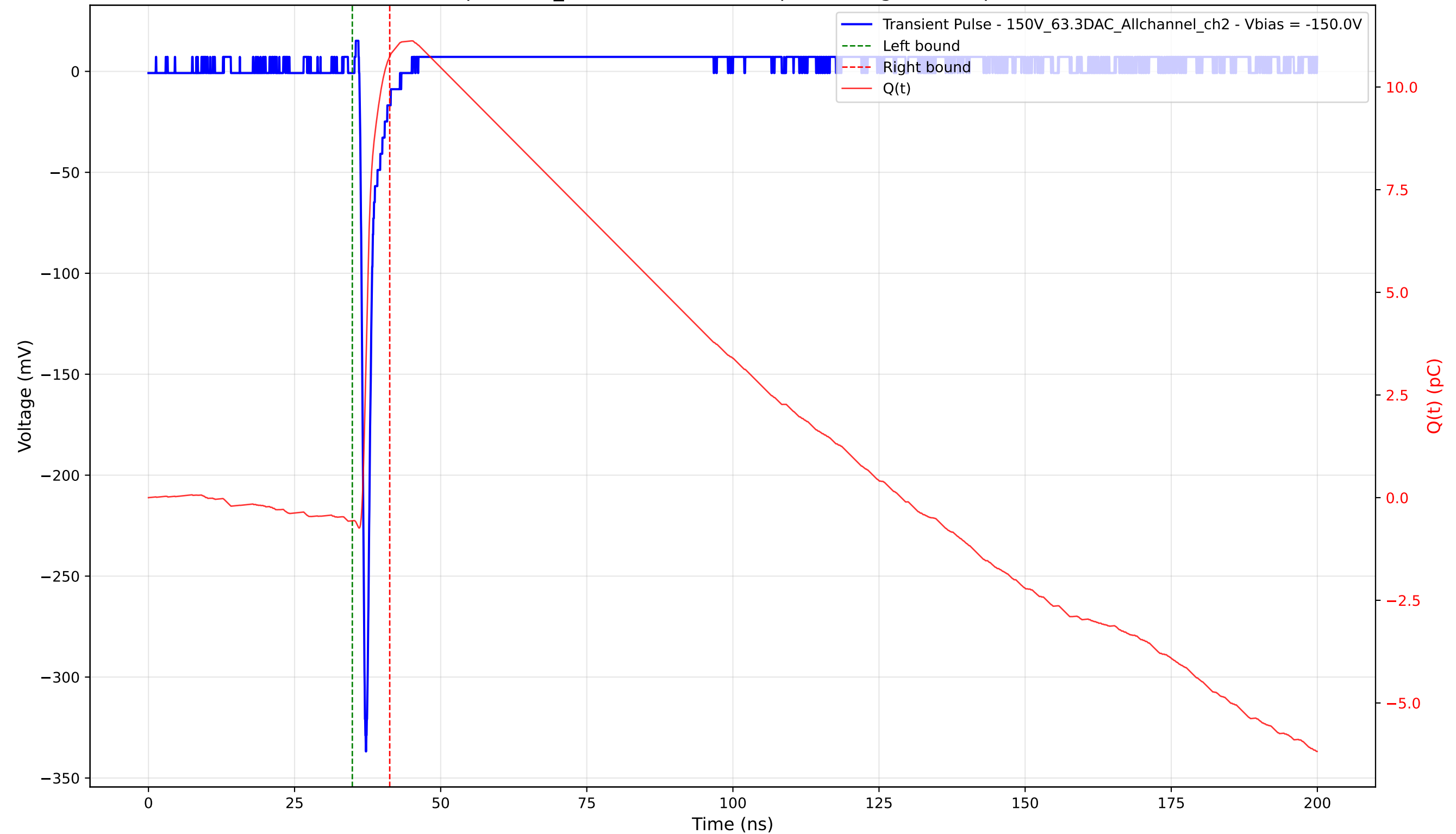
Transient Pulse - Sample: 1cm_42 - Position: 2655.0 \mu\text{m} - Charge: 11.31 pC - Rise Time: 0.75 ns
