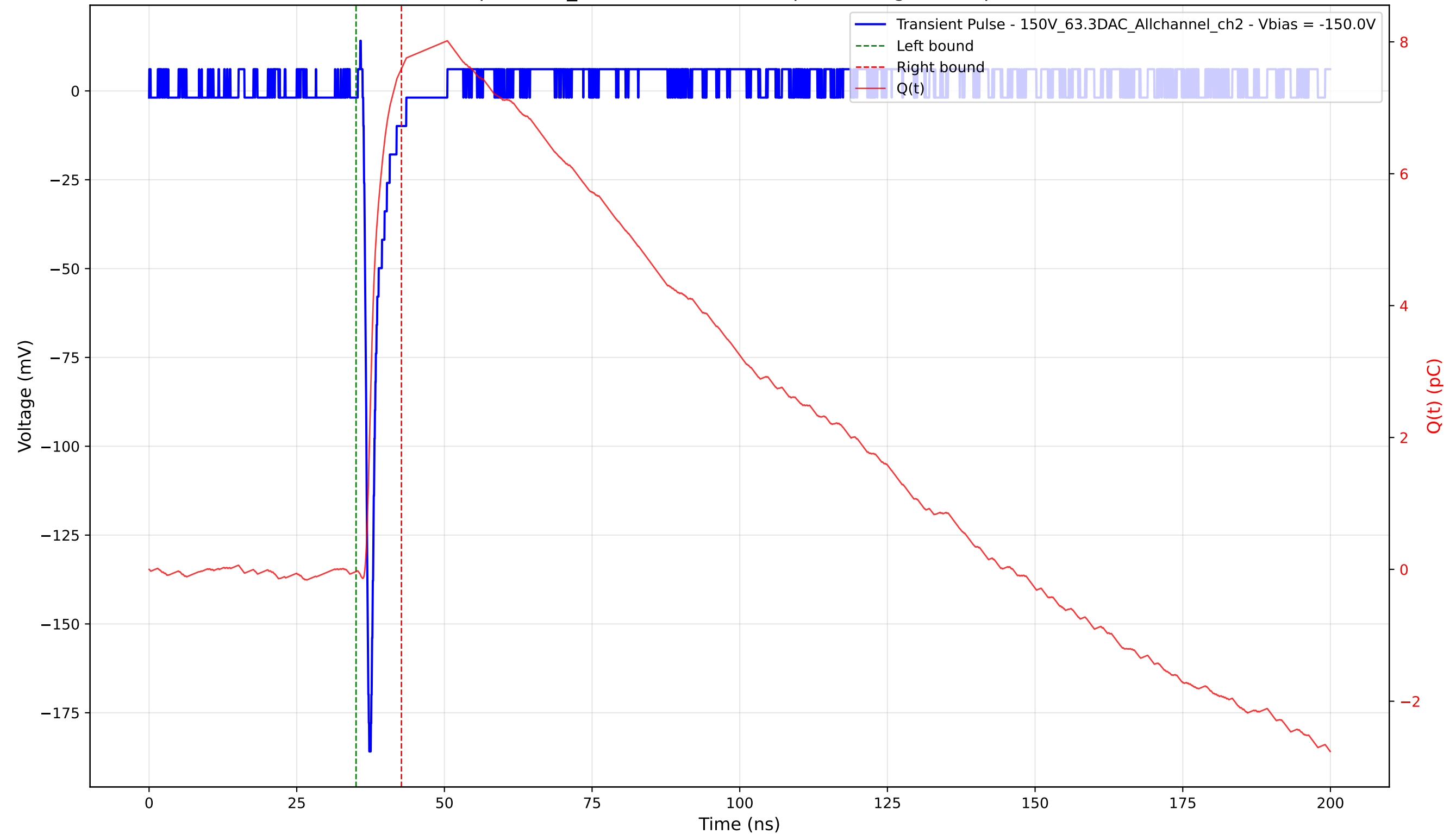
Transient Pulse - Sample: 1cm_42 - Position: 2480.0 \mu\text{m} - Charge: 7.63 pC - Rise Time: 0.76 ns
