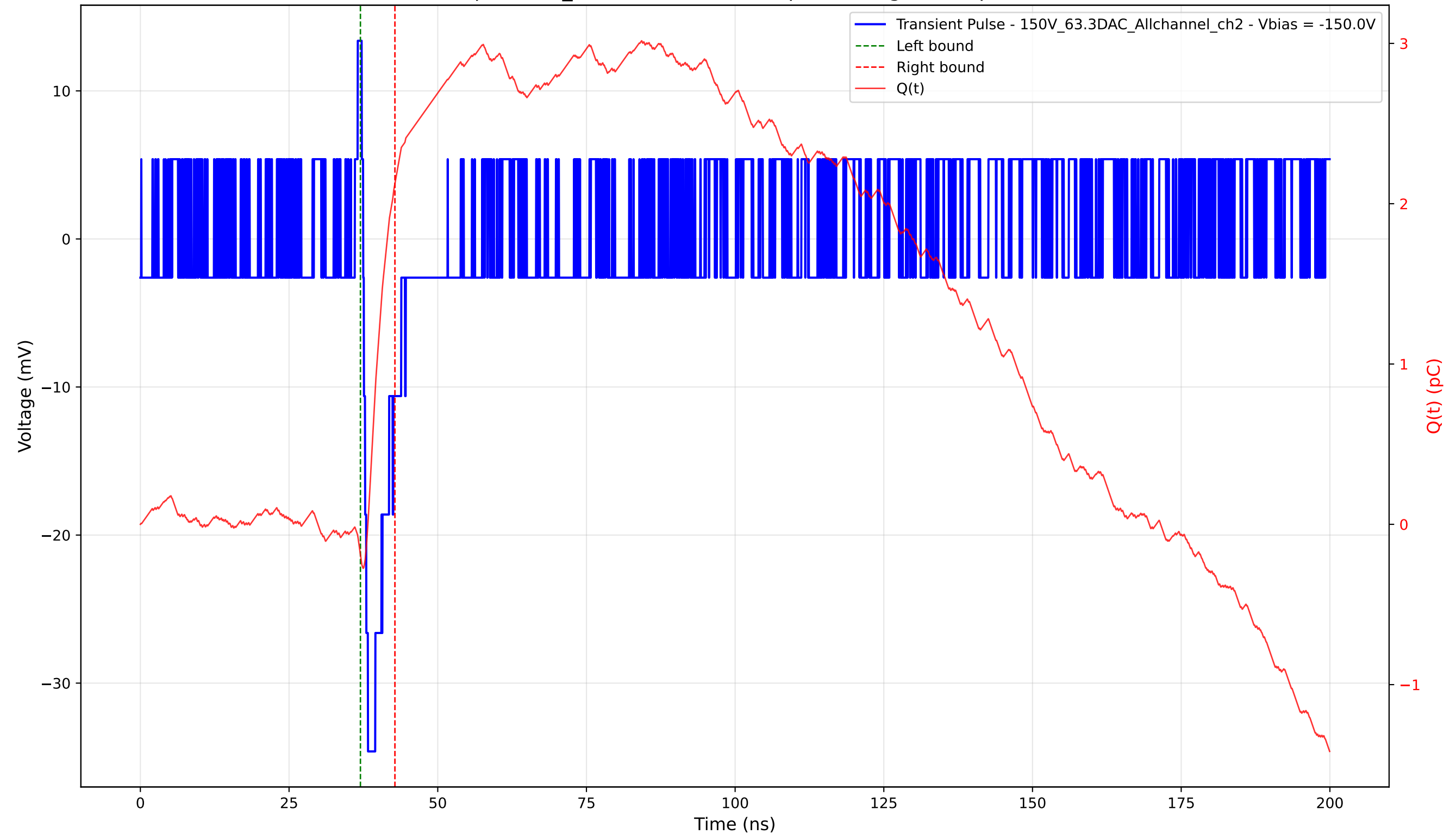
Transient Pulse - Sample: 1cm_42 - Position: 4795.0 \mu\text{m} - Charge: 2.32 pC - Rise Time: 0.72 ns
