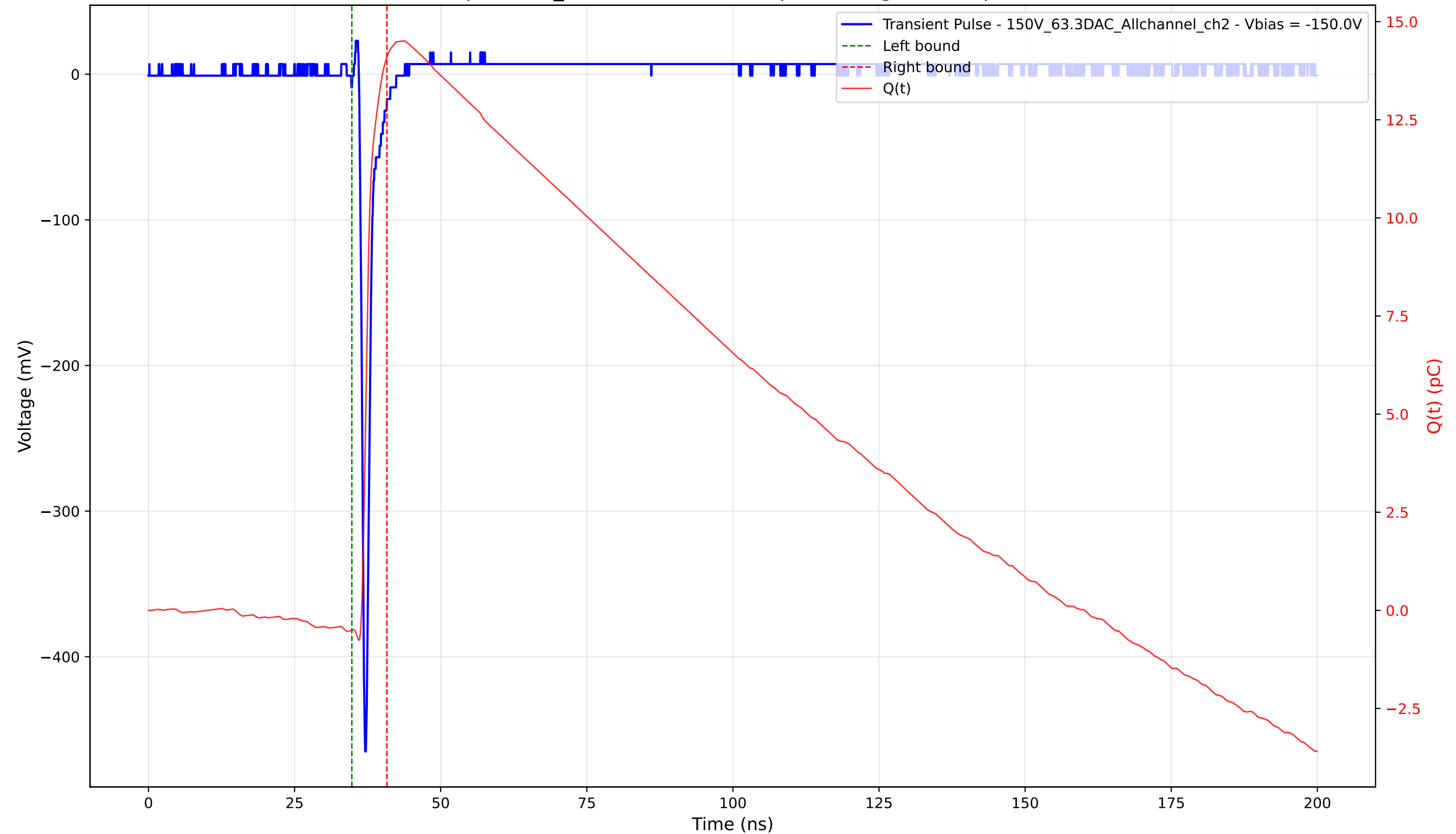
Transient Pulse - Sample: 1cm_42 - Position: 2835.0 \mu\text{m} - Charge: 14.61 pC - Rise Time: 0.73 ns
