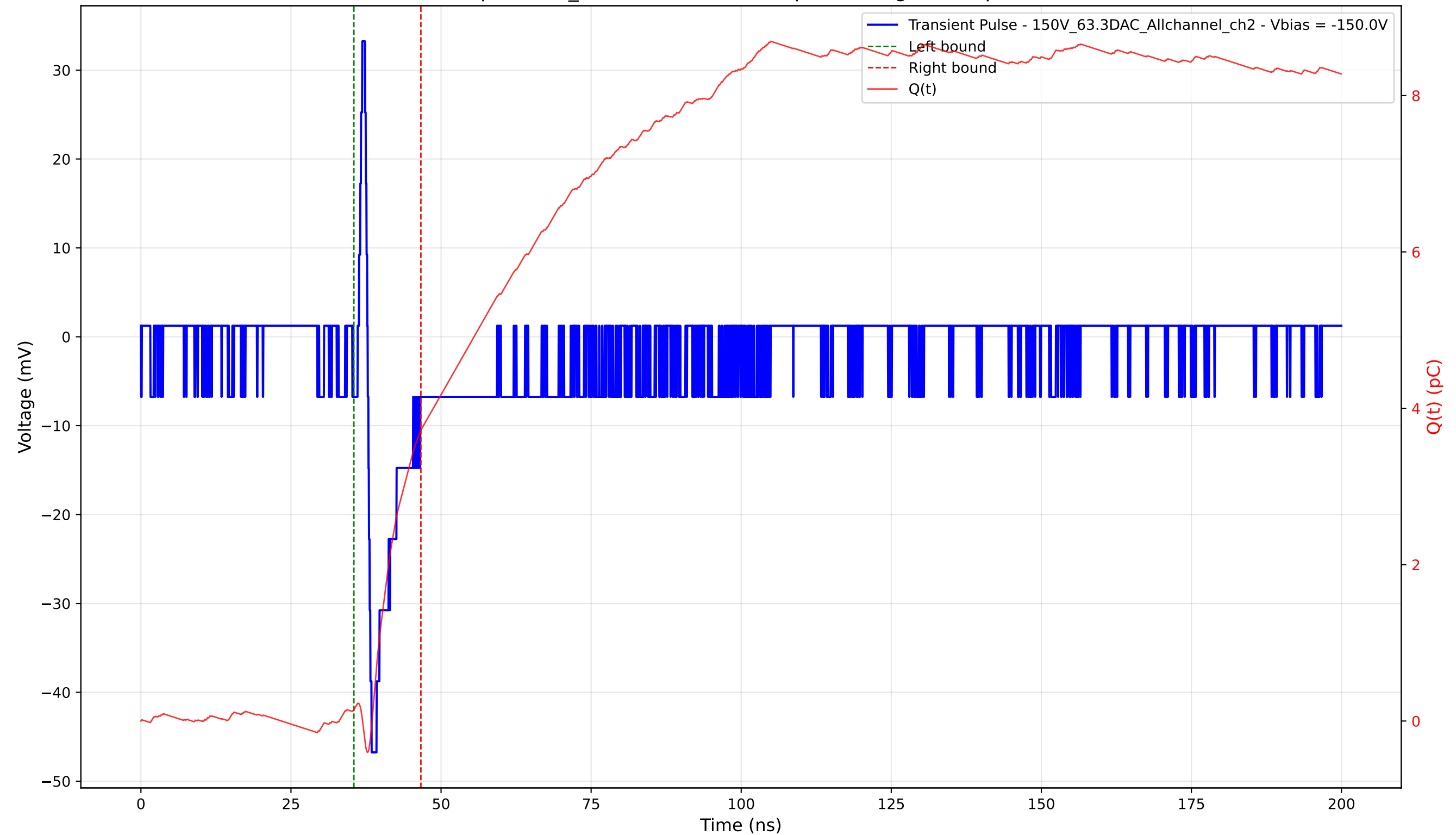
Transient Pulse - Sample: 1cm_42 - Position: 1245.0 \mu\text{m} - Charge: 3.58 pC - Rise Time: 0.66 ns
