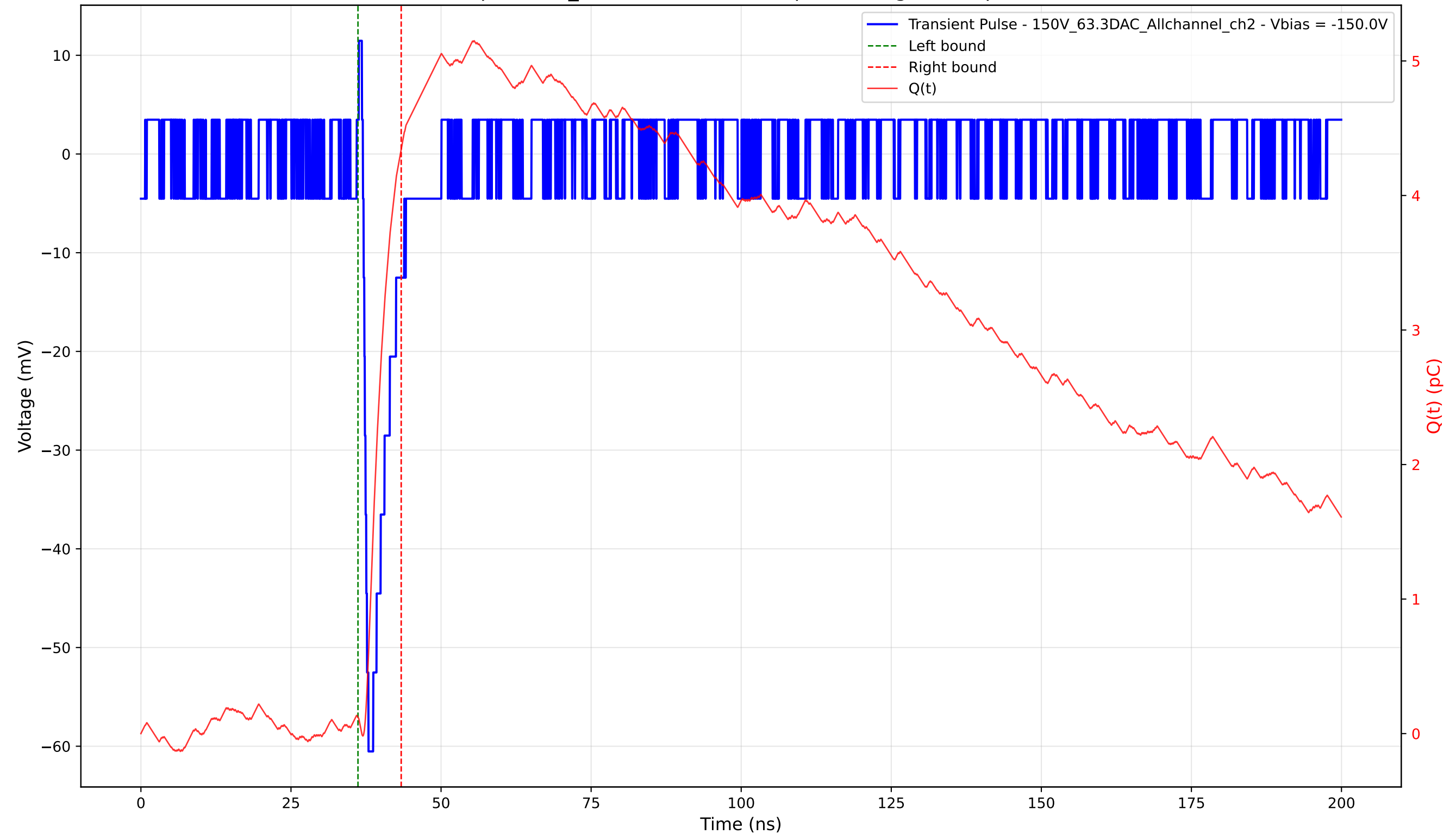
Transient Pulse - Sample: 1cm_42 - Position: 4160.0 \mu\text{m} - Charge: 4.22 pC - Rise Time: 0.83 ns
