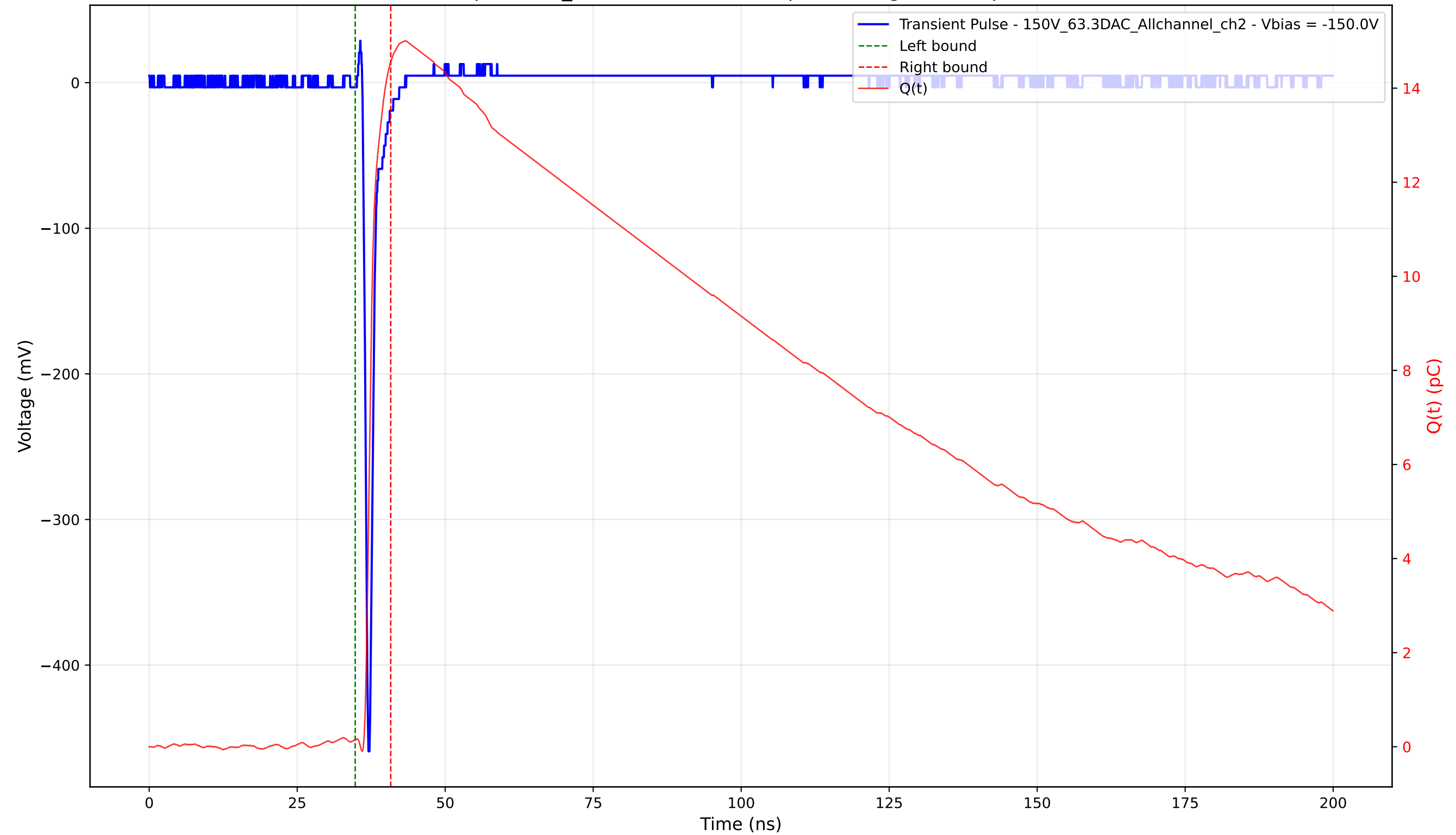
Transient Pulse - Sample: 1cm_42 - Position: 2890.0 \mu\text{m} - Charge: 14.41 pC - Rise Time: 0.72 ns
