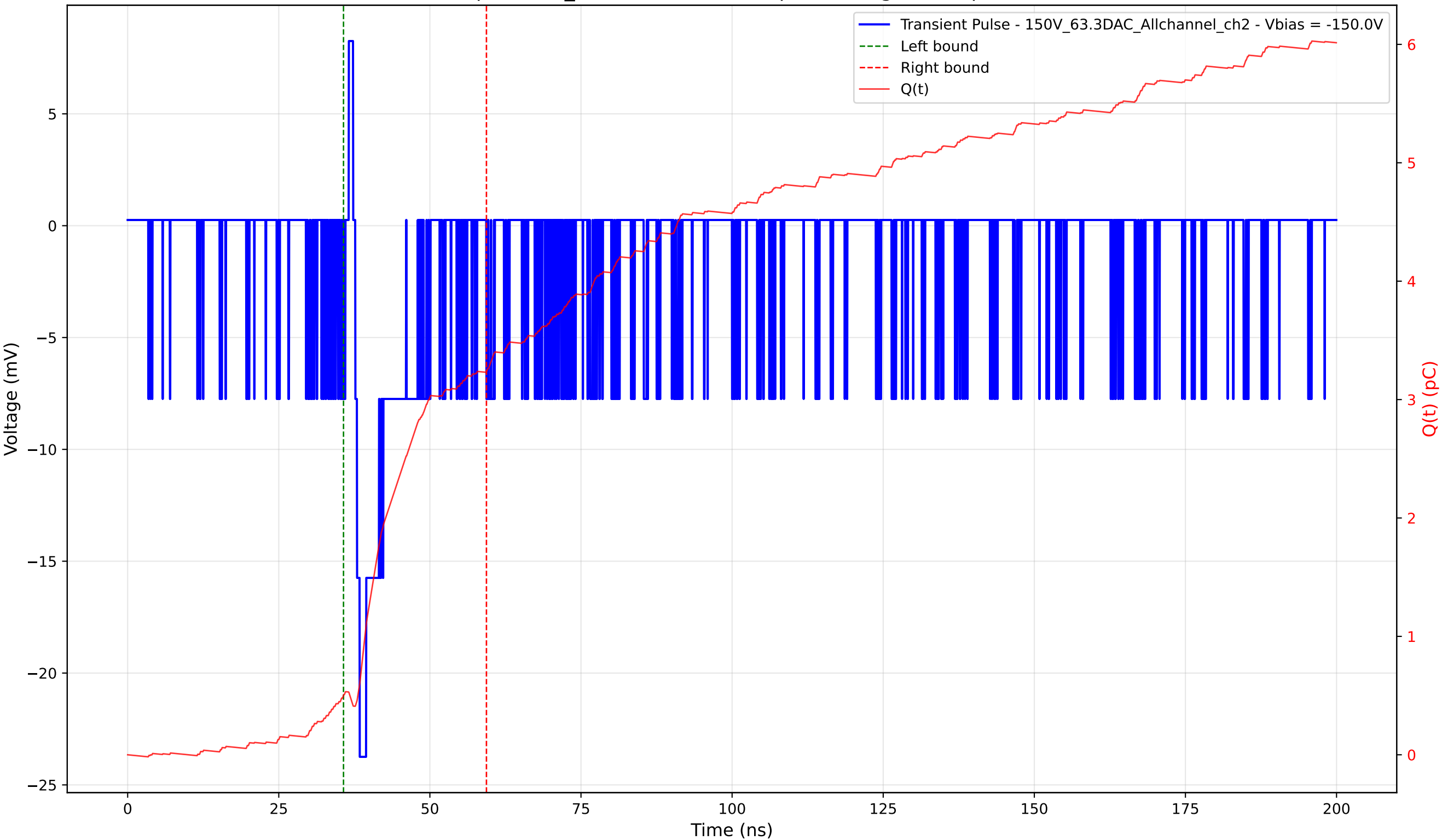
Transient Pulse - Sample: 1cm_42 - Position: 225.0 \mu\text{m} - Charge: 2.72 pC - Rise Time: 0.75 ns
