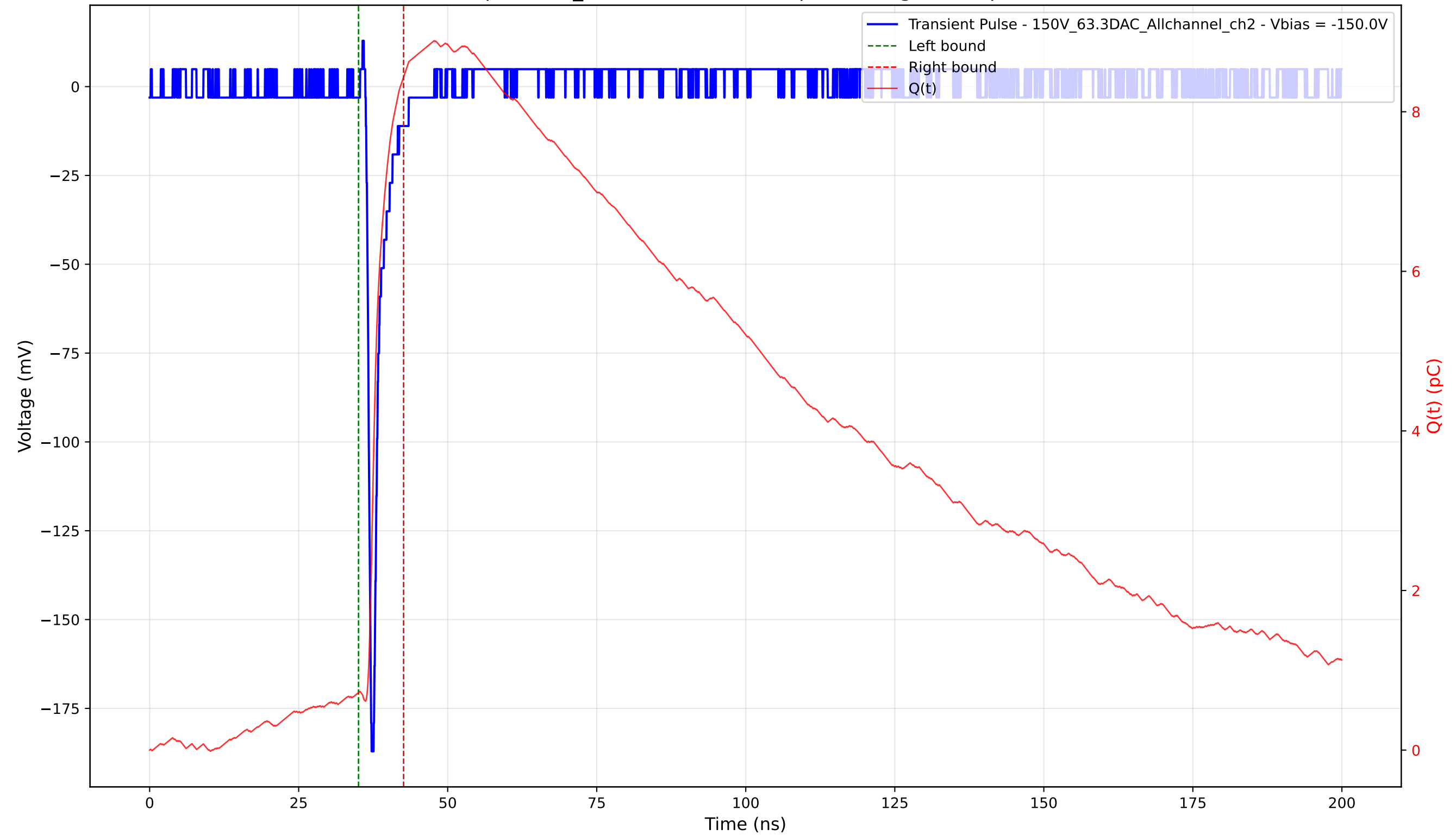
Transient Pulse - Sample: 1cm_42 - Position: 2485.0 \mu\text{m} - Charge: 7.72 pC - Rise Time: 0.75 ns
