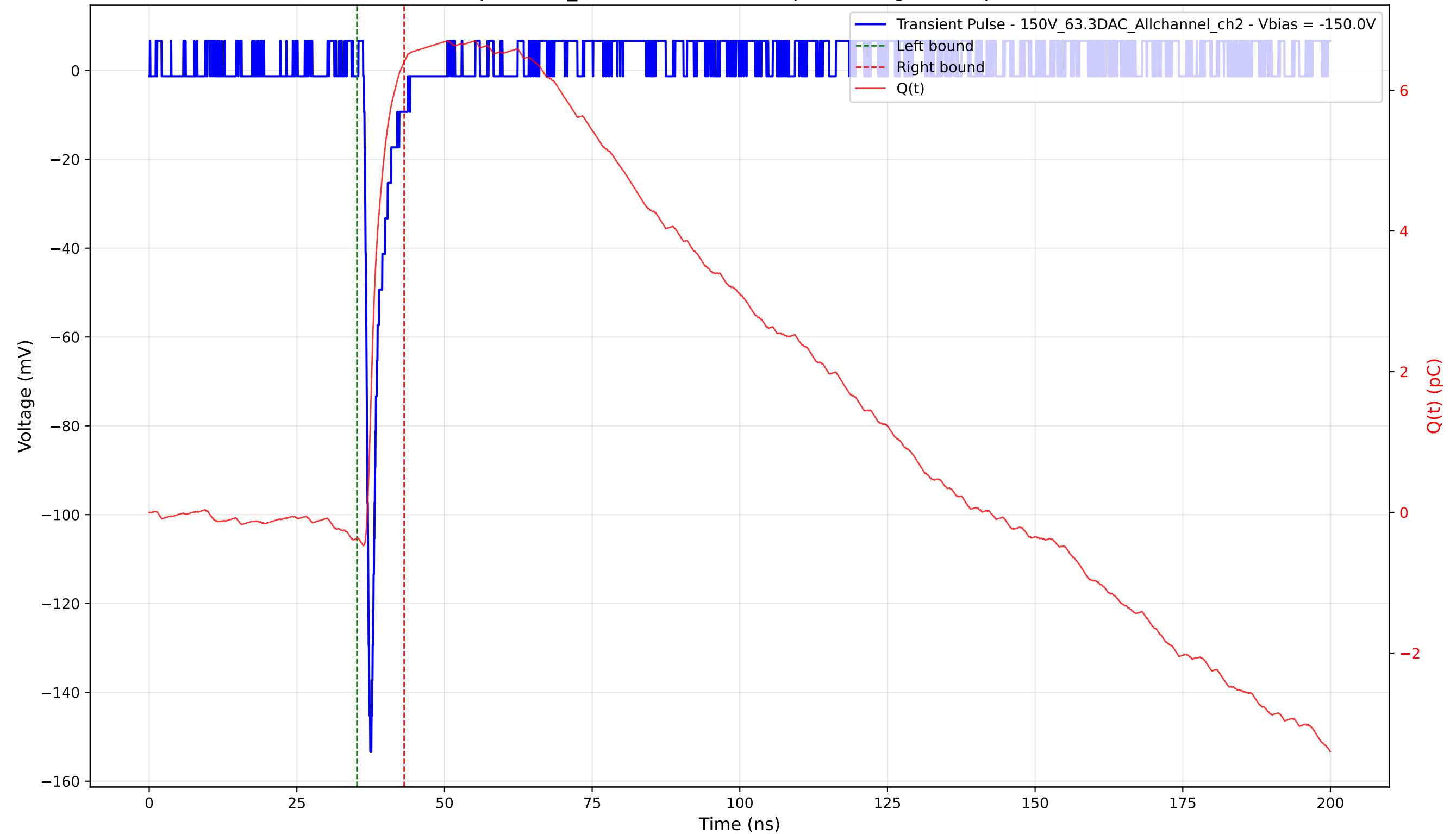
Transient Pulse - Sample: 1cm_42 - Position: 2385.0 \mu\text{m} - Charge: 6.77 pC - Rise Time: 0.85 ns
