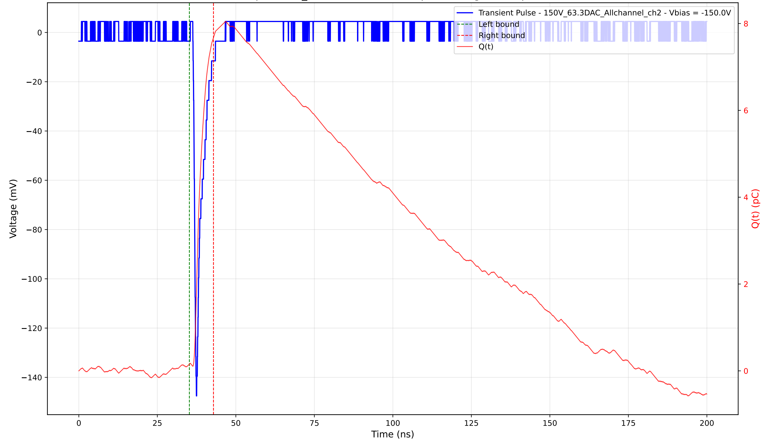
Transient Pulse - Sample: 1cm_42 - Position: 3685.0 \mu\text{m} - Charge: 7.52 pC - Rise Time: 0.86 ns
