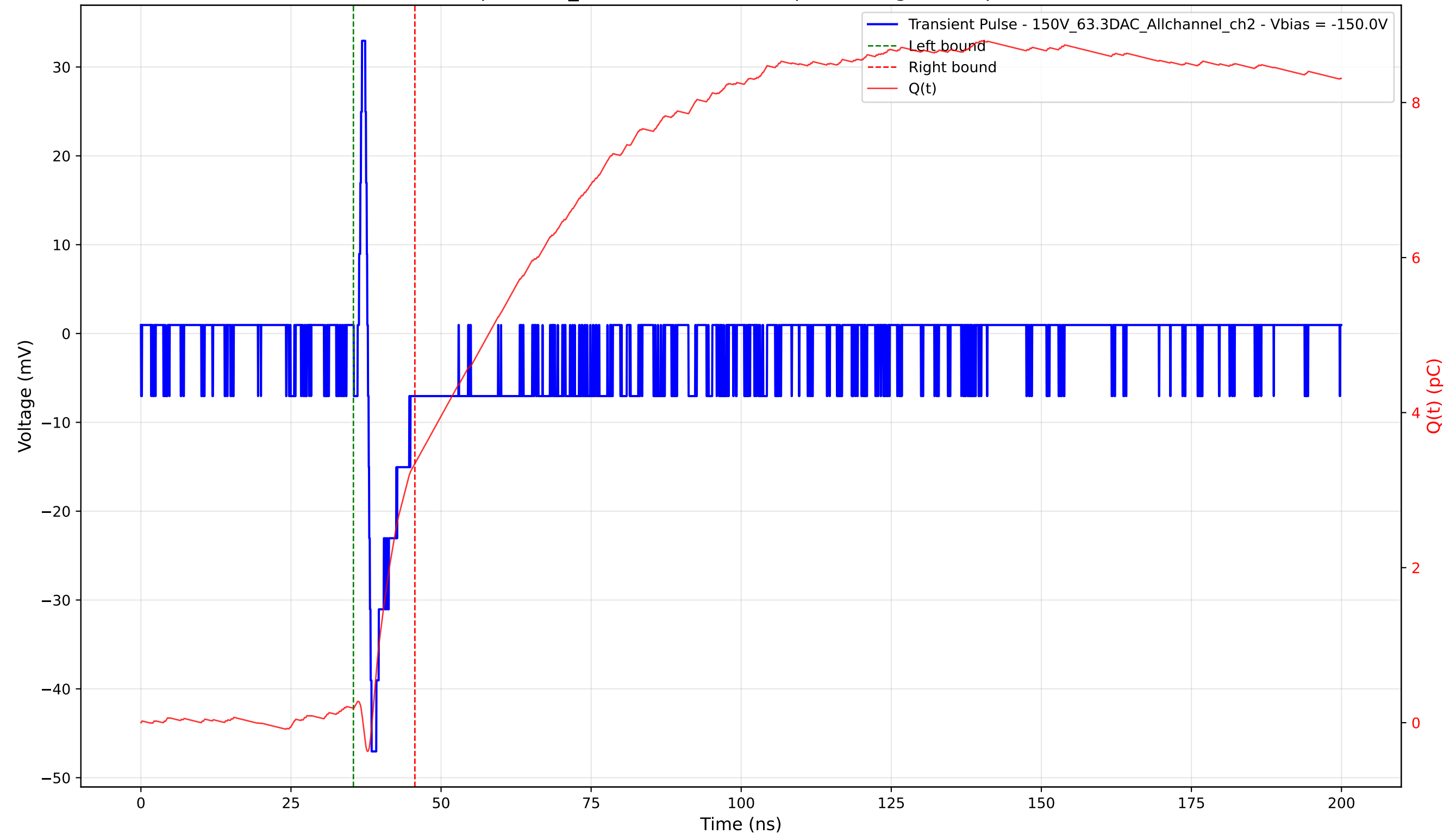
Transient Pulse - Sample: 1cm_42 - Position: 1190.0 \mu\text{m} - Charge: 3.15 pC - Rise Time: 0.62 ns
