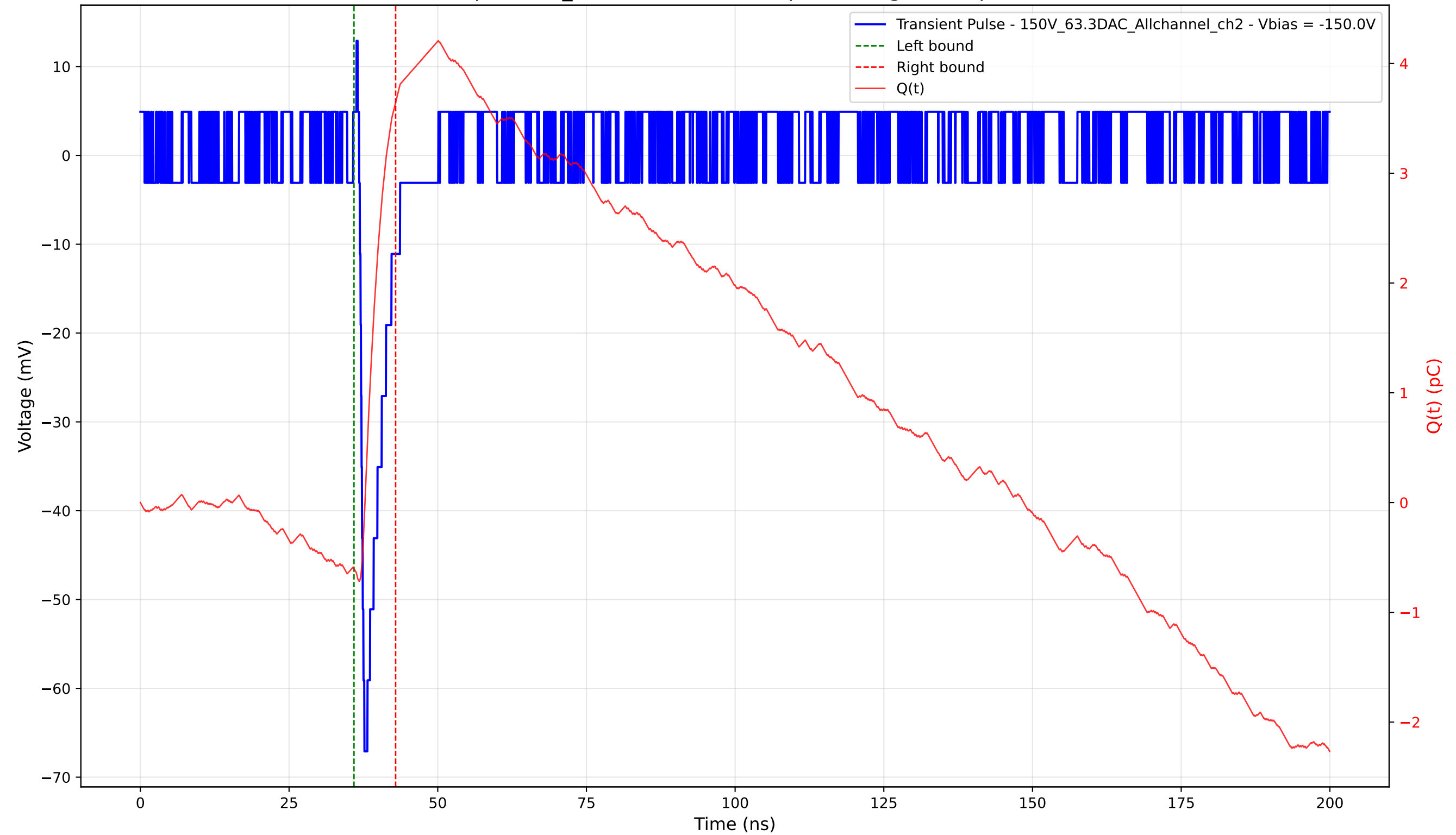
Transient Pulse - Sample: 1cm_42 - Position: 4050.0 \mu\text{m} - Charge: 4.25 pC - Rise Time: 0.78 ns
