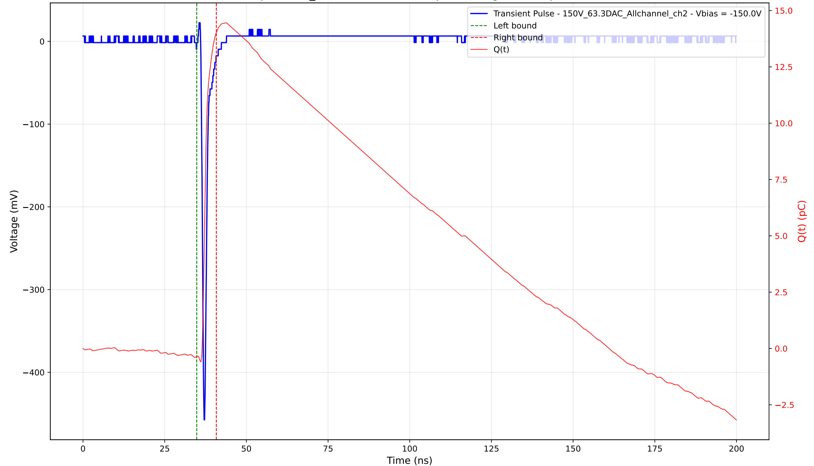
Transient Pulse - Sample: 1cm_42 - Position: 2845.0 \mu\text{m} - Charge: 14.38 pC - Rise Time: 0.68 ns
