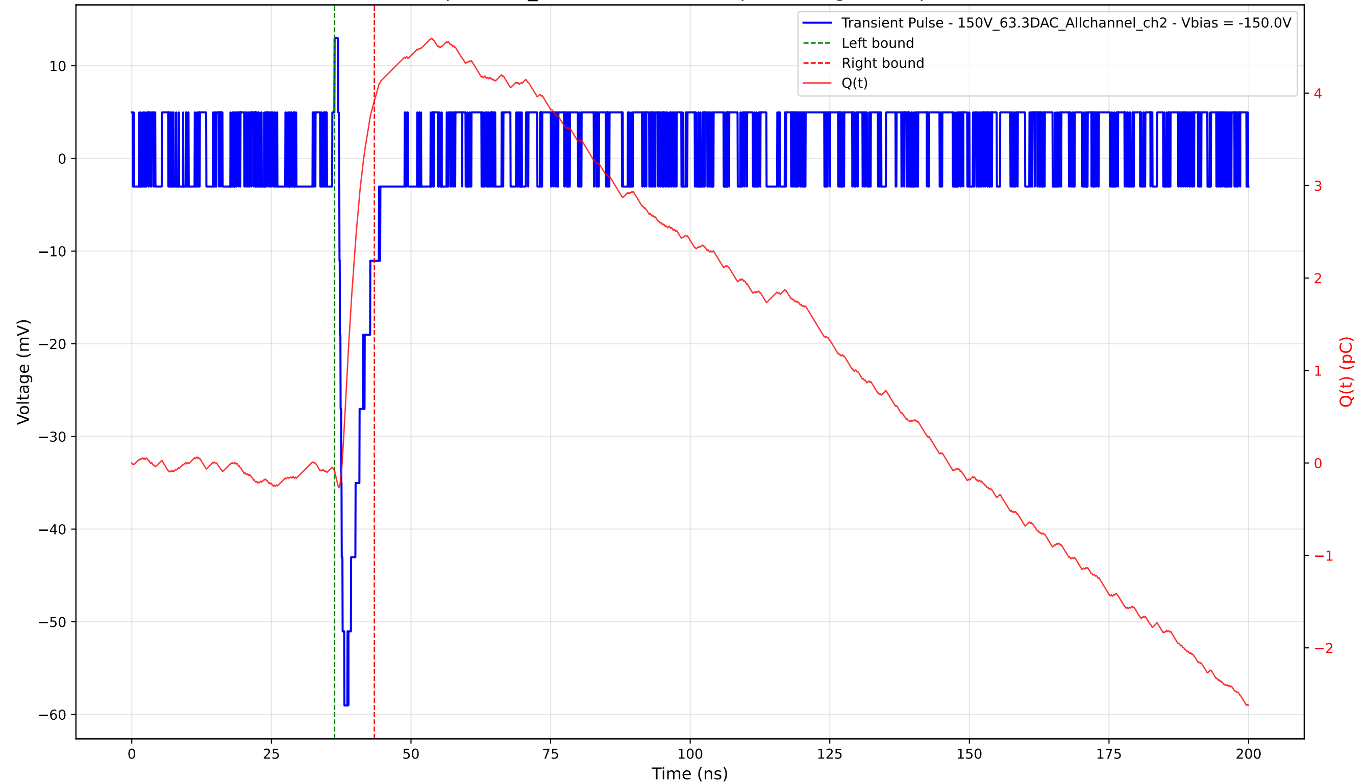
Transient Pulse - Sample: 1cm_42 - Position: 4235.0 \mu\text{m} - Charge: 4.01 pC - Rise Time: 0.91 ns
