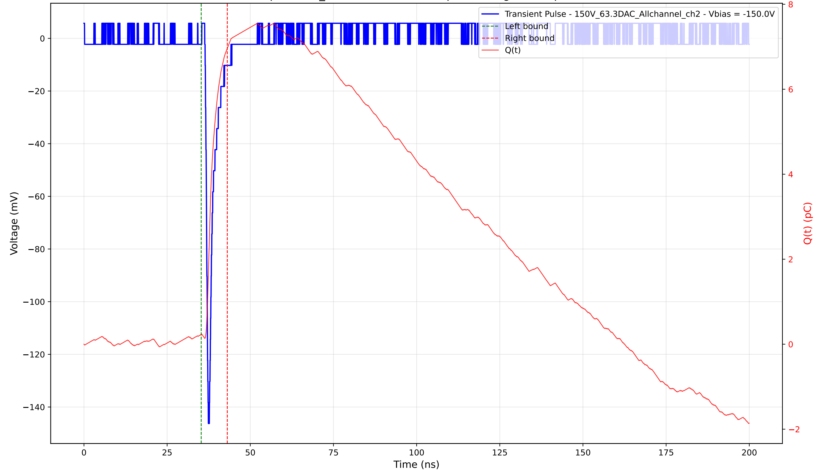
Transient Pulse - Sample: 1cm_42 - Position: 2365.0 \mu\text{m} - Charge: 6.73 pC - Rise Time: 0.82 ns
