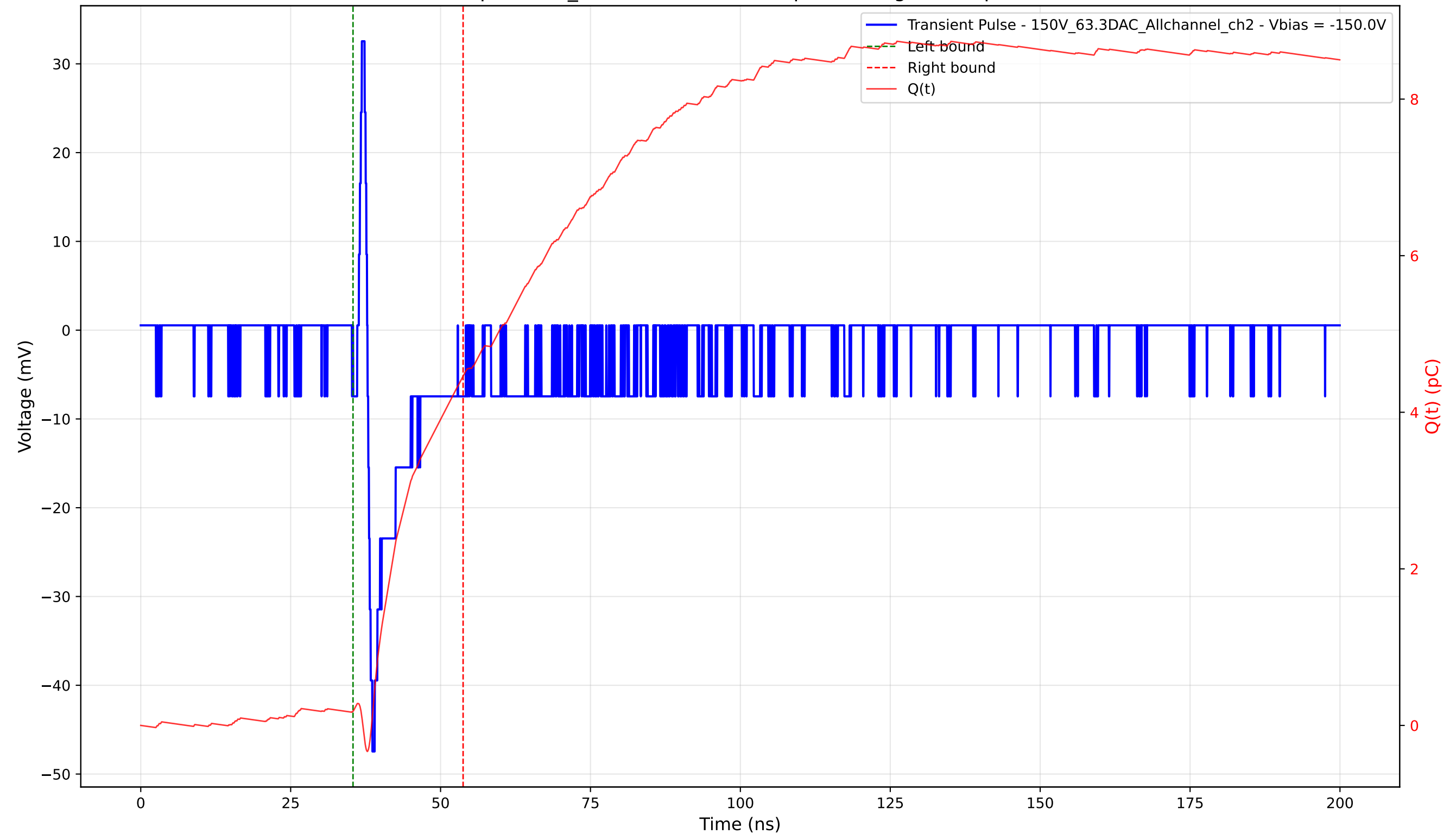
Transient Pulse - Sample: 1cm_42 - Position: 1130.0 \mu\text{m} - Charge: 4.28 pC - Rise Time: 0.82 ns
