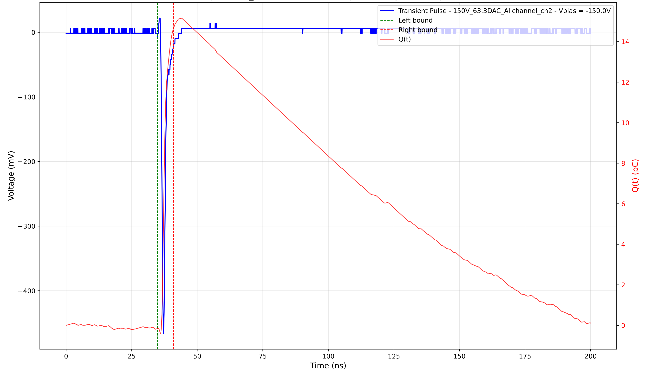
Transient Pulse - Sample: 1cm_42 - Position: 2785.0 \mu\text{m} - Charge: 14.81 pC - Rise Time: 0.72 ns
