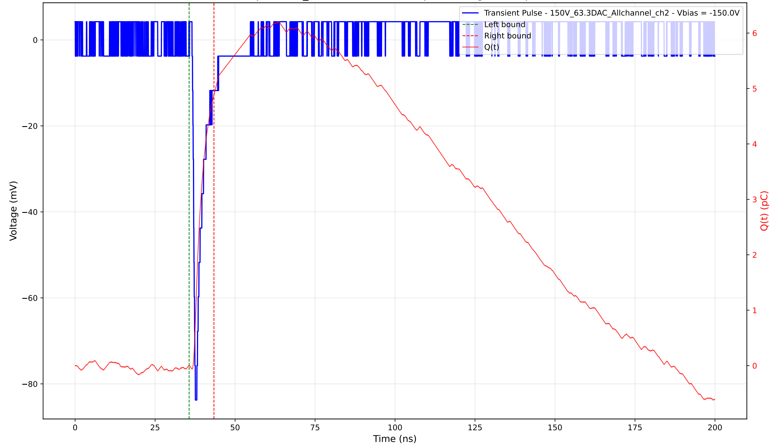
Transient Pulse - Sample: 1cm_42 - Position: 2070.0 \mu\text{m} - Charge: 4.90 pC - Rise Time: 0.74 ns
