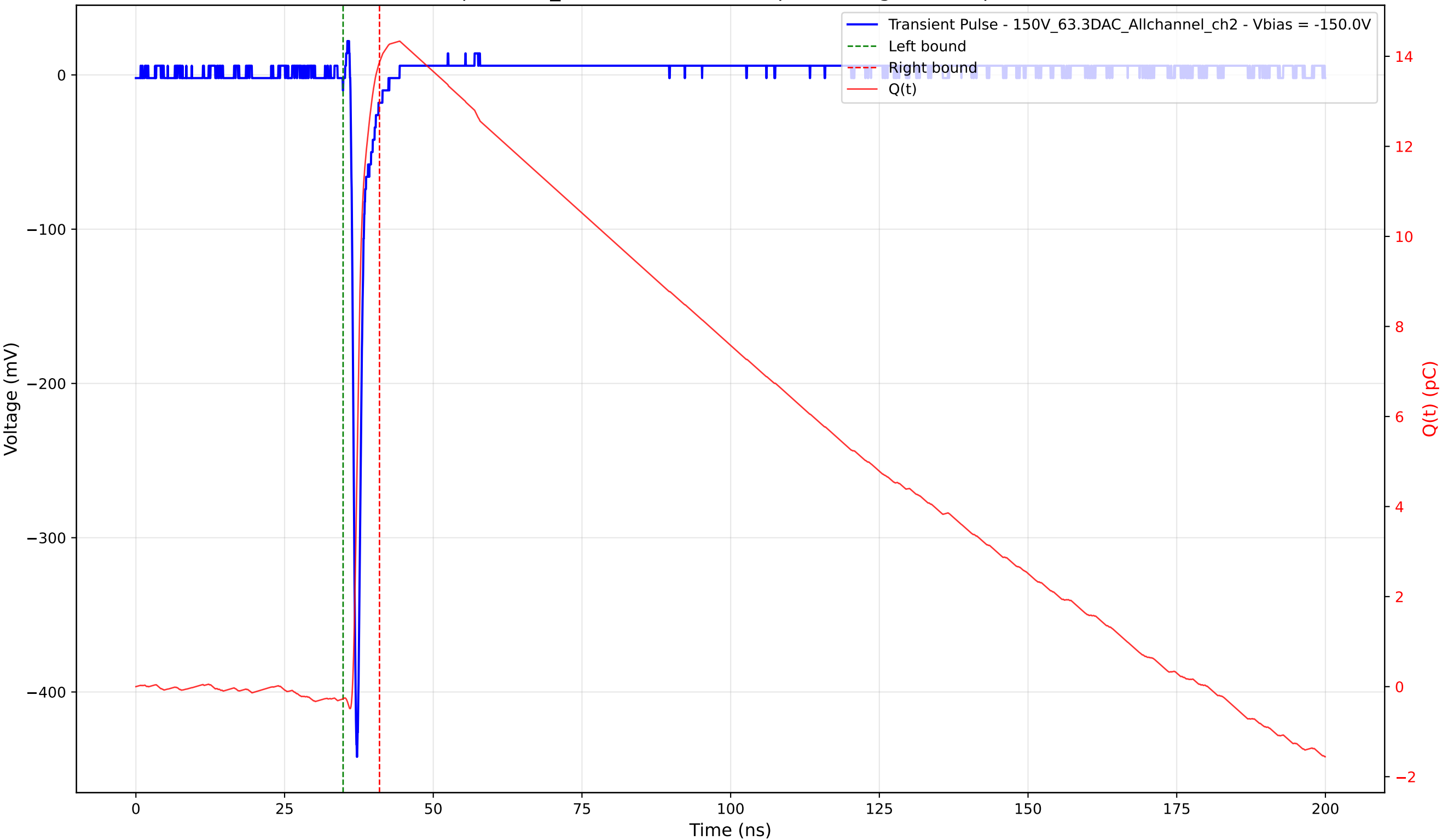
Transient Pulse - Sample: 1cm_42 - Position: 2750.0 \mu\text{m} - Charge: 14.13 pC - Rise Time: 0.71 ns
