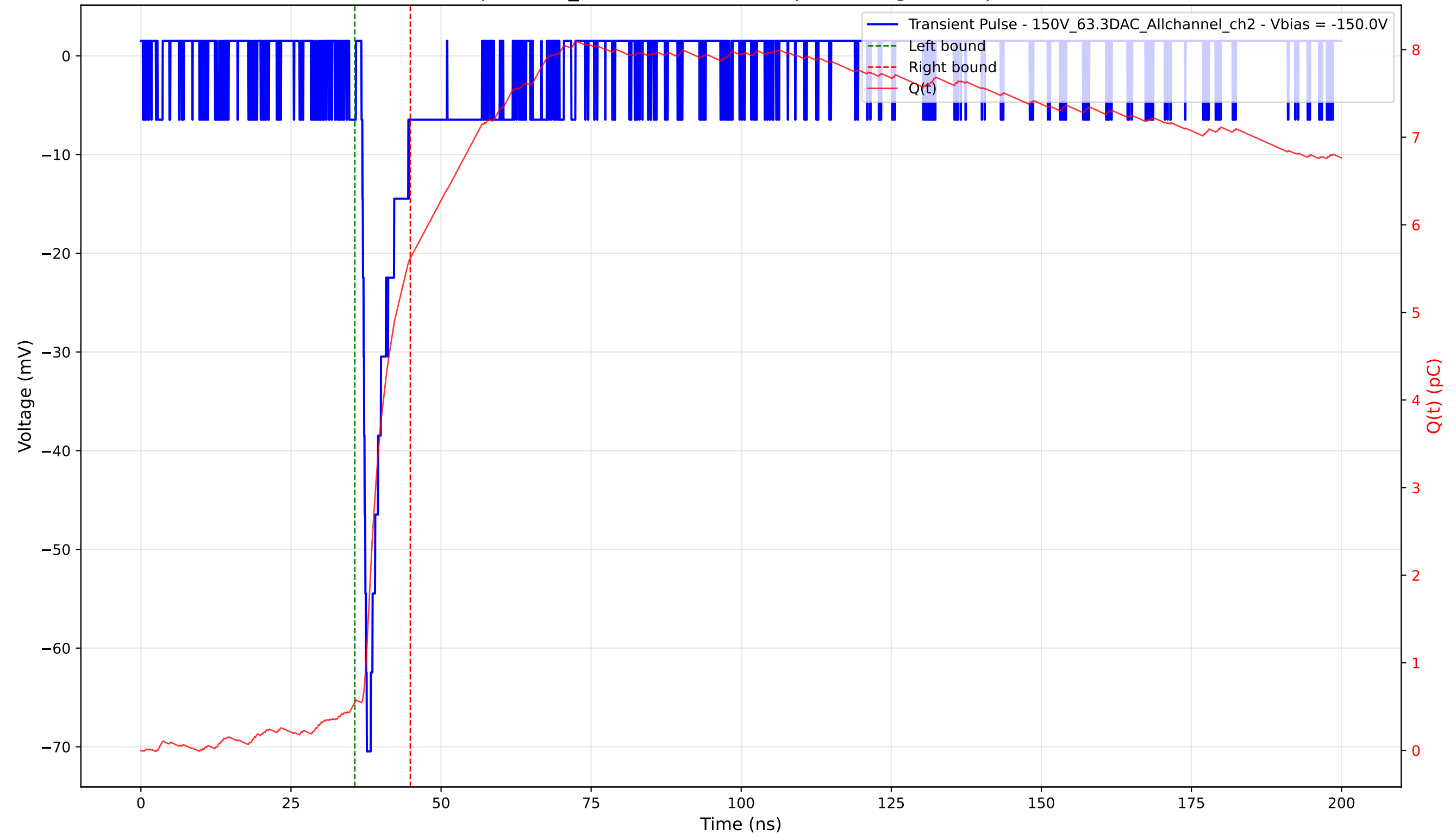
Transient Pulse - Sample: 1cm_42 - Position: 2005.0 \mu\text{m} - Charge: 5.07 pC - Rise Time: 0.76 ns
