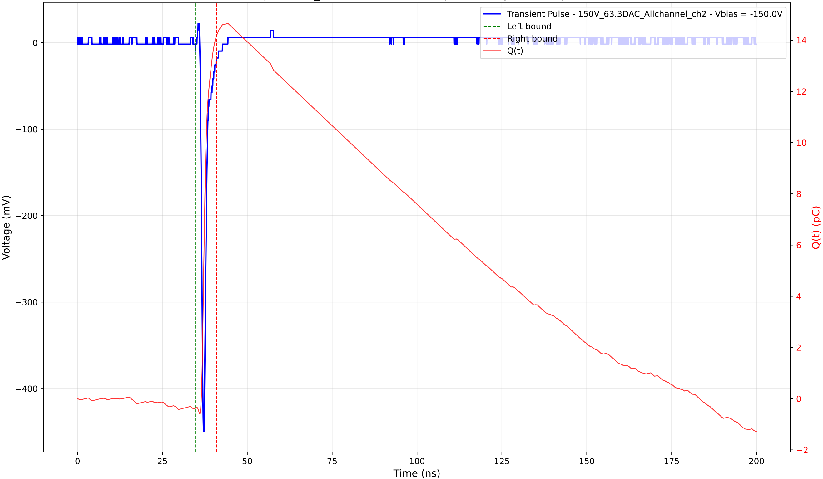
Transient Pulse - Sample: 1cm_42 - Position: 2770.0 \mu\text{m} - Charge: 14.54 pC - Rise Time: 0.73 ns
