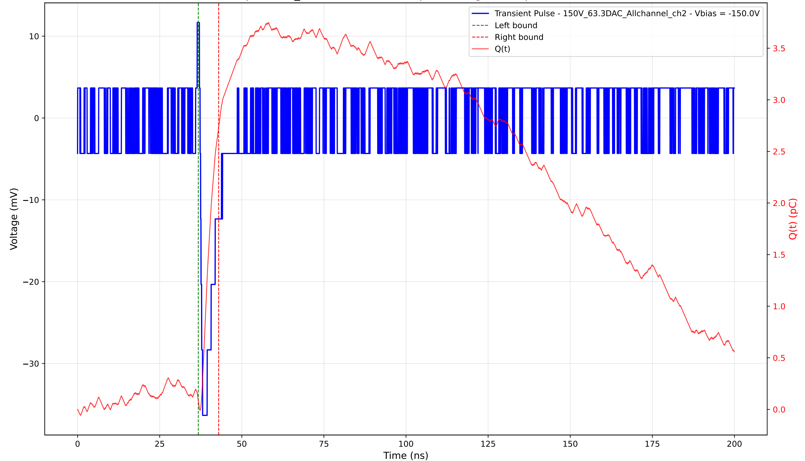
Transient Pulse - Sample: 1cm_42 - Position: 4515.0 \mu\text{m} - Charge: 2.65 pC - Rise Time: 0.00 ns (N/A)
