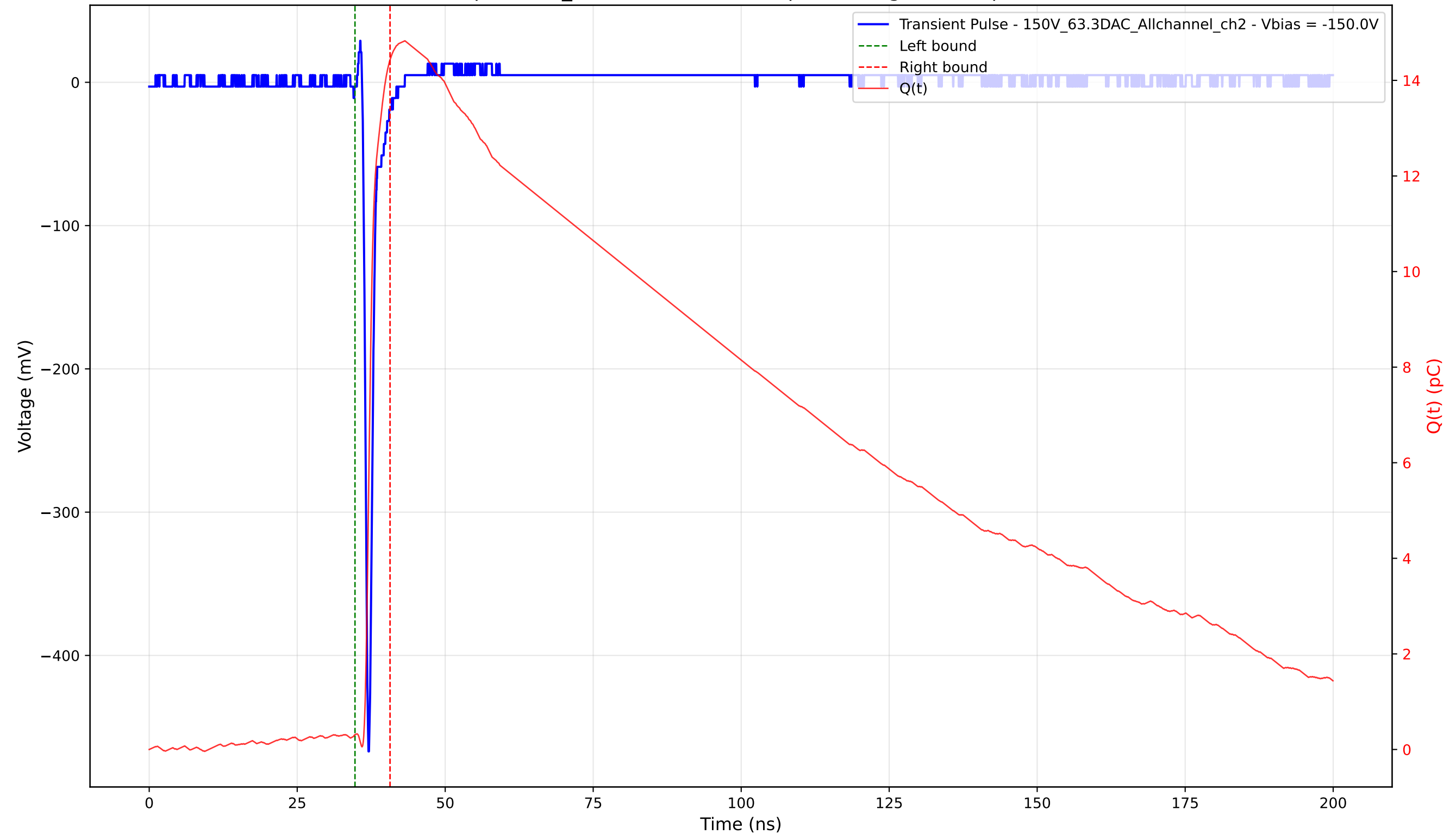
Transient Pulse - Sample: 1cm_42 - Position: 3035.0 \mu\text{m} - Charge: 14.12 pC - Rise Time: 0.73 ns
