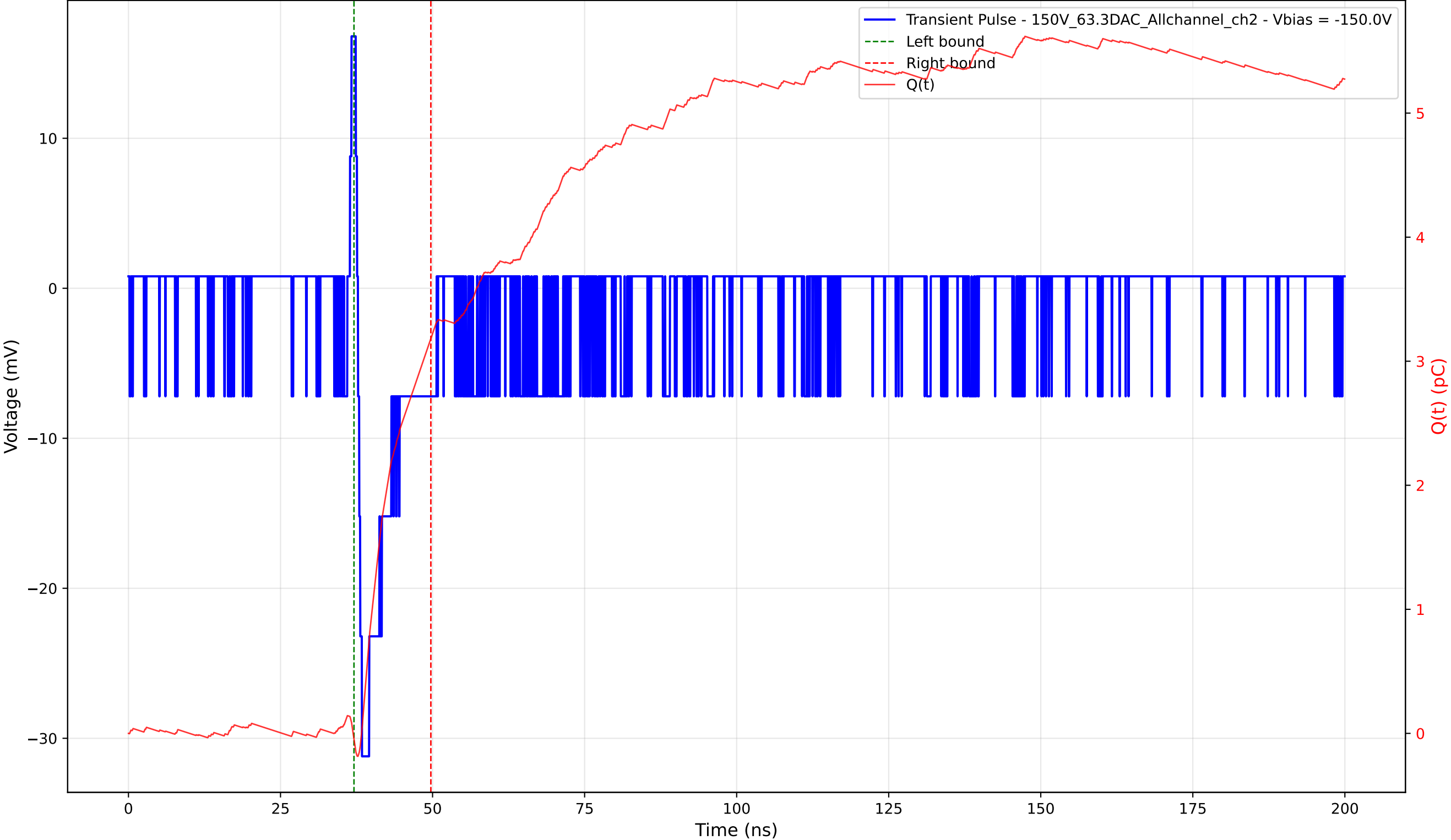
Transient Pulse - Sample: 1cm_42 - Position: 495.0 \mu\text{m} - Charge: 3.23 pC - Rise Time: 0.67 ns
