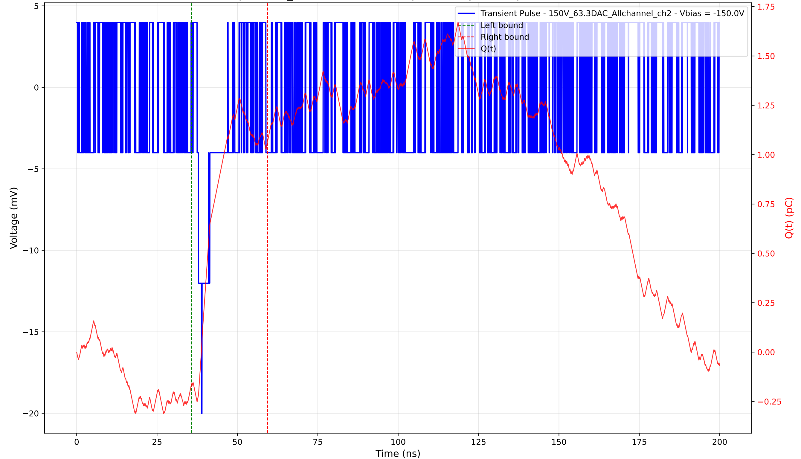
Transient Pulse - Sample: 1cm_42 - Position: 5045.0 \mu\text{m} - Charge: 1.23 pC - Rise Time: 0.00 ns (N/A)
