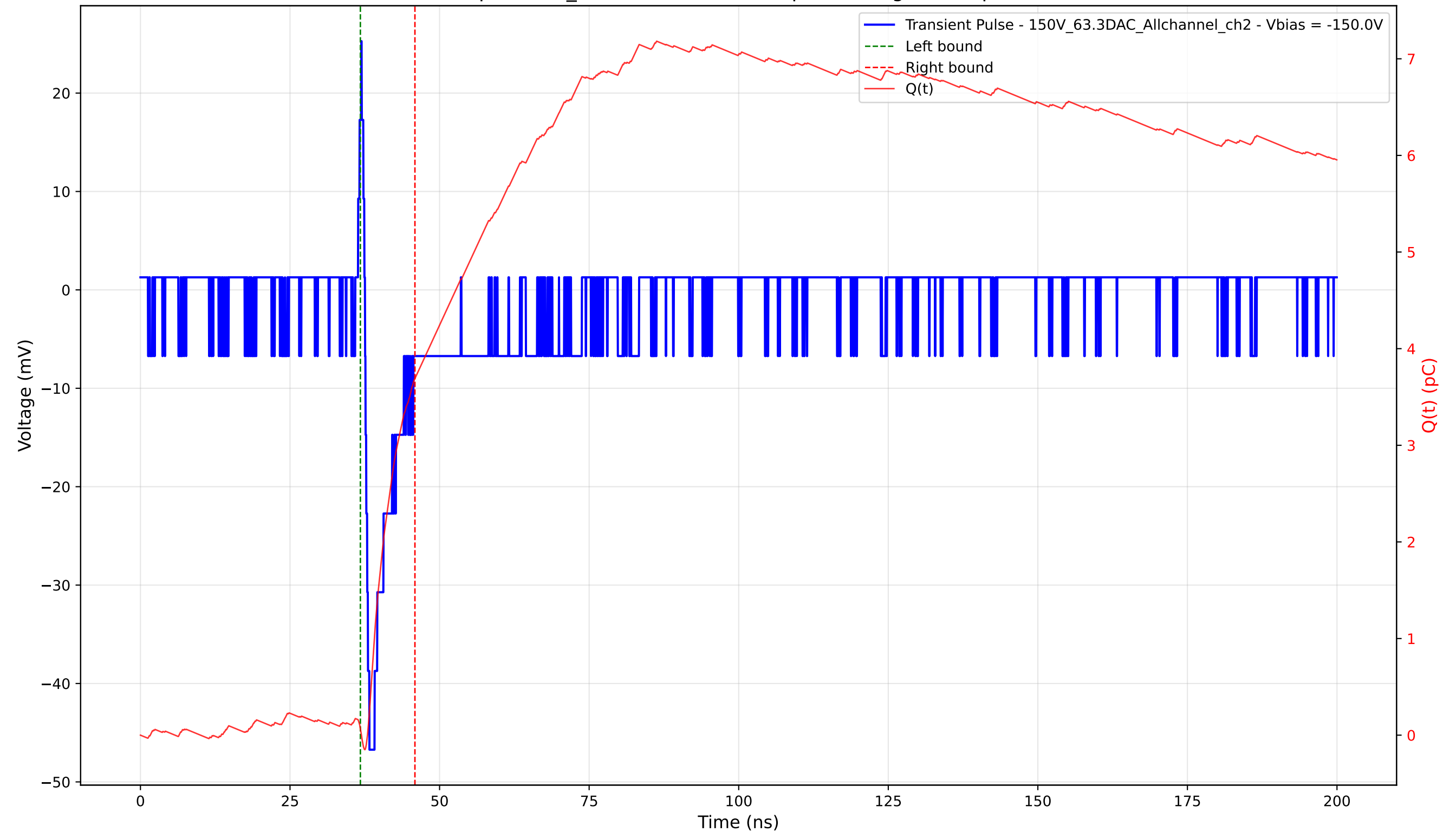
Transient Pulse - Sample: 1cm_42 - Position: 1545.0 \mu\text{m} - Charge: 3.62 pC - Rise Time: 0.74 ns
