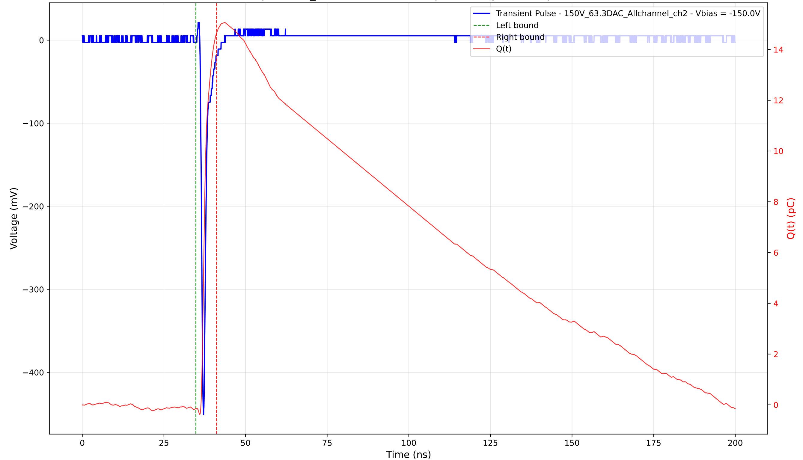
Transient Pulse - Sample: 1cm_42 - Position: 3235.0 \mu\text{m} - Charge: 14.80 pC - Rise Time: 0.69 ns
