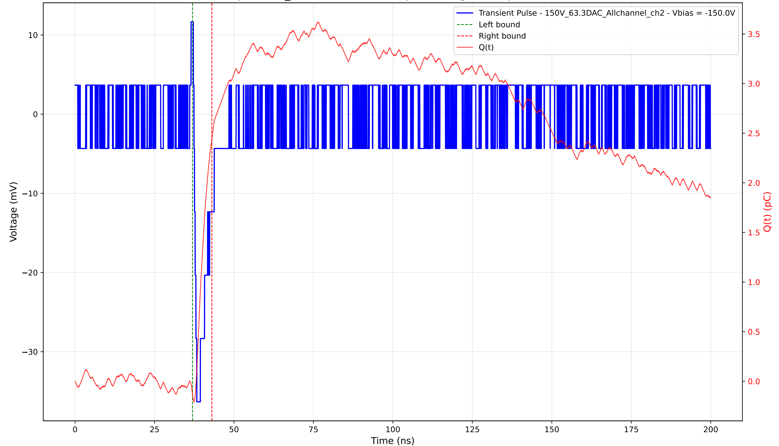
Transient Pulse - Sample: 1cm_42 - Position: 4820.0 \mu\text{m} - Charge: 2.58 pC - Rise Time: 0.00 ns (N/A)
