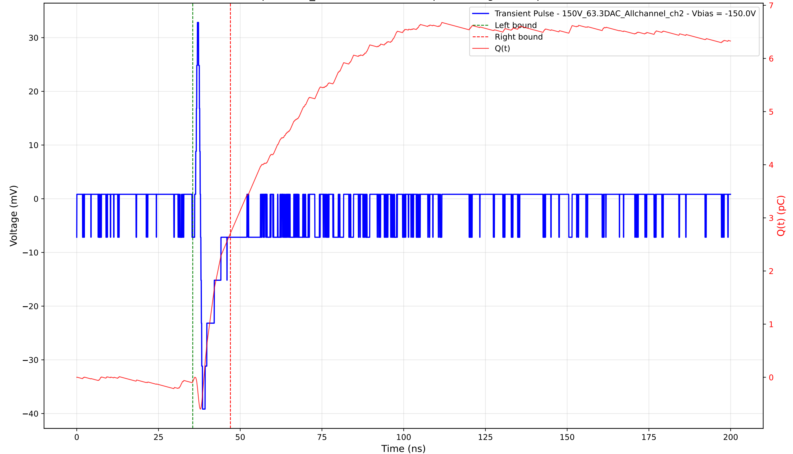
Transient Pulse - Sample: 1cm_42 - Position: 1055.0 \mu\text{m} - Charge: 2.79 pC - Rise Time: 0.62 ns
