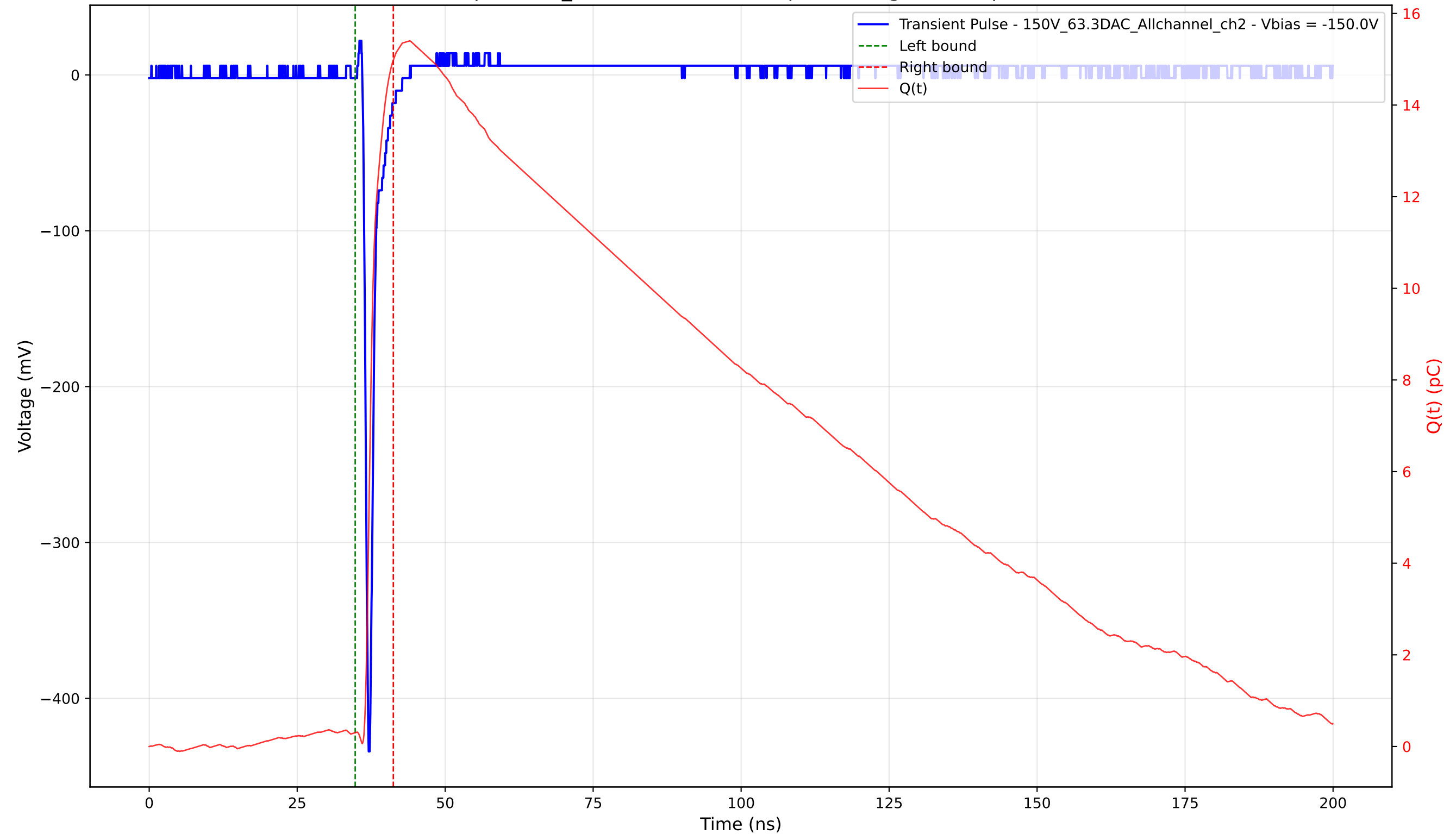
Transient Pulse - Sample: 1cm_42 - Position: 3285.0 \mu\text{m} - Charge: 14.68 pC - Rise Time: 0.73 ns
