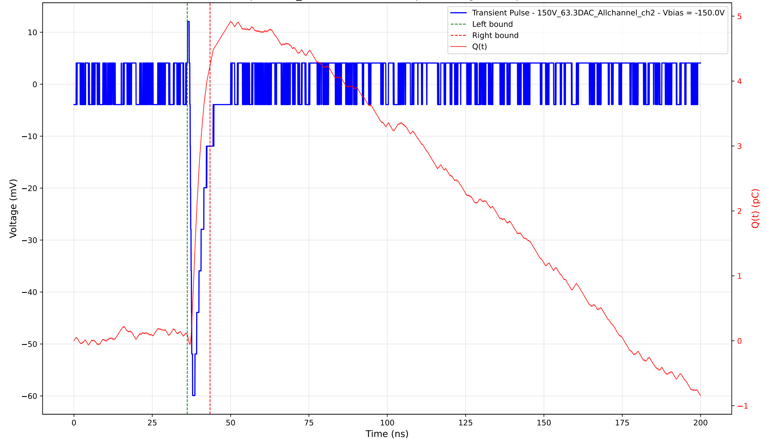
Transient Pulse - Sample: 1cm_42 - Position: 4145.0 \mu\text{m} - Charge: 4.15 pC - Rise Time: 0.79 ns
