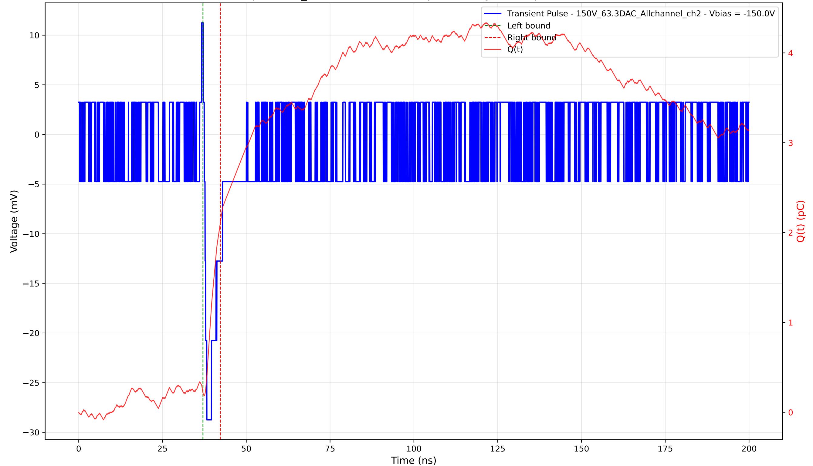
Transient Pulse - Sample: 1cm_42 - Position: 4915.0 \mu\text{m} - Charge: 1.89 pC - Rise Time: 0.00 ns (N/A)
