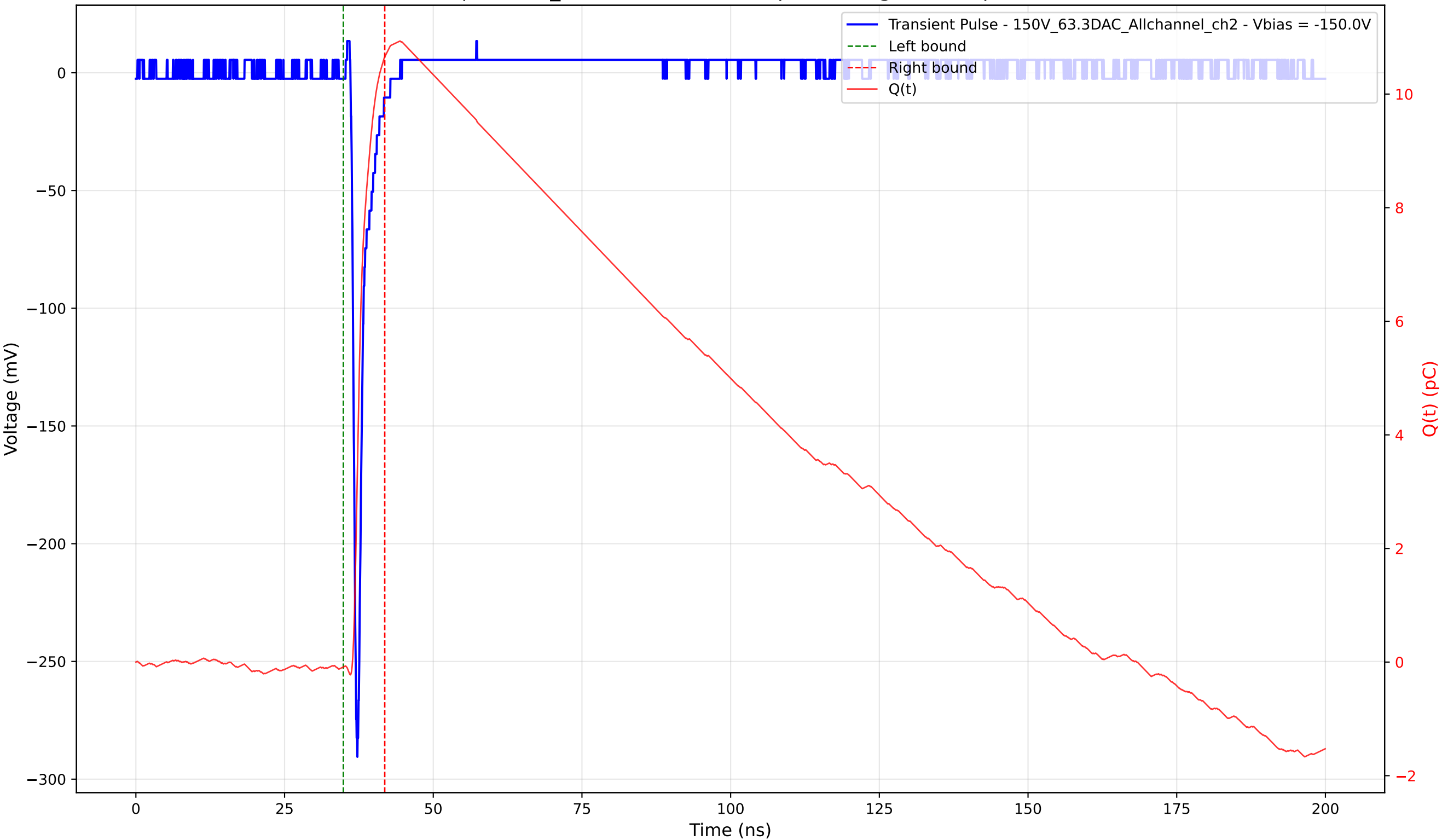
Transient Pulse - Sample: 1cm_42 - Position: 3435.0 \mu\text{m} - Charge: 10.74 pC - Rise Time: 0.79 ns
