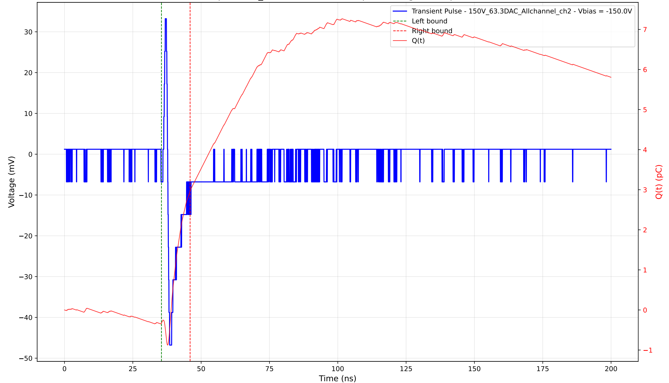
Transient Pulse - Sample: 1cm_42 - Position: 1300.0 \mu\text{m} - Charge: 3.30 pC - Rise Time: 0.70 ns
