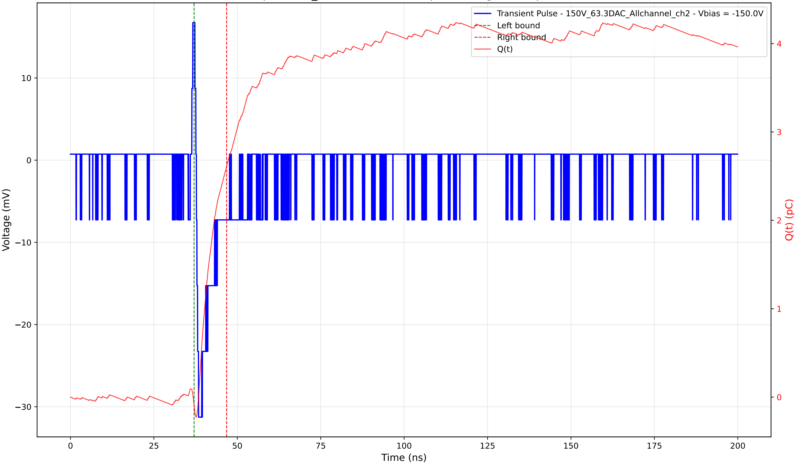
Transient Pulse - Sample: 1cm_42 - Position: 455.0 \mu\text{m} - Charge: 2.70 pC - Rise Time: 0.67 ns
