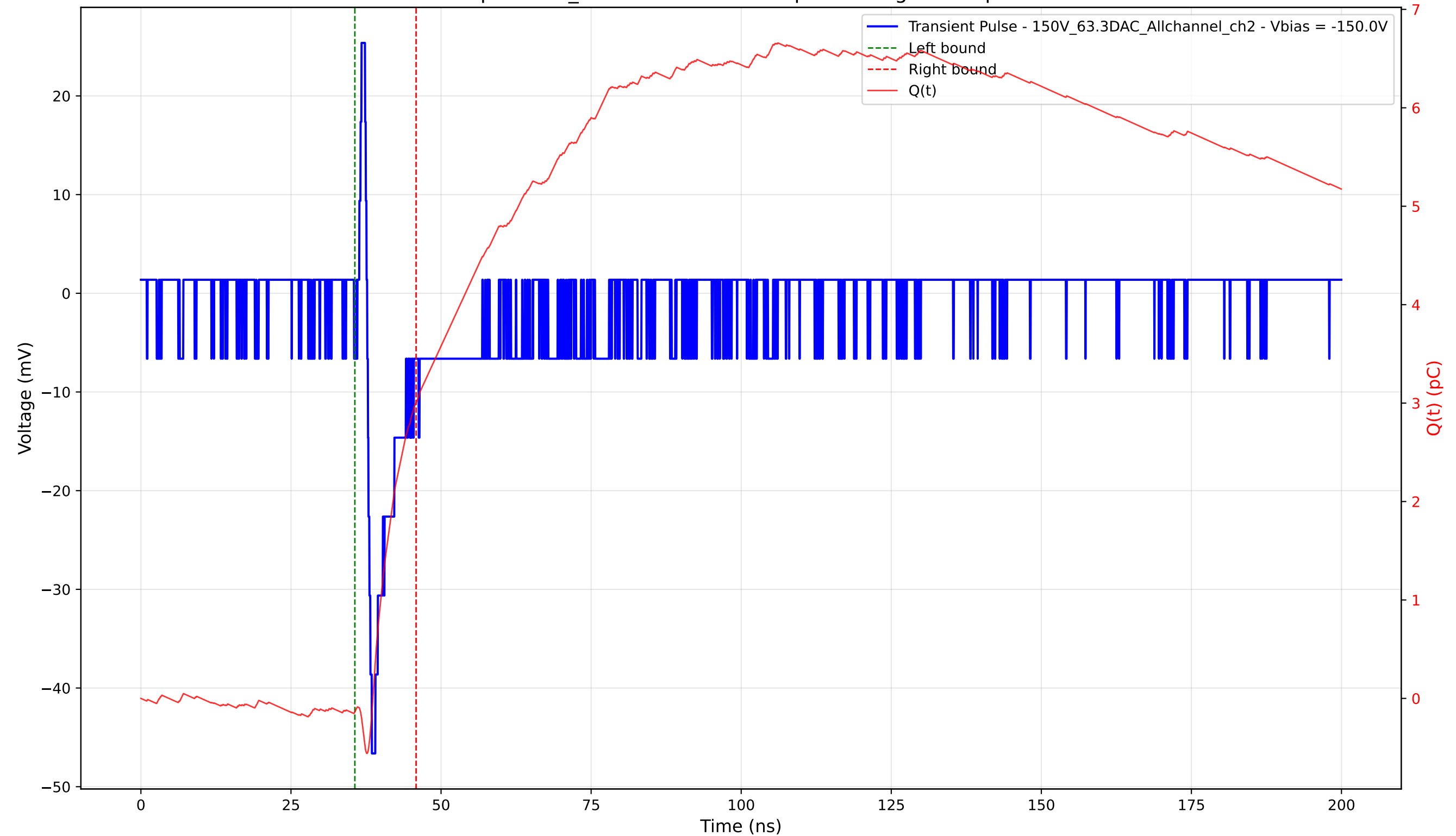
Transient Pulse - Sample: 1cm_42 - Position: 1420.0 \mu\text{m} - Charge: 3.14 pC - Rise Time: 0.77 ns
