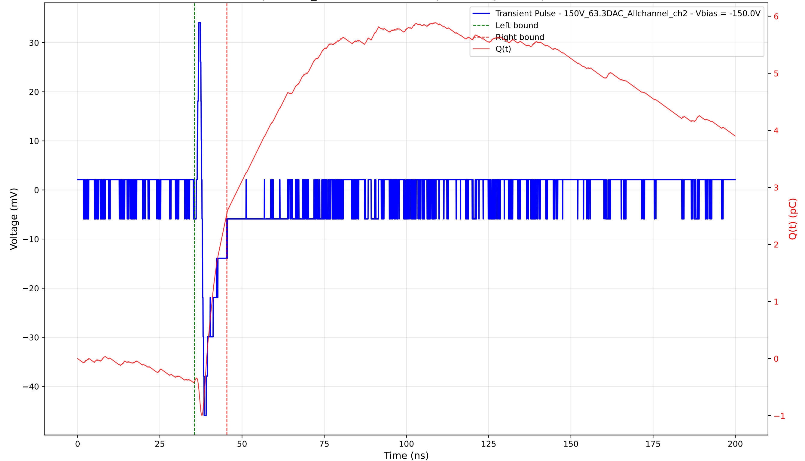
Transient Pulse - Sample: 1cm_42 - Position: 1165.0 \mu\text{m} - Charge: 2.94 pC - Rise Time: 0.65 ns
