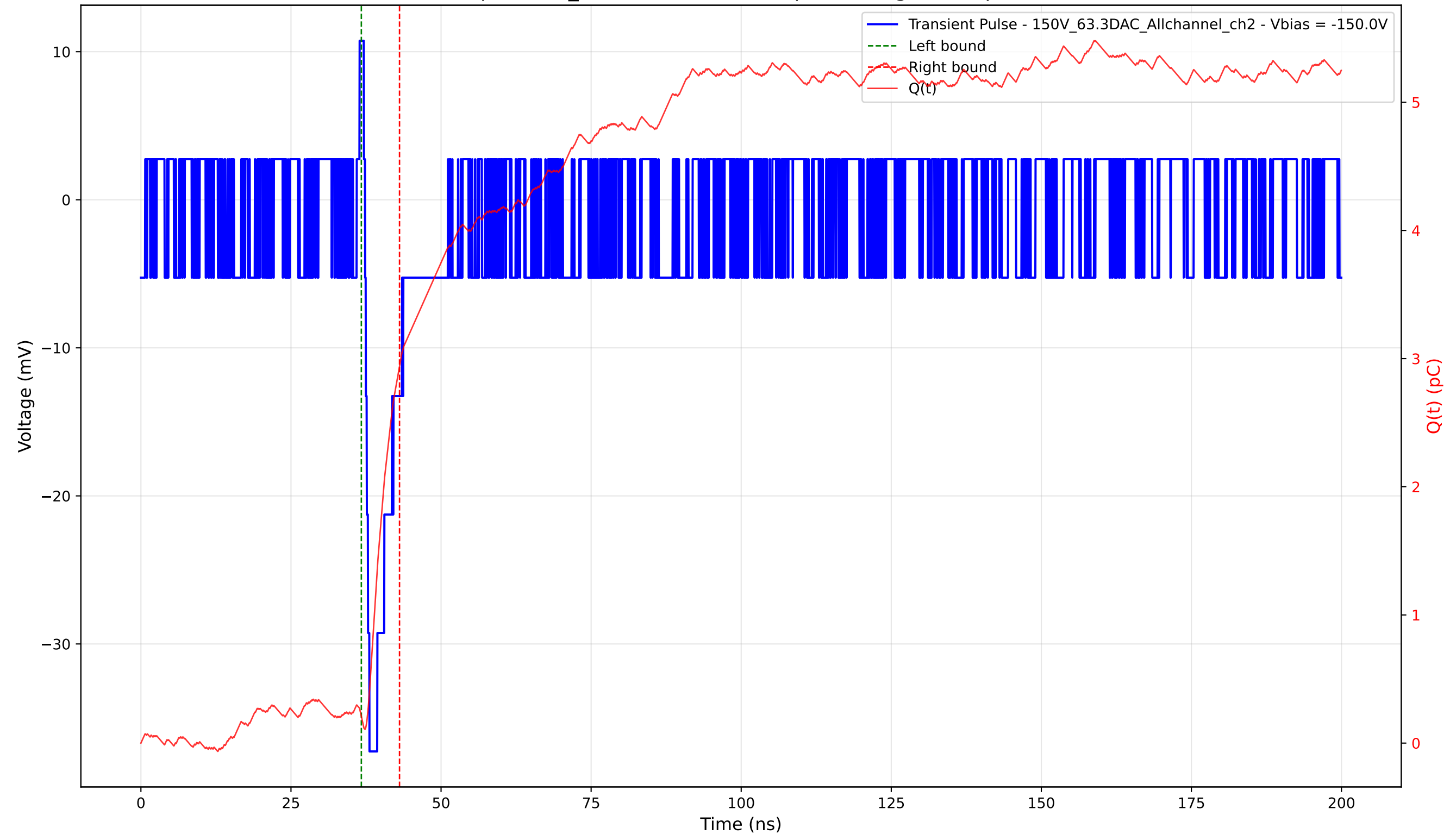
Transient Pulse - Sample: 1cm_42 - Position: 4545.0 \mu\text{m} - Charge: 2.73 pC - Rise Time: 0.74 ns
