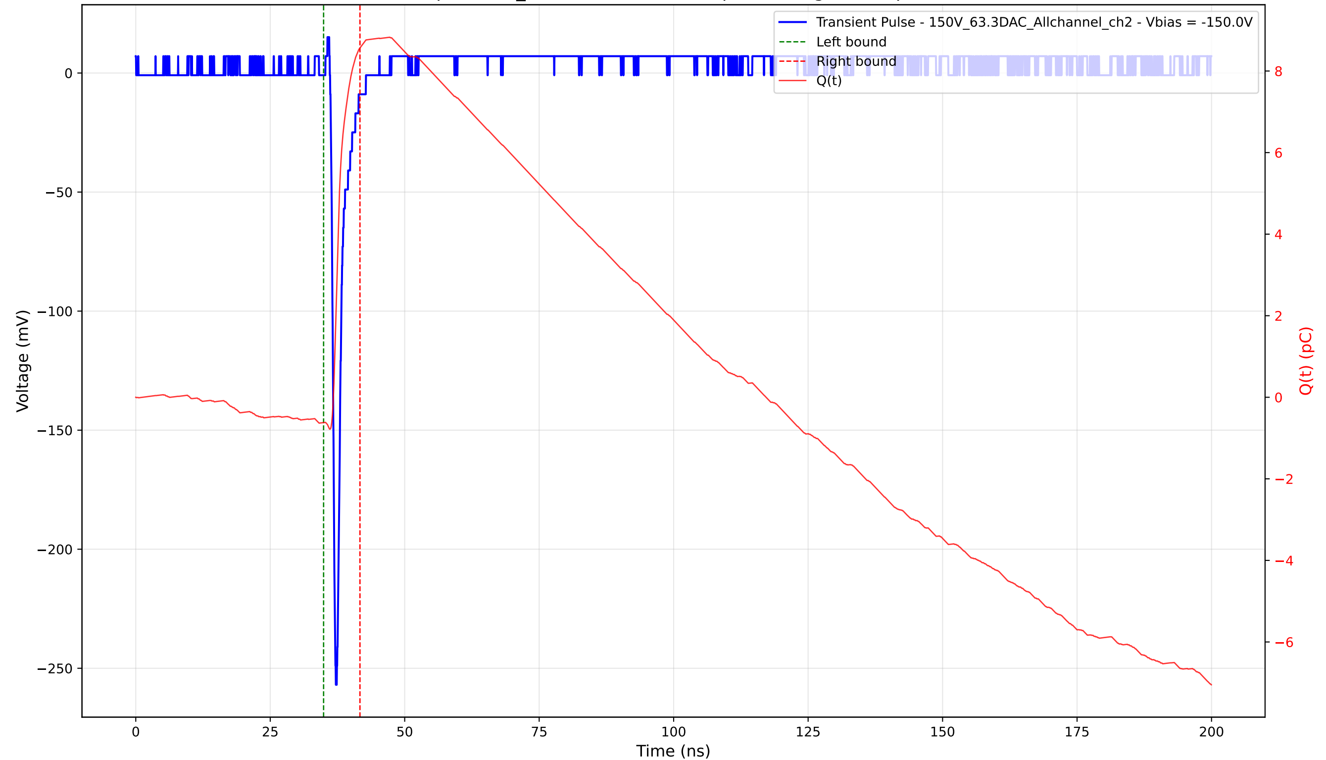
Transient Pulse - Sample: 1cm_42 - Position: 2580.0 \mu\text{m} - Charge: 9.18 pC - Rise Time: 0.75 ns
