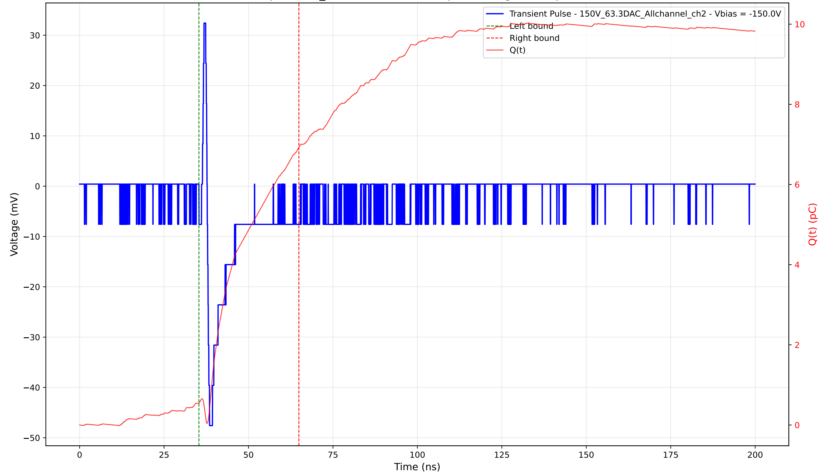
Transient Pulse - Sample: 1cm_42 - Position: 1280.0 \mu\text{m} - Charge: 6.39 pC - Rise Time: 0.70 ns
