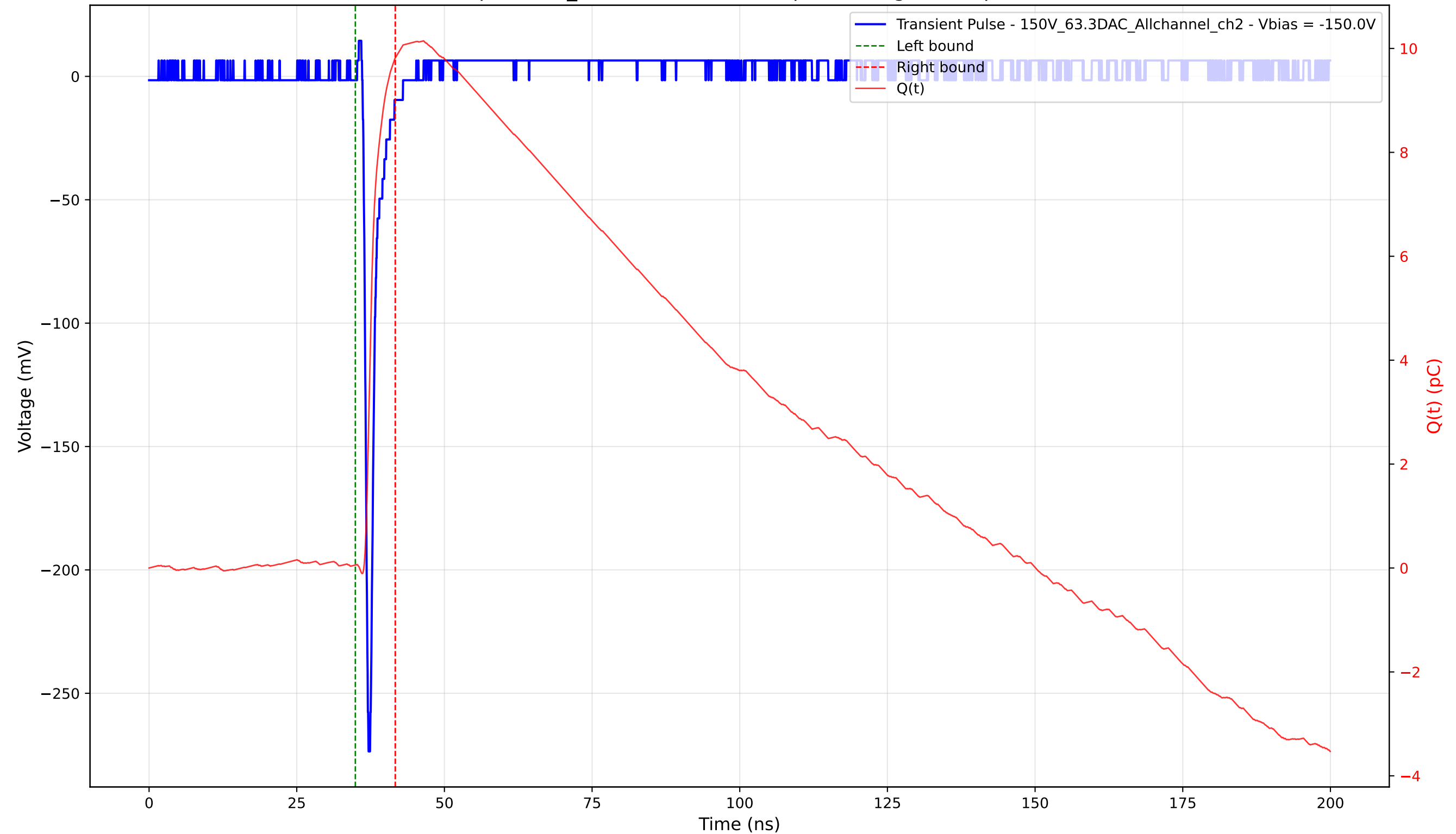
Transient Pulse - Sample: 1cm_42 - Position: 2600.0 \mu\text{m} - Charge: 9.76 pC - Rise Time: 0.76 ns
