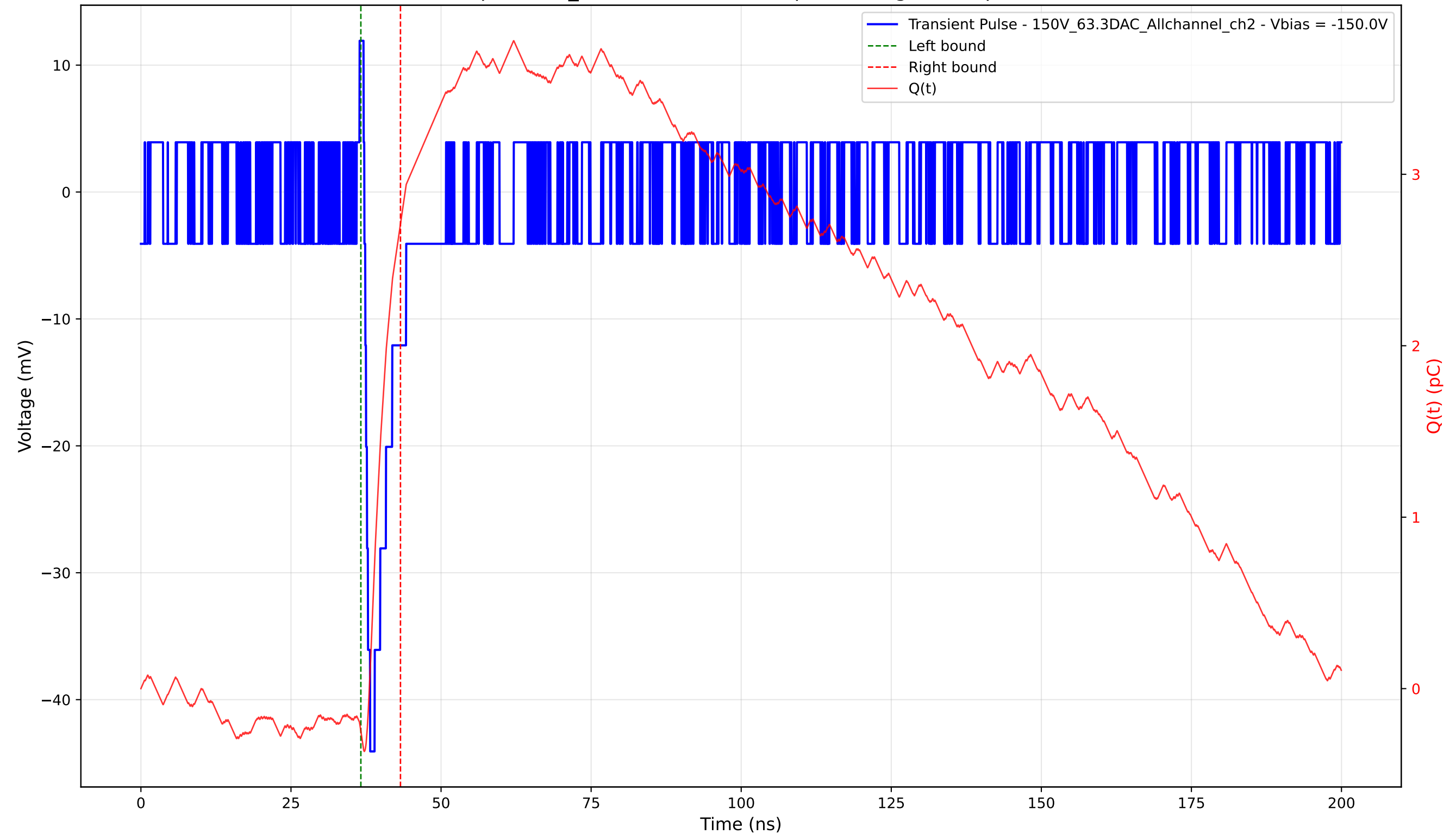
Transient Pulse - Sample: 1cm_42 - Position: 4460.0 \mu\text{m} - Charge: 2.96 pC - Rise Time: 0.84 ns
