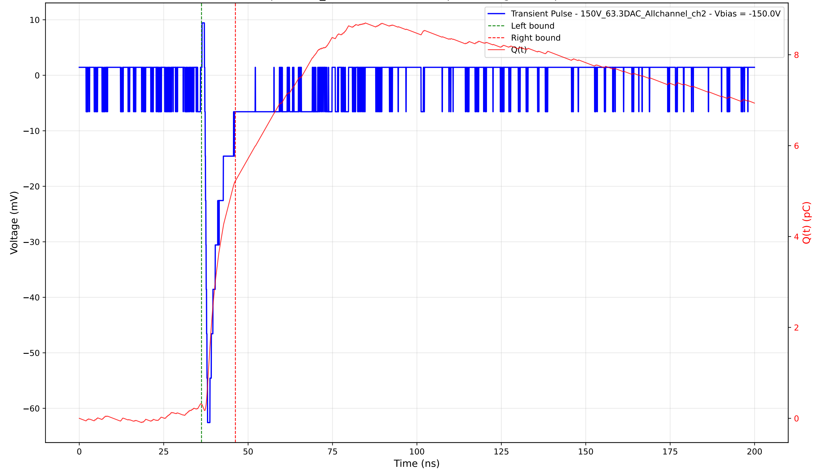
Transient Pulse - Sample: 1cm_42 - Position: 1835.0 \mu\text{m} - Charge: 4.91 pC - Rise Time: 0.80 ns
