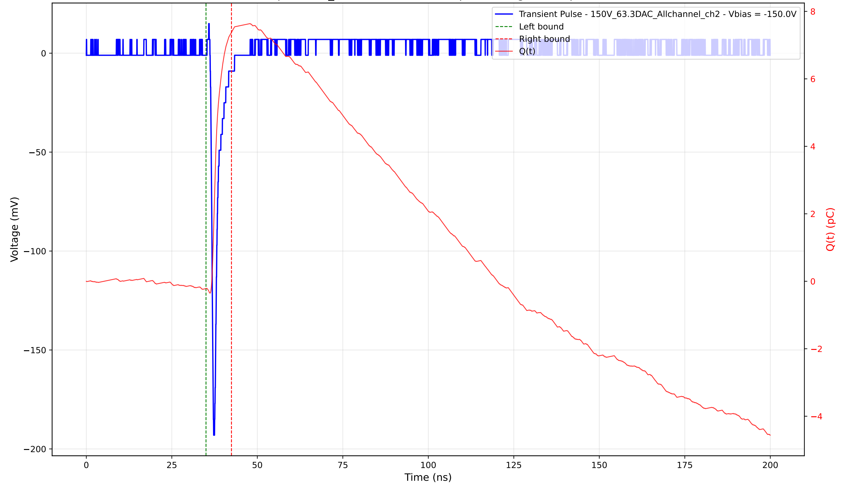
Transient Pulse - Sample: 1cm_42 - Position: 2495.0 \mu\text{m} - Charge: 7.60 pC - Rise Time: 0.73 ns
