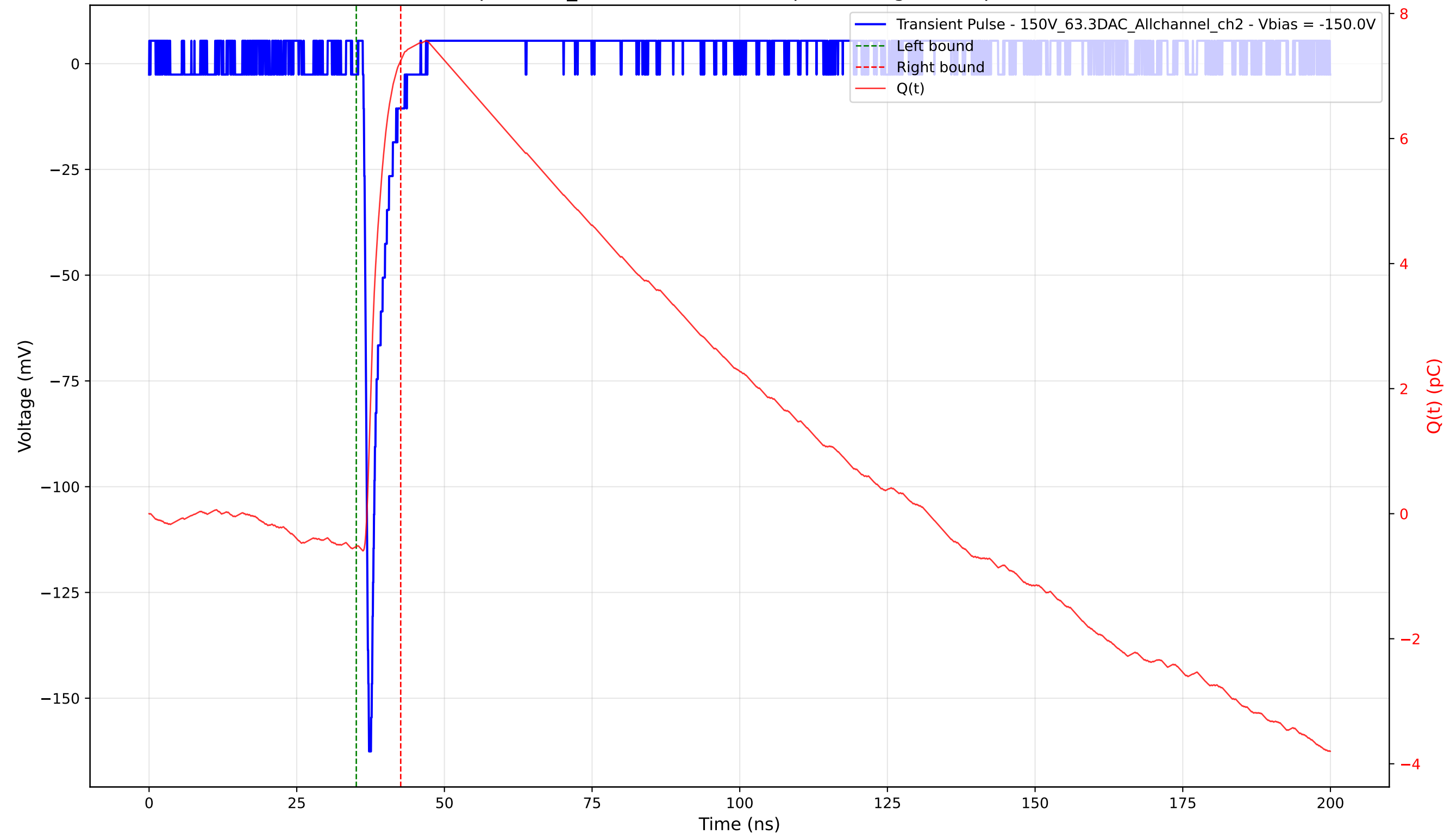
Transient Pulse - Sample: 1cm_42 - Position: 3605.0 \mu\text{m} - Charge: 7.77 pC - Rise Time: 0.73 ns
