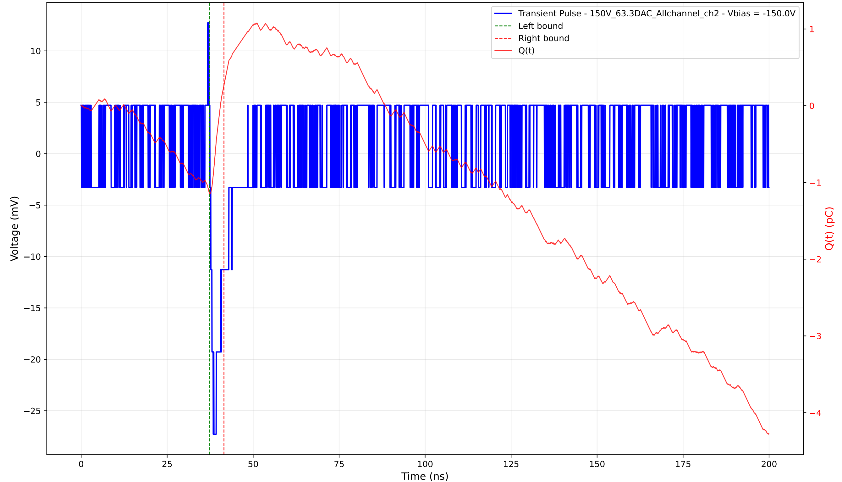
Transient Pulse - Sample: 1cm_42 - Position: 4945.0 \mu\text{m} - Charge: 1.40 pC - Rise Time: 0.00 ns (N/A)
