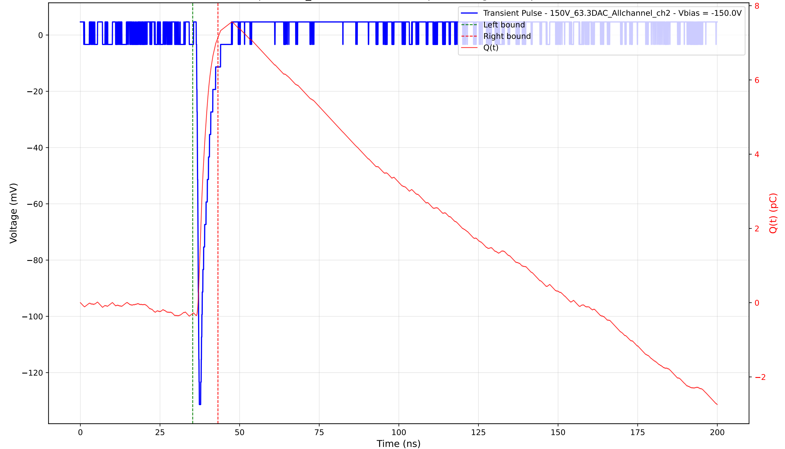
Transient Pulse - Sample: 1cm_42 - Position: 3745.0 \mu\text{m} - Charge: 7.43 pC - Rise Time: 0.75 ns
