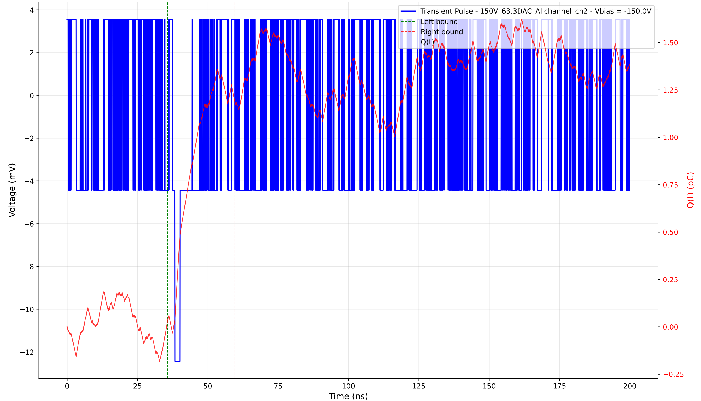
Transient Pulse - Sample: 1cm_42 - Position: 5090.0 \mu\text{m} - Charge: 1.18 pC - Rise Time: 0.00 ns (N/A)
