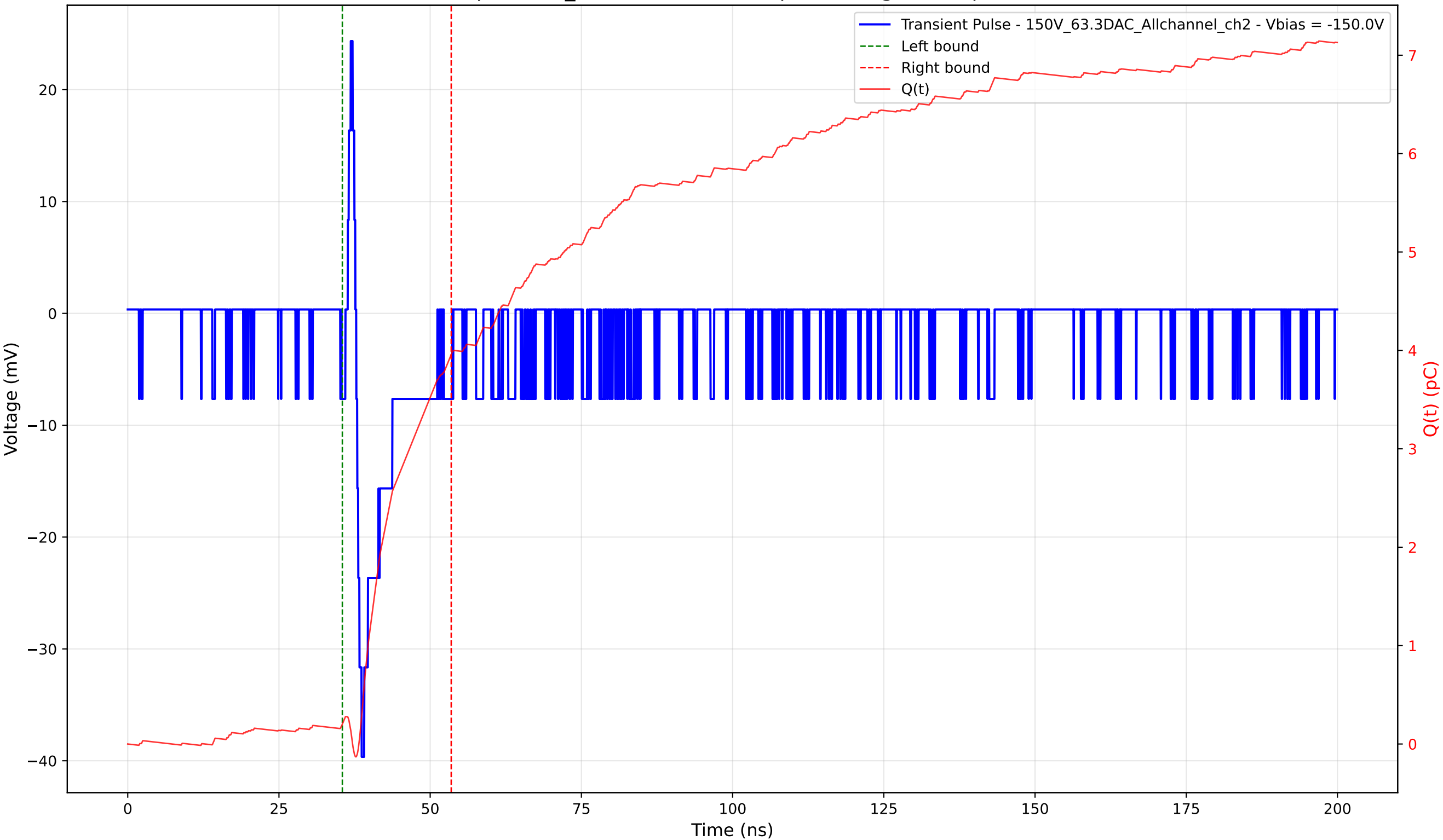
Transient Pulse - Sample: 1cm_42 - Position: 540.0 \mu\text{m} - Charge: 3.76 pC - Rise Time: 0.90 ns
