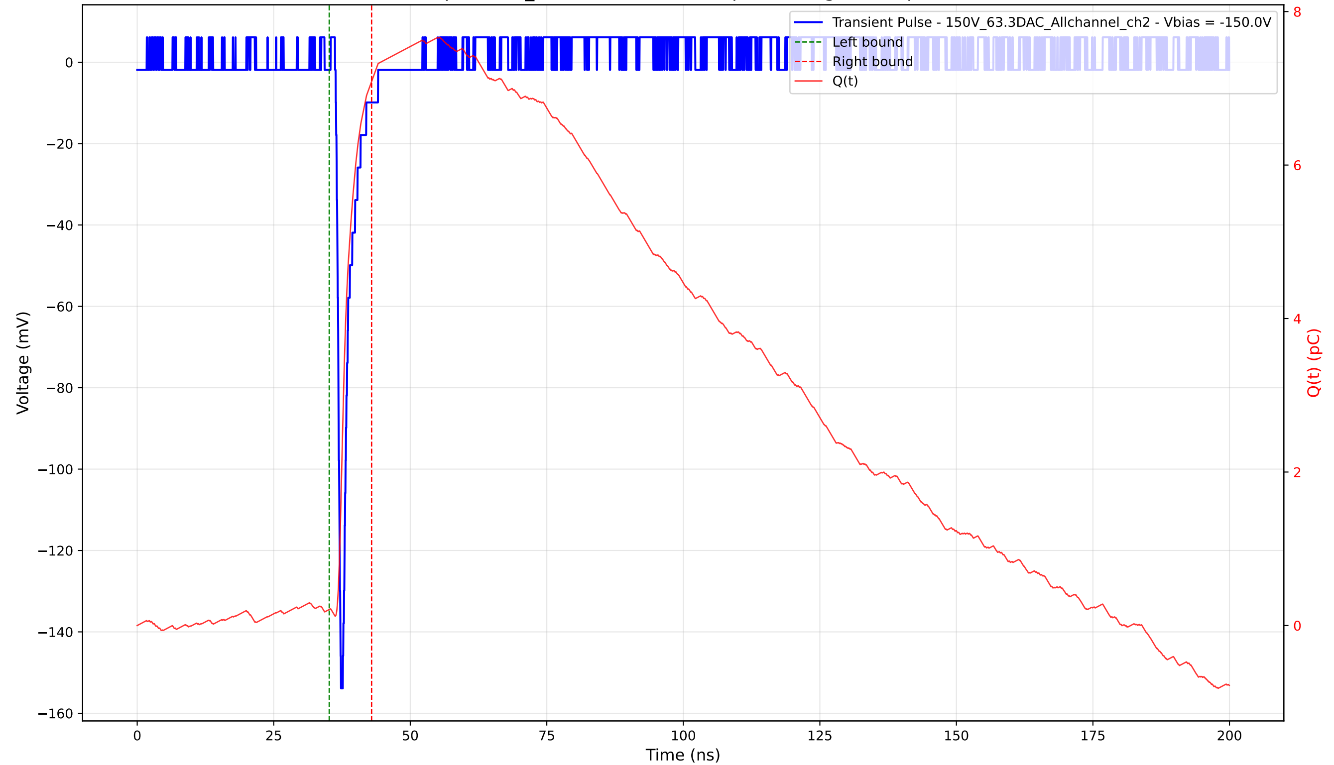
Transient Pulse - Sample: 1cm_42 - Position: 2400.0 \mu\text{m} - Charge: 6.88 pC - Rise Time: 0.81 ns
