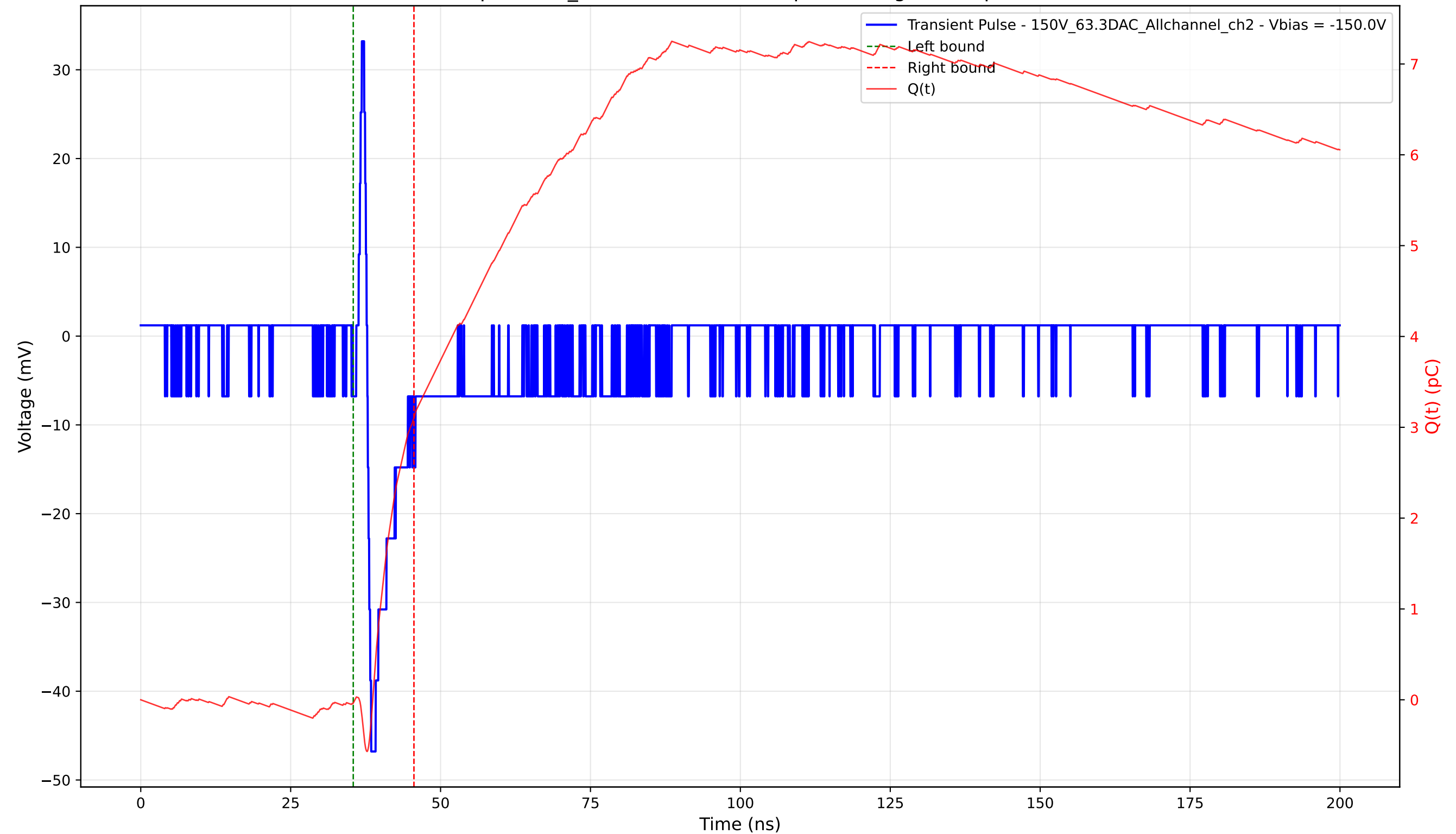
Transient Pulse - Sample: 1cm_42 - Position: 1330.0 \mu\text{m} - Charge: 3.13 pC - Rise Time: 0.66 ns
