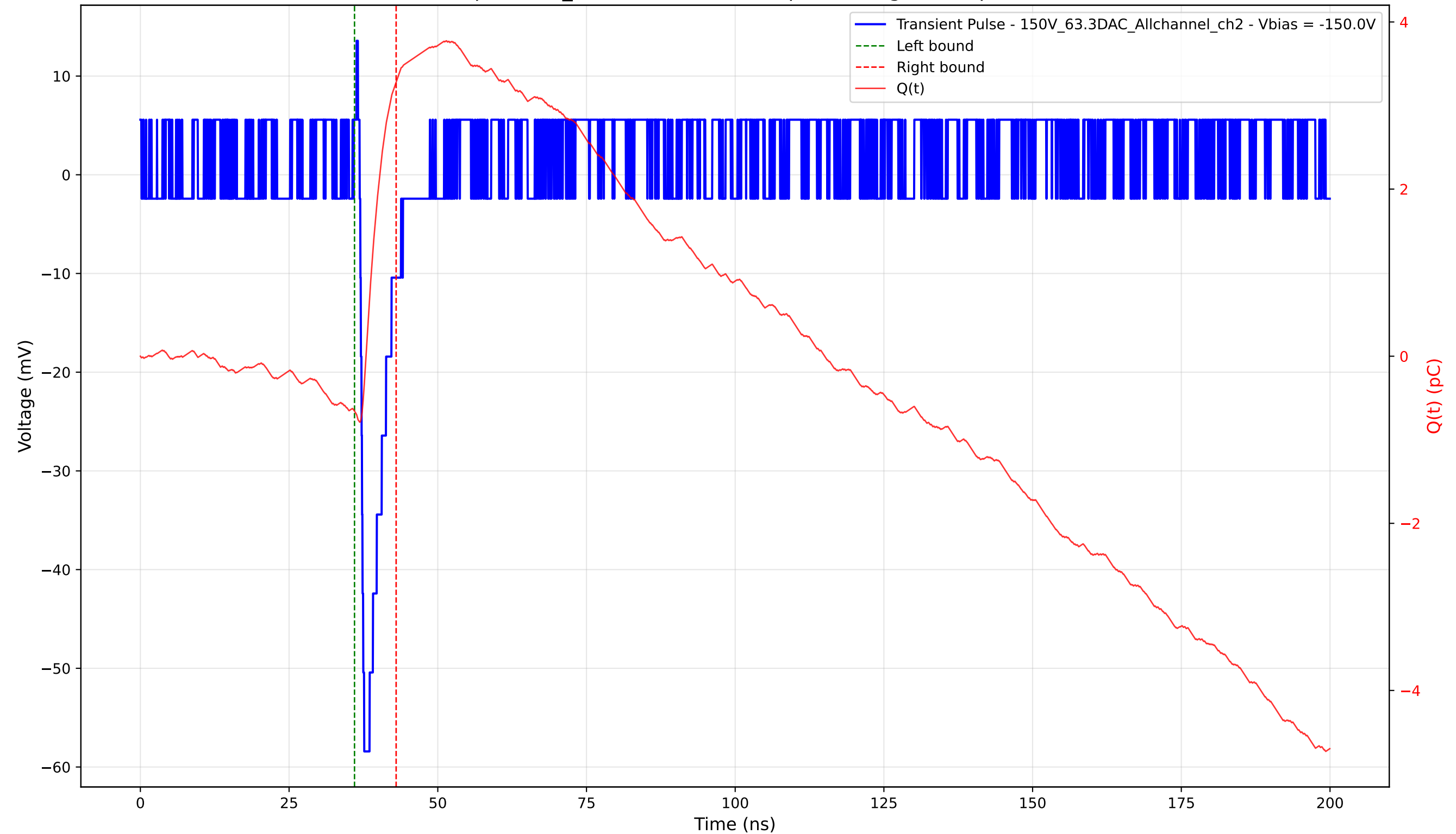
Transient Pulse - Sample: 1cm_42 - Position: 4075.0 \mu\text{m} - Charge: 3.94 pC - Rise Time: 0.66 ns
