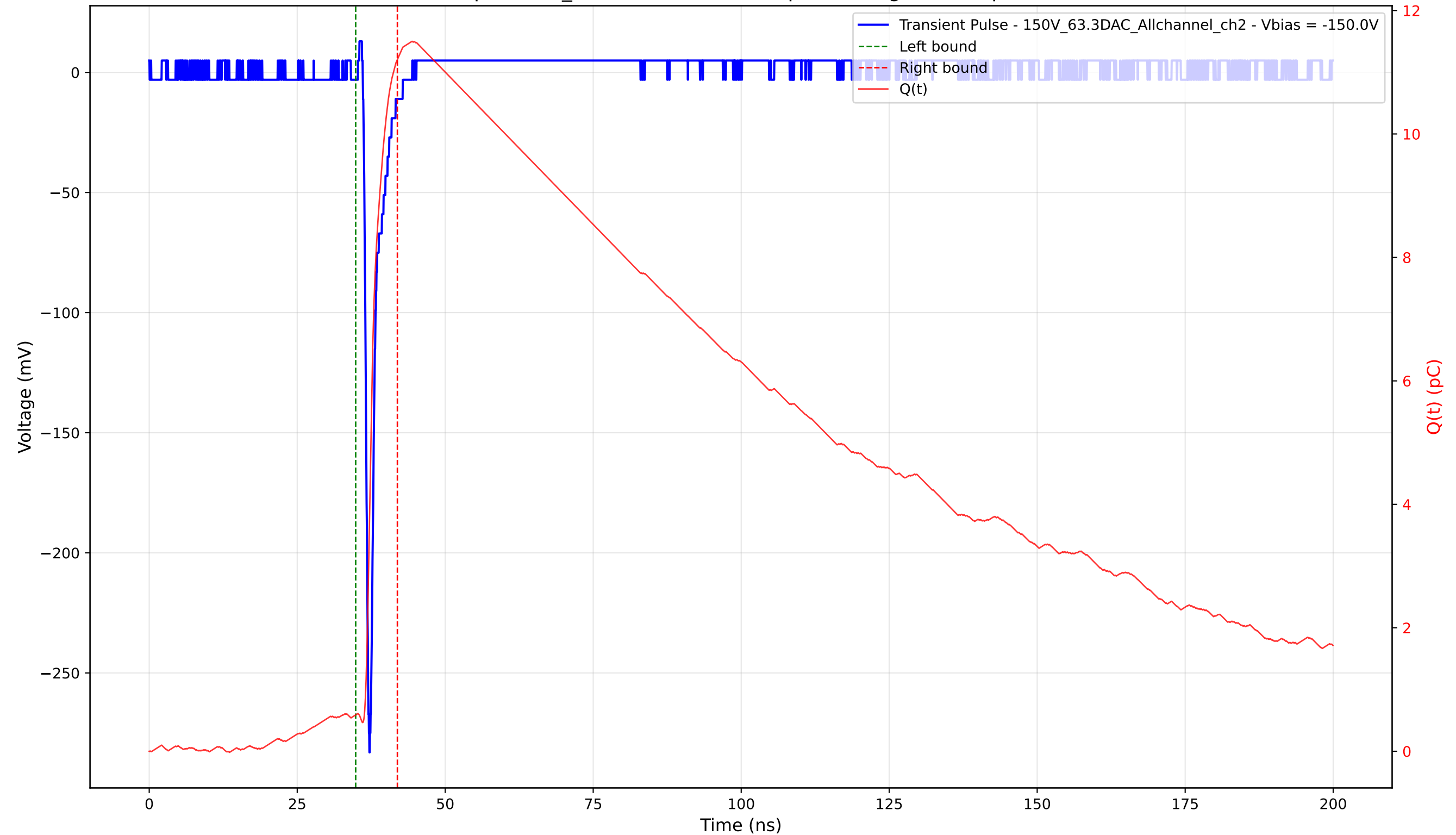
Transient Pulse - Sample: 1cm_42 - Position: 3440.0 \mu\text{m} - Charge: 10.62 pC - Rise Time: 0.73 ns
