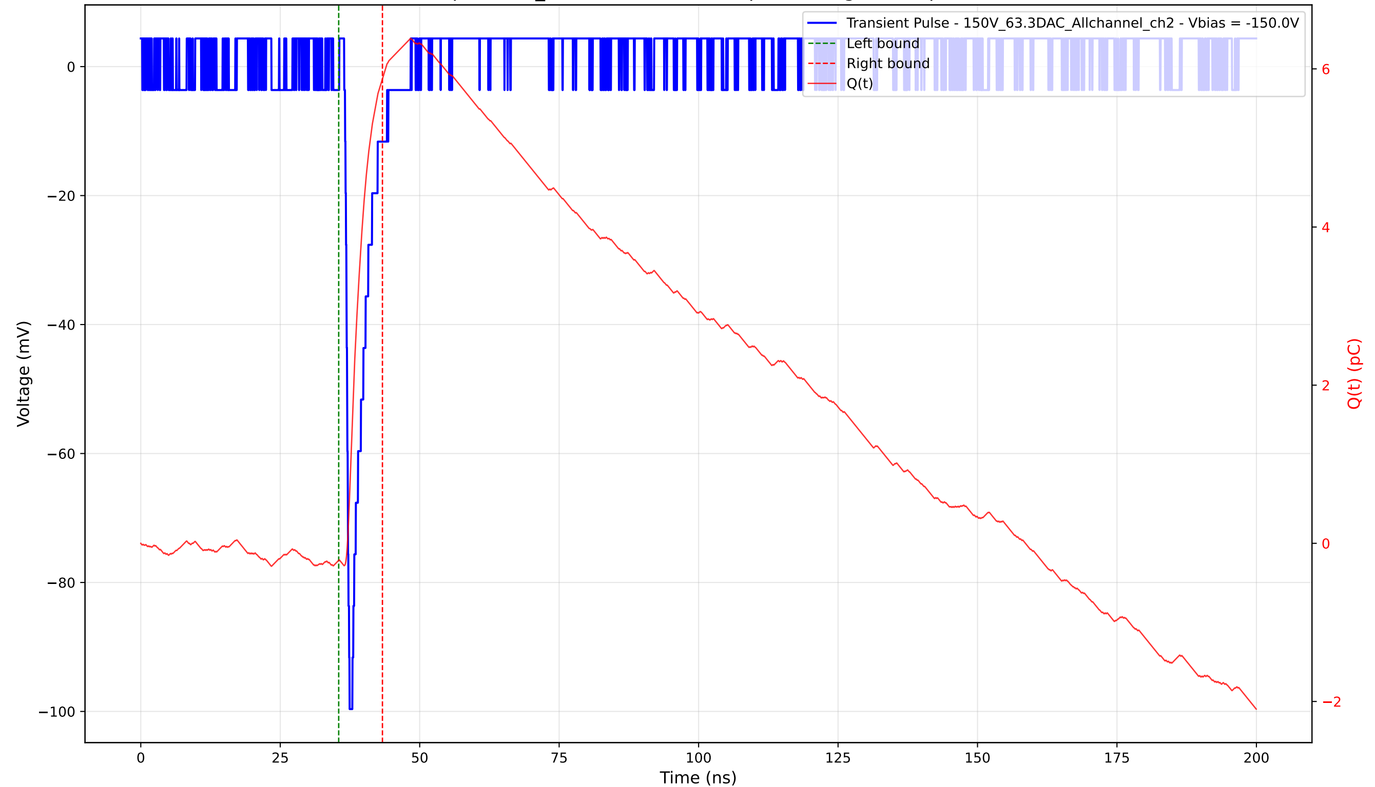
Transient Pulse - Sample: 1cm_42 - Position: 3895.0 \mu\text{m} - Charge: 6.09 pC - Rise Time: 0.73 ns
