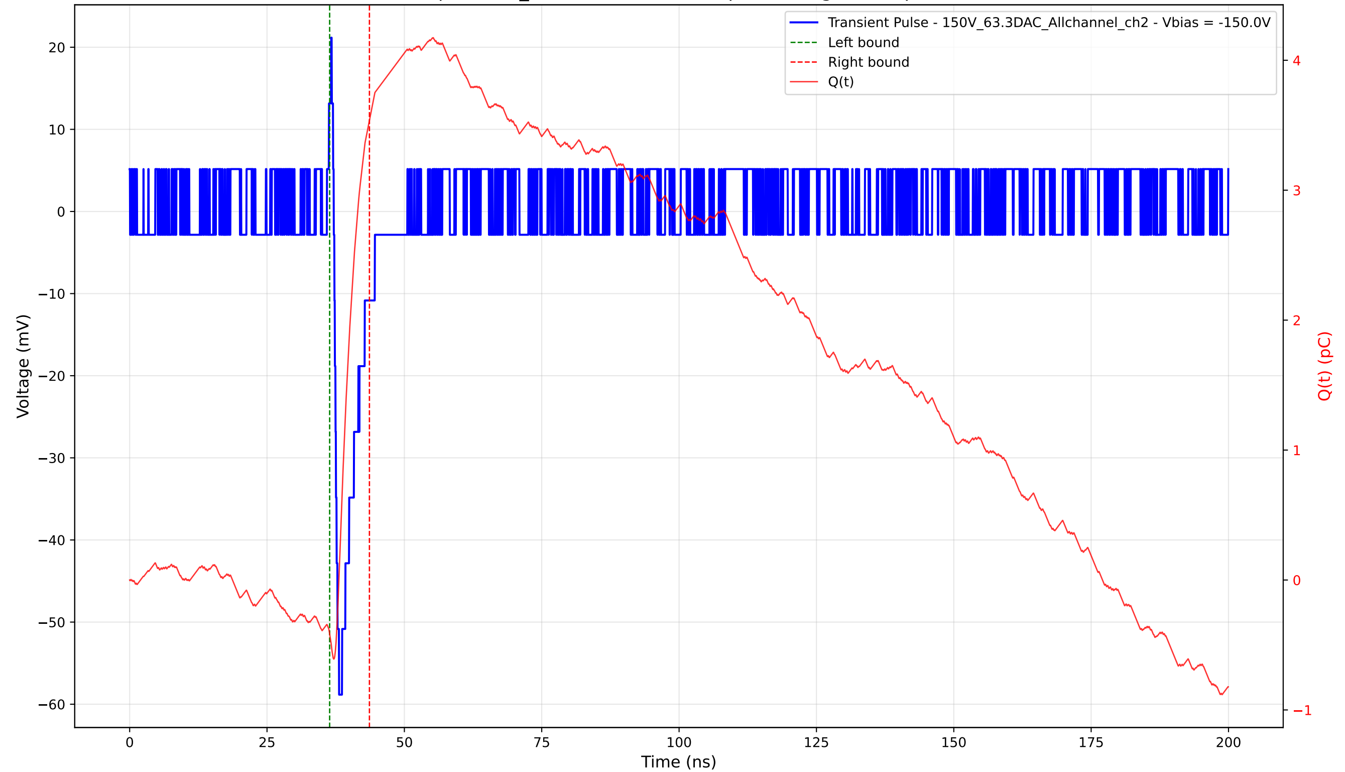
Transient Pulse - Sample: 1cm_42 - Position: 4305.0 \mu\text{m} - Charge: 3.95 pC - Rise Time: 0.86 ns
