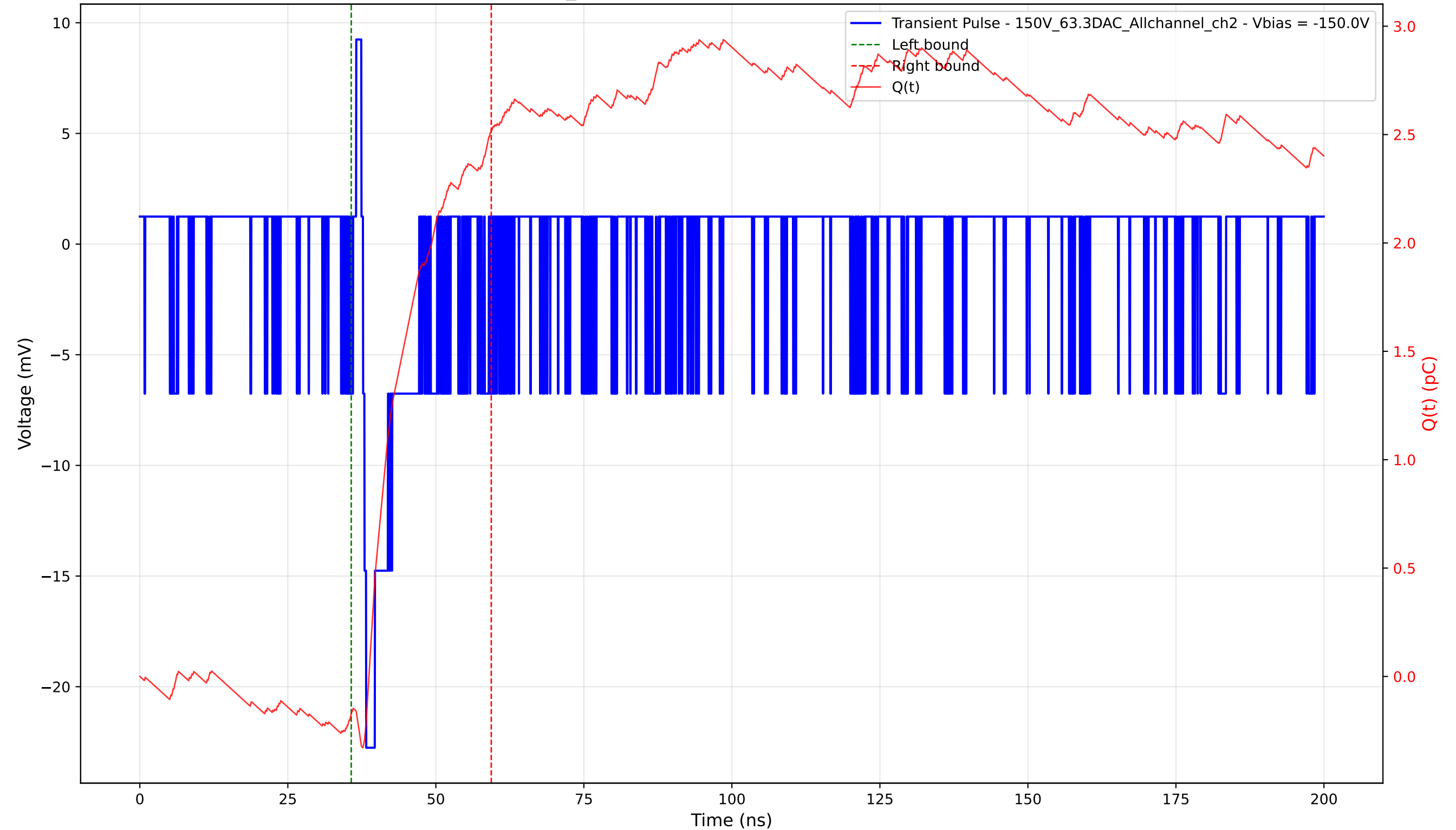
Transient Pulse - Sample: 1cm_42 - Position: 310.0 \mu\text{m} - Charge: 2.68 pC - Rise Time: 0.55 ns
