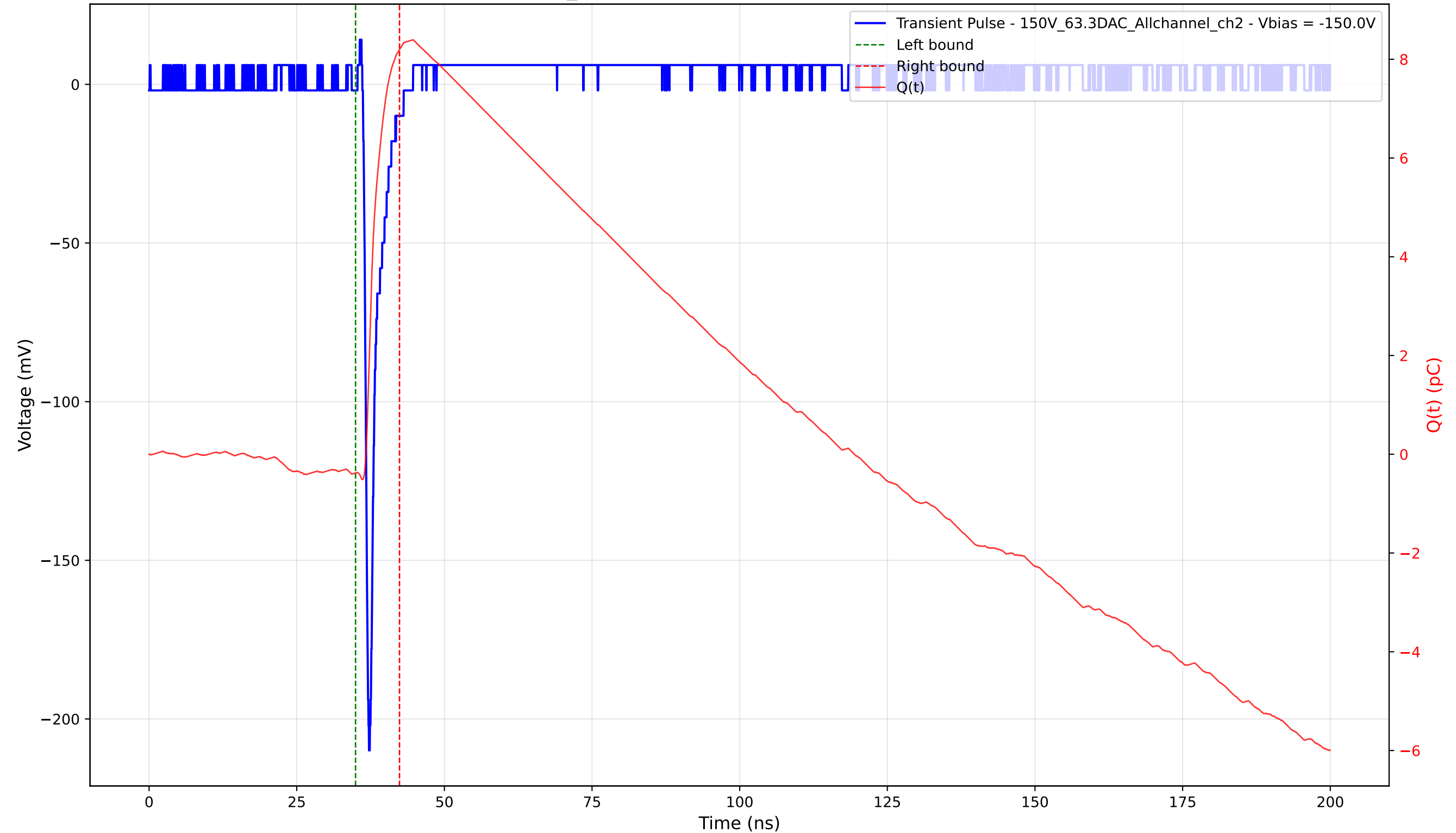
Transient Pulse - Sample: 1cm_42 - Position: 3520.0 \mu\text{m} - Charge: 8.58 pC - Rise Time: 0.74 ns
