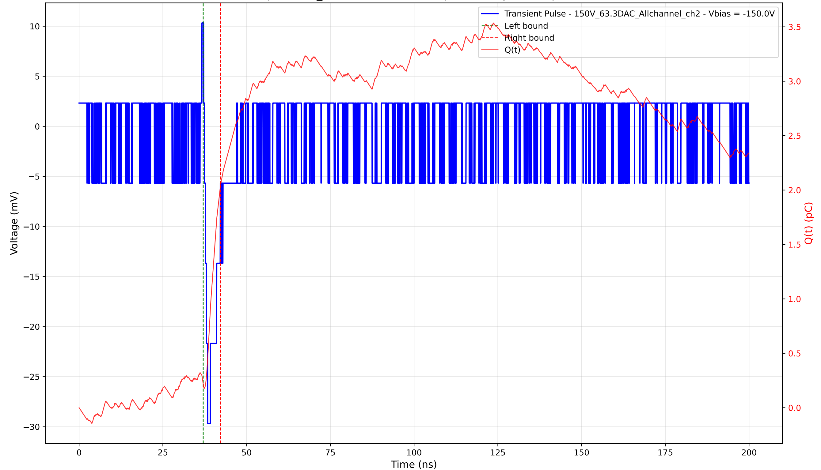
Transient Pulse - Sample: 1cm_42 - Position: 4950.0 \mu\text{m} - Charge: 1.81 pC - Rise Time: 0.95 ns
