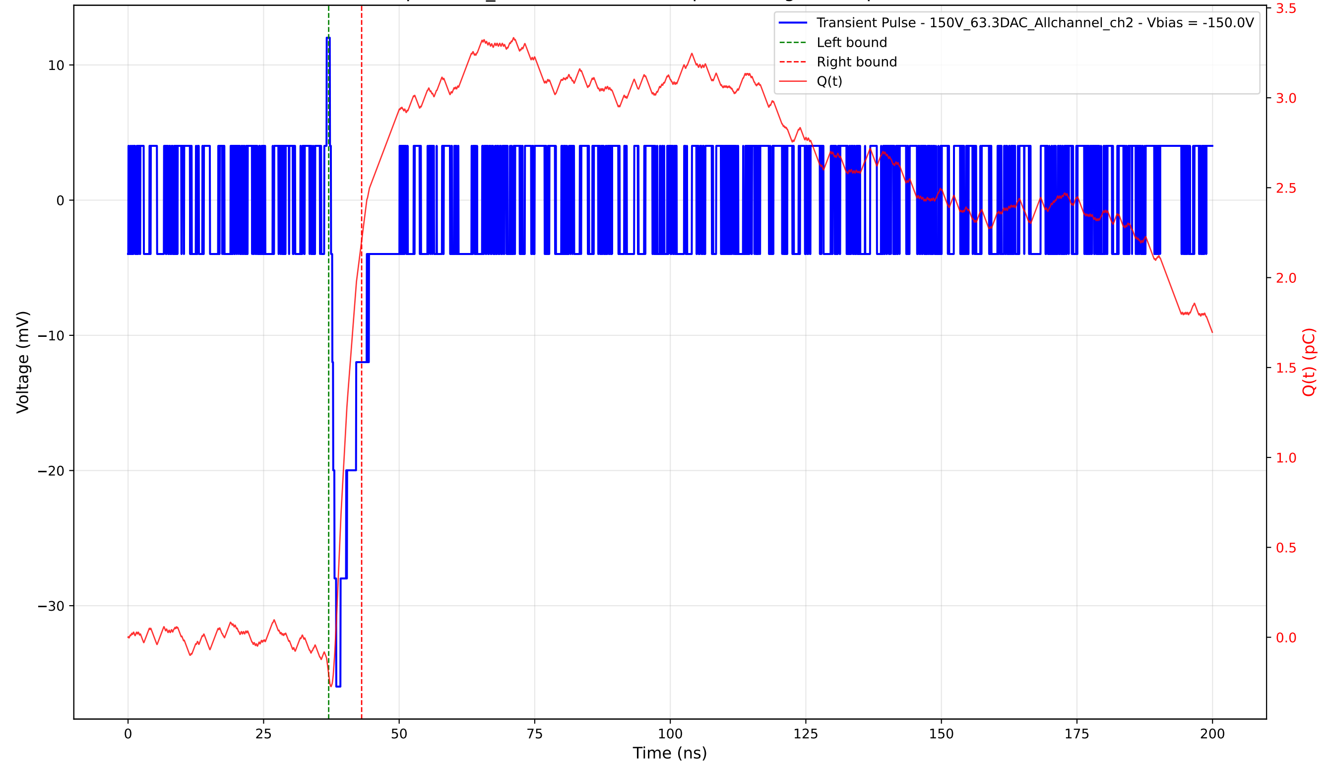
Transient Pulse - Sample: 1cm_42 - Position: 4845.0 \mu\text{m} - Charge: 2.41 pC - Rise Time: 0.00 ns (N/A)
