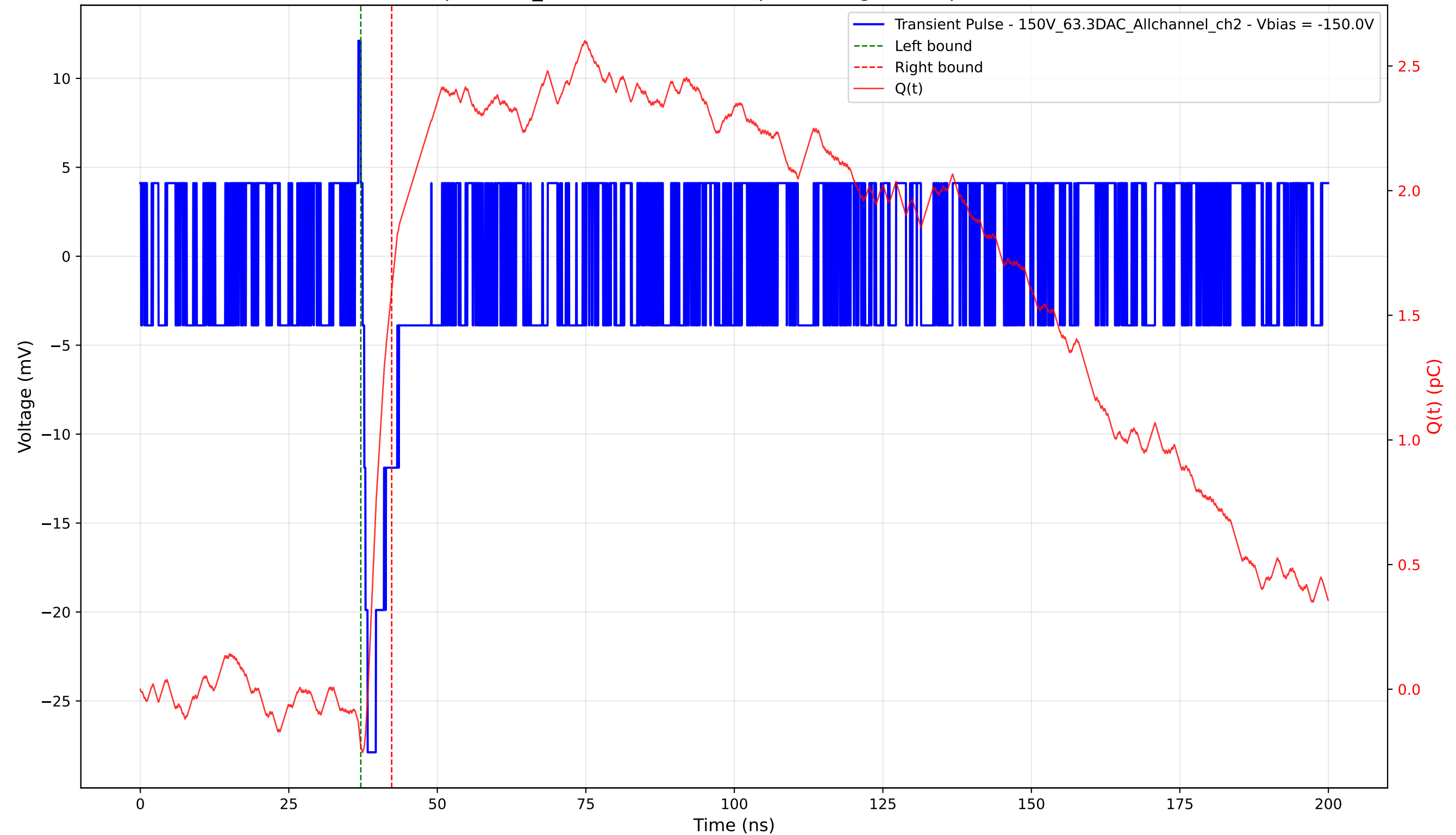
Transient Pulse - Sample: 1cm_42 - Position: 4920.0 \mu\text{m} - Charge: 1.83 pC - Rise Time: 0.00 ns (N/A)
