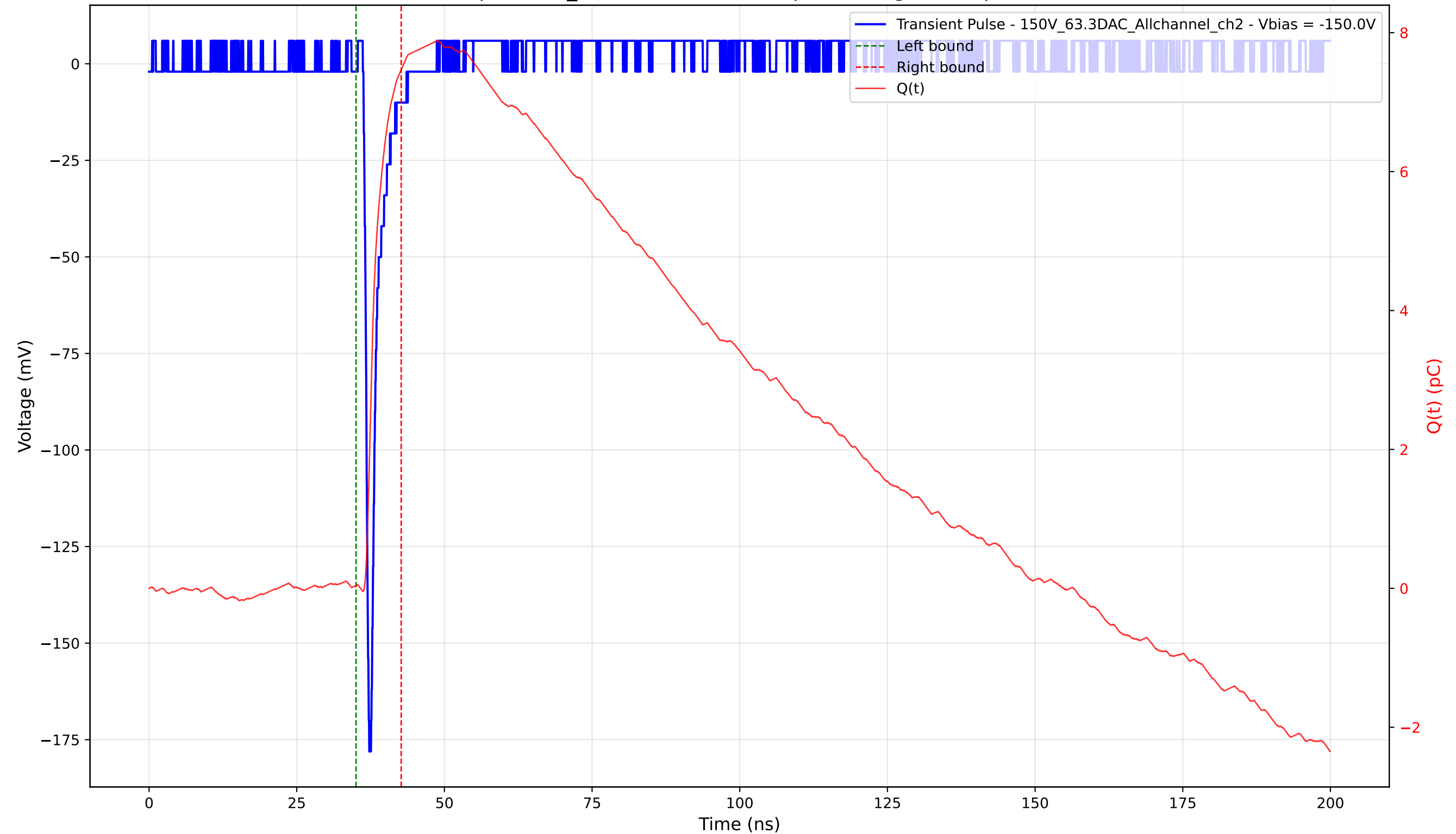
Transient Pulse - Sample: 1cm_42 - Position: 2465.0 \mu\text{m} - Charge: 7.43 pC - Rise Time: 0.79 ns
