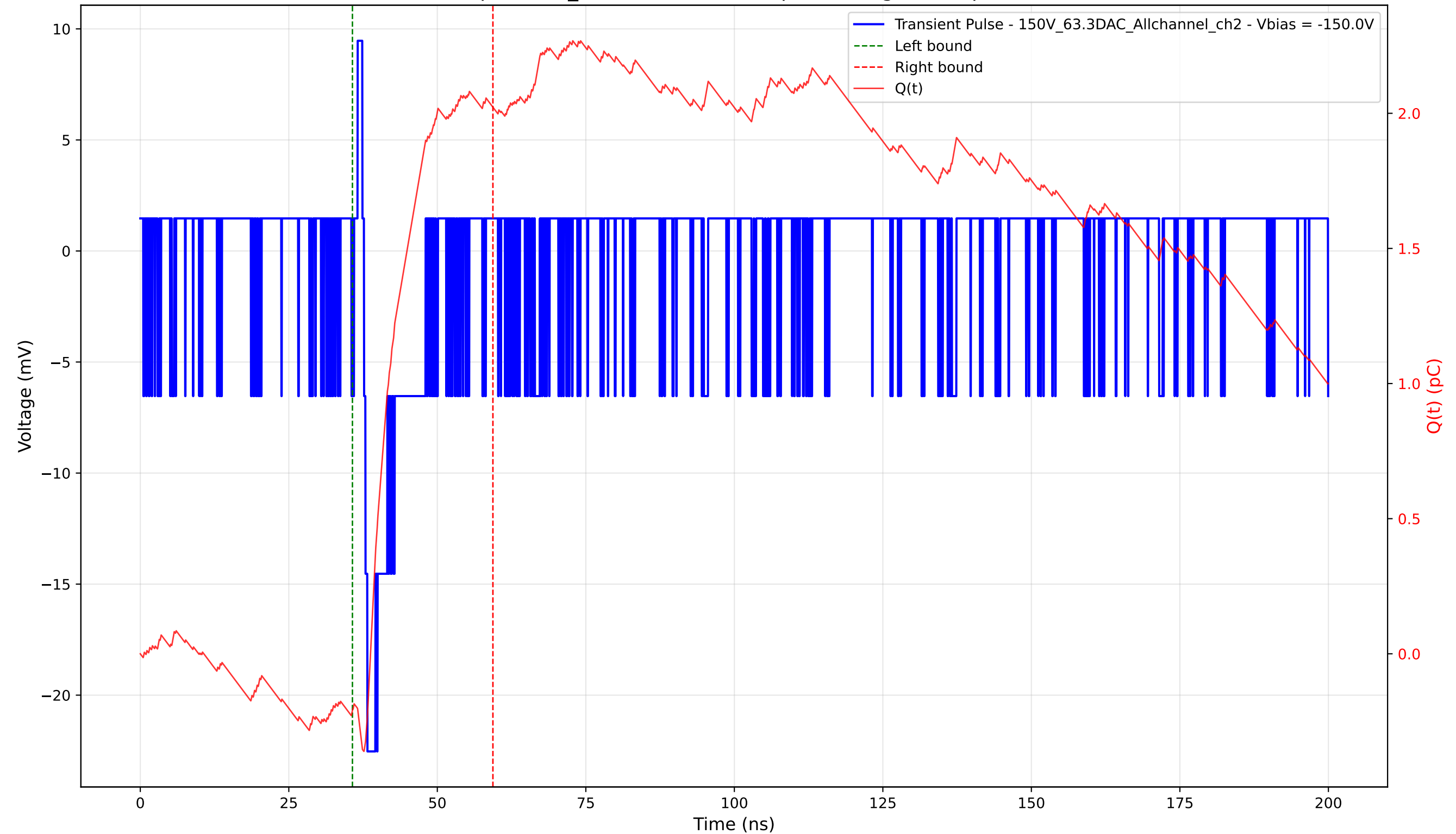
Transient Pulse - Sample: 1cm_42 - Position: 275.0 \mu\text{m} - Charge: 2.23 pC - Rise Time: 0.59 ns
