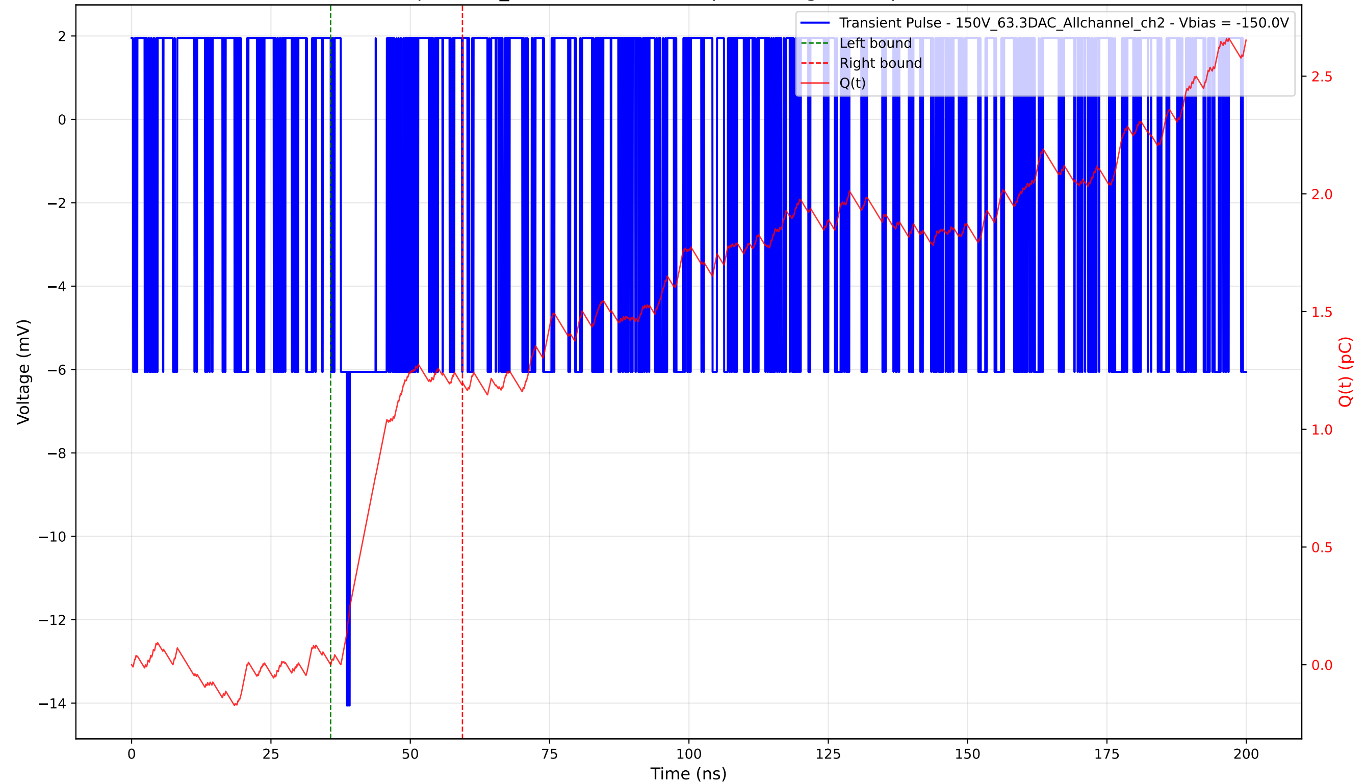
Transient Pulse - Sample: 1cm_42 - Position: 5130.0 \mu\text{m} - Charge: 1.19 pC - Rise Time: 0.00 ns (N/A)
