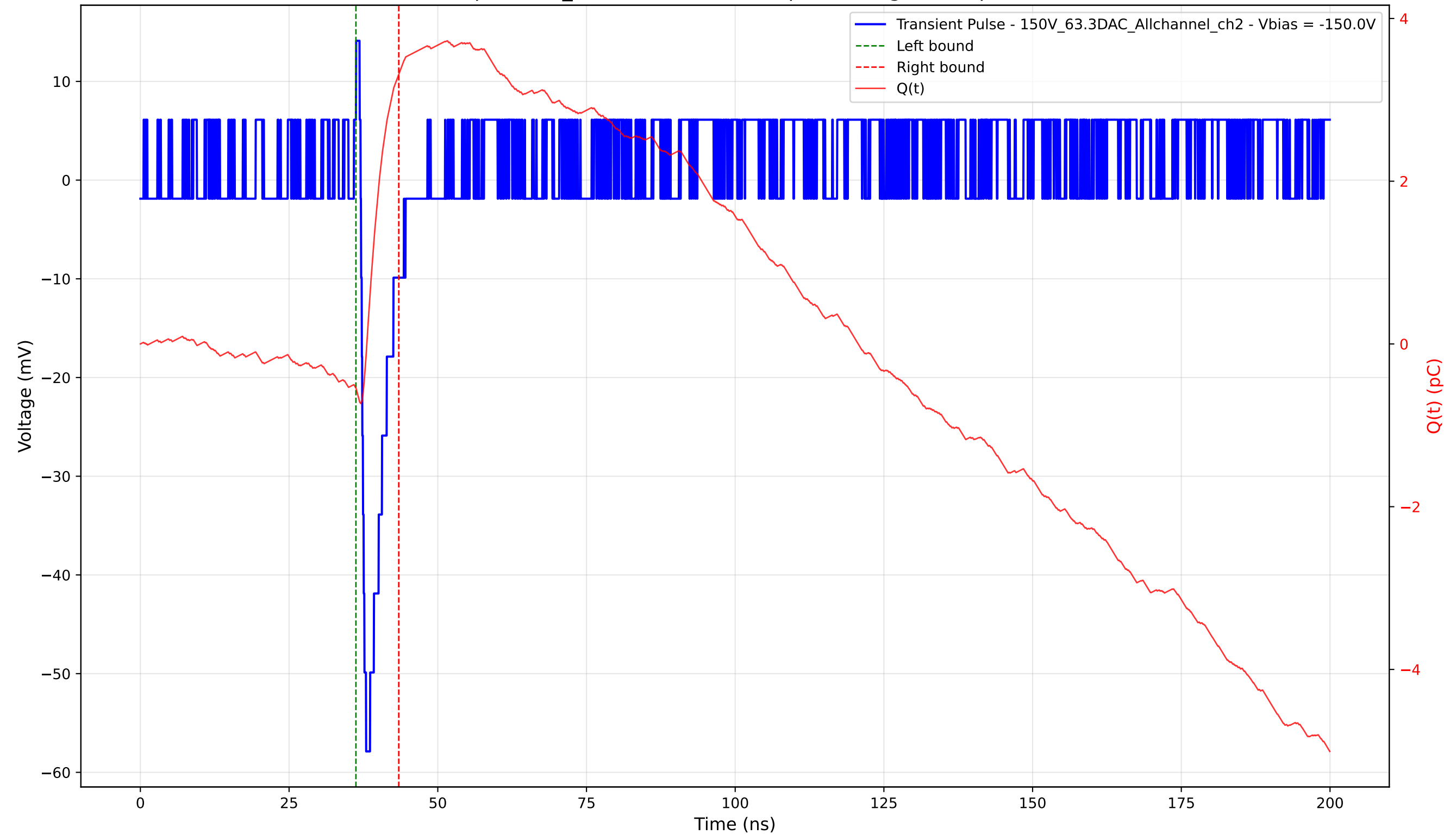
Transient Pulse - Sample: 1cm_42 - Position: 4175.0 \mu\text{m} - Charge: 3.85 pC - Rise Time: 0.86 ns
