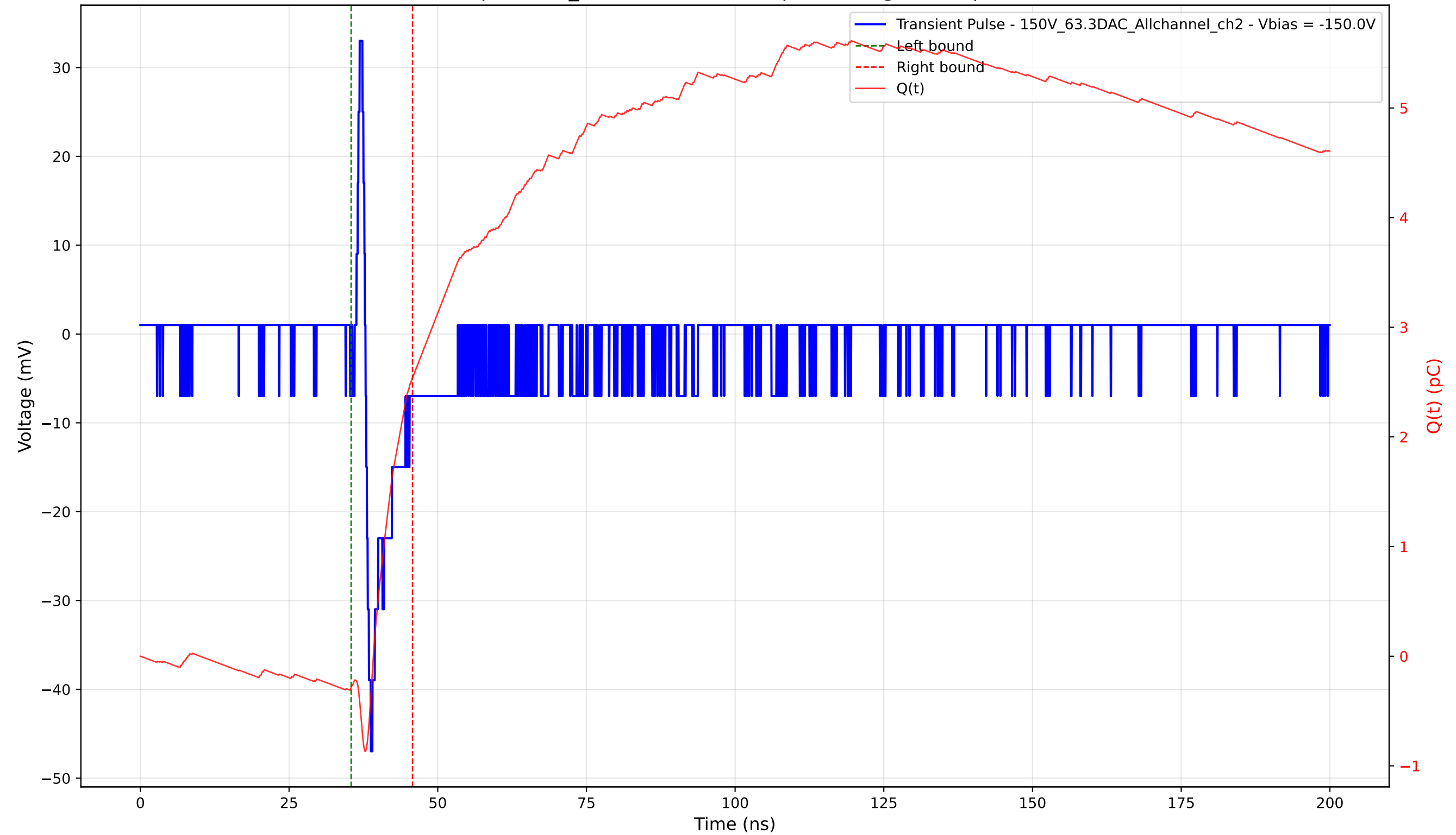
Transient Pulse - Sample: 1cm_42 - Position: 700.0 \mu\text{m} - Charge: 2.82 pC - Rise Time: 0.90 ns
