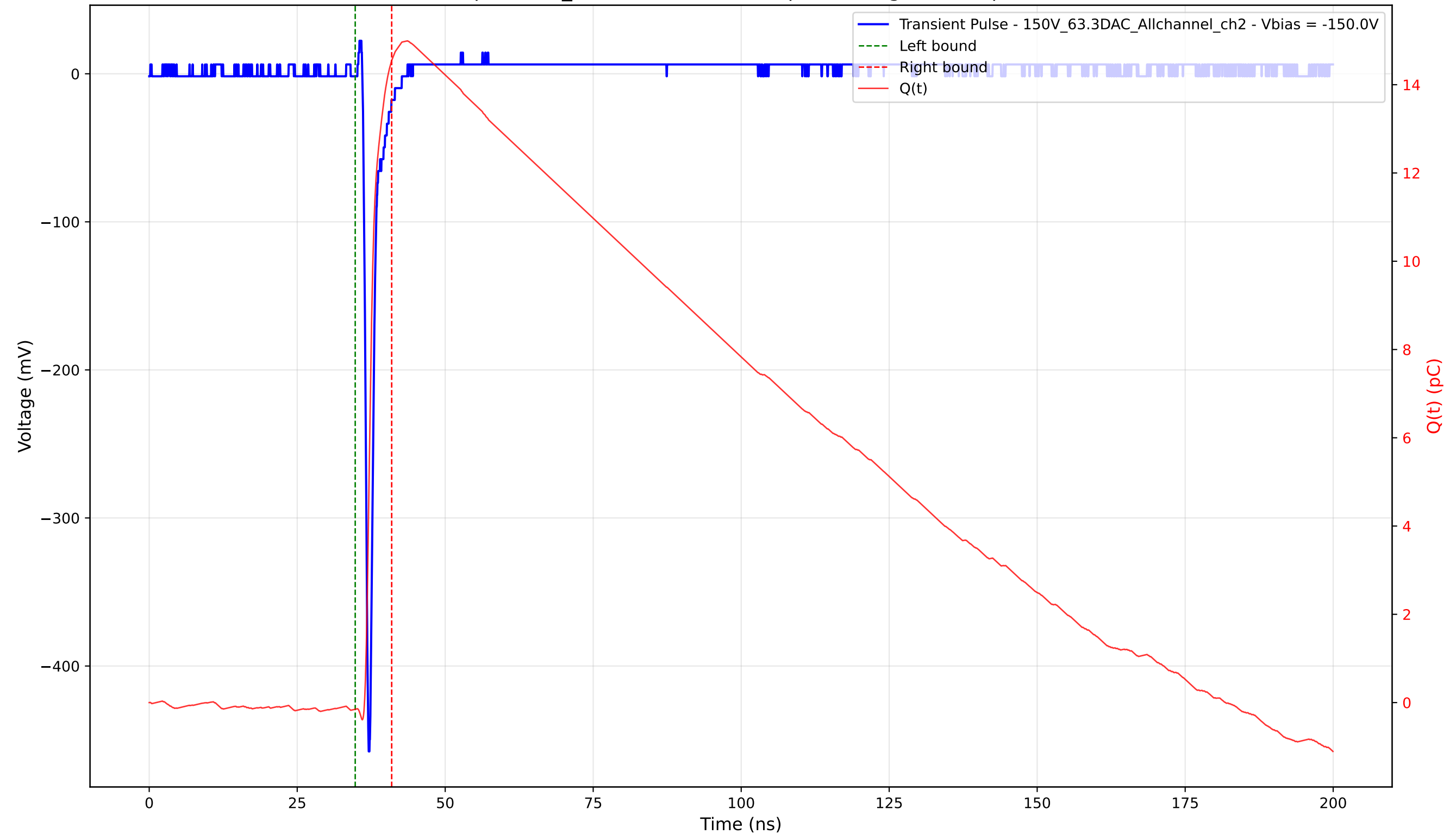
Transient Pulse - Sample: 1cm_42 - Position: 2790.0 \mu\text{m} - Charge: 14.70 pC - Rise Time: 0.73 ns
