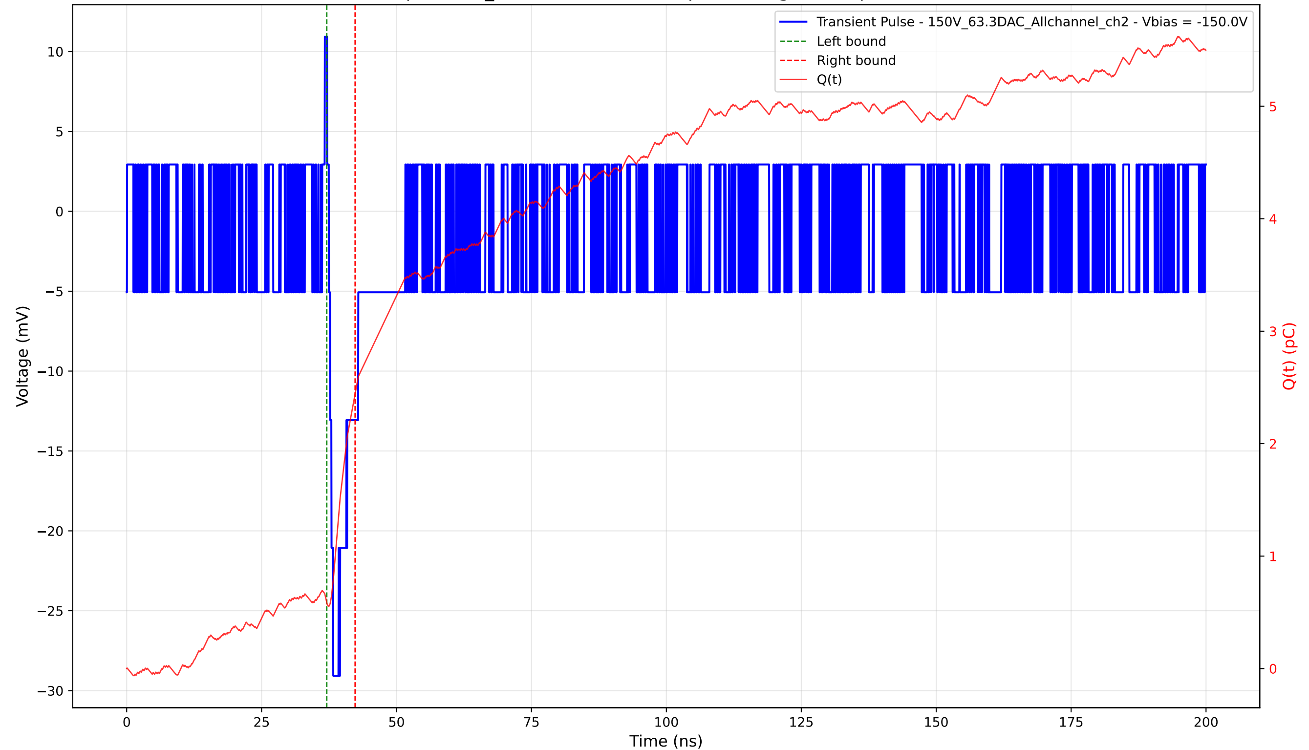
Transient Pulse - Sample: 1cm_42 - Position: 4930.0 \mu\text{m} - Charge: 1.86 pC - Rise Time: 0.00 ns (N/A)
