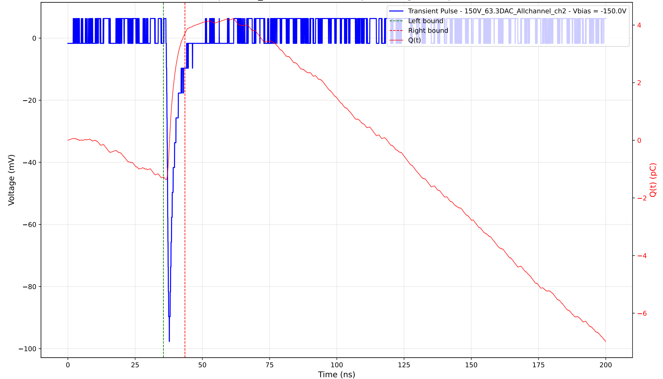
Transient Pulse - Sample: 1cm_42 - Position: 2115.0 \mu\text{m} - Charge: 4.98 pC - Rise Time: 0.76 ns
