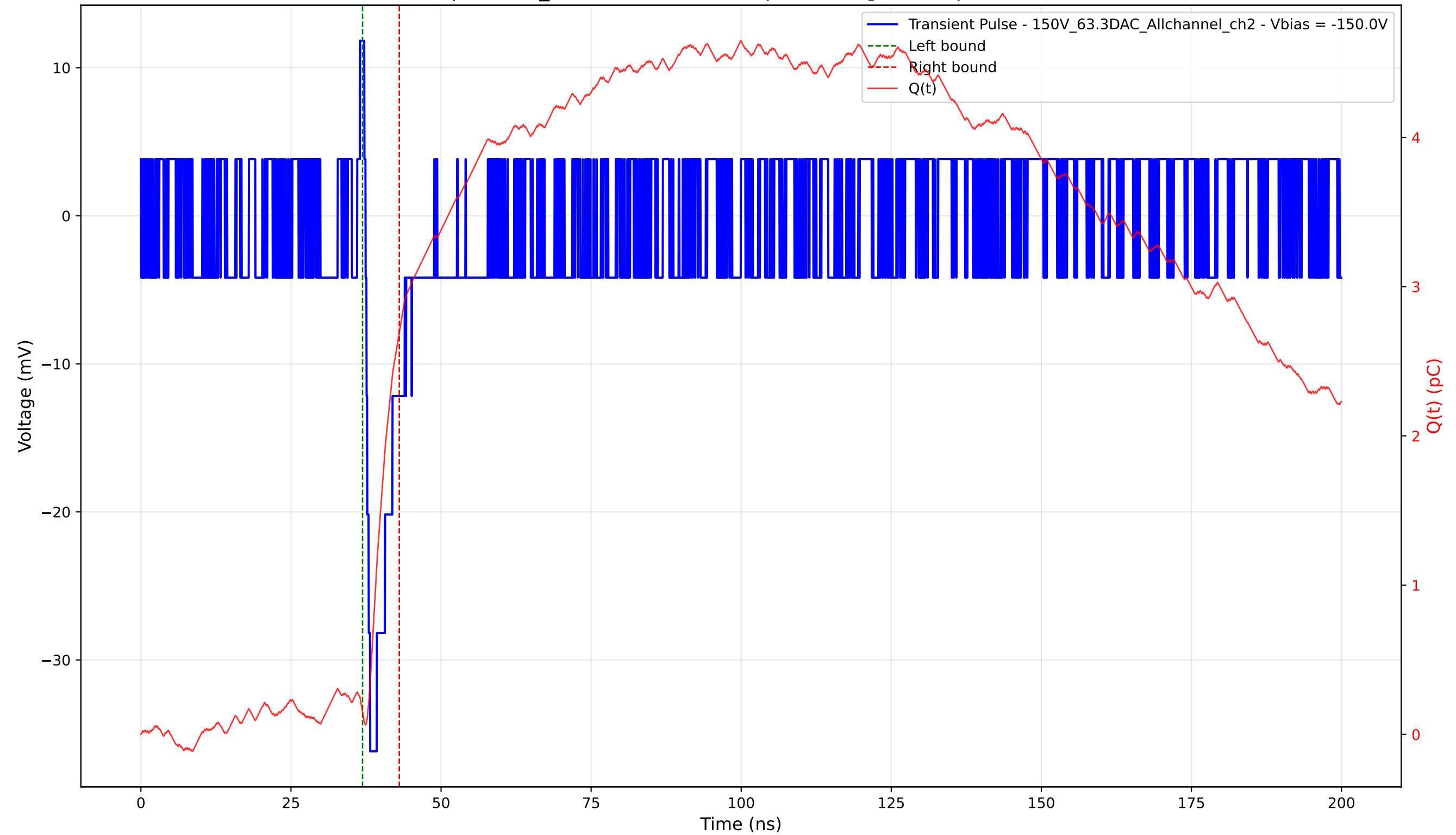
Transient Pulse - Sample: 1cm_42 - Position: 4675.0 \mu\text{m} - Charge: 2.54 pC - Rise Time: 0.00 ns (N/A)
