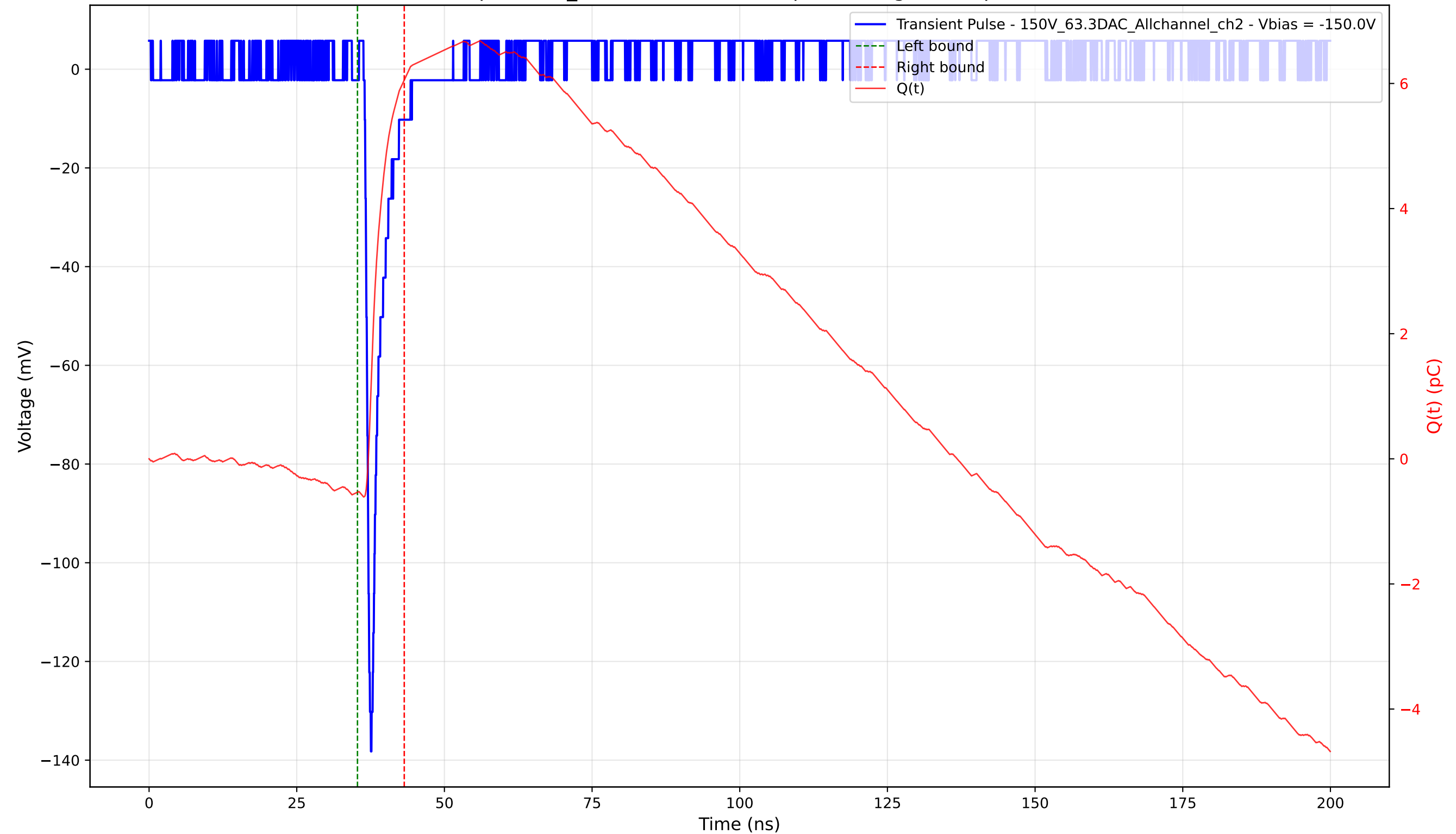
Transient Pulse - Sample: 1cm_42 - Position: 2255.0 \mu\text{m} - Charge: 6.59 pC - Rise Time: 0.82 ns
