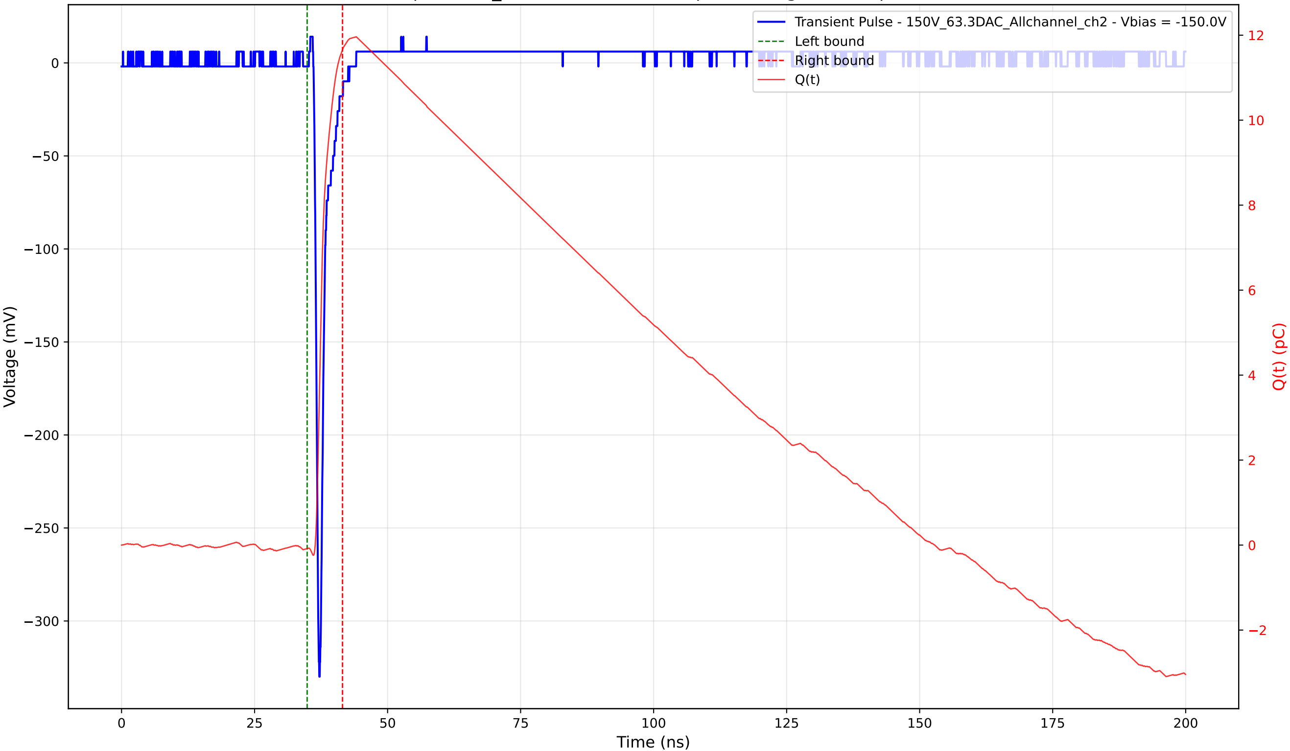
Transient Pulse - Sample: 1cm_42 - Position: 3395.0 \mu\text{m} - Charge: 11.74 pC - Rise Time: 0.72 ns
