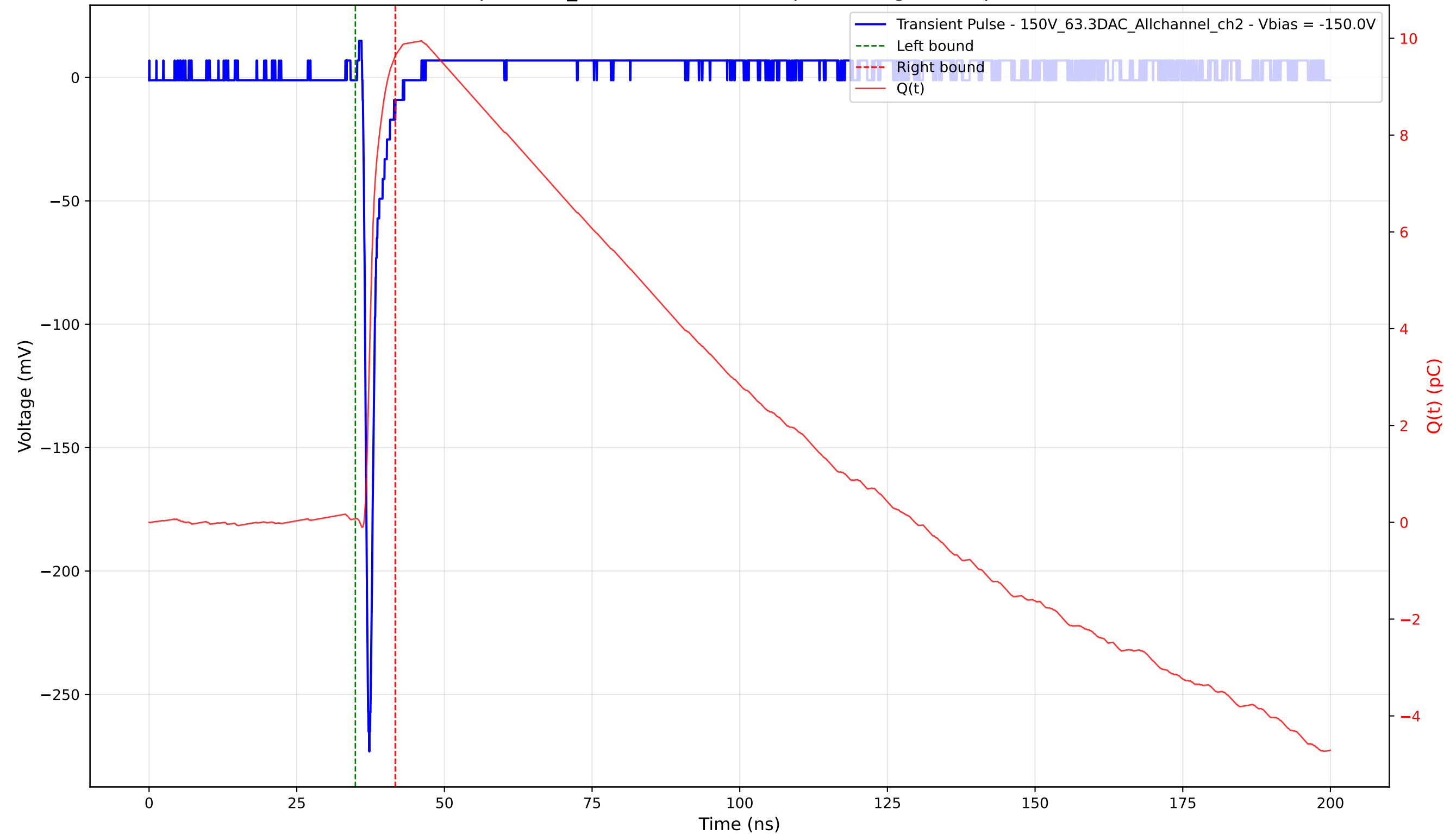
Transient Pulse - Sample: 1cm_42 - Position: 2590.0 \mu\text{m} - Charge: 9.57 pC - Rise Time: 0.73 ns
