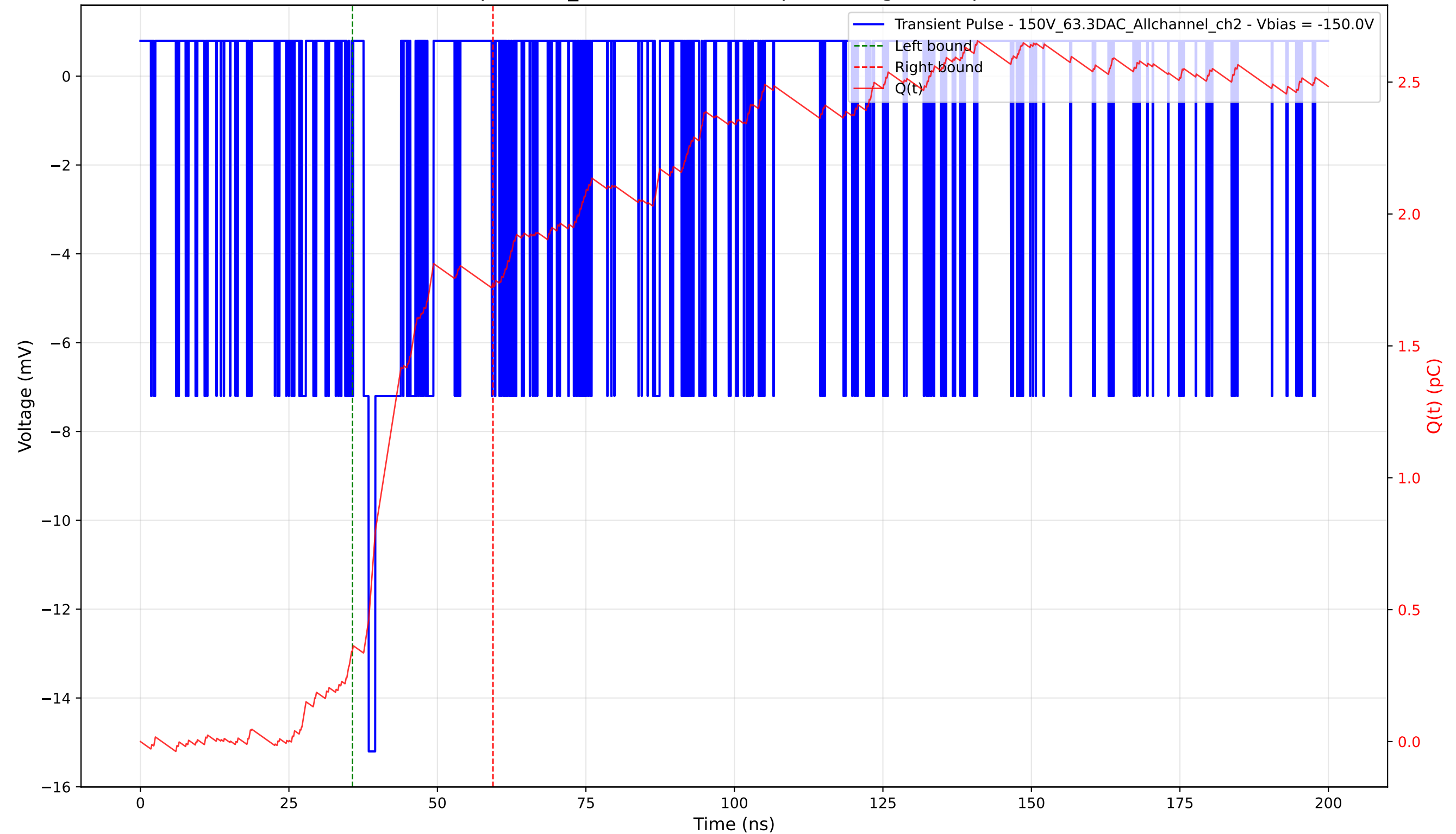
Transient Pulse - Sample: 1cm_42 - Position: 135.0 \mu\text{m} - Charge: 1.38 pC - Rise Time: 0.88 ns
