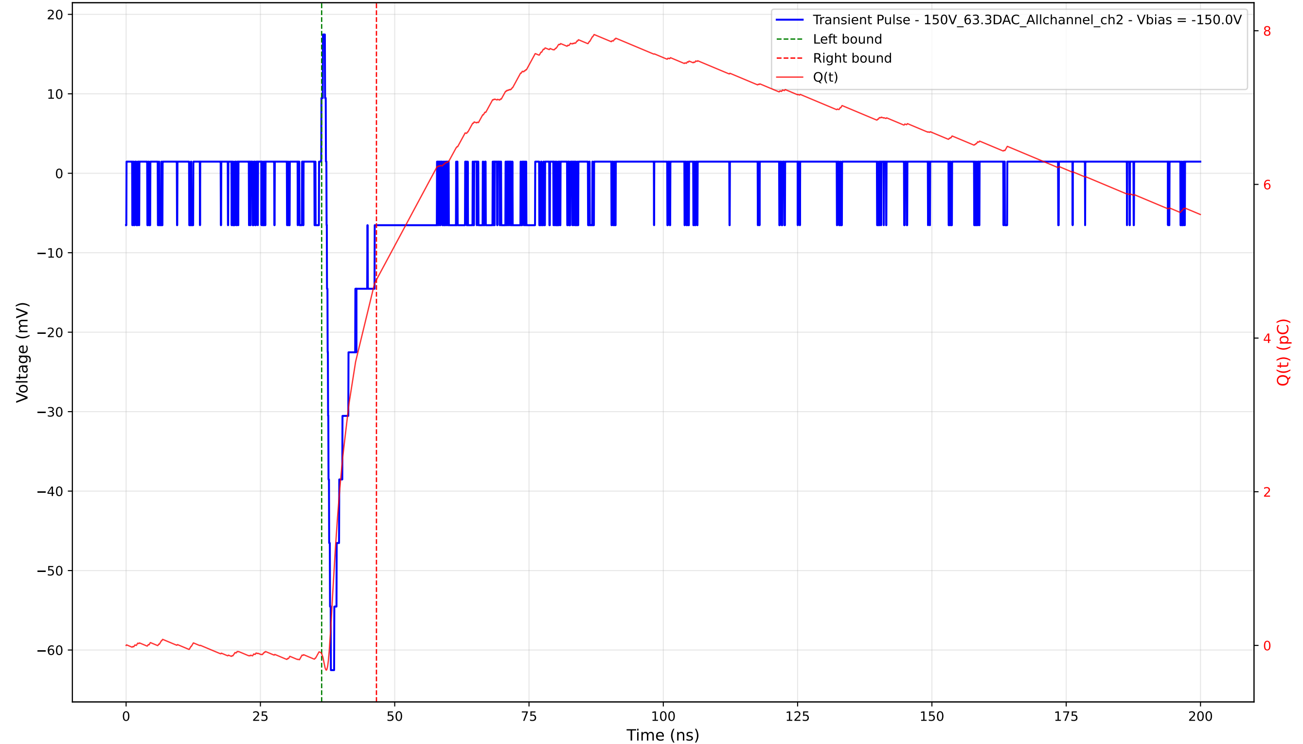
Transient Pulse - Sample: 1cm_42 - Position: 1725.0 \mu\text{m} - Charge: 4.87 pC - Rise Time: 0.80 ns
