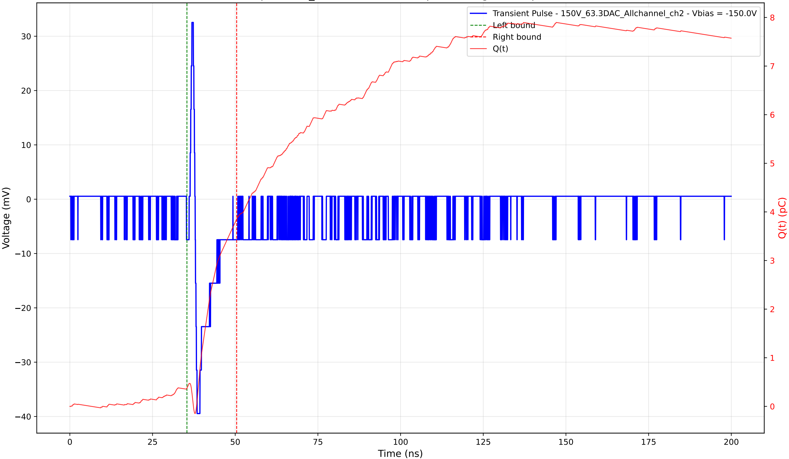
Transient Pulse - Sample: 1cm_42 - Position: 870.0 \mu\text{m} - Charge: 3.48 pC - Rise Time: 0.58 ns
