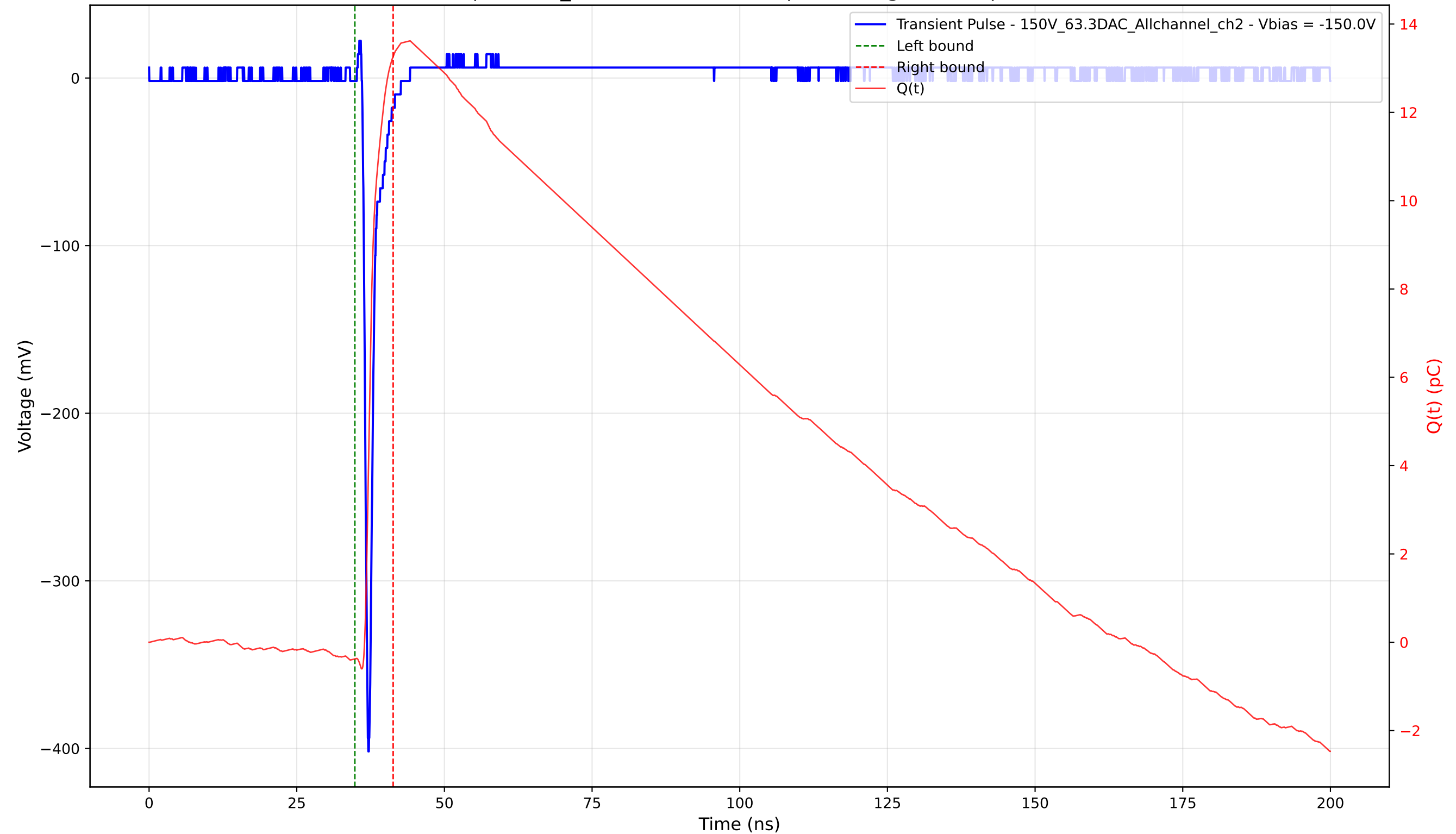
Transient Pulse - Sample: 1cm_42 - Position: 3330.0 \mu\text{m} - Charge: 13.64 pC - Rise Time: 0.73 ns
