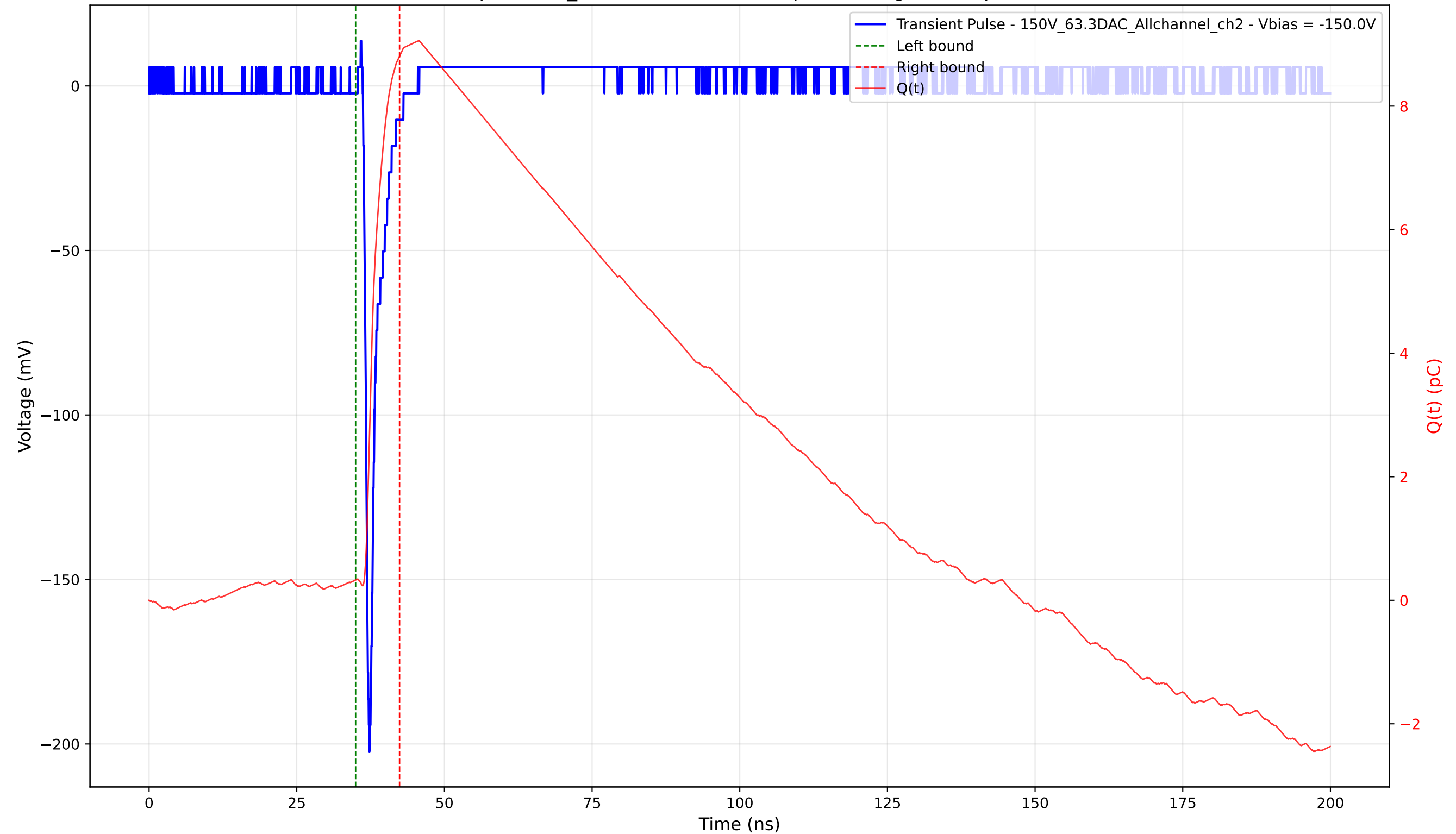
Transient Pulse - Sample: 1cm_42 - Position: 3540.0 \mu\text{m} - Charge: 8.48 pC - Rise Time: 0.79 ns
