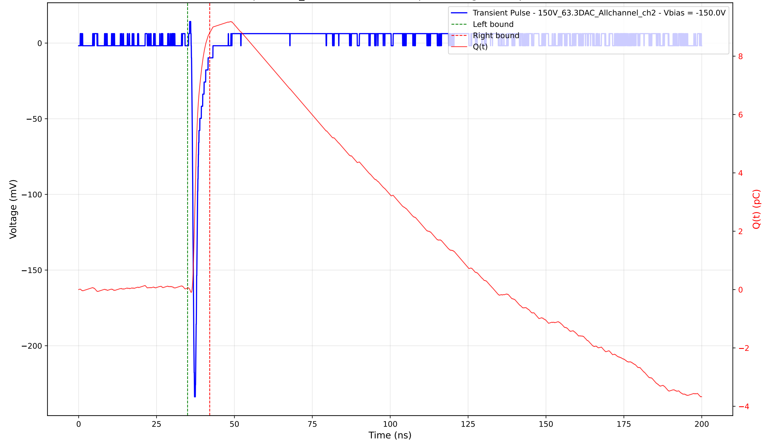
Transient Pulse - Sample: 1cm_42 - Position: 2555.0 \mu\text{m} - Charge: 8.75 pC - Rise Time: 0.77 ns
