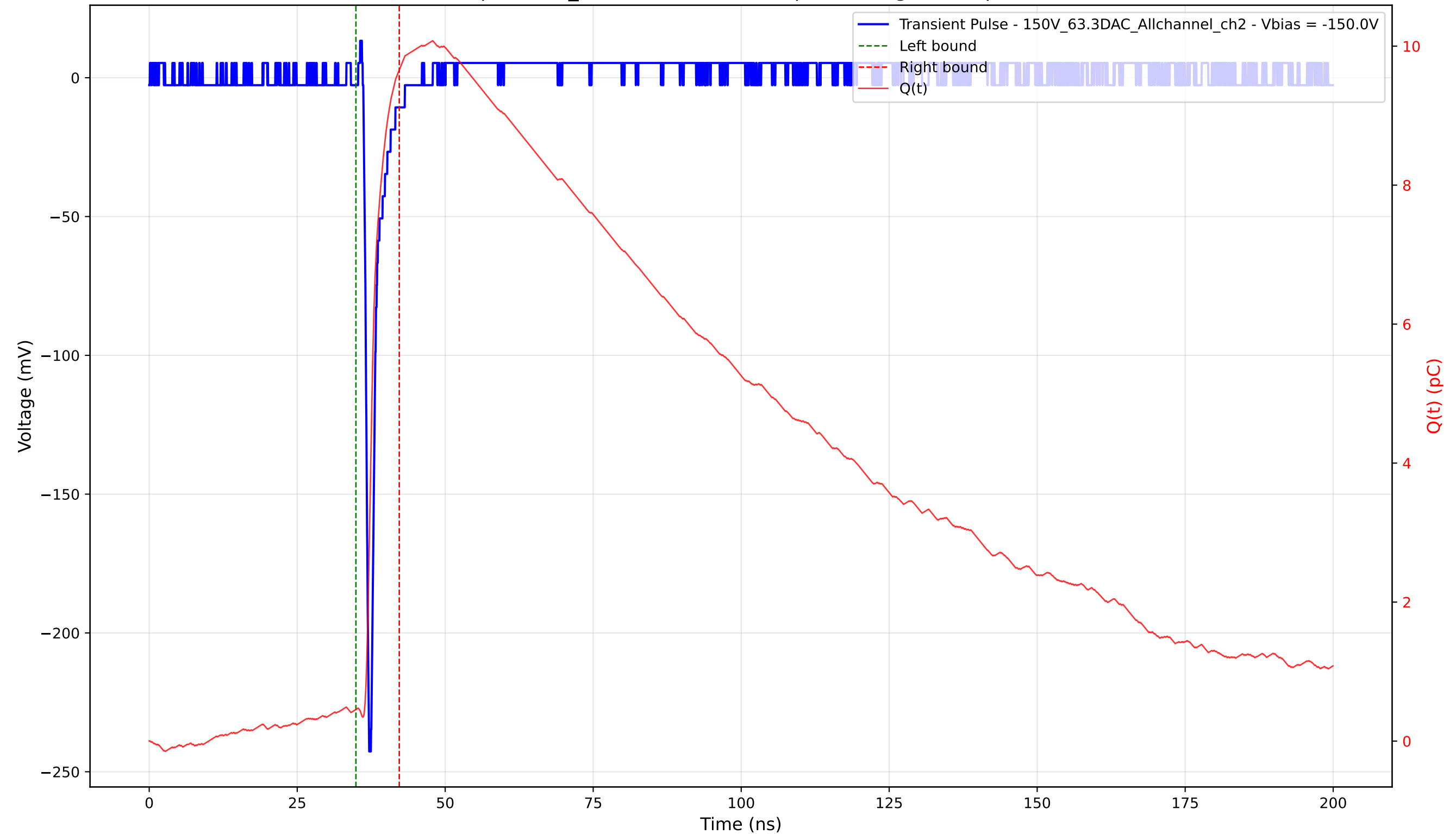
Transient Pulse - Sample: 1cm_42 - Position: 2565.0 \mu\text{m} - Charge: 9.20 pC - Rise Time: 0.77 ns
