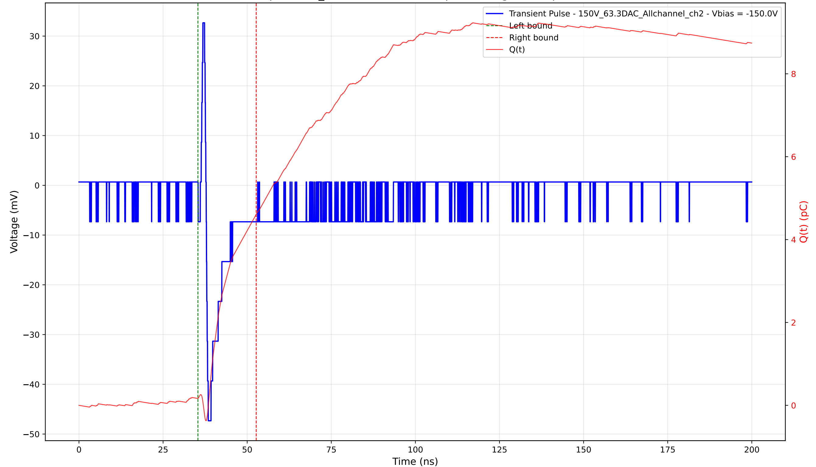
Transient Pulse - Sample: 1cm_42 - Position: 1225.0 \mu\text{m} - Charge: 4.44 pC - Rise Time: 0.62 ns
