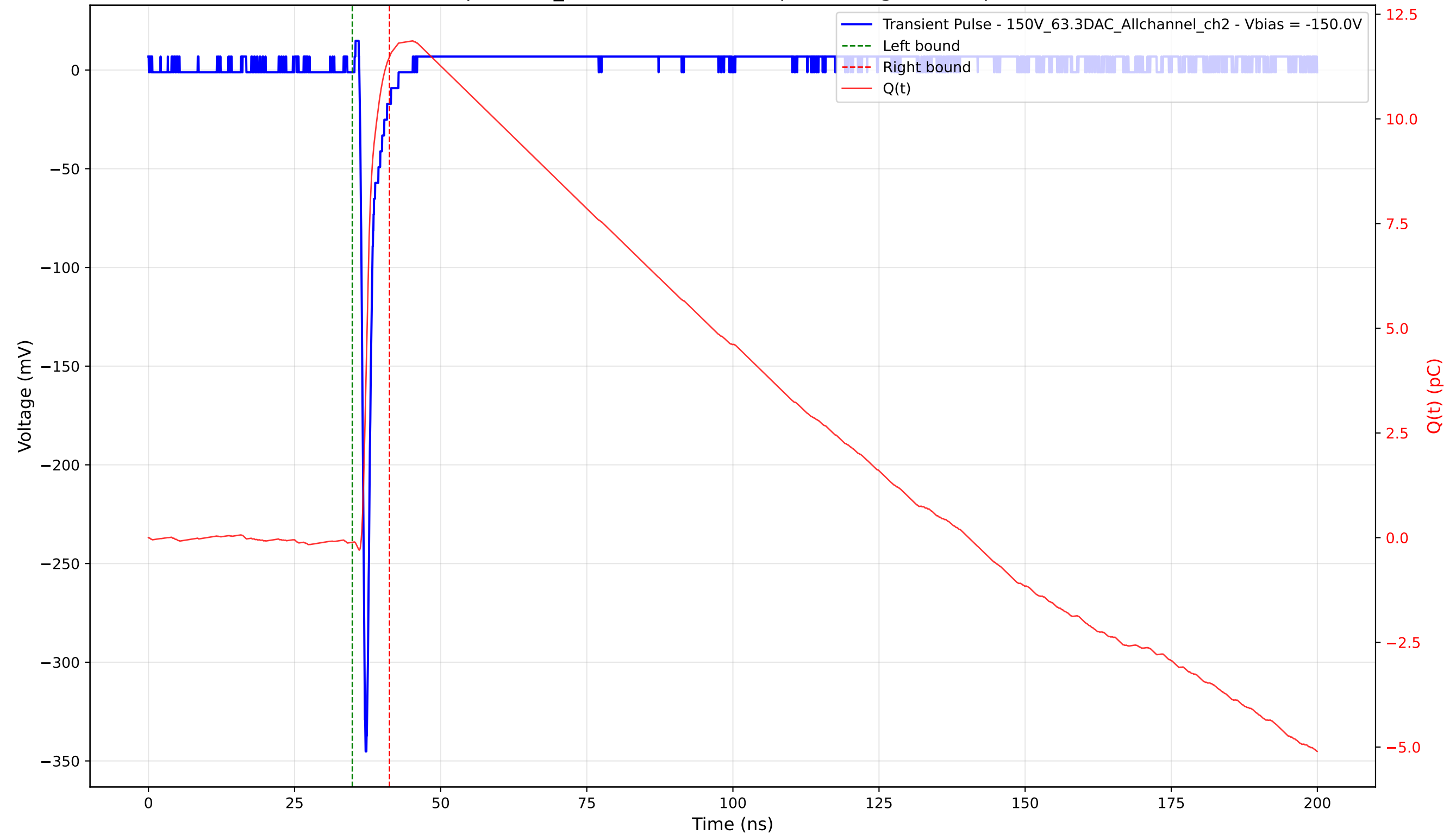
Transient Pulse - Sample: 1cm_42 - Position: 2665.0 \mu\text{m} - Charge: 11.59 pC - Rise Time: 0.75 ns
