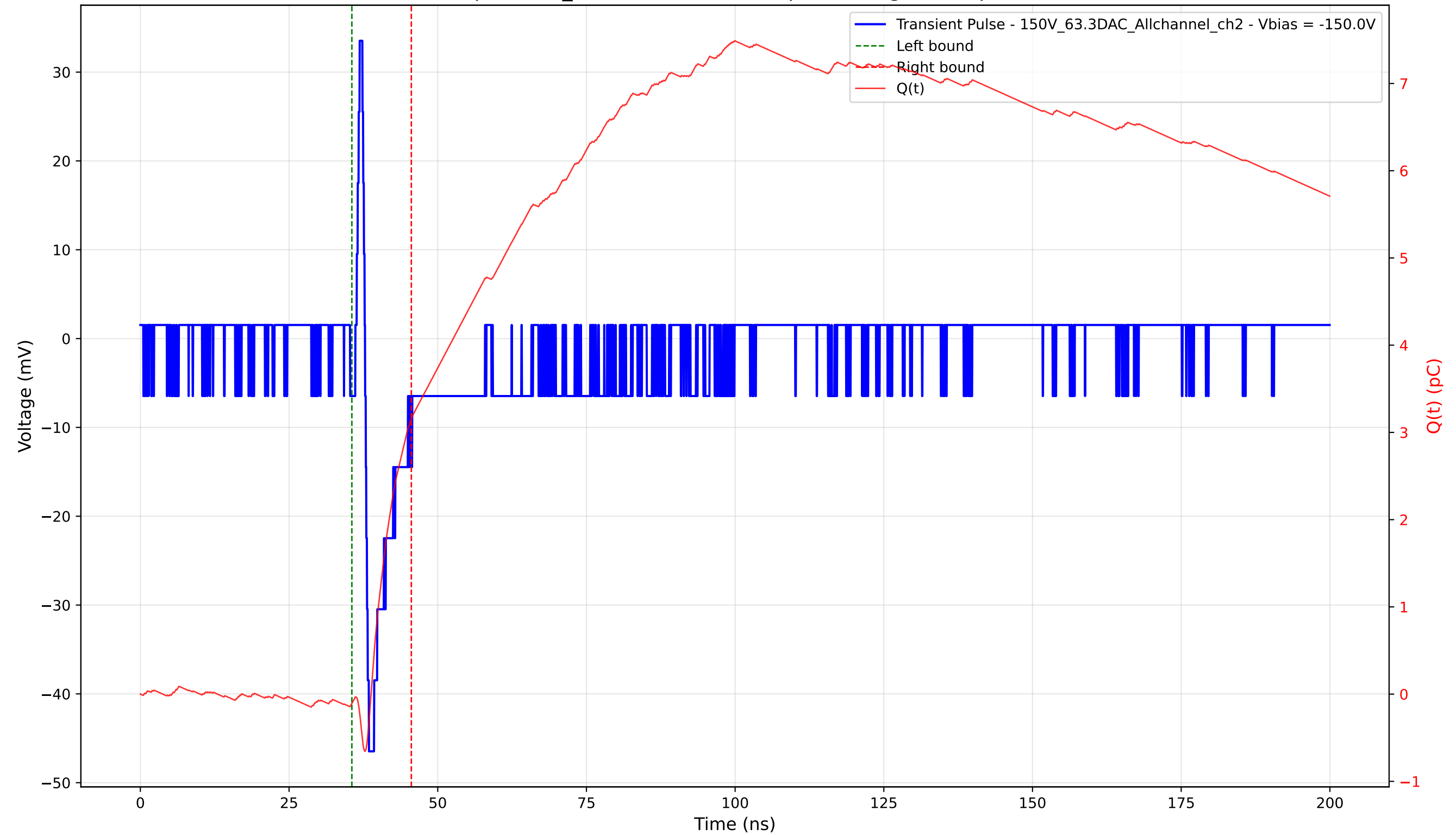
Transient Pulse - Sample: 1cm_42 - Position: 1265.0 \mu\text{m} - Charge: 3.25 pC - Rise Time: 0.65 ns
