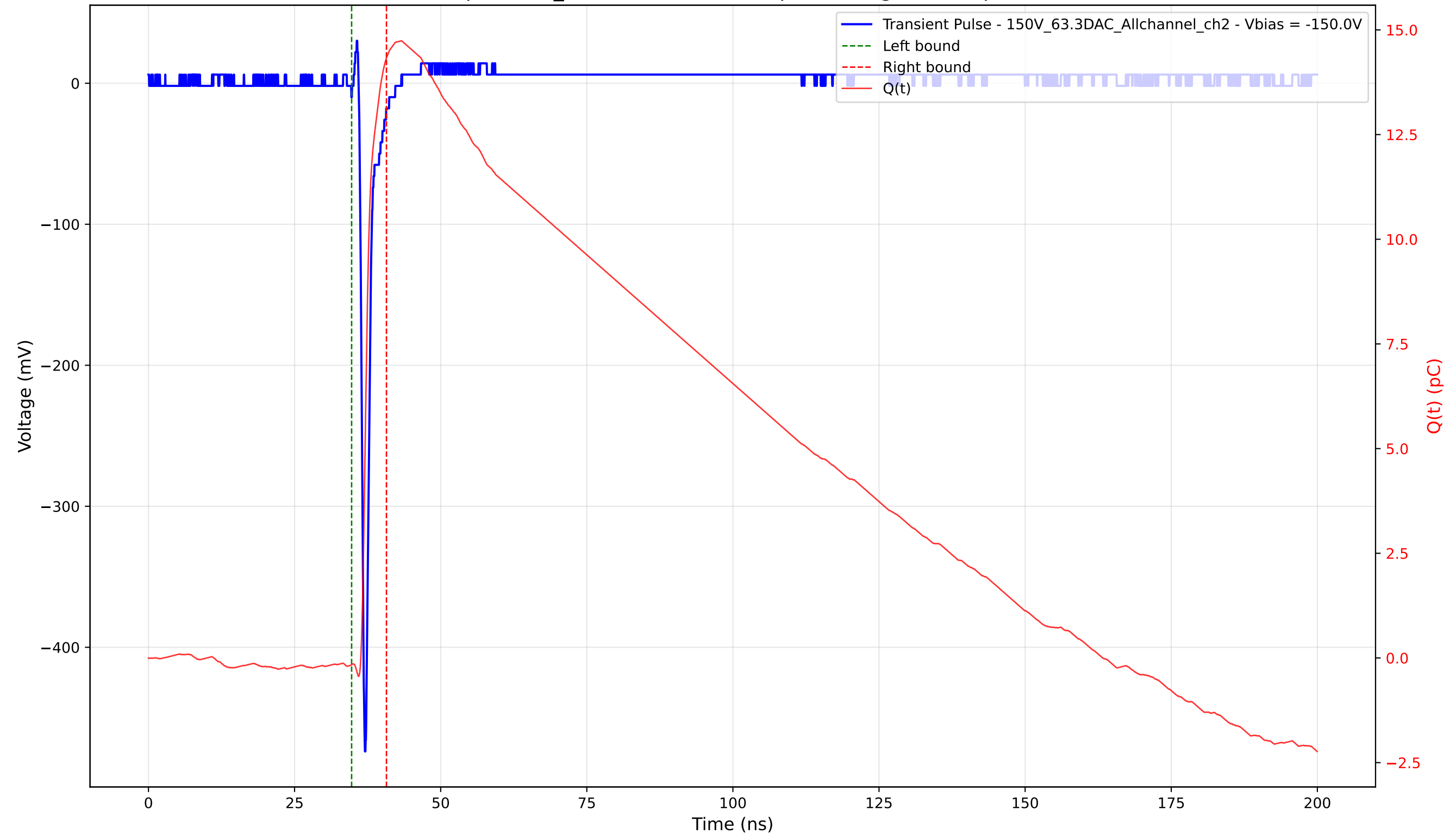
Transient Pulse - Sample: 1cm_42 - Position: 3120.0 \mu\text{m} - Charge: 14.50 pC - Rise Time: 0.73 ns
