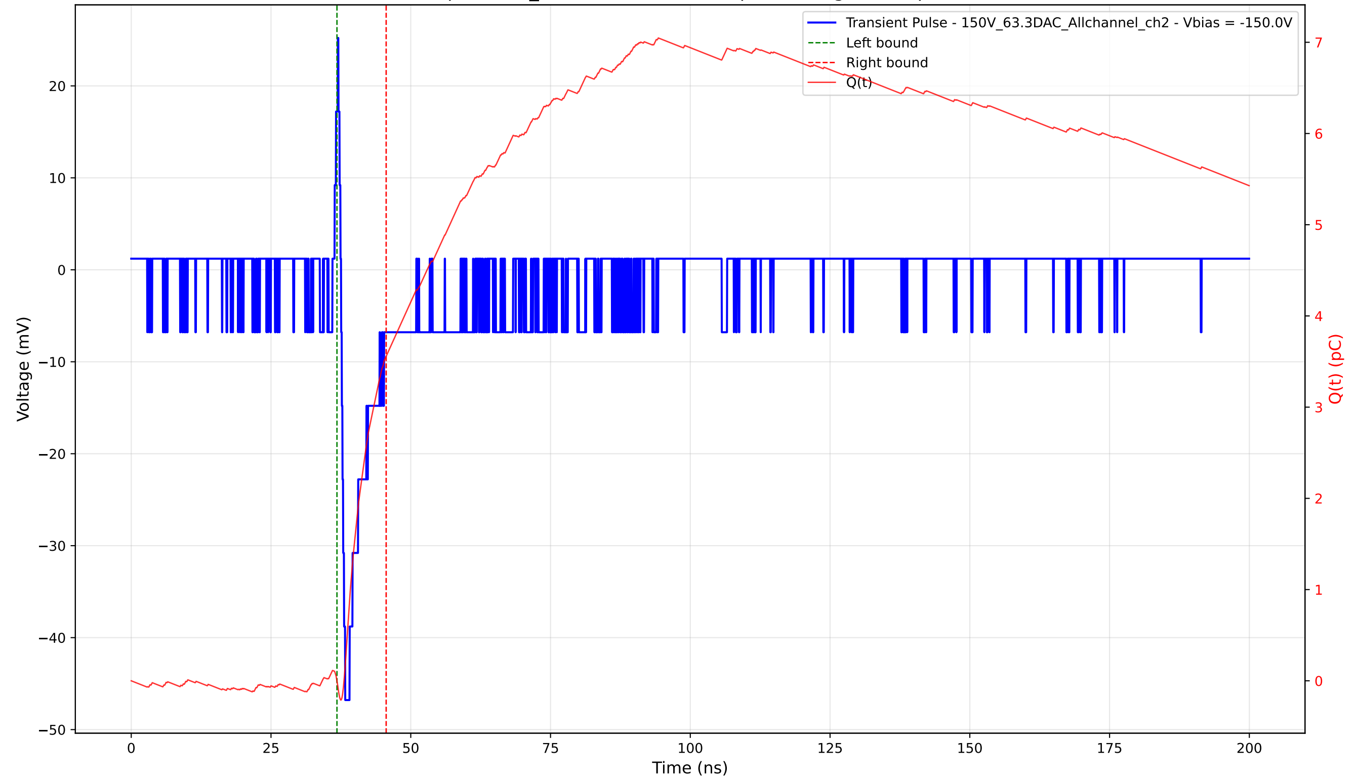
Transient Pulse - Sample: 1cm_42 - Position: 1530.0 \mu\text{m} - Charge: 3.56 pC - Rise Time: 0.74 ns
