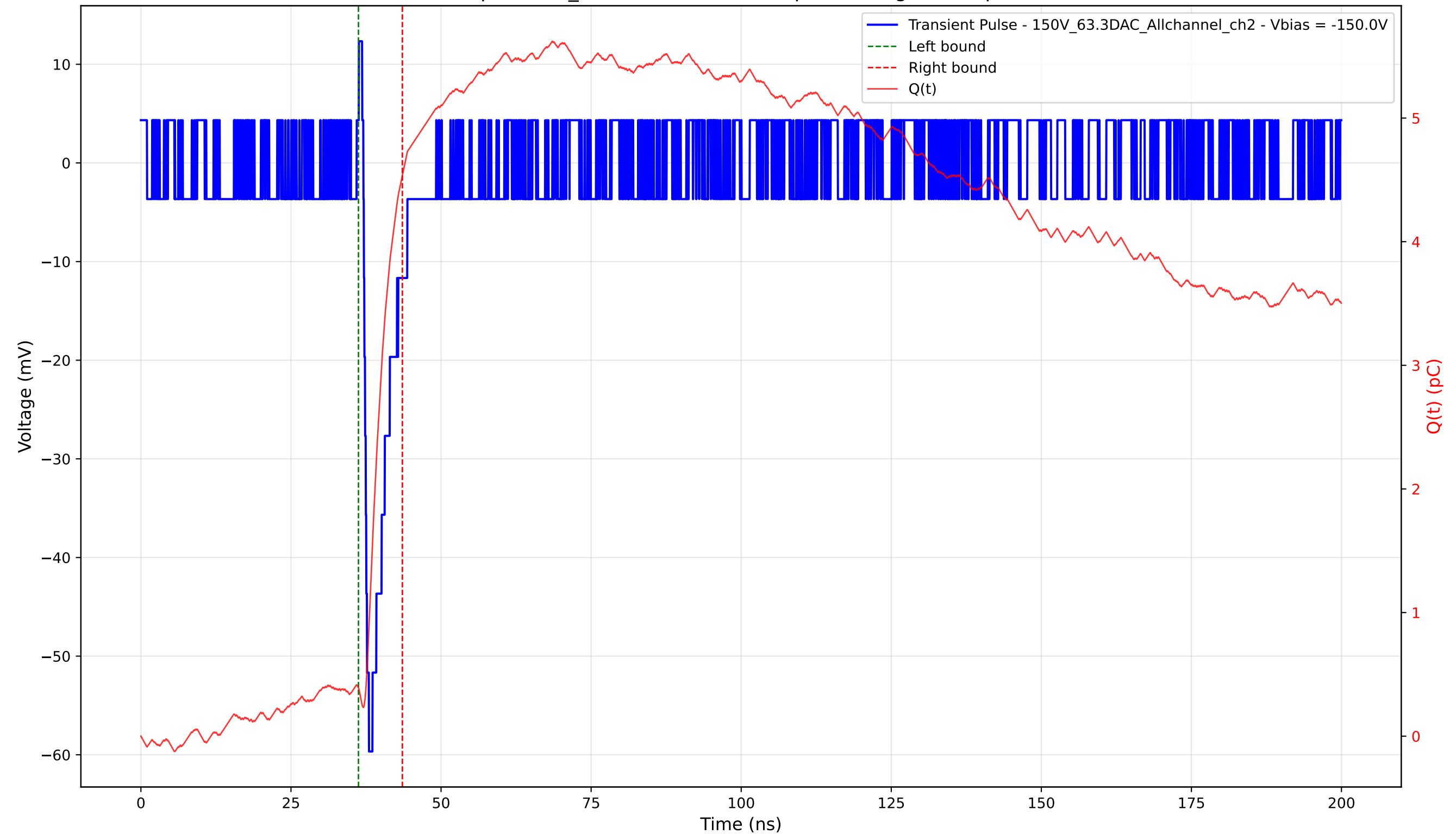
Transient Pulse - Sample: 1cm_42 - Position: 4185.0 \mu\text{m} - Charge: 4.15 pC - Rise Time: 0.87 ns
