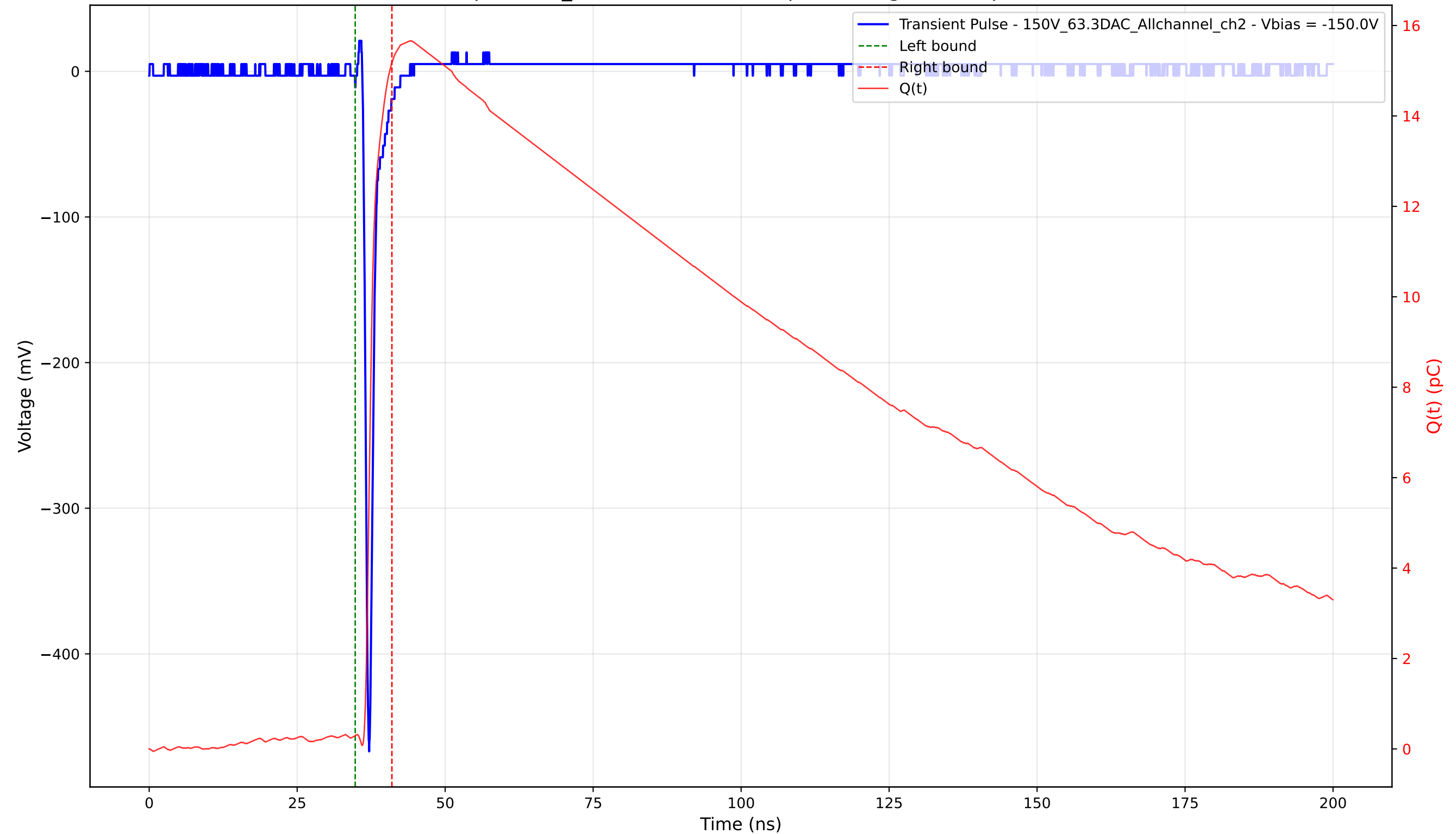
Transient Pulse - Sample: 1cm_42 - Position: 2800.0 \mu\text{m} - Charge: 14.89 pC - Rise Time: 0.71 ns
