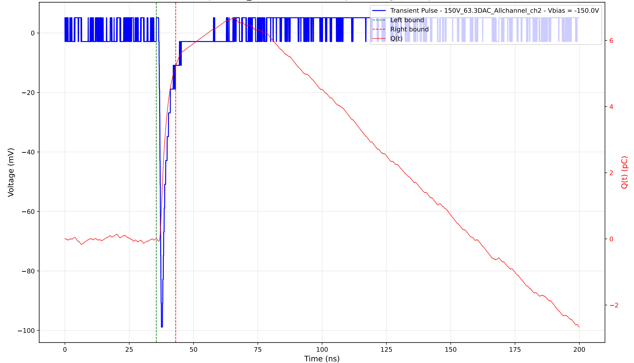
Transient Pulse - Sample: 1cm_42 - Position: 2130.0 \mu\text{m} - Charge: 5.22 pC - Rise Time: 0.76 ns
