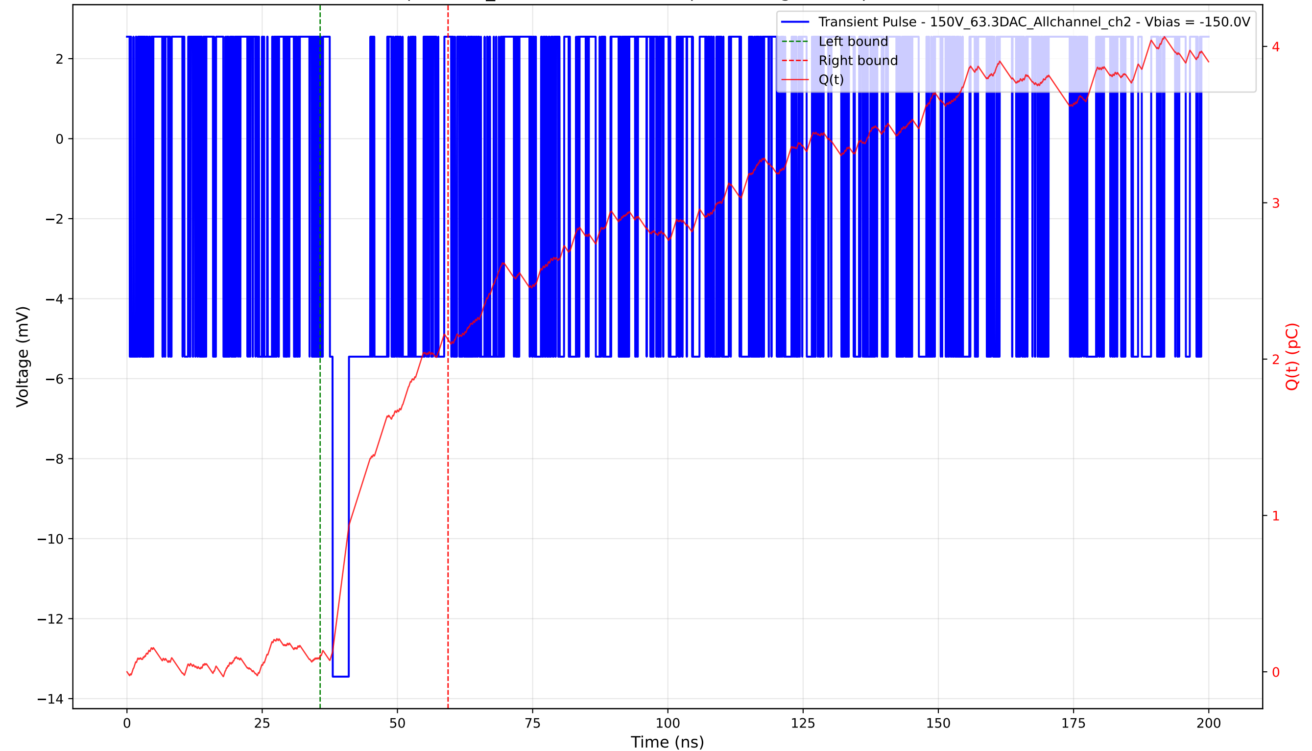
Transient Pulse - Sample: 1cm_42 - Position: 5060.0 \mu\text{m} - Charge: 2.03 pC - Rise Time: 0.00 ns (N/A)
