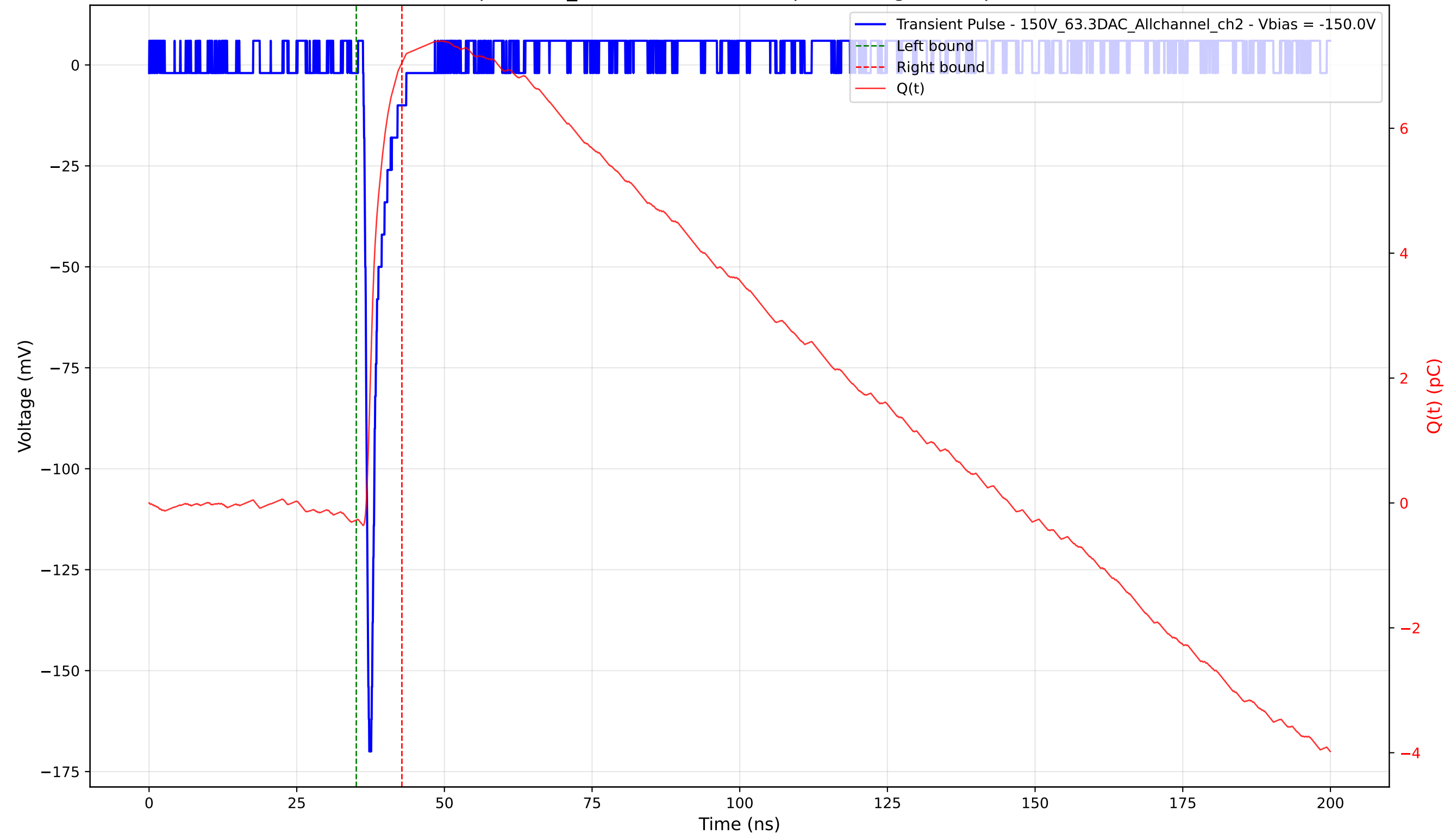
Transient Pulse - Sample: 1cm_42 - Position: 2450.0 \mu\text{m} - Charge: 7.32 pC - Rise Time: 0.73 ns
