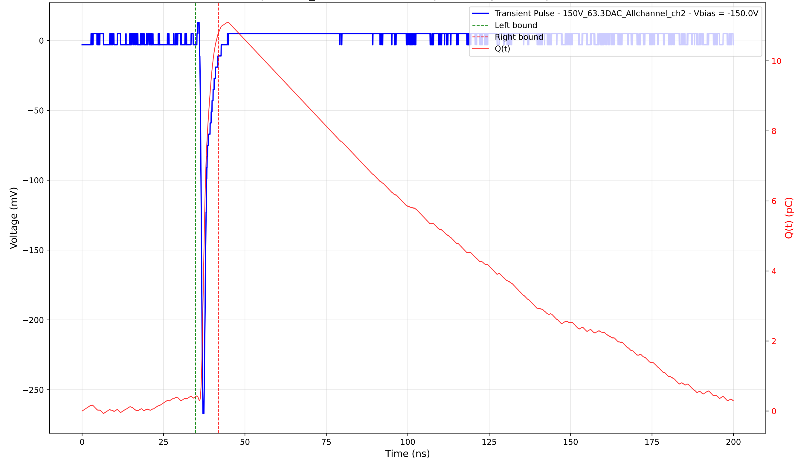
Transient Pulse - Sample: 1cm_42 - Position: 3450.0 \mu\text{m} - Charge: 10.41 pC - Rise Time: 0.75 ns
