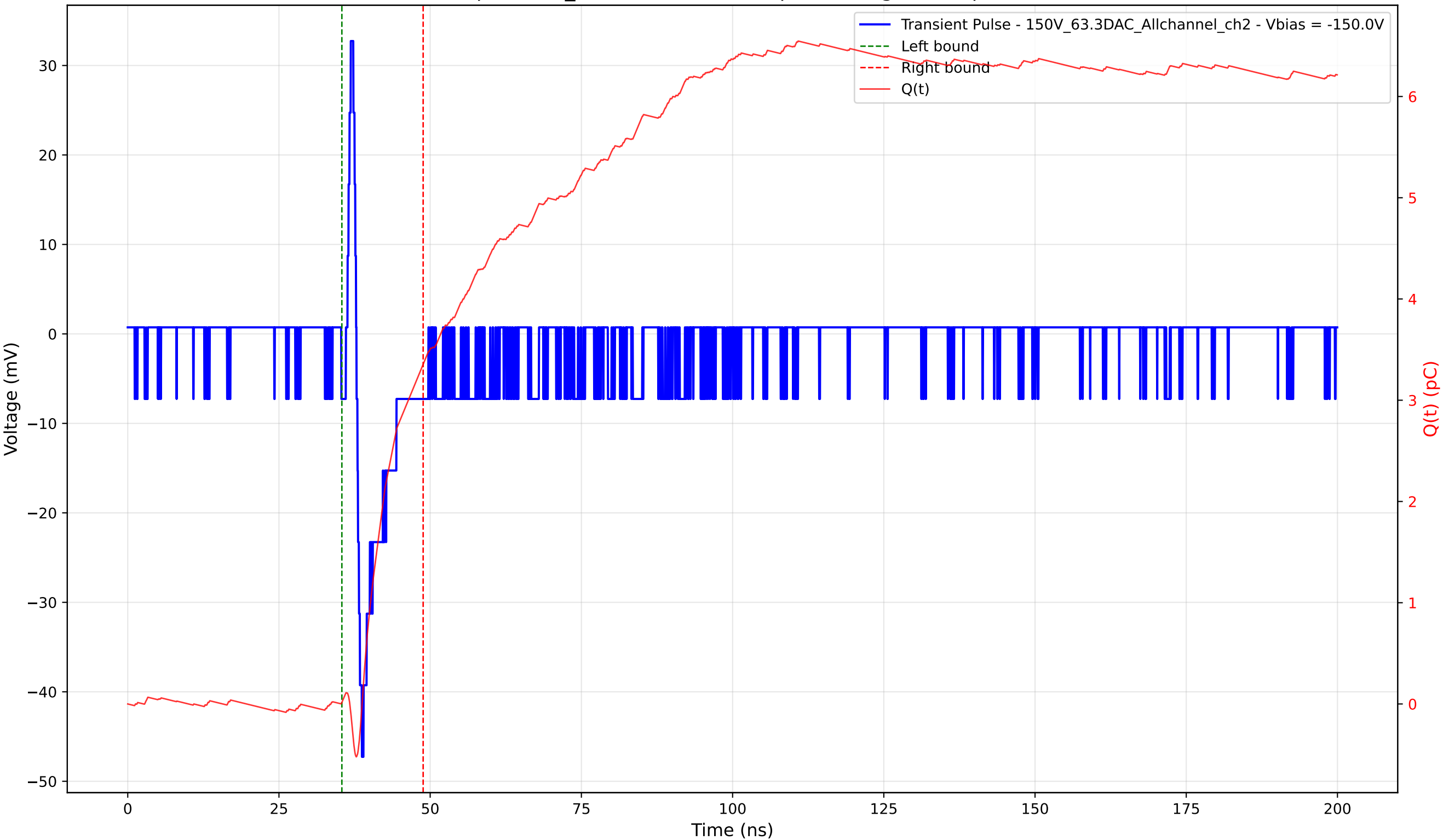
Transient Pulse - Sample: 1cm_42 - Position: 680.0 \mu\text{m} - Charge: 3.34 pC - Rise Time: 0.90 ns
