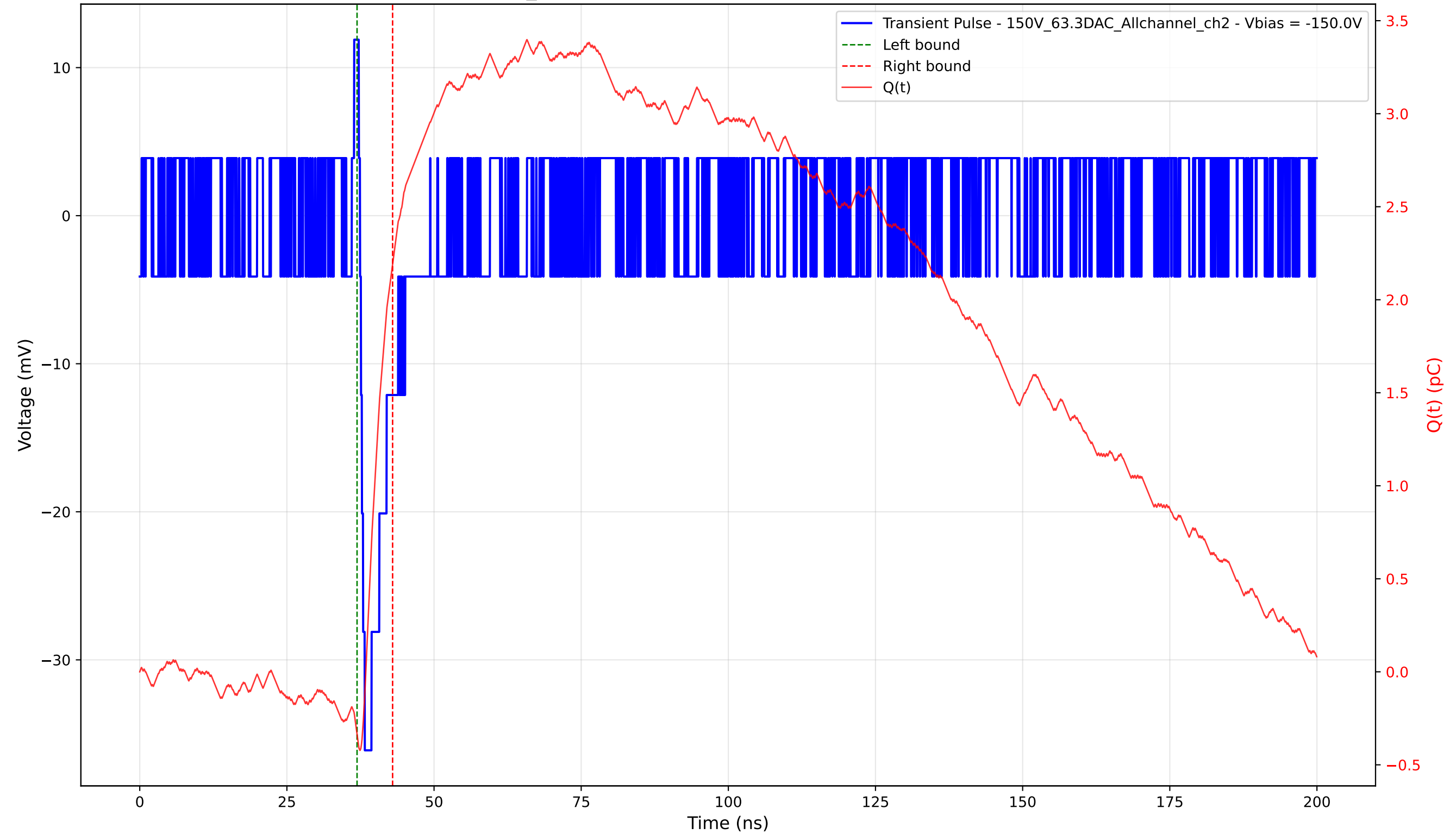
Transient Pulse - Sample: 1cm_42 - Position: 4700.0 \mu\text{m} - Charge: 2.53 pC - Rise Time: 0.00 ns (N/A)
