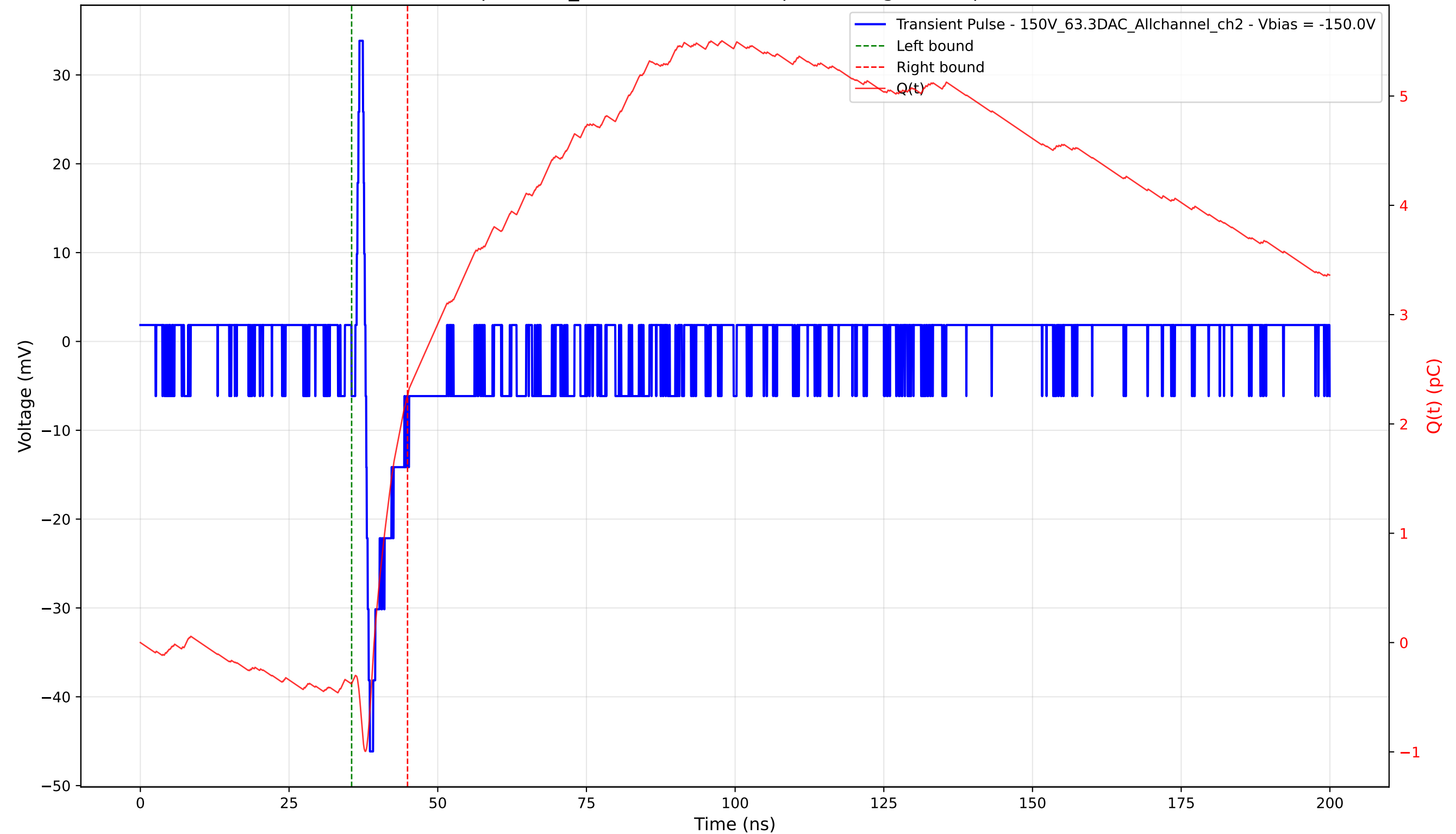
Transient Pulse - Sample: 1cm_42 - Position: 770.0 \mu\text{m} - Charge: 2.63 pC - Rise Time: 0.73 ns
