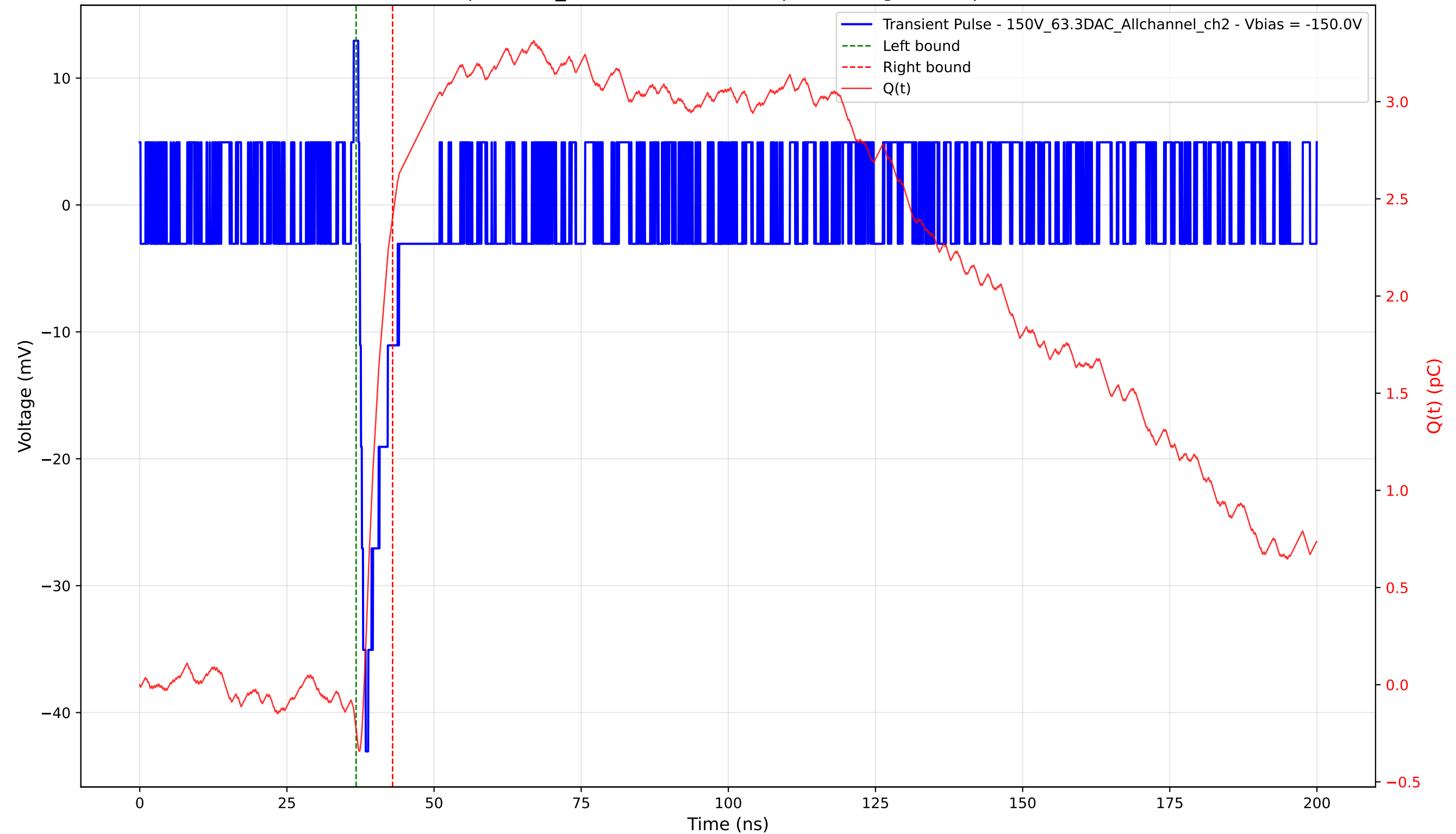
Transient Pulse - Sample: 1cm_42 - Position: 4510.0 \mu\text{m} - Charge: 2.64 pC - Rise Time: 0.99 ns
