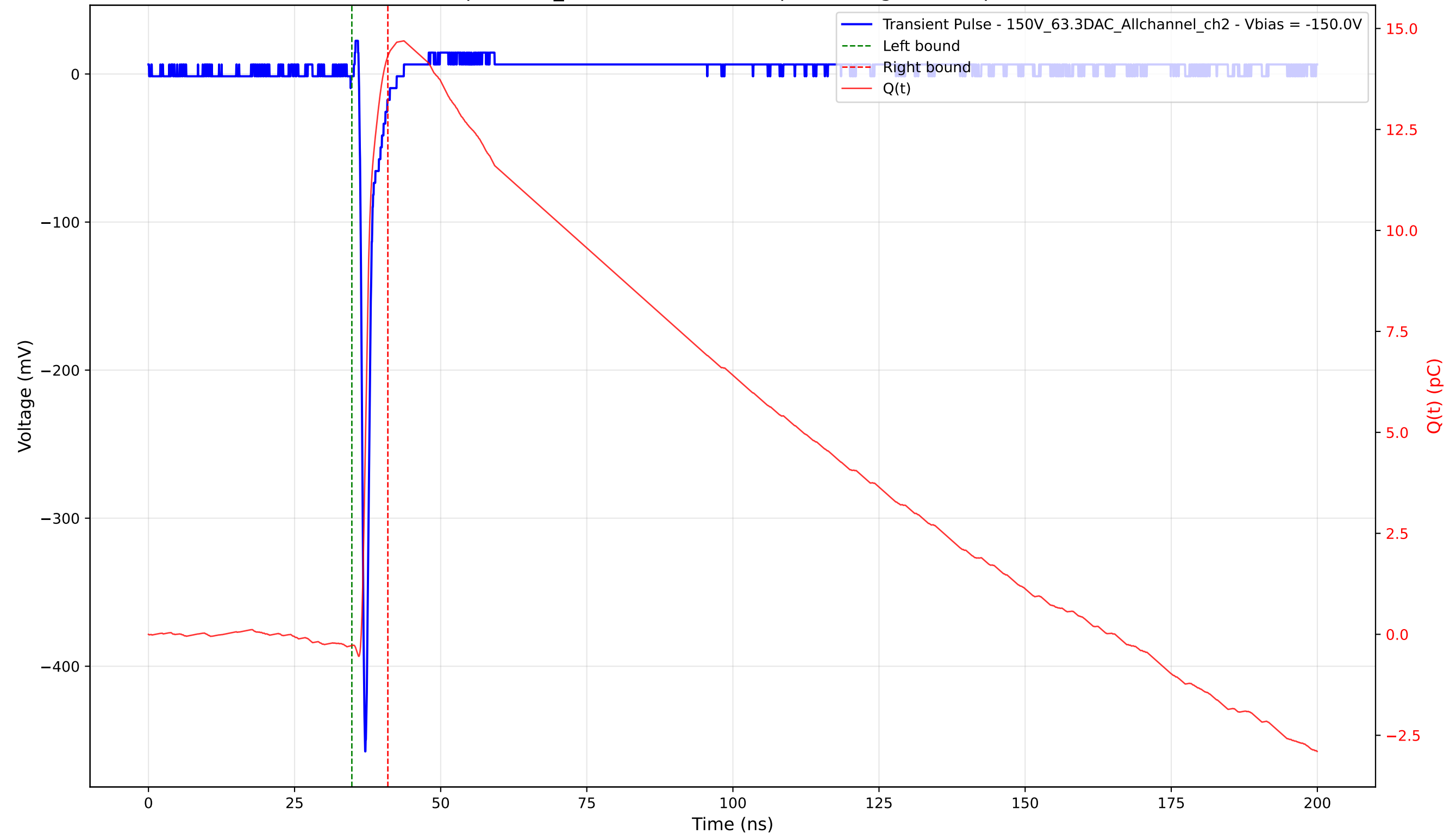
Transient Pulse - Sample: 1cm_42 - Position: 3210.0 \mu\text{m} - Charge: 14.59 pC - Rise Time: 0.70 ns
