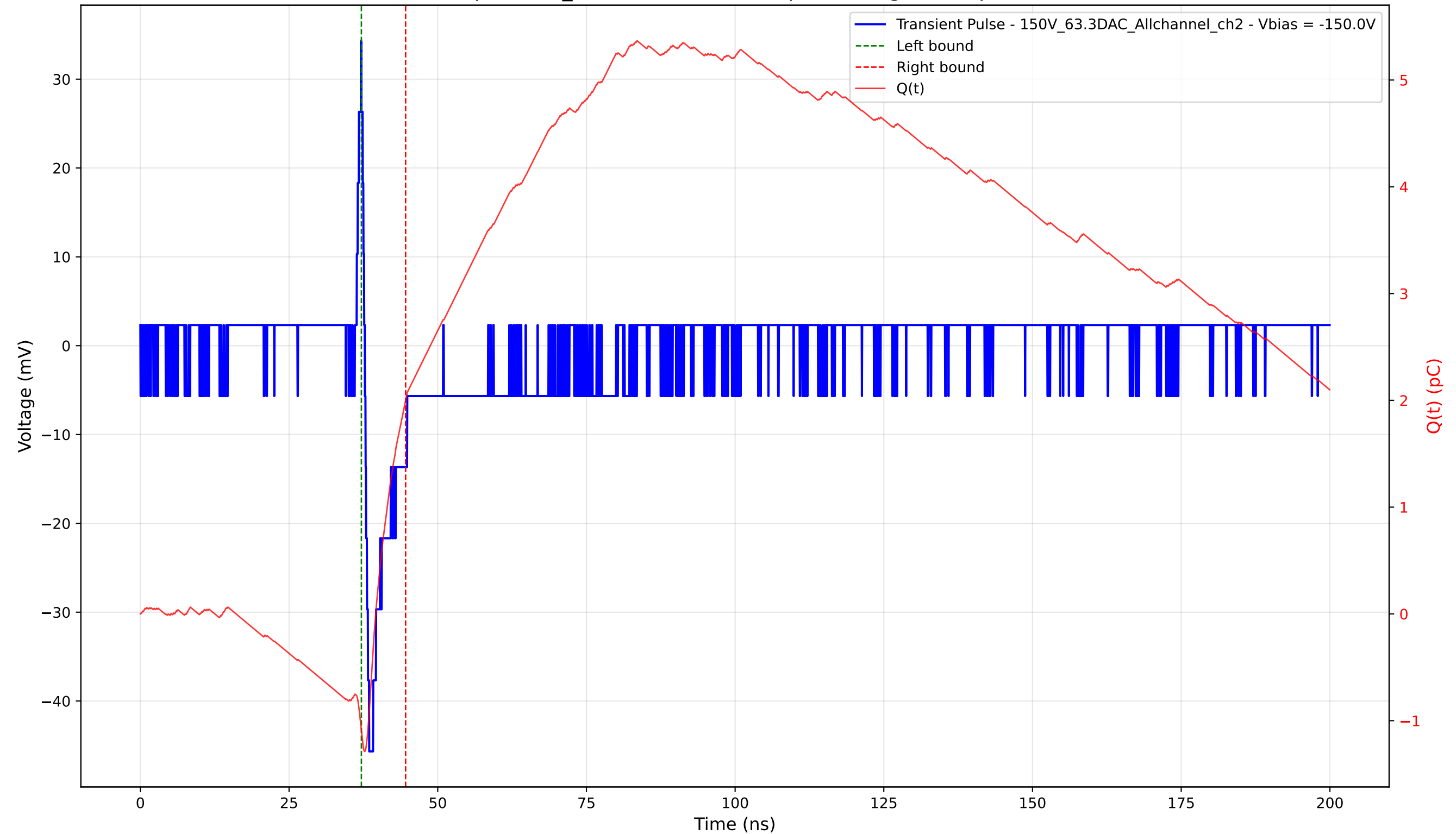
Transient Pulse - Sample: 1cm_42 - Position: 1375.0 \mu\text{m} - Charge: 3.10 pC - Rise Time: 0.73 ns
