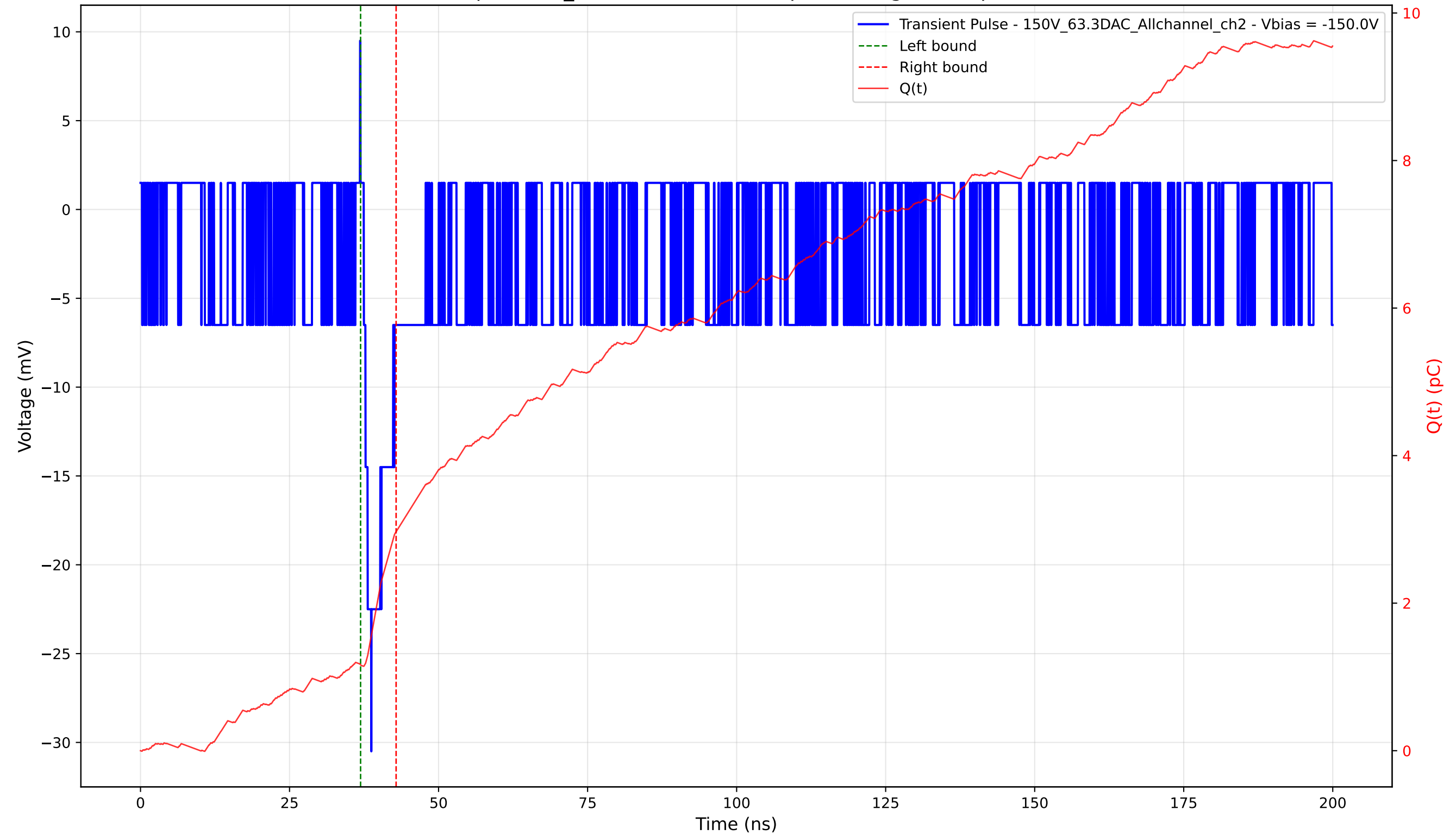
Transient Pulse - Sample: 1cm_42 - Position: 4975.0 \mu\text{m} - Charge: 1.81 pC - Rise Time: 1.27 ns
