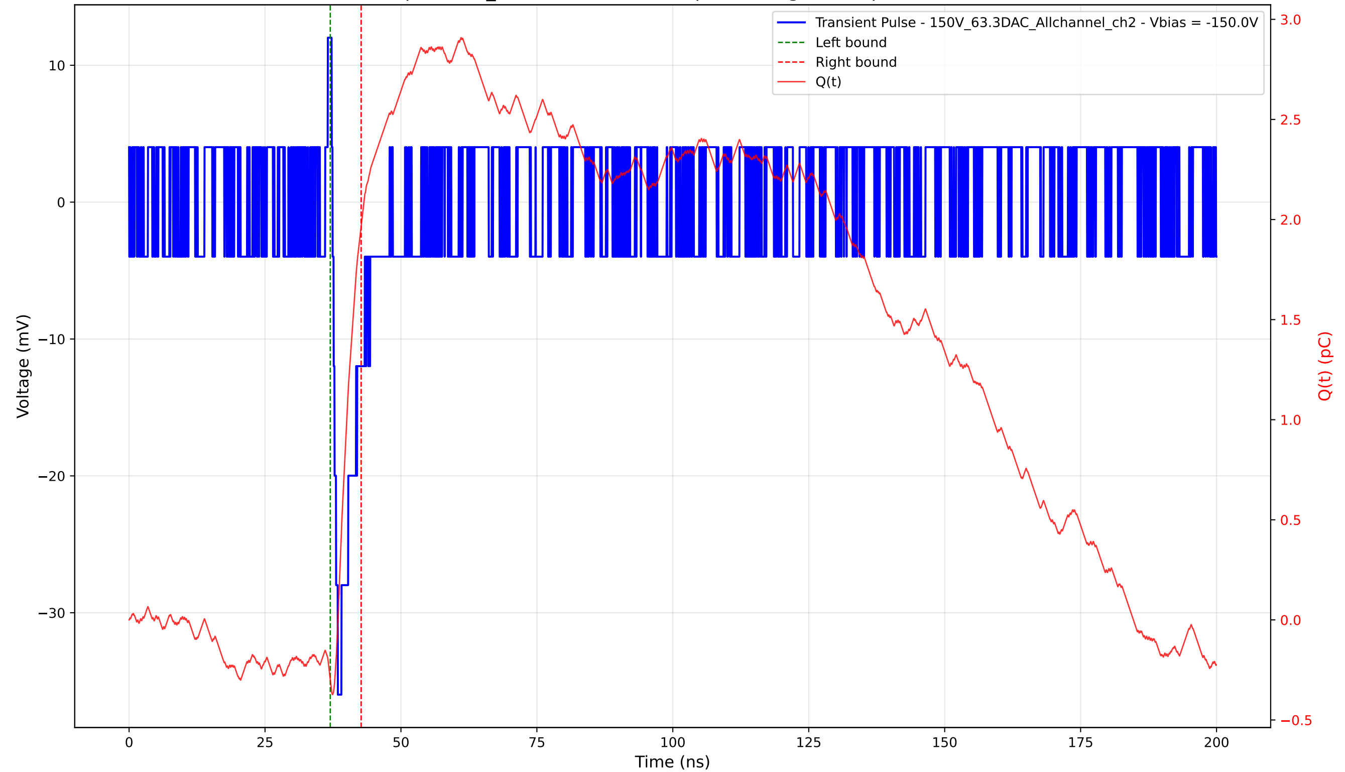
Transient Pulse - Sample: 1cm_42 - Position: 4860.0 \mu\text{m} - Charge: 2.27 pC - Rise Time: 0.00 ns (N/A)
