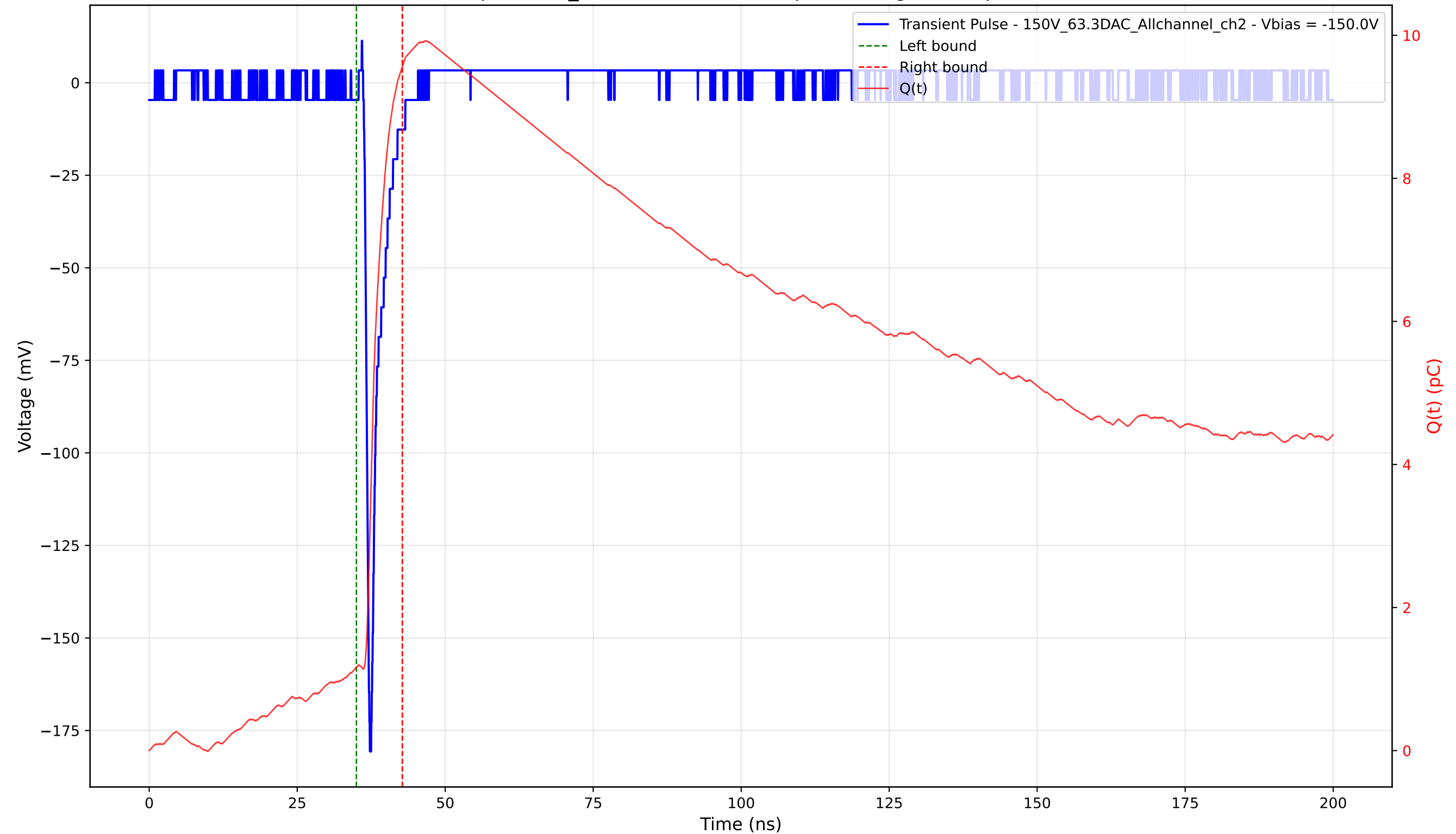
Transient Pulse - Sample: 1cm_42 - Position: 3580.0 \mu\text{m} - Charge: 8.40 pC - Rise Time: 0.77 ns
