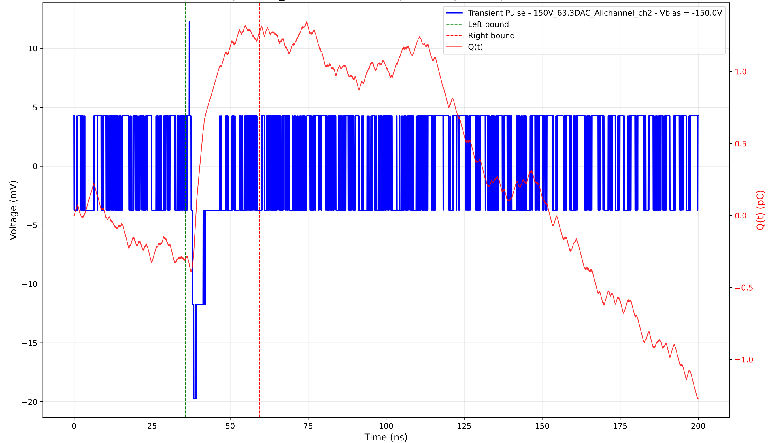
Transient Pulse - Sample: 1cm_42 - Position: 5015.0 \mu\text{m} - Charge: 1.57 pC - Rise Time: 0.00 ns (N/A)
