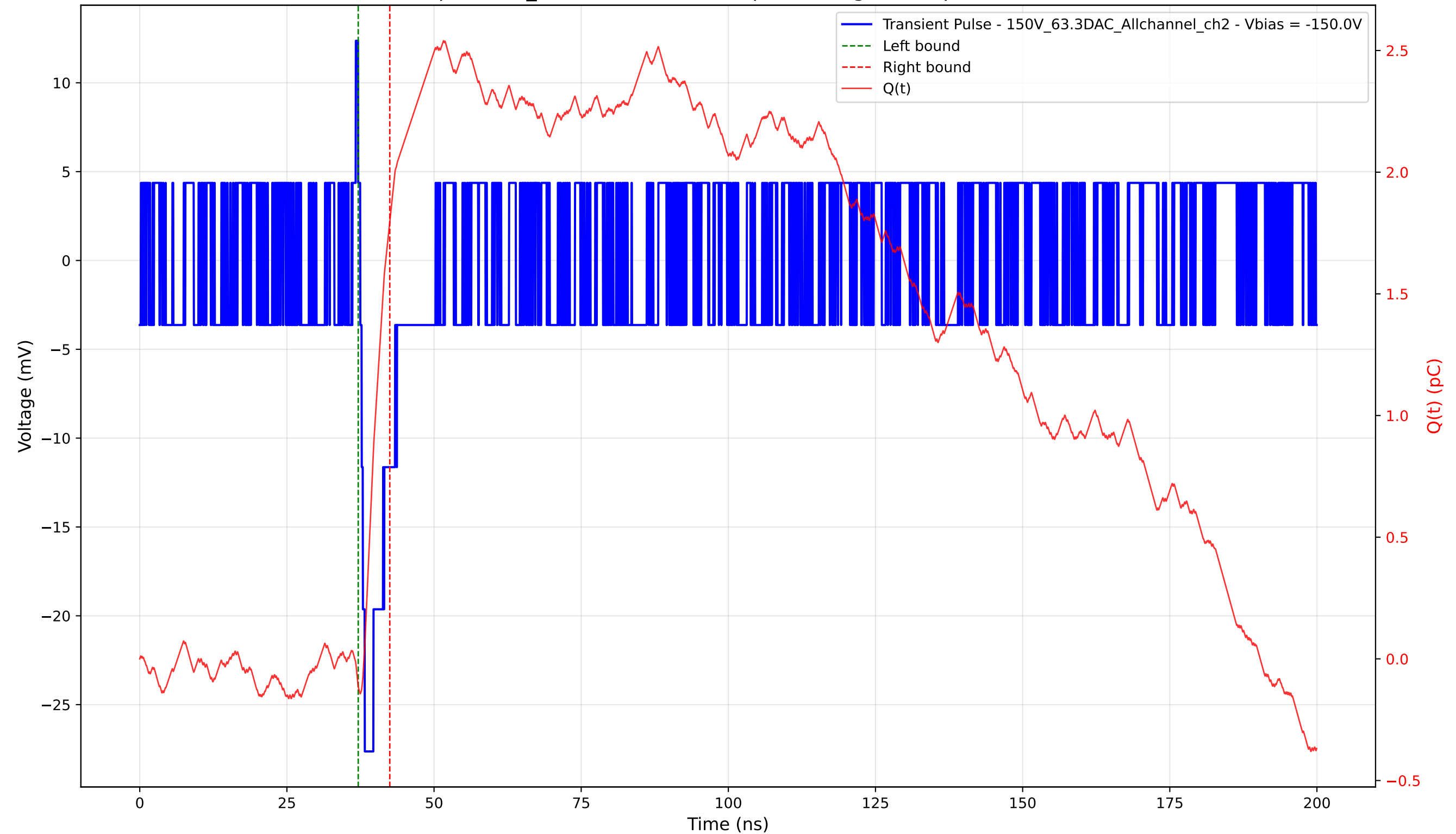
Transient Pulse - Sample: 1cm_42 - Position: 4910.0 \mu\text{m} - Charge: 1.91 pC - Rise Time: 0.00 ns (N/A)
