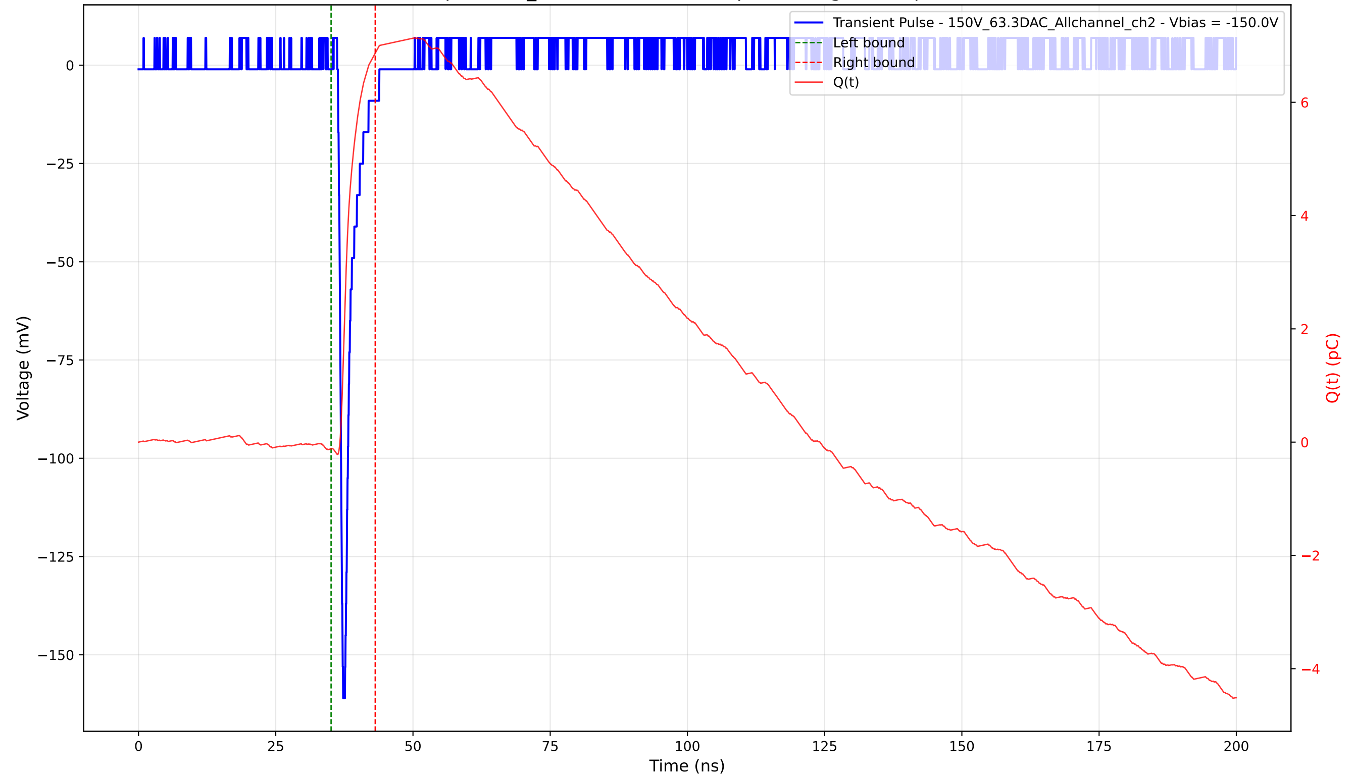
Transient Pulse - Sample: 1cm_42 - Position: 2430.0 \mu\text{m} - Charge: 6.99 pC - Rise Time: 0.76 ns
