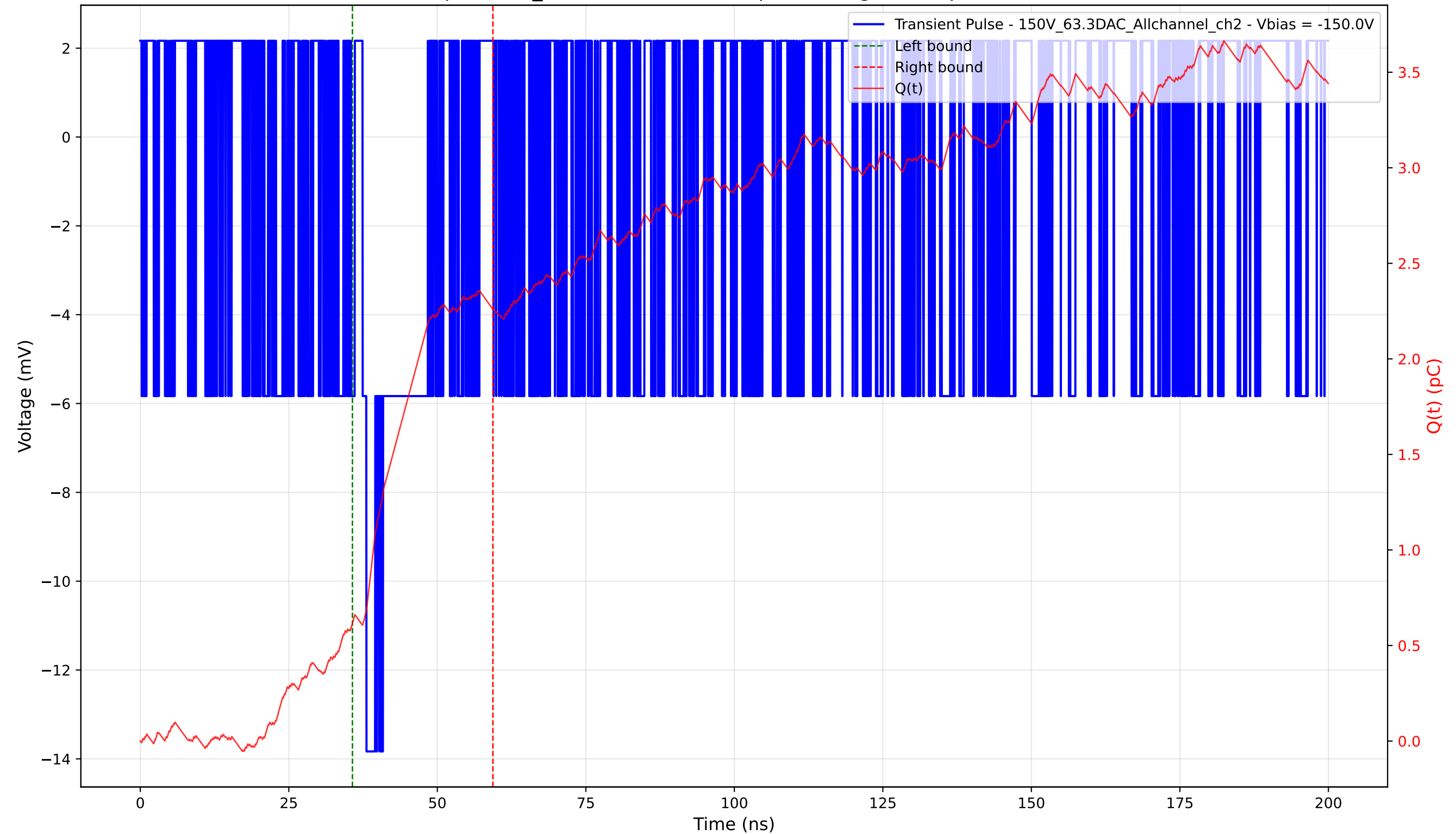
Transient Pulse - Sample: 1cm_42 - Position: 5075.0 \mu\text{m} - Charge: 1.64 pC - Rise Time: 0.00 ns (N/A)
