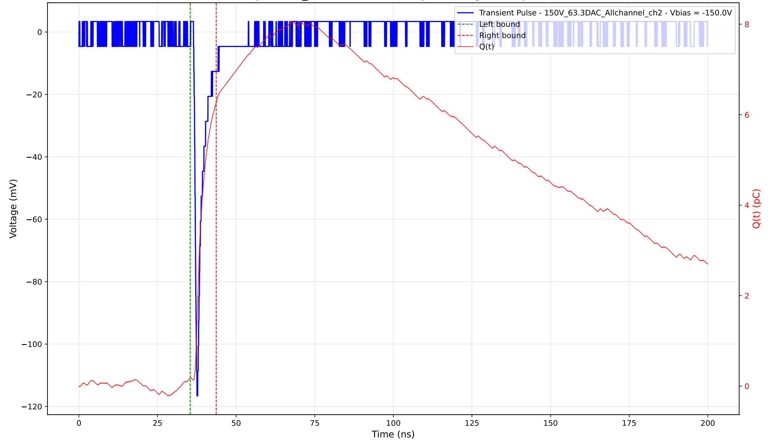
Transient Pulse - Sample: 1cm_42 - Position: 2185.0 \mu\text{m} - Charge: 6.08 pC - Rise Time: 0.84 ns
