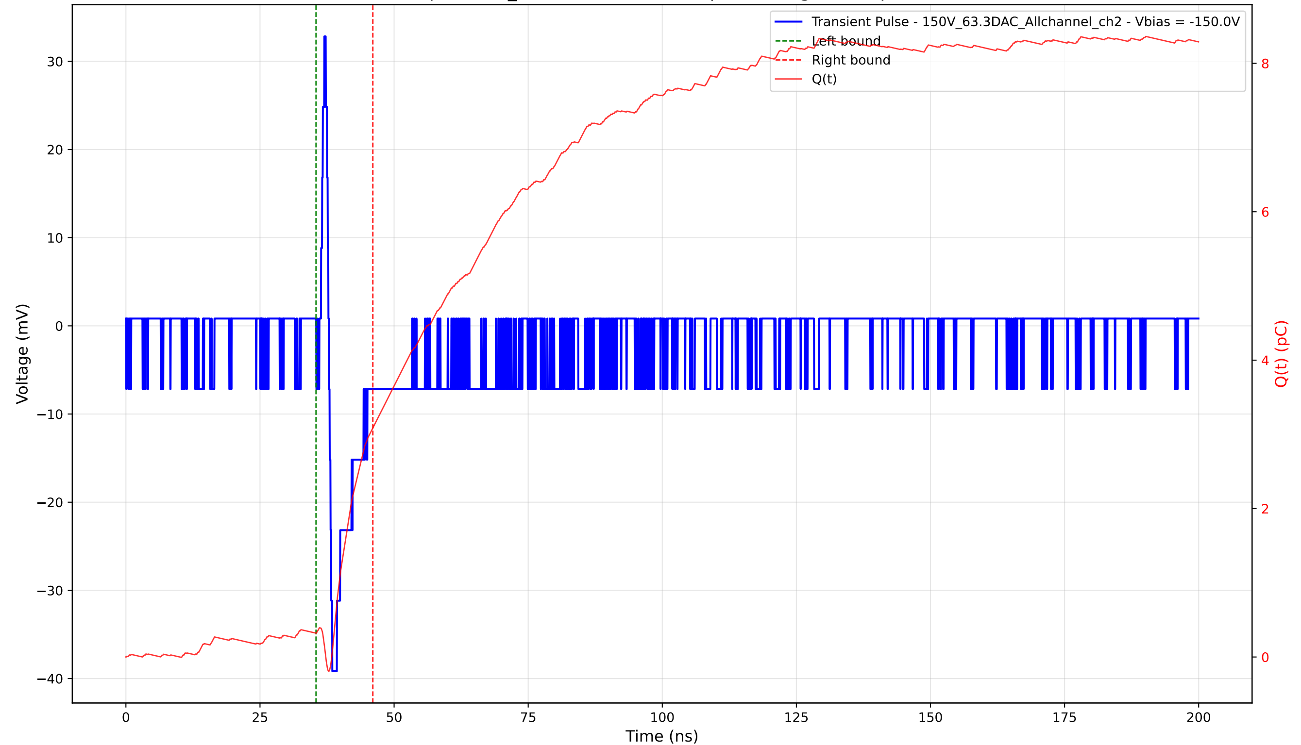
Transient Pulse - Sample: 1cm_42 - Position: 1045.0 \mu\text{m} - Charge: 2.77 pC - Rise Time: 0.62 ns
