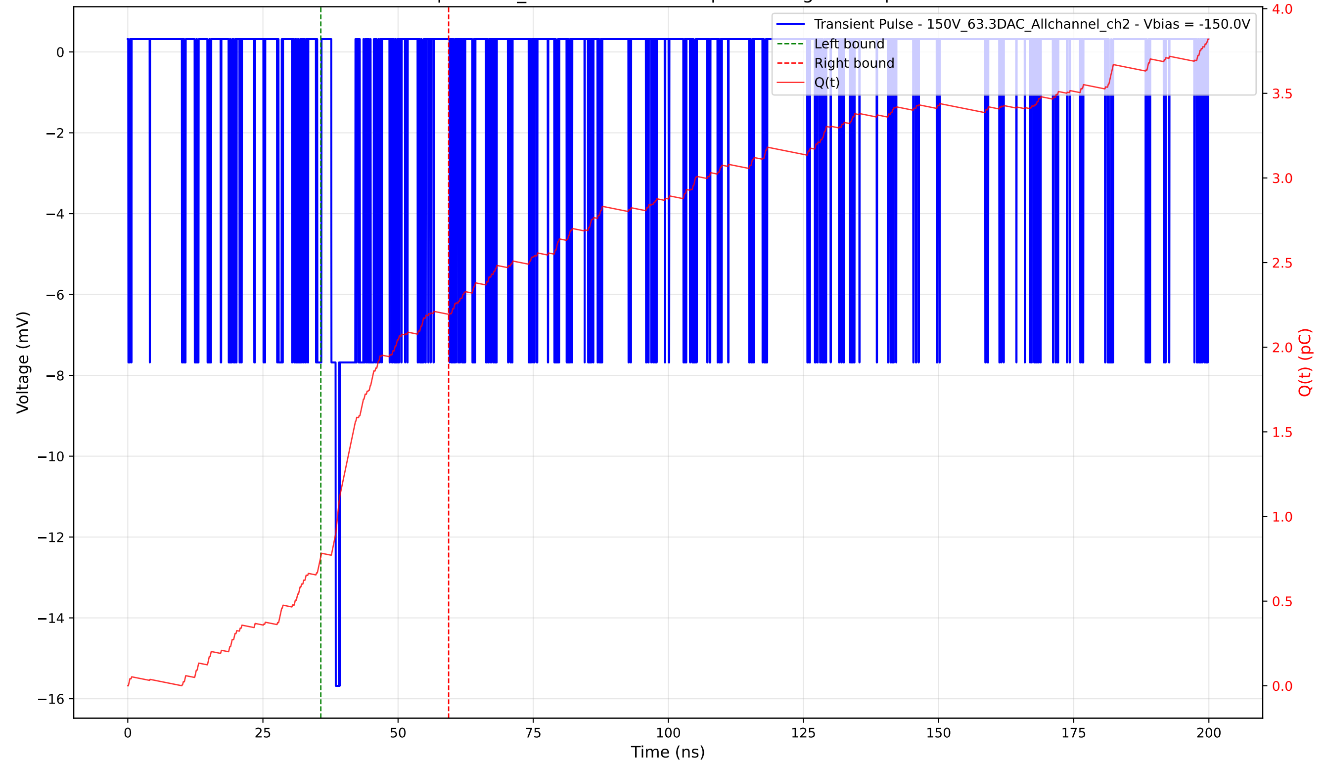
Transient Pulse - Sample: 1cm_42 - Position: 105.0 \mu\text{m} - Charge: 1.43 pC - Rise Time: 0.83 ns
