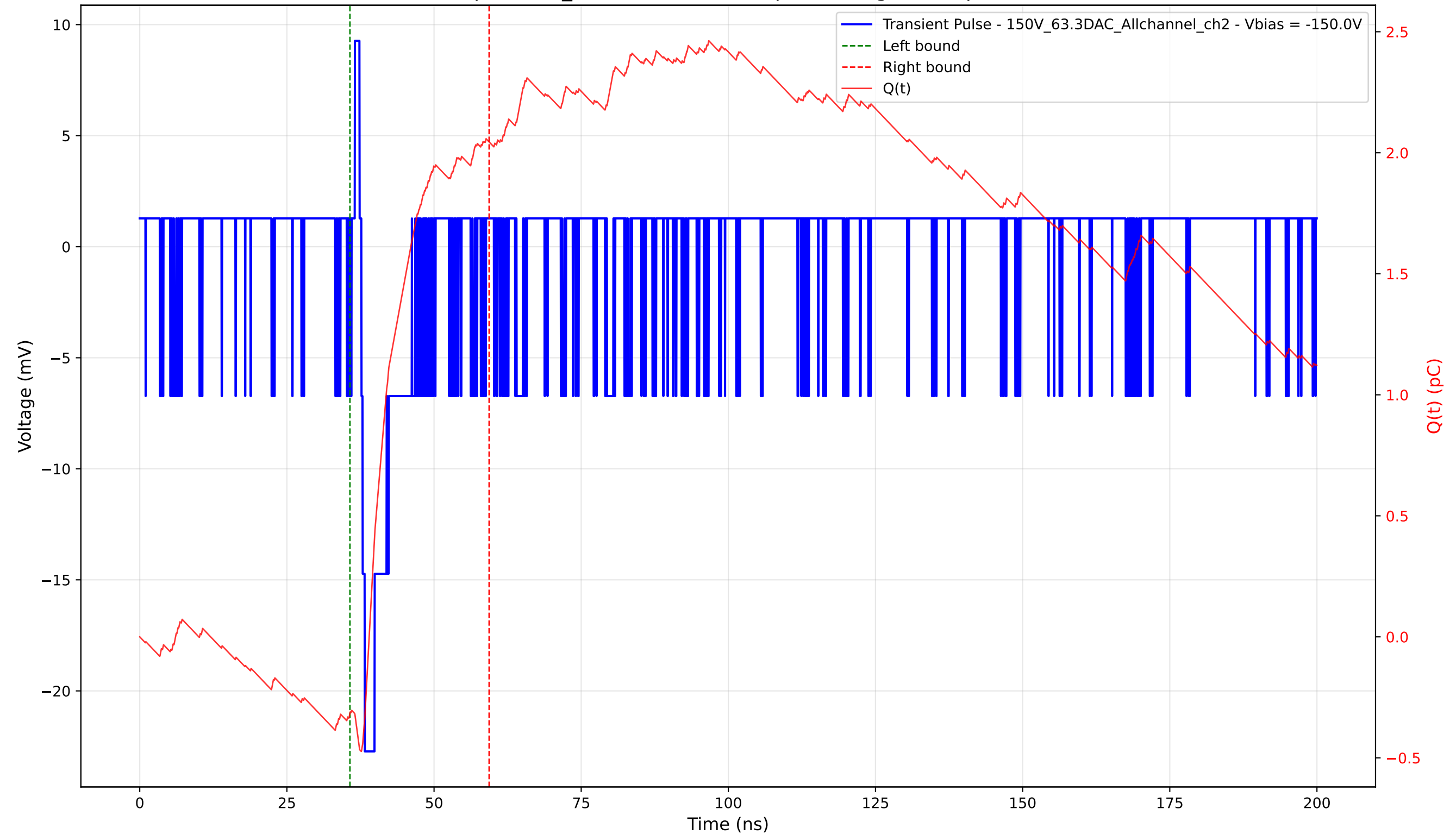
Transient Pulse - Sample: 1cm_42 - Position: 285.0 \mu\text{m} - Charge: 2.36 pC - Rise Time: 0.59 ns
