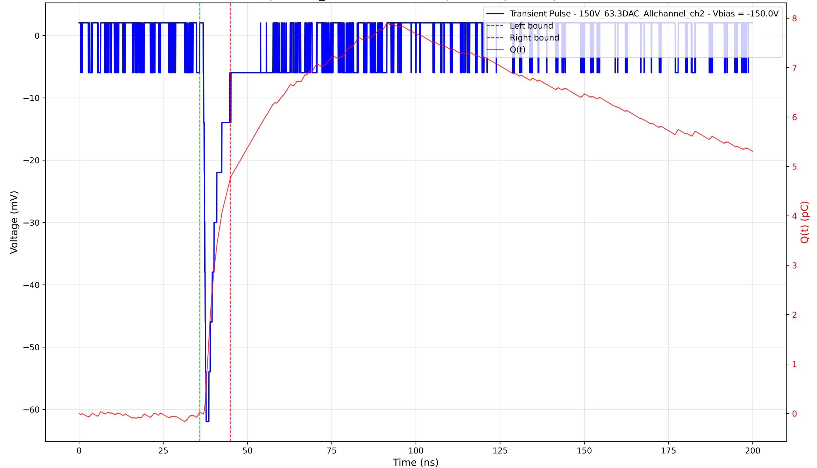
Transient Pulse - Sample: 1cm_42 - Position: 1955.0 \mu\text{m} - Charge: 4.71 pC - Rise Time: 0.72 ns
