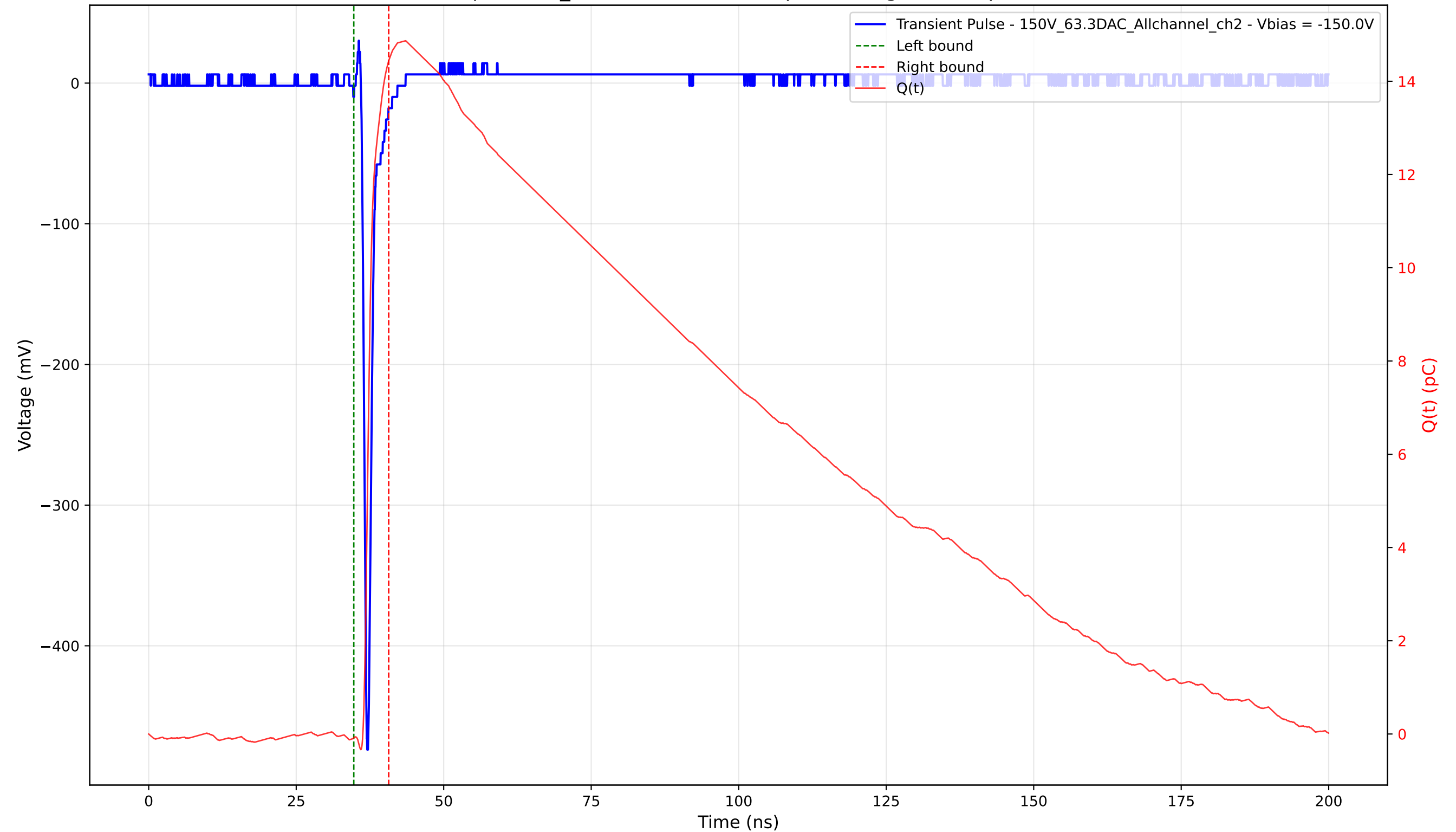
Transient Pulse - Sample: 1cm_42 - Position: 2950.0 \mu\text{m} - Charge: 14.52 pC - Rise Time: 0.67 ns
