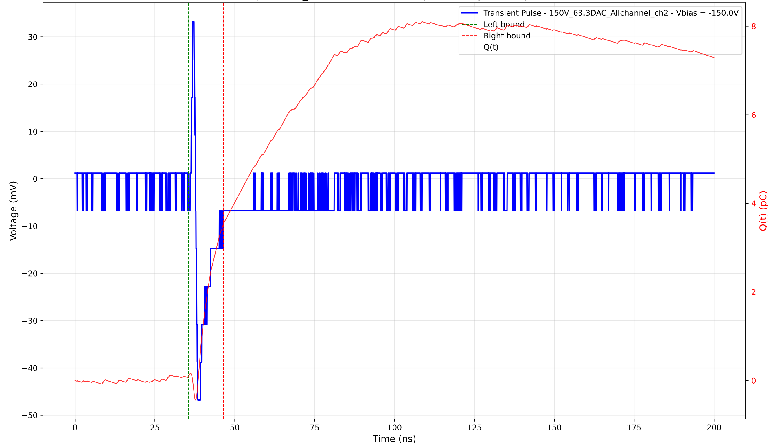
Transient Pulse - Sample: 1cm_42 - Position: 1315.0 \mu\text{m} - Charge: 3.45 pC - Rise Time: 0.66 ns
