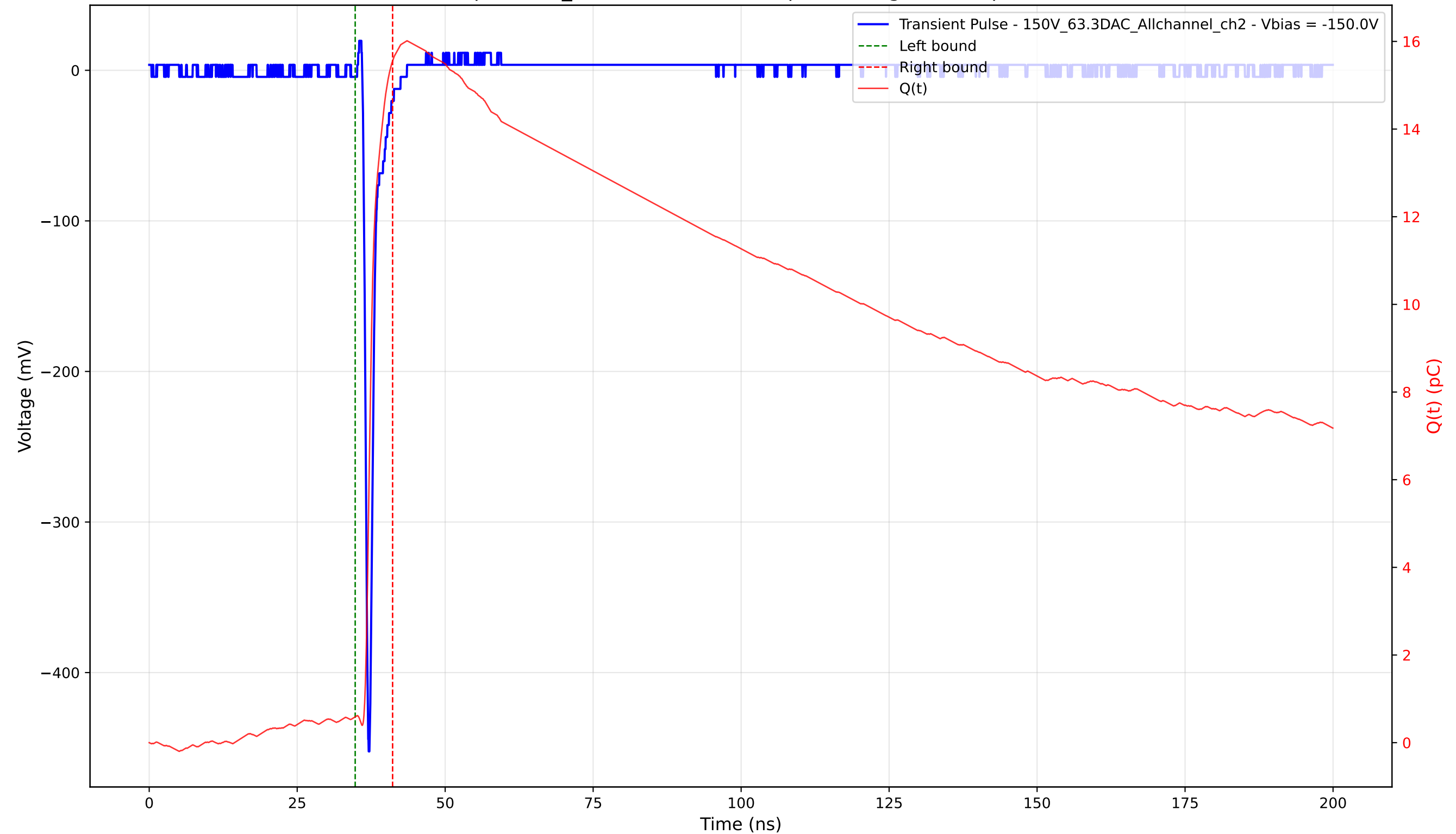
Transient Pulse - Sample: 1cm_42 - Position: 3220.0 \mu\text{m} - Charge: 14.96 pC - Rise Time: 0.69 ns
