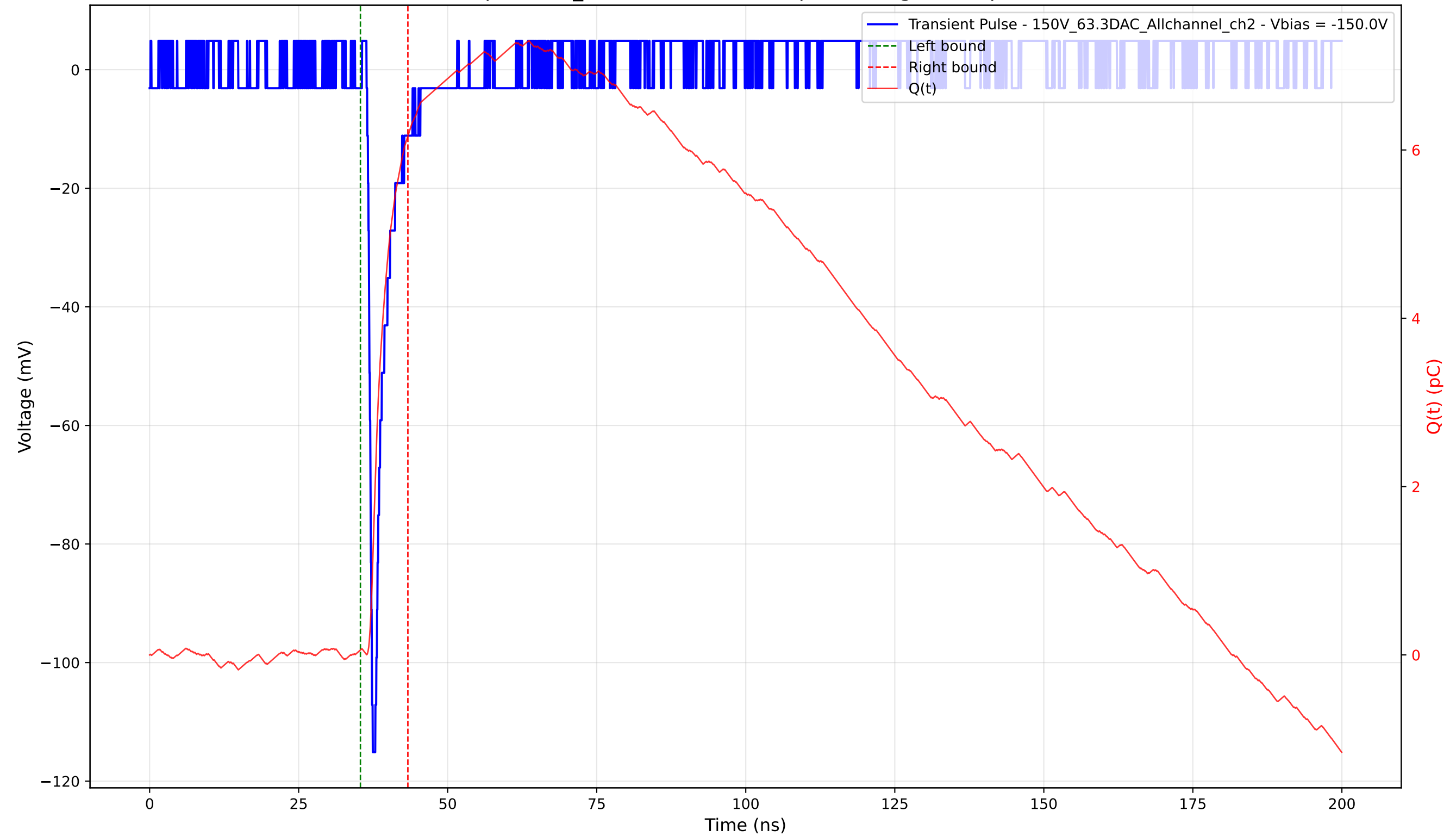
Transient Pulse - Sample: 1cm_42 - Position: 2195.0 \mu\text{m} - Charge: 6.11 pC - Rise Time: 0.72 ns
