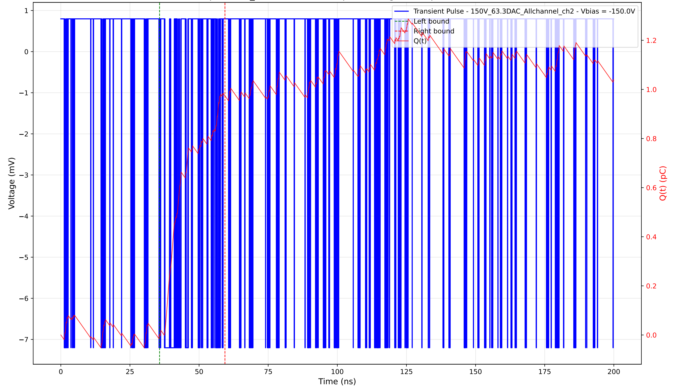
Transient Pulse - Sample: 1cm_42 - Position: 30.0 \mu\text{m} - Charge: 0.97 pC - Rise Time: 0.00 ns (N/A)
