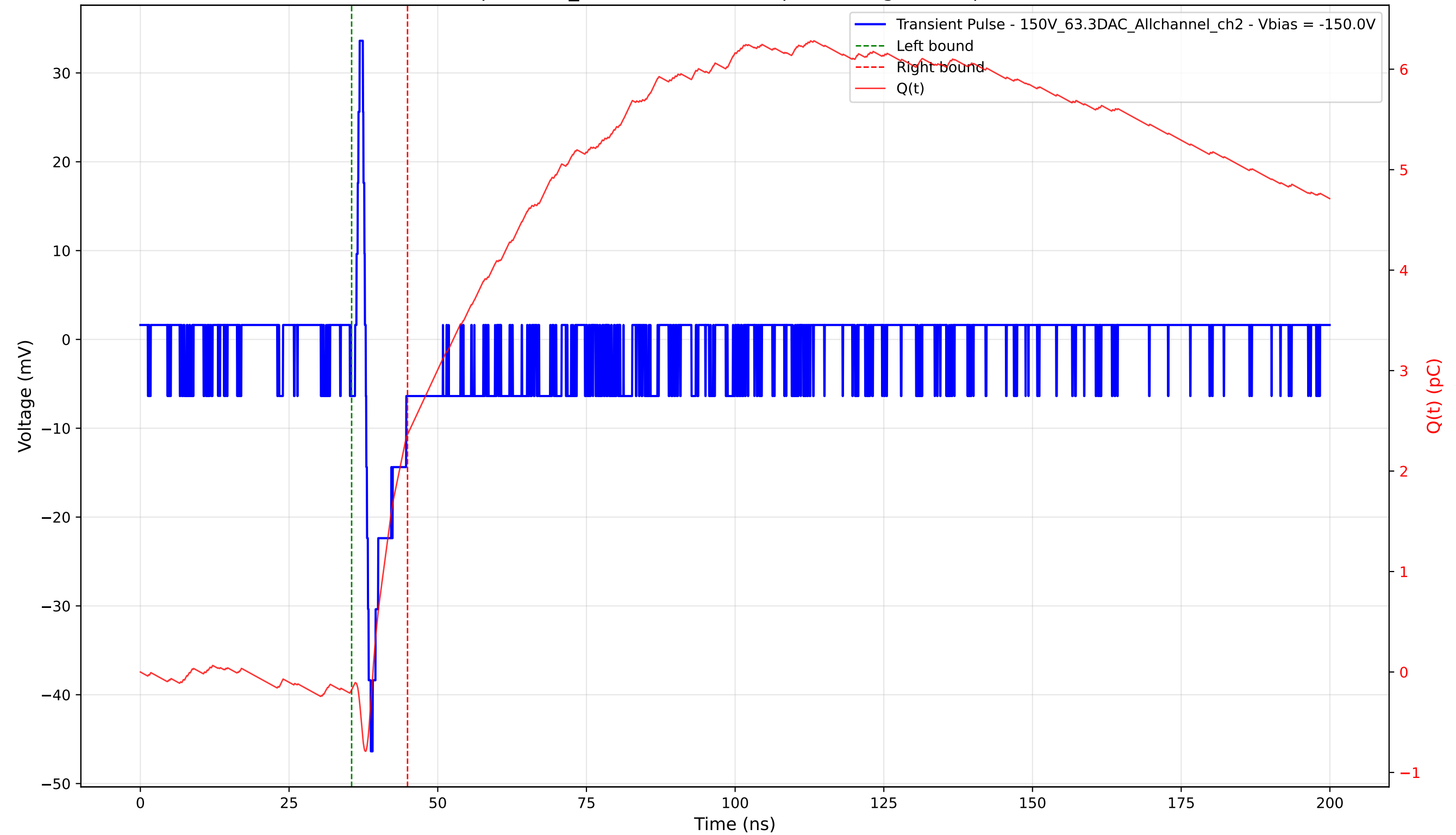
Transient Pulse - Sample: 1cm_42 - Position: 815.0 \mu\text{m} - Charge: 2.54 pC - Rise Time: 0.85 ns
