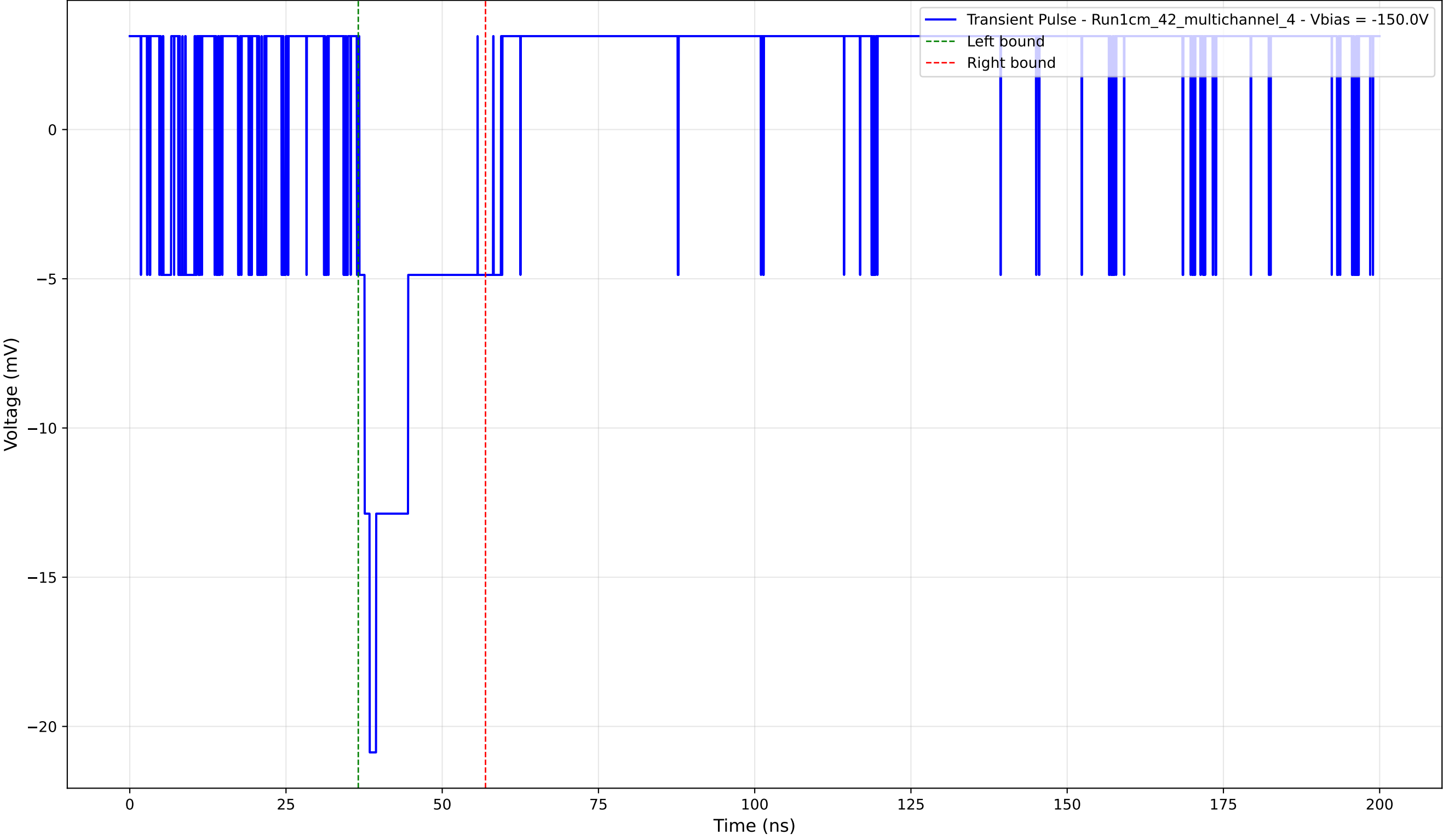
Transient Pulse - Sample: 1cm_42_multichannel - Position: 955.0 \mu\text{m} - Charge: 3.24 pC - Rise Time: 0.00 ns (N/A)
