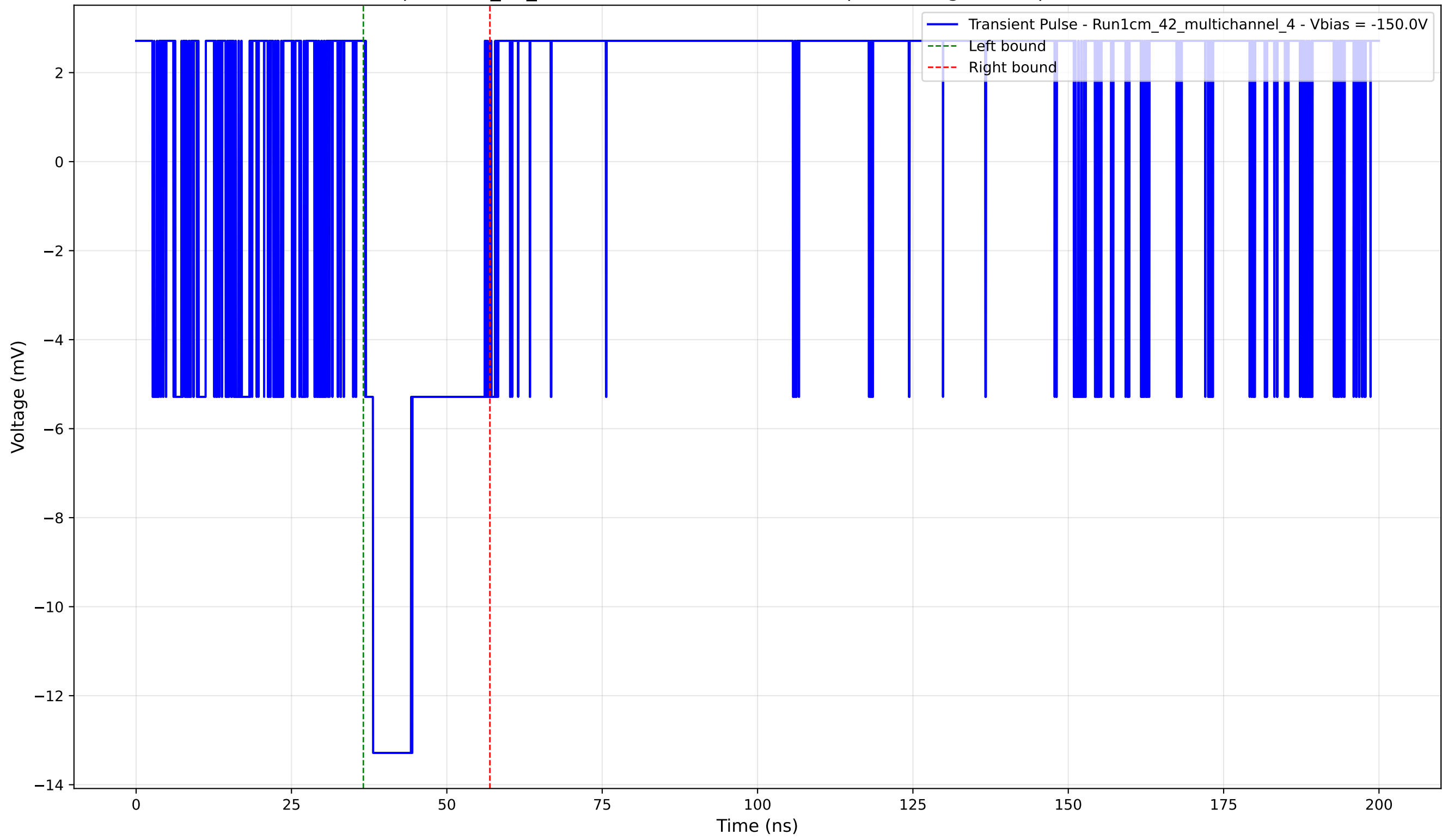
Transient Pulse - Sample: 1cm_42_multichannel - Position: 510.0 \mu\text{m} - Charge: 3.05 pC - Rise Time: 0.00 ns (N/A)
