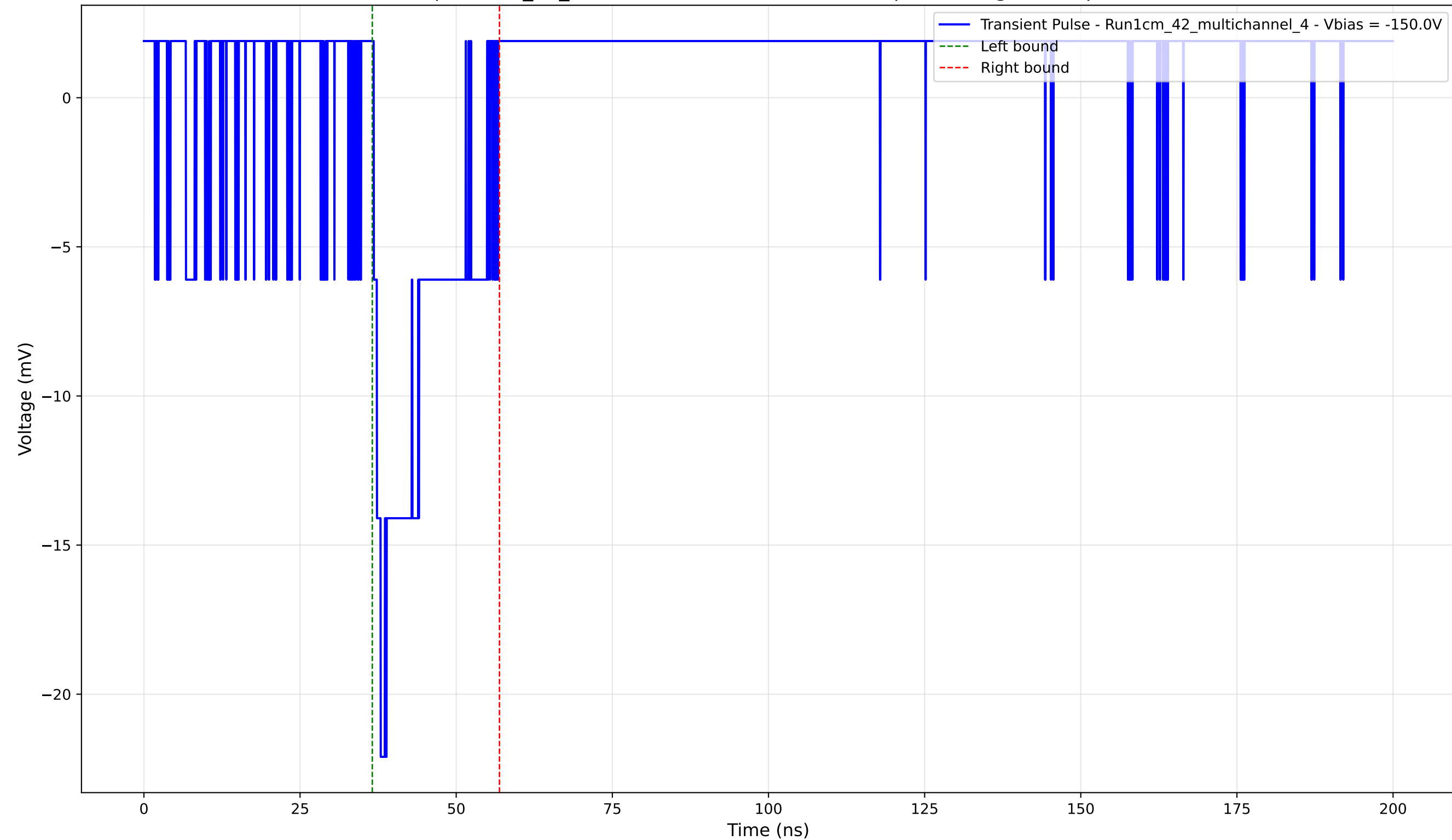
Transient Pulse - Sample: 1cm_42_multichannel - Position: 3575.0 \mu\text{m} - Charge: 3.37 pC - Rise Time: 1.12 ns
