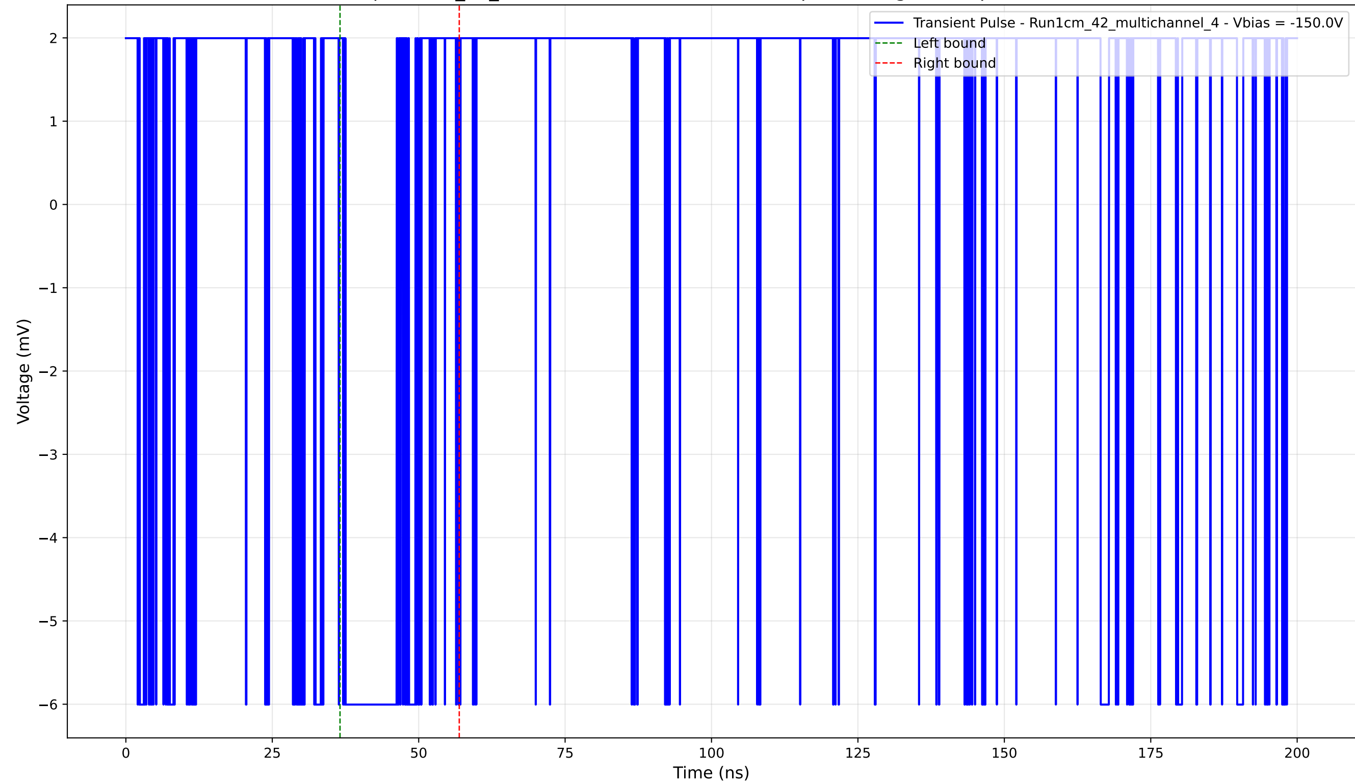
Transient Pulse - Sample: 1cm_42_multichannel - Position: 4865.0 \mu\text{m} - Charge: 1.10 pC - Rise Time: 0.00 ns (N/A)
