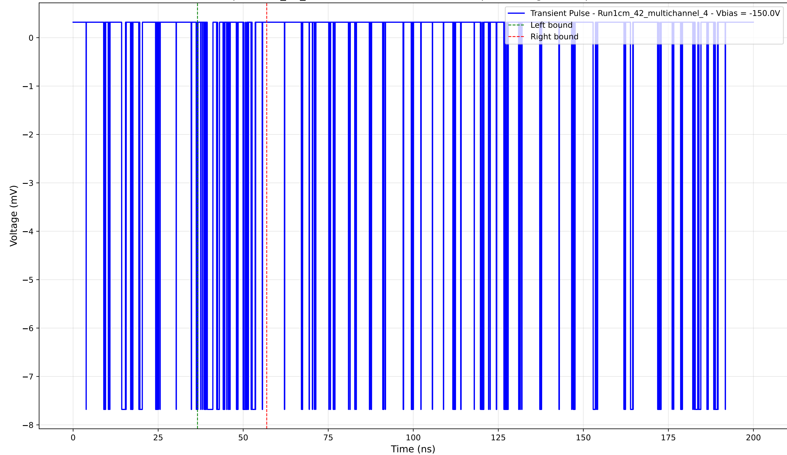
Transient Pulse - Sample: 1cm_42_multichannel - Position: 3920.0 \mu\text{m} - Charge: 0.92 pC - Rise Time: 0.02 ns
