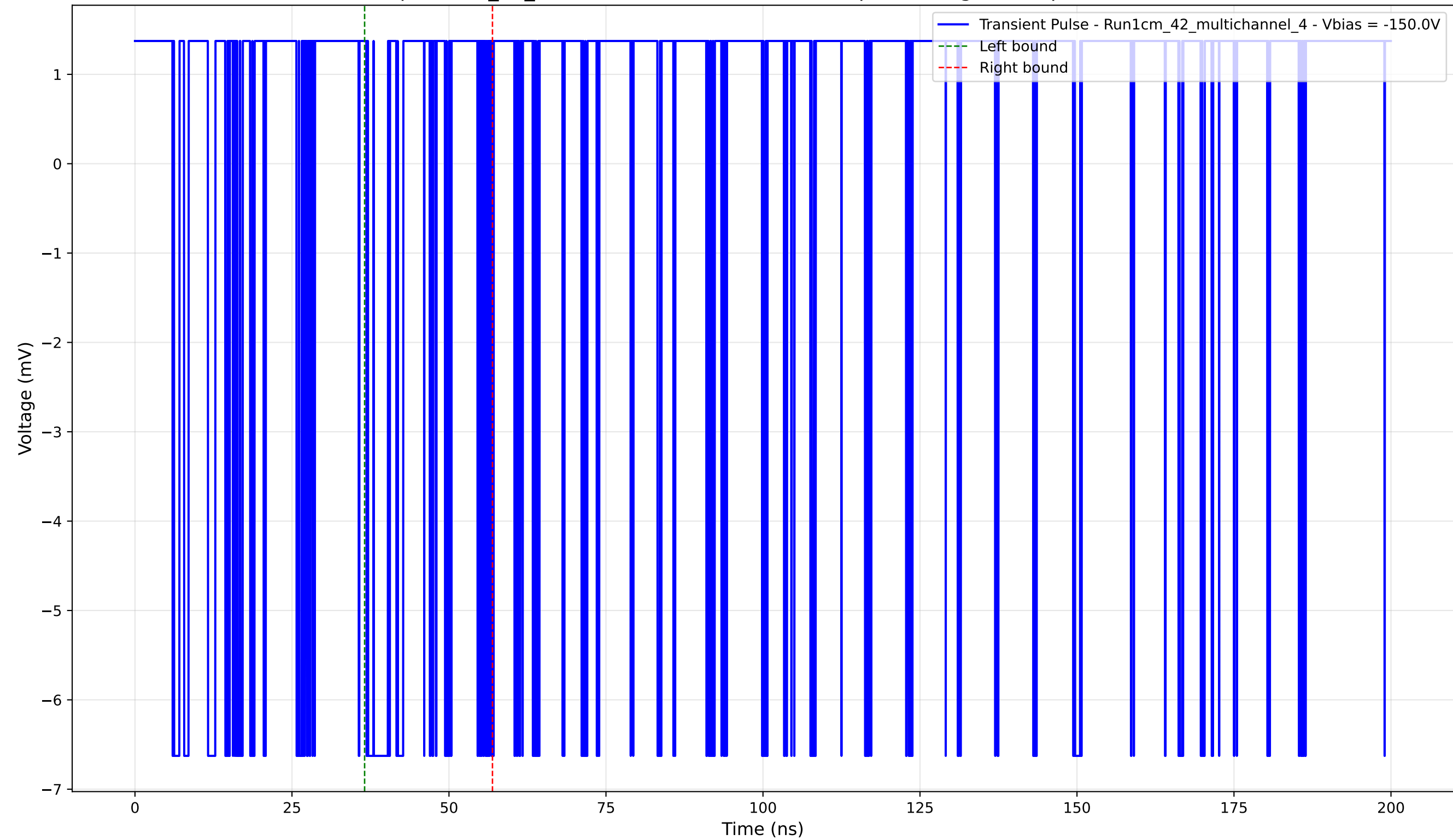
Transient Pulse - Sample: 1cm_42_multichannel - Position: 1870.0 \mu\text{m} - Charge: 0.47 pC - Rise Time: 0.00 ns (N/A)
