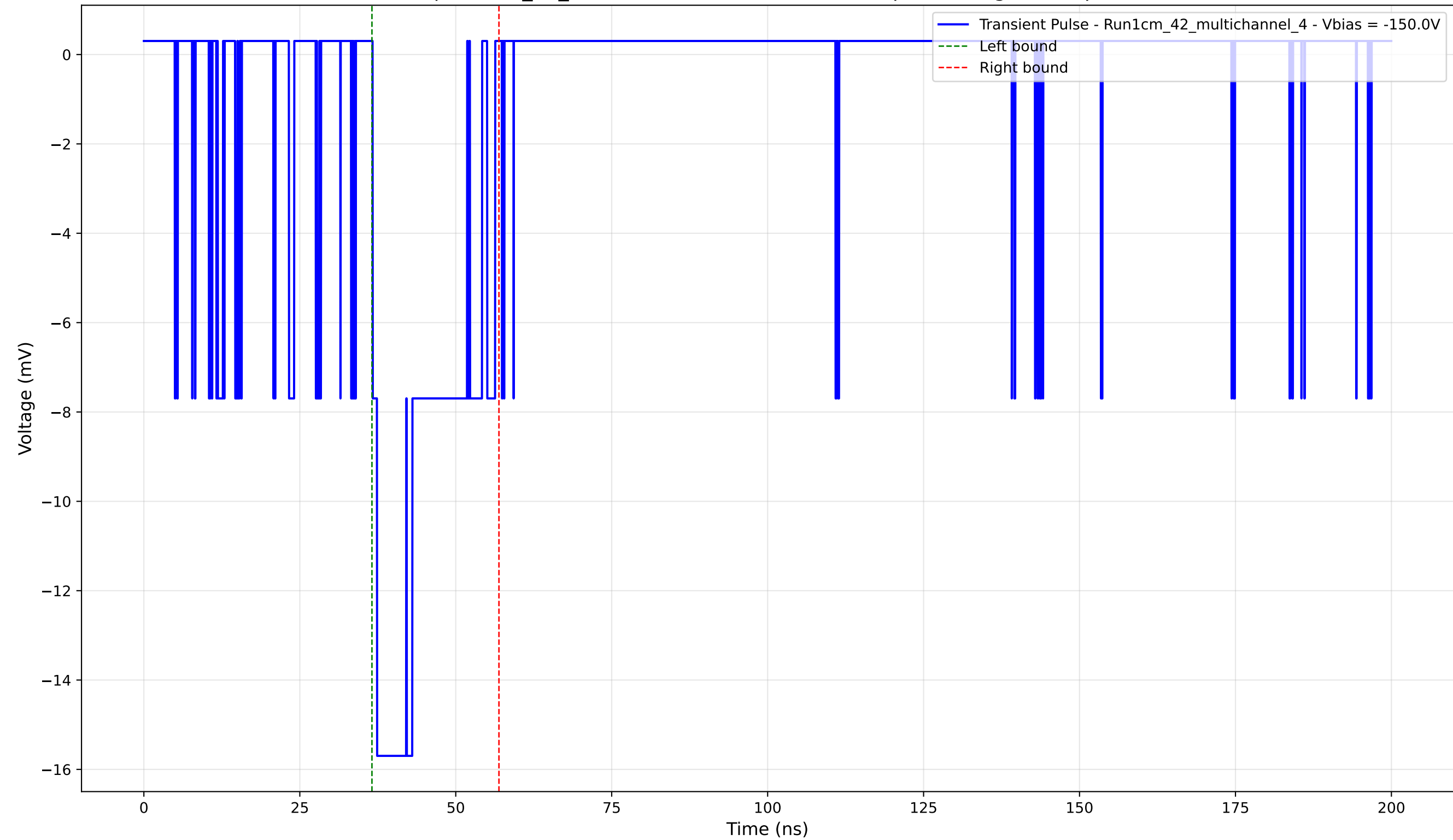
Transient Pulse - Sample: 1cm_42_multichannel - Position: 3600.0 \mu\text{m} - Charge: 3.74 pC - Rise Time: 0.72 ns
