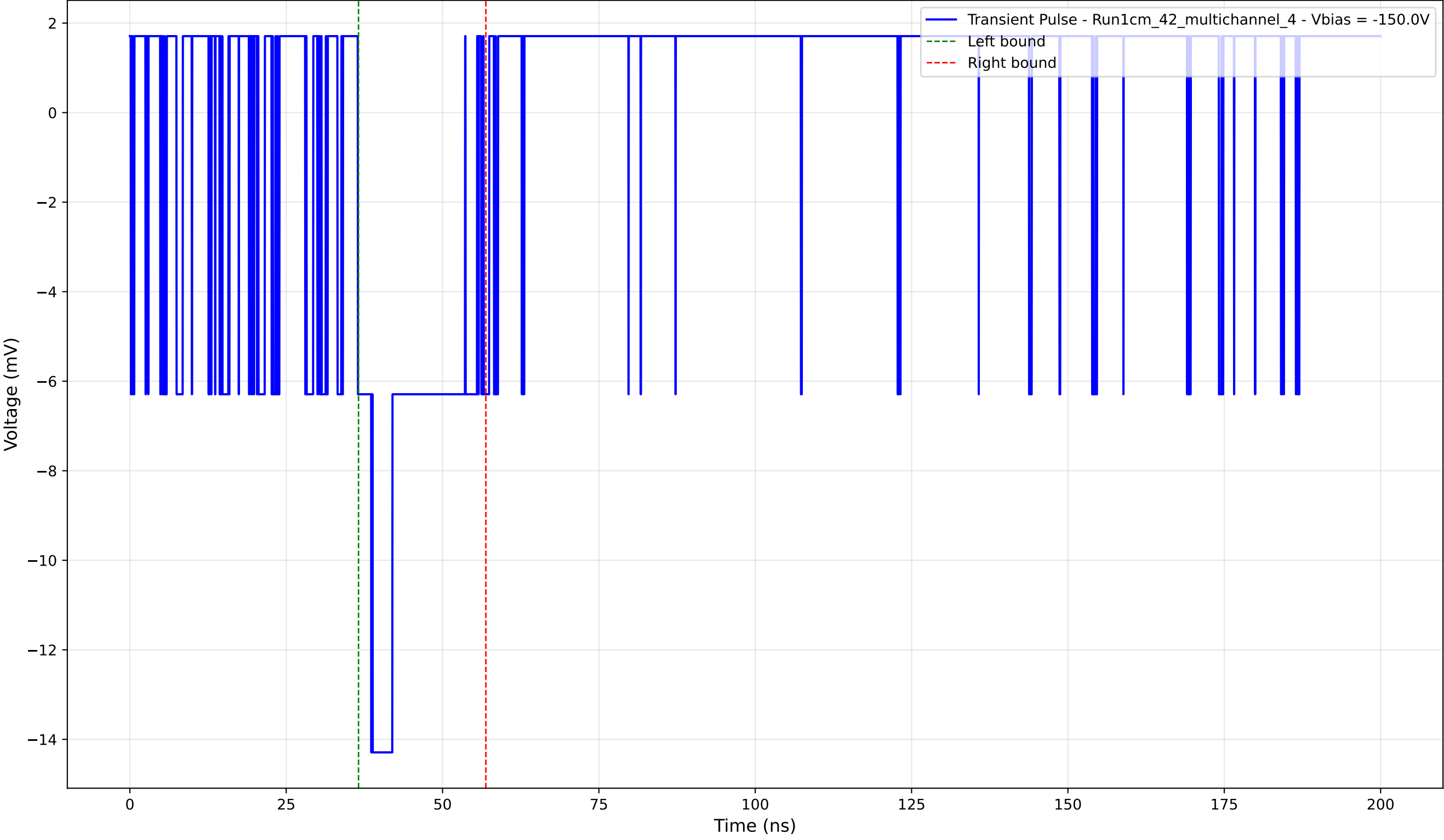
Transient Pulse - Sample: 1cm_42_multichannel - Position: 140.0 \mu\text{m} - Charge: 2.97 pC - Rise Time: 0.00 ns (N/A)
