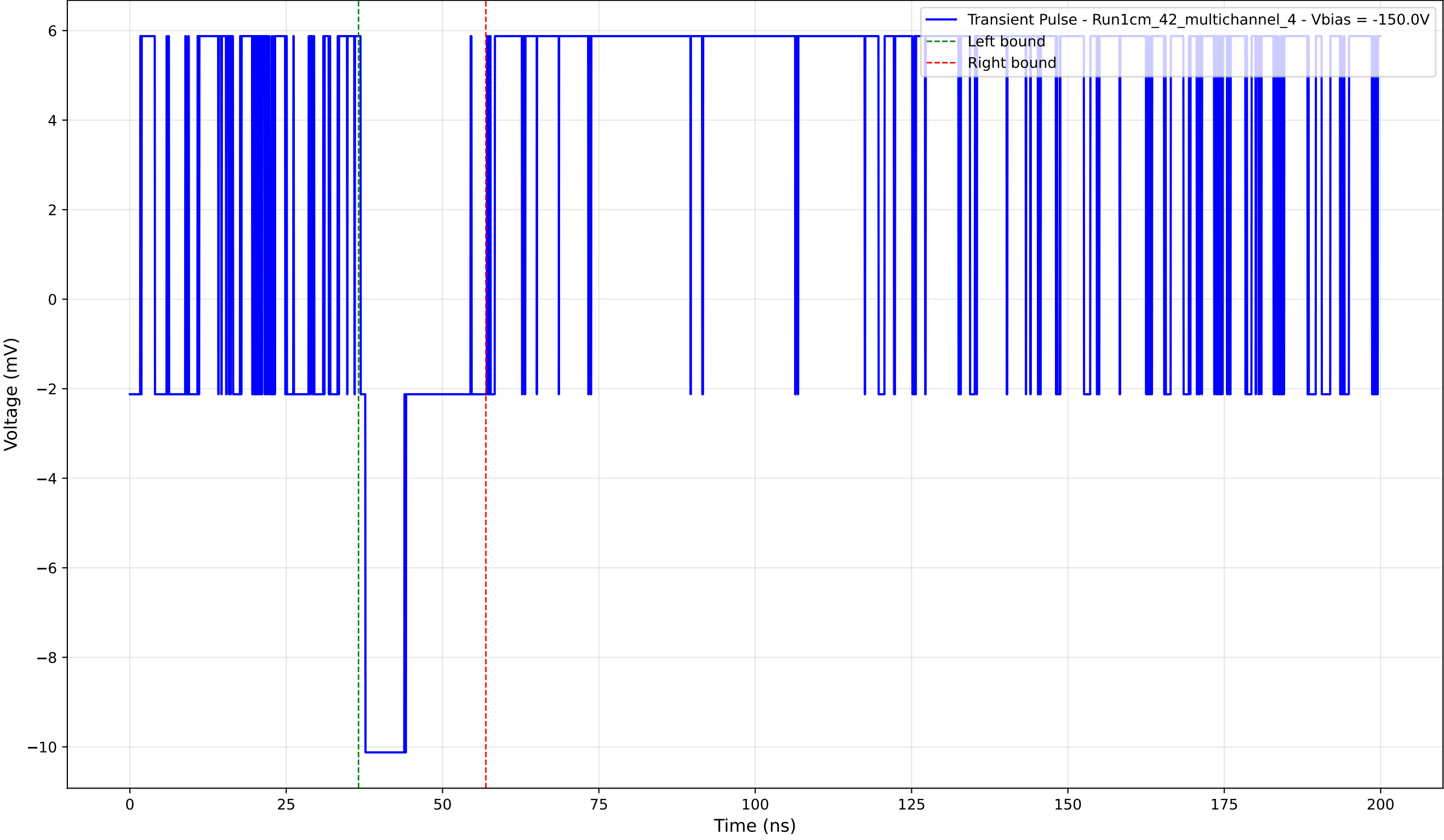
Transient Pulse - Sample: 1cm_42_multichannel - Position: 755.0 \mu\text{m} - Charge: 1.81 pC - Rise Time: 0.00 ns (N/A)
