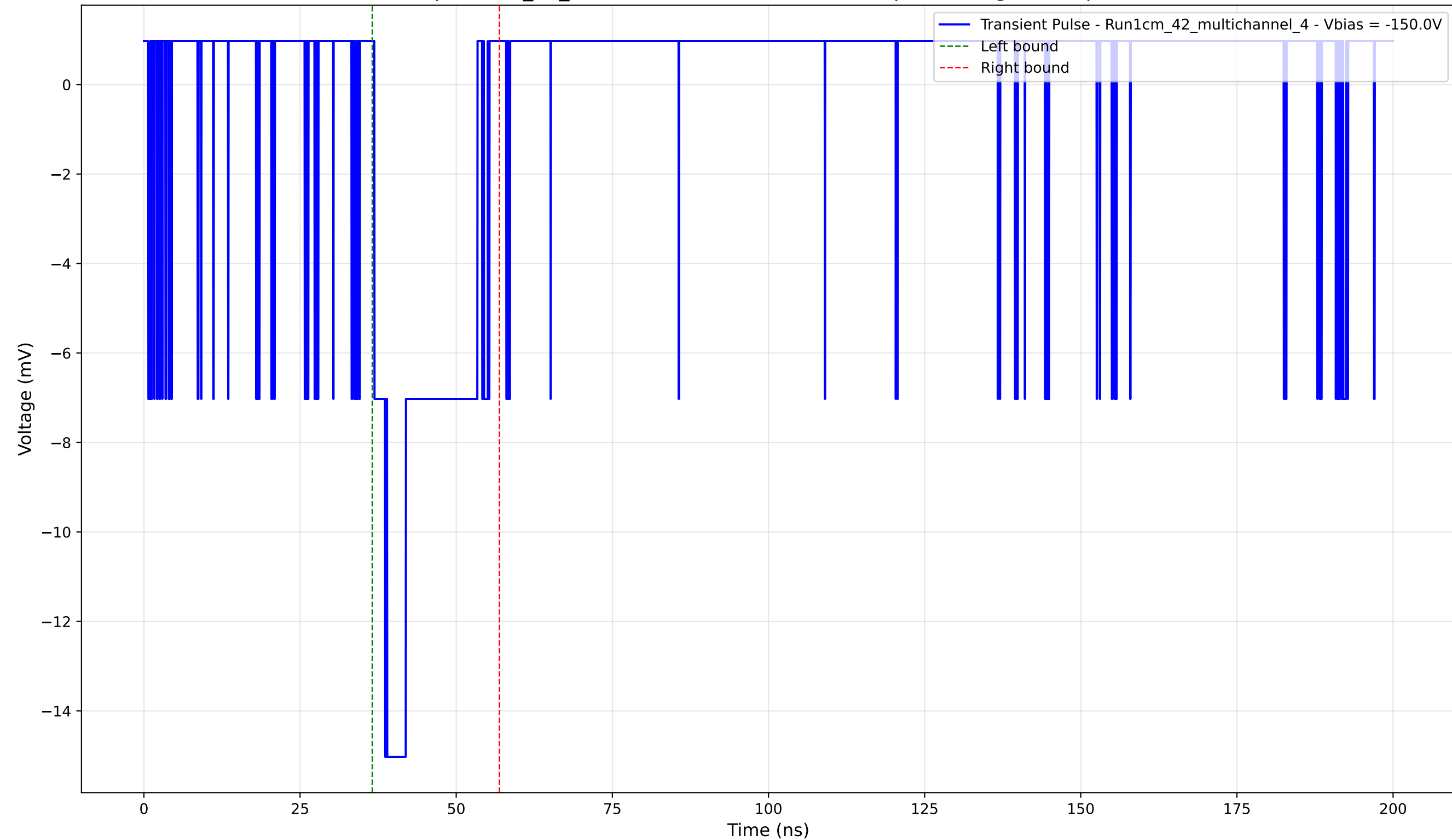
Transient Pulse - Sample: 1cm_42_multichannel - Position: 4765.0 \mu\text{m} - Charge: 2.93 pC - Rise Time: 1.74 ns
