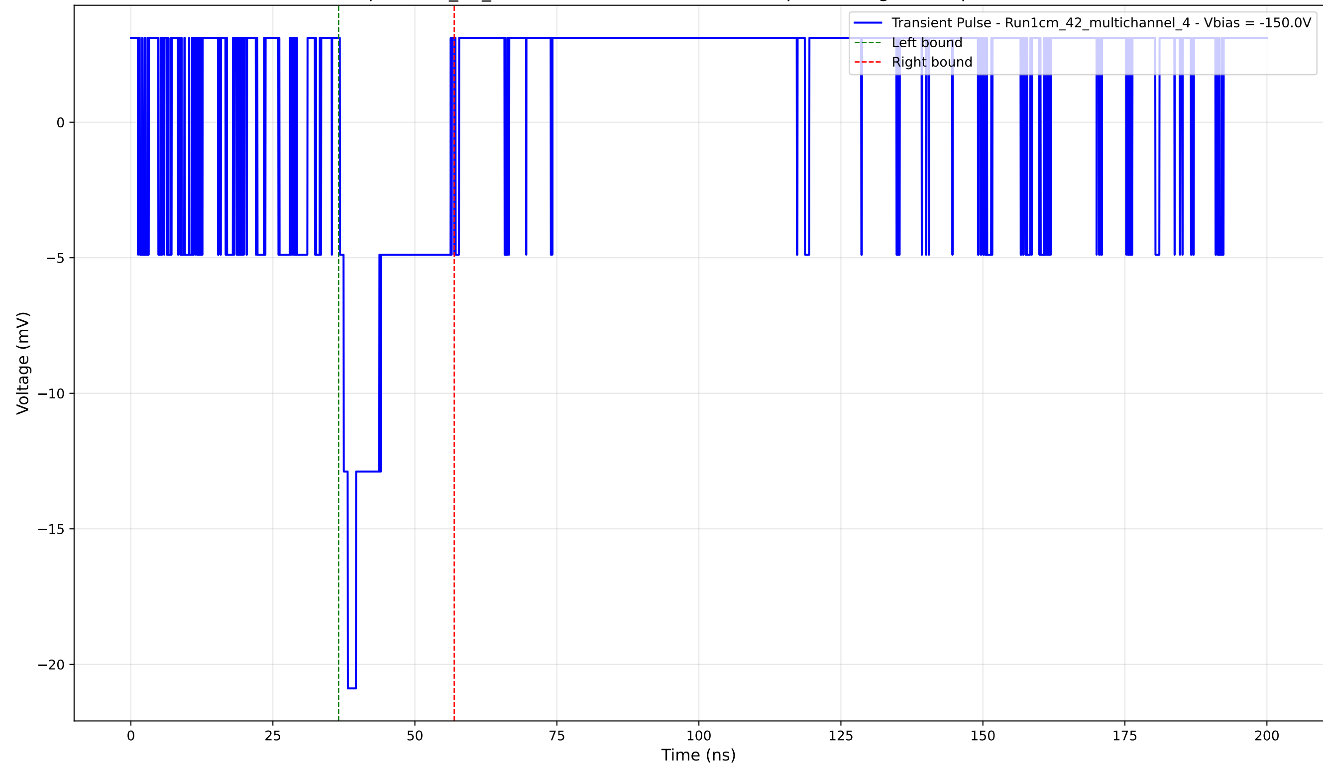
Transient Pulse - Sample: 1cm_42_multichannel - Position: 1050.0 \mu\text{m} - Charge: 3.15 pC - Rise Time: 0.00 ns (N/A)
