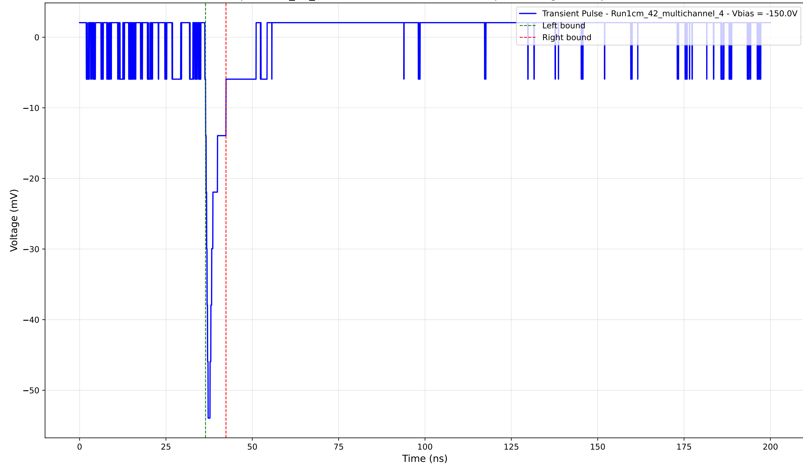
Transient Pulse - Sample: 1cm_42_multichannel - Position: 2760.0 \mu\text{m} - Charge: 2.92 pC - Rise Time: 0.94 ns
