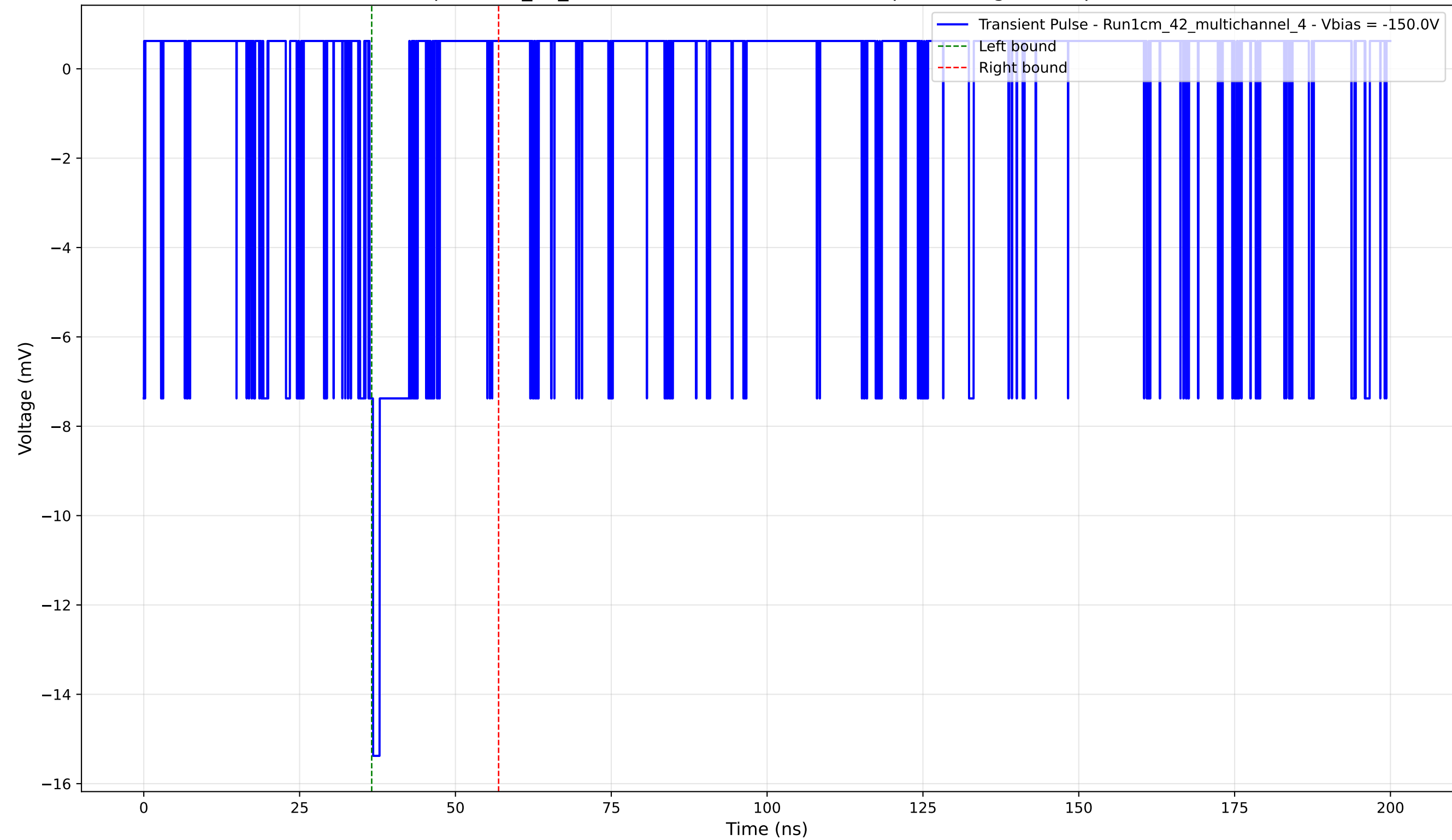
Transient Pulse - Sample: 1cm_42_multichannel - Position: 2350.0 \mu\text{m} - Charge: 1.21 pC - Rise Time: 0.58 ns
