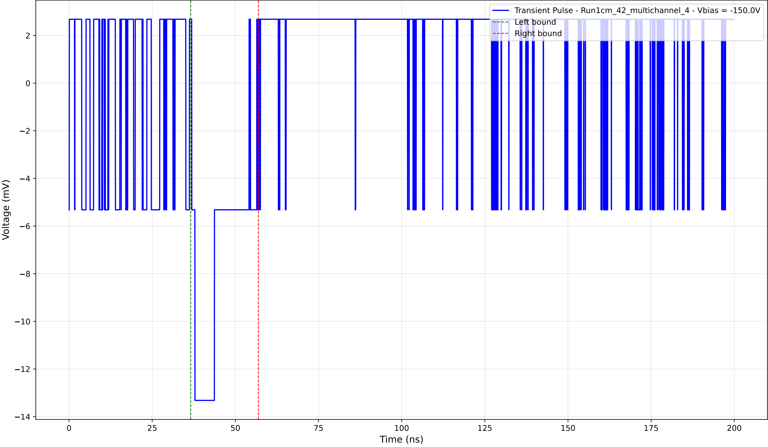
Transient Pulse - Sample: 1cm_42_multichannel - Position: 705.0 \mu\text{m} - Charge: 2.98 pC - Rise Time: 0.00 ns (N/A)
