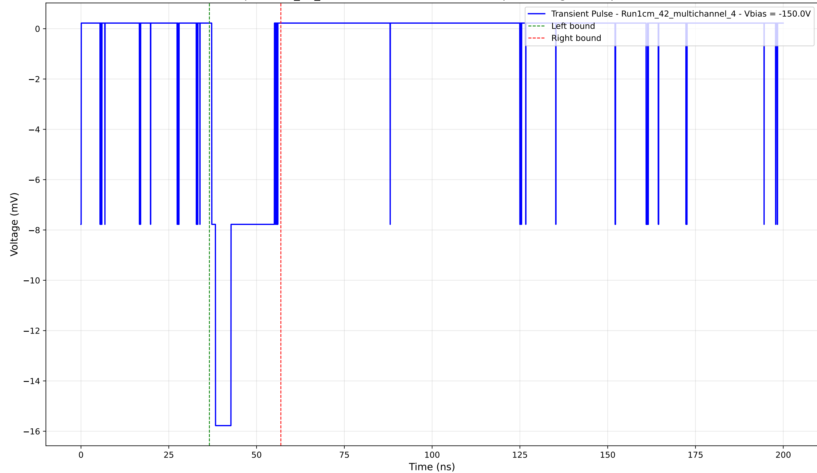
Transient Pulse - Sample: 1cm_42_multichannel - Position: 4140.0 \mu\text{m} - Charge: 3.52 pC - Rise Time: 1.08 ns
