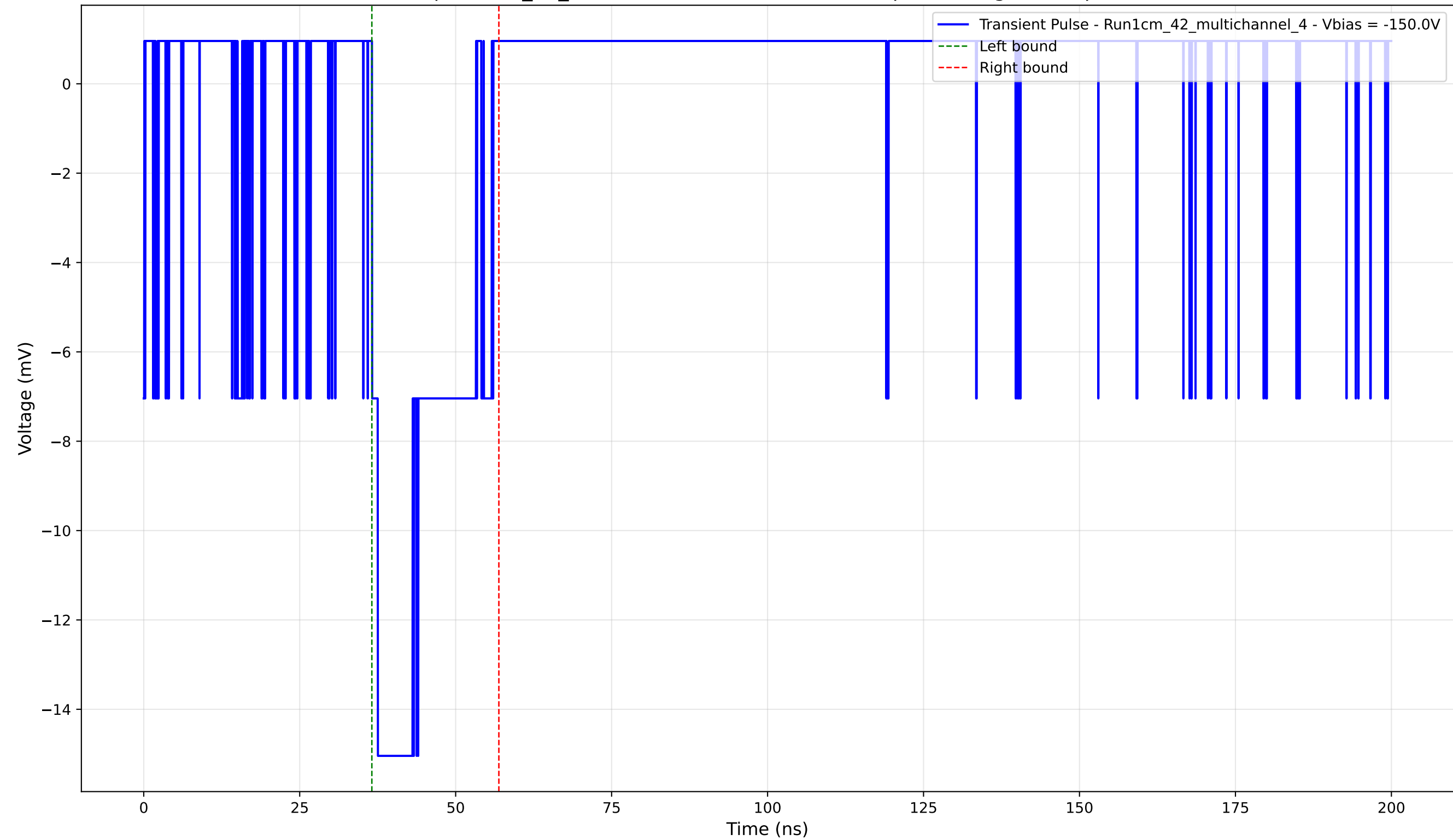
Transient Pulse - Sample: 1cm_42_multichannel - Position: 3750.0 \mu\text{m} - Charge: 3.49 pC - Rise Time: 0.94 ns
