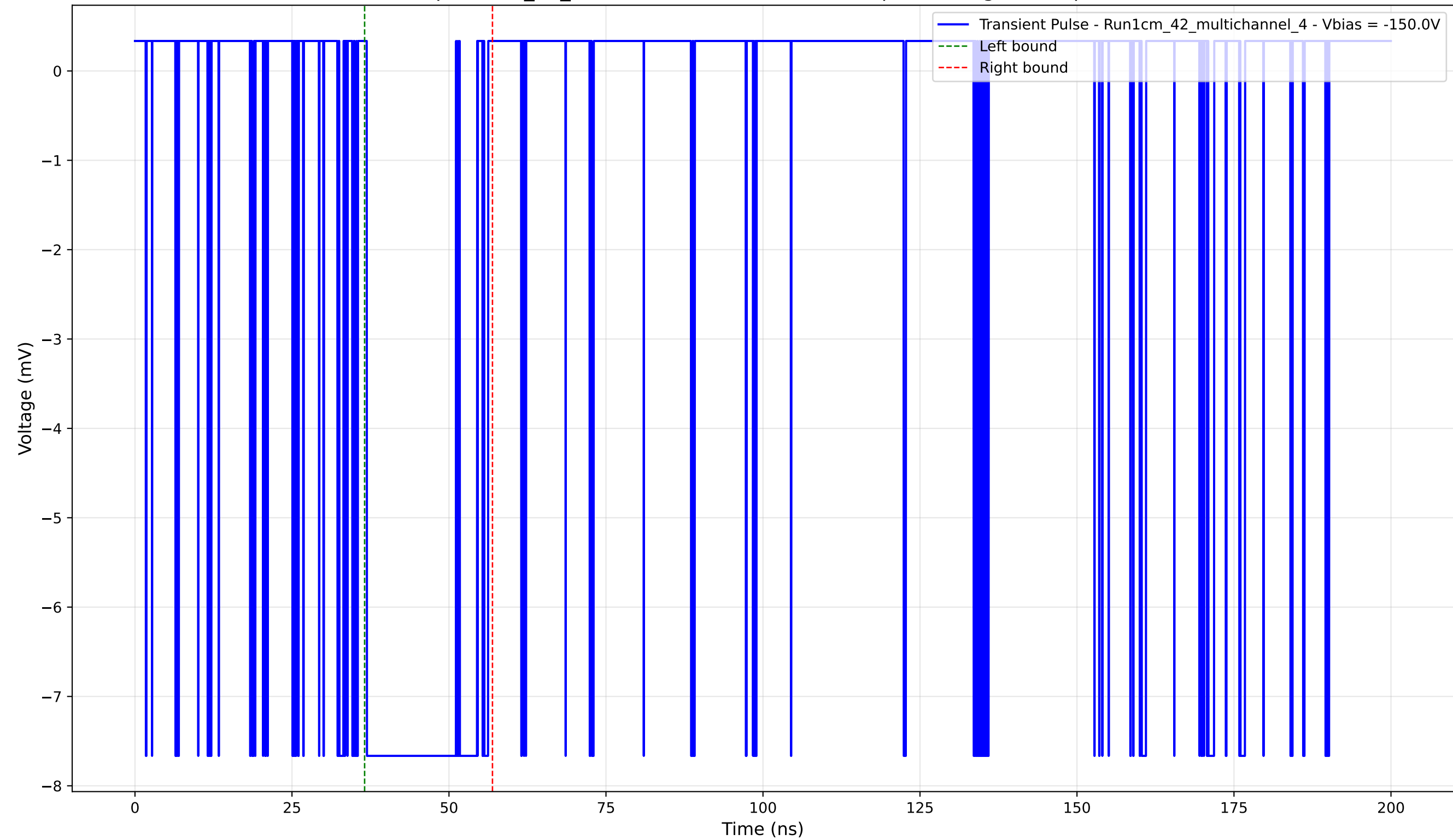
Transient Pulse - Sample: 1cm_42_multichannel - Position: 100.0 \mu\text{m} - Charge: 2.77 pC - Rise Time: 0.02 ns
