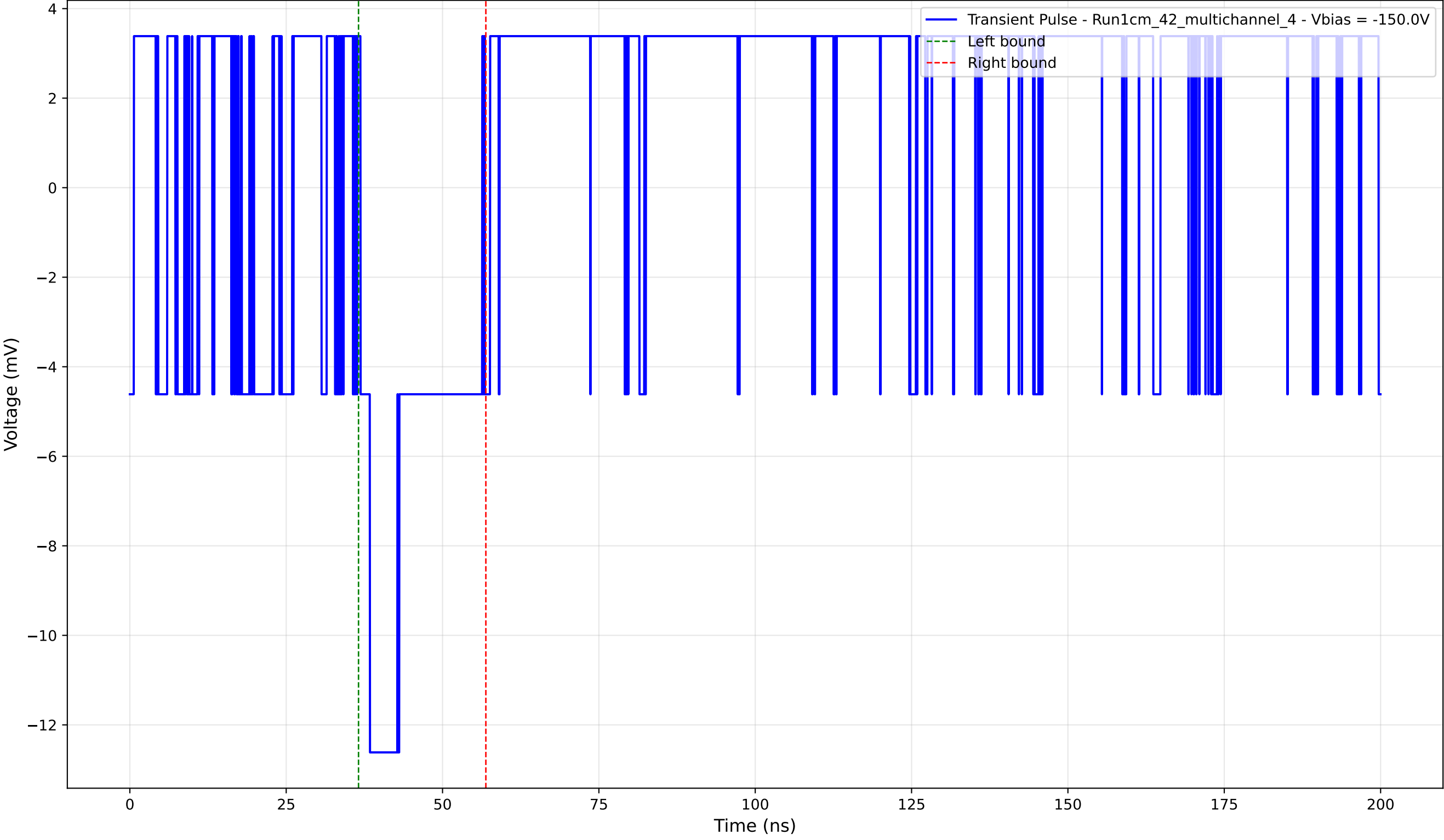
Transient Pulse - Sample: 1cm_42_multichannel - Position: 245.0 \mu\text{m} - Charge: 2.54 pC - Rise Time: 0.00 ns (N/A)
