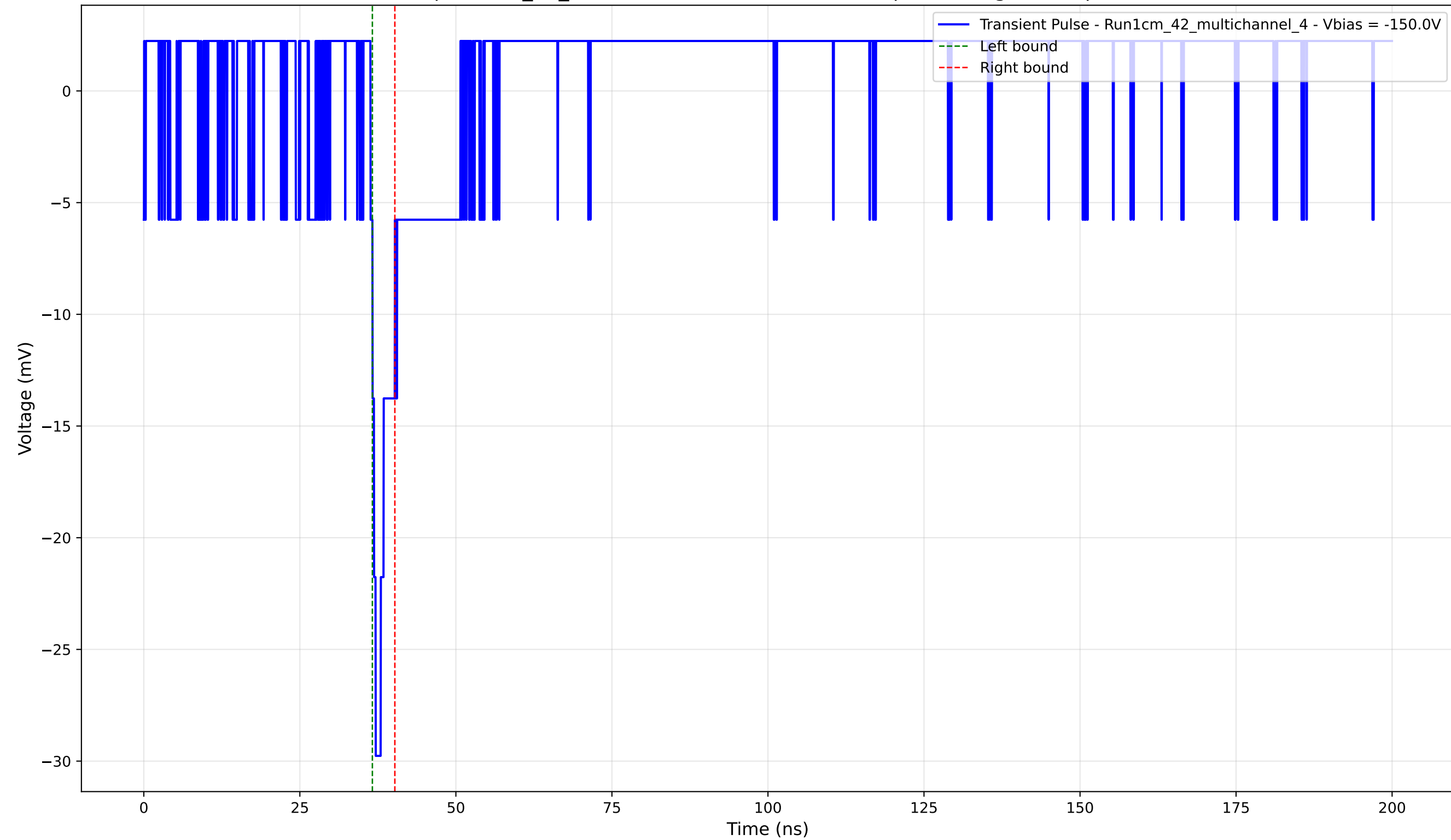
Transient Pulse - Sample: 1cm_42_multichannel - Position: 2835.0 \mu\text{m} - Charge: 1.37 pC - Rise Time: 0.84 ns
