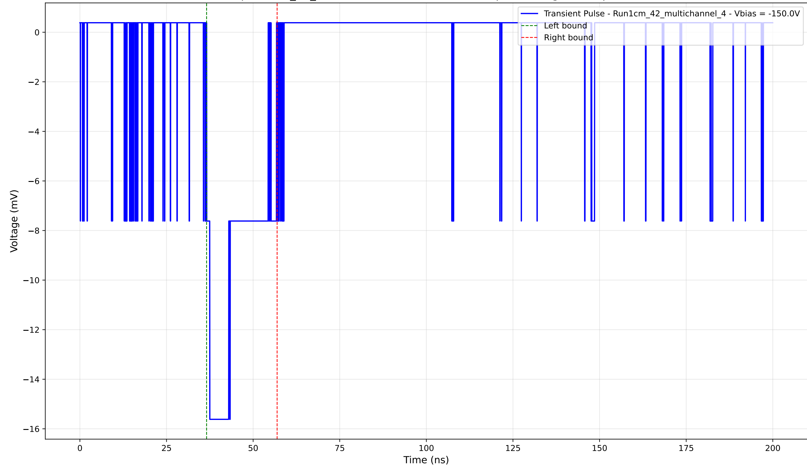
Transient Pulse - Sample: 1cm_42_multichannel - Position: 3620.0 \mu\text{m} - Charge: 3.87 pC - Rise Time: 0.90 ns
