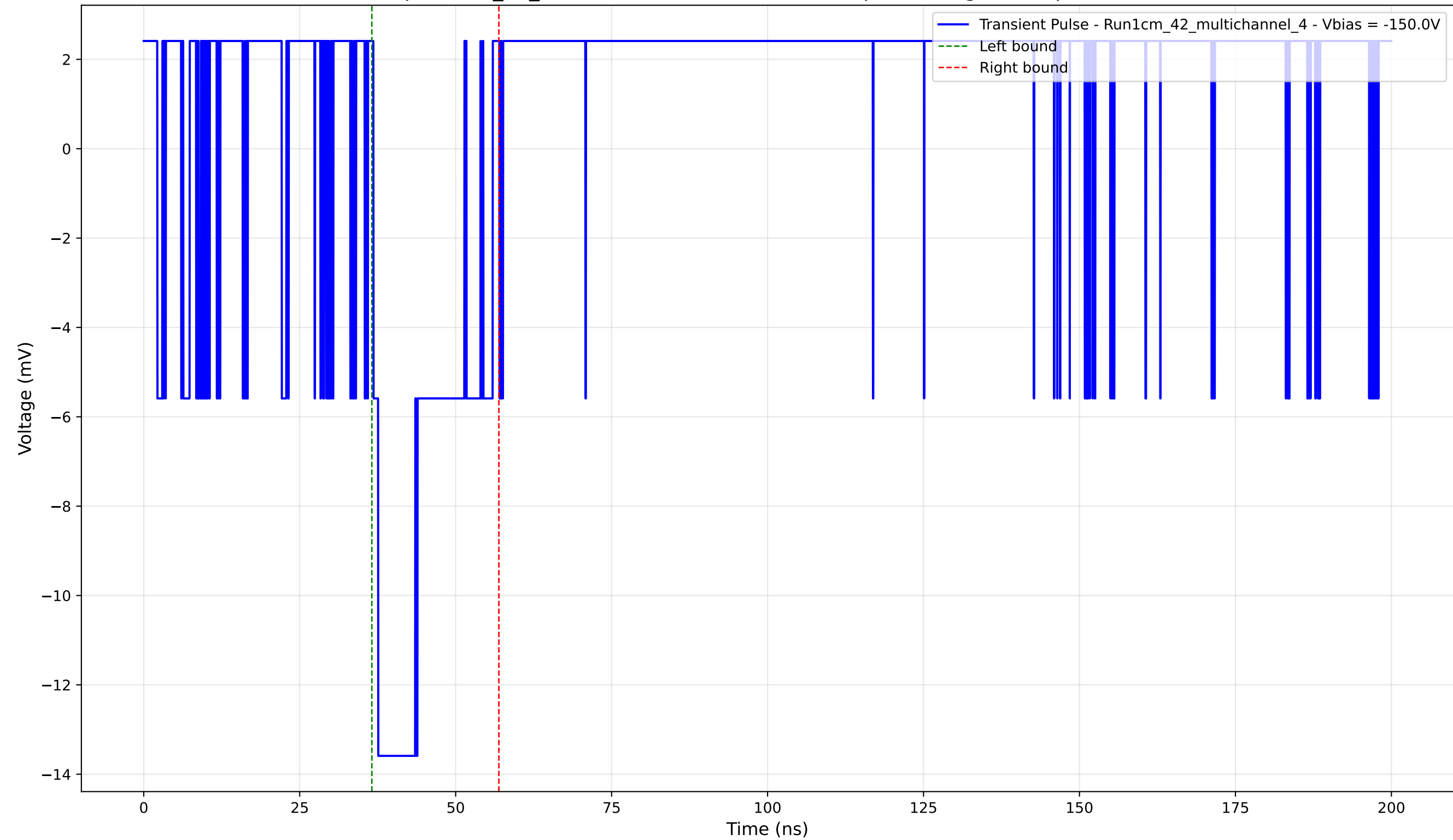
Transient Pulse - Sample: 1cm_42_multichannel - Position: 3770.0 \mu\text{m} - Charge: 2.99 pC - Rise Time: 0.00 ns (N/A)
