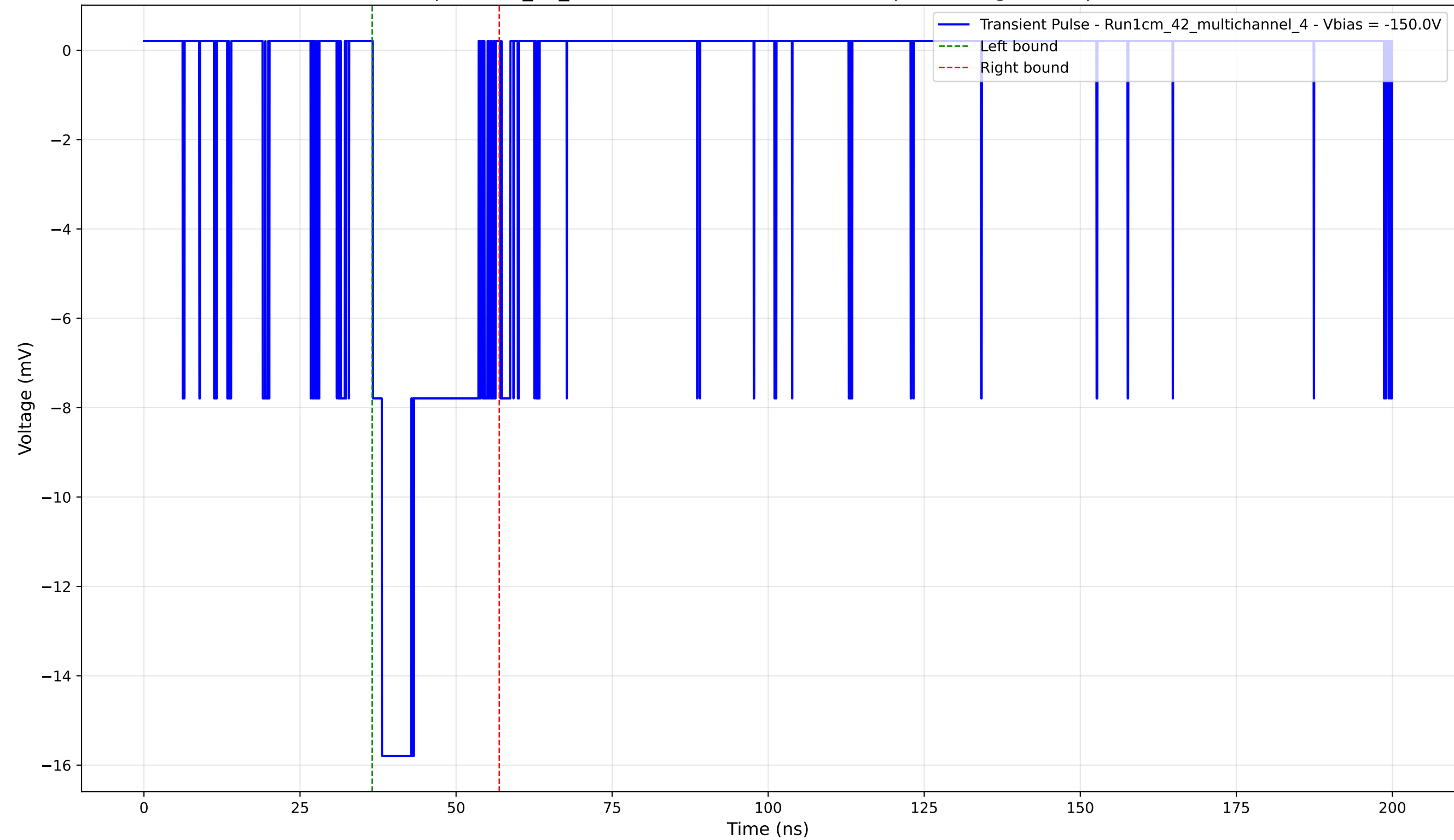
Transient Pulse - Sample: 1cm_42_multichannel - Position: 4125.0 \mu\text{m} - Charge: 3.68 pC - Rise Time: 1.48 ns
