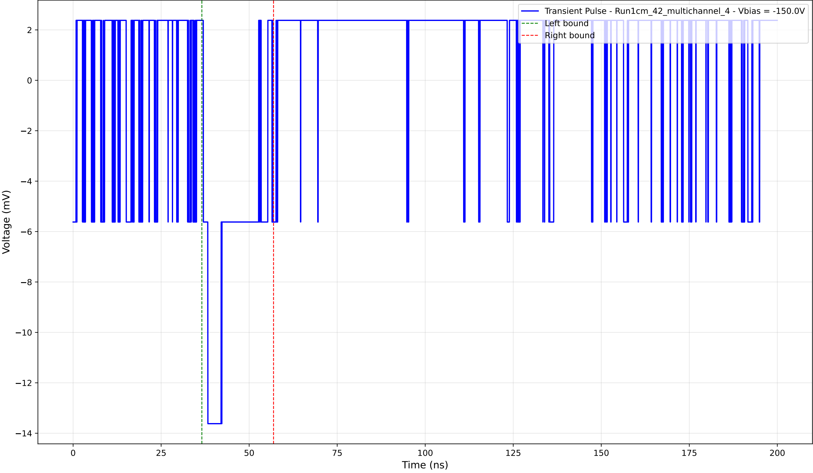
Transient Pulse - Sample: 1cm_42_multichannel - Position: 170.0 \mu\text{m} - Charge: 2.55 pC - Rise Time: 0.00 ns (N/A)
