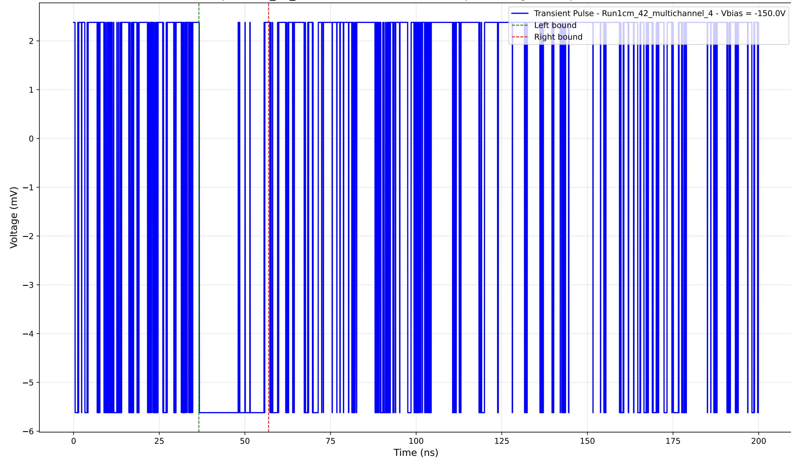
Transient Pulse - Sample: 1cm_42_multichannel - Position: 825.0 \mu\text{m} - Charge: 2.01 pC - Rise Time: 0.00 ns (N/A)
