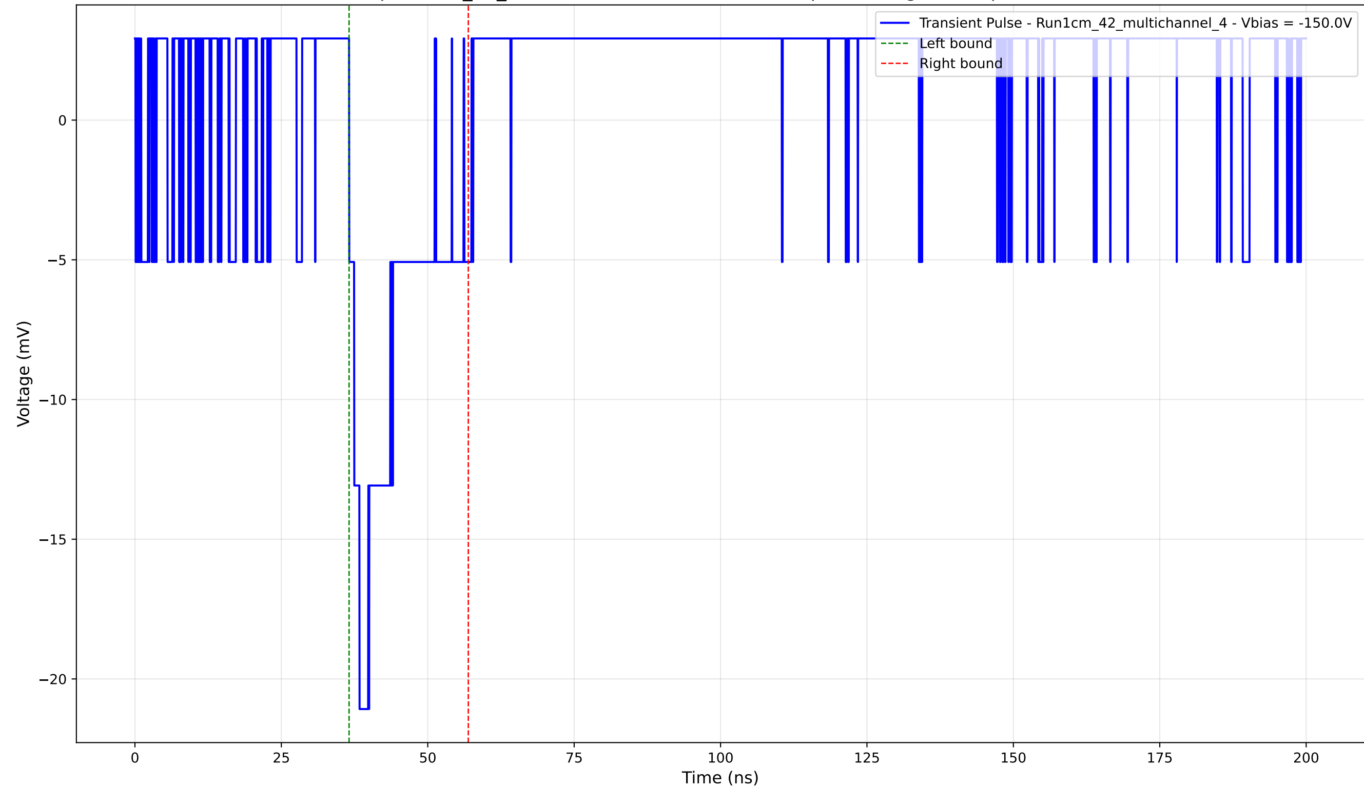
Transient Pulse - Sample: 1cm_42_multichannel - Position: 1040.0 \mu\text{m} - Charge: 3.28 pC - Rise Time: 0.00 ns (N/A)
