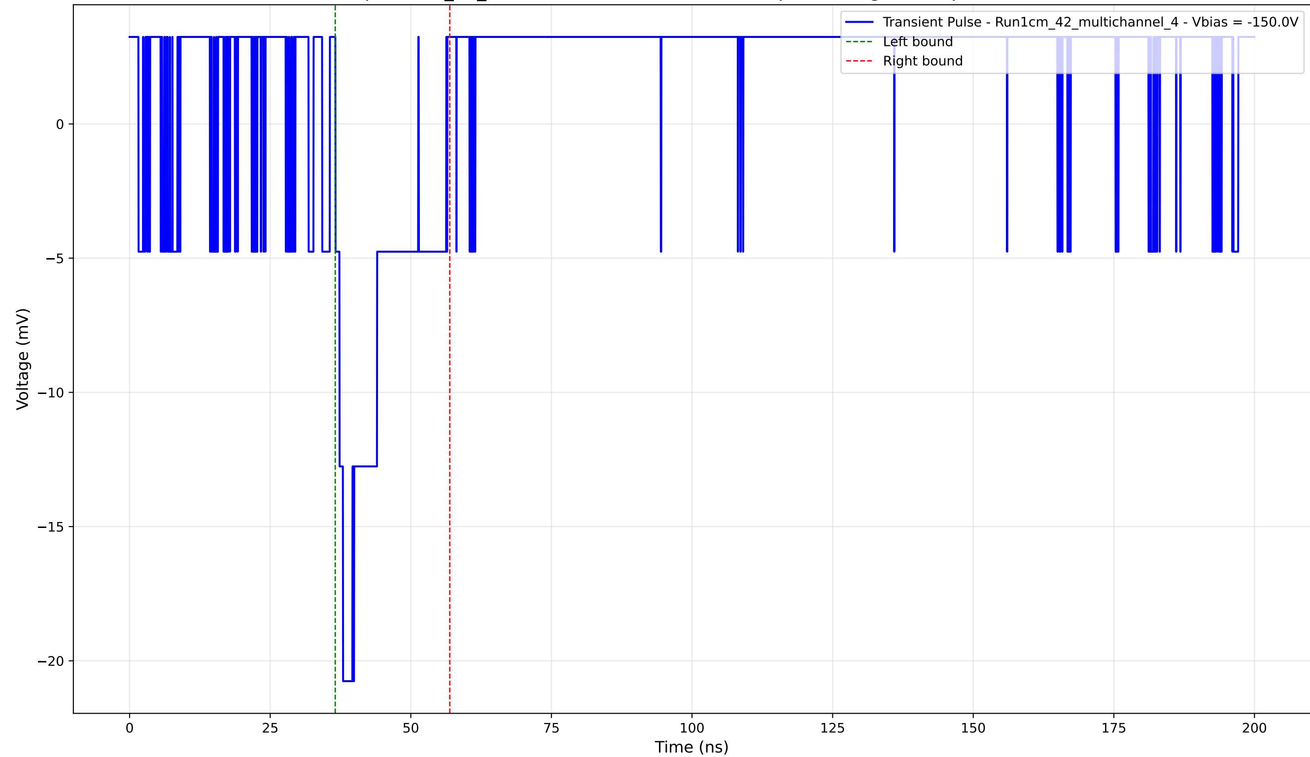
Transient Pulse - Sample: 1cm_42_multichannel - Position: 1095.0 \mu\text{m} - Charge: 3.19 pC - Rise Time: 0.00 ns (N/A)
