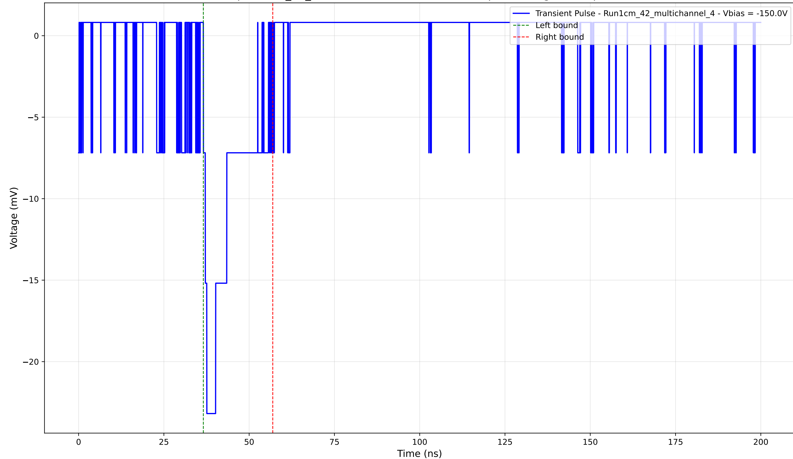
Transient Pulse - Sample: 1cm_42_multichannel - Position: 1290.0 \mu\text{m} - Charge: 4.16 pC - Rise Time: 1.02 ns
