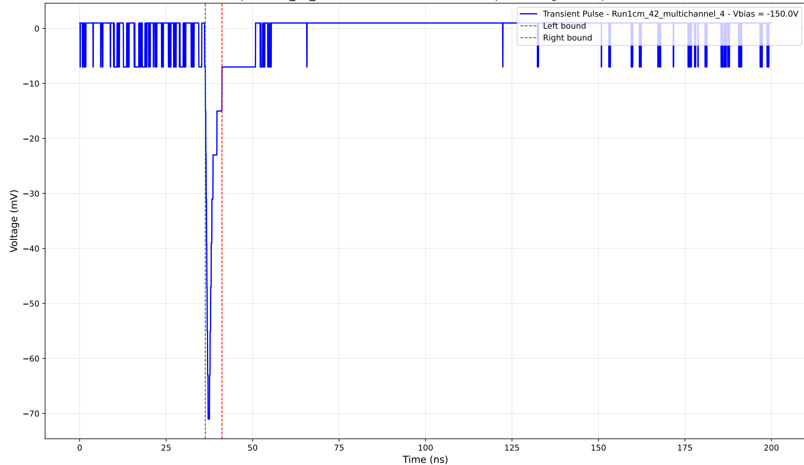
Transient Pulse - Sample: 1cm_42_multichannel - Position: 2190.0 \mu\text{m} - Charge: 3.07 pC - Rise Time: 0.80 ns
