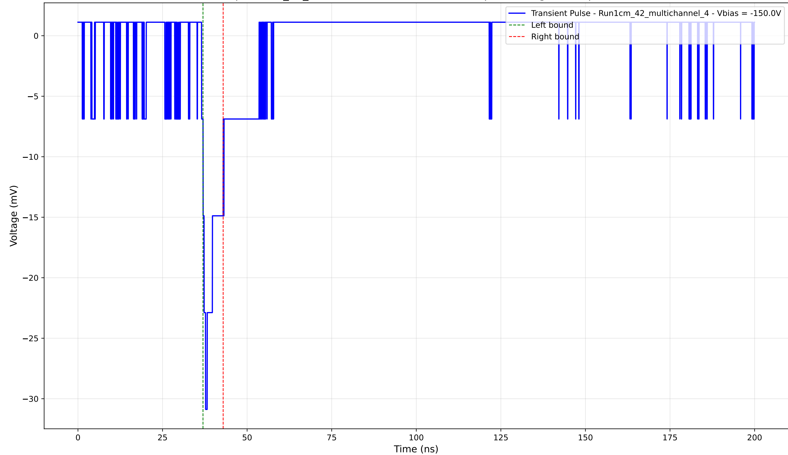
Transient Pulse - Sample: 1cm_42_multichannel - Position: 3255.0 \mu\text{m} - Charge: 2.24 pC - Rise Time: 1.19 ns
