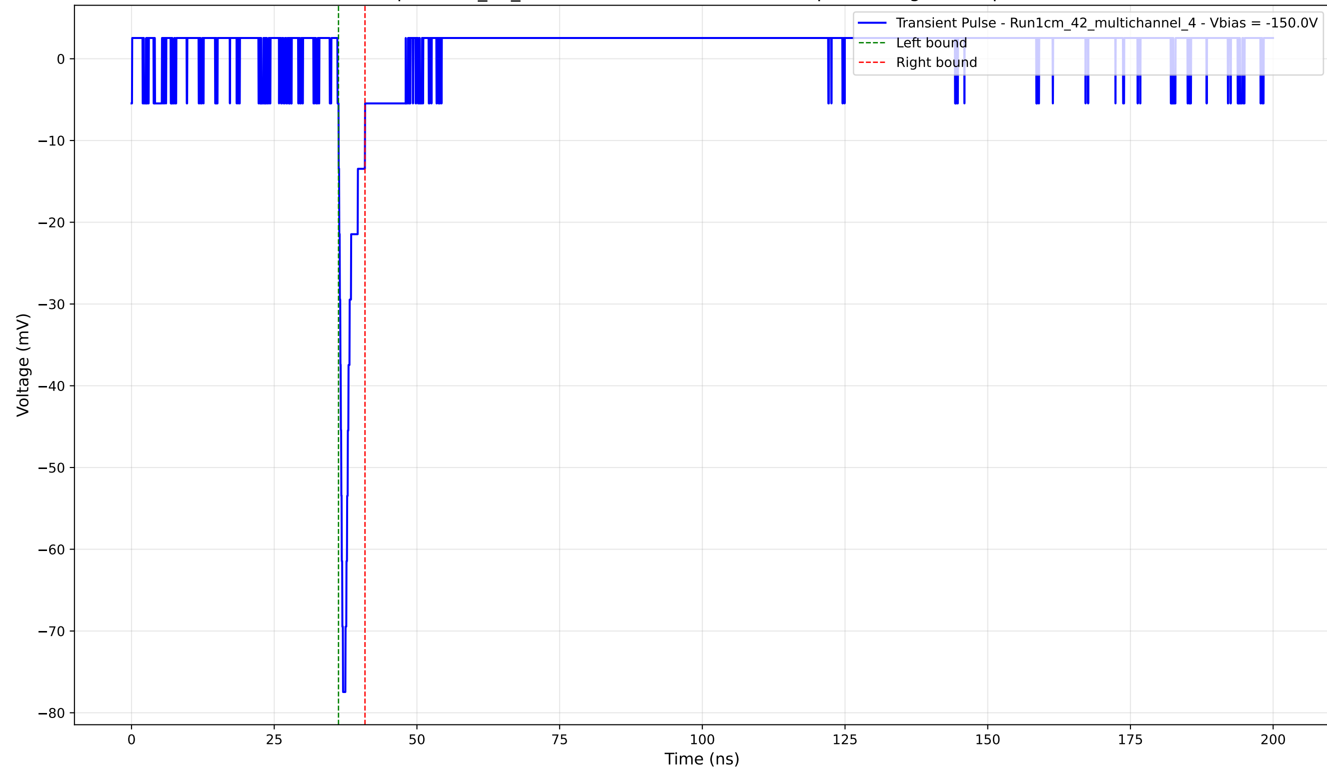
Transient Pulse - Sample: 1cm_42_multichannel - Position: 2500.0 \mu\text{m} - Charge: 3.08 pC - Rise Time: 0.77 ns
