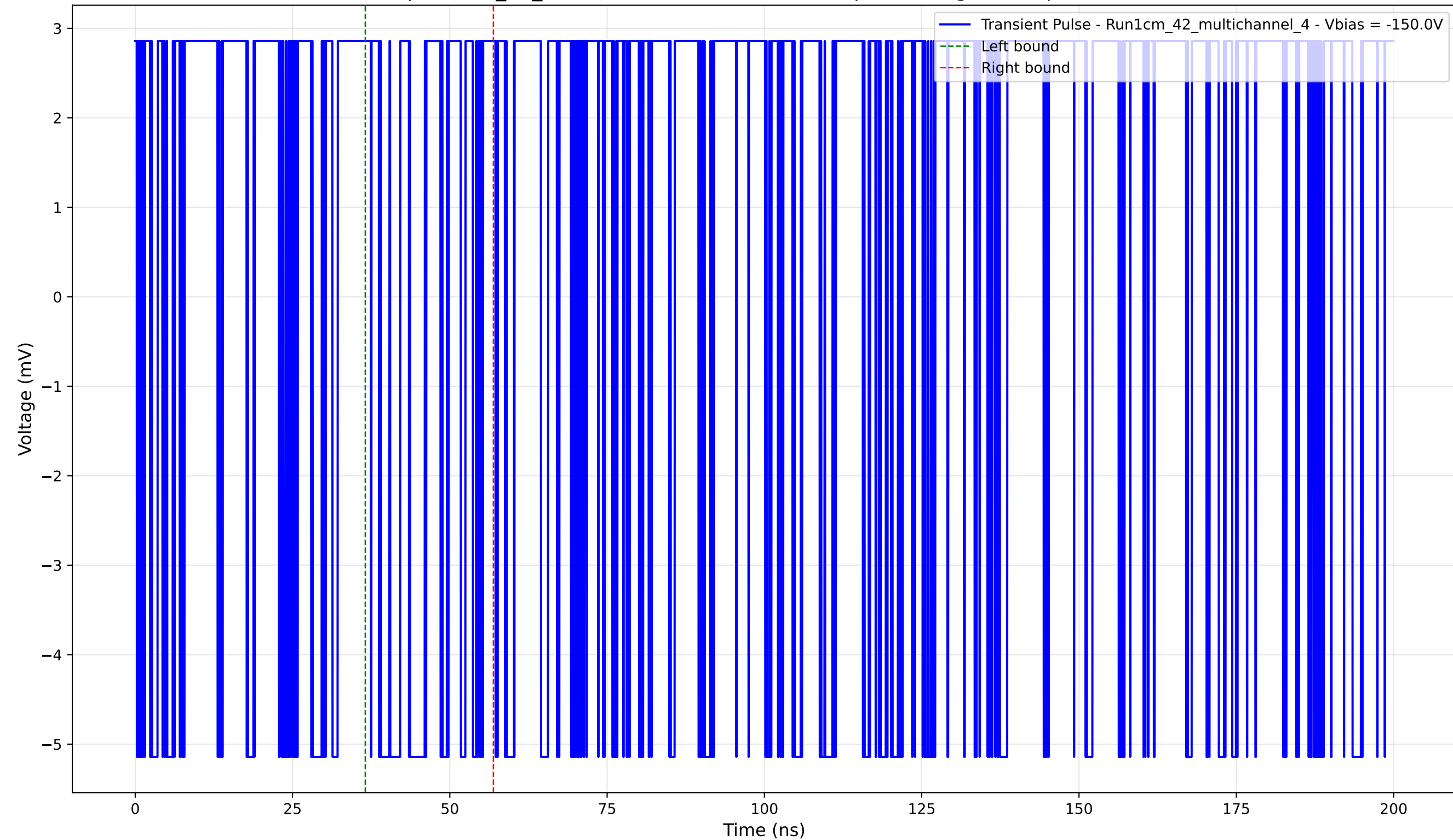
Transient Pulse - Sample: 1cm_42_multichannel - Position: 365.0 \mu\text{m} - Charge: 0.18 pC - Rise Time: 0.00 ns (N/A)
