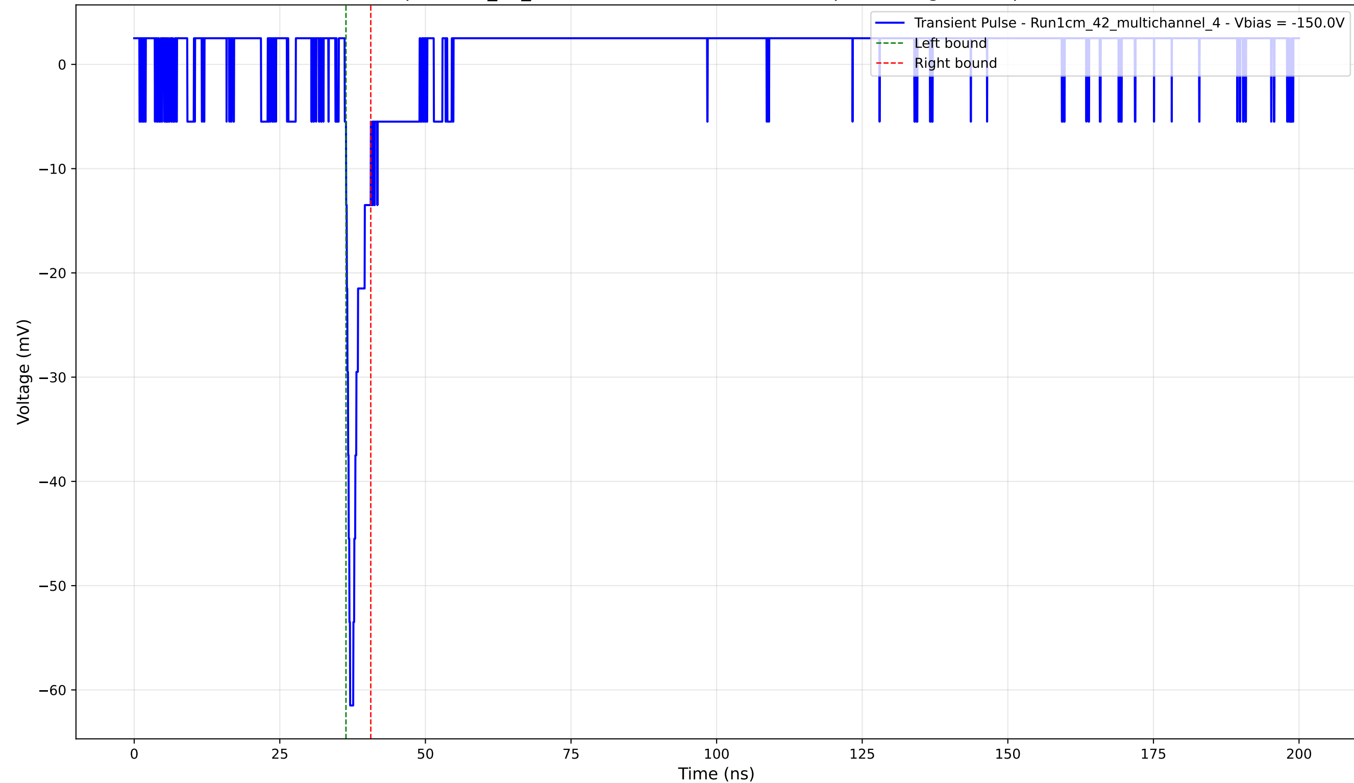
Transient Pulse - Sample: 1cm_42_multichannel - Position: 2595.0 \mu\text{m} - Charge: 2.56 pC - Rise Time: 0.70 ns
