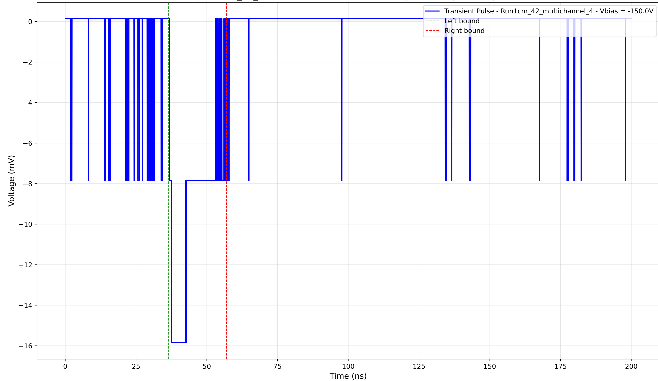
Transient Pulse - Sample: 1cm_42_multichannel - Position: 3625.0 \mu\text{m} - Charge: 3.85 pC - Rise Time: 0.76 ns
