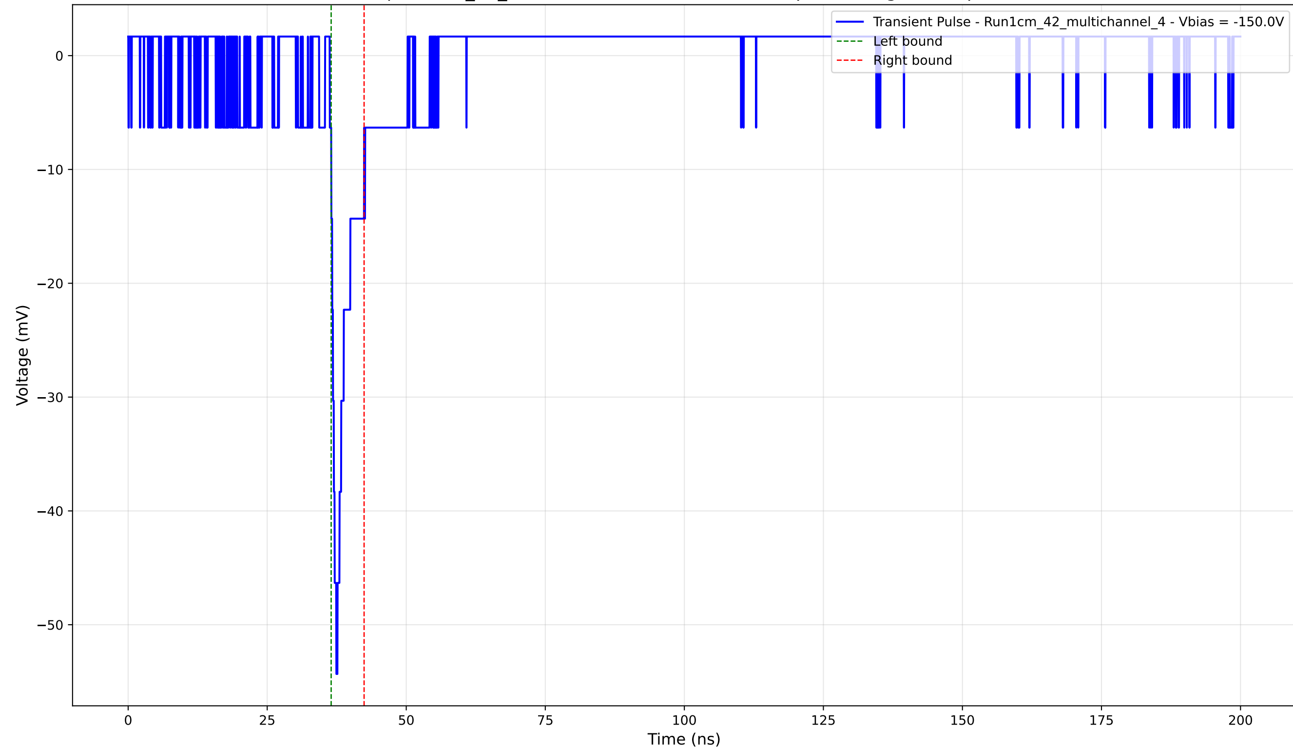
Transient Pulse - Sample: 1cm_42_multichannel - Position: 1960.0 \mu\text{m} - Charge: 2.91 pC - Rise Time: 1.18 ns
