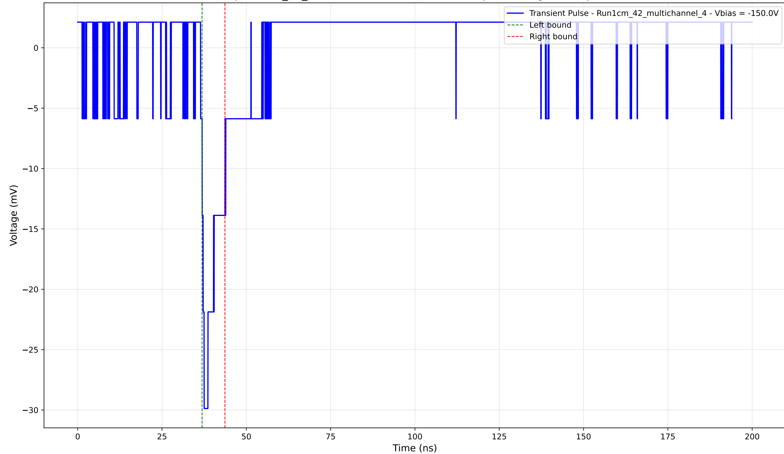
Transient Pulse - Sample: 1cm_42_multichannel - Position: 1510.0 \mu\text{m} - Charge: 2.57 pC - Rise Time: 1.06 ns
