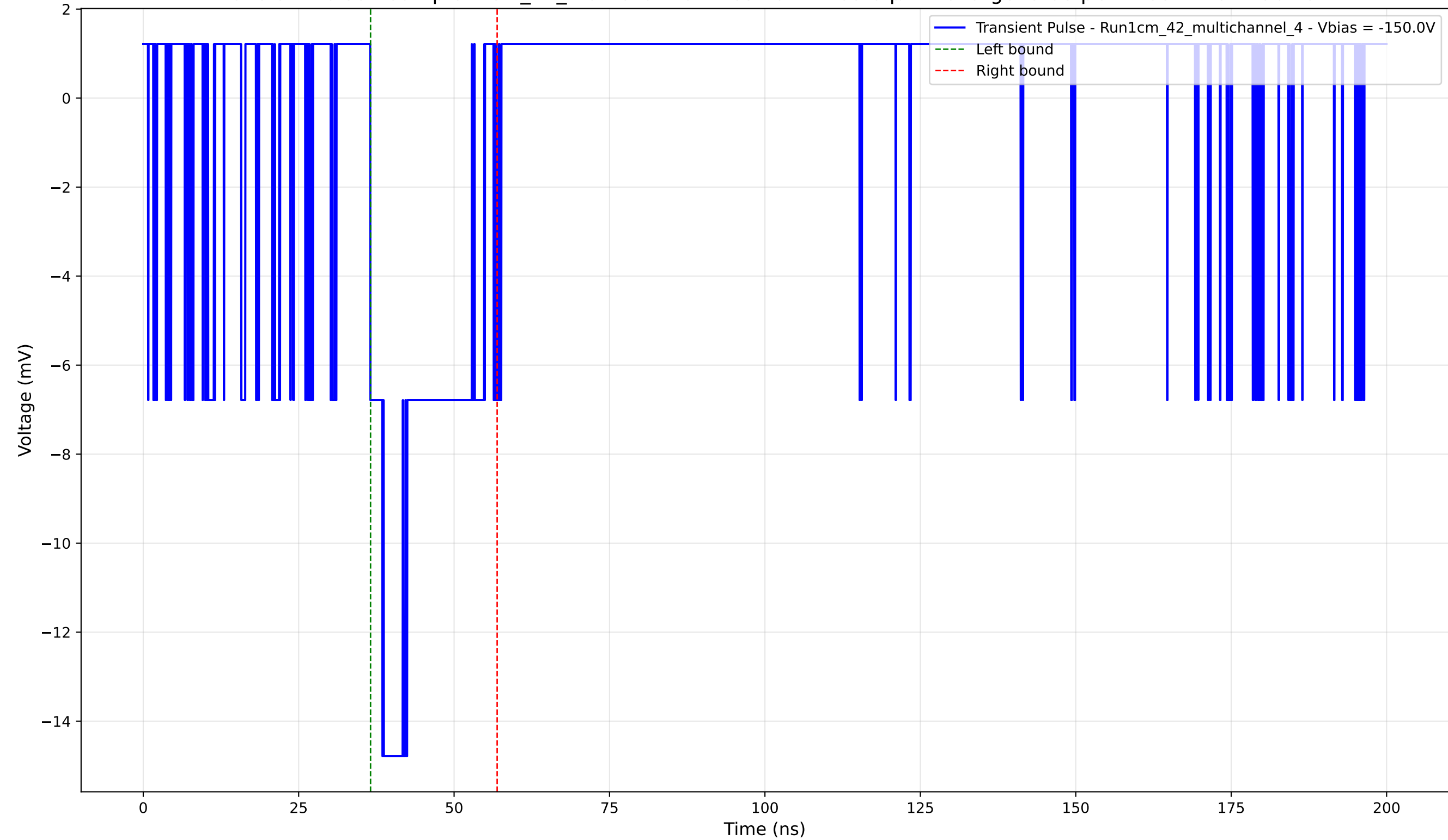
Transient Pulse - Sample: 1cm_42_multichannel - Position: 4785.0 \mu\text{m} - Charge: 3.08 pC - Rise Time: 1.96 ns
