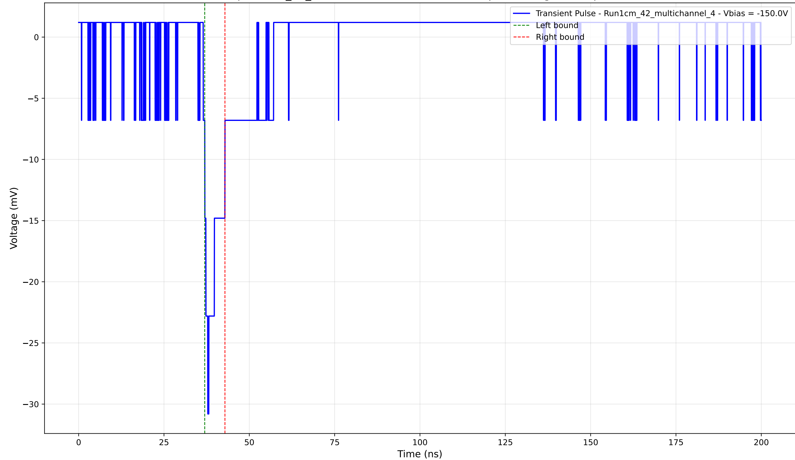
Transient Pulse - Sample: 1cm_42_multichannel - Position: 3285.0 \mu\text{m} - Charge: 2.20 pC - Rise Time: 1.33 ns
