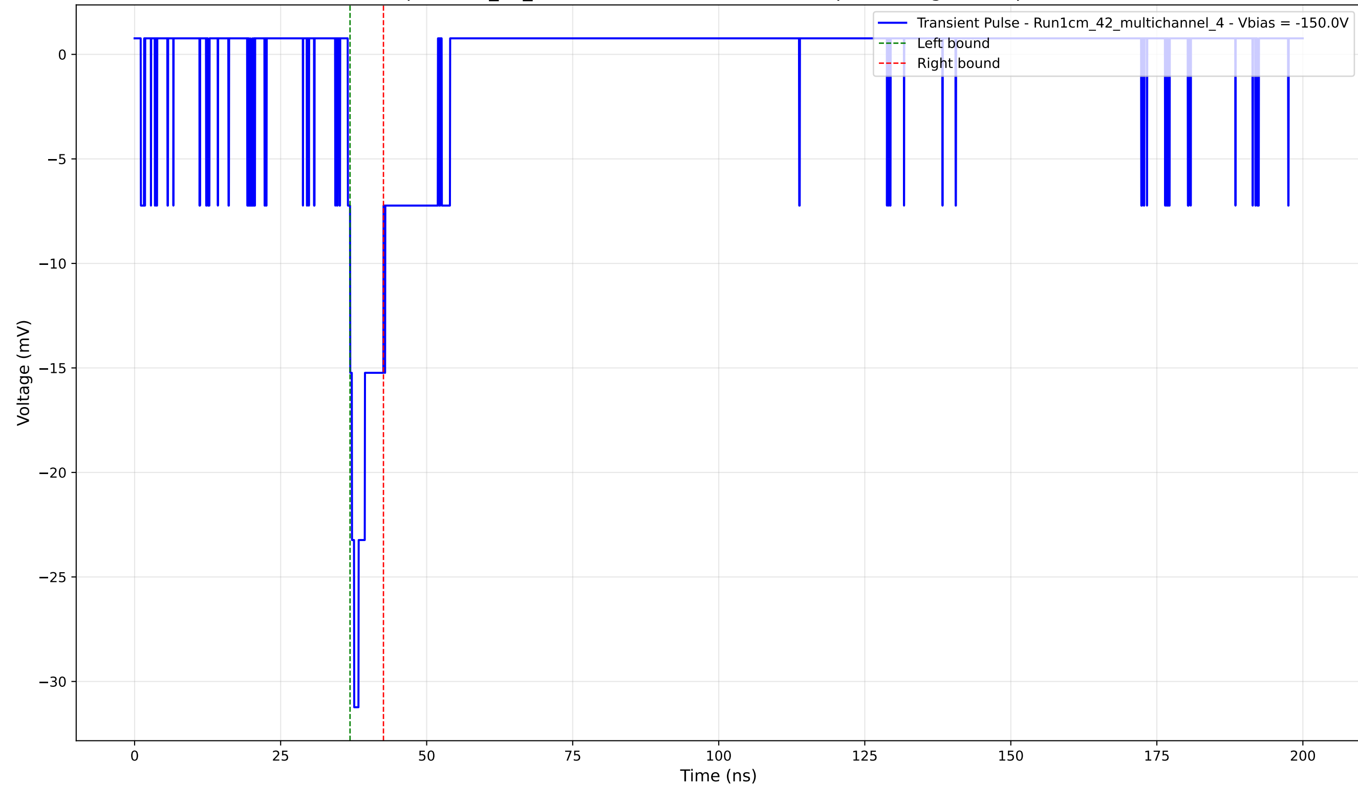
Transient Pulse - Sample: 1cm_42_multichannel - Position: 3200.0 \mu\text{m} - Charge: 2.22 pC - Rise Time: 1.09 ns
