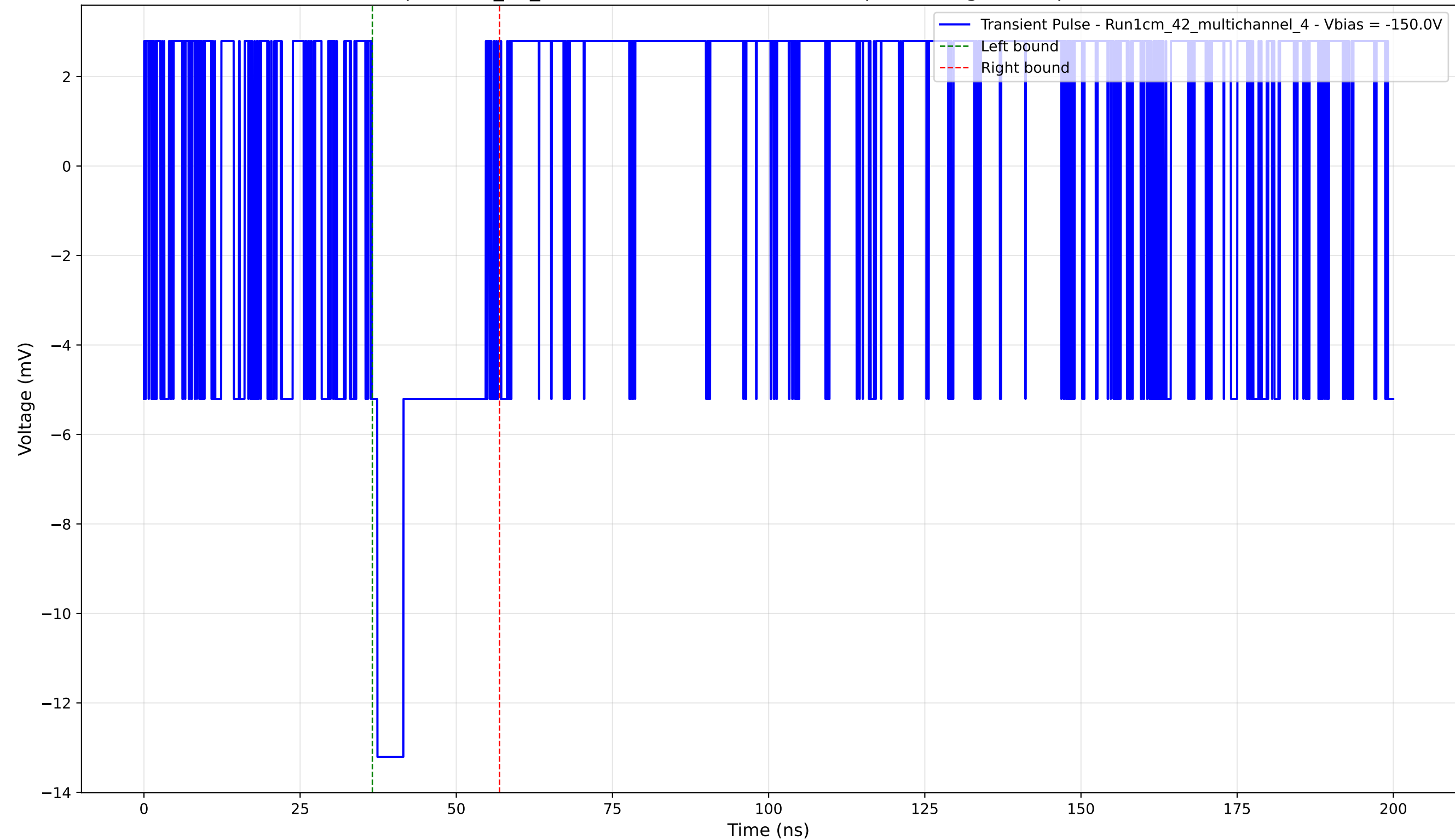
Transient Pulse - Sample: 1cm_42_multichannel - Position: 1320.0 \mu\text{m} - Charge: 2.62 pC - Rise Time: 0.00 ns (N/A)
