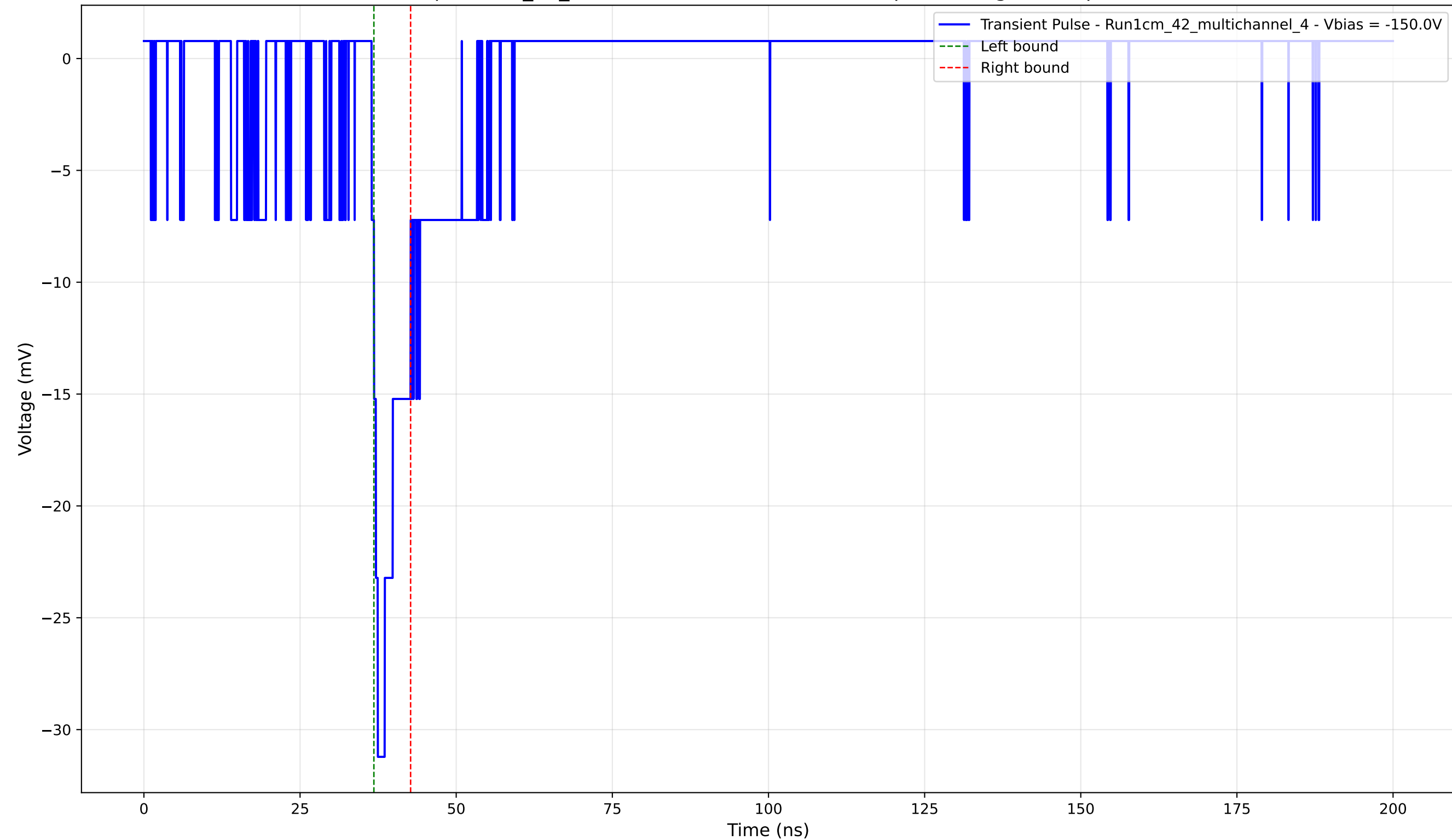
Transient Pulse - Sample: 1cm_42_multichannel - Position: 1560.0 \mu\text{m} - Charge: 2.40 pC - Rise Time: 0.99 ns
