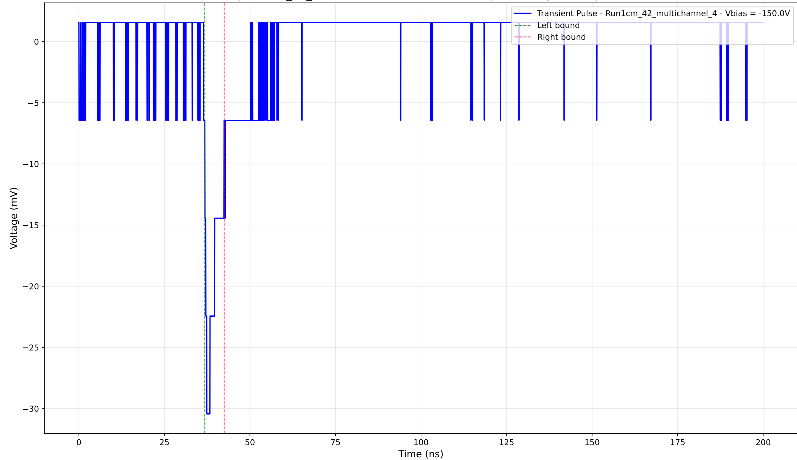
Transient Pulse - Sample: 1cm_42_multichannel - Position: 3130.0 \mu\text{m} - Charge: 2.19 pC - Rise Time: 0.99 ns
