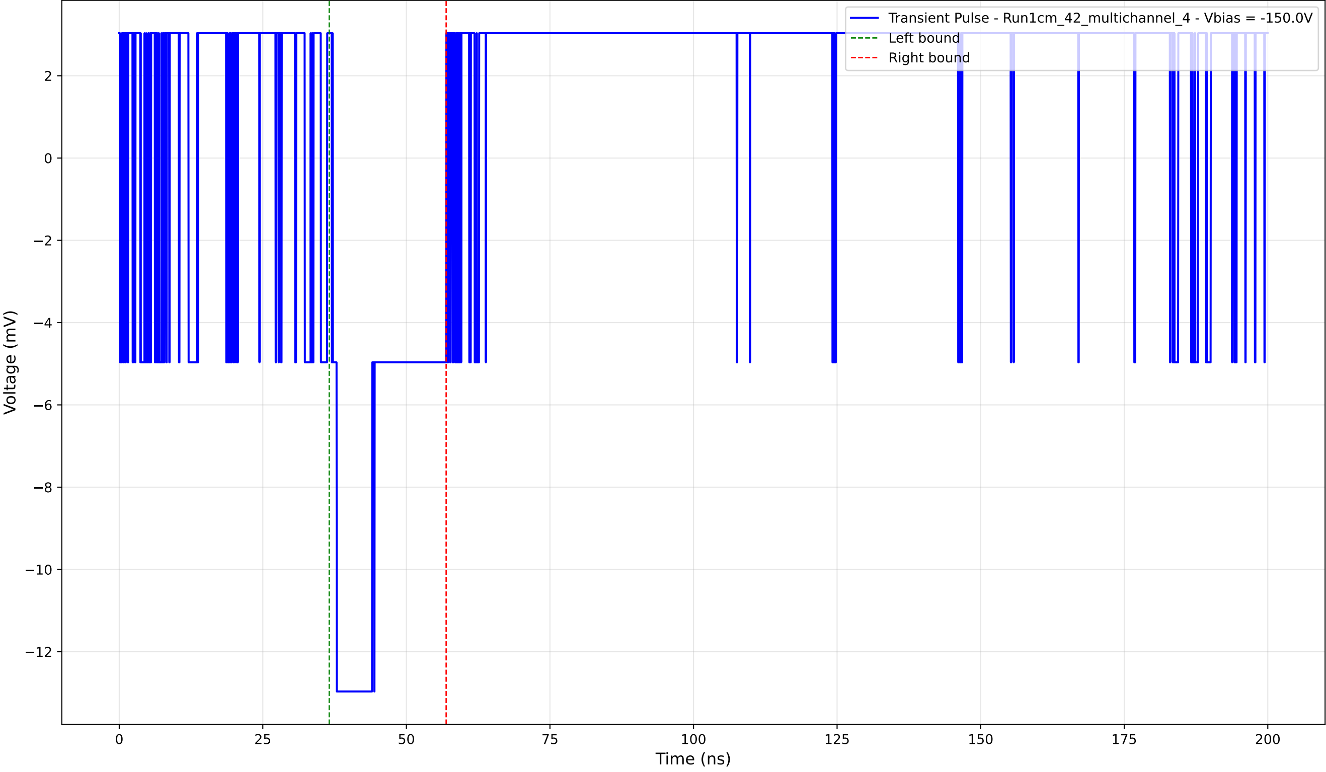
Transient Pulse - Sample: 1cm_42_multichannel - Position: 700.0 \mu\text{m} - Charge: 2.95 pC - Rise Time: 0.00 ns (N/A)
