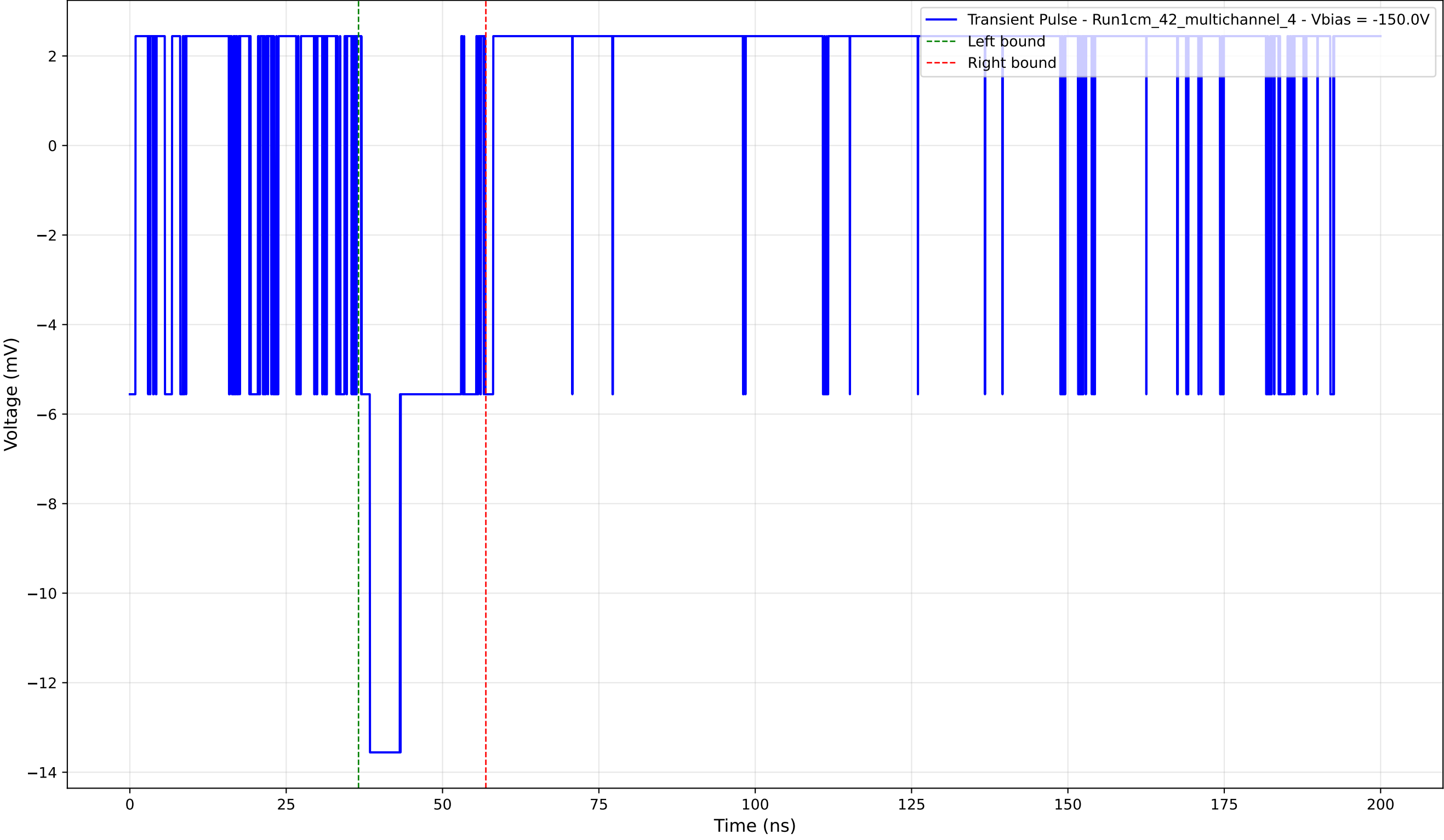
Transient Pulse - Sample: 1cm_42_multichannel - Position: 450.0 \mu\text{m} - Charge: 2.75 pC - Rise Time: 0.00 ns (N/A)
