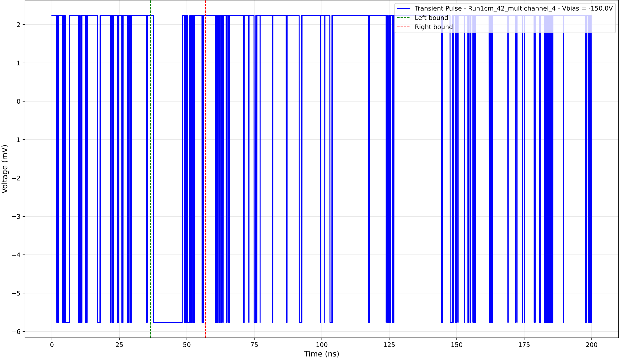
Transient Pulse - Sample: 1cm_42_multichannel - Position: 4440.0 \mu\text{m} - Charge: 1.29 pC - Rise Time: 0.00 ns (N/A)
