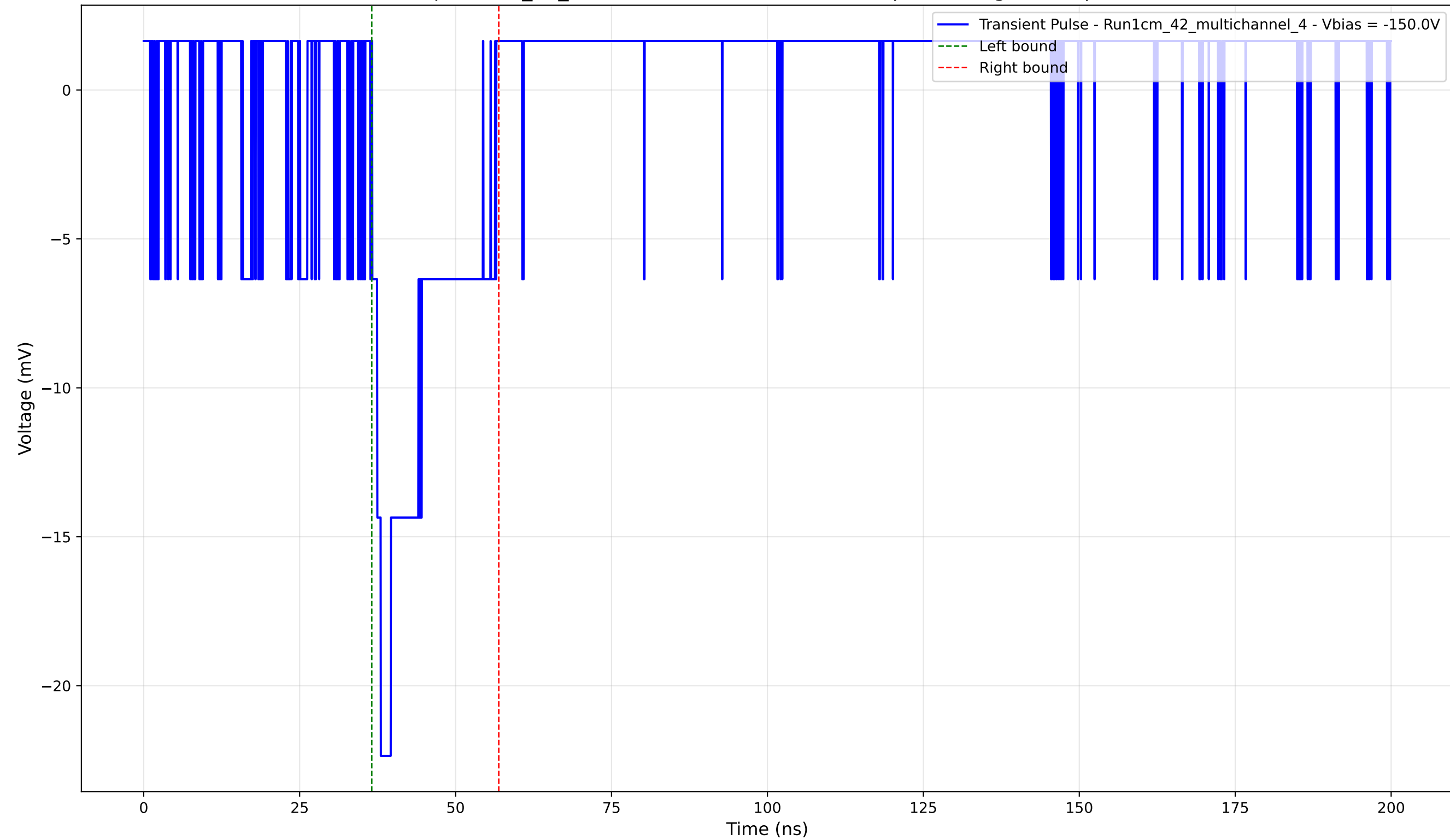
Transient Pulse - Sample: 1cm_42_multichannel - Position: 1070.0 \mu\text{m} - Charge: 3.82 pC - Rise Time: 1.38 ns
