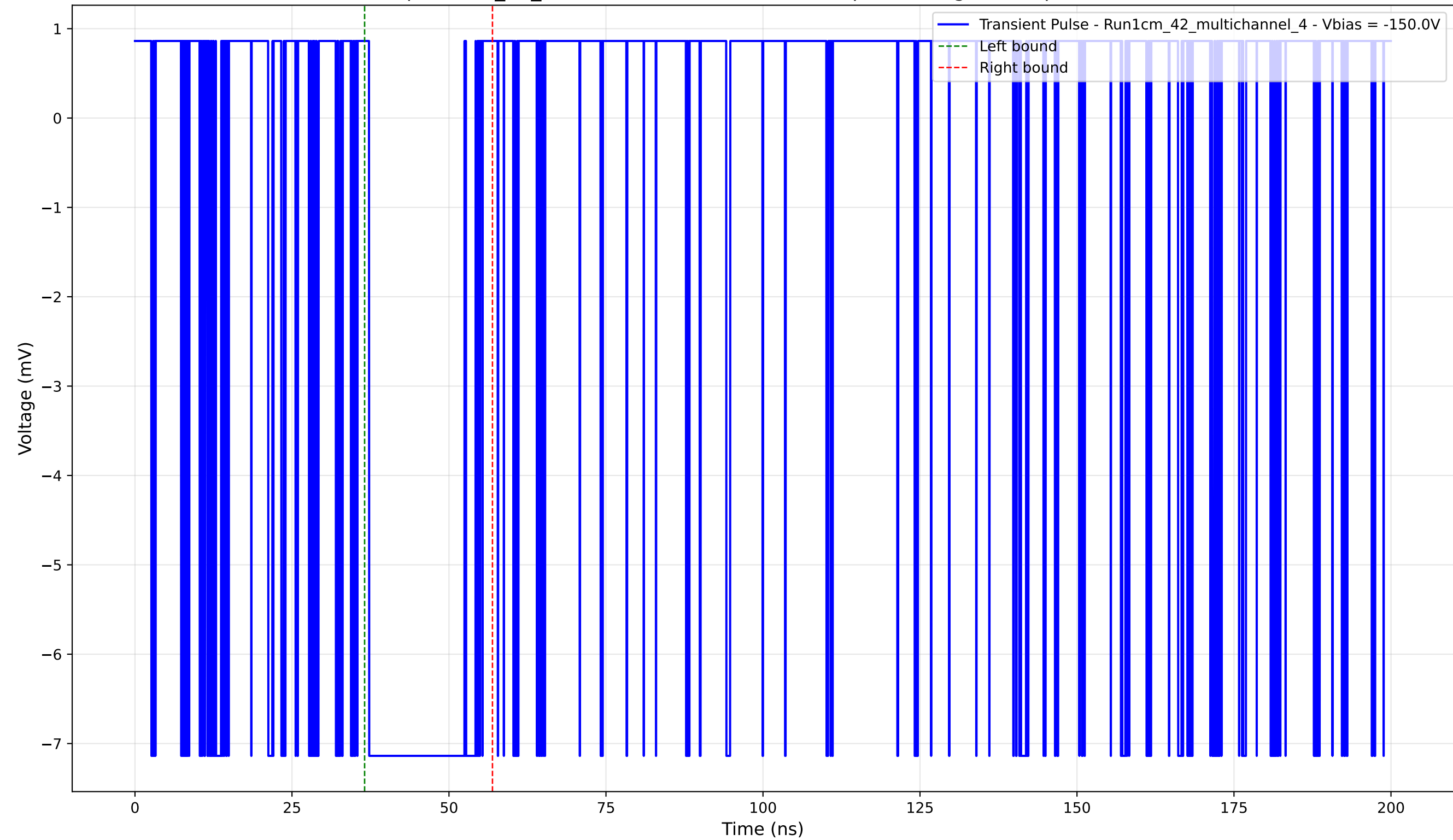
Transient Pulse - Sample: 1cm_42_multichannel - Position: 820.0 \mu\text{m} - Charge: 2.43 pC - Rise Time: 0.00 ns (N/A)
