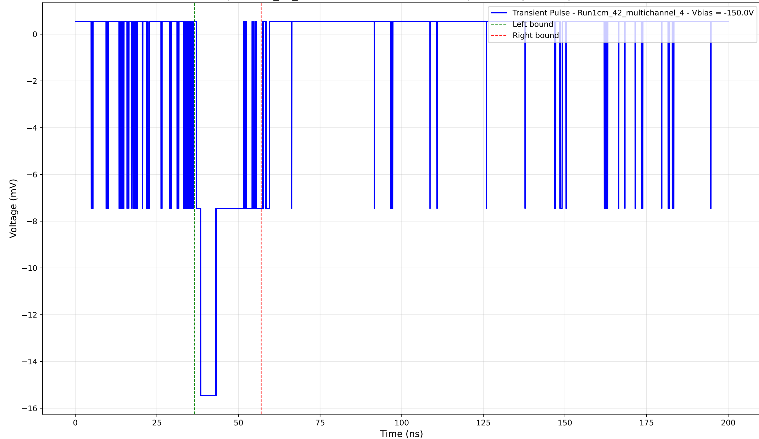
Transient Pulse - Sample: 1cm_42_multichannel - Position: 4325.0 \mu\text{m} - Charge: 3.54 pC - Rise Time: 1.32 ns
