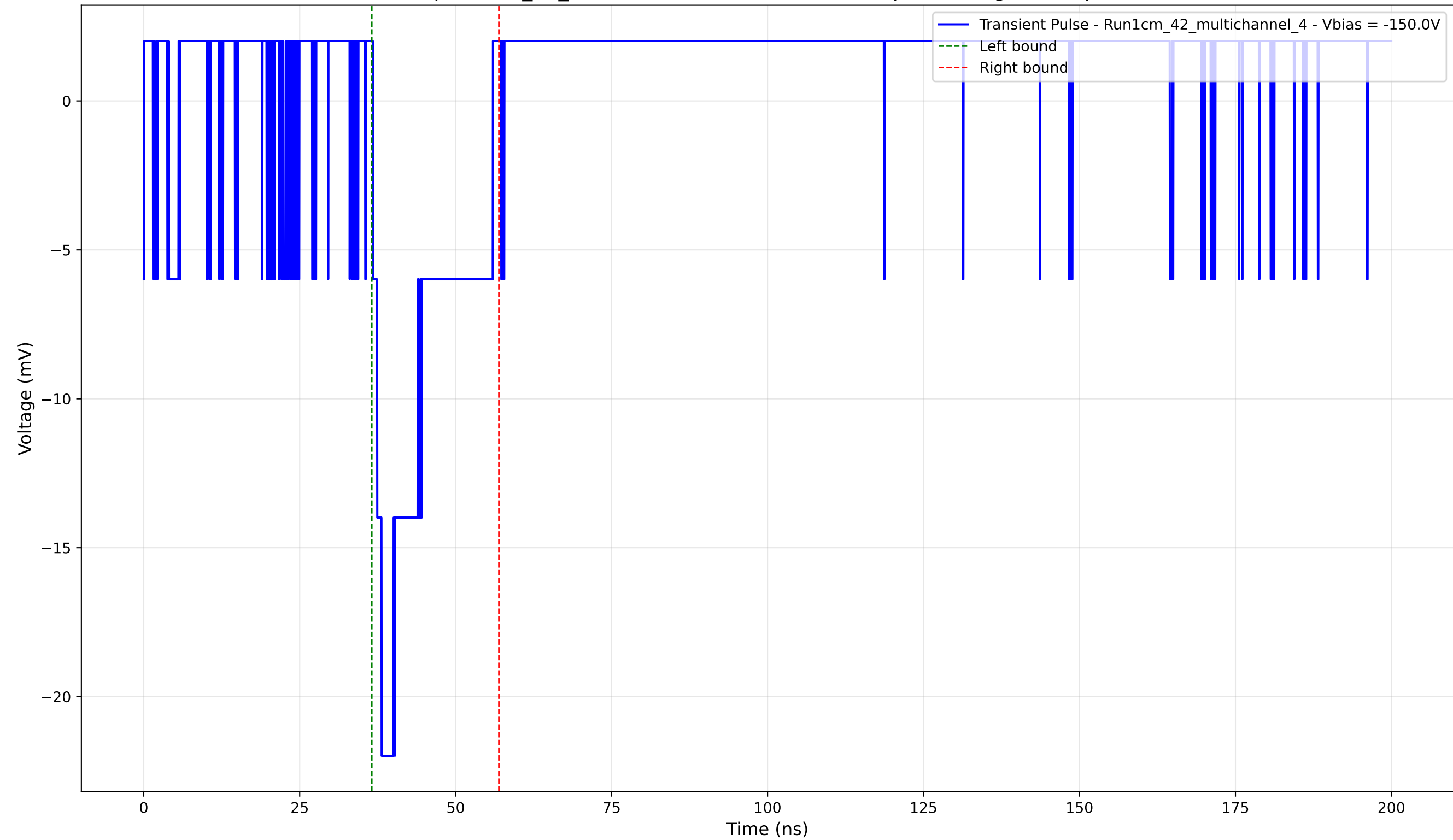
Transient Pulse - Sample: 1cm_42_multichannel - Position: 1005.0 \mu\text{m} - Charge: 3.66 pC - Rise Time: 1.40 ns
