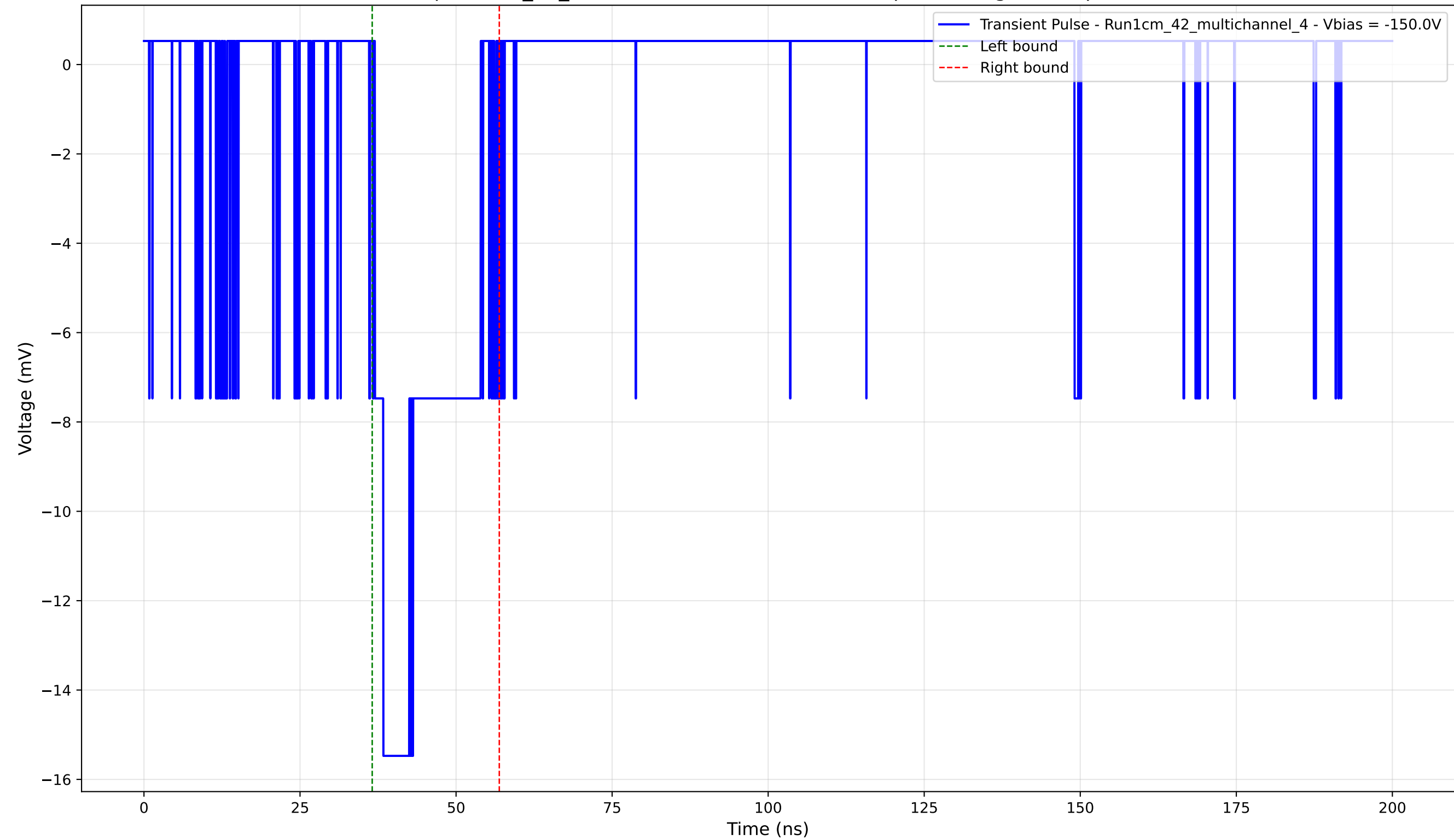
Transient Pulse - Sample: 1cm_42_multichannel - Position: 4200.0 \mu\text{m} - Charge: 3.34 pC - Rise Time: 1.36 ns
