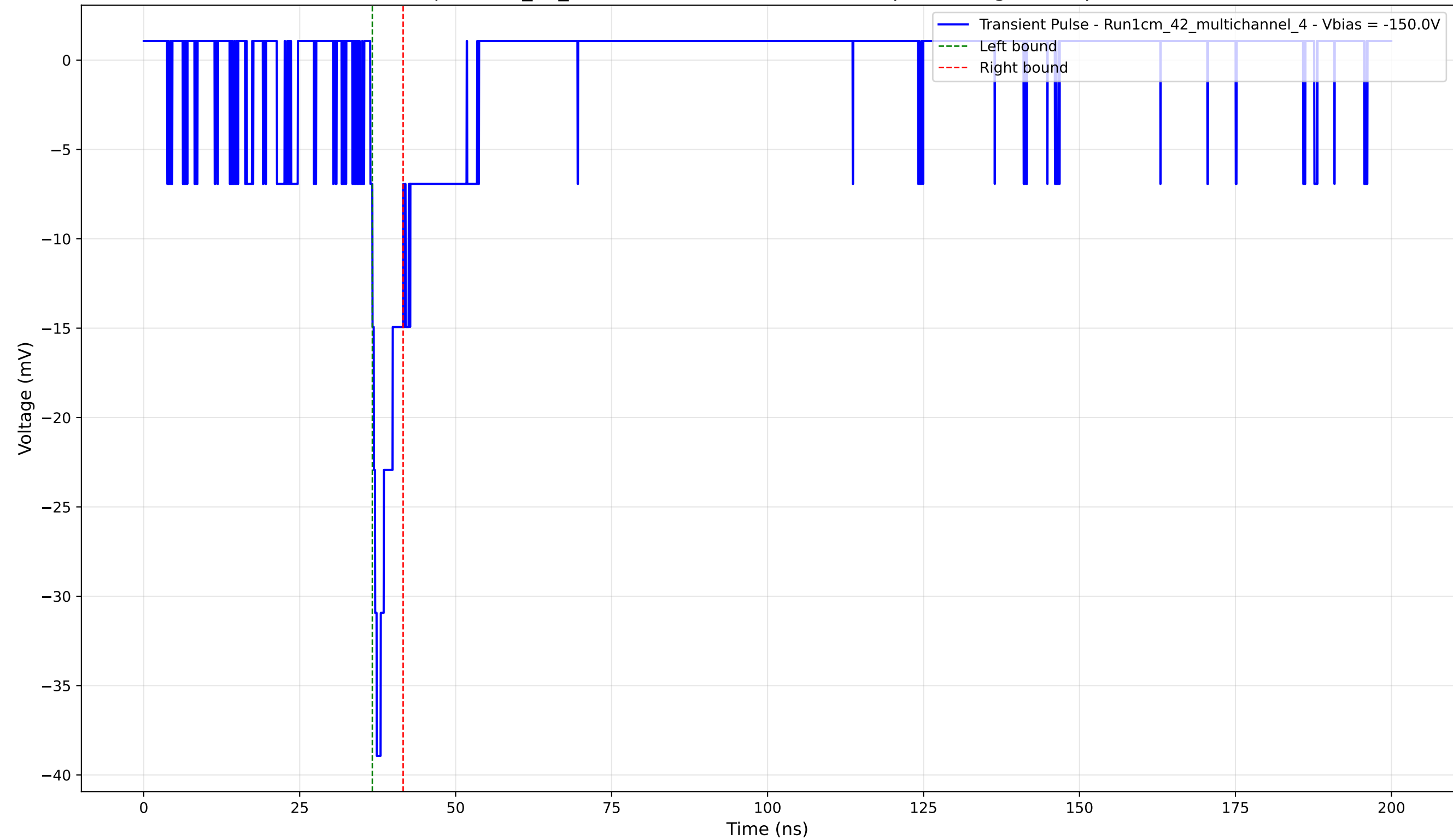
Transient Pulse - Sample: 1cm_42_multichannel - Position: 2975.0 \mu\text{m} - Charge: 2.28 pC - Rise Time: 1.03 ns
