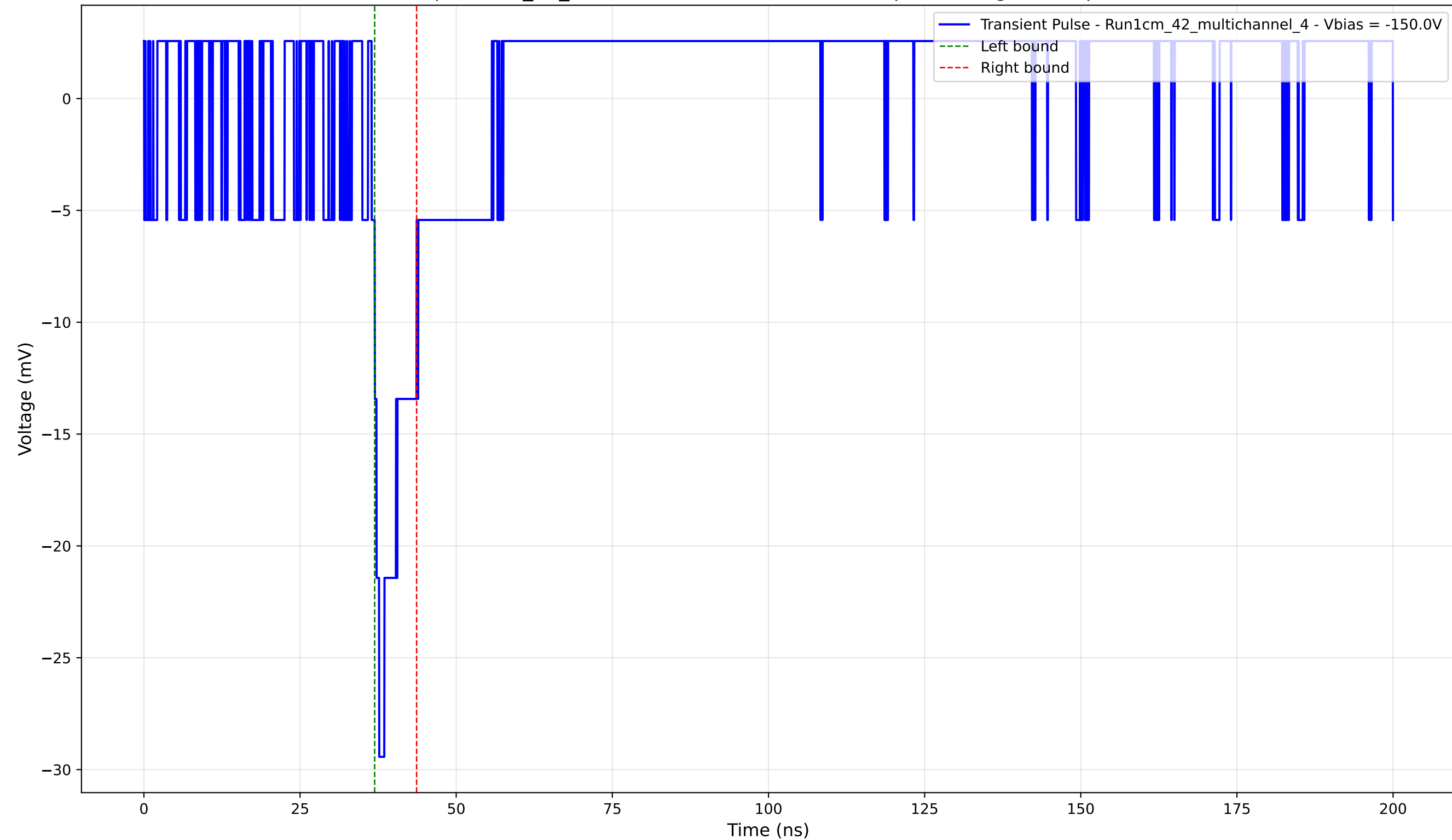
Transient Pulse - Sample: 1cm_42_multichannel - Position: 1460.0 \mu\text{m} - Charge: 2.45 pC - Rise Time: 1.22 ns
