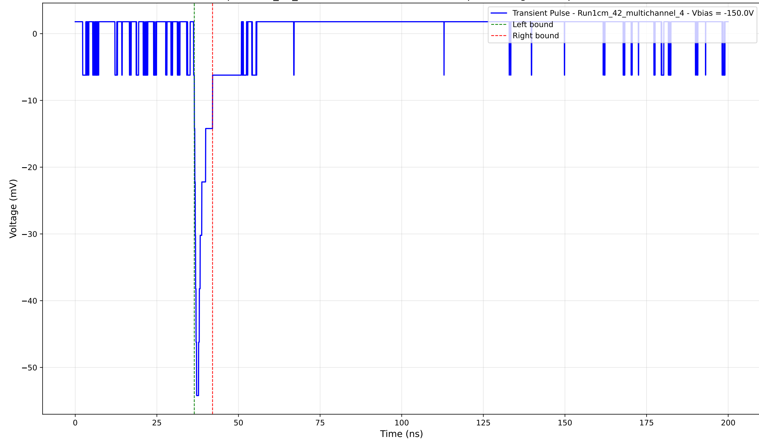
Transient Pulse - Sample: 1cm_42_multichannel - Position: 2745.0 \mu\text{m} - Charge: 2.92 pC - Rise Time: 0.90 ns
