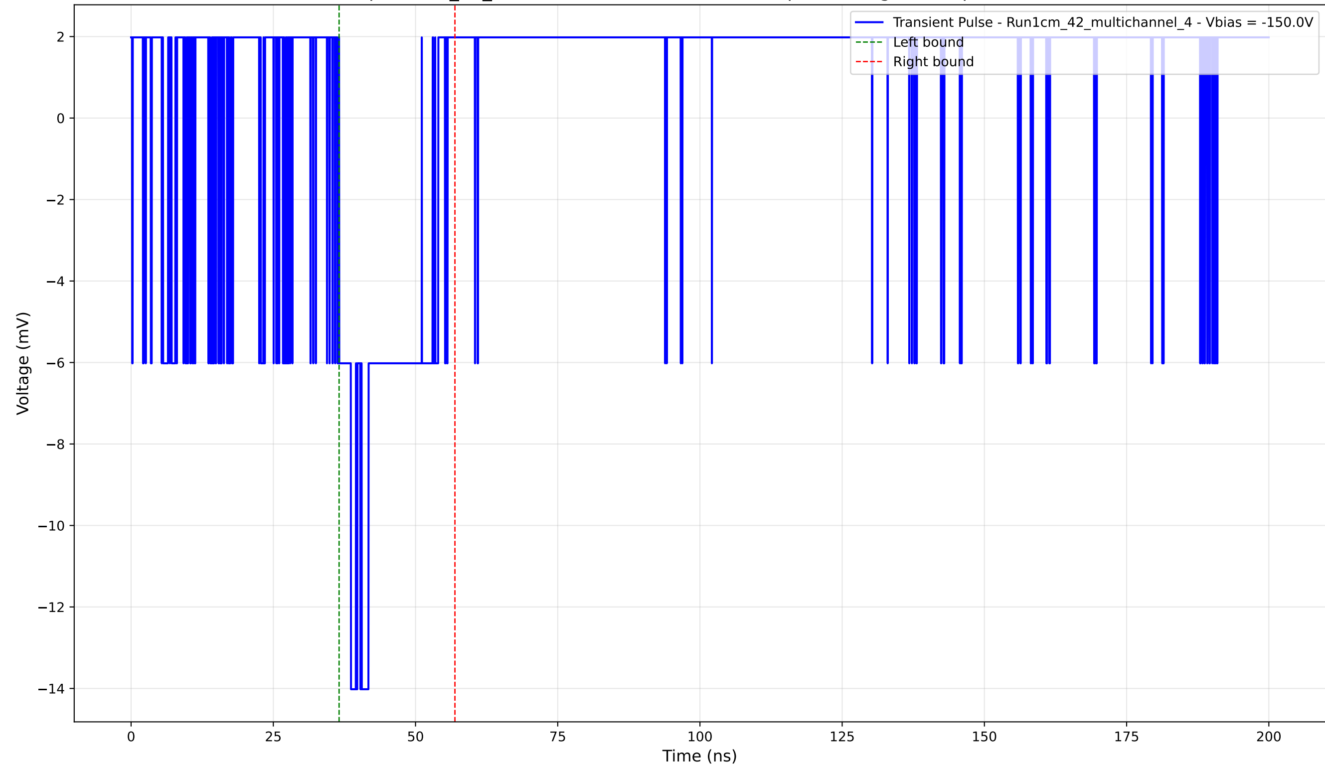
Transient Pulse - Sample: 1cm_42_multichannel - Position: 4820.0 \mu\text{m} - Charge: 2.37 pC - Rise Time: 0.00 ns (N/A)
