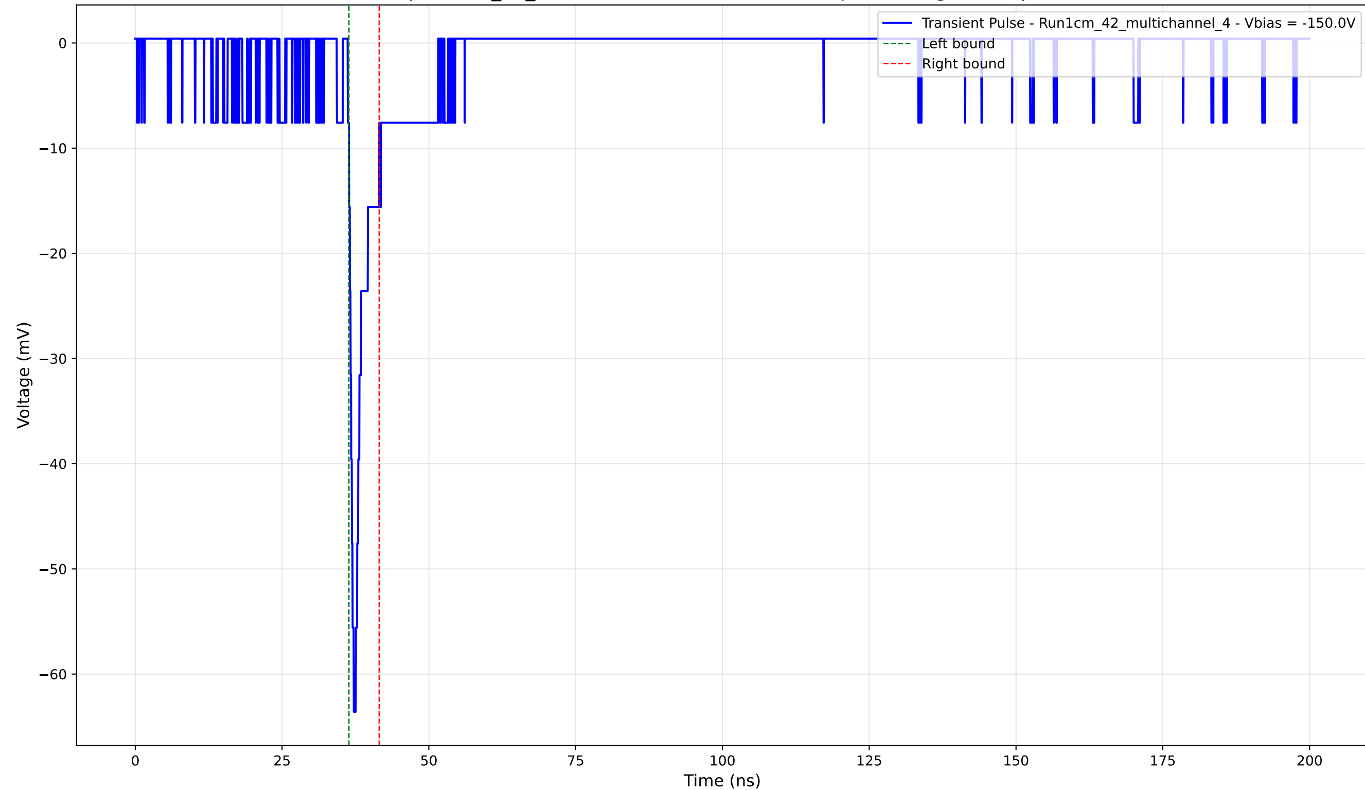
Transient Pulse - Sample: 1cm_42_multichannel - Position: 2645.0 \mu\text{m} - Charge: 2.96 pC - Rise Time: 1.02 ns
