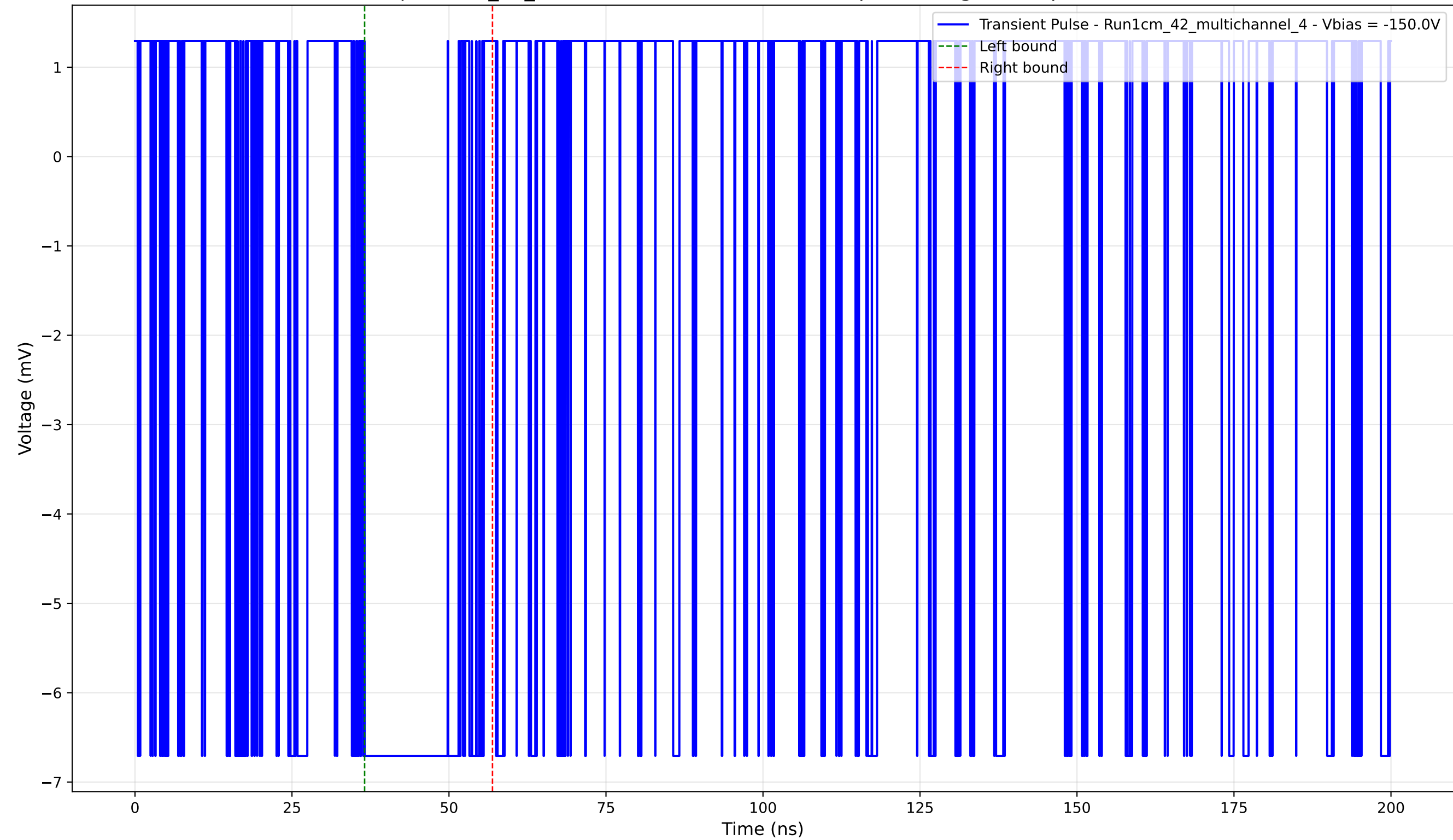
Transient Pulse - Sample: 1cm_42_multichannel - Position: 1415.0 \mu\text{m} - Charge: 2.22 pC - Rise Time: 0.00 ns (N/A)
