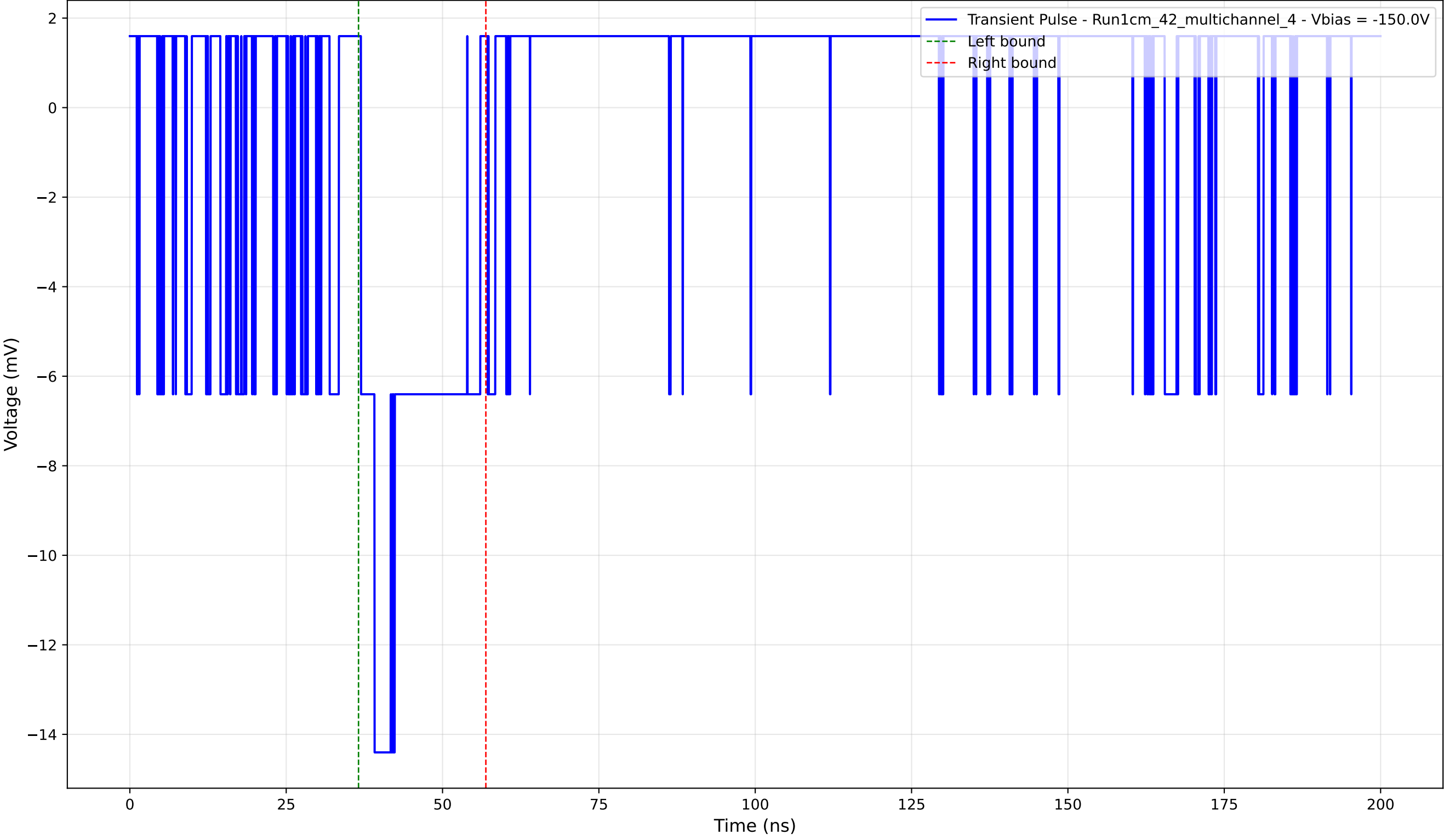
Transient Pulse - Sample: 1cm_42_multichannel - Position: 175.0 \mu\text{m} - Charge: 2.88 pC - Rise Time: 0.00 ns (N/A)
