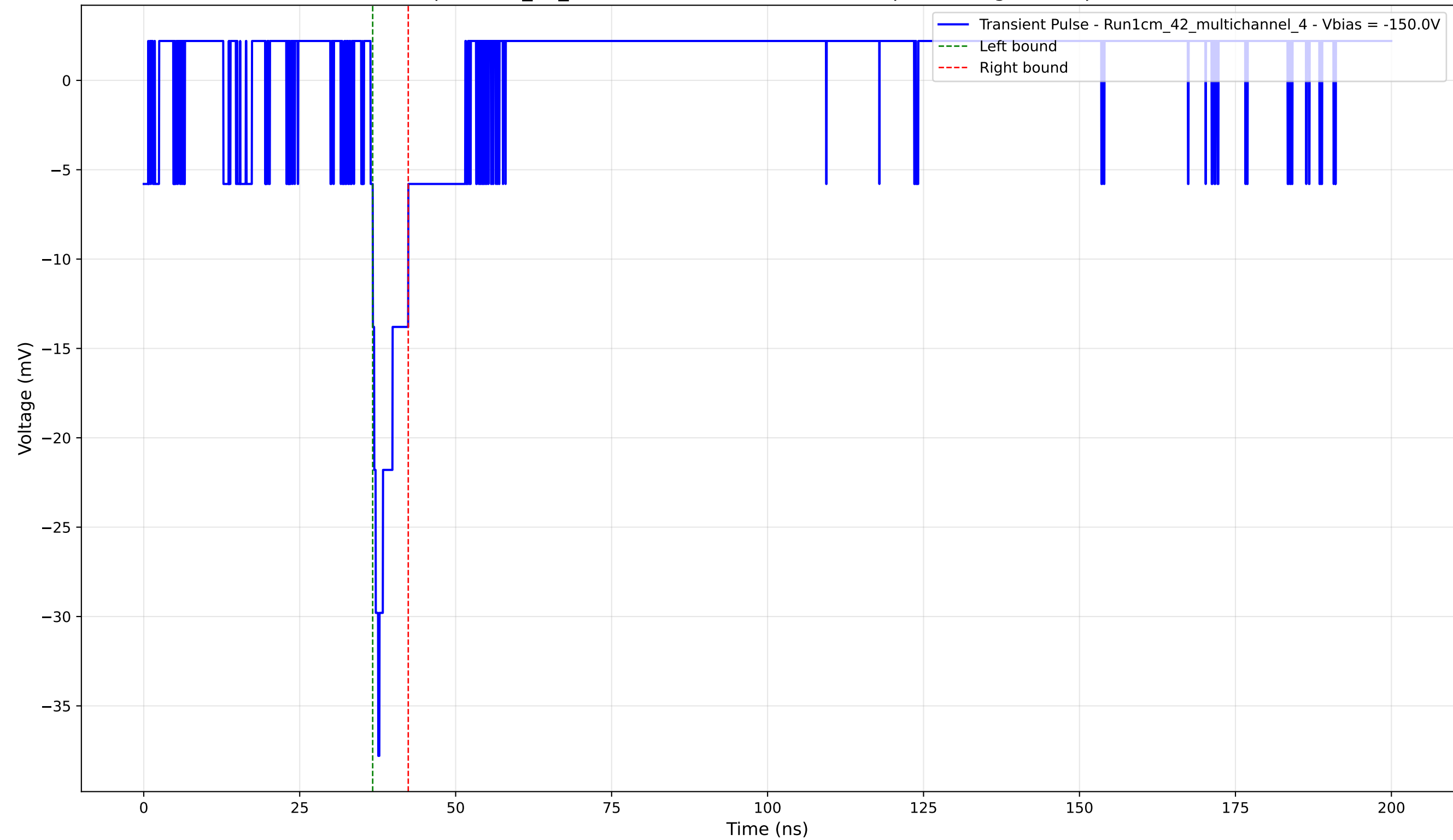
Transient Pulse - Sample: 1cm_42_multichannel - Position: 3040.0 \mu\text{m} - Charge: 2.26 pC - Rise Time: 1.23 ns
