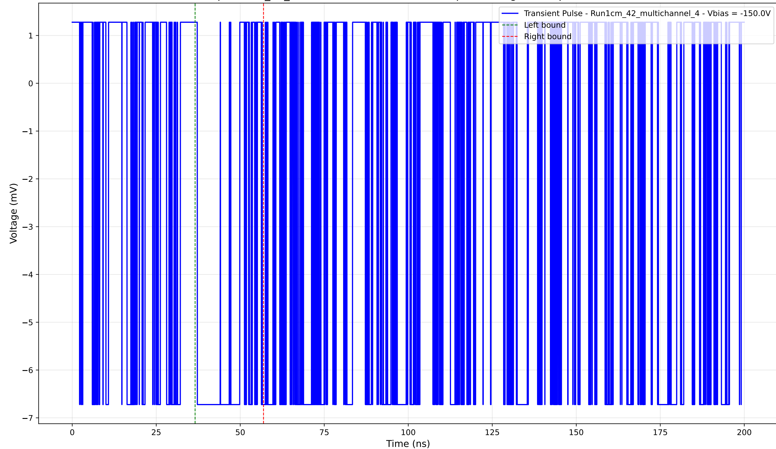
Transient Pulse - Sample: 1cm_42_multichannel - Position: 330.0 \mu\text{m} - Charge: 1.87 pC - Rise Time: 0.00 ns (N/A)
