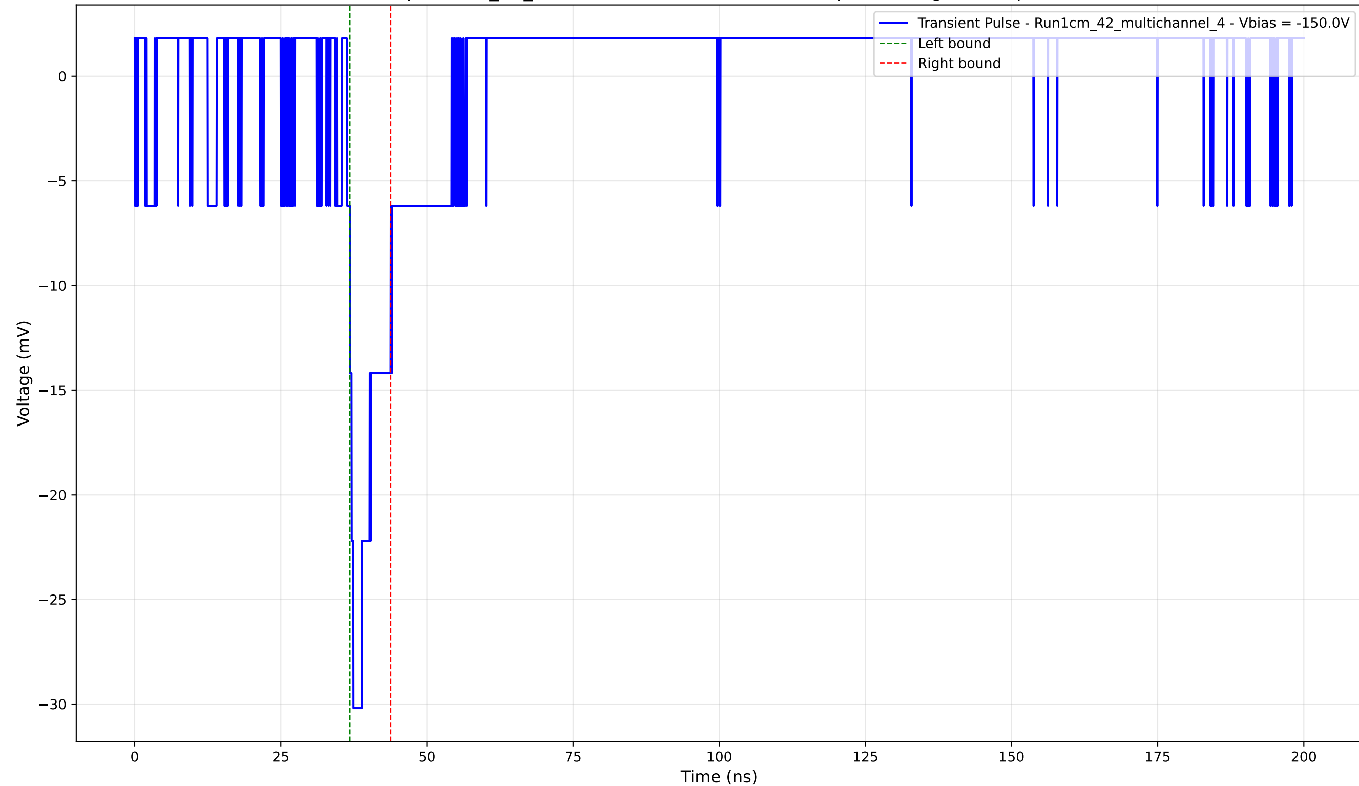
Transient Pulse - Sample: 1cm_42_multichannel - Position: 1535.0 \mu\text{m} - Charge: 2.72 pC - Rise Time: 1.11 ns
