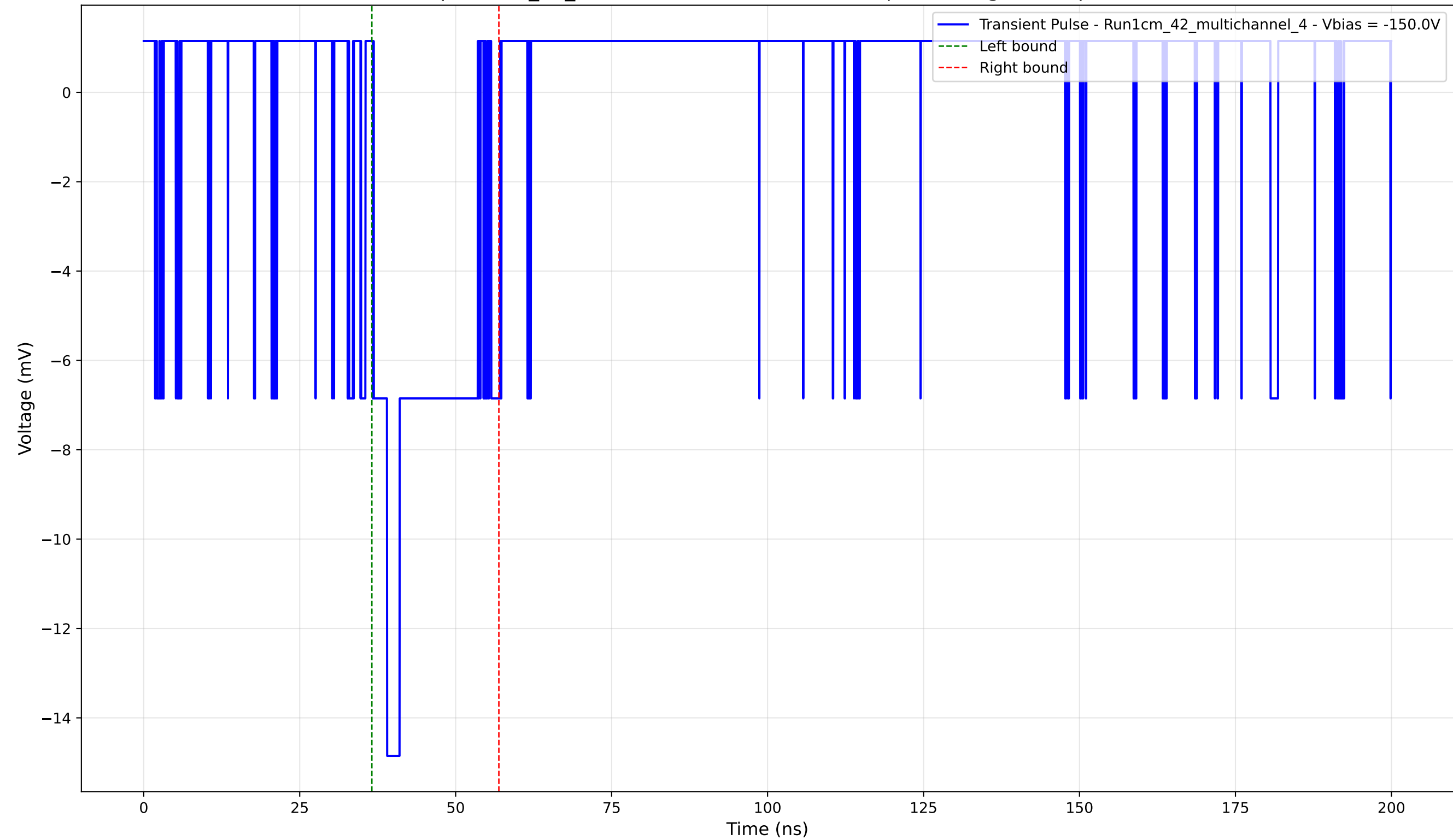
Transient Pulse - Sample: 1cm_42_multichannel - Position: 125.0 \mu\text{m} - Charge: 2.84 pC - Rise Time: 2.16 ns
