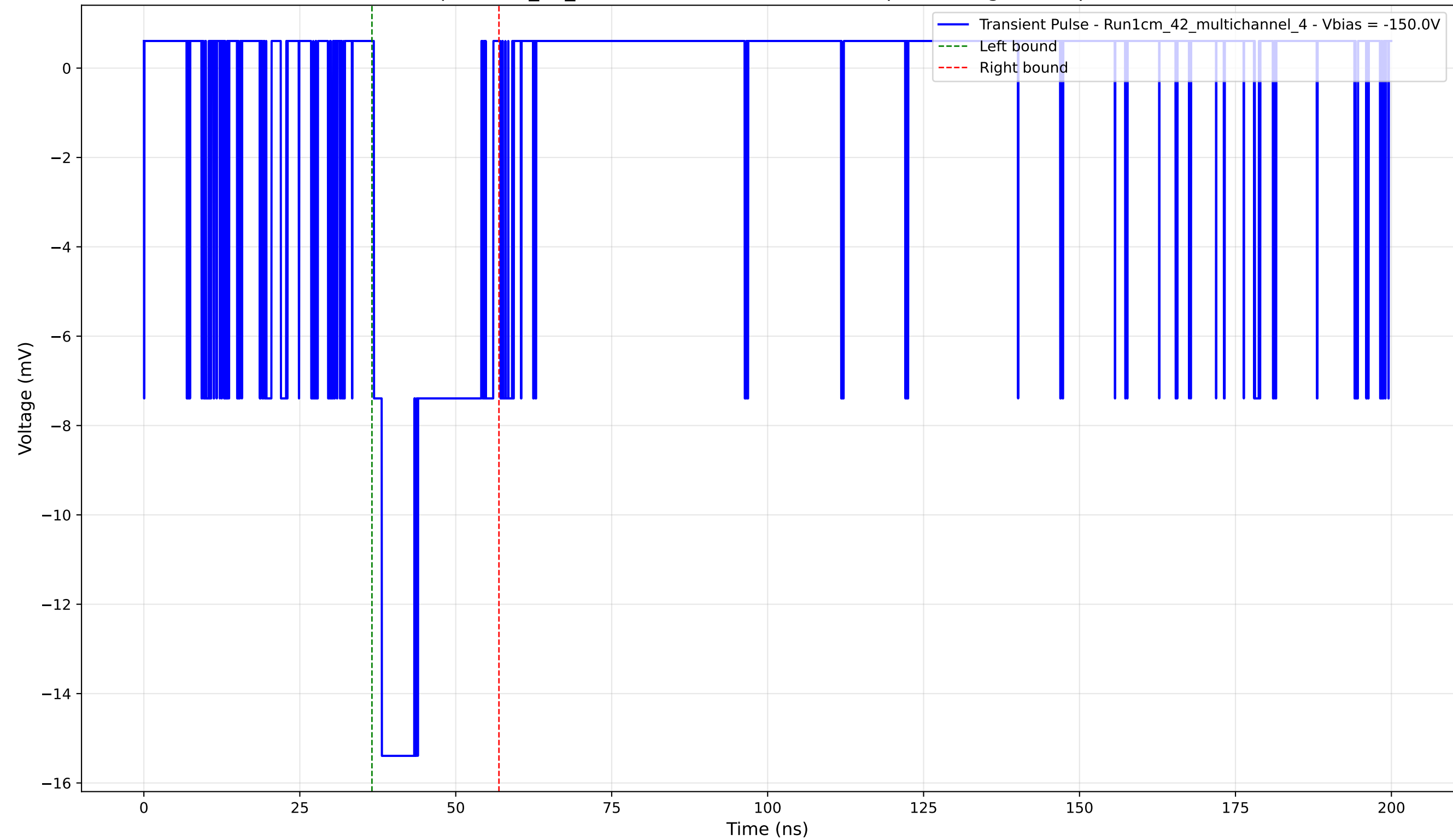
Transient Pulse - Sample: 1cm_42_multichannel - Position: 455.0 \mu\text{m} - Charge: 3.63 pC - Rise Time: 1.28 ns
