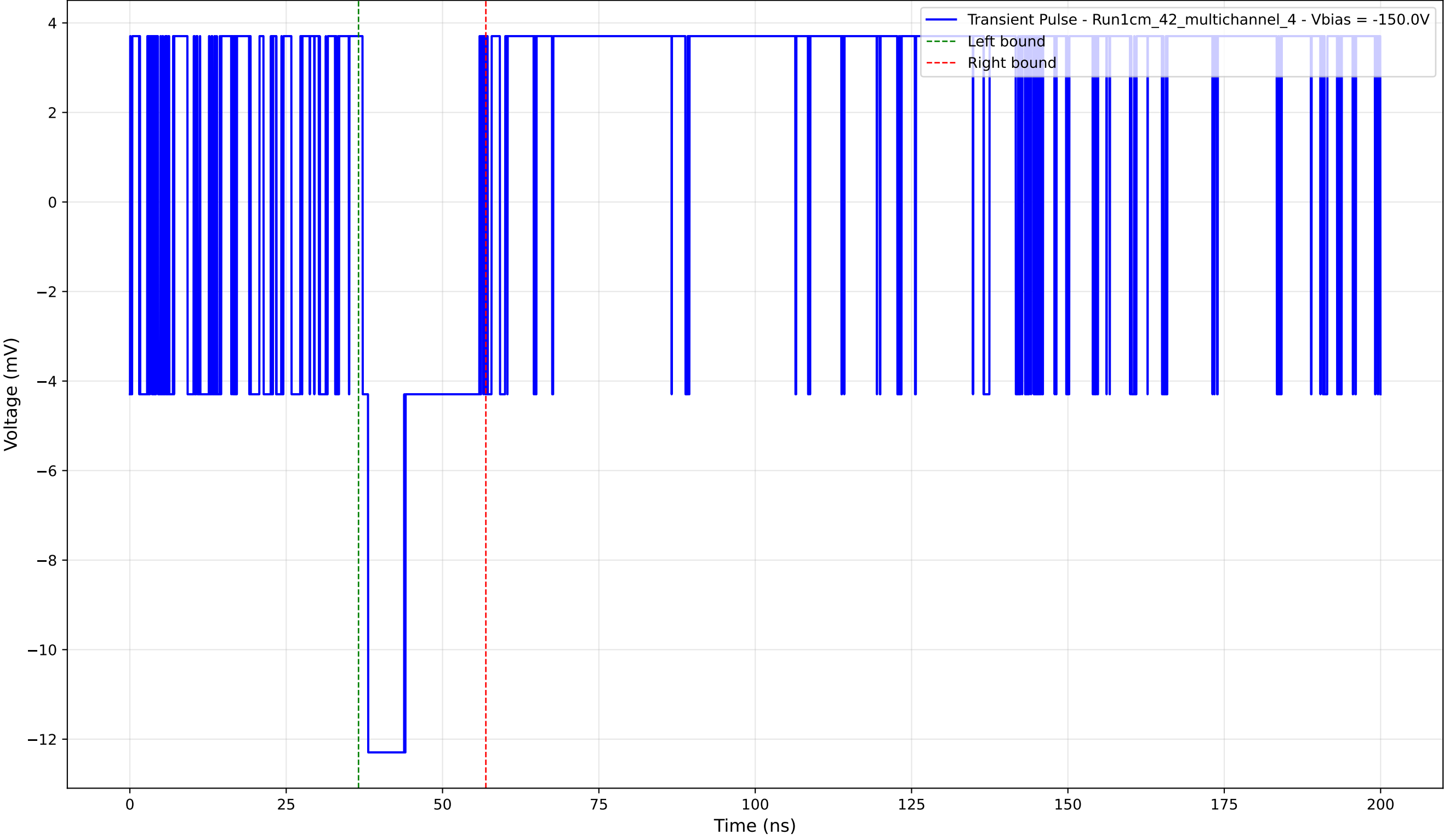
Transient Pulse - Sample: 1cm_42_multichannel - Position: 505.0 \mu\text{m} - Charge: 2.47 pC - Rise Time: 0.00 ns (N/A)
