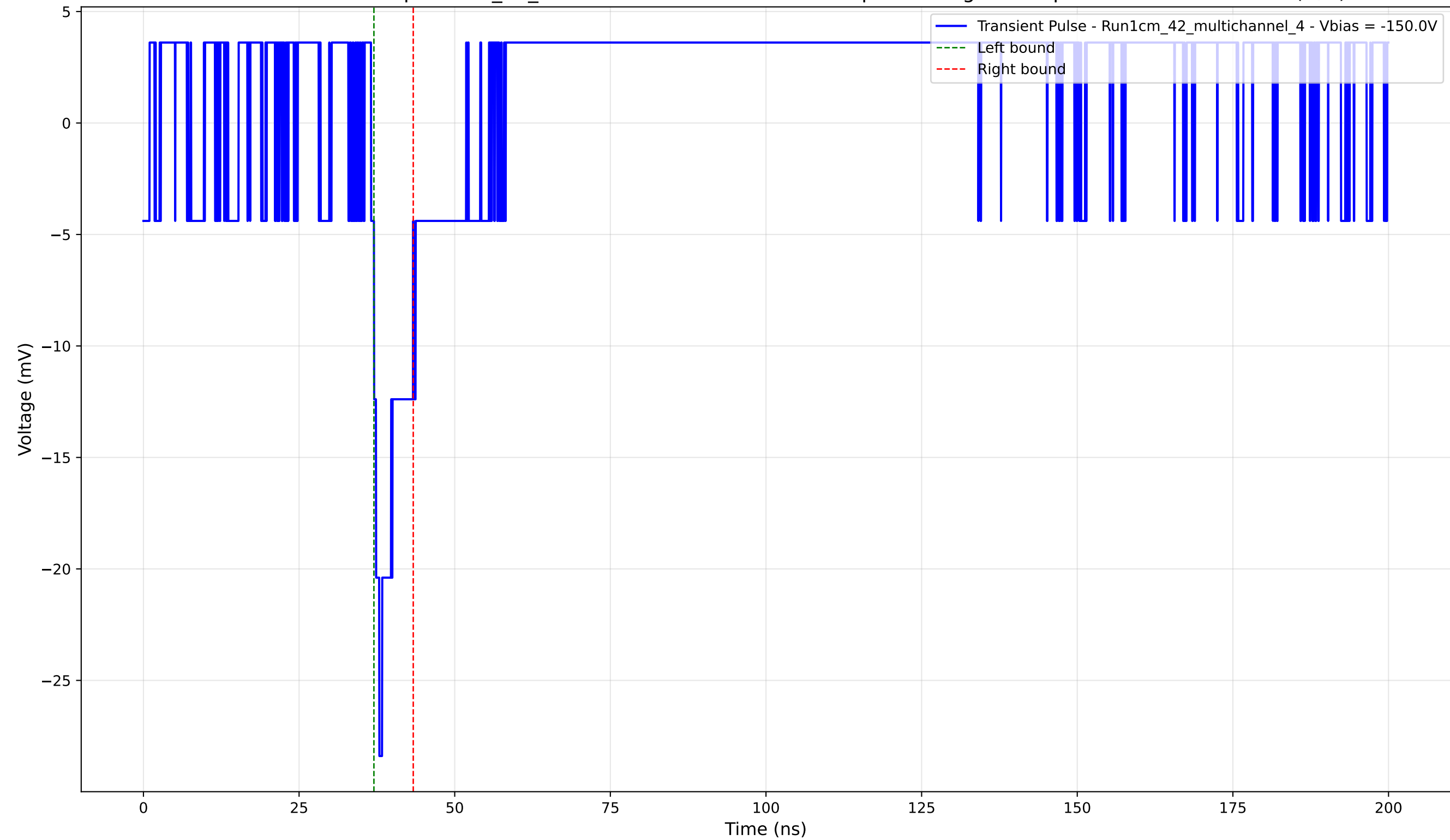
Transient Pulse - Sample: 1cm_42_multichannel - Position: 1445.0 \mu\text{m} - Charge: 2.04 pC - Rise Time: 0.00 ns (N/A)
