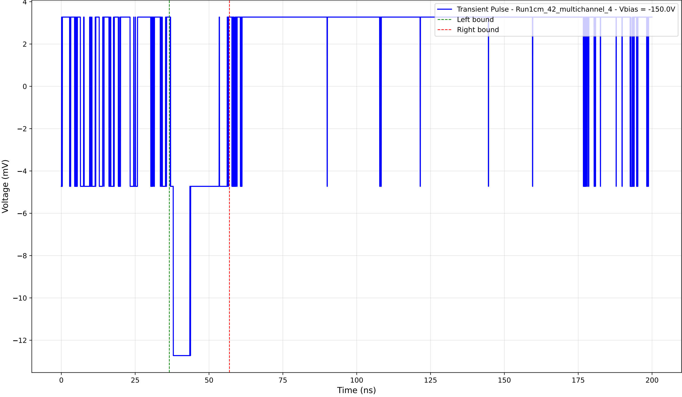
Transient Pulse - Sample: 1cm_42_multichannel - Position: 655.0 \mu\text{m} - Charge: 2.66 pC - Rise Time: 0.00 ns (N/A)
