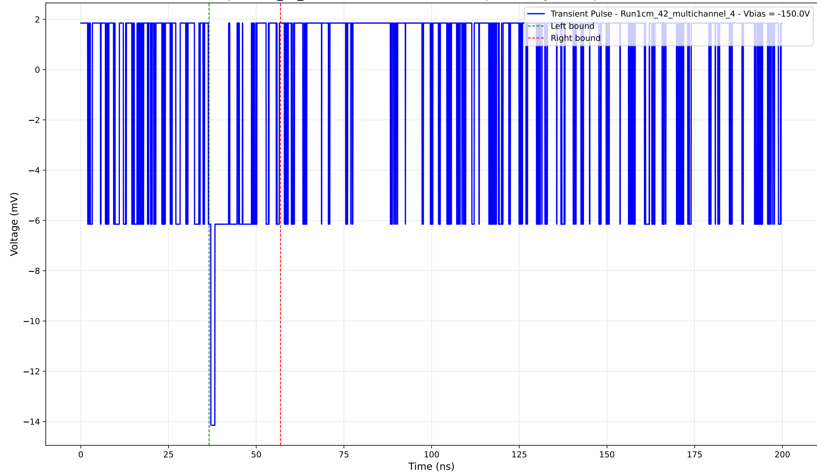
Transient Pulse - Sample: 1cm_42_multichannel - Position: 1920.0 \mu\text{m} - Charge: 1.65 pC - Rise Time: 0.00 ns (N/A)
