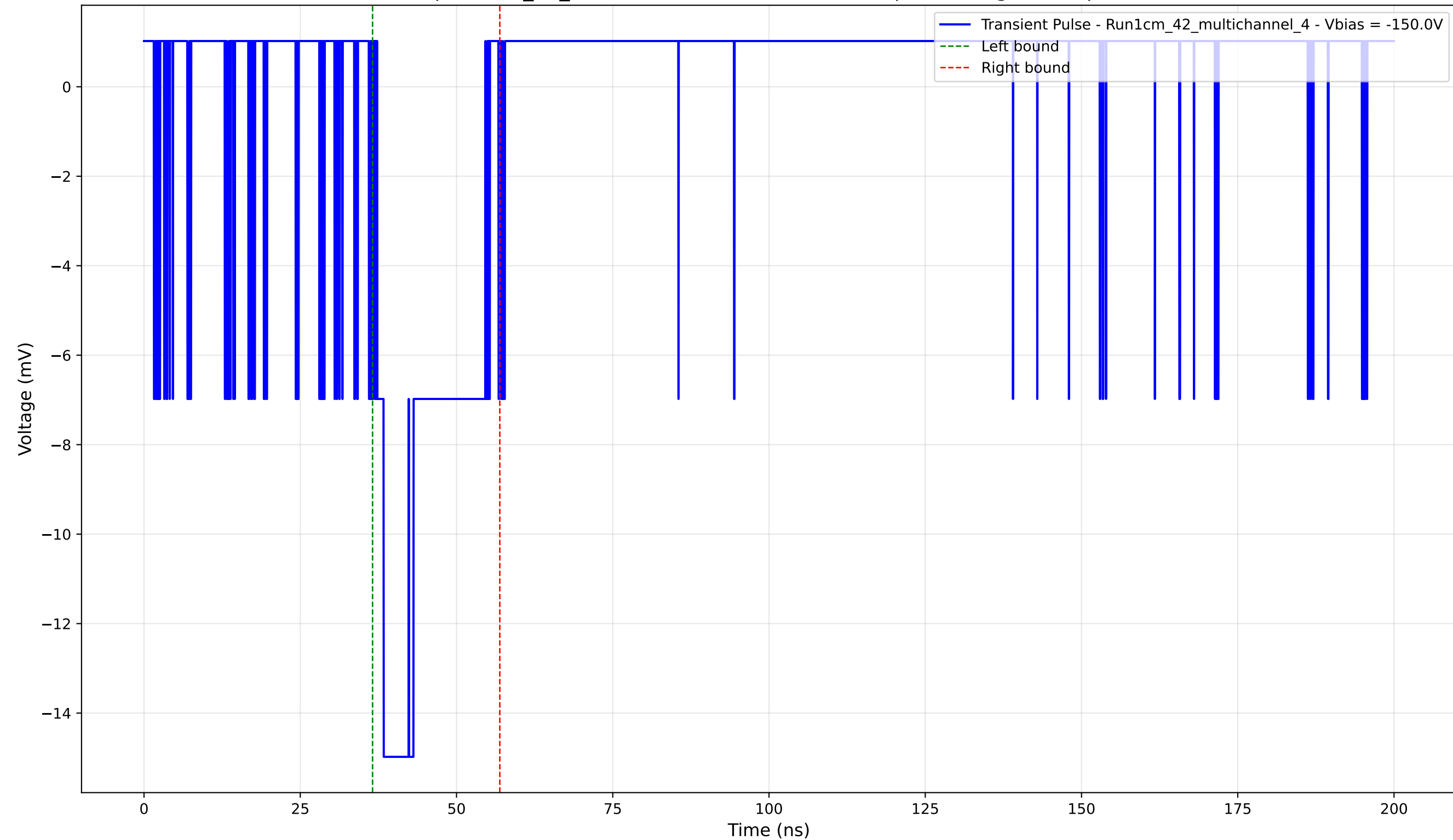
Transient Pulse - Sample: 1cm_42_multichannel - Position: 4520.0 \mu\text{m} - Charge: 3.27 pC - Rise Time: 1.04 ns
