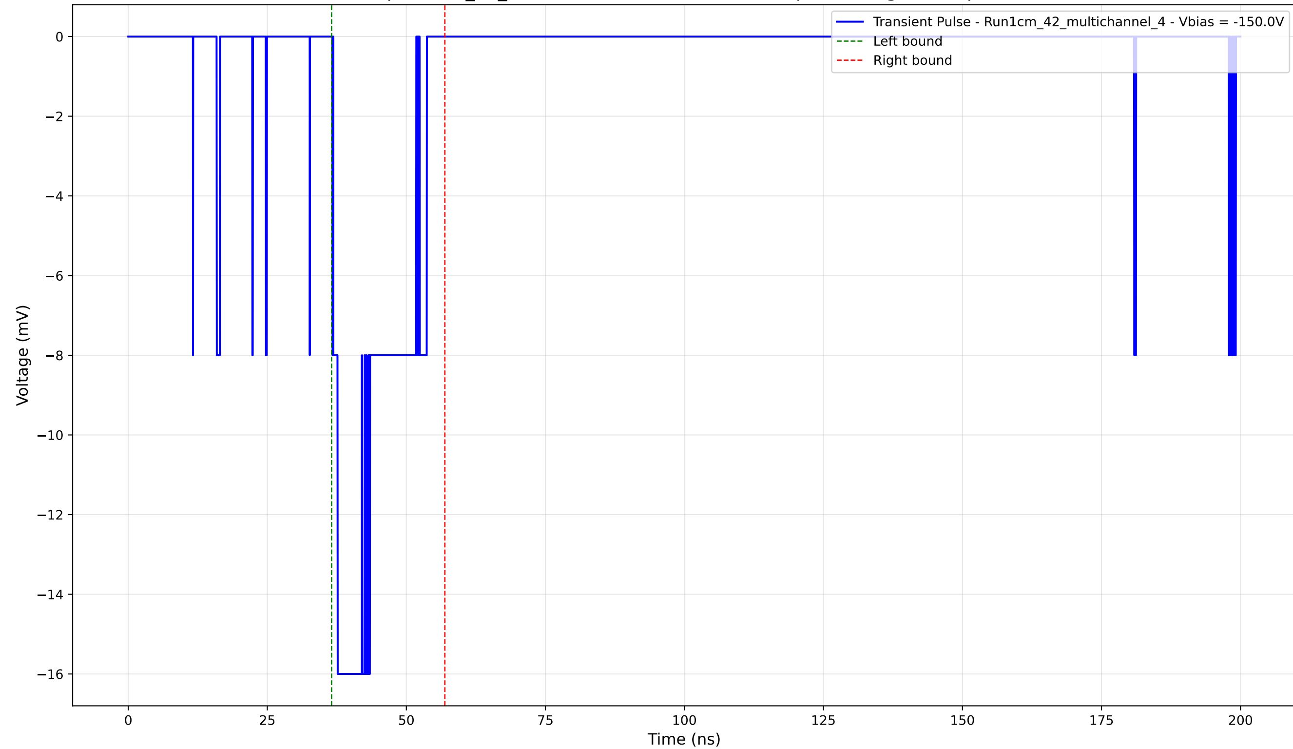
Transient Pulse - Sample: 1cm_42_multichannel - Position: 3795.0 \mu\text{m} - Charge: 3.50 pC - Rise Time: 0.80 ns
