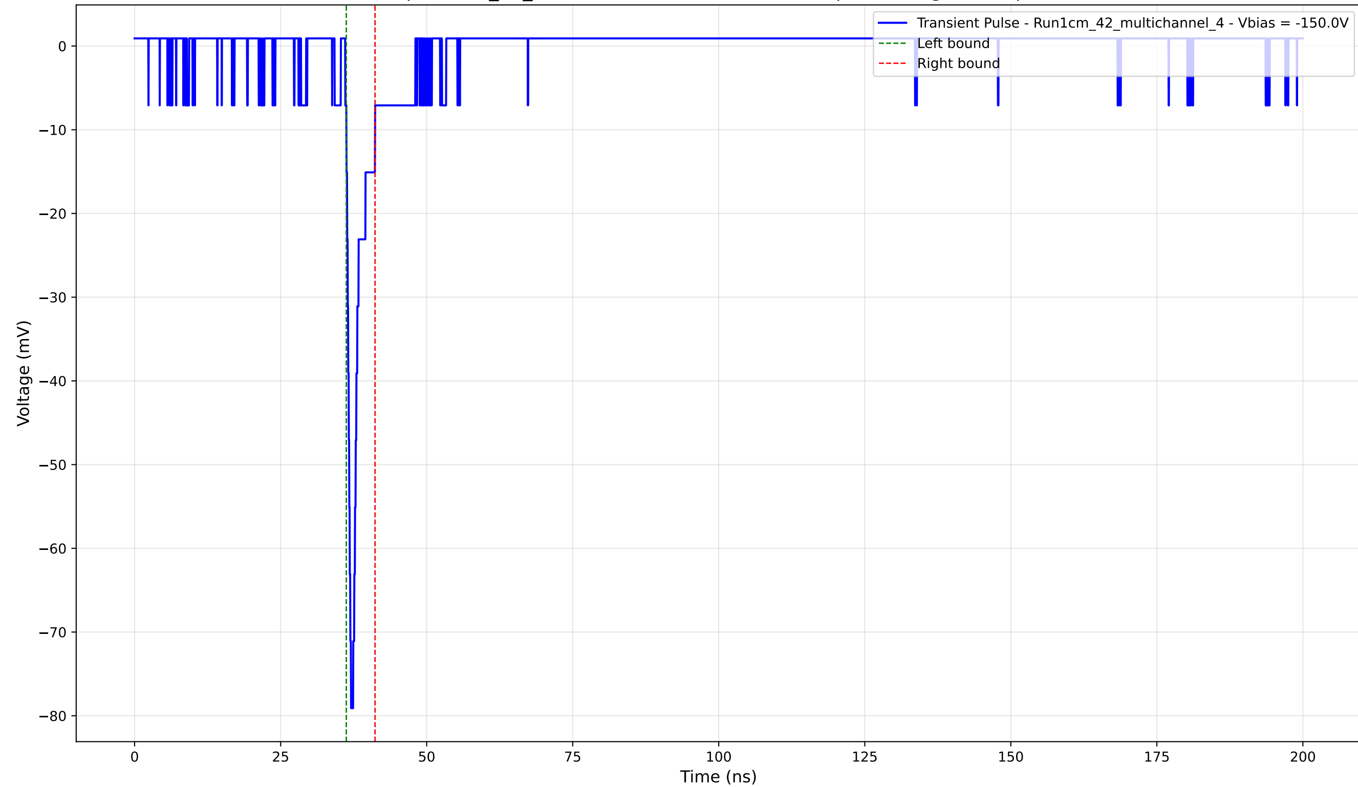
Transient Pulse - Sample: 1cm_42_multichannel - Position: 2305.0 \mu\text{m} - Charge: 3.23 pC - Rise Time: 0.80 ns
