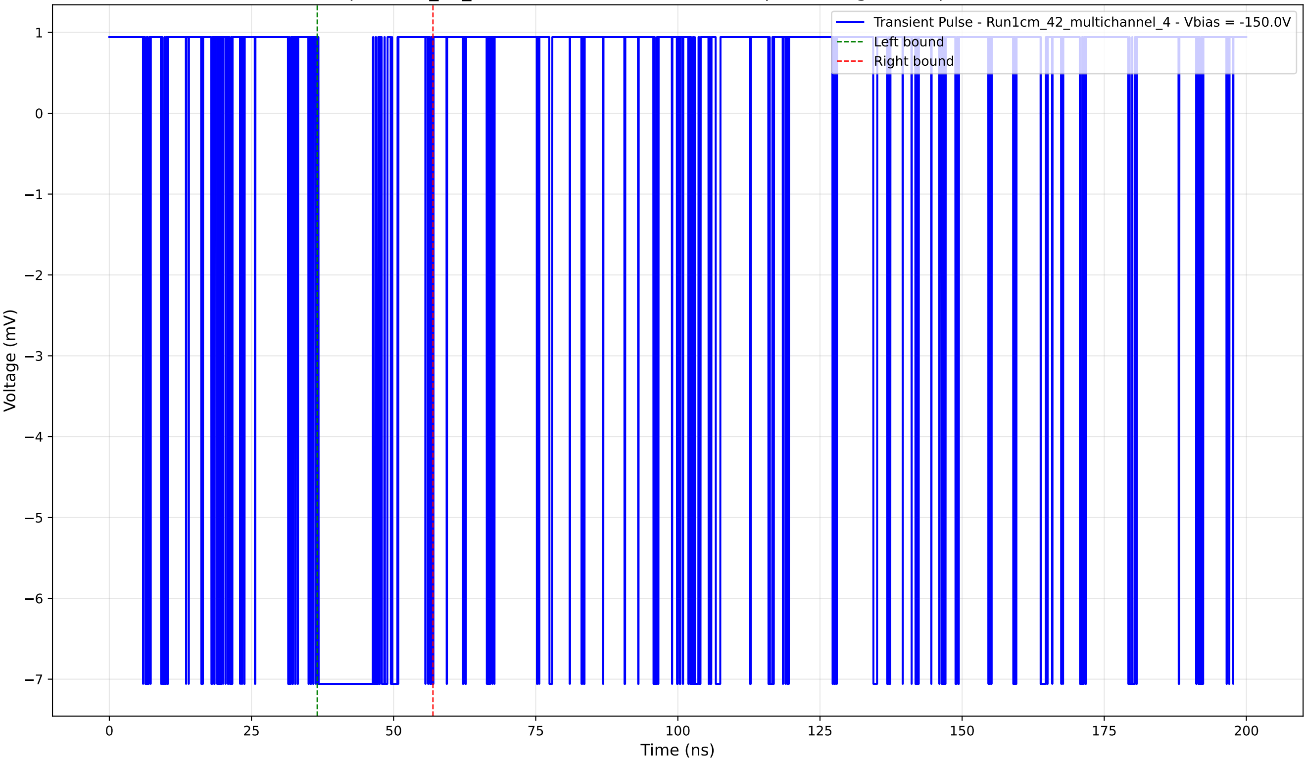
Transient Pulse - Sample: 1cm_42_multichannel - Position: 3435.0 \mu\text{m} - Charge: 1.70 pC - Rise Time: 0.00 ns (N/A)
