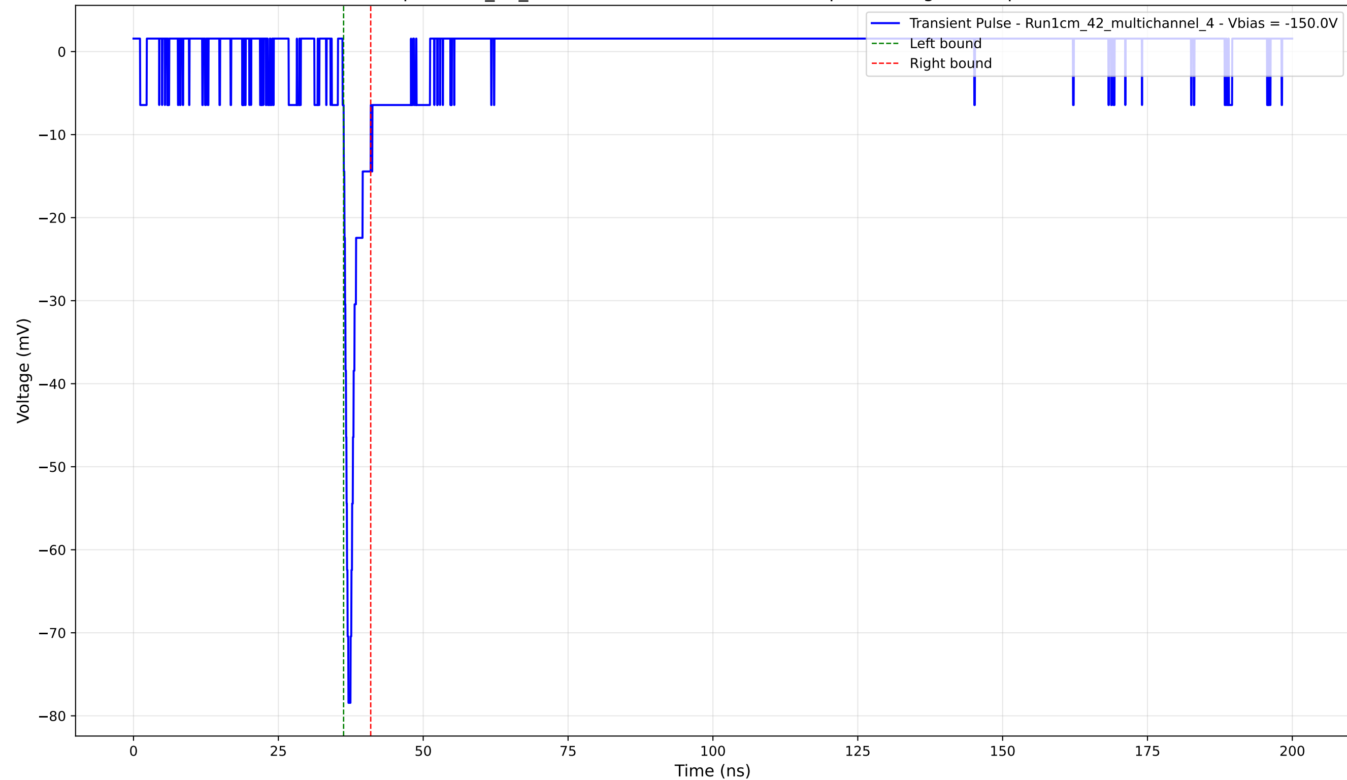
Transient Pulse - Sample: 1cm_42_multichannel - Position: 2275.0 \mu\text{m} - Charge: 3.10 pC - Rise Time: 0.82 ns
