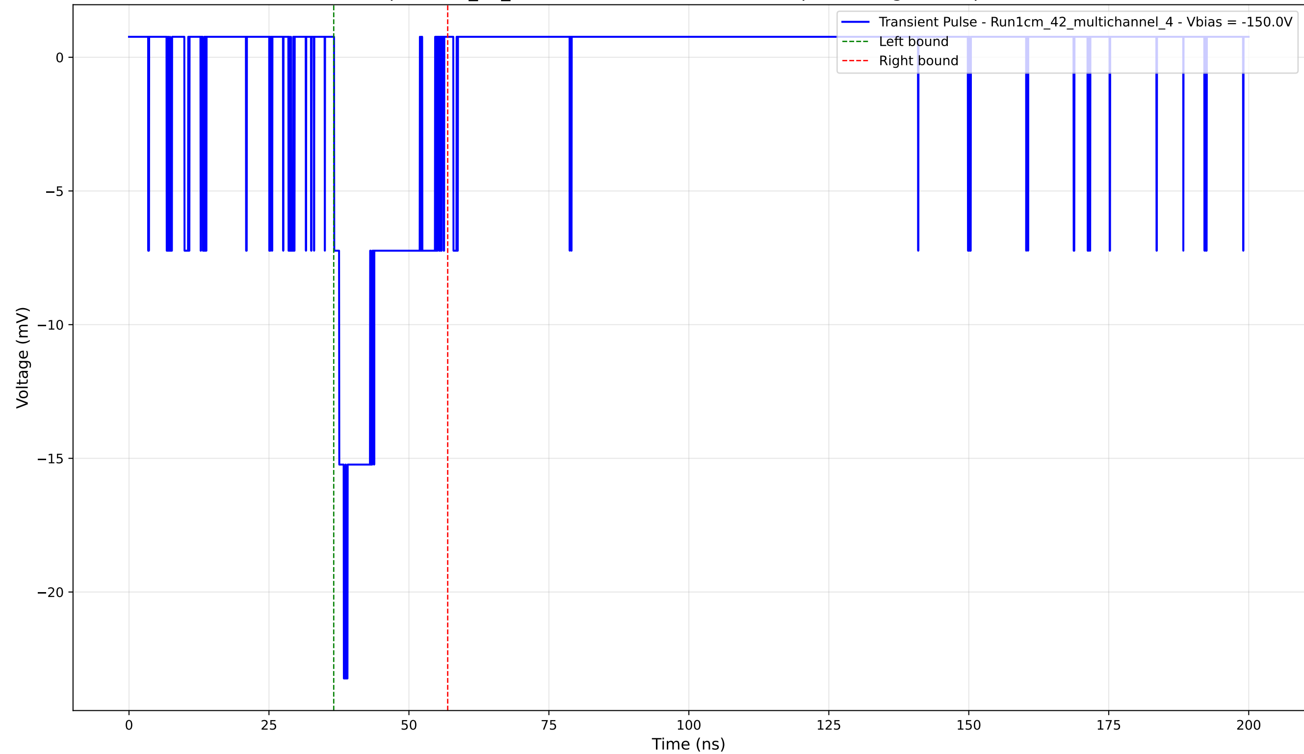
Transient Pulse - Sample: 1cm_42_multichannel - Position: 3670.0 \mu\text{m} - Charge: 3.67 pC - Rise Time: 1.74 ns
