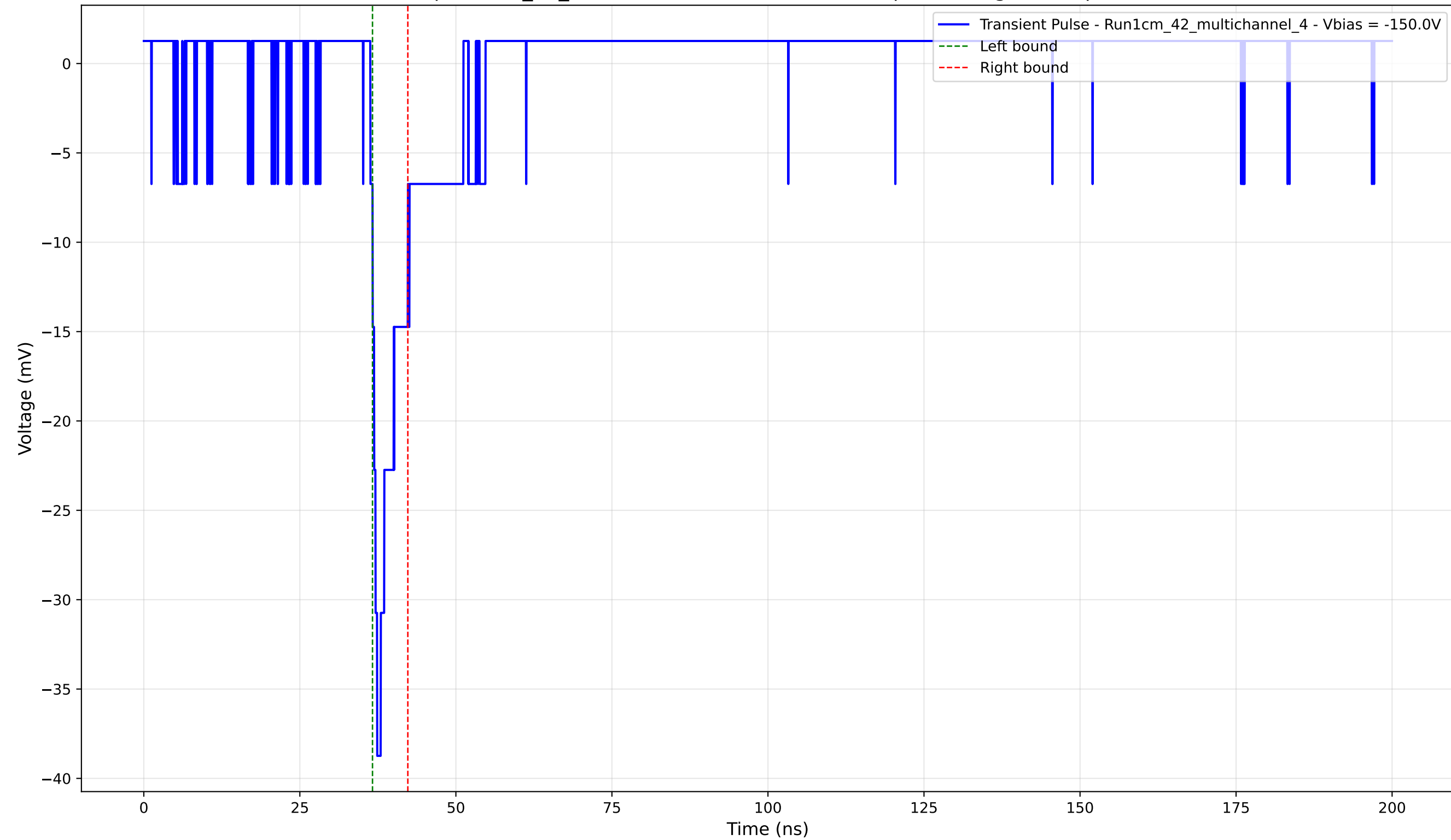
Transient Pulse - Sample: 1cm_42_multichannel - Position: 3025.0 \mu\text{m} - Charge: 2.49 pC - Rise Time: 1.09 ns
