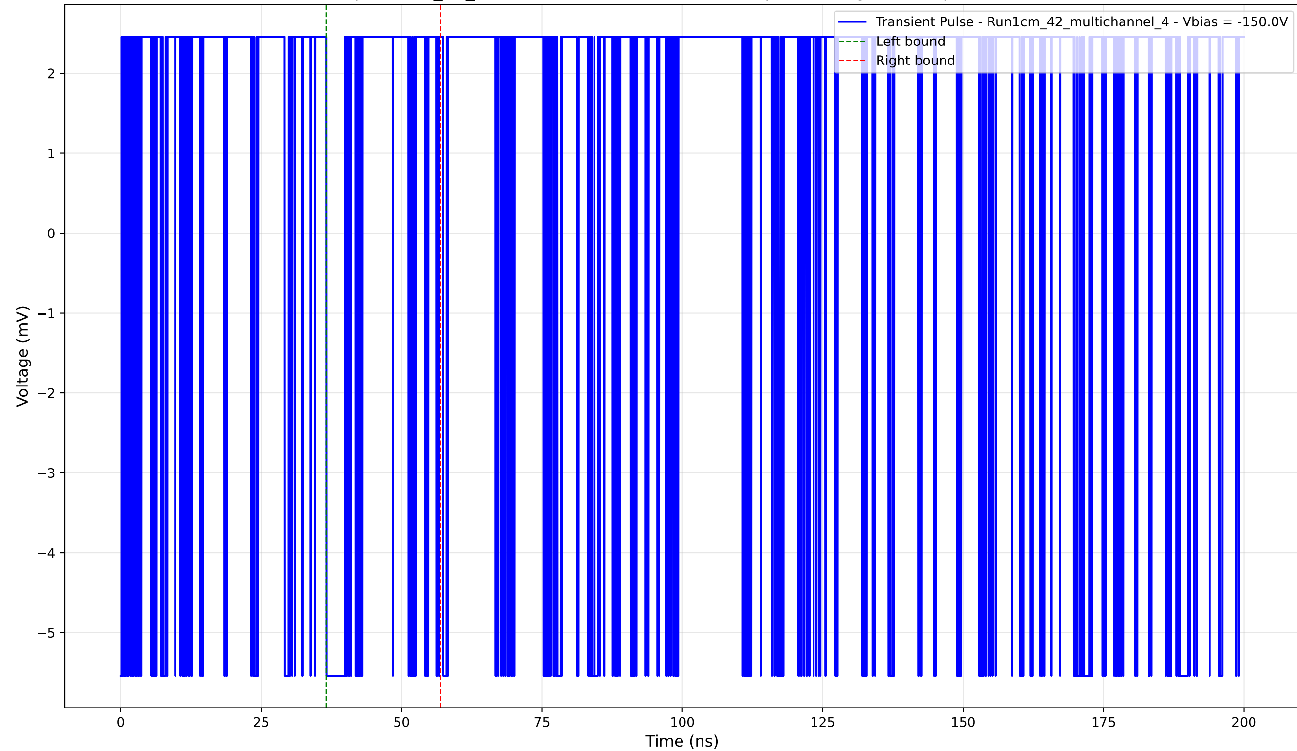
Transient Pulse - Sample: 1cm_42_multichannel - Position: 2880.0 \mu\text{m} - Charge: -0.02 pC - Rise Time: 0.00 ns (N/A)
