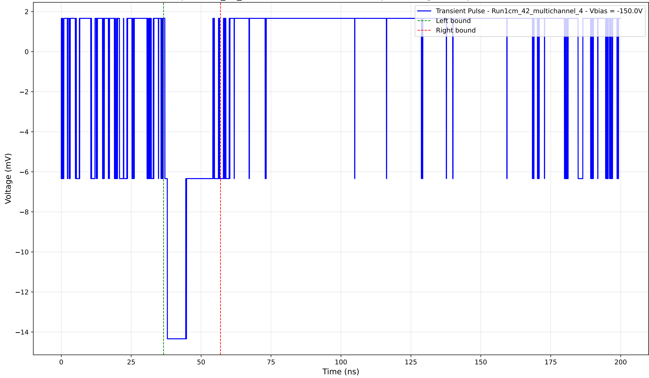
Transient Pulse - Sample: 1cm_42_multichannel - Position: 625.0 \mu\text{m} - Charge: 3.51 pC - Rise Time: 0.00 ns (N/A)
