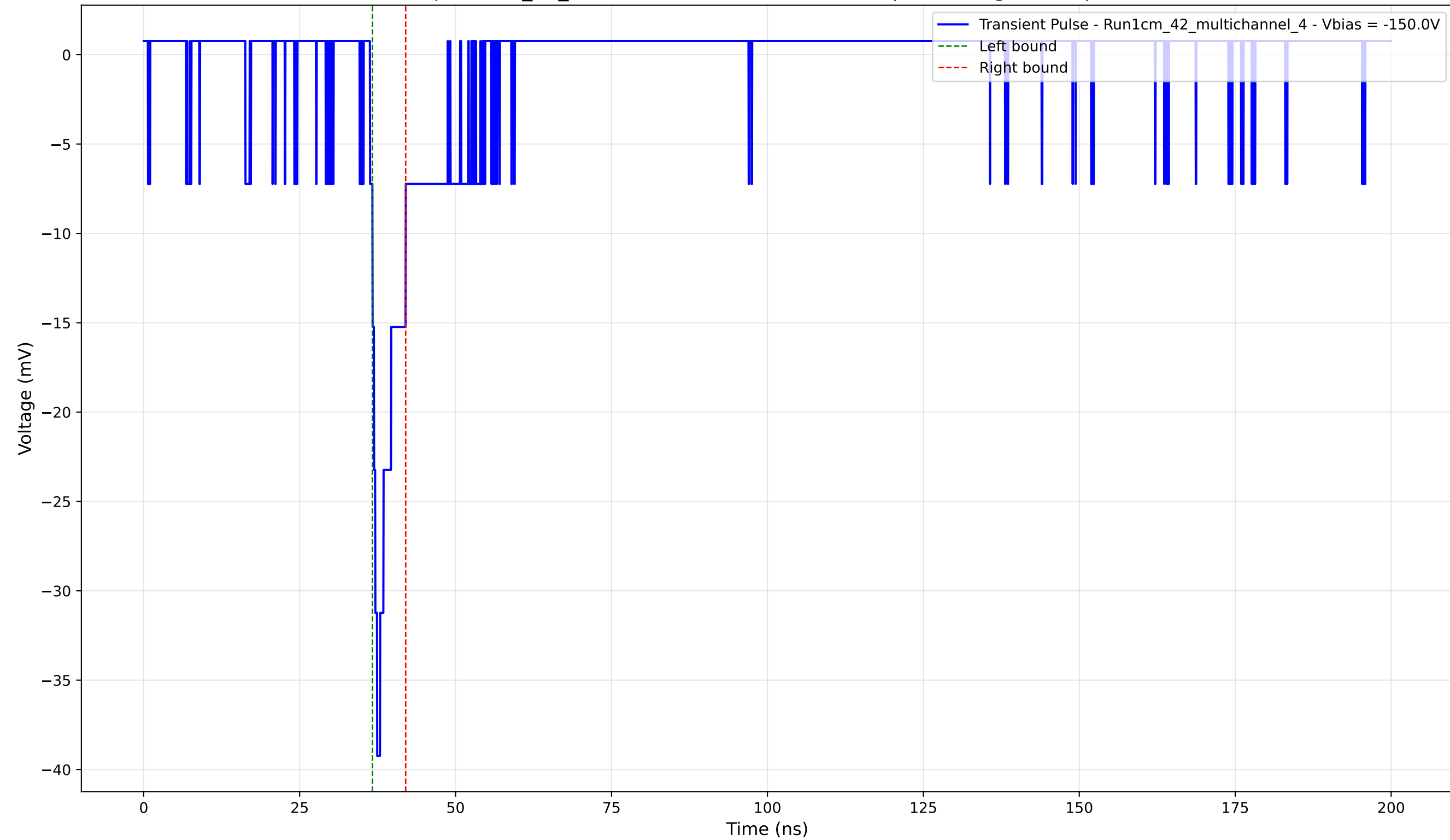
Transient Pulse - Sample: 1cm_42_multichannel - Position: 3020.0 \mu\text{m} - Charge: 2.35 pC - Rise Time: 1.15 ns
