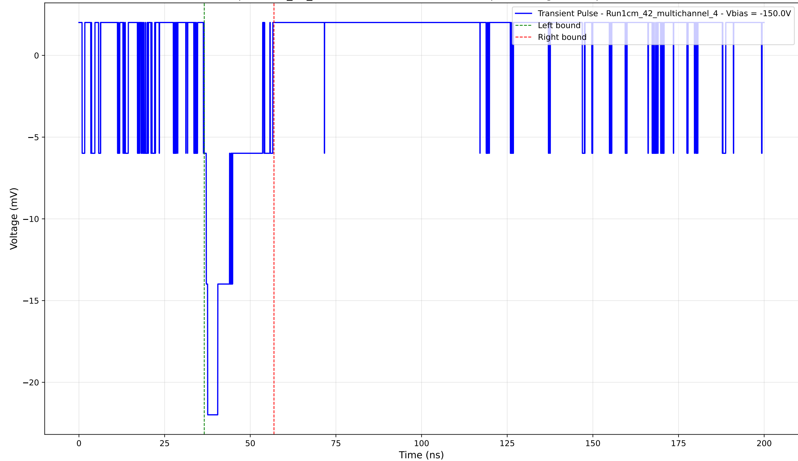
Transient Pulse - Sample: 1cm_42_multichannel - Position: 1260.0 \mu\text{m} - Charge: 3.95 pC - Rise Time: 1.04 ns
