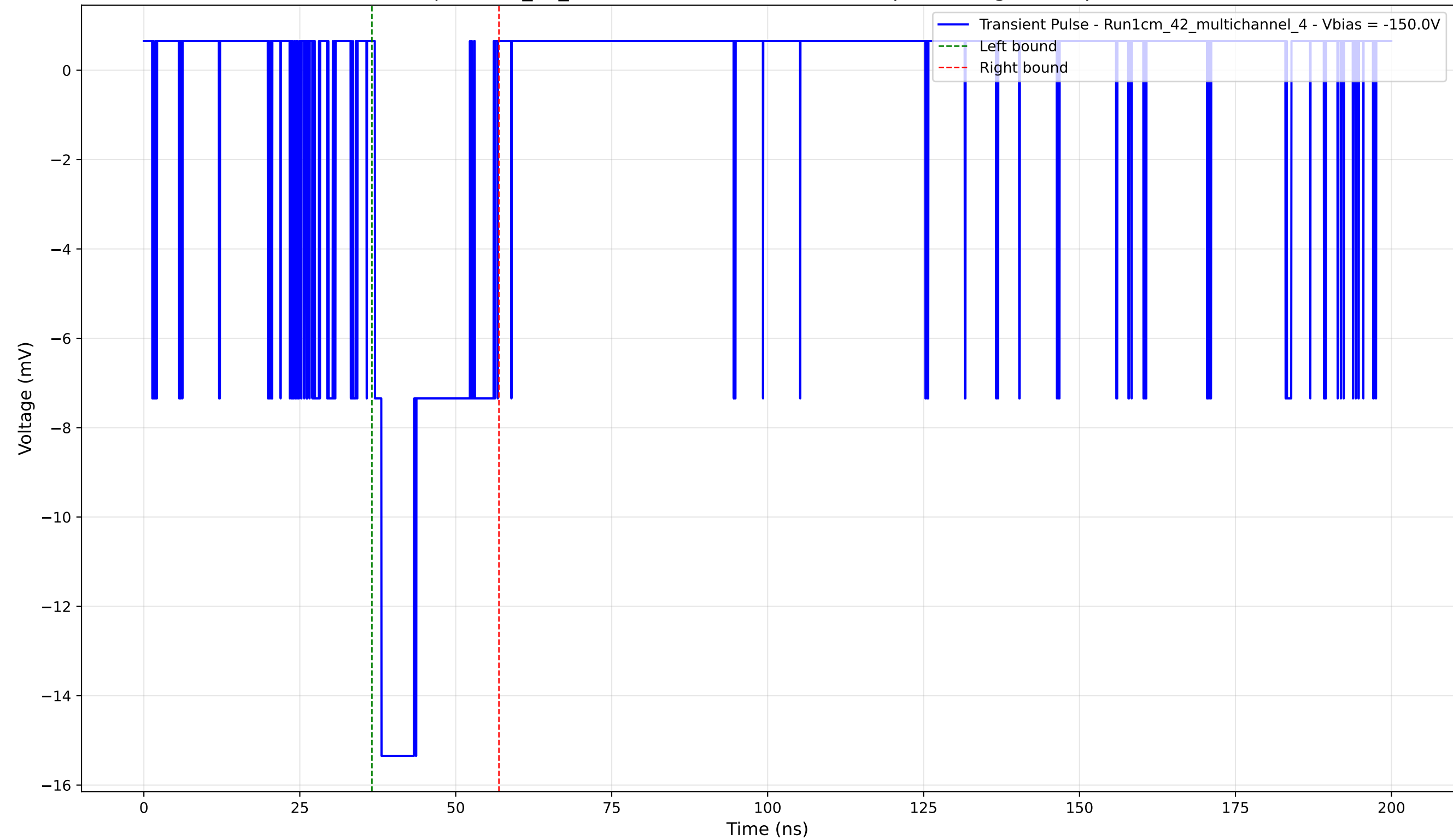
Transient Pulse - Sample: 1cm_42_multichannel - Position: 4120.0 \mu\text{m} - Charge: 3.61 pC - Rise Time: 1.06 ns
