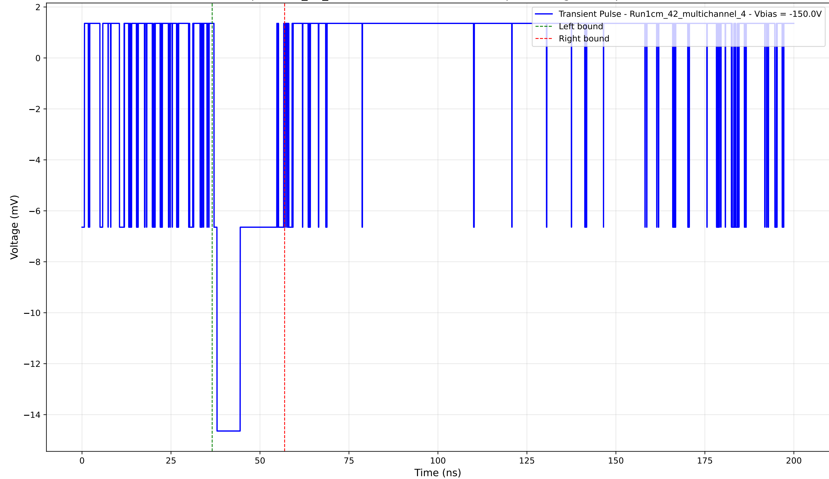
Transient Pulse - Sample: 1cm_42_multichannel - Position: 640.0 \mu\text{m} - Charge: 3.63 pC - Rise Time: 0.86 ns
