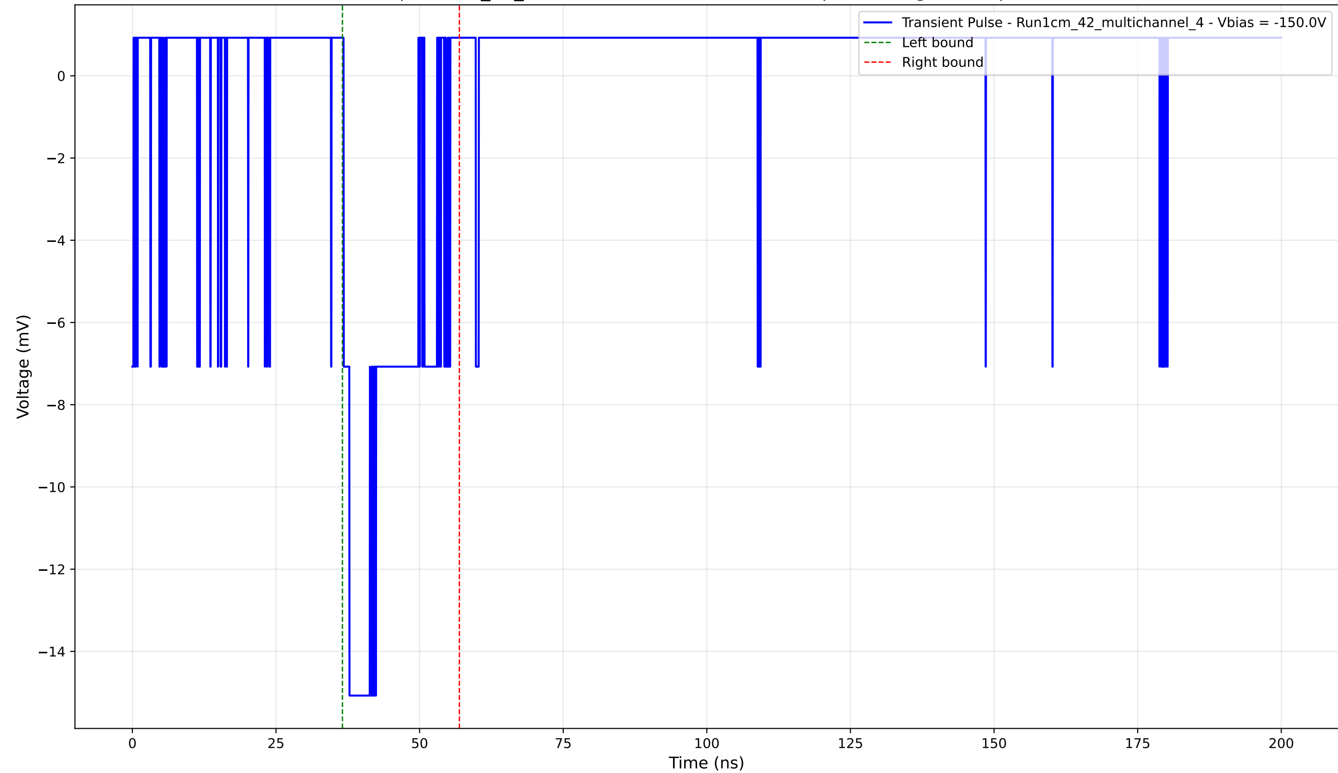
Transient Pulse - Sample: 1cm_42_multichannel - Position: 3835.0 \mu\text{m} - Charge: 2.94 pC - Rise Time: 1.02 ns
