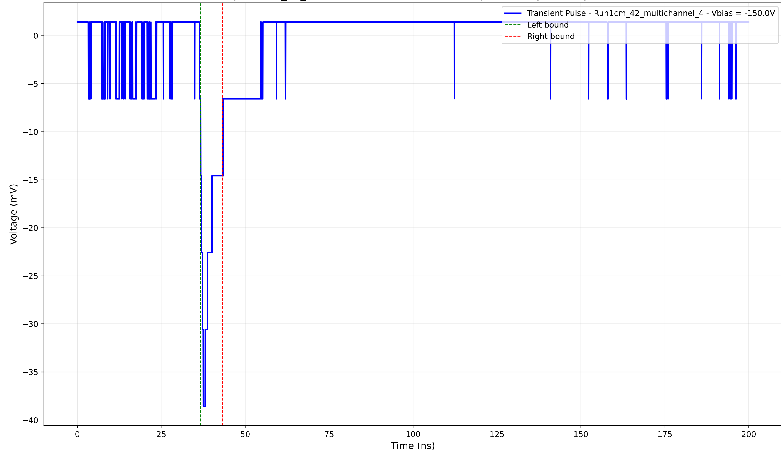
Transient Pulse - Sample: 1cm_42_multichannel - Position: 1690.0 \mu\text{m} - Charge: 2.75 pC - Rise Time: 1.09 ns
