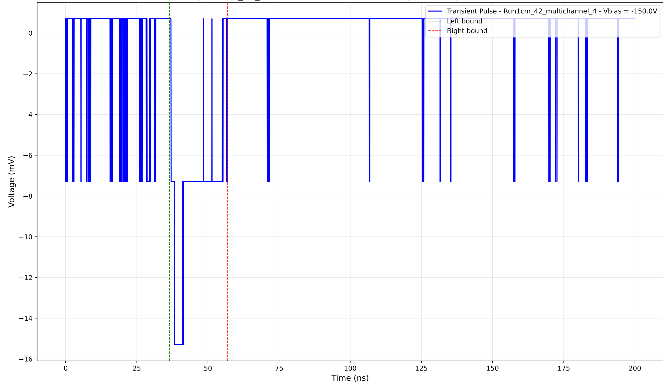
Transient Pulse - Sample: 1cm_42_multichannel - Position: 3965.0 \mu\text{m} - Charge: 3.14 pC - Rise Time: 1.18 ns
