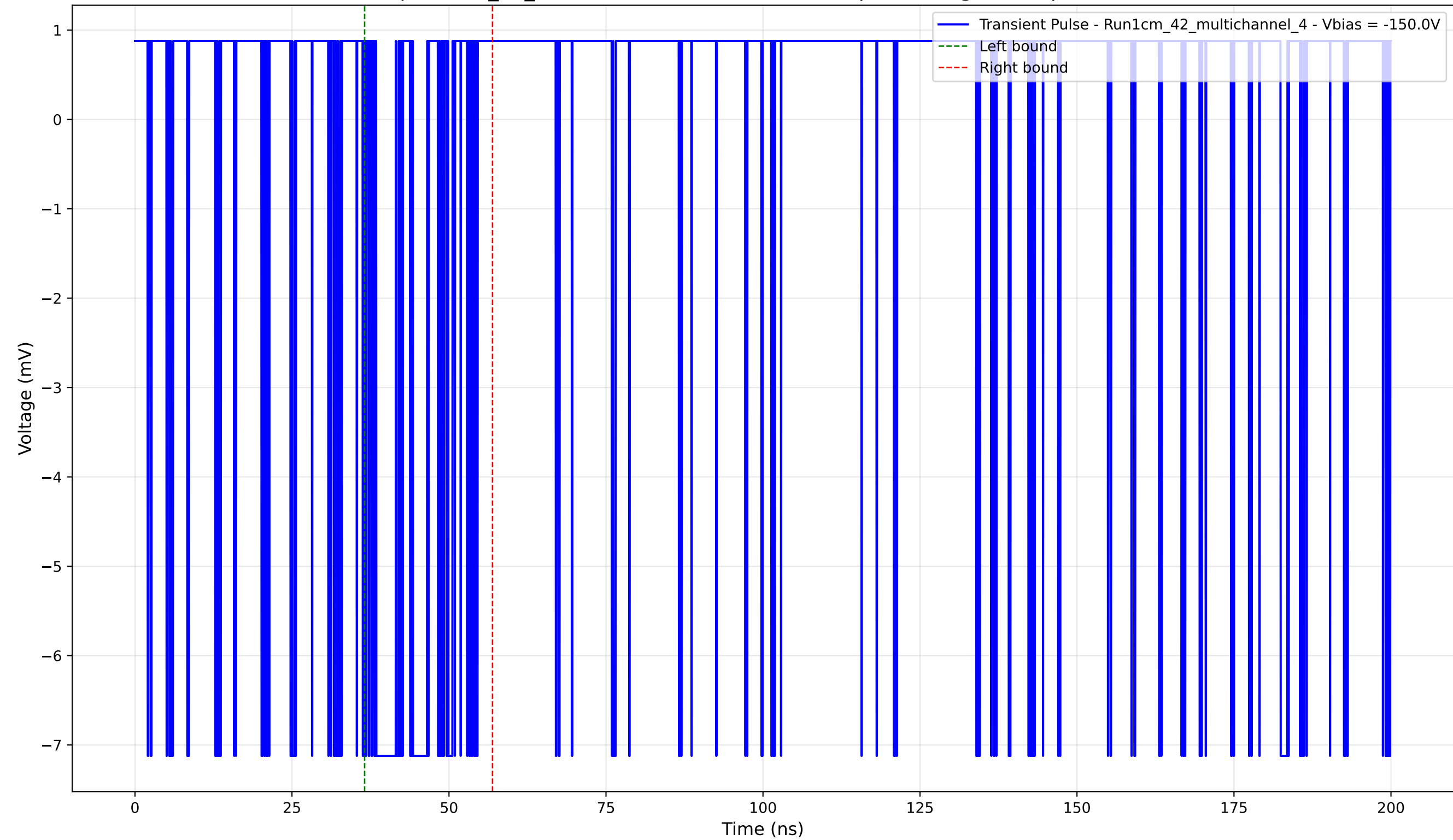
Transient Pulse - Sample: 1cm_42_multichannel - Position: 4875.0 \mu\text{m} - Charge: 1.10 pC - Rise Time: 0.00 ns (N/A)
