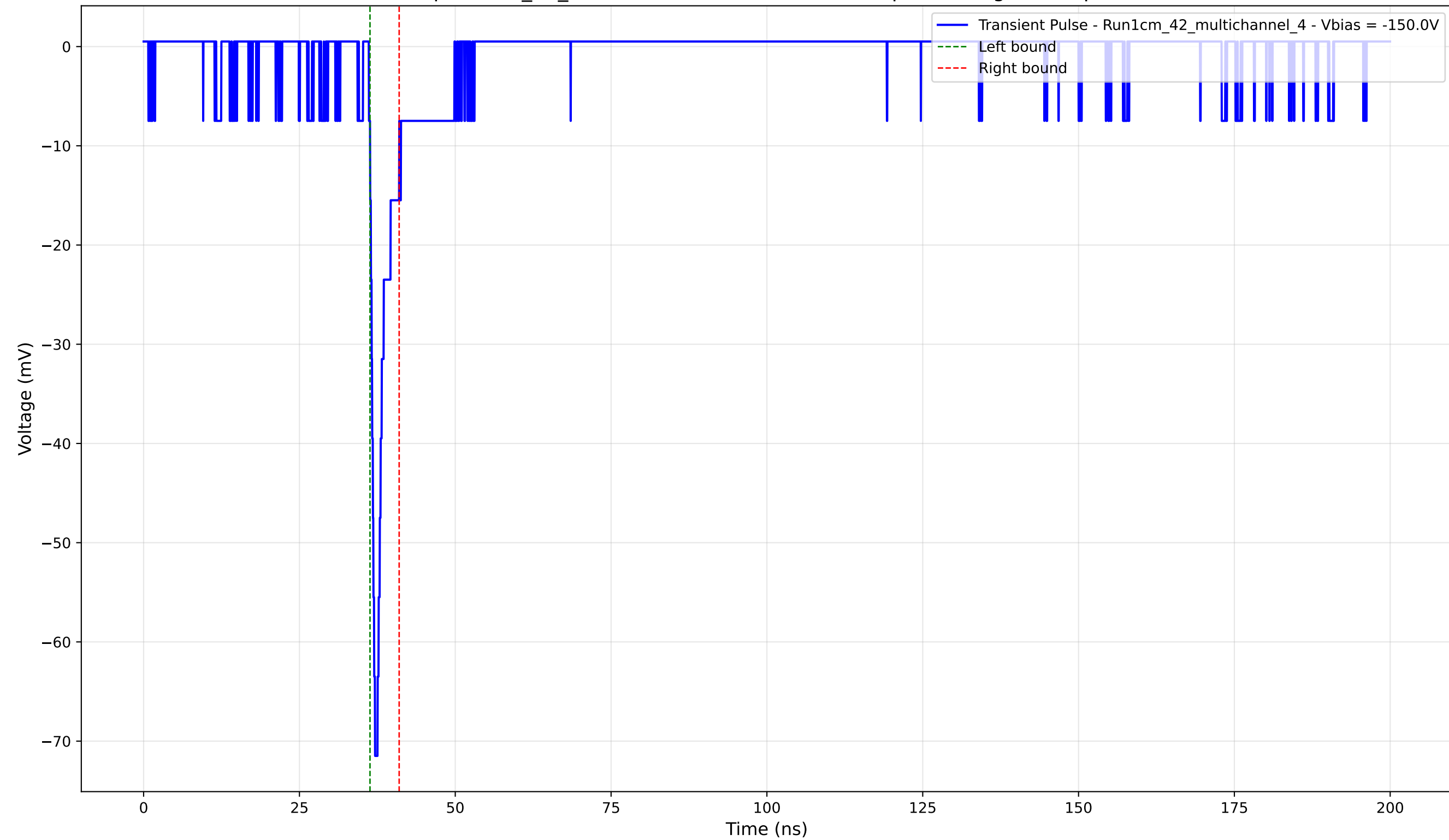
Transient Pulse - Sample: 1cm_42_multichannel - Position: 2195.0 \mu\text{m} - Charge: 3.05 pC - Rise Time: 0.98 ns
