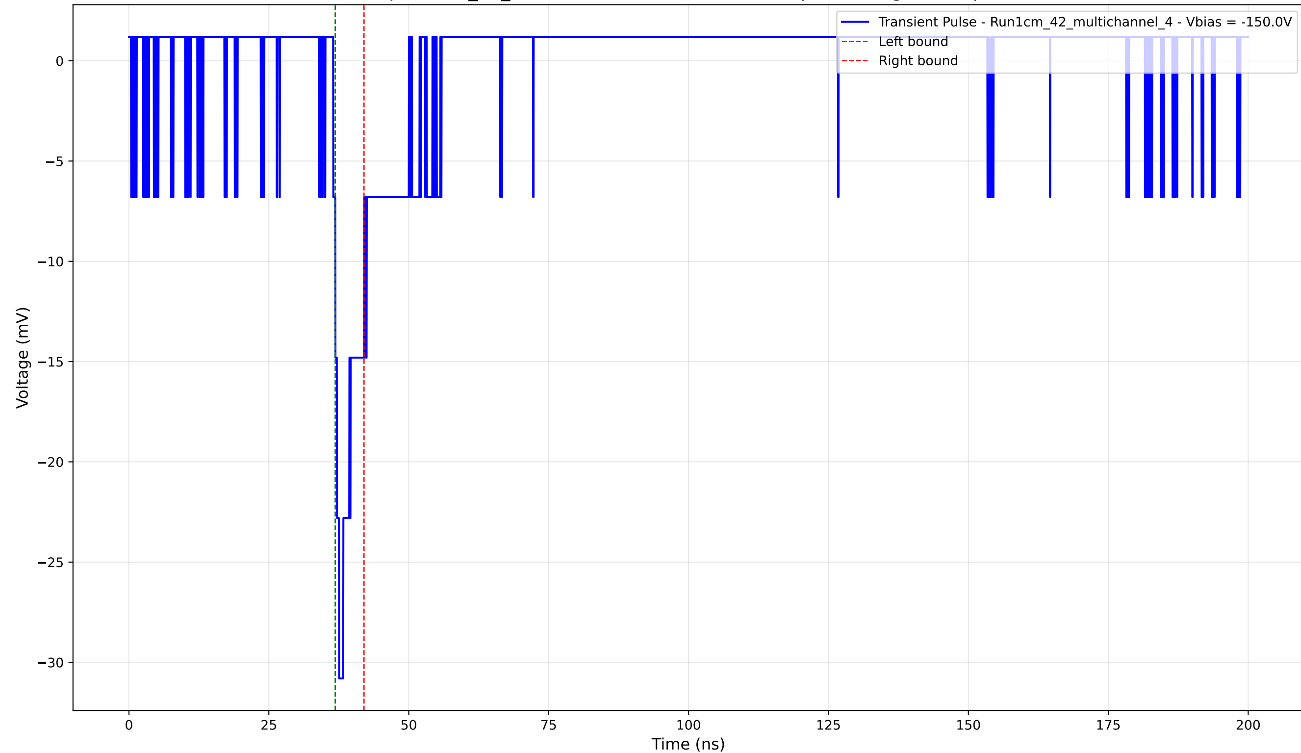
Transient Pulse - Sample: 1cm_42_multichannel - Position: 3185.0 \mu\text{m} - Charge: 2.02 pC - Rise Time: 1.05 ns
