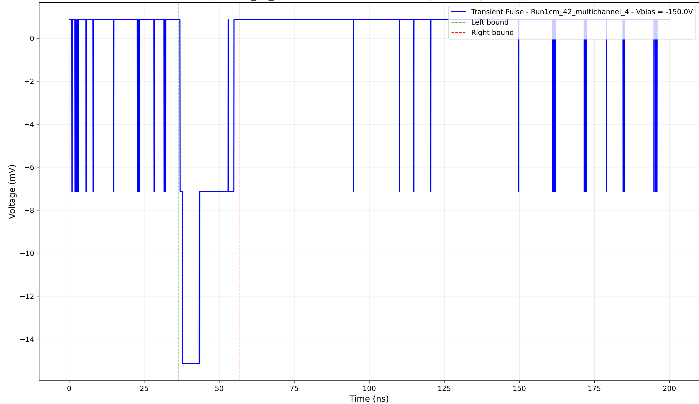
Transient Pulse - Sample: 1cm_42_multichannel - Position: 3820.0 \mu\text{m} - Charge: 3.42 pC - Rise Time: 0.88 ns
