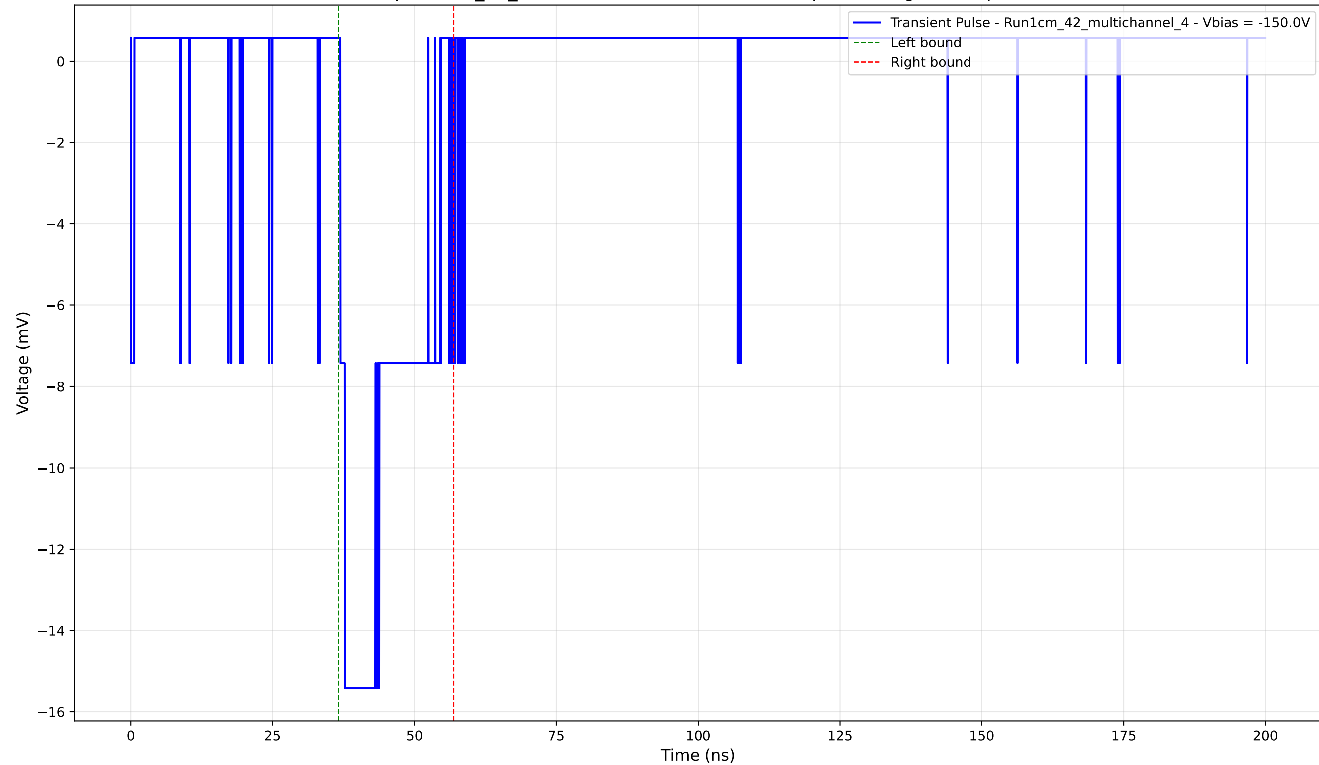
Transient Pulse - Sample: 1cm_42_multichannel - Position: 3805.0 \mu\text{m} - Charge: 3.55 pC - Rise Time: 0.80 ns
