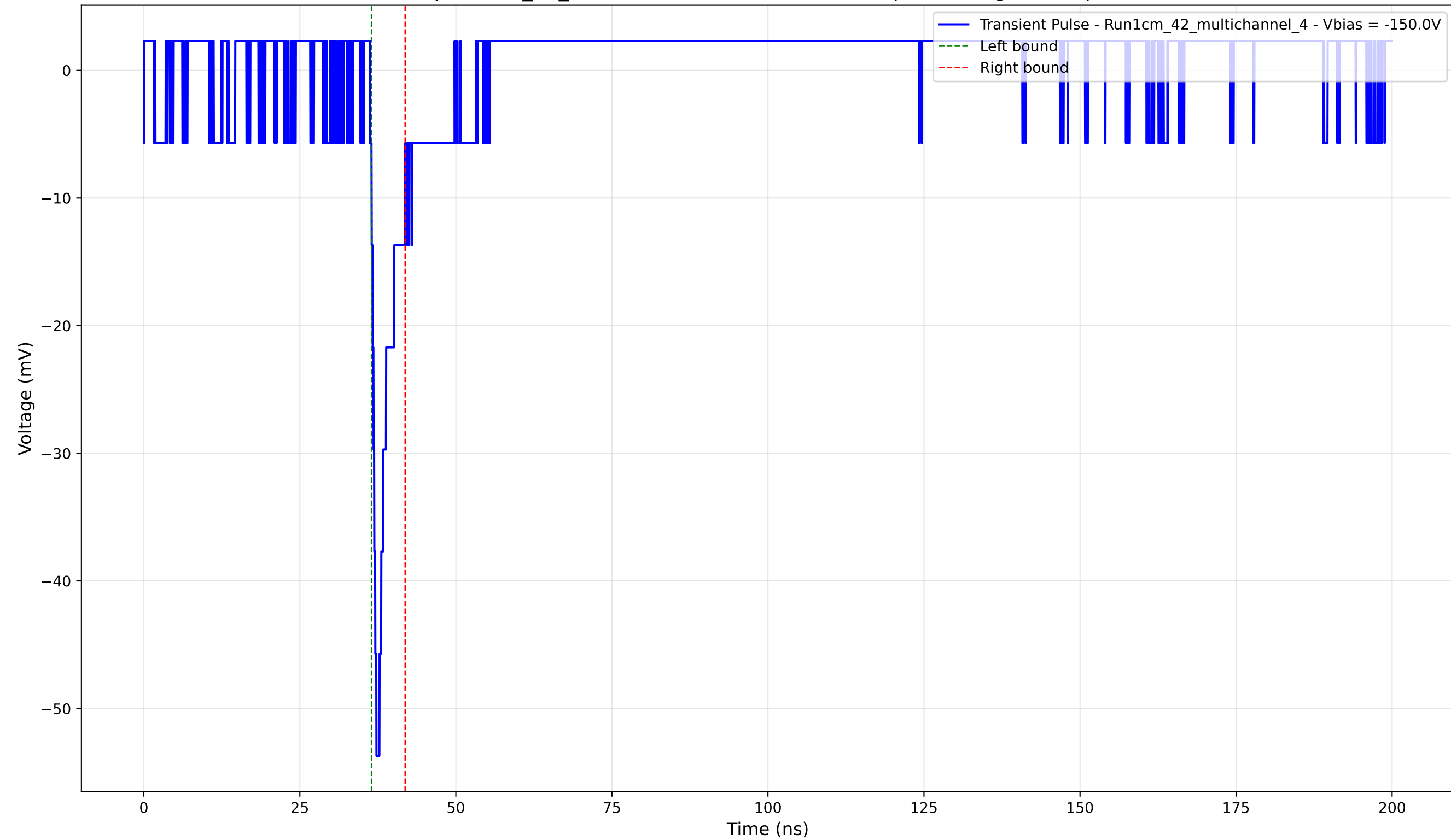
Transient Pulse - Sample: 1cm_42_multichannel - Position: 1975.0 \mu\text{m} - Charge: 2.81 pC - Rise Time: 1.02 ns
