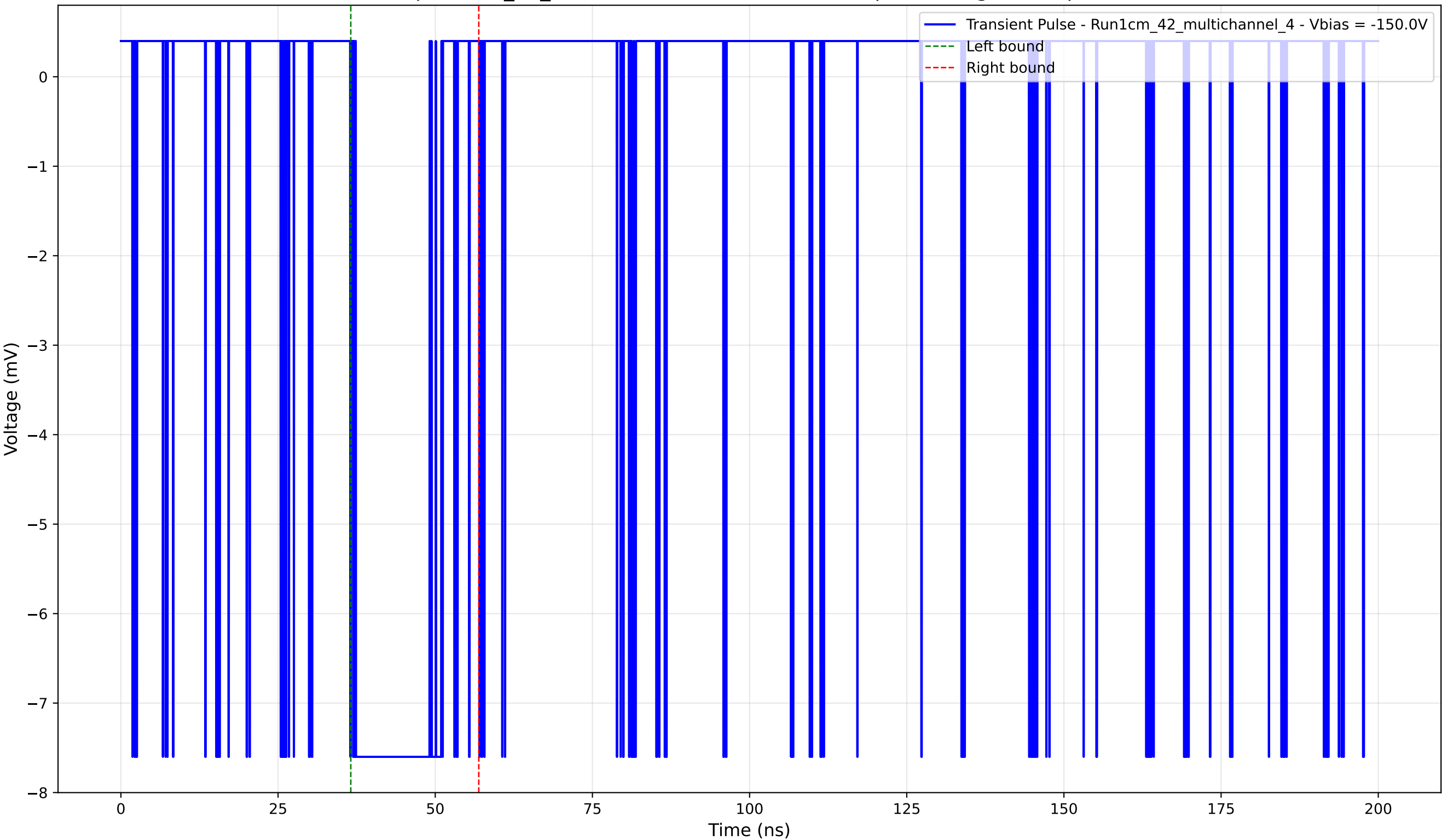
Transient Pulse - Sample: 1cm_42_multichannel - Position: 4445.0 \mu\text{m} - Charge: 2.11 pC - Rise Time: 0.02 ns
