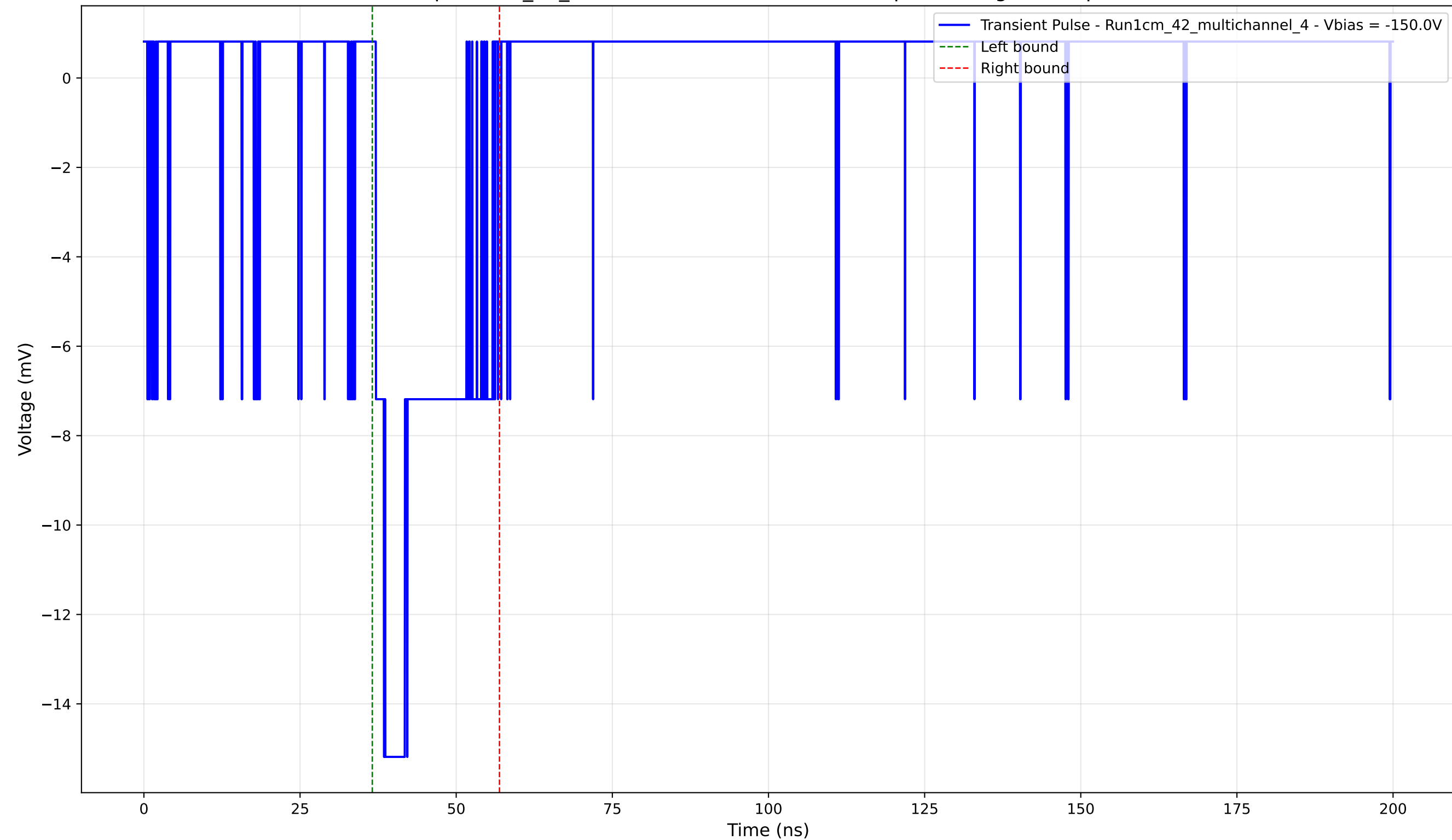
Transient Pulse - Sample: 1cm_42_multichannel - Position: 4660.0 \mu\text{m} - Charge: 3.12 pC - Rise Time: 1.30 ns
