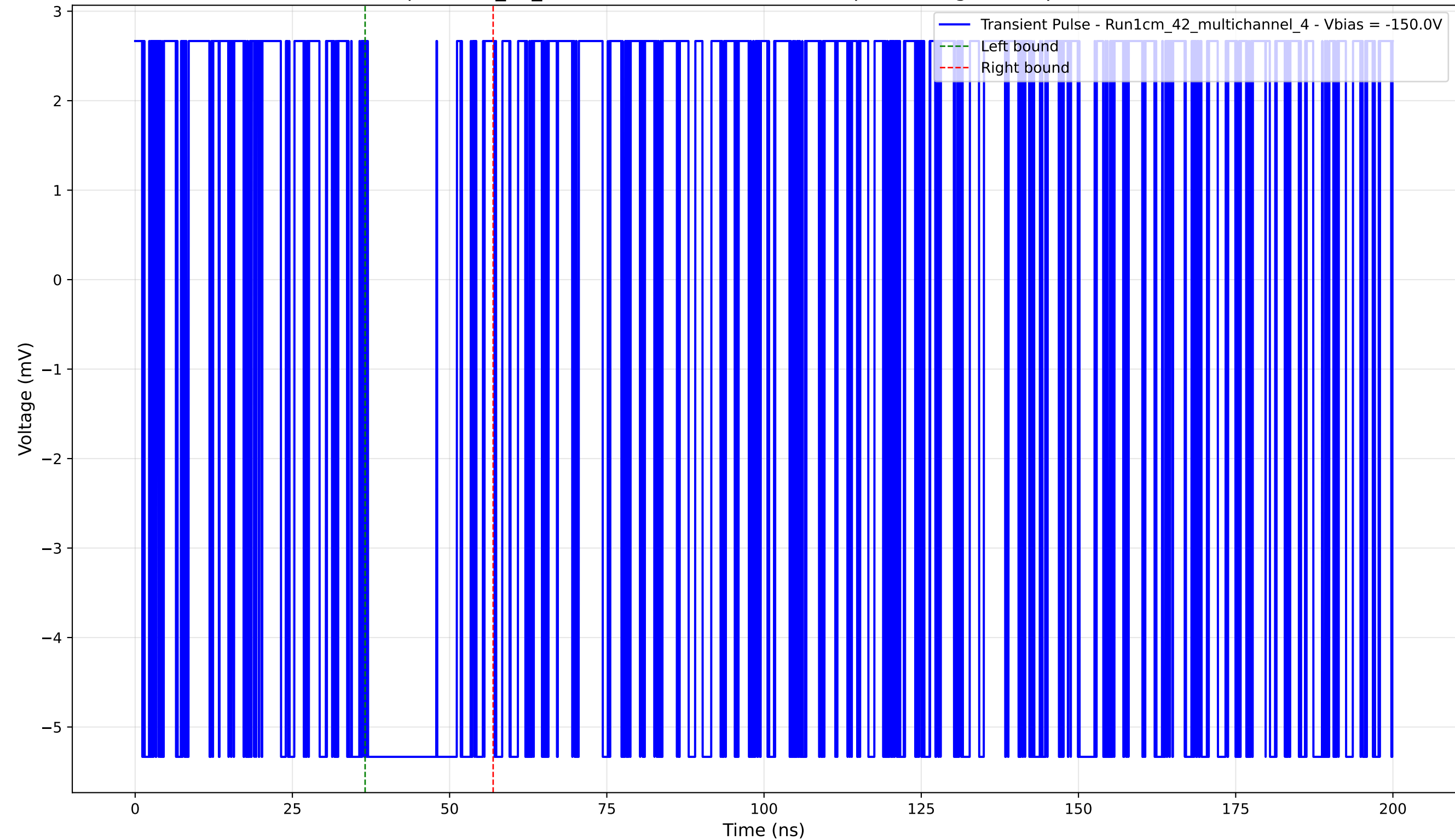
Transient Pulse - Sample: 1cm_42_multichannel - Position: 320.0 \mu\text{m} - Charge: 1.63 pC - Rise Time: 0.00 ns (N/A)
