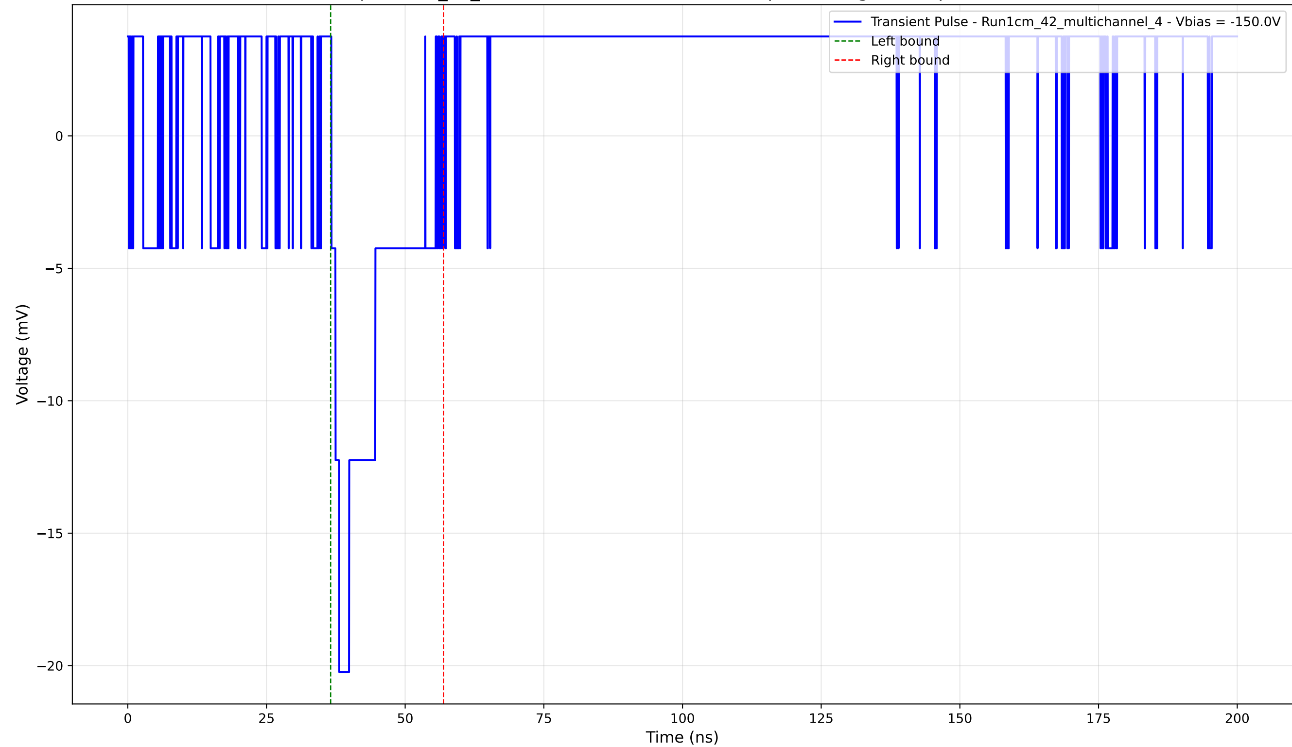
Transient Pulse - Sample: 1cm_42_multichannel - Position: 1030.0 \mu\text{m} - Charge: 3.04 pC - Rise Time: 0.00 ns (N/A)
