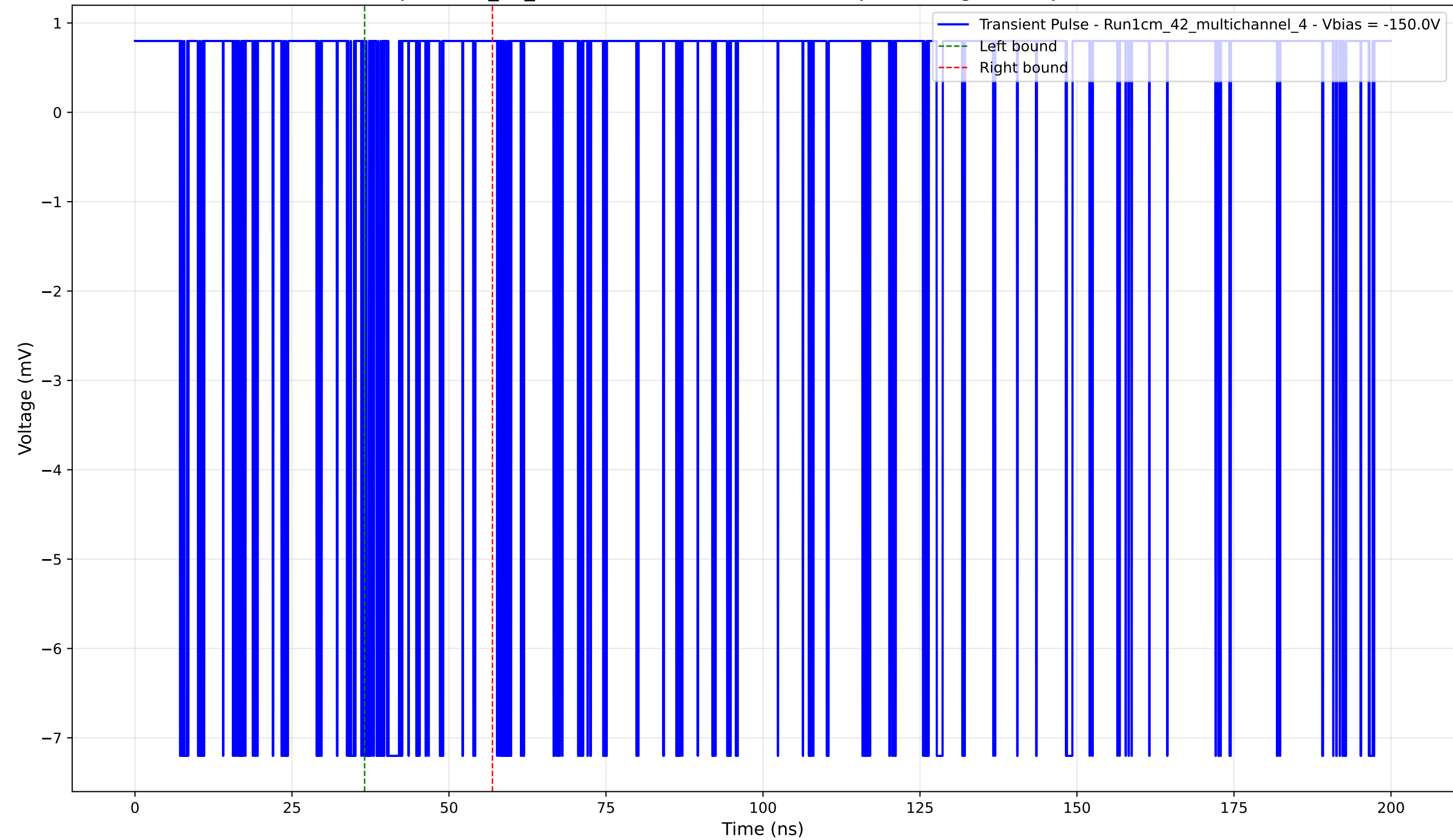
Transient Pulse - Sample: 1cm_42_multichannel - Position: 3380.0 \mu\text{m} - Charge: 0.51 pC - Rise Time: 0.00 ns (N/A)
