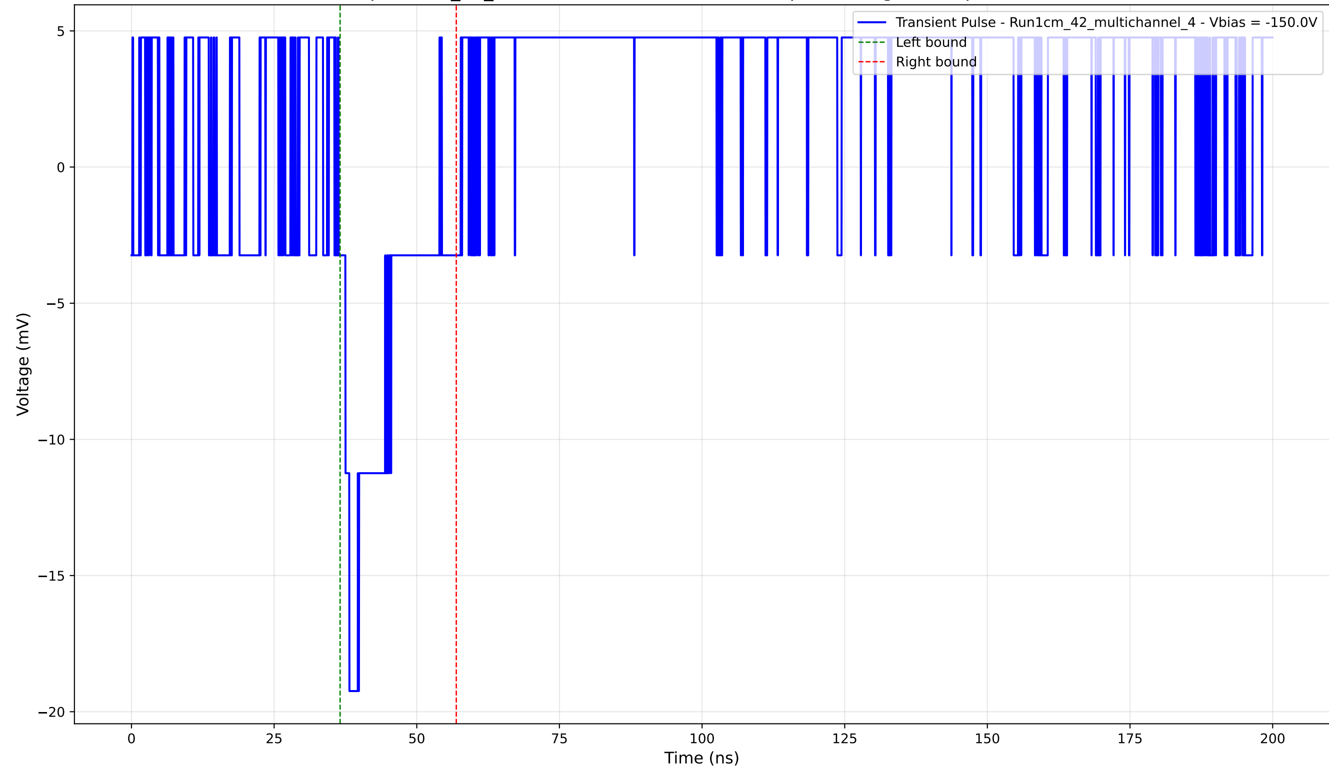
Transient Pulse - Sample: 1cm_42_multichannel - Position: 1010.0 \mu\text{m} - Charge: 2.75 pC - Rise Time: 0.00 ns (N/A)
