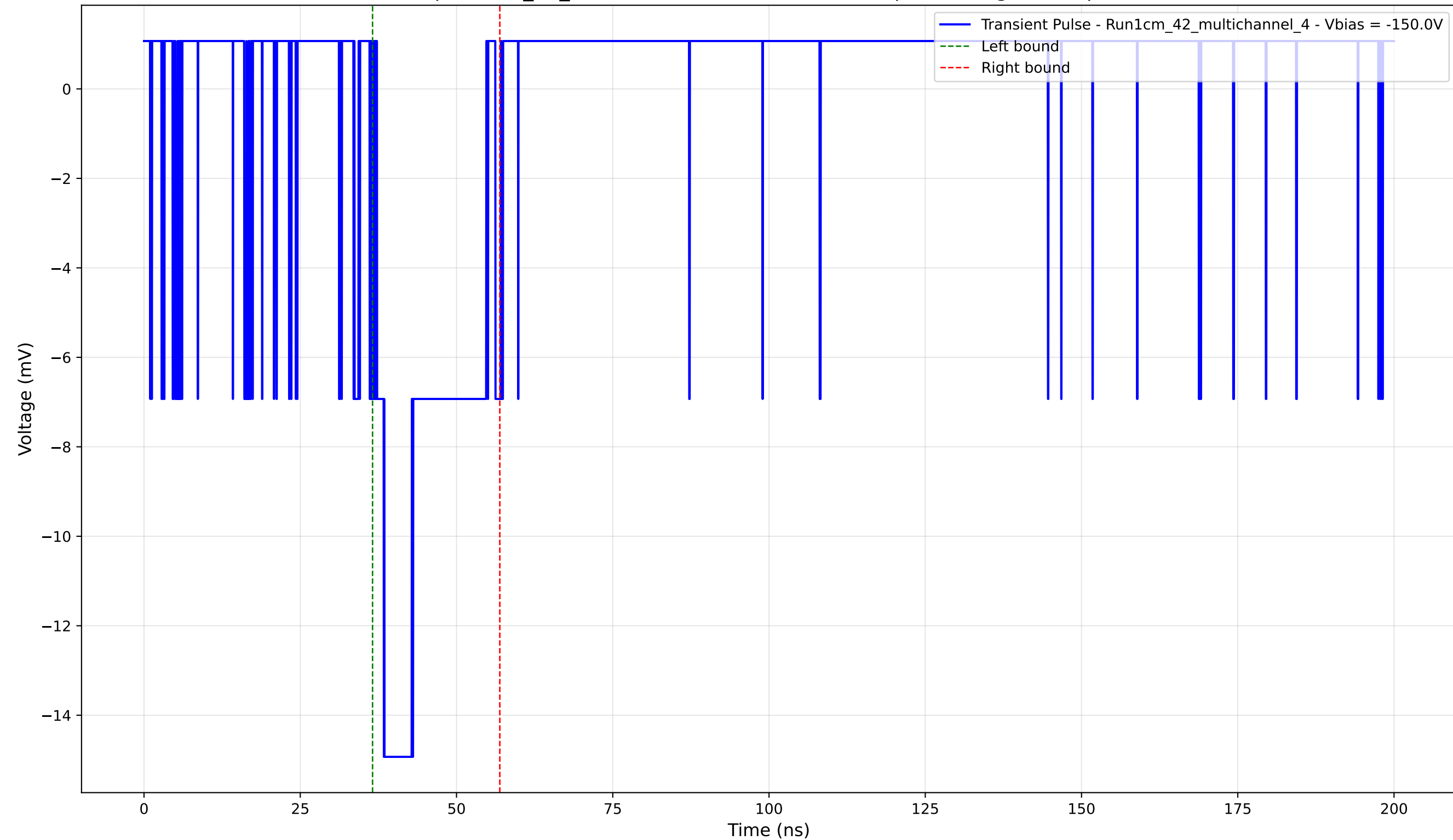
Transient Pulse - Sample: 1cm_42_multichannel - Position: 4245.0 \mu\text{m} - Charge: 3.27 pC - Rise Time: 1.10 ns
