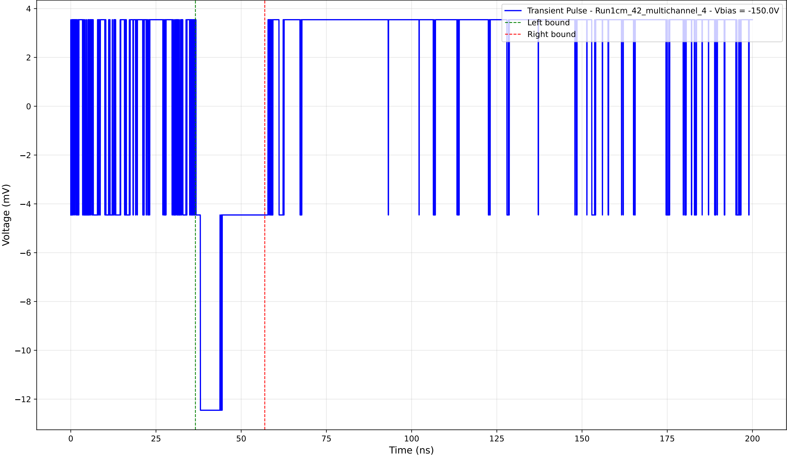
Transient Pulse - Sample: 1cm_42_multichannel - Position: 575.0 \mu\text{m} - Charge: 2.77 pC - Rise Time: 0.00 ns (N/A)
