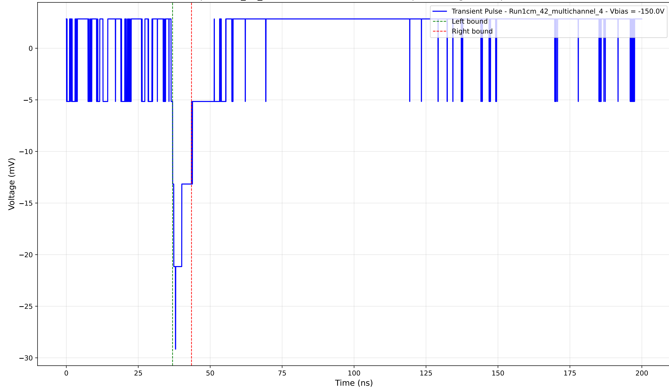
Transient Pulse - Sample: 1cm_42_multichannel - Position: 1450.0 \mu\text{m} - Charge: 2.19 pC - Rise Time: 1.54 ns
