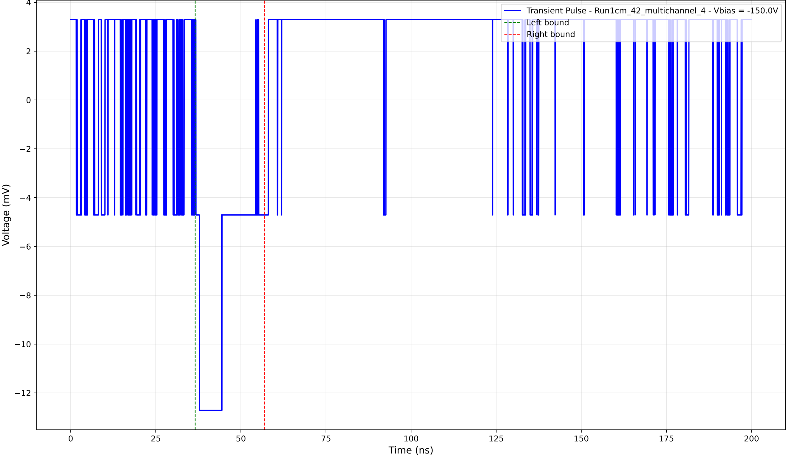
Transient Pulse - Sample: 1cm_42_multichannel - Position: 605.0 \mu\text{m} - Charge: 2.88 pC - Rise Time: 0.00 ns (N/A)
