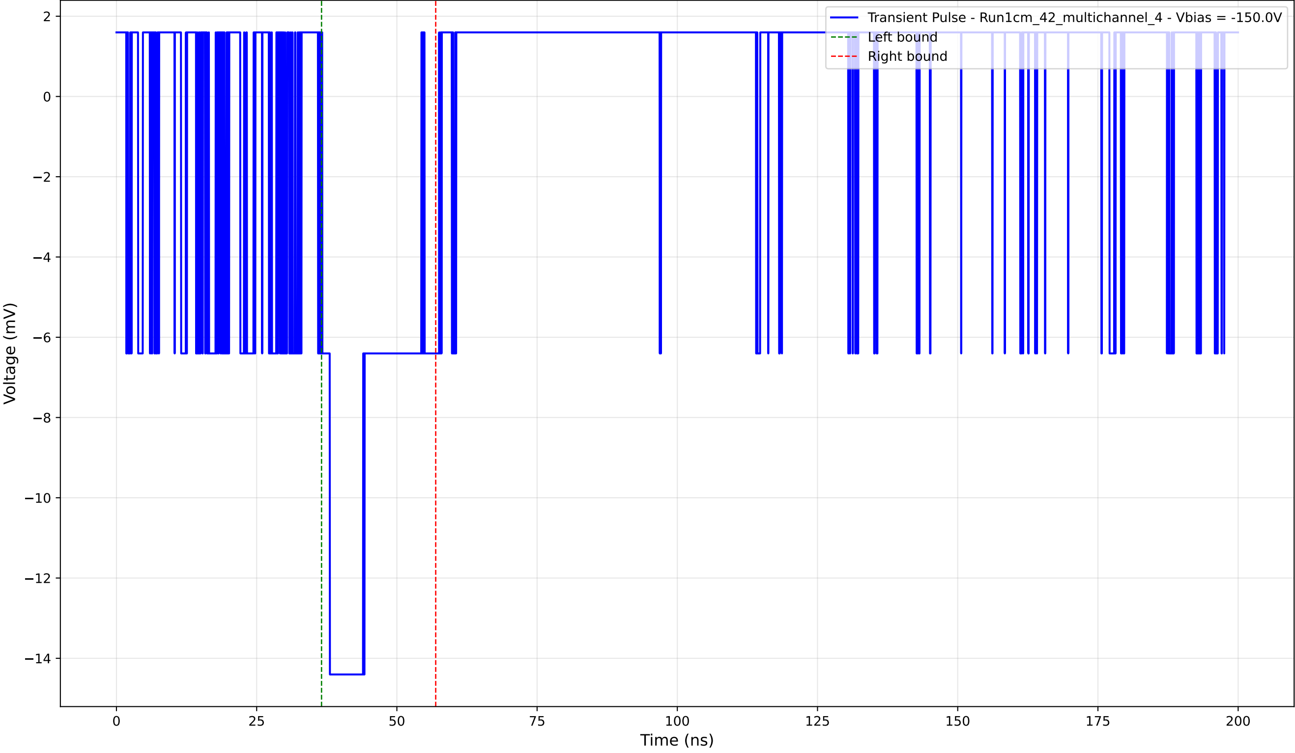
Transient Pulse - Sample: 1cm_42_multichannel - Position: 530.0 \mu\text{m} - Charge: 3.51 pC - Rise Time: 0.00 ns (N/A)
