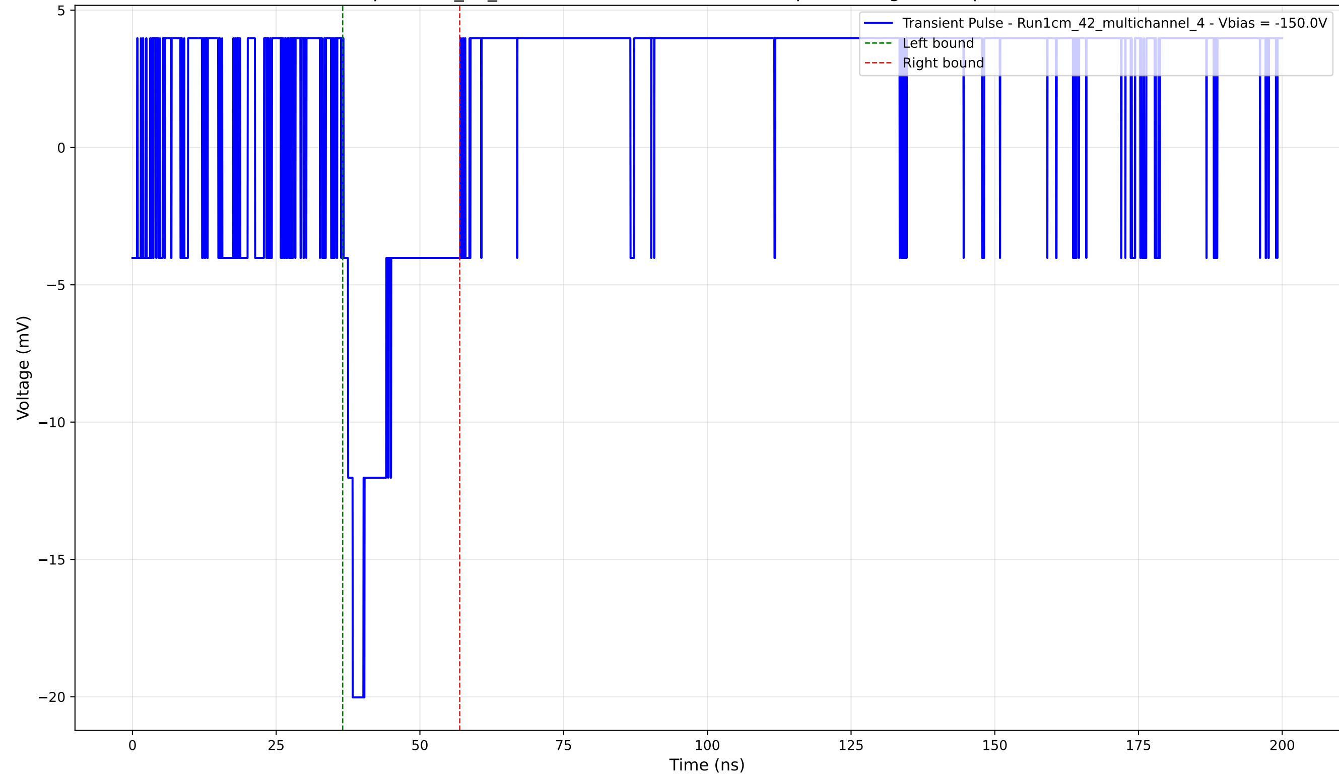
Transient Pulse - Sample: 1cm_42_multichannel - Position: 1000.0 \mu\text{m} - Charge: 3.02 pC - Rise Time: 0.00 ns (N/A)
