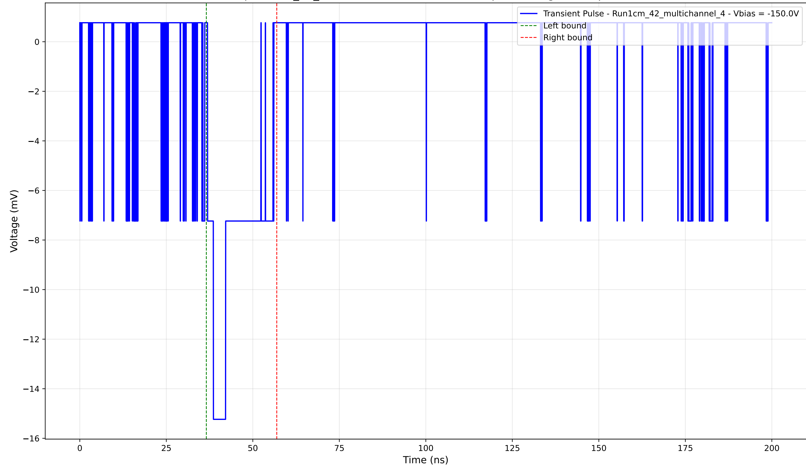
Transient Pulse - Sample: 1cm_42_multichannel - Position: 150.0 \mu\text{m} - Charge: 3.29 pC - Rise Time: 1.70 ns
