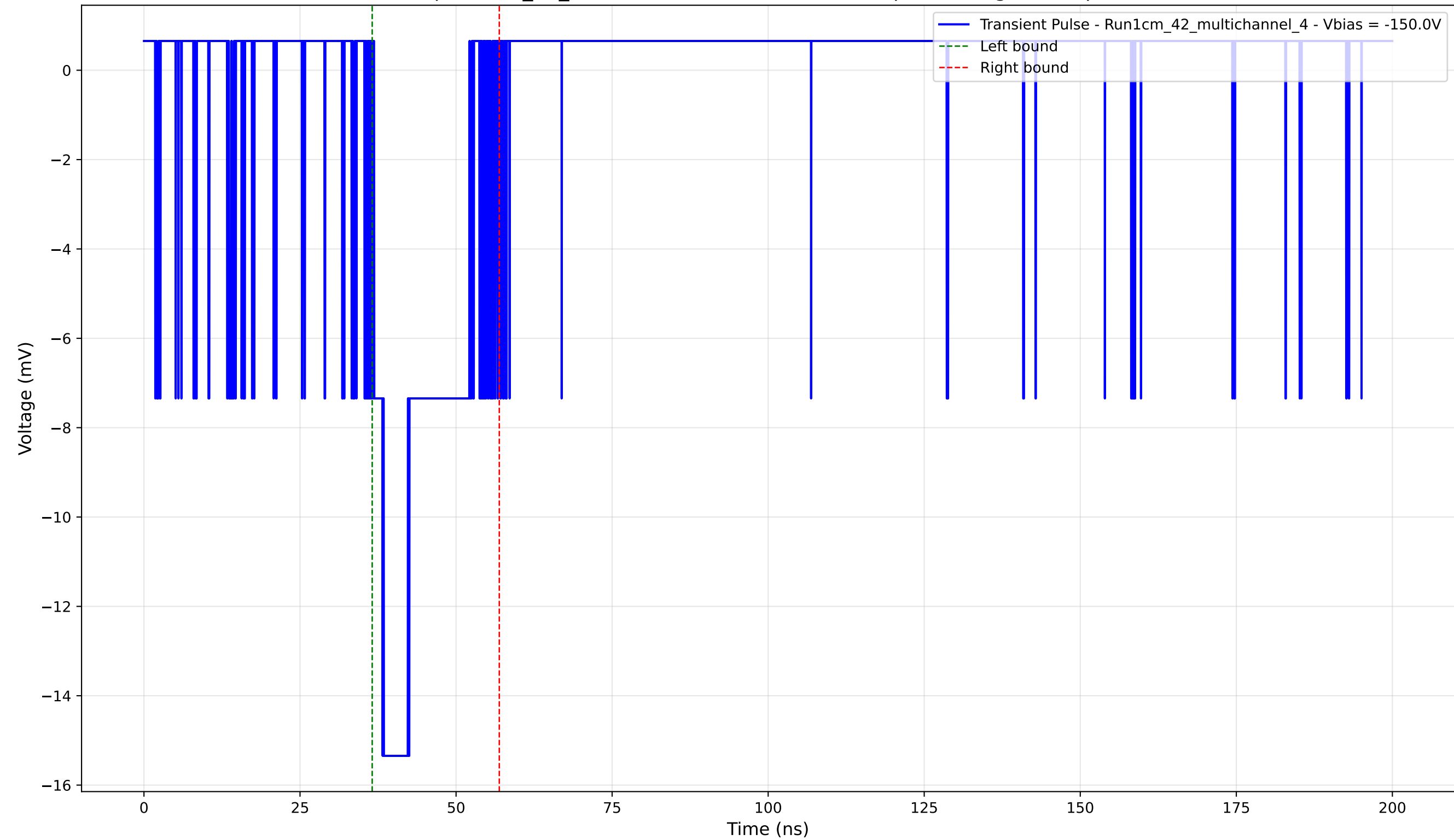
Transient Pulse - Sample: 1cm_42_multichannel - Position: 4160.0 \mu\text{m} - Charge: 3.13 pC - Rise Time: 1.36 ns
