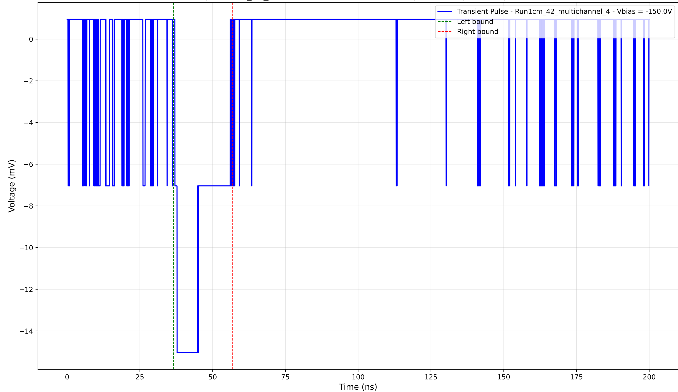
Transient Pulse - Sample: 1cm_42_multichannel - Position: 710.0 \mu\text{m} - Charge: 3.85 pC - Rise Time: 0.76 ns
