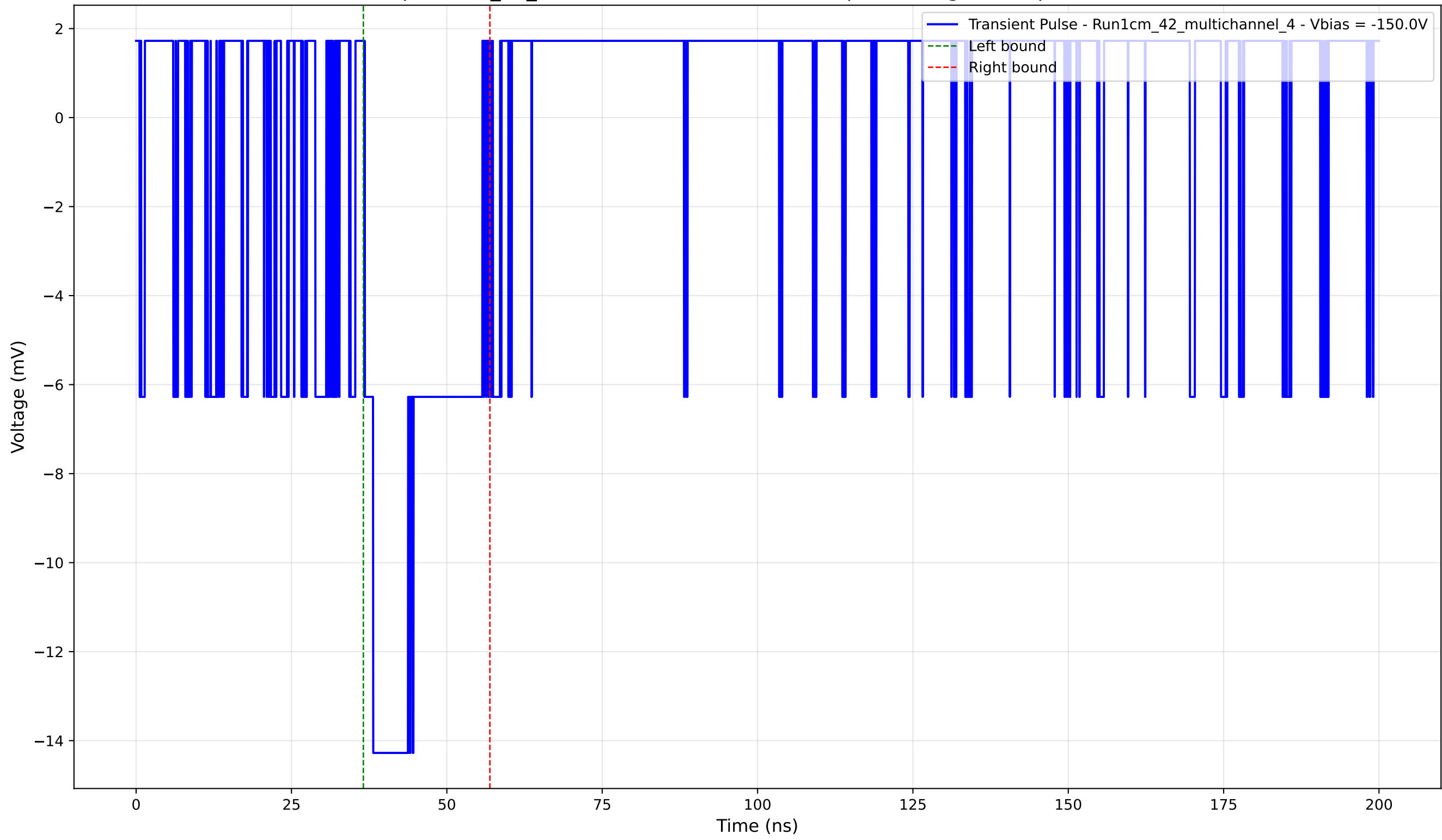
Transient Pulse - Sample: 1cm_42_multichannel - Position: 545.0 \mu\text{m} - Charge: 3.33 pC - Rise Time: 0.00 ns (N/A)
