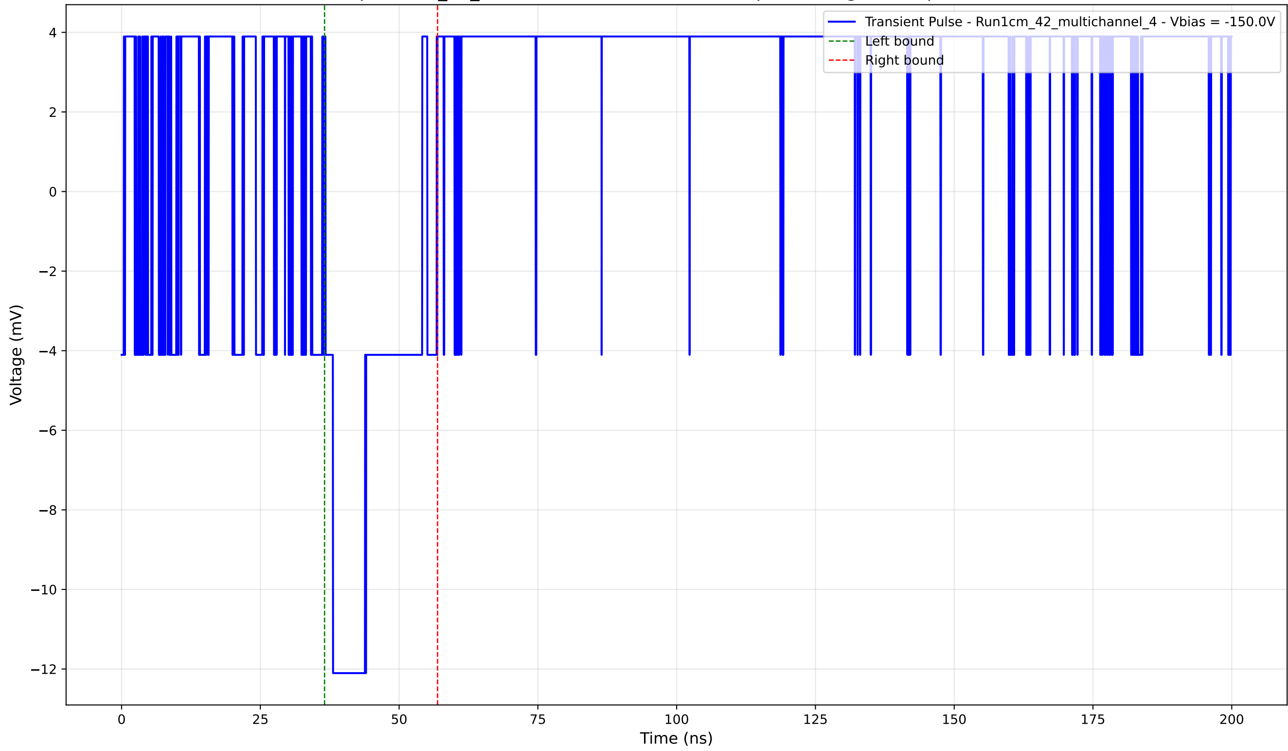
Transient Pulse - Sample: 1cm_42_multichannel - Position: 520.0 \mu\text{m} - Charge: 2.42 pC - Rise Time: 0.00 ns (N/A)
