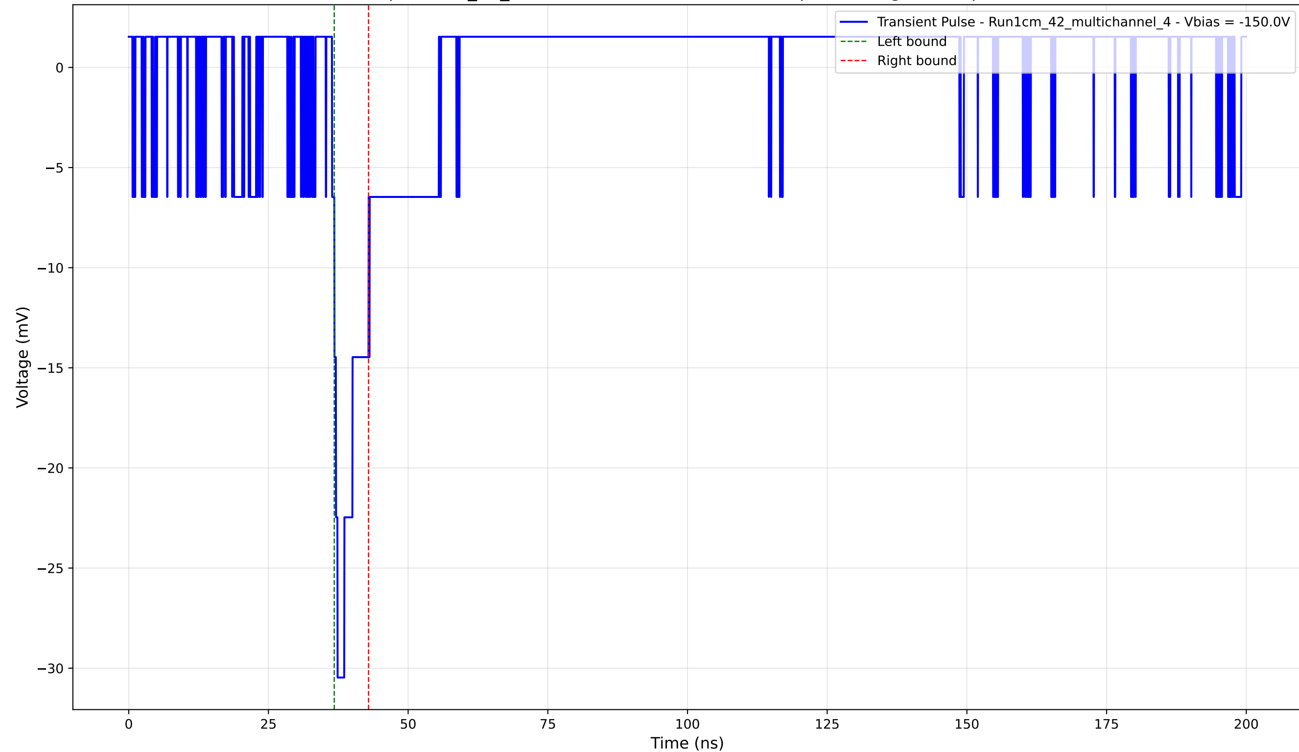
Transient Pulse - Sample: 1cm_42_multichannel - Position: 1590.0 \mu\text{m} - Charge: 2.44 pC - Rise Time: 0.99 ns
