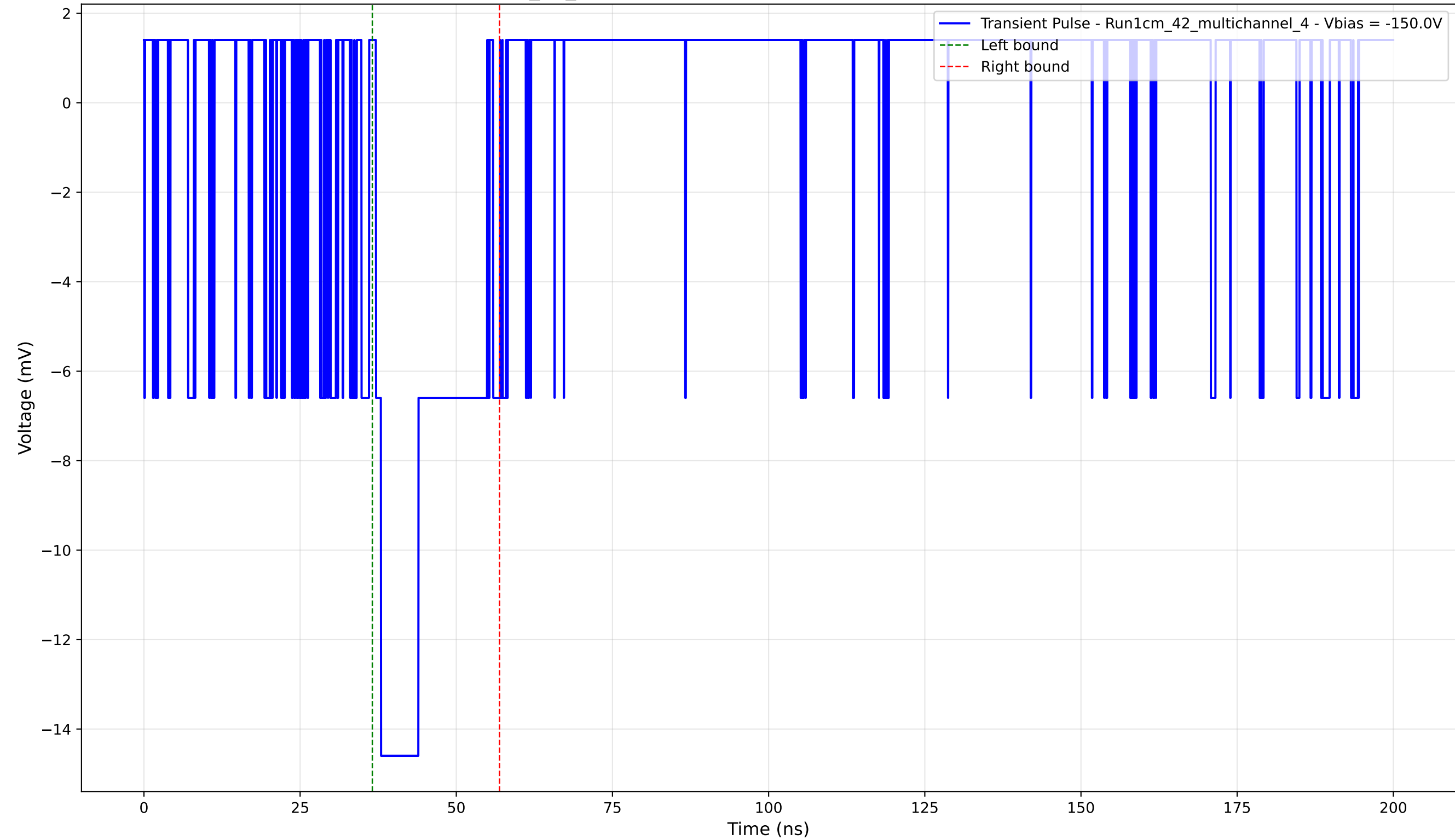
Transient Pulse - Sample: 1cm_42_multichannel - Position: 570.0 \mu\text{m} - Charge: 3.43 pC - Rise Time: 0.82 ns
