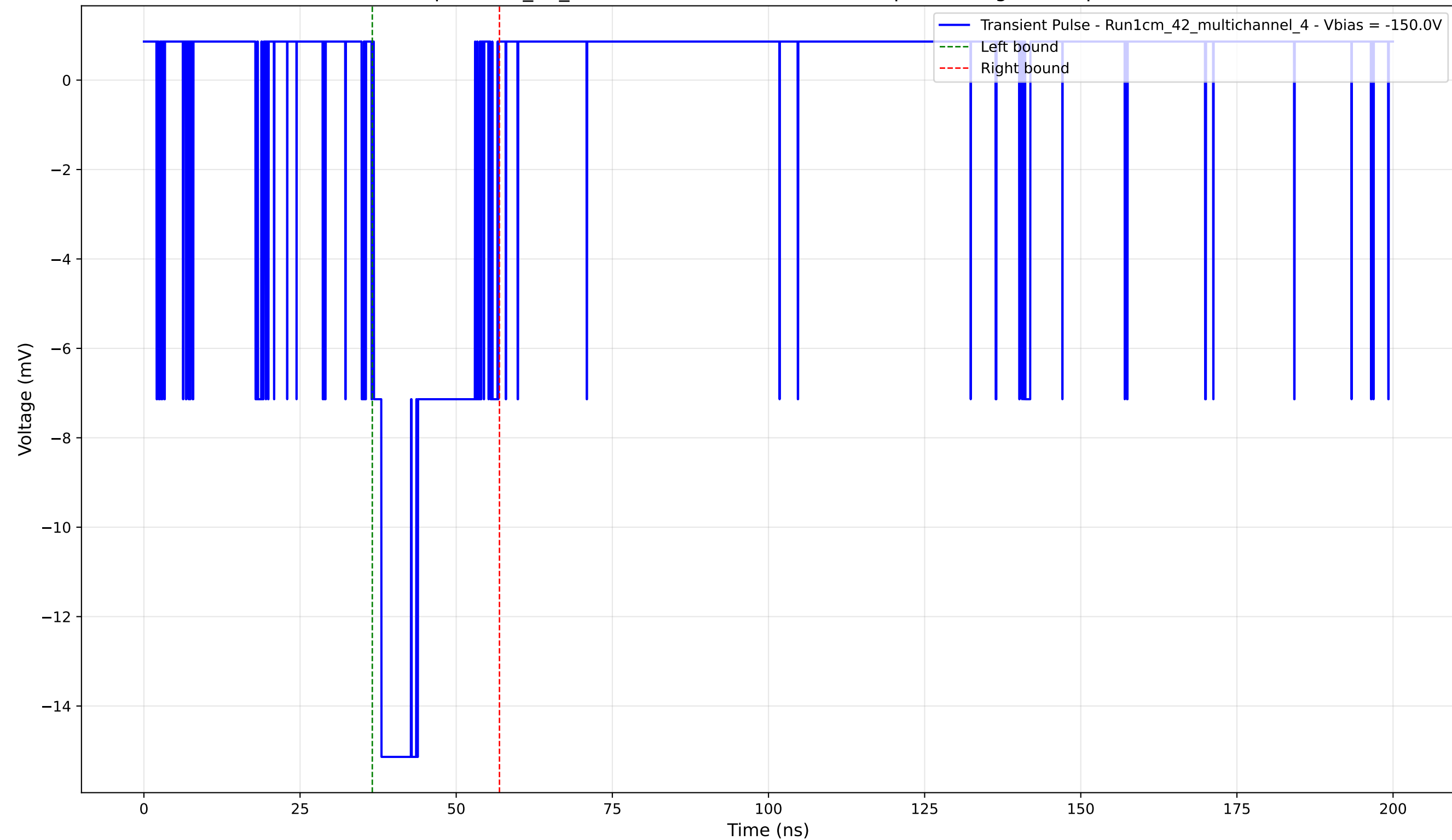
Transient Pulse - Sample: 1cm_42_multichannel - Position: 4020.0 \mu\text{m} - Charge: 3.48 pC - Rise Time: 1.22 ns
