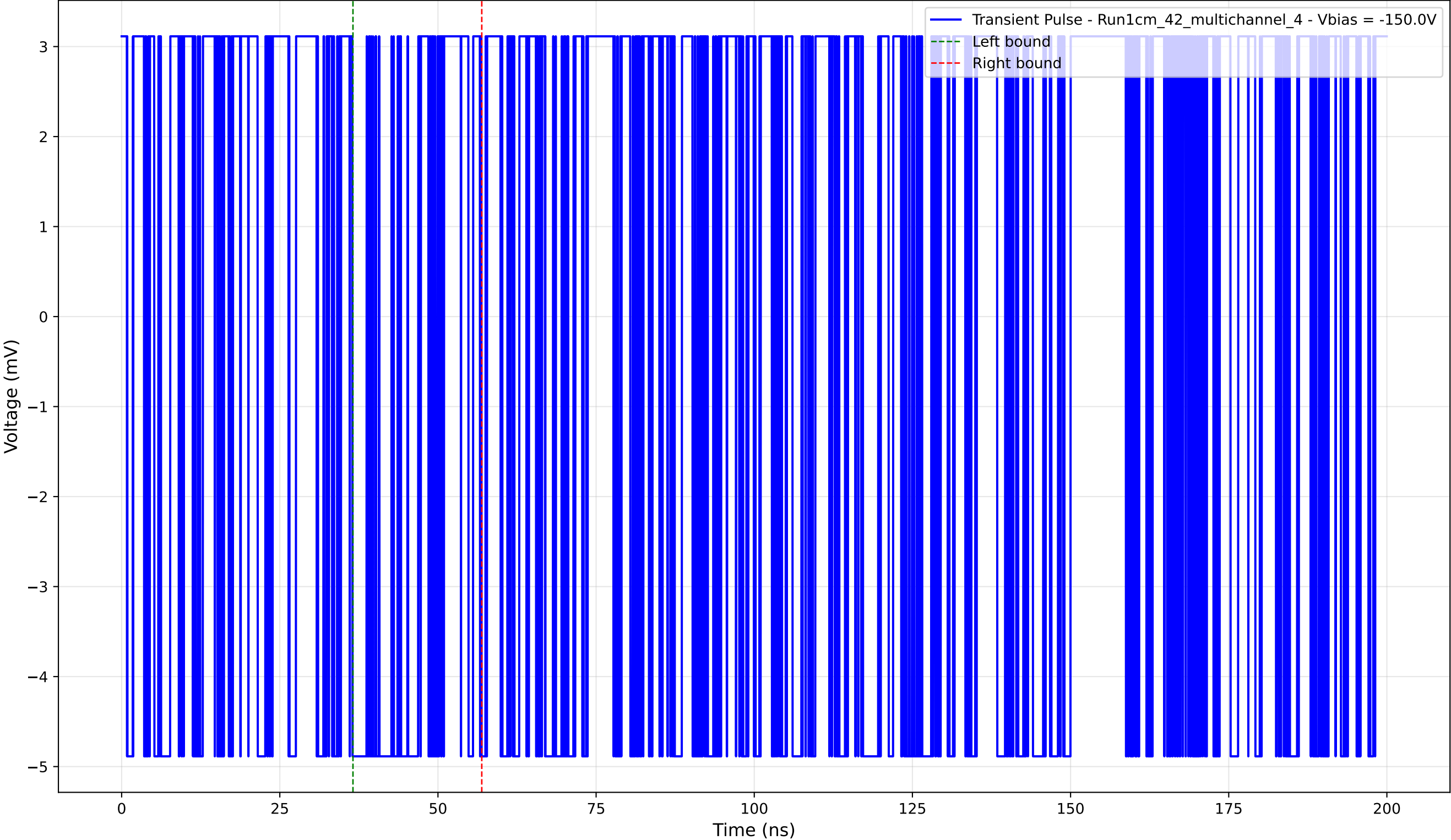
Transient Pulse - Sample: 1cm_42_multichannel - Position: 1365.0 \mu\text{m} - Charge: 0.61 pC - Rise Time: 0.00 ns (N/A)
