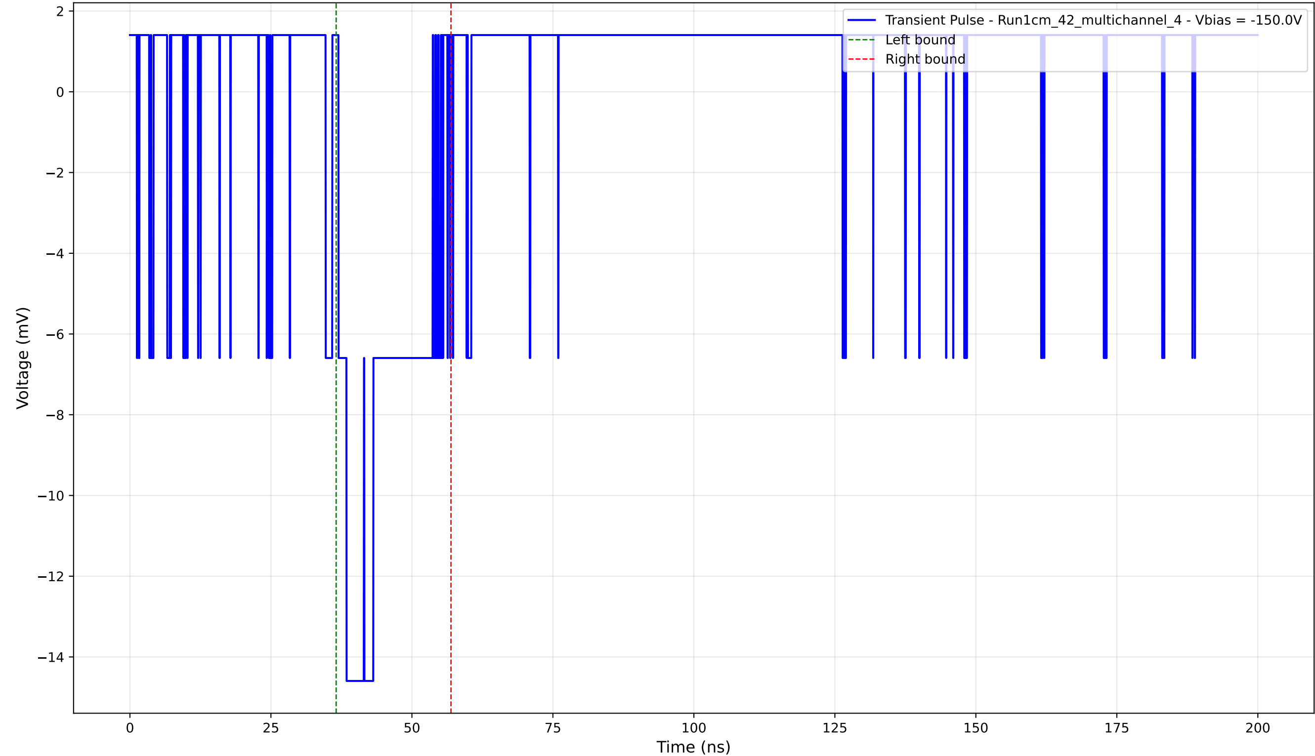
Transient Pulse - Sample: 1cm_42_multichannel - Position: 4155.0 \mu\text{m} - Charge: 3.07 pC - Rise Time: 1.44 ns
