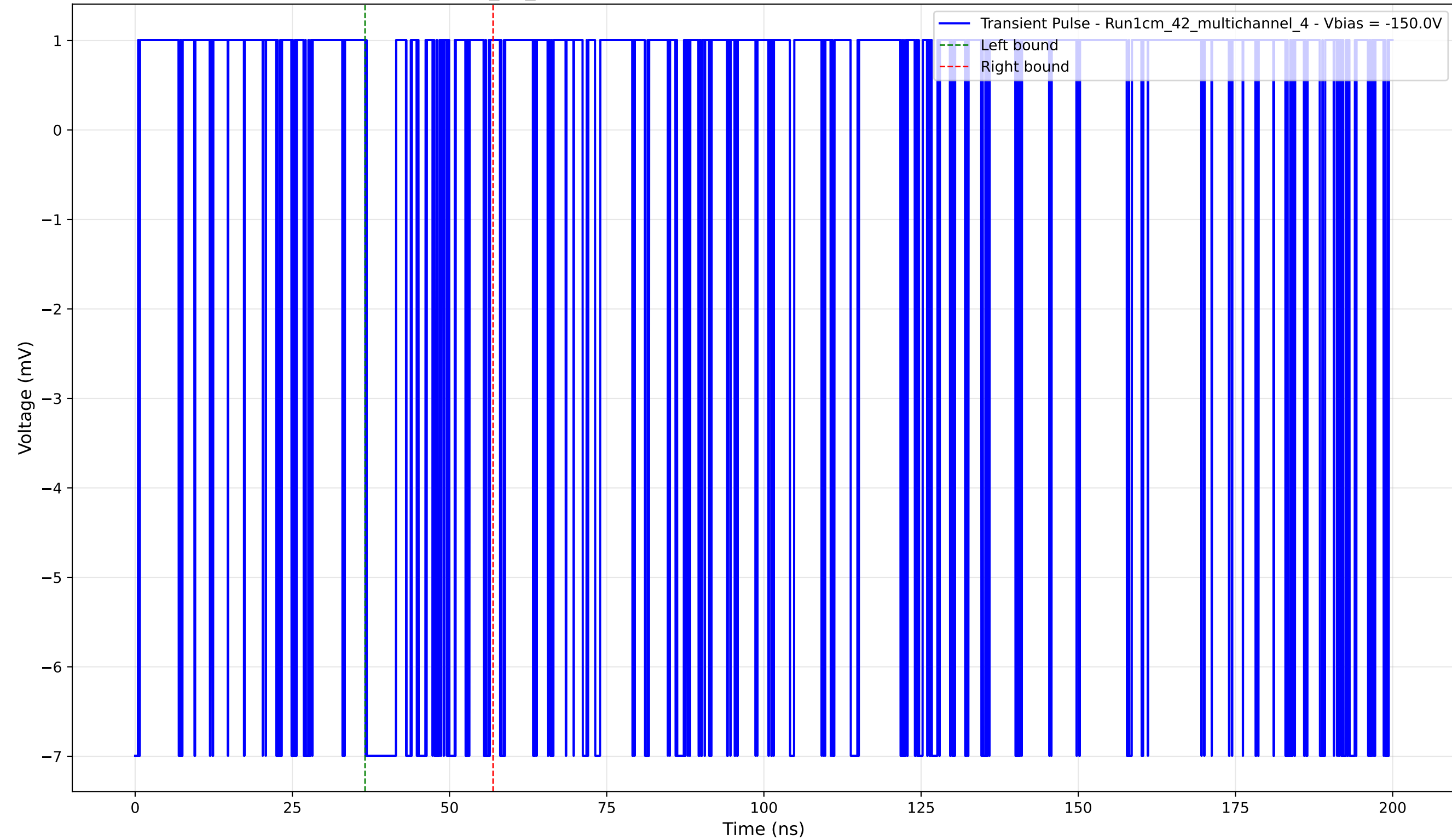
Transient Pulse - Sample: 1cm_42_multichannel - Position: 1400.0 \mu\text{m} - Charge: 1.24 pC - Rise Time: 0.00 ns (N/A)
