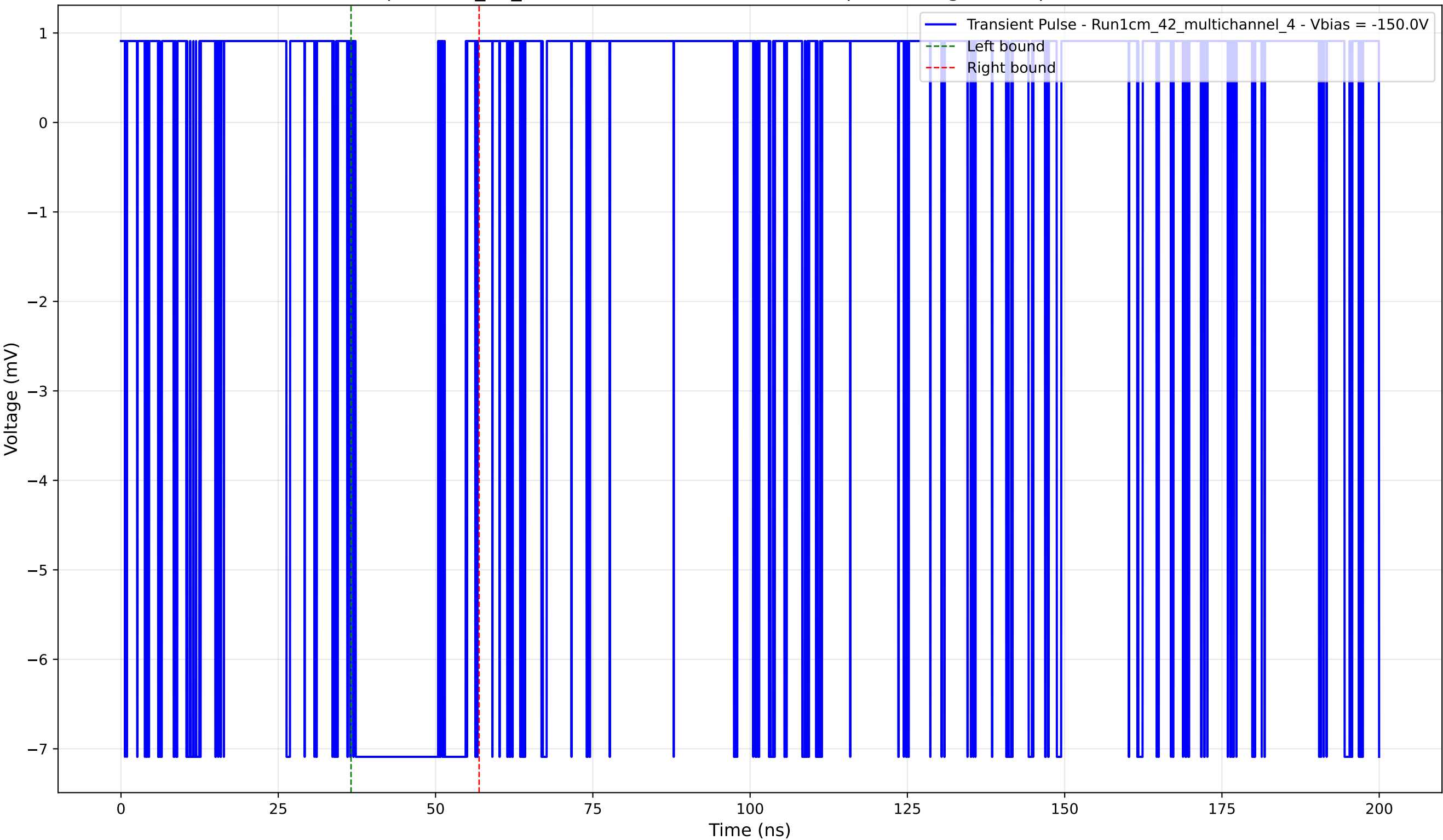
Transient Pulse - Sample: 1cm_42_multichannel - Position: 4355.0 \mu\text{m} - Charge: 2.38 pC - Rise Time: 0.00 ns (N/A)
