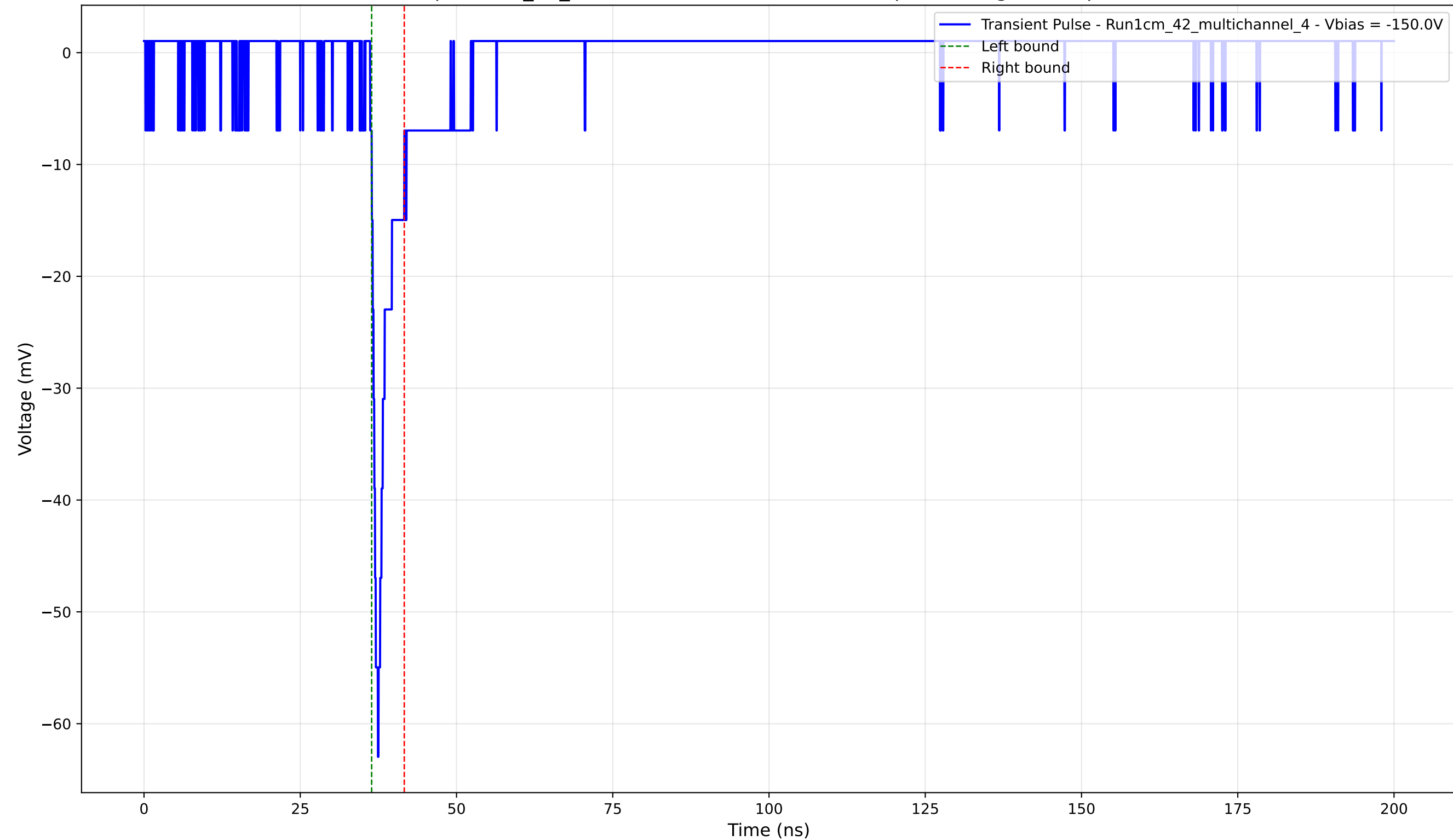
Transient Pulse - Sample: 1cm_42_multichannel - Position: 2690.0 \mu\text{m} - Charge: 2.85 pC - Rise Time: 1.24 ns
