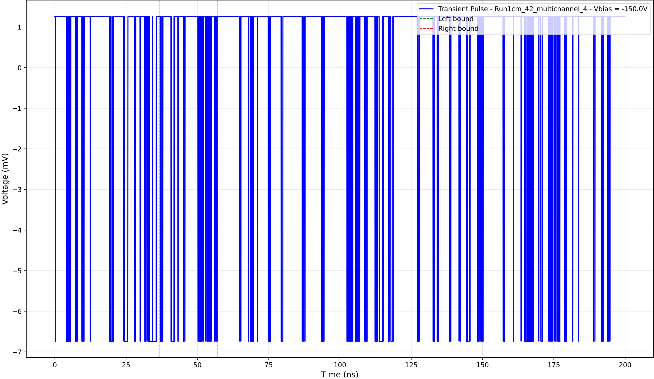
Transient Pulse - Sample: 1cm_42_multichannel - Position: 3405.0 \mu\text{m} - Charge: 0.14 pC - Rise Time: 0.00 ns (N/A)
