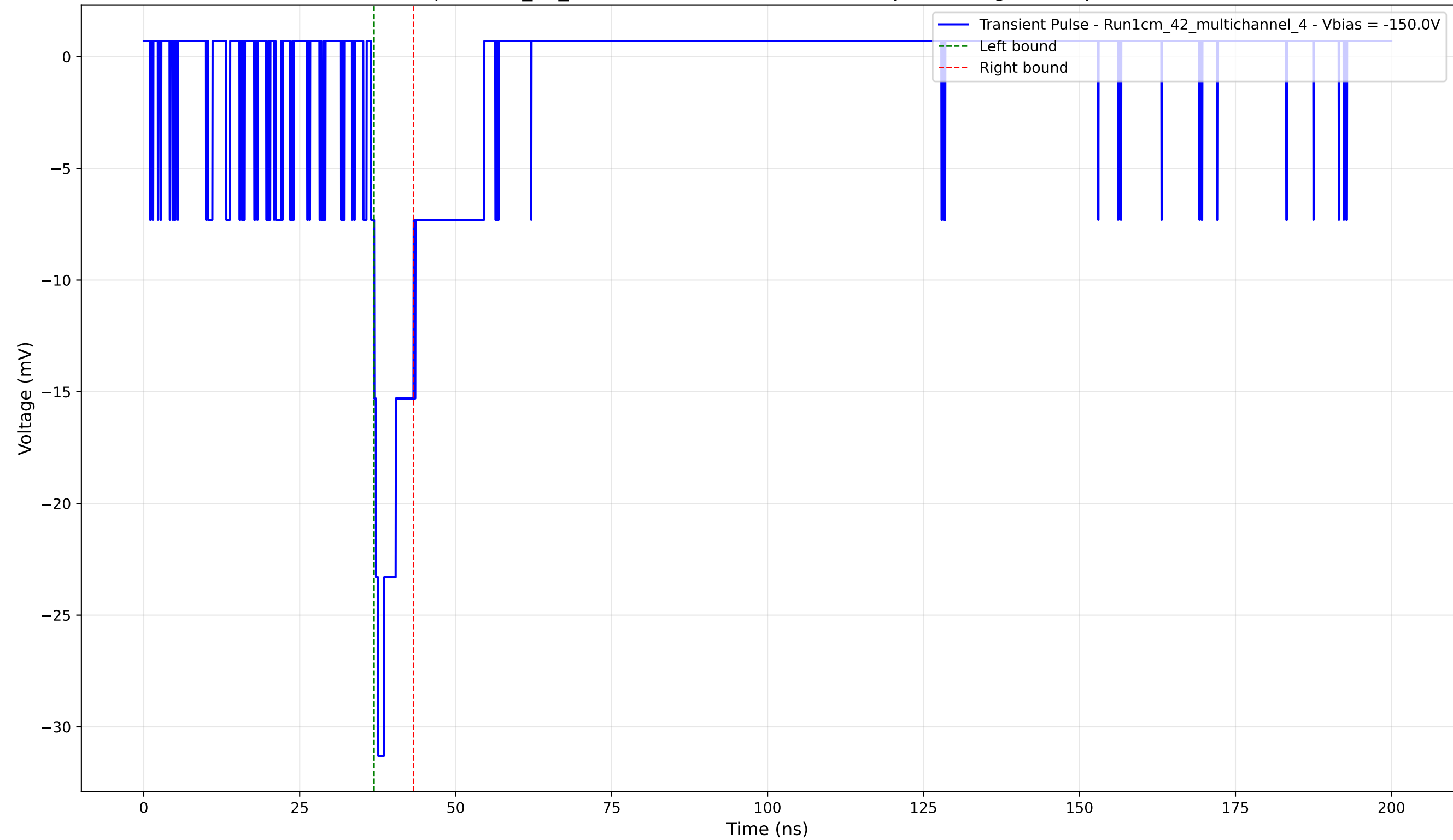
Transient Pulse - Sample: 1cm_42_multichannel - Position: 1495.0 \mu\text{m} - Charge: 2.60 pC - Rise Time: 1.15 ns
