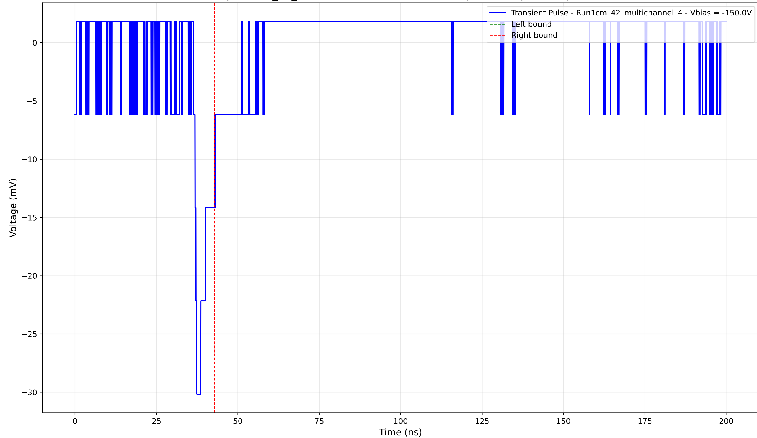
Transient Pulse - Sample: 1cm_42_multichannel - Position: 1580.0 \mu\text{m} - Charge: 2.36 pC - Rise Time: 0.97 ns
