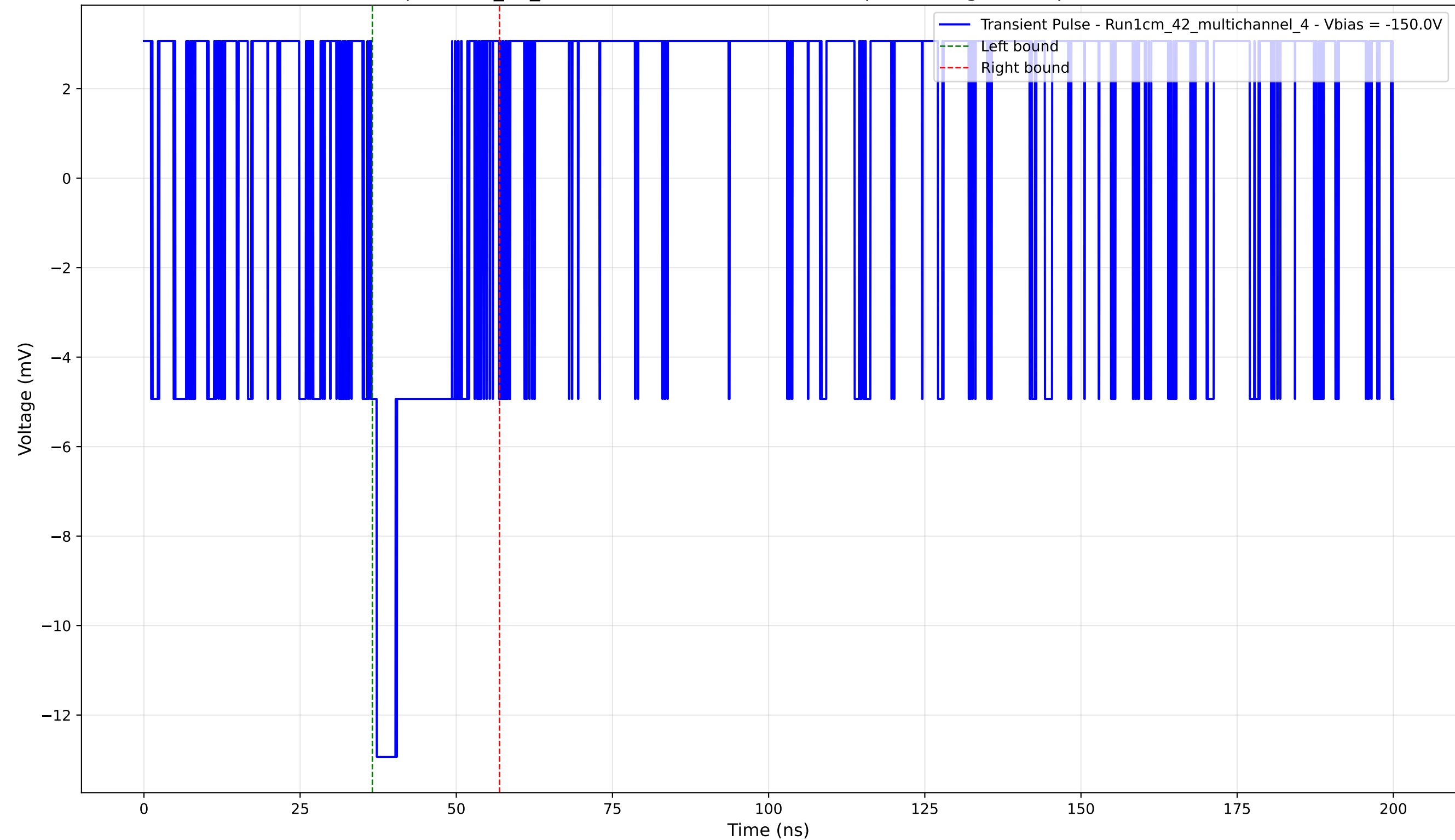
Transient Pulse - Sample: 1cm_42_multichannel - Position: 1425.0 \mu\text{m} - Charge: 1.82 pC - Rise Time: 0.00 ns (N/A)
