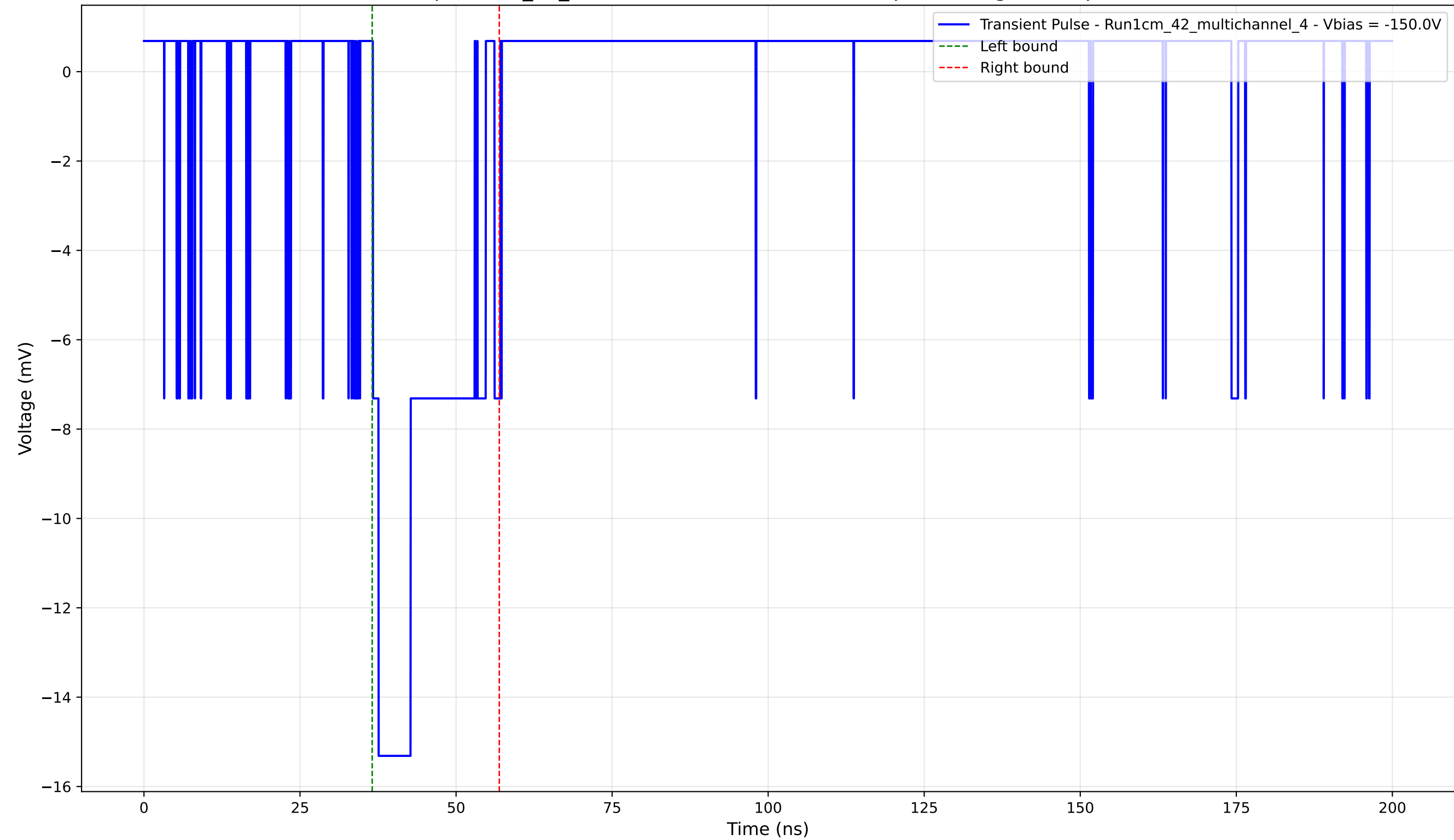
Transient Pulse - Sample: 1cm_42_multichannel - Position: 3705.0 \mu\text{m} - Charge: 3.53 pC - Rise Time: 0.92 ns
