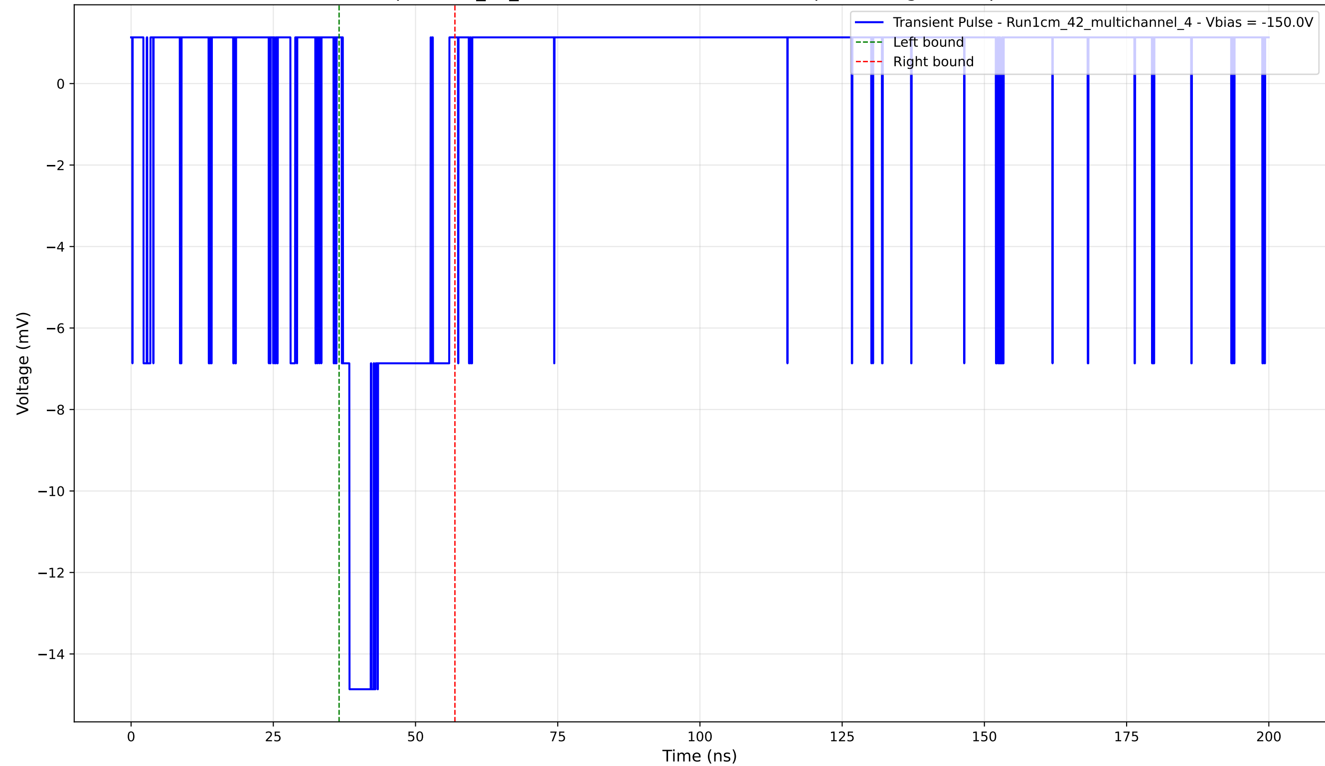
Transient Pulse - Sample: 1cm_42_multichannel - Position: 4185.0 \mu\text{m} - Charge: 3.24 pC - Rise Time: 1.16 ns
