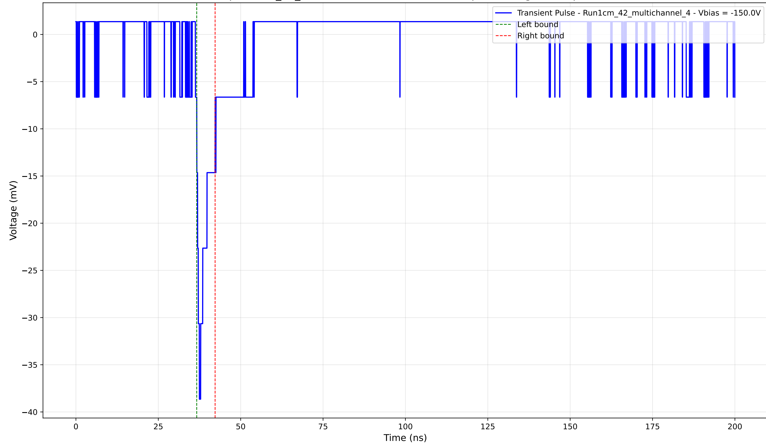
Transient Pulse - Sample: 1cm_42_multichannel - Position: 3030.0 \mu\text{m} - Charge: 2.37 pC - Rise Time: 1.21 ns
