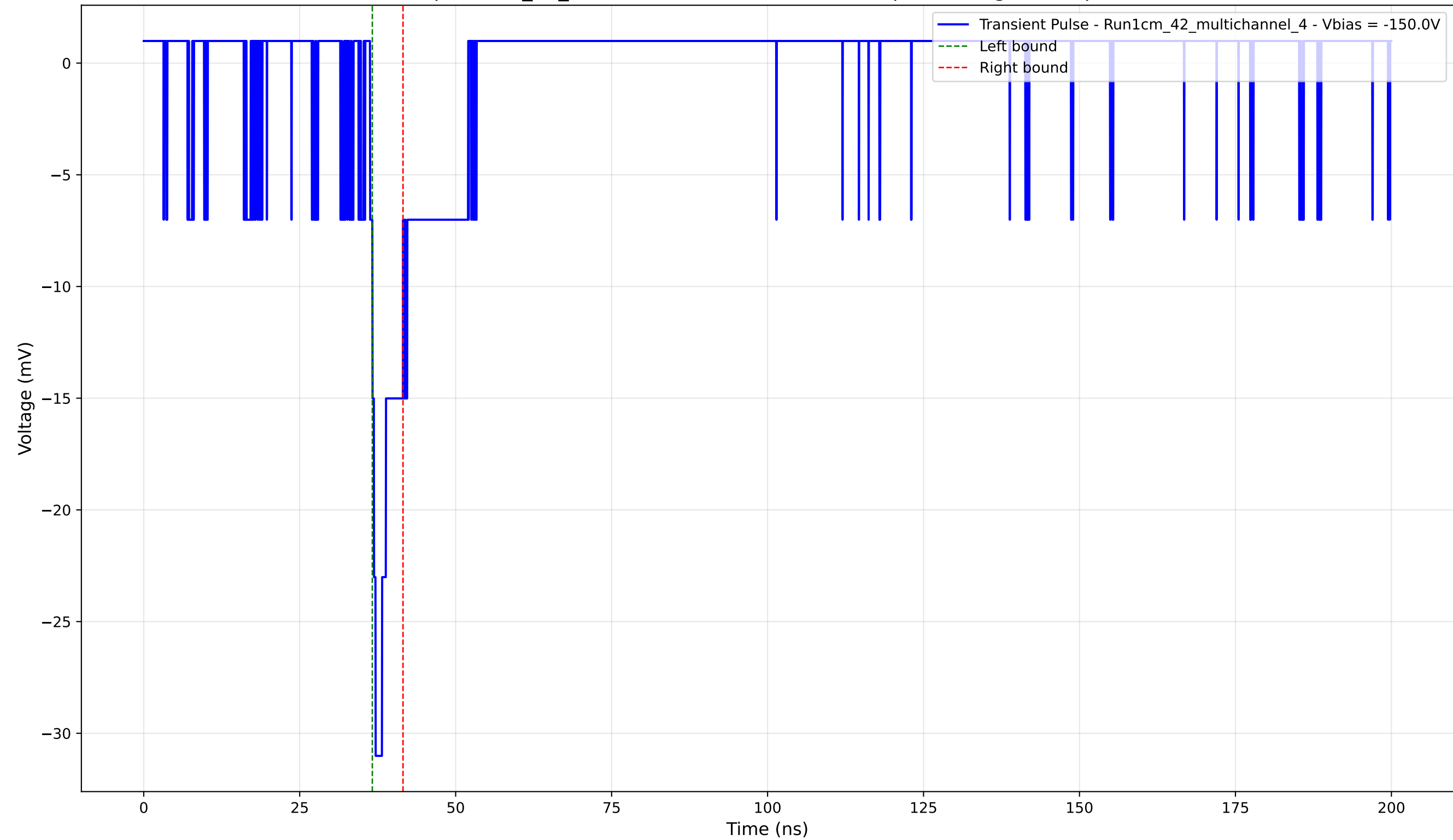
Transient Pulse - Sample: 1cm_42_multichannel - Position: 2955.0 \mu\text{m} - Charge: 1.95 pC - Rise Time: 0.89 ns
