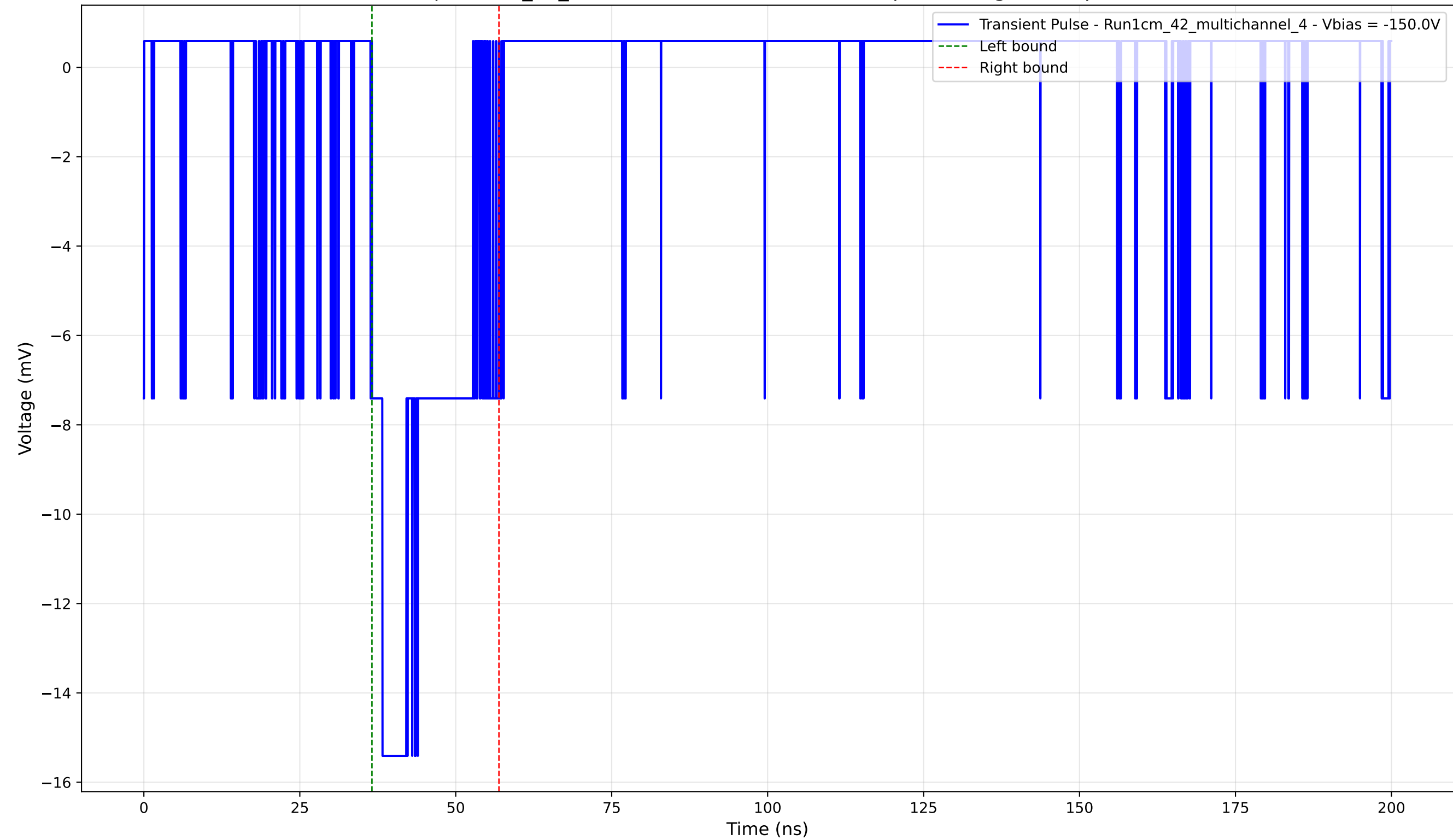
Transient Pulse - Sample: 1cm_42_multichannel - Position: 4320.0 \mu\text{m} - Charge: 3.45 pC - Rise Time: 1.70 ns
