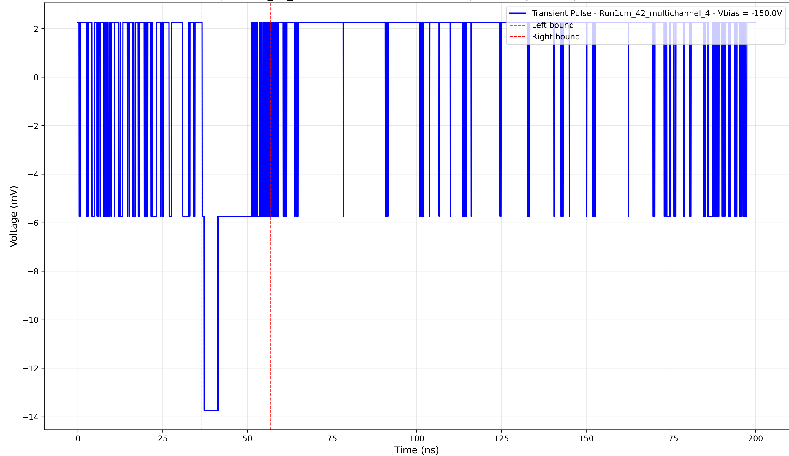
Transient Pulse - Sample: 1cm_42_multichannel - Position: 1430.0 \mu\text{m} - Charge: 2.63 pC - Rise Time: 0.00 ns (N/A)
