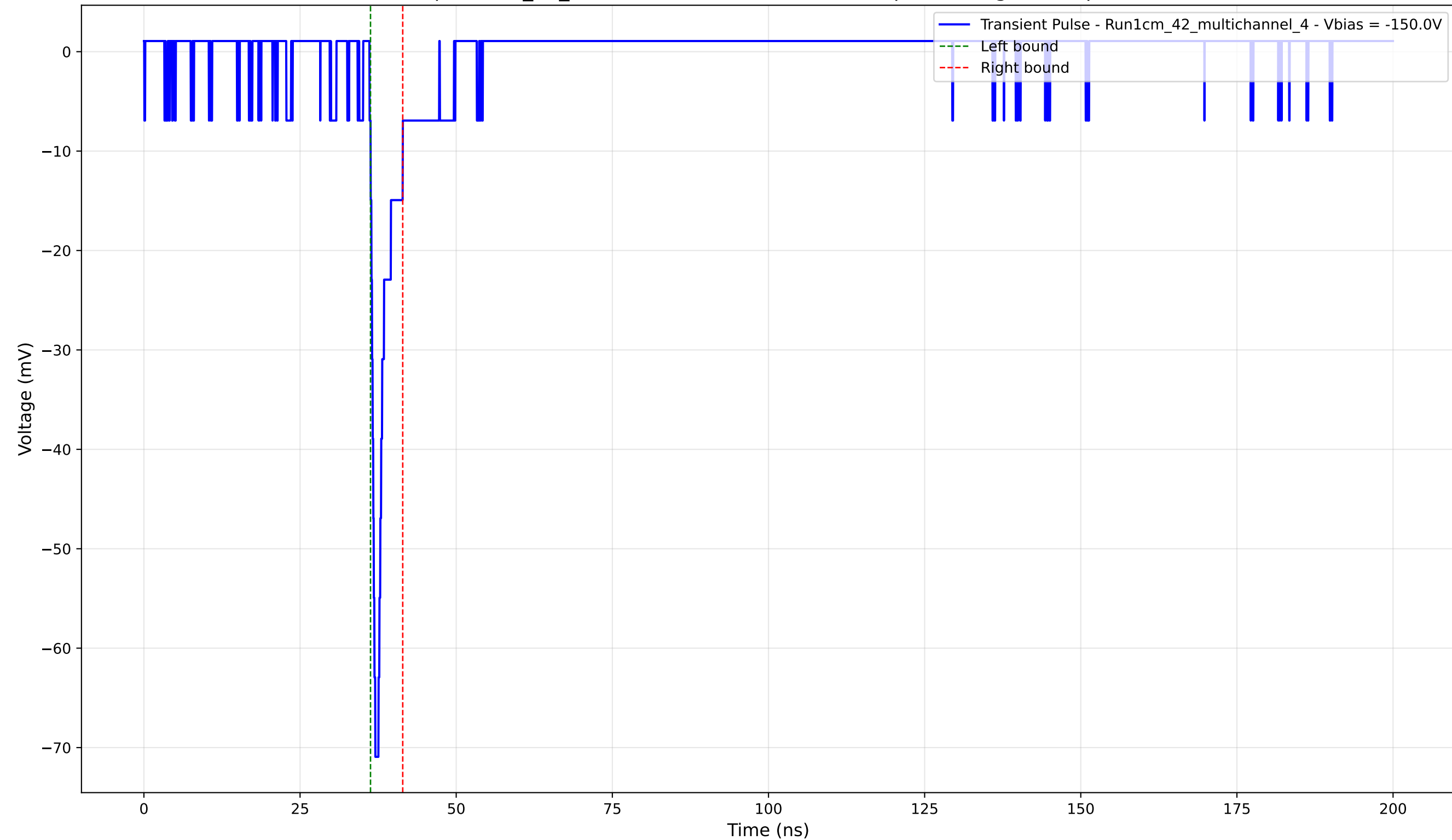
Transient Pulse - Sample: 1cm_42_multichannel - Position: 2530.0 \mu\text{m} - Charge: 3.17 pC - Rise Time: 0.76 ns
