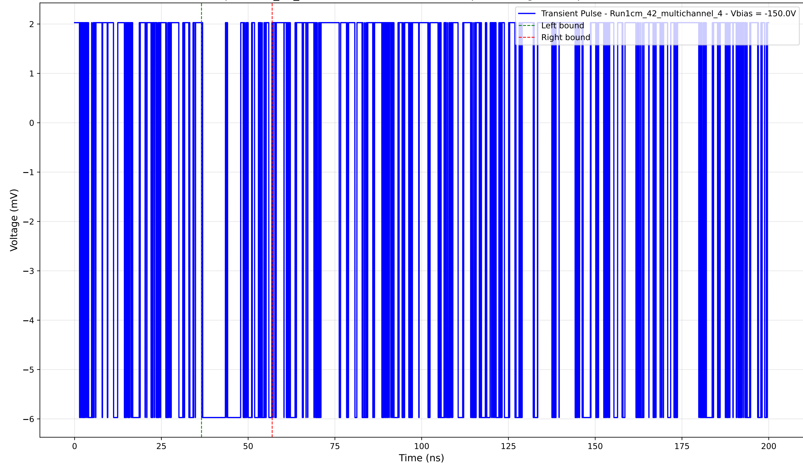
Transient Pulse - Sample: 1cm_42_multichannel - Position: 895.0 \mu\text{m} - Charge: 1.66 pC - Rise Time: 0.00 ns (N/A)
