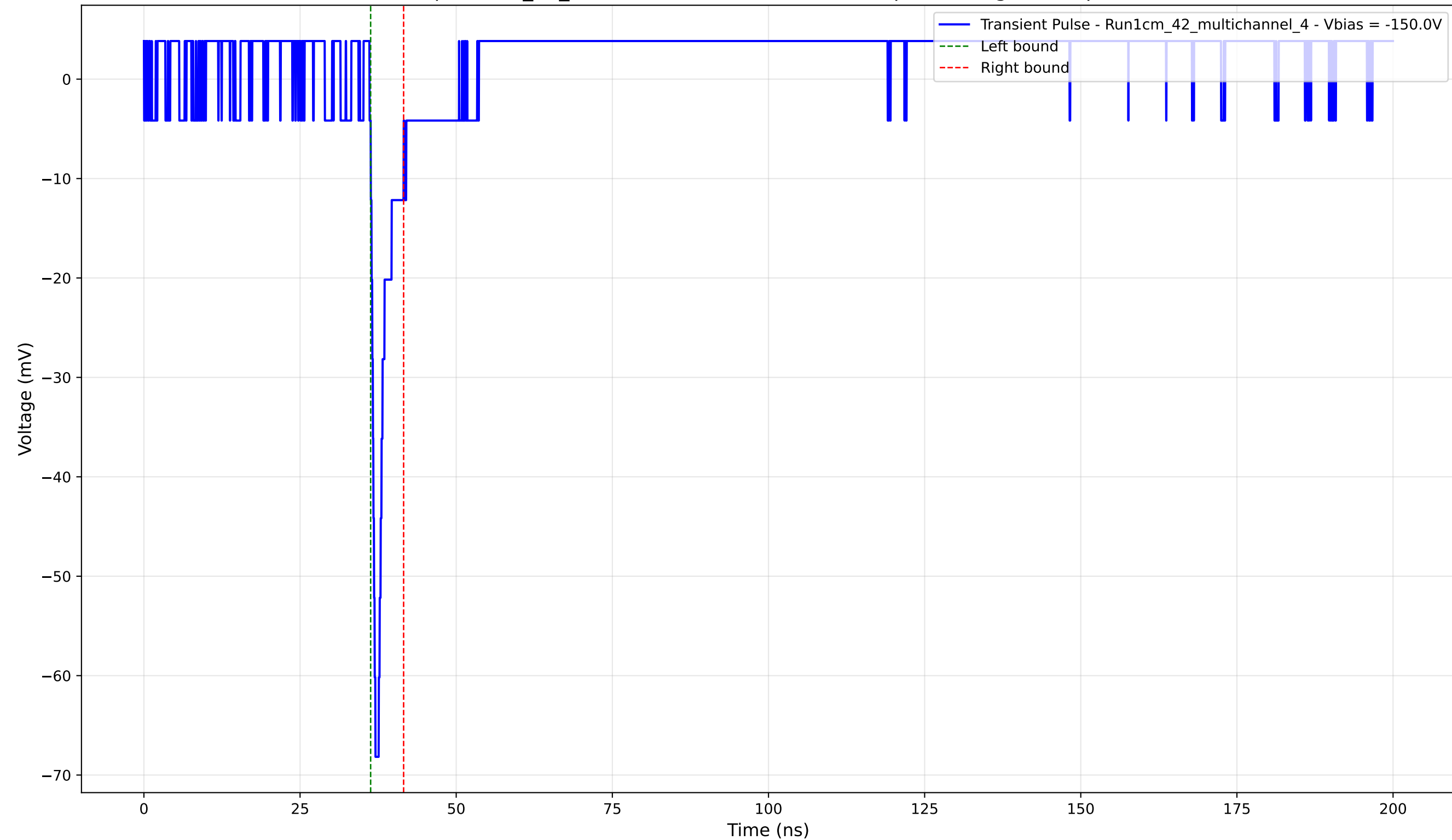
Transient Pulse - Sample: 1cm_42_multichannel - Position: 2200.0 \mu\text{m} - Charge: 2.95 pC - Rise Time: 0.75 ns
