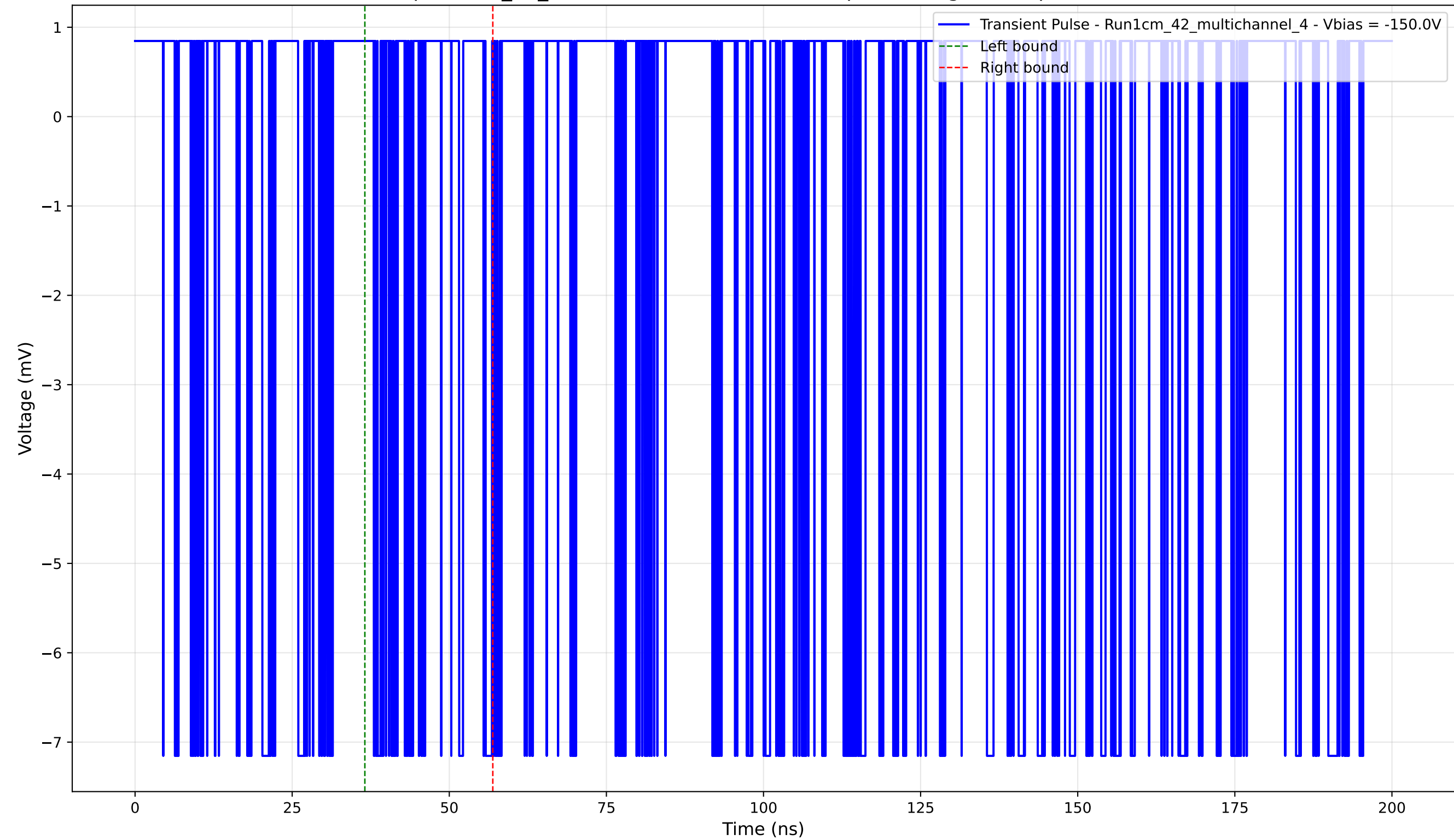
Transient Pulse - Sample: 1cm_42_multichannel - Position: 35.0 \mu\text{m} - Charge: 0.46 pC - Rise Time: 0.00 ns (N/A)
