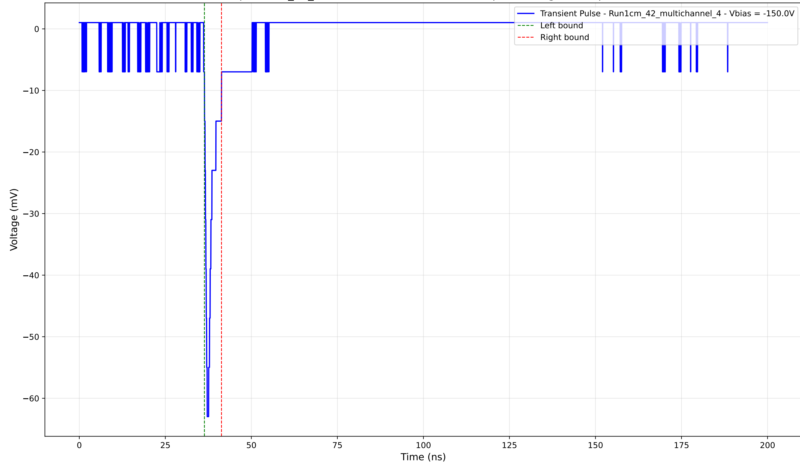
Transient Pulse - Sample: 1cm_42_multichannel - Position: 2120.0 \mu\text{m} - Charge: 2.91 pC - Rise Time: 1.02 ns
