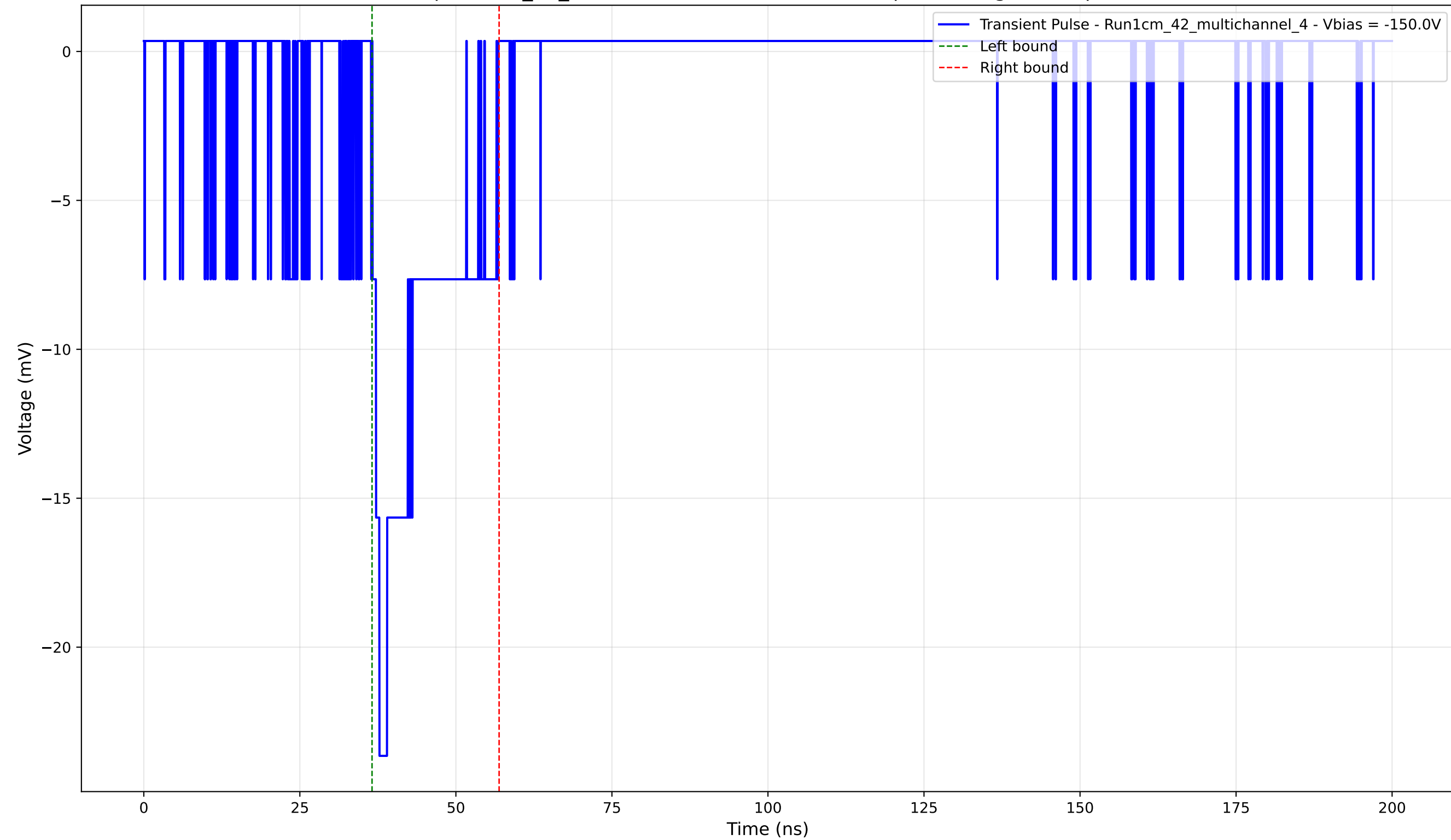
Transient Pulse - Sample: 1cm_42_multichannel - Position: 3475.0 \mu\text{m} - Charge: 4.07 pC - Rise Time: 1.11 ns
