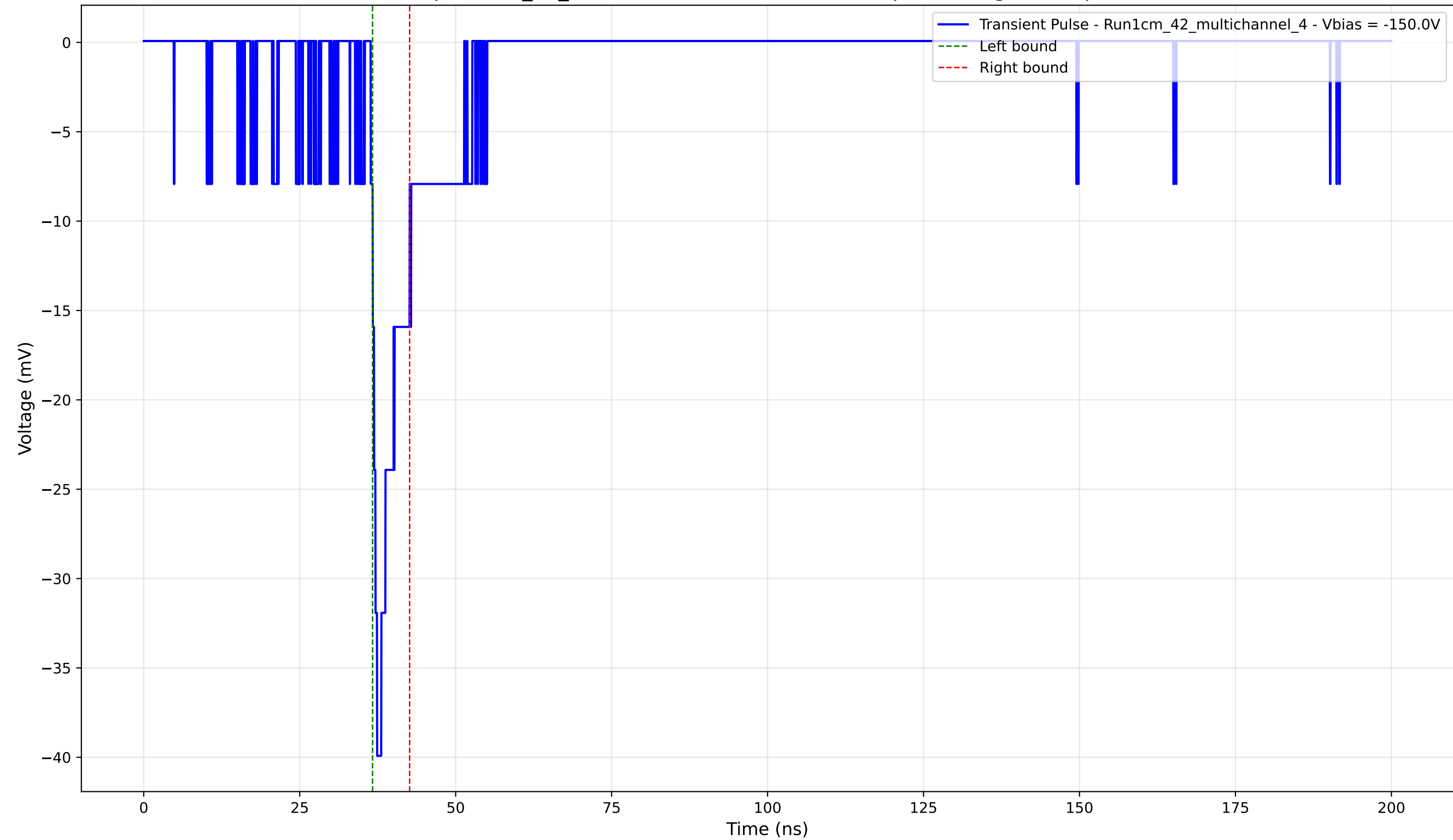
Transient Pulse - Sample: 1cm_42_multichannel - Position: 1705.0 \mu\text{m} - Charge: 2.77 pC - Rise Time: 1.03 ns
