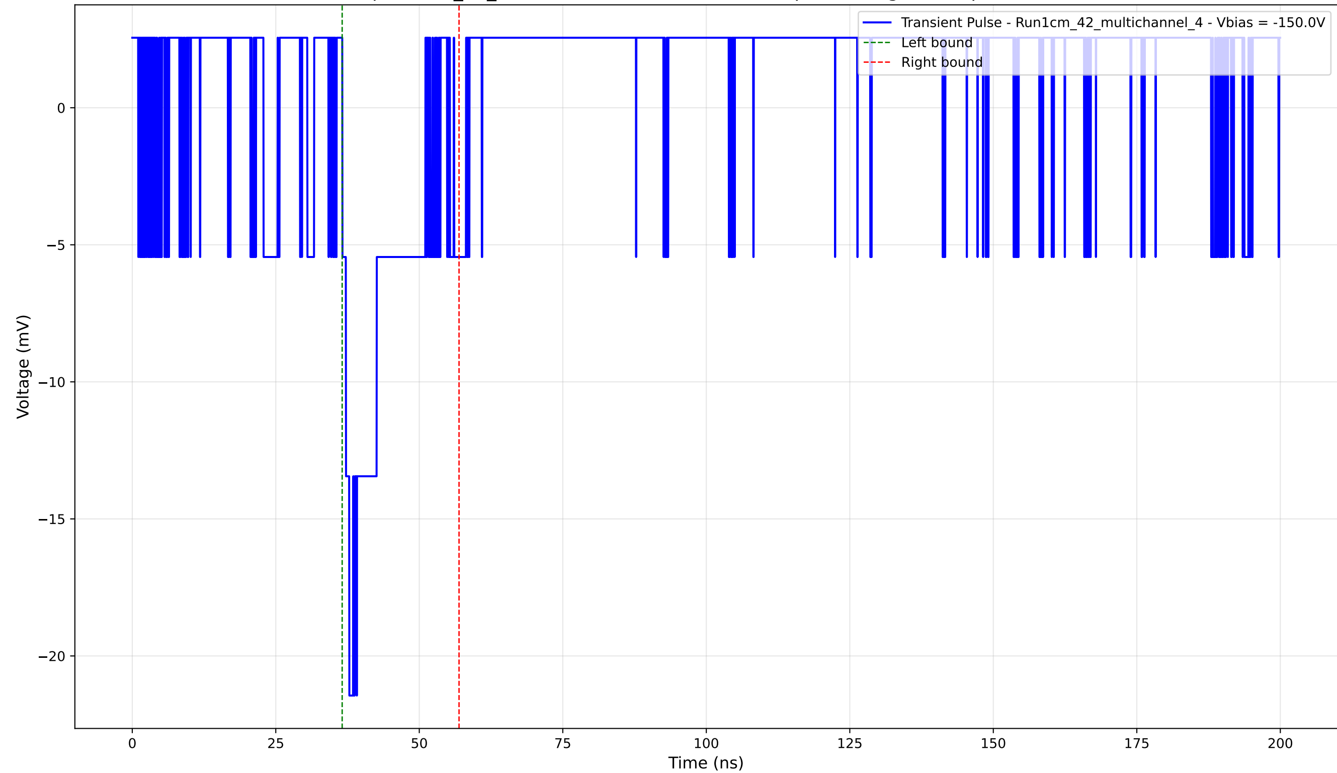
Transient Pulse - Sample: 1cm_42_multichannel - Position: 1310.0 \mu\text{m} - Charge: 2.82 pC - Rise Time: 0.00 ns (N/A)
