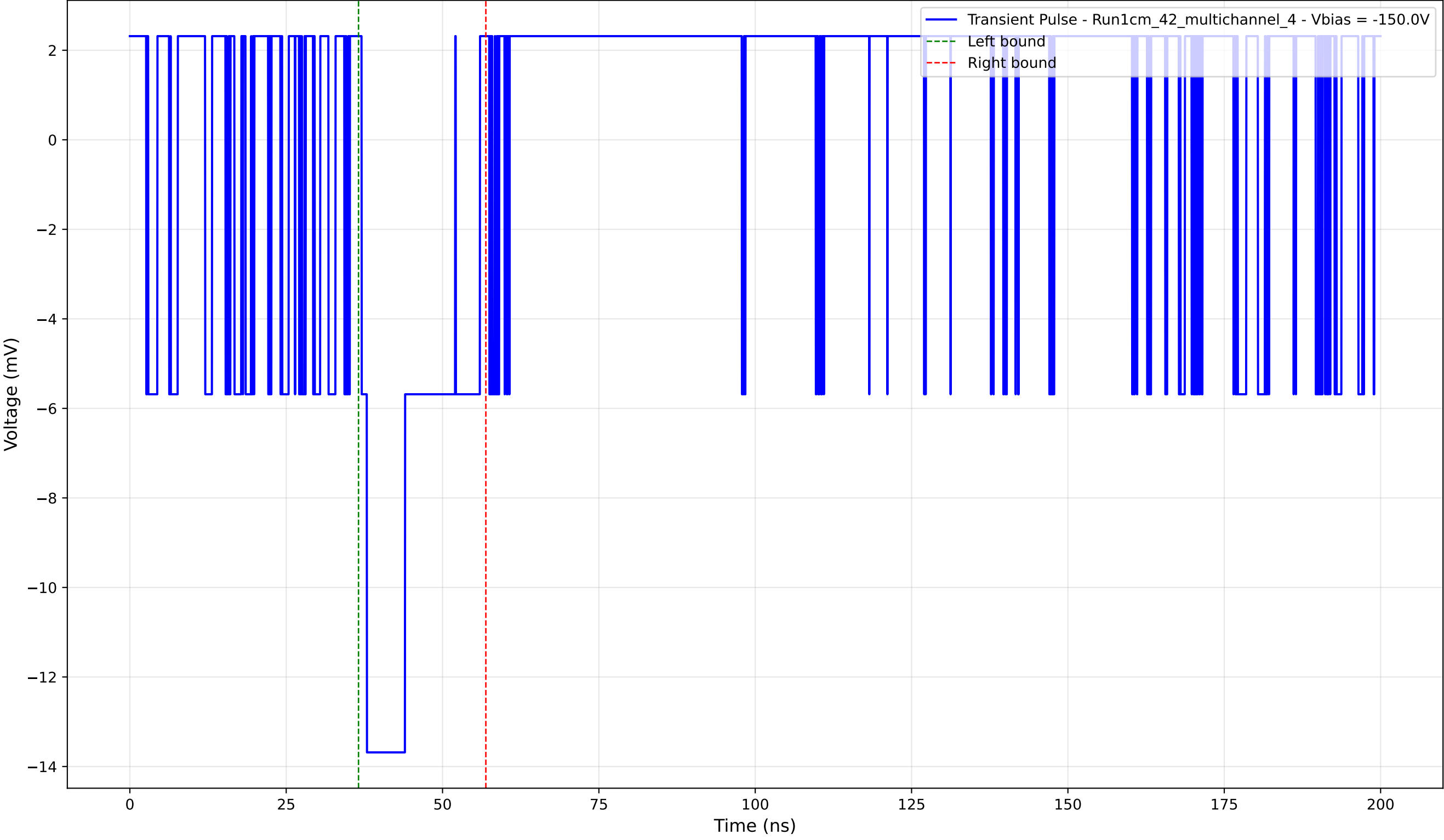
Transient Pulse - Sample: 1cm_42_multichannel - Position: 590.0 \mu\text{m} - Charge: 3.05 pC - Rise Time: 0.00 ns (N/A)
