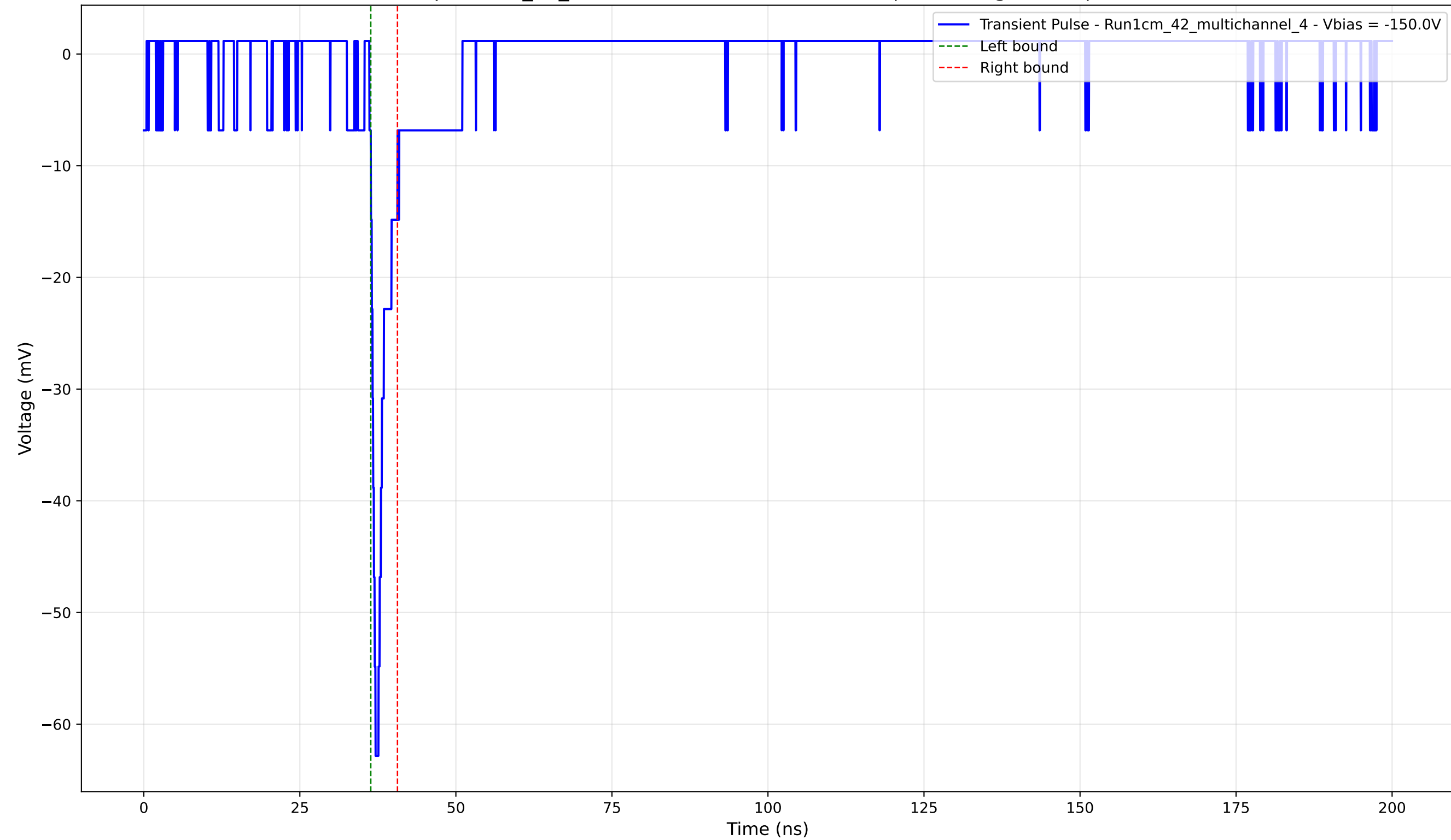
Transient Pulse - Sample: 1cm_42_multichannel - Position: 2615.0 \mu\text{m} - Charge: 2.67 pC - Rise Time: 0.98 ns
