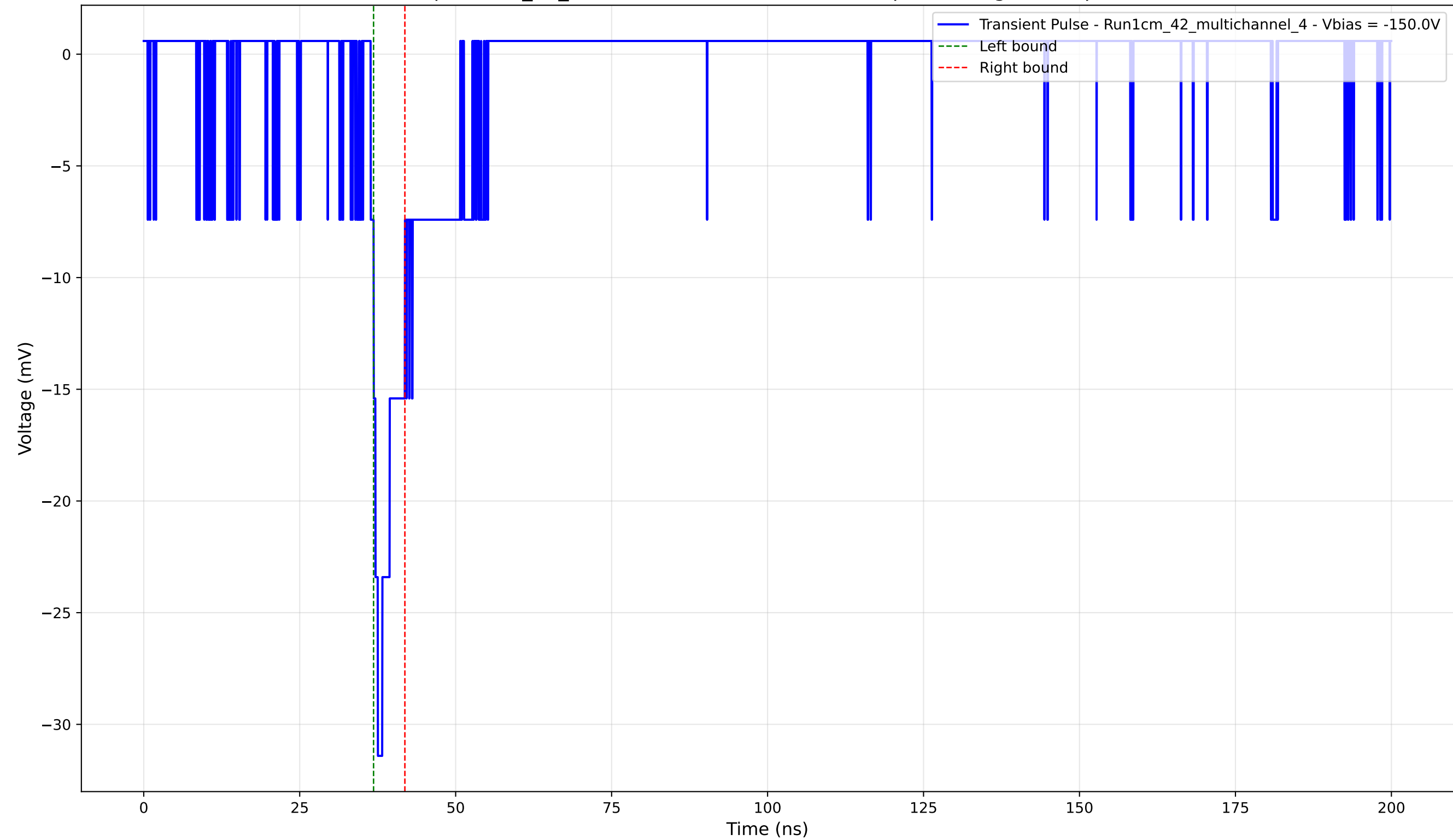
Transient Pulse - Sample: 1cm_42_multichannel - Position: 3165.0 \mu\text{m} - Charge: 2.02 pC - Rise Time: 1.15 ns
