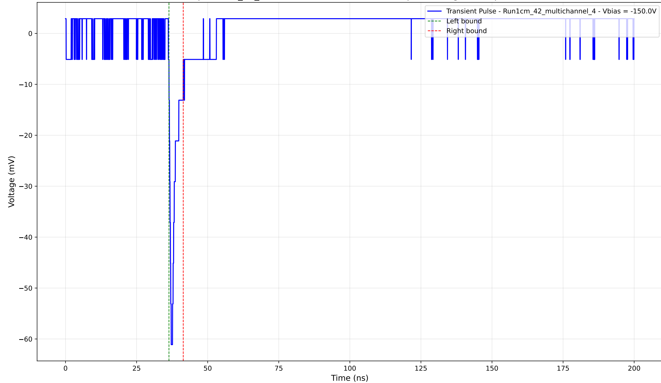
Transient Pulse - Sample: 1cm_42_multichannel - Position: 2110.0 \mu\text{m} - Charge: 2.78 pC - Rise Time: 0.78 ns
