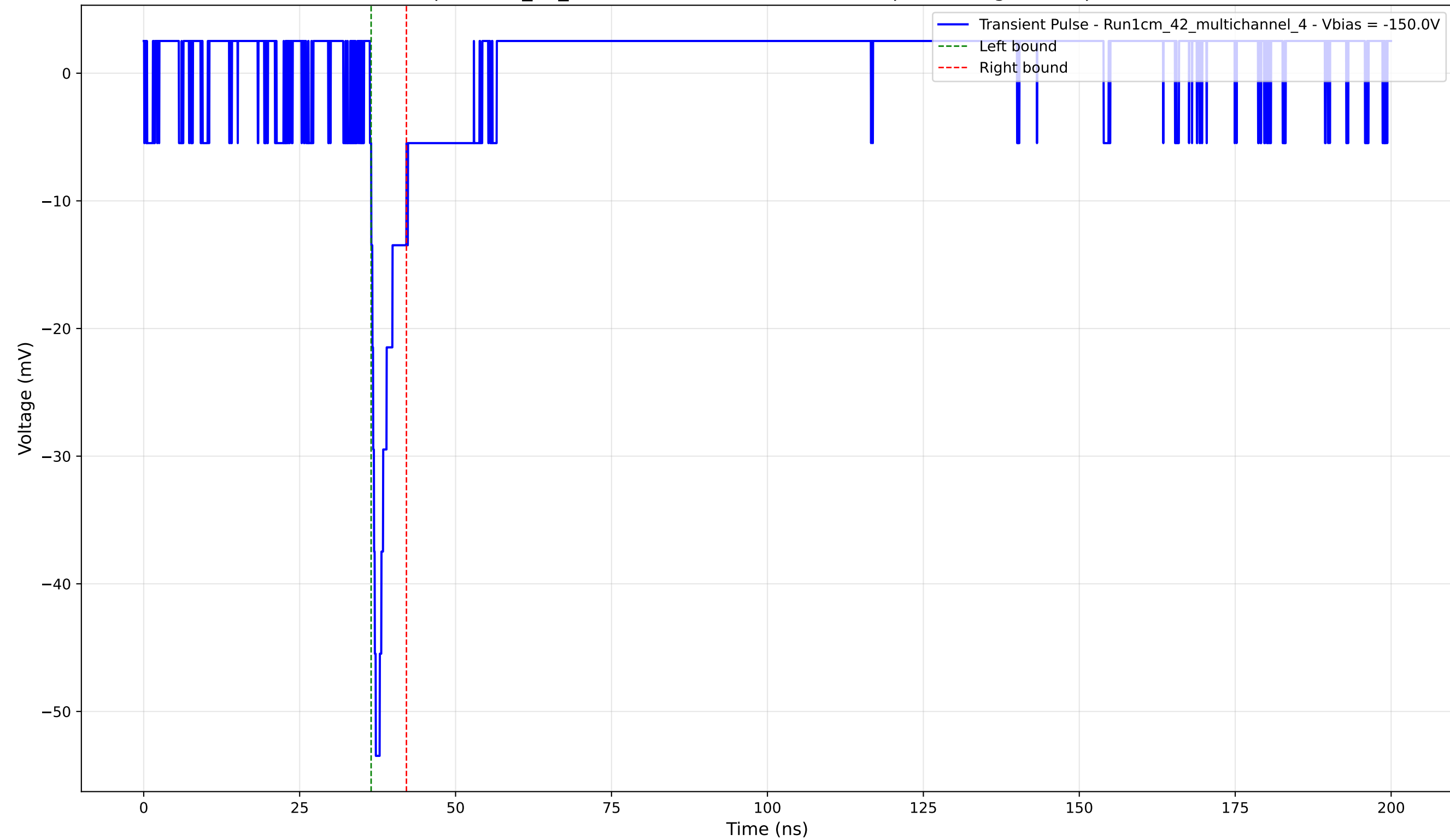
Transient Pulse - Sample: 1cm_42_multichannel - Position: 1985.0 \mu\text{m} - Charge: 2.89 pC - Rise Time: 0.94 ns
