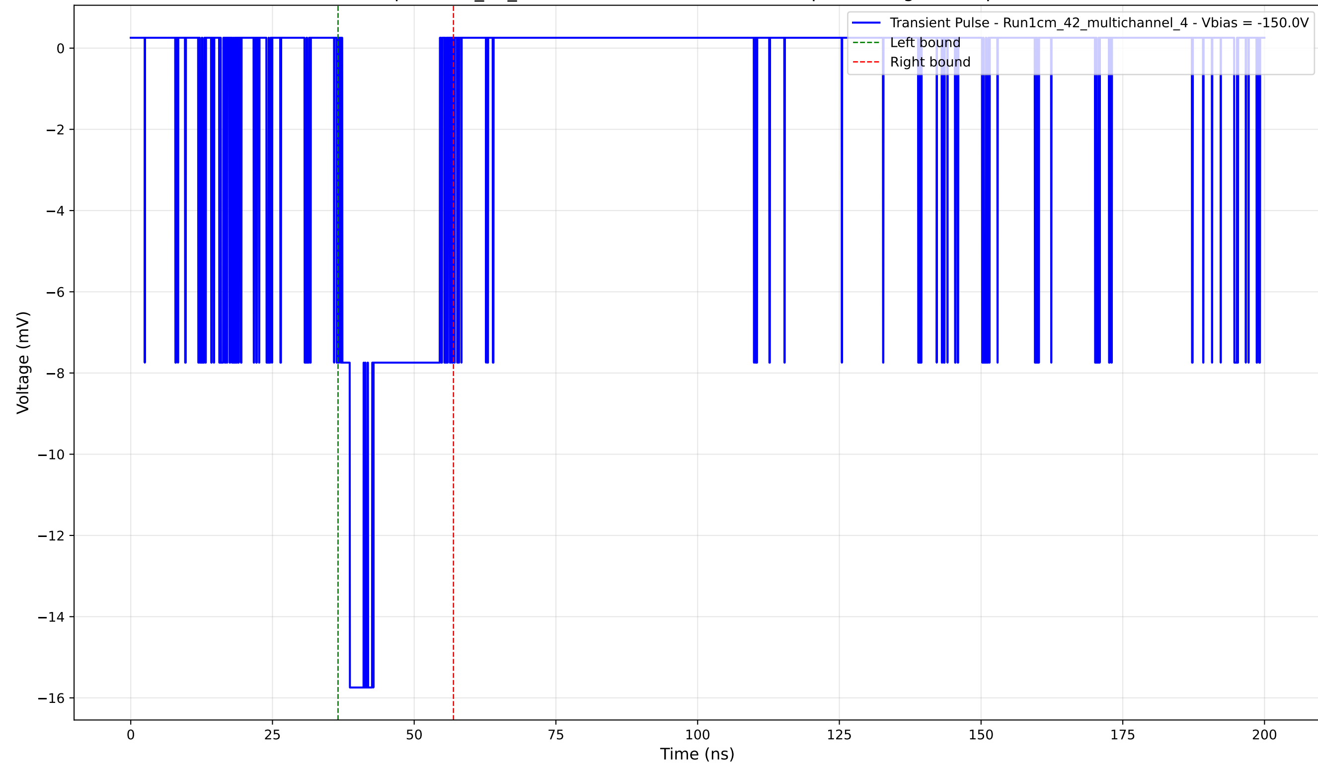
Transient Pulse - Sample: 1cm_42_multichannel - Position: 4475.0 \mu\text{m} - Charge: 3.43 pC - Rise Time: 1.34 ns
