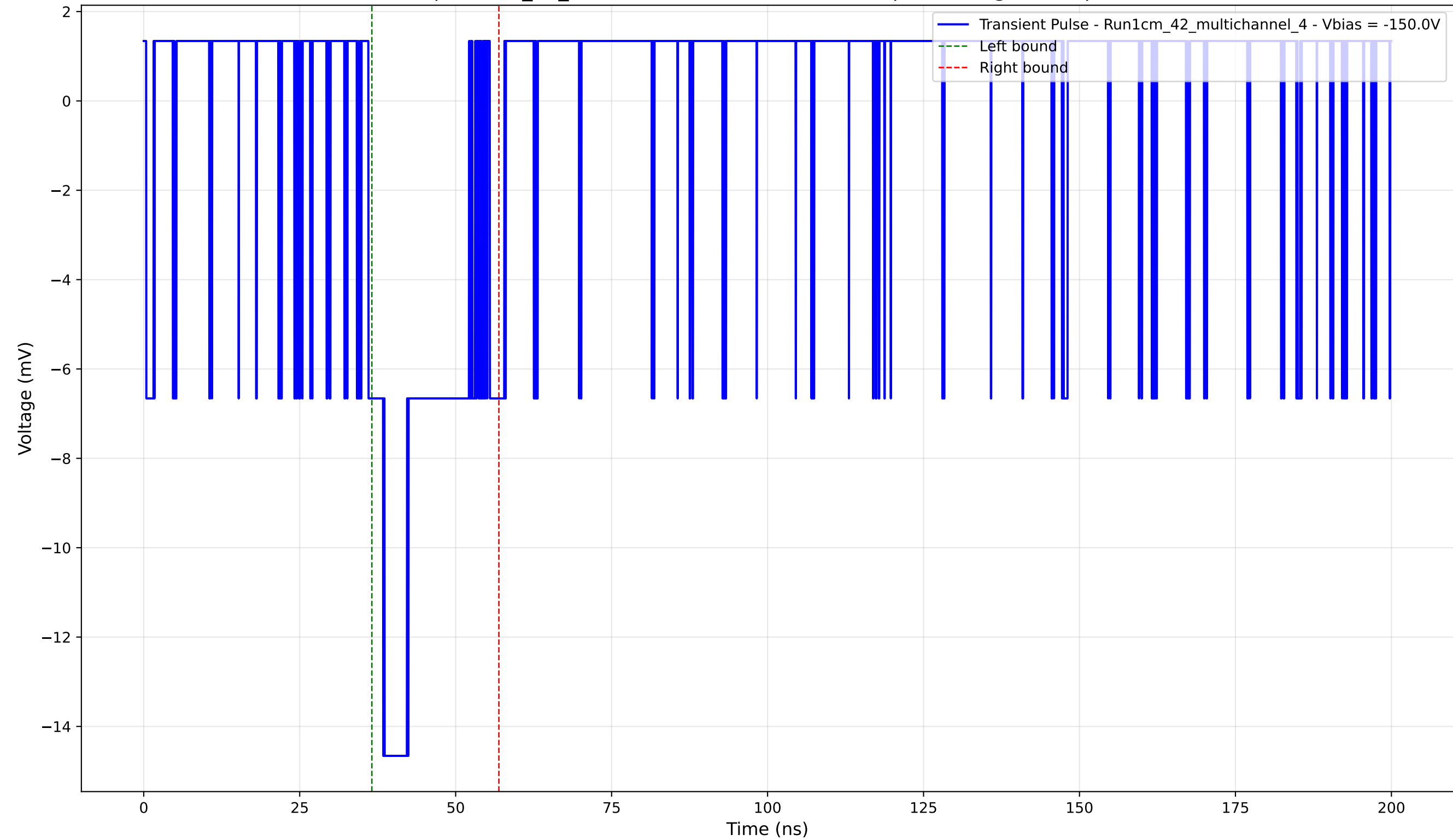
Transient Pulse - Sample: 1cm_42_multichannel - Position: 4795.0 \mu\text{m} - Charge: 3.04 pC - Rise Time: 2.38 ns
