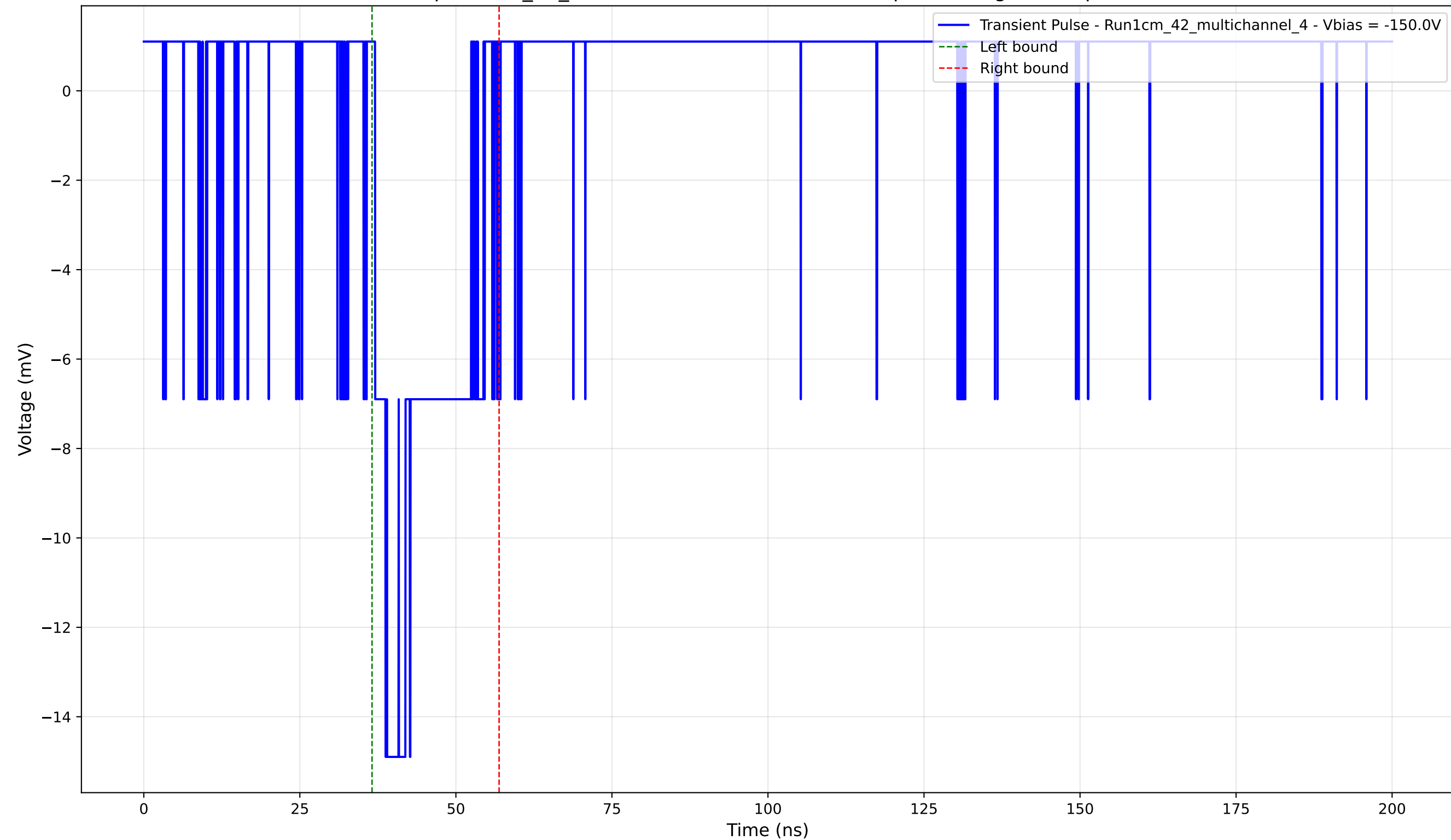
Transient Pulse - Sample: 1cm_42_multichannel - Position: 4805.0 \mu\text{m} - Charge: 2.85 pC - Rise Time: 1.68 ns
