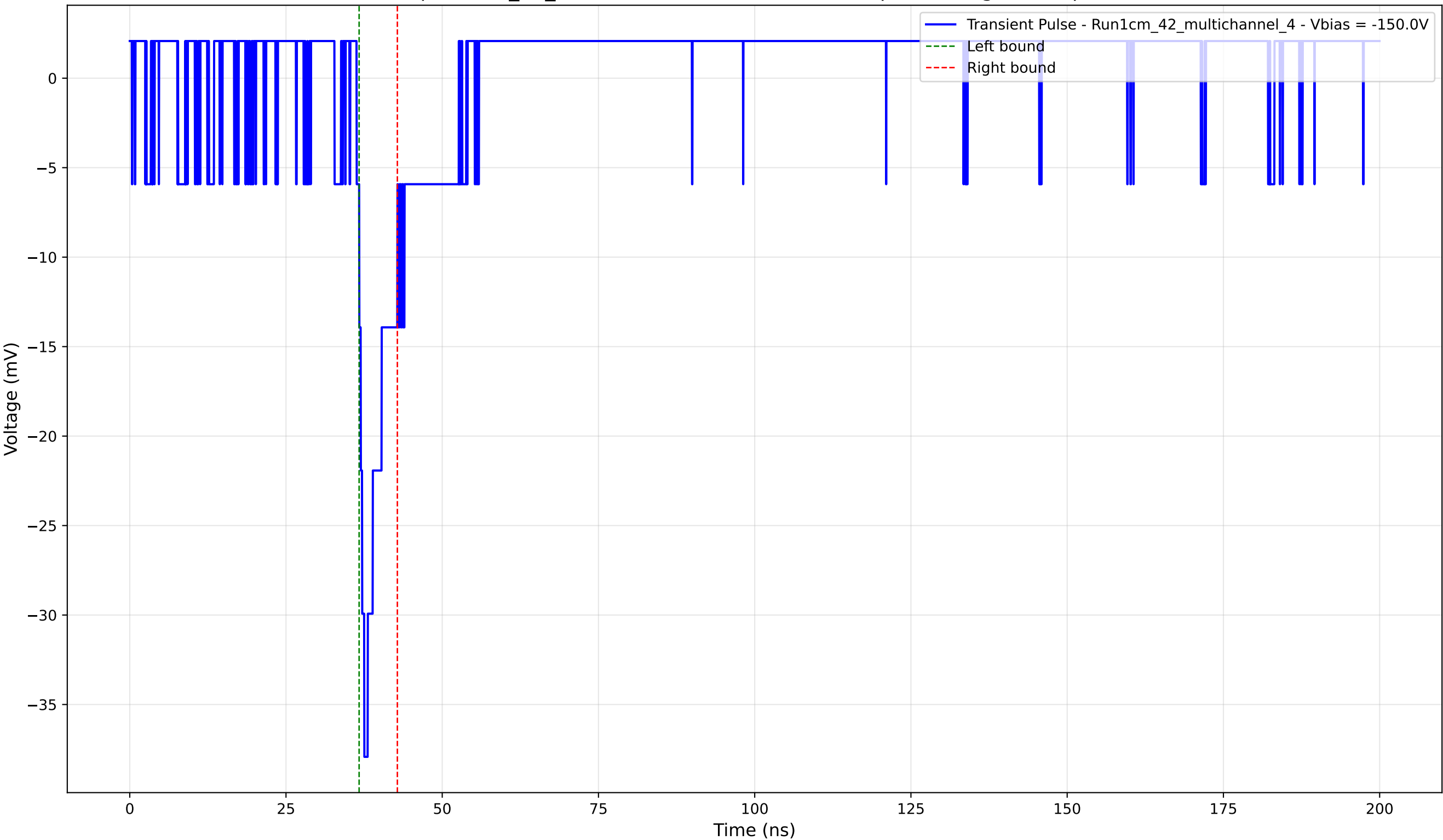
Transient Pulse - Sample: 1cm_42_multichannel - Position: 1680.0 \mu\text{m} - Charge: 2.60 pC - Rise Time: 1.23 ns
