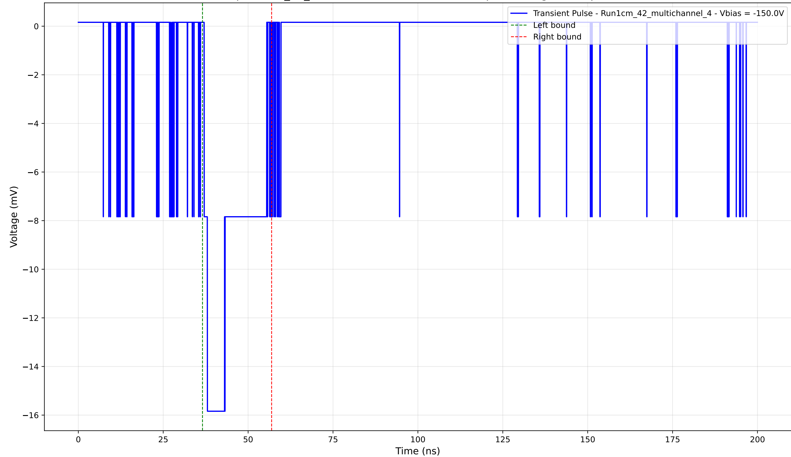
Transient Pulse - Sample: 1cm_42_multichannel - Position: 3995.0 \mu\text{m} - Charge: 3.77 pC - Rise Time: 0.96 ns
