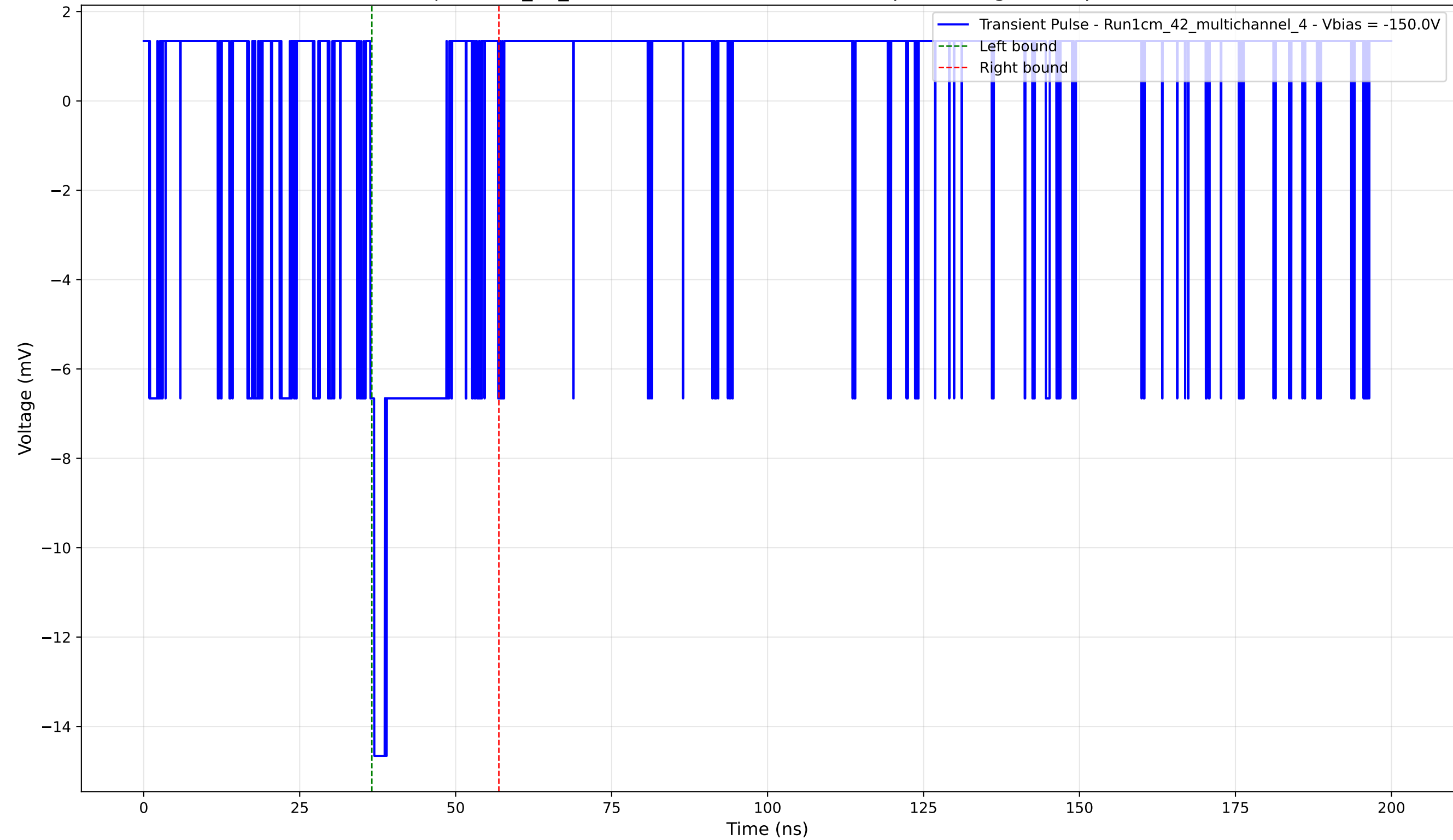
Transient Pulse - Sample: 1cm_42_multichannel - Position: 2940.0 \mu\text{m} - Charge: 1.93 pC - Rise Time: 0.64 ns
