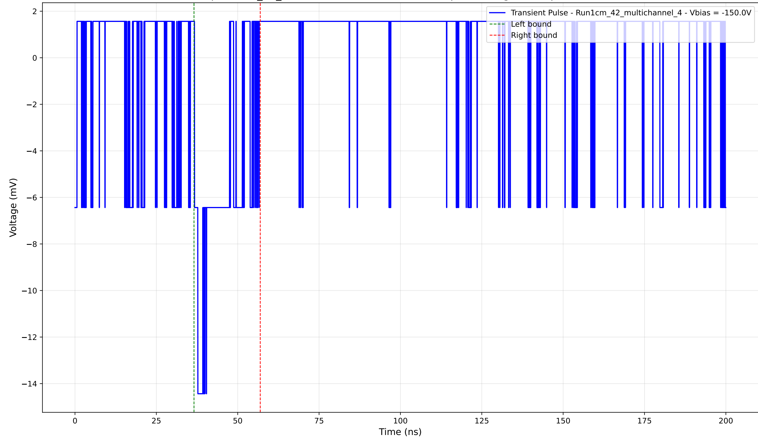
Transient Pulse - Sample: 1cm_42_multichannel - Position: 3450.0 \mu\text{m} - Charge: 2.09 pC - Rise Time: 0.00 ns (N/A)
