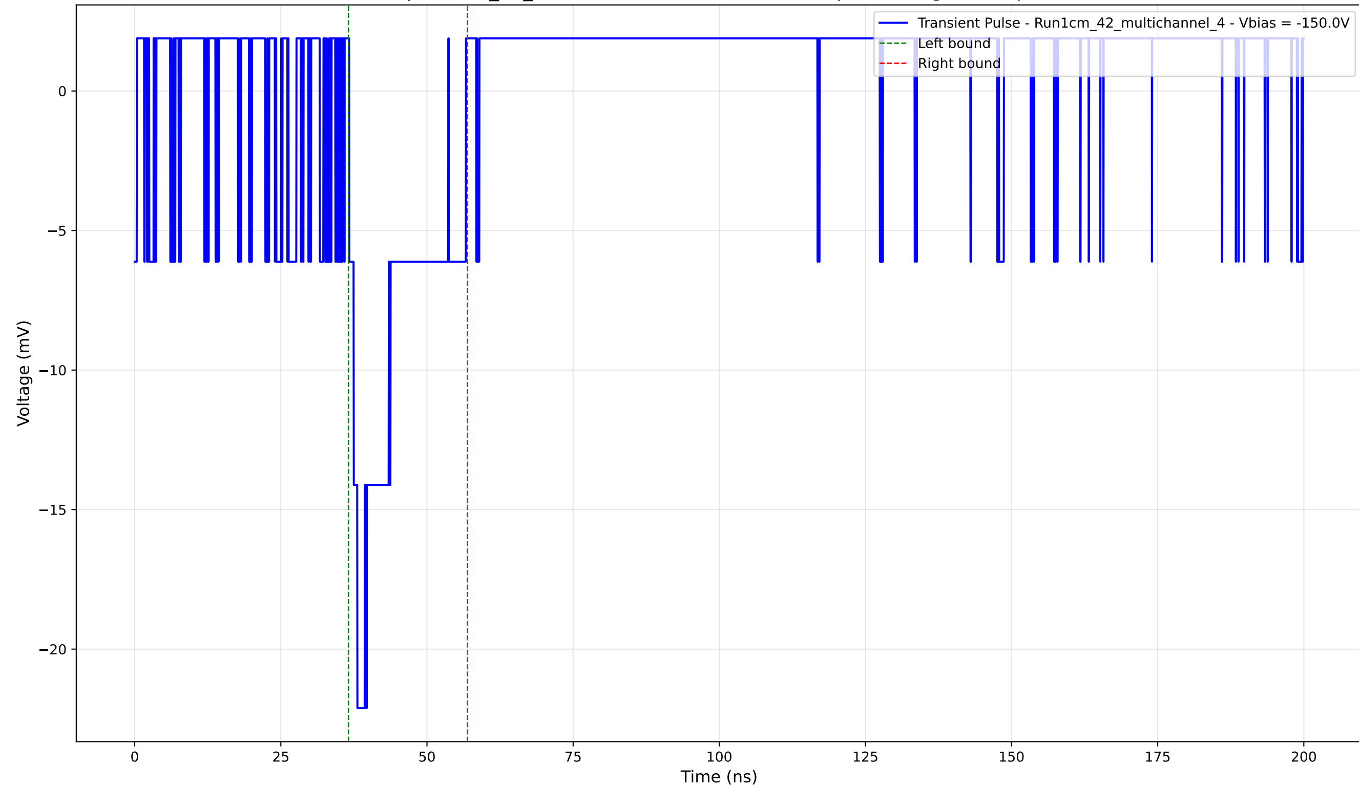
Transient Pulse - Sample: 1cm_42_multichannel - Position: 1115.0 \mu\text{m} - Charge: 3.61 pC - Rise Time: 1.40 ns
