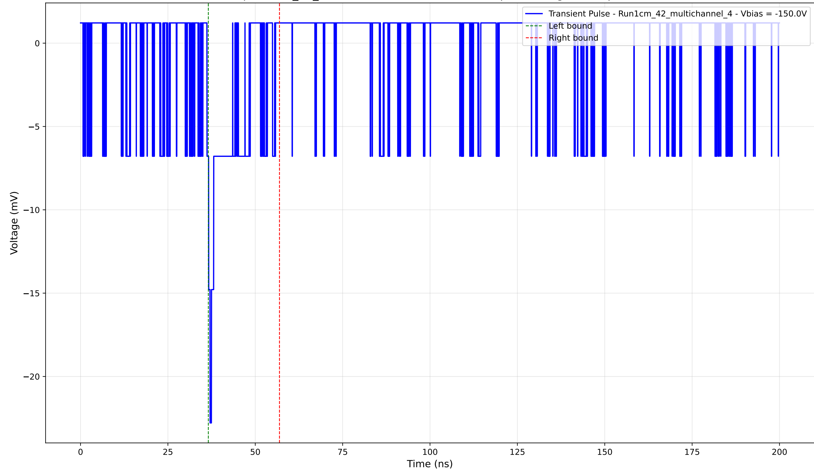
Transient Pulse - Sample: 1cm_42_multichannel - Position: 2425.0 \mu\text{m} - Charge: 1.92 pC - Rise Time: 0.90 ns
