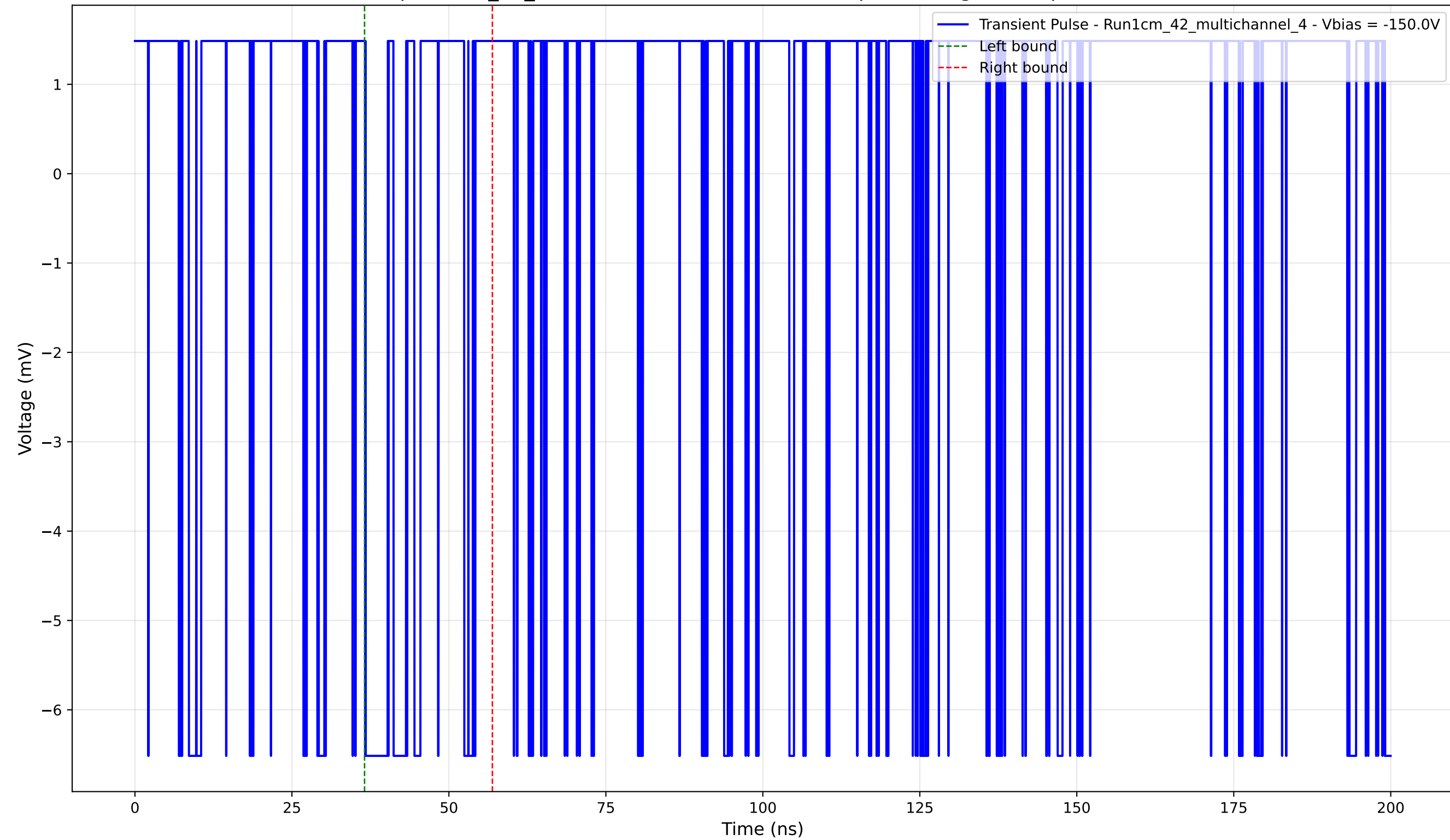
Transient Pulse - Sample: 1cm_42_multichannel - Position: 2920.0 \mu\text{m} - Charge: 0.72 pC - Rise Time: 0.00 ns (N/A)
