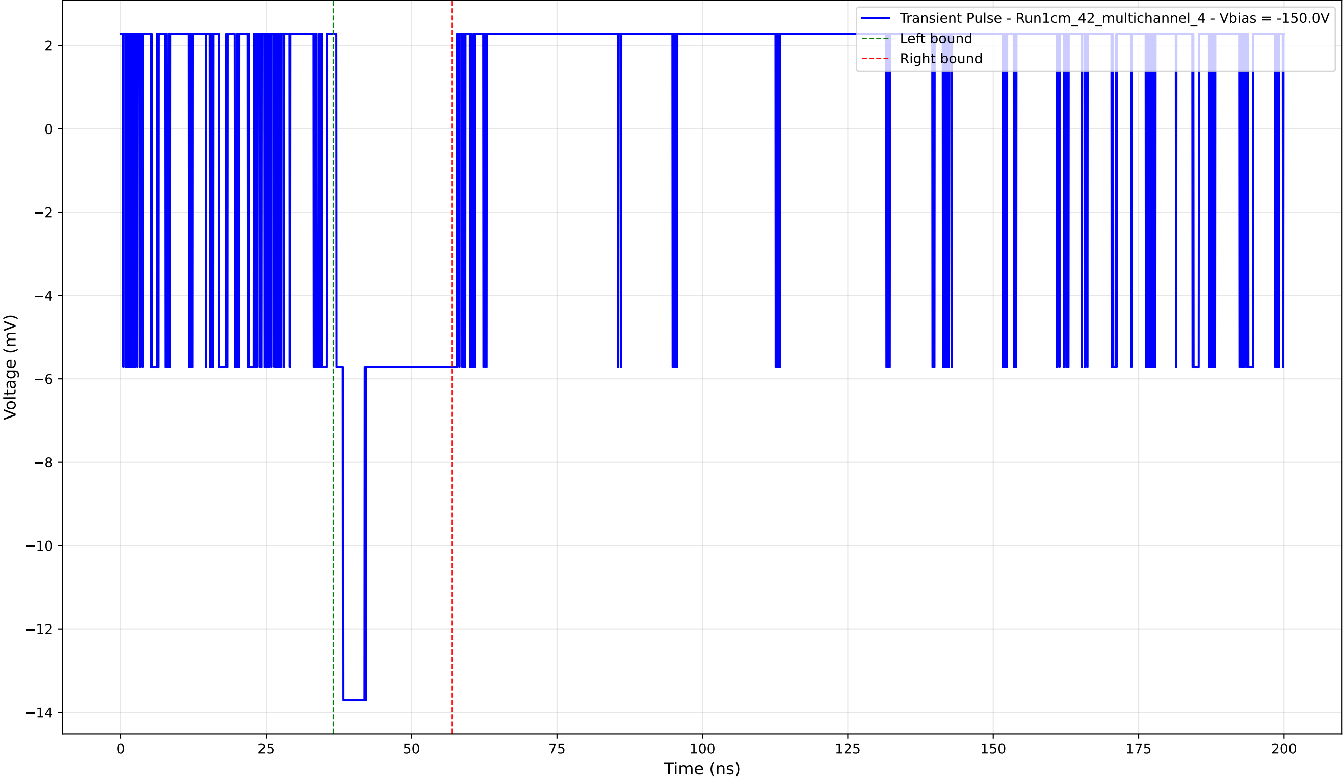
Transient Pulse - Sample: 1cm_42_multichannel - Position: 225.0 \mu\text{m} - Charge: 2.85 pC - Rise Time: 0.00 ns (N/A)
