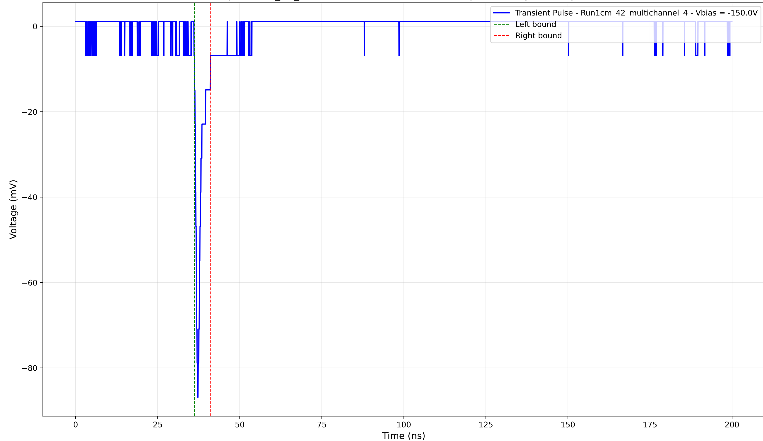
Transient Pulse - Sample: 1cm_42_multichannel - Position: 2480.0 \mu\text{m} - Charge: 3.30 pC - Rise Time: 0.76 ns
