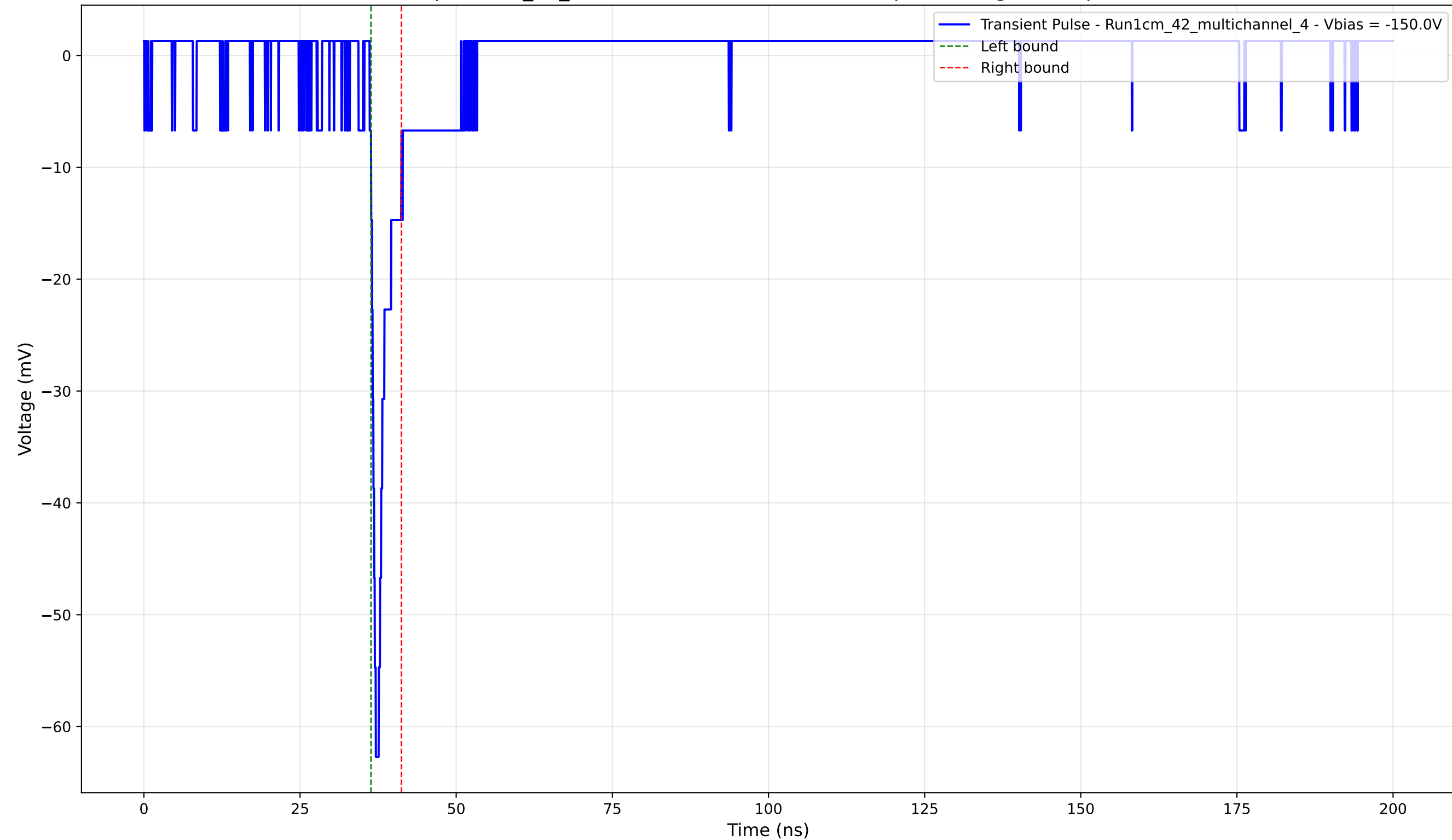
Transient Pulse - Sample: 1cm_42_multichannel - Position: 2610.0 \mu\text{m} - Charge: 2.83 pC - Rise Time: 0.98 ns
