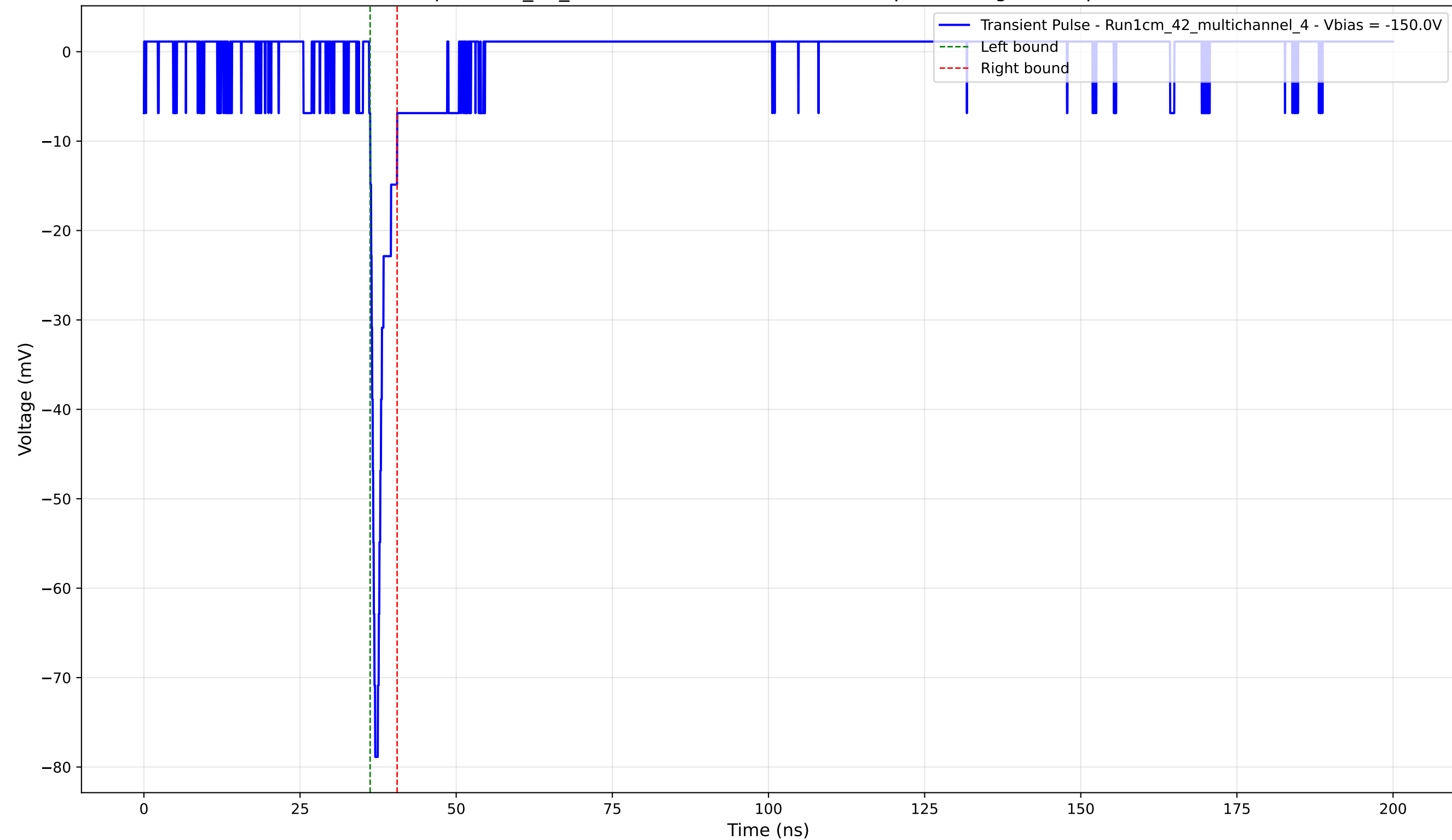
Transient Pulse - Sample: 1cm_42_multichannel - Position: 2465.0 \mu\text{m} - Charge: 3.06 pC - Rise Time: 0.80 ns
