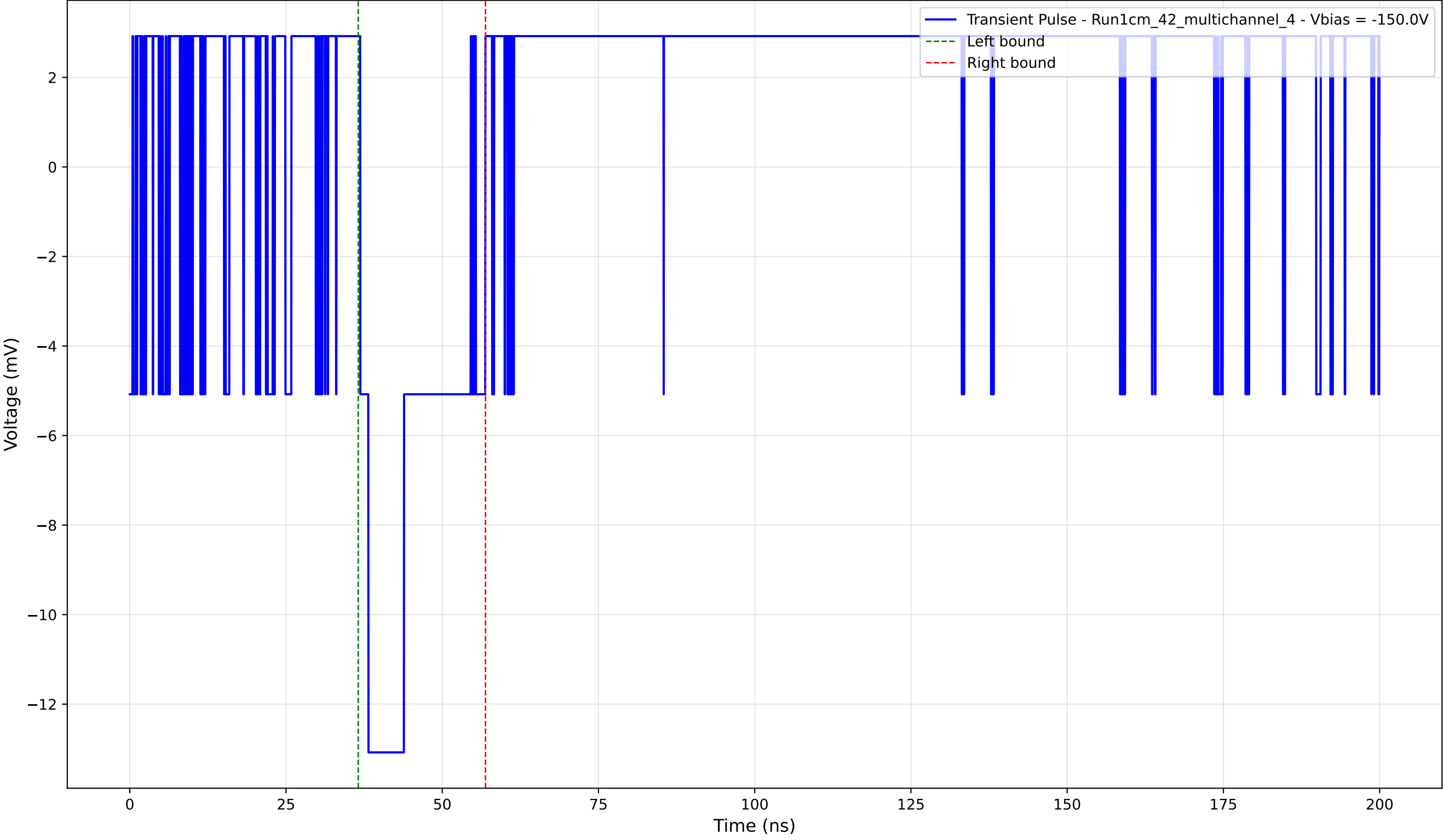
Transient Pulse - Sample: 1cm_42_multichannel - Position: 475.0 \mu\text{m} - Charge: 2.88 pC - Rise Time: 0.00 ns (N/A)
