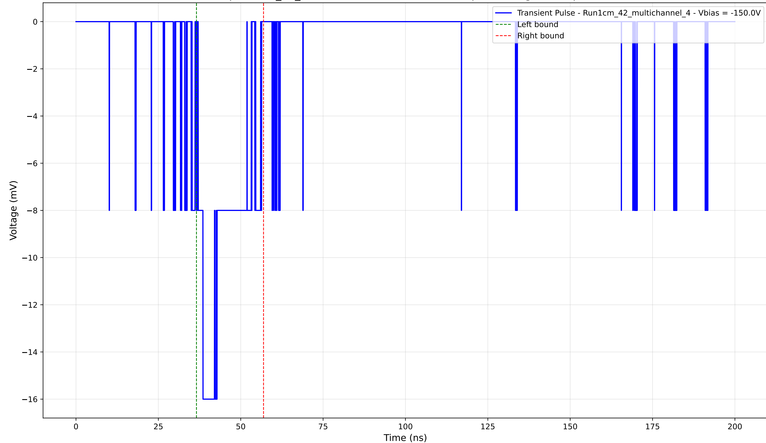
Transient Pulse - Sample: 1cm_42_multichannel - Position: 4770.0 \mu\text{m} - Charge: 3.55 pC - Rise Time: 1.46 ns
