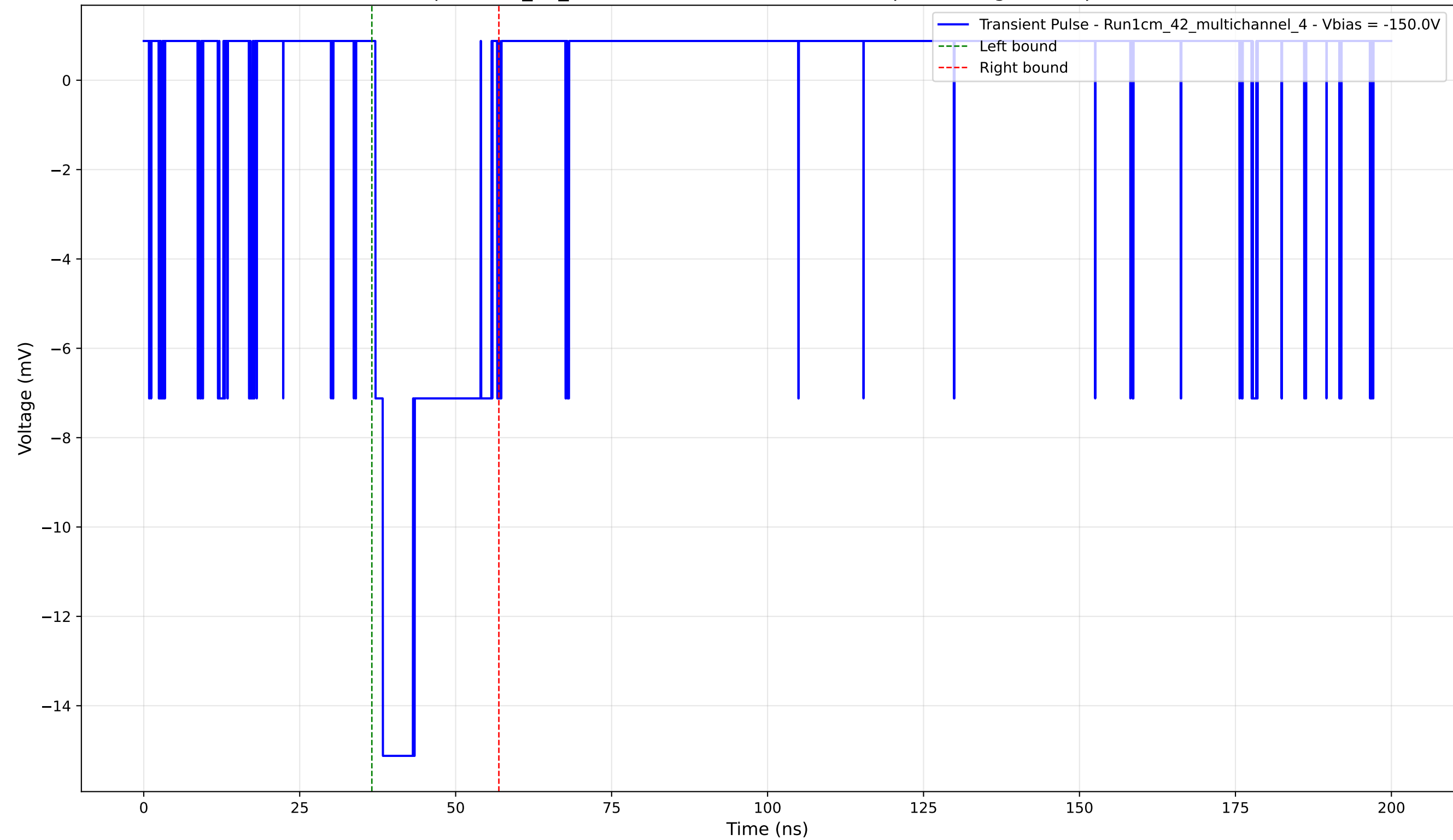
Transient Pulse - Sample: 1cm_42_multichannel - Position: 4145.0 \mu\text{m} - Charge: 3.43 pC - Rise Time: 1.20 ns
