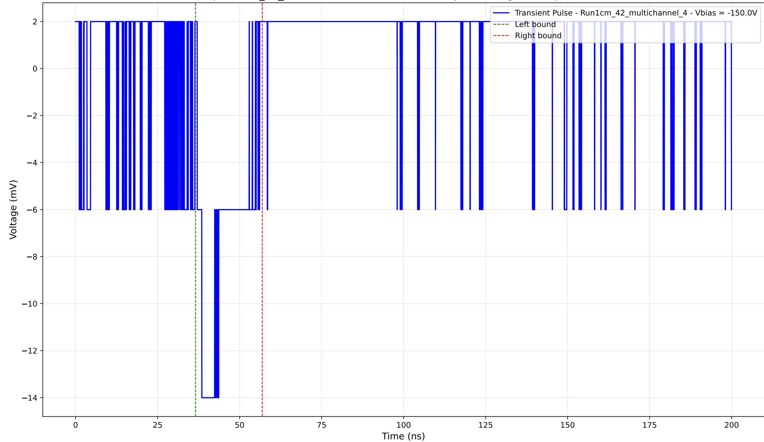
Transient Pulse - Sample: 1cm_42_multichannel - Position: 4550.0 \mu\text{m} - Charge: 2.79 pC - Rise Time: 0.00 ns (N/A)
