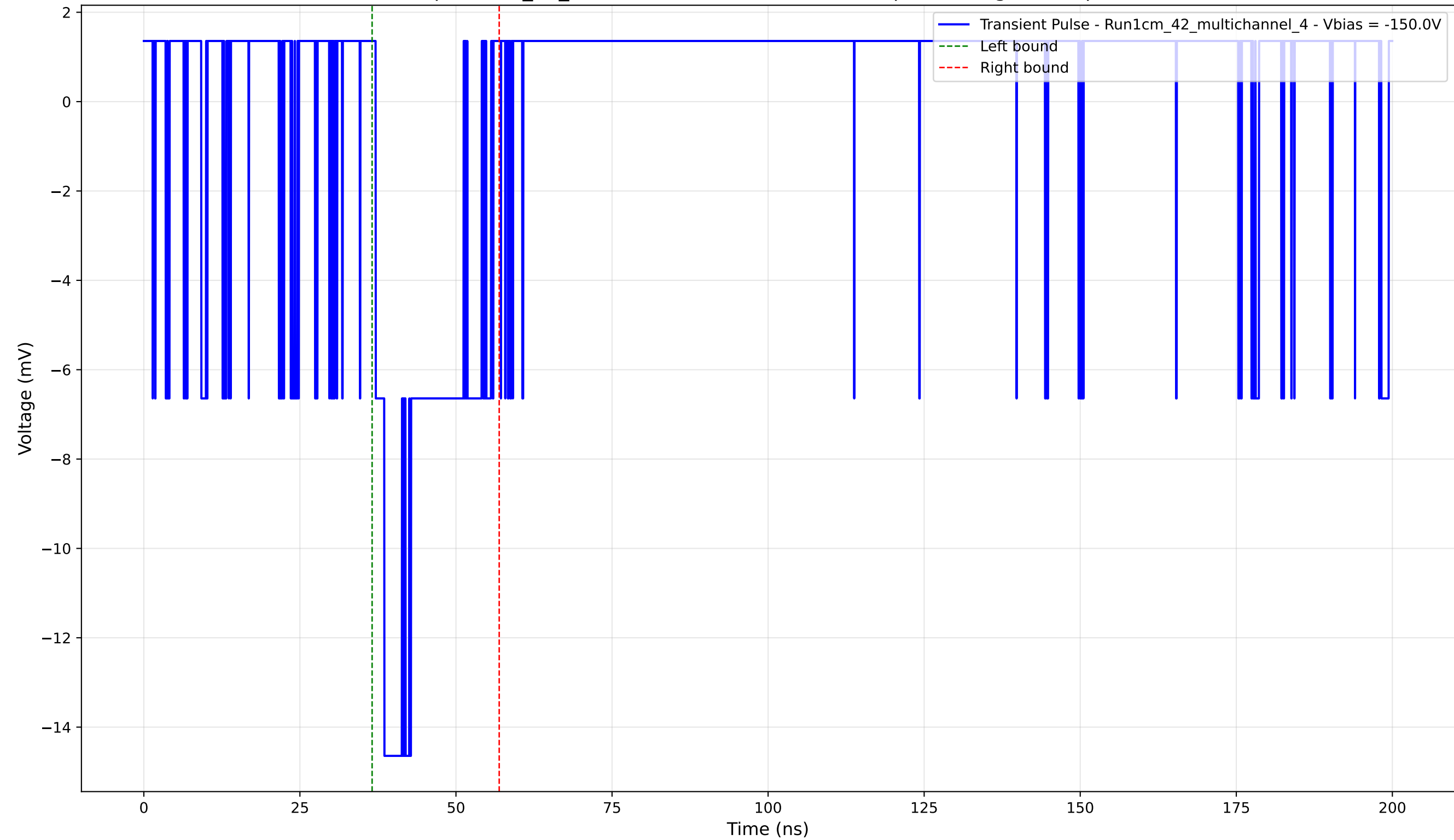
Transient Pulse - Sample: 1cm_42_multichannel - Position: 4730.0 \mu\text{m} - Charge: 2.91 pC - Rise Time: 1.40 ns
