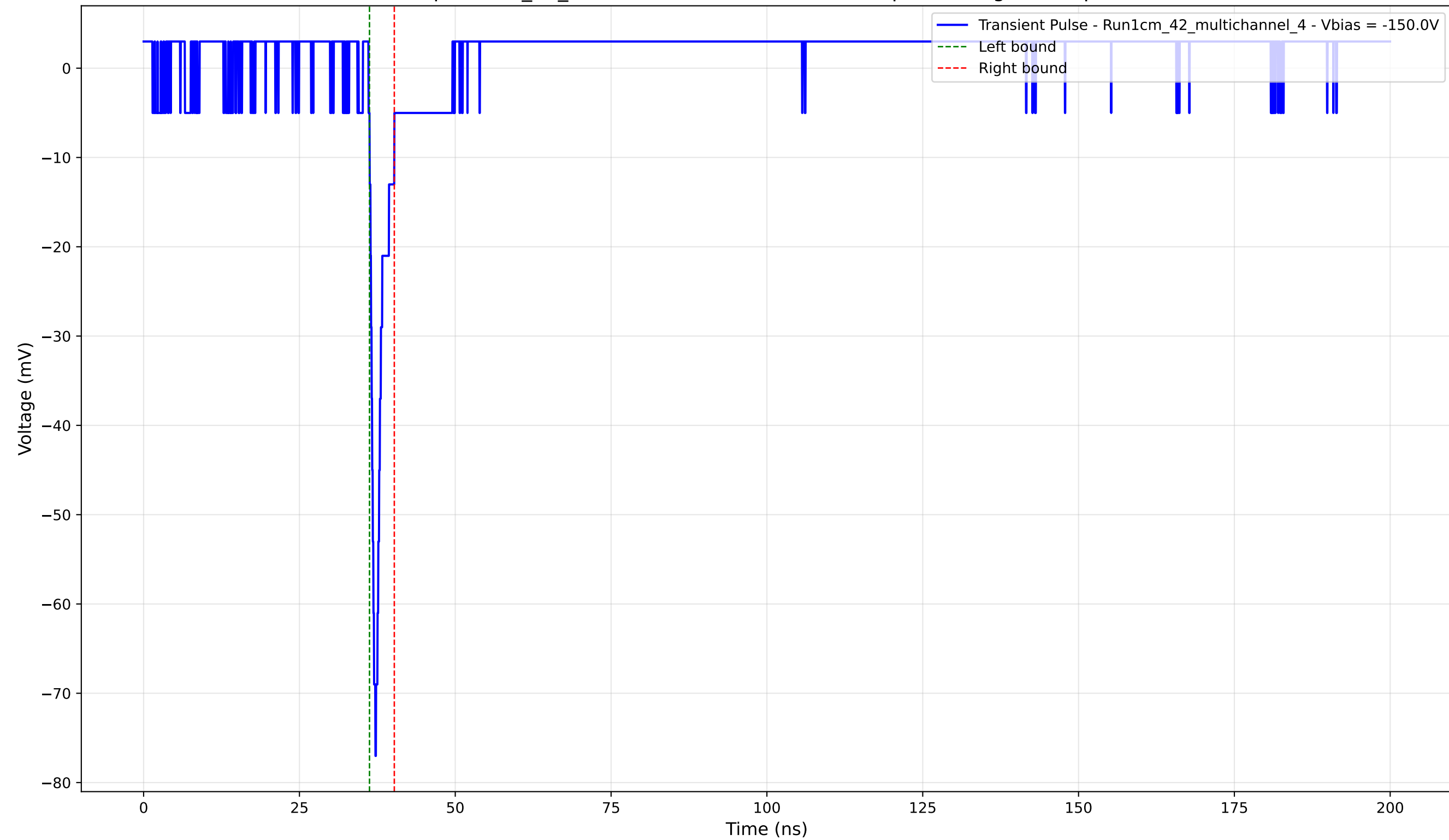
Transient Pulse - Sample: 1cm_42_multichannel - Position: 2455.0 \mu\text{m} - Charge: 2.62 pC - Rise Time: 0.93 ns
