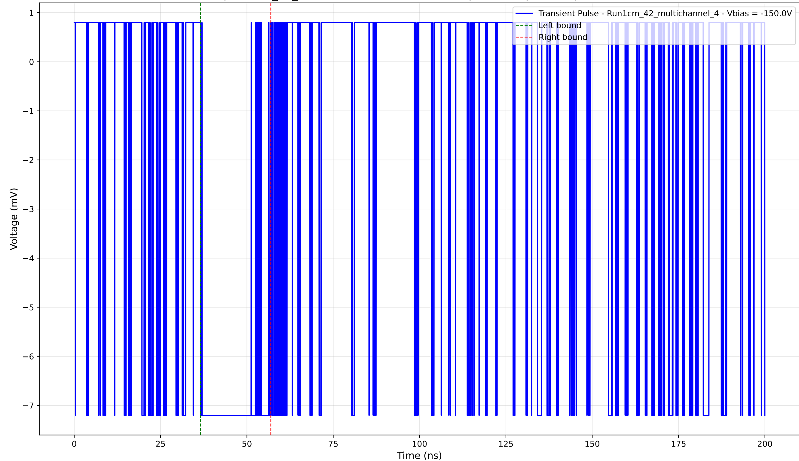
Transient Pulse - Sample: 1cm_42_multichannel - Position: 310.0 \mu\text{m} - Charge: 2.75 pC - Rise Time: 0.00 ns (N/A)
