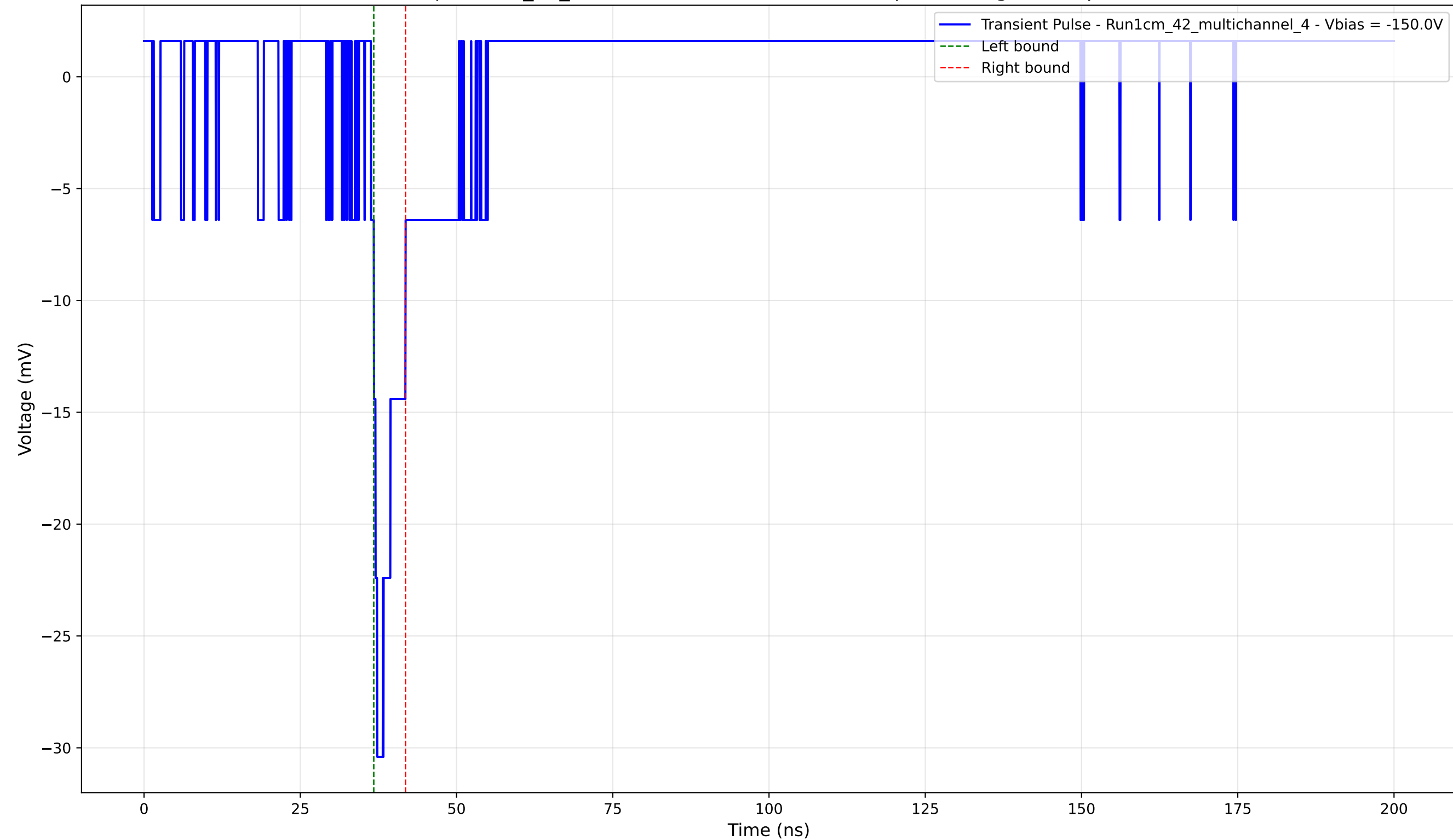
Transient Pulse - Sample: 1cm_42_multichannel - Position: 3080.0 \mu\text{m} - Charge: 2.00 pC - Rise Time: 0.99 ns
