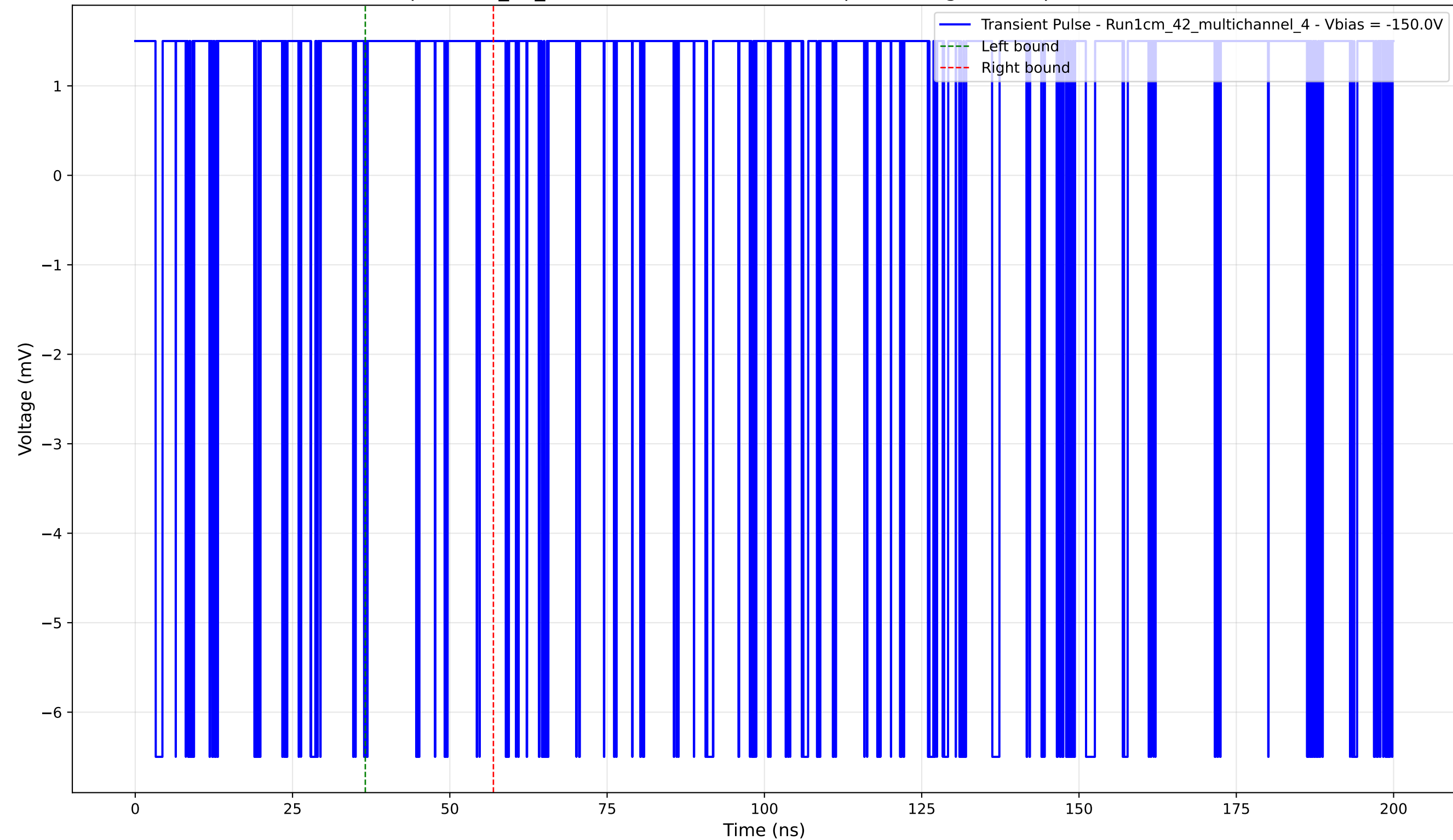
Transient Pulse - Sample: 1cm_42_multichannel - Position: 45.0 \mu\text{m} - Charge: -0.41 pC - Rise Time: 0.00 ns (N/A)
