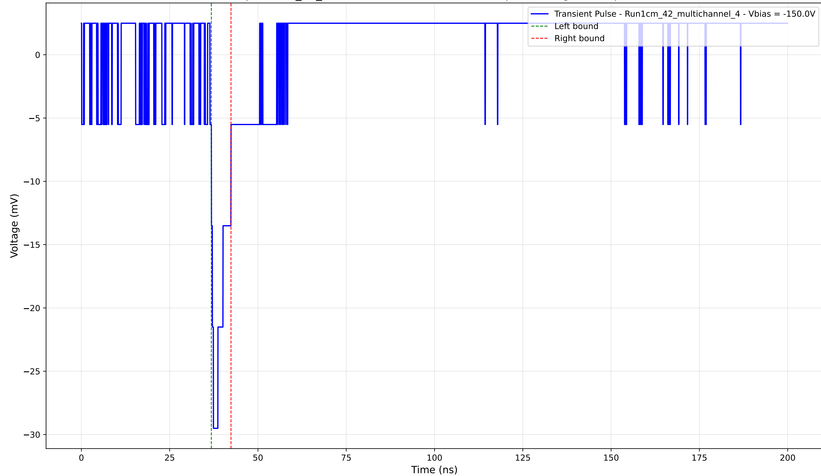
Transient Pulse - Sample: 1cm_42_multichannel - Position: 1585.0 \mu\text{m} - Charge: 2.19 pC - Rise Time: 1.00 ns
