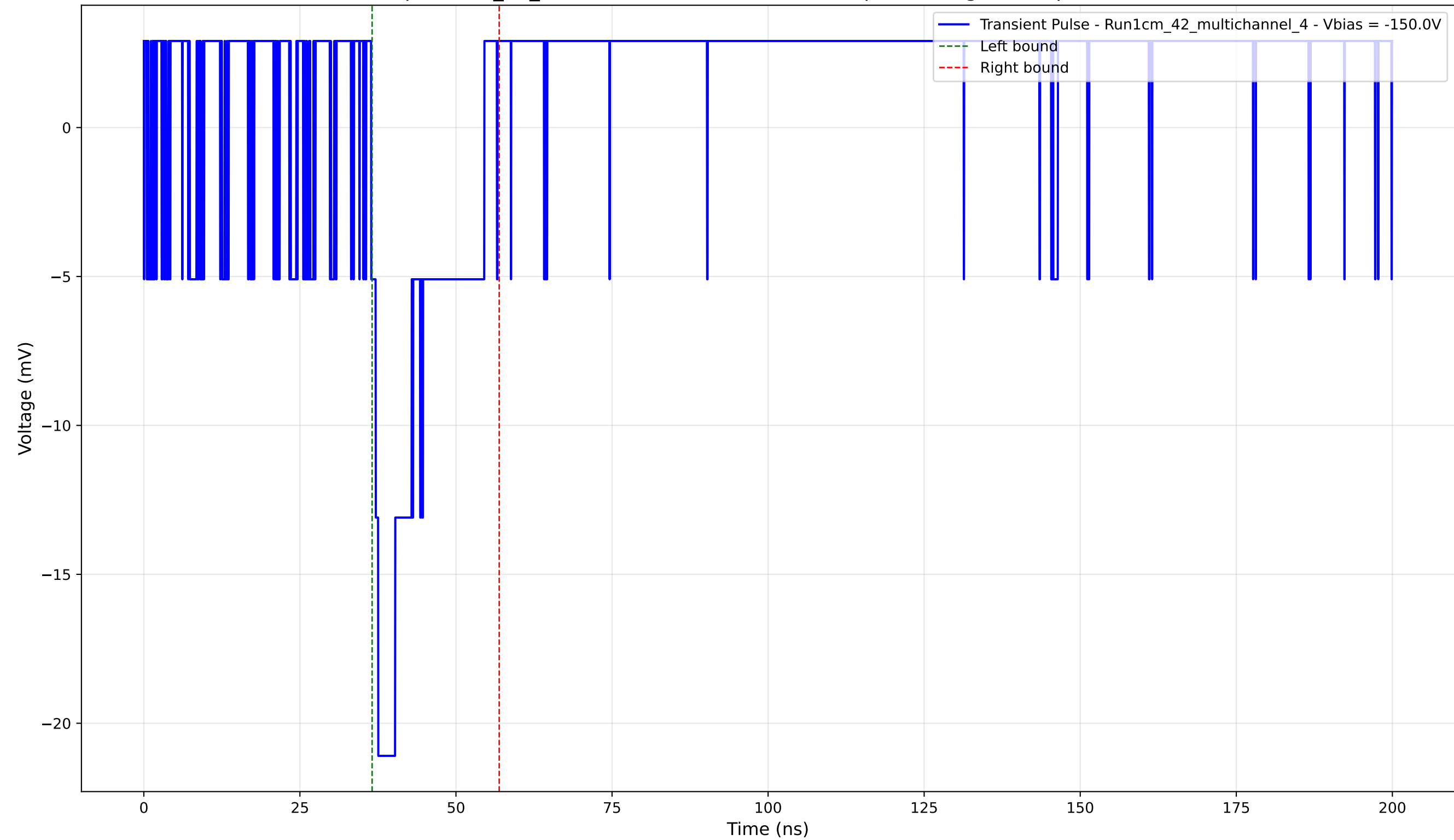
Transient Pulse - Sample: 1cm_42_multichannel - Position: 1280.0 \mu\text{m} - Charge: 3.11 pC - Rise Time: 0.00 ns (N/A)
