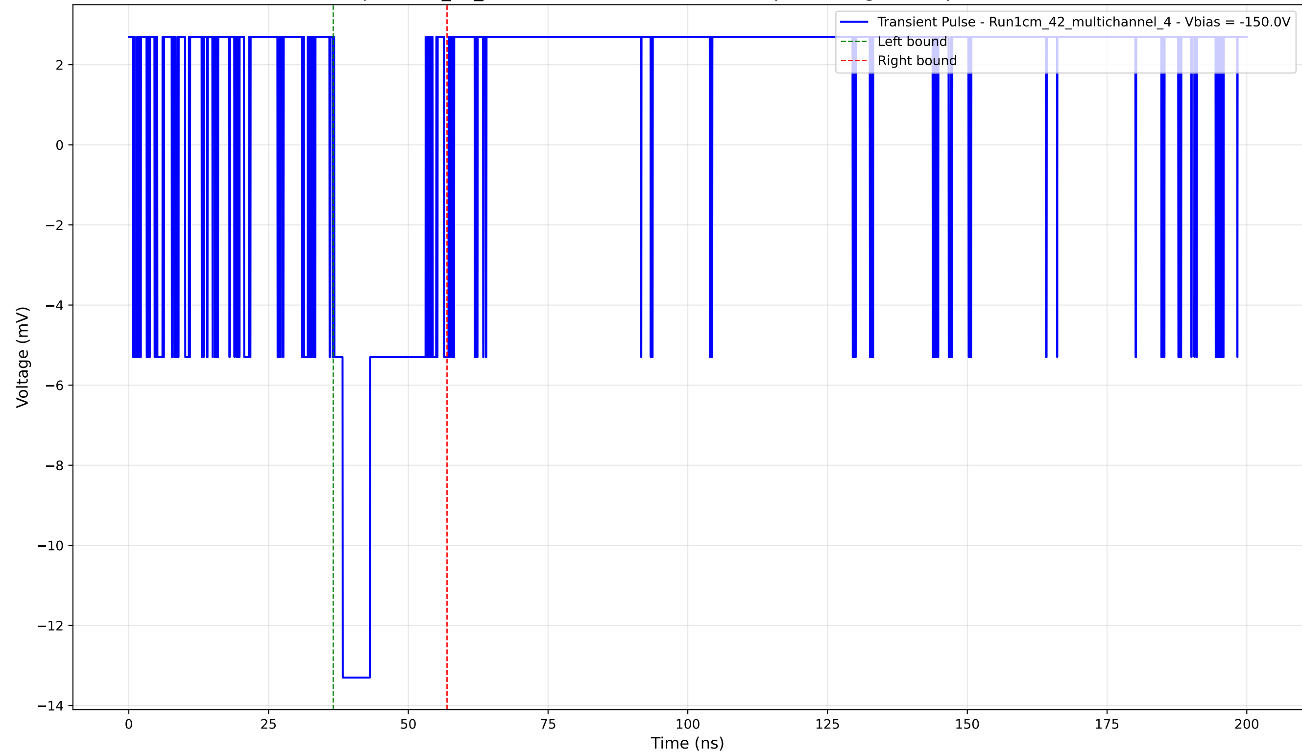
Transient Pulse - Sample: 1cm_42_multichannel - Position: 4190.0 \mu\text{m} - Charge: 2.62 pC - Rise Time: 0.00 ns (N/A)
