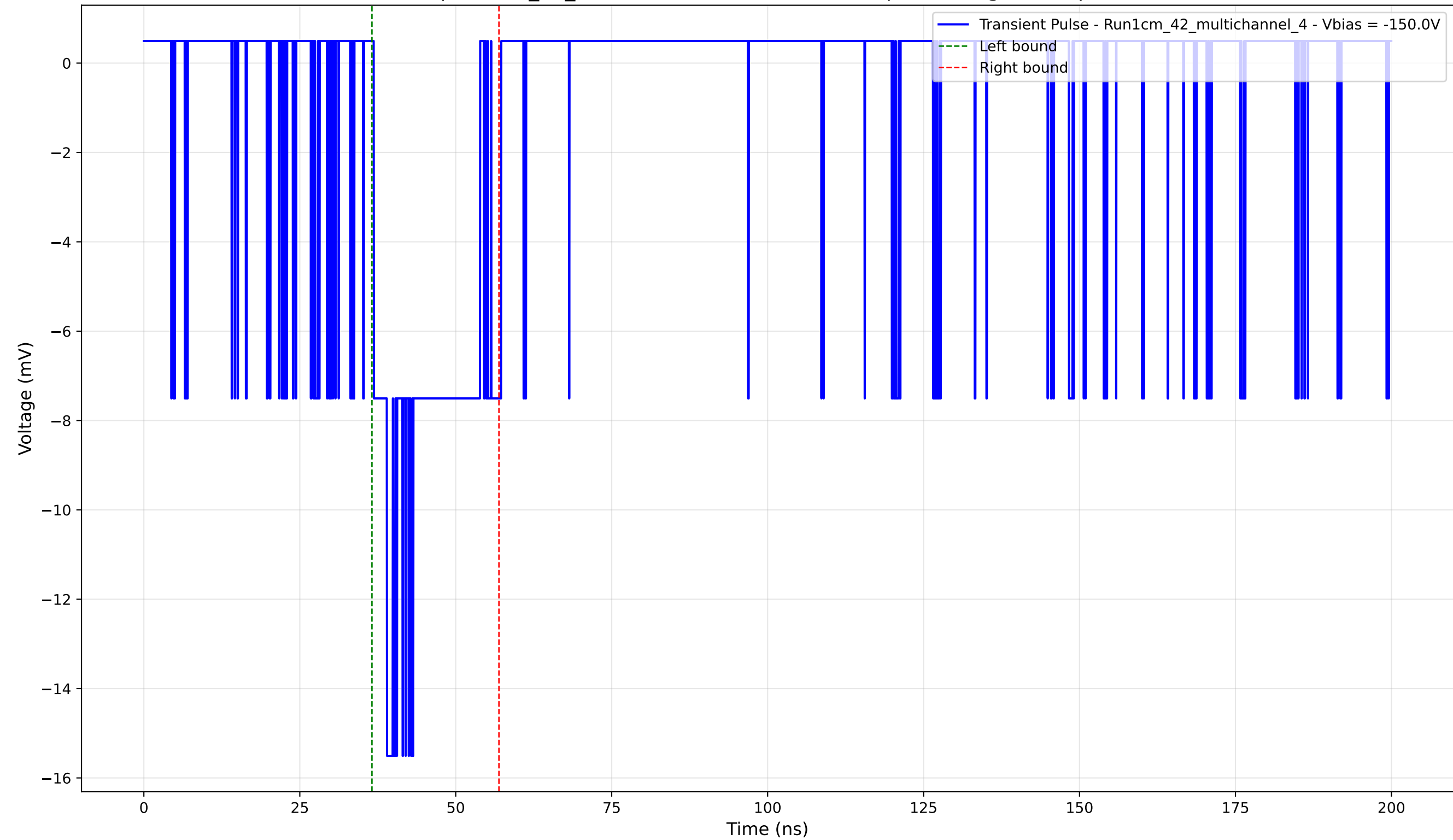
Transient Pulse - Sample: 1cm_42_multichannel - Position: 130.0 \mu\text{m} - Charge: 3.17 pC - Rise Time: 2.12 ns
