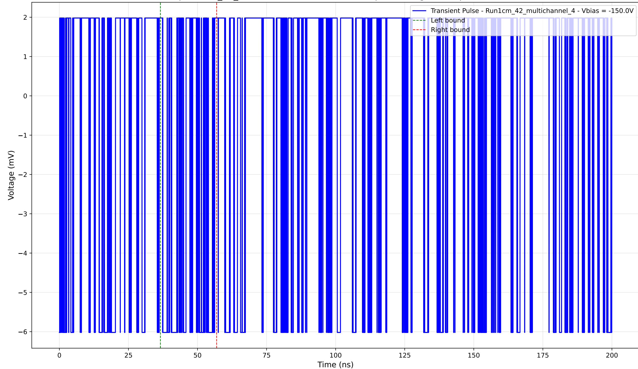
Transient Pulse - Sample: 1cm_42_multichannel - Position: 360.0 \mu\text{m} - Charge: 0.95 pC - Rise Time: 0.00 ns (N/A)
