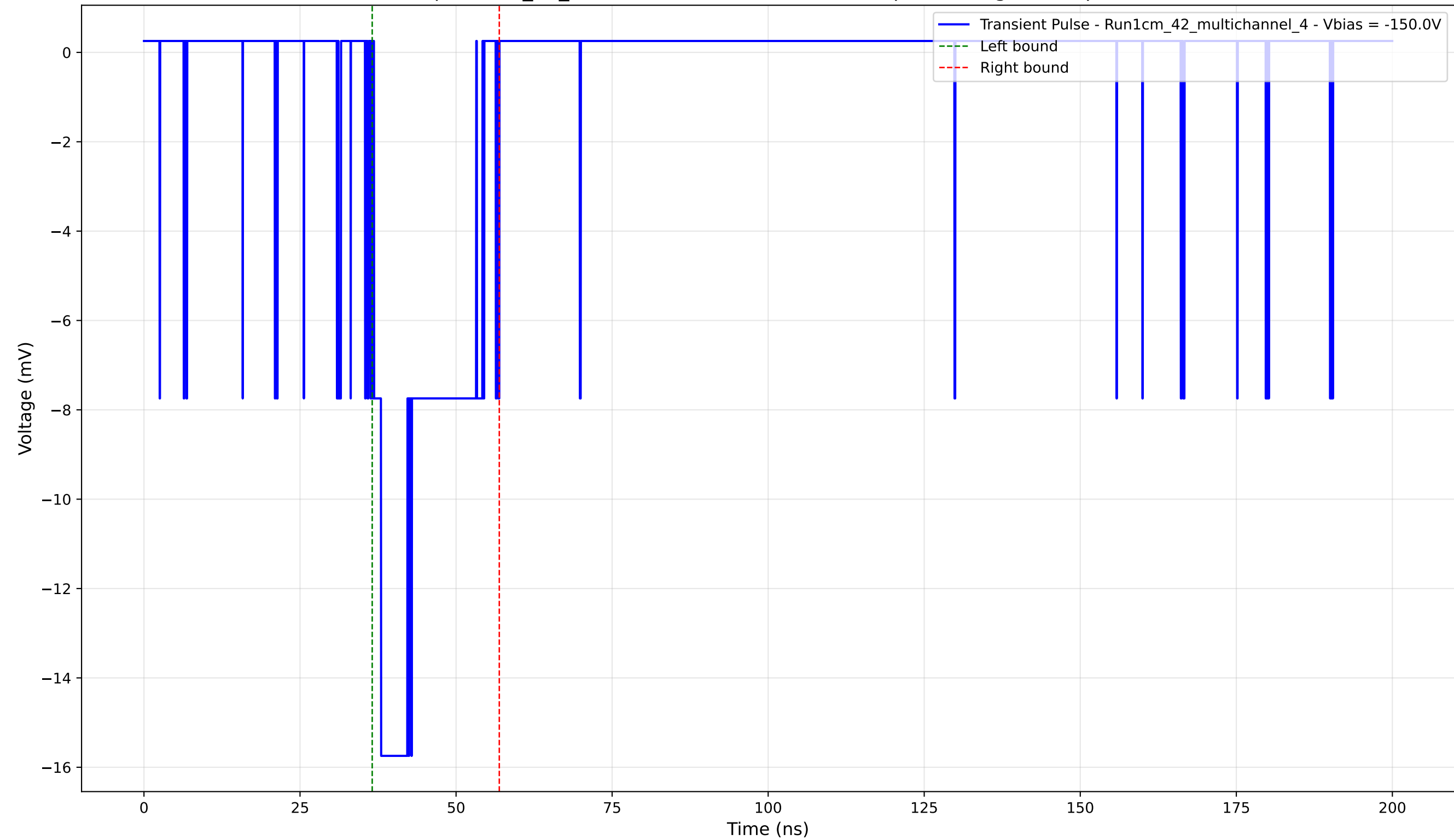
Transient Pulse - Sample: 1cm_42_multichannel - Position: 3830.0 \mu\text{m} - Charge: 3.45 pC - Rise Time: 1.14 ns
