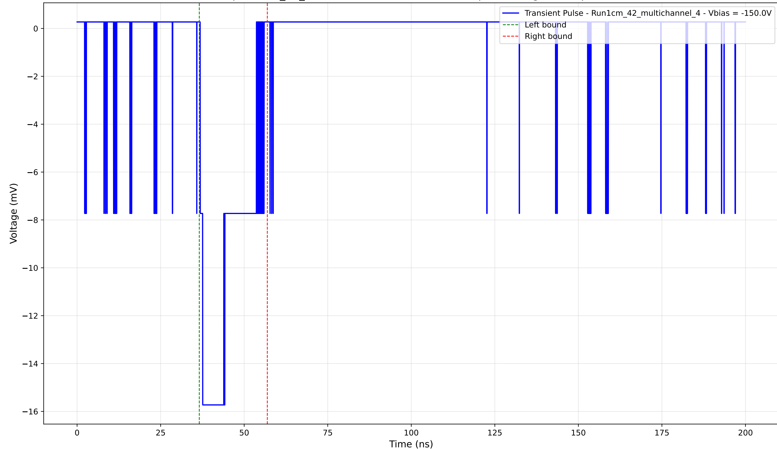
Transient Pulse - Sample: 1cm_42_multichannel - Position: 3745.0 \mu\text{m} - Charge: 3.81 pC - Rise Time: 0.76 ns
