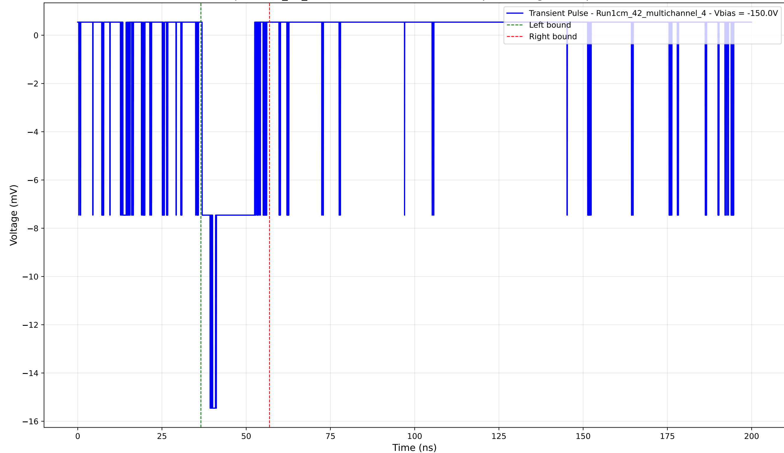
Transient Pulse - Sample: 1cm_42_multichannel - Position: 4810.0 \mu\text{m} - Charge: 2.67 pC - Rise Time: 2.38 ns
