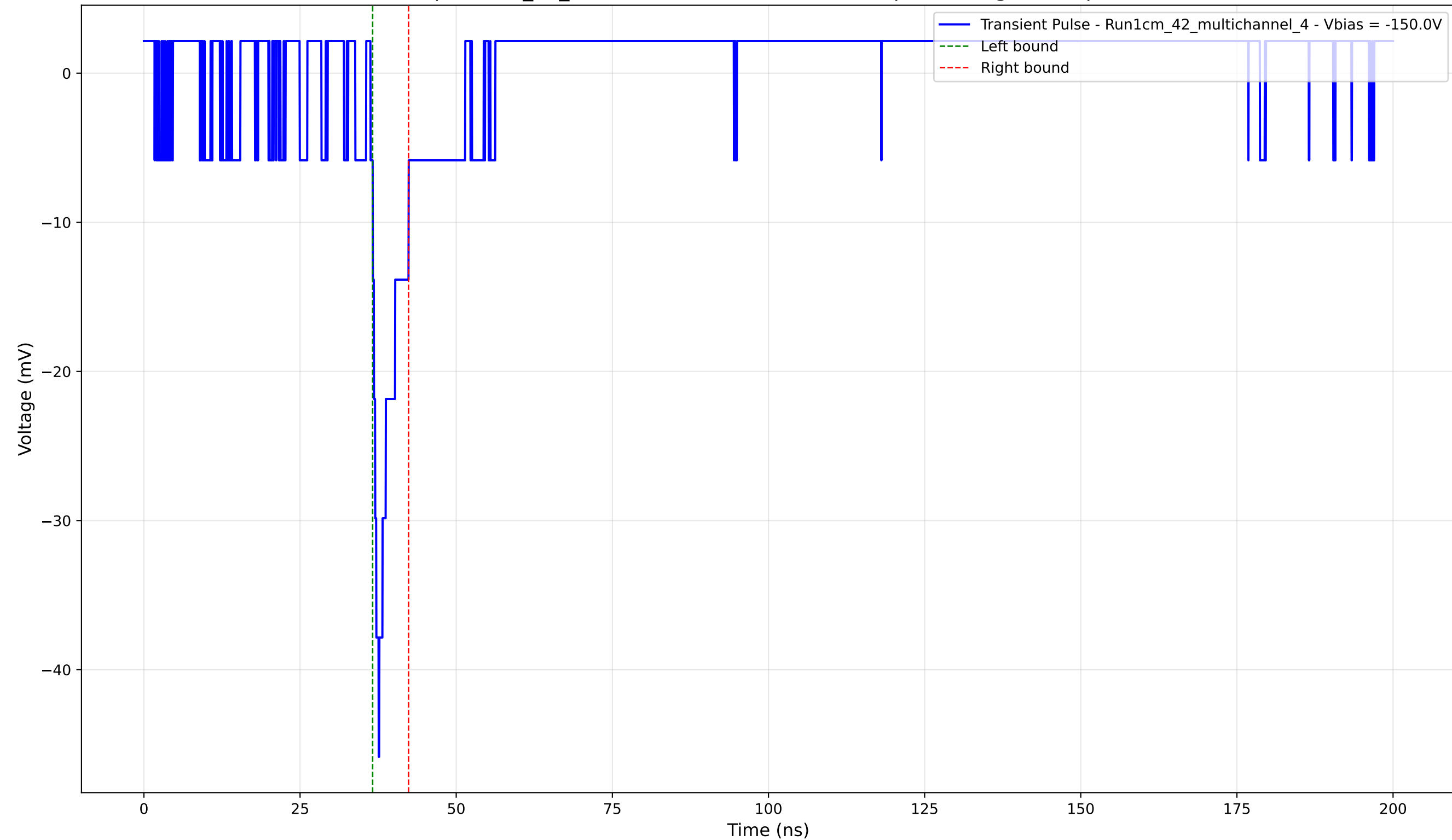
Transient Pulse - Sample: 1cm_42_multichannel - Position: 1795.0 \mu\text{m} - Charge: 2.58 pC - Rise Time: 1.31 ns
