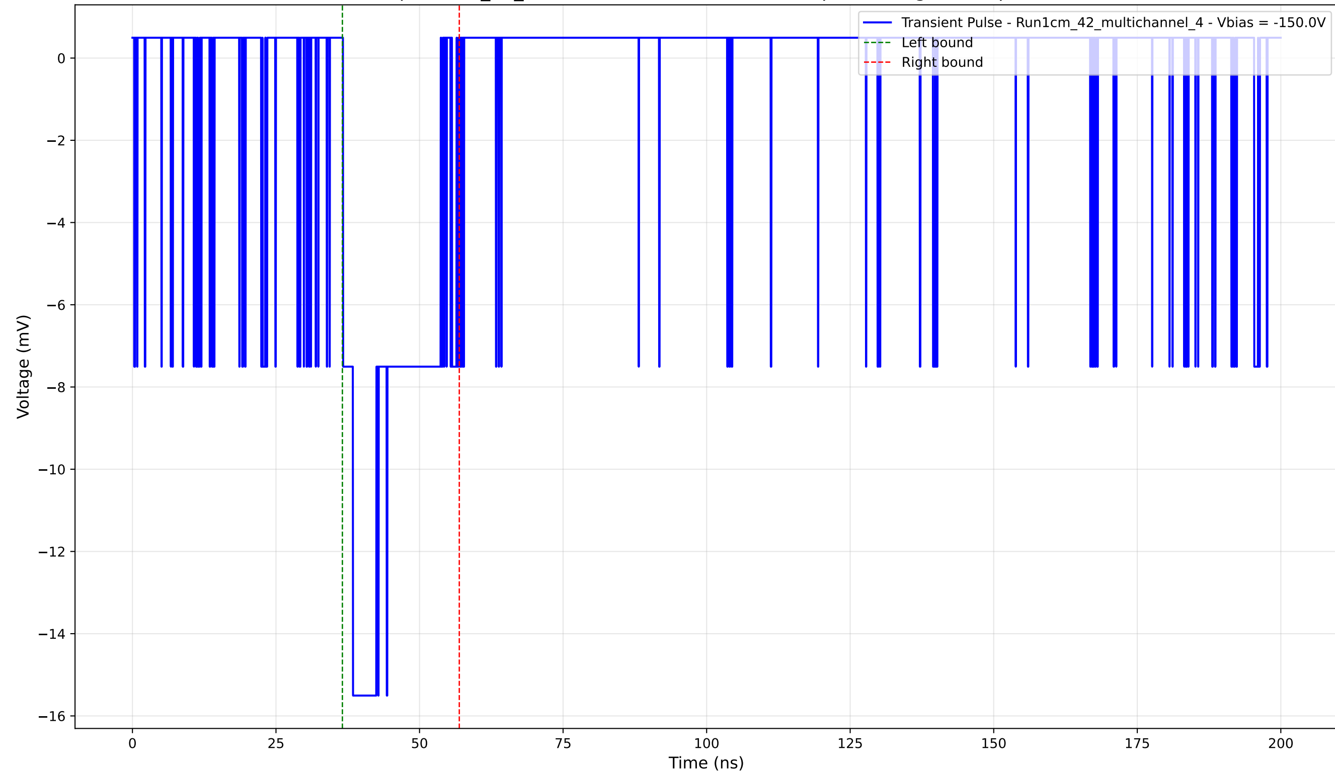
Transient Pulse - Sample: 1cm_42_multichannel - Position: 4570.0 \mu\text{m} - Charge: 3.46 pC - Rise Time: 1.74 ns
