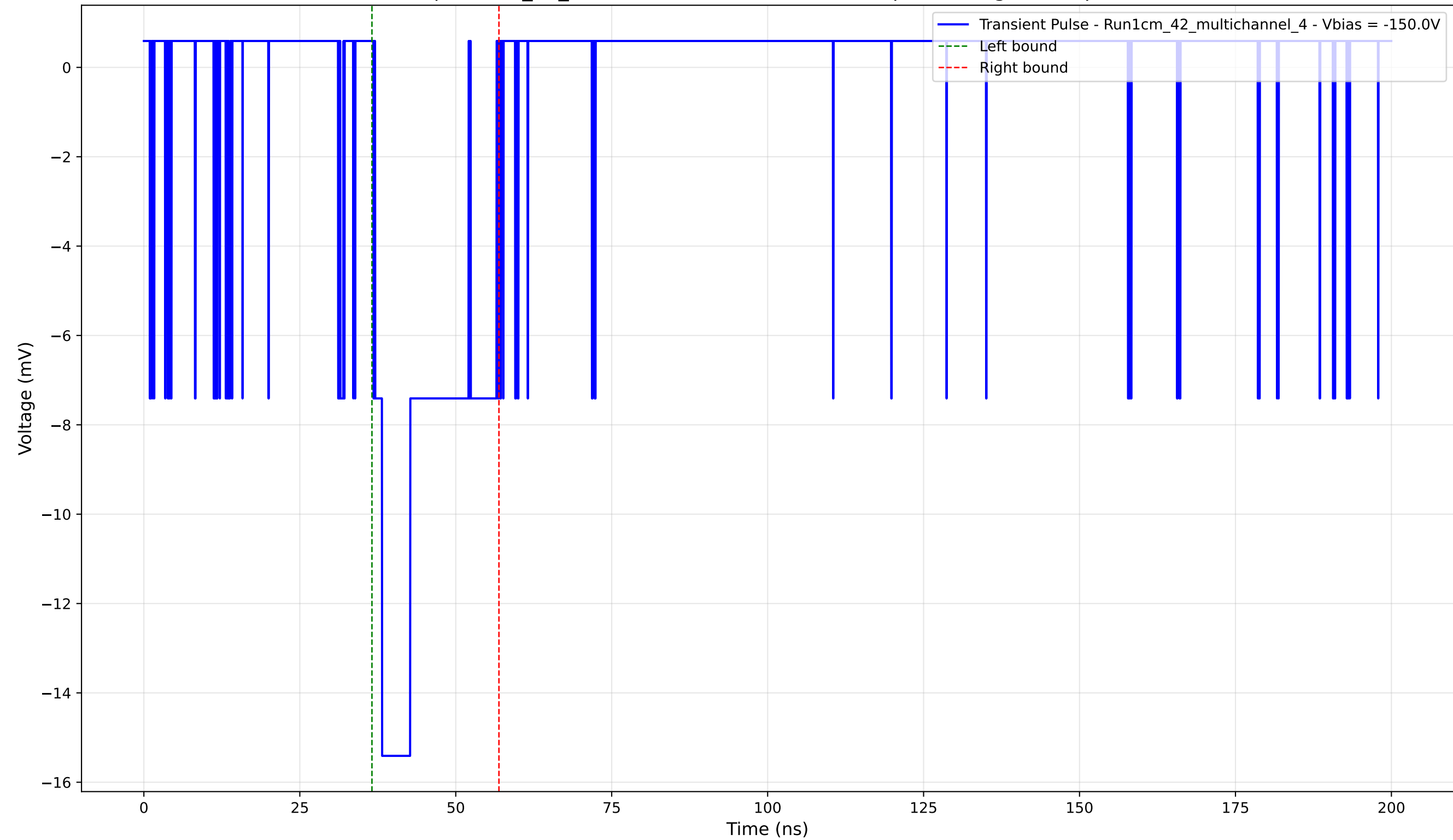
Transient Pulse - Sample: 1cm_42_multichannel - Position: 4135.0 \mu\text{m} - Charge: 3.62 pC - Rise Time: 1.12 ns
