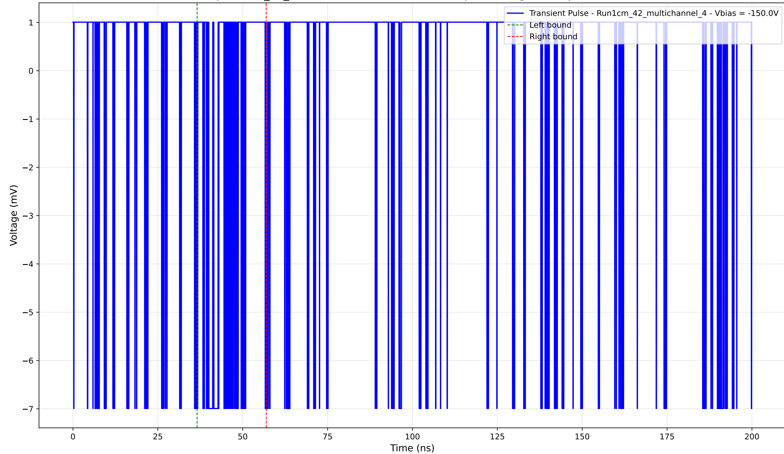
Transient Pulse - Sample: 1cm_42_multichannel - Position: 3895.0 \mu\text{m} - Charge: 0.51 pC - Rise Time: 0.00 ns (N/A)
