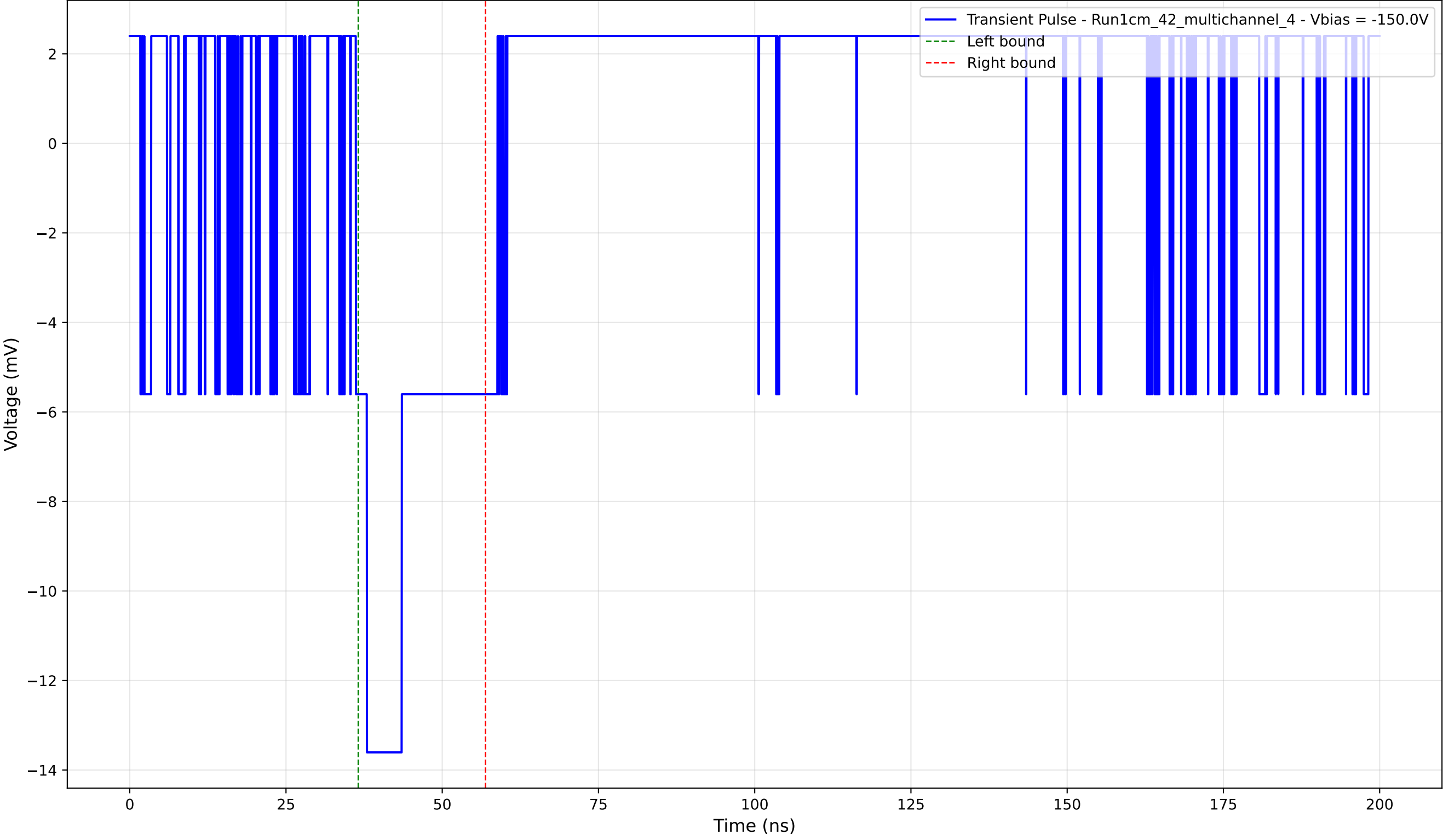
Transient Pulse - Sample: 1cm_42_multichannel - Position: 600.0 \mu\text{m} - Charge: 3.17 pC - Rise Time: 0.00 ns (N/A)
