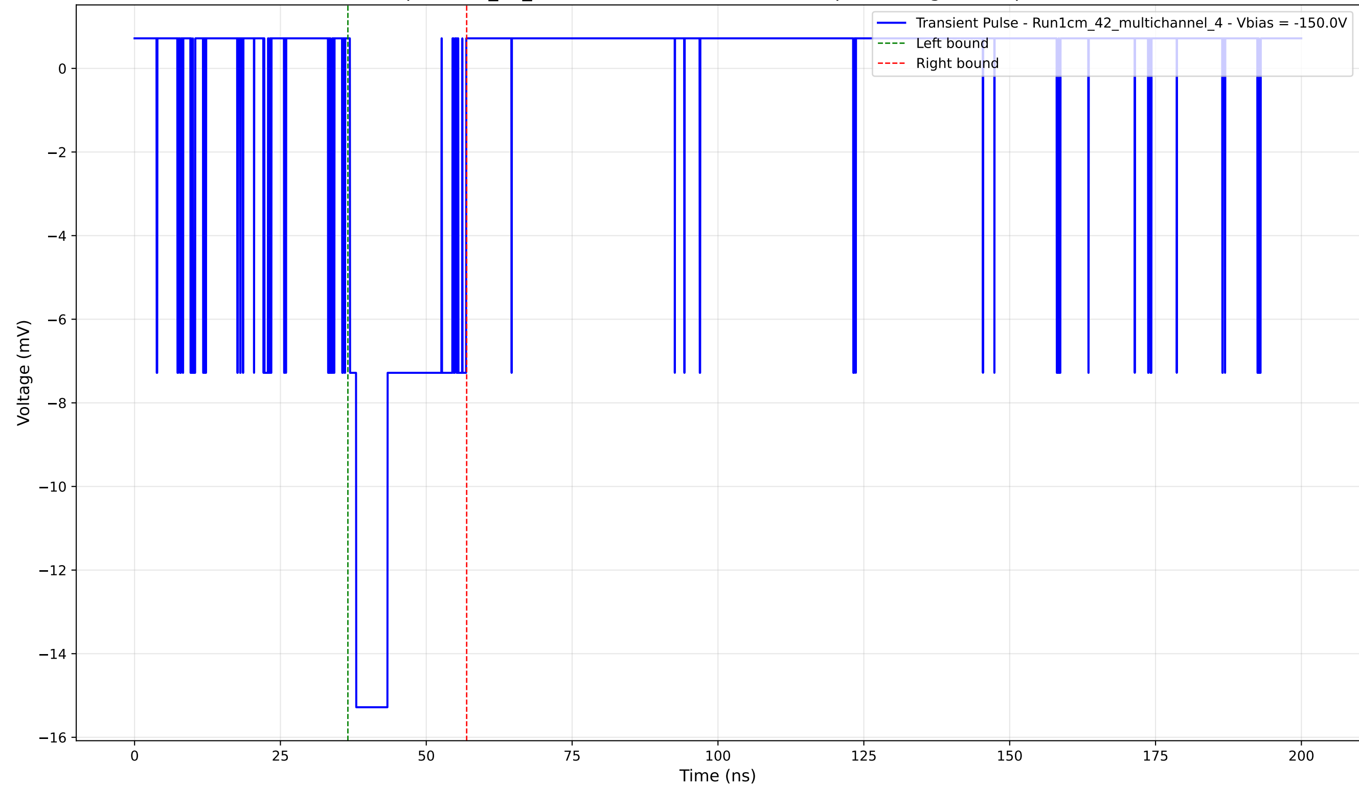
Transient Pulse - Sample: 1cm_42_multichannel - Position: 4075.0 \mu\text{m} - Charge: 3.64 pC - Rise Time: 1.08 ns
