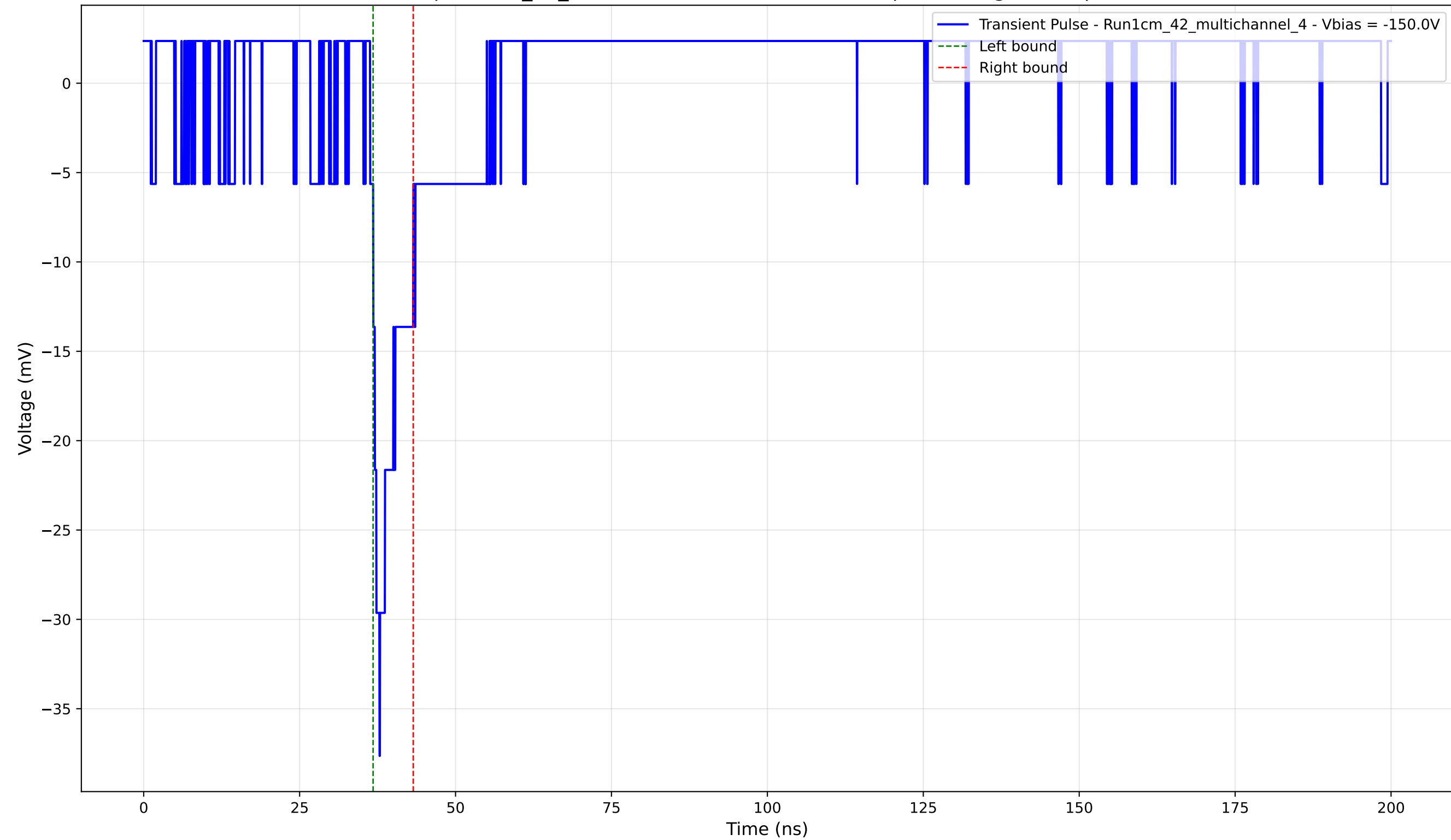
Transient Pulse - Sample: 1cm_42_multichannel - Position: 1625.0 \mu\text{m} - Charge: 2.50 pC - Rise Time: 1.51 ns
