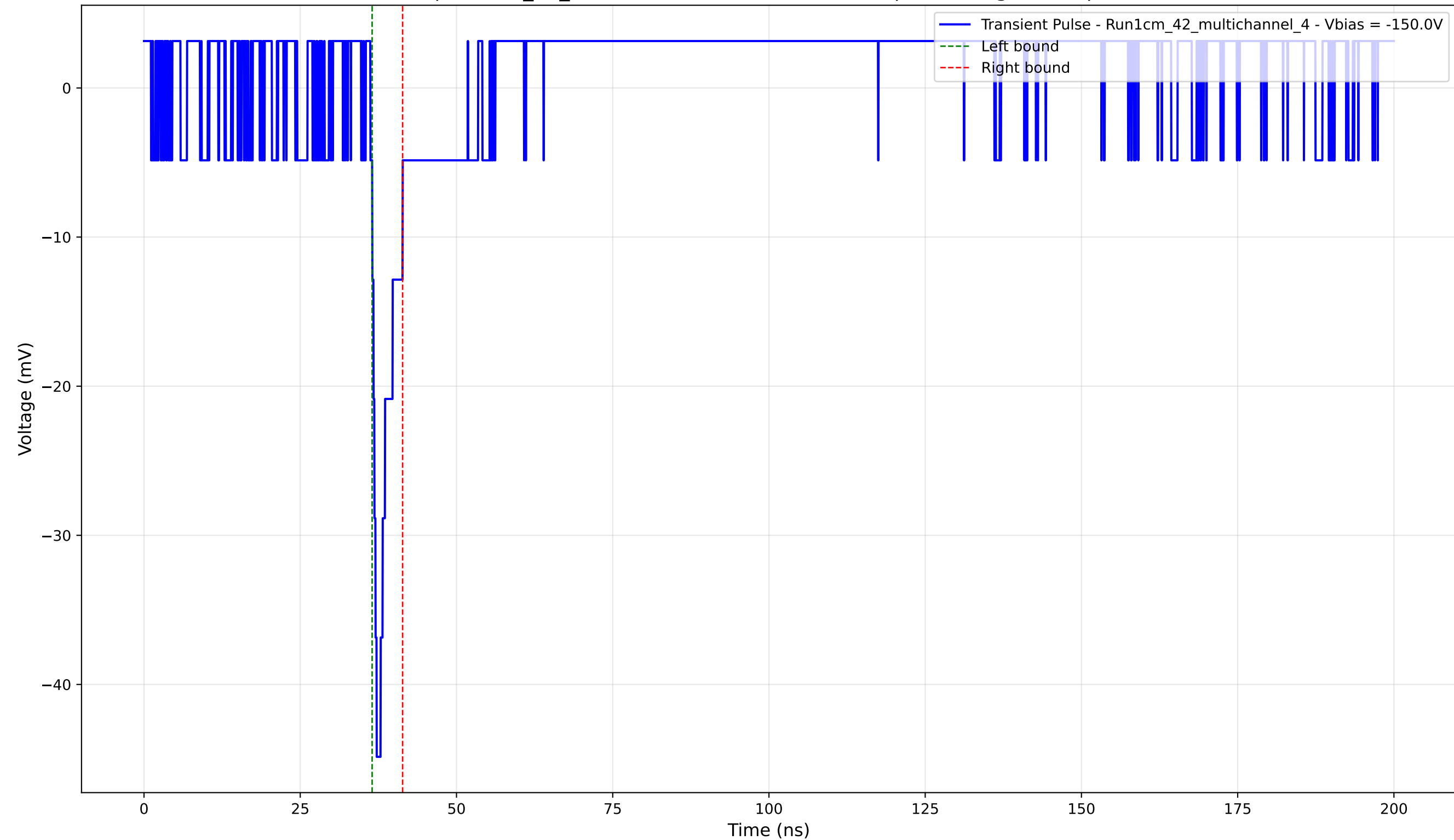
Transient Pulse - Sample: 1cm_42_multichannel - Position: 1950.0 \mu\text{m} - Charge: 2.30 pC - Rise Time: 1.00 ns
