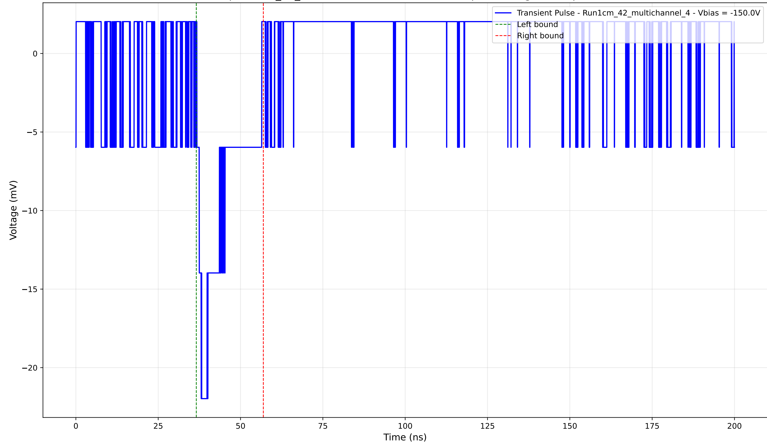
Transient Pulse - Sample: 1cm_42_multichannel - Position: 1045.0 \mu\text{m} - Charge: 3.73 pC - Rise Time: 1.32 ns
