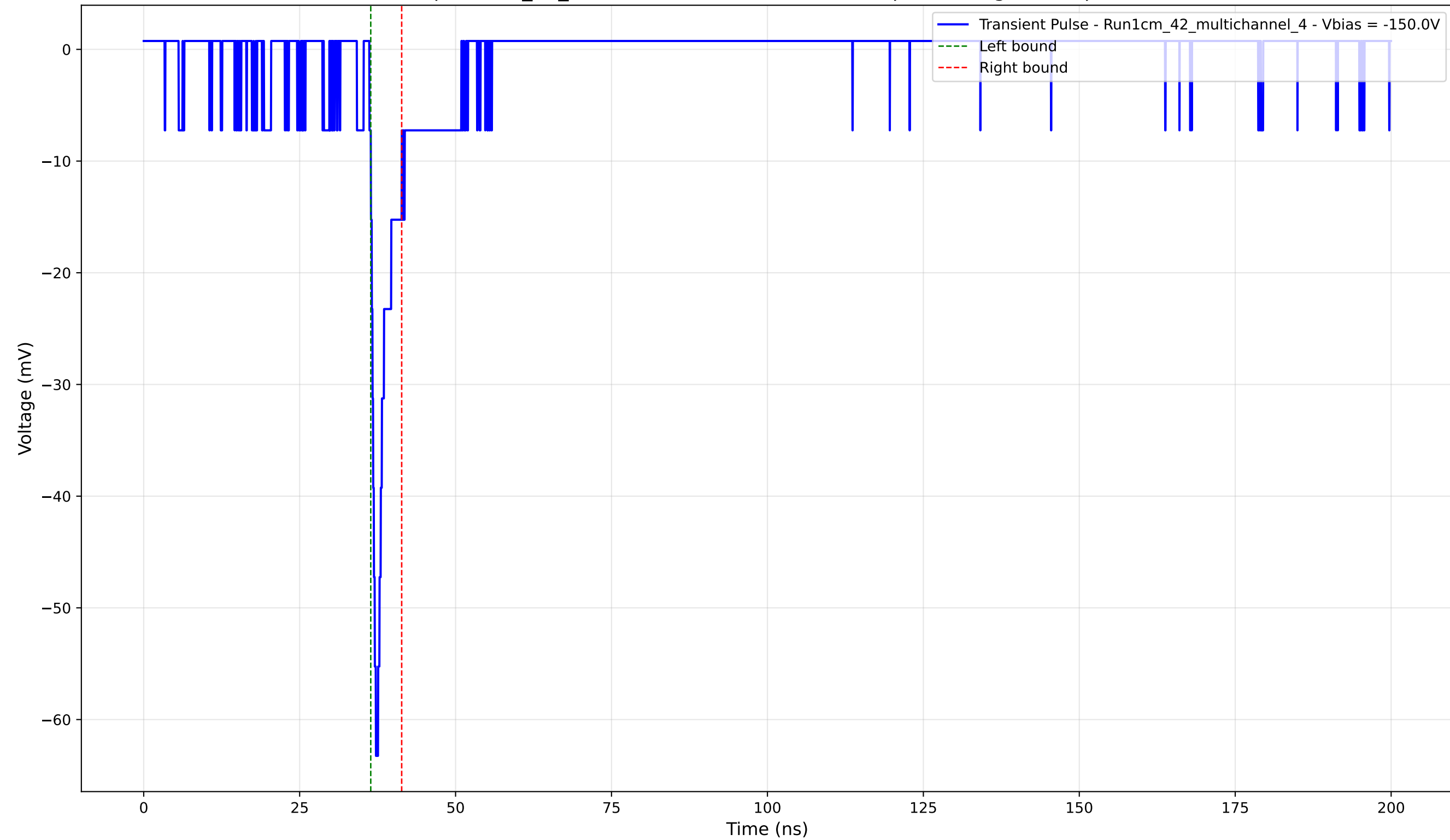
Transient Pulse - Sample: 1cm_42_multichannel - Position: 2105.0 \mu\text{m} - Charge: 2.88 pC - Rise Time: 1.04 ns
