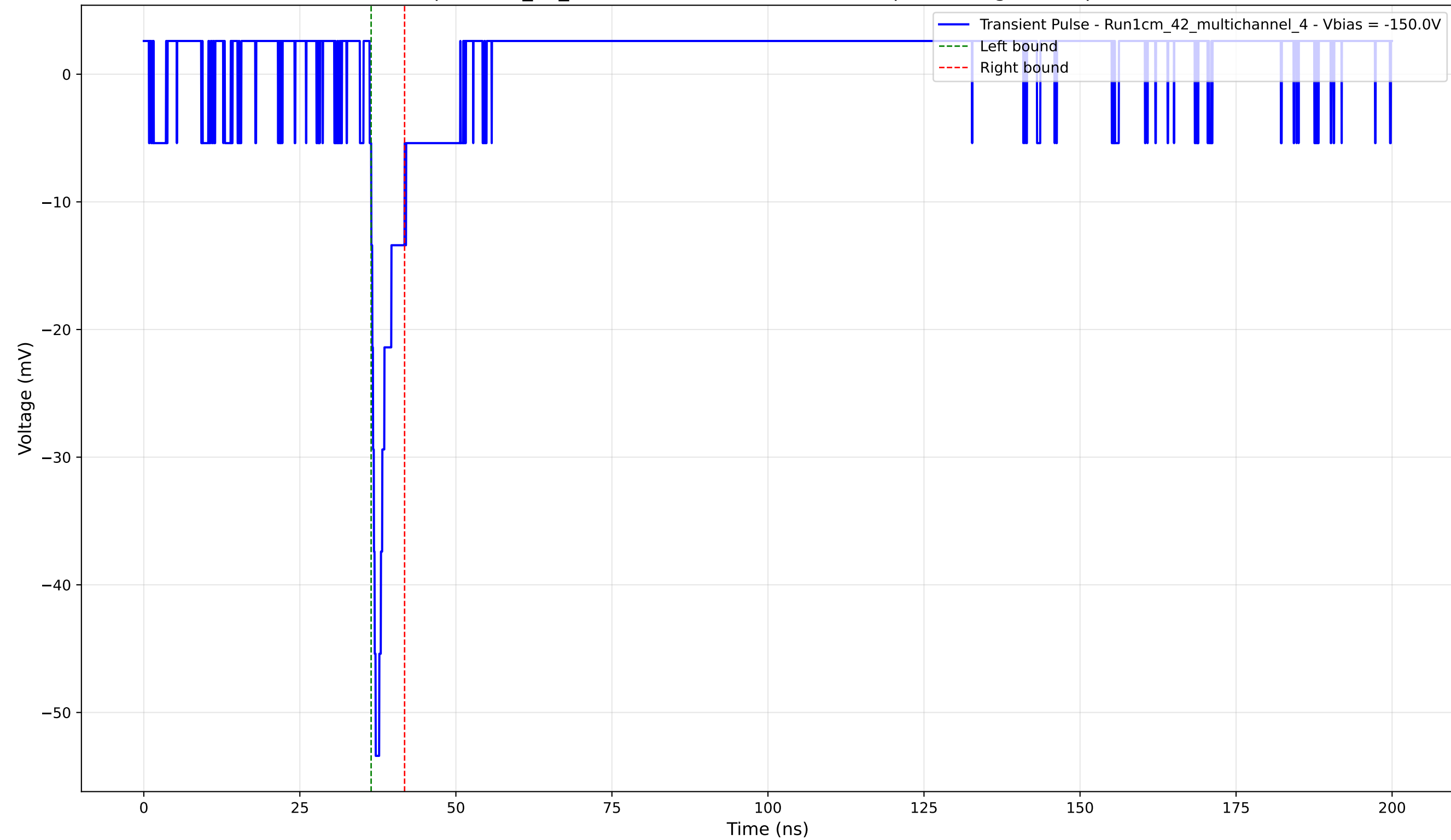
Transient Pulse - Sample: 1cm_42_multichannel - Position: 2715.0 \mu\text{m} - Charge: 2.68 pC - Rise Time: 0.96 ns
