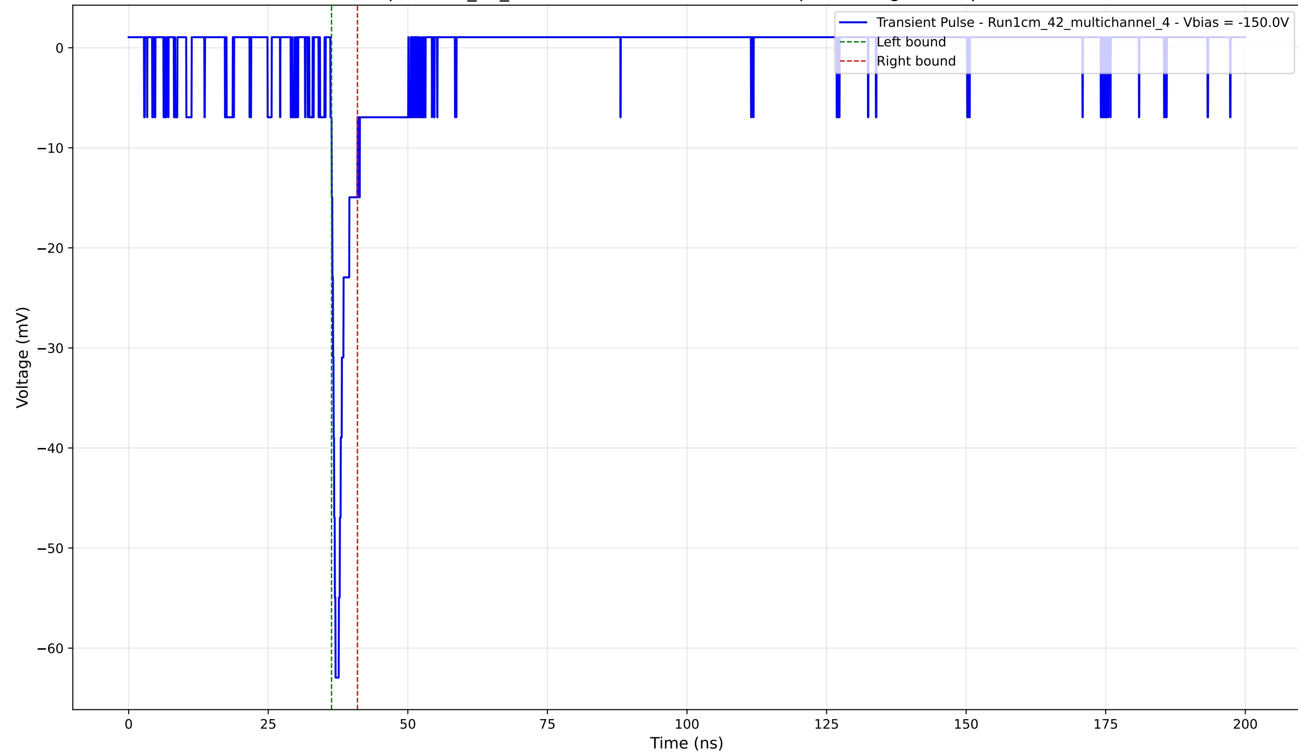
Transient Pulse - Sample: 1cm_42_multichannel - Position: 2590.0 \mu\text{m} - Charge: 2.84 pC - Rise Time: 0.90 ns
