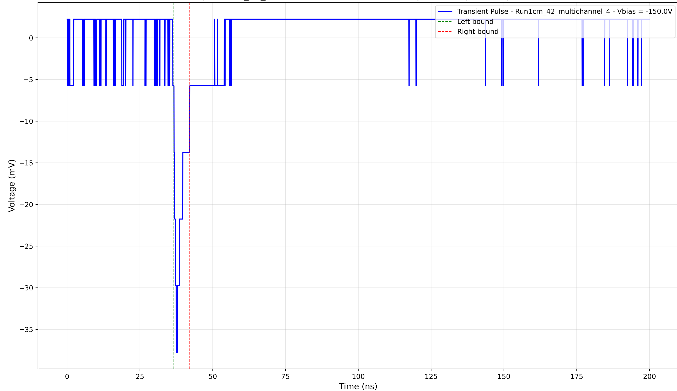
Transient Pulse - Sample: 1cm_42_multichannel - Position: 3050.0 \mu\text{m} - Charge: 2.23 pC - Rise Time: 1.19 ns
