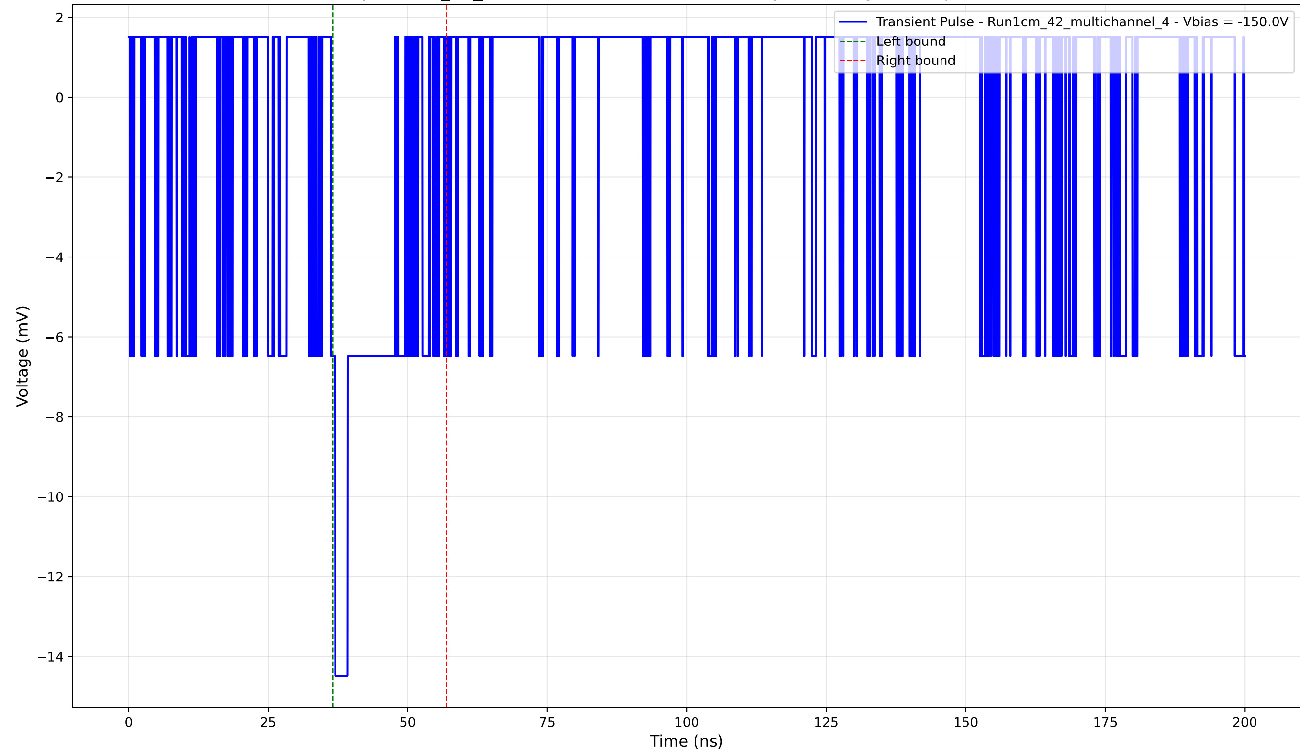
Transient Pulse - Sample: 1cm_42_multichannel - Position: 1835.0 \mu\text{m} - Charge: 2.35 pC - Rise Time: 0.00 ns (N/A)
