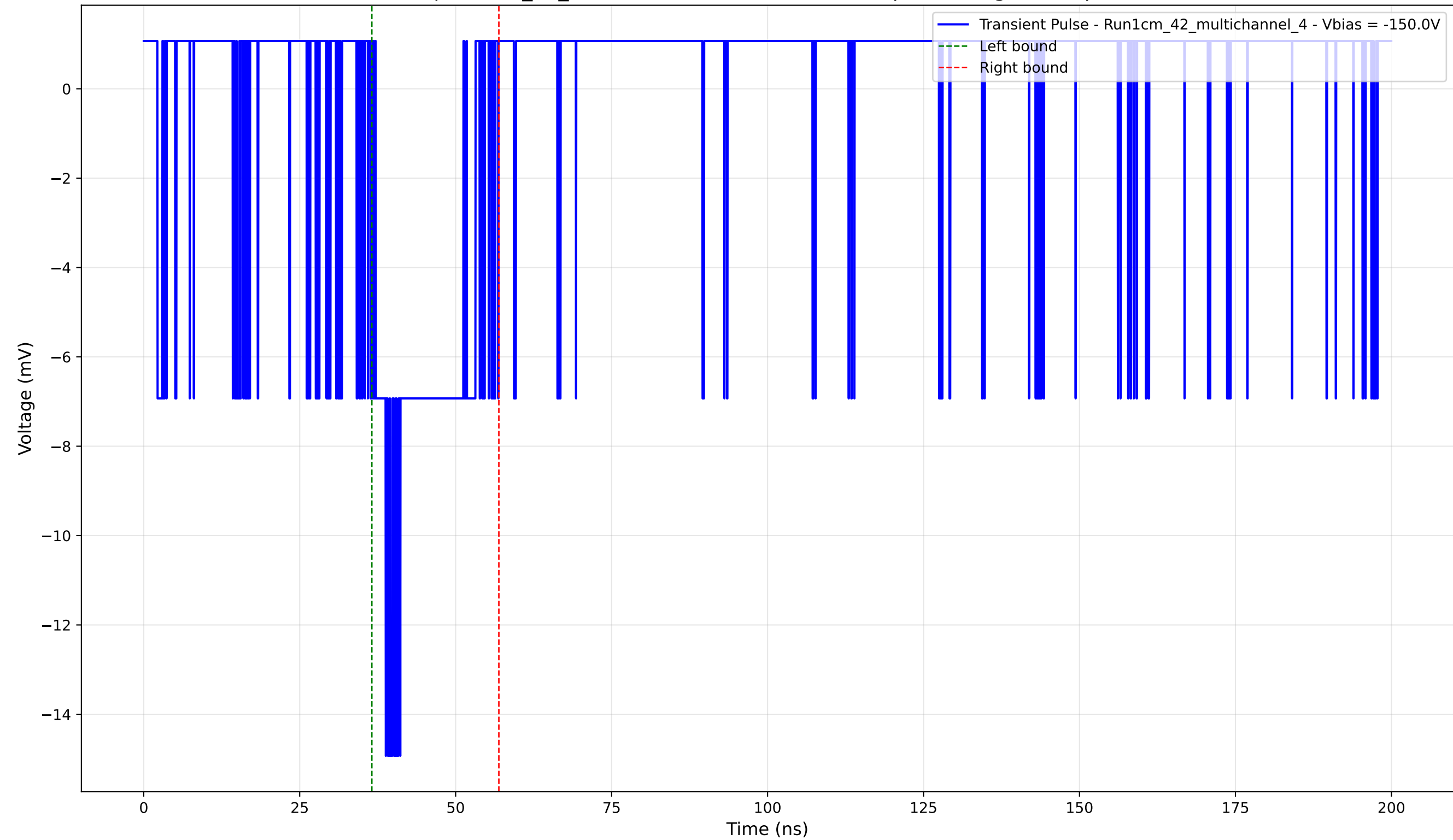
Transient Pulse - Sample: 1cm_42_multichannel - Position: 4460.0 \mu\text{m} - Charge: 2.47 pC - Rise Time: 1.60 ns
