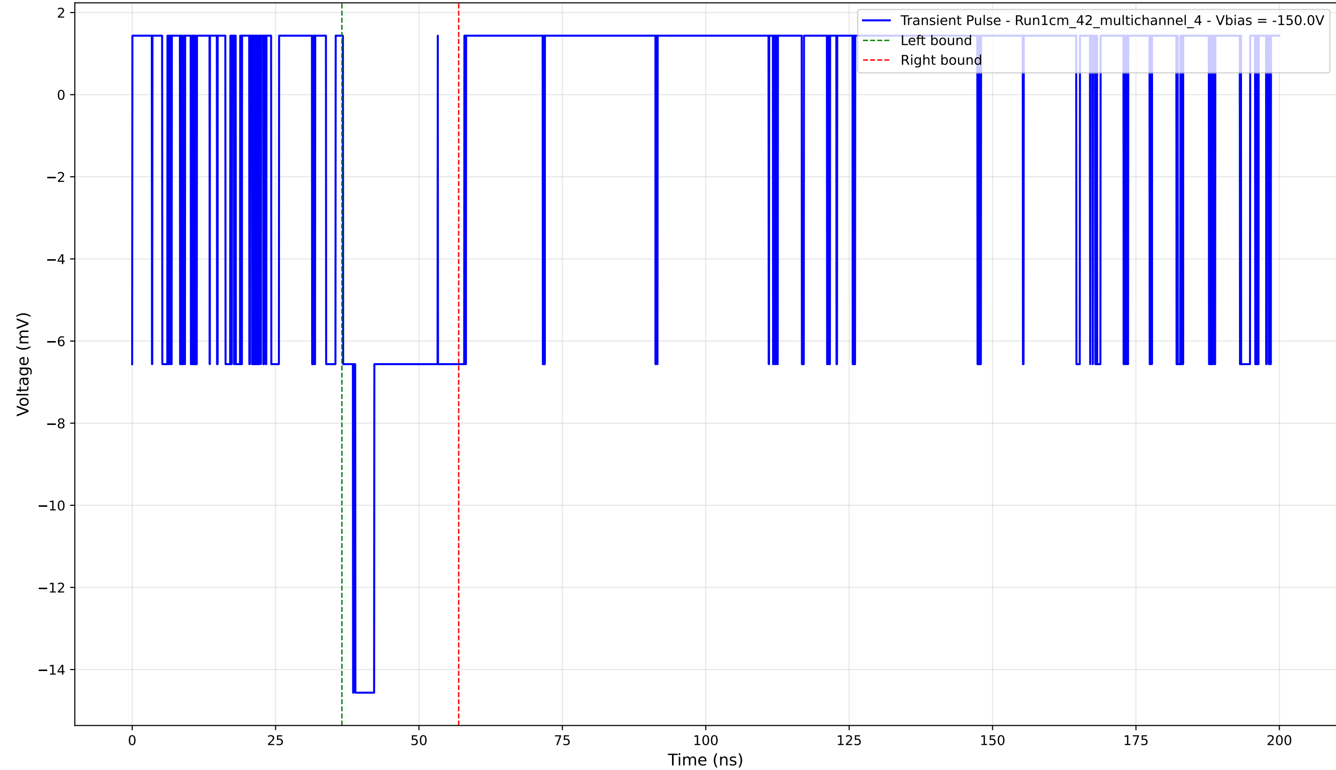
Transient Pulse - Sample: 1cm_42_multichannel - Position: 430.0 \mu\text{m} - Charge: 3.18 pC - Rise Time: 1.76 ns
