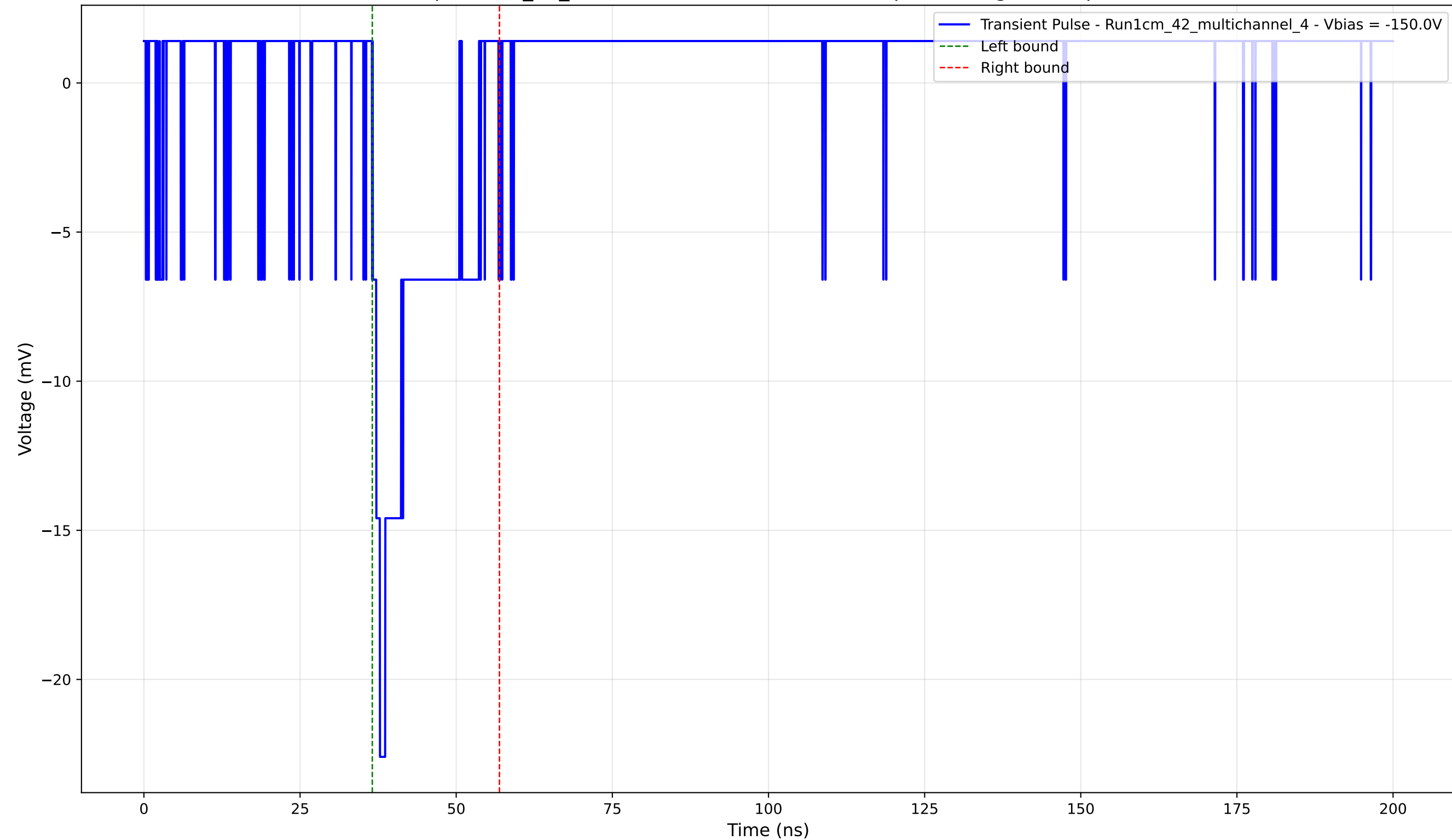
Transient Pulse - Sample: 1cm_42_multichannel - Position: 3335.0 \mu\text{m} - Charge: 2.95 pC - Rise Time: 1.16 ns
