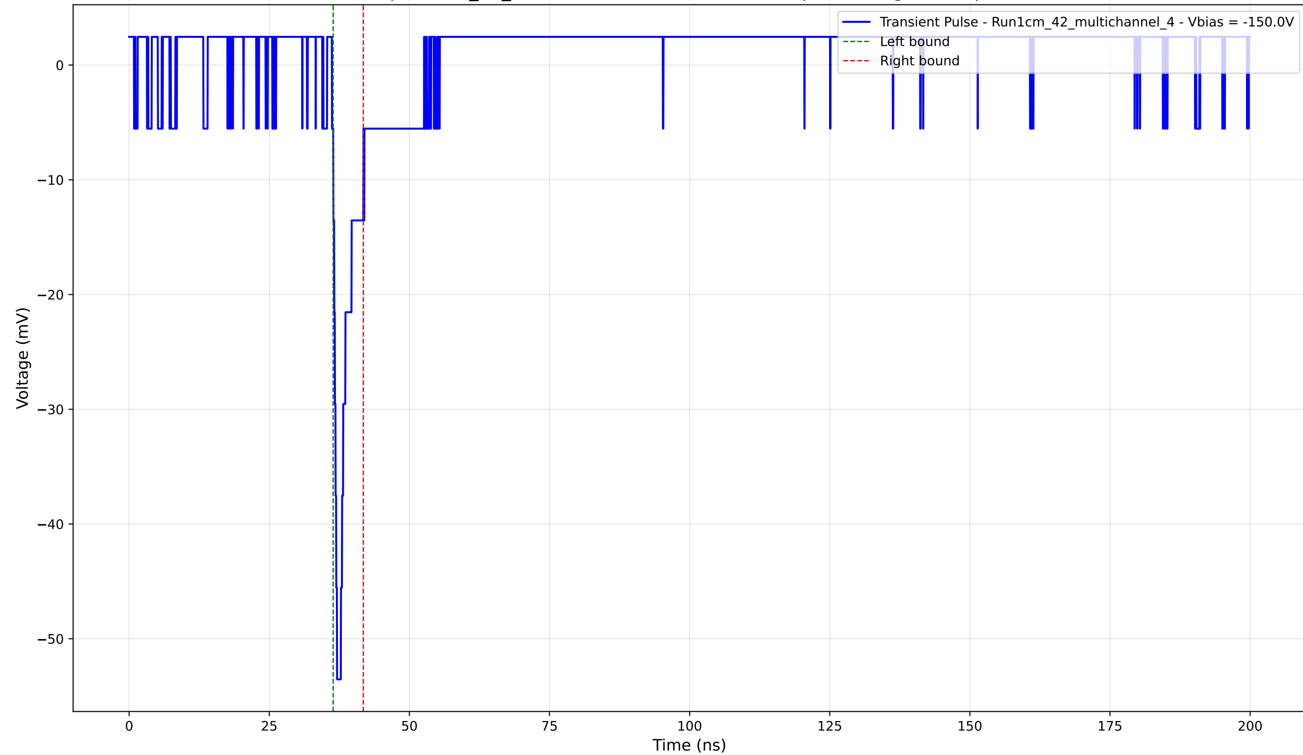
Transient Pulse - Sample: 1cm_42_multichannel - Position: 2685.0 \mu\text{m} - Charge: 2.75 pC - Rise Time: 0.90 ns
