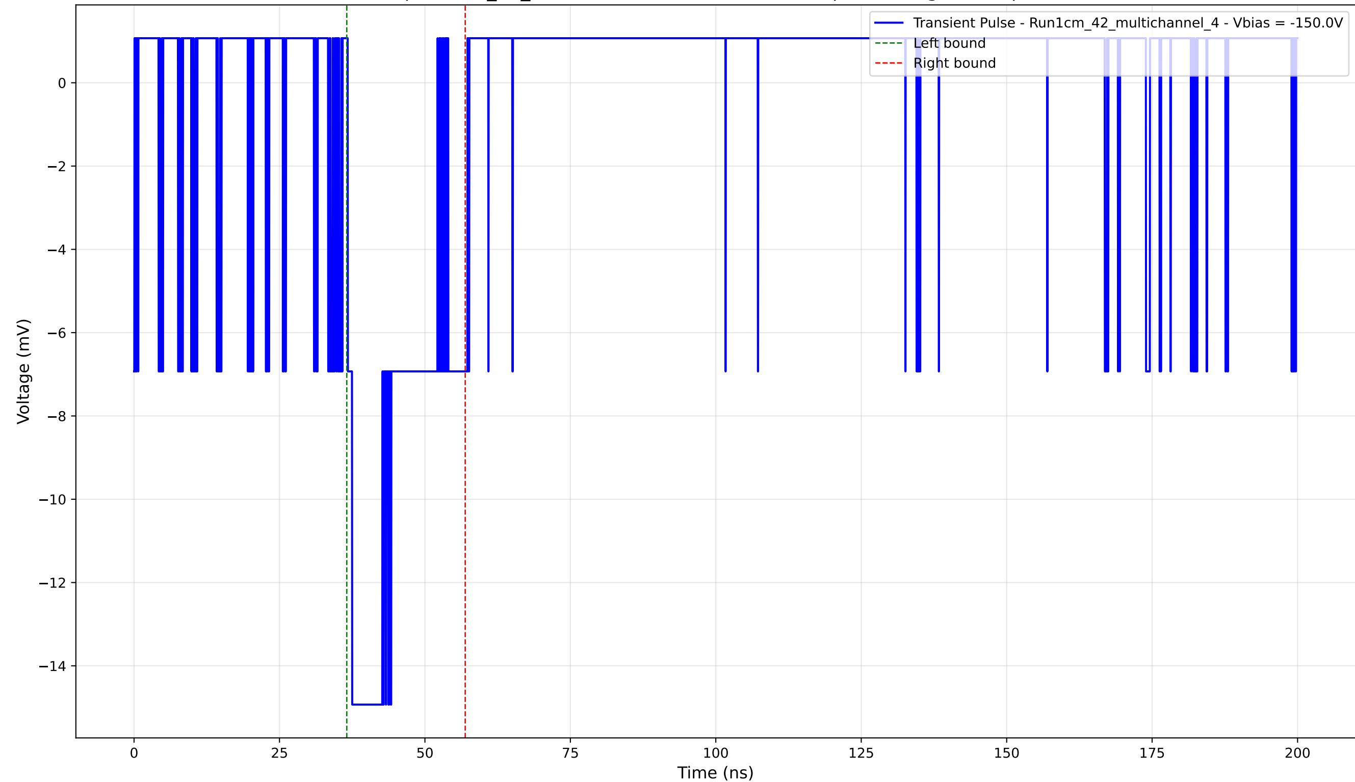
Transient Pulse - Sample: 1cm_42_multichannel - Position: 3655.0 \mu\text{m} - Charge: 3.59 pC - Rise Time: 0.76 ns
