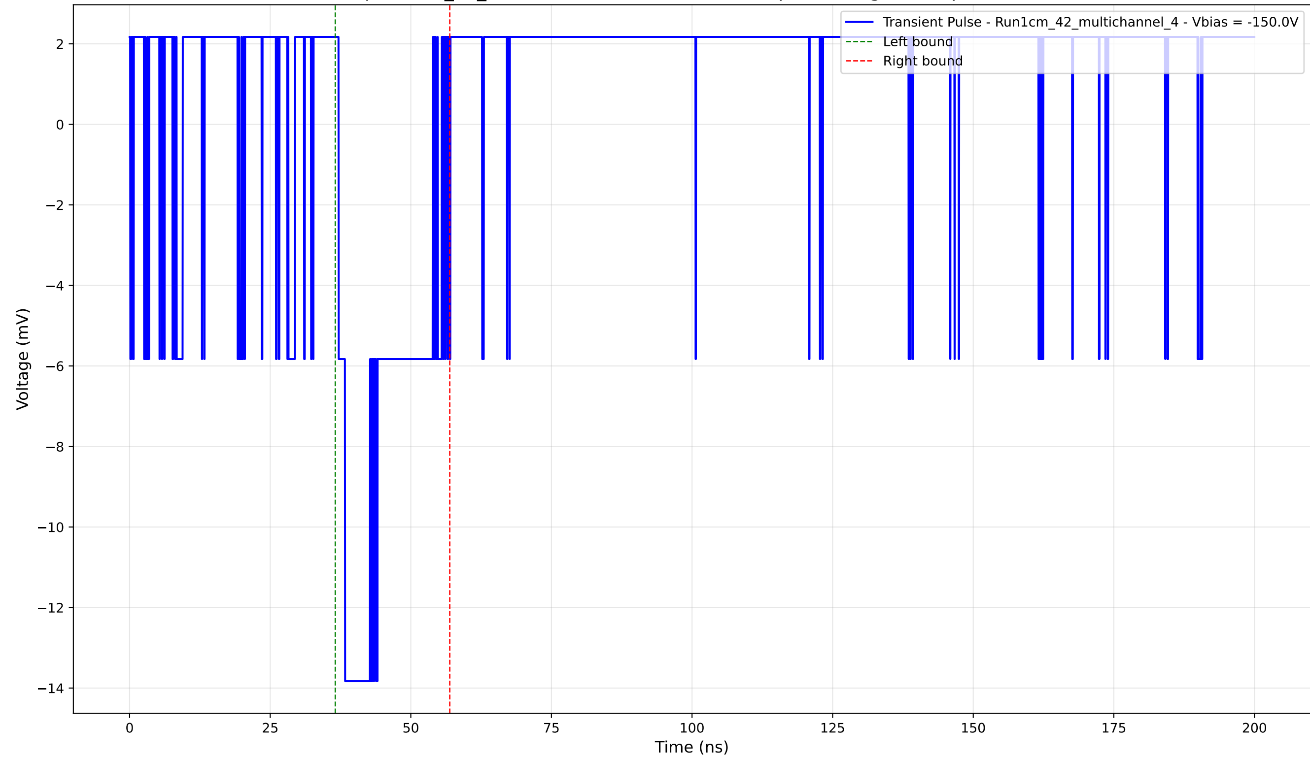
Transient Pulse - Sample: 1cm_42_multichannel - Position: 4295.0 \mu\text{m} - Charge: 2.87 pC - Rise Time: 0.00 ns (N/A)
