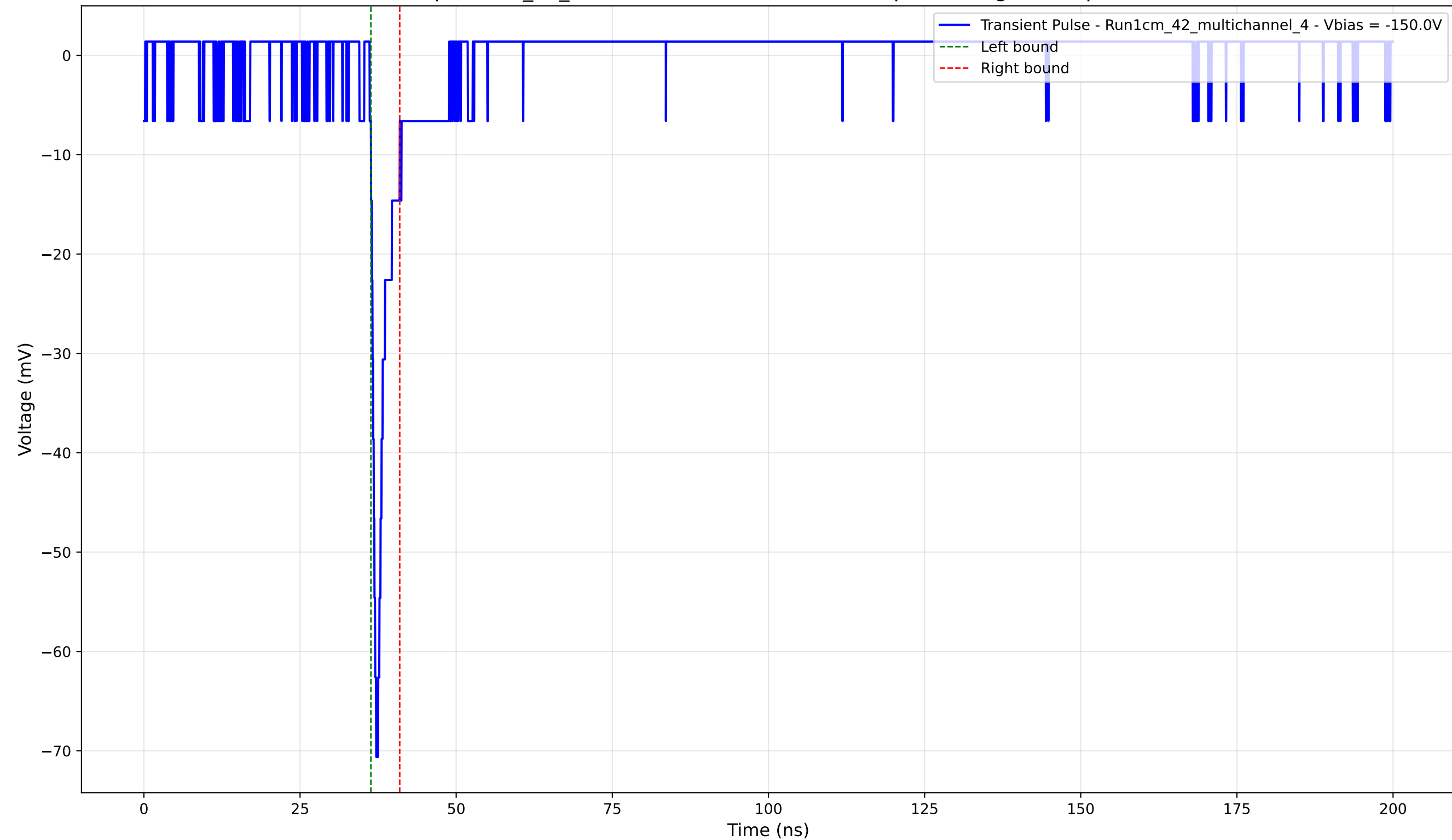
Transient Pulse - Sample: 1cm_42_multichannel - Position: 2175.0 \mu\text{m} - Charge: 2.94 pC - Rise Time: 0.84 ns
