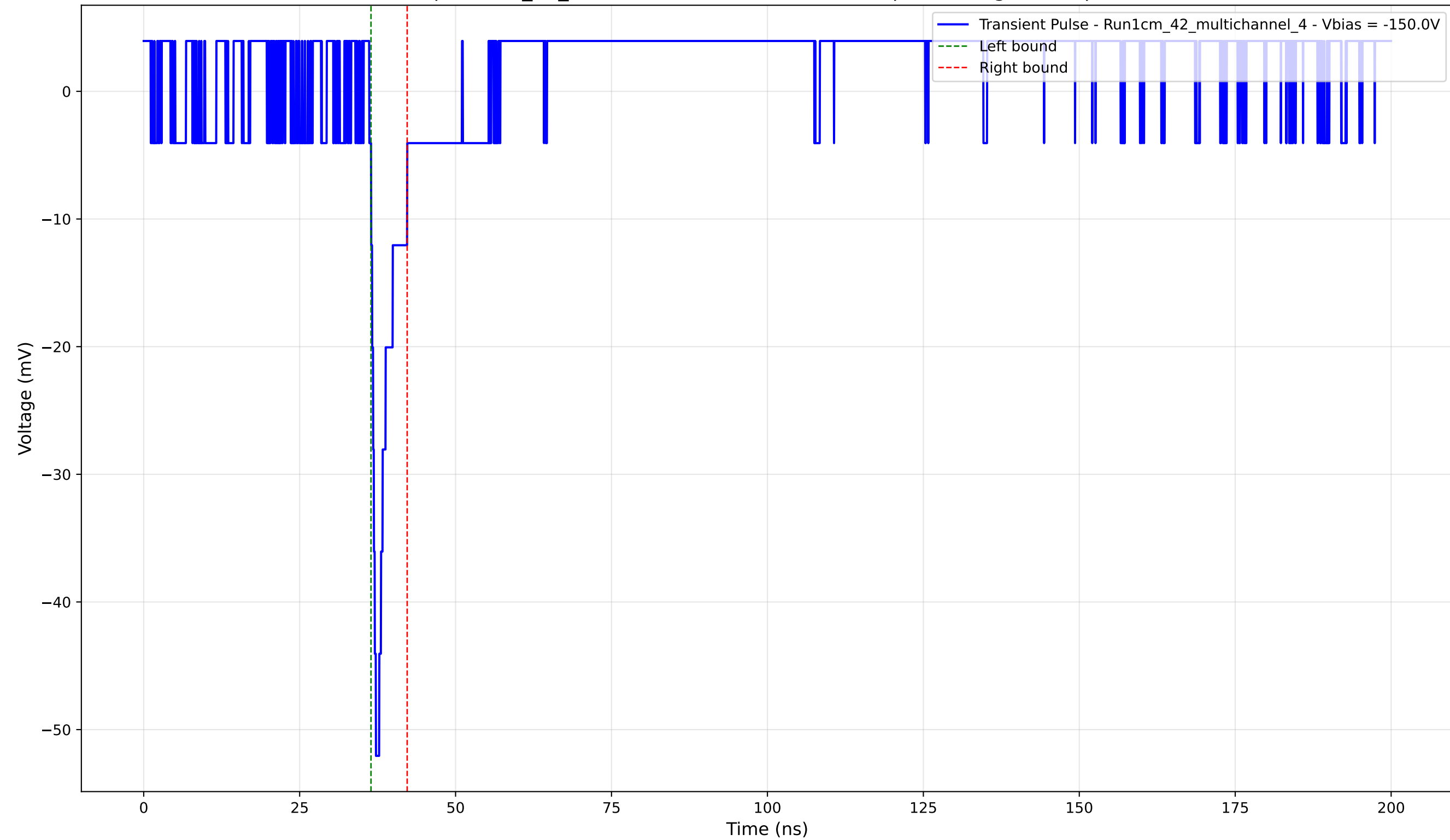
Transient Pulse - Sample: 1cm_42_multichannel - Position: 1990.0 \mu\text{m} - Charge: 2.71 pC - Rise Time: 0.78 ns
