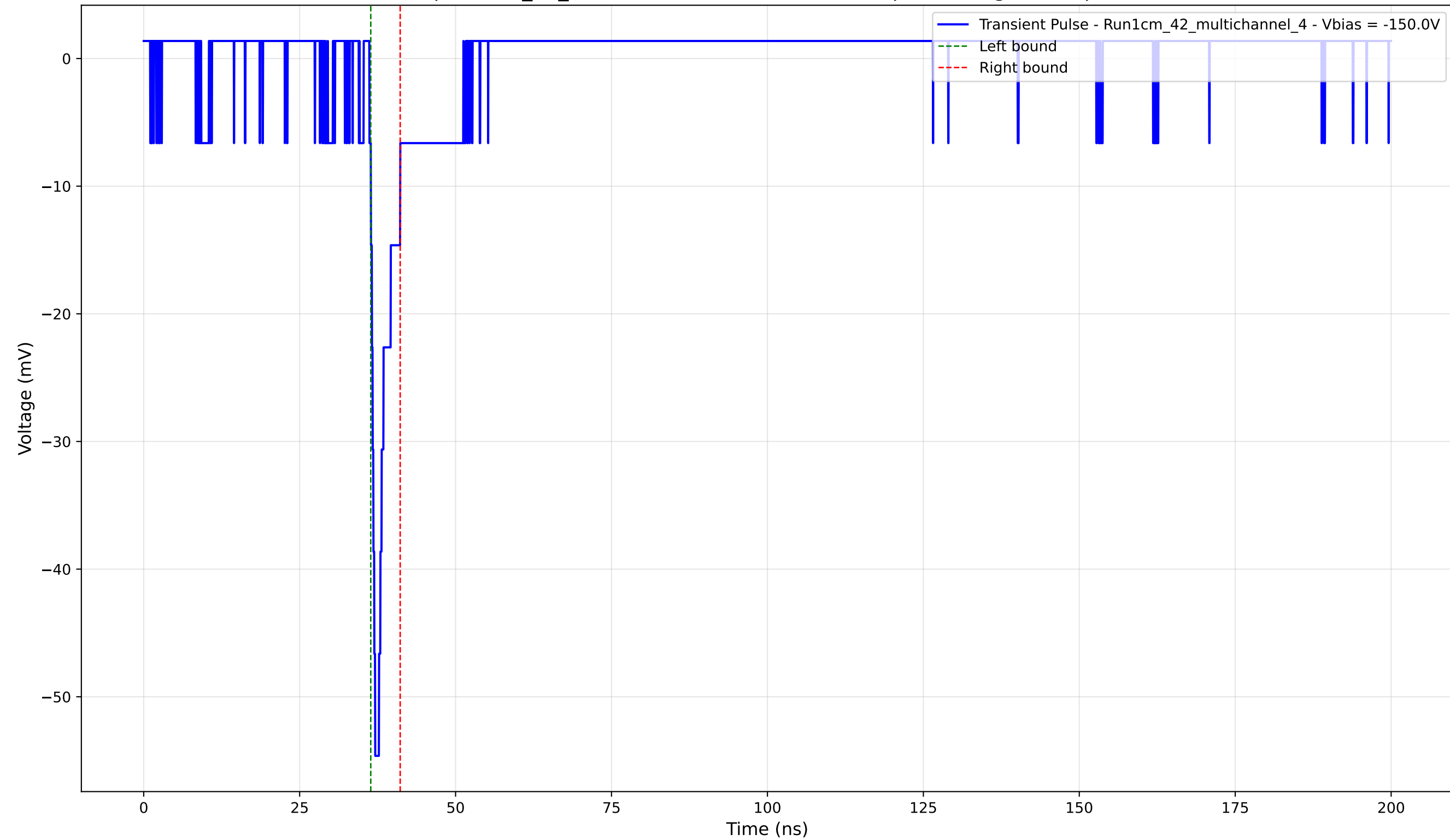
Transient Pulse - Sample: 1cm_42_multichannel - Position: 2680.0 \mu\text{m} - Charge: 2.61 pC - Rise Time: 0.92 ns
