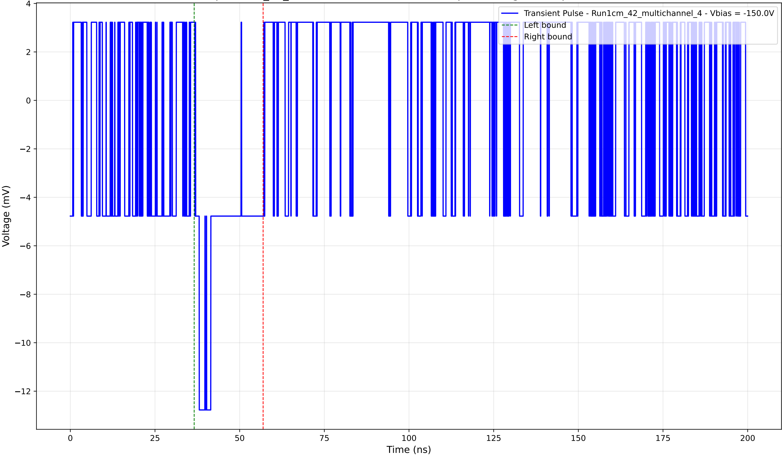
Transient Pulse - Sample: 1cm_42_multichannel - Position: 920.0 \mu\text{m} - Charge: 2.39 pC - Rise Time: 0.00 ns (N/A)
