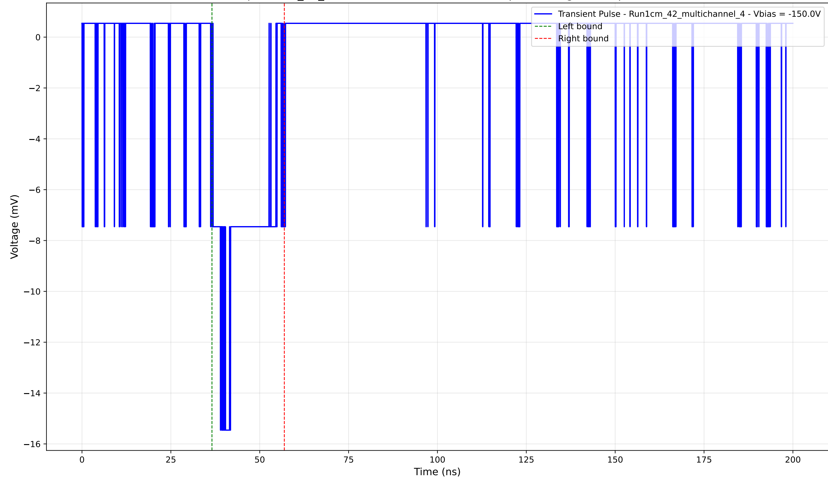
Transient Pulse - Sample: 1cm_42_multichannel - Position: 4465.0 \mu\text{m} - Charge: 3.09 pC - Rise Time: 2.08 ns
