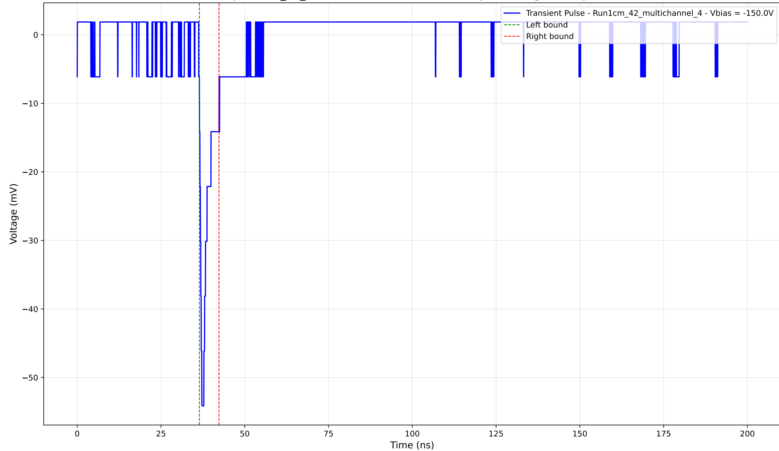
Transient Pulse - Sample: 1cm_42_multichannel - Position: 2005.0 \mu\text{m} - Charge: 2.98 pC - Rise Time: 0.94 ns
