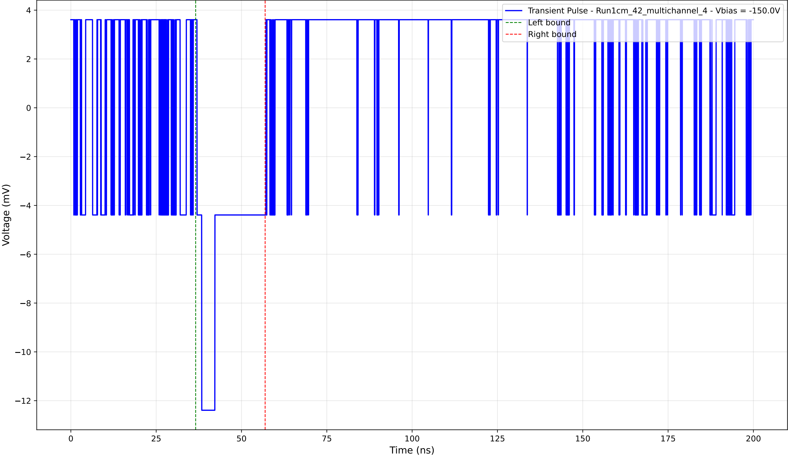
Transient Pulse - Sample: 1cm_42_multichannel - Position: 230.0 \mu\text{m} - Charge: 2.34 pC - Rise Time: 0.00 ns (N/A)
