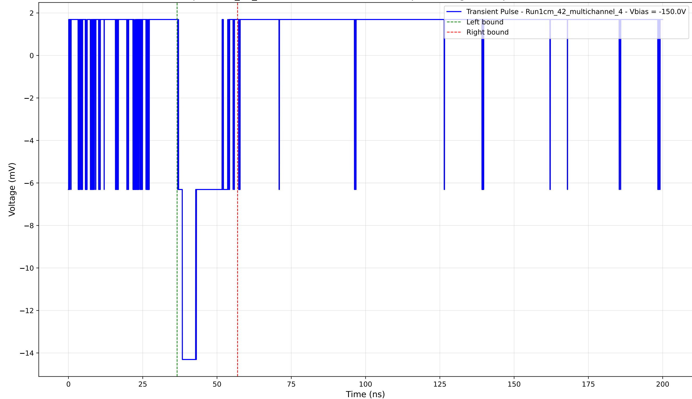
Transient Pulse - Sample: 1cm_42_multichannel - Position: 4170.0 \mu\text{m} - Charge: 2.76 pC - Rise Time: 0.00 ns (N/A)
