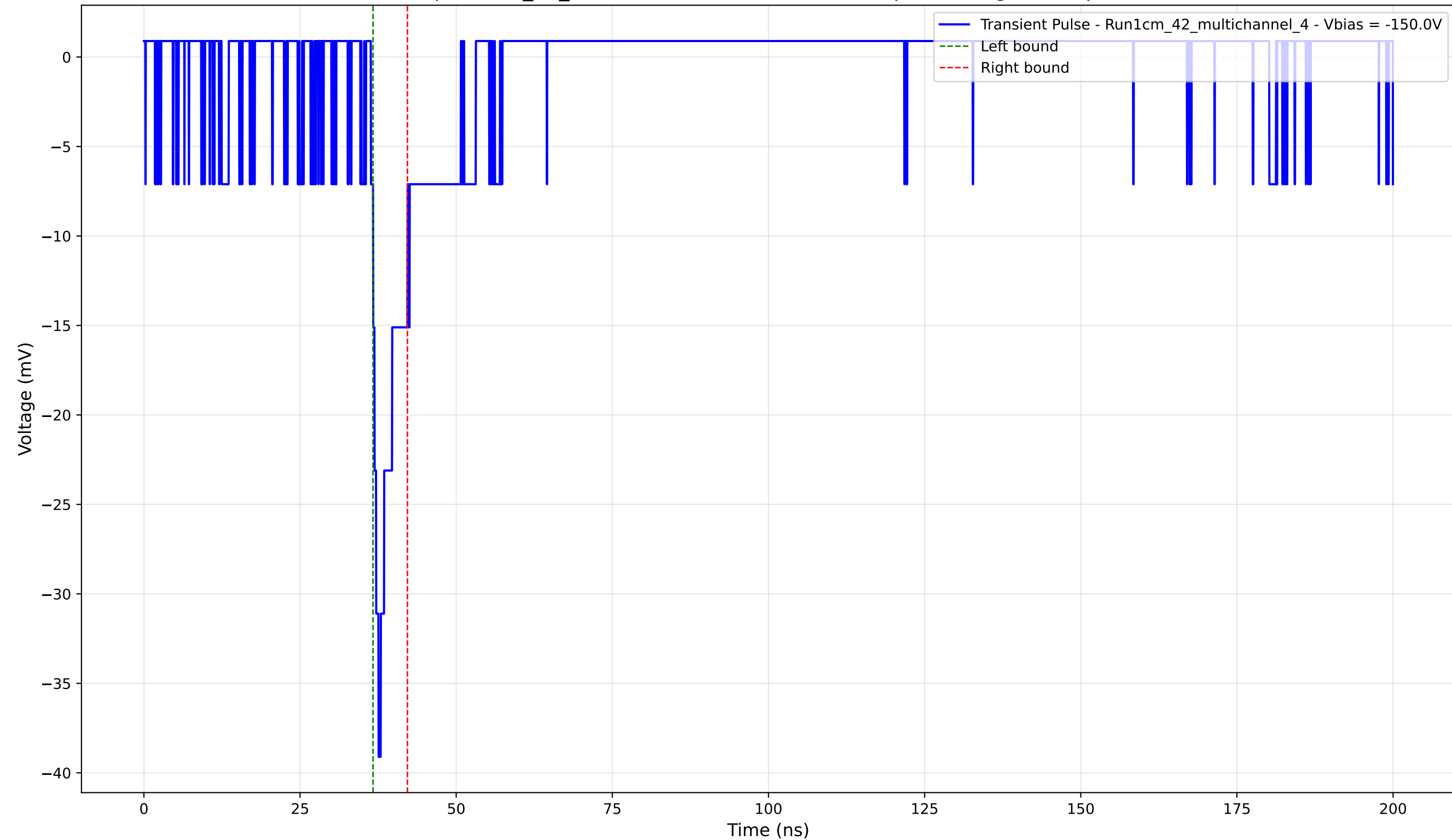
Transient Pulse - Sample: 1cm_42_multichannel - Position: 3045.0 \mu\text{m} - Charge: 2.38 pC - Rise Time: 1.23 ns
