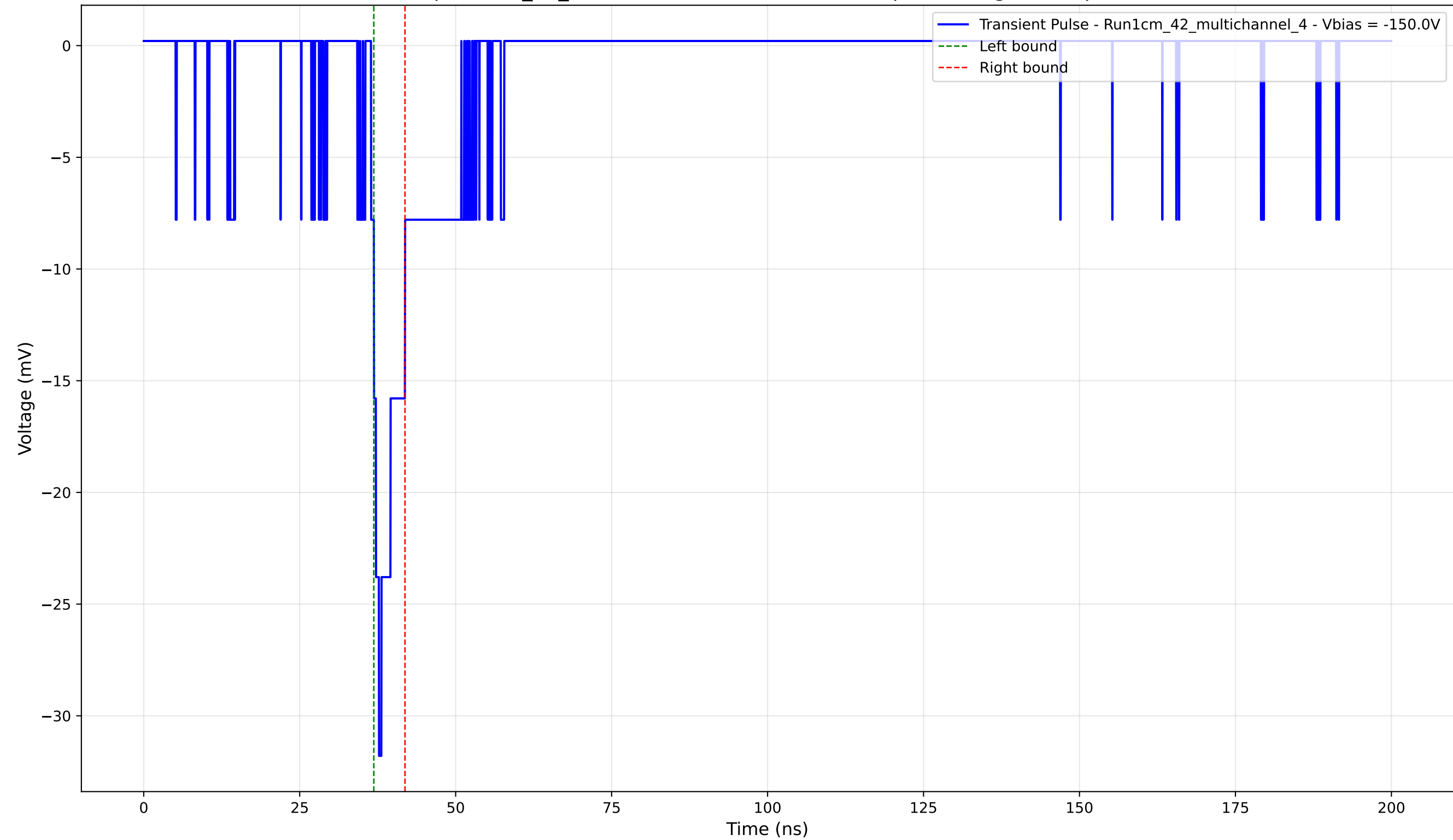
Transient Pulse - Sample: 1cm_42_multichannel - Position: 3175.0 \mu\text{m} - Charge: 2.01 pC - Rise Time: 1.27 ns
