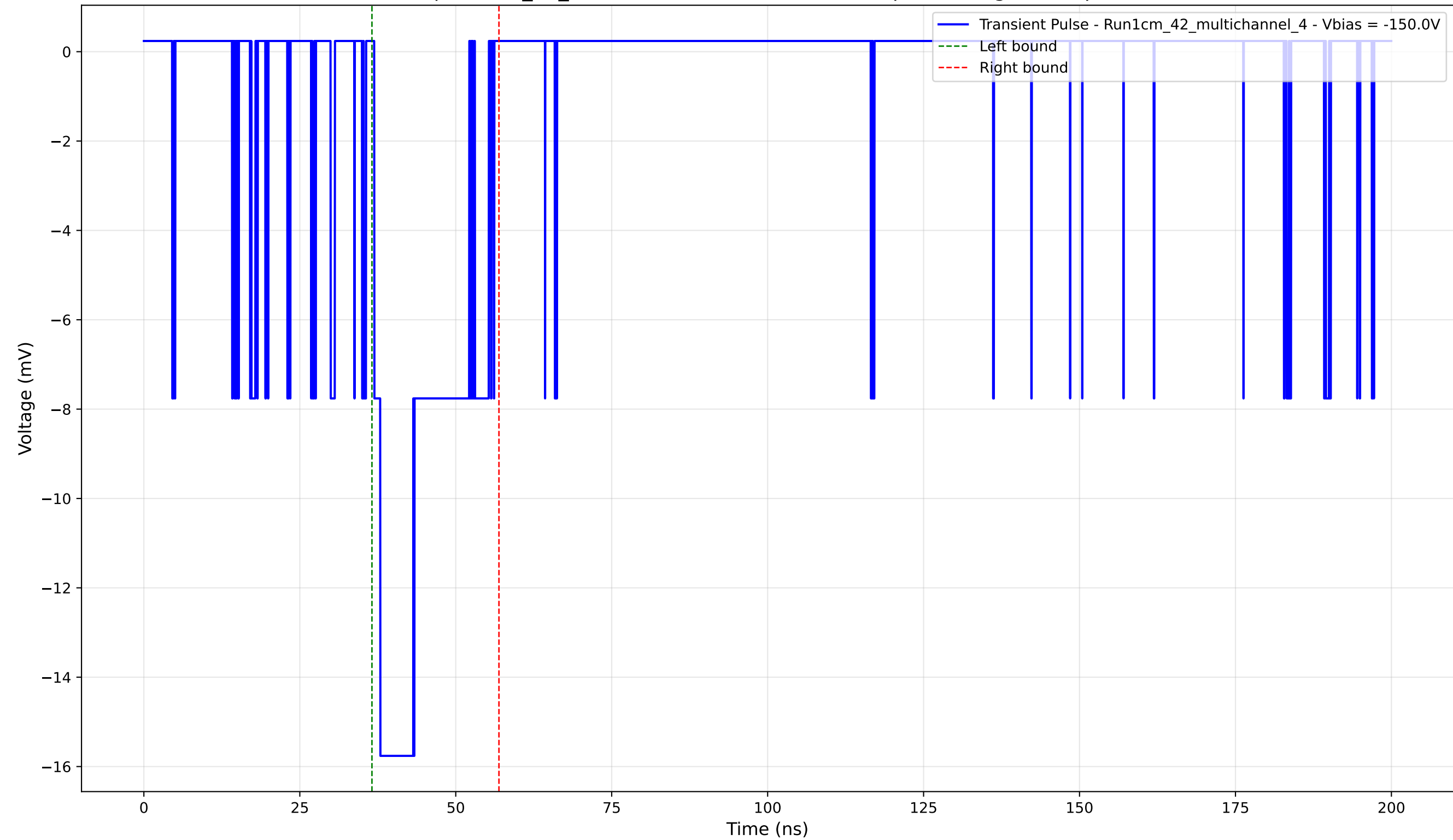
Transient Pulse - Sample: 1cm_42_multichannel - Position: 3990.0 \mu\text{m} - Charge: 3.66 pC - Rise Time: 0.98 ns
