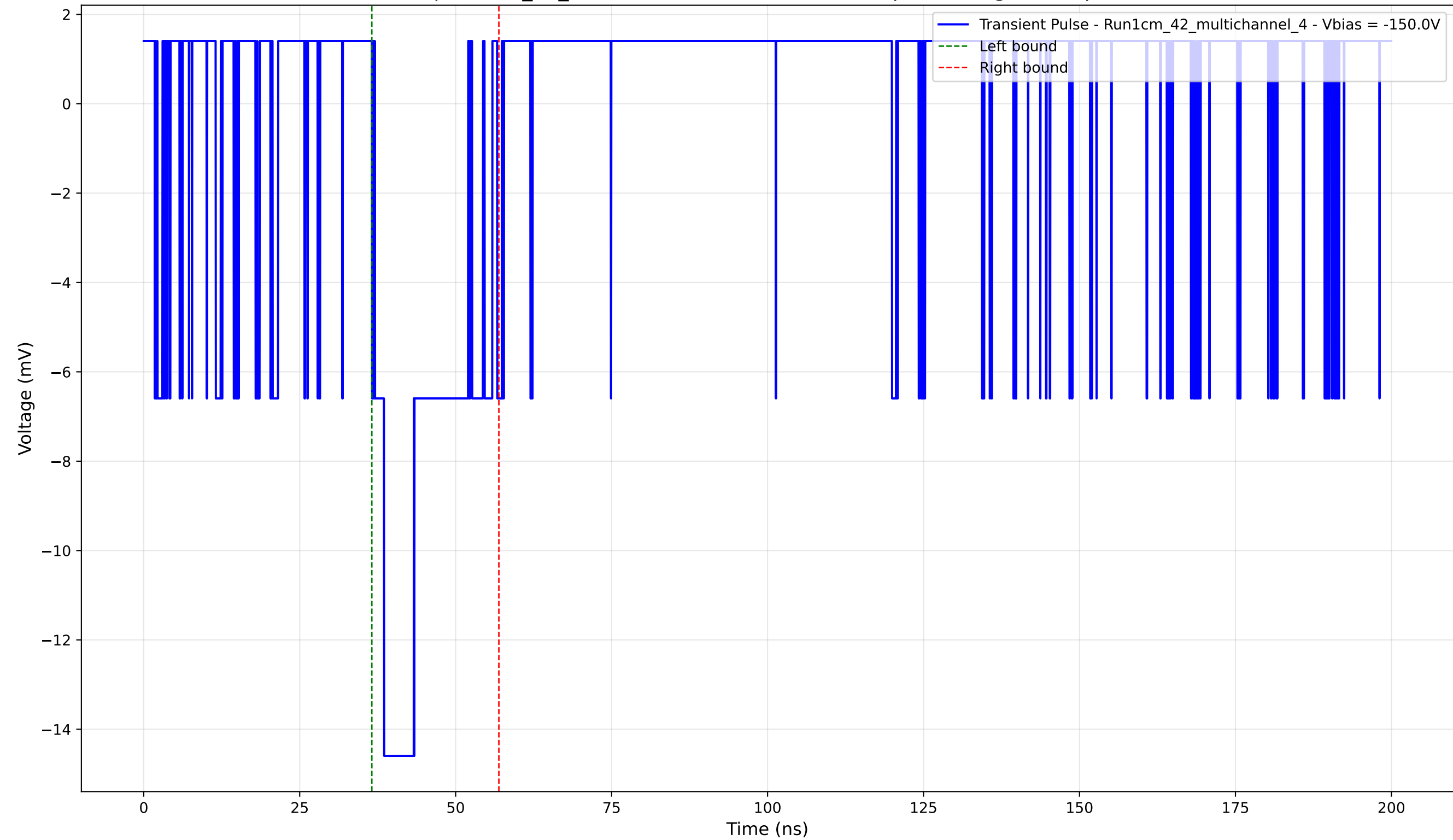
Transient Pulse - Sample: 1cm_42_multichannel - Position: 4625.0 \mu\text{m} - Charge: 3.19 pC - Rise Time: 1.48 ns
