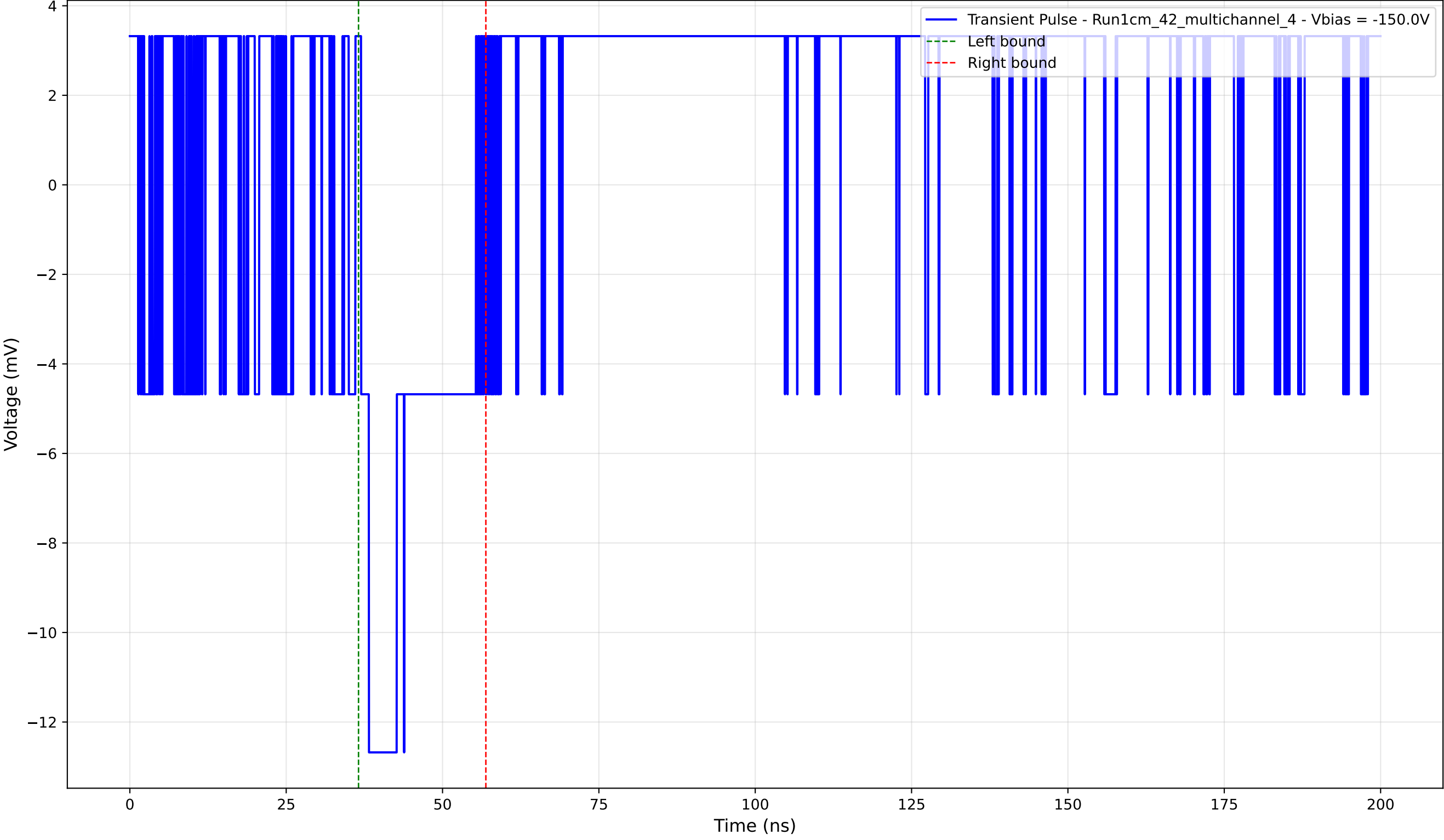
Transient Pulse - Sample: 1cm_42_multichannel - Position: 275.0 \mu\text{m} - Charge: 2.44 pC - Rise Time: 0.00 ns (N/A)
