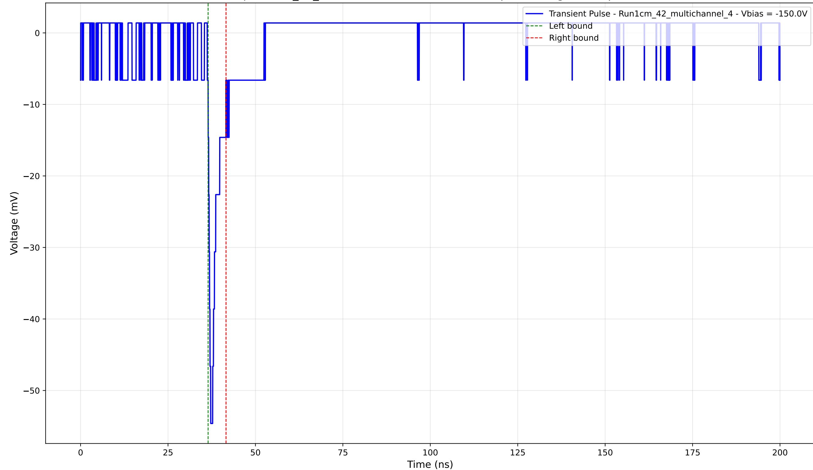
Transient Pulse - Sample: 1cm_42_multichannel - Position: 2740.0 \mu\text{m} - Charge: 2.78 pC - Rise Time: 0.98 ns
