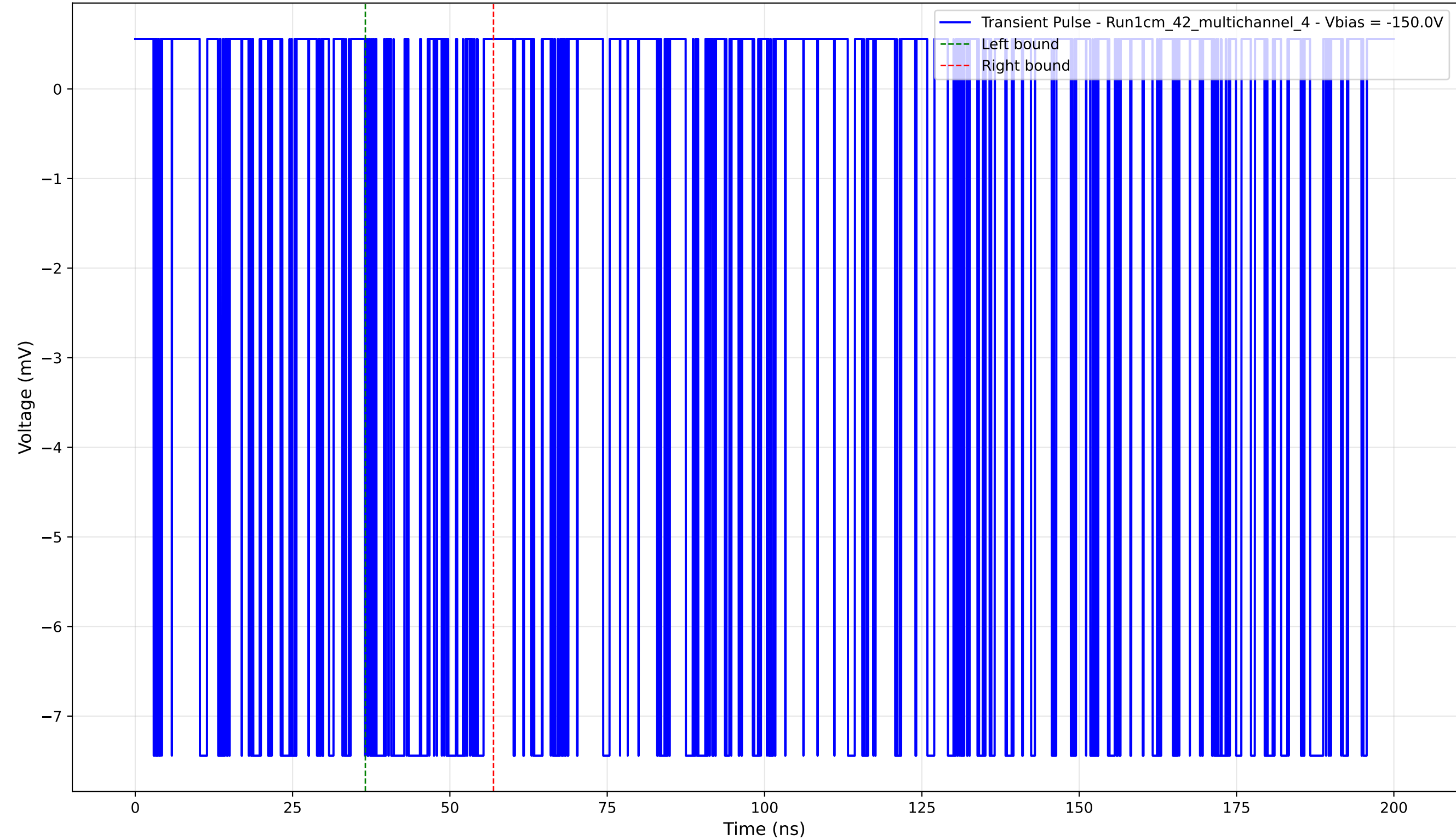
Transient Pulse - Sample: 1cm_42_multichannel - Position: 345.0 \mu\text{m} - Charge: 1.72 pC - Rise Time: 0.02 ns
