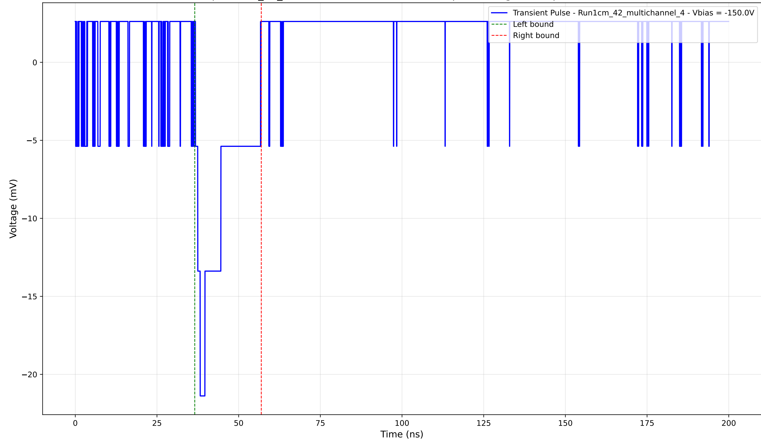
Transient Pulse - Sample: 1cm_42_multichannel - Position: 1015.0 \mu\text{m} - Charge: 3.50 pC - Rise Time: 0.00 ns (N/A)
