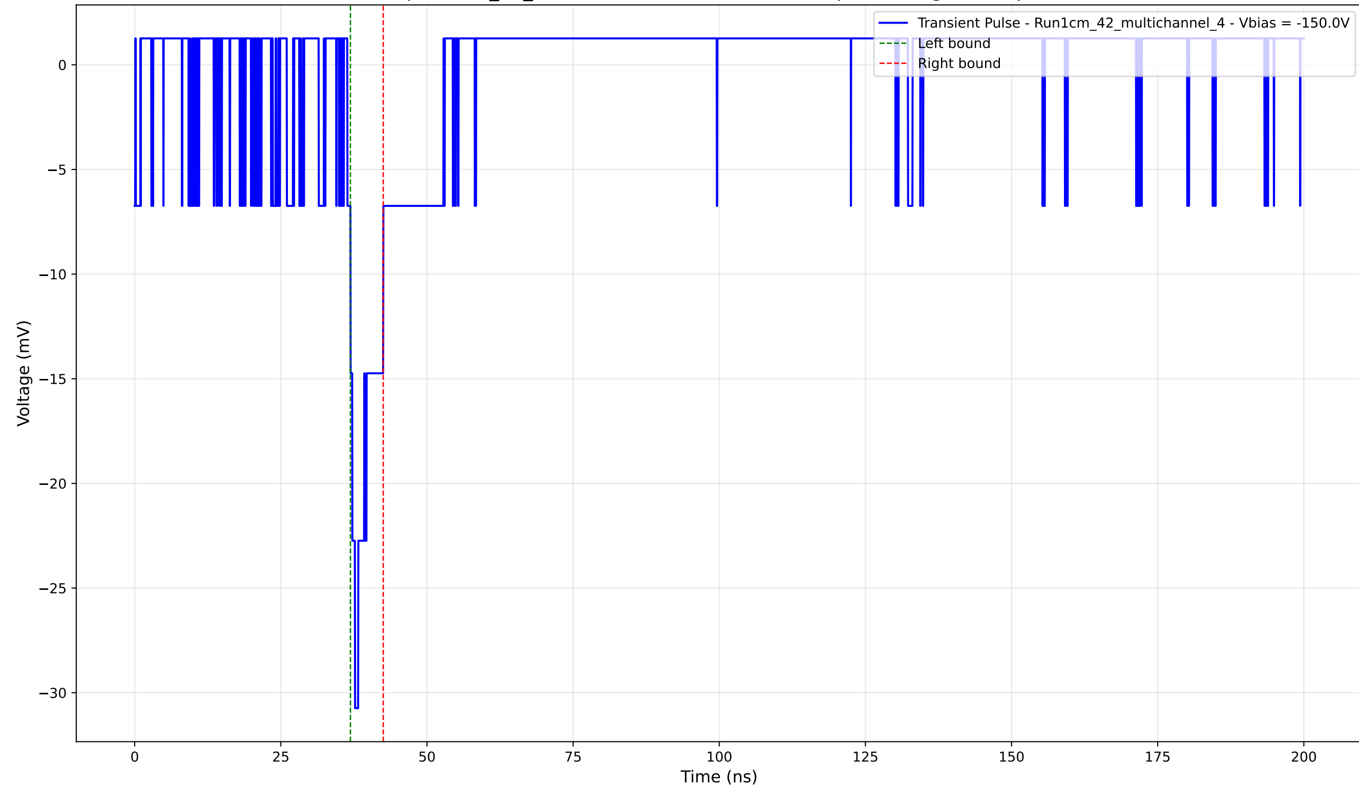
Transient Pulse - Sample: 1cm_42_multichannel - Position: 3230.0 \mu\text{m} - Charge: 2.12 pC - Rise Time: 1.31 ns
