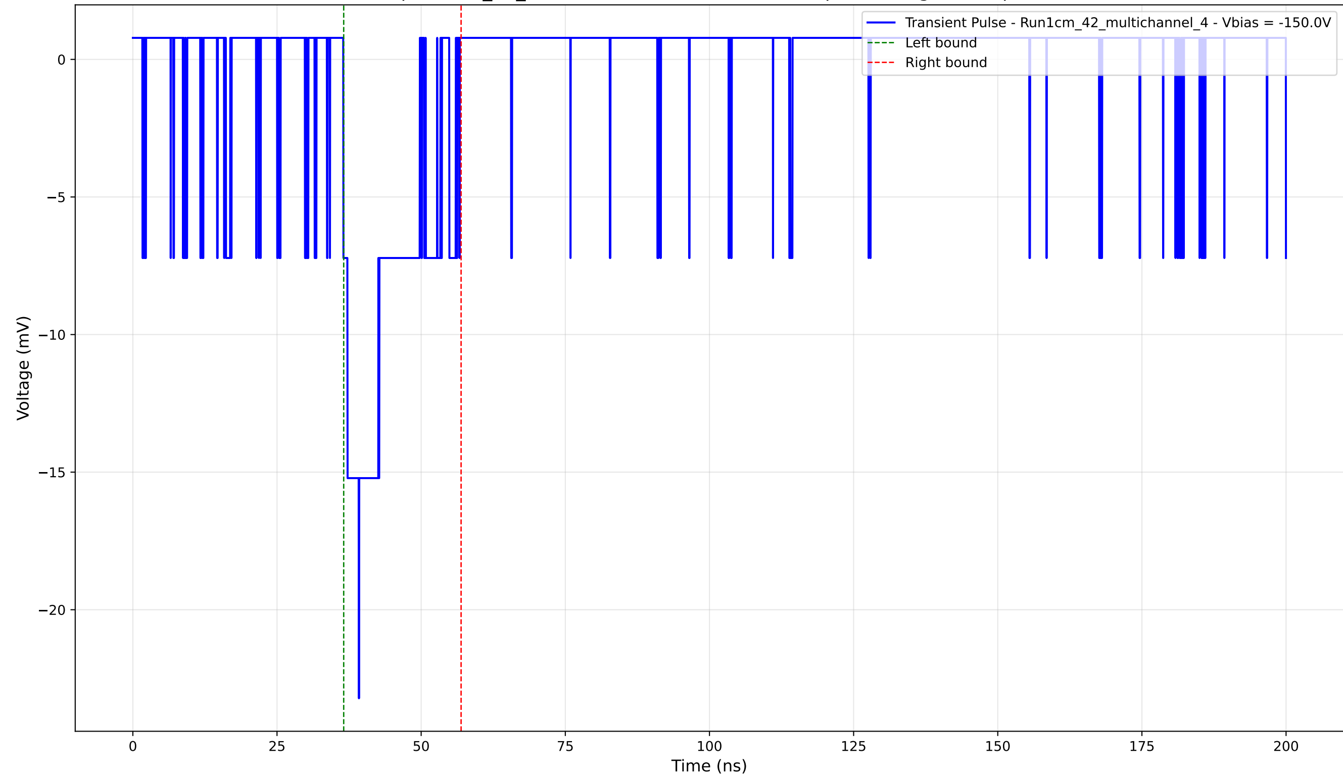
Transient Pulse - Sample: 1cm_42_multichannel - Position: 3470.0 \mu\text{m} - Charge: 3.35 pC - Rise Time: 2.70 ns
