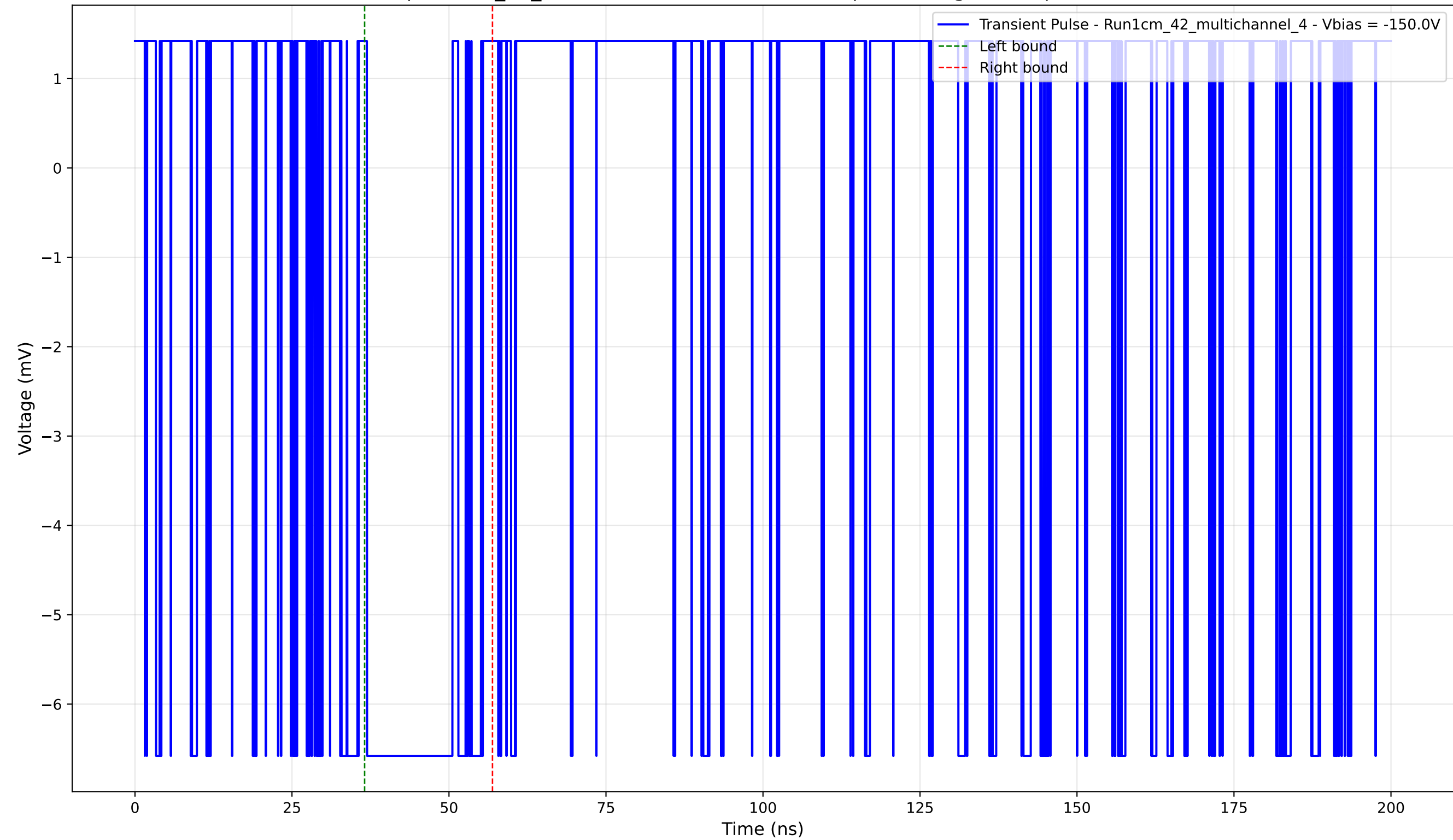
Transient Pulse - Sample: 1cm_42_multichannel - Position: 105.0 \mu\text{m} - Charge: 2.15 pC - Rise Time: 0.00 ns (N/A)
