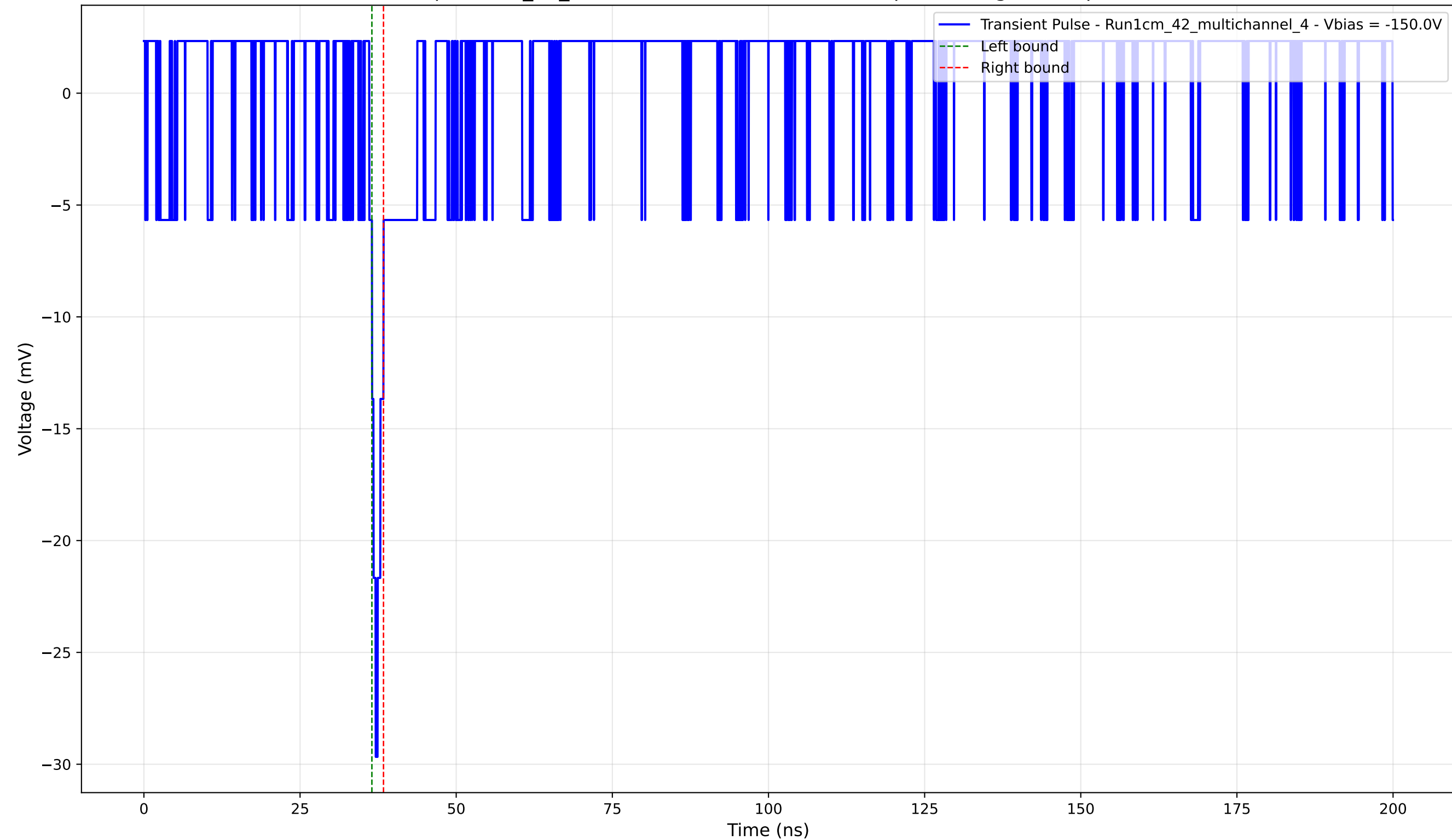
Transient Pulse - Sample: 1cm_42_multichannel - Position: 2430.0 \mu\text{m} - Charge: 0.73 pC - Rise Time: 1.04 ns
