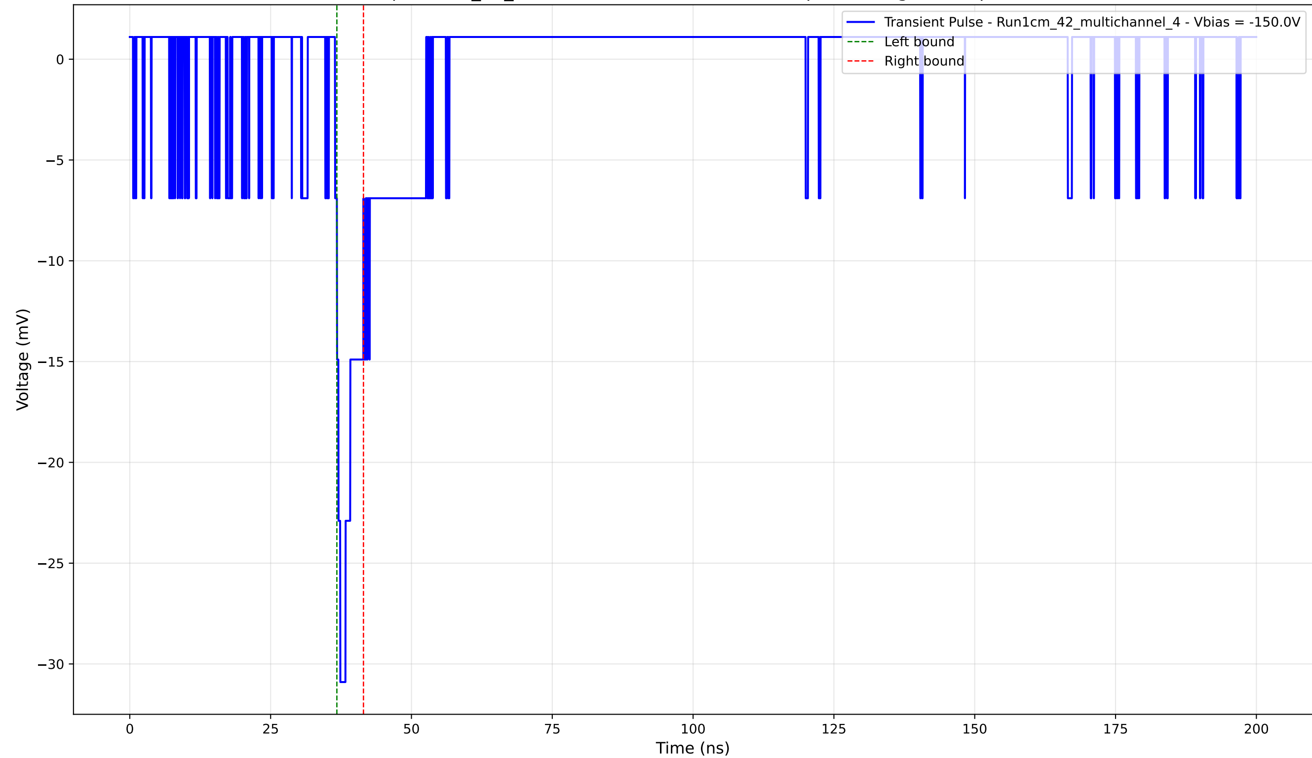
Transient Pulse - Sample: 1cm_42_multichannel - Position: 3105.0 \mu\text{m} - Charge: 1.89 pC - Rise Time: 0.93 ns
