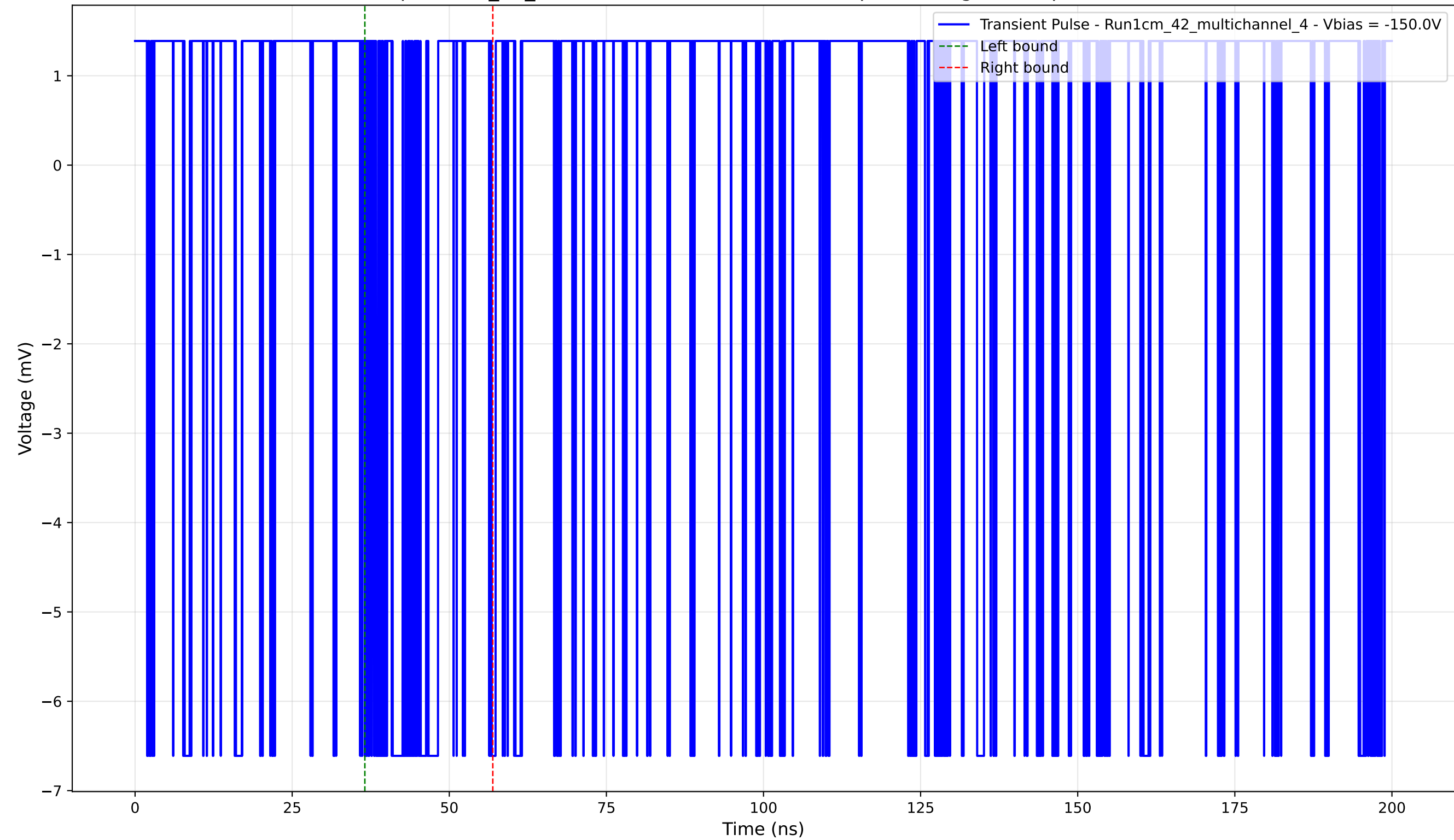
Transient Pulse - Sample: 1cm_42_multichannel - Position: 4380.0 \mu\text{m} - Charge: 0.78 pC - Rise Time: 0.00 ns (N/A)
