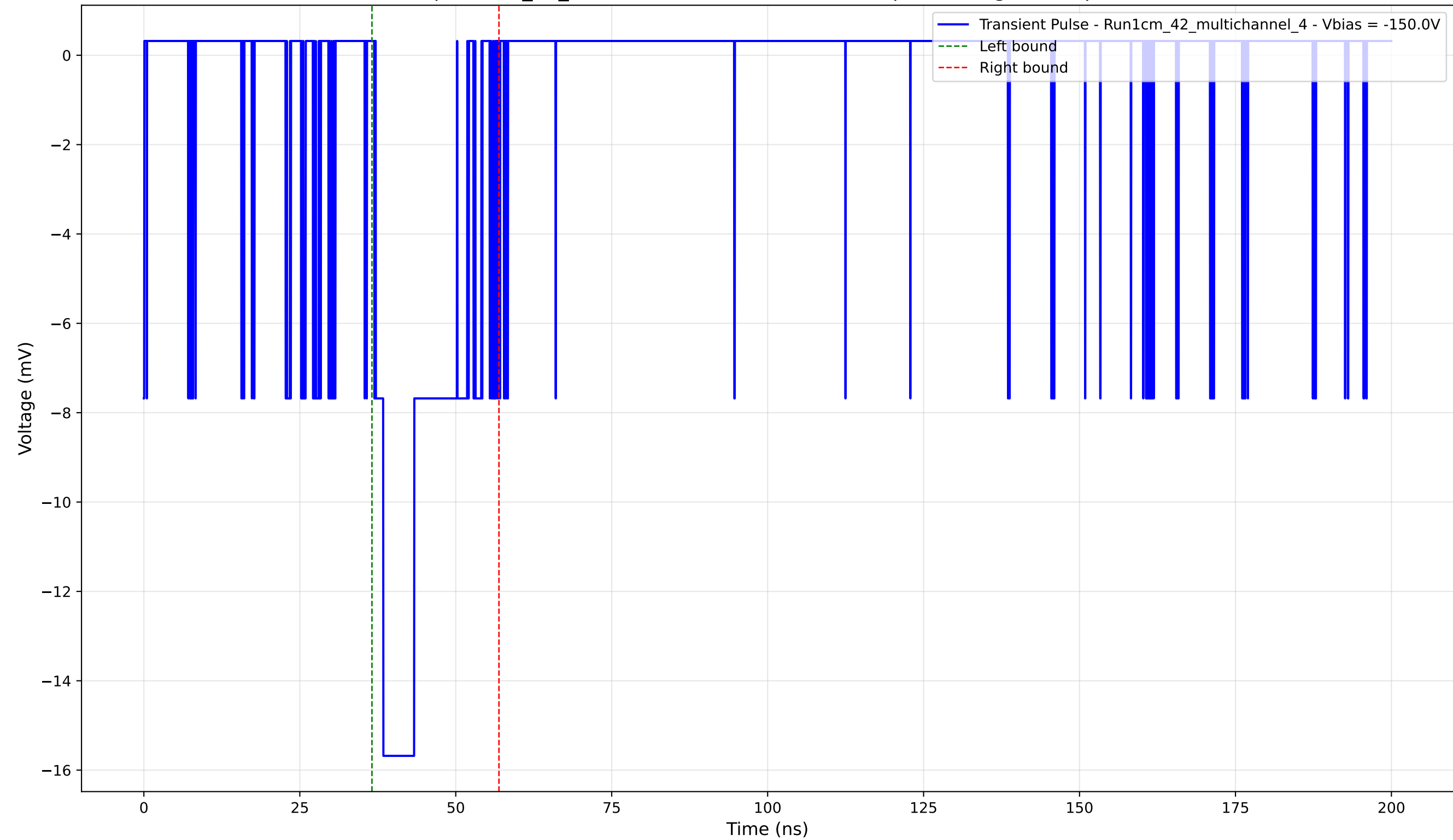
Transient Pulse - Sample: 1cm_42_multichannel - Position: 4535.0 \mu\text{m} - Charge: 3.38 pC - Rise Time: 1.22 ns
