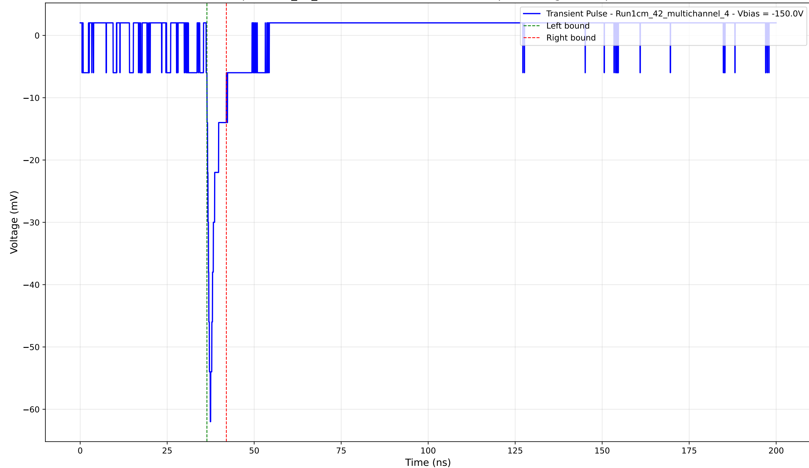
Transient Pulse - Sample: 1cm_42_multichannel - Position: 2040.0 \mu\text{m} - Charge: 2.90 pC - Rise Time: 0.96 ns
