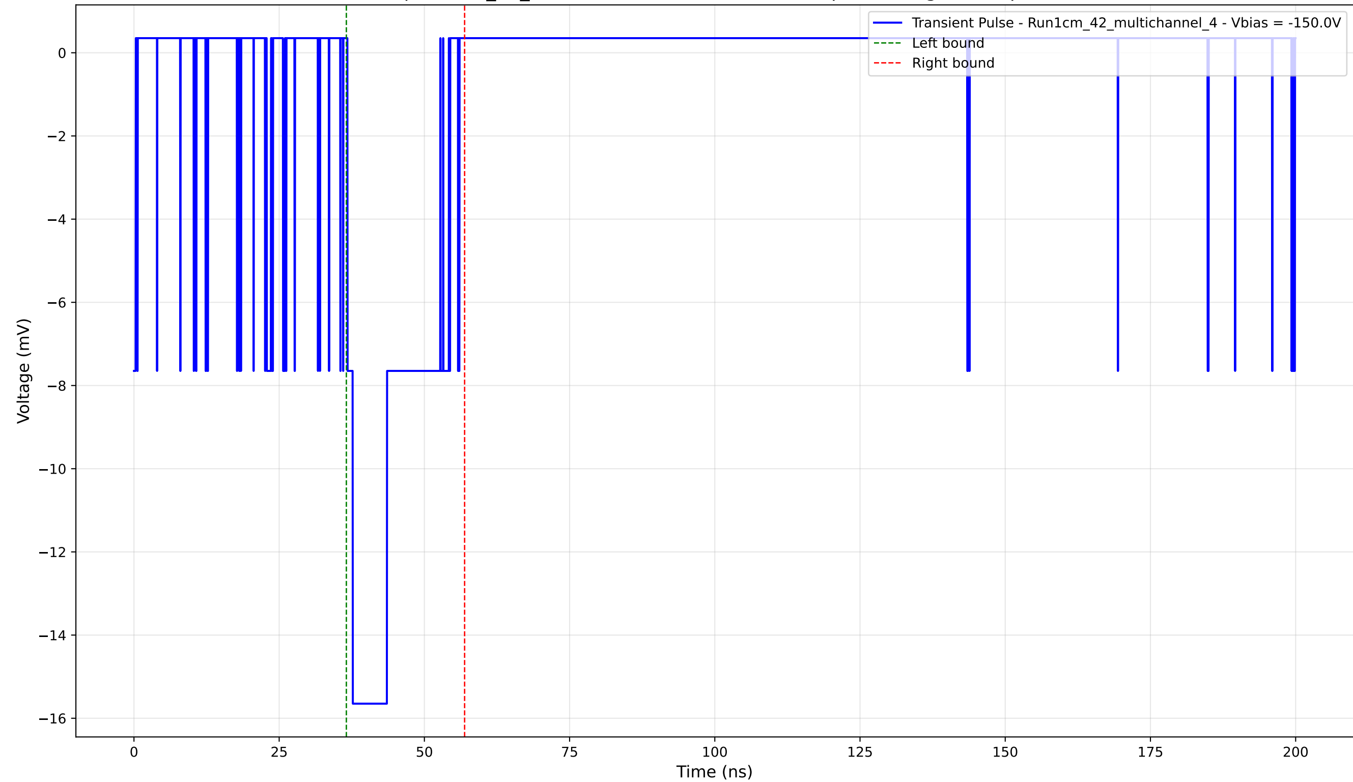
Transient Pulse - Sample: 1cm_42_multichannel - Position: 3760.0 \mu\text{m} - Charge: 3.64 pC - Rise Time: 0.92 ns
