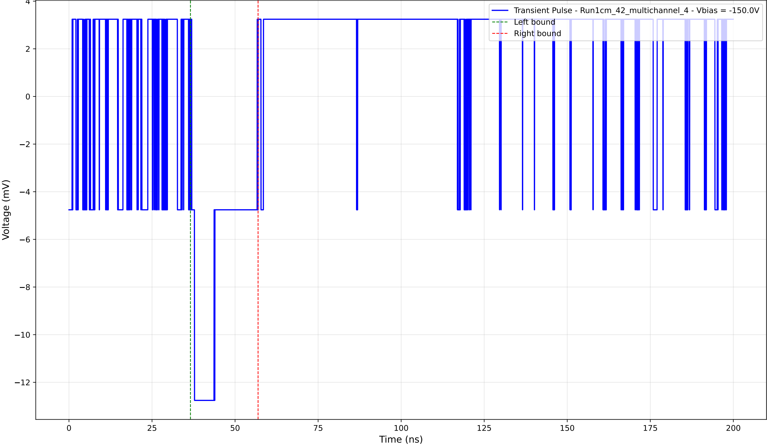
Transient Pulse - Sample: 1cm_42_multichannel - Position: 650.0 \mu\text{m} - Charge: 2.82 pC - Rise Time: 0.00 ns (N/A)
