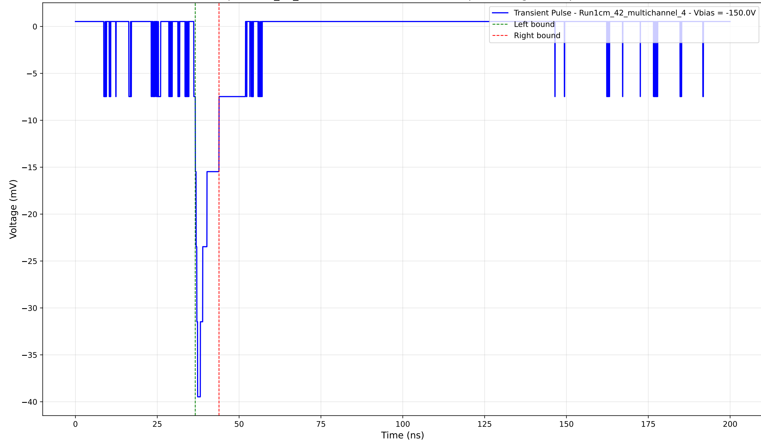
Transient Pulse - Sample: 1cm_42_multichannel - Position: 1730.0 \mu\text{m} - Charge: 3.20 pC - Rise Time: 1.17 ns
