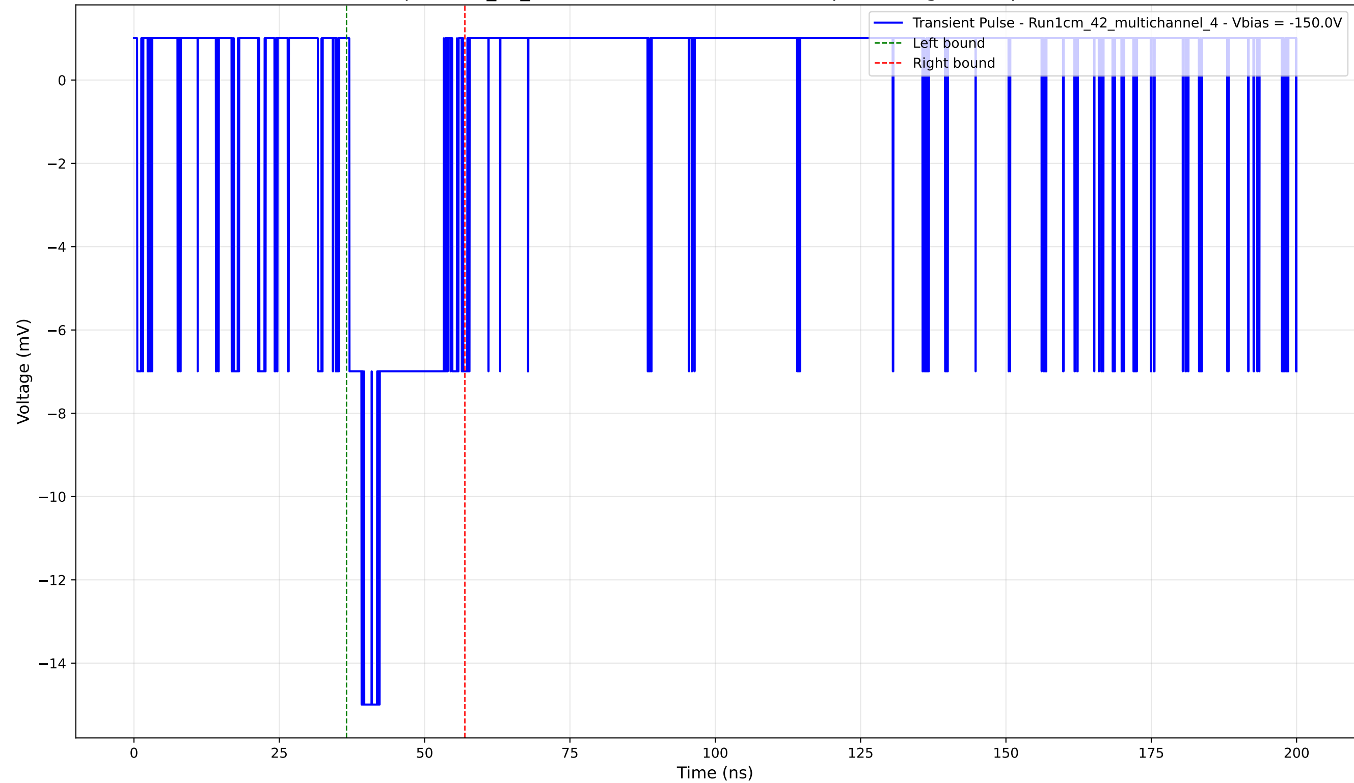
Transient Pulse - Sample: 1cm_42_multichannel - Position: 4340.0 \mu\text{m} - Charge: 2.93 pC - Rise Time: 2.10 ns
