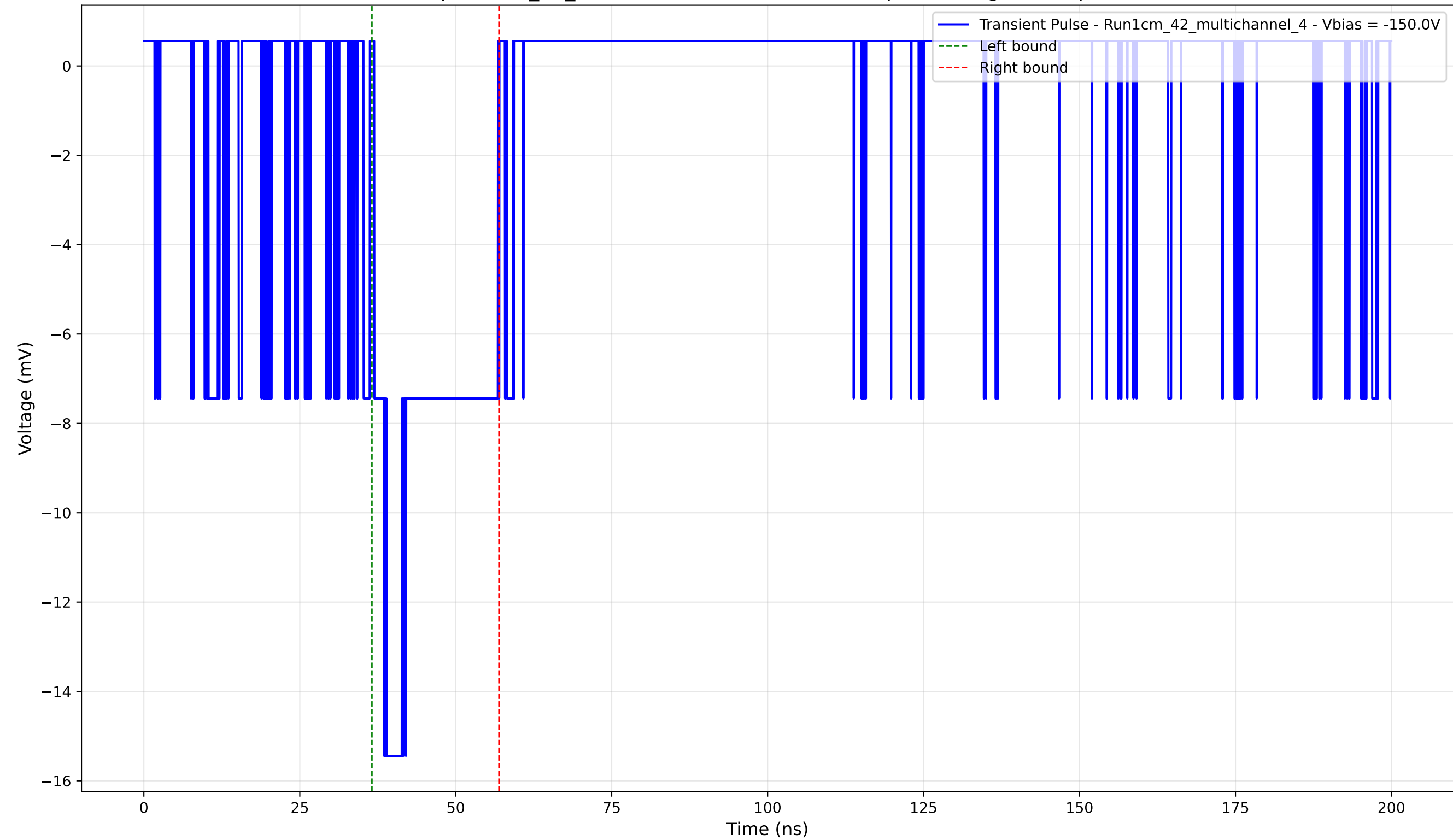
Transient Pulse - Sample: 1cm_42_multichannel - Position: 240.0 \mu\text{m} - Charge: 3.40 pC - Rise Time: 1.58 ns
