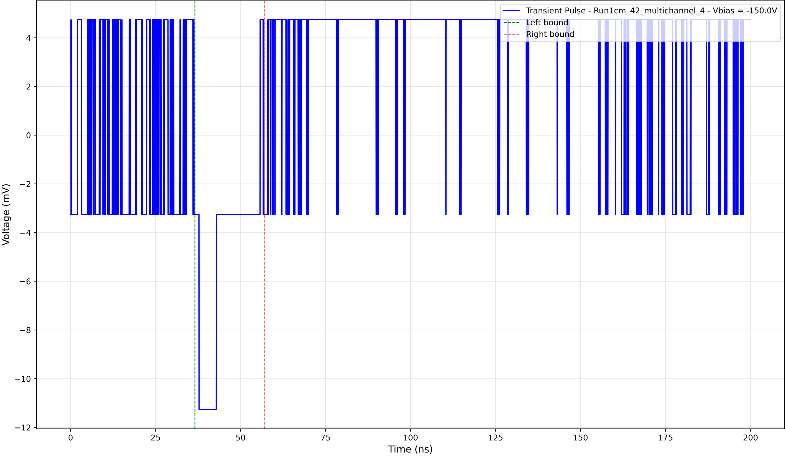
Transient Pulse - Sample: 1cm_42_multichannel - Position: 930.0 \mu\text{m} - Charge: 1.97 pC - Rise Time: 0.00 ns (N/A)
