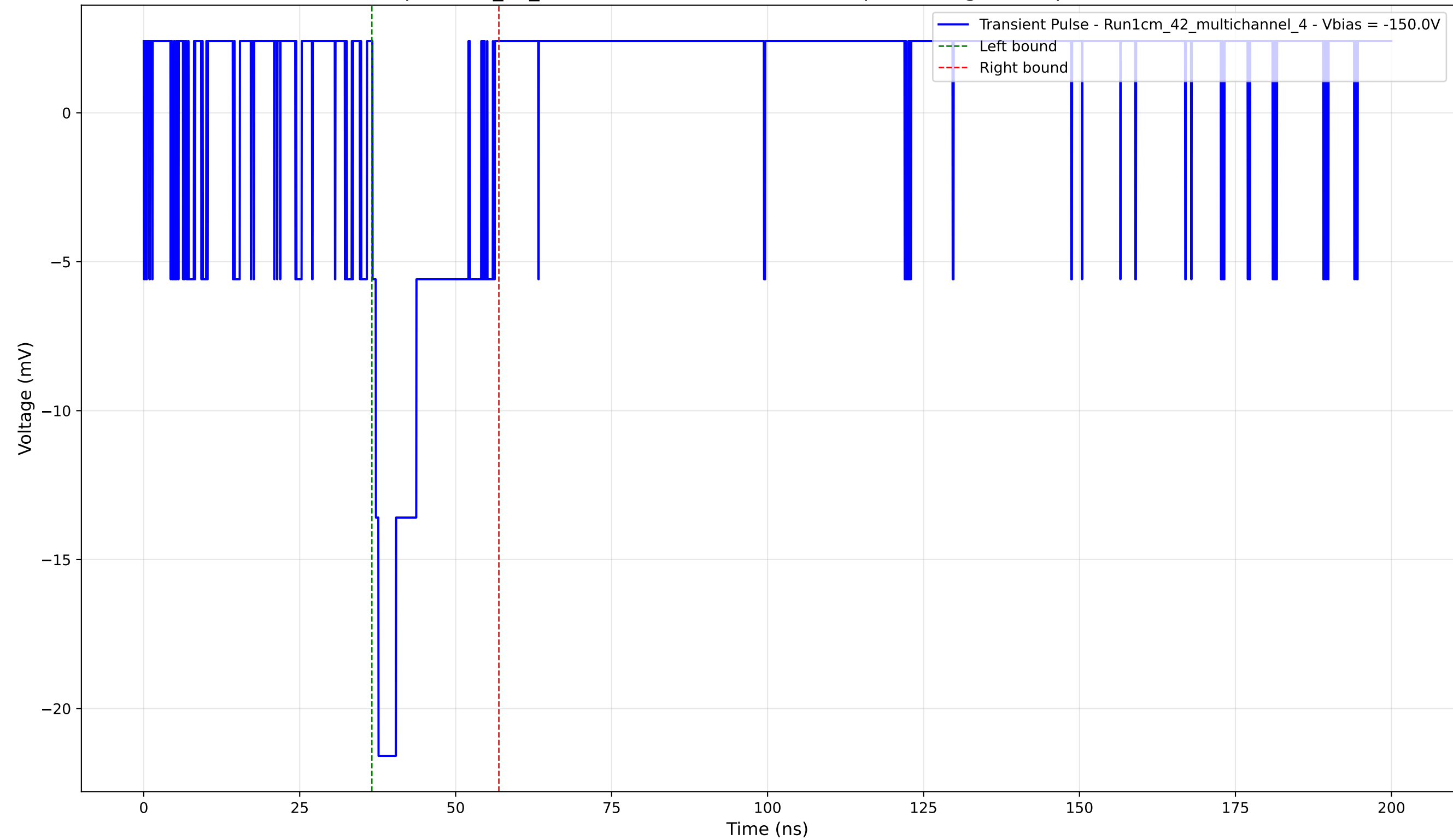
Transient Pulse - Sample: 1cm_42_multichannel - Position: 1245.0 \mu\text{m} - Charge: 3.57 pC - Rise Time: 0.00 ns (N/A)
