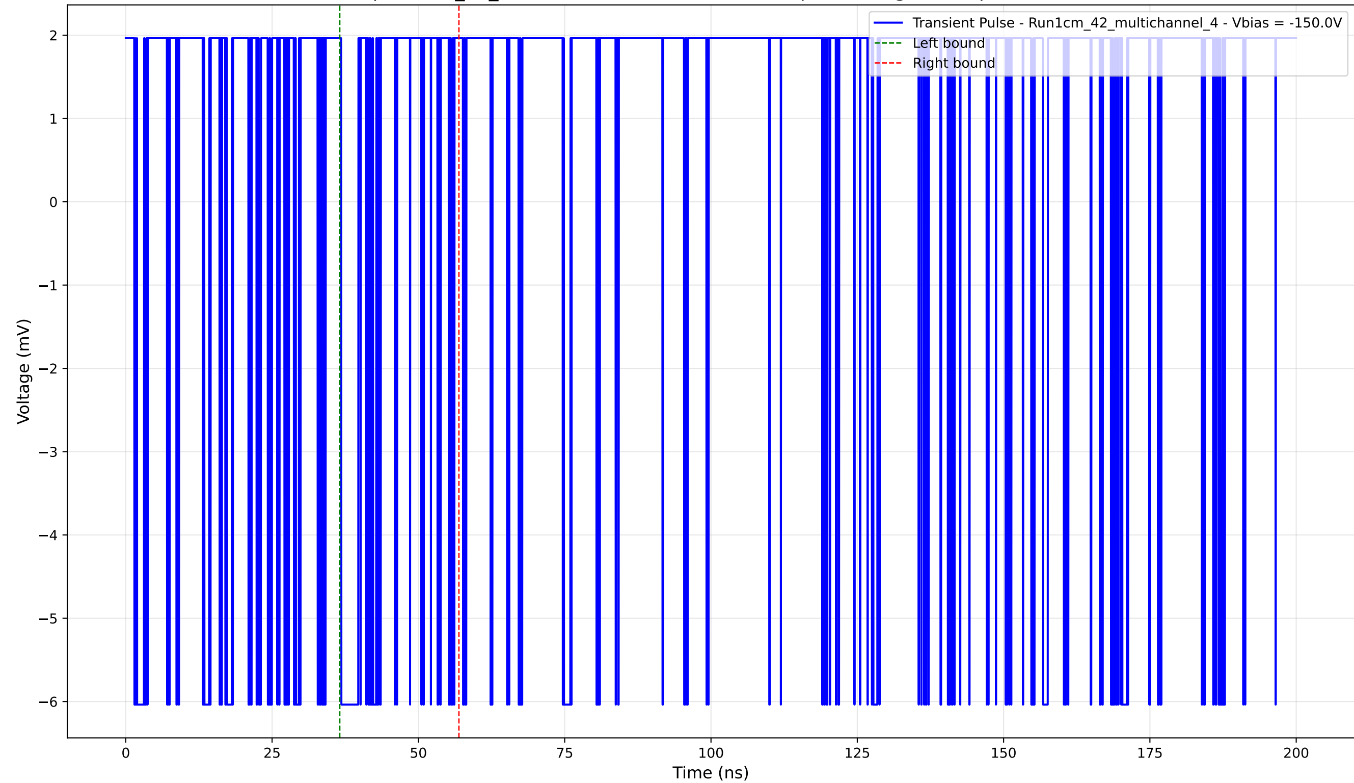
Transient Pulse - Sample: 1cm_42_multichannel - Position: 2890.0 \mu\text{m} - Charge: 0.08 pC - Rise Time: 0.00 ns (N/A)
