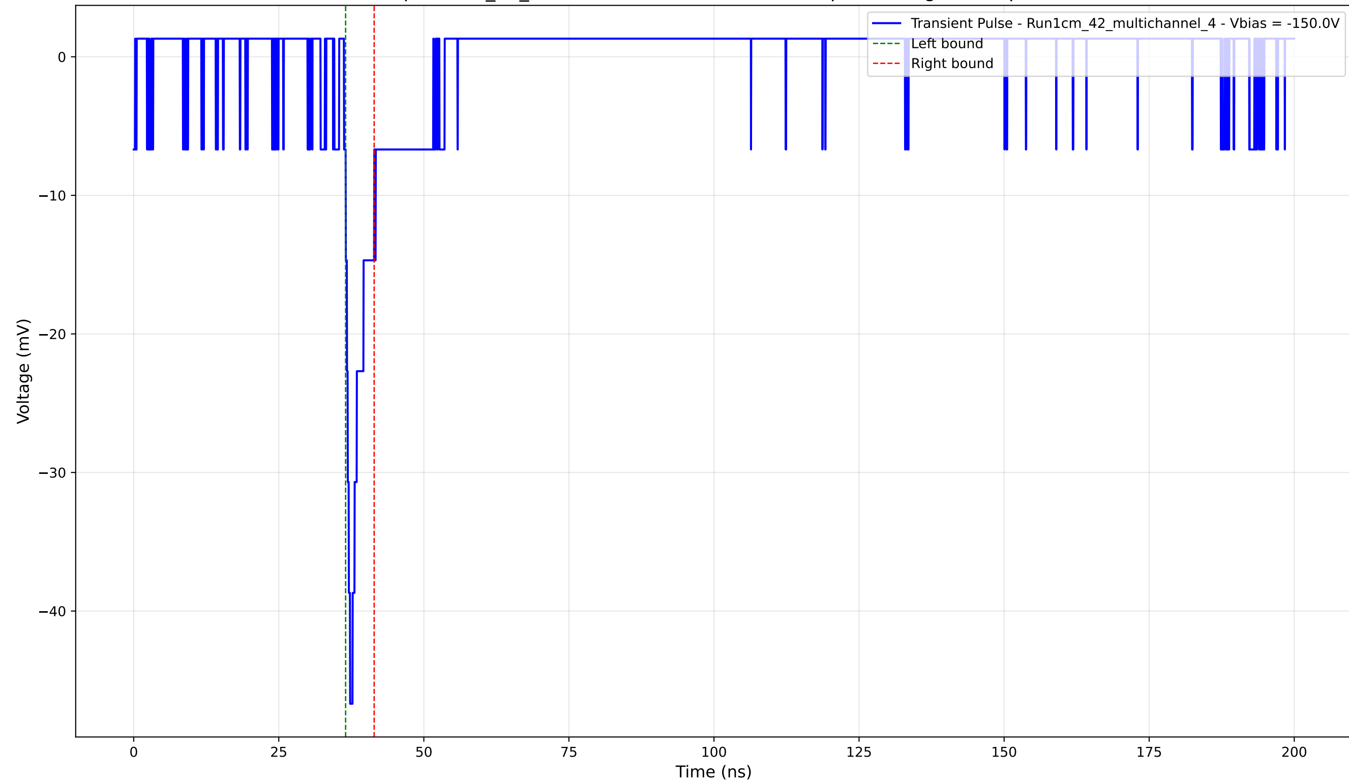
Transient Pulse - Sample: 1cm_42_multichannel - Position: 2815.0 \mu\text{m} - Charge: 2.38 pC - Rise Time: 1.05 ns
