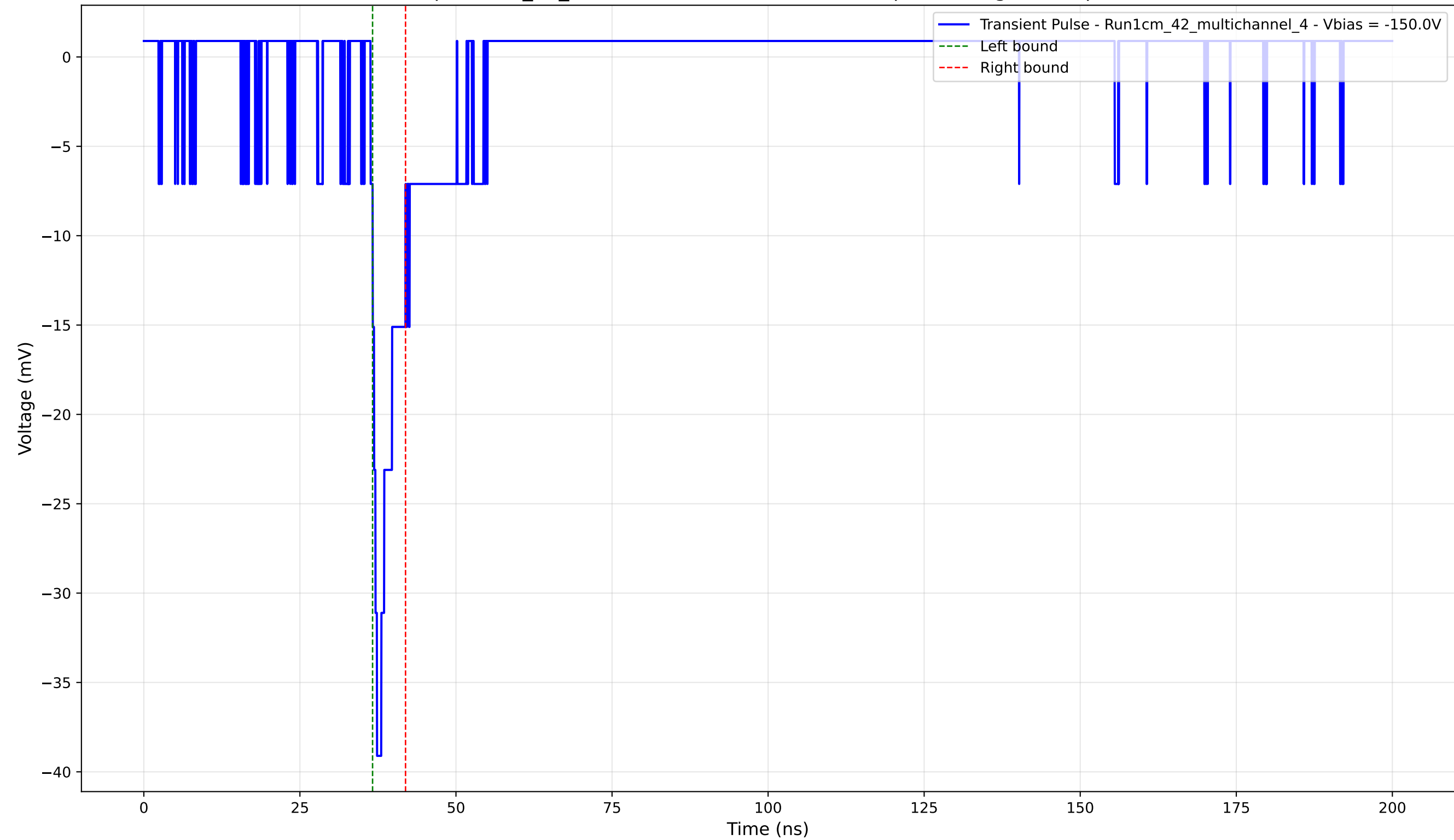
Transient Pulse - Sample: 1cm_42_multichannel - Position: 3010.0 \mu\text{m} - Charge: 2.39 pC - Rise Time: 1.03 ns
