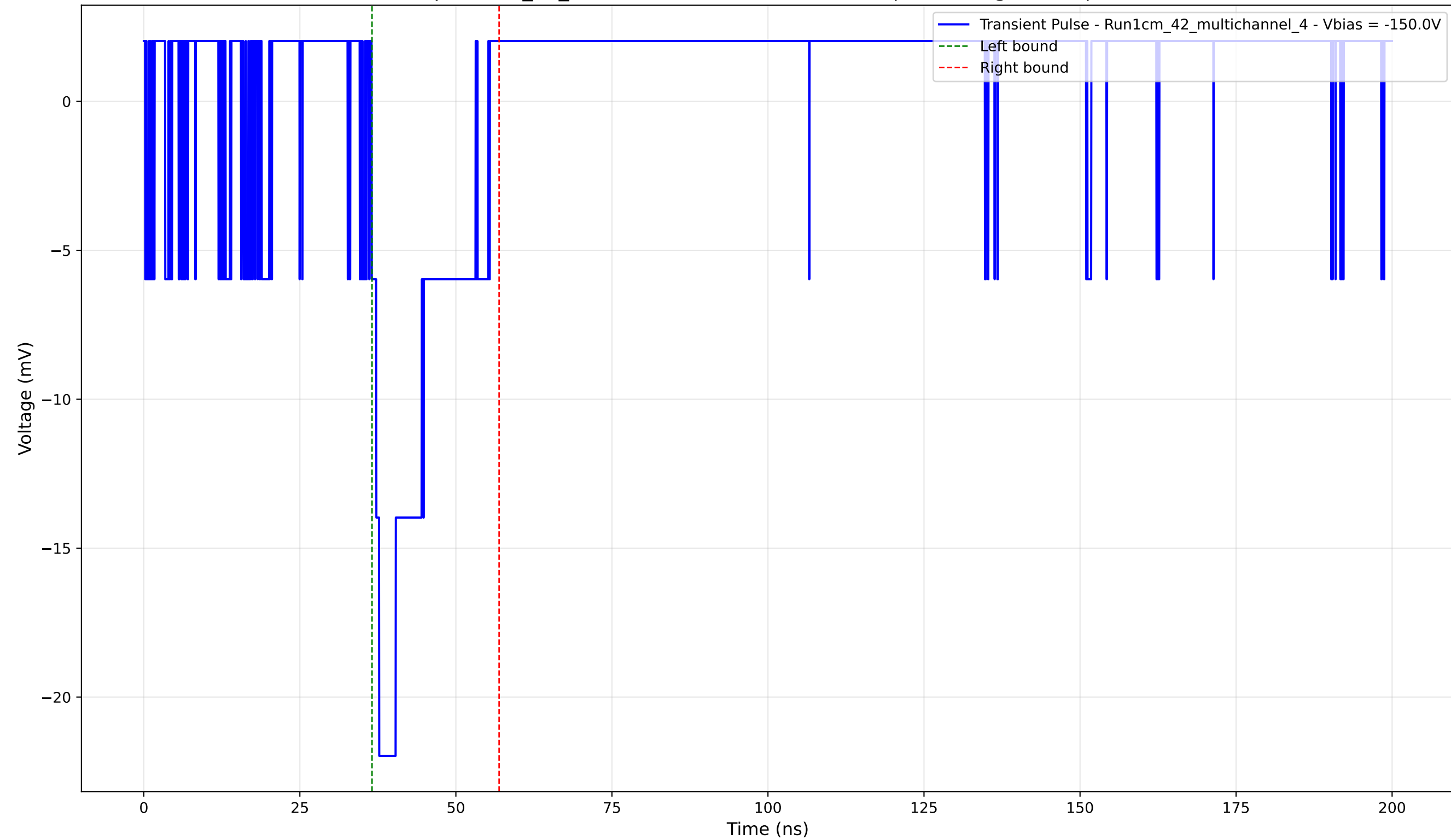
Transient Pulse - Sample: 1cm_42_multichannel - Position: 1225.0 \mu\text{m} - Charge: 3.76 pC - Rise Time: 1.22 ns
