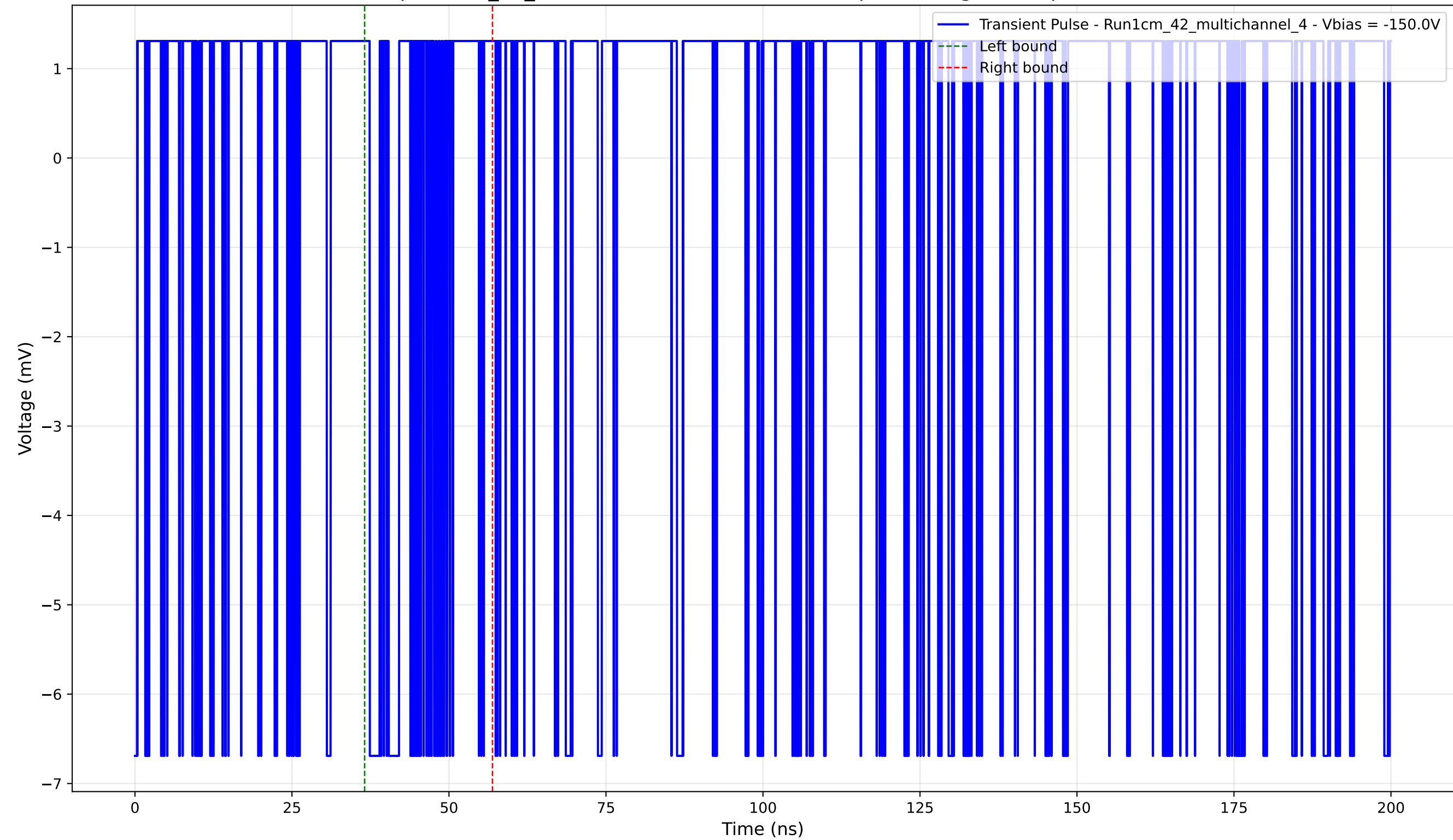
Transient Pulse - Sample: 1cm_42_multichannel - Position: 4425.0 \mu\text{m} - Charge: 0.49 pC - Rise Time: 0.00 ns (N/A)
