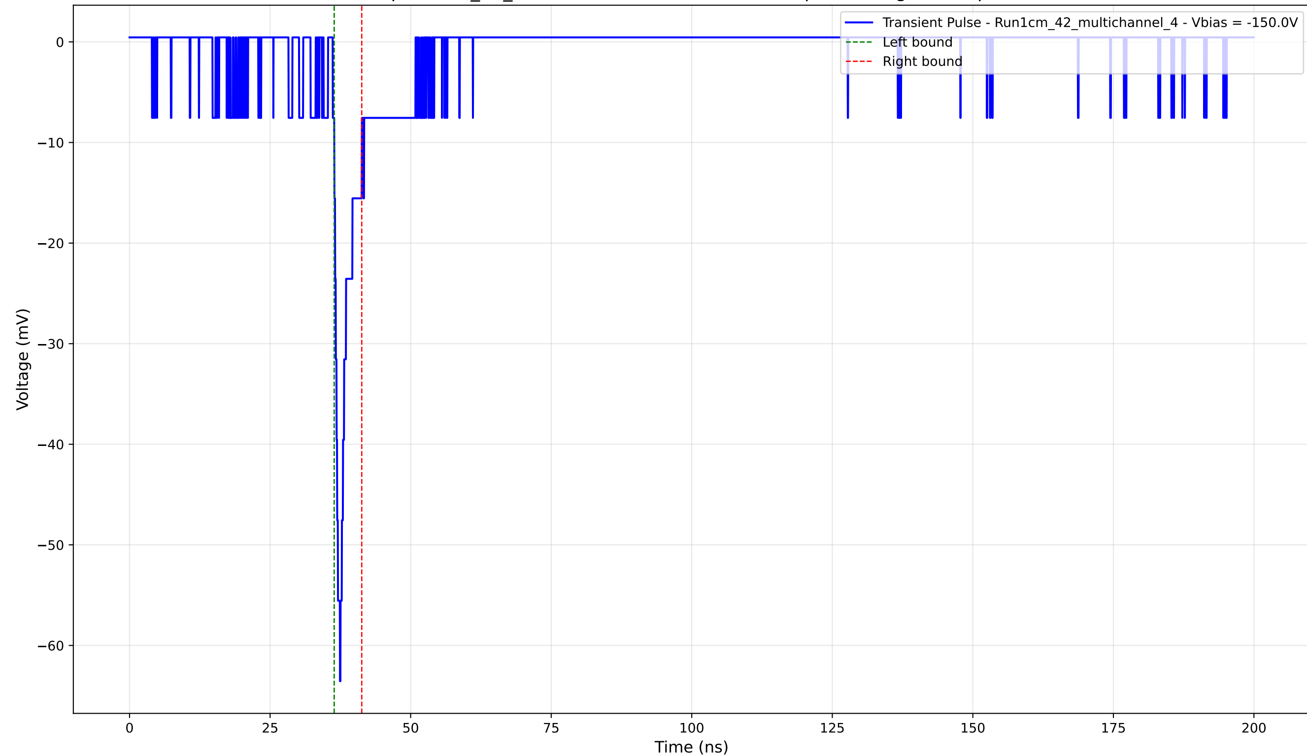
Transient Pulse - Sample: 1cm_42_multichannel - Position: 2670.0 \mu\text{m} - Charge: 2.81 pC - Rise Time: 1.28 ns
