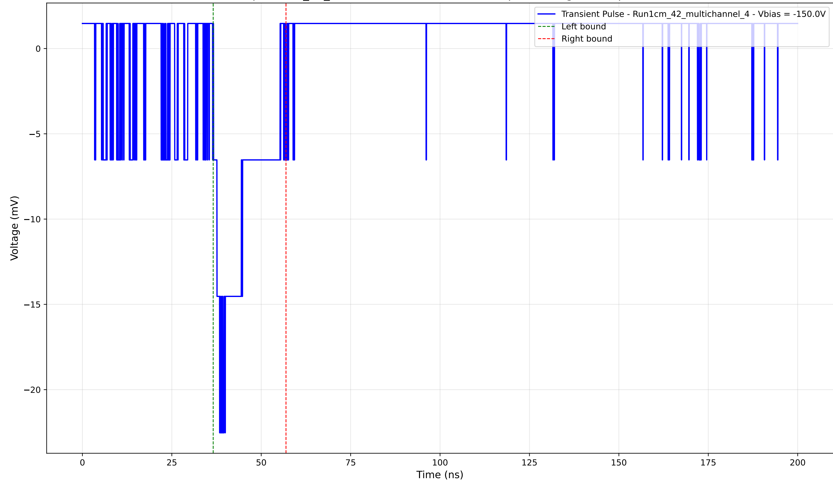
Transient Pulse - Sample: 1cm_42_multichannel - Position: 970.0 \mu\text{m} - Charge: 3.71 pC - Rise Time: 1.74 ns
