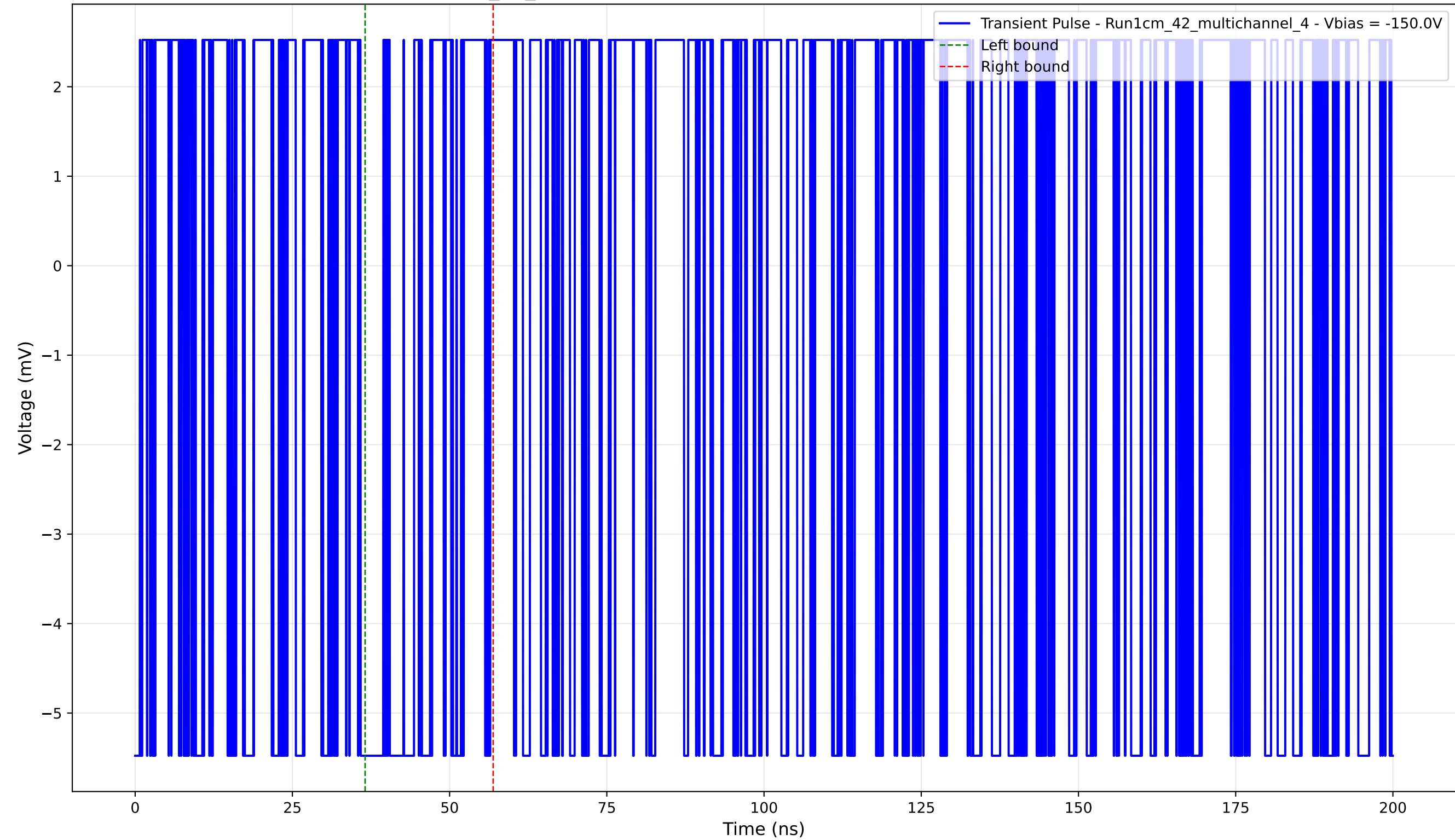
Transient Pulse - Sample: 1cm_42_multichannel - Position: 1890.0 \mu\text{m} - Charge: 0.73 pC - Rise Time: 0.00 ns (N/A)
