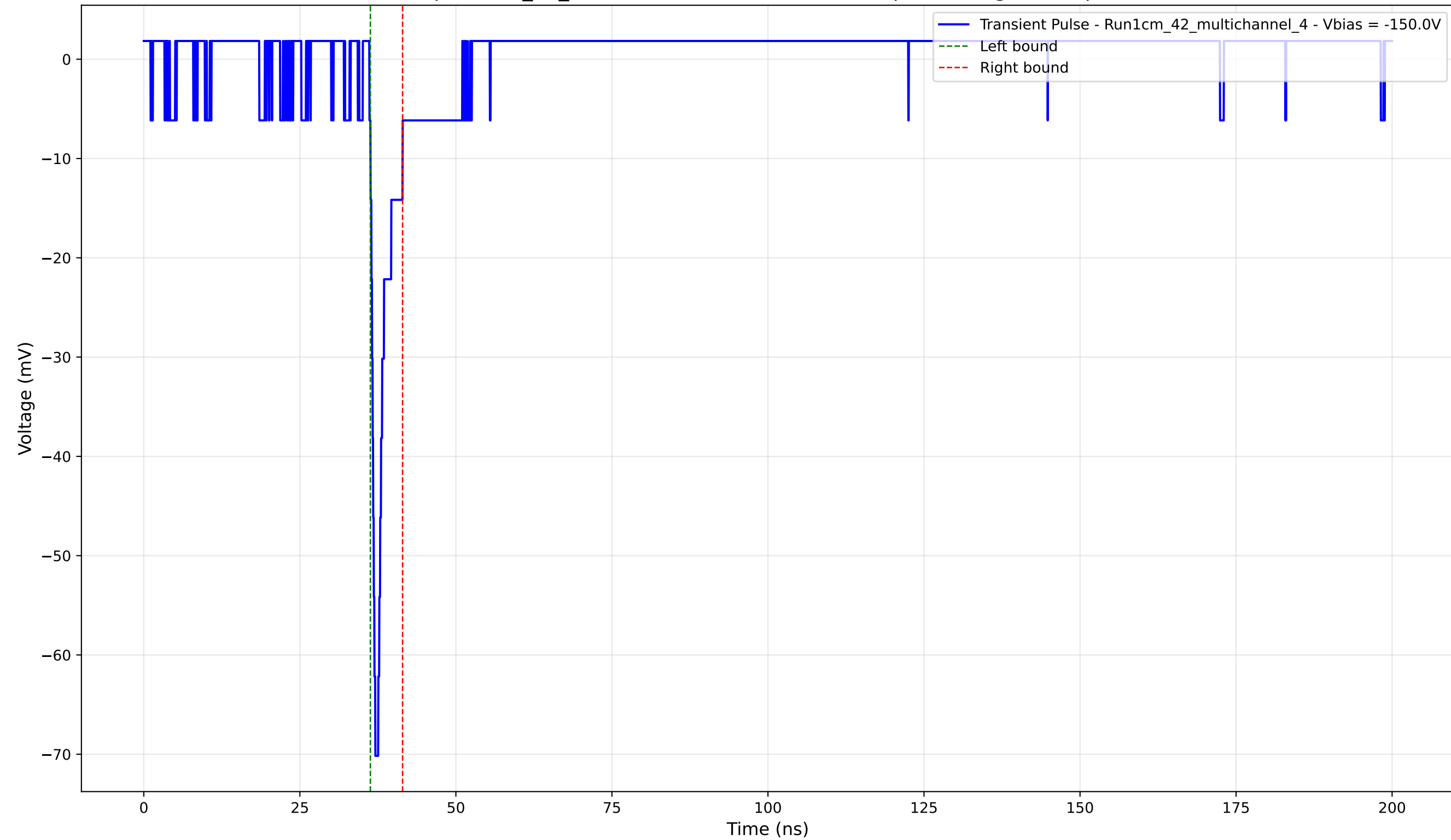
Transient Pulse - Sample: 1cm_42_multichannel - Position: 2565.0 \mu\text{m} - Charge: 3.08 pC - Rise Time: 0.78 ns
