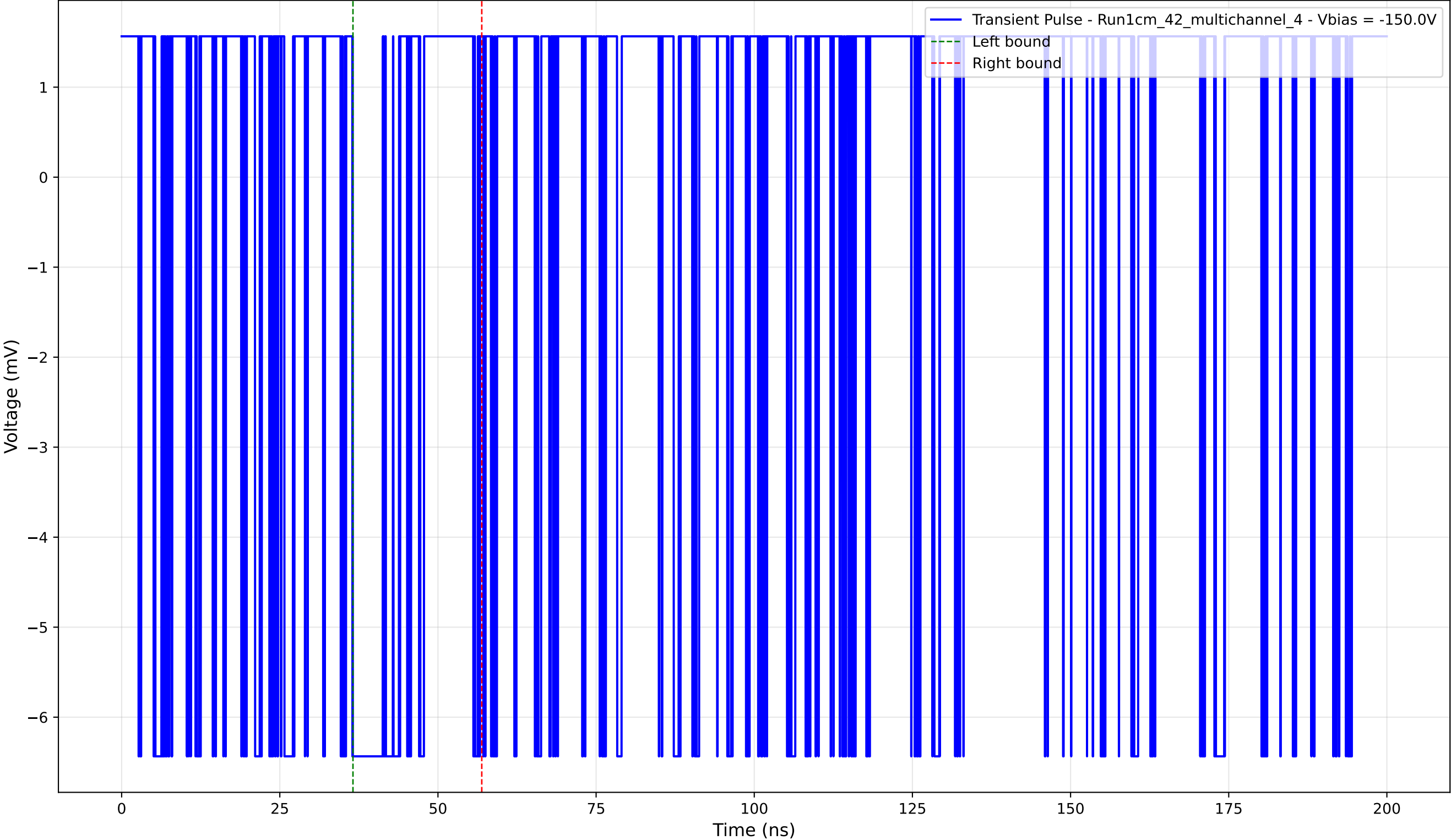
Transient Pulse - Sample: 1cm_42_multichannel - Position: 2860.0 \mu\text{m} - Charge: 0.80 pC - Rise Time: 0.00 ns (N/A)
