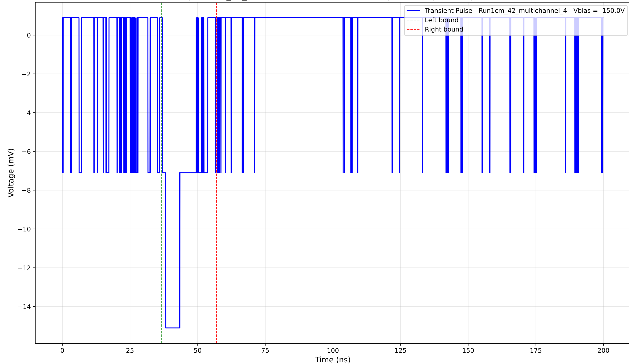
Transient Pulse - Sample: 1cm_42_multichannel - Position: 4530.0 \mu\text{m} - Charge: 3.02 pC - Rise Time: 1.24 ns
