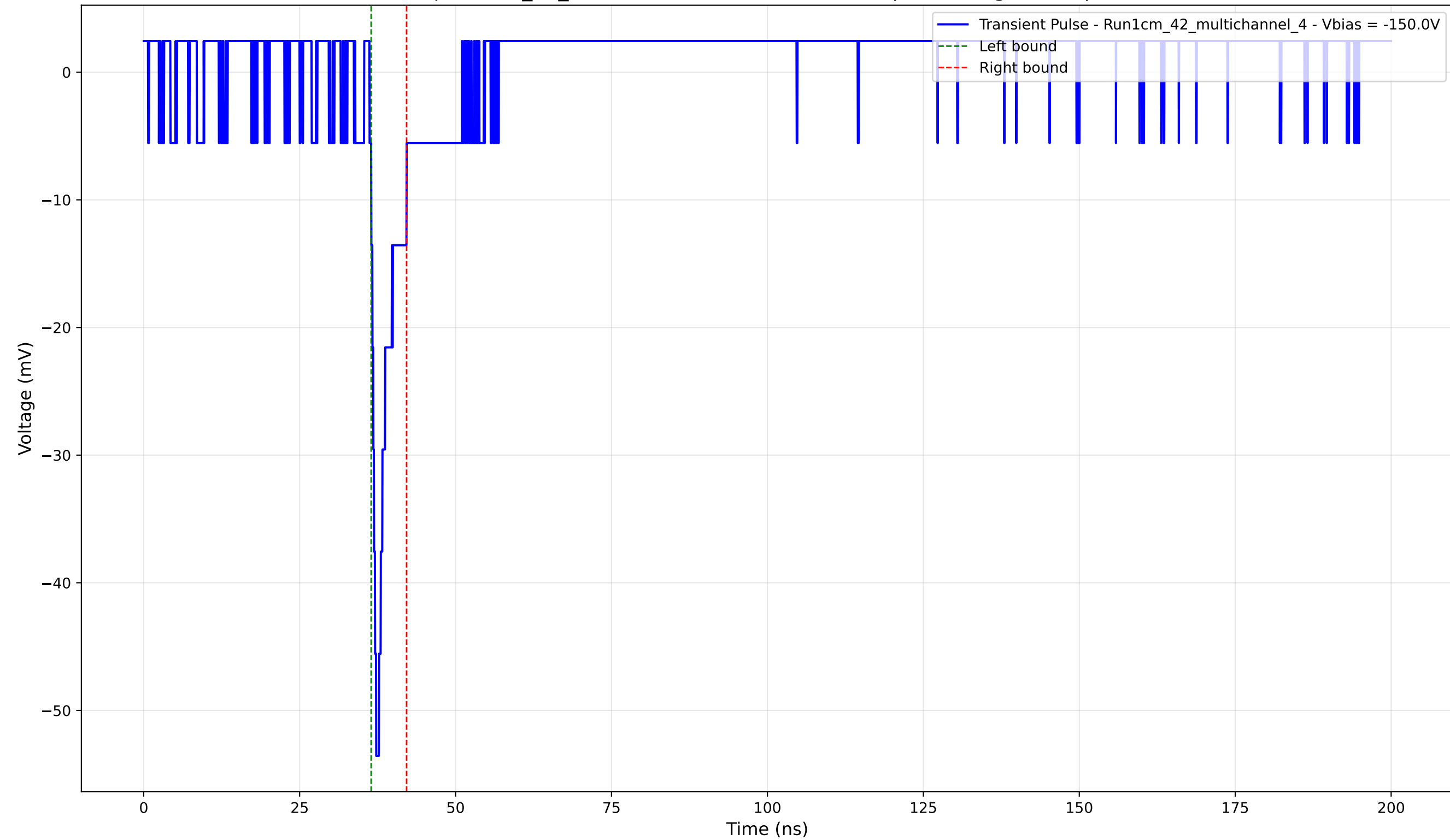
Transient Pulse - Sample: 1cm_42_multichannel - Position: 2775.0 \mu\text{m} - Charge: 2.79 pC - Rise Time: 1.06 ns
