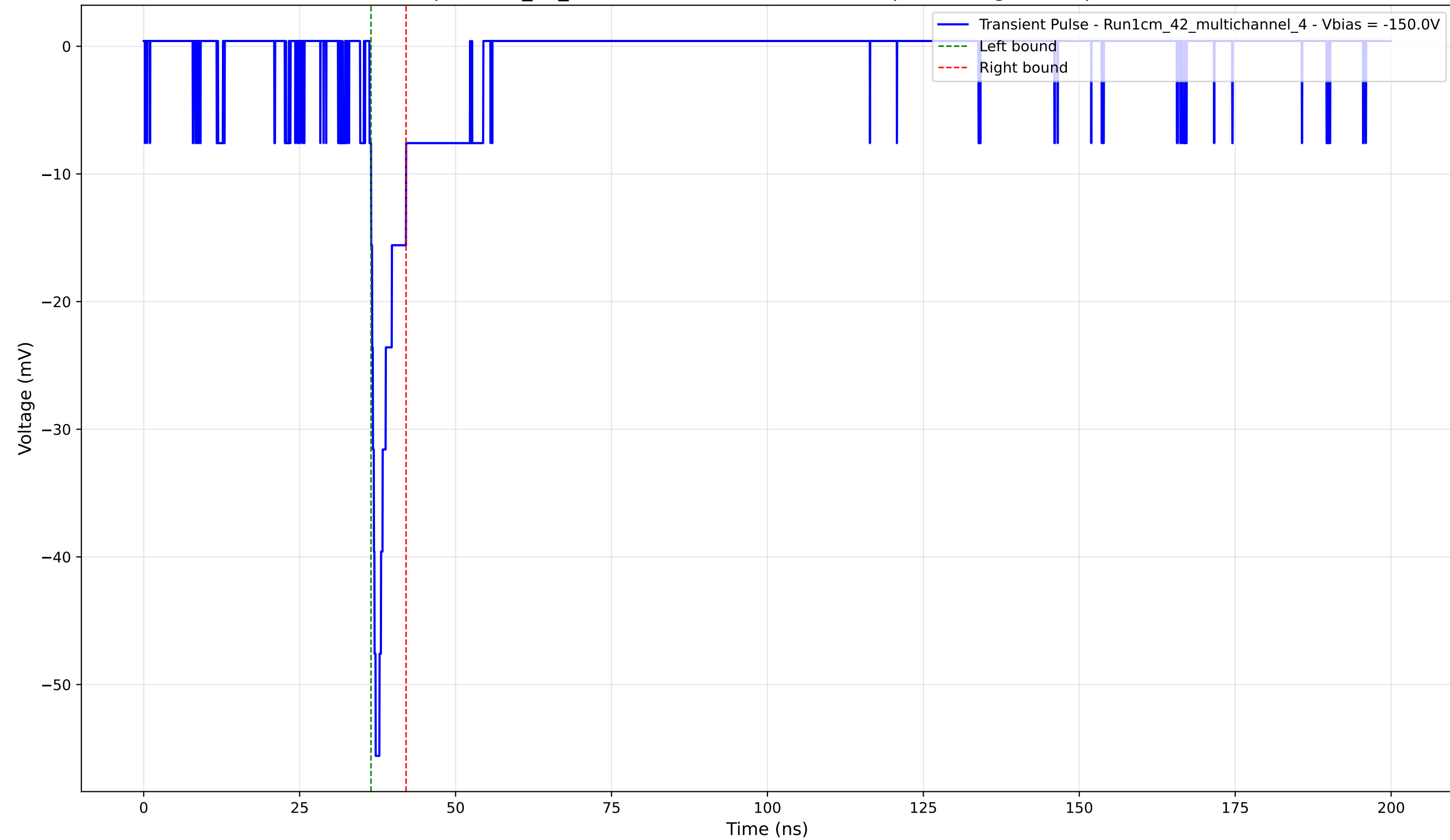
Transient Pulse - Sample: 1cm_42_multichannel - Position: 2025.0 \mu\text{m} - Charge: 3.07 pC - Rise Time: 0.99 ns
