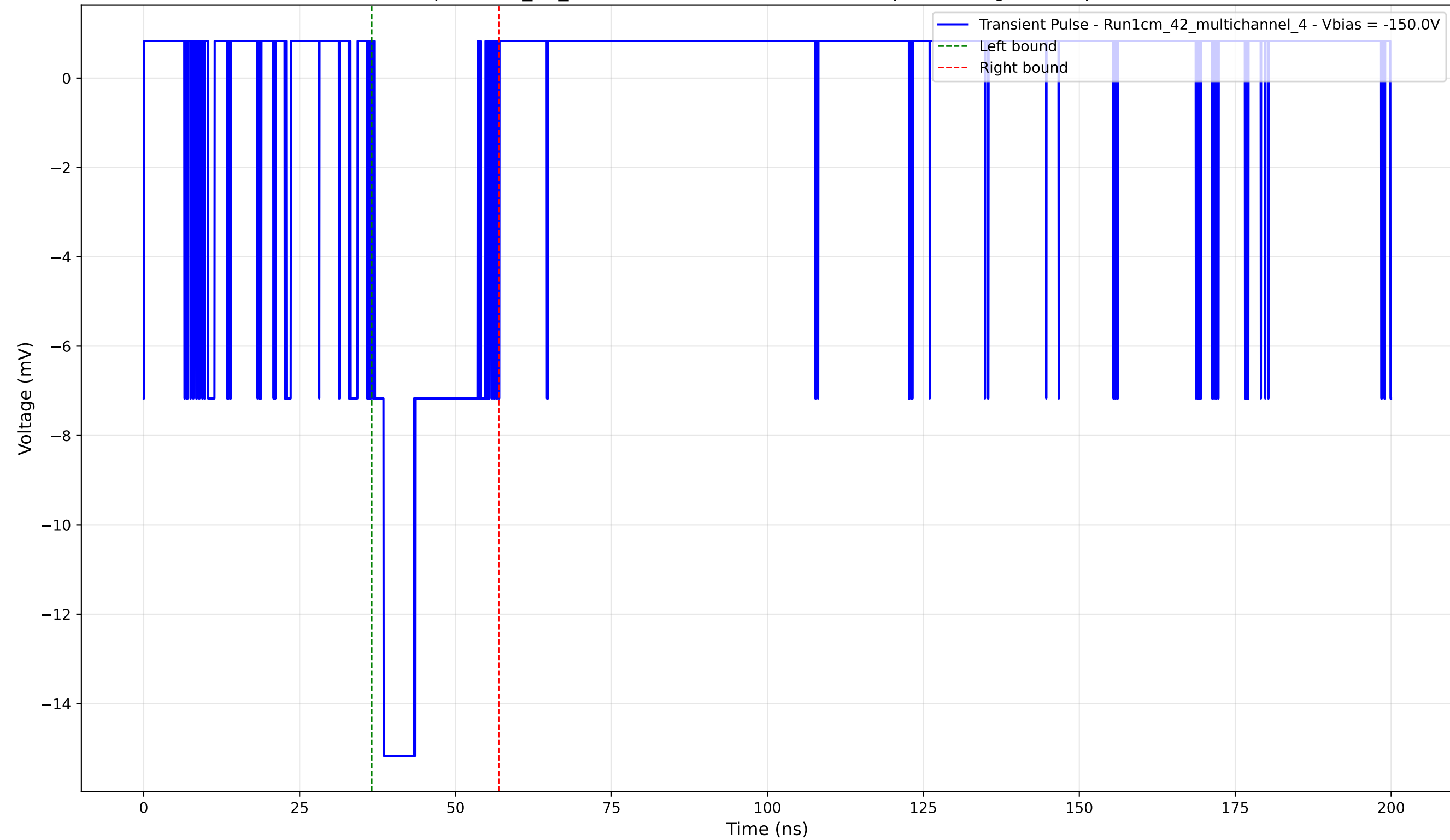
Transient Pulse - Sample: 1cm_42_multichannel - Position: 4500.0 \mu\text{m} - Charge: 3.43 pC - Rise Time: 1.42 ns
