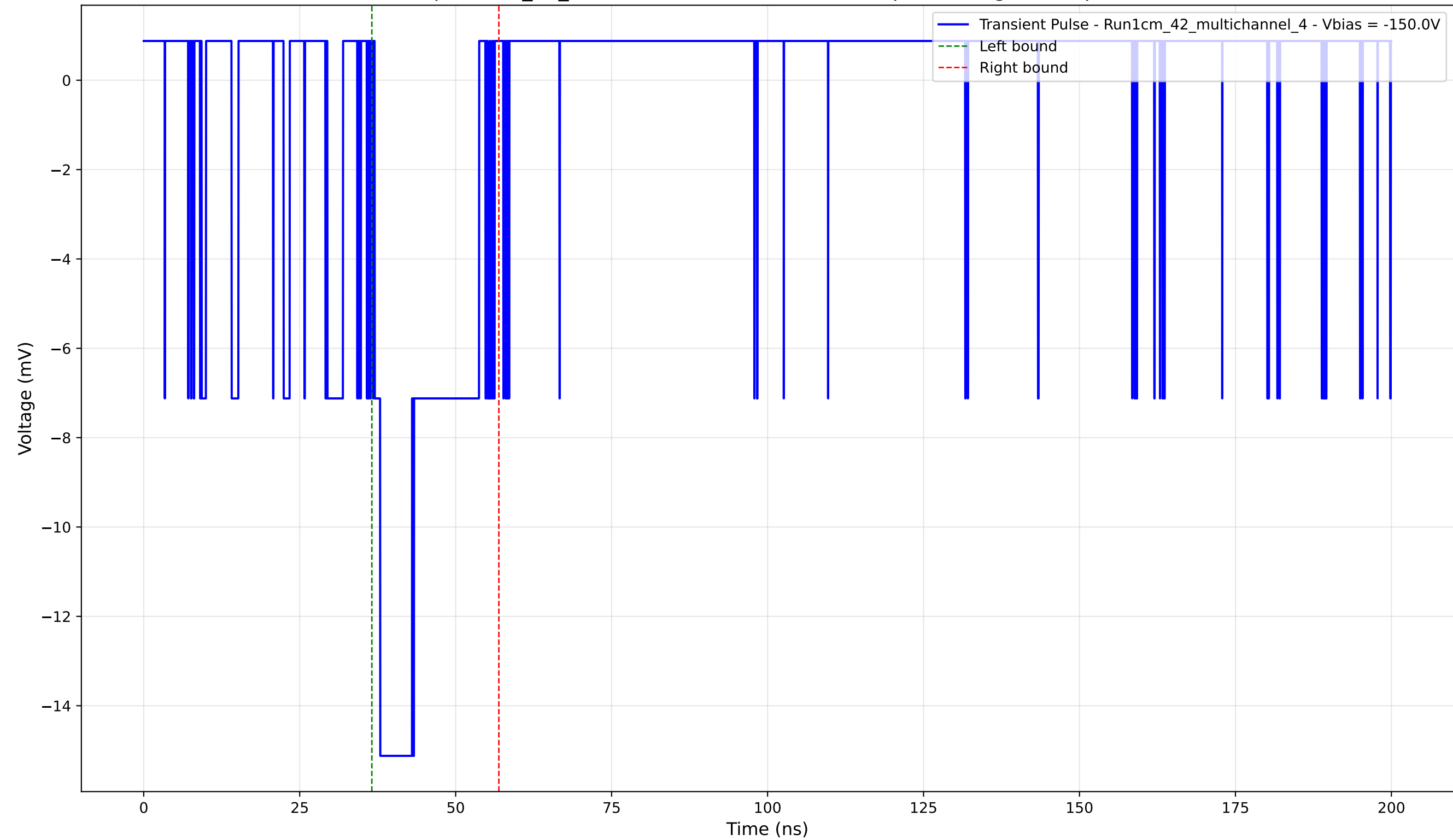
Transient Pulse - Sample: 1cm_42_multichannel - Position: 4015.0 \mu\text{m} - Charge: 3.31 pC - Rise Time: 0.90 ns
