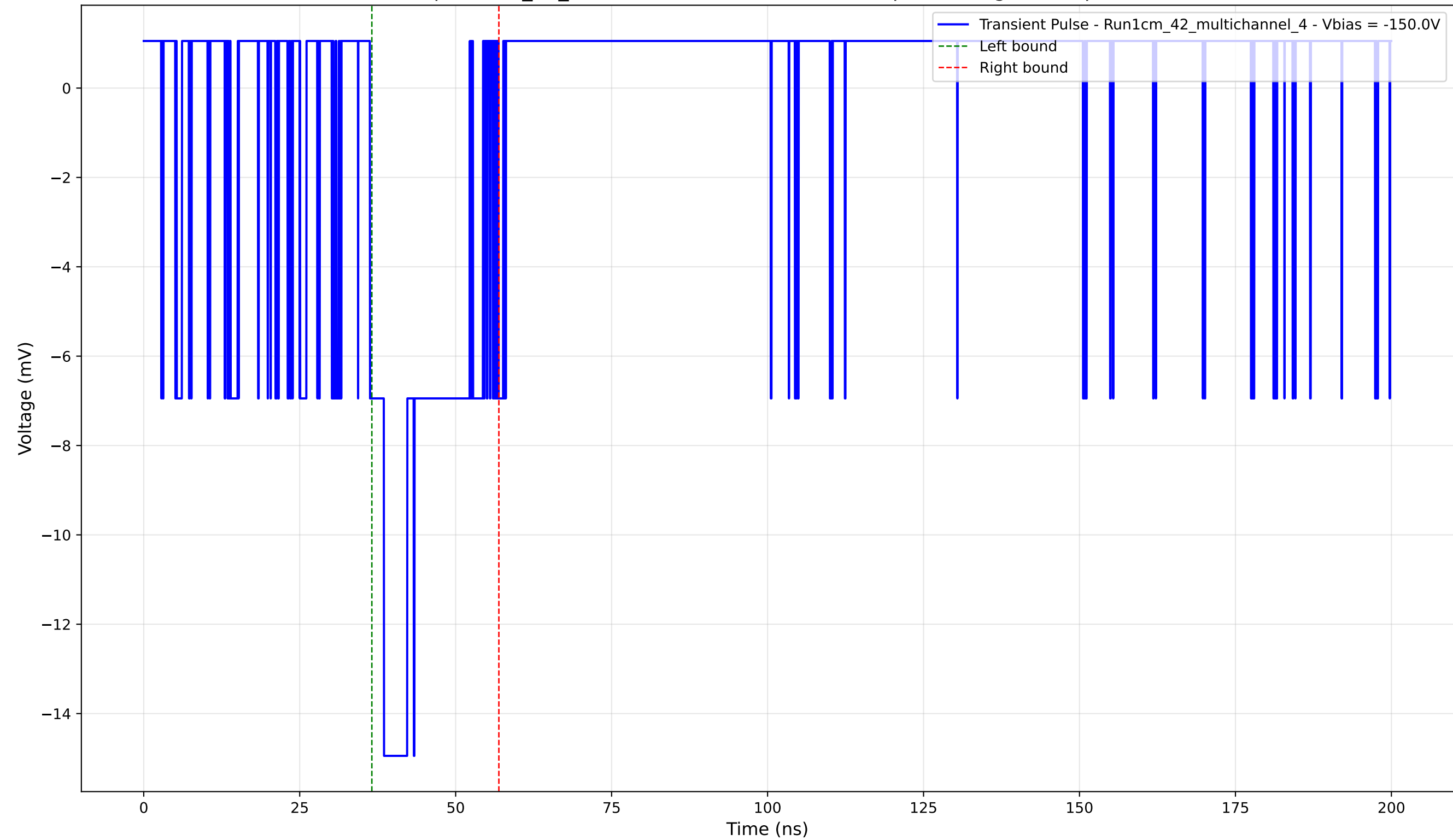
Transient Pulse - Sample: 1cm_42_multichannel - Position: 4650.0 \mu\text{m} - Charge: 3.16 pC - Rise Time: 2.26 ns
