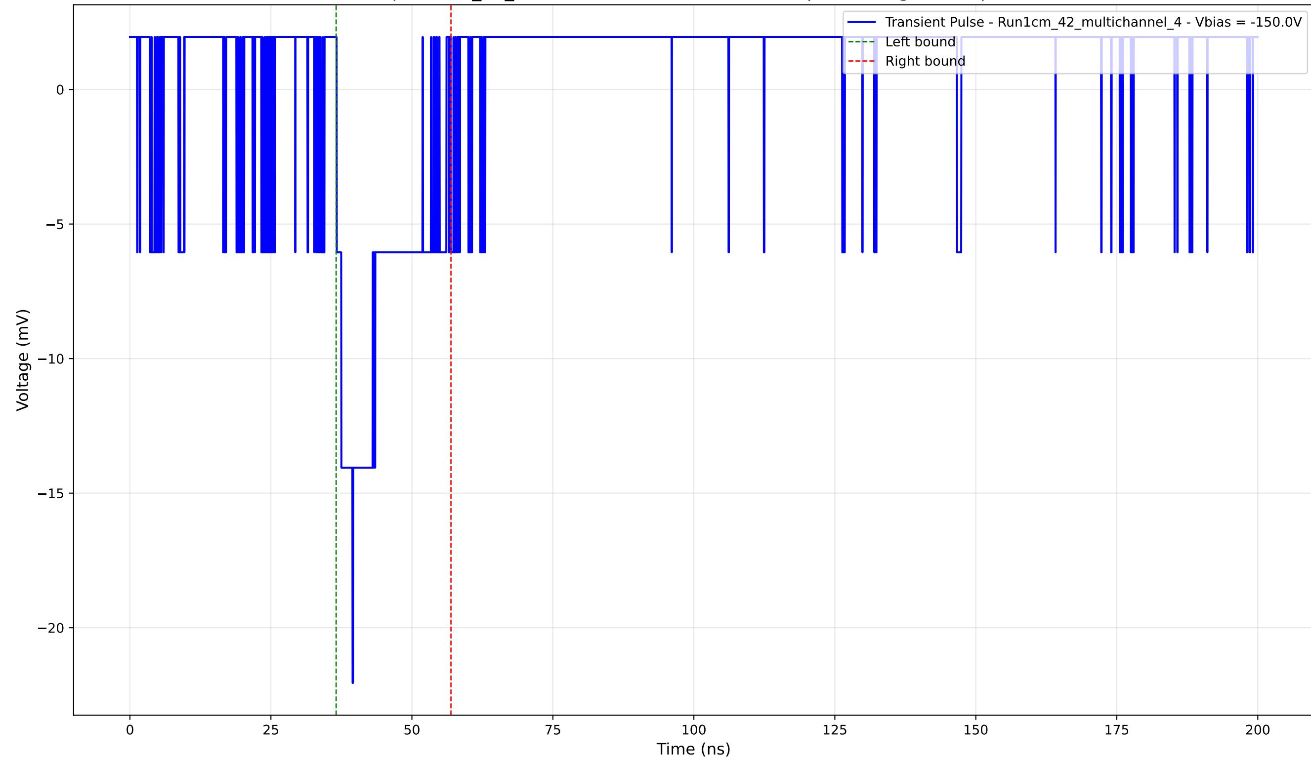
Transient Pulse - Sample: 1cm_42_multichannel - Position: 3690.0 \mu\text{m} - Charge: 3.17 pC - Rise Time: 2.82 ns
