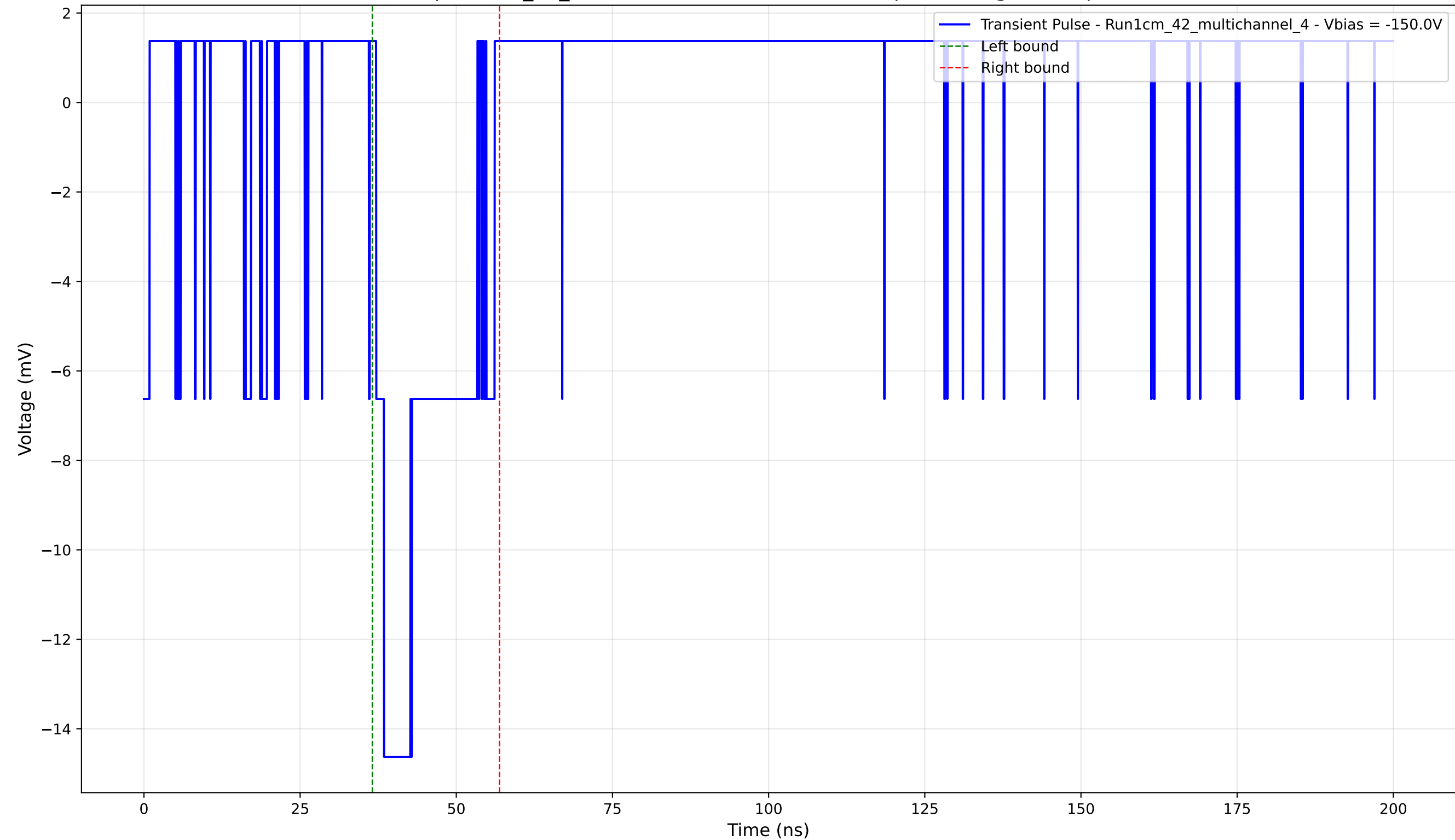
Transient Pulse - Sample: 1cm_42_multichannel - Position: 4230.0 \mu\text{m} - Charge: 3.02 pC - Rise Time: 1.26 ns
