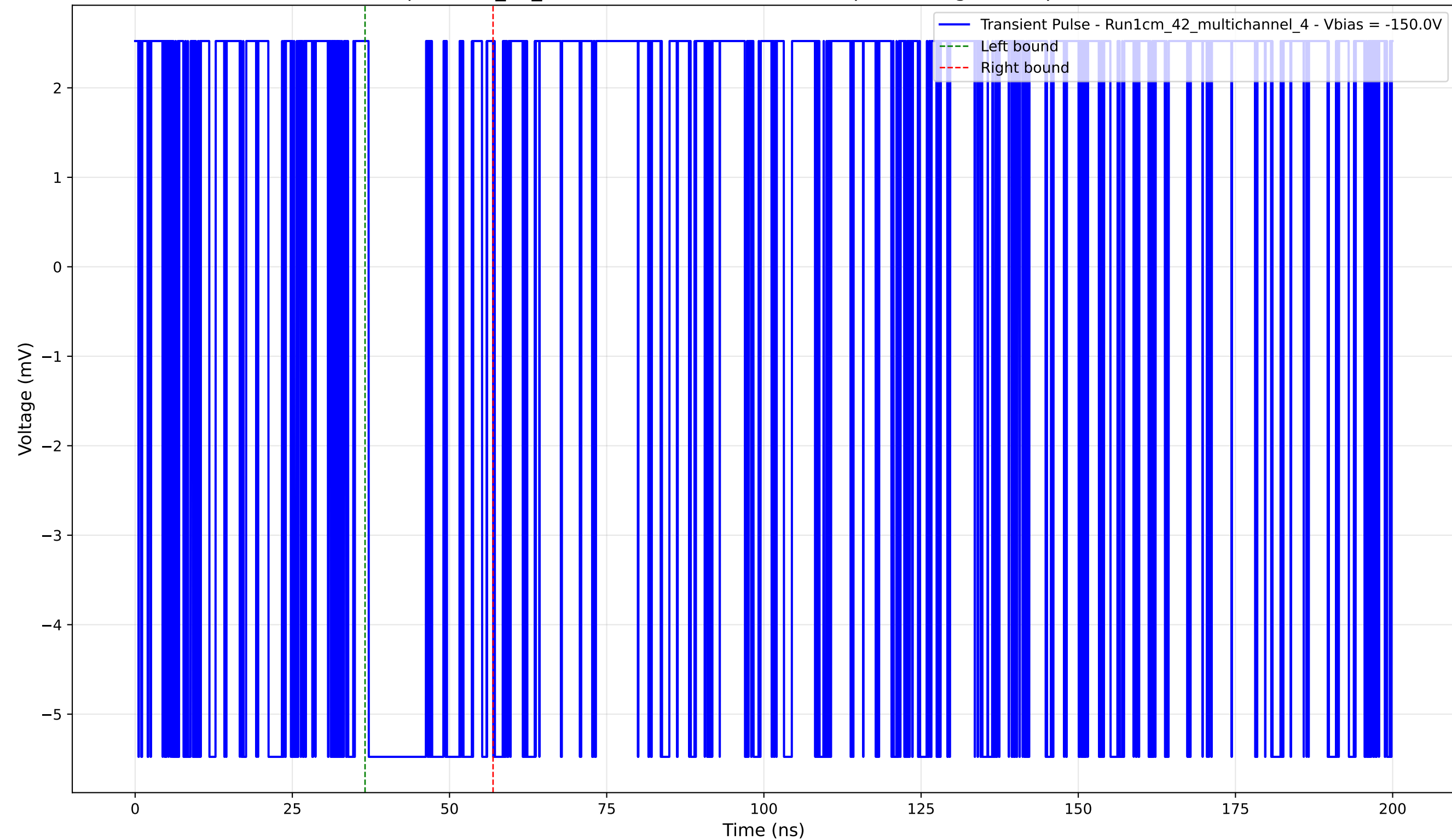
Transient Pulse - Sample: 1cm_42_multichannel - Position: 400.0 \mu\text{m} - Charge: 1.51 pC - Rise Time: 0.00 ns (N/A)
