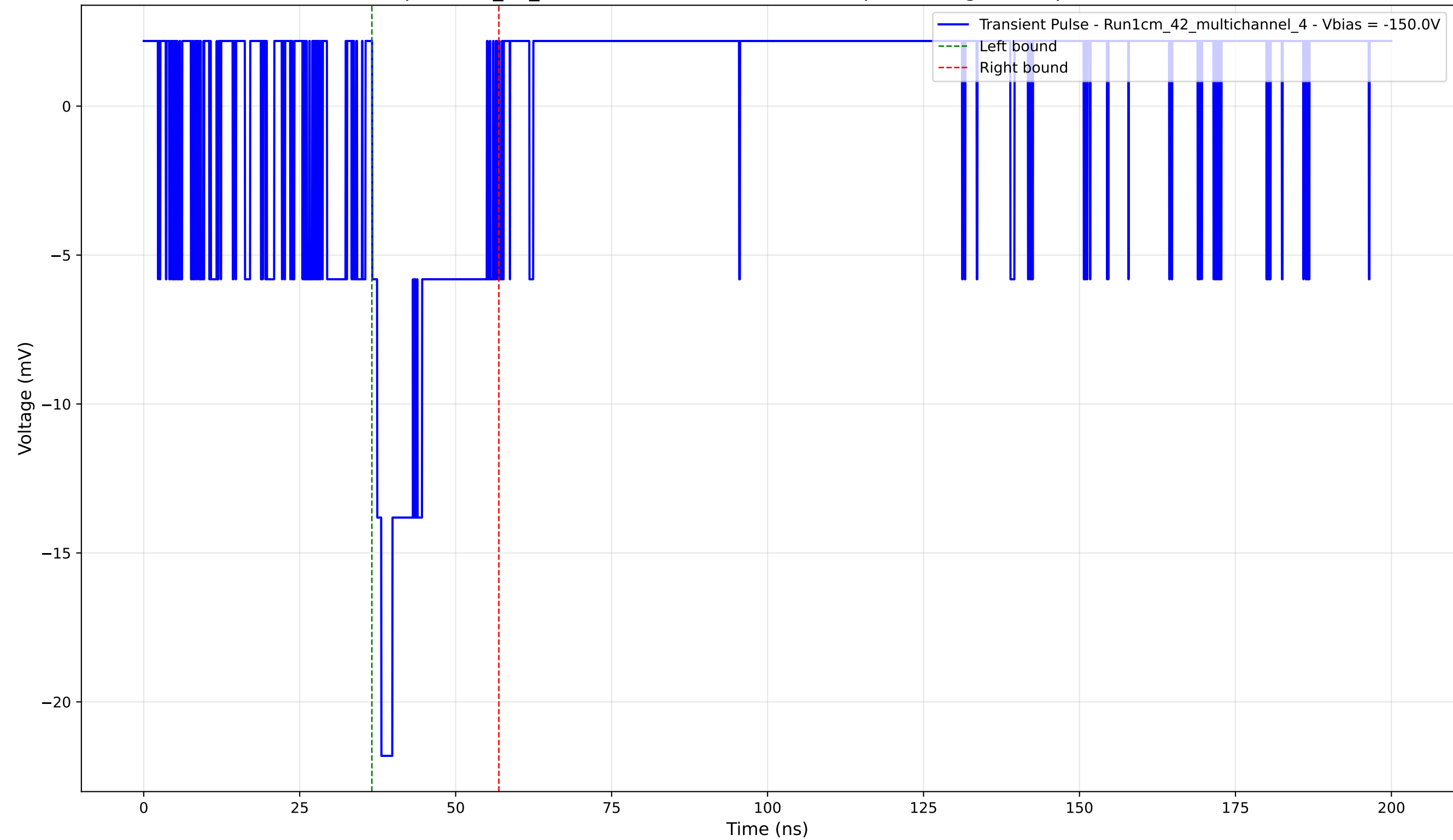
Transient Pulse - Sample: 1cm_42_multichannel - Position: 1065.0 \mu\text{m} - Charge: 3.67 pC - Rise Time: 0.00 ns (N/A)
