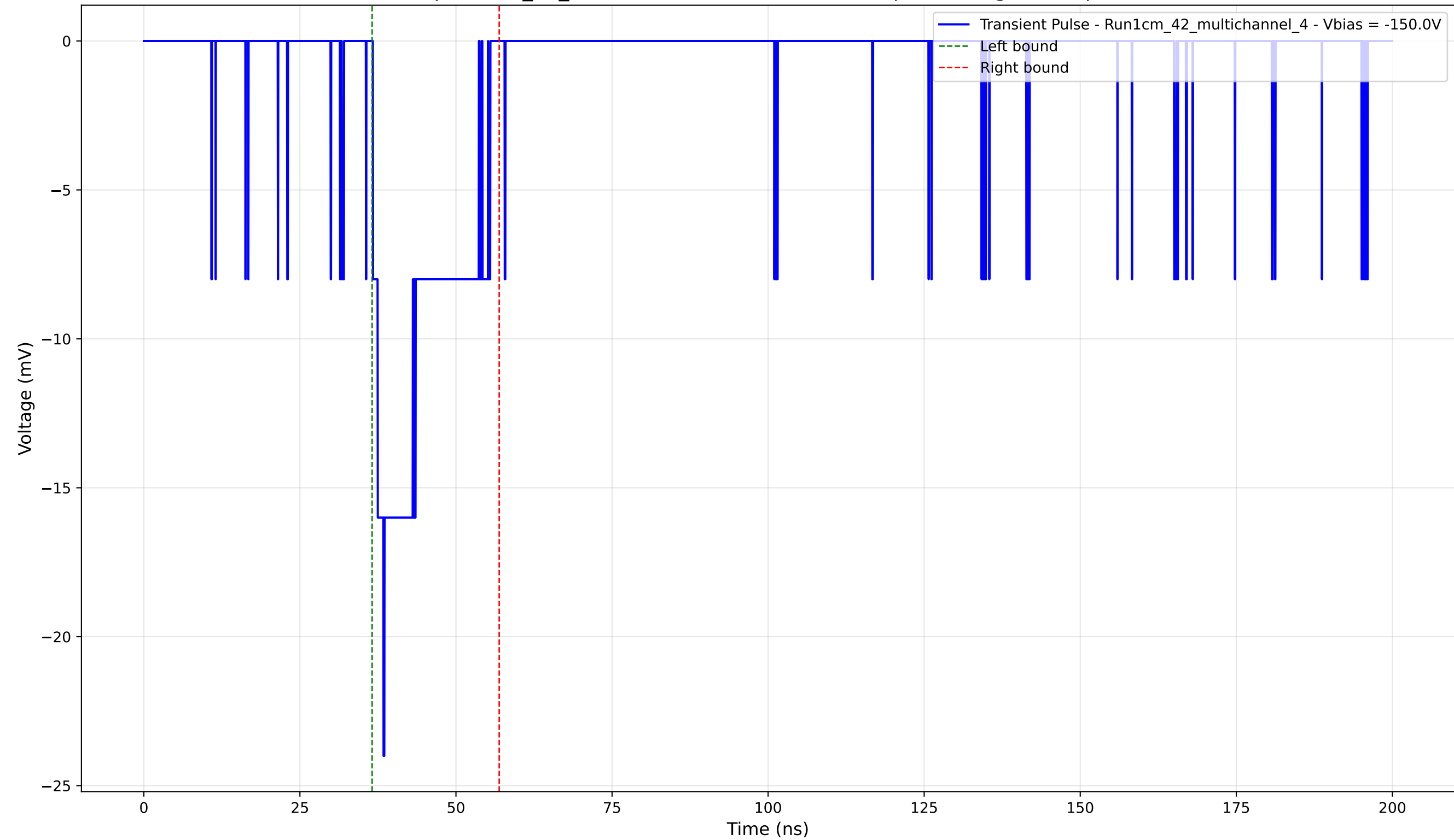
Transient Pulse - Sample: 1cm_42_multichannel - Position: 3660.0 \mu\text{m} - Charge: 3.94 pC - Rise Time: 1.69 ns
