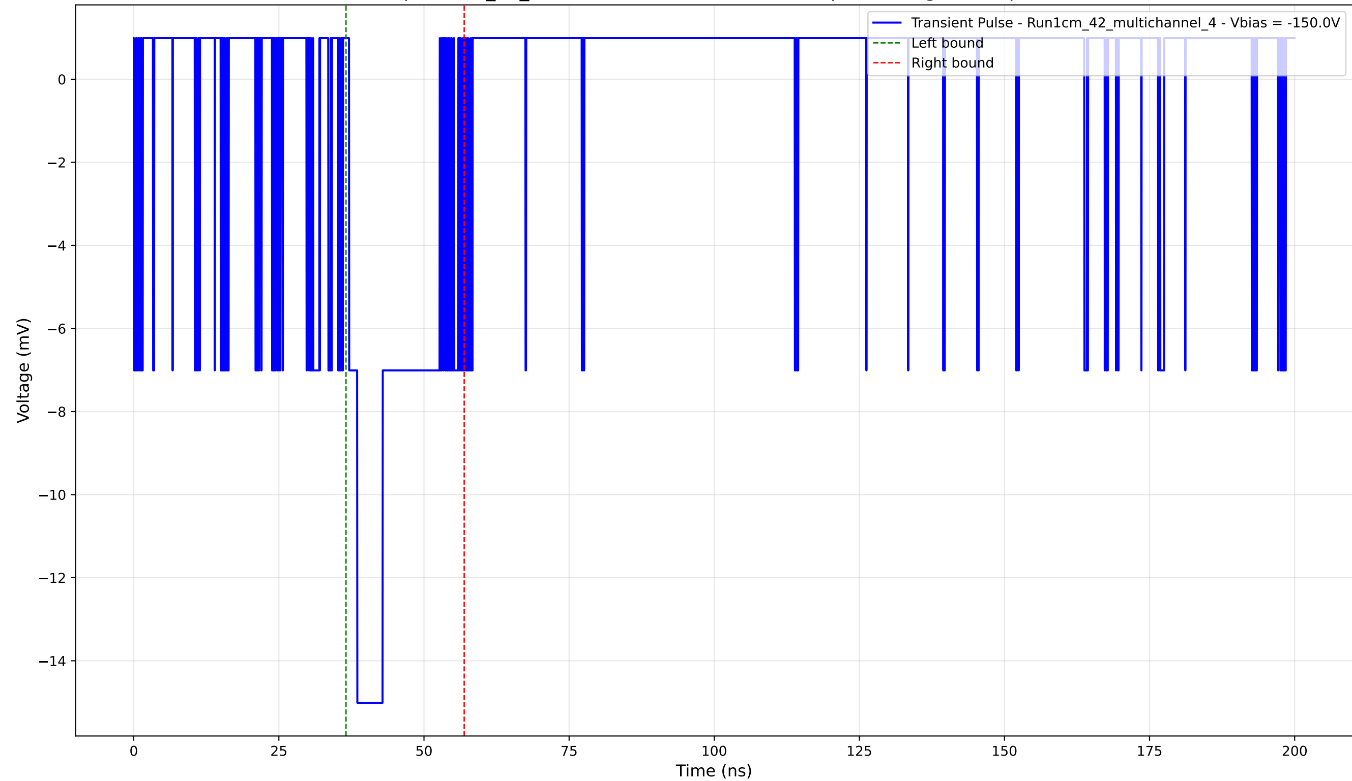
Transient Pulse - Sample: 1cm_42_multichannel - Position: 4315.0 \mu\text{m} - Charge: 3.22 pC - Rise Time: 1.42 ns
