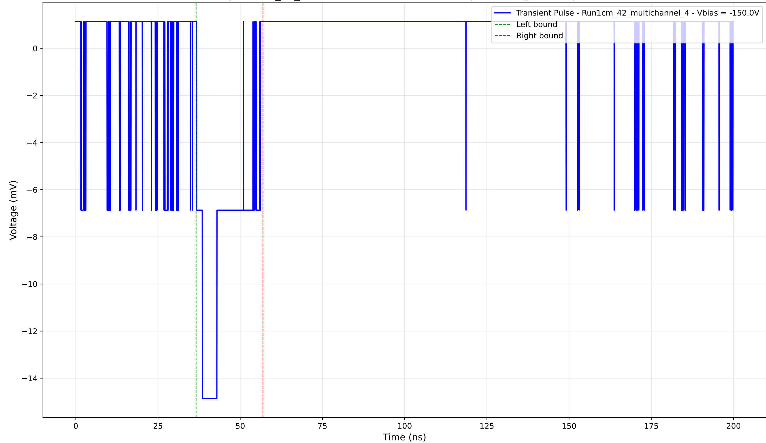
Transient Pulse - Sample: 1cm_42_multichannel - Position: 4560.0 \mu\text{m} - Charge: 3.26 pC - Rise Time: 1.72 ns
