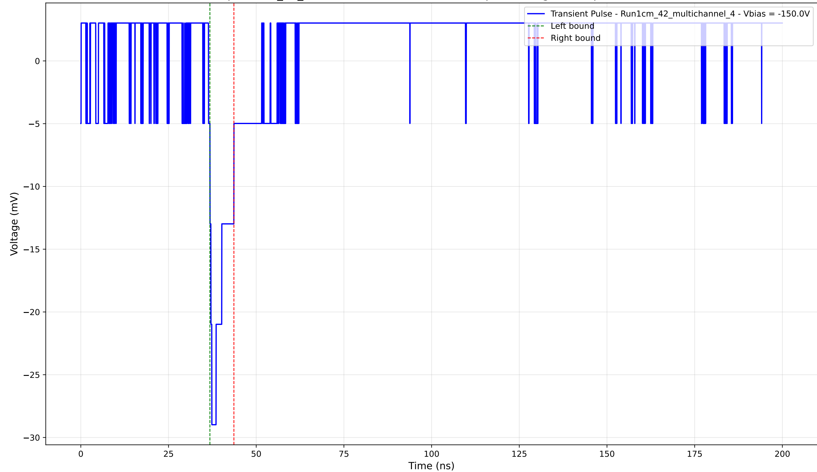
Transient Pulse - Sample: 1cm_42_multichannel - Position: 1605.0 \mu\text{m} - Charge: 2.46 pC - Rise Time: 0.00 ns (N/A)
