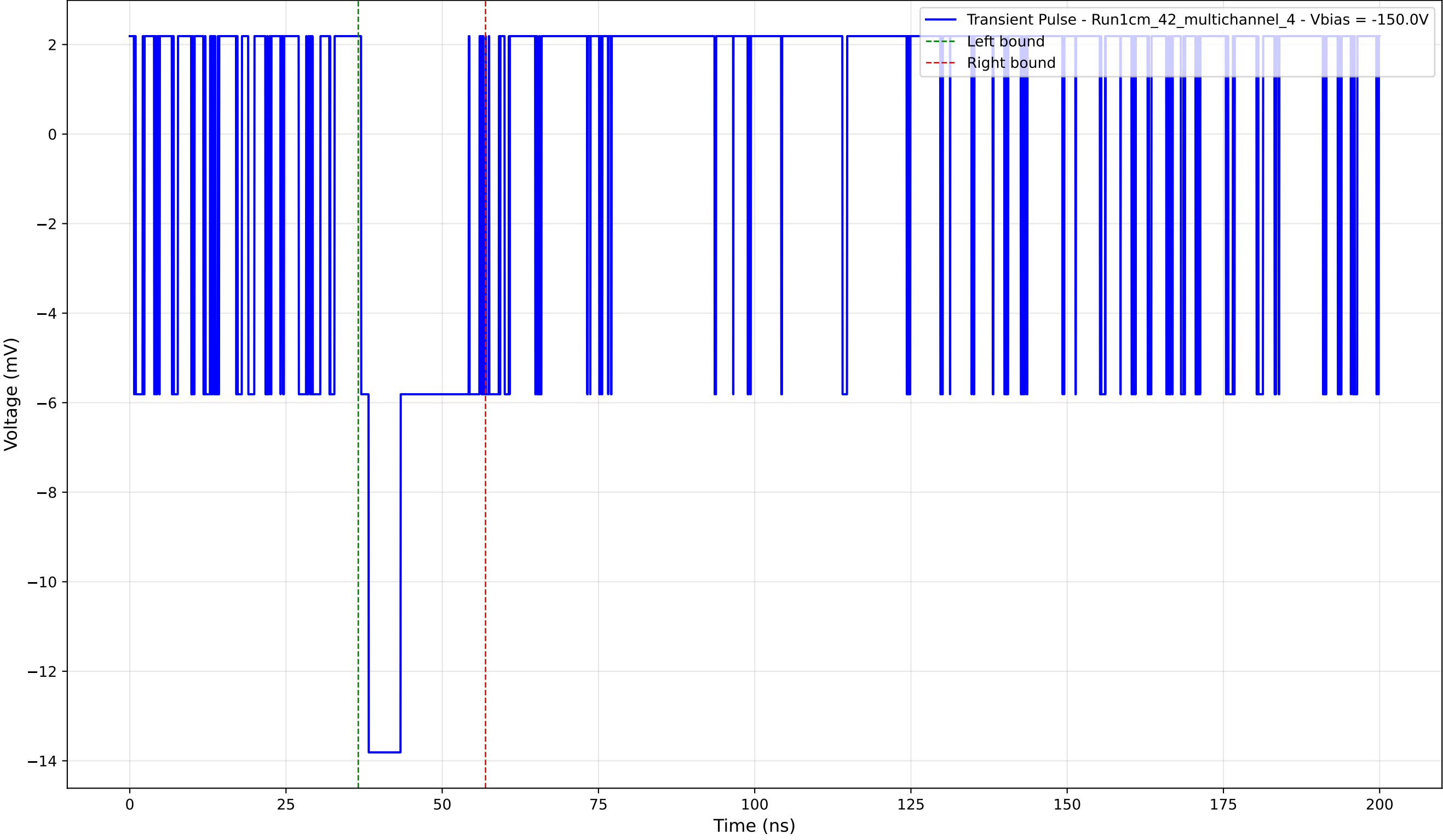
Transient Pulse - Sample: 1cm_42_multichannel - Position: 250.0 \mu\text{m} - Charge: 3.02 pC - Rise Time: 0.00 ns (N/A)
