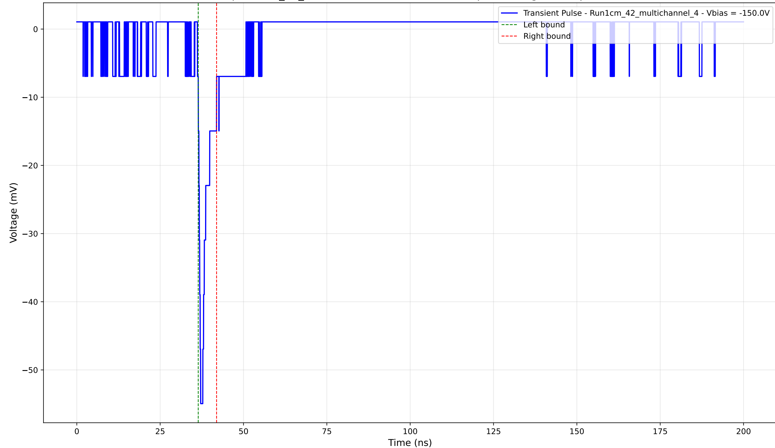
Transient Pulse - Sample: 1cm_42_multichannel - Position: 2045.0 \mu\text{m} - Charge: 2.96 pC - Rise Time: 0.96 ns
