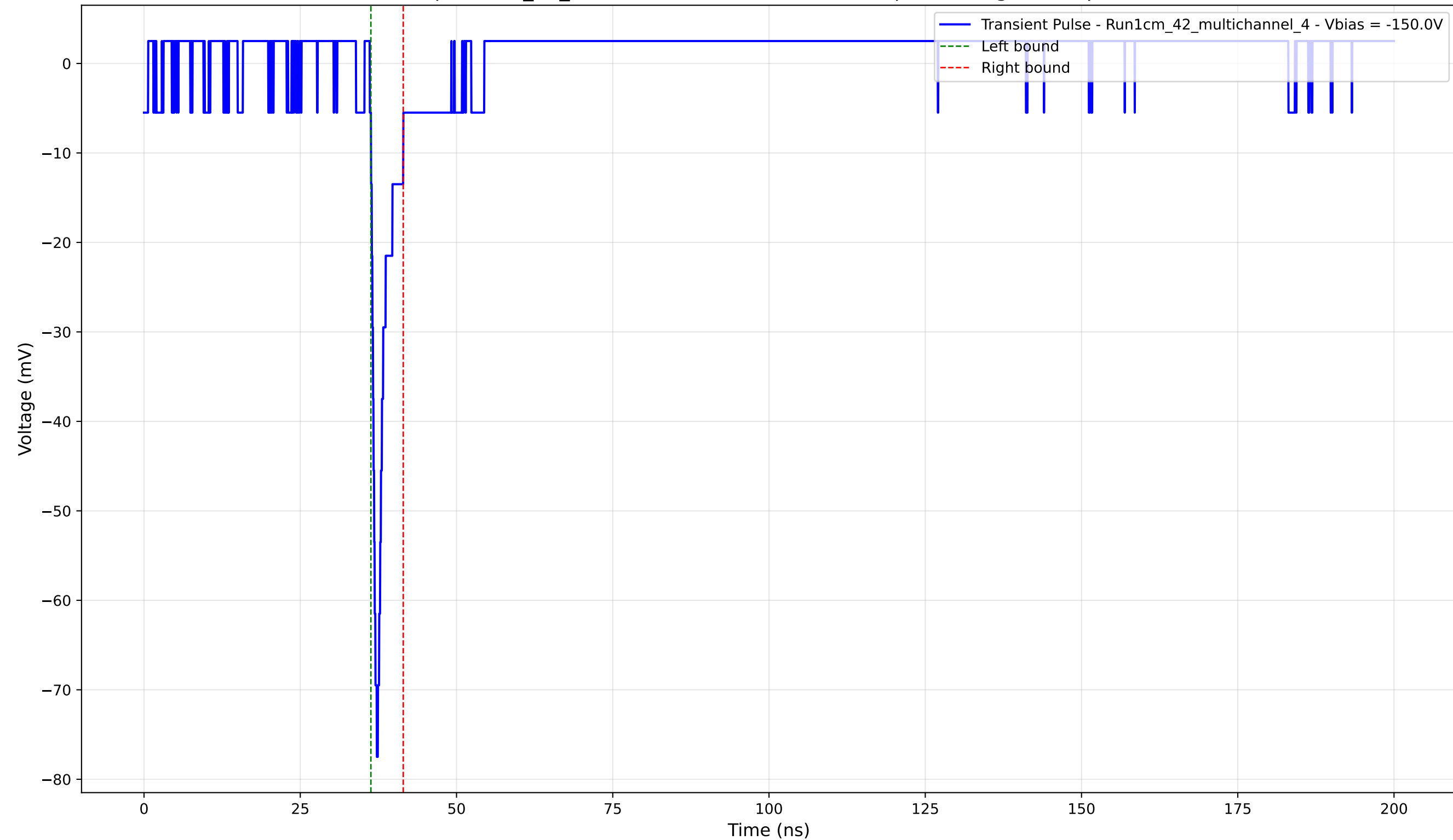
Transient Pulse - Sample: 1cm_42_multichannel - Position: 2210.0 \mu\text{m} - Charge: 3.17 pC - Rise Time: 0.93 ns
