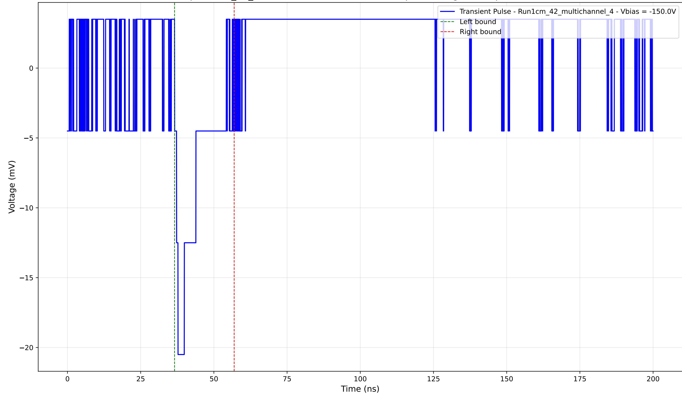
Transient Pulse - Sample: 1cm_42_multichannel - Position: 1195.0 \mu\text{m} - Charge: 3.03 pC - Rise Time: 0.00 ns (N/A)
