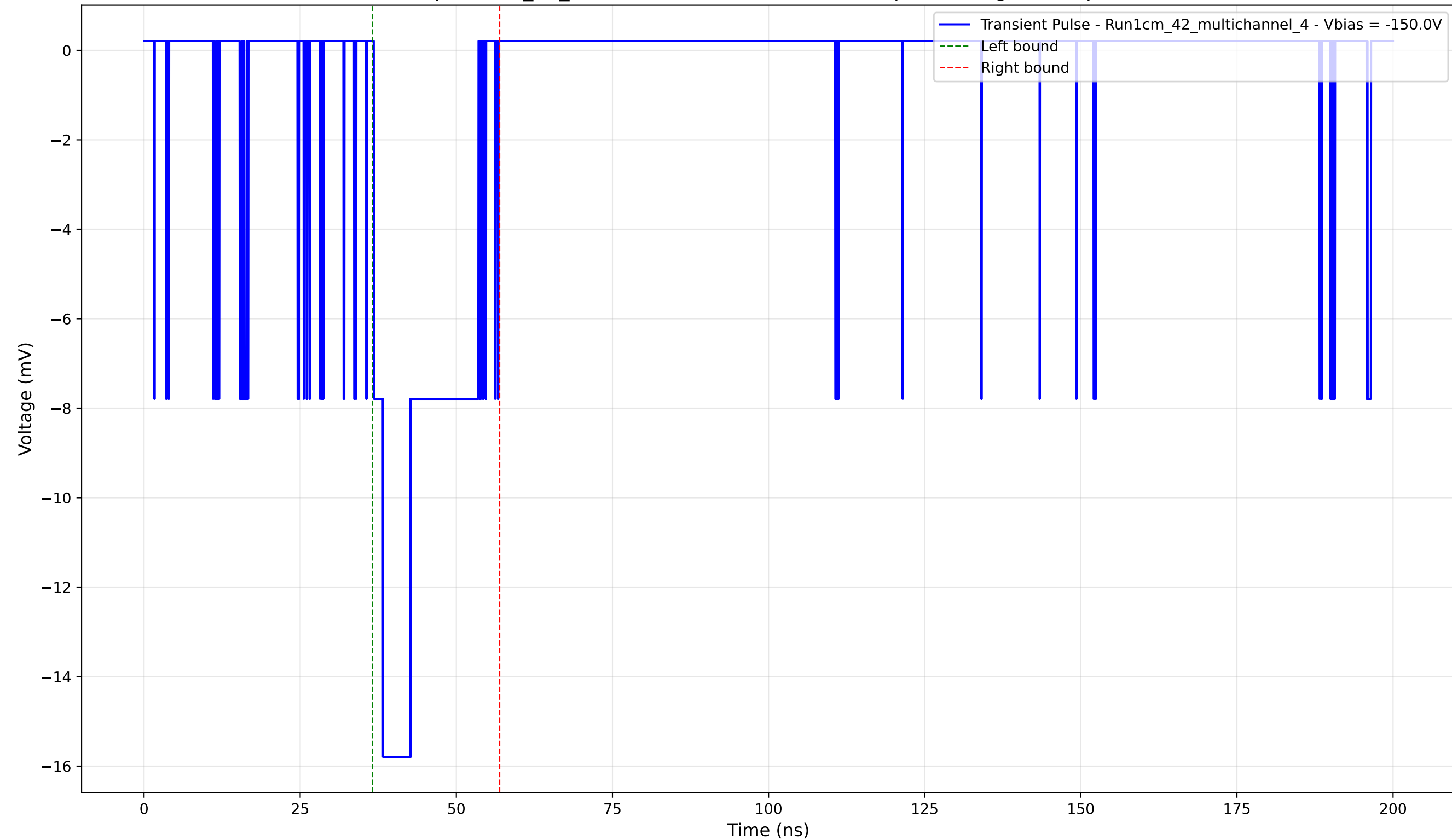
Transient Pulse - Sample: 1cm_42_multichannel - Position: 4100.0 \mu\text{m} - Charge: 3.41 pC - Rise Time: 1.46 ns
