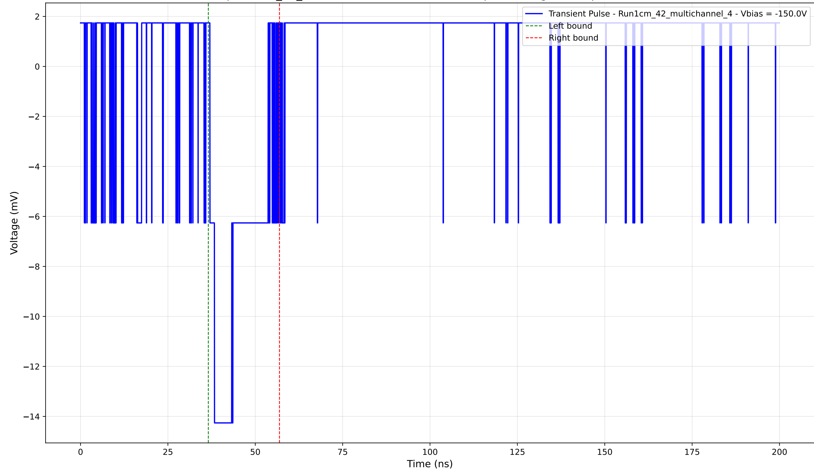
Transient Pulse - Sample: 1cm_42_multichannel - Position: 4290.0 \mu\text{m} - Charge: 2.99 pC - Rise Time: 0.00 ns (N/A)
