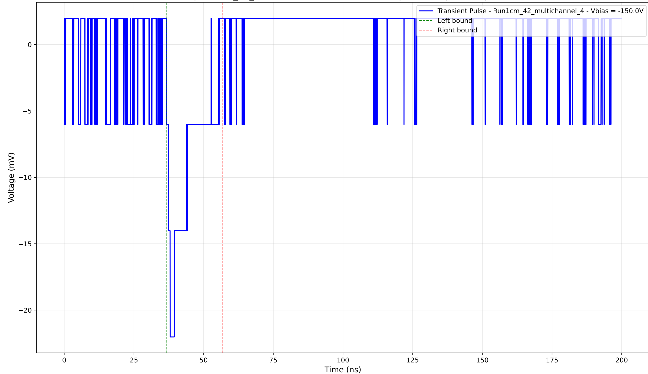
Transient Pulse - Sample: 1cm_42_multichannel - Position: 1100.0 \mu\text{m} - Charge: 3.47 pC - Rise Time: 1.24 ns
