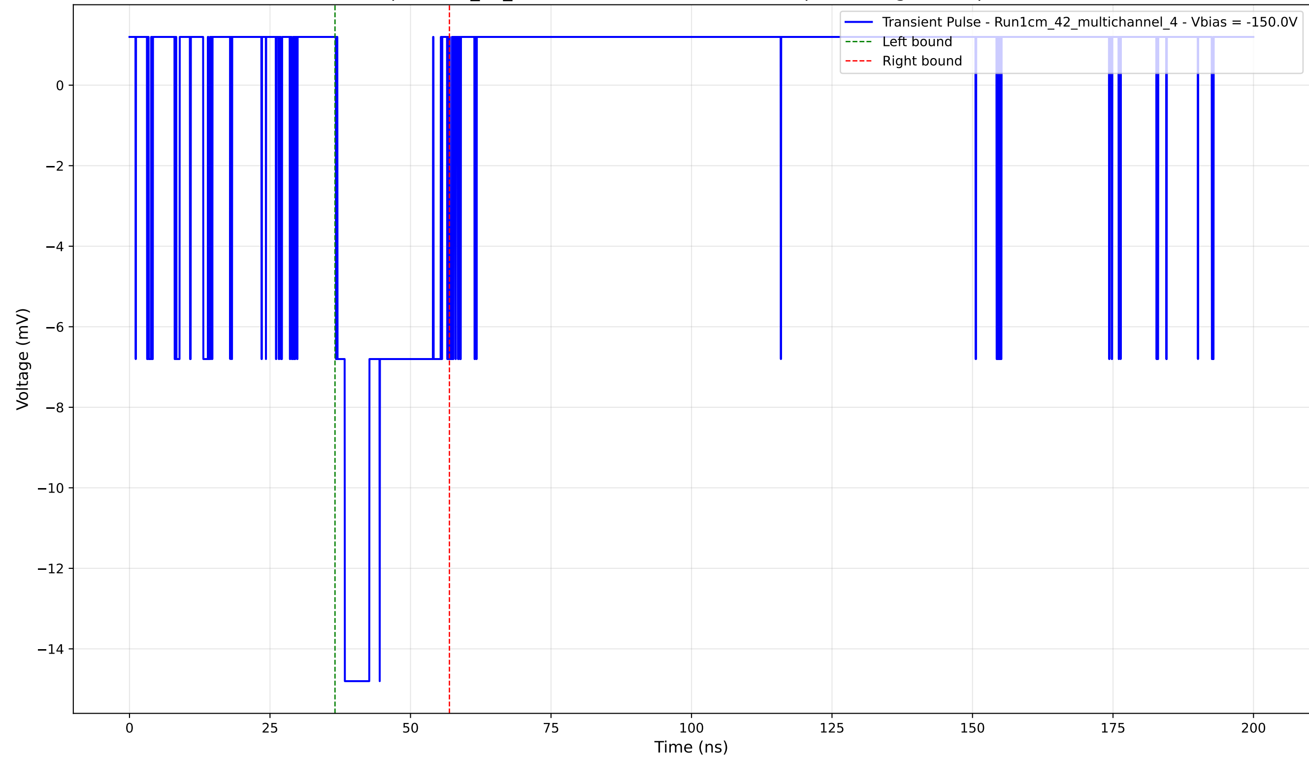
Transient Pulse - Sample: 1cm_42_multichannel - Position: 4210.0 \mu\text{m} - Charge: 3.24 pC - Rise Time: 1.32 ns
