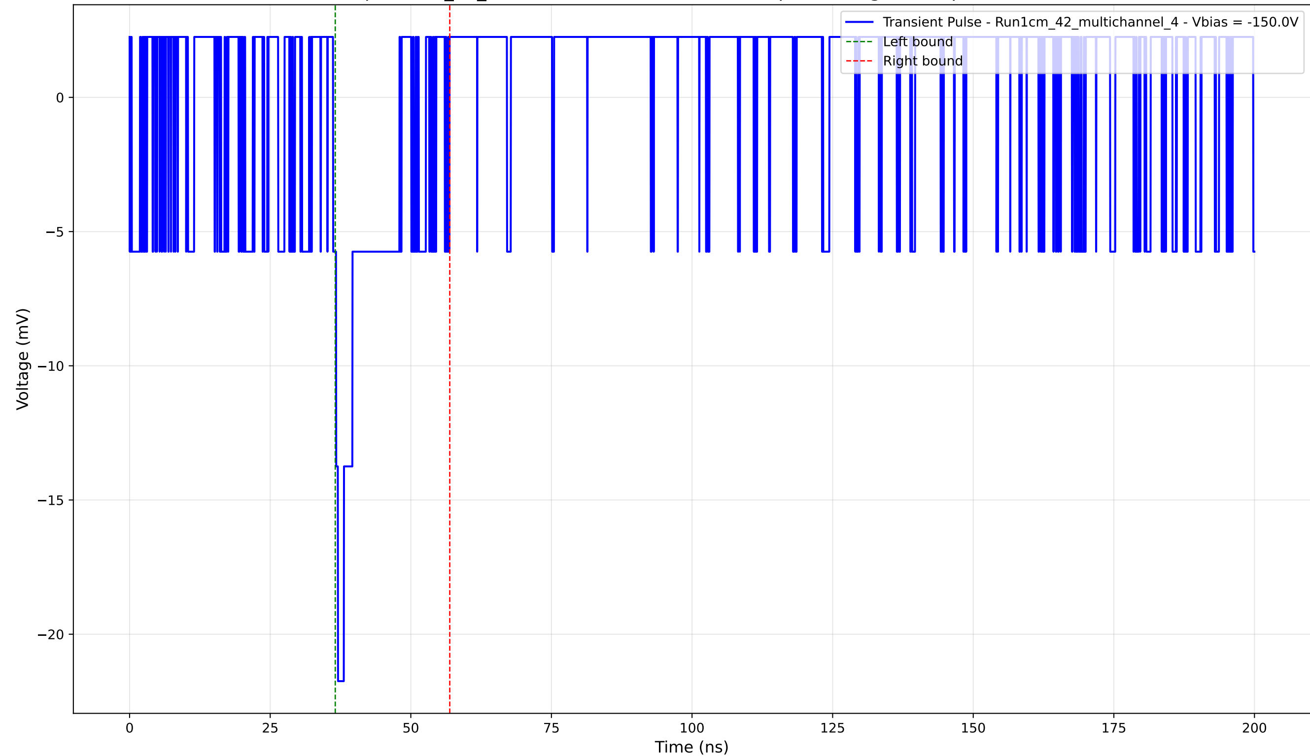
Transient Pulse - Sample: 1cm_42_multichannel - Position: 1930.0 \mu\text{m} - Charge: 2.12 pC - Rise Time: 0.00 ns (N/A)
