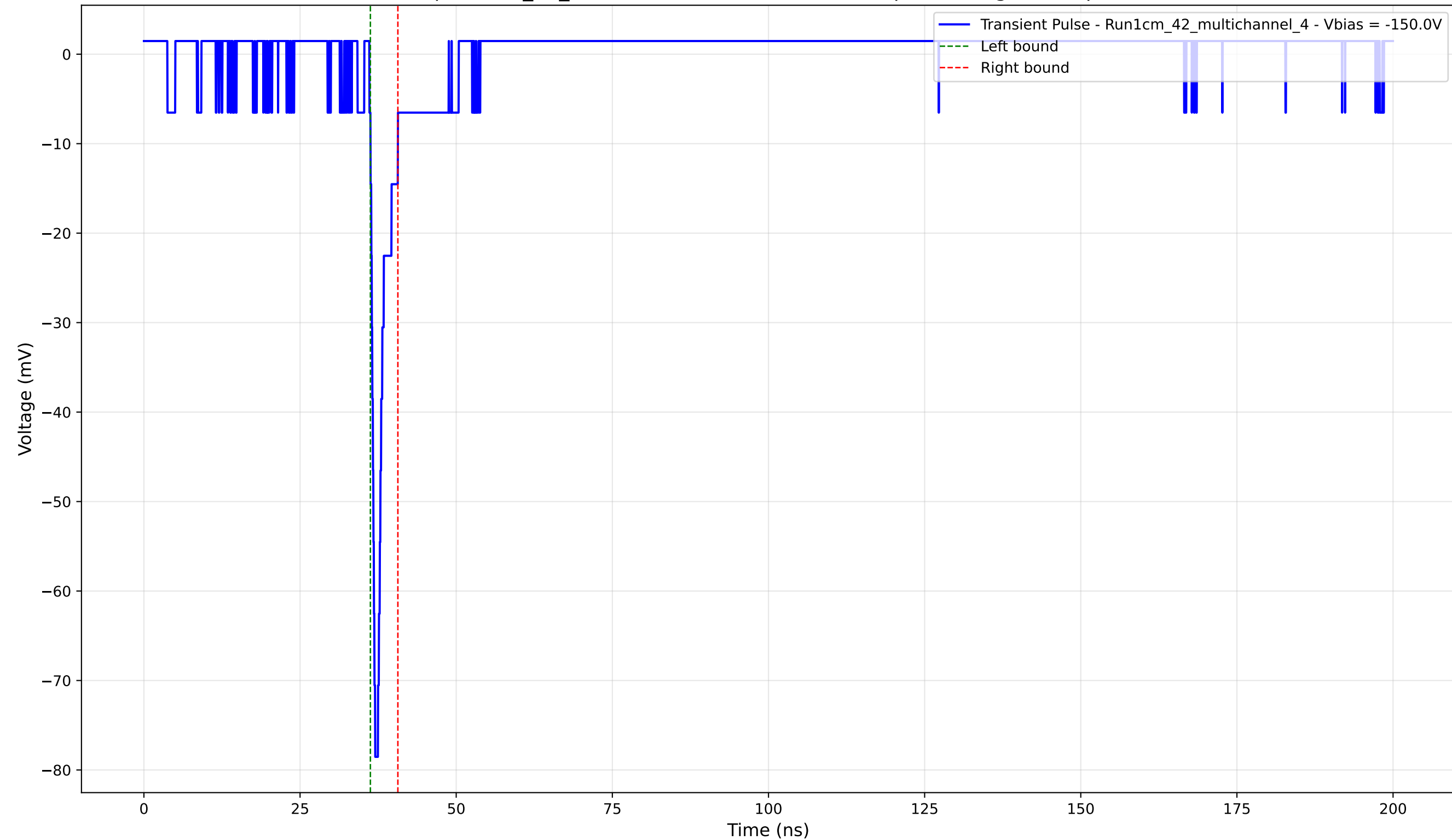
Transient Pulse - Sample: 1cm_42_multichannel - Position: 2290.0 \mu\text{m} - Charge: 3.09 pC - Rise Time: 0.76 ns
