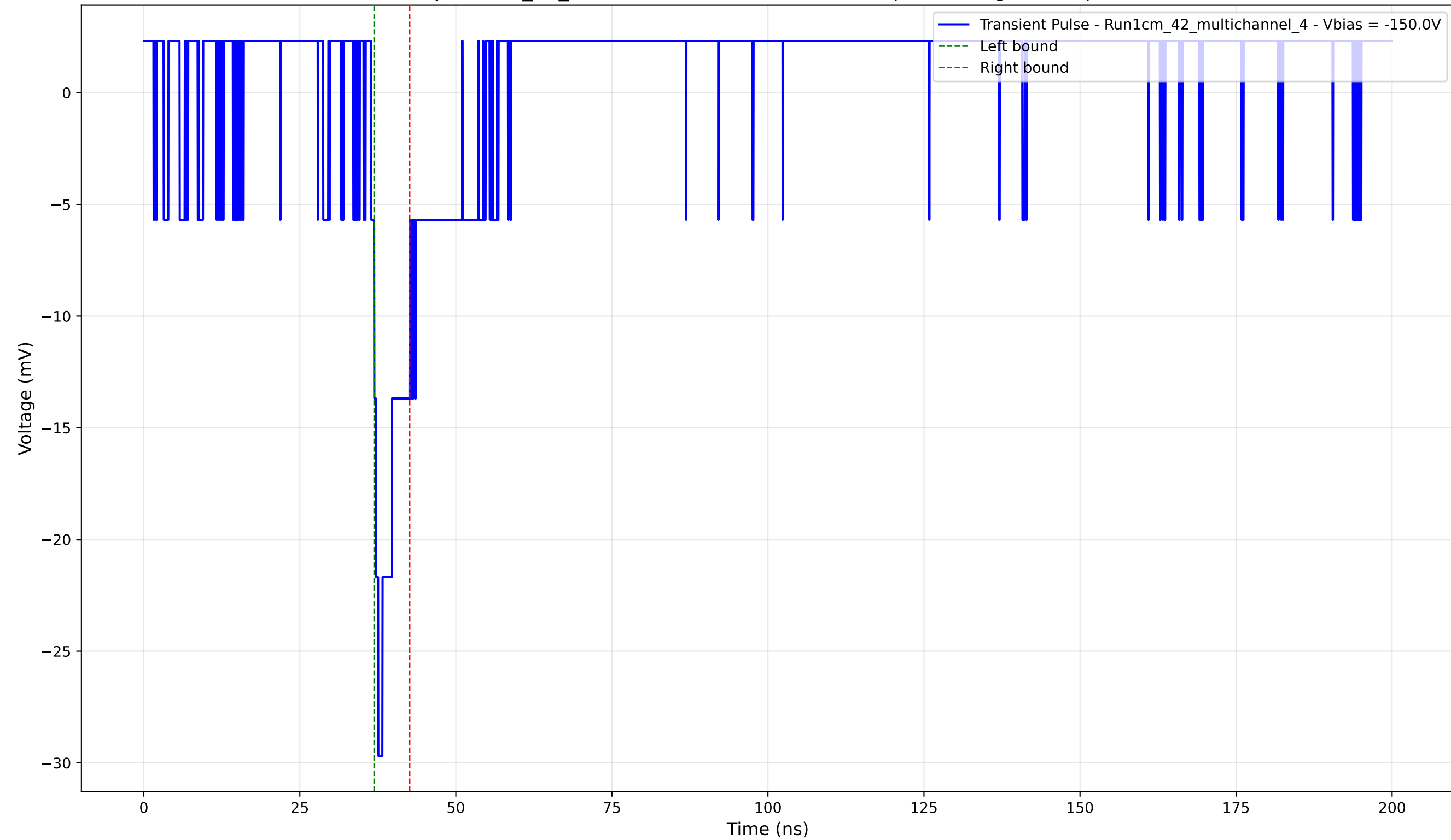
Transient Pulse - Sample: 1cm_42_multichannel - Position: 3225.0 \mu\text{m} - Charge: 2.07 pC - Rise Time: 1.14 ns
