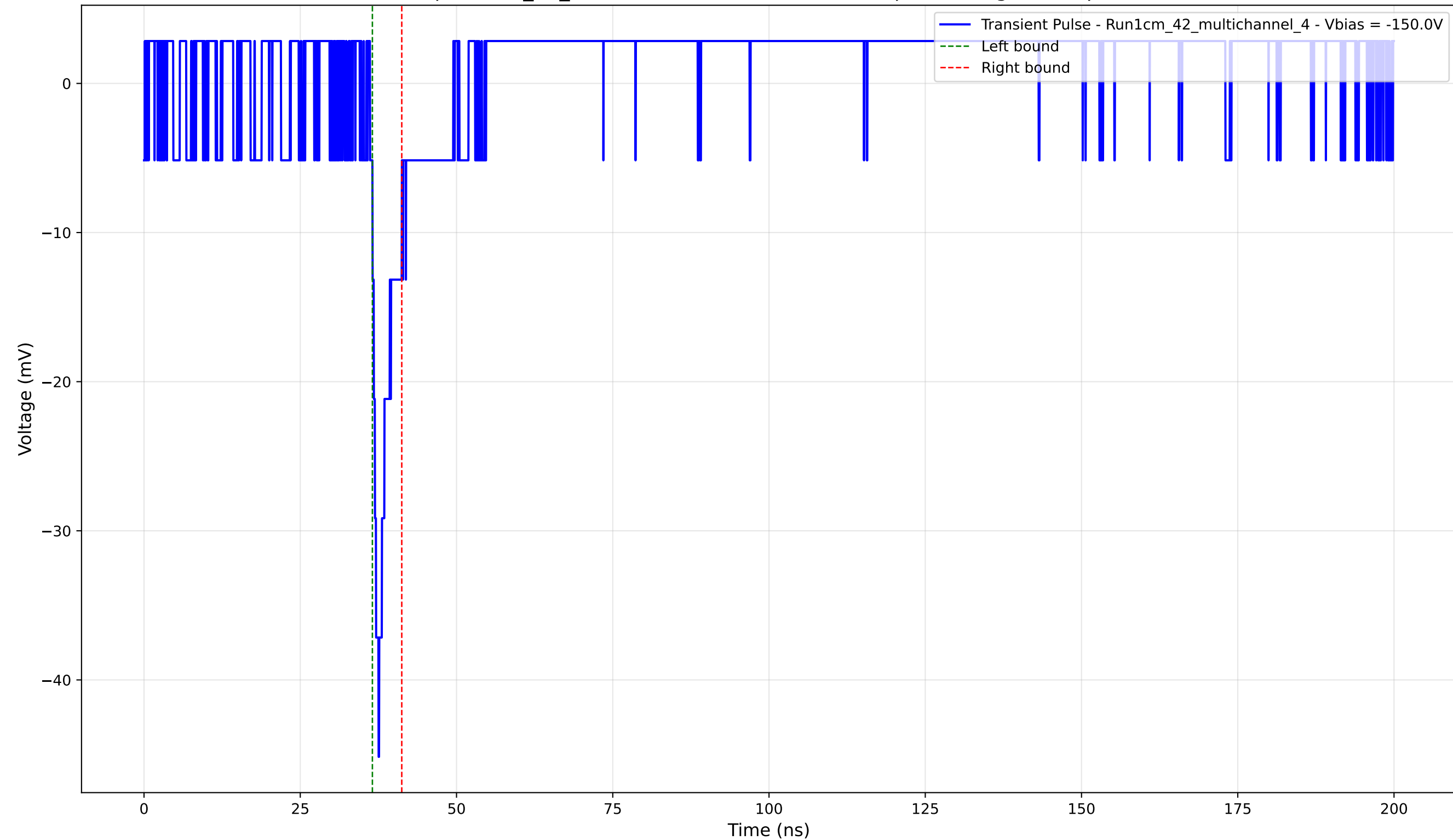
Transient Pulse - Sample: 1cm_42_multichannel - Position: 1945.0 \mu\text{m} - Charge: 2.07 pC - Rise Time: 1.37 ns
