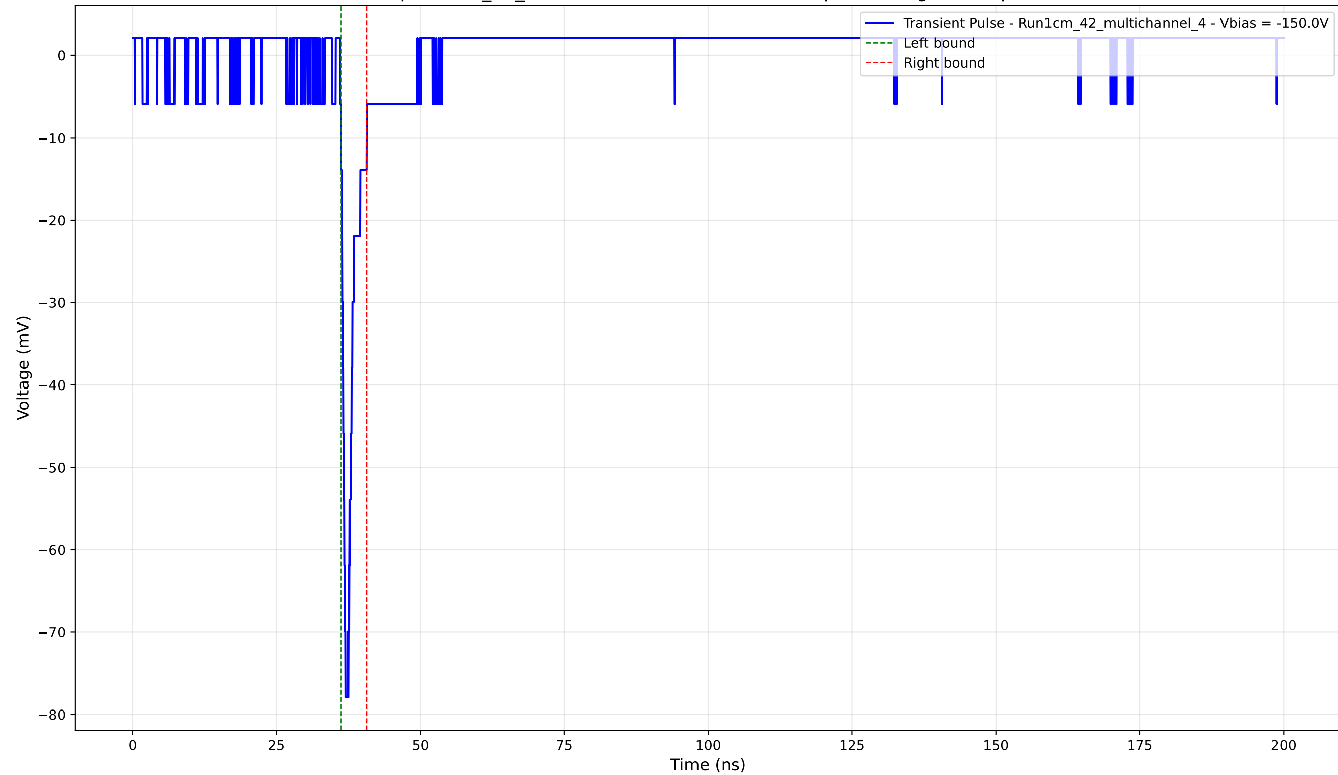
Transient Pulse - Sample: 1cm_42_multichannel - Position: 2285.0 \mu\text{m} - Charge: 3.02 pC - Rise Time: 0.80 ns
