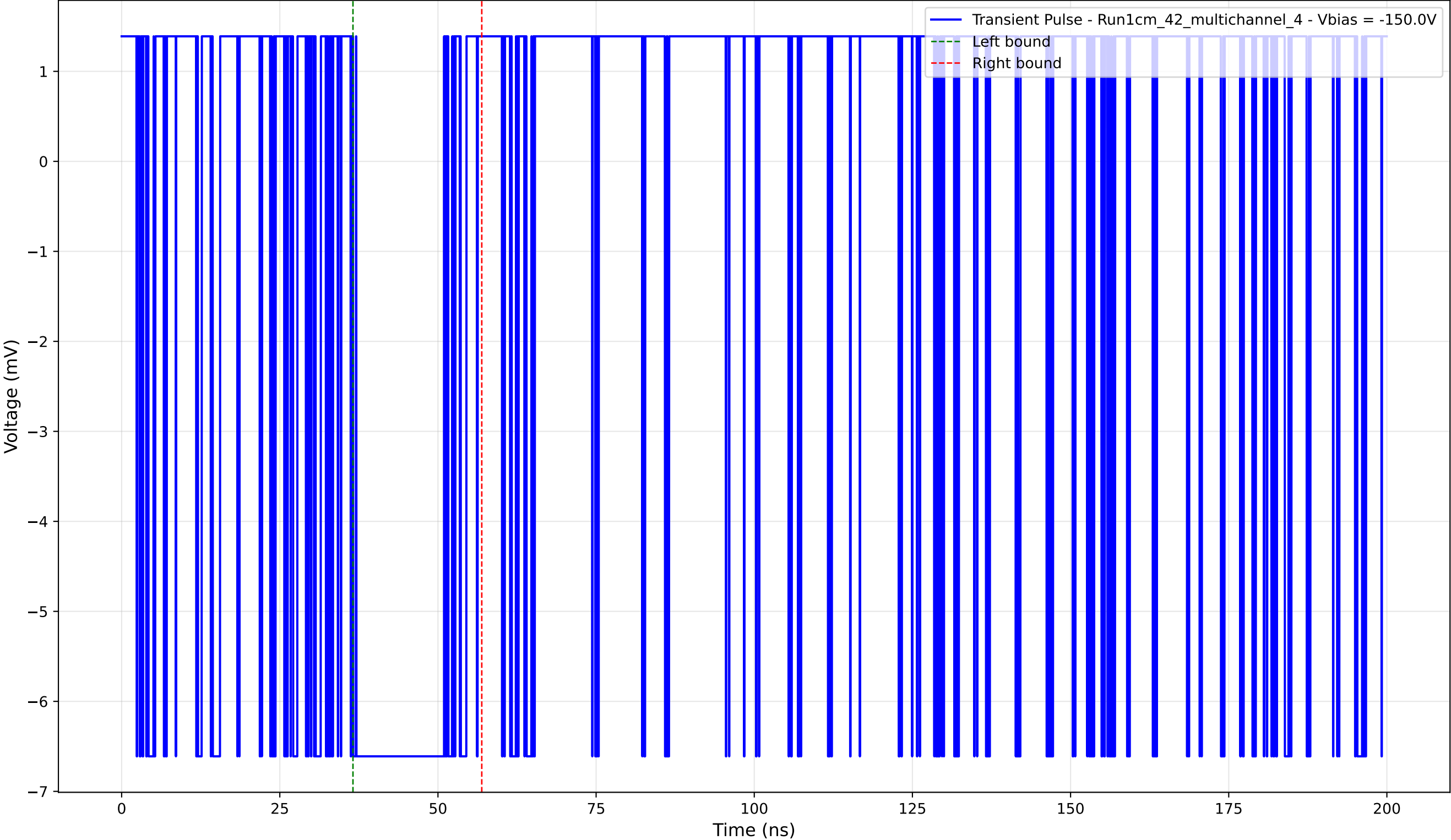
Transient Pulse - Sample: 1cm_42_multichannel - Position: 4450.0 \mu\text{m} - Charge: 2.08 pC - Rise Time: 0.00 ns (N/A)
