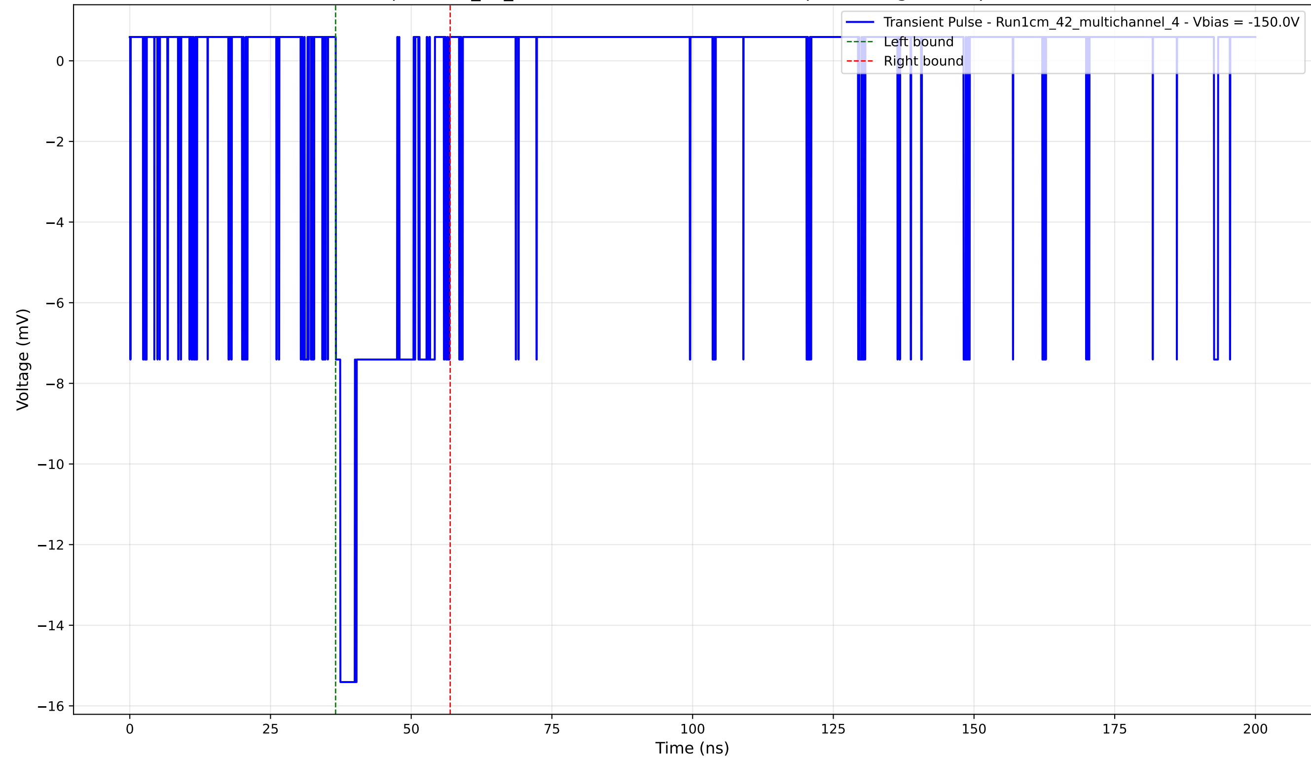
Transient Pulse - Sample: 1cm_42_multichannel - Position: 3345.0 \mu\text{m} - Charge: 2.93 pC - Rise Time: 0.82 ns
