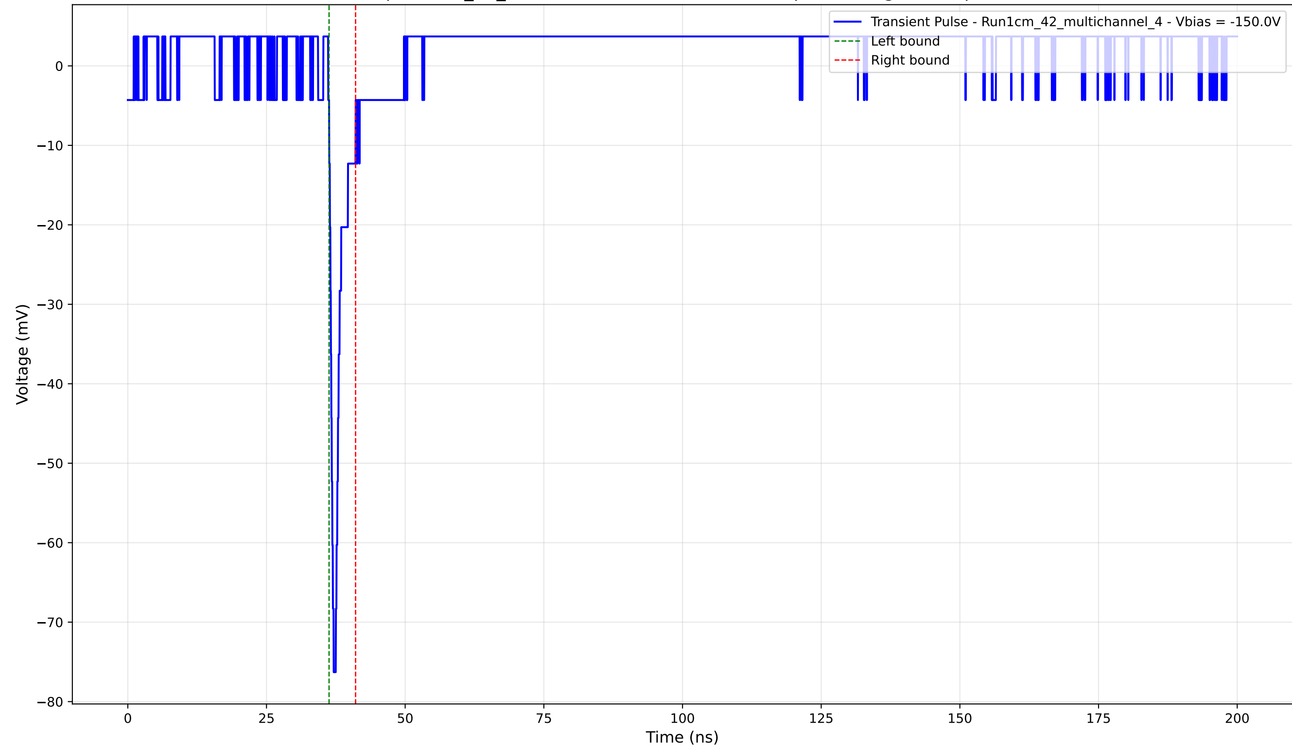
Transient Pulse - Sample: 1cm_42_multichannel - Position: 2255.0 \mu\text{m} - Charge: 2.96 pC - Rise Time: 0.81 ns
