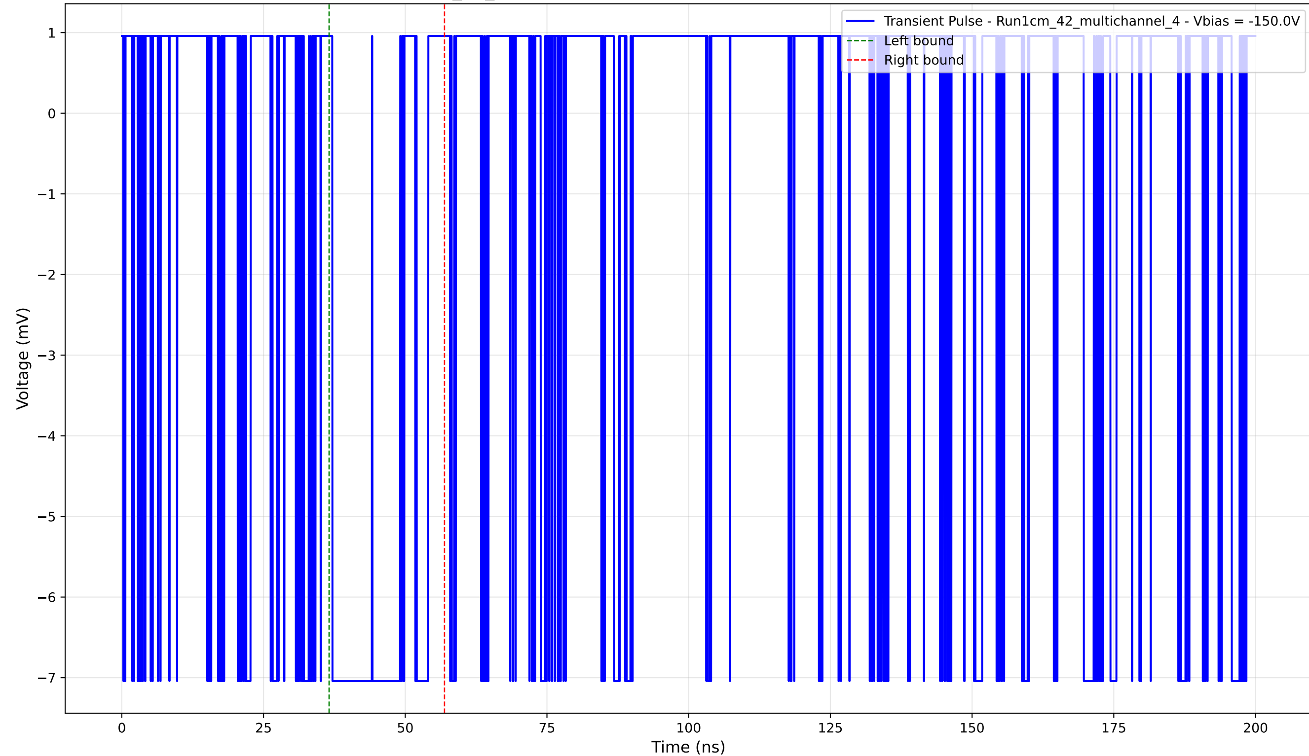
Transient Pulse - Sample: 1cm_42_multichannel - Position: 80.0 \mu\text{m} - Charge: 1.92 pC - Rise Time: 0.00 ns (N/A)
