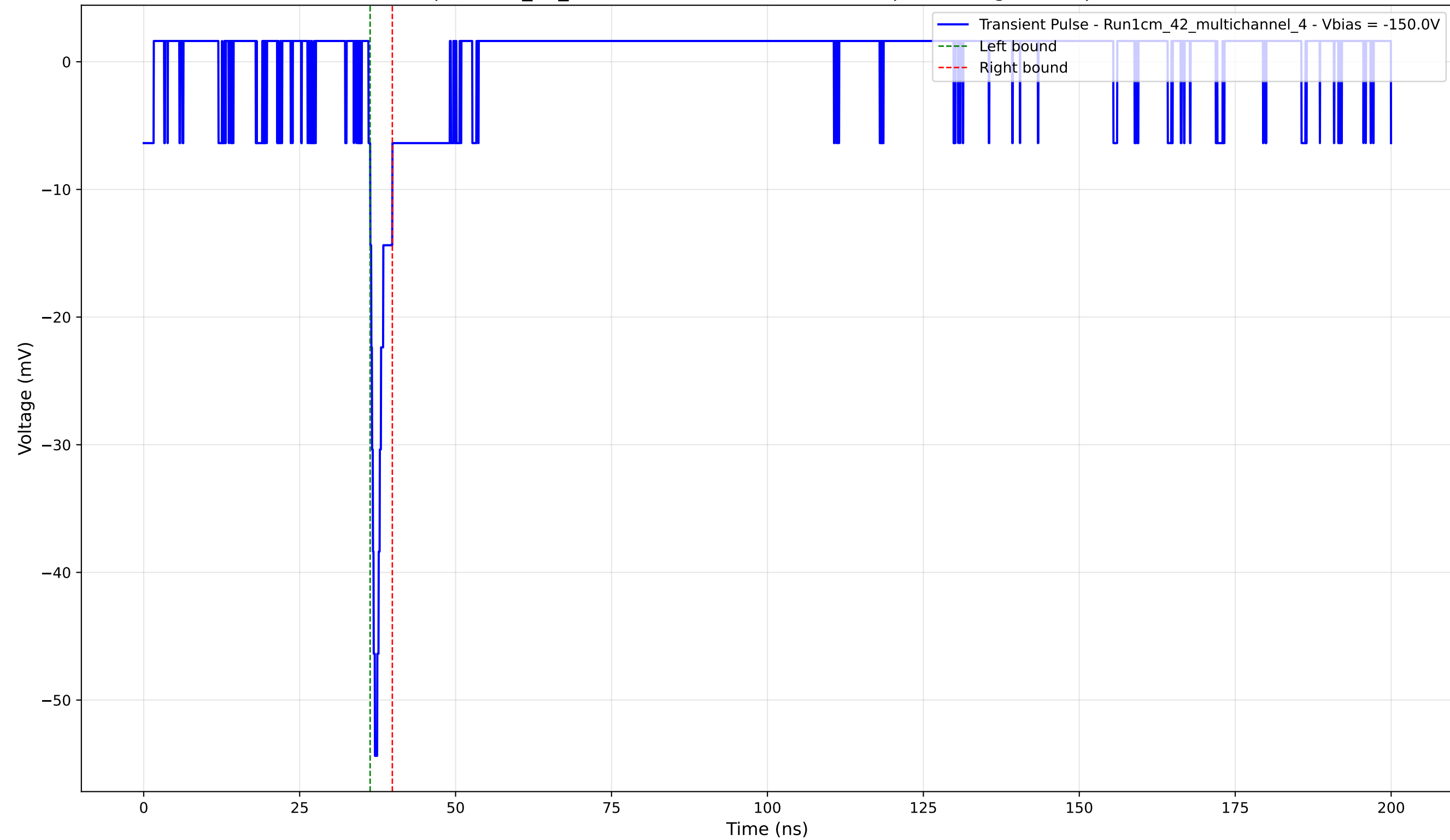
Transient Pulse - Sample: 1cm_42_multichannel - Position: 2330.0 \mu\text{m} - Charge: 1.92 pC - Rise Time: 1.02 ns
