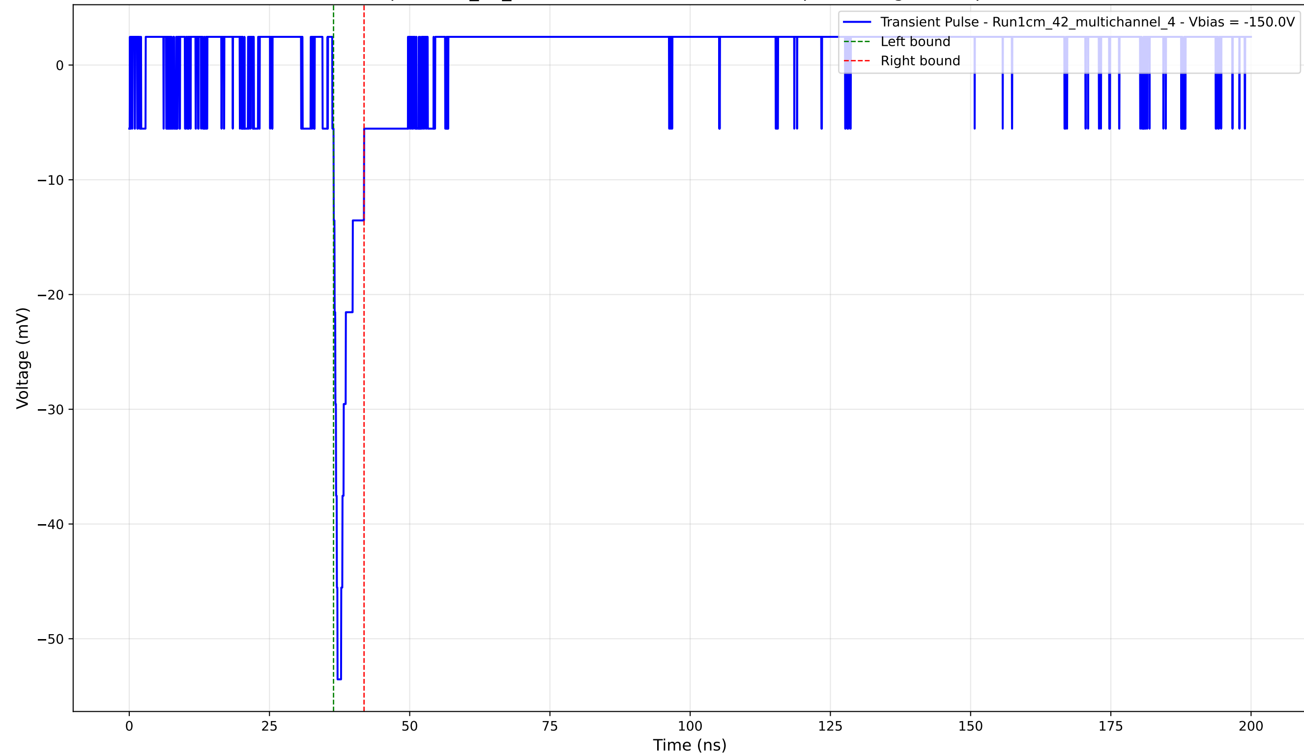
Transient Pulse - Sample: 1cm_42_multichannel - Position: 2725.0 \mu\text{m} - Charge: 2.77 pC - Rise Time: 0.92 ns
