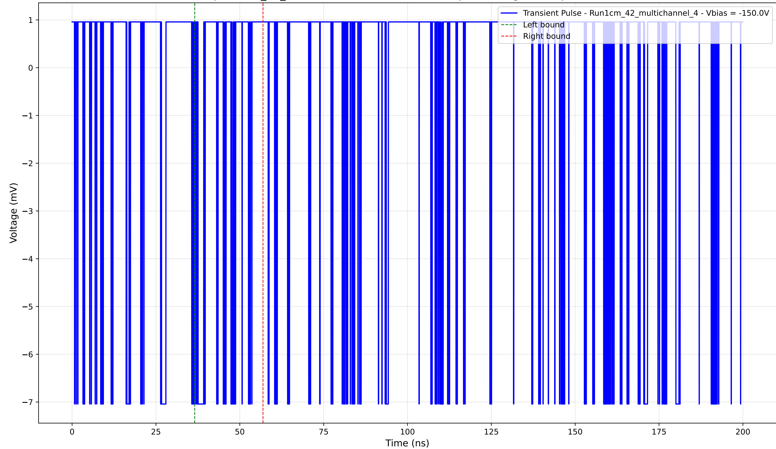
Transient Pulse - Sample: 1cm_42_multichannel - Position: 3395.0 \mu\text{m} - Charge: 0.31 pC - Rise Time: 0.00 ns (N/A)
