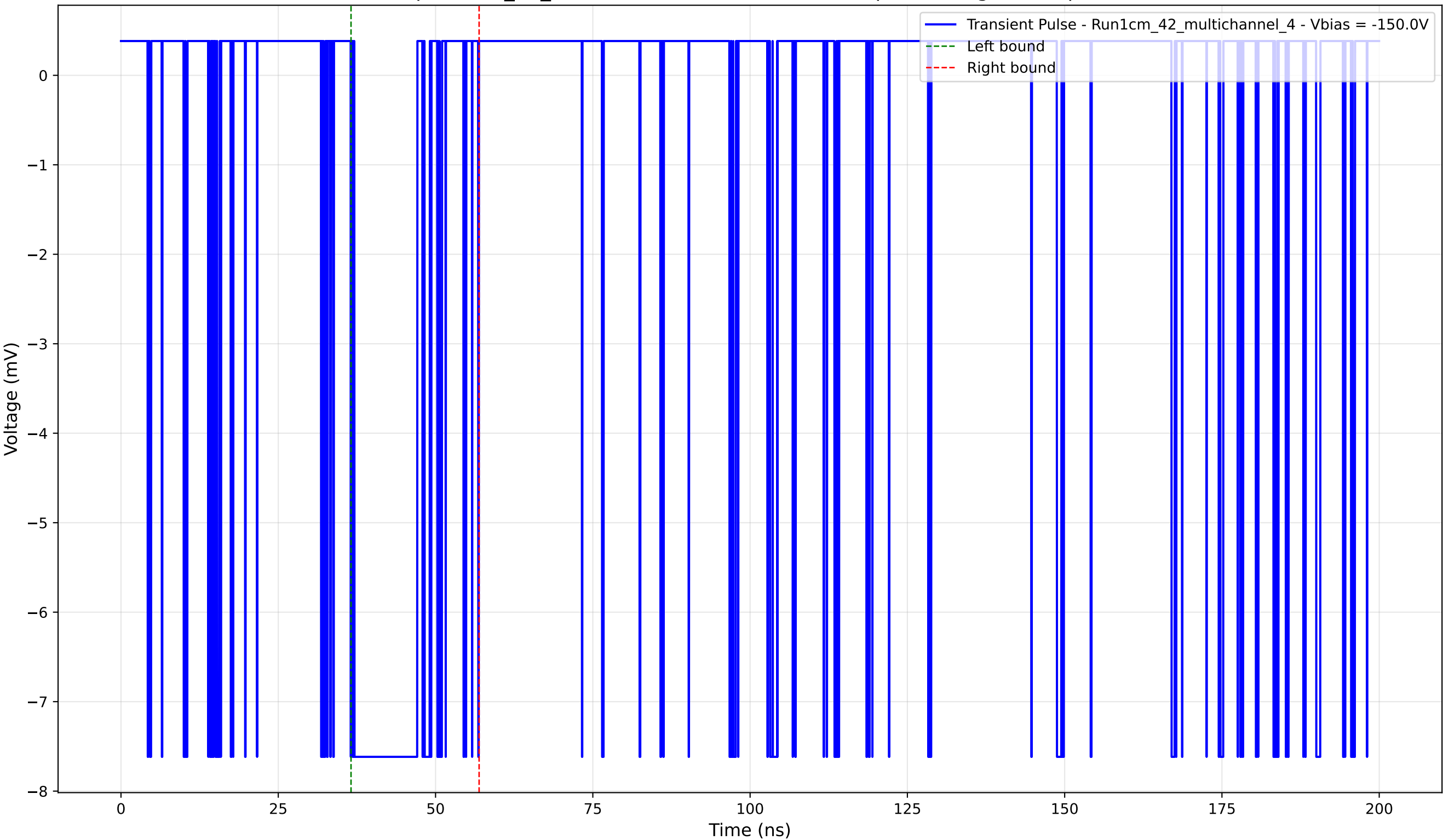
Transient Pulse - Sample: 1cm_42_multichannel - Position: 3865.0 \mu\text{m} - Charge: 1.81 pC - Rise Time: 0.02 ns
