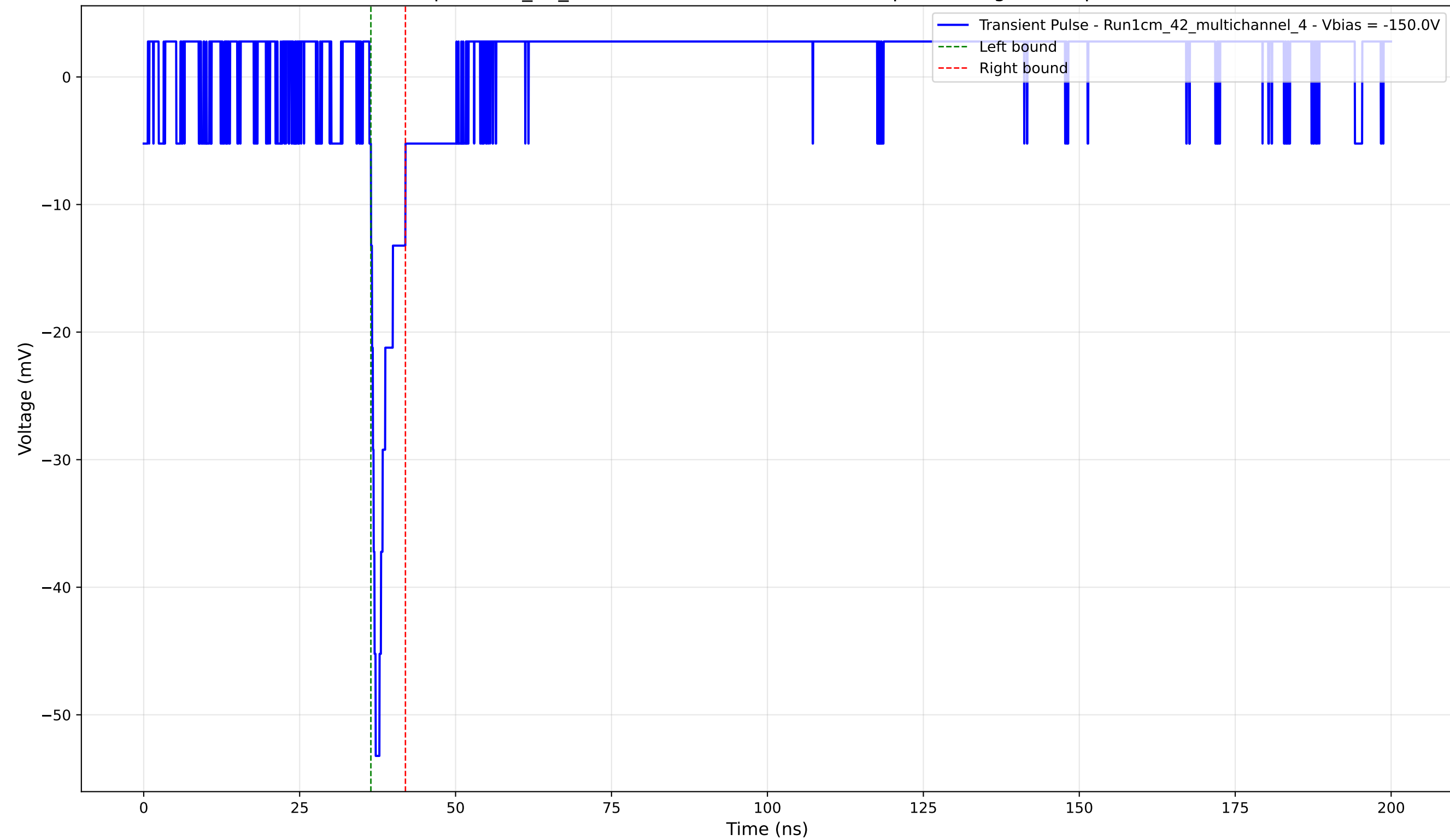
Transient Pulse - Sample: 1cm_42_multichannel - Position: 2020.0 \mu\text{m} - Charge: 2.81 pC - Rise Time: 0.76 ns
