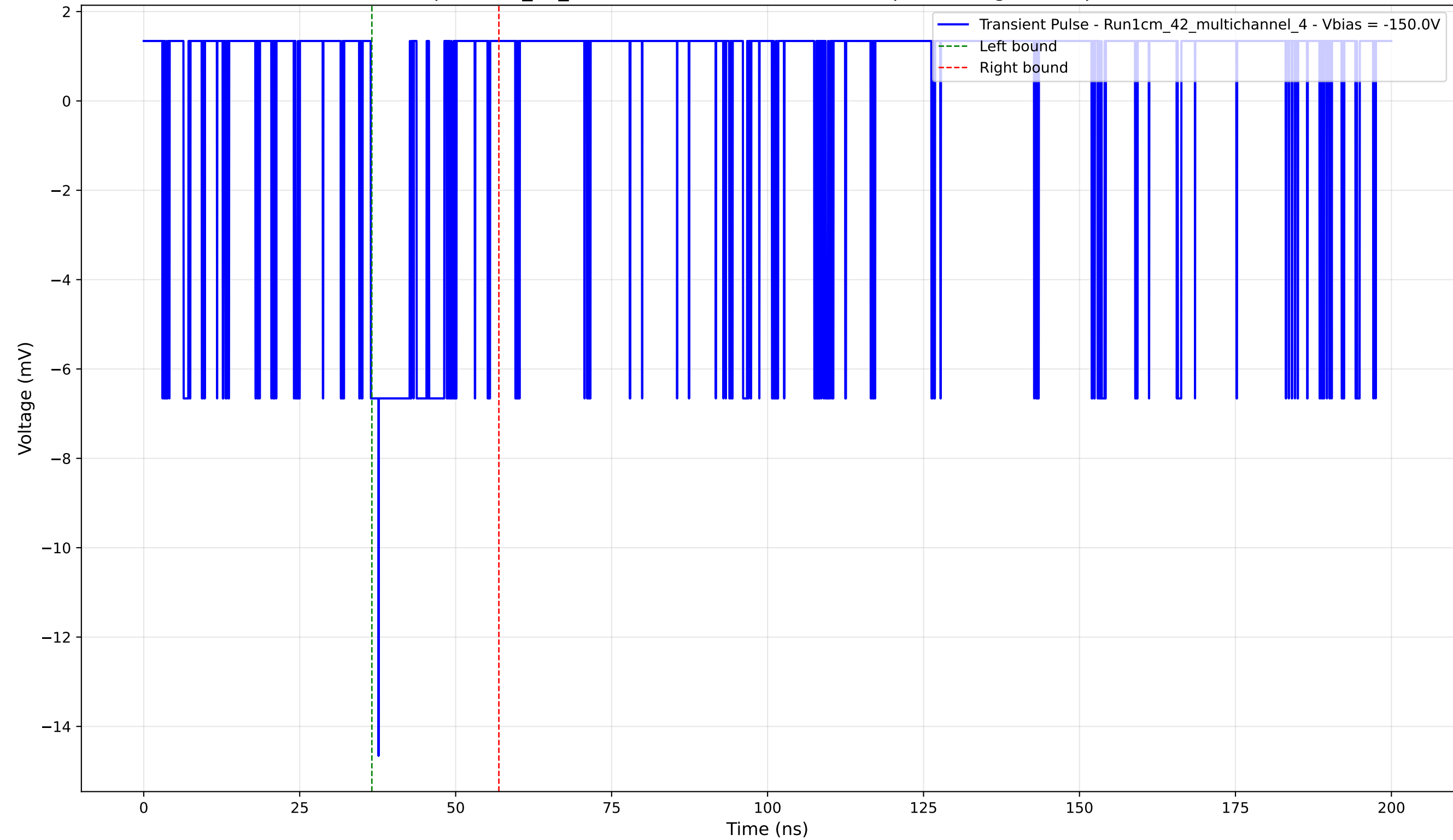
Transient Pulse - Sample: 1cm_42_multichannel - Position: 2855.0 \mu\text{m} - Charge: 1.36 pC - Rise Time: 1.26 ns
