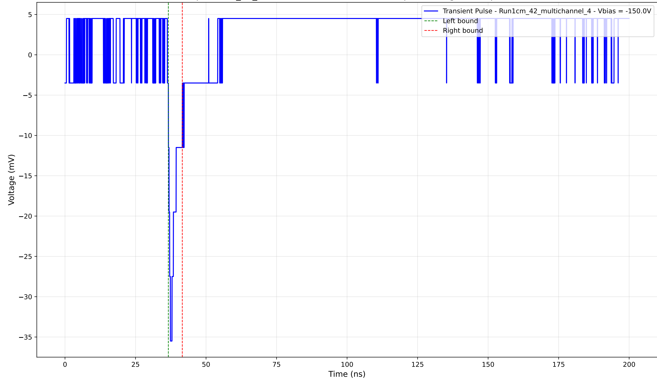
Transient Pulse - Sample: 1cm_42_multichannel - Position: 1810.0 \mu\text{m} - Charge: 1.84 pC - Rise Time: 0.74 ns
