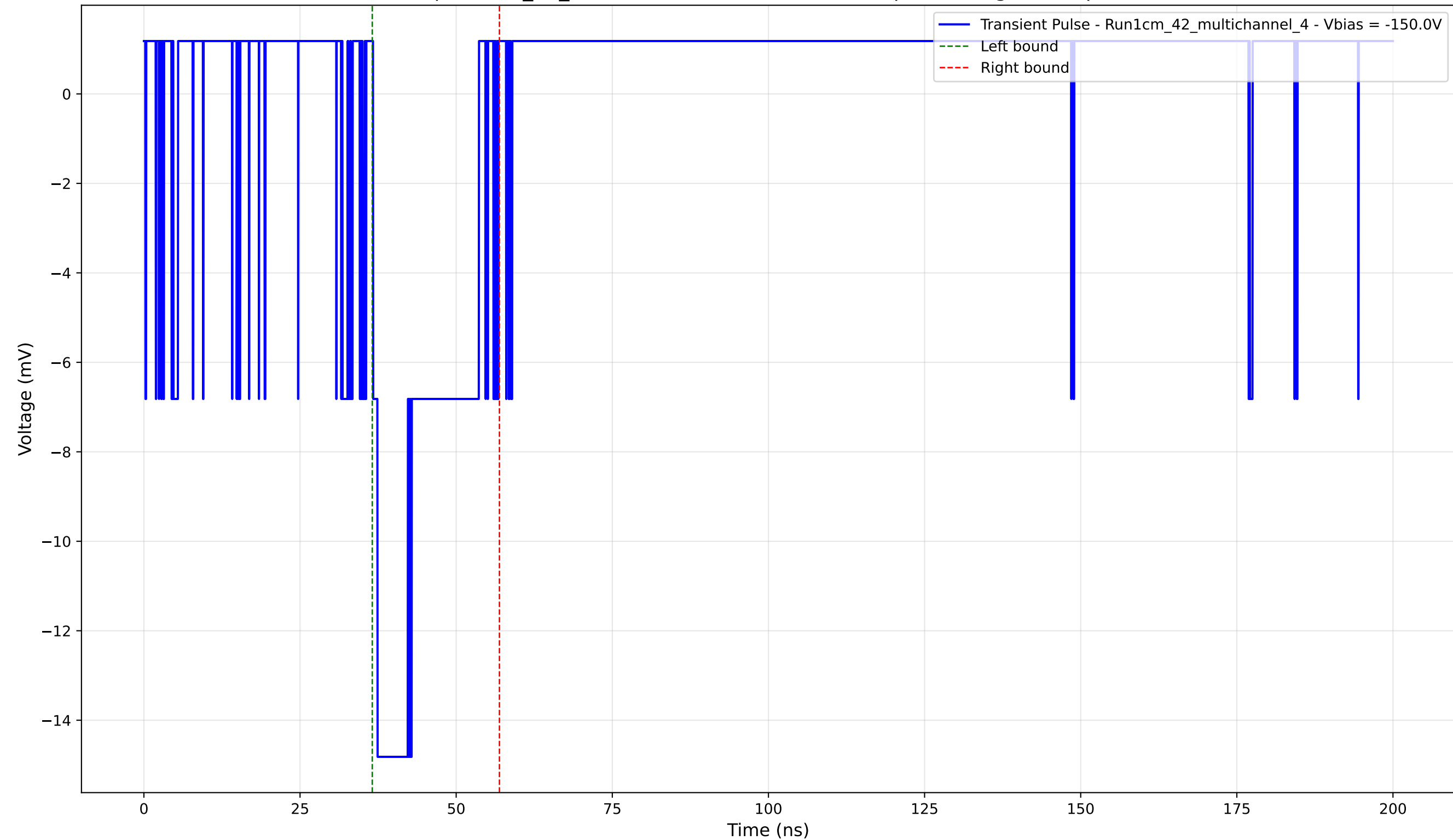
Transient Pulse - Sample: 1cm_42_multichannel - Position: 3605.0 \mu\text{m} - Charge: 3.17 pC - Rise Time: 0.72 ns
