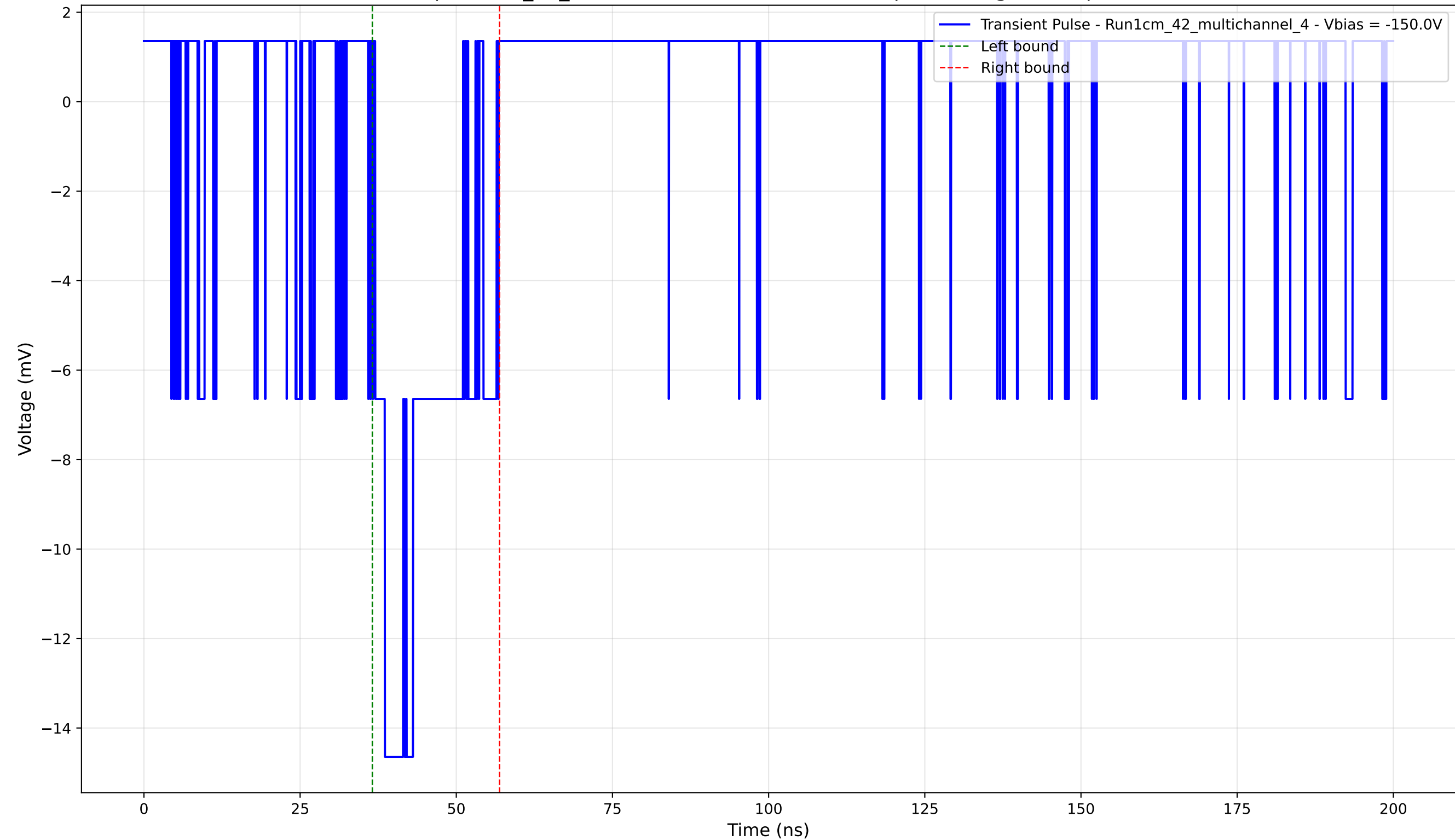
Transient Pulse - Sample: 1cm_42_multichannel - Position: 4485.0 \mu\text{m} - Charge: 3.03 pC - Rise Time: 1.56 ns
