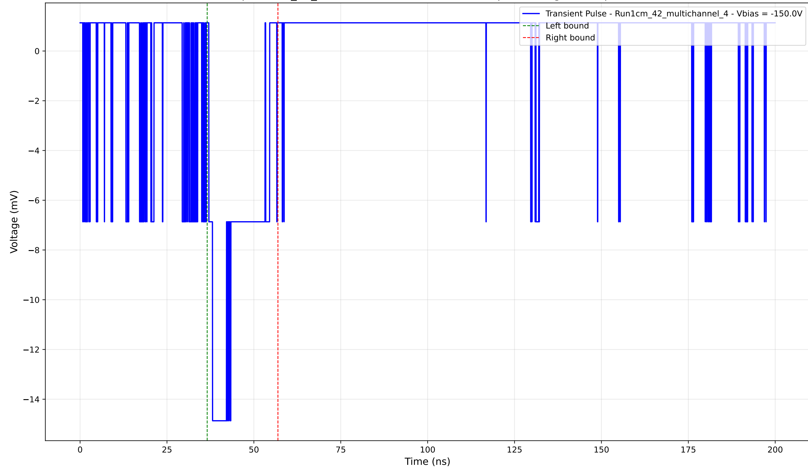
Transient Pulse - Sample: 1cm_42_multichannel - Position: 4070.0 \mu\text{m} - Charge: 3.06 pC - Rise Time: 1.08 ns
