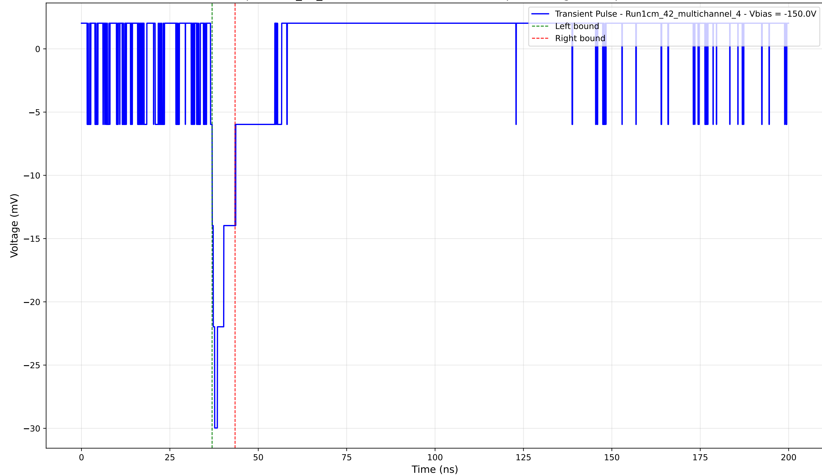
Transient Pulse - Sample: 1cm_42_multichannel - Position: 1475.0 \mu\text{m} - Charge: 2.41 pC - Rise Time: 1.18 ns
