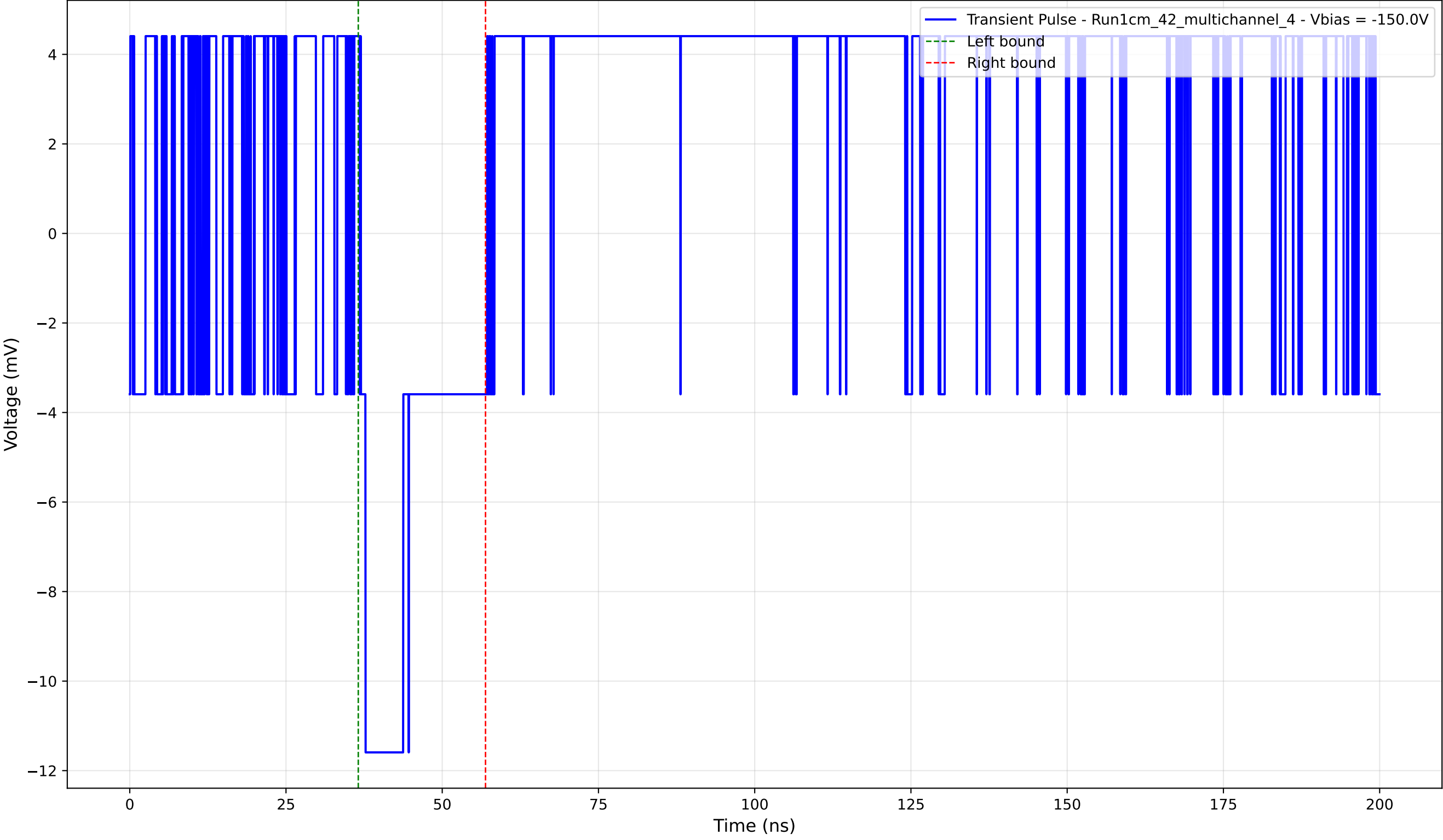
Transient Pulse - Sample: 1cm_42_multichannel - Position: 715.0 \mu\text{m} - Charge: 2.39 pC - Rise Time: 0.00 ns (N/A)
