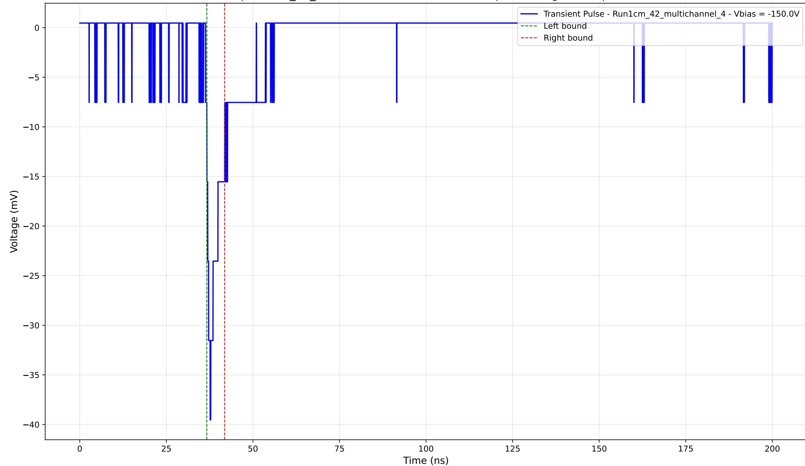
Transient Pulse - Sample: 1cm_42_multichannel - Position: 3060.0 \mu\text{m} - Charge: 2.31 pC - Rise Time: 1.33 ns
