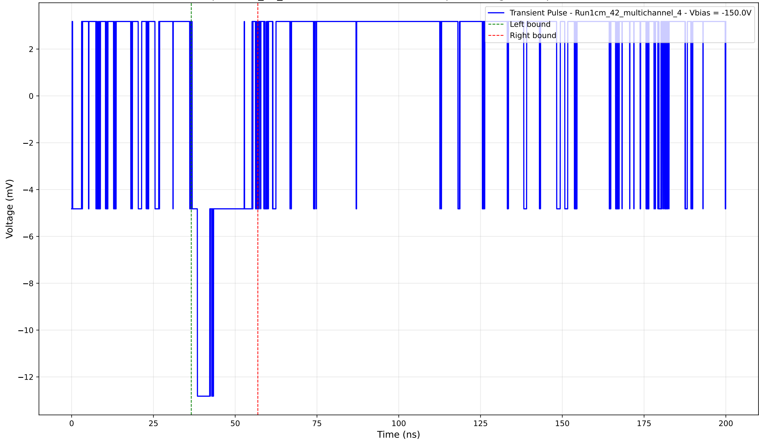
Transient Pulse - Sample: 1cm_42_multichannel - Position: 155.0 \mu\text{m} - Charge: 2.42 pC - Rise Time: 0.00 ns (N/A)
