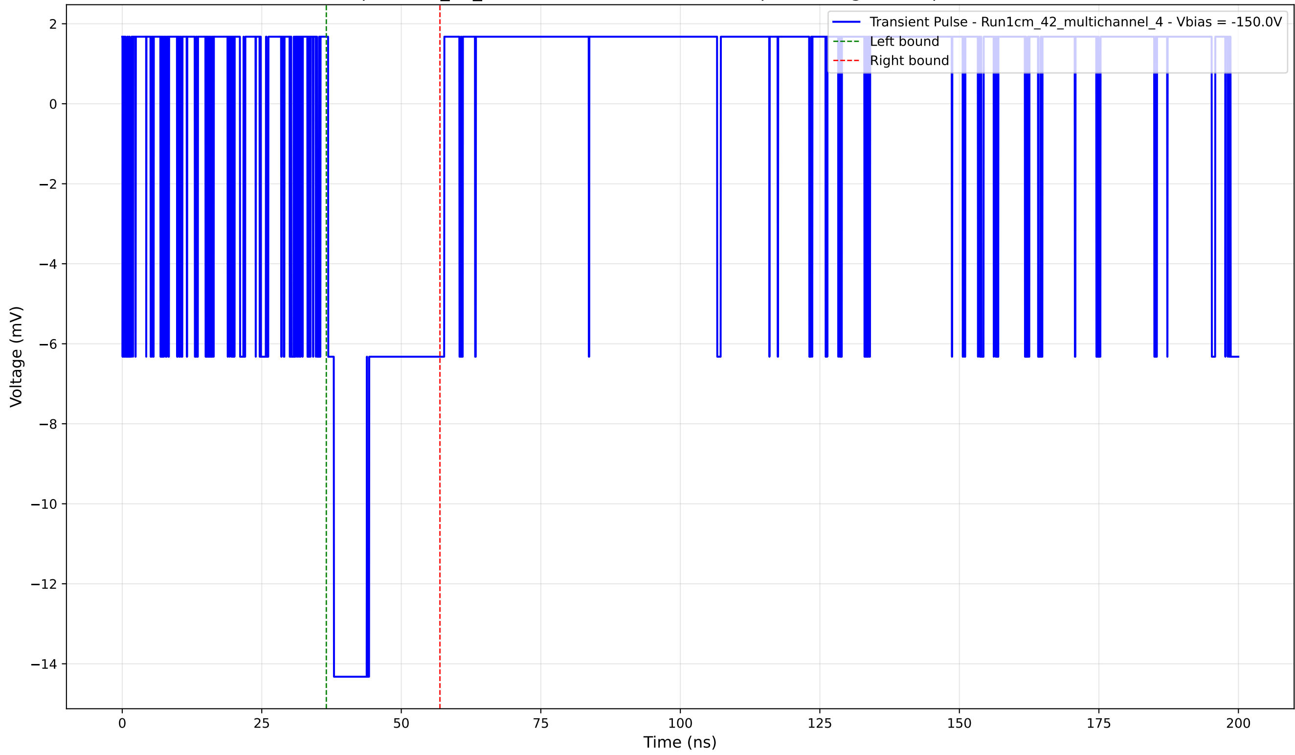
Transient Pulse - Sample: 1cm_42_multichannel - Position: 660.0 \mu\text{m} - Charge: 3.52 pC - Rise Time: 0.00 ns (N/A)
