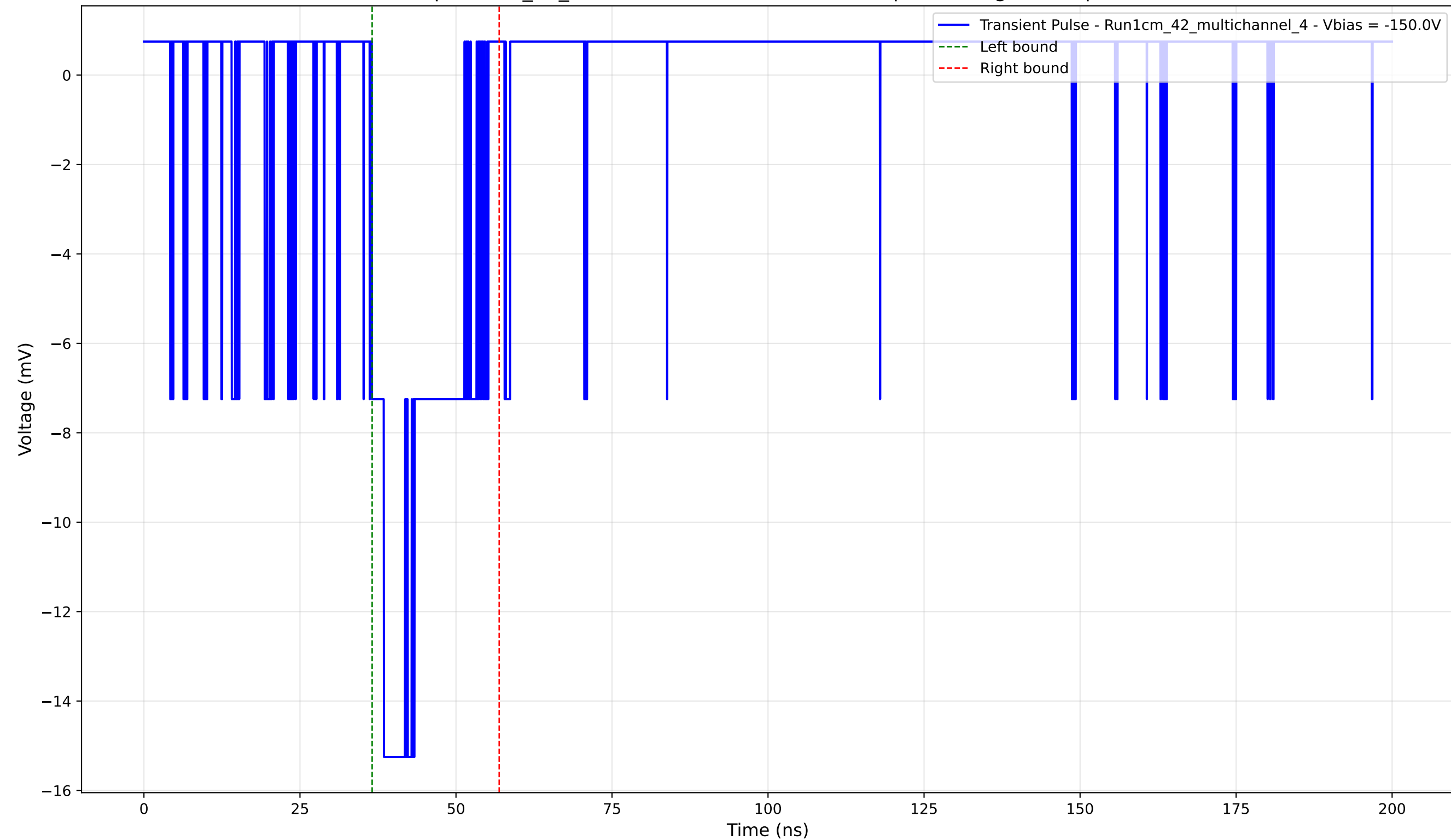
Transient Pulse - Sample: 1cm_42_multichannel - Position: 4680.0 \mu\text{m} - Charge: 3.19 pC - Rise Time: 1.94 ns
