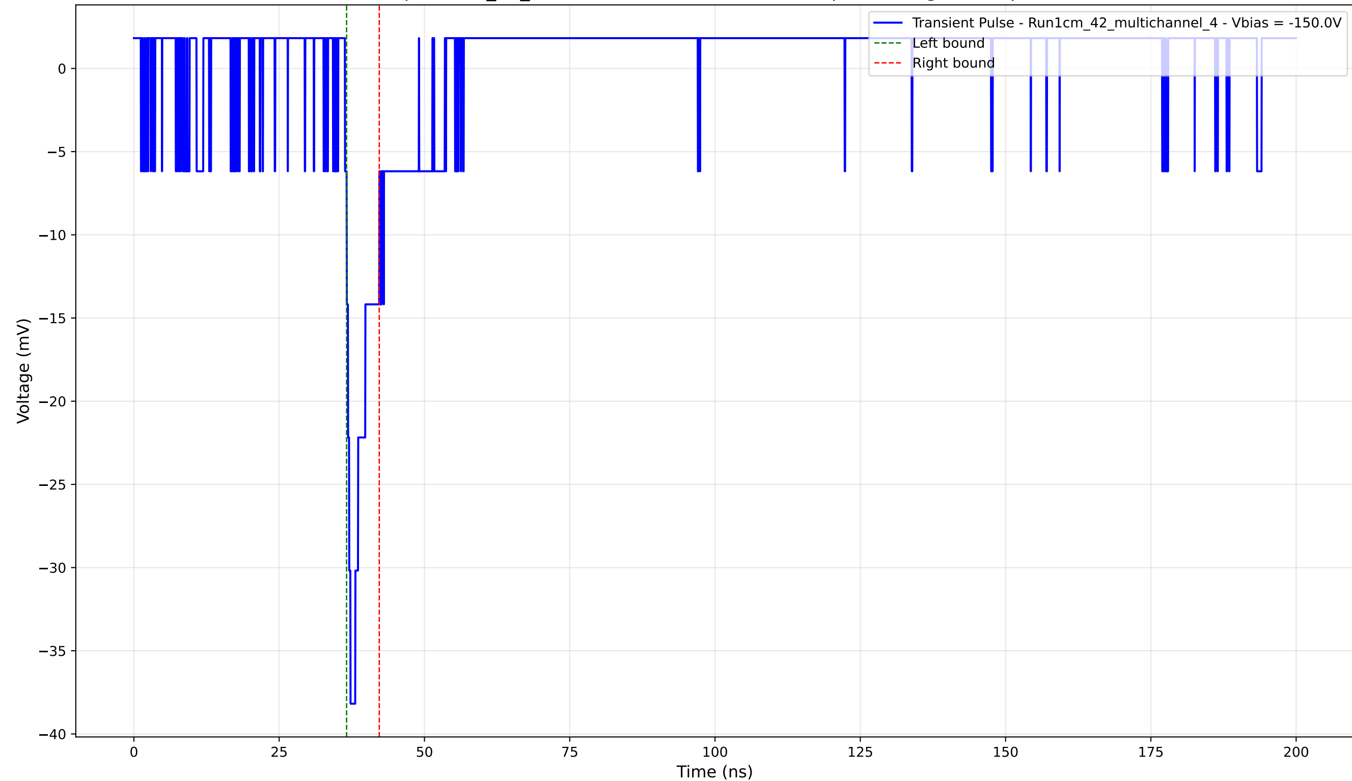
Transient Pulse - Sample: 1cm_42_multichannel - Position: 2985.0 \mu\text{m} - Charge: 2.45 pC - Rise Time: 0.95 ns
