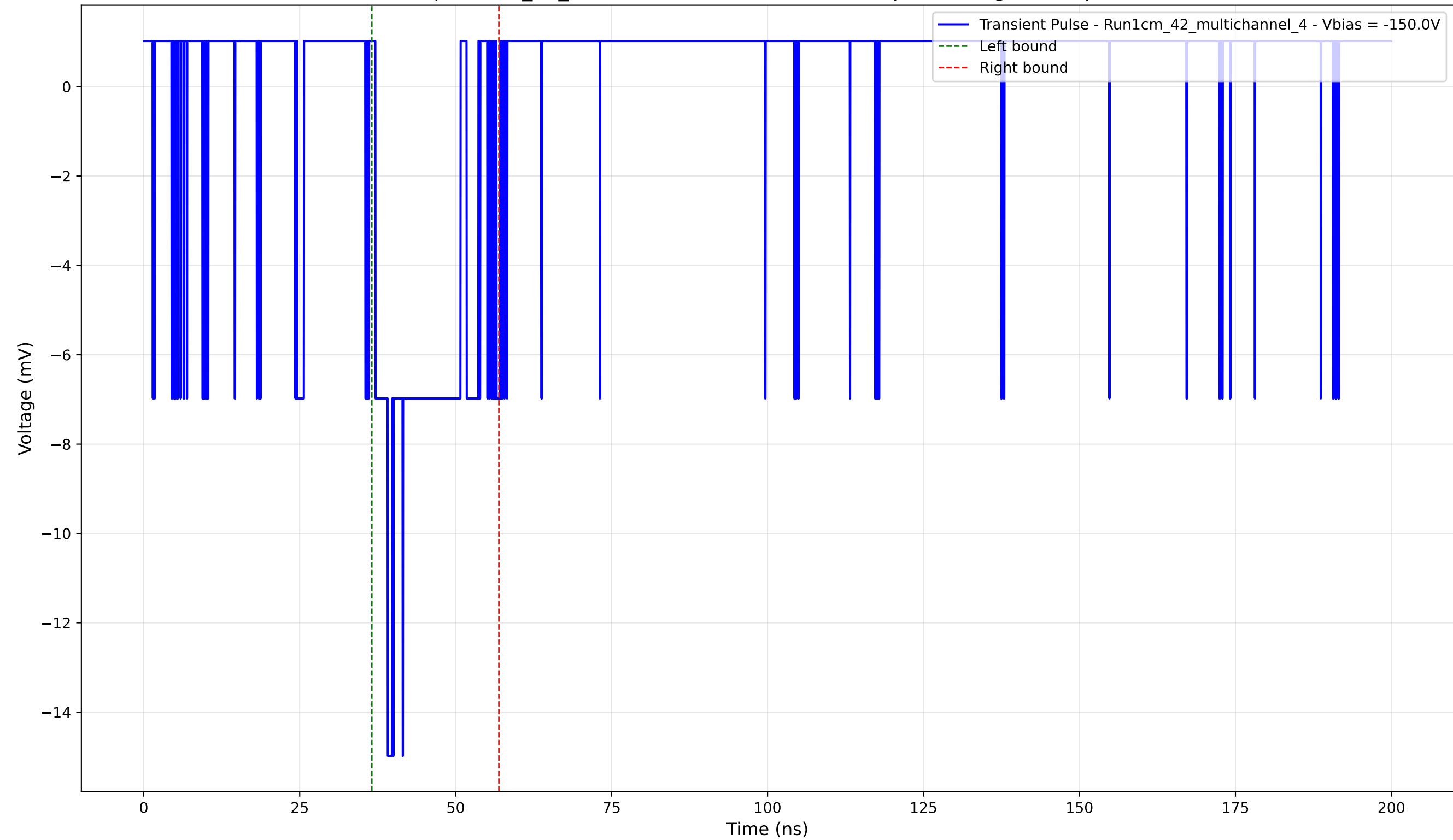
Transient Pulse - Sample: 1cm_42_multichannel - Position: 3960.0 \mu\text{m} - Charge: 2.39 pC - Rise Time: 1.98 ns
