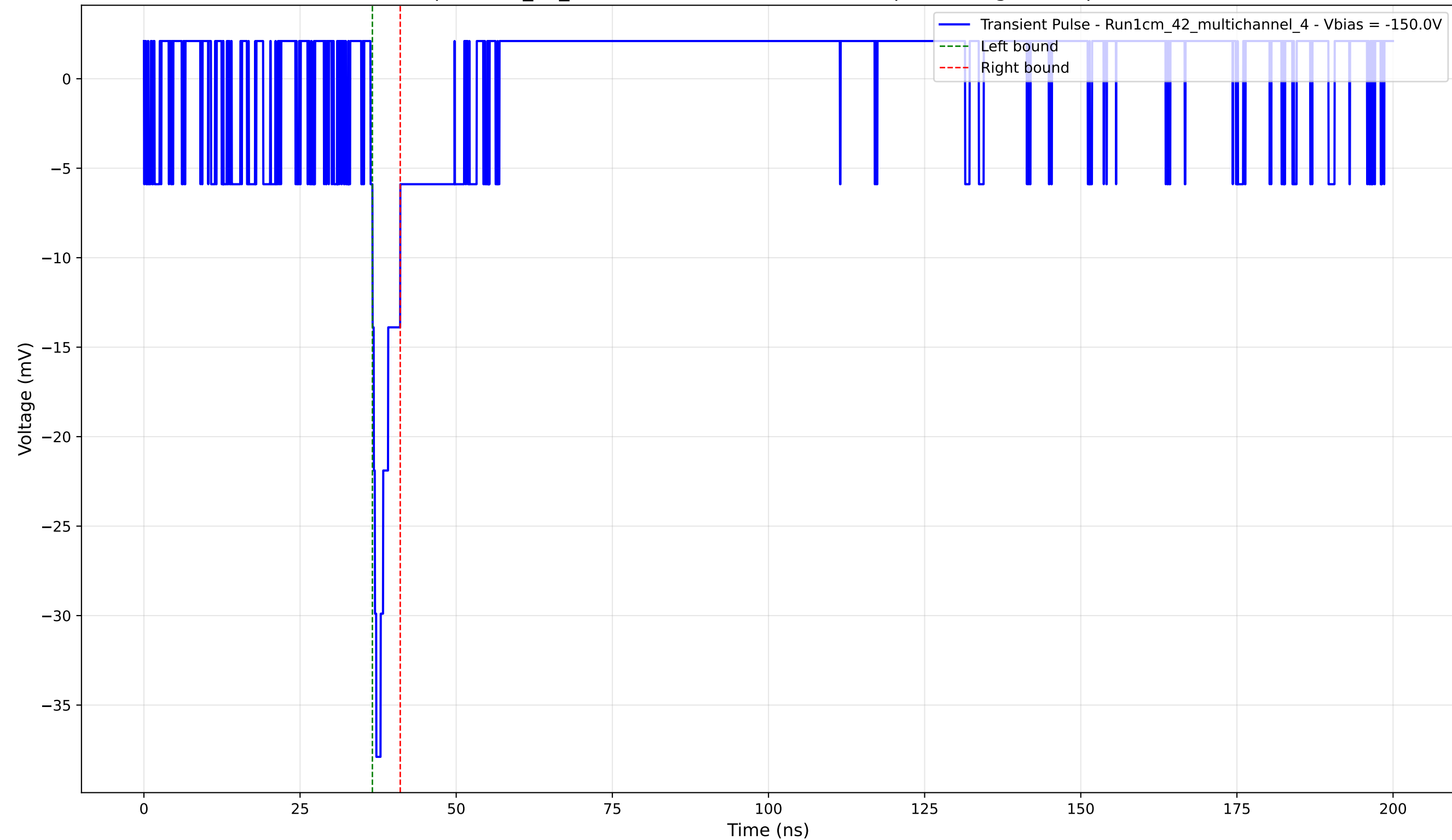
Transient Pulse - Sample: 1cm_42_multichannel - Position: 1940.0 \mu\text{m} - Charge: 1.93 pC - Rise Time: 0.93 ns
