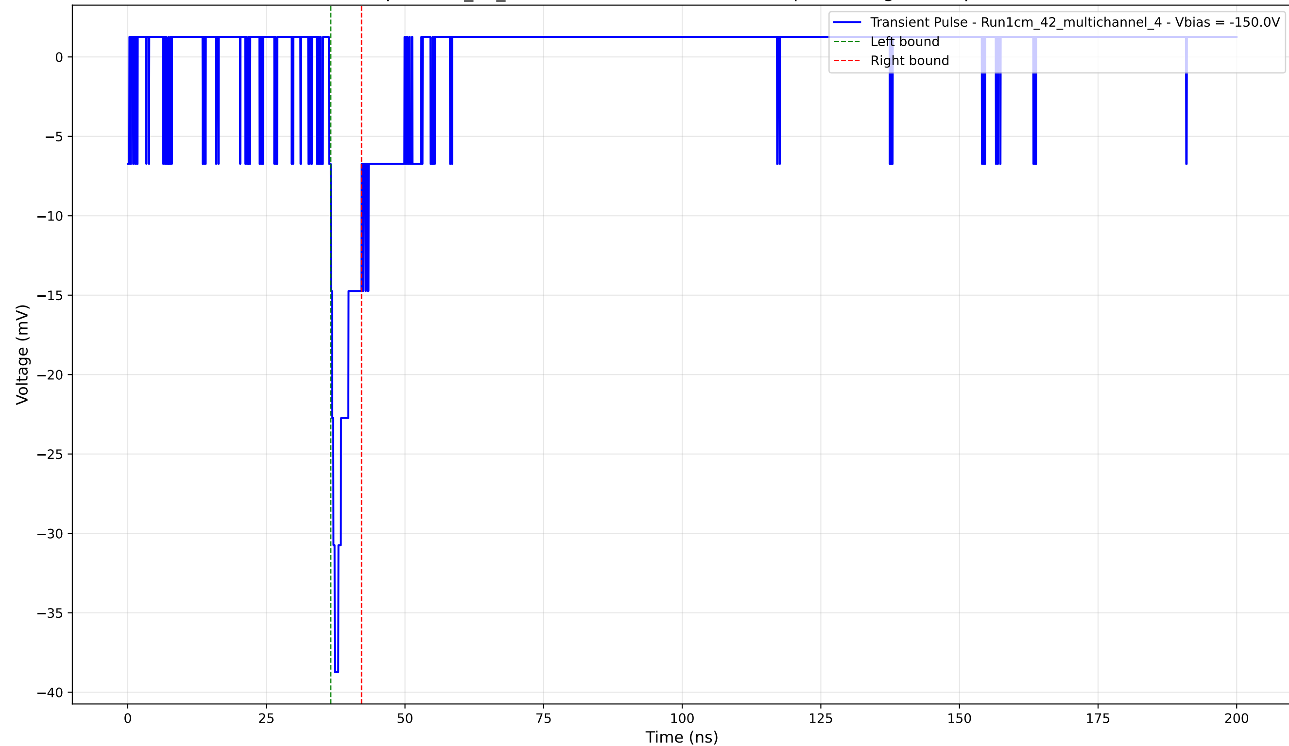
Transient Pulse - Sample: 1cm_42_multichannel - Position: 2995.0 \mu\text{m} - Charge: 2.42 pC - Rise Time: 1.03 ns
