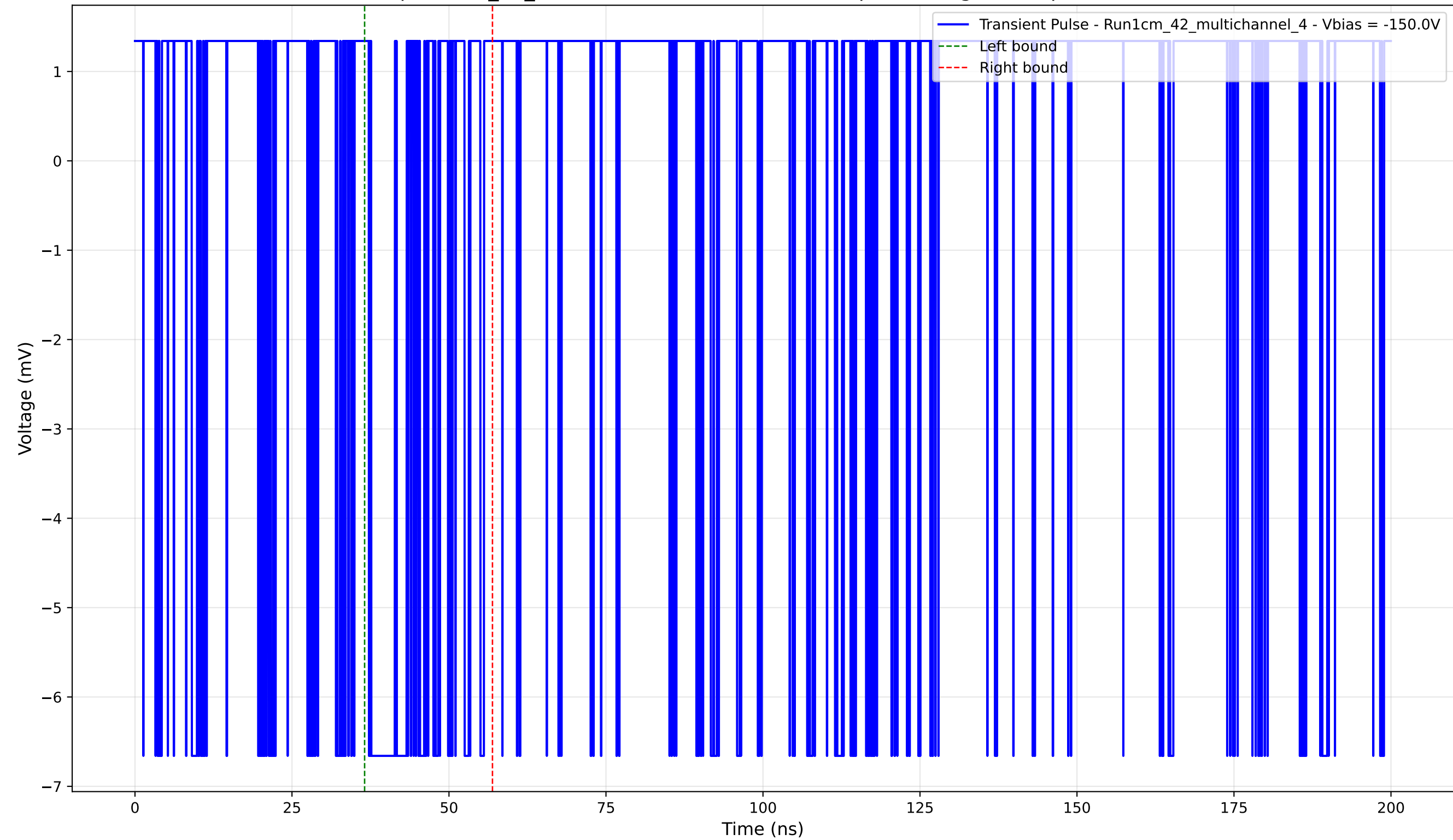
Transient Pulse - Sample: 1cm_42_multichannel - Position: 3370.0 \mu\text{m} - Charge: 1.01 pC - Rise Time: 0.00 ns (N/A)
