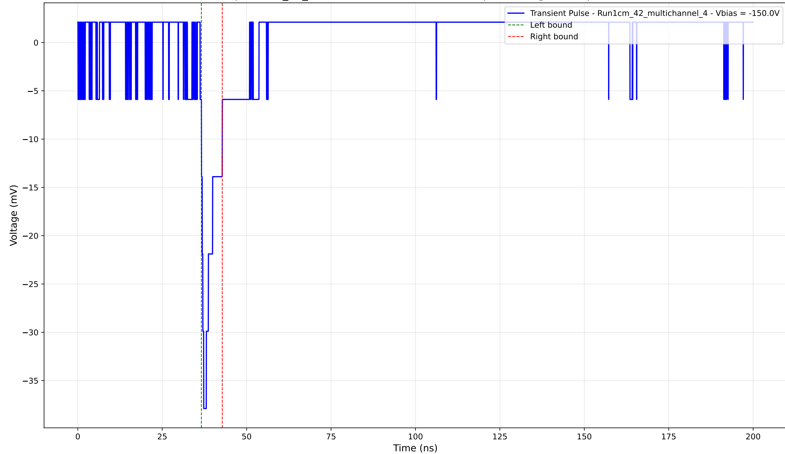
Transient Pulse - Sample: 1cm_42_multichannel - Position: 2980.0 \mu\text{m} - Charge: 2.59 pC - Rise Time: 1.07 ns
