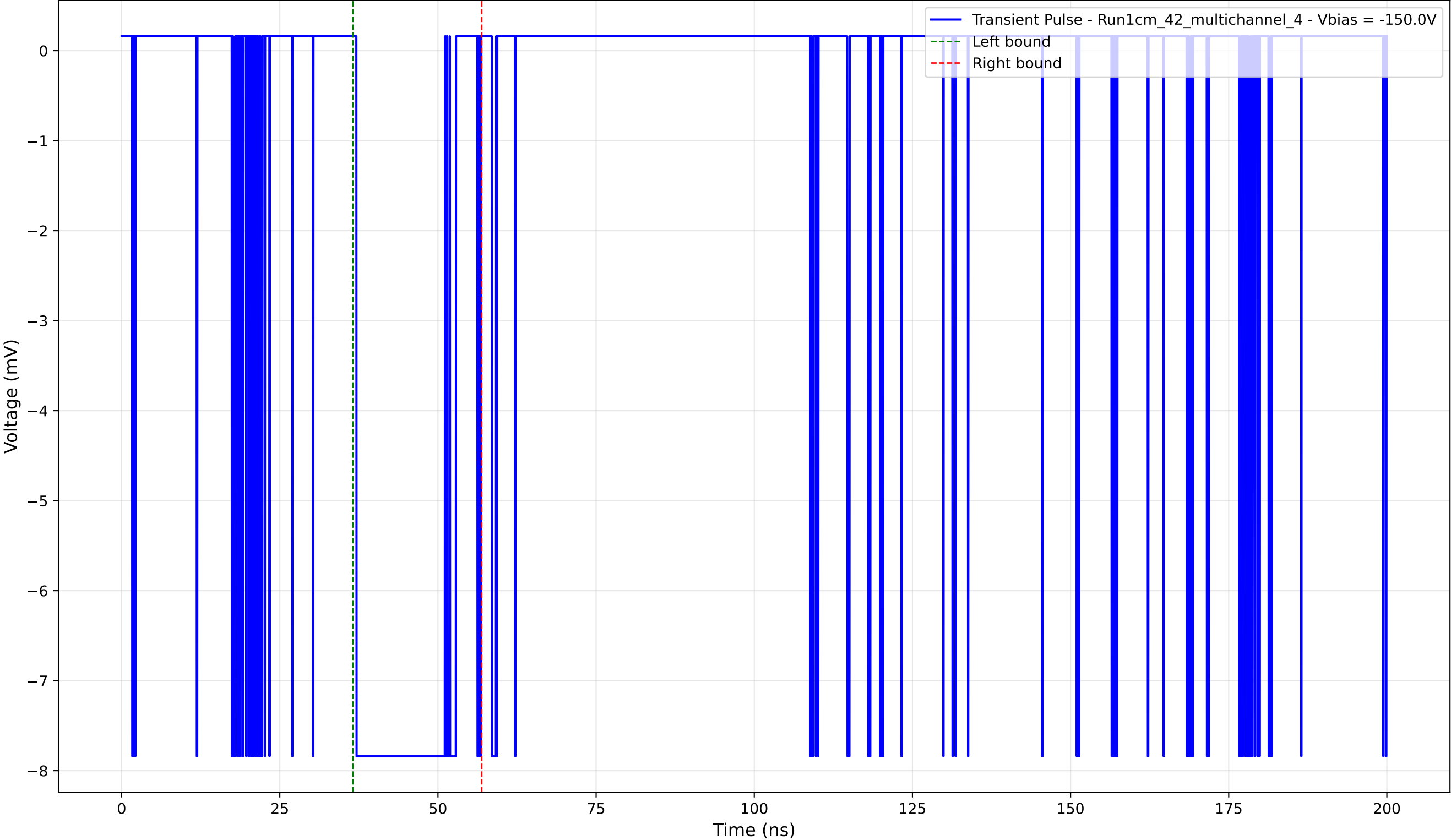
Transient Pulse - Sample: 1cm_42_multichannel - Position: 4855.0 \mu\text{m} - Charge: 2.45 pC - Rise Time: 0.02 ns
