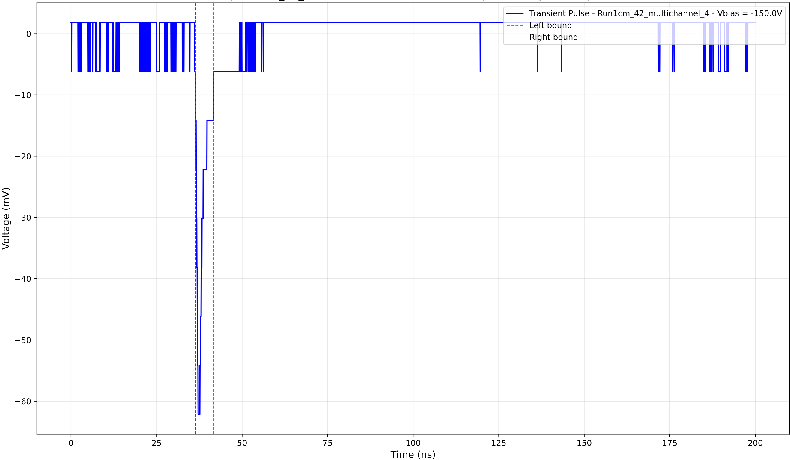
Transient Pulse - Sample: 1cm_42_multichannel - Position: 2130.0 \mu\text{m} - Charge: 2.93 pC - Rise Time: 0.74 ns
