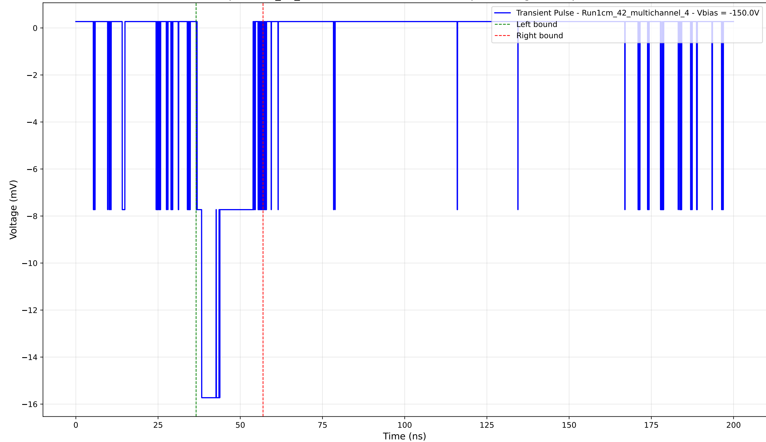
Transient Pulse - Sample: 1cm_42_multichannel - Position: 4110.0 \mu\text{m} - Charge: 3.64 pC - Rise Time: 1.40 ns
