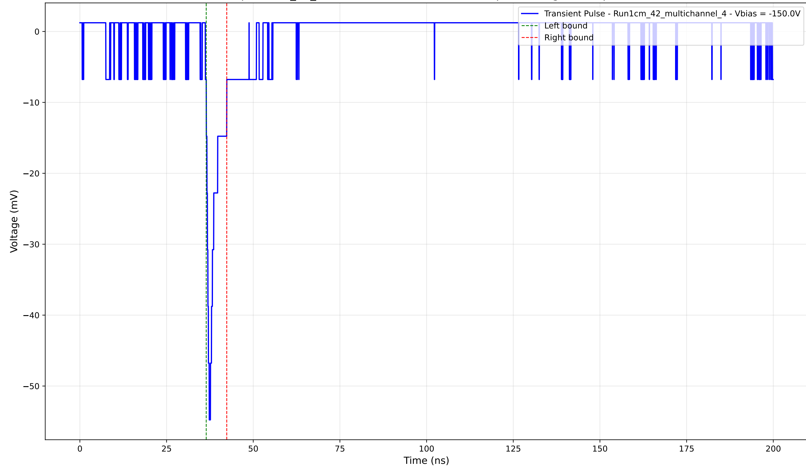
Transient Pulse - Sample: 1cm_42_multichannel - Position: 2765.0 \mu\text{m} - Charge: 2.94 pC - Rise Time: 1.12 ns
