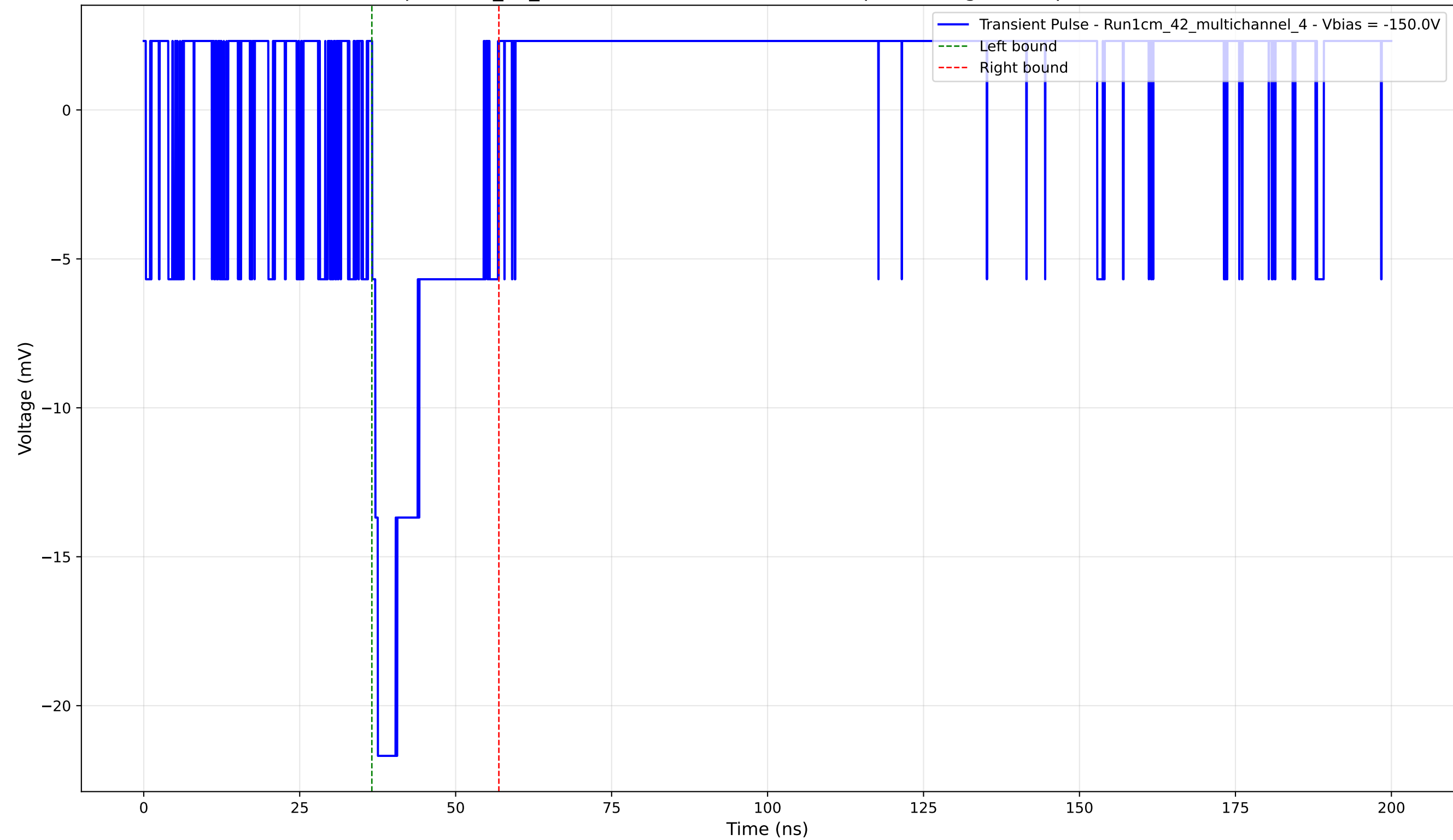
Transient Pulse - Sample: 1cm_42_multichannel - Position: 1275.0 \mu\text{m} - Charge: 3.80 pC - Rise Time: 0.00 ns (N/A)
