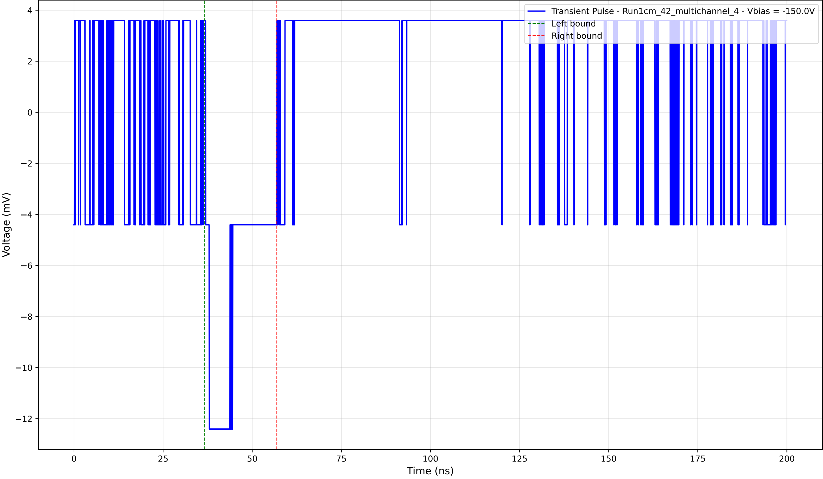
Transient Pulse - Sample: 1cm_42_multichannel - Position: 560.0 \mu\text{m} - Charge: 2.73 pC - Rise Time: 0.00 ns (N/A)
