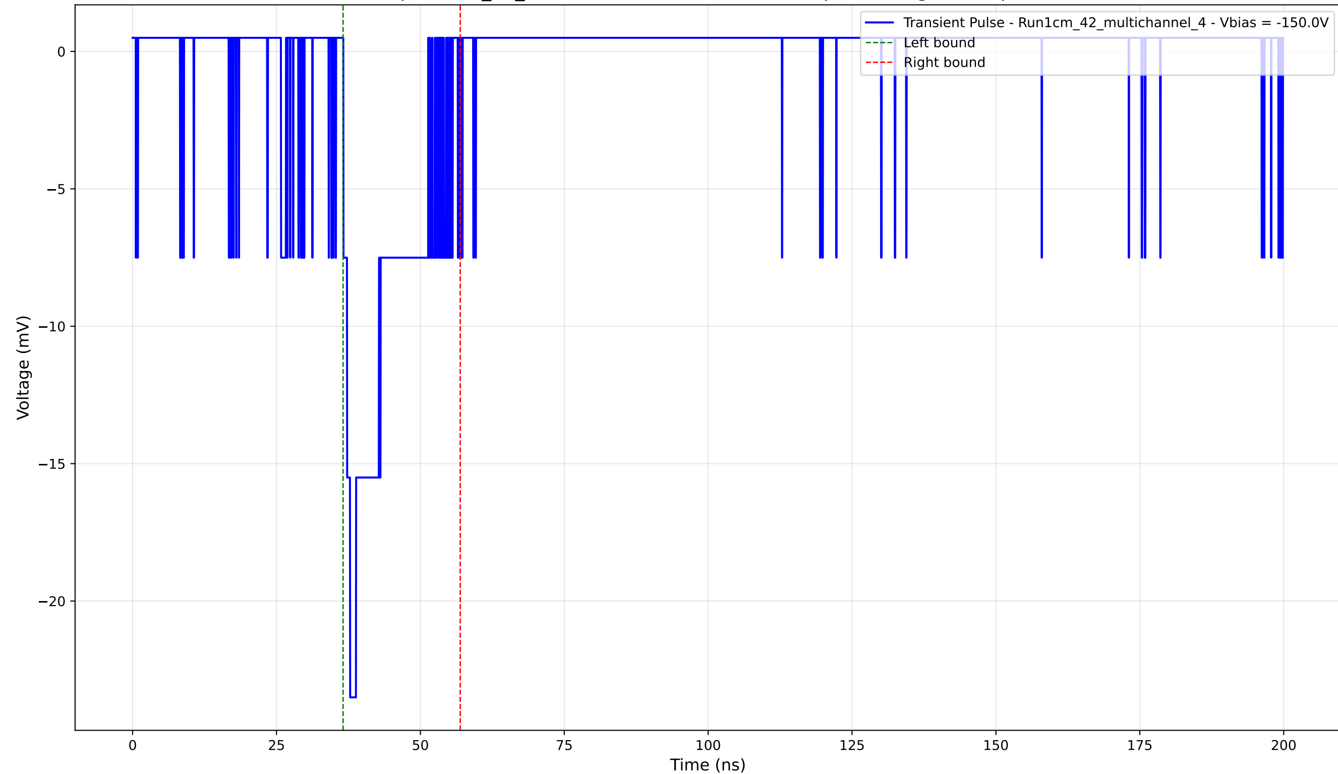
Transient Pulse - Sample: 1cm_42_multichannel - Position: 3530.0 \mu\text{m} - Charge: 3.70 pC - Rise Time: 1.17 ns
