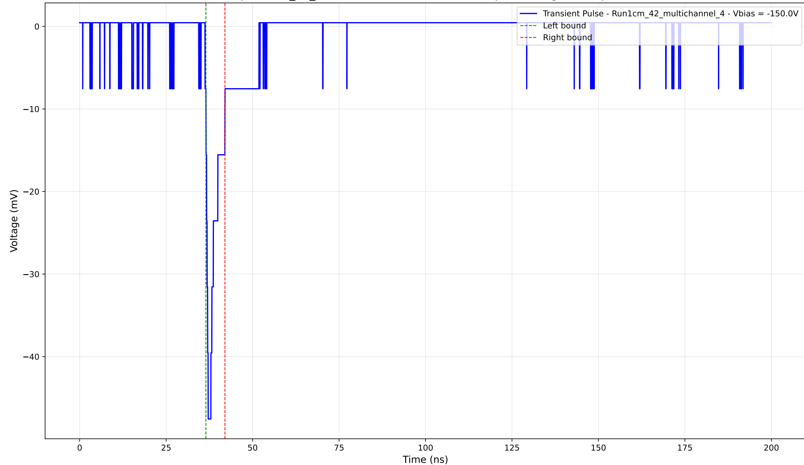
Transient Pulse - Sample: 1cm_42_multichannel - Position: 2810.0 \mu\text{m} - Charge: 2.84 pC - Rise Time: 0.91 ns
