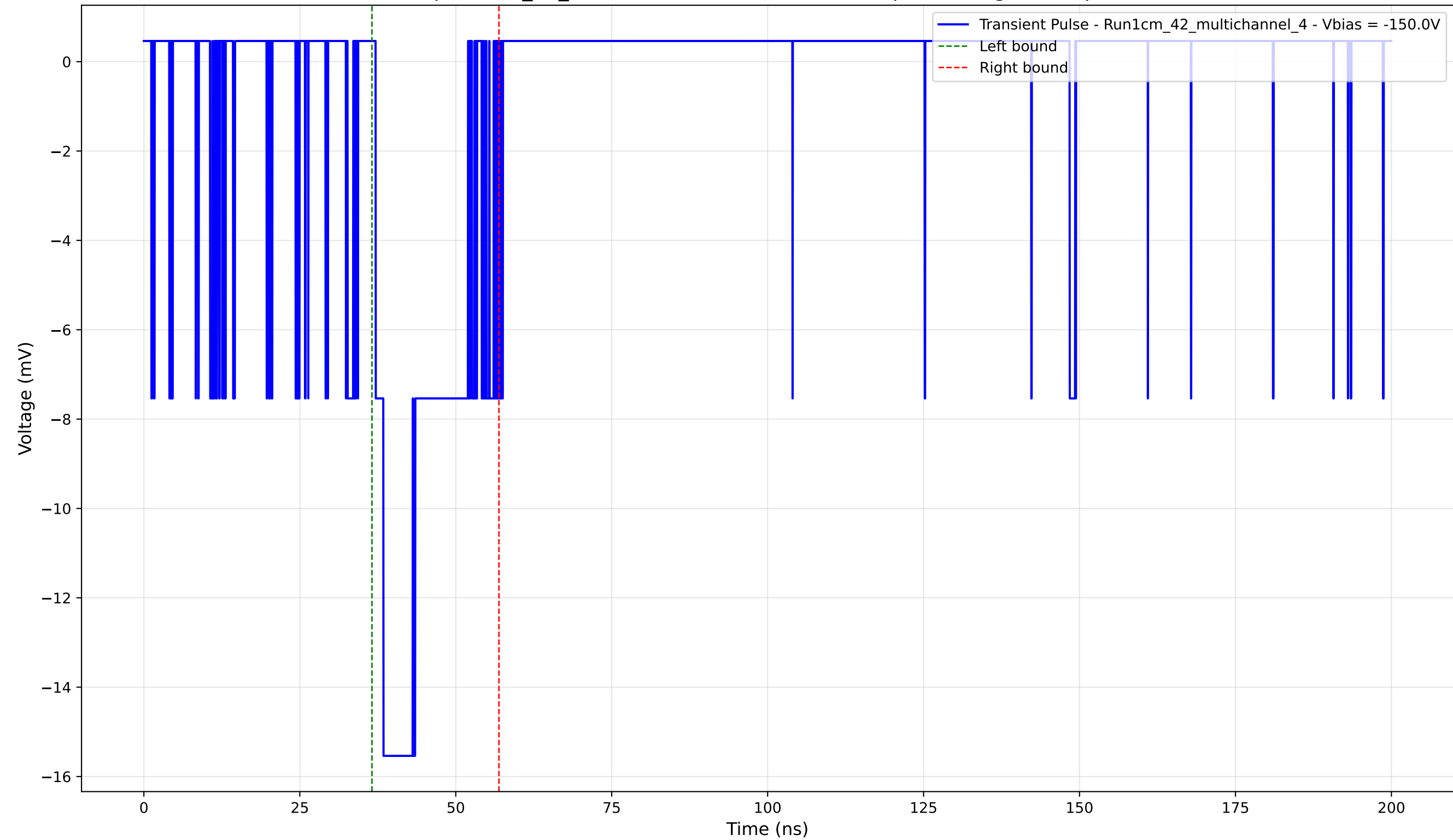
Transient Pulse - Sample: 1cm_42_multichannel - Position: 4615.0 \mu\text{m} - Charge: 3.45 pC - Rise Time: 1.26 ns
