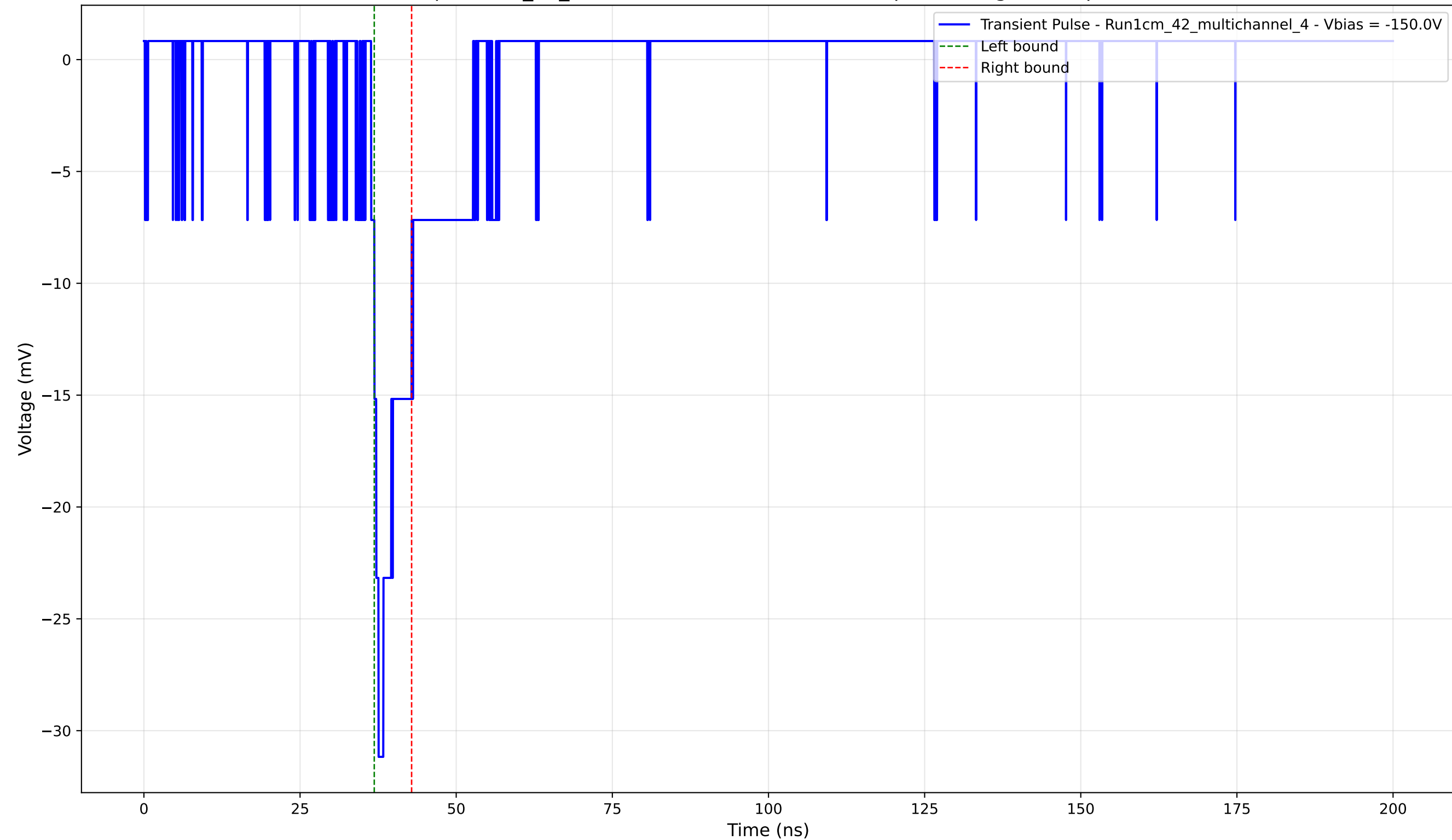
Transient Pulse - Sample: 1cm_42_multichannel - Position: 3220.0 \mu\text{m} - Charge: 2.33 pC - Rise Time: 1.19 ns
