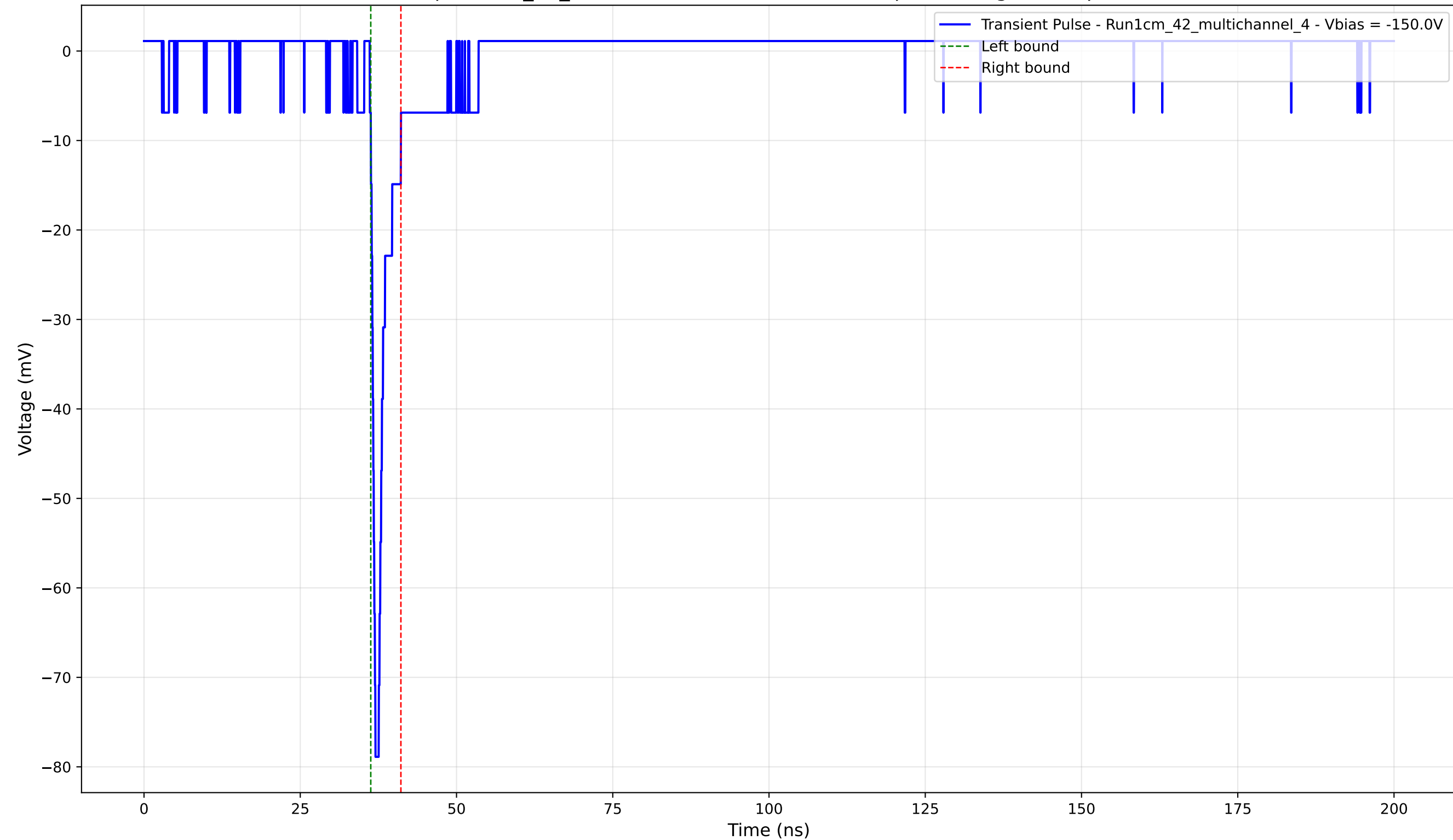
Transient Pulse - Sample: 1cm_42_multichannel - Position: 2250.0 \mu\text{m} - Charge: 3.31 pC - Rise Time: 0.74 ns
