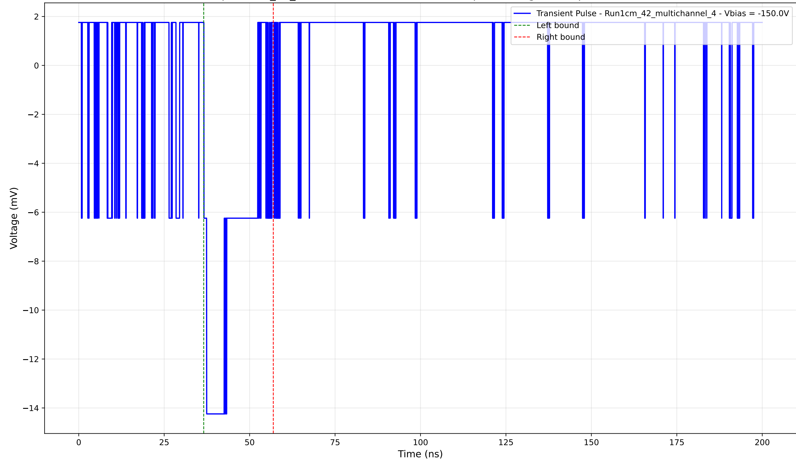
Transient Pulse - Sample: 1cm_42_multichannel - Position: 3645.0 \mu\text{m} - Charge: 2.92 pC - Rise Time: 0.00 ns (N/A)
