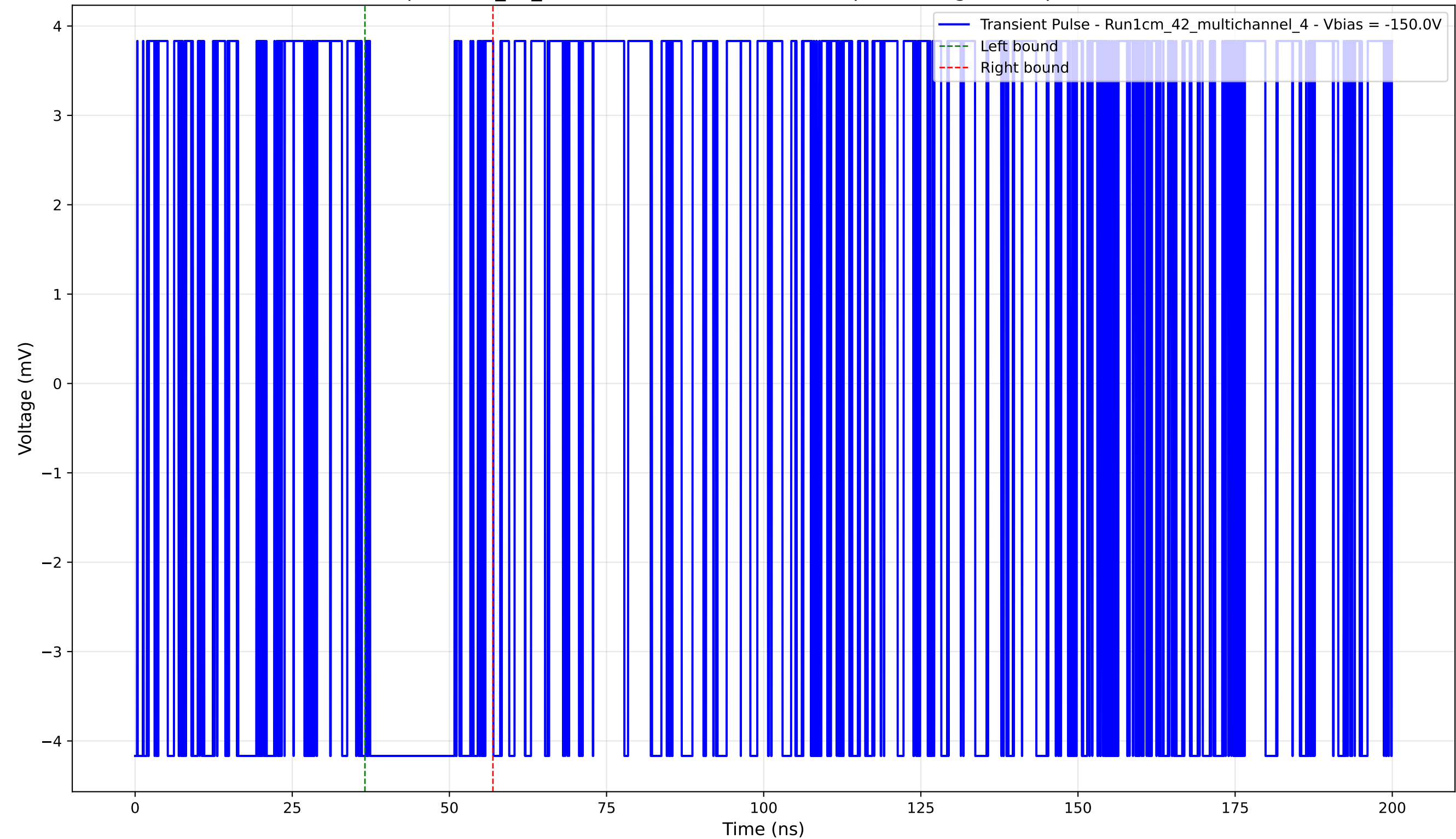
Transient Pulse - Sample: 1cm_42_multichannel - Position: 830.0 \mu\text{m} - Charge: 1.18 pC - Rise Time: 0.00 ns (N/A)
