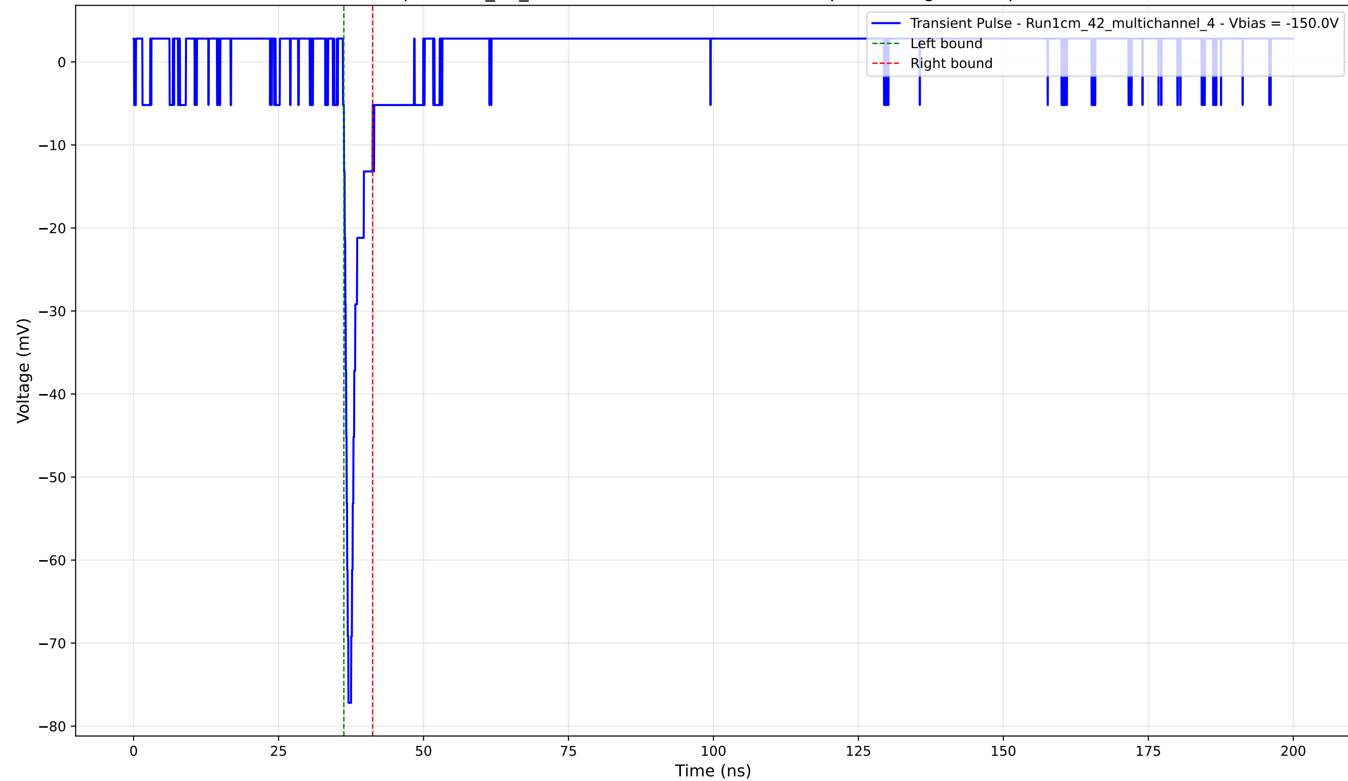
Transient Pulse - Sample: 1cm_42_multichannel - Position: 2270.0 \mu\text{m} - Charge: 3.18 pC - Rise Time: 0.77 ns
