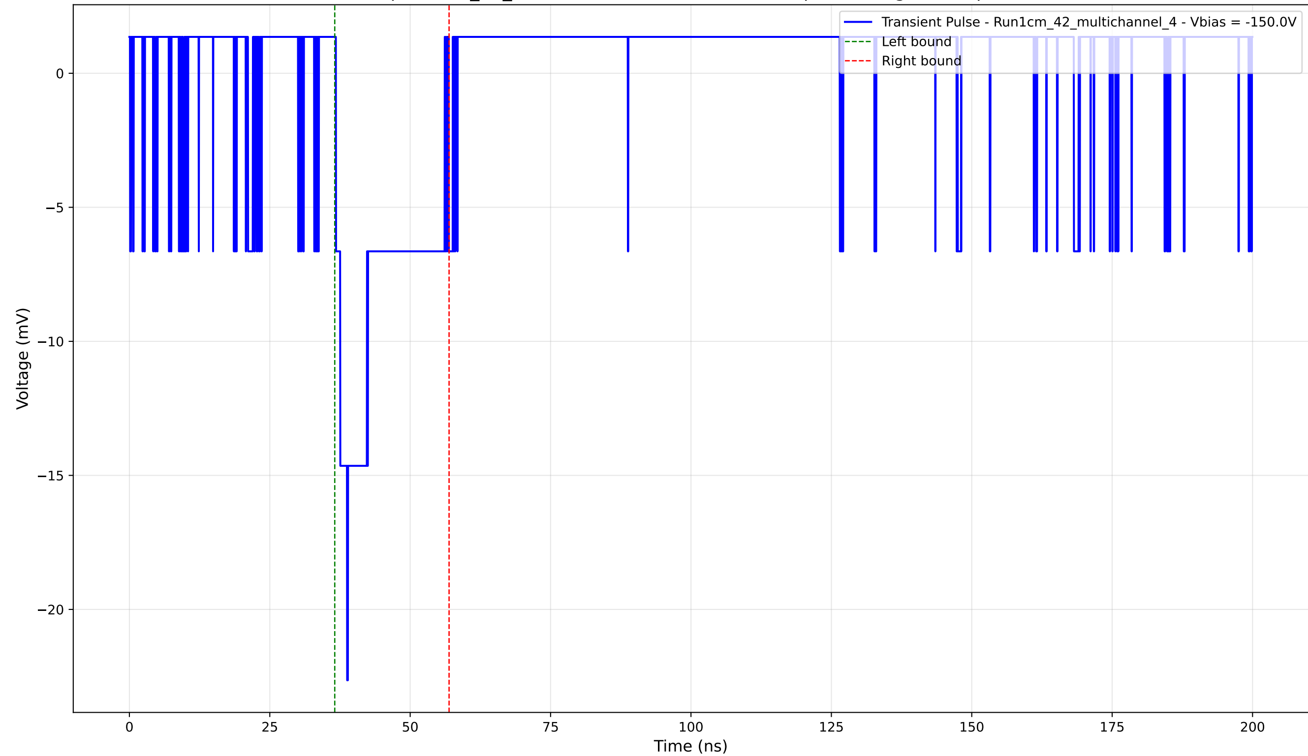
Transient Pulse - Sample: 1cm_42_multichannel - Position: 3685.0 \mu\text{m} - Charge: 3.42 pC - Rise Time: 2.00 ns
