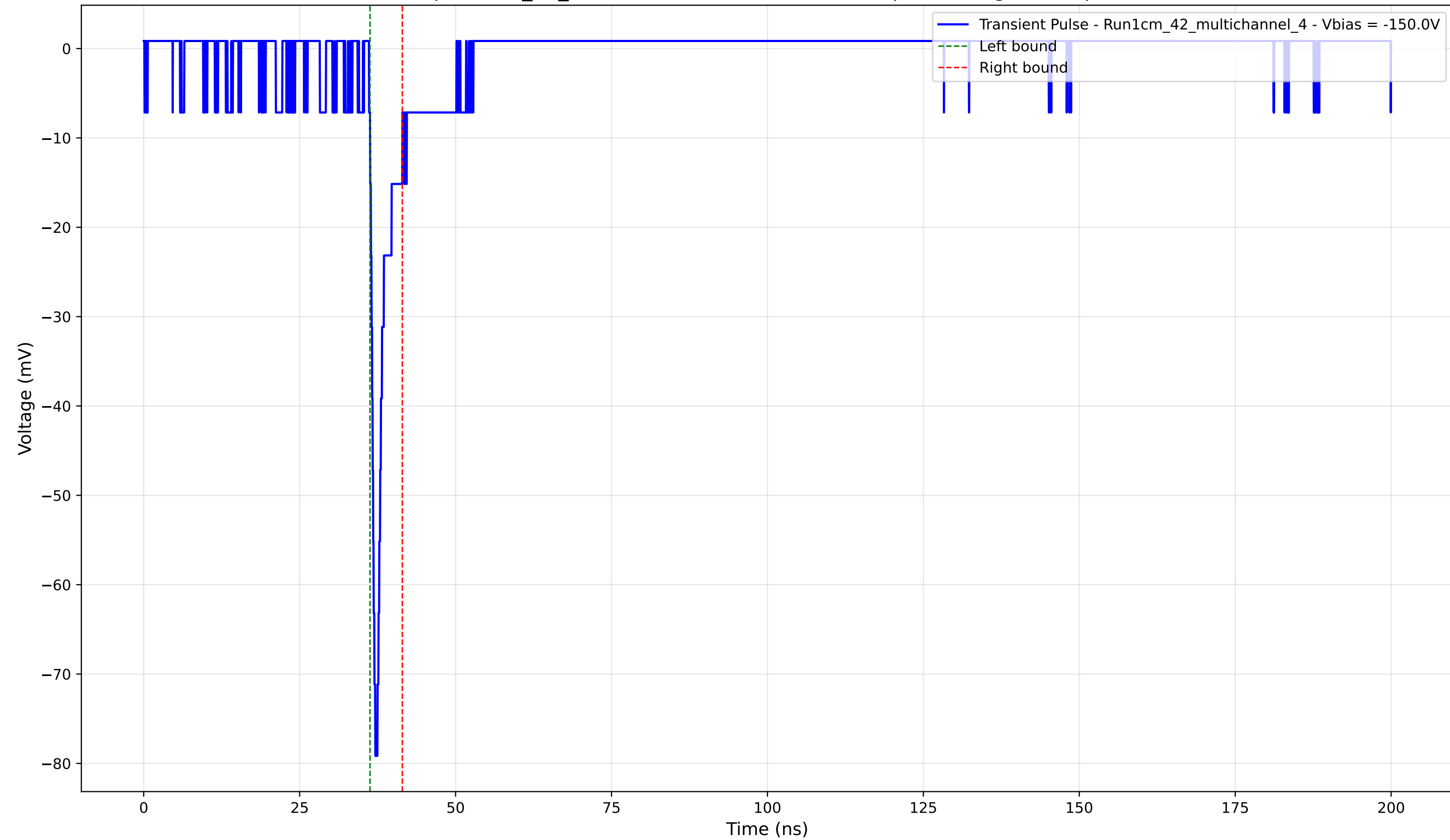
Transient Pulse - Sample: 1cm_42_multichannel - Position: 2240.0 \mu\text{m} - Charge: 3.37 pC - Rise Time: 0.84 ns
