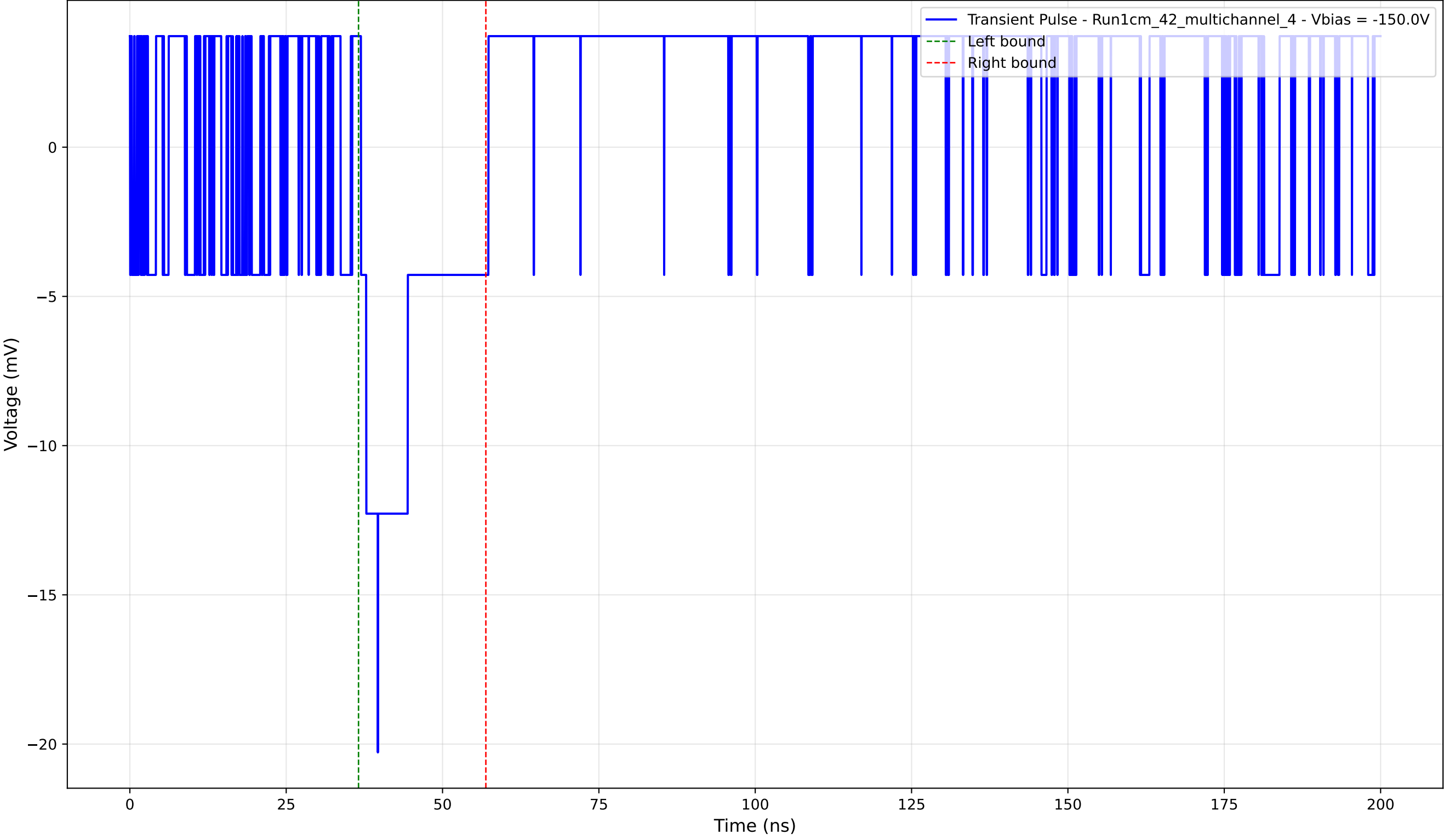
Transient Pulse - Sample: 1cm_42_multichannel - Position: 720.0 \mu\text{m} - Charge: 2.75 pC - Rise Time: 0.00 ns (N/A)
