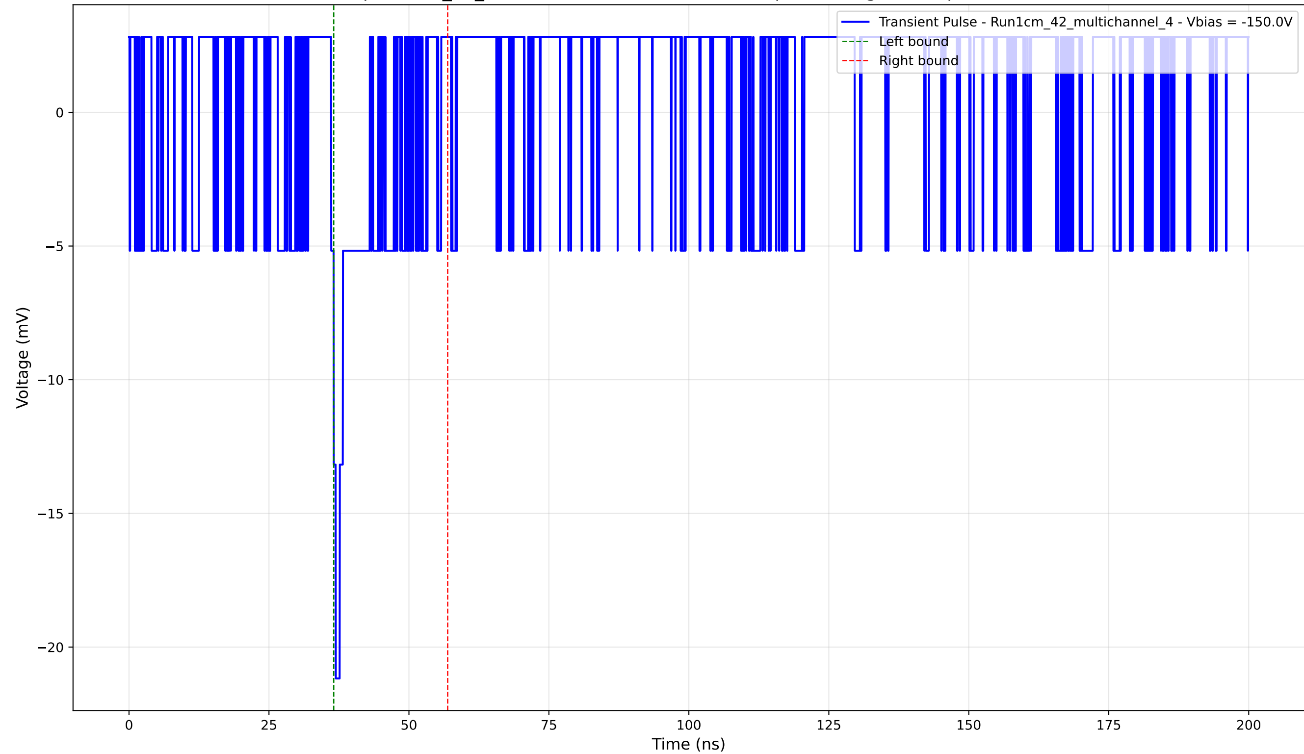
Transient Pulse - Sample: 1cm_42_multichannel - Position: 2345.0 \mu\text{m} - Charge: 1.30 pC - Rise Time: 0.00 ns (N/A)
