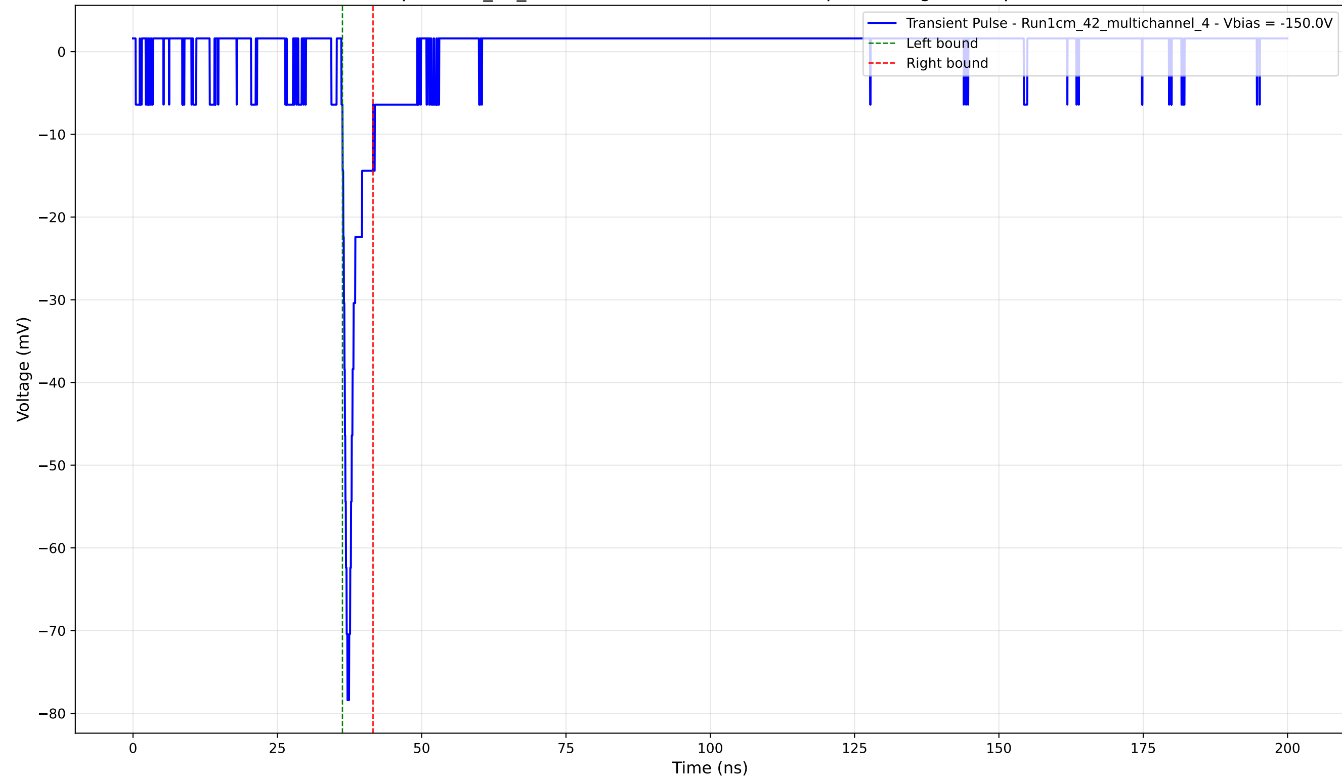
Transient Pulse - Sample: 1cm_42_multichannel - Position: 2535.0 \mu\text{m} - Charge: 3.29 pC - Rise Time: 0.86 ns
