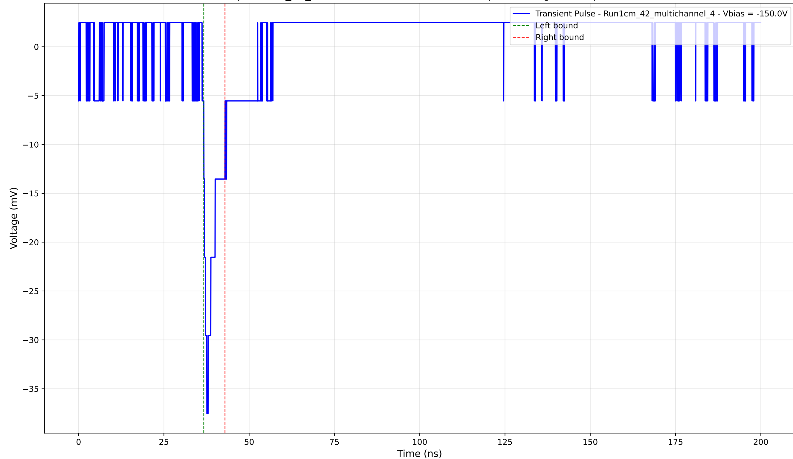
Transient Pulse - Sample: 1cm_42_multichannel - Position: 1675.0 \mu\text{m} - Charge: 2.48 pC - Rise Time: 1.41 ns
