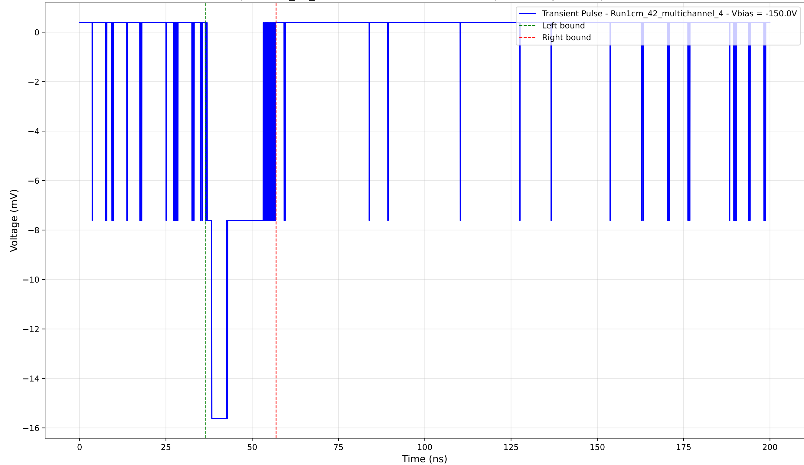
Transient Pulse - Sample: 1cm_42_multichannel - Position: 4275.0 \mu\text{m} - Charge: 3.42 pC - Rise Time: 1.36 ns
