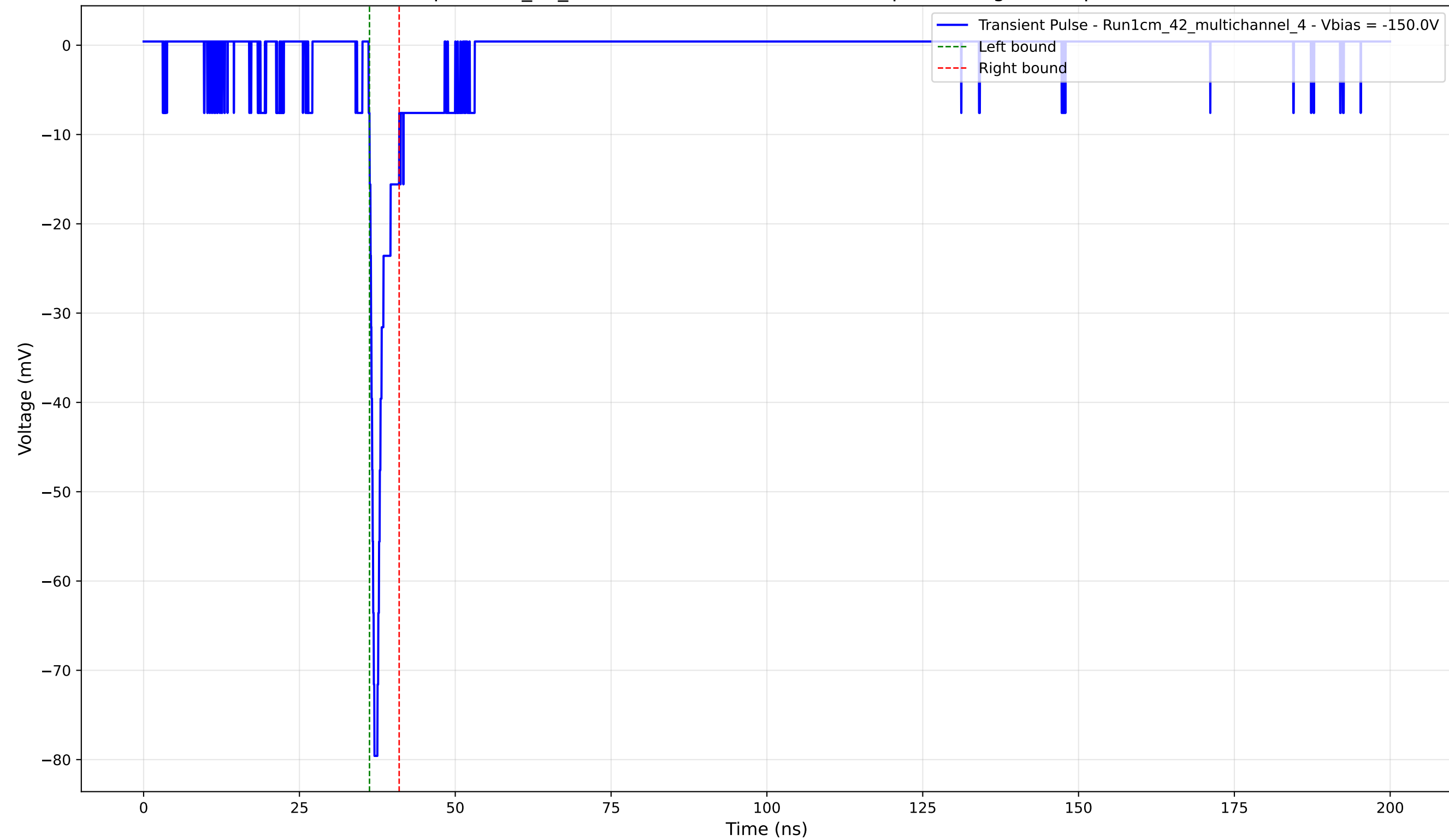
Transient Pulse - Sample: 1cm_42_multichannel - Position: 2280.0 \mu\text{m} - Charge: 3.32 pC - Rise Time: 0.78 ns
