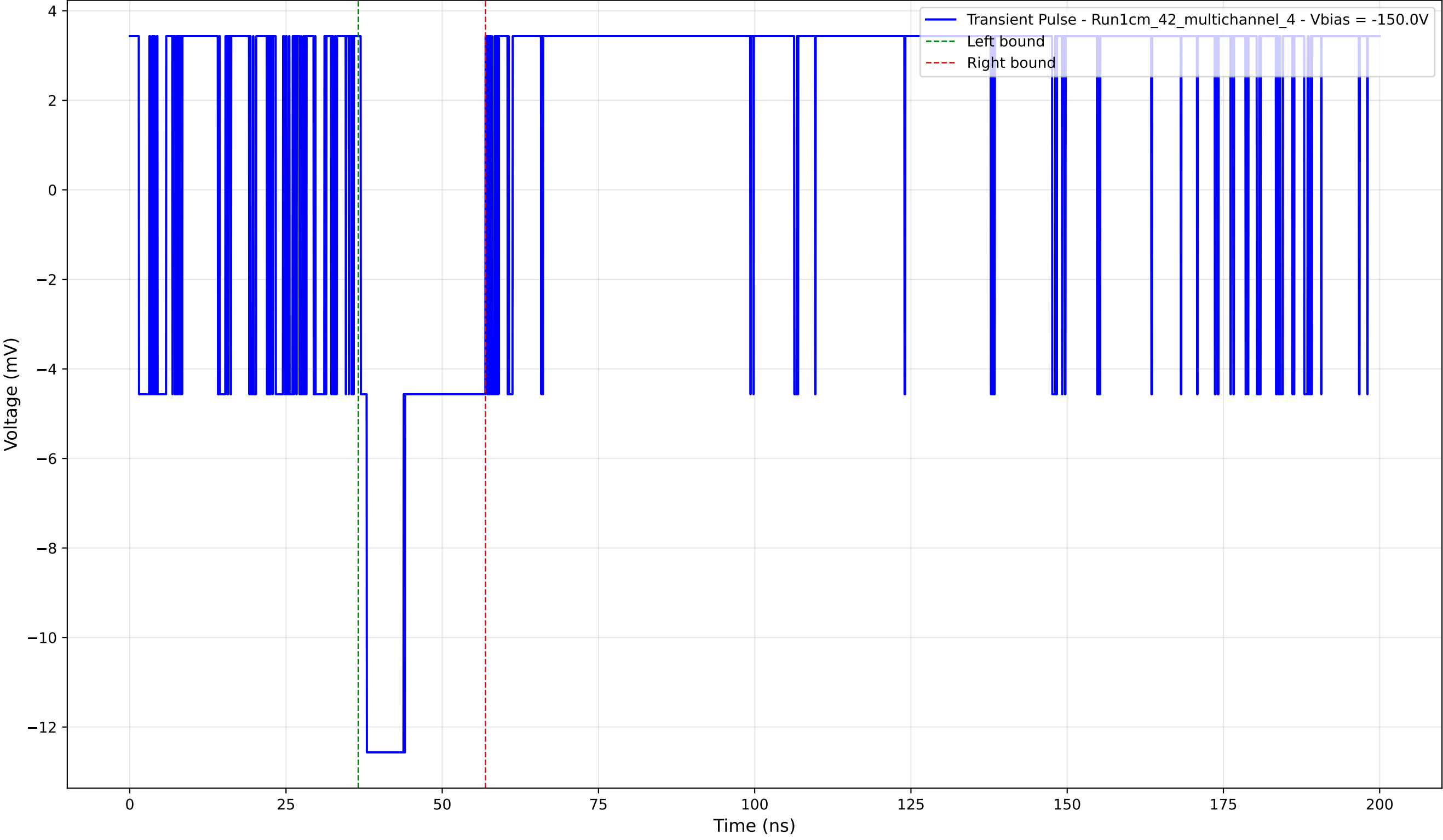
Transient Pulse - Sample: 1cm_42_multichannel - Position: 635.0 \mu\text{m} - Charge: 2.75 pC - Rise Time: 0.00 ns (N/A)
