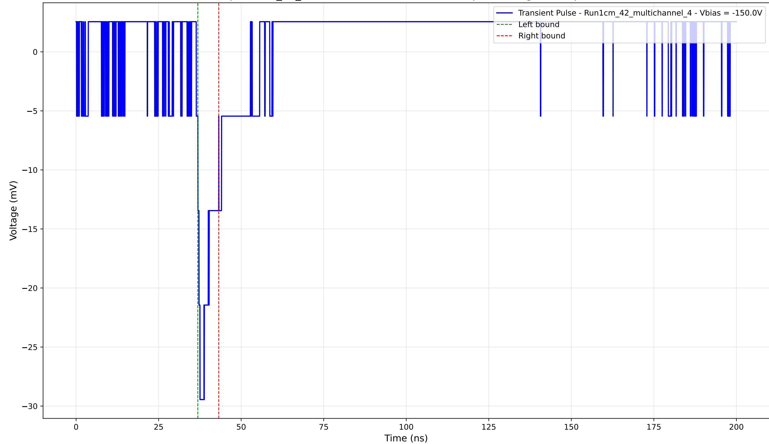
Transient Pulse - Sample: 1cm_42_multichannel - Position: 1500.0 \mu\text{m} - Charge: 2.39 pC - Rise Time: 1.14 ns
