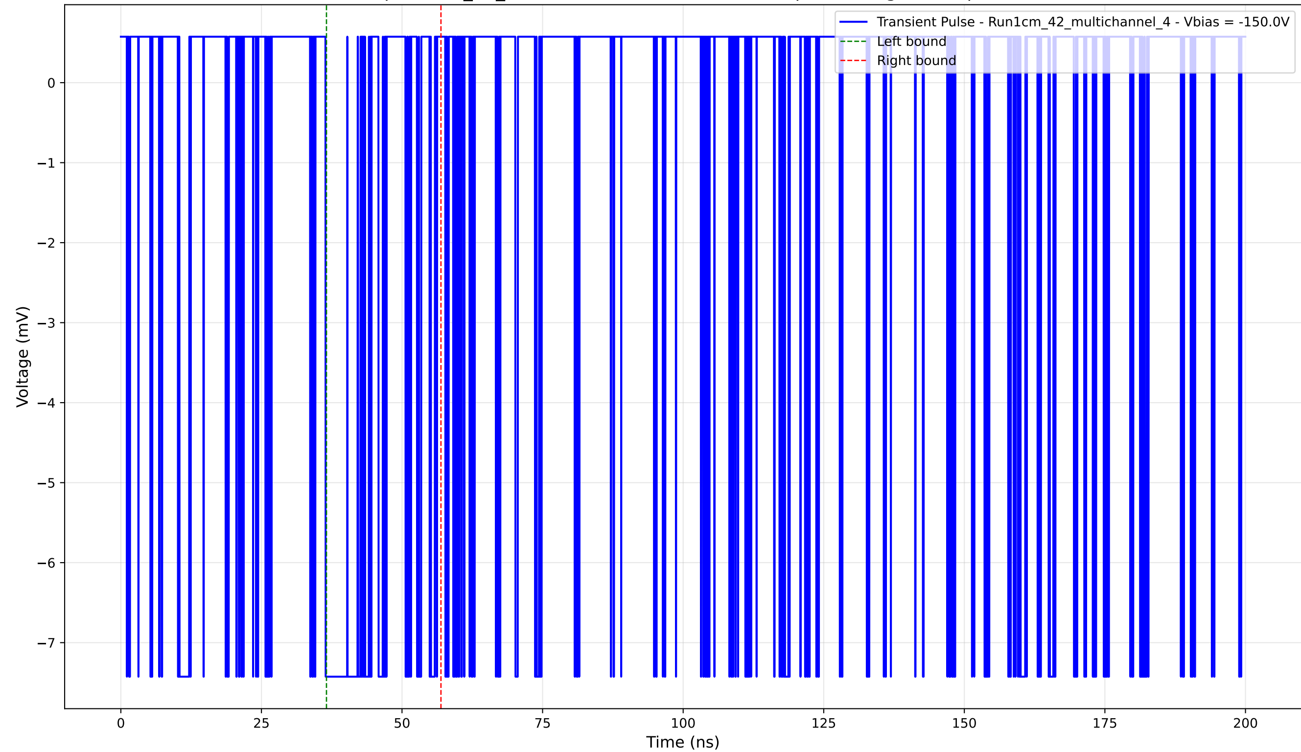
Transient Pulse - Sample: 1cm_42_multichannel - Position: 2865.0 \mu\text{m} - Charge: 1.48 pC - Rise Time: 0.02 ns
