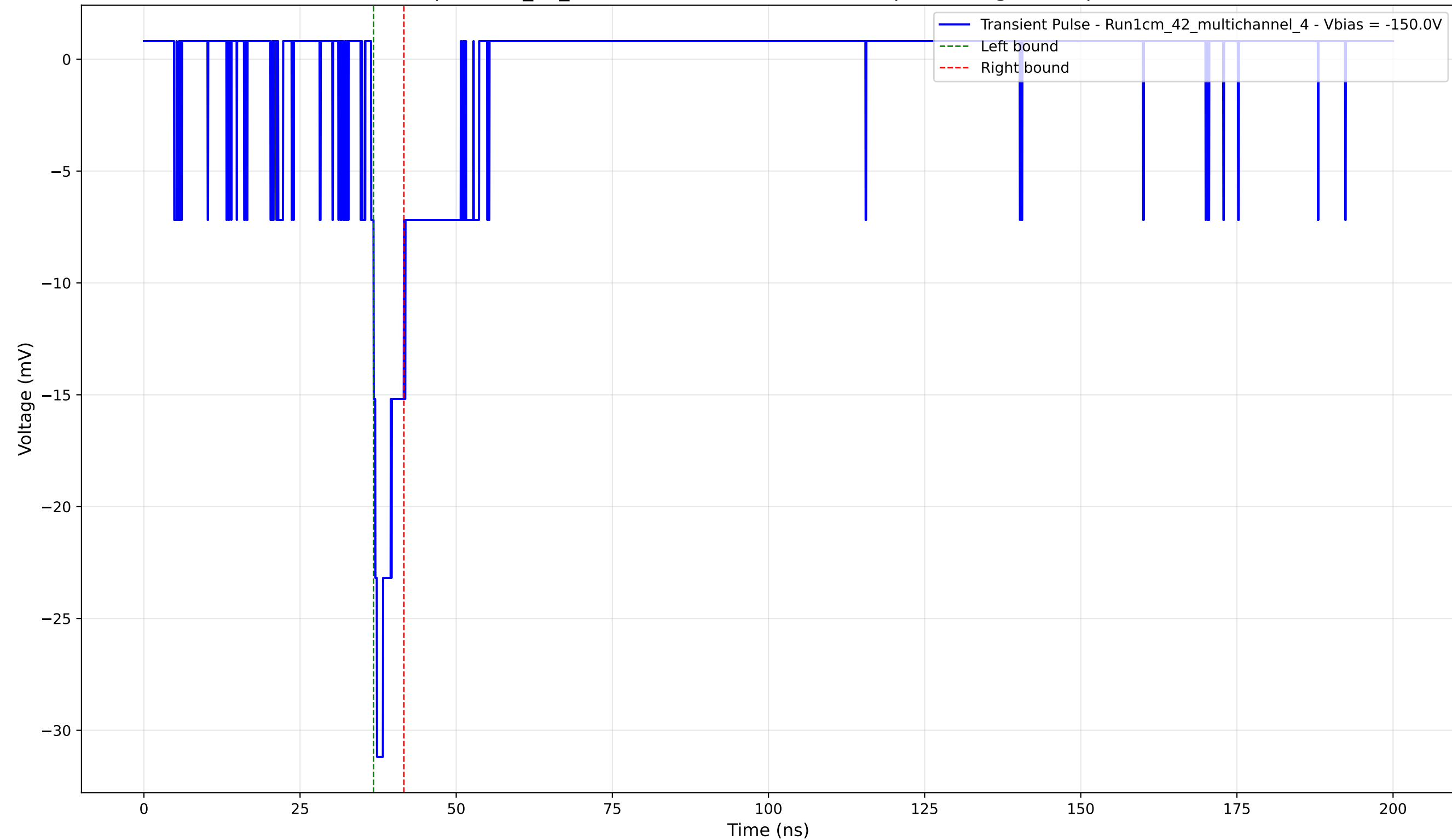
Transient Pulse - Sample: 1cm_42_multichannel - Position: 3100.0 \mu\text{m} - Charge: 2.03 pC - Rise Time: 0.93 ns
