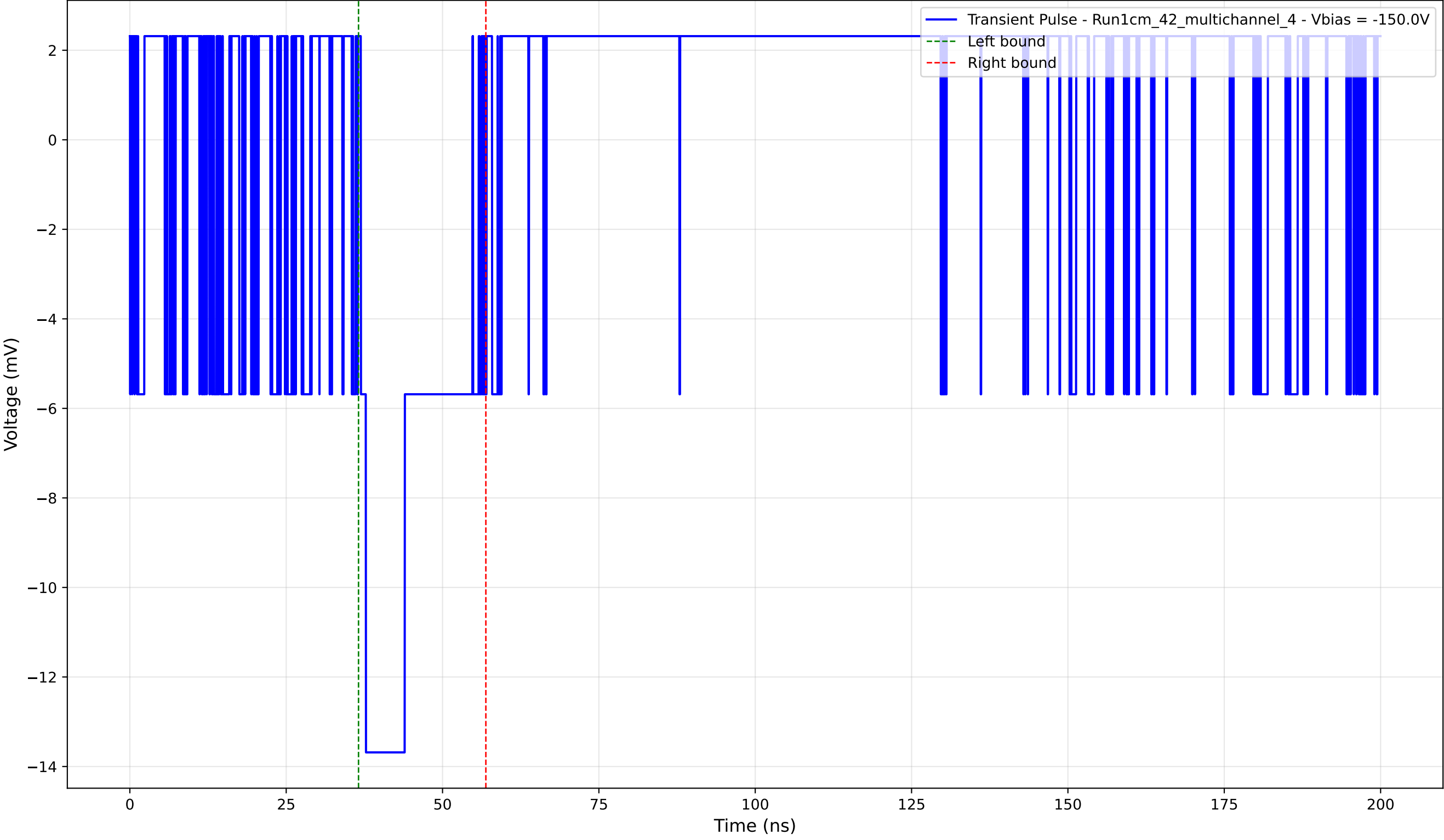
Transient Pulse - Sample: 1cm_42_multichannel - Position: 735.0 \mu\text{m} - Charge: 3.16 pC - Rise Time: 0.00 ns (N/A)
