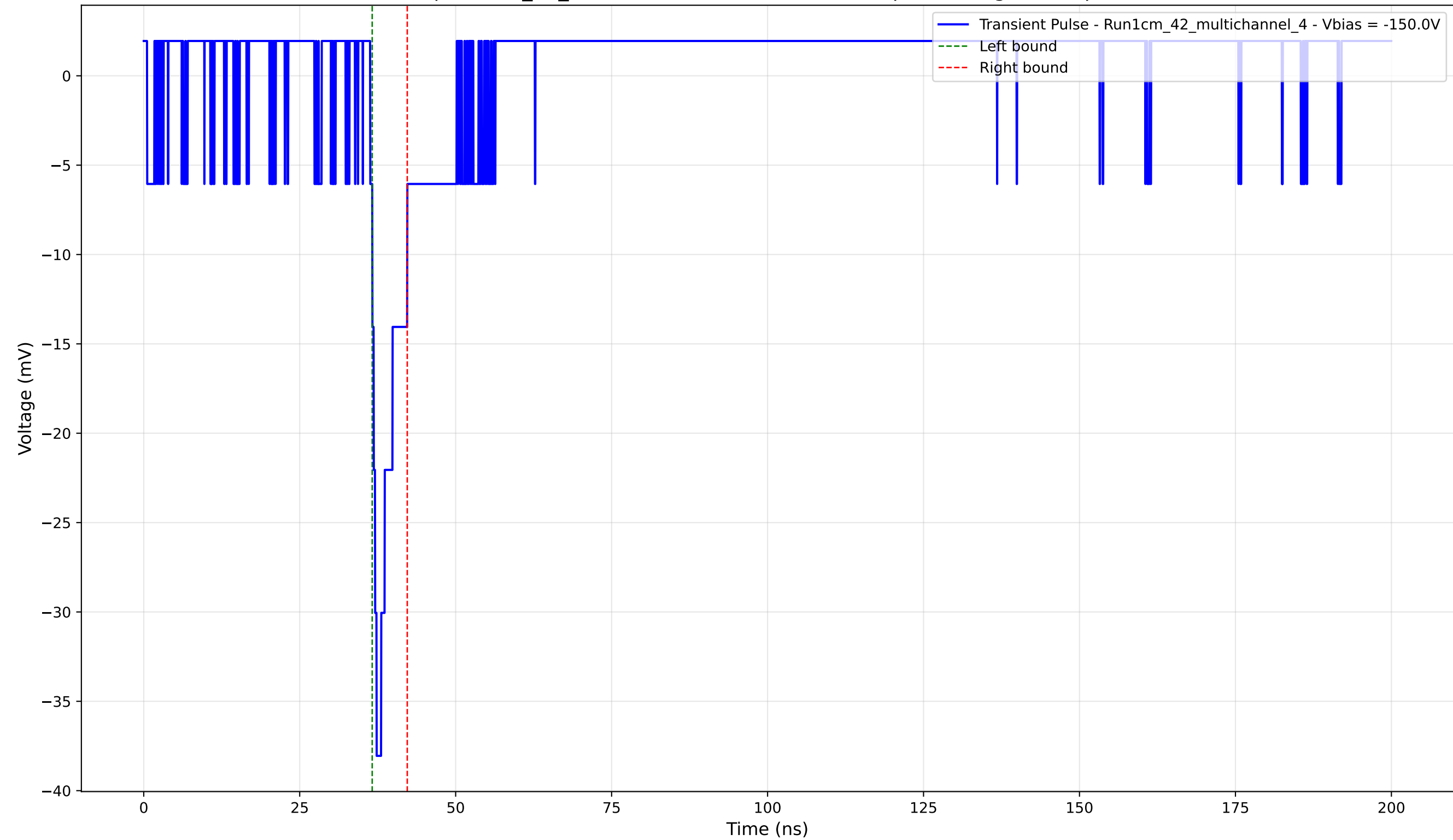
Transient Pulse - Sample: 1cm_42_multichannel - Position: 3005.0 \mu\text{m} - Charge: 2.42 pC - Rise Time: 1.03 ns
