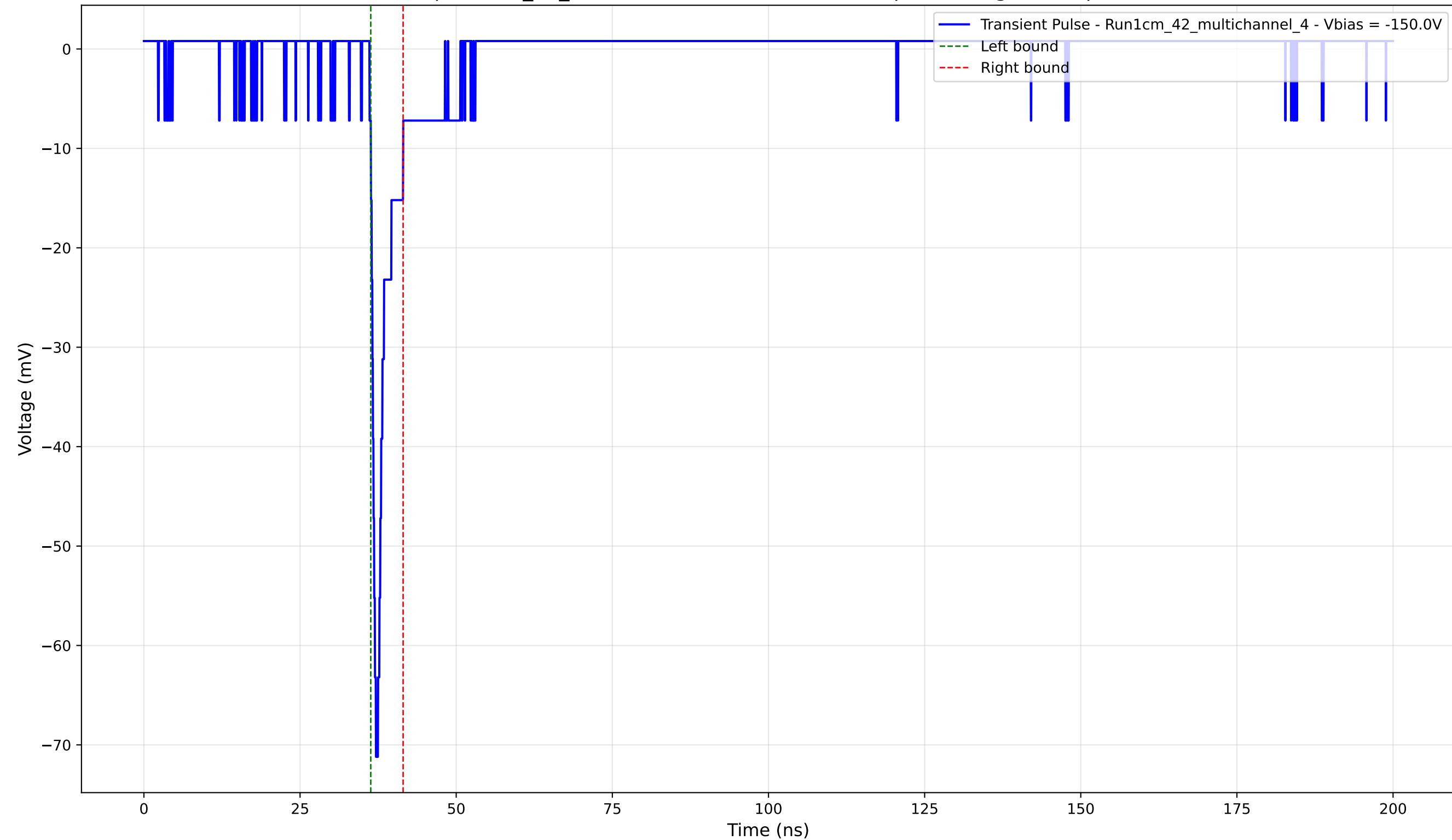
Transient Pulse - Sample: 1cm_42_multichannel - Position: 2570.0 \mu\text{m} - Charge: 3.14 pC - Rise Time: 1.02 ns
