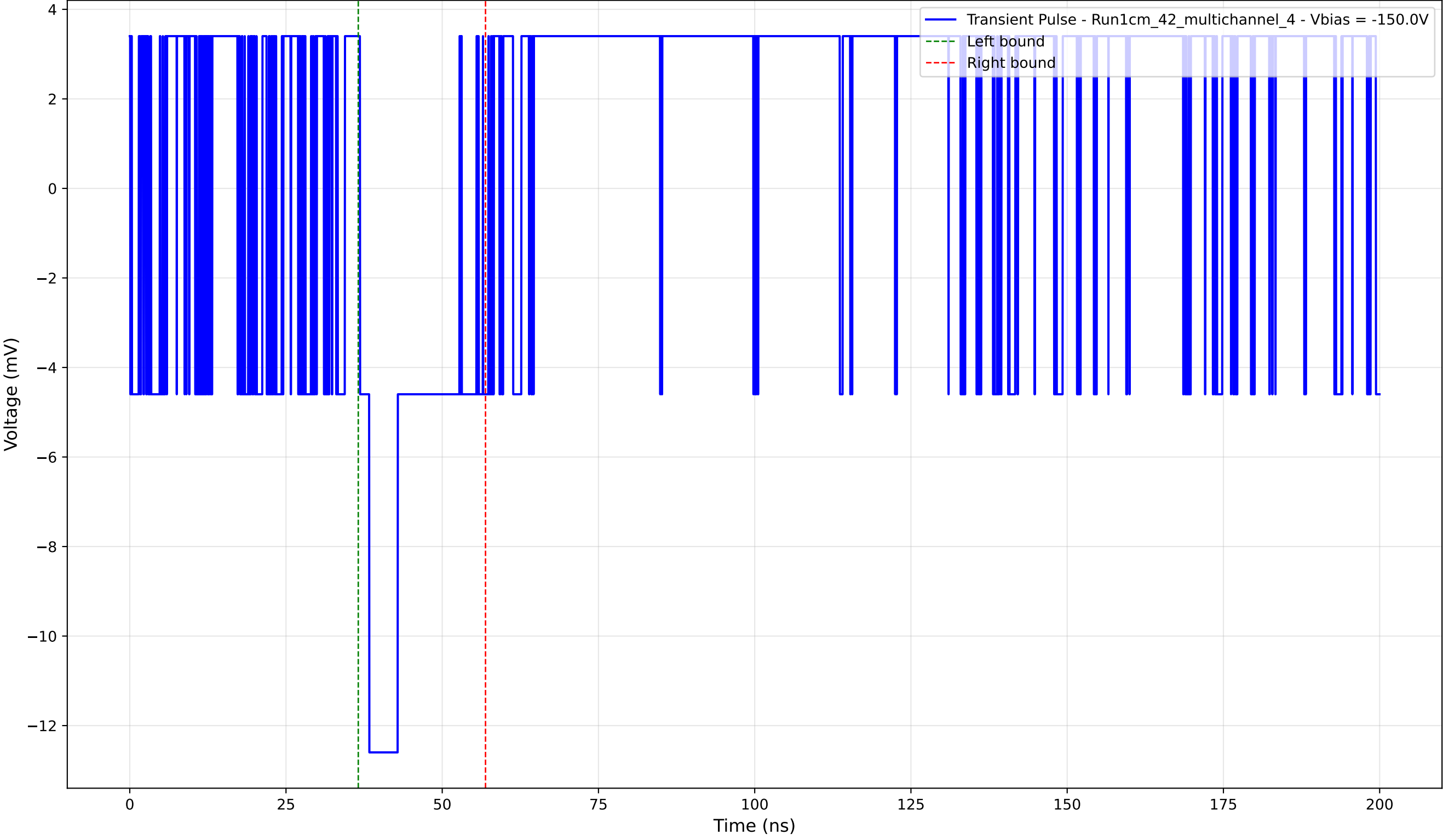
Transient Pulse - Sample: 1cm_42_multichannel - Position: 270.0 \mu\text{m} - Charge: 2.49 pC - Rise Time: 0.00 ns (N/A)
