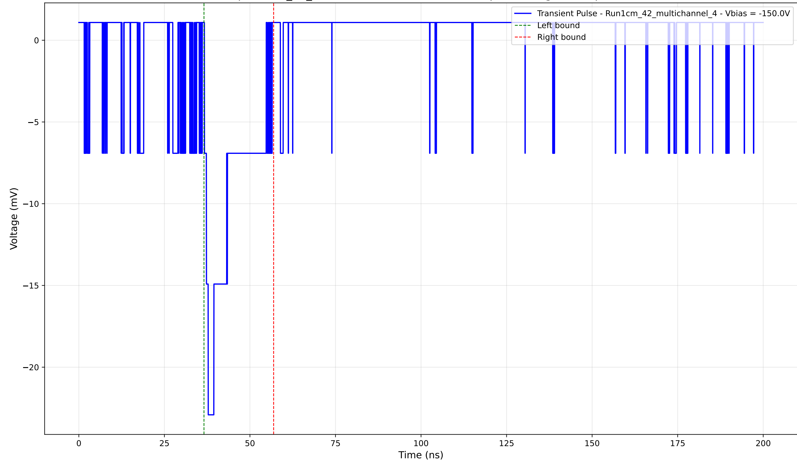
Transient Pulse - Sample: 1cm_42_multichannel - Position: 3515.0 \mu\text{m} - Charge: 3.86 pC - Rise Time: 1.12 ns
