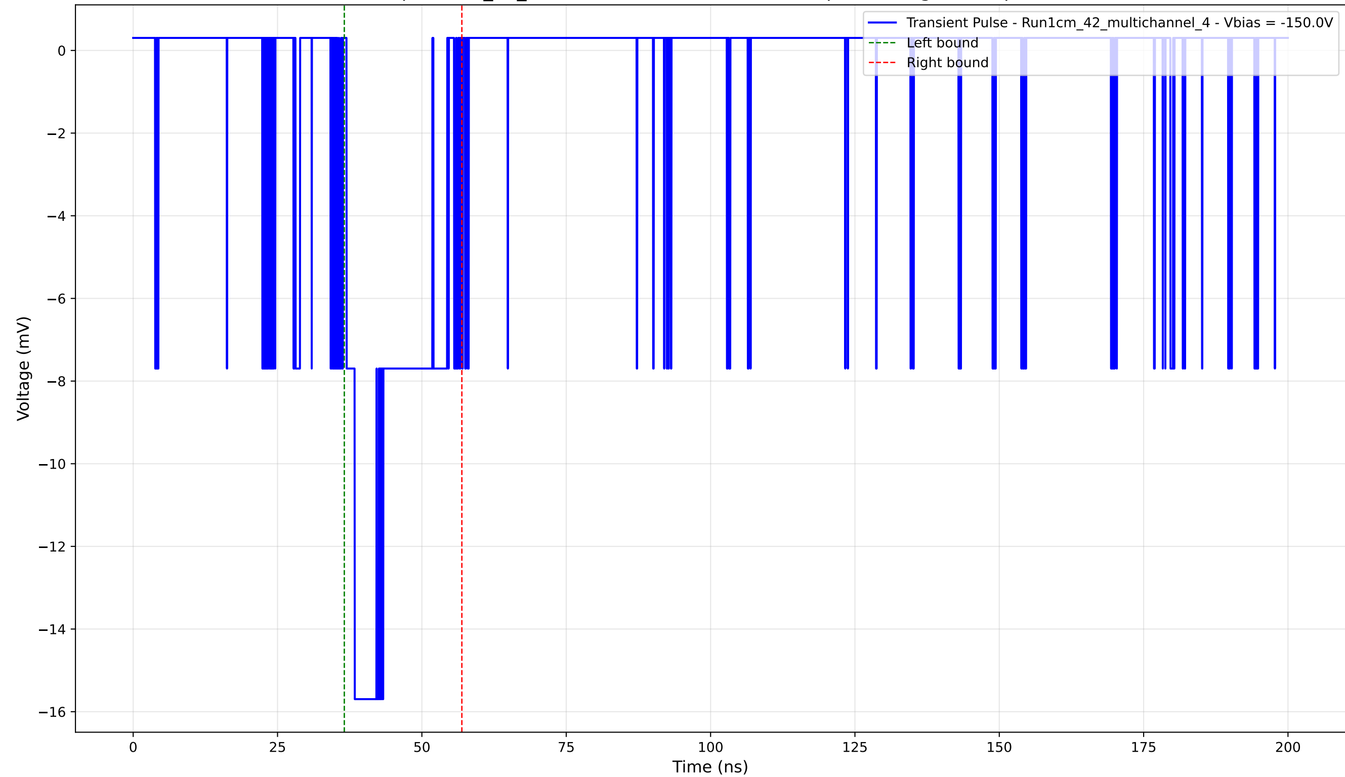
Transient Pulse - Sample: 1cm_42_multichannel - Position: 4755.0 \mu\text{m} - Charge: 3.49 pC - Rise Time: 1.42 ns
