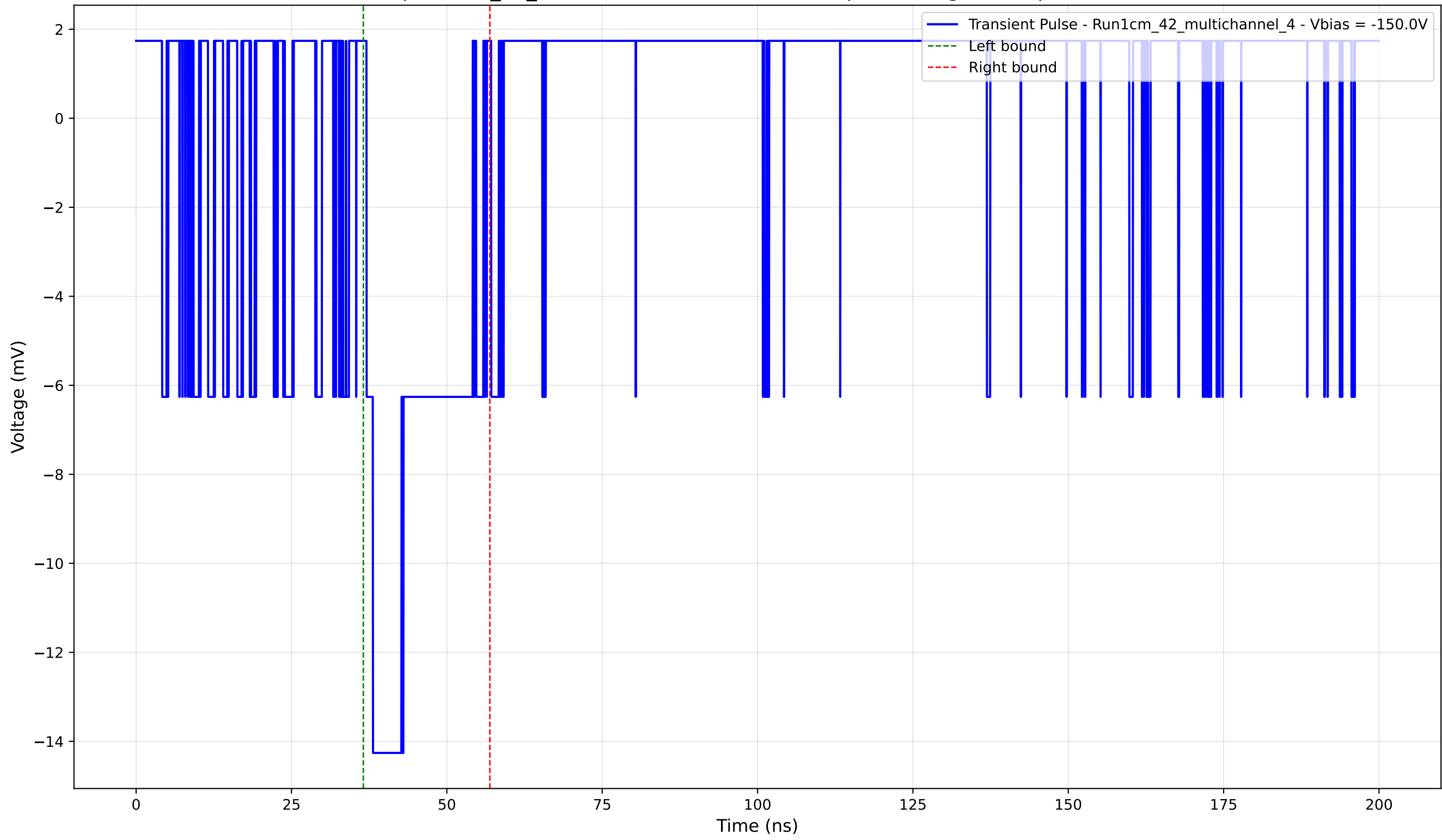
Transient Pulse - Sample: 1cm_42_multichannel - Position: 445.0 \mu\text{m} - Charge: 3.03 pC - Rise Time: 0.00 ns (N/A)
