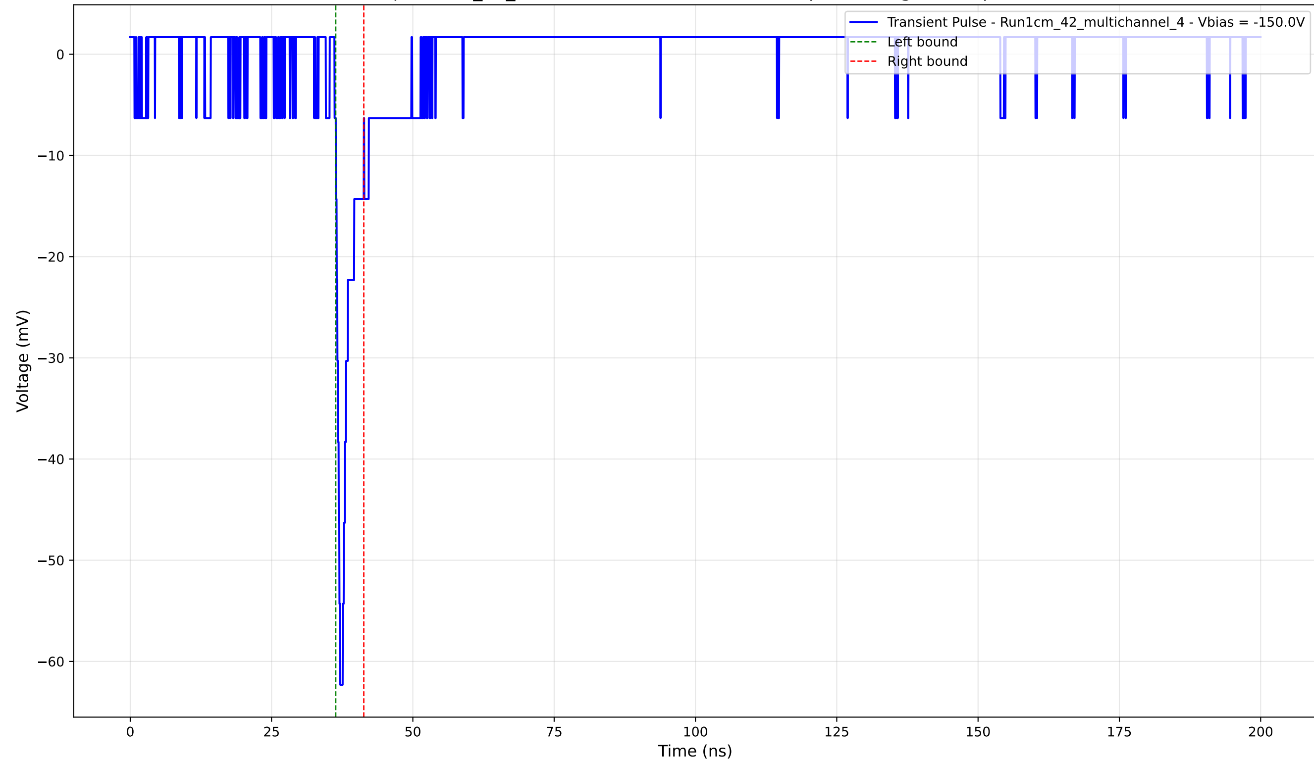
Transient Pulse - Sample: 1cm_42_multichannel - Position: 2640.0 \mu\text{m} - Charge: 2.81 pC - Rise Time: 1.00 ns
