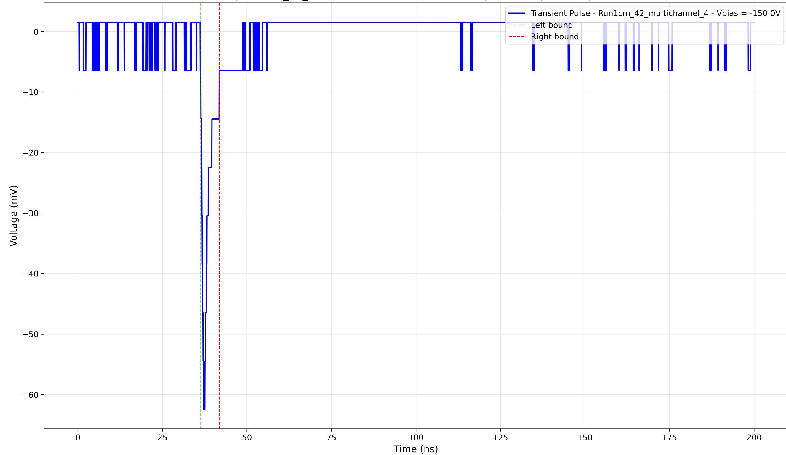
Transient Pulse - Sample: 1cm_42_multichannel - Position: 2135.0 \mu\text{m} - Charge: 2.94 pC - Rise Time: 1.06 ns
