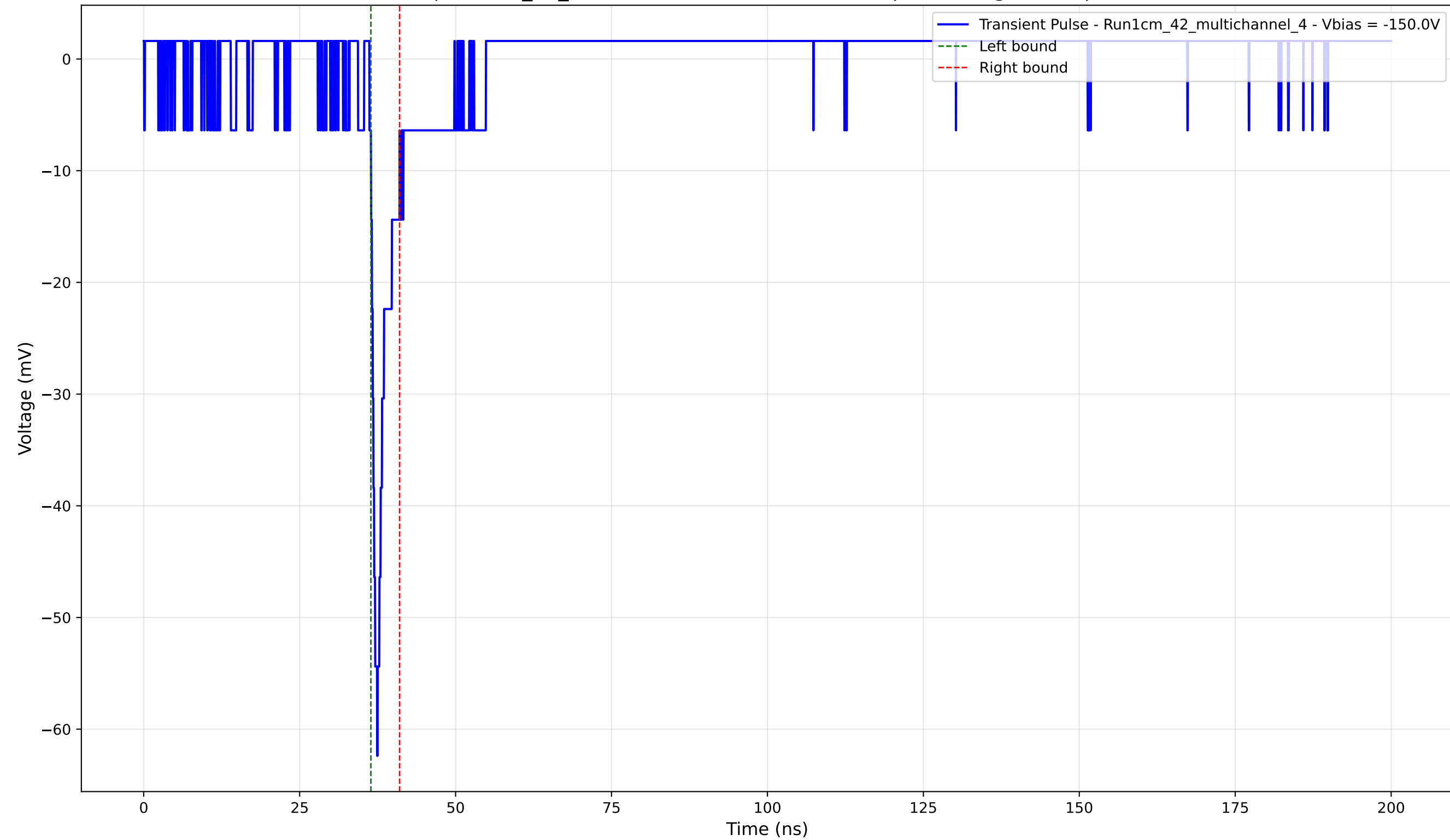
Transient Pulse - Sample: 1cm_42_multichannel - Position: 2075.0 \mu\text{m} - Charge: 2.63 pC - Rise Time: 1.24 ns
