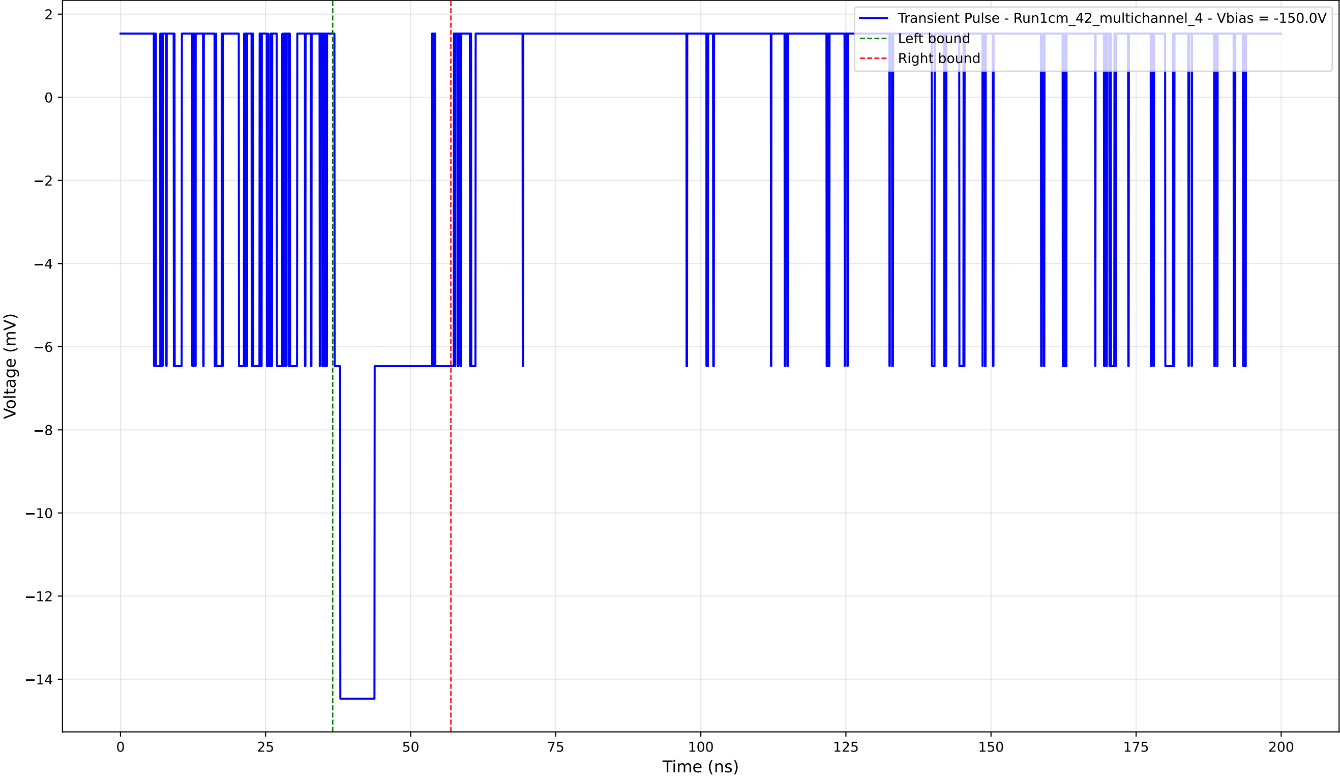
Transient Pulse - Sample: 1cm_42_multichannel - Position: 580.0 \mu\text{m} - Charge: 3.50 pC - Rise Time: 0.00 ns (N/A)
