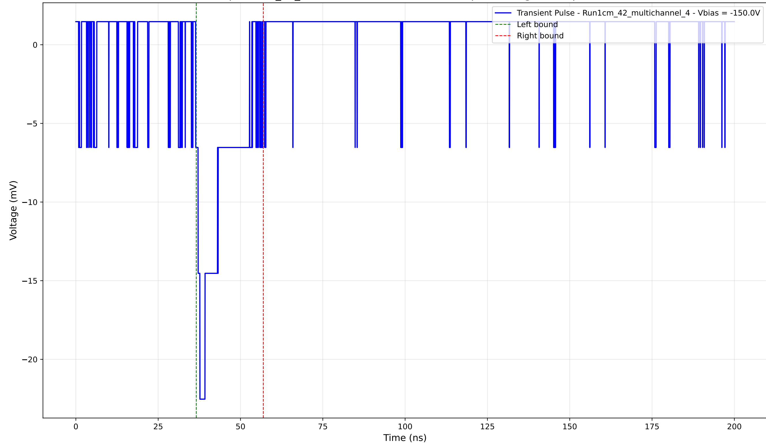
Transient Pulse - Sample: 1cm_42_multichannel - Position: 3480.0 \mu\text{m} - Charge: 3.45 pC - Rise Time: 1.30 ns
