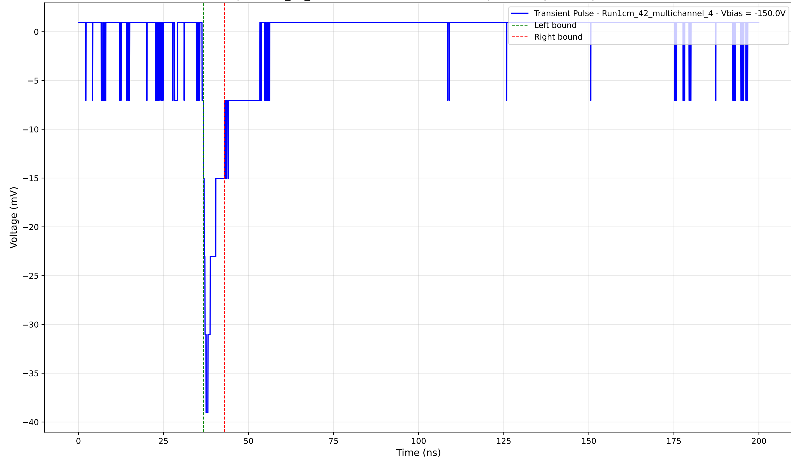
Transient Pulse - Sample: 1cm_42_multichannel - Position: 1660.0 \mu\text{m} - Charge: 2.75 pC - Rise Time: 1.19 ns
