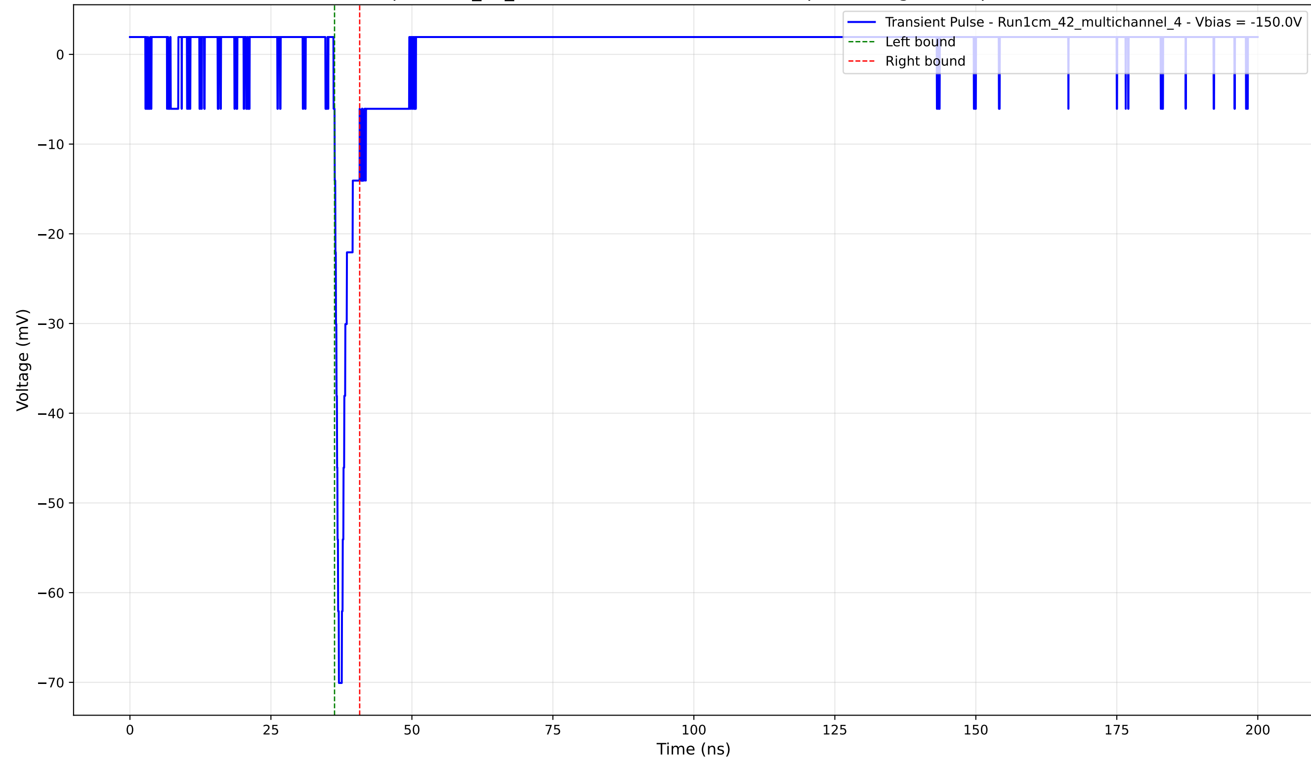
Transient Pulse - Sample: 1cm_42_multichannel - Position: 2540.0 \mu\text{m} - Charge: 2.90 pC - Rise Time: 0.76 ns
