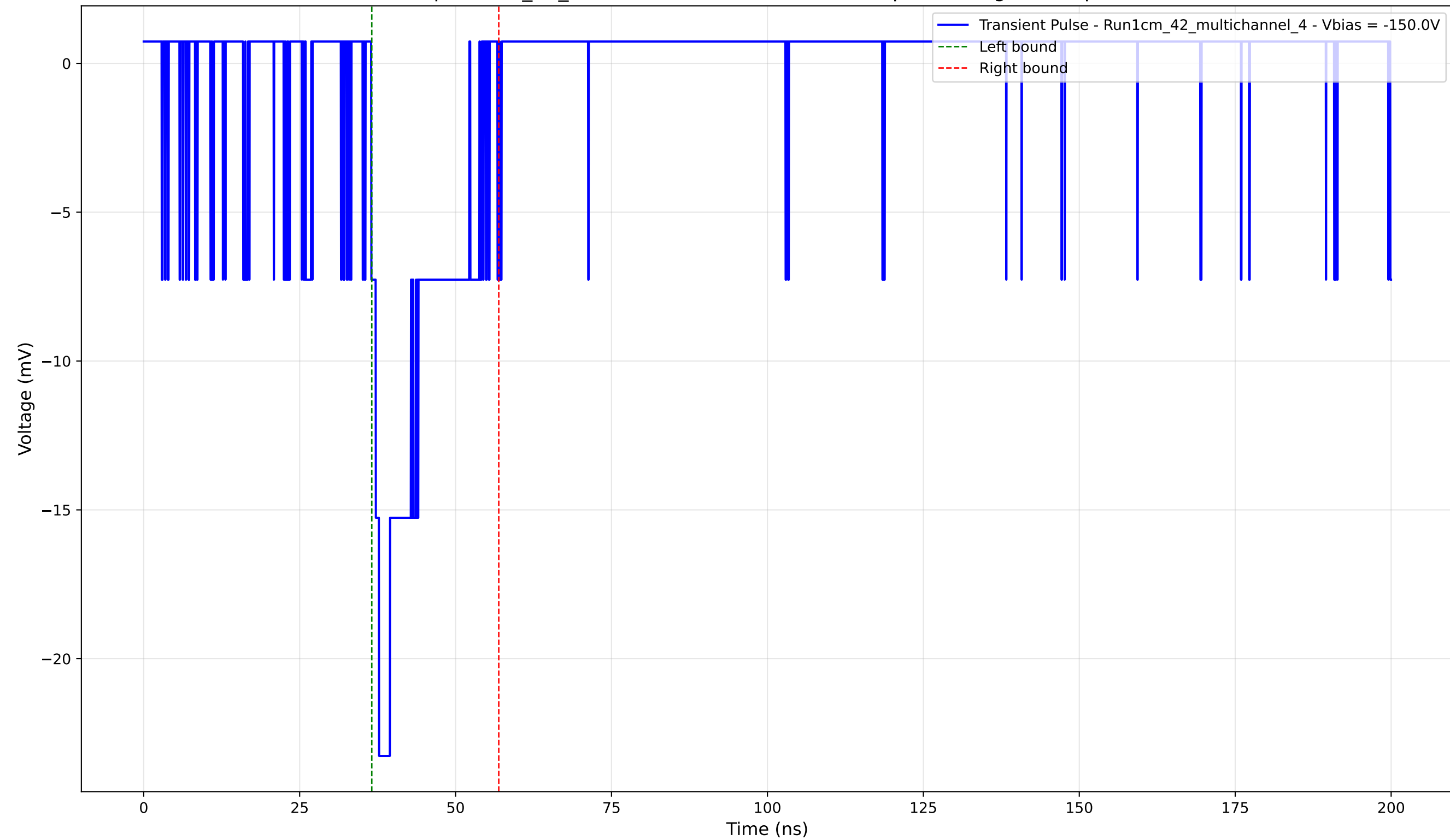
Transient Pulse - Sample: 1cm_42_multichannel - Position: 3495.0 \mu\text{m} - Charge: 3.89 pC - Rise Time: 1.26 ns
