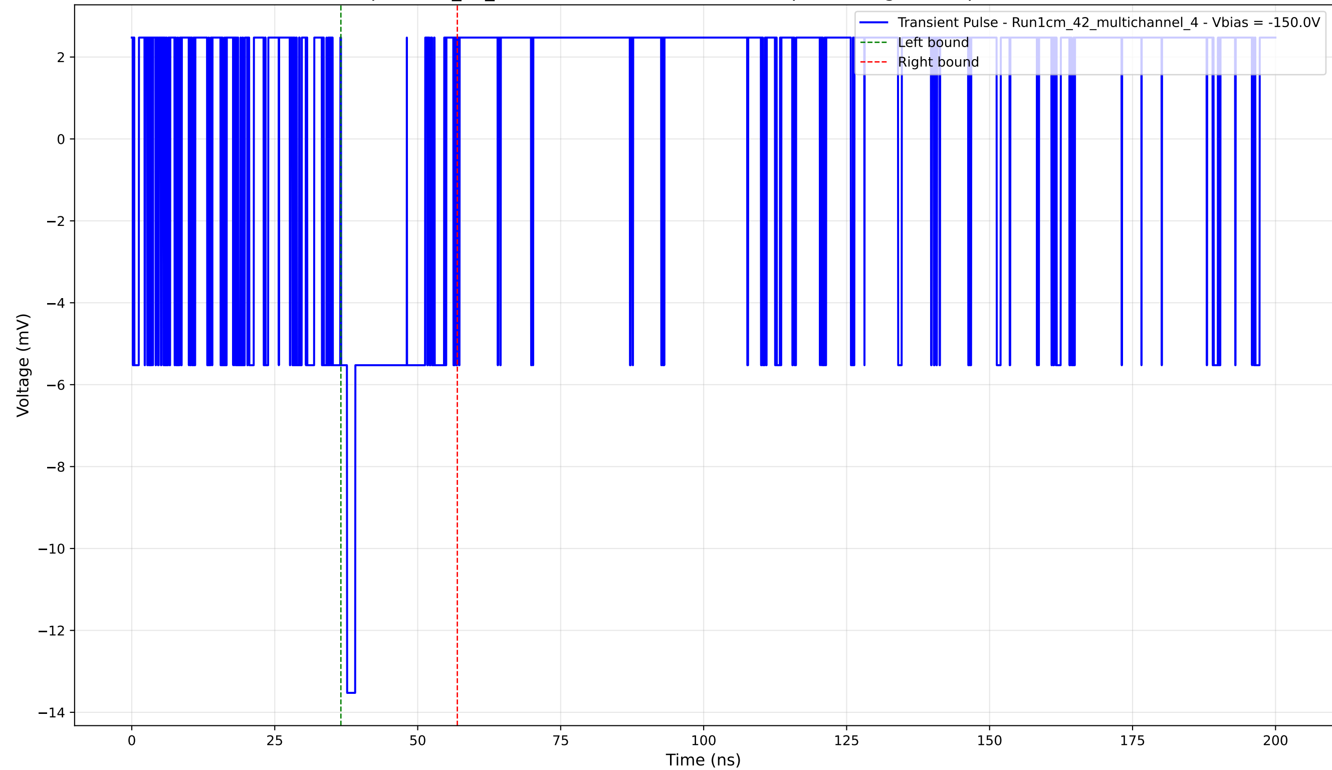
Transient Pulse - Sample: 1cm_42_multichannel - Position: 1420.0 \mu\text{m} - Charge: 2.00 pC - Rise Time: 0.00 ns (N/A)
