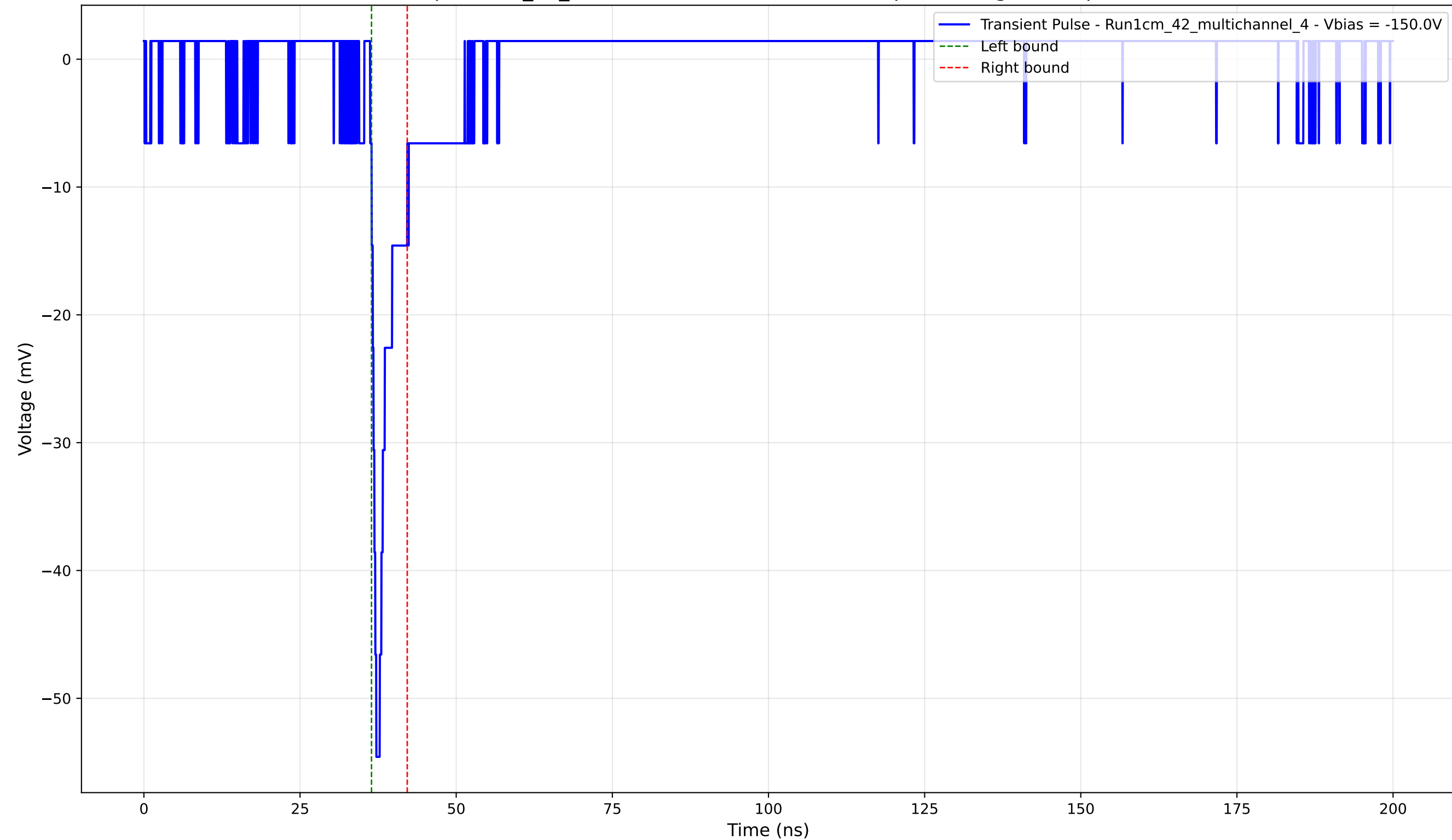
Transient Pulse - Sample: 1cm_42_multichannel - Position: 2755.0 \mu\text{m} - Charge: 2.91 pC - Rise Time: 0.98 ns
