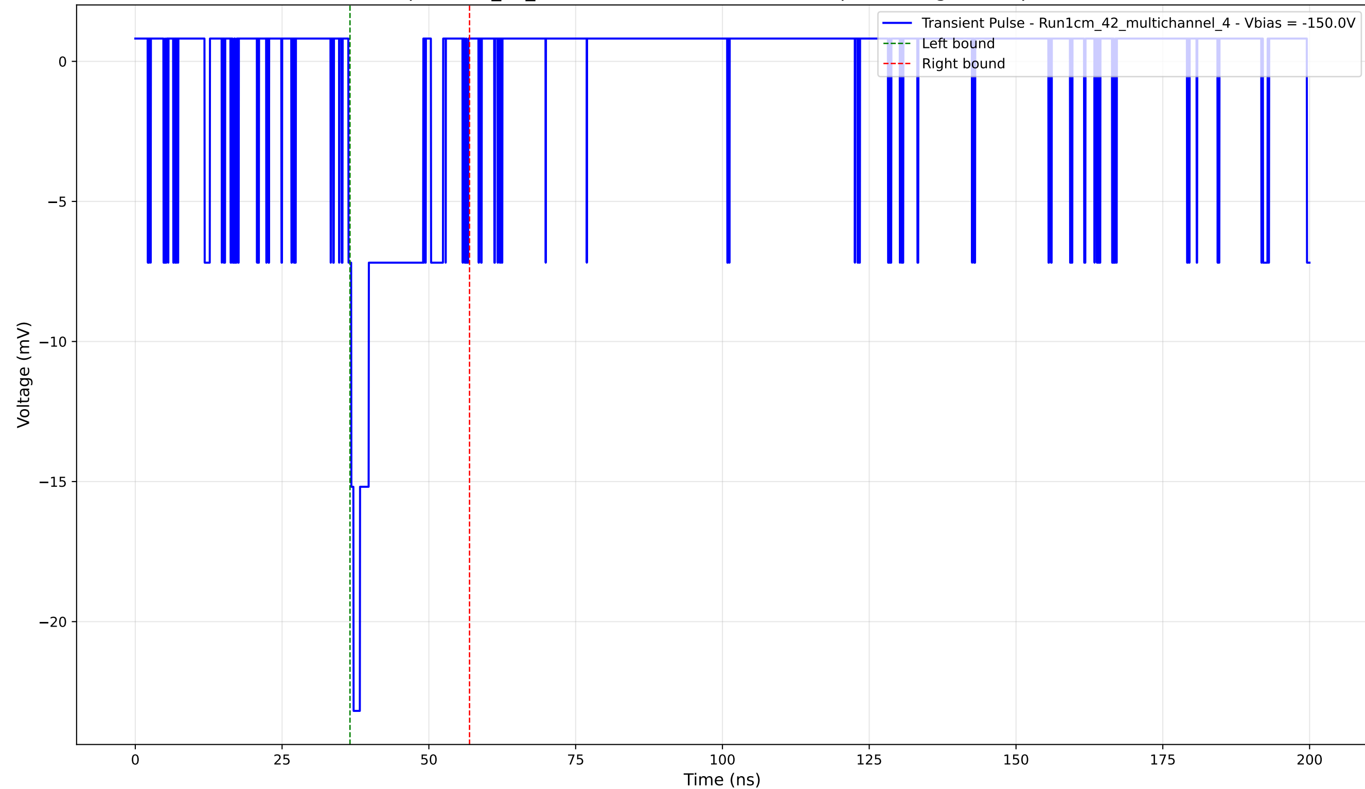
Transient Pulse - Sample: 1cm_42_multichannel - Position: 1830.0 \mu\text{m} - Charge: 2.76 pC - Rise Time: 0.88 ns
