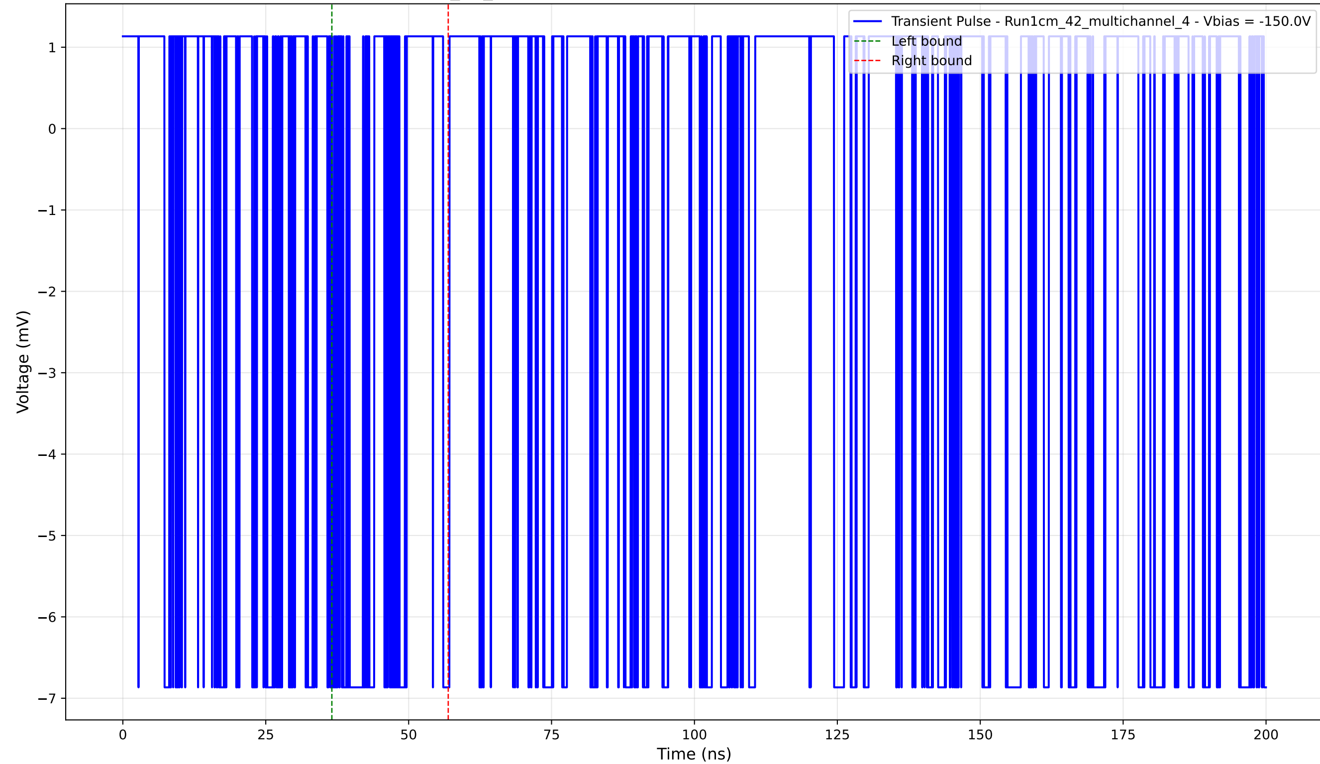
Transient Pulse - Sample: 1cm_42_multichannel - Position: 350.0 \mu\text{m} - Charge: 0.99 pC - Rise Time: 0.00 ns (N/A)
