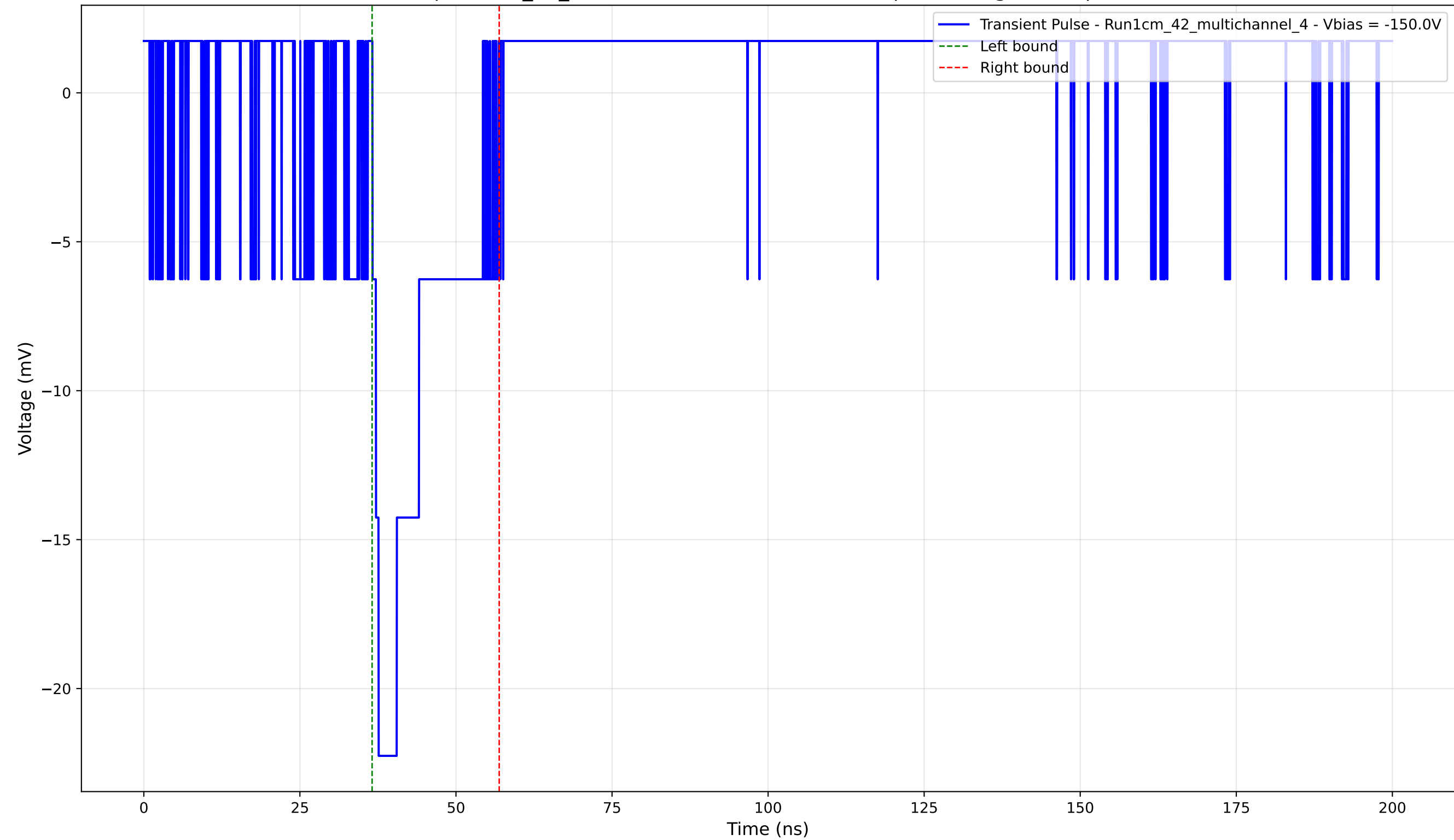
Transient Pulse - Sample: 1cm_42_multichannel - Position: 1270.0 \mu\text{m} - Charge: 3.99 pC - Rise Time: 1.00 ns
