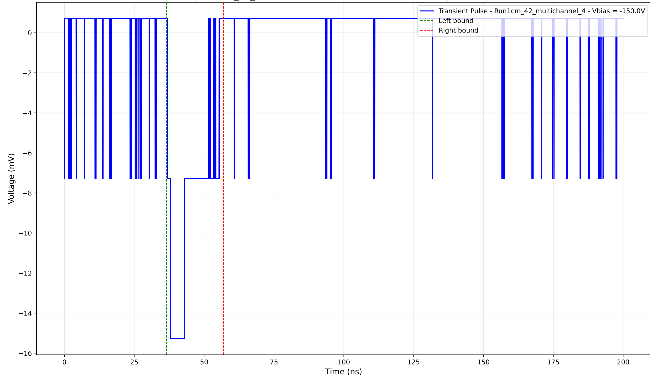
Transient Pulse - Sample: 1cm_42_multichannel - Position: 4050.0 \mu\text{m} - Charge: 3.31 pC - Rise Time: 1.06 ns
