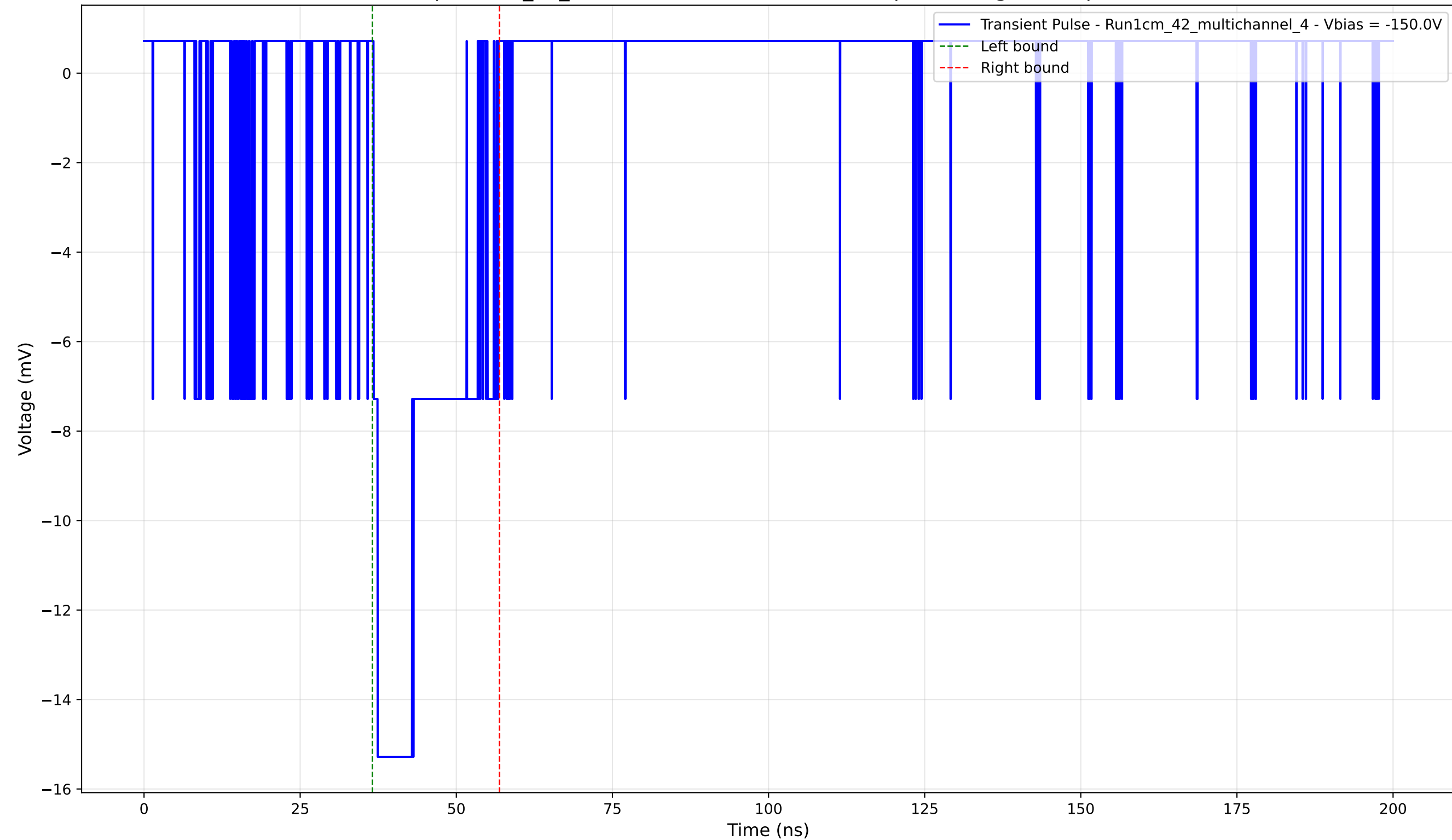
Transient Pulse - Sample: 1cm_42_multichannel - Position: 3610.0 \mu\text{m} - Charge: 3.56 pC - Rise Time: 0.66 ns
