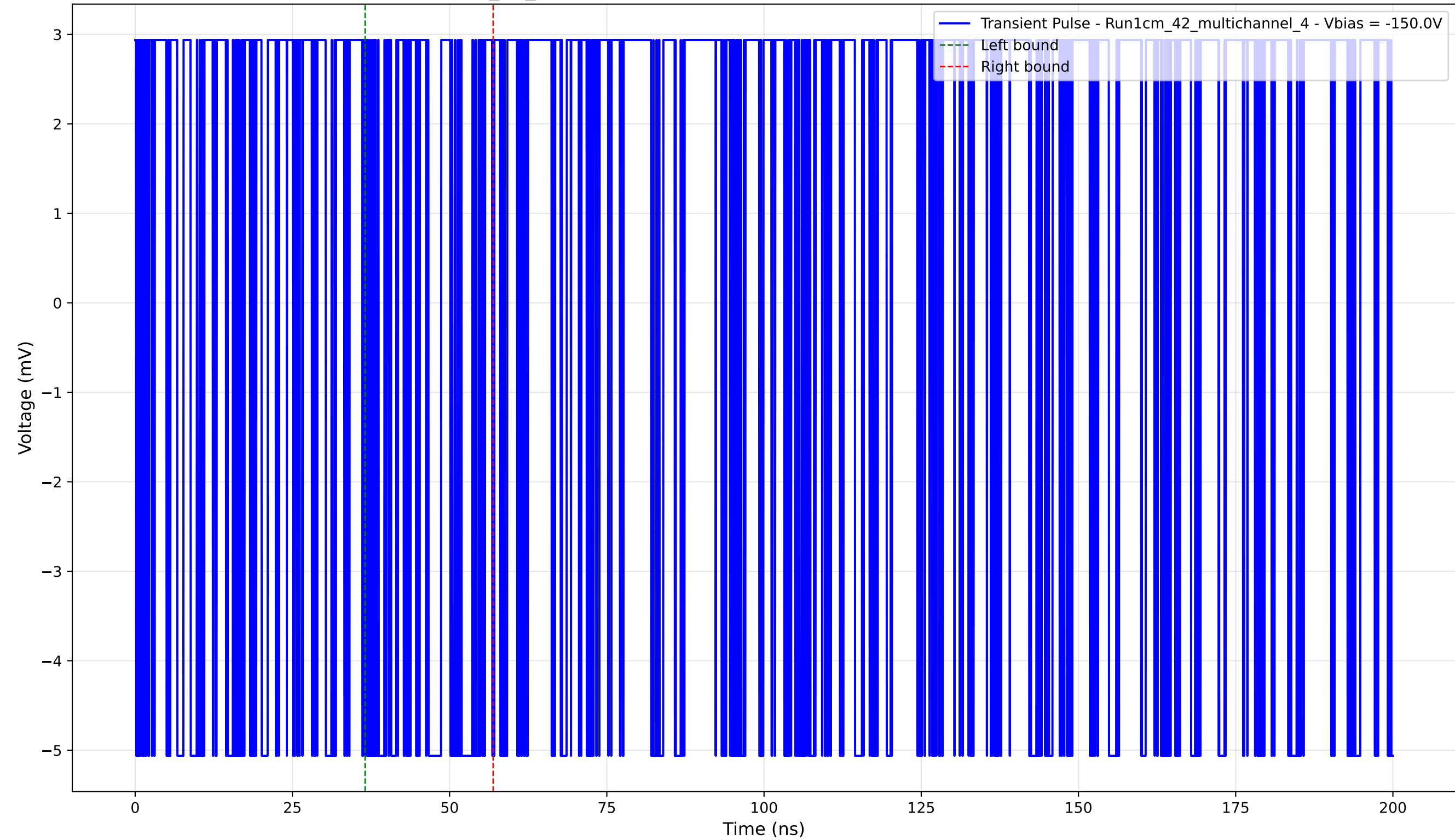
Transient Pulse - Sample: 1cm_42_multichannel - Position: 1385.0 \mu\text{m} - Charge: 0.55 pC - Rise Time: 0.00 ns (N/A)
