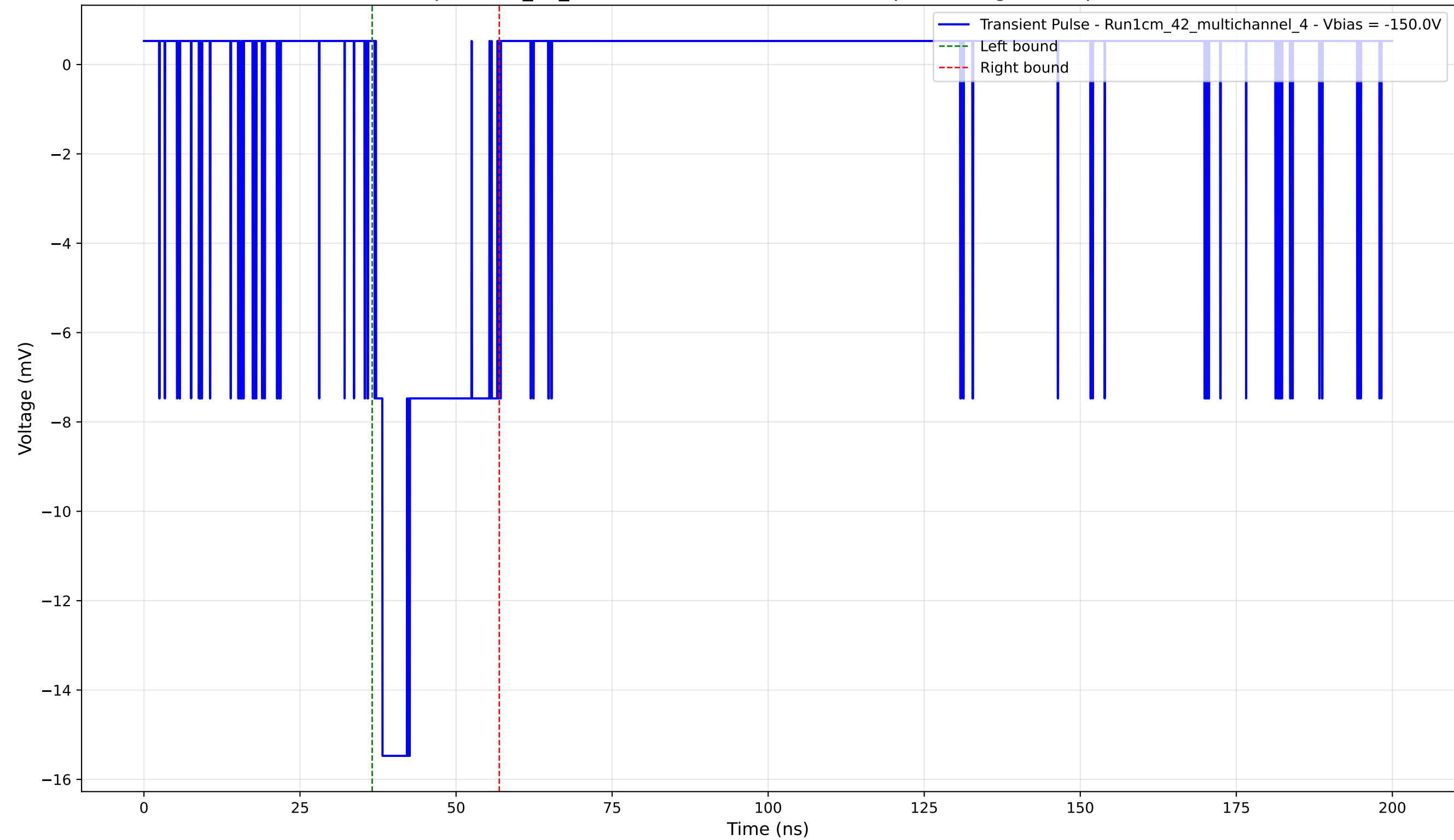
Transient Pulse - Sample: 1cm_42_multichannel - Position: 4105.0 \mu\text{m} - Charge: 3.57 pC - Rise Time: 1.04 ns
