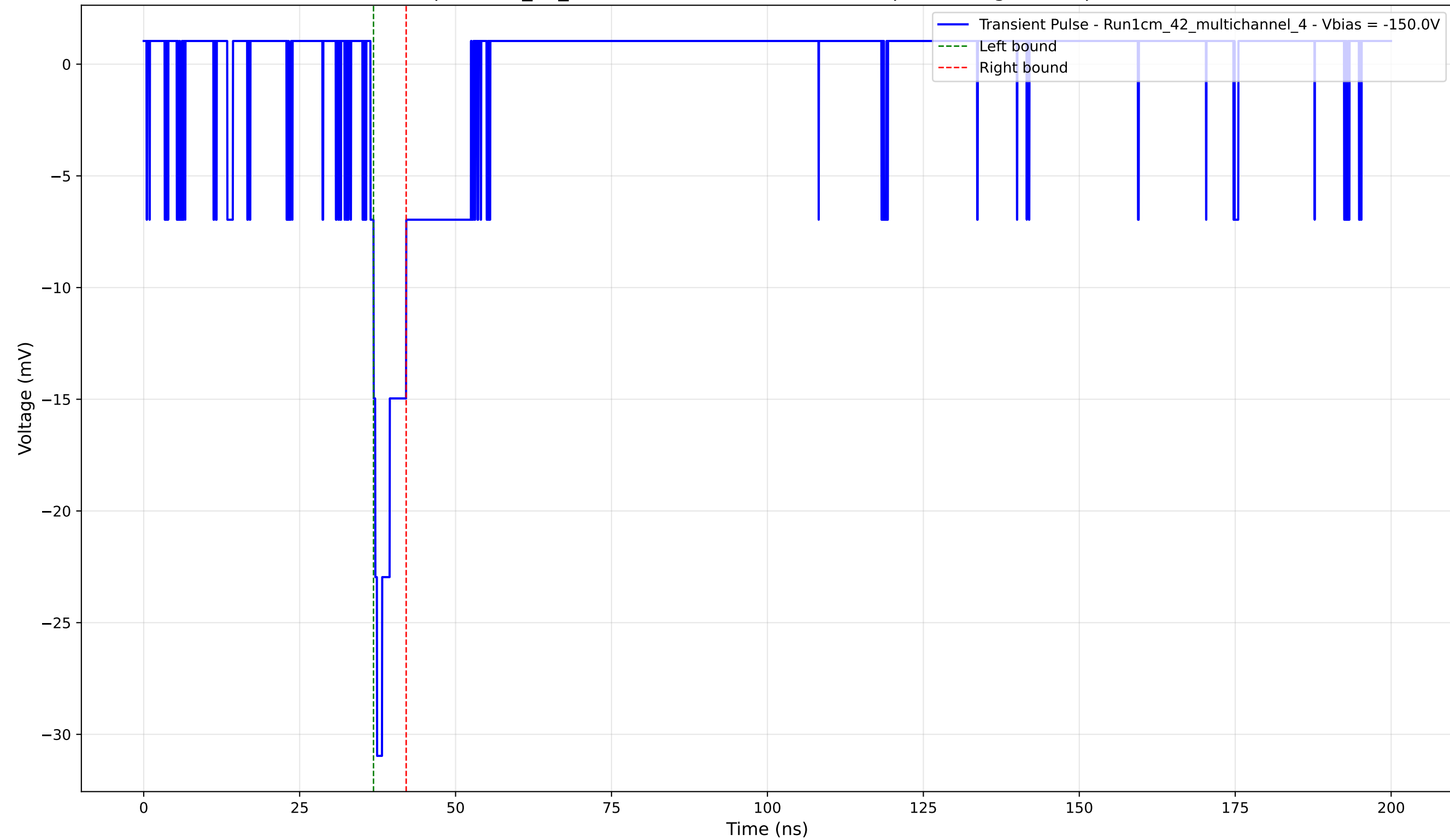
Transient Pulse - Sample: 1cm_42_multichannel - Position: 3115.0 \mu\text{m} - Charge: 2.07 pC - Rise Time: 1.05 ns
