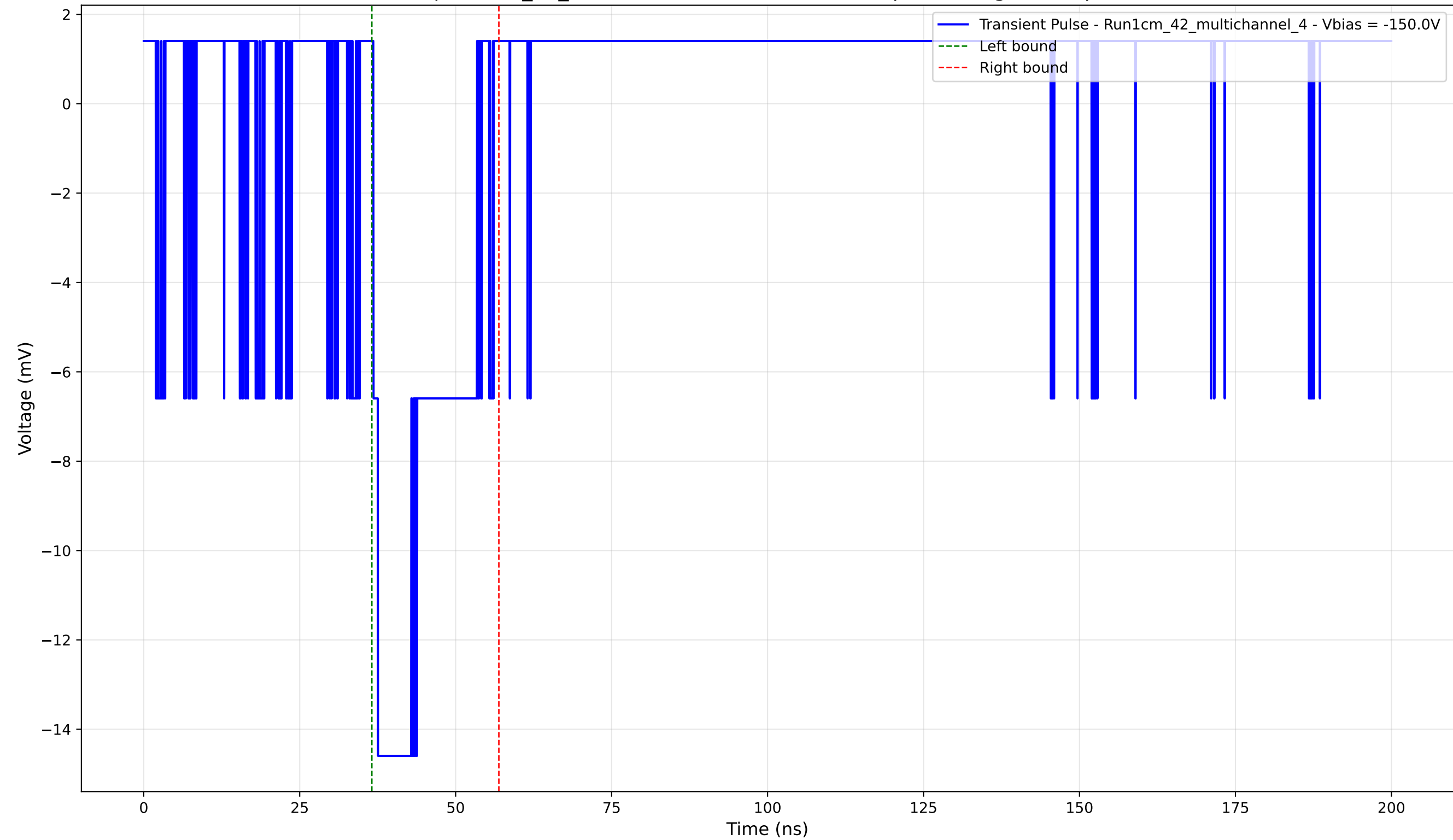
Transient Pulse - Sample: 1cm_42_multichannel - Position: 3730.0 \mu\text{m} - Charge: 3.15 pC - Rise Time: 0.74 ns
