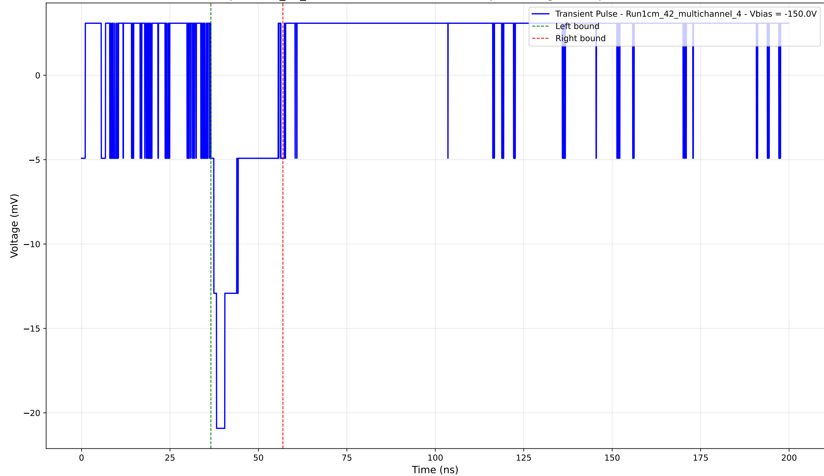
Transient Pulse - Sample: 1cm_42_multichannel - Position: 1035.0 \mu\text{m} - Charge: 3.35 pC - Rise Time: 0.00 ns (N/A)
