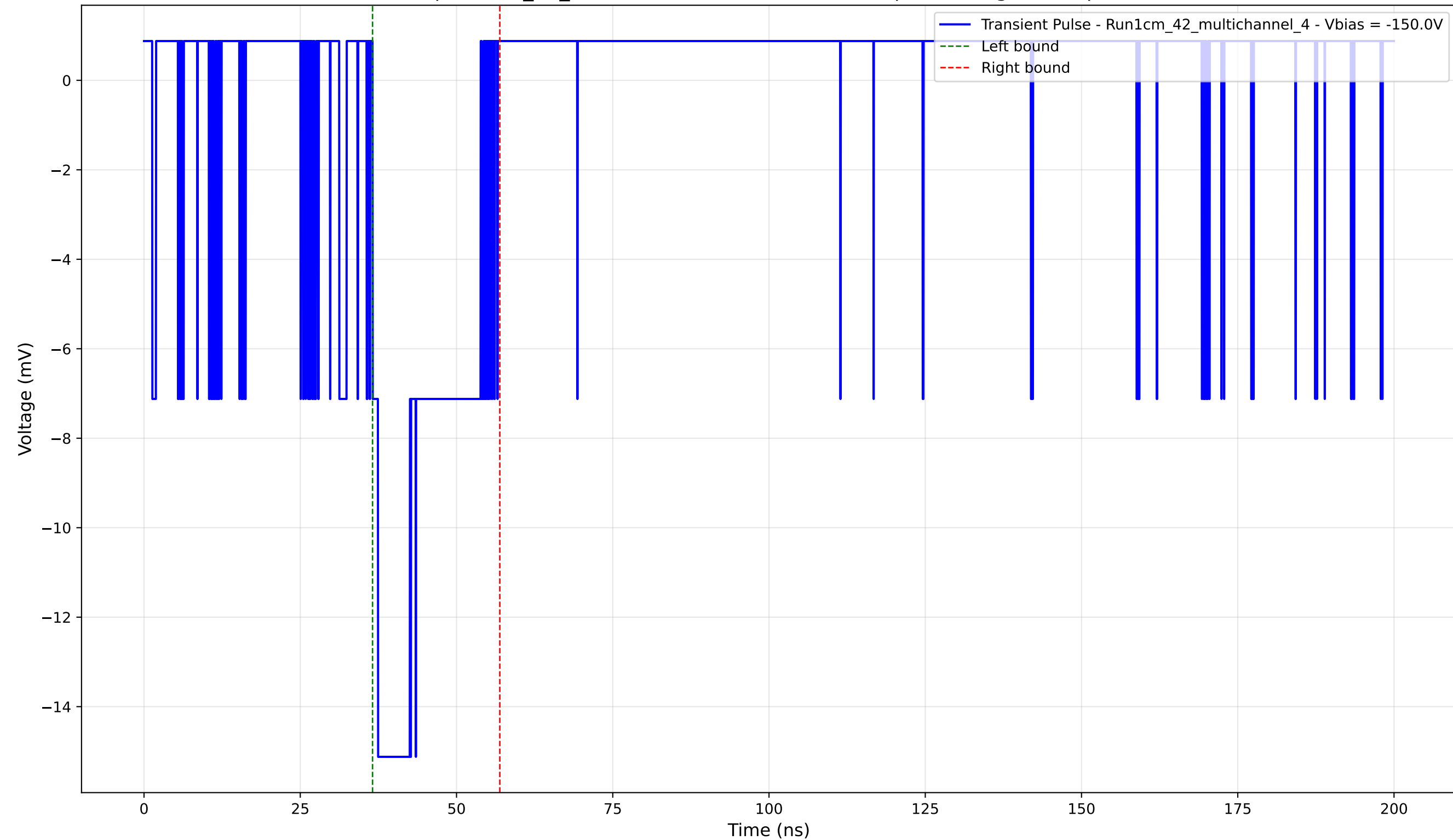
Transient Pulse - Sample: 1cm_42_multichannel - Position: 3700.0 \mu\text{m} - Charge: 3.38 pC - Rise Time: 0.88 ns
