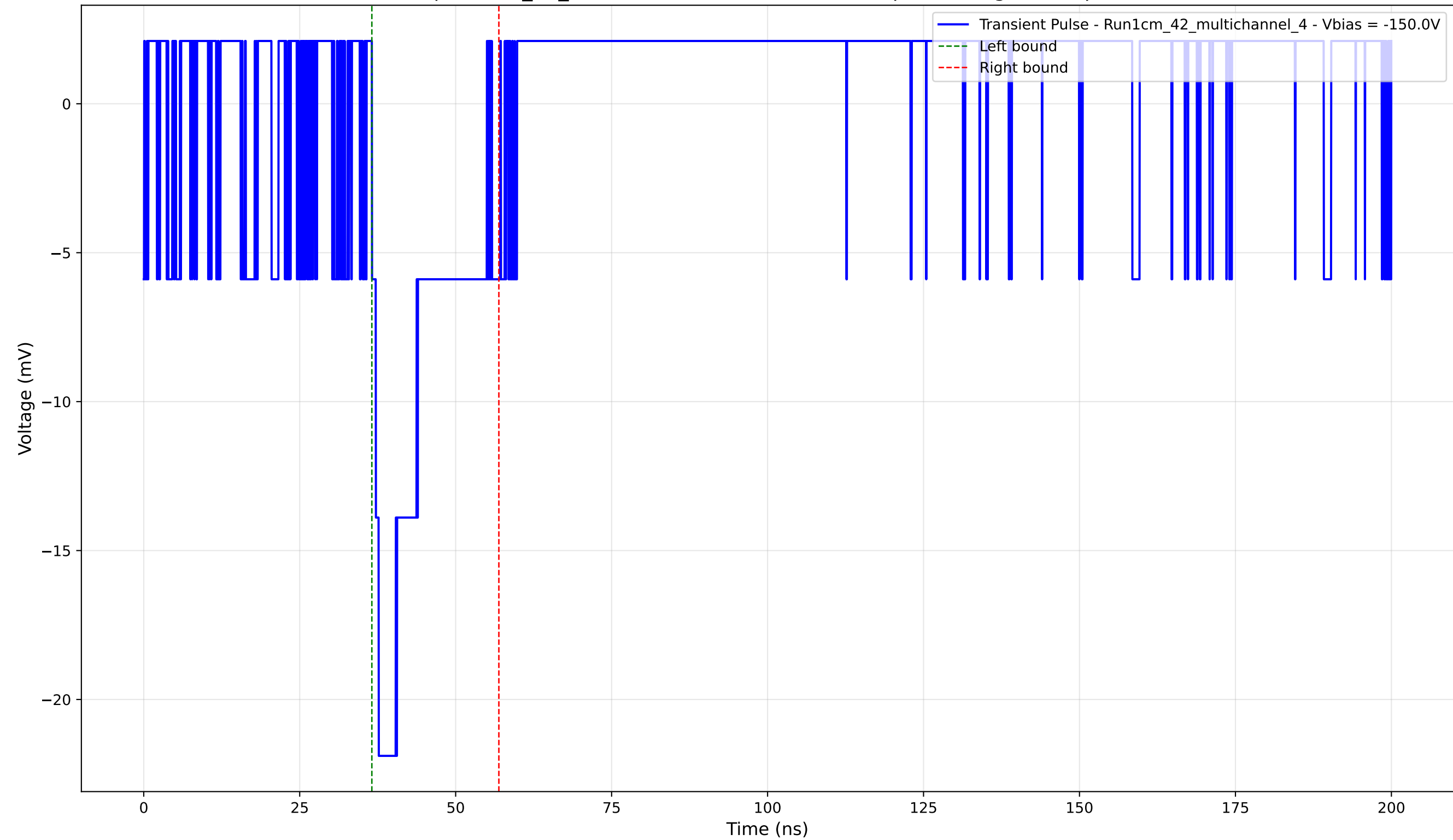
Transient Pulse - Sample: 1cm_42_multichannel - Position: 1205.0 \mu\text{m} - Charge: 3.84 pC - Rise Time: 1.10 ns
