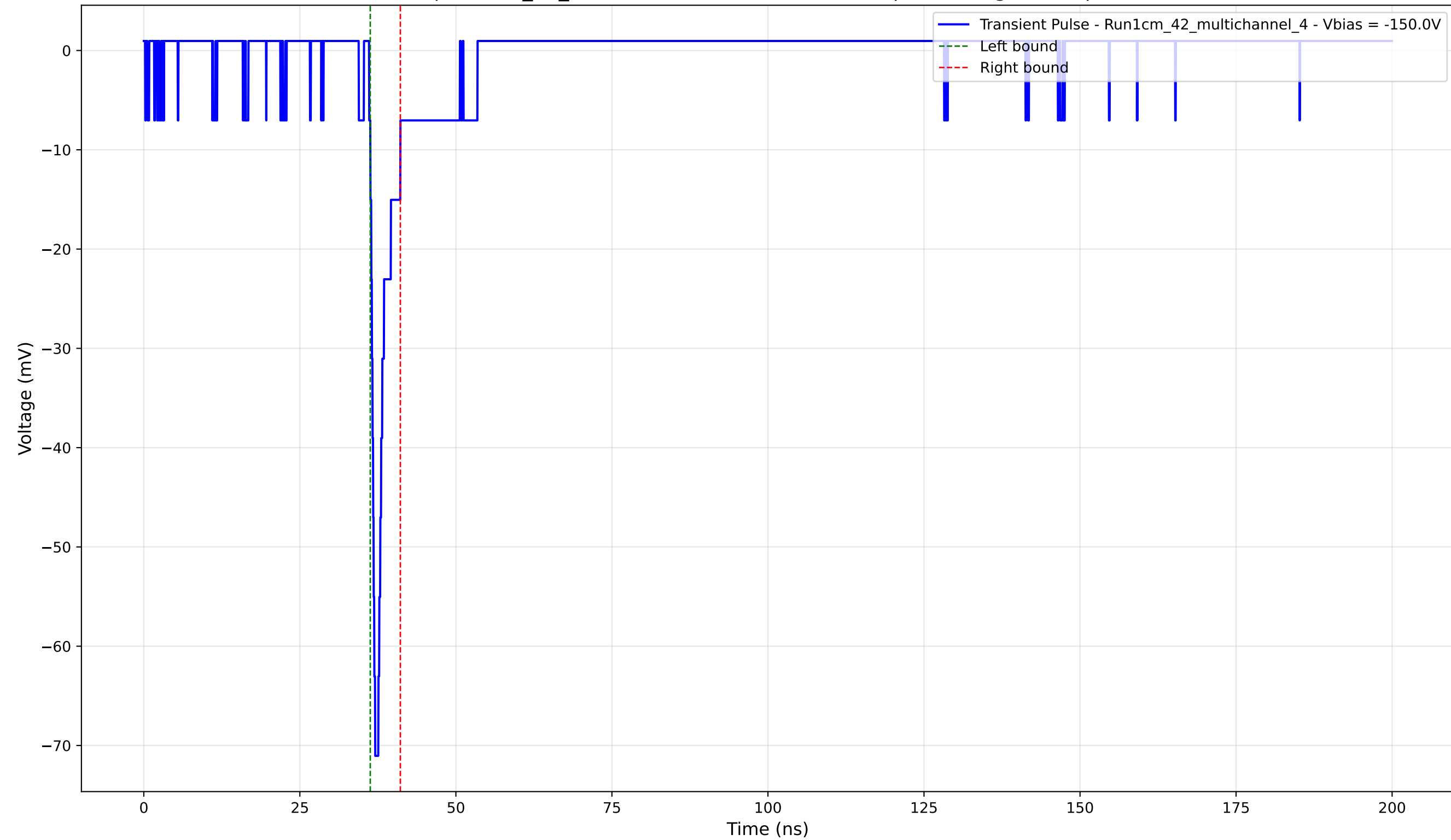
Transient Pulse - Sample: 1cm_42_multichannel - Position: 2220.0 \mu\text{m} - Charge: 3.09 pC - Rise Time: 0.78 ns
