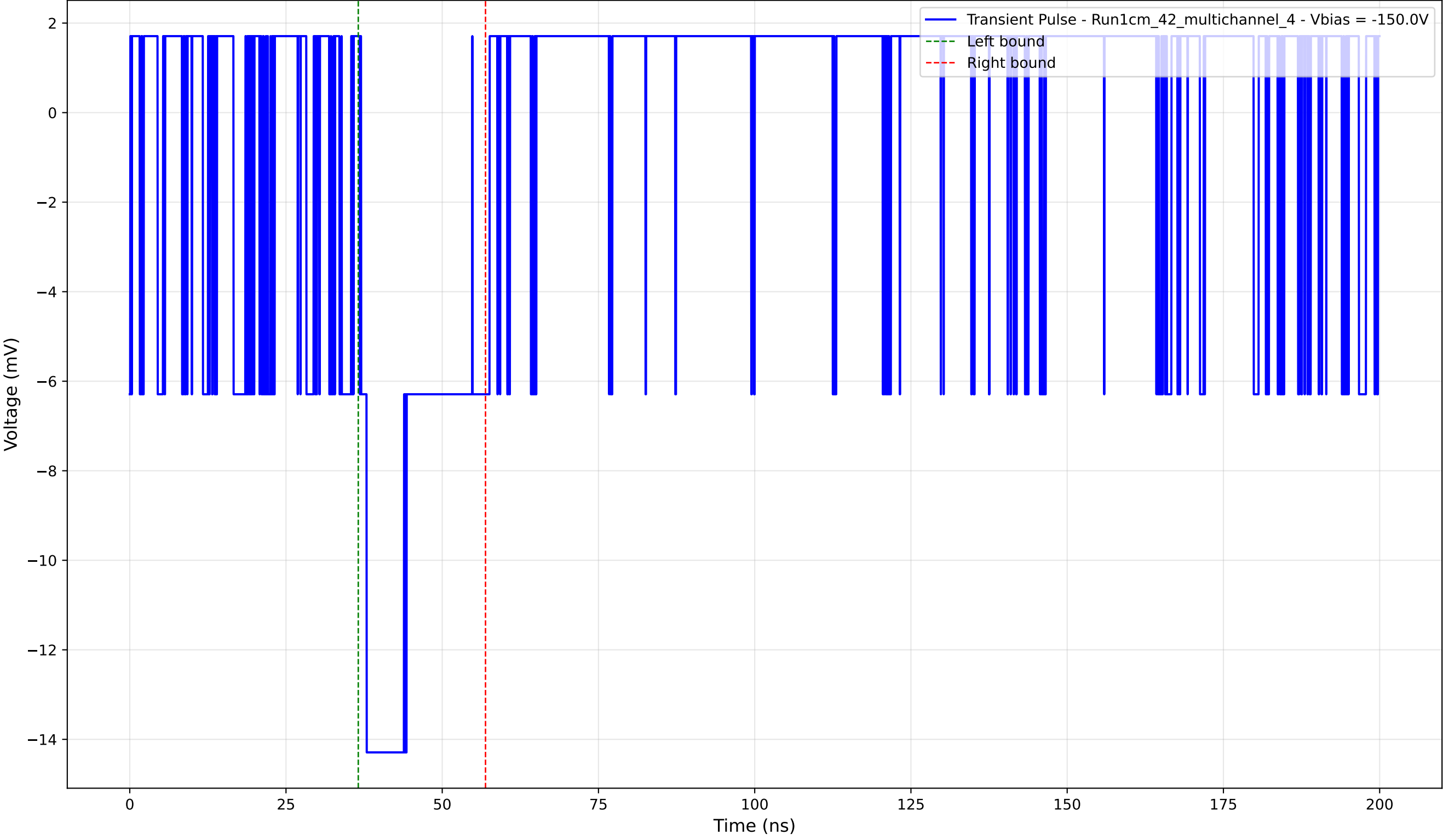
Transient Pulse - Sample: 1cm_42_multichannel - Position: 665.0 \mu\text{m} - Charge: 3.49 pC - Rise Time: 0.00 ns (N/A)
