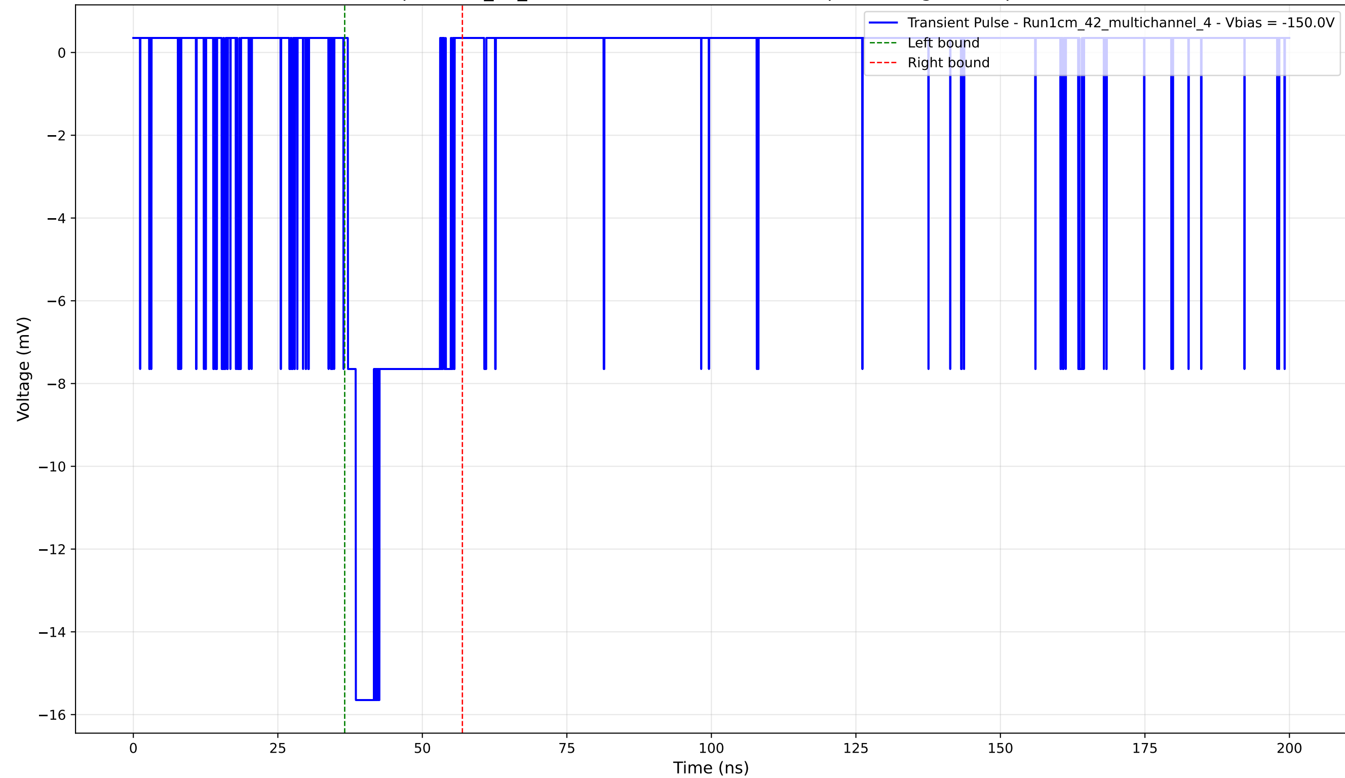
Transient Pulse - Sample: 1cm_42_multichannel - Position: 4665.0 \mu\text{m} - Charge: 3.27 pC - Rise Time: 1.38 ns
