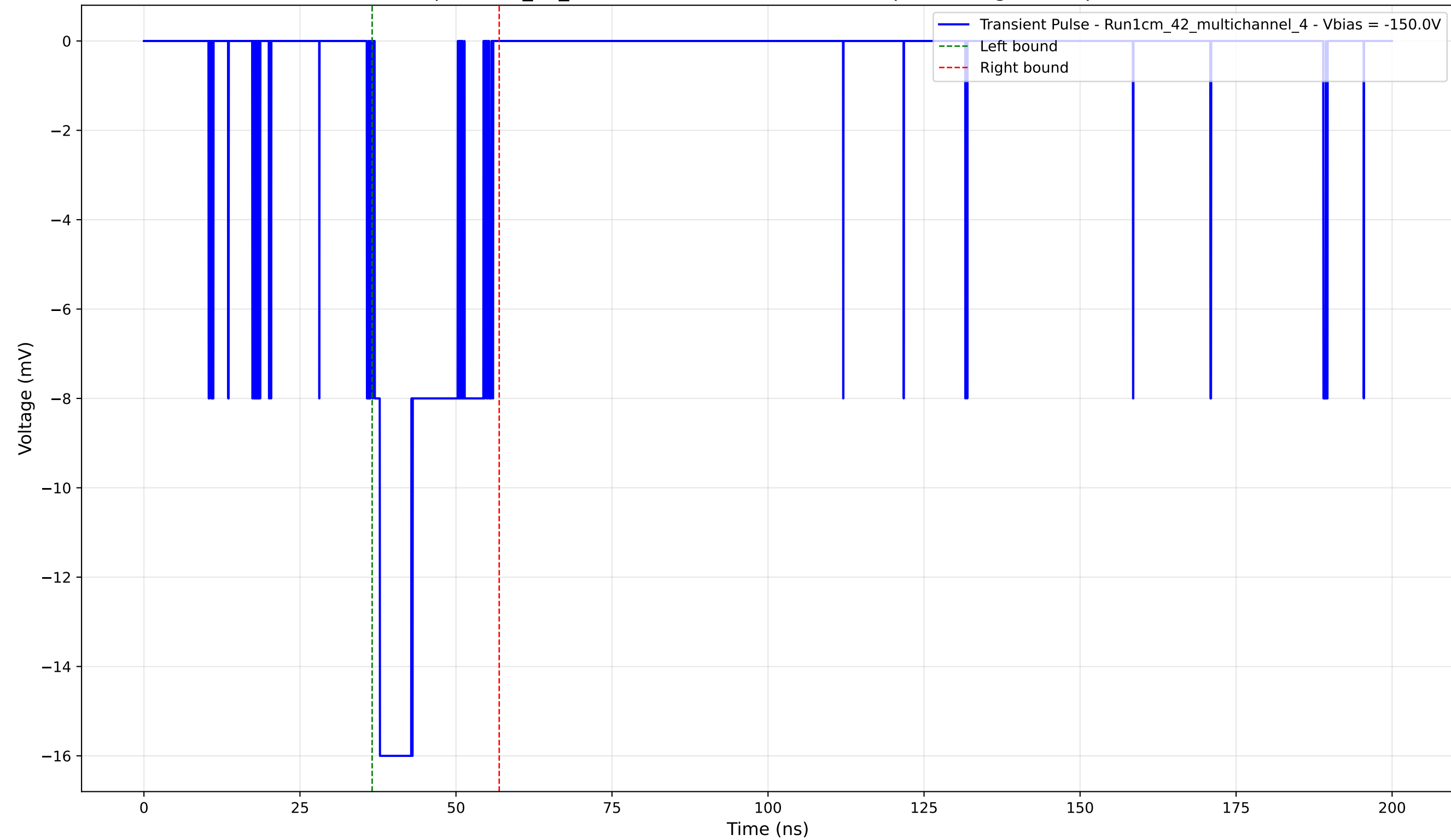
Transient Pulse - Sample: 1cm_42_multichannel - Position: 3825.0 \mu\text{m} - Charge: 3.68 pC - Rise Time: 0.84 ns
