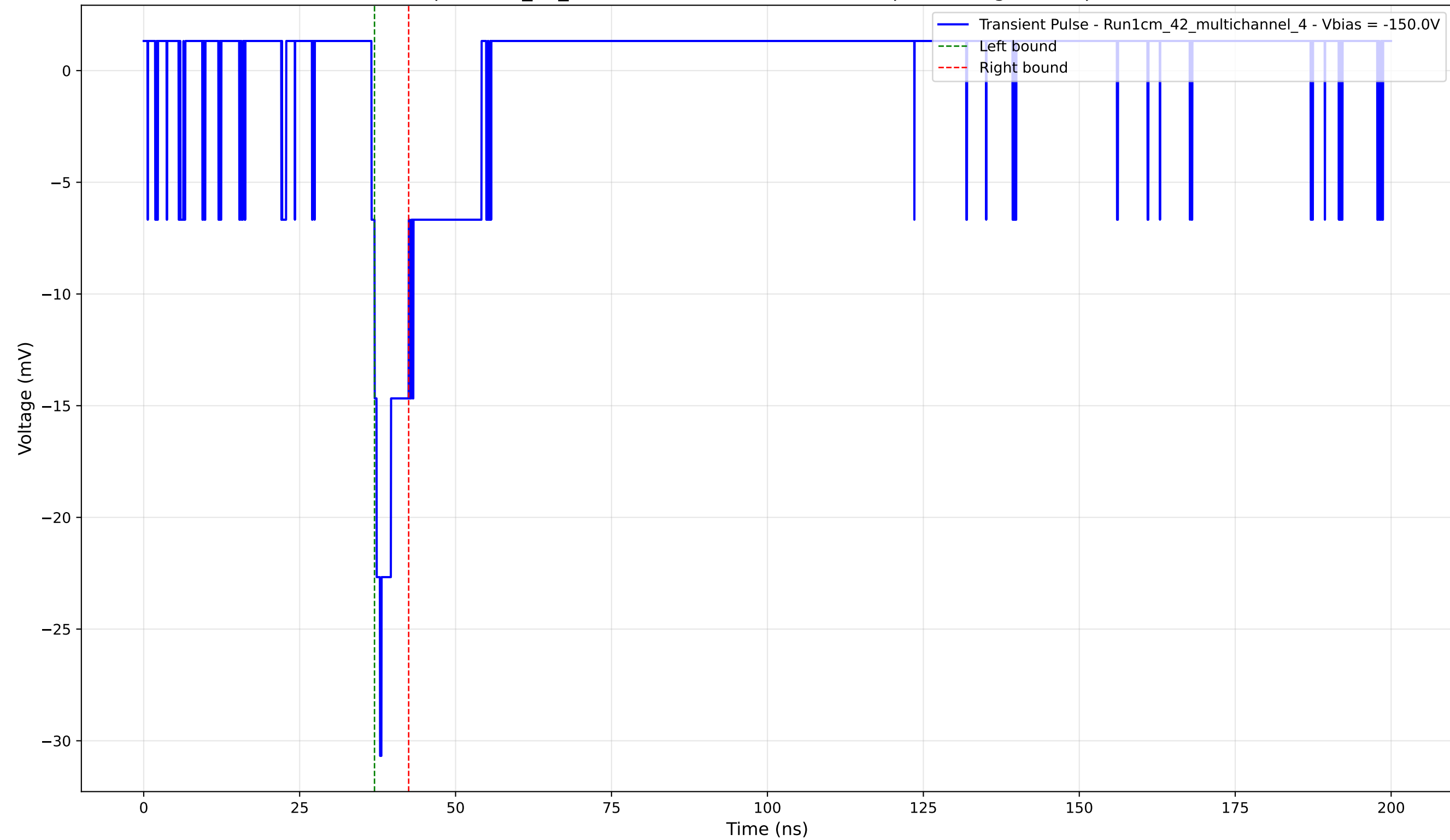
Transient Pulse - Sample: 1cm_42_multichannel - Position: 3305.0 \mu\text{m} - Charge: 2.01 pC - Rise Time: 1.37 ns
