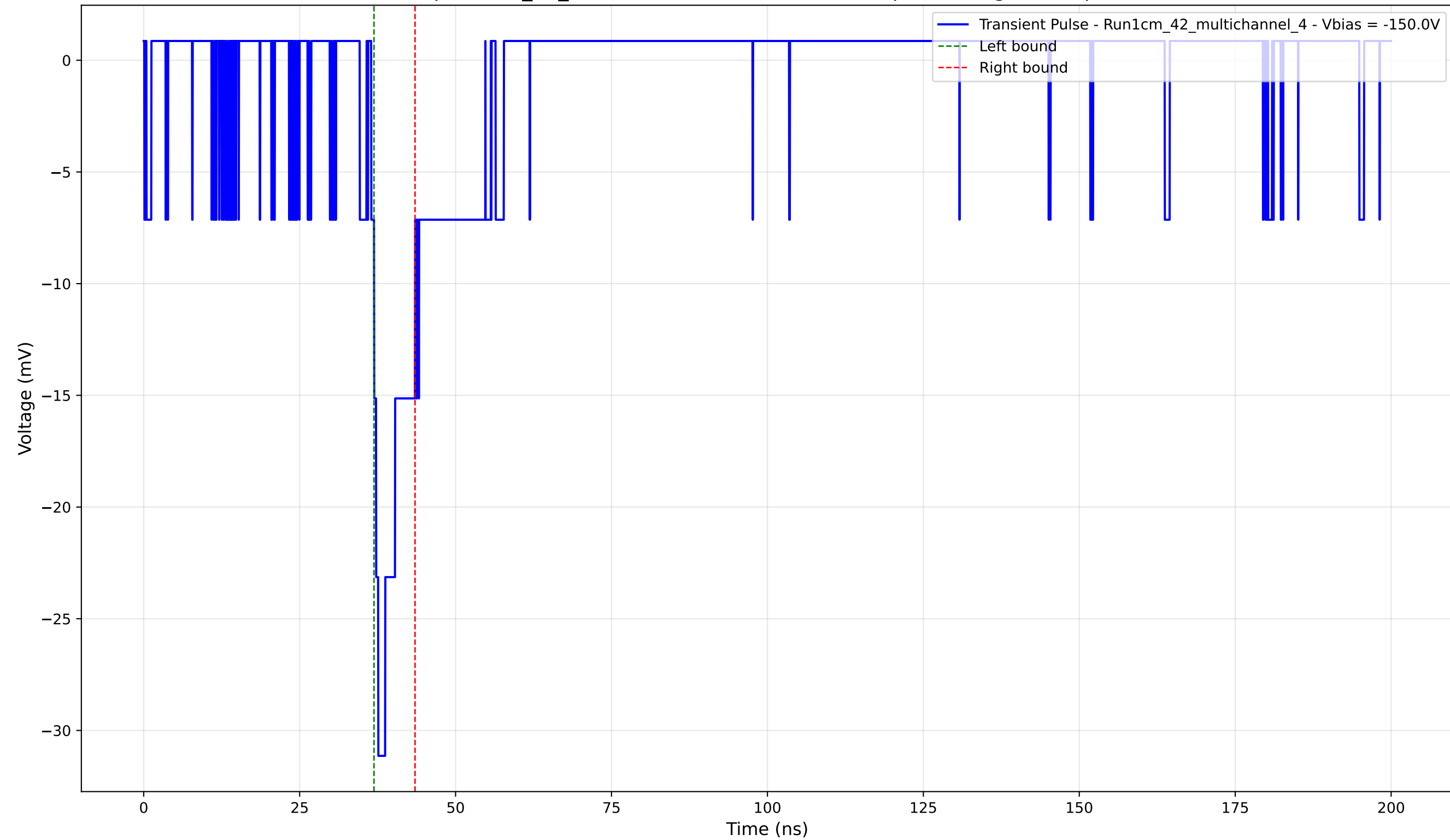
Transient Pulse - Sample: 1cm_42_multichannel - Position: 1480.0 \mu\text{m} - Charge: 2.65 pC - Rise Time: 1.13 ns
