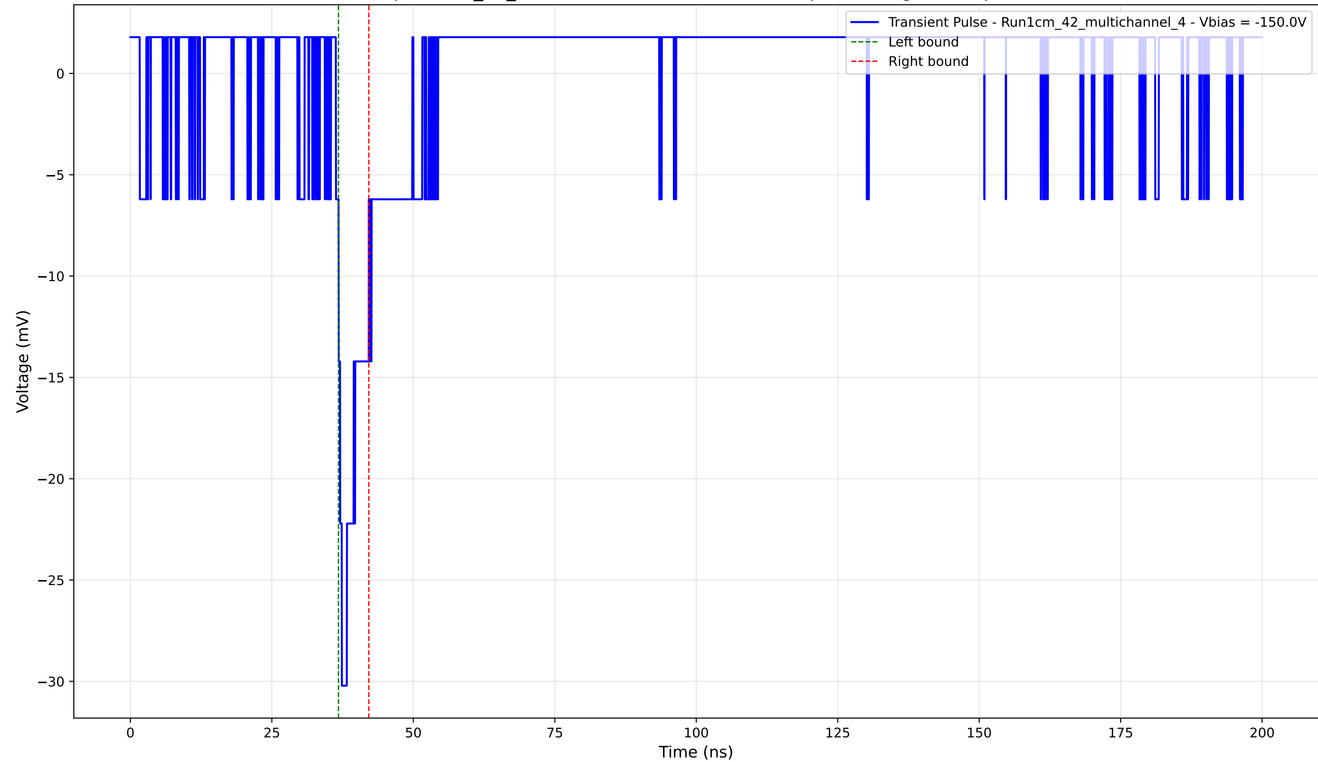
Transient Pulse - Sample: 1cm_42_multichannel - Position: 3090.0 \mu\text{m} - Charge: 2.06 pC - Rise Time: 1.05 ns
