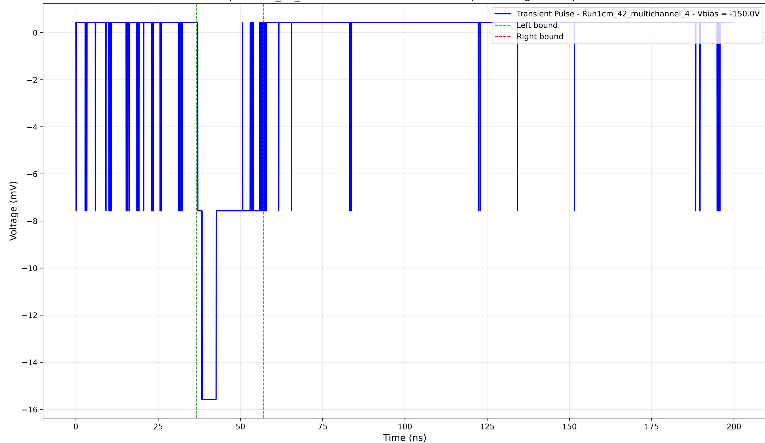
Transient Pulse - Sample: 1cm_42_multichannel - Position: 4265.0 \mu\text{m} - Charge: 3.53 pC - Rise Time: 1.10 ns
