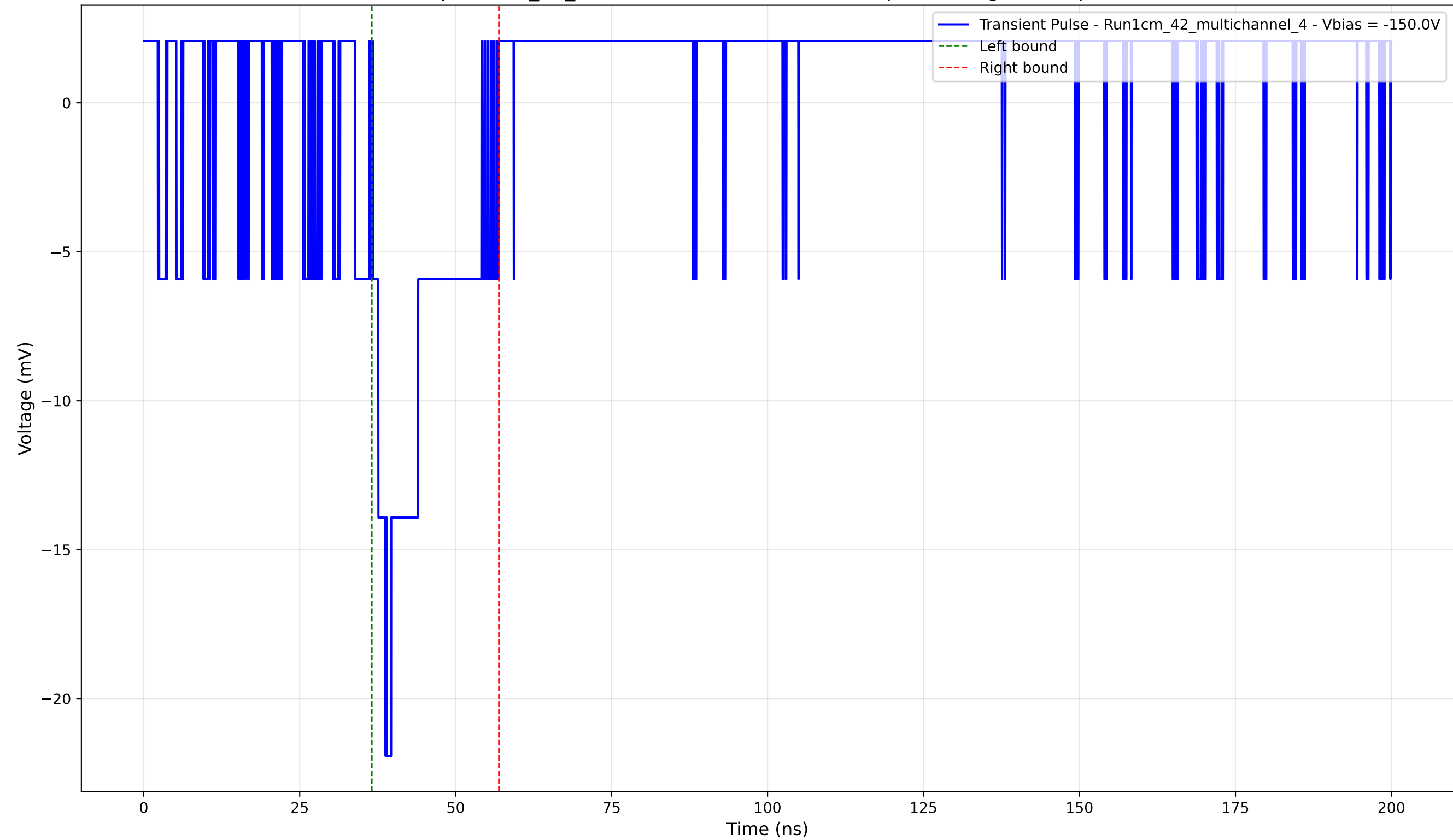
Transient Pulse - Sample: 1cm_42_multichannel - Position: 965.0 \mu\text{m} - Charge: 3.43 pC - Rise Time: 2.00 ns
