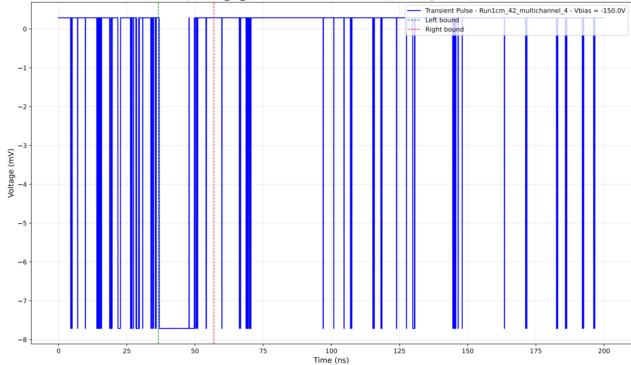
Transient Pulse - Sample: 1cm_42_multichannel - Position: 3445.0 \mu\text{m} - Charge: 2.00 pC - Rise Time: 0.02 ns
