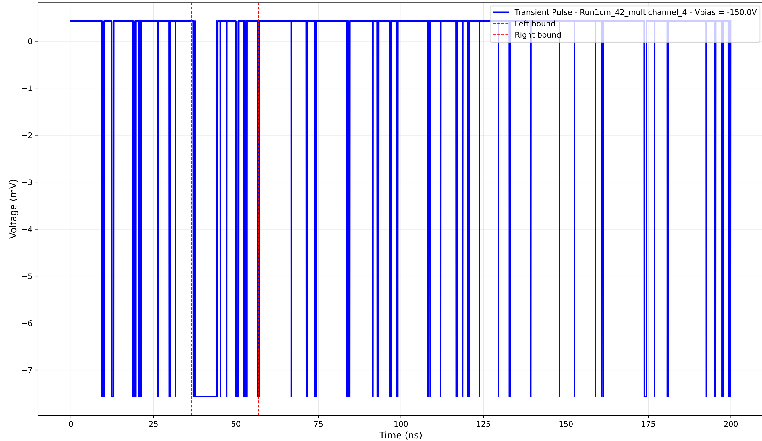
Transient Pulse - Sample: 1cm_42_multichannel - Position: 3940.0 \mu\text{m} - Charge: 1.14 pC - Rise Time: 0.02 ns
