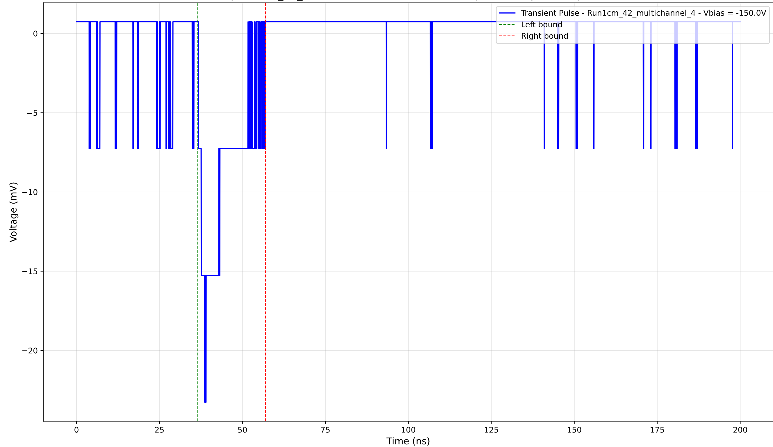
Transient Pulse - Sample: 1cm_42_multichannel - Position: 3735.0 \mu\text{m} - Charge: 3.40 pC - Rise Time: 1.88 ns
