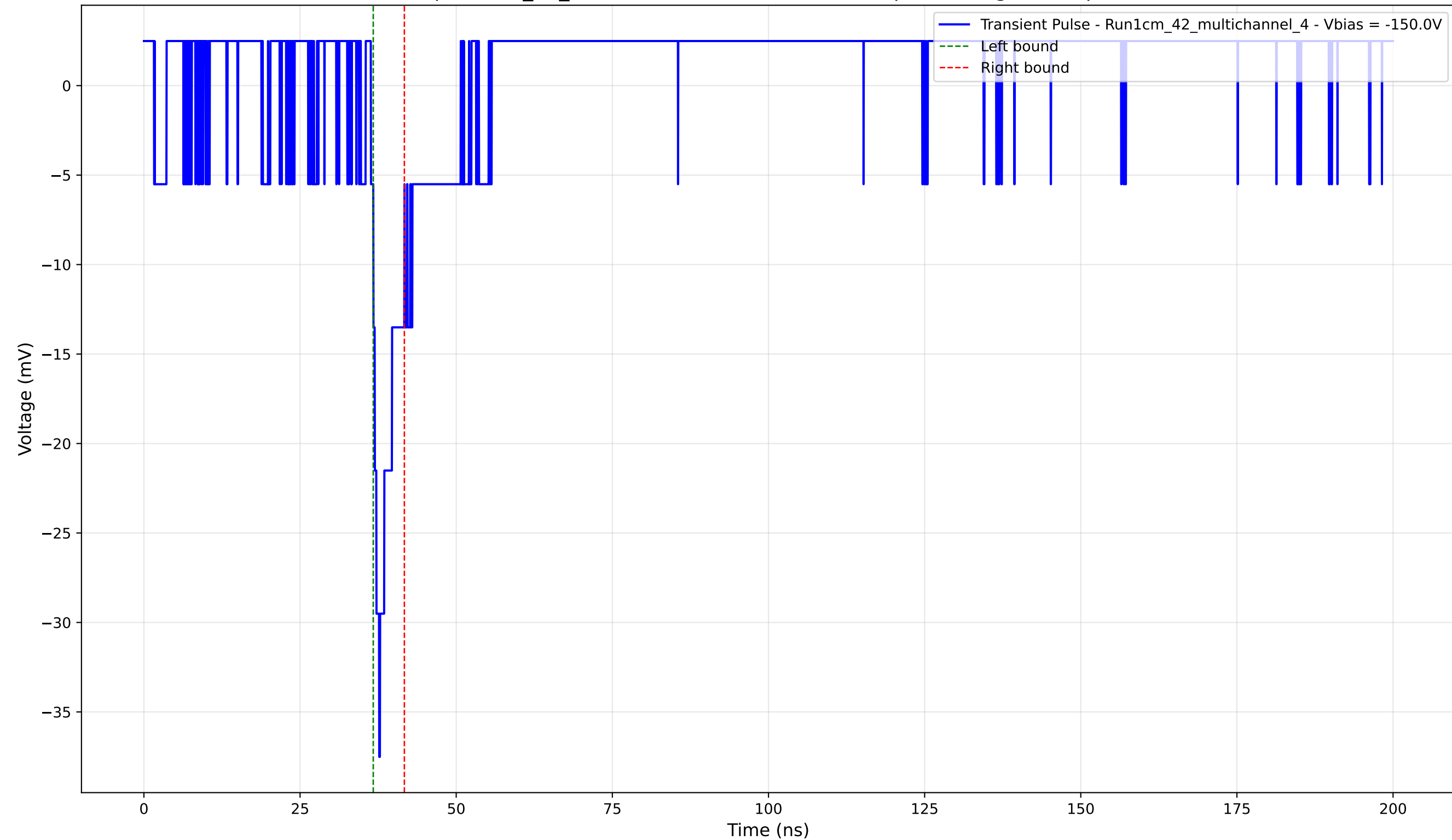
Transient Pulse - Sample: 1cm_42_multichannel - Position: 3065.0 \mu\text{m} - Charge: 2.01 pC - Rise Time: 1.33 ns
