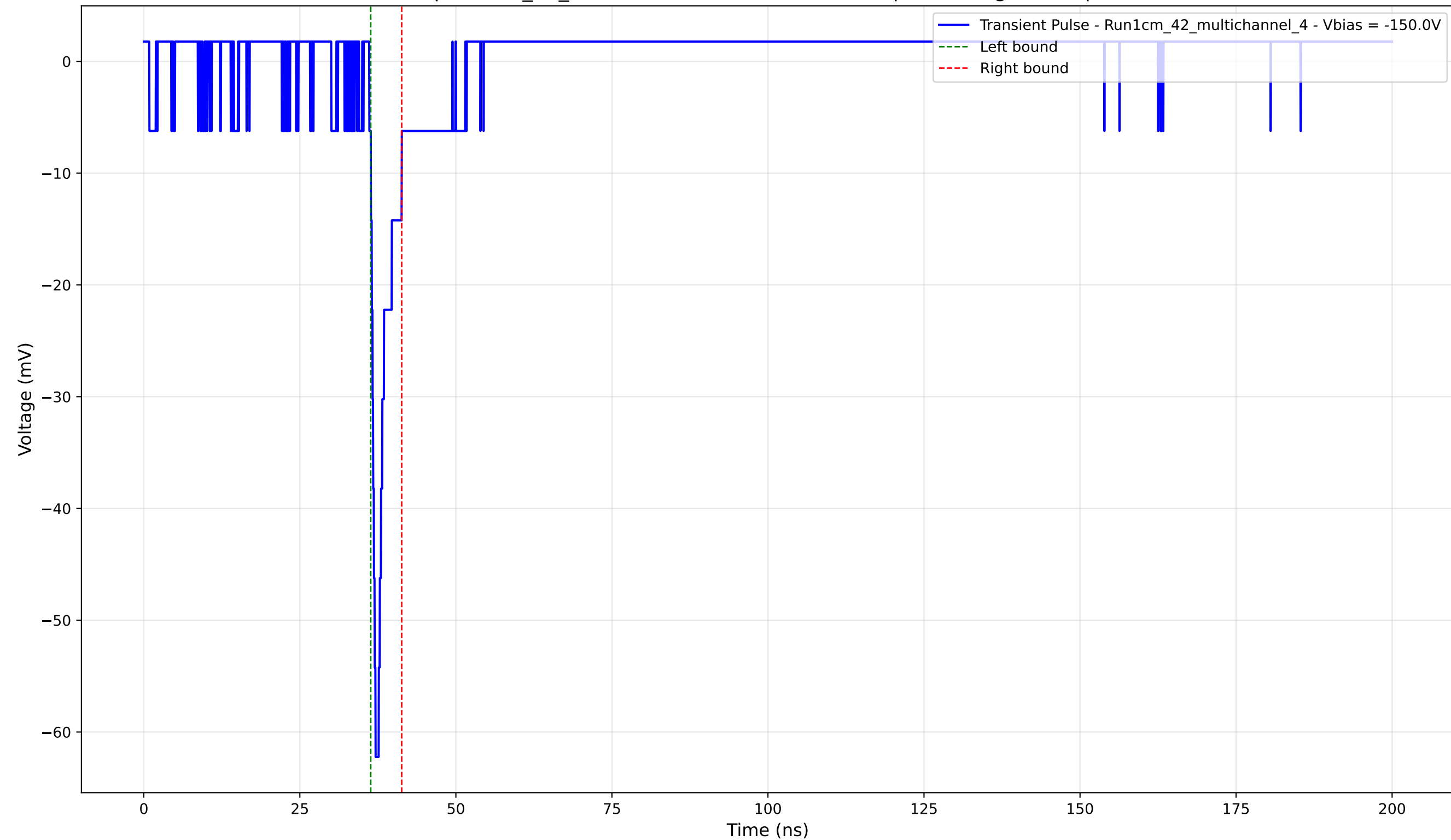
Transient Pulse - Sample: 1cm_42_multichannel - Position: 2155.0 \mu\text{m} - Charge: 2.84 pC - Rise Time: 1.00 ns
