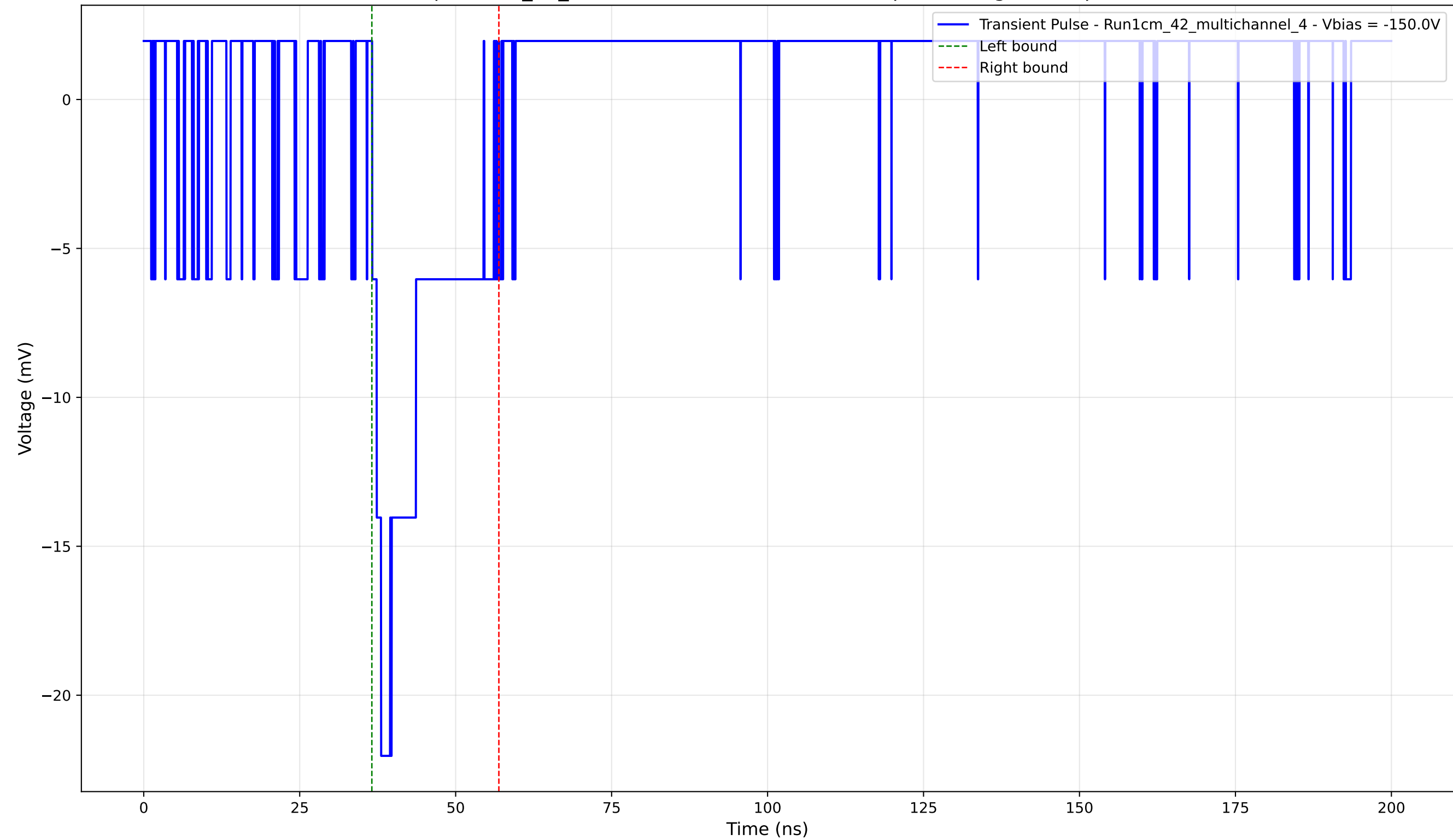
Transient Pulse - Sample: 1cm_42_multichannel - Position: 1130.0 \mu\text{m} - Charge: 3.66 pC - Rise Time: 1.44 ns
