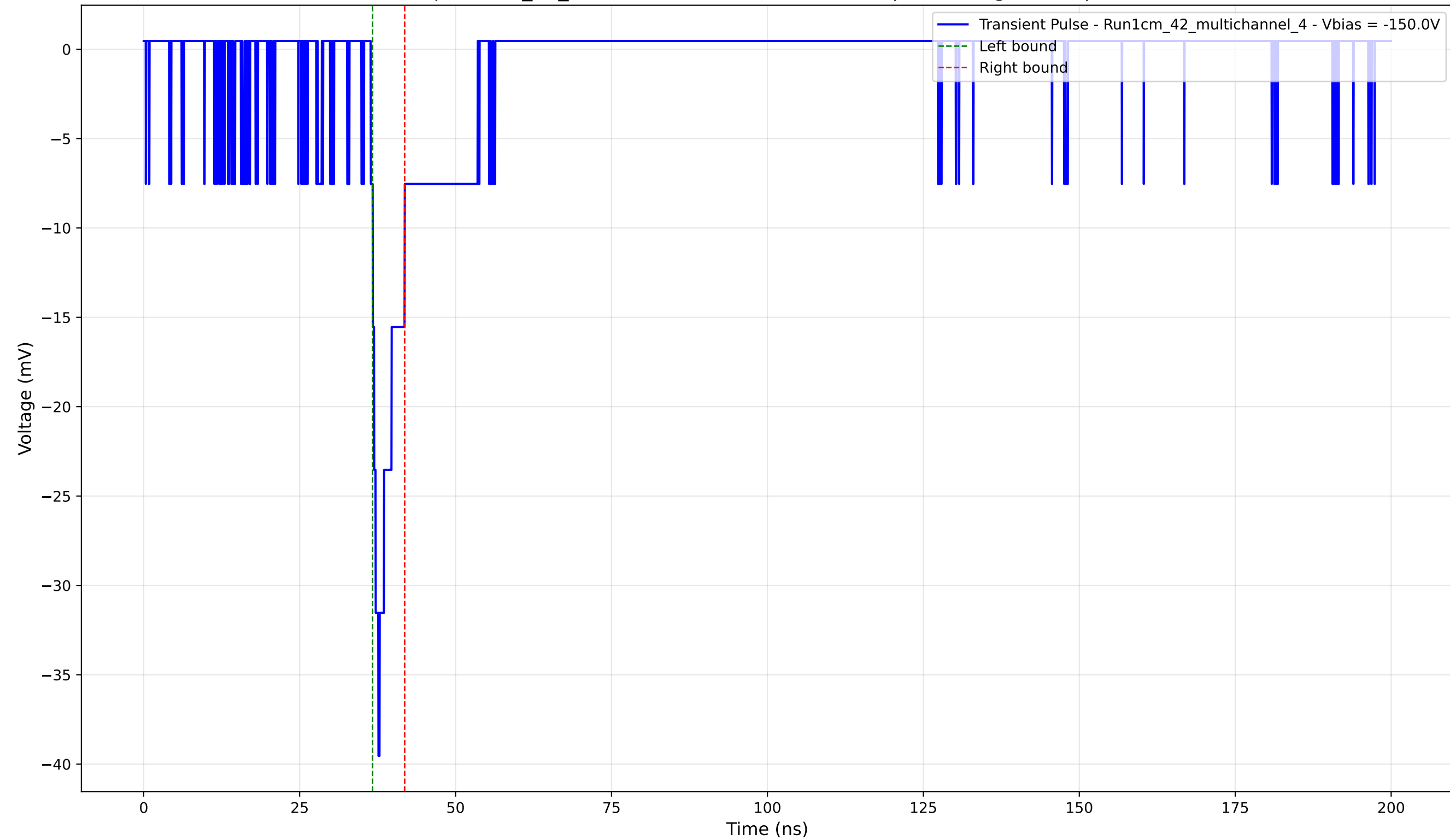
Transient Pulse - Sample: 1cm_42_multichannel - Position: 3035.0 \mu\text{m} - Charge: 2.29 pC - Rise Time: 1.23 ns
