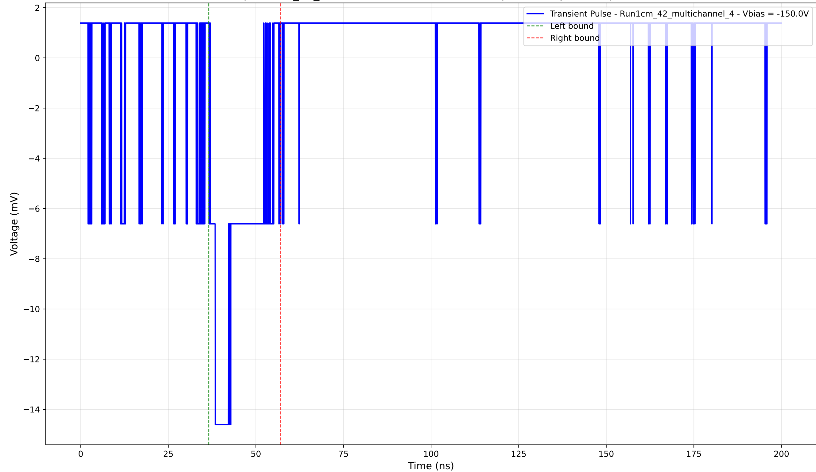
Transient Pulse - Sample: 1cm_42_multichannel - Position: 4670.0 \mu\text{m} - Charge: 2.99 pC - Rise Time: 1.40 ns
