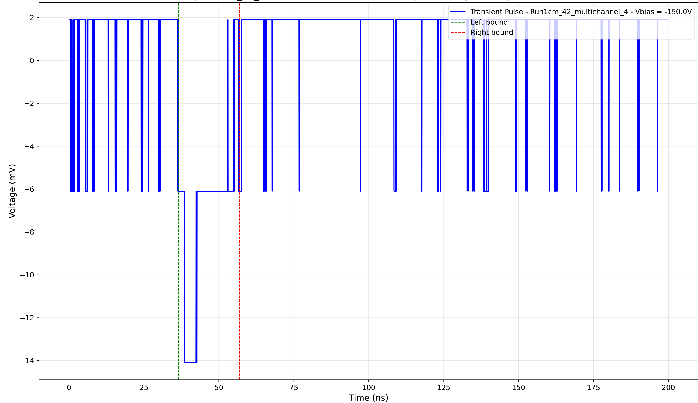
Transient Pulse - Sample: 1cm_42_multichannel - Position: 4740.0 \mu\text{m} - Charge: 2.86 pC - Rise Time: 0.00 ns (N/A)
