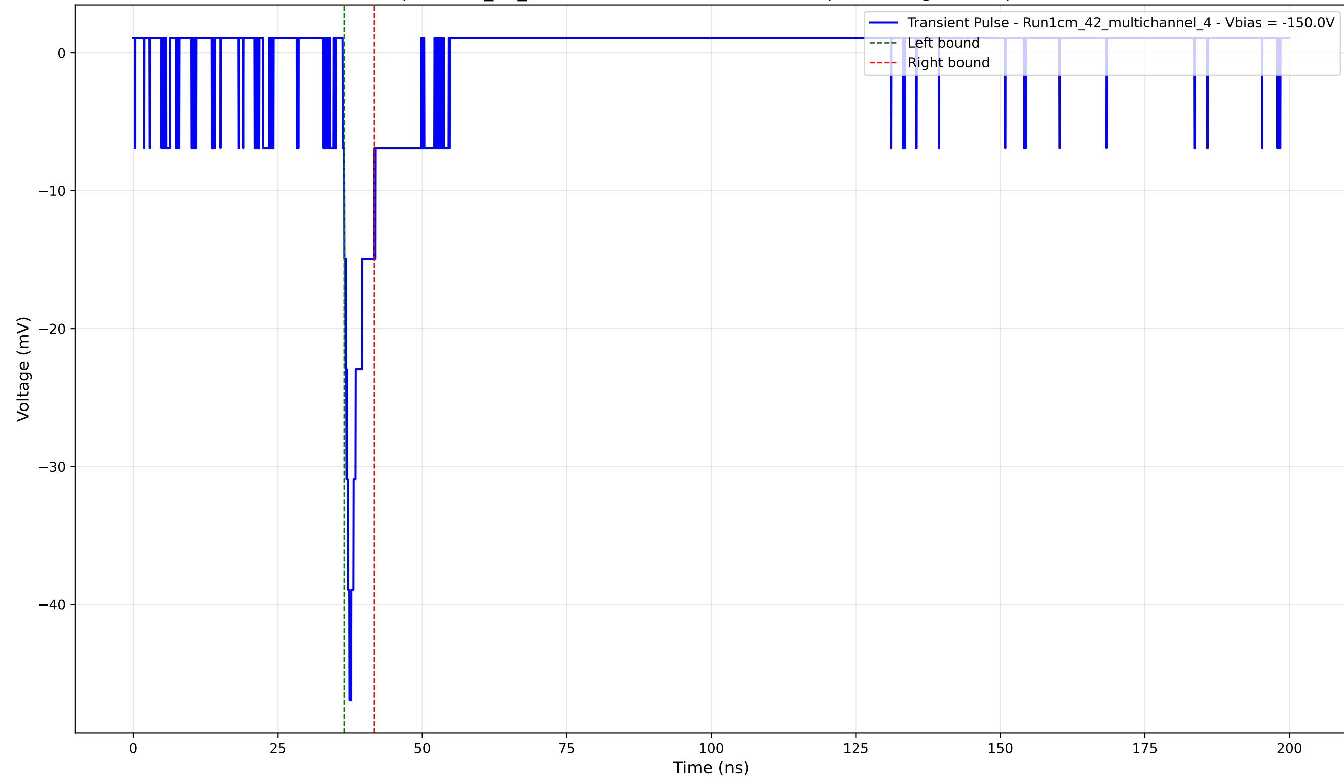
Transient Pulse - Sample: 1cm_42_multichannel - Position: 2820.0 \mu\text{m} - Charge: 2.44 pC - Rise Time: 1.09 ns
