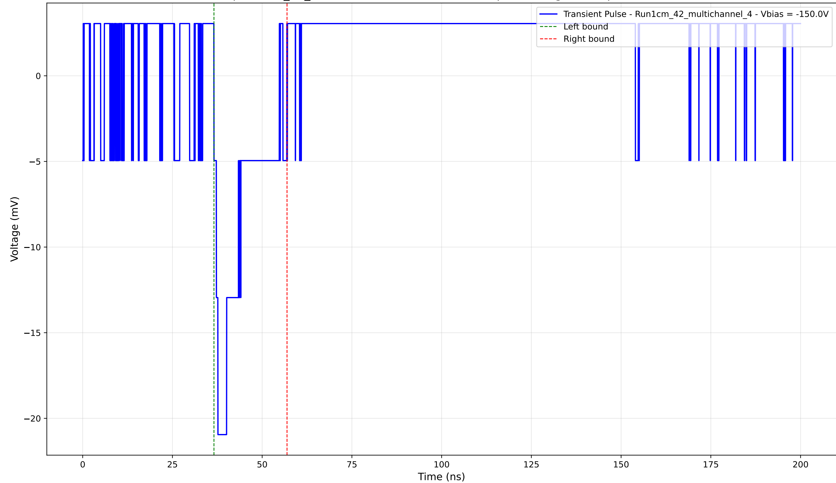
Transient Pulse - Sample: 1cm_42_multichannel - Position: 1250.0 \mu\text{m} - Charge: 3.29 pC - Rise Time: 0.00 ns (N/A)
