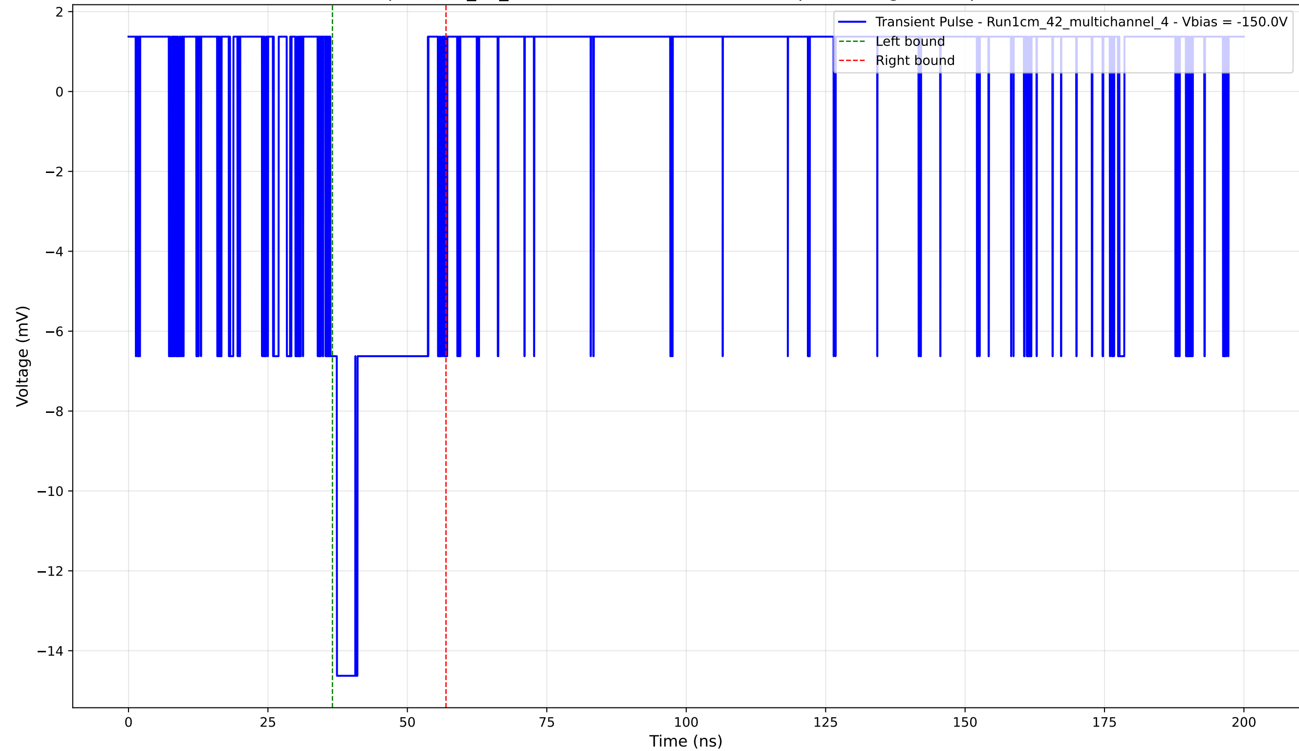
Transient Pulse - Sample: 1cm_42_multichannel - Position: 3455.0 \mu\text{m} - Charge: 2.92 pC - Rise Time: 1.18 ns
