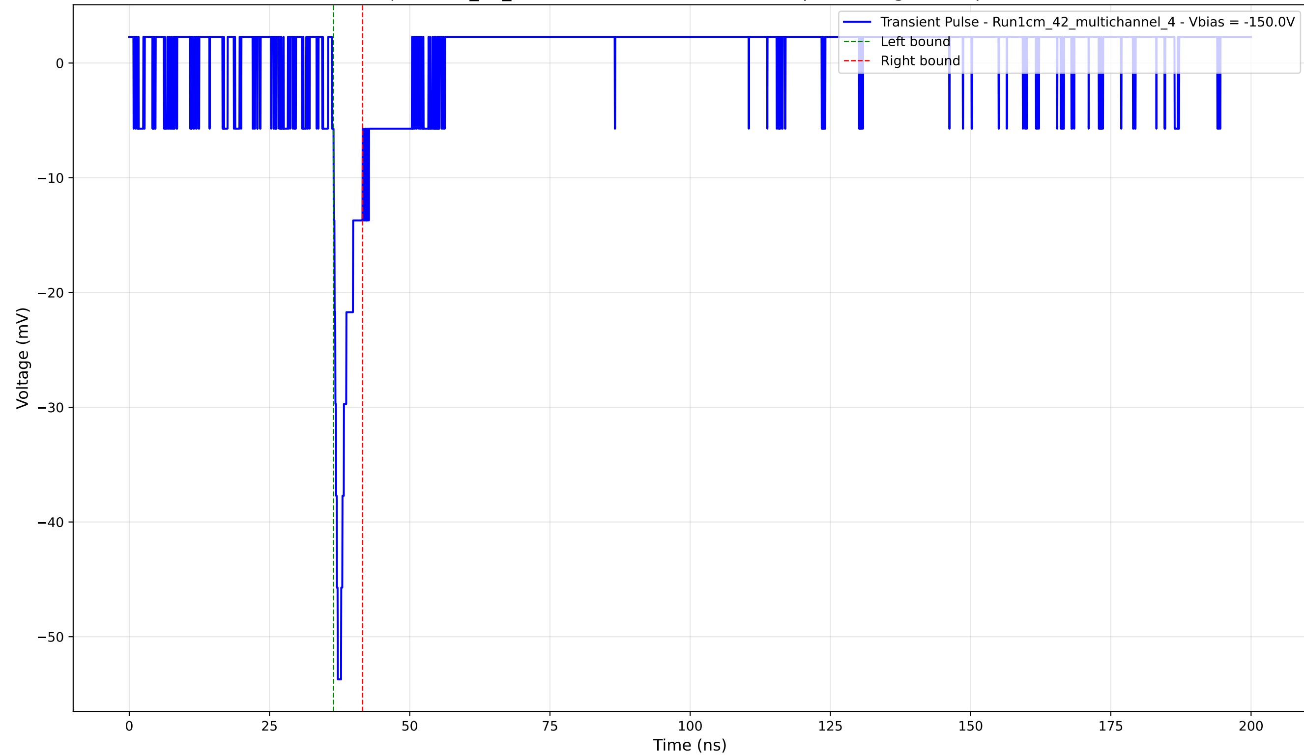
Transient Pulse - Sample: 1cm_42_multichannel - Position: 2730.0 \mu\text{m} - Charge: 2.74 pC - Rise Time: 1.02 ns
