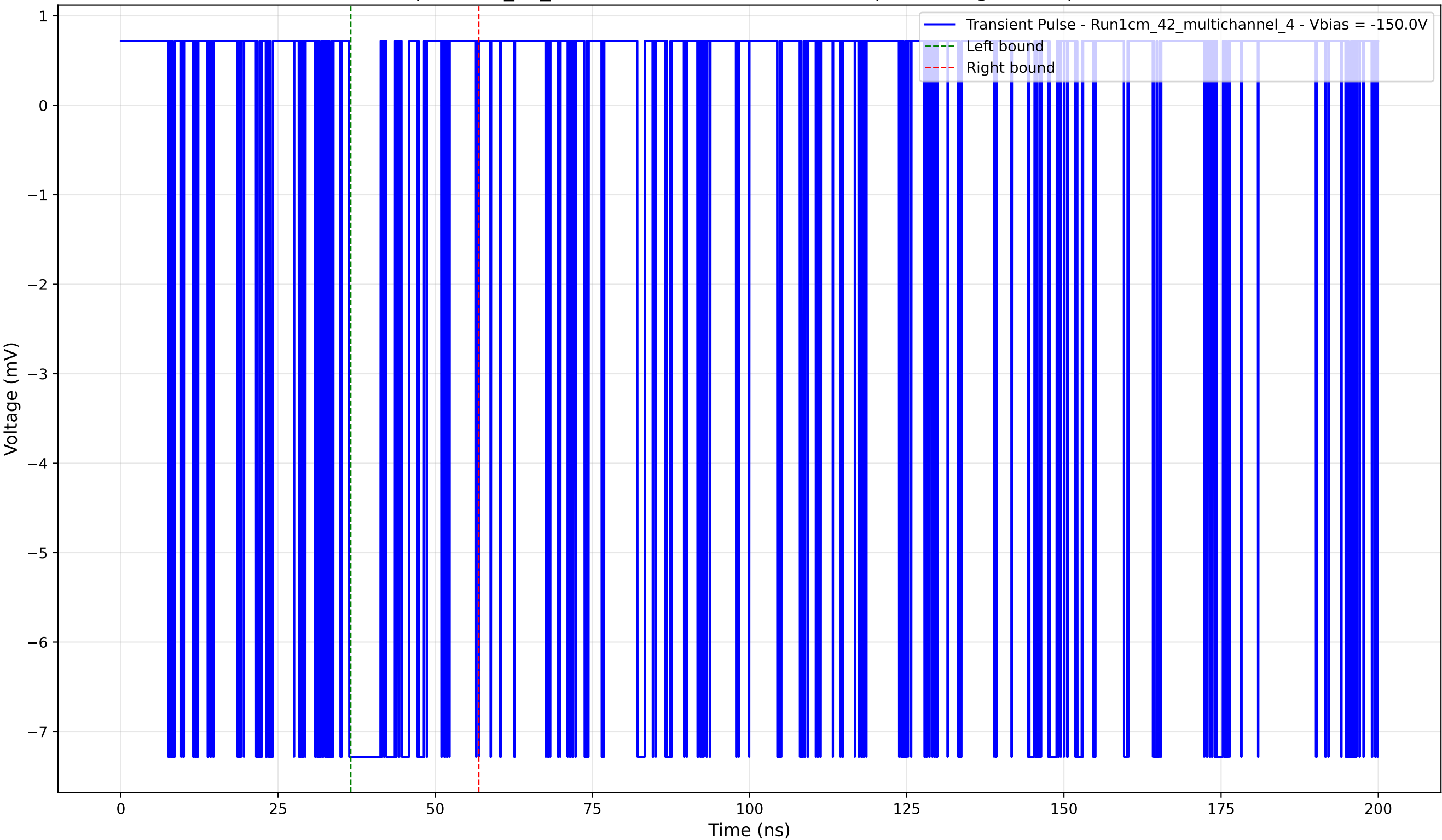
Transient Pulse - Sample: 1cm_42_multichannel - Position: 2415.0 \mu\text{m} - Charge: 1.24 pC - Rise Time: 0.02 ns
