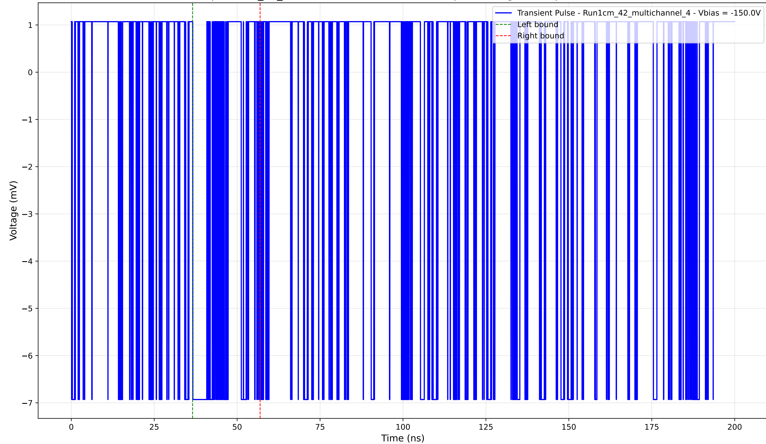
Transient Pulse - Sample: 1cm_42_multichannel - Position: 1905.0 \mu\text{m} - Charge: 1.18 pC - Rise Time: 0.00 ns (N/A)
