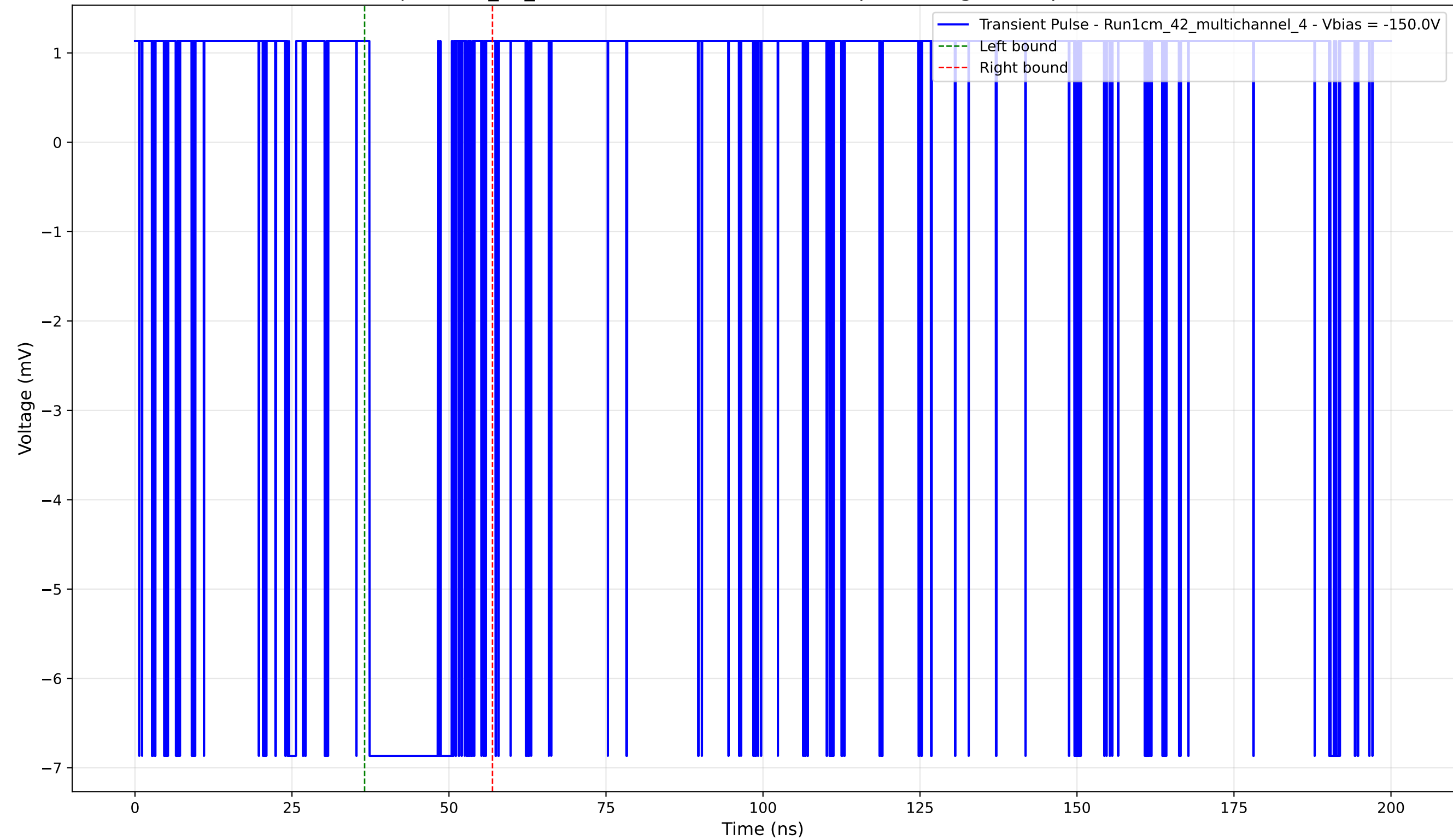
Transient Pulse - Sample: 1cm_42_multichannel - Position: 3945.0 \mu\text{m} - Charge: 1.86 pC - Rise Time: 0.00 ns (N/A)
