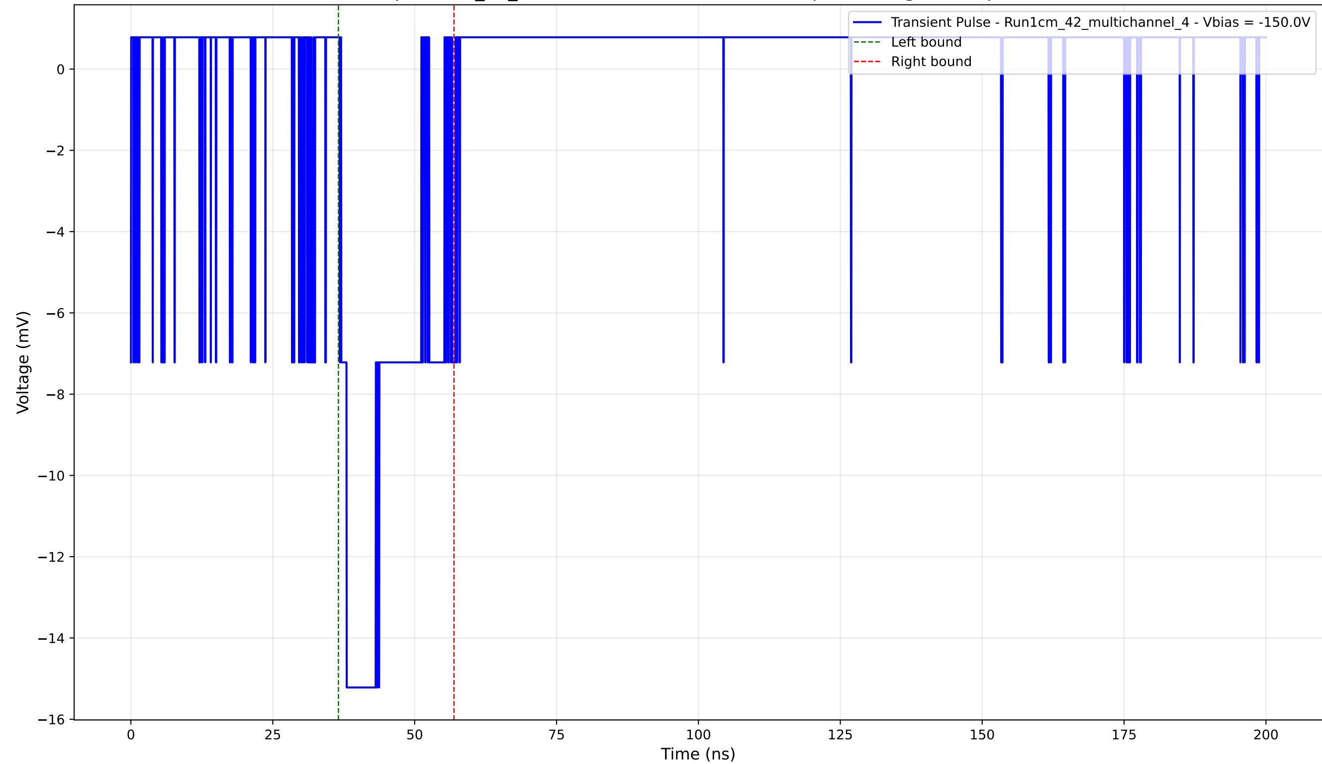
Transient Pulse - Sample: 1cm_42_multichannel - Position: 4010.0 \mu\text{m} - Charge: 3.42 pC - Rise Time: 0.96 ns
