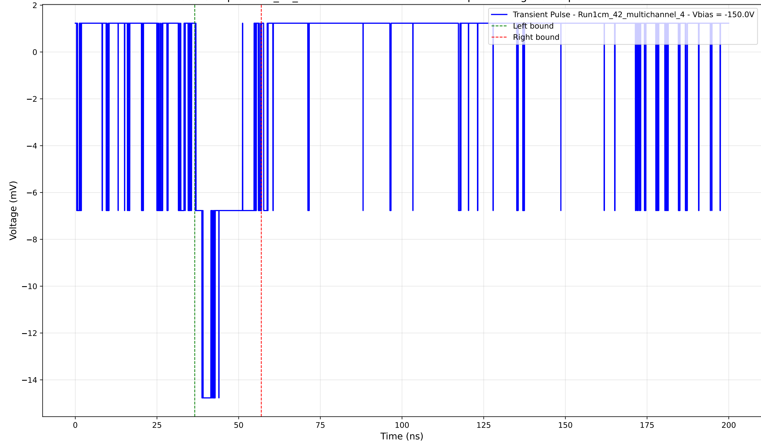
Transient Pulse - Sample: 1cm_42_multichannel - Position: 4480.0 \mu\text{m} - Charge: 3.06 pC - Rise Time: 1.84 ns
