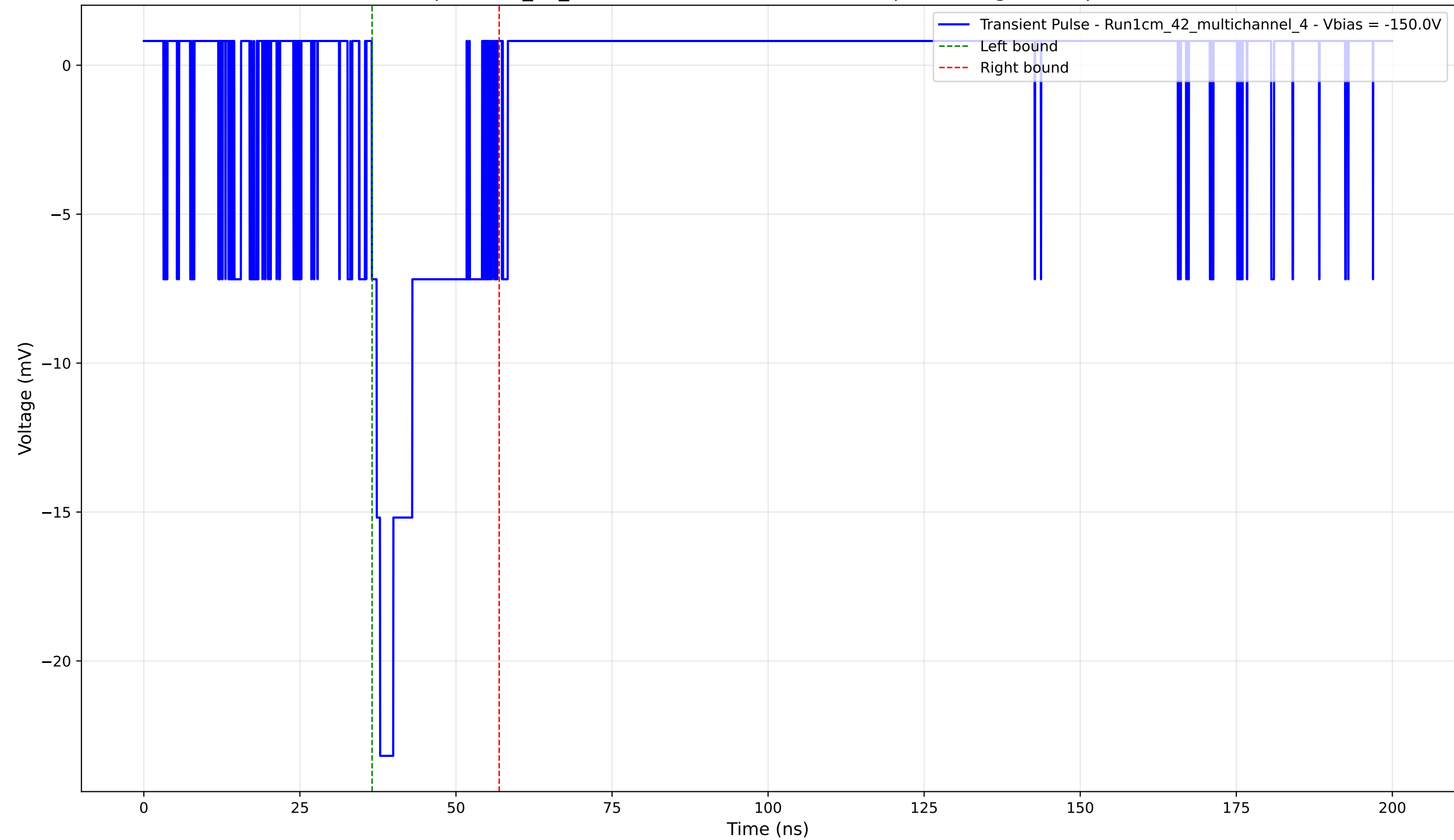
Transient Pulse - Sample: 1cm_42_multichannel - Position: 3565.0 \mu\text{m} - Charge: 3.87 pC - Rise Time: 1.34 ns
