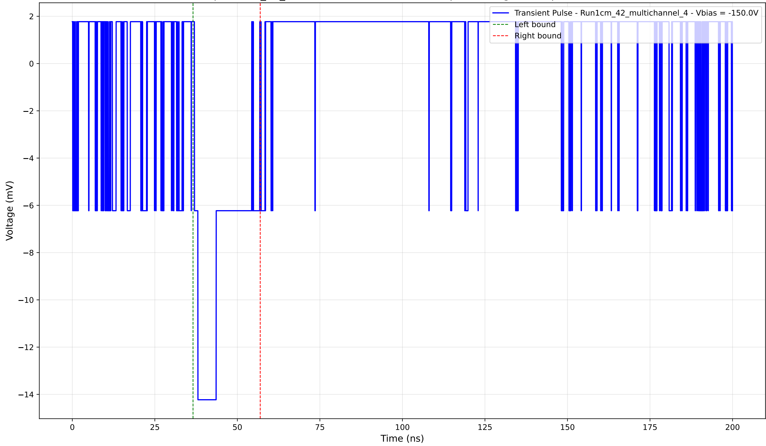
Transient Pulse - Sample: 1cm_42_multichannel - Position: 465.0 \mu\text{m} - Charge: 3.30 pC - Rise Time: 0.00 ns (N/A)
