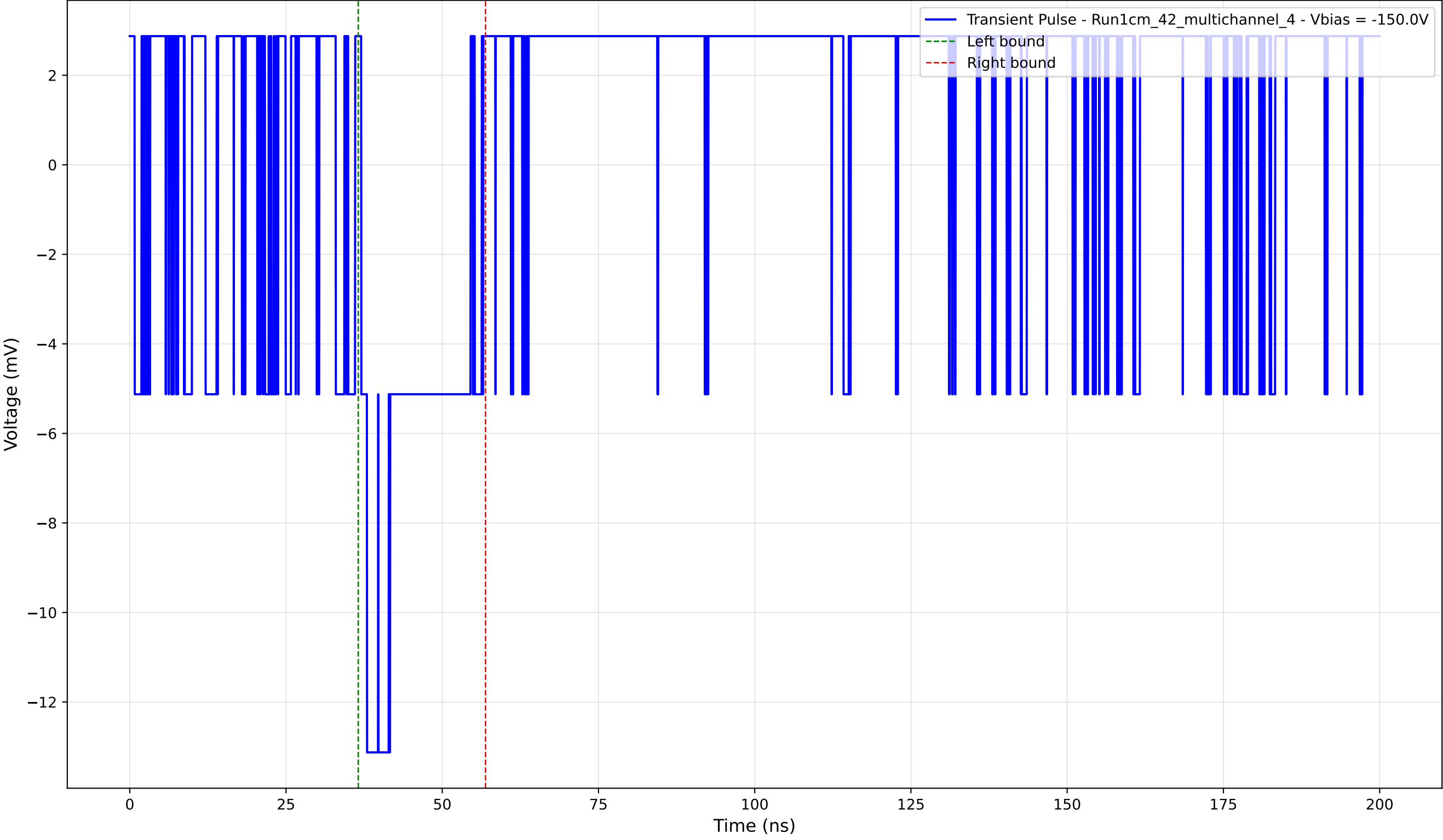
Transient Pulse - Sample: 1cm_42_multichannel - Position: 810.0 \mu\text{m} - Charge: 2.42 pC - Rise Time: 0.00 ns (N/A)
