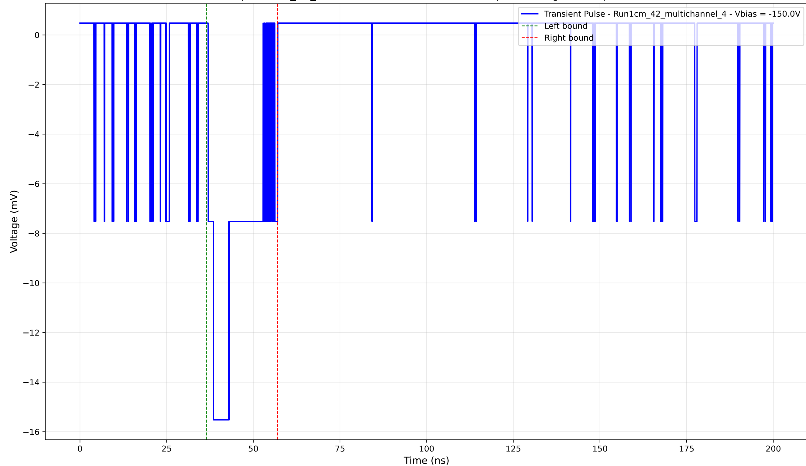
Transient Pulse - Sample: 1cm_42_multichannel - Position: 4260.0 \mu\text{m} - Charge: 3.46 pC - Rise Time: 1.56 ns
