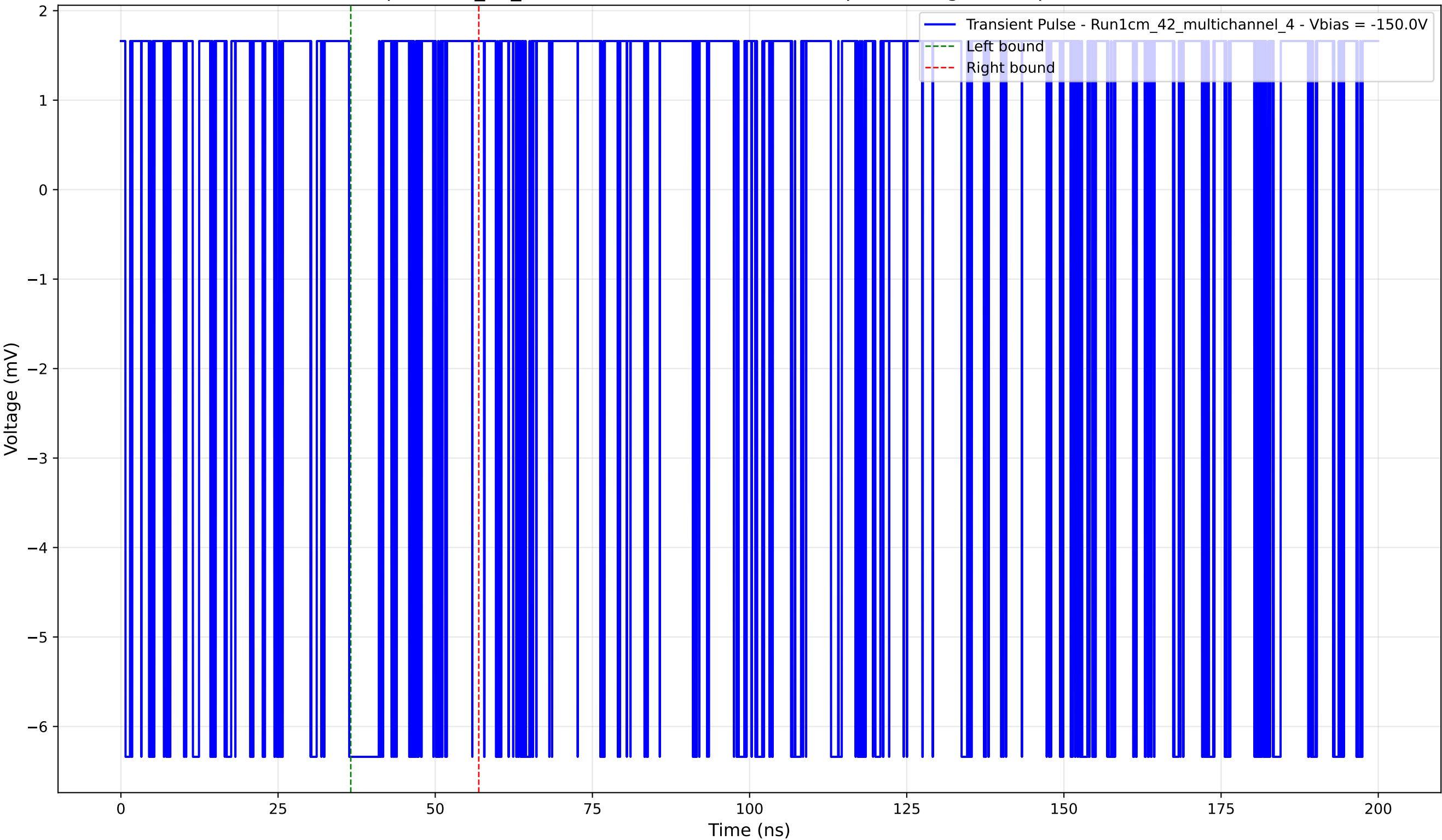
Transient Pulse - Sample: 1cm_42_multichannel - Position: 2870.0 \mu\text{m} - Charge: 0.44 pC - Rise Time: 0.00 ns (N/A)
