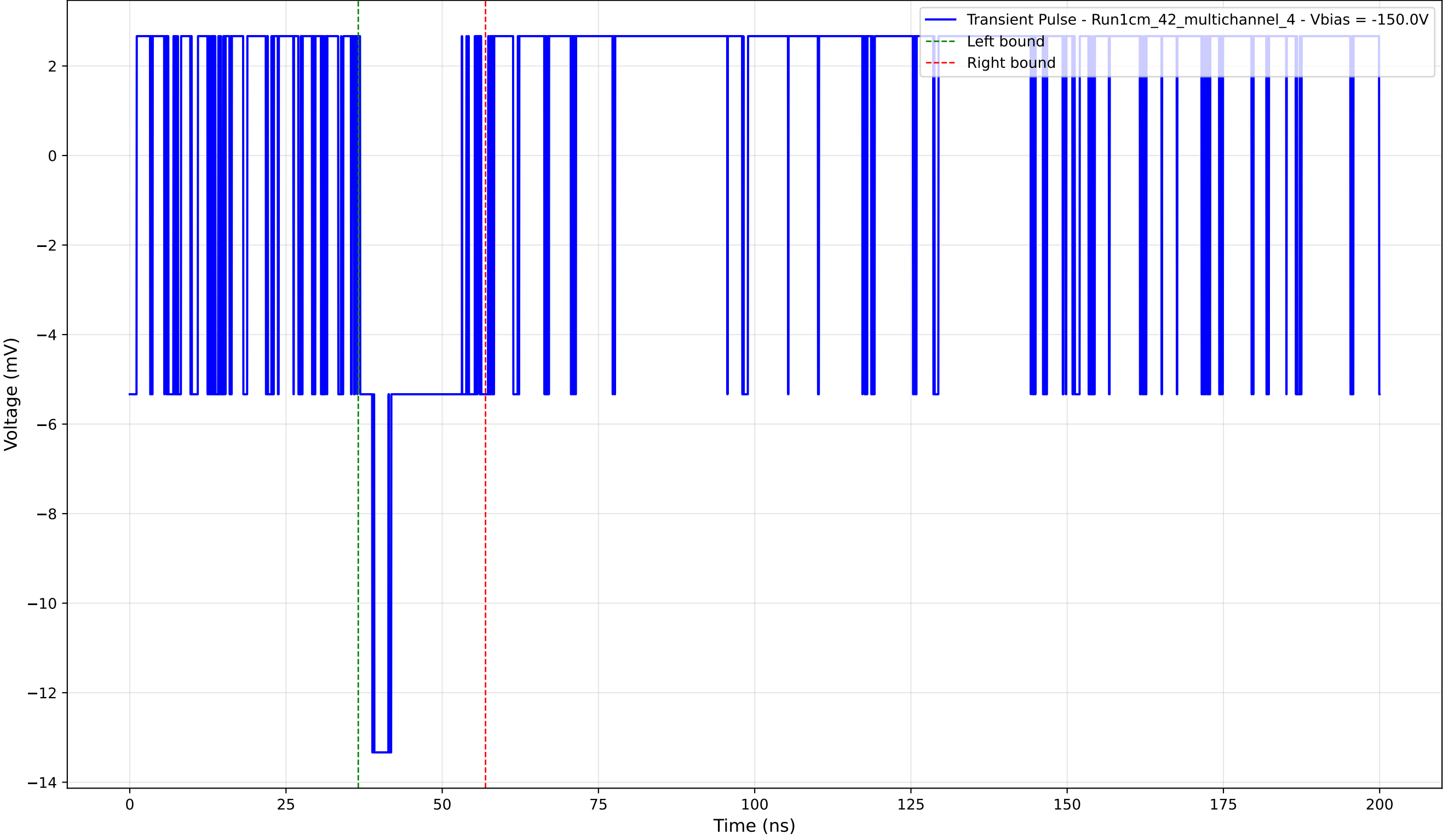
Transient Pulse - Sample: 1cm_42_multichannel - Position: 425.0 \mu\text{m} - Charge: 2.45 pC - Rise Time: 0.00 ns (N/A)
