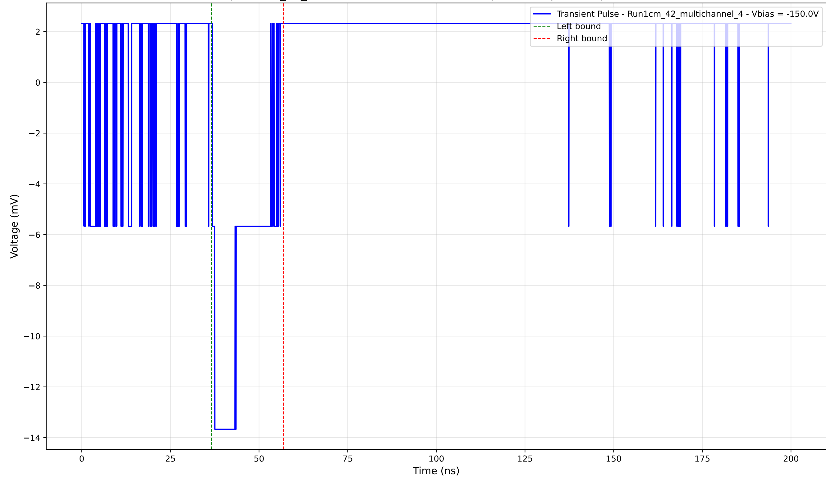
Transient Pulse - Sample: 1cm_42_multichannel - Position: 3675.0 \mu\text{m} - Charge: 2.86 pC - Rise Time: 0.00 ns (N/A)
