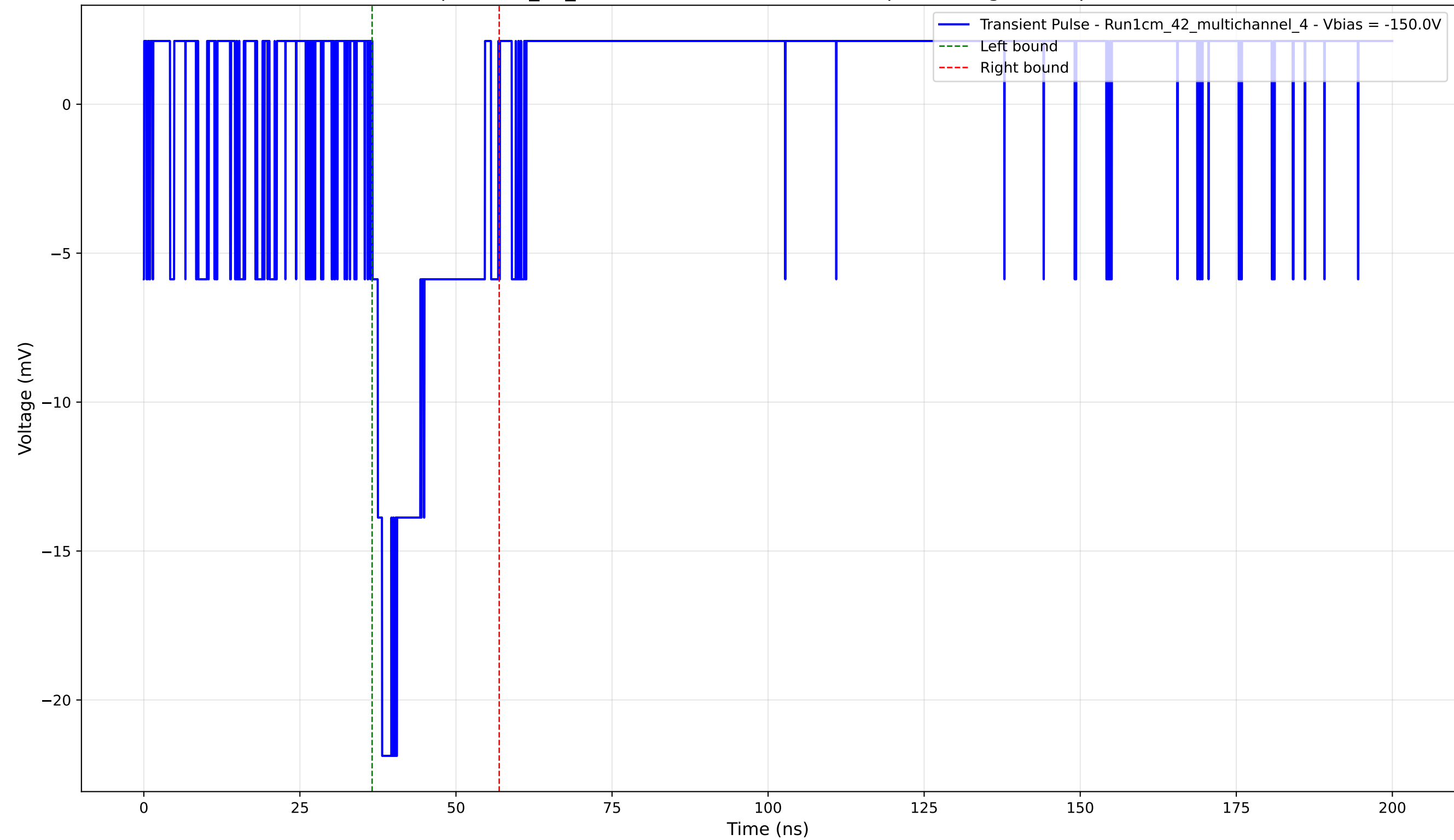
Transient Pulse - Sample: 1cm_42_multichannel - Position: 990.0 \mu\text{m} - Charge: 3.68 pC - Rise Time: 1.56 ns
