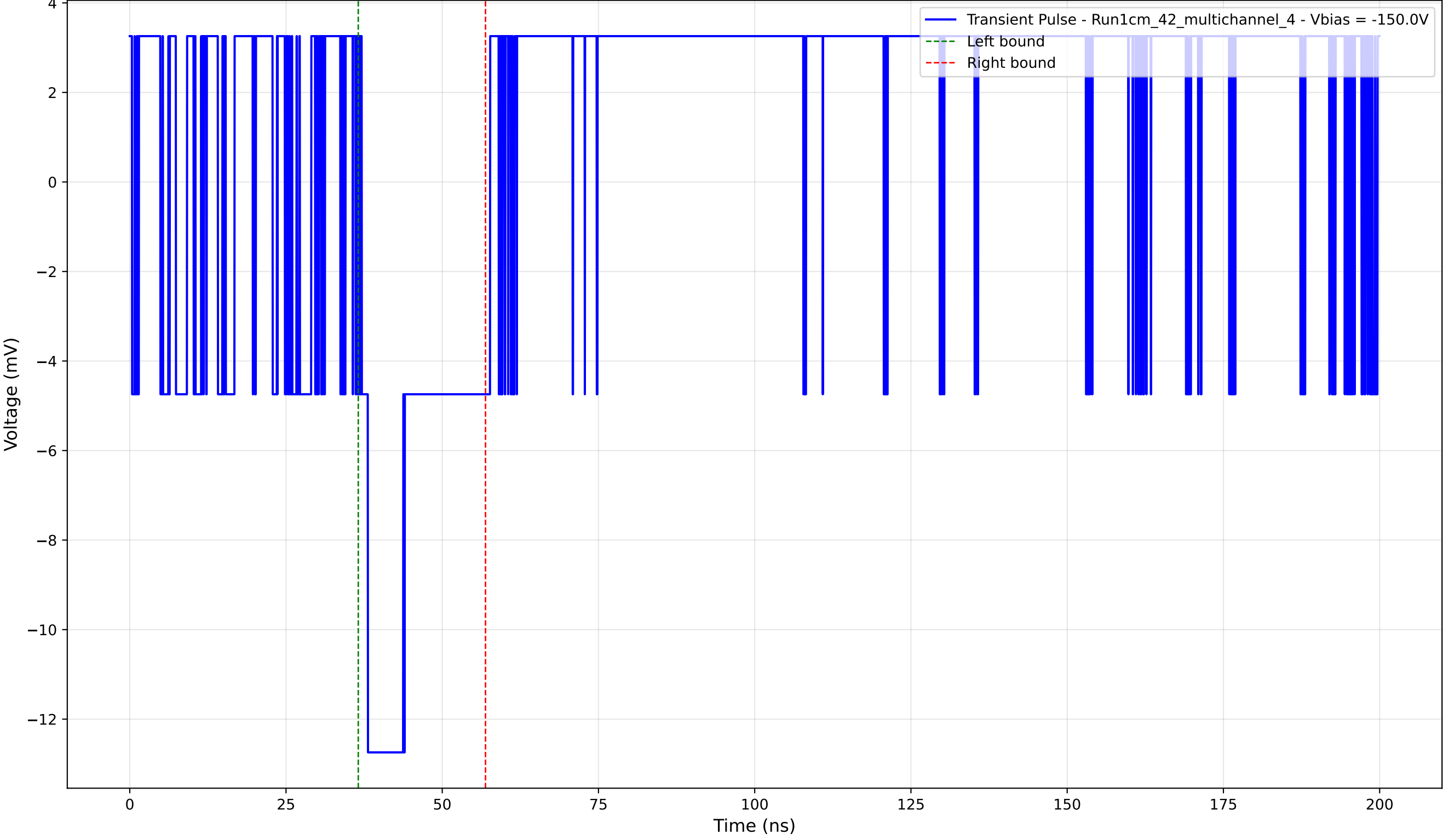
Transient Pulse - Sample: 1cm_42_multichannel - Position: 555.0 \mu\text{m} - Charge: 2.79 pC - Rise Time: 0.00 ns (N/A)
