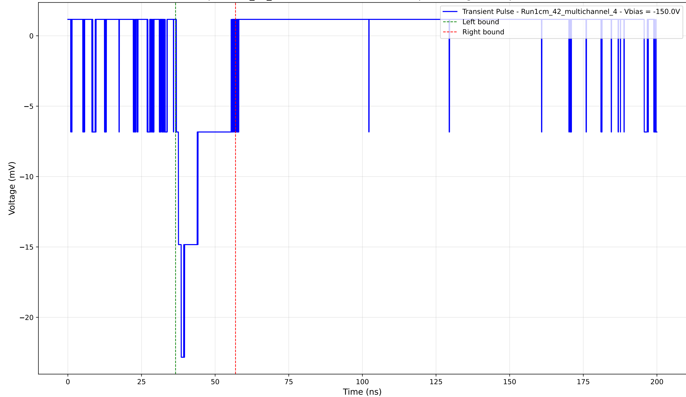
Transient Pulse - Sample: 1cm_42_multichannel - Position: 960.0 \mu\text{m} - Charge: 3.80 pC - Rise Time: 1.66 ns
