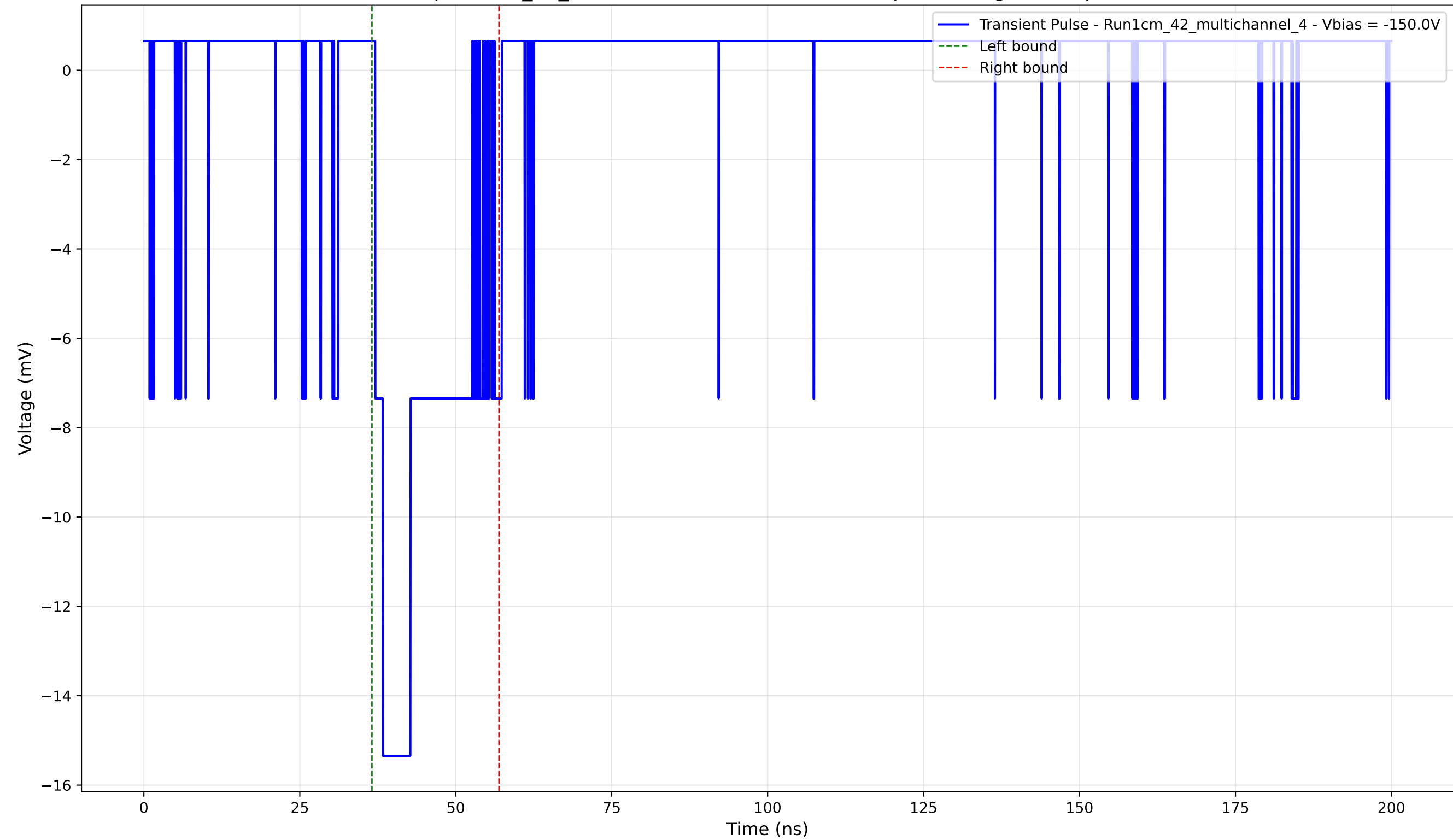
Transient Pulse - Sample: 1cm_42_multichannel - Position: 4215.0 \mu\text{m} - Charge: 3.39 pC - Rise Time: 1.22 ns
