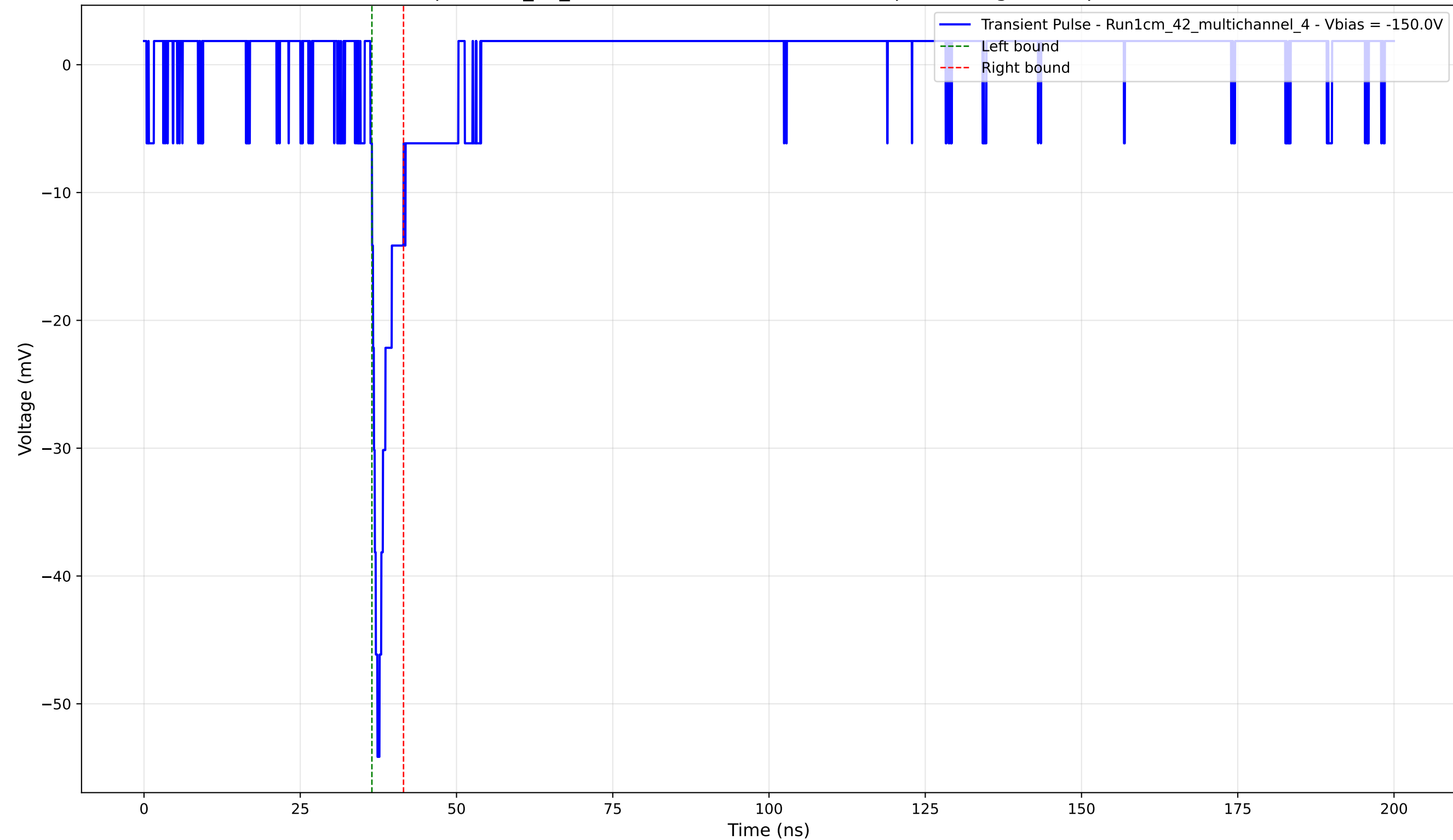
Transient Pulse - Sample: 1cm_42_multichannel - Position: 2770.0 \mu\text{m} - Charge: 2.61 pC - Rise Time: 1.12 ns
