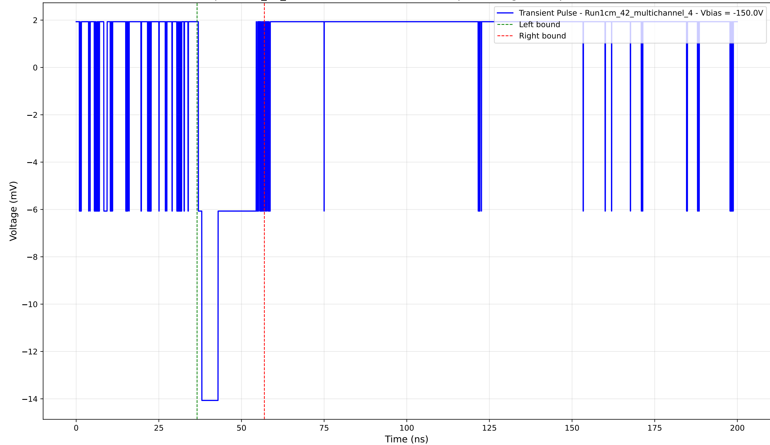
Transient Pulse - Sample: 1cm_42_multichannel - Position: 3975.0 \mu\text{m} - Charge: 3.01 pC - Rise Time: 0.00 ns (N/A)
