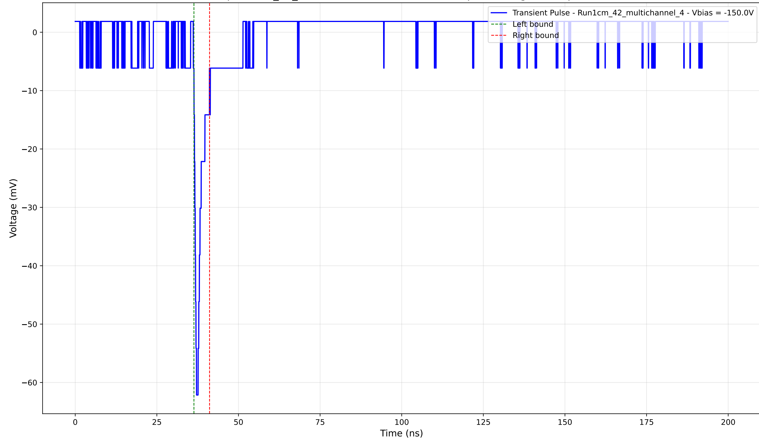
Transient Pulse - Sample: 1cm_42_multichannel - Position: 2140.0 \mu\text{m} - Charge: 2.81 pC - Rise Time: 0.78 ns
