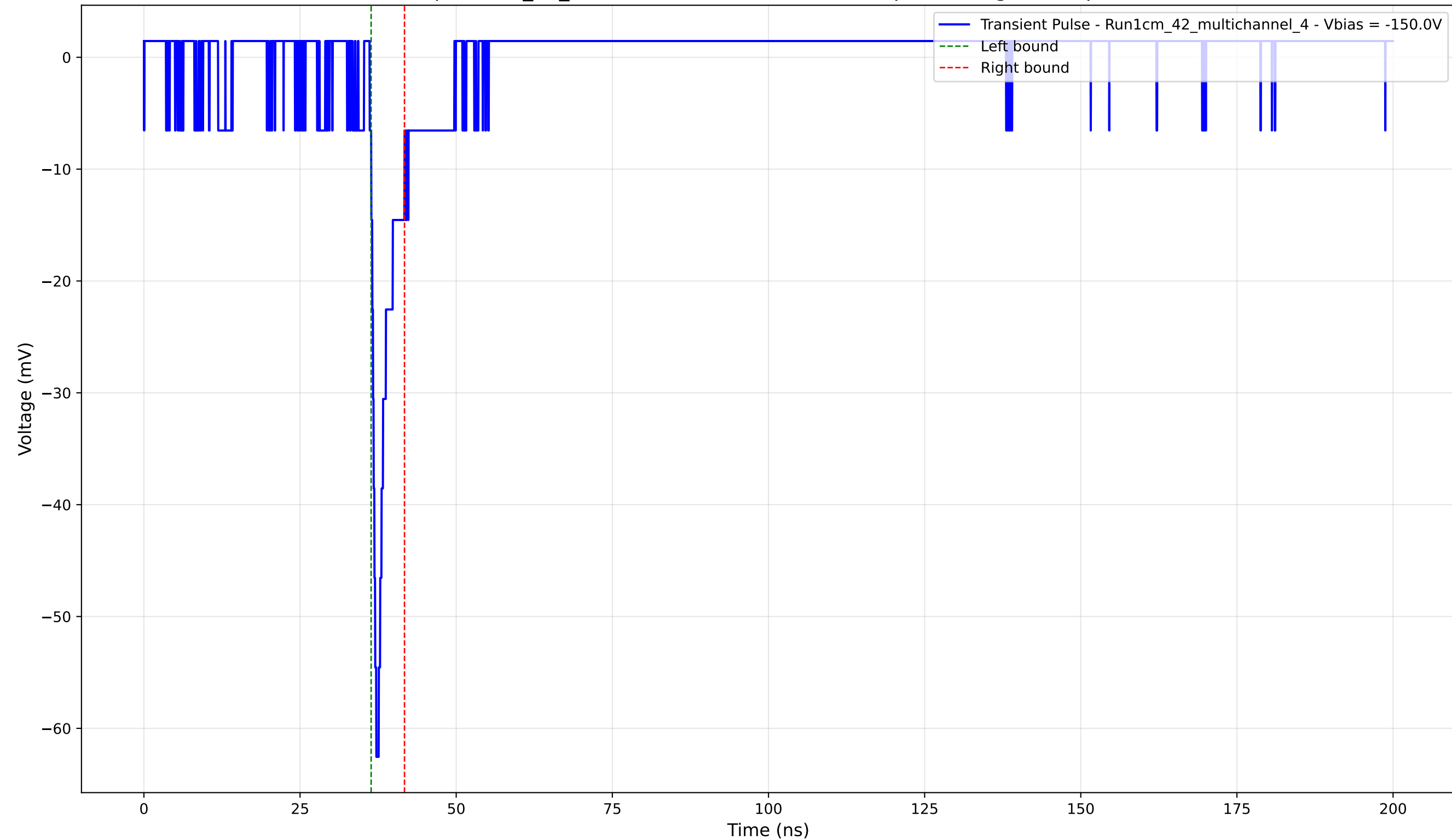
Transient Pulse - Sample: 1cm_42_multichannel - Position: 2095.0 \mu\text{m} - Charge: 3.02 pC - Rise Time: 1.06 ns
