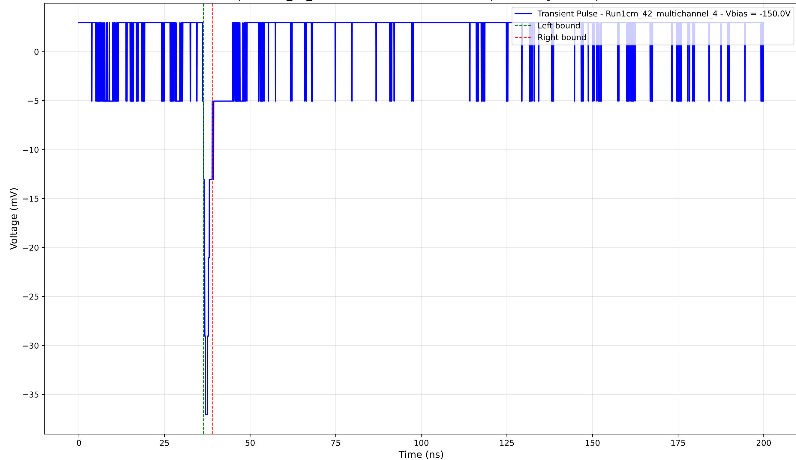
Transient Pulse - Sample: 1cm_42_multichannel - Position: 2435.0 \mu\text{m} - Charge: 1.15 pC - Rise Time: 0.87 ns
