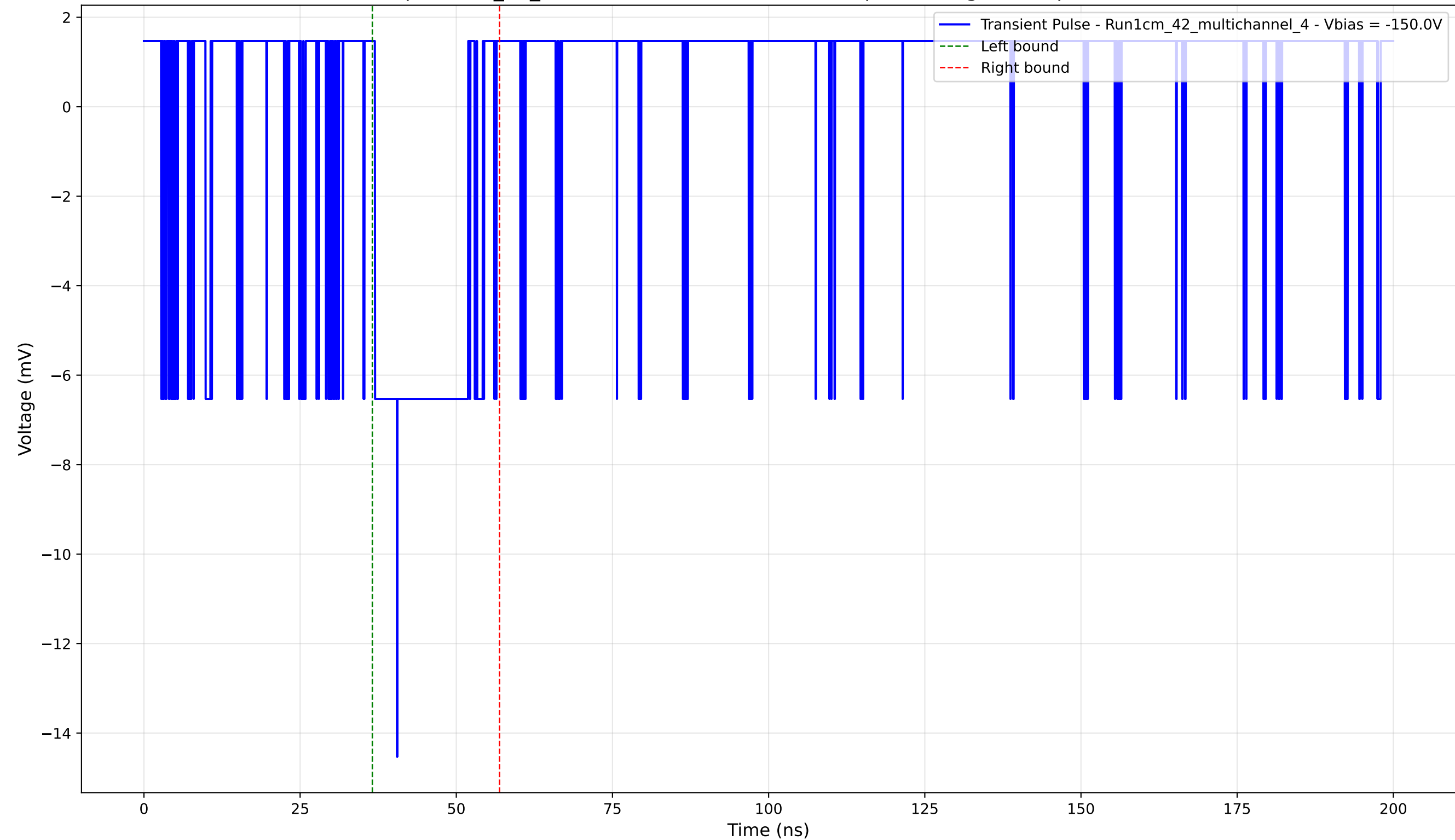
Transient Pulse - Sample: 1cm_42_multichannel - Position: 4840.0 \mu\text{m} - Charge: 2.05 pC - Rise Time: 0.00 ns (N/A)
