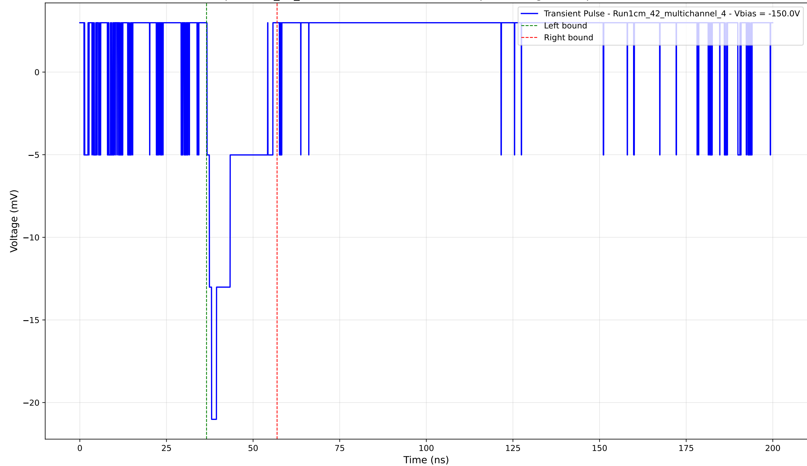
Transient Pulse - Sample: 1cm_42_multichannel - Position: 1140.0 \mu\text{m} - Charge: 3.00 pC - Rise Time: 0.00 ns (N/A)
