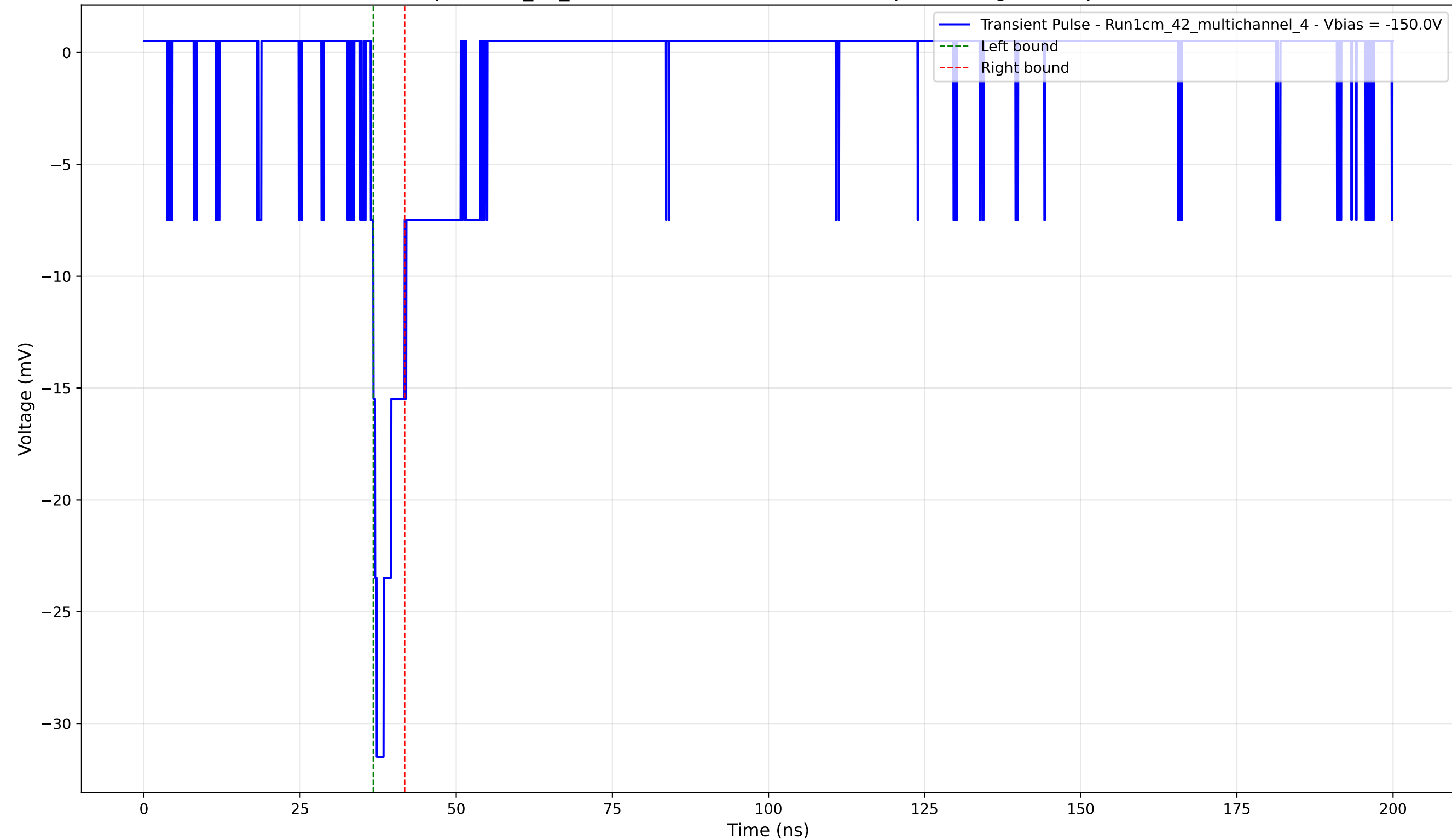
Transient Pulse - Sample: 1cm_42_multichannel - Position: 3075.0 \mu\text{m} - Charge: 2.15 pC - Rise Time: 0.95 ns
