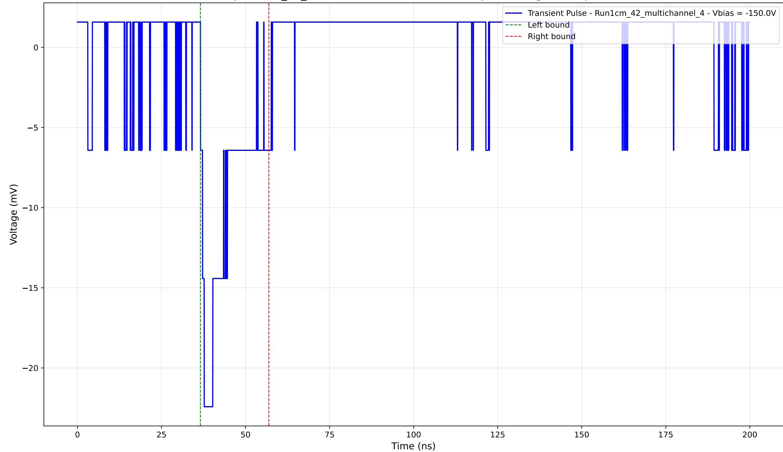
Transient Pulse - Sample: 1cm_42_multichannel - Position: 1235.0 \mu\text{m} - Charge: 4.11 pC - Rise Time: 1.12 ns
