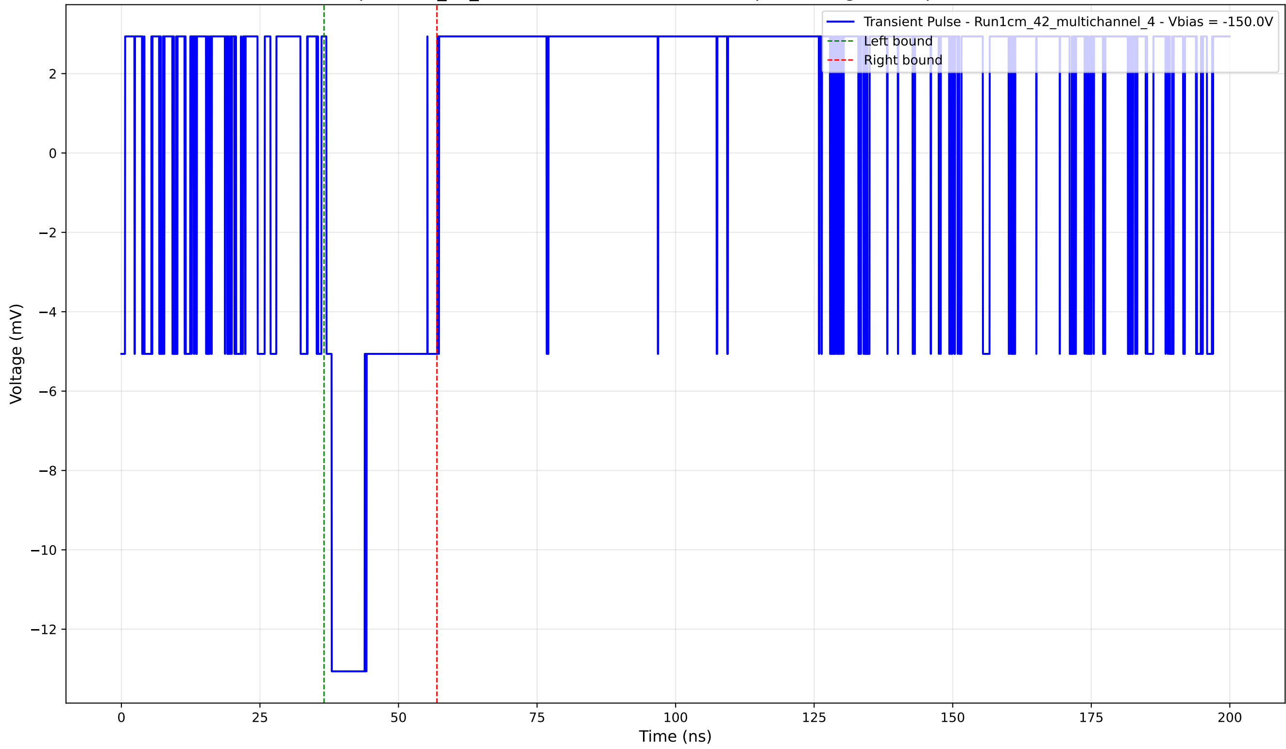
Transient Pulse - Sample: 1cm_42_multichannel - Position: 525.0 \mu\text{m} - Charge: 2.97 pC - Rise Time: 0.00 ns (N/A)
