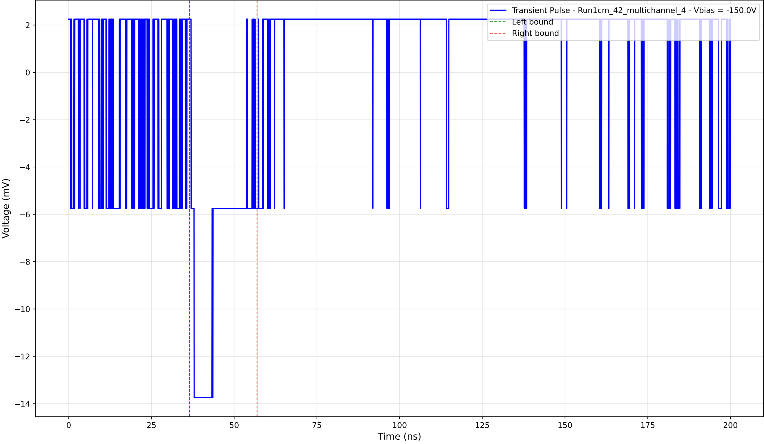
Transient Pulse - Sample: 1cm_42_multichannel - Position: 615.0 \mu\text{m} - Charge: 3.10 pC - Rise Time: 0.00 ns (N/A)
