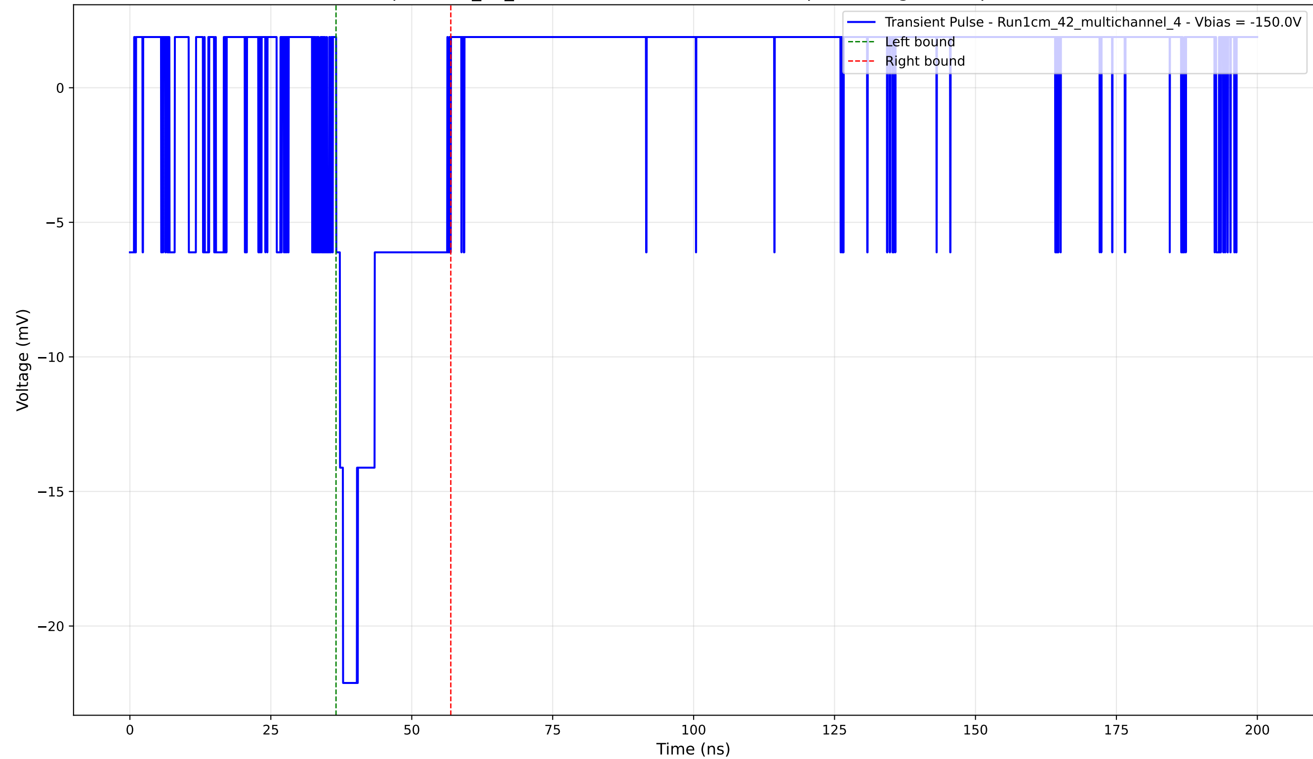
Transient Pulse - Sample: 1cm_42_multichannel - Position: 1185.0 \mu\text{m} - Charge: 3.85 pC - Rise Time: 1.22 ns
