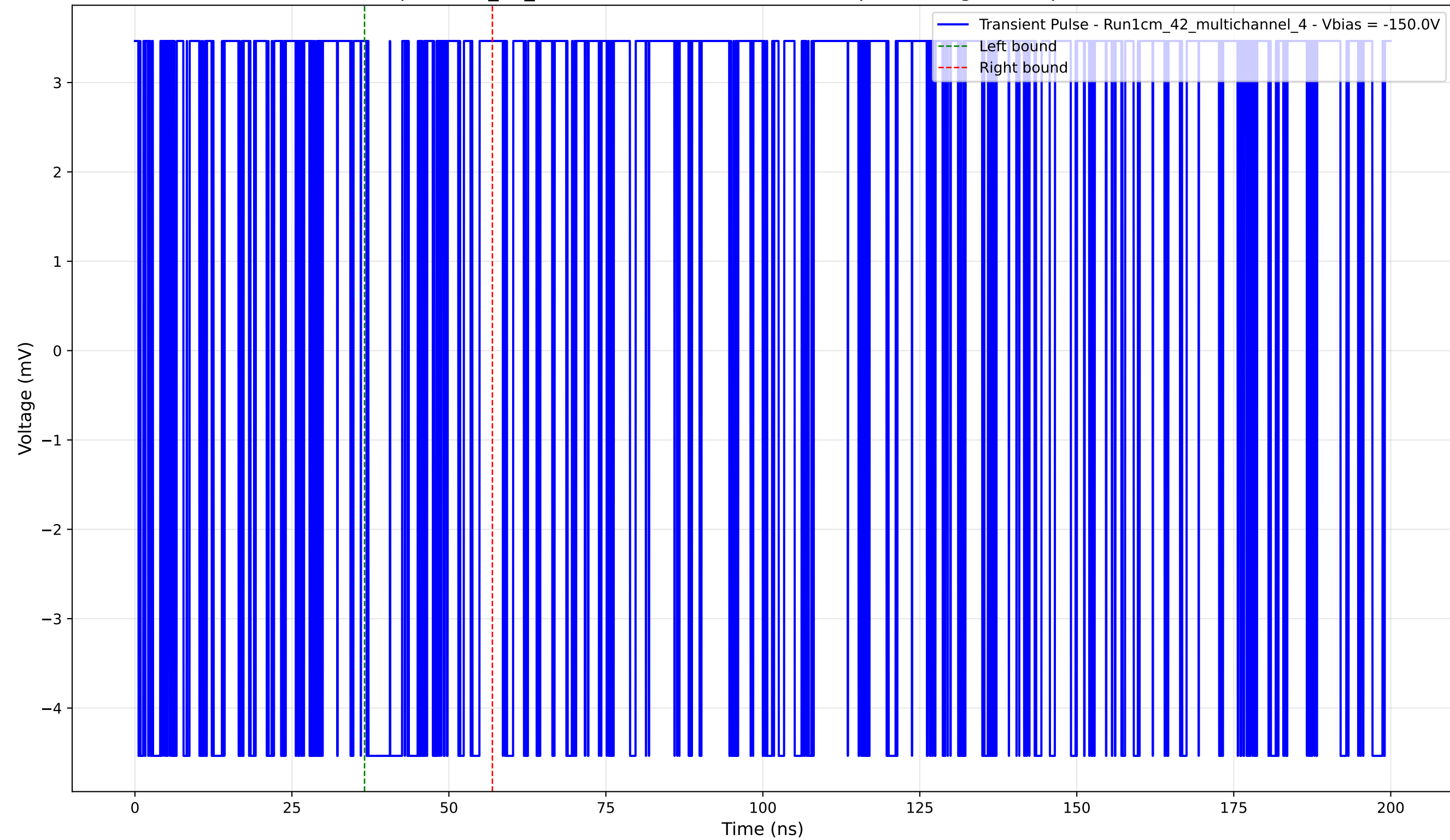
Transient Pulse - Sample: 1cm_42_multichannel - Position: 1345.0 \mu\text{m} - Charge: 0.32 pC - Rise Time: 0.00 ns (N/A)
