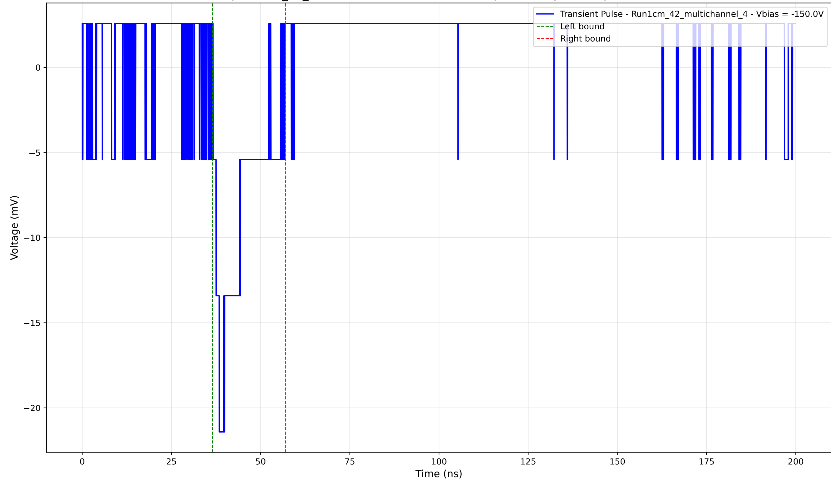
Transient Pulse - Sample: 1cm_42_multichannel - Position: 1060.0 \mu\text{m} - Charge: 3.32 pC - Rise Time: 0.00 ns (N/A)
