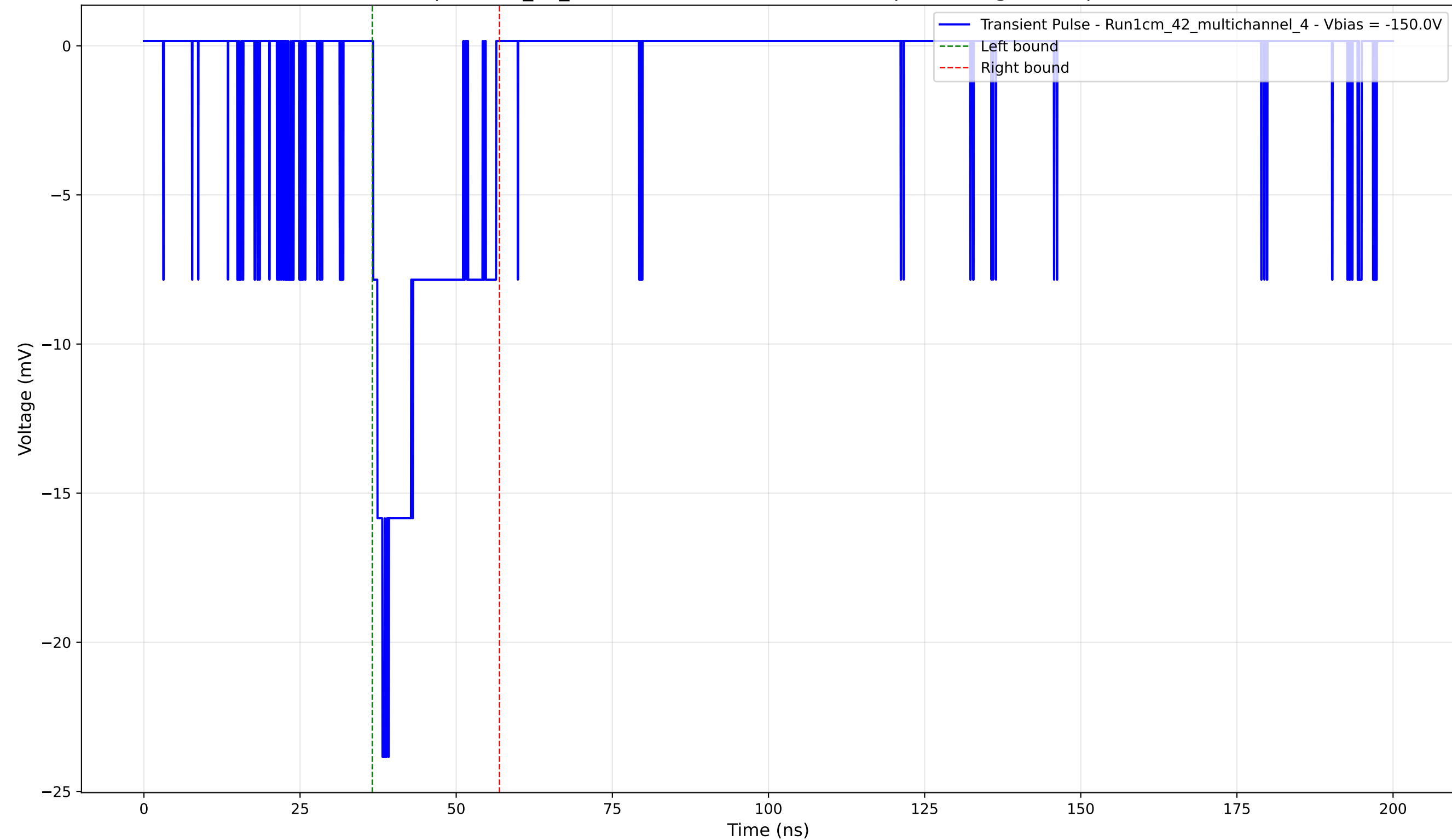
Transient Pulse - Sample: 1cm_42_multichannel - Position: 3590.0 \mu\text{m} - Charge: 3.97 pC - Rise Time: 1.49 ns
