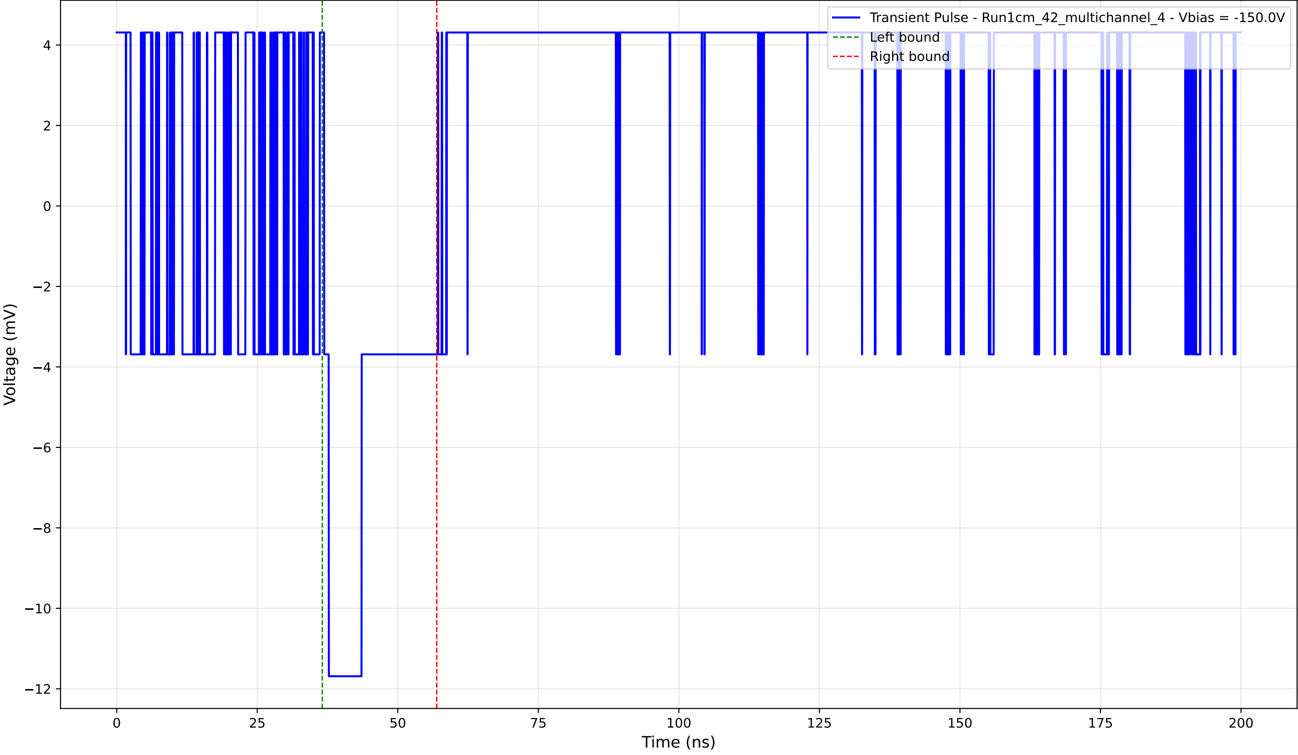
Transient Pulse - Sample: 1cm_42_multichannel - Position: 790.0 \mu\text{m} - Charge: 2.39 pC - Rise Time: 0.00 ns (N/A)
