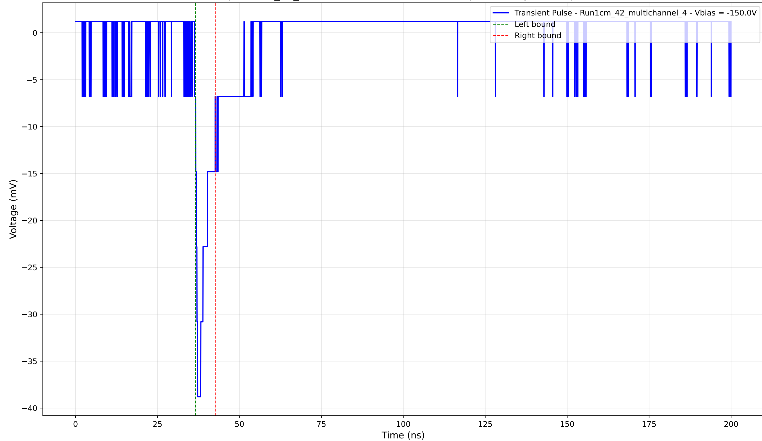
Transient Pulse - Sample: 1cm_42_multichannel - Position: 1760.0 \mu\text{m} - Charge: 2.77 pC - Rise Time: 0.93 ns
