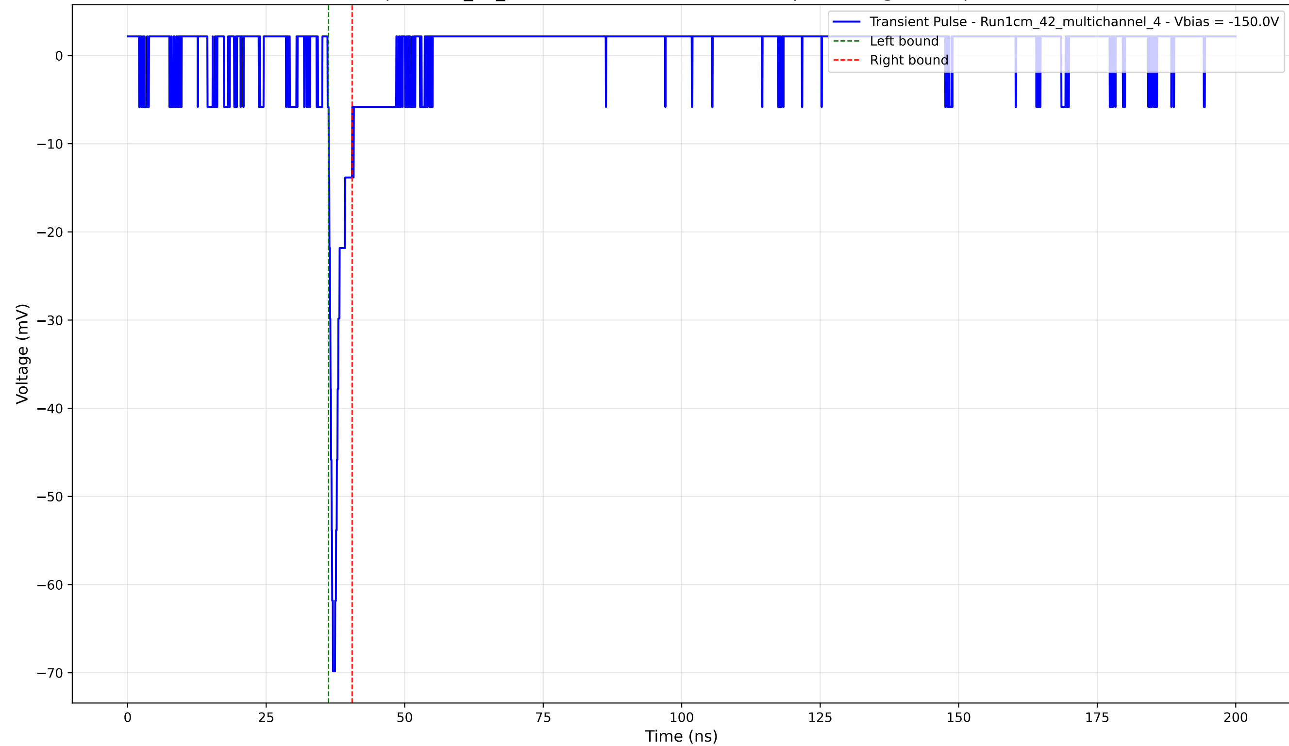
Transient Pulse - Sample: 1cm_42_multichannel - Position: 2315.0 \mu\text{m} - Charge: 2.65 pC - Rise Time: 0.78 ns
