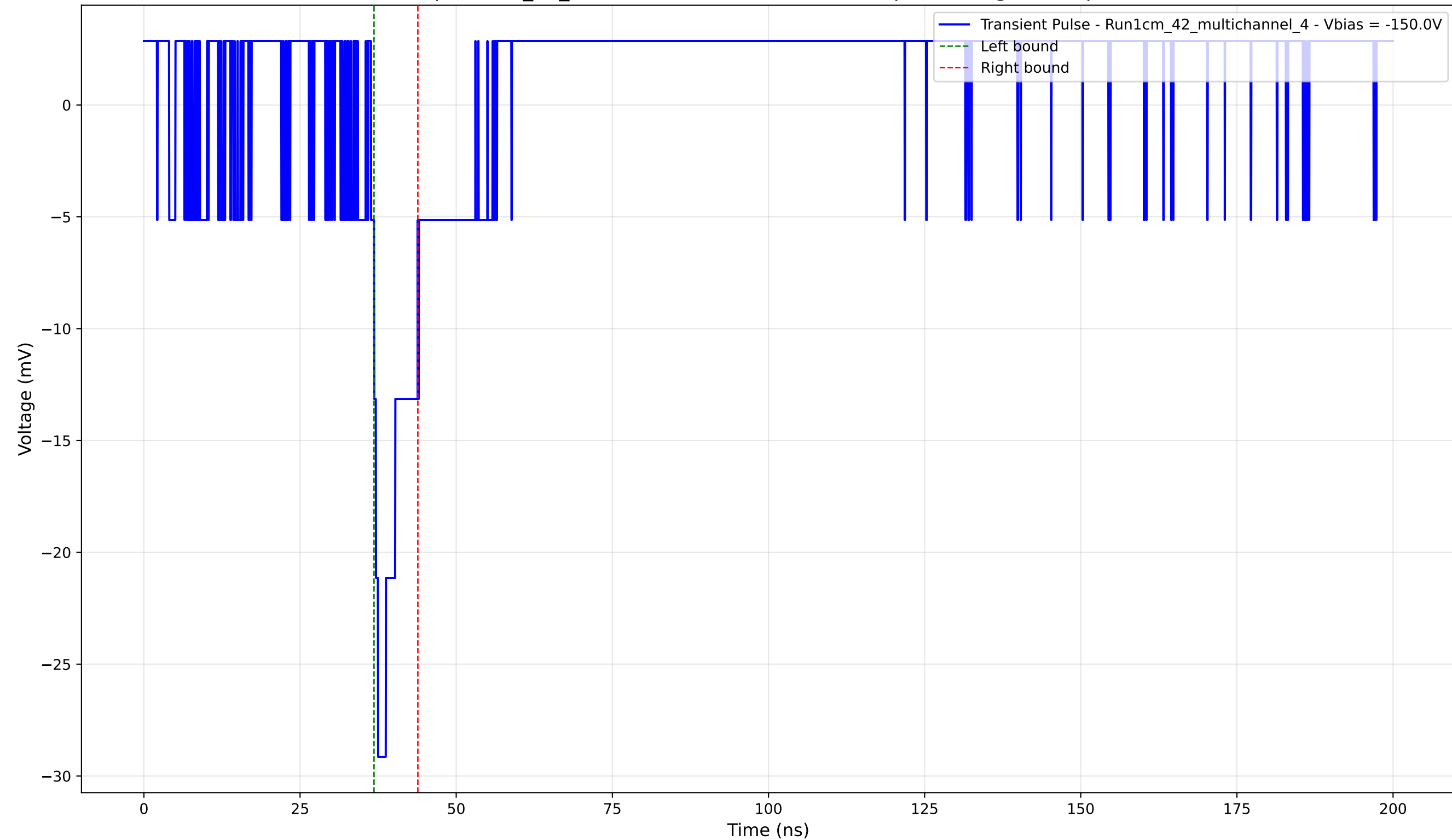
Transient Pulse - Sample: 1cm_42_multichannel - Position: 1525.0 \mu\text{m} - Charge: 2.54 pC - Rise Time: 1.14 ns
