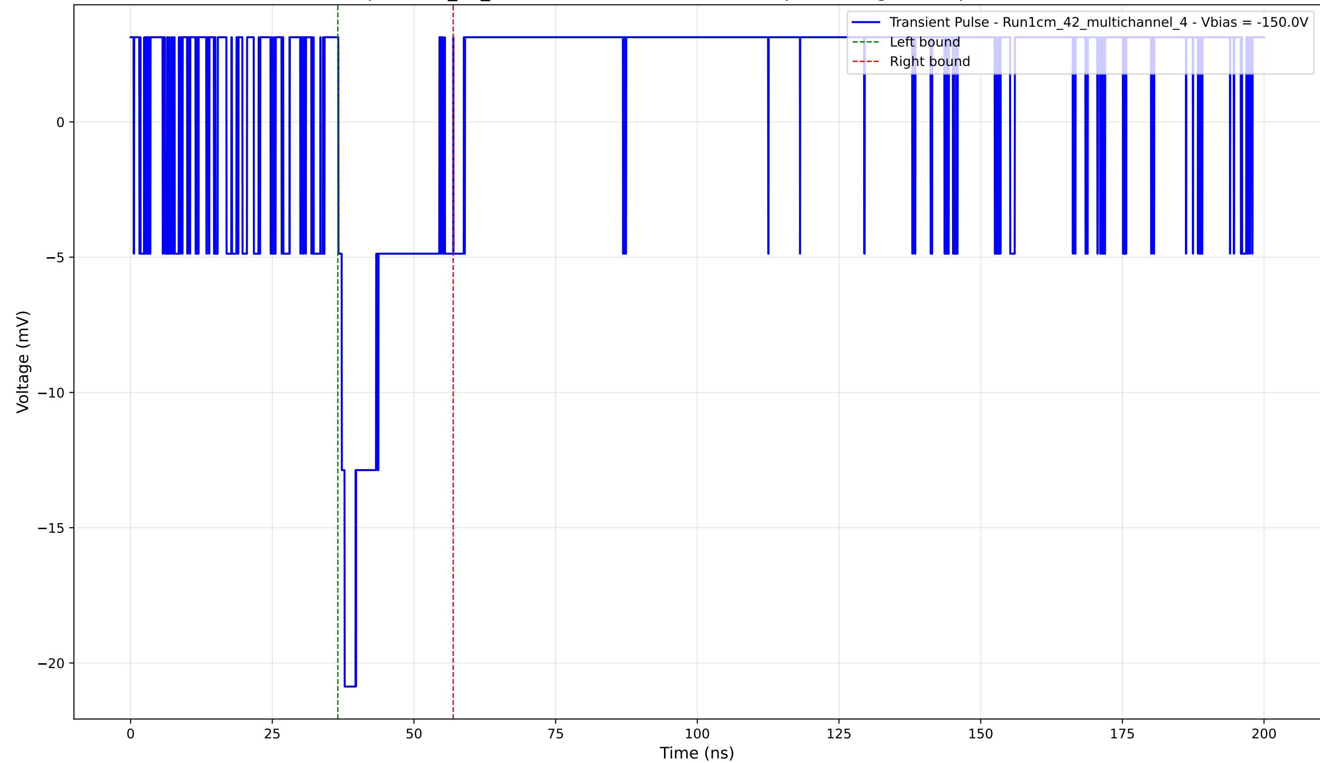
Transient Pulse - Sample: 1cm_42_multichannel - Position: 1180.0 \mu\text{m} - Charge: 3.20 pC - Rise Time: 0.00 ns (N/A)
