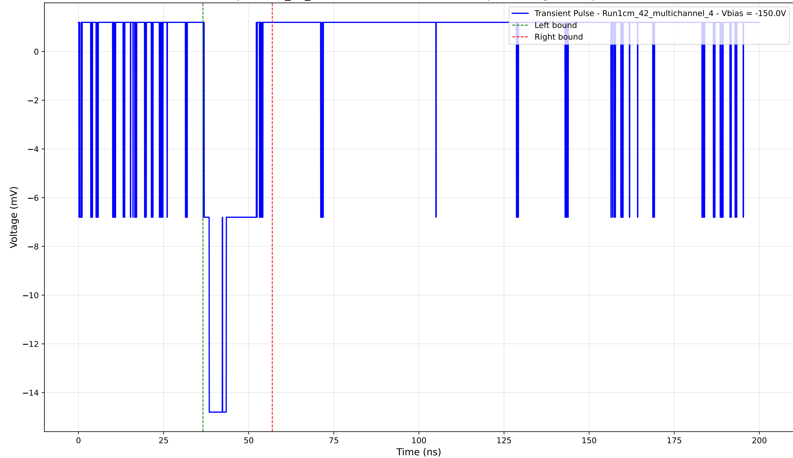
Transient Pulse - Sample: 1cm_42_multichannel - Position: 4225.0 \mu\text{m} - Charge: 2.87 pC - Rise Time: 1.50 ns
