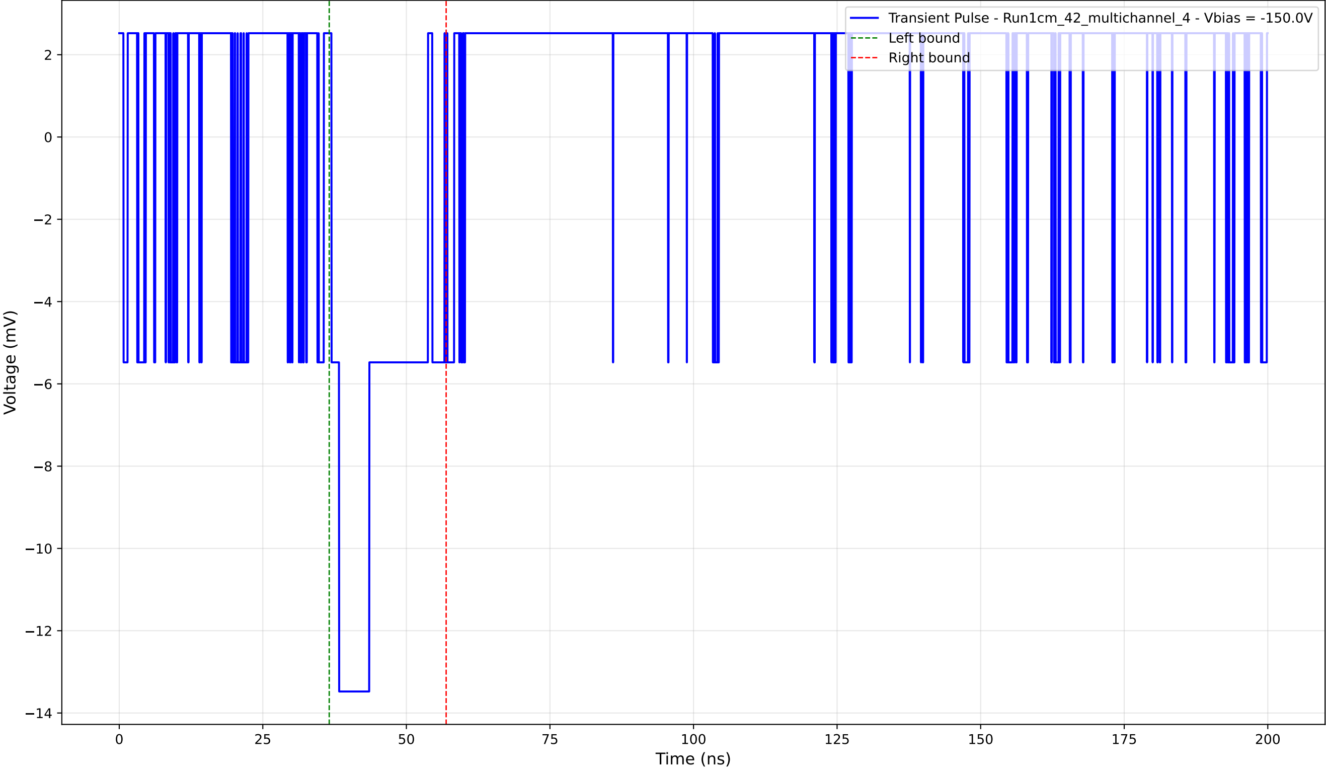
Transient Pulse - Sample: 1cm_42_multichannel - Position: 460.0 \mu\text{m} - Charge: 2.88 pC - Rise Time: 0.00 ns (N/A)
