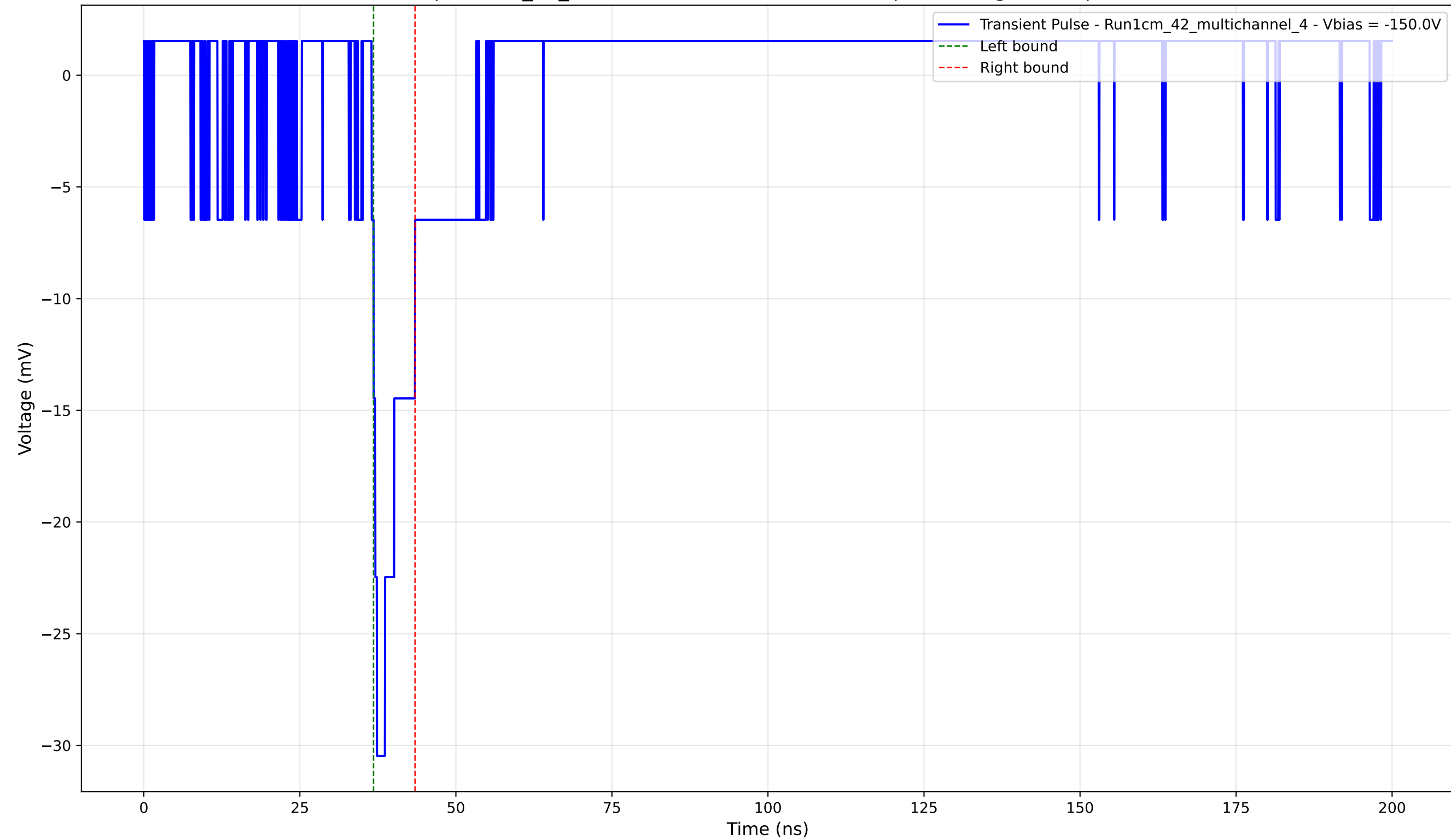
Transient Pulse - Sample: 1cm_42_multichannel - Position: 1615.0 \mu\text{m} - Charge: 2.62 pC - Rise Time: 0.85 ns
