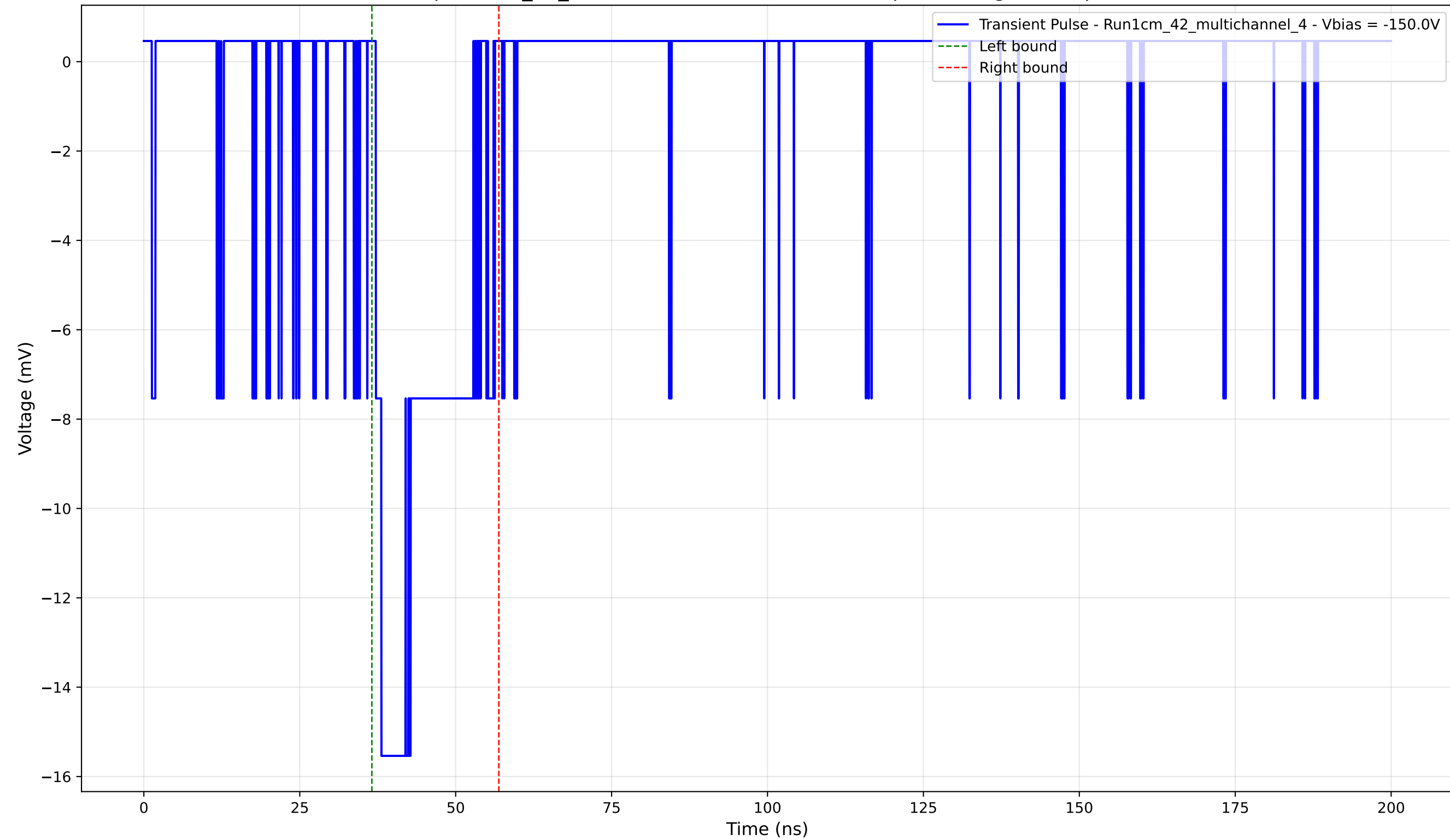
Transient Pulse - Sample: 1cm_42_multichannel - Position: 3970.0 \mu\text{m} - Charge: 3.31 pC - Rise Time: 0.90 ns
