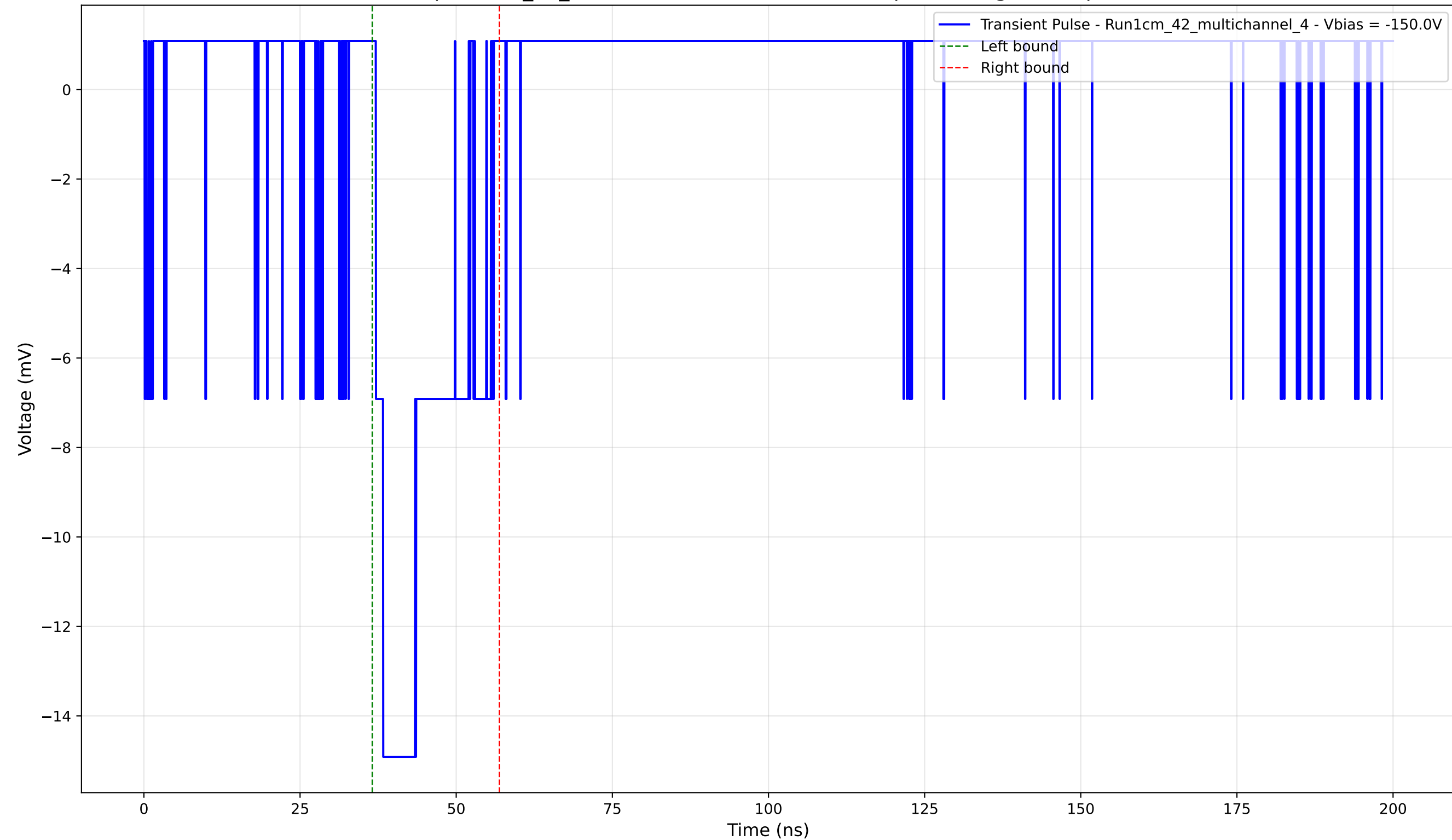
Transient Pulse - Sample: 1cm_42_multichannel - Position: 4205.0 \mu\text{m} - Charge: 3.25 pC - Rise Time: 1.18 ns
