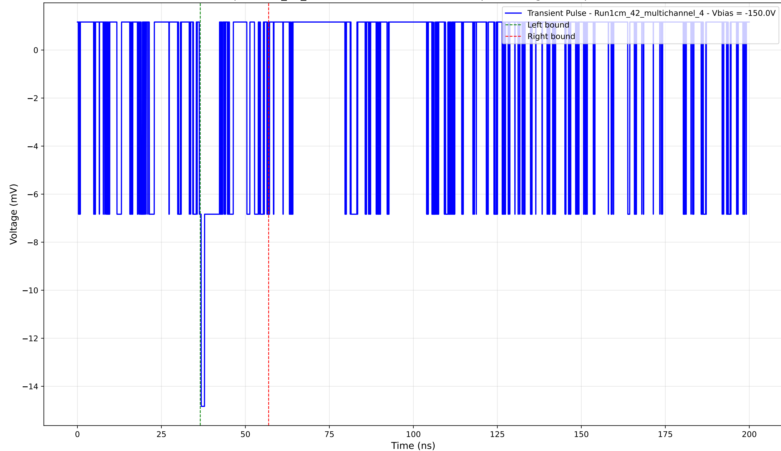
Transient Pulse - Sample: 1cm_42_multichannel - Position: 2420.0 \mu\text{m} - Charge: 1.54 pC - Rise Time: 0.58 ns
