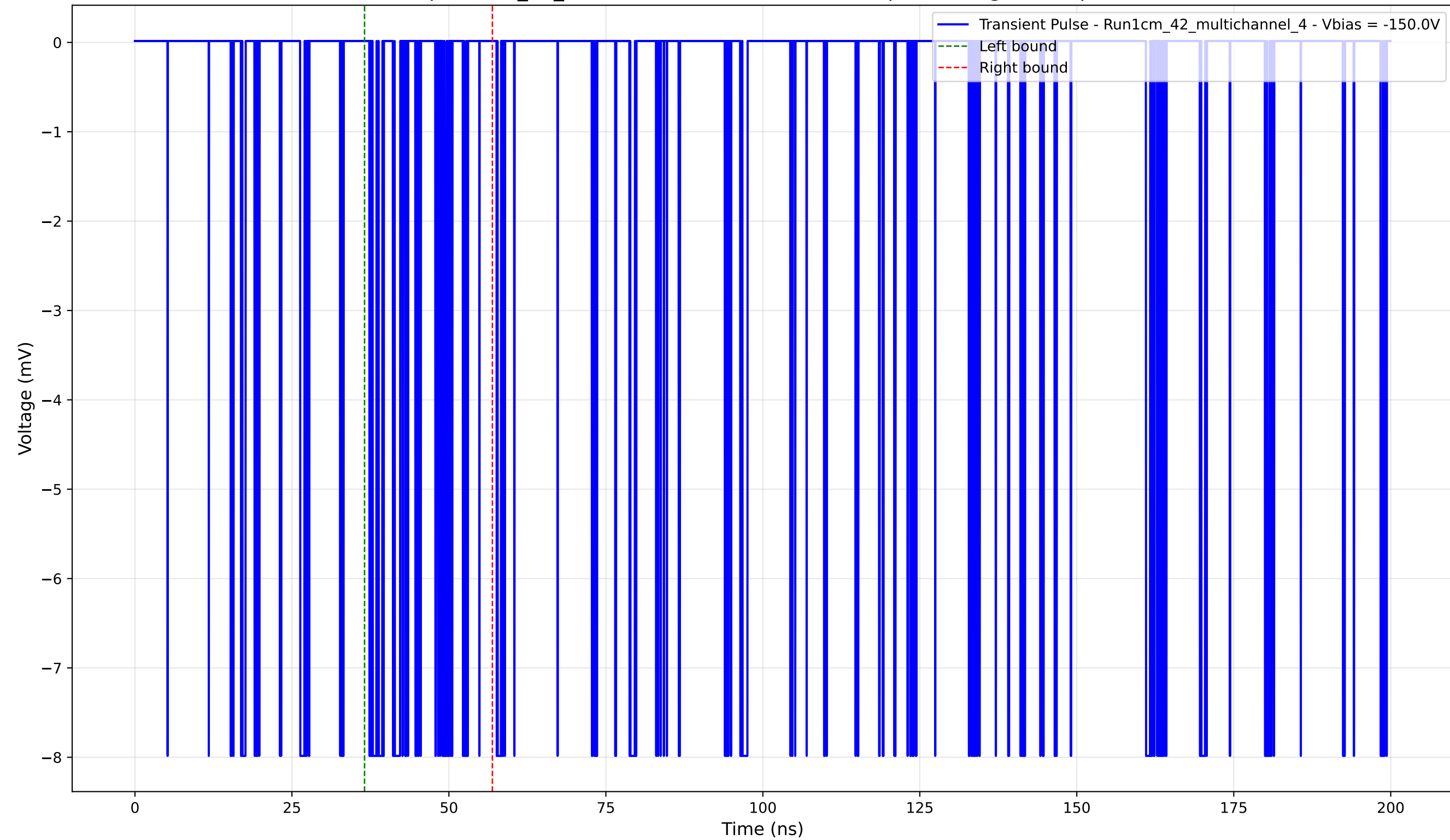
Transient Pulse - Sample: 1cm_42_multichannel - Position: 3890.0 \mu\text{m} - Charge: 0.81 pC - Rise Time: 0.02 ns
