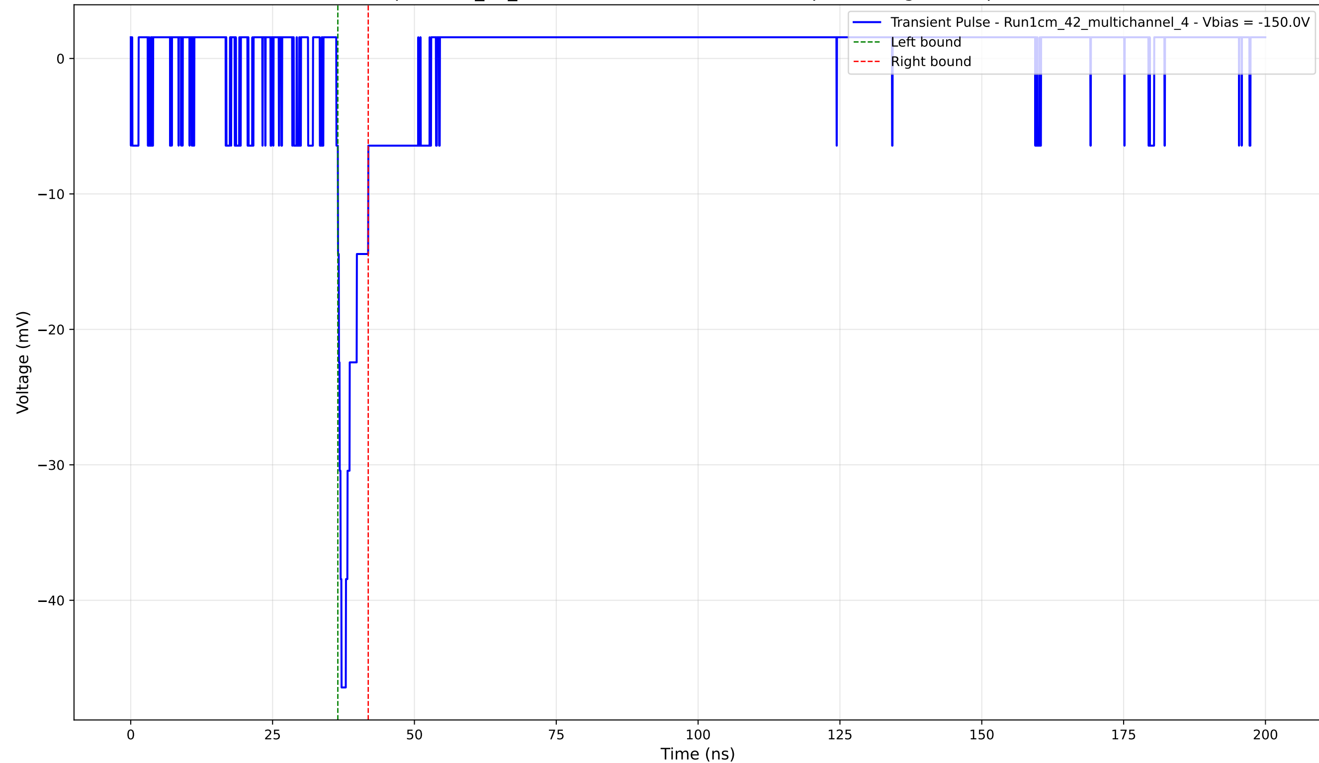
Transient Pulse - Sample: 1cm_42_multichannel - Position: 2805.0 \mu\text{m} - Charge: 2.65 pC - Rise Time: 0.91 ns
