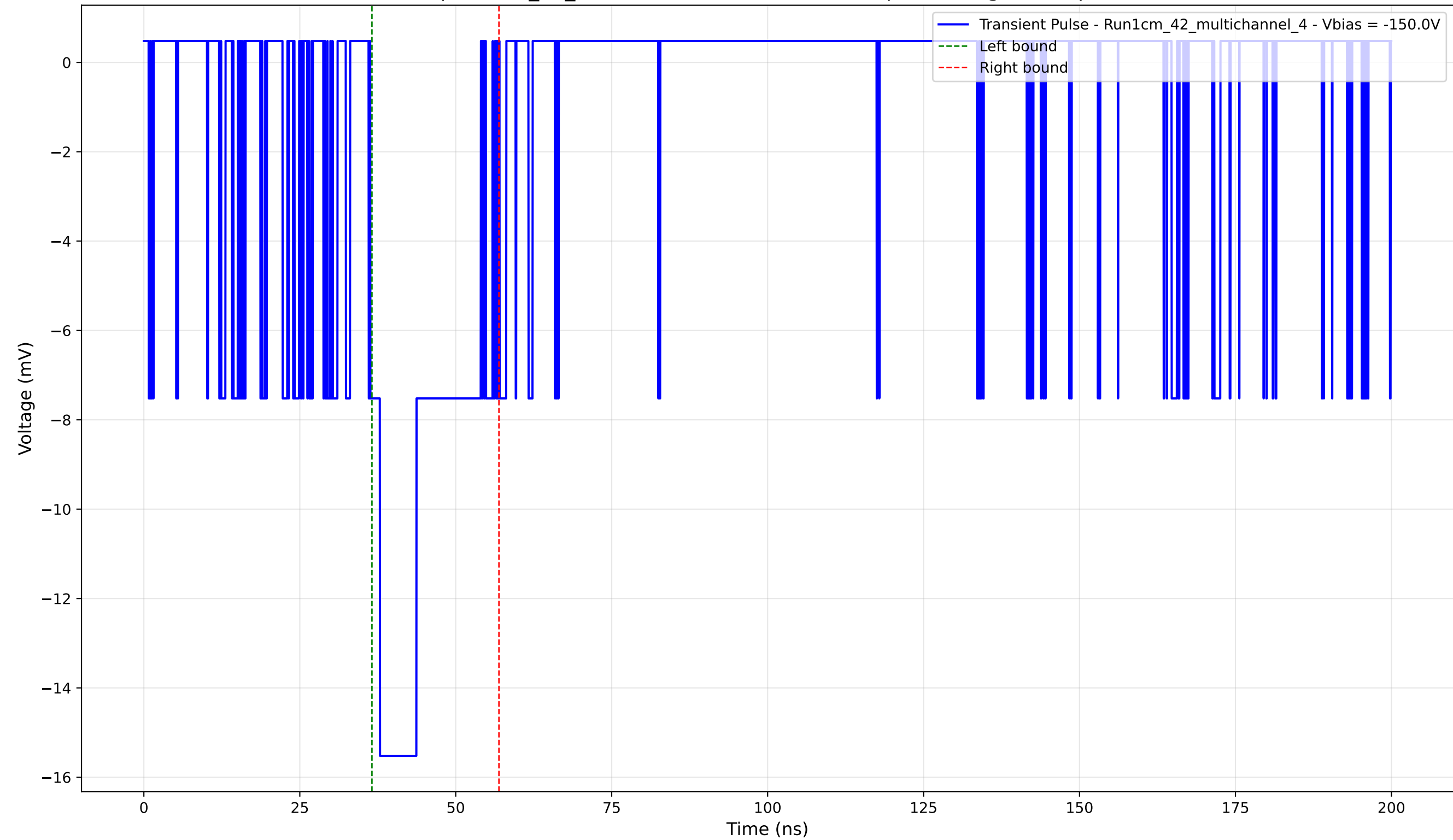
Transient Pulse - Sample: 1cm_42_multichannel - Position: 680.0 \mu\text{m} - Charge: 3.82 pC - Rise Time: 1.56 ns
