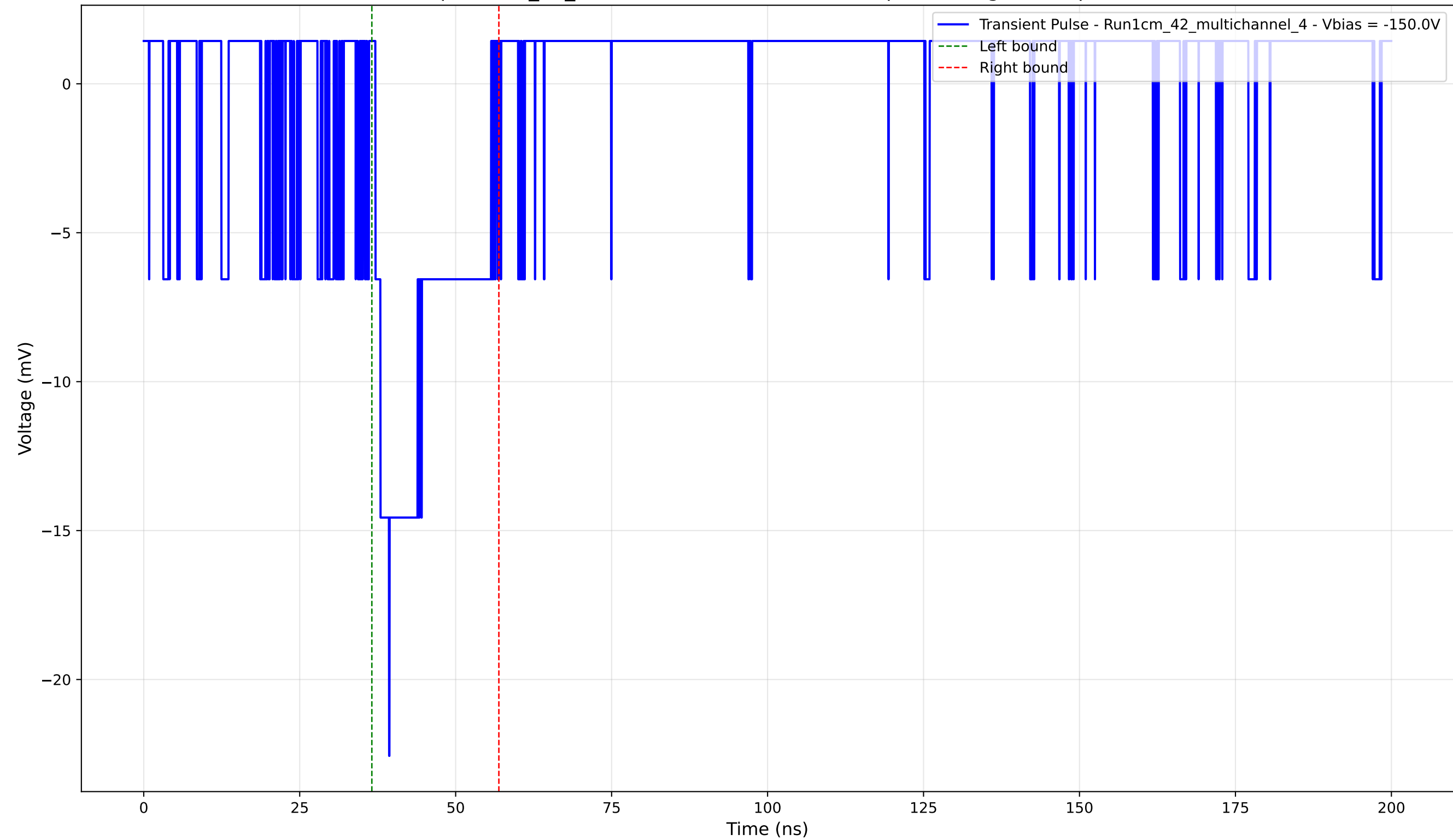
Transient Pulse - Sample: 1cm_42_multichannel - Position: 675.0 \mu\text{m} - Charge: 3.47 pC - Rise Time: 2.20 ns
