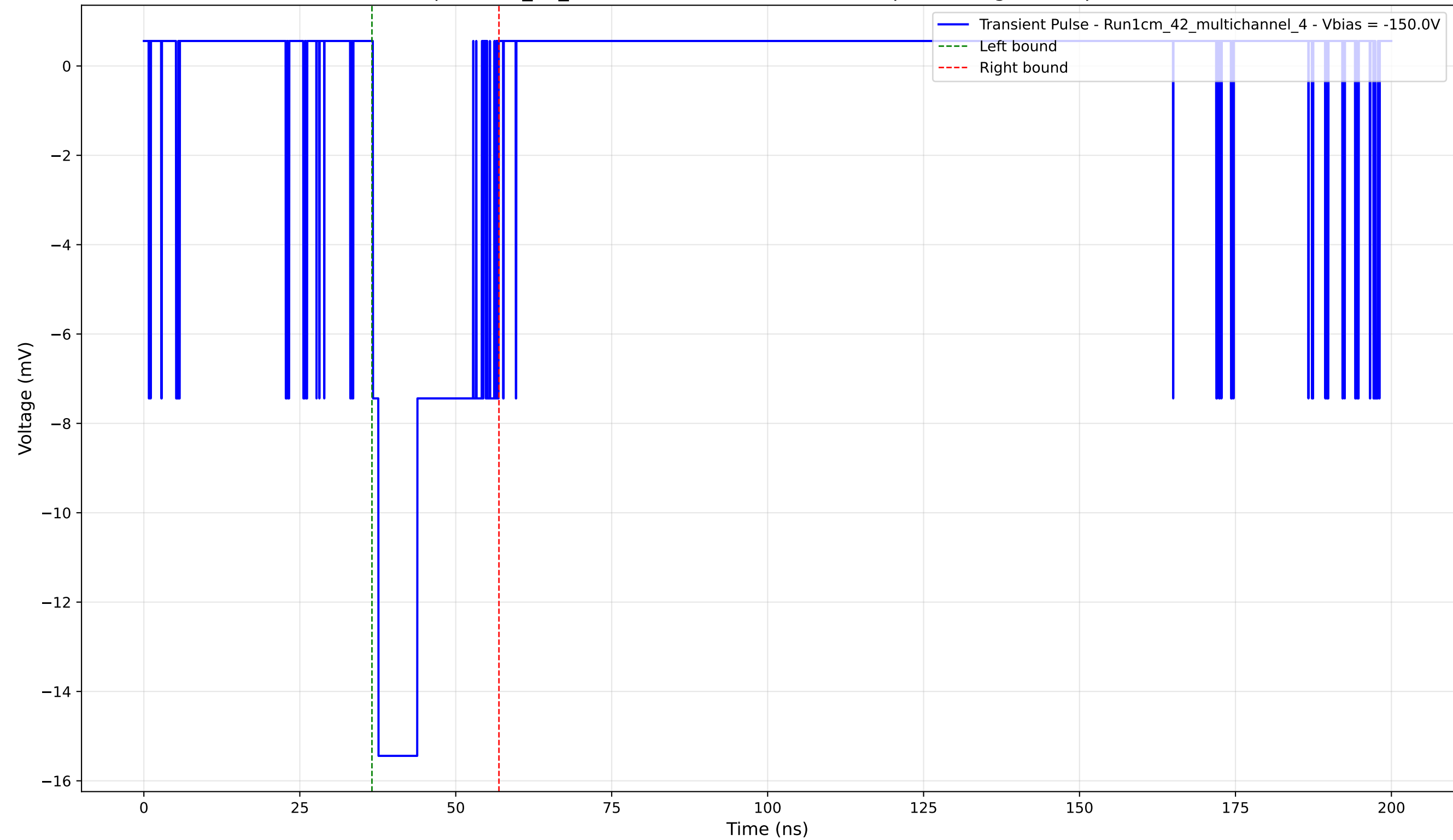
Transient Pulse - Sample: 1cm_42_multichannel - Position: 3775.0 \mu\text{m} - Charge: 3.84 pC - Rise Time: 0.90 ns
