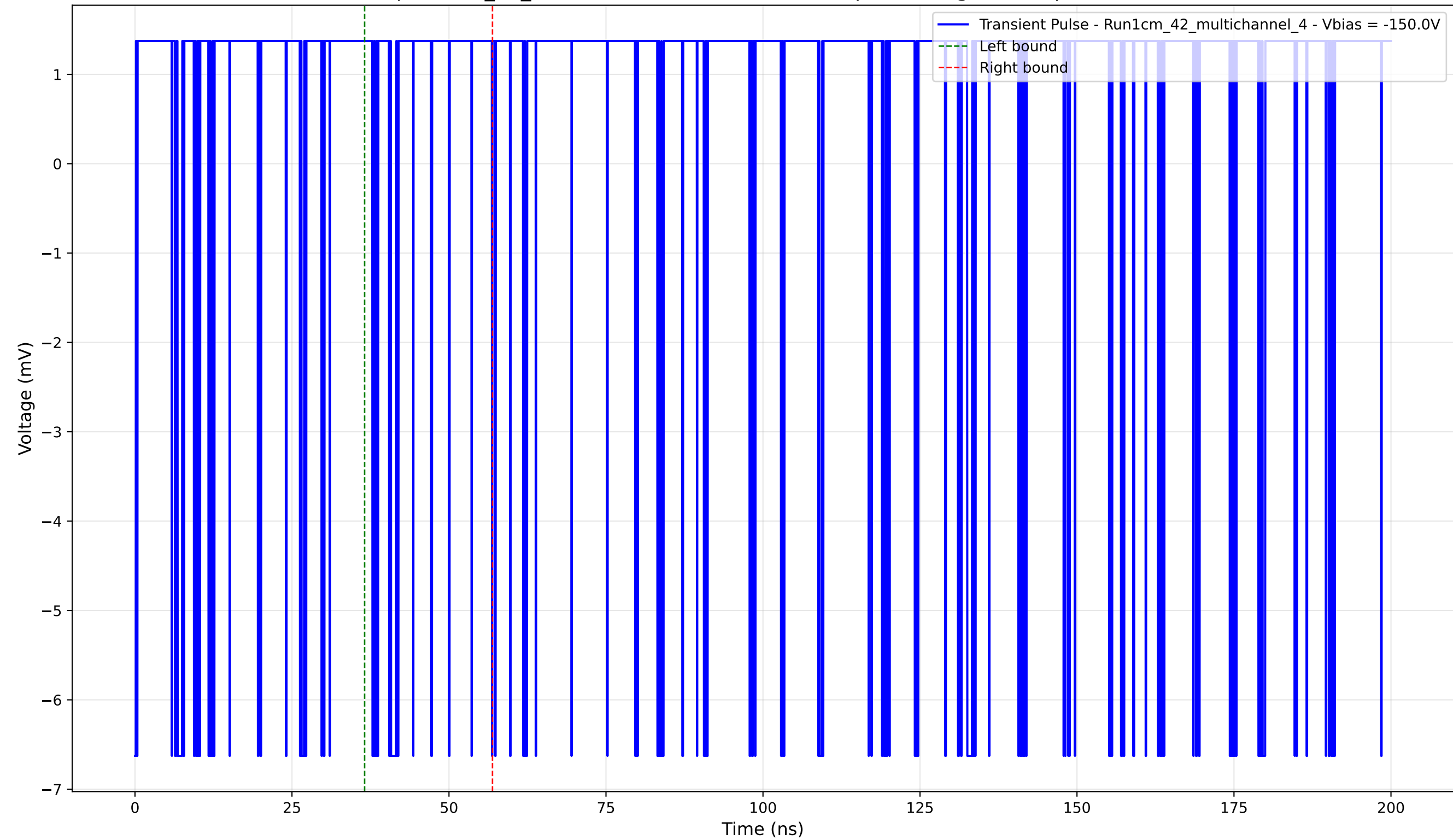
Transient Pulse - Sample: 1cm_42_multichannel - Position: 3910.0 \mu\text{m} - Charge: -0.20 pC - Rise Time: 0.00 ns (N/A)
