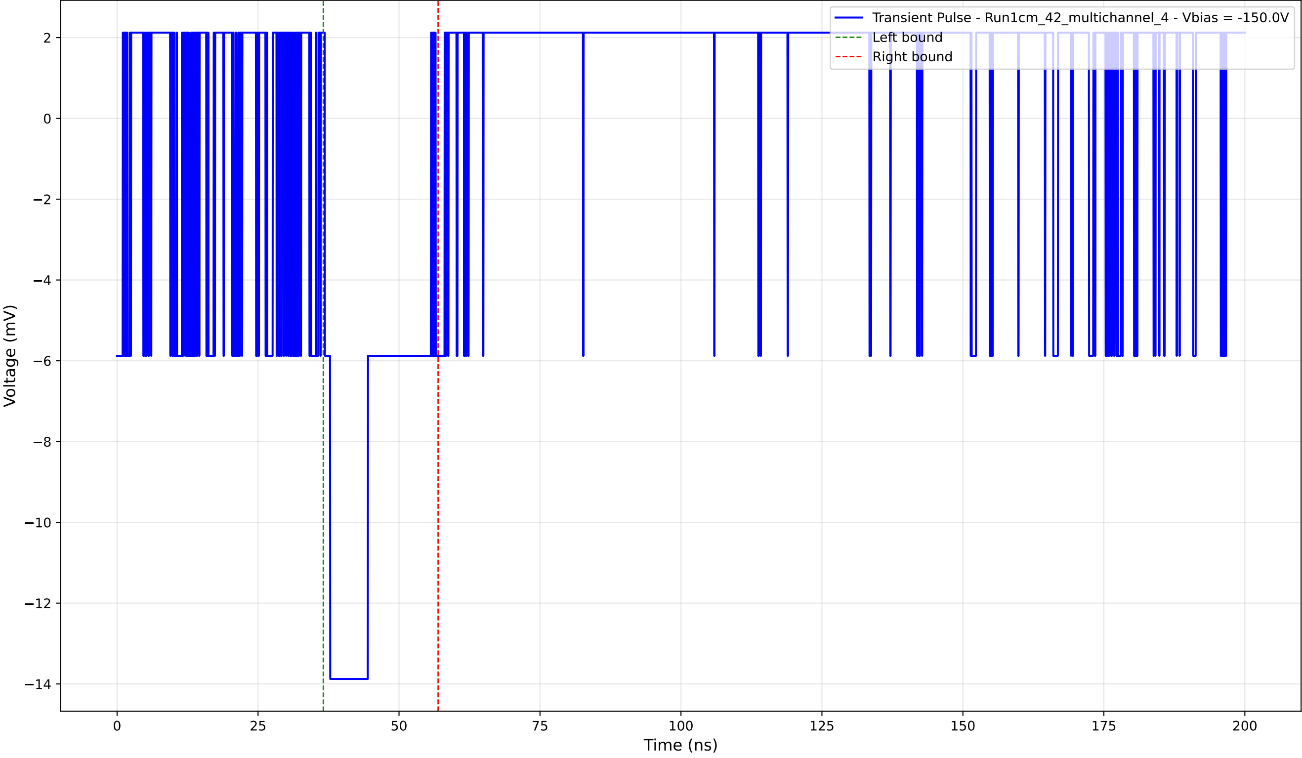
Transient Pulse - Sample: 1cm_42_multichannel - Position: 770.0 \mu\text{m} - Charge: 3.36 pC - Rise Time: 0.00 ns (N/A)
