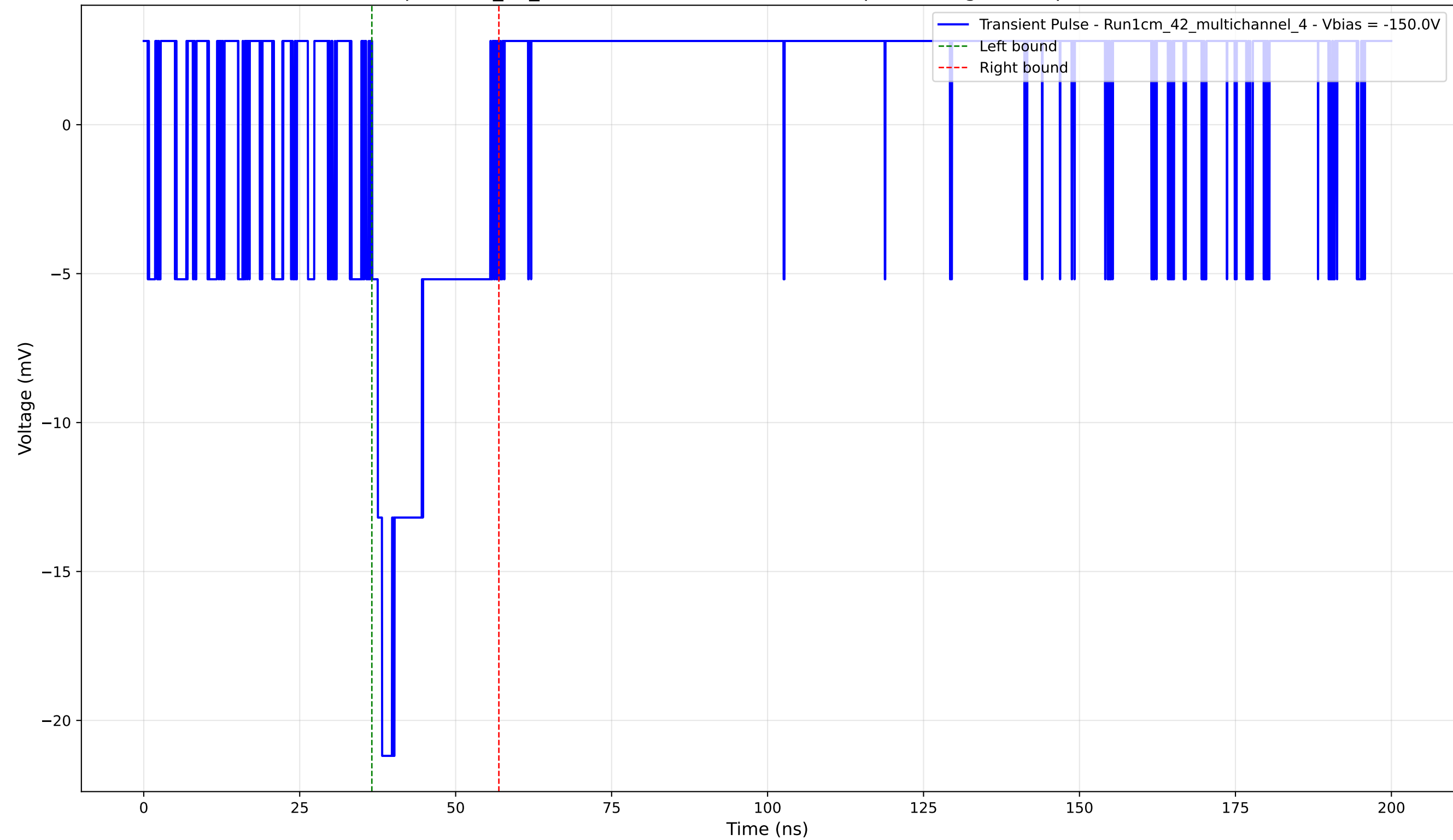
Transient Pulse - Sample: 1cm_42_multichannel - Position: 1020.0 \mu\text{m} - Charge: 3.42 pC - Rise Time: 0.00 ns (N/A)
