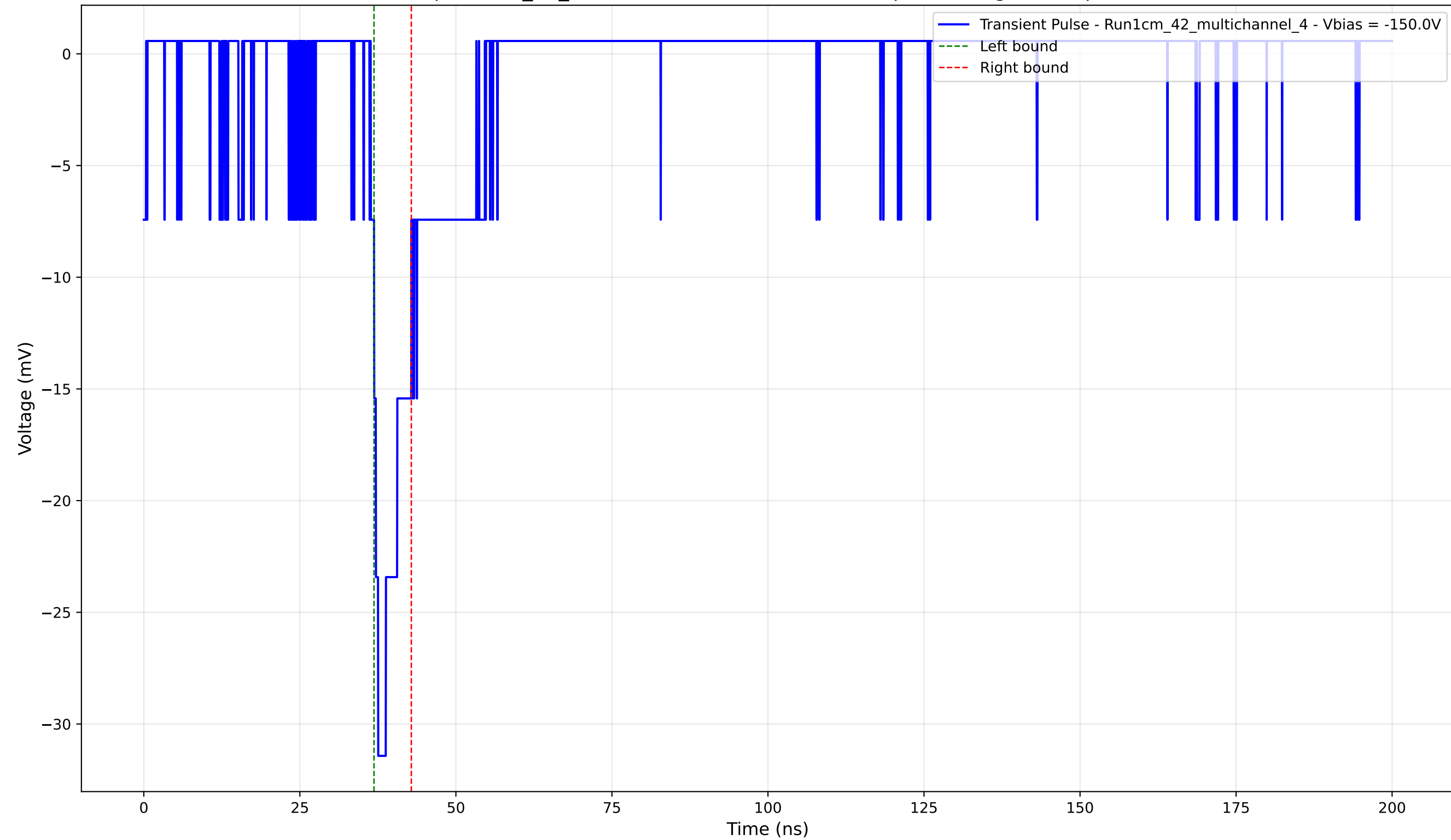
Transient Pulse - Sample: 1cm_42_multichannel - Position: 1515.0 \mu\text{m} - Charge: 2.59 pC - Rise Time: 1.19 ns
