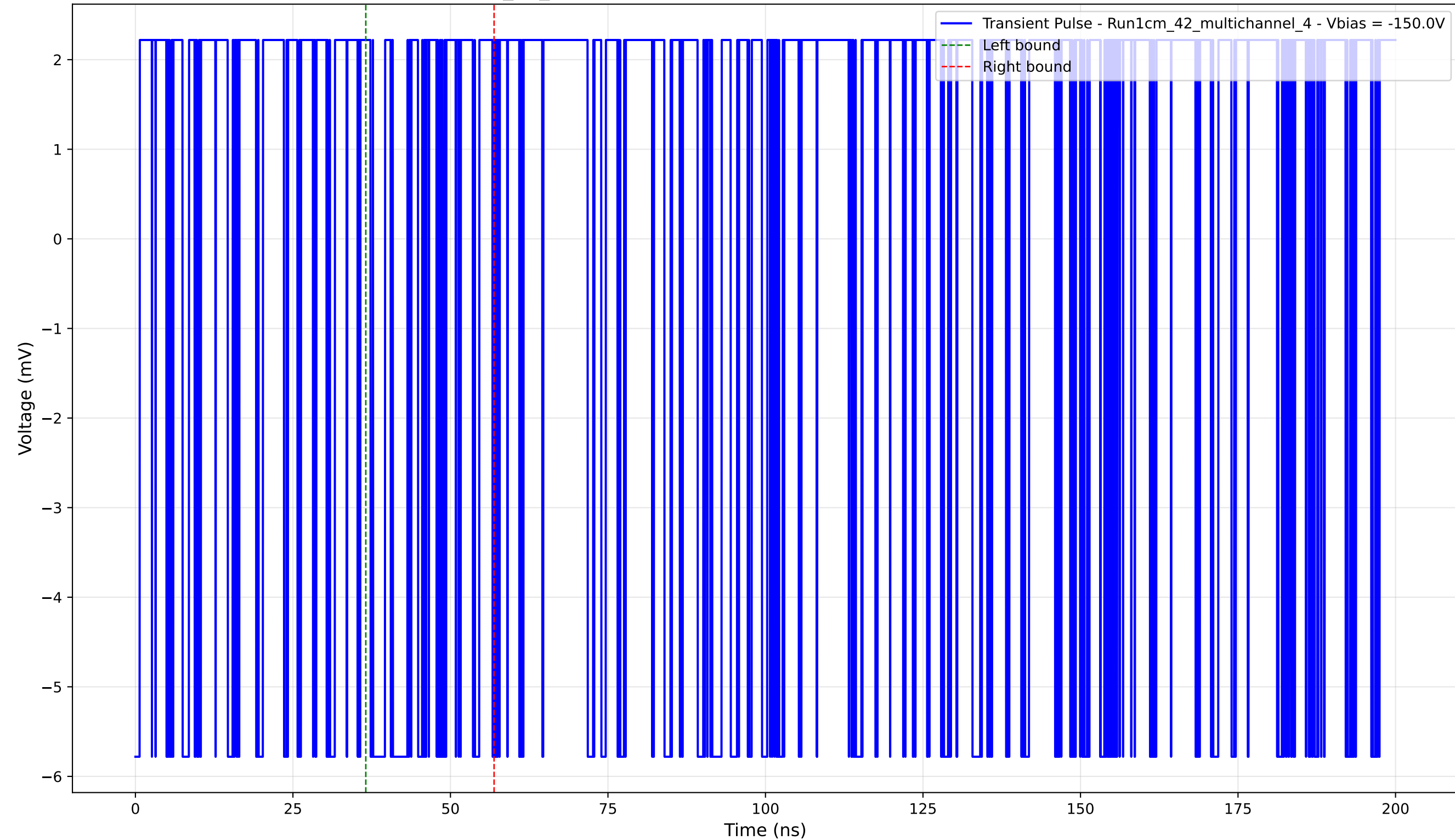
Transient Pulse - Sample: 1cm_42_multichannel - Position: 65.0 \mu\text{m} - Charge: 0.46 pC - Rise Time: 0.00 ns (N/A)
