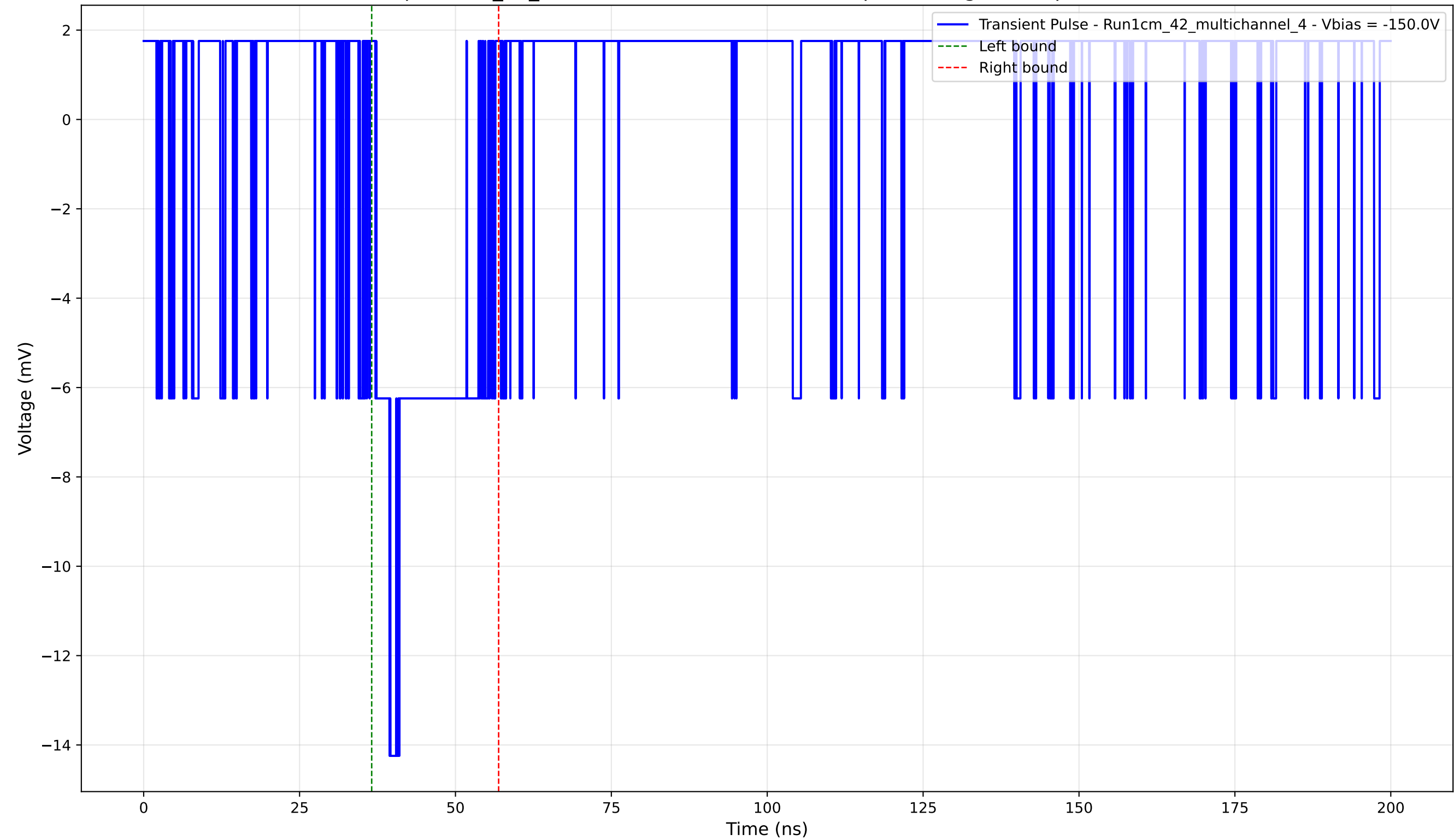
Transient Pulse - Sample: 1cm_42_multichannel - Position: 4345.0 \mu\text{m} - Charge: 2.38 pC - Rise Time: 0.00 ns (N/A)
