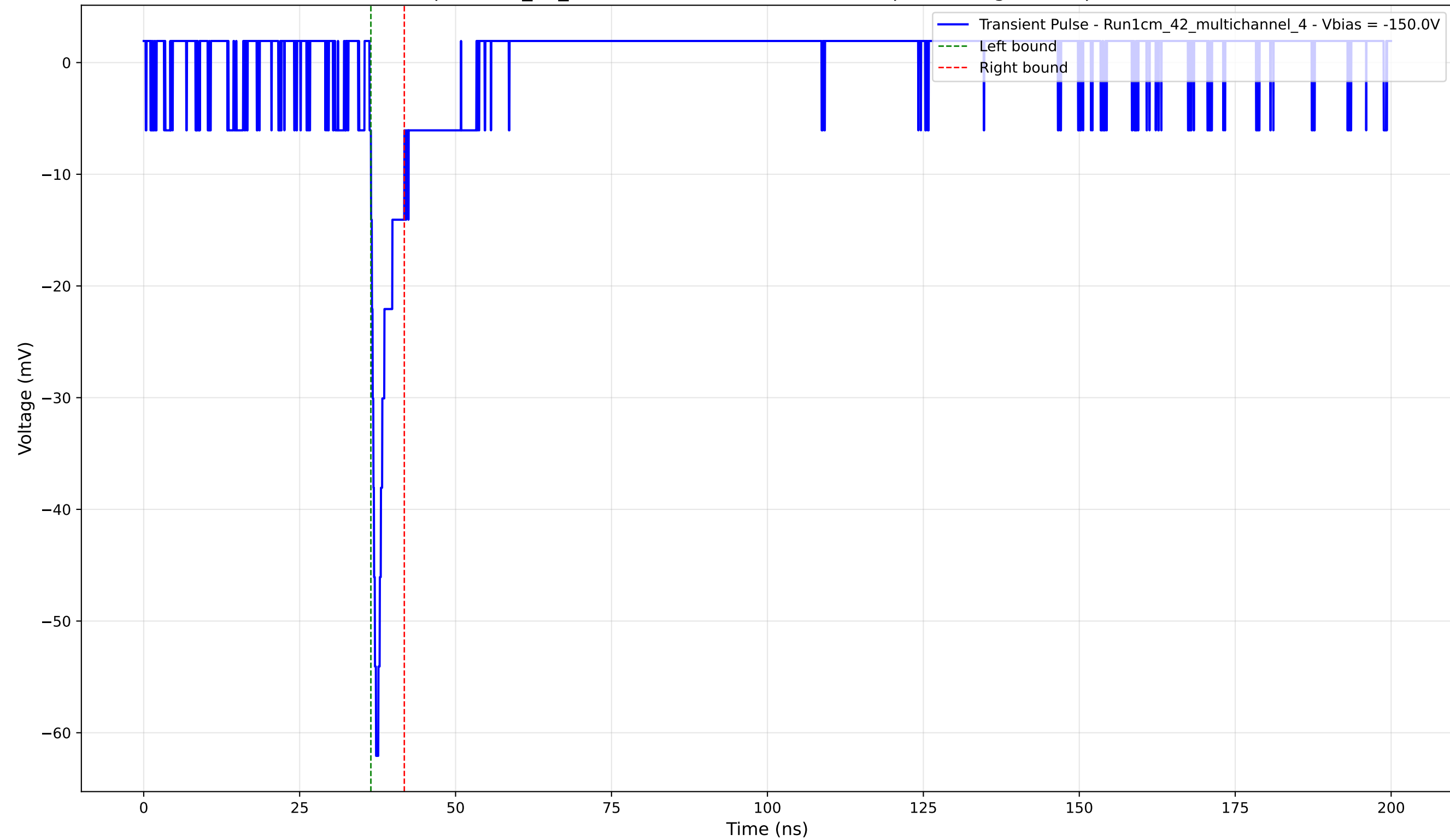
Transient Pulse - Sample: 1cm_42_multichannel - Position: 2080.0 \mu\text{m} - Charge: 2.92 pC - Rise Time: 0.82 ns
