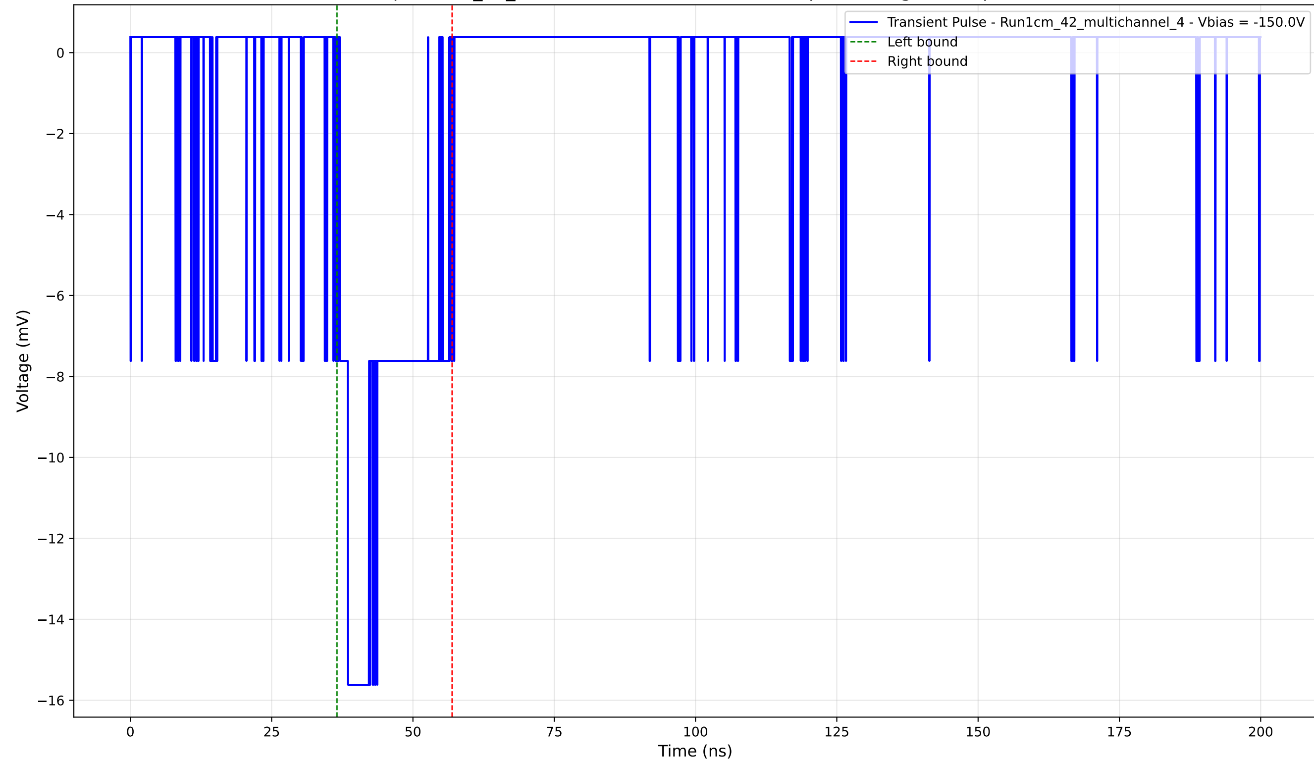
Transient Pulse - Sample: 1cm_42_multichannel - Position: 4590.0 \mu\text{m} - Charge: 3.56 pC - Rise Time: 1.42 ns
