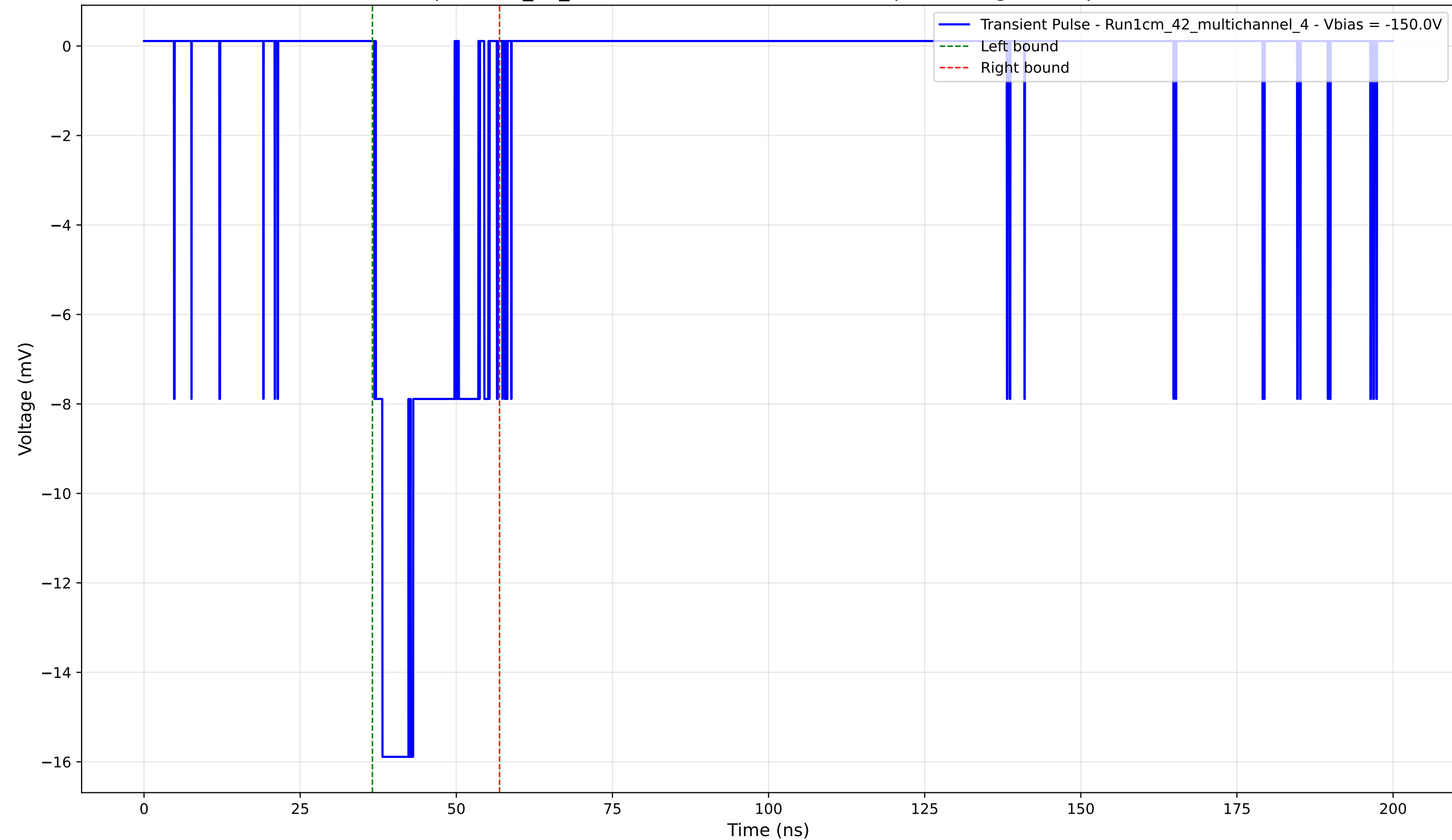
Transient Pulse - Sample: 1cm_42_multichannel - Position: 4060.0 \mu\text{m} - Charge: 3.47 pC - Rise Time: 1.06 ns
