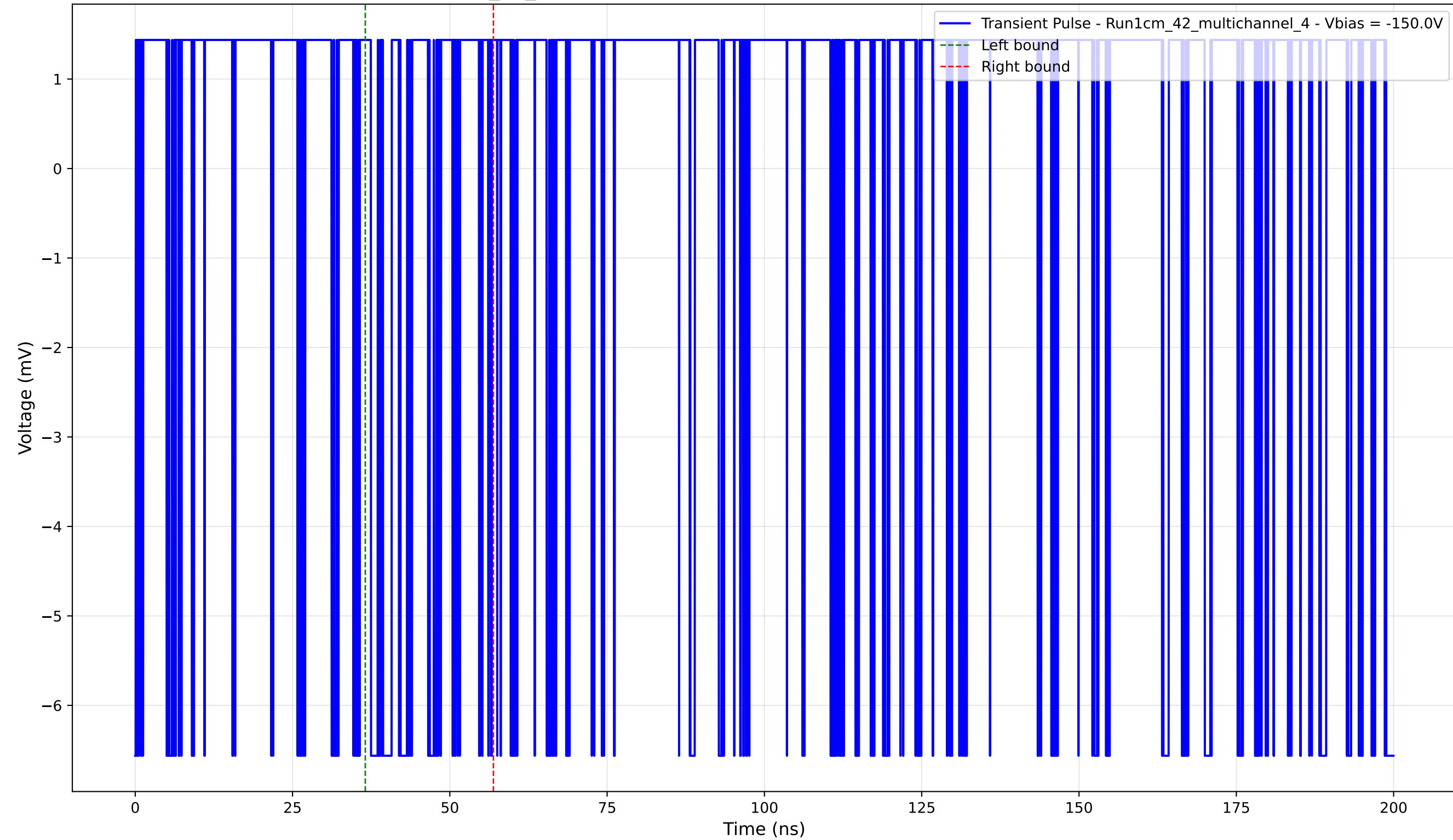
Transient Pulse - Sample: 1cm_42_multichannel - Position: 3385.0 \mu\text{m} - Charge: 0.51 pC - Rise Time: 0.00 ns (N/A)
