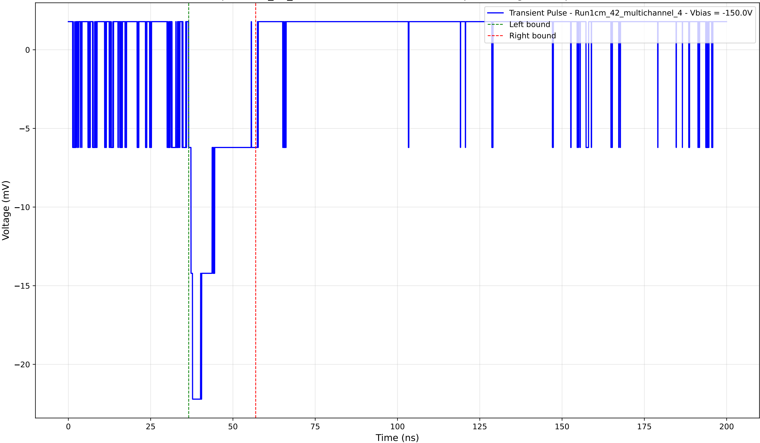
Transient Pulse - Sample: 1cm_42_multichannel - Position: 1220.0 \mu\text{m} - Charge: 4.03 pC - Rise Time: 1.20 ns
