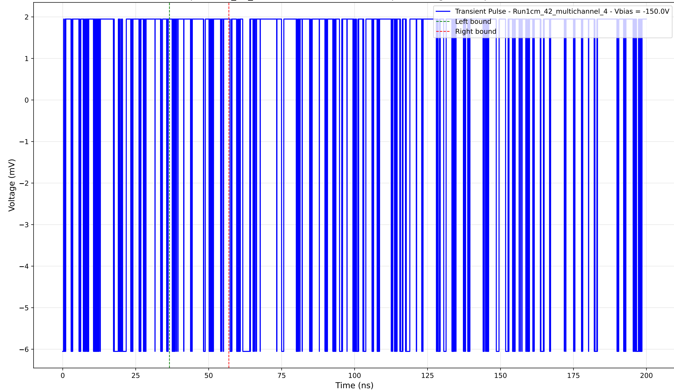
Transient Pulse - Sample: 1cm_42_multichannel - Position: 40.0 \mu\text{m} - Charge: -0.34 pC - Rise Time: 0.00 ns (N/A)
