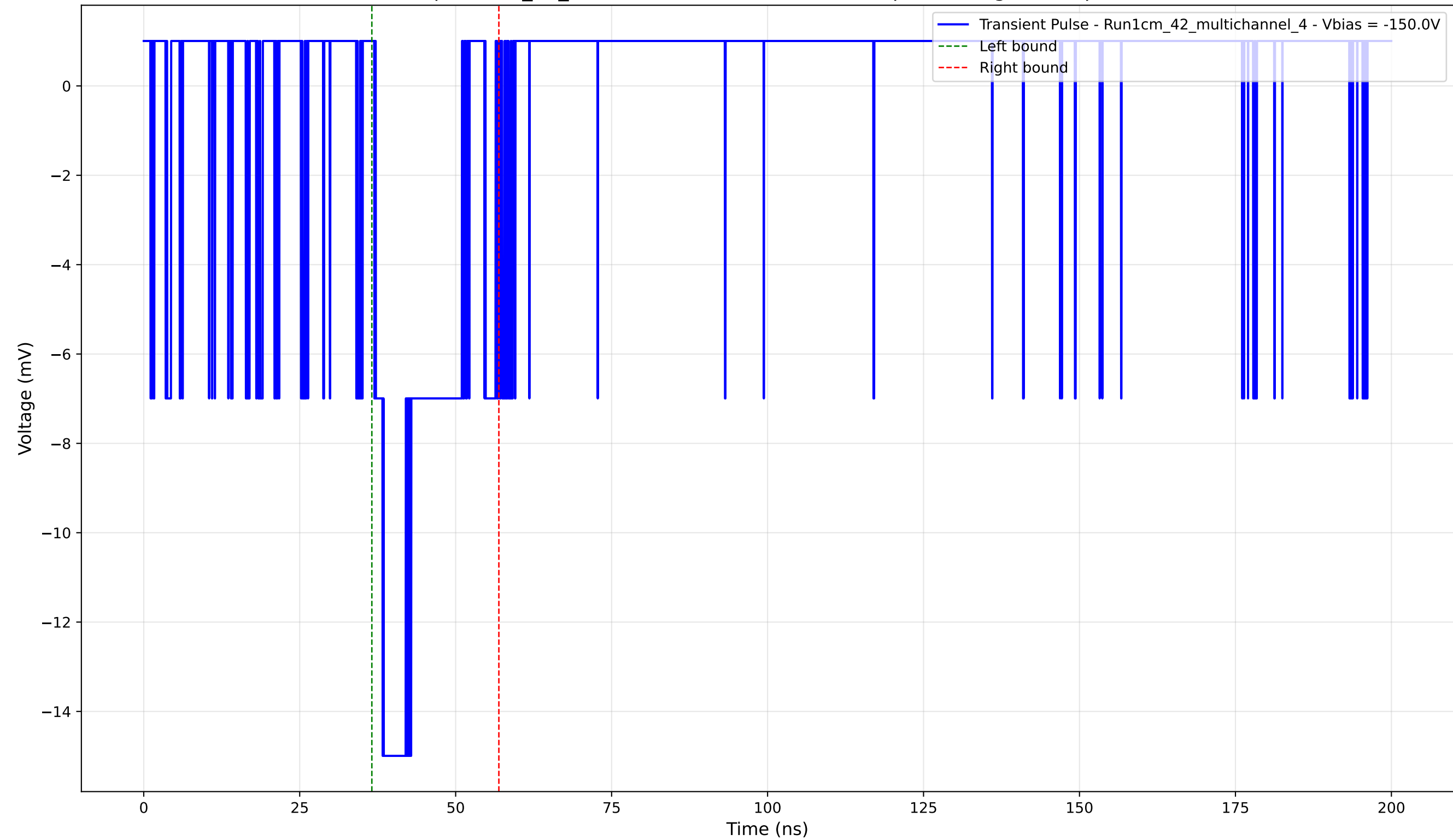
Transient Pulse - Sample: 1cm_42_multichannel - Position: 4635.0 \mu\text{m} - Charge: 2.84 pC - Rise Time: 1.10 ns
