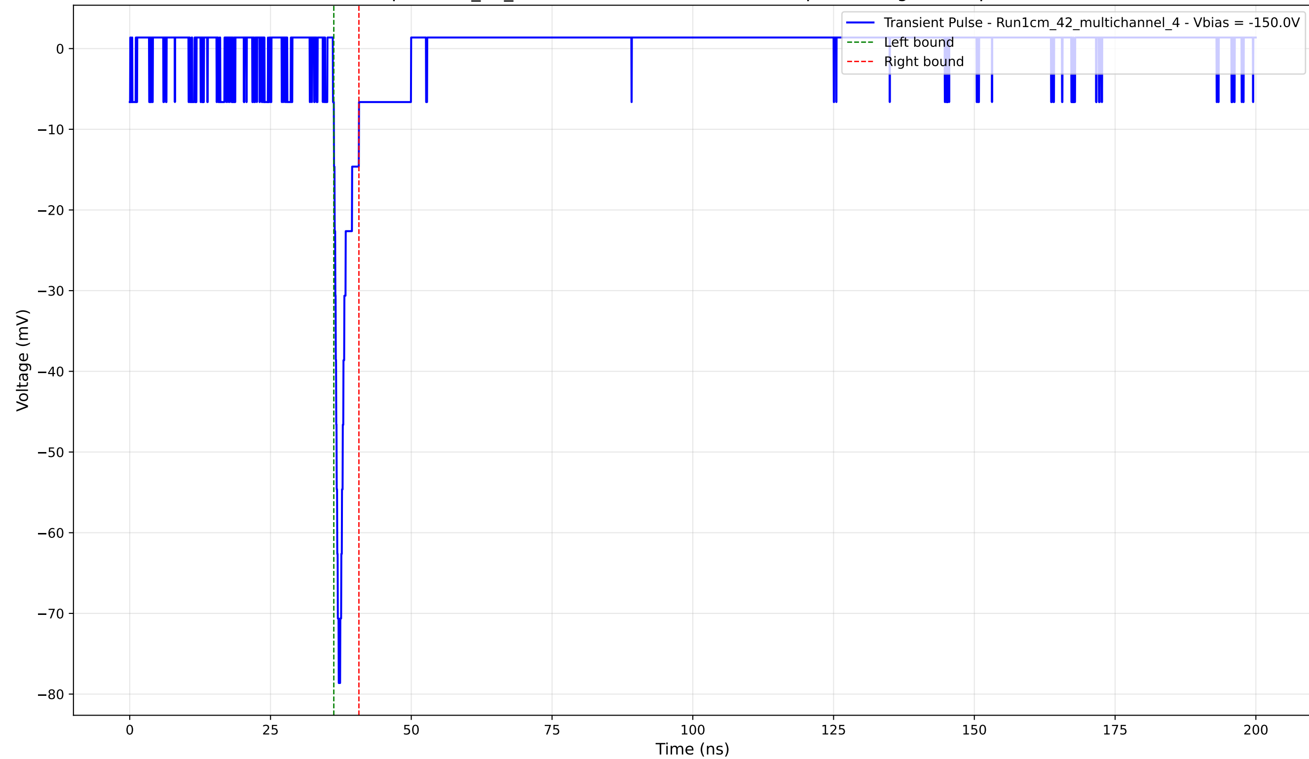
Transient Pulse - Sample: 1cm_42_multichannel - Position: 2310.0 \mu\text{m} - Charge: 2.99 pC - Rise Time: 0.86 ns
