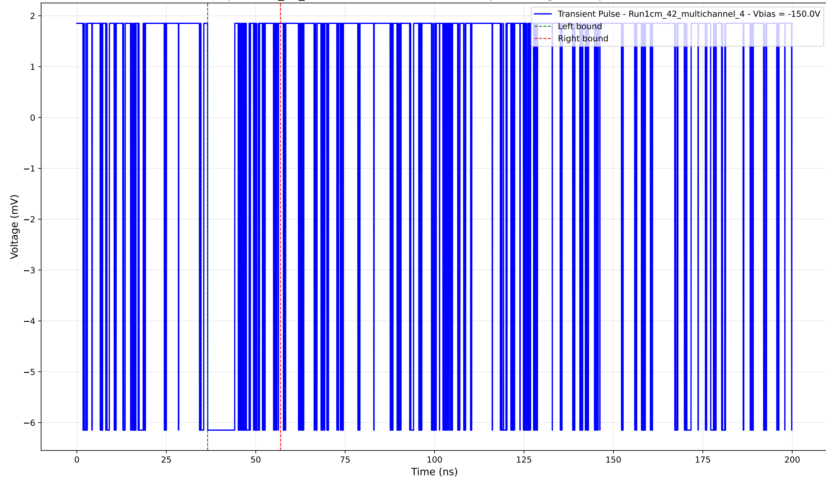
Transient Pulse - Sample: 1cm_42_multichannel - Position: 1850.0 \mu\text{m} - Charge: 1.16 pC - Rise Time: 0.00 ns (N/A)
