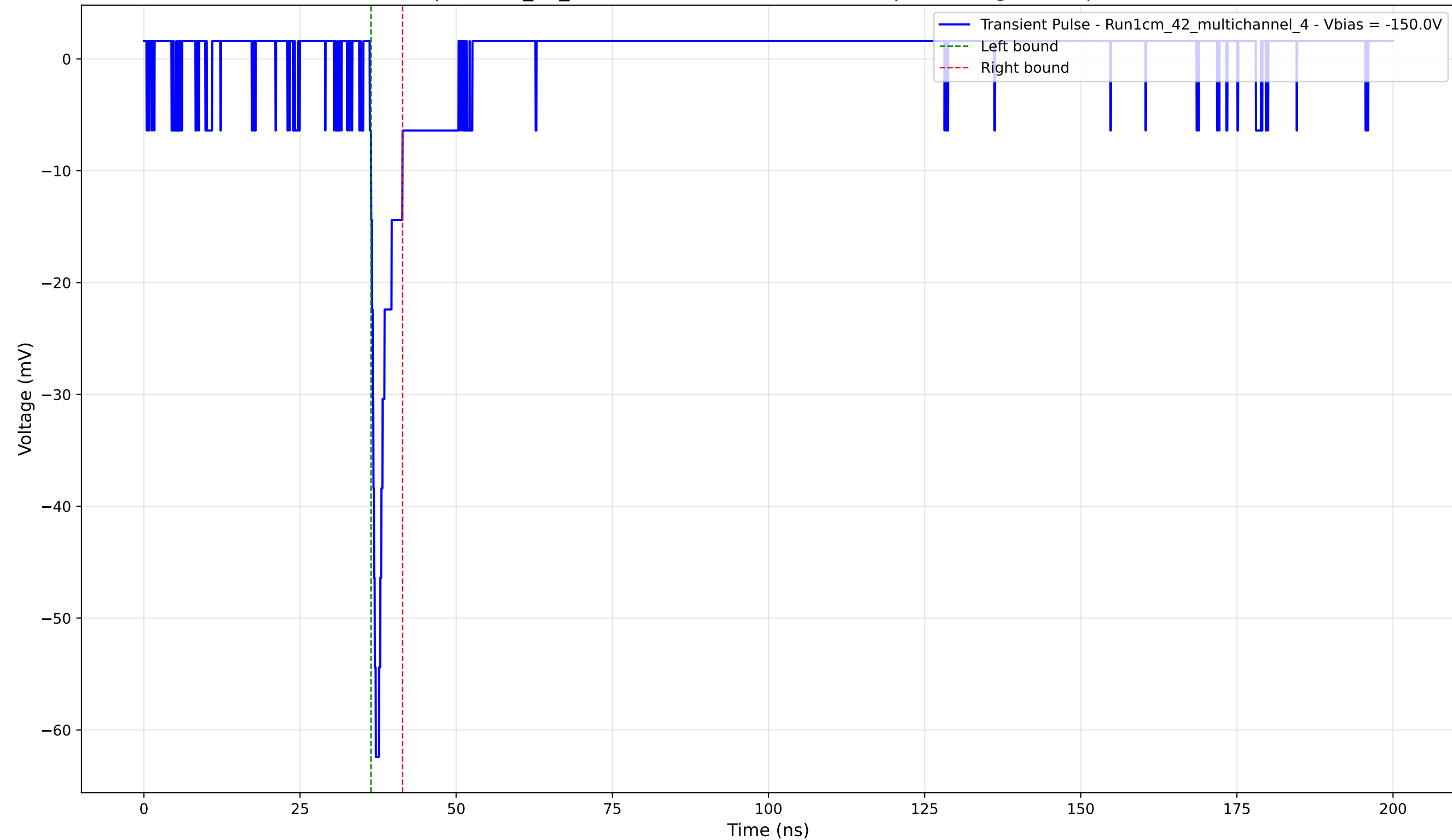
Transient Pulse - Sample: 1cm_42_multichannel - Position: 2145.0 \mu\text{m} - Charge: 2.90 pC - Rise Time: 0.96 ns
