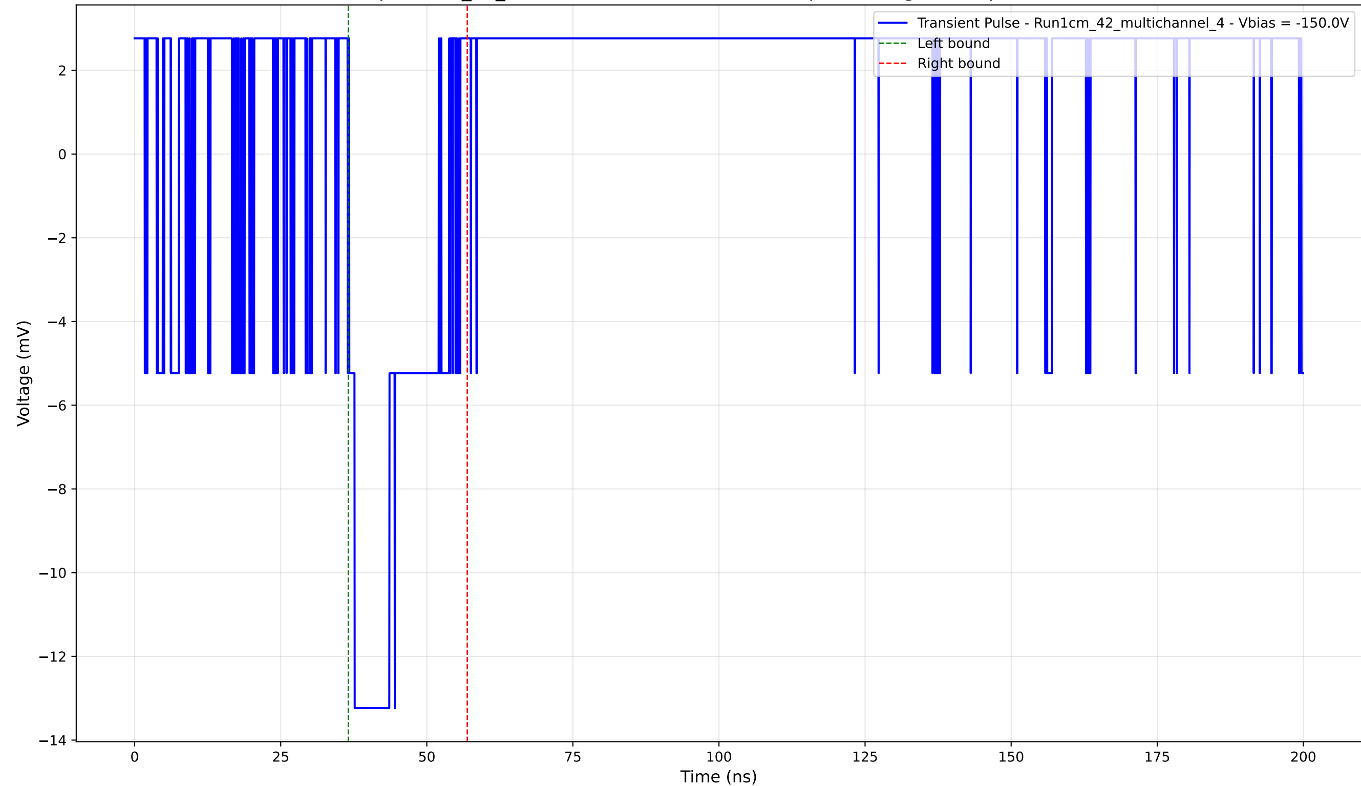
Transient Pulse - Sample: 1cm_42_multichannel - Position: 3780.0 \mu\text{m} - Charge: 2.67 pC - Rise Time: 0.00 ns (N/A)
