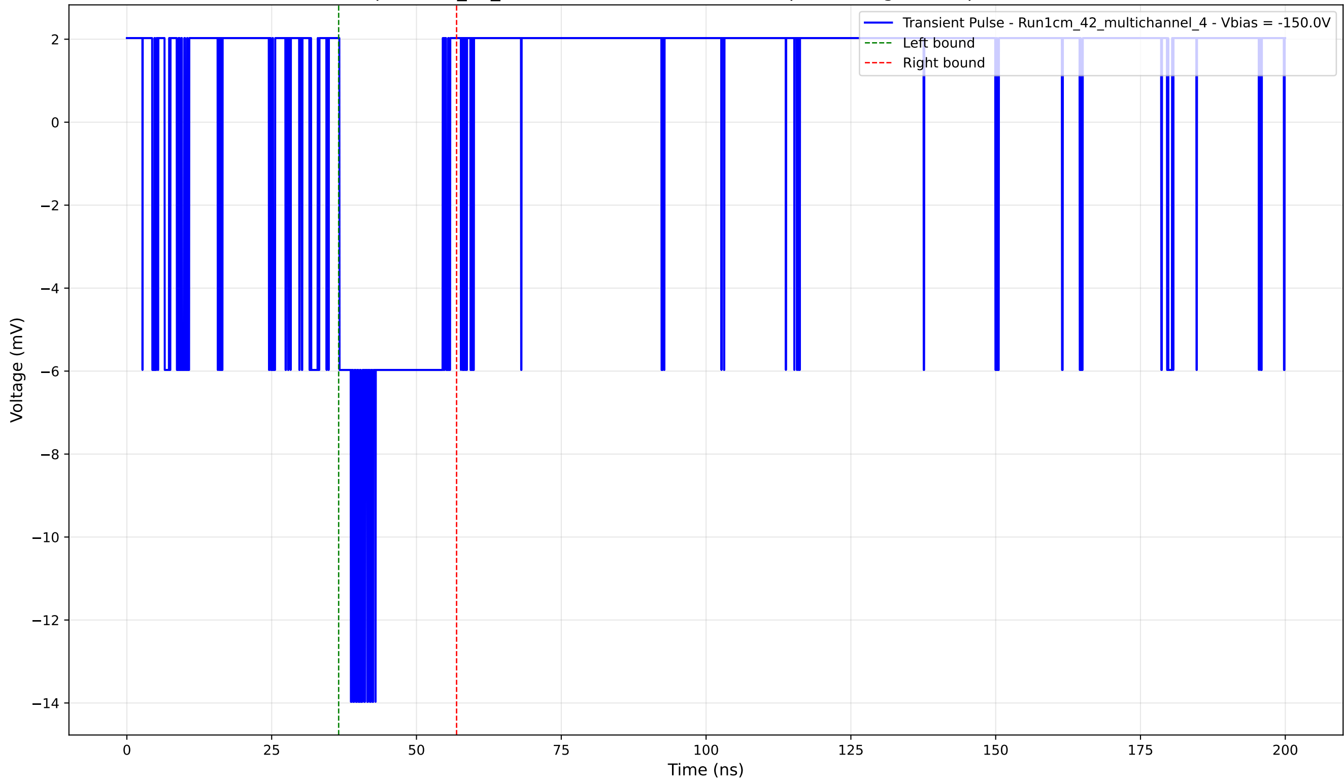
Transient Pulse - Sample: 1cm_42_multichannel - Position: 120.0 \mu\text{m} - Charge: 2.42 pC - Rise Time: 0.00 ns (N/A)
