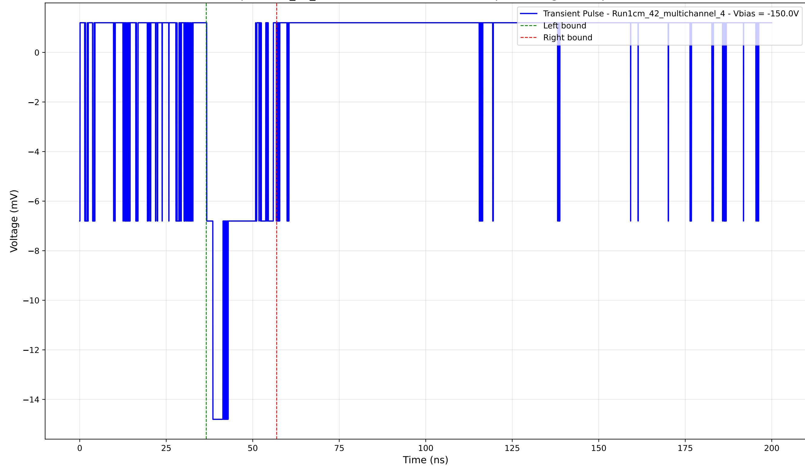
Transient Pulse - Sample: 1cm_42_multichannel - Position: 4735.0 \mu\text{m} - Charge: 2.90 pC - Rise Time: 1.80 ns
