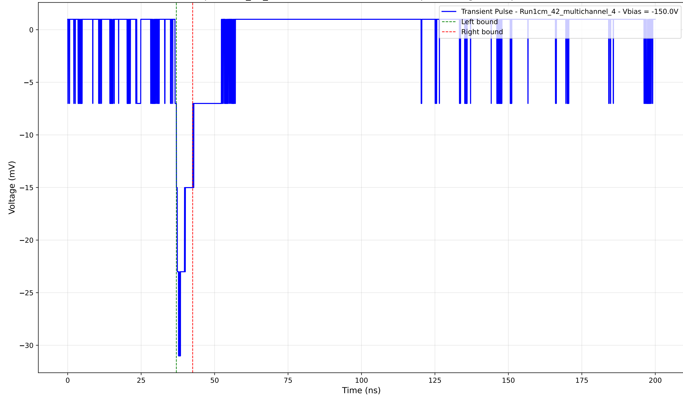
Transient Pulse - Sample: 1cm_42_multichannel - Position: 3295.0 \mu\text{m} - Charge: 2.15 pC - Rise Time: 1.21 ns
