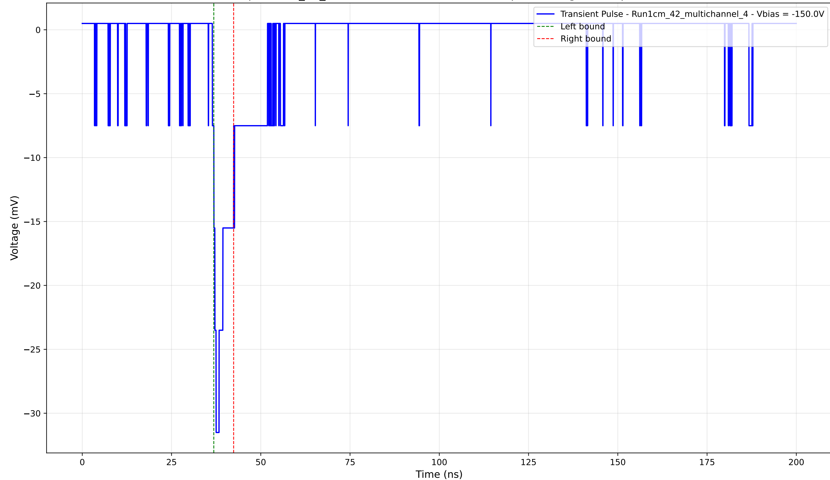
Transient Pulse - Sample: 1cm_42_multichannel - Position: 3155.0 \mu\text{m} - Charge: 2.21 pC - Rise Time: 1.05 ns
