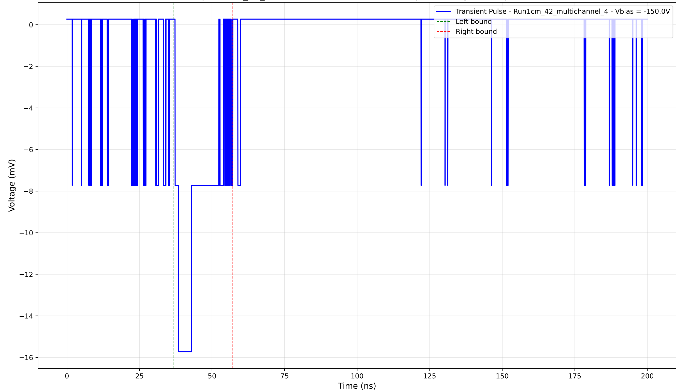
Transient Pulse - Sample: 1cm_42_multichannel - Position: 4280.0 \mu\text{m} - Charge: 3.44 pC - Rise Time: 1.24 ns
