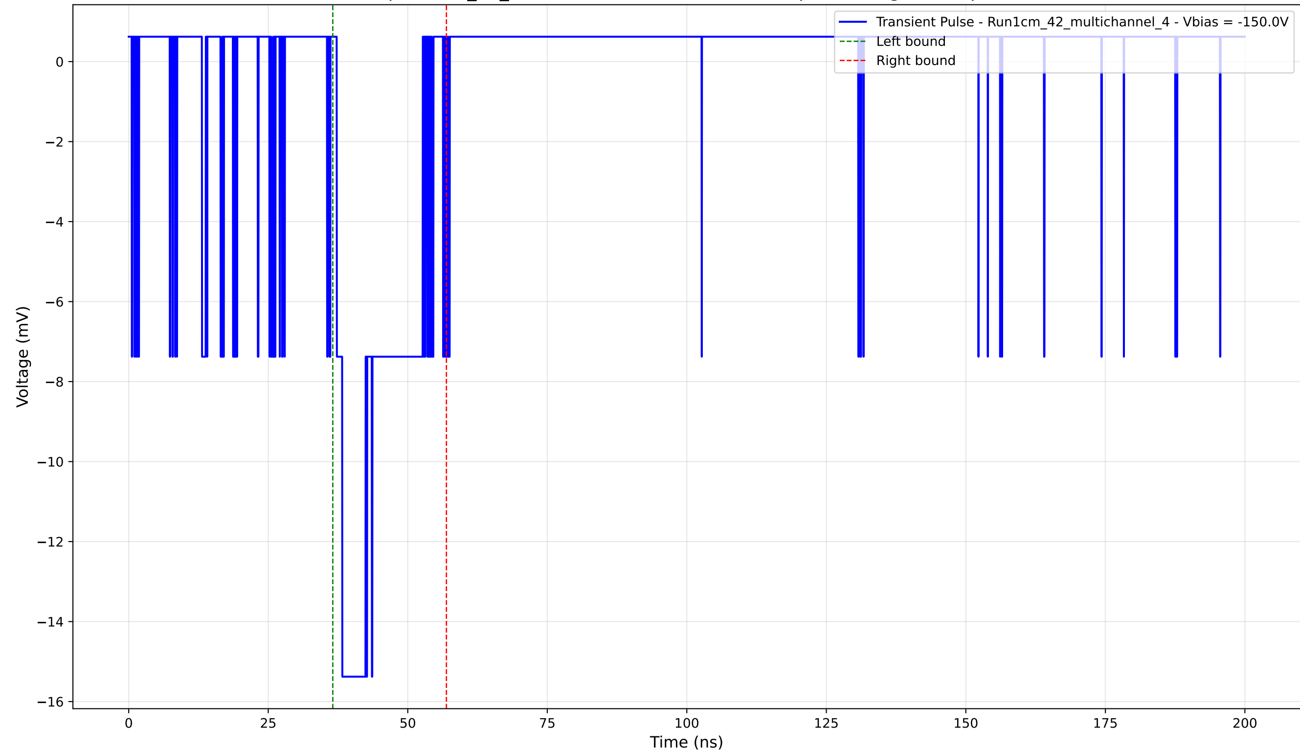
Transient Pulse - Sample: 1cm_42_multichannel - Position: 4165.0 \mu\text{m} - Charge: 3.13 pC - Rise Time: 1.00 ns
