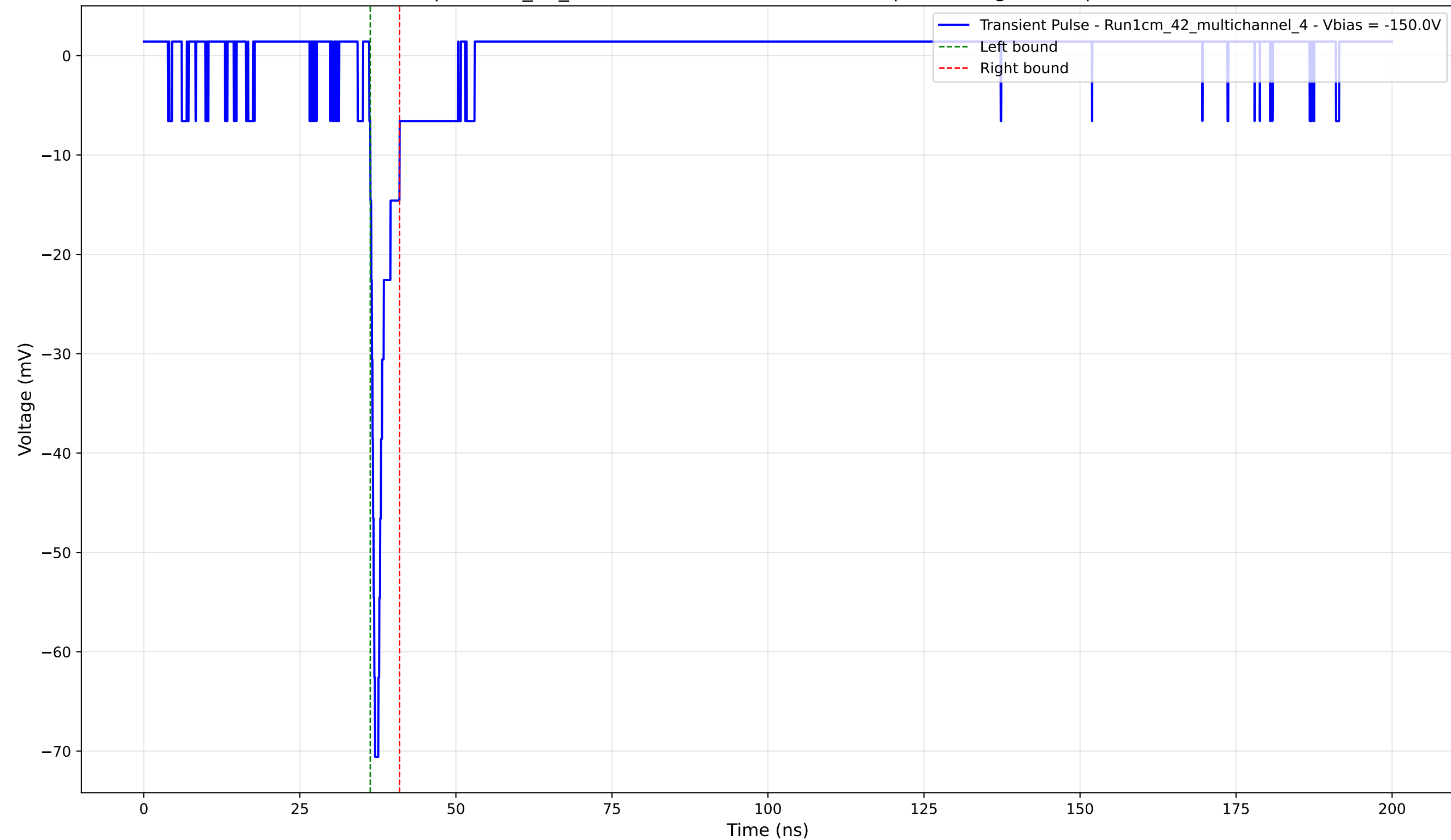
Transient Pulse - Sample: 1cm_42_multichannel - Position: 2545.0 \mu\text{m} - Charge: 3.00 pC - Rise Time: 0.76 ns
