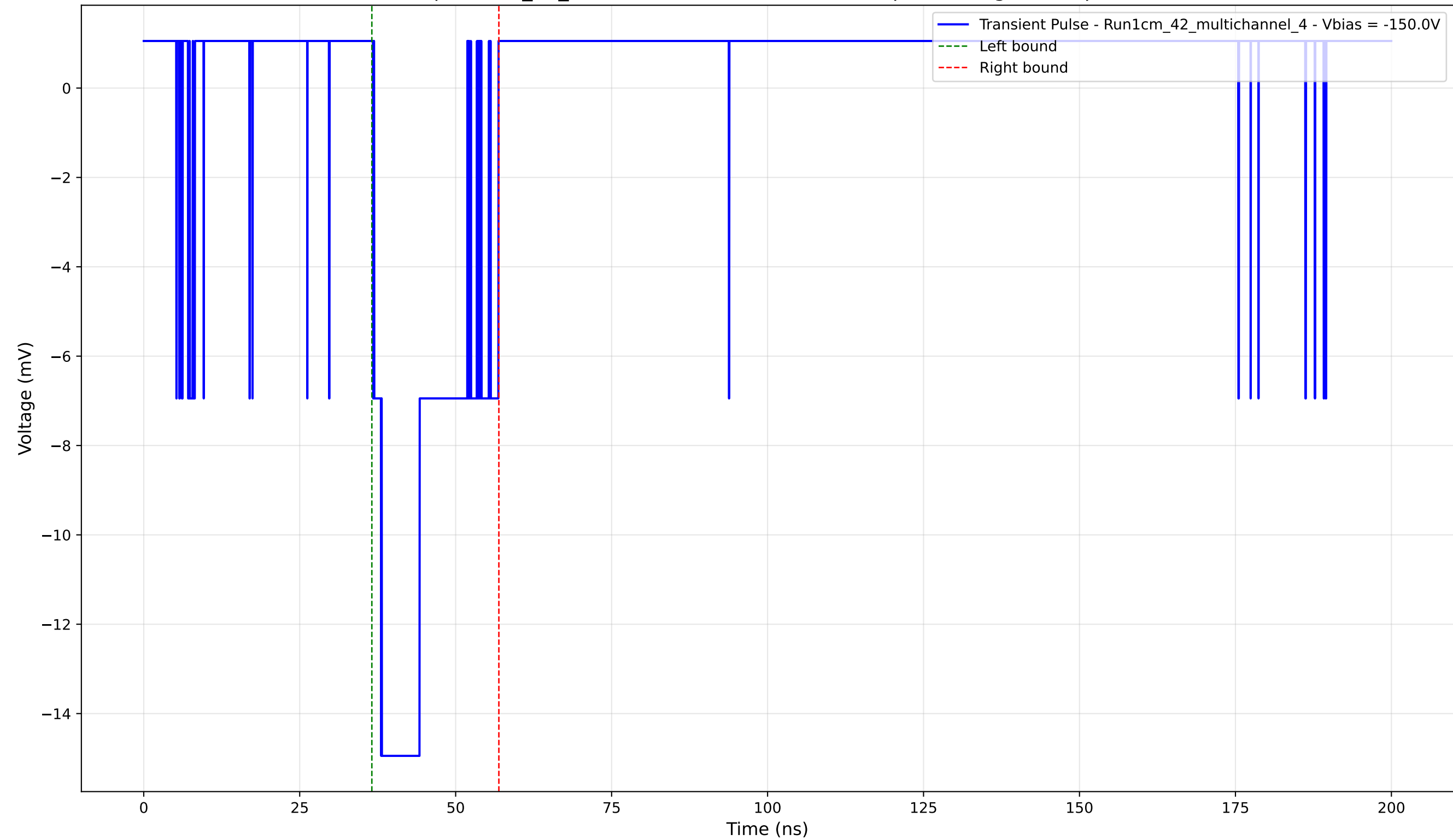
Transient Pulse - Sample: 1cm_42_multichannel - Position: 4030.0 \mu\text{m} - Charge: 3.64 pC - Rise Time: 1.12 ns
