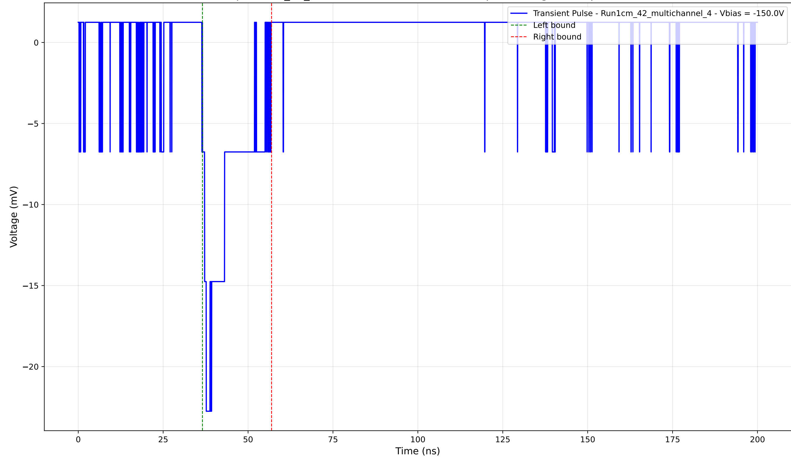
Transient Pulse - Sample: 1cm_42_multichannel - Position: 3500.0 \mu\text{m} - Charge: 3.66 pC - Rise Time: 1.12 ns
