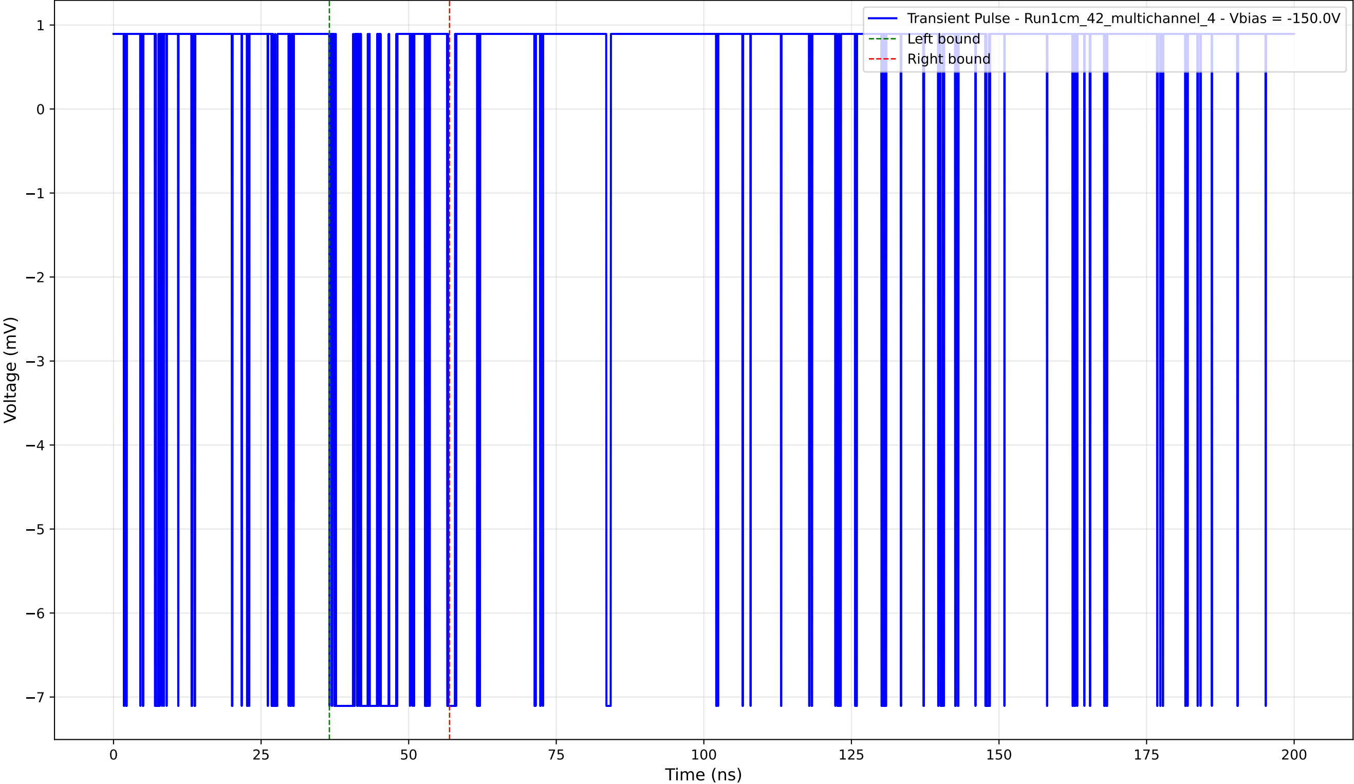
Transient Pulse - Sample: 1cm_42_multichannel - Position: 3870.0 \mu\text{m} - Charge: 1.28 pC - Rise Time: 0.00 ns (N/A)
