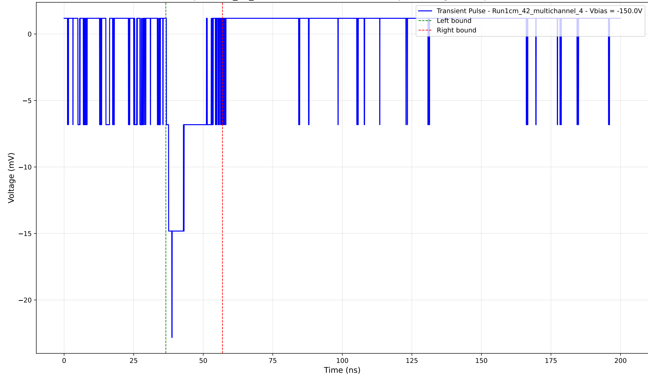
Transient Pulse - Sample: 1cm_42_multichannel - Position: 3695.0 \mu\text{m} - Charge: 3.23 pC - Rise Time: 1.98 ns
