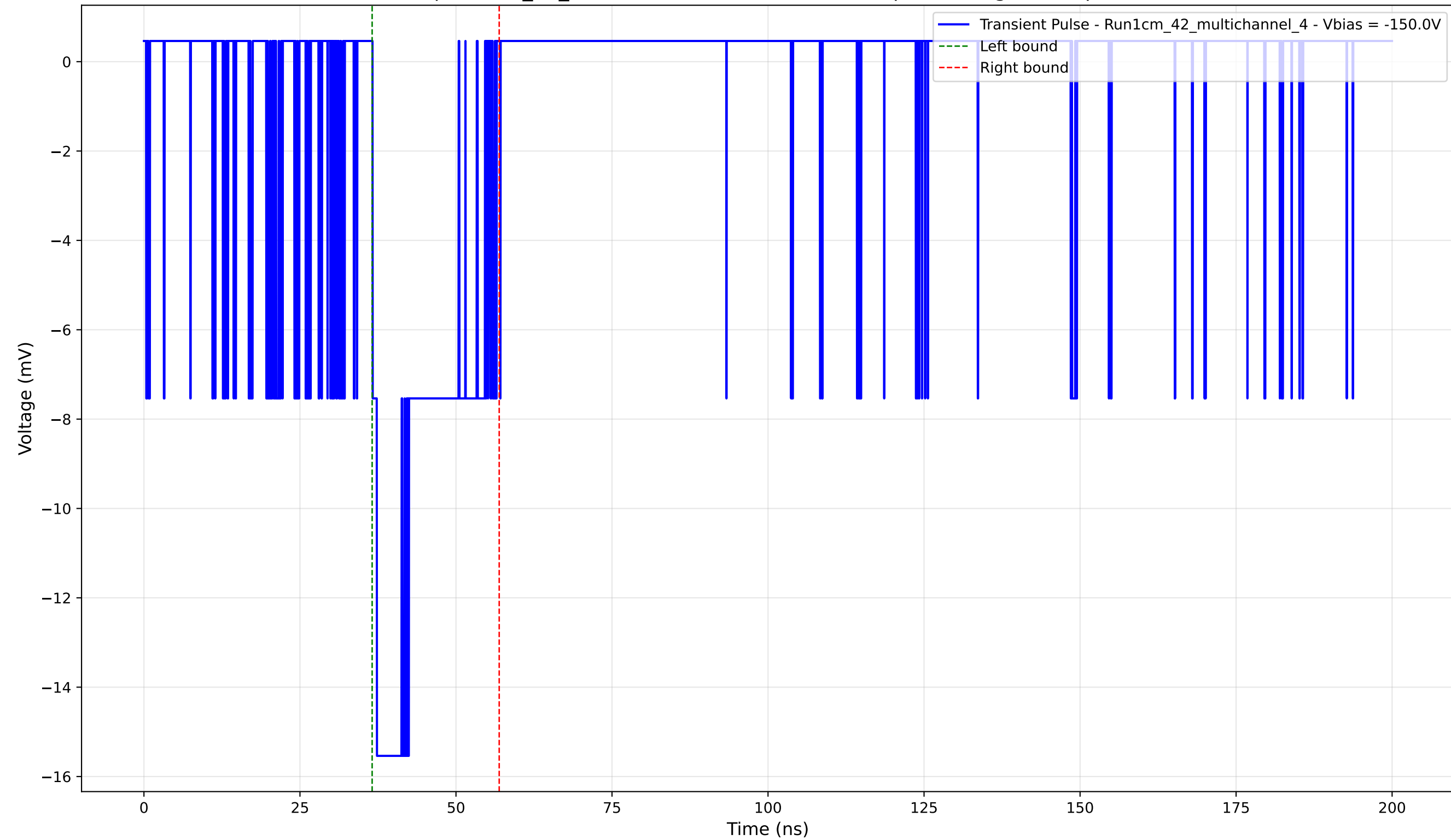
Transient Pulse - Sample: 1cm_42_multichannel - Position: 3460.0 \mu\text{m} - Charge: 3.53 pC - Rise Time: 0.70 ns
