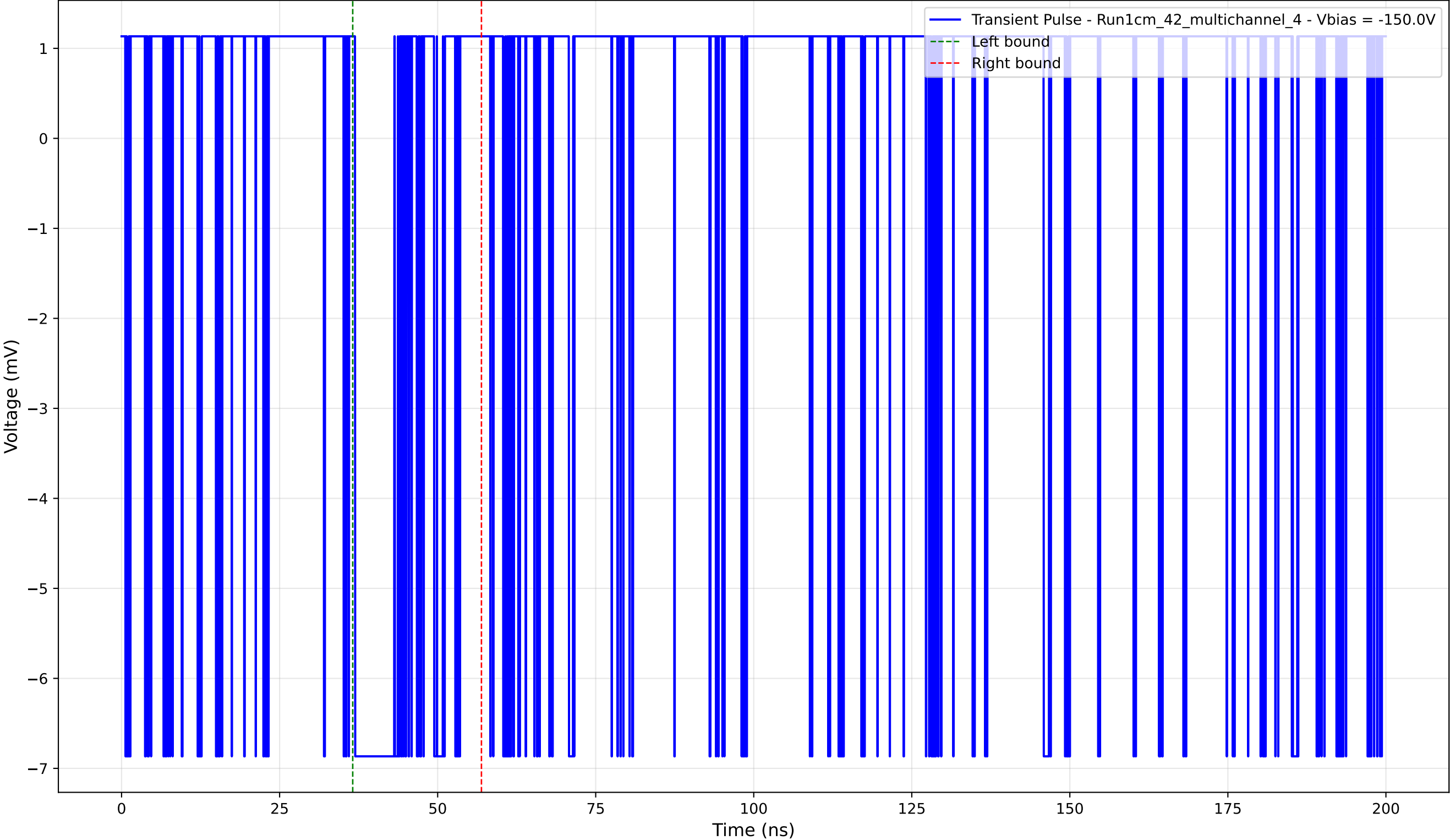
Transient Pulse - Sample: 1cm_42_multichannel - Position: 3430.0 \mu\text{m} - Charge: 1.16 pC - Rise Time: 0.00 ns (N/A)
