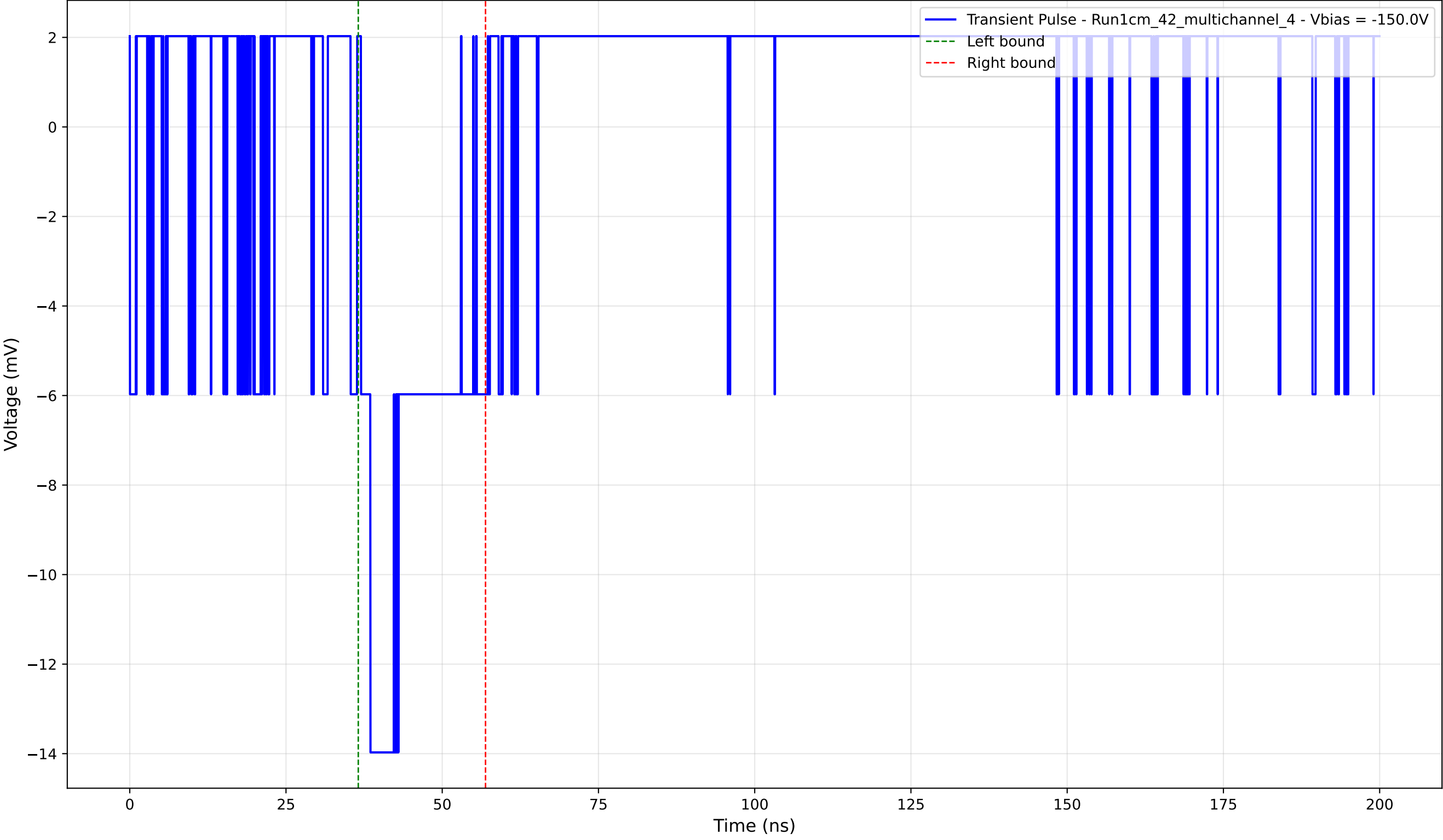
Transient Pulse - Sample: 1cm_42_multichannel - Position: 280.0 \mu\text{m} - Charge: 2.98 pC - Rise Time: 0.00 ns (N/A)
