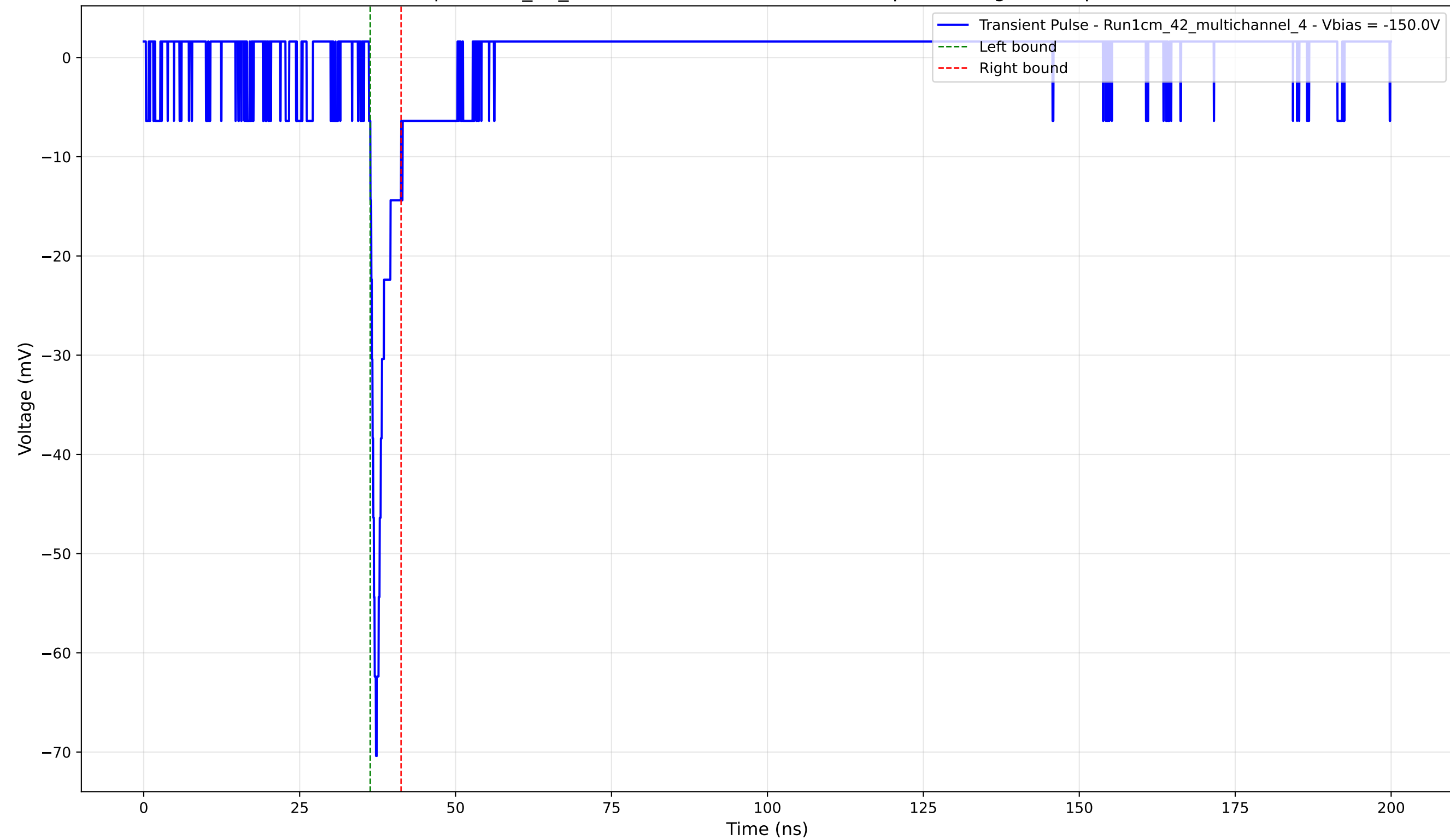
Transient Pulse - Sample: 1cm_42_multichannel - Position: 2575.0 \mu\text{m} - Charge: 2.93 pC - Rise Time: 0.90 ns
