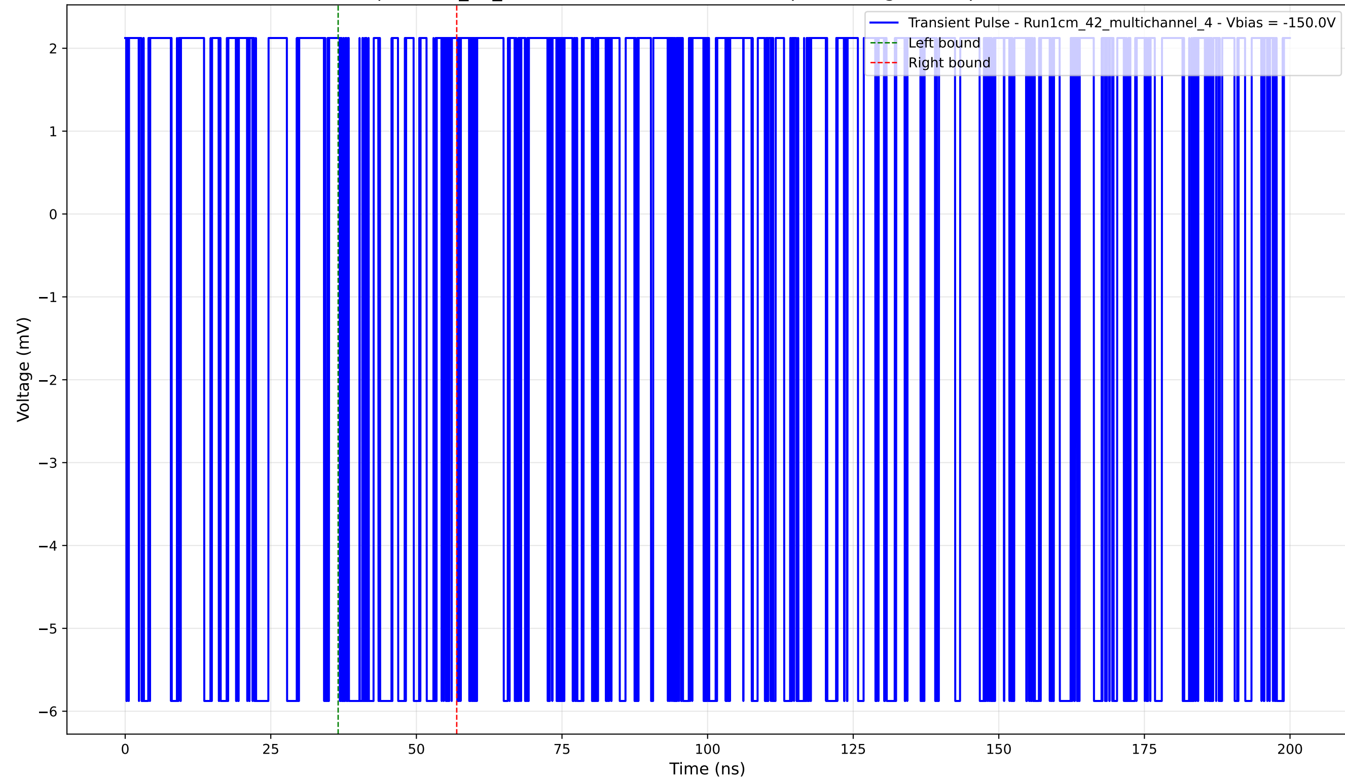
Transient Pulse - Sample: 1cm_42_multichannel - Position: 355.0 \mu\text{m} - Charge: 0.96 pC - Rise Time: 0.00 ns (N/A)
