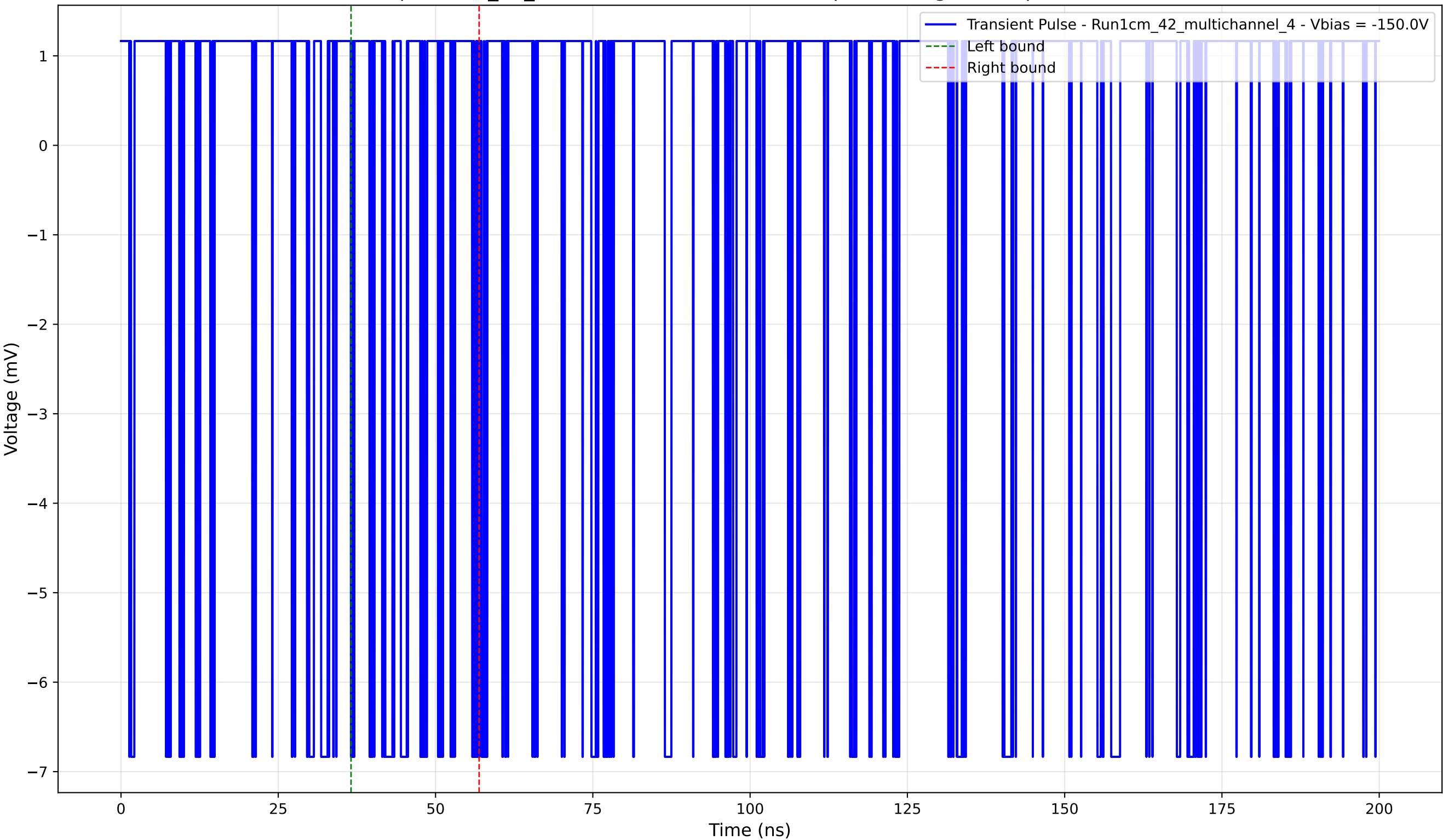
Transient Pulse - Sample: 1cm_42_multichannel - Position: 50.0 \mu\text{m} - Charge: 0.40 pC - Rise Time: 0.00 ns (N/A)
