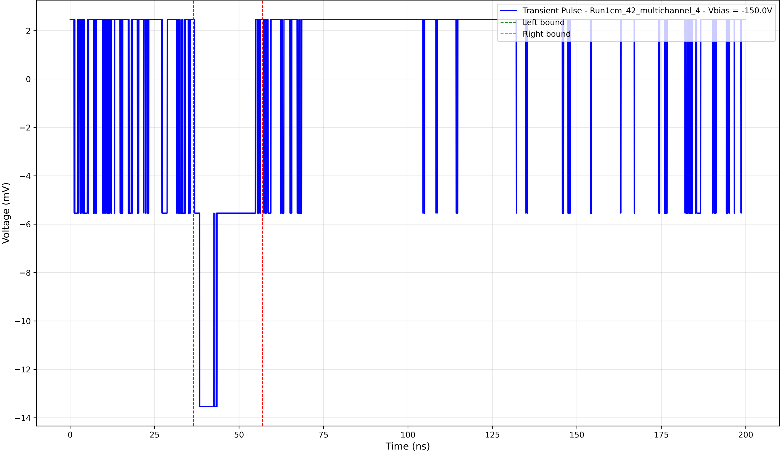
Transient Pulse - Sample: 1cm_42_multichannel - Position: 220.0 \mu\text{m} - Charge: 2.75 pC - Rise Time: 0.00 ns (N/A)
