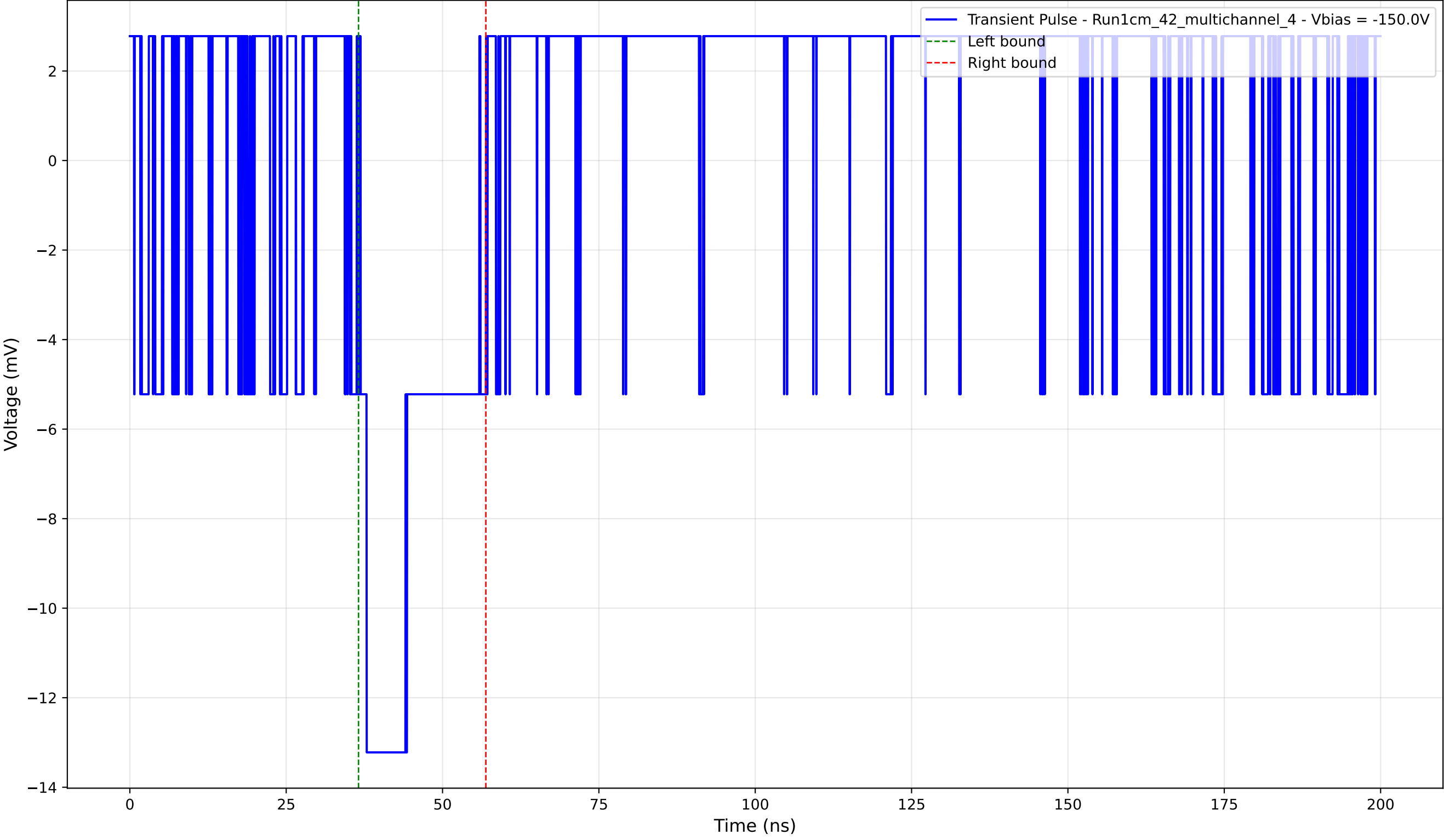
Transient Pulse - Sample: 1cm_42_multichannel - Position: 685.0 \mu\text{m} - Charge: 3.09 pC - Rise Time: 0.00 ns (N/A)
