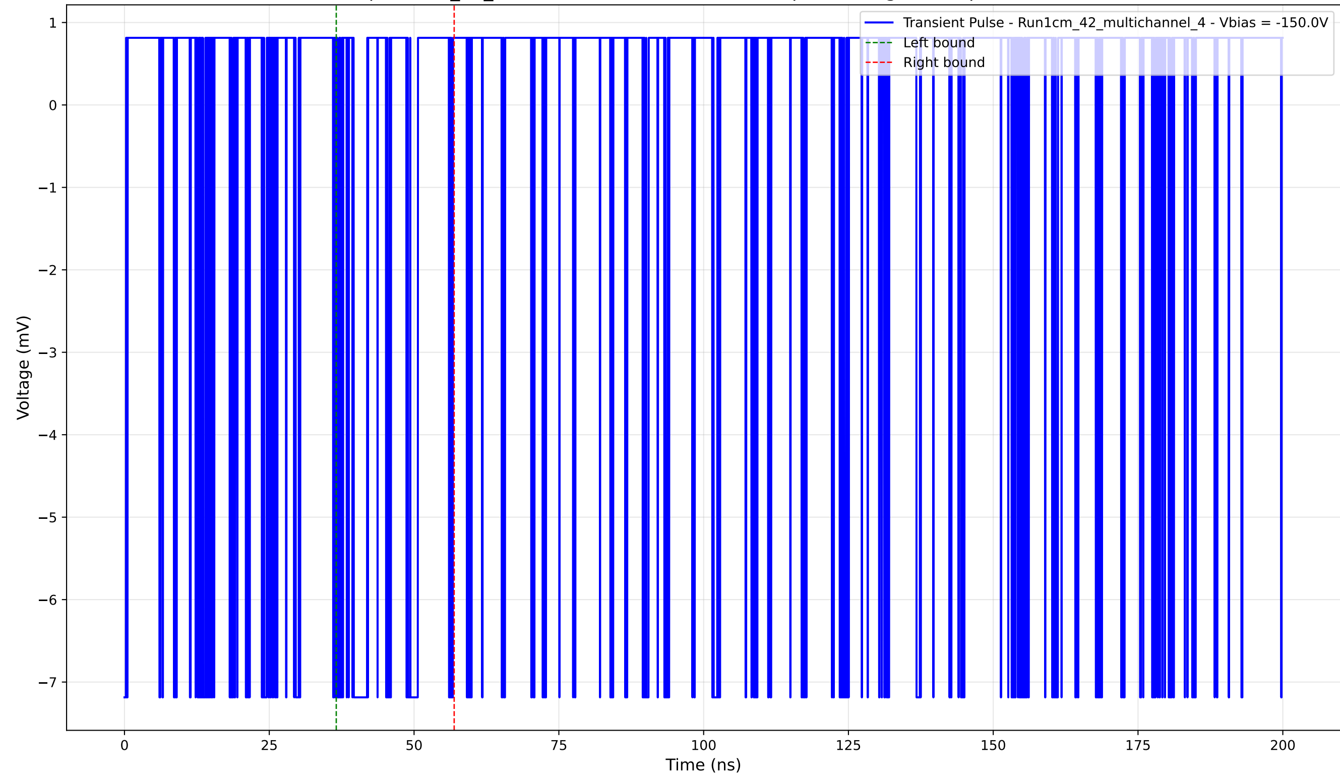
Transient Pulse - Sample: 1cm_42_multichannel - Position: 4405.0 \mu\text{m} - Charge: 0.65 pC - Rise Time: 0.00 ns (N/A)
