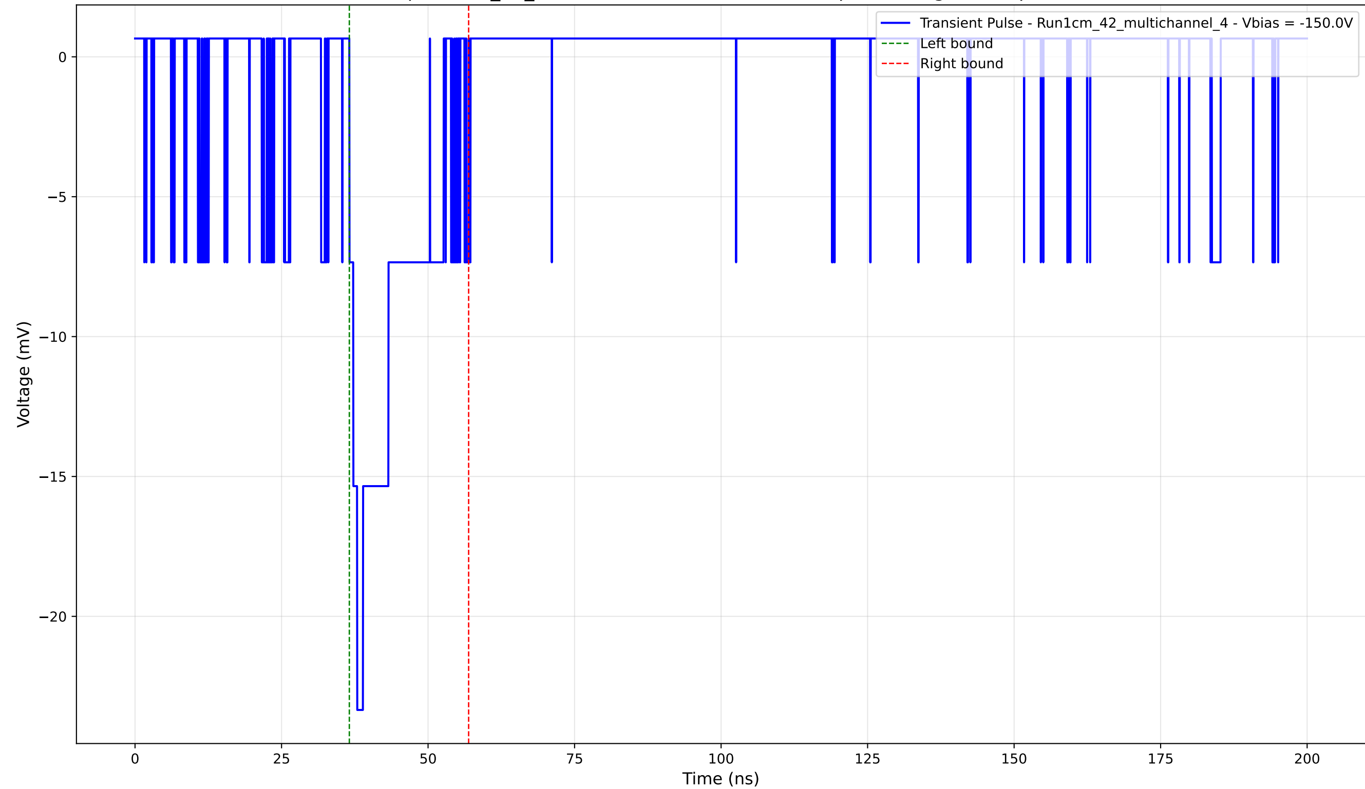
Transient Pulse - Sample: 1cm_42_multichannel - Position: 3550.0 \mu\text{m} - Charge: 3.70 pC - Rise Time: 1.33 ns
