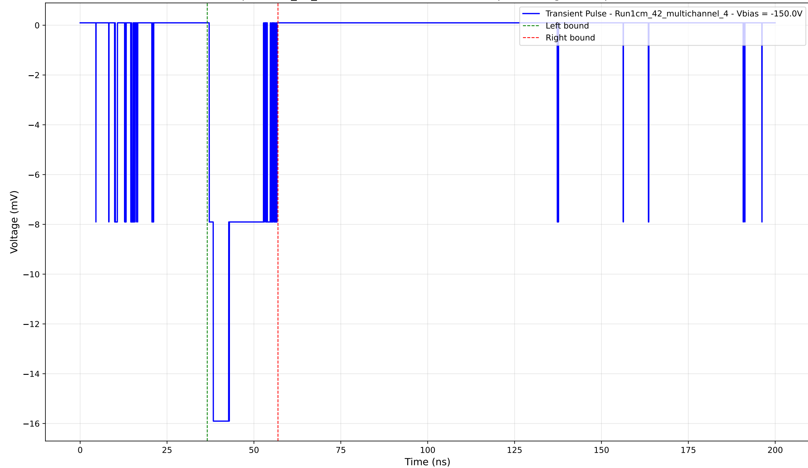
Transient Pulse - Sample: 1cm_42_multichannel - Position: 4195.0 \mu\text{m} - Charge: 3.60 pC - Rise Time: 1.18 ns
