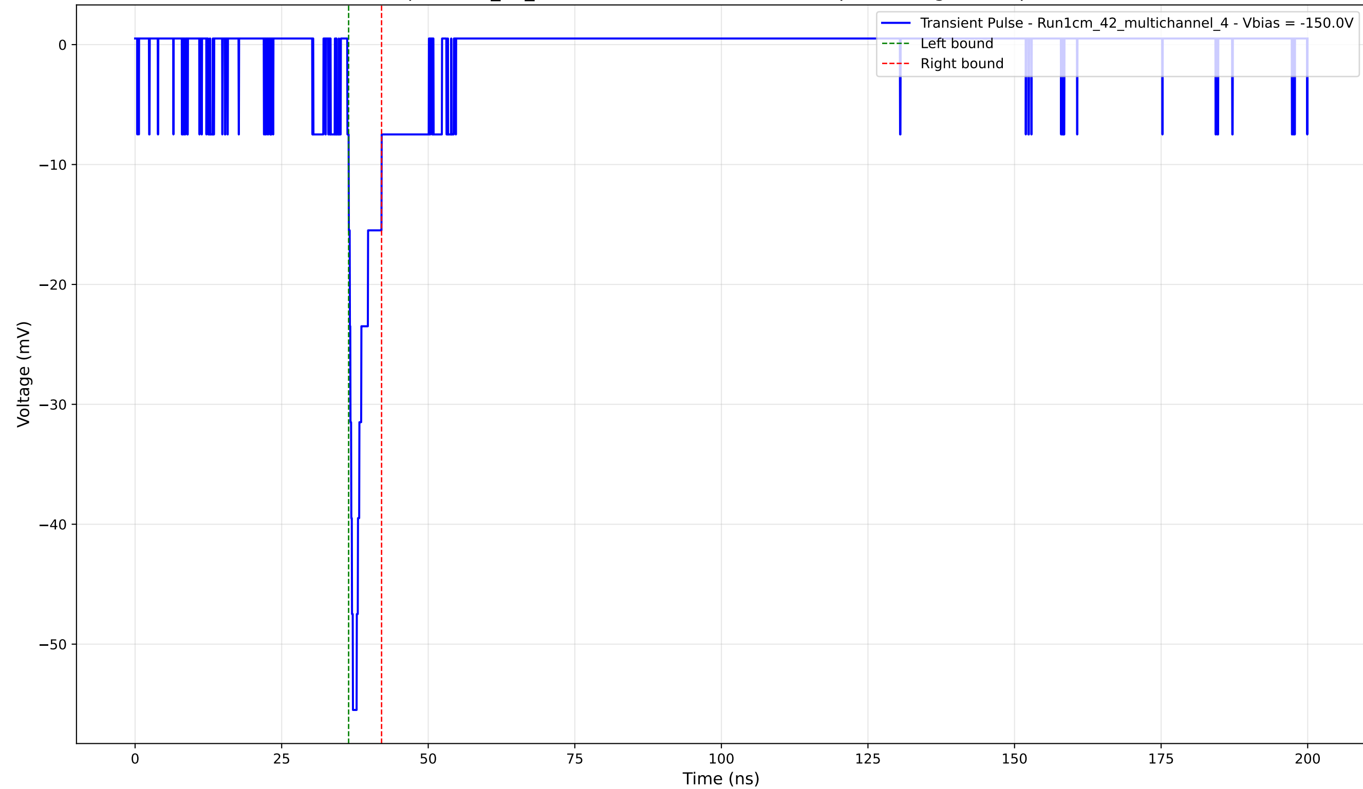
Transient Pulse - Sample: 1cm_42_multichannel - Position: 2055.0 \mu\text{m} - Charge: 3.02 pC - Rise Time: 0.95 ns
