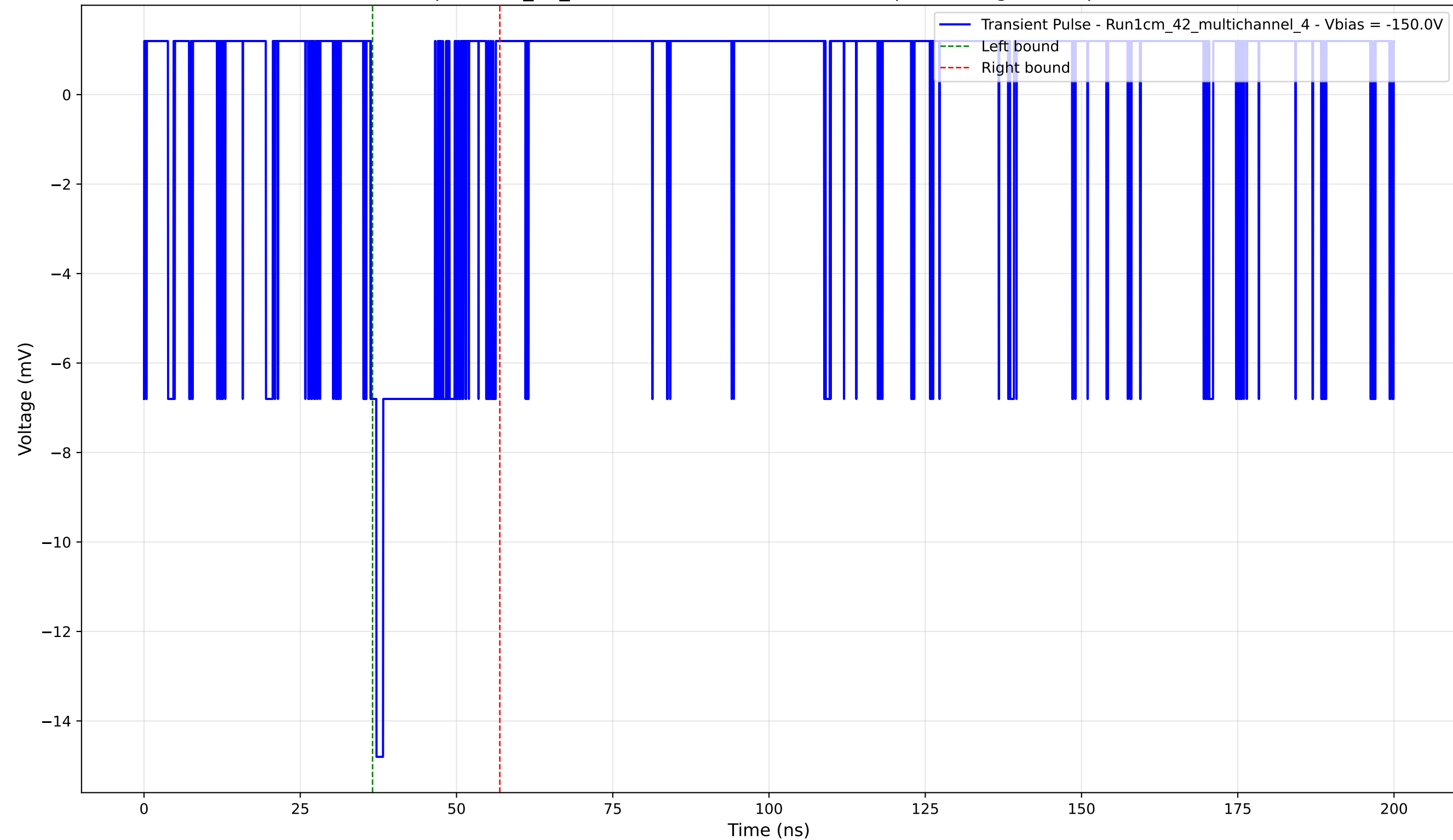
Transient Pulse - Sample: 1cm_42_multichannel - Position: 2935.0 \mu\text{m} - Charge: 2.00 pC - Rise Time: 0.90 ns
