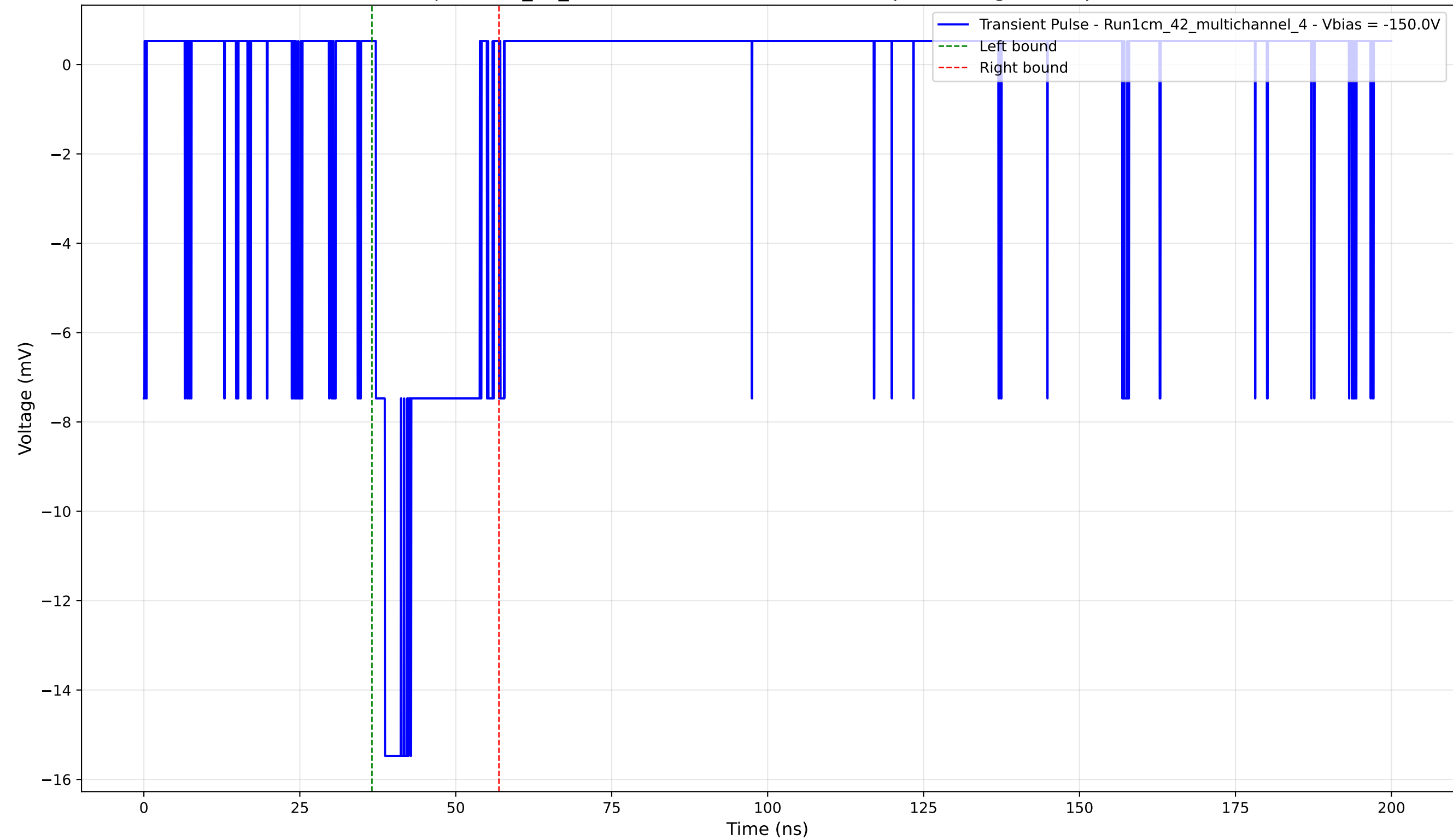
Transient Pulse - Sample: 1cm_42_multichannel - Position: 4715.0 \mu\text{m} - Charge: 3.24 pC - Rise Time: 1.46 ns
