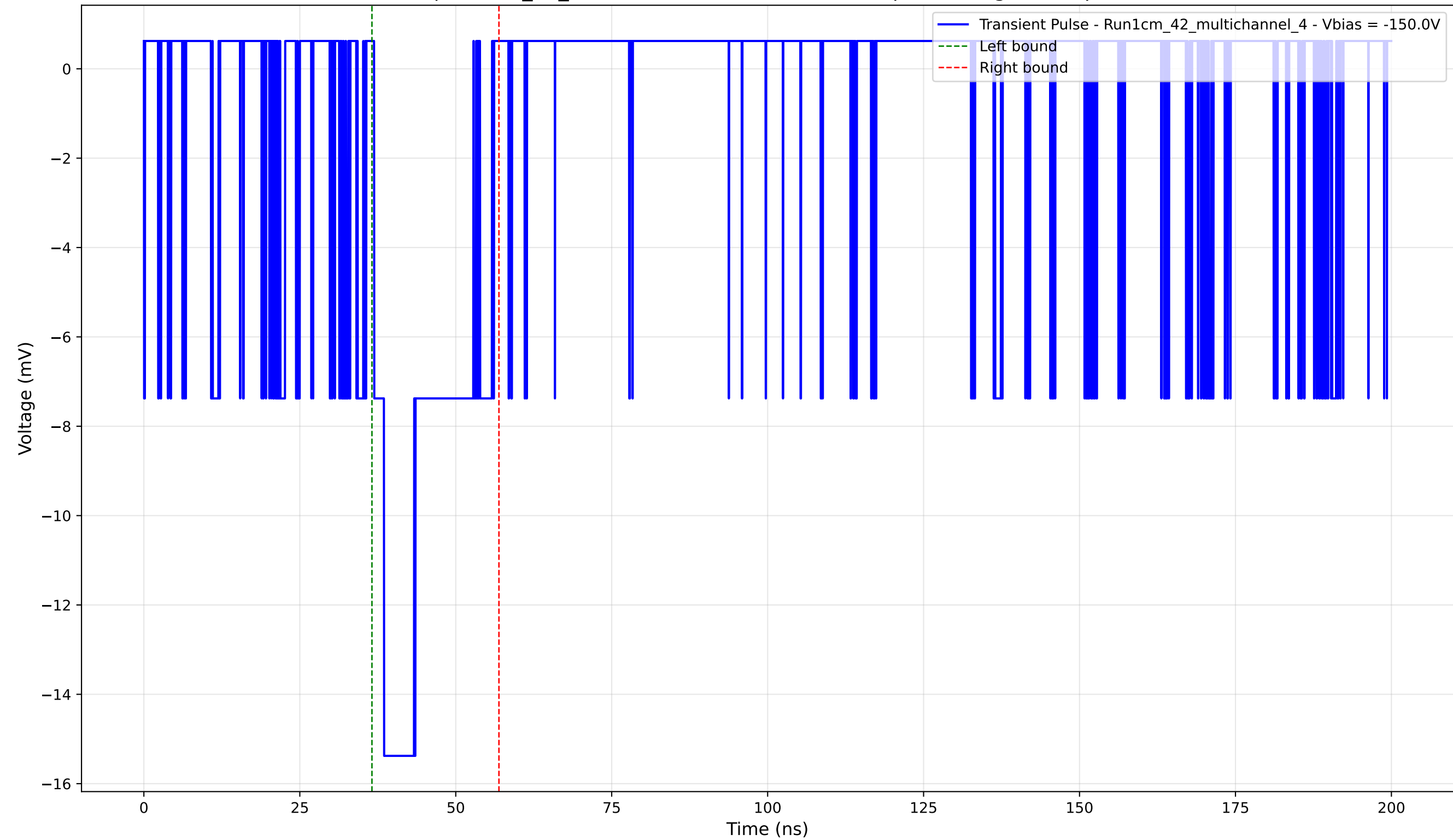
Transient Pulse - Sample: 1cm_42_multichannel - Position: 4555.0 \mu\text{m} - Charge: 3.50 pC - Rise Time: 1.60 ns
