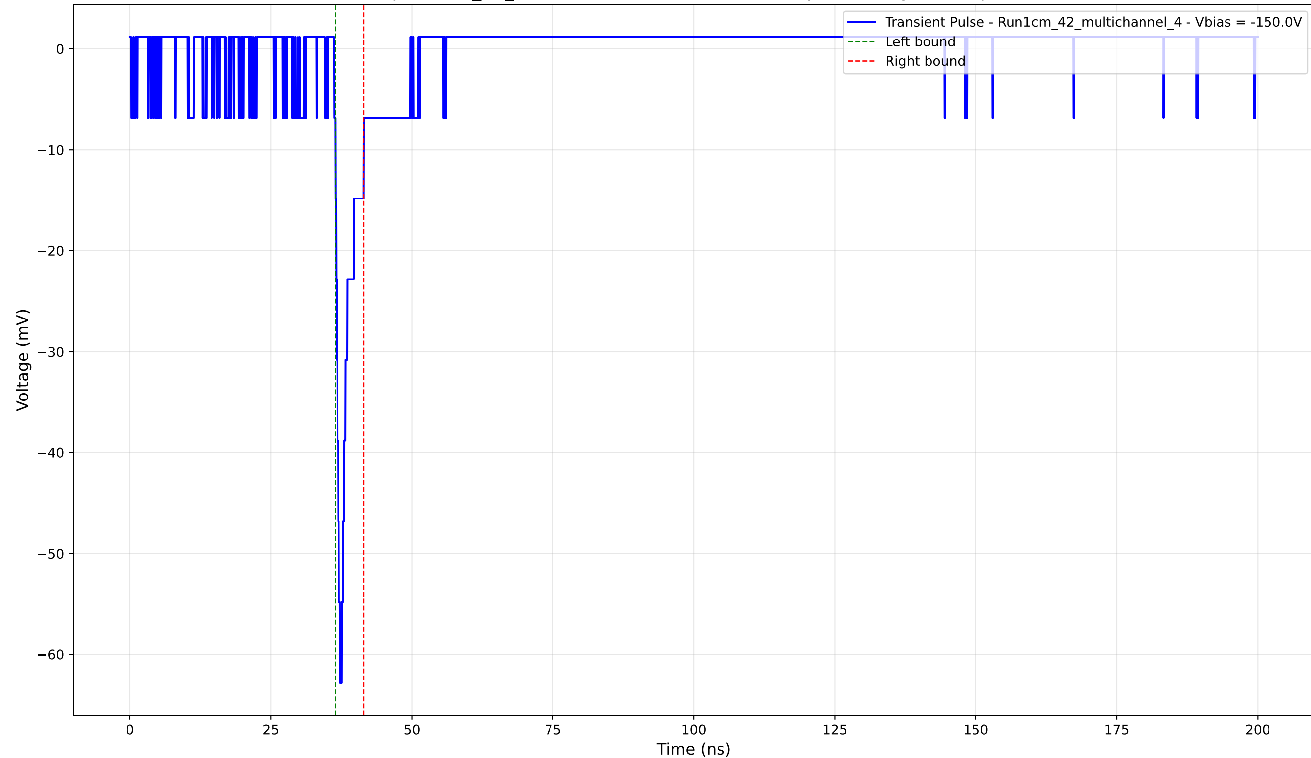
Transient Pulse - Sample: 1cm_42_multichannel - Position: 2090.0 \mu\text{m} - Charge: 2.89 pC - Rise Time: 1.06 ns
