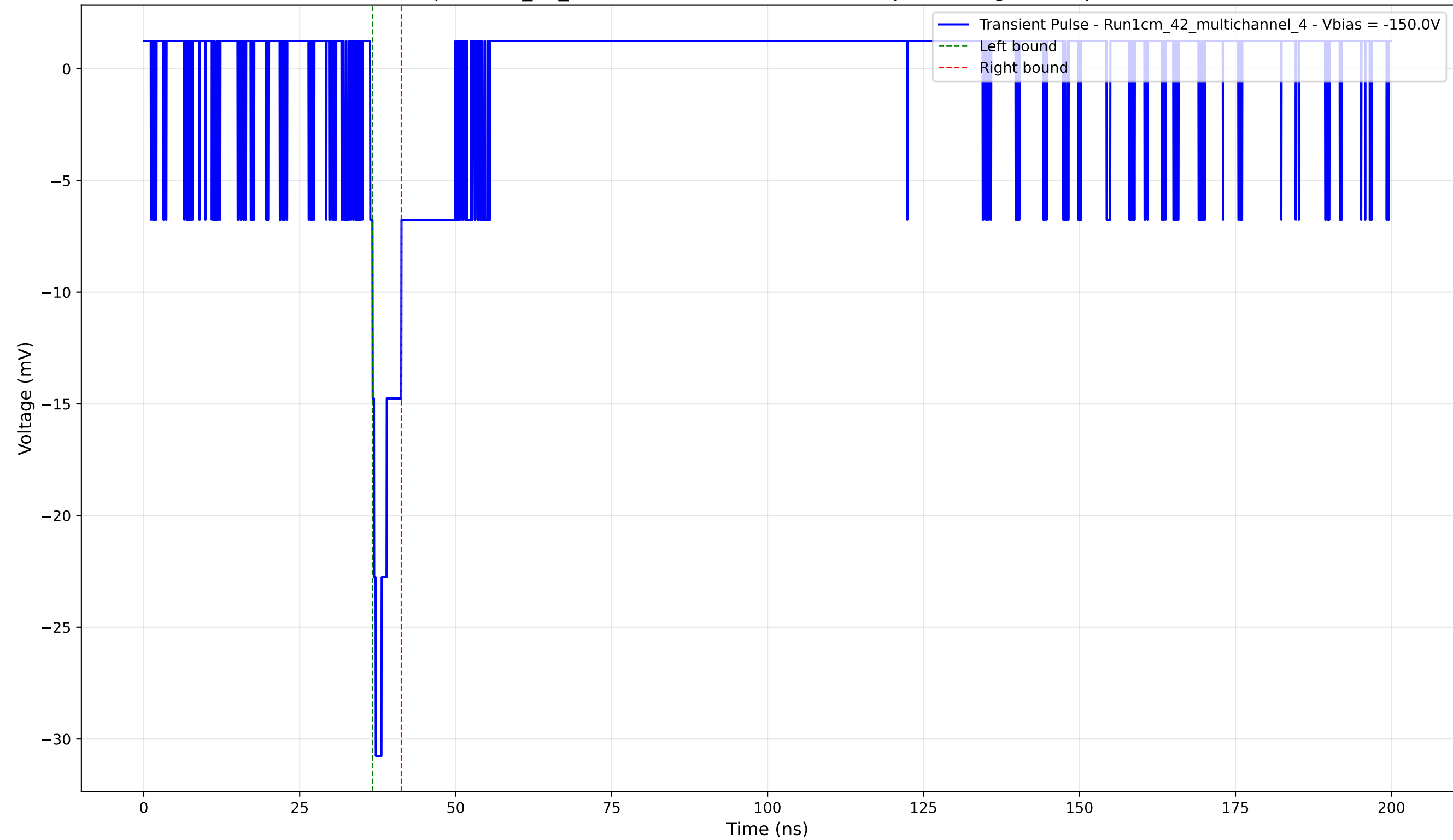
Transient Pulse - Sample: 1cm_42_multichannel - Position: 1820.0 \mu\text{m} - Charge: 1.84 pC - Rise Time: 0.89 ns
