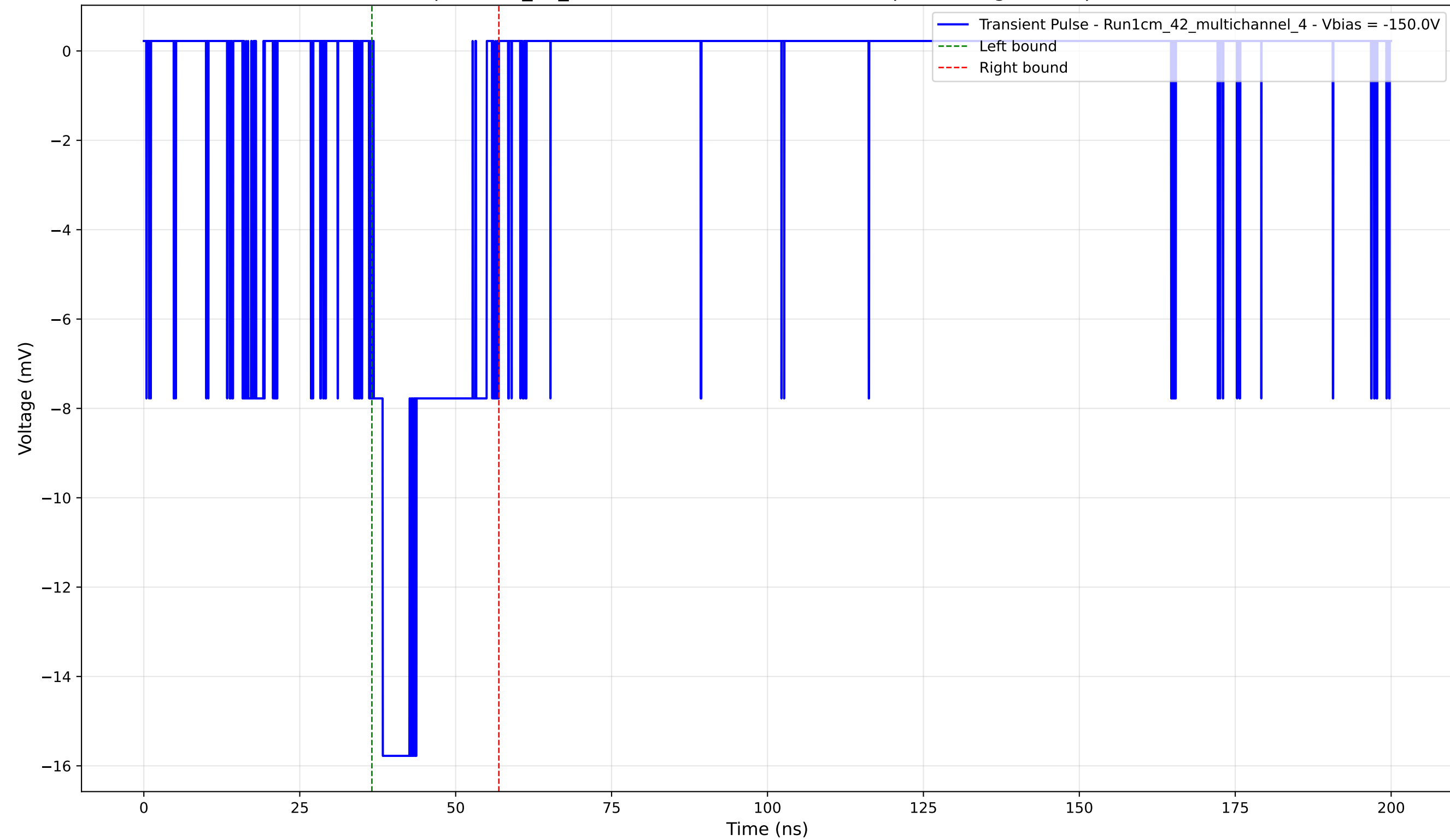
Transient Pulse - Sample: 1cm_42_multichannel - Position: 4285.0 \mu\text{m} - Charge: 3.71 pC - Rise Time: 1.46 ns
