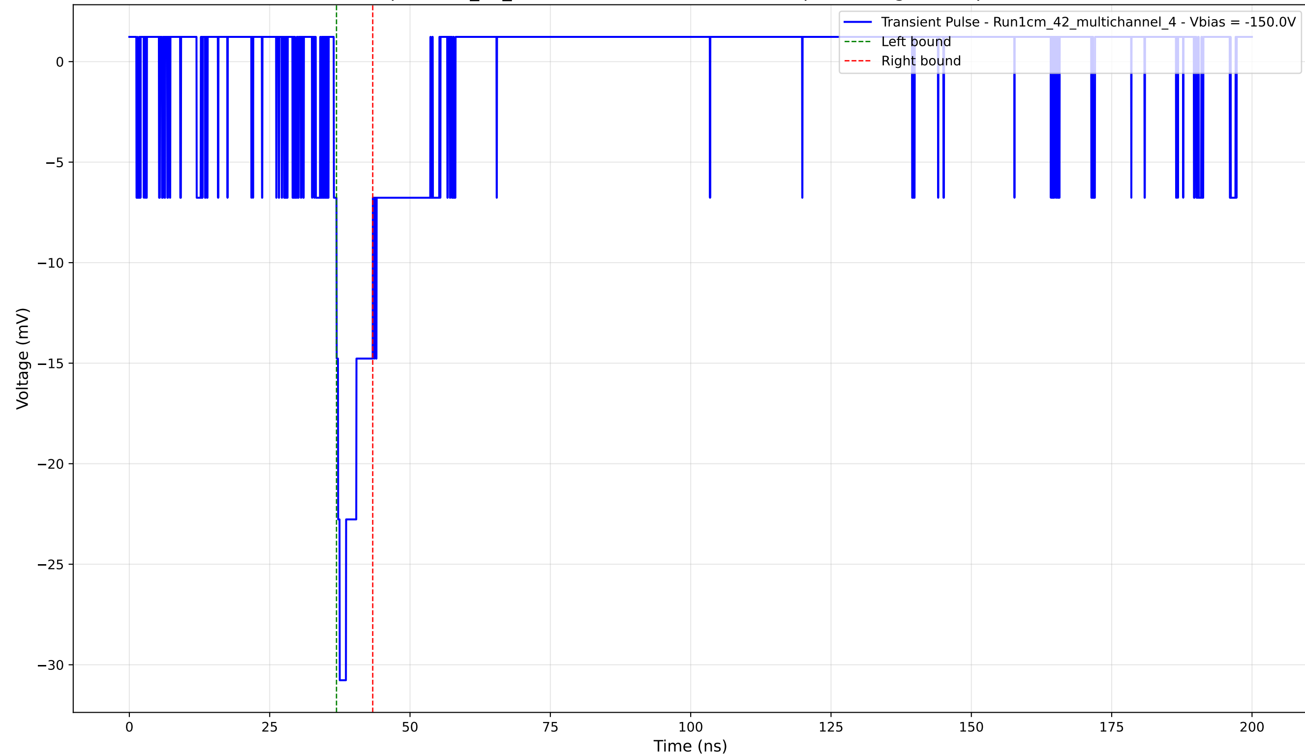
Transient Pulse - Sample: 1cm_42_multichannel - Position: 1520.0 \mu\text{m} - Charge: 2.61 pC - Rise Time: 1.05 ns
