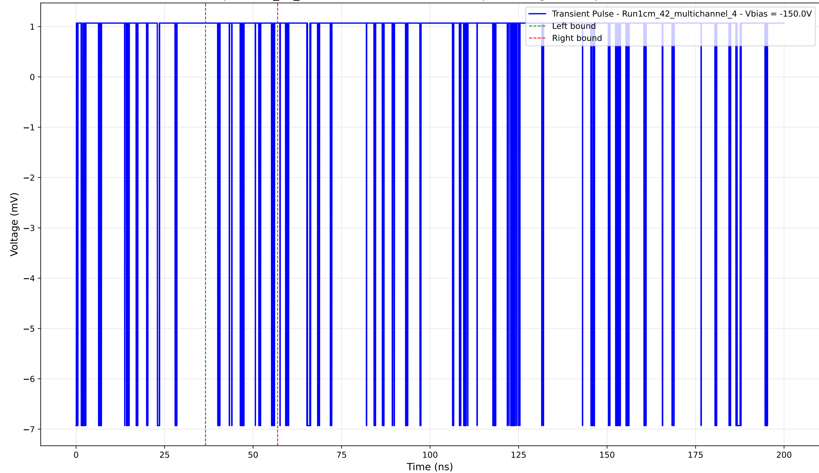
Transient Pulse - Sample: 1cm_42_multichannel - Position: 3905.0 \mu\text{m} - Charge: -0.12 pC - Rise Time: 0.00 ns (N/A)
