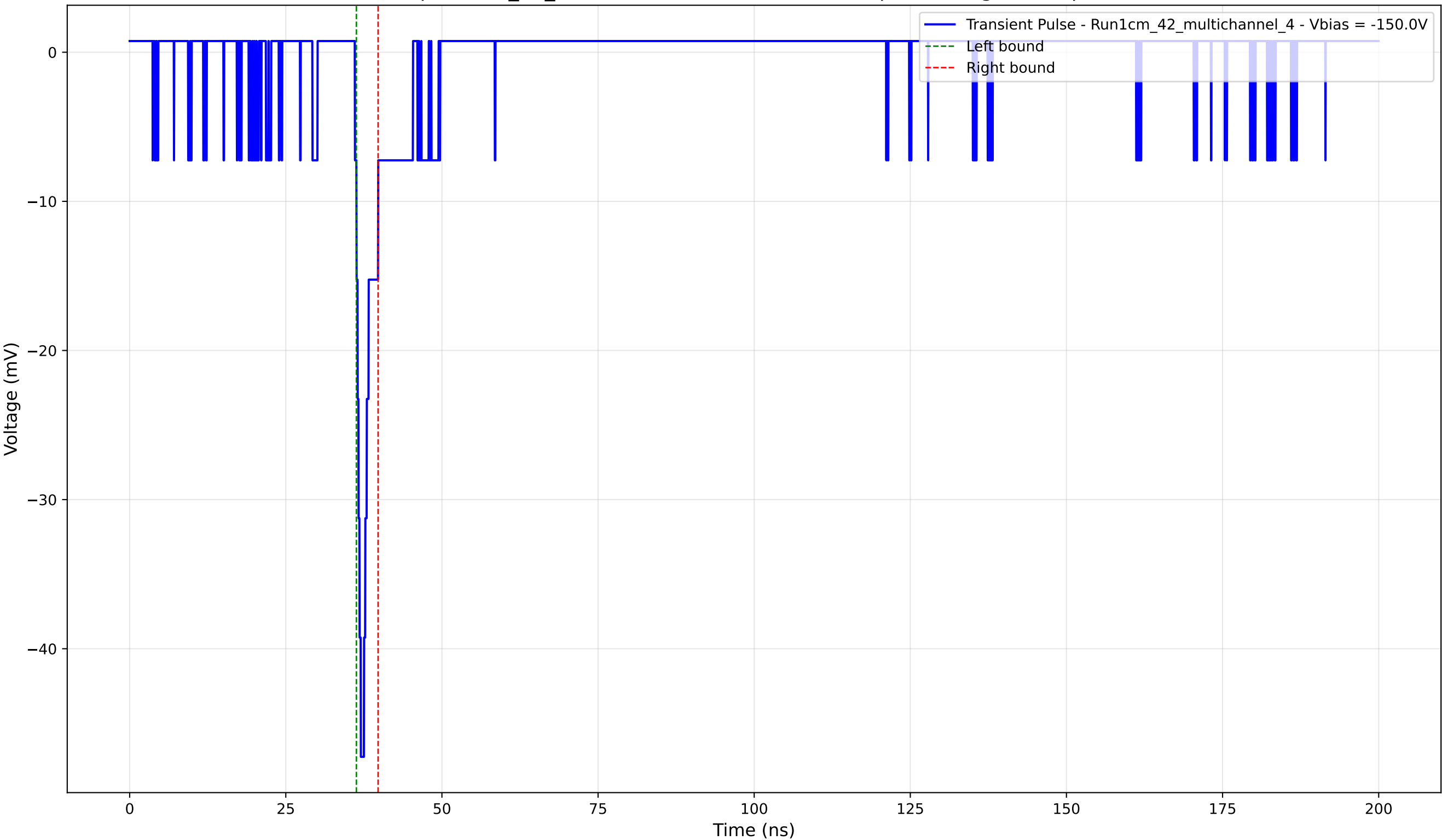
Transient Pulse - Sample: 1cm_42_multichannel - Position: 2440.0 \mu\text{m} - Charge: 1.78 pC - Rise Time: 0.95 ns
