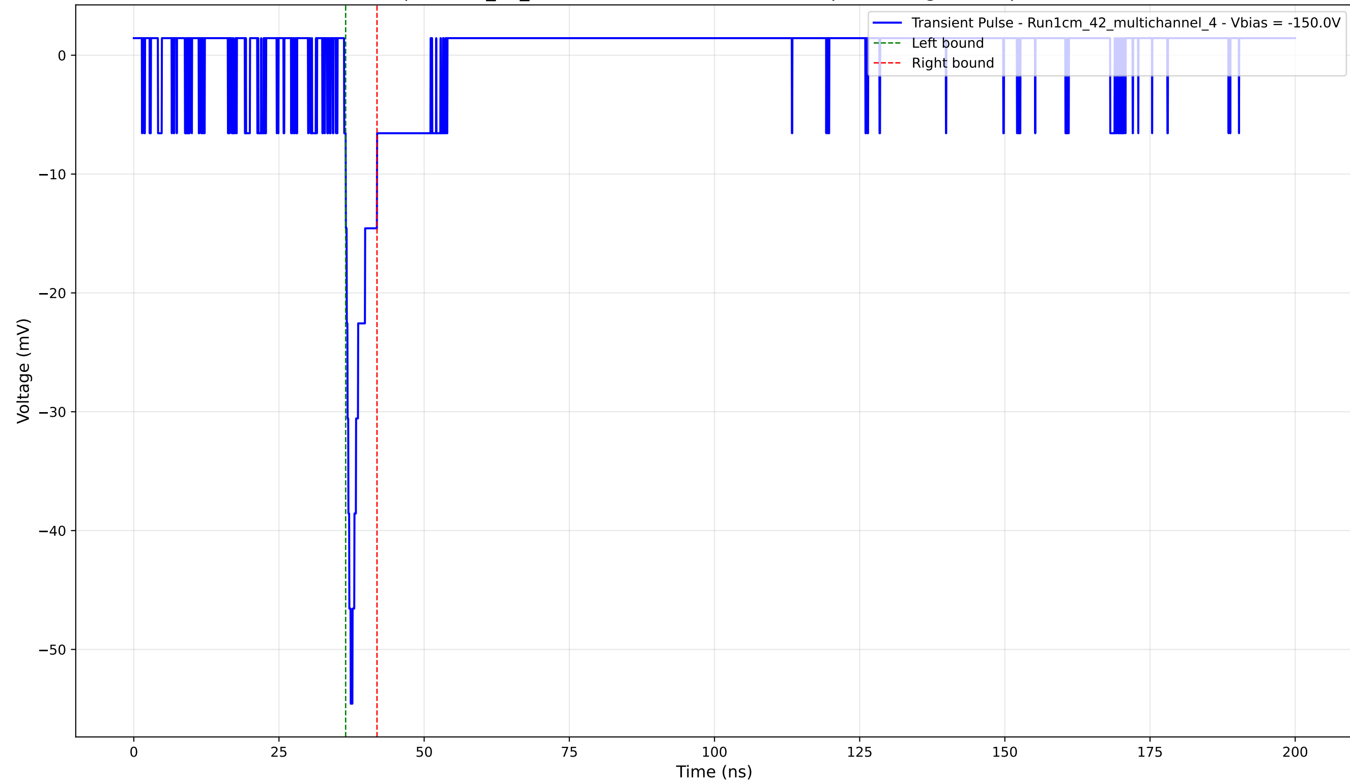
Transient Pulse - Sample: 1cm_42_multichannel - Position: 2790.0 \mu\text{m} - Charge: 2.77 pC - Rise Time: 1.12 ns
