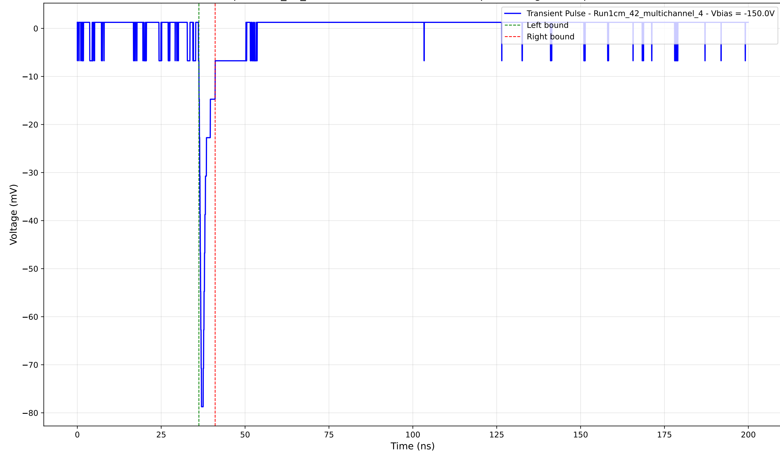
Transient Pulse - Sample: 1cm_42_multichannel - Position: 2485.0 \mu\text{m} - Charge: 3.29 pC - Rise Time: 0.76 ns
