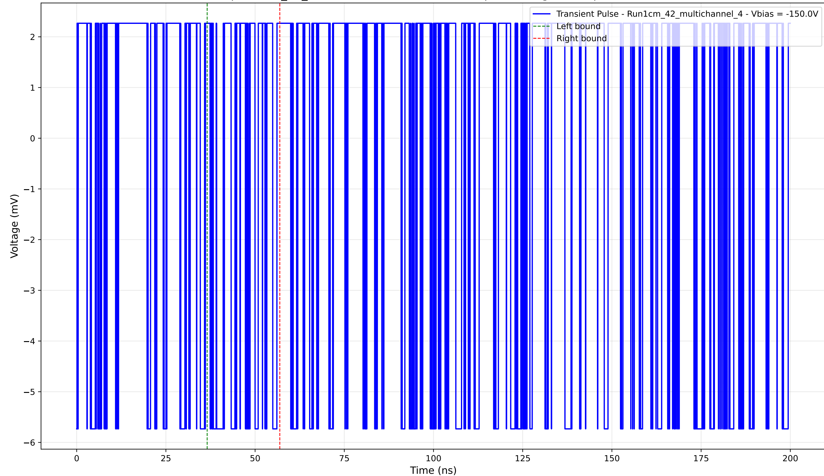
Transient Pulse - Sample: 1cm_42_multichannel - Position: 885.0 \mu\text{m} - Charge: 0.35 pC - Rise Time: 0.00 ns (N/A)
