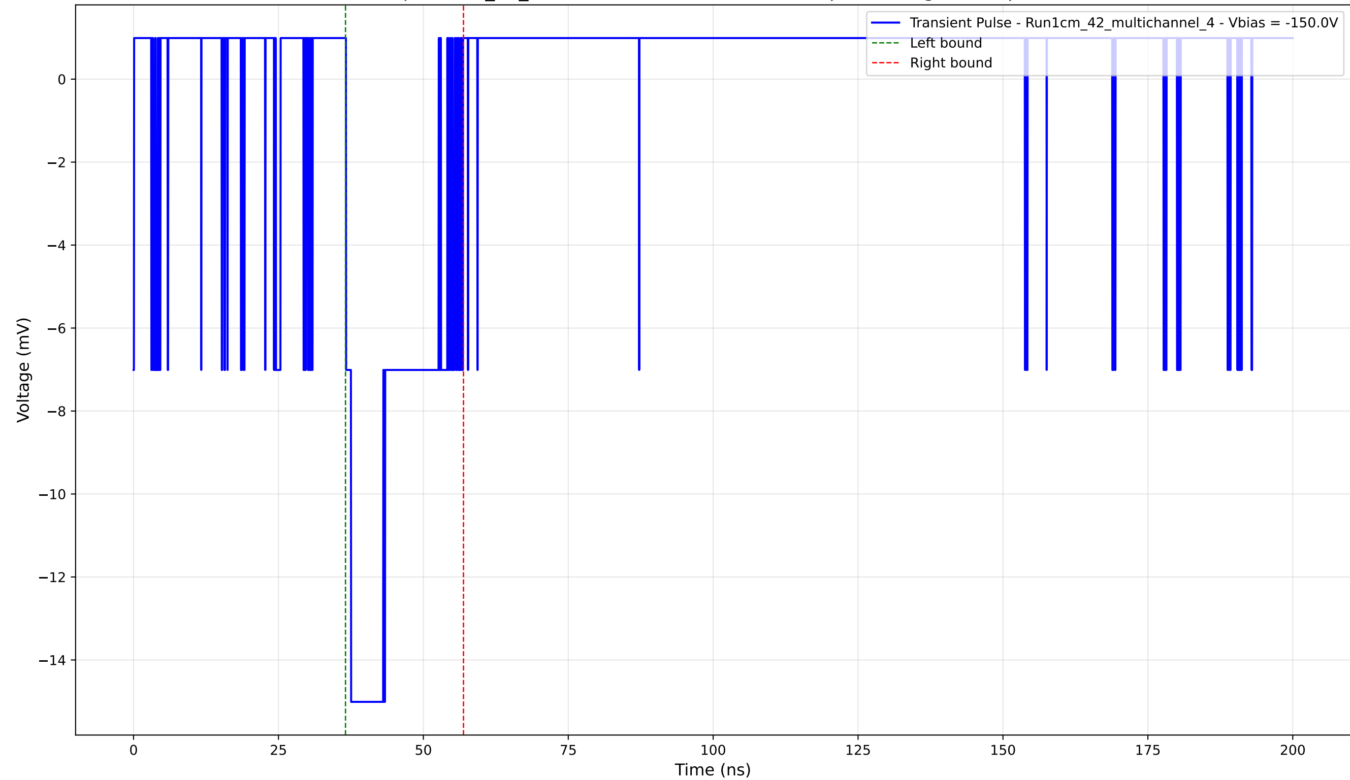
Transient Pulse - Sample: 1cm_42_multichannel - Position: 3710.0 \mu\text{m} - Charge: 3.52 pC - Rise Time: 0.88 ns
