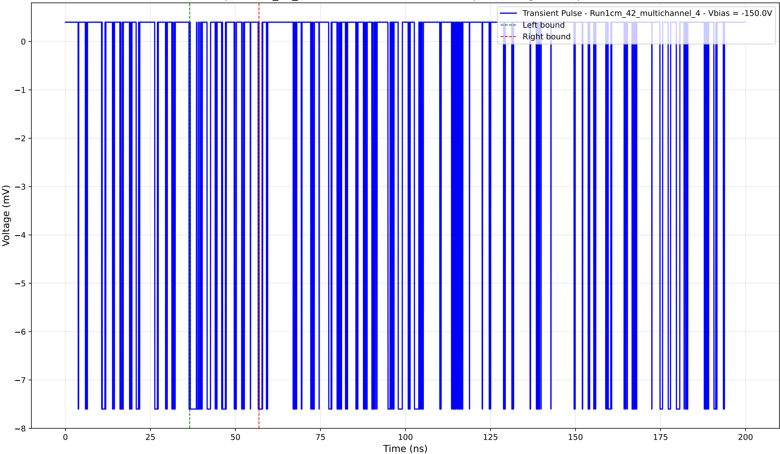
Transient Pulse - Sample: 1cm_42_multichannel - Position: 1895.0 \mu\text{m} - Charge: 0.91 pC - Rise Time: 0.02 ns
