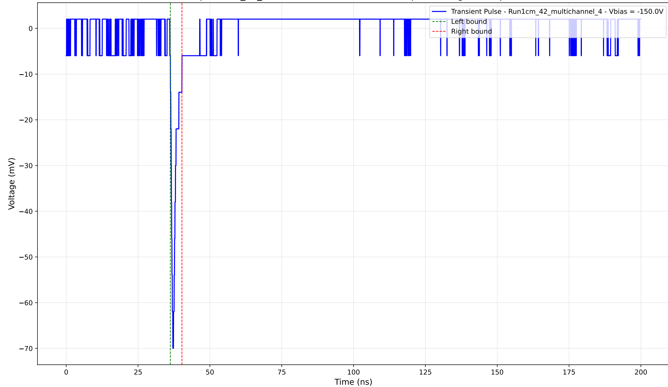
Transient Pulse - Sample: 1cm_42_multichannel - Position: 2450.0 \mu\text{m} - Charge: 2.54 pC - Rise Time: 0.86 ns
