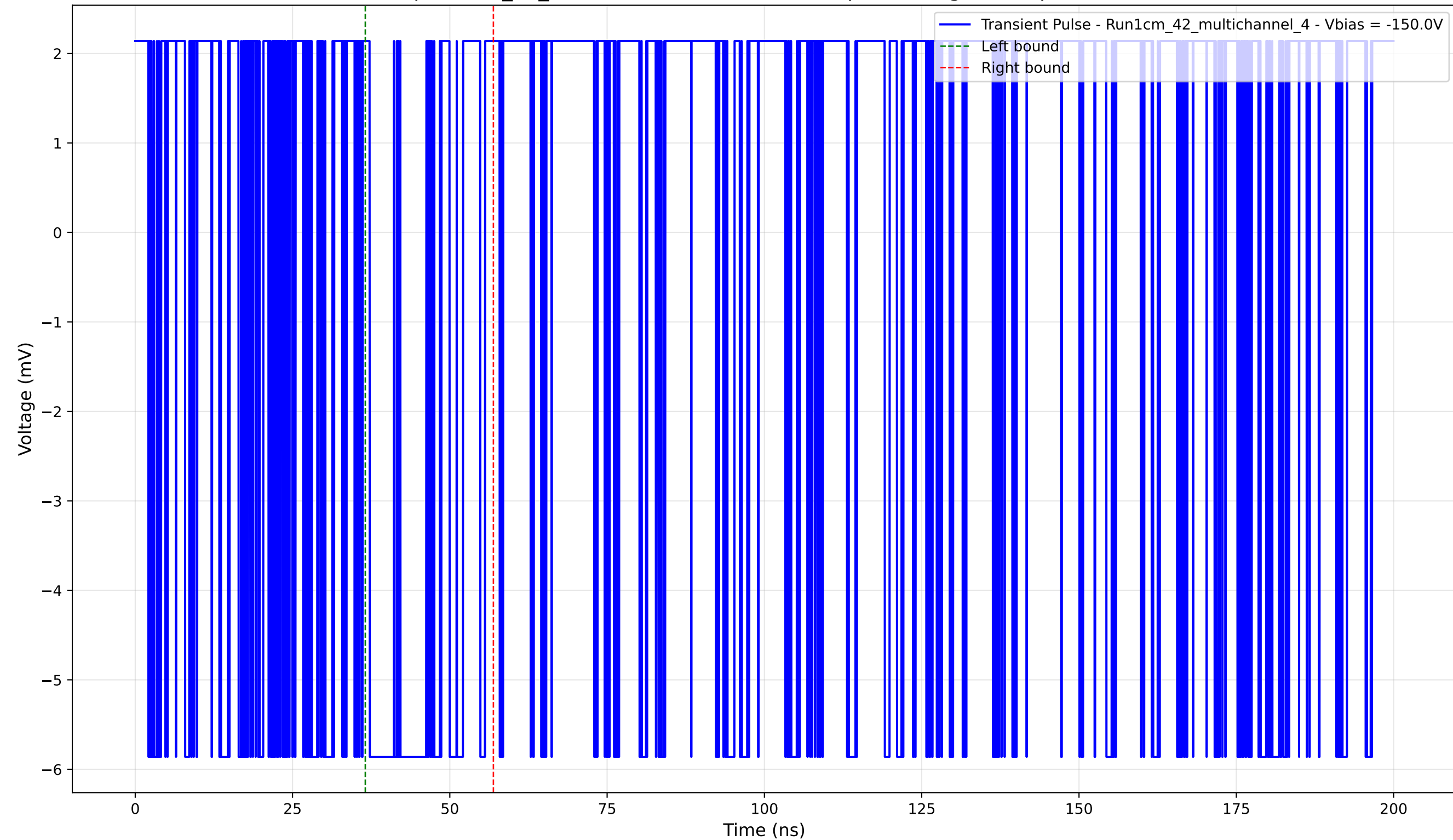
Transient Pulse - Sample: 1cm_42_multichannel - Position: 75.0 \mu\text{m} - Charge: 1.26 pC - Rise Time: 0.00 ns (N/A)
