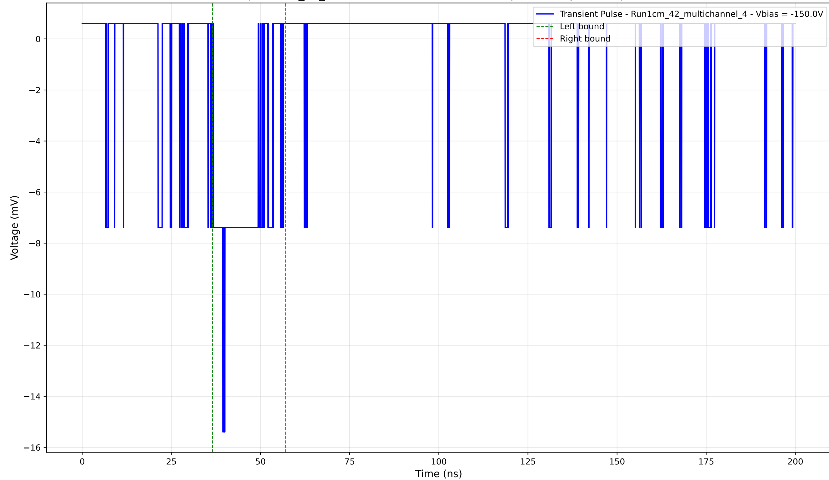
Transient Pulse - Sample: 1cm_42_multichannel - Position: 3850.0 \mu\text{m} - Charge: 2.24 pC - Rise Time: 2.60 ns
