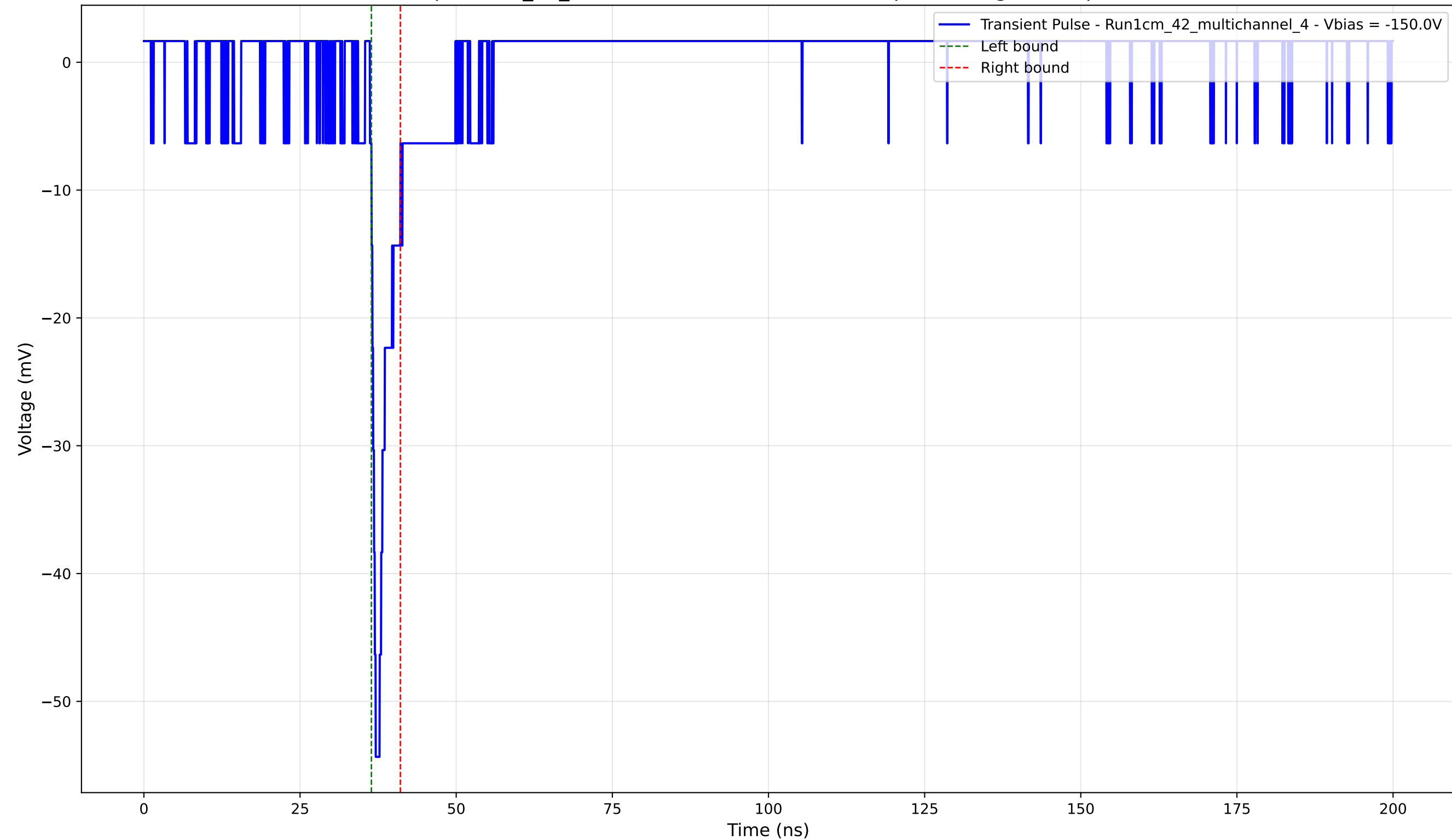
Transient Pulse - Sample: 1cm_42_multichannel - Position: 2705.0 \mu\text{m} - Charge: 2.62 pC - Rise Time: 0.92 ns
