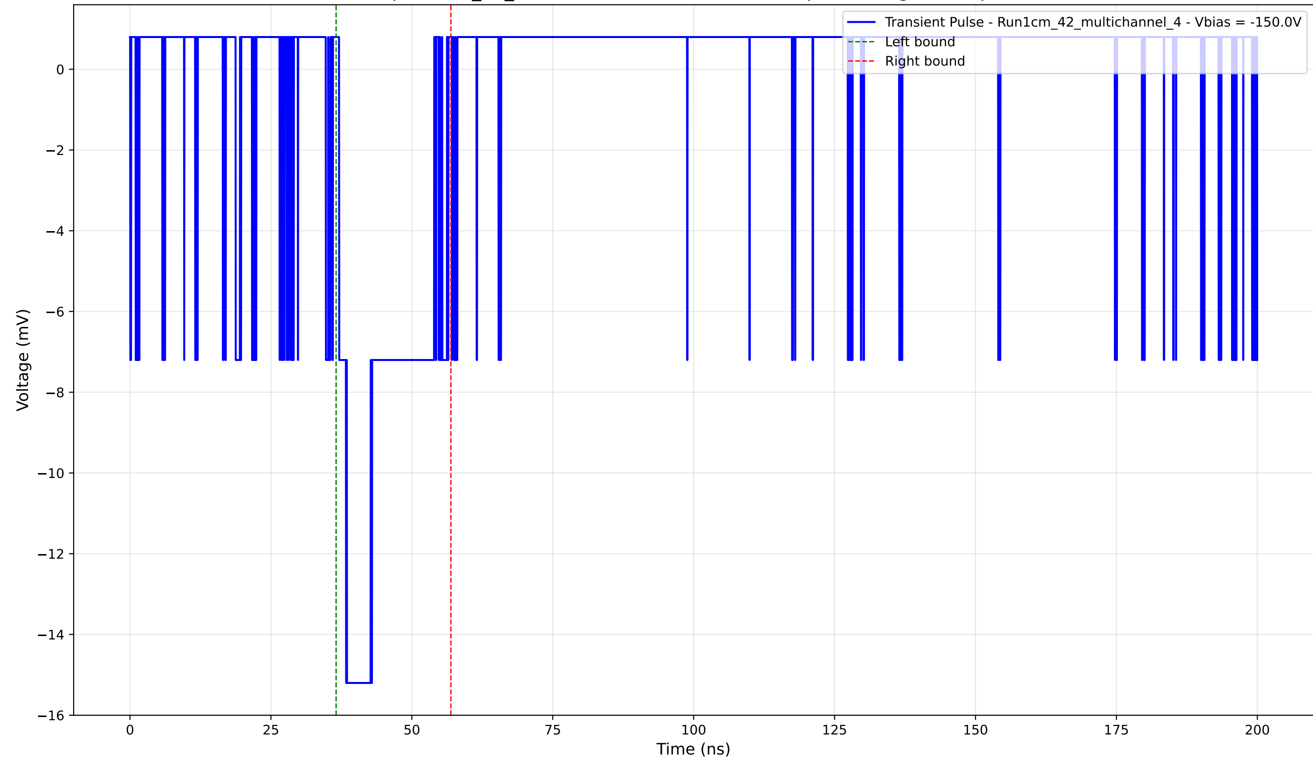
Transient Pulse - Sample: 1cm_42_multichannel - Position: 4505.0 \mu\text{m} - Charge: 3.34 pC - Rise Time: 1.24 ns
