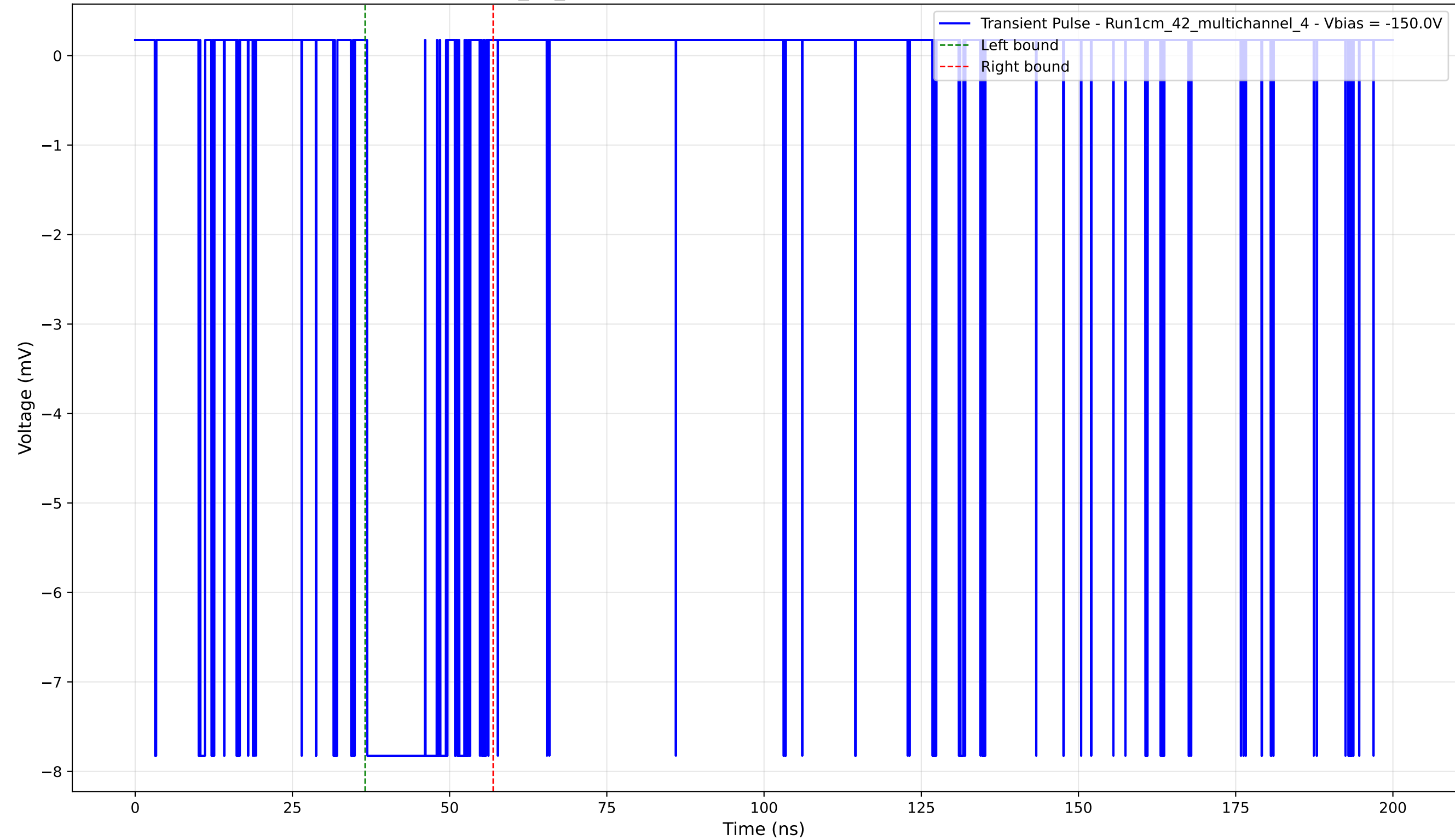
Transient Pulse - Sample: 1cm_42_multichannel - Position: 3950.0 \mu\text{m} - Charge: 2.28 pC - Rise Time: 0.02 ns
