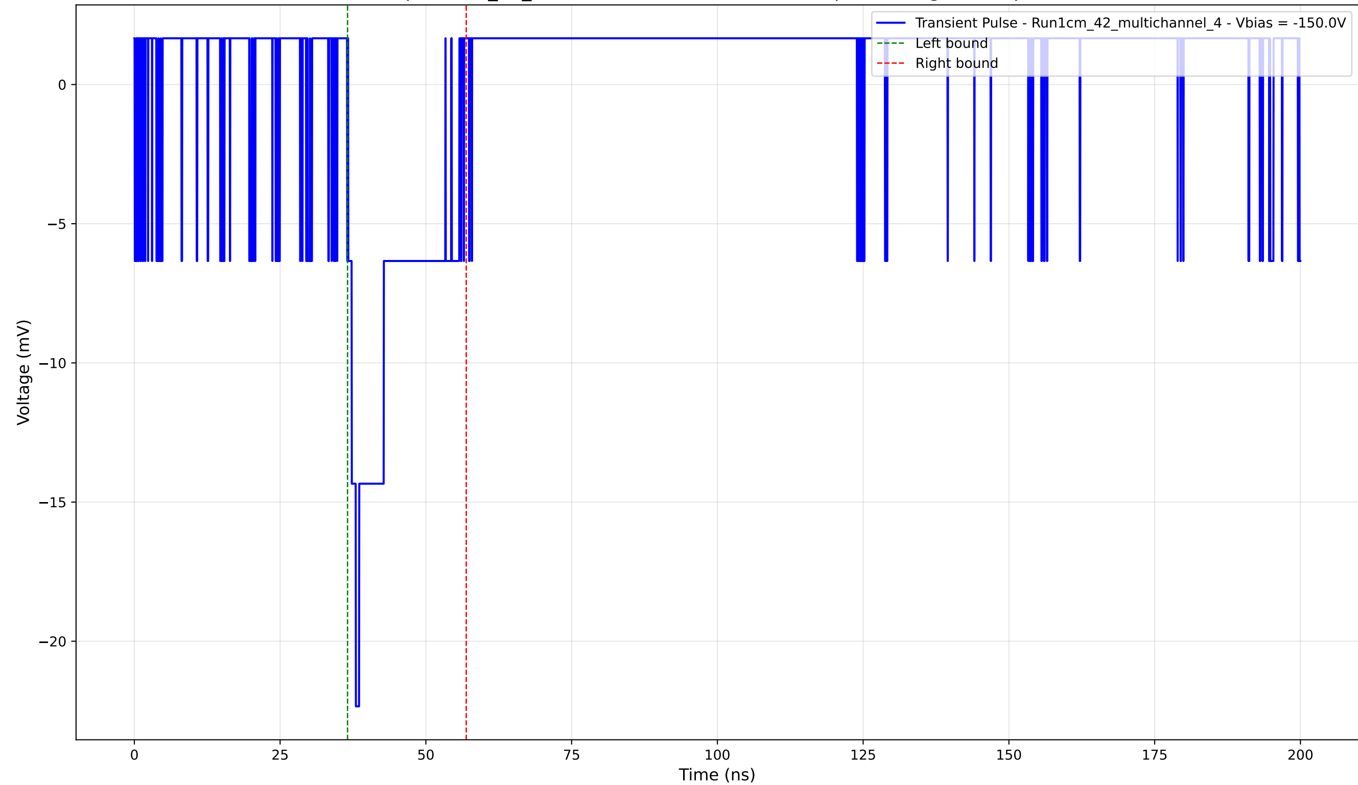
Transient Pulse - Sample: 1cm_42_multichannel - Position: 3570.0 \mu\text{m} - Charge: 3.36 pC - Rise Time: 1.32 ns
