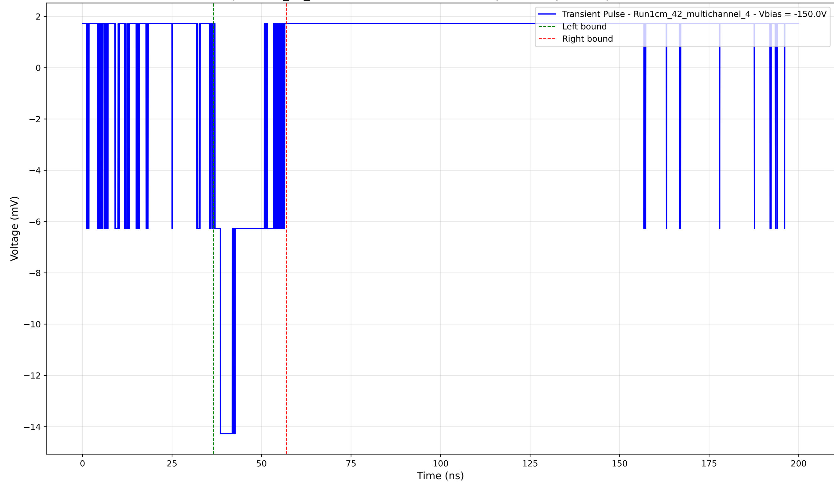
Transient Pulse - Sample: 1cm_42_multichannel - Position: 4175.0 \mu\text{m} - Charge: 2.68 pC - Rise Time: 0.00 ns (N/A)
