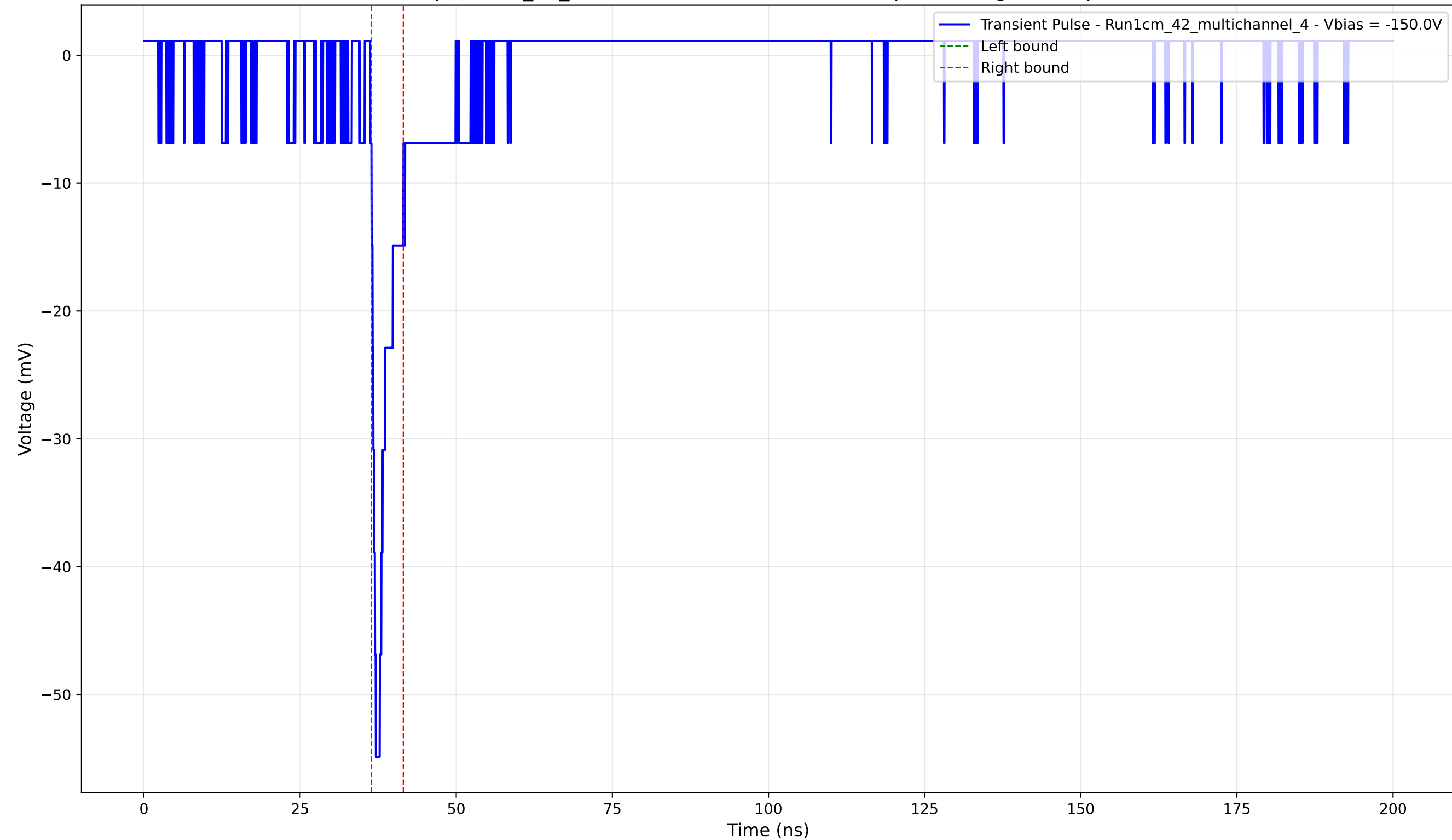
Transient Pulse - Sample: 1cm_42_multichannel - Position: 2700.0 \mu\text{m} - Charge: 2.82 pC - Rise Time: 0.90 ns
