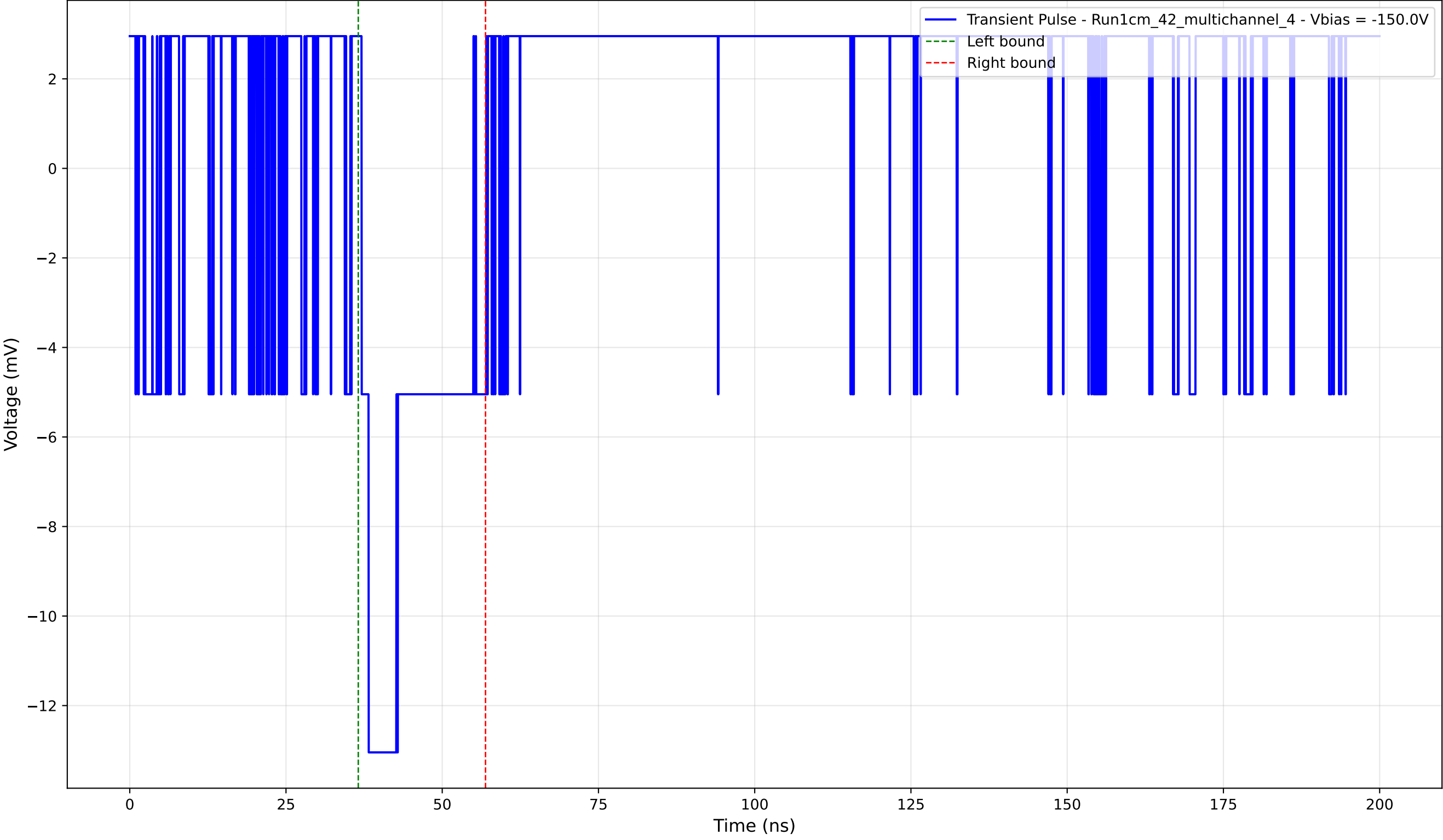
Transient Pulse - Sample: 1cm_42_multichannel - Position: 435.0 \mu\text{m} - Charge: 2.66 pC - Rise Time: 0.00 ns (N/A)
