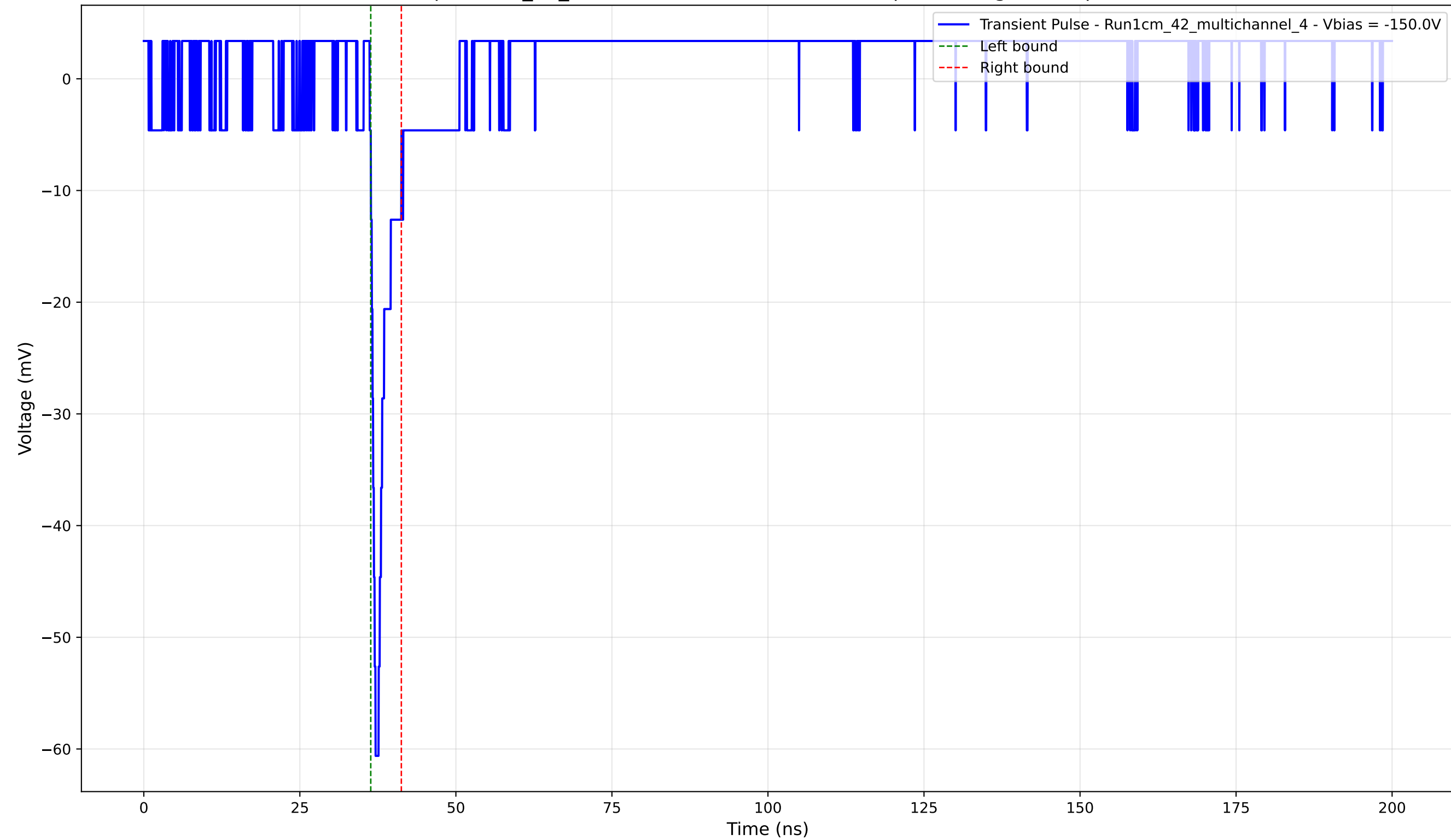
Transient Pulse - Sample: 1cm_42_multichannel - Position: 2620.0 \mu\text{m} - Charge: 2.64 pC - Rise Time: 0.76 ns
