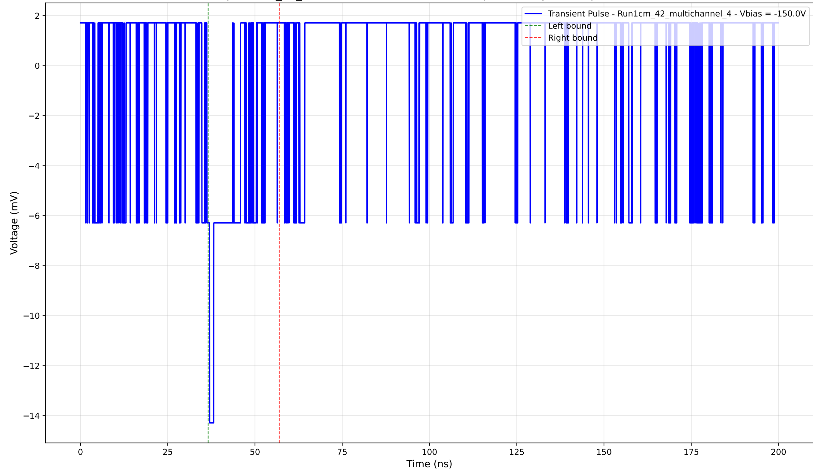
Transient Pulse - Sample: 1cm_42_multichannel - Position: 2850.0 \mu\text{m} - Charge: 1.47 pC - Rise Time: 0.00 ns (N/A)
