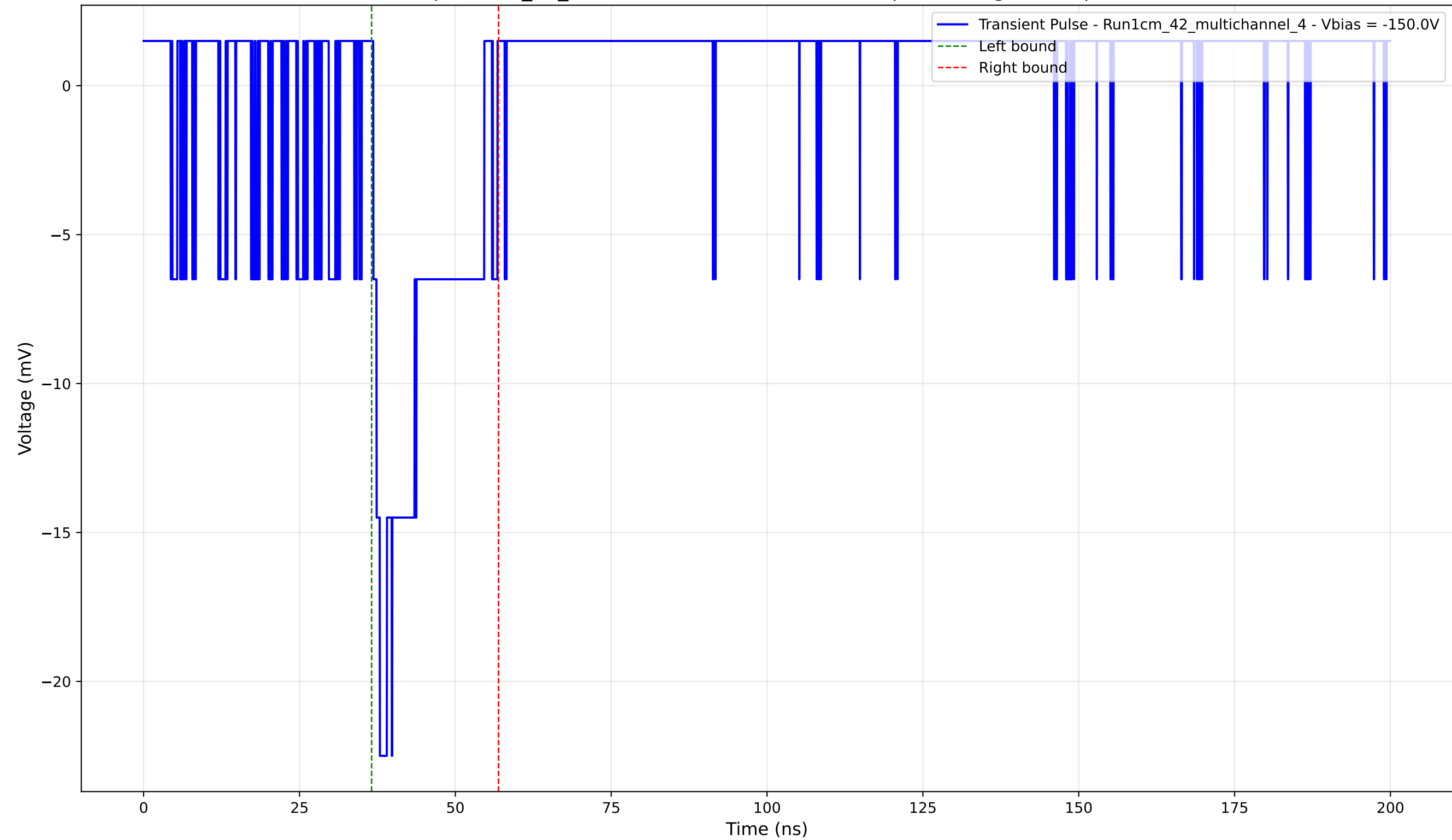
Transient Pulse - Sample: 1cm_42_multichannel - Position: 1120.0 \mu\text{m} - Charge: 3.57 pC - Rise Time: 1.06 ns
