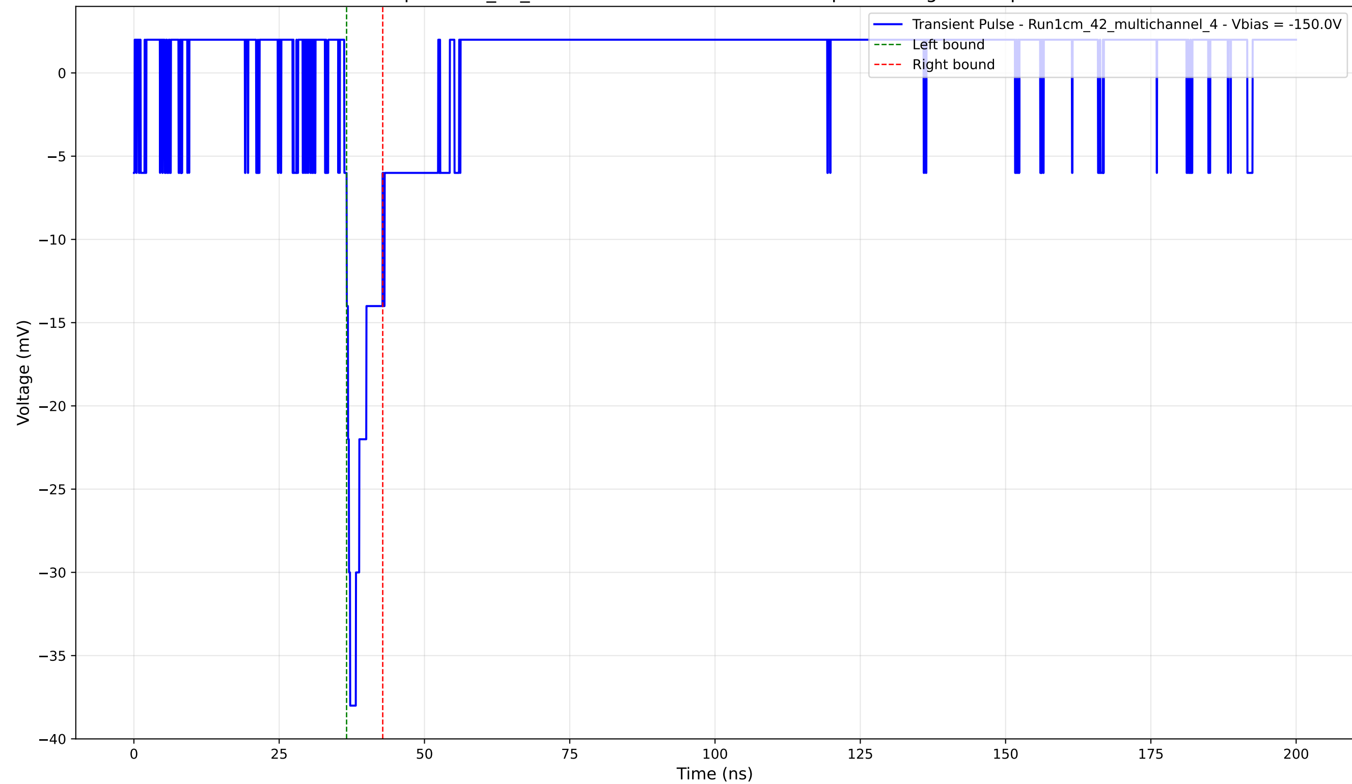
Transient Pulse - Sample: 1cm_42_multichannel - Position: 1800.0 \mu\text{m} - Charge: 2.69 pC - Rise Time: 1.01 ns
