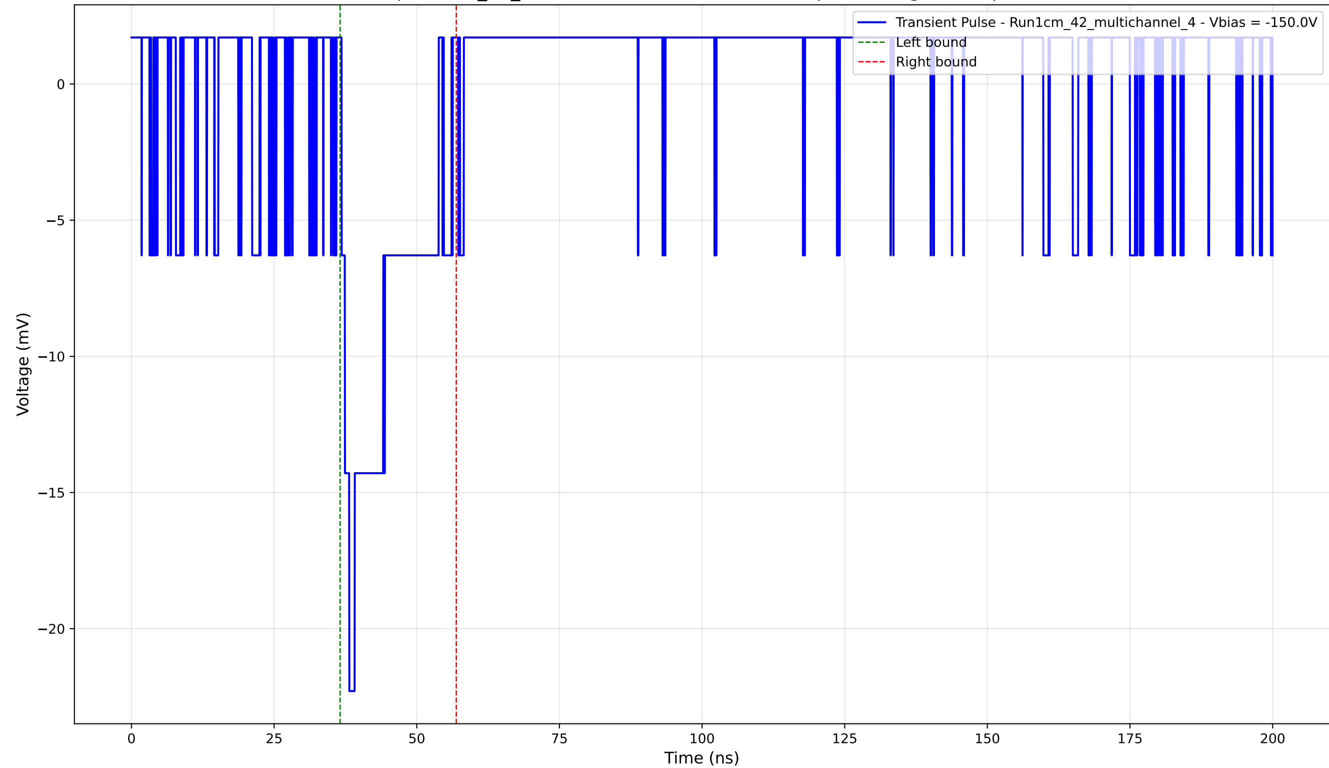
Transient Pulse - Sample: 1cm_42_multichannel - Position: 1085.0 \mu\text{m} - Charge: 3.55 pC - Rise Time: 1.36 ns
