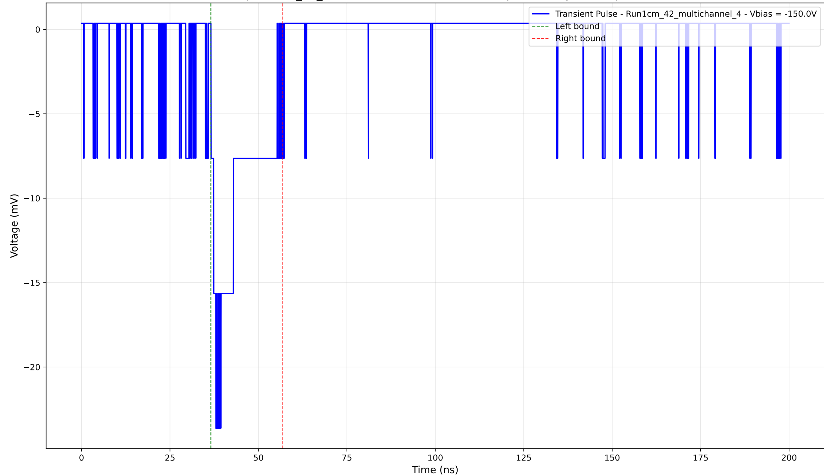
Transient Pulse - Sample: 1cm_42_multichannel - Position: 3545.0 \mu\text{m} - Charge: 4.06 pC - Rise Time: 1.39 ns
