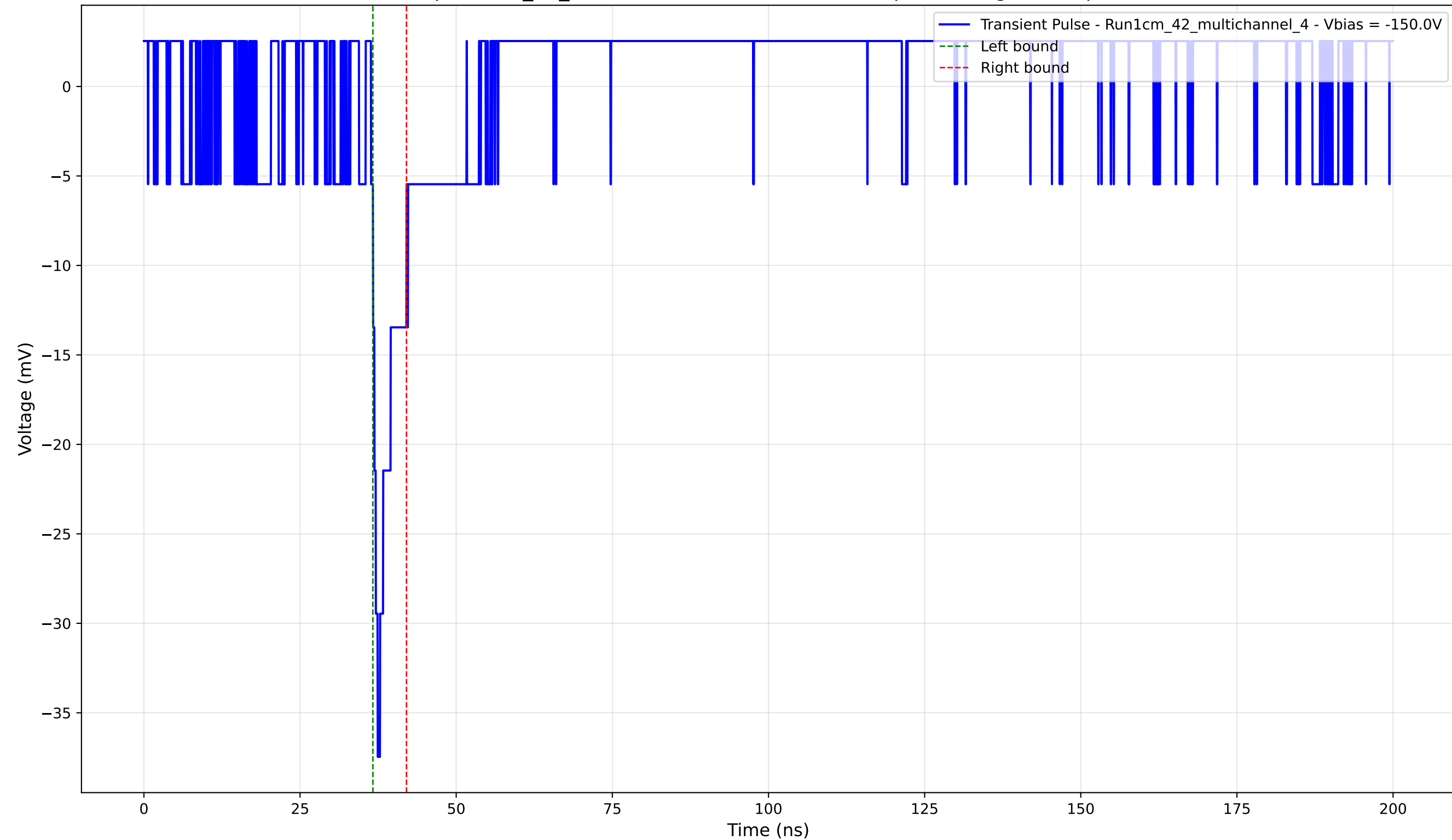
Transient Pulse - Sample: 1cm_42_multichannel - Position: 1815.0 \mu\text{m} - Charge: 2.11 pC - Rise Time: 1.07 ns
