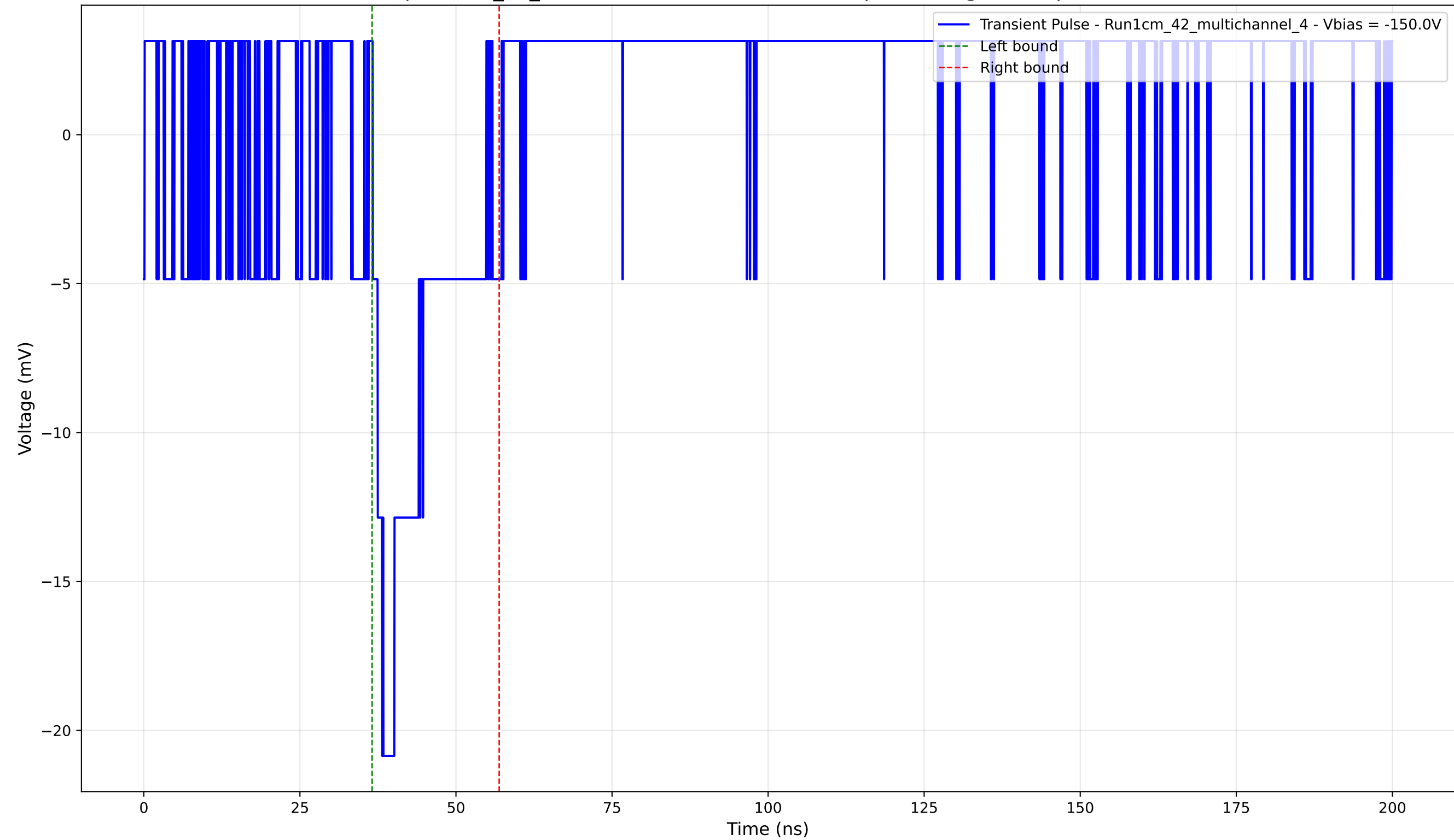
Transient Pulse - Sample: 1cm_42_multichannel - Position: 1055.0 \mu\text{m} - Charge: 3.23 pC - Rise Time: 0.00 ns (N/A)
