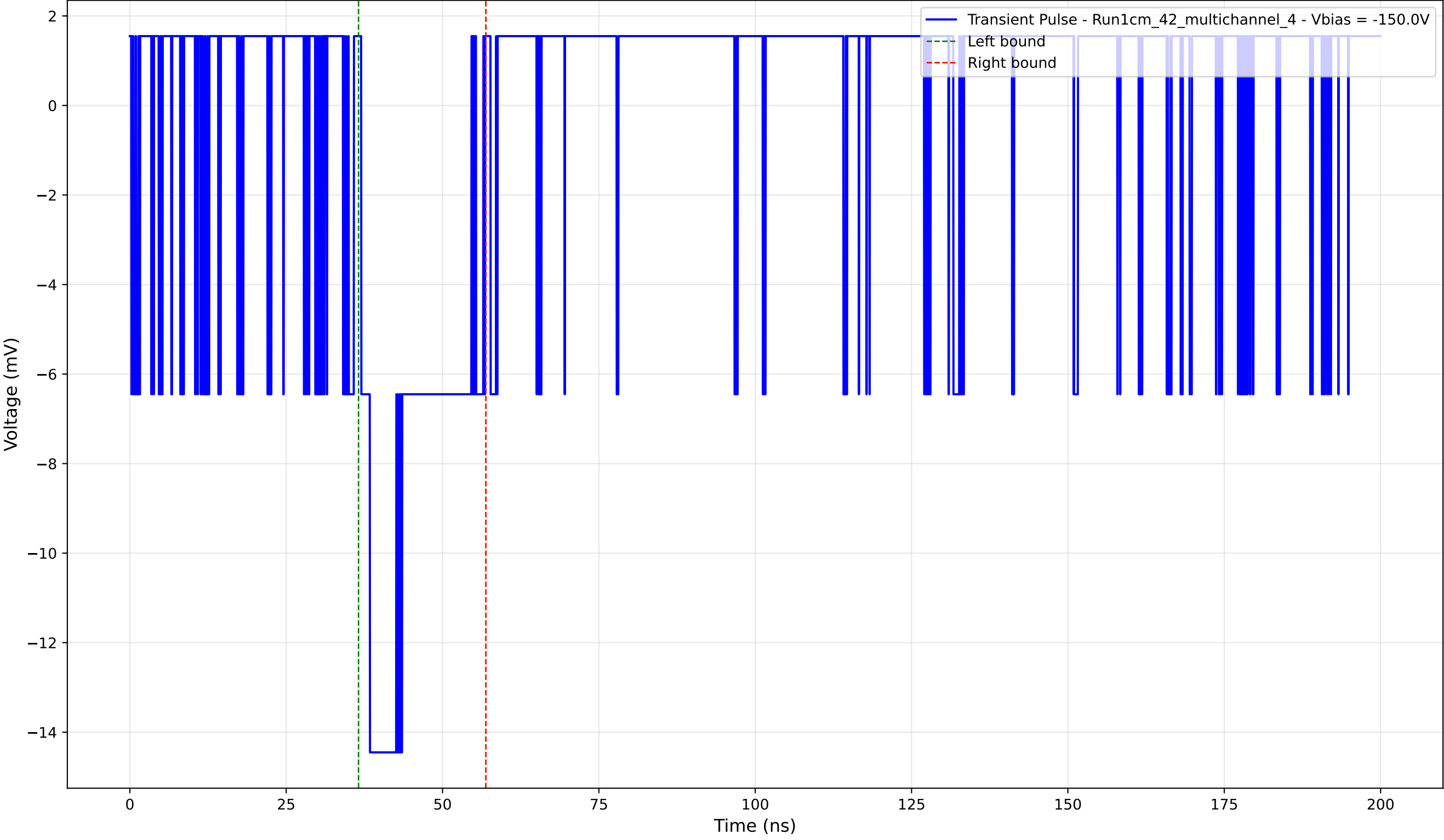
Transient Pulse - Sample: 1cm_42_multichannel - Position: 210.0 \mu\text{m} - Charge: 3.21 pC - Rise Time: 0.00 ns (N/A)
