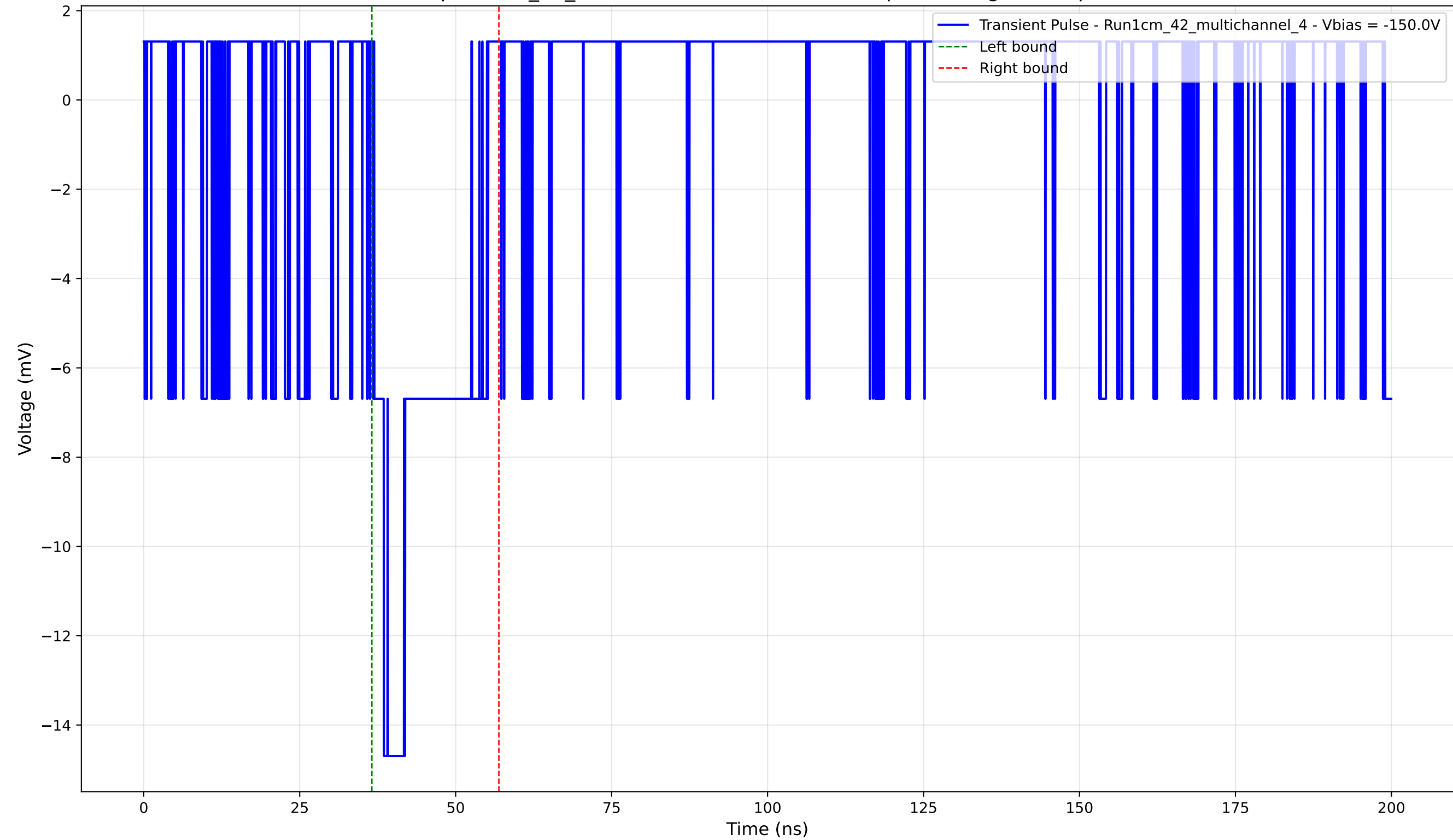
Transient Pulse - Sample: 1cm_42_multichannel - Position: 295.0 \mu\text{m} - Charge: 2.89 pC - Rise Time: 1.54 ns
