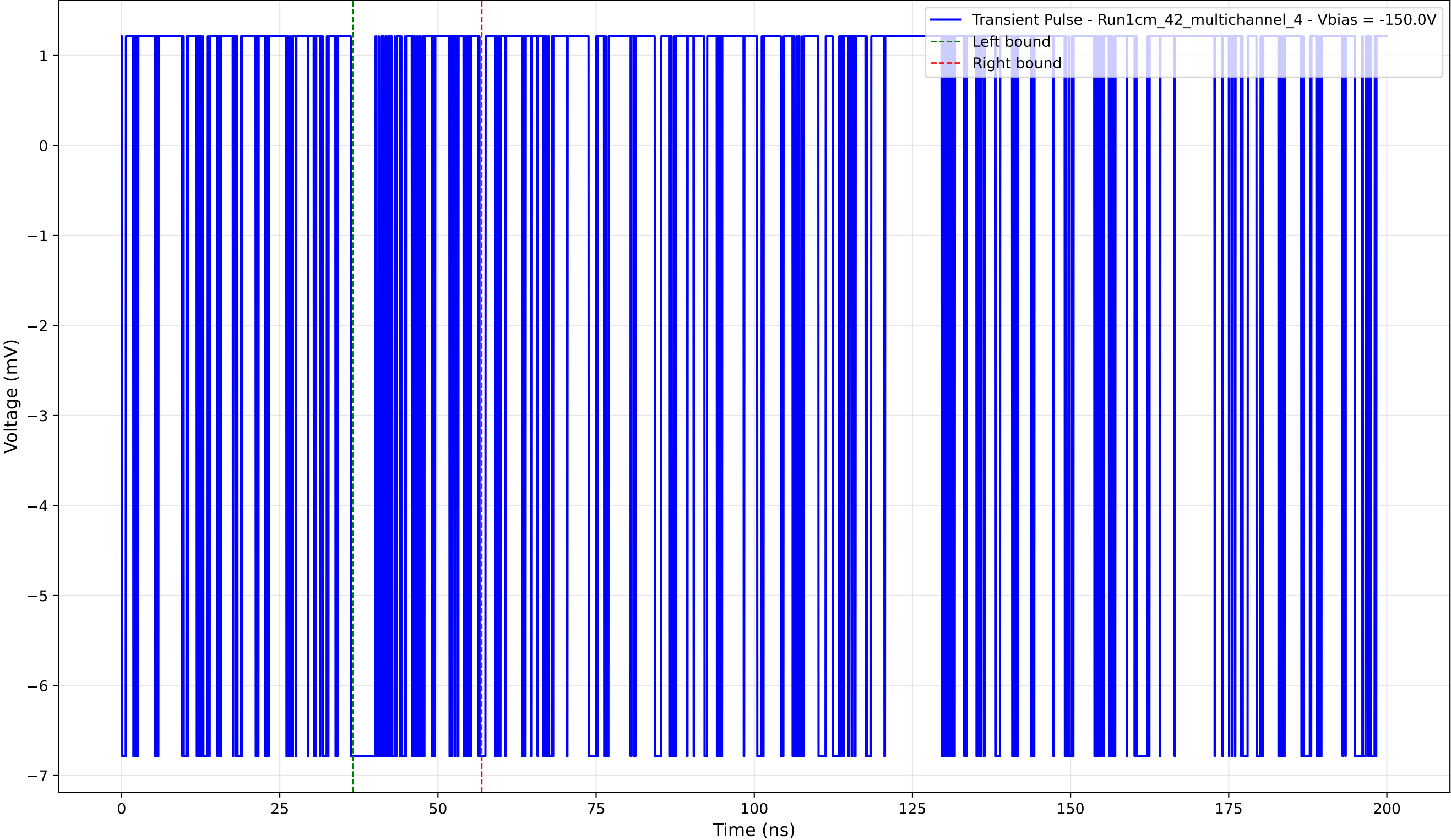
Transient Pulse - Sample: 1cm_42_multichannel - Position: 2360.0 \mu\text{m} - Charge: 1.03 pC - Rise Time: 0.00 ns (N/A)
