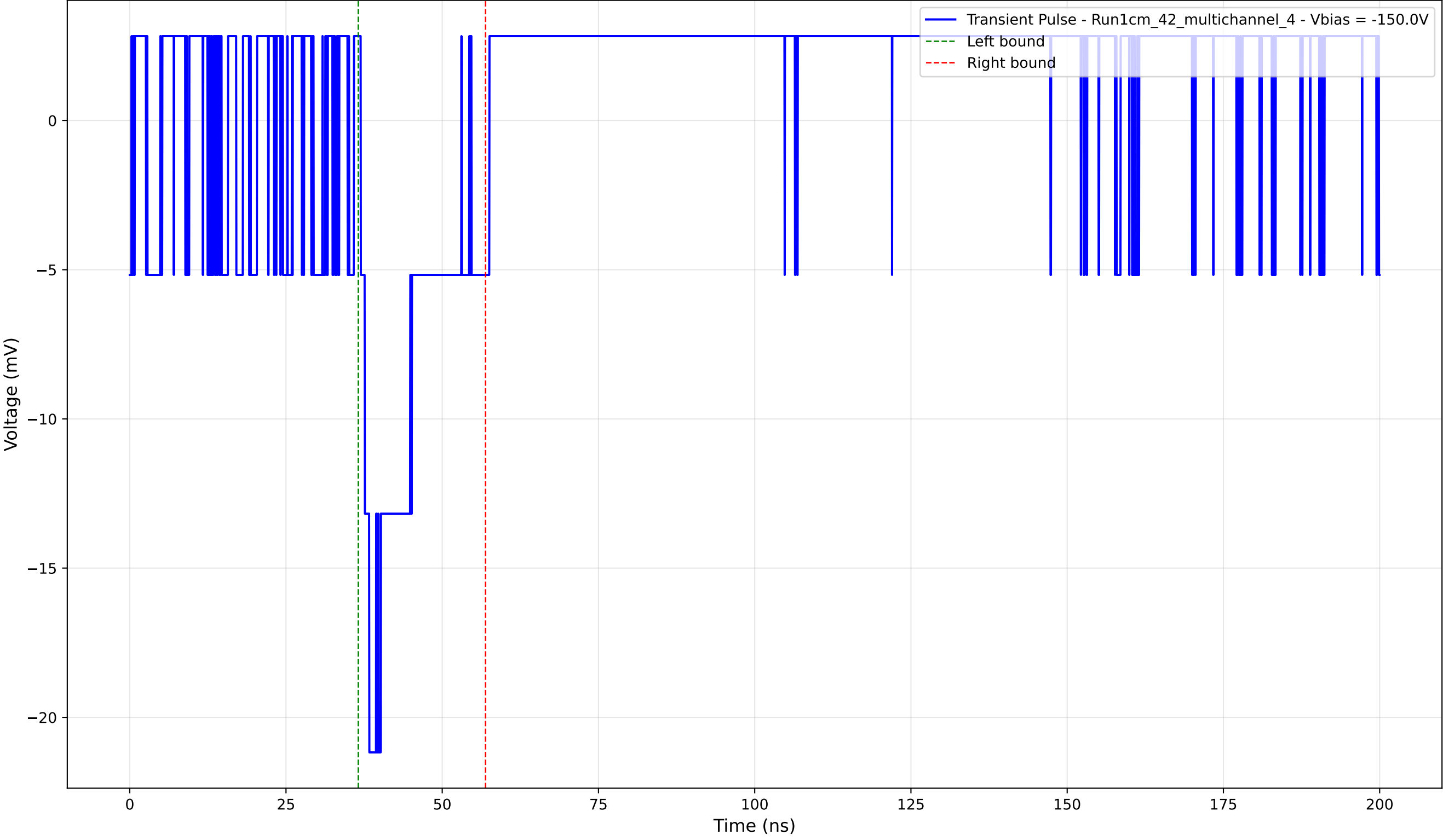
Transient Pulse - Sample: 1cm_42_multichannel - Position: 985.0 \mu\text{m} - Charge: 3.46 pC - Rise Time: 0.00 ns (N/A)
