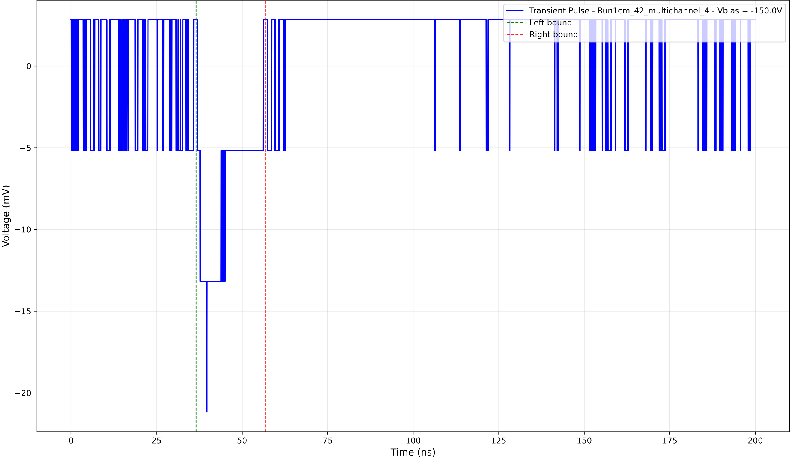
Transient Pulse - Sample: 1cm_42_multichannel - Position: 765.0 \mu\text{m} - Charge: 3.01 pC - Rise Time: 0.00 ns (N/A)
