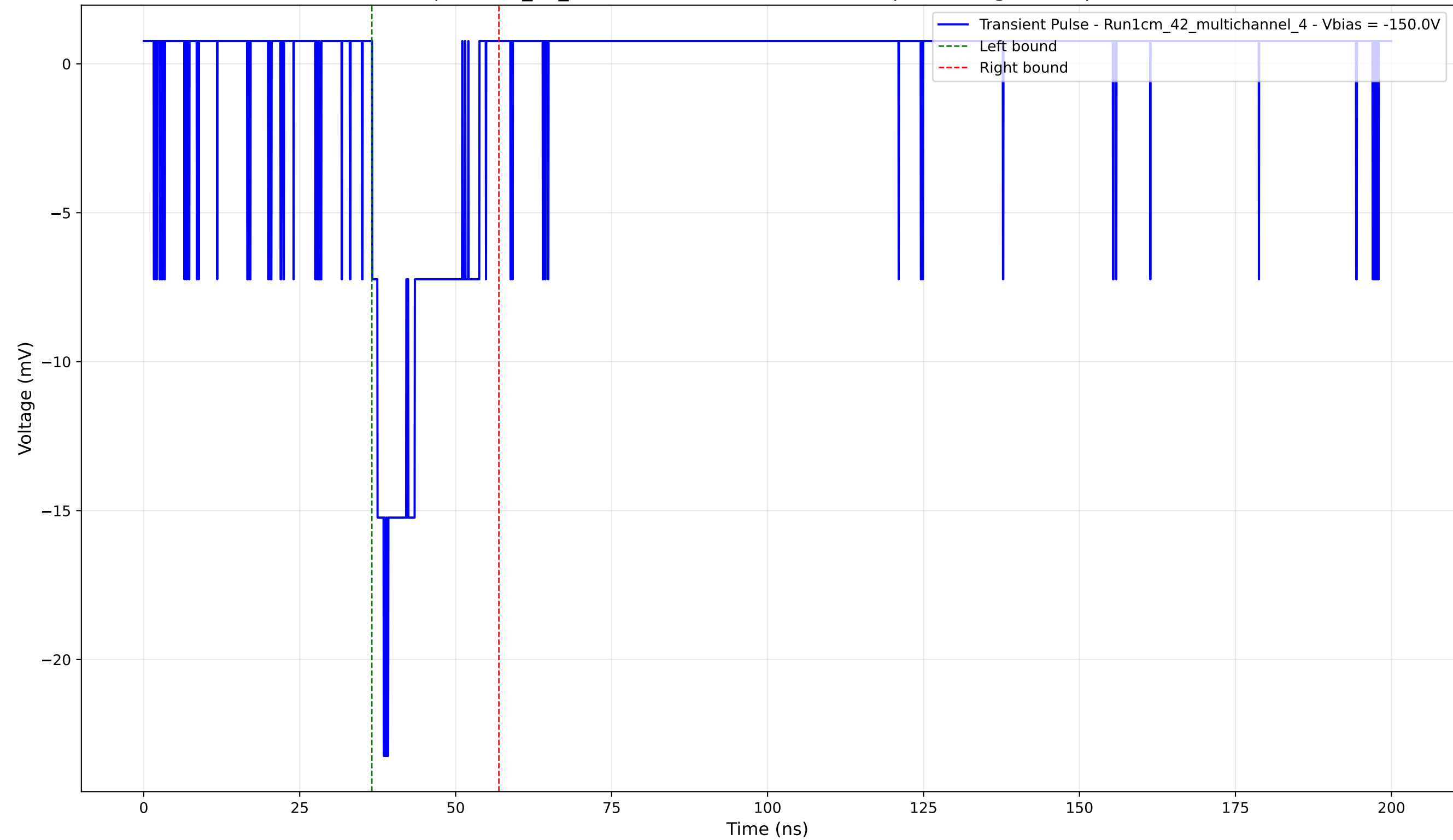
Transient Pulse - Sample: 1cm_42_multichannel - Position: 3615.0 \mu\text{m} - Charge: 3.44 pC - Rise Time: 1.86 ns
