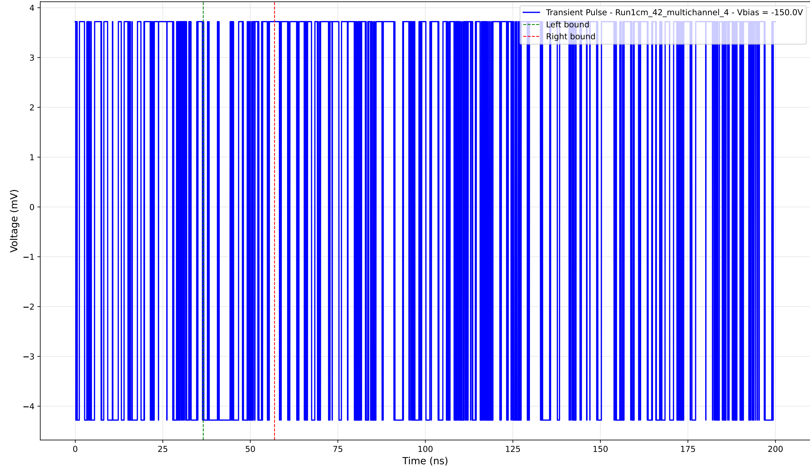
Transient Pulse - Sample: 1cm_42_multichannel - Position: 850.0 \mu\text{m} - Charge: 0.56 pC - Rise Time: 0.00 ns (N/A)
