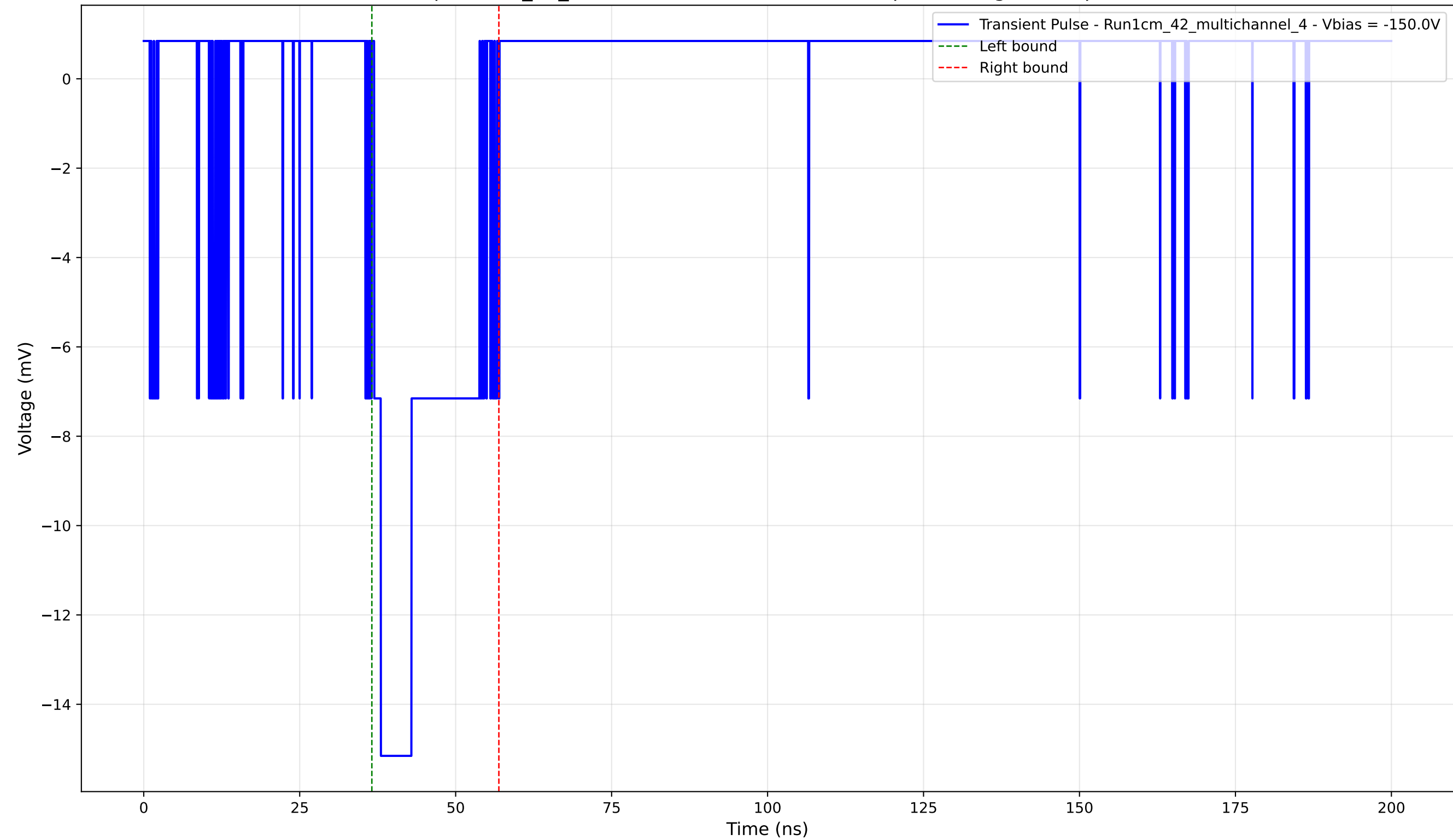
Transient Pulse - Sample: 1cm_42_multichannel - Position: 4065.0 \mu\text{m} - Charge: 3.39 pC - Rise Time: 1.08 ns
