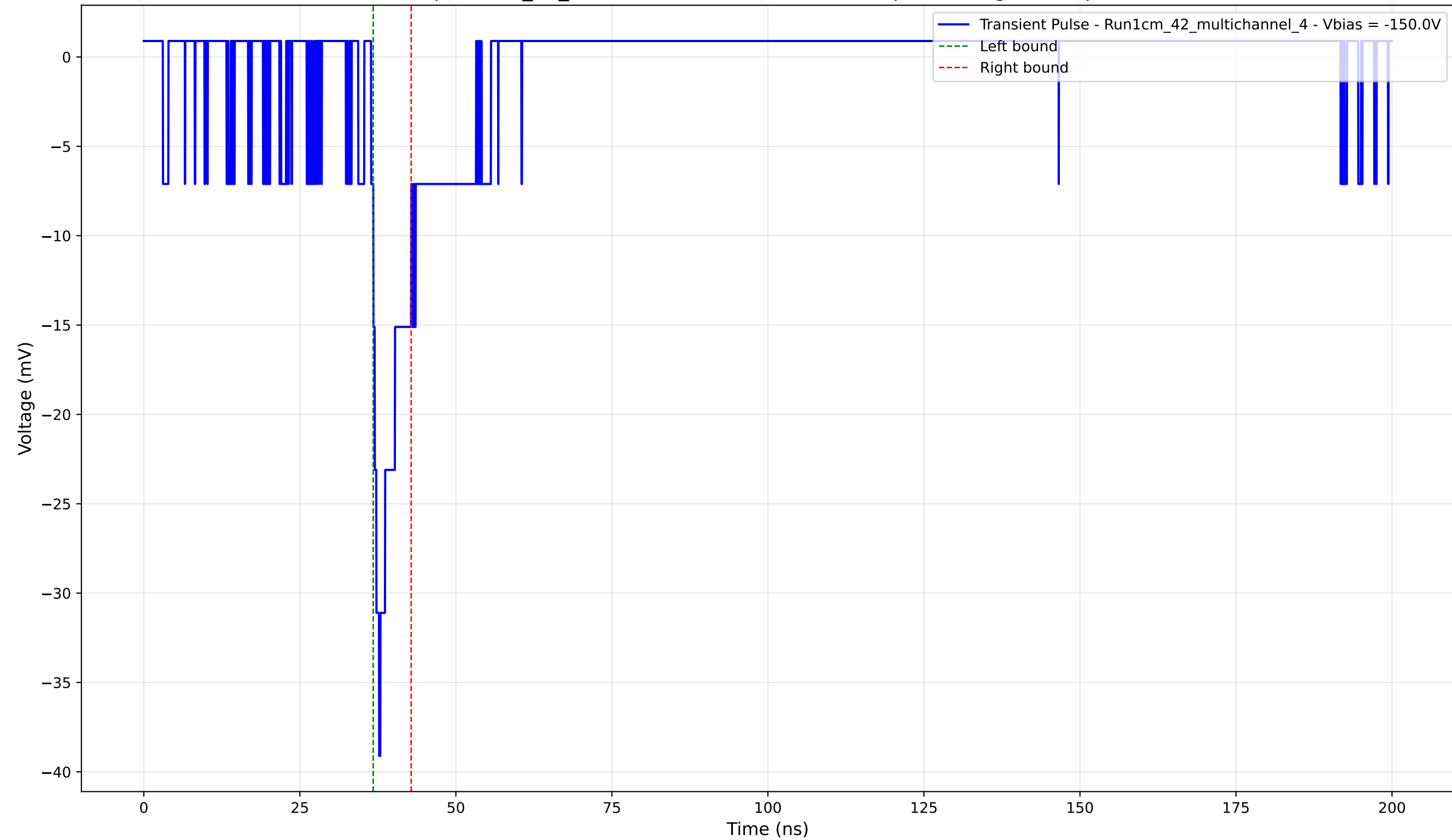
Transient Pulse - Sample: 1cm_42_multichannel - Position: 1640.0 \mu\text{m} - Charge: 2.61 pC - Rise Time: 1.29 ns
