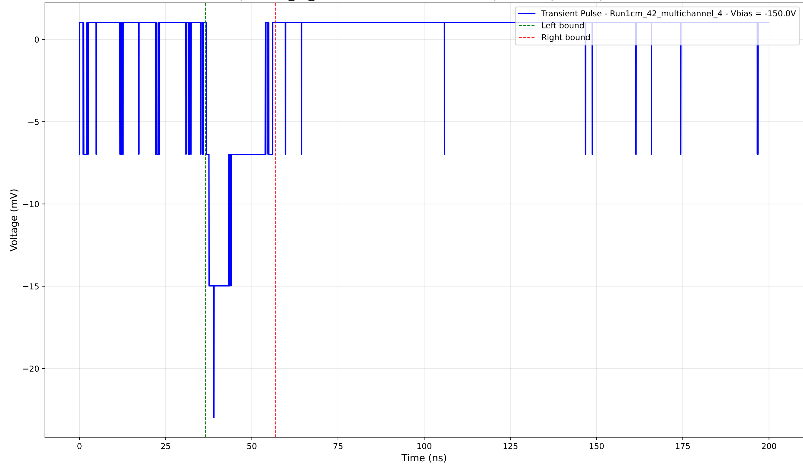
Transient Pulse - Sample: 1cm_42_multichannel - Position: 3790.0 \mu\text{m} - Charge: 3.49 pC - Rise Time: 2.18 ns
