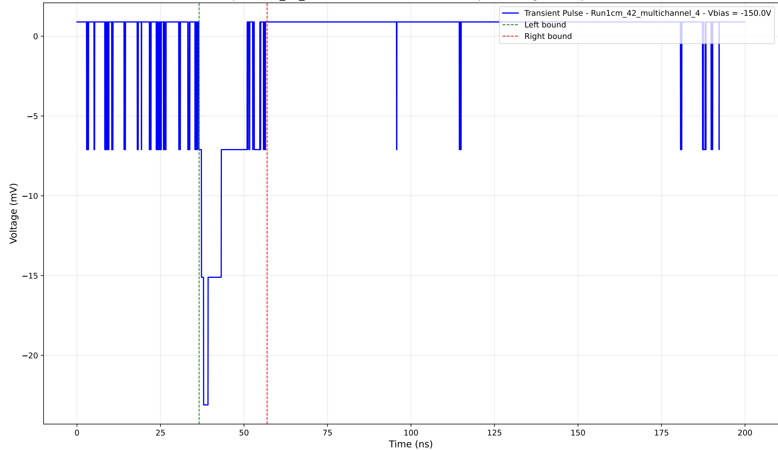
Transient Pulse - Sample: 1cm_42_multichannel - Position: 3525.0 \mu\text{m} - Charge: 3.45 pC - Rise Time: 1.42 ns
