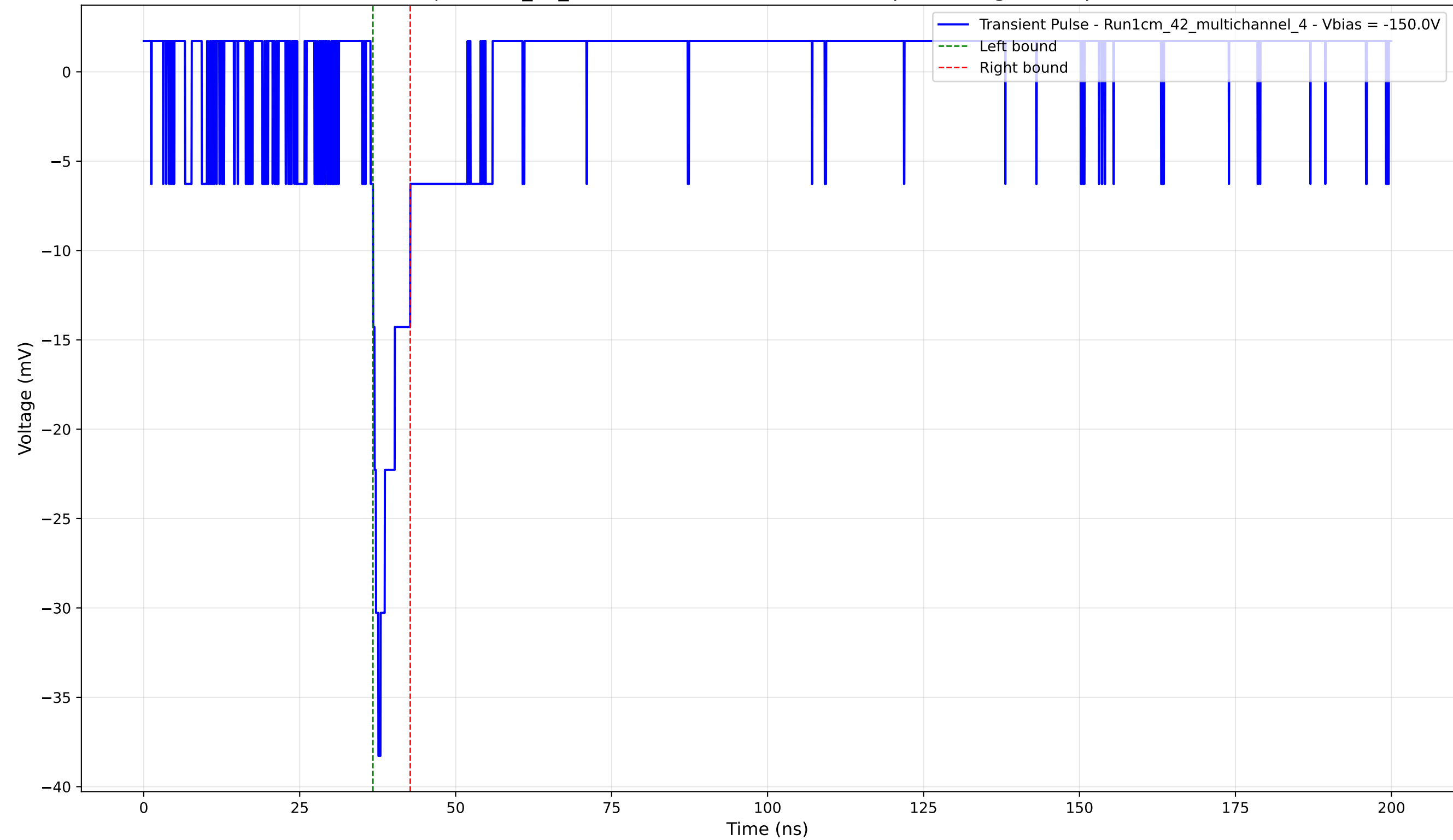
Transient Pulse - Sample: 1cm_42_multichannel - Position: 1665.0 \mu\text{m} - Charge: 2.51 pC - Rise Time: 1.25 ns
