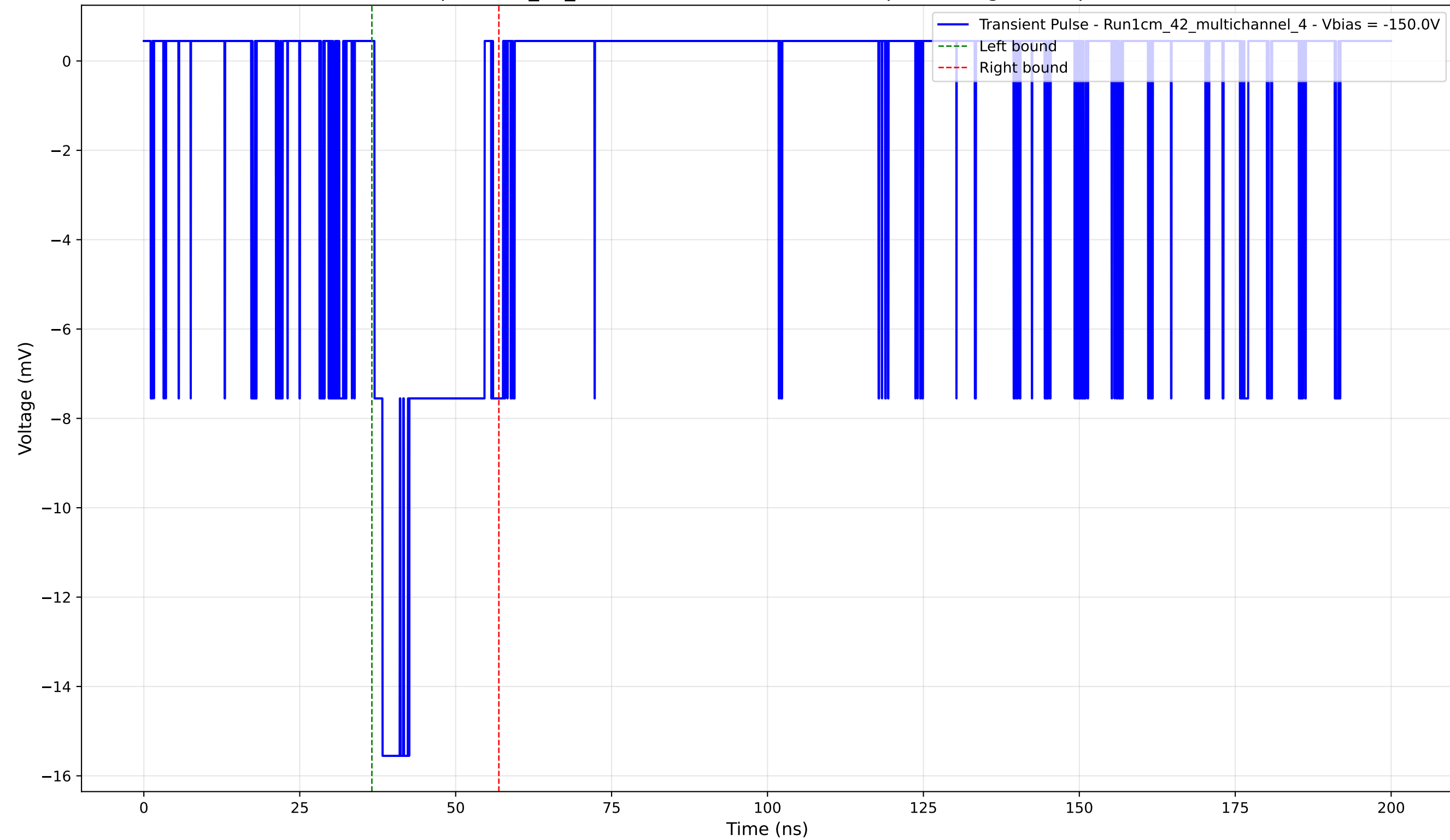
Transient Pulse - Sample: 1cm_42_multichannel - Position: 185.0 \mu\text{m} - Charge: 3.44 pC - Rise Time: 1.30 ns
