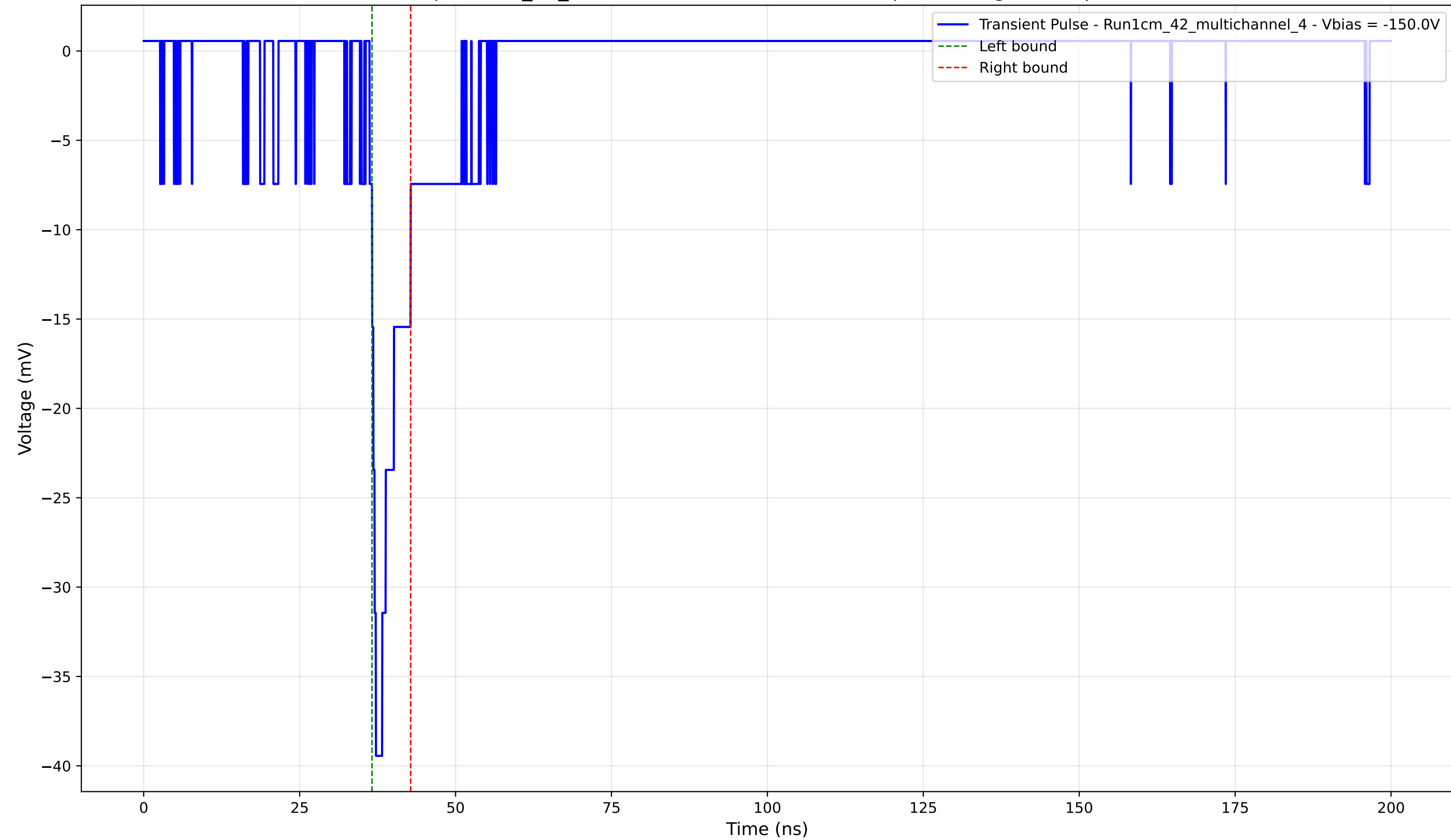
Transient Pulse - Sample: 1cm_42_multichannel - Position: 1775.0 \mu\text{m} - Charge: 2.89 pC - Rise Time: 1.01 ns
