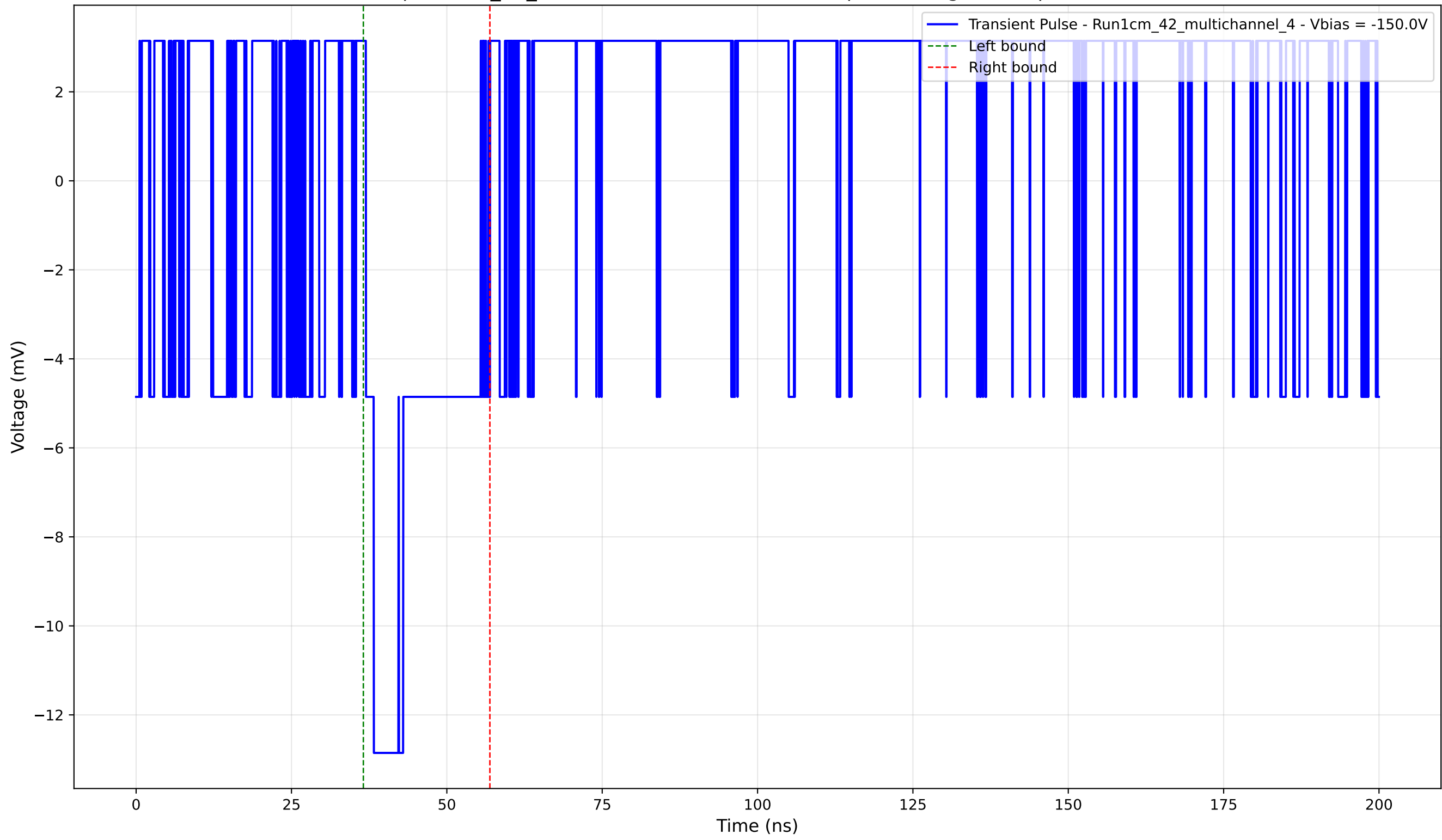
Transient Pulse - Sample: 1cm_42_multichannel - Position: 255.0 \mu\text{m} - Charge: 2.57 pC - Rise Time: 0.00 ns (N/A)
