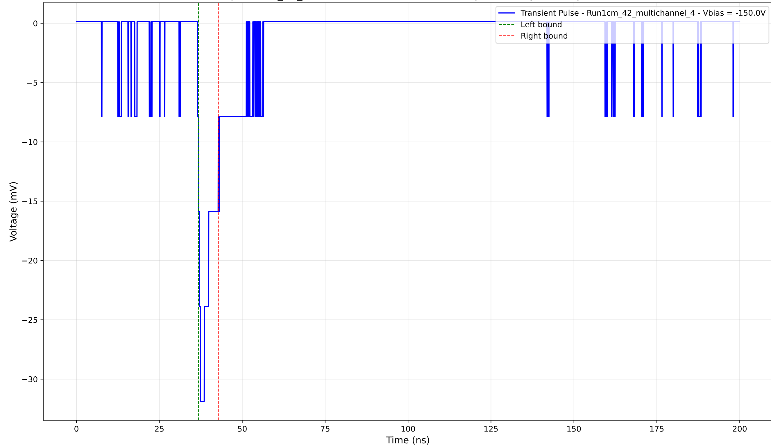
Transient Pulse - Sample: 1cm_42_multichannel - Position: 1610.0 \mu\text{m} - Charge: 2.51 pC - Rise Time: 0.91 ns
