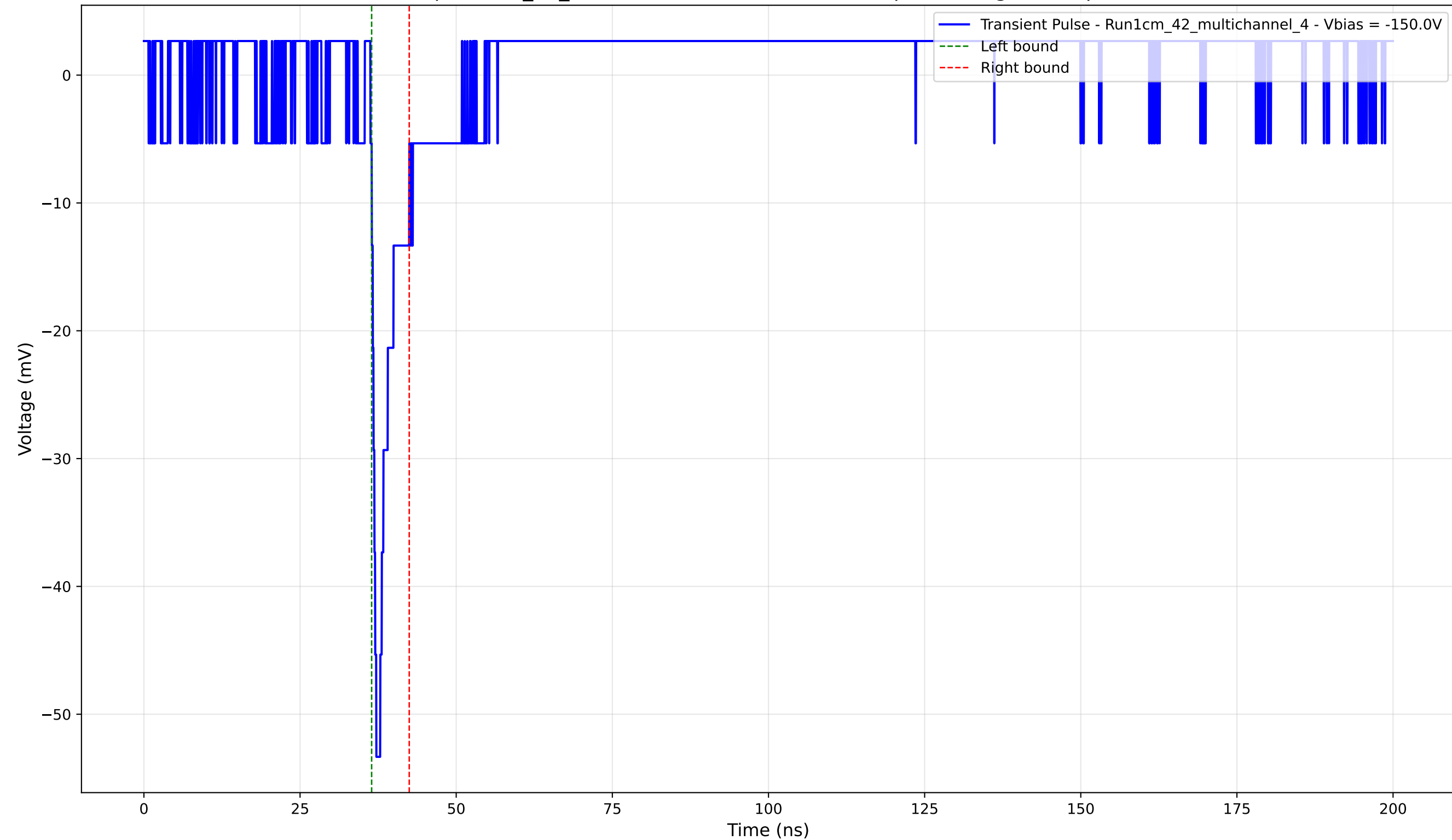
Transient Pulse - Sample: 1cm_42_multichannel - Position: 2000.0 \mu\text{m} - Charge: 3.00 pC - Rise Time: 0.74 ns
