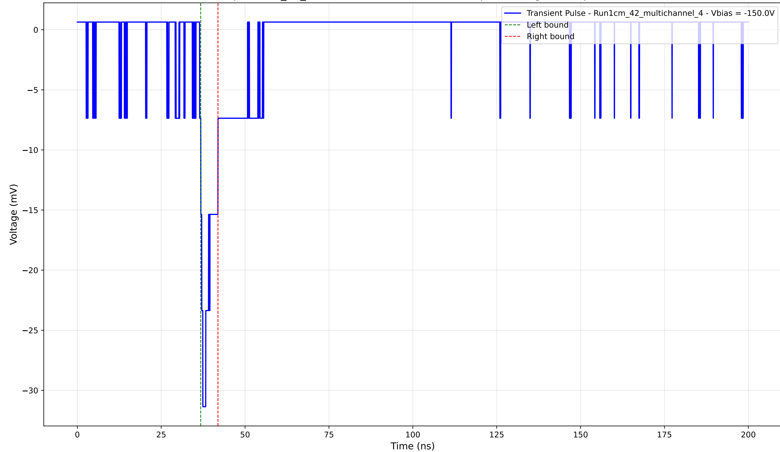
Transient Pulse - Sample: 1cm_42_multichannel - Position: 3120.0 \mu\text{m} - Charge: 2.08 pC - Rise Time: 0.95 ns
