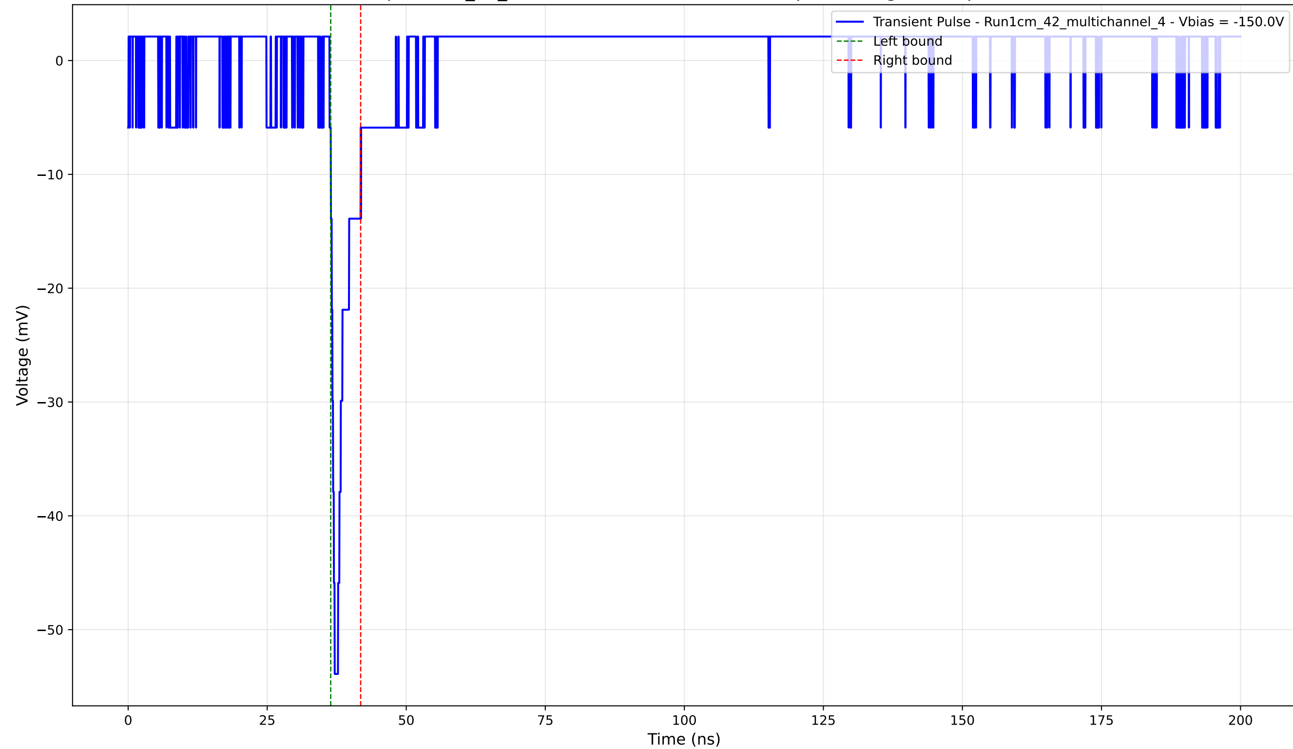
Transient Pulse - Sample: 1cm_42_multichannel - Position: 2710.0 \mu\text{m} - Charge: 2.76 pC - Rise Time: 0.92 ns
