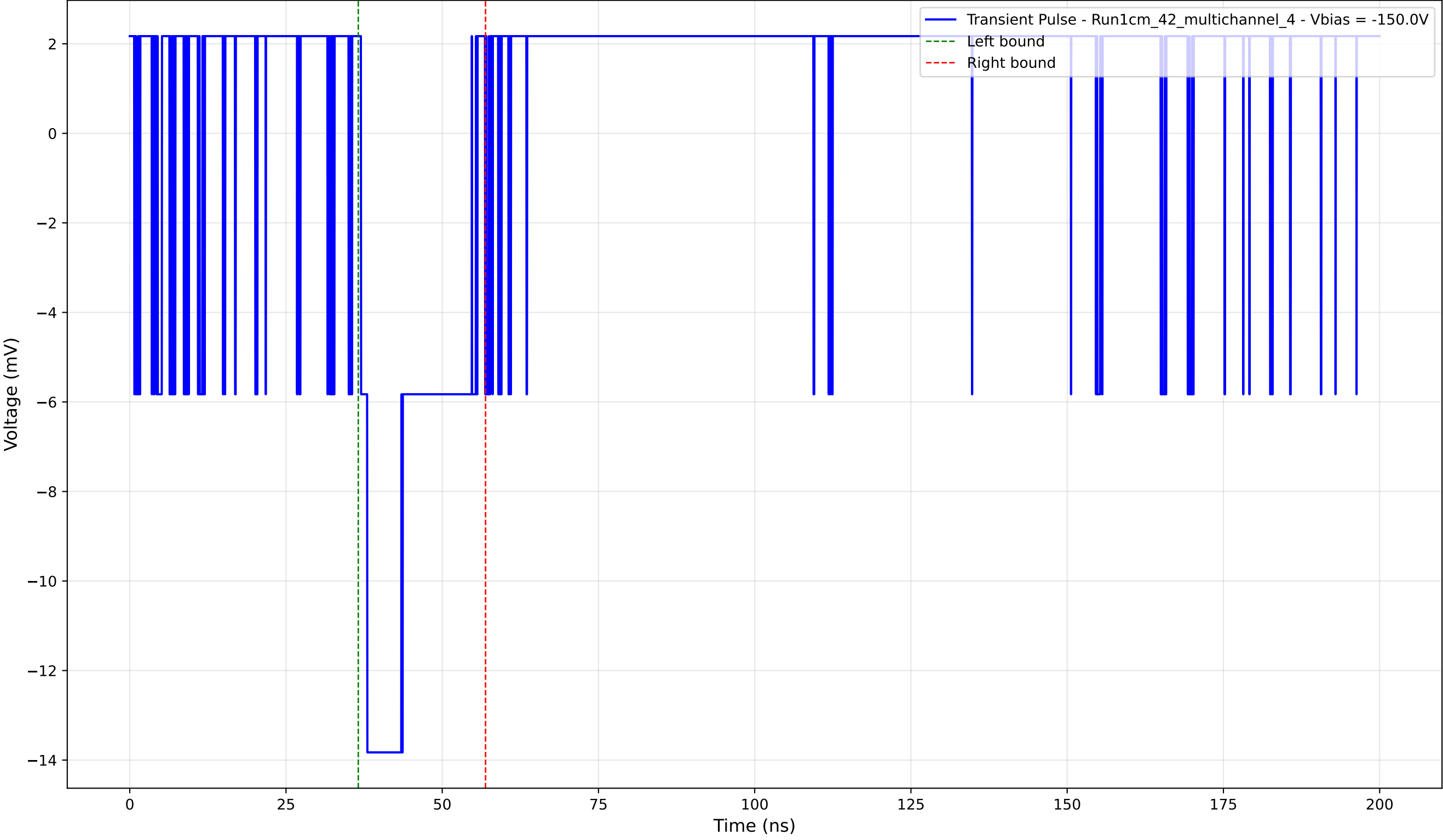
Transient Pulse - Sample: 1cm_42_multichannel - Position: 470.0 \mu\text{m} - Charge: 3.00 pC - Rise Time: 0.00 ns (N/A)
