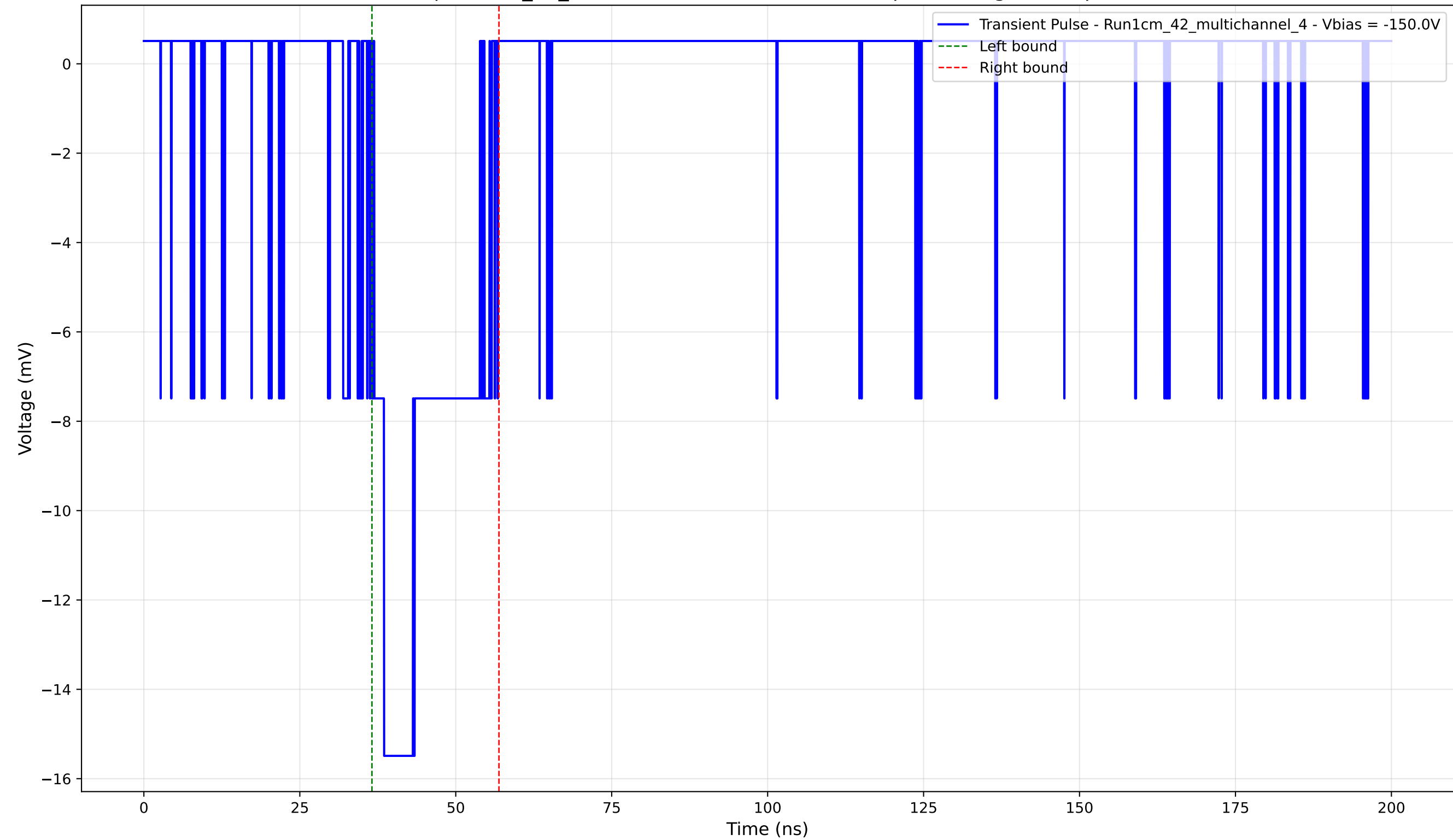
Transient Pulse - Sample: 1cm_42_multichannel - Position: 4595.0 \mu\text{m} - Charge: 3.55 pC - Rise Time: 1.58 ns
