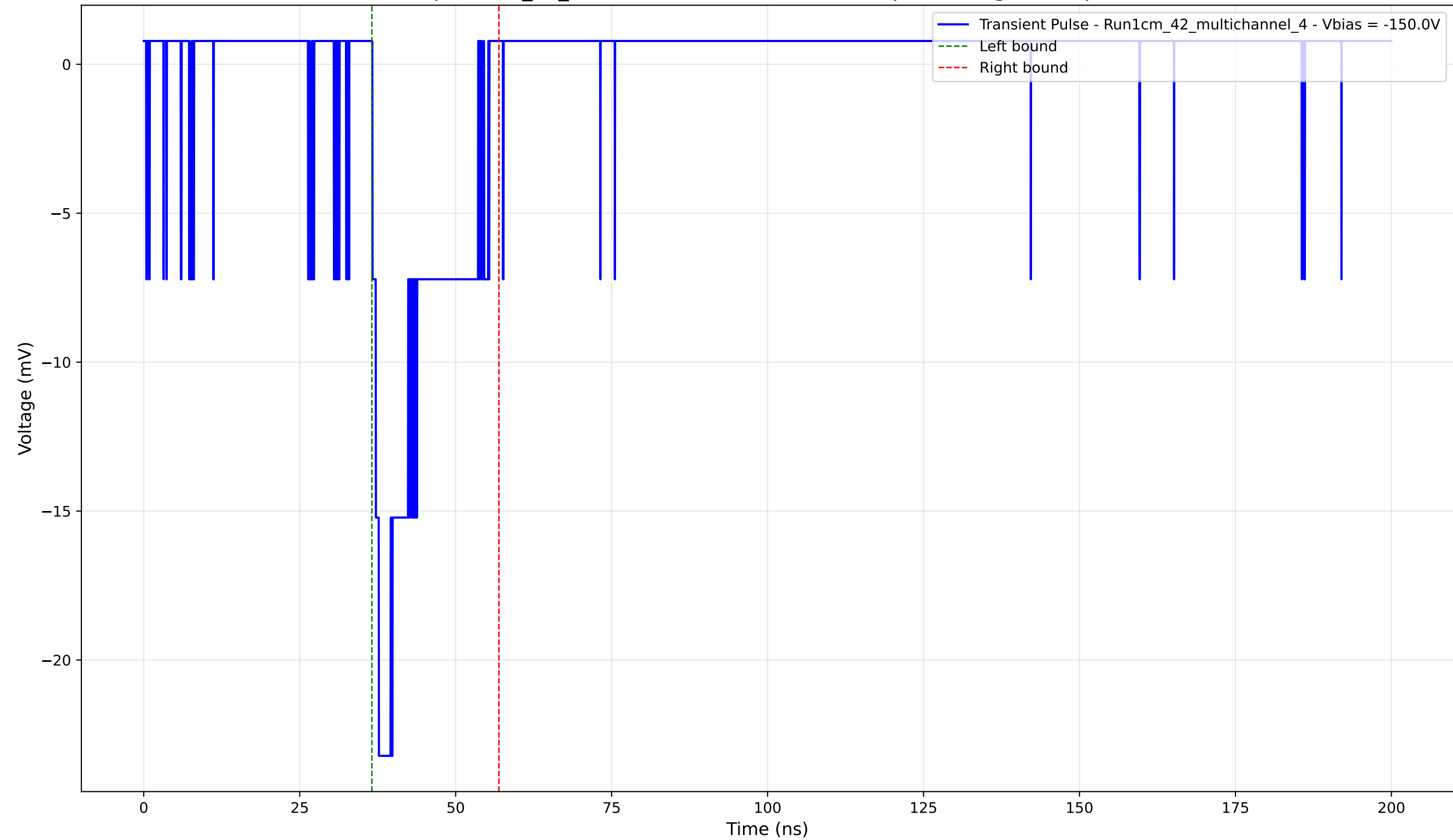
Transient Pulse - Sample: 1cm_42_multichannel - Position: 3505.0 \mu\text{m} - Charge: 3.83 pC - Rise Time: 1.04 ns
