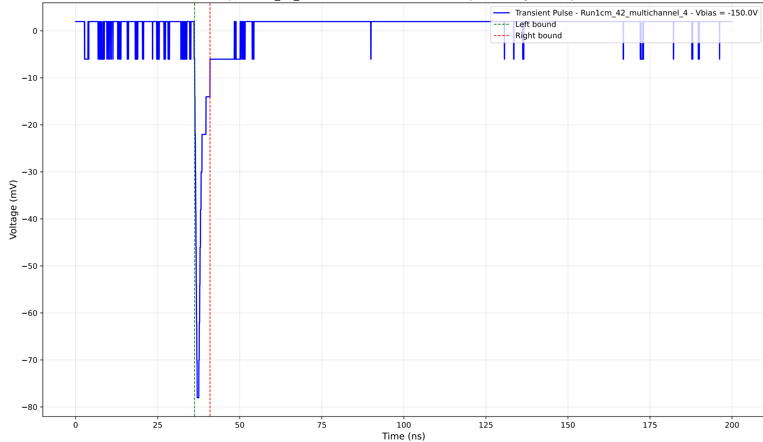
Transient Pulse - Sample: 1cm_42_multichannel - Position: 2265.0 \mu\text{m} - Charge: 3.19 pC - Rise Time: 0.76 ns
