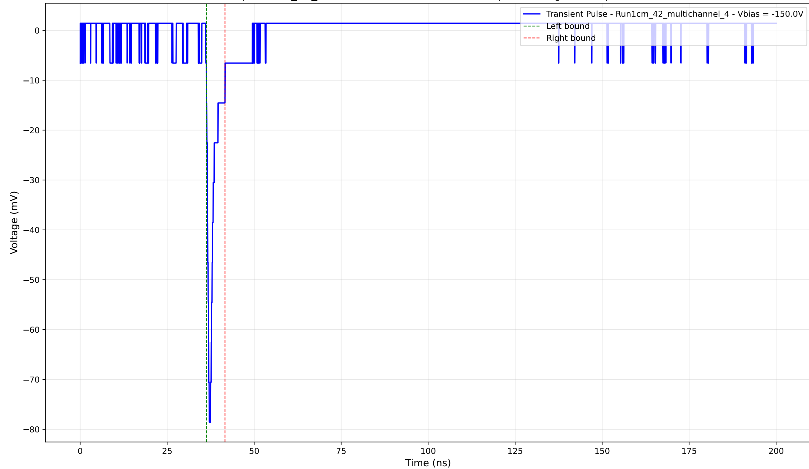
Transient Pulse - Sample: 1cm_42_multichannel - Position: 2505.0 \mu\text{m} - Charge: 3.38 pC - Rise Time: 0.80 ns
