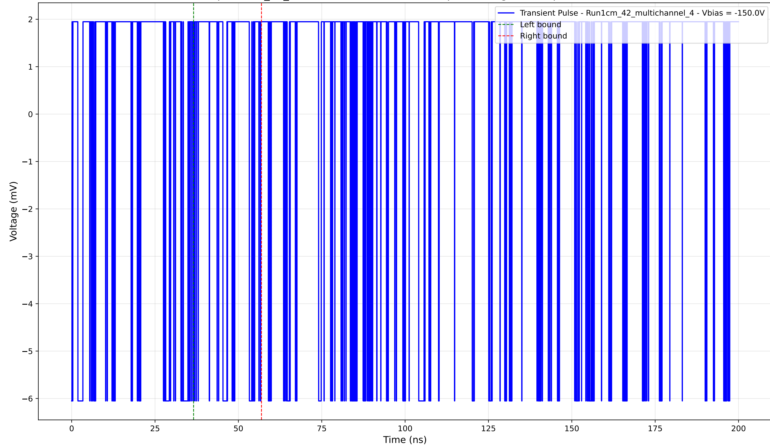
Transient Pulse - Sample: 1cm_42_multichannel - Position: 30.0 \mu\text{m} - Charge: -0.23 pC - Rise Time: 0.00 ns (N/A)
