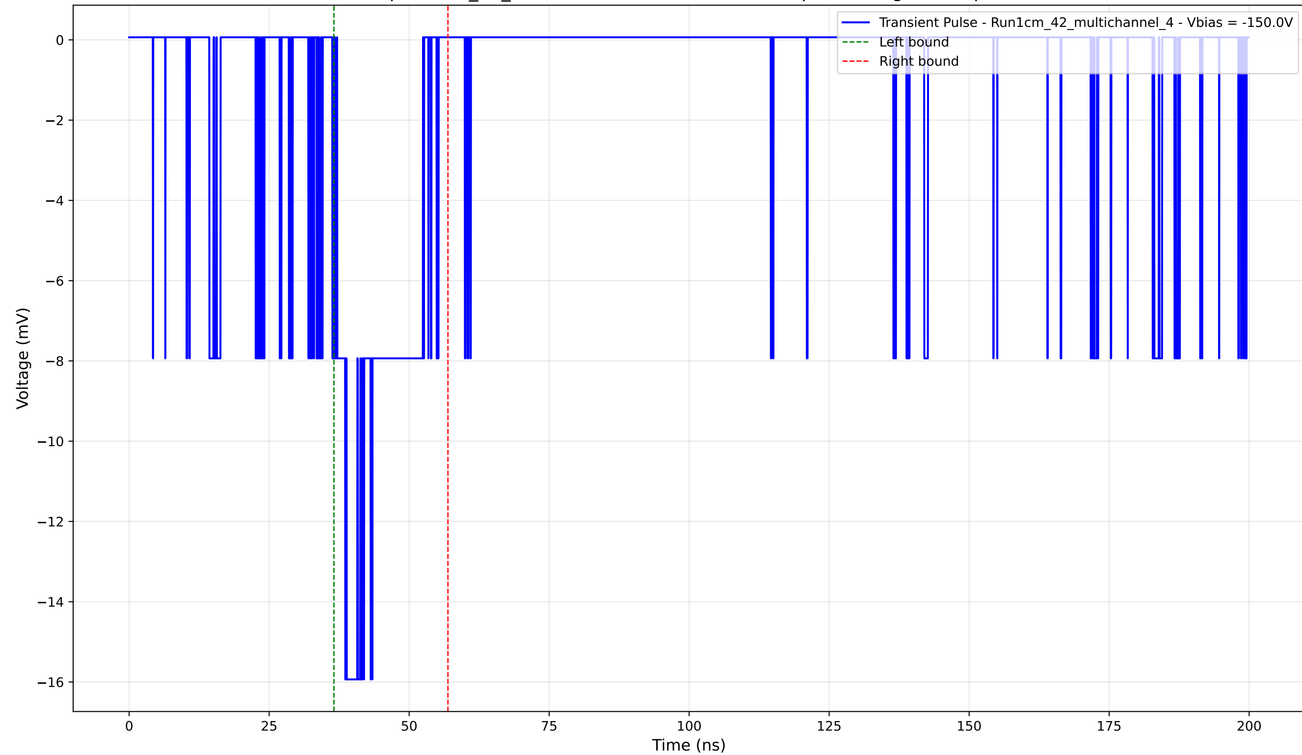
Transient Pulse - Sample: 1cm_42_multichannel - Position: 4800.0 \mu\text{m} - Charge: 3.04 pC - Rise Time: 1.44 ns
