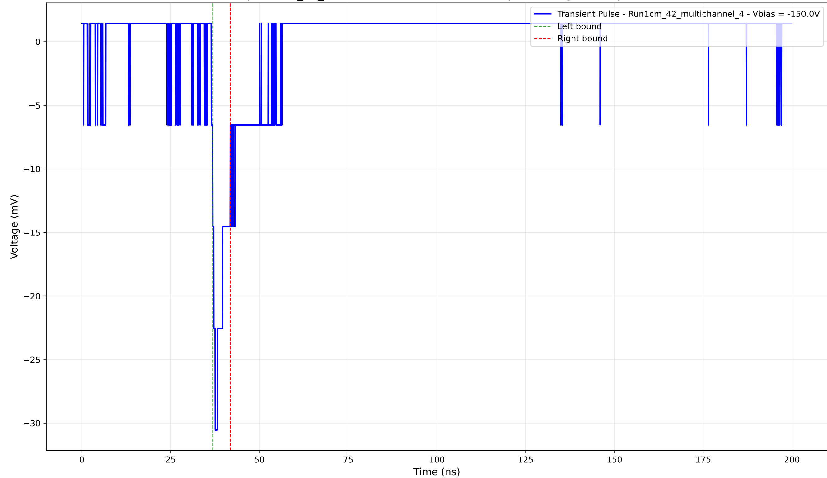
Transient Pulse - Sample: 1cm_42_multichannel - Position: 3195.0 \mu\text{m} - Charge: 1.92 pC - Rise Time: 1.11 ns
