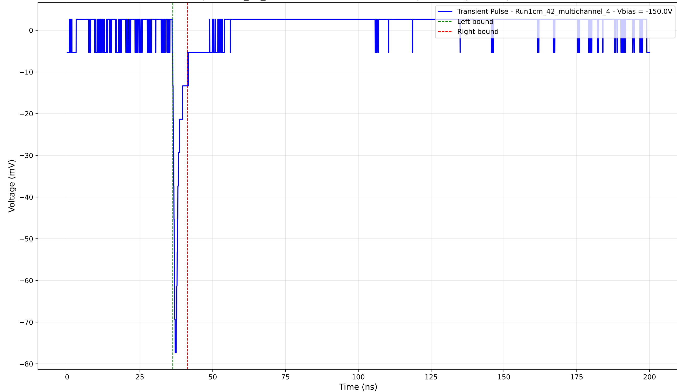
Transient Pulse - Sample: 1cm_42_multichannel - Position: 2525.0 \mu\text{m} - Charge: 3.16 pC - Rise Time: 0.81 ns
