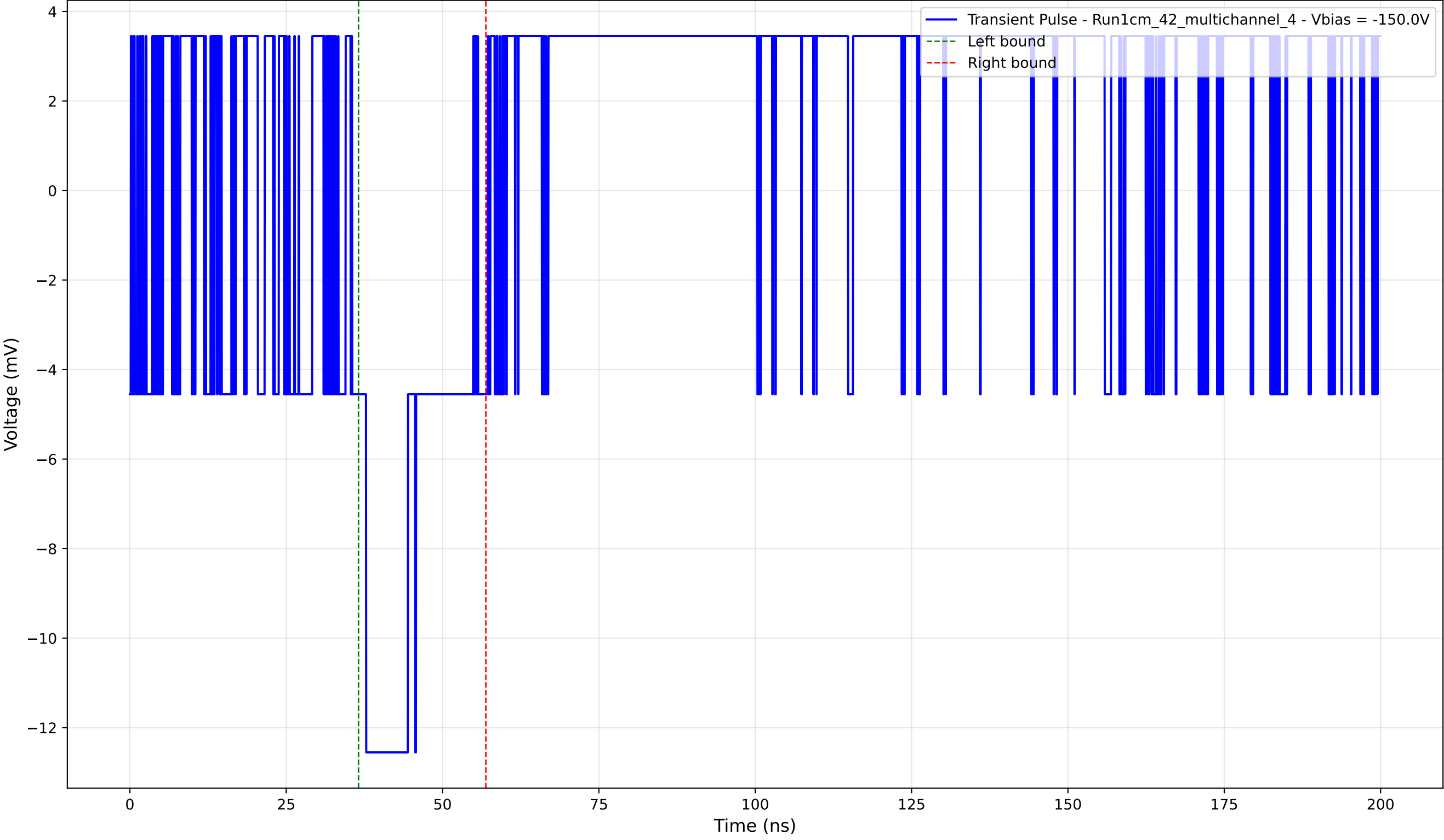
Transient Pulse - Sample: 1cm_42_multichannel - Position: 750.0 \mu\text{m} - Charge: 2.88 pC - Rise Time: 0.00 ns (N/A)
