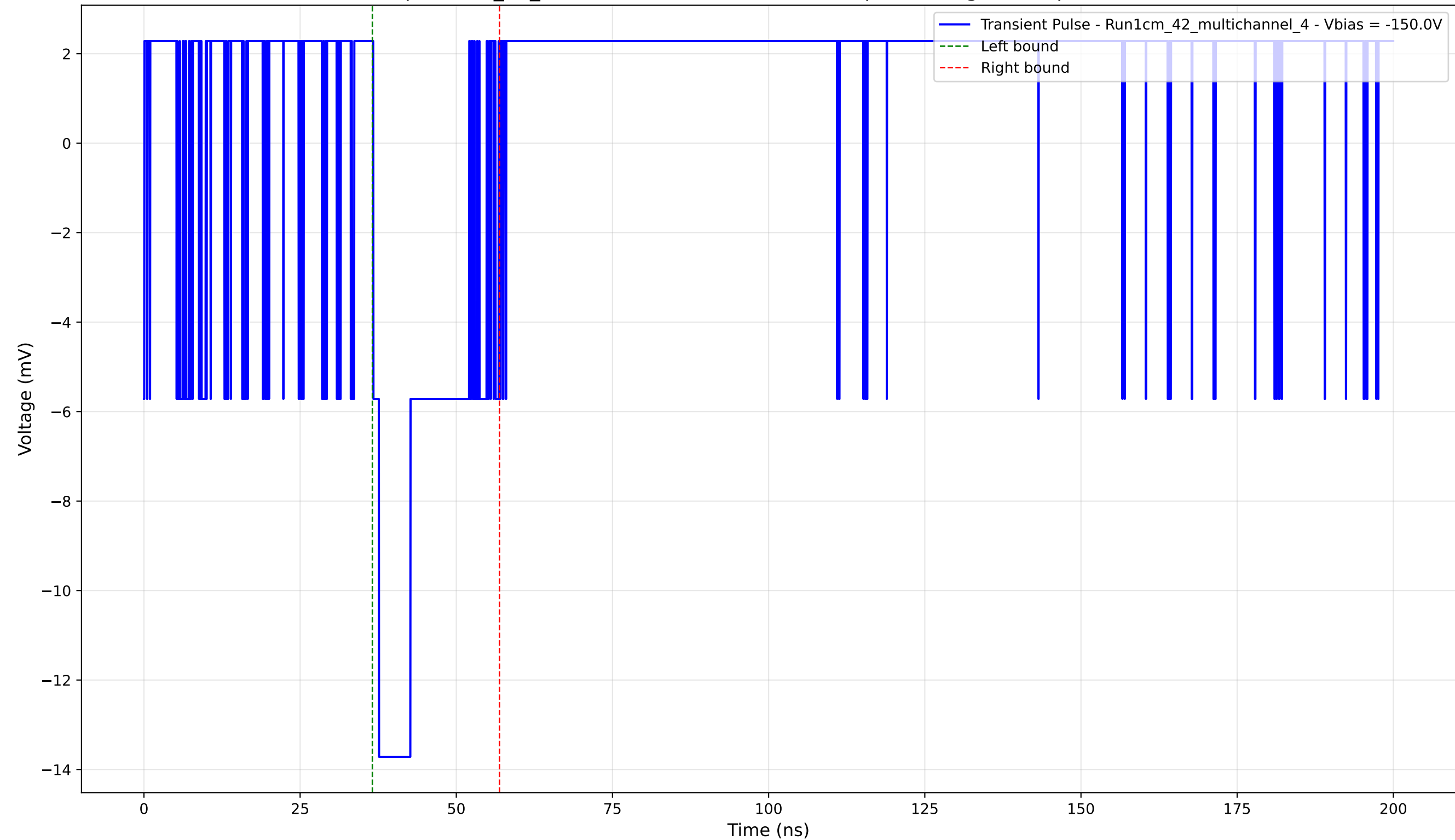
Transient Pulse - Sample: 1cm_42_multichannel - Position: 3720.0 \mu\text{m} - Charge: 2.84 pC - Rise Time: 0.00 ns (N/A)
