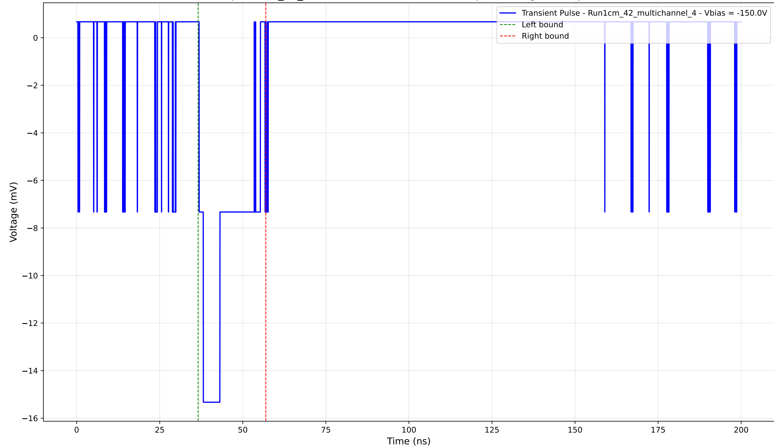
Transient Pulse - Sample: 1cm_42_multichannel - Position: 4025.0 \mu\text{m} - Charge: 3.49 pC - Rise Time: 1.28 ns
