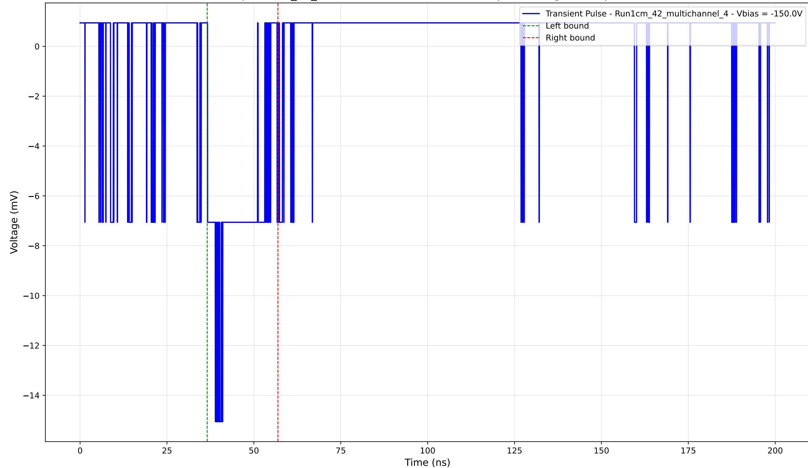
Transient Pulse - Sample: 1cm_42_multichannel - Position: 4815.0 \mu\text{m} - Charge: 2.62 pC - Rise Time: 2.24 ns
