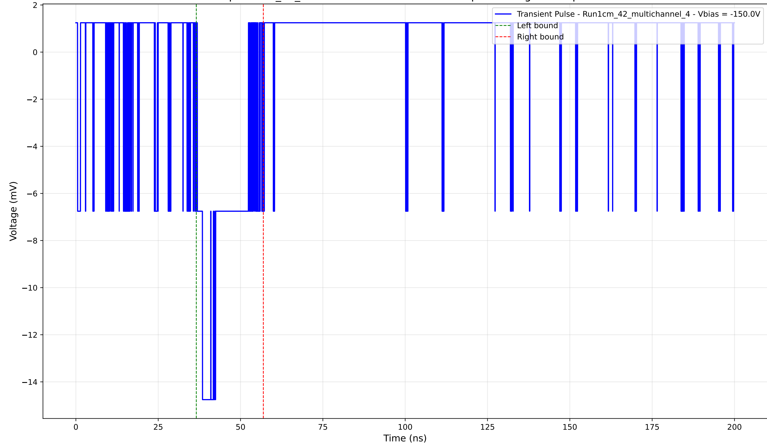
Transient Pulse - Sample: 1cm_42_multichannel - Position: 4775.0 \mu\text{m} - Charge: 2.93 pC - Rise Time: 1.58 ns
