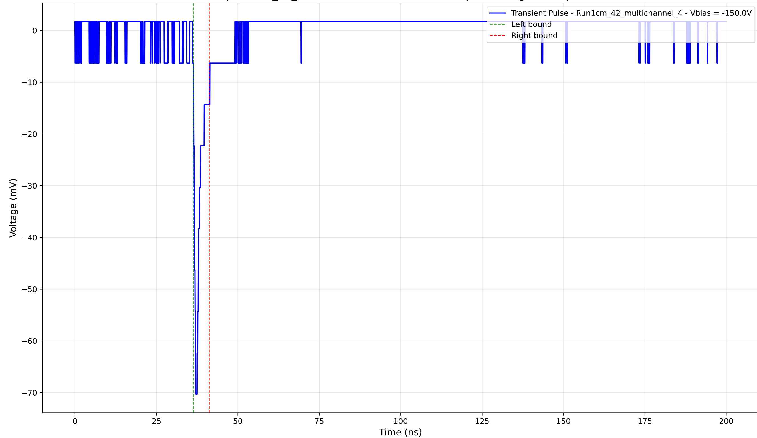
Transient Pulse - Sample: 1cm_42_multichannel - Position: 2205.0 \mu\text{m} - Charge: 3.00 pC - Rise Time: 0.80 ns
