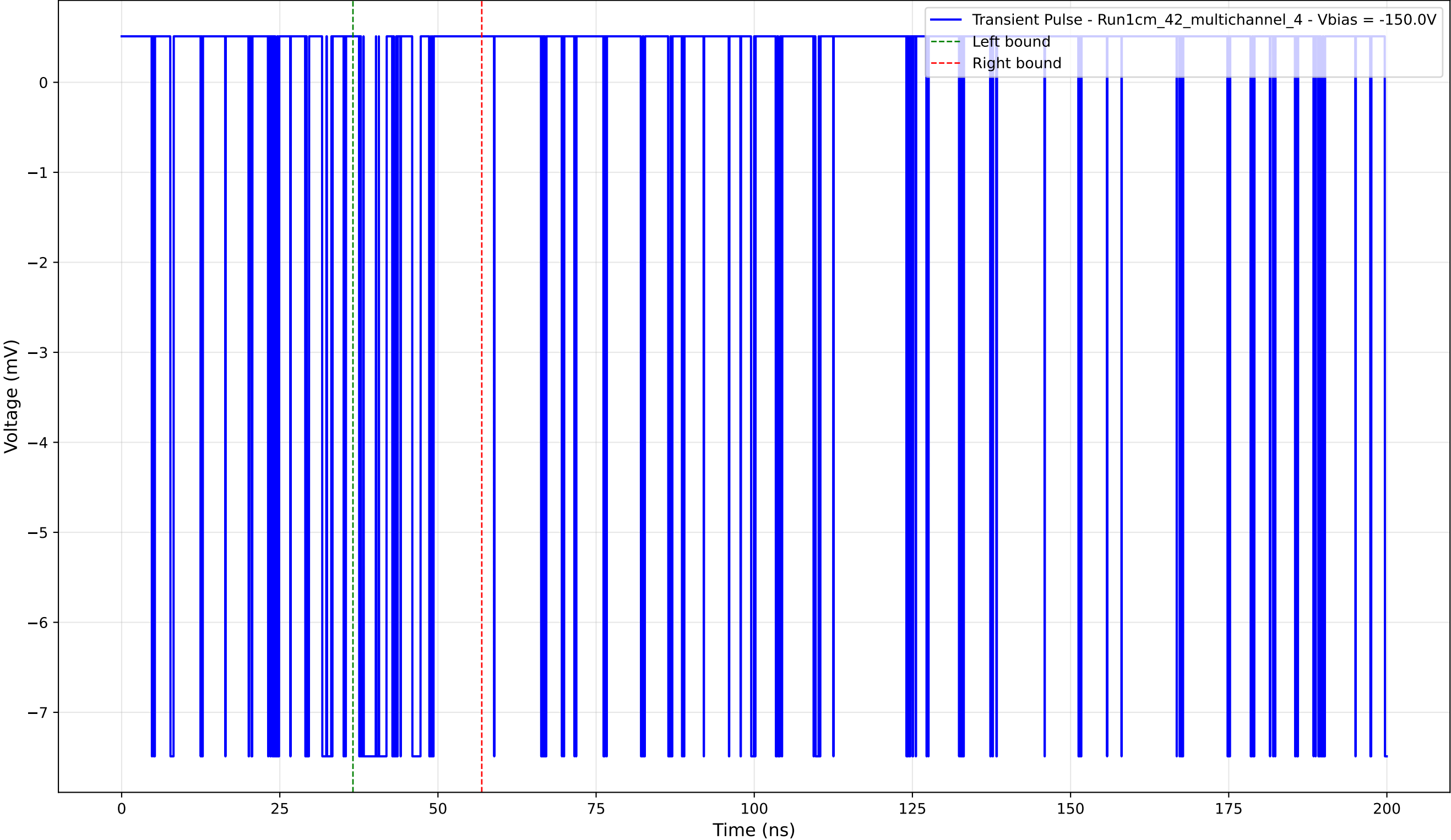
Transient Pulse - Sample: 1cm_42_multichannel - Position: 3930.0 \mu\text{m} - Charge: 0.84 pC - Rise Time: 0.02 ns
