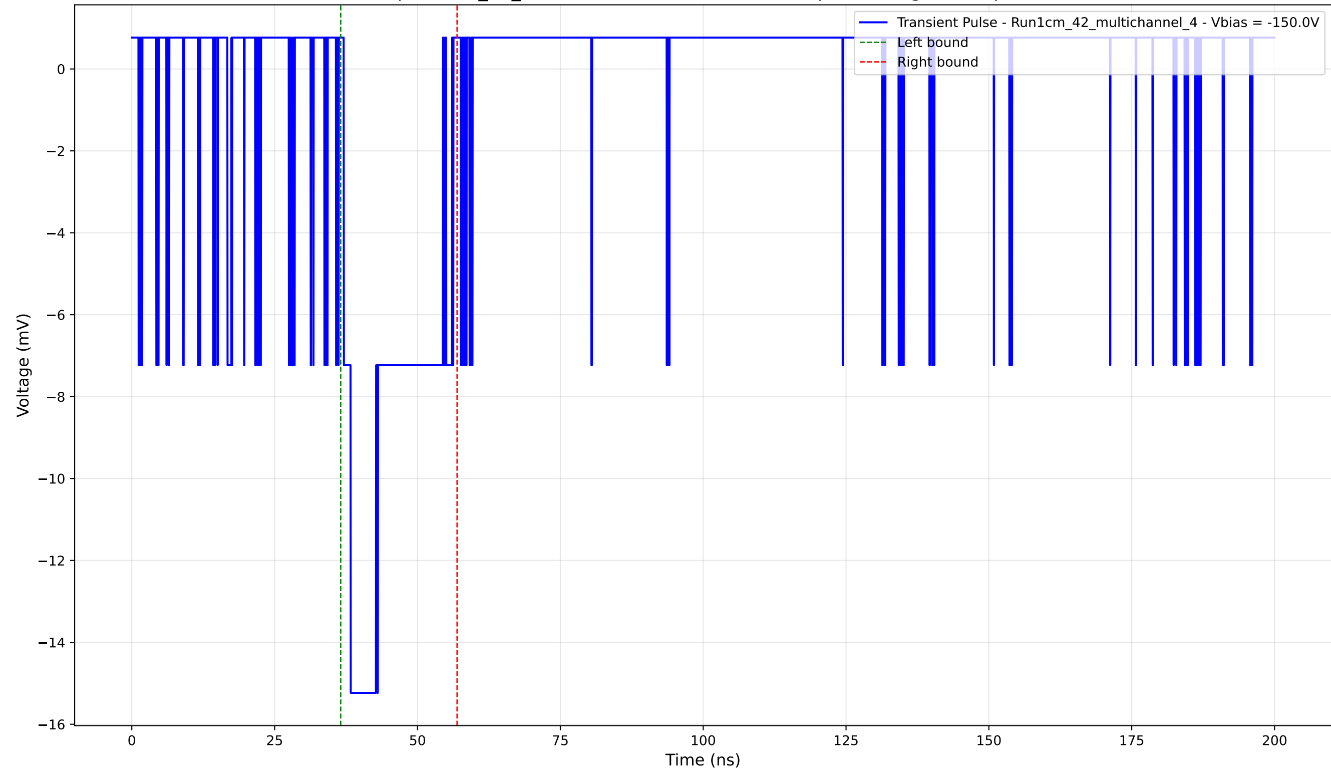
Transient Pulse - Sample: 1cm_42_multichannel - Position: 4630.0 \mu\text{m} - Charge: 3.41 pC - Rise Time: 1.22 ns
