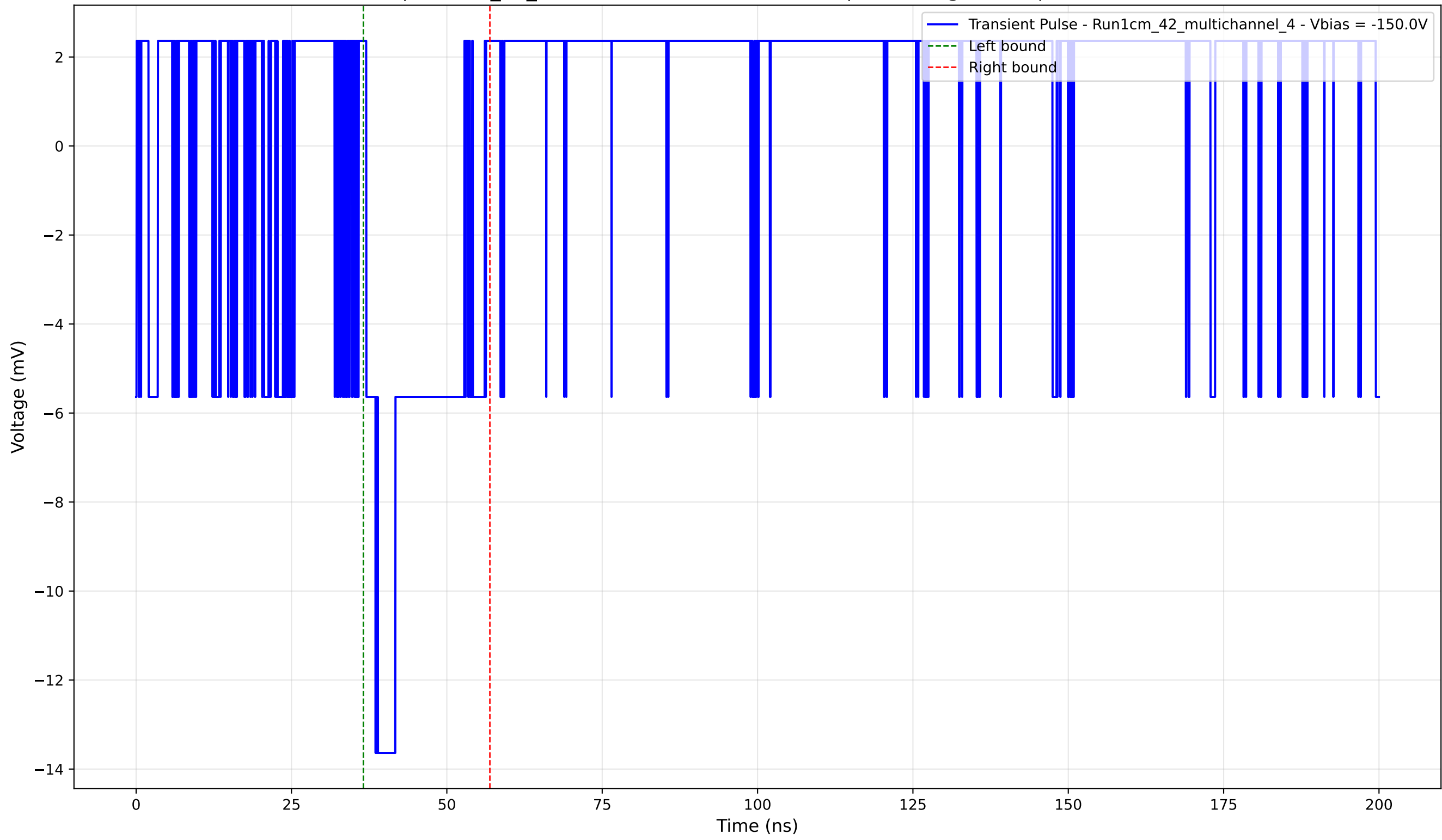
Transient Pulse - Sample: 1cm_42_multichannel - Position: 195.0 \mu\text{m} - Charge: 2.45 pC - Rise Time: 0.00 ns (N/A)
