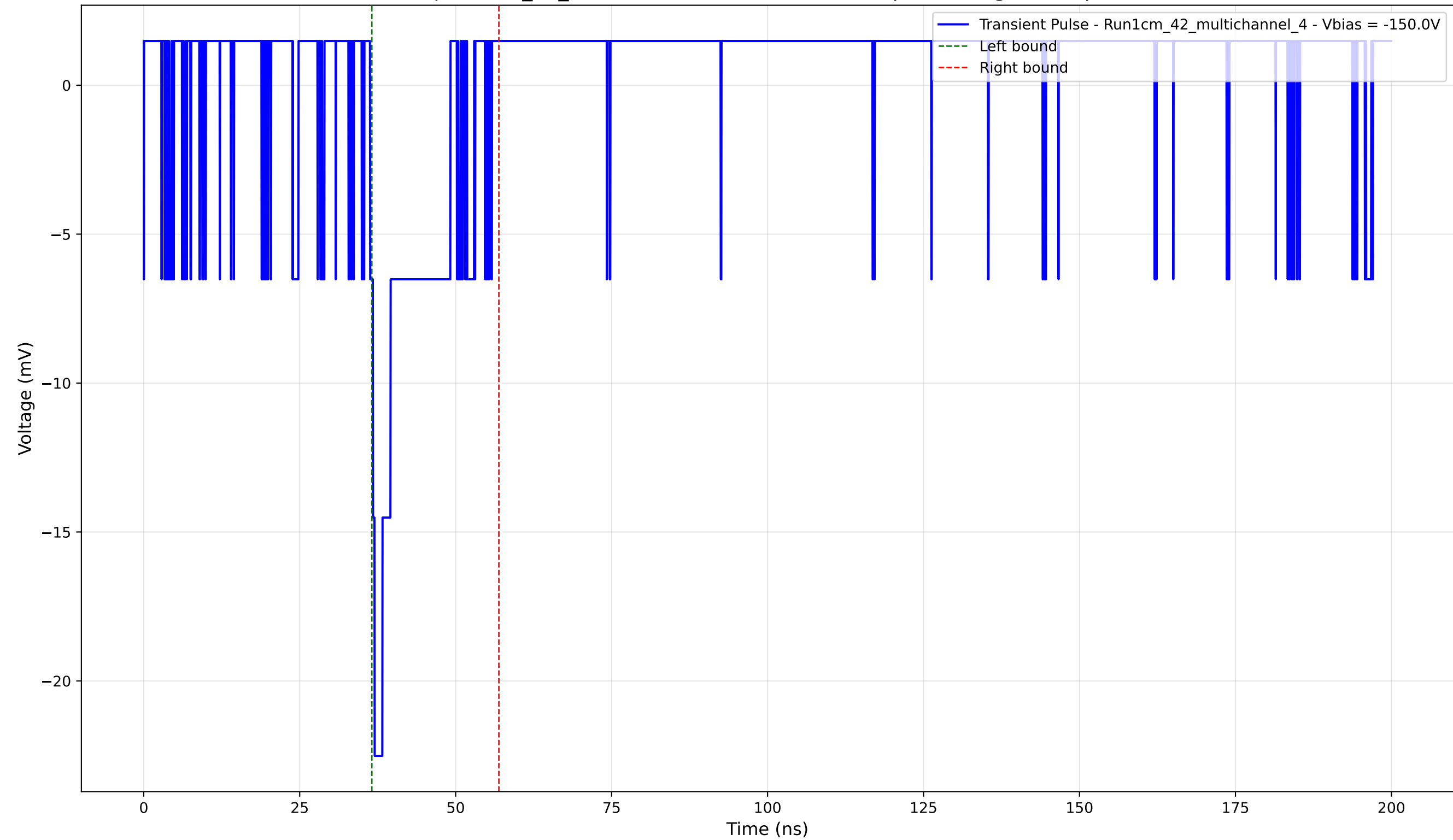
Transient Pulse - Sample: 1cm_42_multichannel - Position: 2840.0 \mu\text{m} - Charge: 2.47 pC - Rise Time: 0.74 ns
