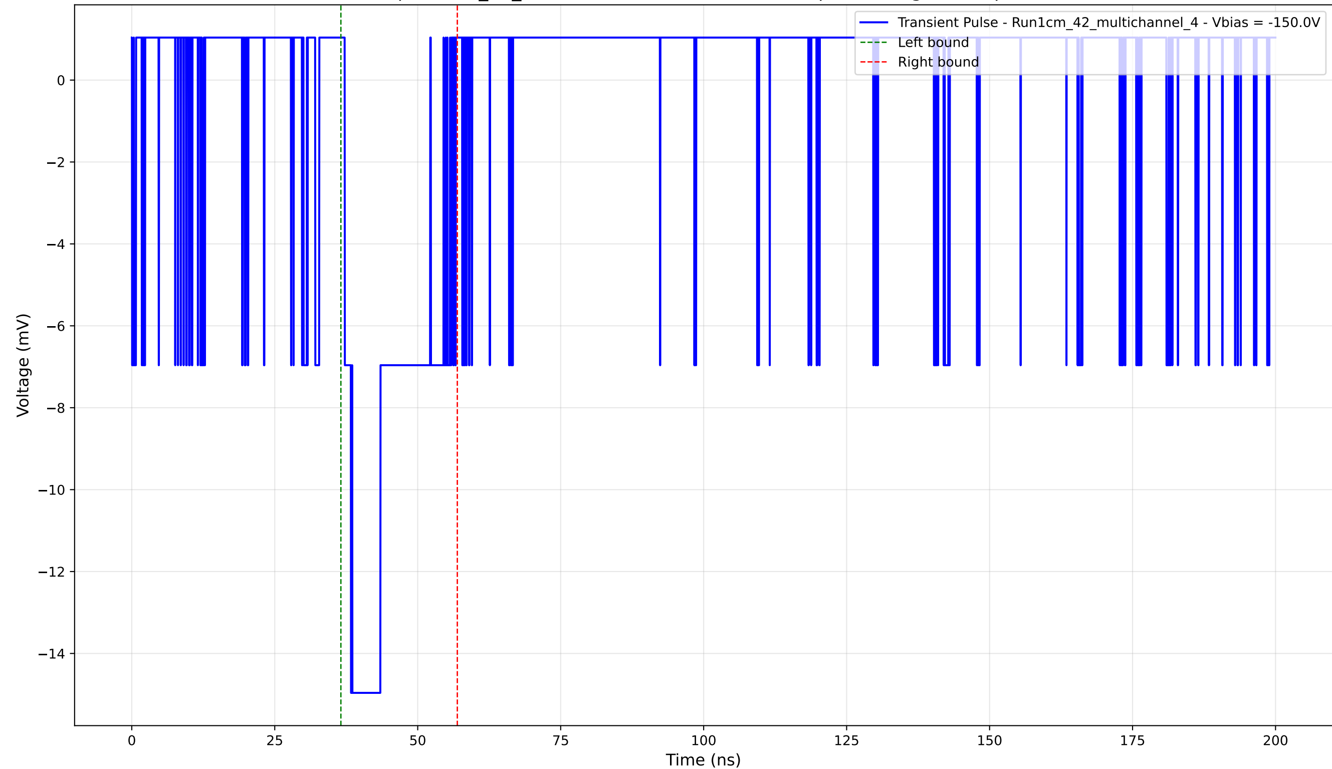
Transient Pulse - Sample: 1cm_42_multichannel - Position: 4580.0 \mu\text{m} - Charge: 3.38 pC - Rise Time: 1.10 ns
