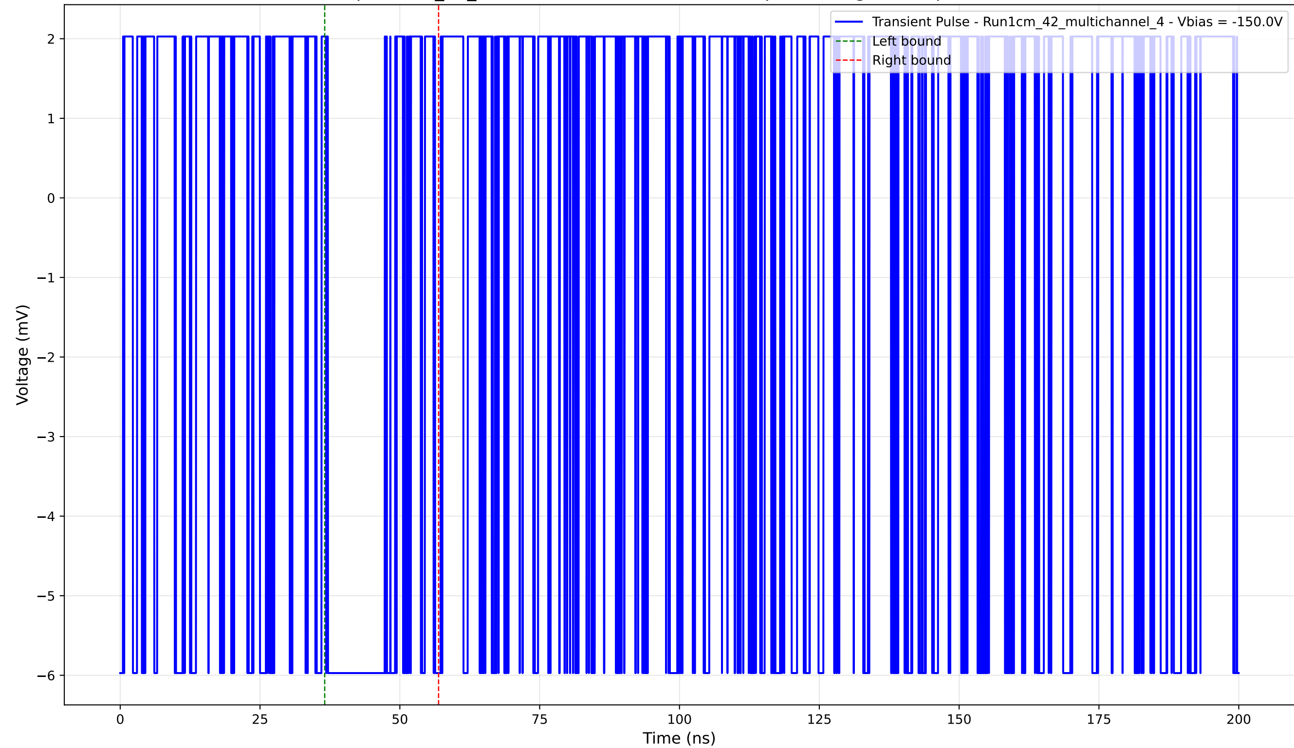
Transient Pulse - Sample: 1cm_42_multichannel - Position: 1340.0 \mu\text{m} - Charge: 1.47 pC - Rise Time: 0.00 ns (N/A)
