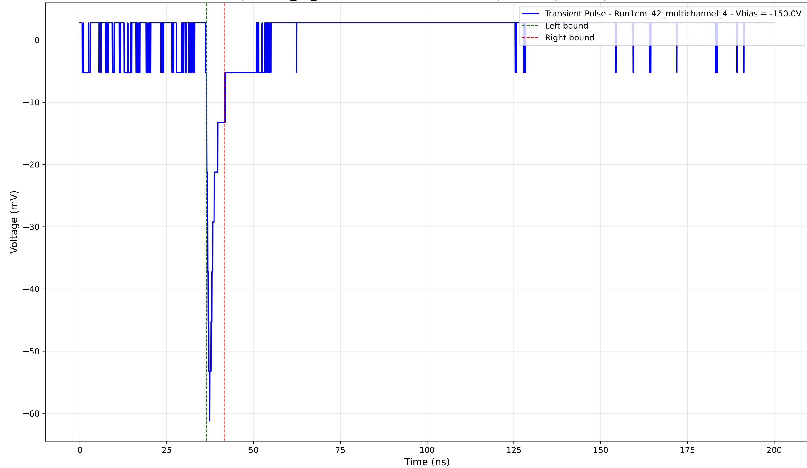
Transient Pulse - Sample: 1cm_42_multichannel - Position: 2065.0 \mu\text{m} - Charge: 2.69 pC - Rise Time: 0.98 ns
