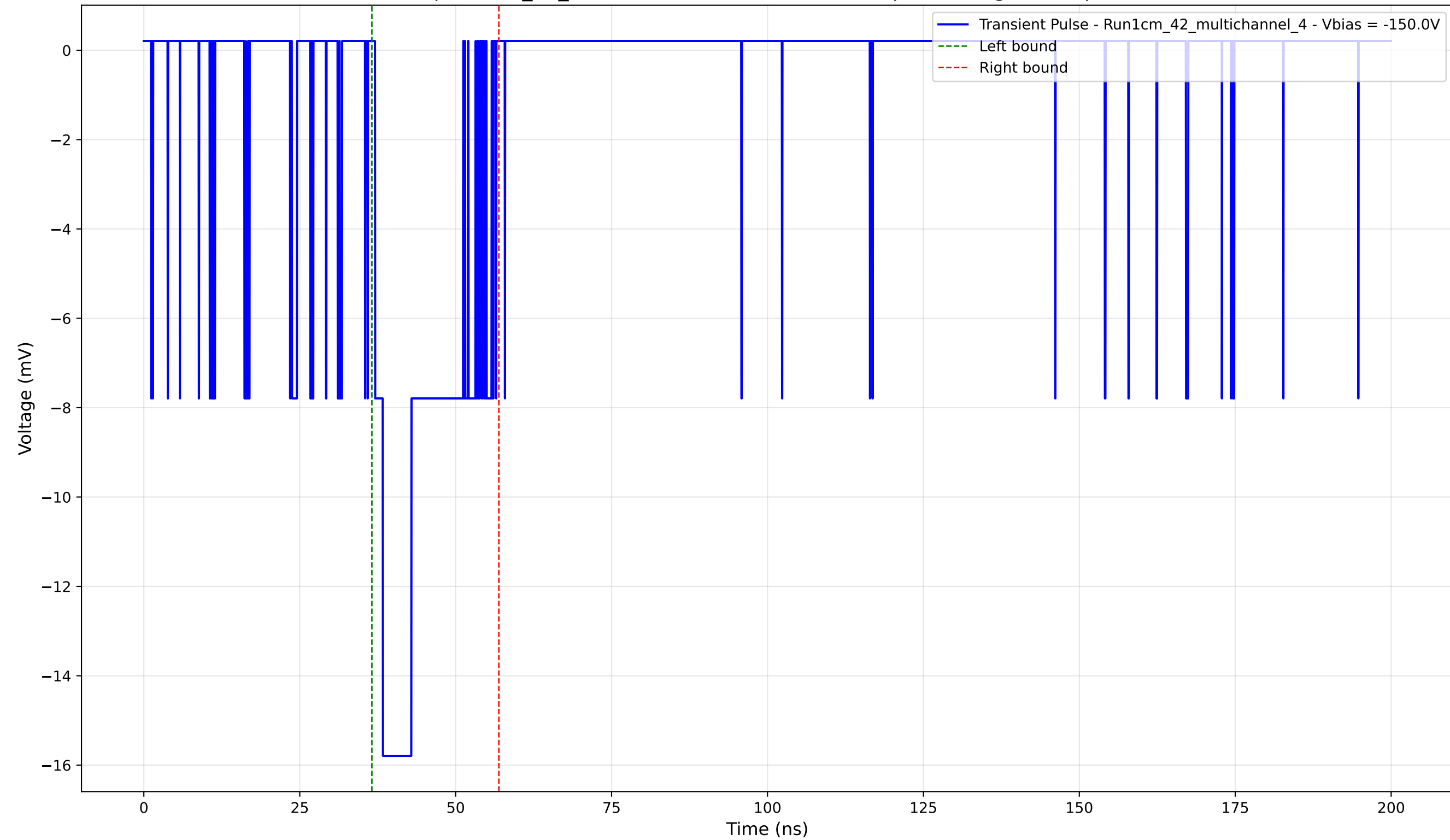
Transient Pulse - Sample: 1cm_42_multichannel - Position: 4220.0 \mu\text{m} - Charge: 3.49 pC - Rise Time: 1.26 ns
