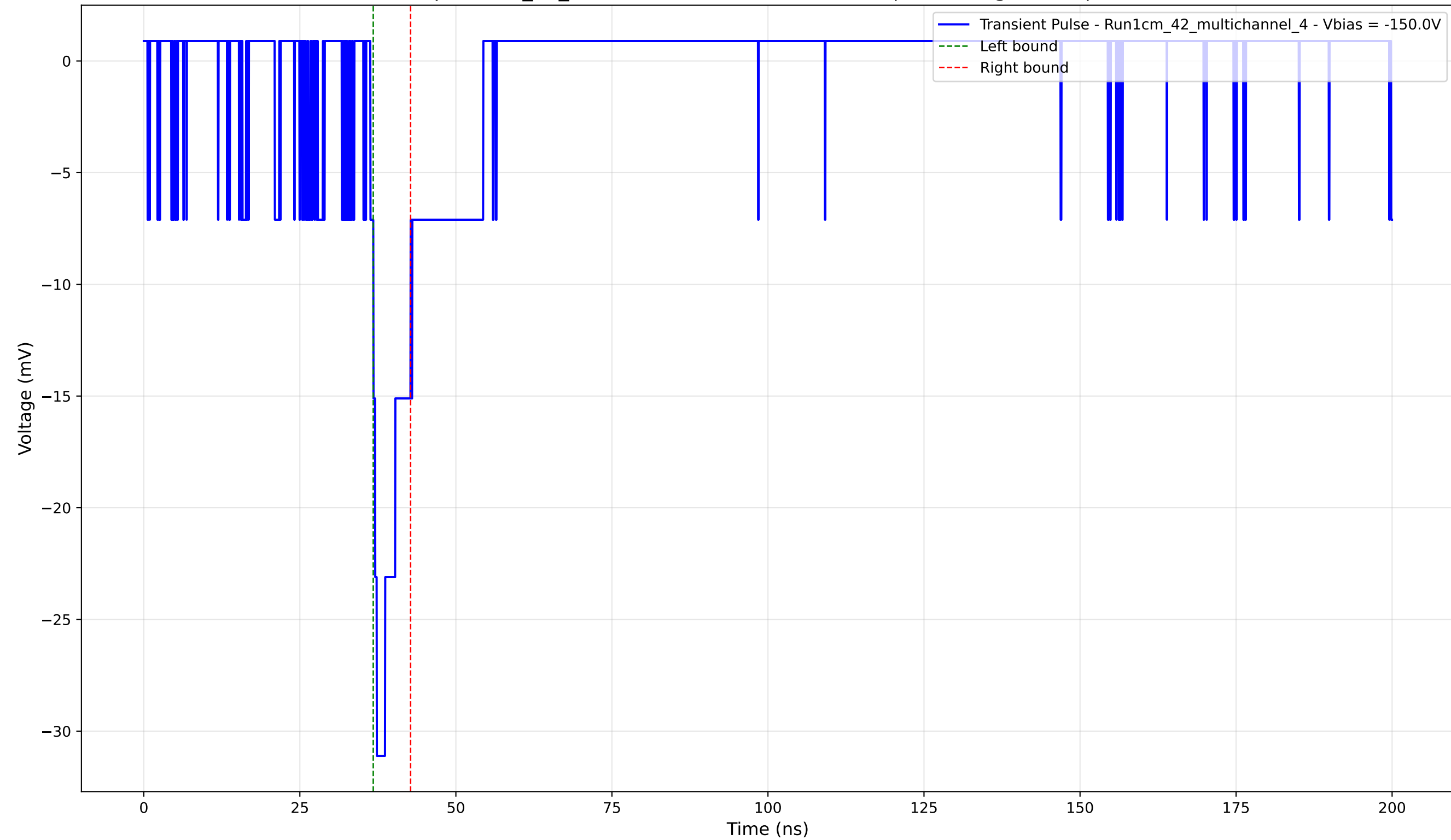
Transient Pulse - Sample: 1cm_42_multichannel - Position: 1620.0 \mu\text{m} - Charge: 2.53 pC - Rise Time: 1.03 ns
