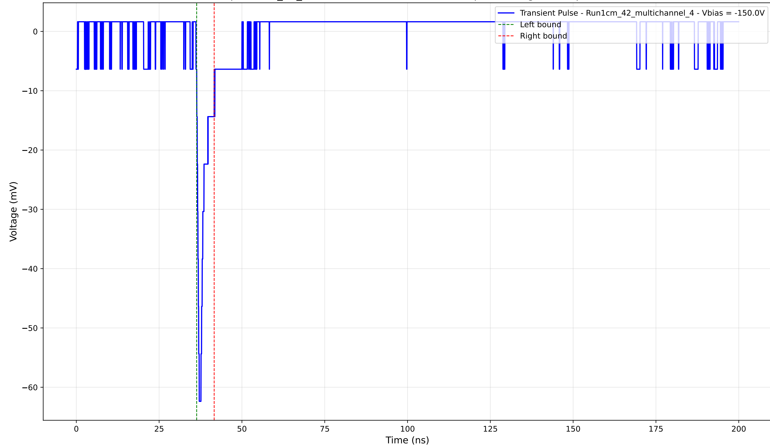
Transient Pulse - Sample: 1cm_42_multichannel - Position: 2150.0 \mu\text{m} - Charge: 2.99 pC - Rise Time: 0.98 ns
