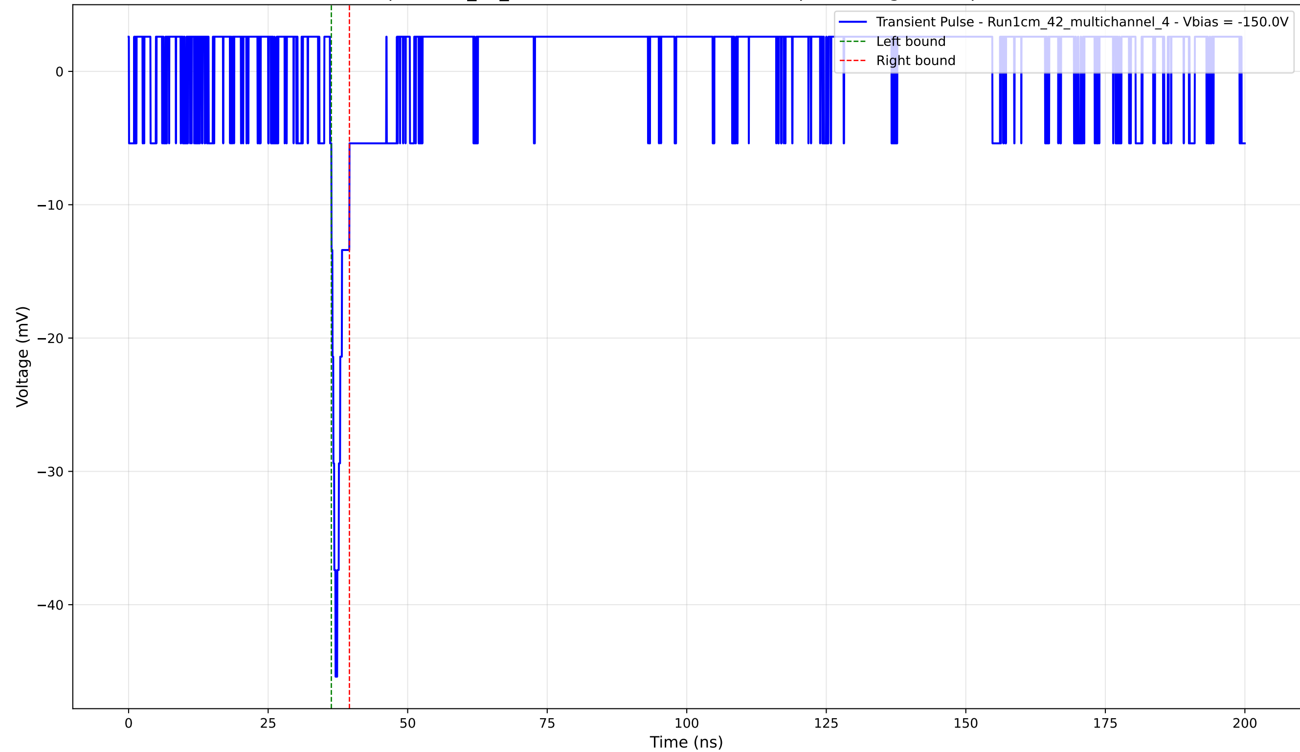
Transient Pulse - Sample: 1cm_42_multichannel - Position: 2335.0 \mu\text{m} - Charge: 1.51 pC - Rise Time: 0.99 ns
