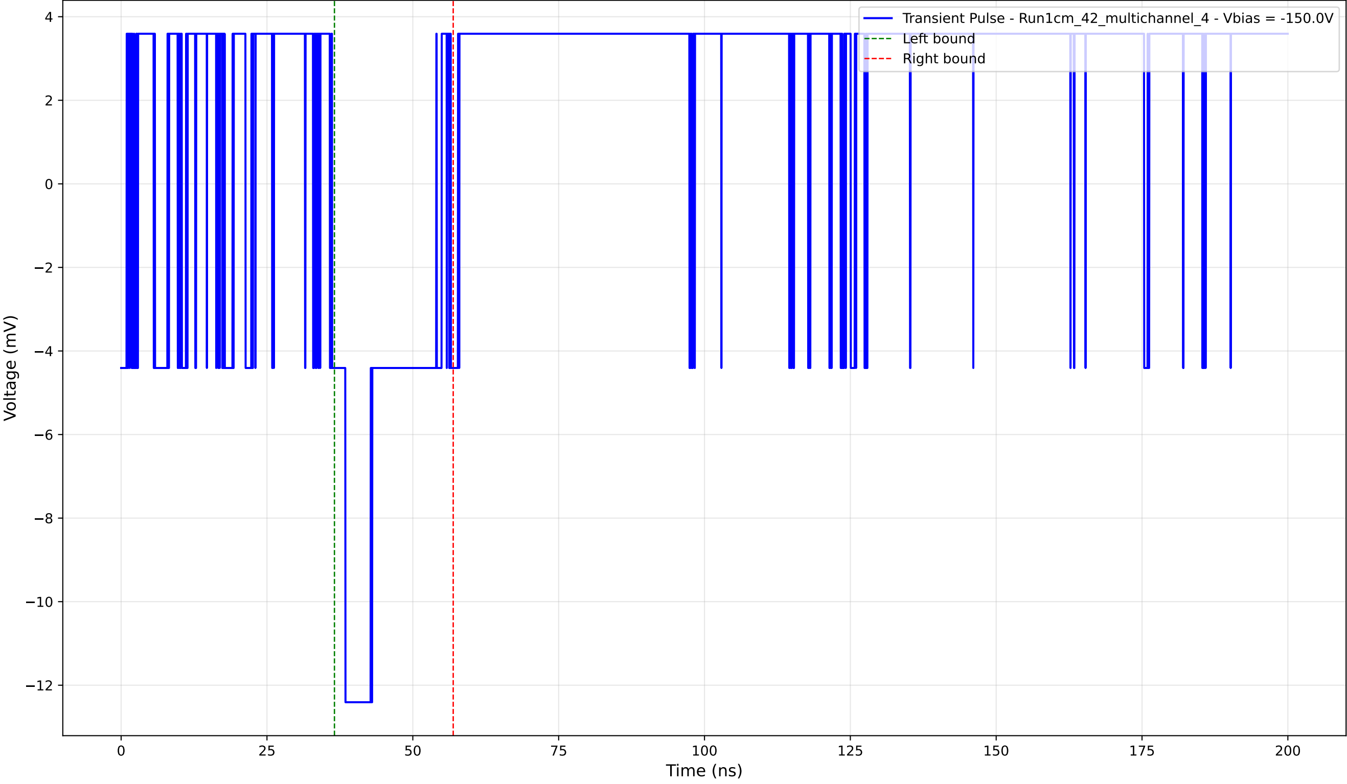
Transient Pulse - Sample: 1cm_42_multichannel - Position: 160.0 \mu\text{m} - Charge: 2.27 pC - Rise Time: 0.00 ns (N/A)
