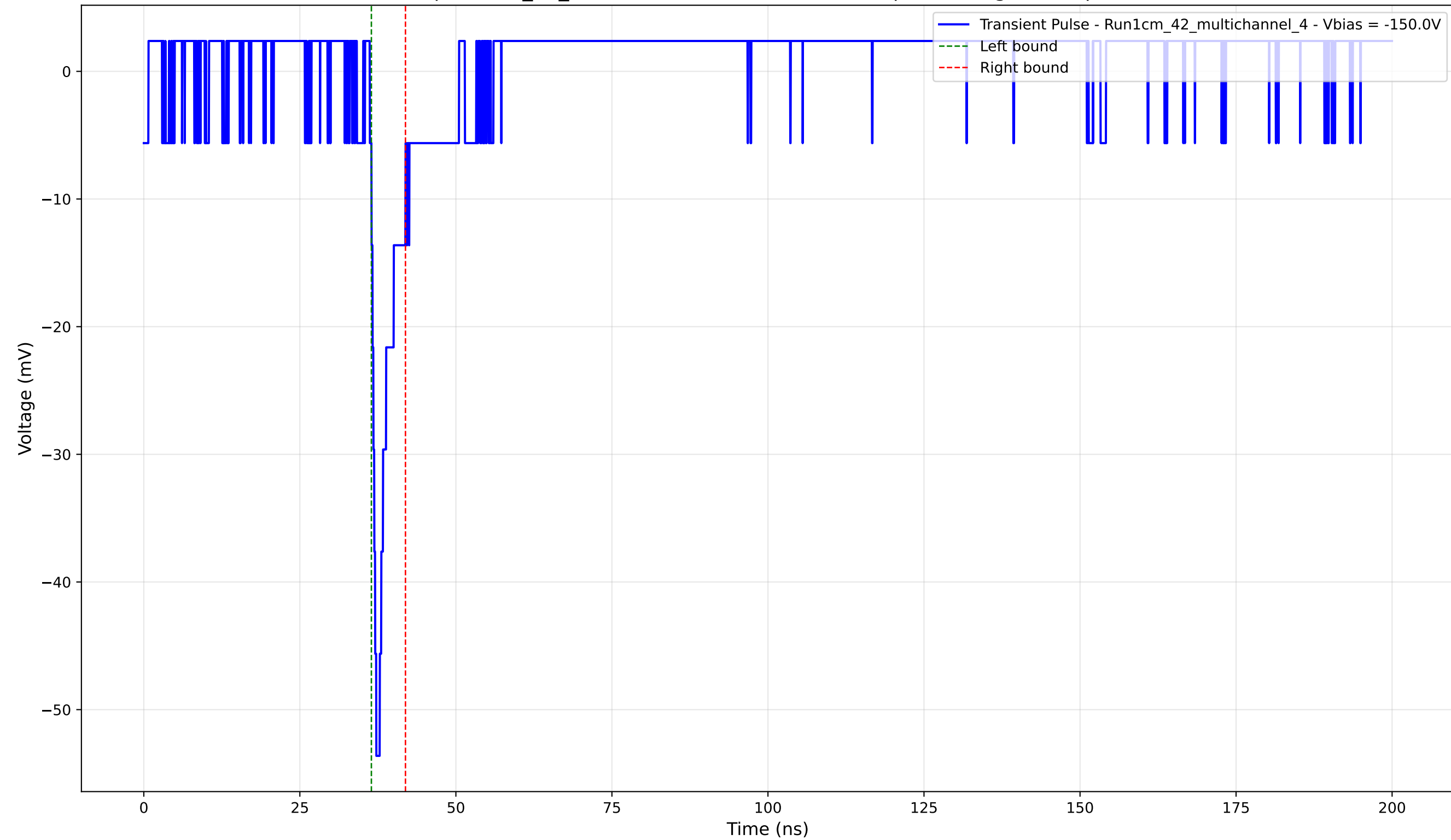
Transient Pulse - Sample: 1cm_42_multichannel - Position: 1980.0 \mu\text{m} - Charge: 2.82 pC - Rise Time: 1.04 ns
