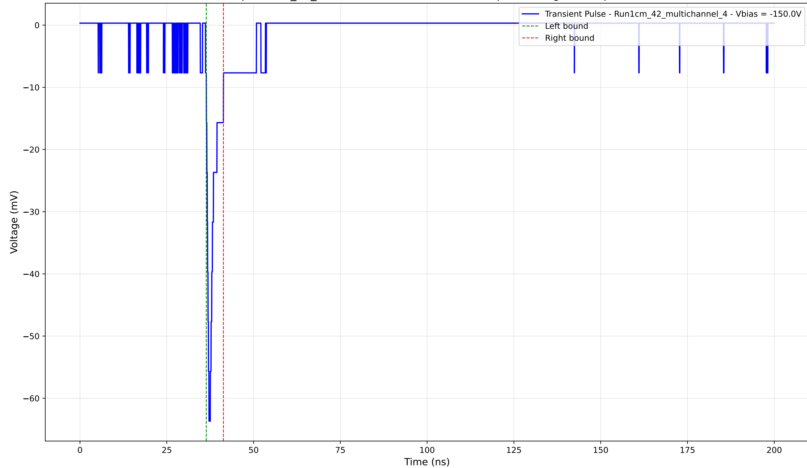
Transient Pulse - Sample: 1cm_42_multichannel - Position: 2630.0 \mu\text{m} - Charge: 2.87 pC - Rise Time: 1.00 ns
