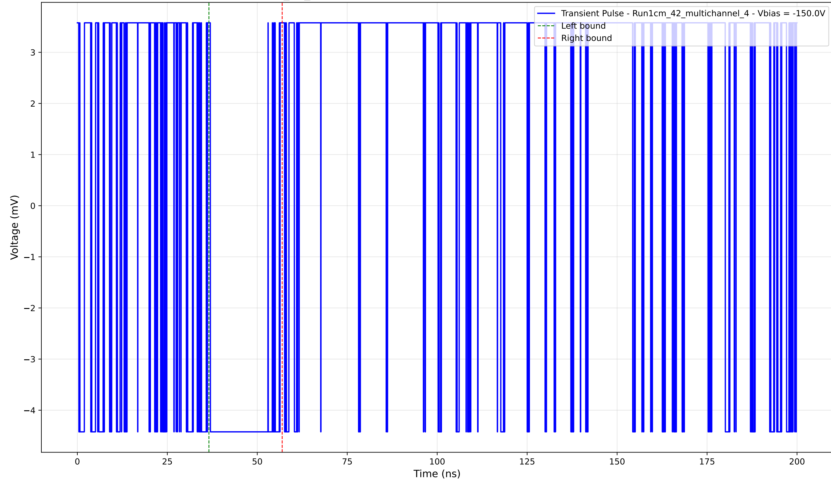
Transient Pulse - Sample: 1cm_42_multichannel - Position: 305.0 \mu\text{m} - Charge: 1.58 pC - Rise Time: 0.00 ns (N/A)
