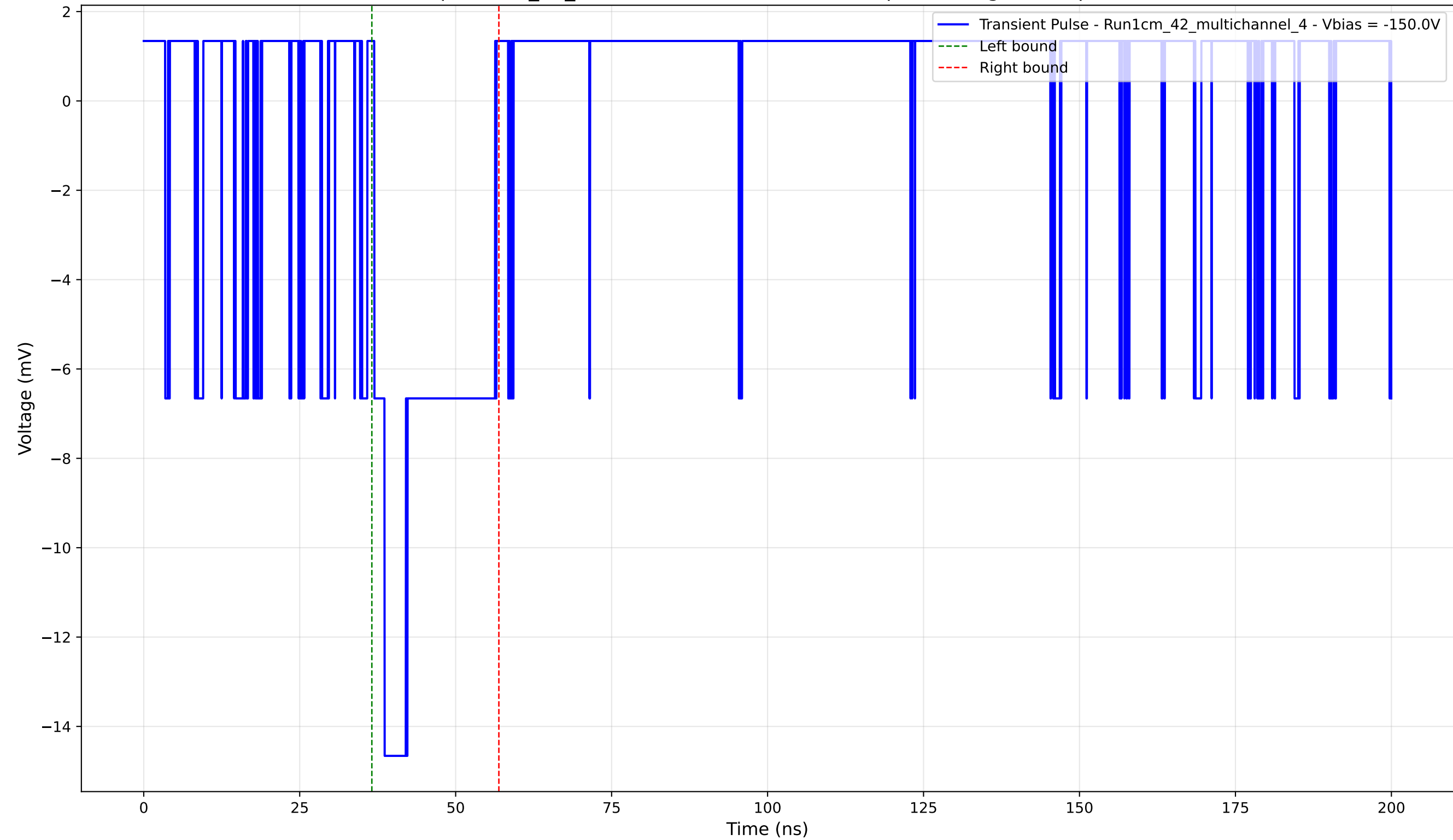
Transient Pulse - Sample: 1cm_42_multichannel - Position: 165.0 \mu\text{m} - Charge: 3.14 pC - Rise Time: 1.66 ns
