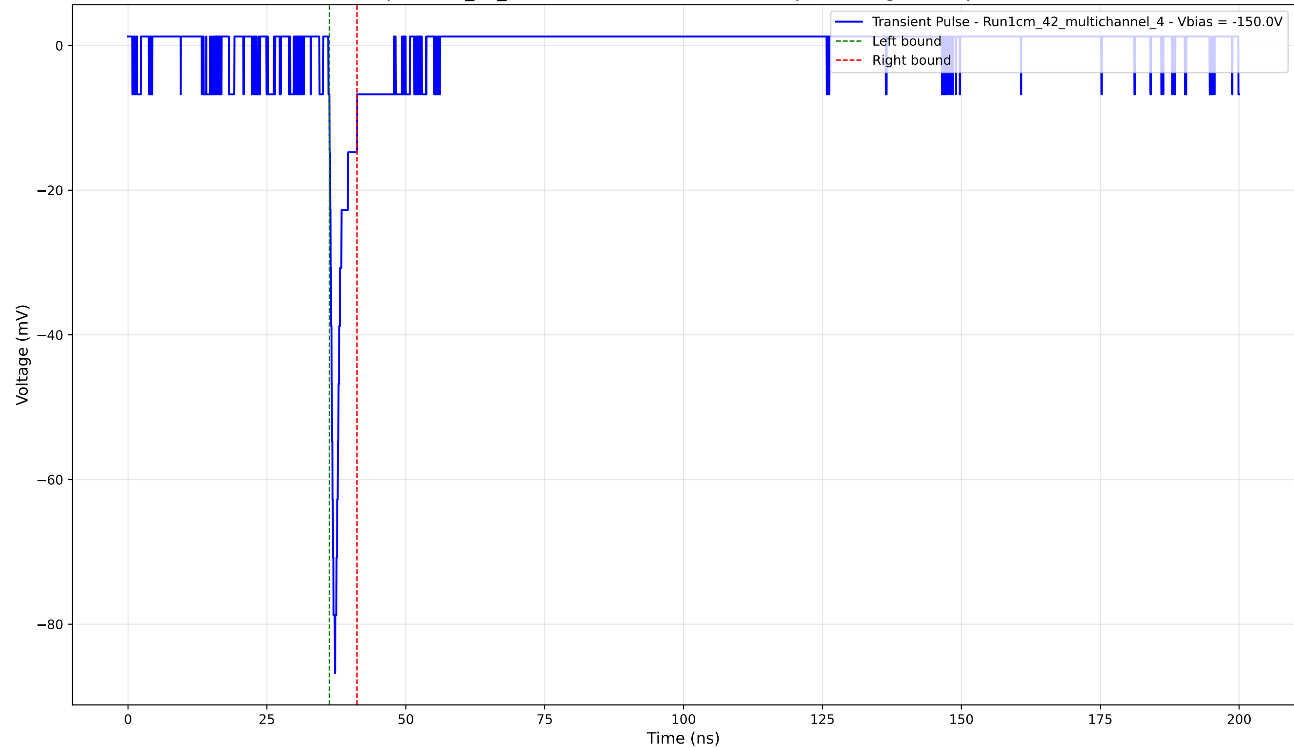
Transient Pulse - Sample: 1cm_42_multichannel - Position: 2475.0 \mu\text{m} - Charge: 3.34 pC - Rise Time: 0.74 ns
