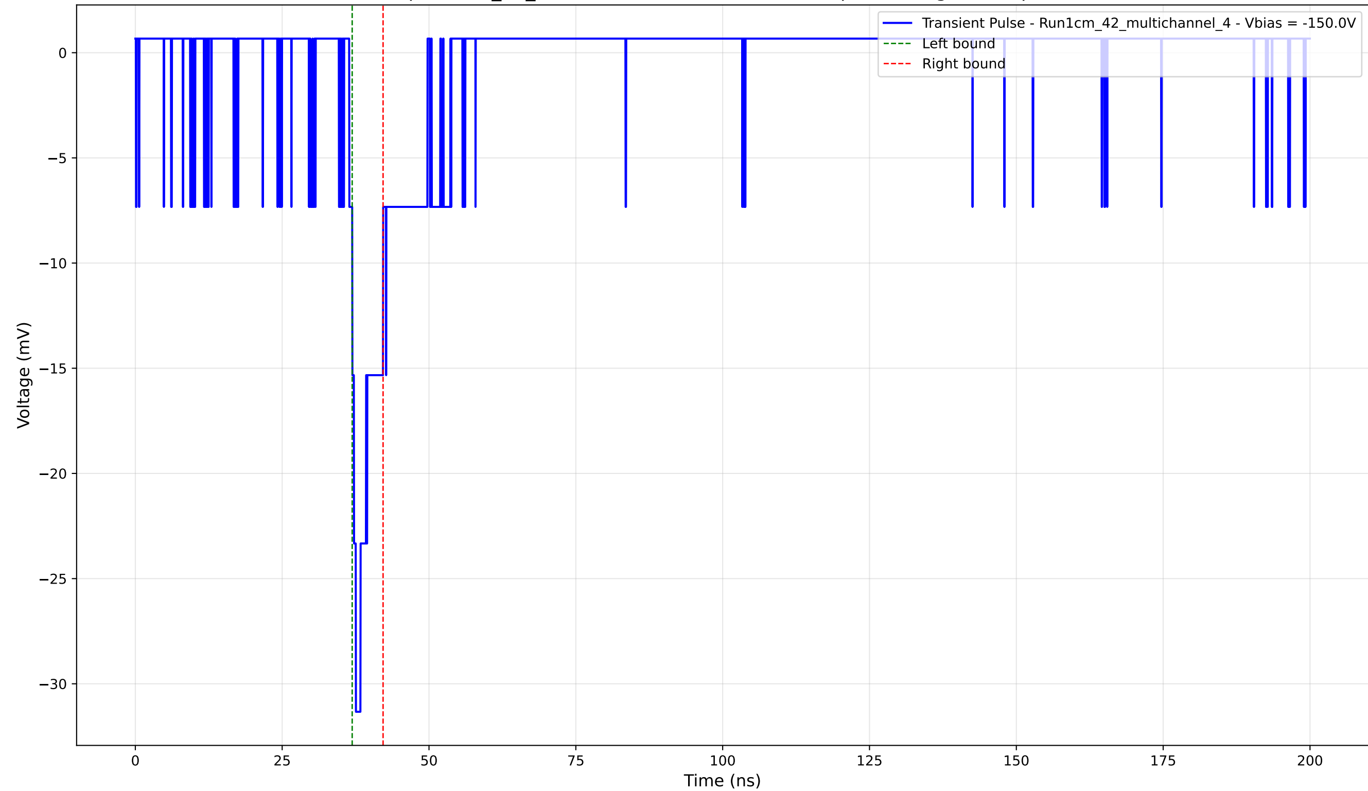
Transient Pulse - Sample: 1cm_42_multichannel - Position: 3215.0 \mu\text{m} - Charge: 2.08 pC - Rise Time: 1.13 ns
