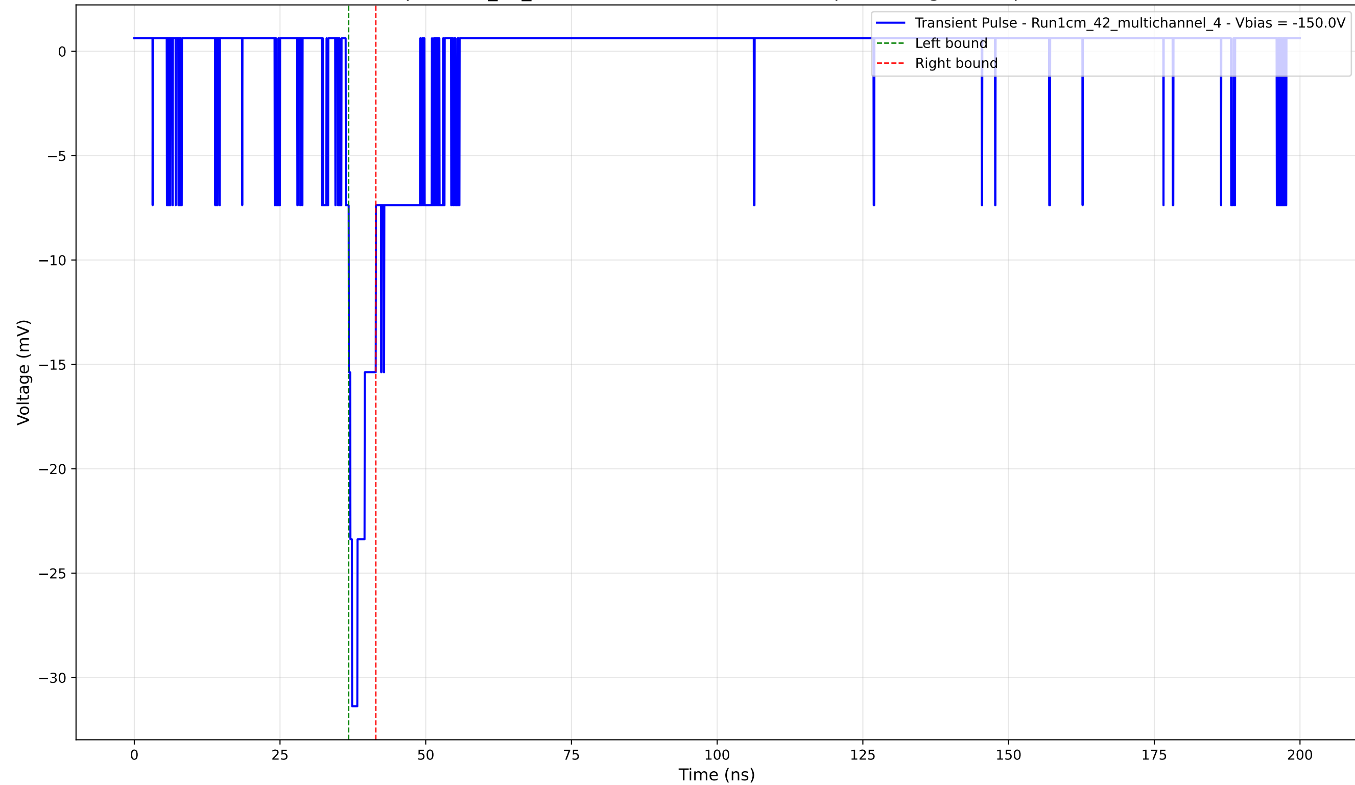
Transient Pulse - Sample: 1cm_42_multichannel - Position: 3095.0 \mu\text{m} - Charge: 1.97 pC - Rise Time: 1.09 ns
