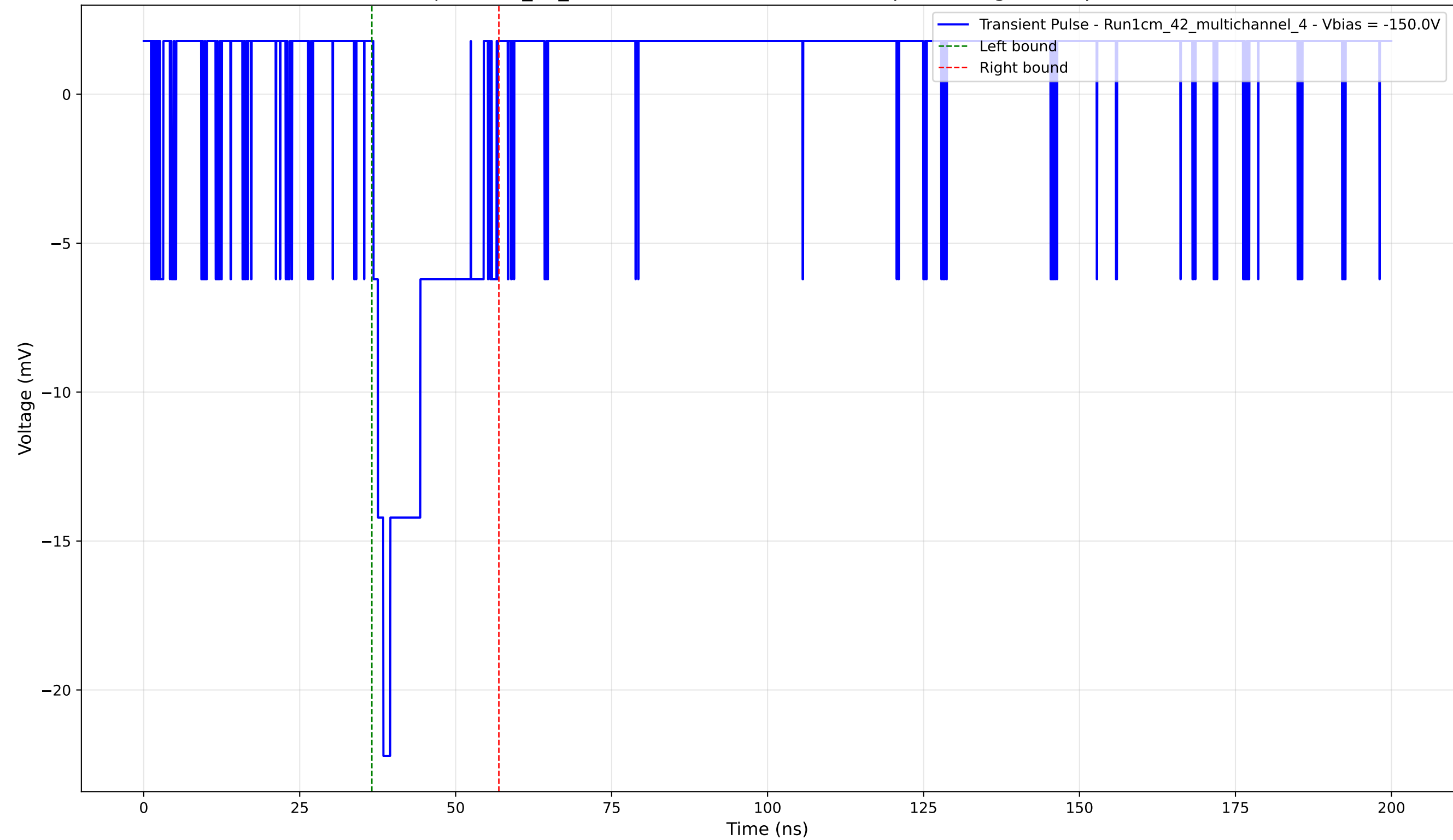
Transient Pulse - Sample: 1cm_42_multichannel - Position: 3680.0 \mu\text{m} - Charge: 3.54 pC - Rise Time: 1.60 ns
