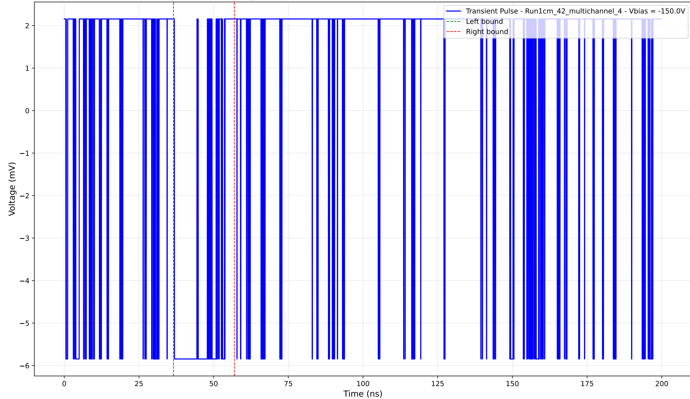
Transient Pulse - Sample: 1cm_42_multichannel - Position: 3440.0 \mu\text{m} - Charge: 1.37 pC - Rise Time: 0.00 ns (N/A)
