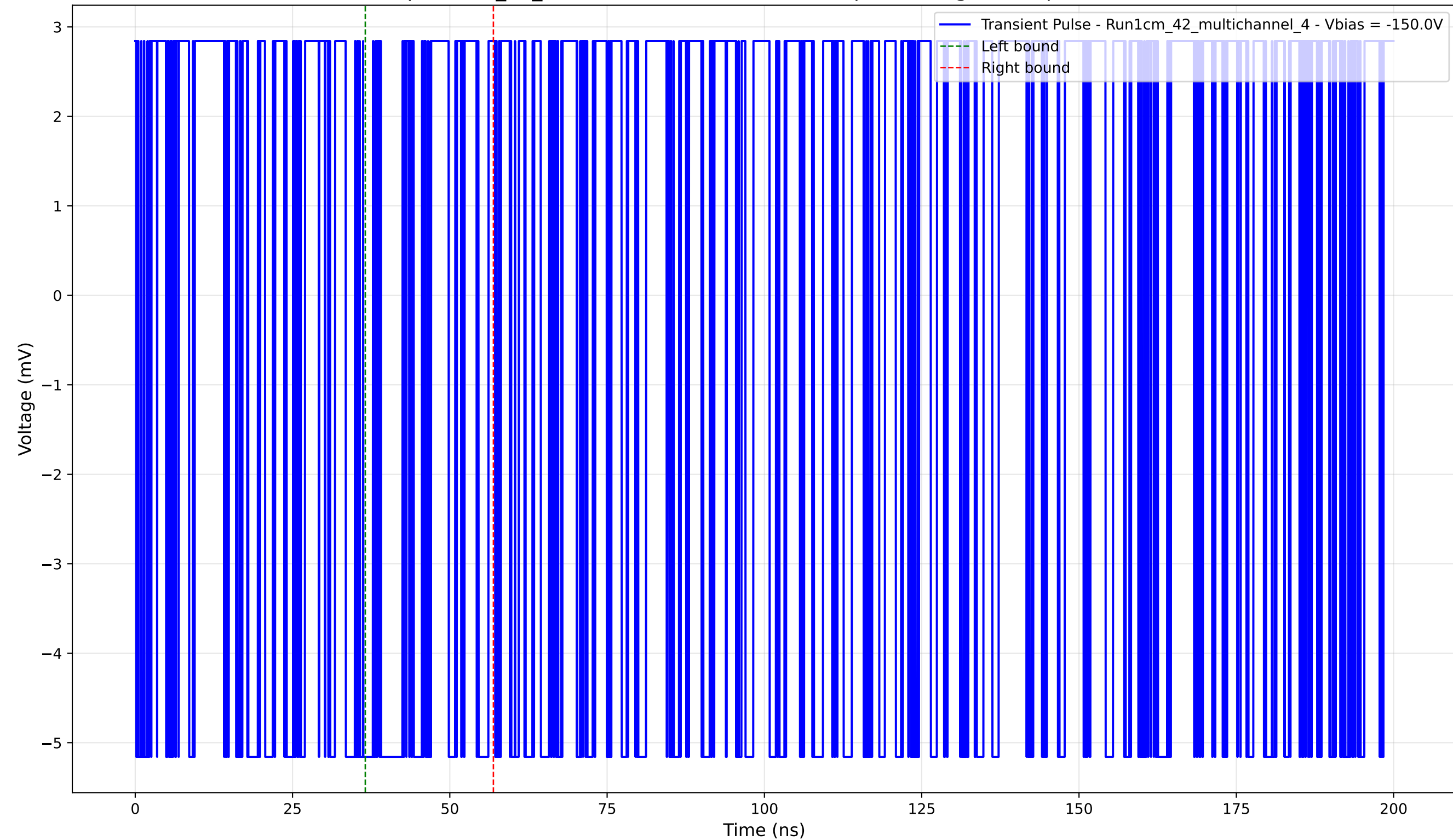
Transient Pulse - Sample: 1cm_42_multichannel - Position: 875.0 \mu\text{m} - Charge: 0.61 pC - Rise Time: 0.00 ns (N/A)
