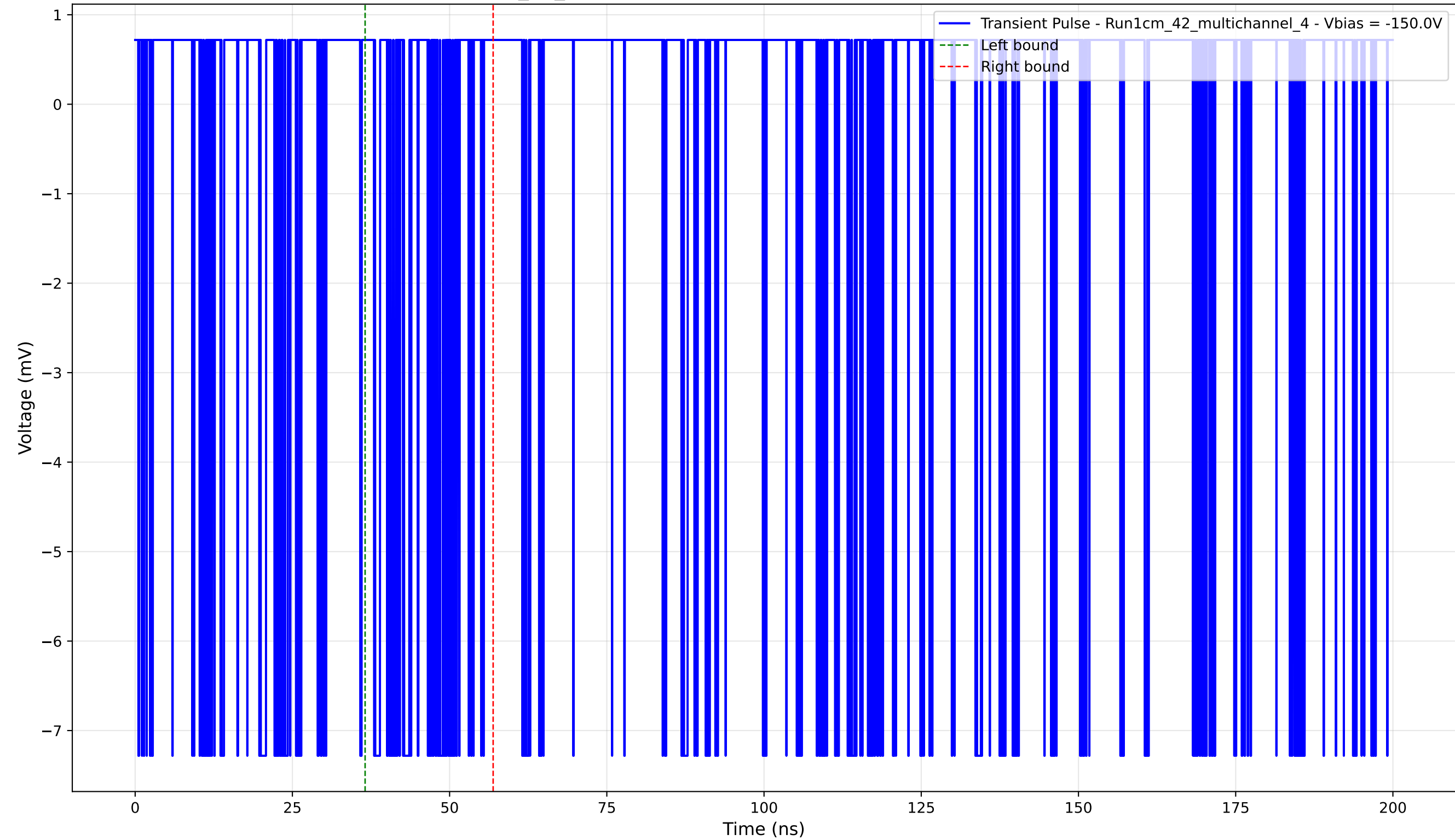
Transient Pulse - Sample: 1cm_42_multichannel - Position: 4395.0 \mu\text{m} - Charge: 0.81 pC - Rise Time: 0.02 ns
