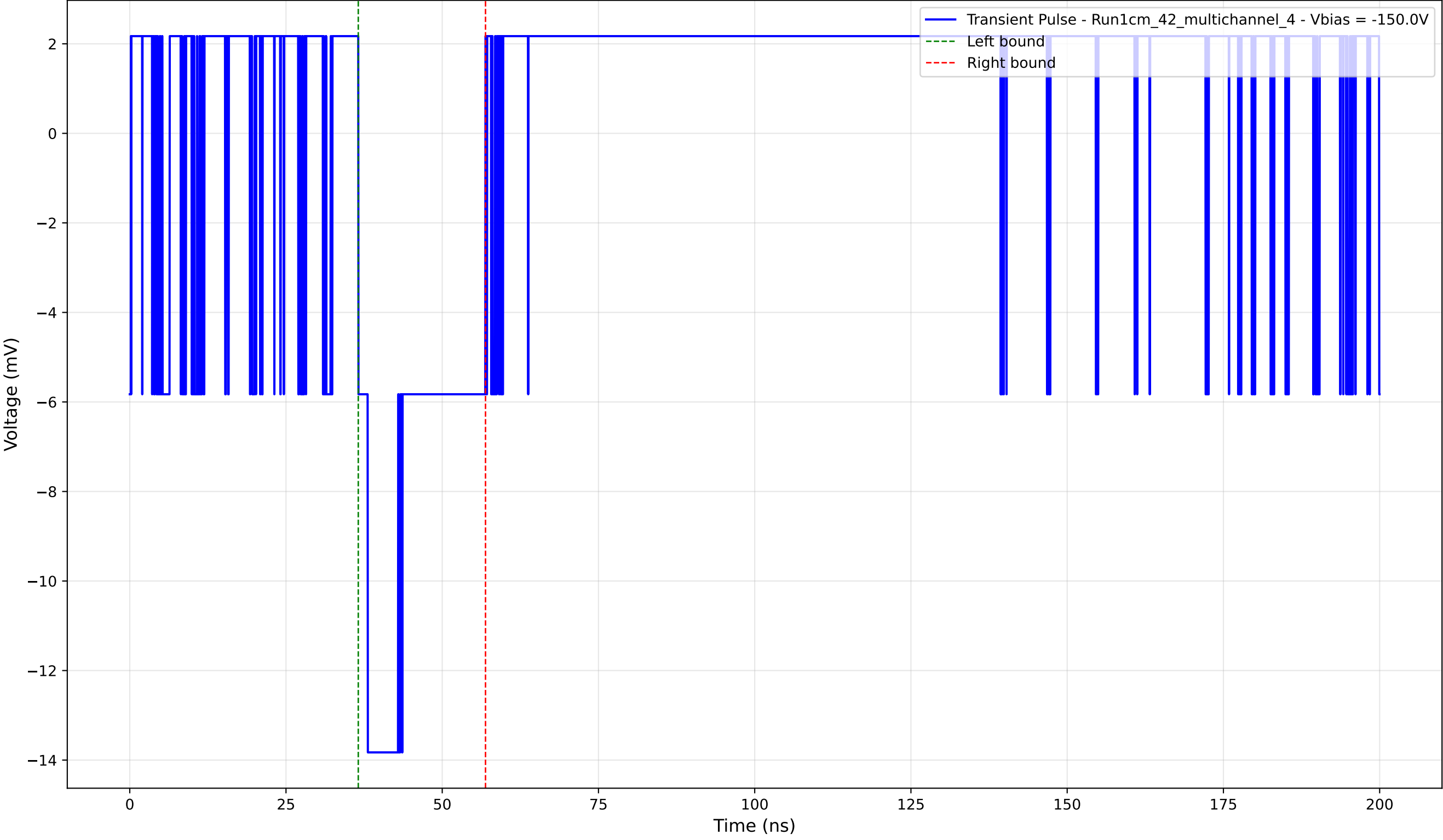
Transient Pulse - Sample: 1cm_42_multichannel - Position: 540.0 \mu\text{m} - Charge: 3.19 pC - Rise Time: 0.00 ns (N/A)
