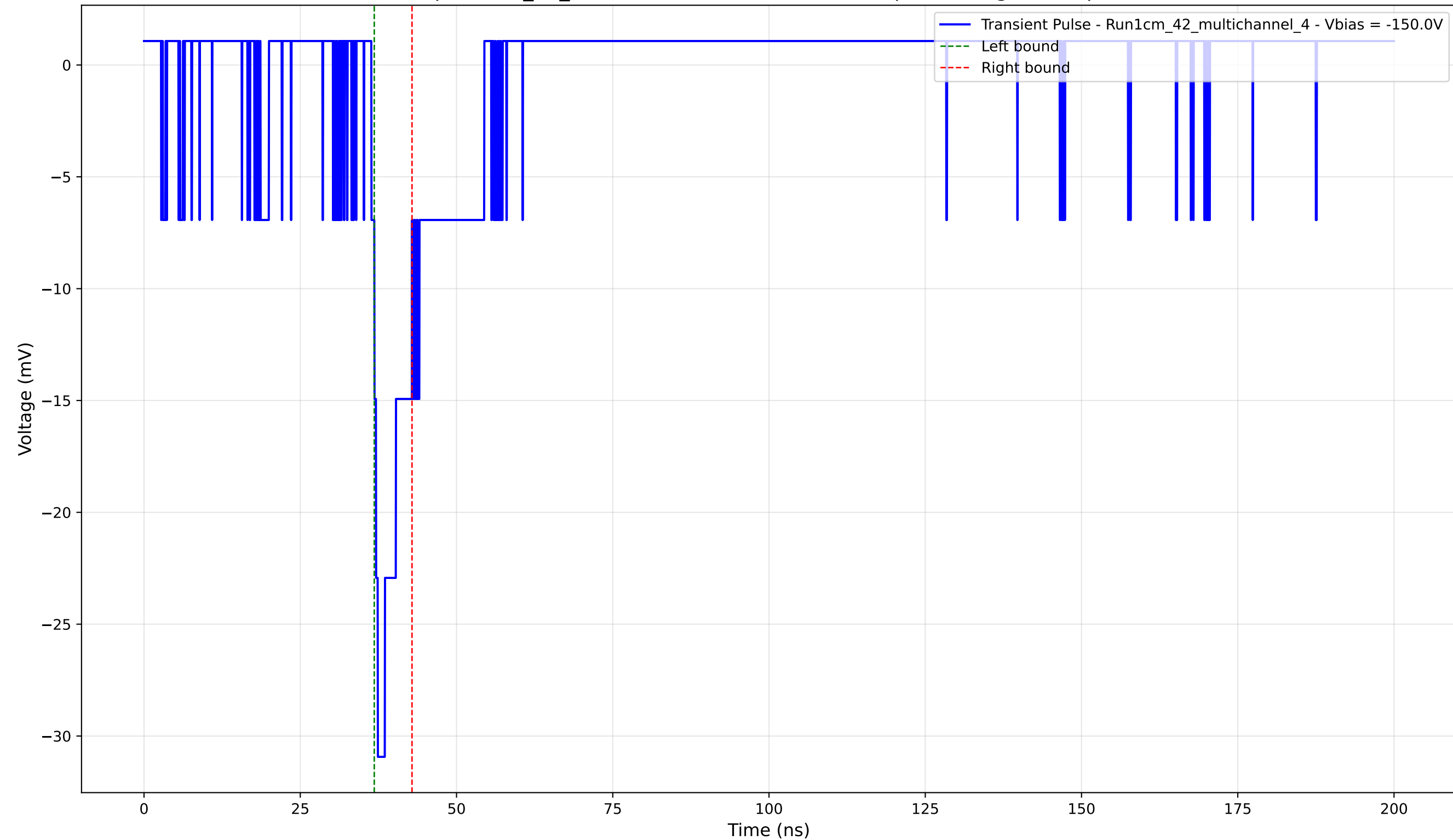
Transient Pulse - Sample: 1cm_42_multichannel - Position: 1565.0 \mu\text{m} - Charge: 2.49 pC - Rise Time: 1.03 ns
