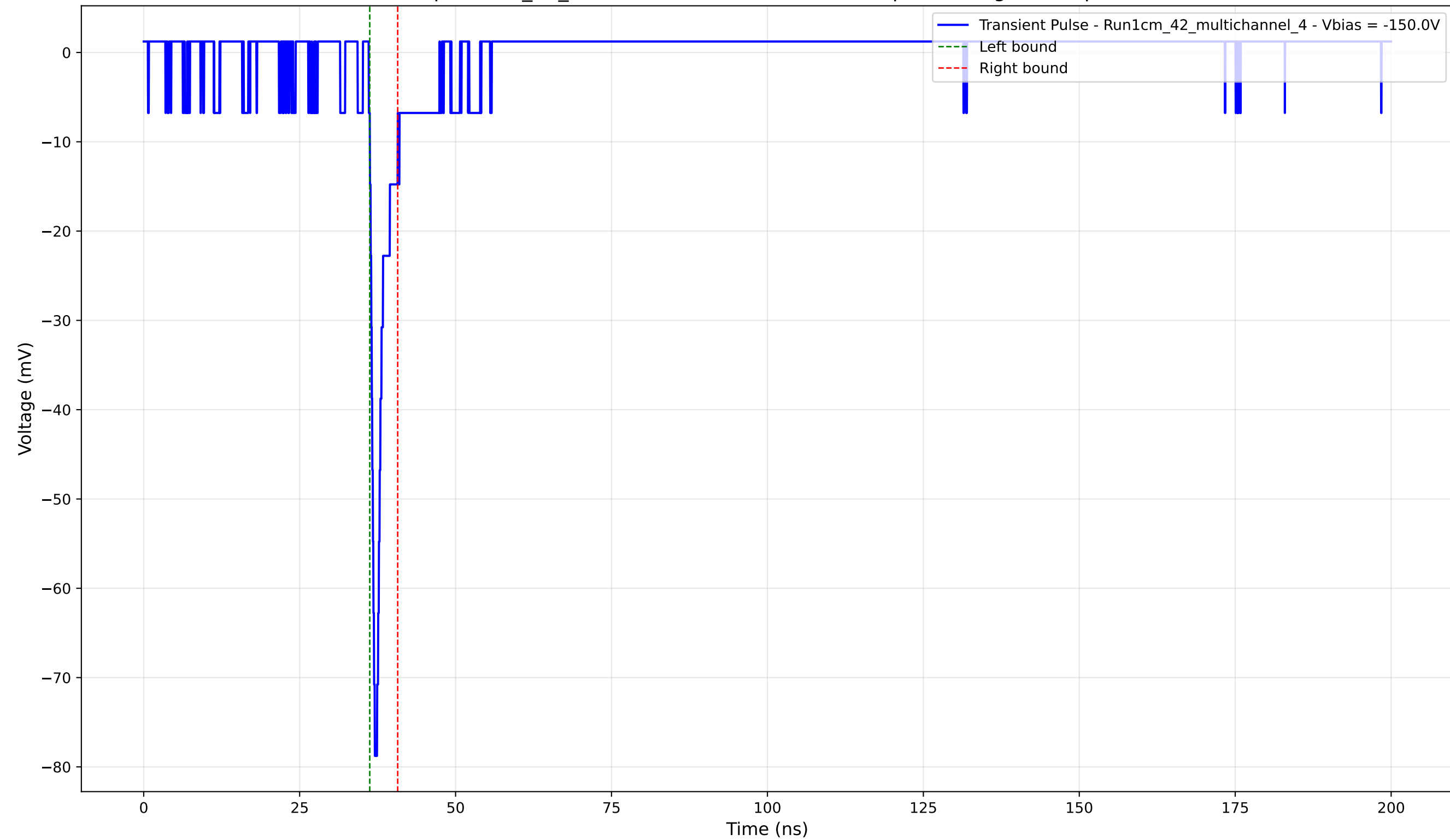
Transient Pulse - Sample: 1cm_42_multichannel - Position: 2460.0 \mu\text{m} - Charge: 3.05 pC - Rise Time: 0.80 ns
