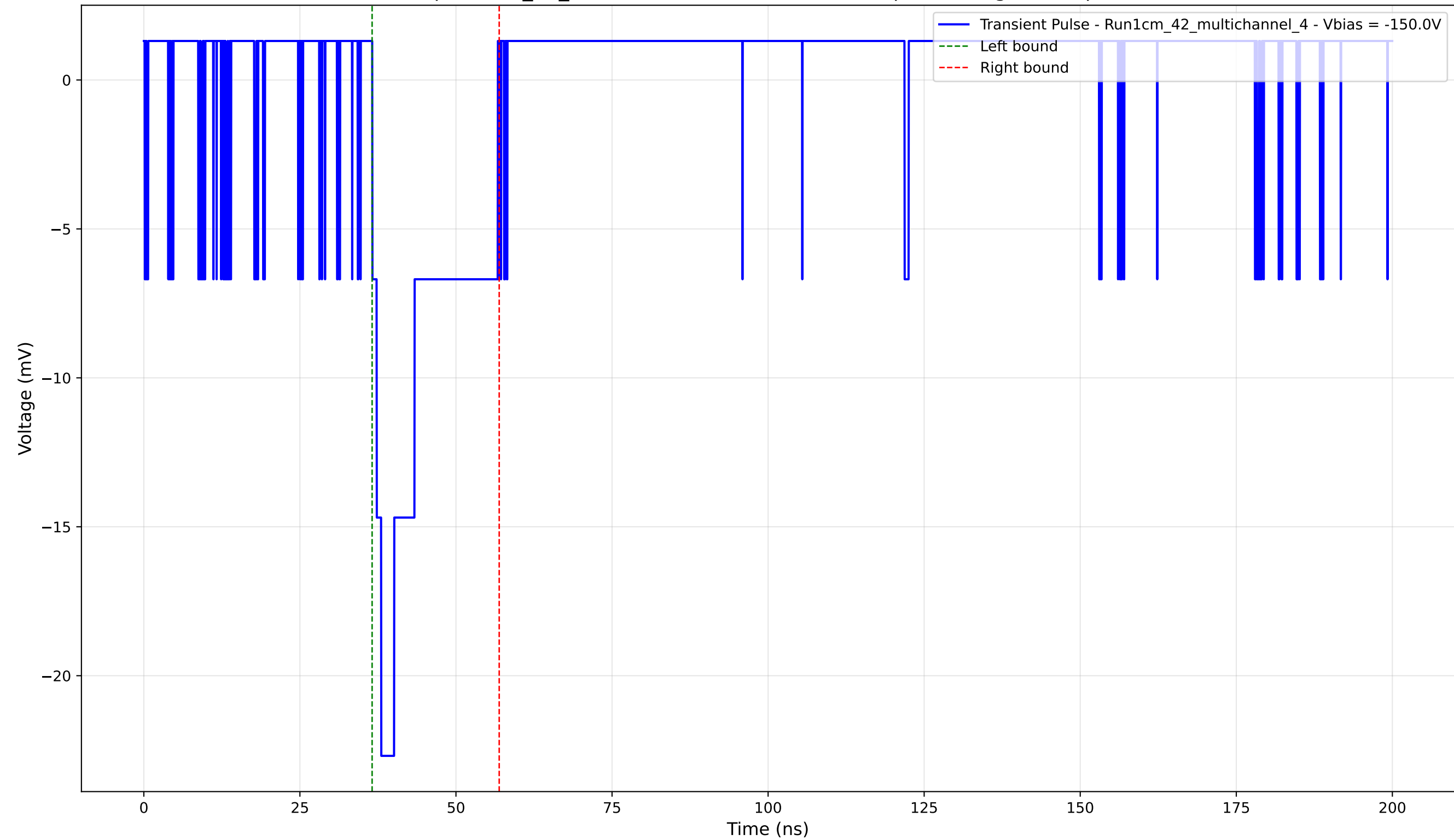
Transient Pulse - Sample: 1cm_42_multichannel - Position: 1150.0 \mu\text{m} - Charge: 4.00 pC - Rise Time: 1.44 ns
