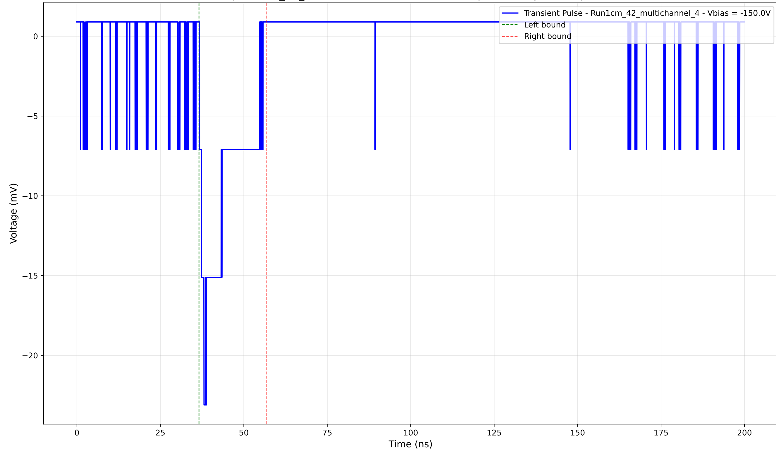
Transient Pulse - Sample: 1cm_42_multichannel - Position: 3635.0 \mu\text{m} - Charge: 3.65 pC - Rise Time: 1.34 ns
