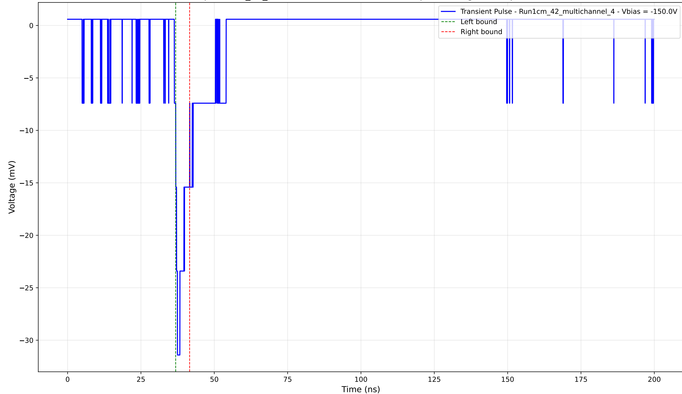
Transient Pulse - Sample: 1cm_42_multichannel - Position: 3180.0 \mu\text{m} - Charge: 2.01 pC - Rise Time: 1.07 ns
