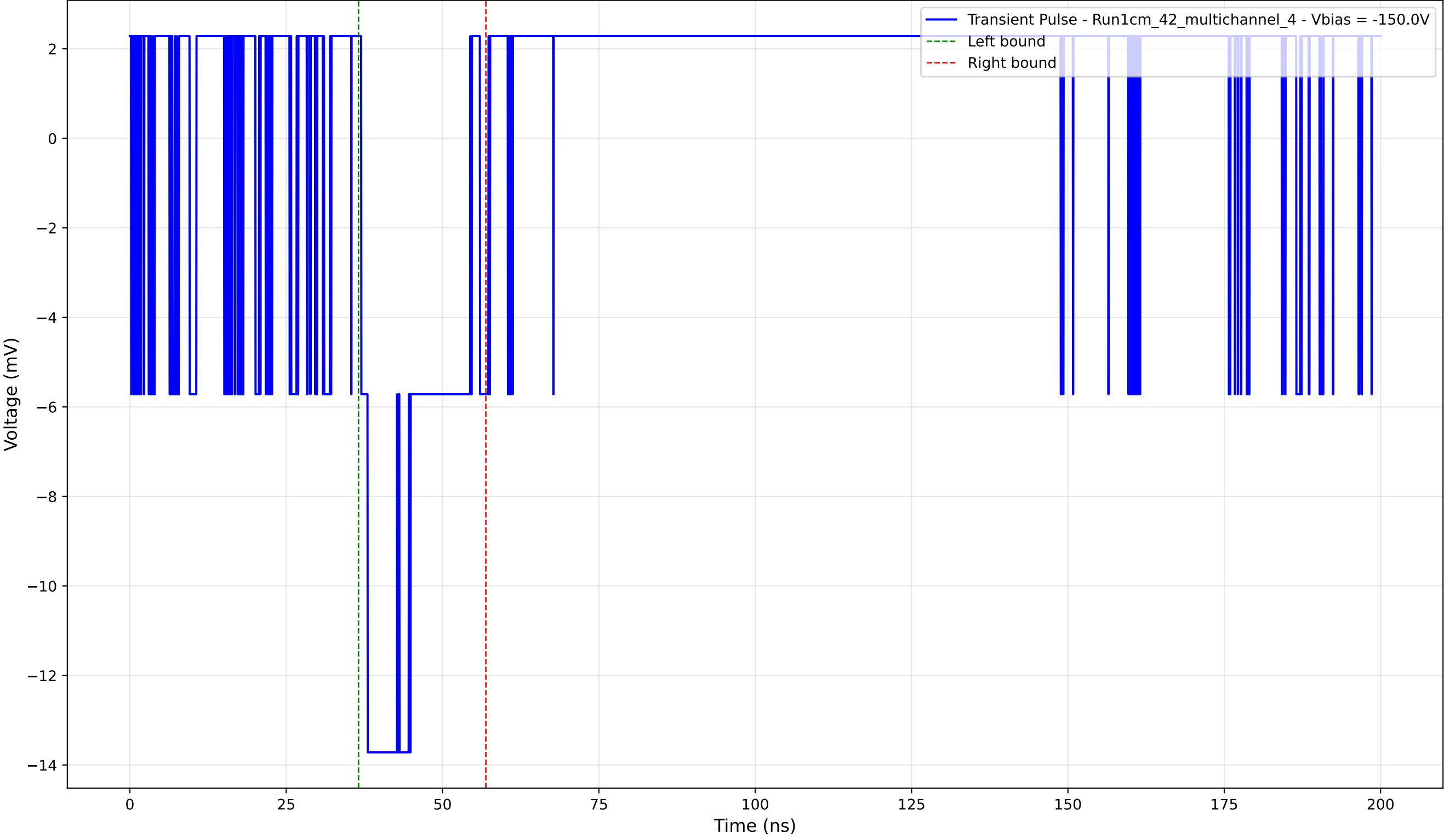
Transient Pulse - Sample: 1cm_42_multichannel - Position: 490.0 \mu\text{m} - Charge: 3.09 pC - Rise Time: 0.00 ns (N/A)
