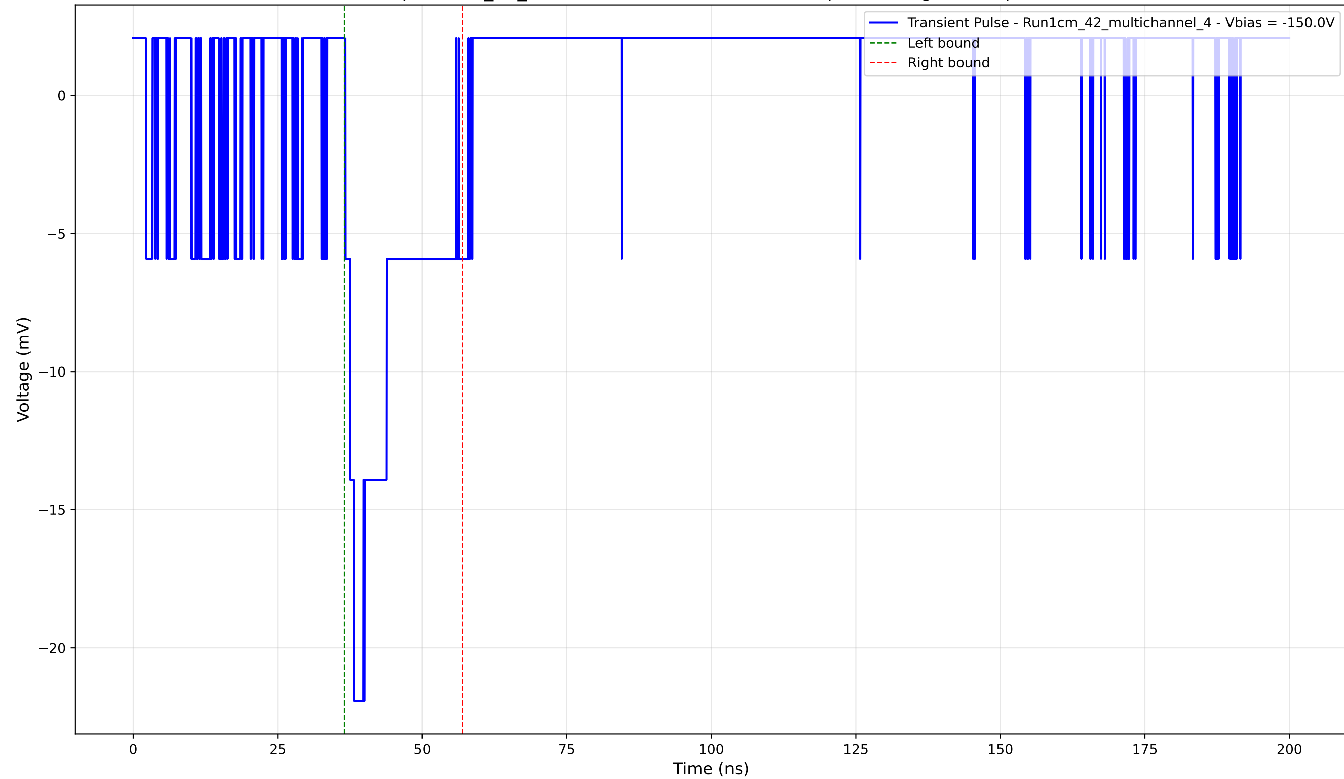
Transient Pulse - Sample: 1cm_42_multichannel - Position: 1105.0 \mu\text{m} - Charge: 3.69 pC - Rise Time: 1.50 ns
