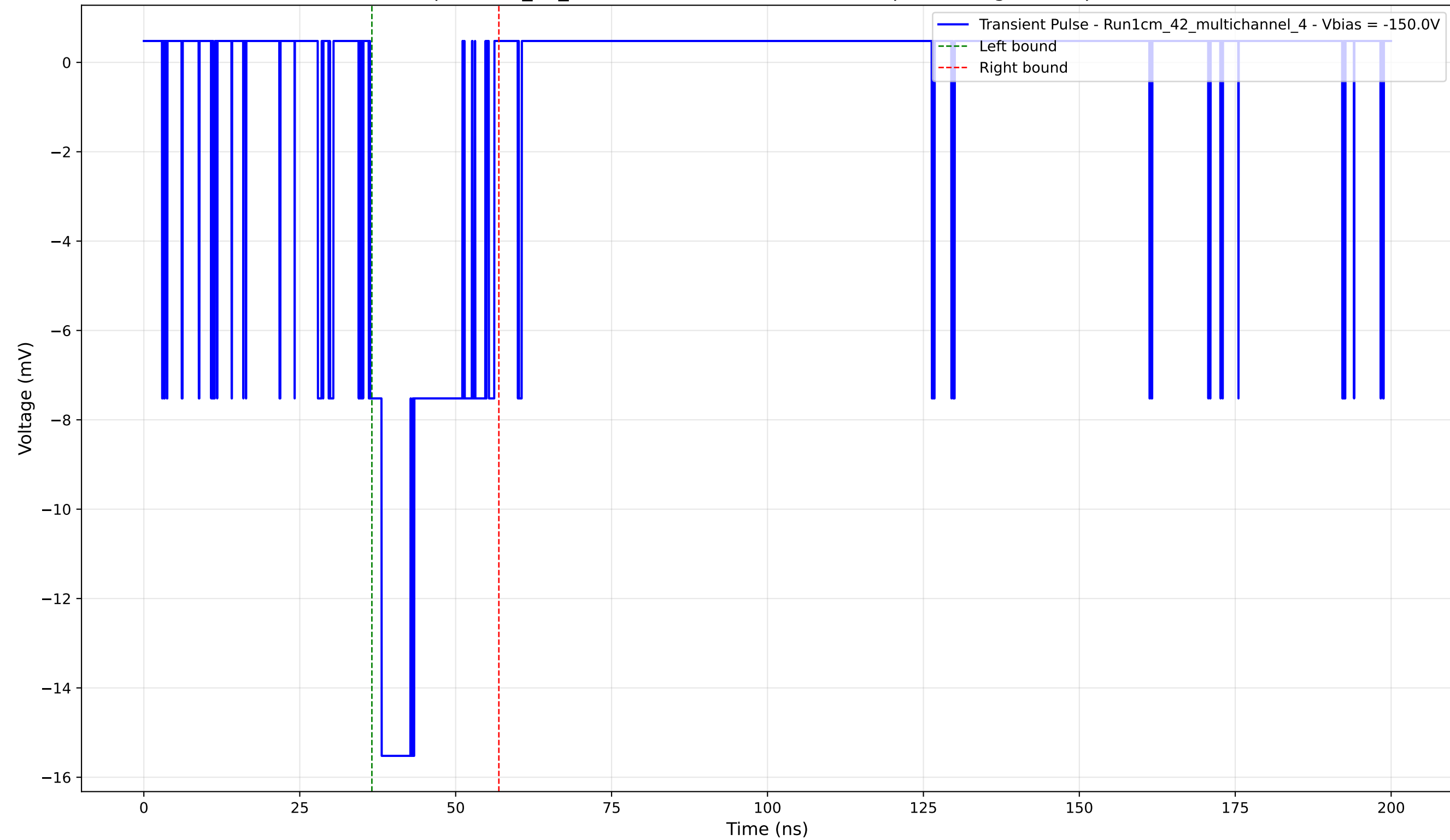
Transient Pulse - Sample: 1cm_42_multichannel - Position: 4080.0 \mu\text{m} - Charge: 3.63 pC - Rise Time: 1.86 ns
