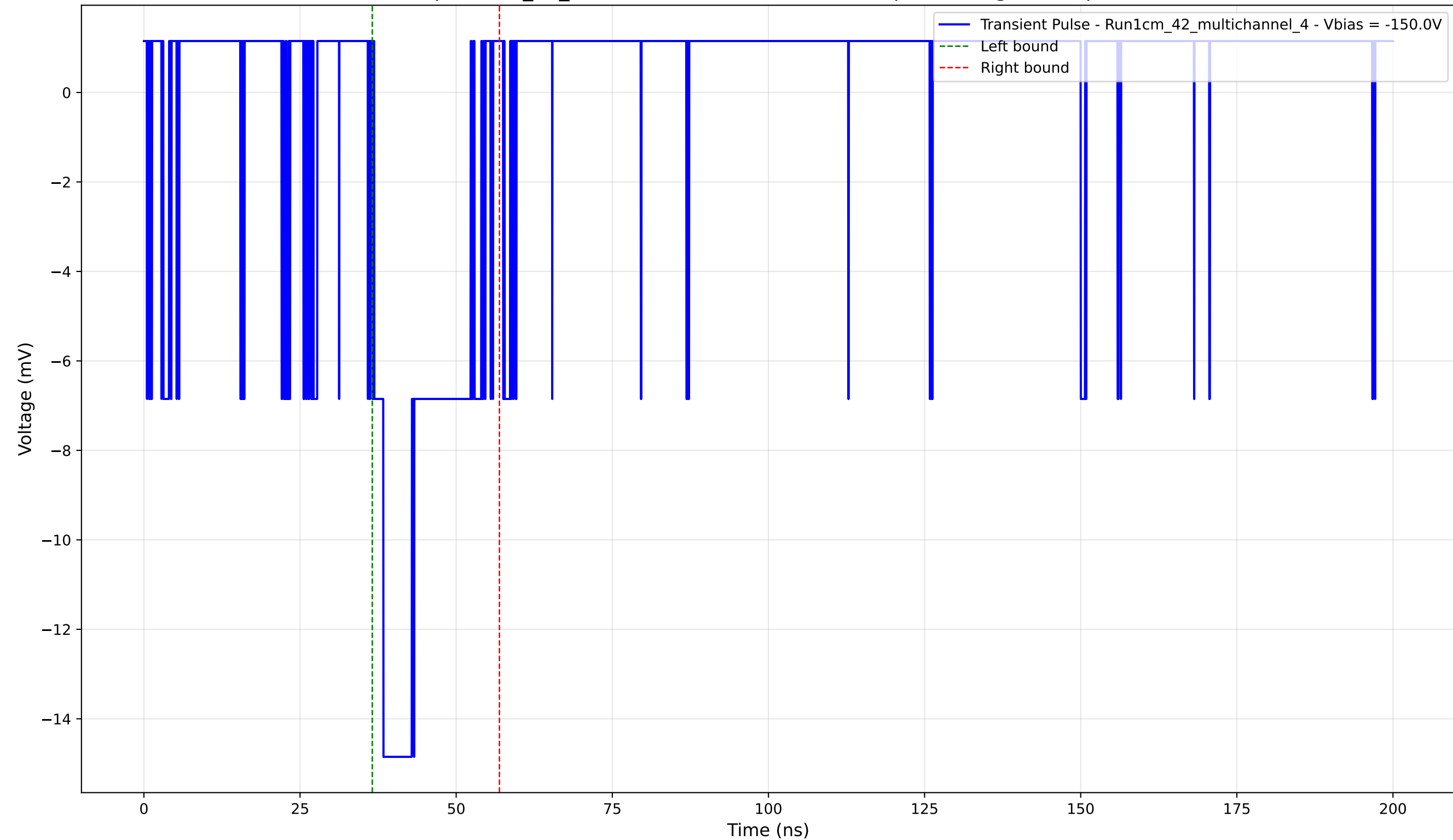
Transient Pulse - Sample: 1cm_42_multichannel - Position: 4240.0 \mu\text{m} - Charge: 3.04 pC - Rise Time: 1.48 ns
