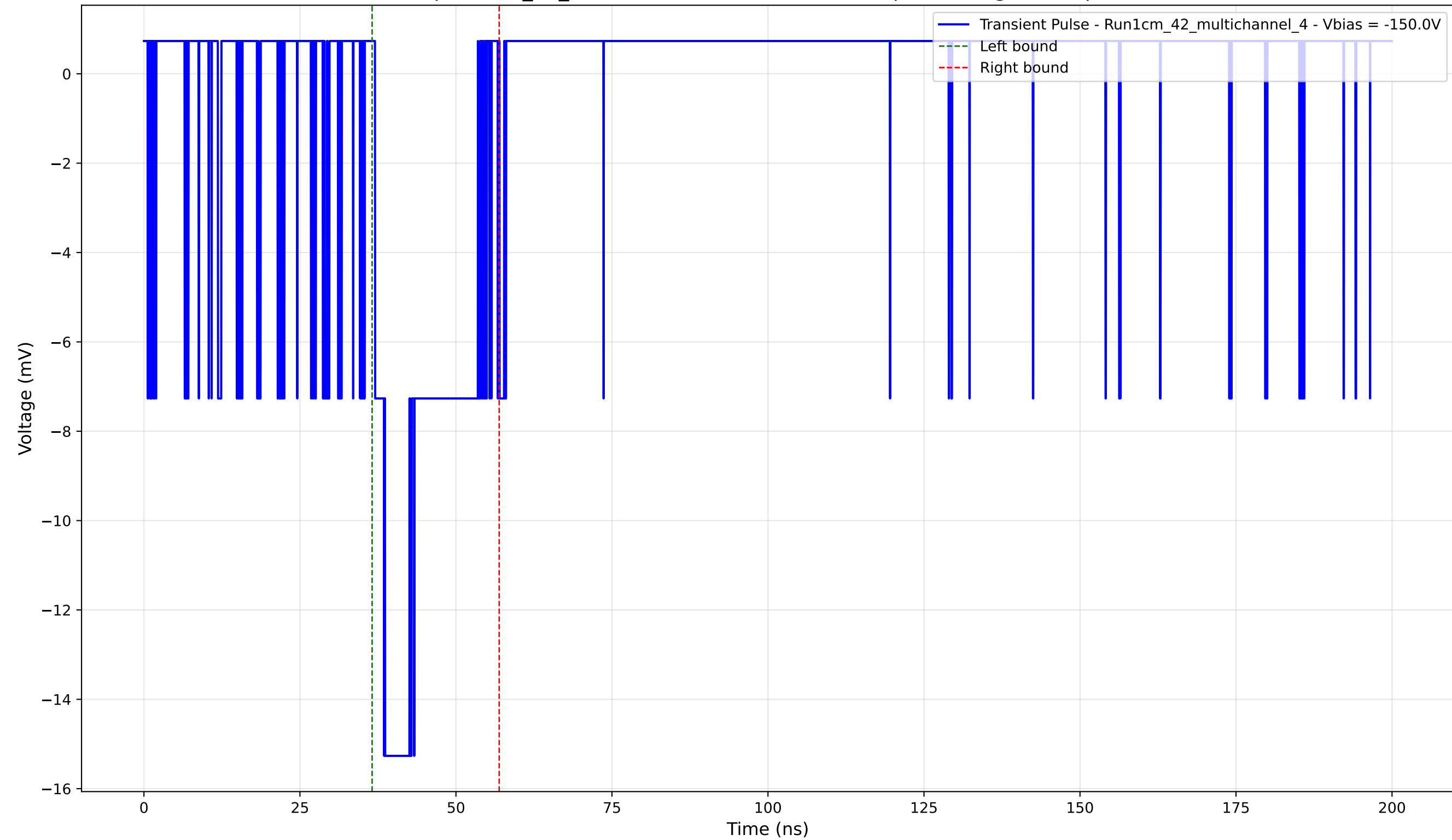
Transient Pulse - Sample: 1cm_42_multichannel - Position: 4600.0 \mu\text{m} - Charge: 3.17 pC - Rise Time: 1.48 ns
