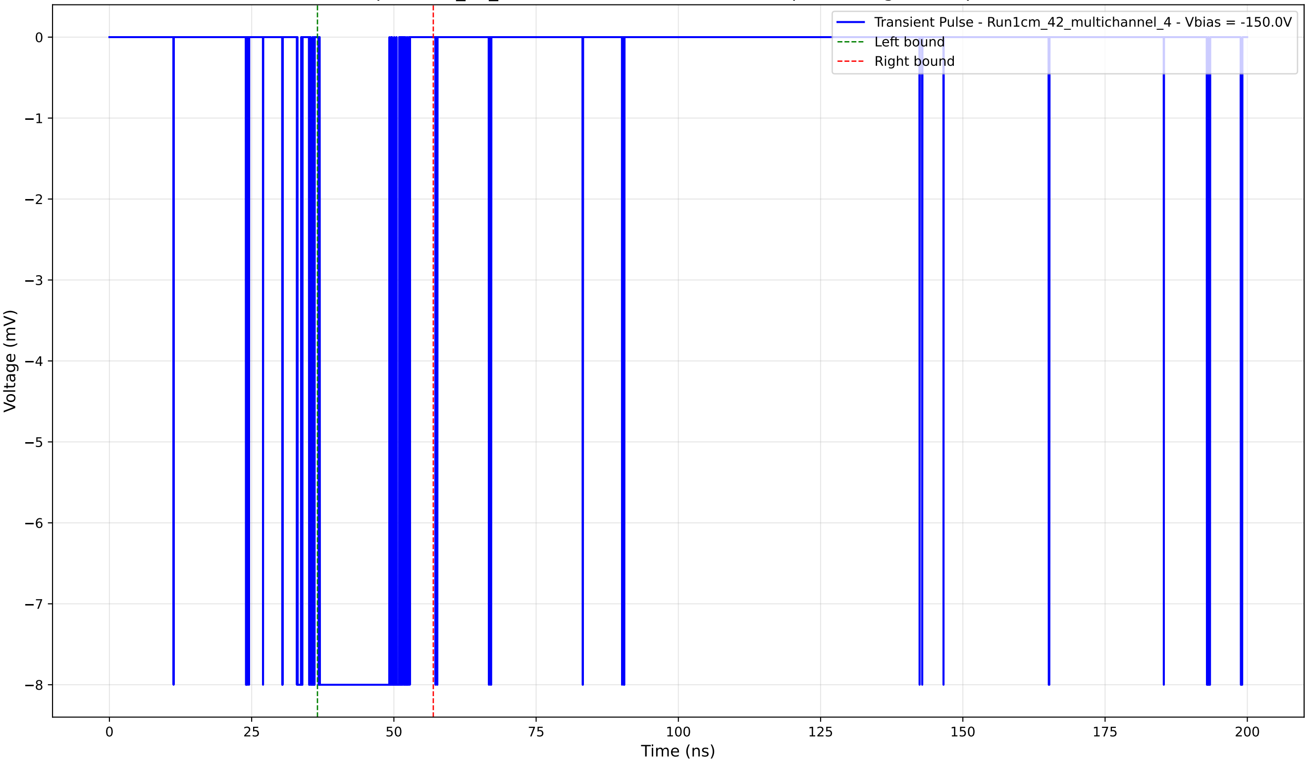
Transient Pulse - Sample: 1cm_42_multichannel - Position: 3955.0 \mu\text{m} - Charge: 2.33 pC - Rise Time: 0.02 ns
