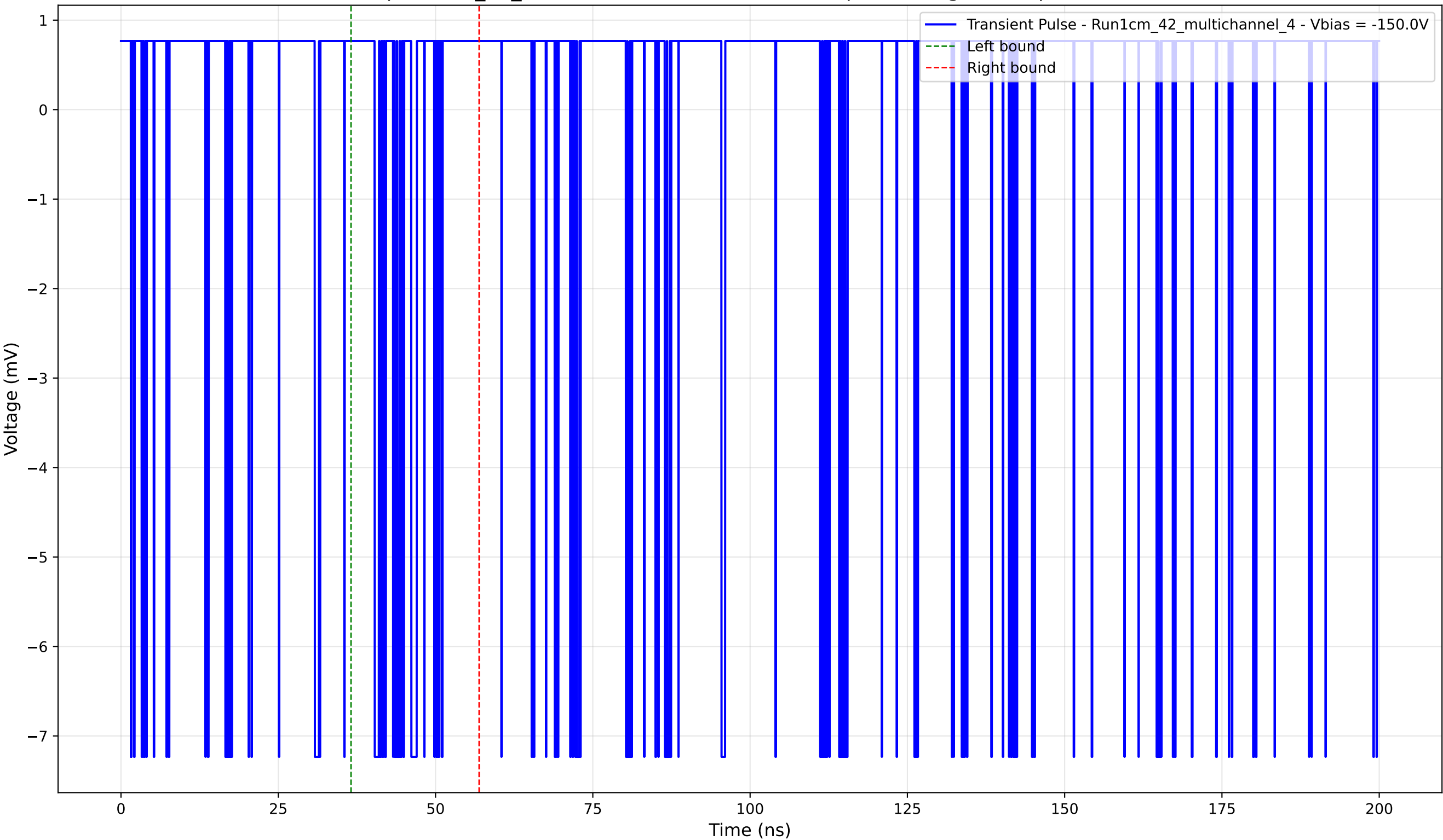
Transient Pulse - Sample: 1cm_42_multichannel - Position: 3885.0 \mu\text{m} - Charge: 0.30 pC - Rise Time: 0.00 ns (N/A)
