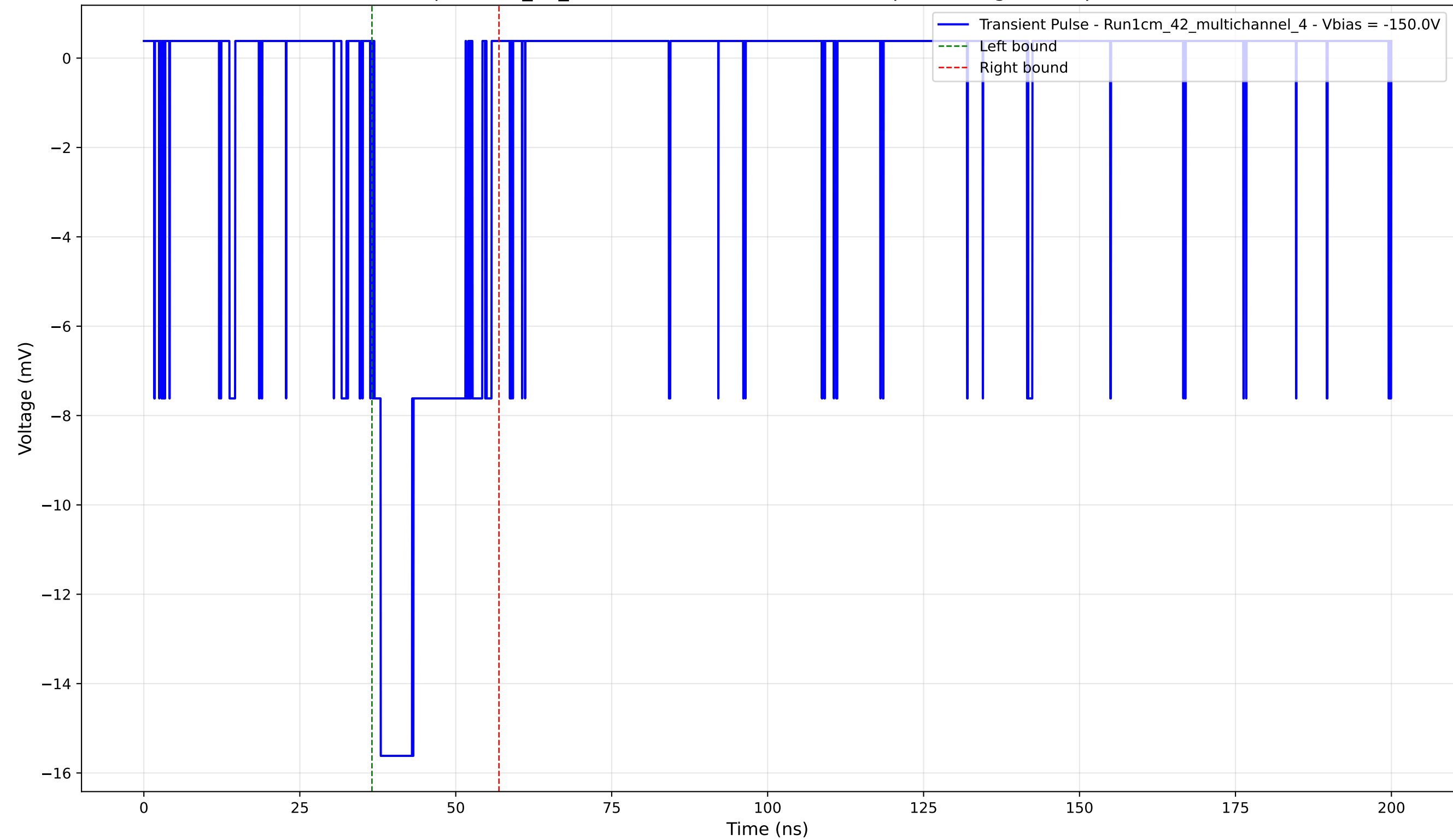
Transient Pulse - Sample: 1cm_42_multichannel - Position: 3980.0 \mu\text{m} - Charge: 3.51 pC - Rise Time: 1.02 ns
