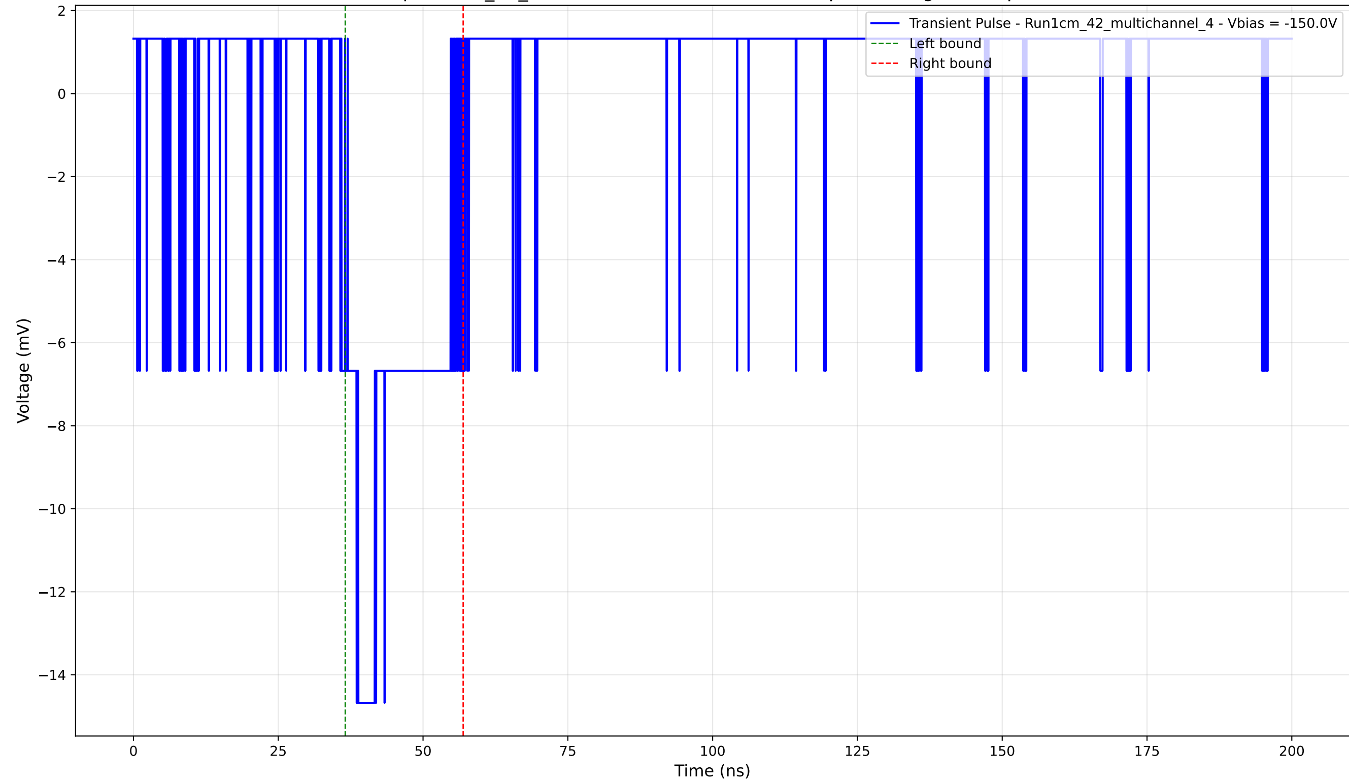
Transient Pulse - Sample: 1cm_42_multichannel - Position: 4725.0 \mu\text{m} - Charge: 3.04 pC - Rise Time: 1.54 ns
