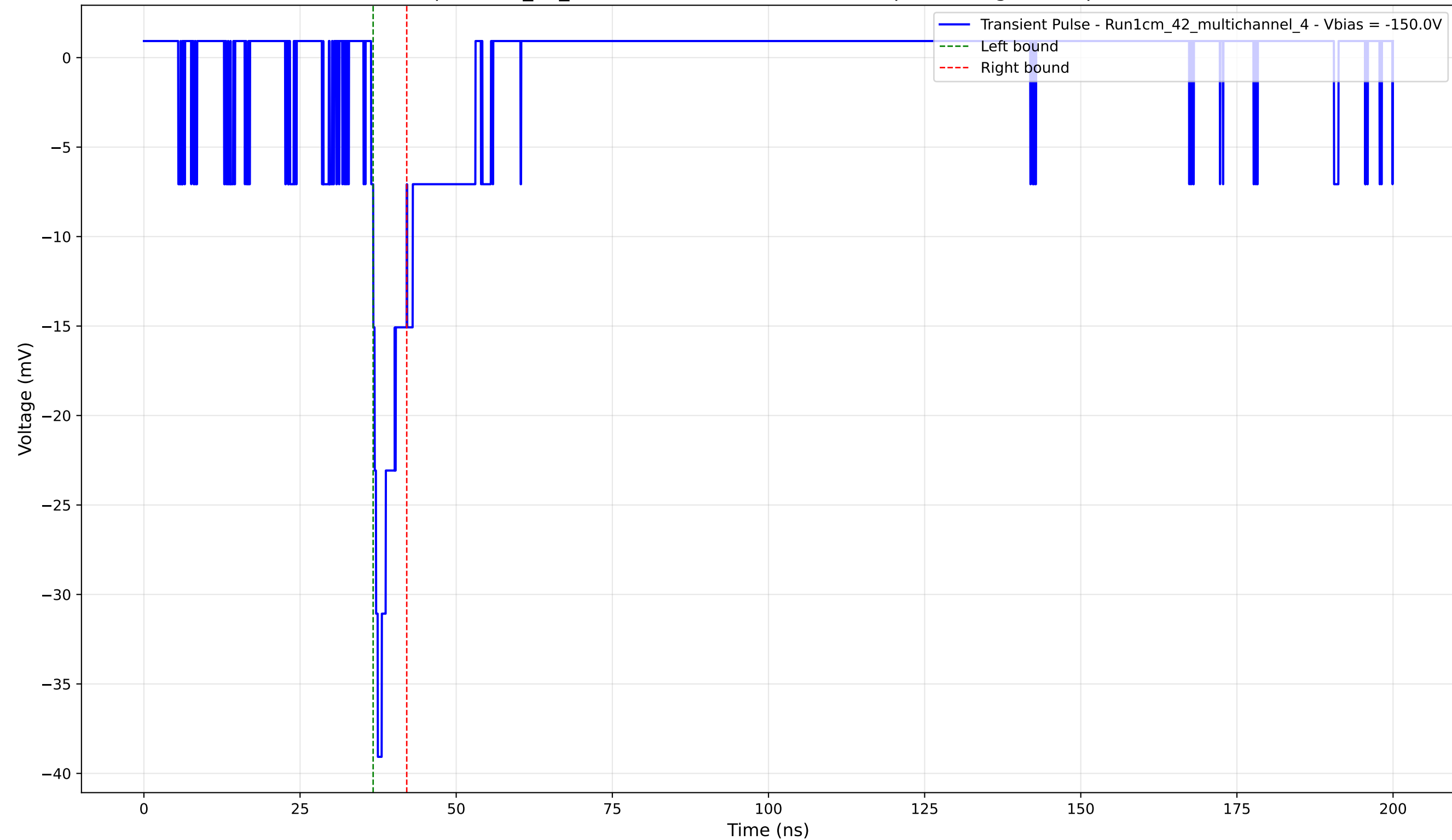
Transient Pulse - Sample: 1cm_42_multichannel - Position: 1710.0 \mu\text{m} - Charge: 2.51 pC - Rise Time: 1.07 ns
