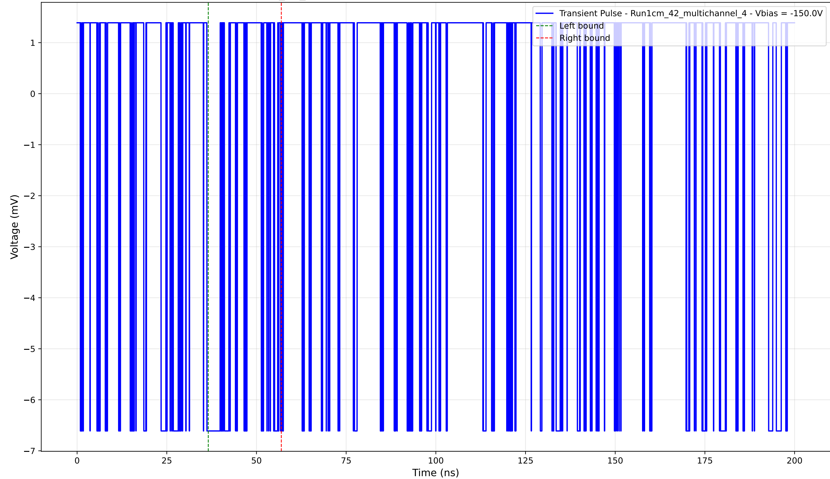
Transient Pulse - Sample: 1cm_42_multichannel - Position: 2370.0 \mu\text{m} - Charge: 0.72 pC - Rise Time: 0.00 ns (N/A)
