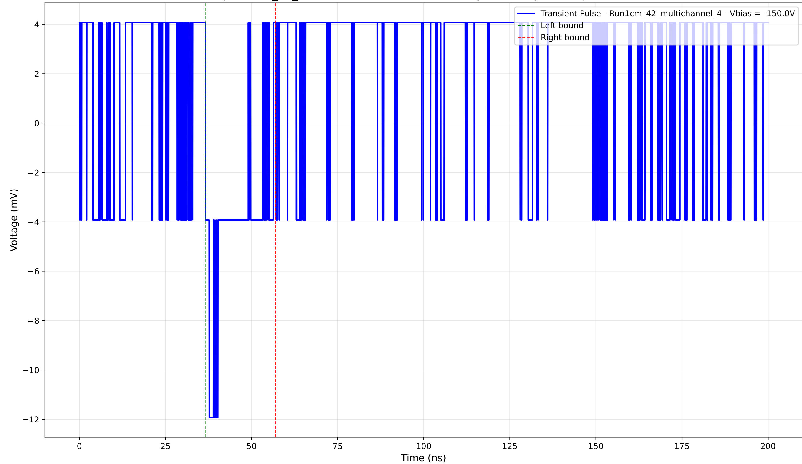
Transient Pulse - Sample: 1cm_42_multichannel - Position: 1325.0 \mu\text{m} - Charge: 1.53 pC - Rise Time: 0.00 ns (N/A)
