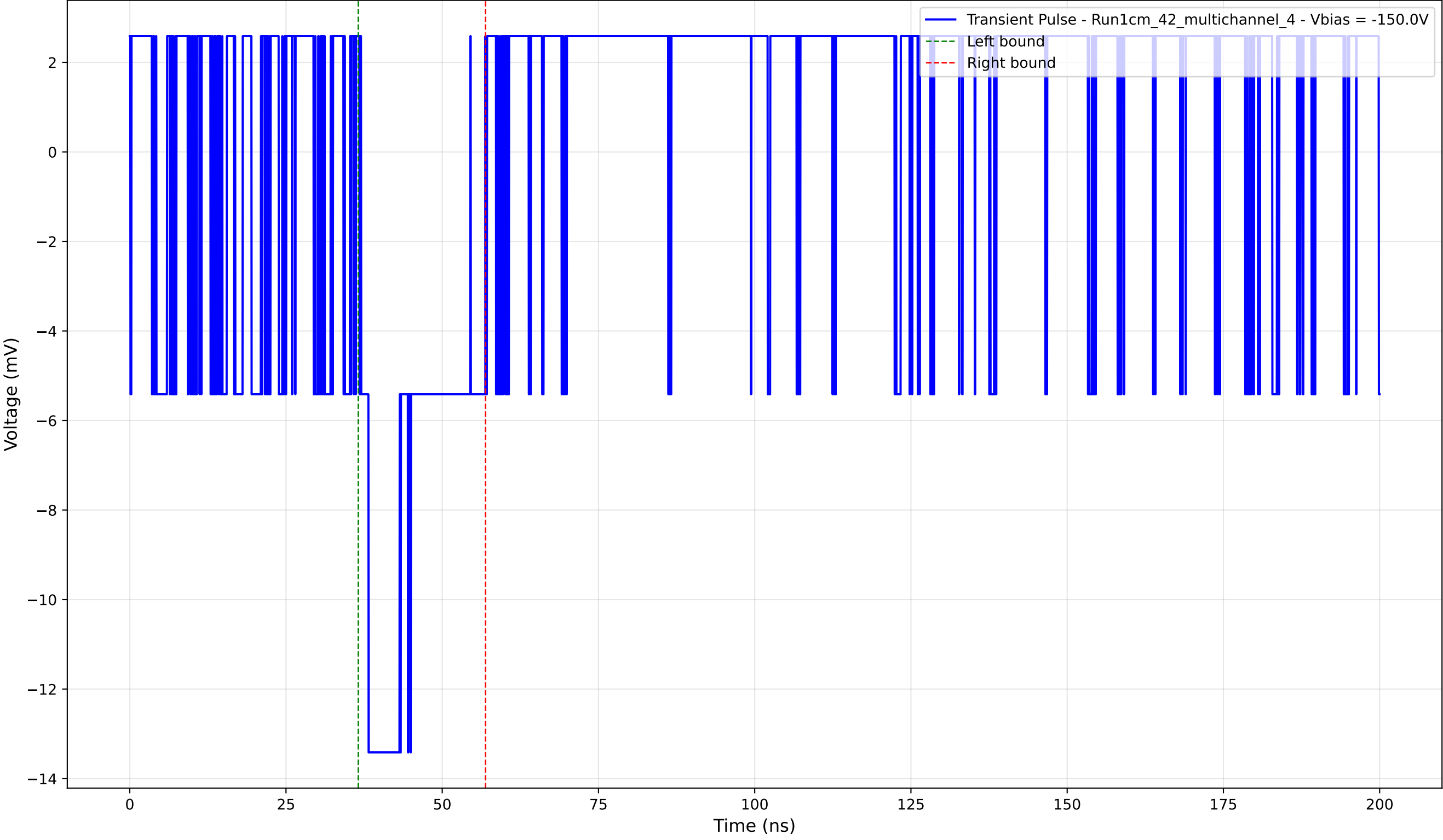
Transient Pulse - Sample: 1cm_42_multichannel - Position: 515.0 \mu\text{m} - Charge: 2.99 pC - Rise Time: 0.00 ns (N/A)
