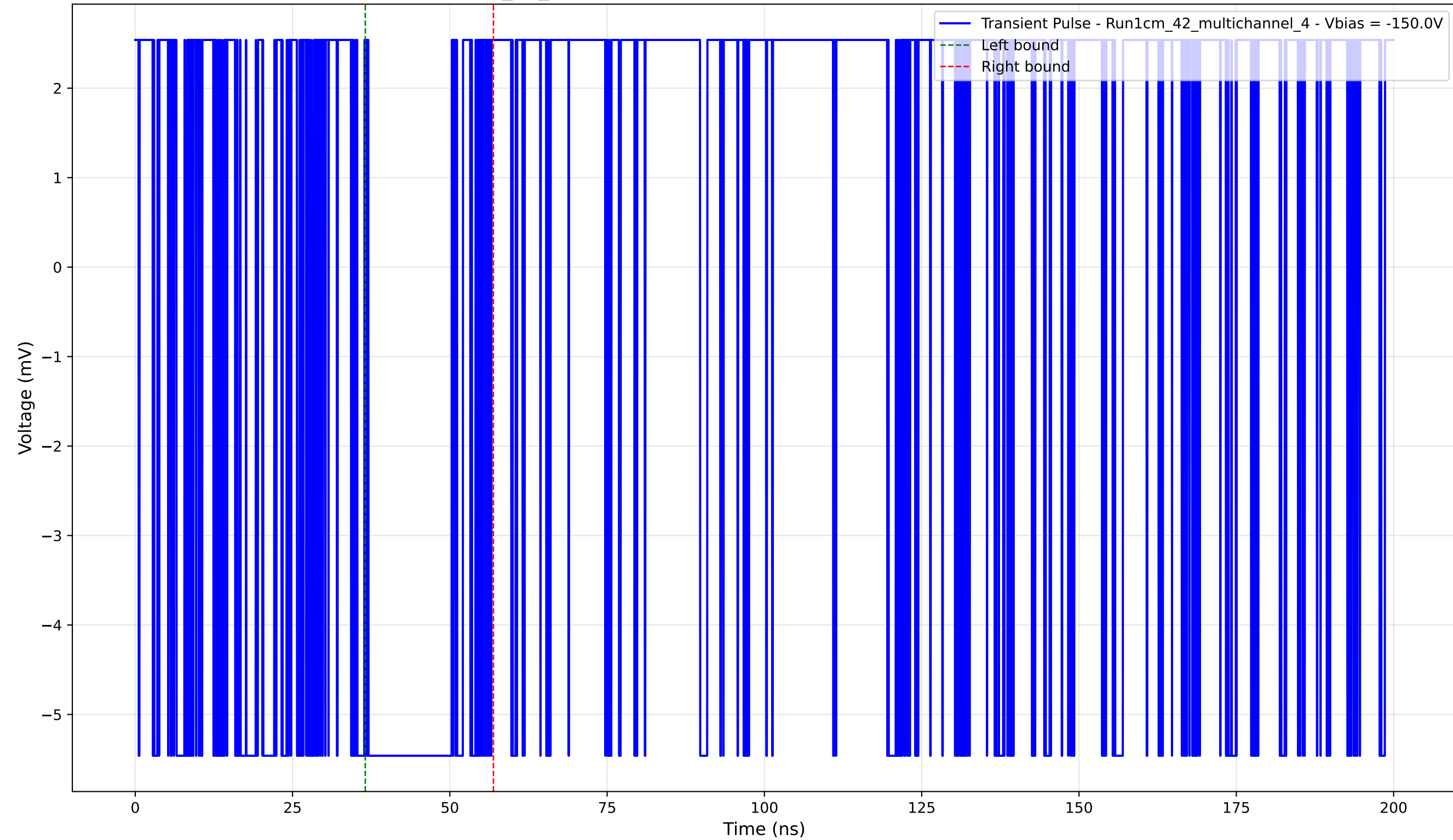
Transient Pulse - Sample: 1cm_42_multichannel - Position: 85.0 \mu\text{m} - Charge: 1.56 pC - Rise Time: 0.00 ns (N/A)
