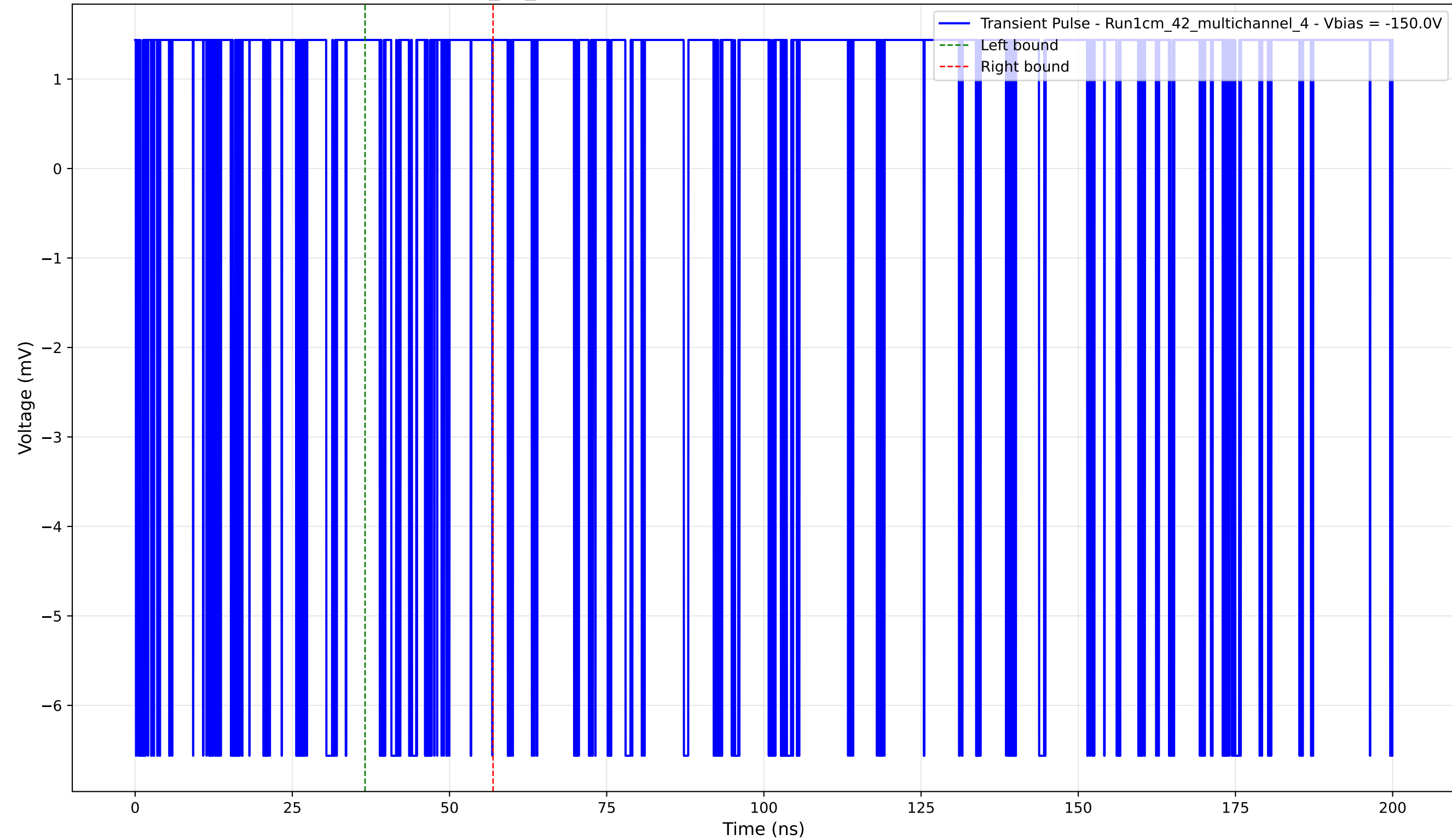
Transient Pulse - Sample: 1cm_42_multichannel - Position: 4400.0 \mu\text{m} - Charge: 0.06 pC - Rise Time: 0.00 ns (N/A)
