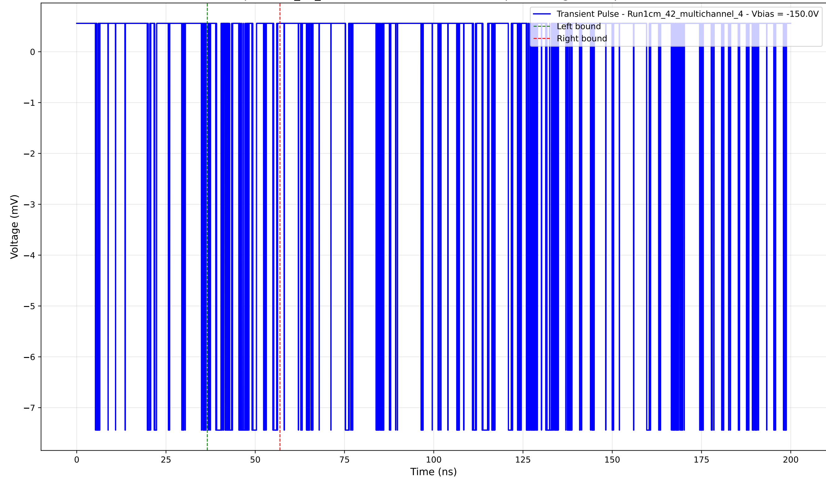
Transient Pulse - Sample: 1cm_42_multichannel - Position: 4415.0 \mu\text{m} - Charge: 1.03 pC - Rise Time: 0.02 ns
