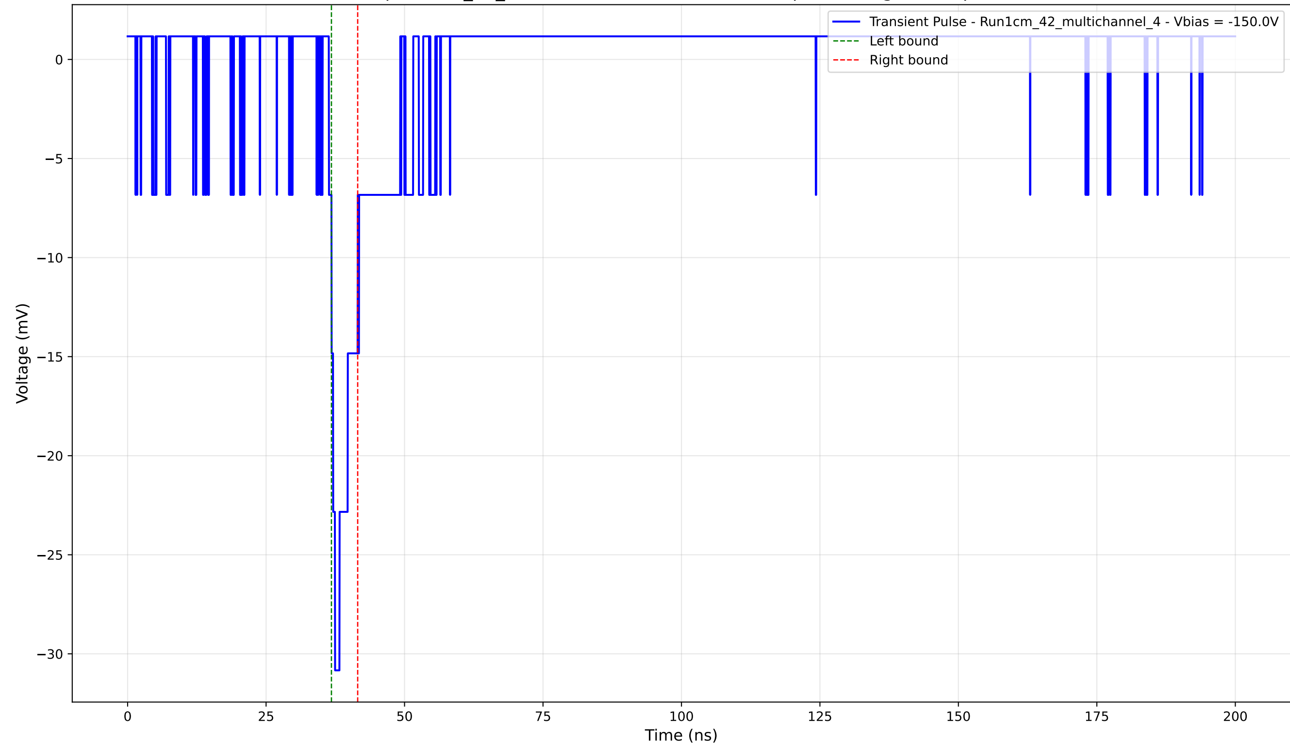
Transient Pulse - Sample: 1cm_42_multichannel - Position: 3125.0 \mu\text{m} - Charge: 1.96 pC - Rise Time: 1.11 ns
