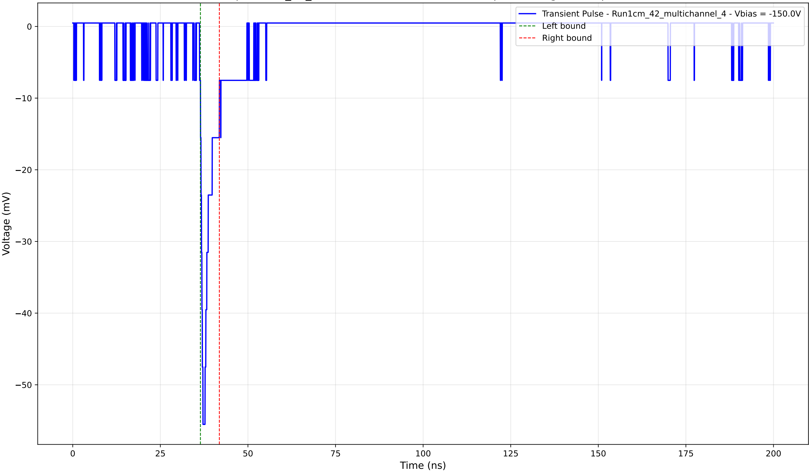
Transient Pulse - Sample: 1cm_42_multichannel - Position: 2735.0 \mu\text{m} - Charge: 2.97 pC - Rise Time: 0.99 ns
