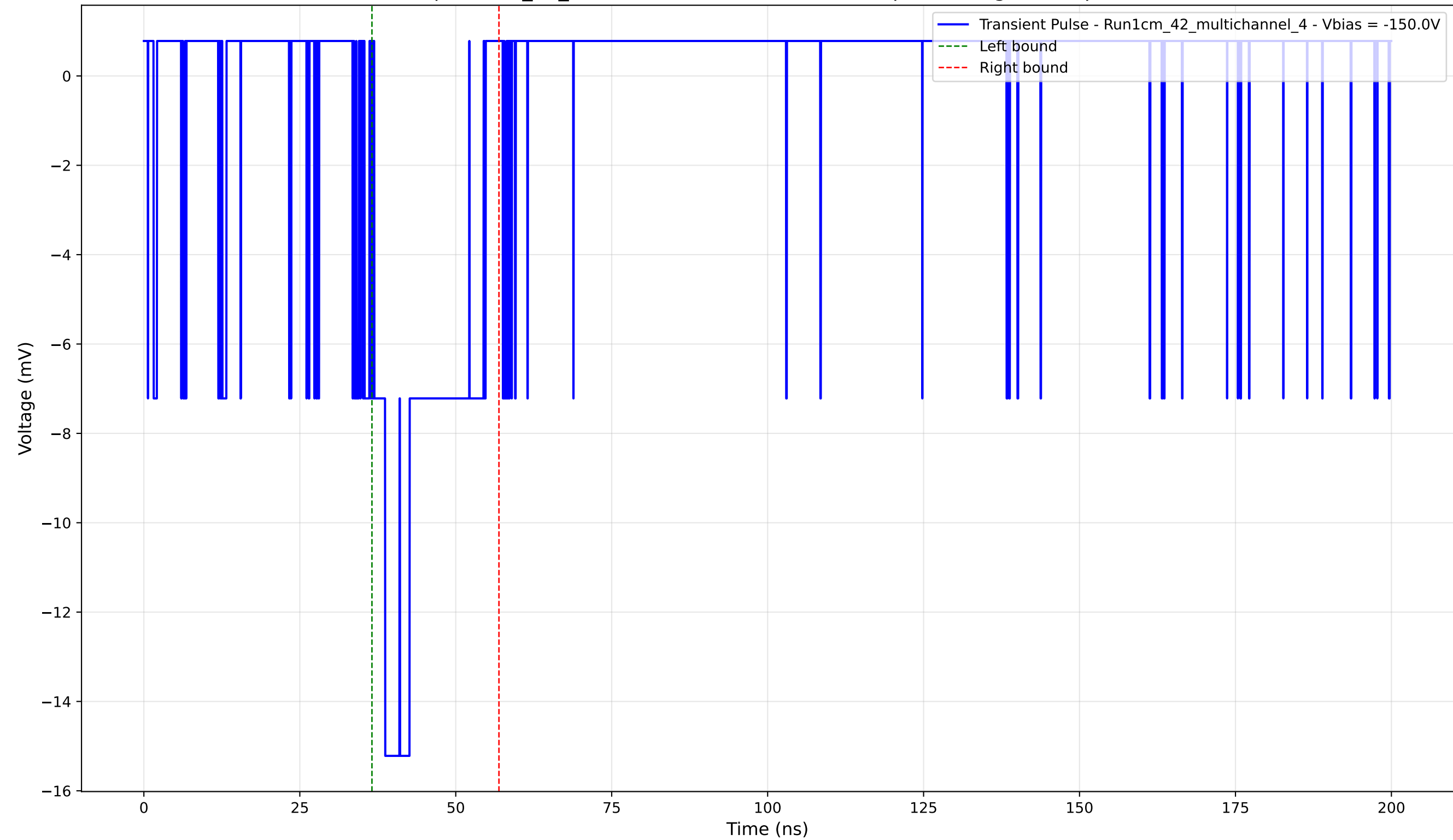
Transient Pulse - Sample: 1cm_42_multichannel - Position: 4640.0 \mu\text{m} - Charge: 3.15 pC - Rise Time: 1.76 ns
