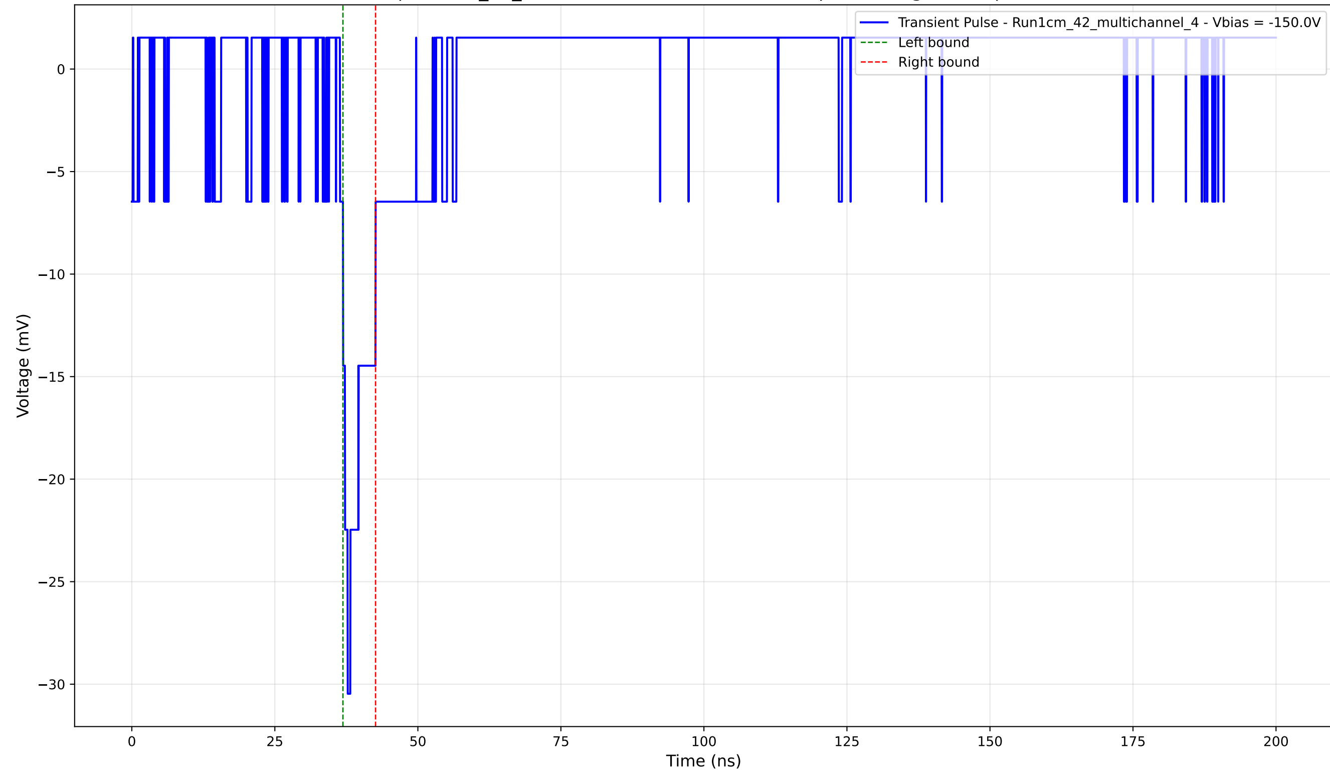
Transient Pulse - Sample: 1cm_42_multichannel - Position: 3245.0 \mu\text{m} - Charge: 2.10 pC - Rise Time: 1.35 ns
