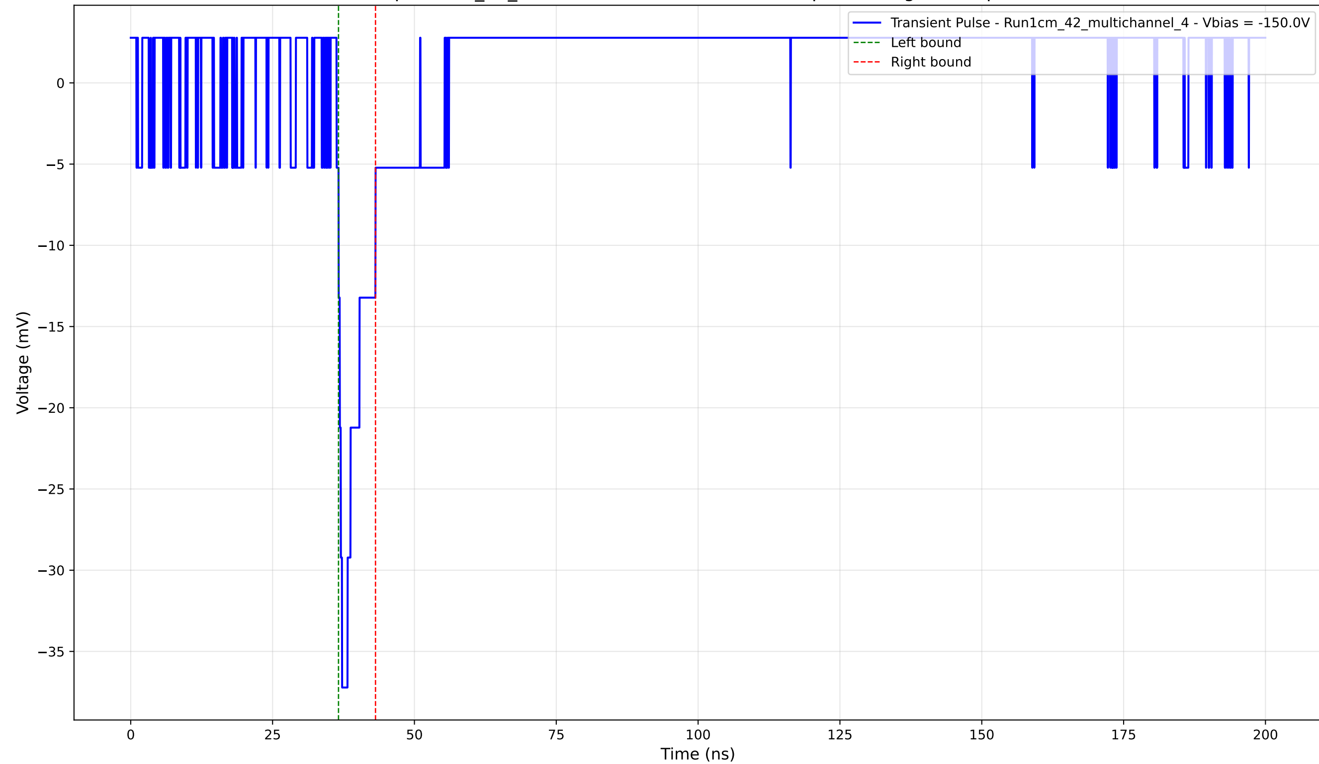
Transient Pulse - Sample: 1cm_42_multichannel - Position: 1755.0 \mu\text{m} - Charge: 2.71 pC - Rise Time: 0.97 ns
