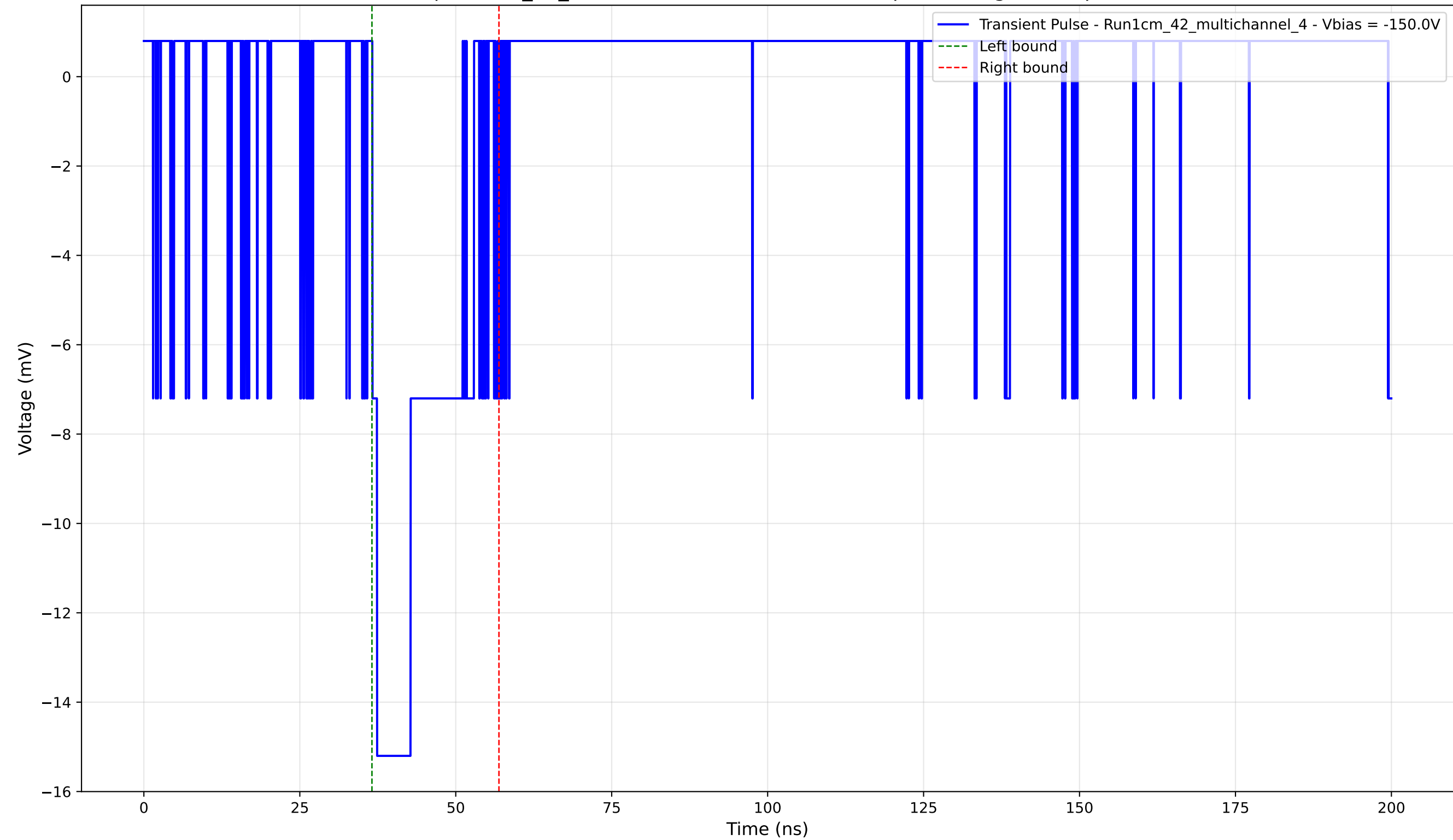
Transient Pulse - Sample: 1cm_42_multichannel - Position: 3595.0 \mu\text{m} - Charge: 3.28 pC - Rise Time: 0.76 ns
