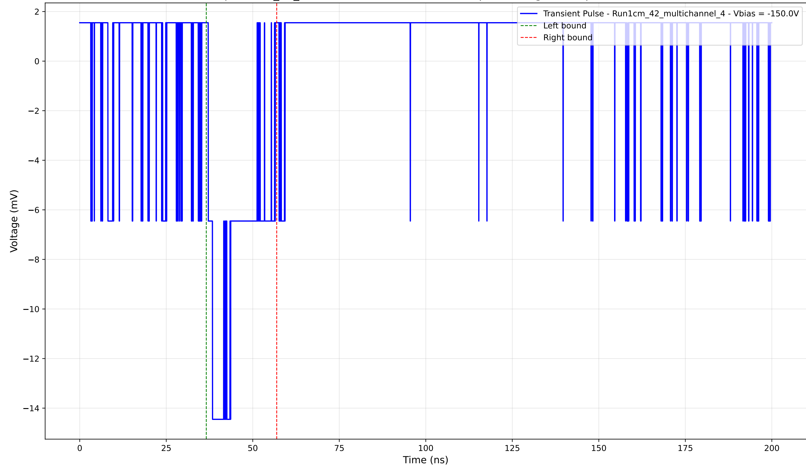
Transient Pulse - Sample: 1cm_42_multichannel - Position: 4565.0 \mu\text{m} - Charge: 3.15 pC - Rise Time: 0.00 ns (N/A)
