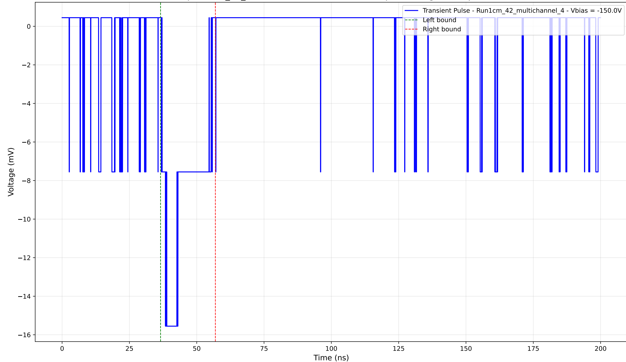
Transient Pulse - Sample: 1cm_42_multichannel - Position: 4700.0 \mu\text{m} - Charge: 3.41 pC - Rise Time: 1.28 ns
