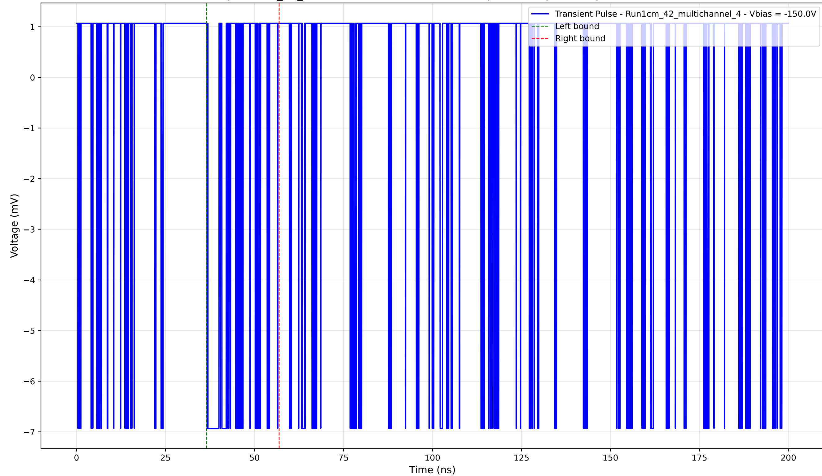
Transient Pulse - Sample: 1cm_42_multichannel - Position: 3420.0 \mu\text{m} - Charge: 0.79 pC - Rise Time: 0.00 ns (N/A)
