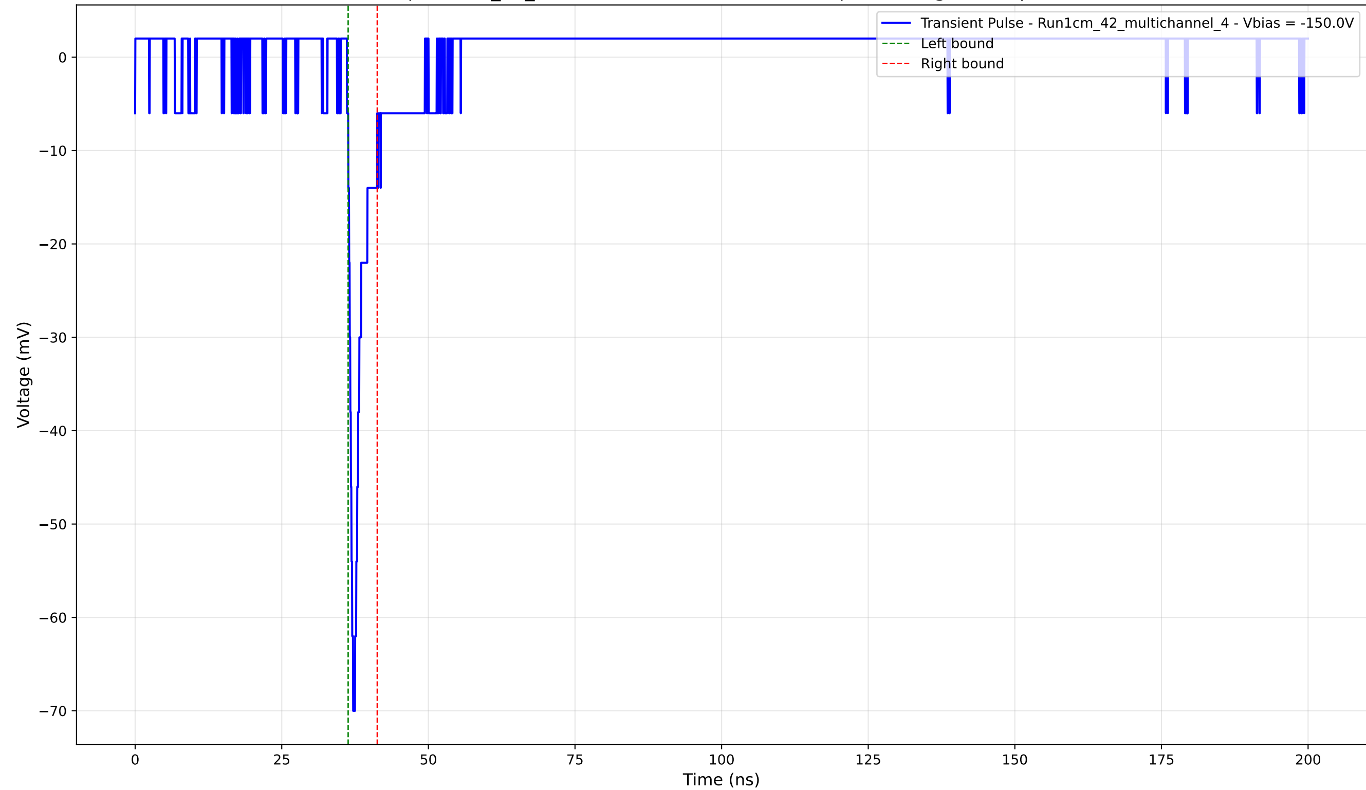
Transient Pulse - Sample: 1cm_42_multichannel - Position: 2185.0 \mu\text{m} - Charge: 2.97 pC - Rise Time: 0.84 ns
