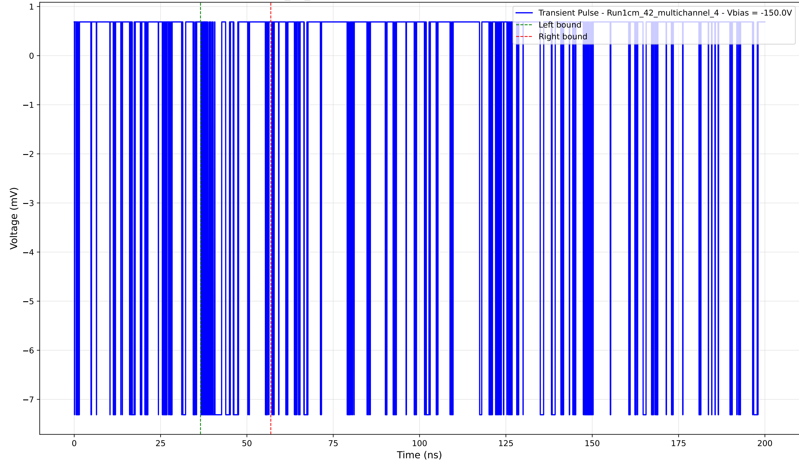
Transient Pulse - Sample: 1cm_42_multichannel - Position: 4375.0 \mu\text{m} - Charge: 1.00 pC - Rise Time: 0.02 ns
