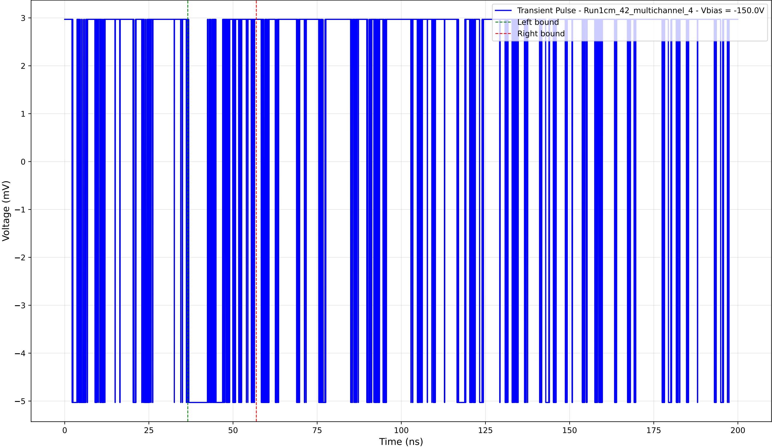
Transient Pulse - Sample: 1cm_42_multichannel - Position: 3425.0 \mu\text{m} - Charge: 0.67 pC - Rise Time: 0.00 ns (N/A)
