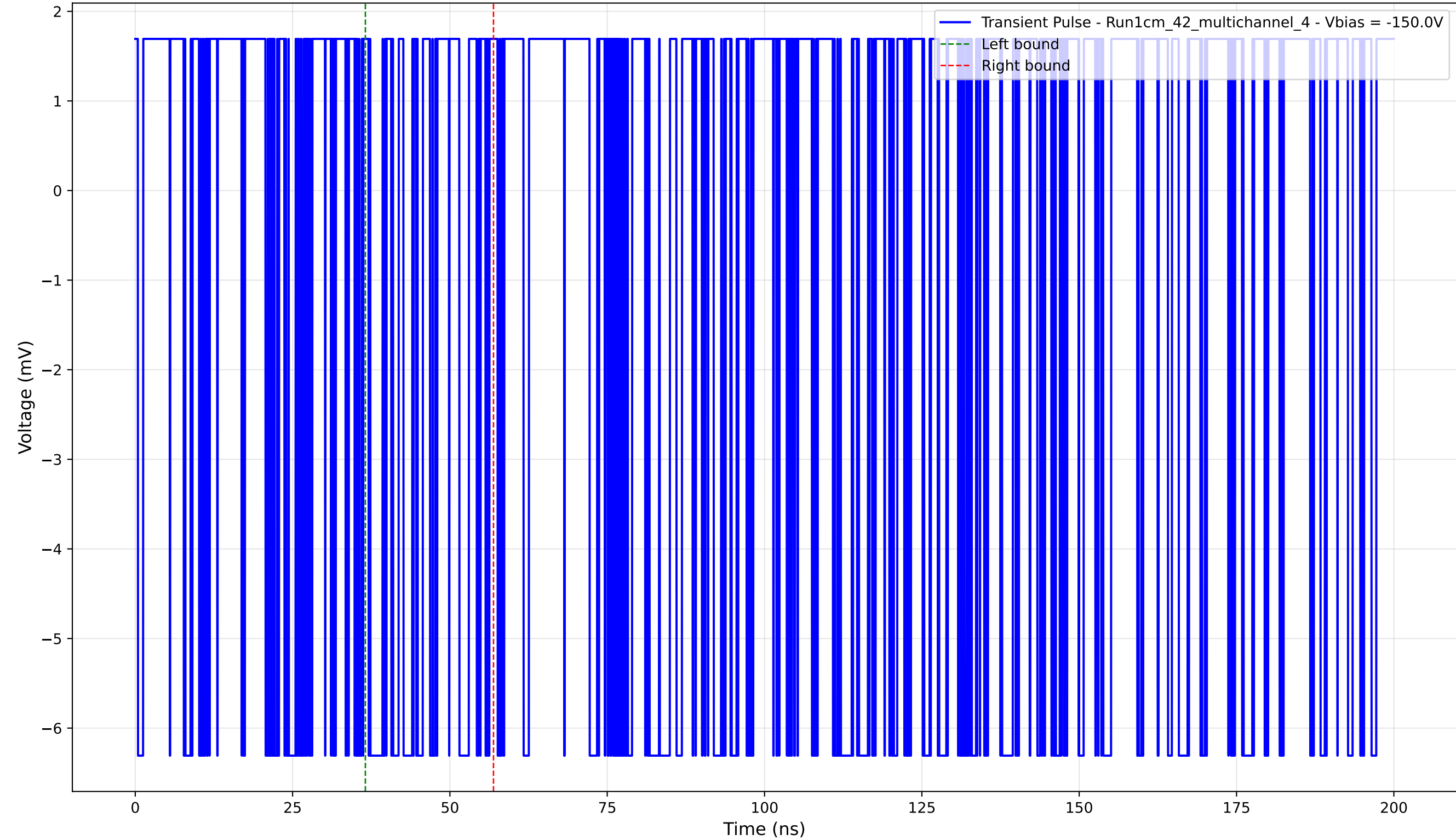
Transient Pulse - Sample: 1cm_42_multichannel - Position: 1370.0 \mu\text{m} - Charge: 0.79 pC - Rise Time: 0.00 ns (N/A)
