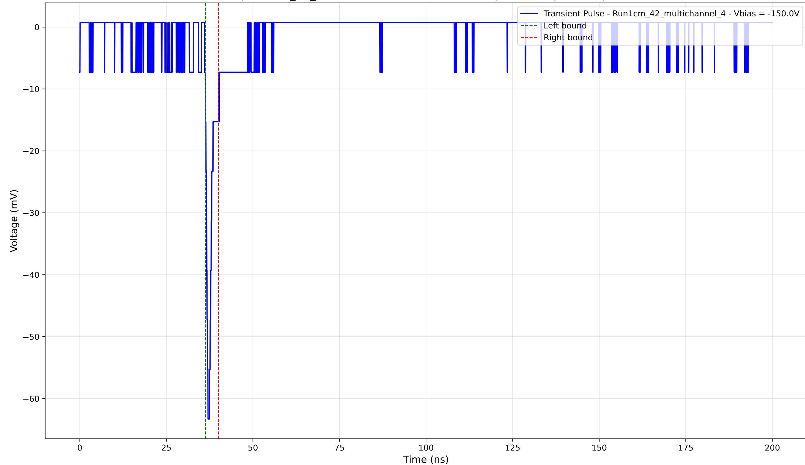
Transient Pulse - Sample: 1cm_42_multichannel - Position: 2325.0 \mu\text{m} - Charge: 2.32 pC - Rise Time: 0.96 ns
