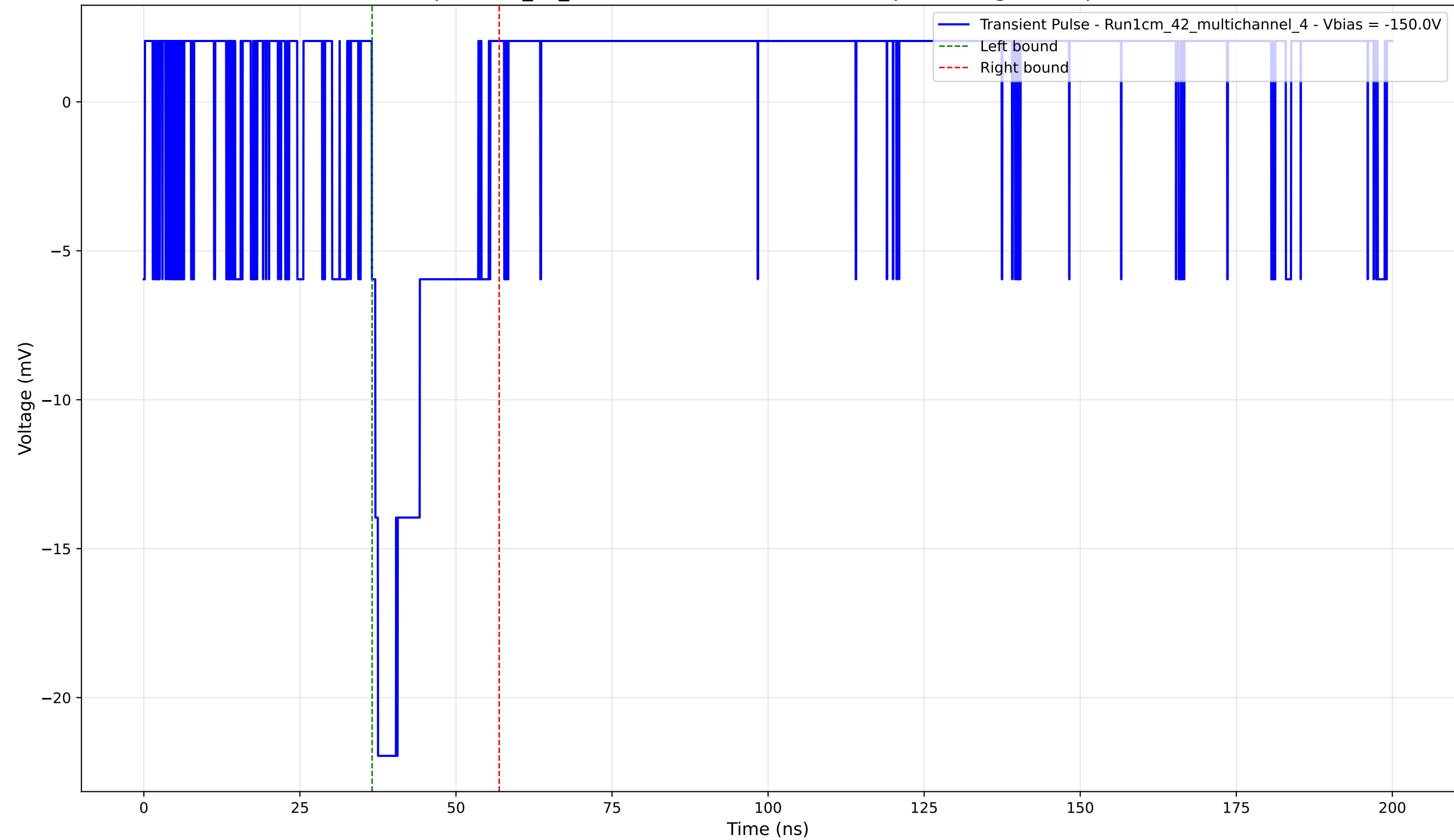
Transient Pulse - Sample: 1cm_42_multichannel - Position: 1285.0 \mu\text{m} - Charge: 3.78 pC - Rise Time: 1.00 ns
