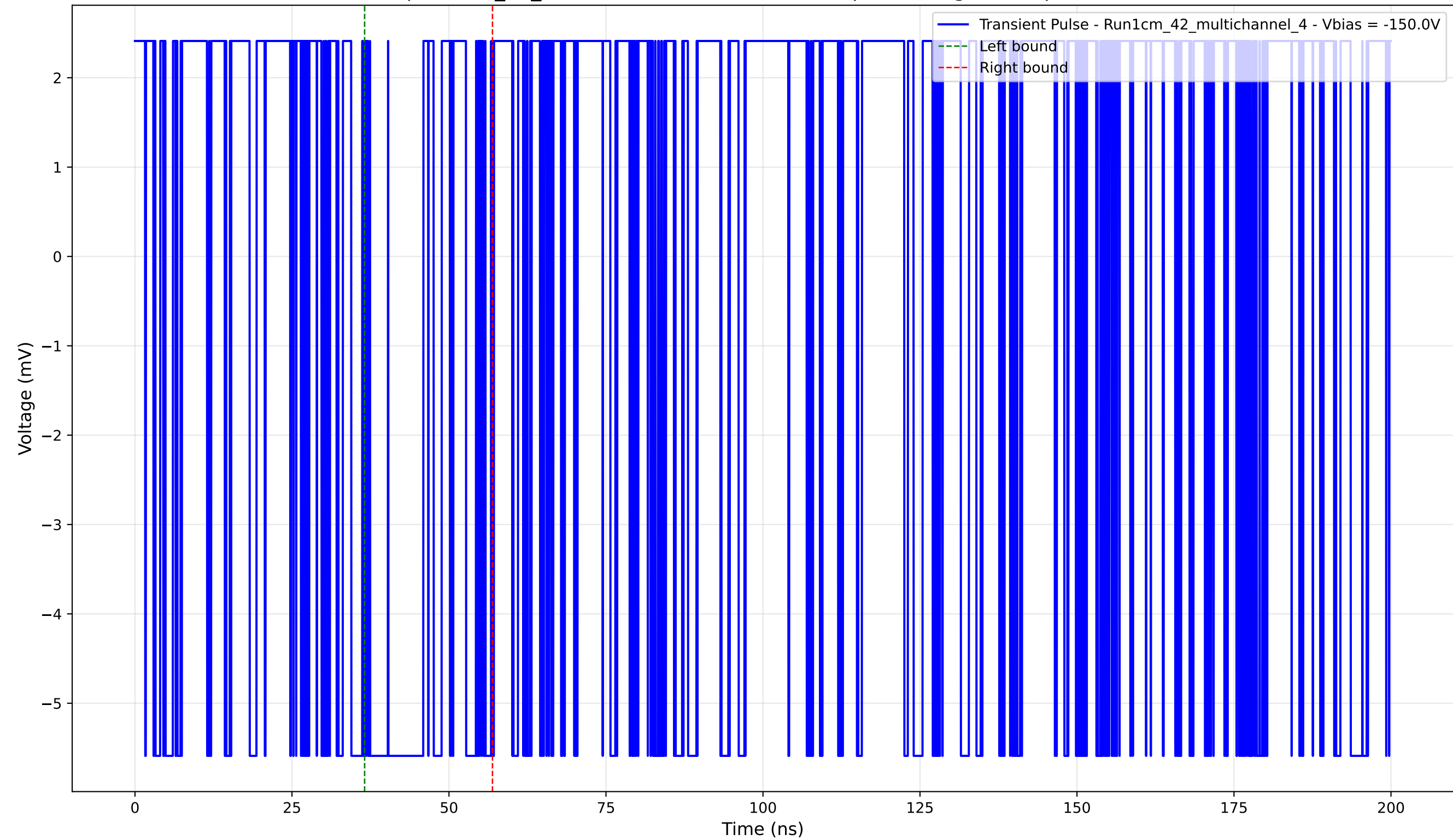
Transient Pulse - Sample: 1cm_42_multichannel - Position: 335.0 \mu\text{m} - Charge: 1.21 pC - Rise Time: 0.00 ns (N/A)
