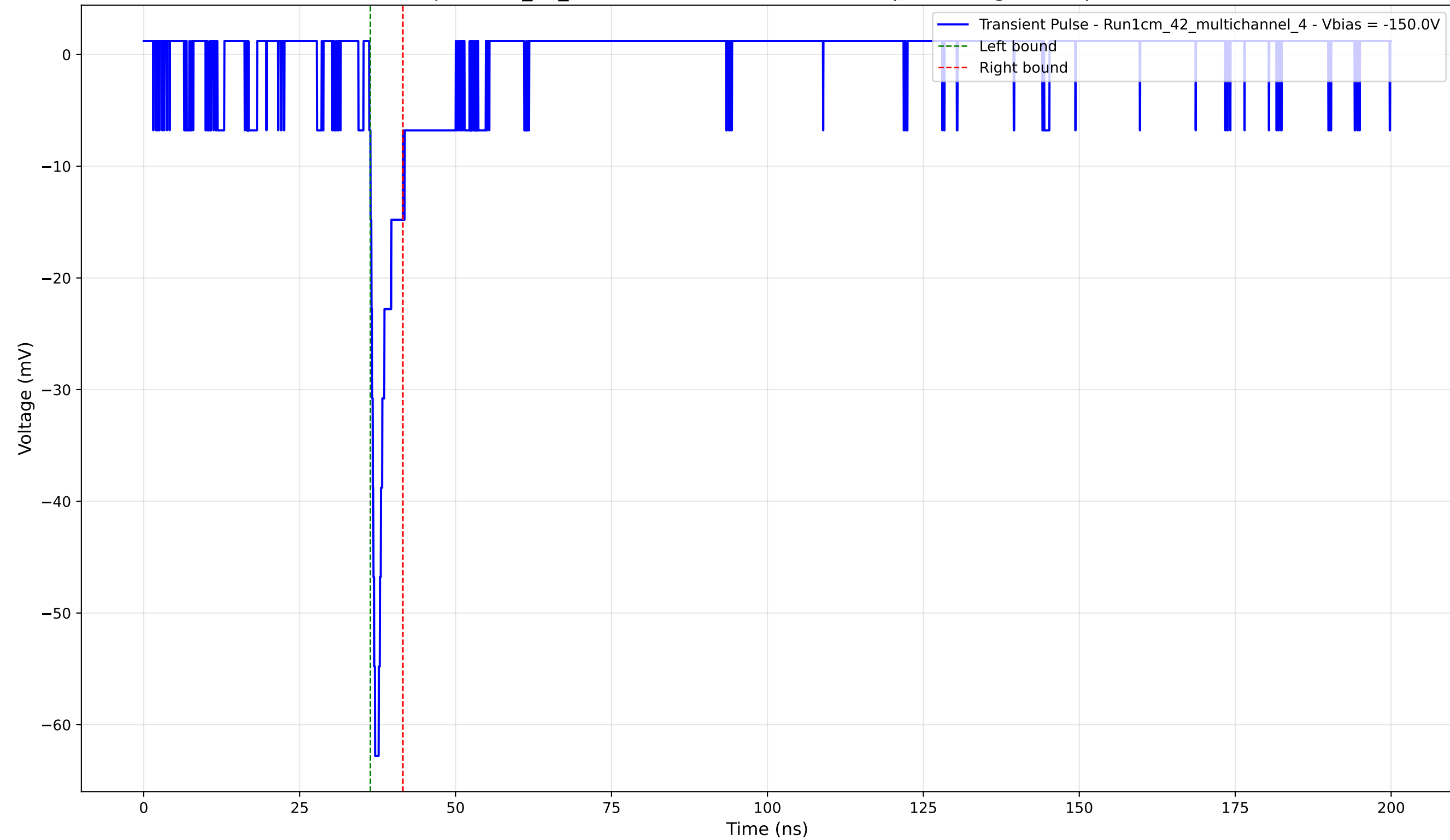
Transient Pulse - Sample: 1cm_42_multichannel - Position: 2160.0 \mu\text{m} - Charge: 3.04 pC - Rise Time: 0.92 ns
