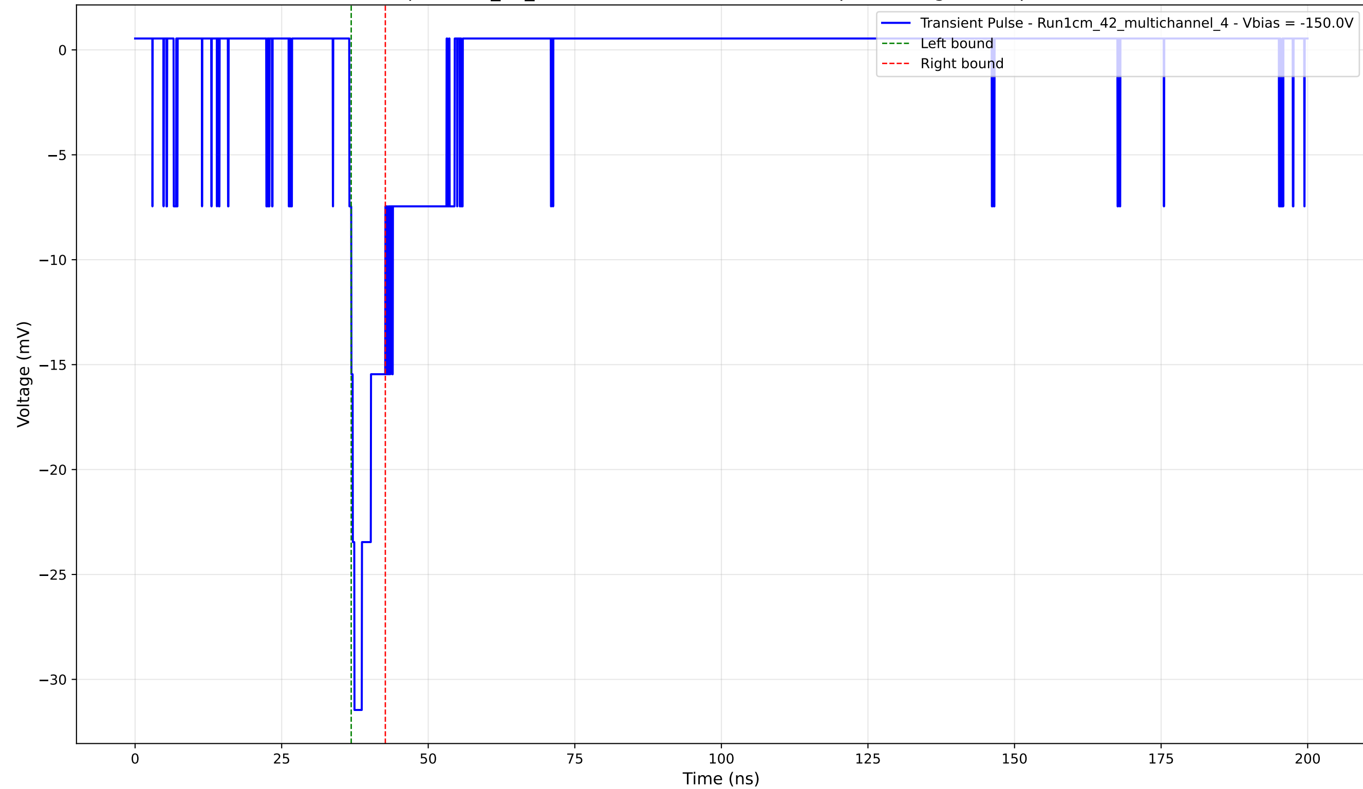
Transient Pulse - Sample: 1cm_42_multichannel - Position: 1550.0 \mu\text{m} - Charge: 2.50 pC - Rise Time: 0.87 ns
