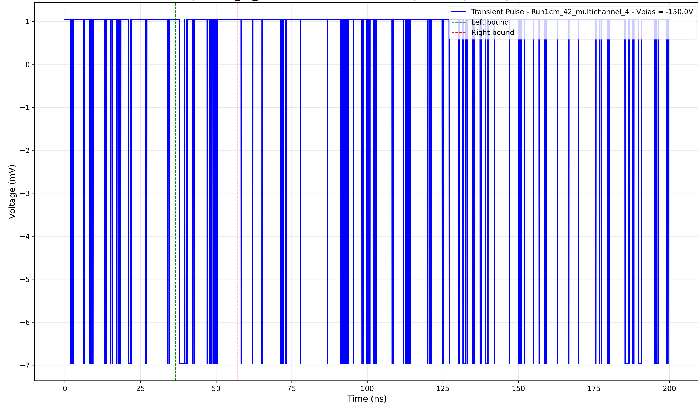
Transient Pulse - Sample: 1cm_42_multichannel - Position: 4420.0 \mu\text{m} - Charge: 0.14 pC - Rise Time: 0.00 ns (N/A)
