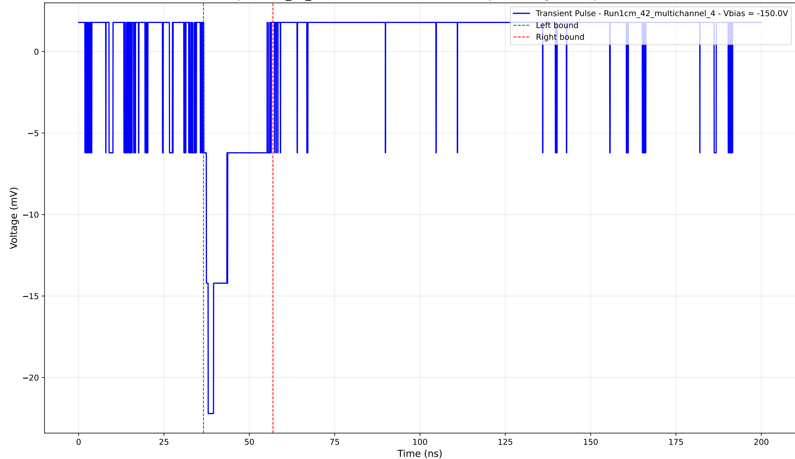
Transient Pulse - Sample: 1cm_42_multichannel - Position: 1145.0 \mu\text{m} - Charge: 3.66 pC - Rise Time: 1.30 ns
