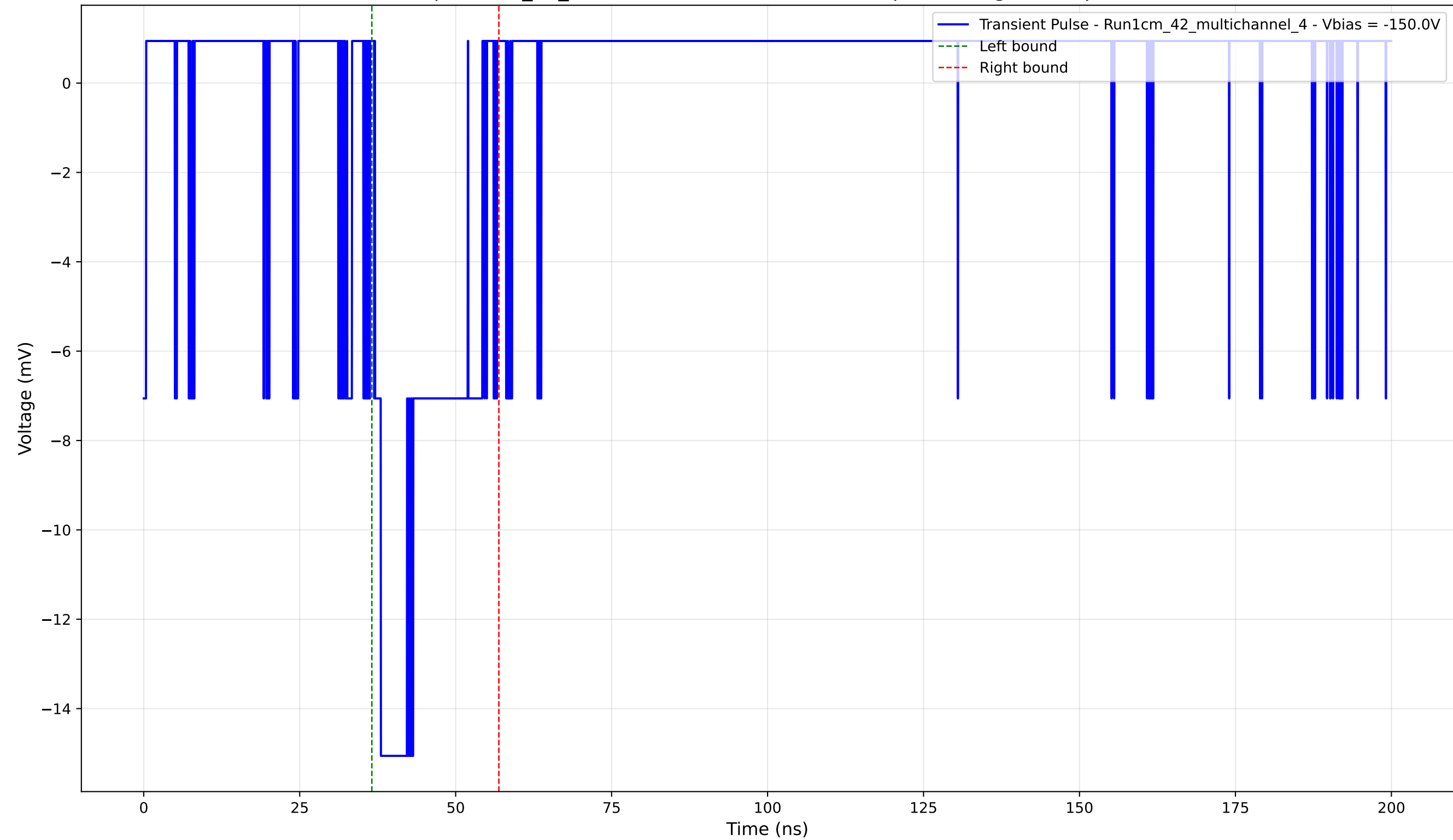
Transient Pulse - Sample: 1cm_42_multichannel - Position: 4085.0 \mu\text{m} - Charge: 3.20 pC - Rise Time: 0.94 ns
