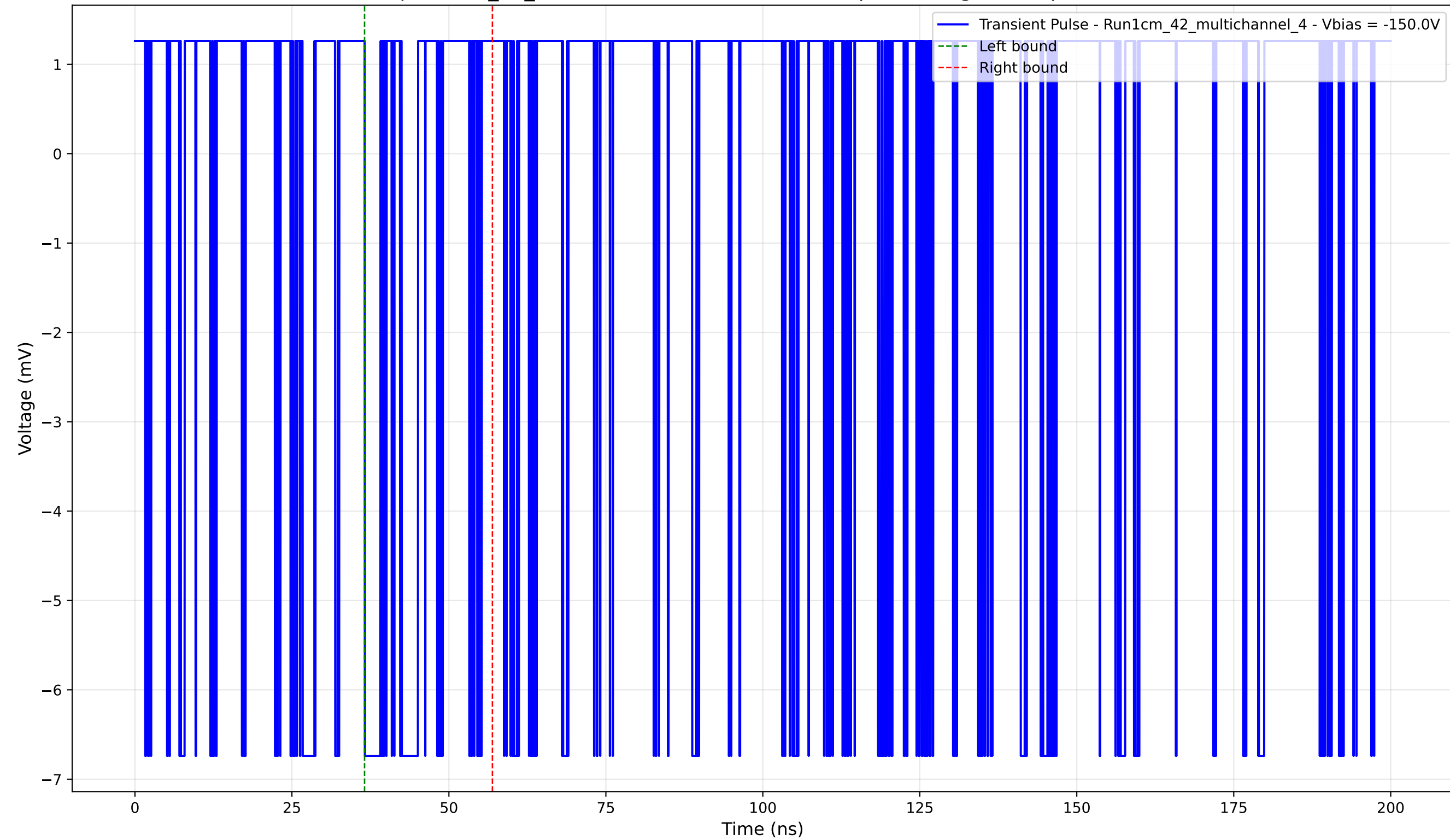
Transient Pulse - Sample: 1cm_42_multichannel - Position: 2390.0 \mu\text{m} - Charge: 0.65 pC - Rise Time: 0.00 ns (N/A)
