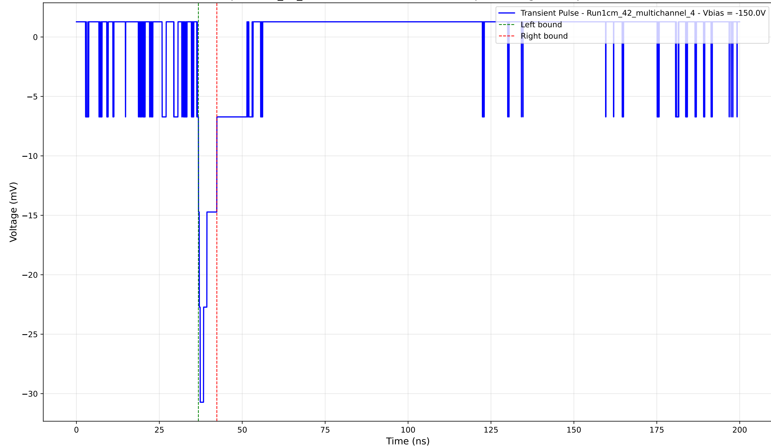
Transient Pulse - Sample: 1cm_42_multichannel - Position: 3110.0 \mu\text{m} - Charge: 2.17 pC - Rise Time: 0.85 ns
