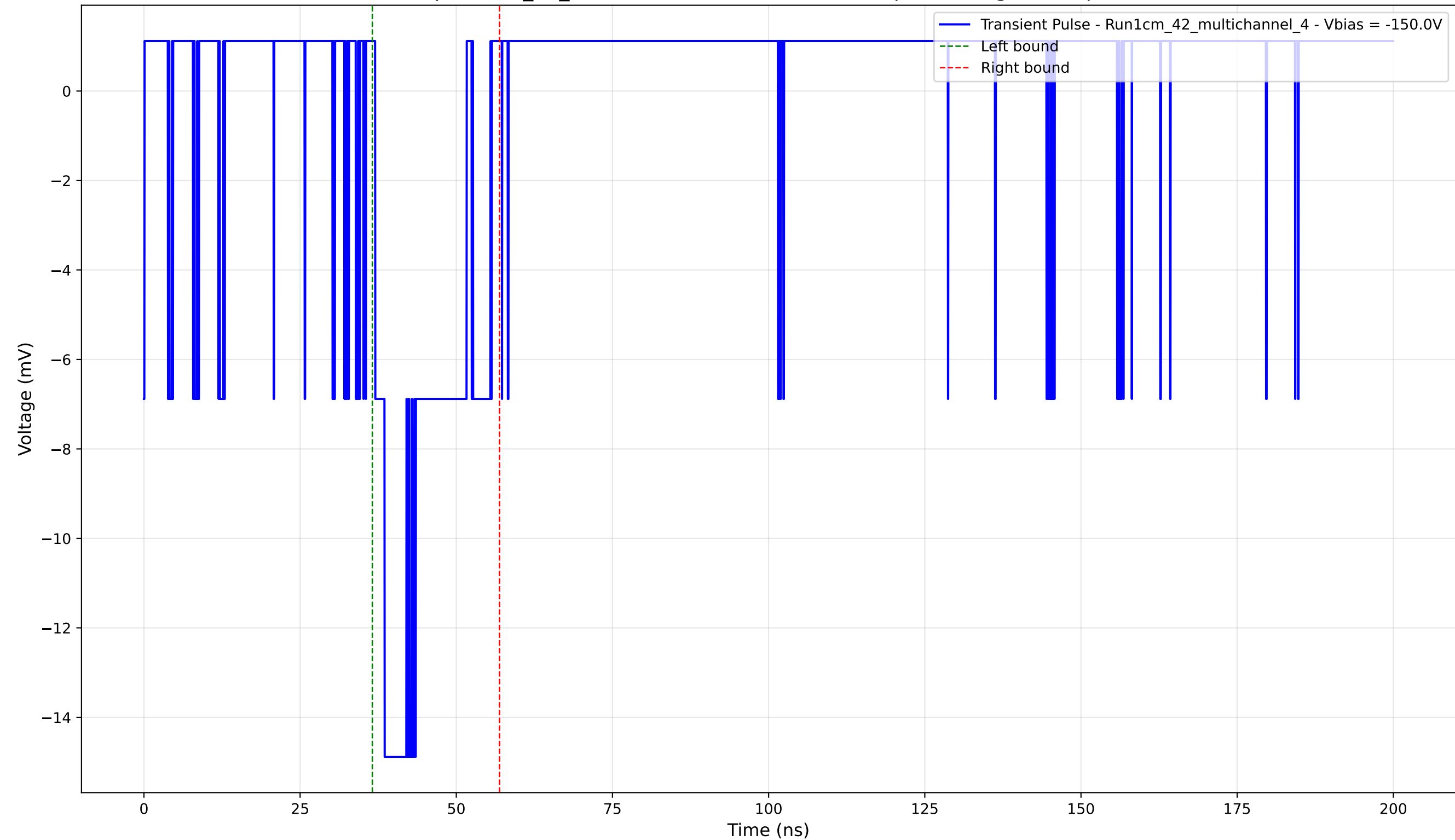
Transient Pulse - Sample: 1cm_42_multichannel - Position: 4750.0 \mu\text{m} - Charge: 3.10 pC - Rise Time: 1.52 ns
