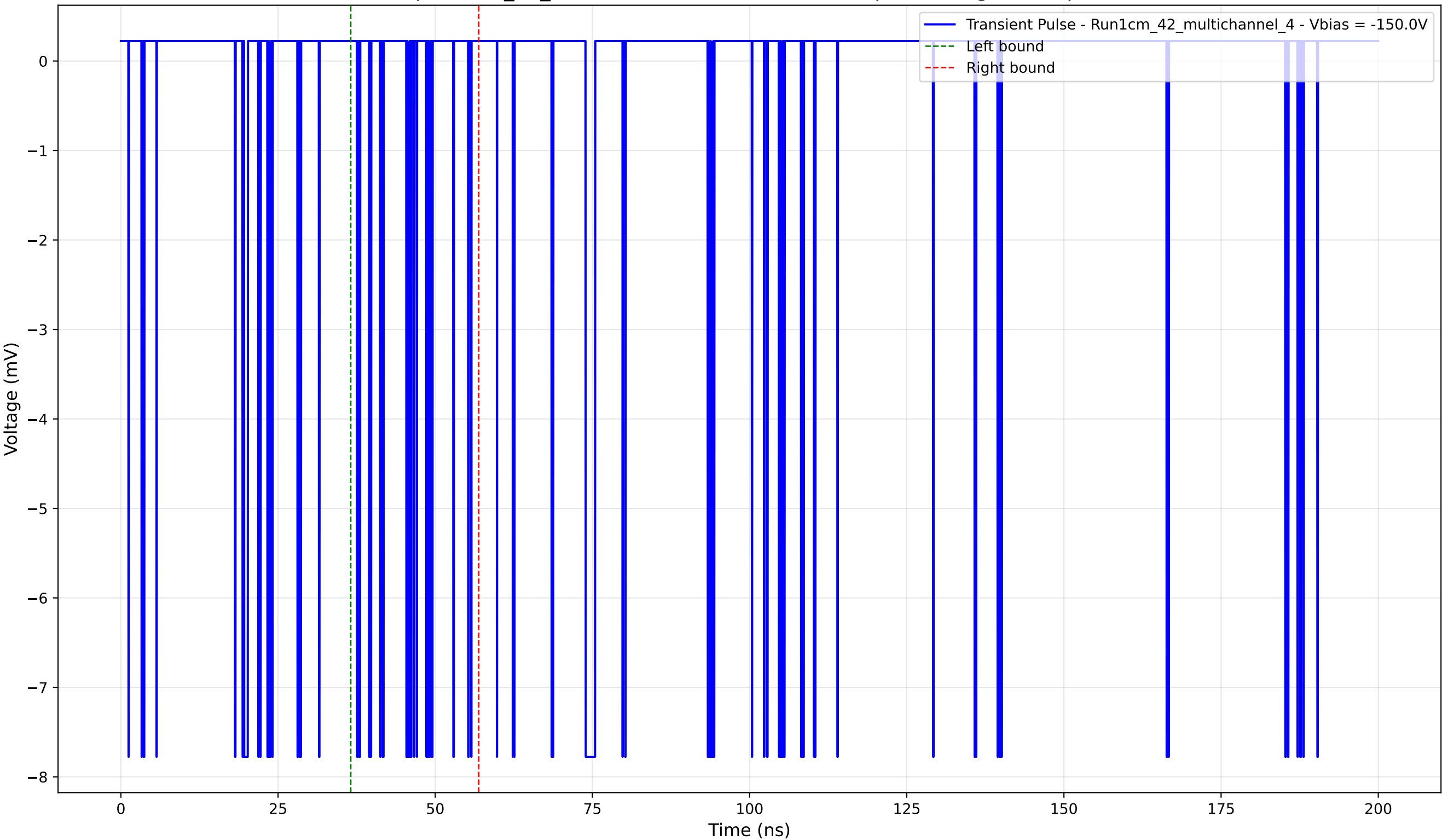
Transient Pulse - Sample: 1cm_42_multichannel - Position: 3915.0 \mu\text{m} - Charge: 0.25 pC - Rise Time: 0.02 ns
