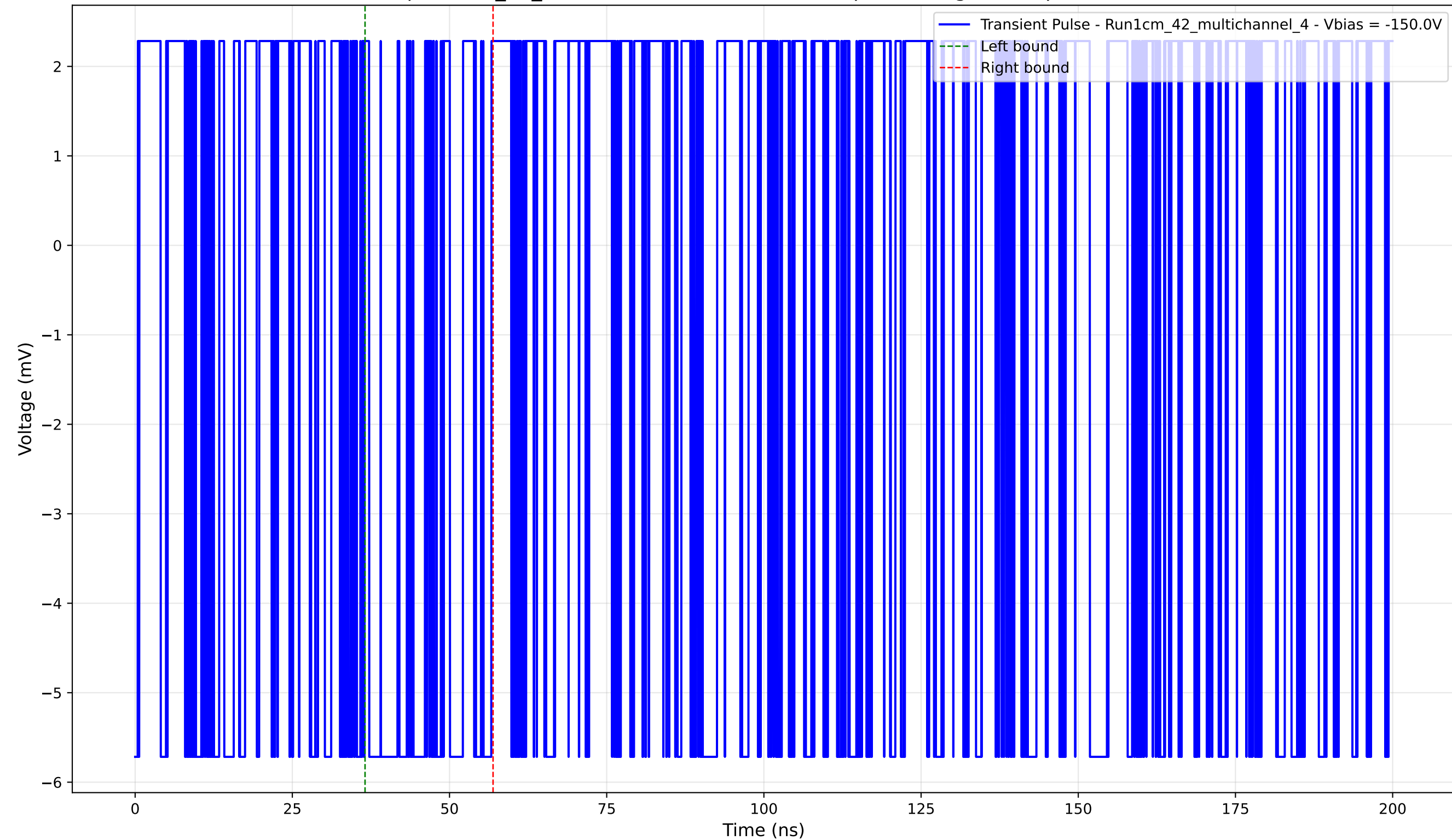
Transient Pulse - Sample: 1cm_42_multichannel - Position: 840.0 \mu\text{m} - Charge: 1.39 pC - Rise Time: 0.00 ns (N/A)
