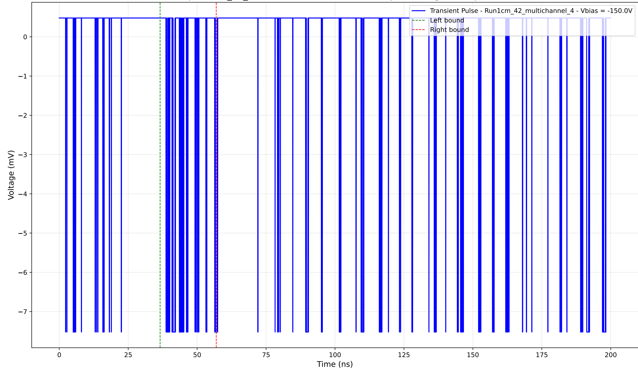
Transient Pulse - Sample: 1cm_42_multichannel - Position: 3880.0 \mu\text{m} - Charge: 0.44 pC - Rise Time: 0.02 ns
