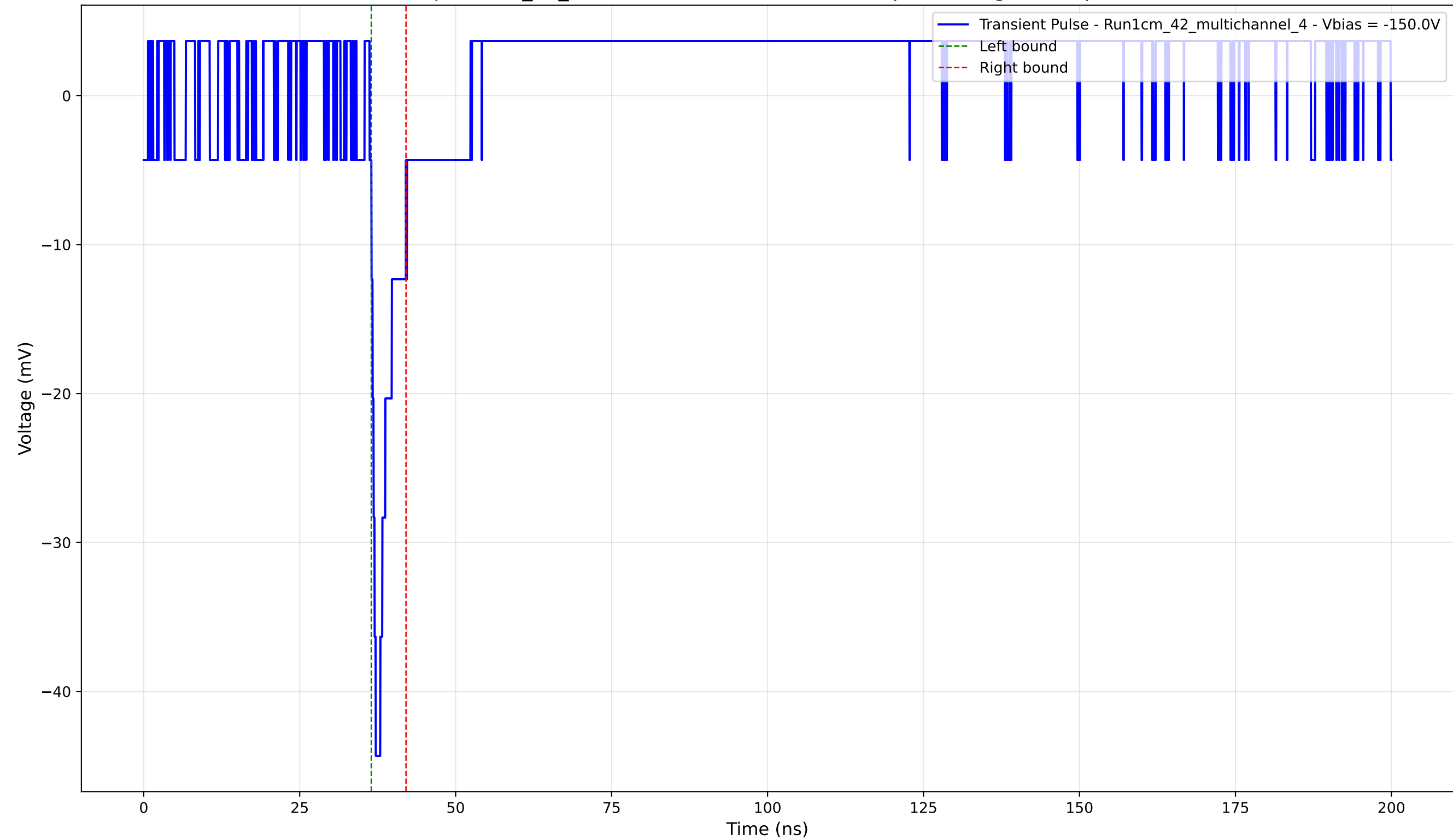
Transient Pulse - Sample: 1cm_42_multichannel - Position: 1955.0 \mu\text{m} - Charge: 2.48 pC - Rise Time: 0.70 ns
