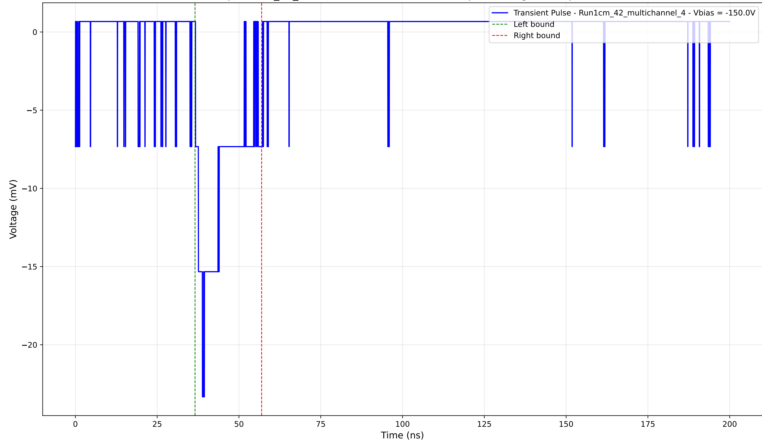
Transient Pulse - Sample: 1cm_42_multichannel - Position: 3740.0 \mu\text{m} - Charge: 3.83 pC - Rise Time: 2.12 ns
