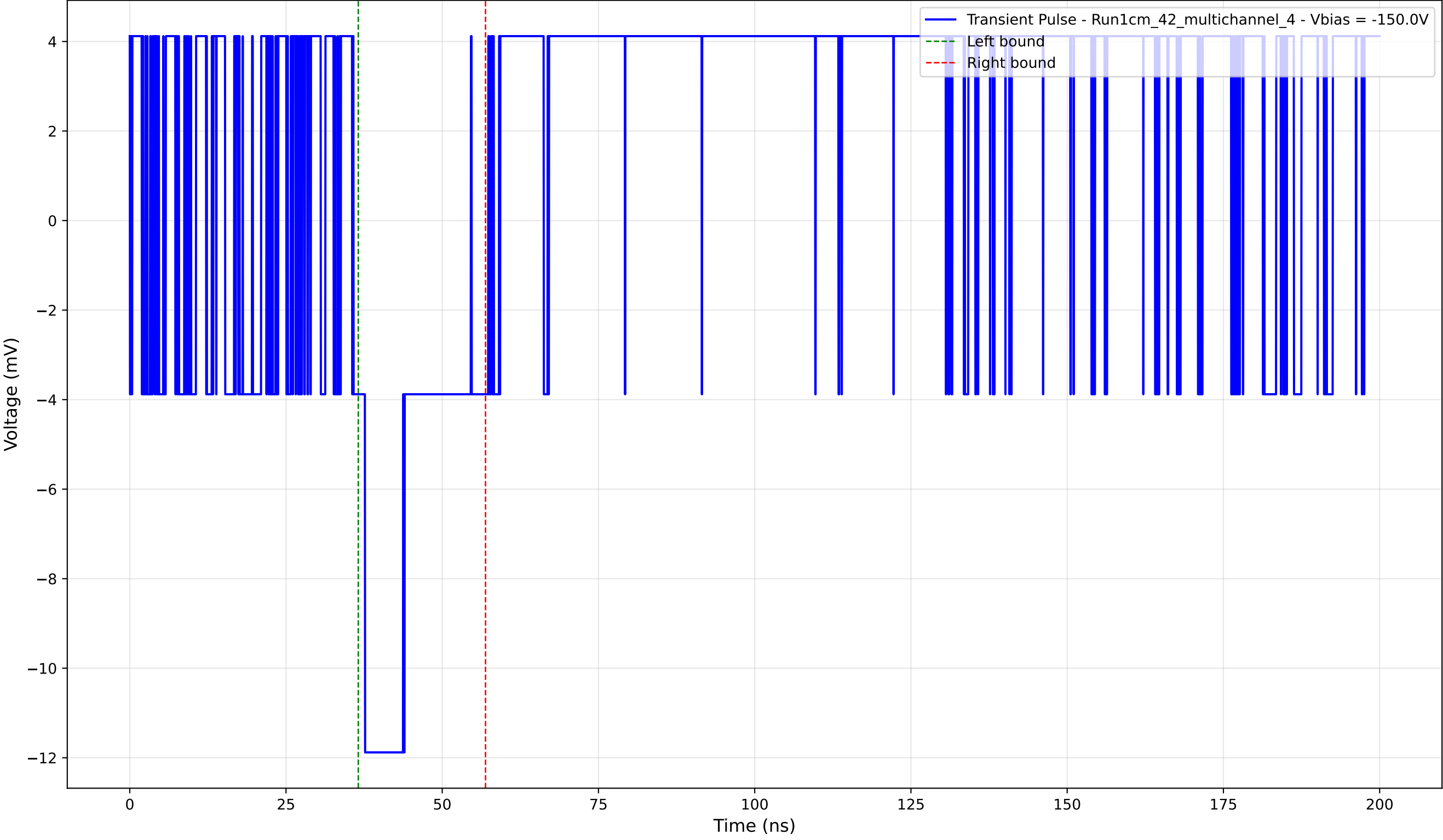
Transient Pulse - Sample: 1cm_42_multichannel - Position: 935.0 \mu\text{m} - Charge: 2.56 pC - Rise Time: 0.00 ns (N/A)
