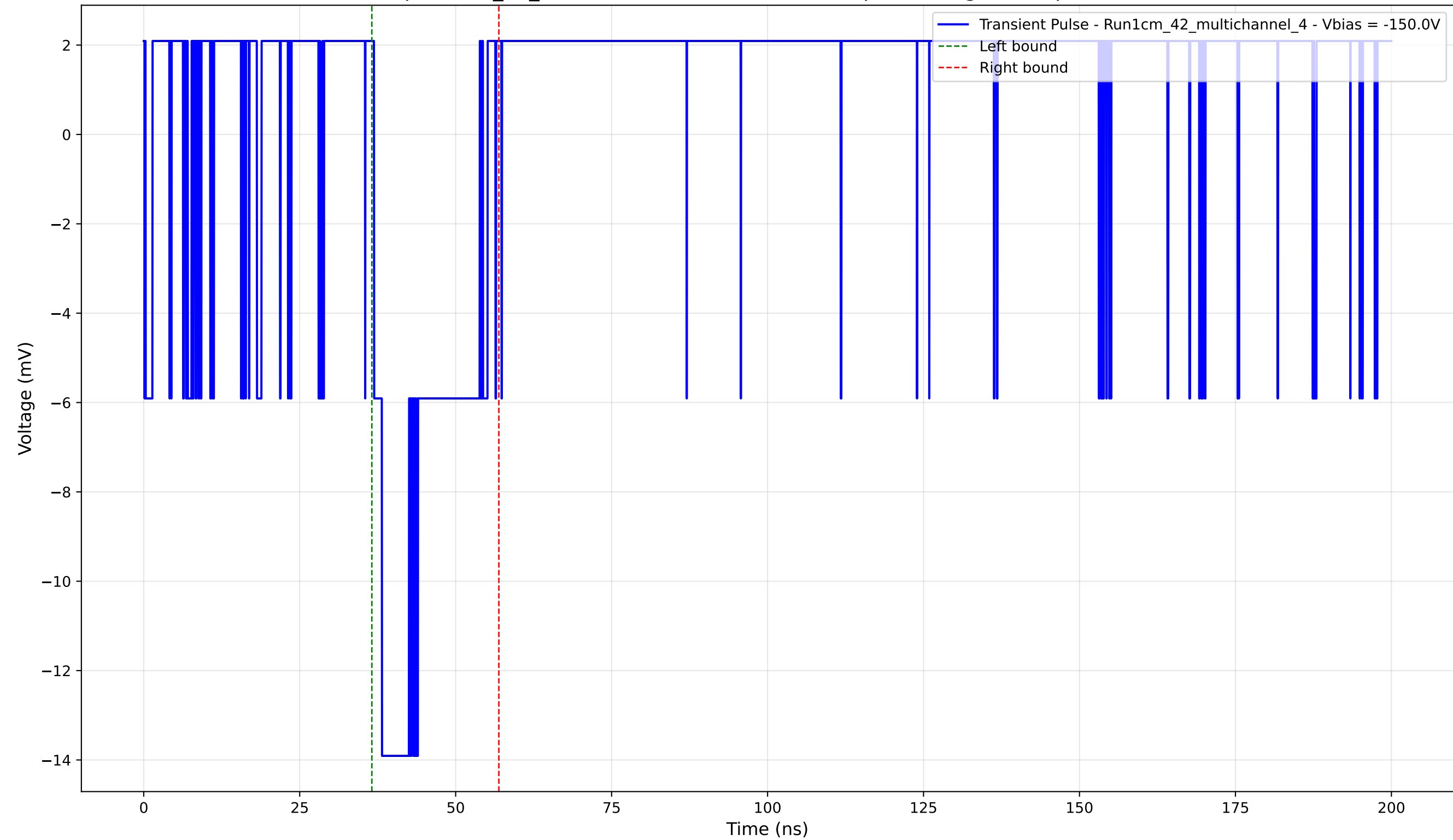
Transient Pulse - Sample: 1cm_42_multichannel - Position: 4090.0 \mu\text{m} - Charge: 2.83 pC - Rise Time: 0.00 ns (N/A)
