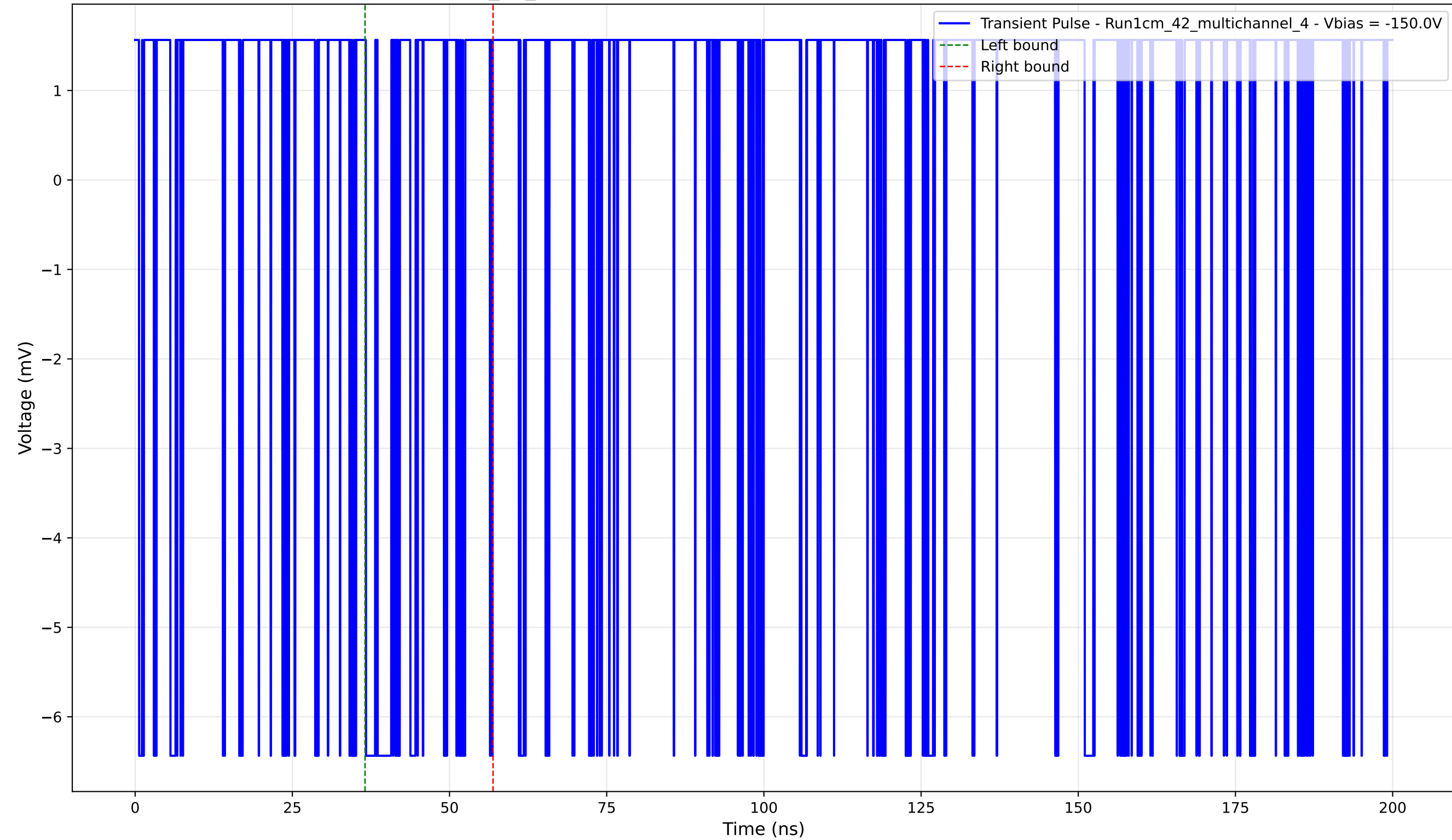
Transient Pulse - Sample: 1cm_42_multichannel - Position: 2395.0 \mu\text{m} - Charge: 0.45 pC - Rise Time: 0.00 ns (N/A)
