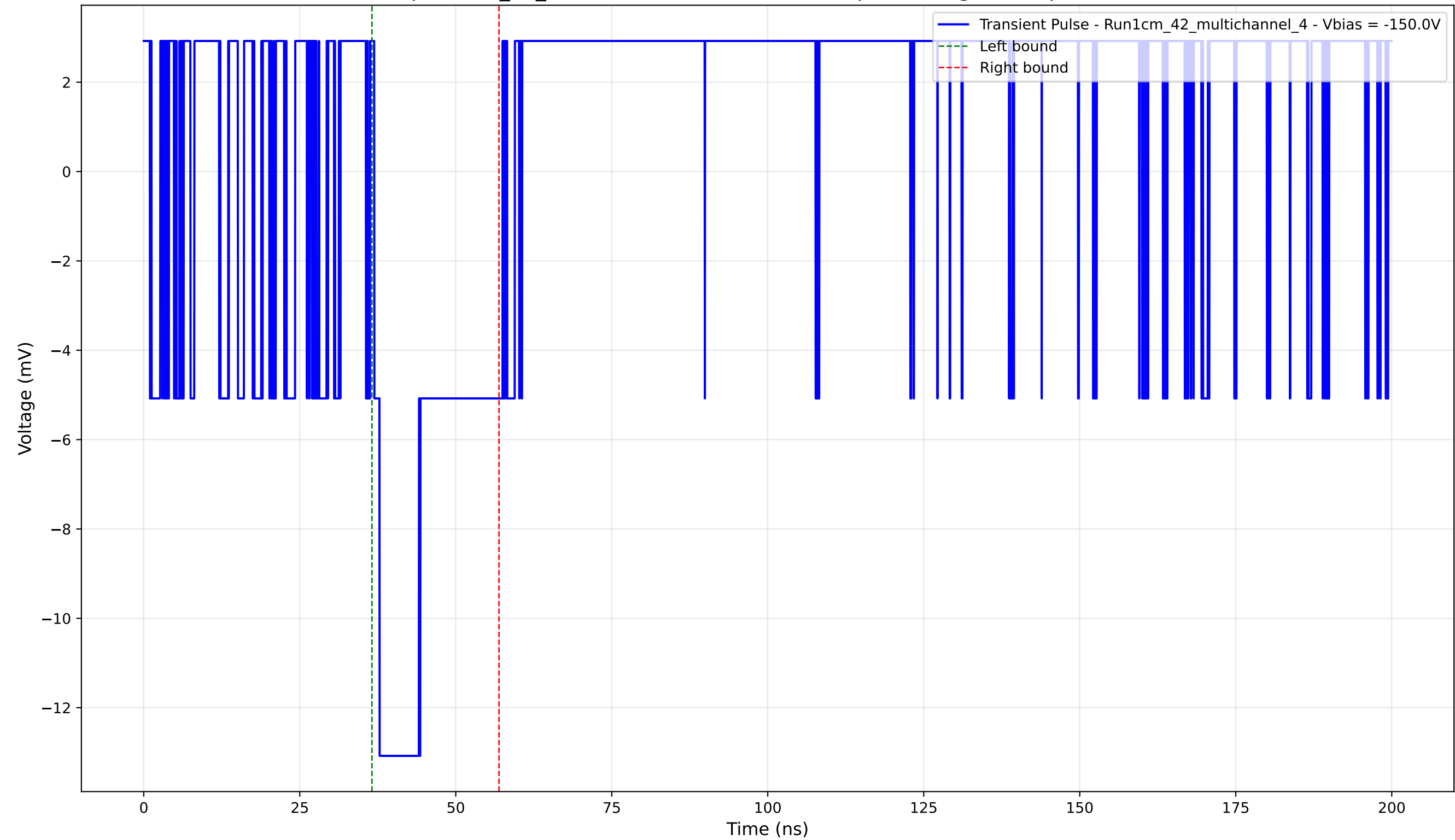
Transient Pulse - Sample: 1cm_42_multichannel - Position: 730.0 \mu\text{m} - Charge: 3.04 pC - Rise Time: 0.00 ns (N/A)
