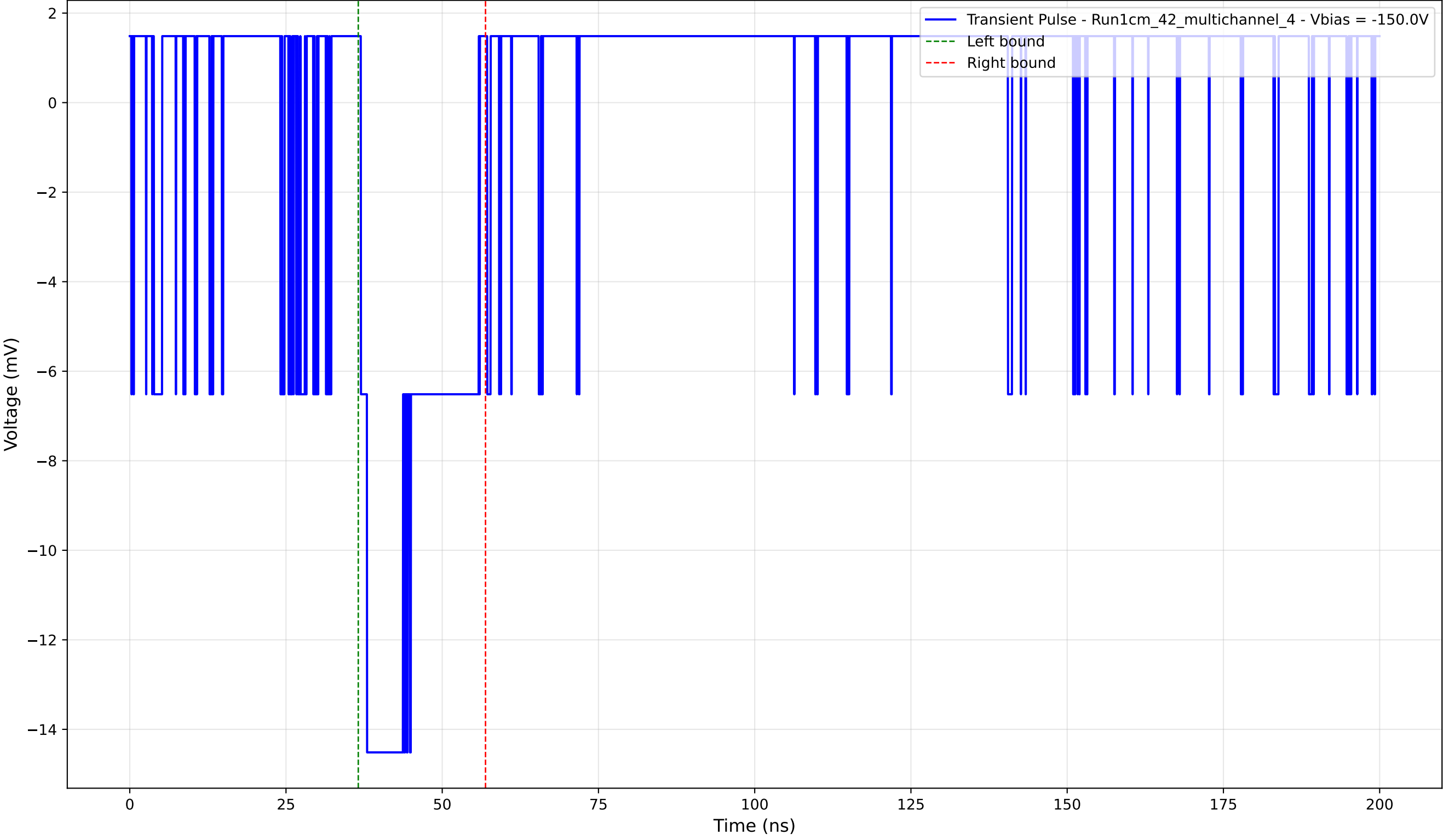
Transient Pulse - Sample: 1cm_42_multichannel - Position: 595.0 \mu\text{m} - Charge: 3.42 pC - Rise Time: 0.00 ns (N/A)
