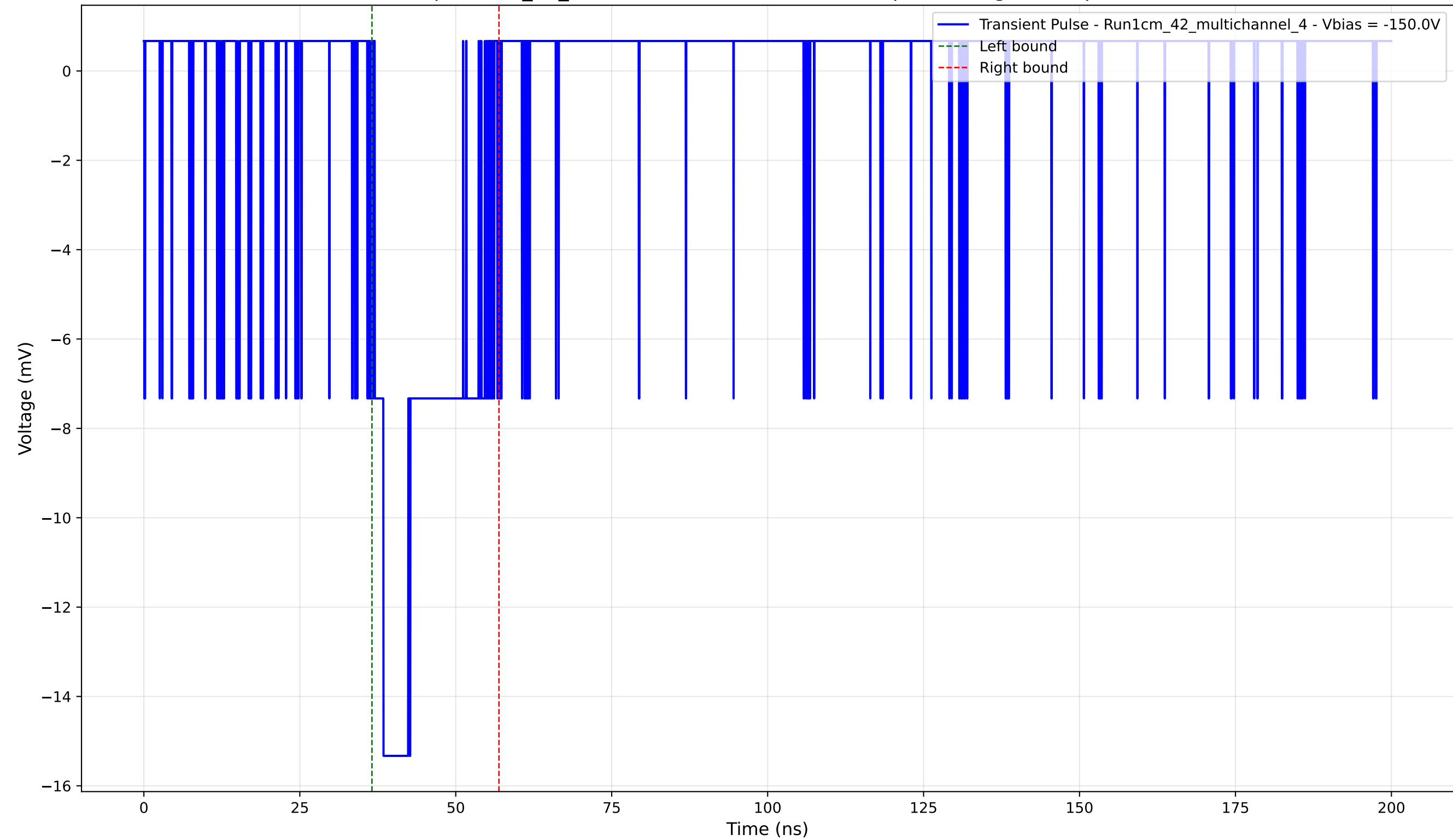
Transient Pulse - Sample: 1cm_42_multichannel - Position: 4605.0 \mu\text{m} - Charge: 3.35 pC - Rise Time: 1.40 ns
