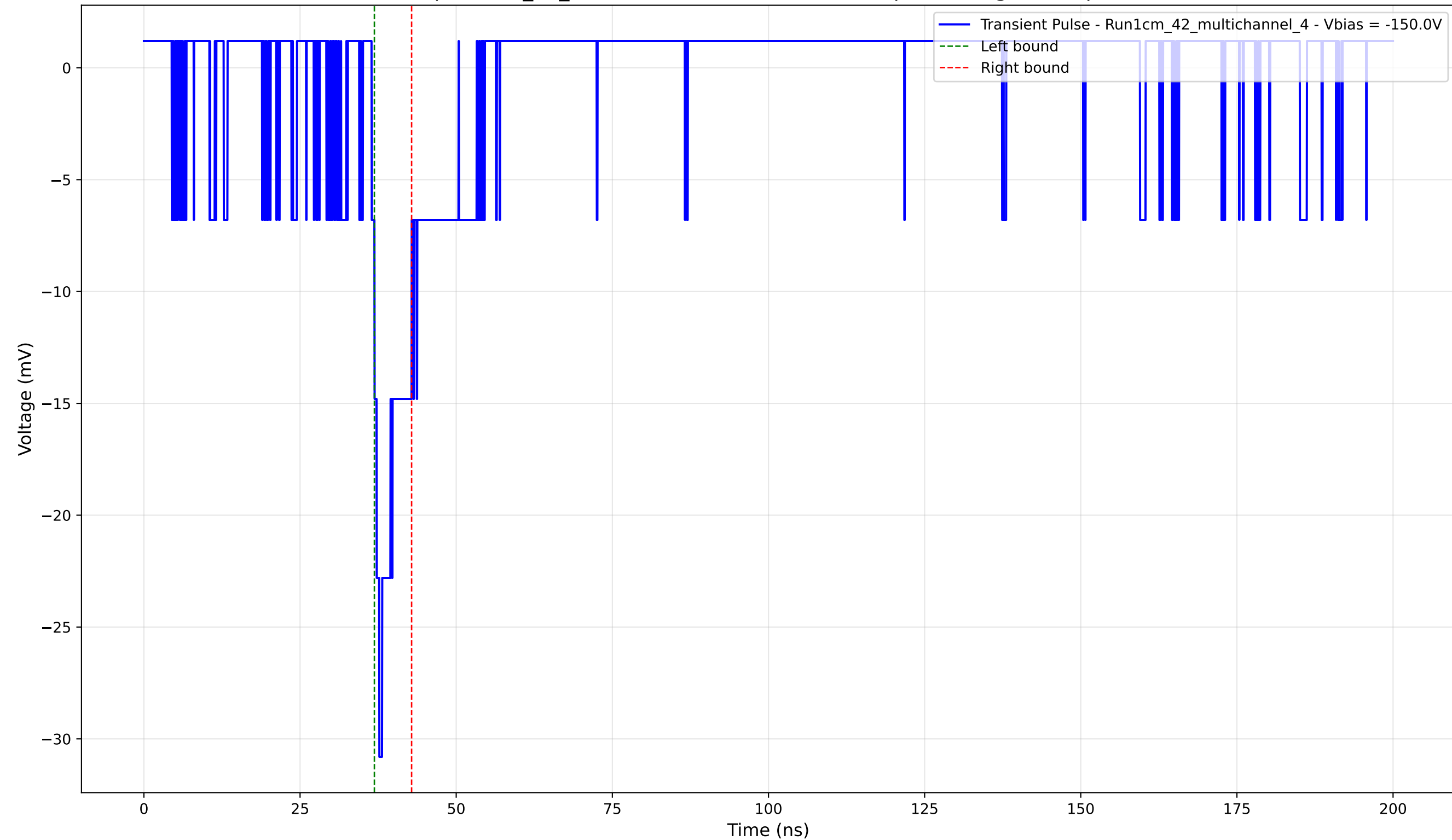
Transient Pulse - Sample: 1cm_42_multichannel - Position: 3265.0 \mu\text{m} - Charge: 2.21 pC - Rise Time: 1.23 ns
