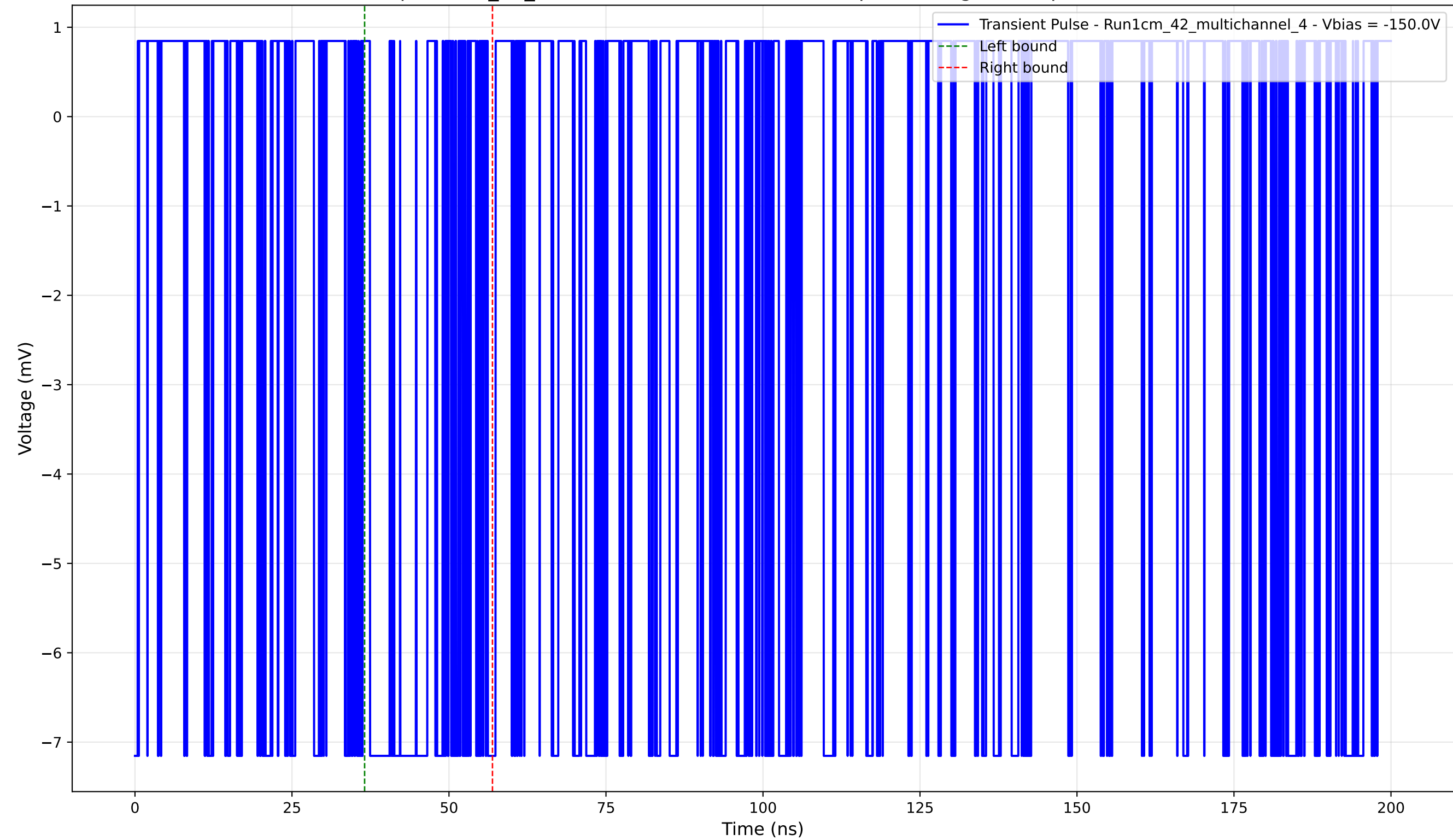
Transient Pulse - Sample: 1cm_42_multichannel - Position: 1395.0 \mu\text{m} - Charge: 1.83 pC - Rise Time: 0.00 ns (N/A)
