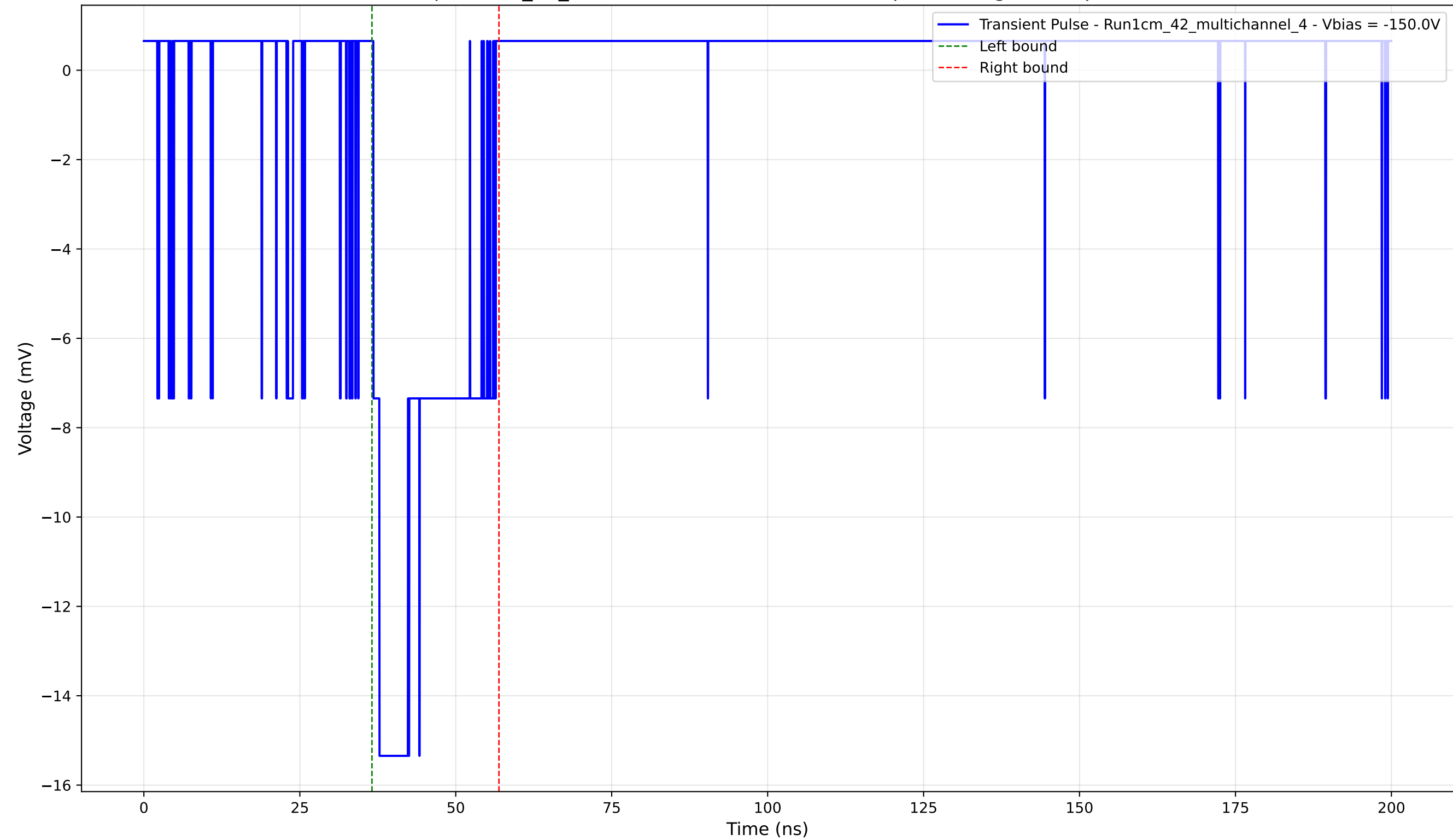
Transient Pulse - Sample: 1cm_42_multichannel - Position: 3815.0 \mu\text{m} - Charge: 3.56 pC - Rise Time: 0.98 ns
