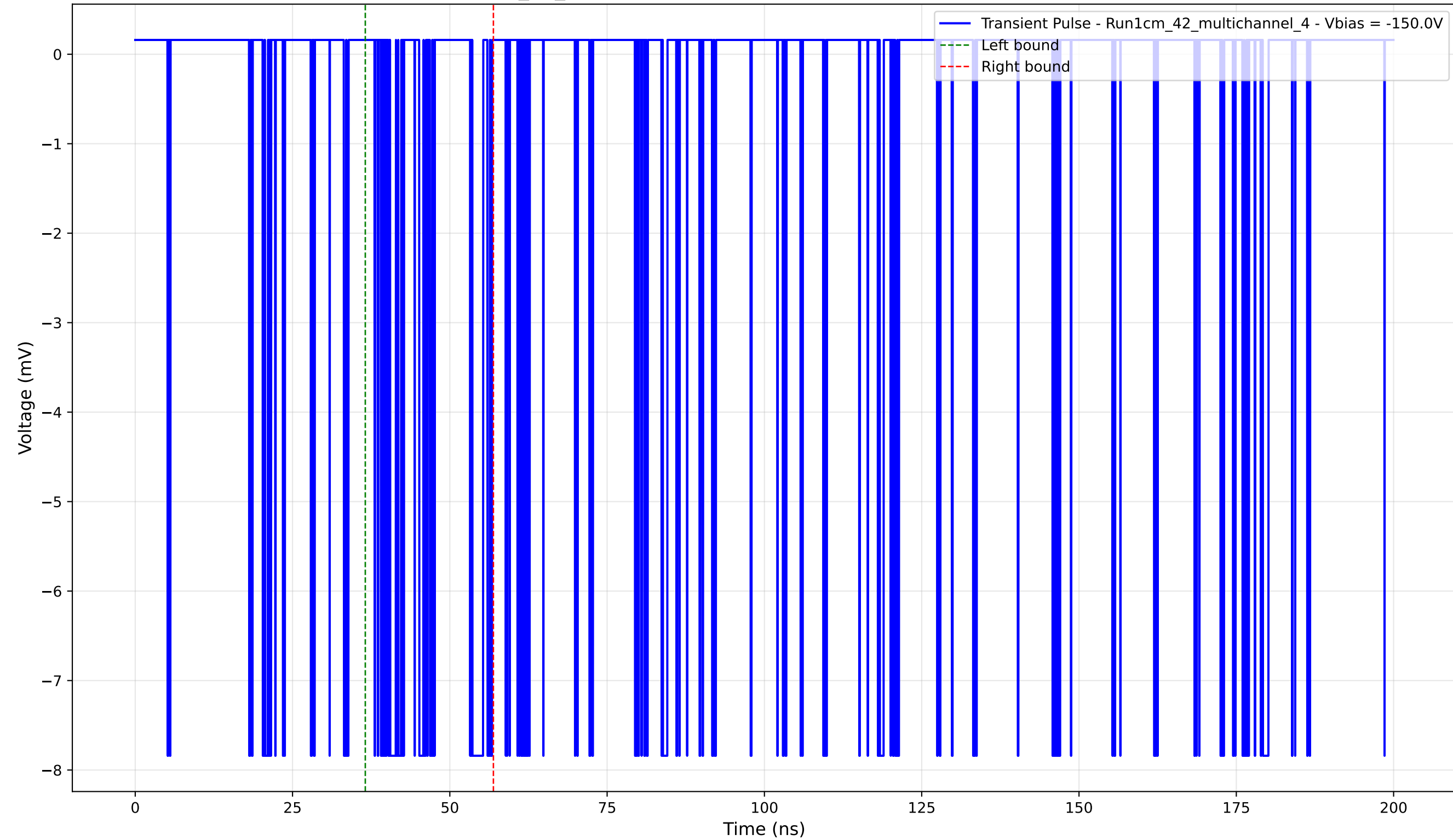
Transient Pulse - Sample: 1cm_42_multichannel - Position: 3925.0 \mu\text{m} - Charge: 1.04 pC - Rise Time: 0.02 ns
