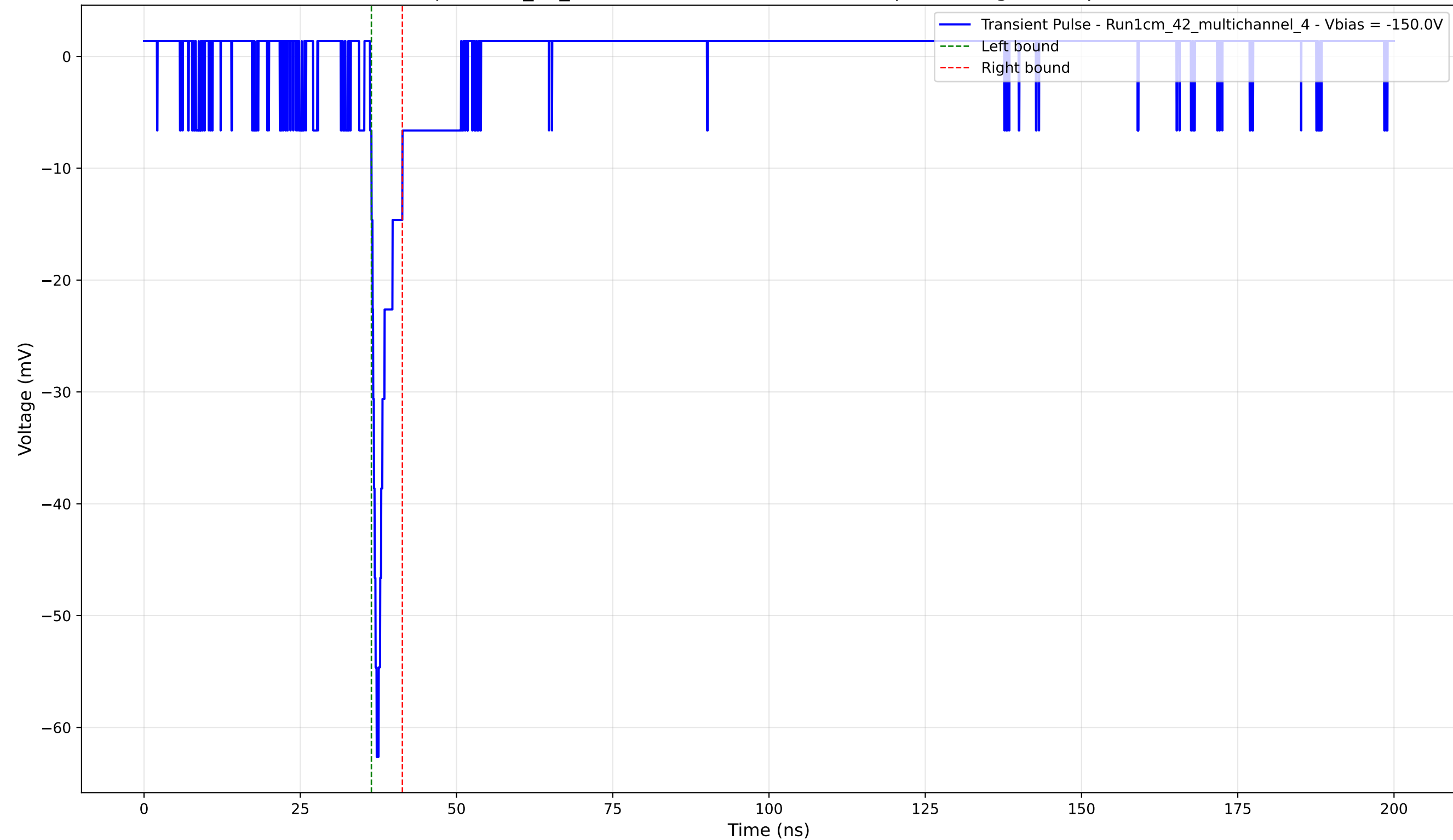
Transient Pulse - Sample: 1cm_42_multichannel - Position: 2650.0 \mu\text{m} - Charge: 2.80 pC - Rise Time: 1.06 ns
