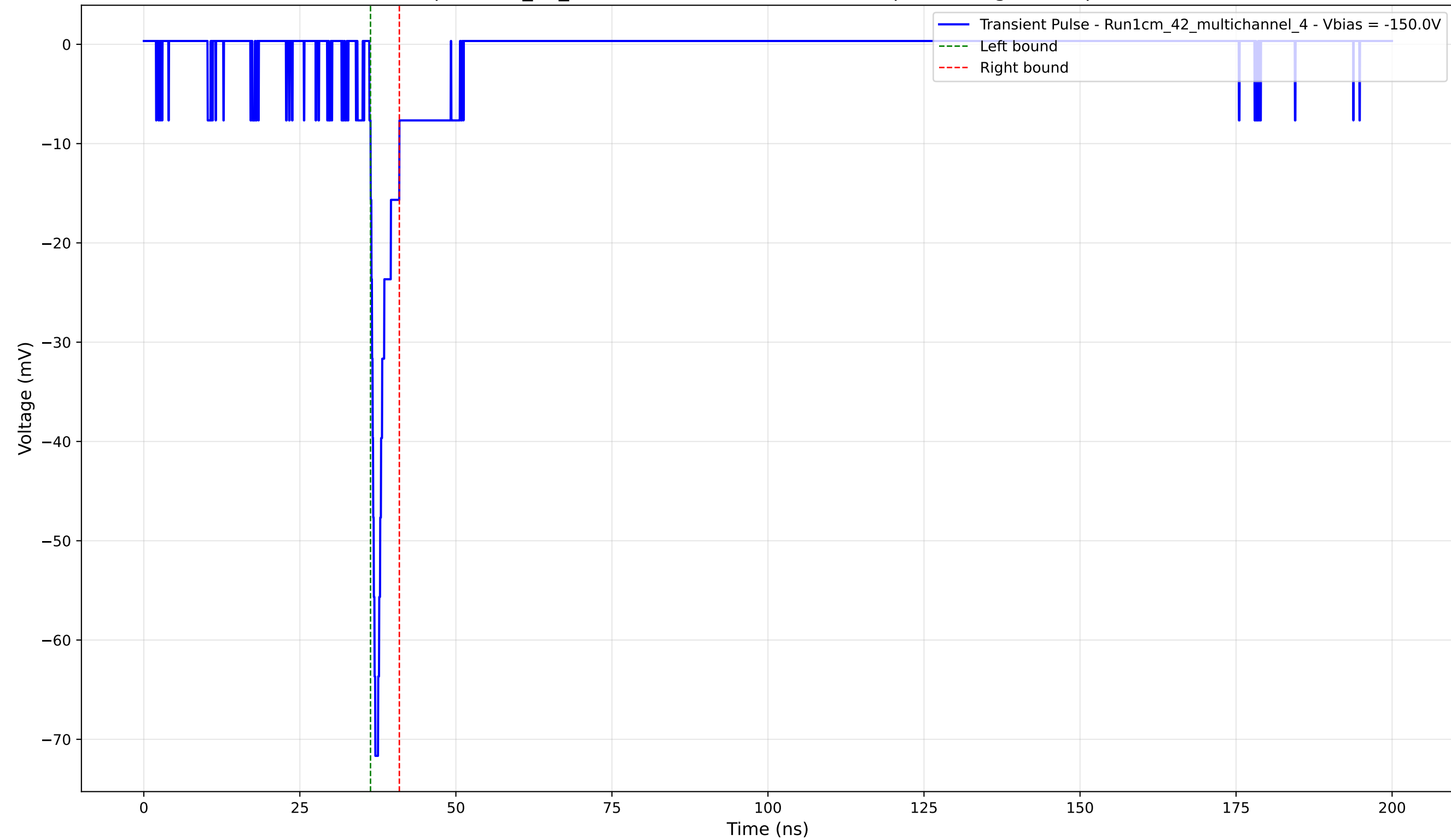
Transient Pulse - Sample: 1cm_42_multichannel - Position: 2560.0 \mu\text{m} - Charge: 3.06 pC - Rise Time: 0.94 ns
