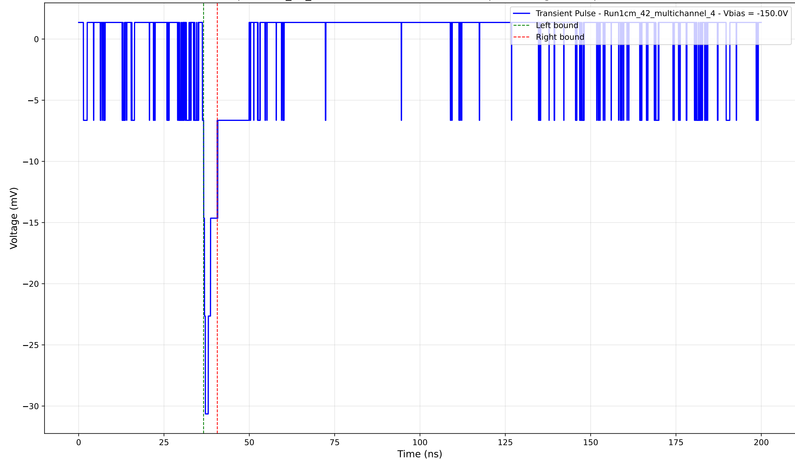
Transient Pulse - Sample: 1cm_42_multichannel - Position: 1935.0 \mu\text{m} - Charge: 1.60 pC - Rise Time: 0.87 ns
