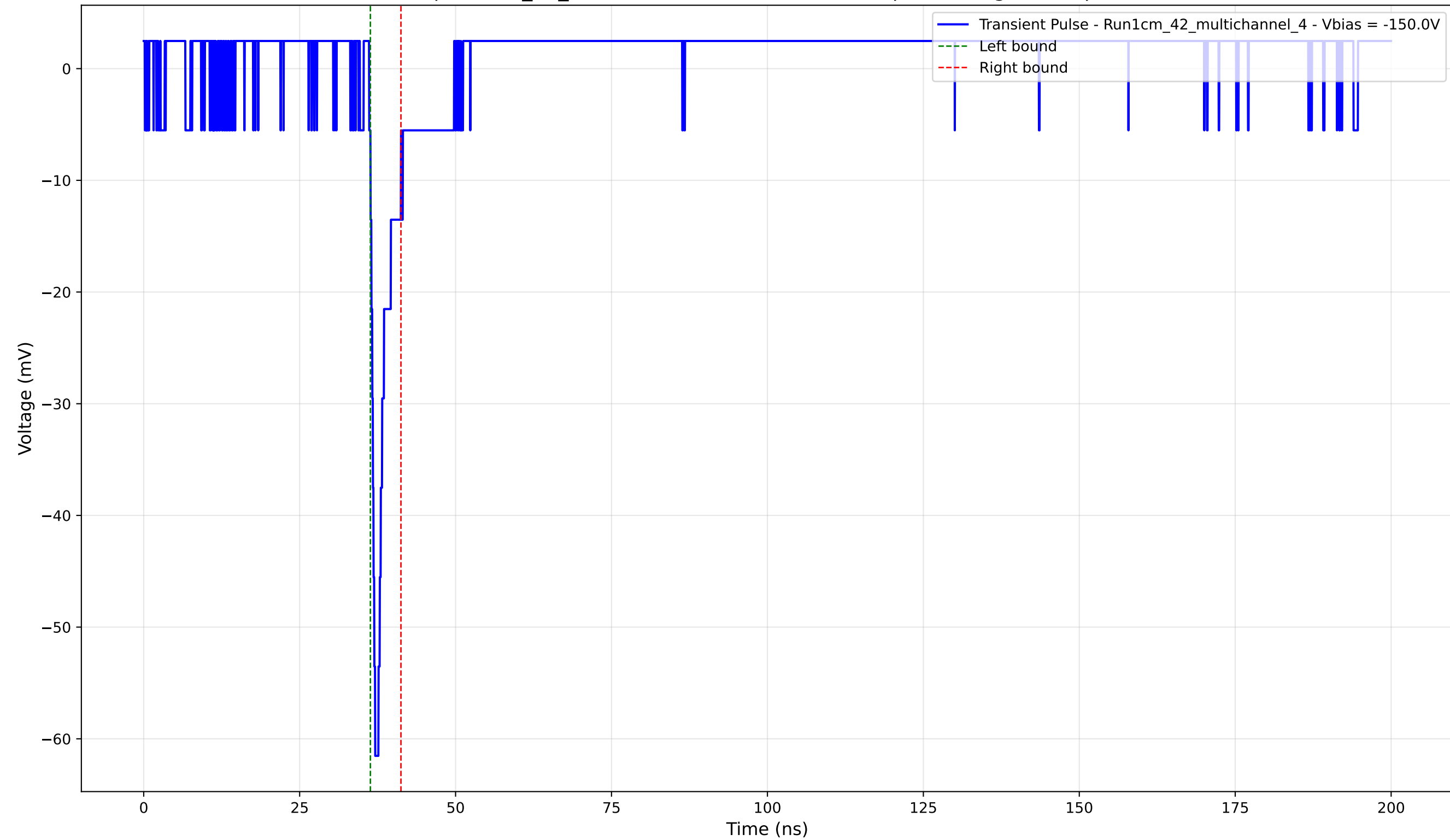
Transient Pulse - Sample: 1cm_42_multichannel - Position: 2625.0 \mu\text{m} - Charge: 2.77 pC - Rise Time: 0.76 ns
