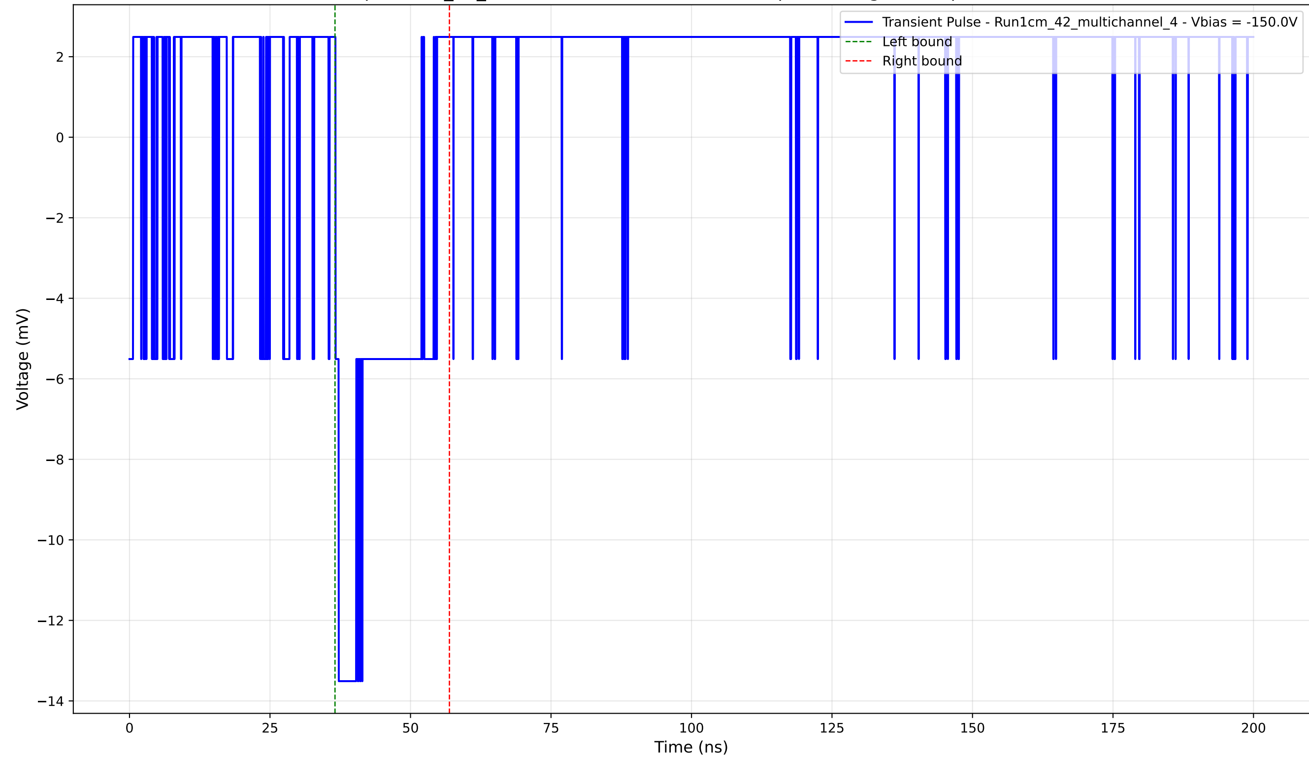
Transient Pulse - Sample: 1cm_42_multichannel - Position: 3340.0 \mu\text{m} - Charge: 2.35 pC - Rise Time: 0.00 ns (N/A)
