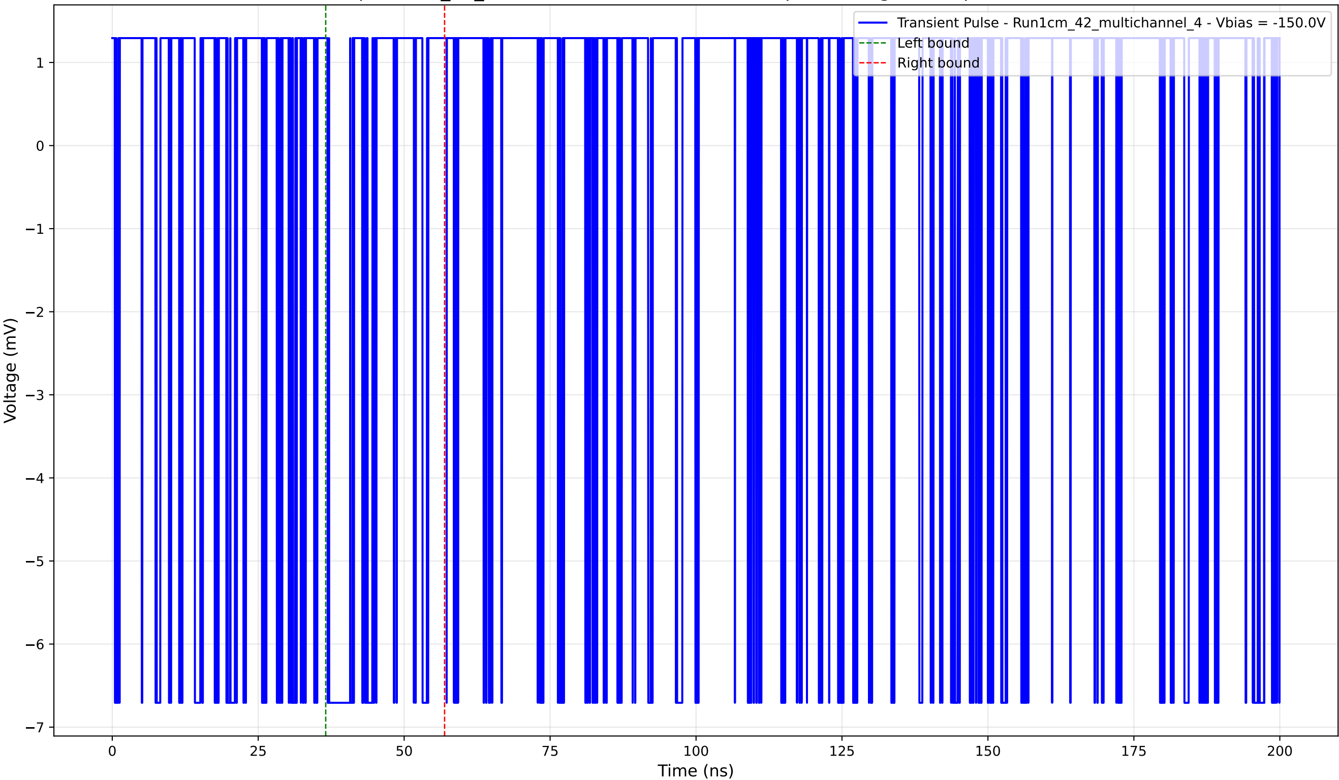
Transient Pulse - Sample: 1cm_42_multichannel - Position: 1865.0 \mu\text{m} - Charge: 0.60 pC - Rise Time: 0.00 ns (N/A)
