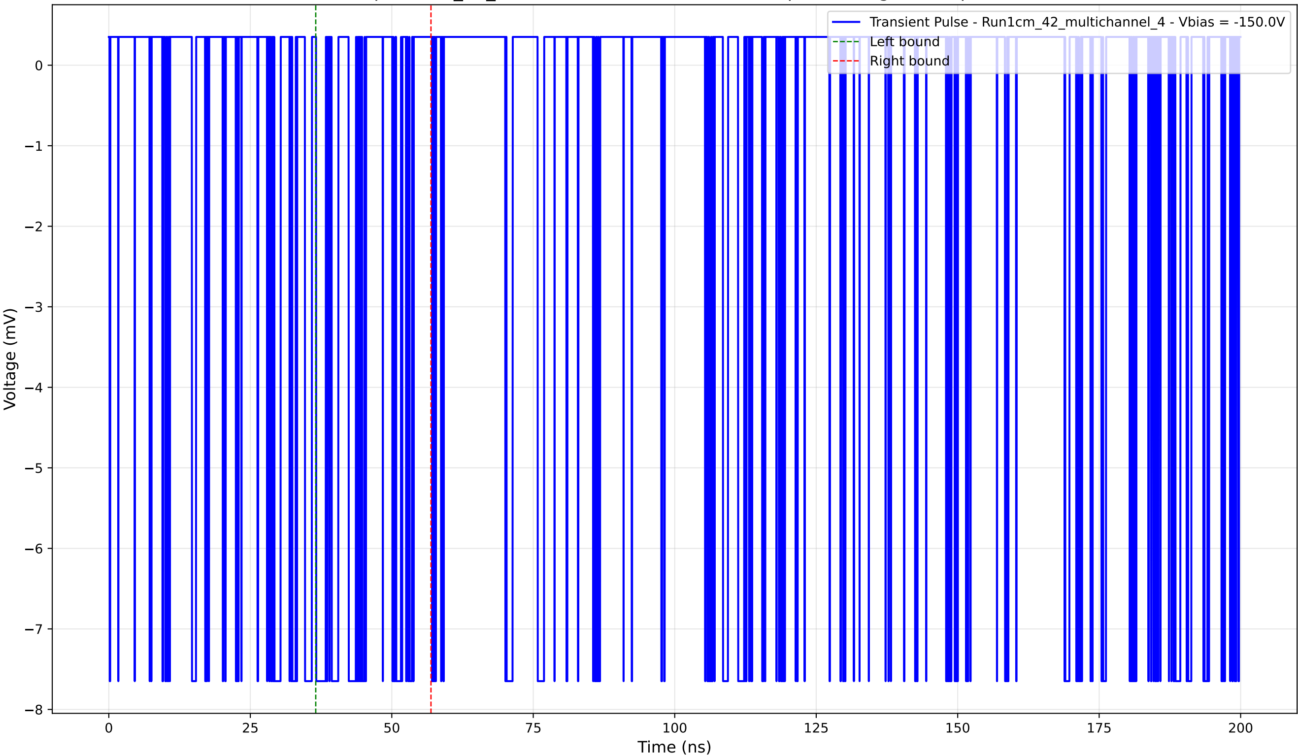
Transient Pulse - Sample: 1cm_42_multichannel - Position: 1885.0 \mu\text{m} - Charge: 1.12 pC - Rise Time: 0.02 ns
