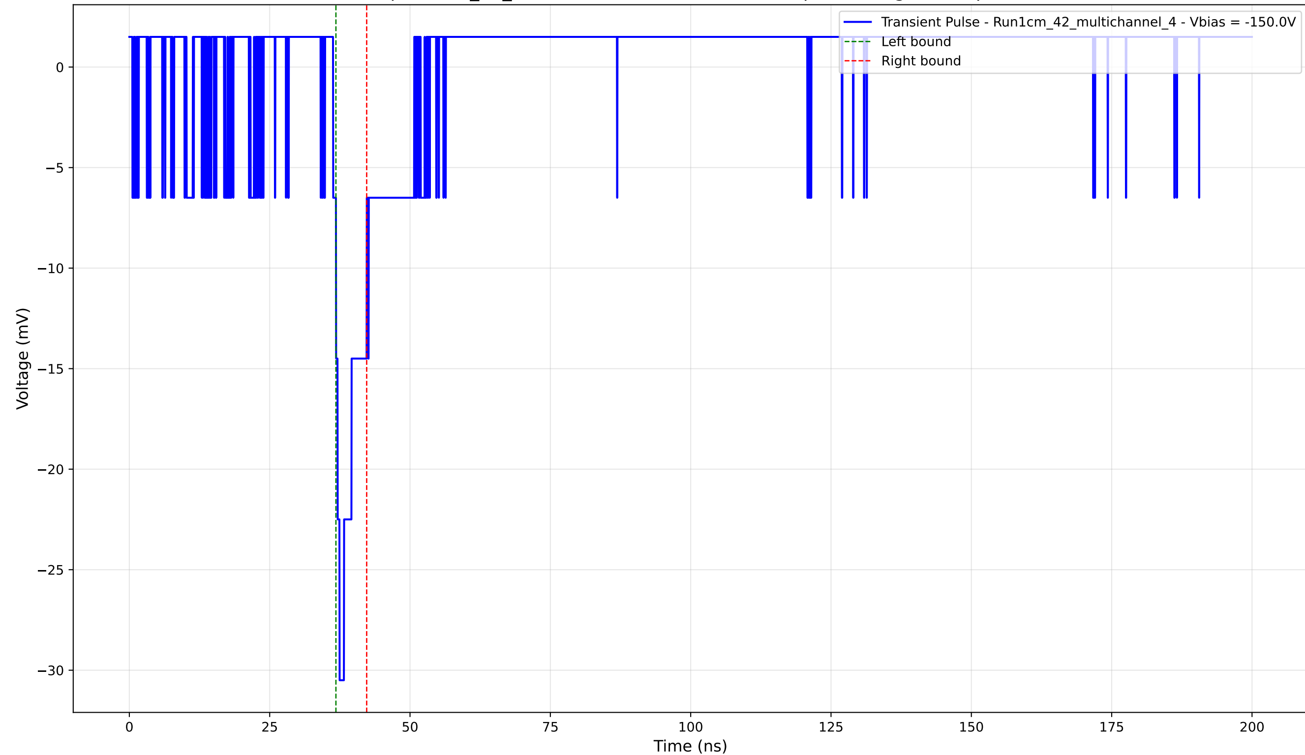
Transient Pulse - Sample: 1cm_42_multichannel - Position: 3145.0 \mu\text{m} - Charge: 2.11 pC - Rise Time: 1.15 ns
