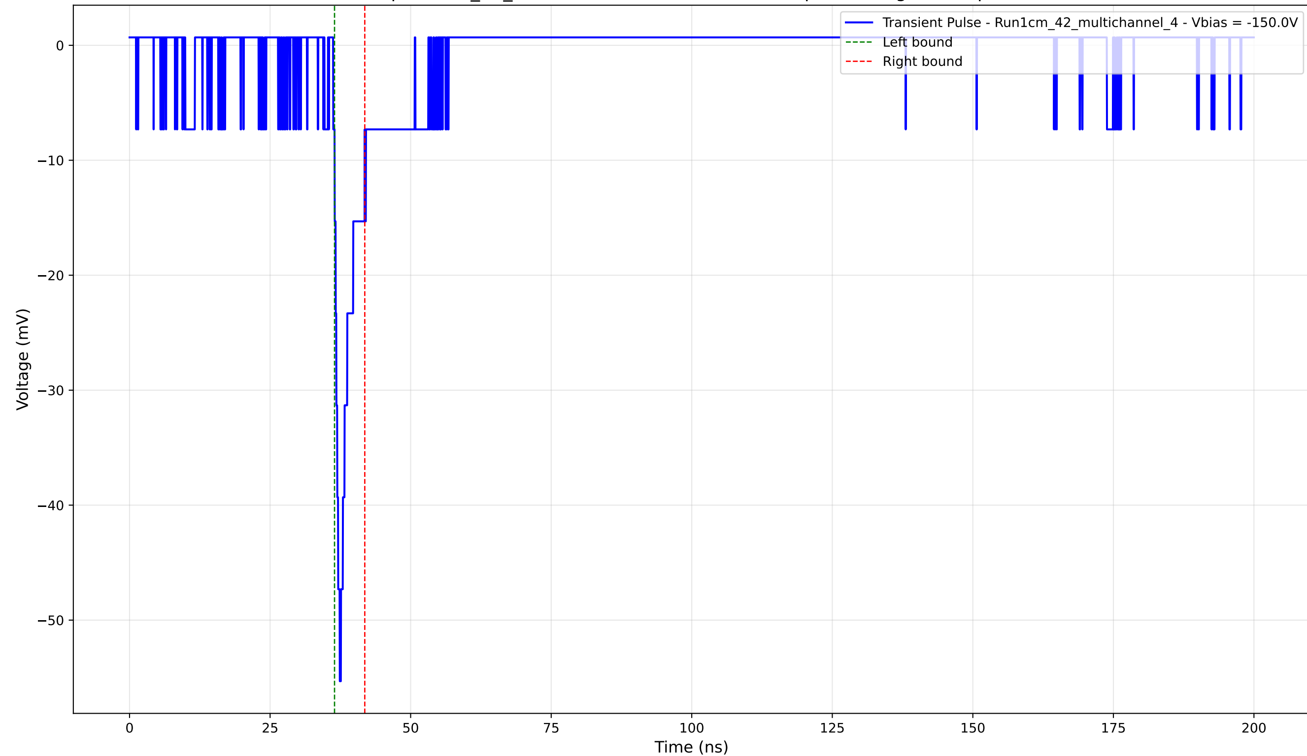
Transient Pulse - Sample: 1cm_42_multichannel - Position: 2785.0 \mu\text{m} - Charge: 2.83 pC - Rise Time: 1.17 ns
