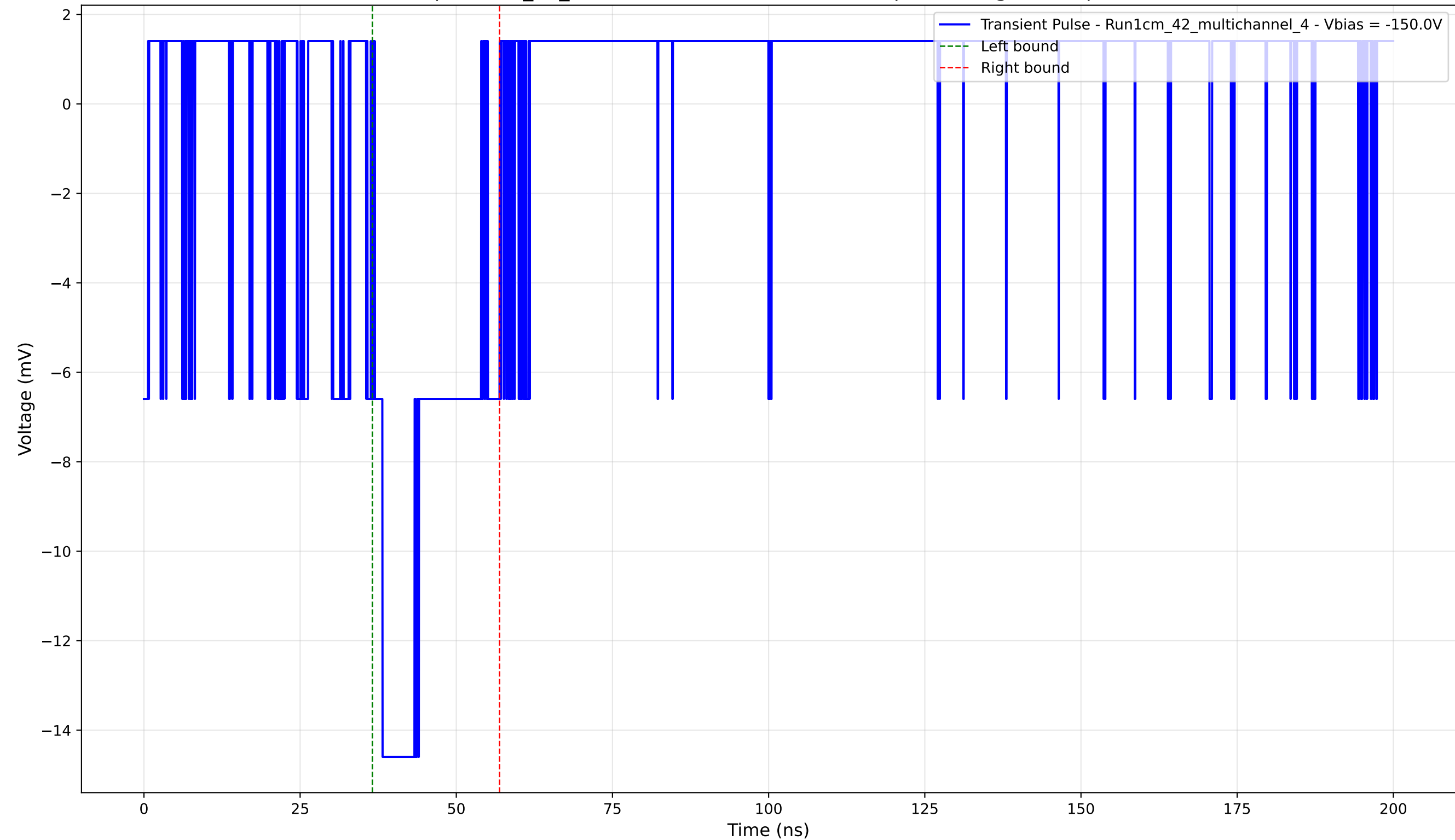
Transient Pulse - Sample: 1cm_42_multichannel - Position: 4300.0 \mu\text{m} - Charge: 3.42 pC - Rise Time: 1.24 ns
