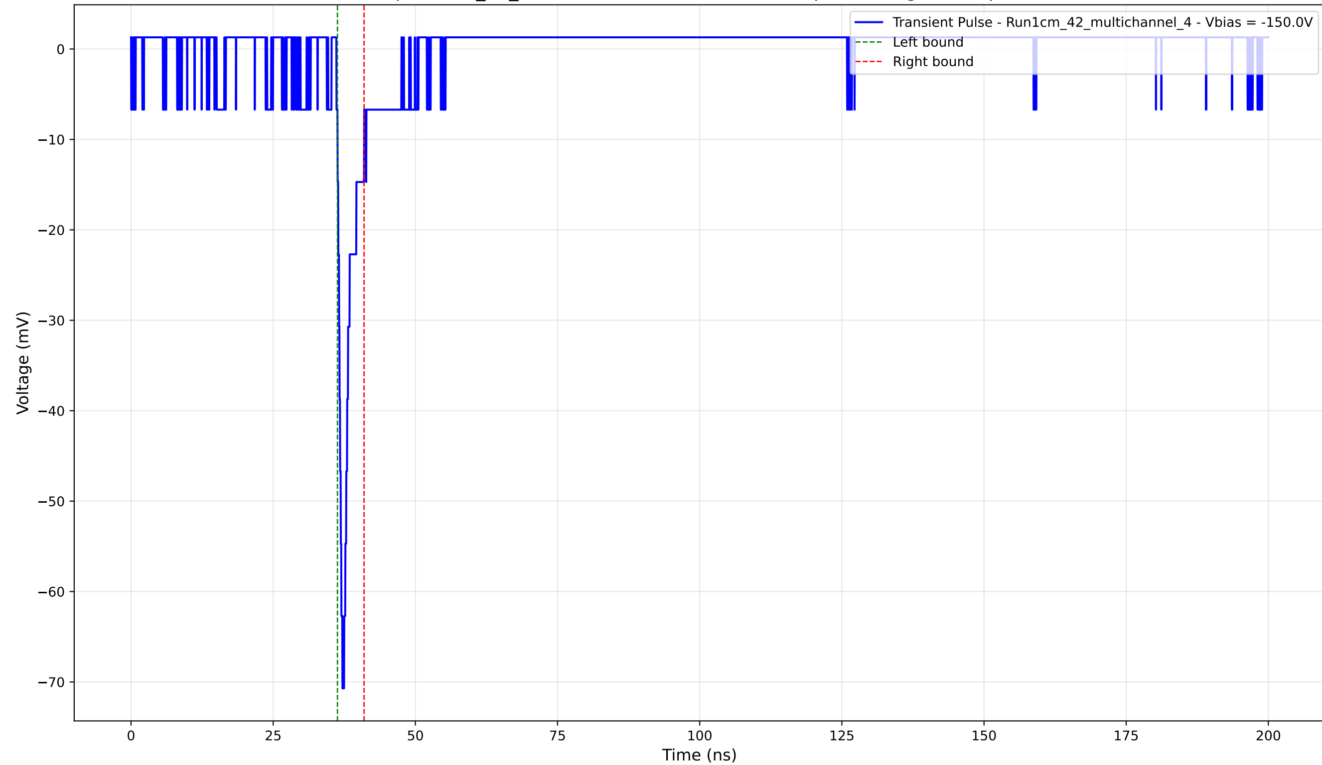
Transient Pulse - Sample: 1cm_42_multichannel - Position: 2580.0 \mu\text{m} - Charge: 2.93 pC - Rise Time: 0.86 ns
