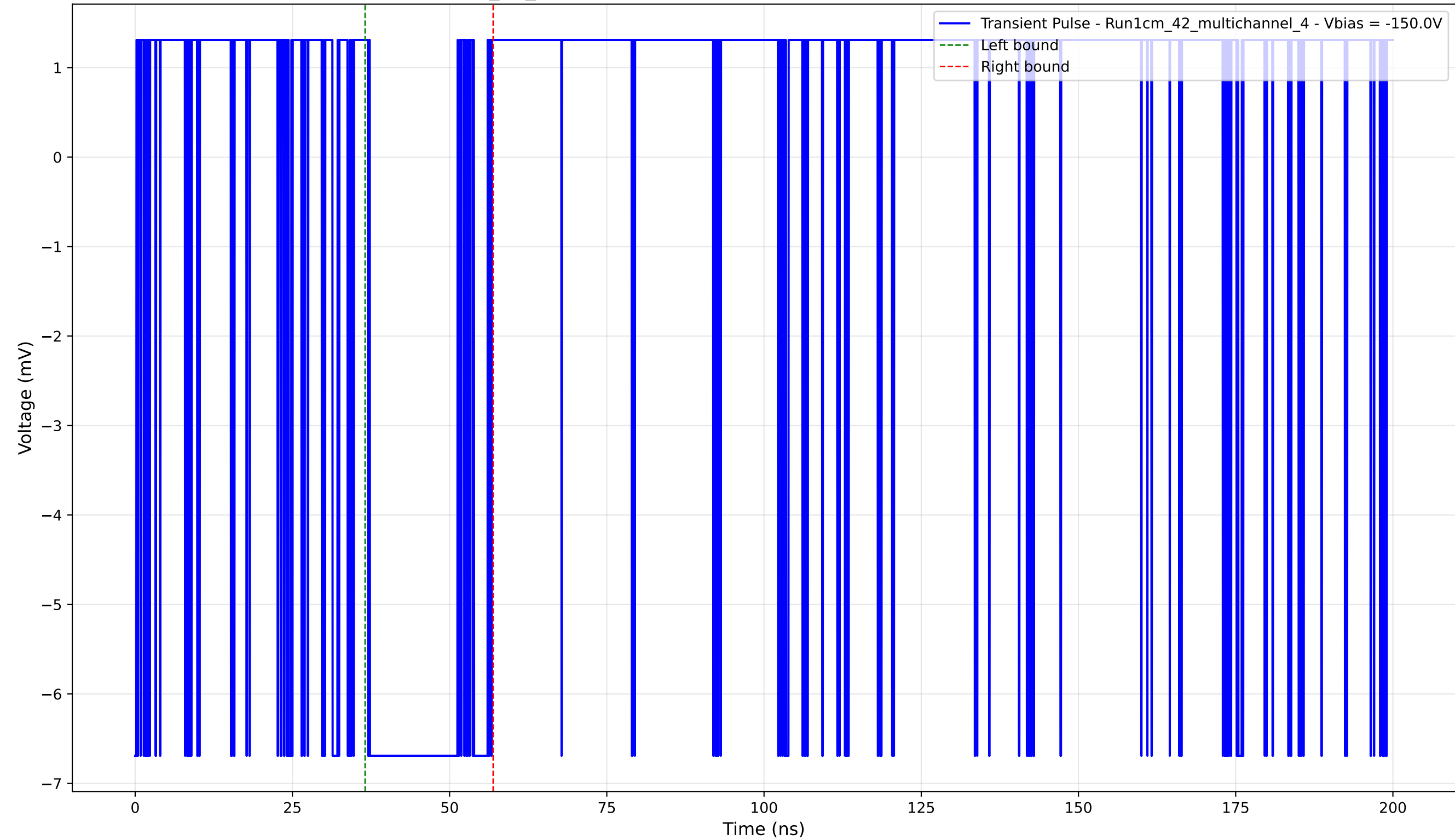
Transient Pulse - Sample: 1cm_42_multichannel - Position: 4455.0 \mu\text{m} - Charge: 2.26 pC - Rise Time: 0.00 ns (N/A)
