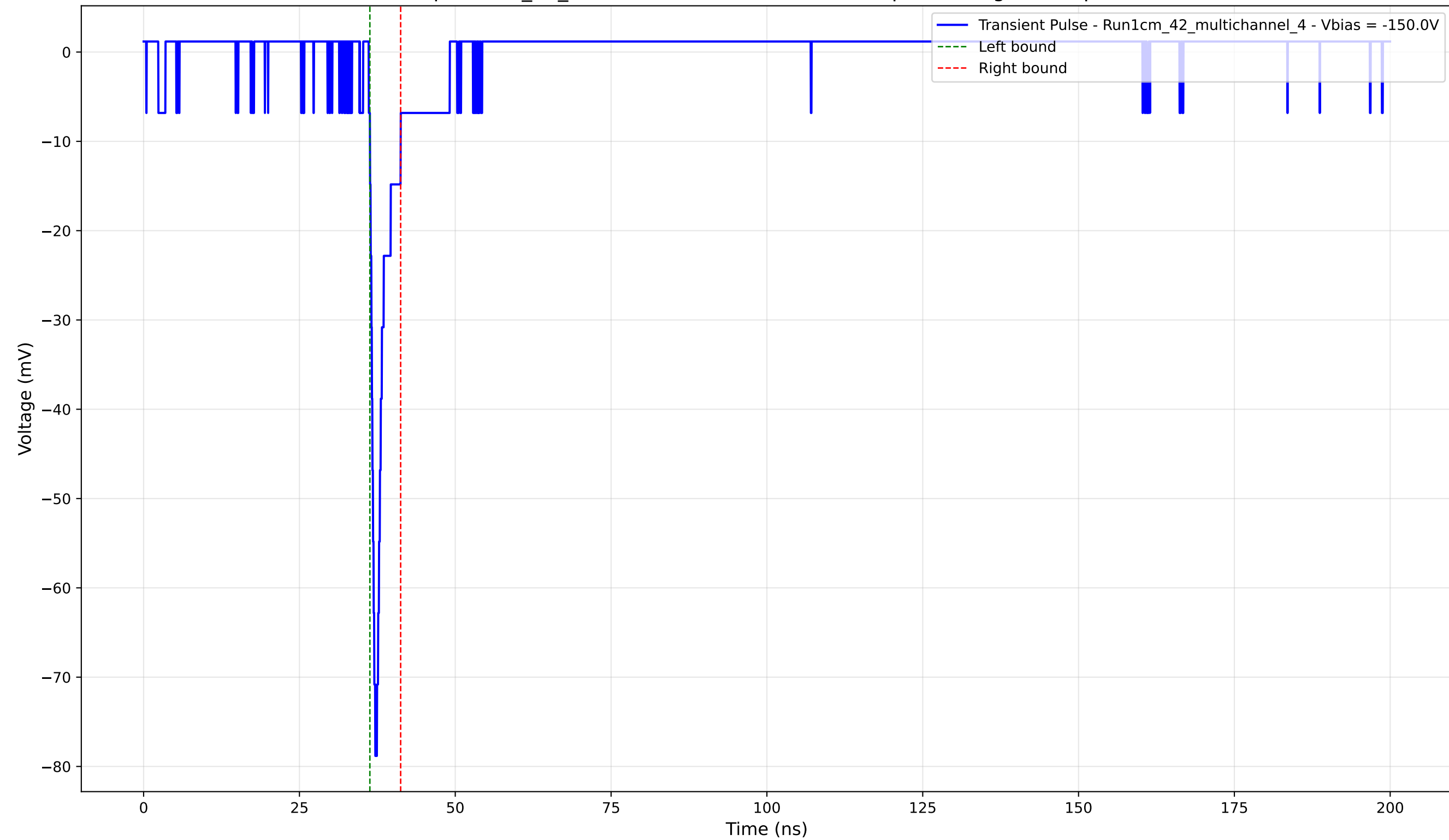
Transient Pulse - Sample: 1cm_42_multichannel - Position: 2225.0 \mu\text{m} - Charge: 3.22 pC - Rise Time: 0.86 ns
