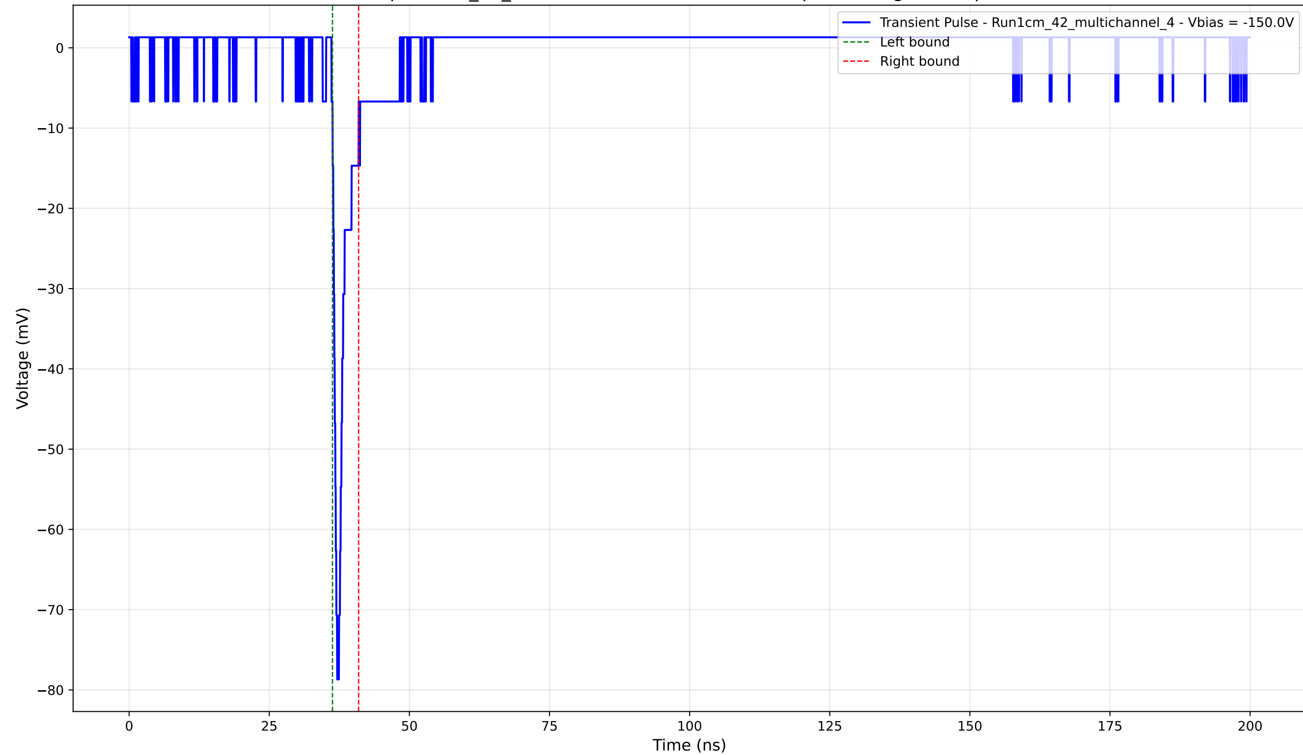
Transient Pulse - Sample: 1cm_42_multichannel - Position: 2520.0 \mu\text{m} - Charge: 3.14 pC - Rise Time: 0.82 ns
