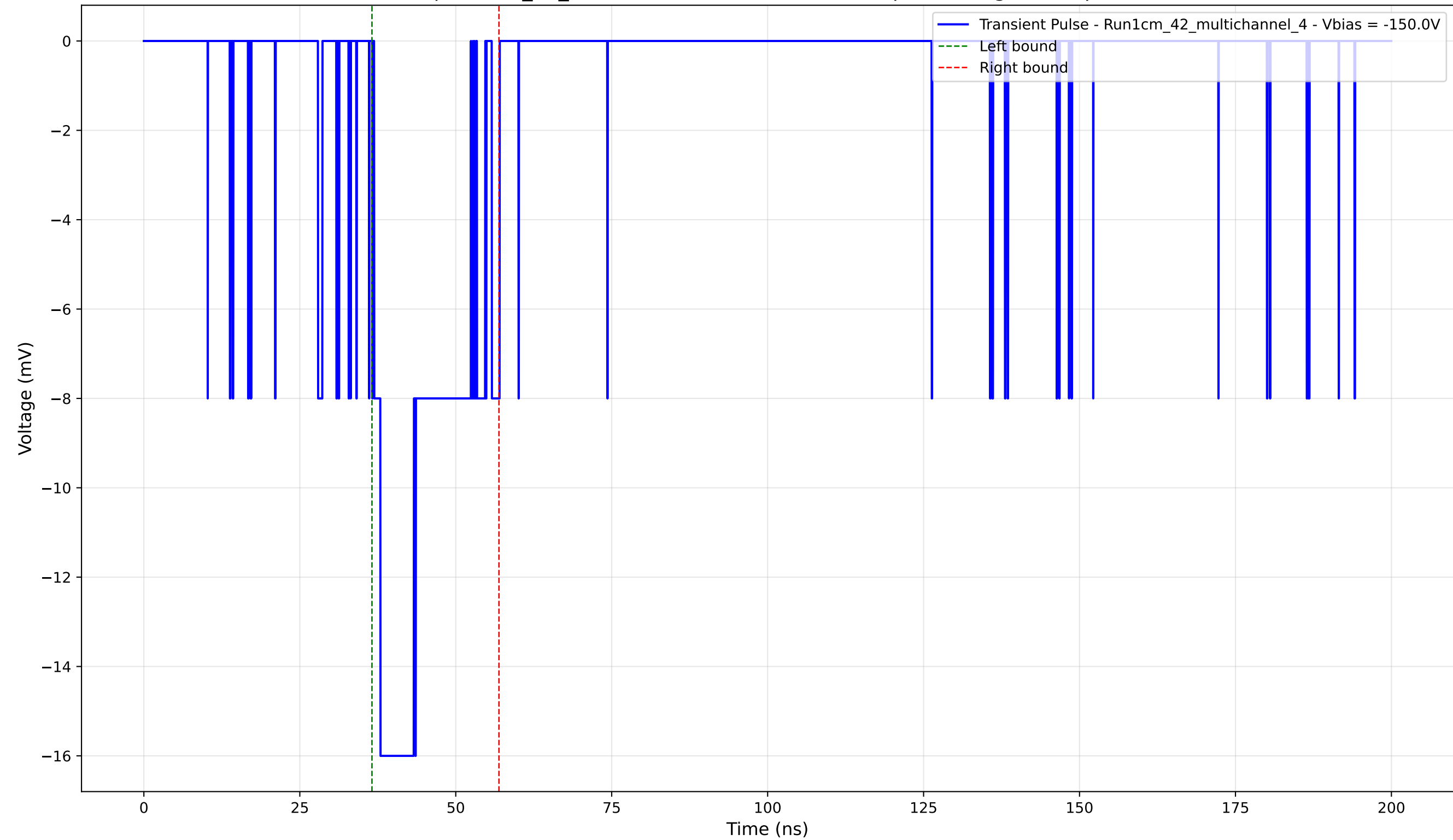
Transient Pulse - Sample: 1cm_42_multichannel - Position: 3985.0 \mu\text{m} - Charge: 3.89 pC - Rise Time: 1.02 ns
