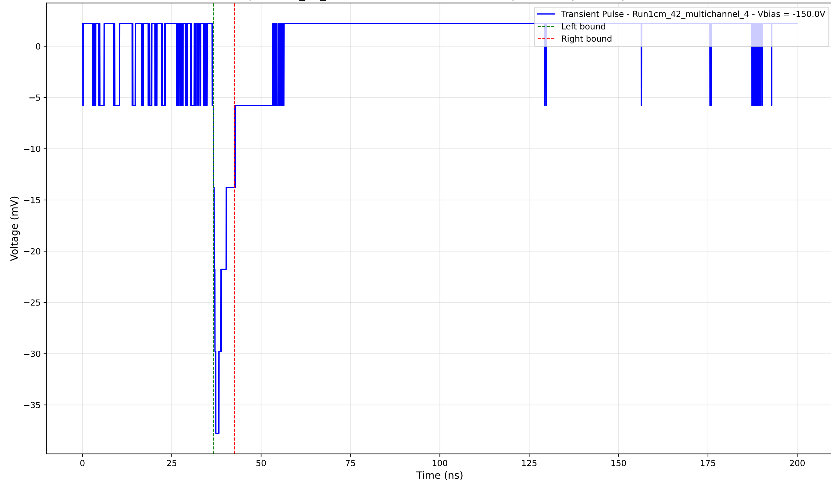
Transient Pulse - Sample: 1cm_42_multichannel - Position: 1740.0 \mu\text{m} - Charge: 2.57 pC - Rise Time: 1.01 ns
