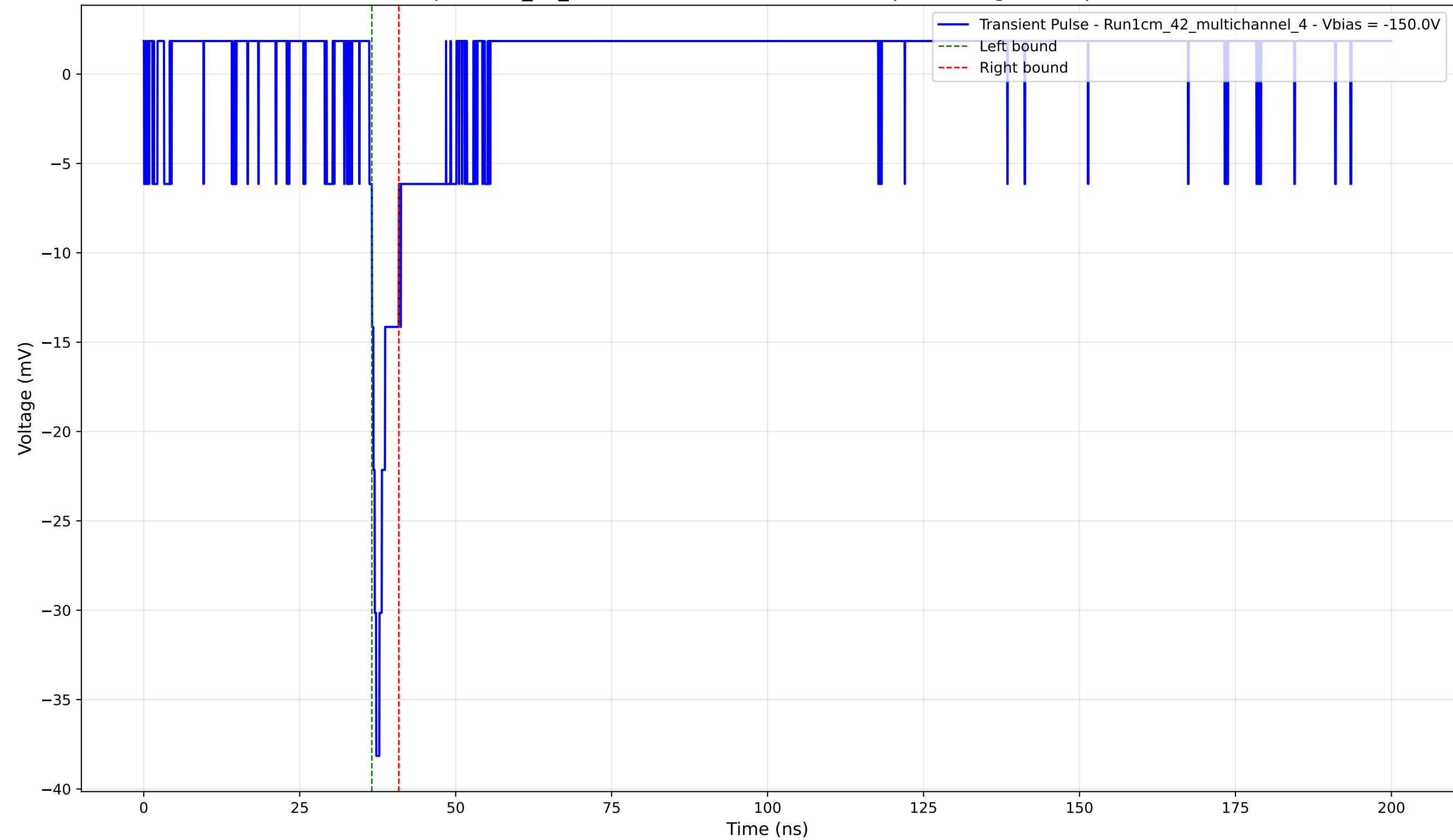
Transient Pulse - Sample: 1cm_42_multichannel - Position: 2830.0 \mu\text{m} - Charge: 1.79 pC - Rise Time: 1.11 ns
