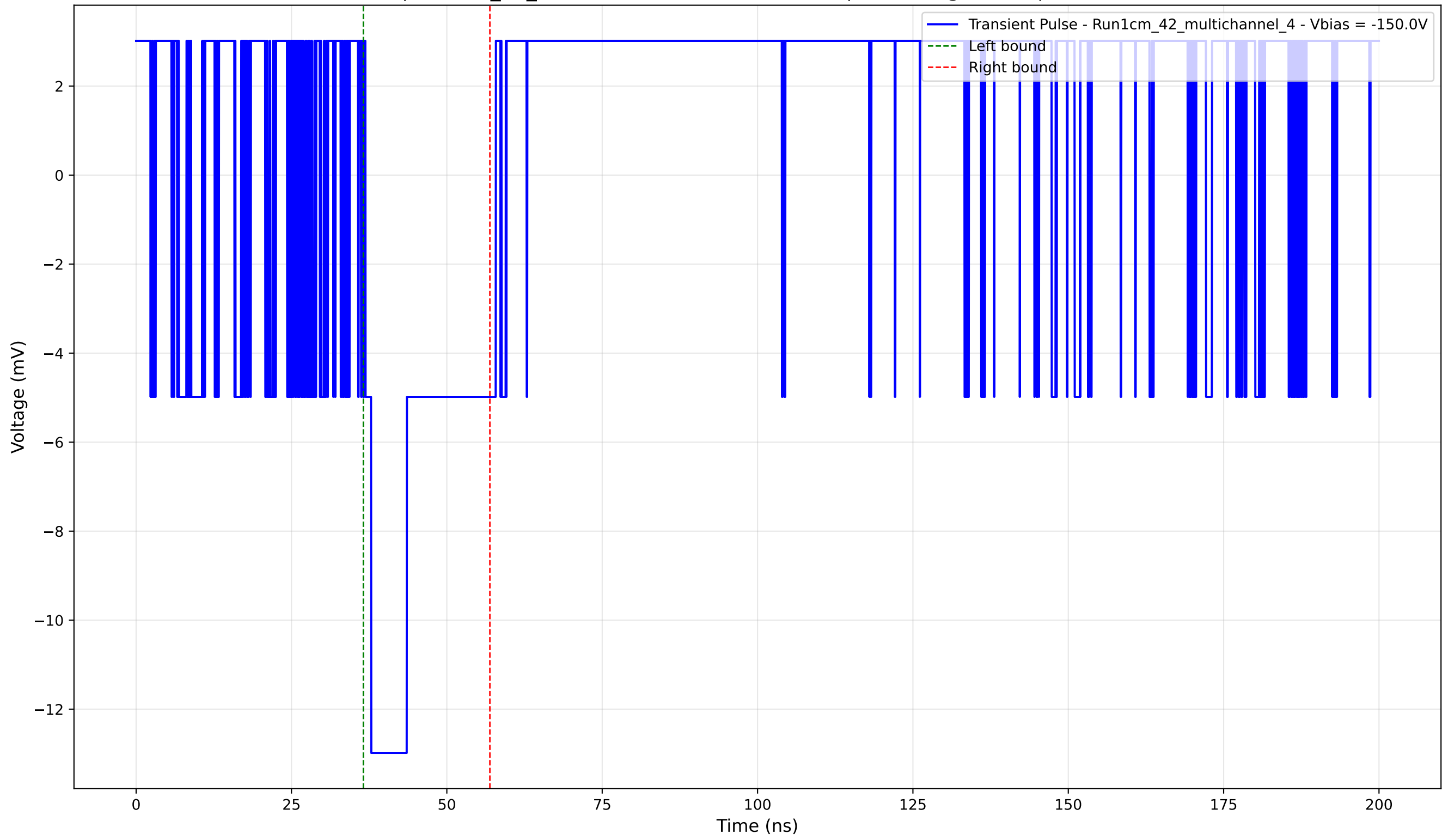
Transient Pulse - Sample: 1cm_42_multichannel - Position: 775.0 \mu\text{m} - Charge: 2.91 pC - Rise Time: 0.00 ns (N/A)
