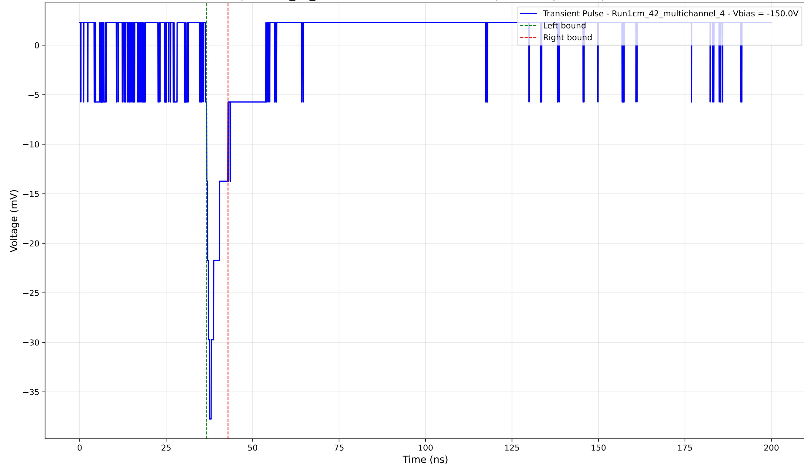
Transient Pulse - Sample: 1cm_42_multichannel - Position: 1670.0 \mu\text{m} - Charge: 2.57 pC - Rise Time: 1.21 ns
