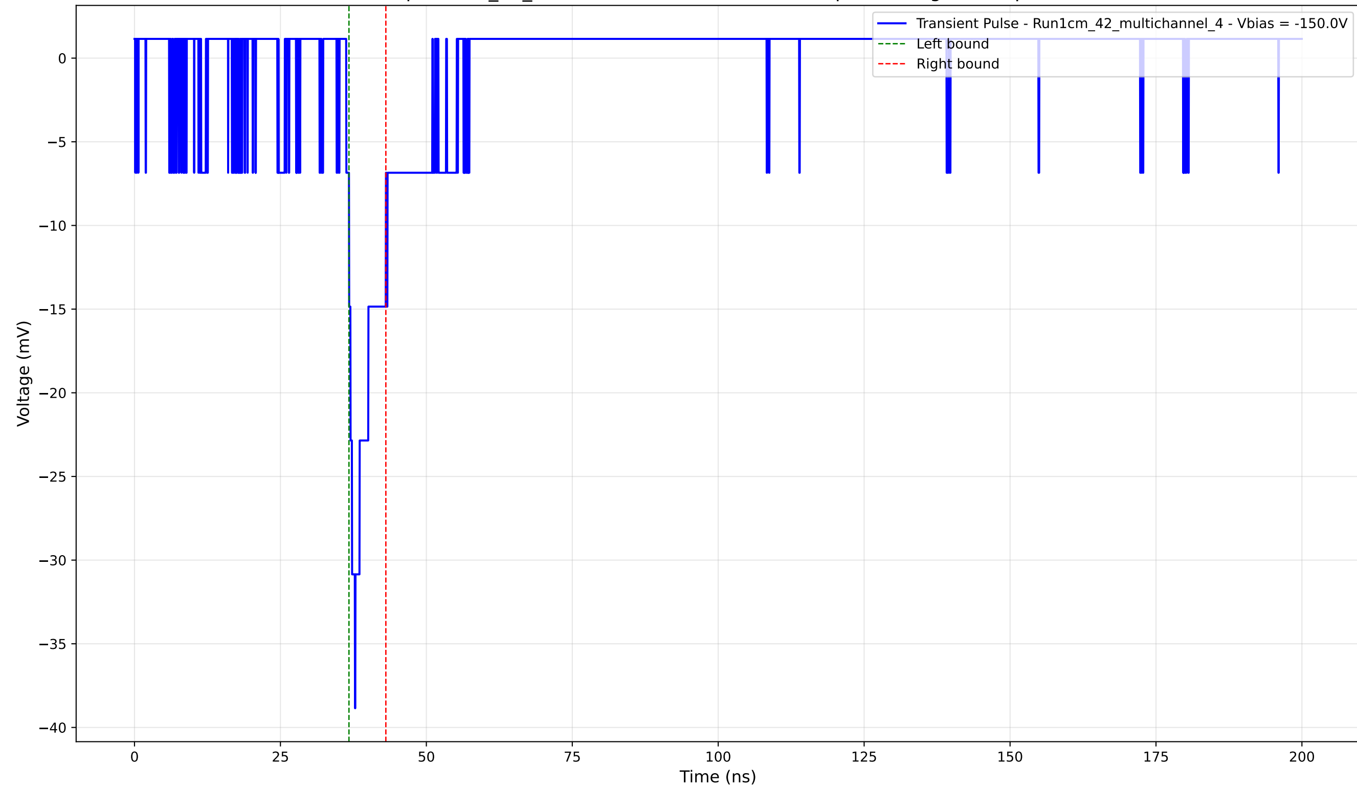
Transient Pulse - Sample: 1cm_42_multichannel - Position: 1650.0 \mu\text{m} - Charge: 2.58 pC - Rise Time: 1.49 ns
