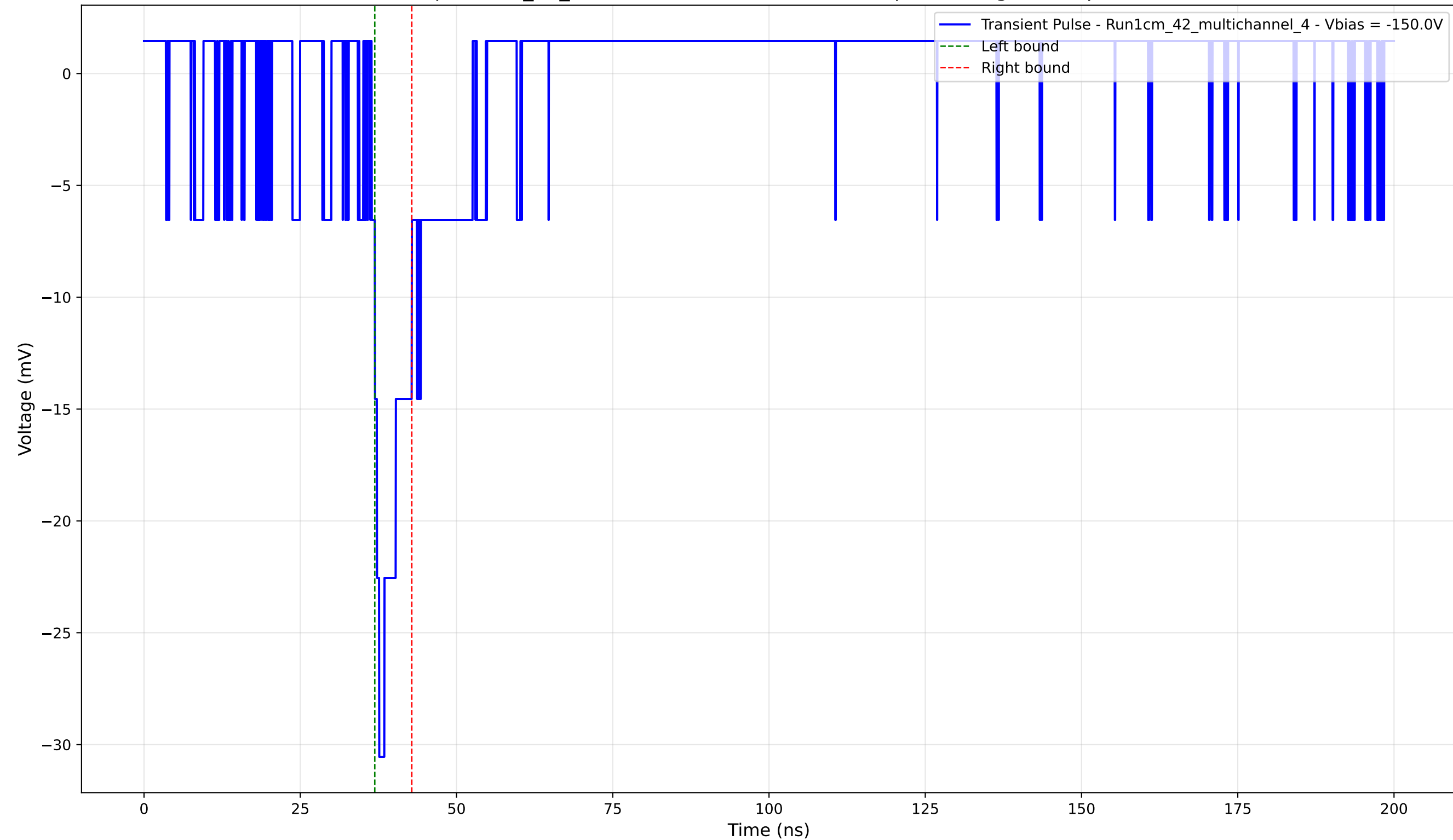
Transient Pulse - Sample: 1cm_42_multichannel - Position: 1470.0 \mu\text{m} - Charge: 2.34 pC - Rise Time: 1.21 ns
