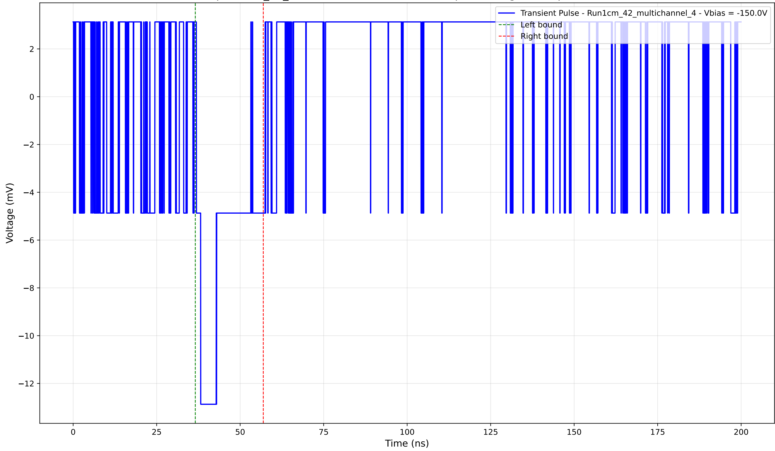
Transient Pulse - Sample: 1cm_42_multichannel - Position: 265.0 \mu\text{m} - Charge: 2.65 pC - Rise Time: 0.00 ns (N/A)
