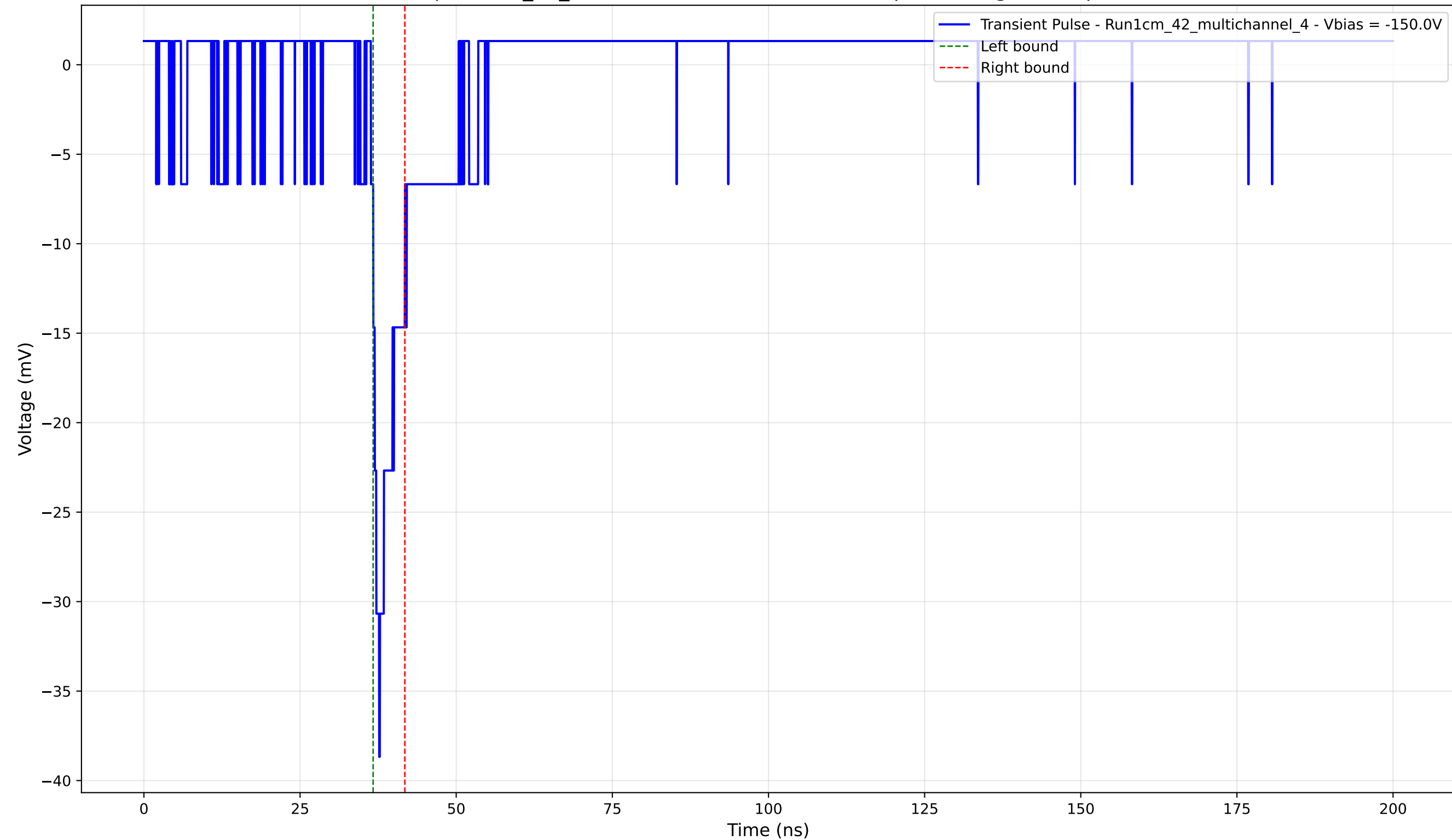
Transient Pulse - Sample: 1cm_42_multichannel - Position: 3055.0 \mu\text{m} - Charge: 2.18 pC - Rise Time: 1.33 ns
