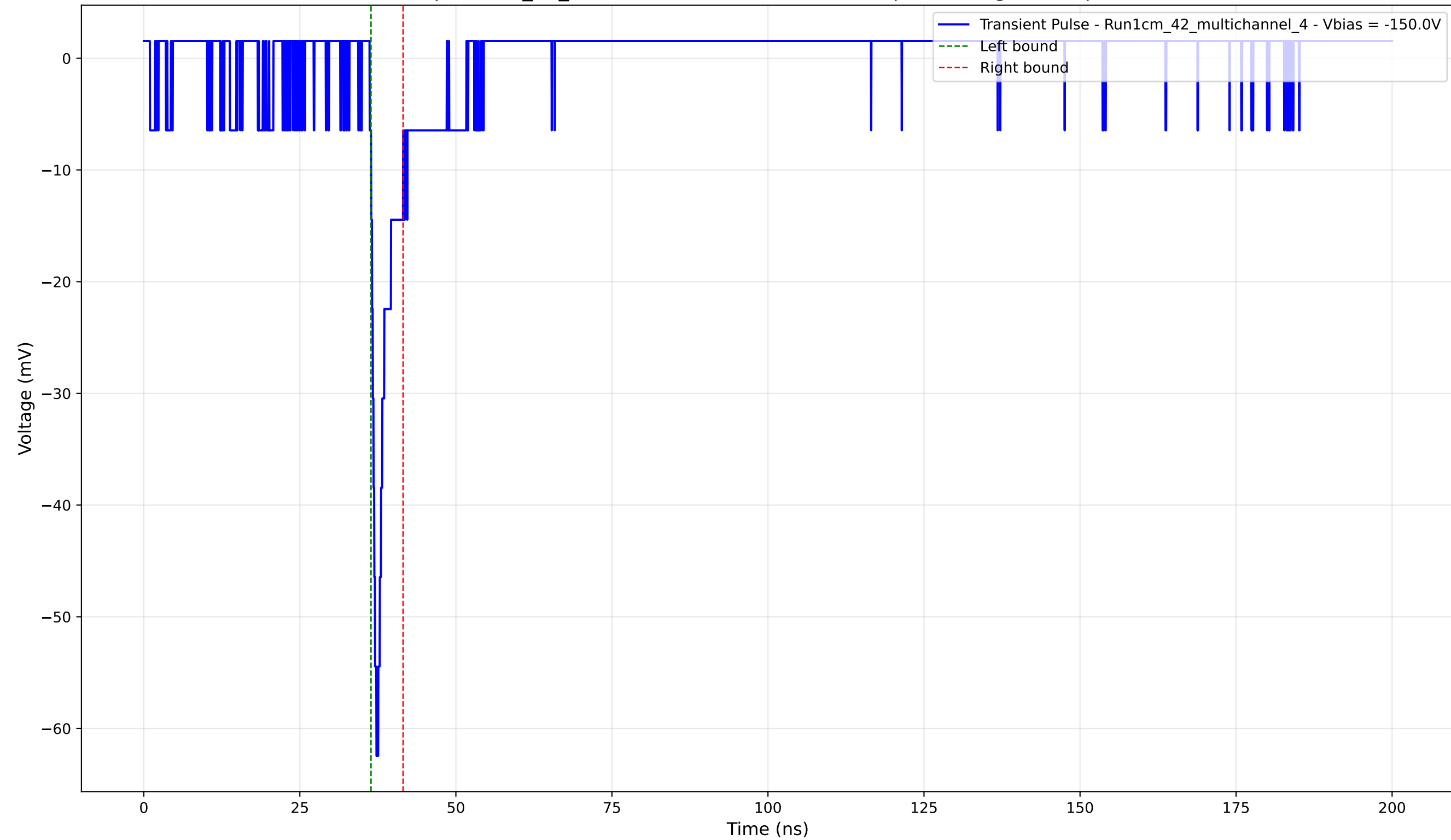
Transient Pulse - Sample: 1cm_42_multichannel - Position: 2675.0 \mu\text{m} - Charge: 2.83 pC - Rise Time: 1.08 ns
