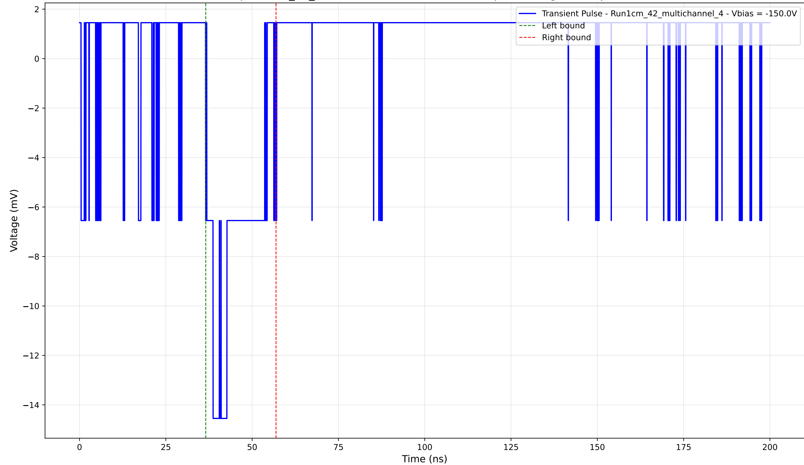
Transient Pulse - Sample: 1cm_42_multichannel - Position: 4790.0 \mu\text{m} - Charge: 2.84 pC - Rise Time: 1.84 ns
