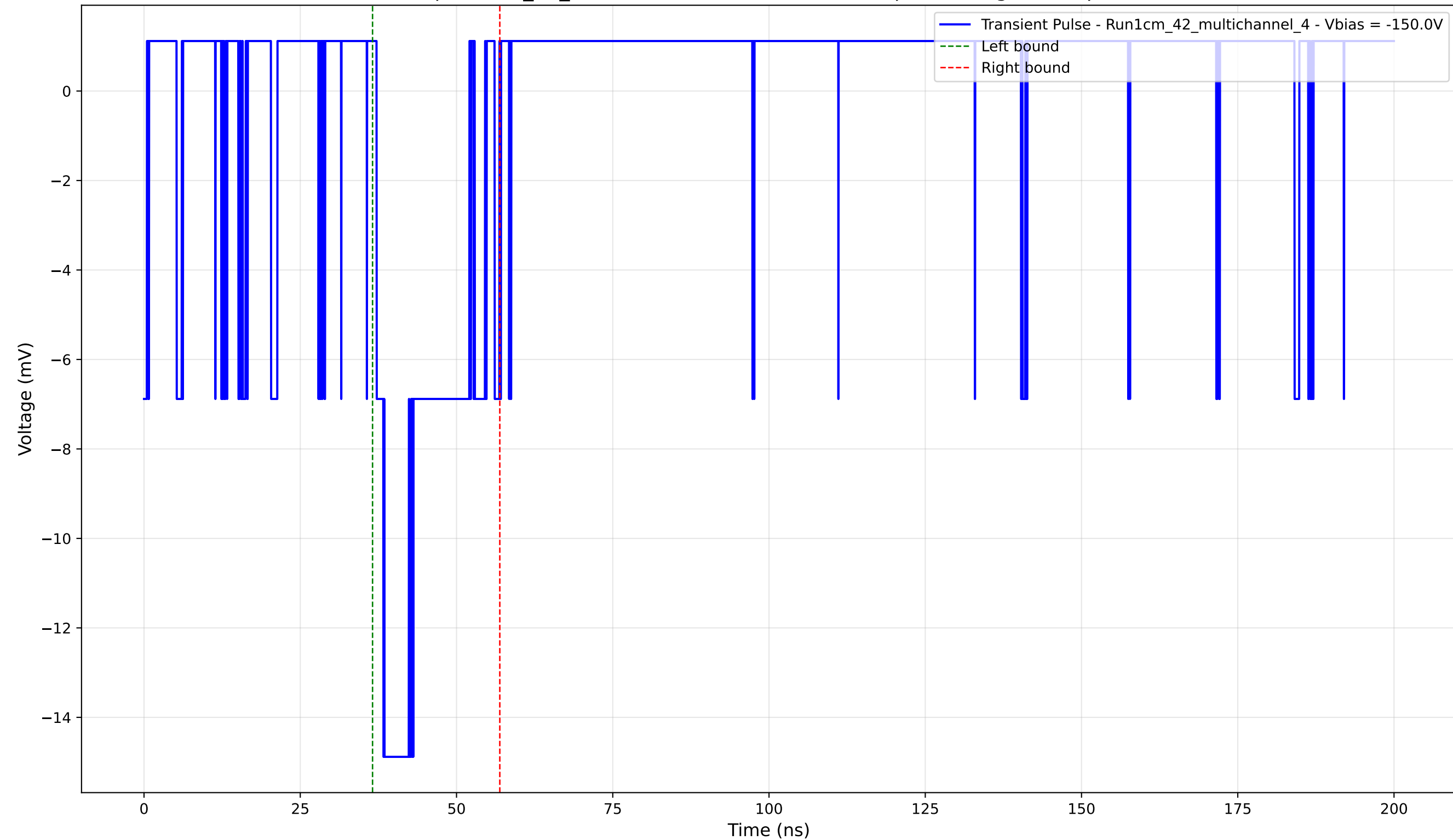
Transient Pulse - Sample: 1cm_42_multichannel - Position: 4235.0 \mu\text{m} - Charge: 3.07 pC - Rise Time: 1.10 ns
