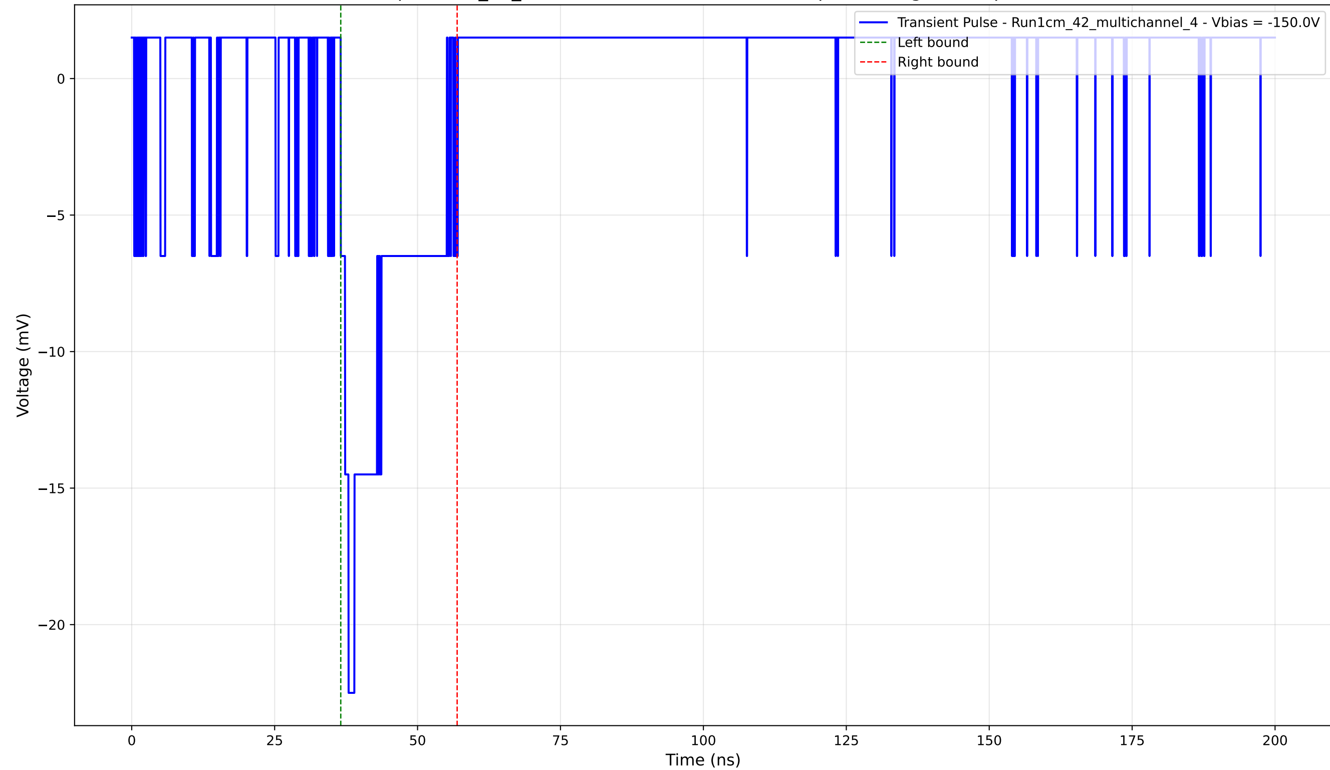
Transient Pulse - Sample: 1cm_42_multichannel - Position: 3540.0 \mu\text{m} - Charge: 3.63 pC - Rise Time: 1.38 ns
