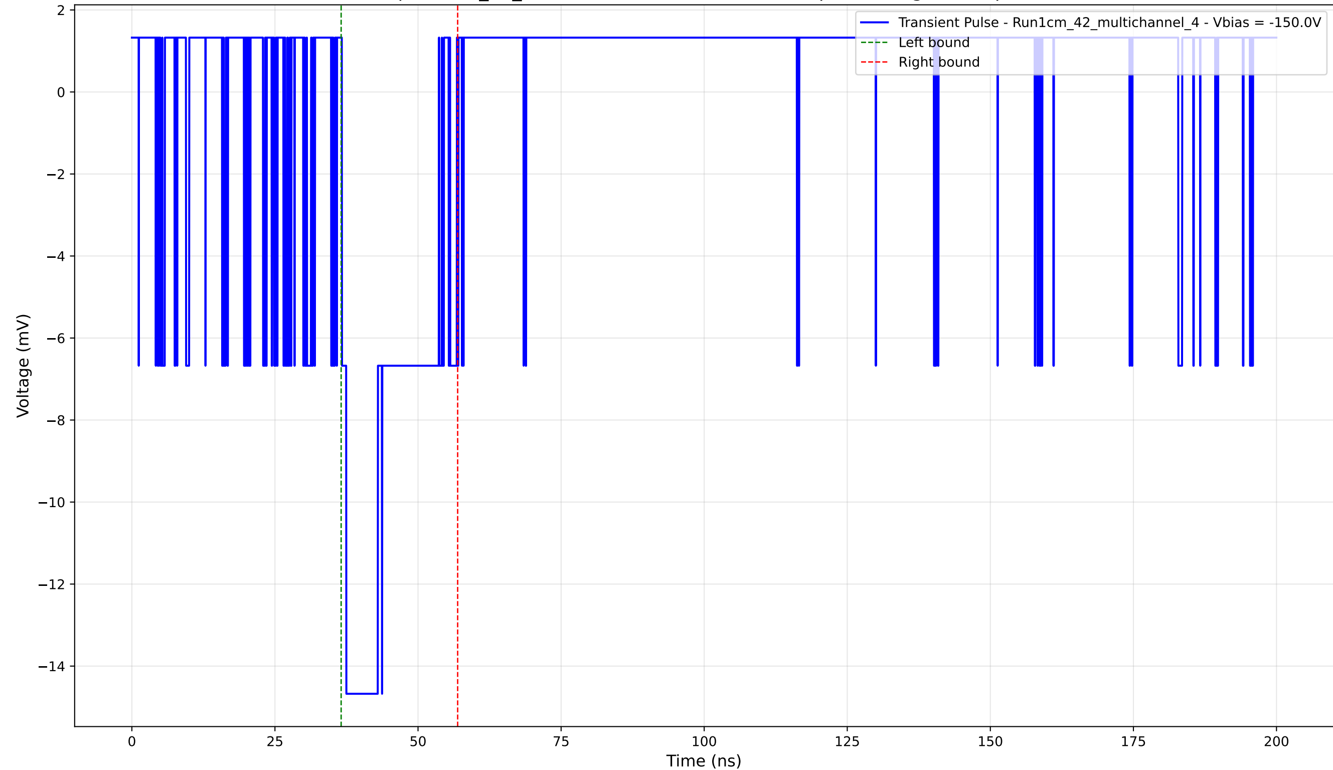
Transient Pulse - Sample: 1cm_42_multichannel - Position: 3665.0 \mu\text{m} - Charge: 3.39 pC - Rise Time: 0.78 ns
