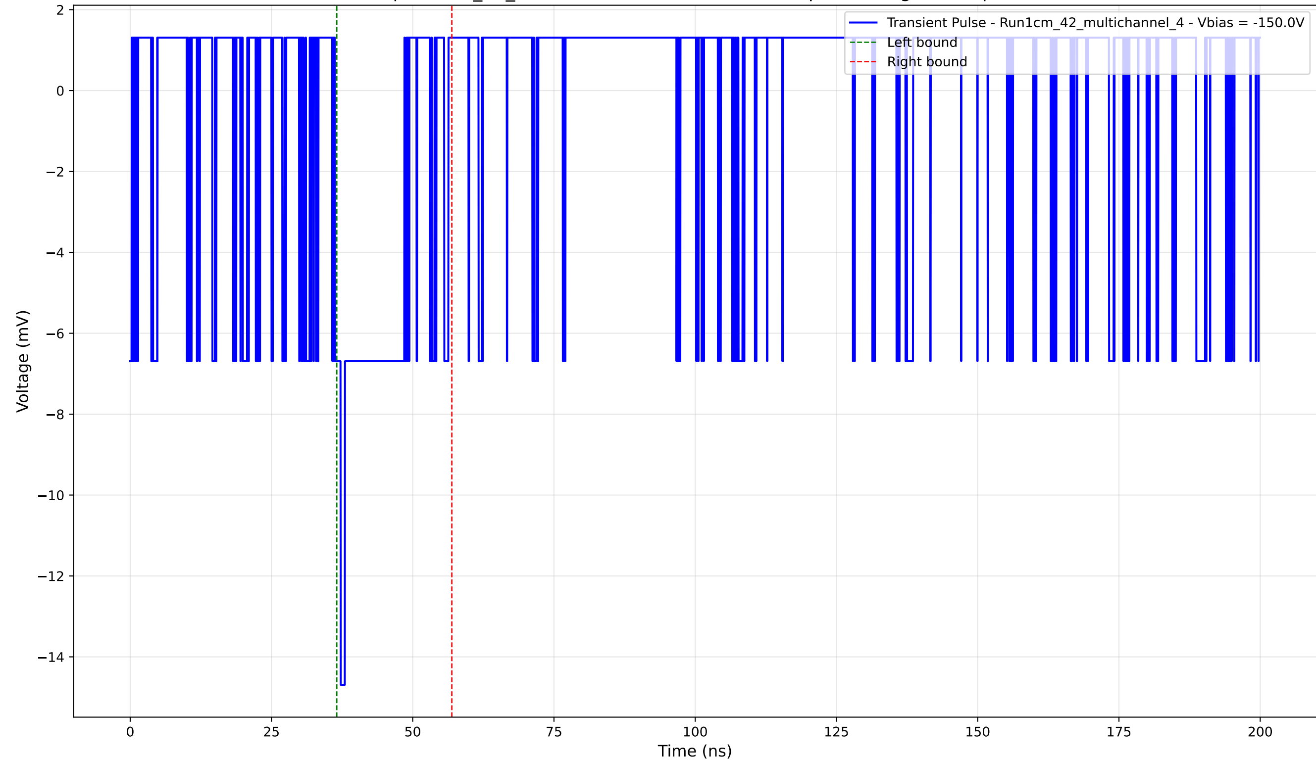
Transient Pulse - Sample: 1cm_42_multichannel - Position: 1840.0 \mu\text{m} - Charge: 1.86 pC - Rise Time: 1.02 ns
