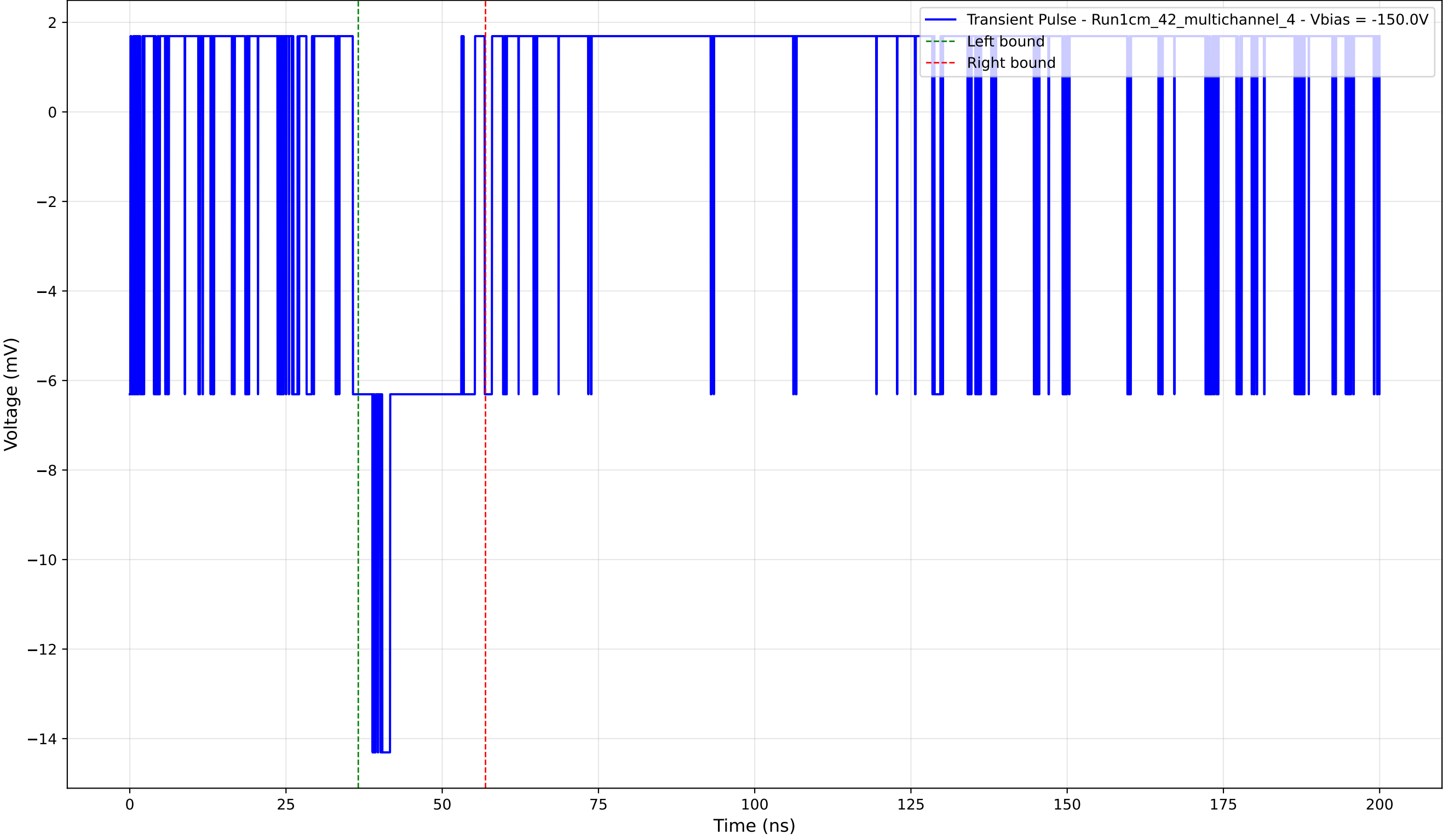
Transient Pulse - Sample: 1cm_42_multichannel - Position: 420.0 \mu\text{m} - Charge: 2.57 pC - Rise Time: 0.00 ns (N/A)
