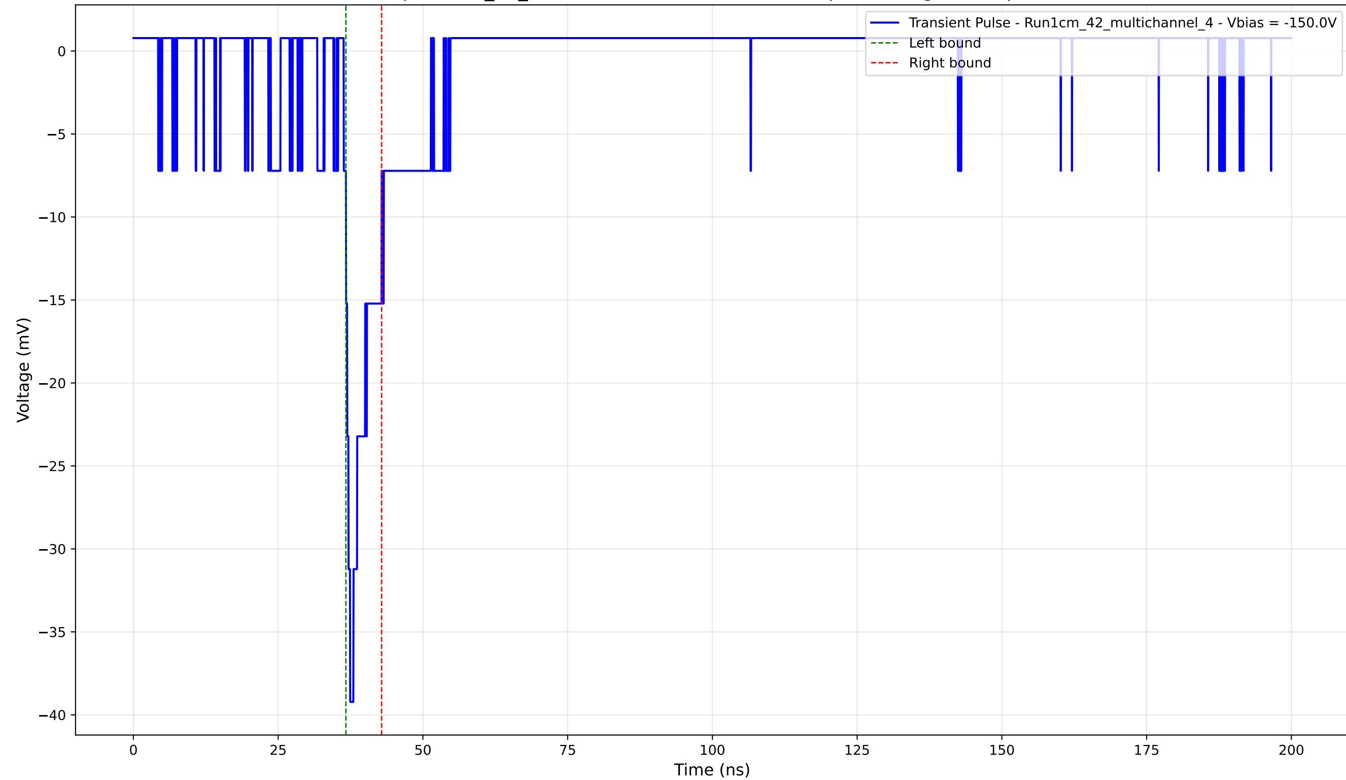
Transient Pulse - Sample: 1cm_42_multichannel - Position: 1700.0 \mu\text{m} - Charge: 2.72 pC - Rise Time: 1.11 ns
