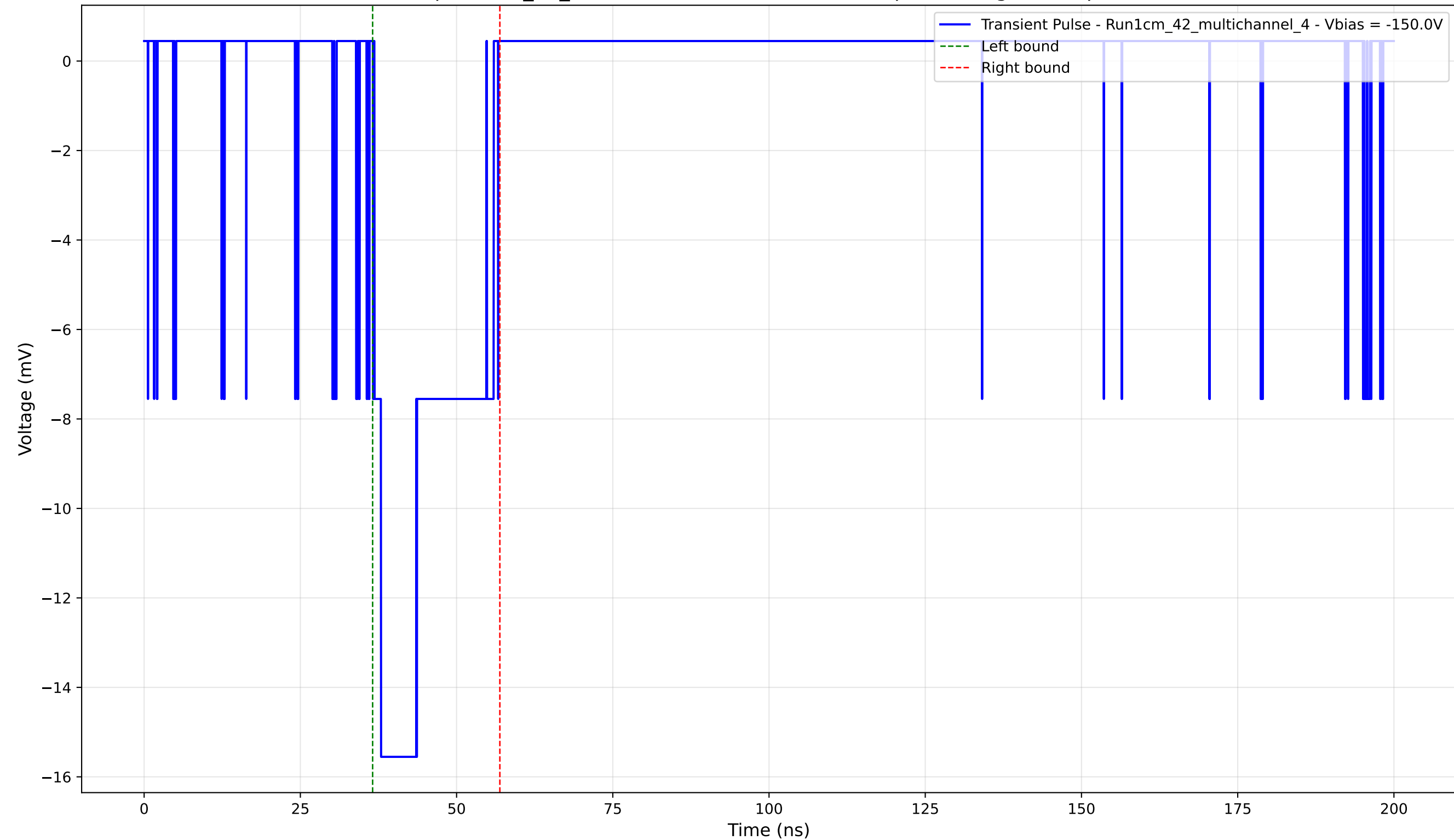
Transient Pulse - Sample: 1cm_42_multichannel - Position: 4000.0 \mu\text{m} - Charge: 3.80 pC - Rise Time: 1.06 ns
