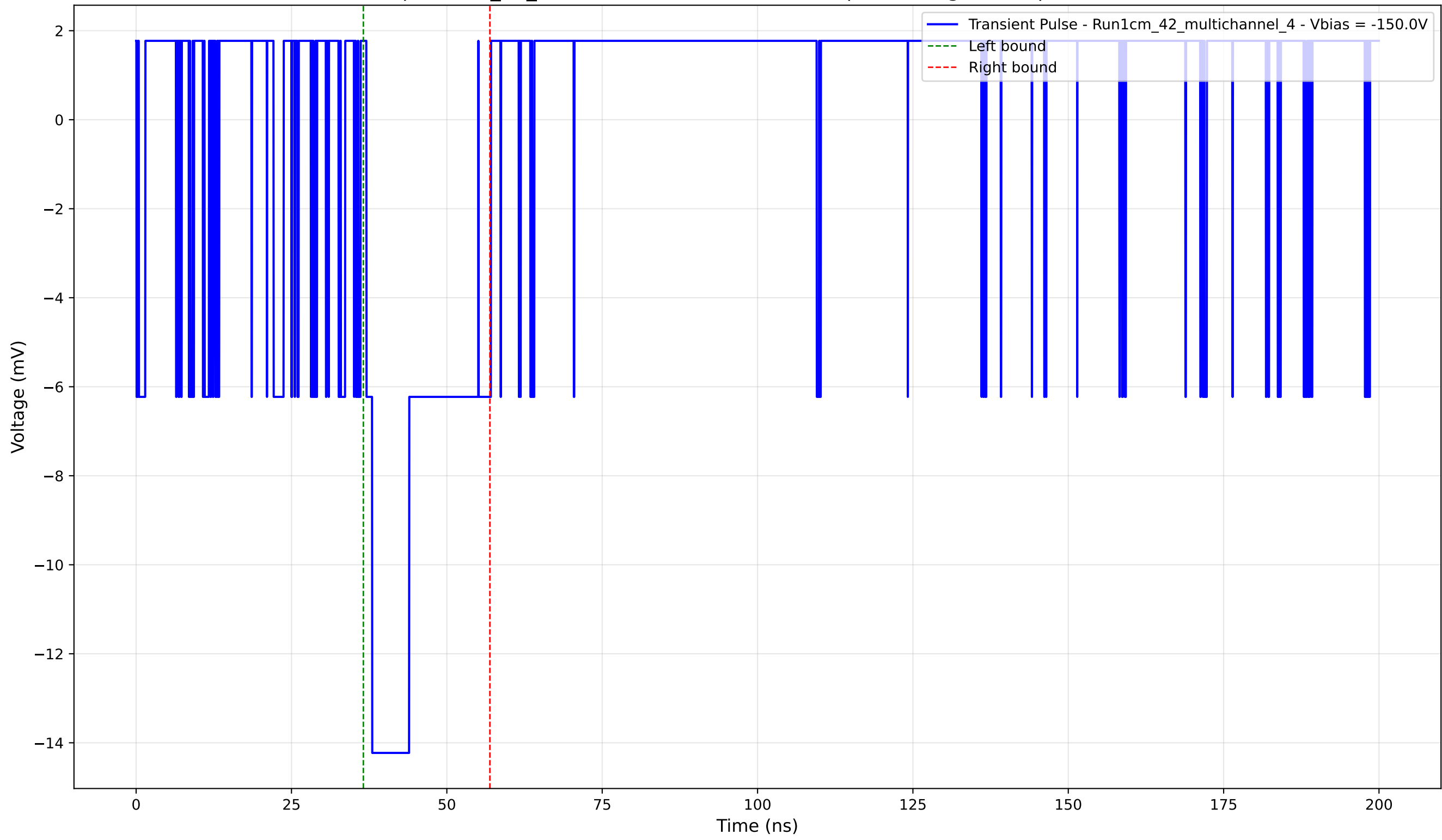
Transient Pulse - Sample: 1cm_42_multichannel - Position: 500.0 \mu\text{m} - Charge: 3.41 pC - Rise Time: 0.00 ns (N/A)
