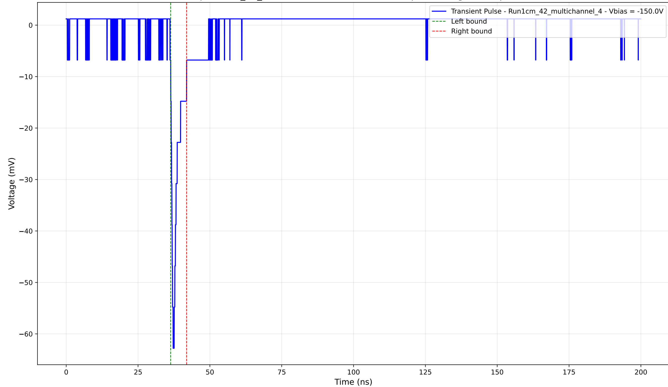
Transient Pulse - Sample: 1cm_42_multichannel - Position: 2115.0 \mu\text{m} - Charge: 3.07 pC - Rise Time: 1.08 ns
