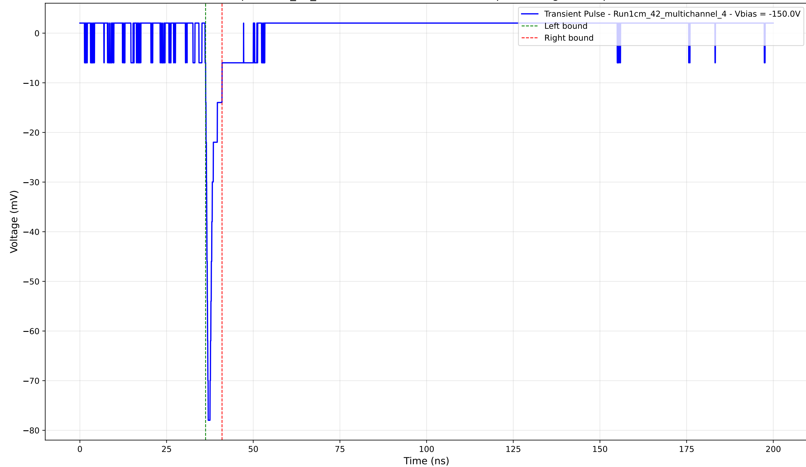
Transient Pulse - Sample: 1cm_42_multichannel - Position: 2490.0 \mu\text{m} - Charge: 3.19 pC - Rise Time: 0.74 ns
