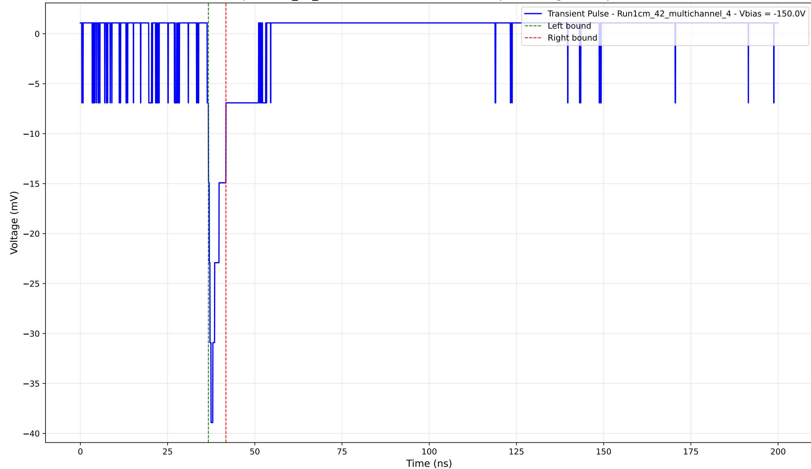
Transient Pulse - Sample: 1cm_42_multichannel - Position: 3015.0 \mu\text{m} - Charge: 2.25 pC - Rise Time: 1.11 ns
