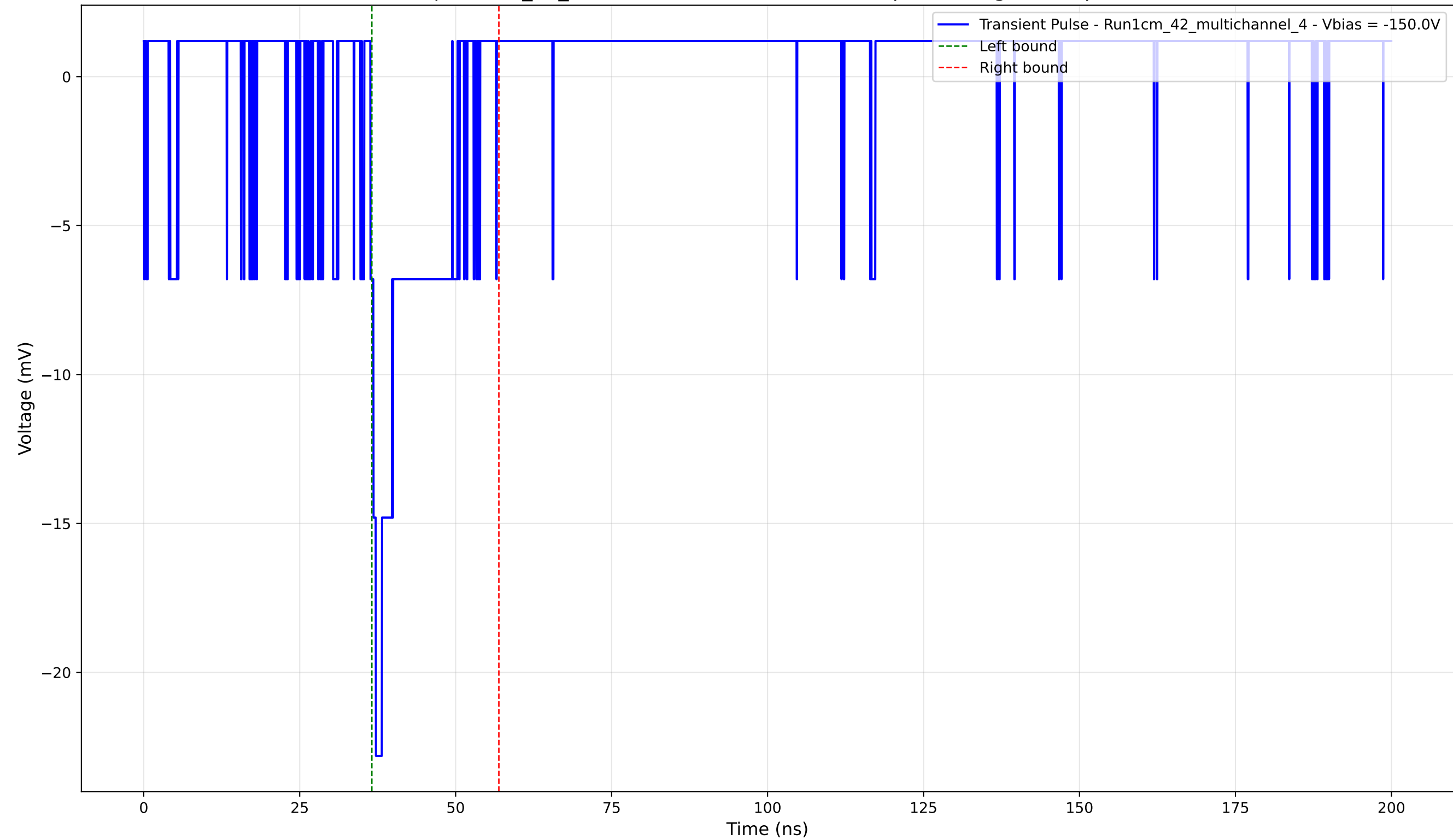
Transient Pulse - Sample: 1cm_42_multichannel - Position: 2945.0 \mu\text{m} - Charge: 2.46 pC - Rise Time: 0.88 ns
