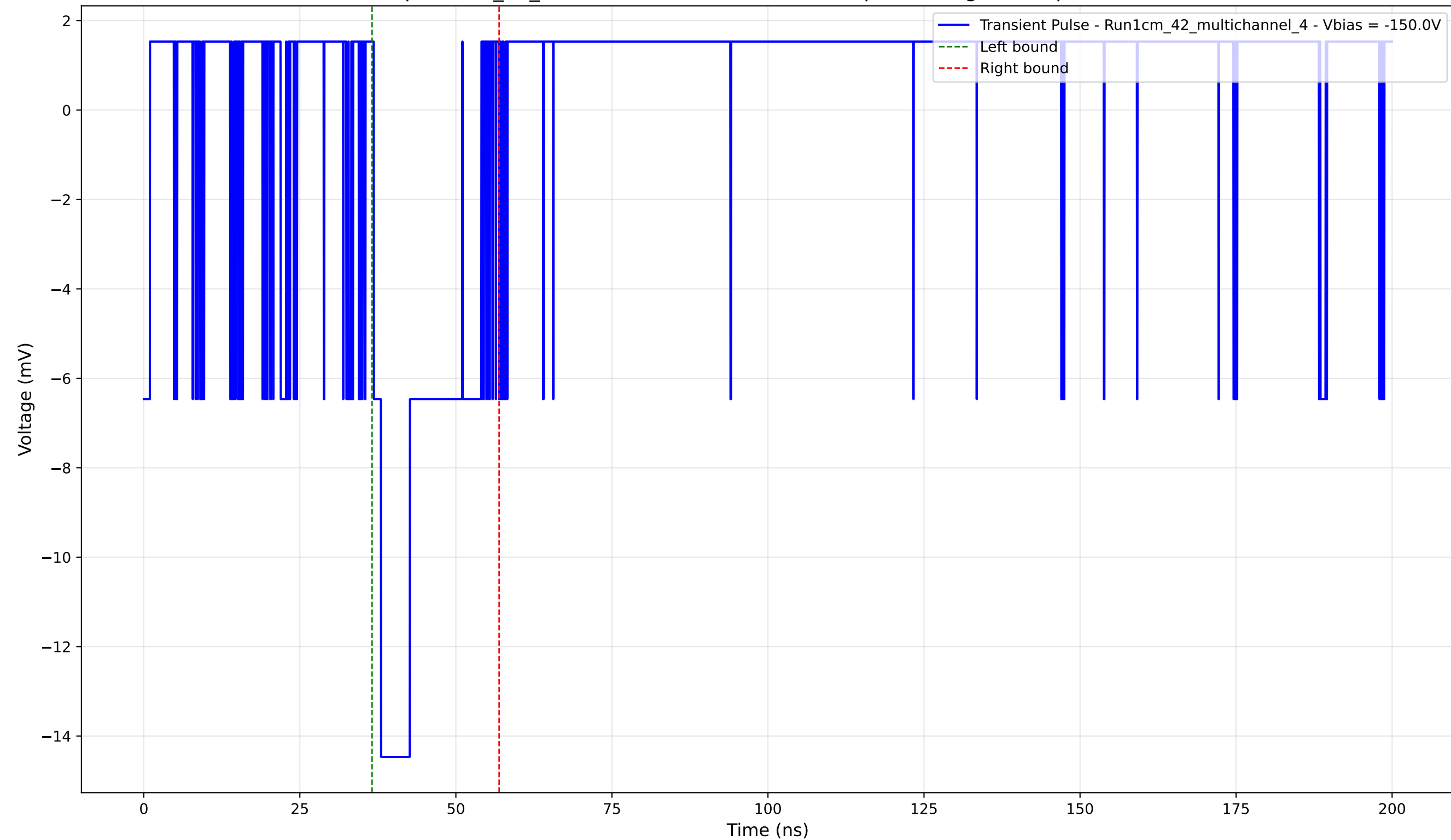
Transient Pulse - Sample: 1cm_42_multichannel - Position: 4040.0 \mu\text{m} - Charge: 2.96 pC - Rise Time: 0.00 ns (N/A)
