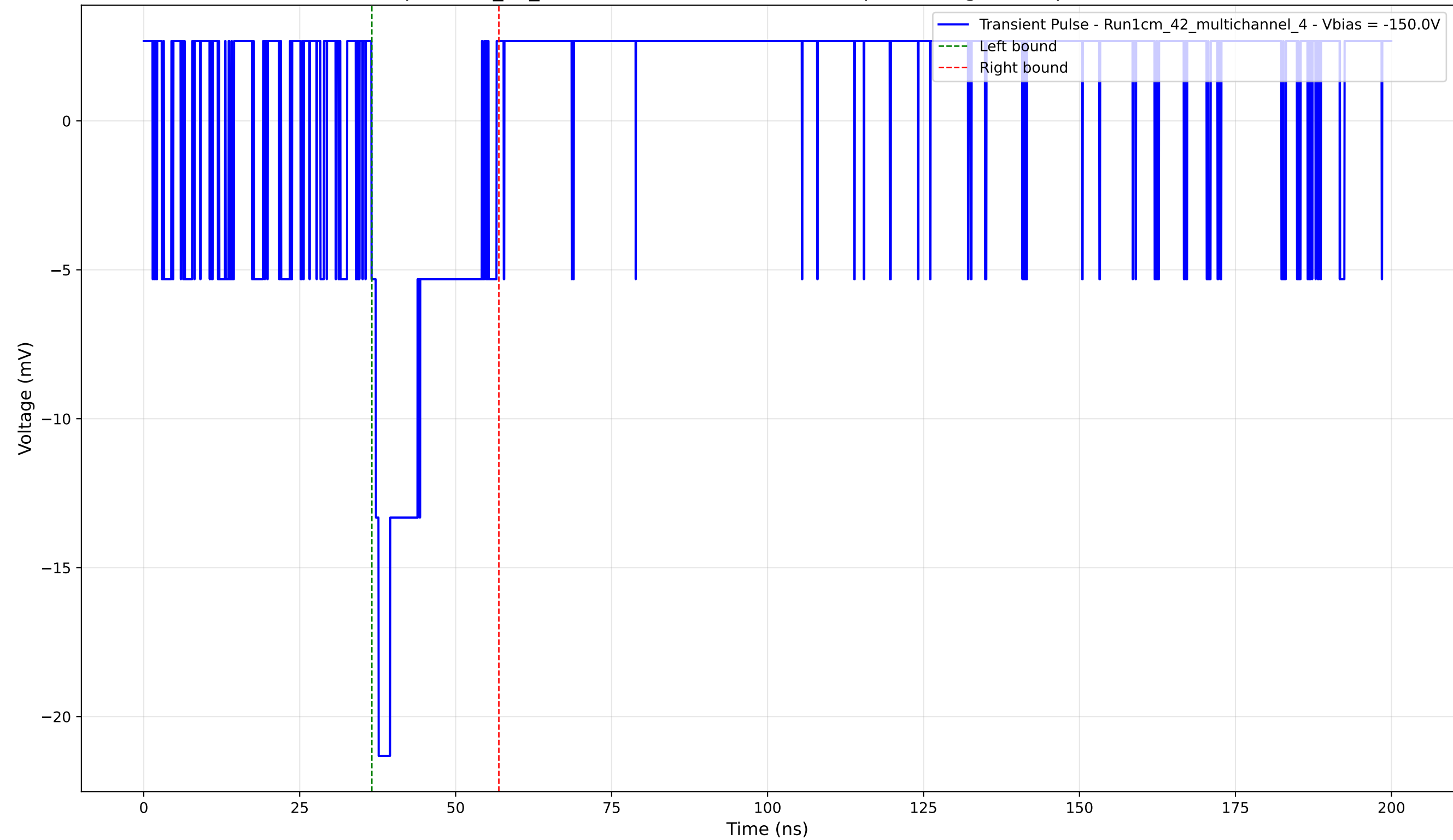
Transient Pulse - Sample: 1cm_42_multichannel - Position: 1300.0 \mu\text{m} - Charge: 3.40 pC - Rise Time: 0.00 ns (N/A)
