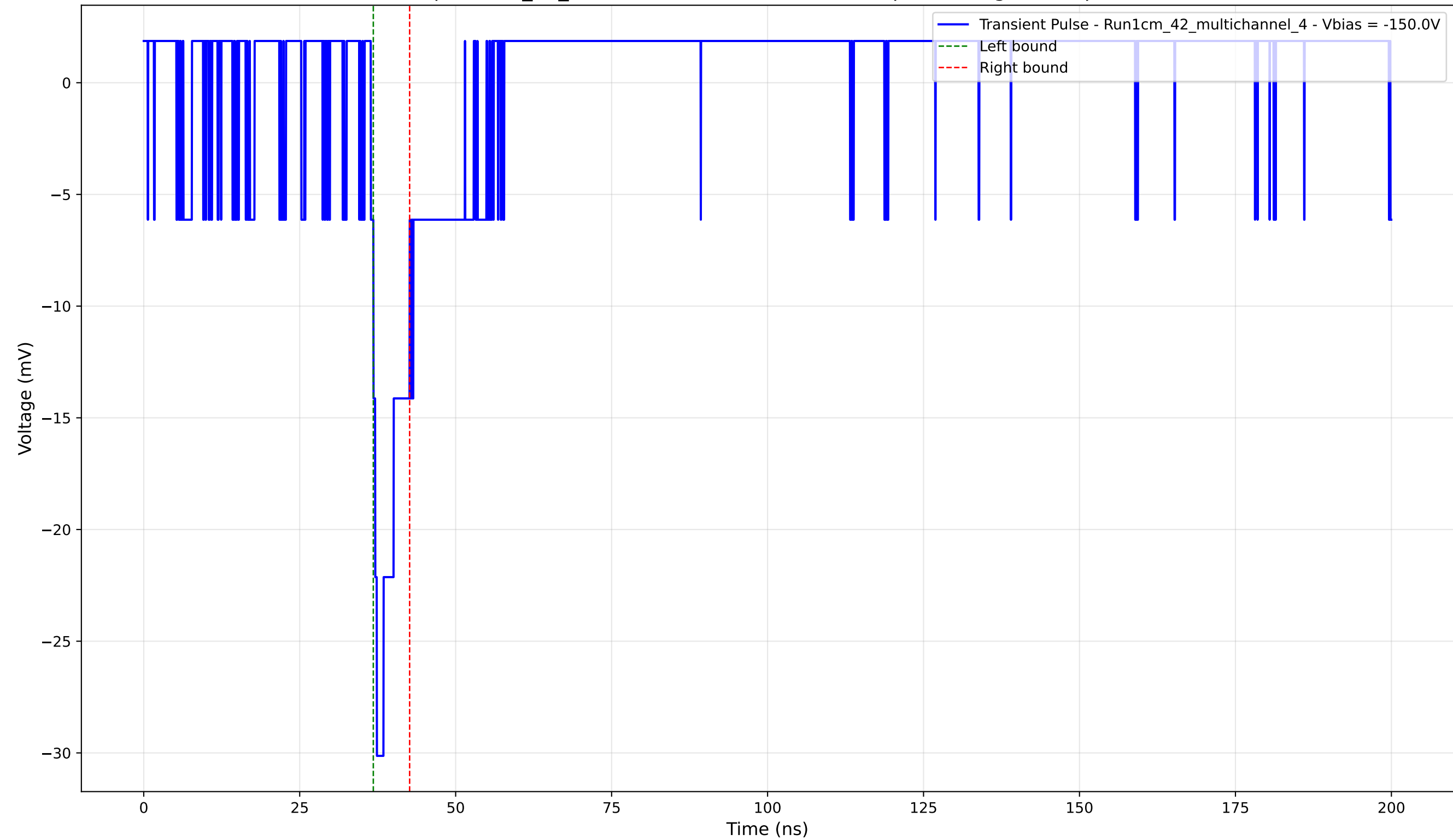
Transient Pulse - Sample: 1cm_42_multichannel - Position: 1600.0 \mu\text{m} - Charge: 2.29 pC - Rise Time: 0.97 ns
