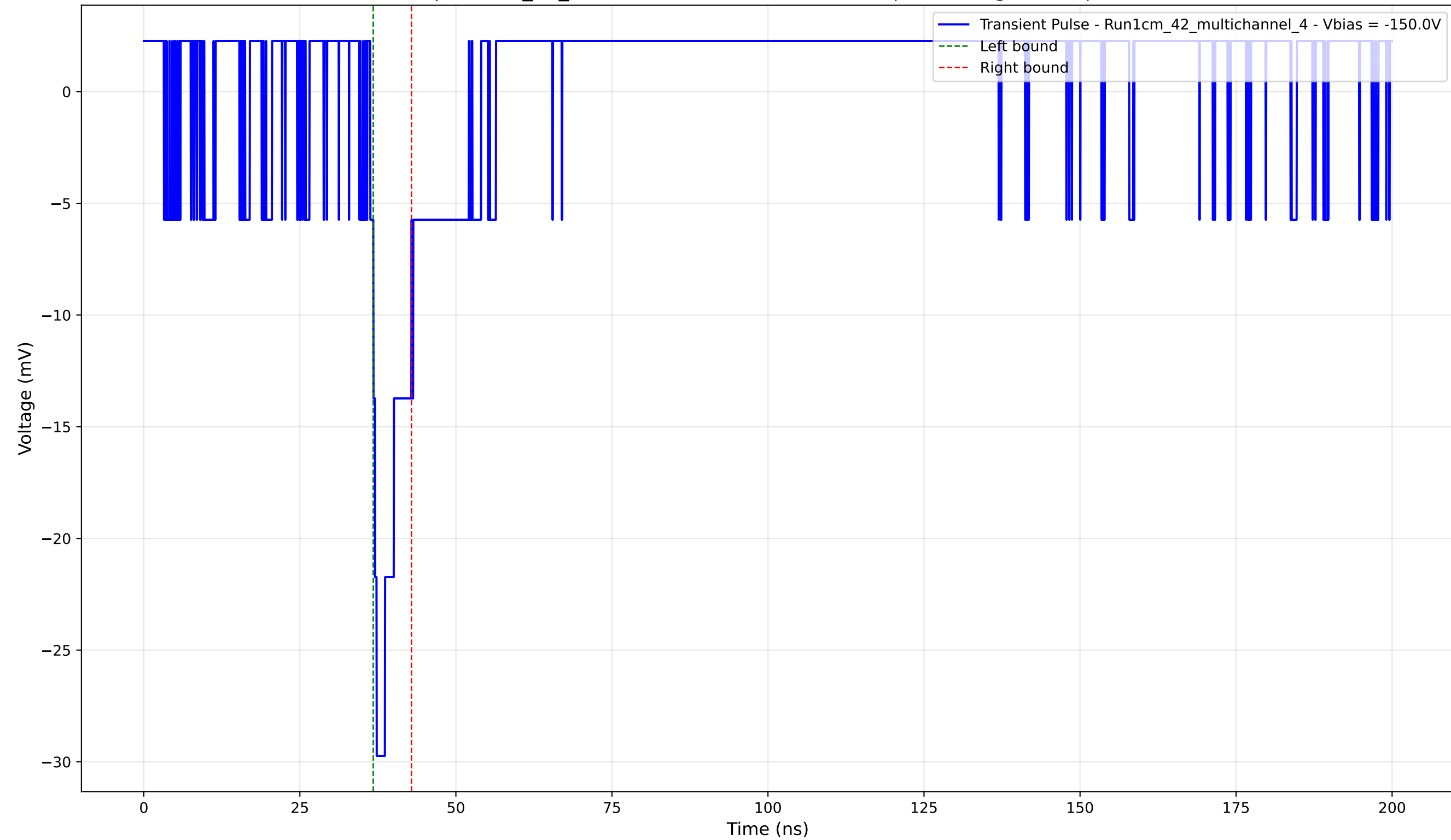
Transient Pulse - Sample: 1cm_42_multichannel - Position: 1635.0 \mu\text{m} - Charge: 2.38 pC - Rise Time: 1.04 ns
