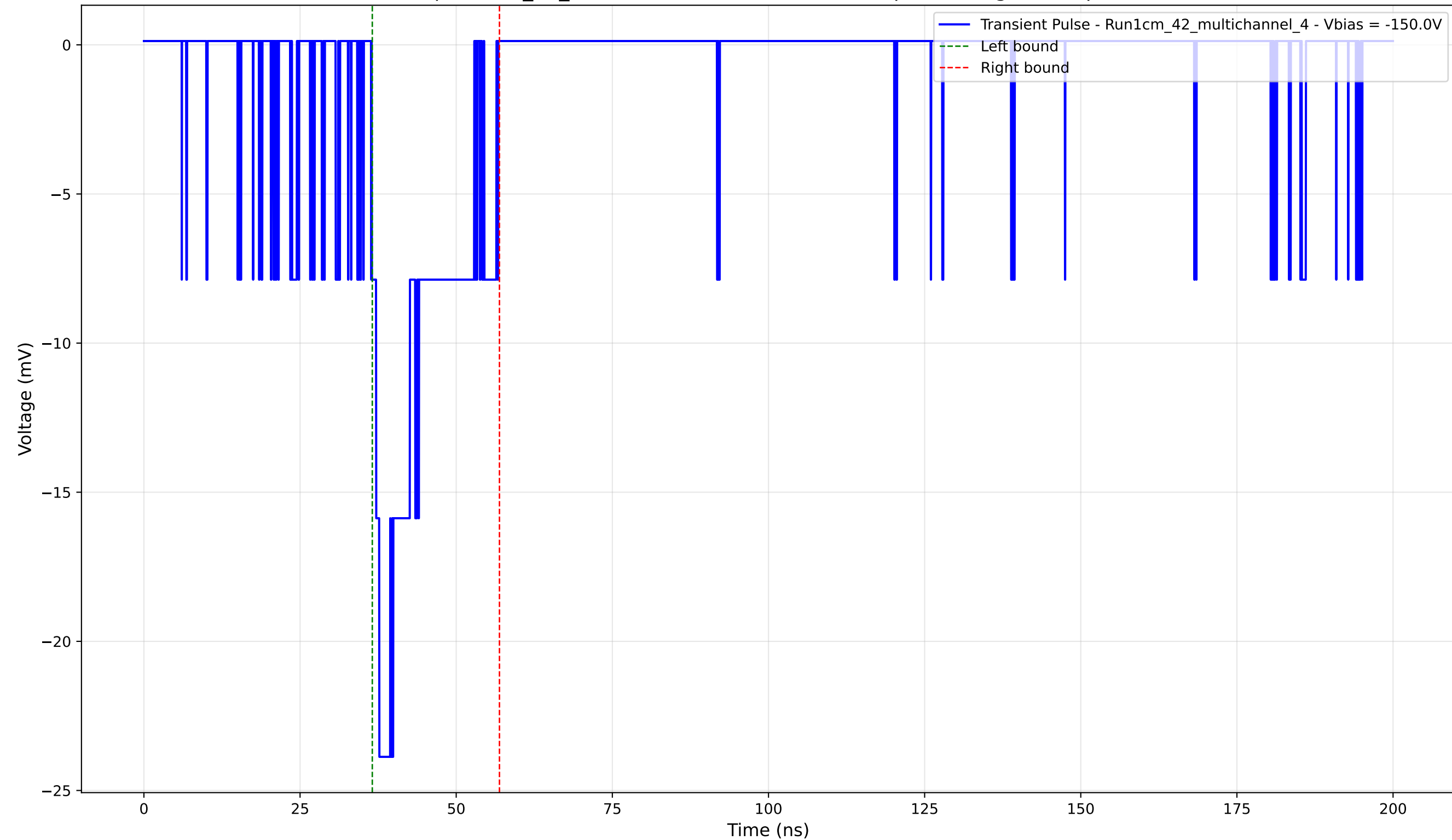
Transient Pulse - Sample: 1cm_42_multichannel - Position: 3490.0 \mu\text{m} - Charge: 4.23 pC - Rise Time: 1.21 ns
