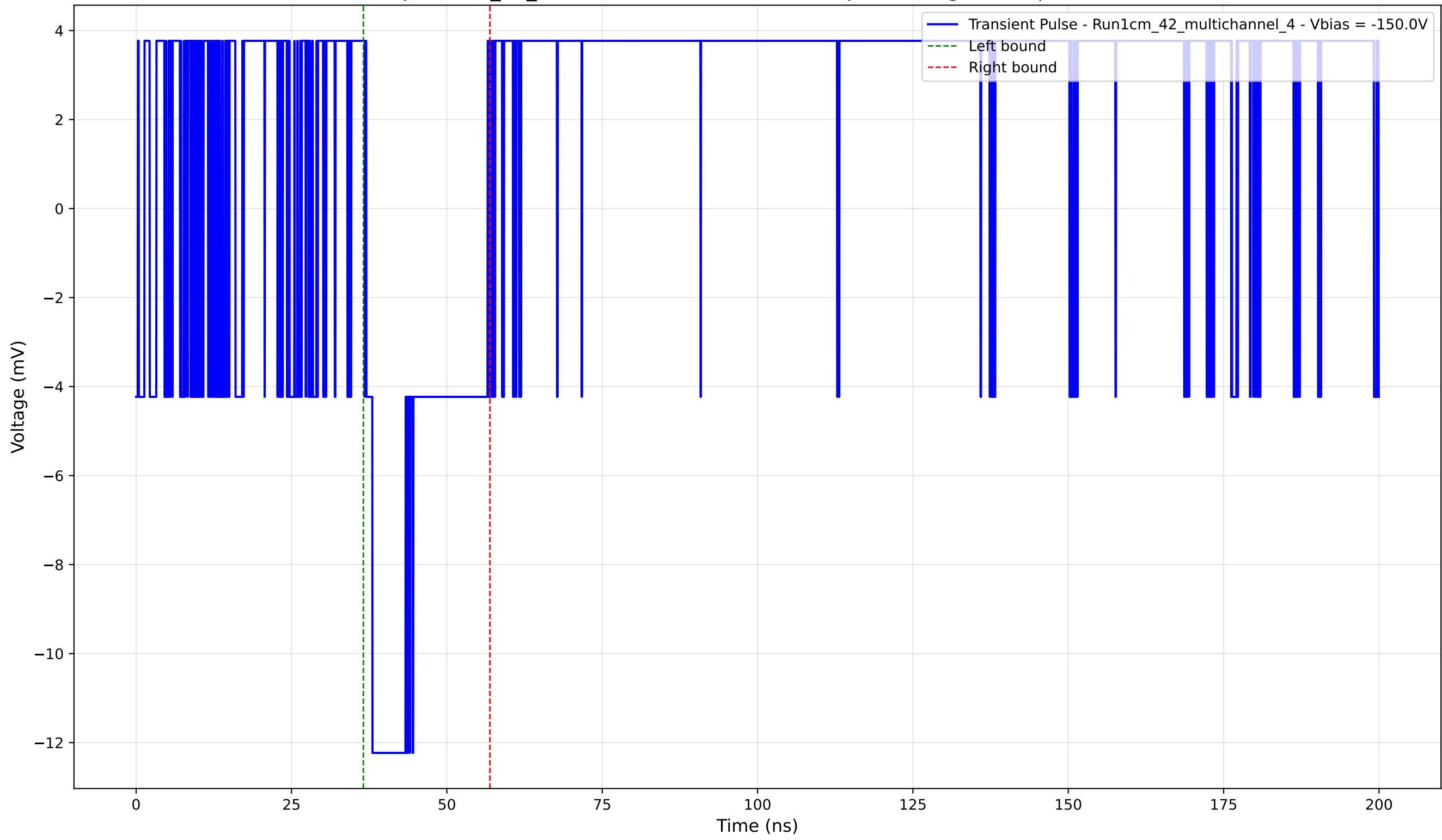
Transient Pulse - Sample: 1cm_42_multichannel - Position: 550.0 \mu\text{m} - Charge: 2.53 pC - Rise Time: 0.00 ns (N/A)
