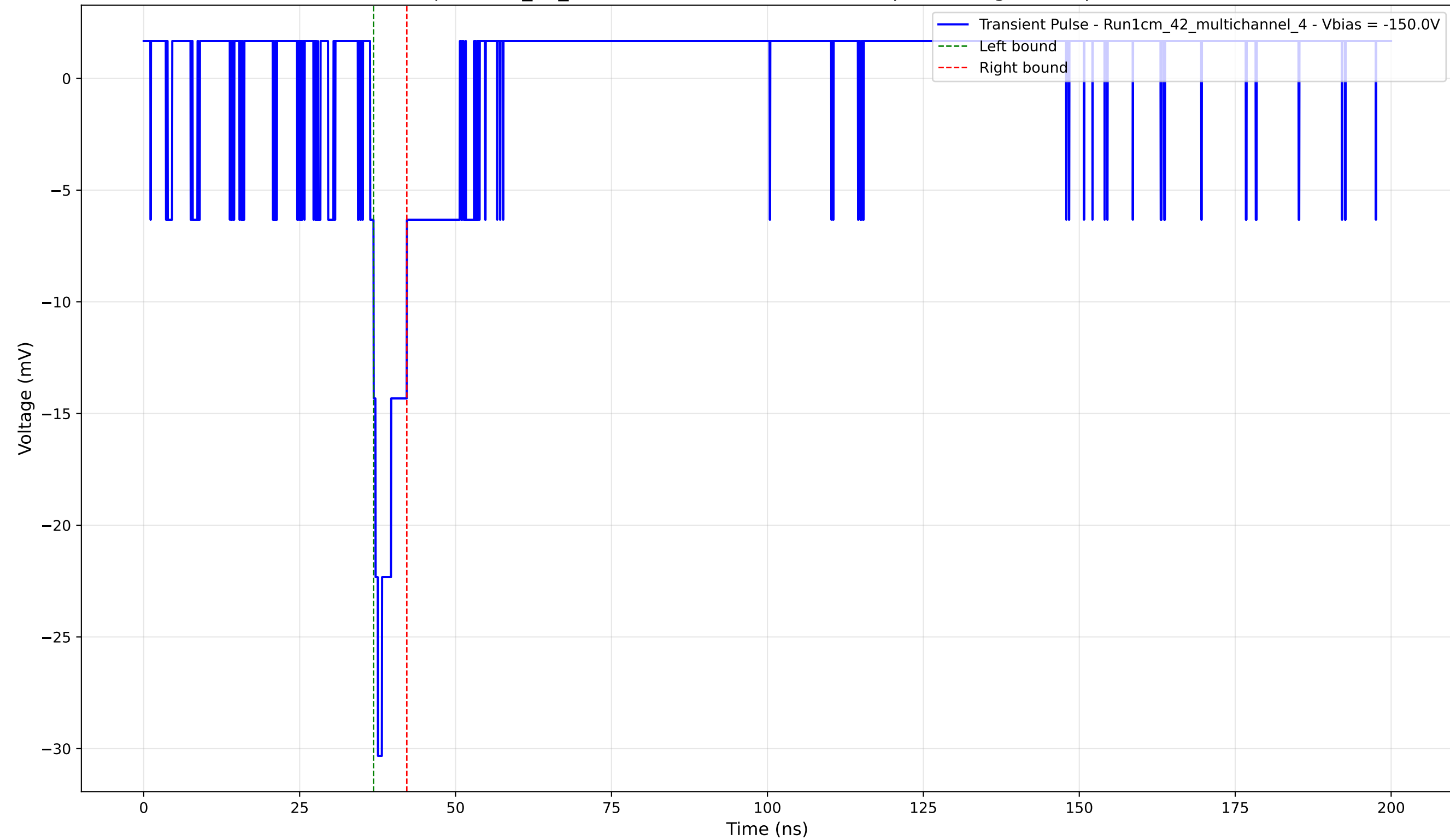
Transient Pulse - Sample: 1cm_42_multichannel - Position: 3170.0 \mu\text{m} - Charge: 2.03 pC - Rise Time: 1.25 ns
