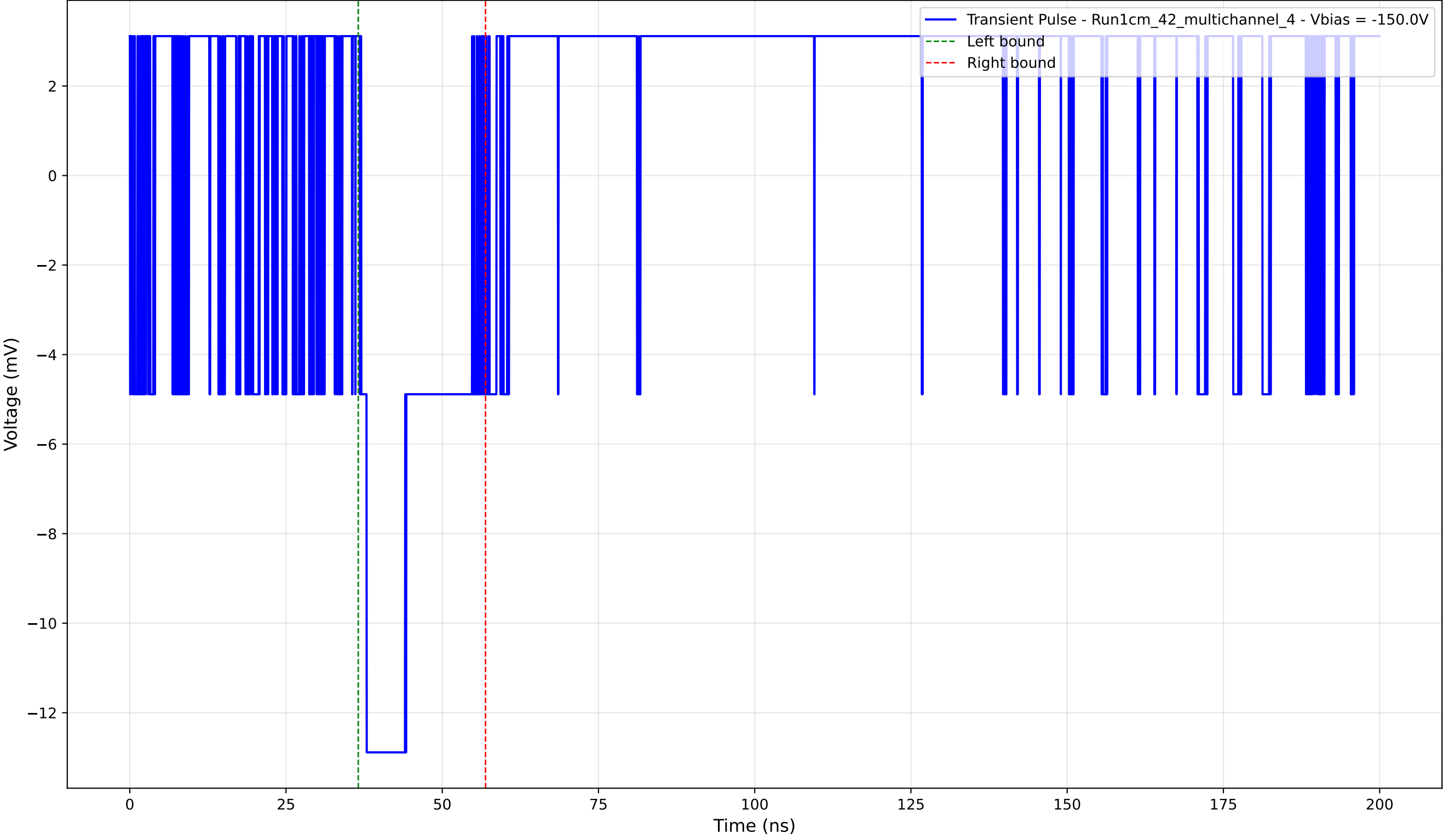
Transient Pulse - Sample: 1cm_42_multichannel - Position: 630.0 \mu\text{m} - Charge: 2.84 pC - Rise Time: 0.00 ns (N/A)
