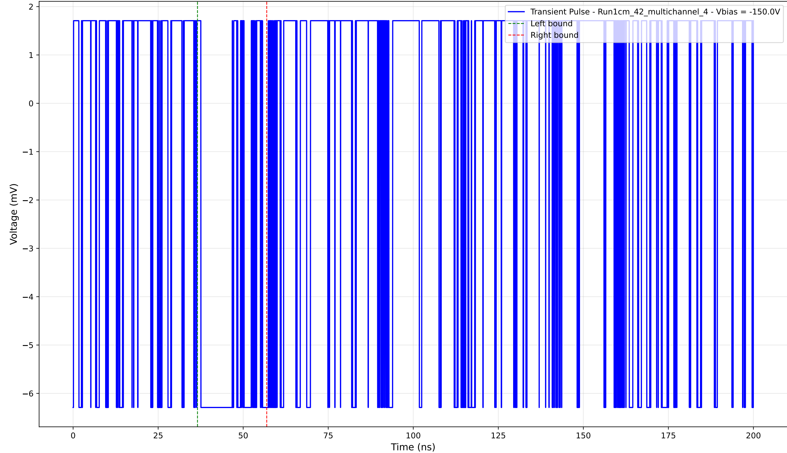
Transient Pulse - Sample: 1cm_42_multichannel - Position: 905.0 \mu\text{m} - Charge: 1.74 pC - Rise Time: 0.00 ns (N/A)
