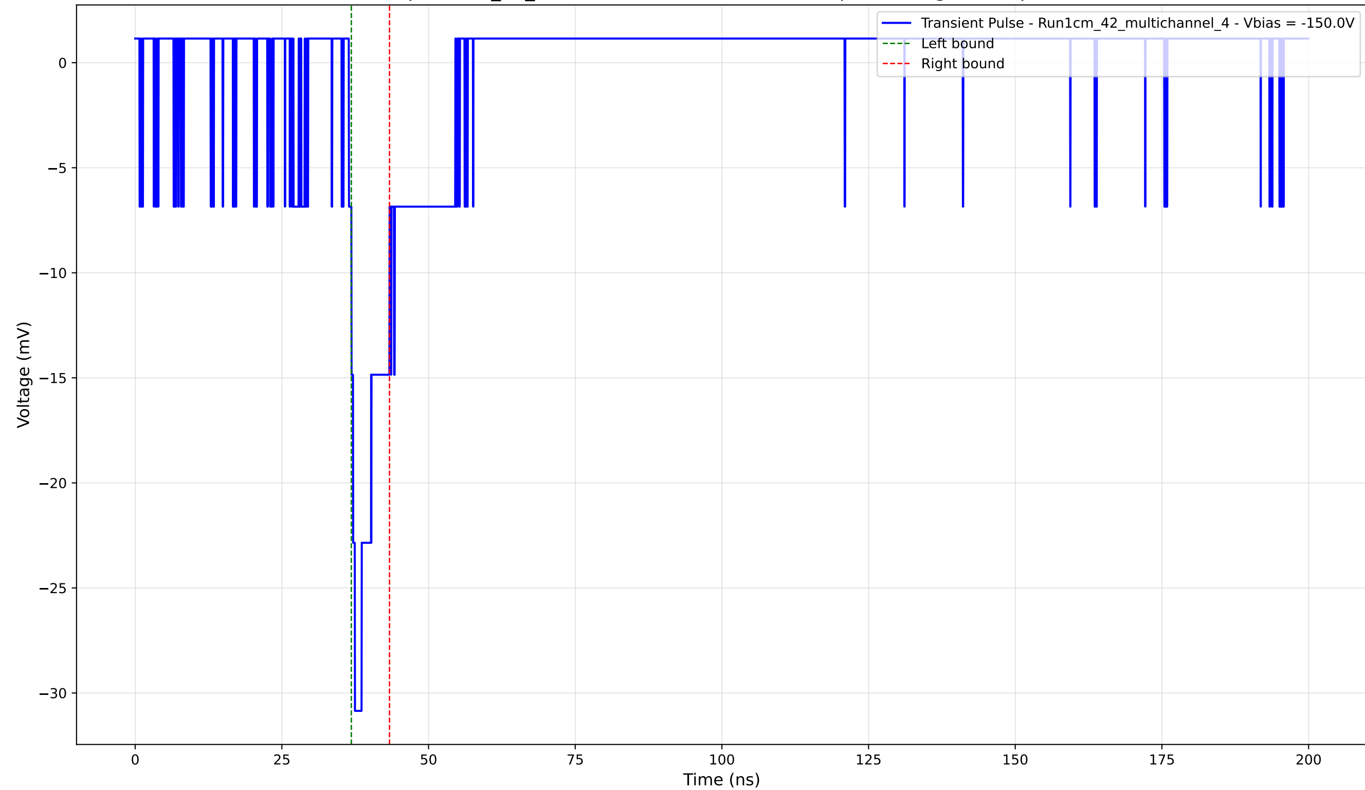
Transient Pulse - Sample: 1cm_42_multichannel - Position: 1555.0 \mu\text{m} - Charge: 2.61 pC - Rise Time: 1.03 ns
