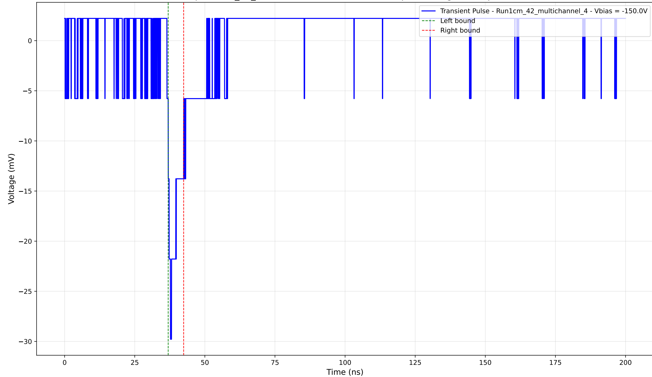
Transient Pulse - Sample: 1cm_42_multichannel - Position: 3240.0 \mu\text{m} - Charge: 1.97 pC - Rise Time: 1.28 ns
