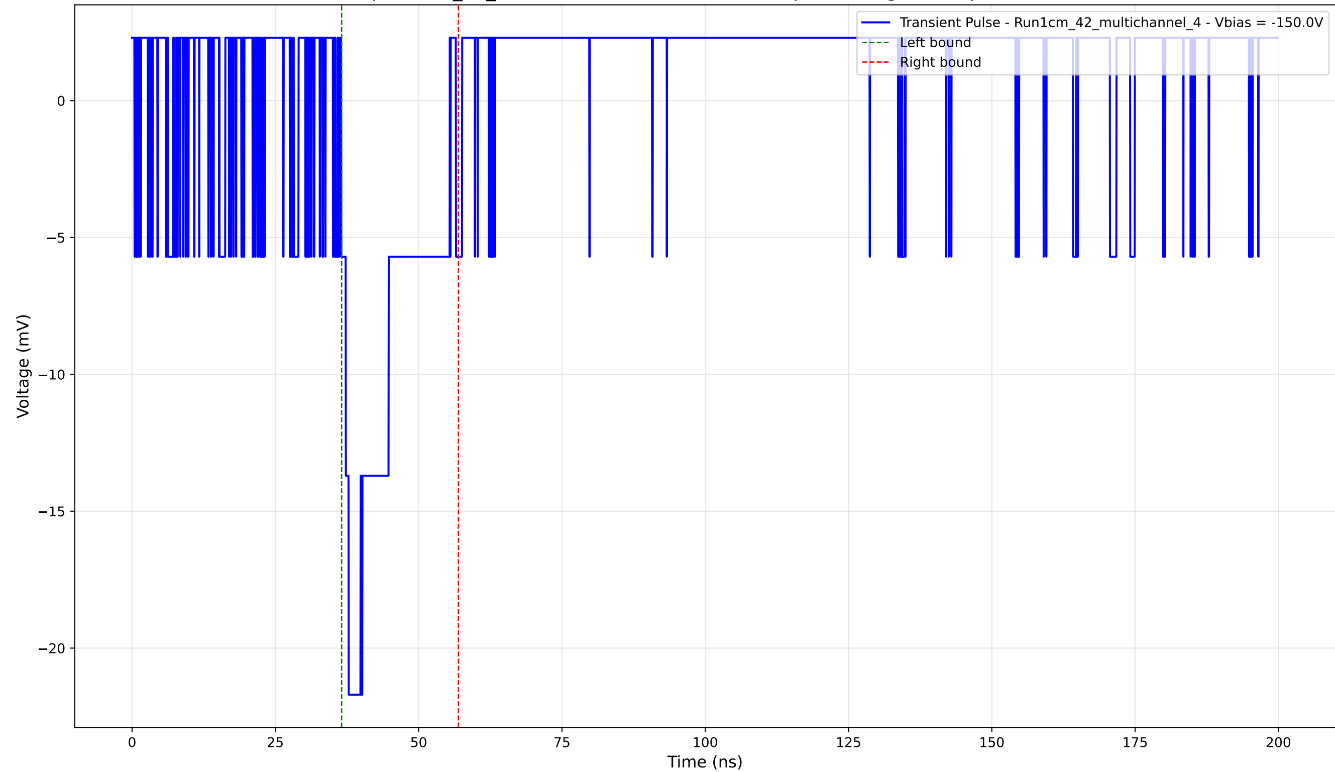
Transient Pulse - Sample: 1cm_42_multichannel - Position: 1160.0 \mu\text{m} - Charge: 3.72 pC - Rise Time: 0.00 ns (N/A)
