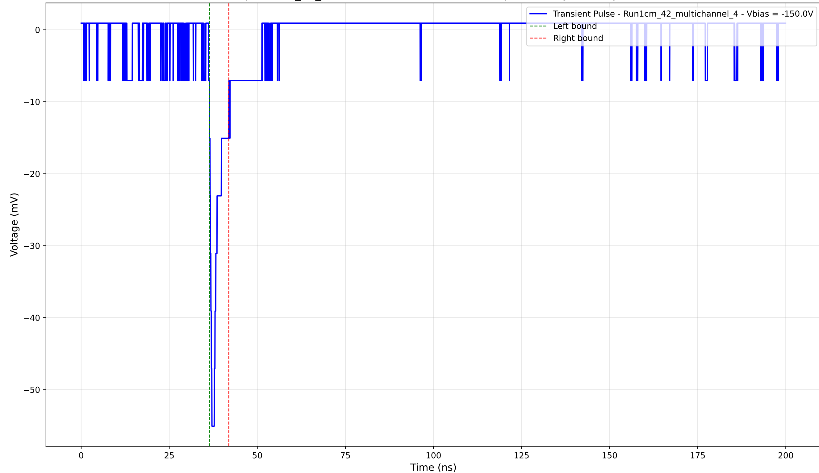
Transient Pulse - Sample: 1cm_42_multichannel - Position: 2695.0 \mu\text{m} - Charge: 2.97 pC - Rise Time: 0.93 ns
