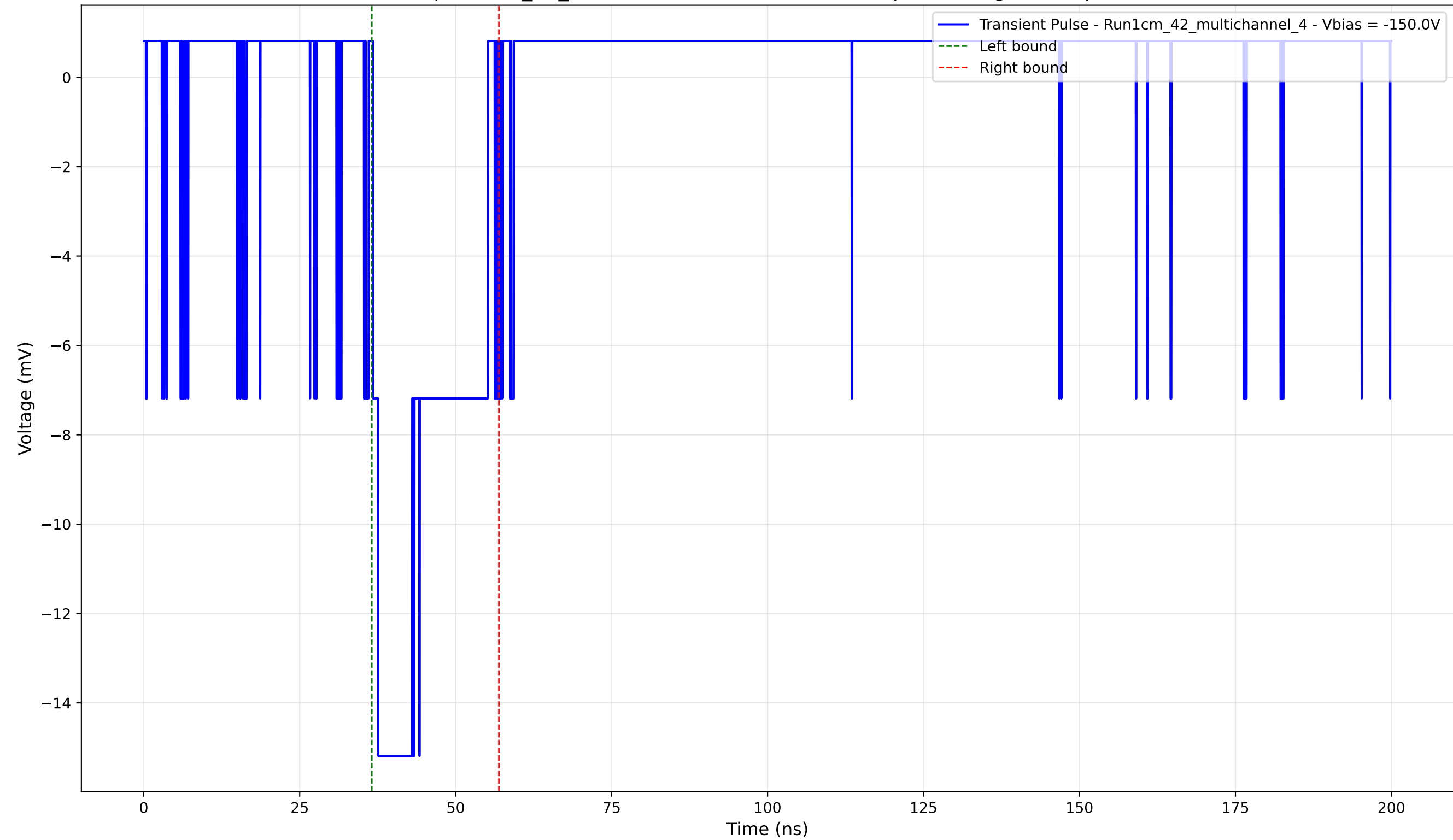
Transient Pulse - Sample: 1cm_42_multichannel - Position: 3785.0 \mu\text{m} - Charge: 3.57 pC - Rise Time: 0.84 ns
