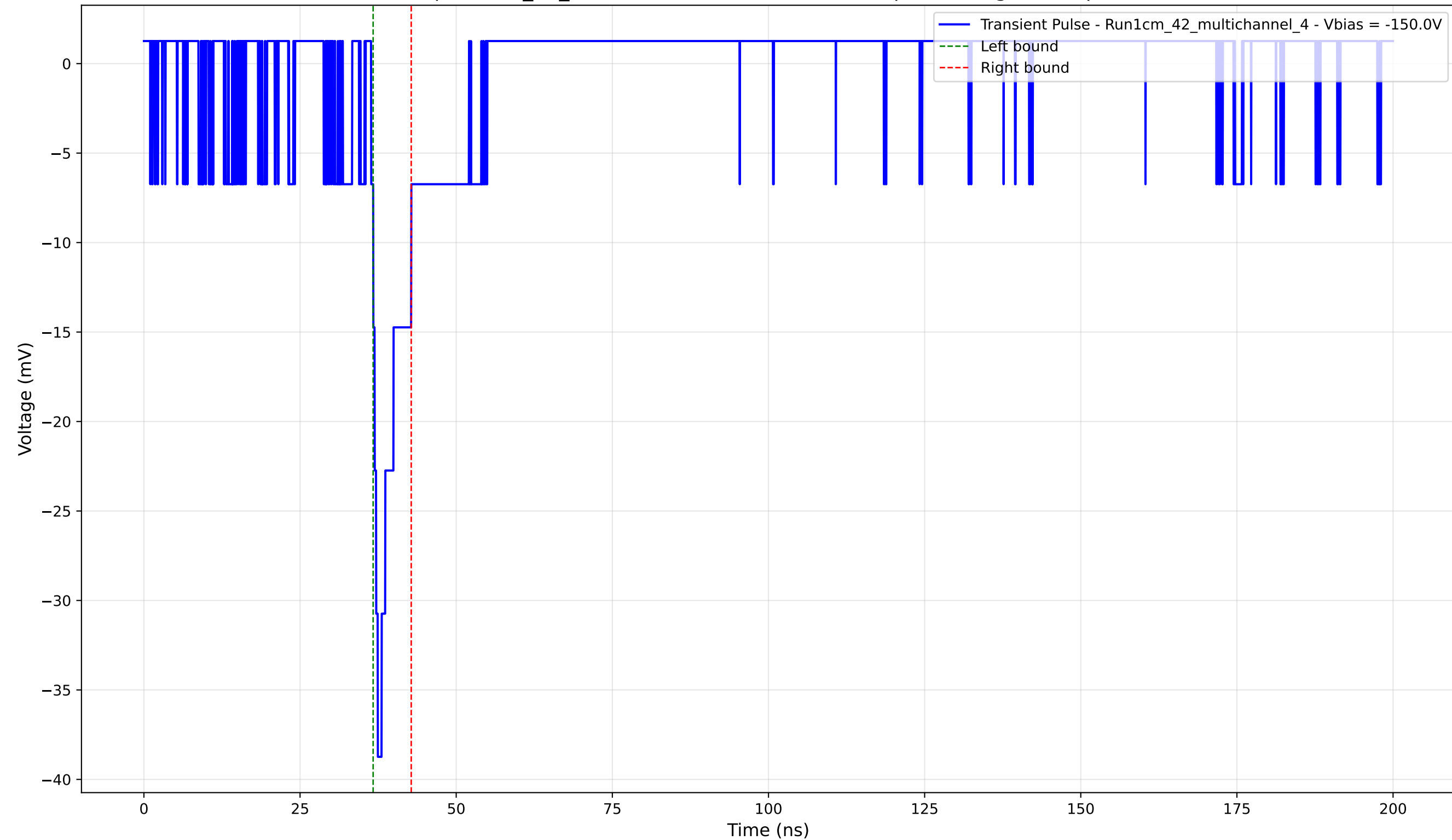
Transient Pulse - Sample: 1cm_42_multichannel - Position: 1695.0 \mu\text{m} - Charge: 2.61 pC - Rise Time: 1.07 ns
