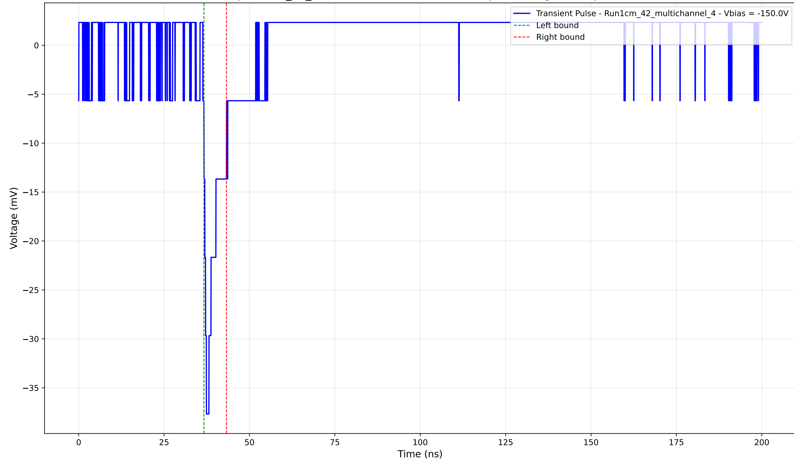
Transient Pulse - Sample: 1cm_42_multichannel - Position: 1715.0 \mu\text{m} - Charge: 2.70 pC - Rise Time: 1.05 ns
