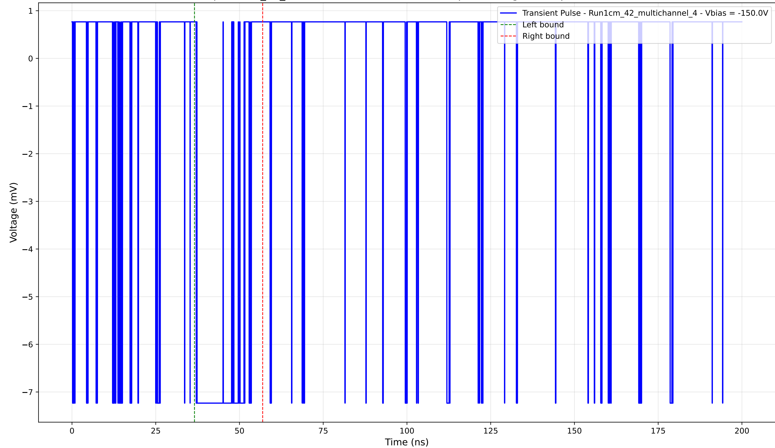
Transient Pulse - Sample: 1cm_42_multichannel - Position: 3860.0 \mu\text{m} - Charge: 1.98 pC - Rise Time: 0.00 ns (N/A)
