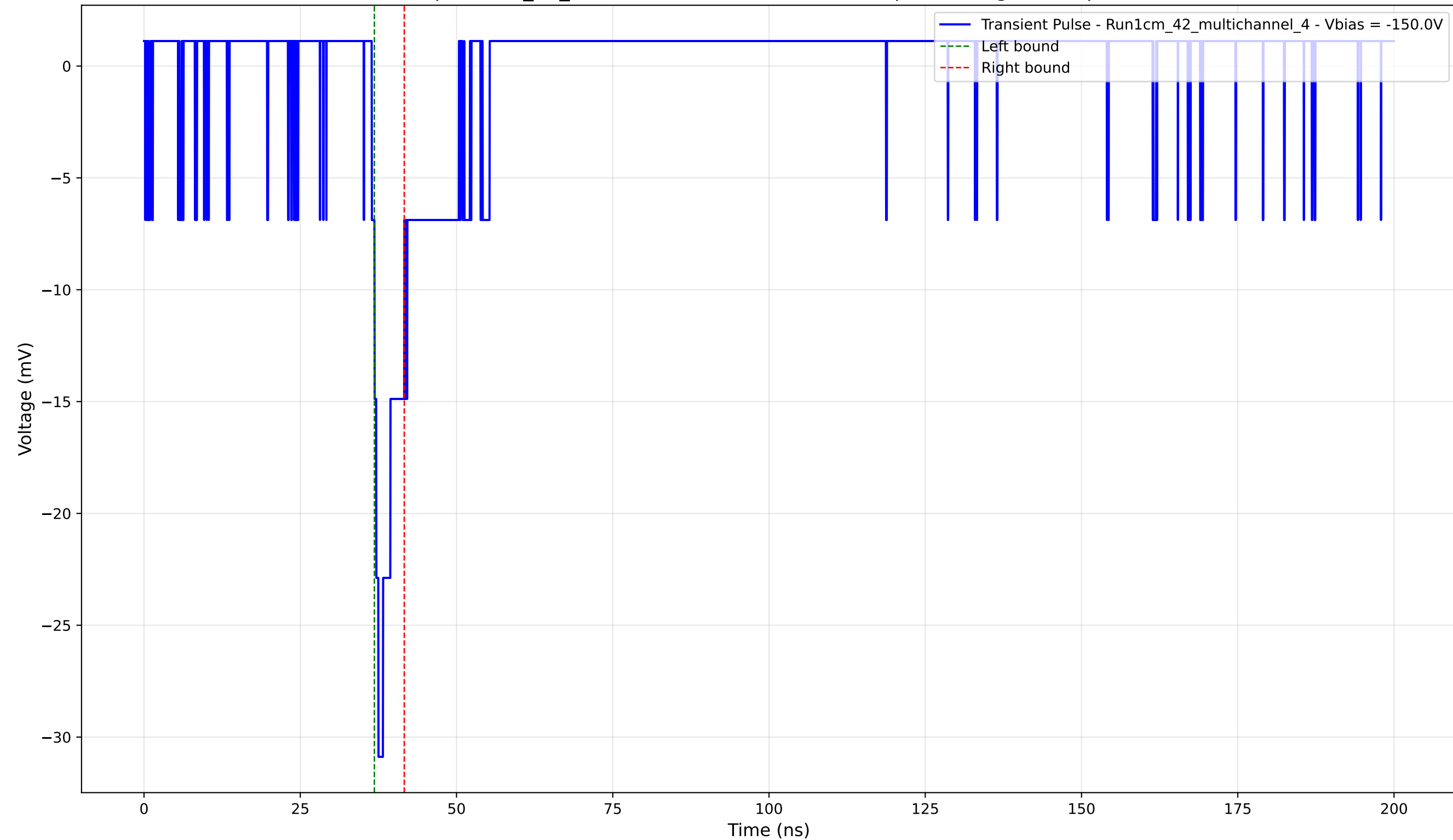
Transient Pulse - Sample: 1cm_42_multichannel - Position: 3150.0 \mu\text{m} - Charge: 1.90 pC - Rise Time: 1.07 ns
