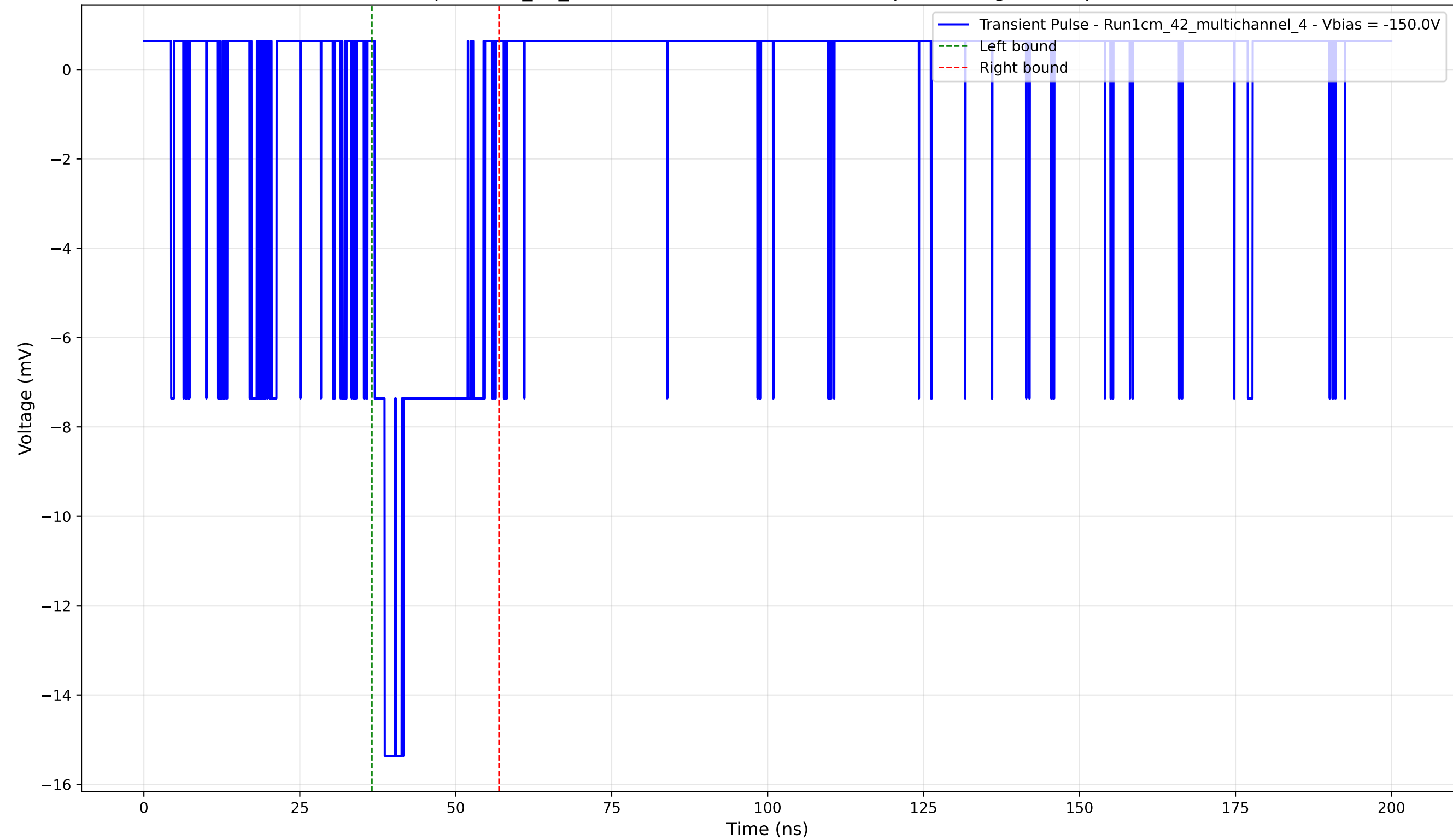
Transient Pulse - Sample: 1cm_42_multichannel - Position: 4780.0 \mu\text{m} - Charge: 3.00 pC - Rise Time: 1.62 ns
