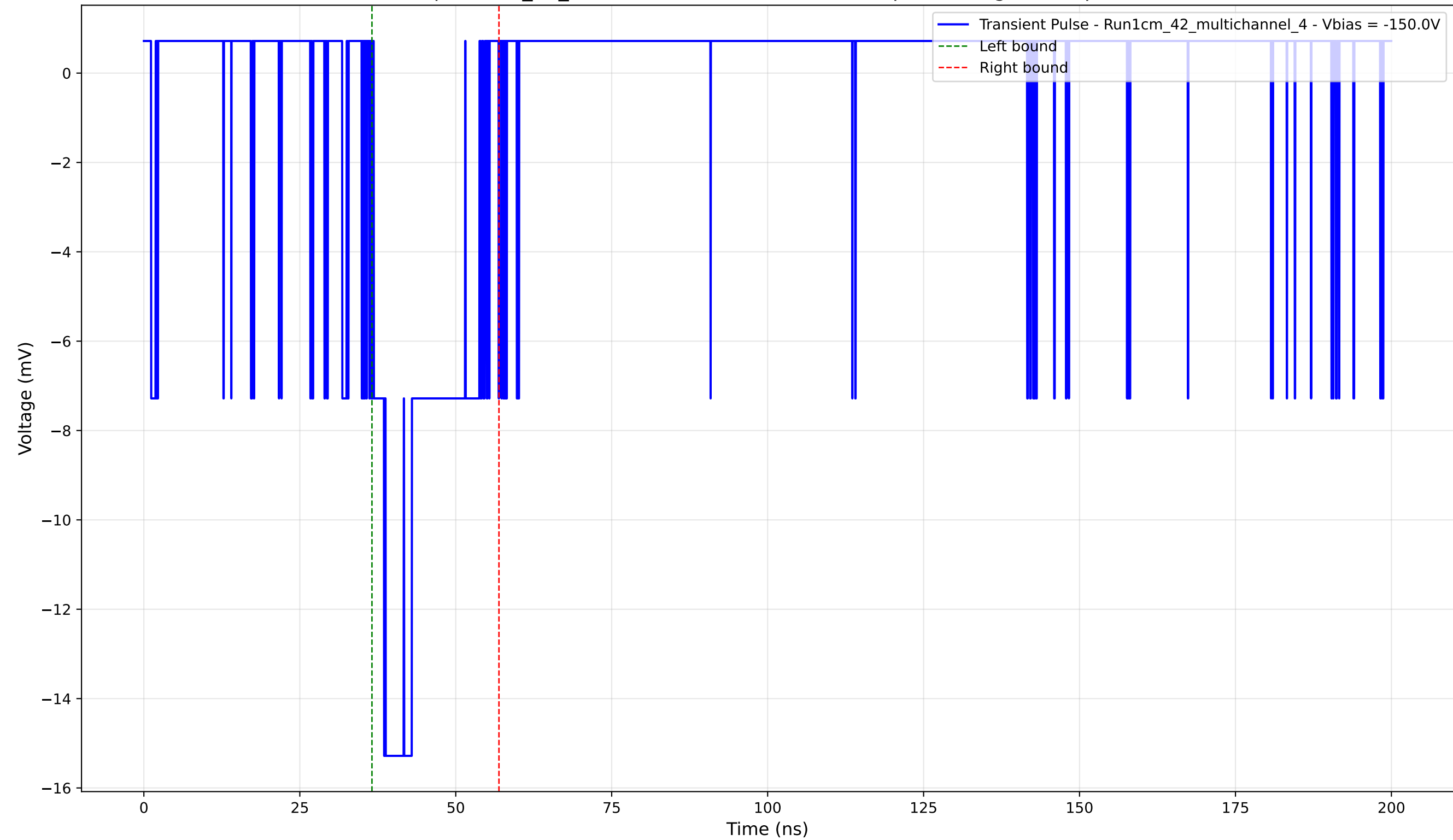
Transient Pulse - Sample: 1cm_42_multichannel - Position: 4690.0 \mu\text{m} - Charge: 3.22 pC - Rise Time: 1.66 ns
