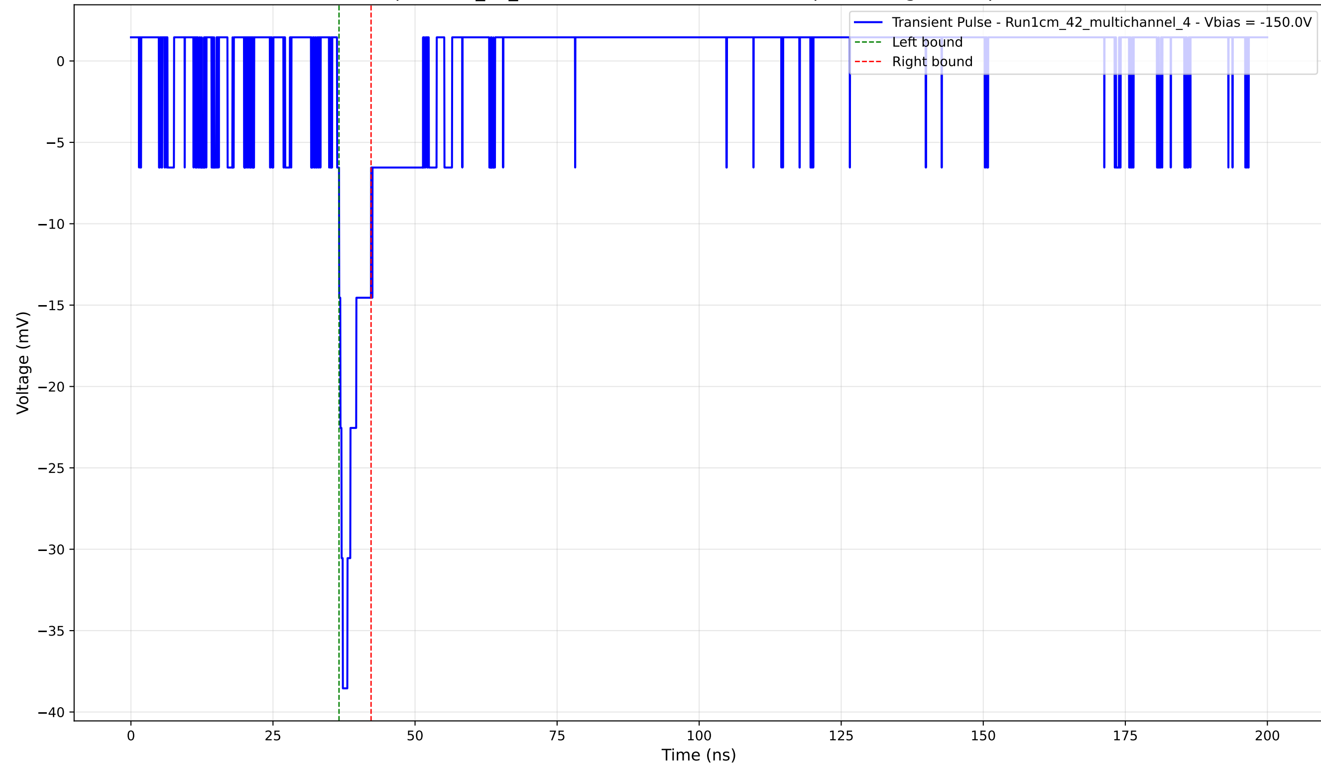
Transient Pulse - Sample: 1cm_42_multichannel - Position: 2990.0 \mu\text{m} - Charge: 2.47 pC - Rise Time: 1.01 ns
