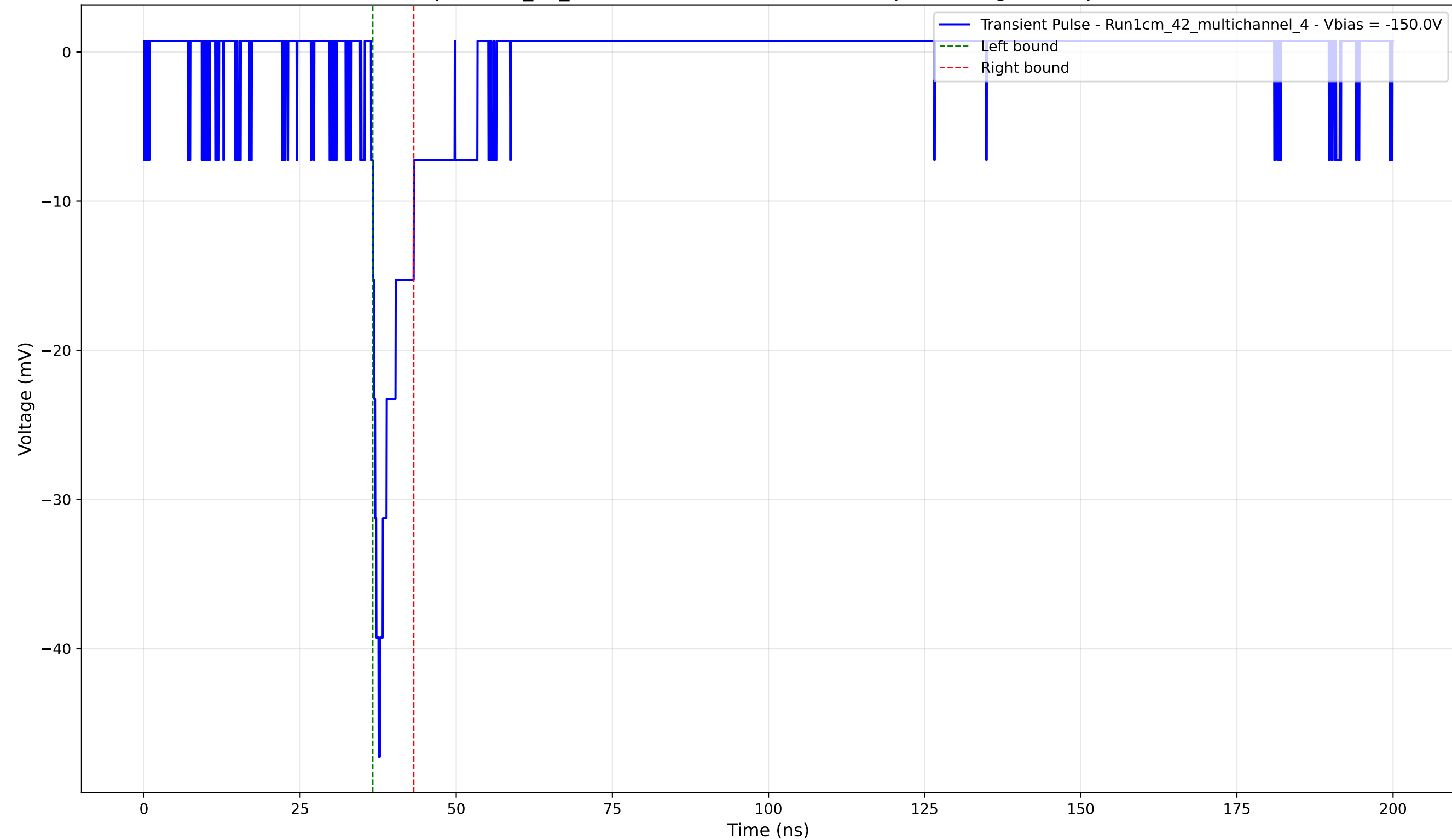
Transient Pulse - Sample: 1cm_42_multichannel - Position: 1780.0 \mu\text{m} - Charge: 3.05 pC - Rise Time: 1.23 ns
