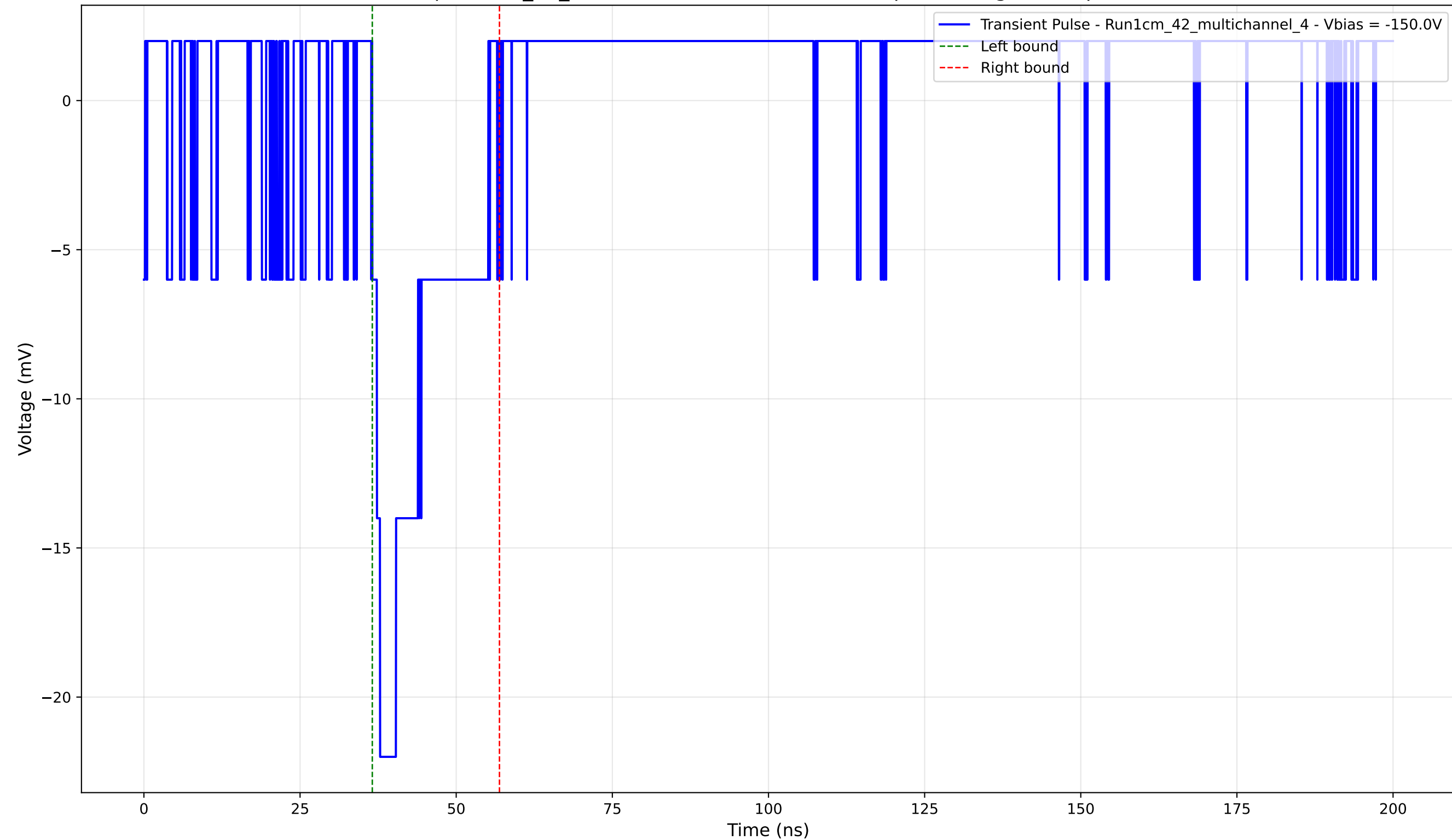
Transient Pulse - Sample: 1cm_42_multichannel - Position: 1175.0 \mu\text{m} - Charge: 3.68 pC - Rise Time: 1.26 ns
