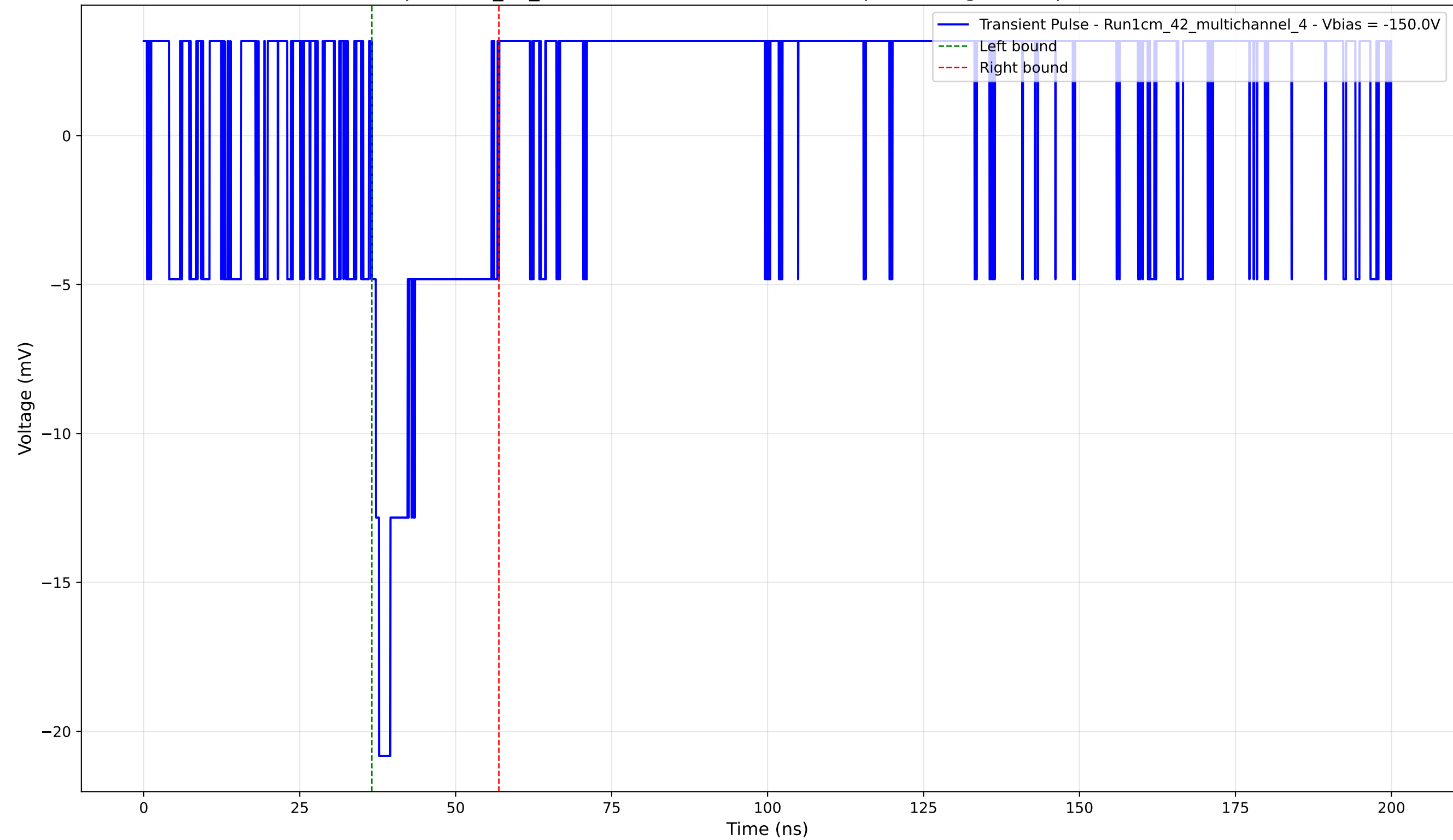
Transient Pulse - Sample: 1cm_42_multichannel - Position: 1305.0 \mu\text{m} - Charge: 3.06 pC - Rise Time: 0.00 ns (N/A)
