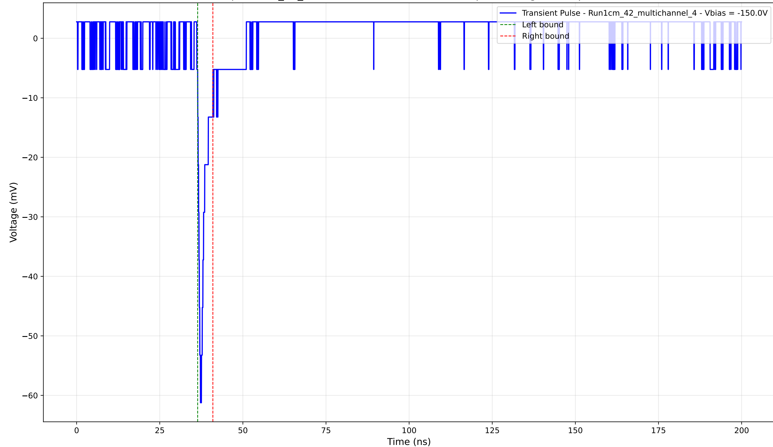
Transient Pulse - Sample: 1cm_42_multichannel - Position: 2655.0 \mu\text{m} - Charge: 2.55 pC - Rise Time: 0.84 ns
