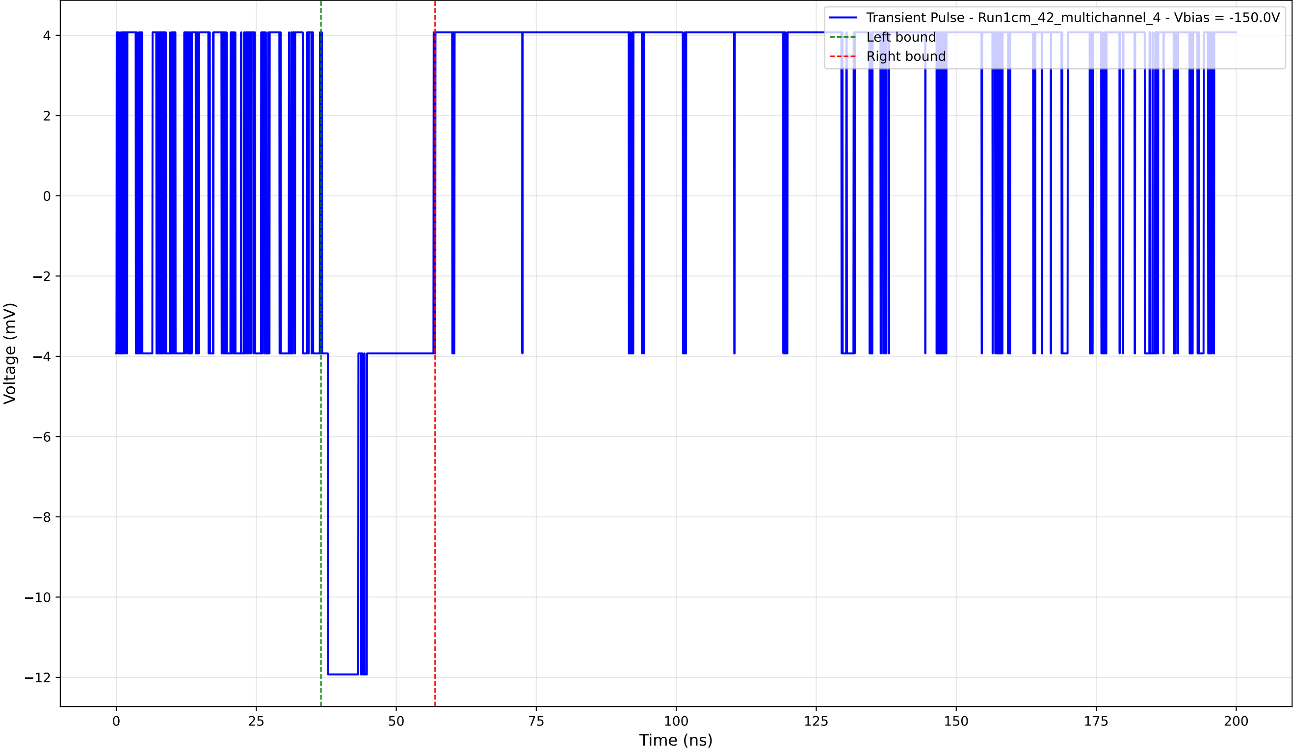
Transient Pulse - Sample: 1cm_42_multichannel - Position: 785.0 \mu\text{m} - Charge: 2.56 pC - Rise Time: 0.00 ns (N/A)
