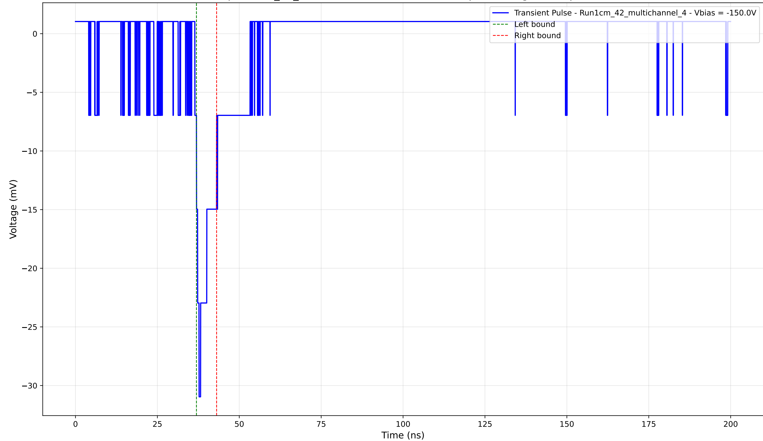
Transient Pulse - Sample: 1cm_42_multichannel - Position: 3290.0 \mu\text{m} - Charge: 2.36 pC - Rise Time: 1.29 ns
