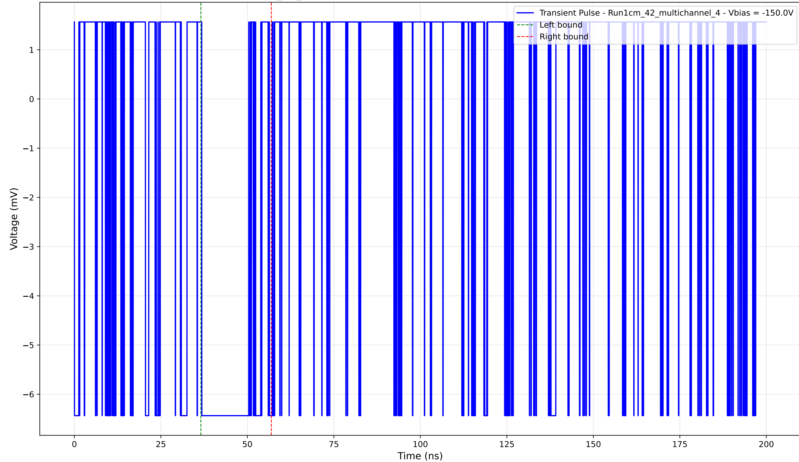
Transient Pulse - Sample: 1cm_42_multichannel - Position: 90.0 \mu\text{m} - Charge: 2.10 pC - Rise Time: 0.00 ns (N/A)
