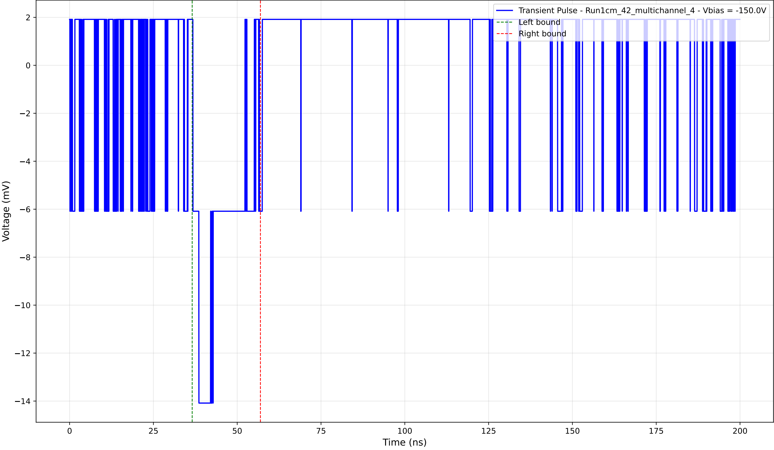
Transient Pulse - Sample: 1cm_42_multichannel - Position: 190.0 \mu\text{m} - Charge: 2.81 pC - Rise Time: 0.00 ns (N/A)
