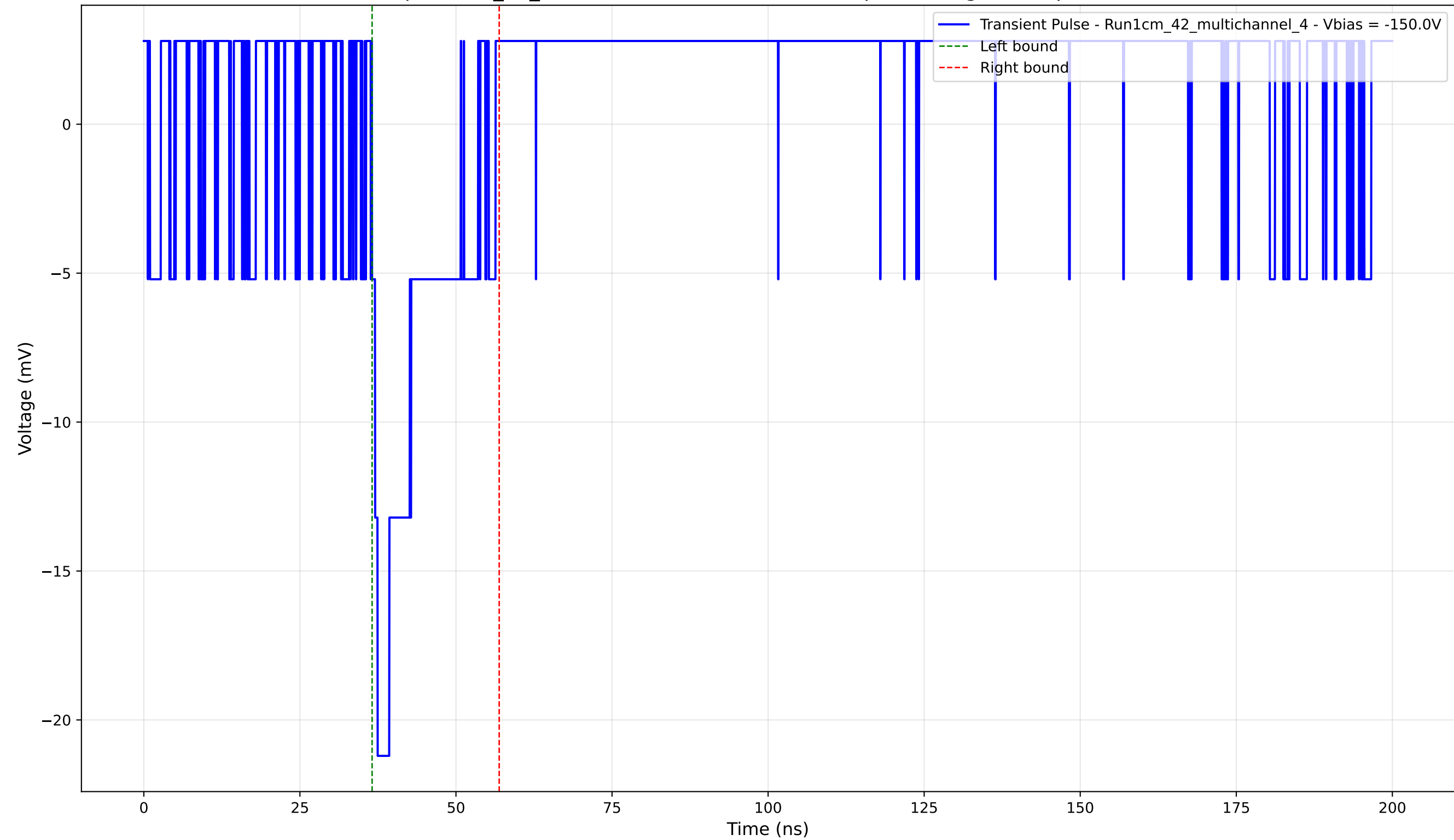
Transient Pulse - Sample: 1cm_42_multichannel - Position: 1440.0 \mu\text{m} - Charge: 2.98 pC - Rise Time: 0.00 ns (N/A)
