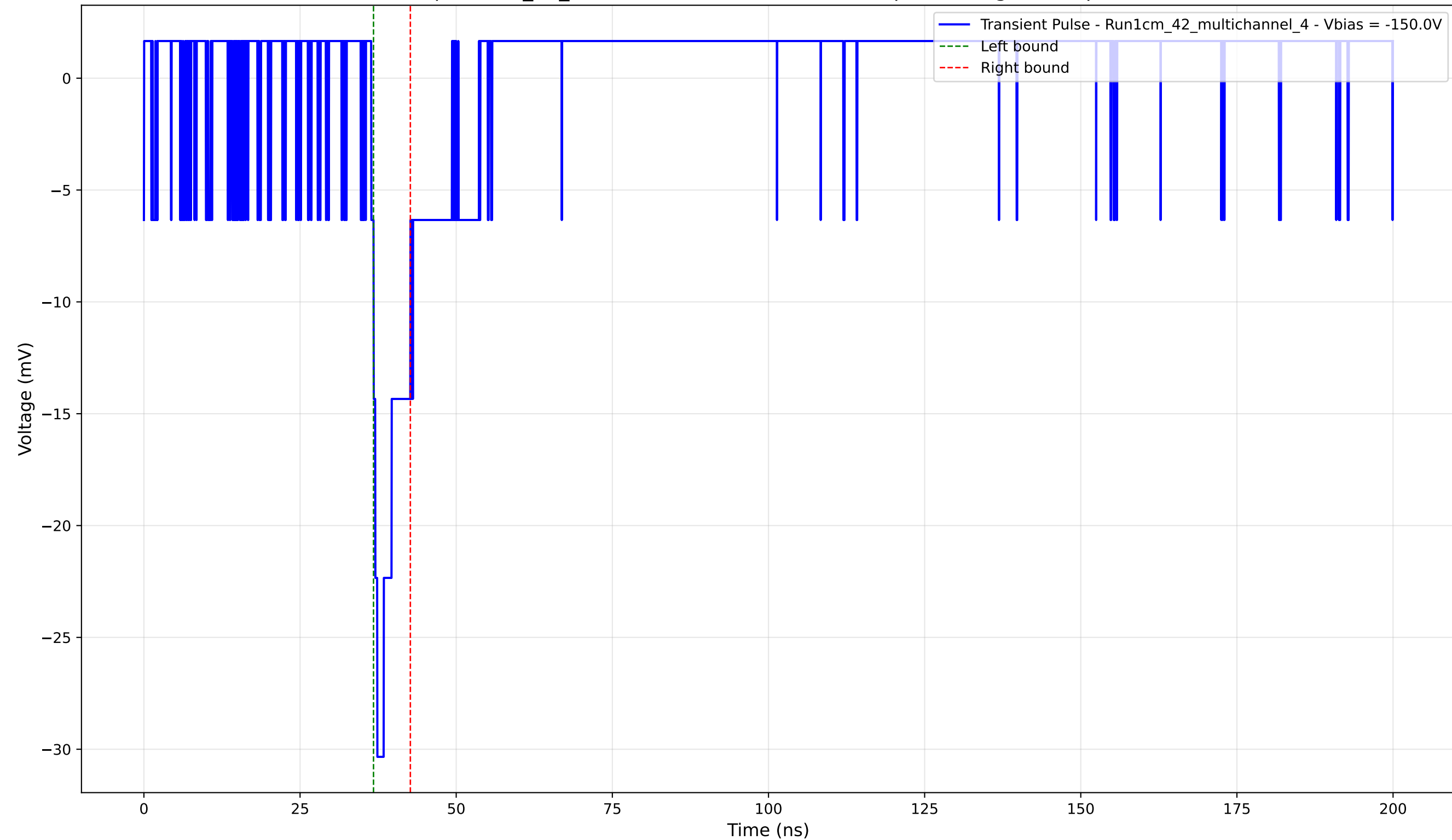
Transient Pulse - Sample: 1cm_42_multichannel - Position: 3140.0 \mu\text{m} - Charge: 2.27 pC - Rise Time: 0.97 ns
