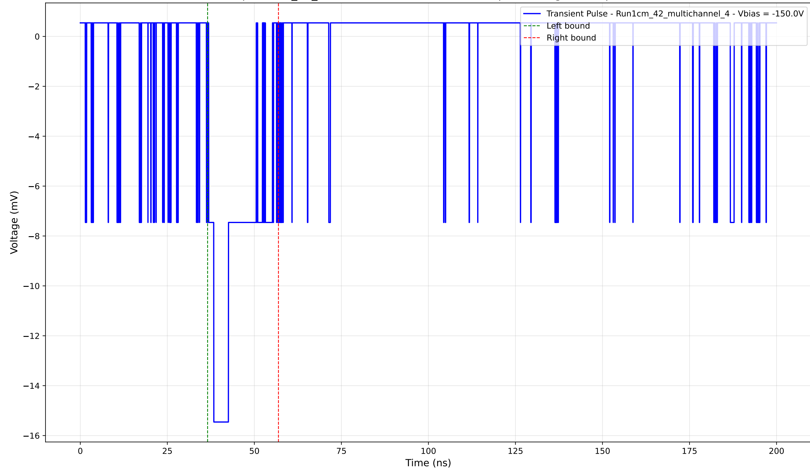
Transient Pulse - Sample: 1cm_42_multichannel - Position: 4695.0 \mu\text{m} - Charge: 3.36 pC - Rise Time: 1.48 ns
