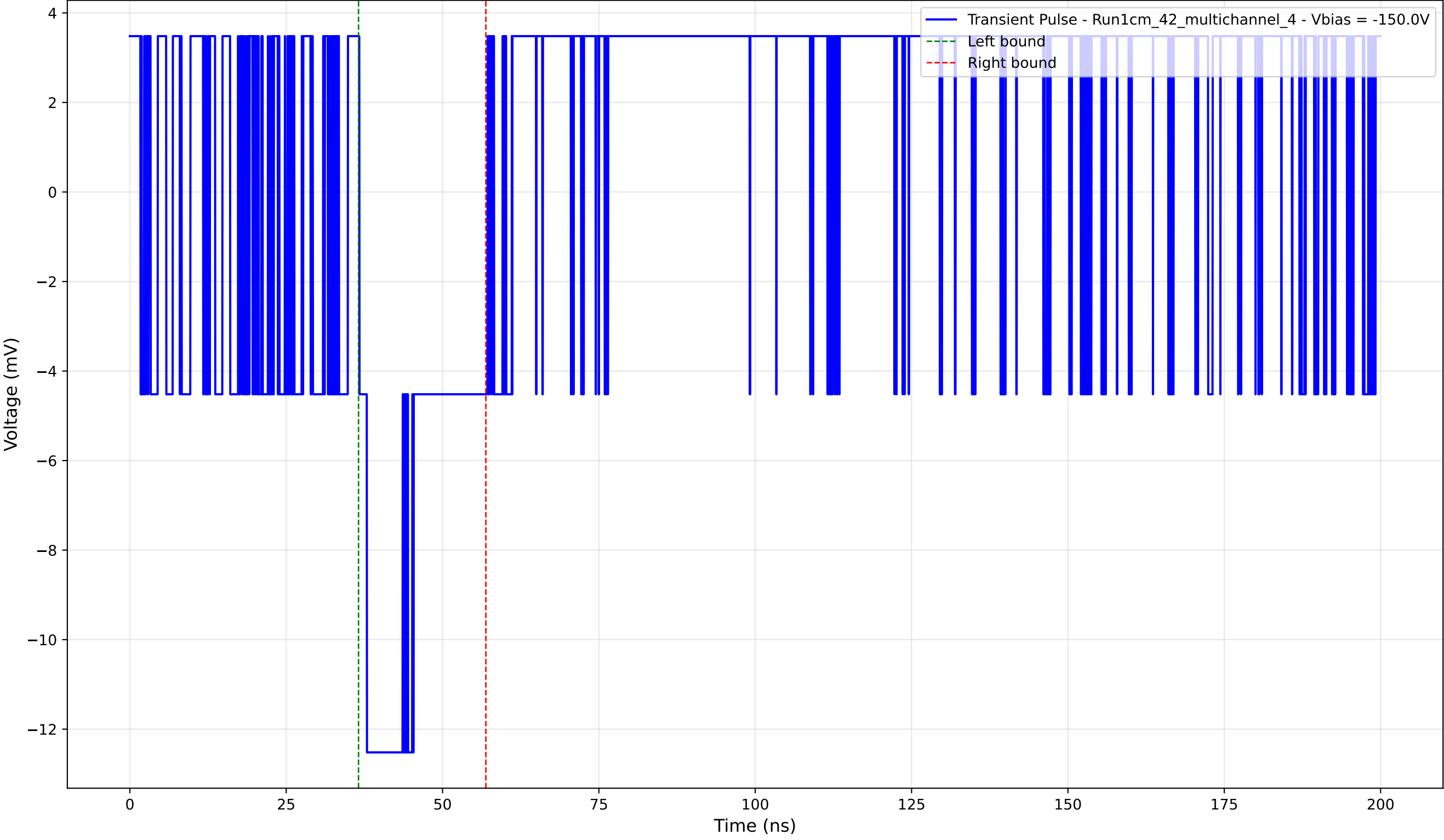
Transient Pulse - Sample: 1cm_42_multichannel - Position: 760.0 \mu\text{m} - Charge: 2.90 pC - Rise Time: 0.00 ns (N/A)
