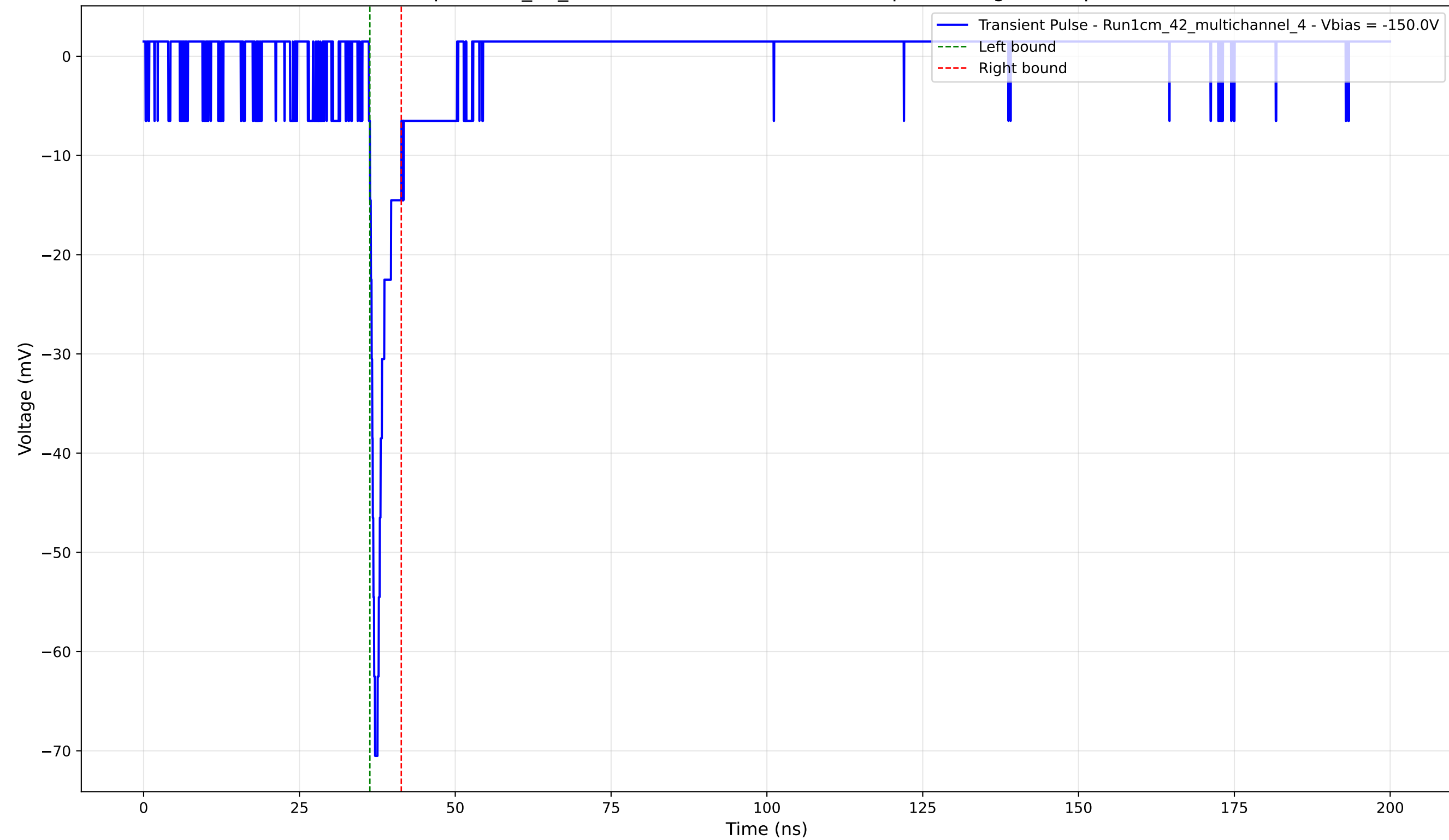
Transient Pulse - Sample: 1cm_42_multichannel - Position: 2180.0 \mu\text{m} - Charge: 3.10 pC - Rise Time: 0.82 ns
