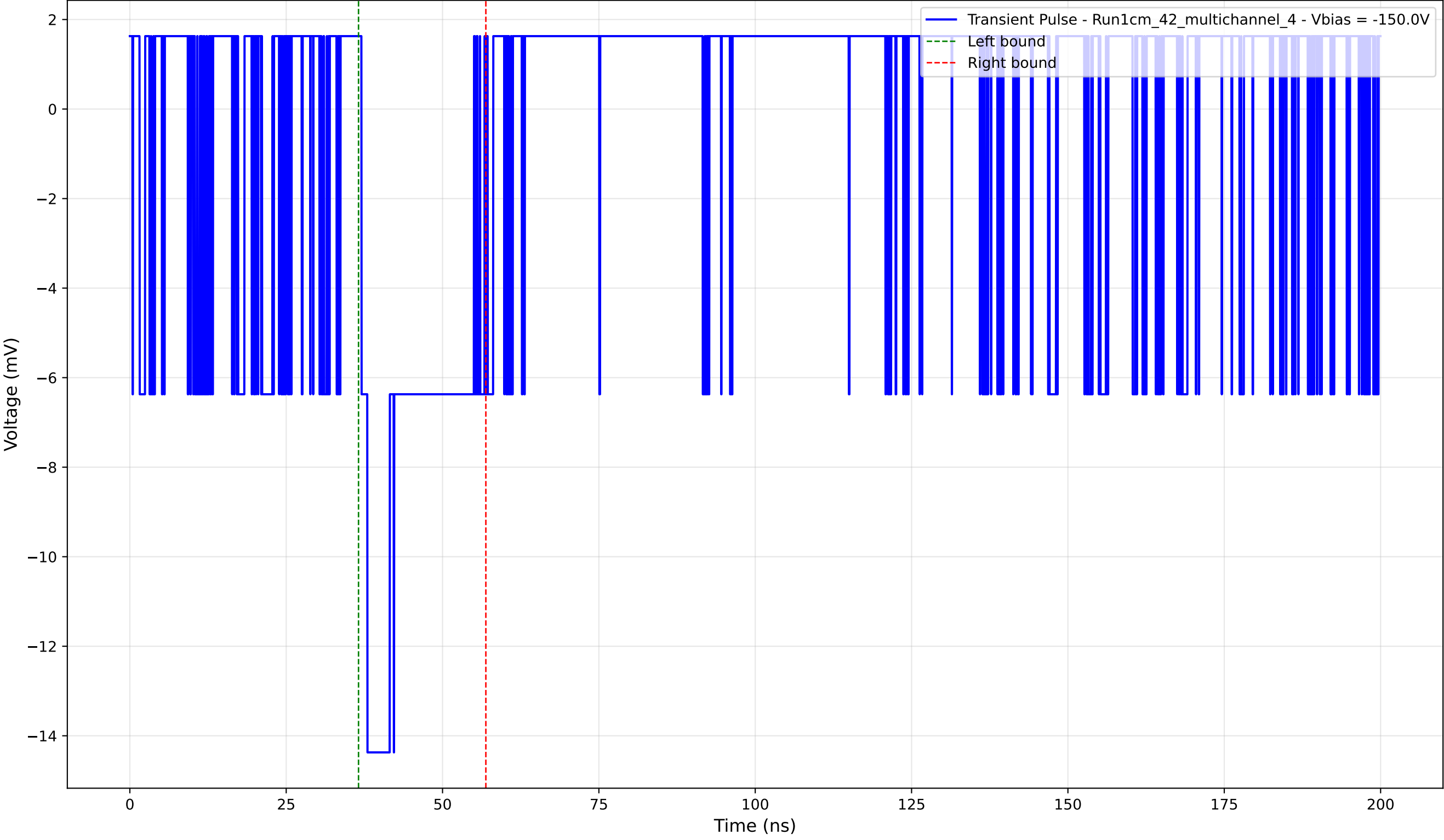
Transient Pulse - Sample: 1cm_42_multichannel - Position: 925.0 \mu\text{m} - Charge: 3.03 pC - Rise Time: 0.00 ns (N/A)
