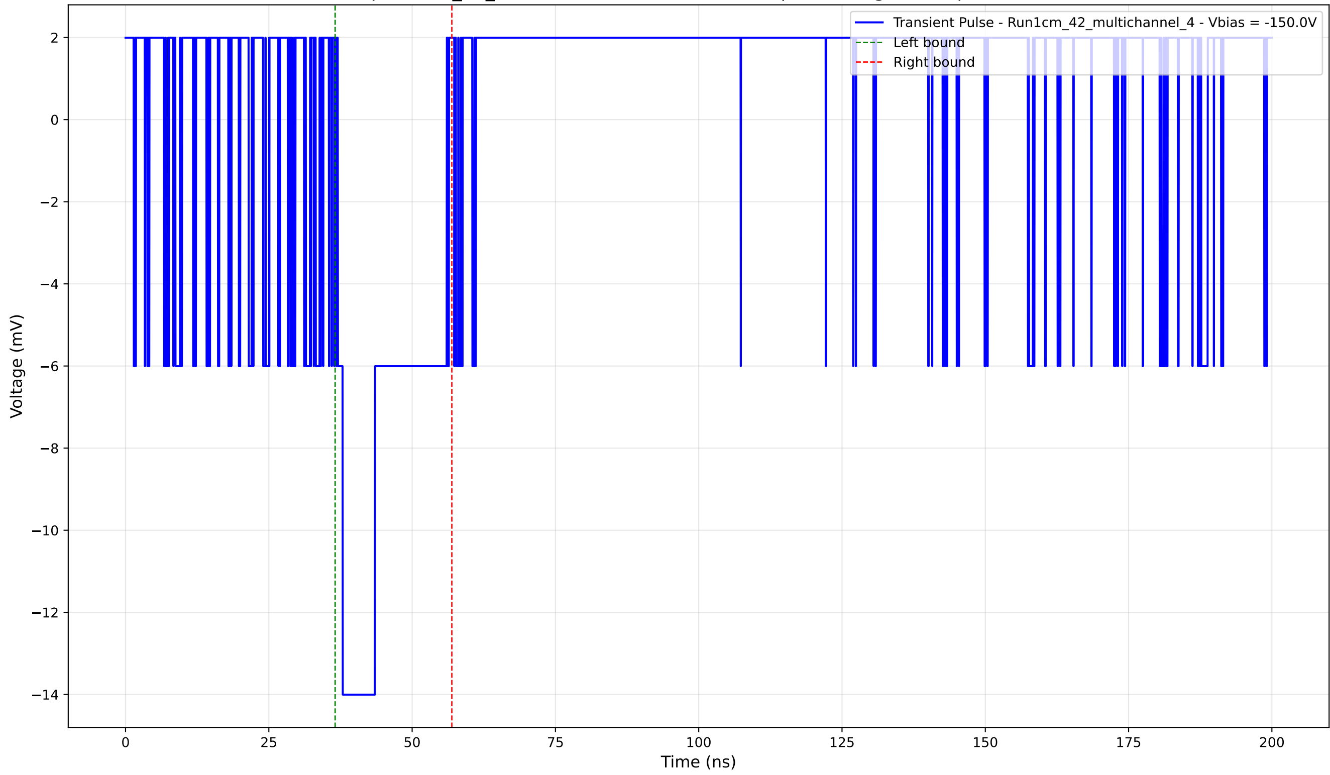
Transient Pulse - Sample: 1cm_42_multichannel - Position: 645.0 \mu\text{m} - Charge: 3.18 pC - Rise Time: 0.00 ns (N/A)
