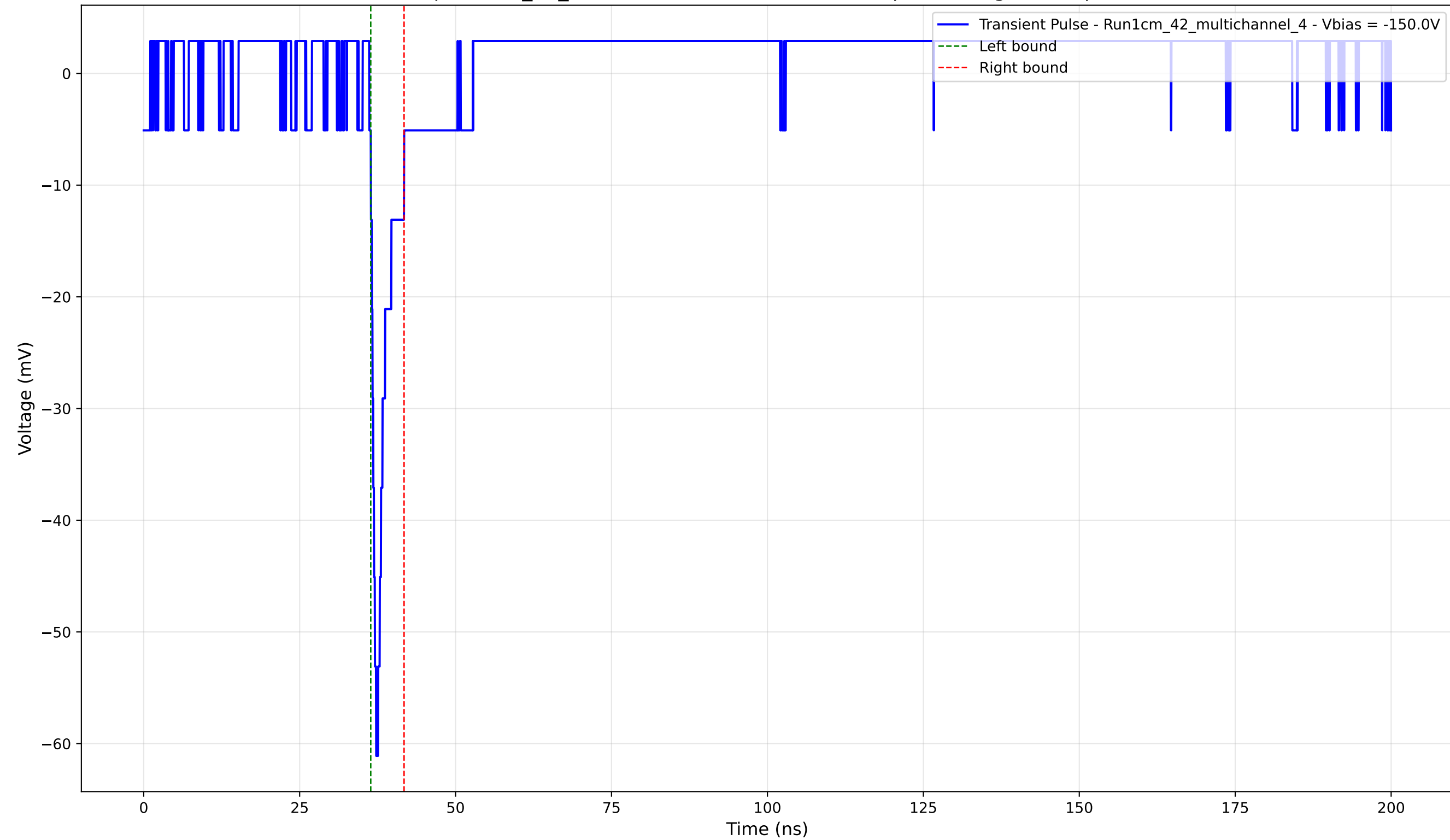
Transient Pulse - Sample: 1cm_42_multichannel - Position: 2085.0 \mu\text{m} - Charge: 2.81 pC - Rise Time: 0.86 ns
