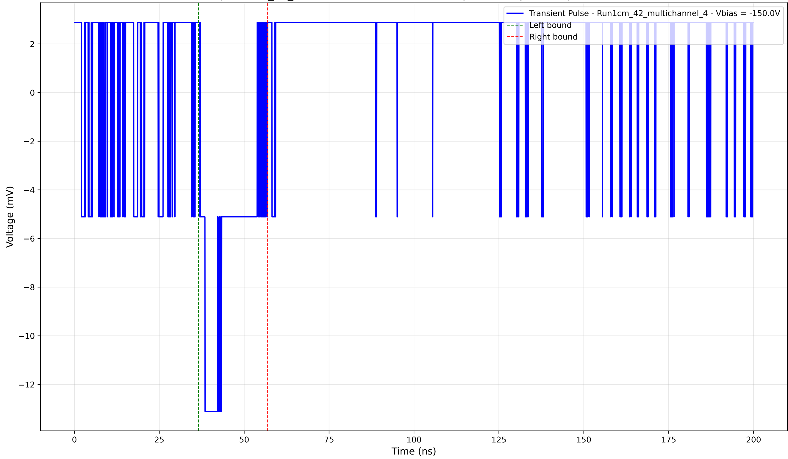
Transient Pulse - Sample: 1cm_42_multichannel - Position: 235.0 \mu\text{m} - Charge: 2.45 pC - Rise Time: 0.00 ns (N/A)
