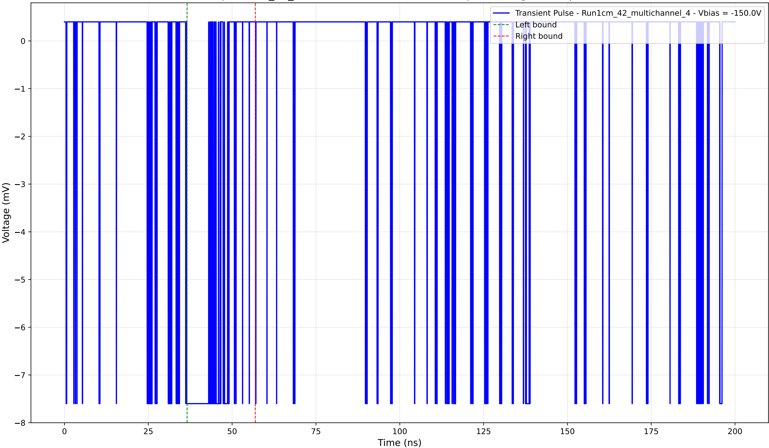
Transient Pulse - Sample: 1cm_42_multichannel - Position: 2930.0 \mu\text{m} - Charge: 1.59 pC - Rise Time: 0.02 ns
