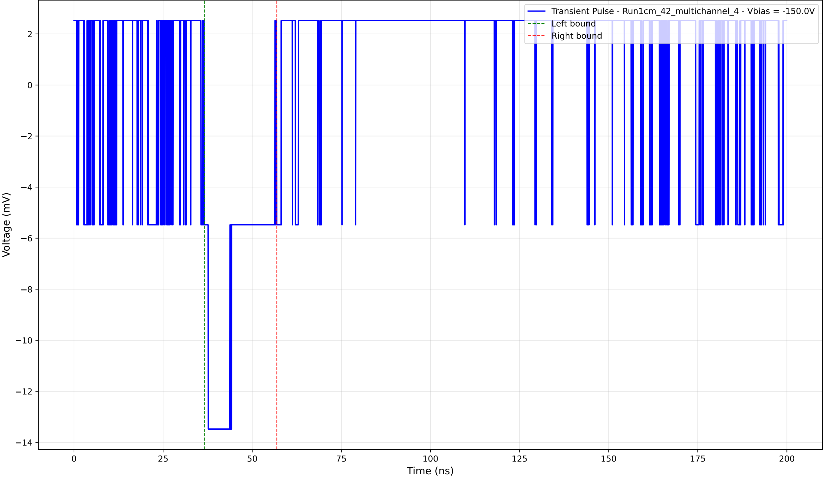
Transient Pulse - Sample: 1cm_42_multichannel - Position: 940.0 \mu\text{m} - Charge: 3.20 pC - Rise Time: 0.00 ns (N/A)
