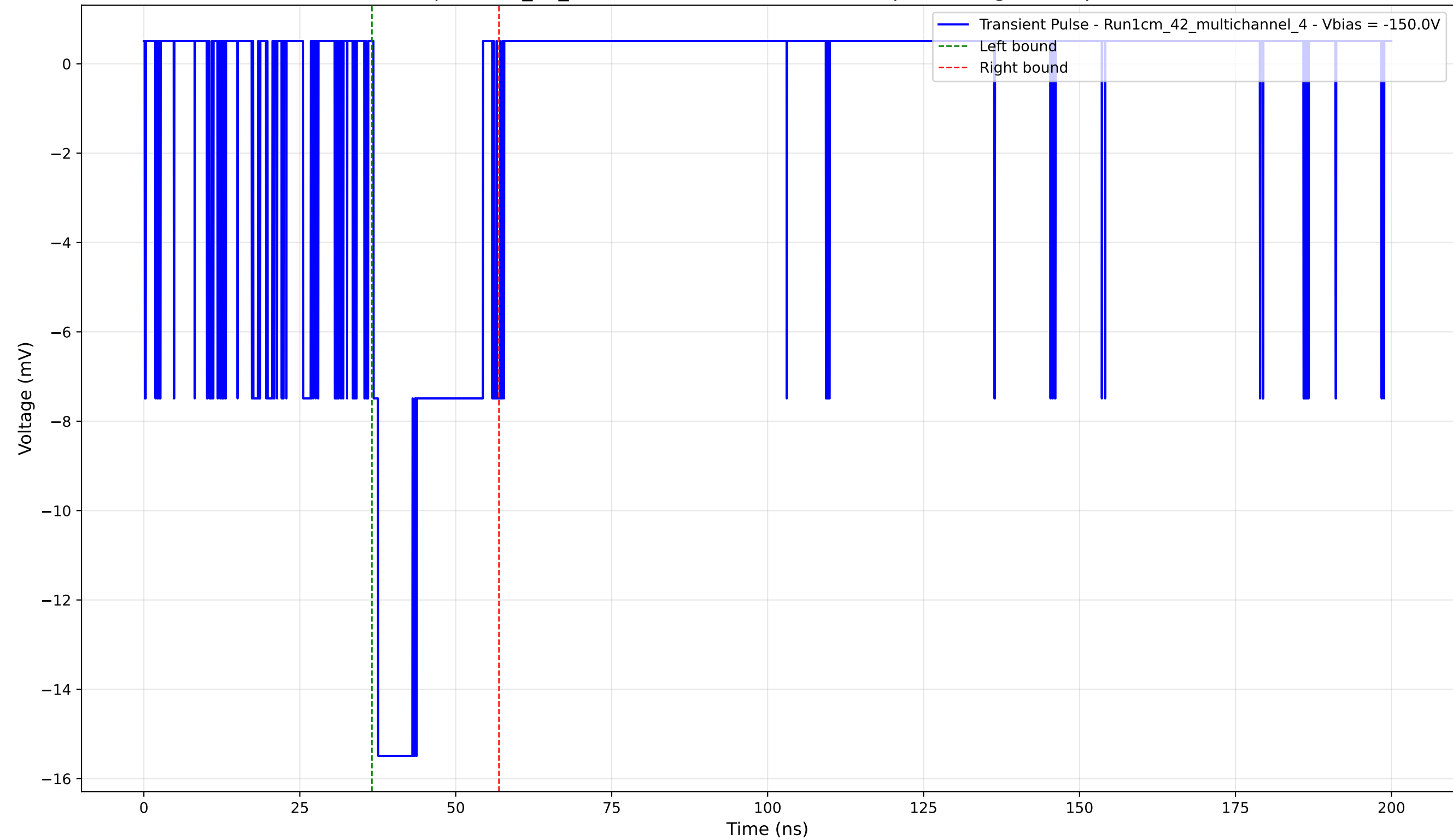
Transient Pulse - Sample: 1cm_42_multichannel - Position: 3755.0 \mu\text{m} - Charge: 3.68 pC - Rise Time: 0.74 ns
