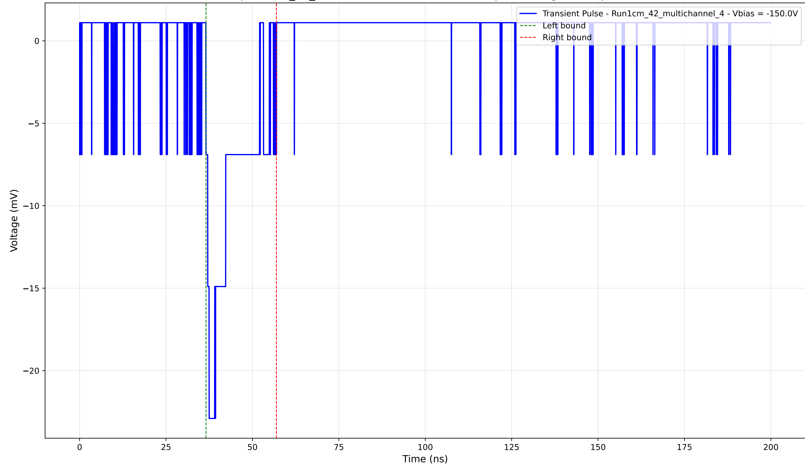
Transient Pulse - Sample: 1cm_42_multichannel - Position: 3325.0 \mu\text{m} - Charge: 3.51 pC - Rise Time: 0.94 ns
