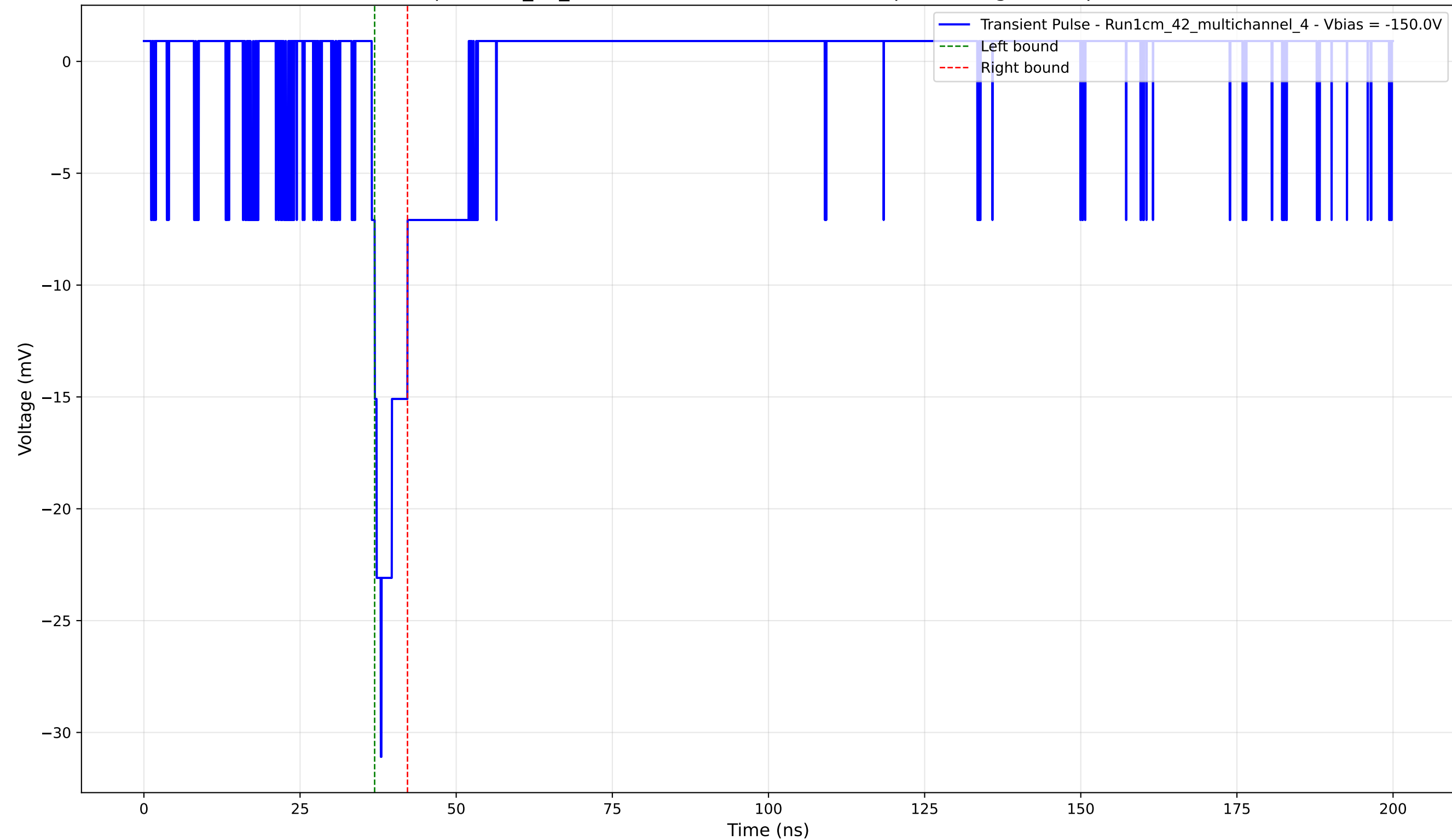
Transient Pulse - Sample: 1cm_42_multichannel - Position: 3260.0 \mu\text{m} - Charge: 1.99 pC - Rise Time: 1.45 ns
