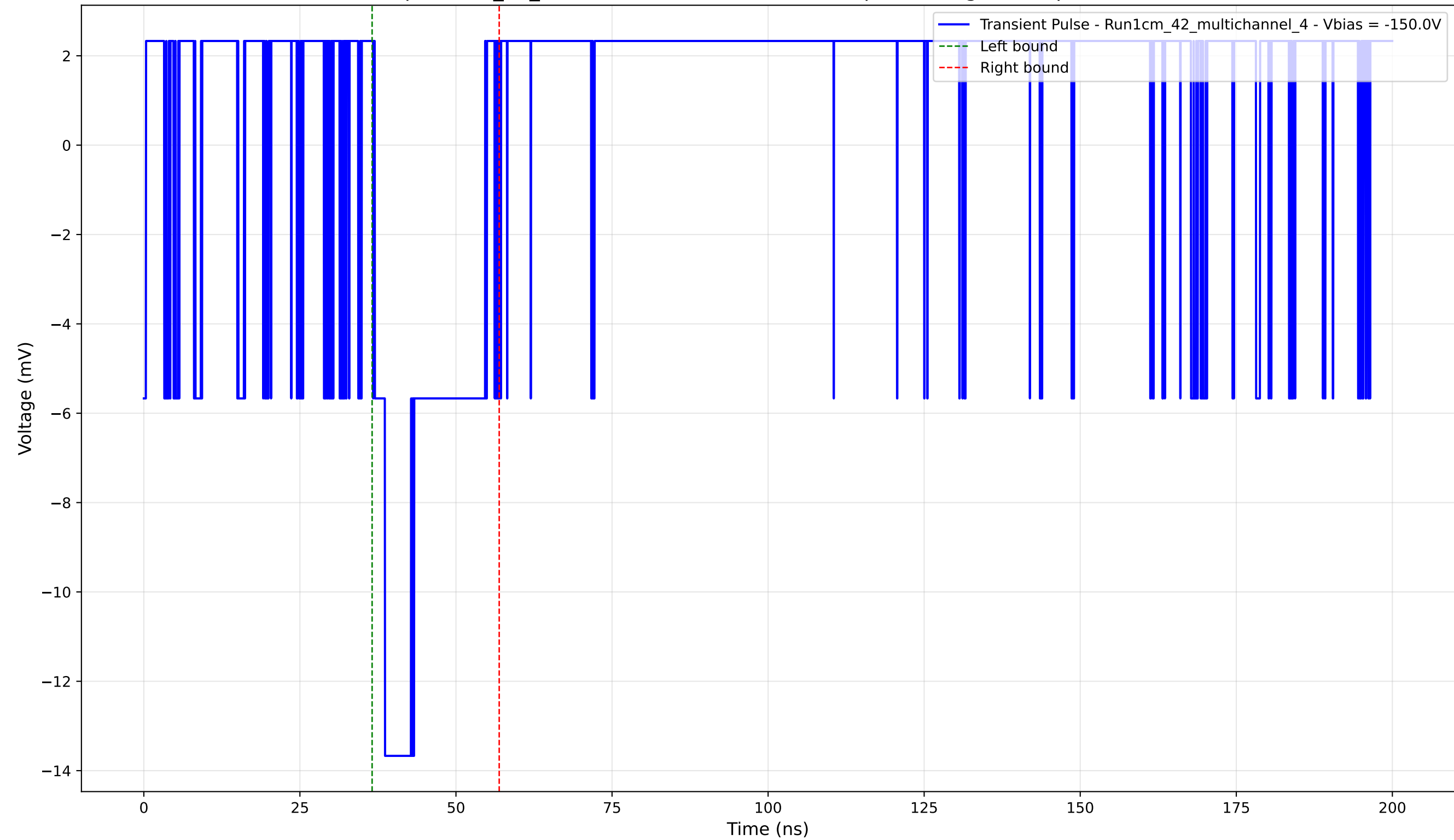
Transient Pulse - Sample: 1cm_42_multichannel - Position: 4510.0 \mu\text{m} - Charge: 2.70 pC - Rise Time: 0.00 ns (N/A)
