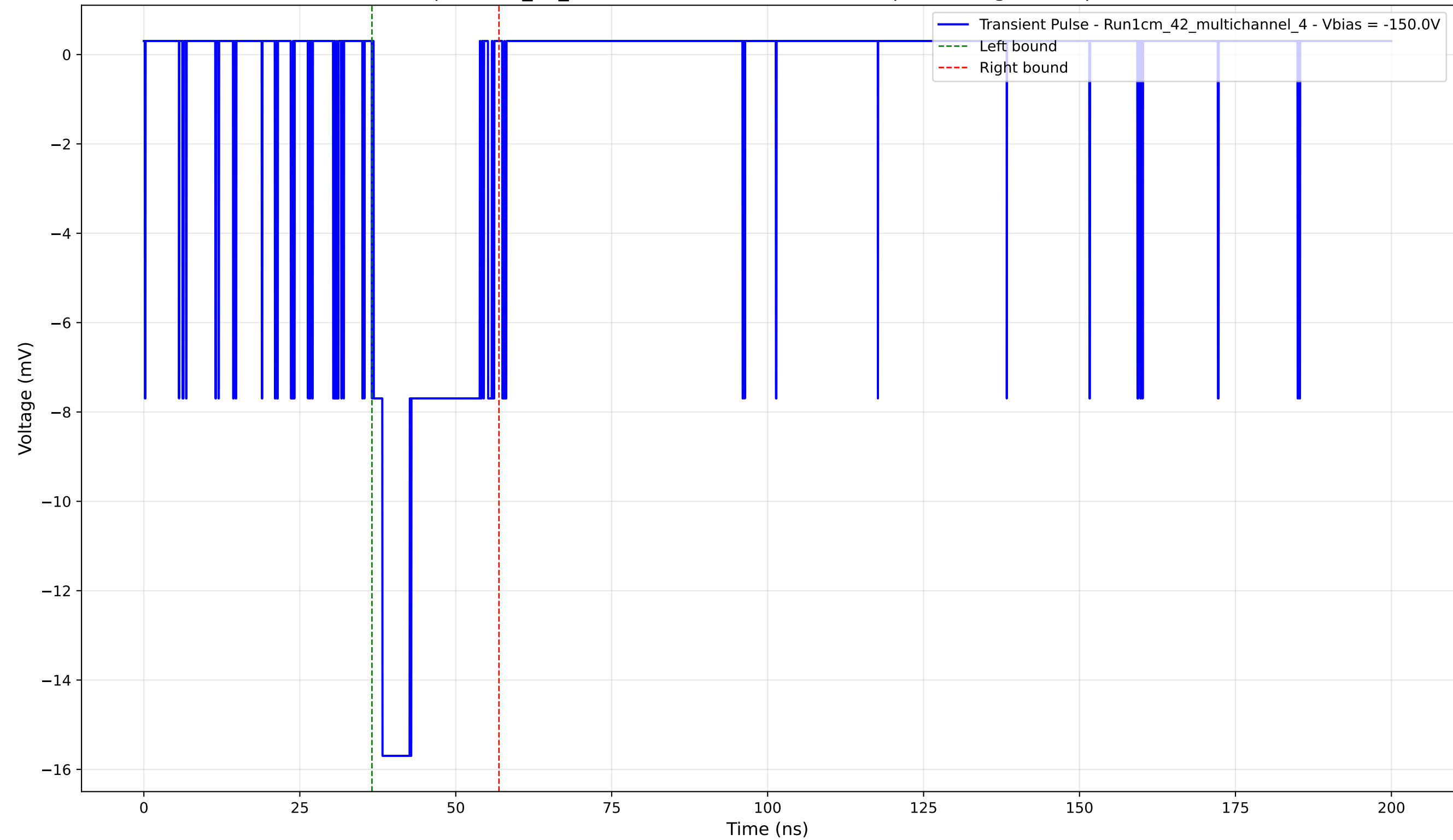
Transient Pulse - Sample: 1cm_42_multichannel - Position: 4150.0 \mu\text{m} - Charge: 3.50 pC - Rise Time: 1.42 ns
