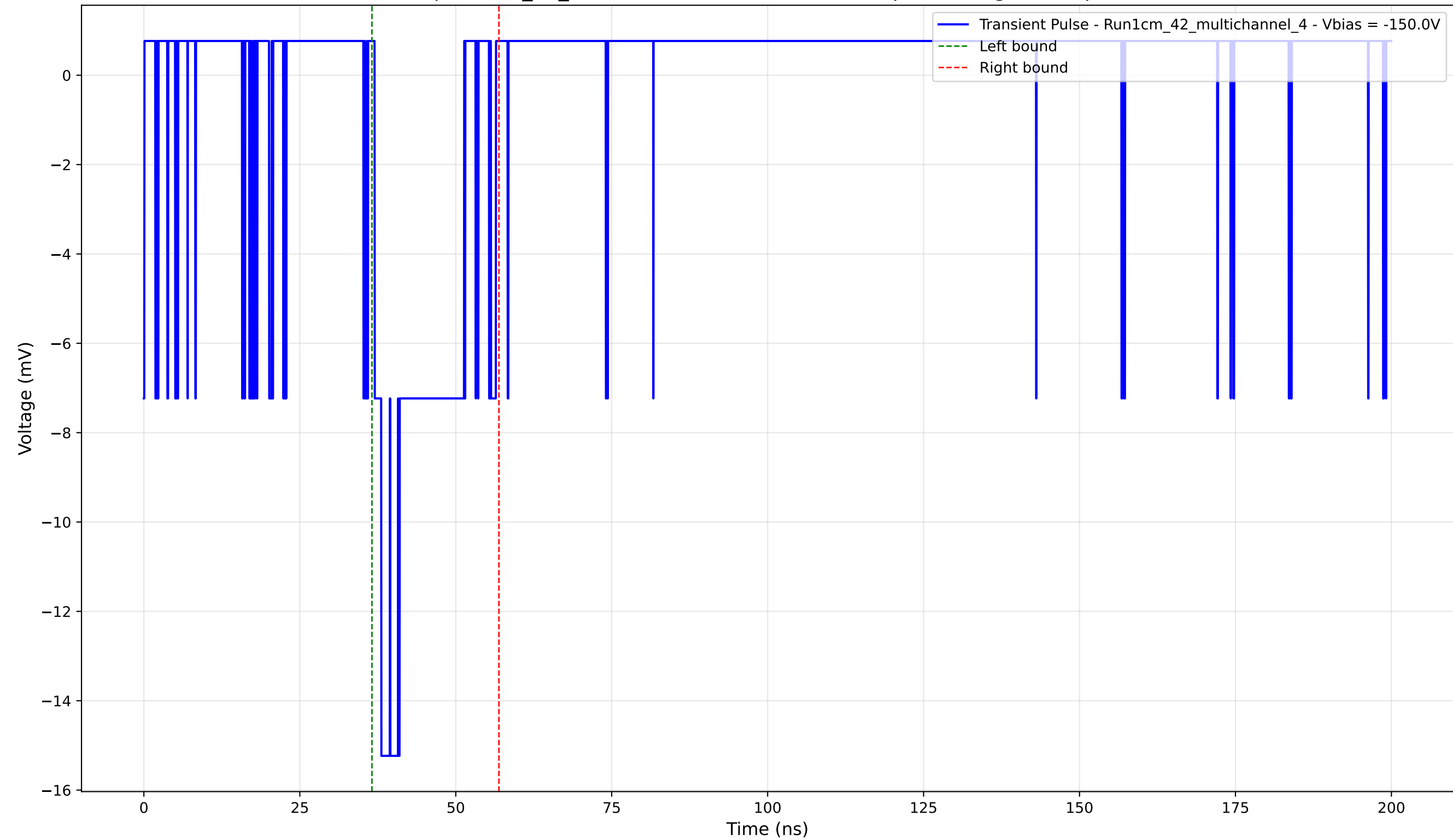
Transient Pulse - Sample: 1cm_42_multichannel - Position: 3845.0 \mu\text{m} - Charge: 2.63 pC - Rise Time: 1.08 ns
