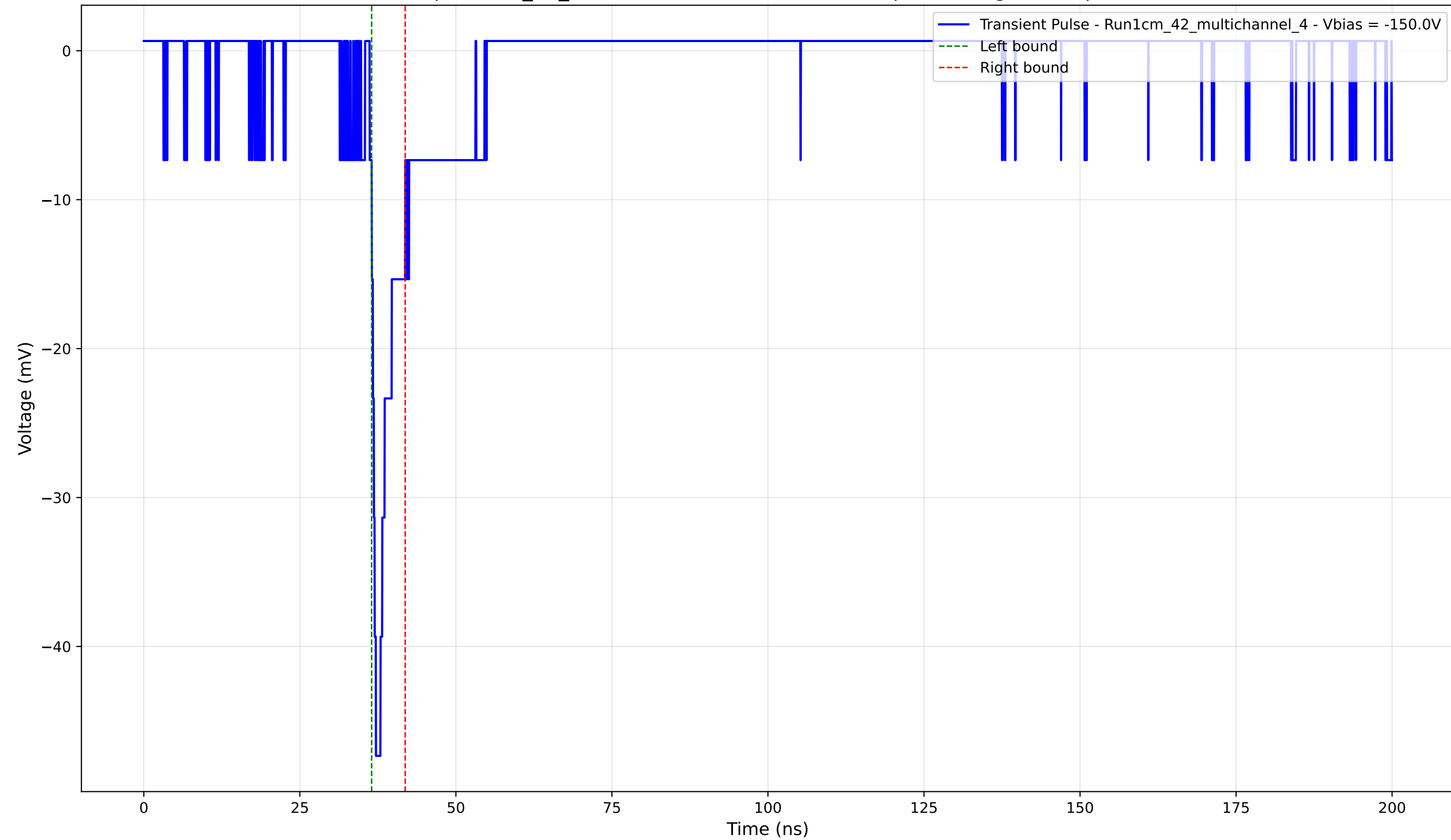
Transient Pulse - Sample: 1cm_42_multichannel - Position: 2795.0 \mu\text{m} - Charge: 2.72 pC - Rise Time: 1.01 ns
