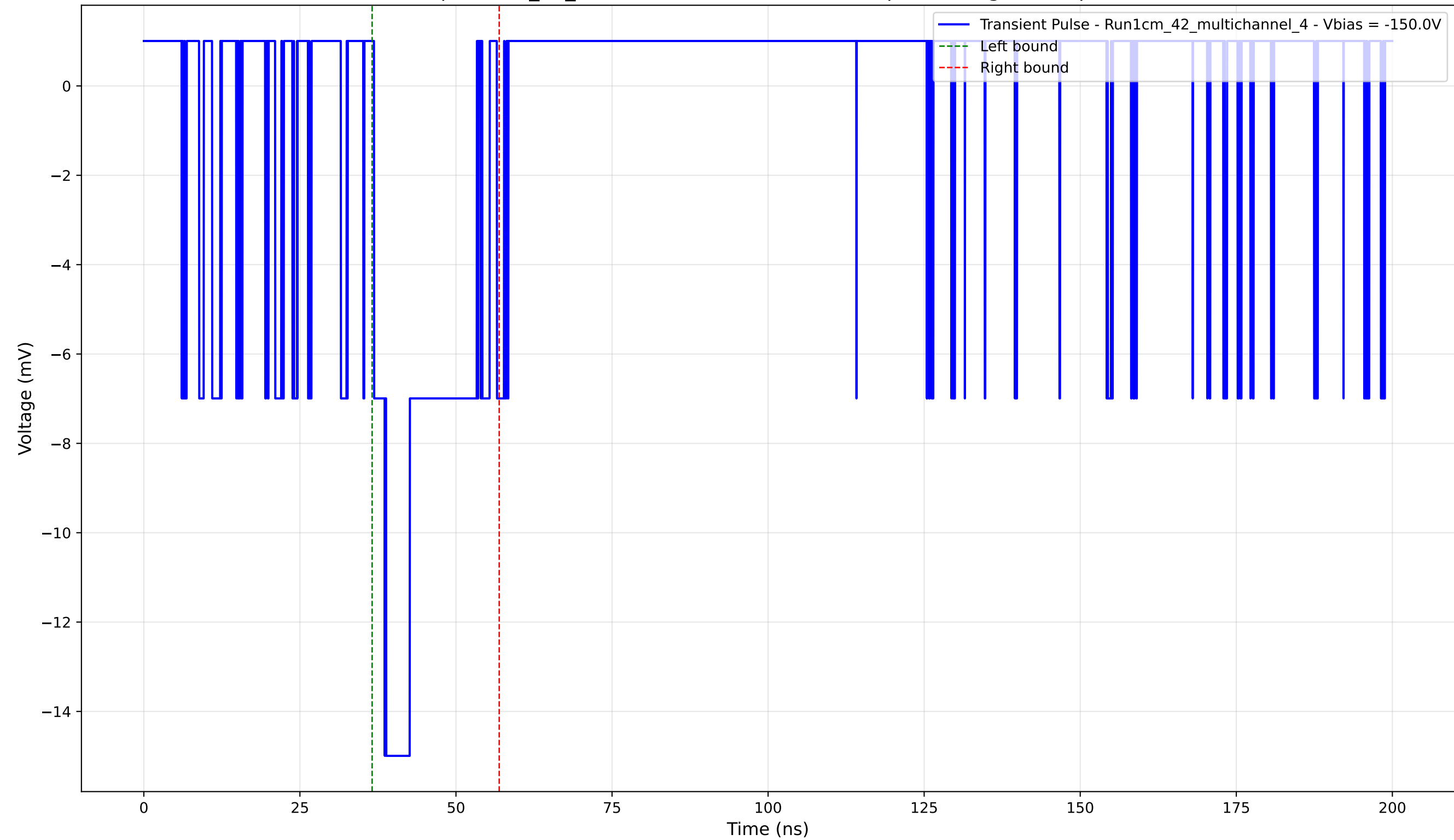
Transient Pulse - Sample: 1cm_42_multichannel - Position: 215.0 \mu\text{m} - Charge: 3.12 pC - Rise Time: 1.74 ns
