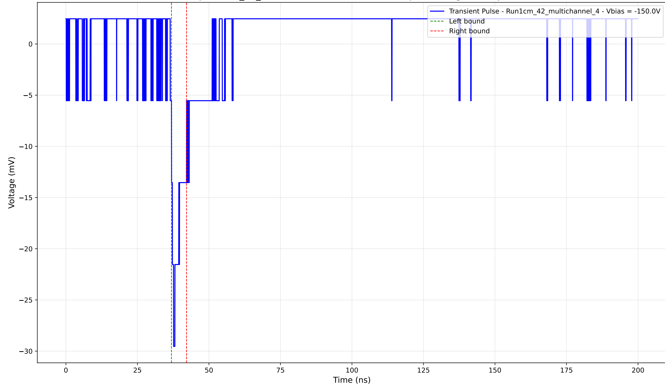
Transient Pulse - Sample: 1cm_42_multichannel - Position: 3235.0 \mu\text{m} - Charge: 1.88 pC - Rise Time: 1.20 ns
