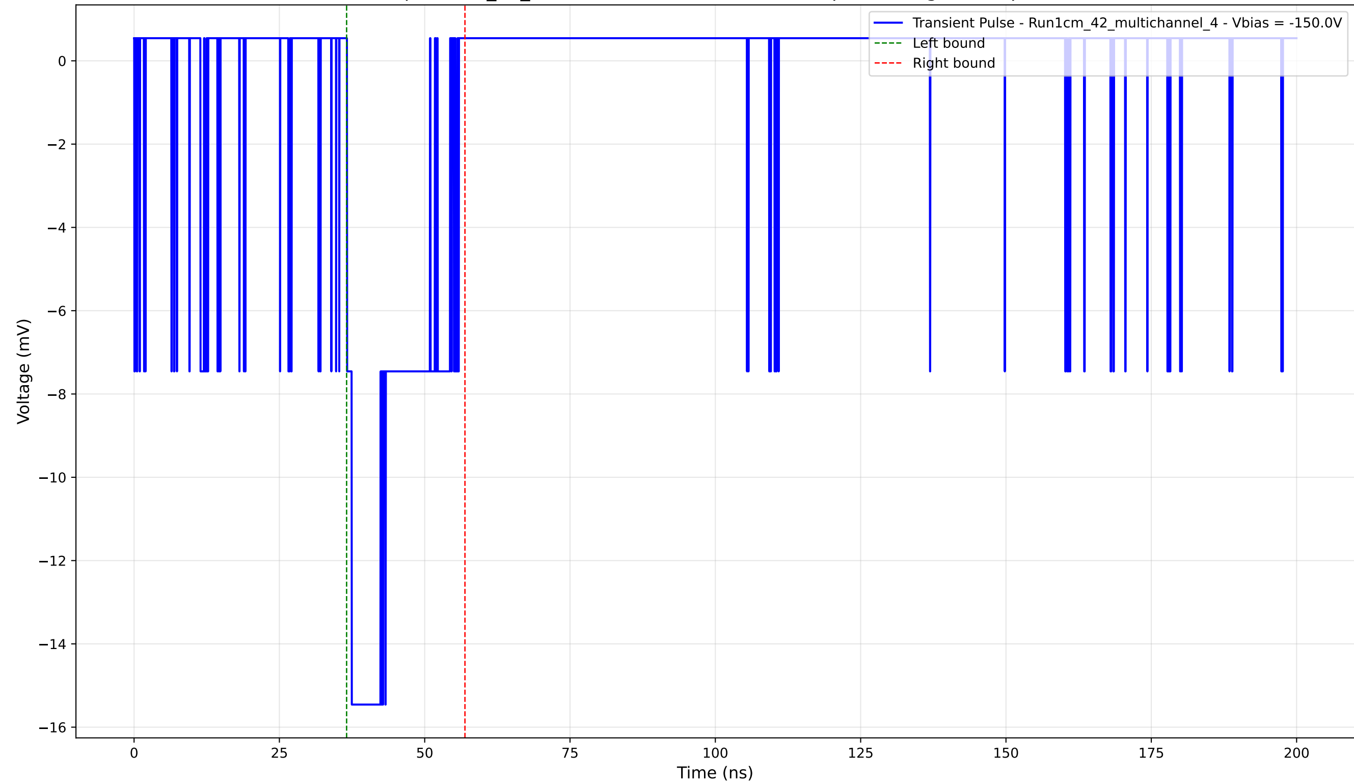
Transient Pulse - Sample: 1cm_42_multichannel - Position: 3640.0 \mu\text{m} - Charge: 3.51 pC - Rise Time: 0.82 ns
