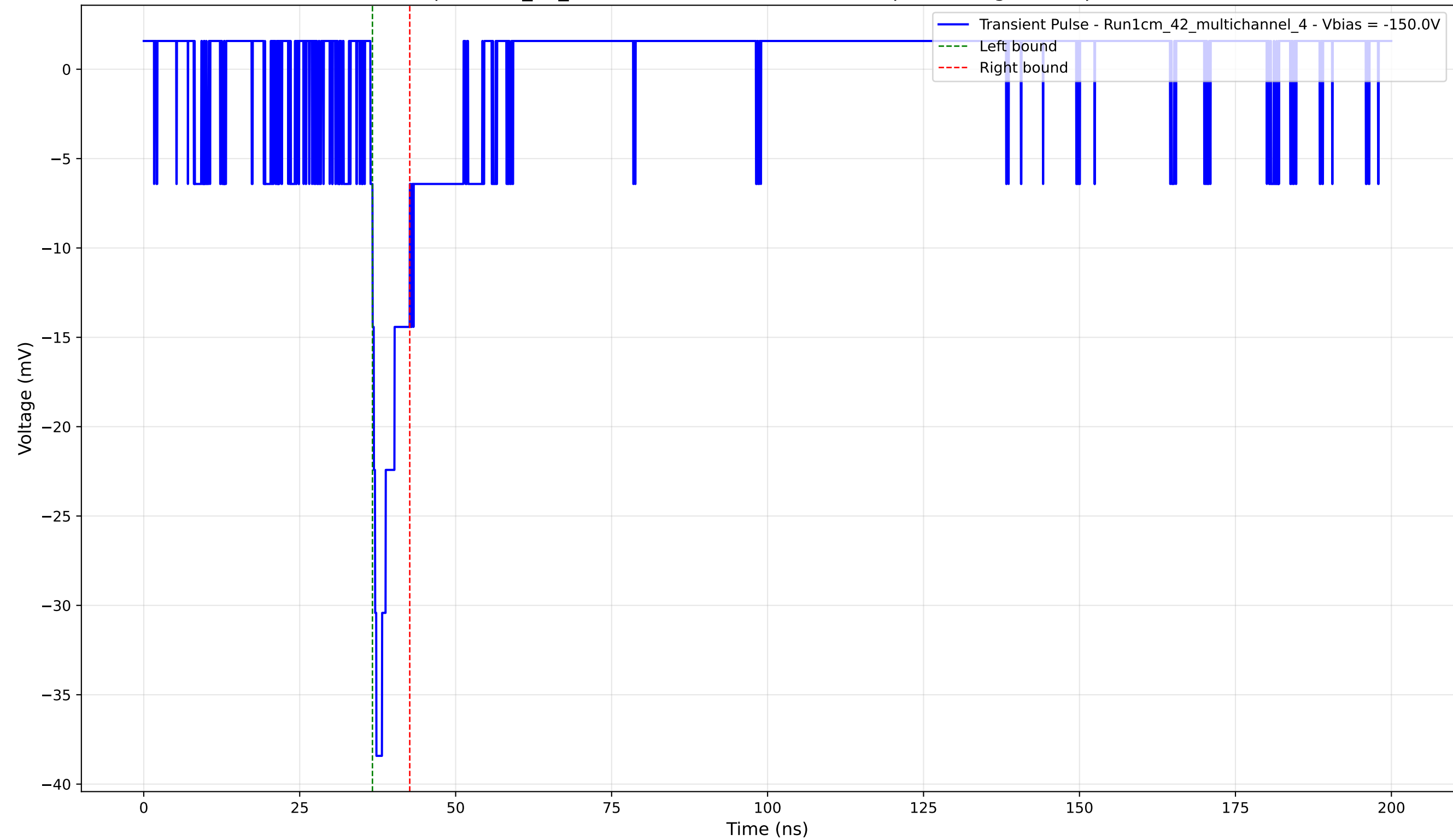
Transient Pulse - Sample: 1cm_42_multichannel - Position: 1745.0 \mu\text{m} - Charge: 2.67 pC - Rise Time: 0.95 ns
