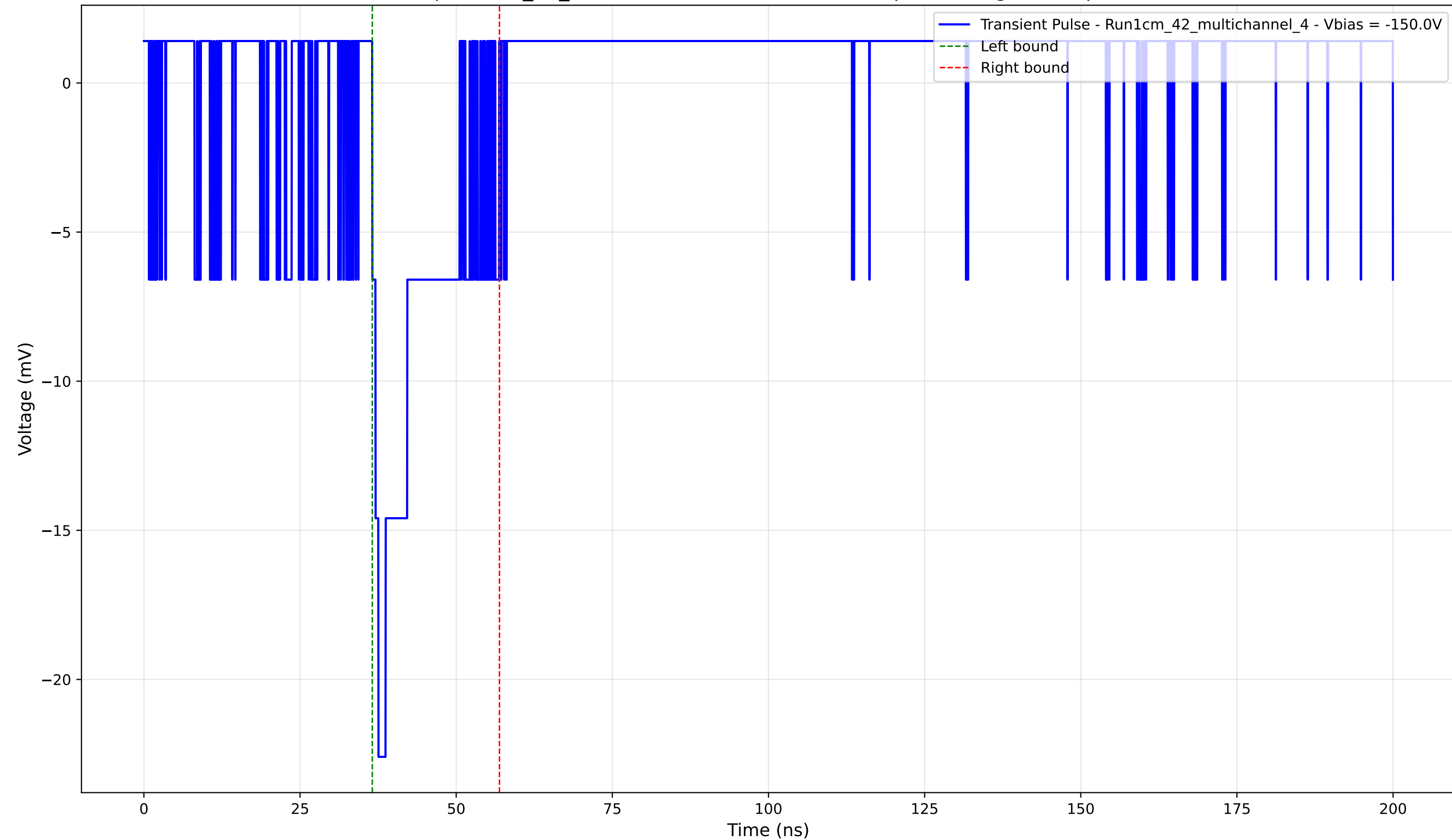
Transient Pulse - Sample: 1cm_42_multichannel - Position: 3330.0 \mu\text{m} - Charge: 3.32 pC - Rise Time: 1.00 ns
