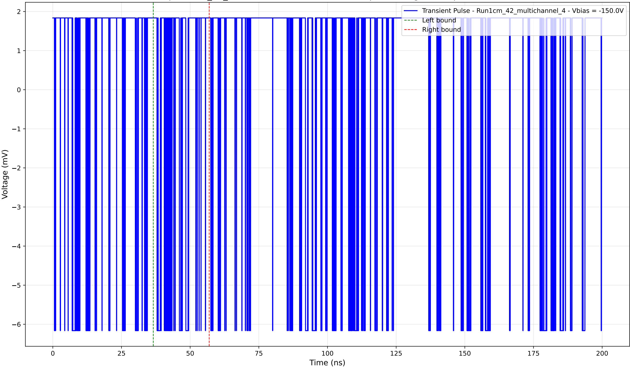
Transient Pulse - Sample: 1cm_42_multichannel - Position: 3415.0 \mu\text{m} - Charge: 0.02 pC - Rise Time: 0.00 ns (N/A)
