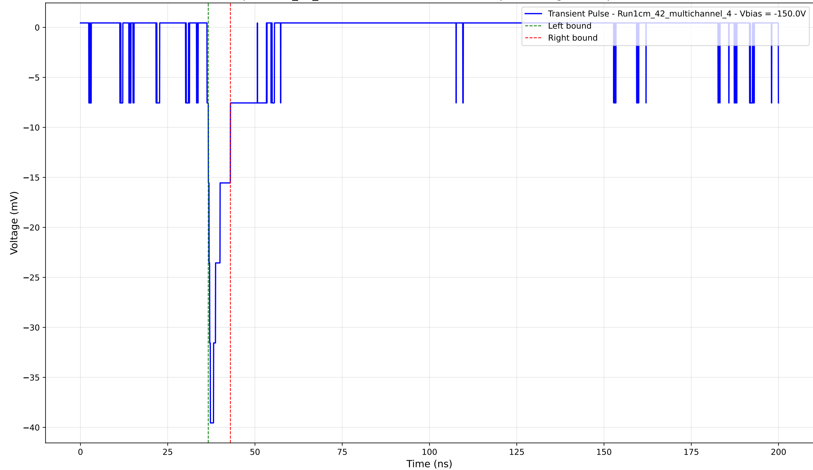
Transient Pulse - Sample: 1cm_42_multichannel - Position: 1790.0 \mu\text{m} - Charge: 2.89 pC - Rise Time: 0.97 ns
