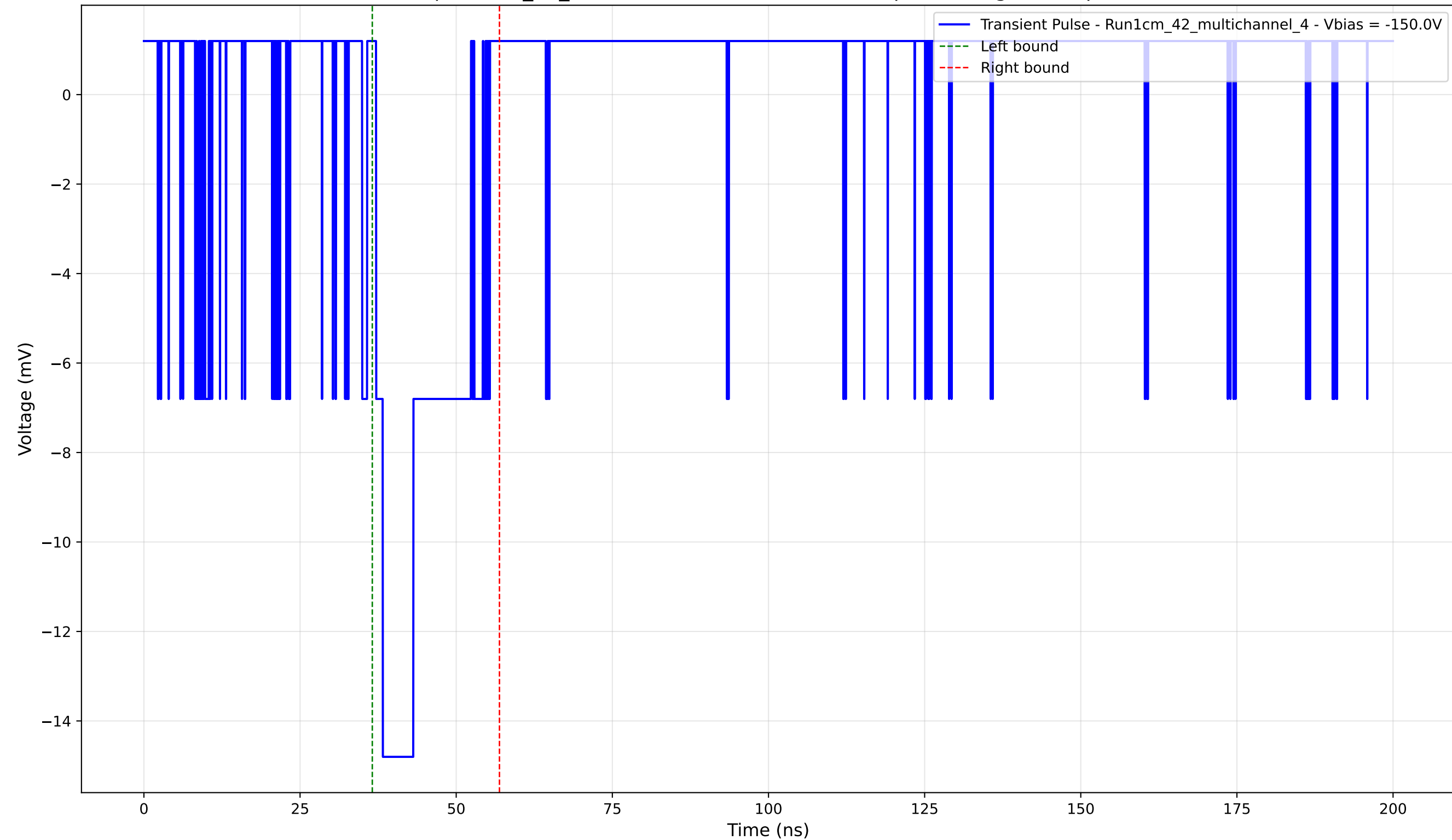
Transient Pulse - Sample: 1cm_42_multichannel - Position: 4310.0 \mu\text{m} - Charge: 3.09 pC - Rise Time: 1.08 ns
