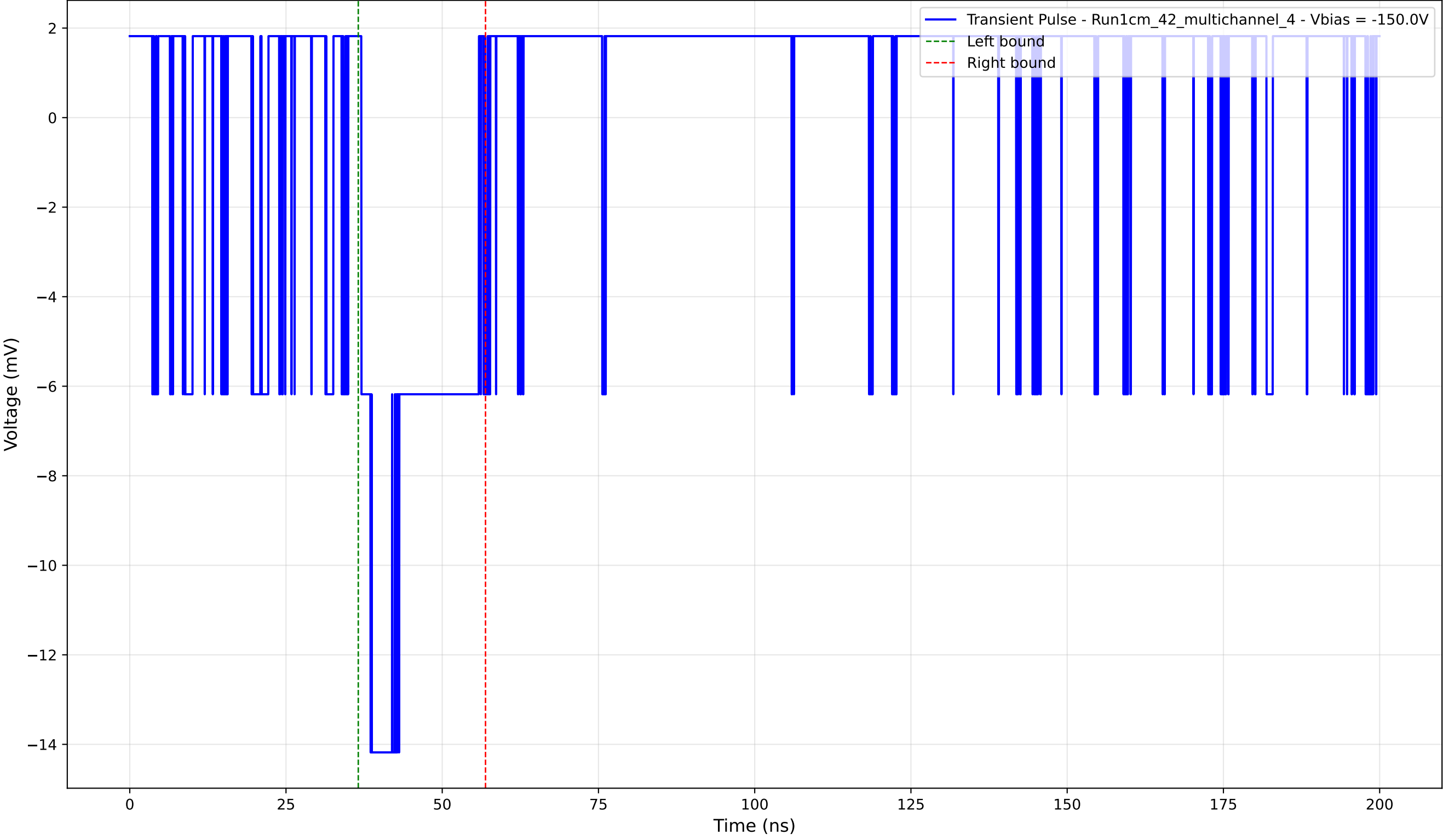
Transient Pulse - Sample: 1cm_42_multichannel - Position: 290.0 \mu\text{m} - Charge: 2.97 pC - Rise Time: 0.00 ns (N/A)
