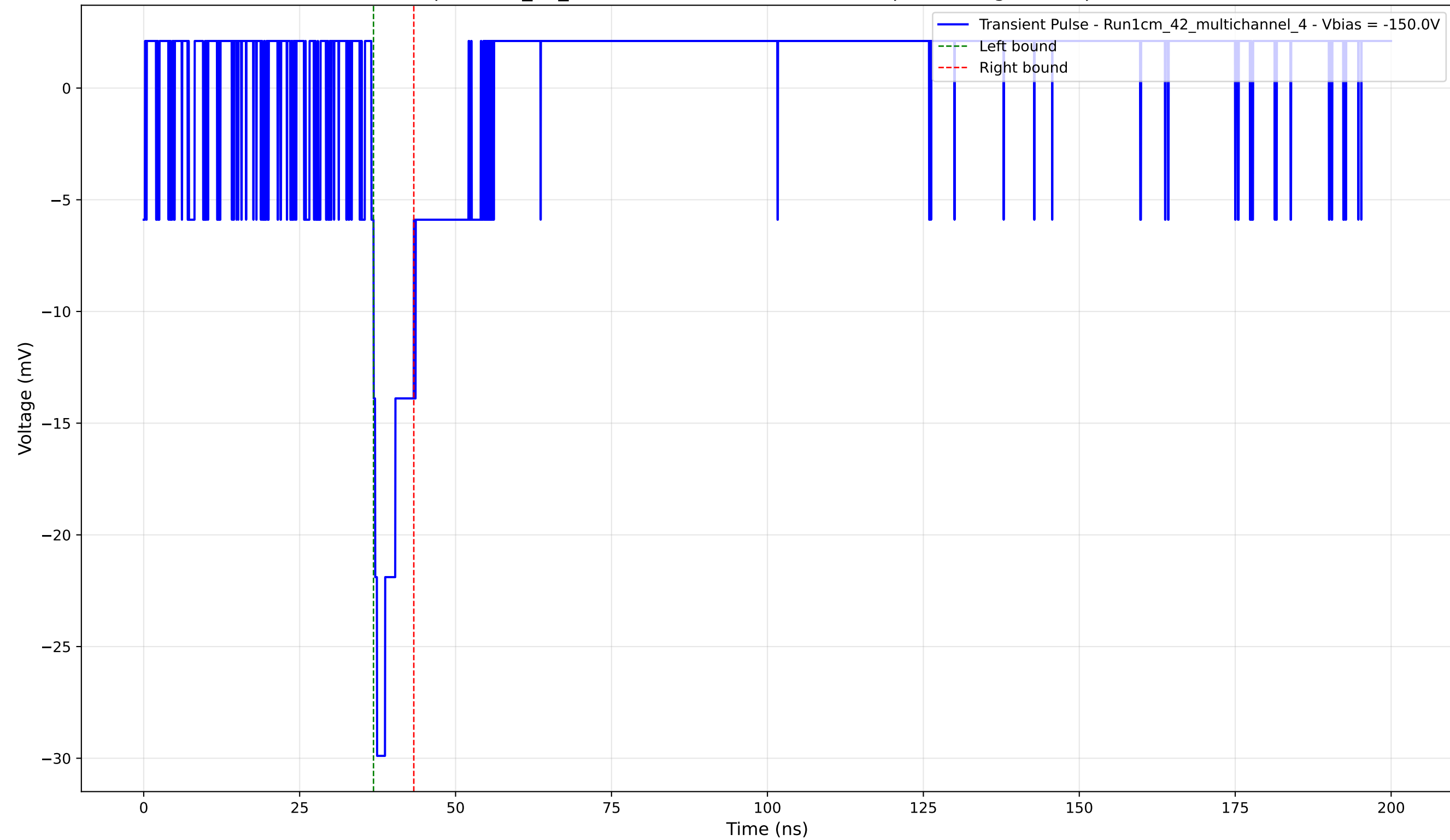
Transient Pulse - Sample: 1cm_42_multichannel - Position: 1570.0 \mu\text{m} - Charge: 2.52 pC - Rise Time: 0.92 ns
