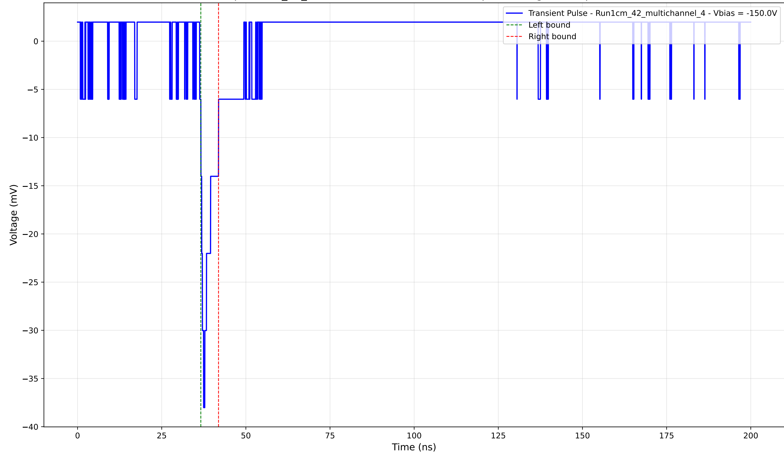
Transient Pulse - Sample: 1cm_42_multichannel - Position: 2960.0 \mu\text{m} - Charge: 2.15 pC - Rise Time: 1.17 ns
