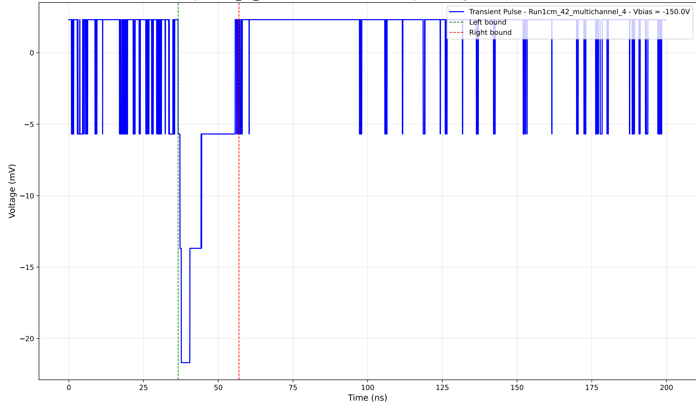
Transient Pulse - Sample: 1cm_42_multichannel - Position: 1255.0 \mu\text{m} - Charge: 3.77 pC - Rise Time: 0.00 ns (N/A)
