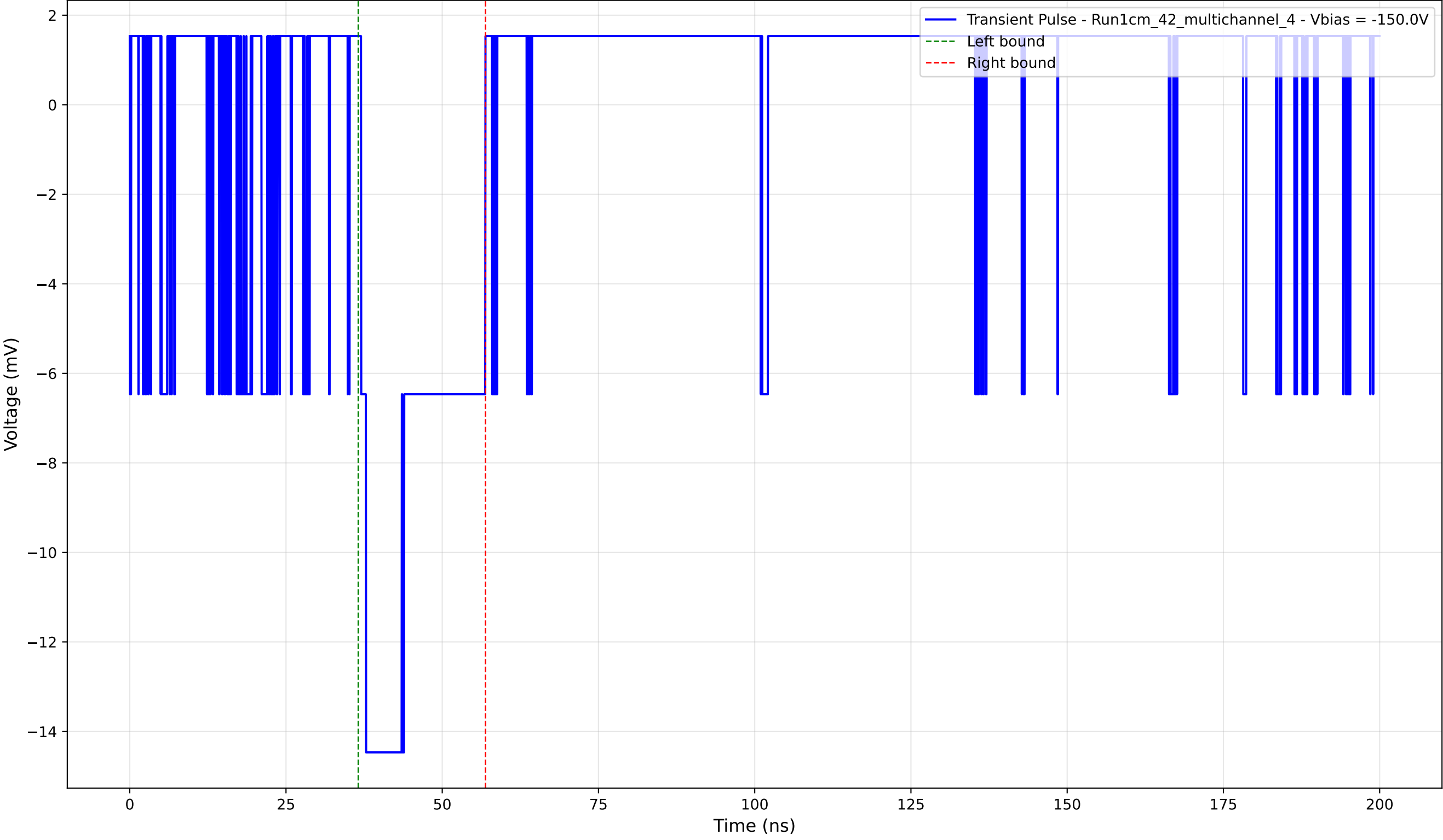
Transient Pulse - Sample: 1cm_42_multichannel - Position: 695.0 \mu\text{m} - Charge: 3.52 pC - Rise Time: 0.00 ns (N/A)
