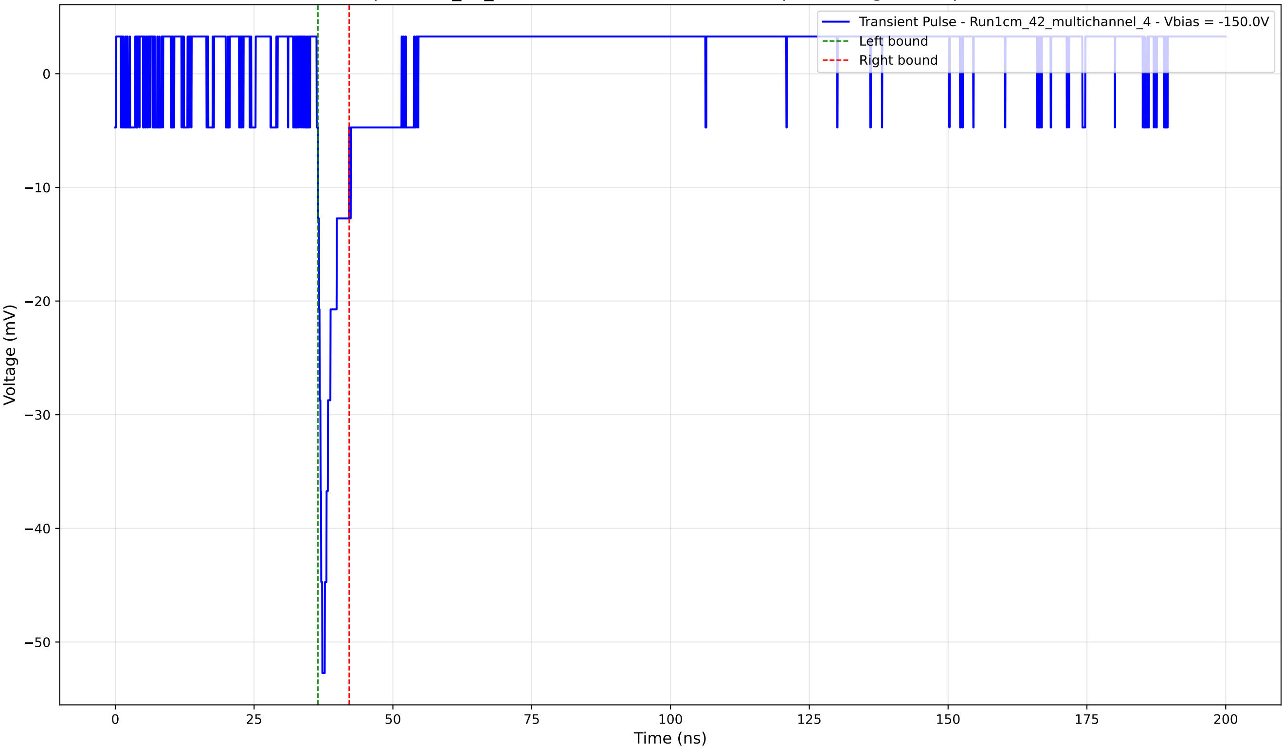
Transient Pulse - Sample: 1cm_42_multichannel - Position: 1970.0 \mu\text{m} - Charge: 2.69 pC - Rise Time: 0.78 ns
