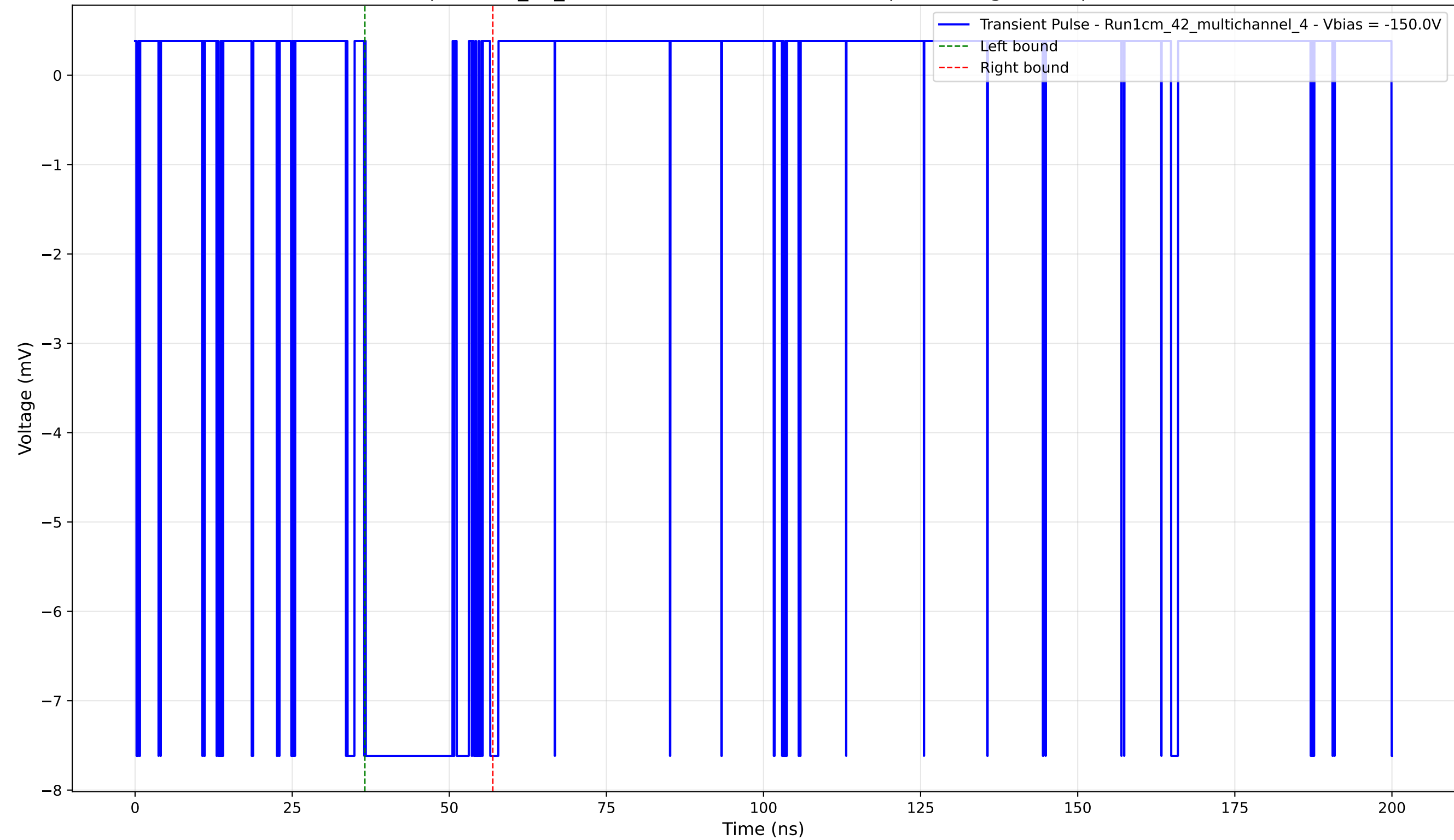
Transient Pulse - Sample: 1cm_42_multichannel - Position: 4845.0 \mu\text{m} - Charge: 2.63 pC - Rise Time: 0.02 ns
