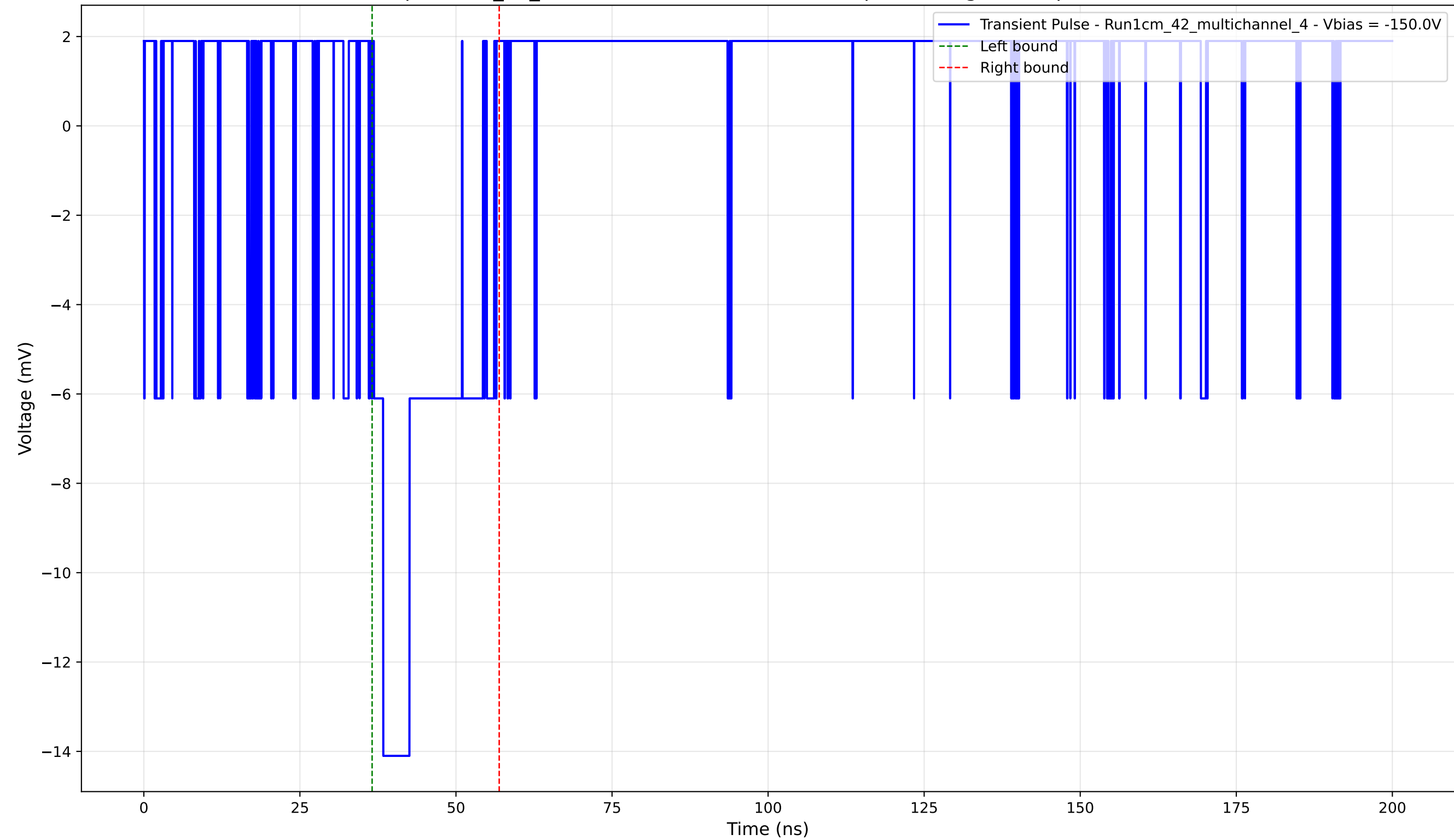
Transient Pulse - Sample: 1cm_42_multichannel - Position: 4760.0 \mu\text{m} - Charge: 2.91 pC - Rise Time: 0.00 ns (N/A)
