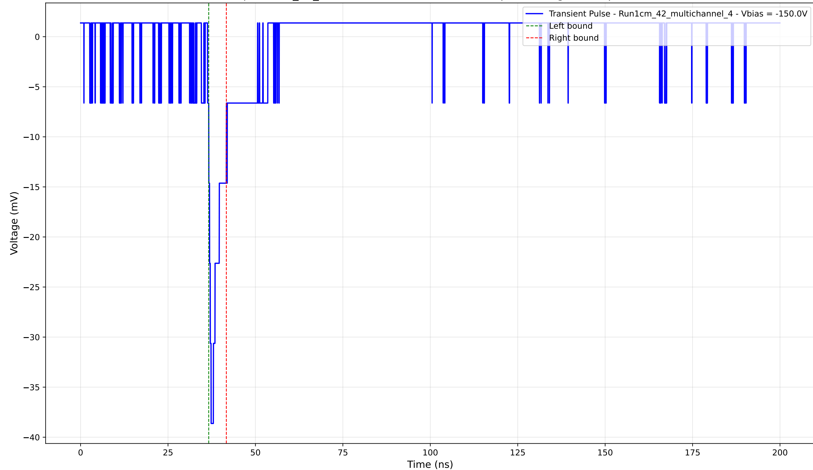
Transient Pulse - Sample: 1cm_42_multichannel - Position: 2970.0 \mu\text{m} - Charge: 2.24 pC - Rise Time: 1.01 ns
