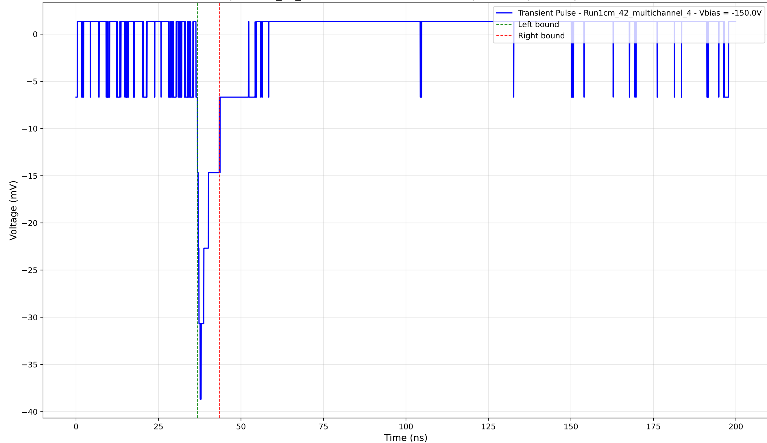
Transient Pulse - Sample: 1cm_42_multichannel - Position: 1655.0 \mu\text{m} - Charge: 2.72 pC - Rise Time: 1.27 ns
