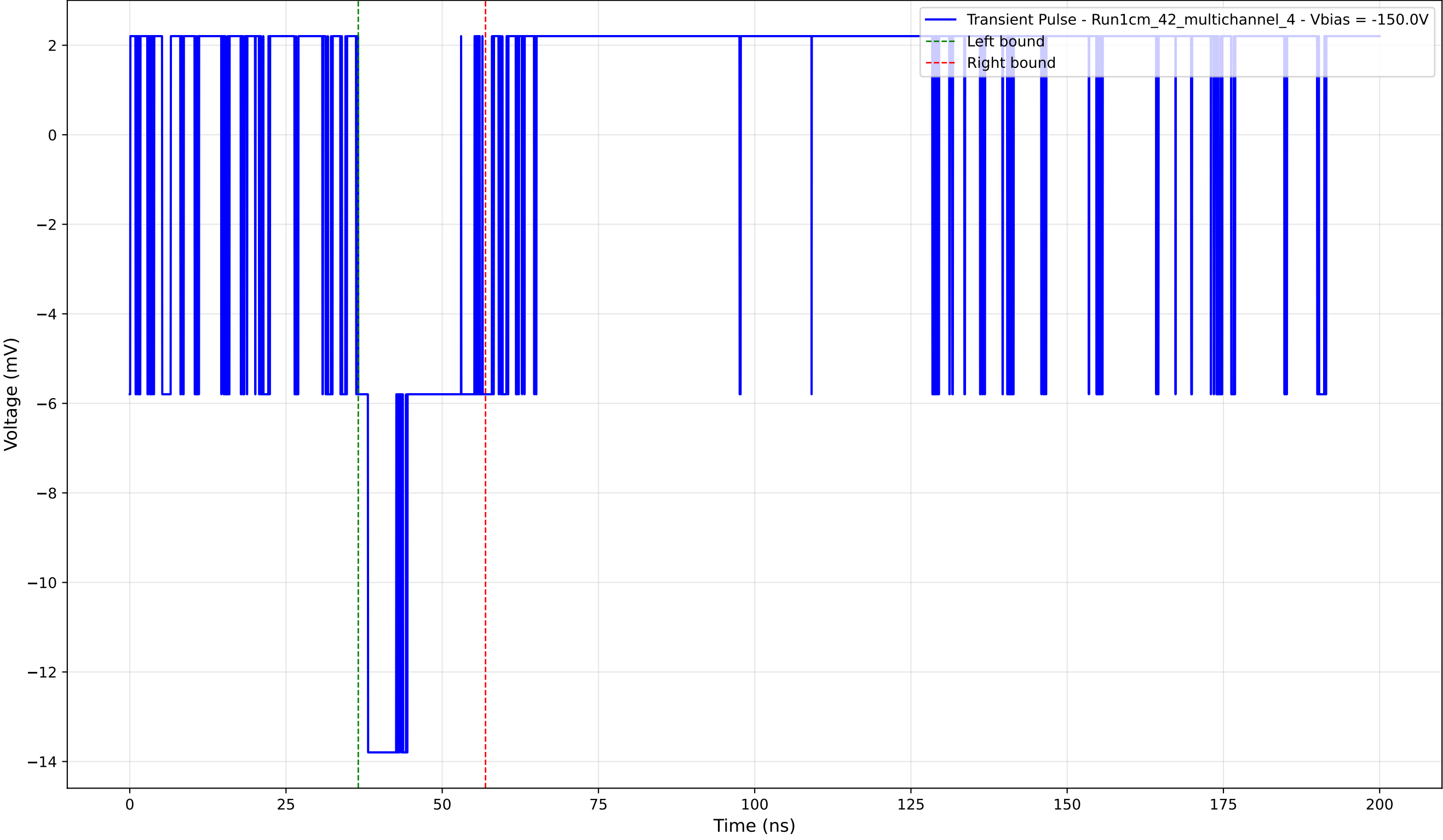
Transient Pulse - Sample: 1cm_42_multichannel - Position: 480.0 \mu\text{m} - Charge: 3.20 pC - Rise Time: 0.00 ns (N/A)
