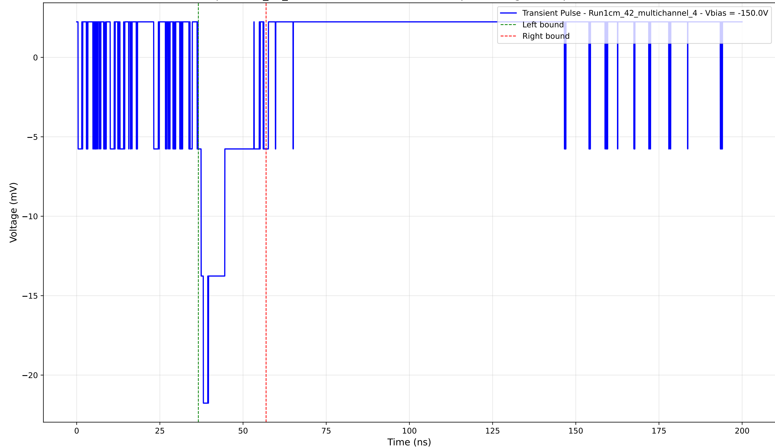
Transient Pulse - Sample: 1cm_42_multichannel - Position: 1125.0 \mu\text{m} - Charge: 3.54 pC - Rise Time: 0.00 ns (N/A)
