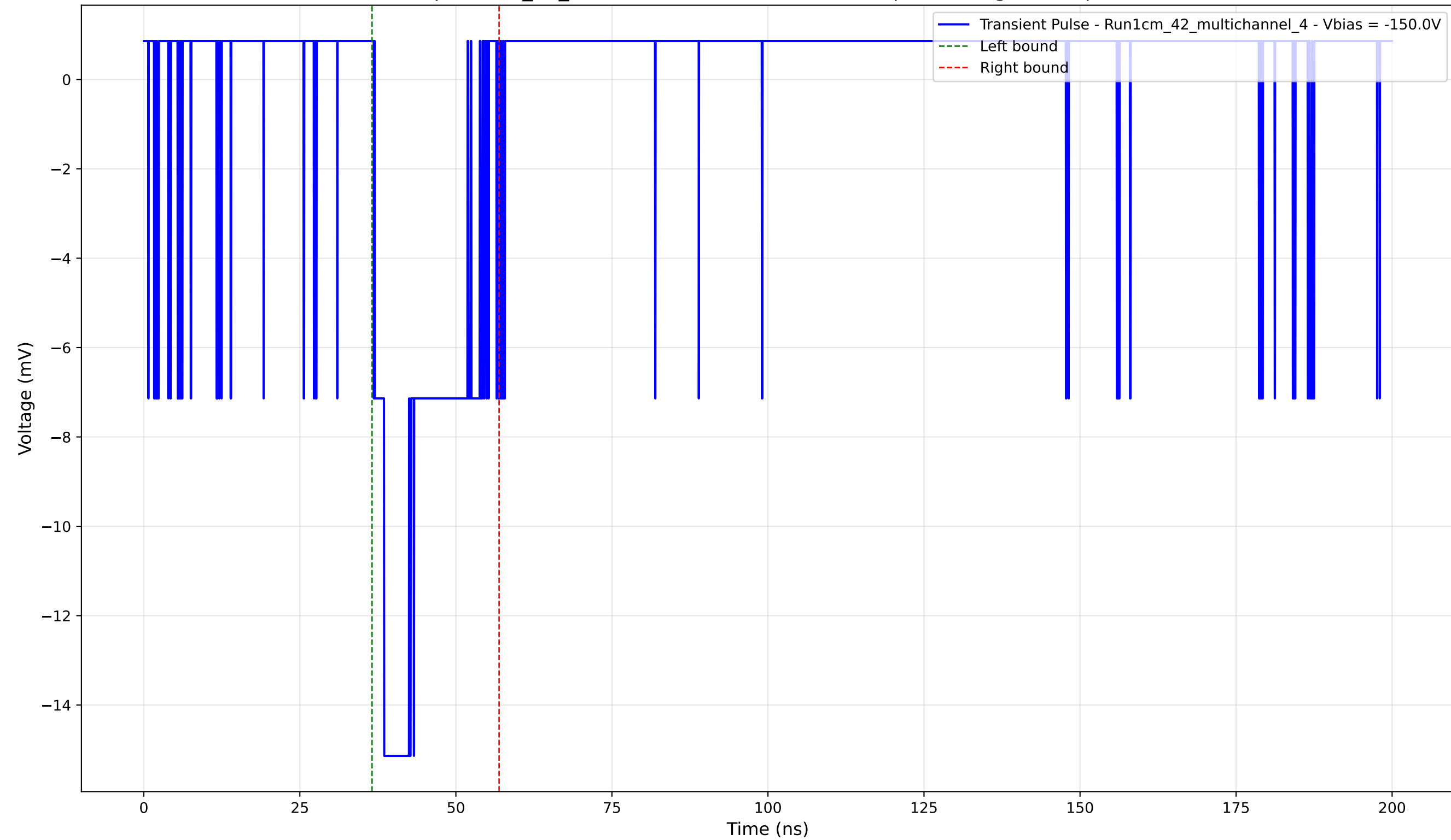
Transient Pulse - Sample: 1cm_42_multichannel - Position: 4685.0 \mu\text{m} - Charge: 3.12 pC - Rise Time: 1.52 ns
