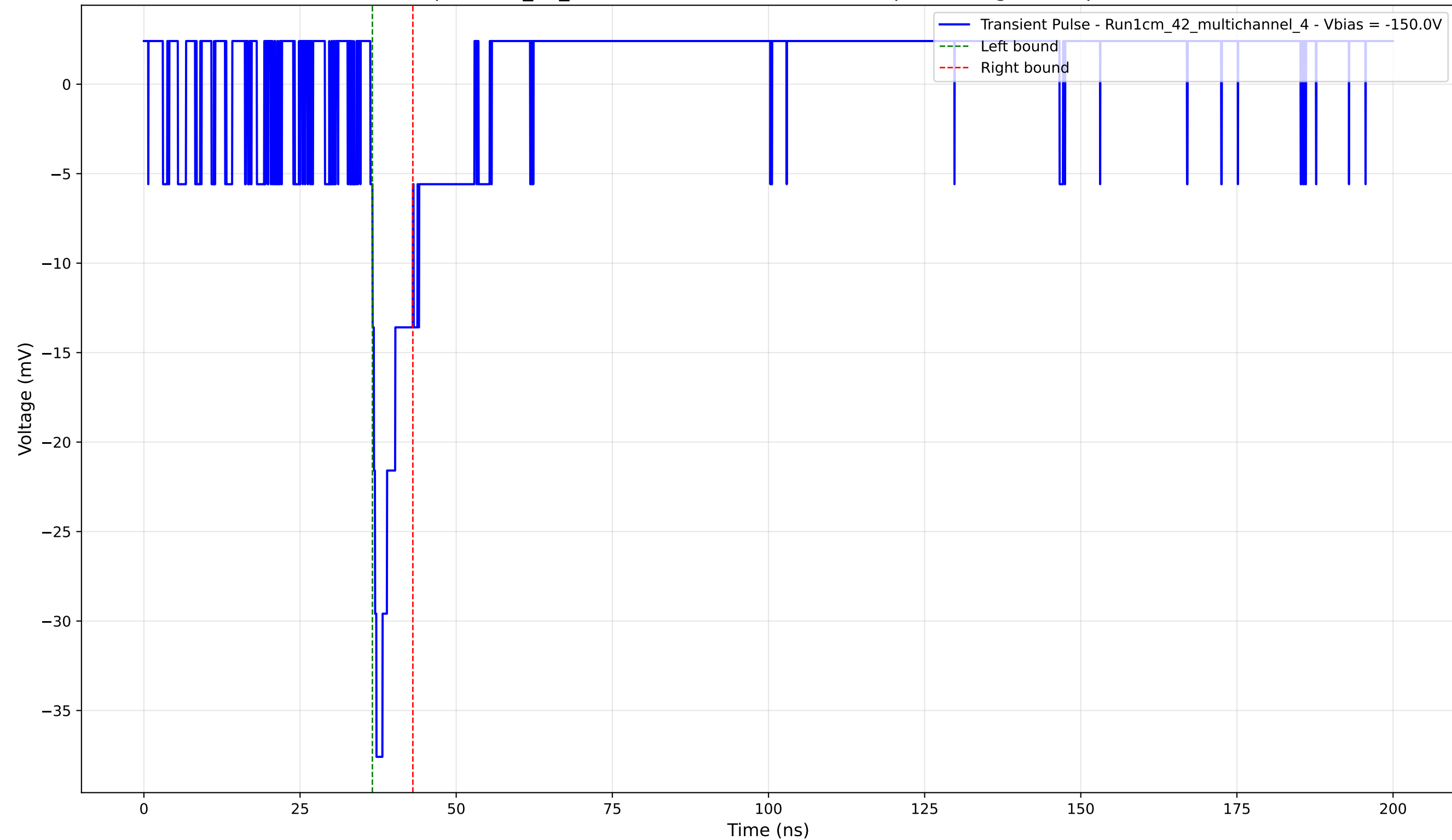
Transient Pulse - Sample: 1cm_42_multichannel - Position: 1765.0 \mu\text{m} - Charge: 2.77 pC - Rise Time: 0.97 ns
