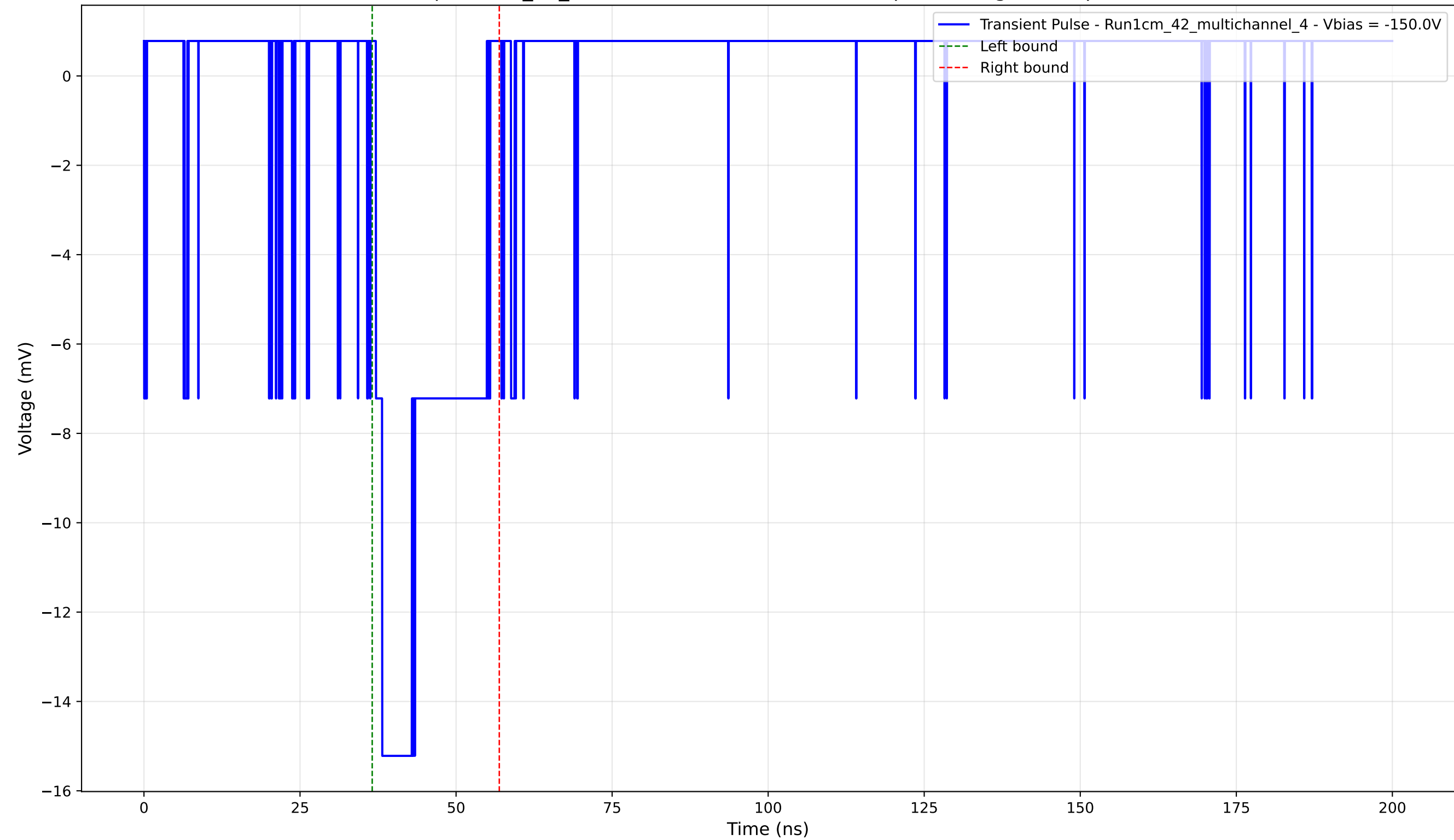
Transient Pulse - Sample: 1cm_42_multichannel - Position: 4130.0 \mu\text{m} - Charge: 3.36 pC - Rise Time: 1.02 ns
