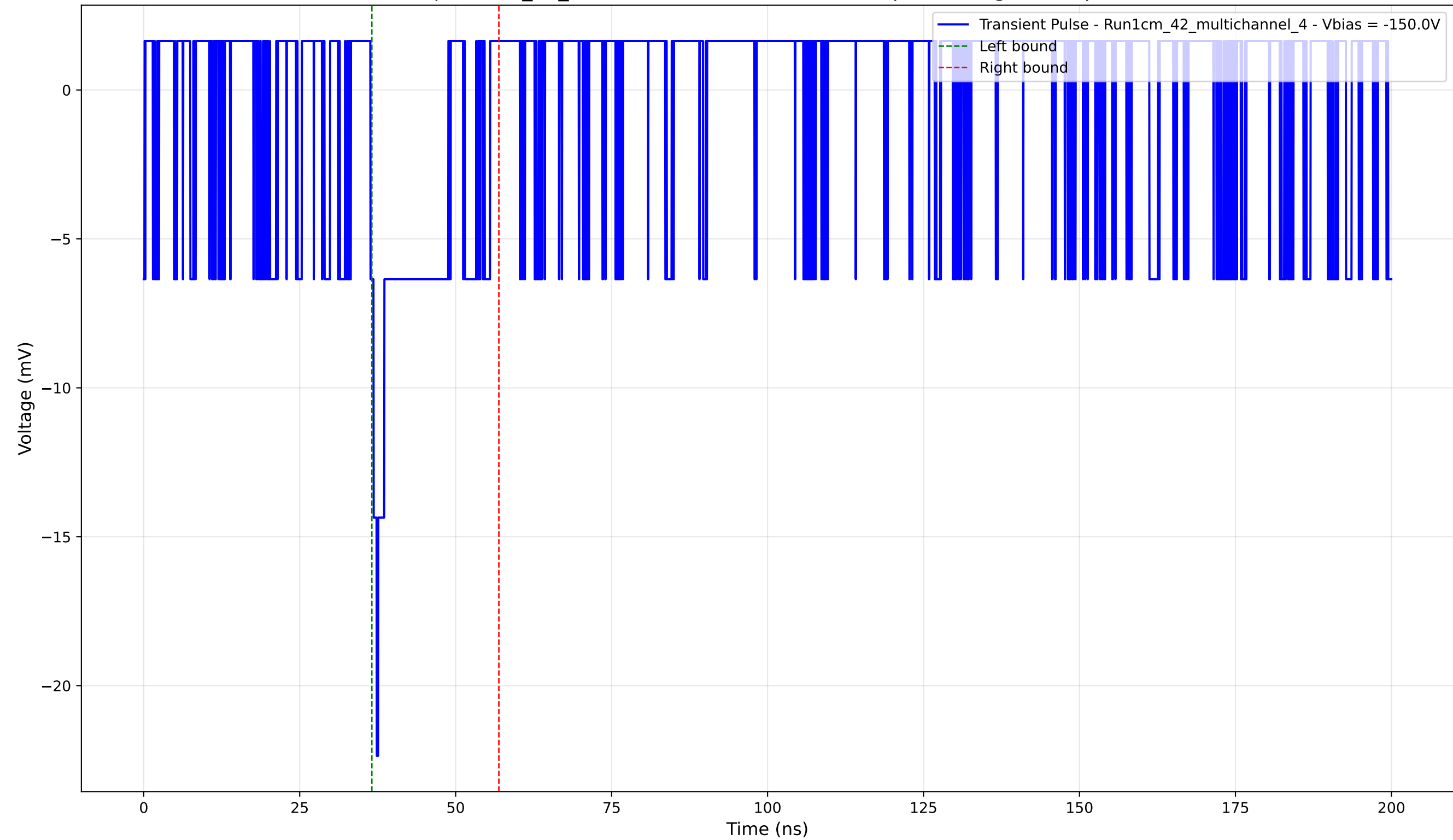
Transient Pulse - Sample: 1cm_42_multichannel - Position: 1925.0 \mu\text{m} - Charge: 2.13 pC - Rise Time: 1.02 ns
