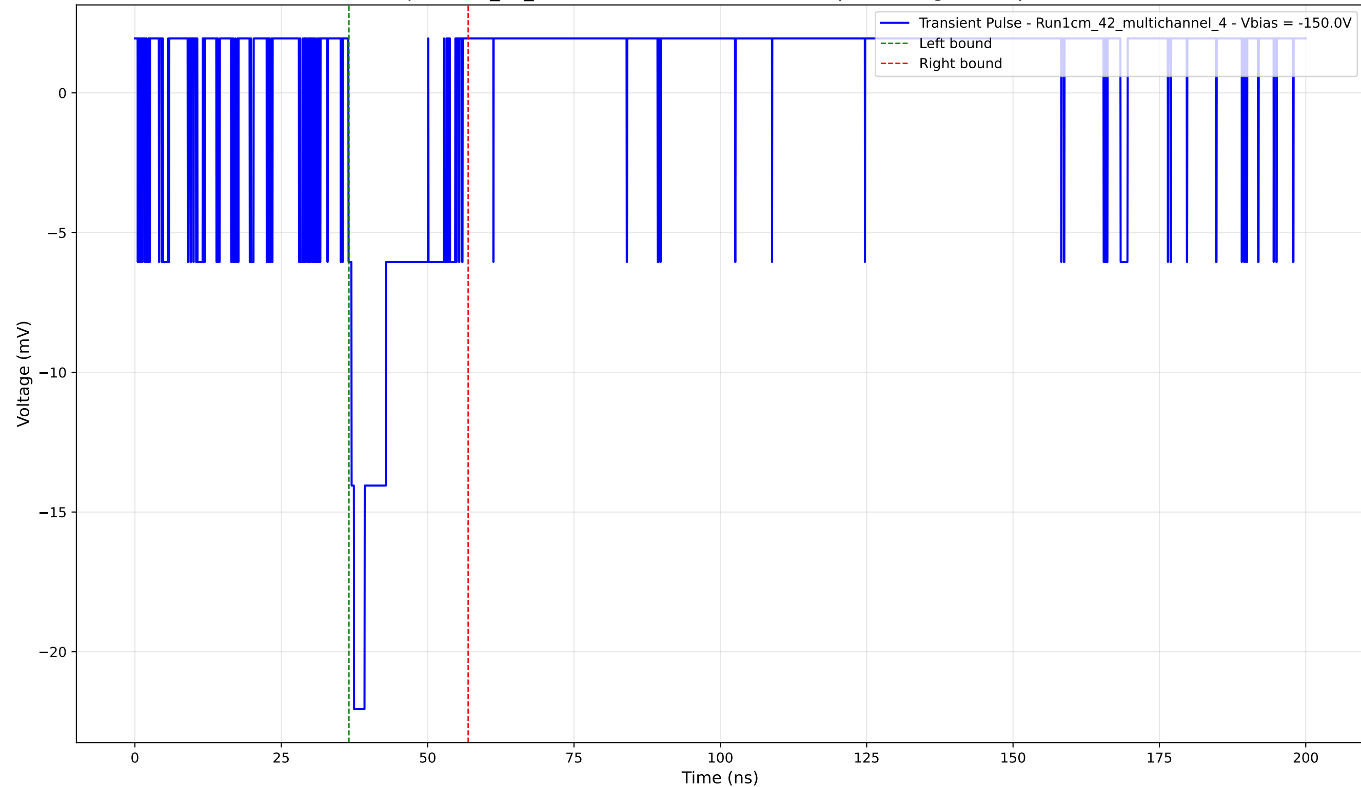
Transient Pulse - Sample: 1cm_42_multichannel - Position: 3315.0 \mu\text{m} - Charge: 3.30 pC - Rise Time: 0.96 ns
