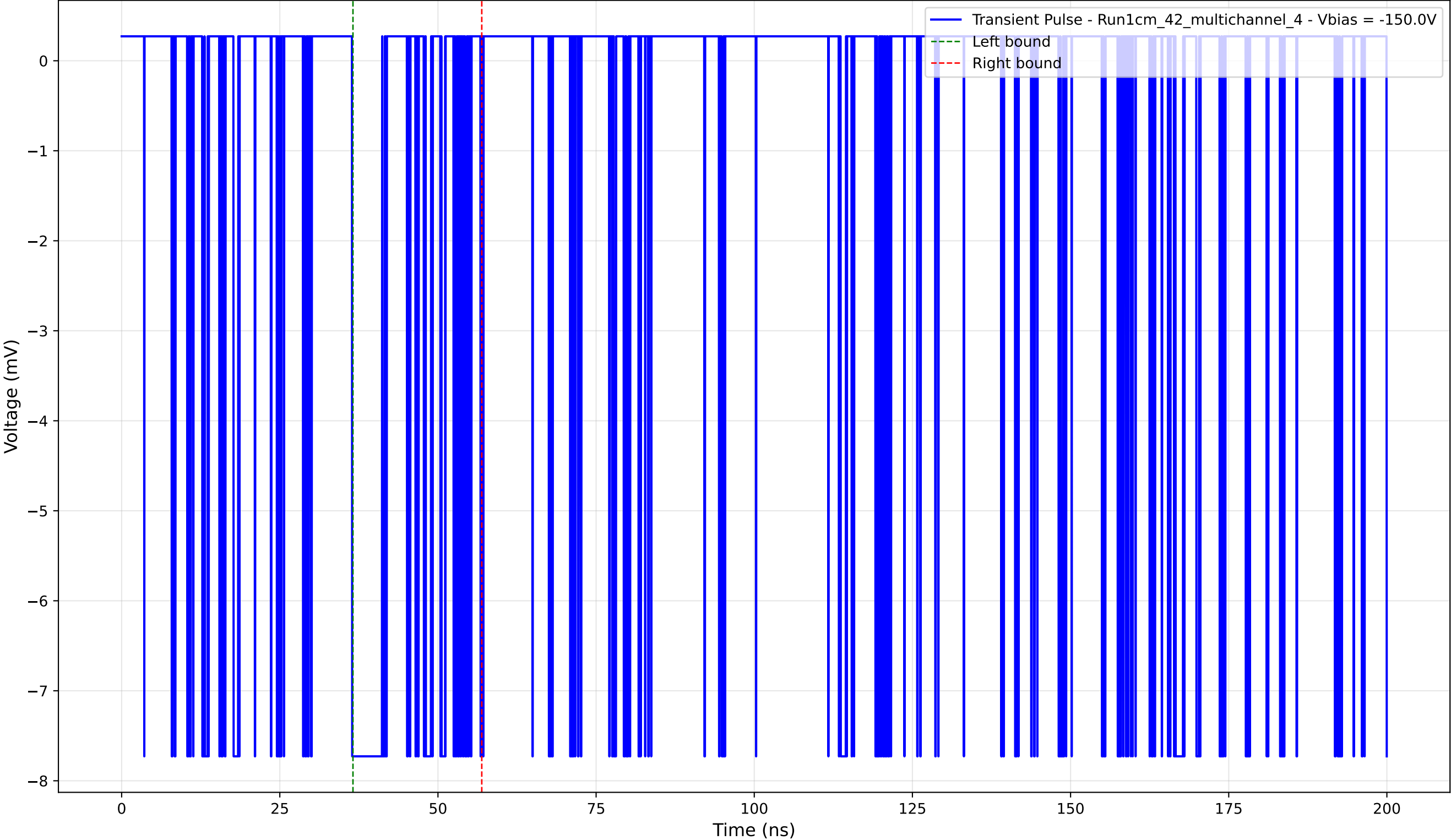
Transient Pulse - Sample: 1cm_42_multichannel - Position: 1880.0 \mu\text{m} - Charge: 1.31 pC - Rise Time: 0.02 ns
