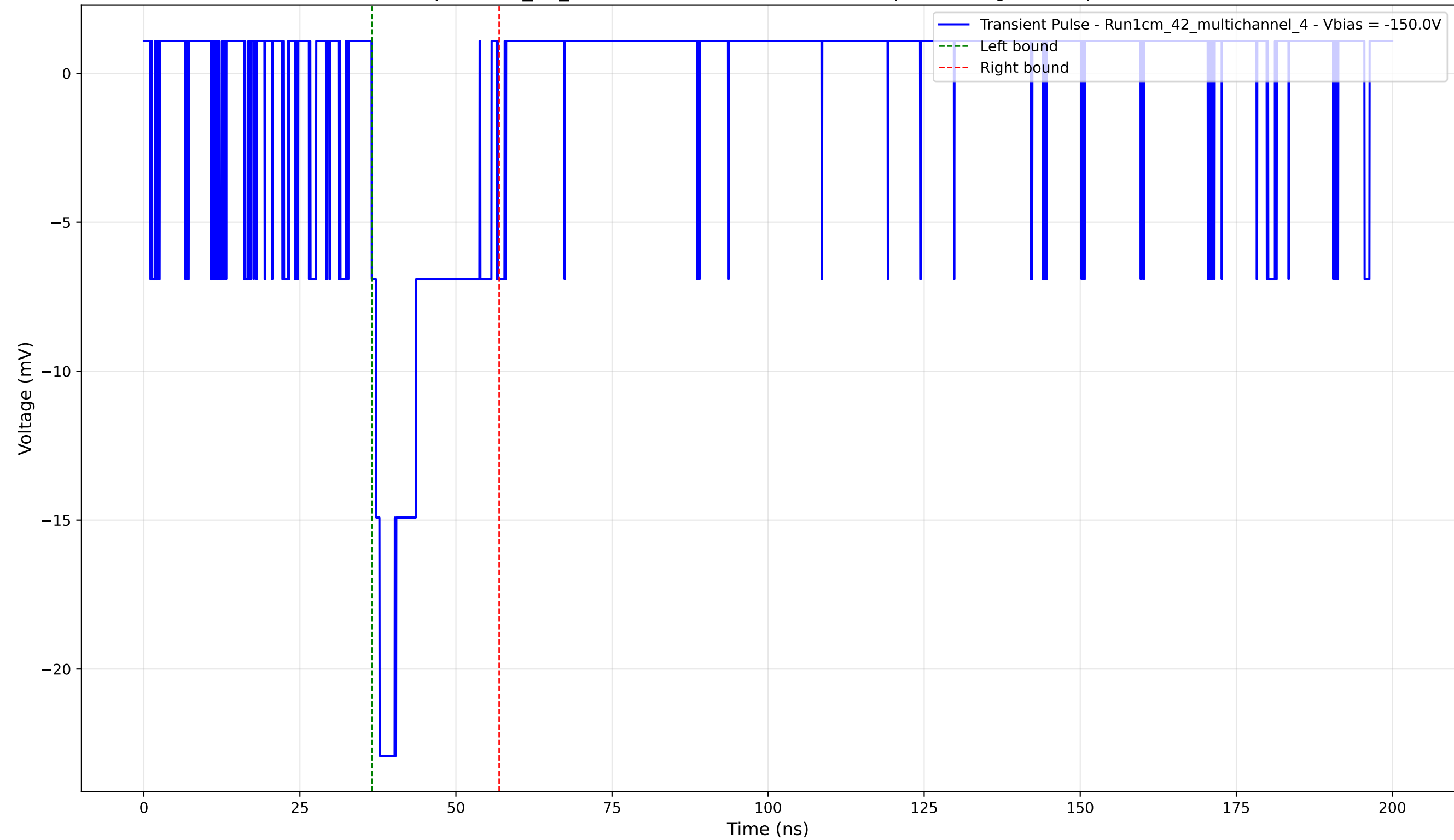
Transient Pulse - Sample: 1cm_42_multichannel - Position: 1200.0 \mu\text{m} - Charge: 4.07 pC - Rise Time: 1.28 ns
