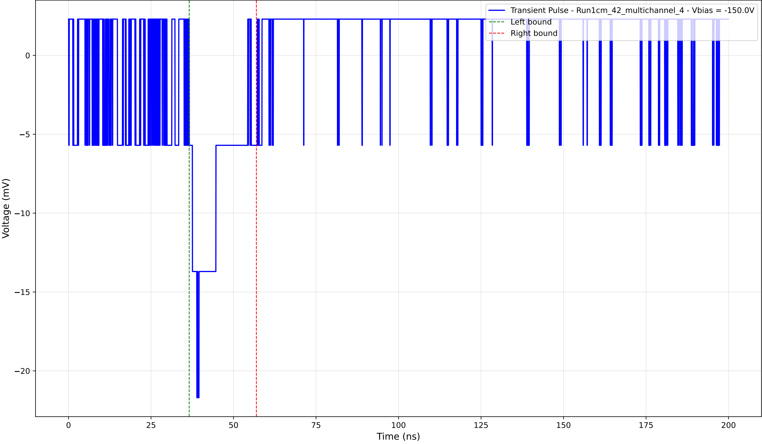
Transient Pulse - Sample: 1cm_42_multichannel - Position: 950.0 \mu\text{m} - Charge: 3.42 pC - Rise Time: 0.00 ns (N/A)
