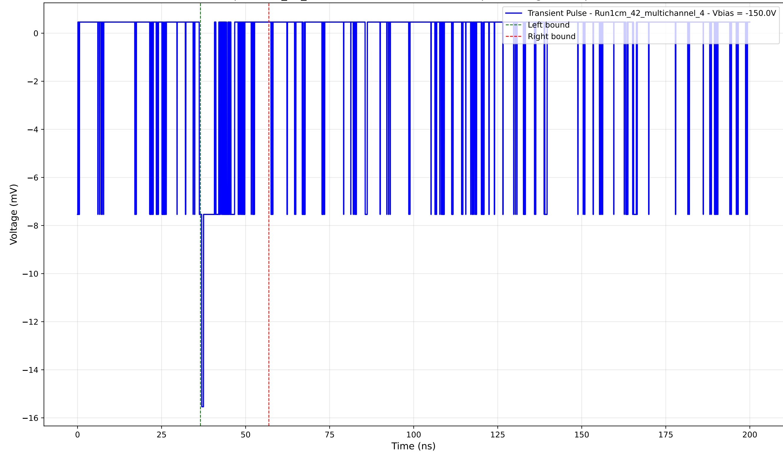
Transient Pulse - Sample: 1cm_42_multichannel - Position: 2355.0 \mu\text{m} - Charge: 1.34 pC - Rise Time: 0.74 ns
