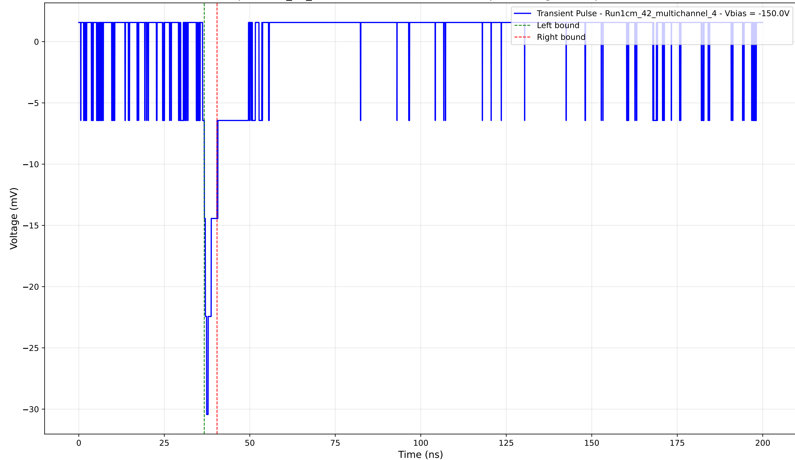
Transient Pulse - Sample: 1cm_42_multichannel - Position: 2950.0 \mu\text{m} - Charge: 1.42 pC - Rise Time: 1.19 ns
