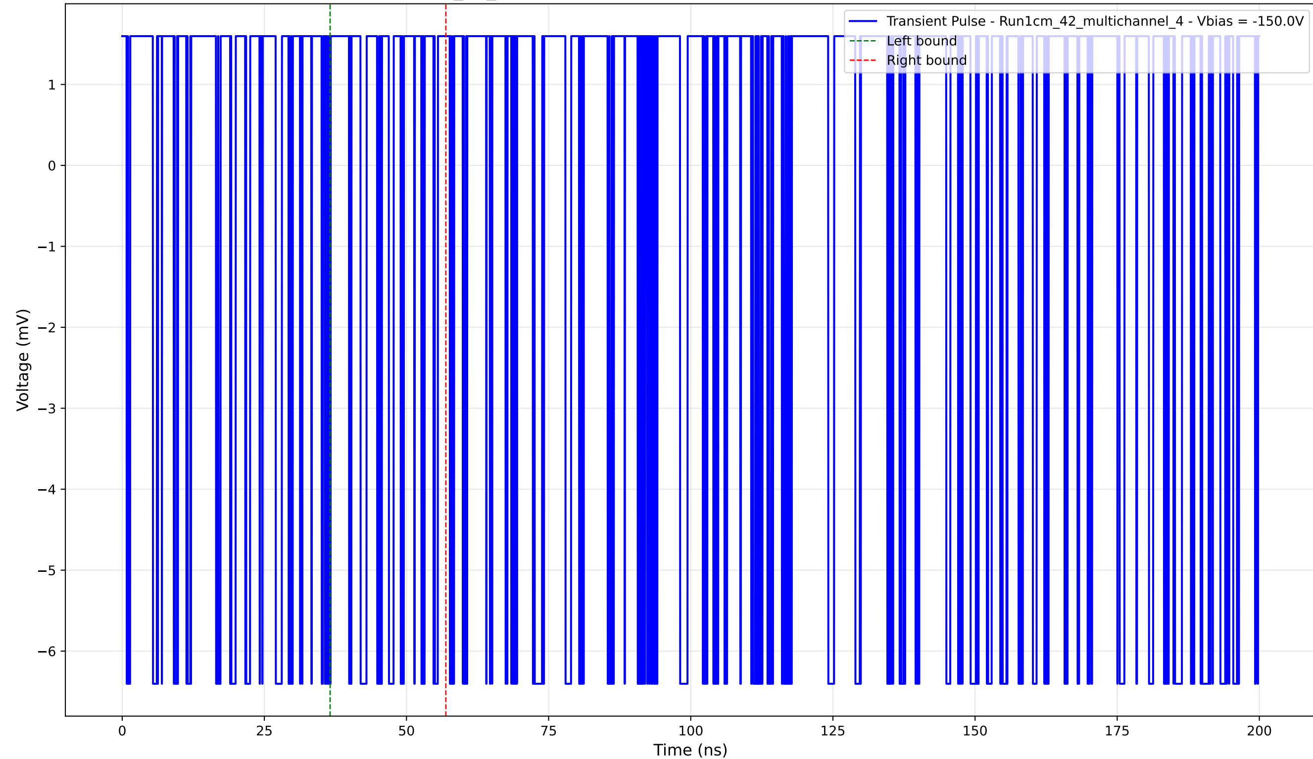
Transient Pulse - Sample: 1cm_42_multichannel - Position: 25.0 \mu\text{m} - Charge: 0.02 pC - Rise Time: 0.00 ns (N/A)
