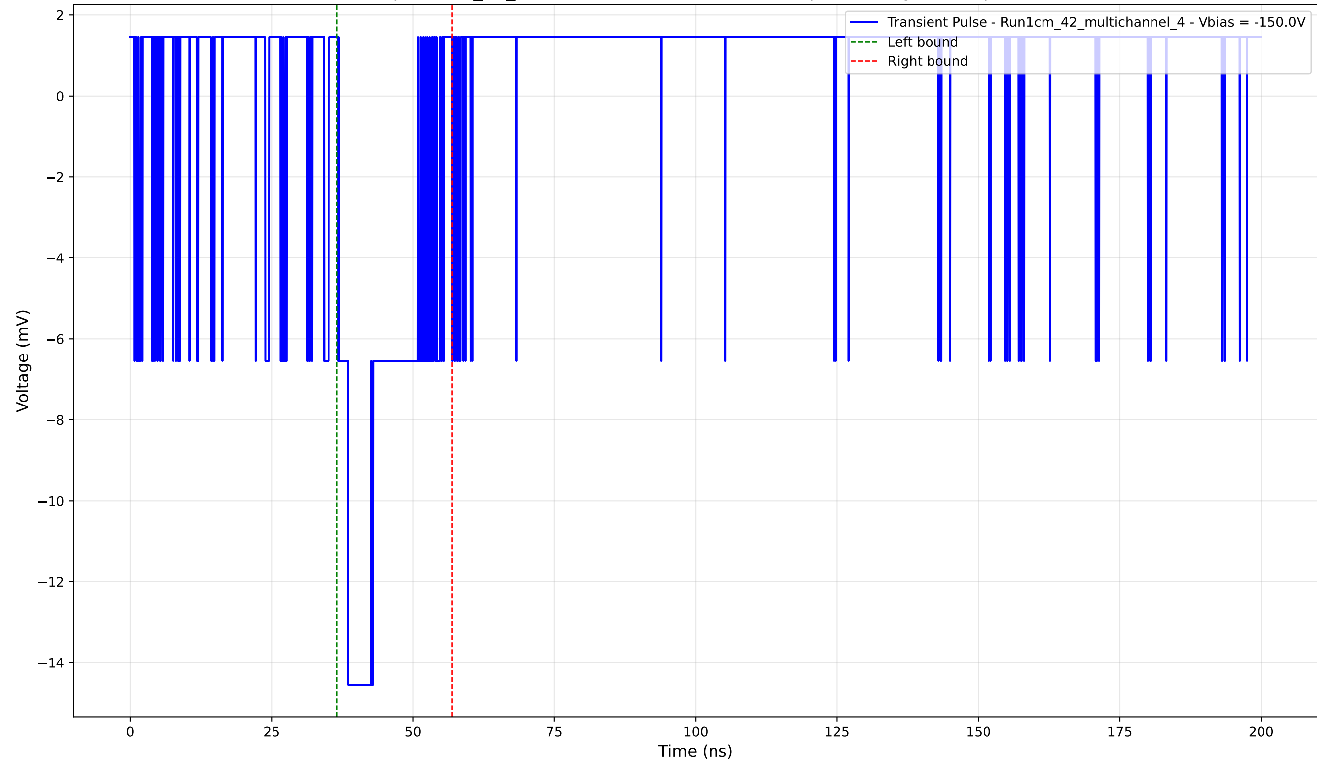
Transient Pulse - Sample: 1cm_42_multichannel - Position: 4655.0 \mu\text{m} - Charge: 2.88 pC - Rise Time: 1.64 ns
