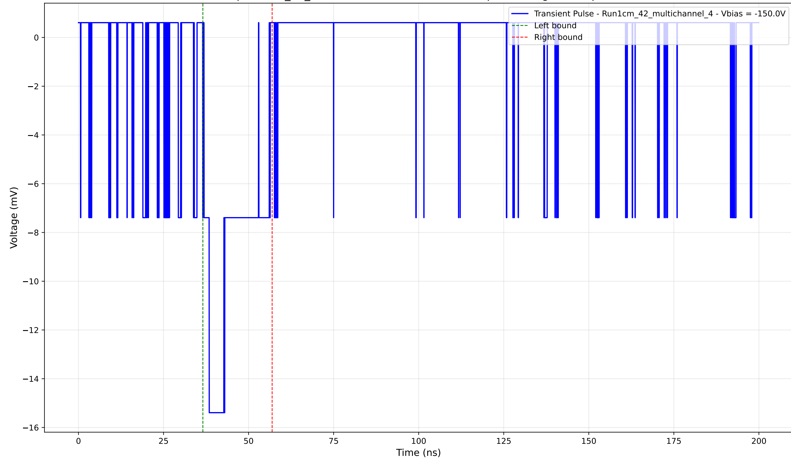
Transient Pulse - Sample: 1cm_42_multichannel - Position: 4270.0 \mu\text{m} - Charge: 3.55 pC - Rise Time: 1.54 ns
