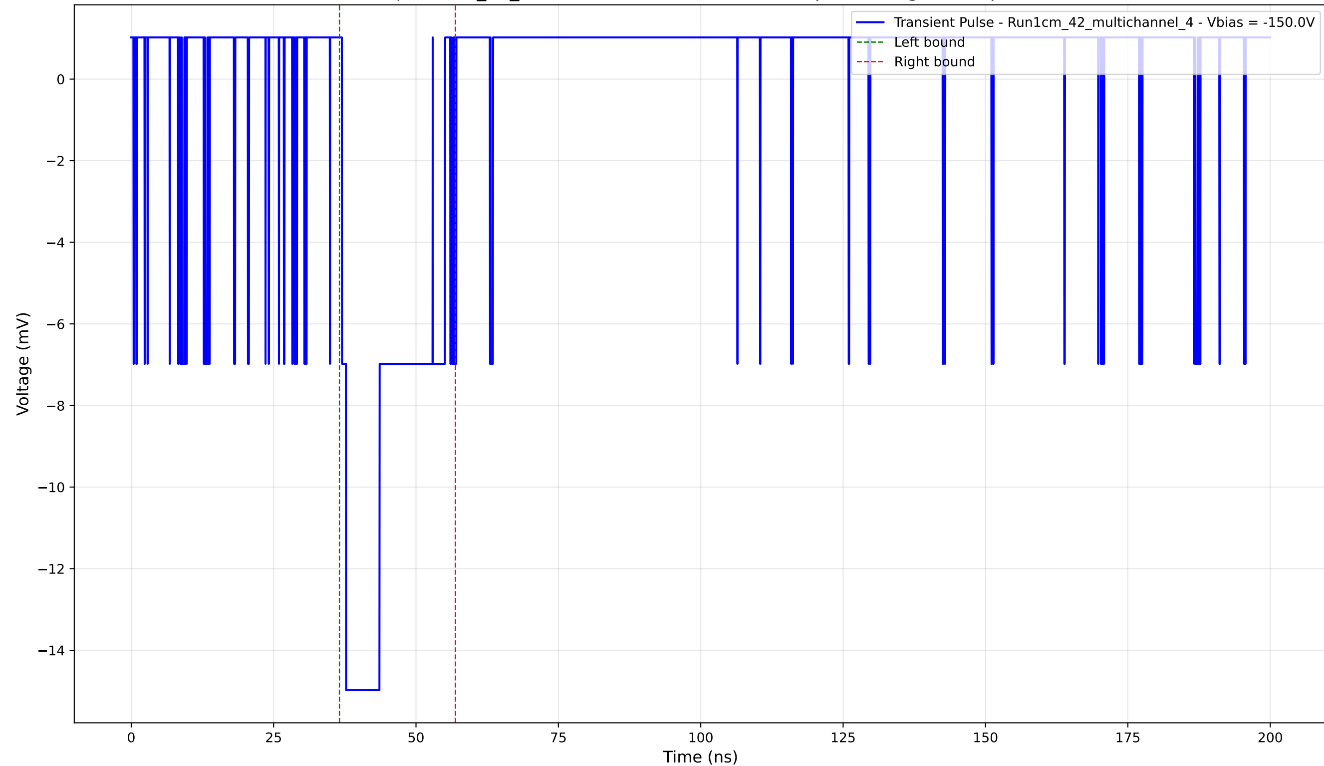
Transient Pulse - Sample: 1cm_42_multichannel - Position: 3810.0 \mu\text{m} - Charge: 3.49 pC - Rise Time: 0.74 ns
