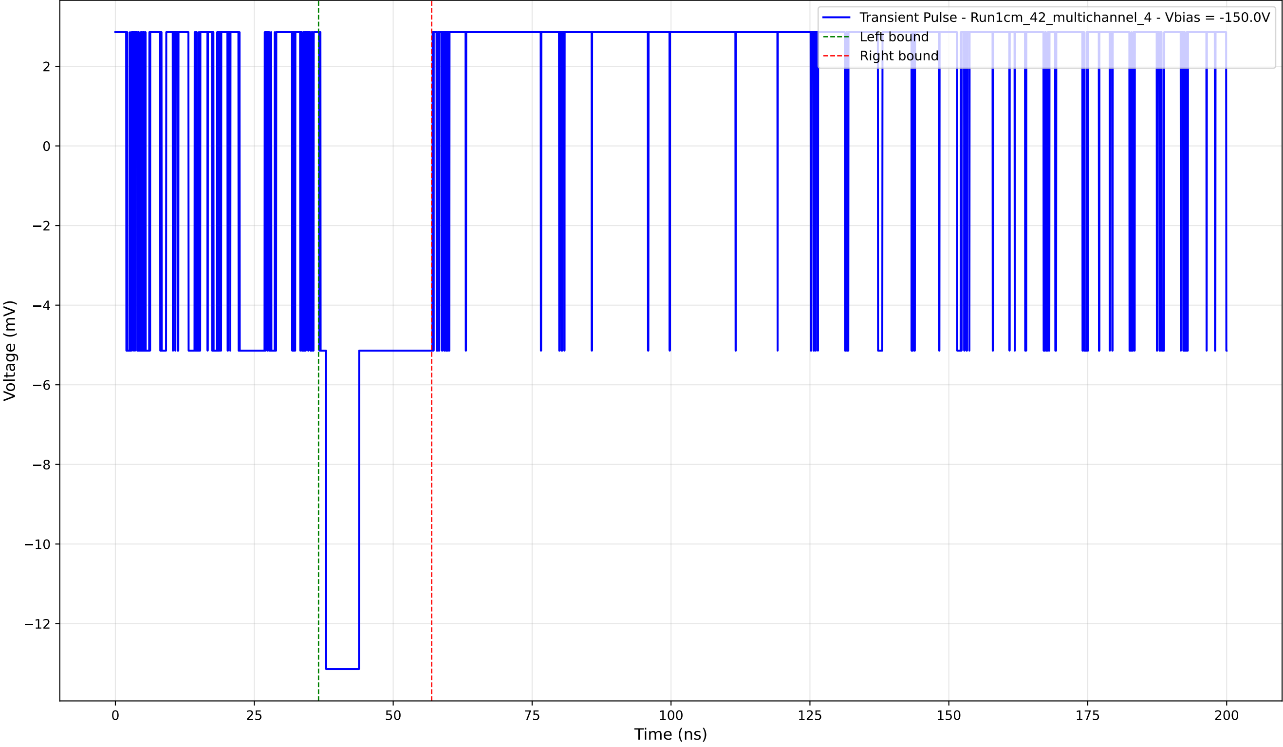
Transient Pulse - Sample: 1cm_42_multichannel - Position: 565.0 \mu\text{m} - Charge: 3.00 pC - Rise Time: 0.00 ns (N/A)
