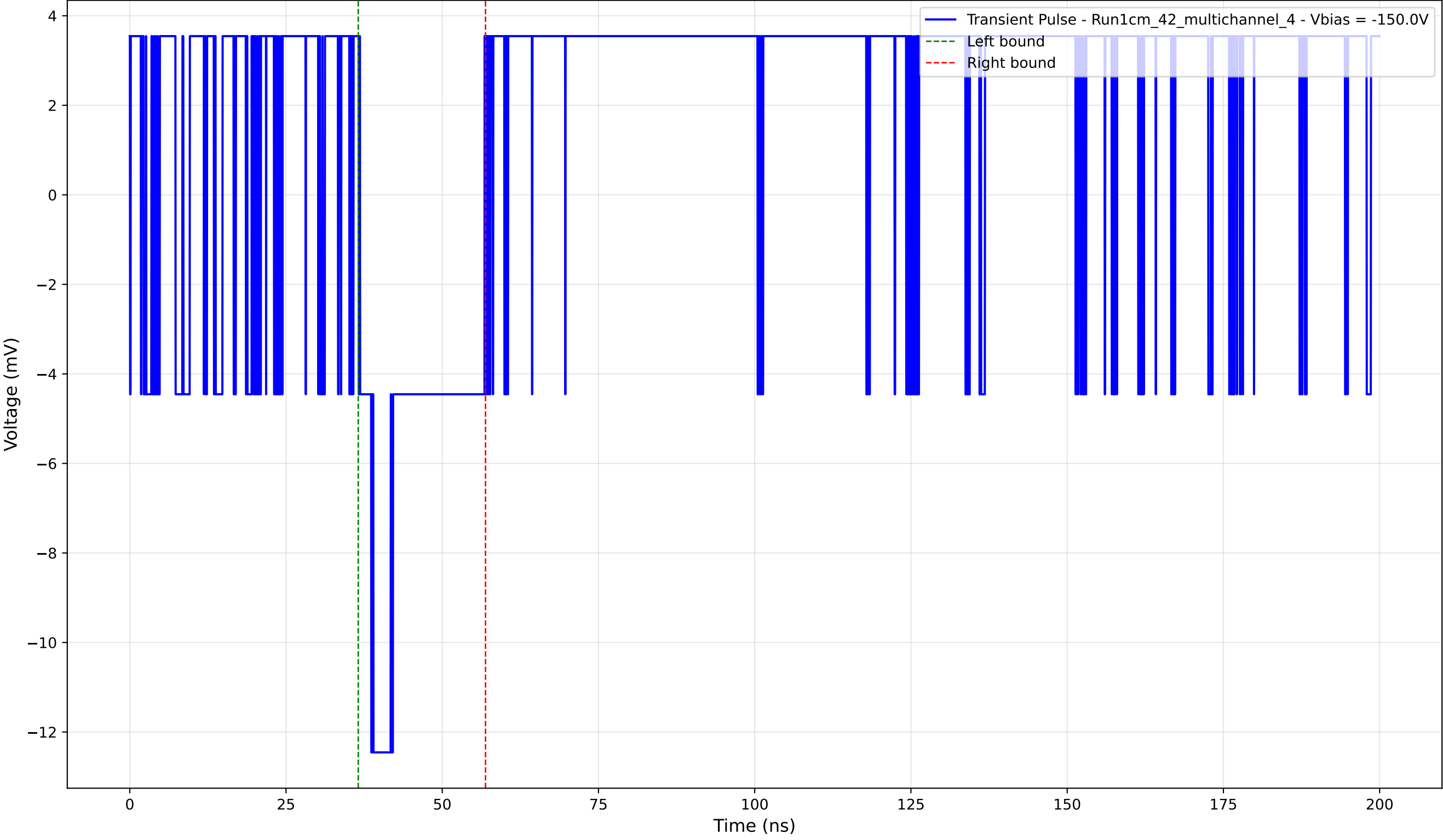
Transient Pulse - Sample: 1cm_42_multichannel - Position: 200.0 \mu\text{m} - Charge: 2.31 pC - Rise Time: 0.00 ns (N/A)
