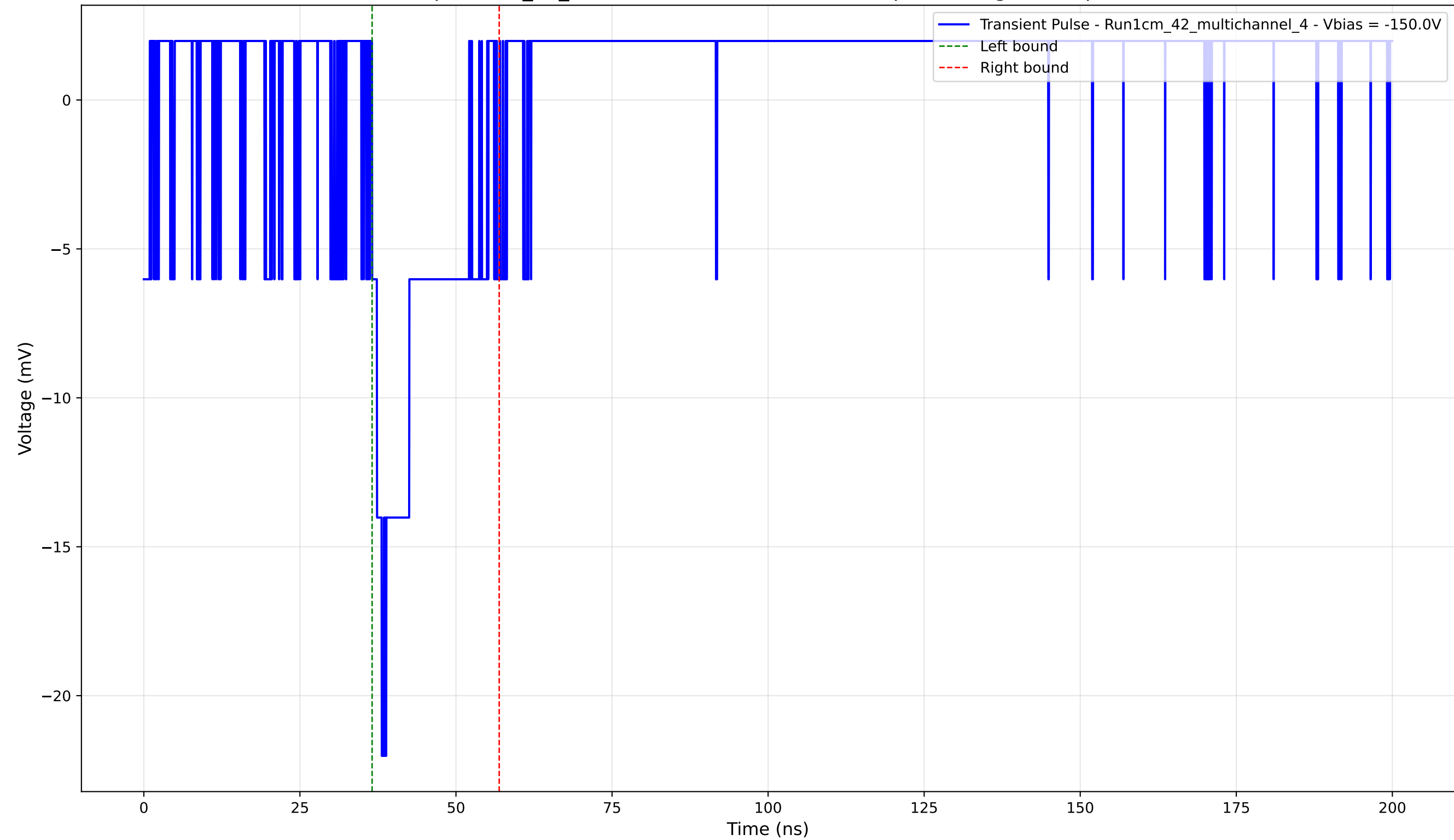
Transient Pulse - Sample: 1cm_42_multichannel - Position: 3585.0 \mu\text{m} - Charge: 3.08 pC - Rise Time: 1.56 ns
