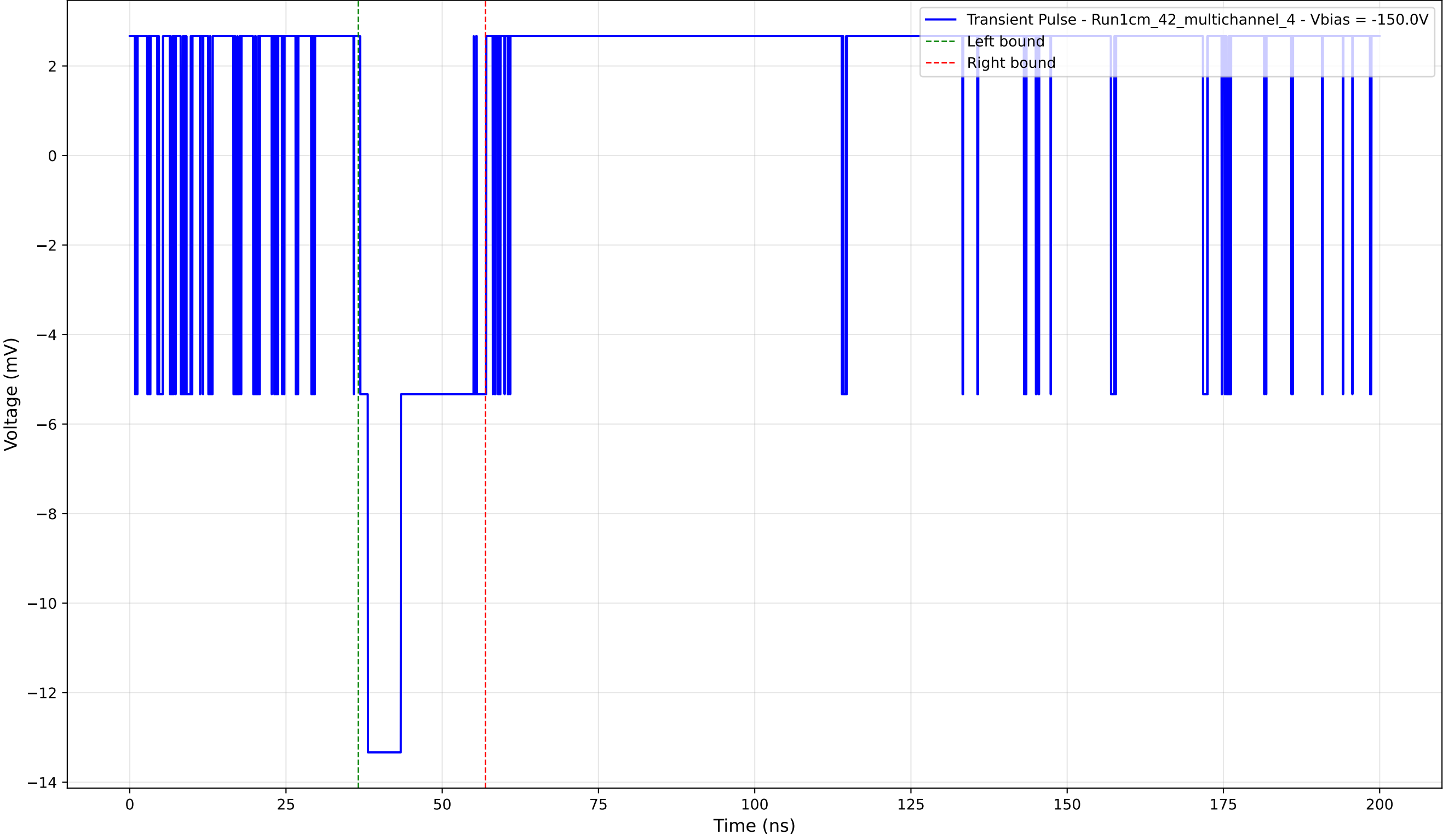
Transient Pulse - Sample: 1cm_42_multichannel - Position: 495.0 \mu\text{m} - Charge: 2.94 pC - Rise Time: 0.00 ns (N/A)
