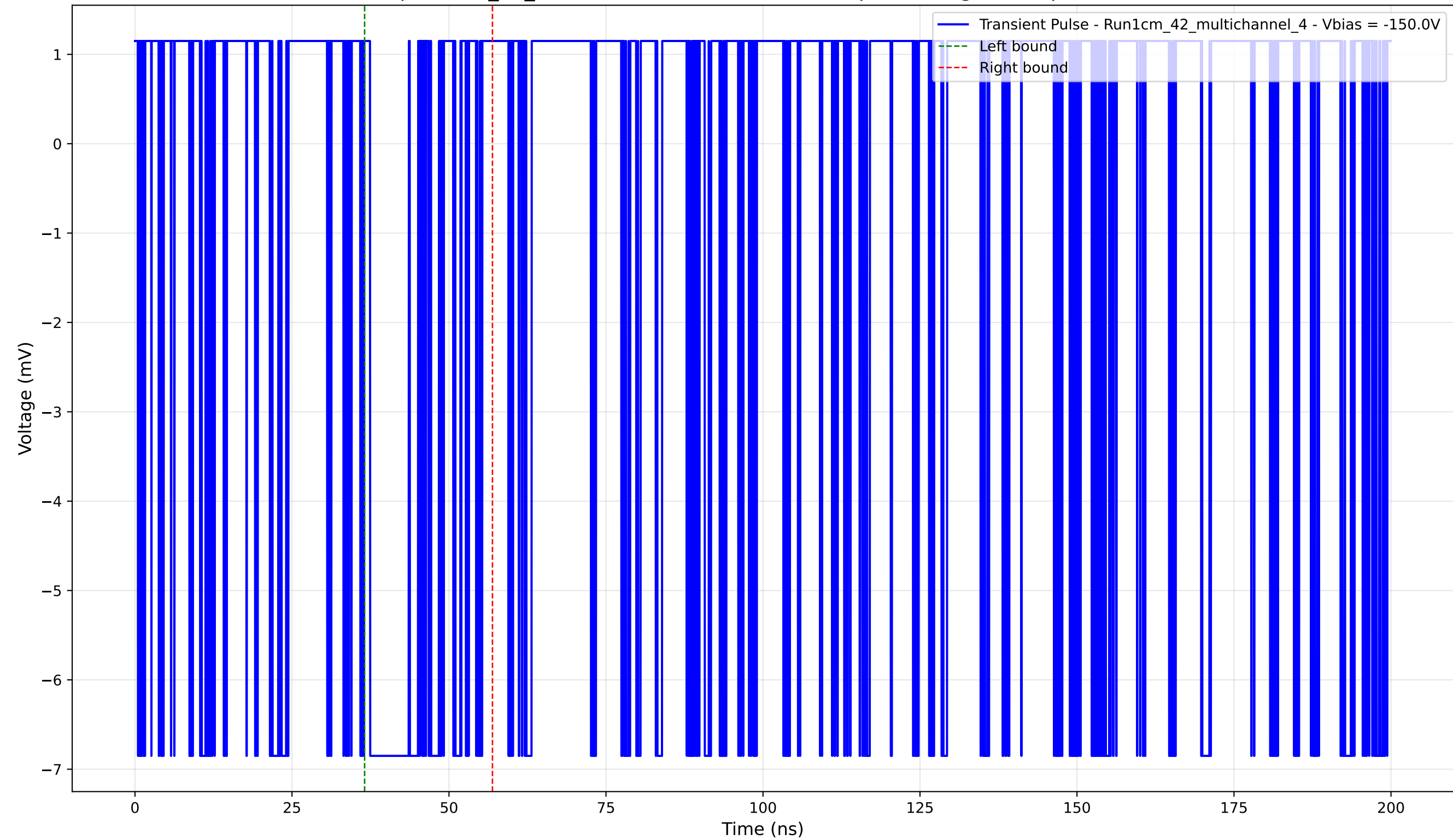
Transient Pulse - Sample: 1cm_42_multichannel - Position: 4435.0 \mu\text{m} - Charge: 1.37 pC - Rise Time: 0.00 ns (N/A)
