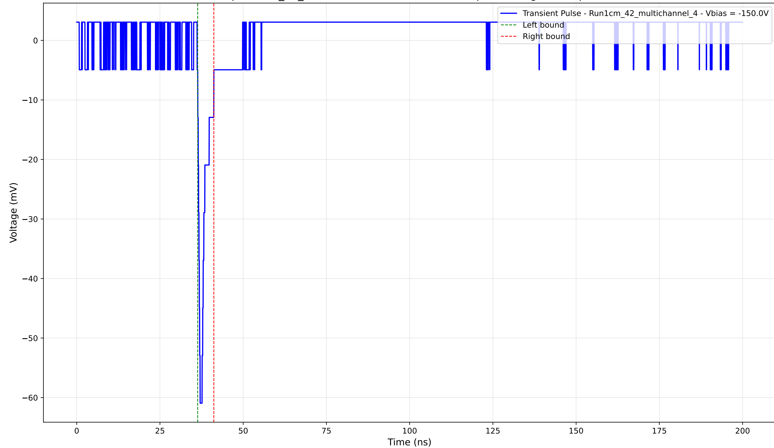
Transient Pulse - Sample: 1cm_42_multichannel - Position: 2605.0 \mu\text{m} - Charge: 2.74 pC - Rise Time: 0.72 ns
