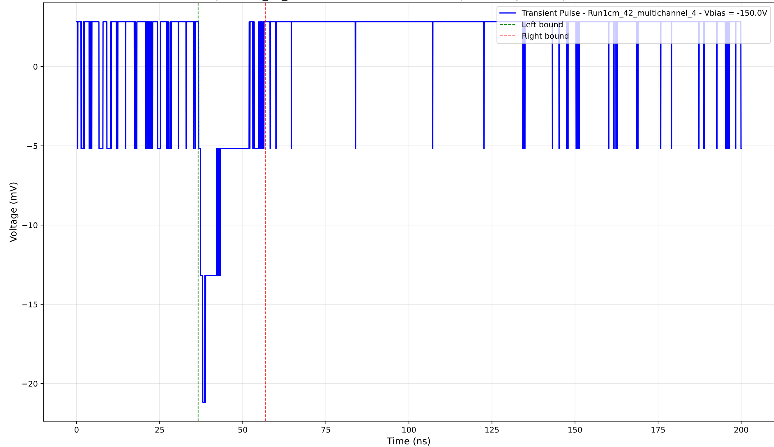
Transient Pulse - Sample: 1cm_42_multichannel - Position: 3555.0 \mu\text{m} - Charge: 2.65 pC - Rise Time: 0.00 ns (N/A)
