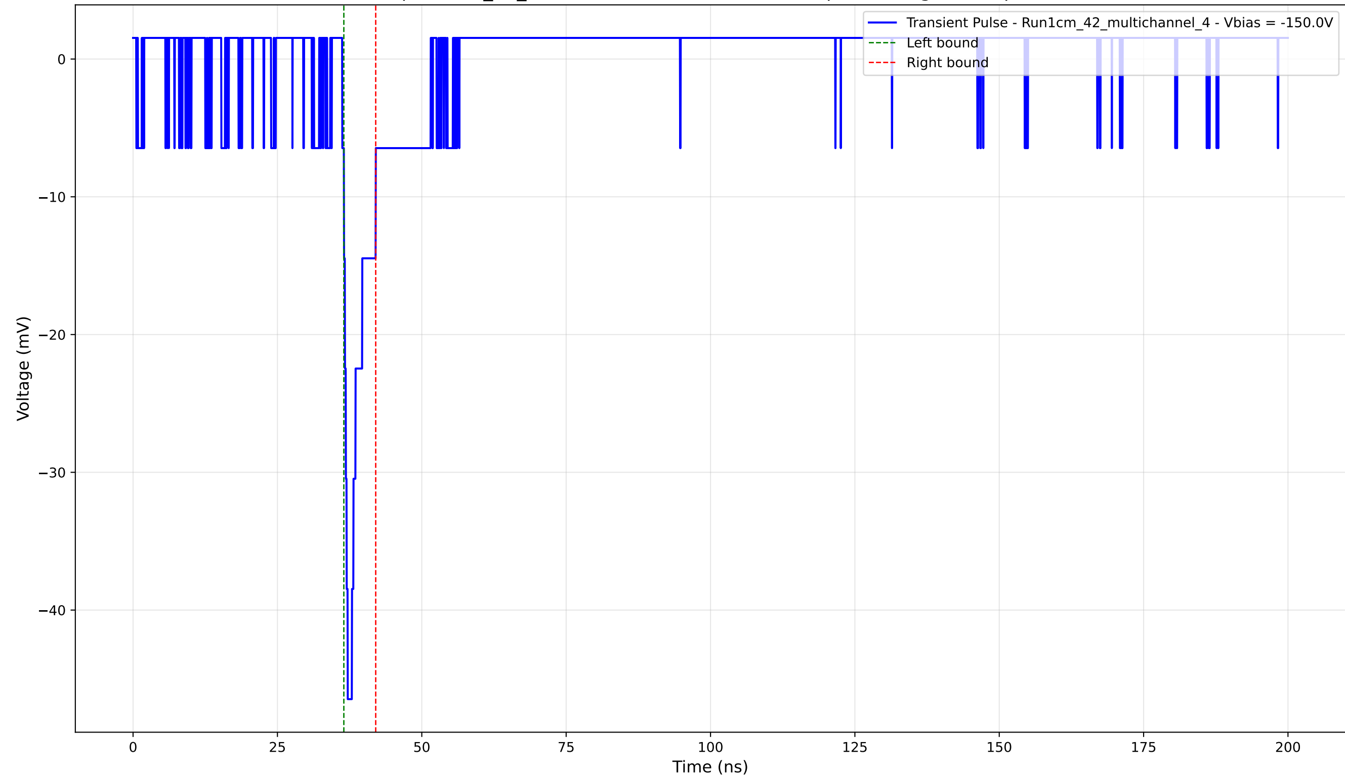
Transient Pulse - Sample: 1cm_42_multichannel - Position: 2800.0 \mu\text{m} - Charge: 2.65 pC - Rise Time: 0.95 ns
