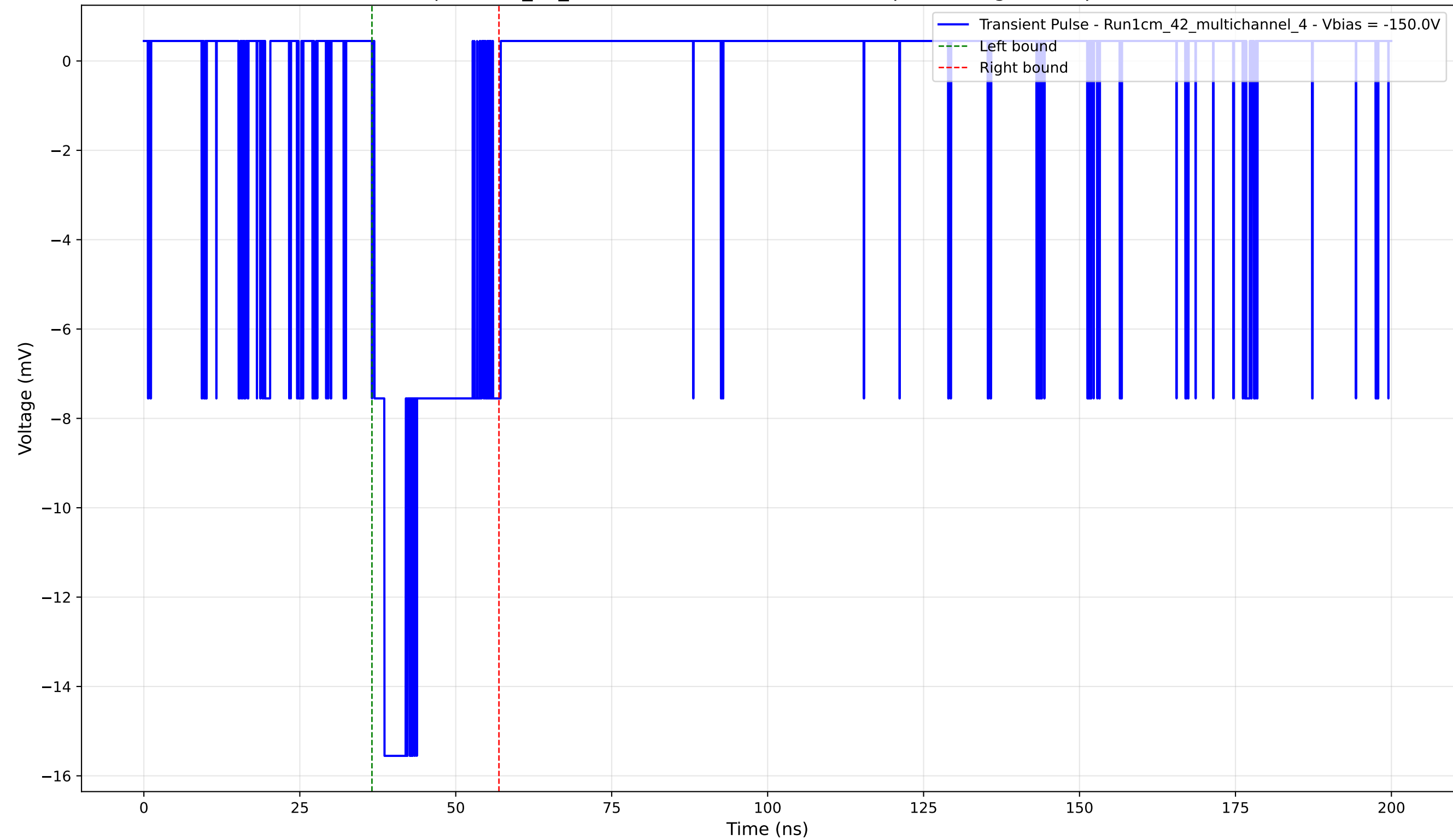
Transient Pulse - Sample: 1cm_42_multichannel - Position: 4705.0 \mu\text{m} - Charge: 3.46 pC - Rise Time: 1.62 ns
