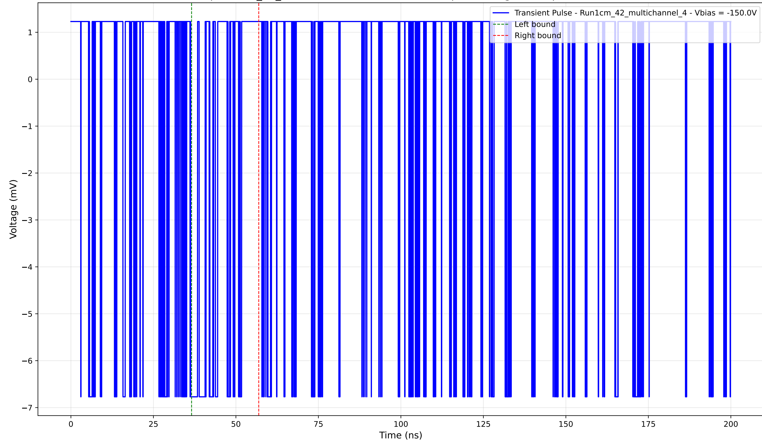
Transient Pulse - Sample: 1cm_42_multichannel - Position: 2365.0 \mu\text{m} - Charge: 0.67 pC - Rise Time: 0.00 ns (N/A)
