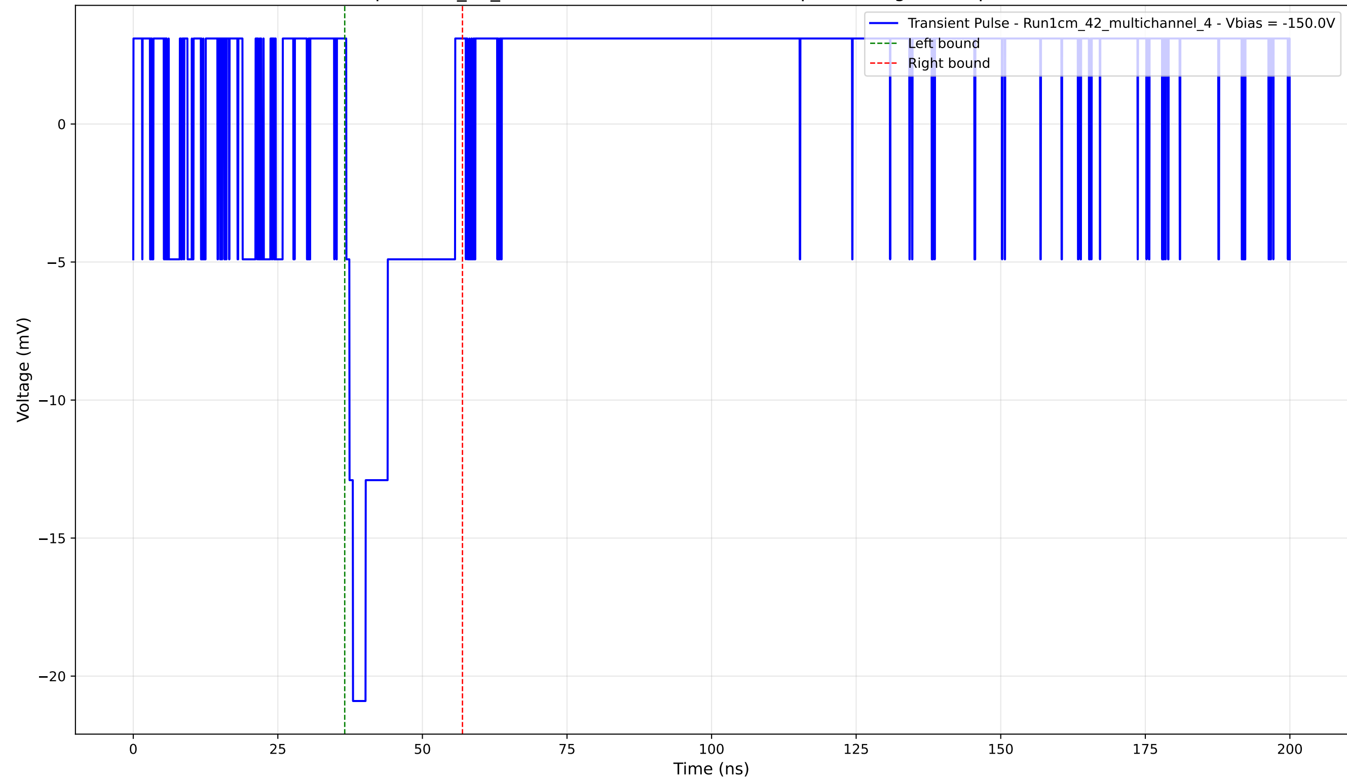
Transient Pulse - Sample: 1cm_42_multichannel - Position: 1090.0 \mu\text{m} - Charge: 3.16 pC - Rise Time: 0.00 ns (N/A)
