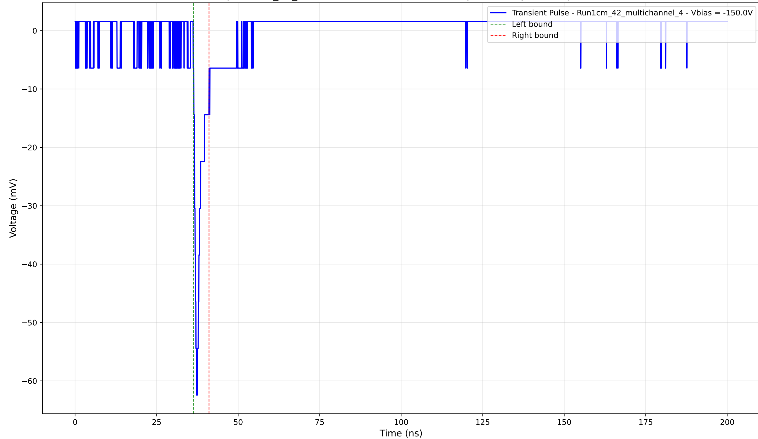
Transient Pulse - Sample: 1cm_42_multichannel - Position: 2660.0 \mu\text{m} - Charge: 2.68 pC - Rise Time: 1.06 ns
