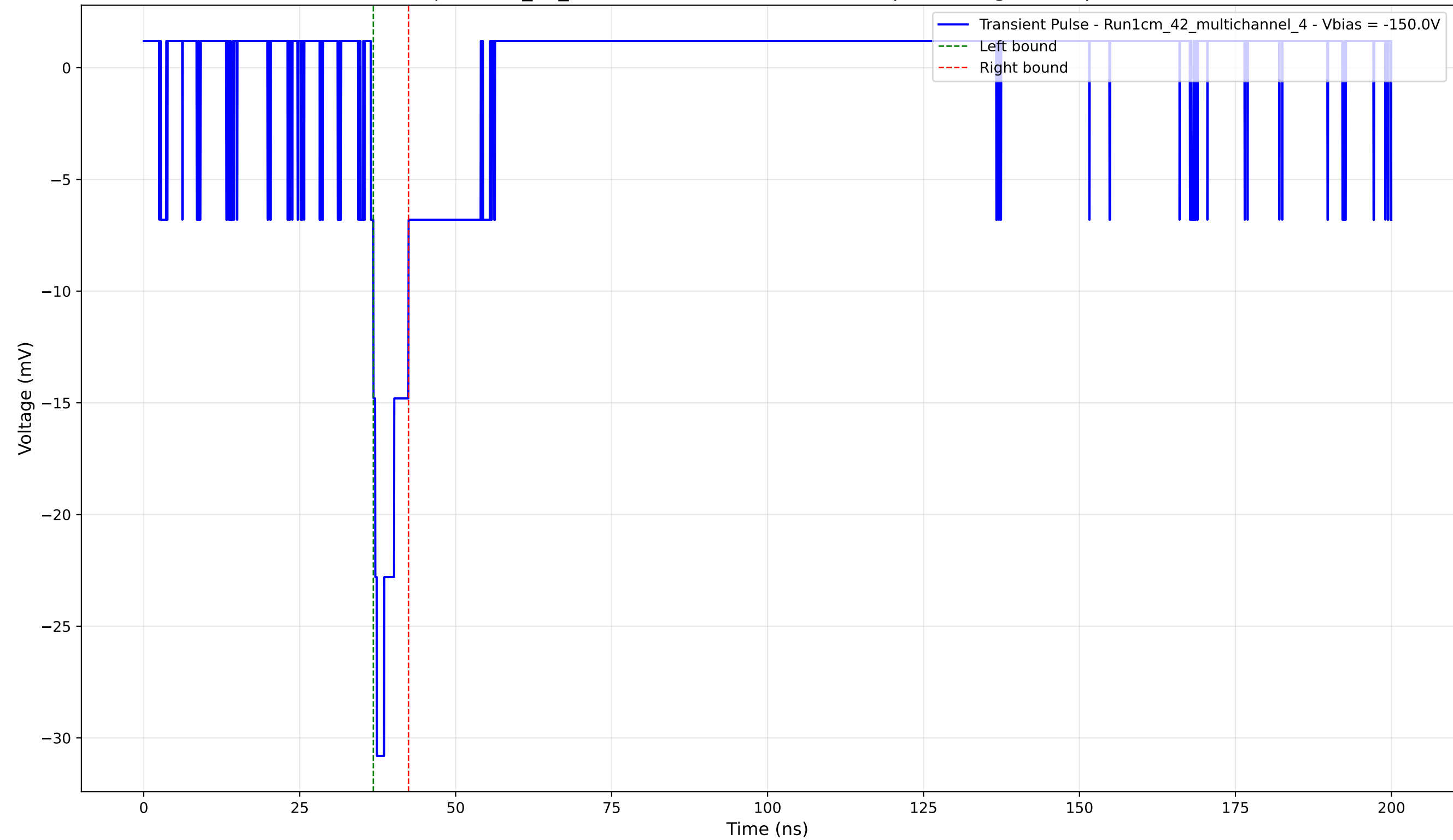
Transient Pulse - Sample: 1cm_42_multichannel - Position: 1575.0 \mu\text{m} - Charge: 2.34 pC - Rise Time: 0.95 ns
