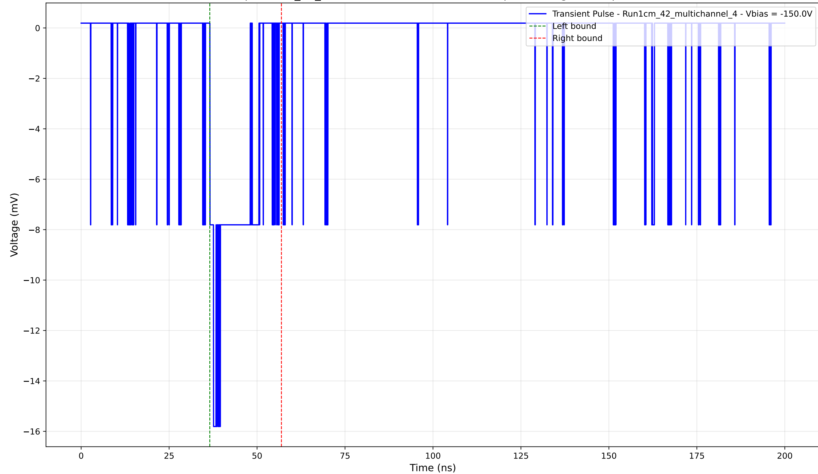
Transient Pulse - Sample: 1cm_42_multichannel - Position: 3350.0 \mu\text{m} - Charge: 2.44 pC - Rise Time: 1.04 ns
