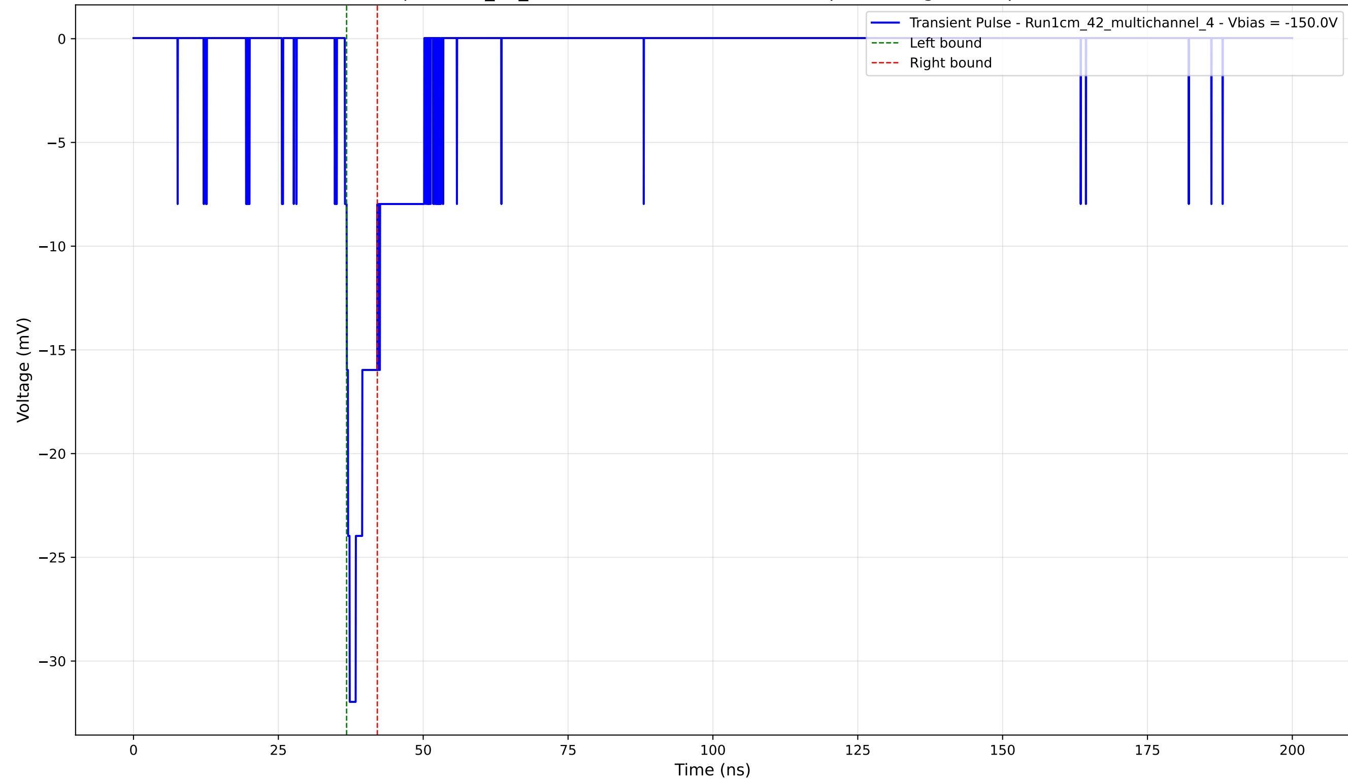
Transient Pulse - Sample: 1cm_42_multichannel - Position: 3085.0 \mu\text{m} - Charge: 2.25 pC - Rise Time: 0.83 ns
