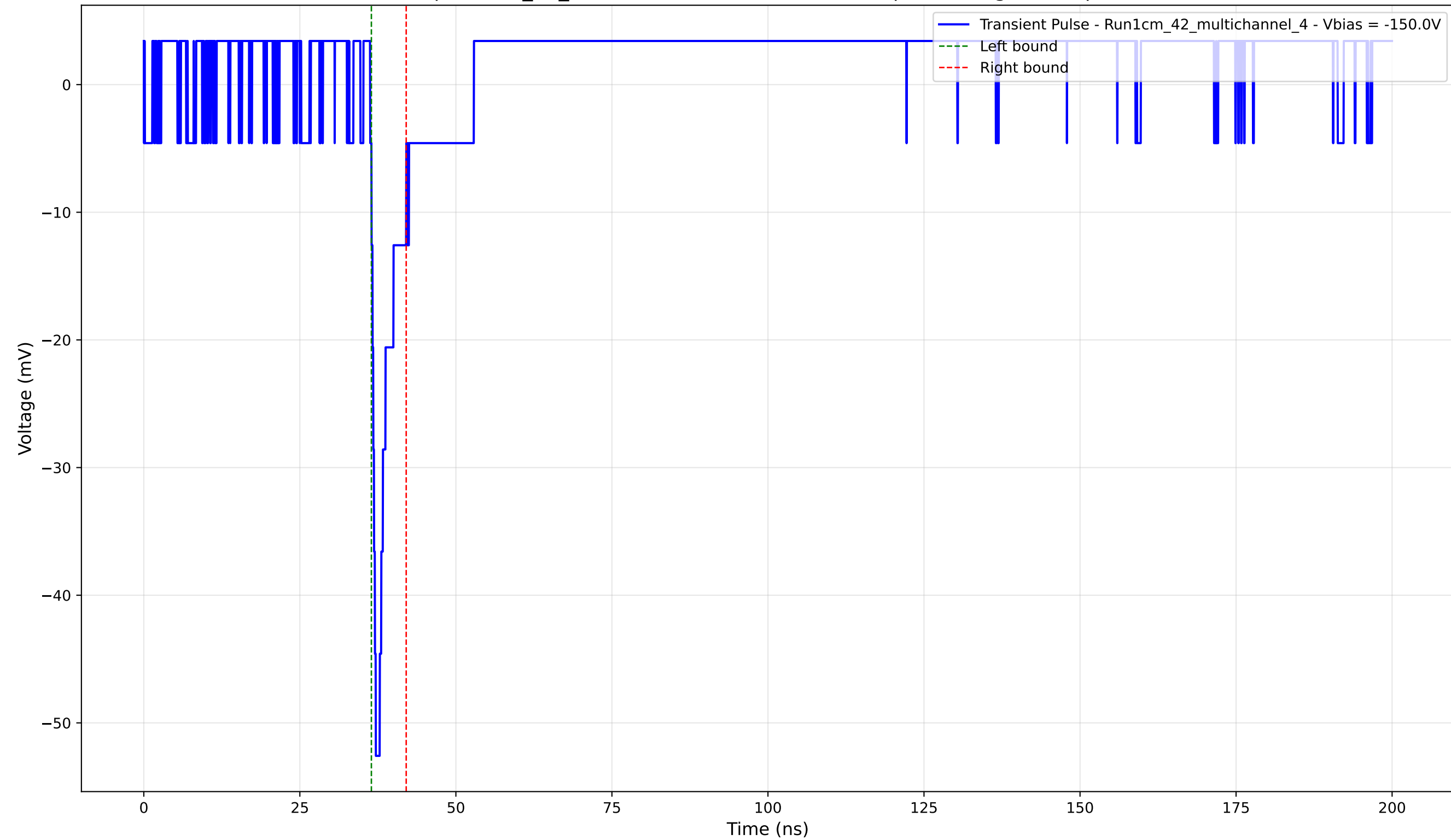
Transient Pulse - Sample: 1cm_42_multichannel - Position: 2015.0 \mu\text{m} - Charge: 2.75 pC - Rise Time: 0.70 ns
