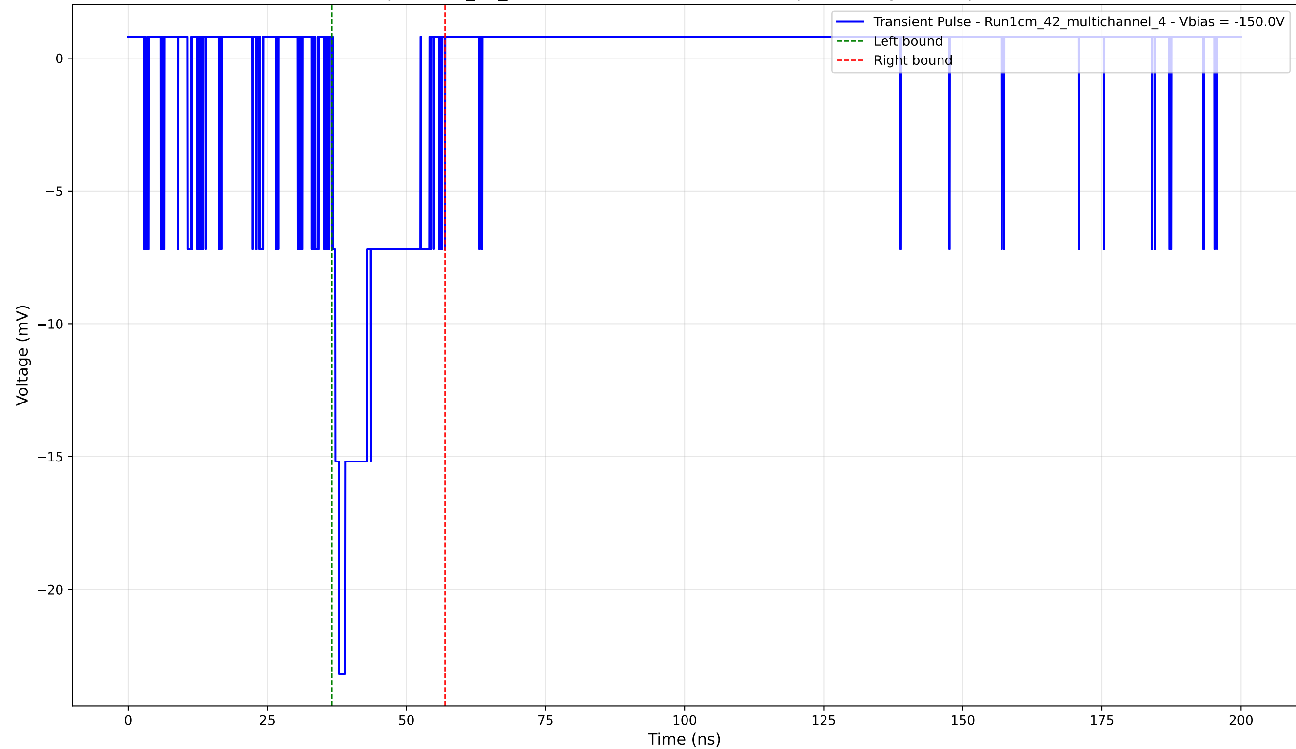
Transient Pulse - Sample: 1cm_42_multichannel - Position: 3535.0 \mu\text{m} - Charge: 3.61 pC - Rise Time: 1.16 ns
