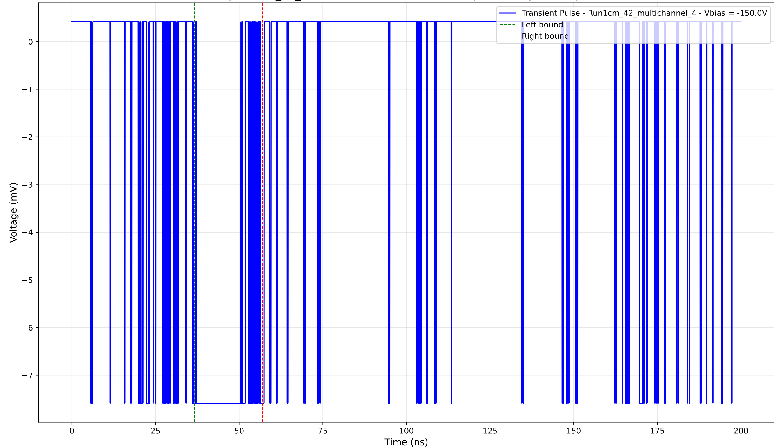
Transient Pulse - Sample: 1cm_42_multichannel - Position: 4850.0 \mu\text{m} - Charge: 2.61 pC - Rise Time: 0.02 ns
