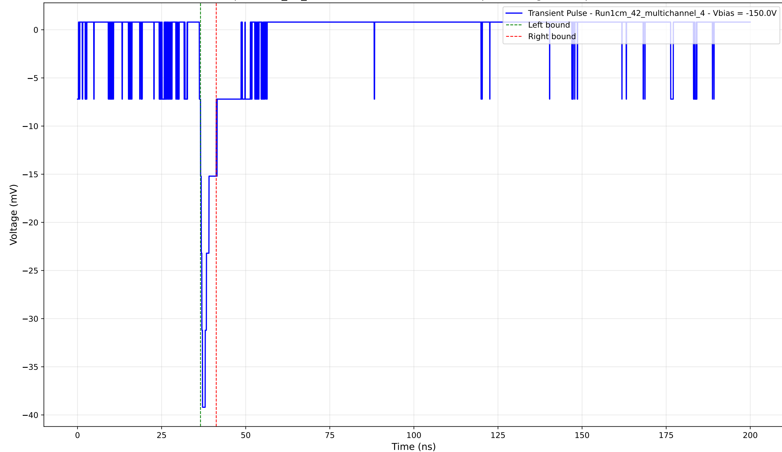
Transient Pulse - Sample: 1cm_42_multichannel - Position: 2825.0 \mu\text{m} - Charge: 2.13 pC - Rise Time: 0.95 ns
