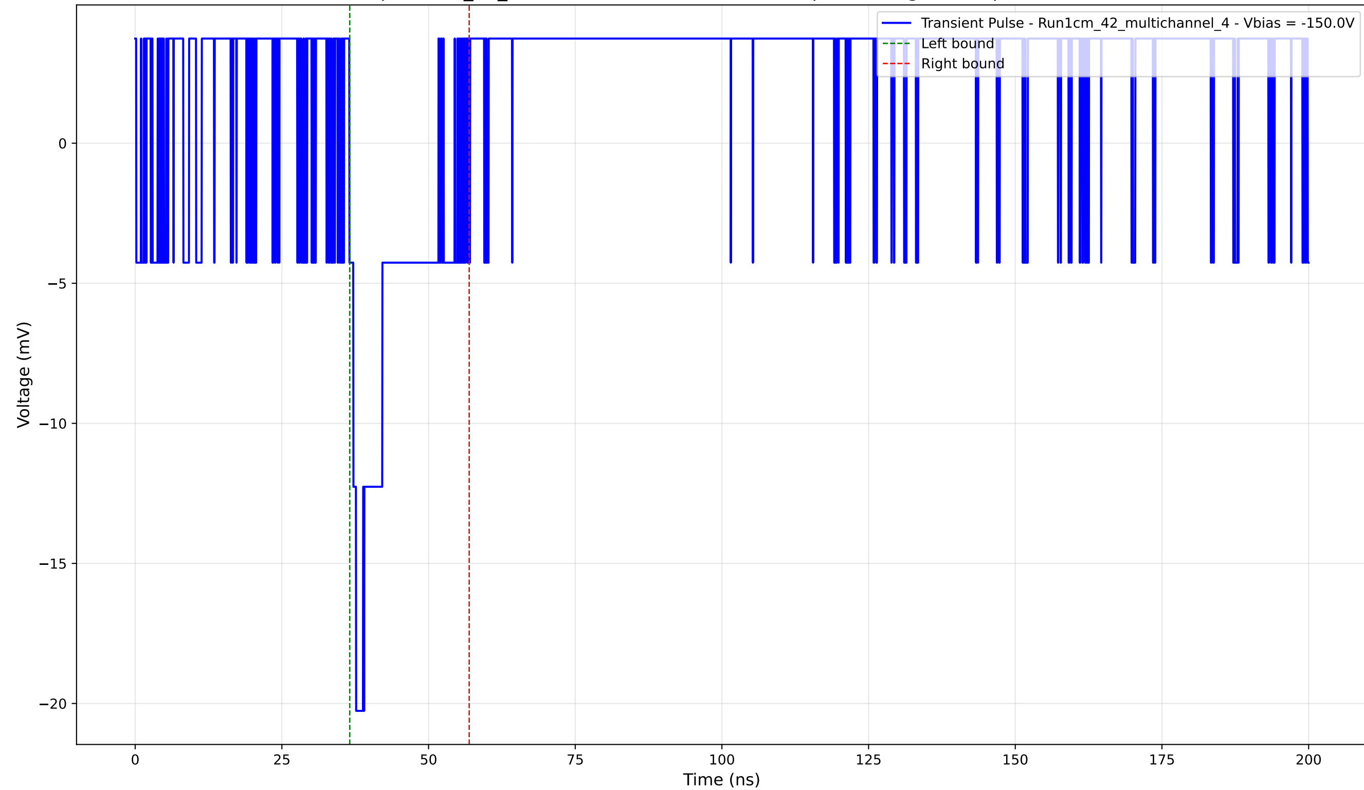
Transient Pulse - Sample: 1cm_42_multichannel - Position: 1435.0 \mu\text{m} - Charge: 2.51 pC - Rise Time: 0.00 ns (N/A)
