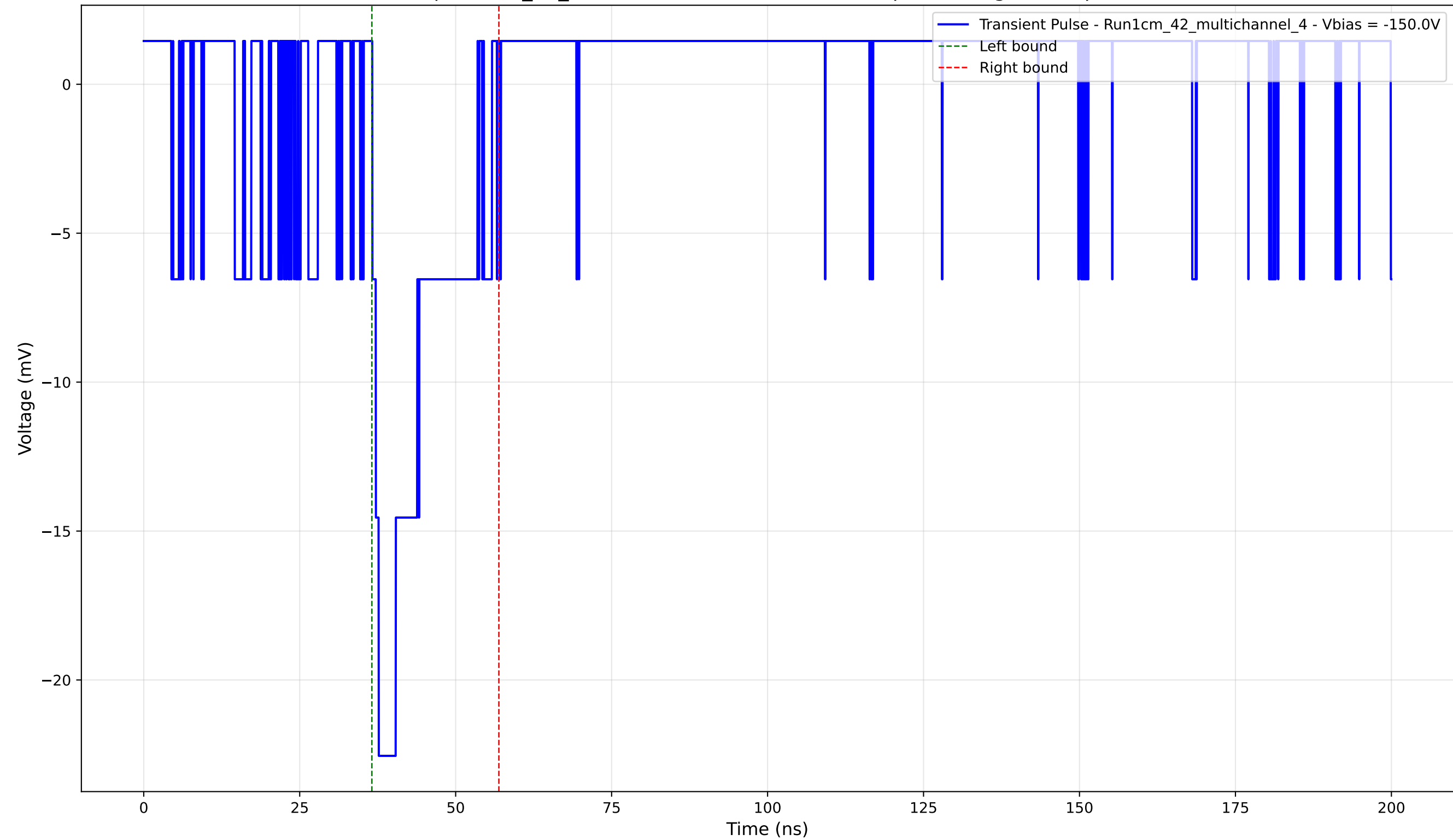
Transient Pulse - Sample: 1cm_42_multichannel - Position: 1240.0 \mu\text{m} - Charge: 3.89 pC - Rise Time: 1.04 ns
