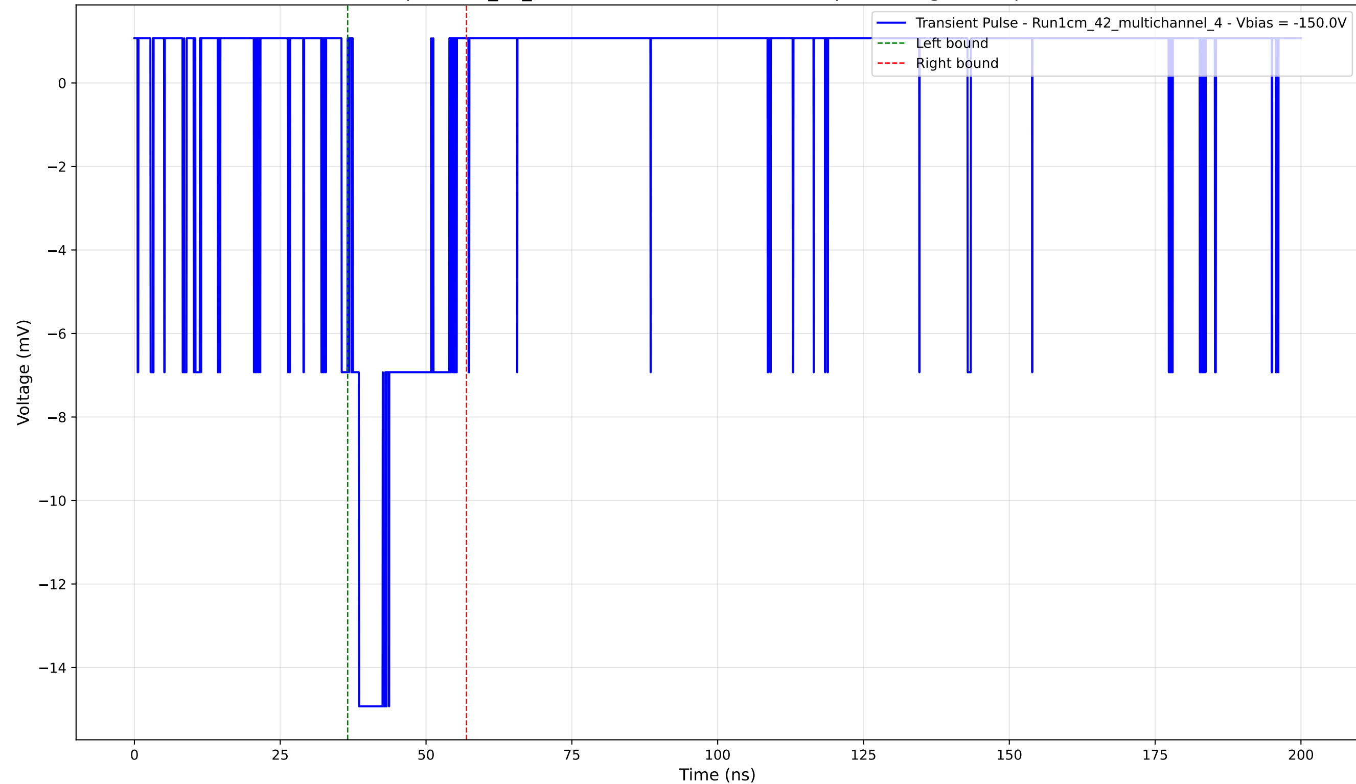
Transient Pulse - Sample: 1cm_42_multichannel - Position: 4525.0 \mu\text{m} - Charge: 3.03 pC - Rise Time: 1.08 ns
