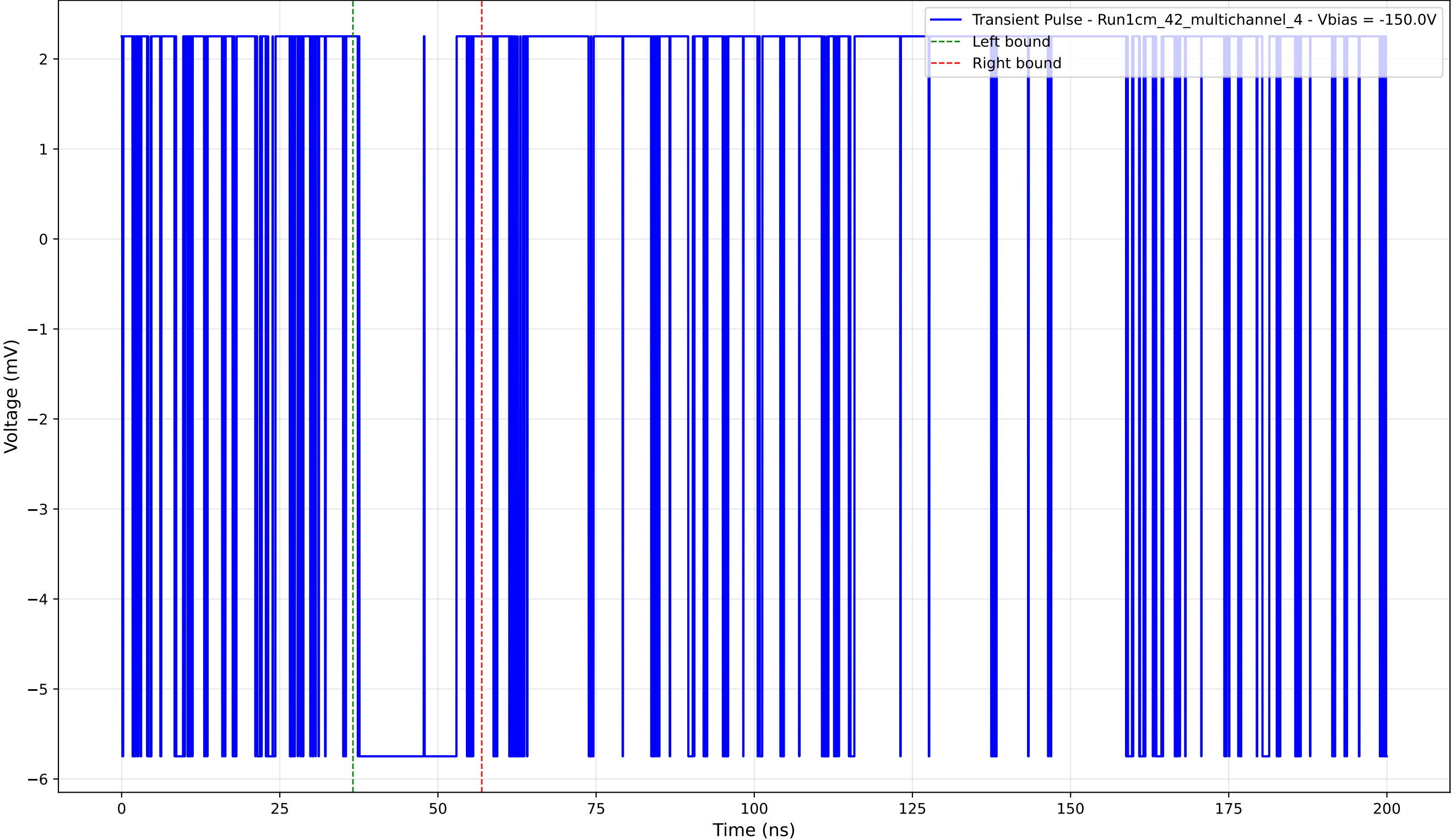
Transient Pulse - Sample: 1cm_42_multichannel - Position: 4360.0 \mu\text{m} - Charge: 1.60 pC - Rise Time: 0.00 ns (N/A)
