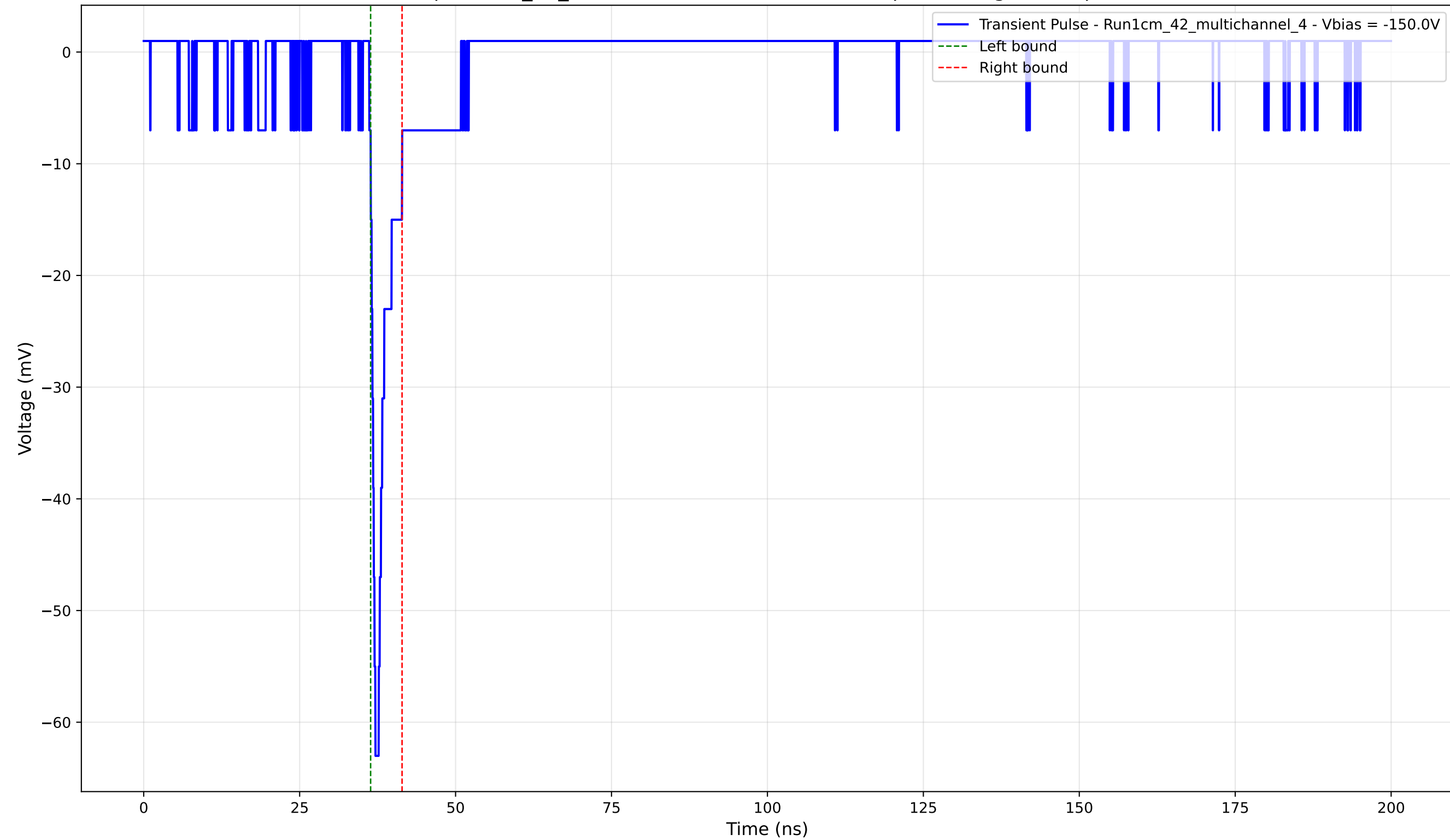
Transient Pulse - Sample: 1cm_42_multichannel - Position: 2125.0 \mu\text{m} - Charge: 2.97 pC - Rise Time: 0.98 ns
