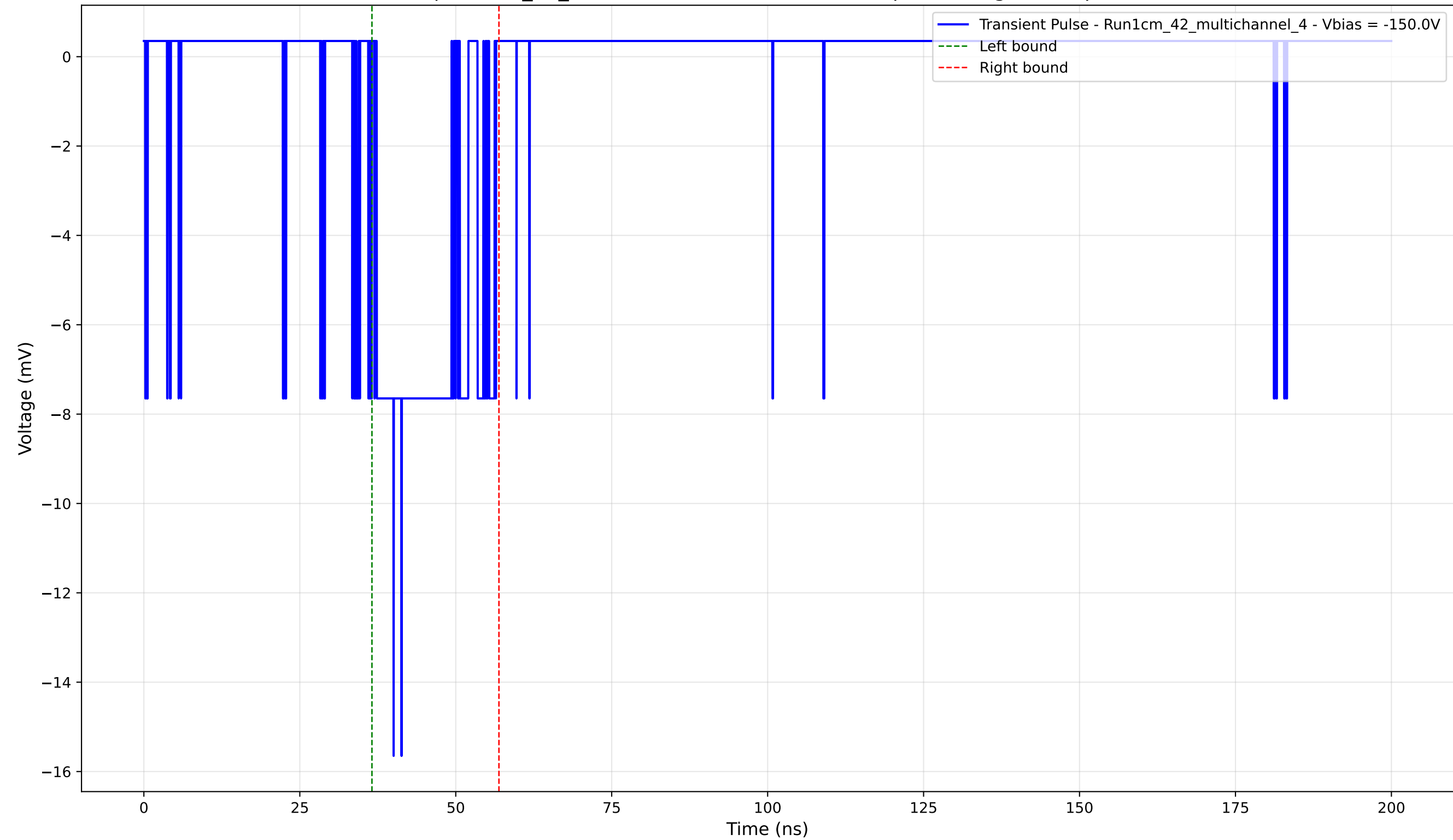
Transient Pulse - Sample: 1cm_42_multichannel - Position: 4830.0 \mu\text{m} - Charge: 2.45 pC - Rise Time: 2.70 ns
