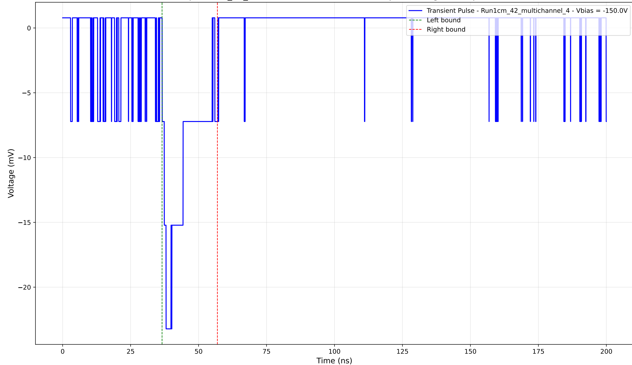
Transient Pulse - Sample: 1cm_42_multichannel - Position: 1110.0 \mu\text{m} - Charge: 4.21 pC - Rise Time: 1.46 ns
