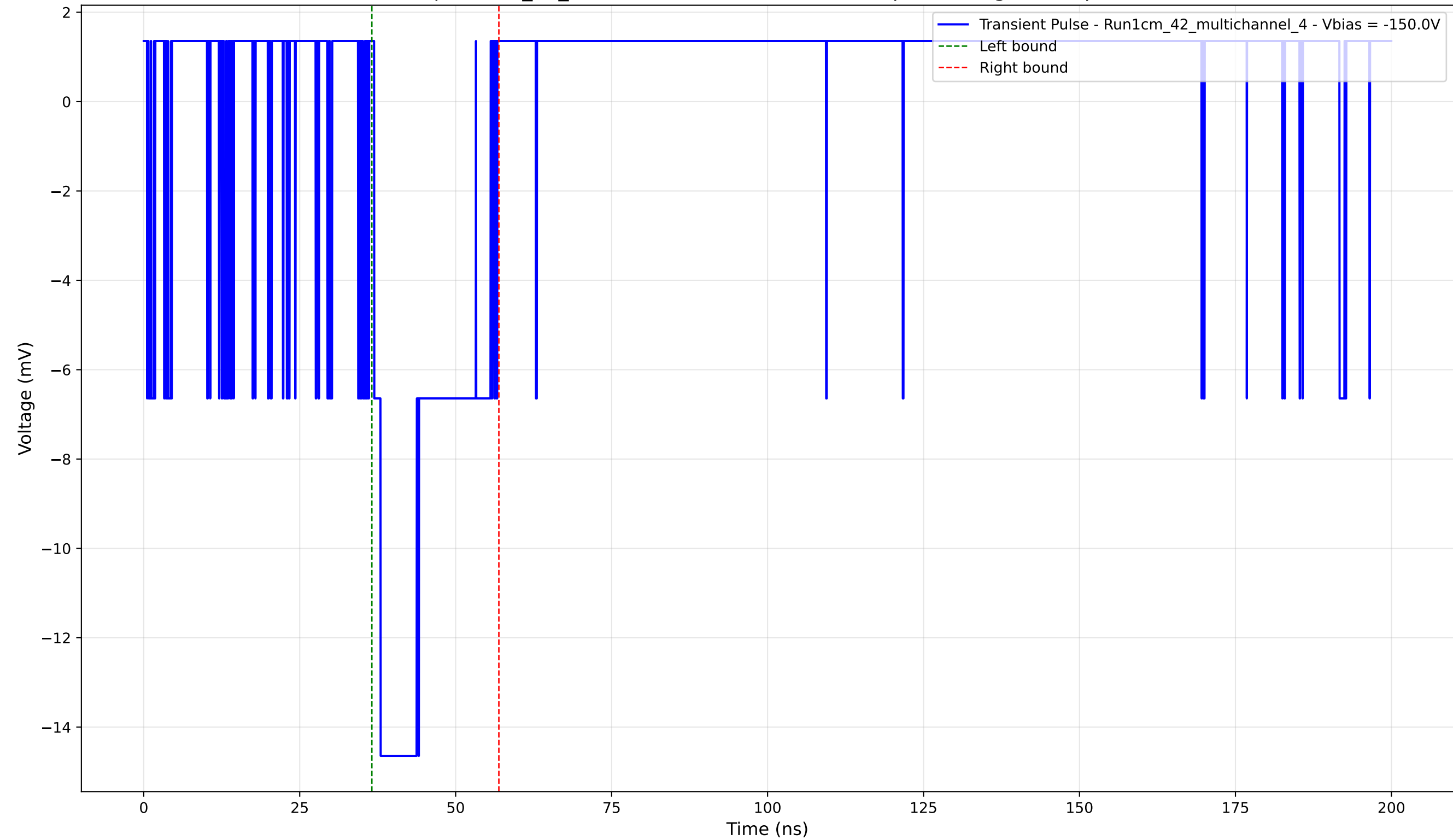
Transient Pulse - Sample: 1cm_42_multichannel - Position: 4055.0 \mu\text{m} - Charge: 3.43 pC - Rise Time: 1.04 ns
