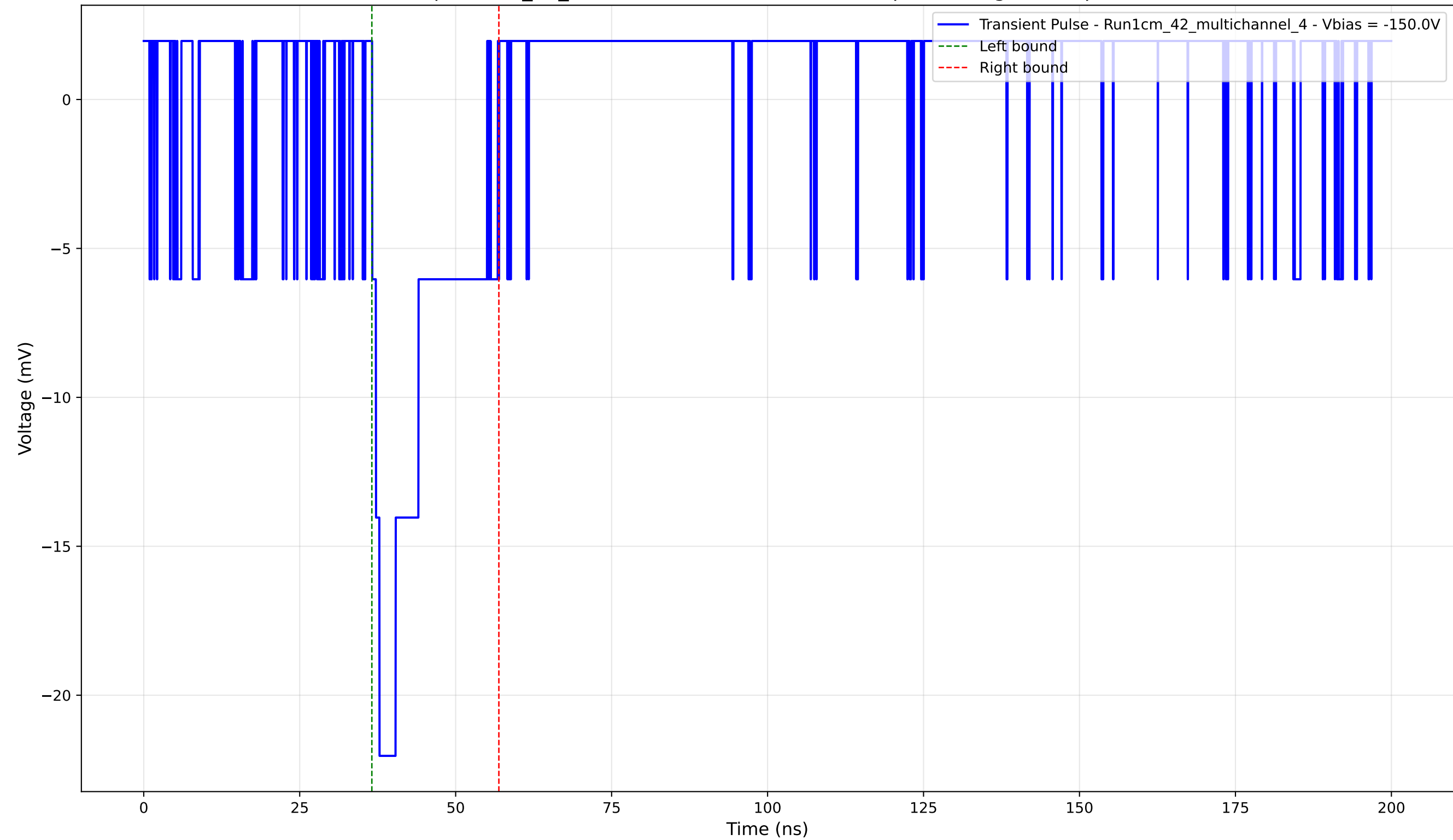
Transient Pulse - Sample: 1cm_42_multichannel - Position: 1190.0 \mu\text{m} - Charge: 3.89 pC - Rise Time: 1.18 ns
