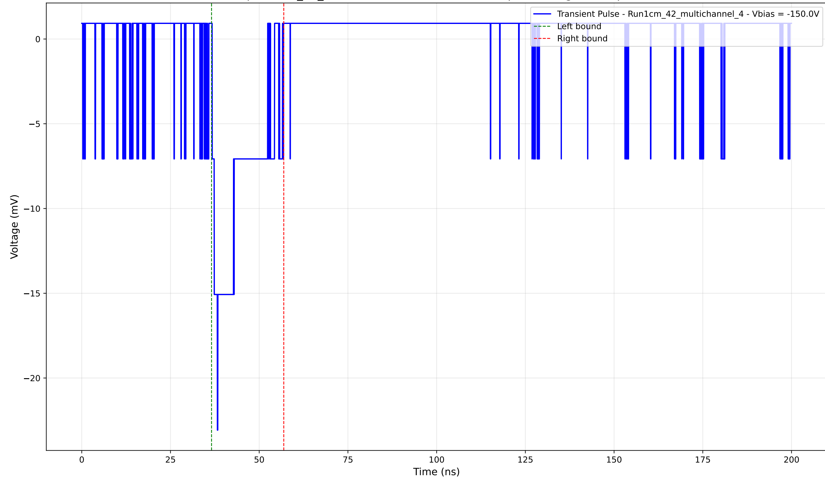
Transient Pulse - Sample: 1cm_42_multichannel - Position: 3580.0 \mu\text{m} - Charge: 3.42 pC - Rise Time: 1.48 ns
