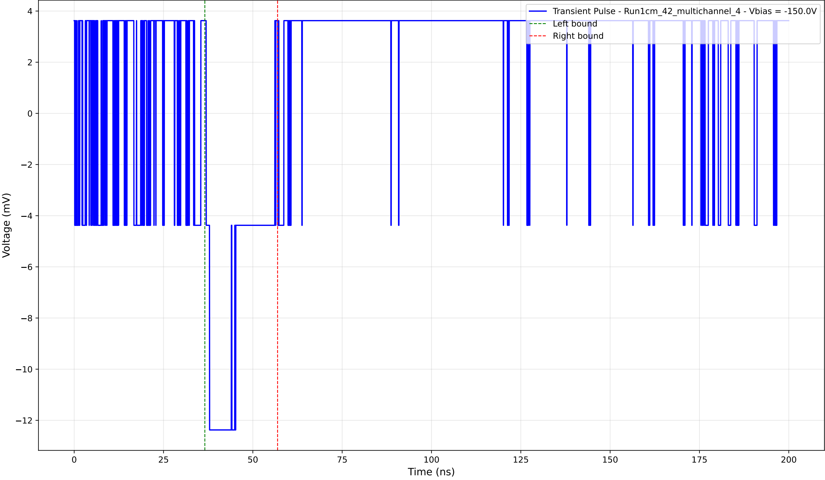
Transient Pulse - Sample: 1cm_42_multichannel - Position: 670.0 \mu\text{m} - Charge: 2.73 pC - Rise Time: 0.00 ns (N/A)
