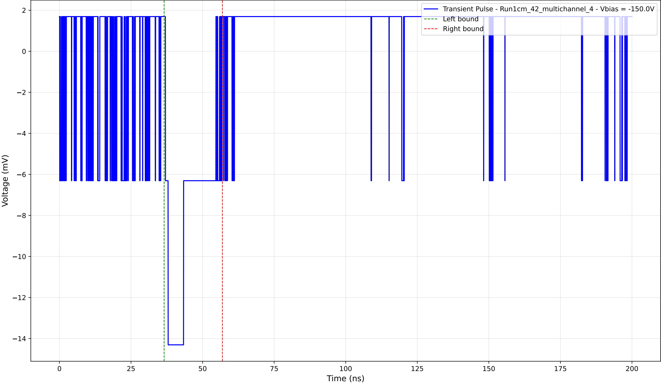
Transient Pulse - Sample: 1cm_42_multichannel - Position: 620.0 \mu\text{m} - Charge: 3.20 pC - Rise Time: 0.00 ns (N/A)
