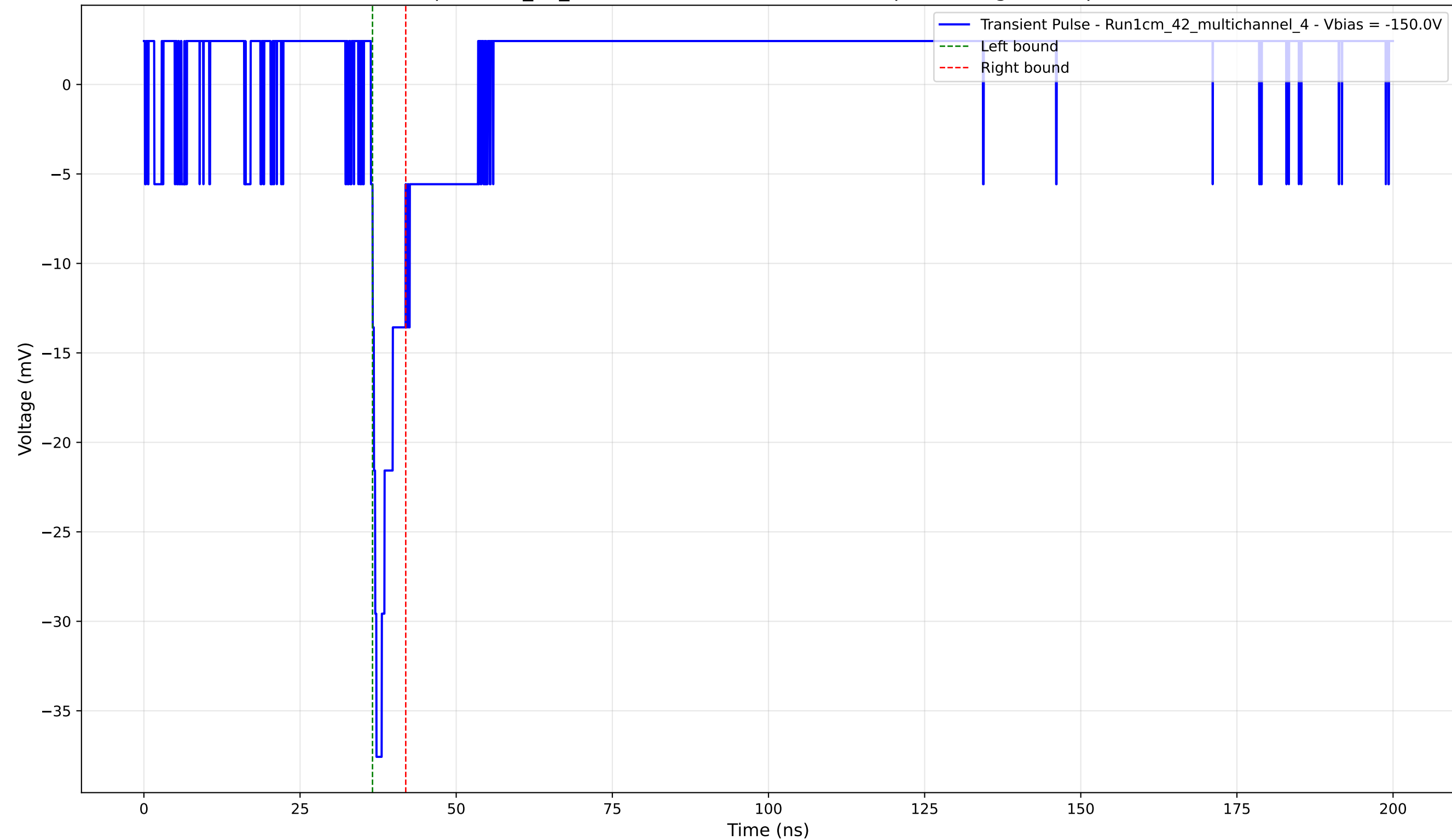
Transient Pulse - Sample: 1cm_42_multichannel - Position: 1805.0 \mu\text{m} - Charge: 2.30 pC - Rise Time: 0.89 ns
