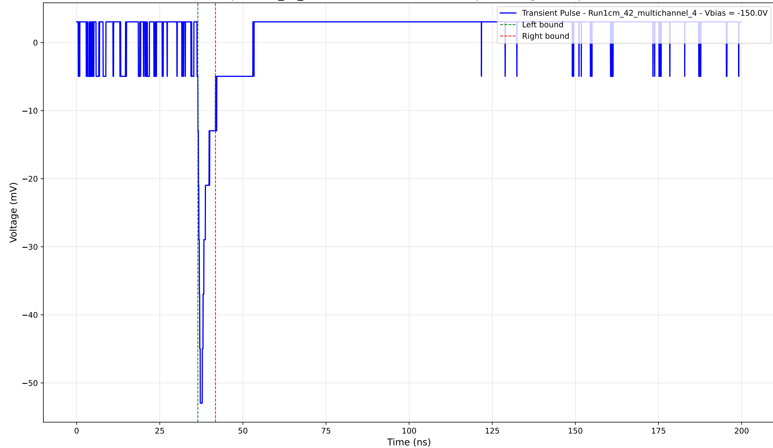
Transient Pulse - Sample: 1cm_42_multichannel - Position: 2010.0 \mu\text{m} - Charge: 2.69 pC - Rise Time: 0.72 ns
