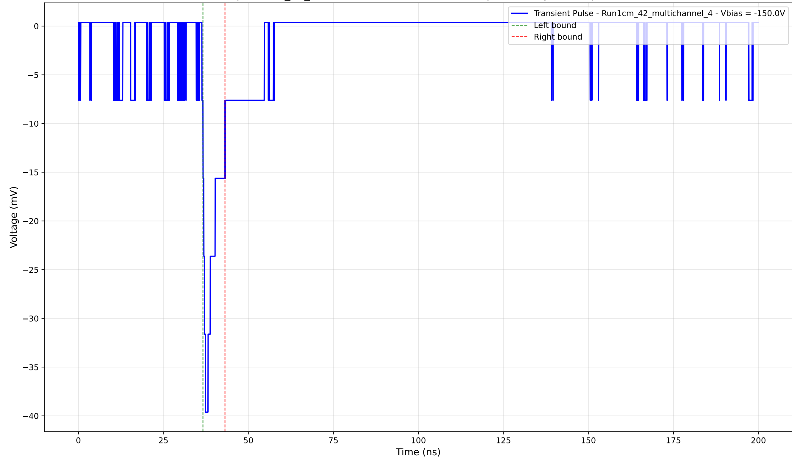
Transient Pulse - Sample: 1cm_42_multichannel - Position: 1725.0 \mu\text{m} - Charge: 2.95 pC - Rise Time: 1.03 ns
