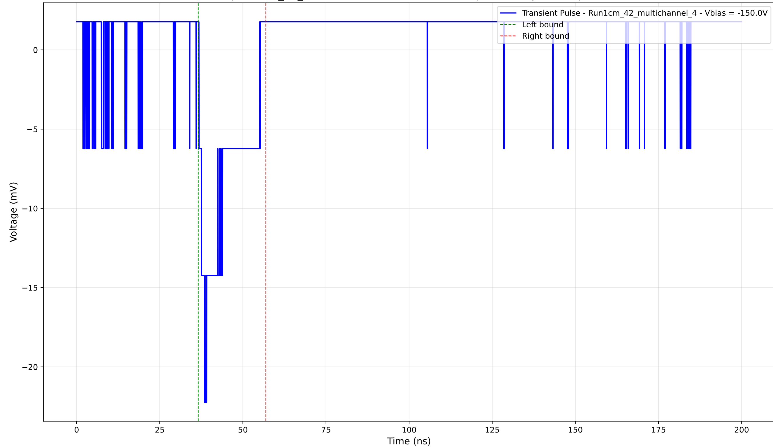
Transient Pulse - Sample: 1cm_42_multichannel - Position: 3715.0 \mu\text{m} - Charge: 3.29 pC - Rise Time: 1.64 ns
