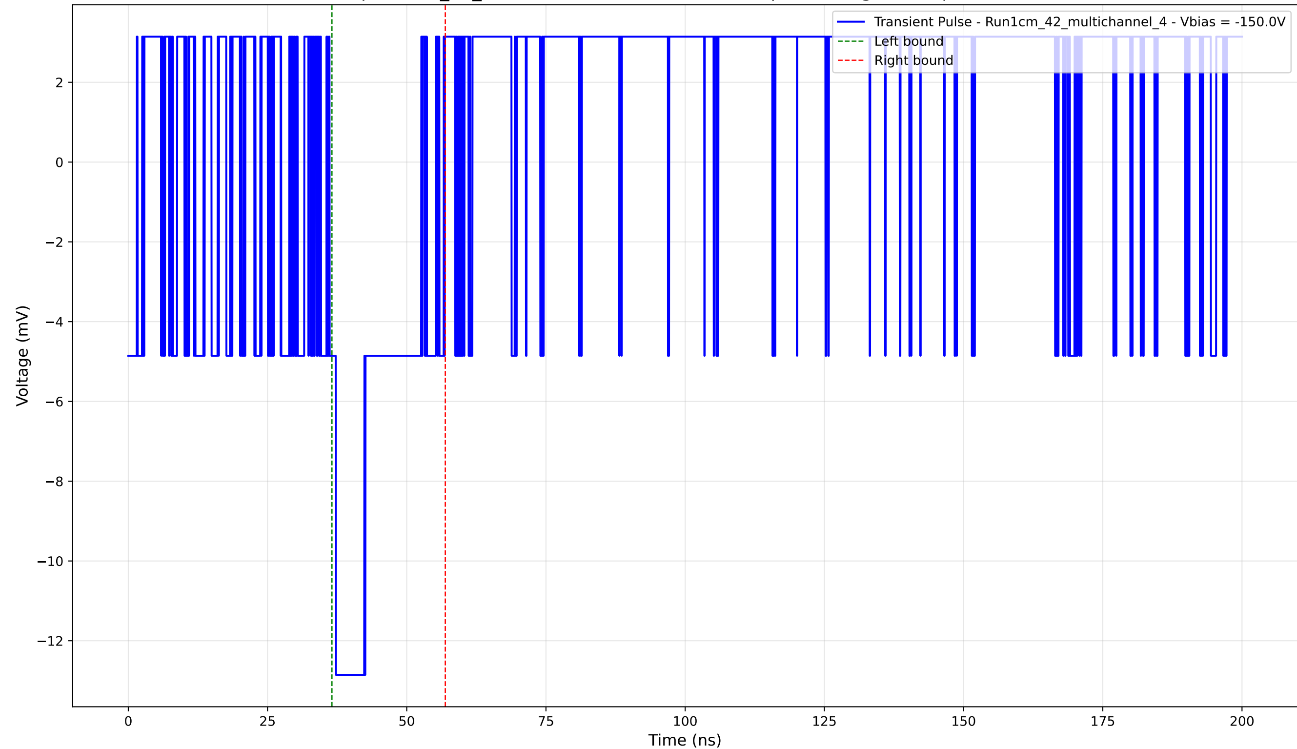
Transient Pulse - Sample: 1cm_42_multichannel - Position: 1315.0 \mu\text{m} - Charge: 2.61 pC - Rise Time: 0.00 ns (N/A)
