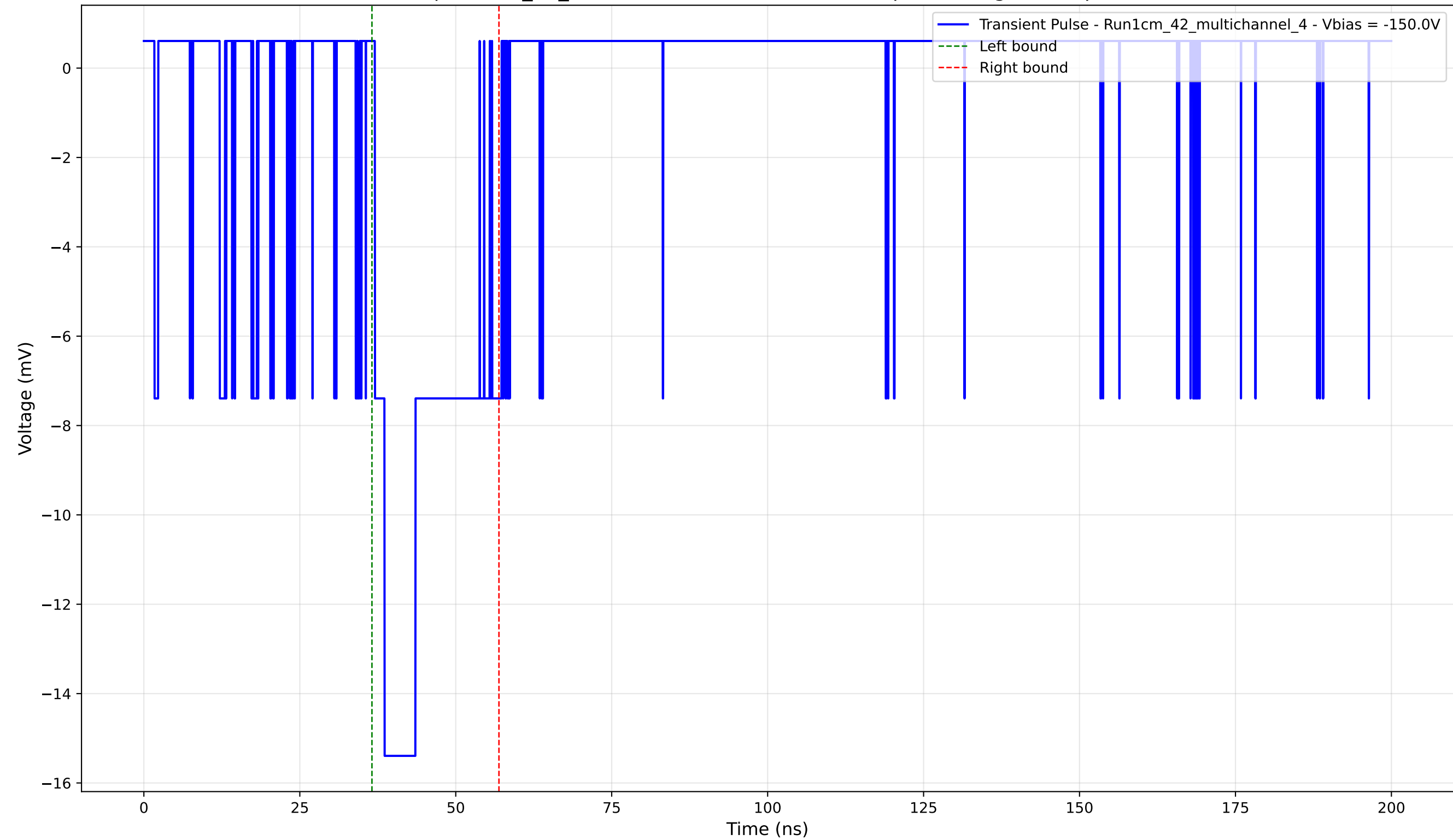
Transient Pulse - Sample: 1cm_42_multichannel - Position: 4710.0 \mu\text{m} - Charge: 3.69 pC - Rise Time: 1.56 ns
