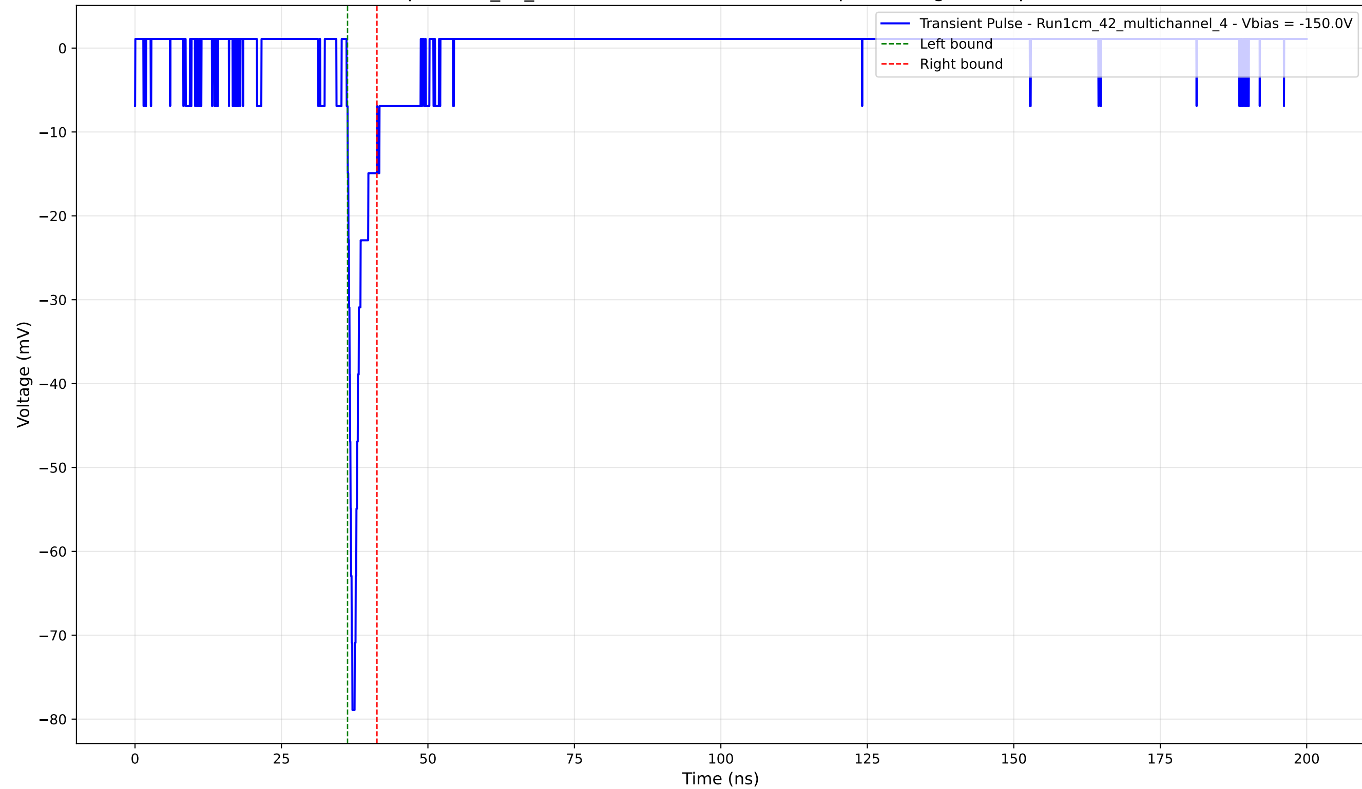
Transient Pulse - Sample: 1cm_42_multichannel - Position: 2230.0 \mu\text{m} - Charge: 3.32 pC - Rise Time: 0.82 ns
