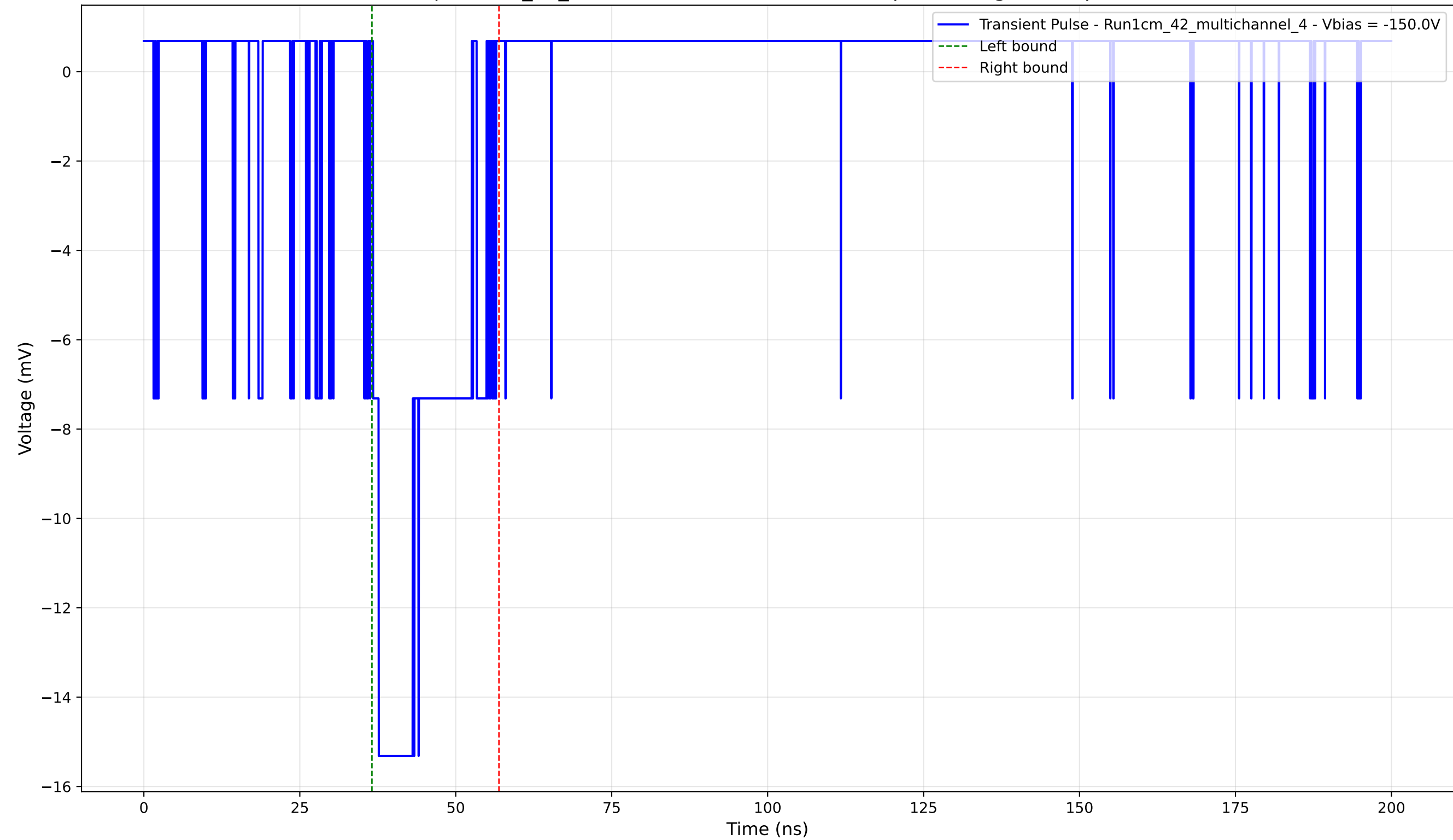
Transient Pulse - Sample: 1cm_42_multichannel - Position: 3765.0 \mu\text{m} - Charge: 3.56 pC - Rise Time: 0.92 ns
