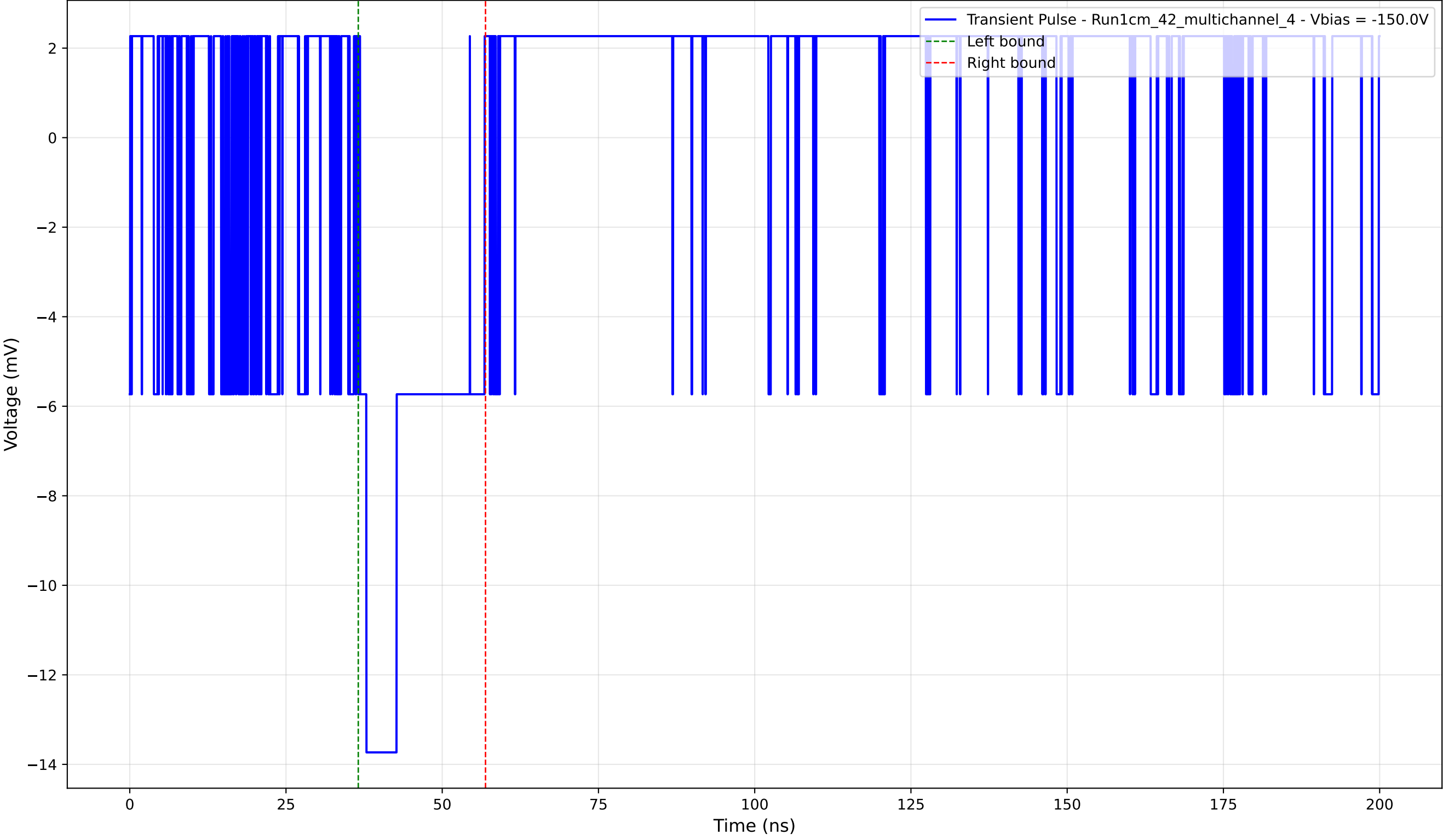
Transient Pulse - Sample: 1cm_42_multichannel - Position: 800.0 \mu\text{m} - Charge: 3.05 pC - Rise Time: 0.00 ns (N/A)
