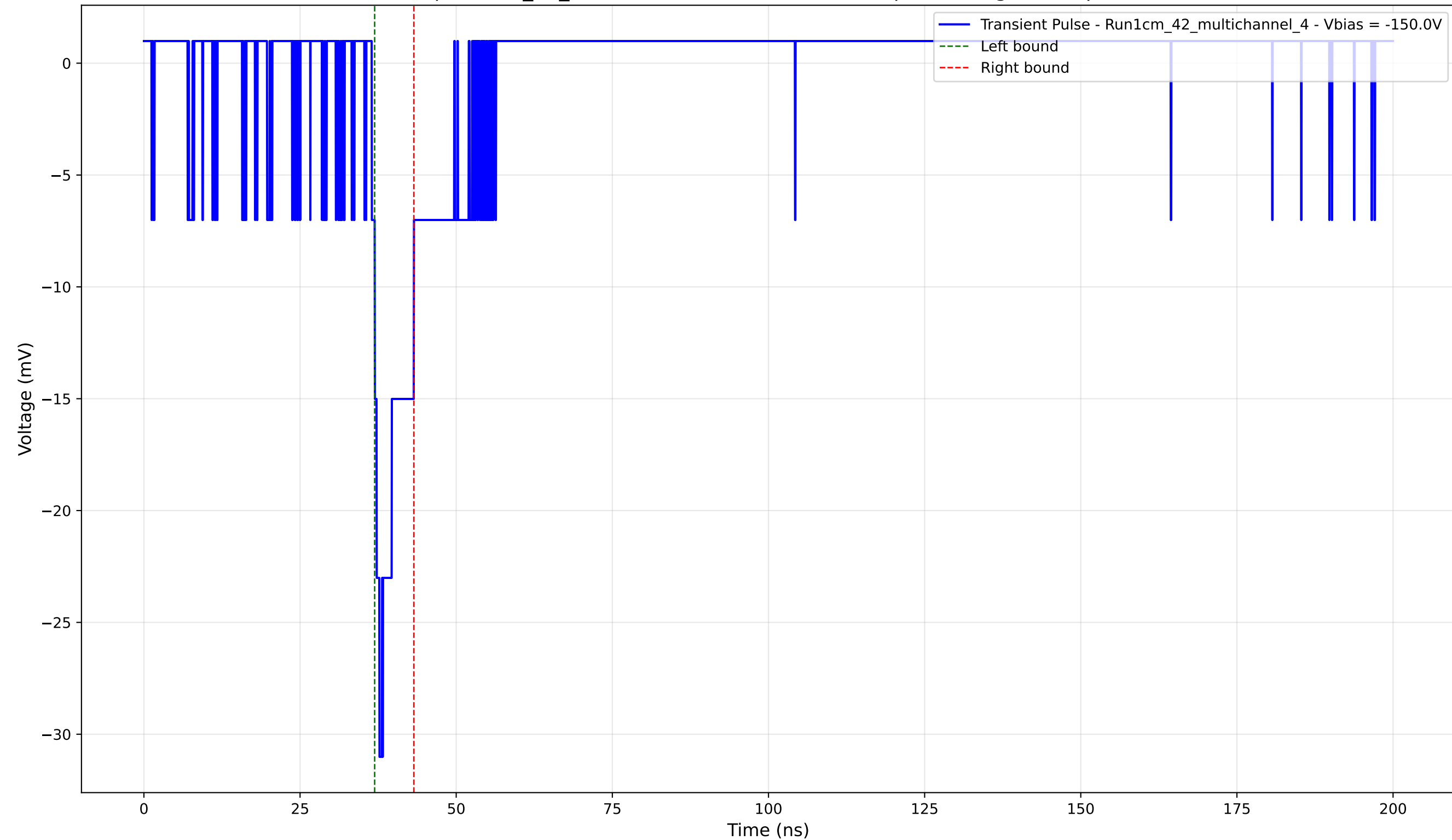
Transient Pulse - Sample: 1cm_42_multichannel - Position: 3250.0 \mu\text{m} - Charge: 2.34 pC - Rise Time: 1.23 ns
