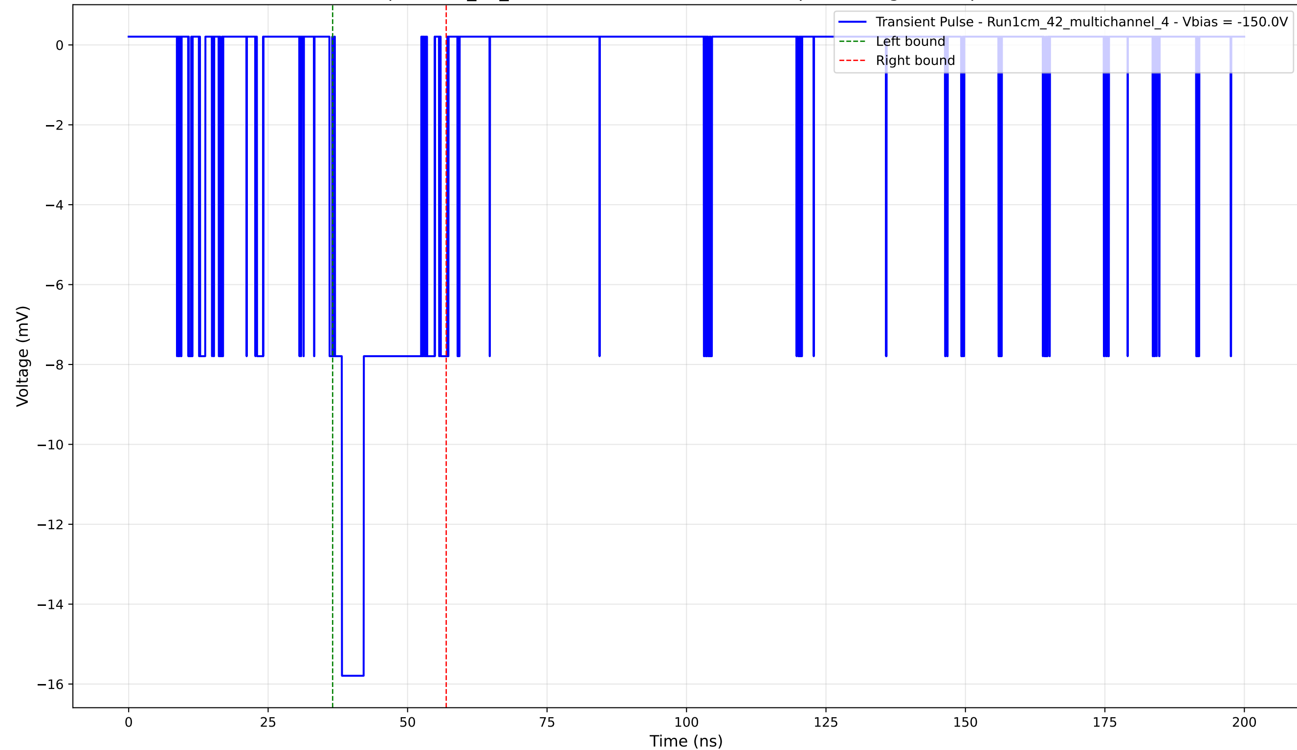
Transient Pulse - Sample: 1cm_42_multichannel - Position: 4745.0 \mu\text{m} - Charge: 3.53 pC - Rise Time: 1.26 ns
