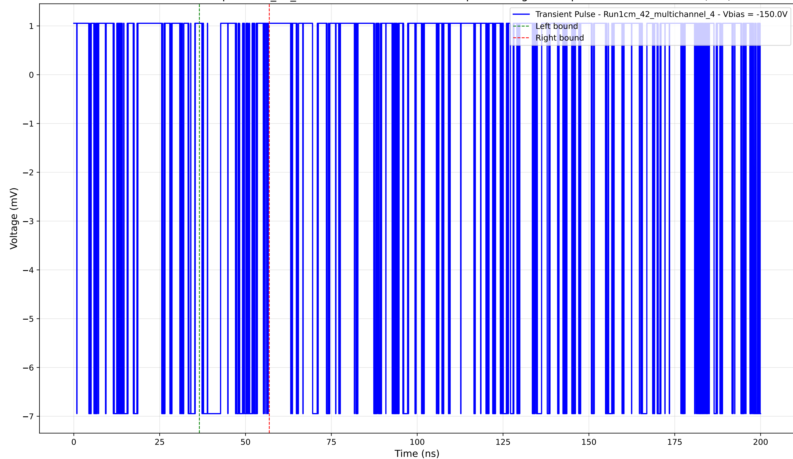
Transient Pulse - Sample: 1cm_42_multichannel - Position: 845.0 \mu\text{m} - Charge: 1.18 pC - Rise Time: 0.00 ns (N/A)
