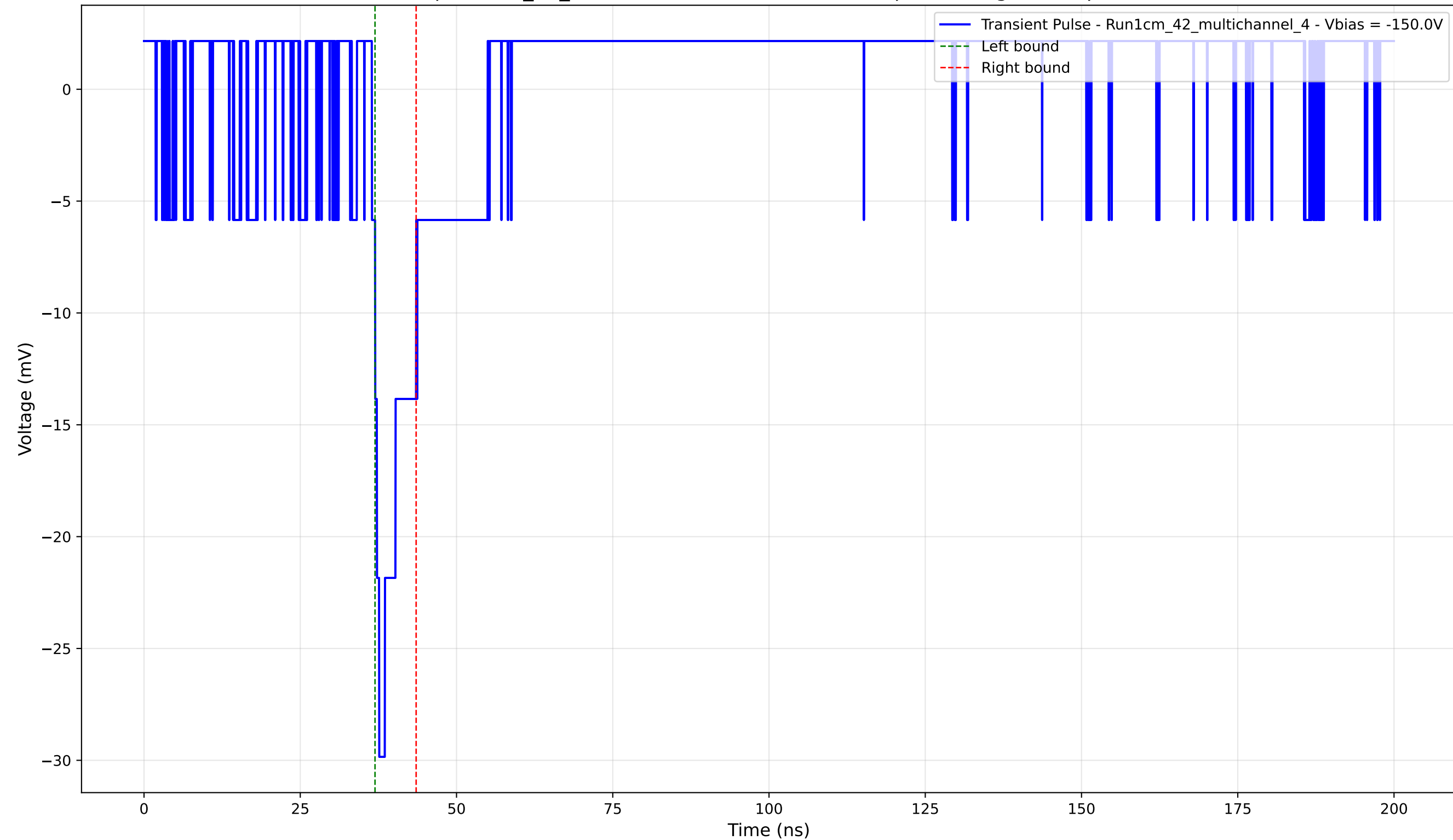
Transient Pulse - Sample: 1cm_42_multichannel - Position: 1465.0 \mu\text{m} - Charge: 2.44 pC - Rise Time: 1.18 ns
