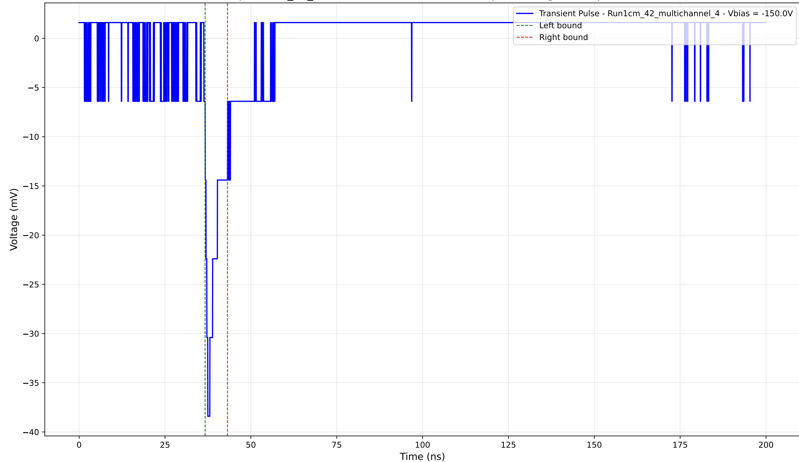
Transient Pulse - Sample: 1cm_42_multichannel - Position: 1685.0 \mu\text{m} - Charge: 2.77 pC - Rise Time: 1.15 ns
