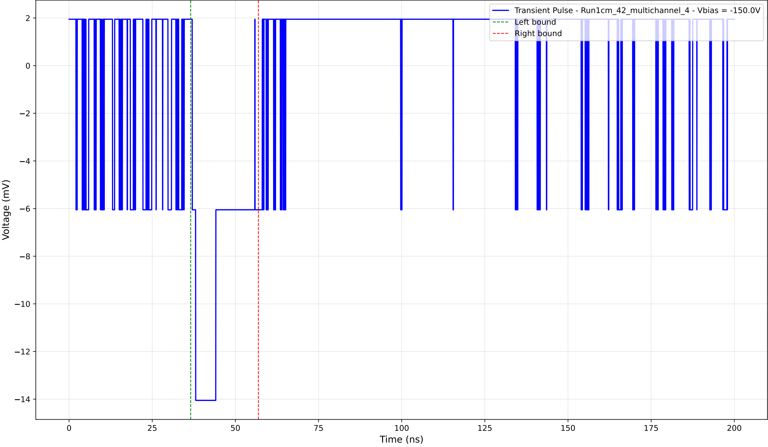
Transient Pulse - Sample: 1cm_42_multichannel - Position: 485.0 \mu\text{m} - Charge: 3.35 pC - Rise Time: 0.00 ns (N/A)
