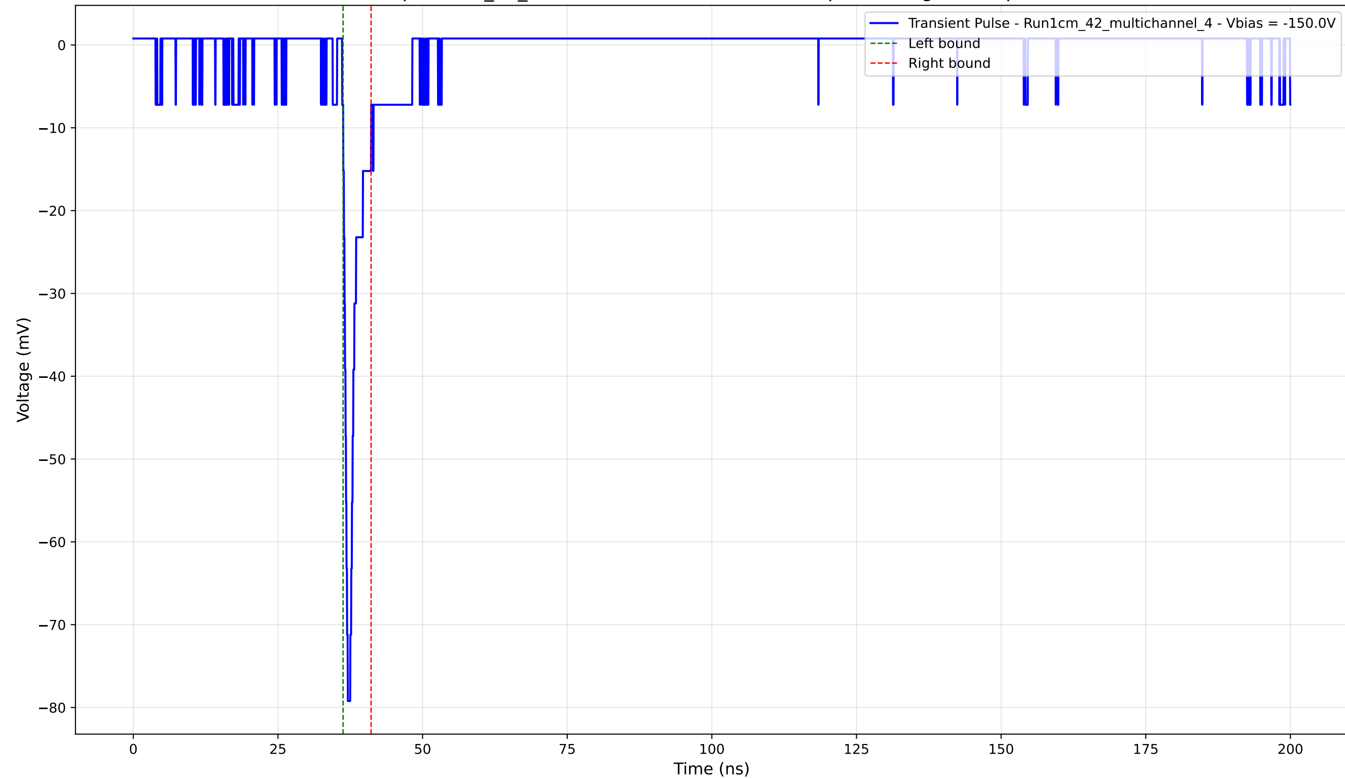
Transient Pulse - Sample: 1cm_42_multichannel - Position: 2515.0 \mu\text{m} - Charge: 3.31 pC - Rise Time: 0.80 ns
