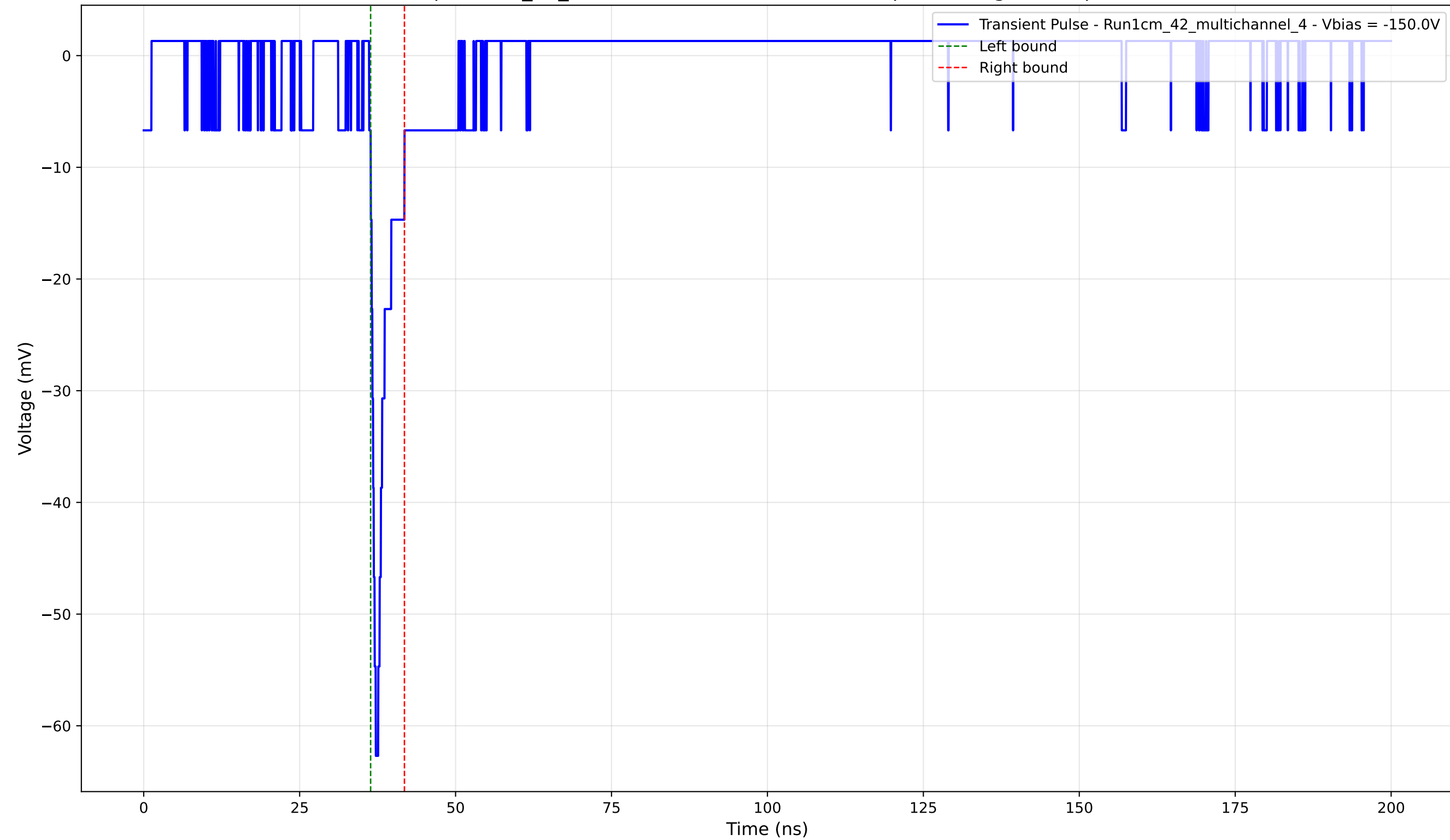
Transient Pulse - Sample: 1cm_42_multichannel - Position: 2100.0 \mu\text{m} - Charge: 3.01 pC - Rise Time: 1.06 ns
