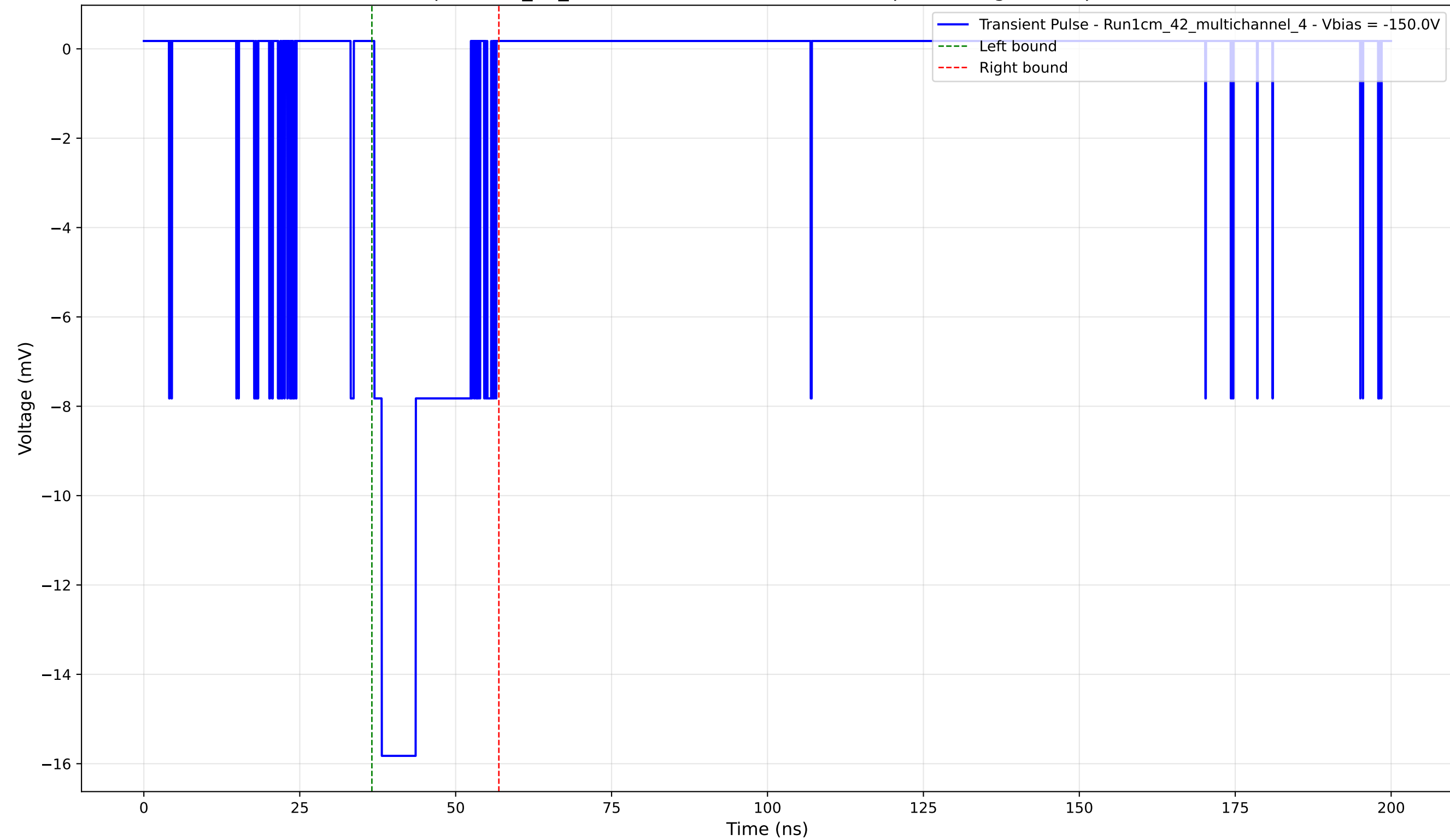
Transient Pulse - Sample: 1cm_42_multichannel - Position: 4045.0 \mu\text{m} - Charge: 3.58 pC - Rise Time: 1.20 ns
