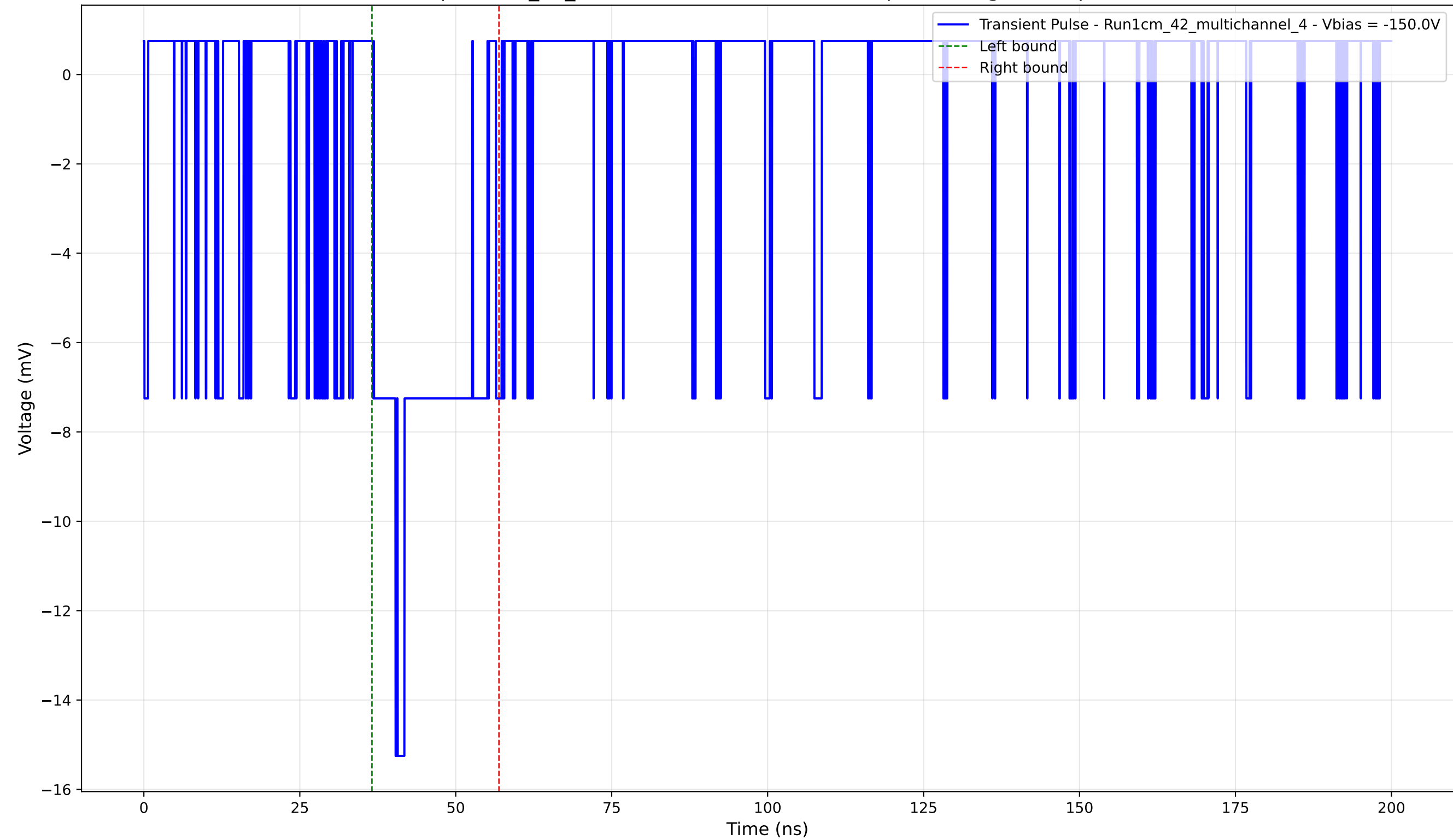
Transient Pulse - Sample: 1cm_42_multichannel - Position: 115.0 \mu\text{m} - Charge: 2.91 pC - Rise Time: 3.48 ns
