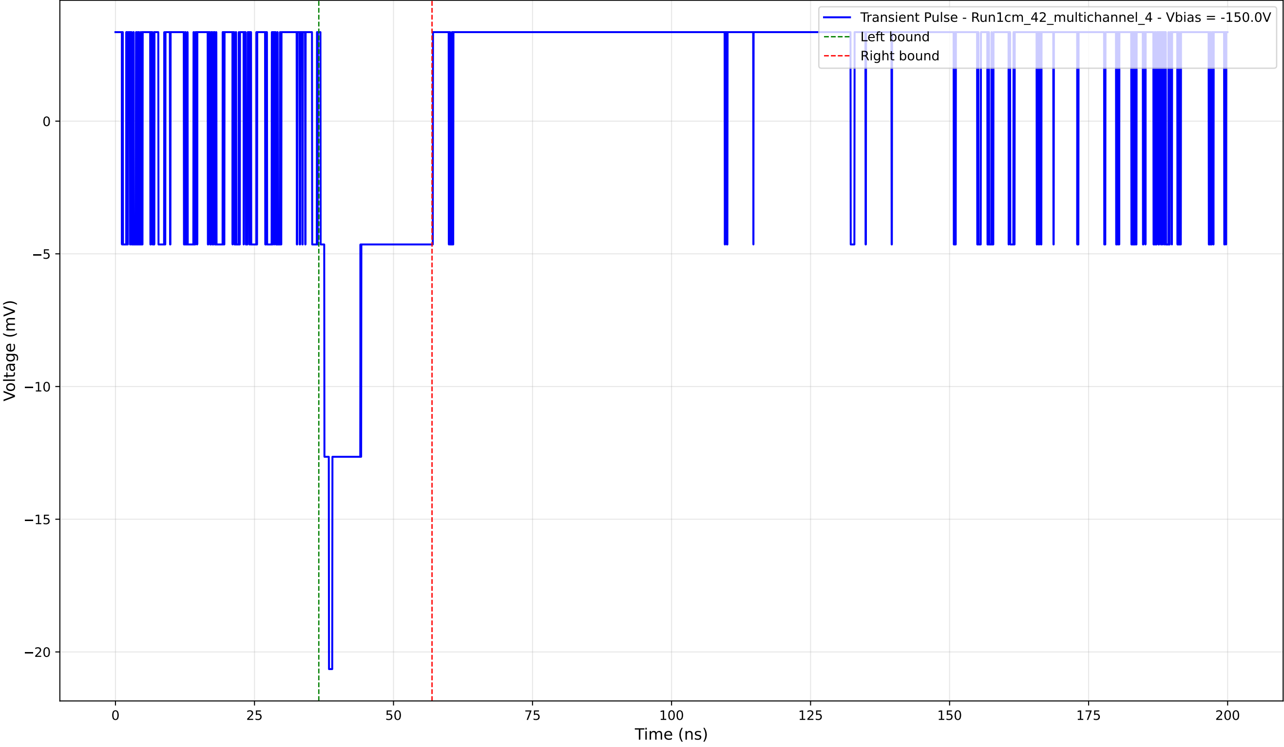
Transient Pulse - Sample: 1cm_42_multichannel - Position: 995.0 \mu\text{m} - Charge: 3.00 pC - Rise Time: 0.00 ns (N/A)
