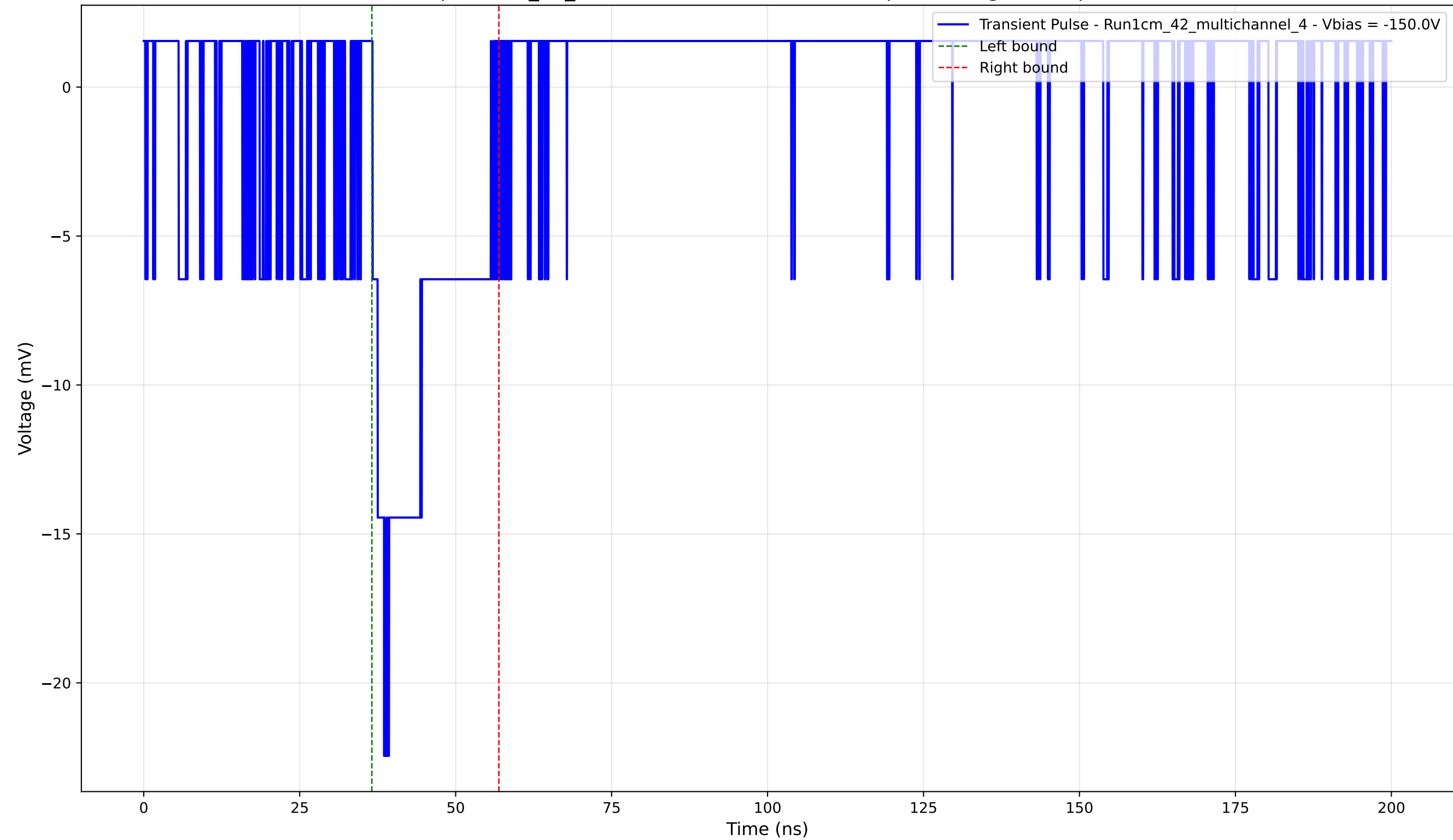
Transient Pulse - Sample: 1cm_42_multichannel - Position: 975.0 \mu\text{m} - Charge: 3.76 pC - Rise Time: 1.88 ns
