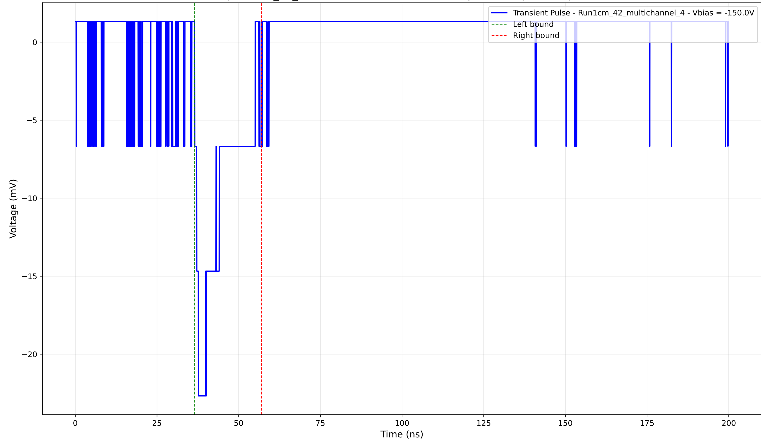
Transient Pulse - Sample: 1cm_42_multichannel - Position: 1295.0 \mu\text{m} - Charge: 3.98 pC - Rise Time: 1.12 ns
