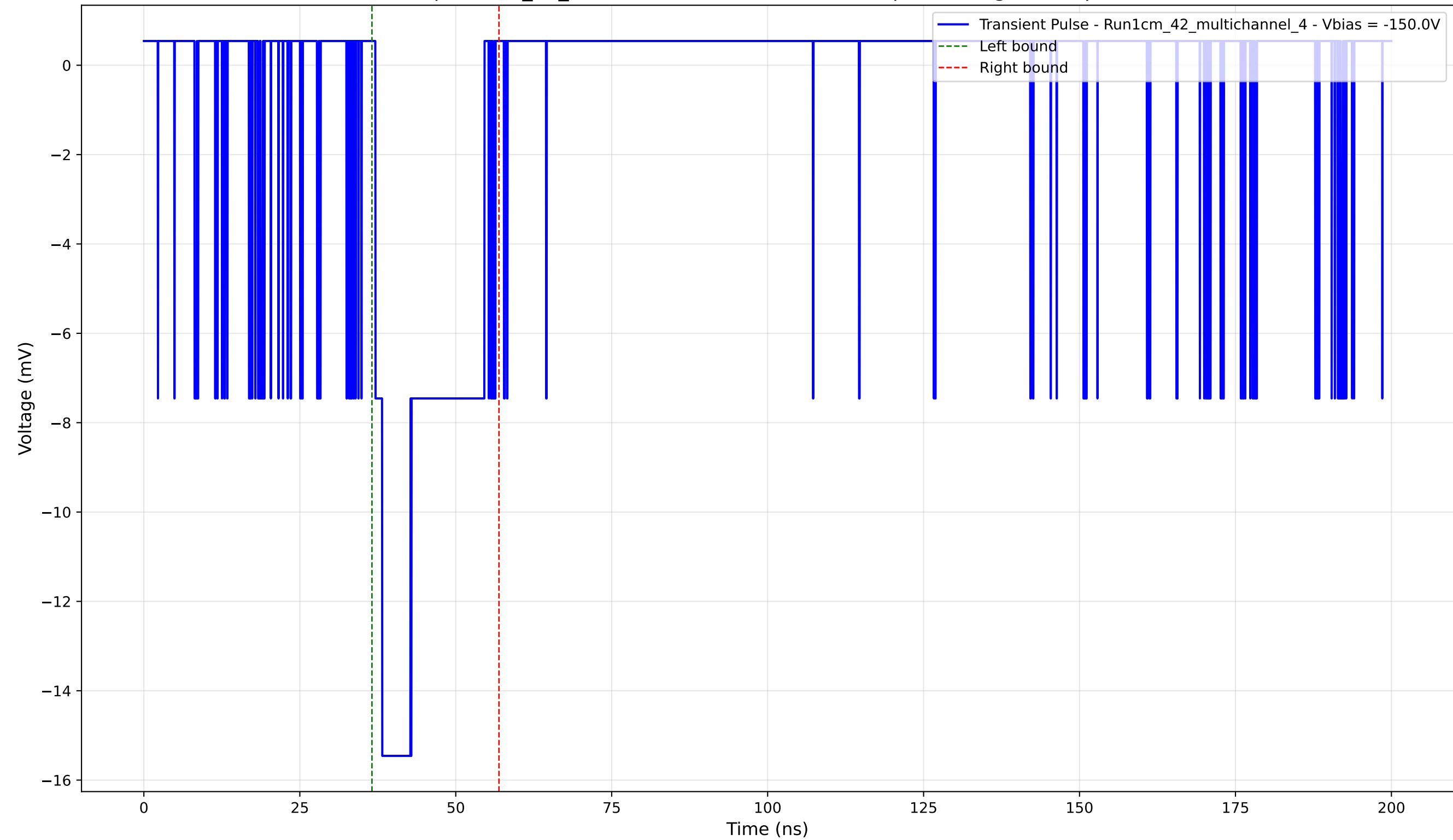
Transient Pulse - Sample: 1cm_42_multichannel - Position: 4545.0 \mu\text{m} - Charge: 3.42 pC - Rise Time: 1.10 ns
