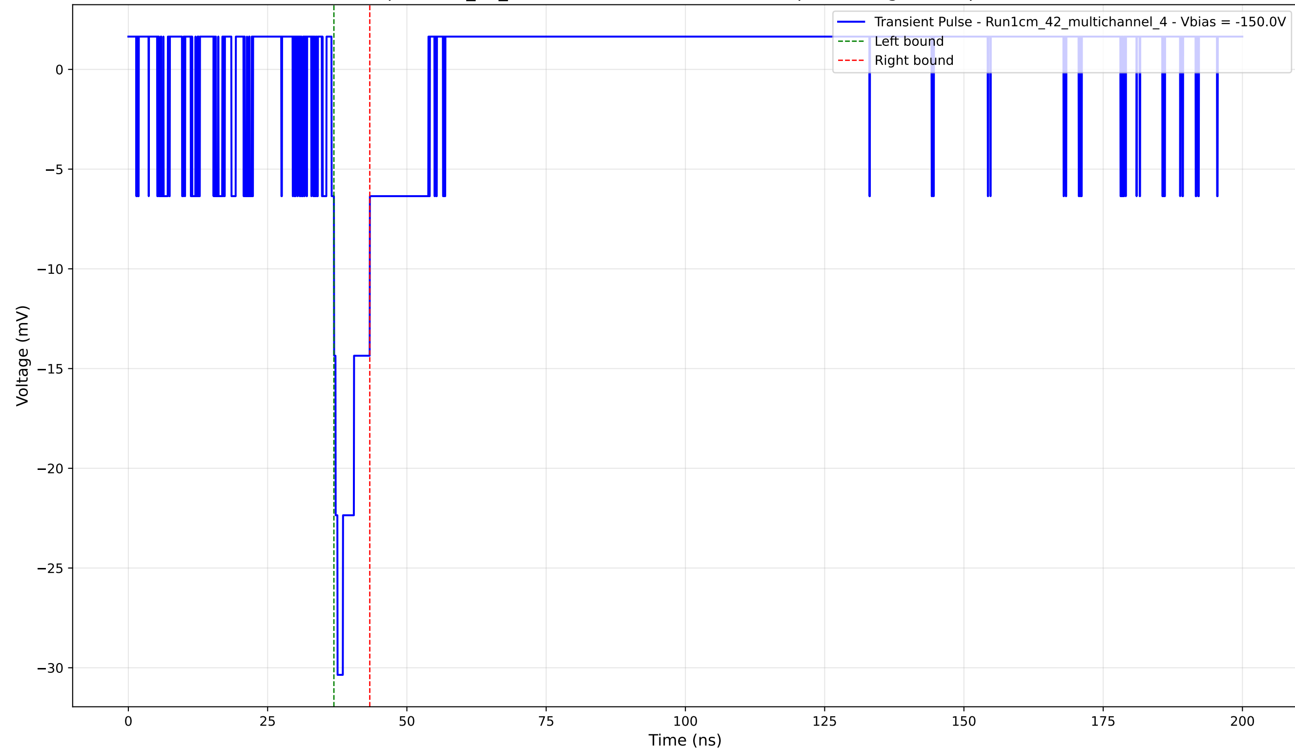
Transient Pulse - Sample: 1cm_42_multichannel - Position: 1490.0 \mu\text{m} - Charge: 2.53 pC - Rise Time: 1.07 ns
