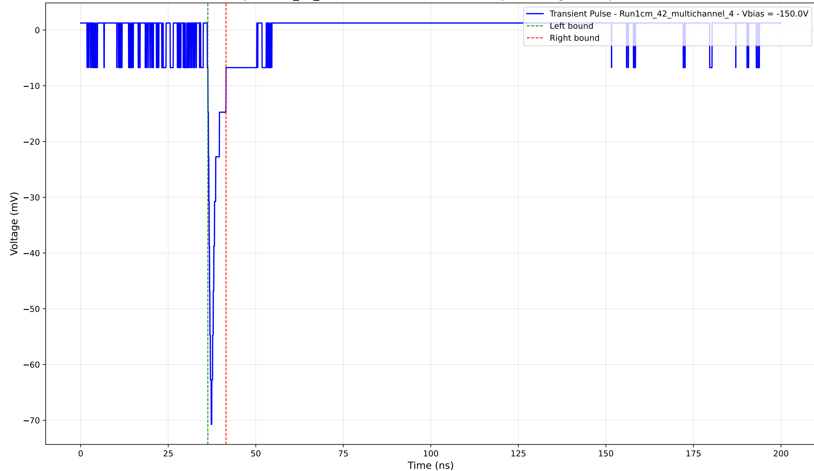
Transient Pulse - Sample: 1cm_42_multichannel - Position: 2165.0 \mu\text{m} - Charge: 3.06 pC - Rise Time: 0.96 ns
