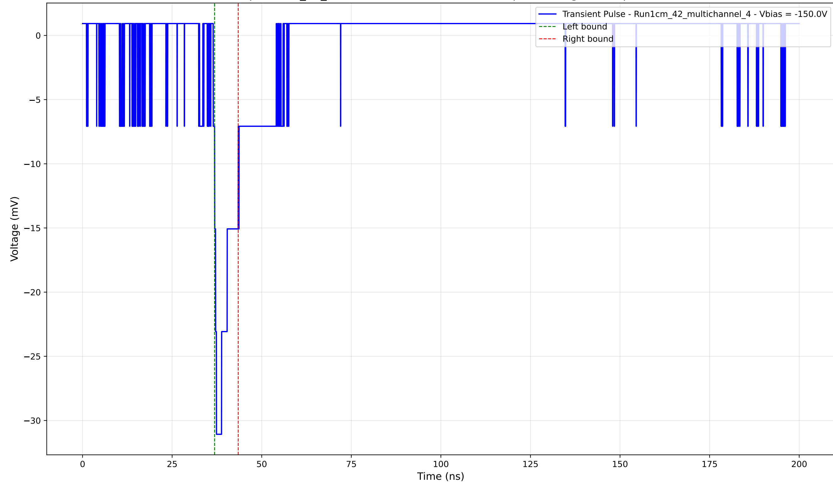
Transient Pulse - Sample: 1cm_42_multichannel - Position: 1540.0 \mu\text{m} - Charge: 2.74 pC - Rise Time: 0.91 ns
