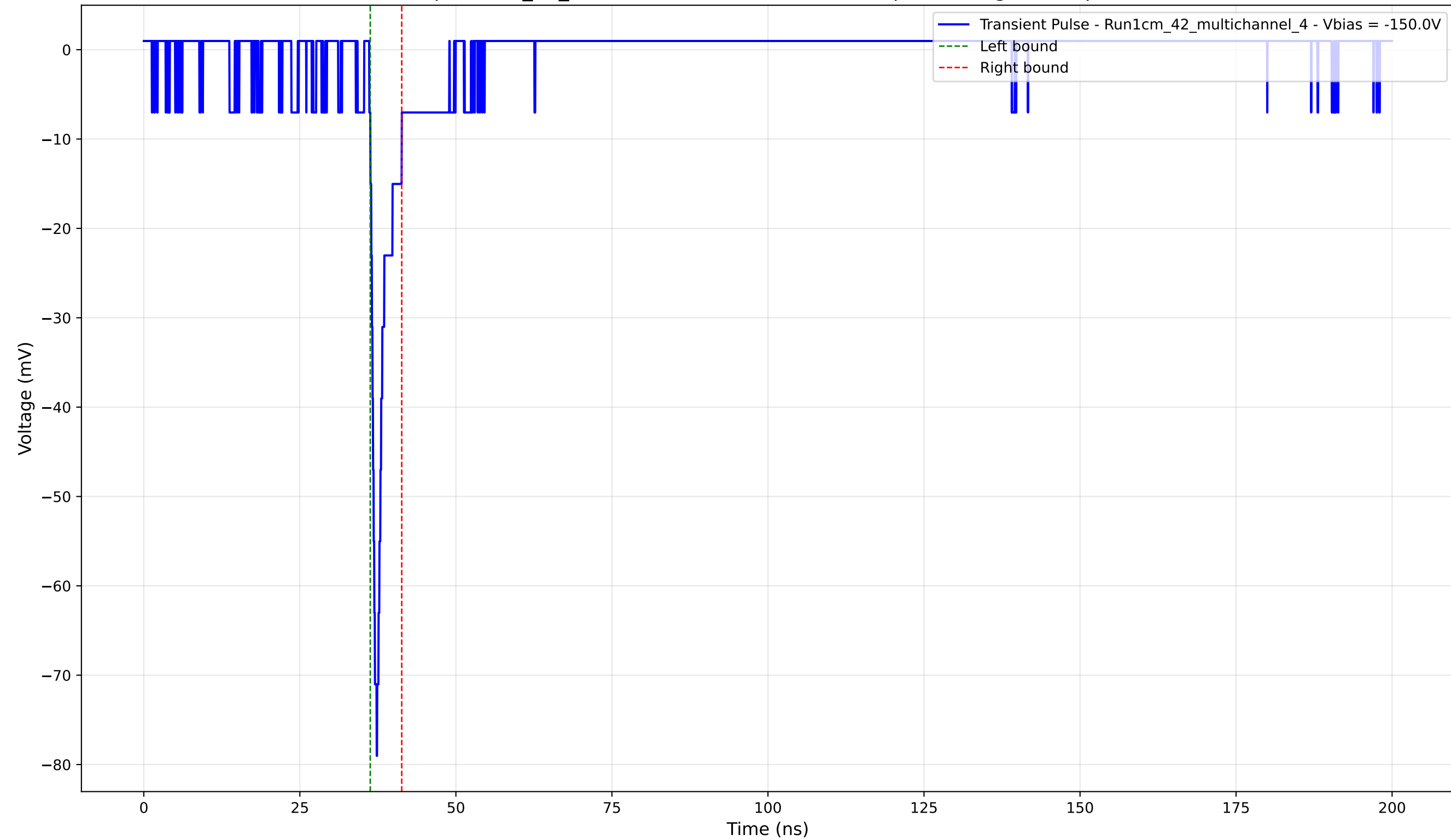
Transient Pulse - Sample: 1cm_42_multichannel - Position: 2215.0 \mu\text{m} - Charge: 3.24 pC - Rise Time: 1.02 ns
