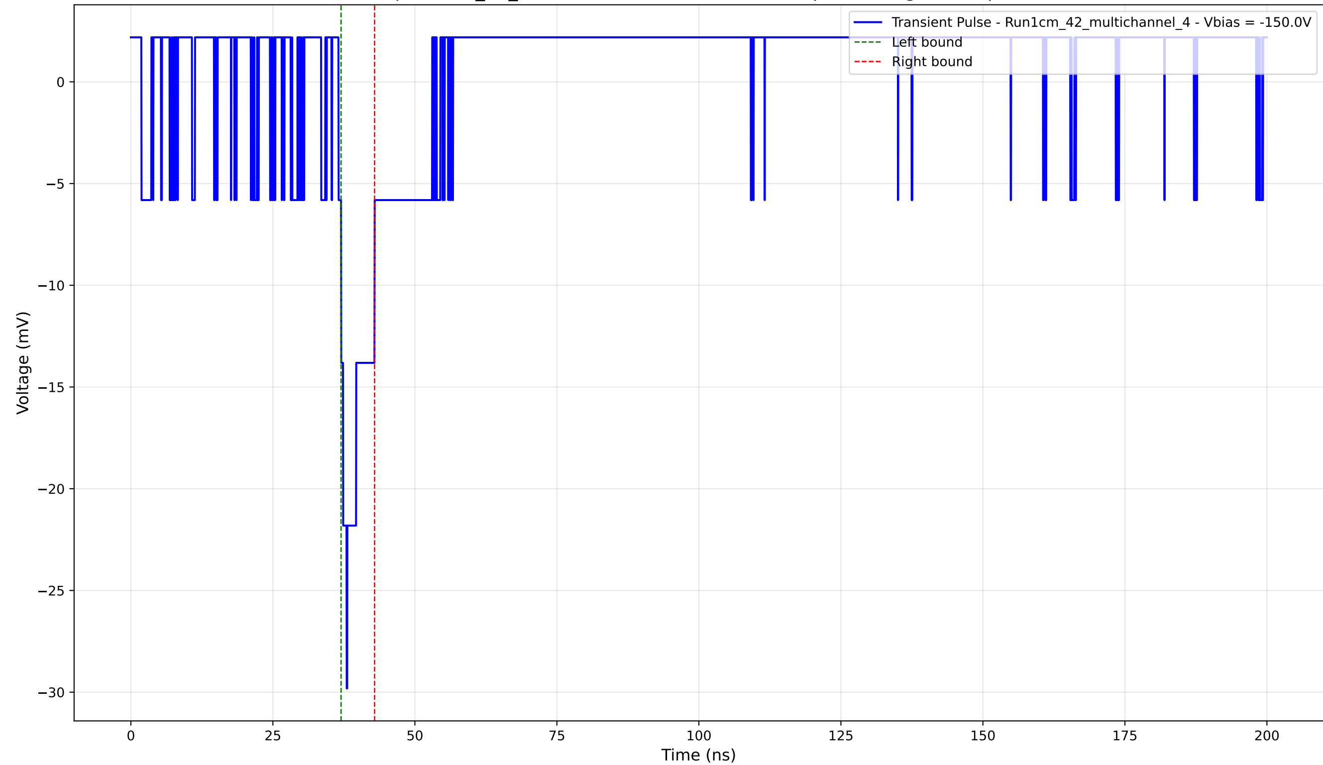
Transient Pulse - Sample: 1cm_42_multichannel - Position: 3310.0 \mu\text{m} - Charge: 2.01 pC - Rise Time: 1.44 ns
