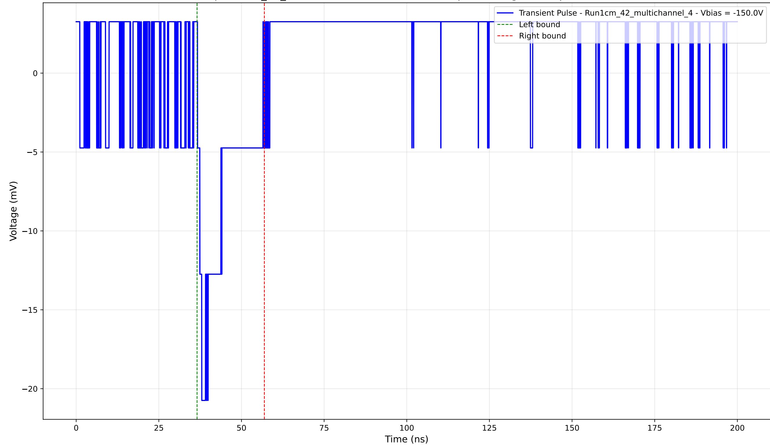
Transient Pulse - Sample: 1cm_42_multichannel - Position: 1080.0 \mu\text{m} - Charge: 3.13 pC - Rise Time: 0.00 ns (N/A)
