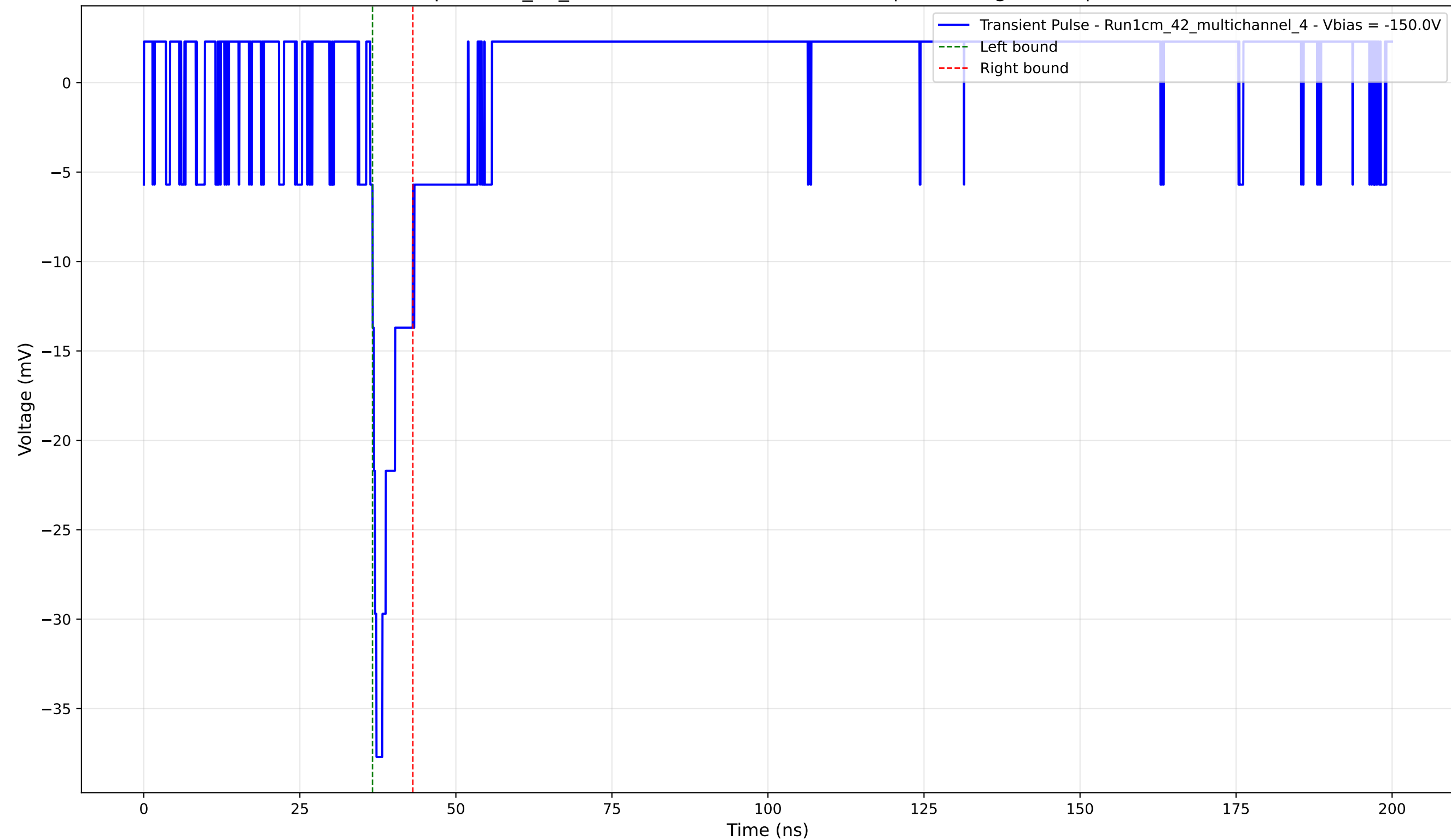
Transient Pulse - Sample: 1cm_42_multichannel - Position: 1750.0 \mu\text{m} - Charge: 2.74 pC - Rise Time: 0.99 ns
