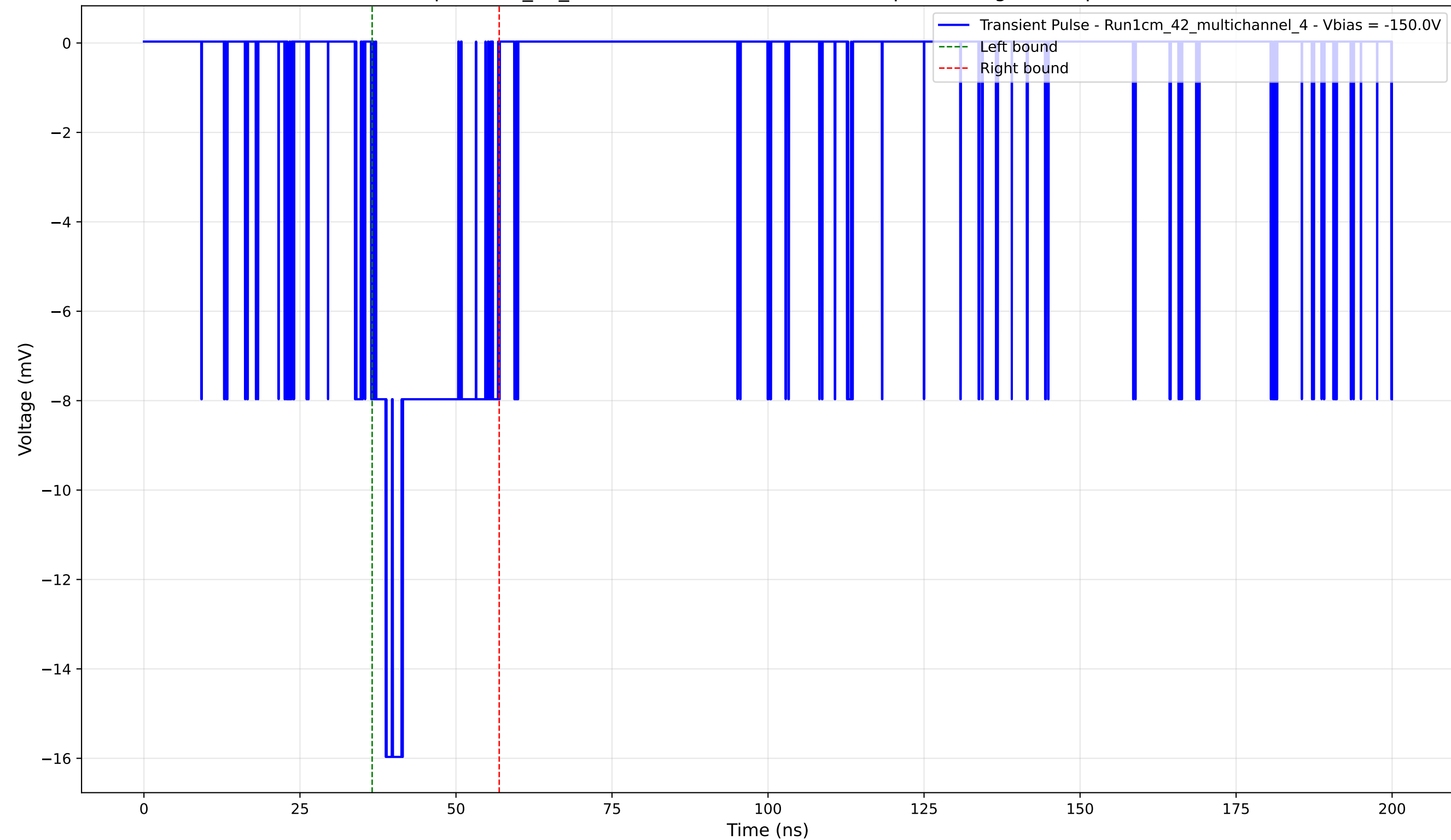
Transient Pulse - Sample: 1cm_42_multichannel - Position: 4470.0 \mu\text{m} - Charge: 3.45 pC - Rise Time: 1.52 ns
