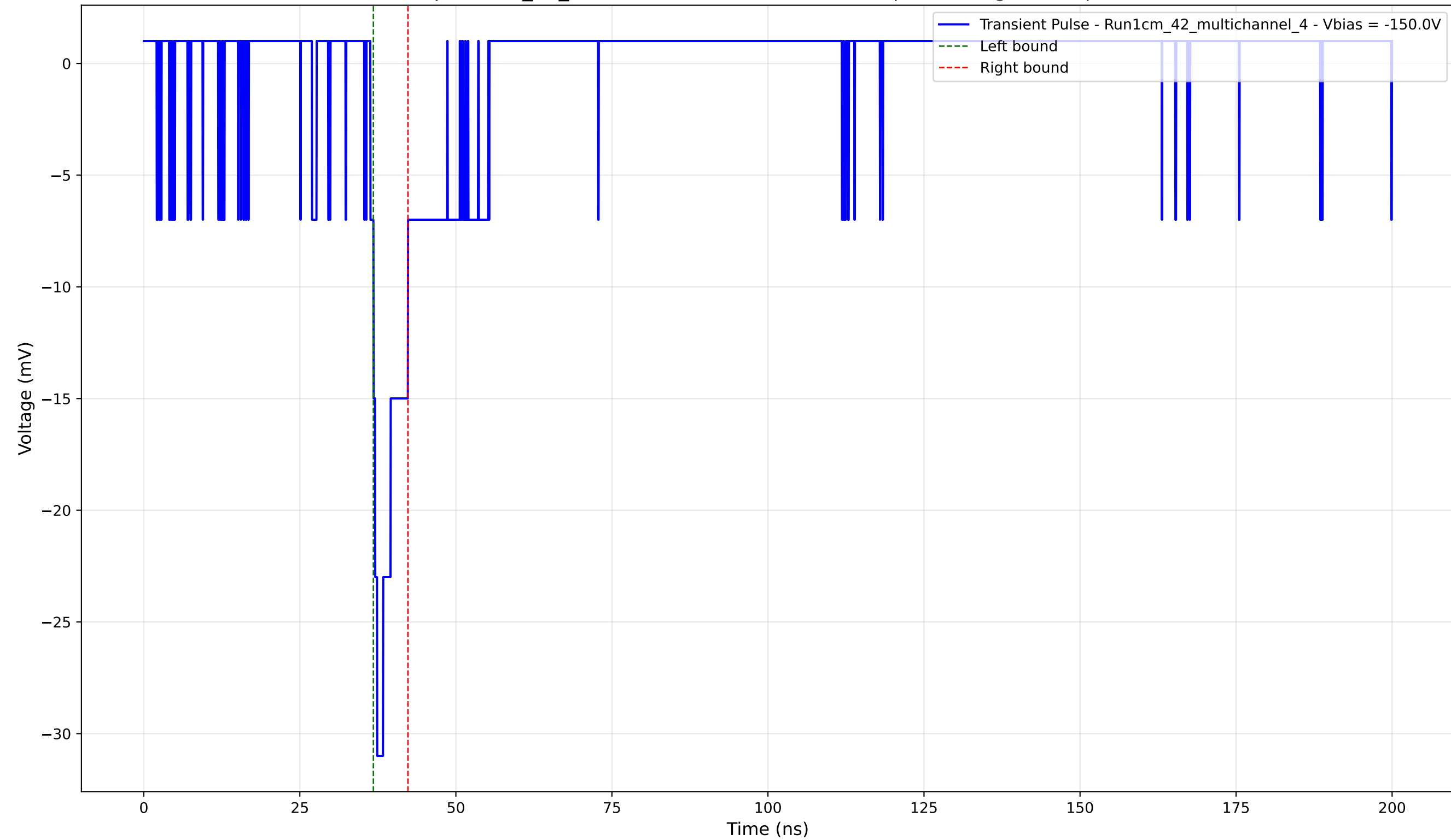
Transient Pulse - Sample: 1cm_42_multichannel - Position: 3135.0 \mu\text{m} - Charge: 2.21 pC - Rise Time: 1.09 ns
