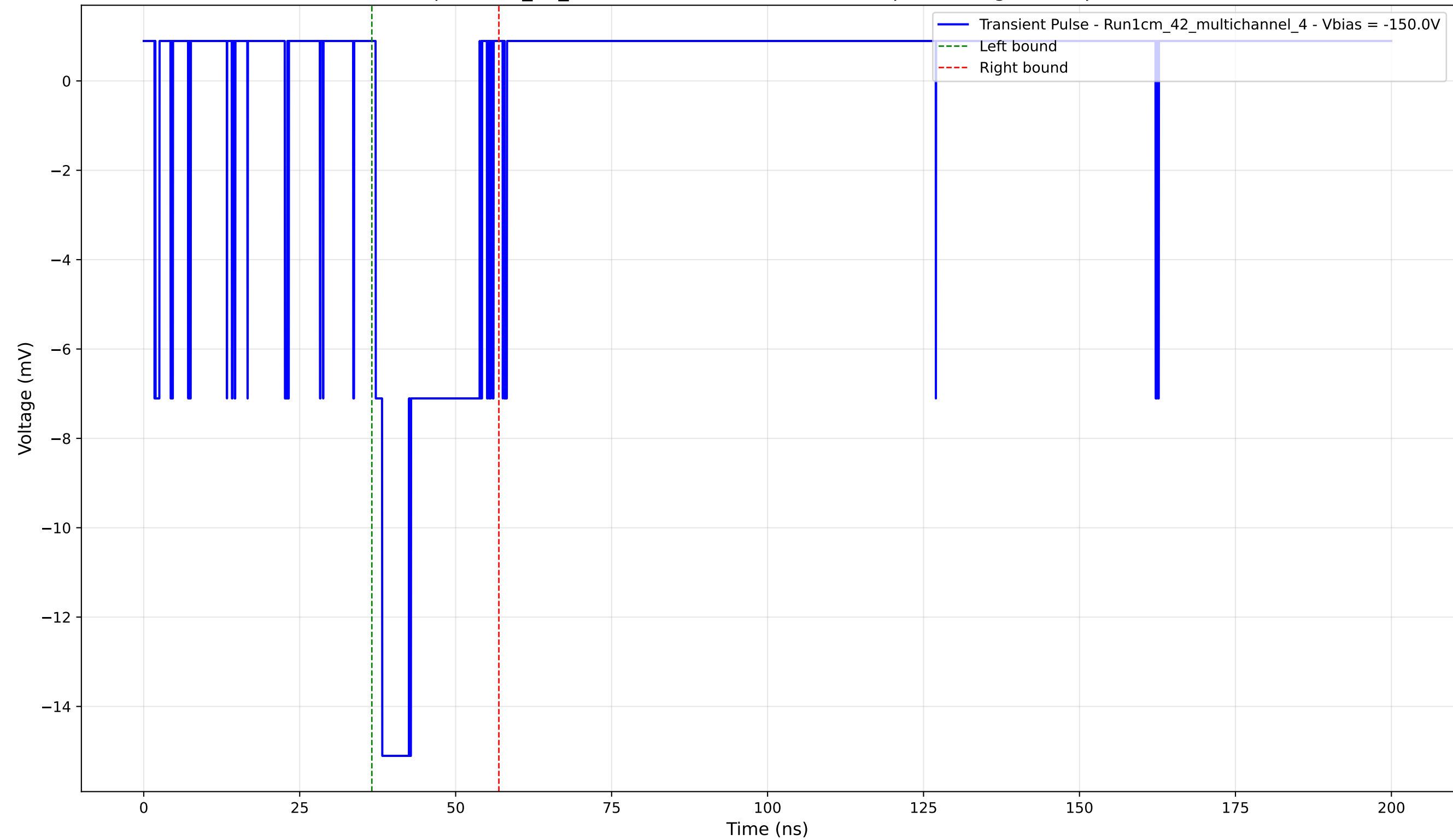
Transient Pulse - Sample: 1cm_42_multichannel - Position: 4180.0 \mu\text{m} - Charge: 3.16 pC - Rise Time: 1.06 ns
