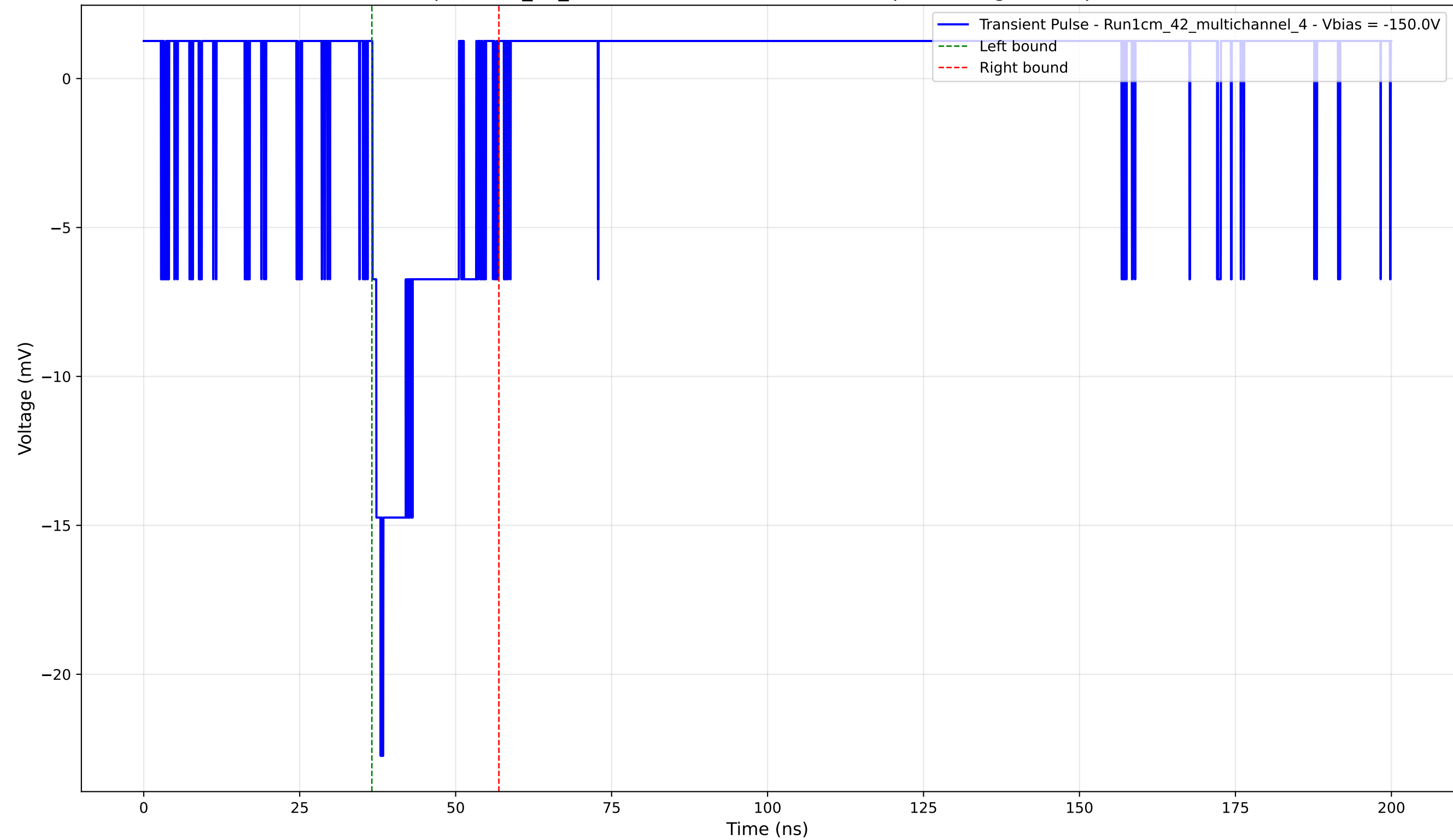
Transient Pulse - Sample: 1cm_42_multichannel - Position: 3465.0 \mu\text{m} - Charge: 3.16 pC - Rise Time: 1.34 ns
