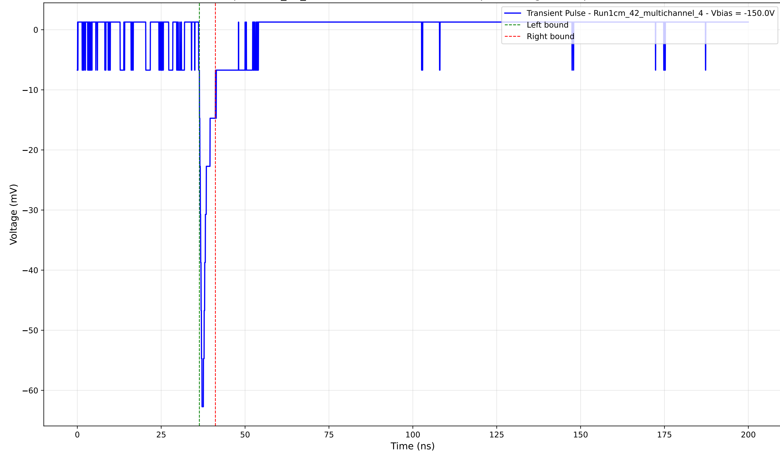
Transient Pulse - Sample: 1cm_42_multichannel - Position: 2635.0 \mu\text{m} - Charge: 2.77 pC - Rise Time: 1.00 ns
