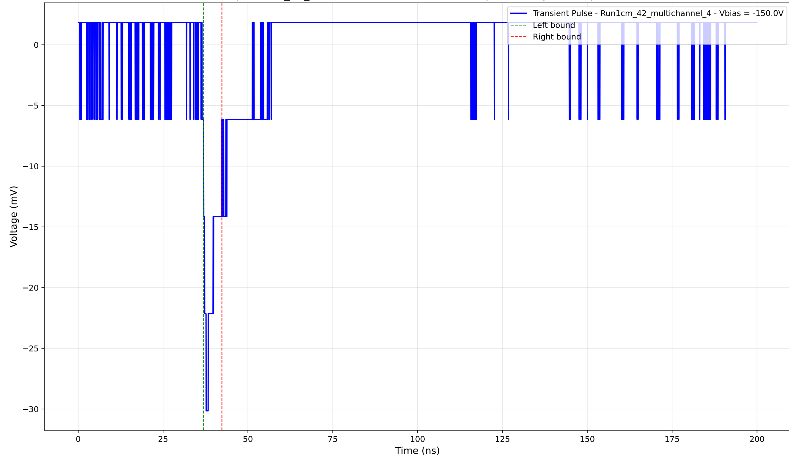
Transient Pulse - Sample: 1cm_42_multichannel - Position: 3275.0 \mu\text{m} - Charge: 2.03 pC - Rise Time: 1.19 ns
