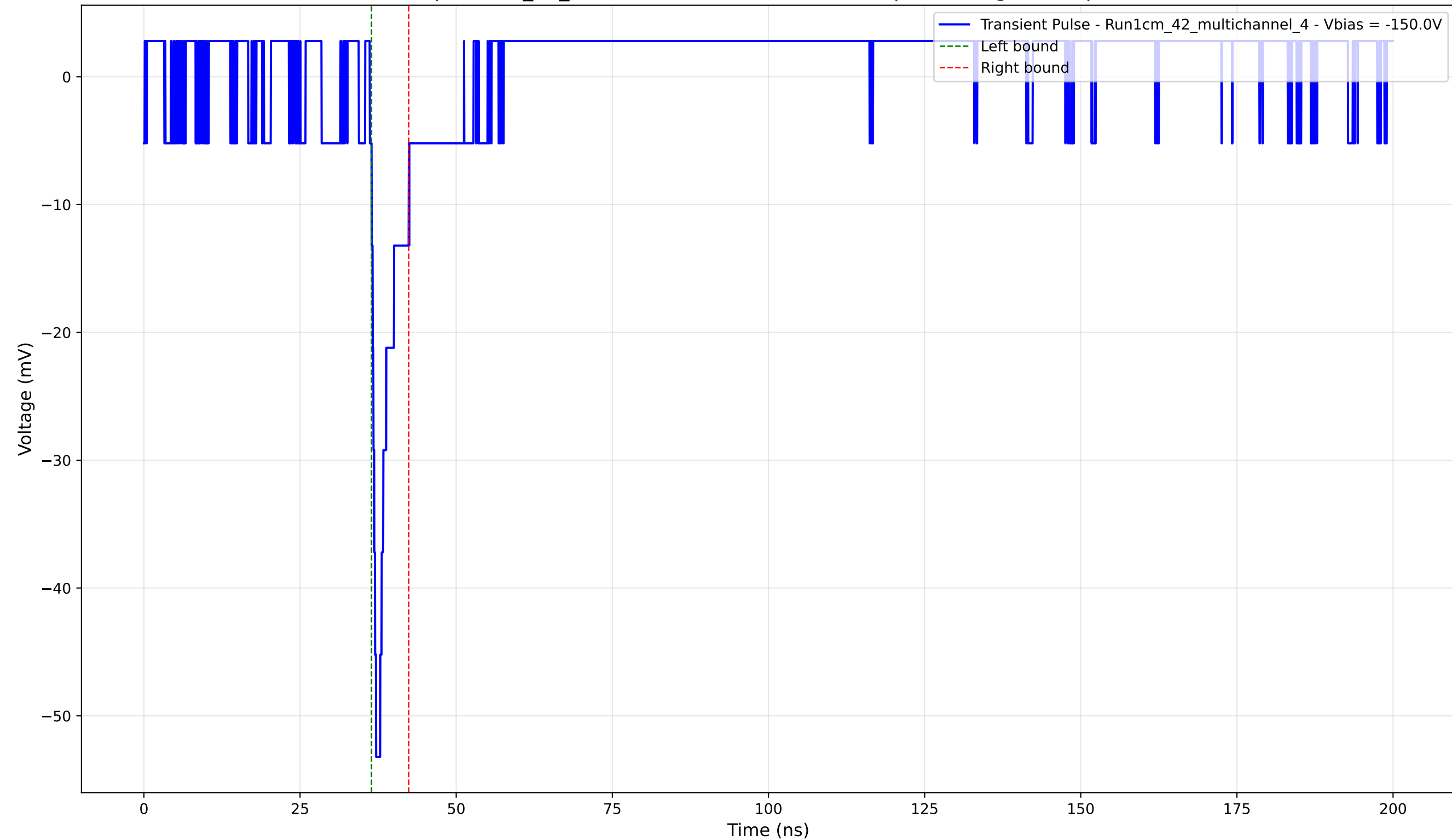
Transient Pulse - Sample: 1cm_42_multichannel - Position: 1995.0 \mu\text{m} - Charge: 2.96 pC - Rise Time: 0.72 ns
