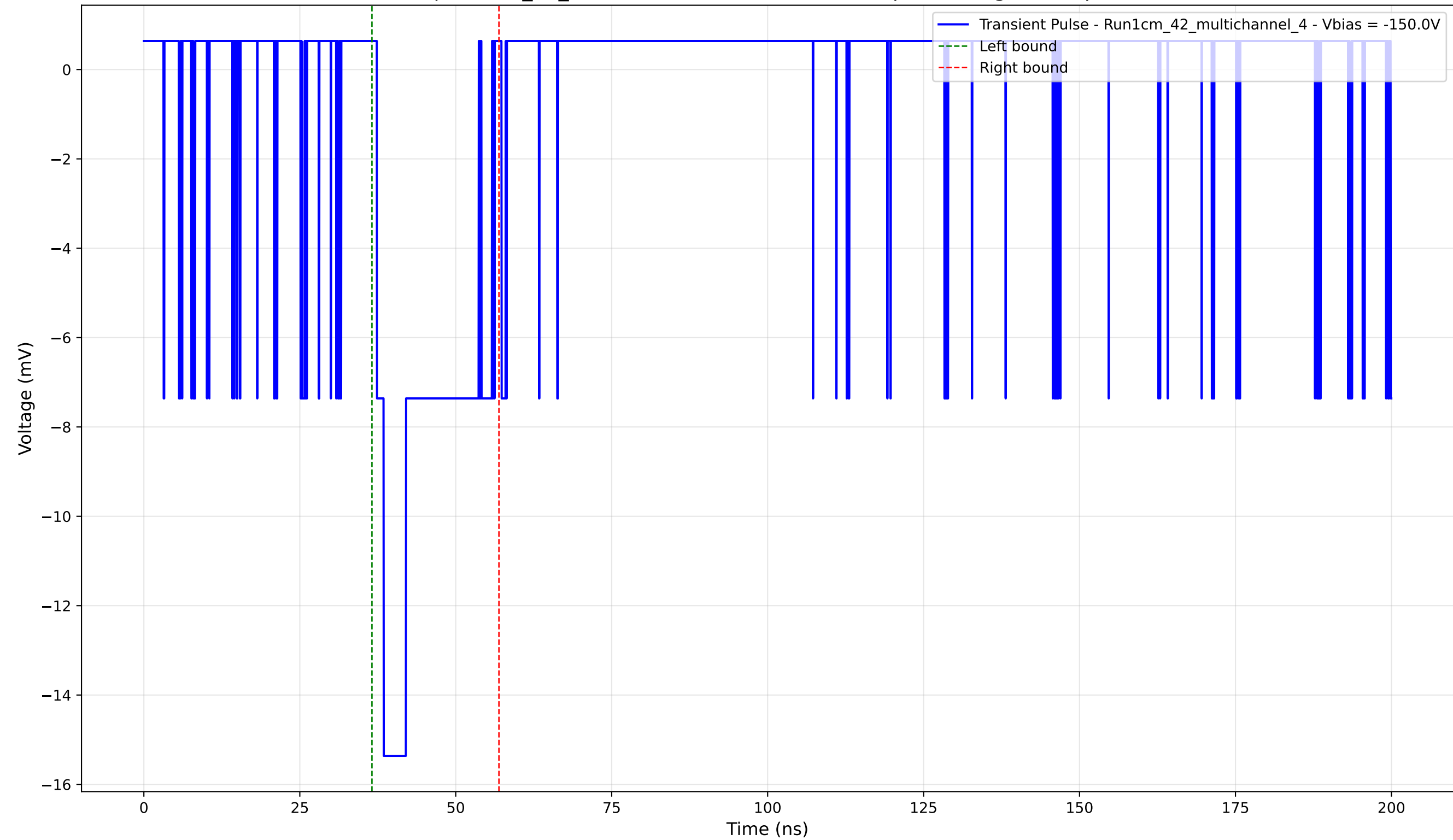
Transient Pulse - Sample: 1cm_42_multichannel - Position: 4330.0 \mu\text{m} - Charge: 3.24 pC - Rise Time: 1.10 ns
