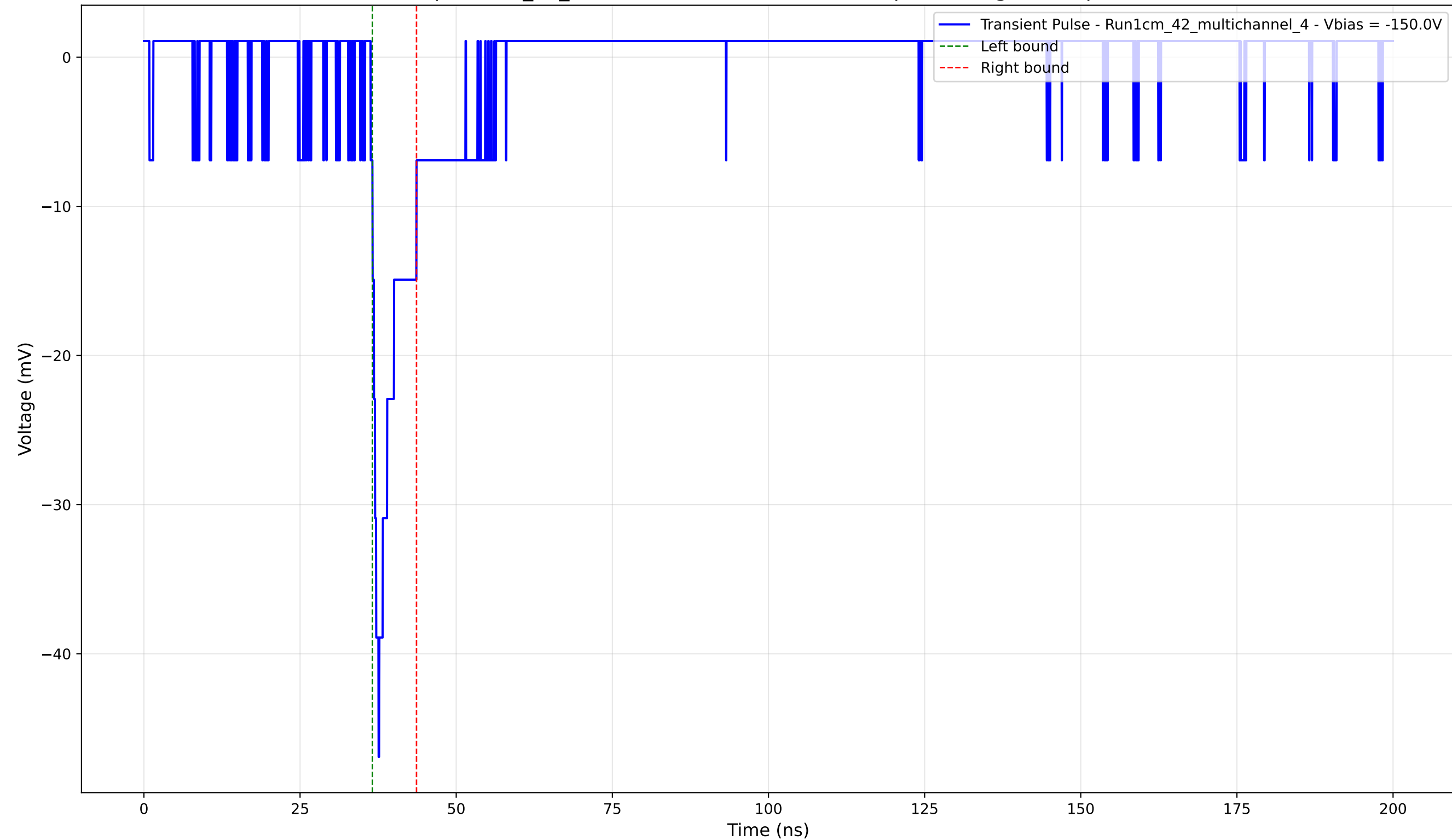
Transient Pulse - Sample: 1cm_42_multichannel - Position: 1785.0 \mu\text{m} - Charge: 3.12 pC - Rise Time: 1.27 ns
