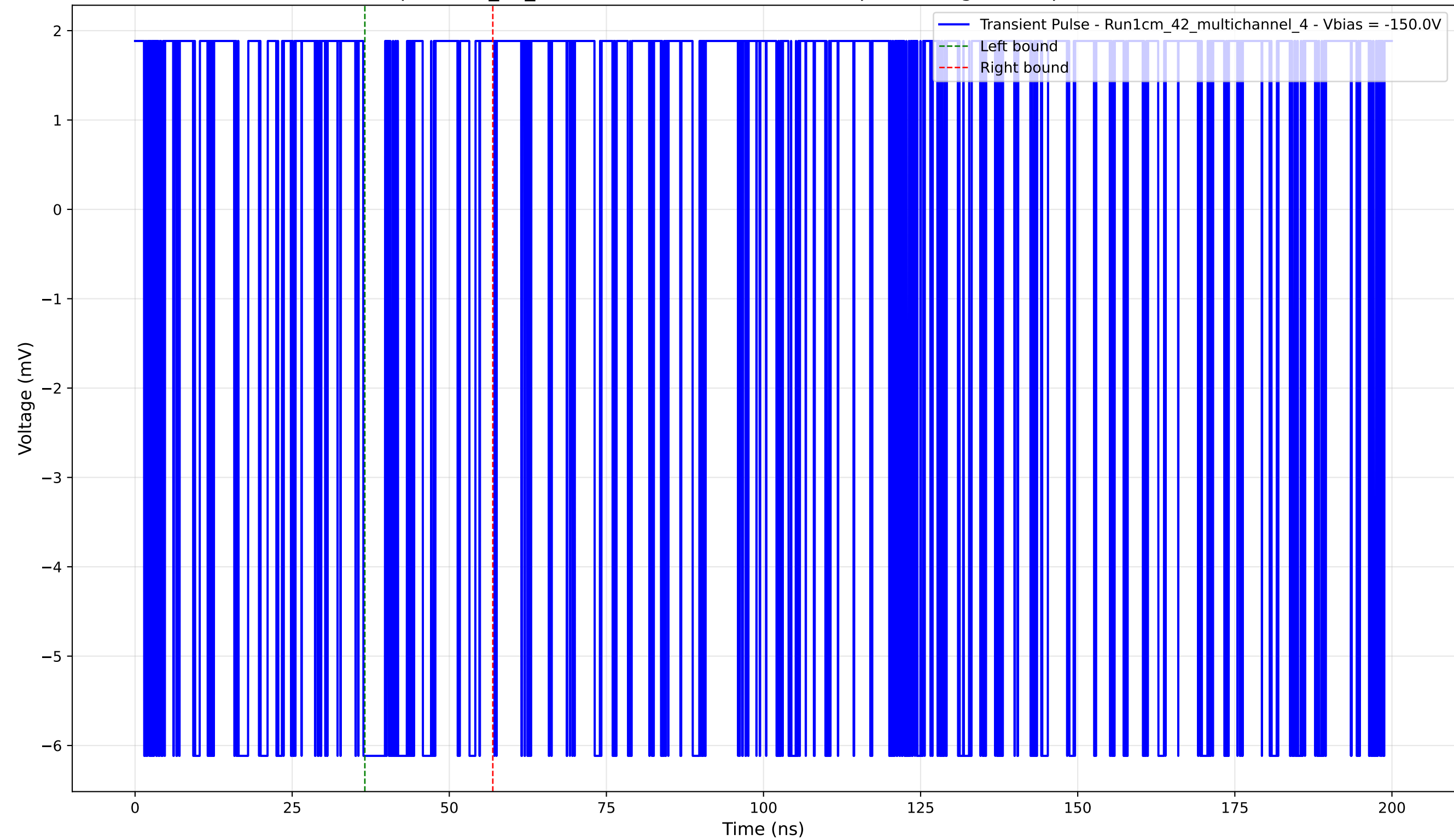
Transient Pulse - Sample: 1cm_42_multichannel - Position: 2405.0 \mu\text{m} - Charge: 0.75 pC - Rise Time: 0.00 ns (N/A)
