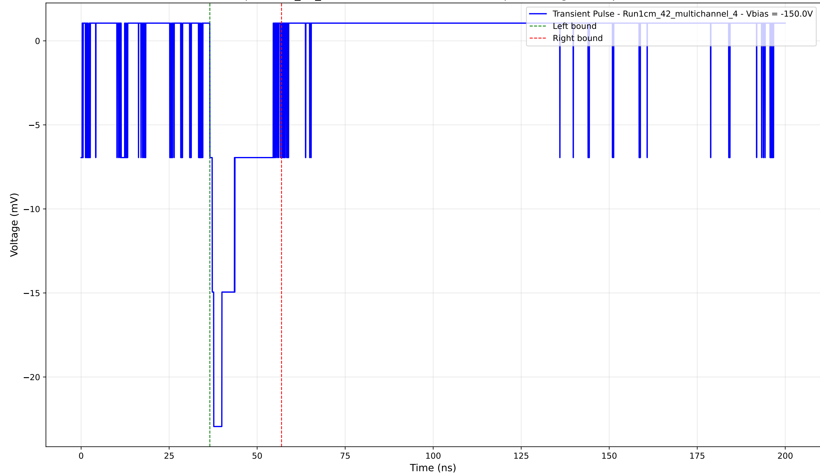
Transient Pulse - Sample: 1cm_42_multichannel - Position: 1230.0 \mu\text{m} - Charge: 3.96 pC - Rise Time: 1.12 ns
