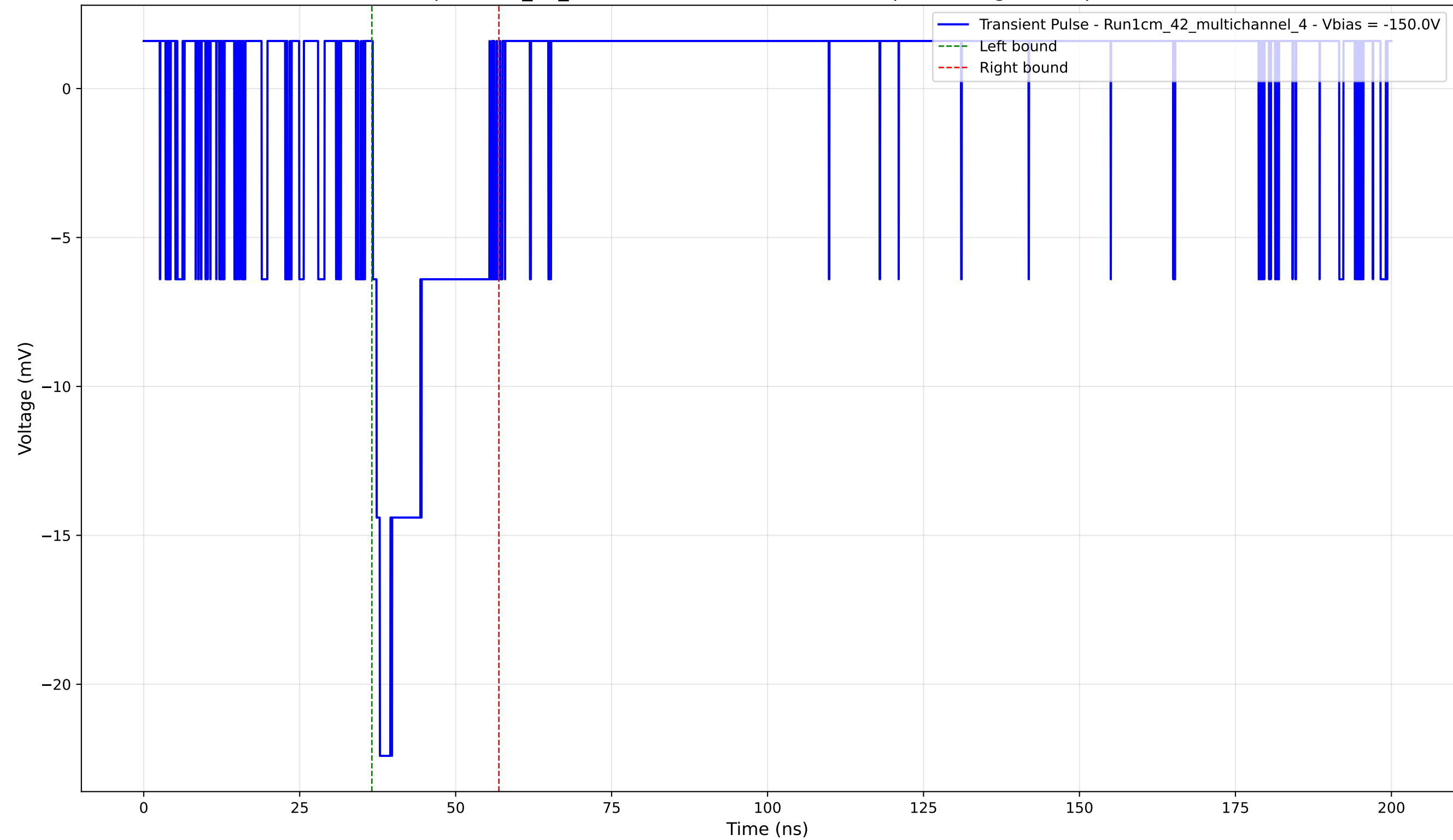
Transient Pulse - Sample: 1cm_42_multichannel - Position: 1135.0 \mu\text{m} - Charge: 3.95 pC - Rise Time: 1.14 ns
