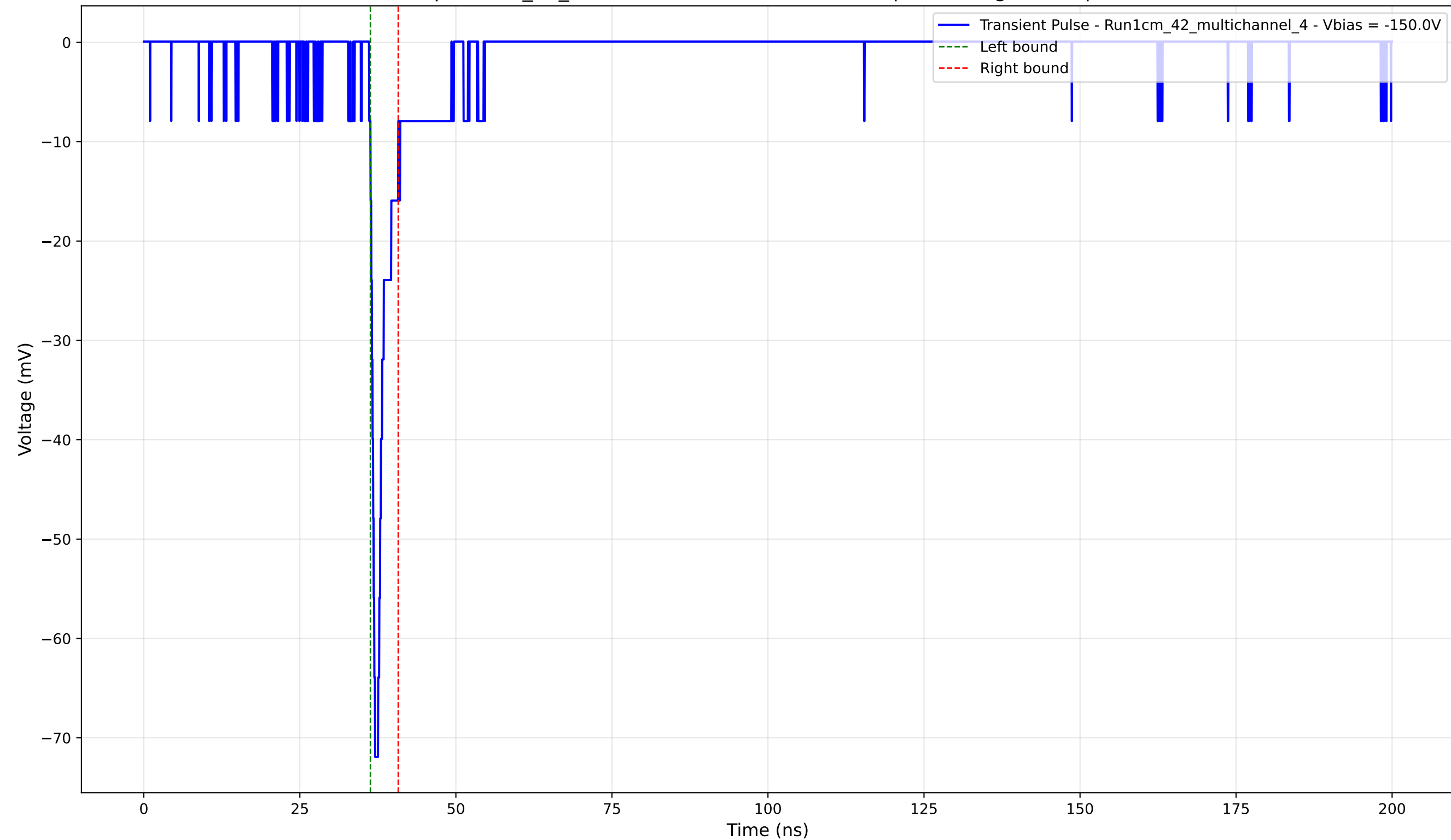
Transient Pulse - Sample: 1cm_42_multichannel - Position: 2550.0 \mu\text{m} - Charge: 3.05 pC - Rise Time: 0.94 ns
