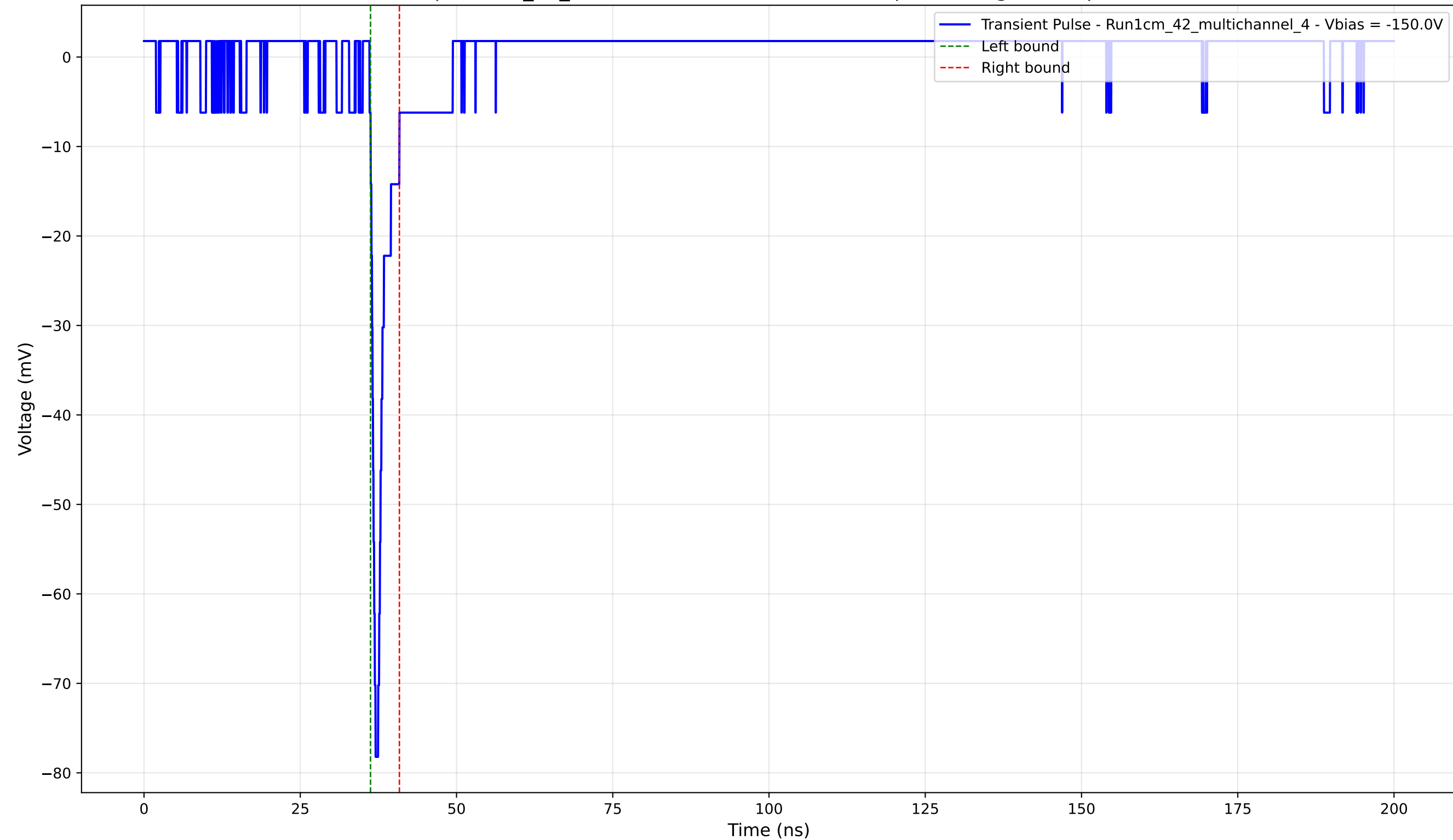
Transient Pulse - Sample: 1cm_42_multichannel - Position: 2300.0 \mu\text{m} - Charge: 3.09 pC - Rise Time: 0.80 ns
