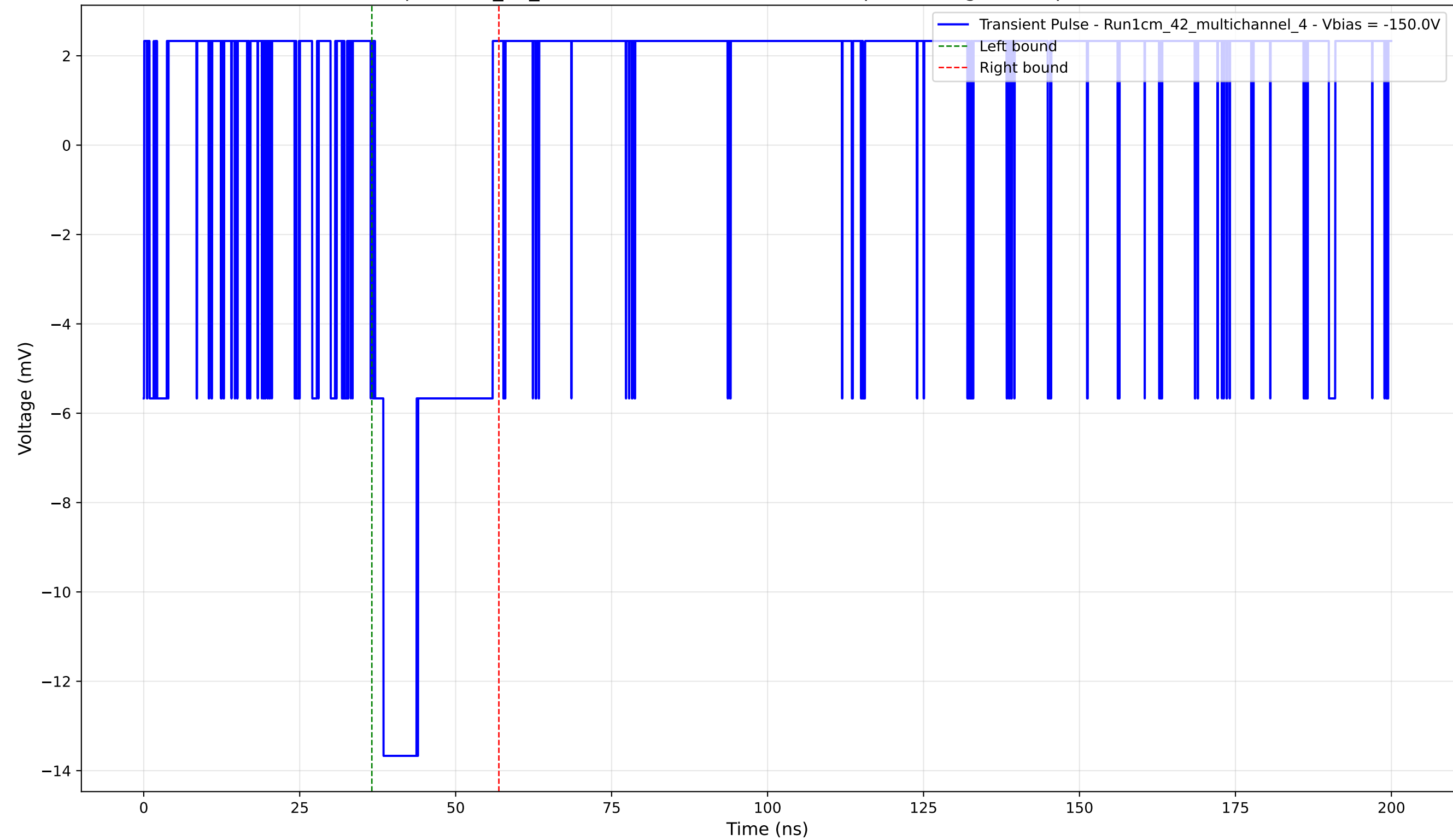
Transient Pulse - Sample: 1cm_42_multichannel - Position: 4495.0 \mu\text{m} - Charge: 2.96 pC - Rise Time: 0.00 ns (N/A)
