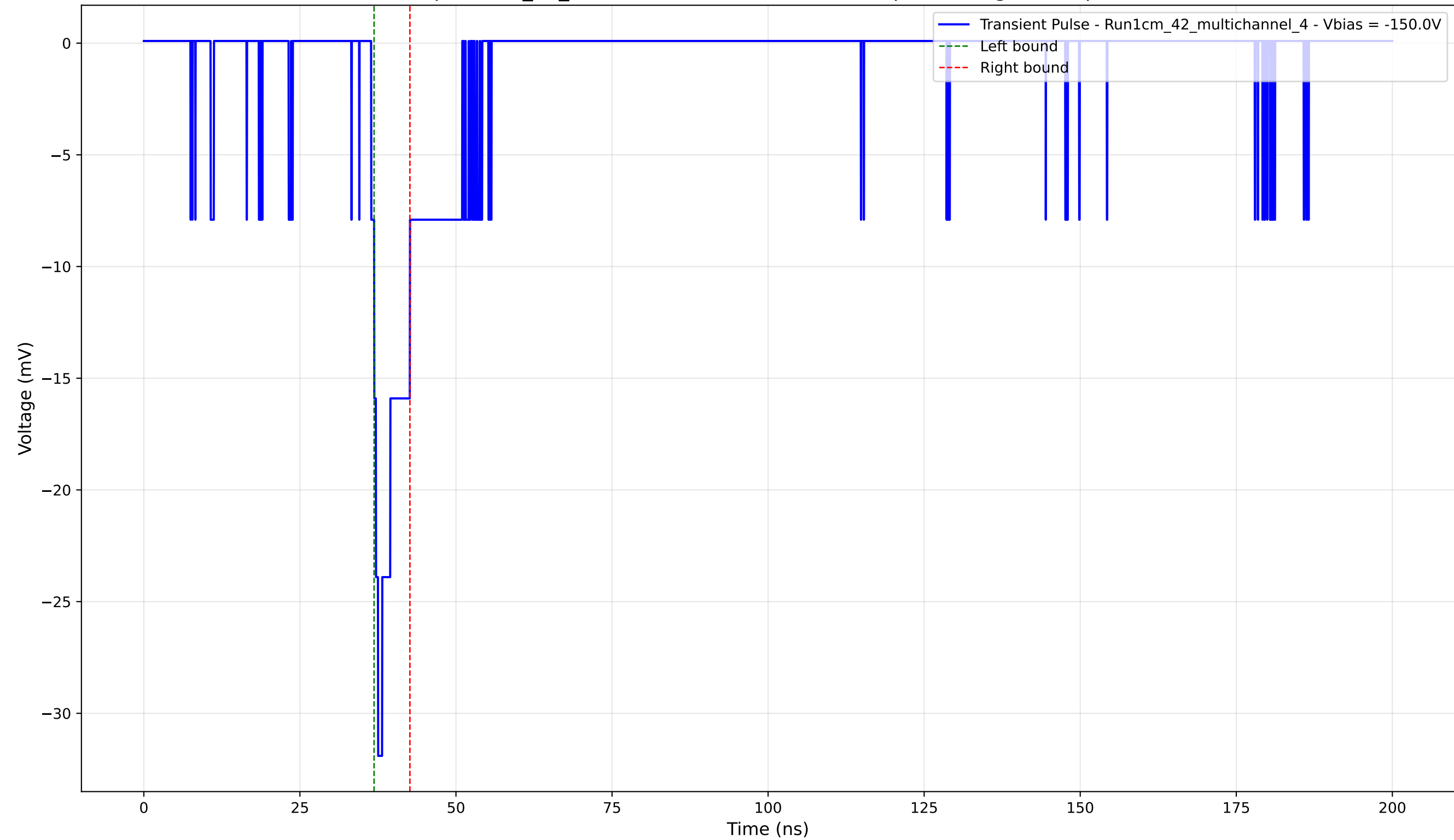
Transient Pulse - Sample: 1cm_42_multichannel - Position: 3205.0 \mu\text{m} - Charge: 2.30 pC - Rise Time: 1.11 ns
