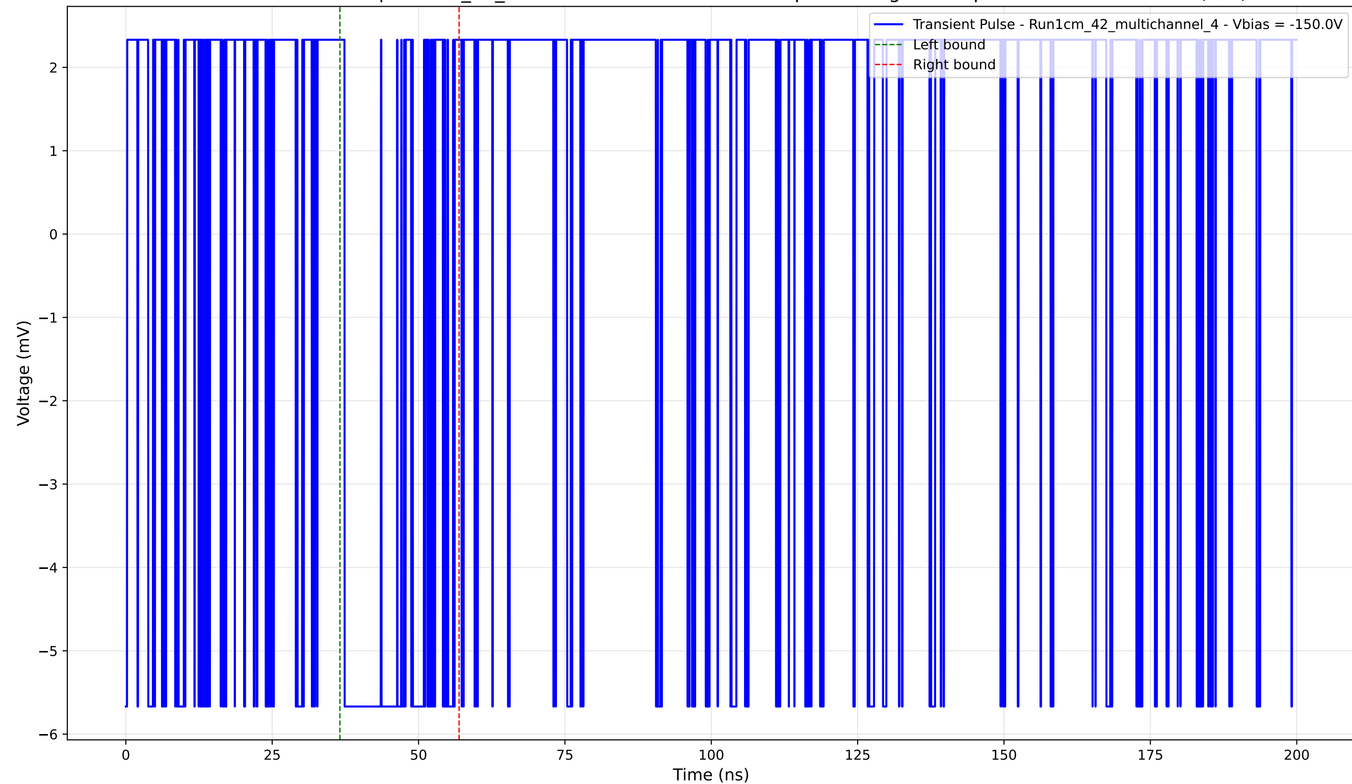
Transient Pulse - Sample: 1cm_42_multichannel - Position: 405.0 \mu\text{m} - Charge: 1.45 pC - Rise Time: 0.00 ns (N/A)
