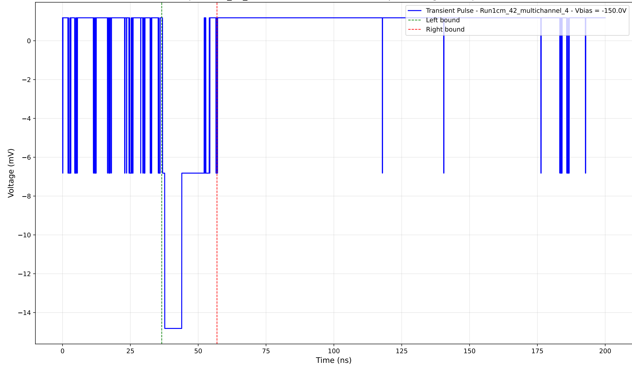
Transient Pulse - Sample: 1cm_42_multichannel - Position: 3800.0 \mu\text{m} - Charge: 3.28 pC - Rise Time: 0.82 ns
