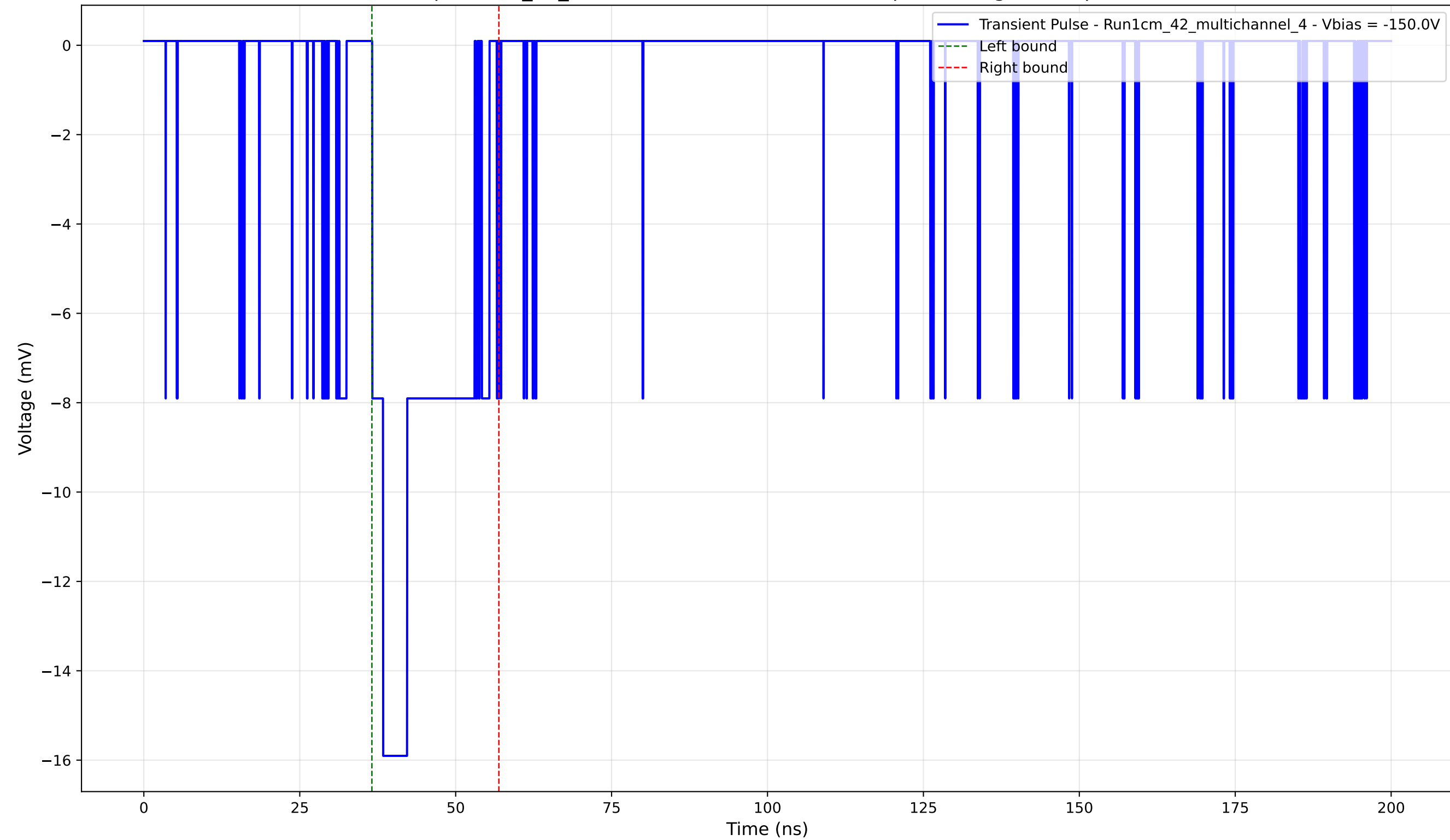
Transient Pulse - Sample: 1cm_42_multichannel - Position: 4720.0 \mu\text{m} - Charge: 3.49 pC - Rise Time: 1.76 ns
