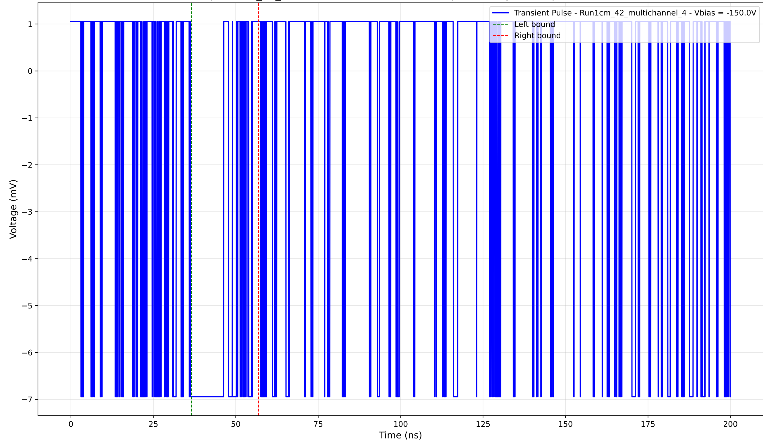
Transient Pulse - Sample: 1cm_42_multichannel - Position: 1410.0 \mu\text{m} - Charge: 1.77 pC - Rise Time: 0.00 ns (N/A)
