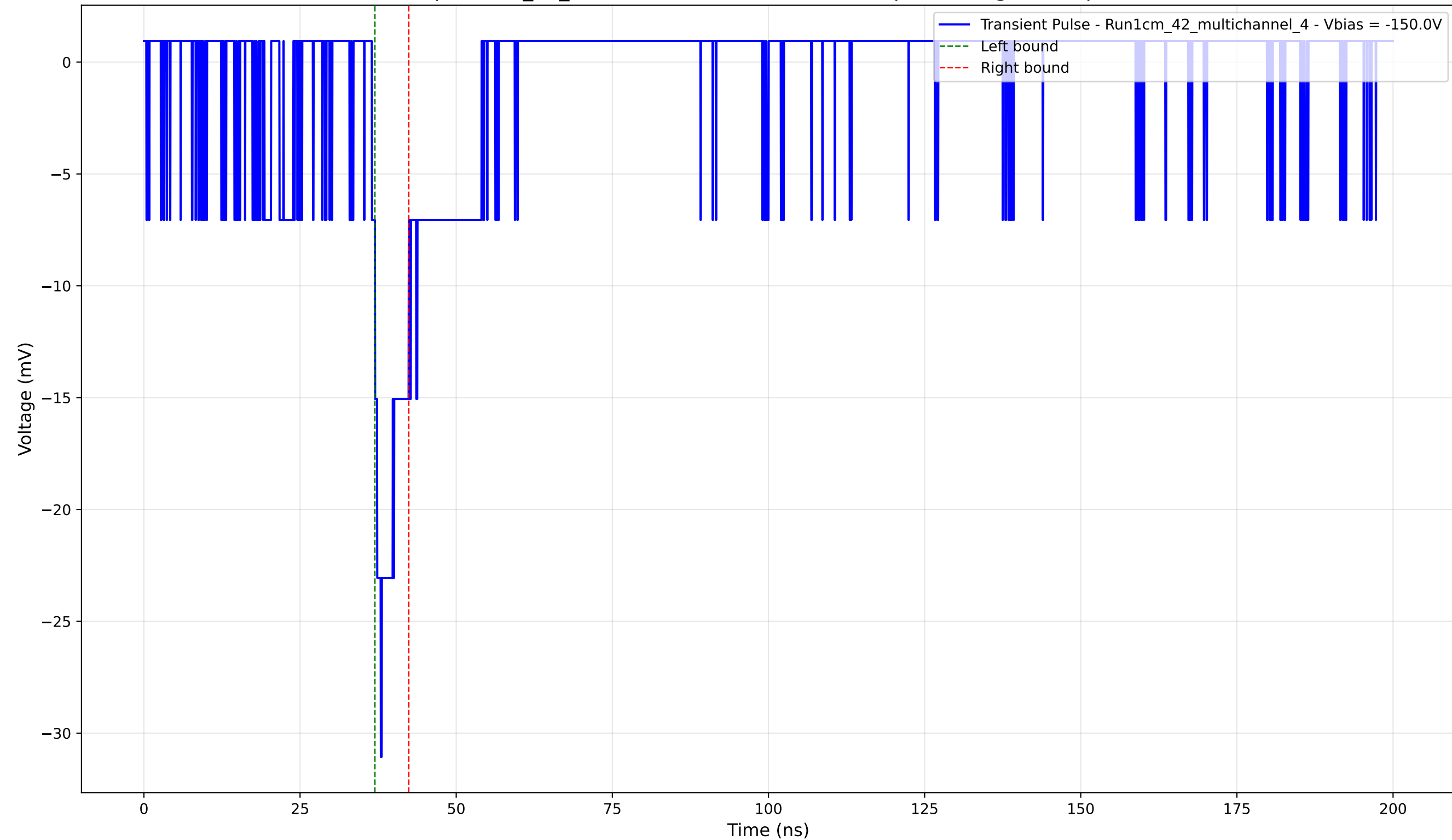
Transient Pulse - Sample: 1cm_42_multichannel - Position: 3280.0 \mu\text{m} - Charge: 2.08 pC - Rise Time: 1.43 ns
