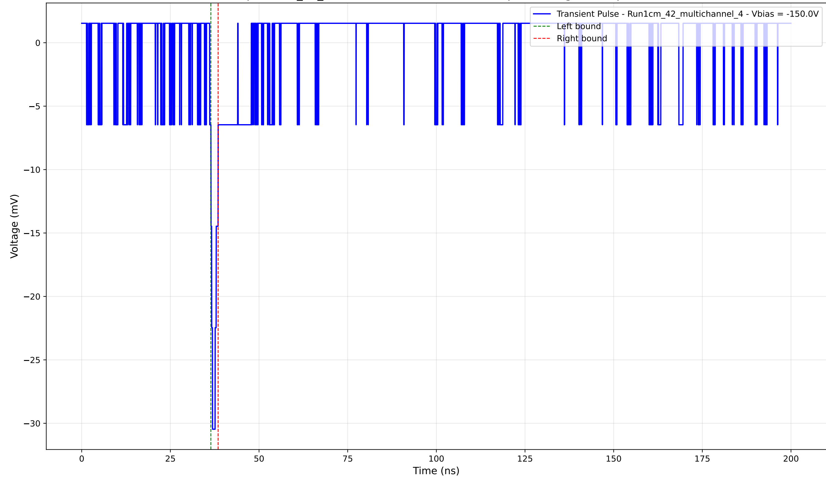
Transient Pulse - Sample: 1cm_42_multichannel - Position: 2340.0 \mu\text{m} - Charge: 0.91 pC - Rise Time: 0.81 ns
