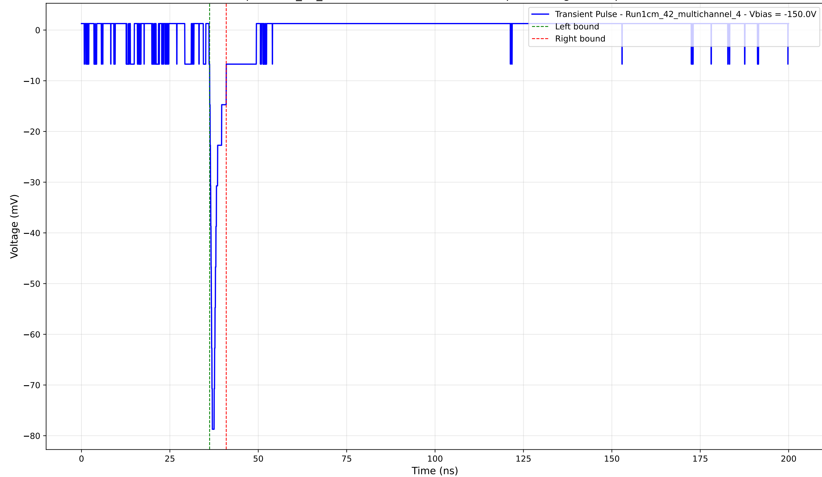
Transient Pulse - Sample: 1cm_42_multichannel - Position: 2295.0 \mu\text{m} - Charge: 3.24 pC - Rise Time: 0.76 ns
