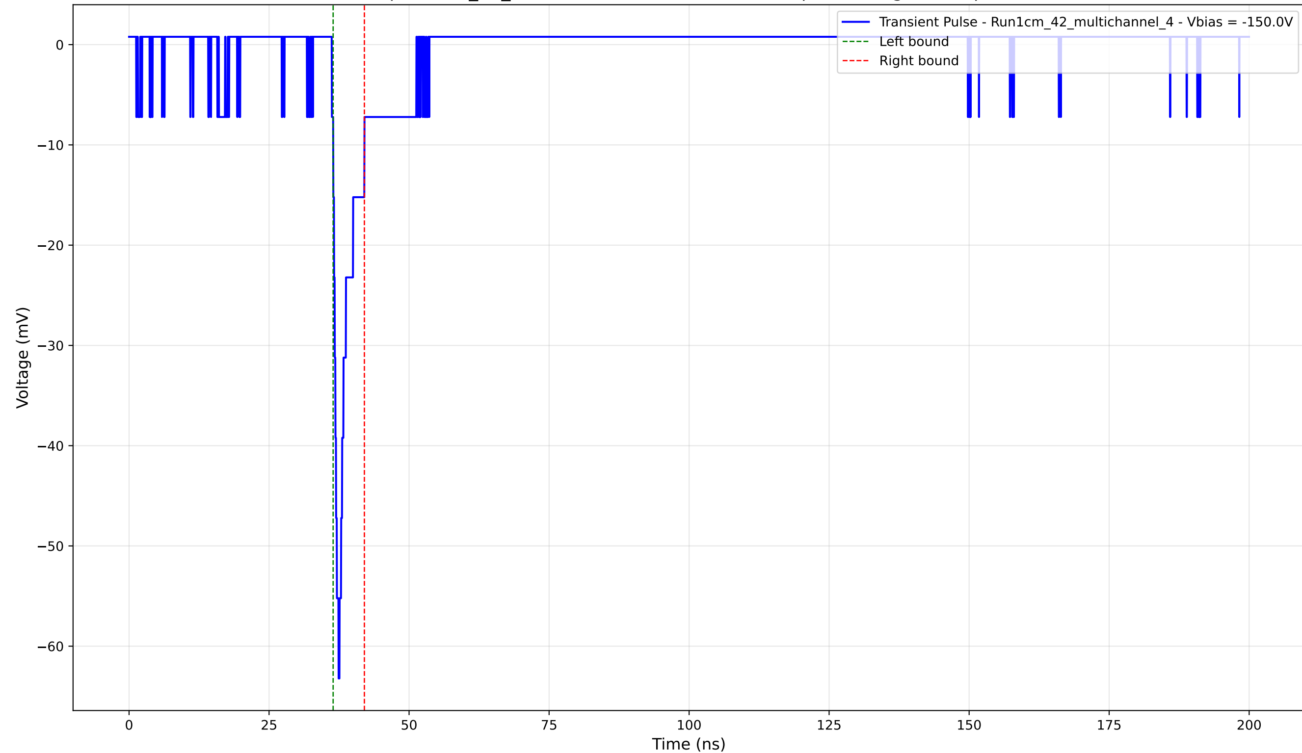
Transient Pulse - Sample: 1cm_42_multichannel - Position: 2060.0 \mu\text{m} - Charge: 3.11 pC - Rise Time: 1.20 ns
