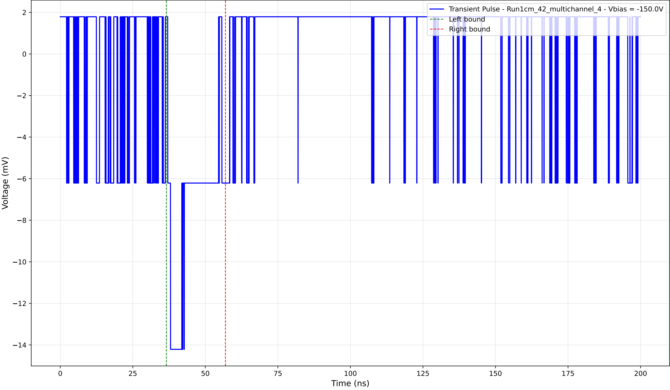
Transient Pulse - Sample: 1cm_42_multichannel - Position: 805.0 \mu\text{m} - Charge: 3.01 pC - Rise Time: 0.00 ns (N/A)
