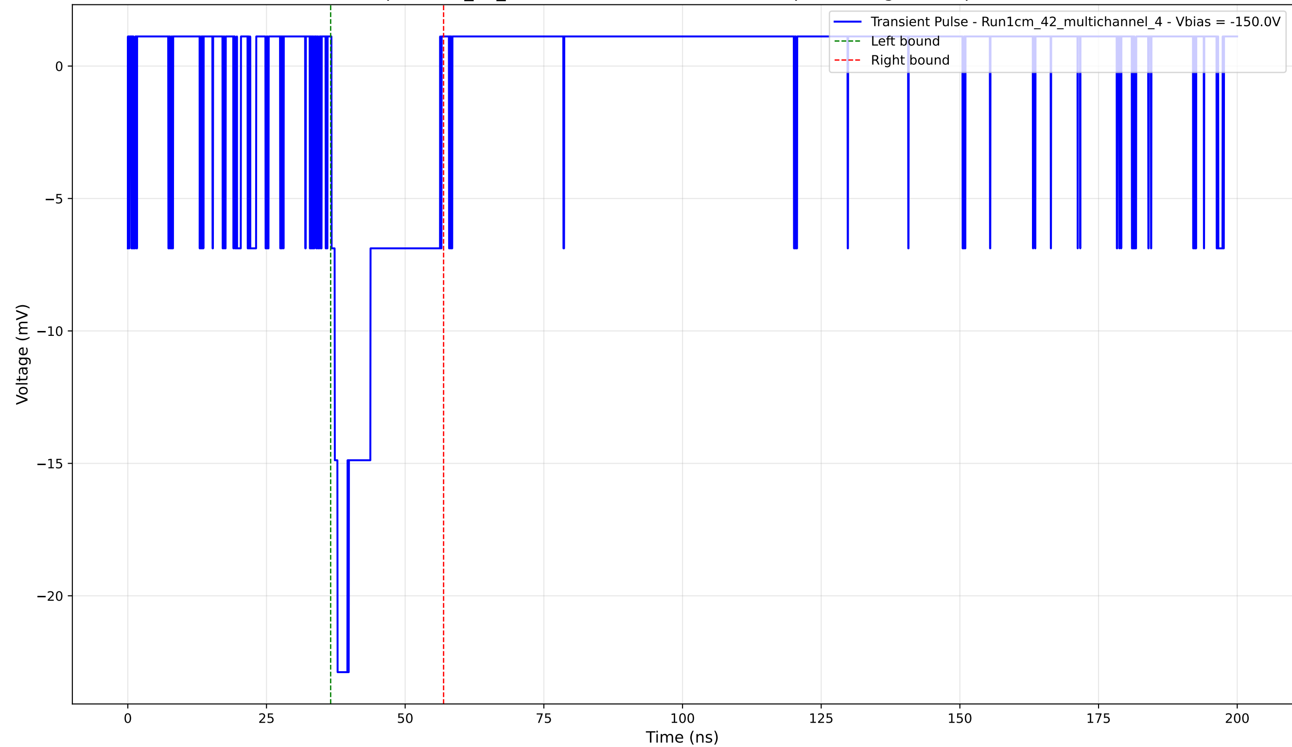
Transient Pulse - Sample: 1cm_42_multichannel - Position: 1165.0 \mu\text{m} - Charge: 4.05 pC - Rise Time: 1.10 ns
