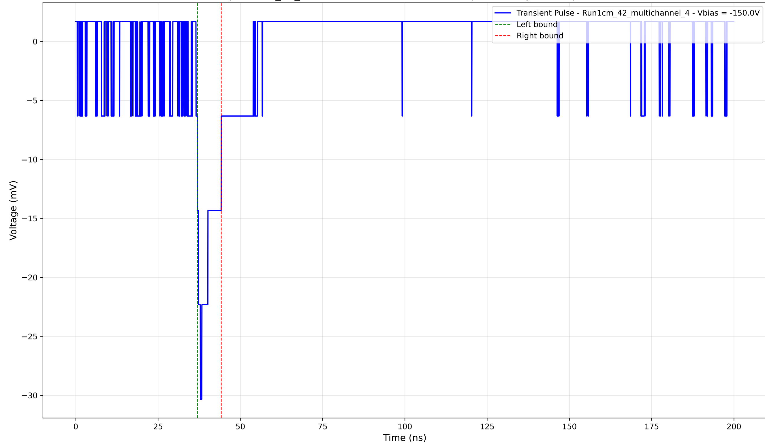
Transient Pulse - Sample: 1cm_42_multichannel - Position: 1455.0 \mu\text{m} - Charge: 2.60 pC - Rise Time: 1.33 ns
