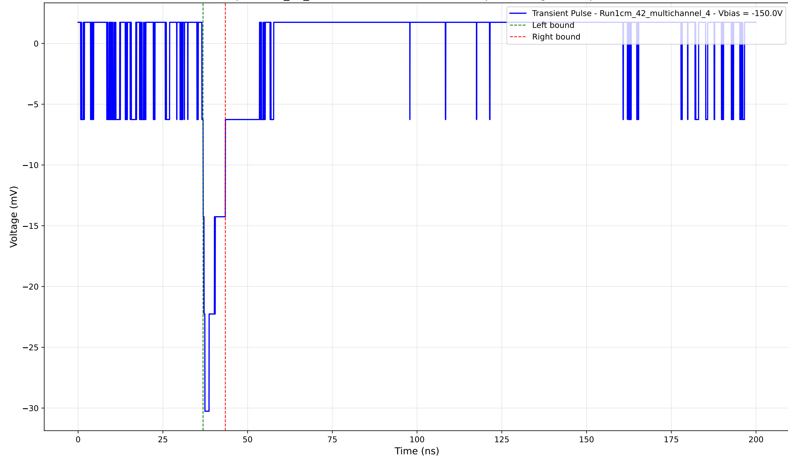
Transient Pulse - Sample: 1cm_42_multichannel - Position: 1545.0 \mu\text{m} - Charge: 2.59 pC - Rise Time: 0.89 ns
