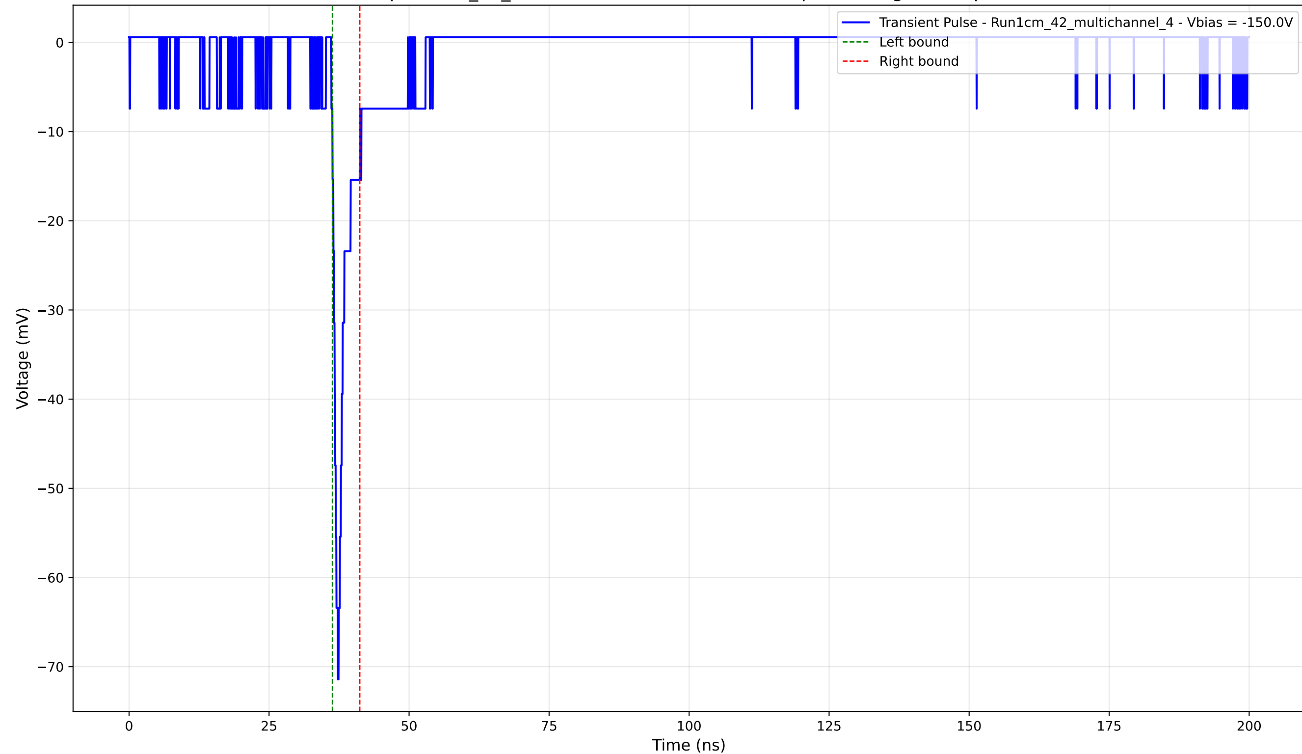
Transient Pulse - Sample: 1cm_42_multichannel - Position: 2585.0 \mu\text{m} - Charge: 2.98 pC - Rise Time: 1.16 ns
