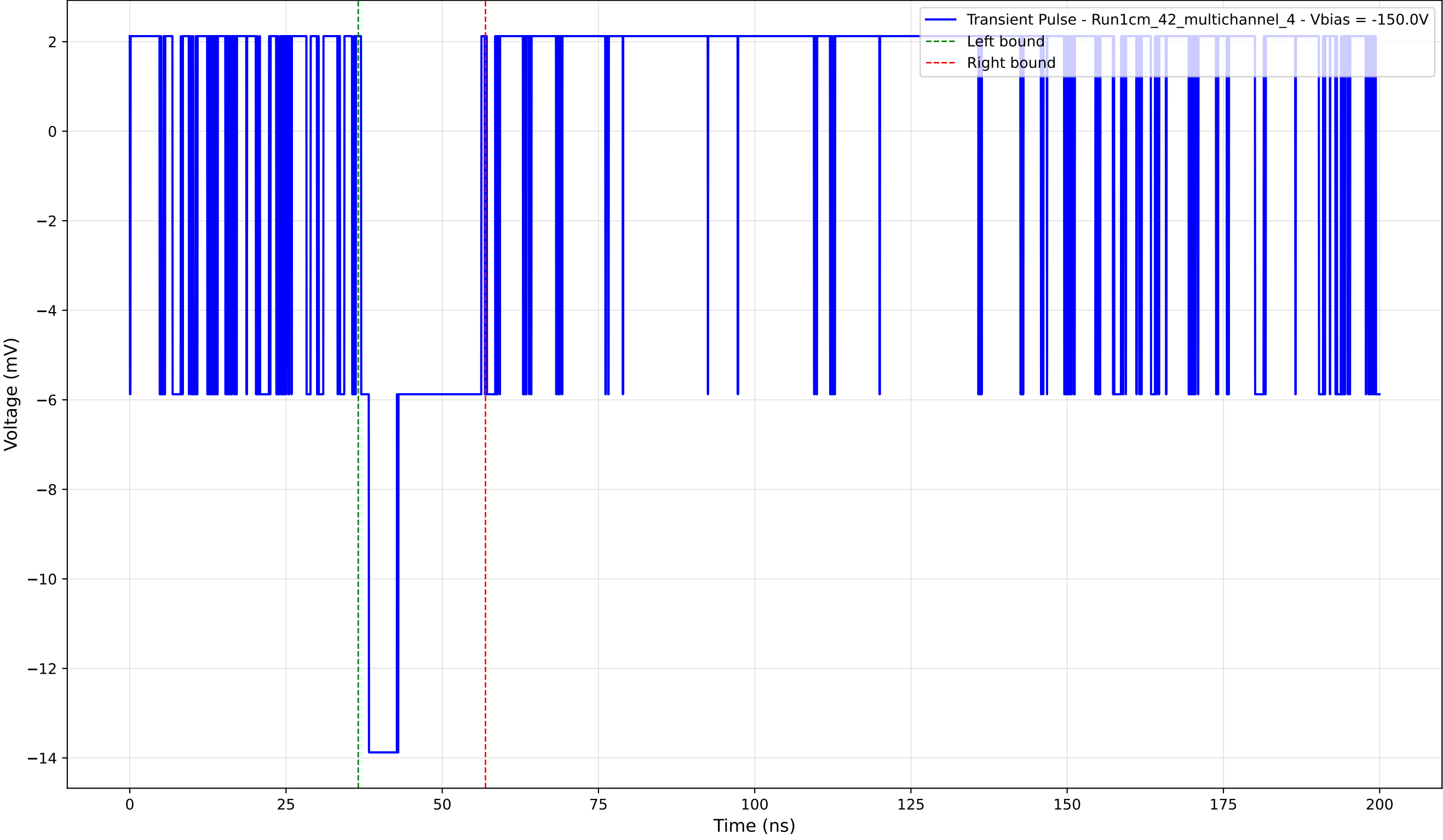
Transient Pulse - Sample: 1cm_42_multichannel - Position: 285.0 \mu\text{m} - Charge: 2.98 pC - Rise Time: 0.00 ns (N/A)
