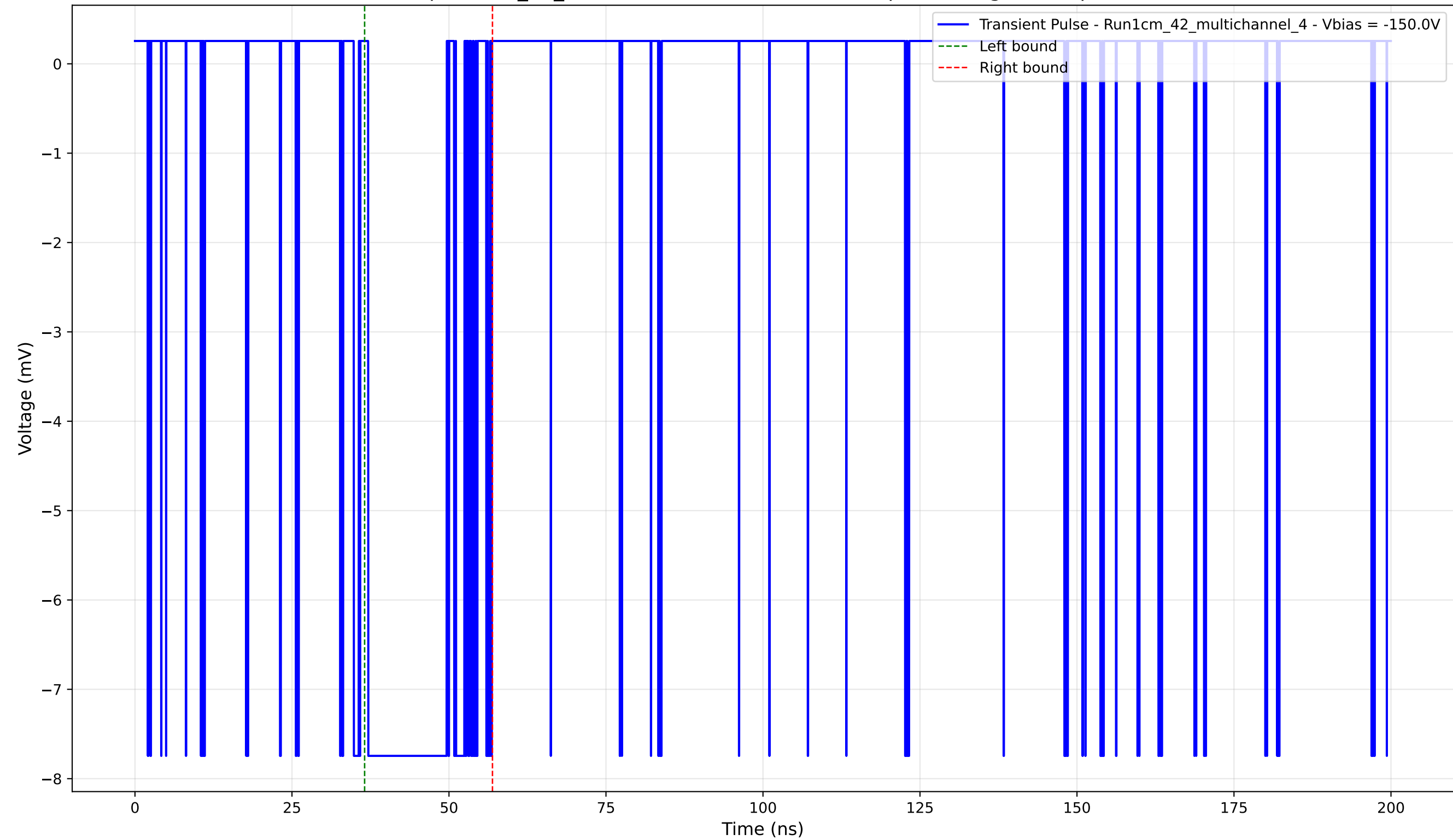
Transient Pulse - Sample: 1cm_42_multichannel - Position: 3855.0 \mu\text{m} - Charge: 2.45 pC - Rise Time: 0.02 ns
