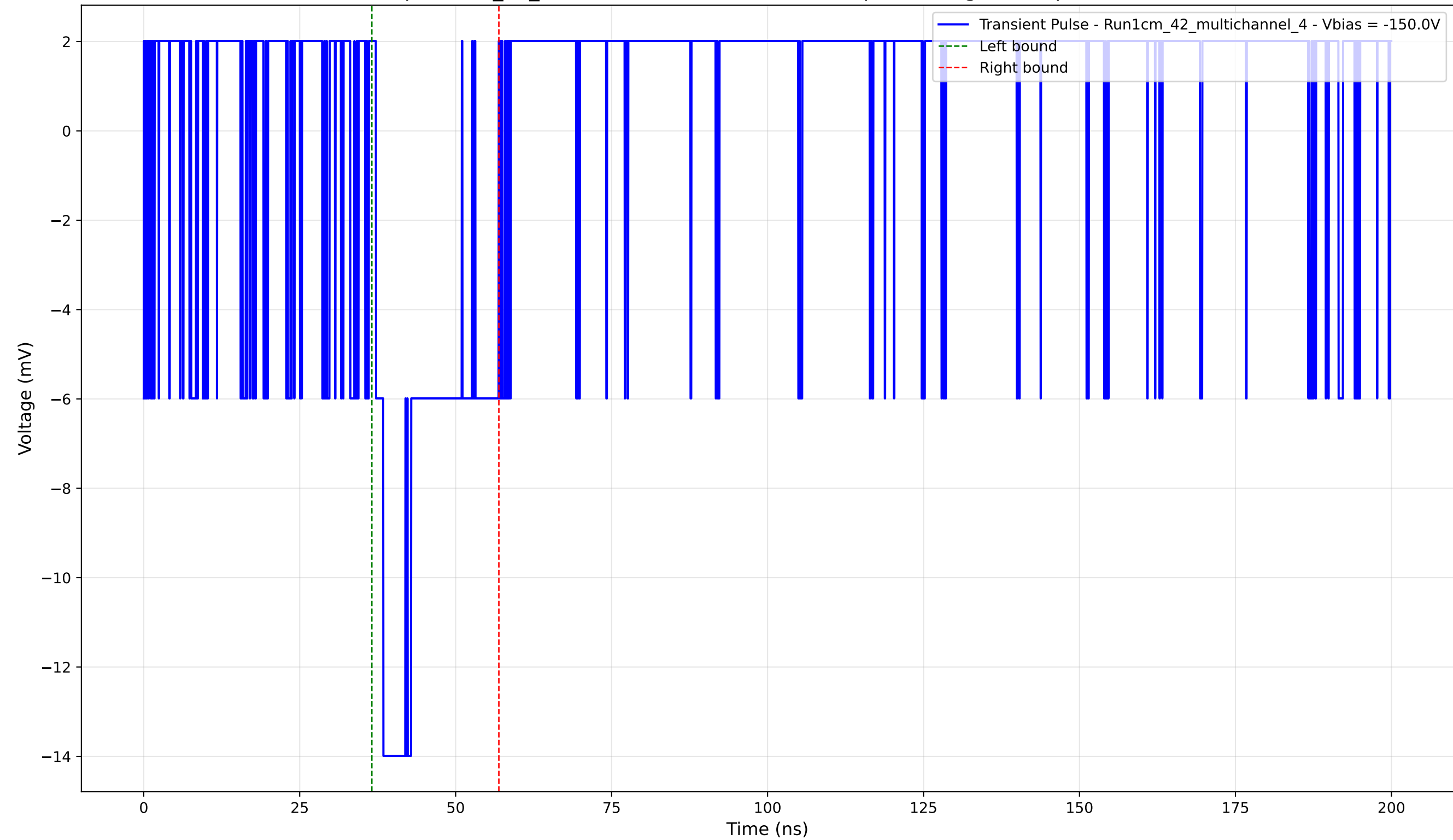
Transient Pulse - Sample: 1cm_42_multichannel - Position: 4335.0 \mu\text{m} - Charge: 2.97 pC - Rise Time: 0.00 ns (N/A)
