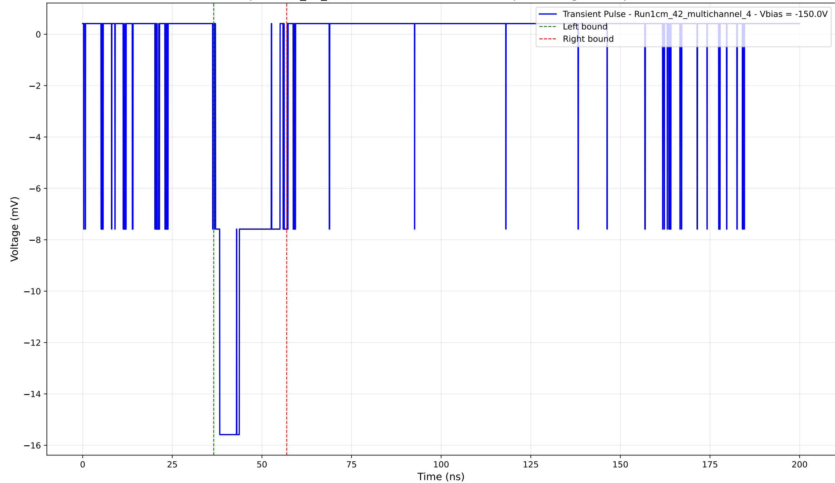
Transient Pulse - Sample: 1cm_42_multichannel - Position: 4095.0 \mu\text{m} - Charge: 3.72 pC - Rise Time: 1.18 ns
