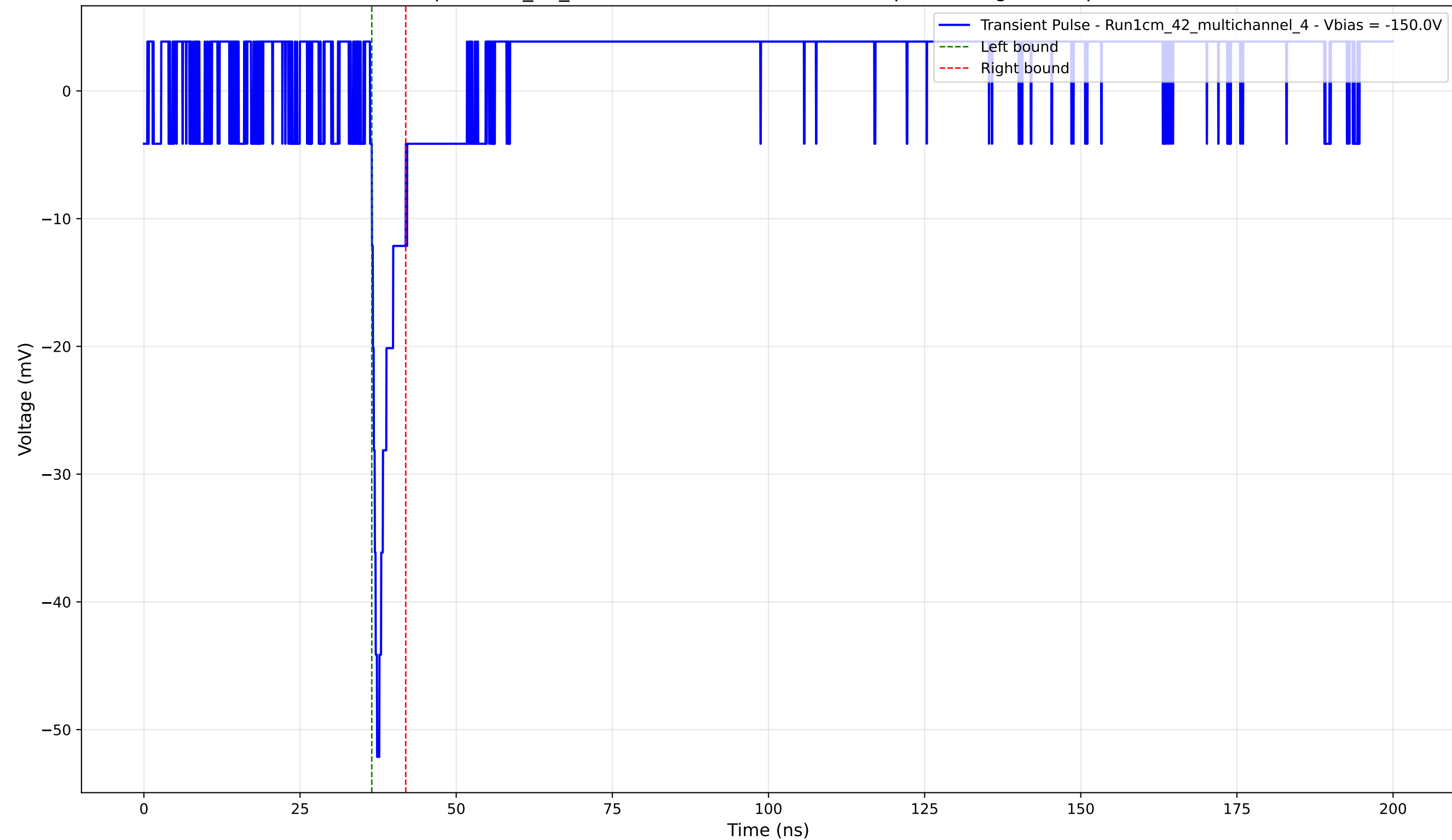
Transient Pulse - Sample: 1cm_42_multichannel - Position: 1965.0 \mu\text{m} - Charge: 2.57 pC - Rise Time: 0.84 ns
