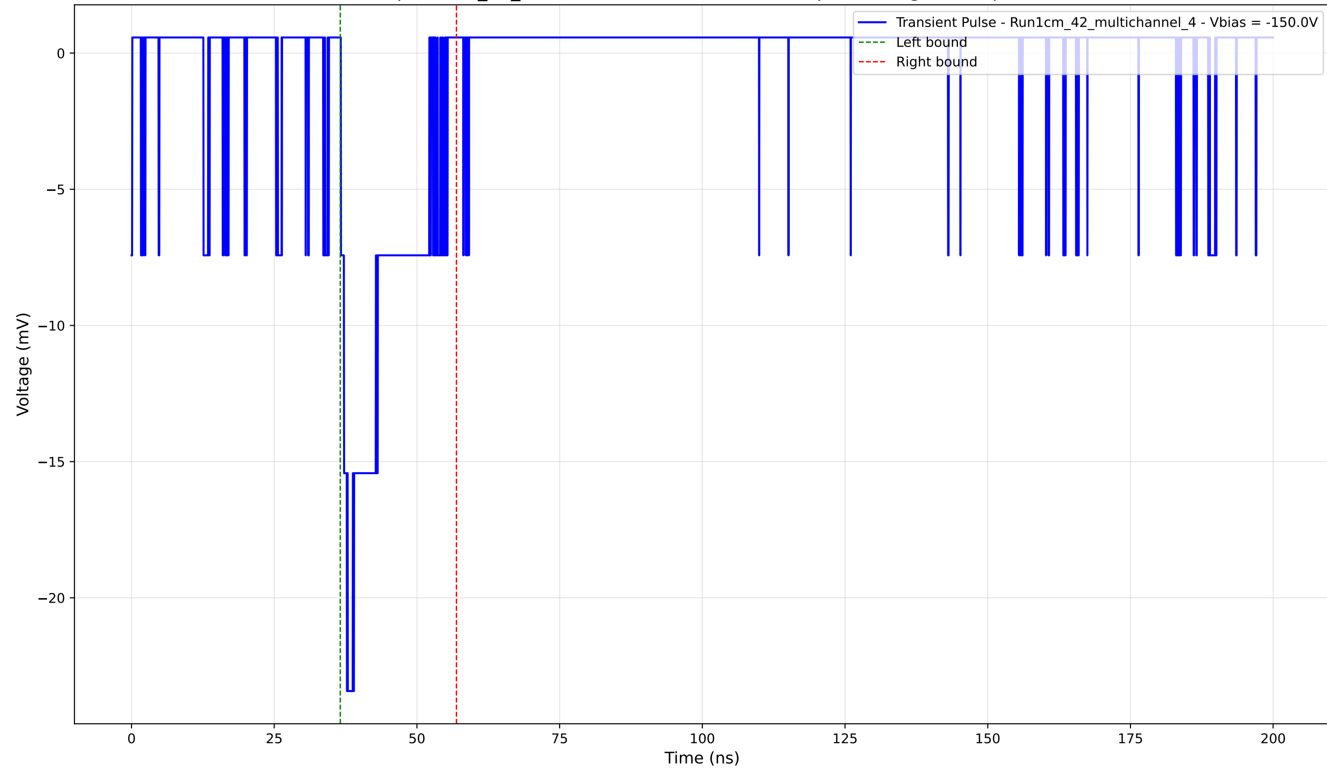
Transient Pulse - Sample: 1cm_42_multichannel - Position: 3485.0 \mu\text{m} - Charge: 3.66 pC - Rise Time: 1.05 ns
