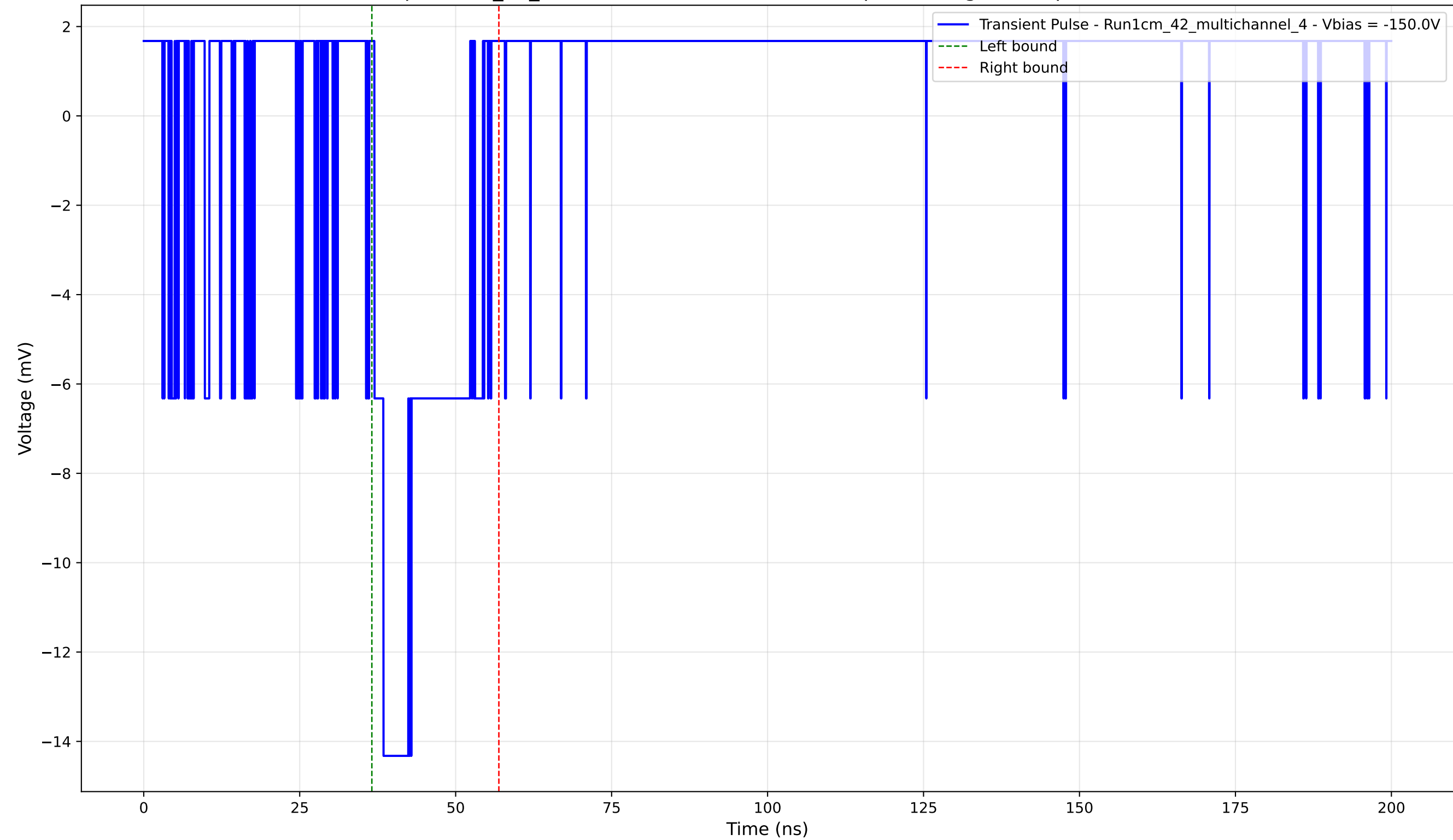
Transient Pulse - Sample: 1cm_42_multichannel - Position: 4675.0 \mu\text{m} - Charge: 2.73 pC - Rise Time: 0.00 ns (N/A)
