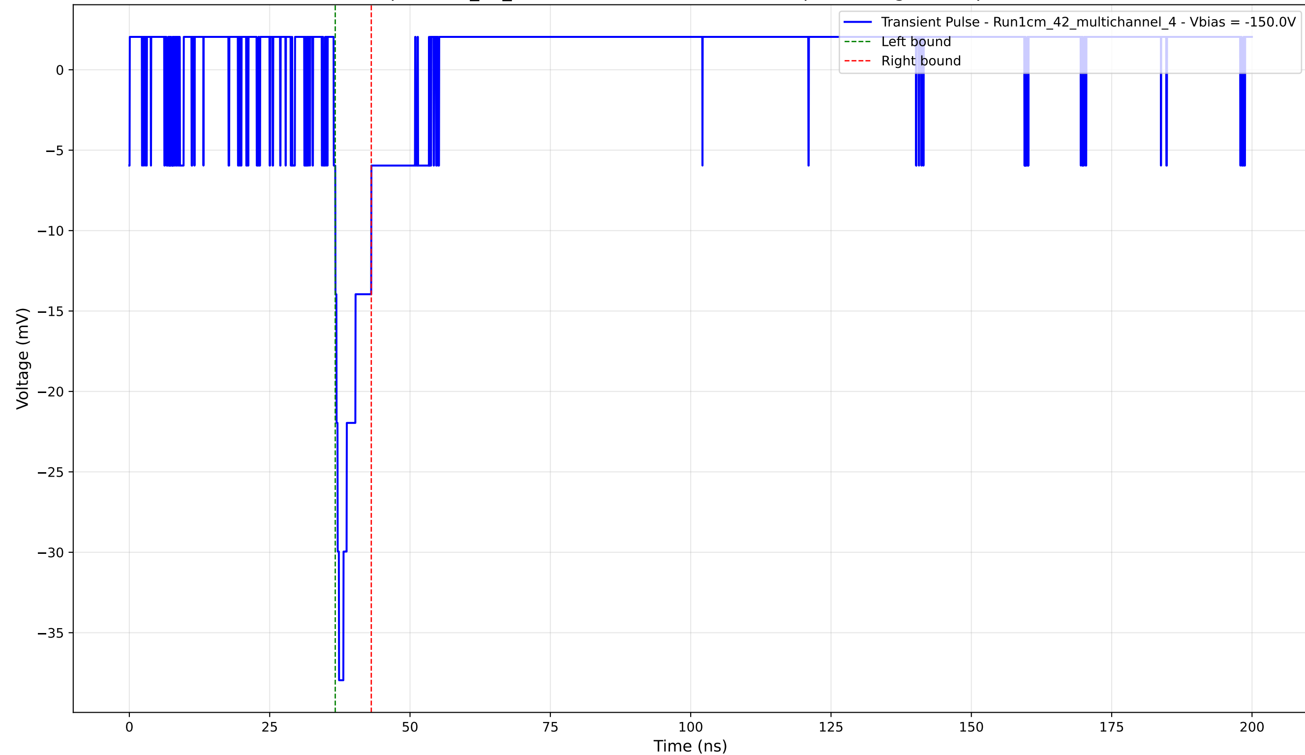
Transient Pulse - Sample: 1cm_42_multichannel - Position: 1735.0 \mu\text{m} - Charge: 2.72 pC - Rise Time: 0.95 ns
