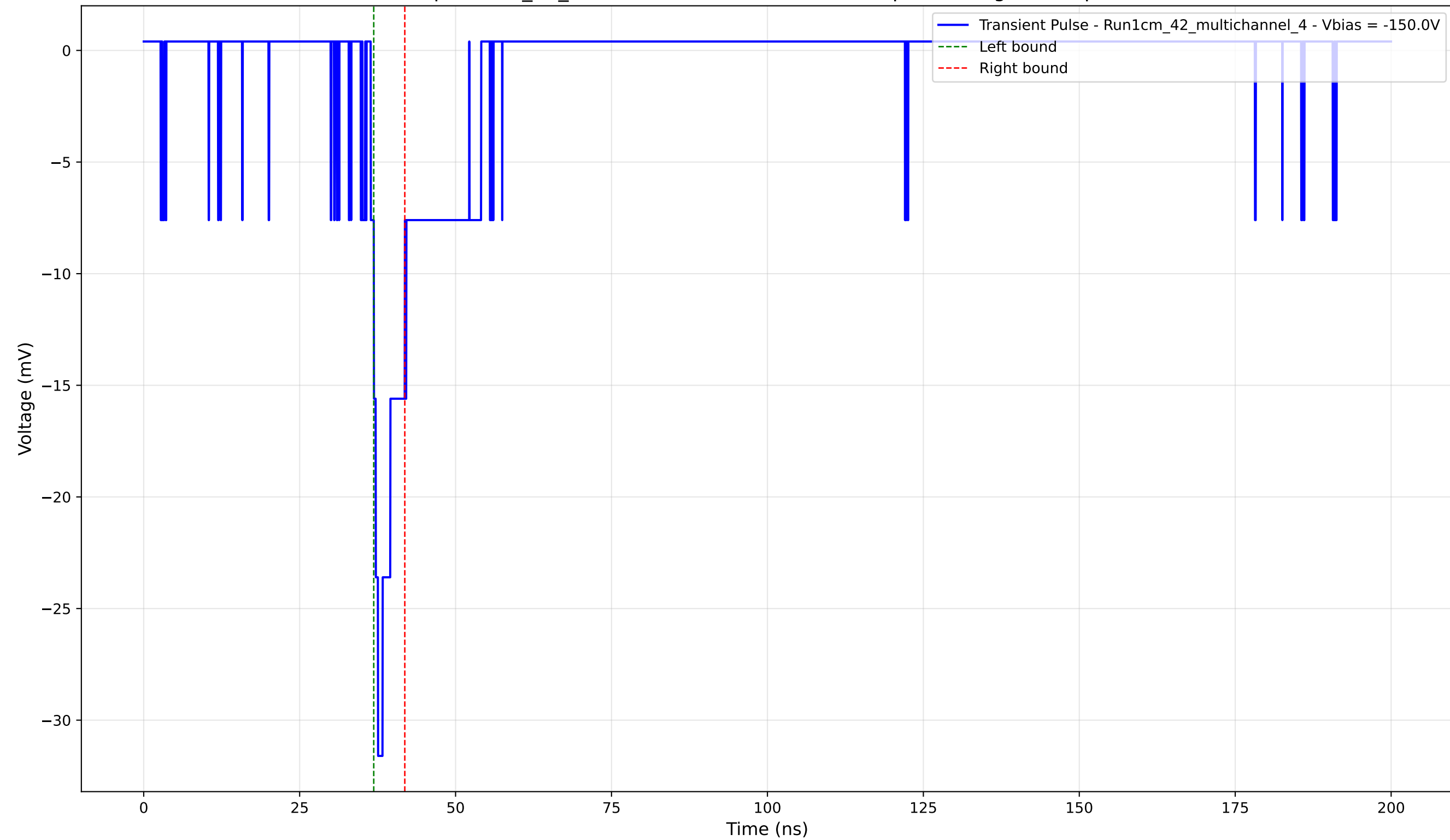
Transient Pulse - Sample: 1cm_42_multichannel - Position: 3190.0 \mu\text{m} - Charge: 2.04 pC - Rise Time: 1.17 ns
