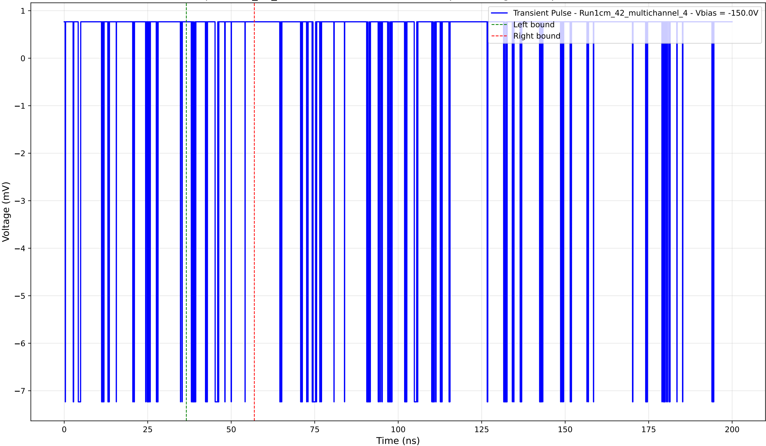
Transient Pulse - Sample: 1cm_42_multichannel - Position: 3900.0 \mu\text{m} - Charge: 0.02 pC - Rise Time: 0.00 ns (N/A)
