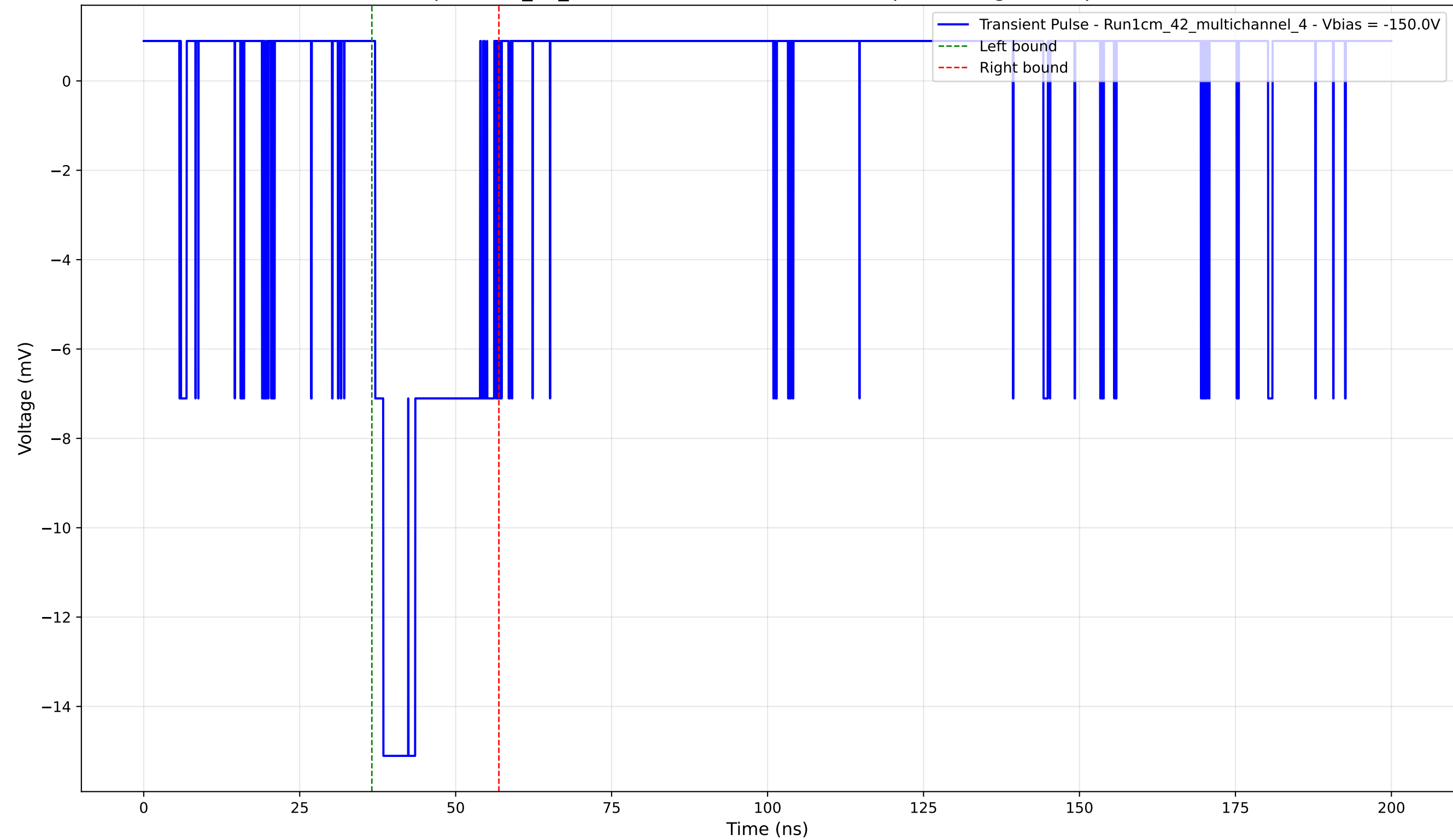
Transient Pulse - Sample: 1cm_42_multichannel - Position: 4255.0 \mu\text{m} - Charge: 3.51 pC - Rise Time: 1.32 ns
