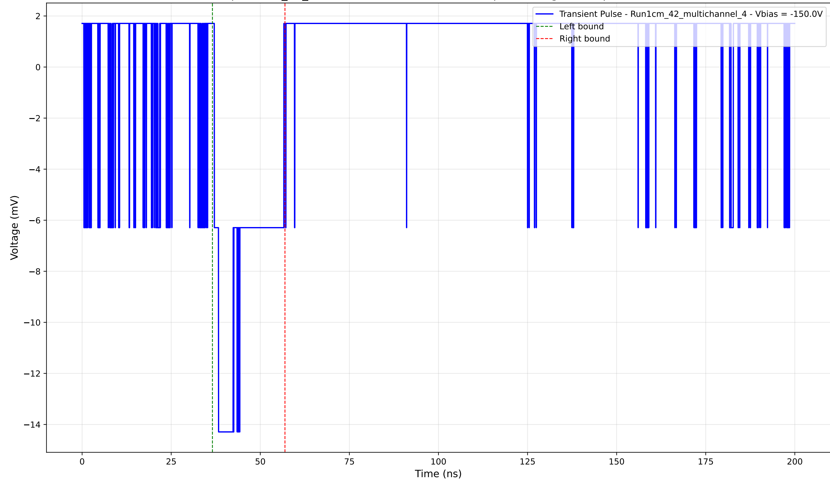
Transient Pulse - Sample: 1cm_42_multichannel - Position: 4515.0 \mu\text{m} - Charge: 3.14 pC - Rise Time: 0.00 ns (N/A)
