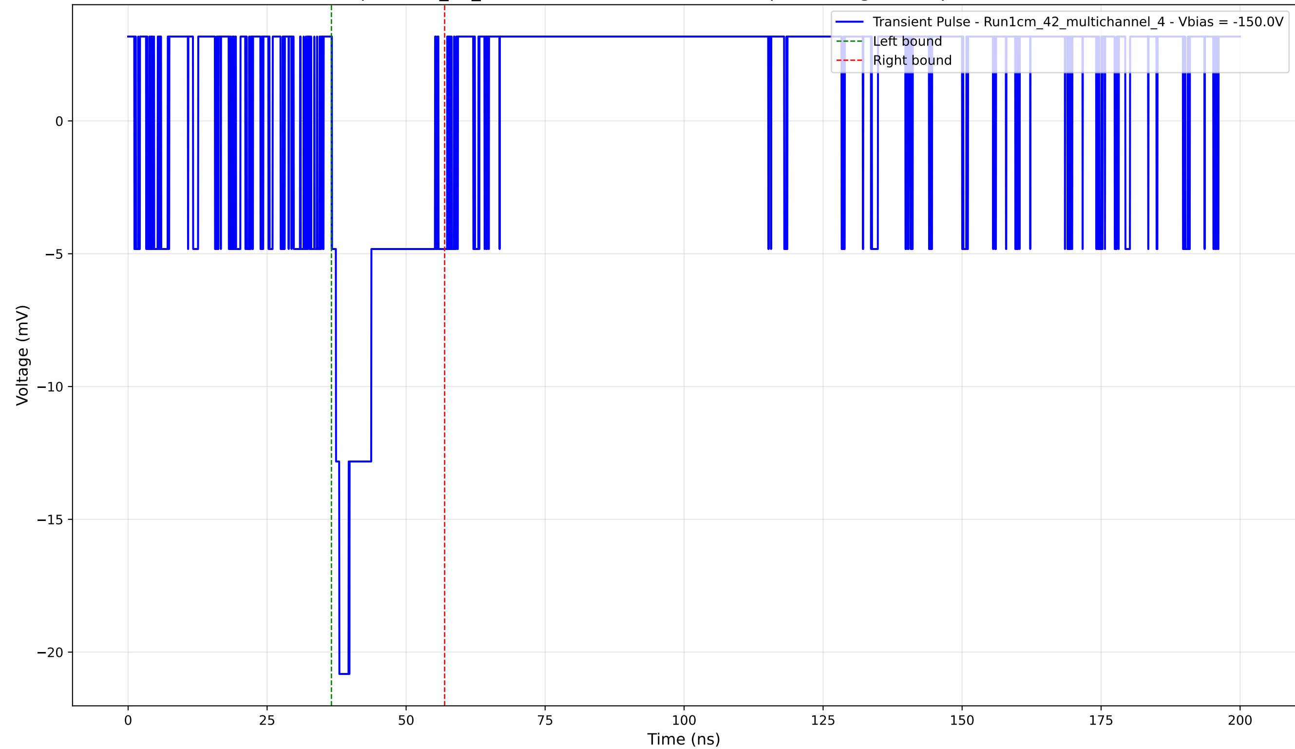
Transient Pulse - Sample: 1cm_42_multichannel - Position: 1075.0 \mu\text{m} - Charge: 3.19 pC - Rise Time: 0.00 ns (N/A)
