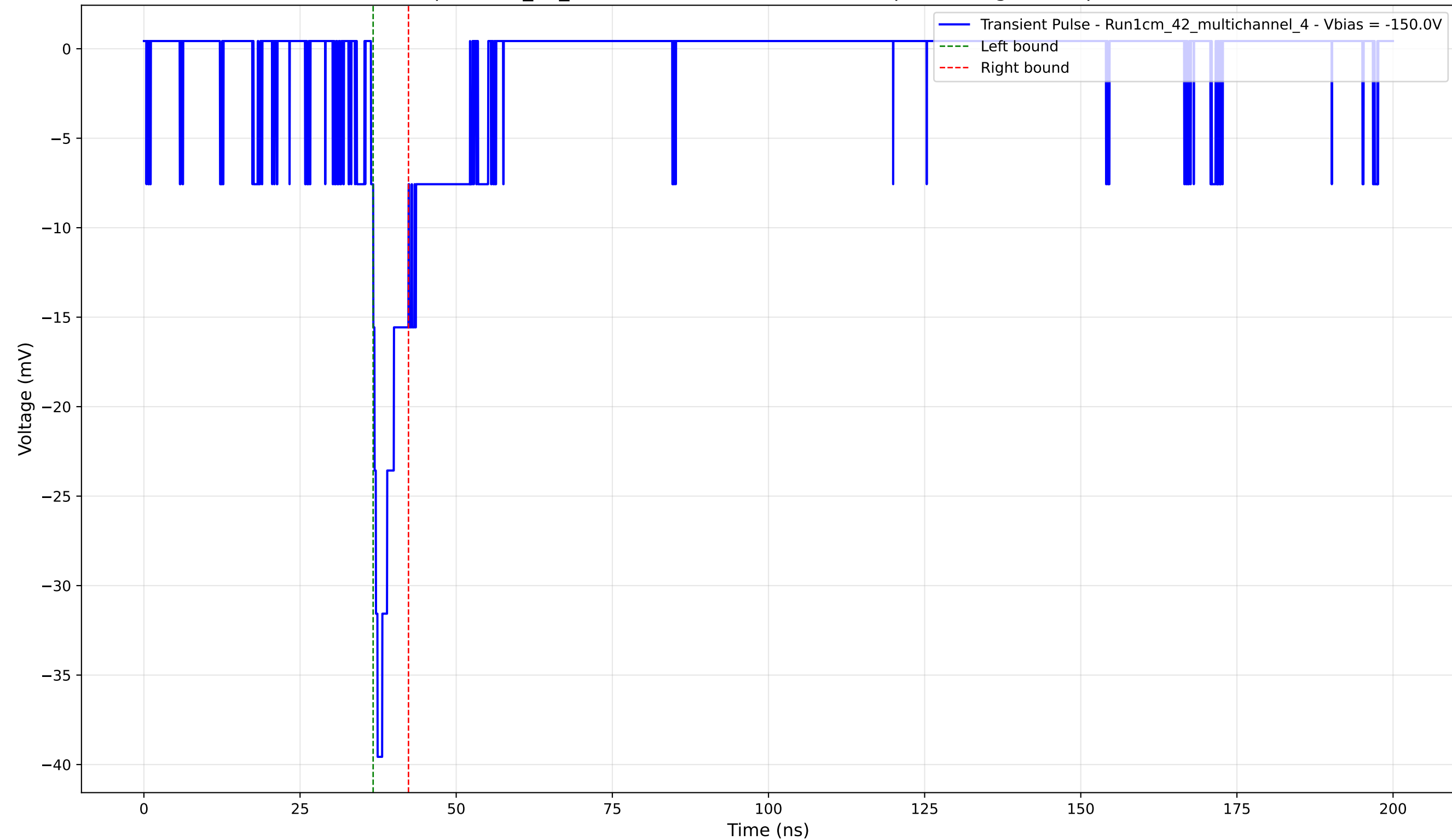
Transient Pulse - Sample: 1cm_42_multichannel - Position: 1720.0 \mu\text{m} - Charge: 2.66 pC - Rise Time: 1.05 ns
