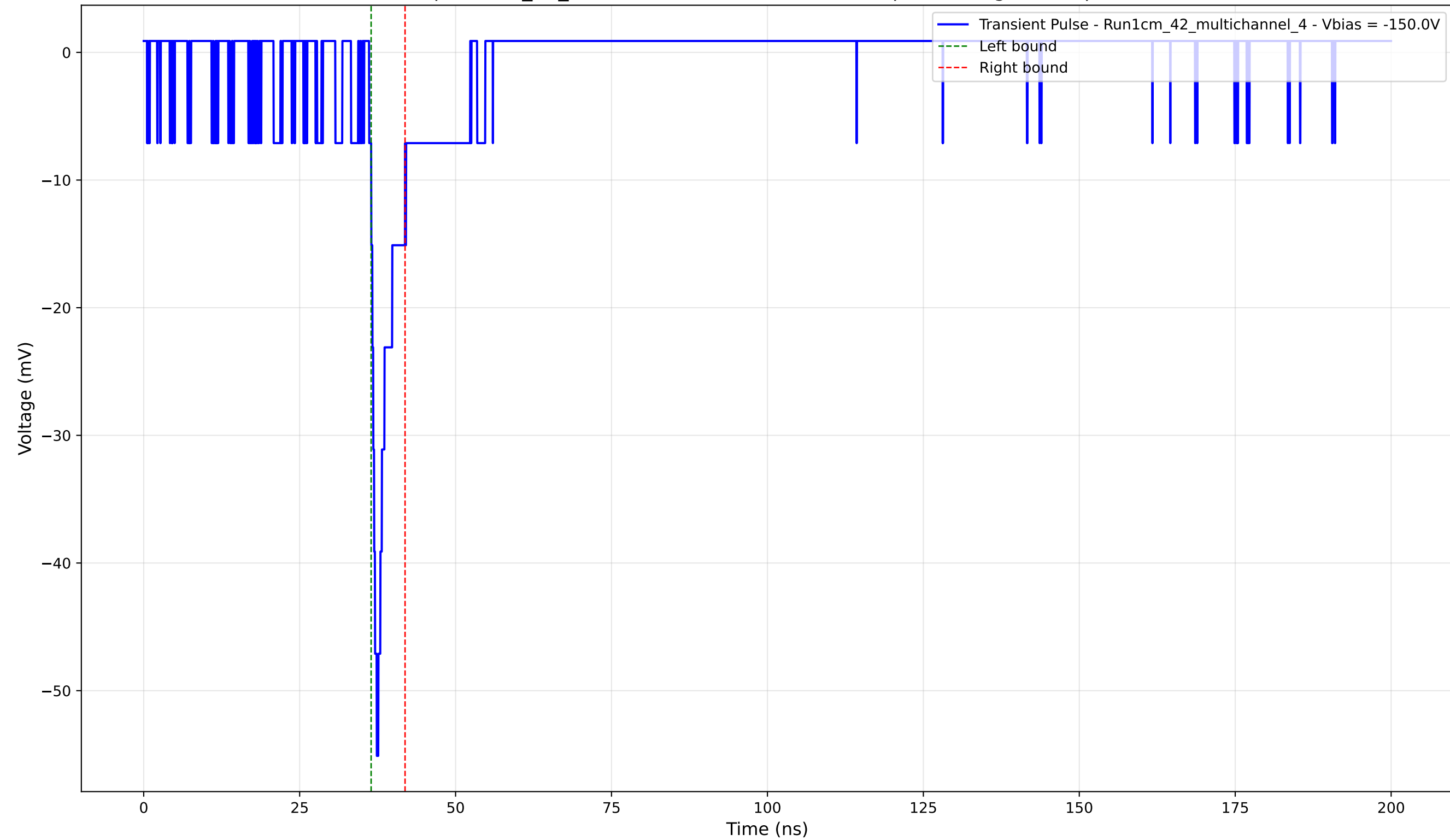
Transient Pulse - Sample: 1cm_42_multichannel - Position: 2780.0 \mu\text{m} - Charge: 2.81 pC - Rise Time: 1.23 ns
