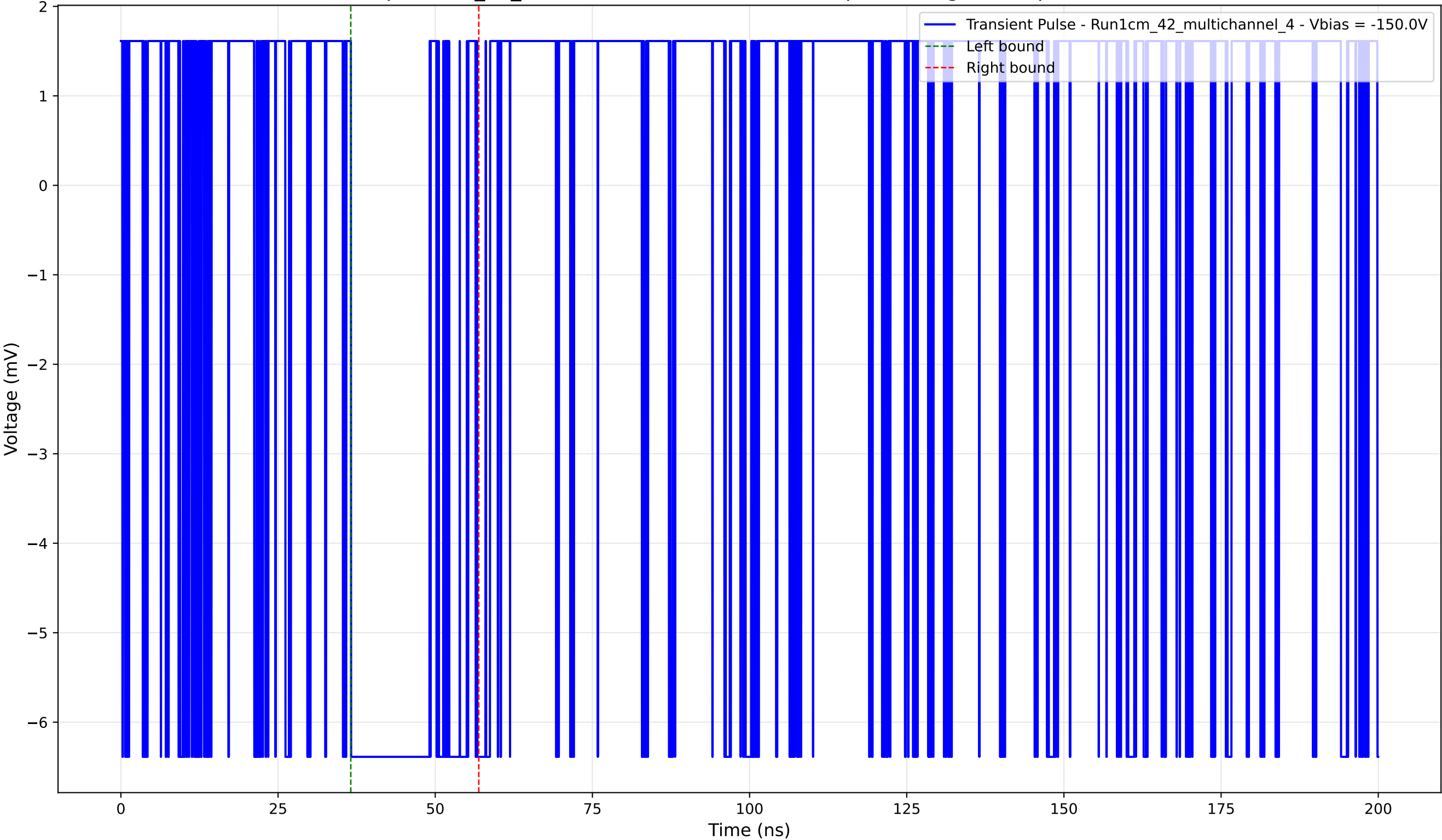
Transient Pulse - Sample: 1cm_42_multichannel - Position: 1335.0 \mu\text{m} - Charge: 2.13 pC - Rise Time: 0.00 ns (N/A)
