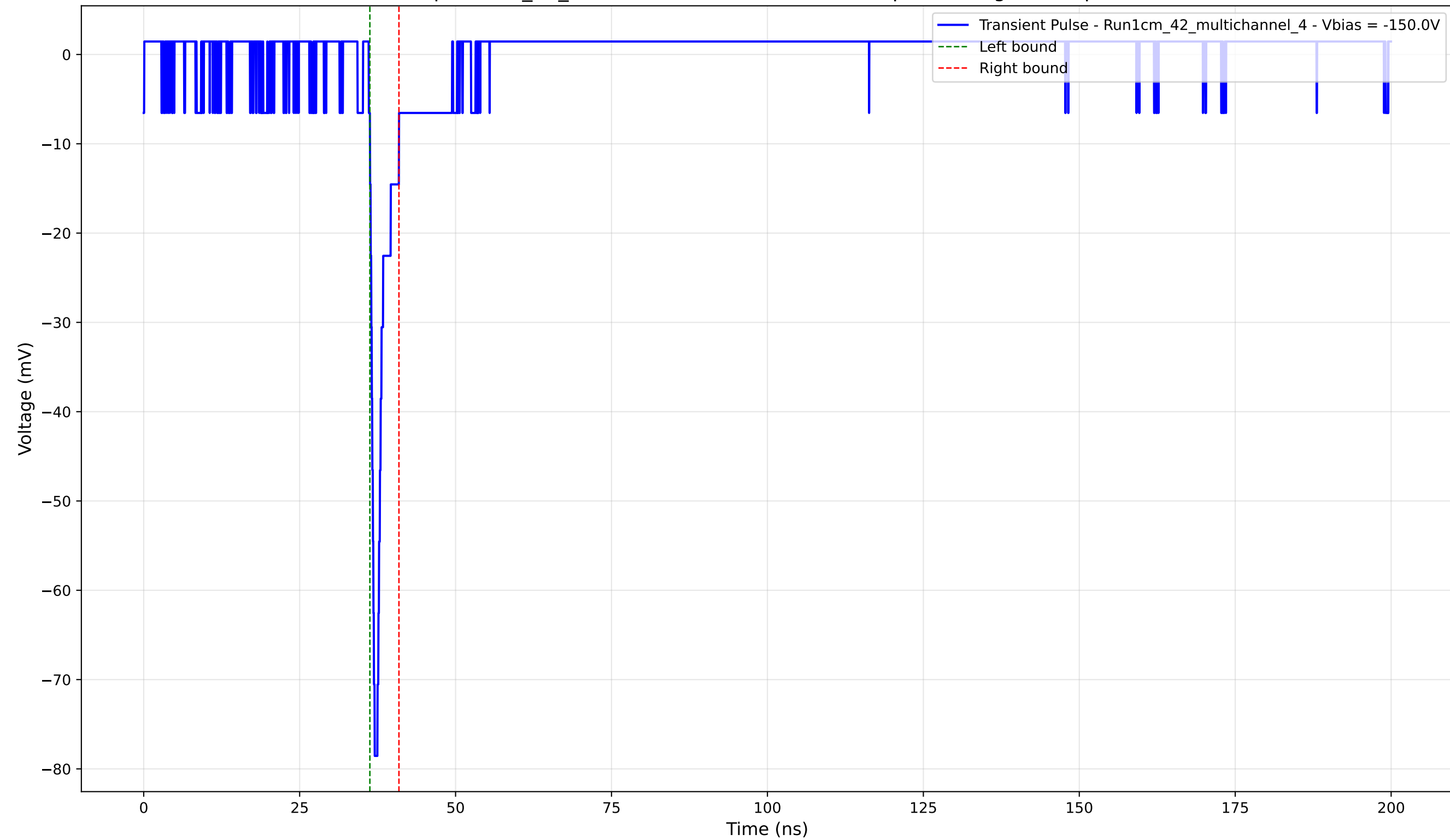
Transient Pulse - Sample: 1cm_42_multichannel - Position: 2470.0 \mu\text{m} - Charge: 3.15 pC - Rise Time: 0.76 ns
