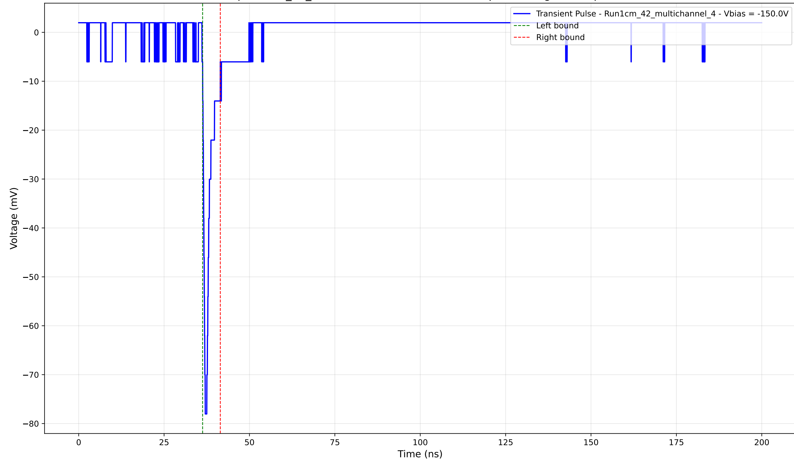
Transient Pulse - Sample: 1cm_42_multichannel - Position: 2245.0 \mu\text{m} - Charge: 3.37 pC - Rise Time: 0.76 ns
