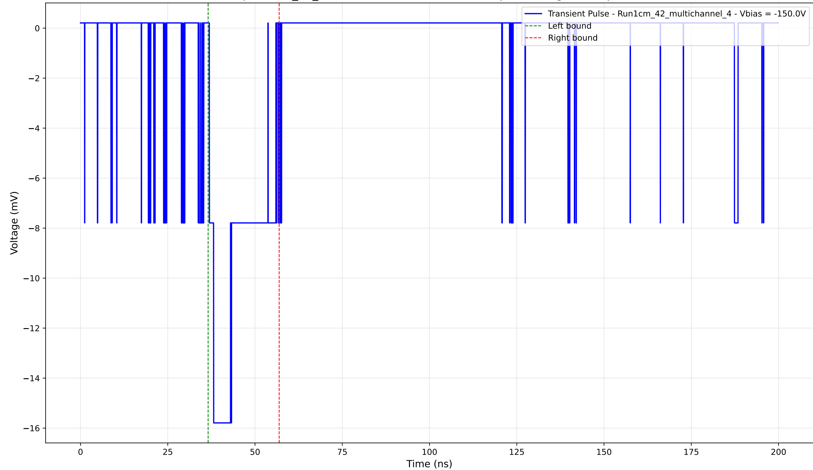
Transient Pulse - Sample: 1cm_42_multichannel - Position: 4035.0 \mu\text{m} - Charge: 3.81 pC - Rise Time: 1.24 ns
