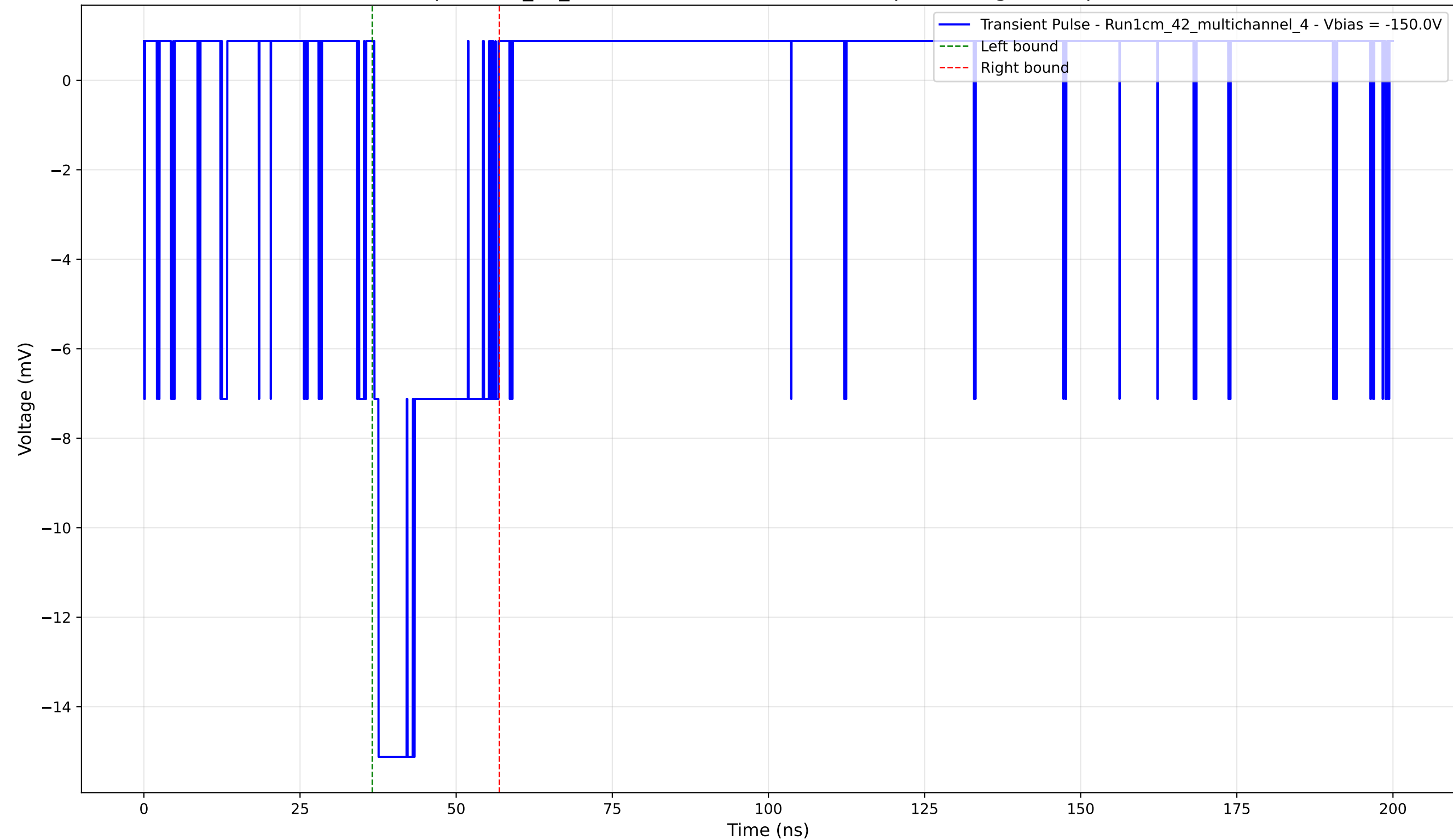
Transient Pulse - Sample: 1cm_42_multichannel - Position: 3725.0 \mu\text{m} - Charge: 3.60 pC - Rise Time: 0.68 ns
