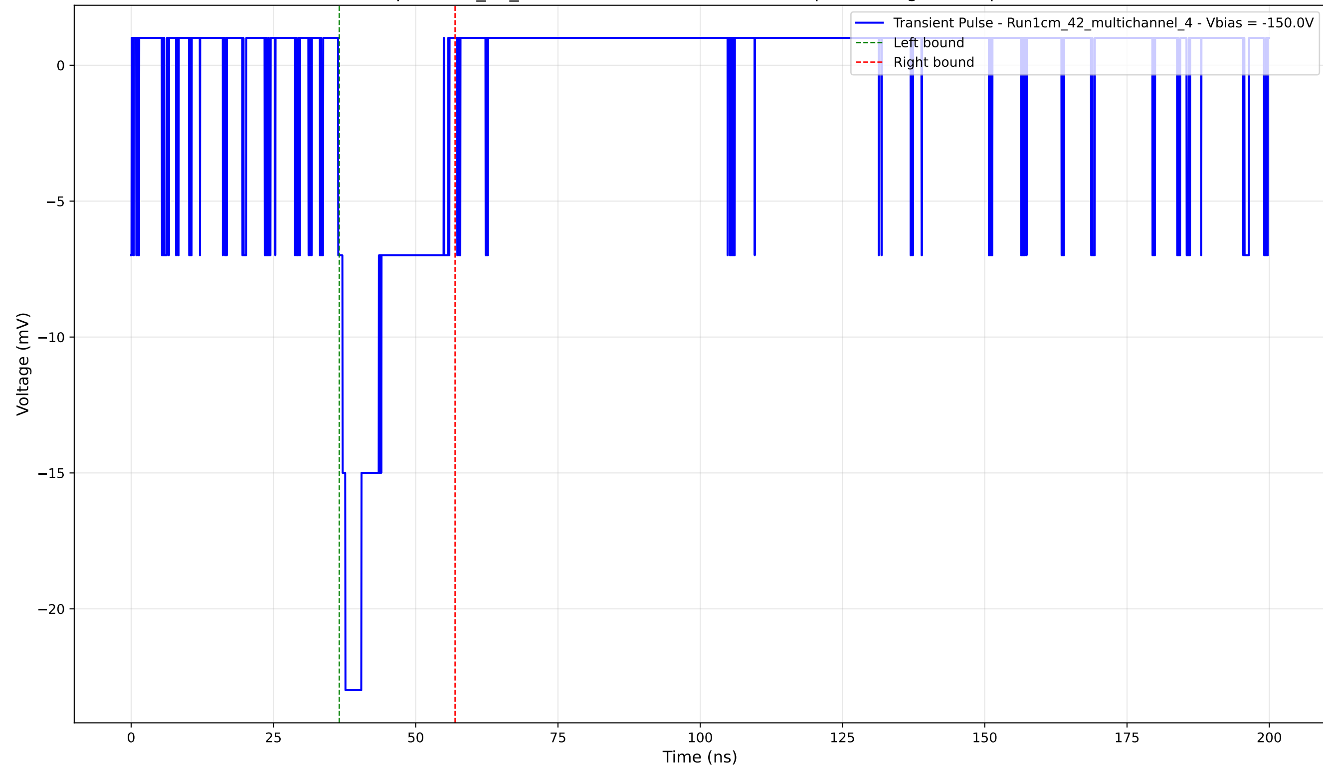
Transient Pulse - Sample: 1cm_42_multichannel - Position: 1265.0 \mu\text{m} - Charge: 4.14 pC - Rise Time: 1.28 ns
