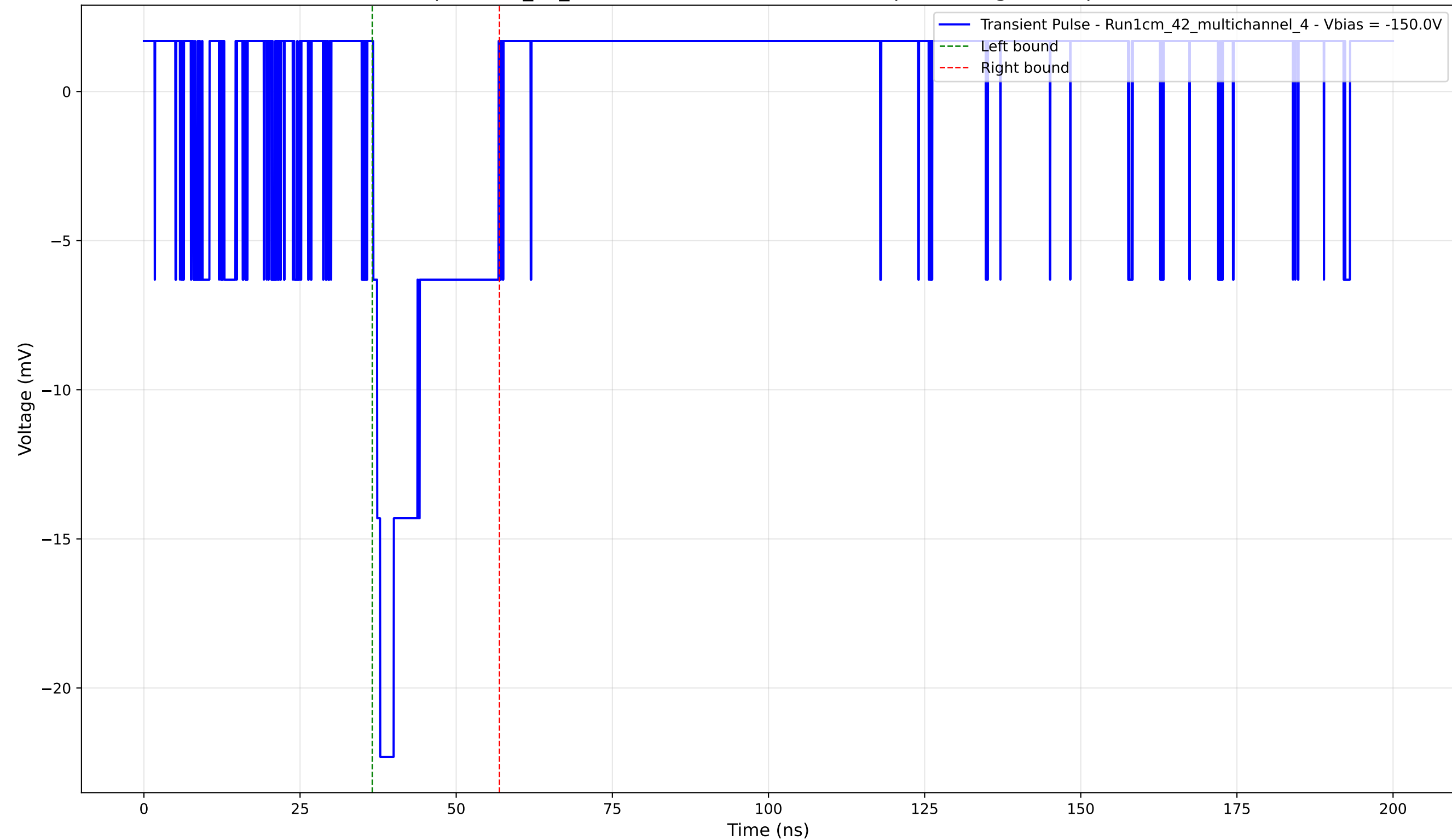
Transient Pulse - Sample: 1cm_42_multichannel - Position: 1155.0 \mu\text{m} - Charge: 3.95 pC - Rise Time: 1.12 ns
