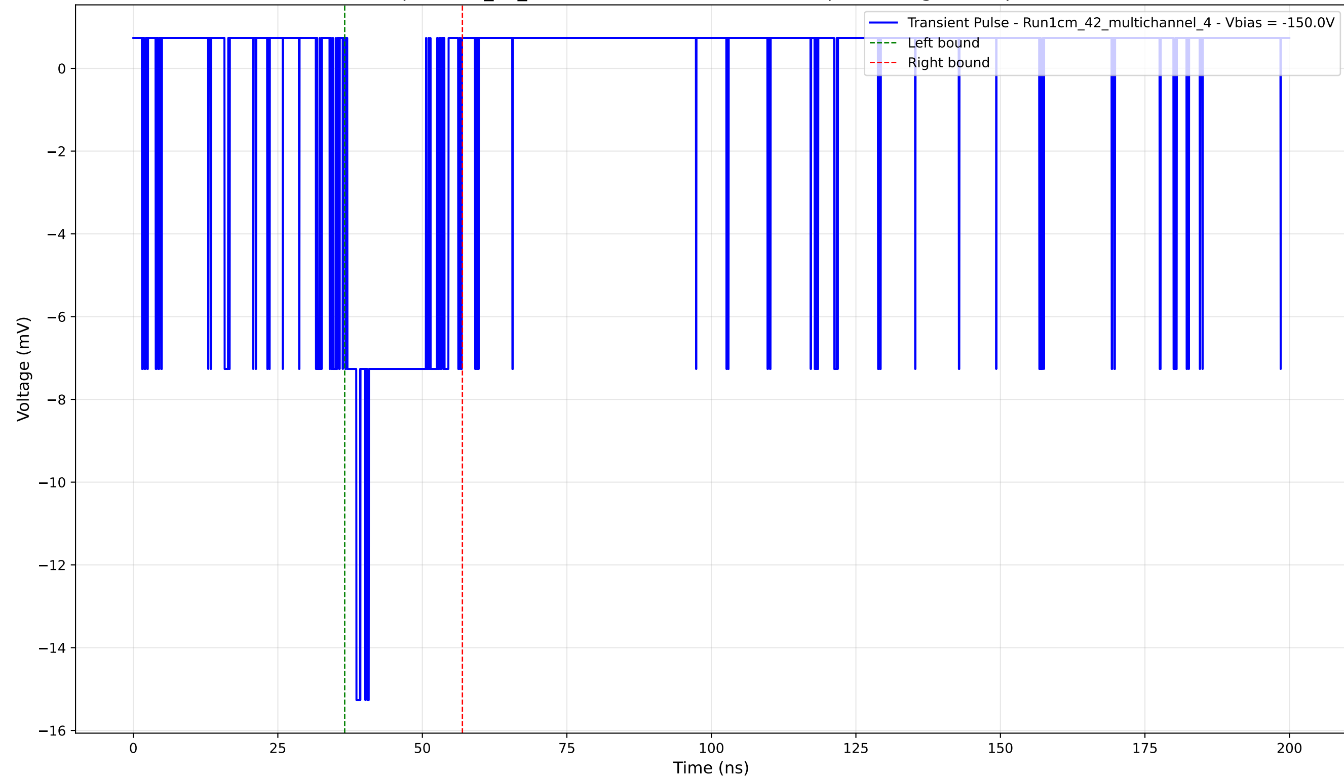
Transient Pulse - Sample: 1cm_42_multichannel - Position: 4825.0 \mu\text{m} - Charge: 2.61 pC - Rise Time: 1.58 ns
