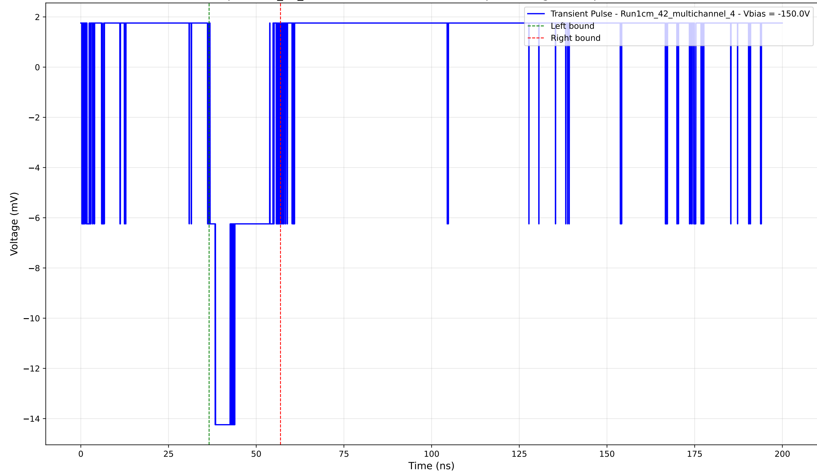
Transient Pulse - Sample: 1cm_42_multichannel - Position: 4540.0 \mu\text{m} - Charge: 3.10 pC - Rise Time: 0.00 ns (N/A)
