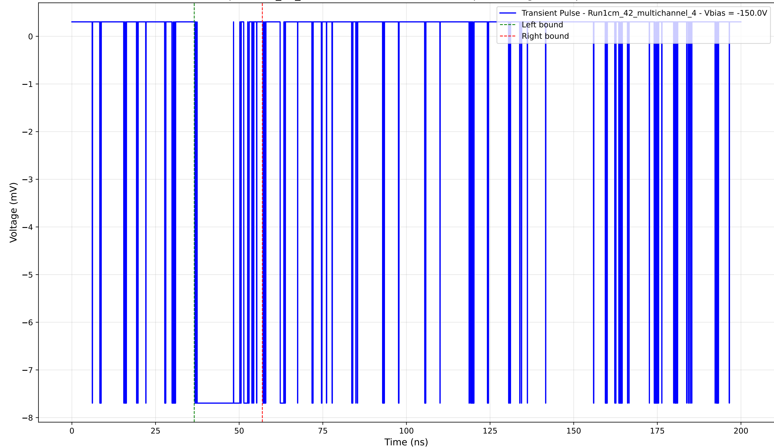
Transient Pulse - Sample: 1cm_42_multichannel - Position: 4860.0 \mu\text{m} - Charge: 2.31 pC - Rise Time: 0.02 ns
