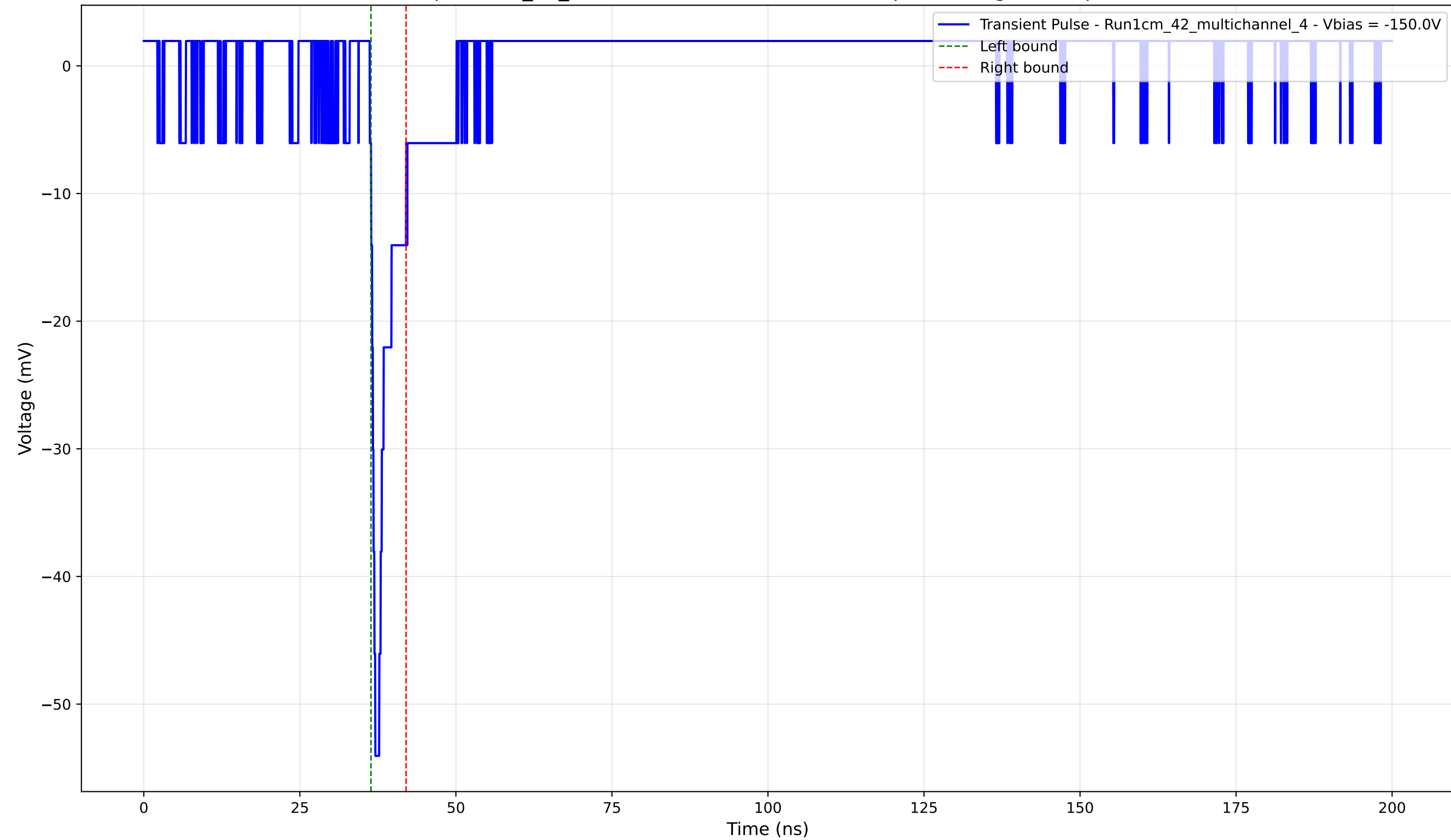
Transient Pulse - Sample: 1cm_42_multichannel - Position: 2665.0 \mu\text{m} - Charge: 2.82 pC - Rise Time: 0.88 ns
