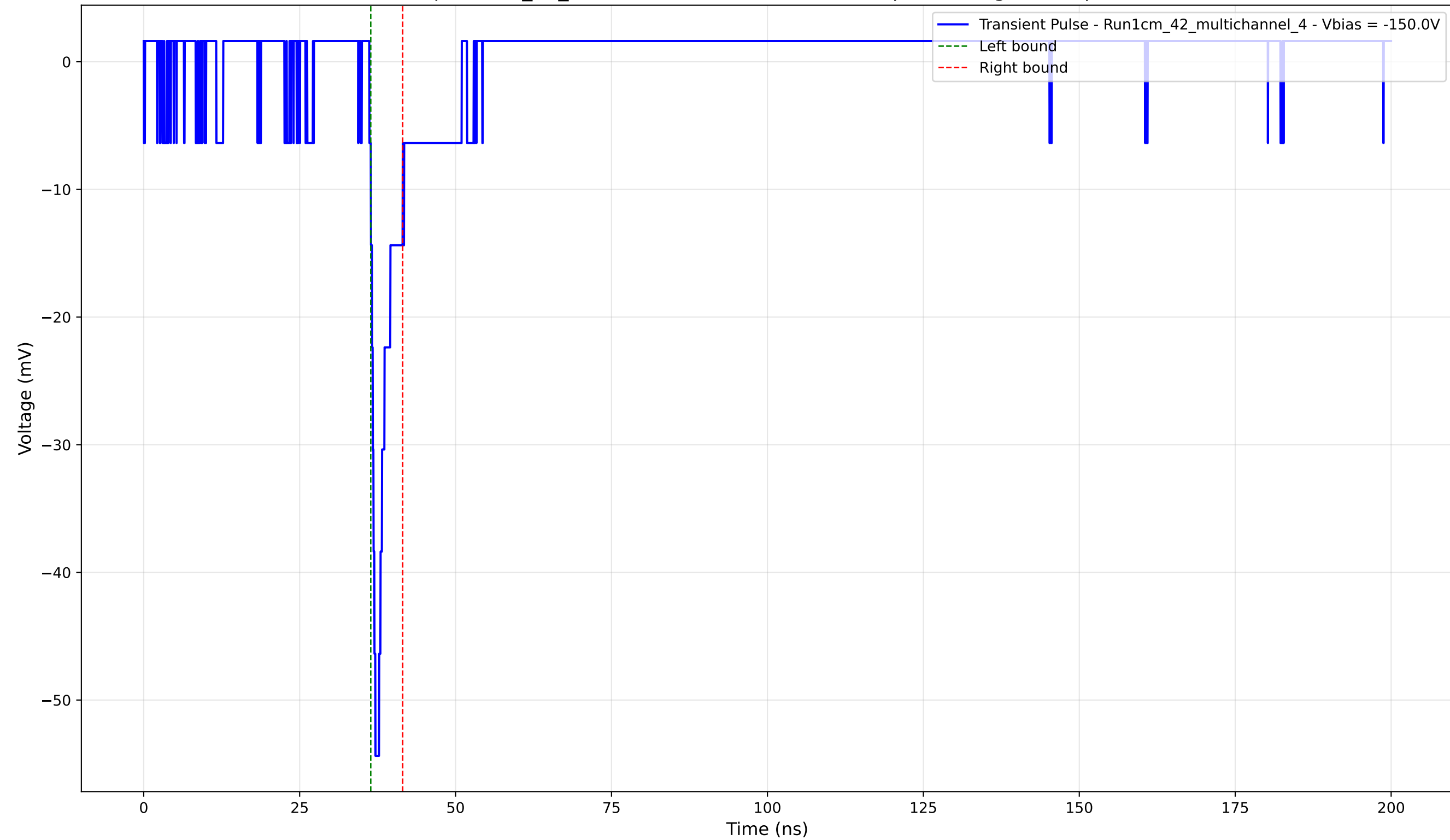
Transient Pulse - Sample: 1cm_42_multichannel - Position: 2070.0 \mu\text{m} - Charge: 2.71 pC - Rise Time: 0.96 ns
