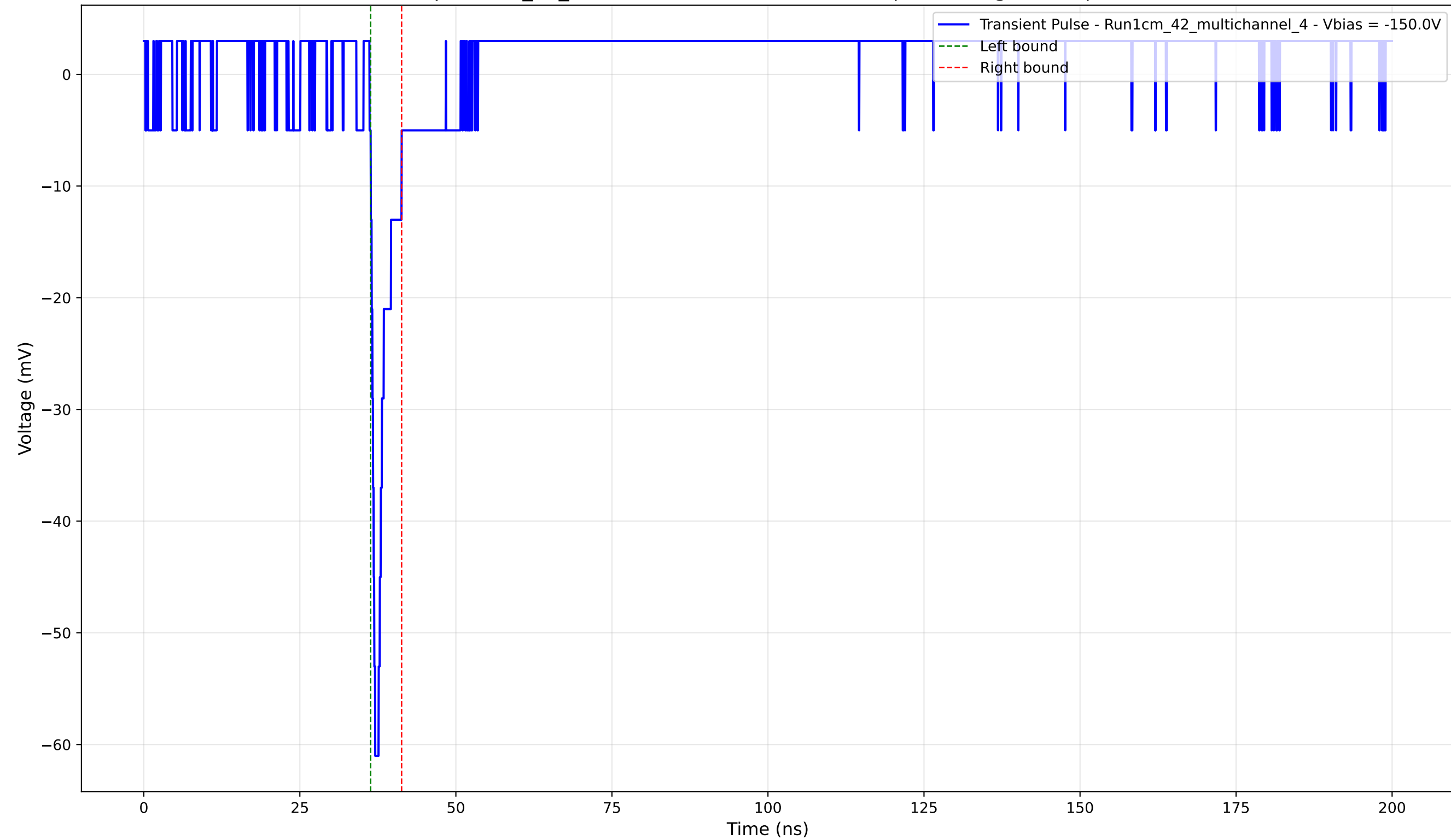
Transient Pulse - Sample: 1cm_42_multichannel - Position: 2600.0 \mu\text{m} - Charge: 2.71 pC - Rise Time: 0.72 ns
