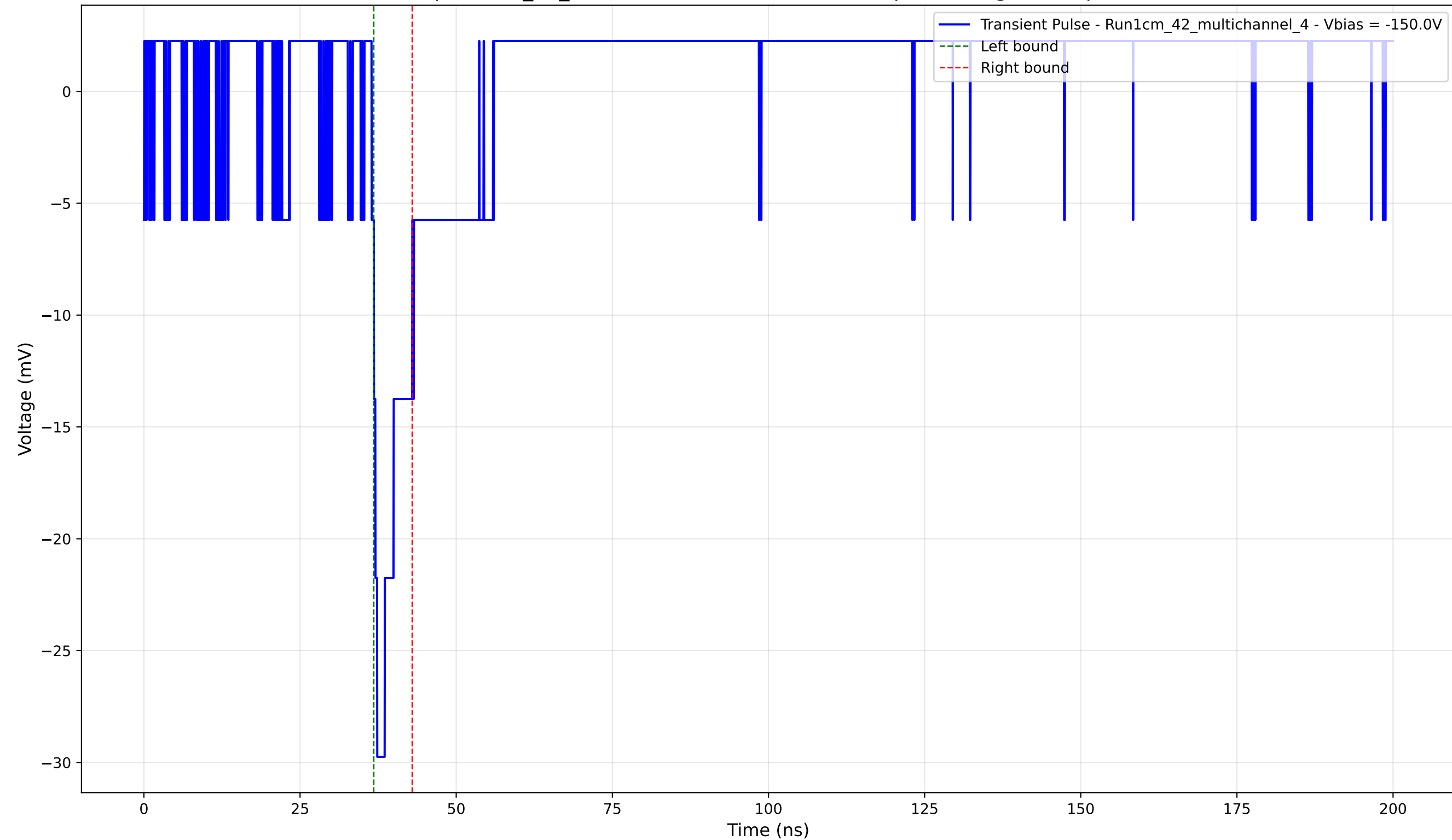
Transient Pulse - Sample: 1cm_42_multichannel - Position: 1630.0 \mu\text{m} - Charge: 2.35 pC - Rise Time: 0.90 ns
