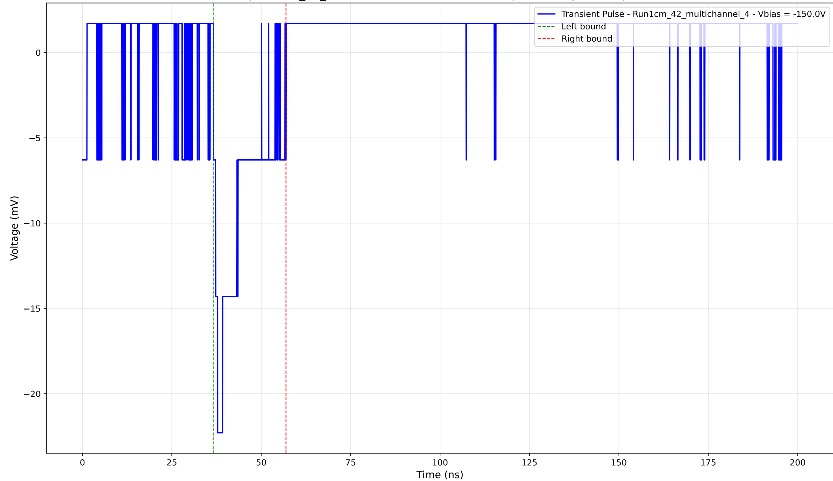
Transient Pulse - Sample: 1cm_42_multichannel - Position: 3520.0 \mu\text{m} - Charge: 3.58 pC - Rise Time: 1.14 ns
