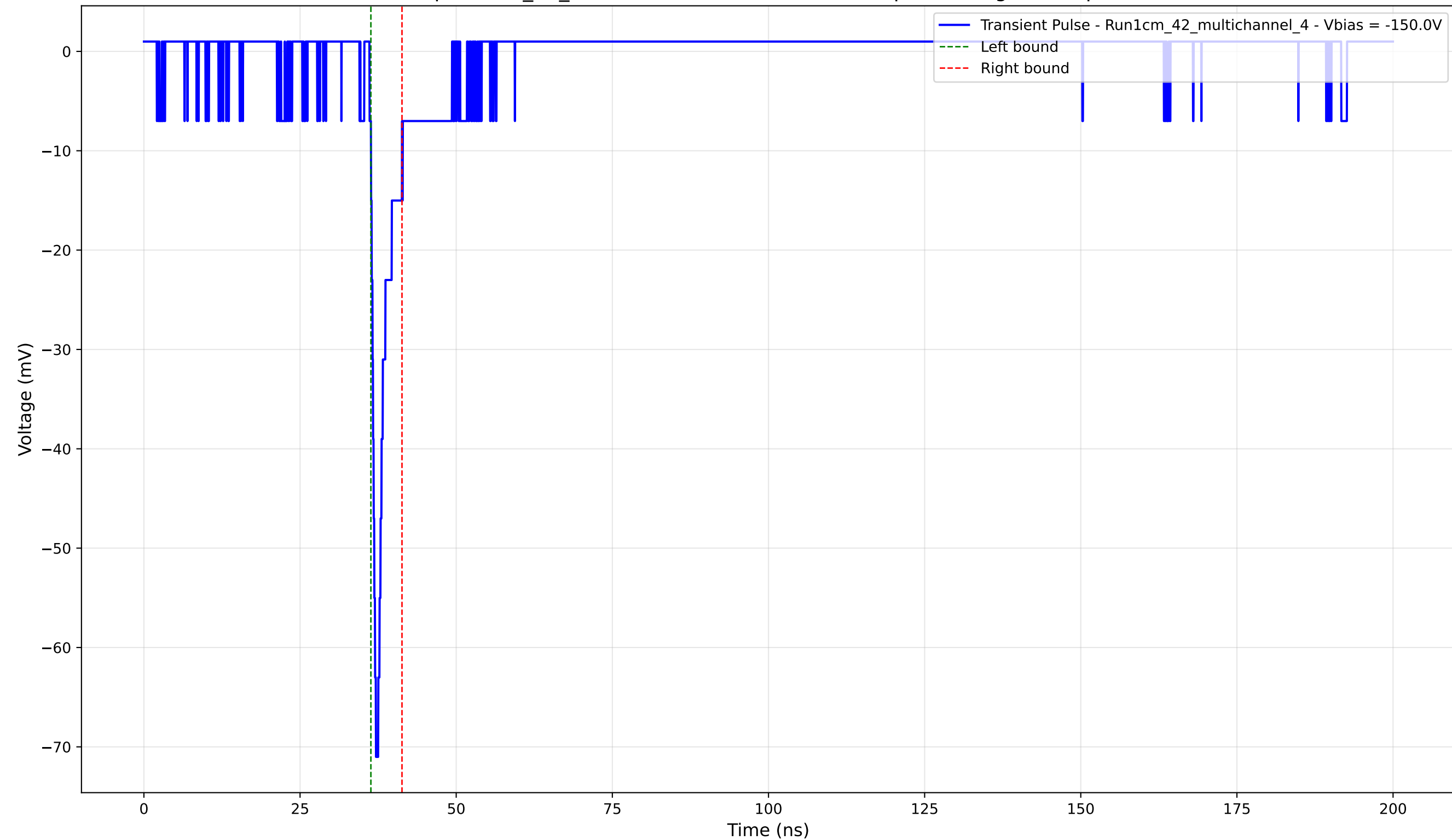
Transient Pulse - Sample: 1cm_42_multichannel - Position: 2170.0 \mu\text{m} - Charge: 3.12 pC - Rise Time: 0.80 ns
