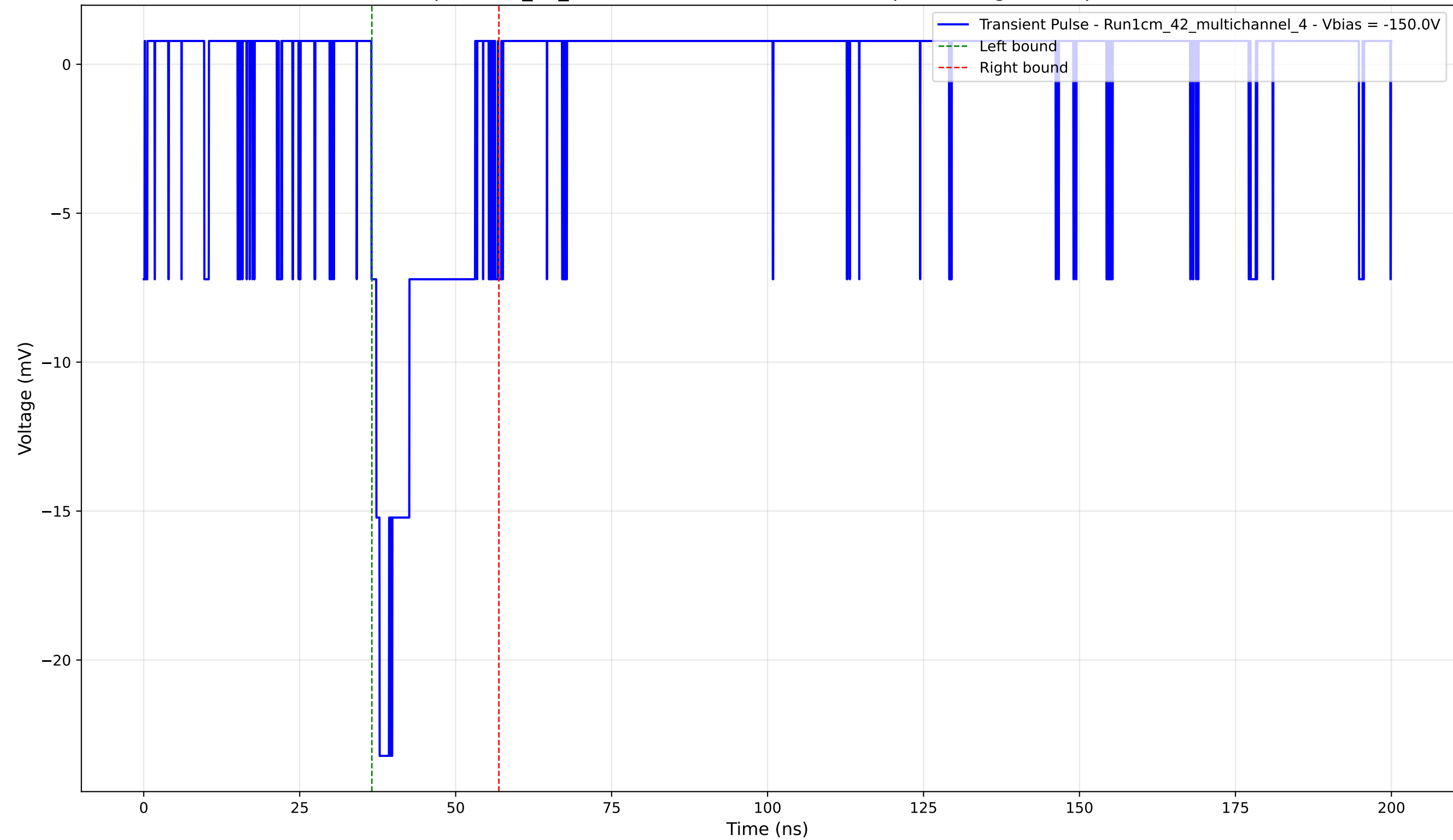
Transient Pulse - Sample: 1cm_42_multichannel - Position: 3510.0 \mu\text{m} - Charge: 3.62 pC - Rise Time: 1.32 ns
