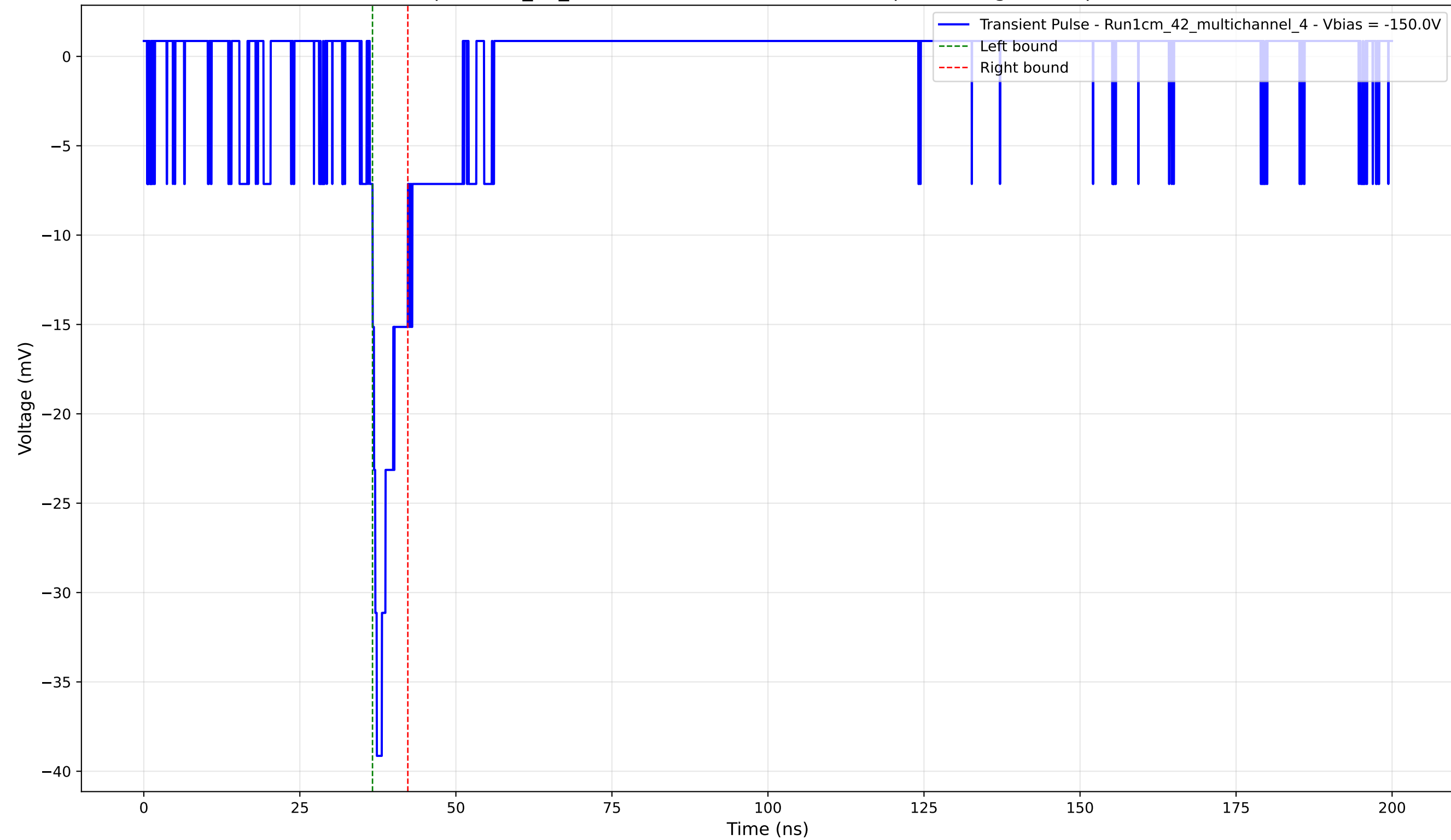
Transient Pulse - Sample: 1cm_42_multichannel - Position: 3000.0 \mu\text{m} - Charge: 2.61 pC - Rise Time: 1.13 ns
