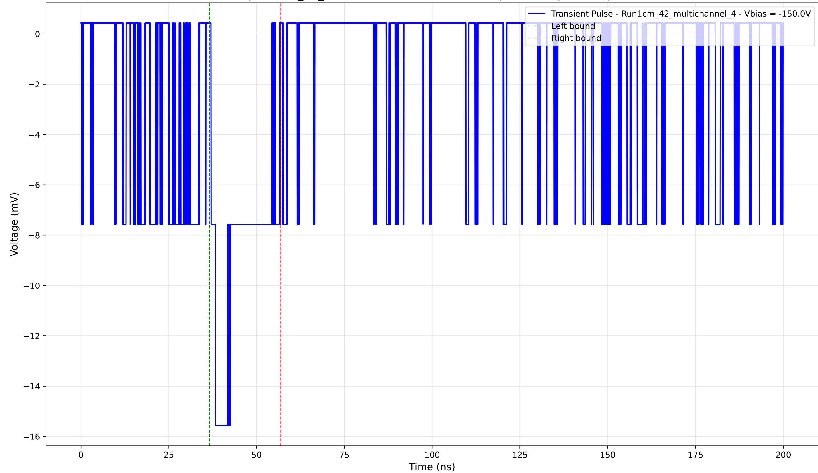
Transient Pulse - Sample: 1cm_42_multichannel - Position: 180.0 \mu\text{m} - Charge: 3.47 pC - Rise Time: 1.26 ns
