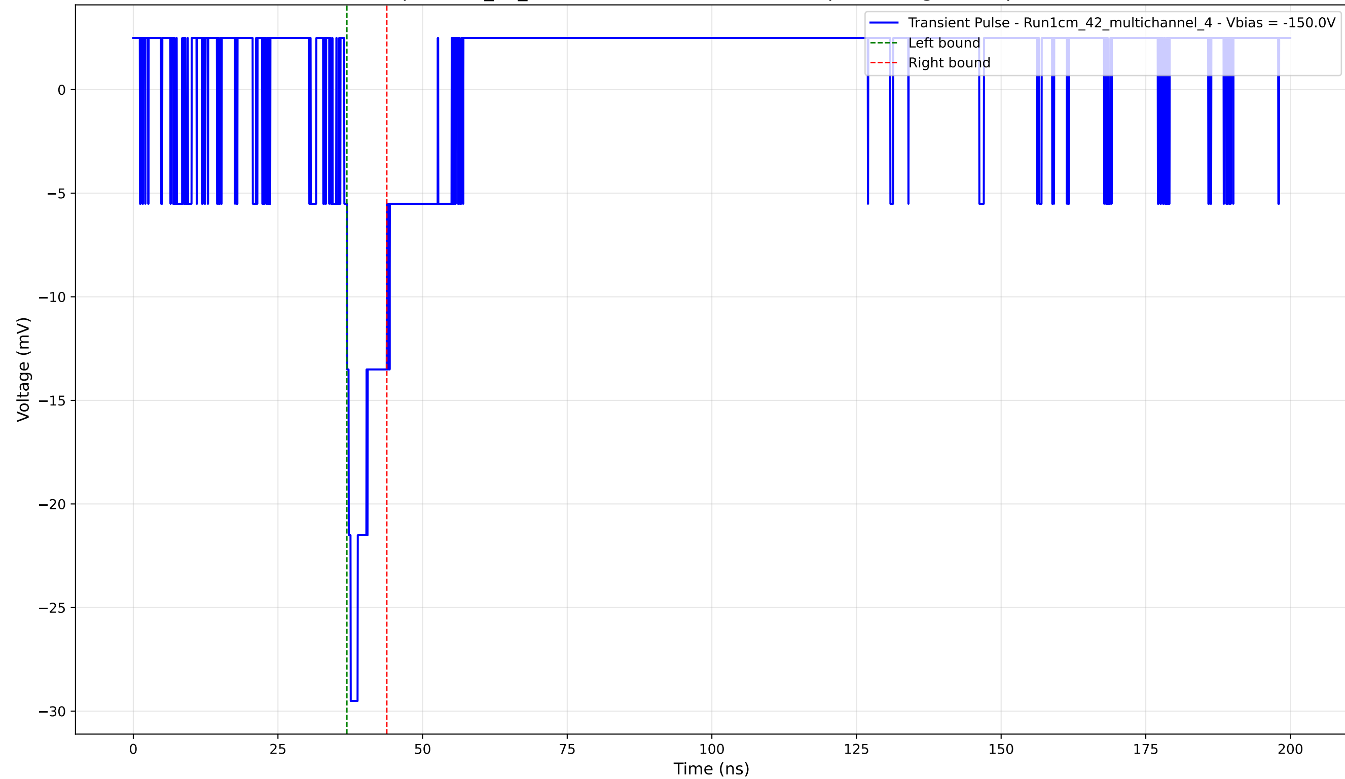
Transient Pulse - Sample: 1cm_42_multichannel - Position: 1485.0 \mu\text{m} - Charge: 2.57 pC - Rise Time: 1.12 ns
