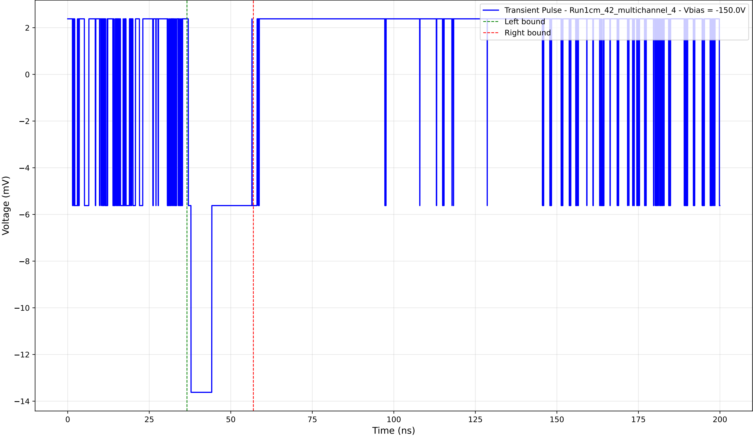
Transient Pulse - Sample: 1cm_42_multichannel - Position: 780.0 \mu\text{m} - Charge: 3.24 pC - Rise Time: 0.00 ns (N/A)
