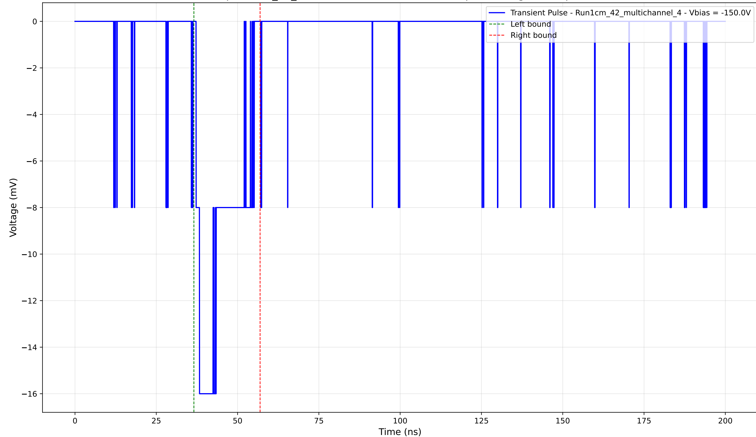
Transient Pulse - Sample: 1cm_42_multichannel - Position: 4250.0 \mu\text{m} - Charge: 3.56 pC - Rise Time: 1.06 ns
