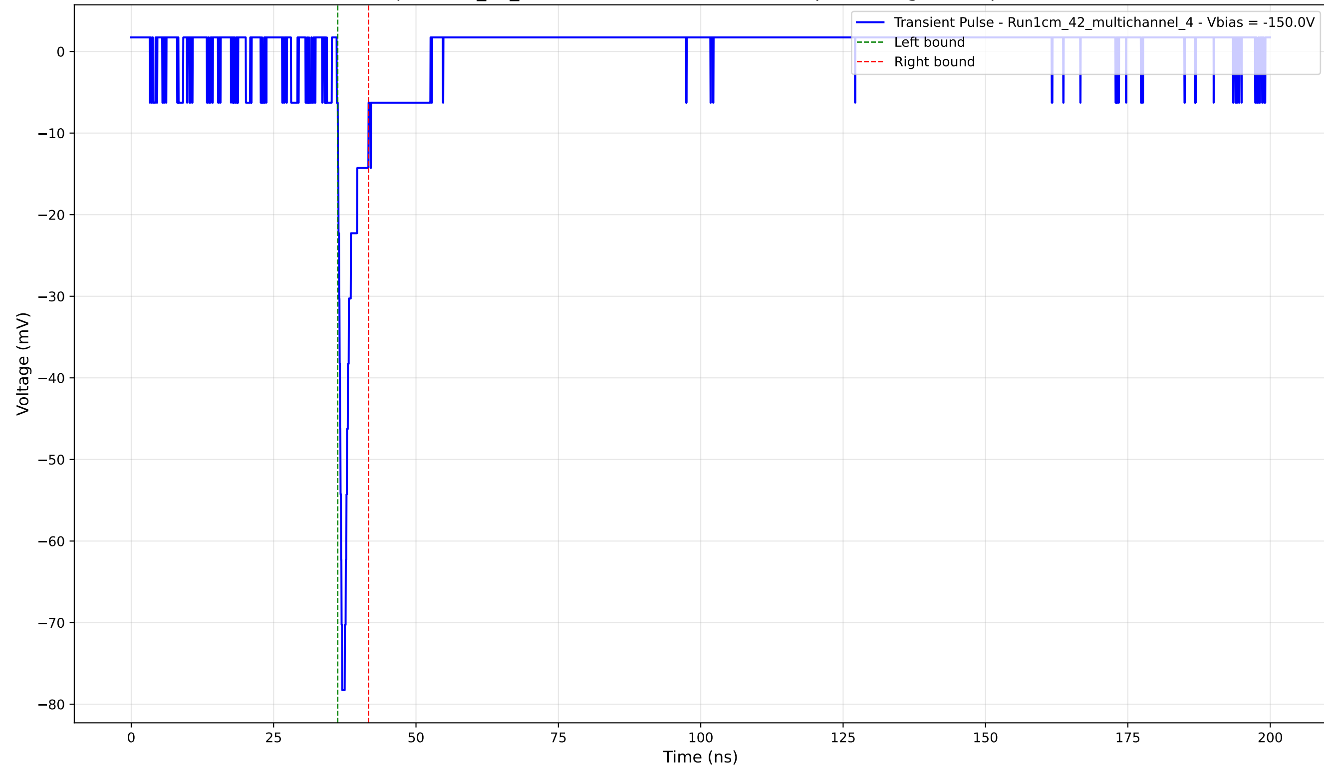
Transient Pulse - Sample: 1cm_42_multichannel - Position: 2260.0 \mu\text{m} - Charge: 3.40 pC - Rise Time: 0.78 ns
