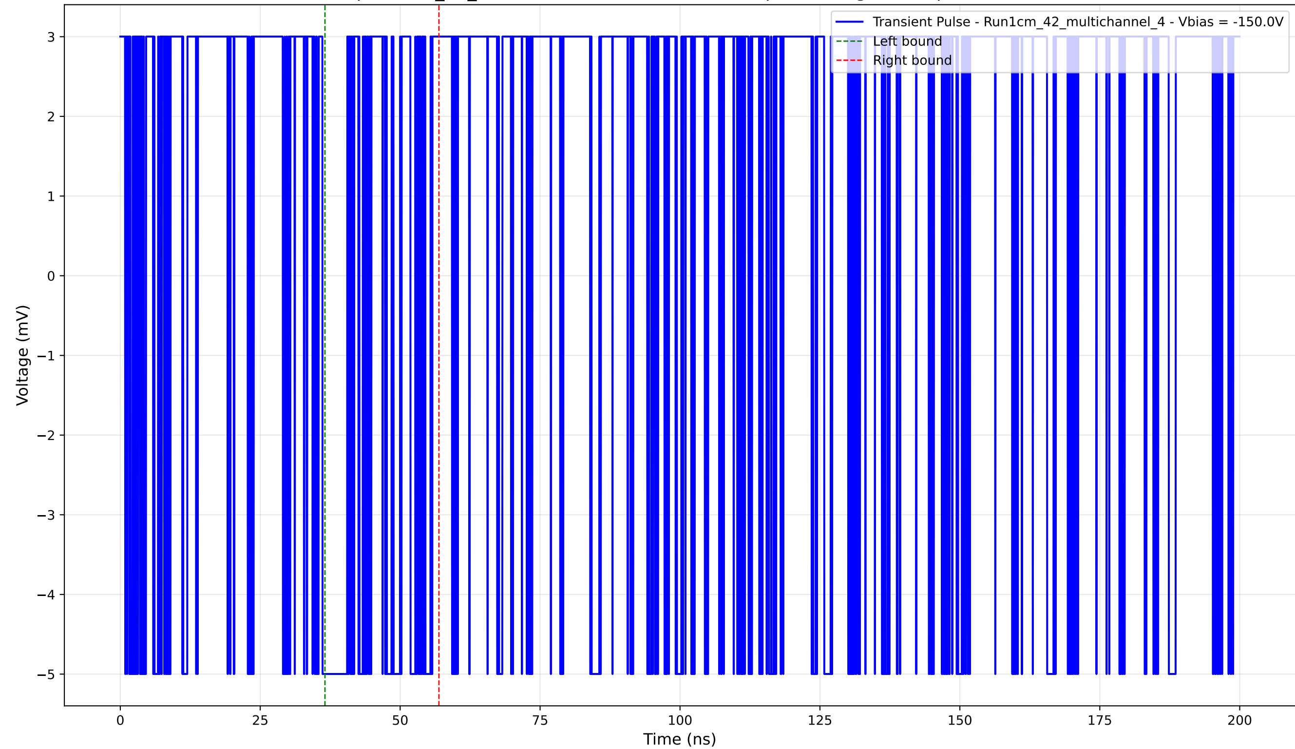
Transient Pulse - Sample: 1cm_42_multichannel - Position: 2410.0 \mu\text{m} - Charge: 0.64 pC - Rise Time: 0.00 ns (N/A)
