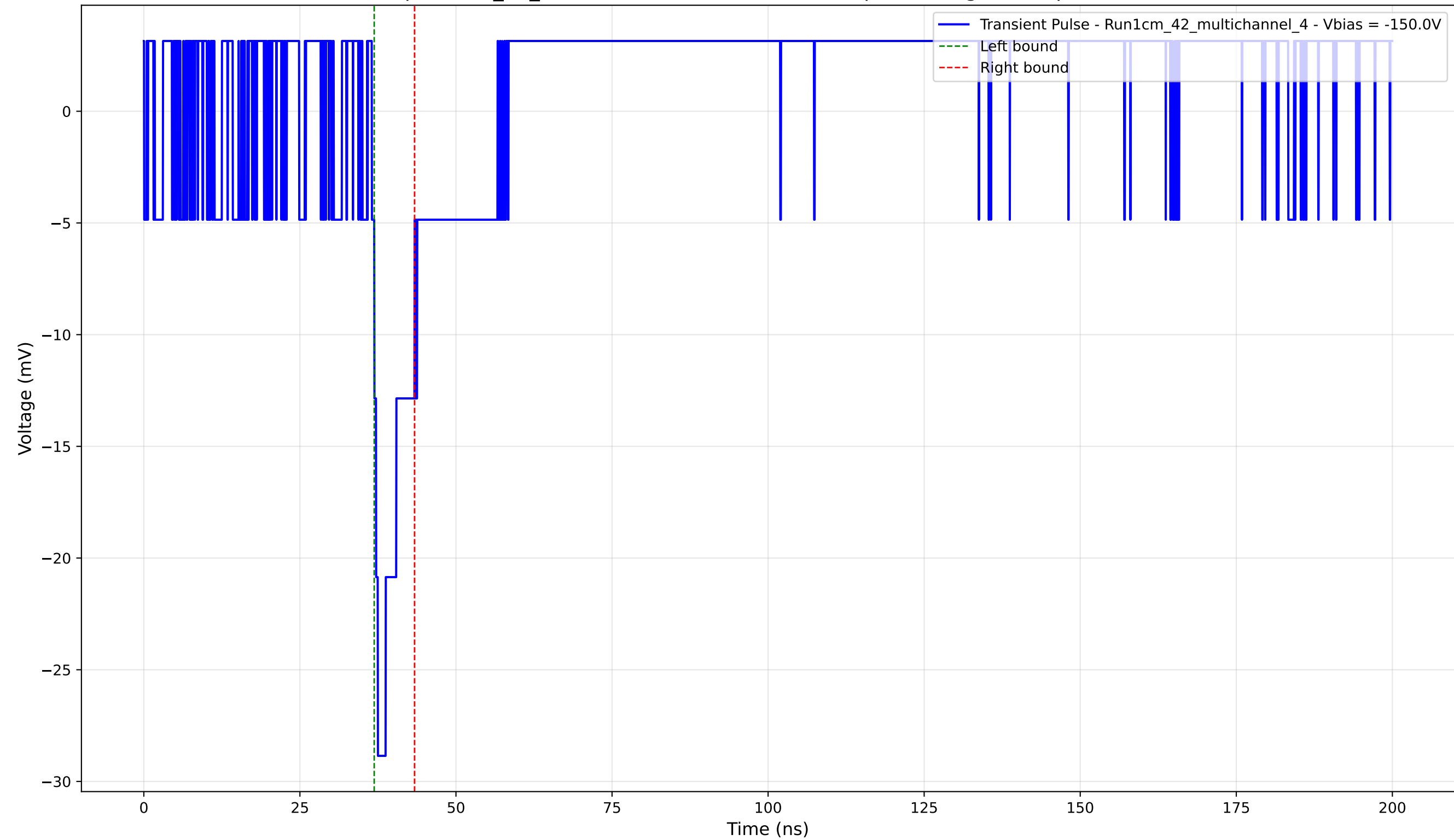
Transient Pulse - Sample: 1cm_42_multichannel - Position: 1505.0 \mu\text{m} - Charge: 2.38 pC - Rise Time: 0.00 ns (N/A)
