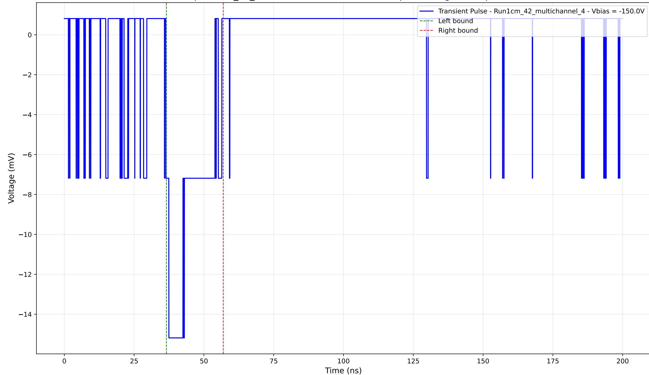
Transient Pulse - Sample: 1cm_42_multichannel - Position: 3650.0 \mu\text{m} - Charge: 3.52 pC - Rise Time: 1.12 ns
