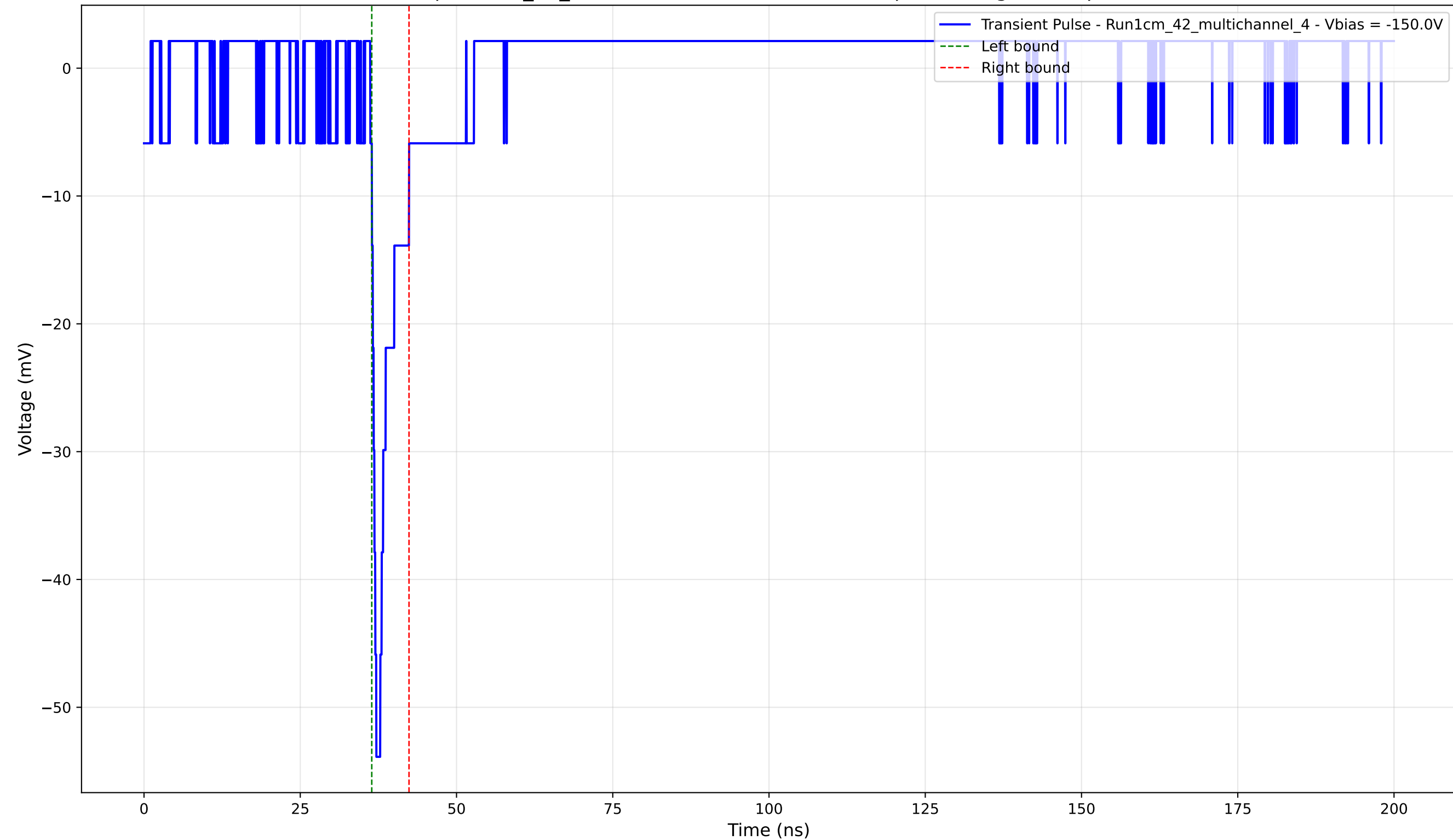
Transient Pulse - Sample: 1cm_42_multichannel - Position: 2030.0 \mu\text{m} - Charge: 3.00 pC - Rise Time: 0.96 ns
