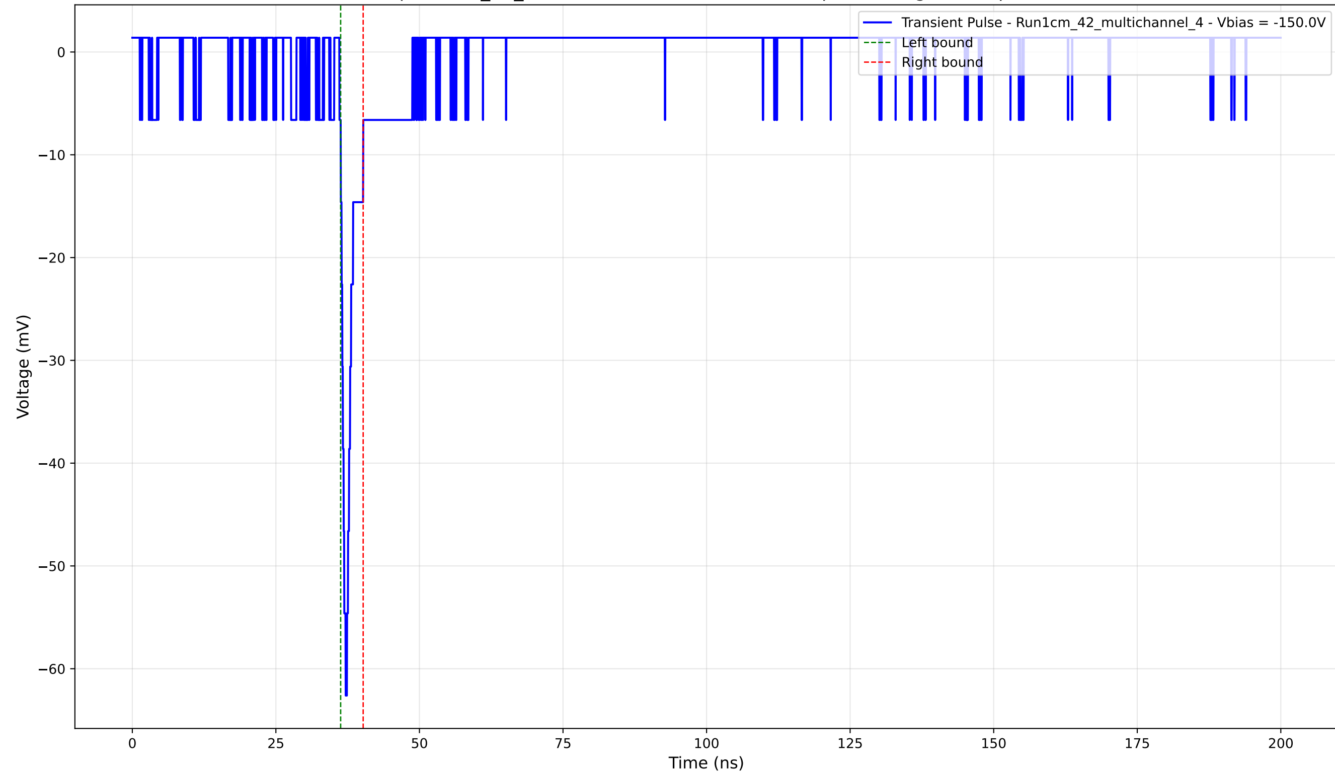
Transient Pulse - Sample: 1cm_42_multichannel - Position: 2445.0 \mu\text{m} - Charge: 2.20 pC - Rise Time: 1.08 ns
