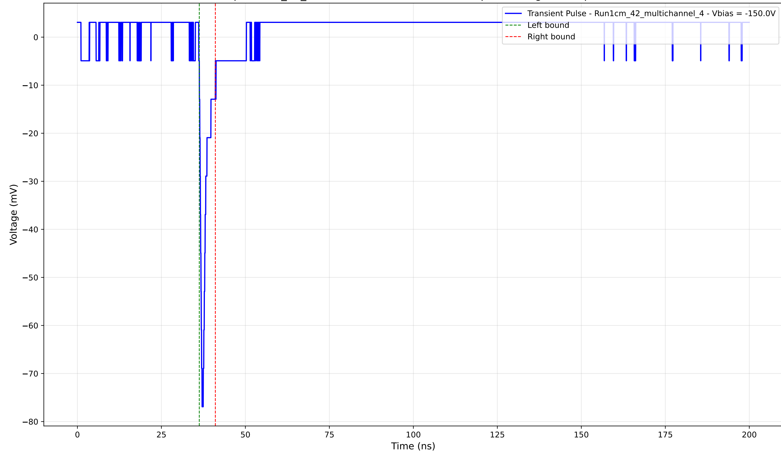
Transient Pulse - Sample: 1cm_42_multichannel - Position: 2235.0 \mu\text{m} - Charge: 3.05 pC - Rise Time: 0.81 ns
