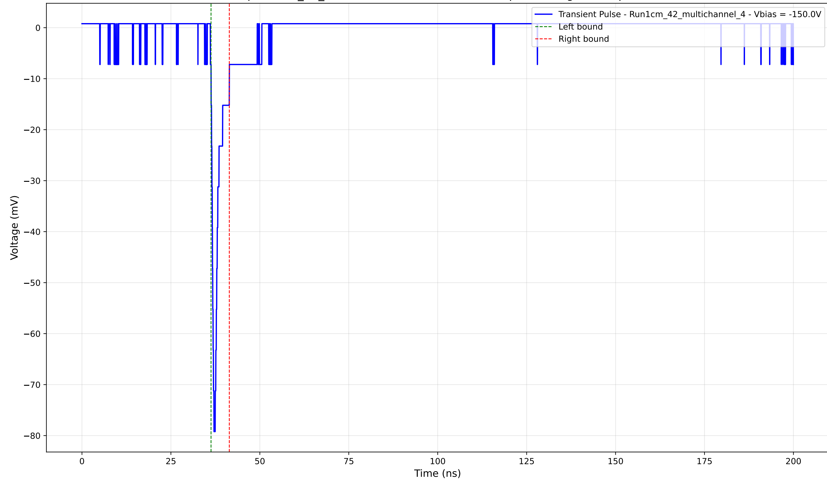
Transient Pulse - Sample: 1cm_42_multichannel - Position: 2510.0 \mu\text{m} - Charge: 3.33 pC - Rise Time: 0.82 ns
