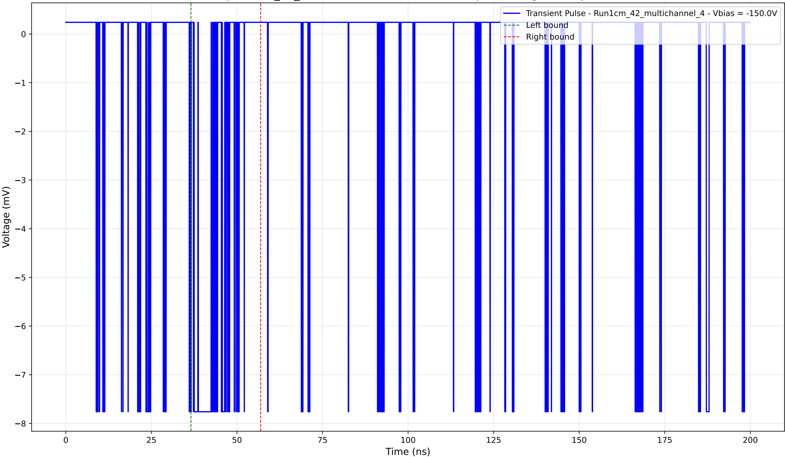
Transient Pulse - Sample: 1cm_42_multichannel - Position: 3875.0 \mu\text{m} - Charge: 1.17 pC - Rise Time: 0.02 ns
