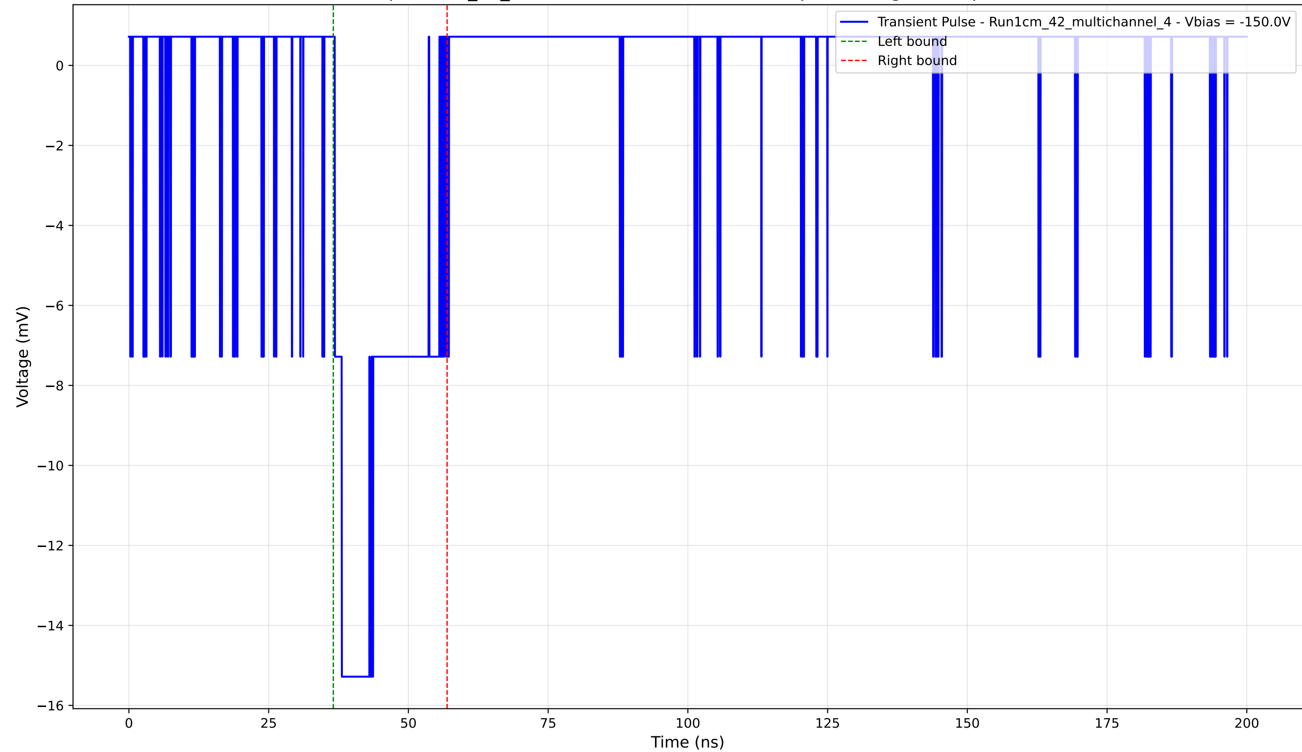
Transient Pulse - Sample: 1cm_42_multichannel - Position: 4115.0 \mu\text{m} - Charge: 3.62 pC - Rise Time: 1.26 ns
