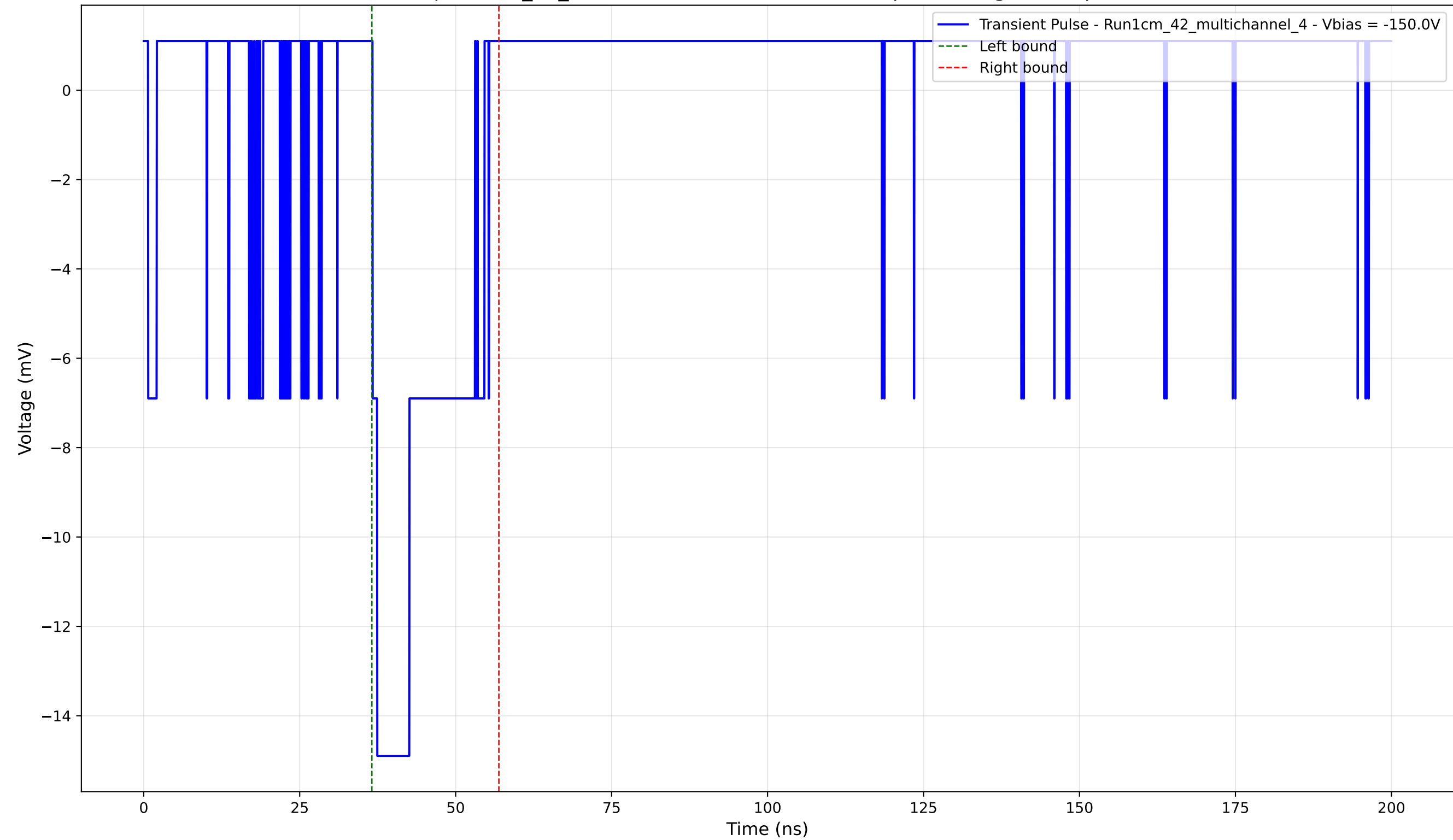
Transient Pulse - Sample: 1cm_42_multichannel - Position: 3630.0 \mu\text{m} - Charge: 3.23 pC - Rise Time: 0.76 ns
