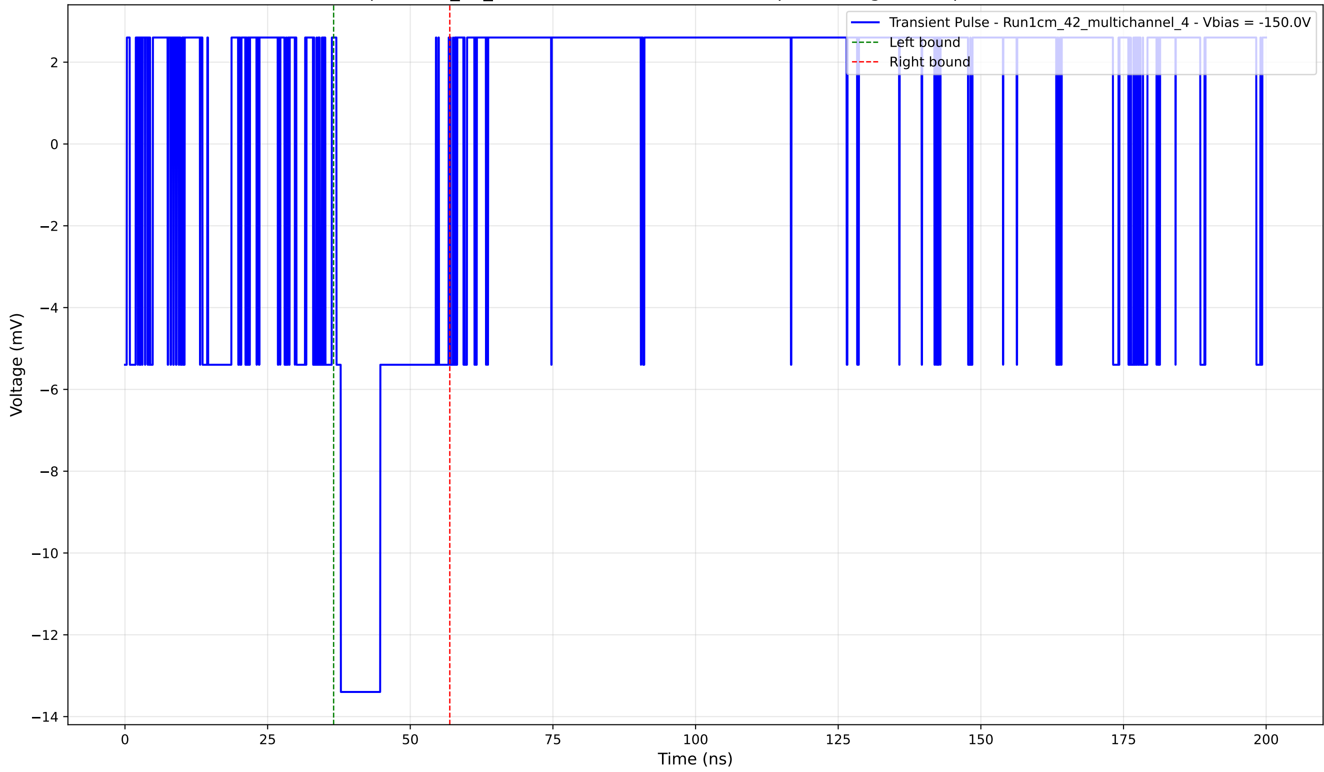
Transient Pulse - Sample: 1cm_42_multichannel - Position: 745.0 \mu\text{m} - Charge: 3.17 pC - Rise Time: 0.00 ns (N/A)
