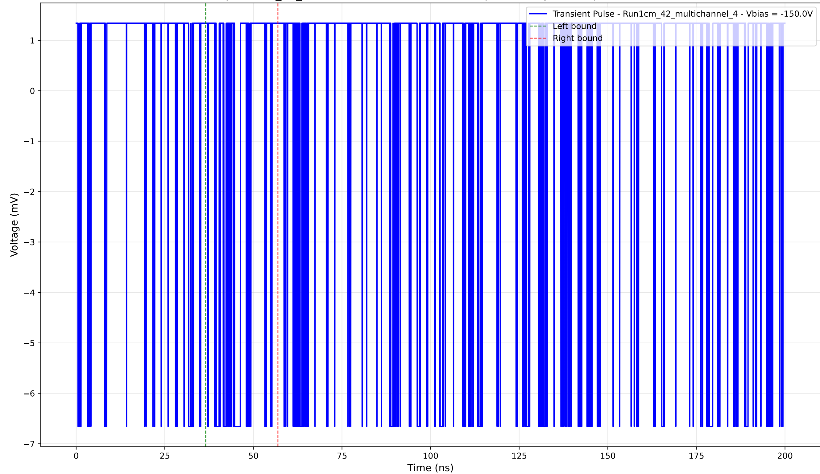
Transient Pulse - Sample: 1cm_42_multichannel - Position: 4390.0 \mu\text{m} - Charge: 0.38 pC - Rise Time: 0.00 ns (N/A)
