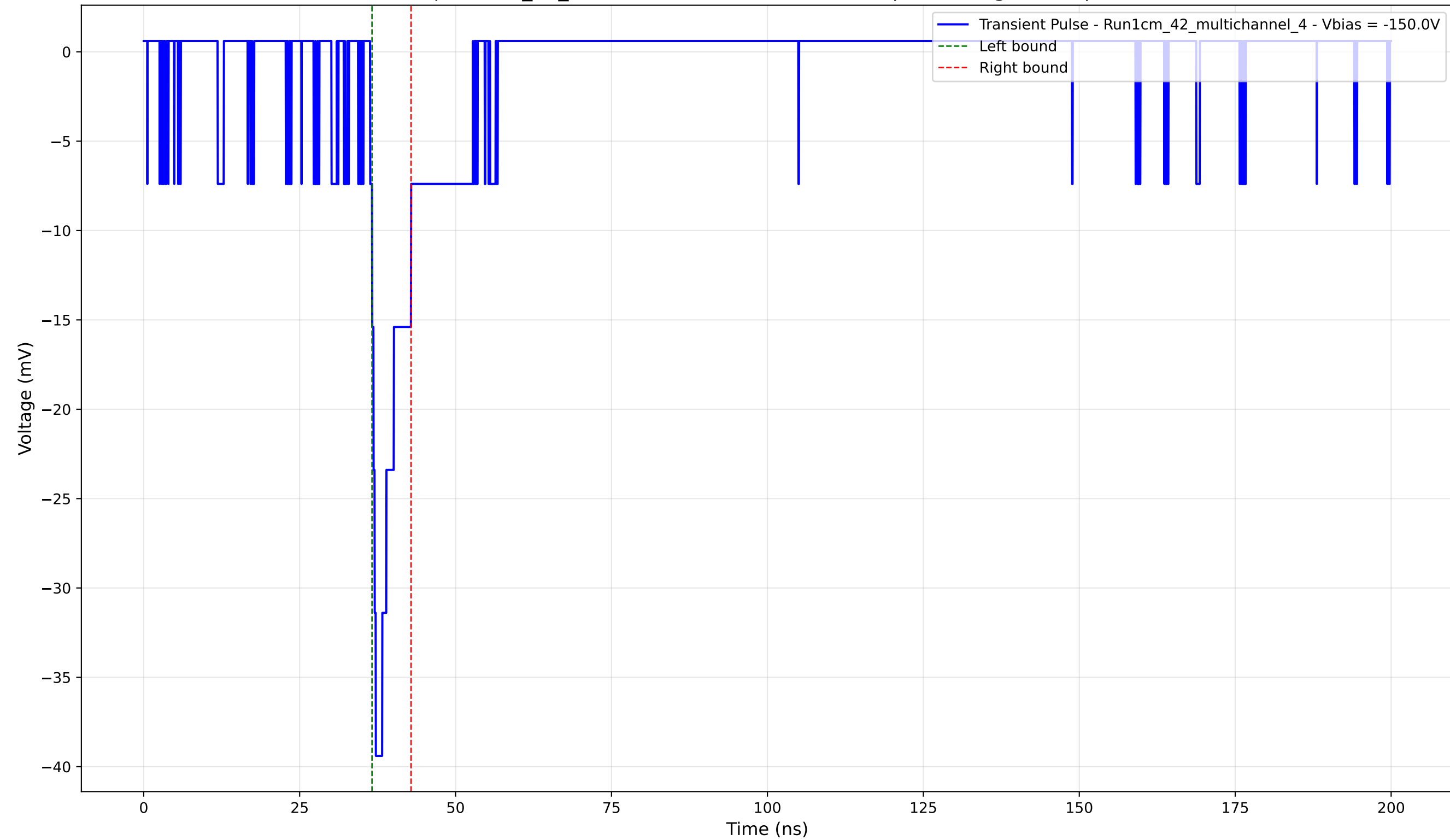
Transient Pulse - Sample: 1cm_42_multichannel - Position: 1770.0 \mu\text{m} - Charge: 2.91 pC - Rise Time: 0.91 ns
