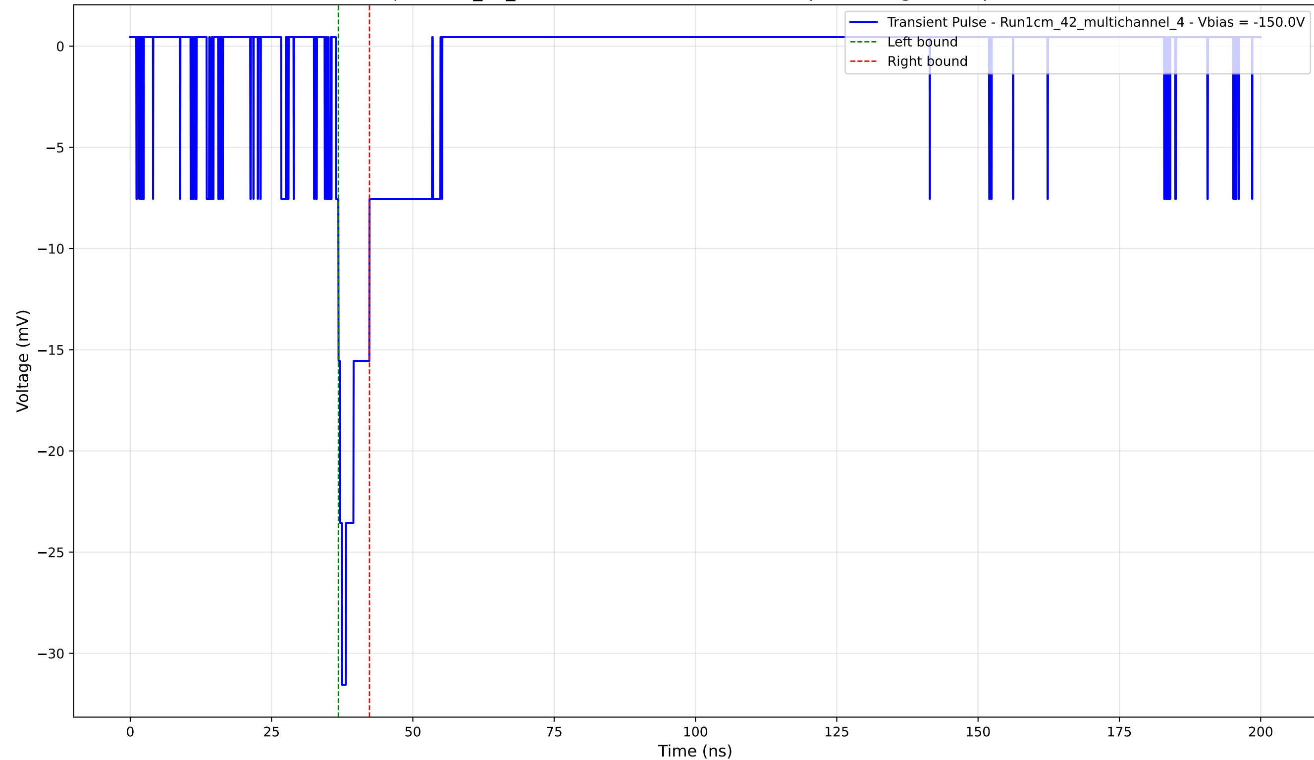
Transient Pulse - Sample: 1cm_42_multichannel - Position: 3160.0 \mu\text{m} - Charge: 2.21 pC - Rise Time: 1.05 ns
