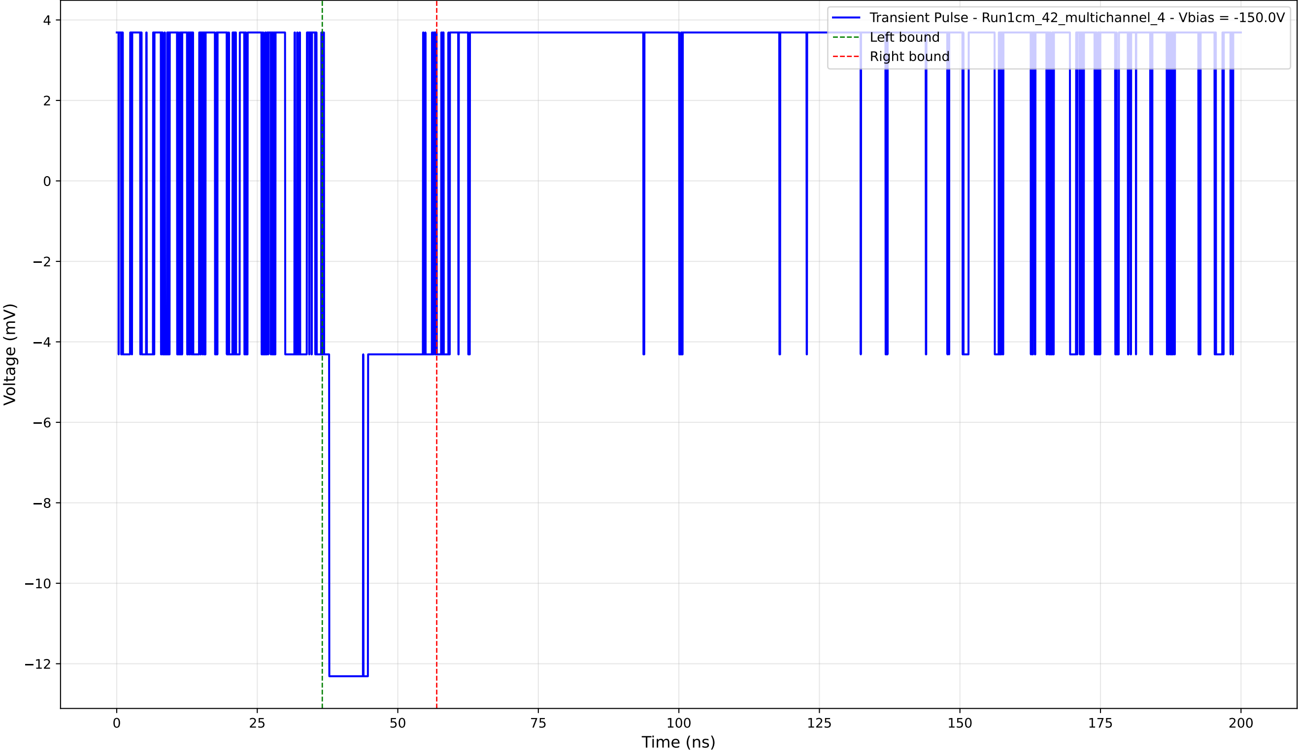
Transient Pulse - Sample: 1cm_42_multichannel - Position: 725.0 \mu\text{m} - Charge: 2.72 pC - Rise Time: 0.00 ns (N/A)
