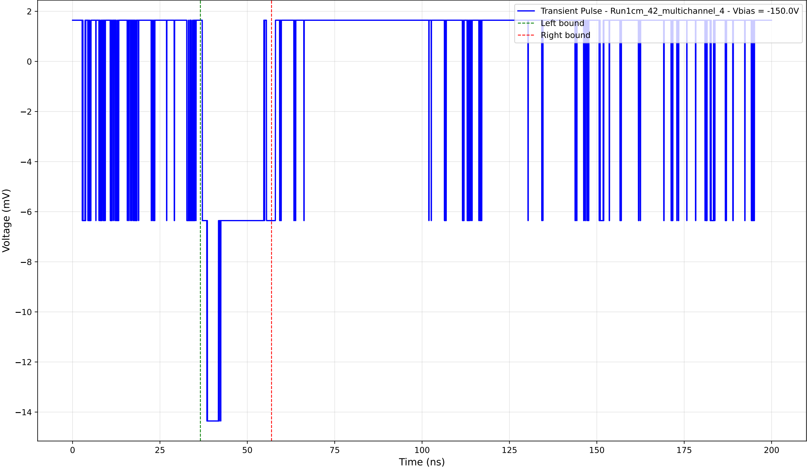
Transient Pulse - Sample: 1cm_42_multichannel - Position: 145.0 \mu\text{m} - Charge: 2.95 pC - Rise Time: 0.00 ns (N/A)
