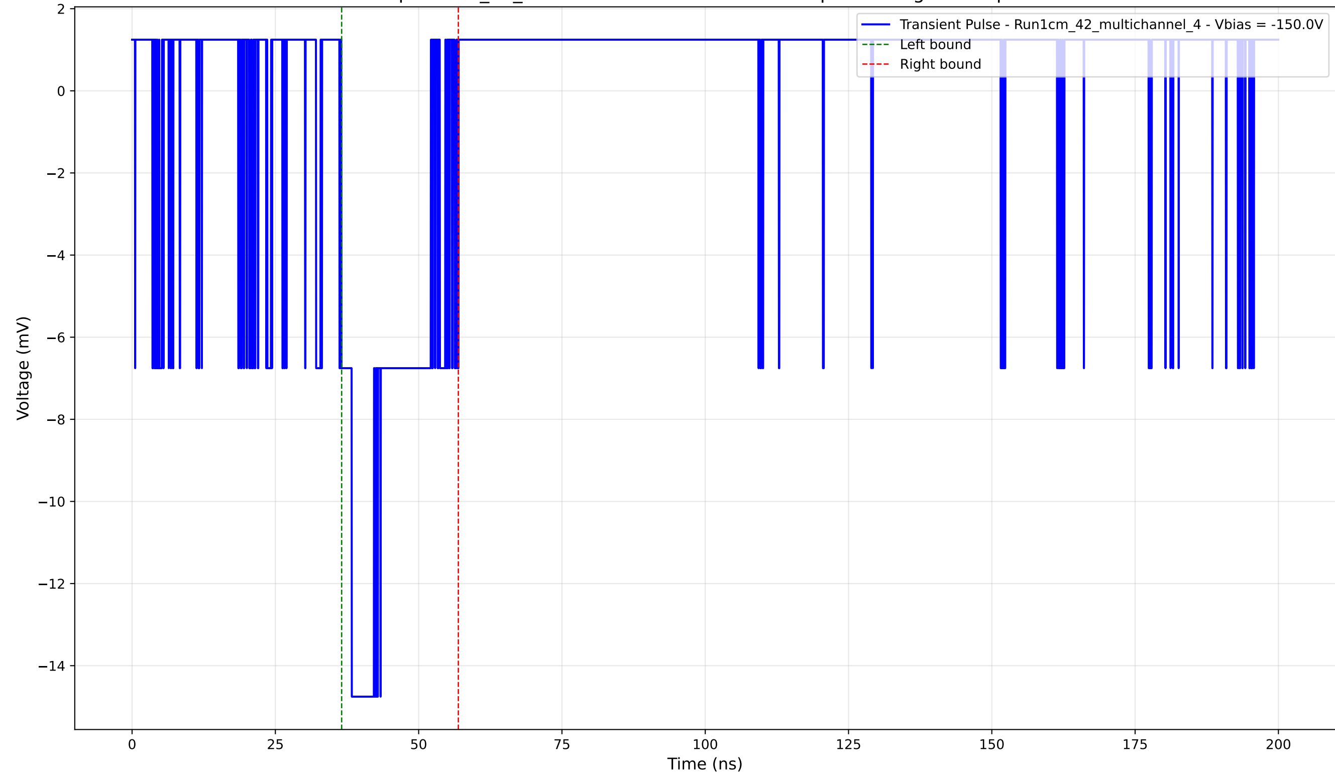
Transient Pulse - Sample: 1cm_42_multichannel - Position: 4575.0 \mu\text{m} - Charge: 3.02 pC - Rise Time: 1.82 ns
