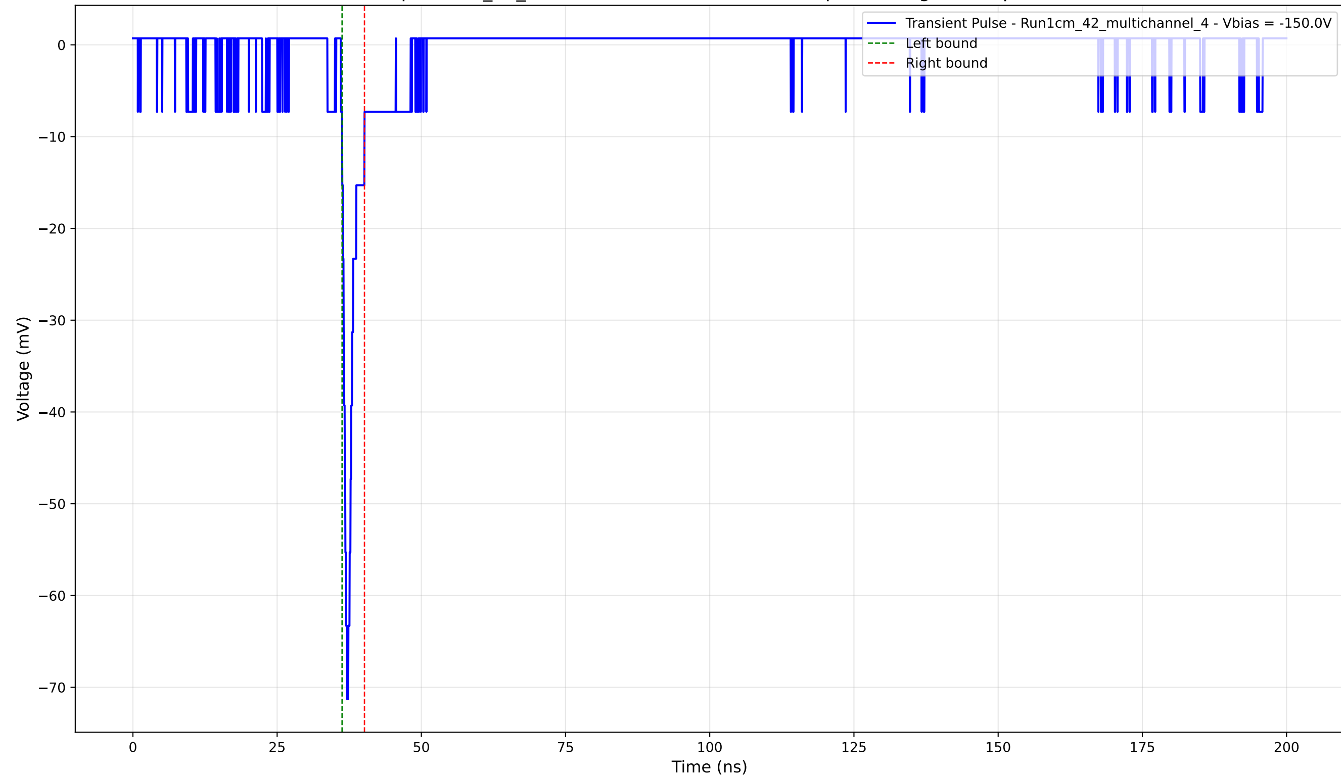
Transient Pulse - Sample: 1cm_42_multichannel - Position: 2320.0 \mu\text{m} - Charge: 2.50 pC - Rise Time: 1.06 ns
