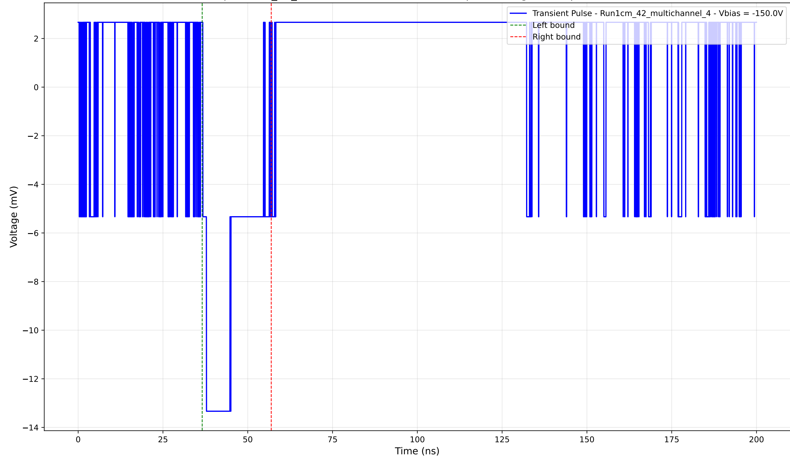
Transient Pulse - Sample: 1cm_42_multichannel - Position: 690.0 \mu\text{m} - Charge: 3.18 pC - Rise Time: 0.00 ns (N/A)
