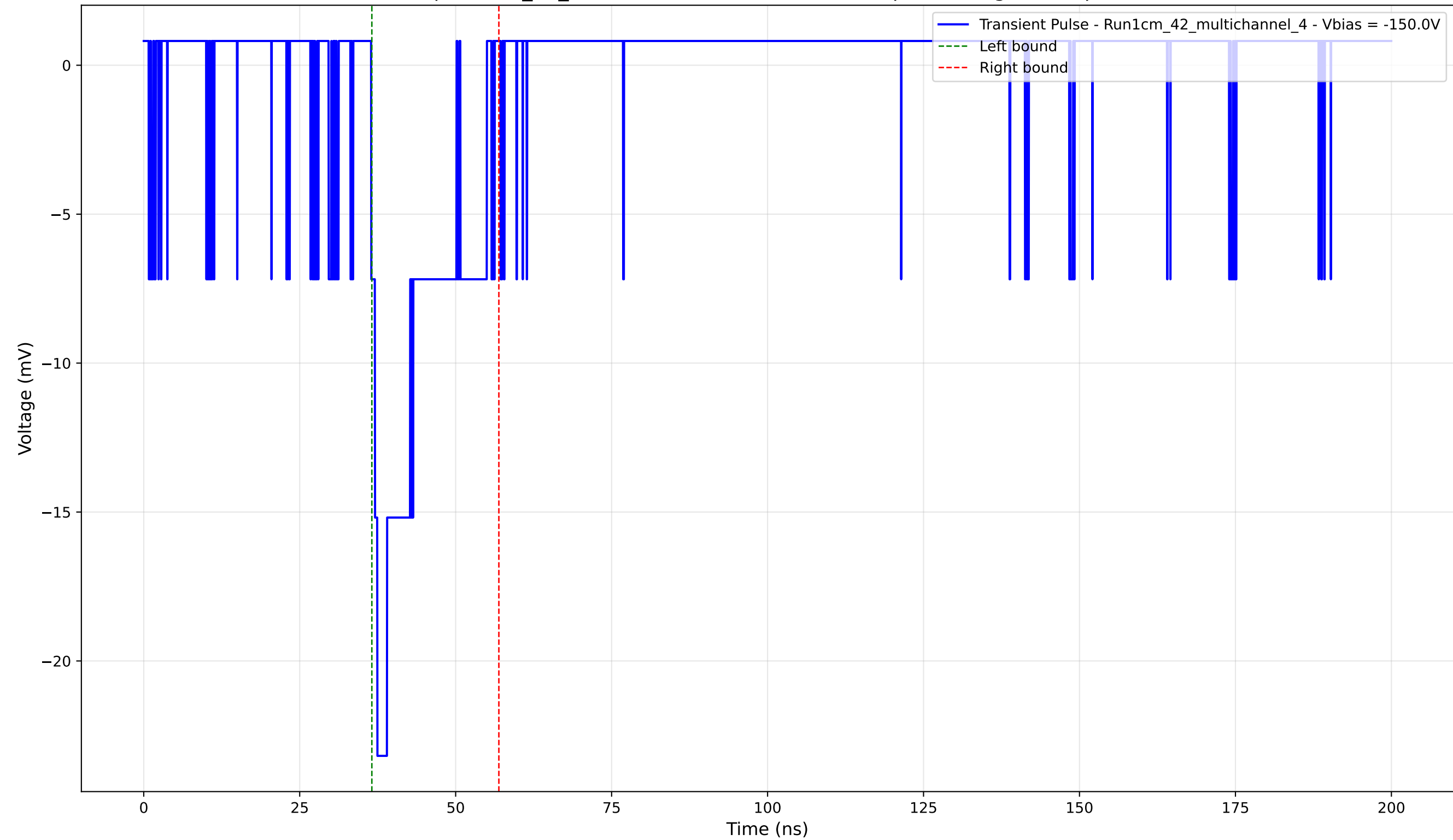
Transient Pulse - Sample: 1cm_42_multichannel - Position: 3320.0 \mu\text{m} - Charge: 3.80 pC - Rise Time: 1.00 ns
