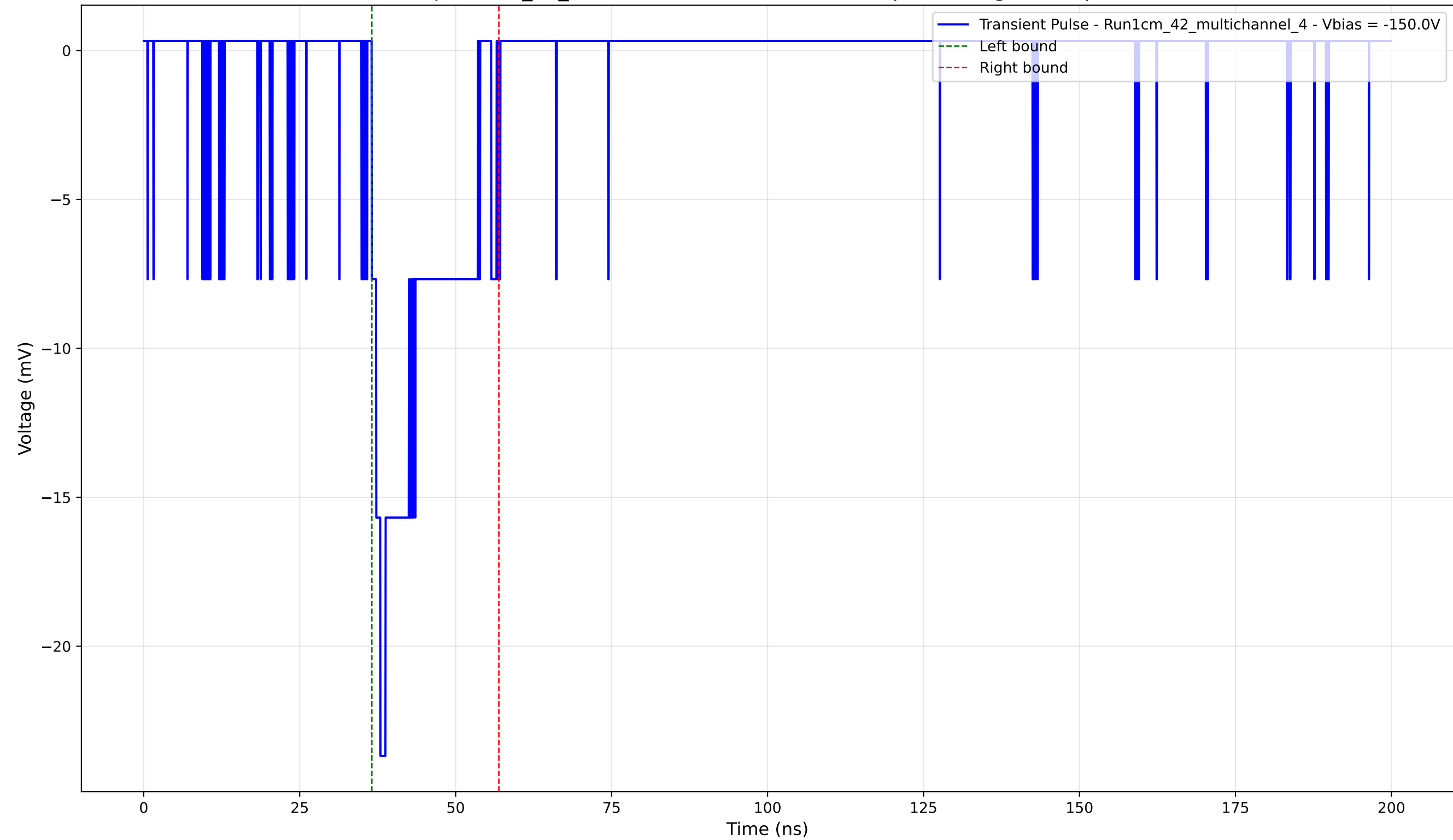
Transient Pulse - Sample: 1cm_42_multichannel - Position: 3560.0 \mu\text{m} - Charge: 3.80 pC - Rise Time: 1.39 ns
