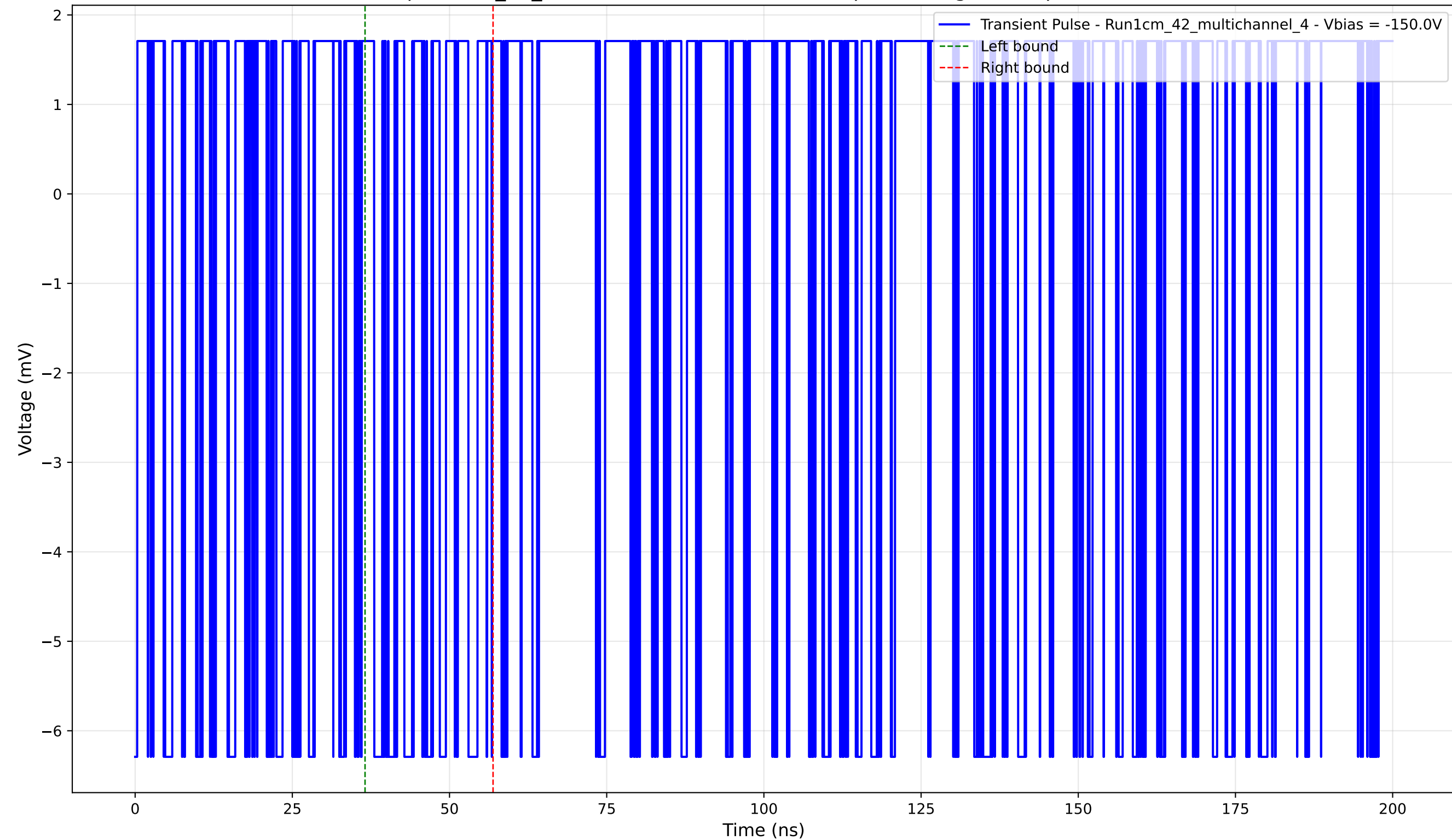
Transient Pulse - Sample: 1cm_42_multichannel - Position: 375.0 \mu\text{m} - Charge: 0.70 pC - Rise Time: 0.00 ns (N/A)
