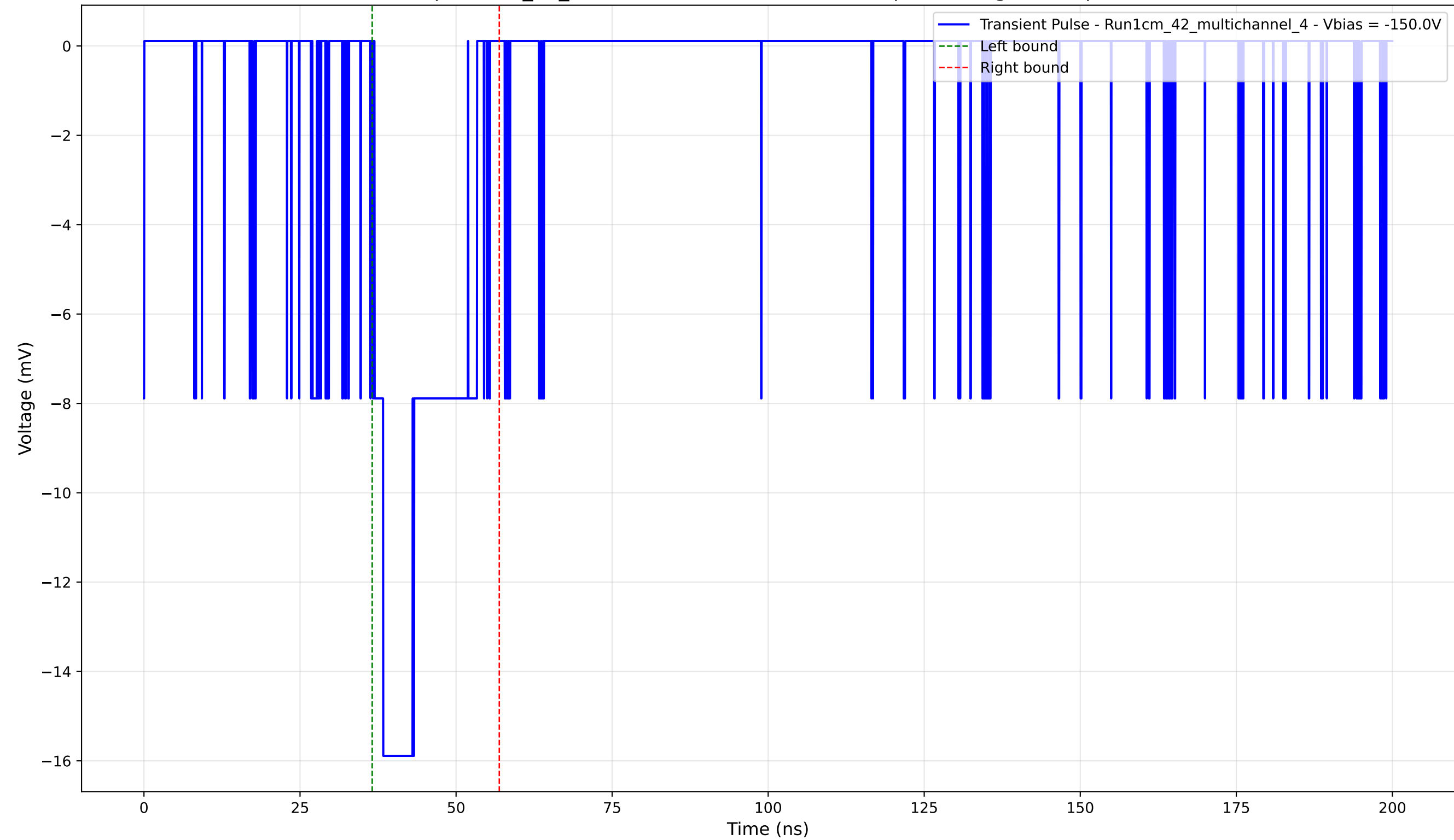
Transient Pulse - Sample: 1cm_42_multichannel - Position: 4490.0 \mu\text{m} - Charge: 3.40 pC - Rise Time: 1.40 ns
