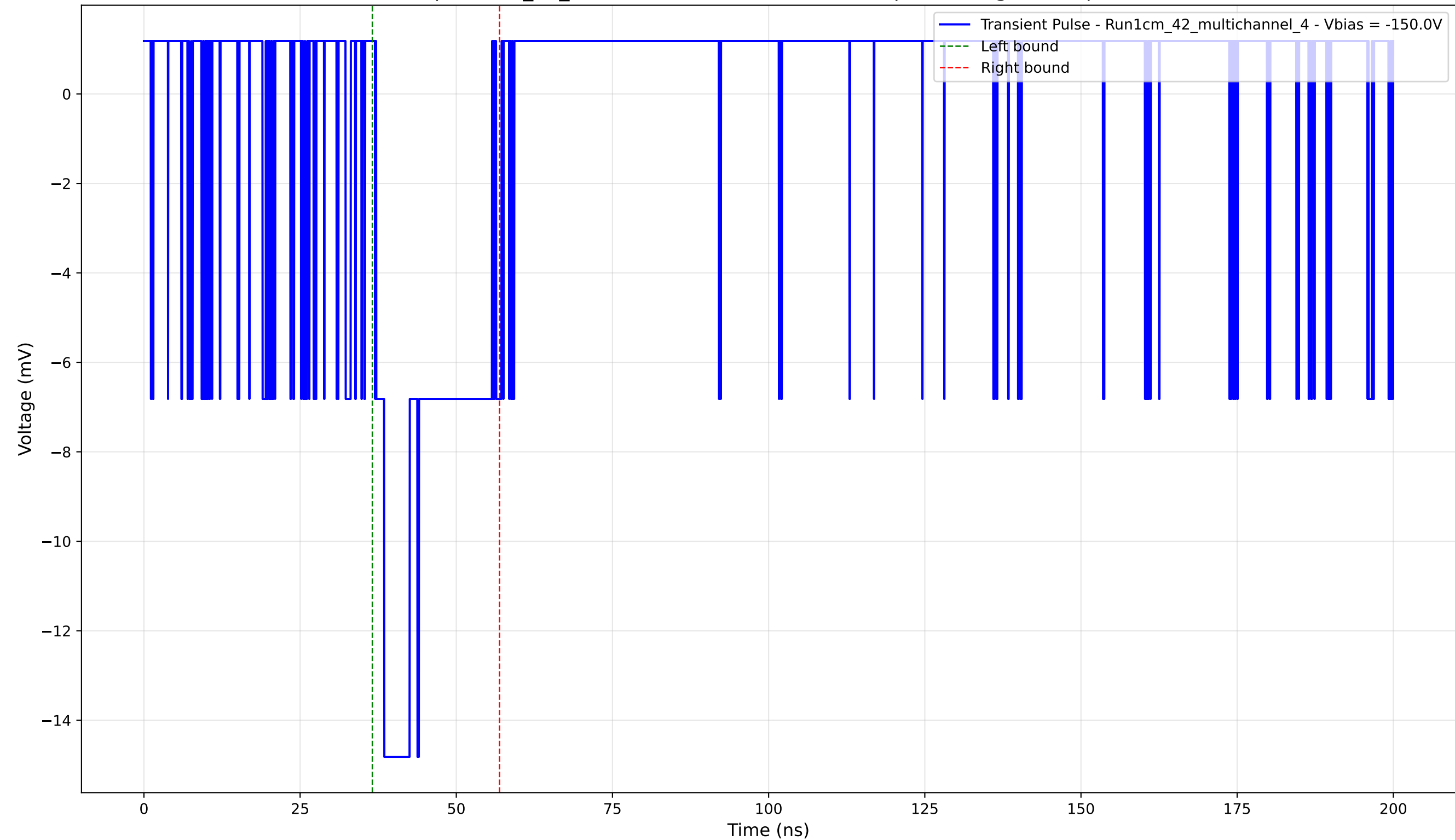
Transient Pulse - Sample: 1cm_42_multichannel - Position: 4585.0 \mu\text{m} - Charge: 3.31 pC - Rise Time: 1.30 ns
