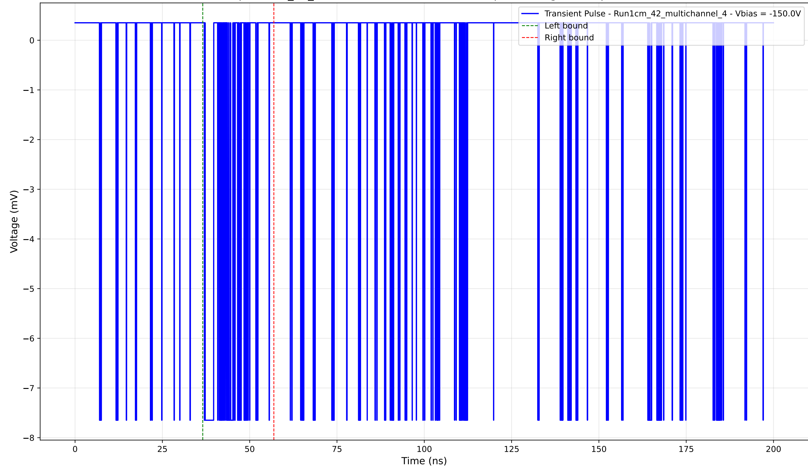
Transient Pulse - Sample: 1cm_42_multichannel - Position: 3375.0 \mu\text{m} - Charge: 1.03 pC - Rise Time: 0.02 ns
