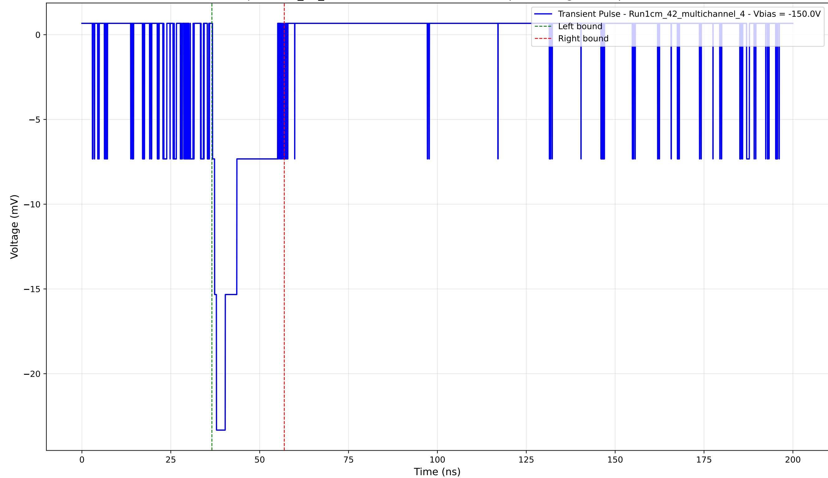
Transient Pulse - Sample: 1cm_42_multichannel - Position: 1170.0 \mu\text{m} - Charge: 4.22 pC - Rise Time: 1.12 ns
