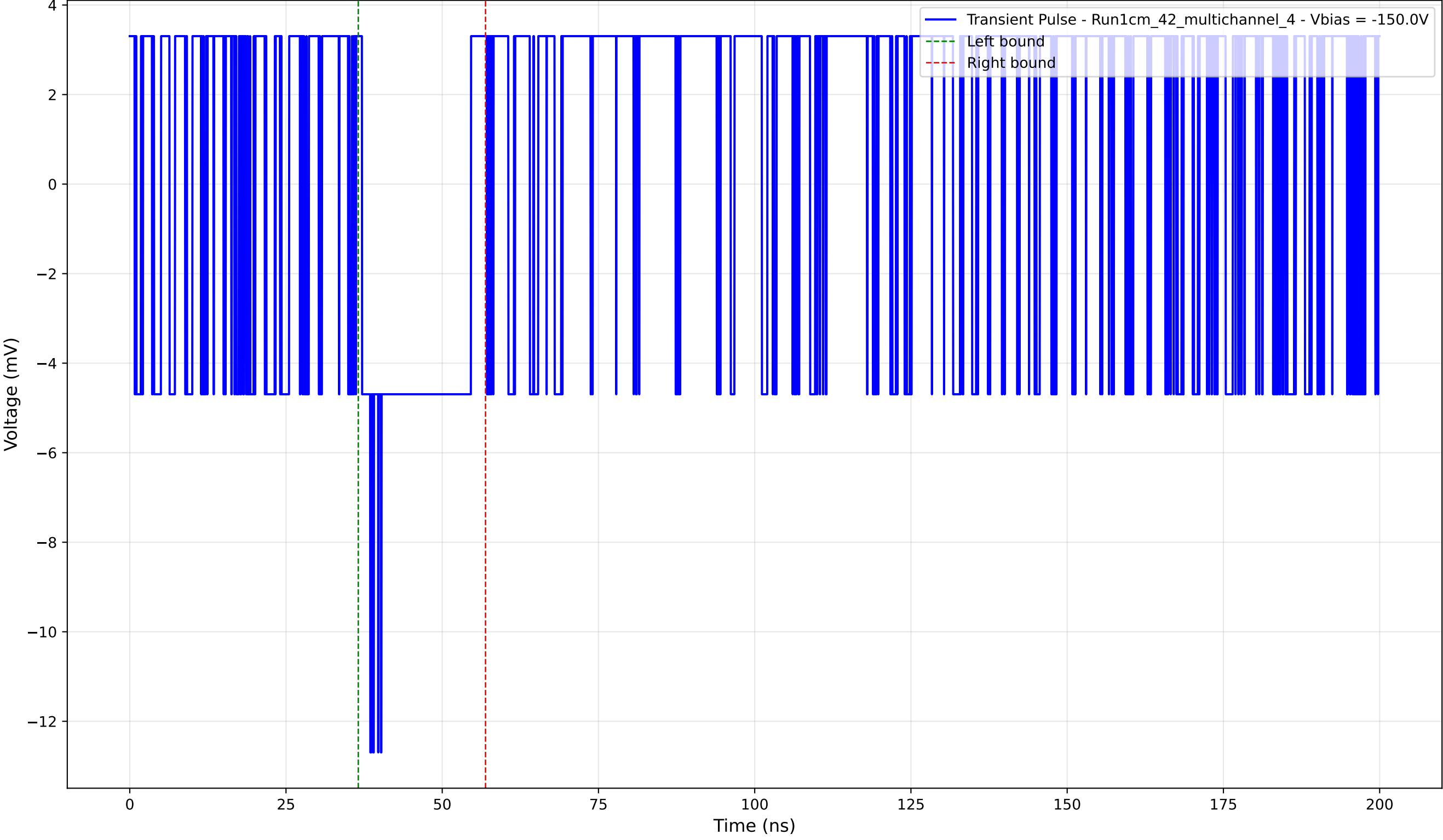
Transient Pulse - Sample: 1cm_42_multichannel - Position: 815.0 \mu\text{m} - Charge: 1.52 pC - Rise Time: 0.00 ns (N/A)
