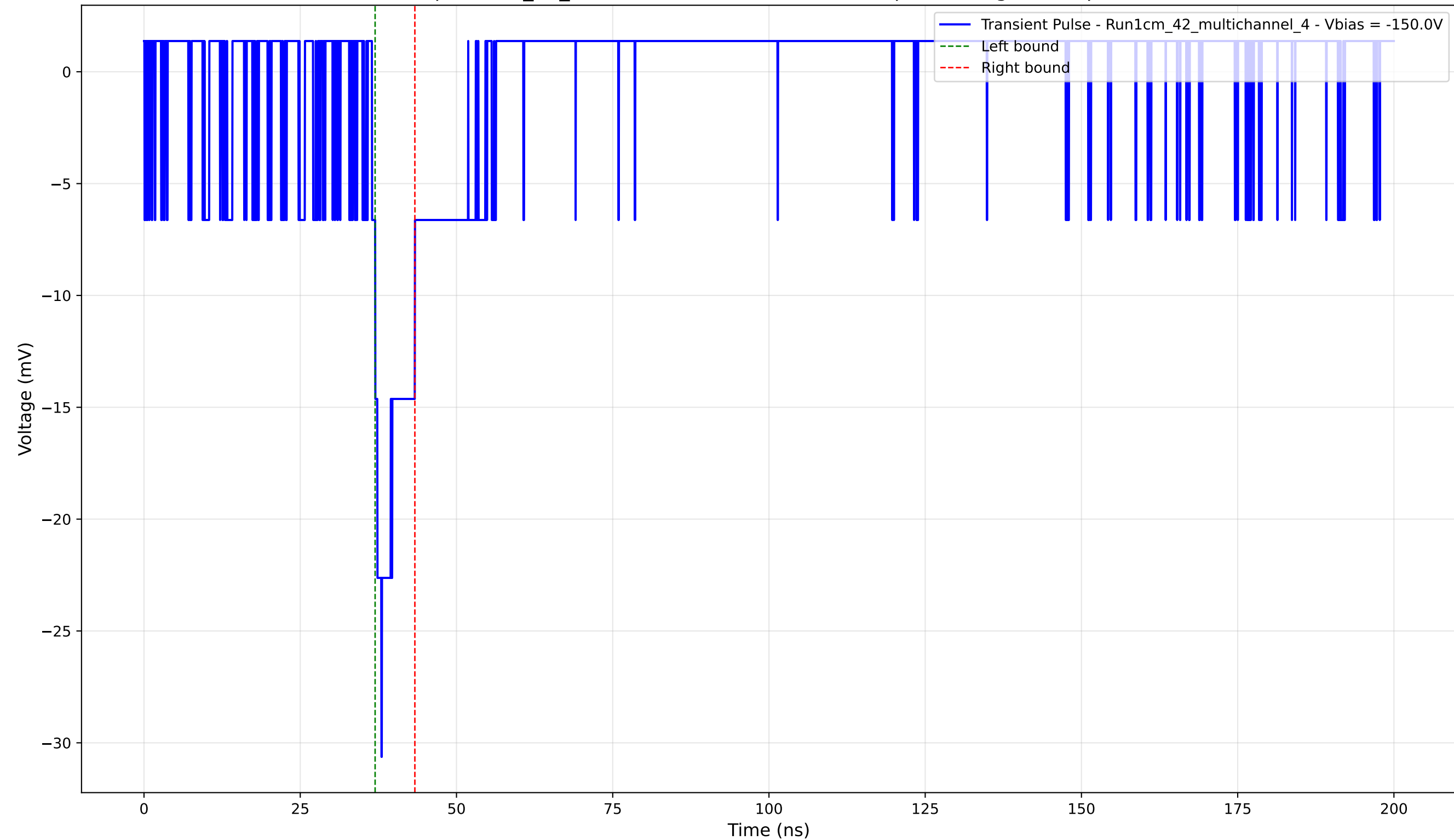
Transient Pulse - Sample: 1cm_42_multichannel - Position: 3300.0 \mu\text{m} - Charge: 2.23 pC - Rise Time: 1.51 ns
