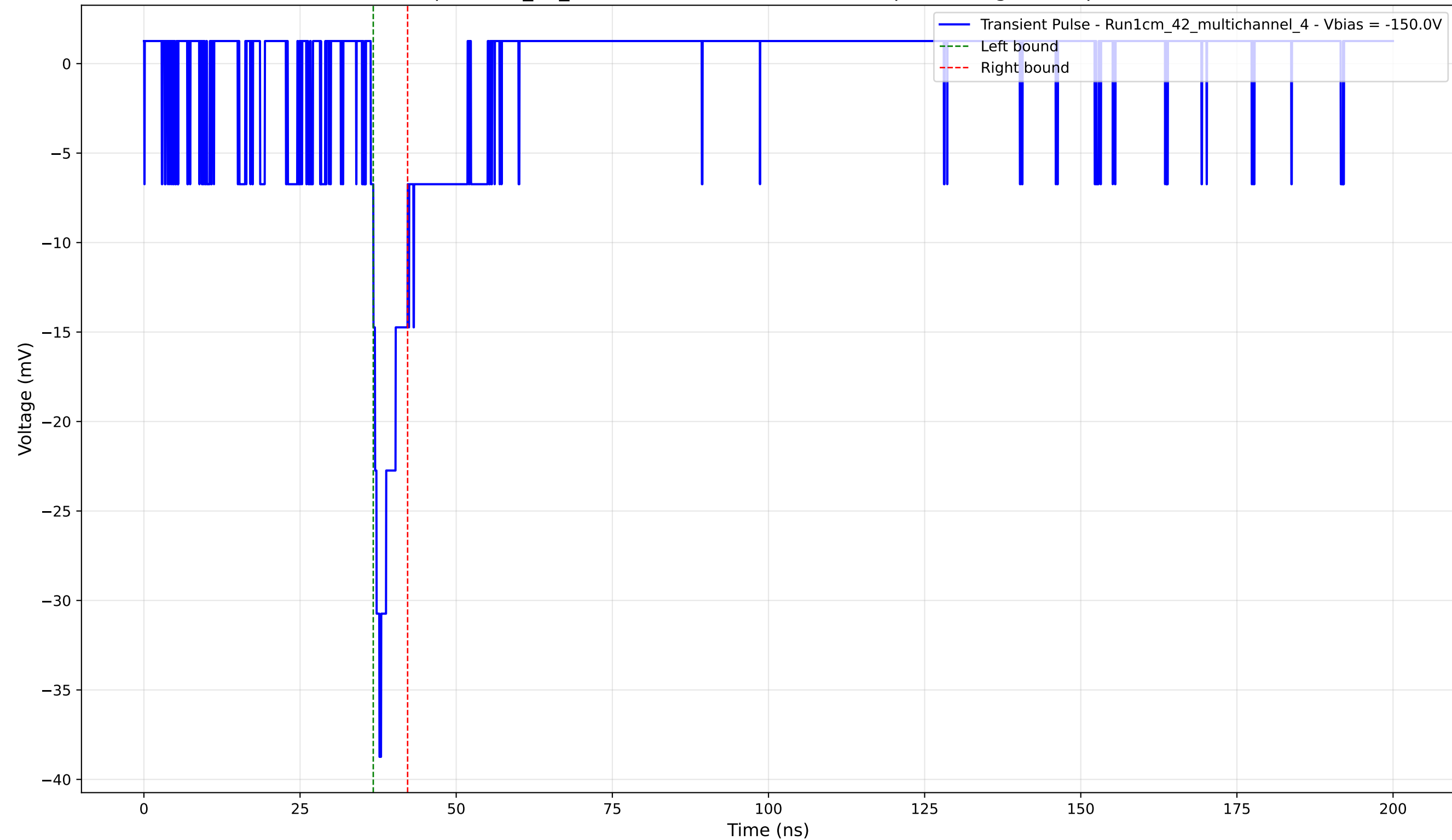
Transient Pulse - Sample: 1cm_42_multichannel - Position: 1645.0 \mu\text{m} - Charge: 2.44 pC - Rise Time: 1.39 ns
