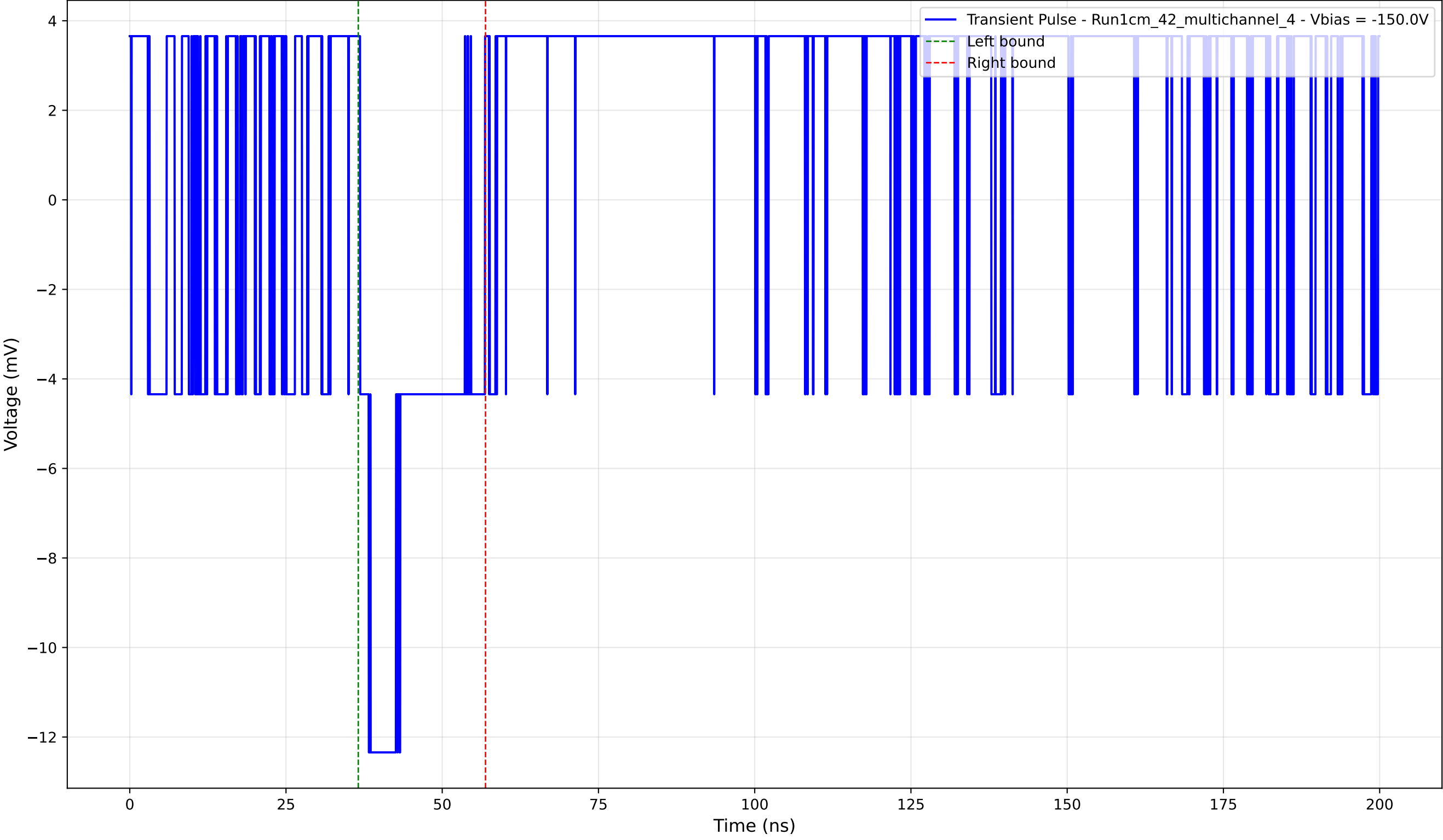
Transient Pulse - Sample: 1cm_42_multichannel - Position: 260.0 \mu\text{m} - Charge: 2.38 pC - Rise Time: 0.00 ns (N/A)
