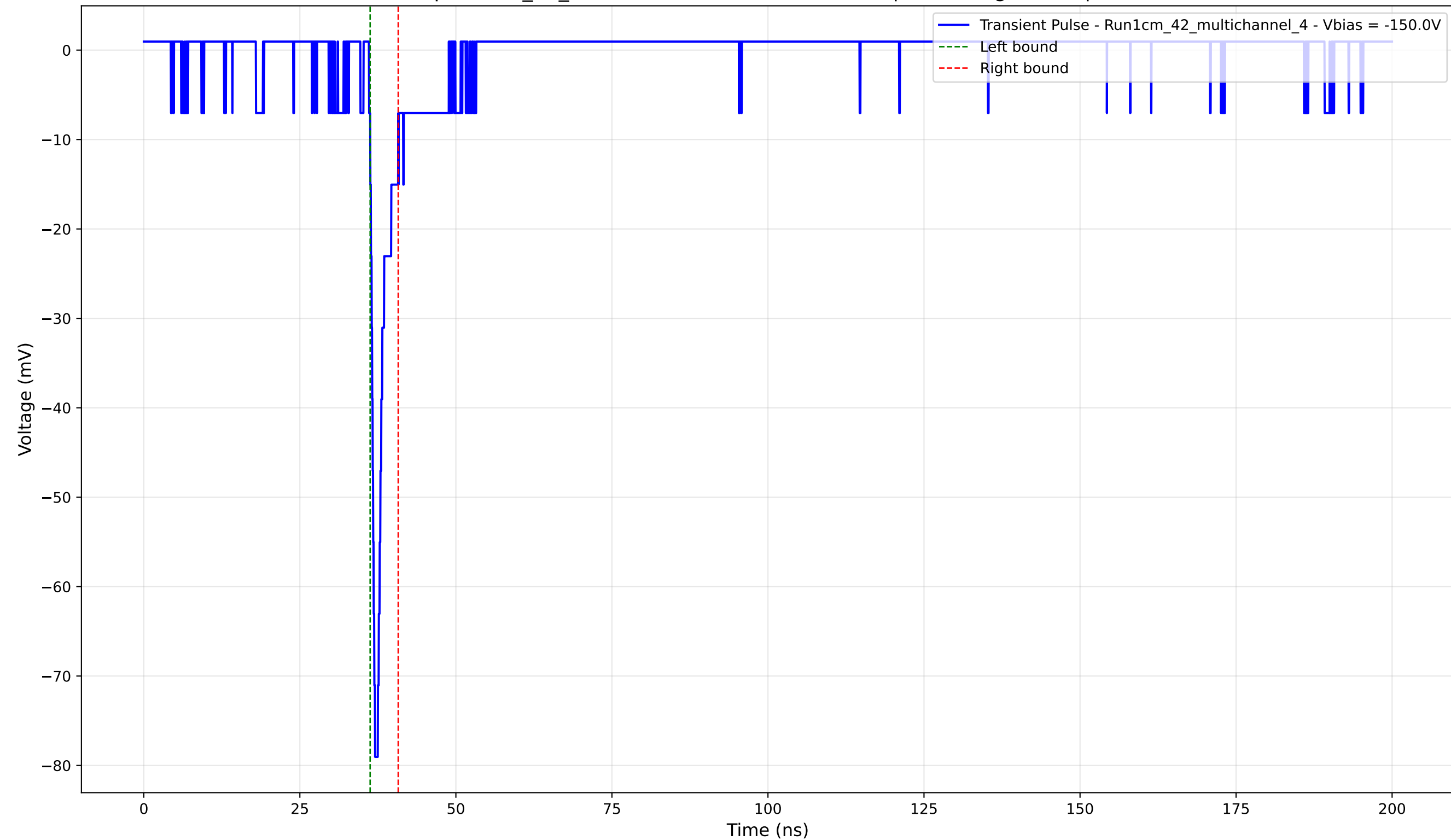
Transient Pulse - Sample: 1cm_42_multichannel - Position: 2495.0 \mu\text{m} - Charge: 3.20 pC - Rise Time: 0.78 ns
