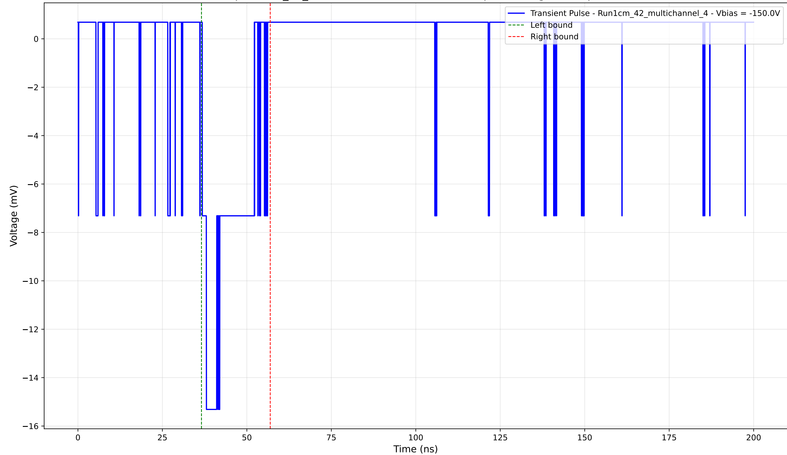
Transient Pulse - Sample: 1cm_42_multichannel - Position: 3840.0 \mu\text{m} - Charge: 2.81 pC - Rise Time: 1.24 ns
