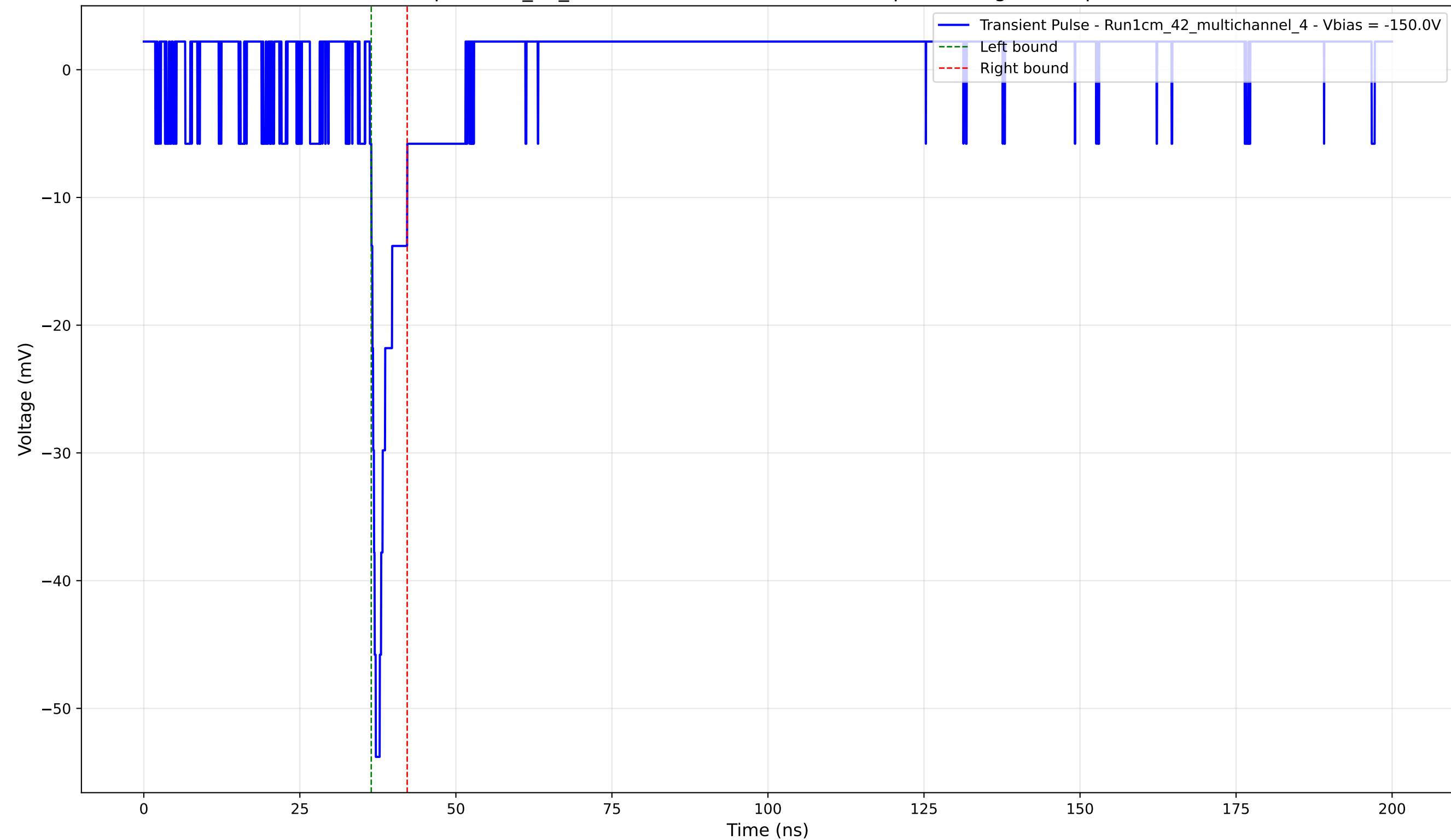
Transient Pulse - Sample: 1cm_42_multichannel - Position: 2035.0 \mu\text{m} - Charge: 2.89 pC - Rise Time: 0.96 ns
