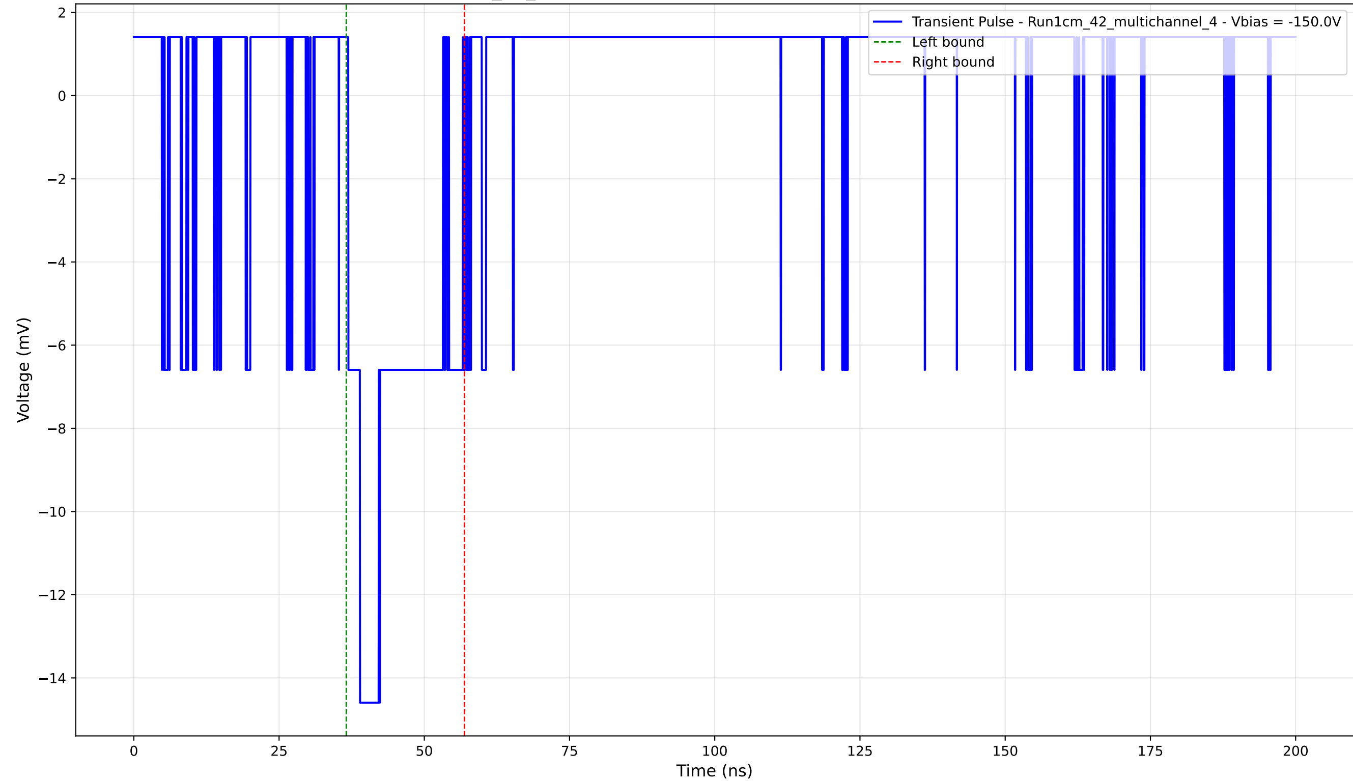
Transient Pulse - Sample: 1cm_42_multichannel - Position: 135.0 \mu\text{m} - Charge: 3.04 pC - Rise Time: 2.02 ns
