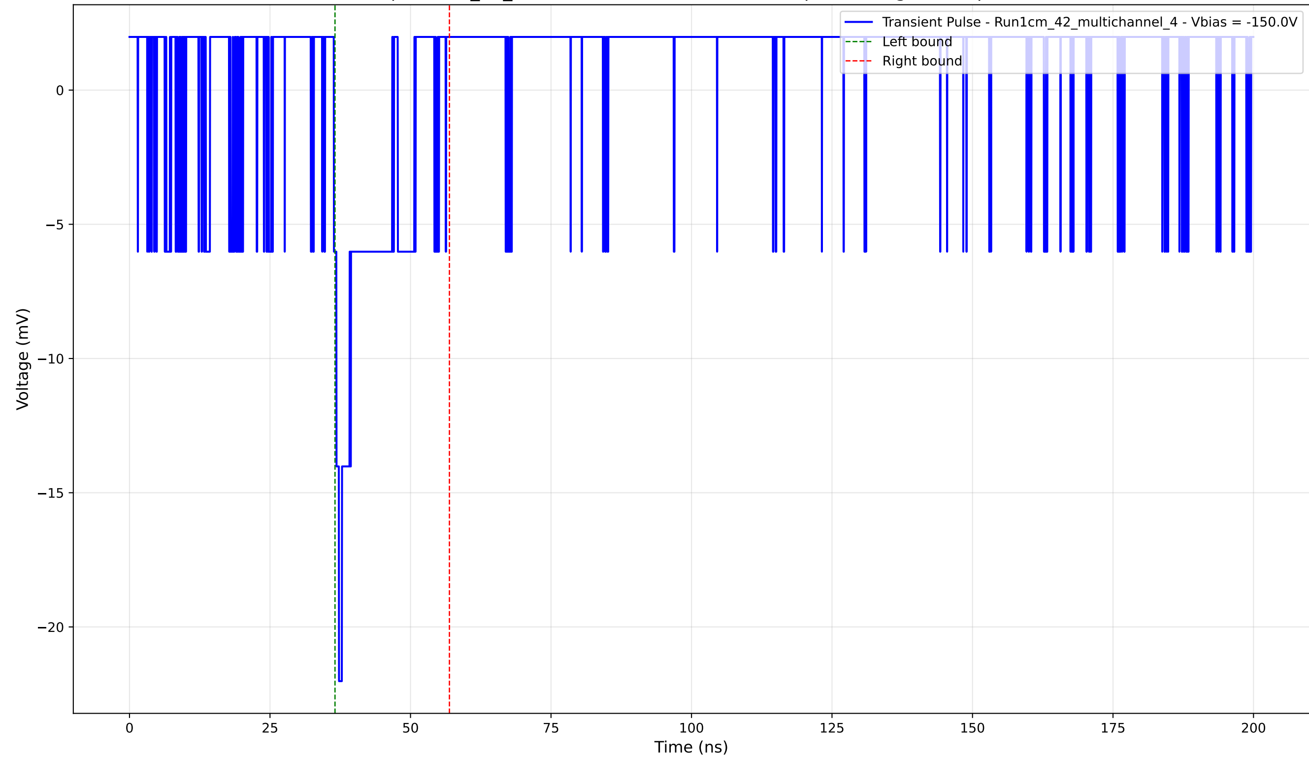
Transient Pulse - Sample: 1cm_42_multichannel - Position: 2845.0 \mu\text{m} - Charge: 1.92 pC - Rise Time: 0.92 ns
