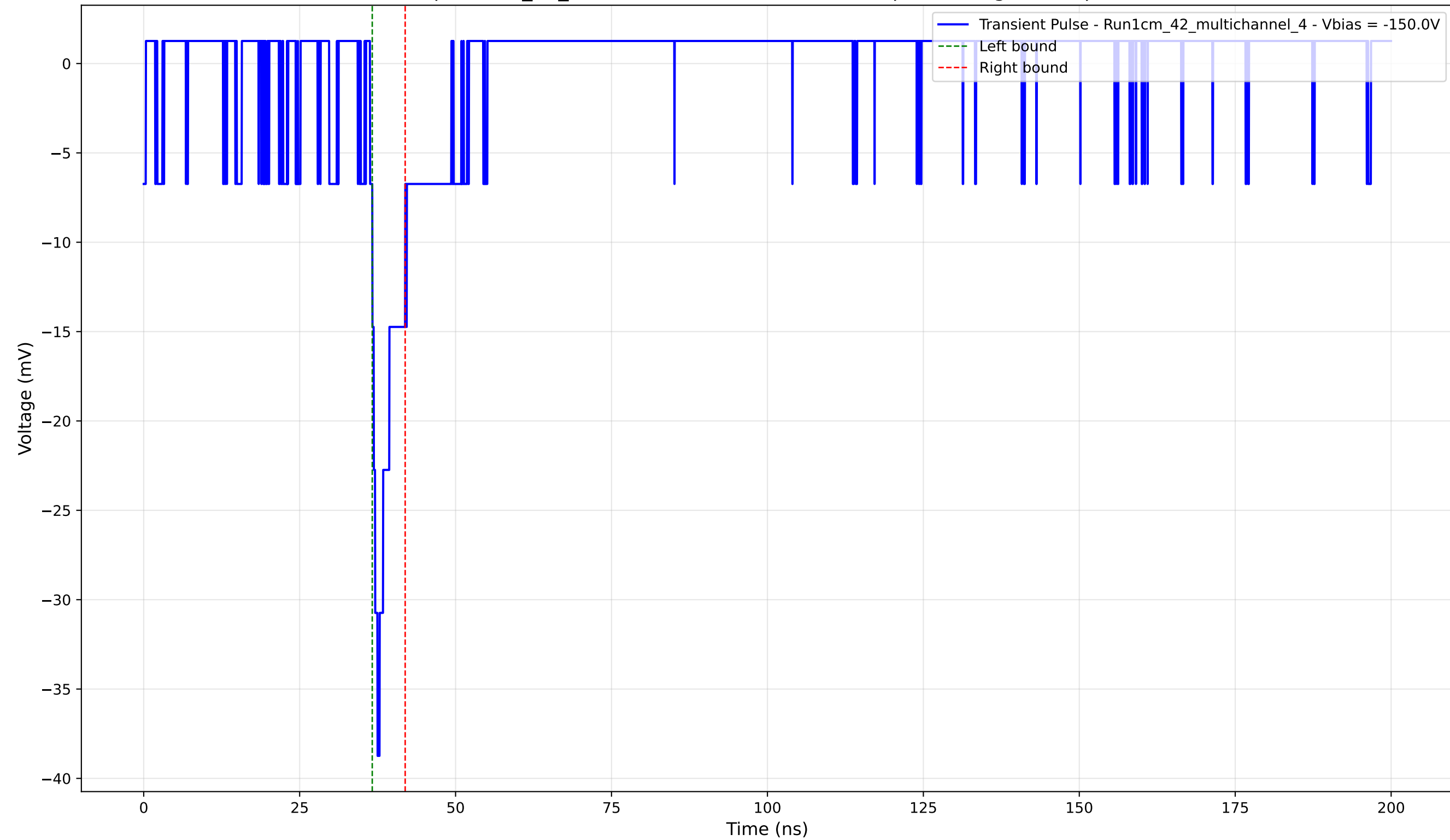
Transient Pulse - Sample: 1cm_42_multichannel - Position: 2965.0 \mu\text{m} - Charge: 2.21 pC - Rise Time: 1.21 ns
