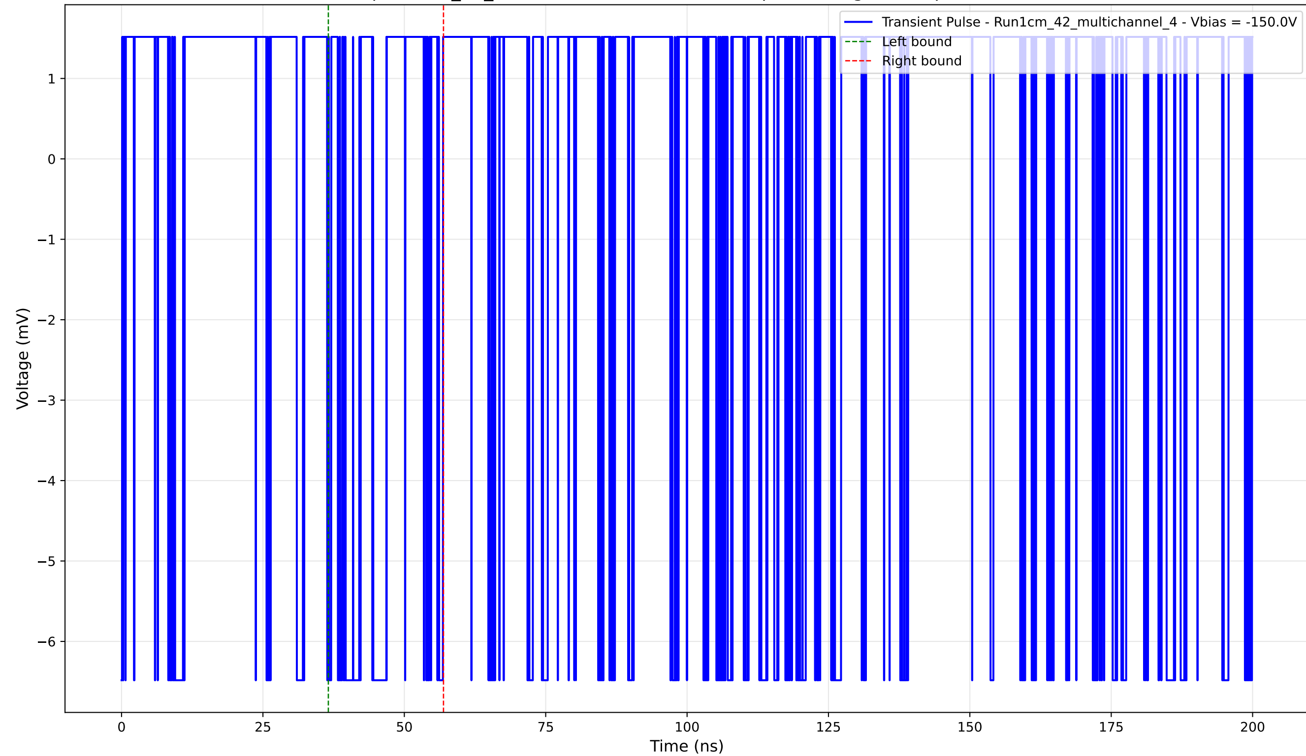
Transient Pulse - Sample: 1cm_42_multichannel - Position: 55.0 \mu\text{m} - Charge: 0.63 pC - Rise Time: 0.00 ns (N/A)
