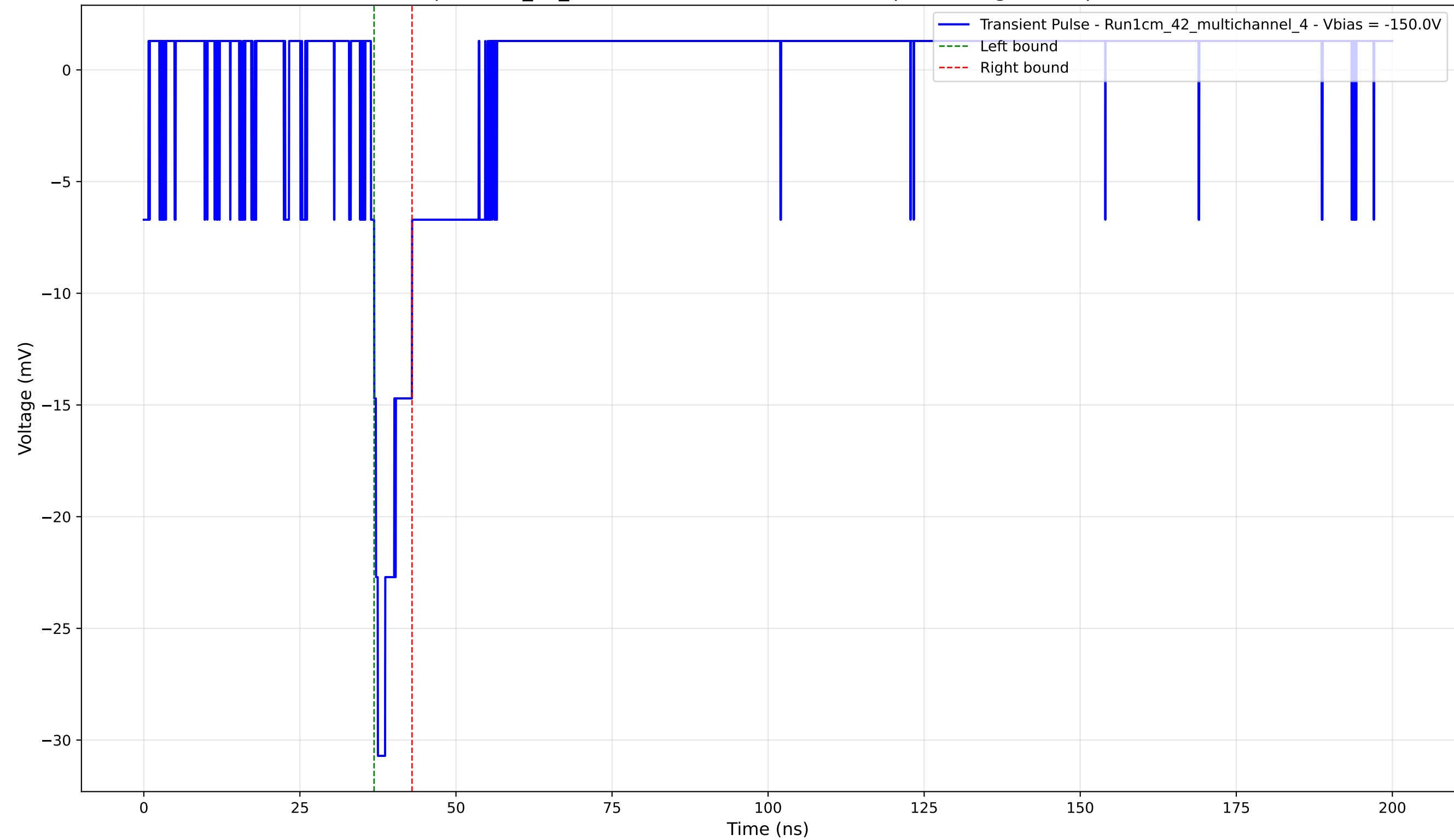
Transient Pulse - Sample: 1cm_42_multichannel - Position: 1530.0 \mu\text{m} - Charge: 2.46 pC - Rise Time: 1.11 ns
