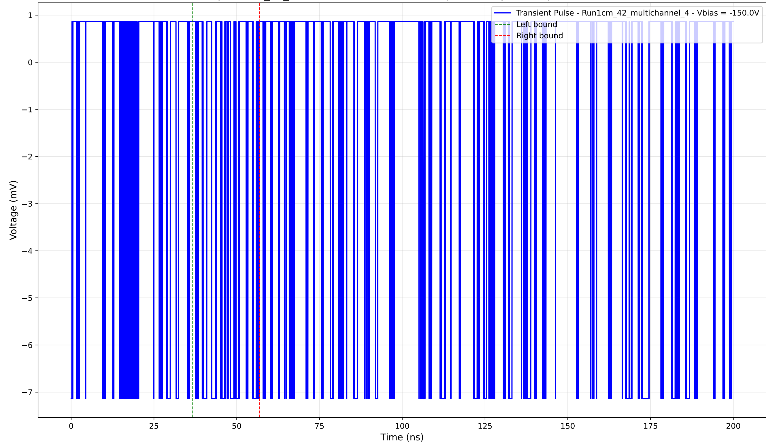
Transient Pulse - Sample: 1cm_42_multichannel - Position: 15.0 \mu\text{m} - Charge: 0.96 pC - Rise Time: 0.00 ns (N/A)
