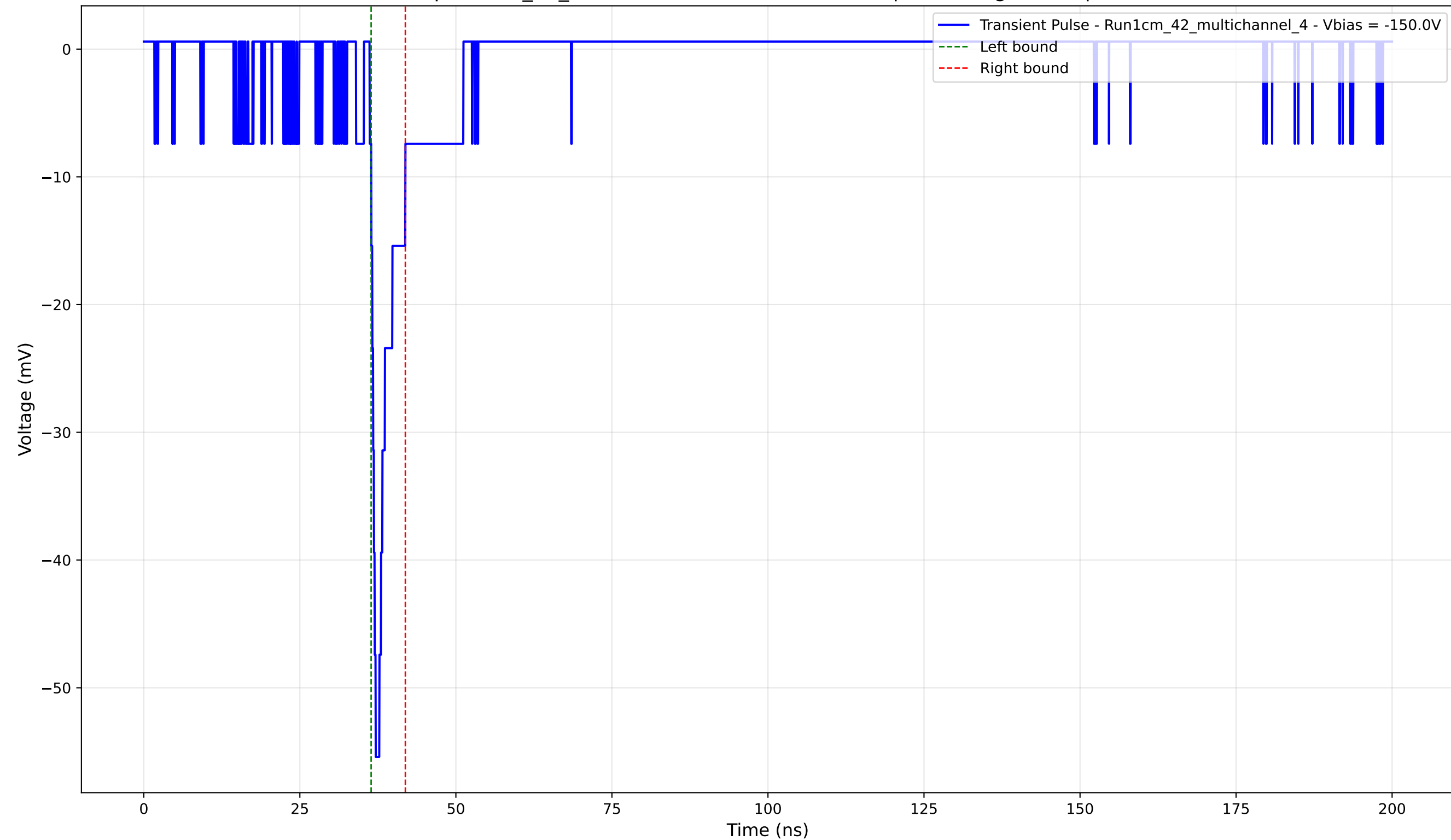
Transient Pulse - Sample: 1cm_42_multichannel - Position: 2050.0 \mu\text{m} - Charge: 2.98 pC - Rise Time: 0.97 ns
