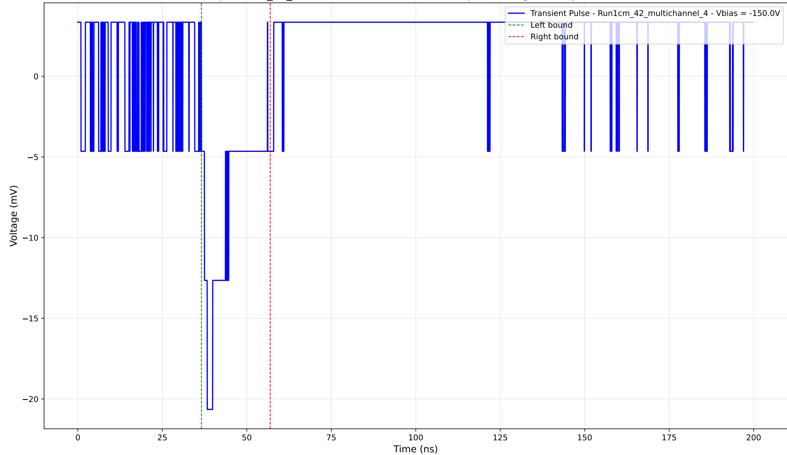
Transient Pulse - Sample: 1cm_42_multichannel - Position: 1025.0 \mu\text{m} - Charge: 3.22 pC - Rise Time: 0.00 ns (N/A)
