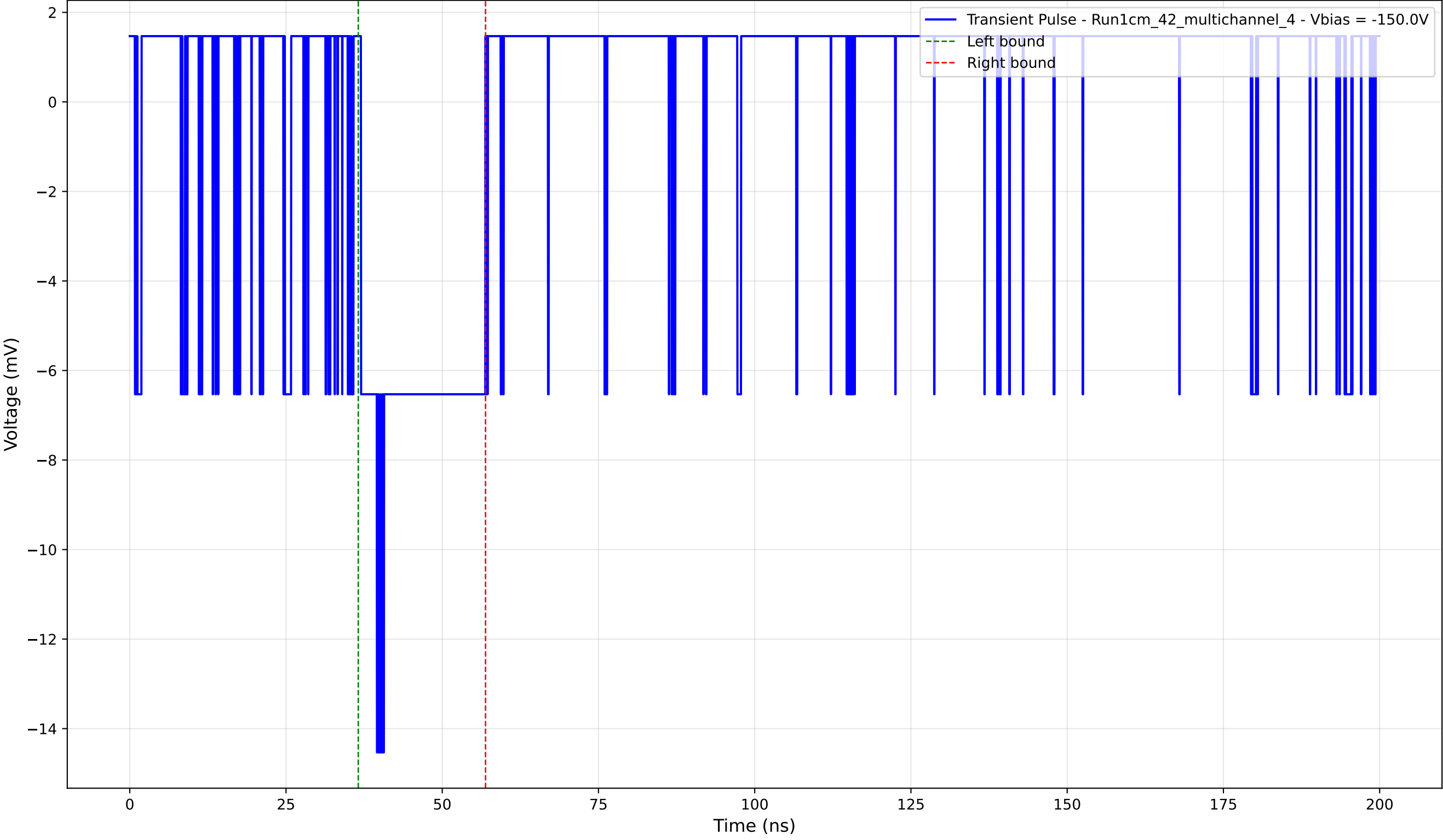
Transient Pulse - Sample: 1cm_42_multichannel - Position: 110.0 \mu\text{m} - Charge: 2.72 pC - Rise Time: 0.00 ns (N/A)
