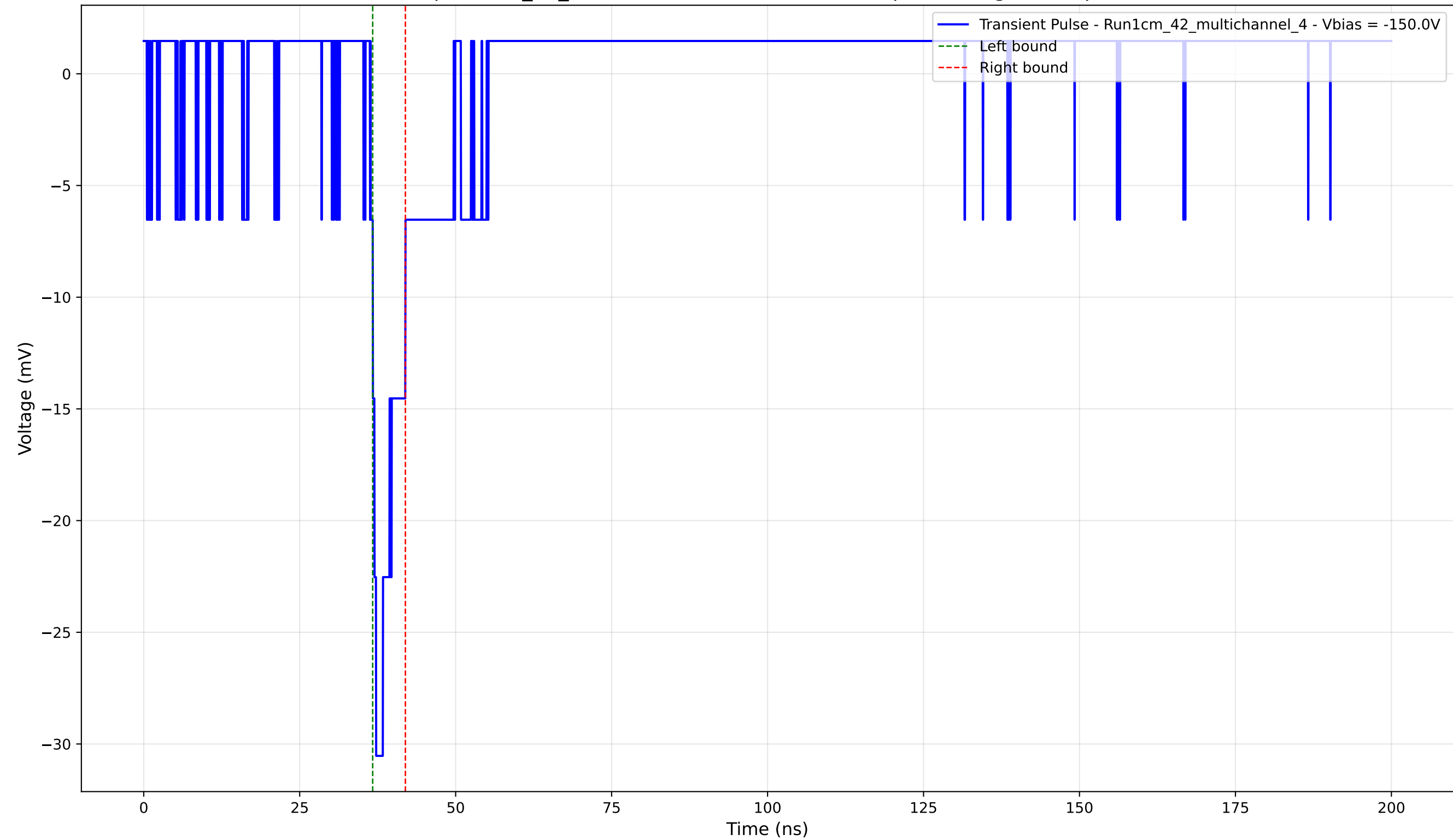
Transient Pulse - Sample: 1cm_42_multichannel - Position: 3070.0 \mu\text{m} - Charge: 2.11 pC - Rise Time: 0.89 ns
