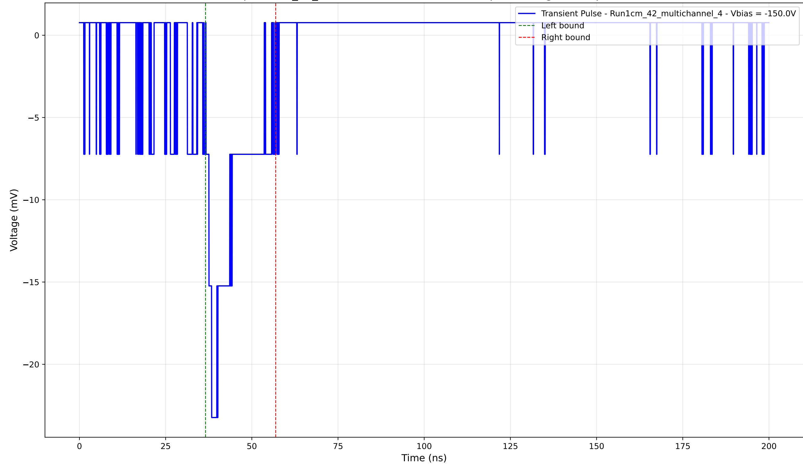
Transient Pulse - Sample: 1cm_42_multichannel - Position: 980.0 \mu\text{m} - Charge: 4.08 pC - Rise Time: 1.66 ns
