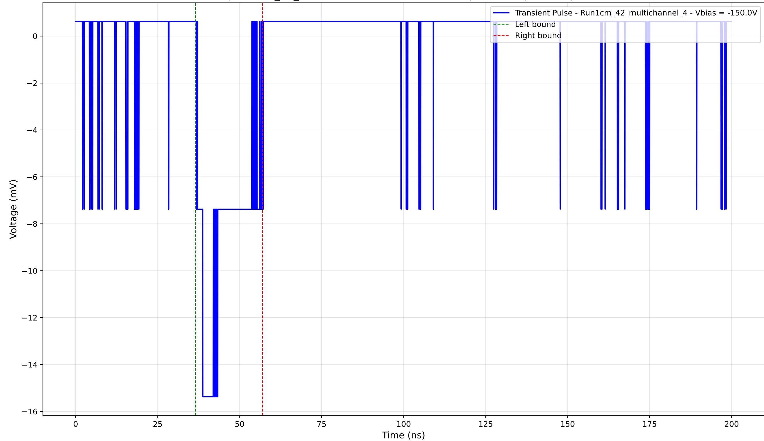
Transient Pulse - Sample: 1cm_42_multichannel - Position: 4645.0 \mu\text{m} - Charge: 3.40 pC - Rise Time: 1.62 ns
