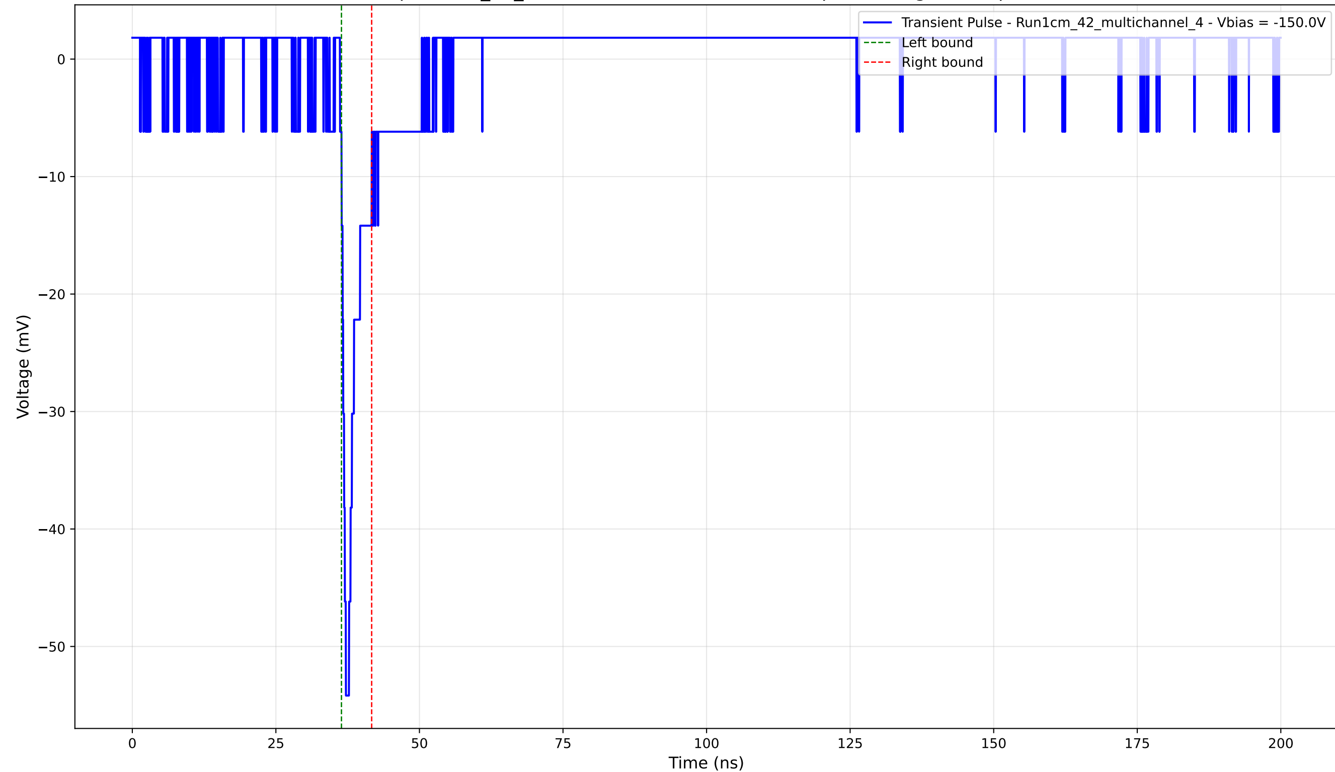
Transient Pulse - Sample: 1cm_42_multichannel - Position: 2750.0 \mu\text{m} - Charge: 2.74 pC - Rise Time: 1.02 ns
