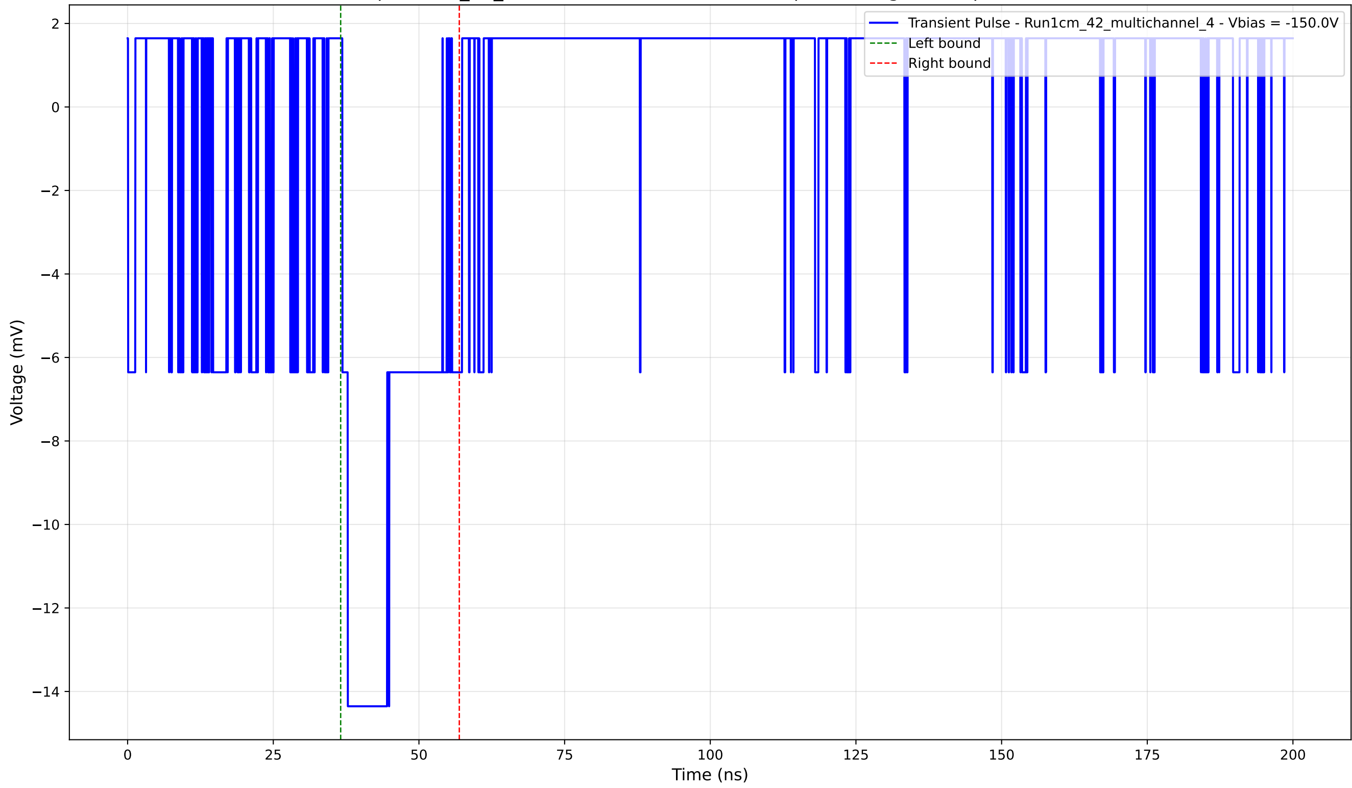
Transient Pulse - Sample: 1cm_42_multichannel - Position: 740.0 \mu\text{m} - Charge: 3.53 pC - Rise Time: 0.00 ns (N/A)
