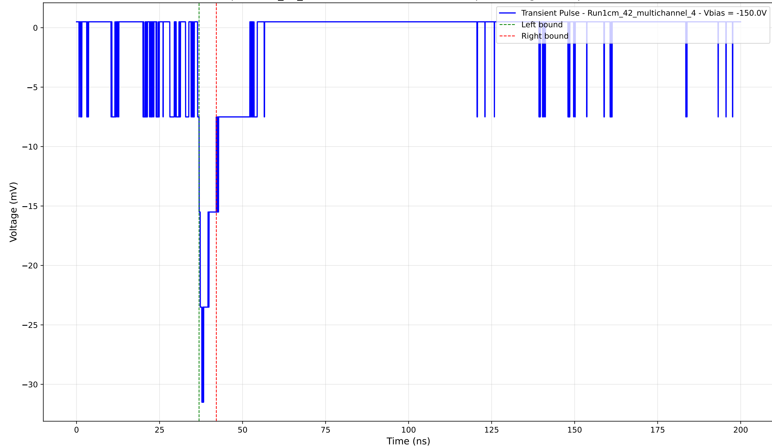
Transient Pulse - Sample: 1cm_42_multichannel - Position: 3270.0 \mu\text{m} - Charge: 2.08 pC - Rise Time: 1.29 ns
