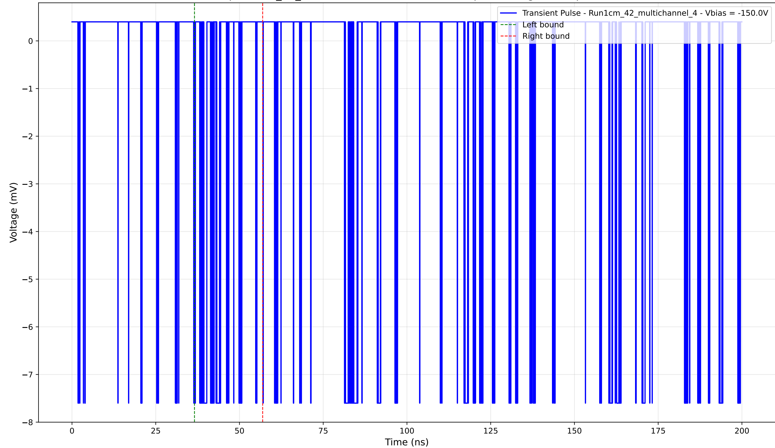
Transient Pulse - Sample: 1cm_42_multichannel - Position: 3410.0 \mu\text{m} - Charge: 0.57 pC - Rise Time: 0.02 ns
