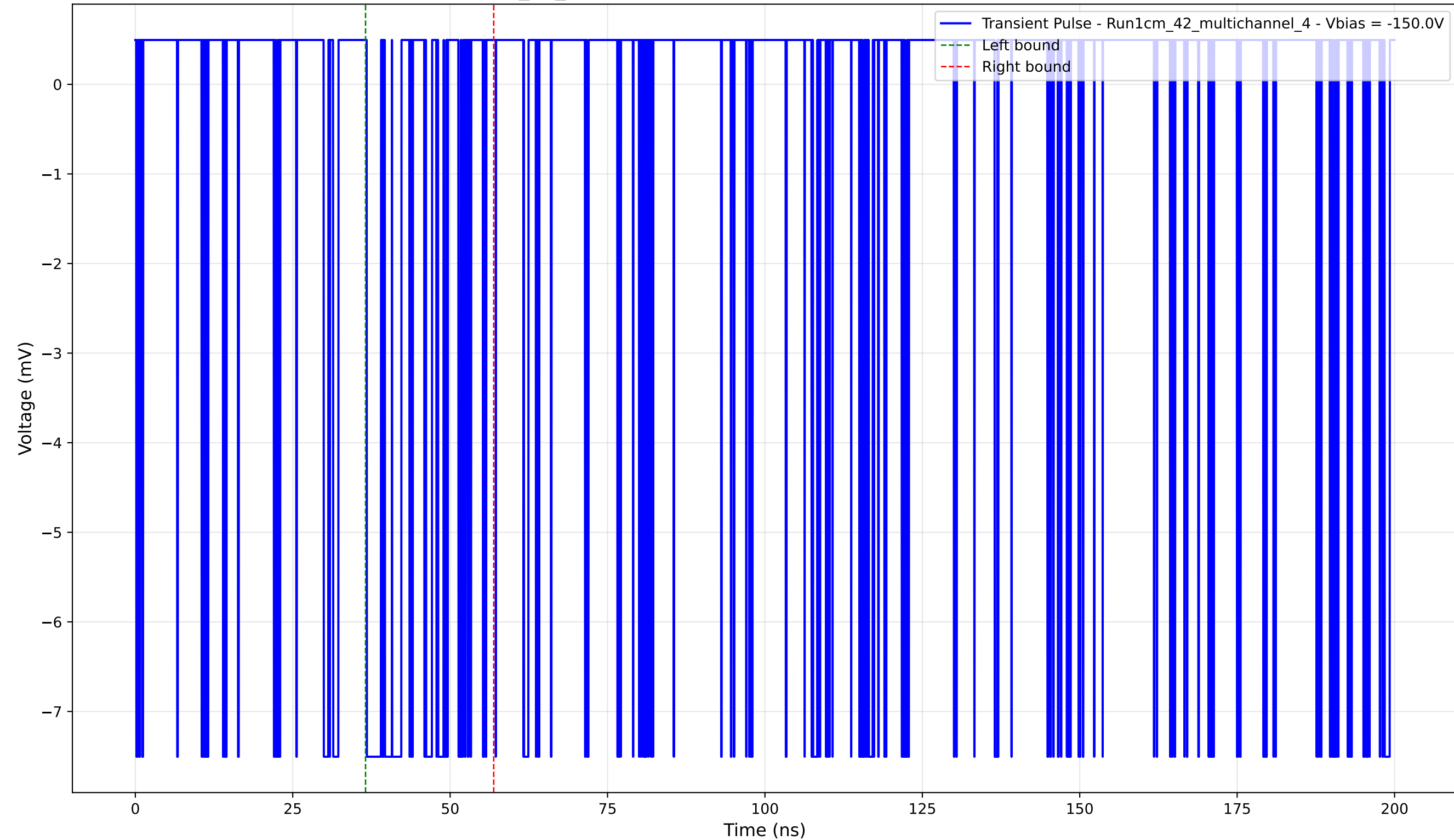
Transient Pulse - Sample: 1cm_42_multichannel - Position: 2905.0 \mu\text{m} - Charge: 1.23 pC - Rise Time: 0.02 ns
