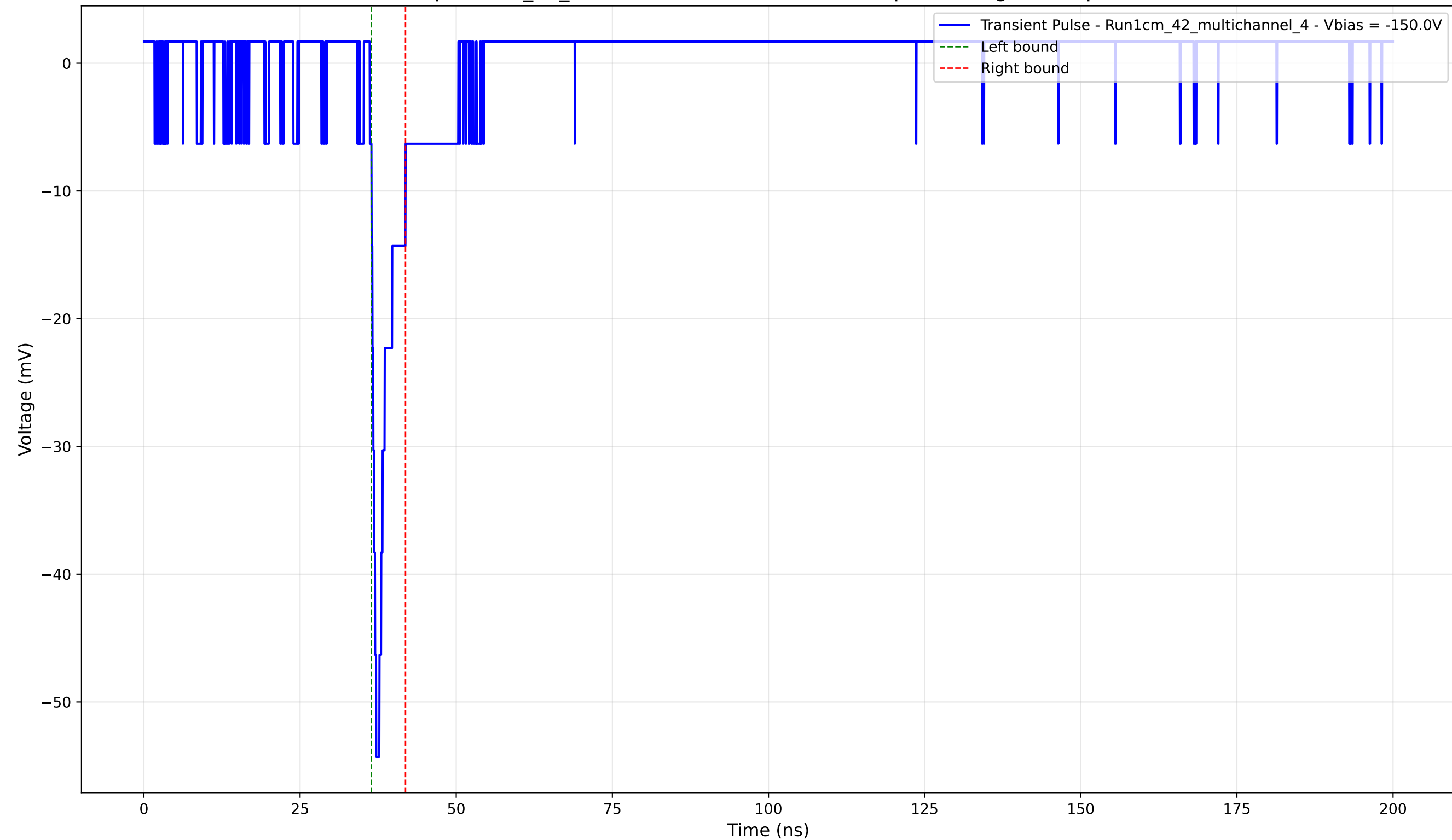
Transient Pulse - Sample: 1cm_42_multichannel - Position: 2720.0 \mu\text{m} - Charge: 2.81 pC - Rise Time: 1.02 ns
