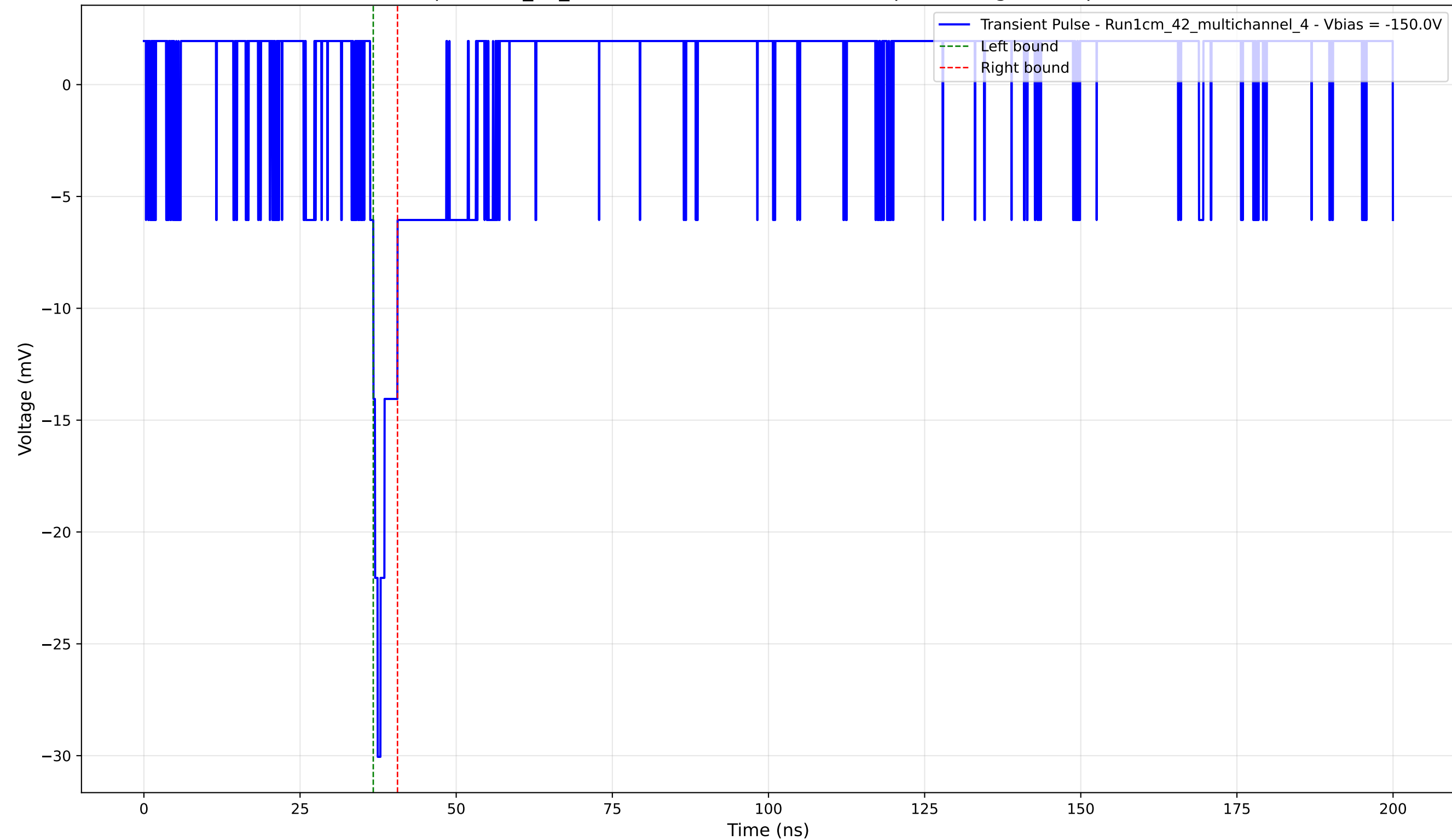
Transient Pulse - Sample: 1cm_42_multichannel - Position: 1825.0 \mu\text{m} - Charge: 1.40 pC - Rise Time: 1.21 ns
