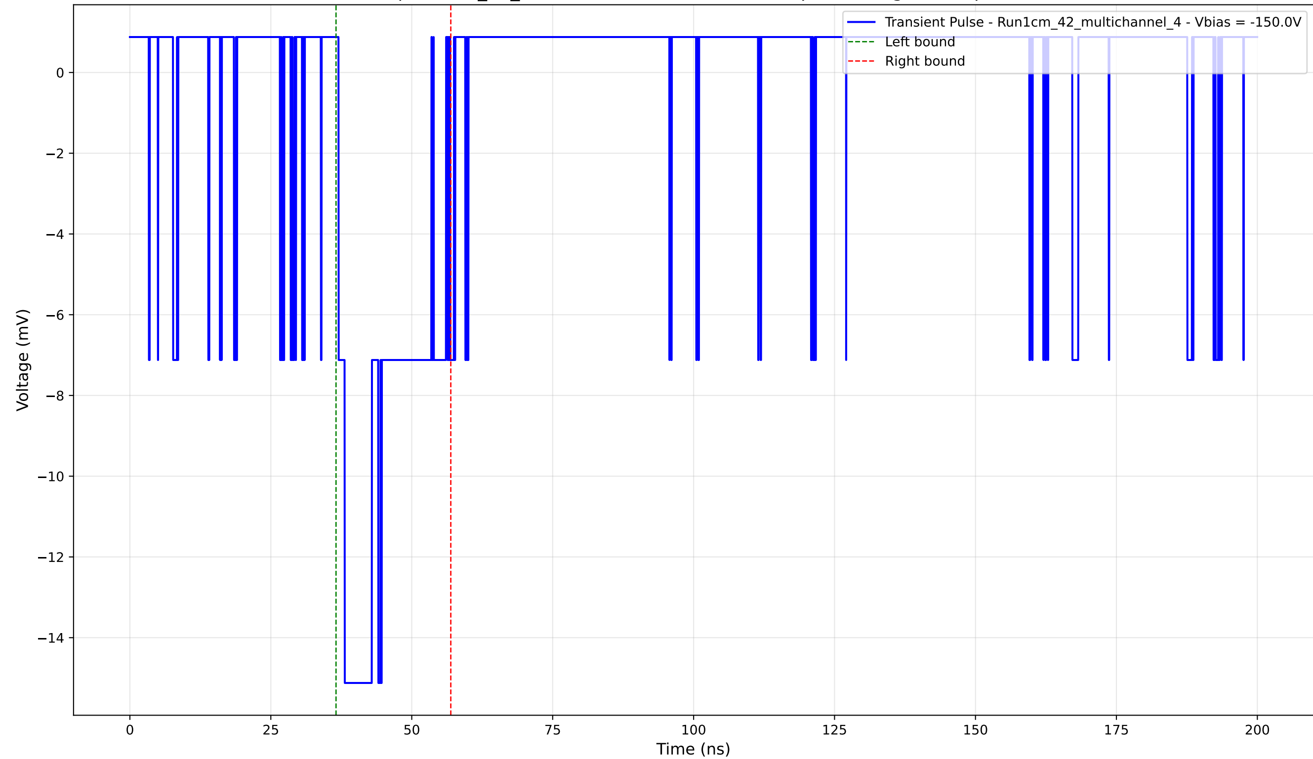
Transient Pulse - Sample: 1cm_42_multichannel - Position: 610.0 \mu\text{m} - Charge: 3.60 pC - Rise Time: 1.10 ns
