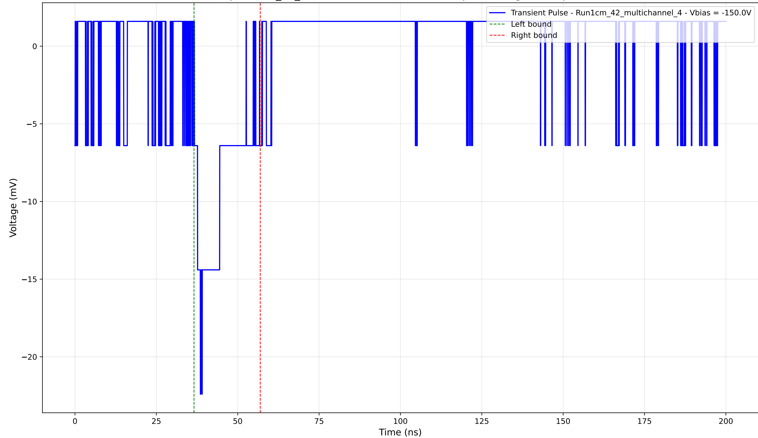
Transient Pulse - Sample: 1cm_42_multichannel - Position: 945.0 \mu\text{m} - Charge: 3.61 pC - Rise Time: 1.84 ns
