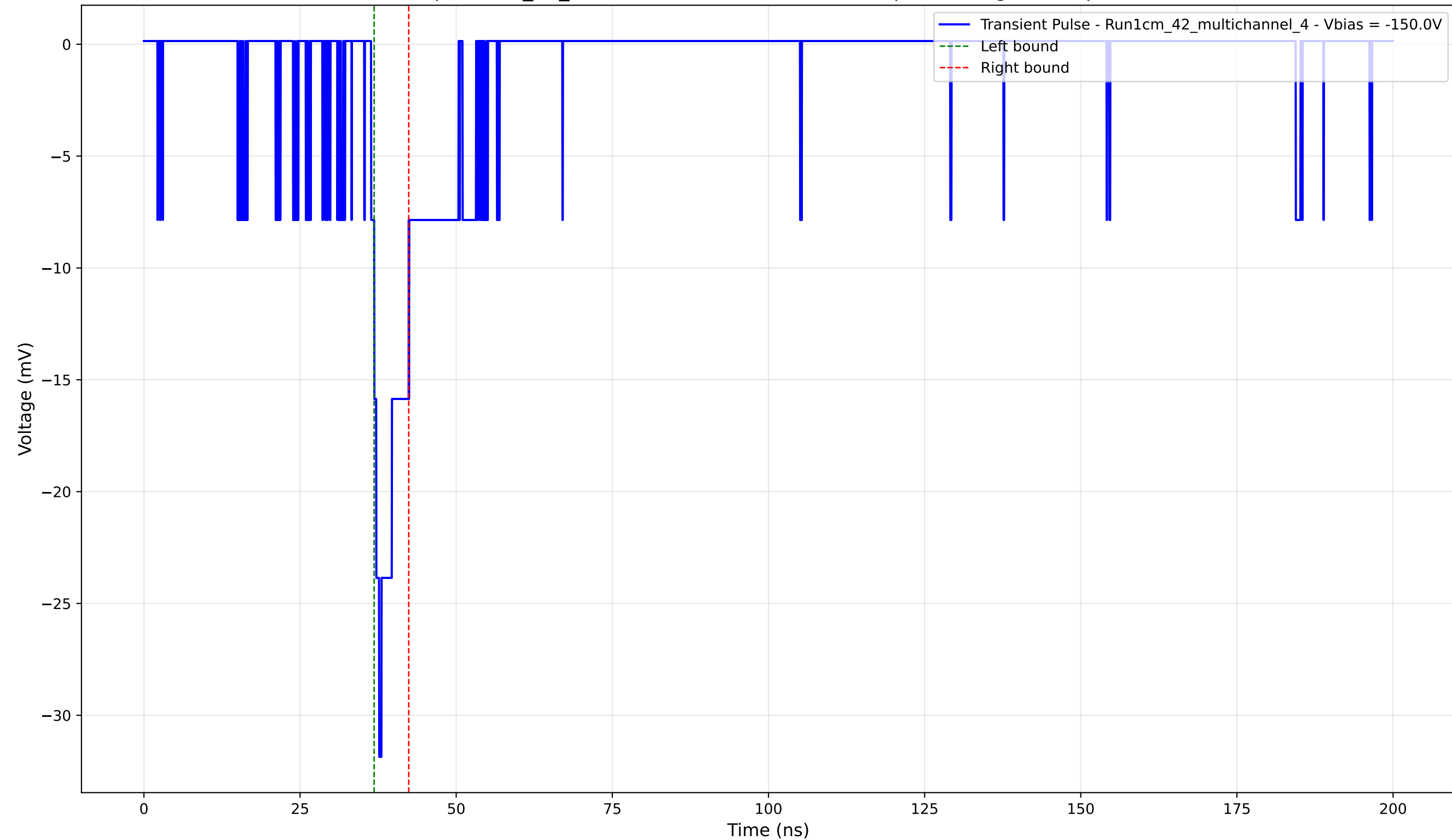
Transient Pulse - Sample: 1cm_42_multichannel - Position: 3210.0 \mu\text{m} - Charge: 2.21 pC - Rise Time: 1.29 ns
