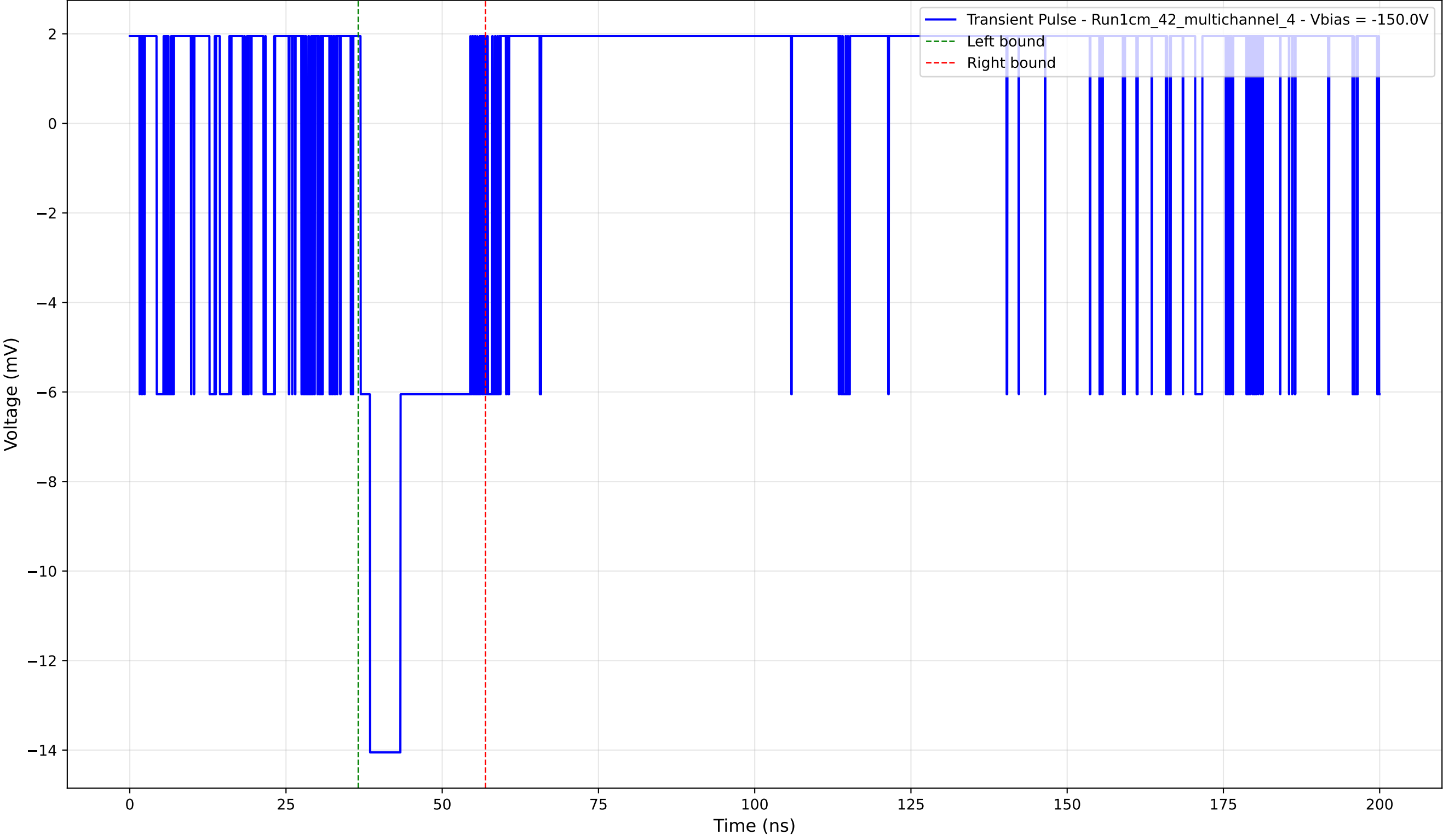
Transient Pulse - Sample: 1cm_42_multichannel - Position: 440.0 \mu\text{m} - Charge: 3.03 pC - Rise Time: 0.00 ns (N/A)
