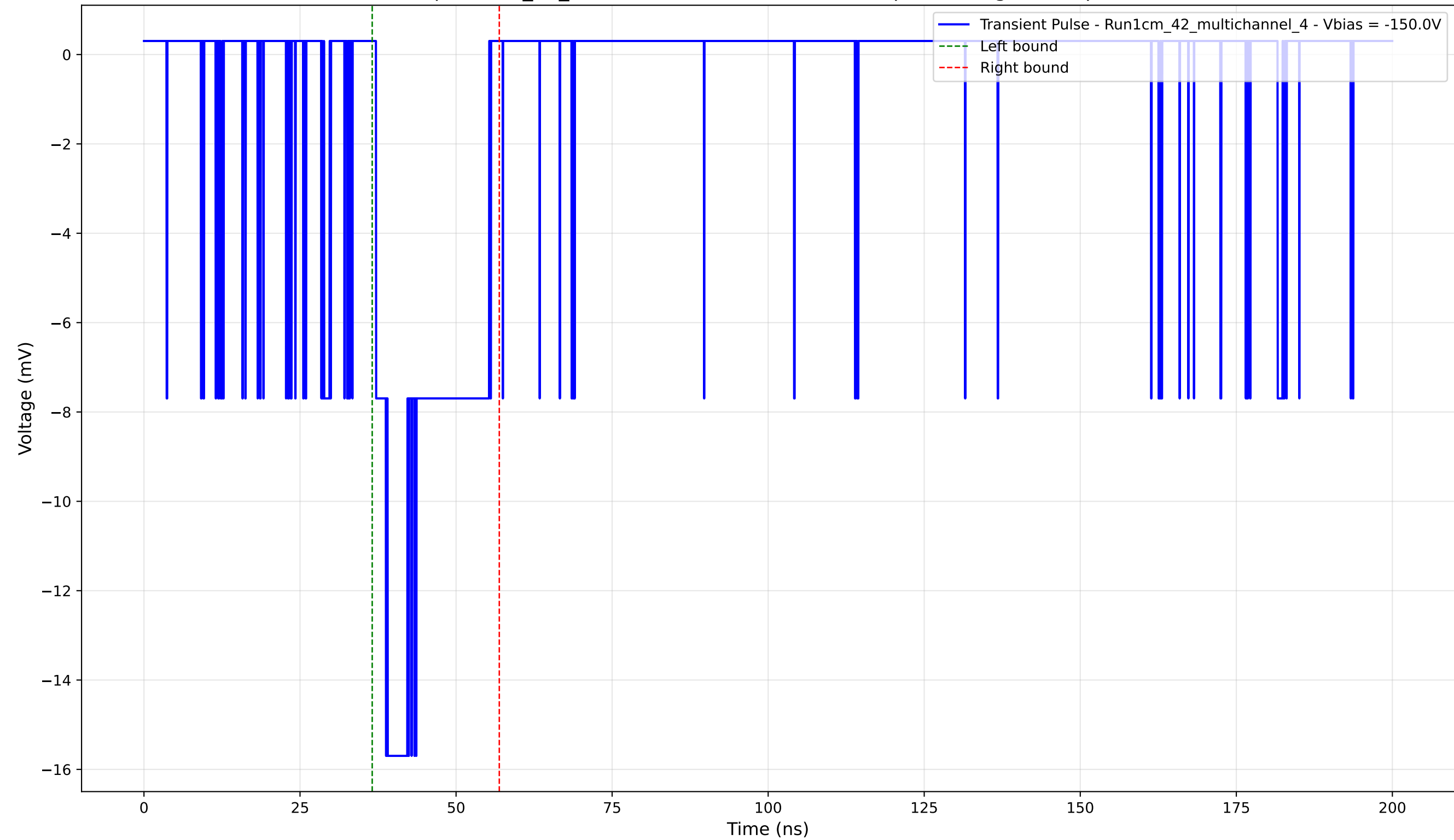
Transient Pulse - Sample: 1cm_42_multichannel - Position: 4620.0 \mu\text{m} - Charge: 3.36 pC - Rise Time: 1.60 ns
