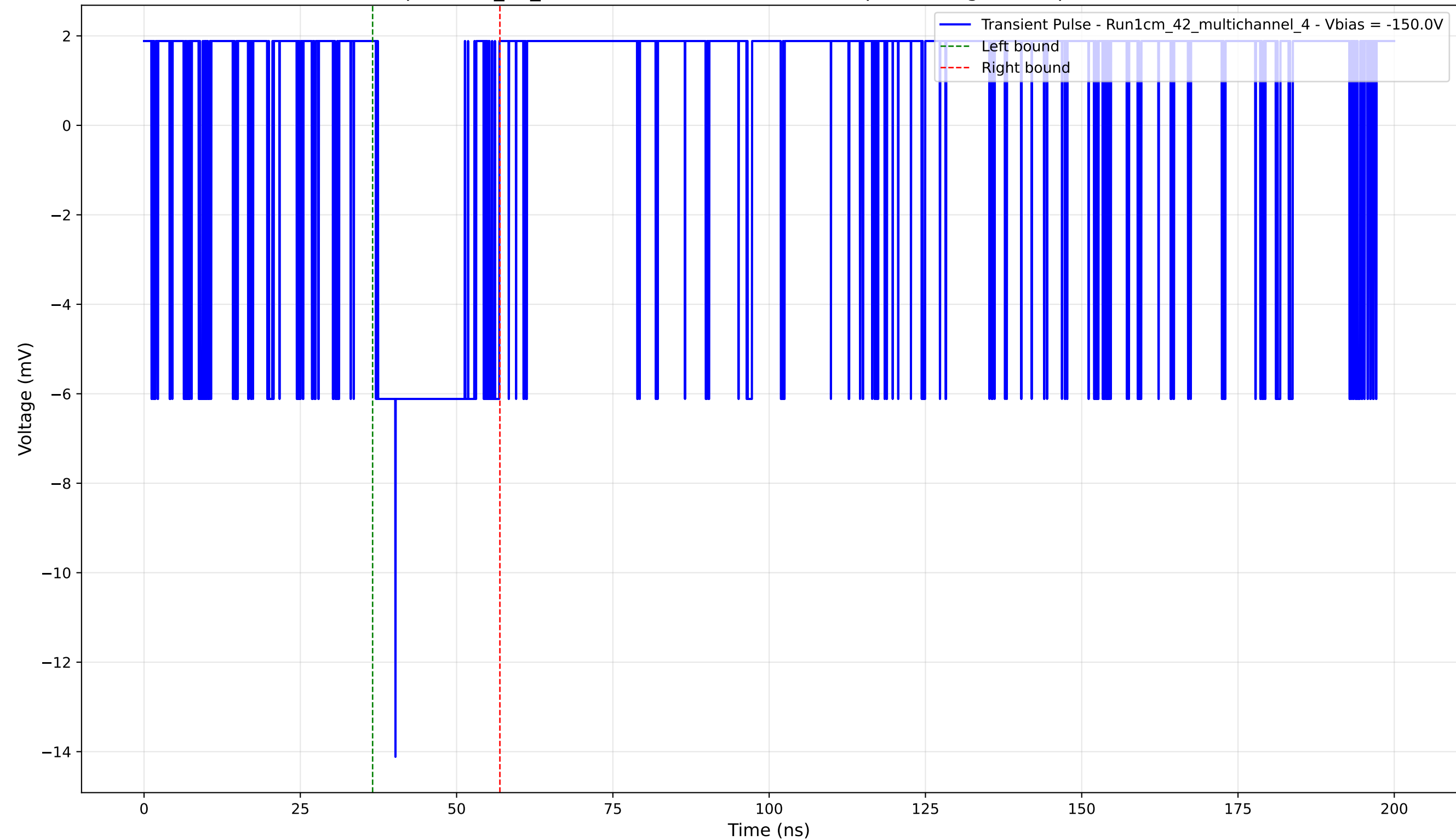
Transient Pulse - Sample: 1cm_42_multichannel - Position: 4350.0 \mu\text{m} - Charge: 2.04 pC - Rise Time: 0.00 ns (N/A)
