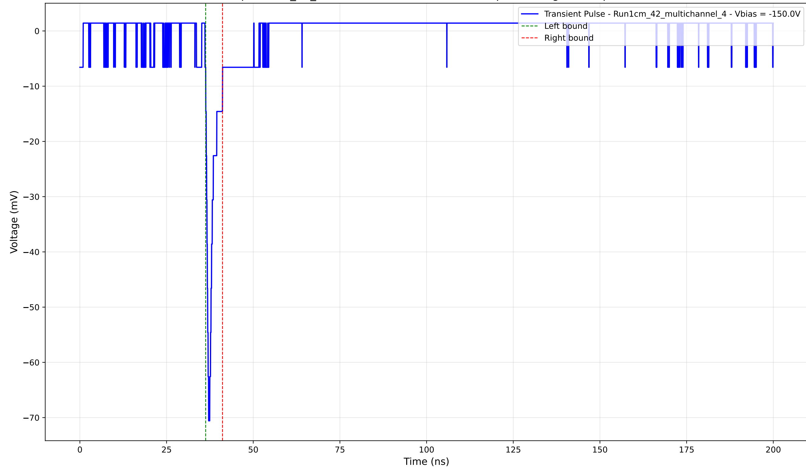
Transient Pulse - Sample: 1cm_42_multichannel - Position: 2555.0 \mu\text{m} - Charge: 2.97 pC - Rise Time: 0.84 ns
