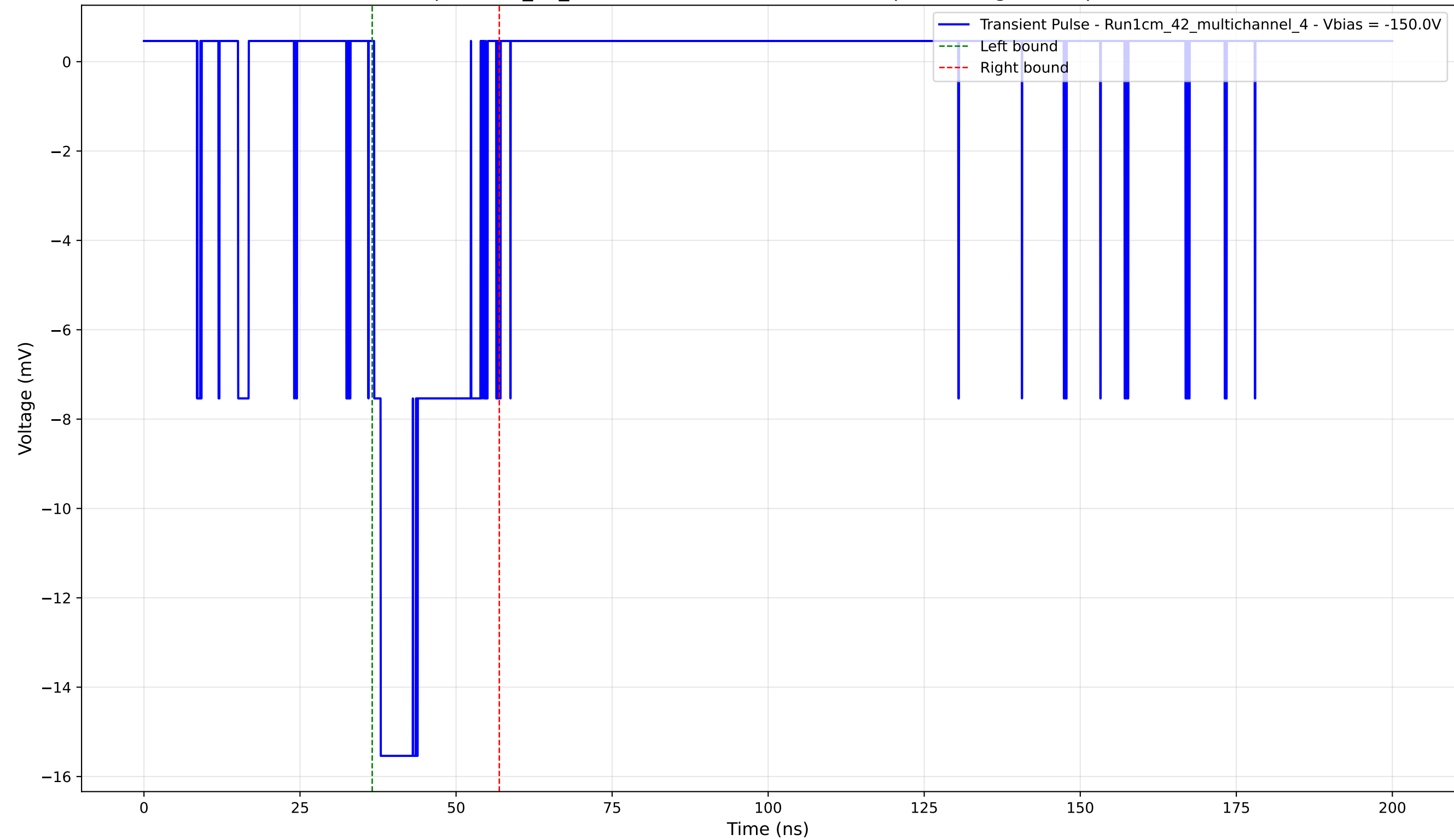
Transient Pulse - Sample: 1cm_42_multichannel - Position: 4005.0 \mu\text{m} - Charge: 3.59 pC - Rise Time: 1.06 ns
