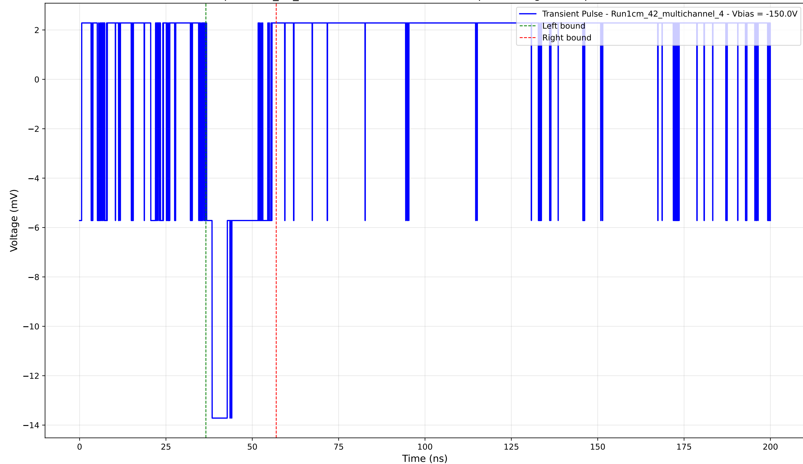
Transient Pulse - Sample: 1cm_42_multichannel - Position: 4305.0 \mu\text{m} - Charge: 2.69 pC - Rise Time: 0.00 ns (N/A)
