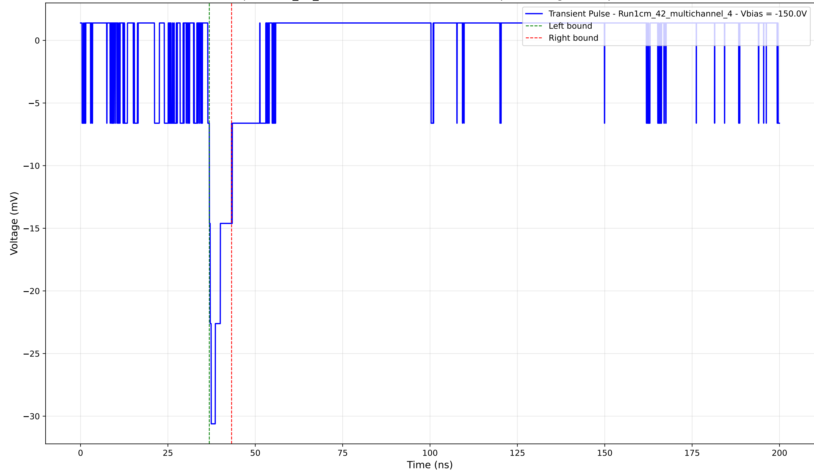
Transient Pulse - Sample: 1cm_42_multichannel - Position: 1595.0 \mu\text{m} - Charge: 2.51 pC - Rise Time: 0.97 ns
