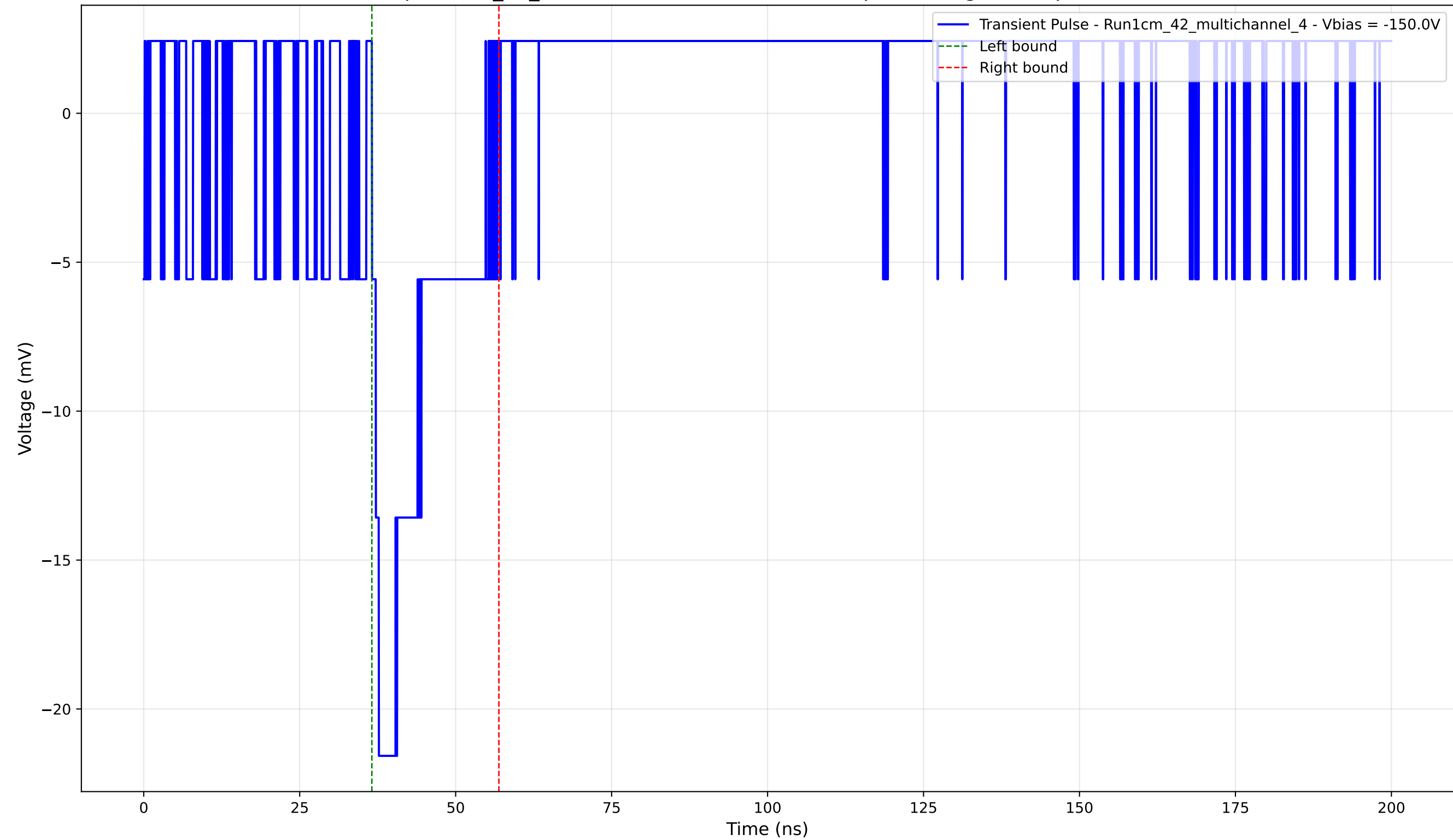
Transient Pulse - Sample: 1cm_42_multichannel - Position: 1210.0 \mu\text{m} - Charge: 3.73 pC - Rise Time: 0.00 ns (N/A)
