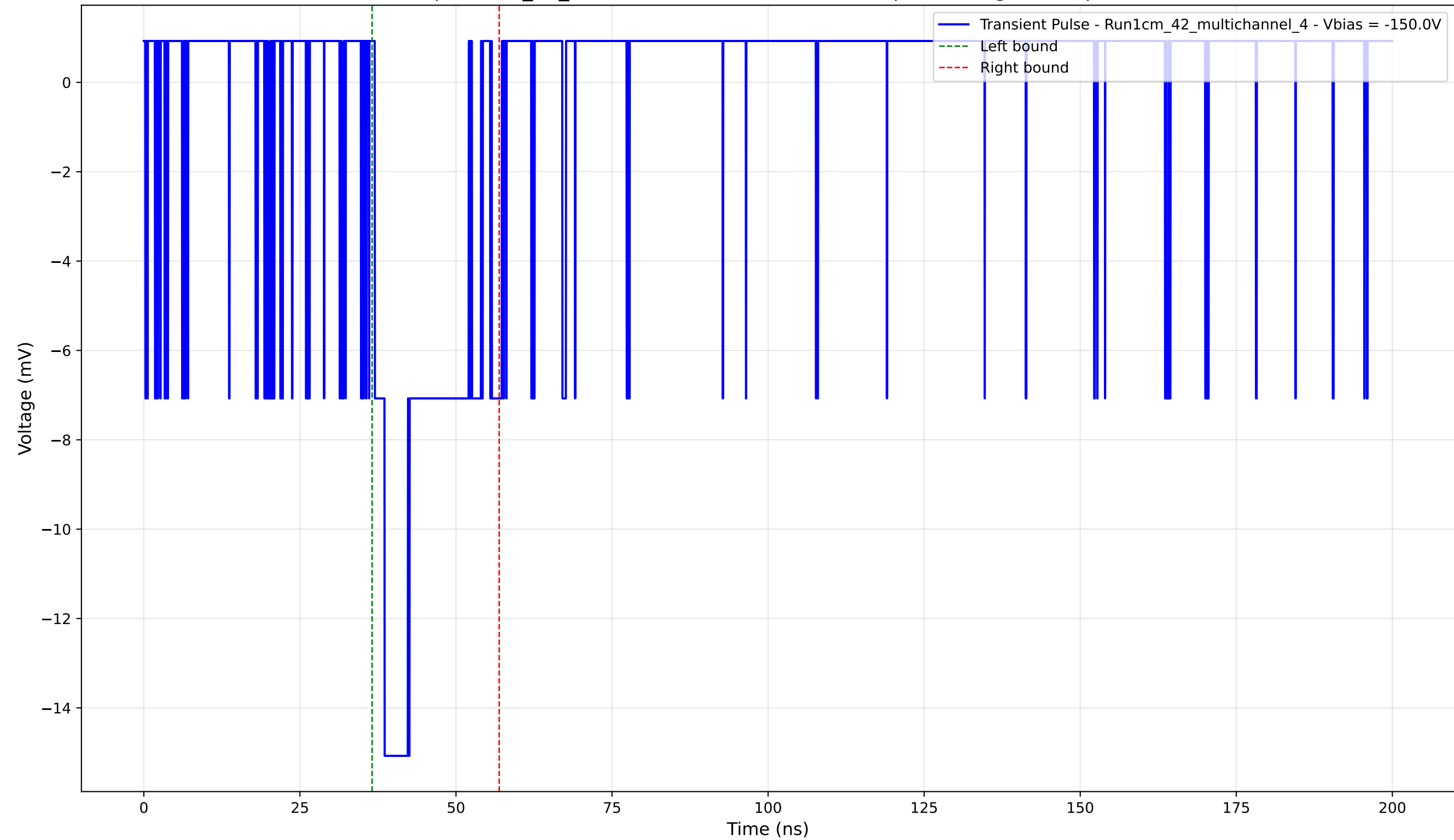
Transient Pulse - Sample: 1cm_42_multichannel - Position: 4610.0 \mu\text{m} - Charge: 3.17 pC - Rise Time: 1.58 ns
