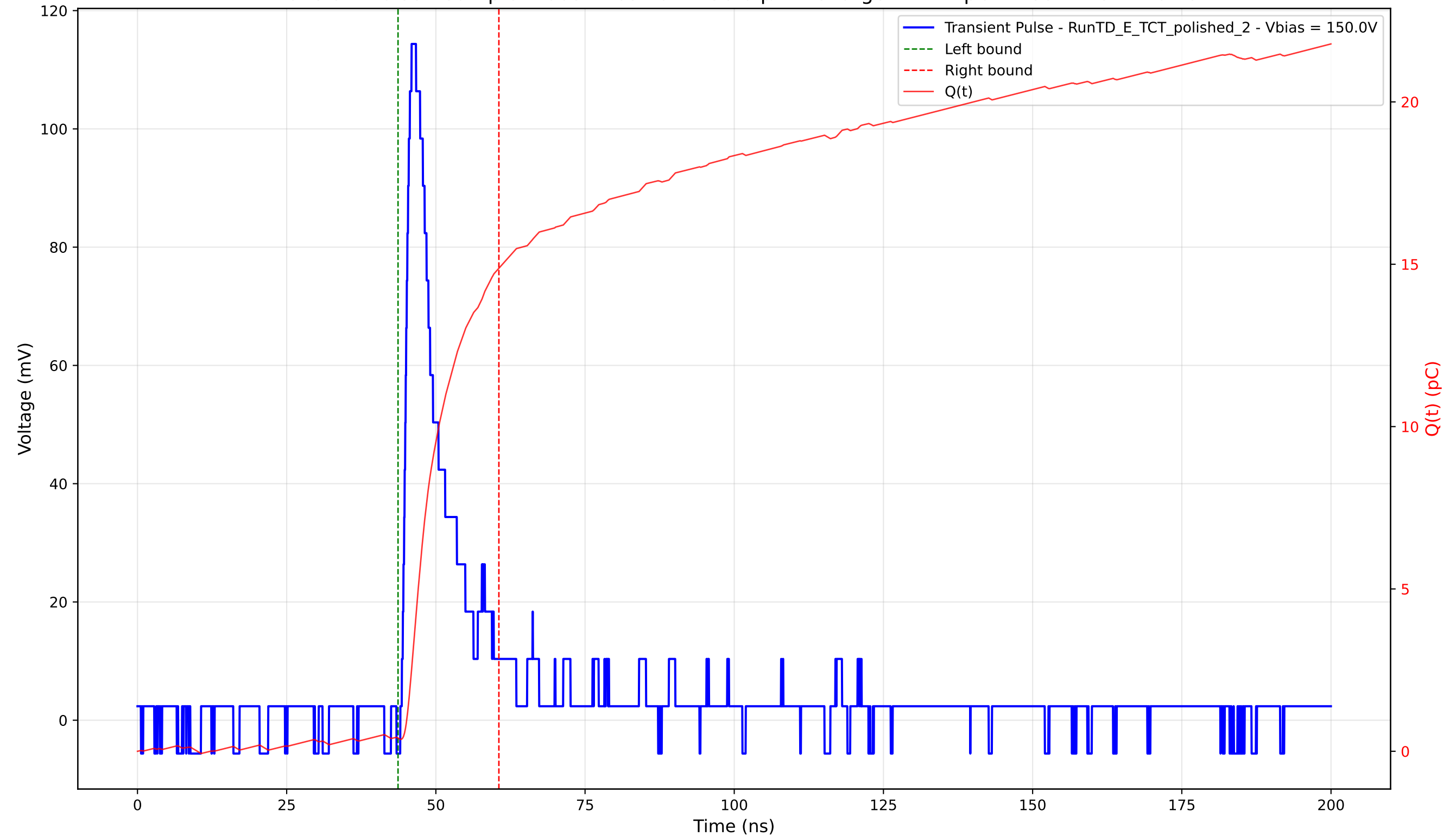
Transient Pulse - Sample: 4003 - Position: 430.0 \mu\text{m} - Charge: 14.47 pC - Rise Time: 1.20 ns
