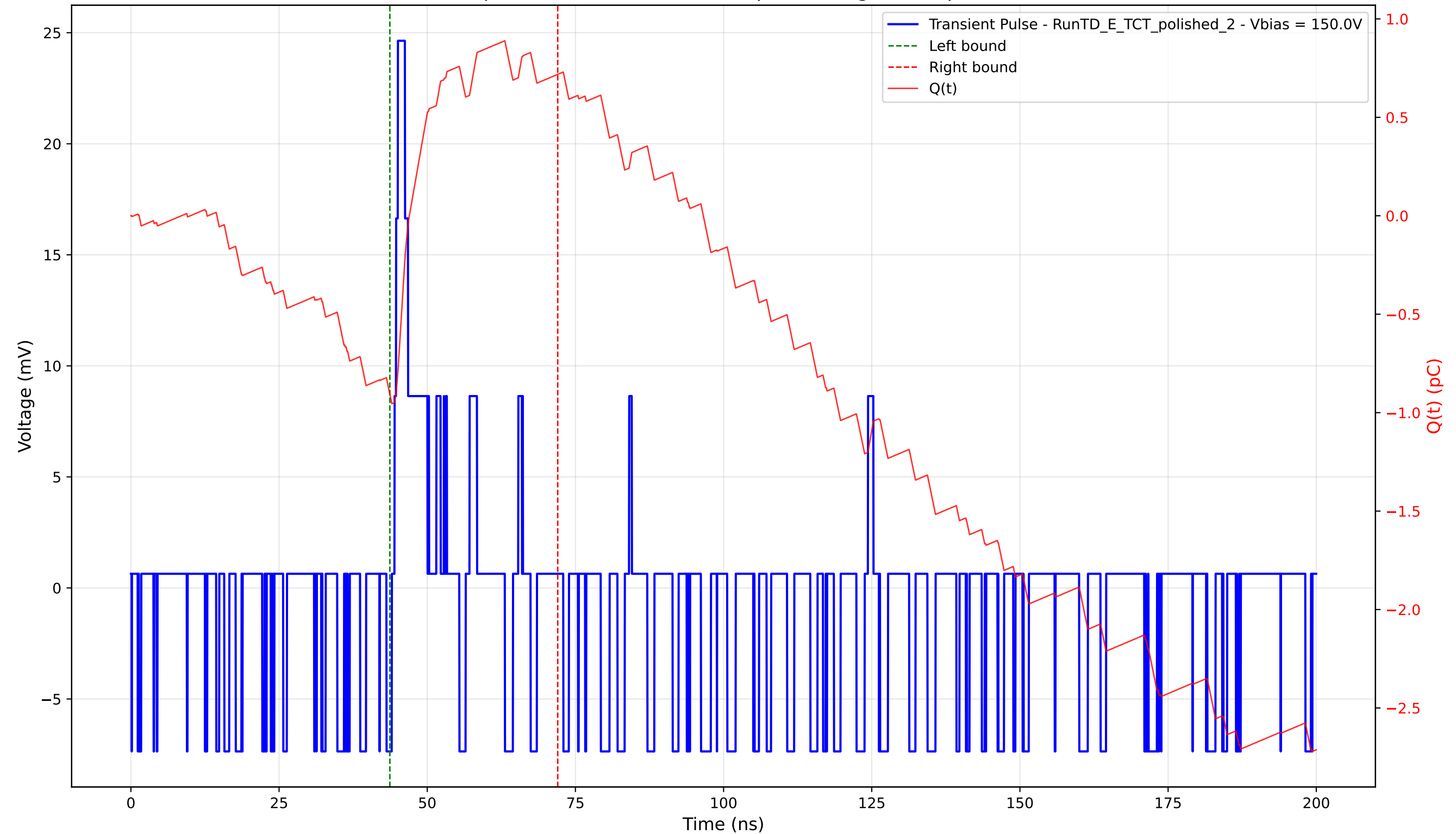
Transient Pulse - Sample: 4003 - Position: 695.0 \mu\text{m} - Charge: 1.63 pC - Rise Time: 0.58 ns
