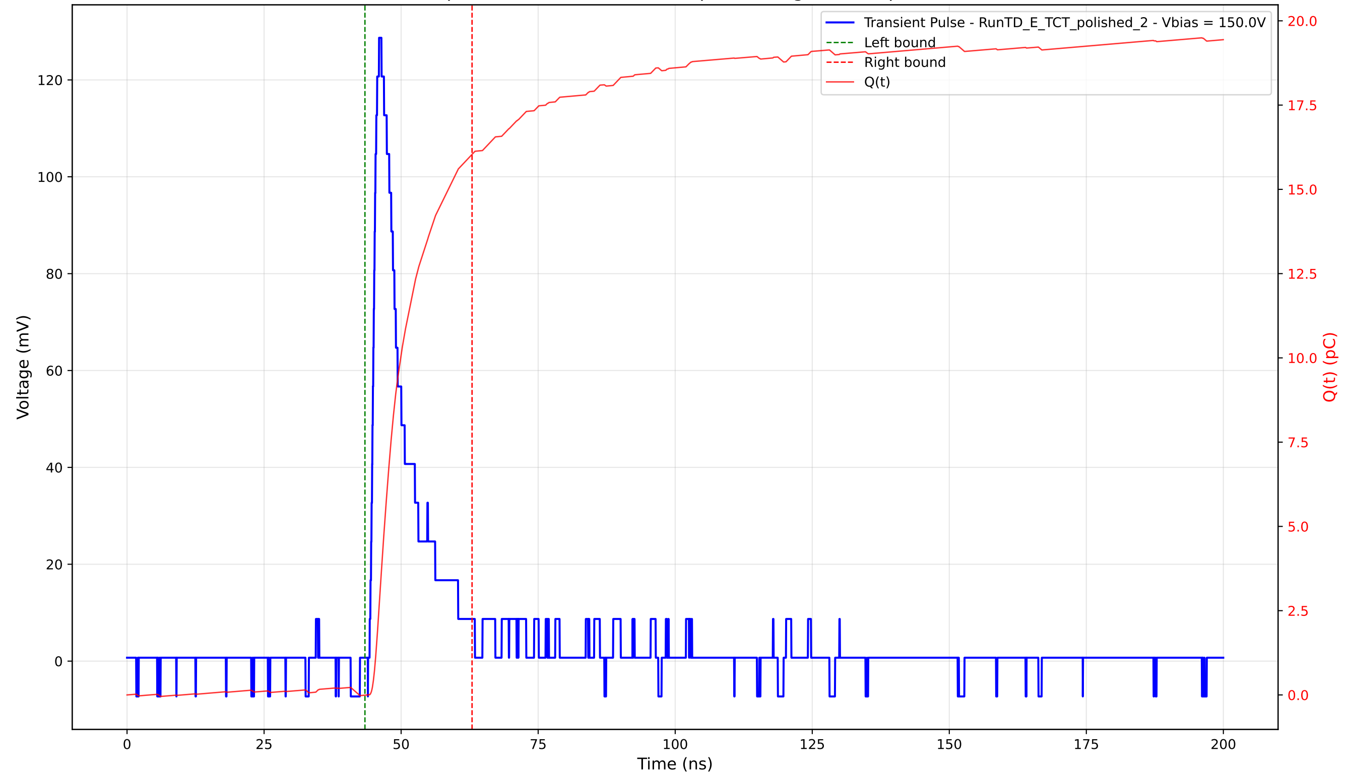
Transient Pulse - Sample: 4003 - Position: 420.0 \mu\text{m} - Charge: 16.05 pC - Rise Time: 1.23 ns
