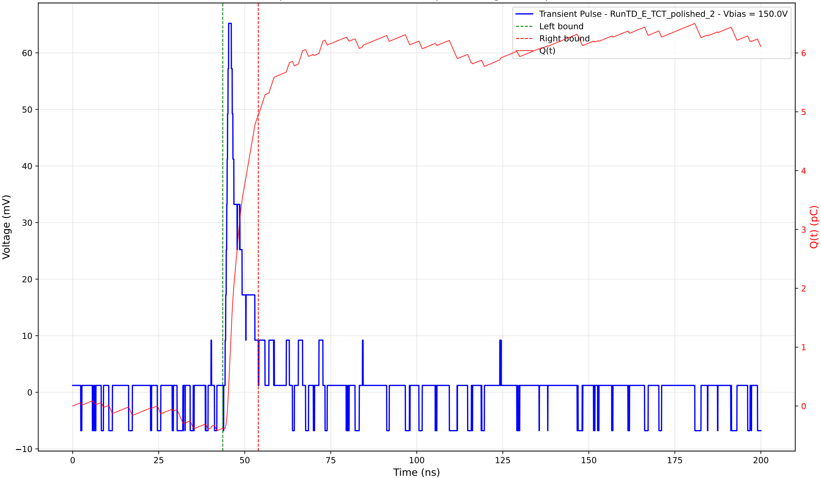
Transient Pulse - Sample: 4003 - Position: 125.0 \mu\text{m} - Charge: 5.34 pC - Rise Time: 1.03 ns
