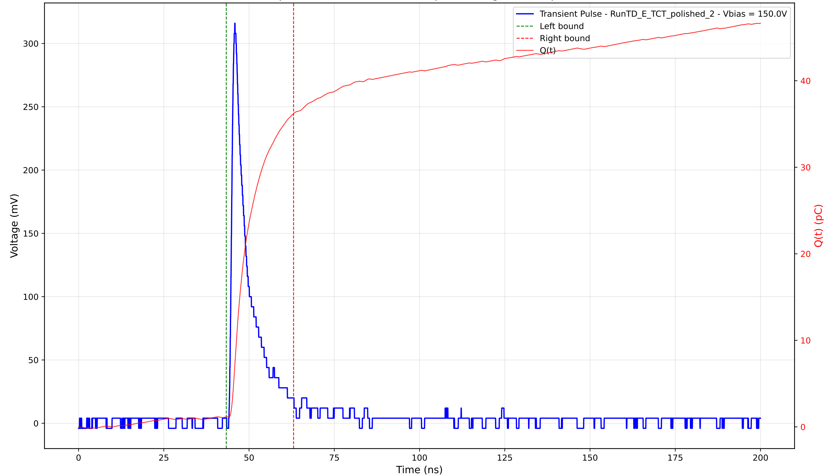
Transient Pulse - Sample: 4003 - Position: 330.0 \mu\text{m} - Charge: 35.07 pC - Rise Time: 1.15 ns
