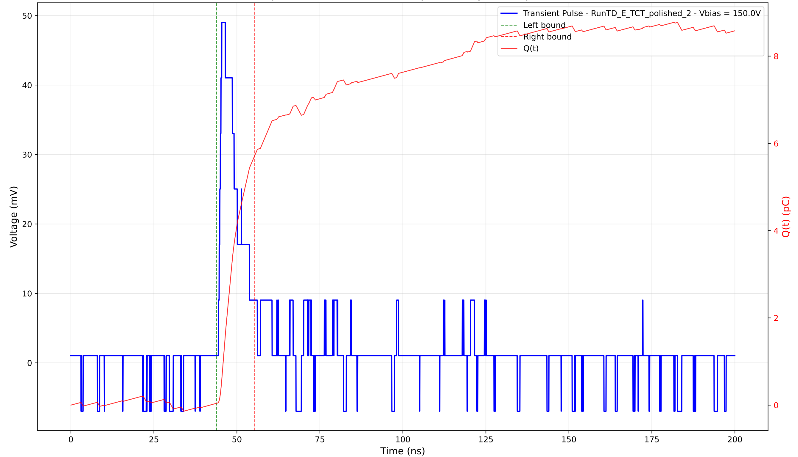
Transient Pulse - Sample: 4003 - Position: 490.0 \mu\text{m} - Charge: 5.69 pC - Rise Time: 1.03 ns
