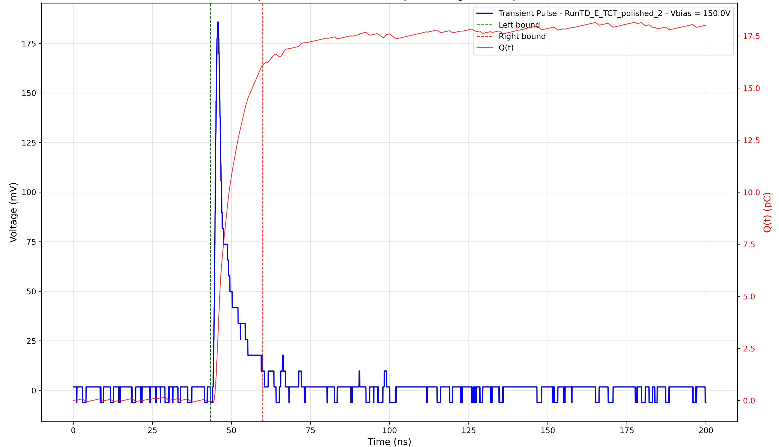
Transient Pulse - Sample: 4003 - Position: 170.0 \mu\text{m} - Charge: 16.13 pC - Rise Time: 0.96 ns
