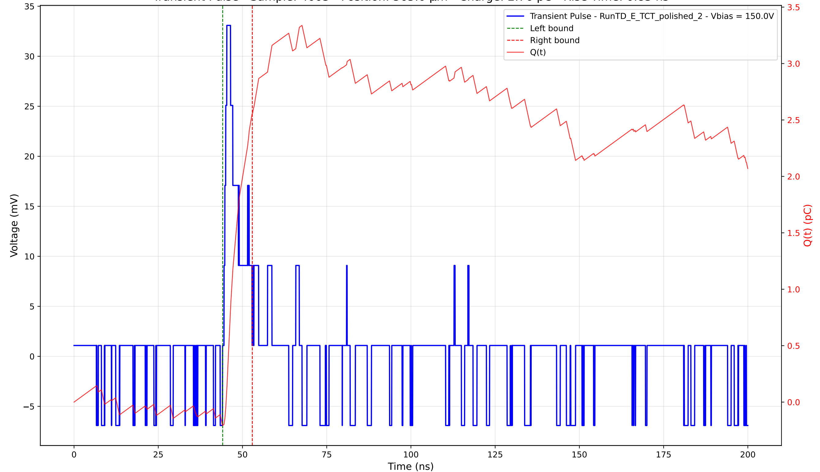
Transient Pulse - Sample: 4003 - Position: 565.0 \mu\text{m} - Charge: 2.76 pC - Rise Time: 0.83 ns
