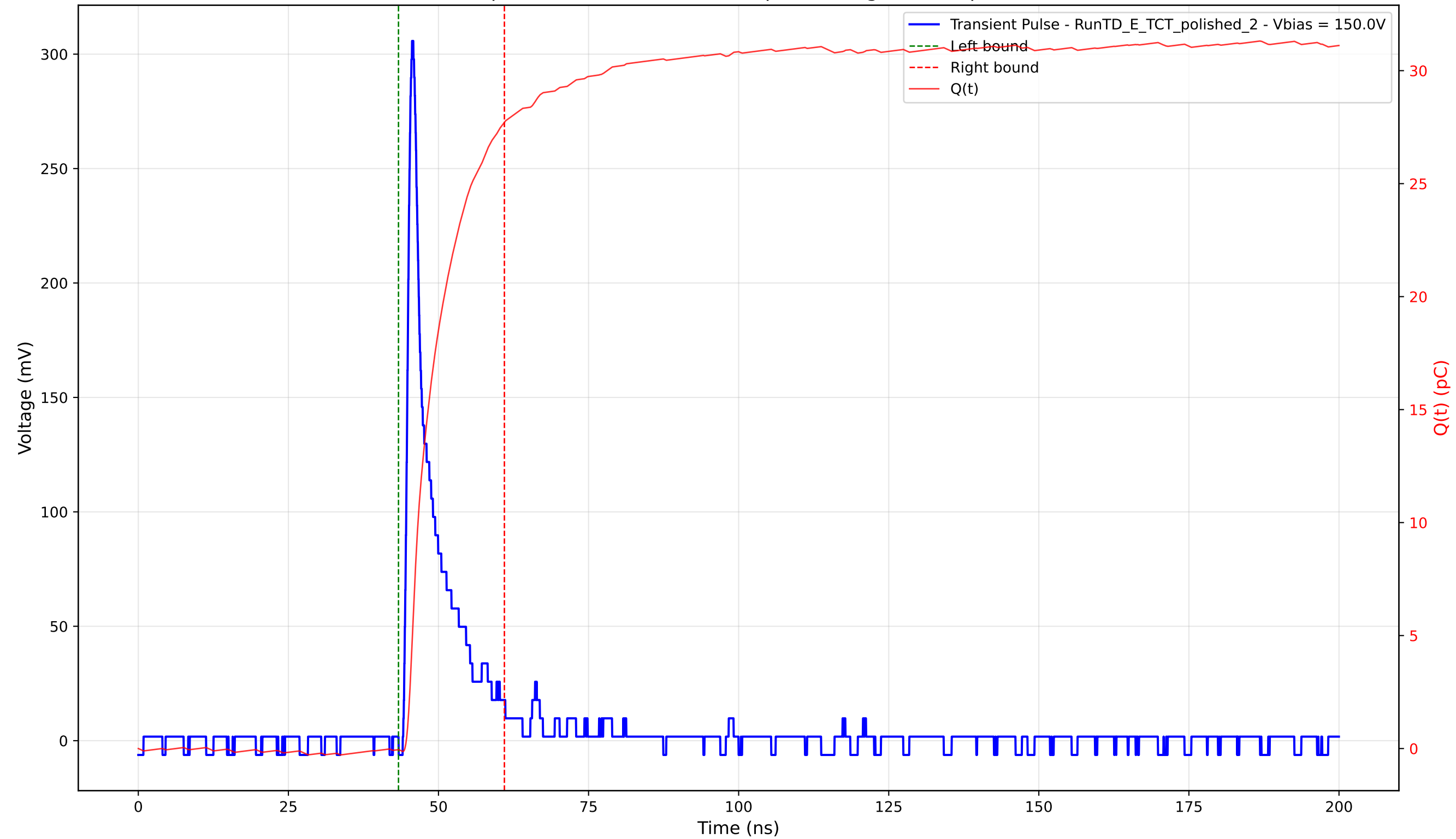
Transient Pulse - Sample: 4003 - Position: 210.0 \mu\text{m} - Charge: 27.76 pC - Rise Time: 1.03 ns
