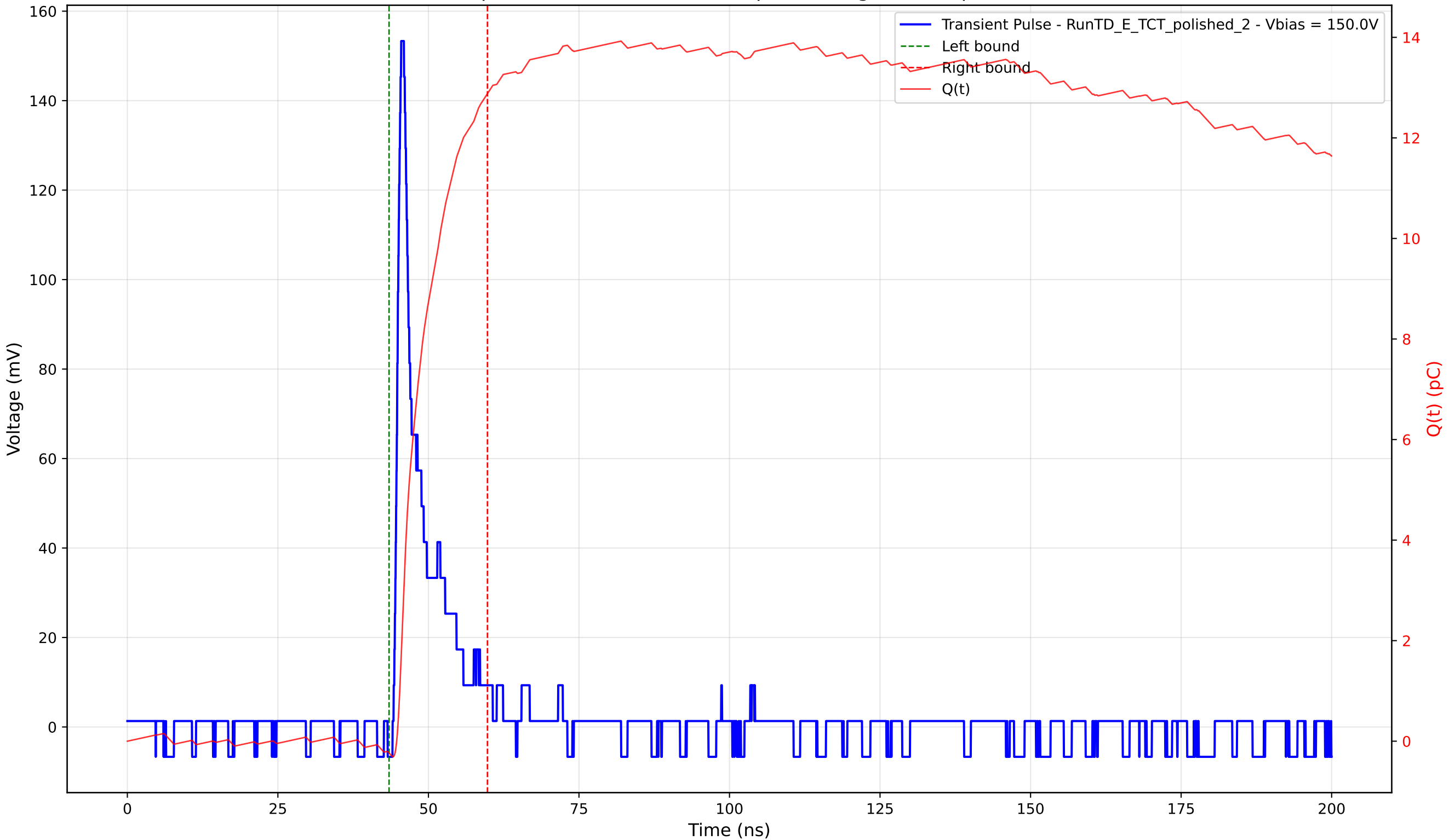
Transient Pulse - Sample: 4003 - Position: 160.0 \mu\text{m} - Charge: 13.12 pC - Rise Time: 1.02 ns
