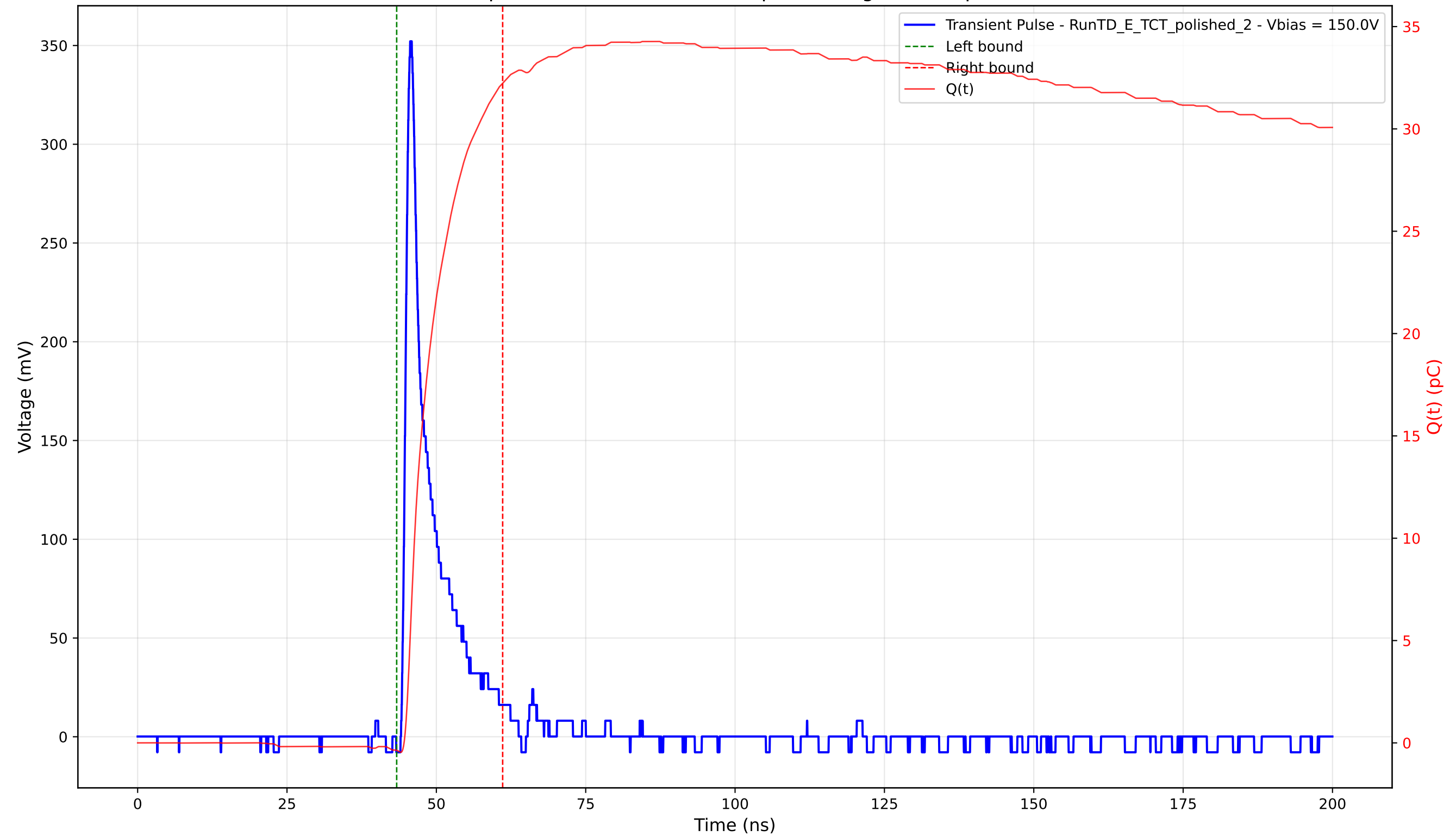
Transient Pulse - Sample: 4003 - Position: 235.0 \mu\text{m} - Charge: 32.59 pC - Rise Time: 1.03 ns
