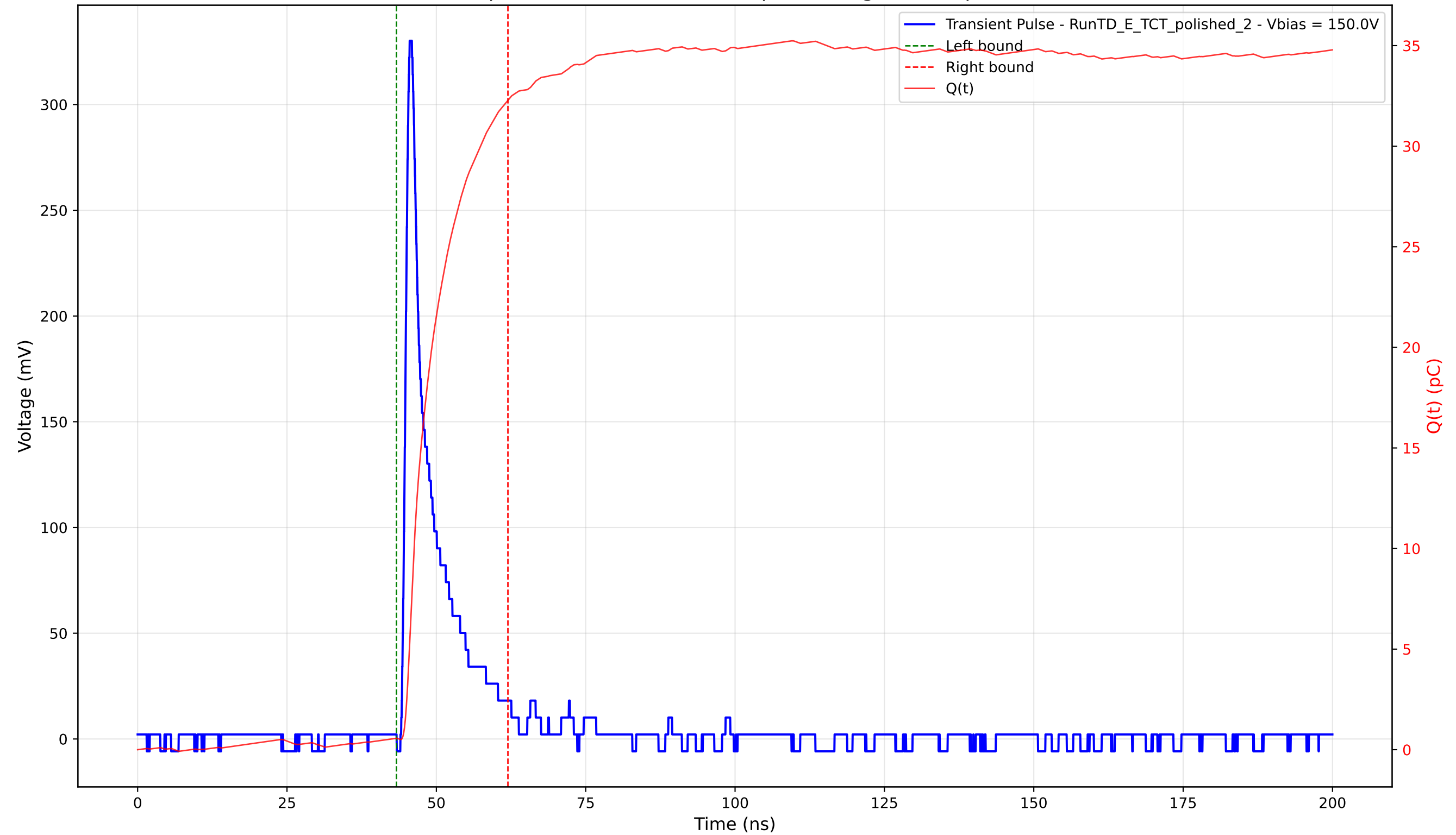
Transient Pulse - Sample: 4003 - Position: 225.0 \mu\text{m} - Charge: 31.71 pC - Rise Time: 1.00 ns
