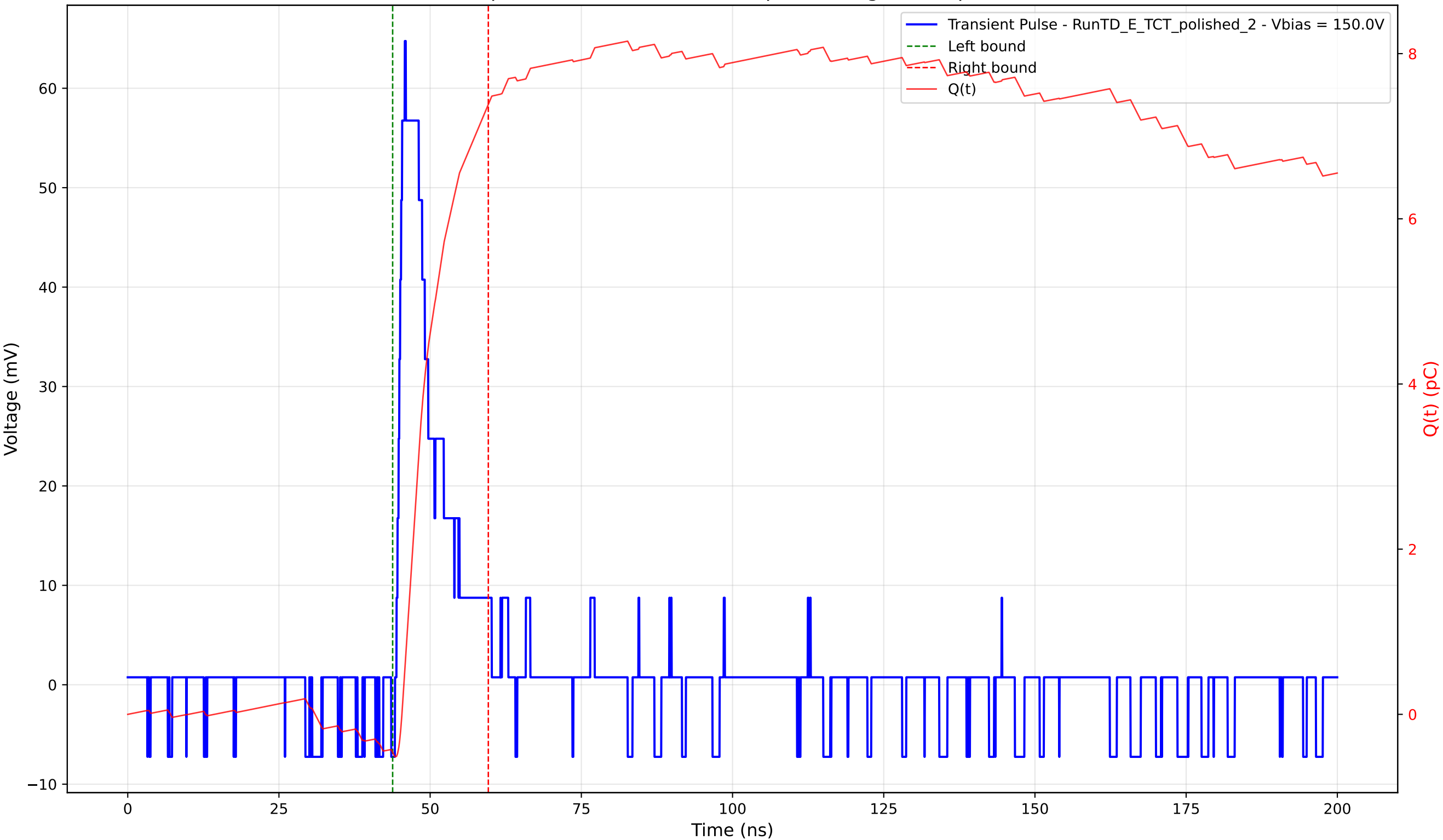
Transient Pulse - Sample: 4003 - Position: 470.0 \mu\text{m} - Charge: 7.85 pC - Rise Time: 1.37 ns
