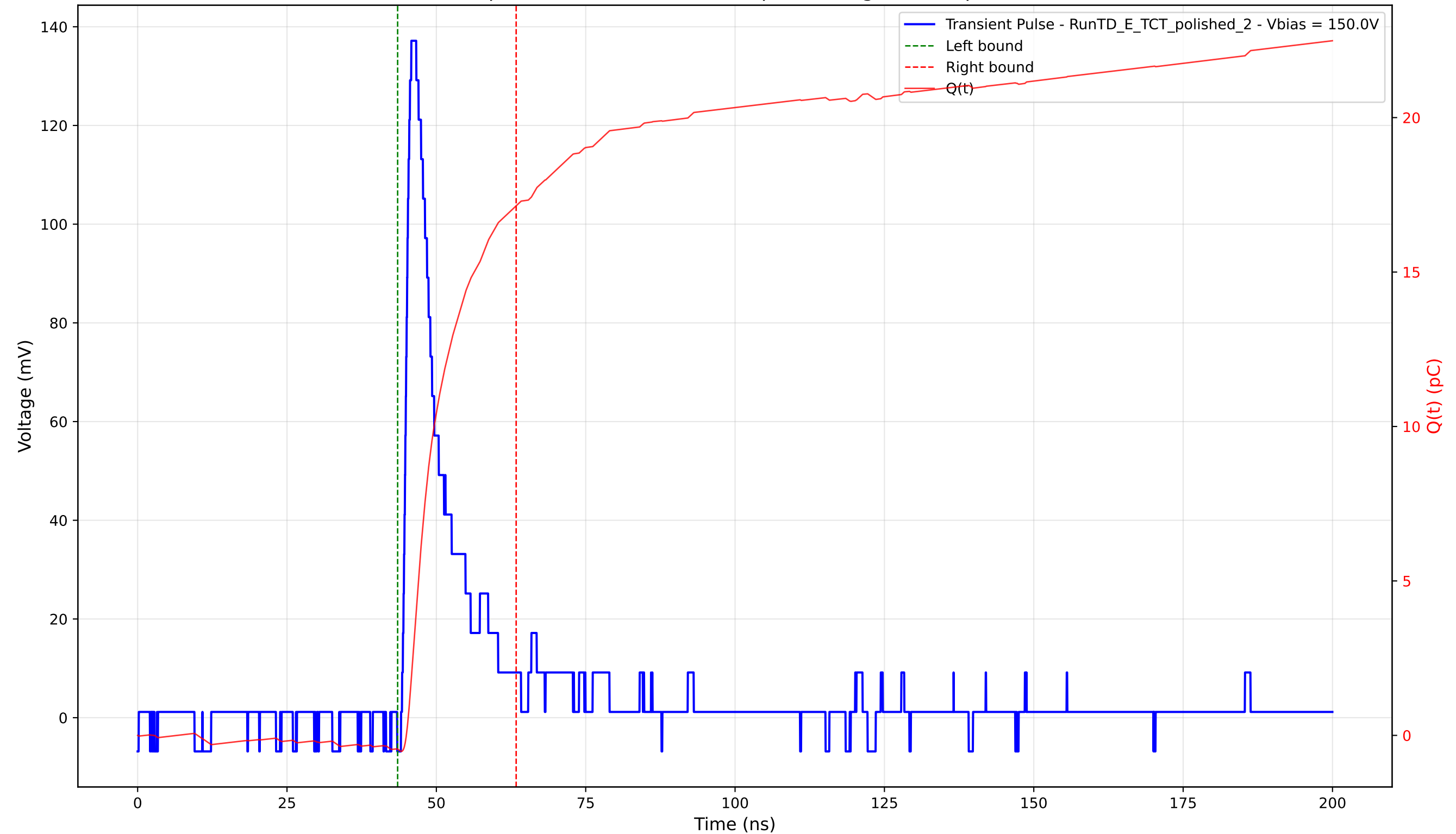
Transient Pulse - Sample: 4003 - Position: 415.0 \mu\text{m} - Charge: 17.59 pC - Rise Time: 1.19 ns
