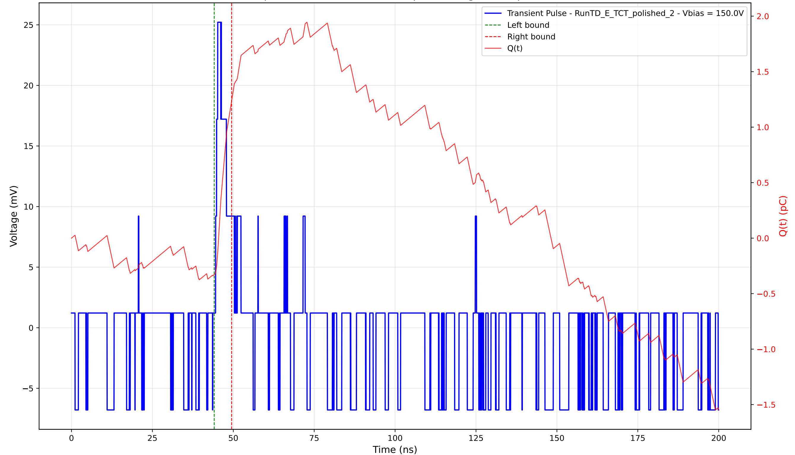
Transient Pulse - Sample: 4003 - Position: 100.0 \mu\text{m} - Charge: 1.57 pC - Rise Time: 0.66 ns
