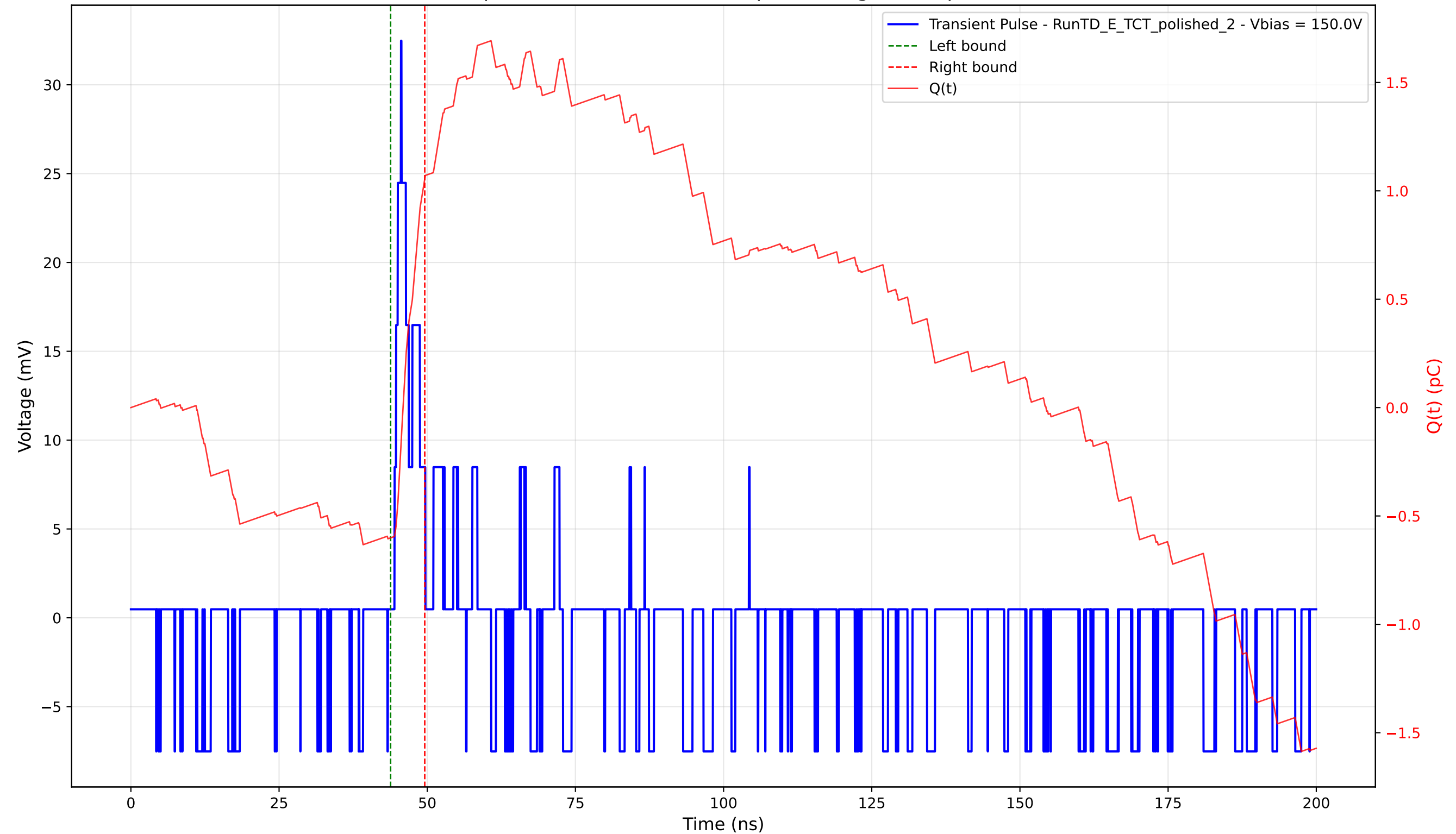
Transient Pulse - Sample: 4003 - Position: 610.0 \mu\text{m} - Charge: 1.66 pC - Rise Time: 1.09 ns
