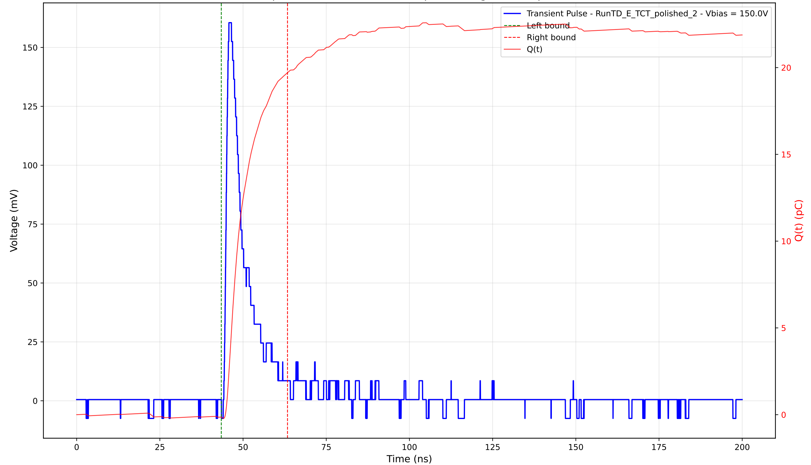
Transient Pulse - Sample: 4003 - Position: 400.0 \mu\text{m} - Charge: 19.84 pC - Rise Time: 1.10 ns
