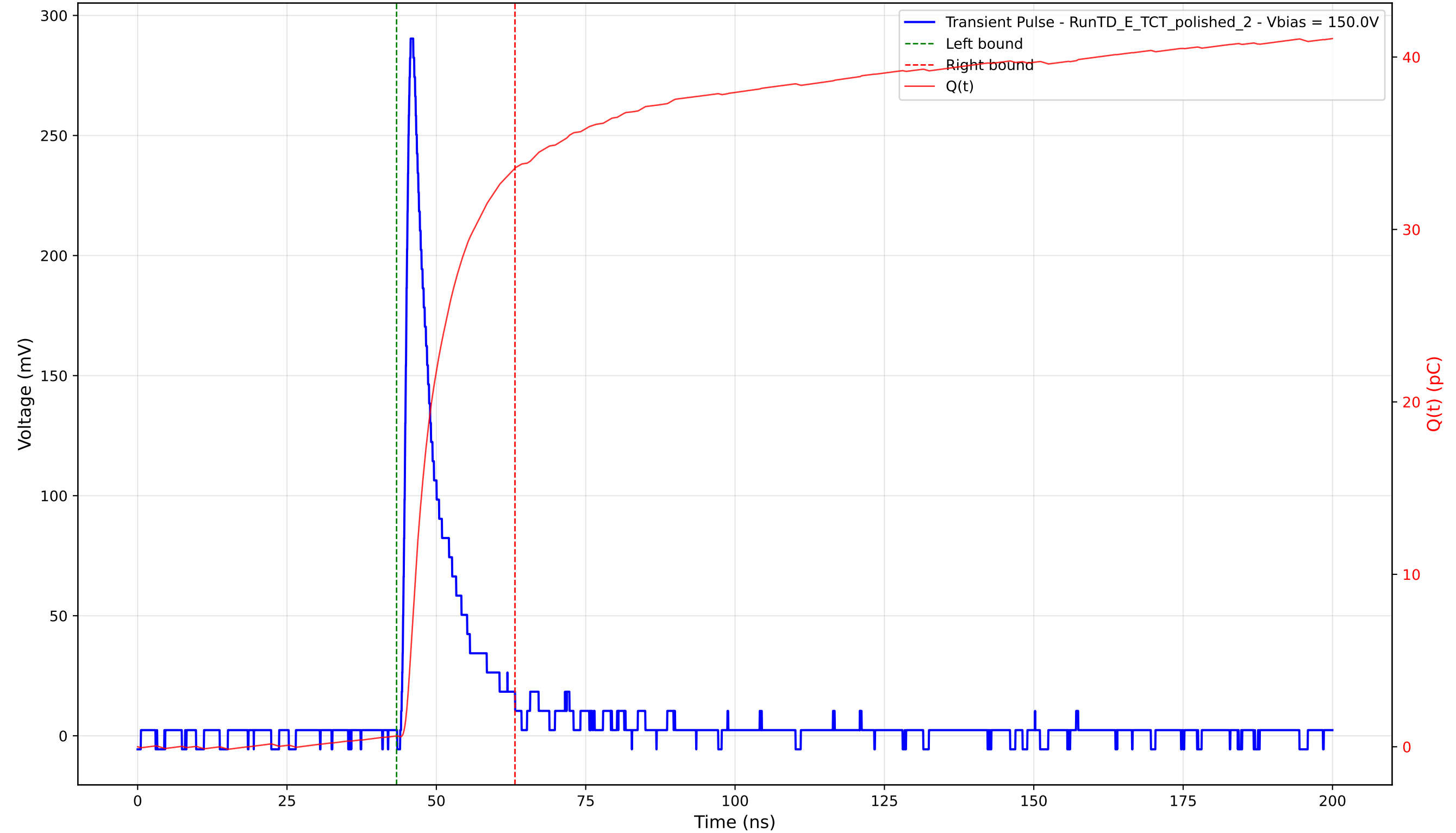
Transient Pulse - Sample: 4003 - Position: 340.0 \mu\text{m} - Charge: 32.93 pC - Rise Time: 1.11 ns
