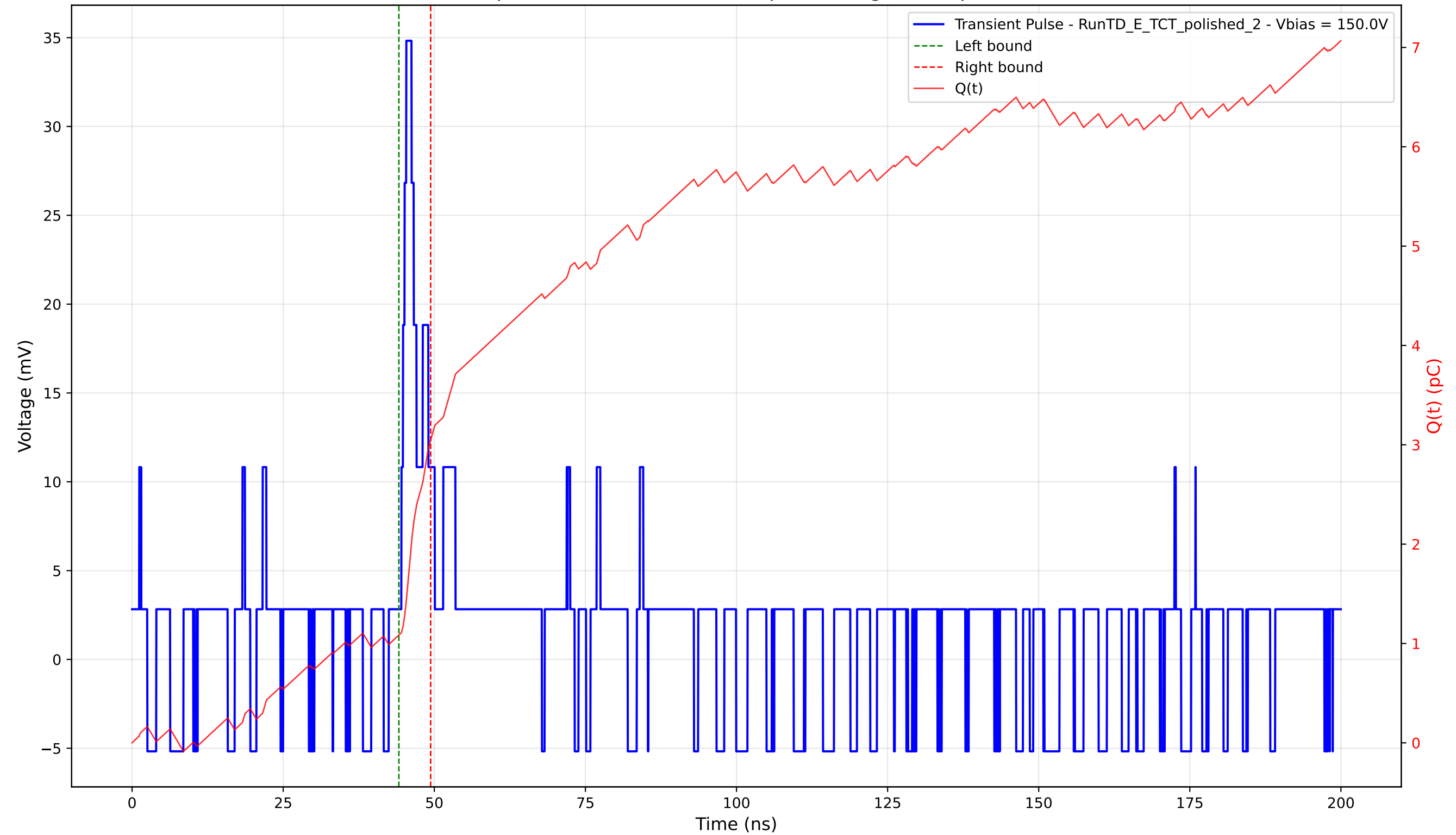
Transient Pulse - Sample: 4003 - Position: 105.0 \mu\text{m} - Charge: 1.97 pC - Rise Time: 0.82 ns
