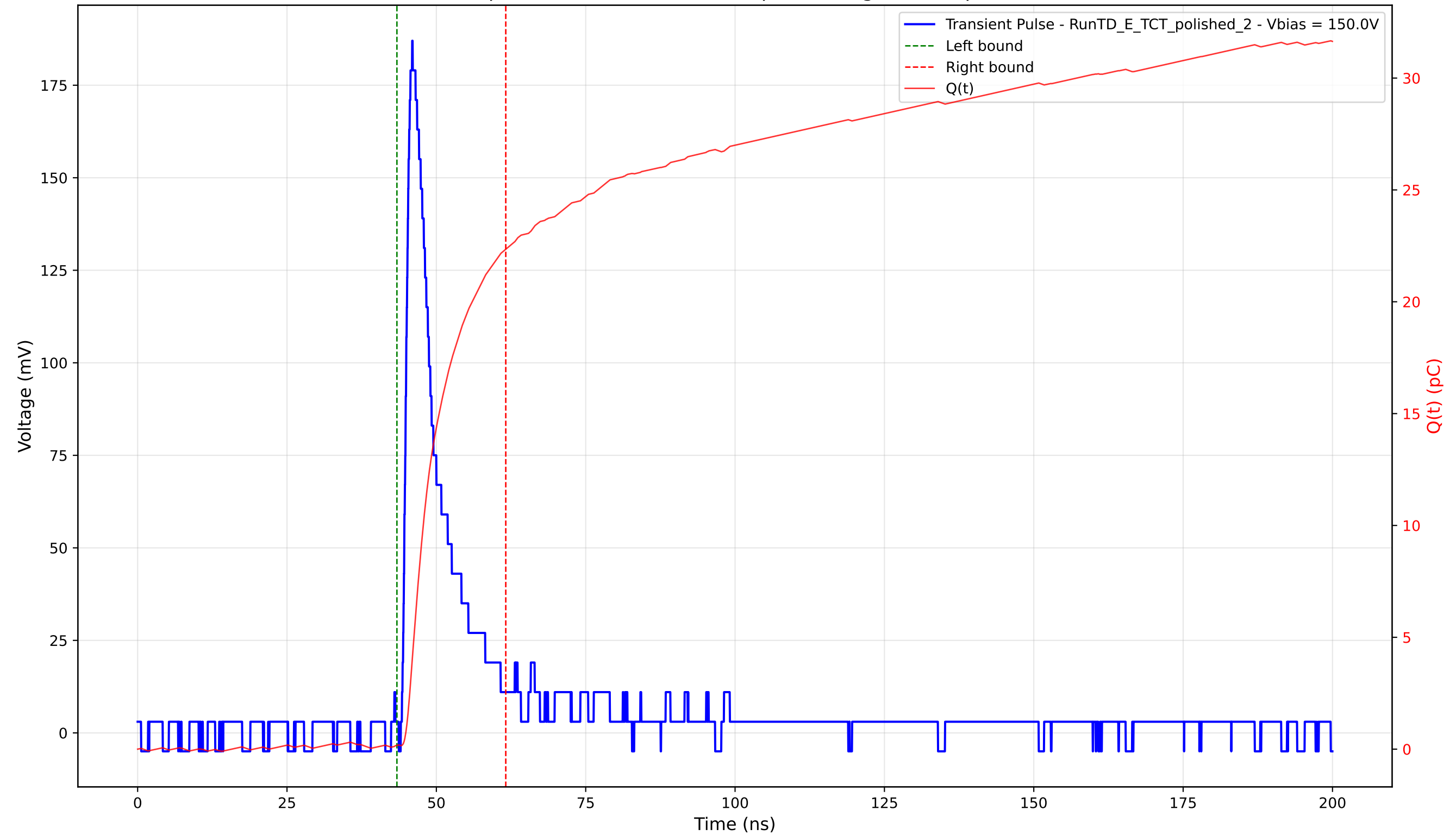
Transient Pulse - Sample: 4003 - Position: 390.0 \mu\text{m} - Charge: 22.17 pC - Rise Time: 1.20 ns
