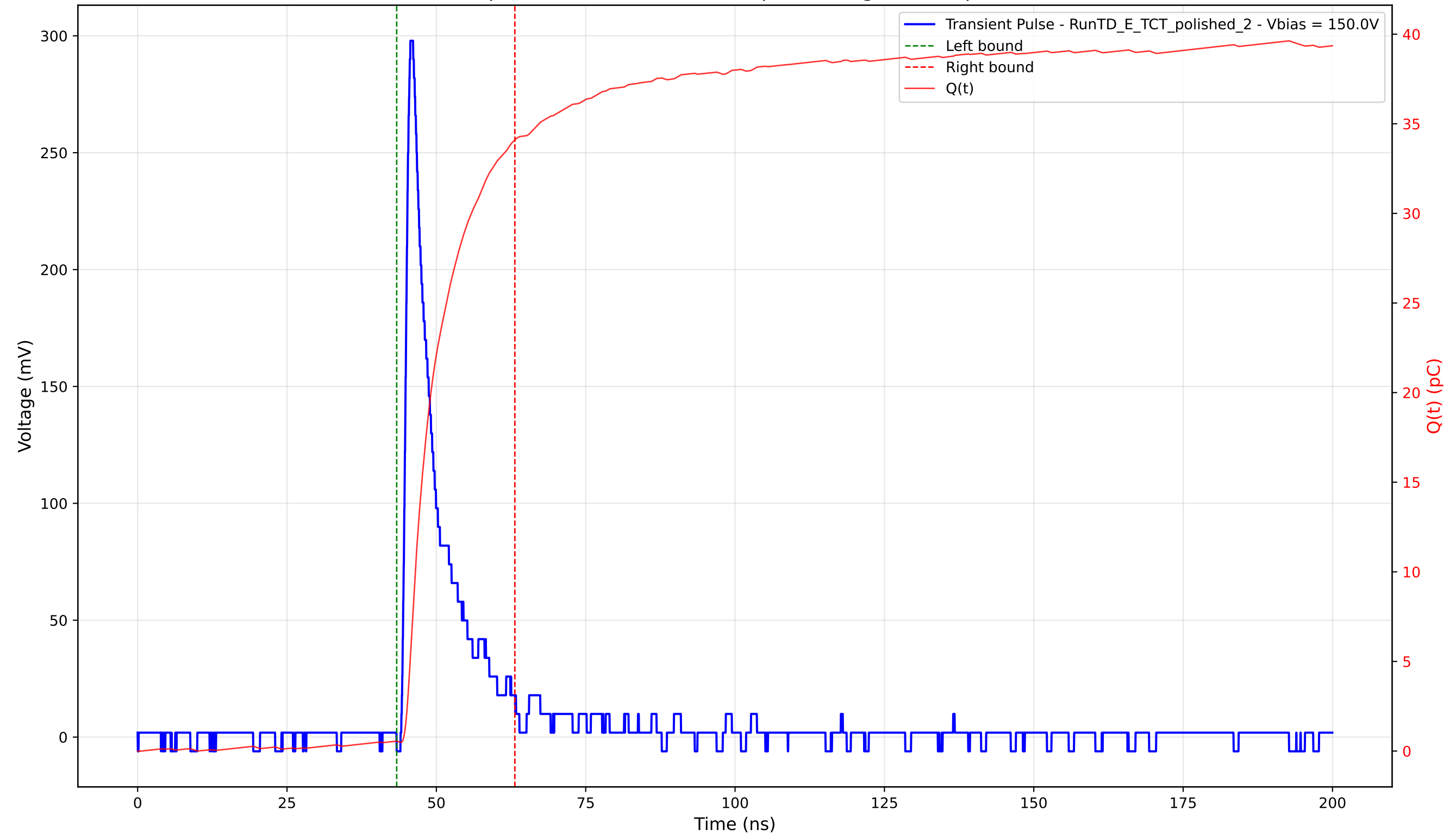
Transient Pulse - Sample: 4003 - Position: 335.0 \mu\text{m} - Charge: 33.55 pC - Rise Time: 1.09 ns
