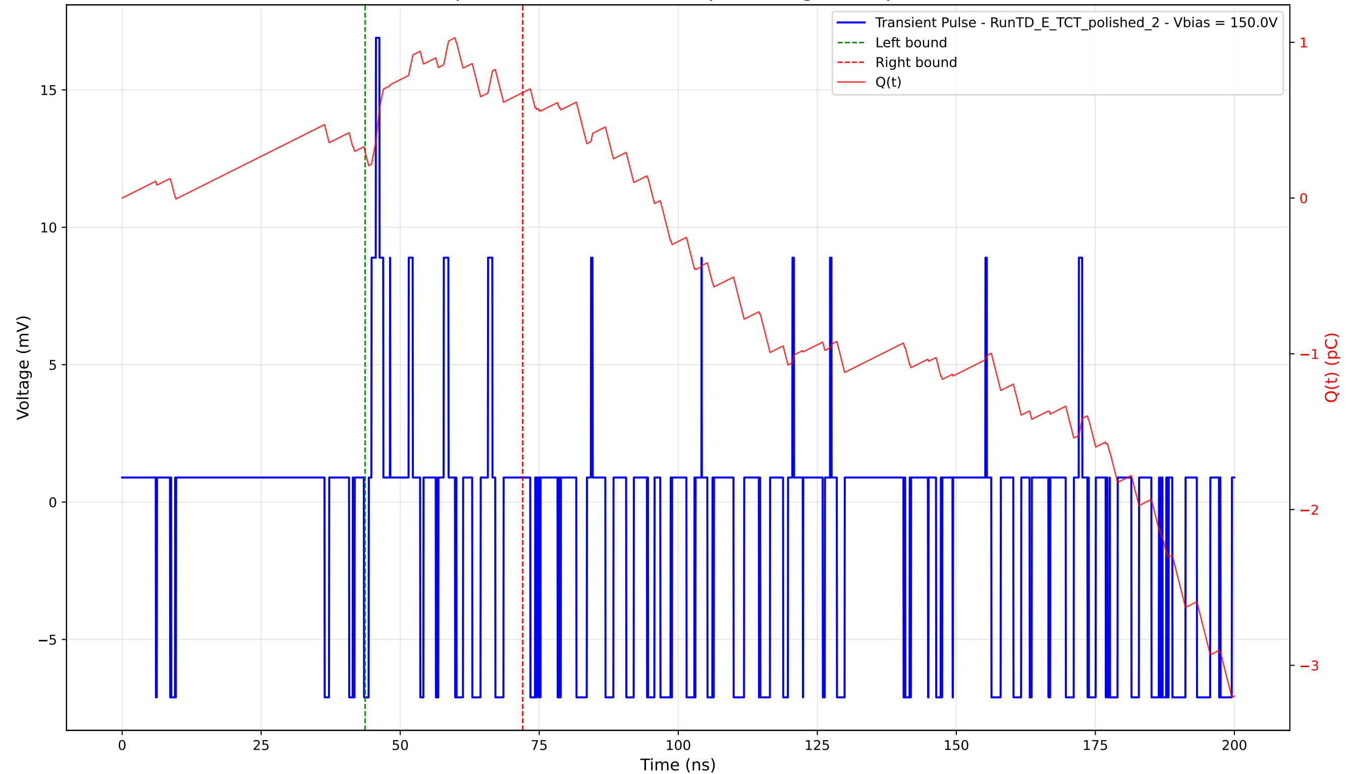
Transient Pulse - Sample: 4003 - Position: 725.0 \mu\text{m} - Charge: 0.38 pC - Rise Time: 0.80 ns
