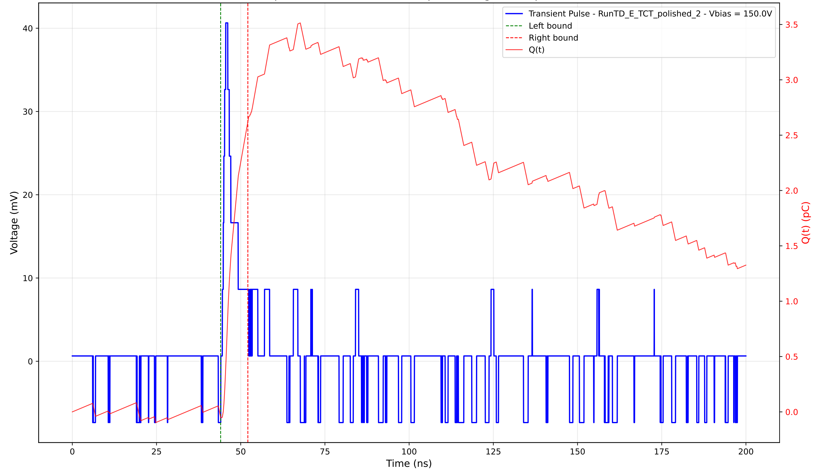
Transient Pulse - Sample: 4003 - Position: 540.0 \mu\text{m} - Charge: 2.67 pC - Rise Time: 1.01 ns
