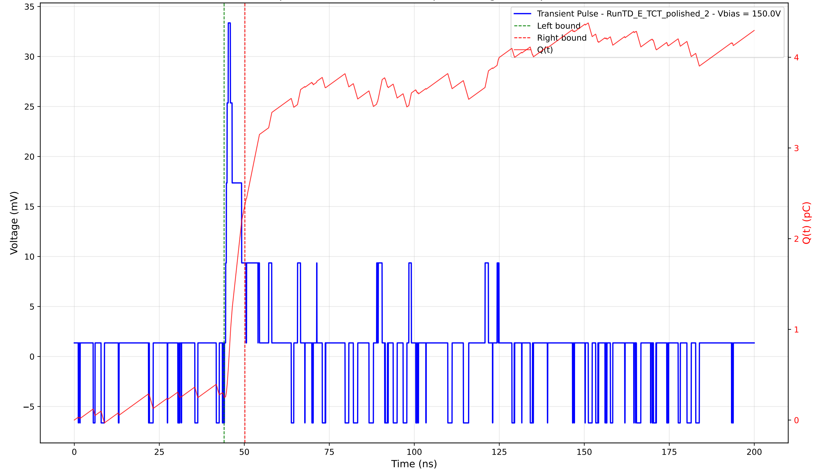
Transient Pulse - Sample: 4003 - Position: 670.0 \mu\text{m} - Charge: 2.11 pC - Rise Time: 0.78 ns
