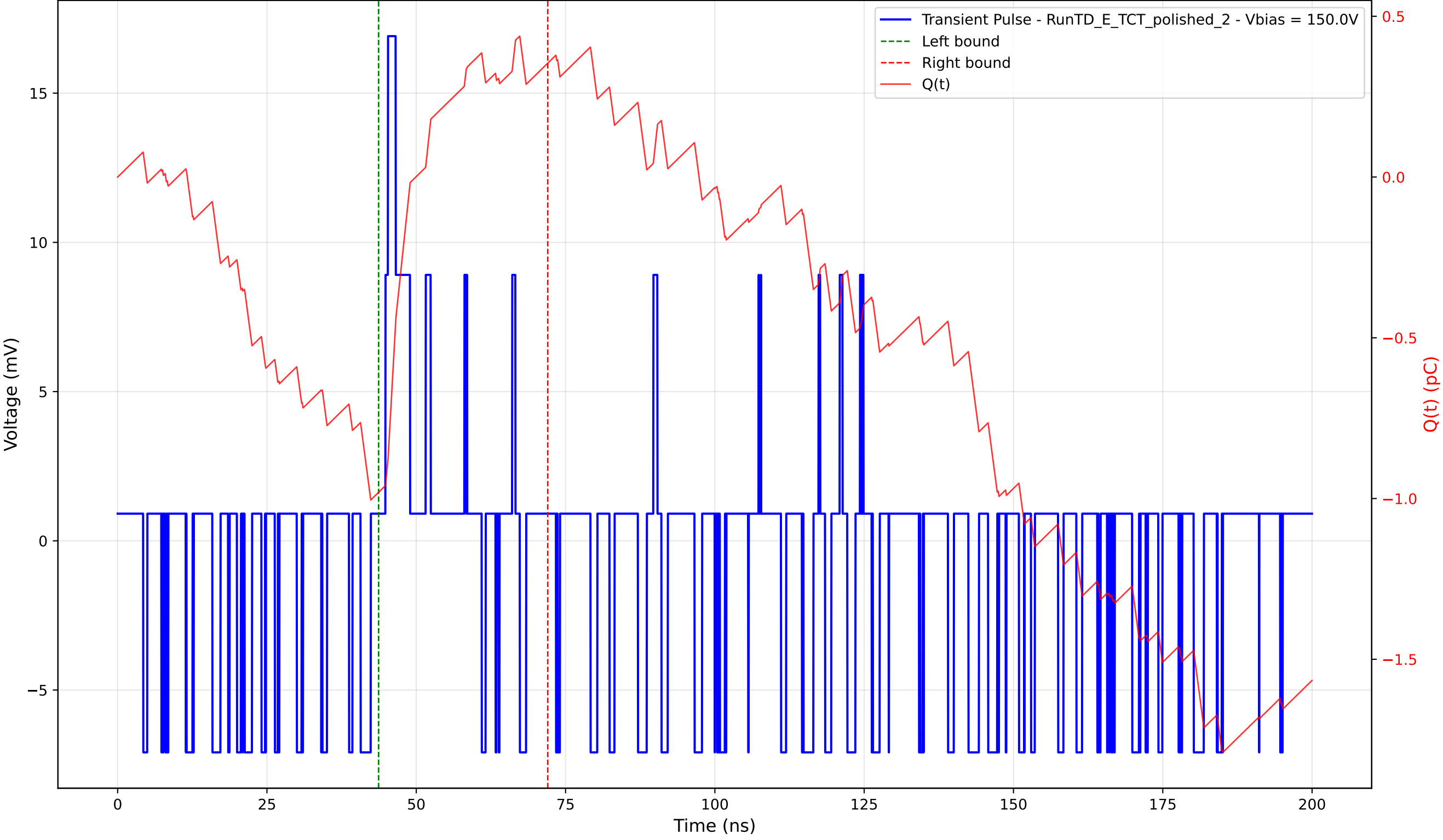
Transient Pulse - Sample: 4003 - Position: 80.0 \mu\text{m} - Charge: 1.33 pC - Rise Time: 0.44 ns
