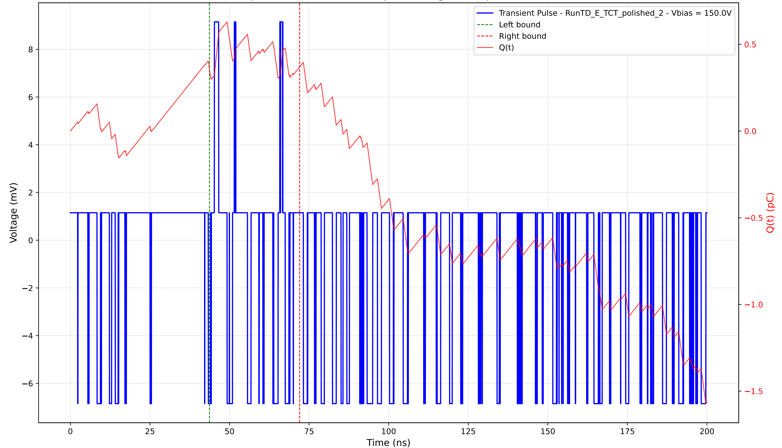
Transient Pulse - Sample: 4003 - Position: 5.0 \mu\text{m} - Charge: 0.02 pC - Rise Time: 0.00 ns (N/A)
