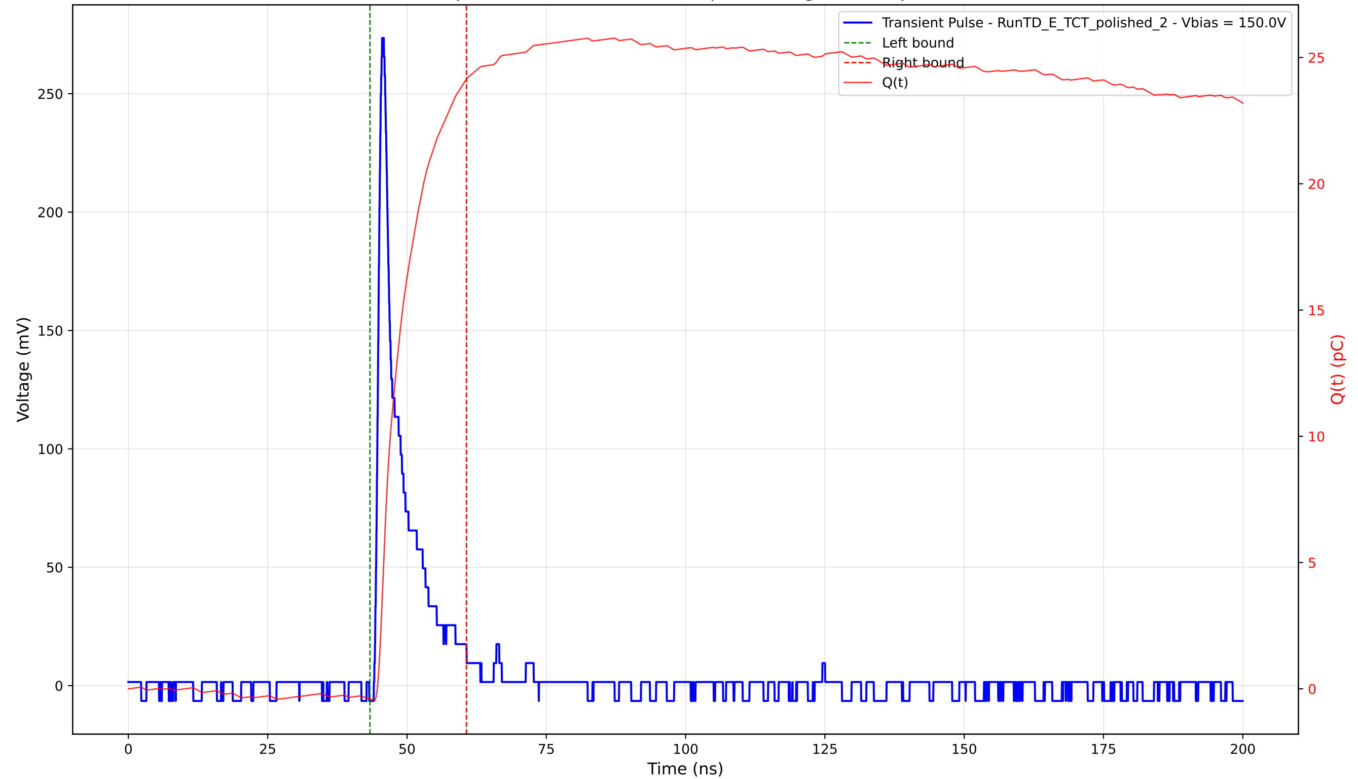
Transient Pulse - Sample: 4003 - Position: 200.0 \mu\text{m} - Charge: 24.55 pC - Rise Time: 0.98 ns
