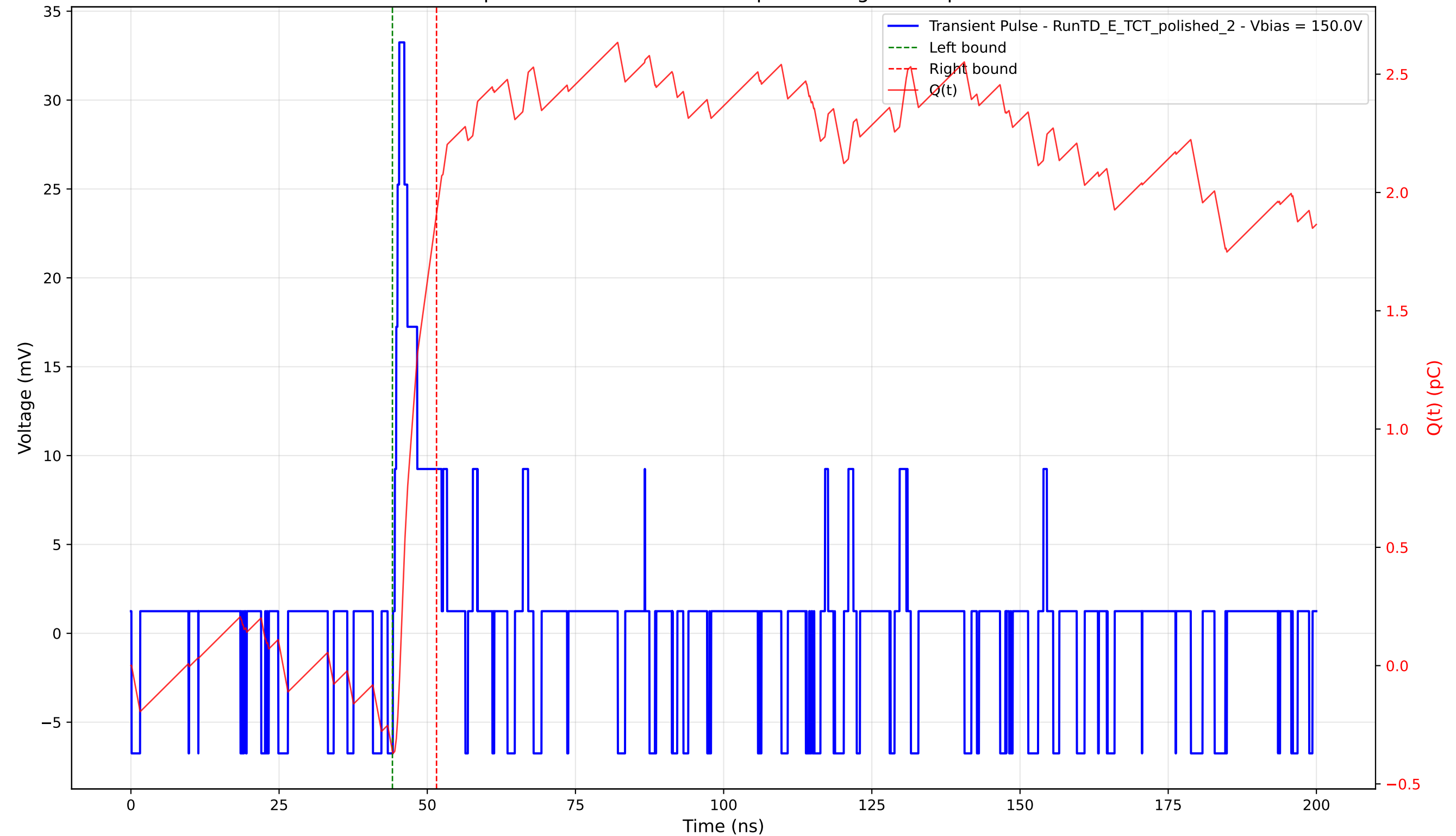
Transient Pulse - Sample: 4003 - Position: 630.0 \mu\text{m} - Charge: 2.27 pC - Rise Time: 0.75 ns
