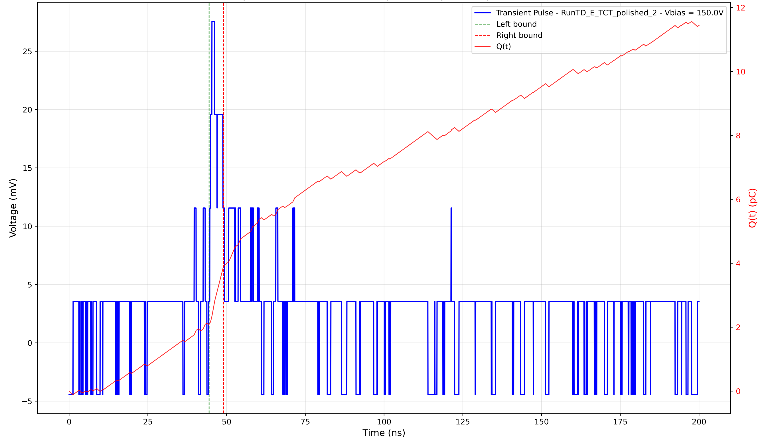
Transient Pulse - Sample: 4003 - Position: 710.0 \mu\text{m} - Charge: 1.79 pC - Rise Time: 0.00 ns (N/A)
