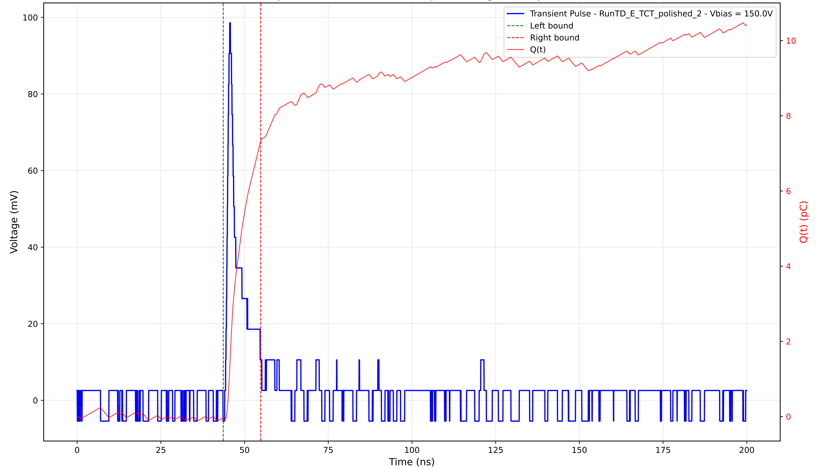
Transient Pulse - Sample: 4003 - Position: 135.0 \mu\text{m} - Charge: 7.36 pC - Rise Time: 1.02 ns
