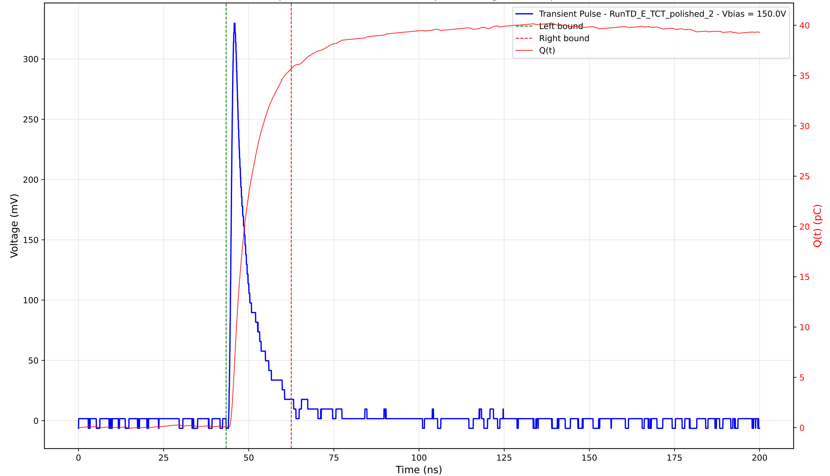
Transient Pulse - Sample: 4003 - Position: 320.0 \mu\text{m} - Charge: 35.60 pC - Rise Time: 1.06 ns
