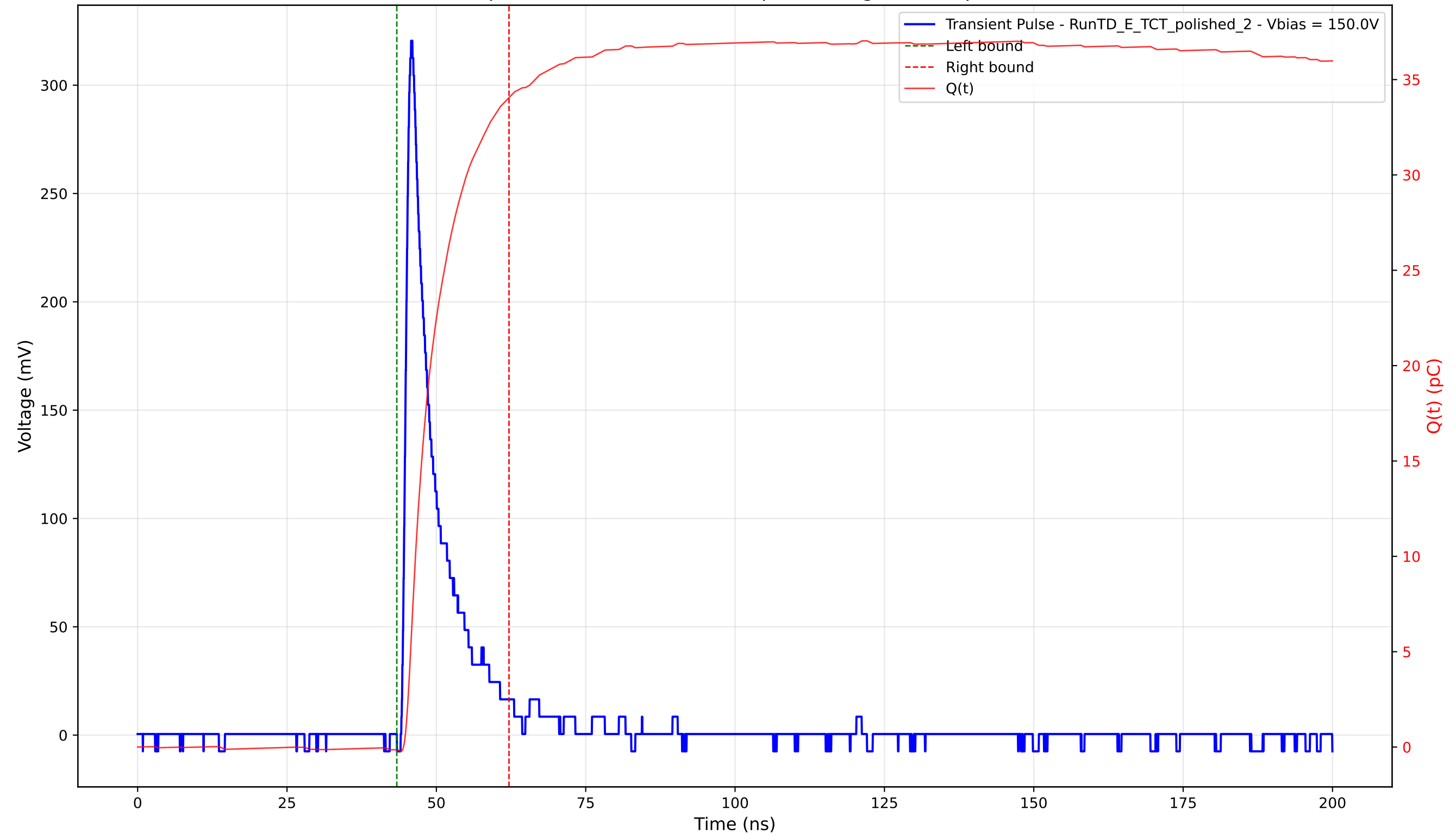
Transient Pulse - Sample: 4003 - Position: 325.0 \mu\text{m} - Charge: 34.19 pC - Rise Time: 1.10 ns
