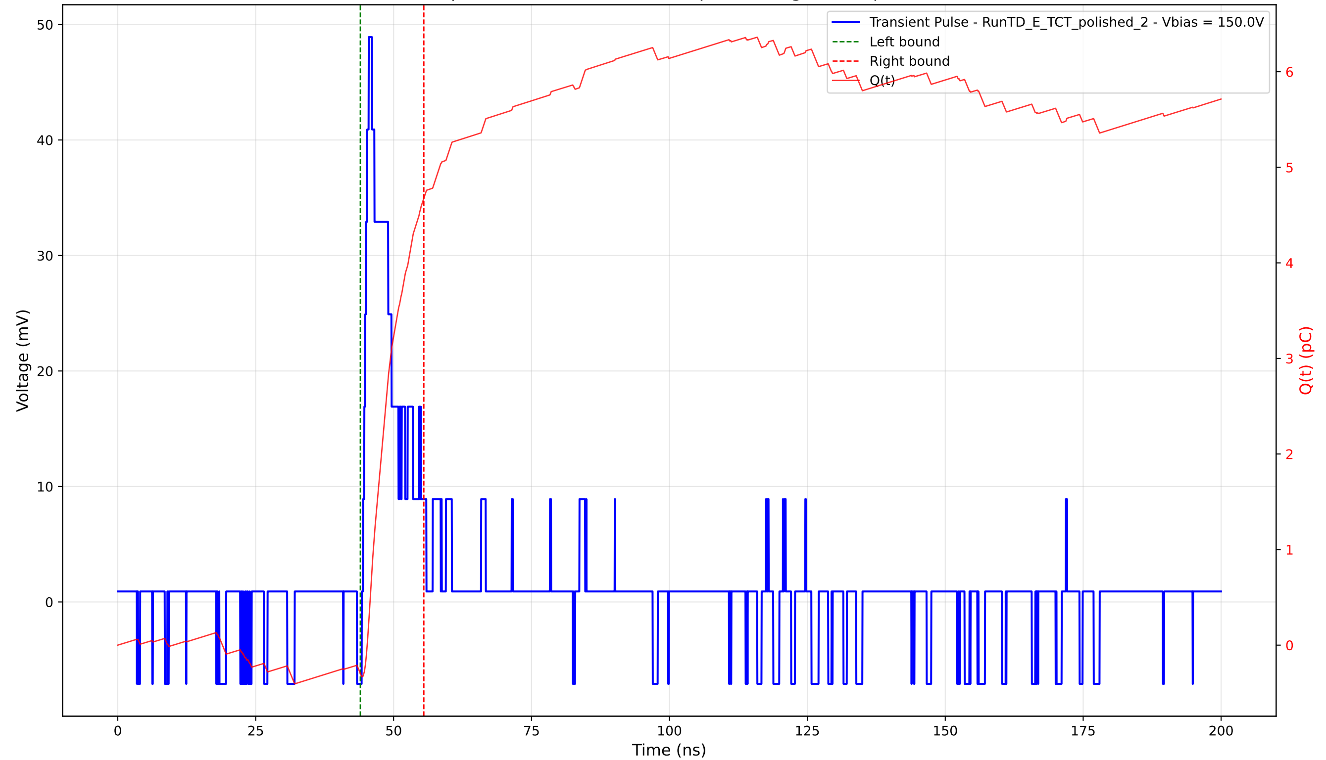
Transient Pulse - Sample: 4003 - Position: 500.0 \mu\text{m} - Charge: 4.97 pC - Rise Time: 1.03 ns
