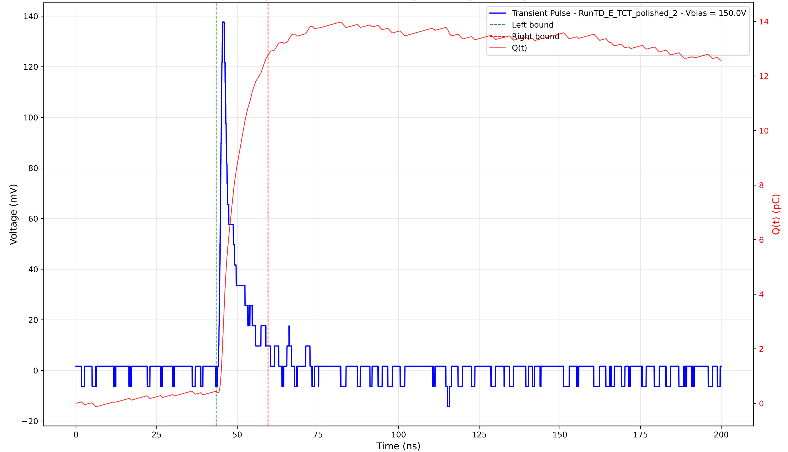
Transient Pulse - Sample: 4003 - Position: 155.0 \mu\text{m} - Charge: 12.33 pC - Rise Time: 1.01 ns
