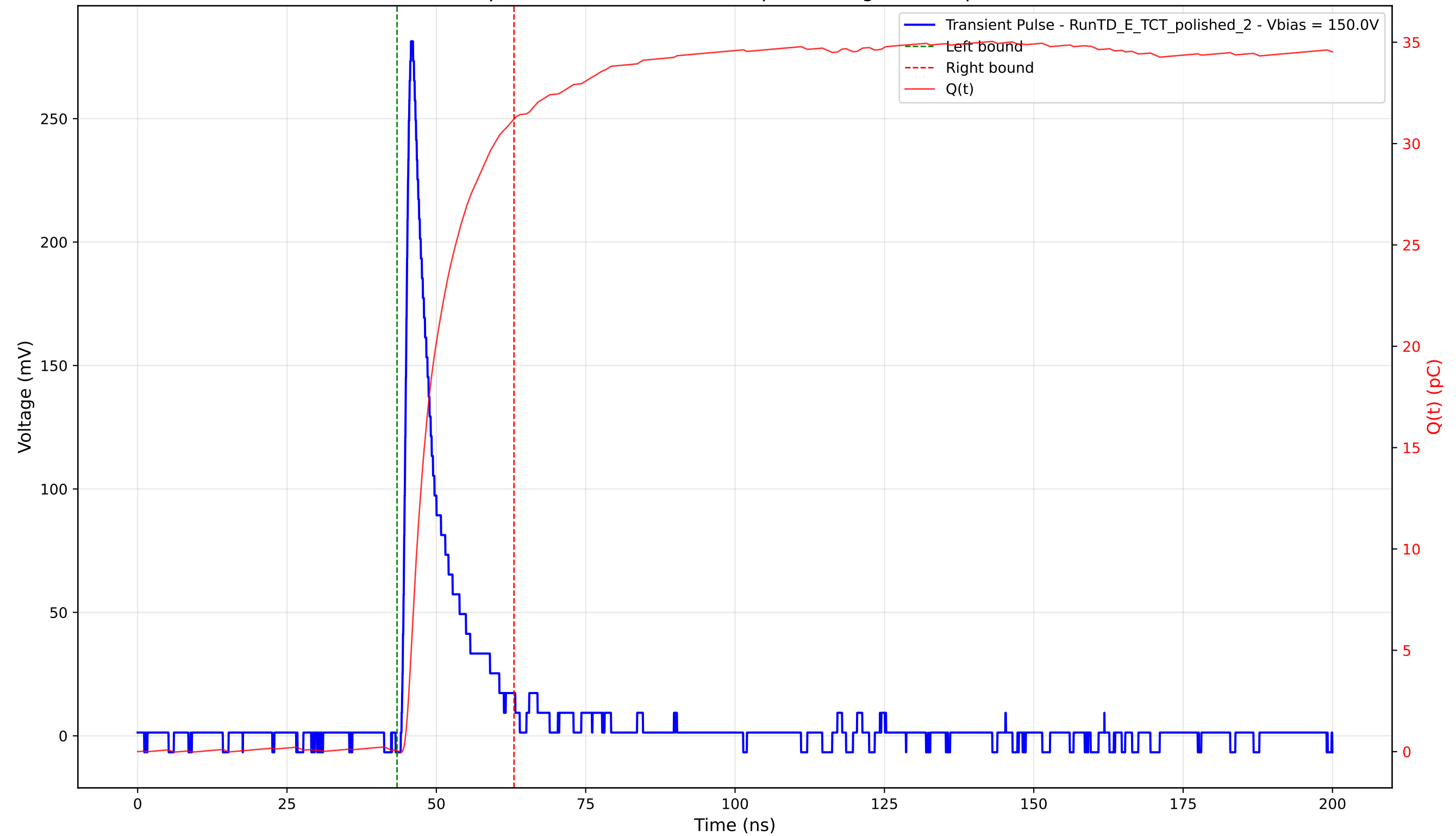
Transient Pulse - Sample: 4003 - Position: 345.0 \mu\text{m} - Charge: 31.17 pC - Rise Time: 1.09 ns
