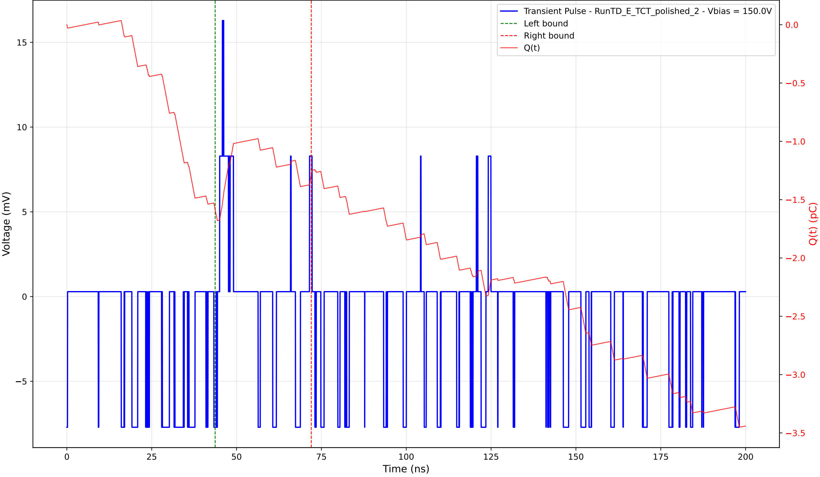
Transient Pulse - Sample: 4003 - Position: 65.0 \mu\text{m} - Charge: 0.30 pC - Rise Time: 0.82 ns
