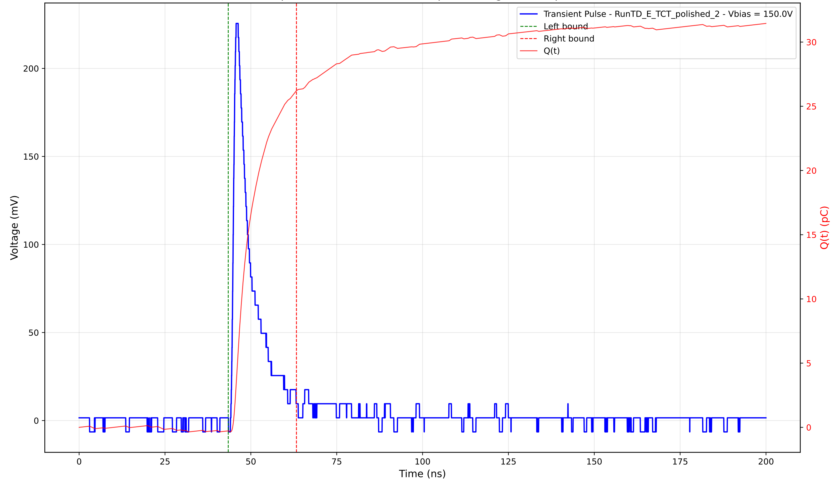
Transient Pulse - Sample: 4003 - Position: 370.0 \mu\text{m} - Charge: 26.49 pC - Rise Time: 1.13 ns
