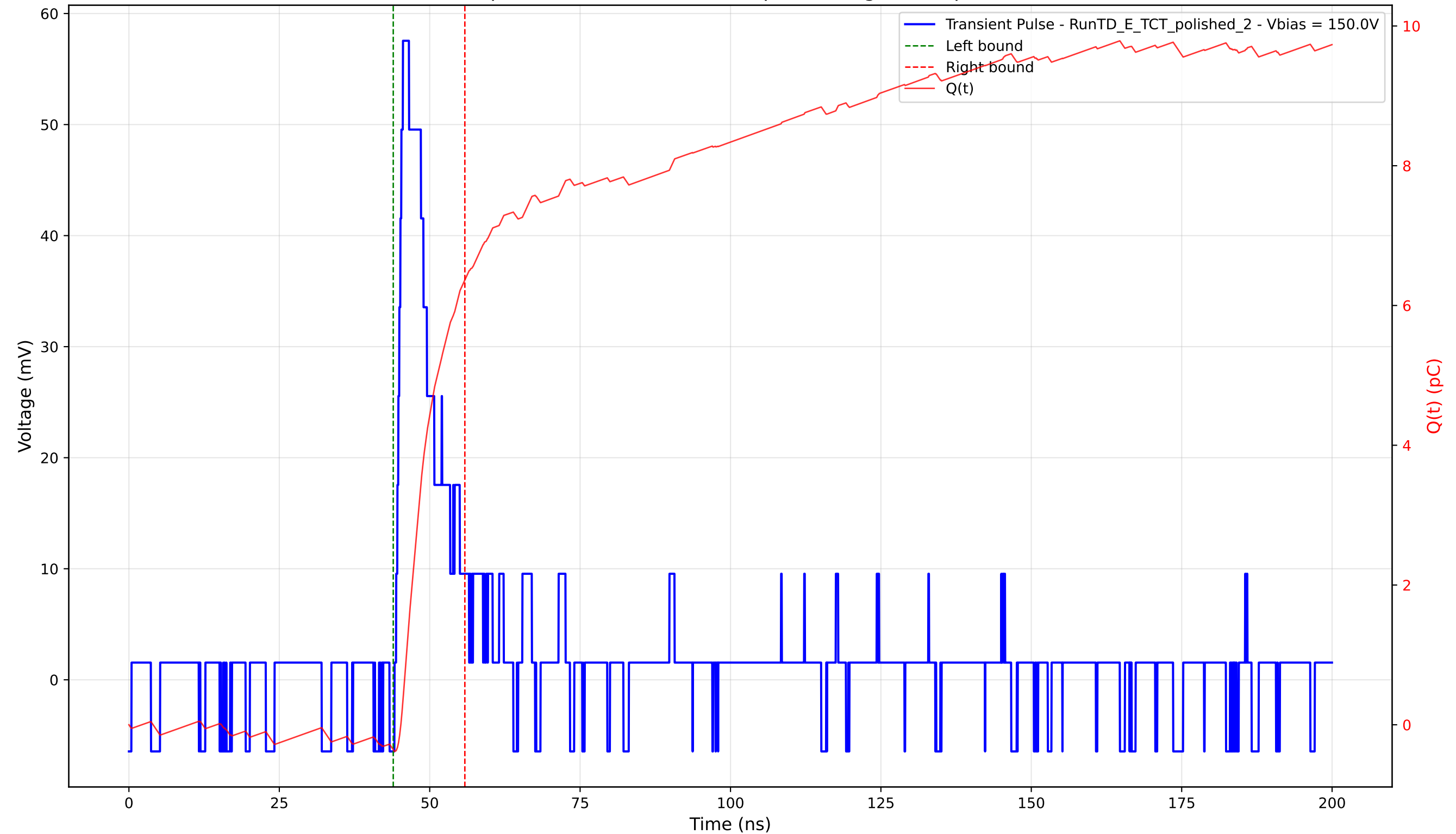
Transient Pulse - Sample: 4003 - Position: 475.0 \mu\text{m} - Charge: 6.72 pC - Rise Time: 1.13 ns
