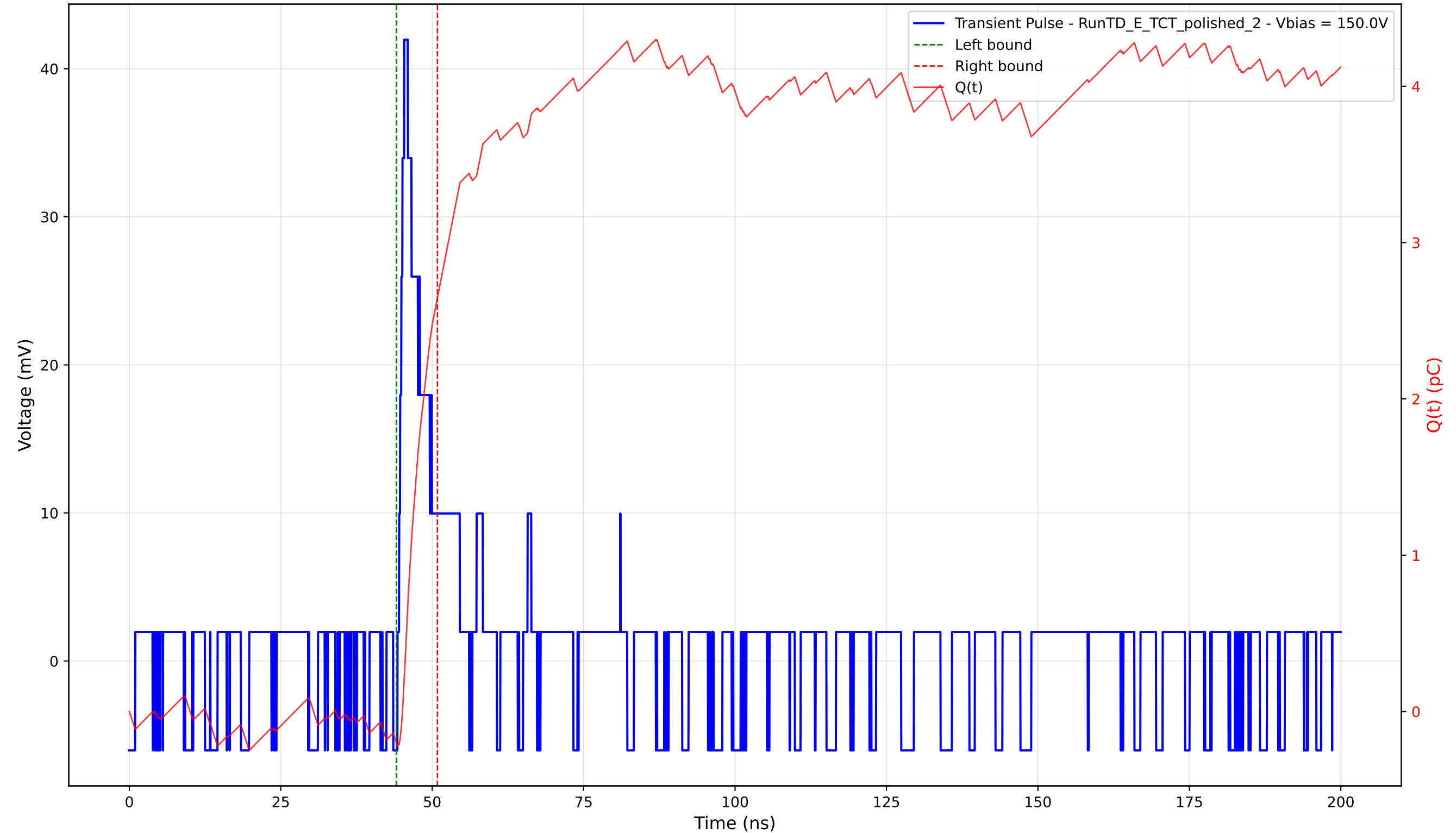
Transient Pulse - Sample: 4003 - Position: 525.0 \mu\text{m} - Charge: 2.85 pC - Rise Time: 0.85 ns
