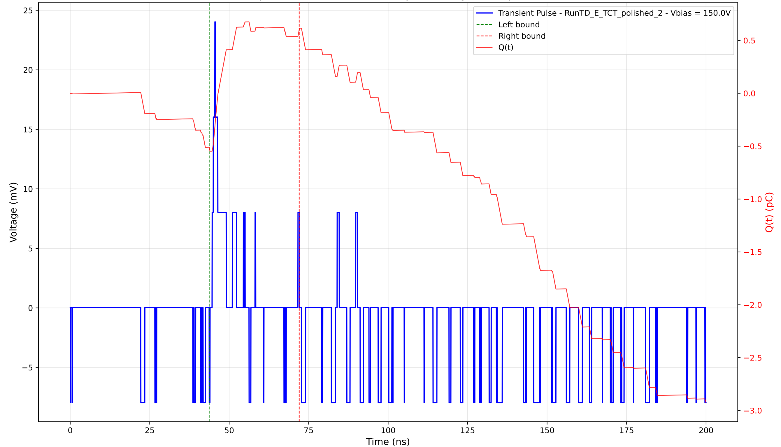
Transient Pulse - Sample: 4003 - Position: 795.0 \mu\text{m} - Charge: 1.11 pC - Rise Time: 0.87 ns
