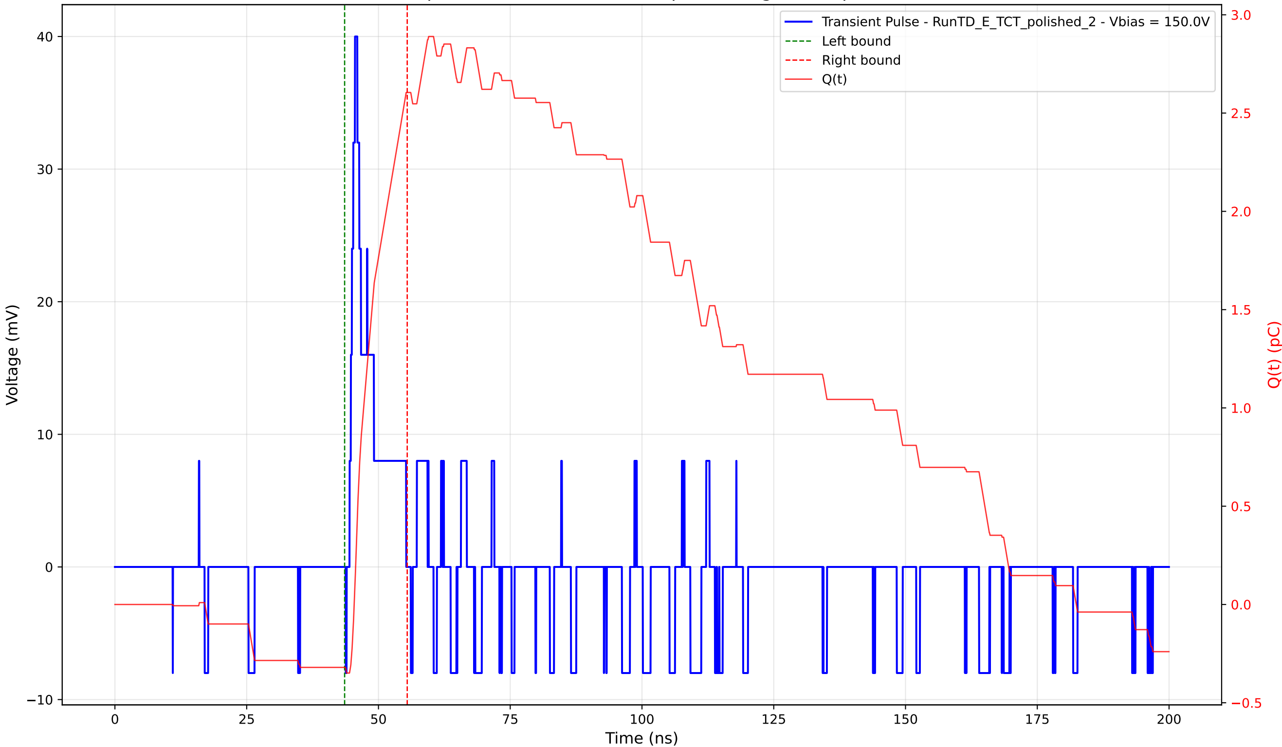
Transient Pulse - Sample: 4003 - Position: 560.0 \mu\text{m} - Charge: 2.92 pC - Rise Time: 1.03 ns
