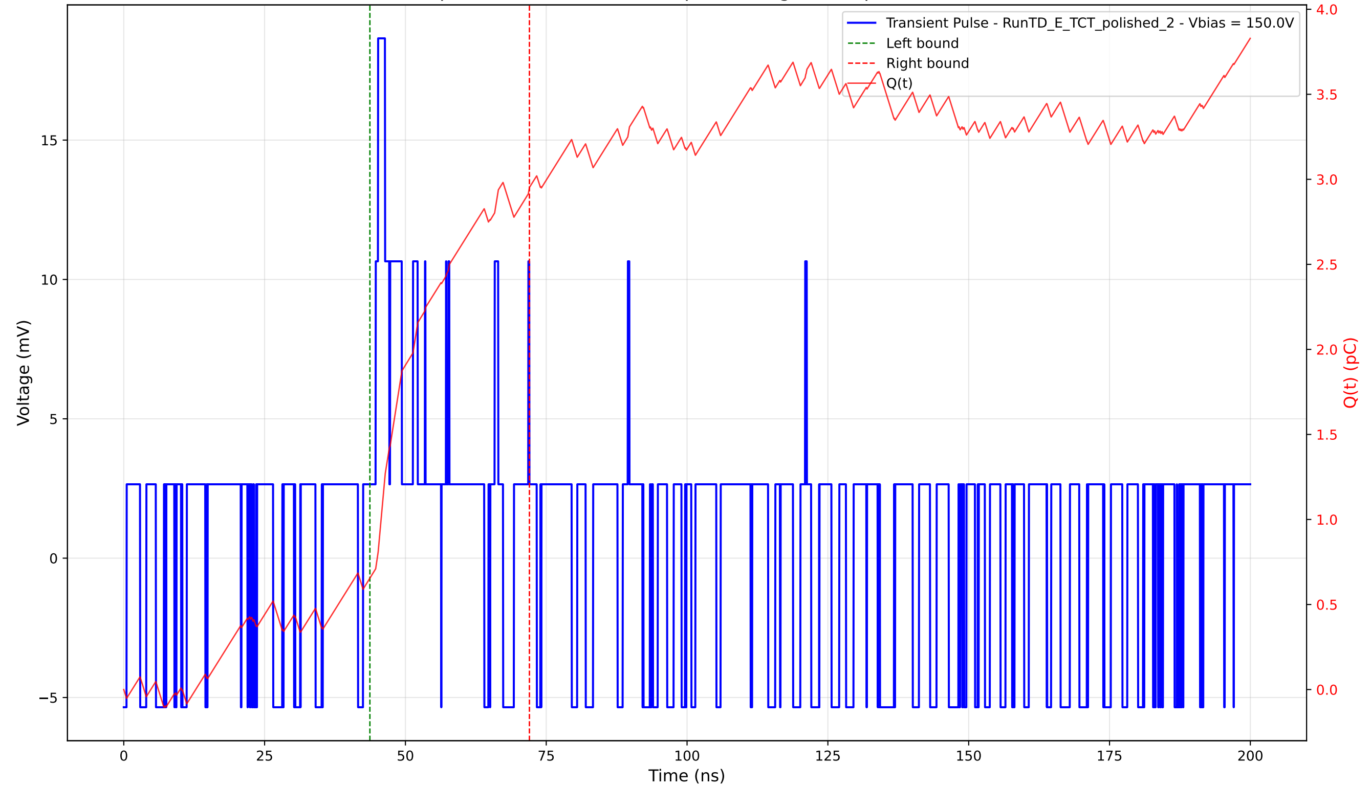
Transient Pulse - Sample: 4003 - Position: 60.0 \mu\text{m} - Charge: 2.30 pC - Rise Time: 0.00 ns (N/A)
