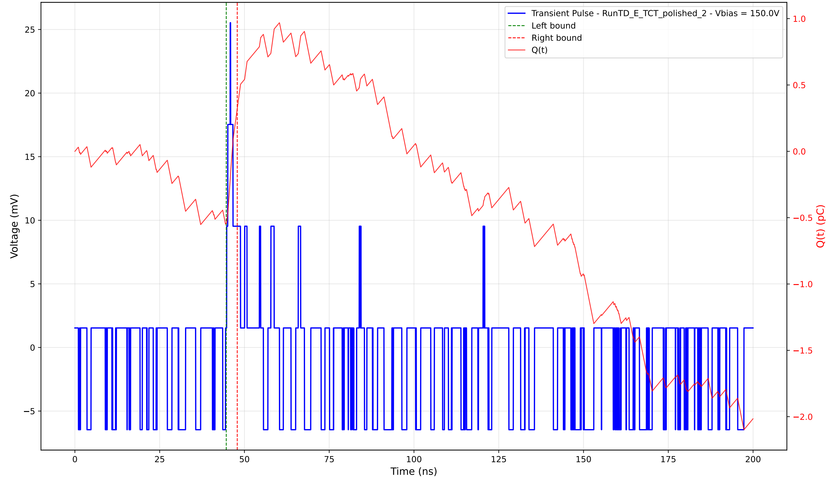
Transient Pulse - Sample: 4003 - Position: 665.0 \mu\text{m} - Charge: 0.87 pC - Rise Time: 1.06 ns
