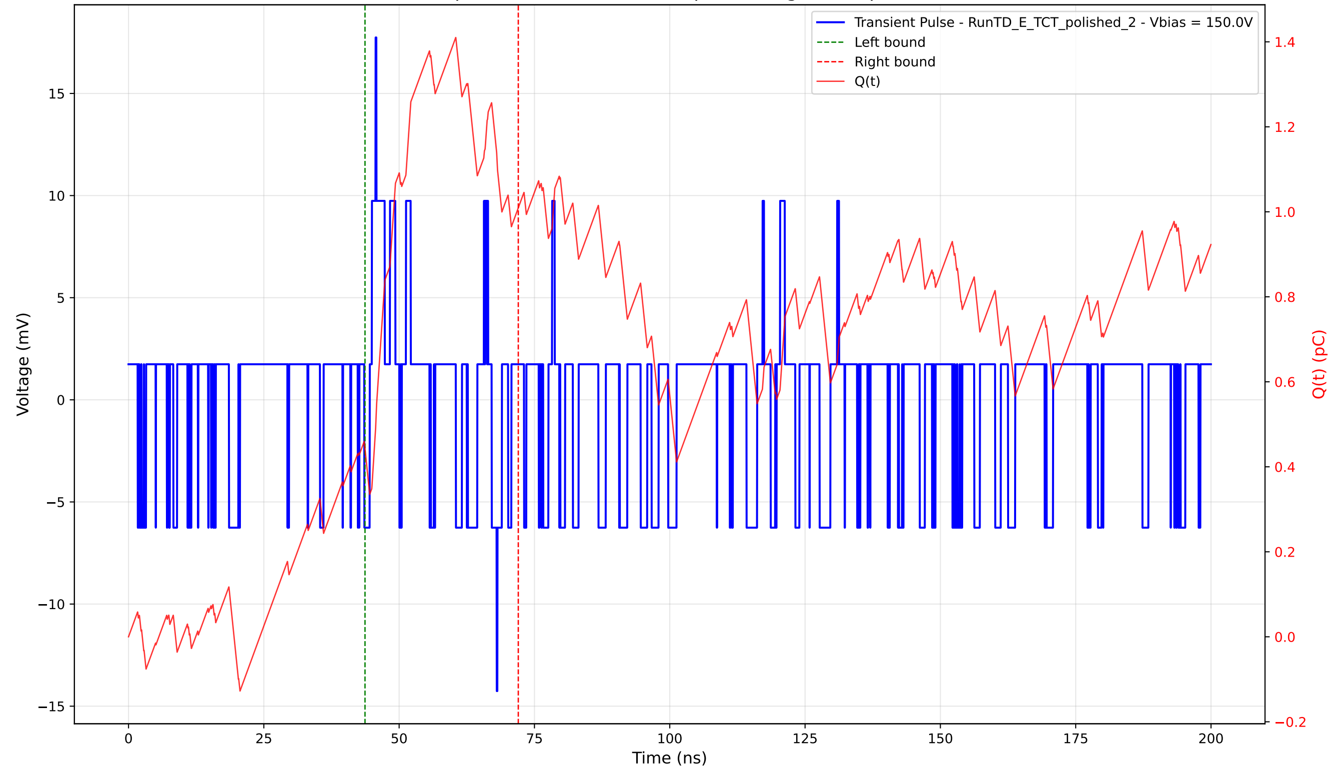
Transient Pulse - Sample: 4003 - Position: 30.0 \mu\text{m} - Charge: 0.57 pC - Rise Time: 0.70 ns
