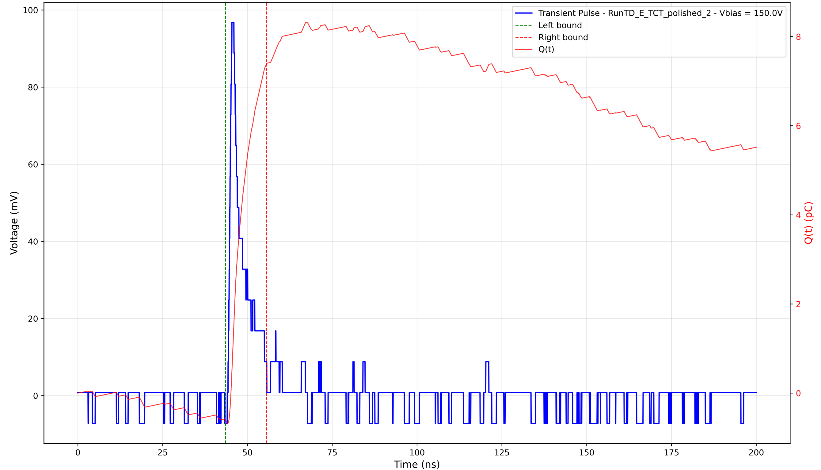
Transient Pulse - Sample: 4003 - Position: 140.0 \mu\text{m} - Charge: 7.99 pC - Rise Time: 0.86 ns
