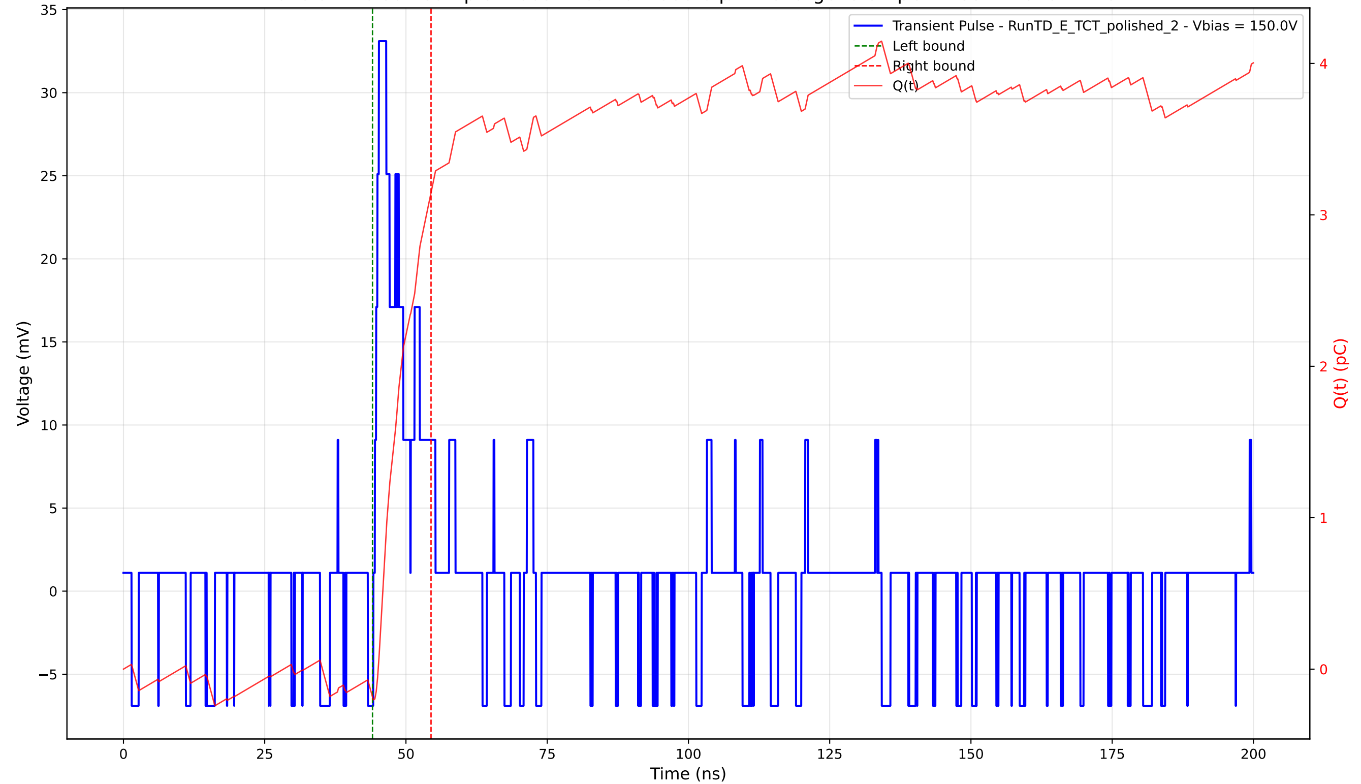
Transient Pulse - Sample: 4003 - Position: 535.0 \mu\text{m} - Charge: 3.34 pC - Rise Time: 0.71 ns
