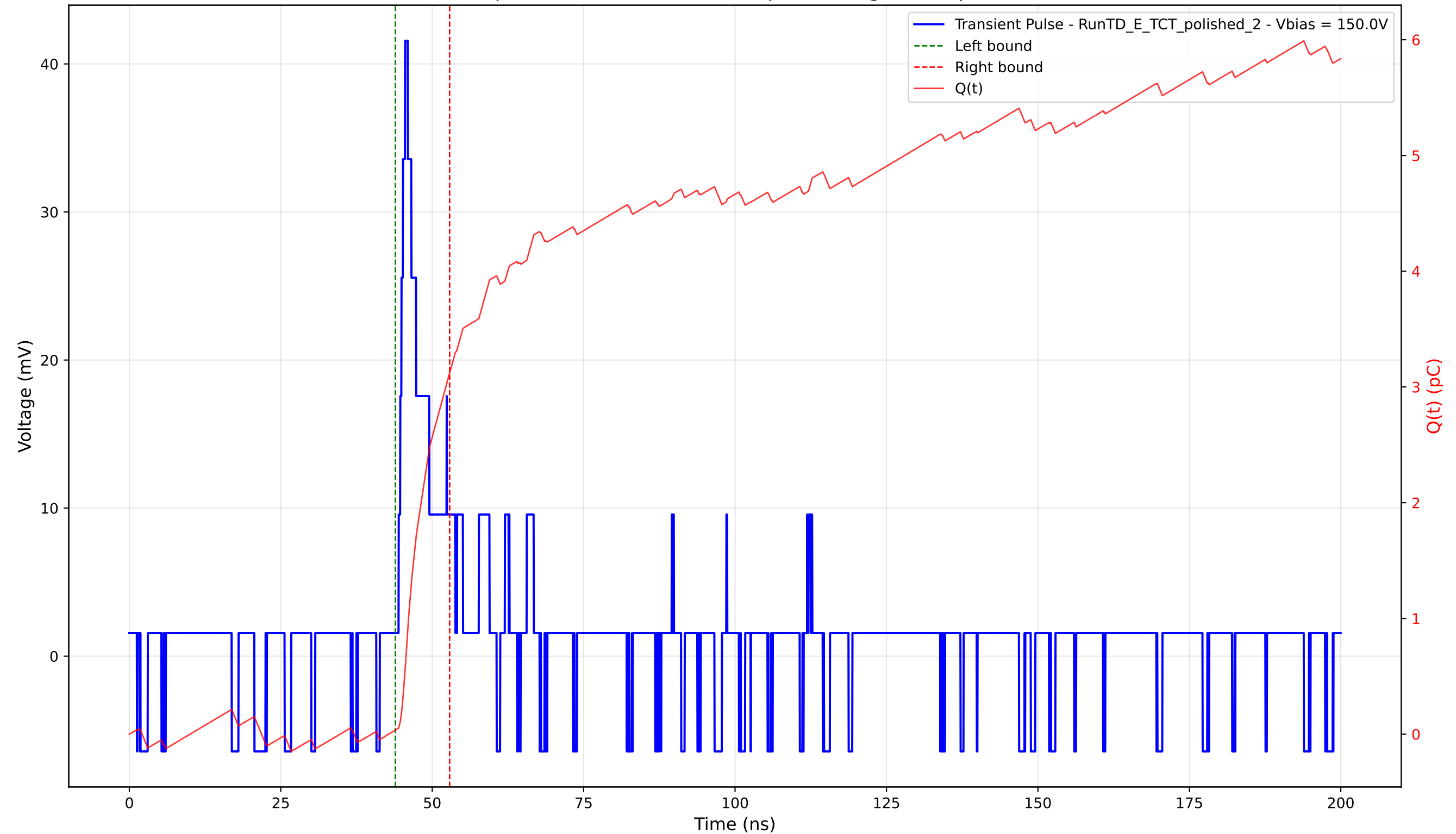
Transient Pulse - Sample: 4003 - Position: 530.0 \mu\text{m} - Charge: 3.09 pC - Rise Time: 1.07 ns
