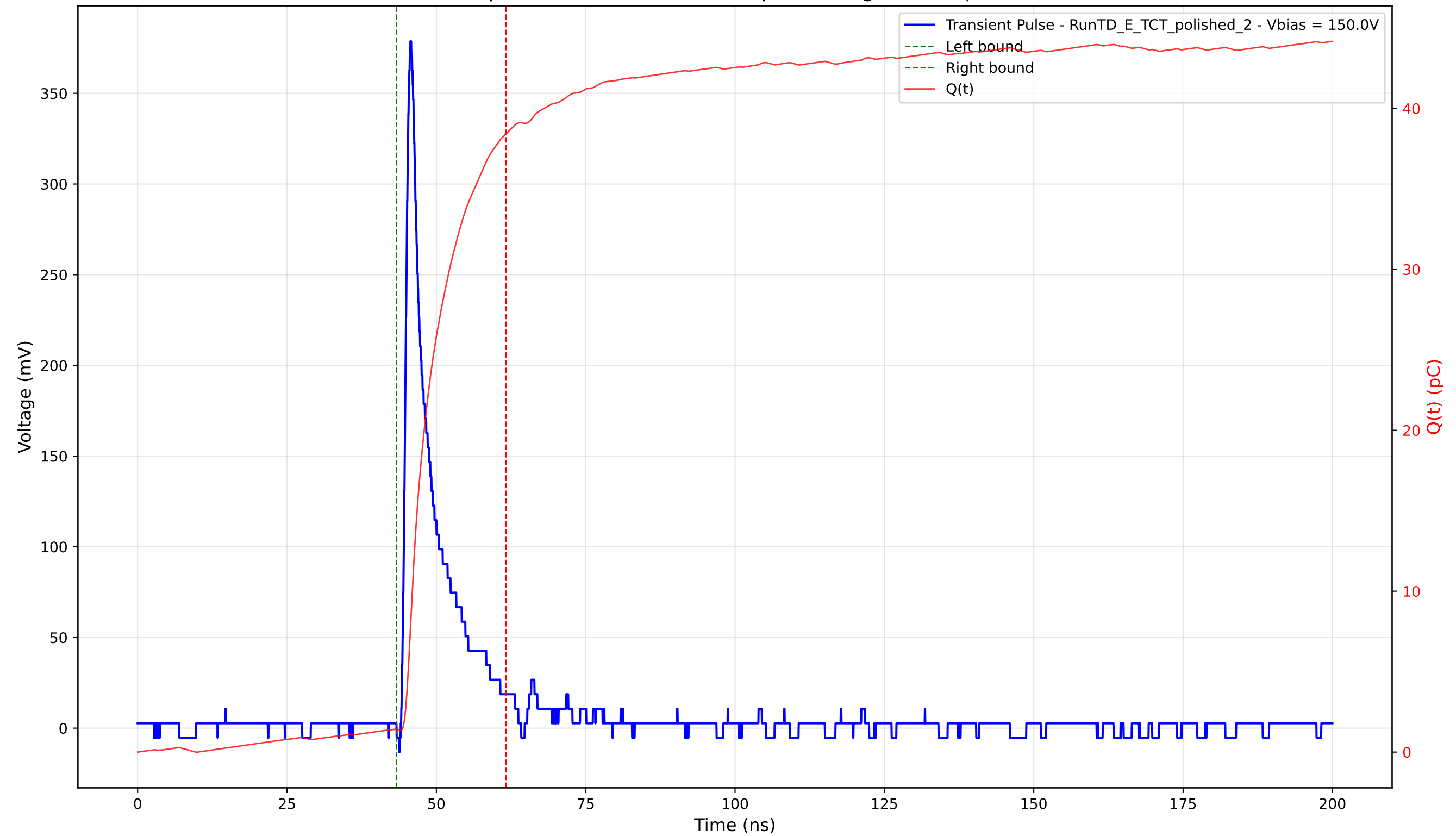
Transient Pulse - Sample: 4003 - Position: 255.0 \mu\text{m} - Charge: 36.98 pC - Rise Time: 1.05 ns
