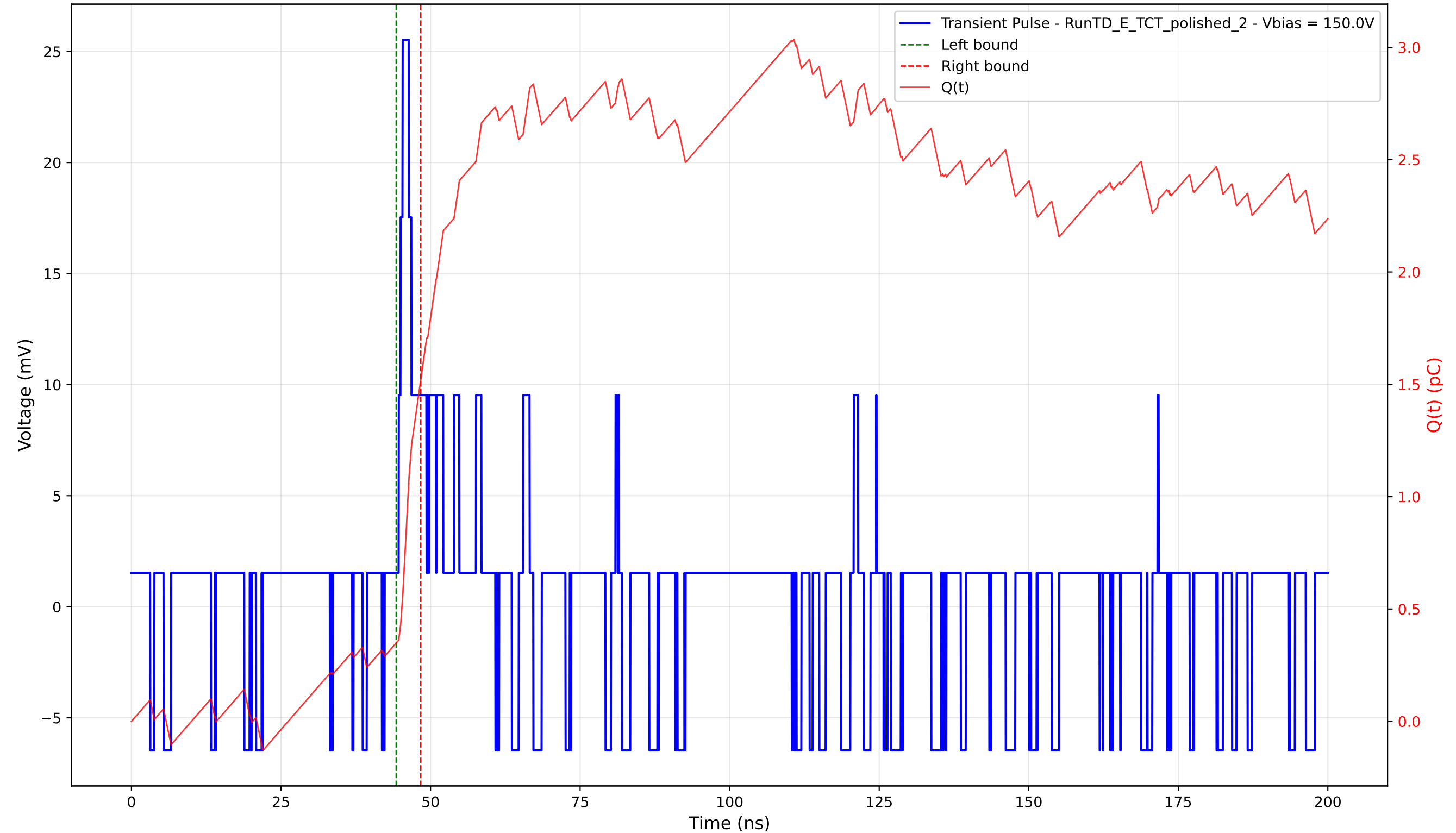
Transient Pulse - Sample: 4003 - Position: 595.0 \mu\text{m} - Charge: 1.17 pC - Rise Time: 0.66 ns
