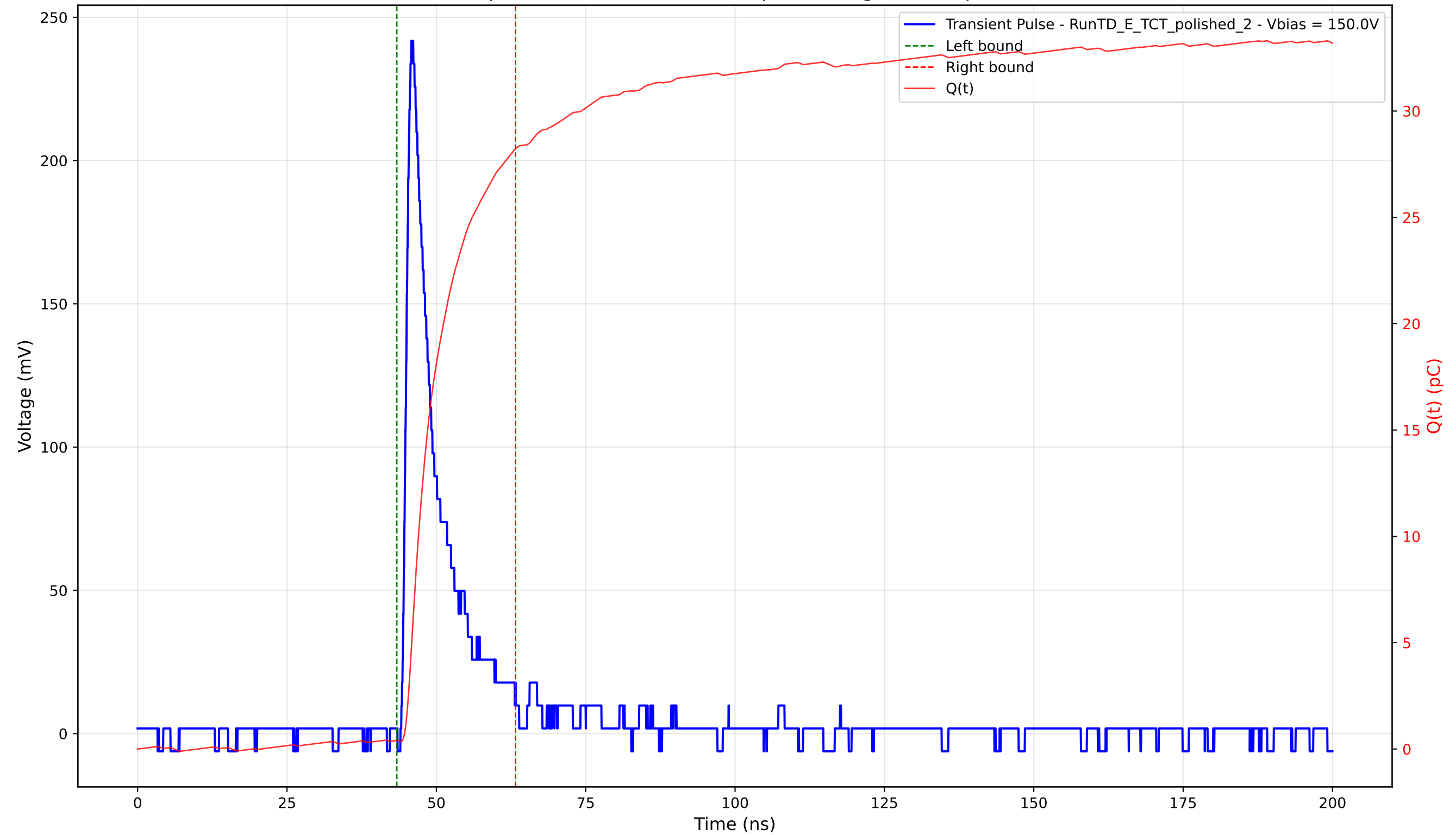
Transient Pulse - Sample: 4003 - Position: 365.0 \mu\text{m} - Charge: 27.84 pC - Rise Time: 1.14 ns
