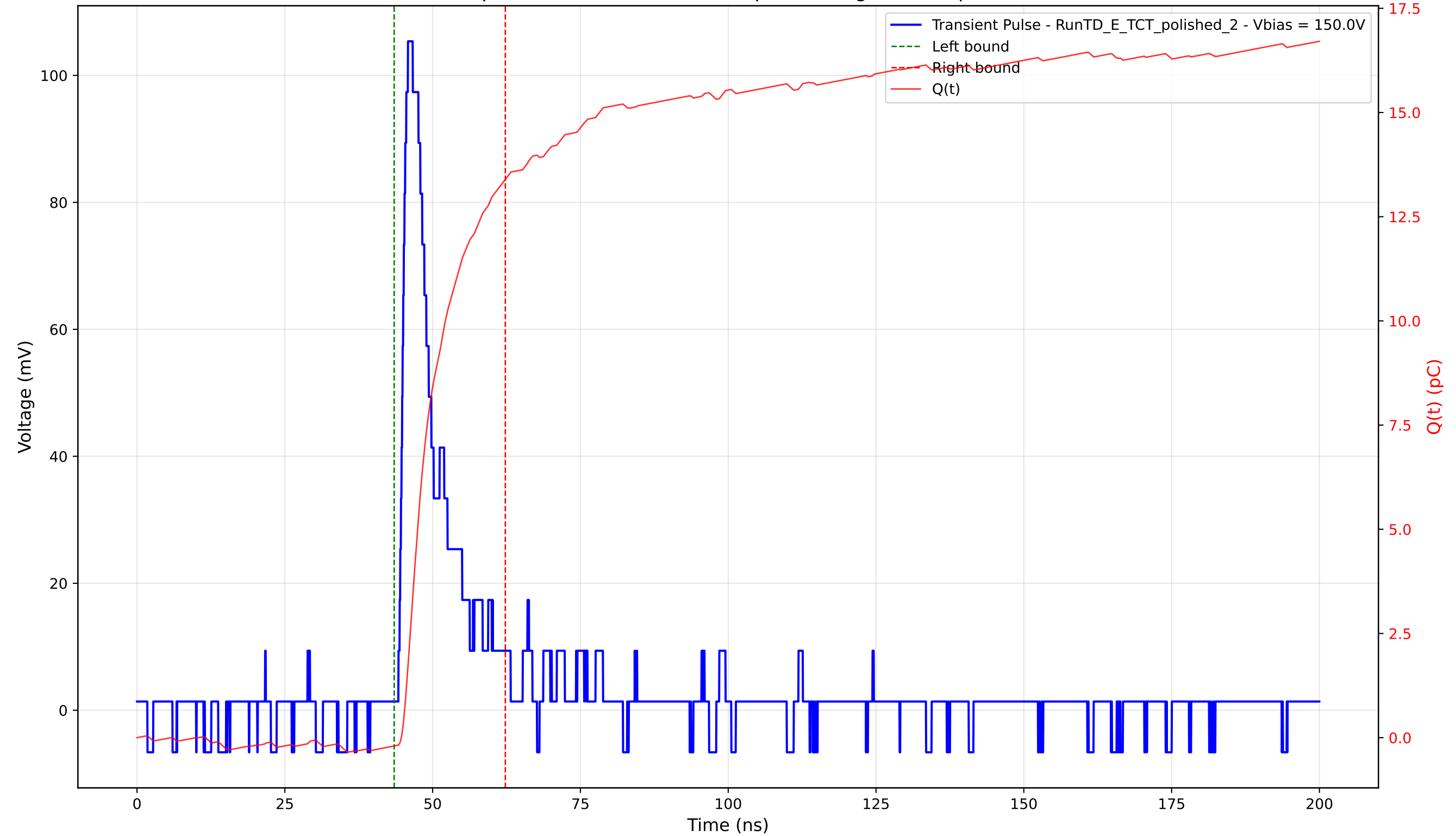
Transient Pulse - Sample: 4003 - Position: 435.0 \mu\text{m} - Charge: 13.60 pC - Rise Time: 1.14 ns
