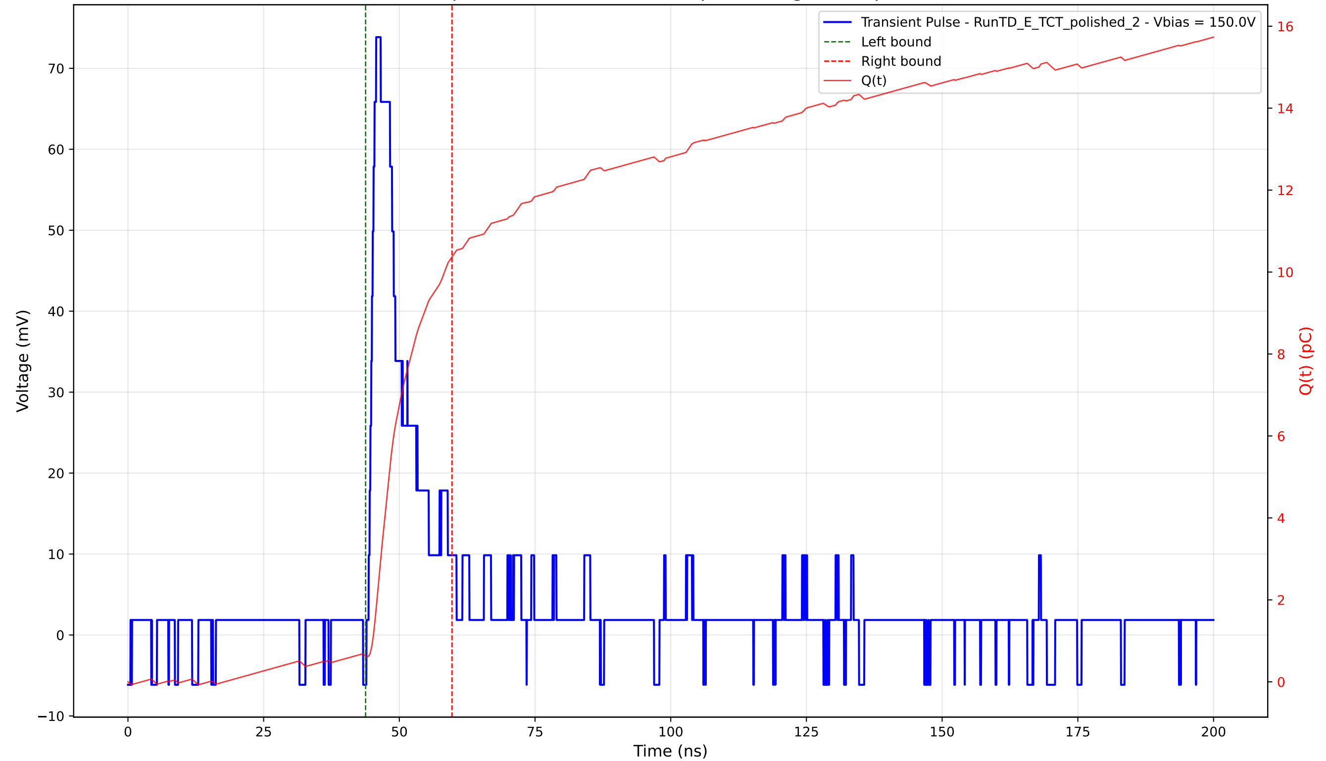
Transient Pulse - Sample: 4003 - Position: 460.0 \mu\text{m} - Charge: 9.74 pC - Rise Time: 1.39 ns
