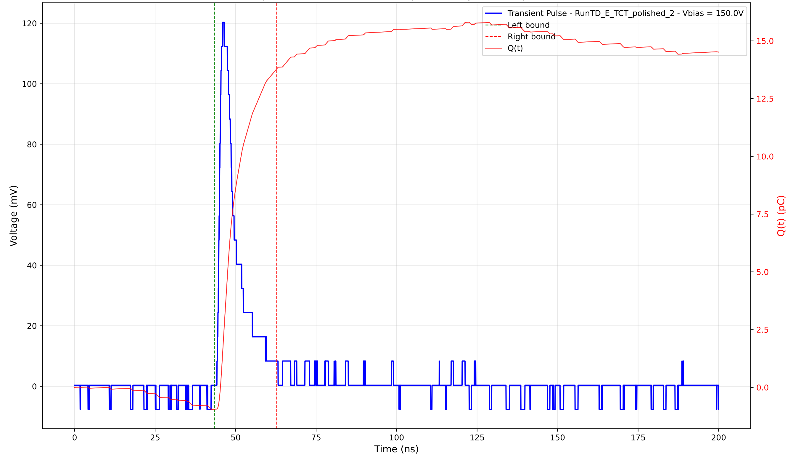
Transient Pulse - Sample: 4003 - Position: 425.0 \mu\text{m} - Charge: 14.74 pC - Rise Time: 1.25 ns
