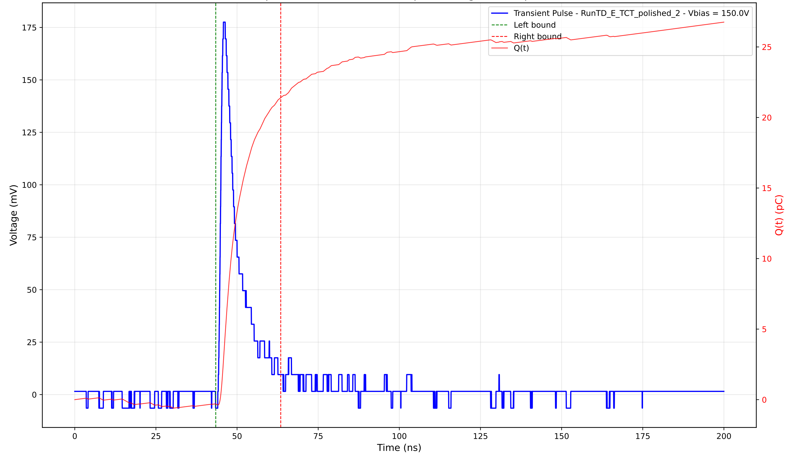
Transient Pulse - Sample: 4003 - Position: 395.0 \mu\text{m} - Charge: 21.71 pC - Rise Time: 1.08 ns
