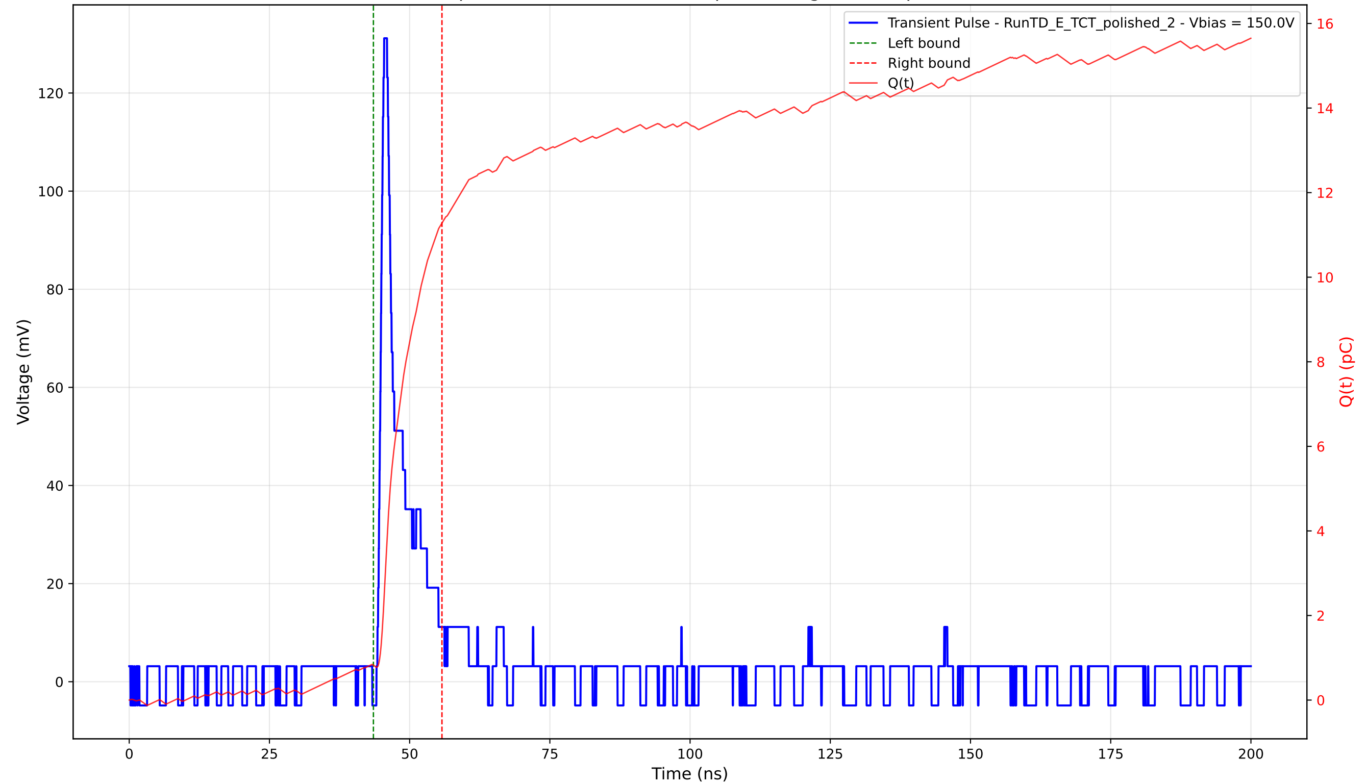
Transient Pulse - Sample: 4003 - Position: 150.0 \mu\text{m} - Charge: 10.46 pC - Rise Time: 0.96 ns
