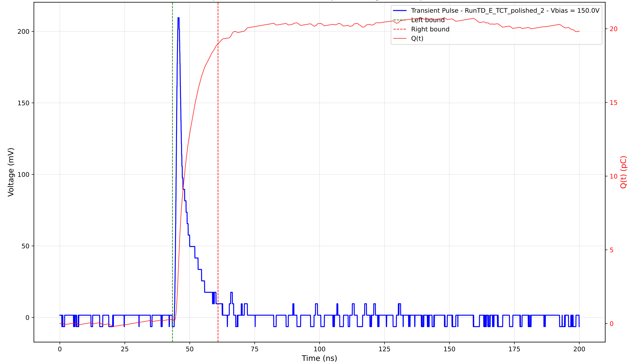
Transient Pulse - Sample: 4003 - Position: 180.0 \mu\text{m} - Charge: 18.70 pC - Rise Time: 0.99 ns
