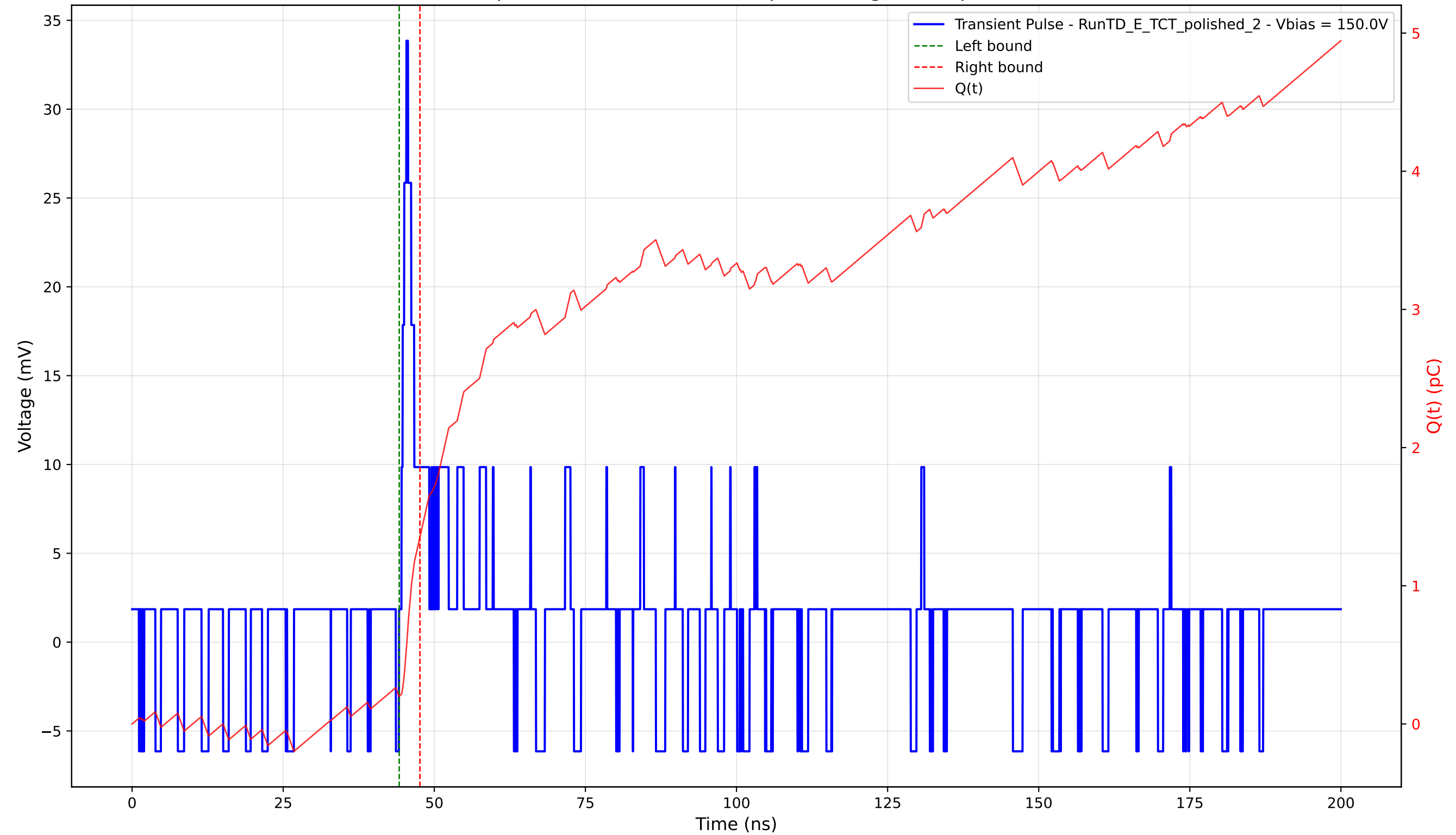
Transient Pulse - Sample: 4003 - Position: 600.0 \mu\text{m} - Charge: 1.15 pC - Rise Time: 0.82 ns
