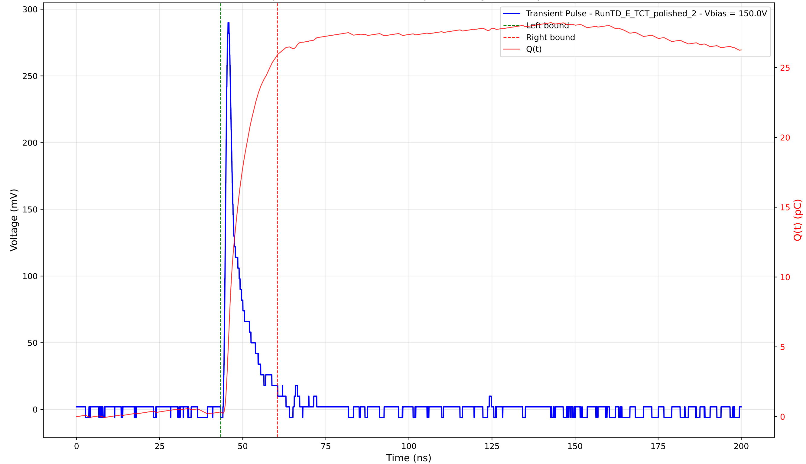
Transient Pulse - Sample: 4003 - Position: 205.0 \mu\text{m} - Charge: 25.58 pC - Rise Time: 1.01 ns
