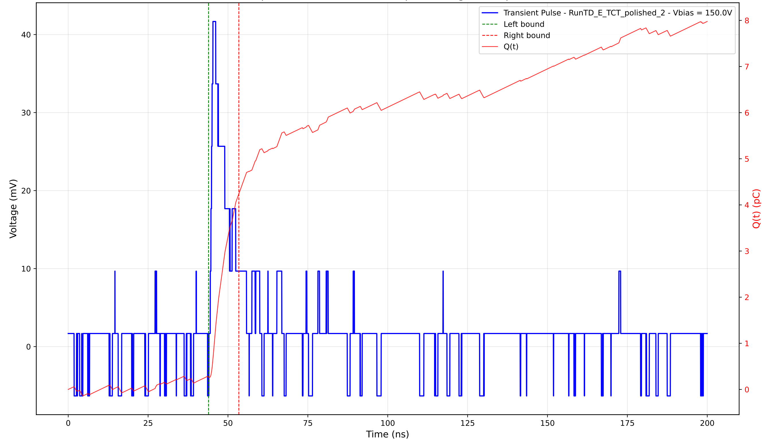
Transient Pulse - Sample: 4003 - Position: 520.0 \mu\text{m} - Charge: 3.98 pC - Rise Time: 0.83 ns
