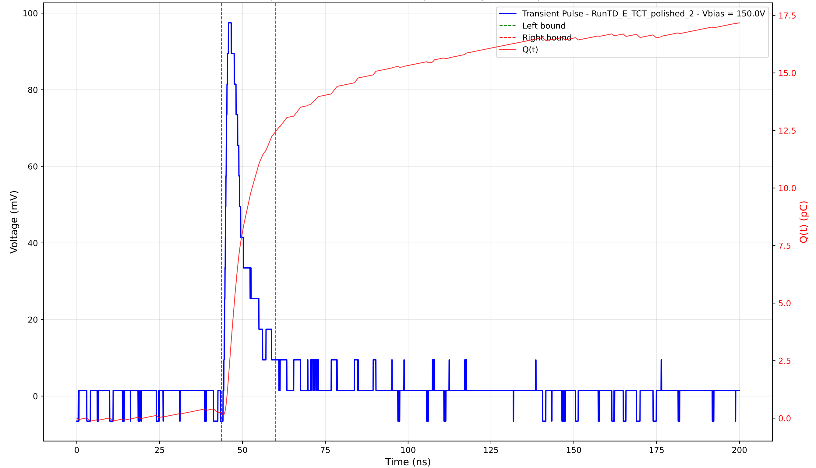
Transient Pulse - Sample: 4003 - Position: 440.0 \mu\text{m} - Charge: 12.26 pC - Rise Time: 1.00 ns
