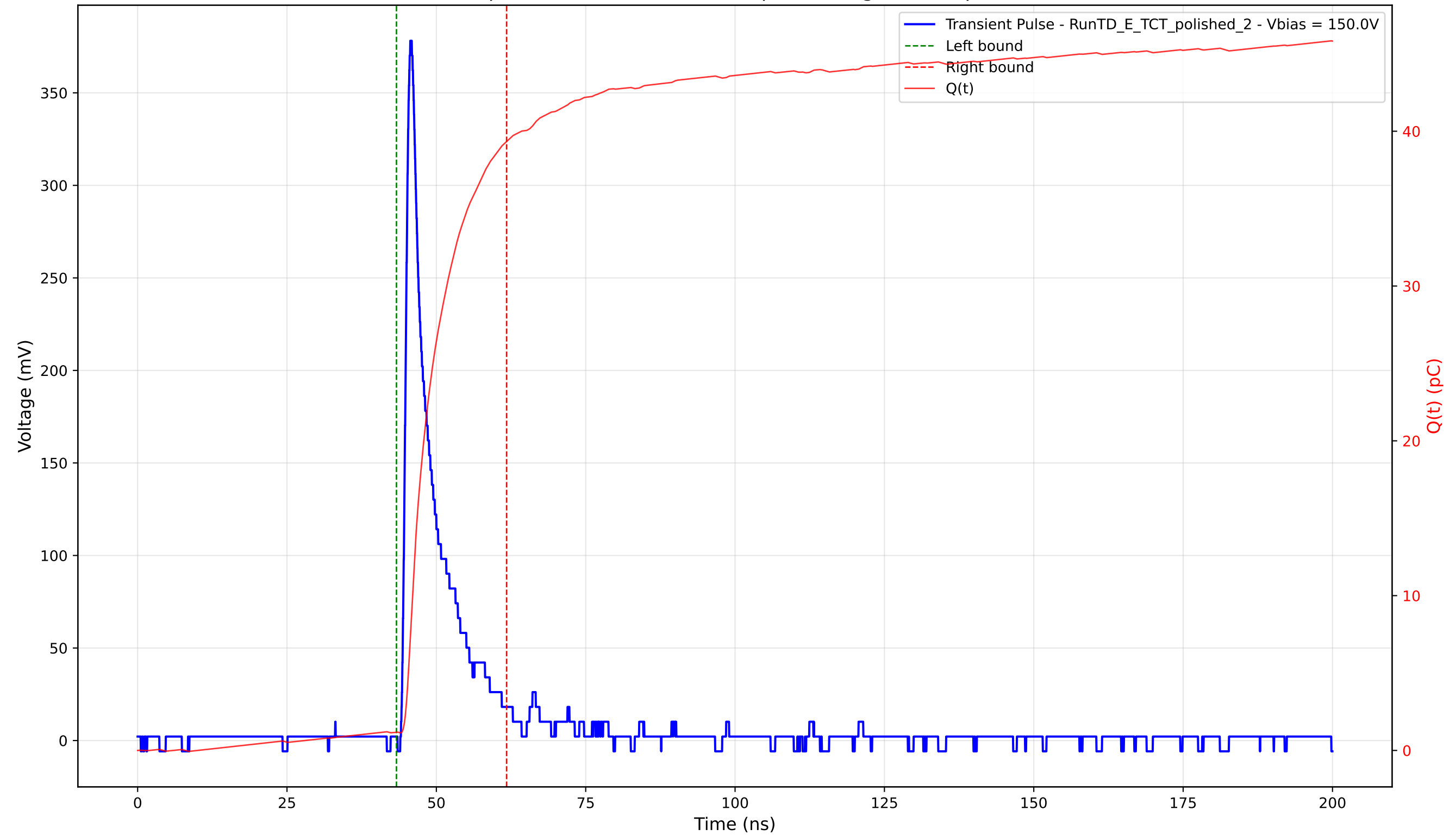
Transient Pulse - Sample: 4003 - Position: 270.0 \mu\text{m} - Charge: 38.16 pC - Rise Time: 1.05 ns
