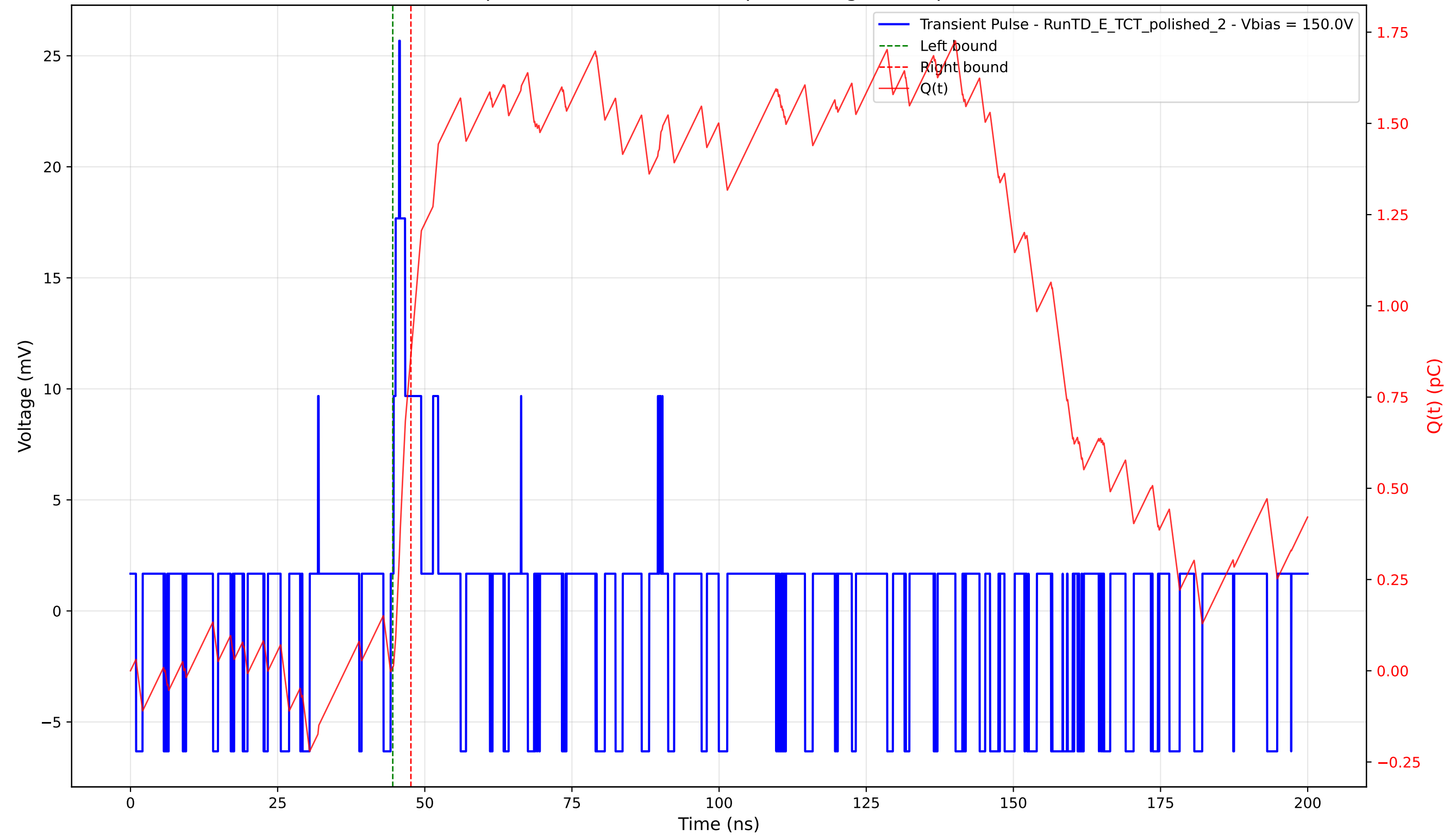
Transient Pulse - Sample: 4003 - Position: 85.0 \mu\text{m} - Charge: 0.86 pC - Rise Time: 0.96 ns
