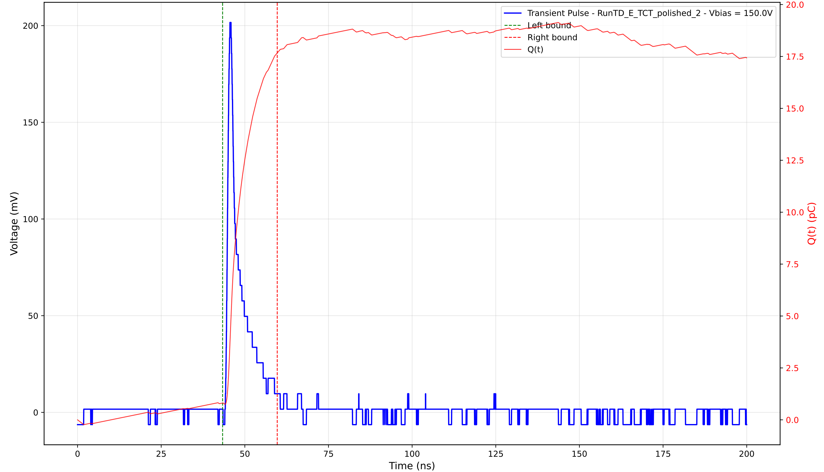
Transient Pulse - Sample: 4003 - Position: 175.0 \mu\text{m} - Charge: 16.86 pC - Rise Time: 0.99 ns
