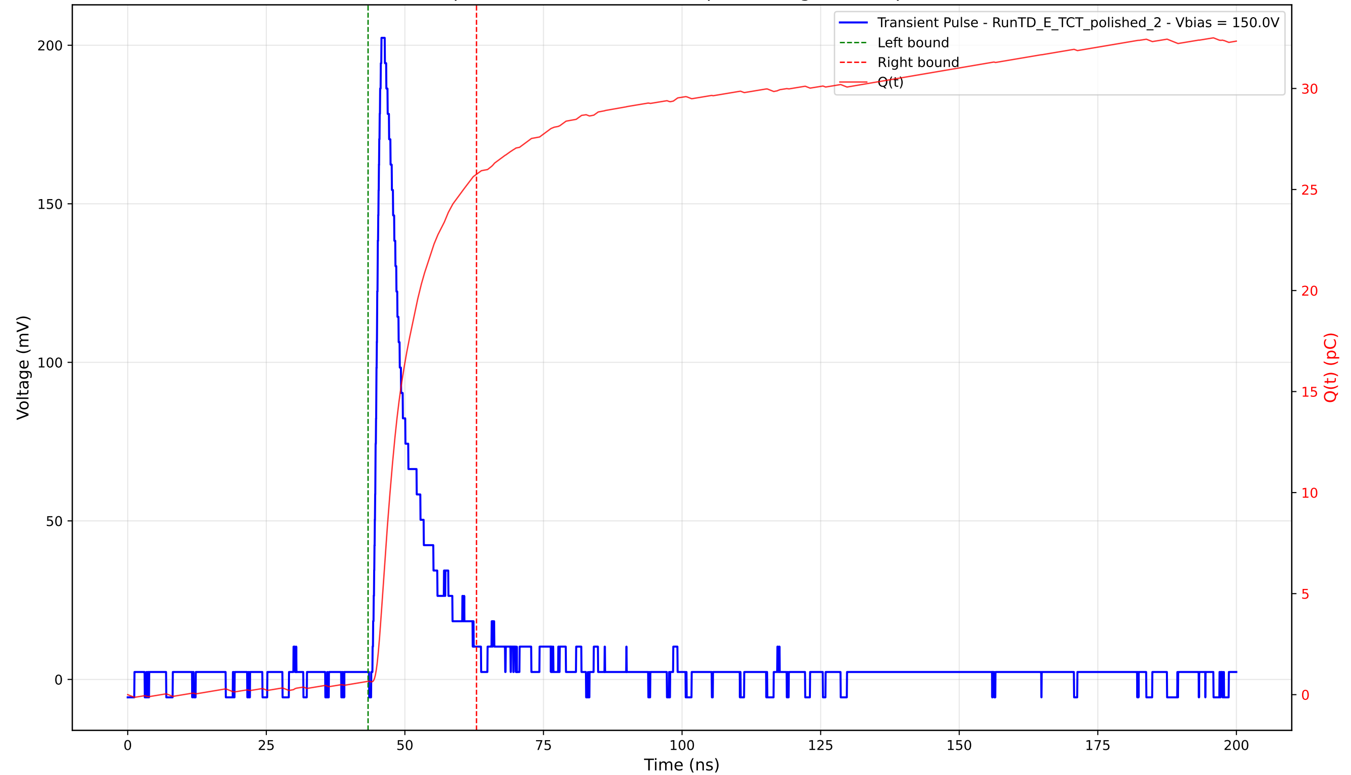
Transient Pulse - Sample: 4003 - Position: 380.0 \mu\text{m} - Charge: 25.10 pC - Rise Time: 1.18 ns
