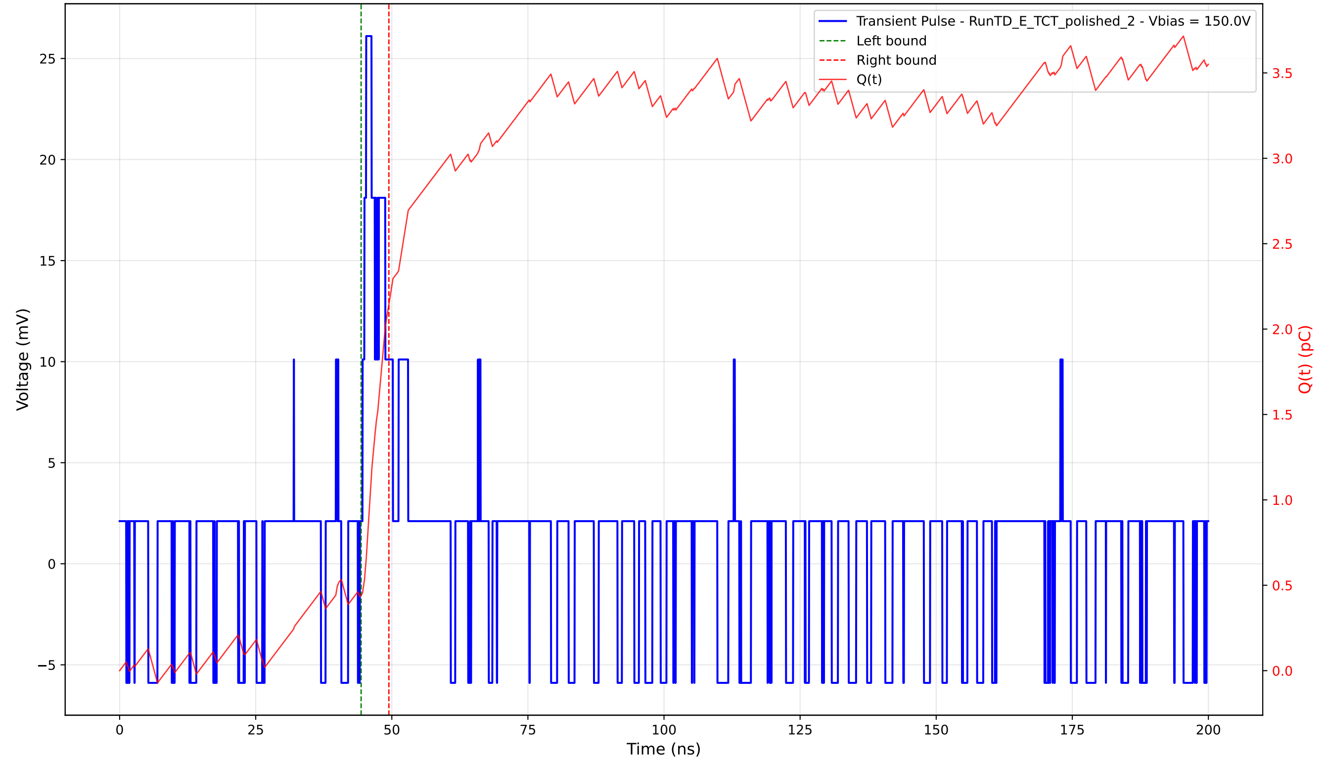
Transient Pulse - Sample: 4003 - Position: 590.0 \mu\text{m} - Charge: 1.70 pC - Rise Time: 0.68 ns
