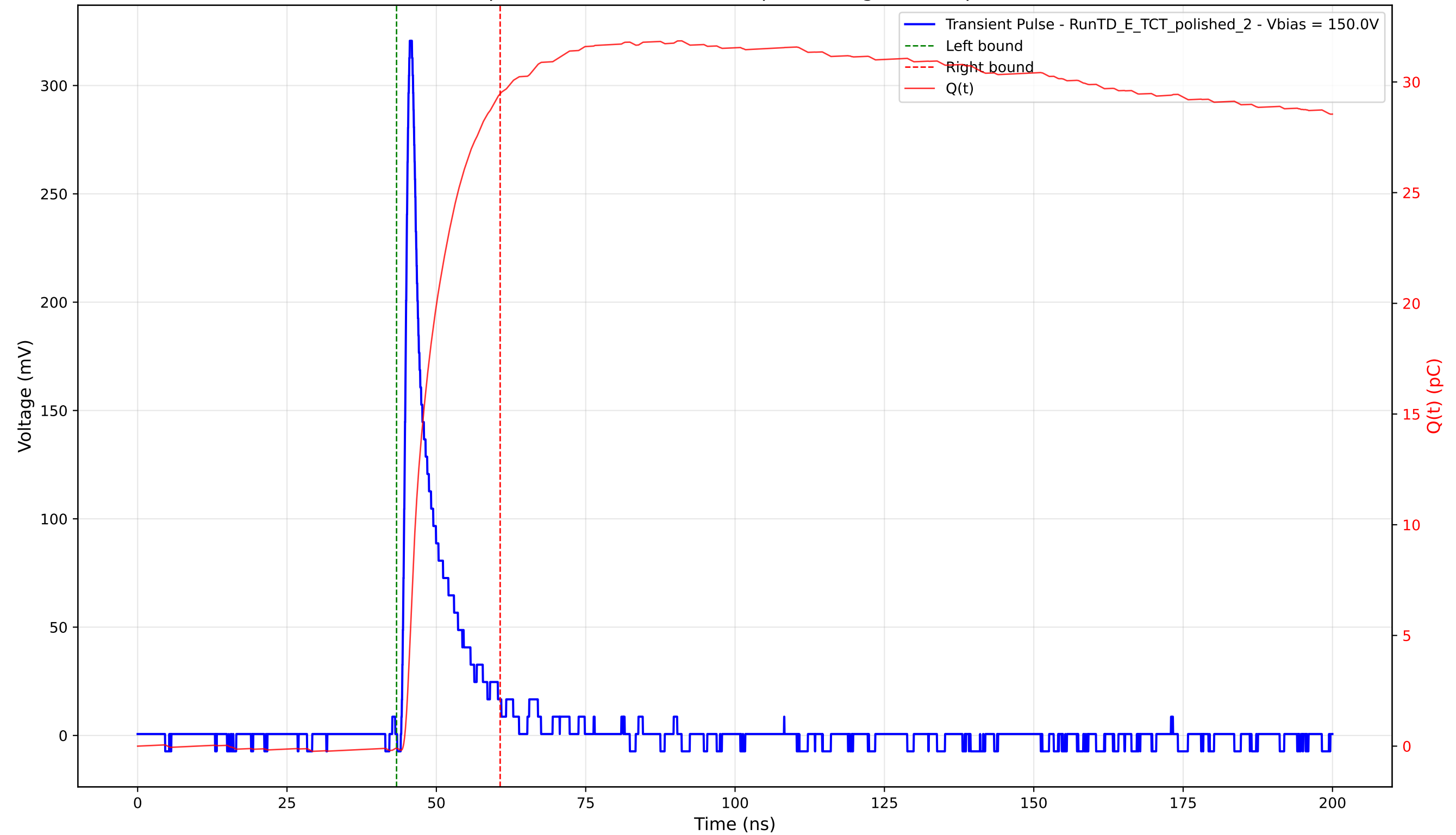
Transient Pulse - Sample: 4003 - Position: 220.0 \mu\text{m} - Charge: 29.57 pC - Rise Time: 0.98 ns
