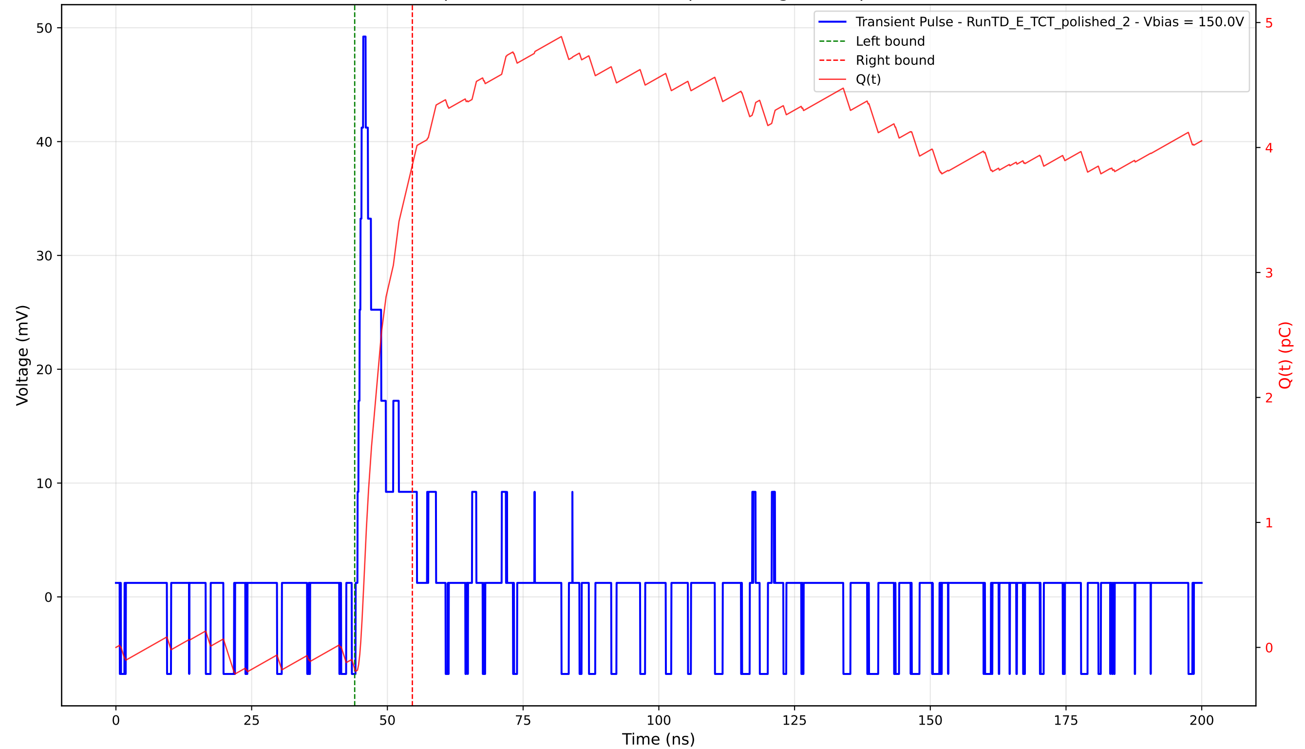
Transient Pulse - Sample: 4003 - Position: 685.0 \mu\text{m} - Charge: 4.03 pC - Rise Time: 1.05 ns
