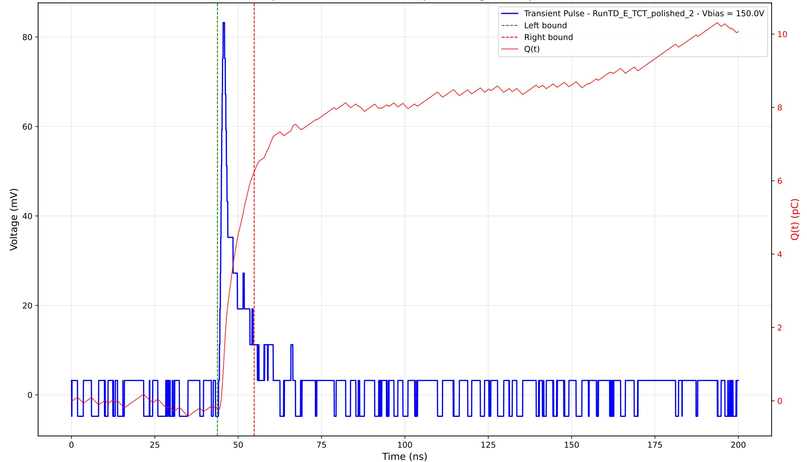
Transient Pulse - Sample: 4003 - Position: 130.0 \mu\text{m} - Charge: 6.46 pC - Rise Time: 0.93 ns
