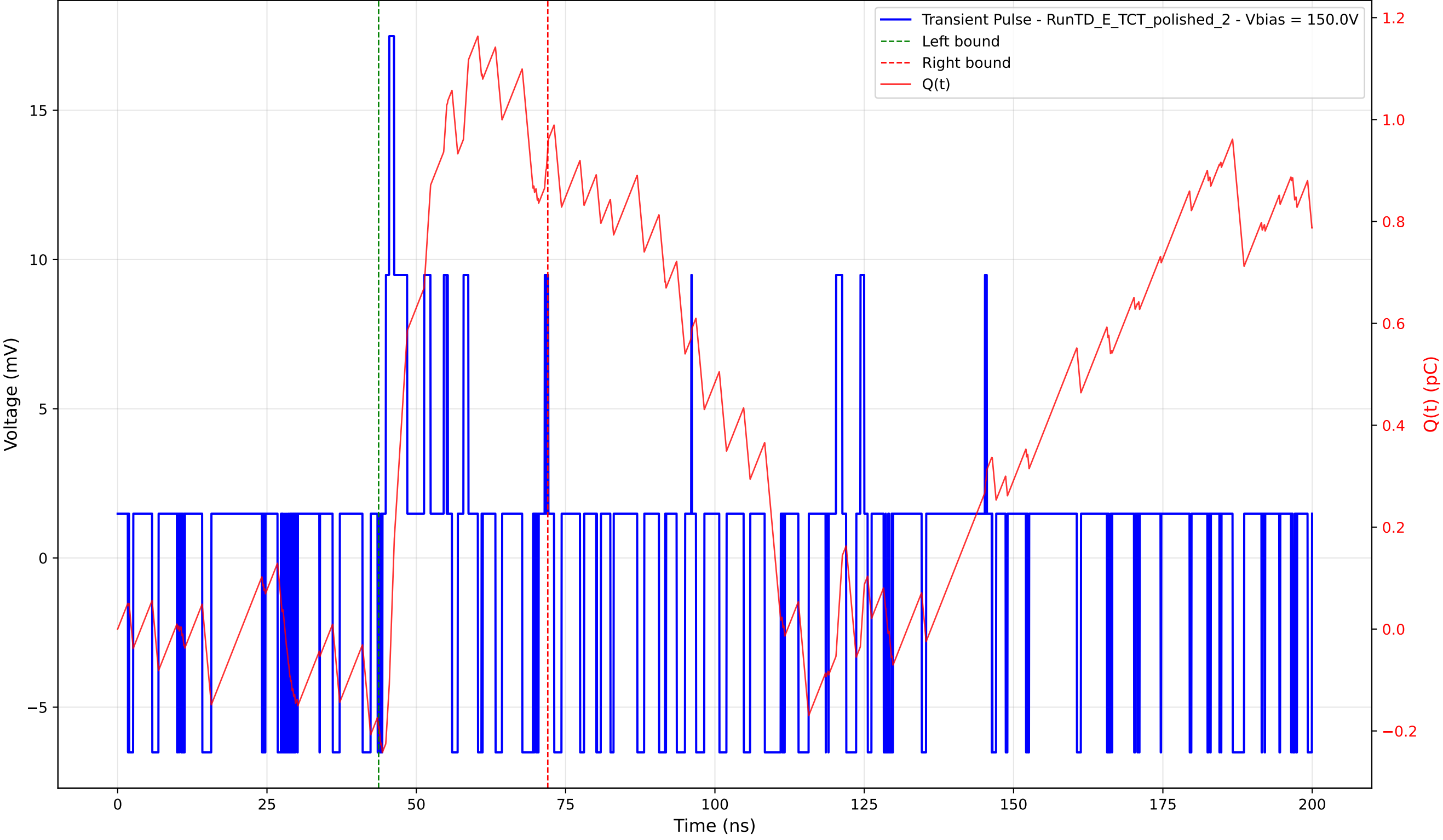
Transient Pulse - Sample: 4003 - Position: 40.0 \mu\text{m} - Charge: 1.14 pC - Rise Time: 0.58 ns
