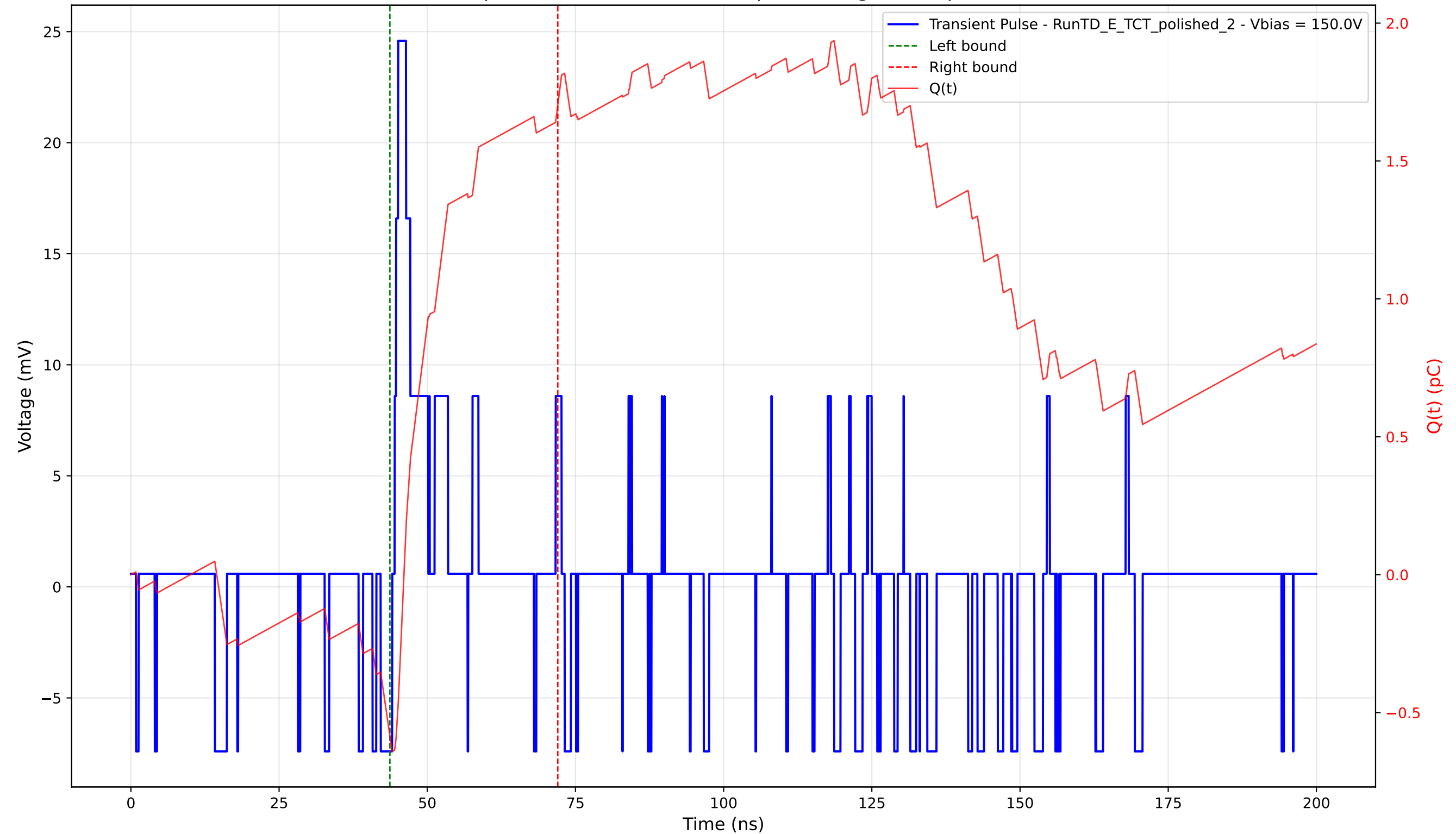
Transient Pulse - Sample: 4003 - Position: 650.0 \mu\text{m} - Charge: 2.29 pC - Rise Time: 0.60 ns
