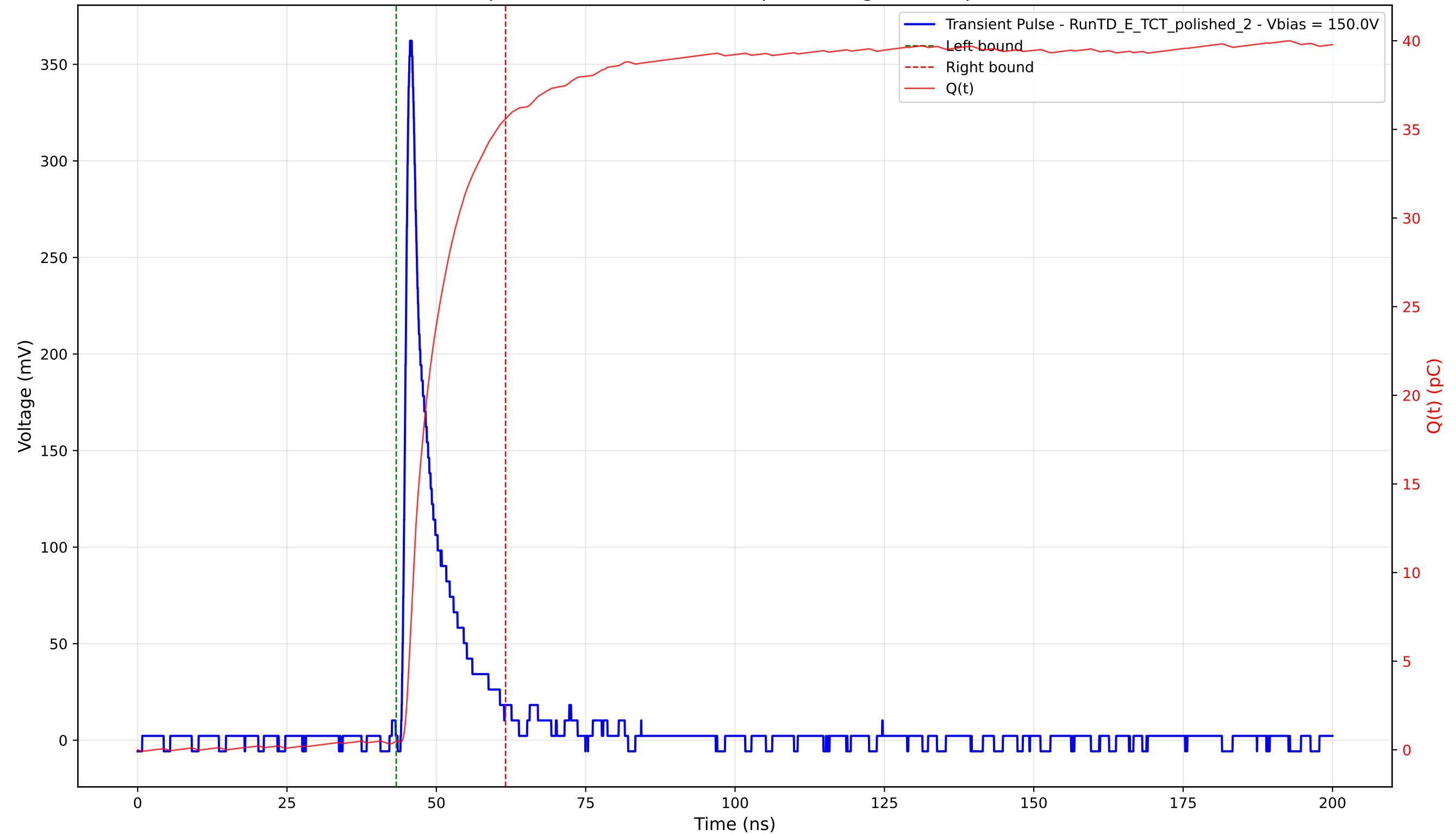
Transient Pulse - Sample: 4003 - Position: 245.0 \mu\text{m} - Charge: 35.11 pC - Rise Time: 1.02 ns
