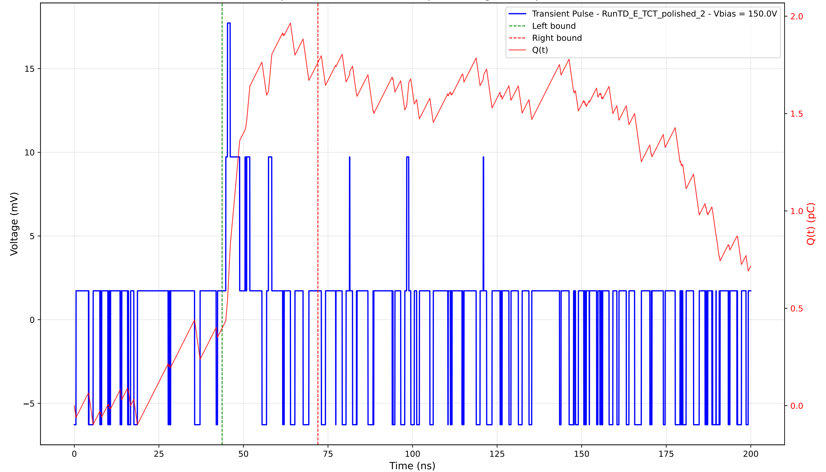
Transient Pulse - Sample: 4003 - Position: 70.0 \mu\text{m} - Charge: 1.36 pC - Rise Time: 0.52 ns
