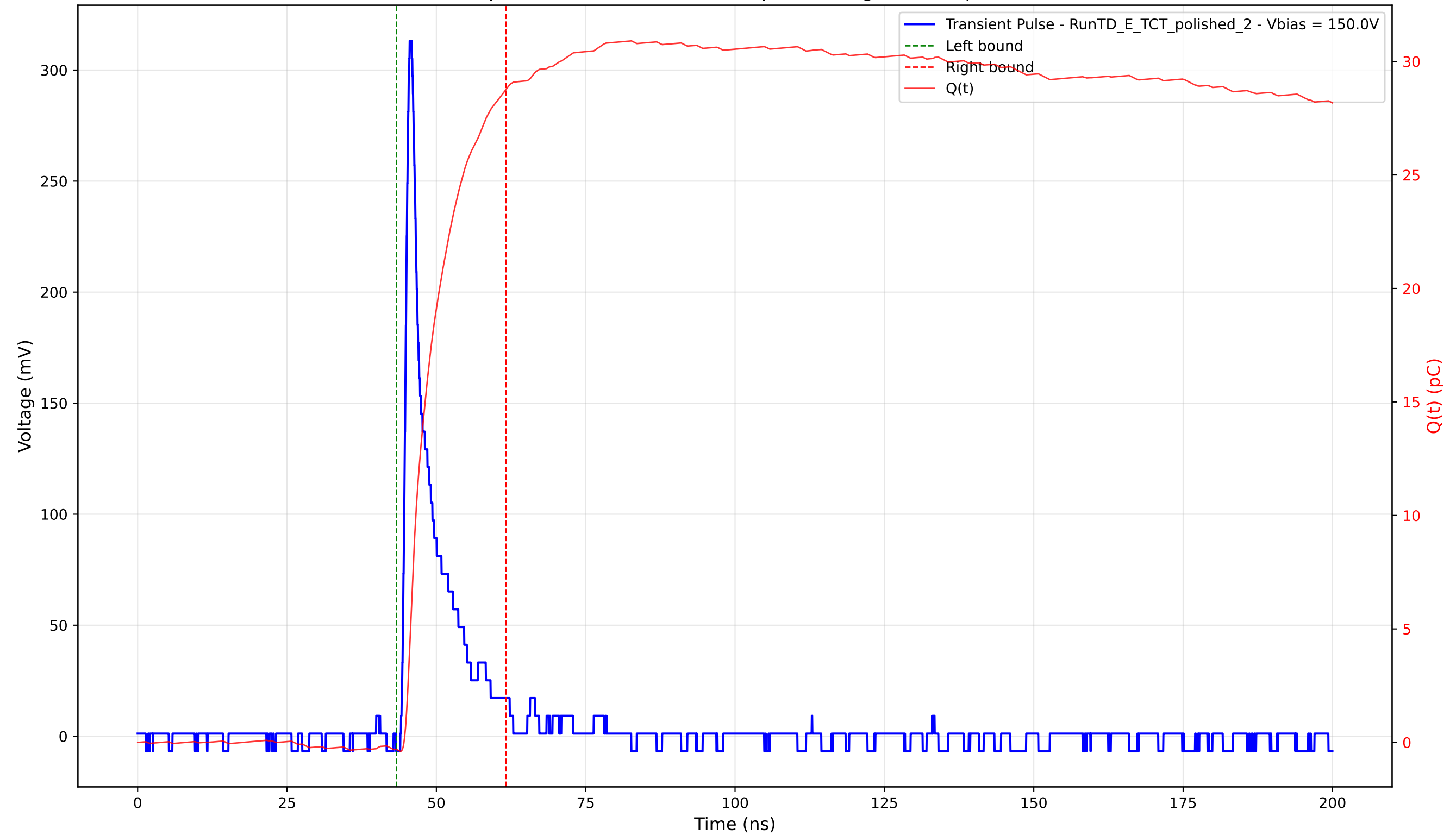
Transient Pulse - Sample: 4003 - Position: 215.0 \mu\text{m} - Charge: 29.09 pC - Rise Time: 1.04 ns
