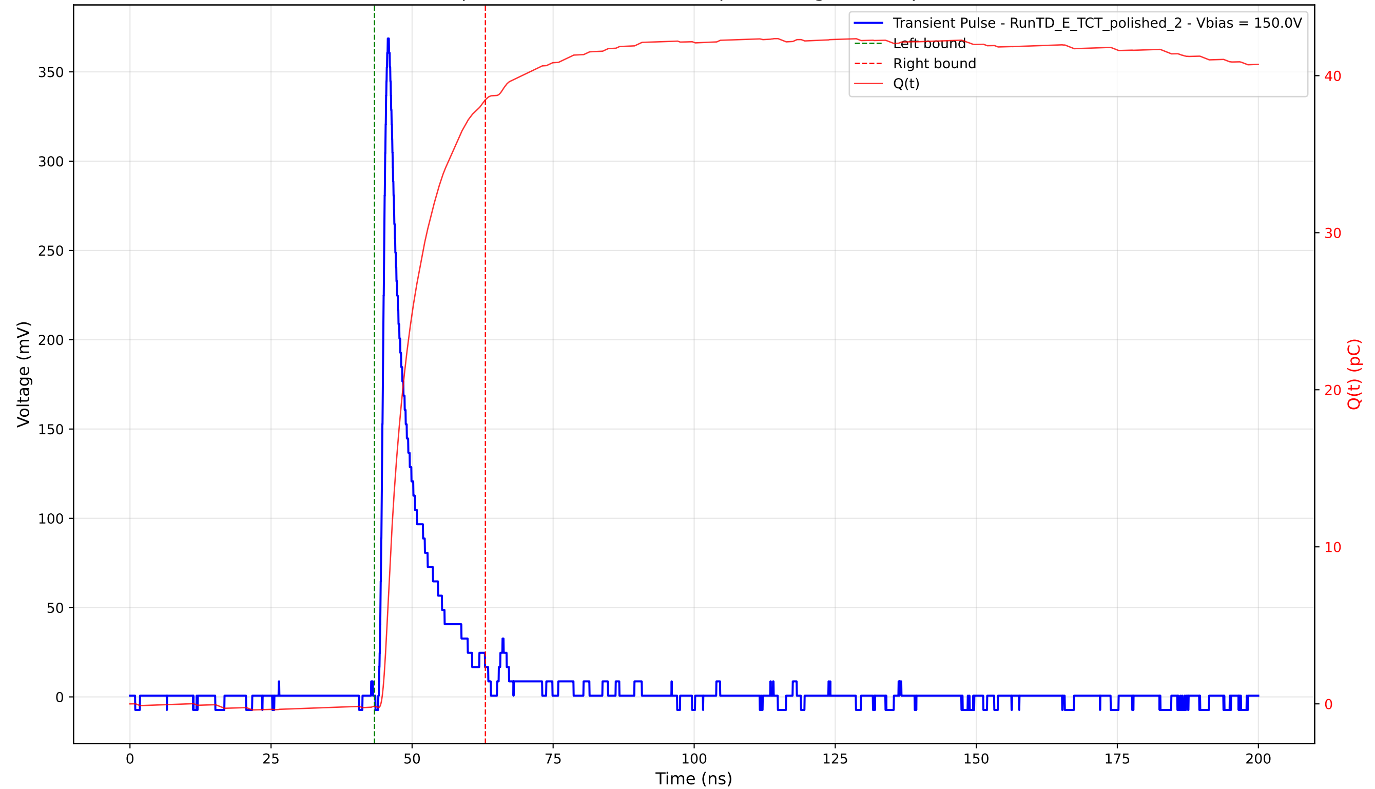
Transient Pulse - Sample: 4003 - Position: 295.0 \mu\text{m} - Charge: 38.63 pC - Rise Time: 1.07 ns
