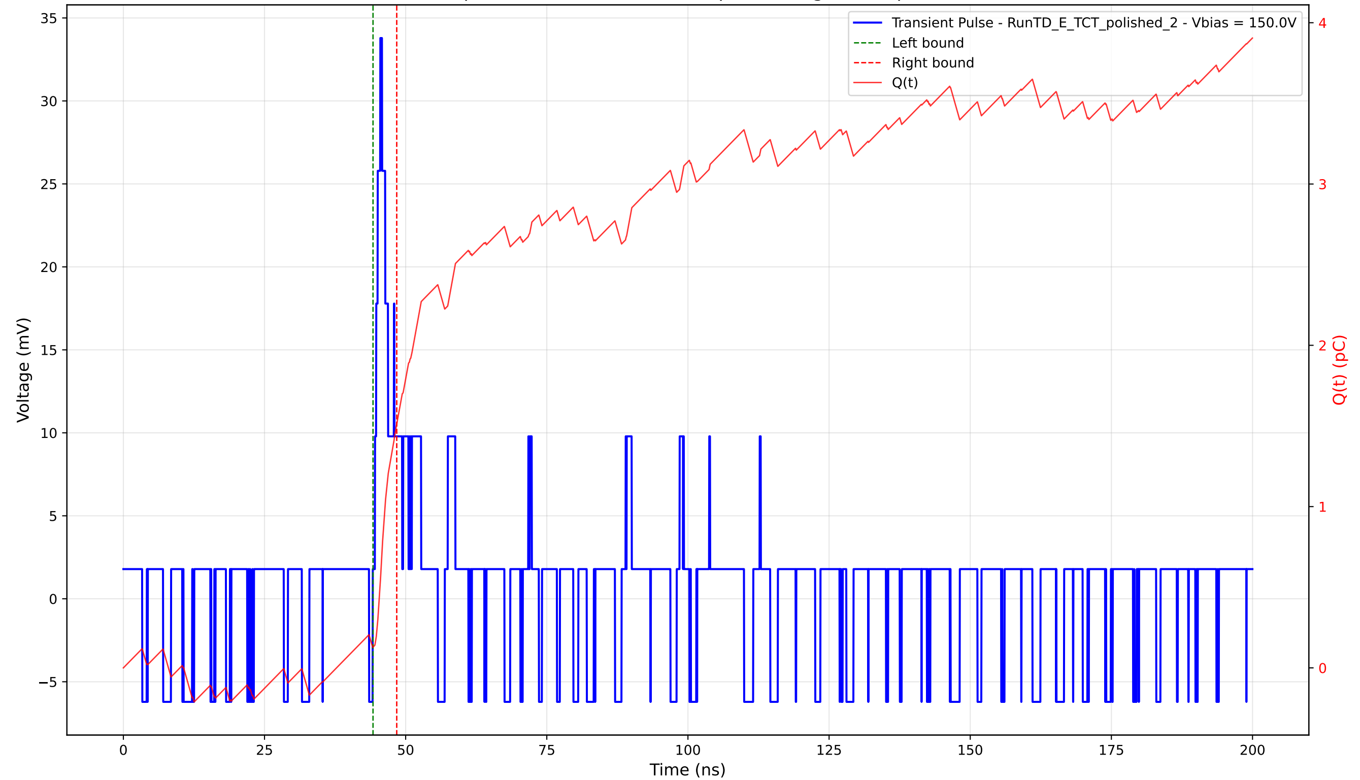
Transient Pulse - Sample: 4003 - Position: 615.0 \mu\text{m} - Charge: 1.38 pC - Rise Time: 0.96 ns
