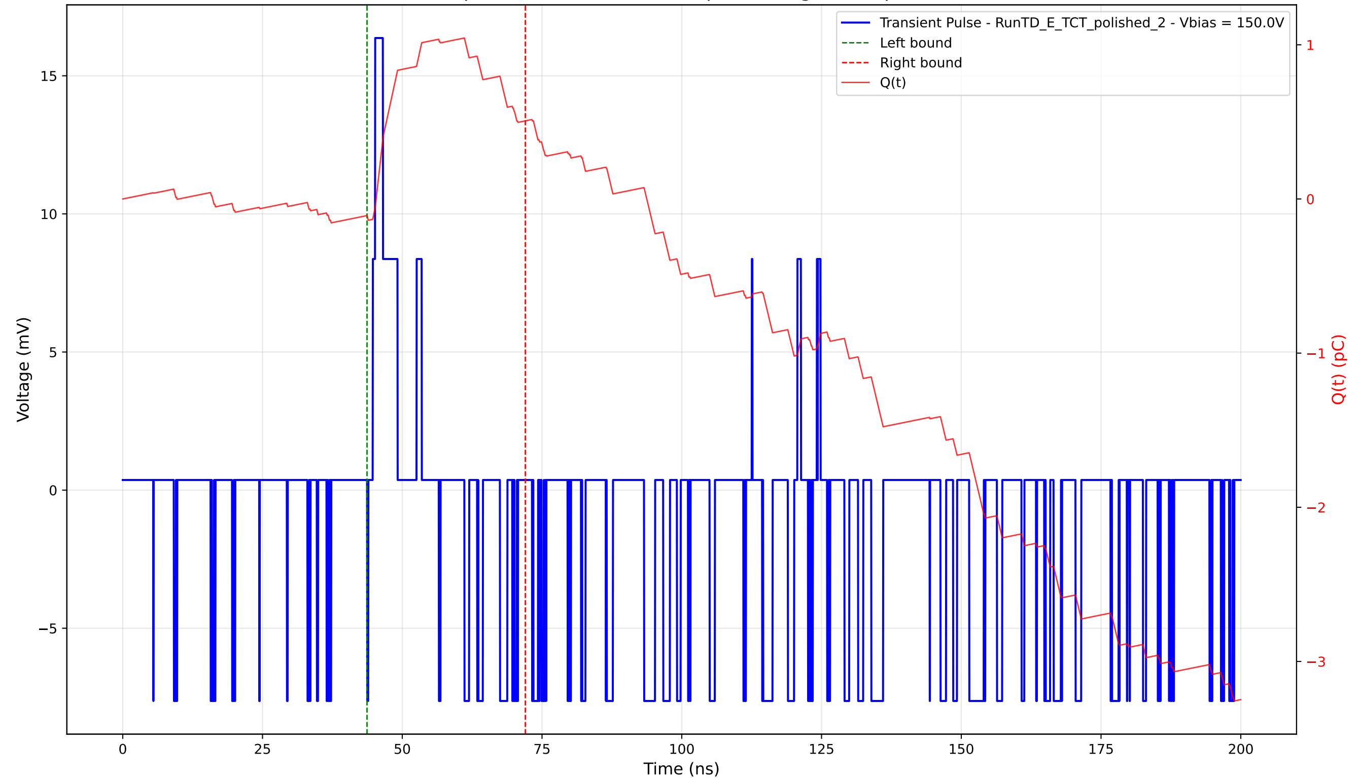
Transient Pulse - Sample: 4003 - Position: 75.0 \mu\text{m} - Charge: 0.61 pC - Rise Time: 0.44 ns
