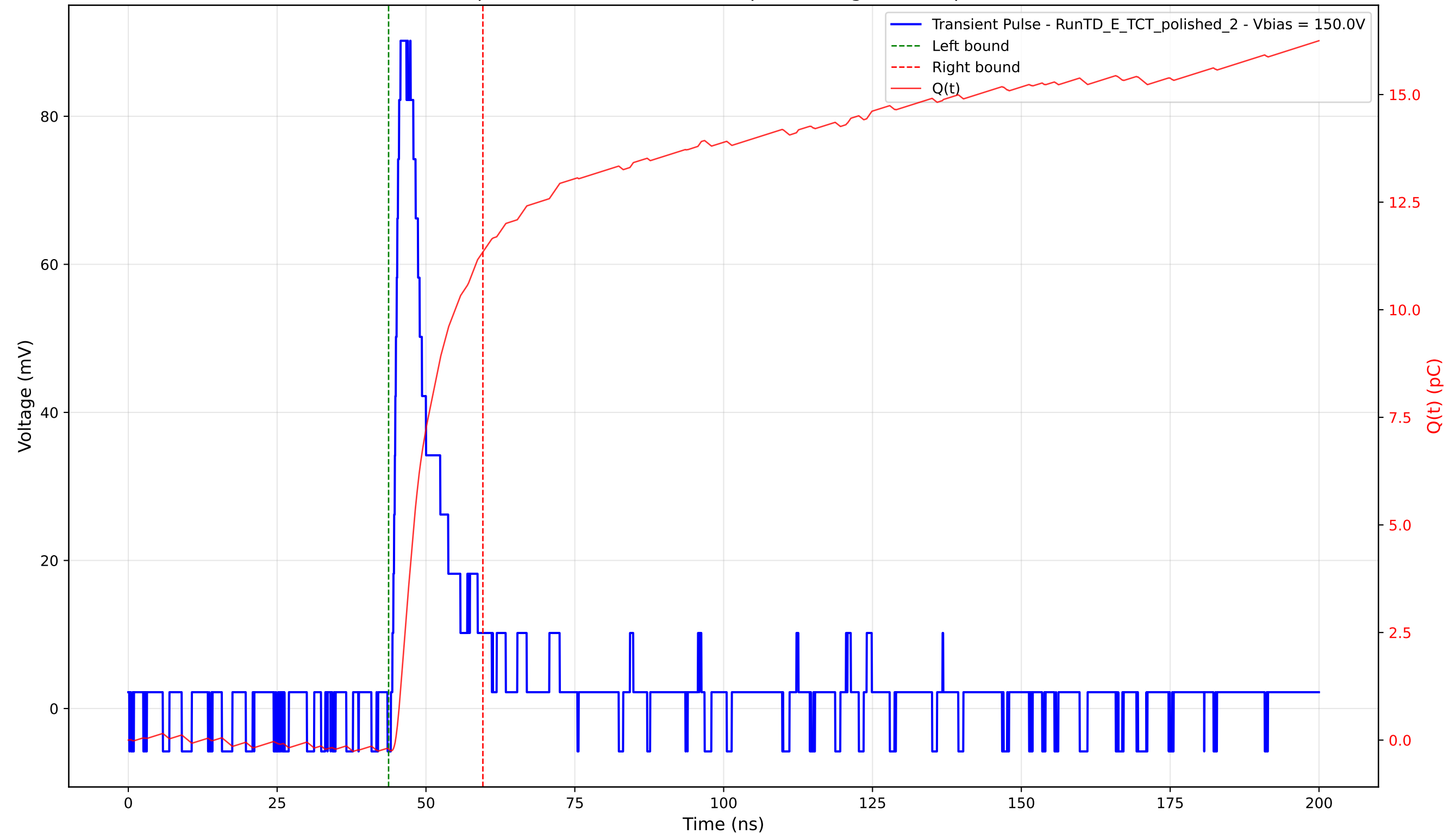
Transient Pulse - Sample: 4003 - Position: 445.0 \mu\text{m} - Charge: 11.55 pC - Rise Time: 1.12 ns
