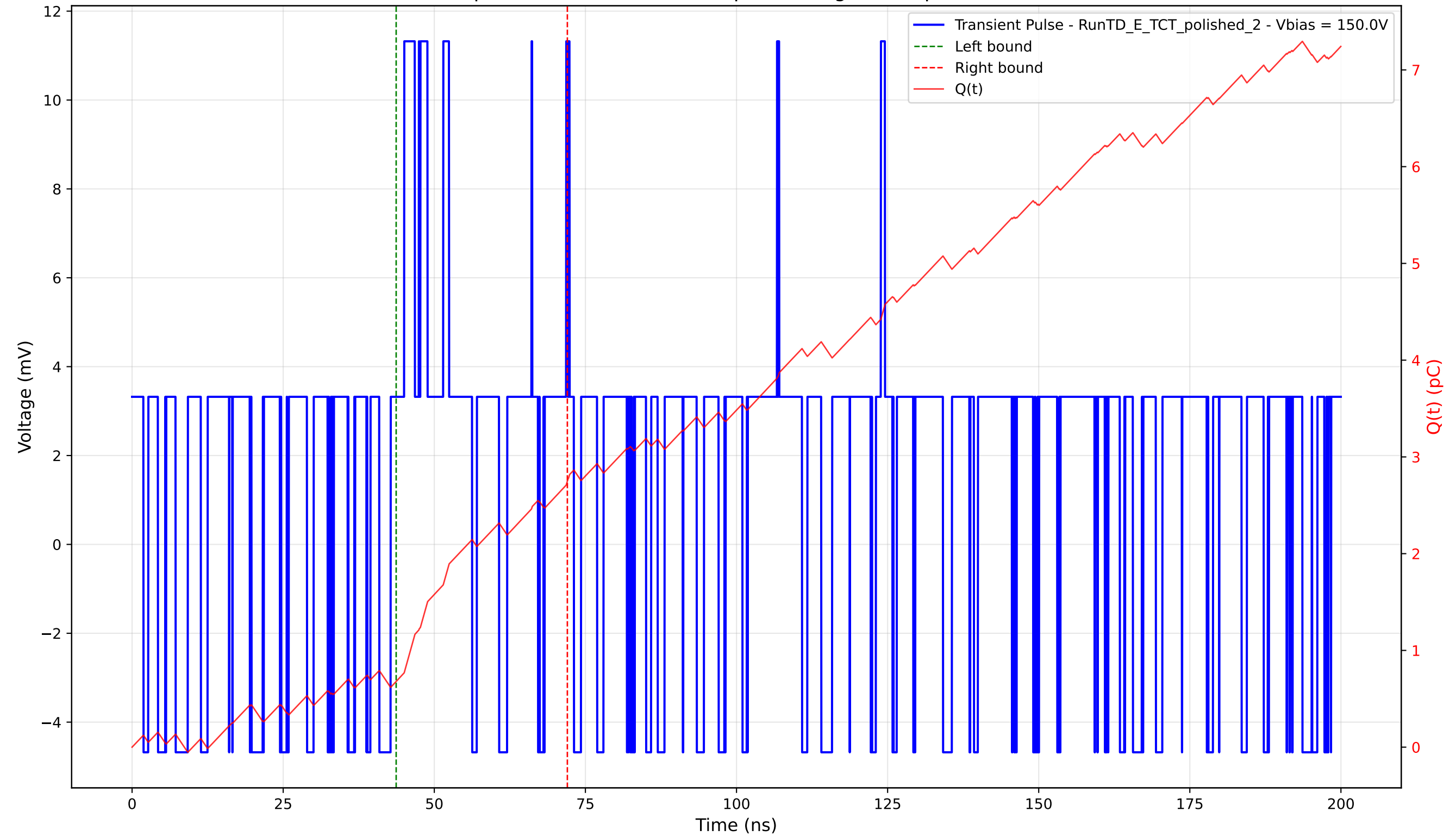
Transient Pulse - Sample: 4003 - Position: 25.0 \mu\text{m} - Charge: 2.07 pC - Rise Time: 0.00 ns (N/A)
