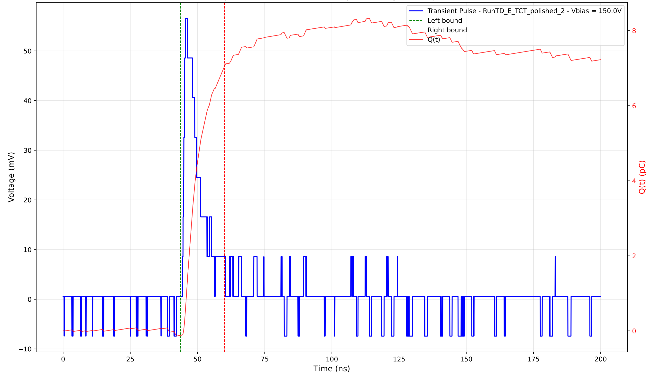
Transient Pulse - Sample: 4003 - Position: 480.0 \mu\text{m} - Charge: 7.16 pC - Rise Time: 1.13 ns
