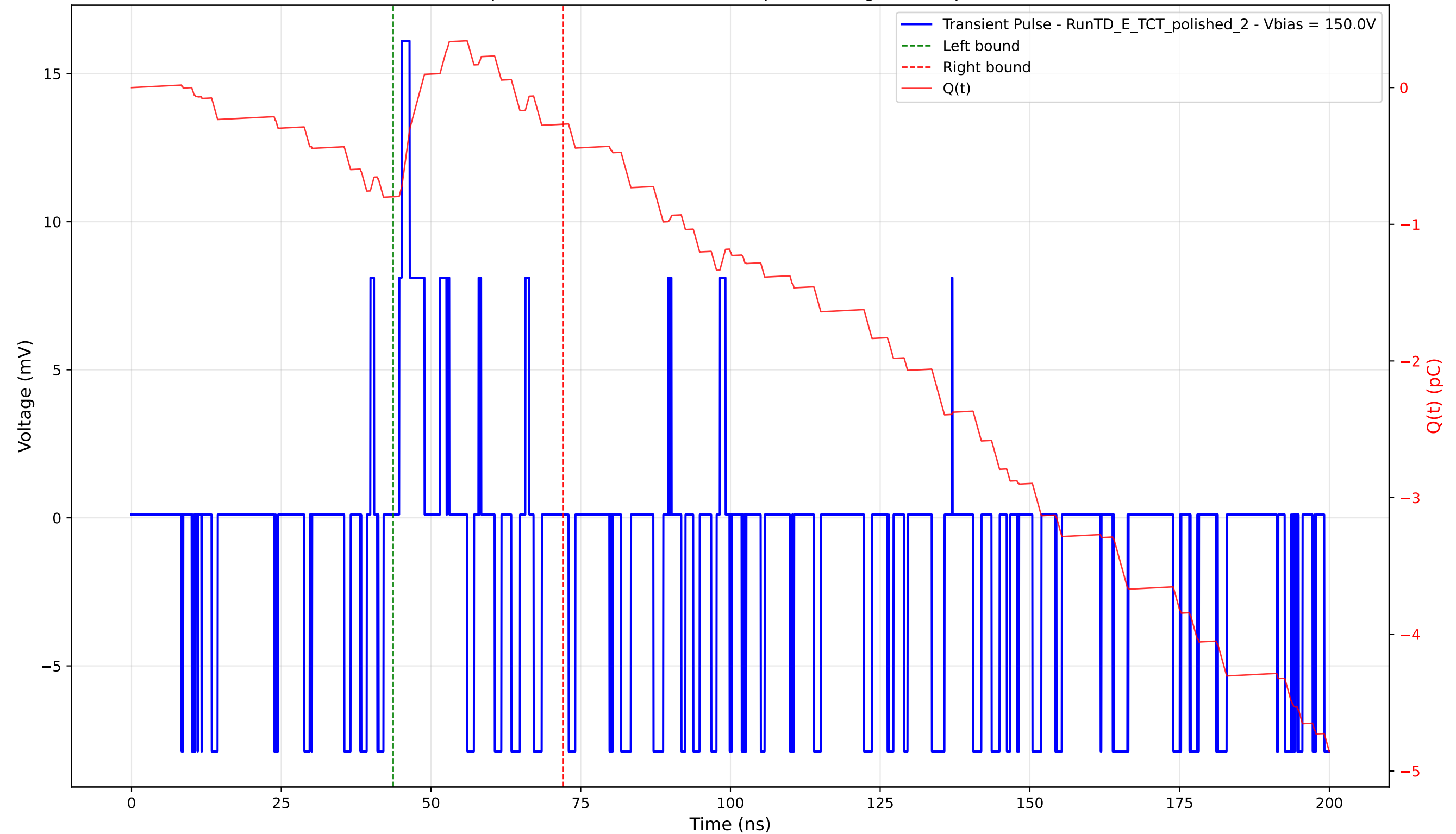
Transient Pulse - Sample: 4003 - Position: 785.0 \mu\text{m} - Charge: 0.53 pC - Rise Time: 0.46 ns
