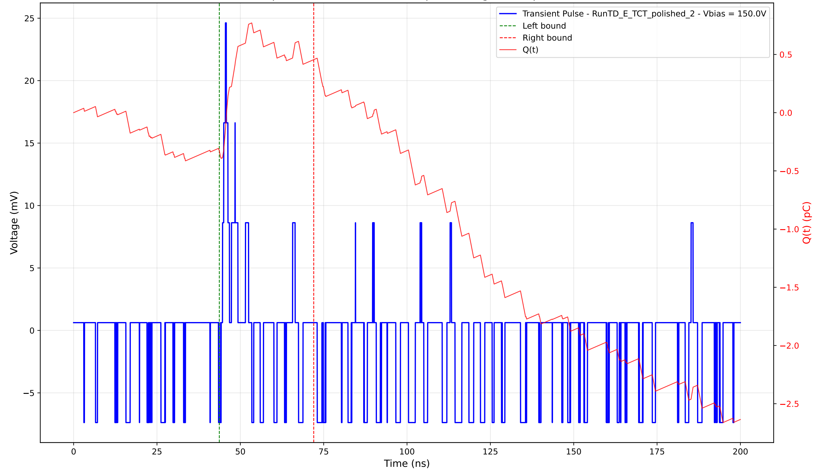
Transient Pulse - Sample: 4003 - Position: 735.0 \mu\text{m} - Charge: 0.78 pC - Rise Time: 0.88 ns
