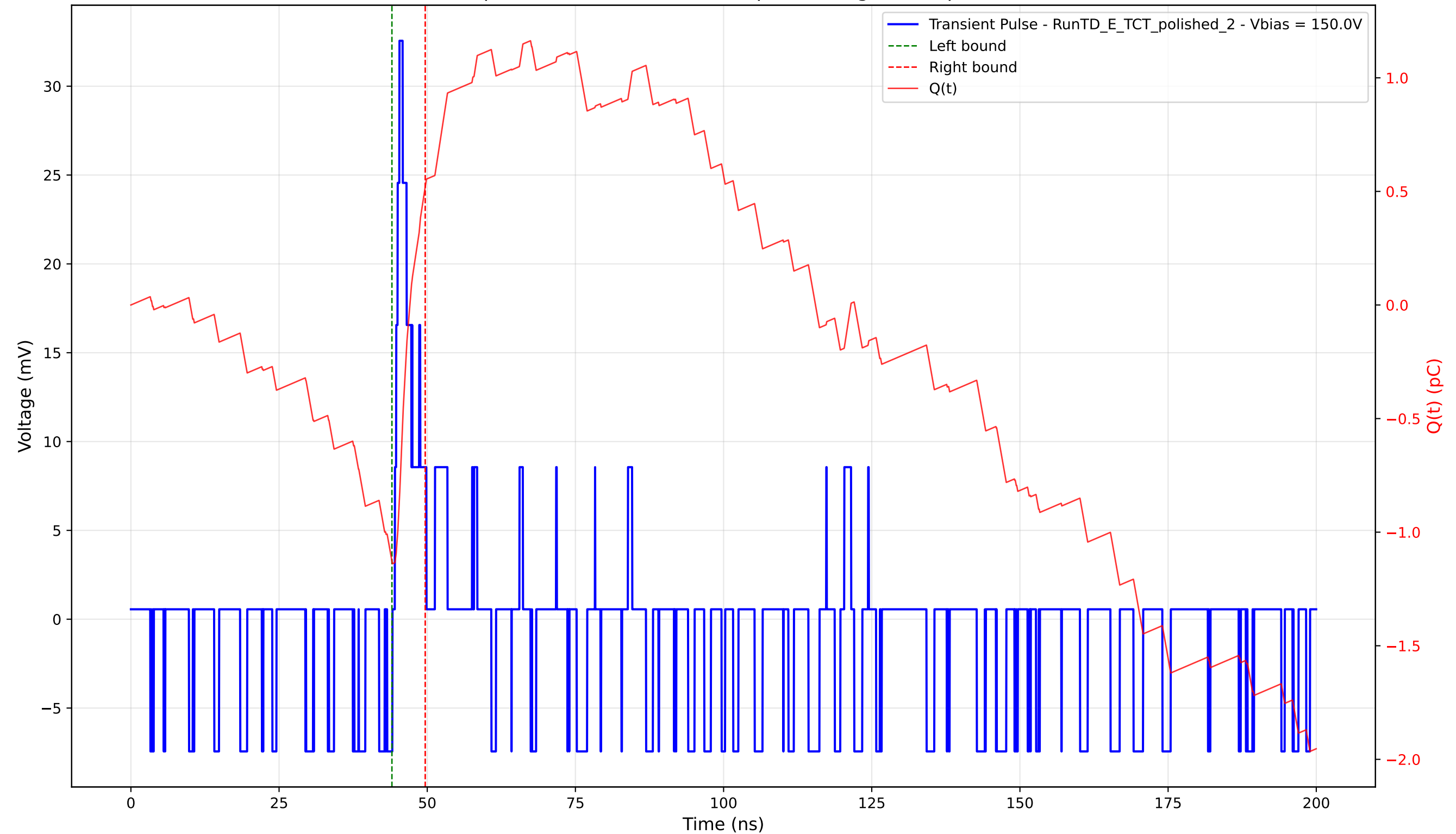
Transient Pulse - Sample: 4003 - Position: 580.0 \mu\text{m} - Charge: 1.65 pC - Rise Time: 0.77 ns
