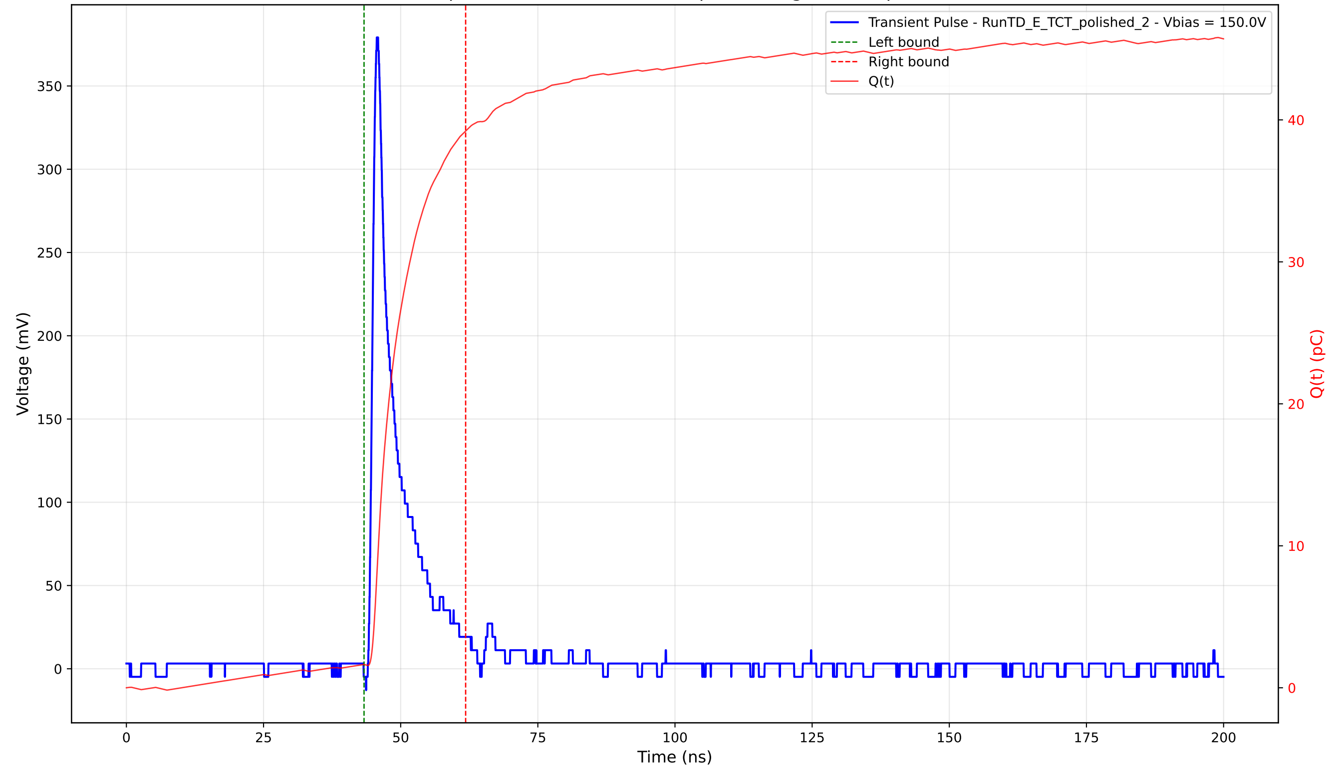
Transient Pulse - Sample: 4003 - Position: 260.0 \mu\text{m} - Charge: 37.58 pC - Rise Time: 1.05 ns
