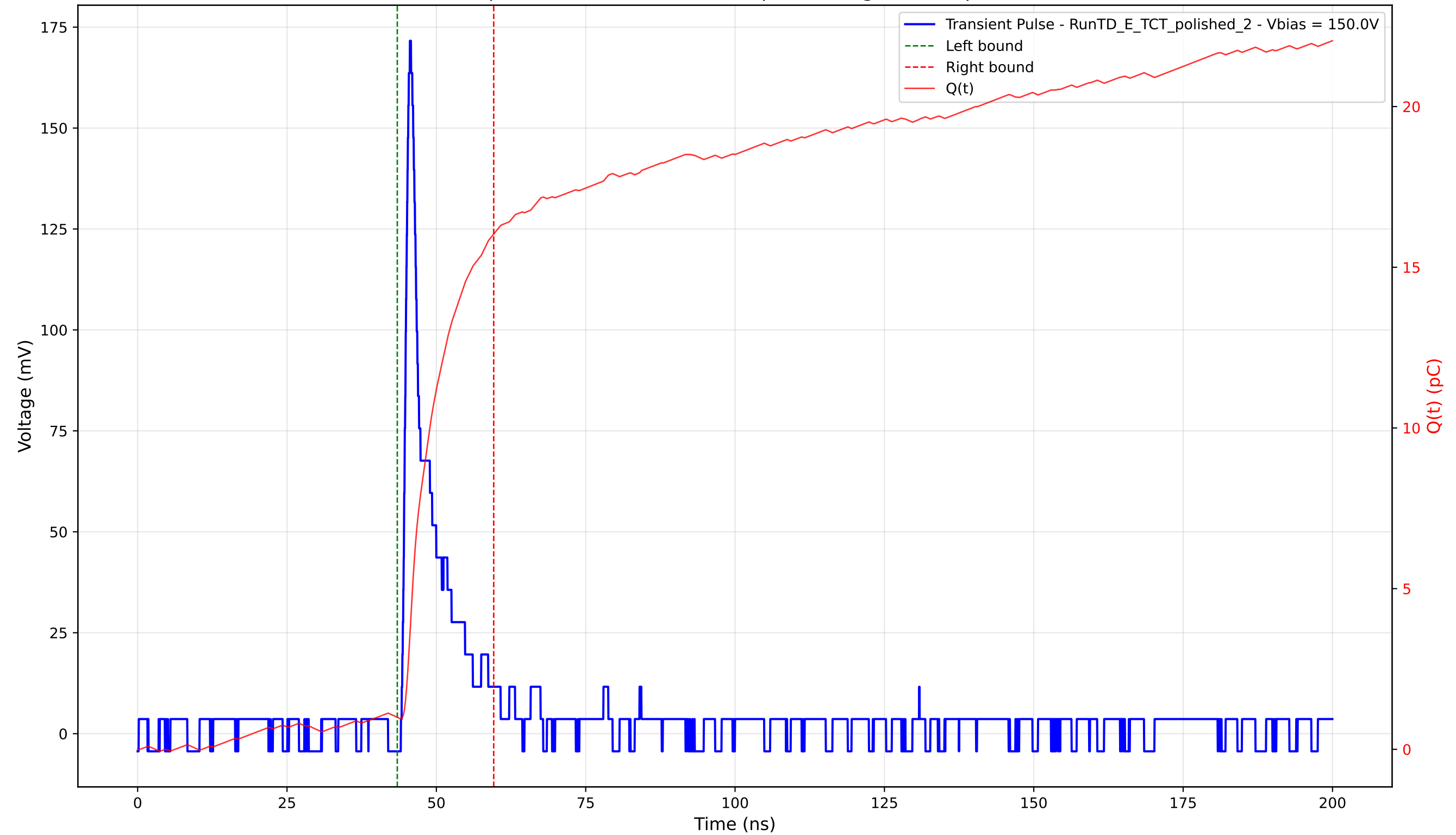
Transient Pulse - Sample: 4003 - Position: 165.0 \mu\text{m} - Charge: 15.04 pC - Rise Time: 1.01 ns
