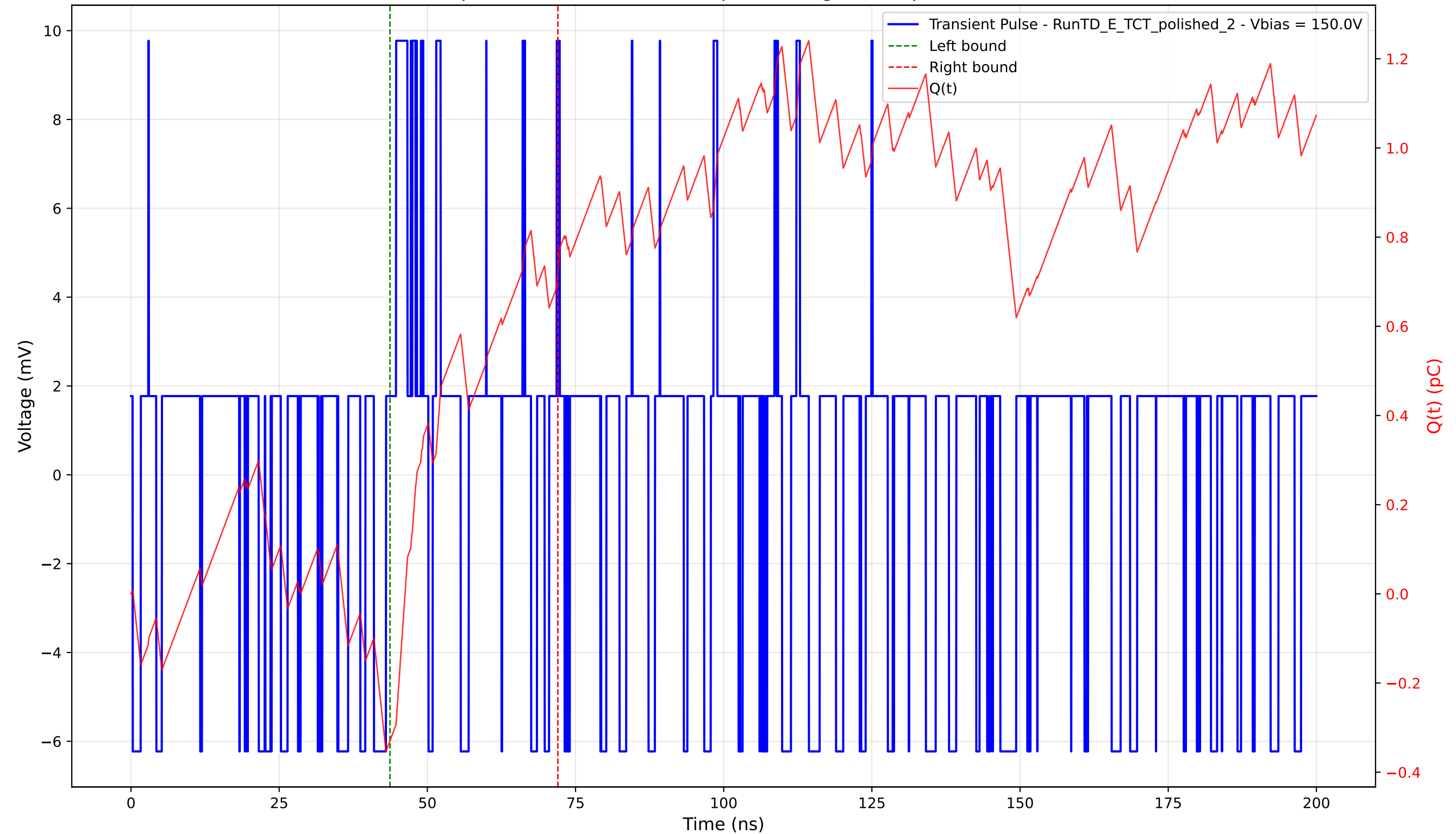
Transient Pulse - Sample: 4003 - Position: 20.0 \mu\text{m} - Charge: 1.05 pC - Rise Time: 0.00 ns (N/A)
