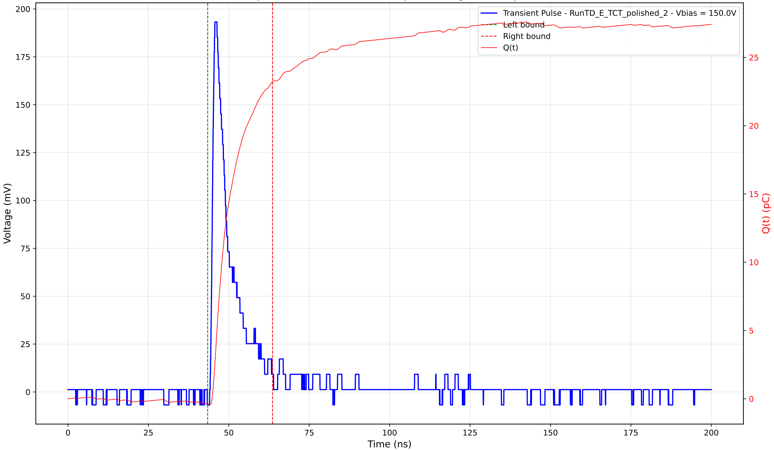
Transient Pulse - Sample: 4003 - Position: 385.0 \mu\text{m} - Charge: 23.59 pC - Rise Time: 1.05 ns
