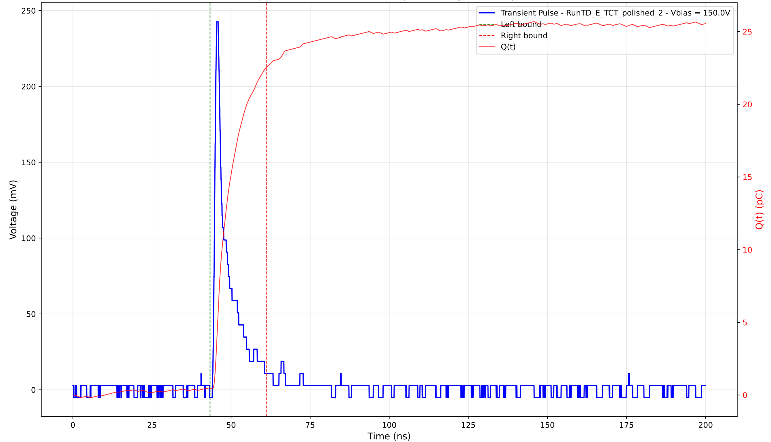
Transient Pulse - Sample: 4003 - Position: 190.0 \mu\text{m} - Charge: 22.08 pC - Rise Time: 0.95 ns
