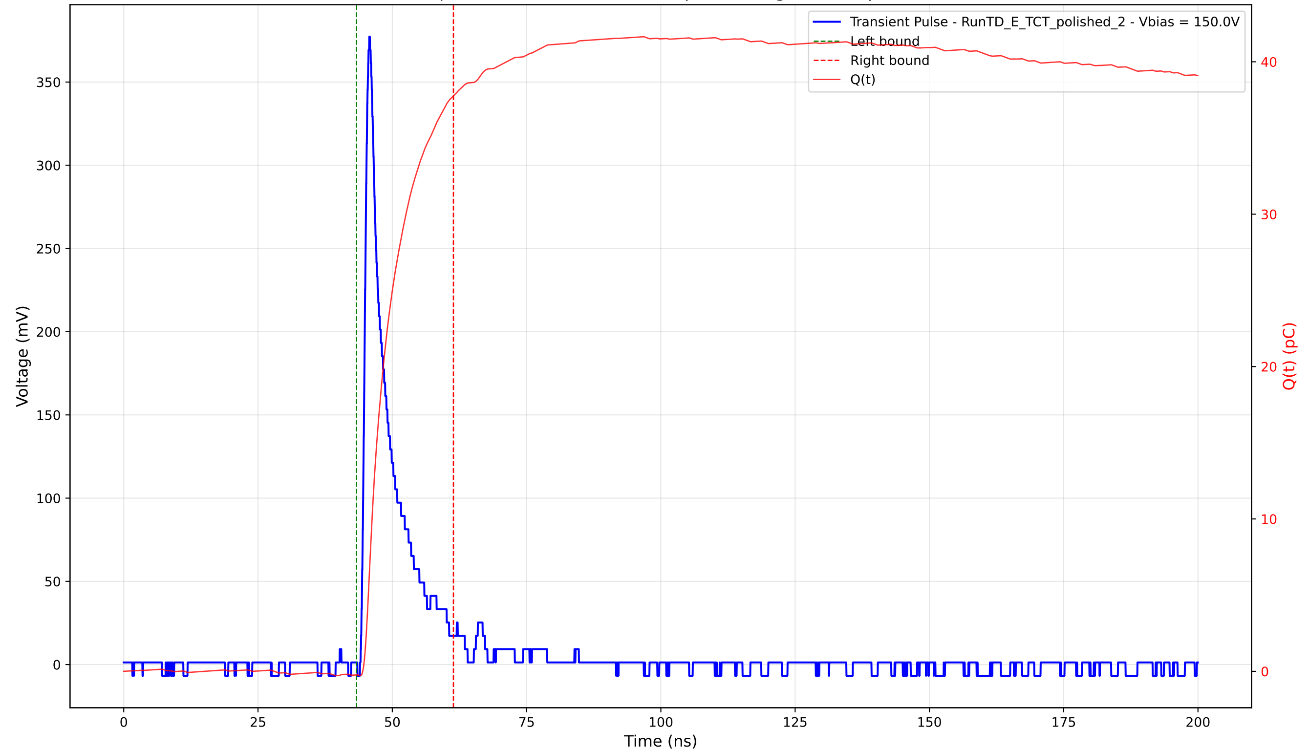
Transient Pulse - Sample: 4003 - Position: 285.0 \mu\text{m} - Charge: 37.98 pC - Rise Time: 1.05 ns
