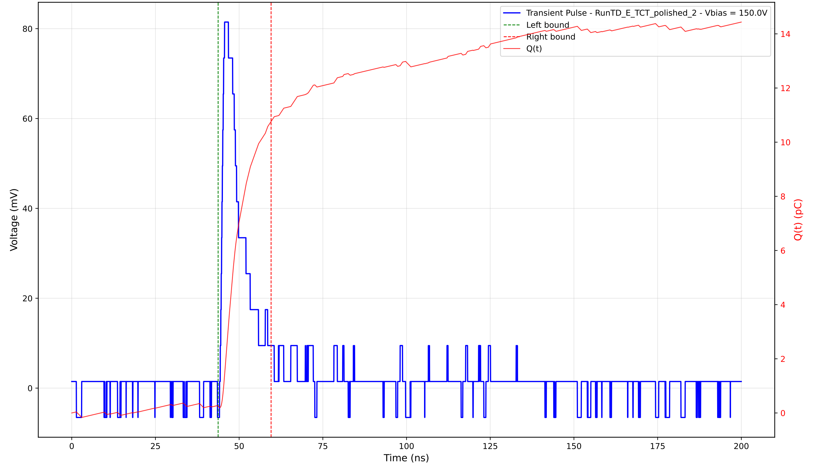
Transient Pulse - Sample: 4003 - Position: 450.0 \mu\text{m} - Charge: 10.52 pC - Rise Time: 1.00 ns
