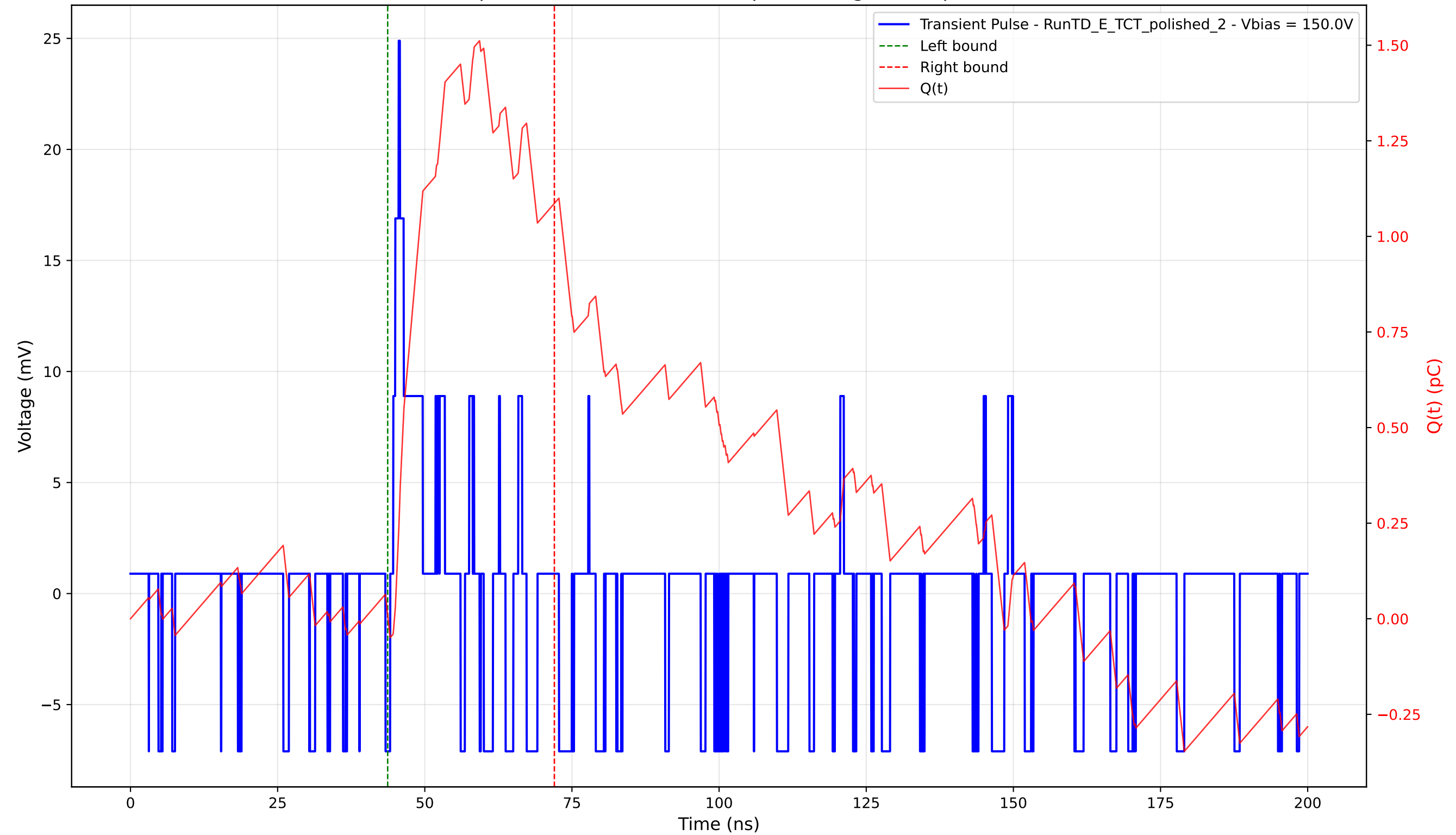
Transient Pulse - Sample: 4003 - Position: 740.0 \mu\text{m} - Charge: 1.08 pC - Rise Time: 0.94 ns
