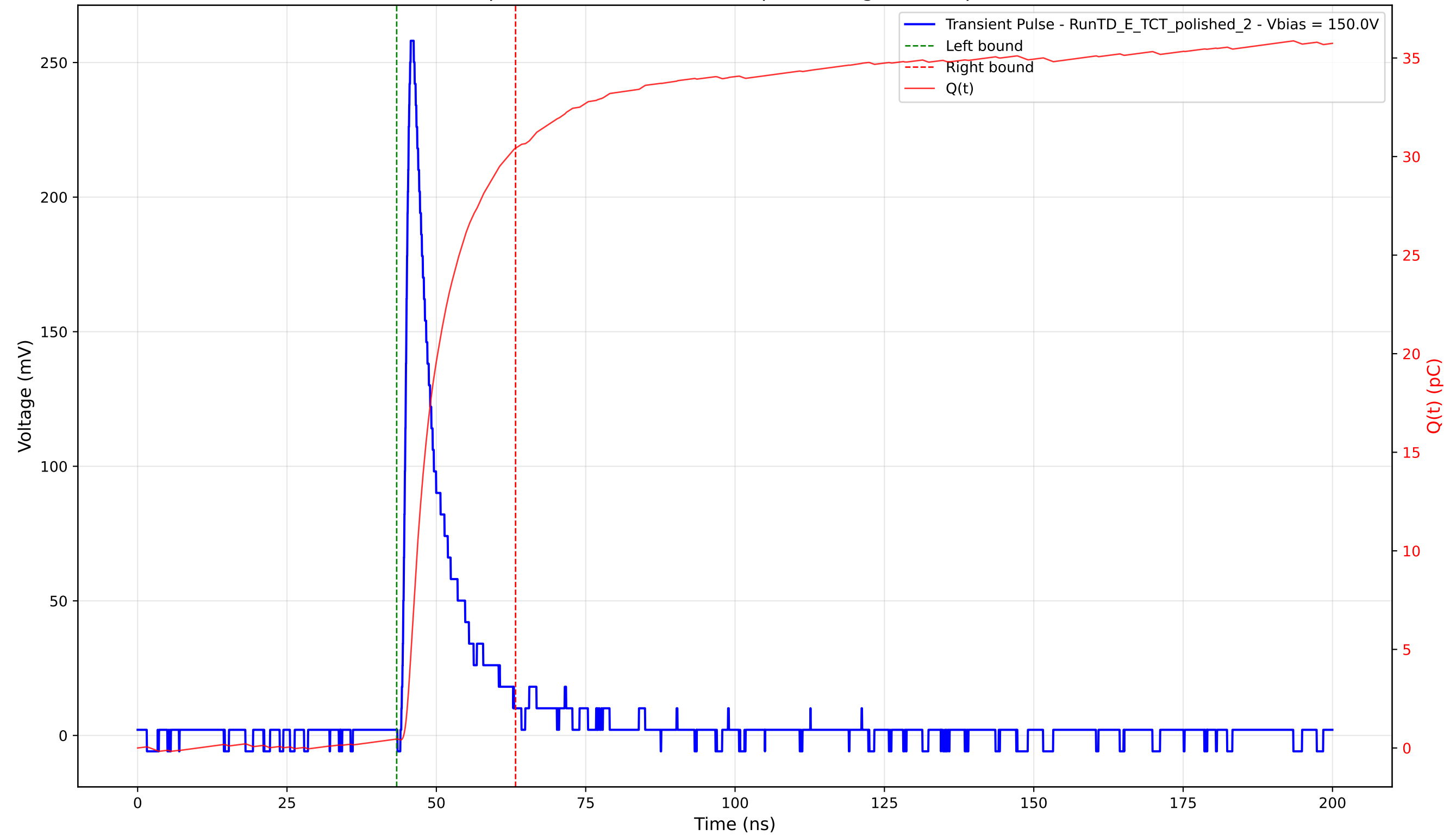
Transient Pulse - Sample: 4003 - Position: 355.0 \mu\text{m} - Charge: 29.96 pC - Rise Time: 1.12 ns
