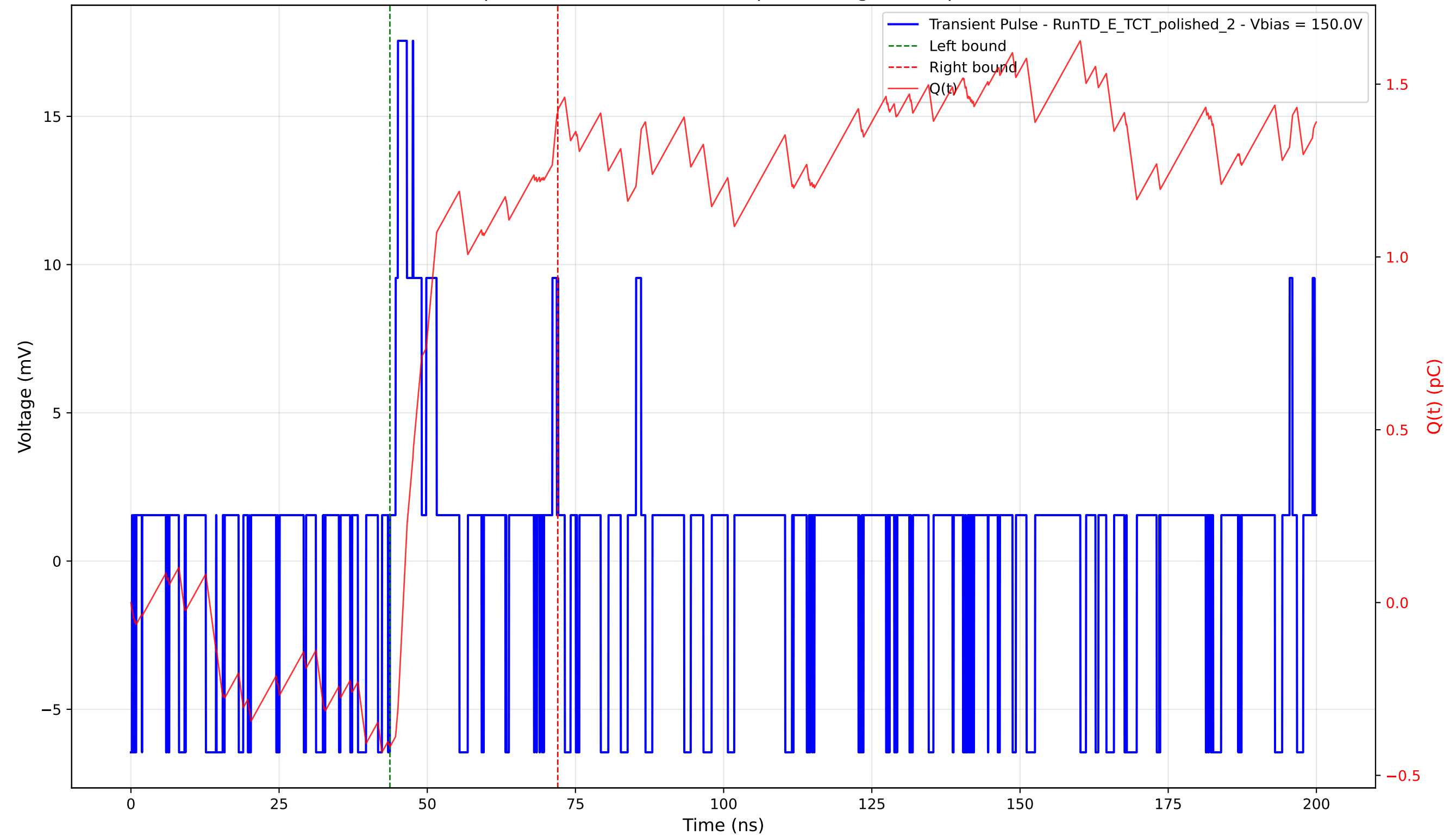
Transient Pulse - Sample: 4003 - Position: 790.0 \mu\text{m} - Charge: 1.83 pC - Rise Time: 0.40 ns
