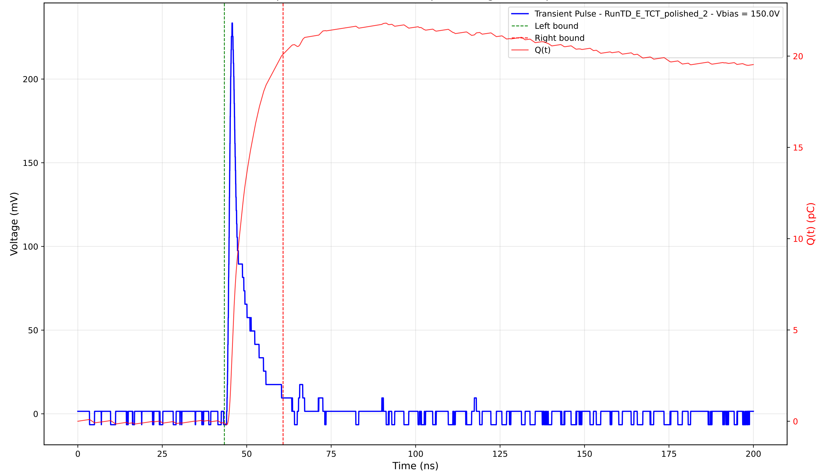
Transient Pulse - Sample: 4003 - Position: 185.0 \mu\text{m} - Charge: 20.21 pC - Rise Time: 1.07 ns
