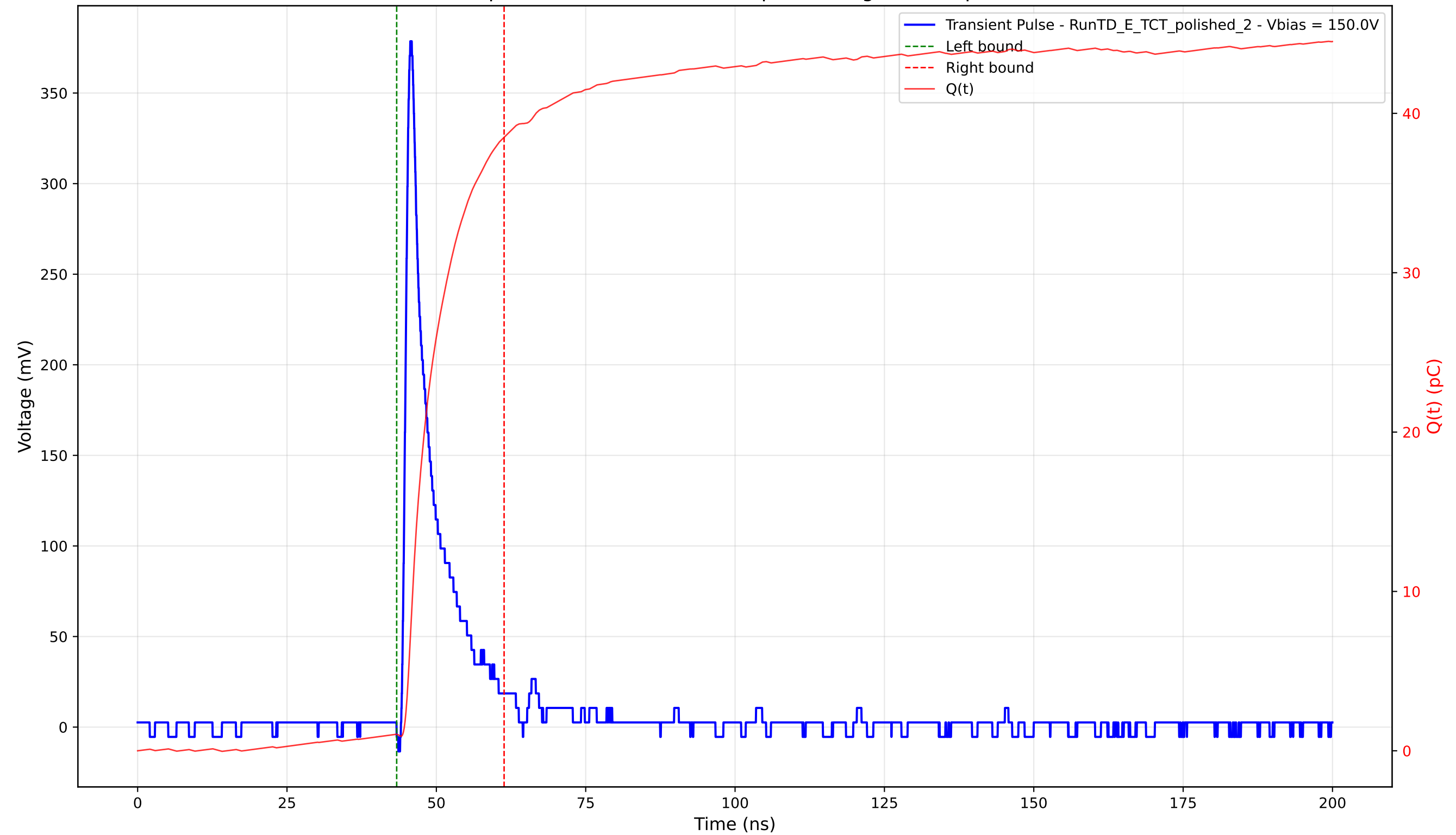
Transient Pulse - Sample: 4003 - Position: 265.0 \mu\text{m} - Charge: 37.46 pC - Rise Time: 1.03 ns
