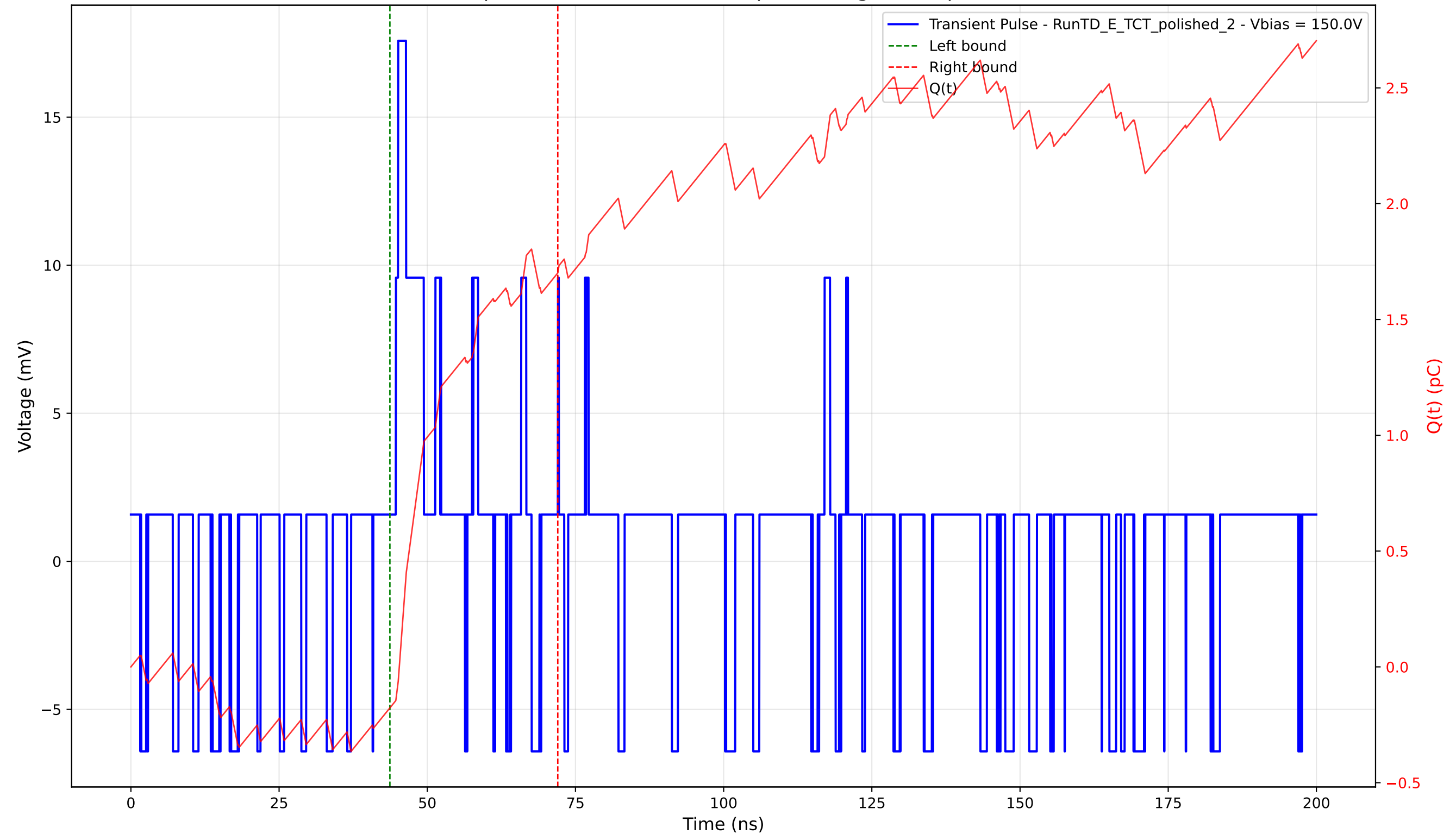
Transient Pulse - Sample: 4003 - Position: 655.0 \mu\text{m} - Charge: 1.88 pC - Rise Time: 0.40 ns
