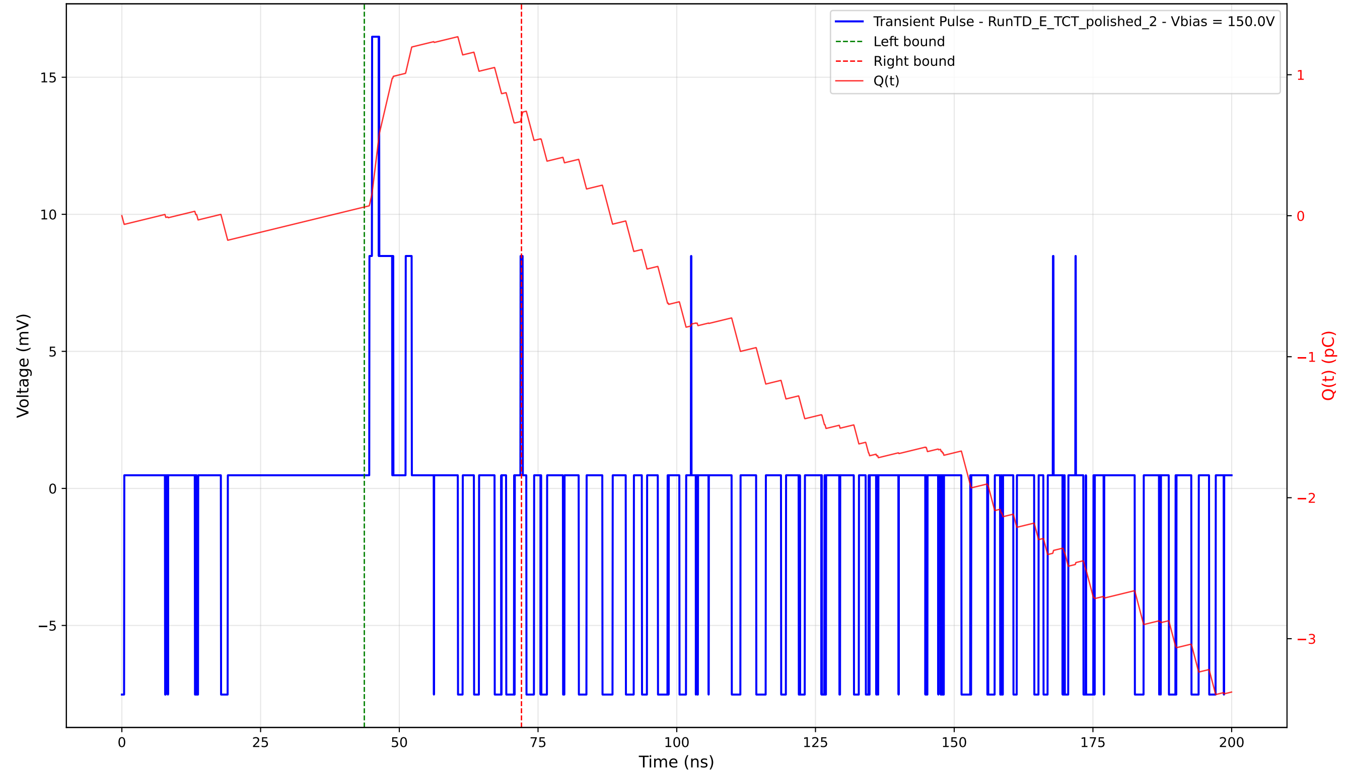
Transient Pulse - Sample: 4003 - Position: 55.0 \mu\text{m} - Charge: 0.63 pC - Rise Time: 0.50 ns
