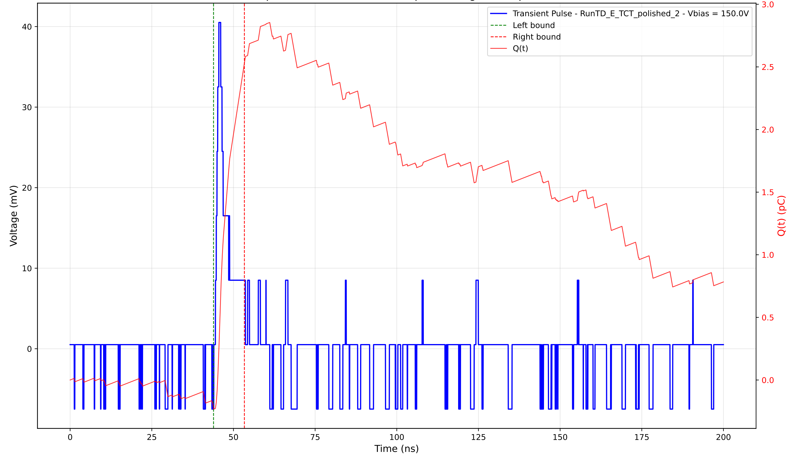
Transient Pulse - Sample: 4003 - Position: 640.0 \mu\text{m} - Charge: 2.75 pC - Rise Time: 1.05 ns
