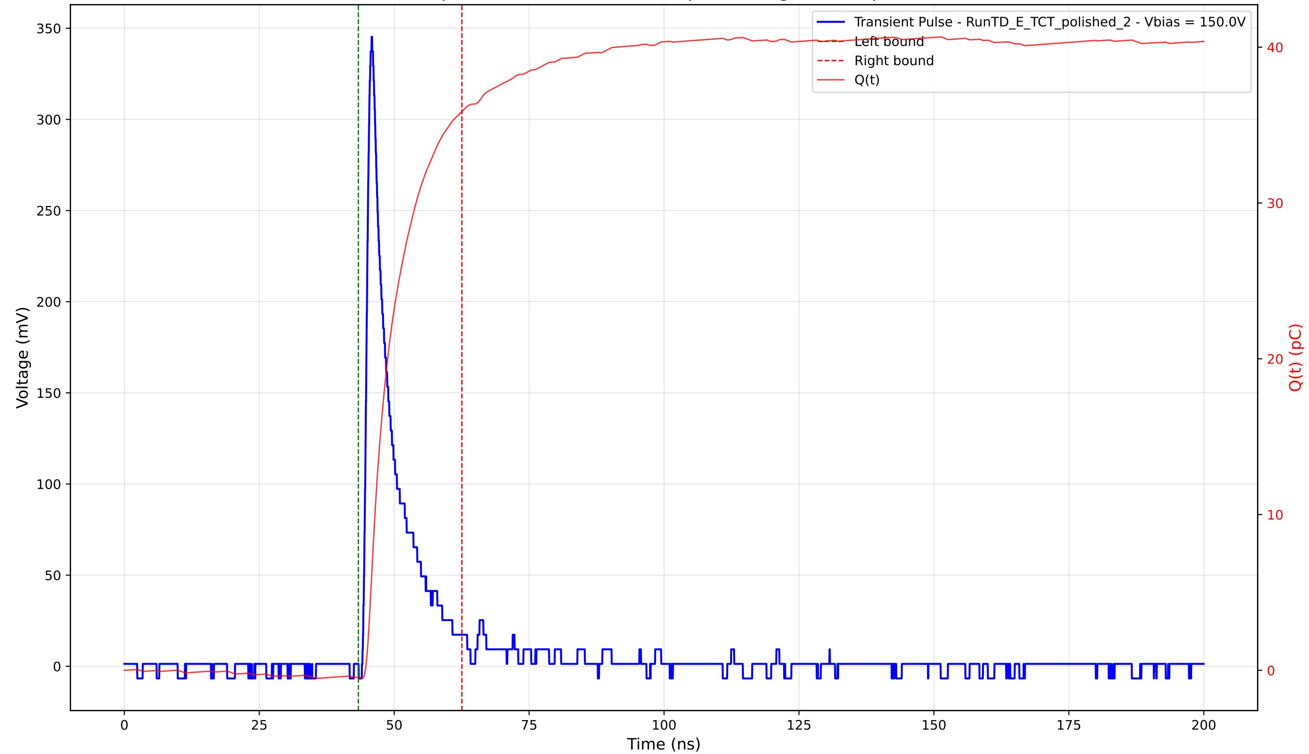
Transient Pulse - Sample: 4003 - Position: 315.0 \mu\text{m} - Charge: 36.31 pC - Rise Time: 1.08 ns
