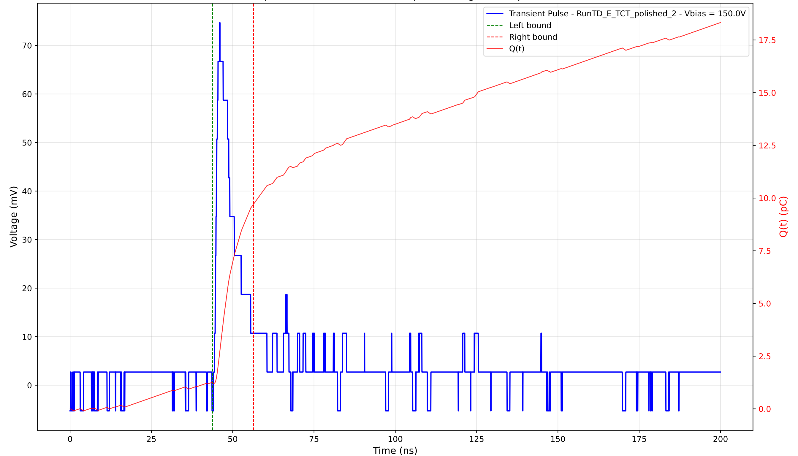
Transient Pulse - Sample: 4003 - Position: 465.0 \mu\text{m} - Charge: 8.47 pC - Rise Time: 1.59 ns
