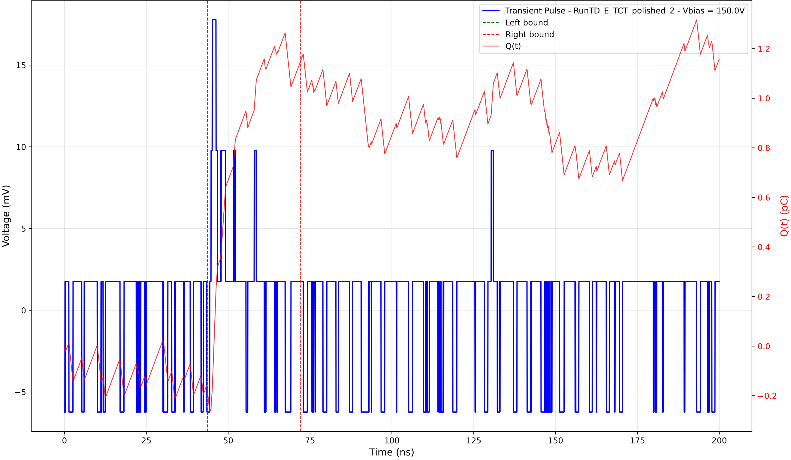
Transient Pulse - Sample: 4003 - Position: 50.0 \mu\text{m} - Charge: 1.33 pC - Rise Time: 0.38 ns
