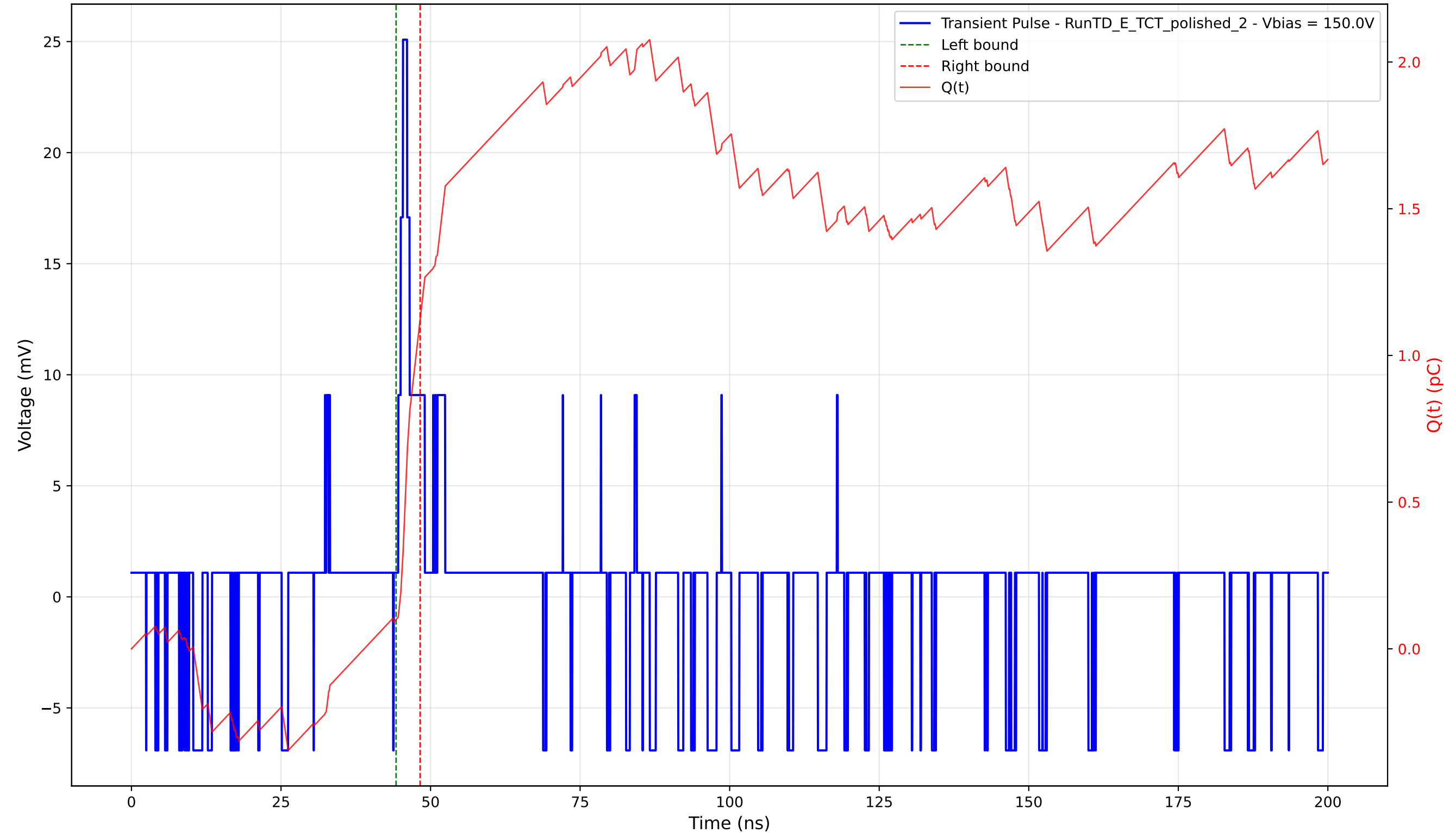
Transient Pulse - Sample: 4003 - Position: 800.0 \mu\text{m} - Charge: 1.03 pC - Rise Time: 0.80 ns
