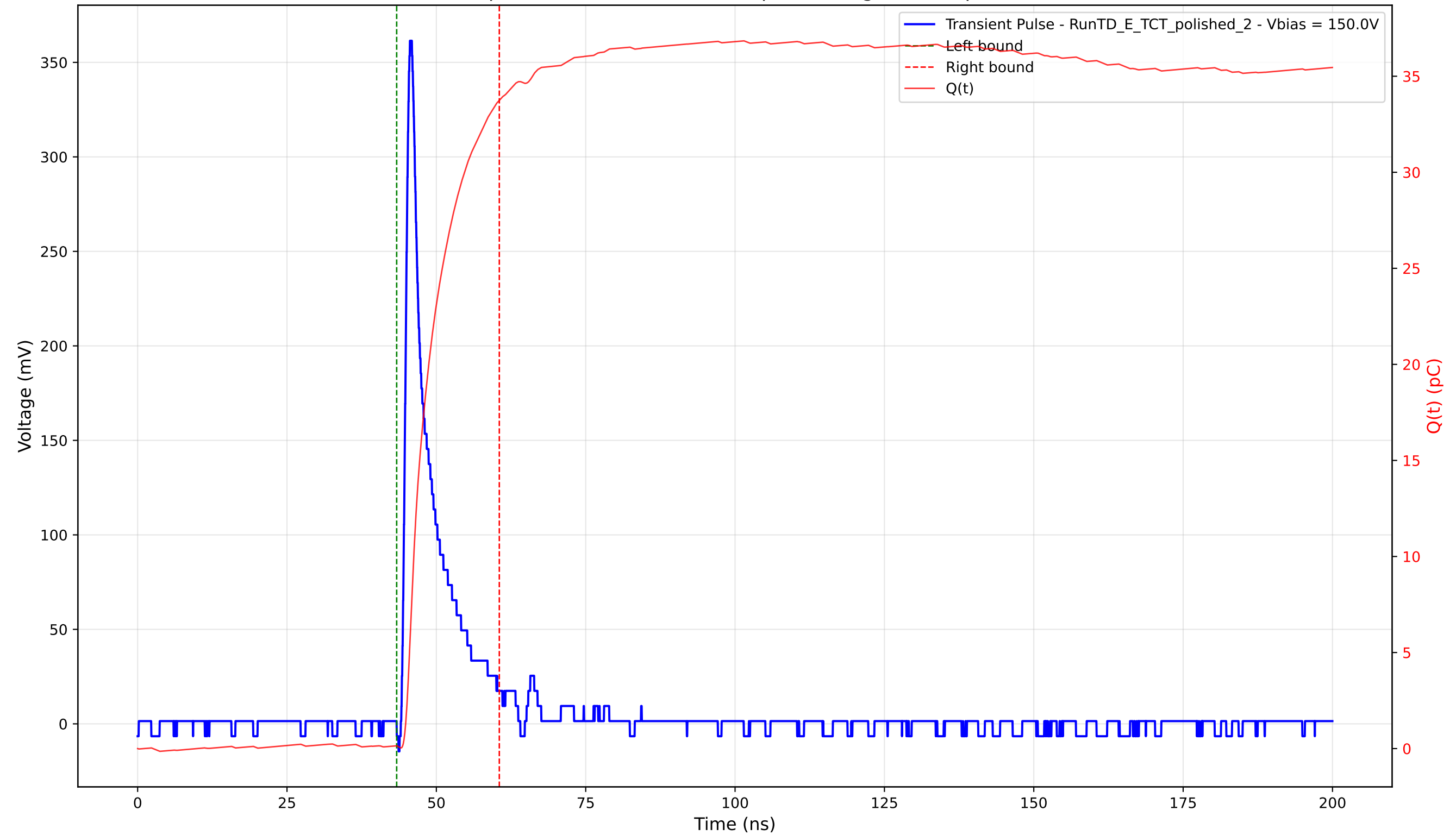
Transient Pulse - Sample: 4003 - Position: 240.0 \mu\text{m} - Charge: 33.60 pC - Rise Time: 1.01 ns
