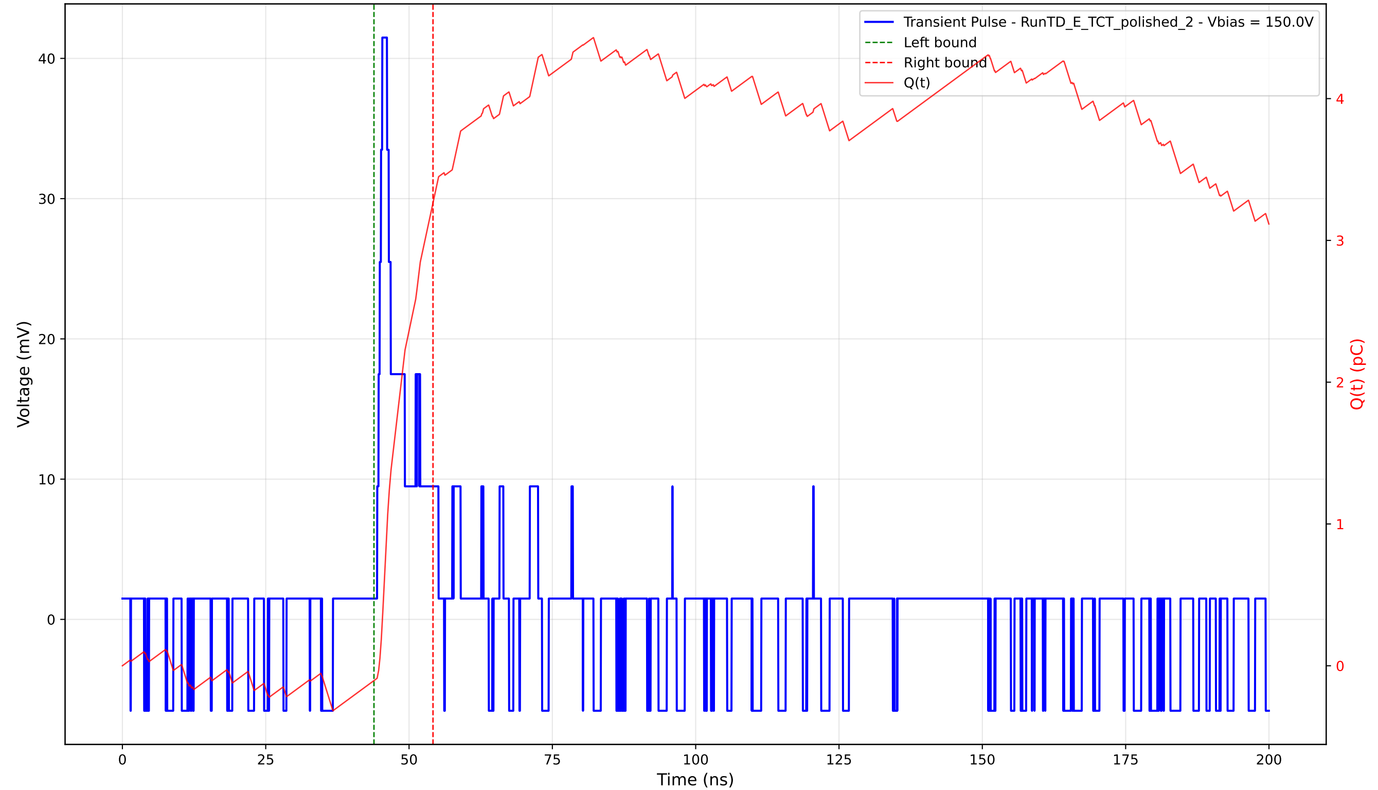
Transient Pulse - Sample: 4003 - Position: 110.0 \mu\text{m} - Charge: 3.37 pC - Rise Time: 0.89 ns
