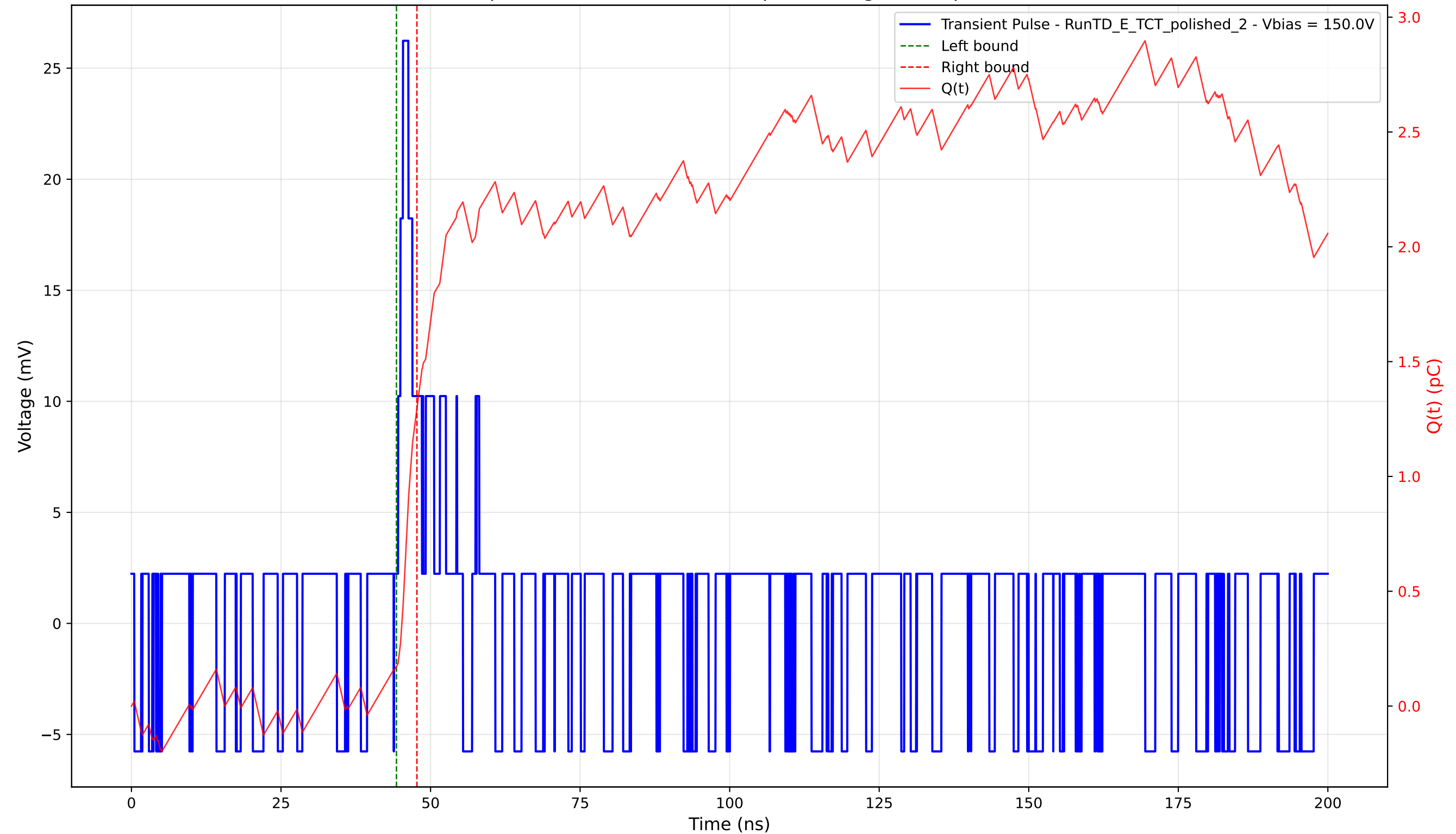
Transient Pulse - Sample: 4003 - Position: 605.0 \mu\text{m} - Charge: 1.12 pC - Rise Time: 0.82 ns
