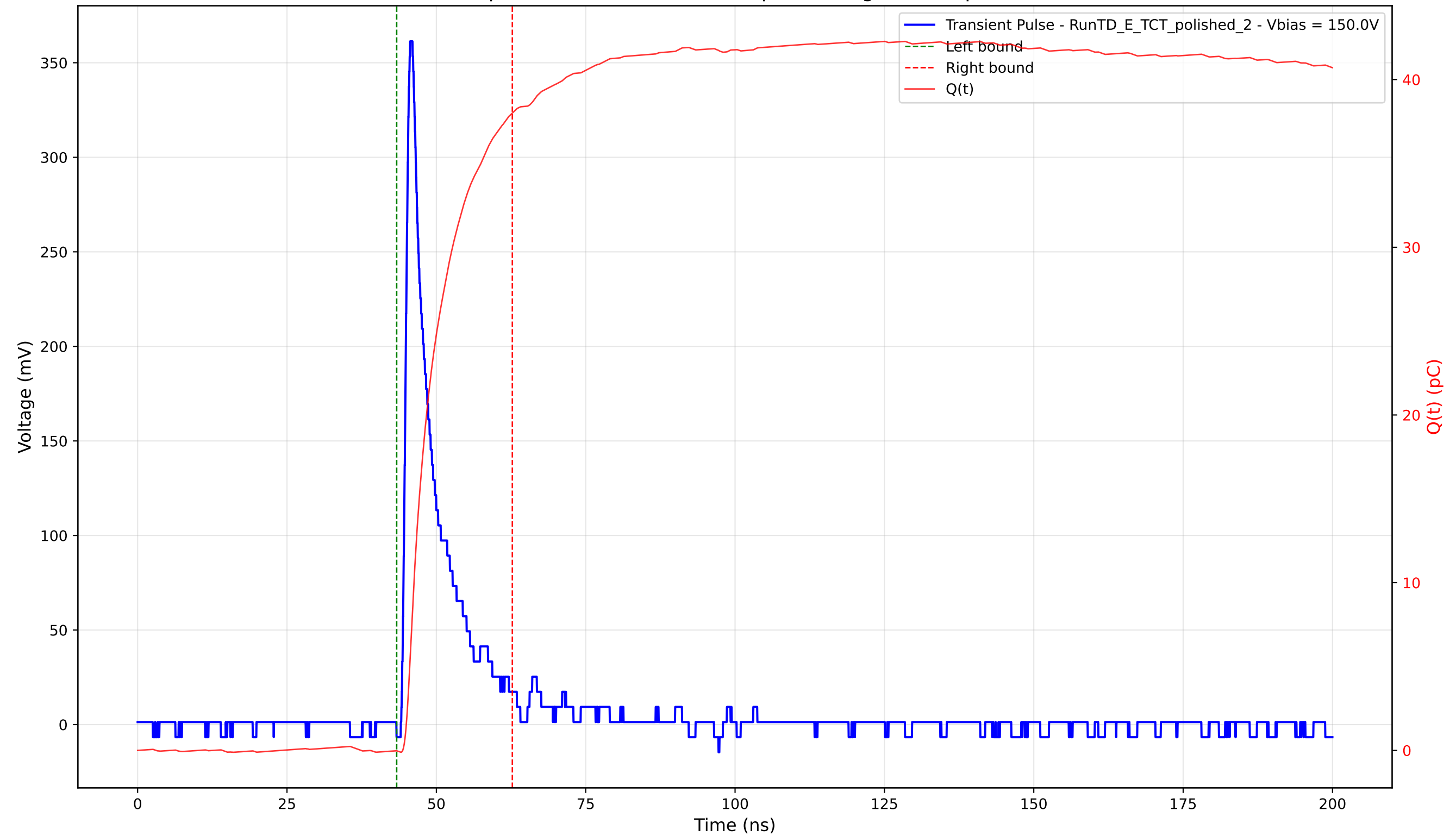
Transient Pulse - Sample: 4003 - Position: 300.0 \mu\text{m} - Charge: 38.03 pC - Rise Time: 1.01 ns
