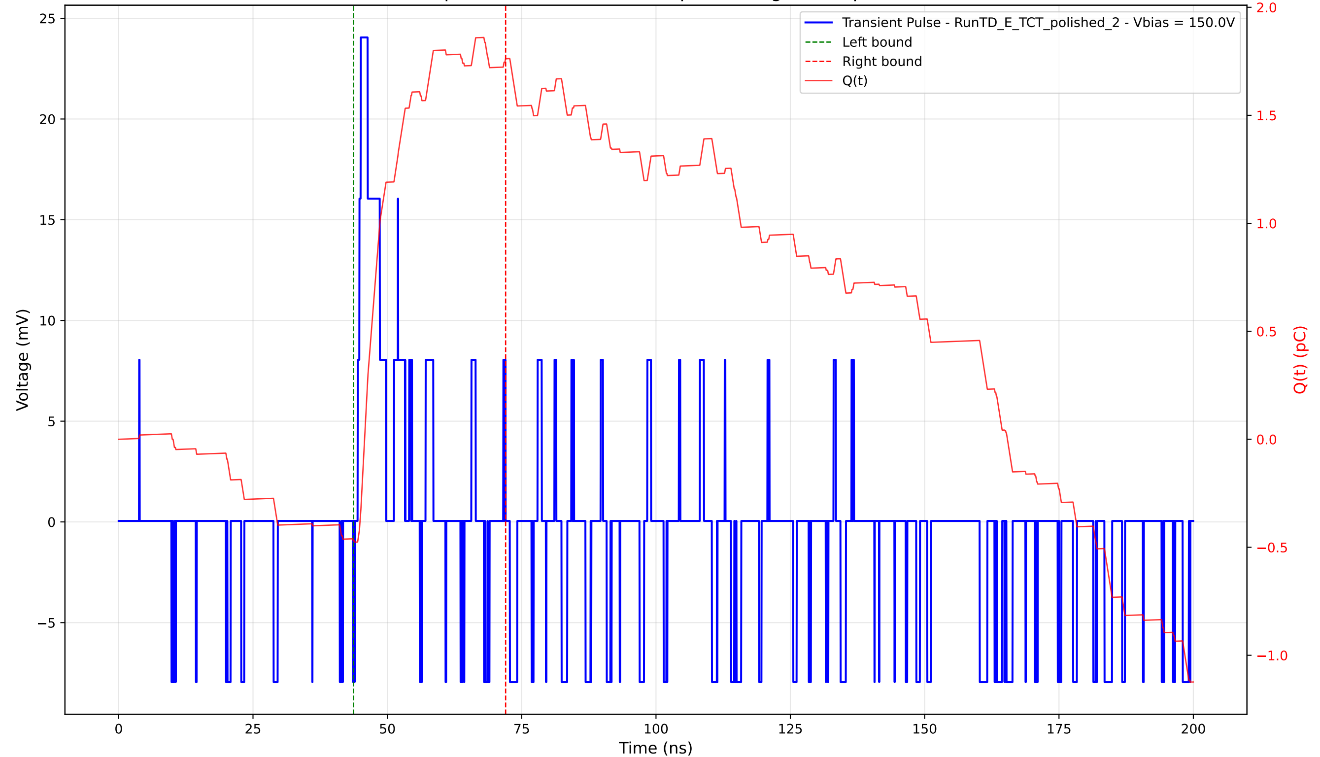
Transient Pulse - Sample: 4003 - Position: 95.0 \mu\text{m} - Charge: 2.23 pC - Rise Time: 0.57 ns
