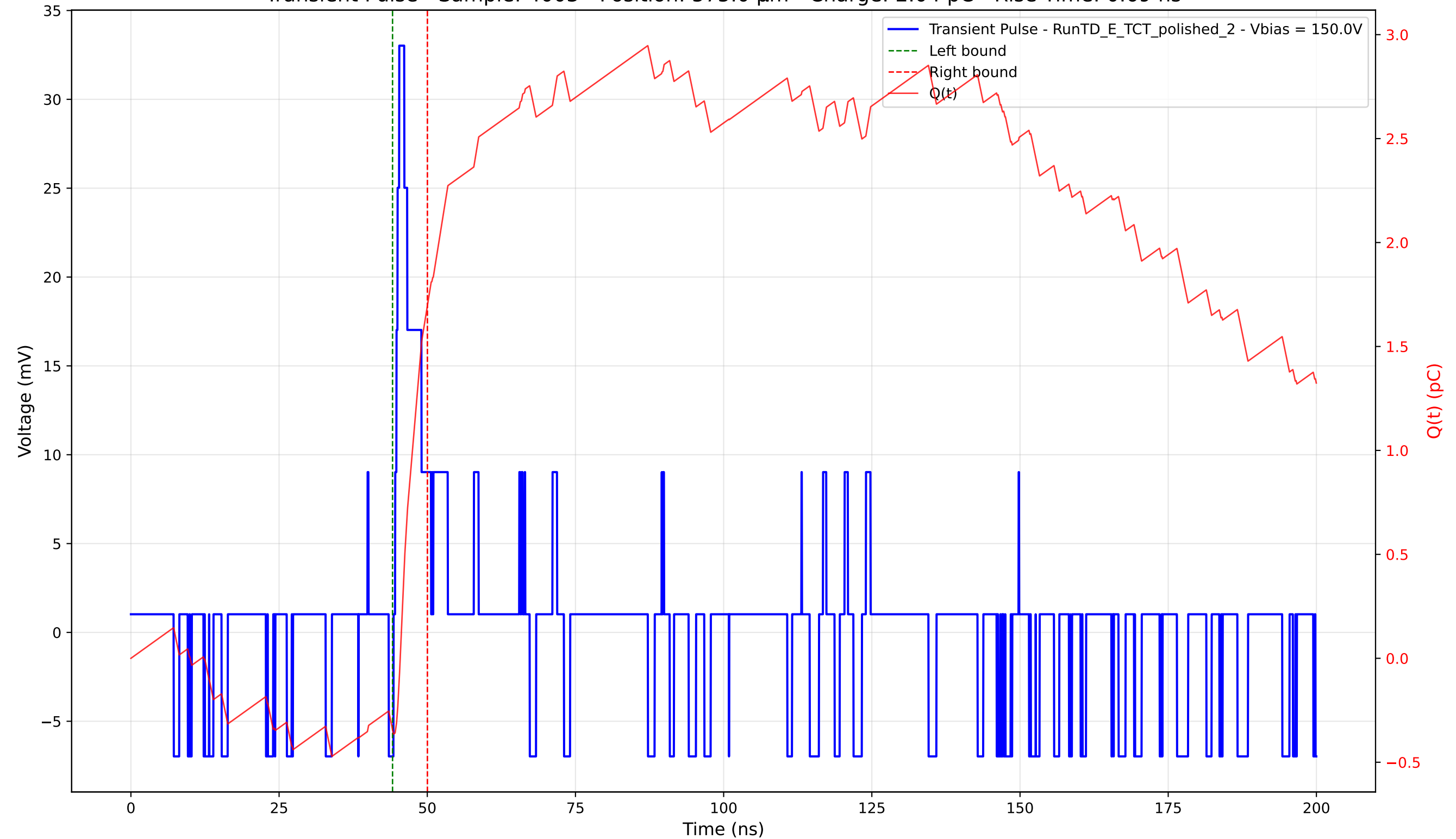
Transient Pulse - Sample: 4003 - Position: 575.0 \mu\text{m} - Charge: 2.04 pC - Rise Time: 0.69 ns
