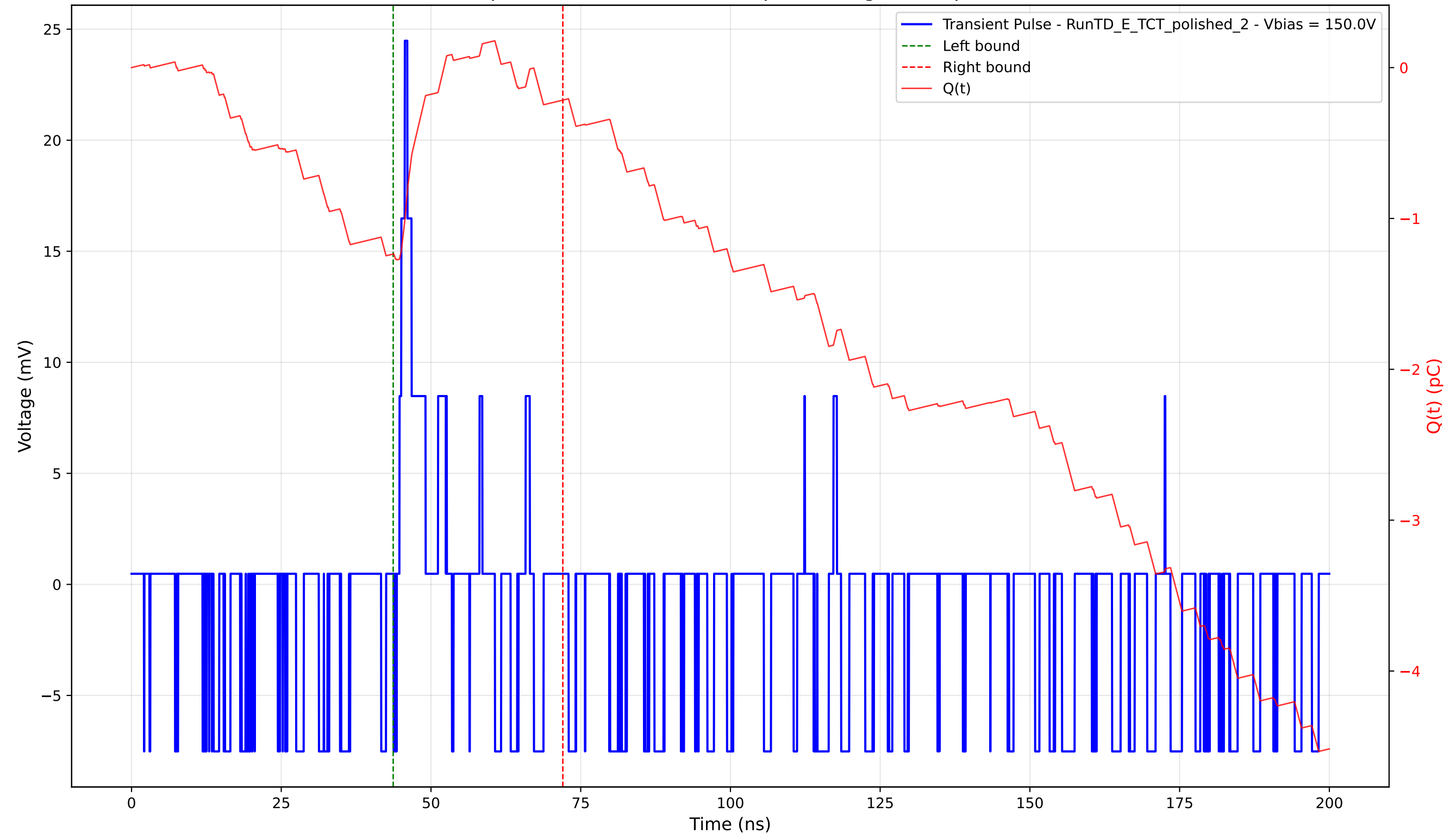
Transient Pulse - Sample: 4003 - Position: 745.0 \mu\text{m} - Charge: 1.02 pC - Rise Time: 0.90 ns
