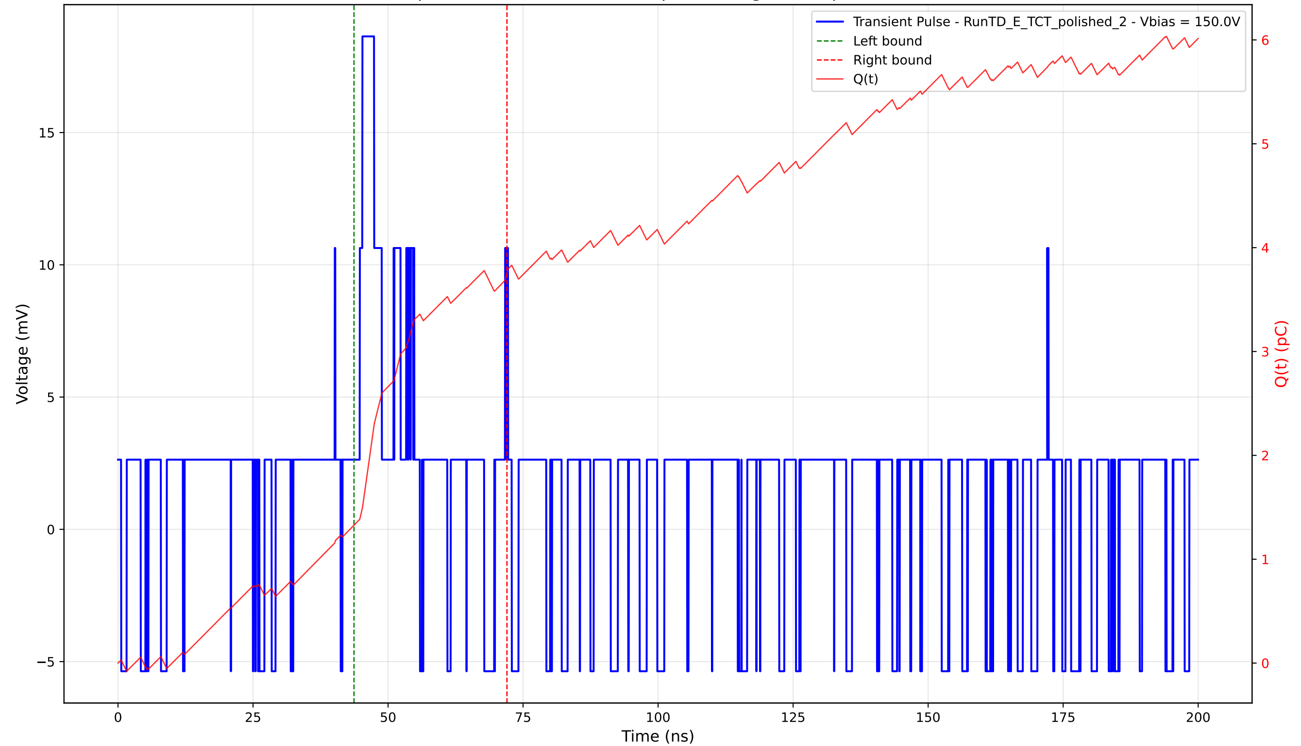
Transient Pulse - Sample: 4003 - Position: 780.0 \mu\text{m} - Charge: 2.42 pC - Rise Time: 0.00 ns (N/A)
