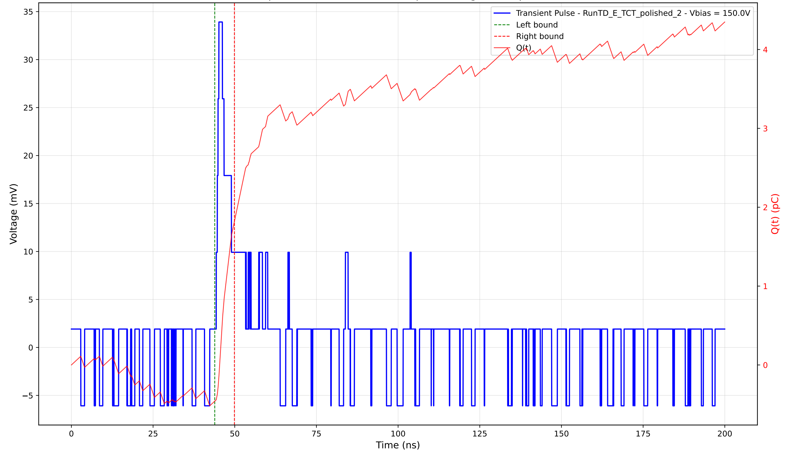
Transient Pulse - Sample: 4003 - Position: 635.0 \mu\text{m} - Charge: 2.28 pC - Rise Time: 0.82 ns
