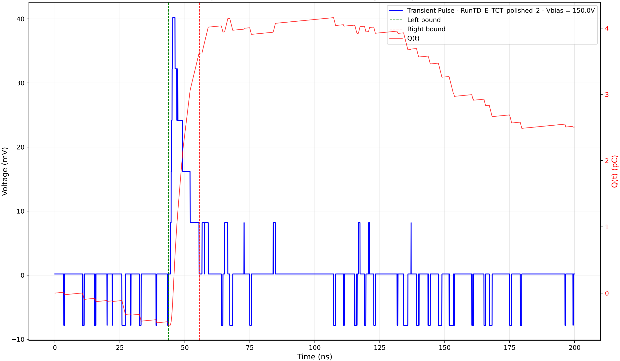
Transient Pulse - Sample: 4003 - Position: 510.0 \mu\text{m} - Charge: 4.11 pC - Rise Time: 0.89 ns
