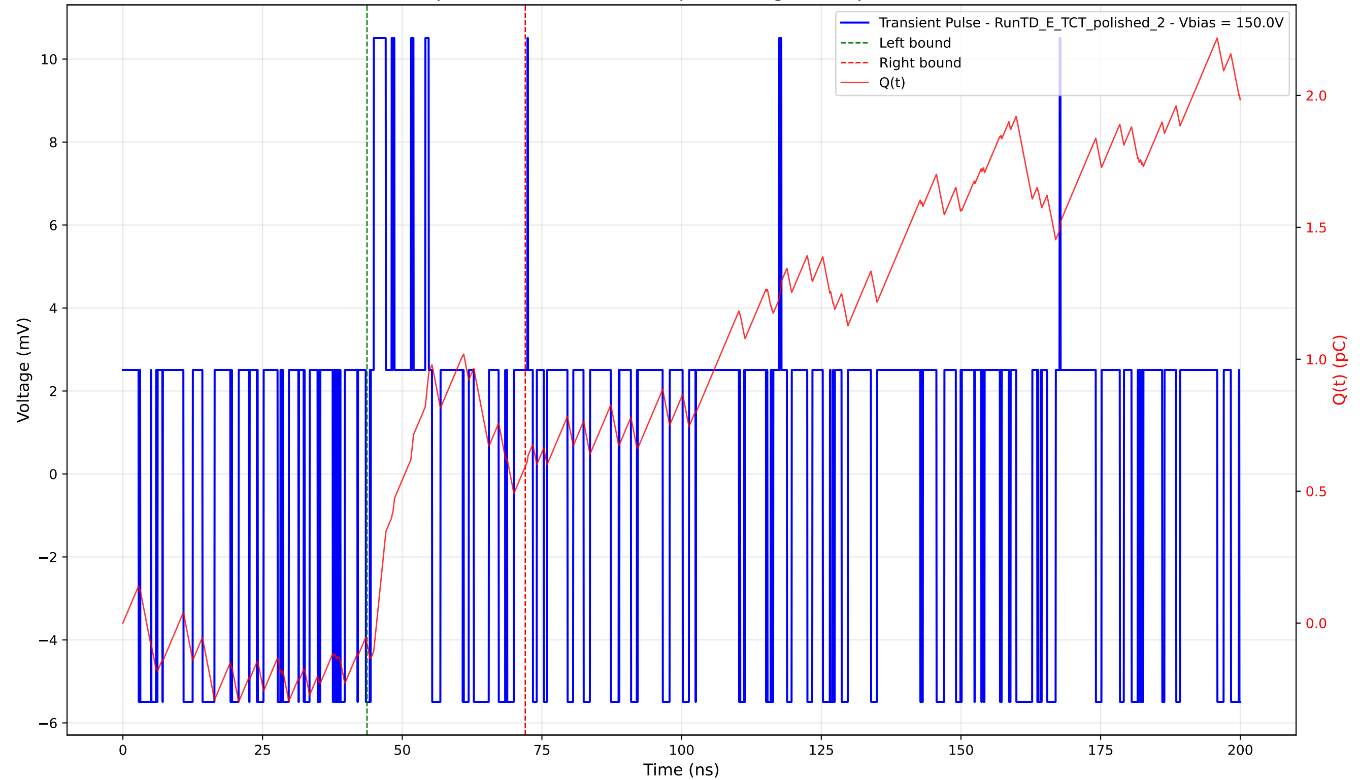
Transient Pulse - Sample: 4003 - Position: 35.0 \mu\text{m} - Charge: 0.67 pC - Rise Time: 0.00 ns (N/A)
