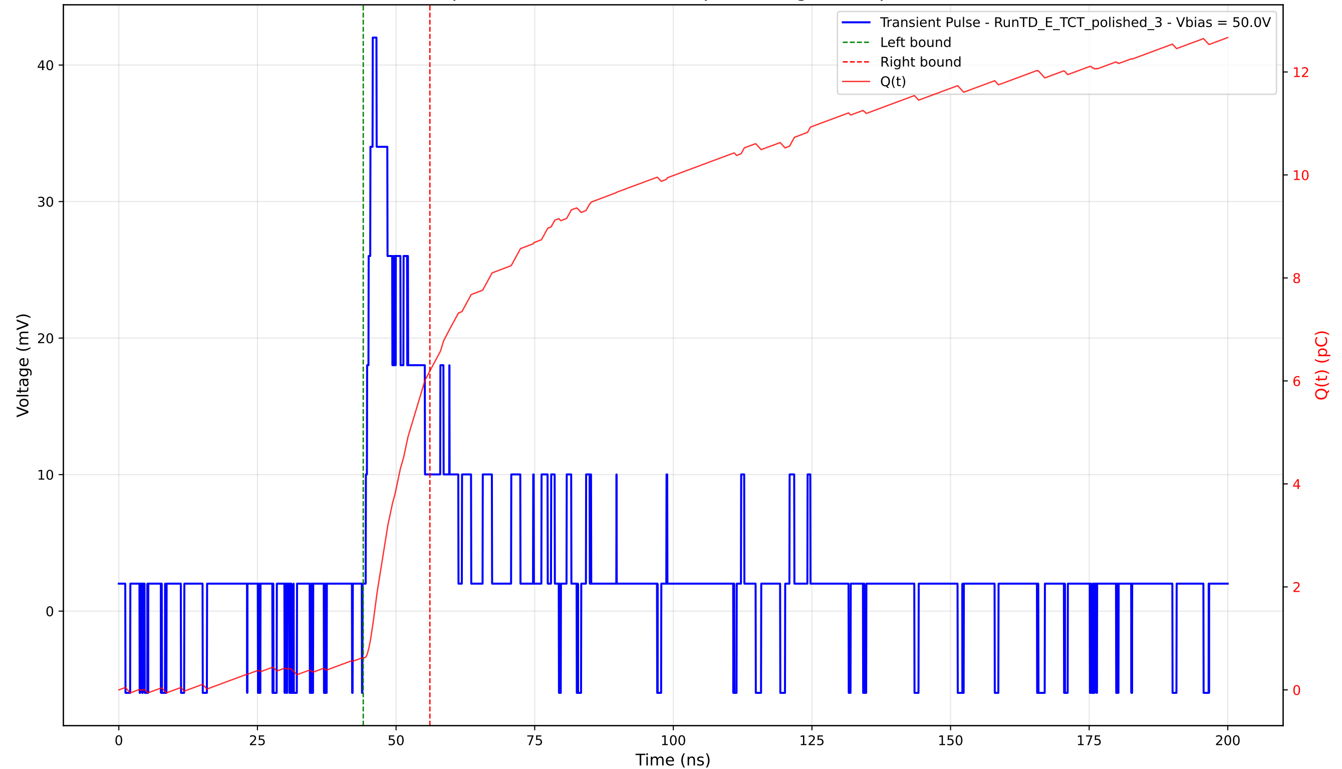
Transient Pulse - Sample: 4003 - Position: 380.0 \mu\text{m} - Charge: 5.58 pC - Rise Time: 1.25 ns
