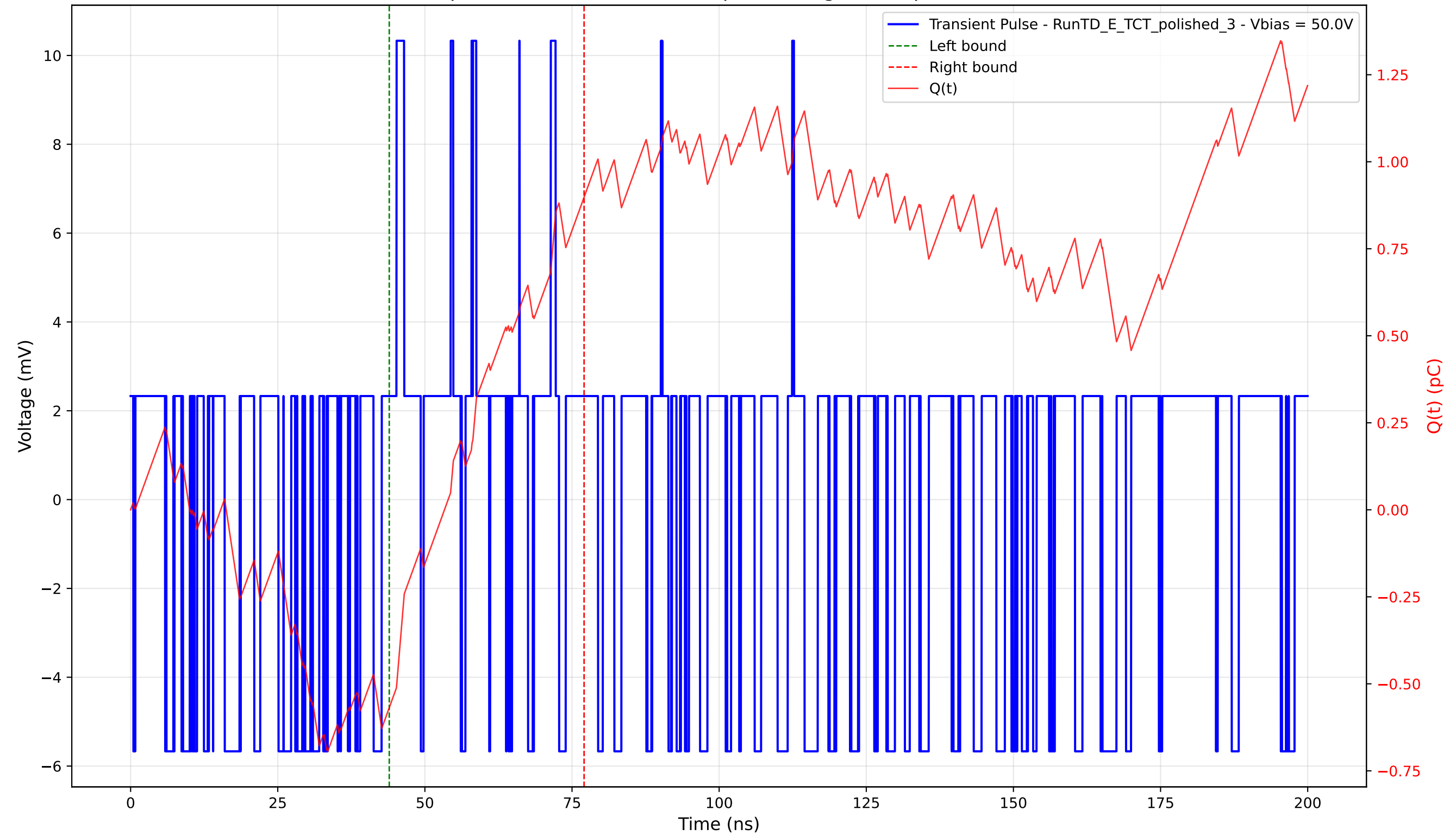
Transient Pulse - Sample: 4003 - Position: 755.0 \mu\text{m} - Charge: 1.47 pC - Rise Time: 0.00 ns (N/A)
