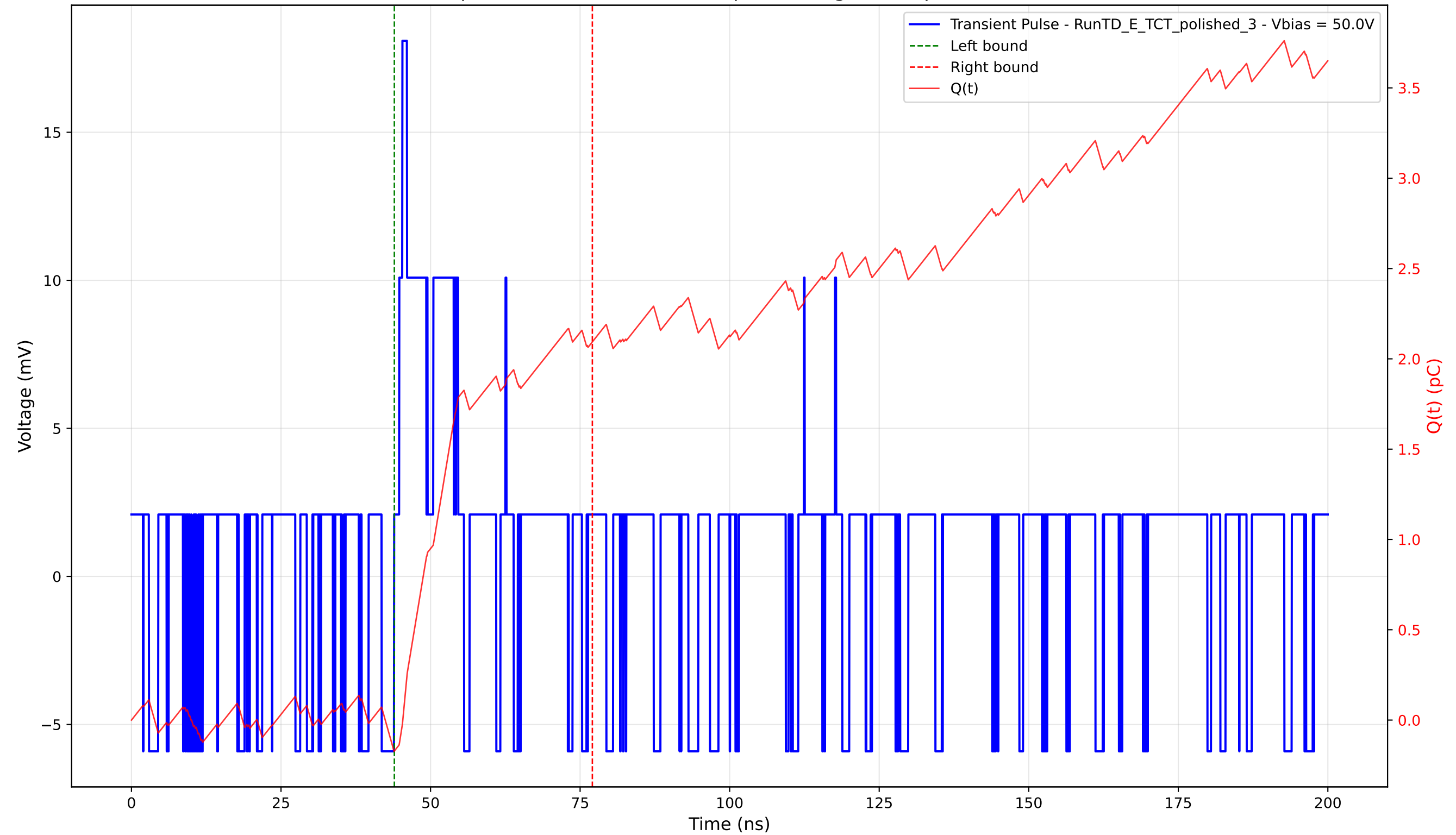
Transient Pulse - Sample: 4003 - Position: 450.0 \mu\text{m} - Charge: 2.26 pC - Rise Time: 0.00 ns (N/A)
