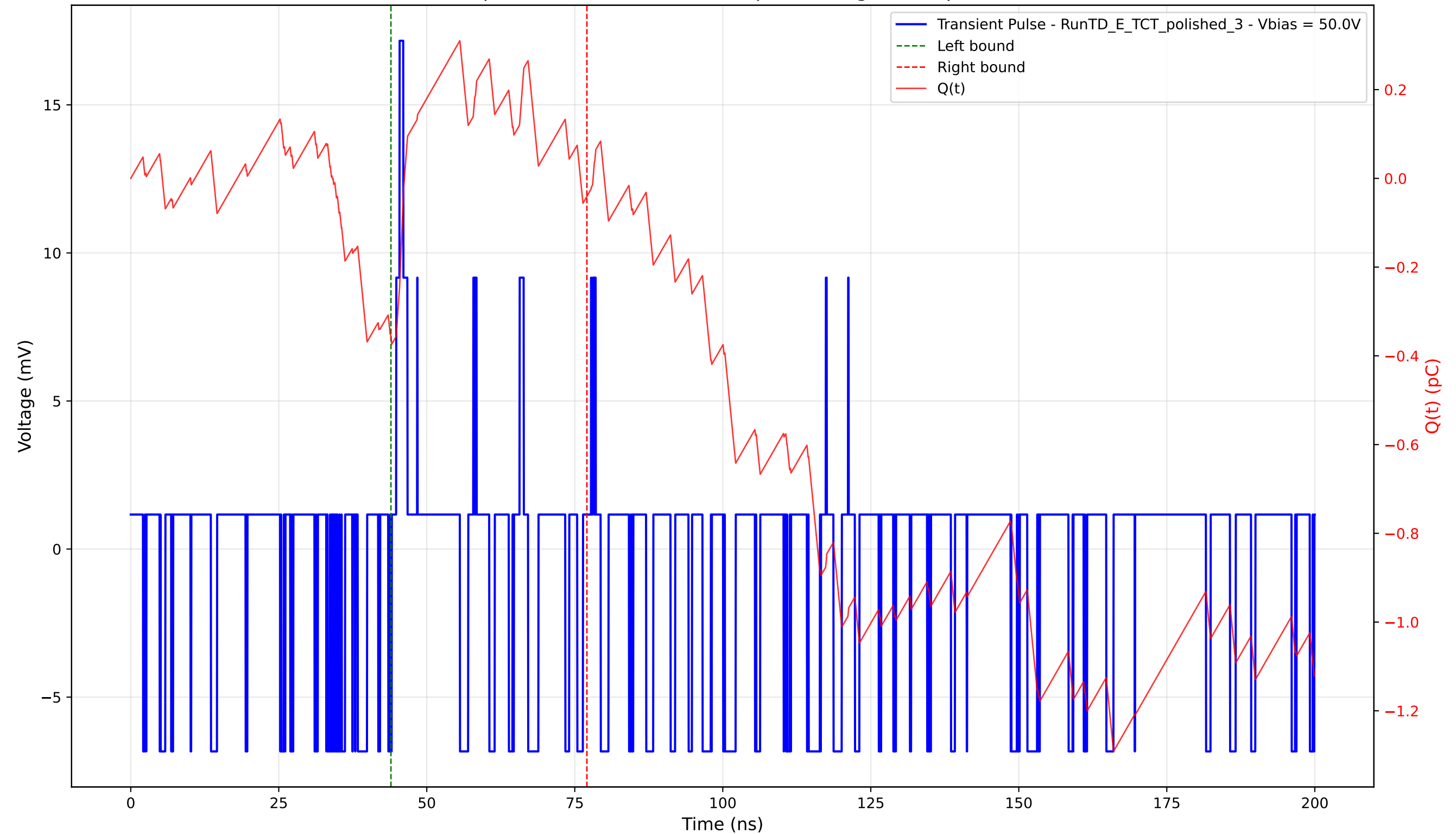
Transient Pulse - Sample: 4003 - Position: 665.0 \mu\text{m} - Charge: 0.32 pC - Rise Time: 0.58 ns
