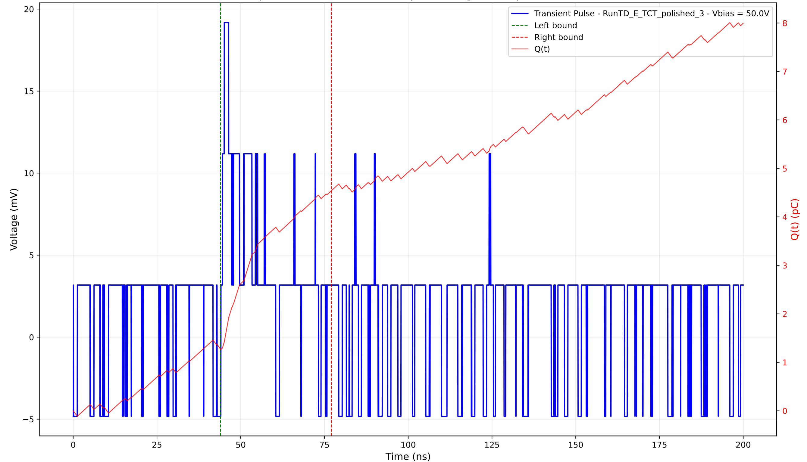
Transient Pulse - Sample: 4003 - Position: 480.0 \mu\text{m} - Charge: 3.27 pC - Rise Time: 0.00 ns (N/A)
