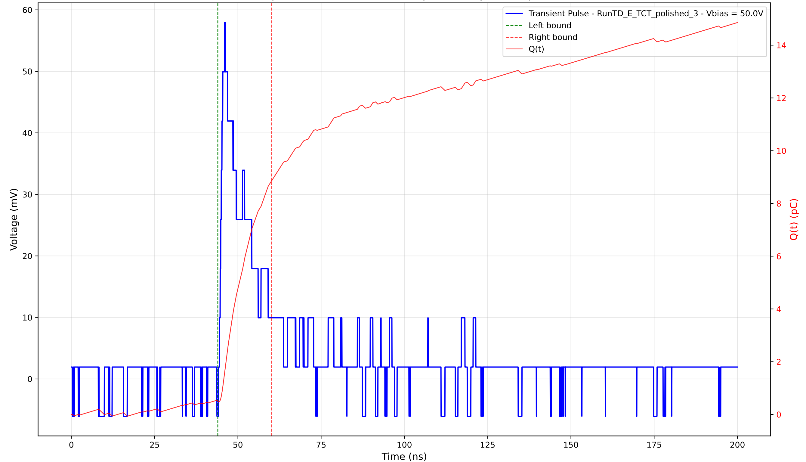
Transient Pulse - Sample: 4003 - Position: 365.0 \mu\text{m} - Charge: 8.33 pC - Rise Time: 1.51 ns
