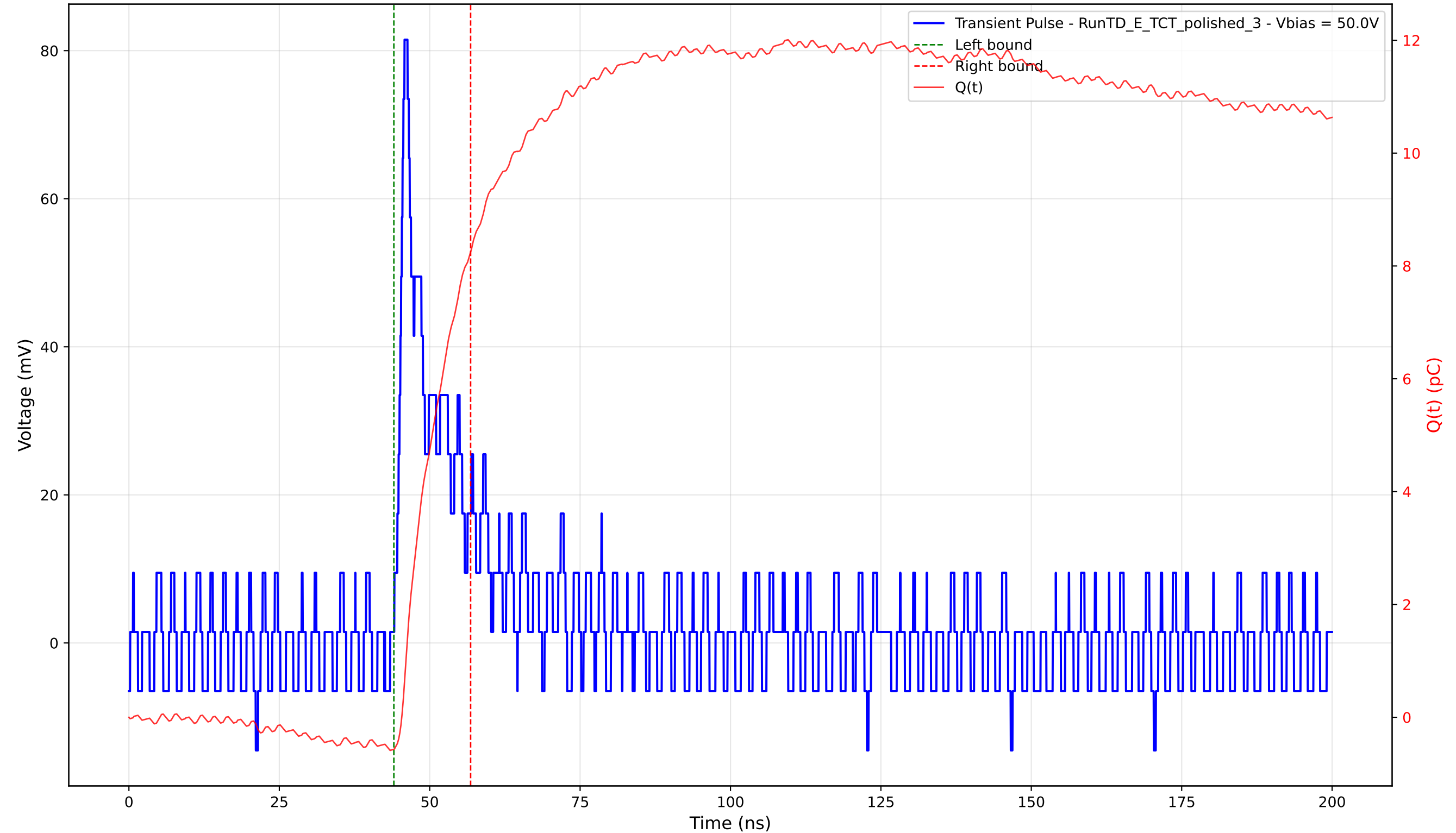
Transient Pulse - Sample: 4003 - Position: 155.0 \mu\text{m} - Charge: 8.81 pC - Rise Time: 1.50 ns
