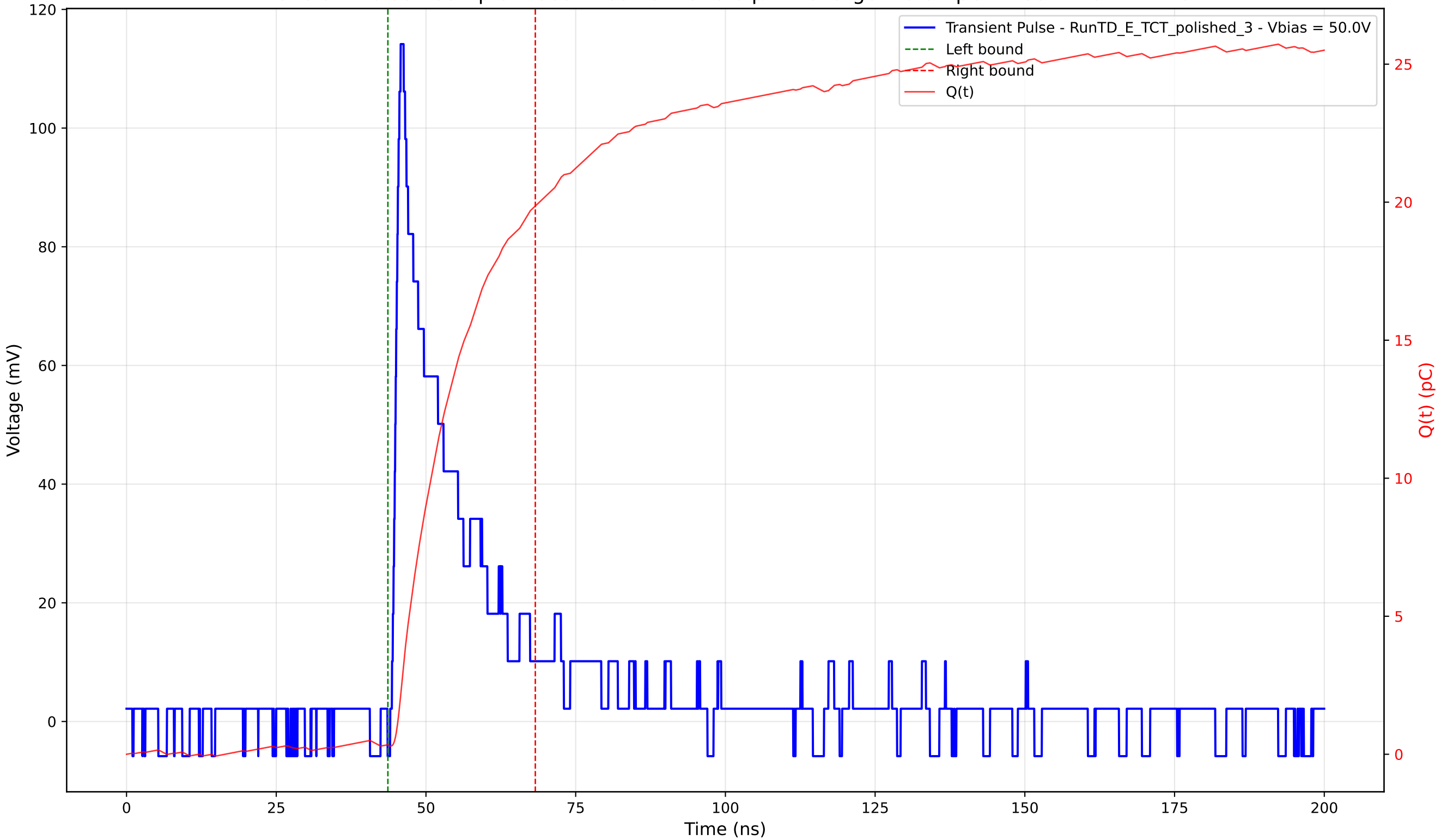
Transient Pulse - Sample: 4003 - Position: 310.0 \mu\text{m} - Charge: 19.52 pC - Rise Time: 1.12 ns
