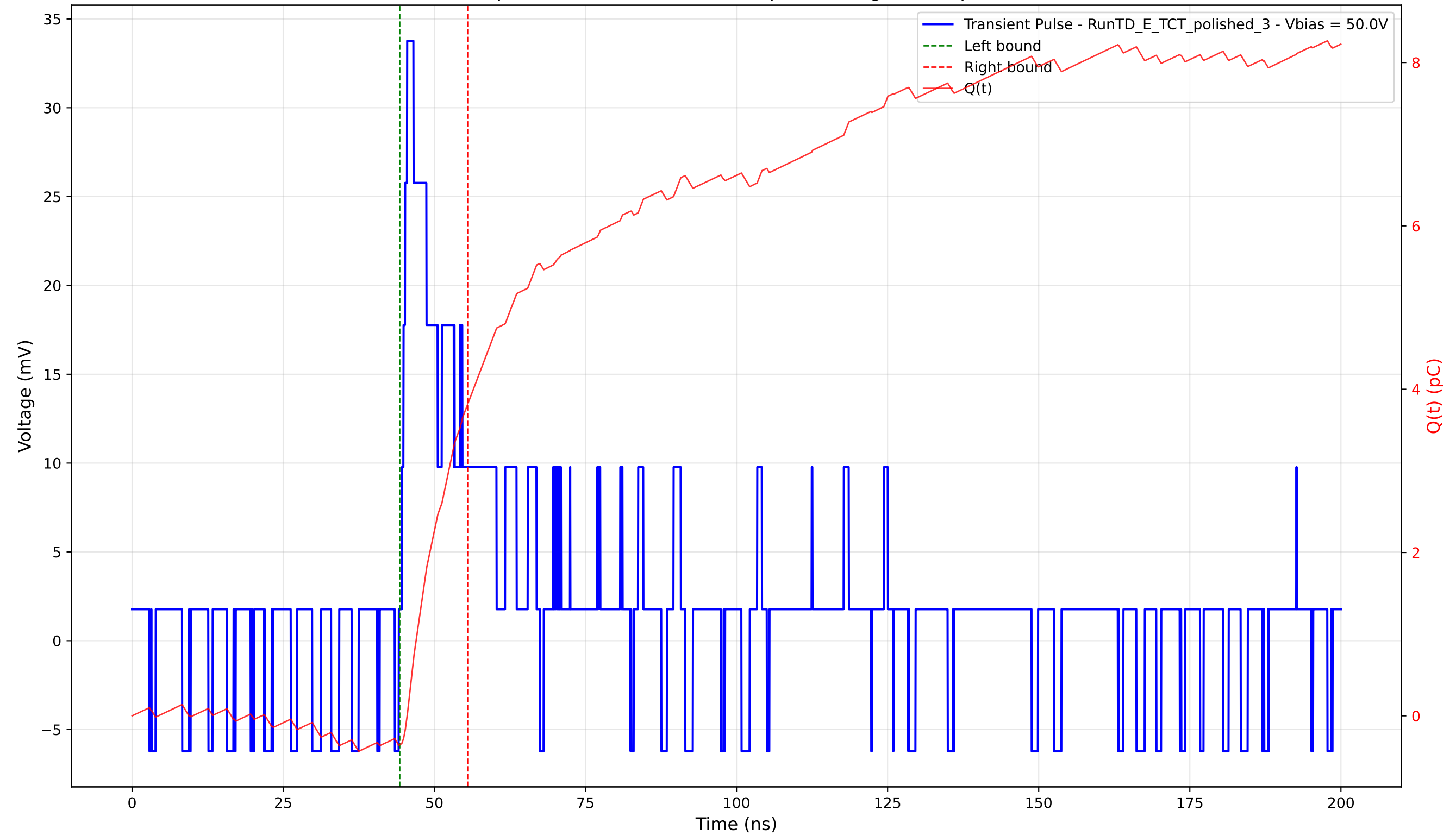
Transient Pulse - Sample: 4003 - Position: 395.0 \mu\text{m} - Charge: 4.19 pC - Rise Time: 0.90 ns
