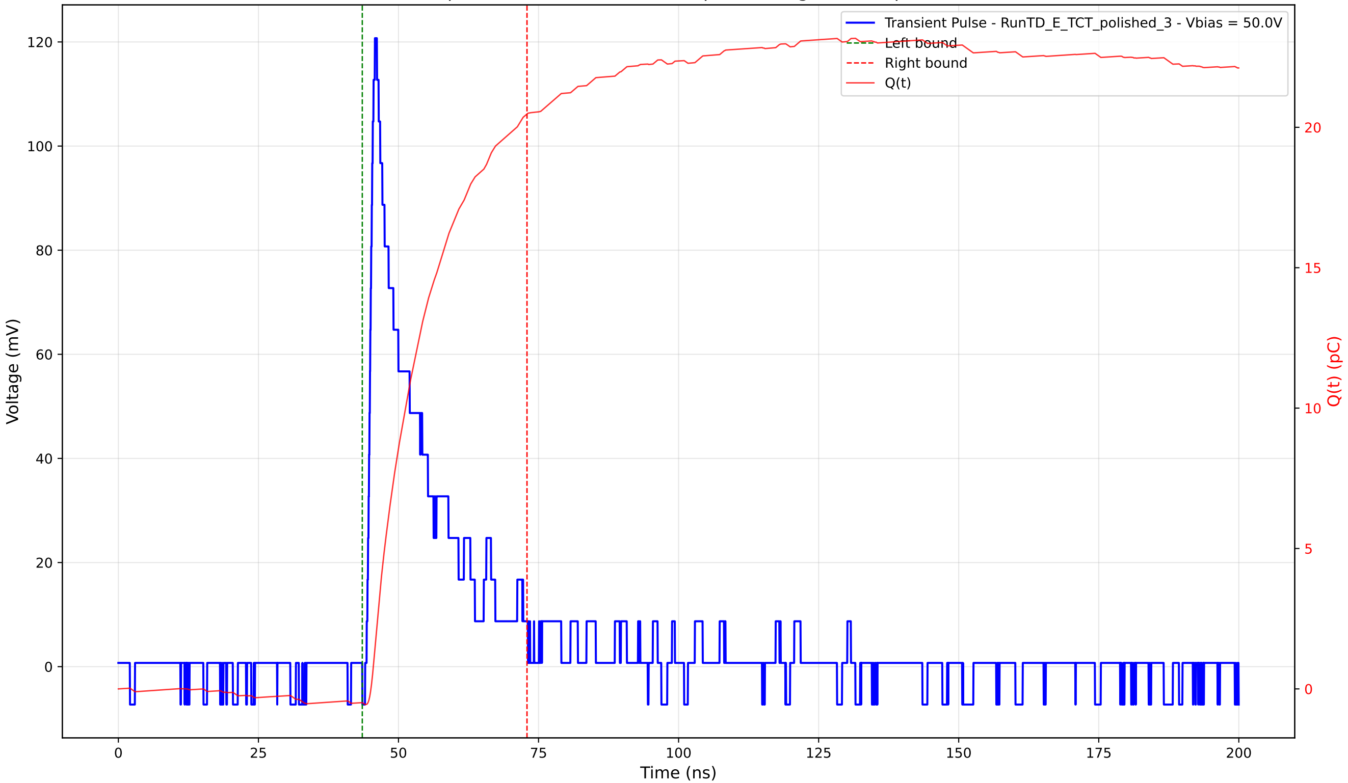
Transient Pulse - Sample: 4003 - Position: 305.0 \mu\text{m} - Charge: 20.96 pC - Rise Time: 1.09 ns
