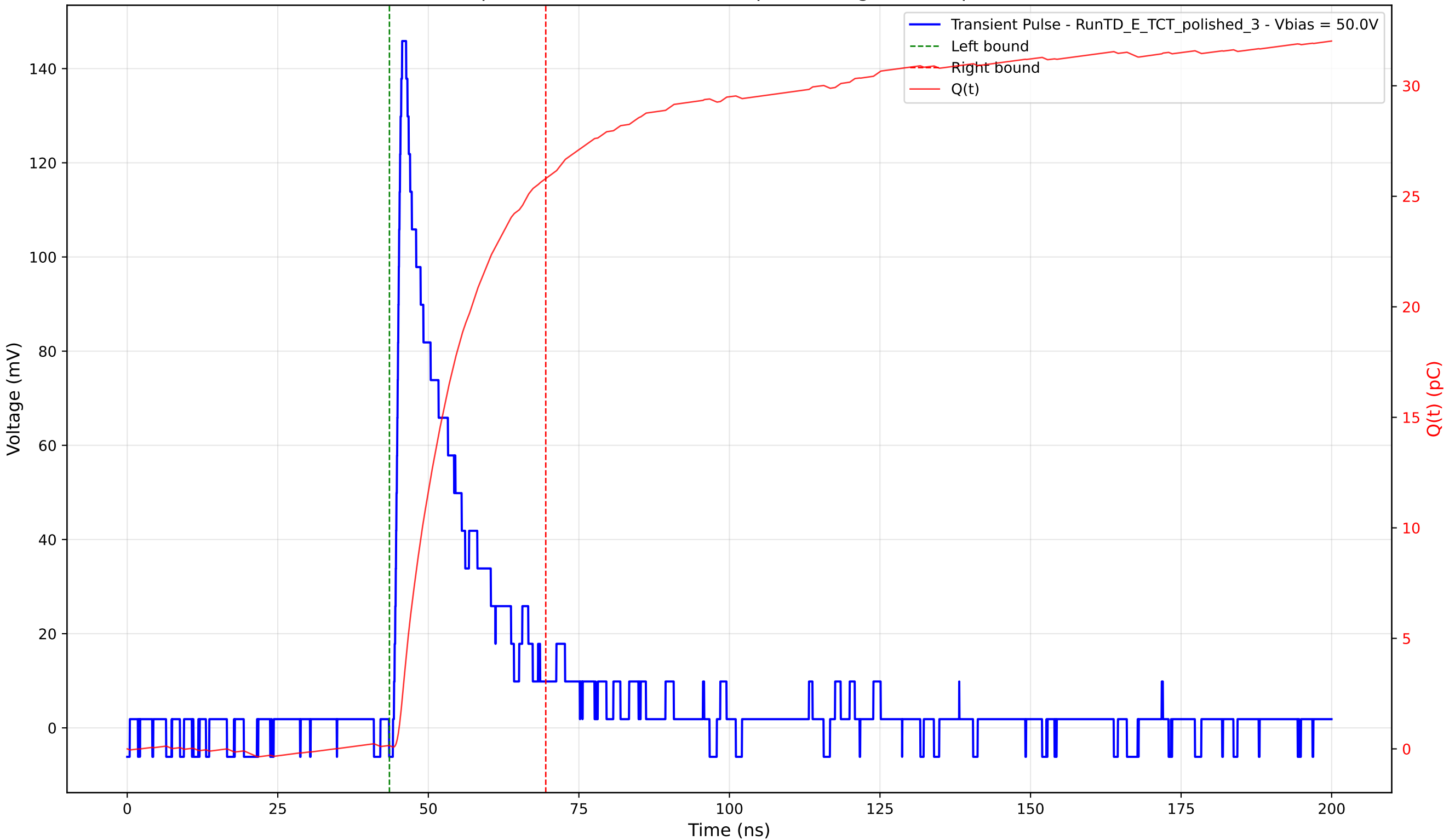
Transient Pulse - Sample: 4003 - Position: 255.0 \mu\text{m} - Charge: 25.65 pC - Rise Time: 1.11 ns
