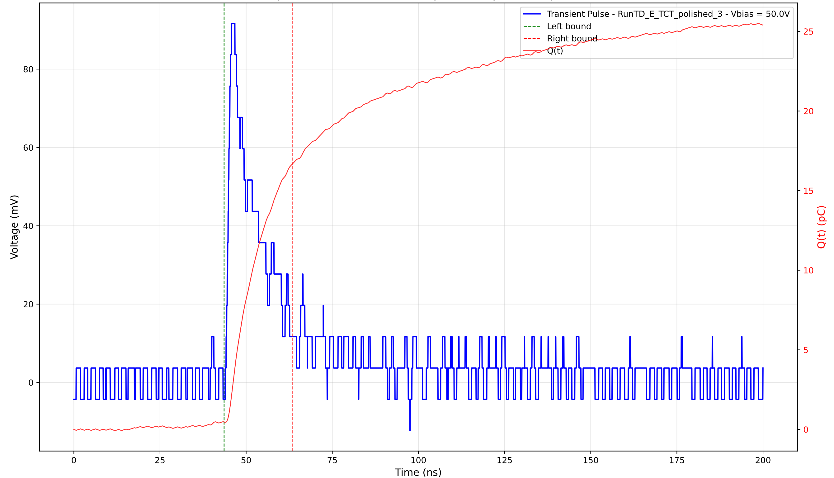
Transient Pulse - Sample: 4003 - Position: 325.0 \mu\text{m} - Charge: 16.24 pC - Rise Time: 1.29 ns
