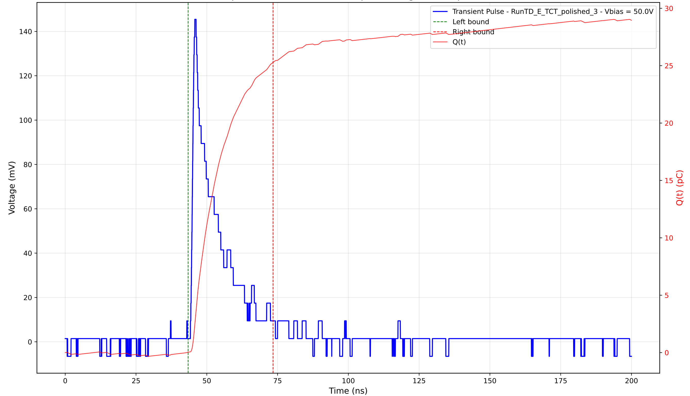
Transient Pulse - Sample: 4003 - Position: 220.0 \mu\text{m} - Charge: 25.25 pC - Rise Time: 1.21 ns
