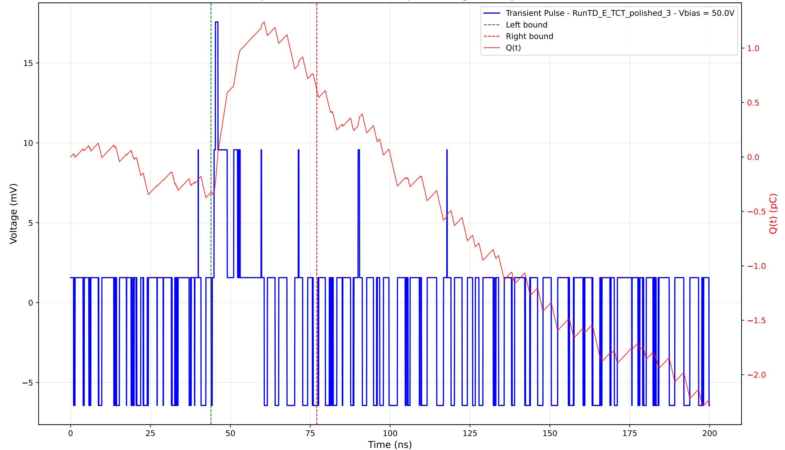
Transient Pulse - Sample: 4003 - Position: 490.0 \mu\text{m} - Charge: 0.94 pC - Rise Time: 0.44 ns
