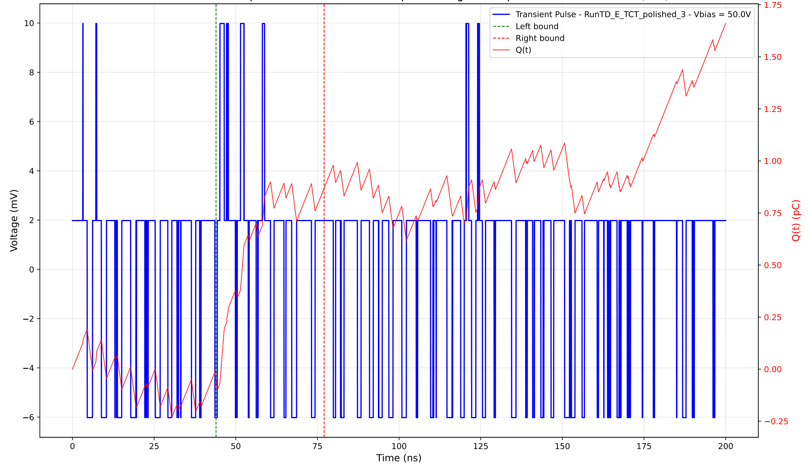
Transient Pulse - Sample: 4003 - Position: 750.0 \mu\text{m} - Charge: 0.93 pC - Rise Time: 0.00 ns (N/A)
