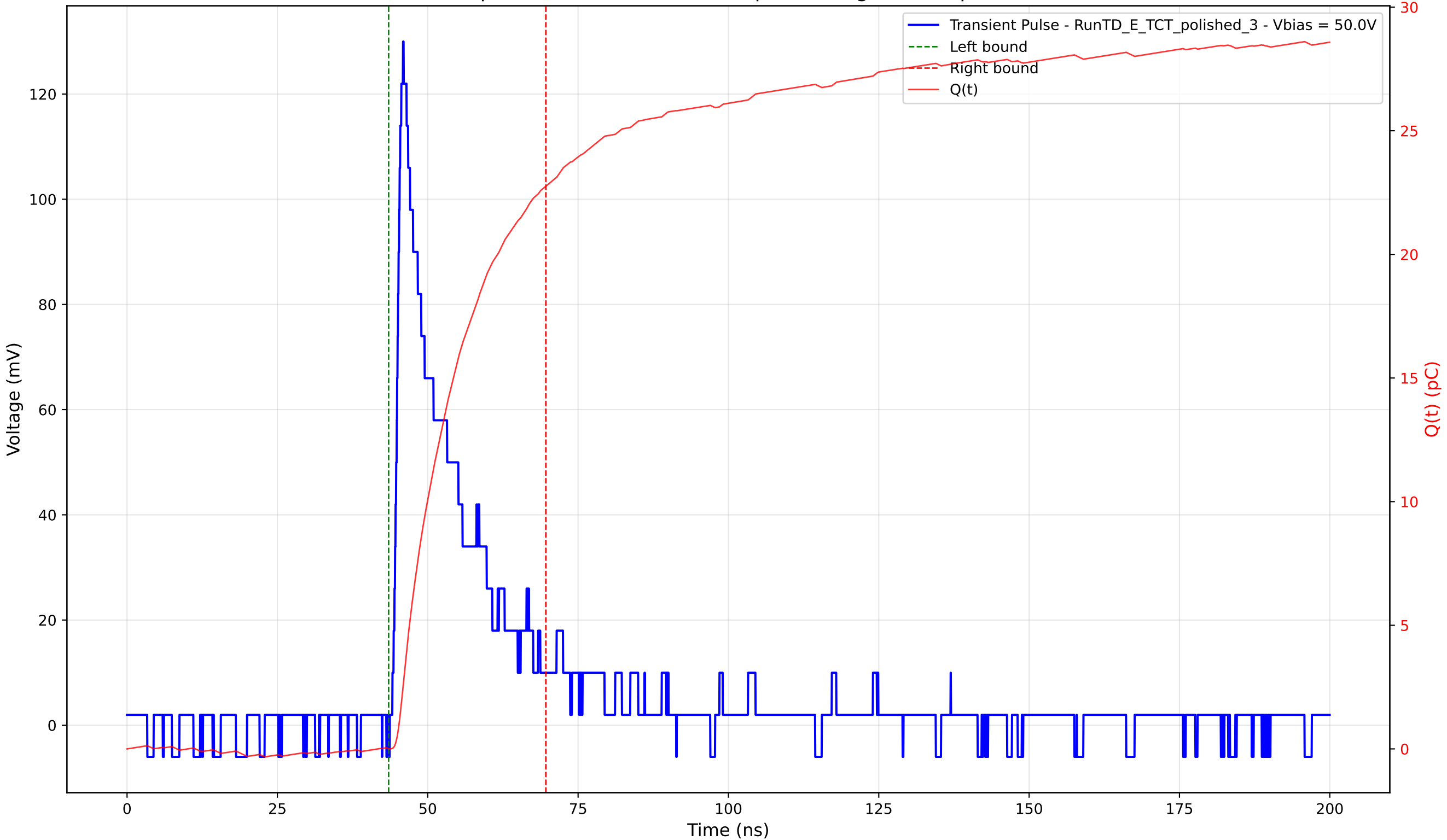
Transient Pulse - Sample: 4003 - Position: 295.0 \mu\text{m} - Charge: 22.74 pC - Rise Time: 1.29 ns
