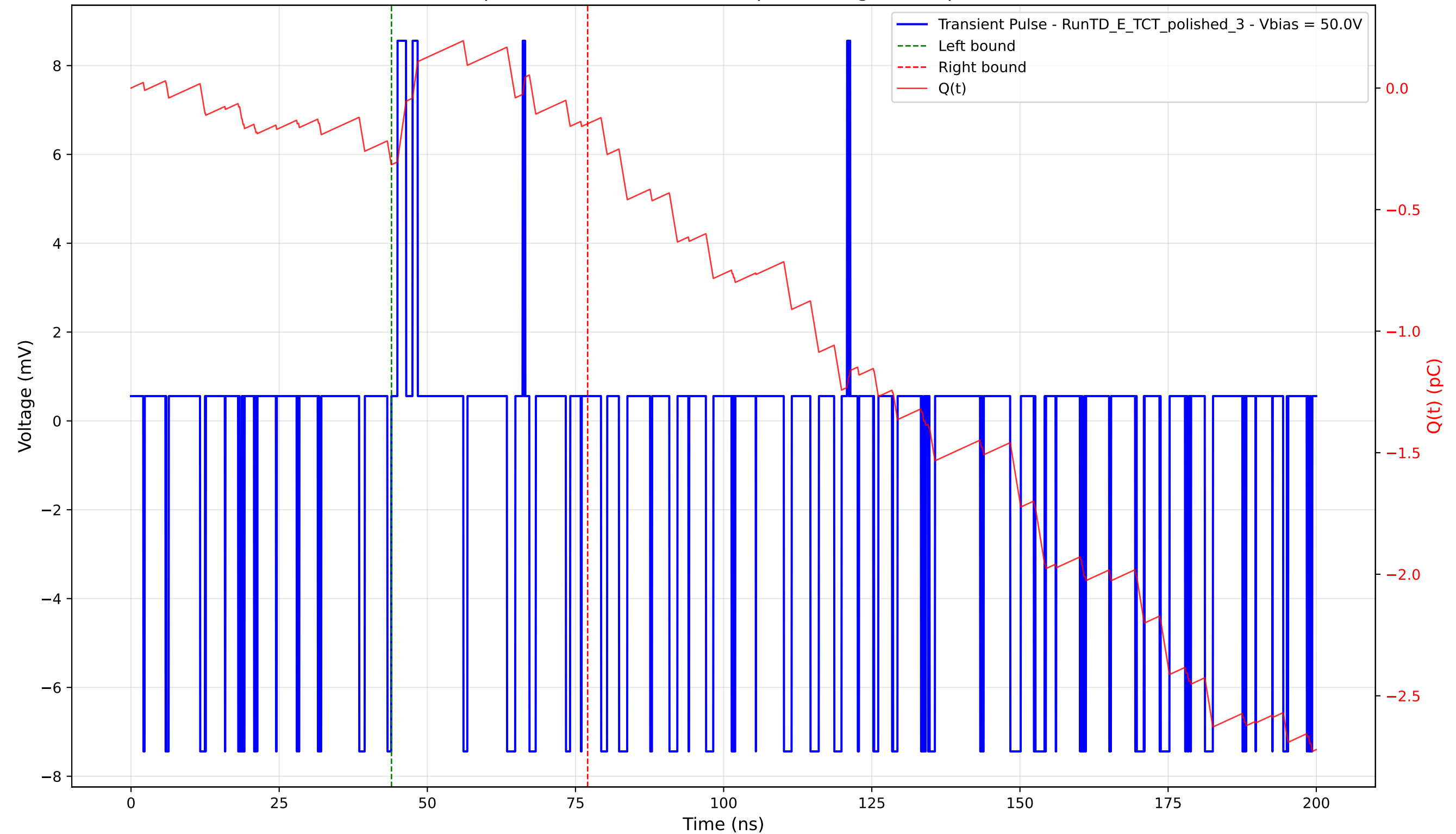
Transient Pulse - Sample: 4003 - Position: 760.0 \mu\text{m} - Charge: 0.17 pC - Rise Time: 0.02 ns
