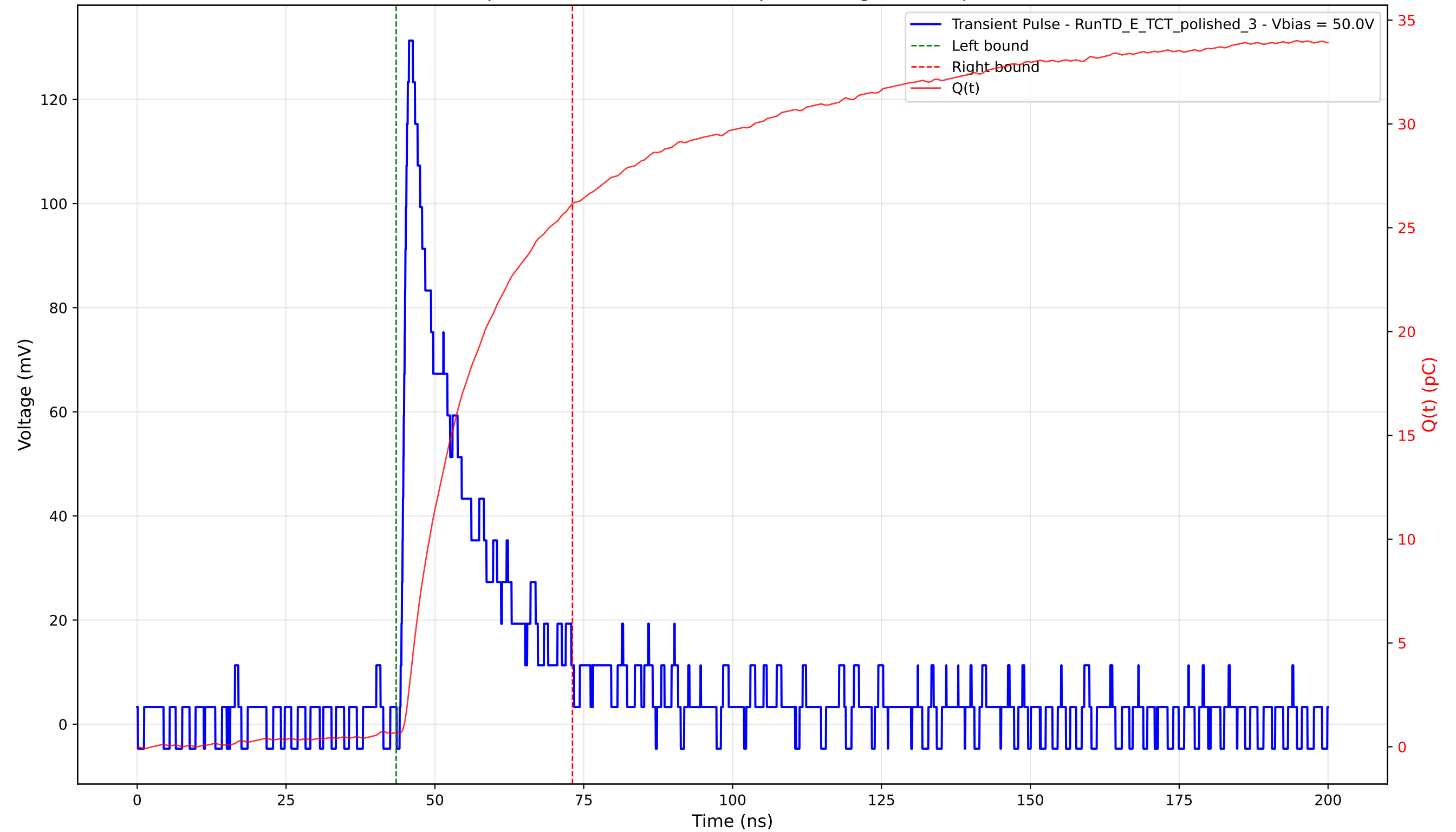
Transient Pulse - Sample: 4003 - Position: 285.0 \mu\text{m} - Charge: 25.46 pC - Rise Time: 1.08 ns
