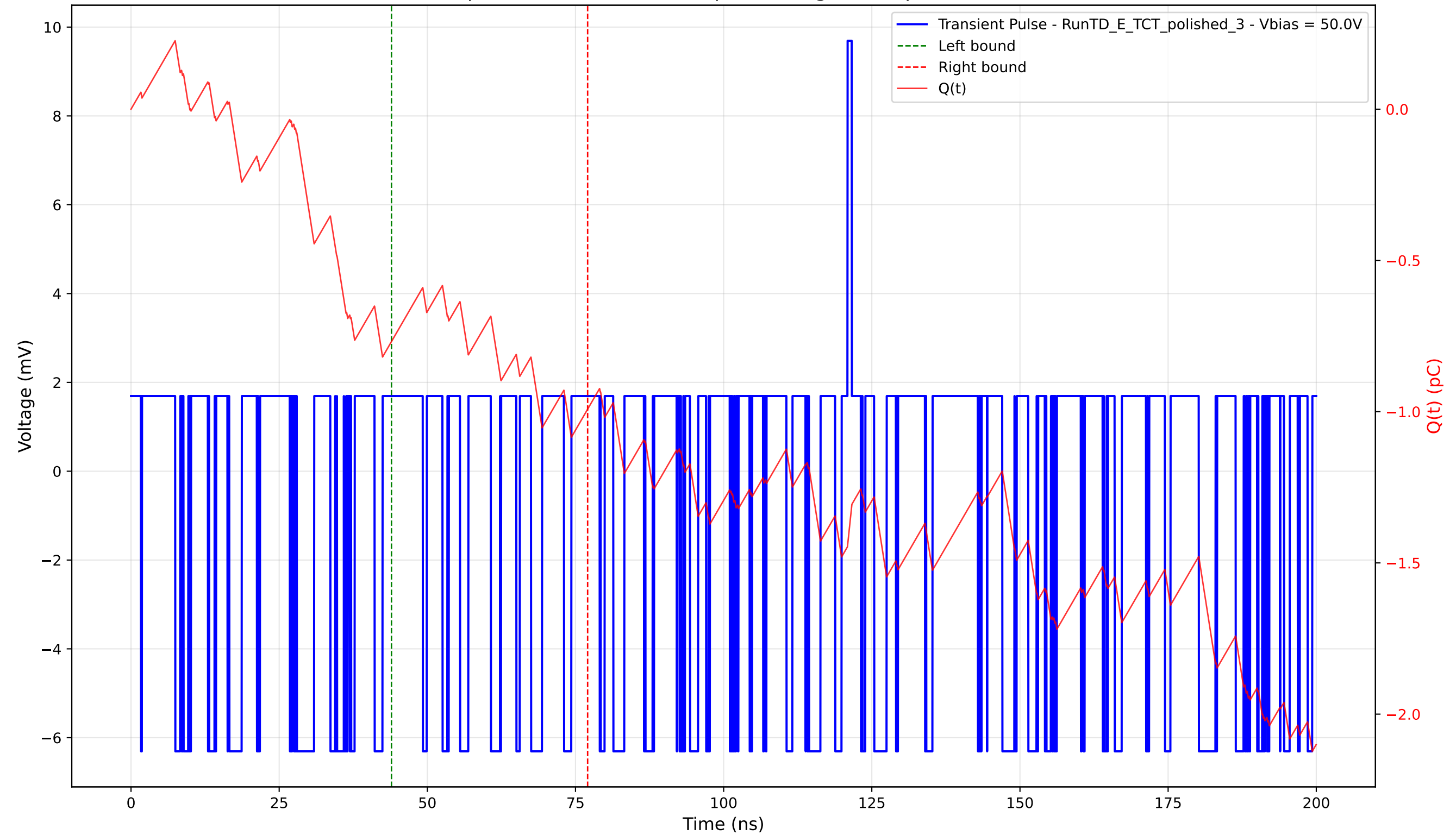
Transient Pulse - Sample: 4003 - Position: 5.0 \mu\text{m} - Charge: 0.22 pC - Rise Time: 0.00 ns (N/A)
