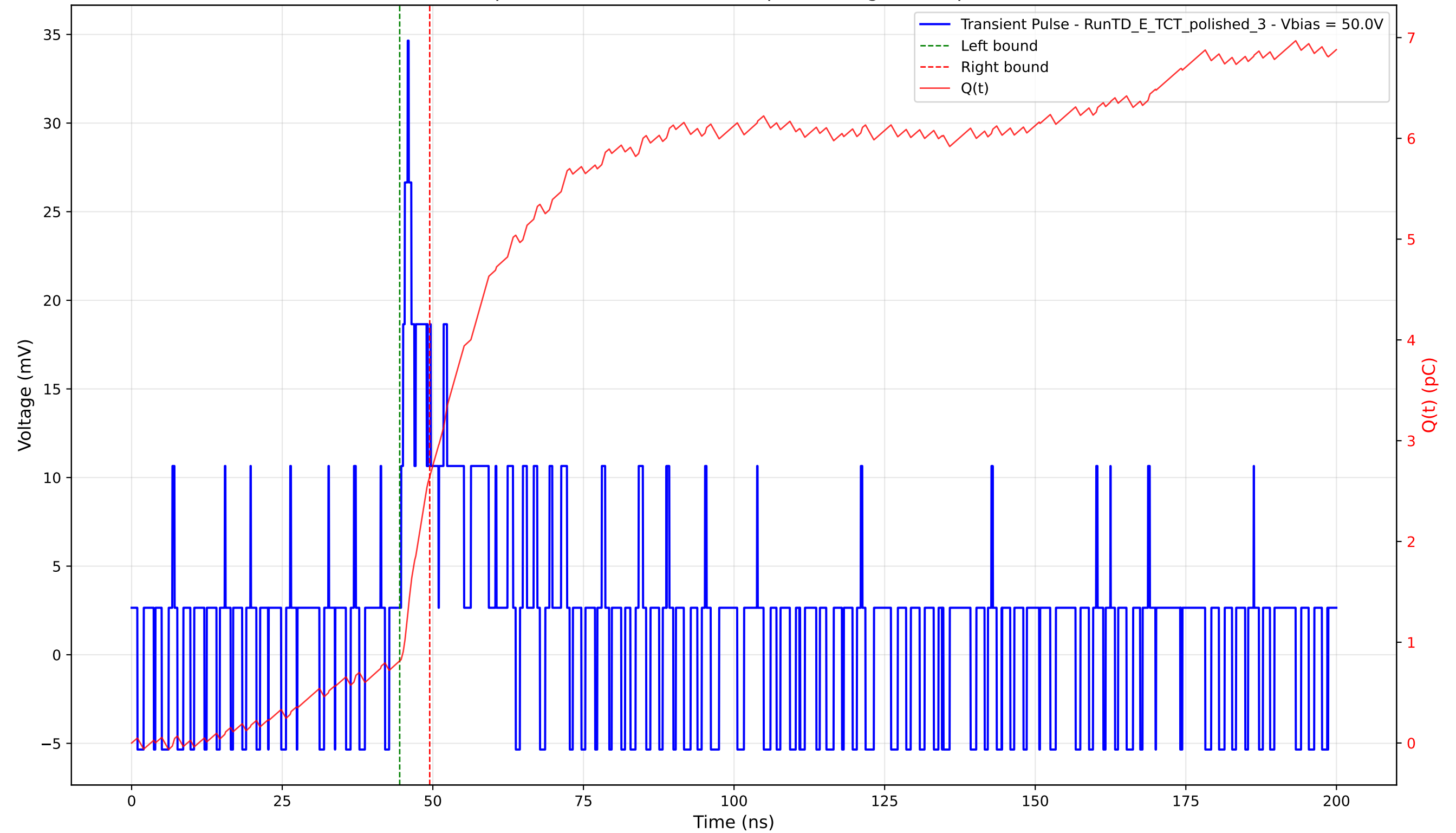
Transient Pulse - Sample: 4003 - Position: 115.0 \mu\text{m} - Charge: 1.83 pC - Rise Time: 1.10 ns
