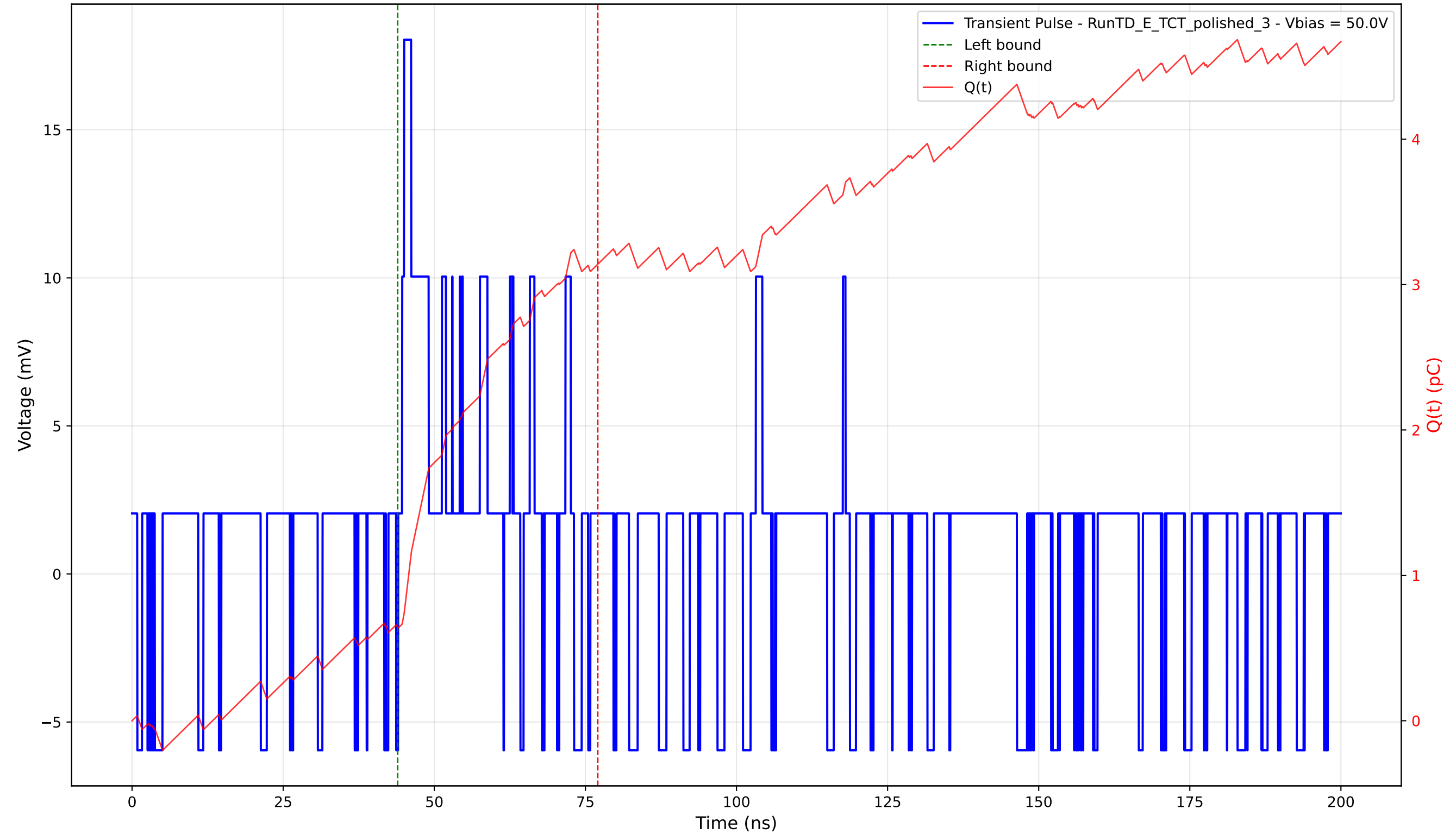
Transient Pulse - Sample: 4003 - Position: 565.0 \mu\text{m} - Charge: 2.50 pC - Rise Time: 0.00 ns (N/A)
