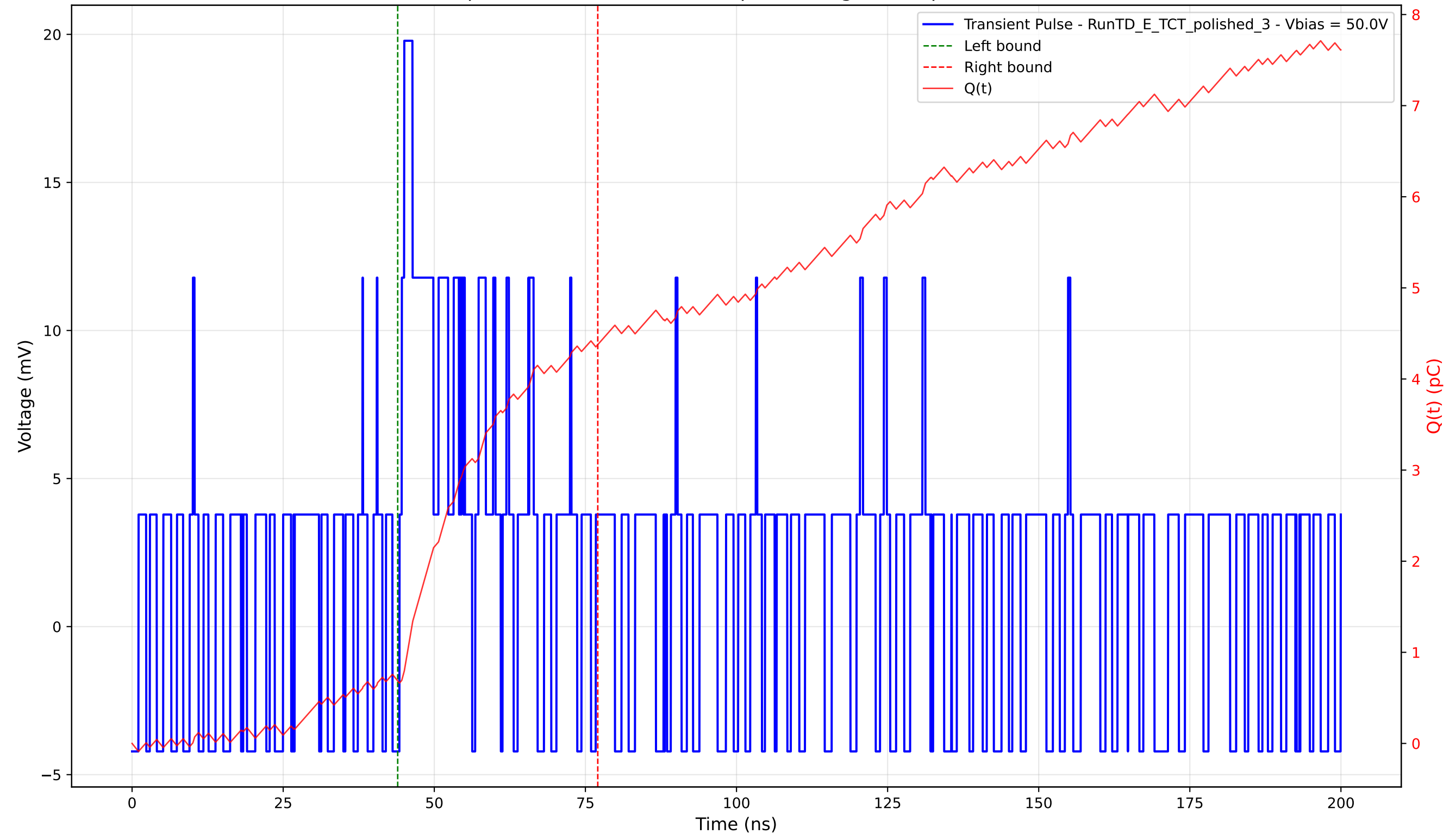
Transient Pulse - Sample: 4003 - Position: 105.0 \mu\text{m} - Charge: 3.69 pC - Rise Time: 0.00 ns (N/A)
