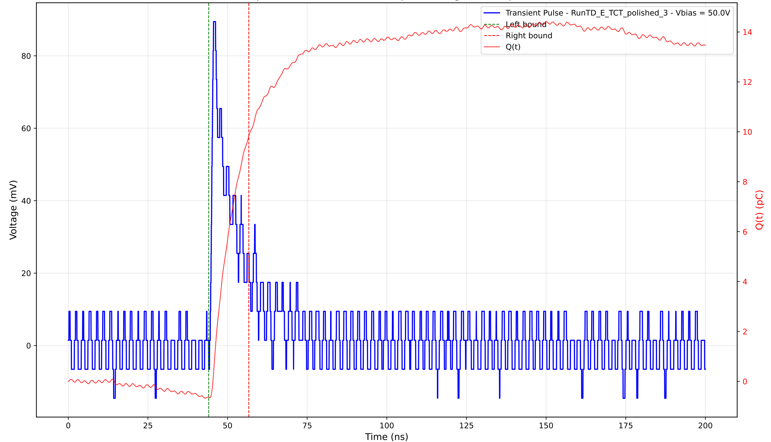
Transient Pulse - Sample: 4003 - Position: 165.0 \mu\text{m} - Charge: 10.47 pC - Rise Time: 0.88 ns
