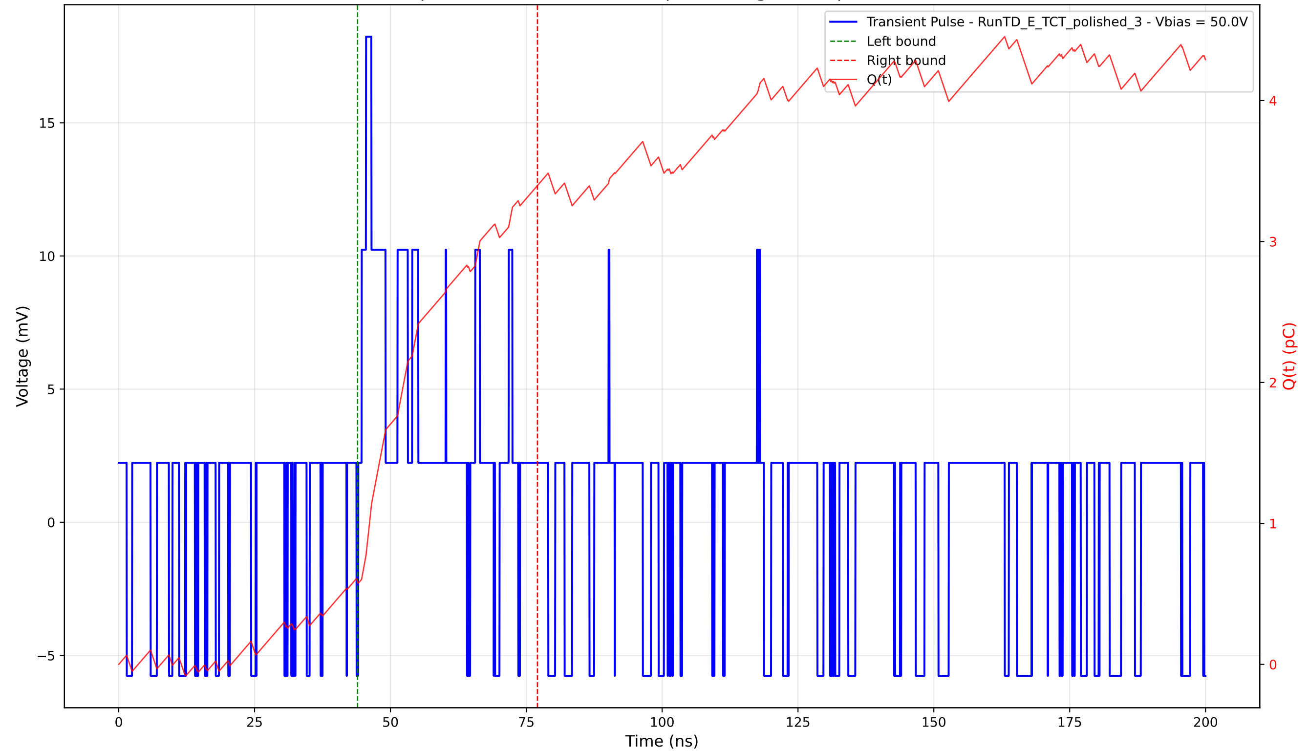
Transient Pulse - Sample: 4003 - Position: 535.0 \mu\text{m} - Charge: 2.81 pC - Rise Time: 0.00 ns (N/A)
