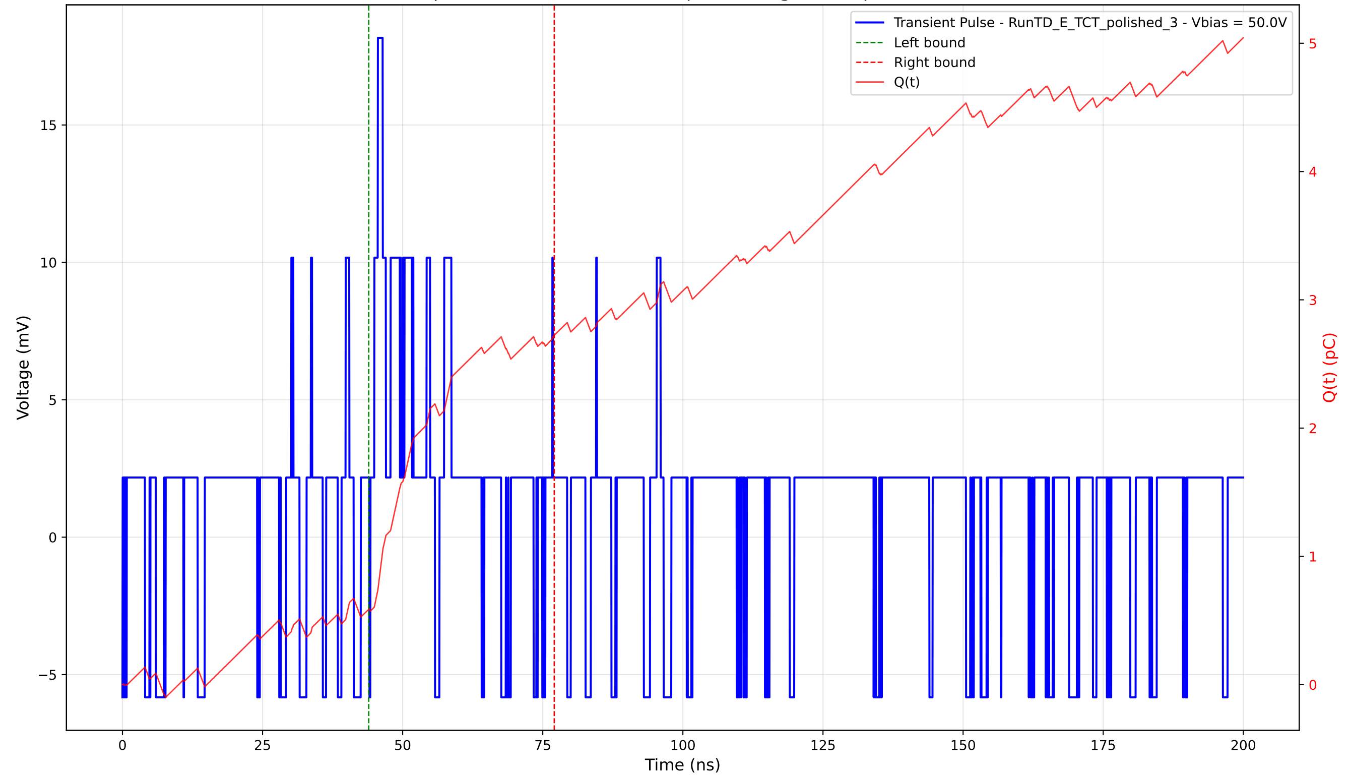
Transient Pulse - Sample: 4003 - Position: 570.0 \mu\text{m} - Charge: 2.13 pC - Rise Time: 0.00 ns (N/A)
