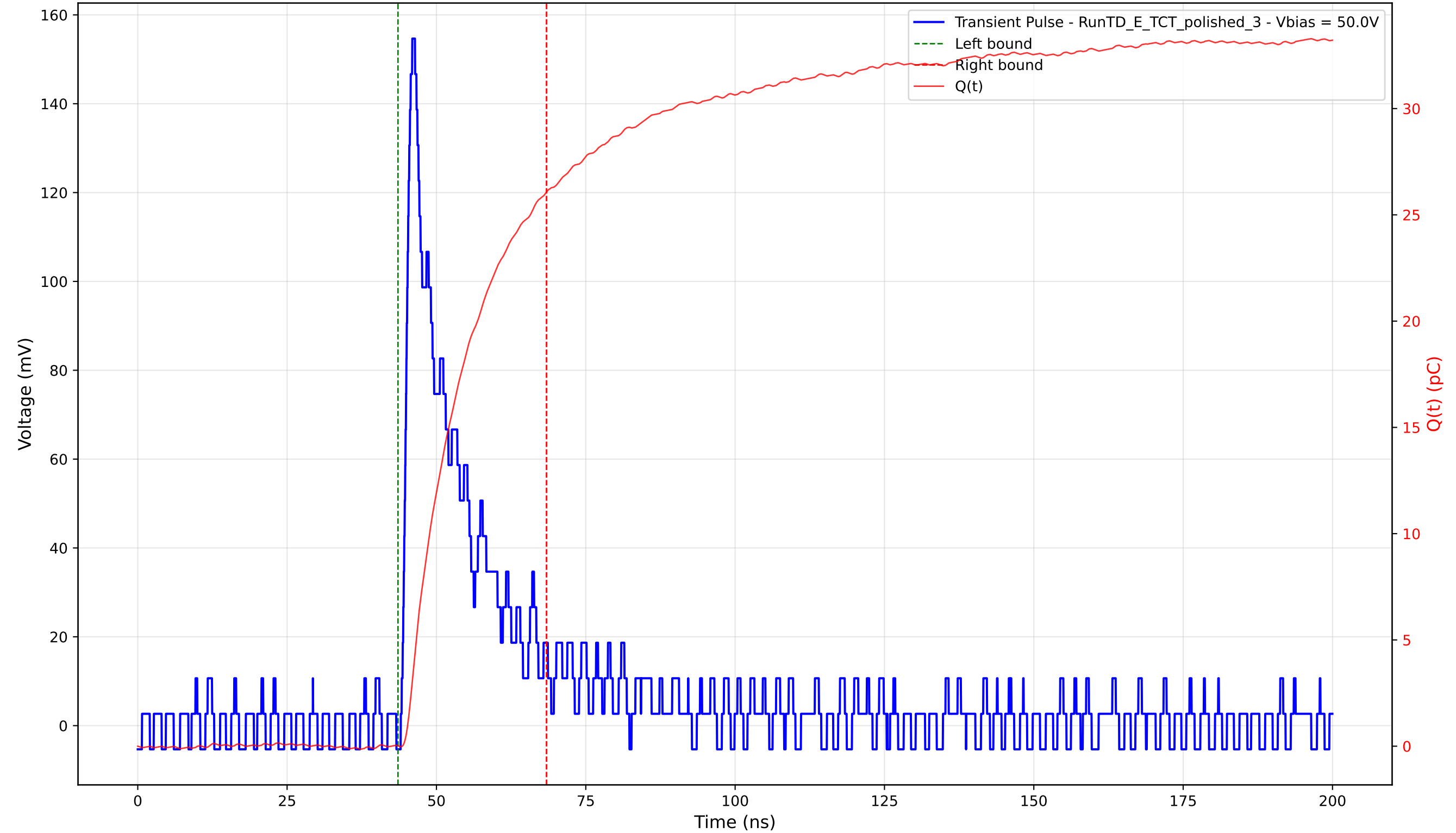
Transient Pulse - Sample: 4003 - Position: 240.0 \mu\text{m} - Charge: 26.06 pC - Rise Time: 1.35 ns
