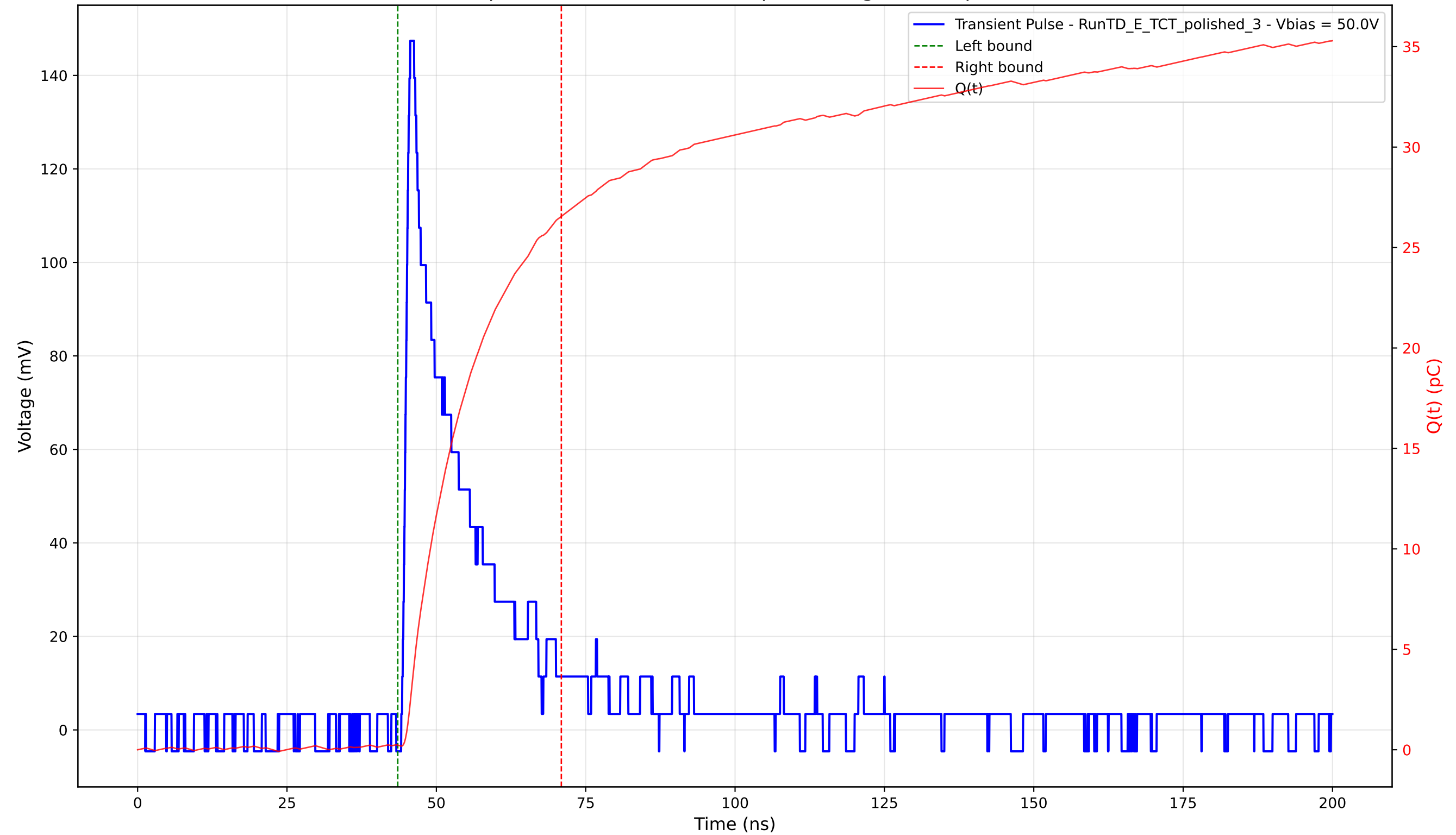
Transient Pulse - Sample: 4003 - Position: 260.0 \mu\text{m} - Charge: 26.32 pC - Rise Time: 1.11 ns
