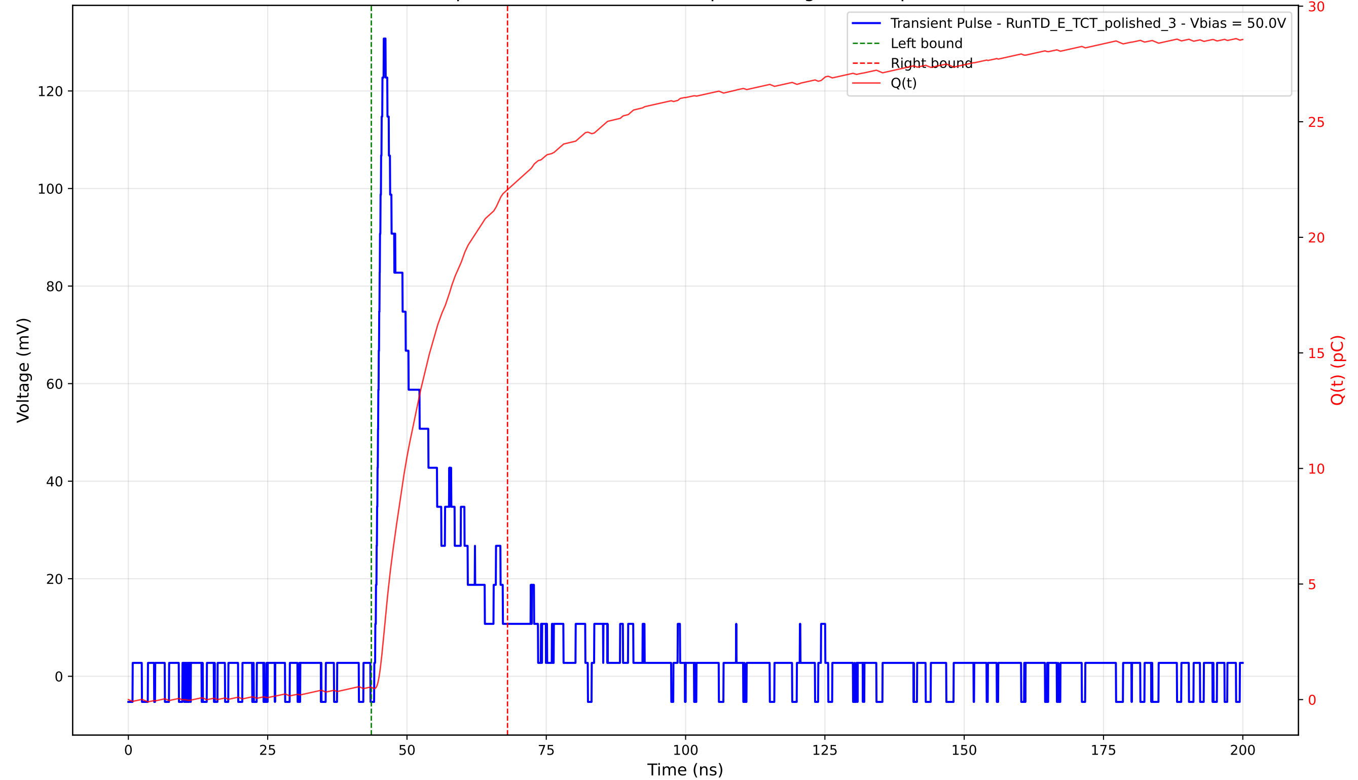
Transient Pulse - Sample: 4003 - Position: 200.0 \mu\text{m} - Charge: 21.53 pC - Rise Time: 1.17 ns
