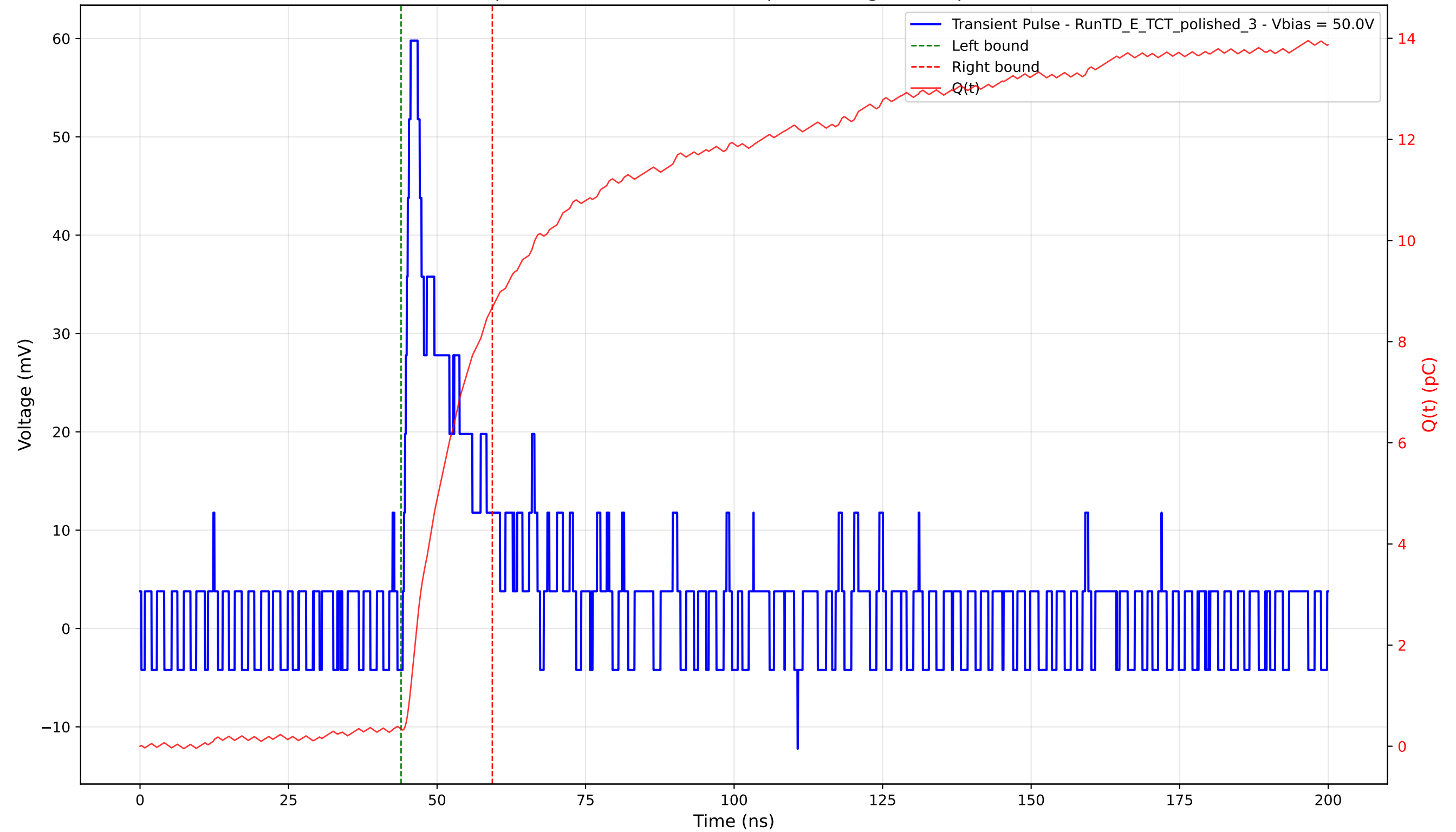
Transient Pulse - Sample: 4003 - Position: 145.0 \mu\text{m} - Charge: 8.34 pC - Rise Time: 1.13 ns
