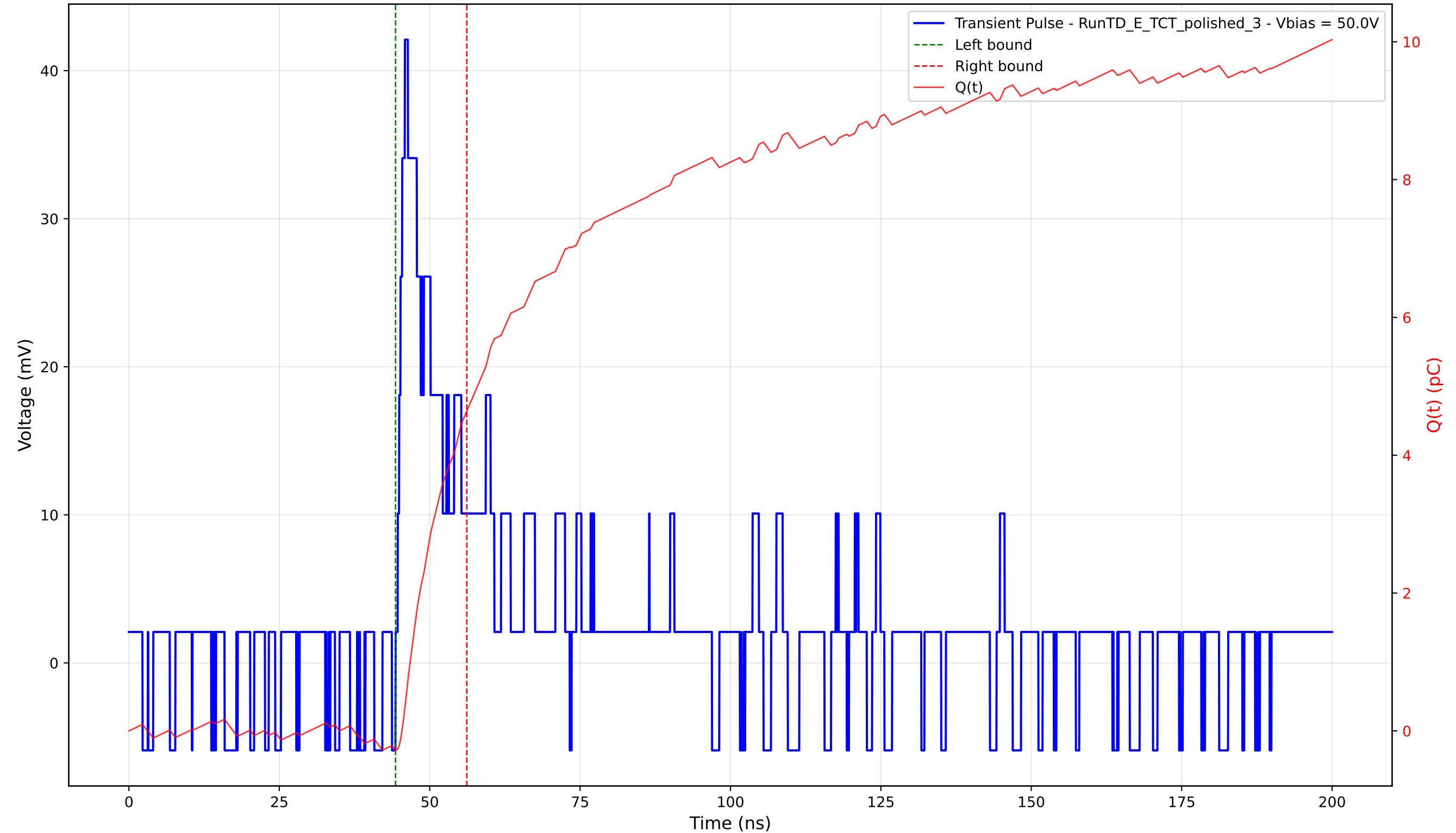
Transient Pulse - Sample: 4003 - Position: 385.0 \mu\text{m} - Charge: 4.92 pC - Rise Time: 1.19 ns
