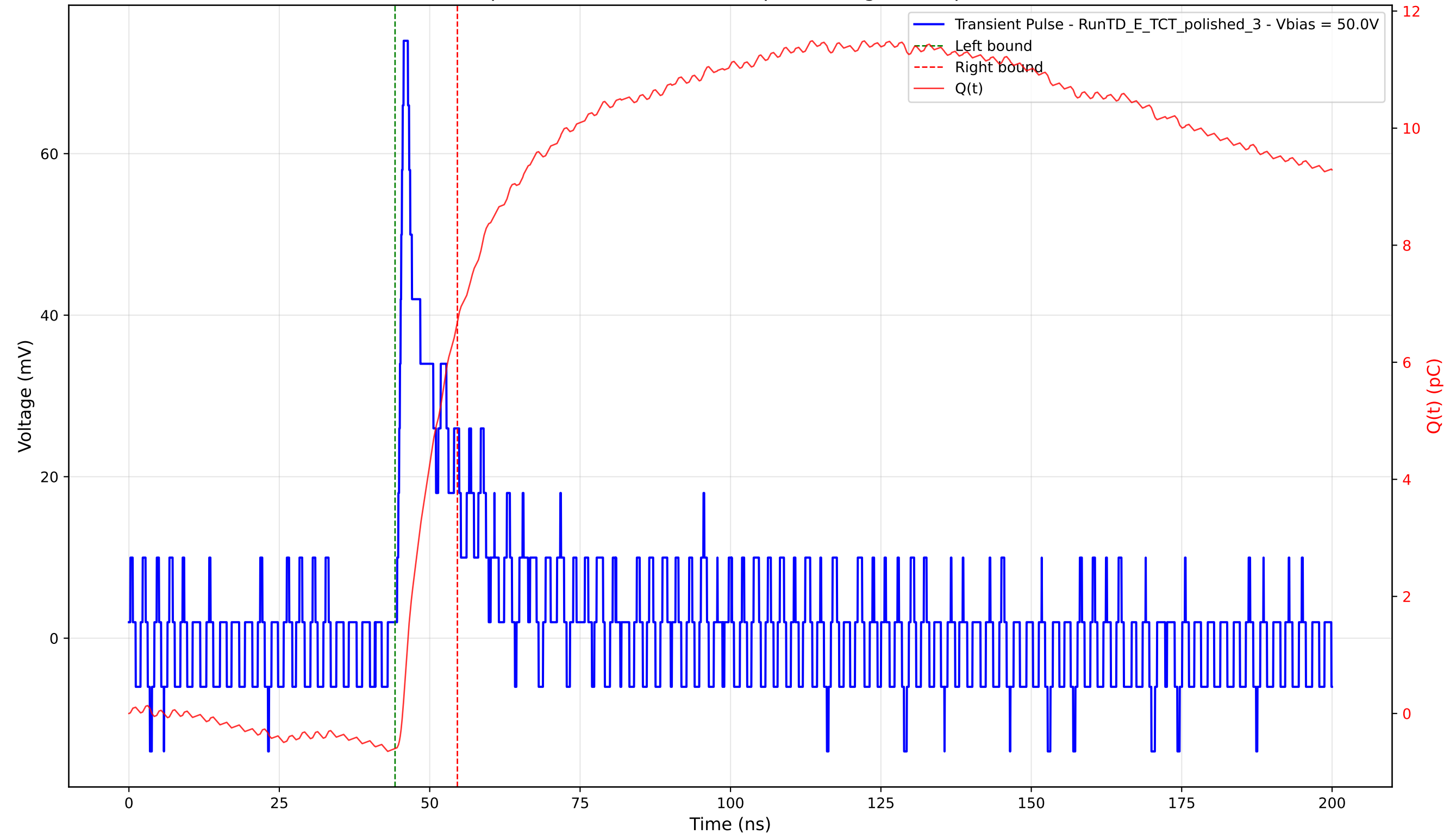
Transient Pulse - Sample: 4003 - Position: 150.0 \mu\text{m} - Charge: 7.29 pC - Rise Time: 1.09 ns
