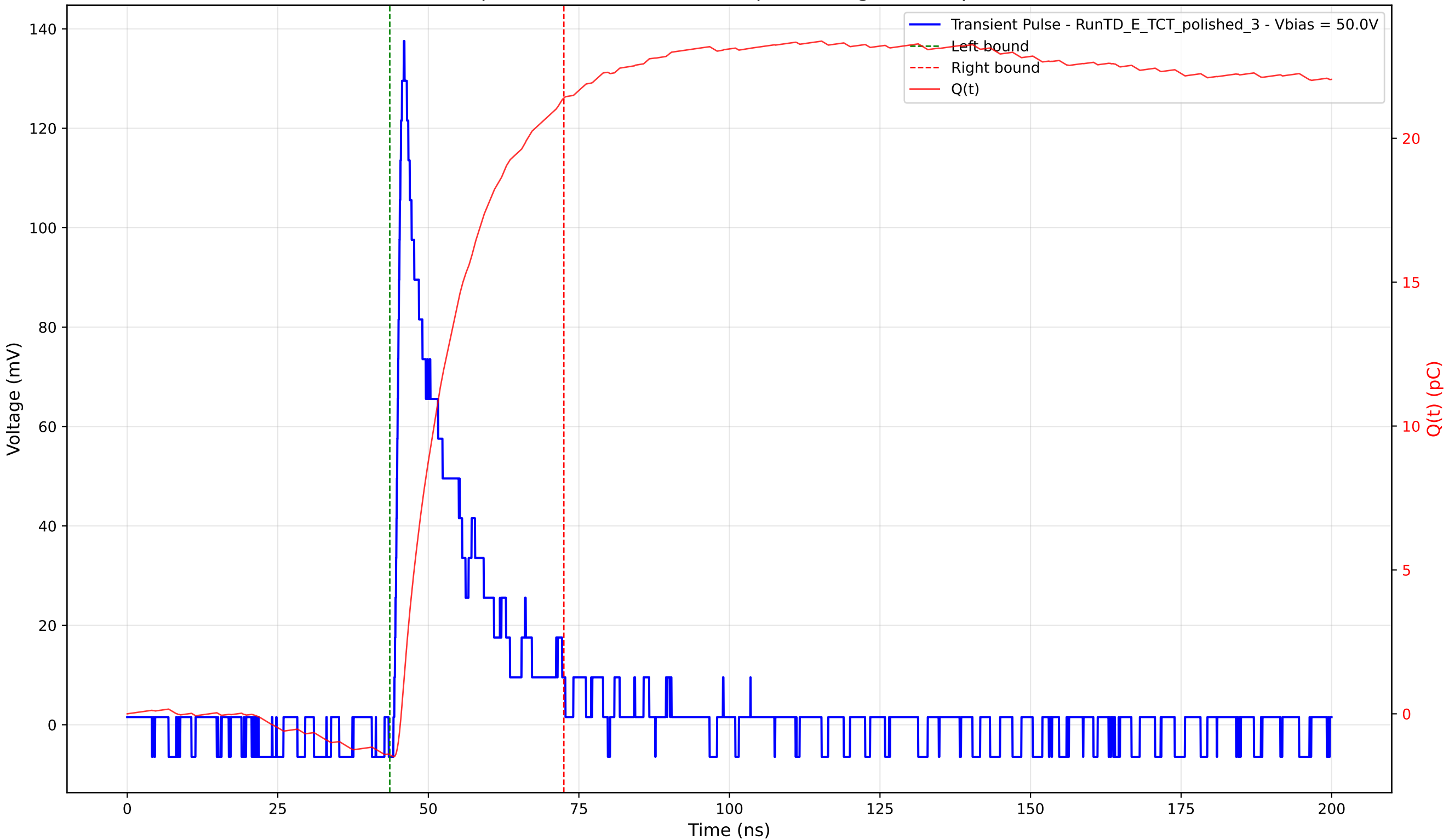
Transient Pulse - Sample: 4003 - Position: 210.0 \mu\text{m} - Charge: 22.82 pC - Rise Time: 1.17 ns
