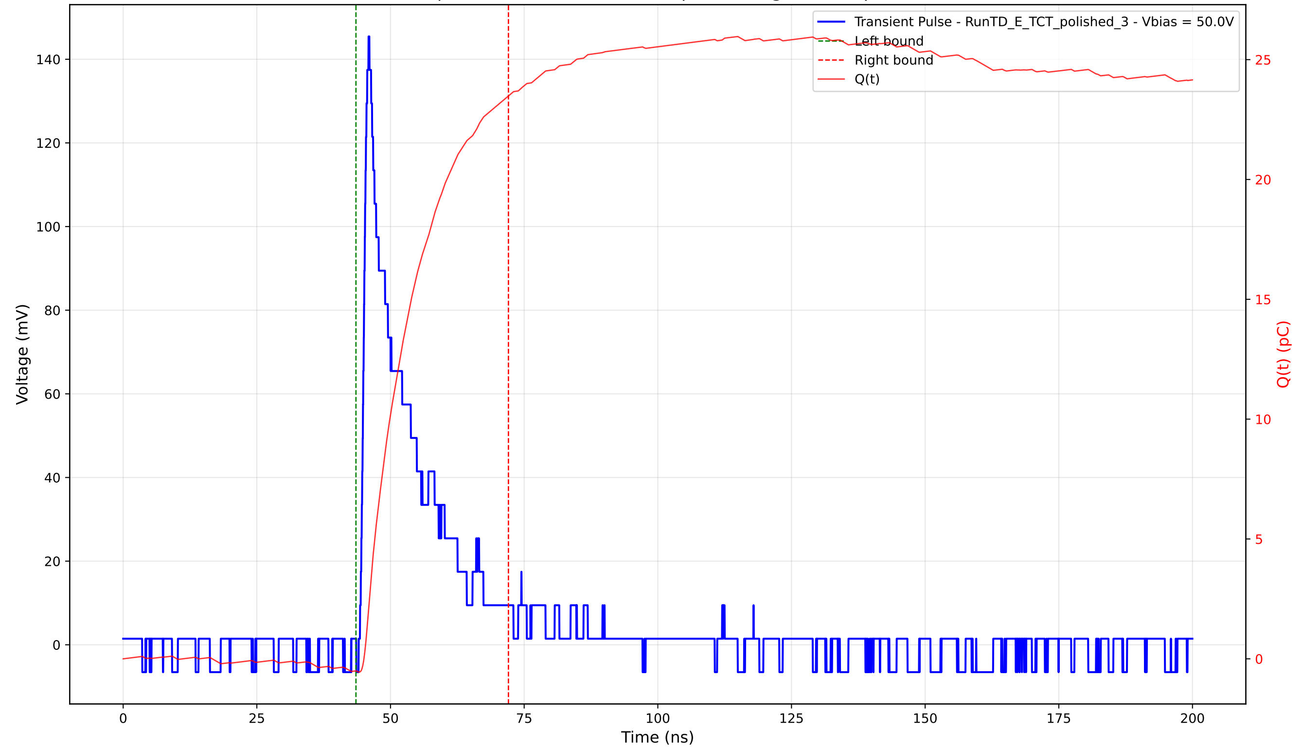
Transient Pulse - Sample: 4003 - Position: 215.0 \mu\text{m} - Charge: 23.99 pC - Rise Time: 1.21 ns
