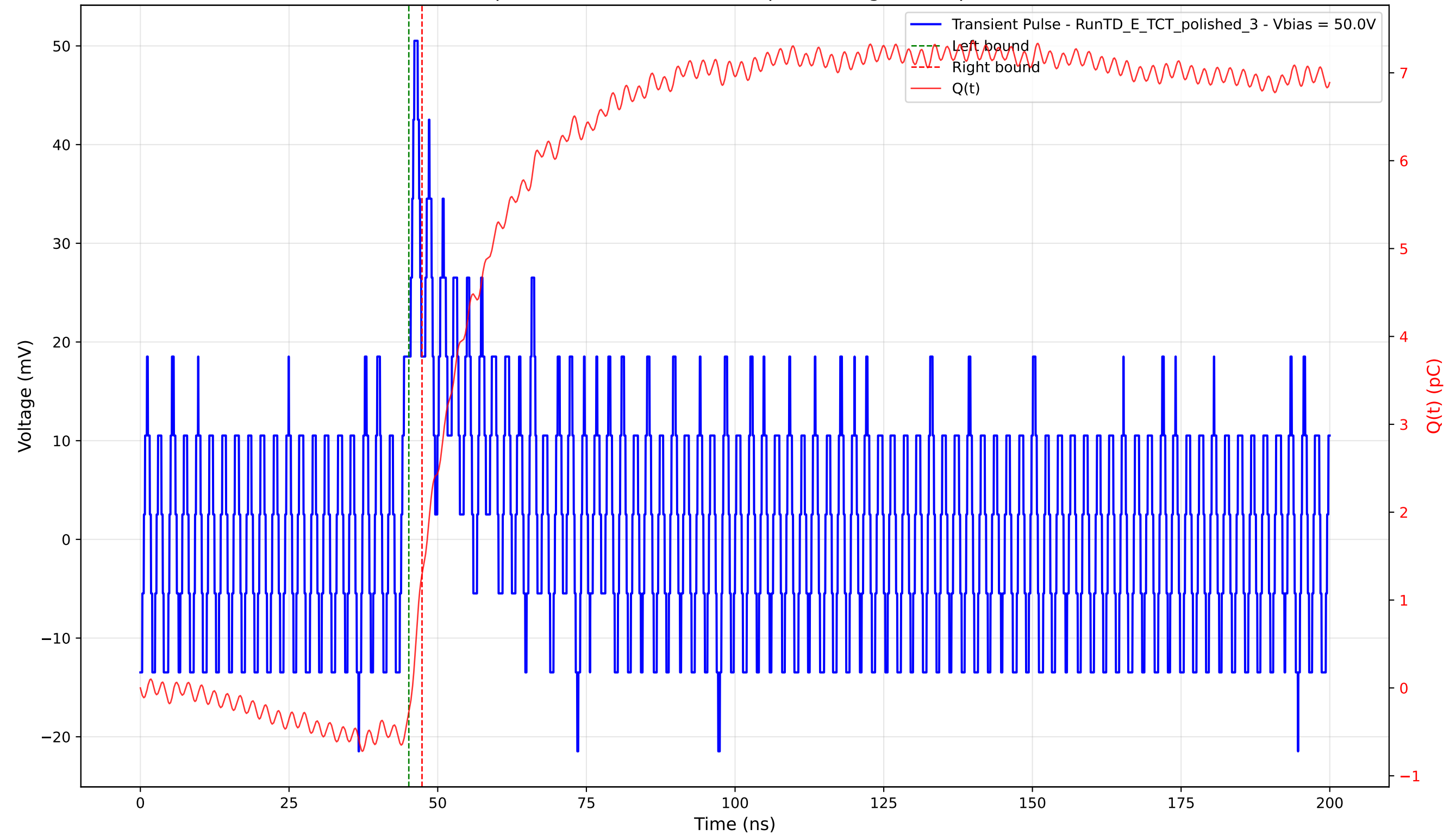
Transient Pulse - Sample: 4003 - Position: 130.0 \mu\text{m} - Charge: 1.57 pC - Rise Time: 2.01 ns
