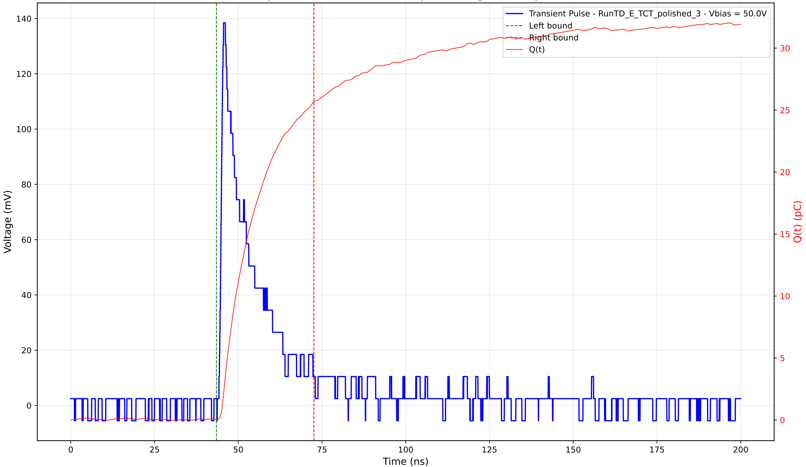
Transient Pulse - Sample: 4003 - Position: 280.0 \mu\text{m} - Charge: 25.58 pC - Rise Time: 1.09 ns
