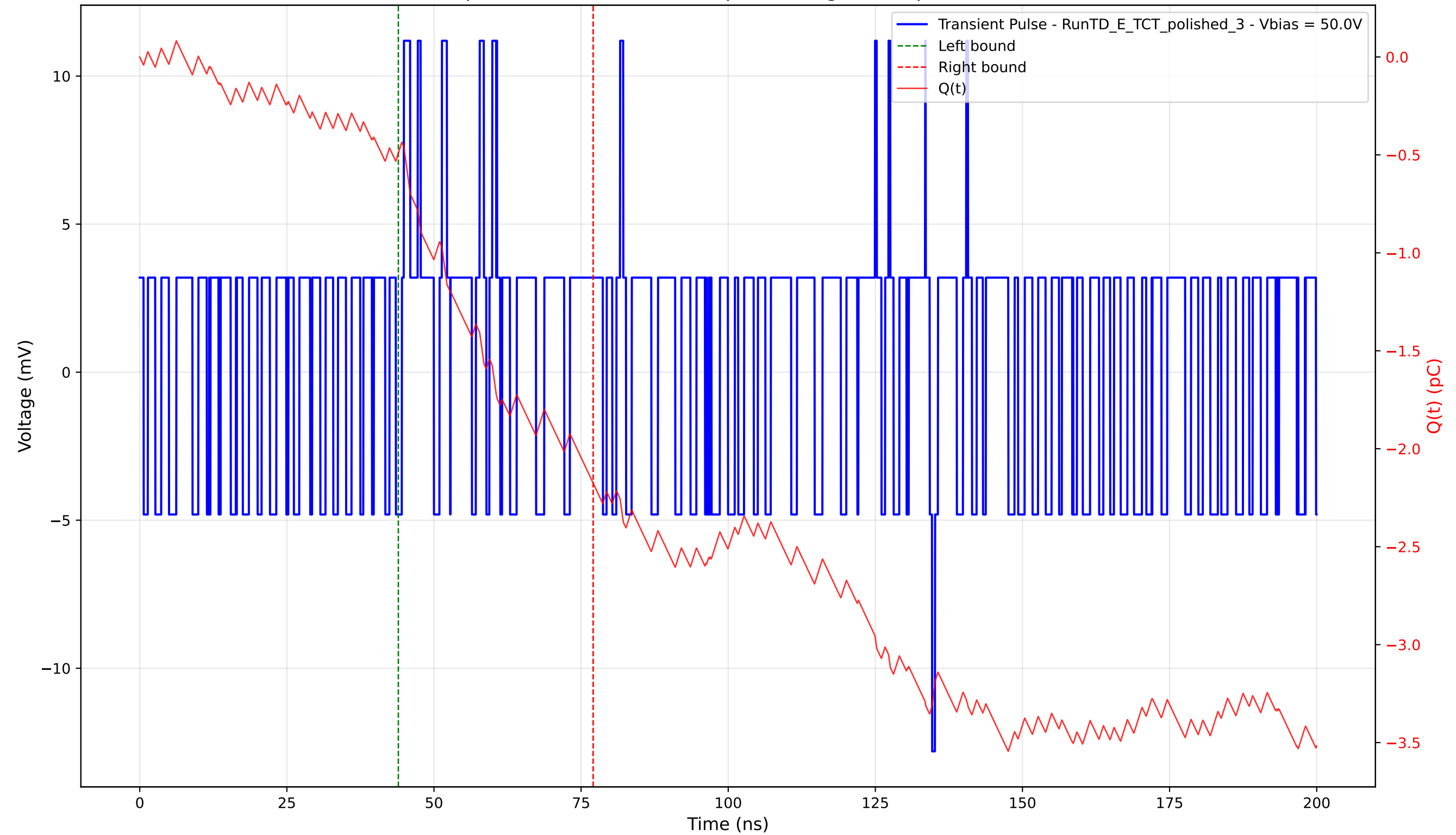
Transient Pulse - Sample: 4003 - Position: 35.0 \mu\text{m} - Charge: 1.69 pC - Rise Time: 0.00 ns (N/A)
