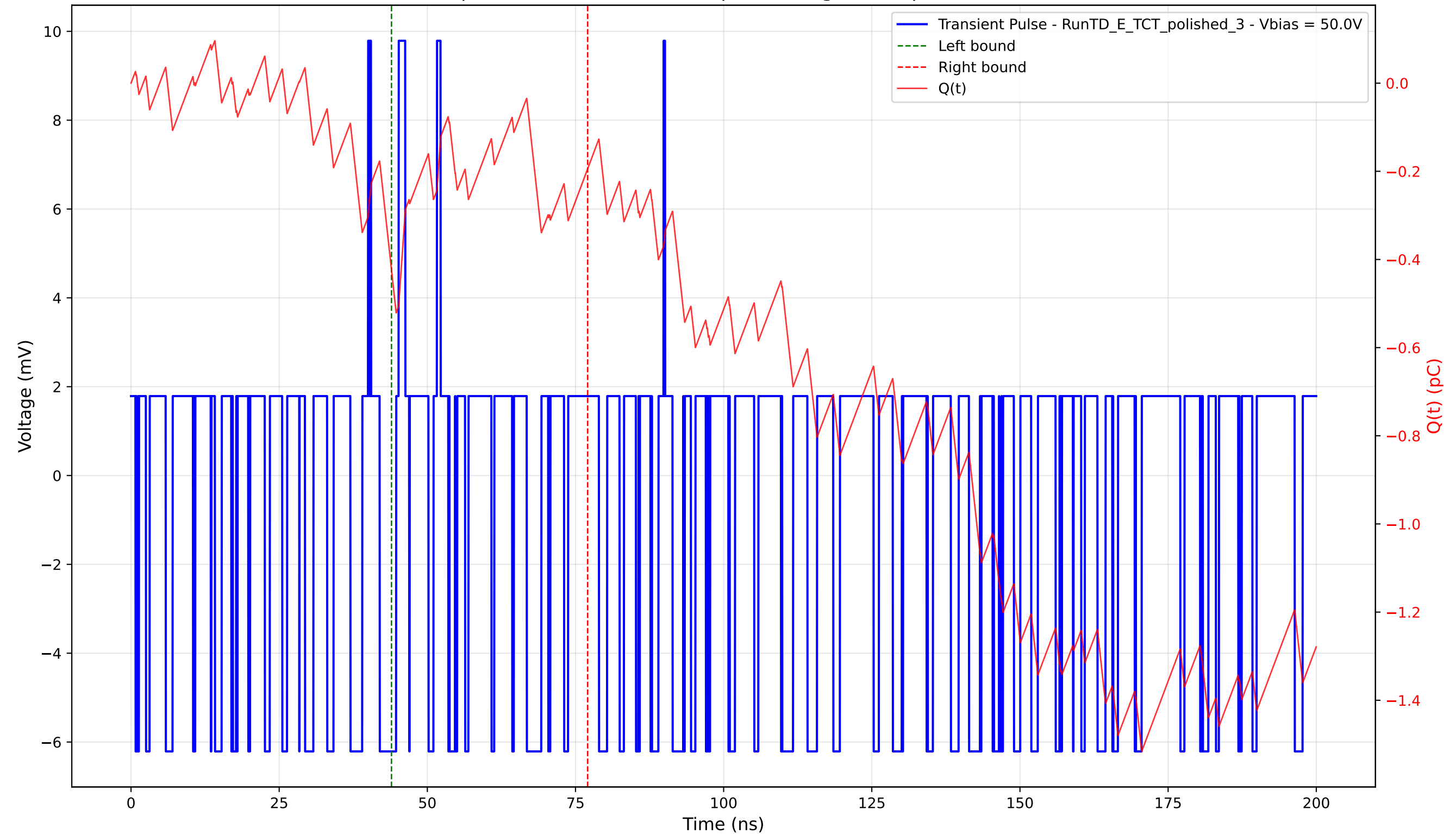
Transient Pulse - Sample: 4003 - Position: 15.0 \mu\text{m} - Charge: 0.23 pC - Rise Time: 0.00 ns (N/A)
