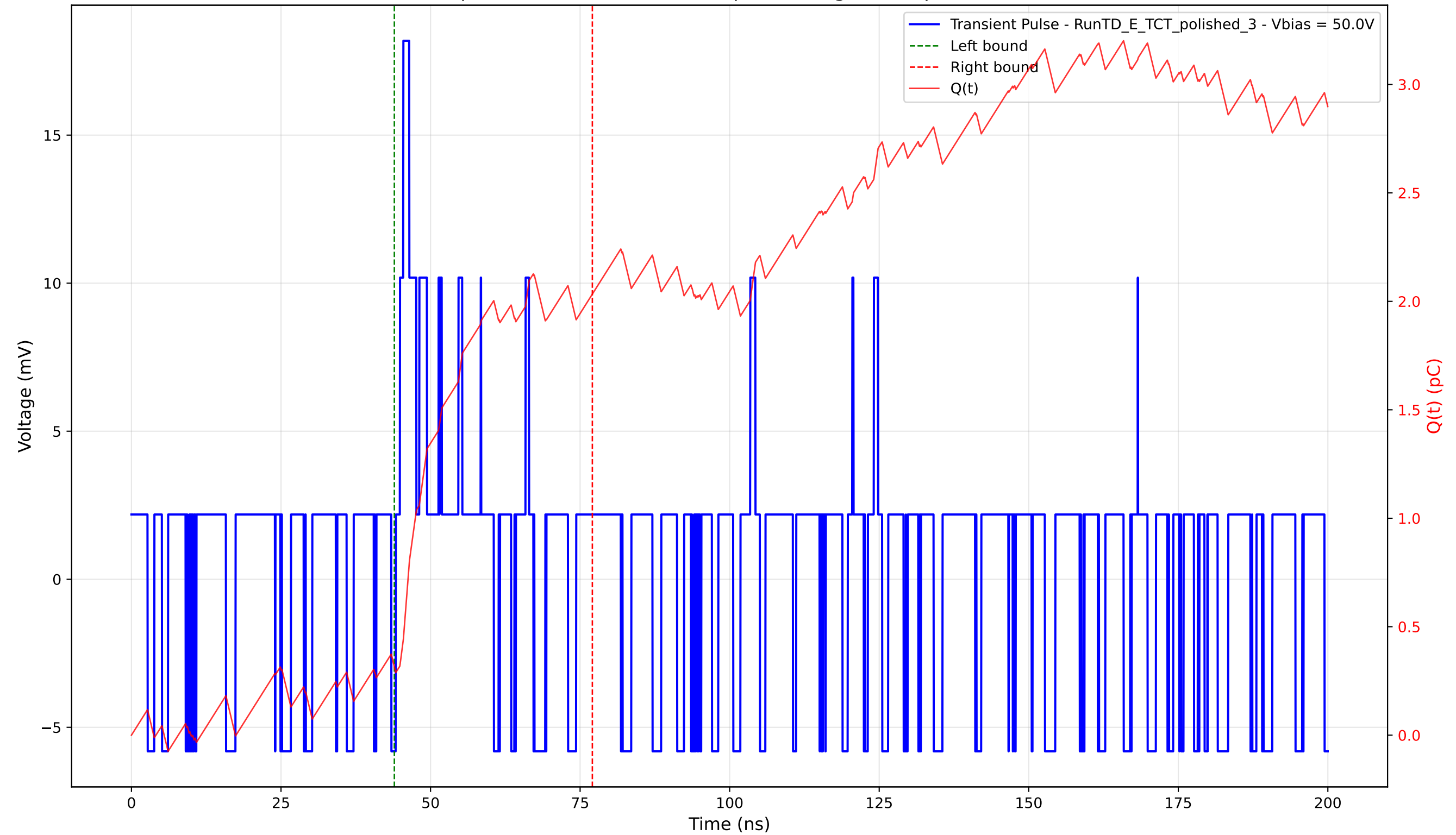
Transient Pulse - Sample: 4003 - Position: 670.0 \mu\text{m} - Charge: 1.72 pC - Rise Time: 0.00 ns (N/A)
