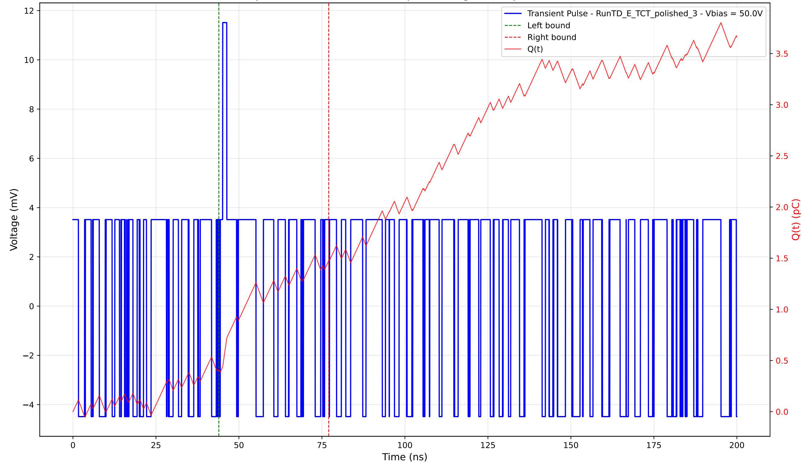
Transient Pulse - Sample: 4003 - Position: 780.0 \mu\text{m} - Charge: 1.07 pC - Rise Time: 0.00 ns (N/A)
