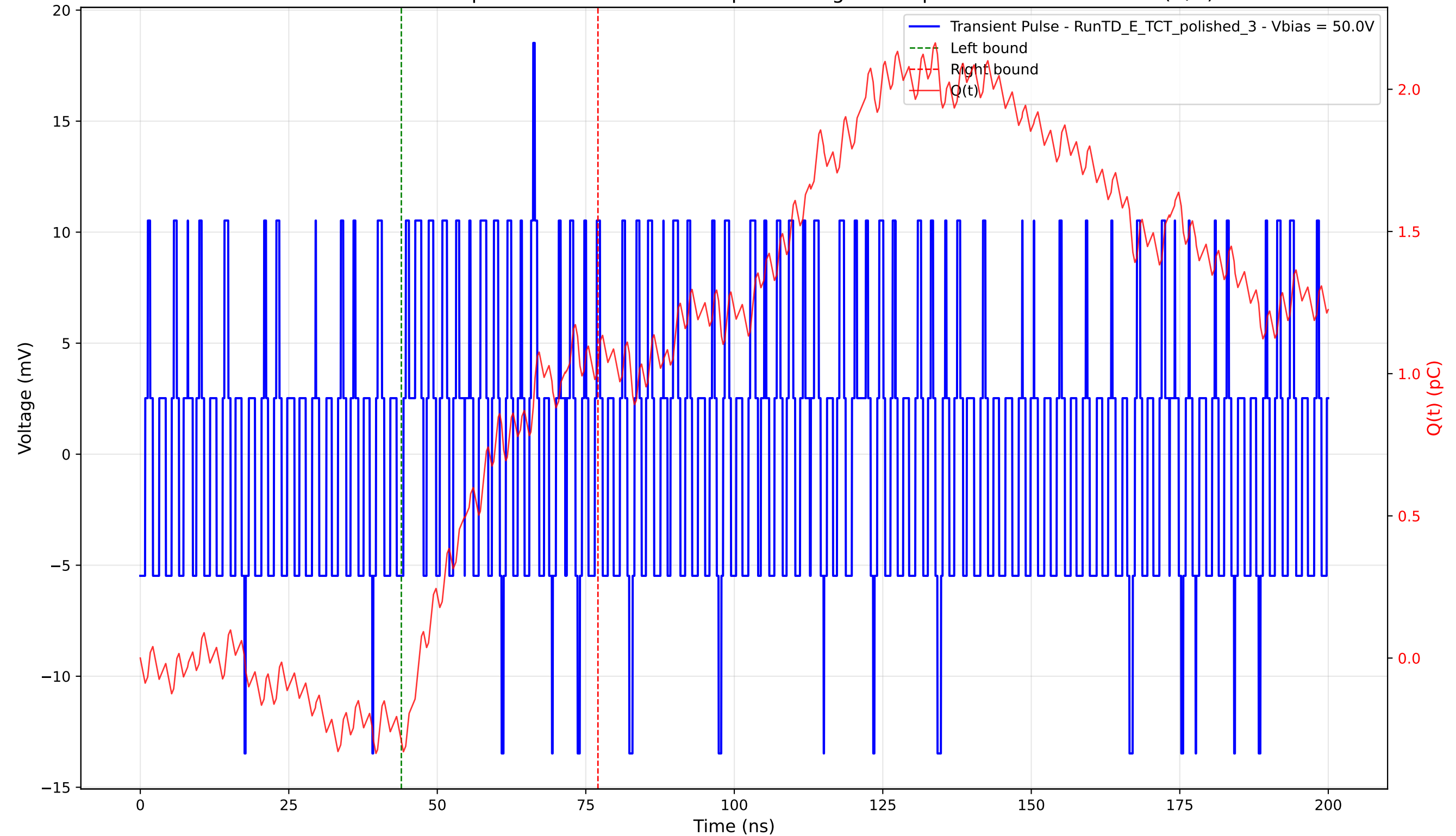
Transient Pulse - Sample: 4003 - Position: 65.0 \mu\text{m} - Charge: 1.33 pC - Rise Time: 0.00 ns (N/A)
