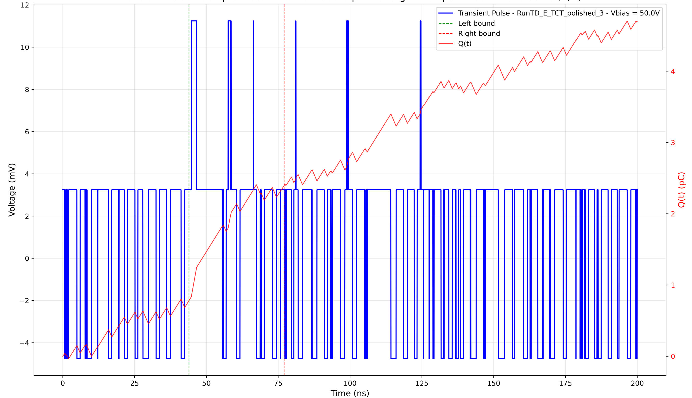
Transient Pulse - Sample: 4003 - Position: 690.0 \mu\text{m} - Charge: 1.61 pC - Rise Time: 0.00 ns (N/A)
