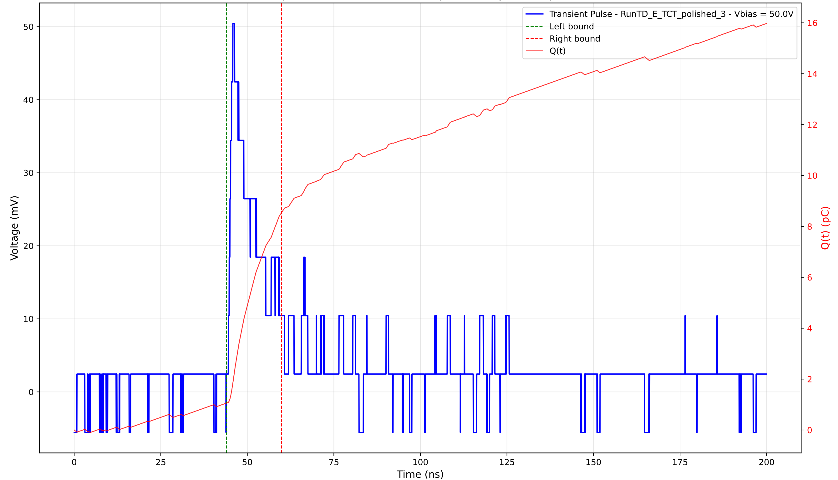
Transient Pulse - Sample: 4003 - Position: 375.0 \mu\text{m} - Charge: 7.49 pC - Rise Time: 1.31 ns
