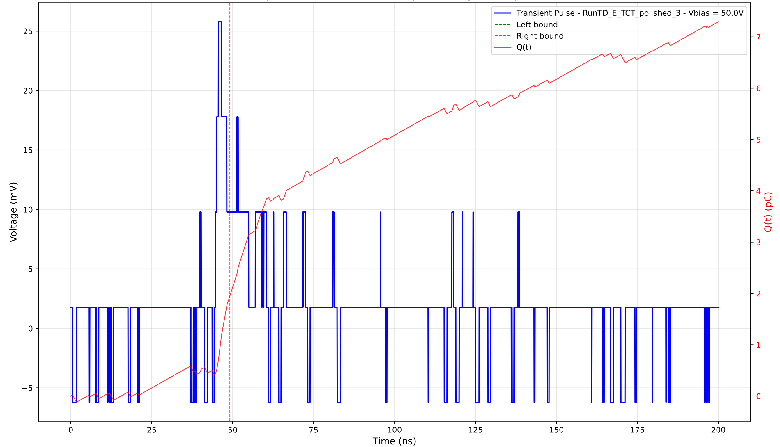
Transient Pulse - Sample: 4003 - Position: 415.0 \mu\text{m} - Charge: 1.52 pC - Rise Time: 0.86 ns
