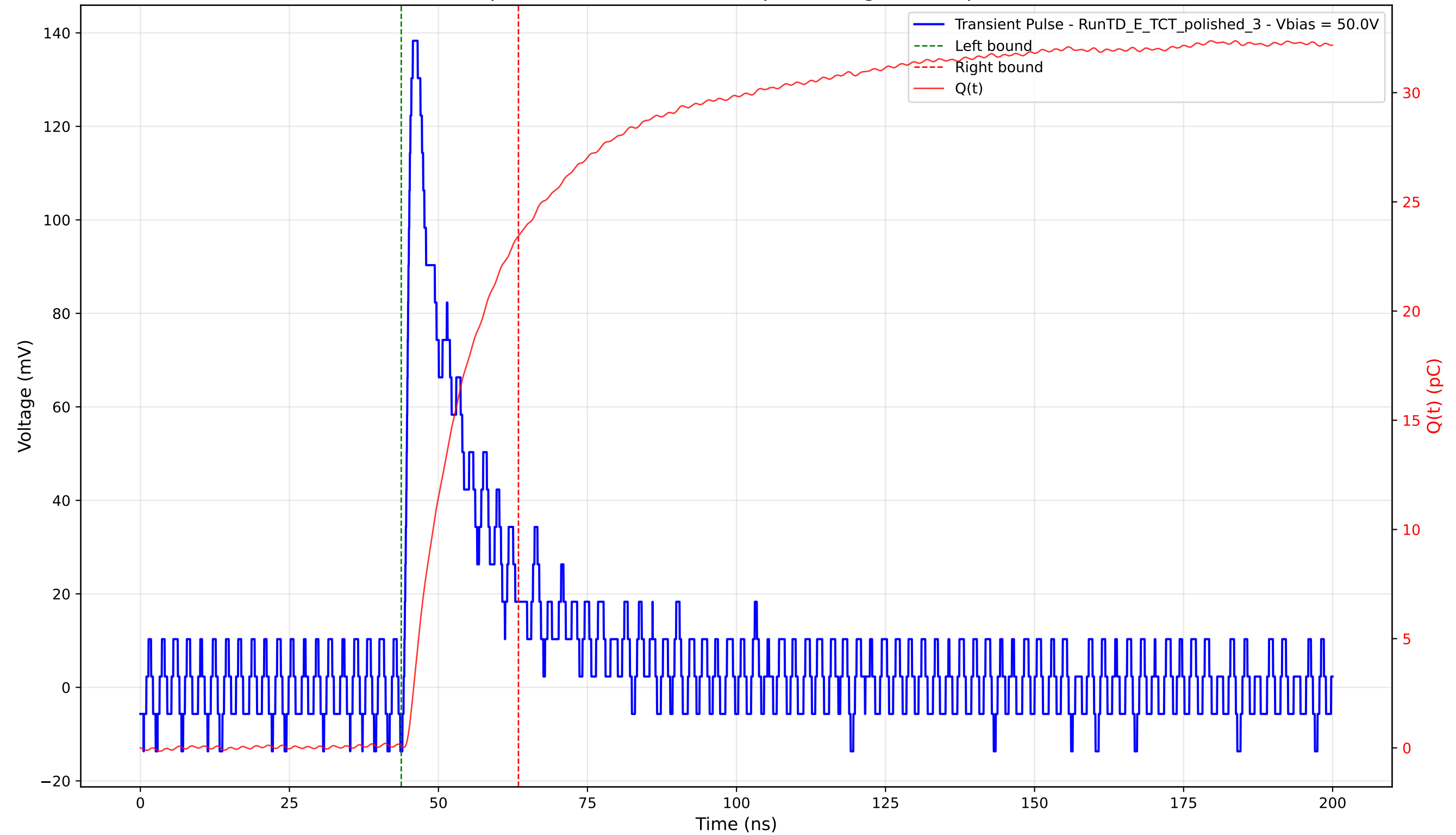
Transient Pulse - Sample: 4003 - Position: 265.0 \mu\text{m} - Charge: 23.35 pC - Rise Time: 1.11 ns
