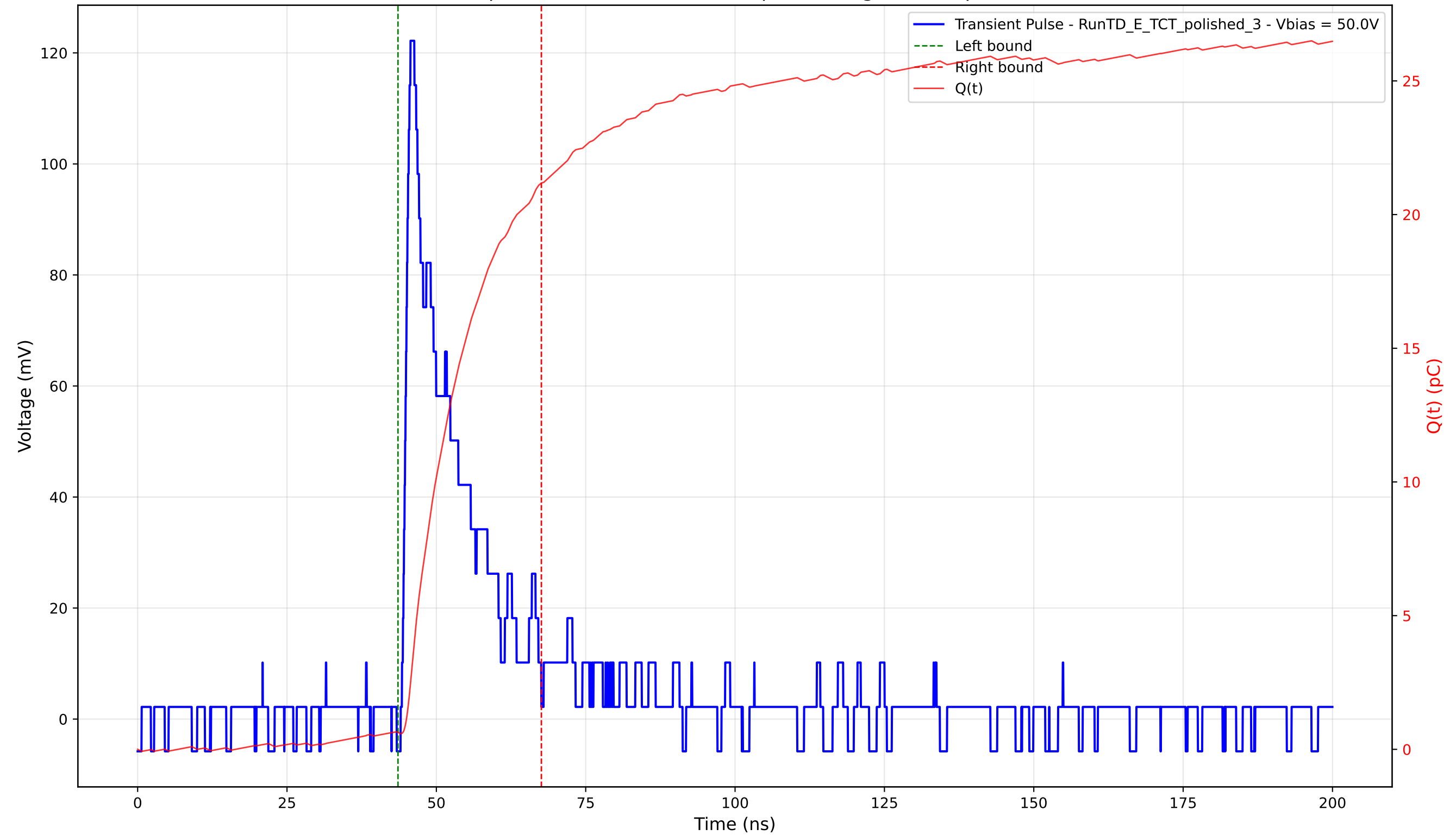
Transient Pulse - Sample: 4003 - Position: 195.0 \mu\text{m} - Charge: 20.55 pC - Rise Time: 1.11 ns
