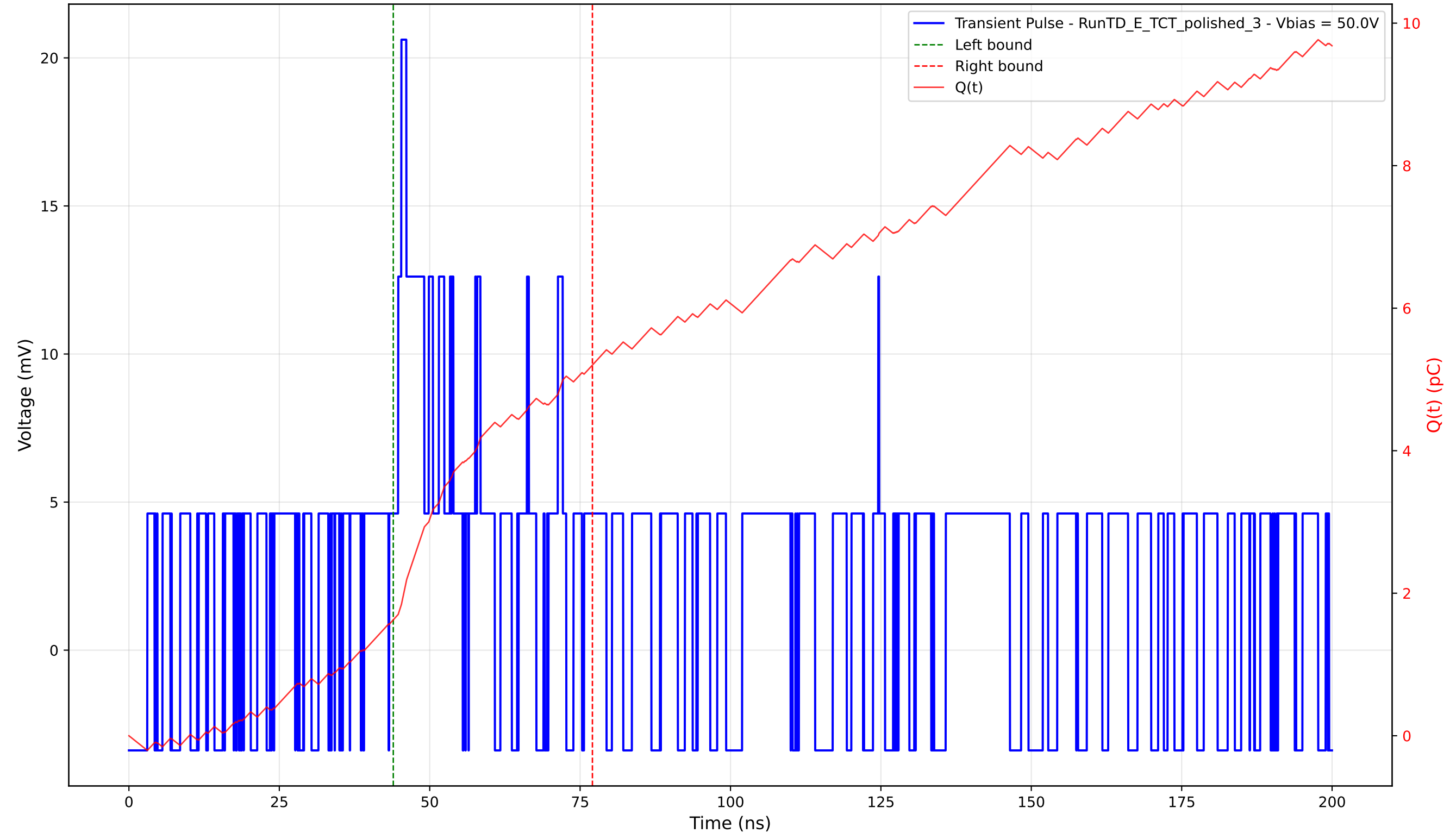
Transient Pulse - Sample: 4003 - Position: 545.0 \mu\text{m} - Charge: 3.57 pC - Rise Time: 0.00 ns (N/A)
