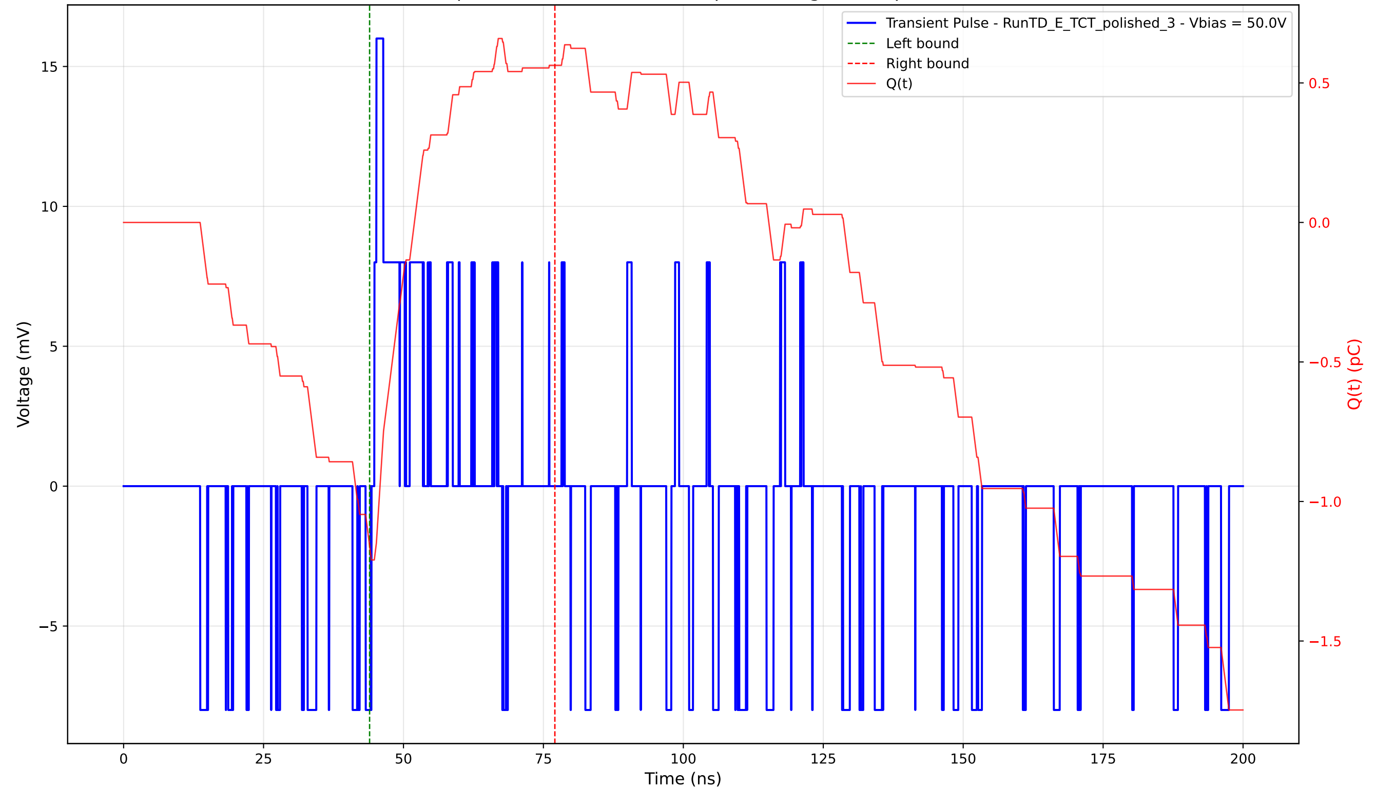
Transient Pulse - Sample: 4003 - Position: 435.0 \mu\text{m} - Charge: 1.73 pC - Rise Time: 0.38 ns
