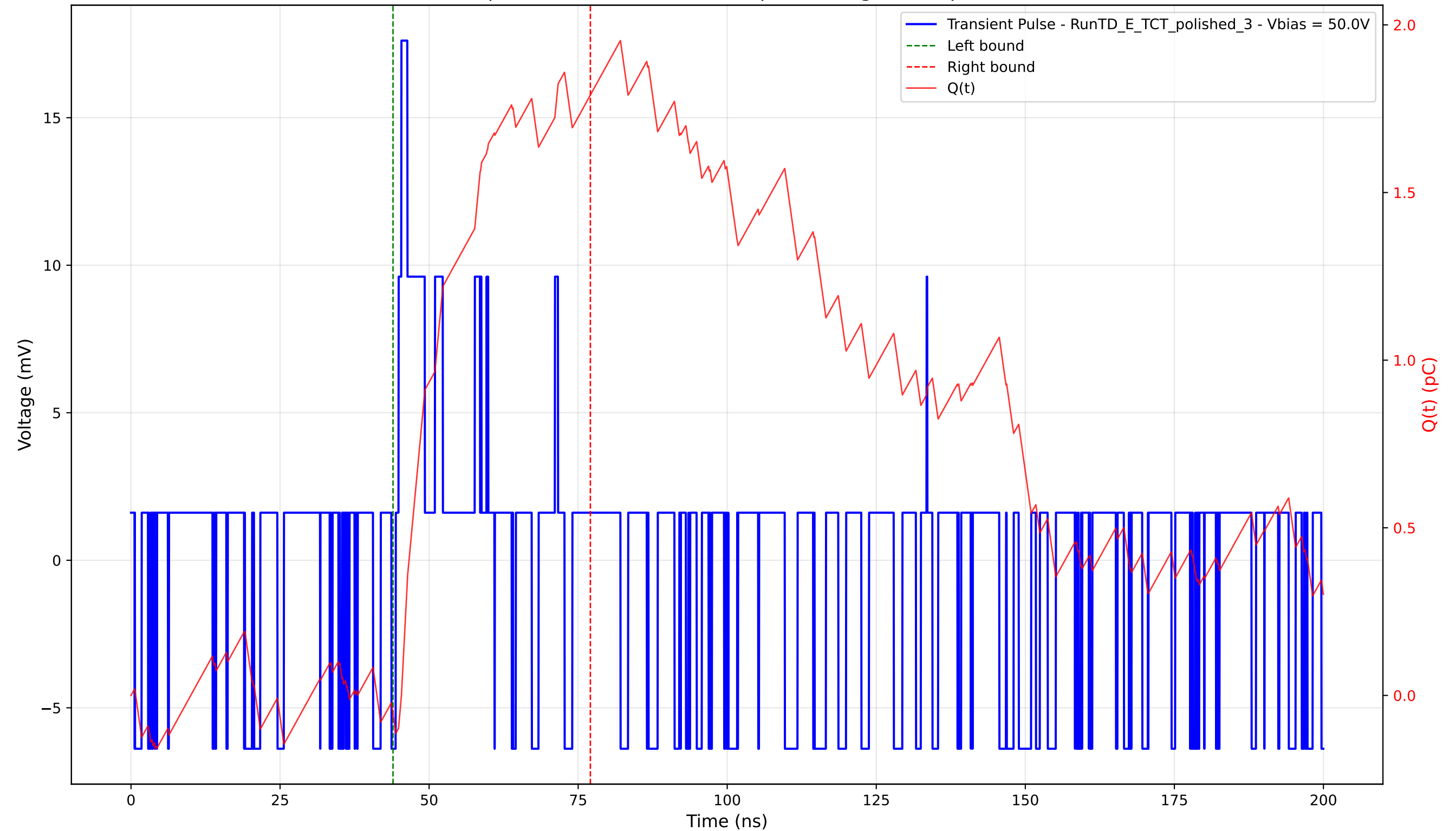
Transient Pulse - Sample: 4003 - Position: 515.0 \mu\text{m} - Charge: 1.85 pC - Rise Time: 0.48 ns
