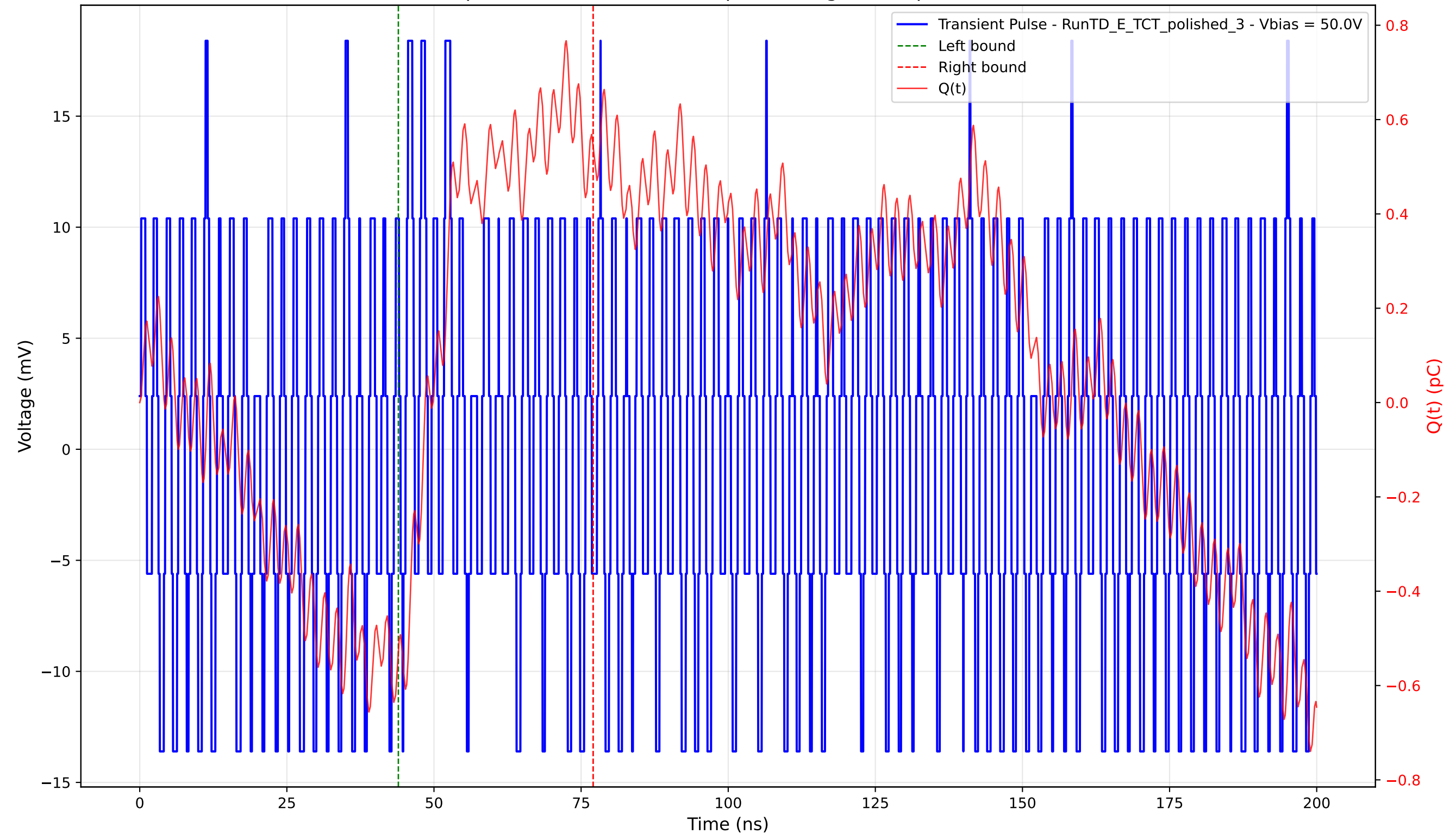
Transient Pulse - Sample: 4003 - Position: 85.0 \mu\text{m} - Charge: 1.07 pC - Rise Time: 0.00 ns (N/A)
