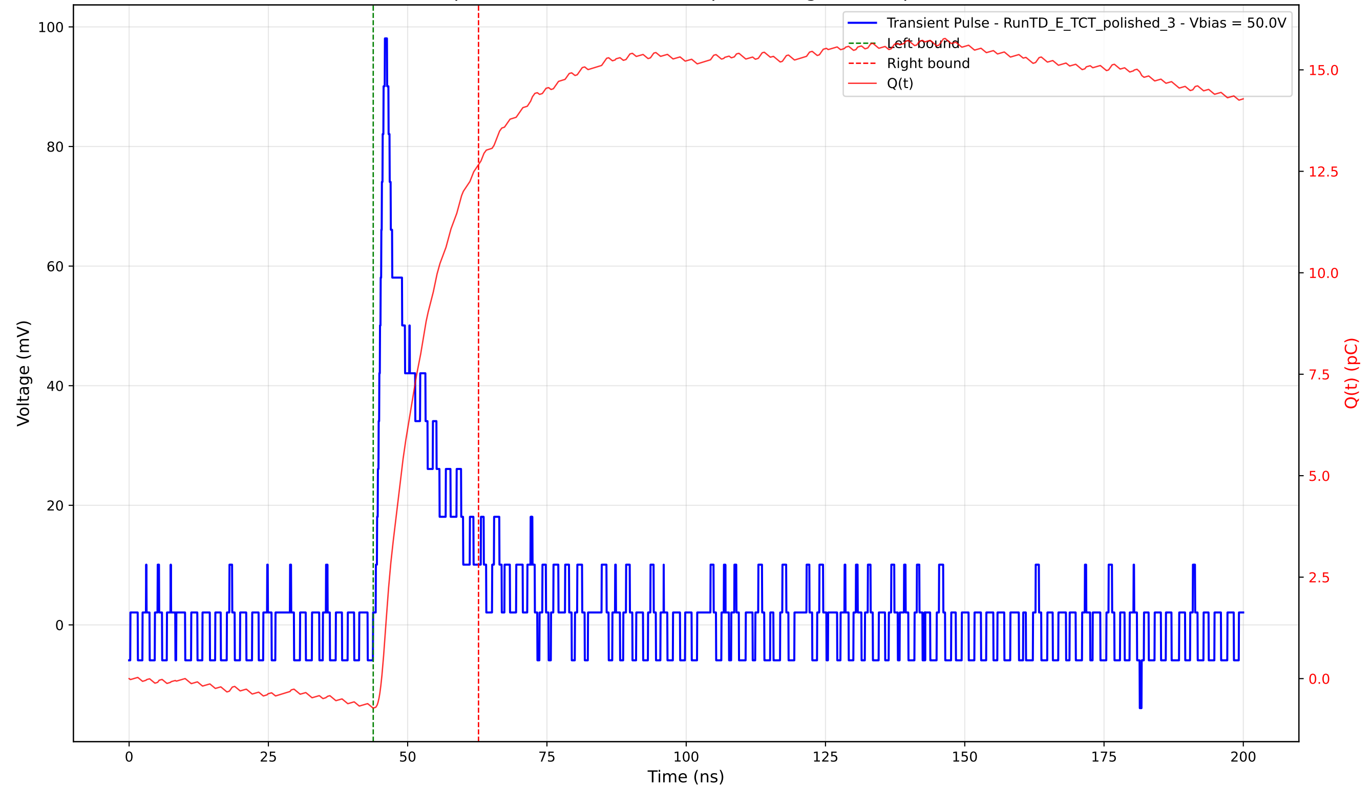
Transient Pulse - Sample: 4003 - Position: 170.0 \mu\text{m} - Charge: 13.39 pC - Rise Time: 1.38 ns
