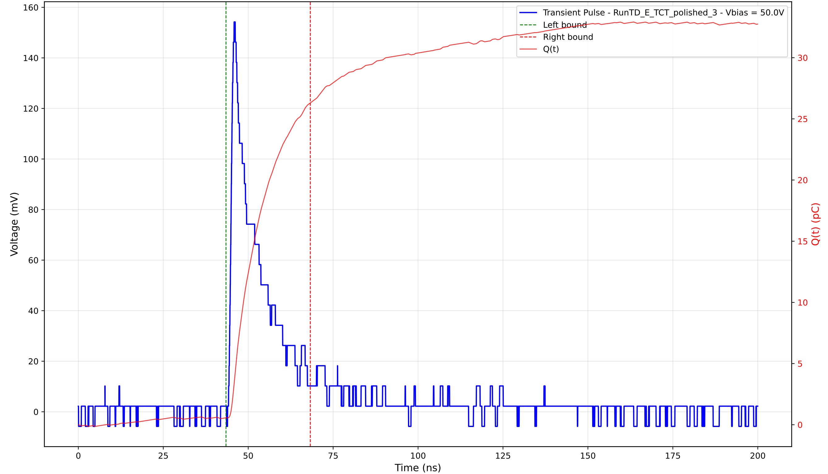
Transient Pulse - Sample: 4003 - Position: 250.0 \mu\text{m} - Charge: 25.73 pC - Rise Time: 1.27 ns
