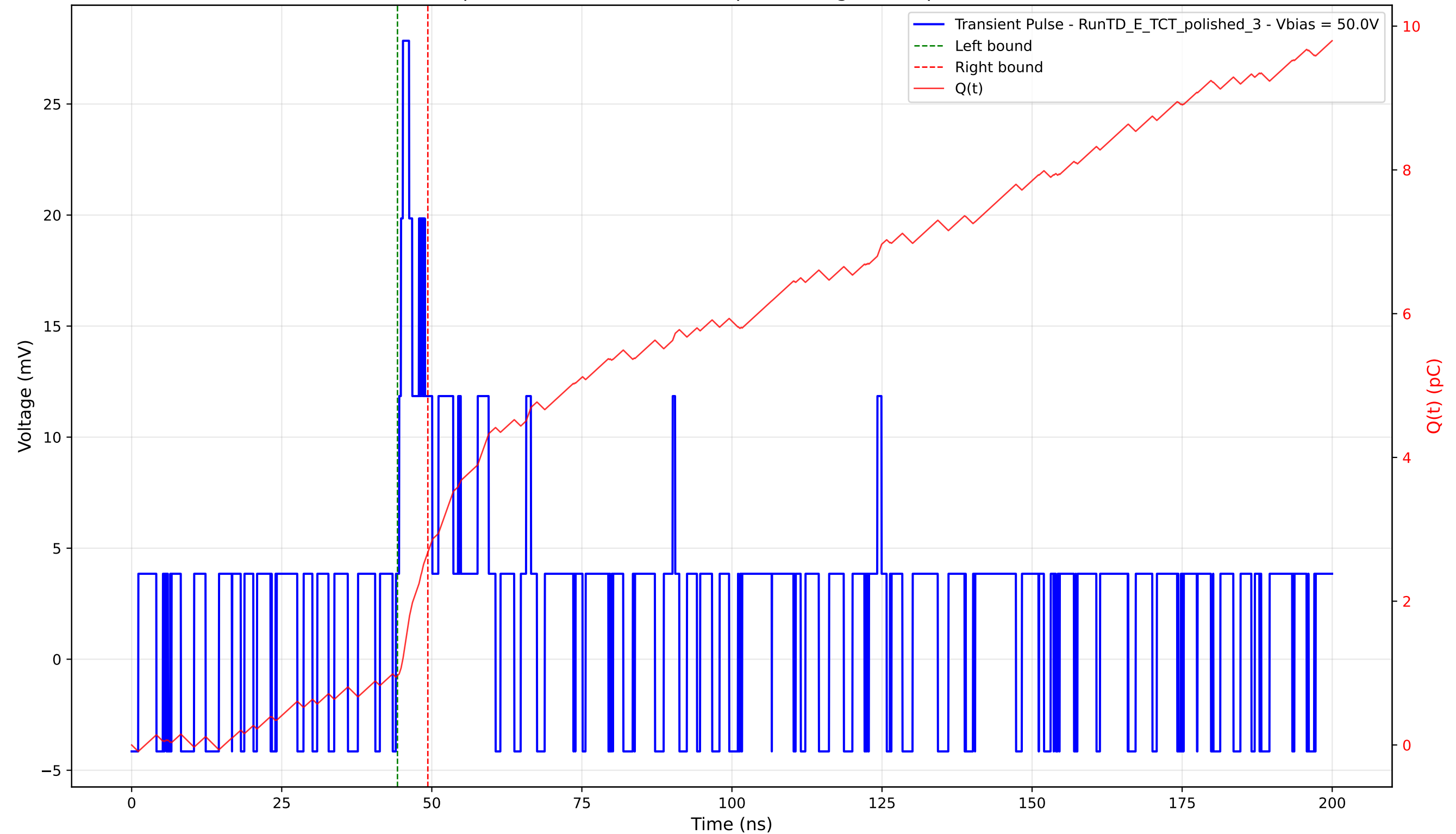
Transient Pulse - Sample: 4003 - Position: 640.0 \mu\text{m} - Charge: 1.72 pC - Rise Time: 0.00 ns (N/A)
