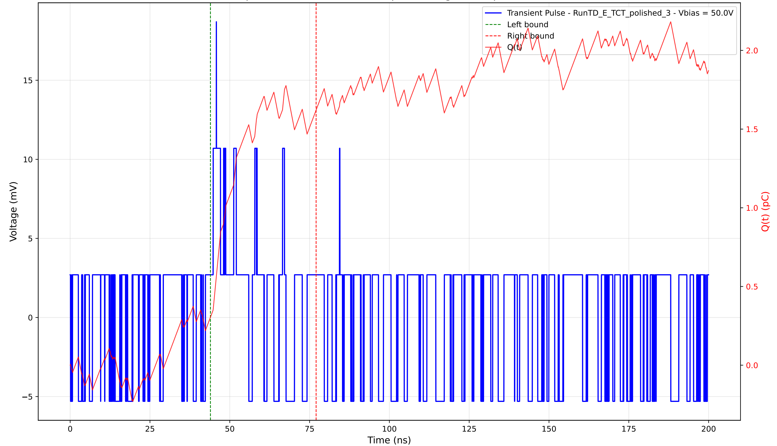
Transient Pulse - Sample: 4003 - Position: 585.0 \mu\text{m} - Charge: 1.31 pC - Rise Time: 0.00 ns (N/A)
