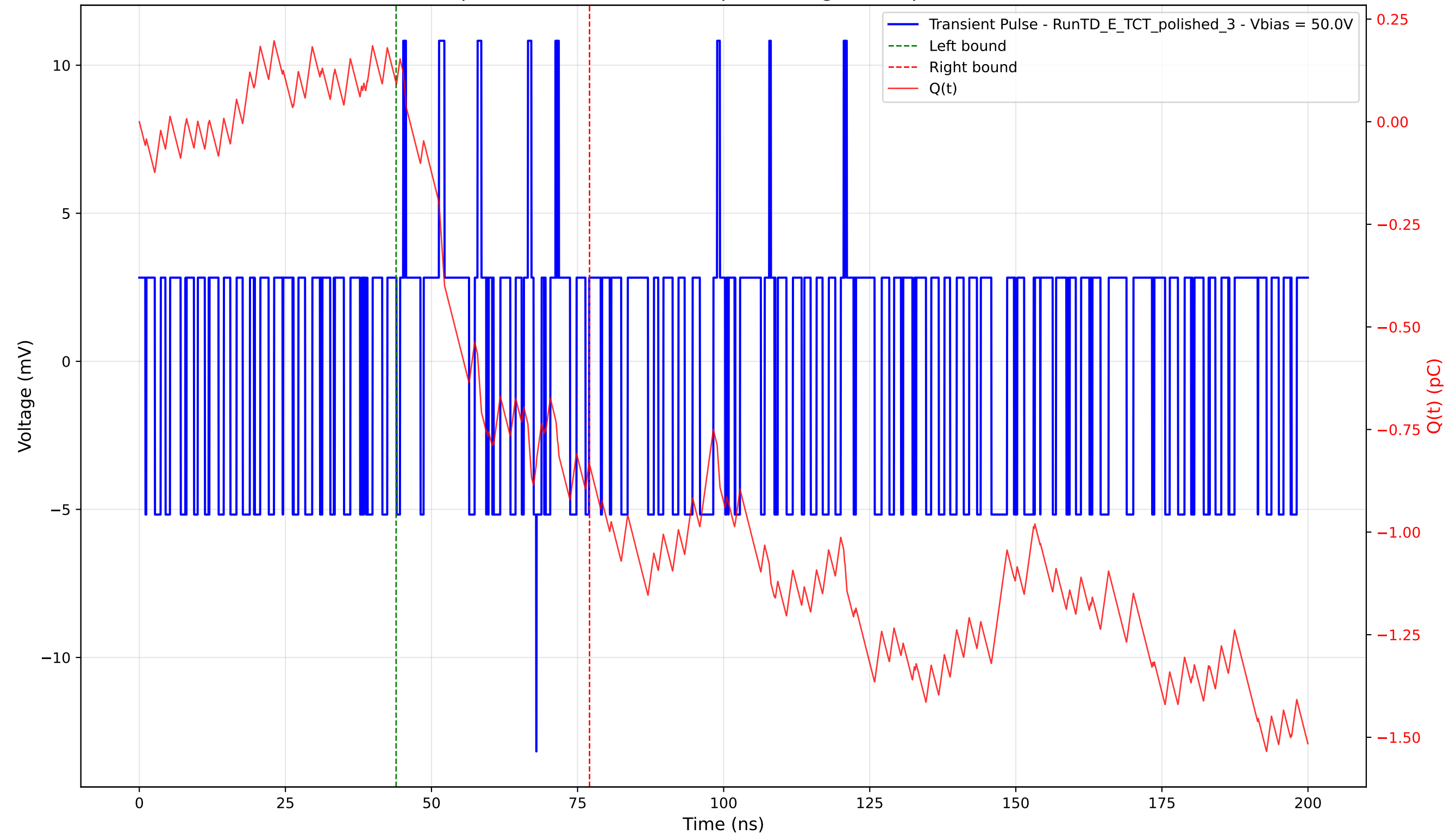
Transient Pulse - Sample: 4003 - Position: 25.0 \mu\text{m} - Charge: 0.93 pC - Rise Time: 0.00 ns (N/A)
