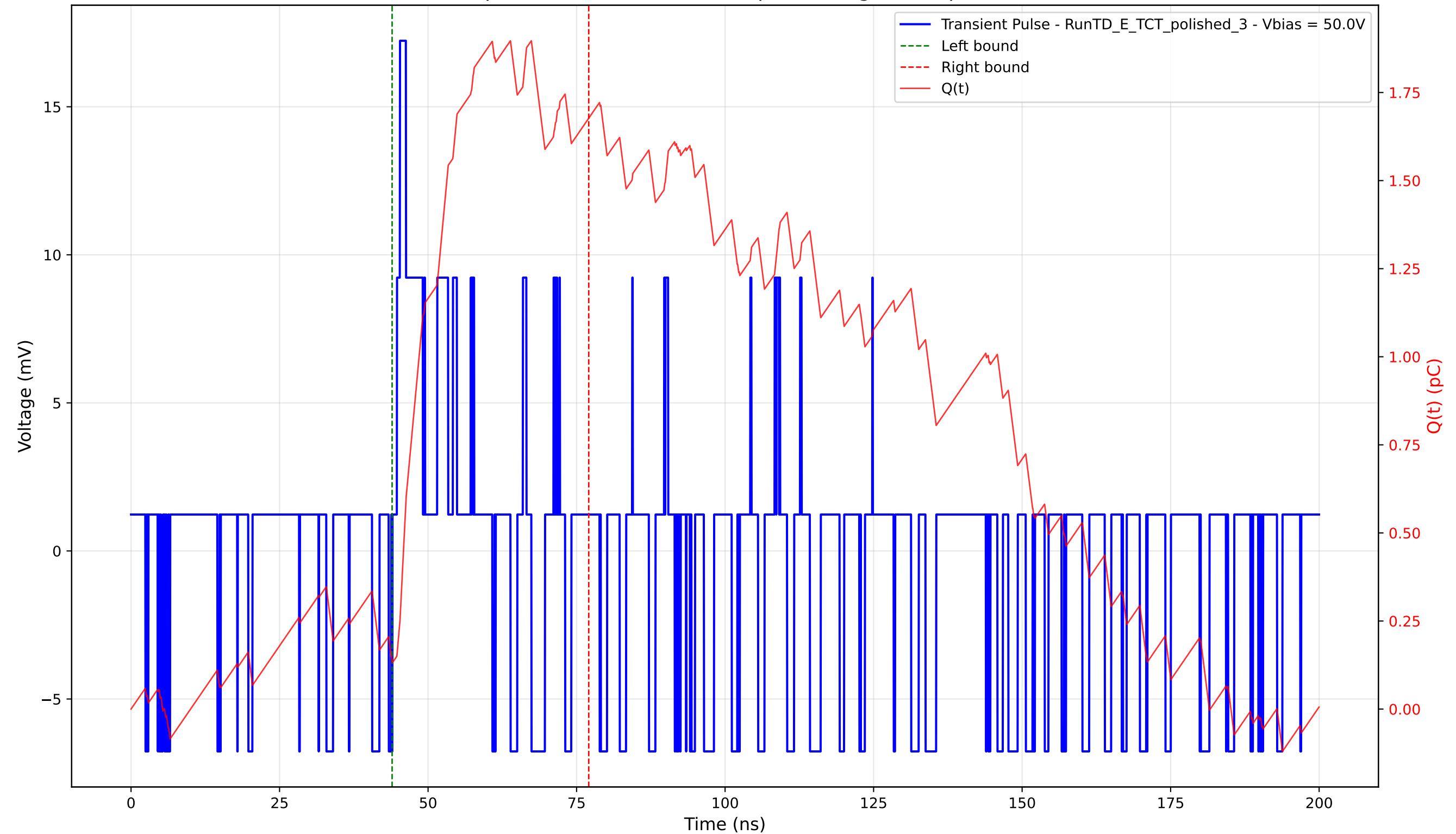
Transient Pulse - Sample: 4003 - Position: 705.0 \mu\text{m} - Charge: 1.54 pC - Rise Time: 0.52 ns
