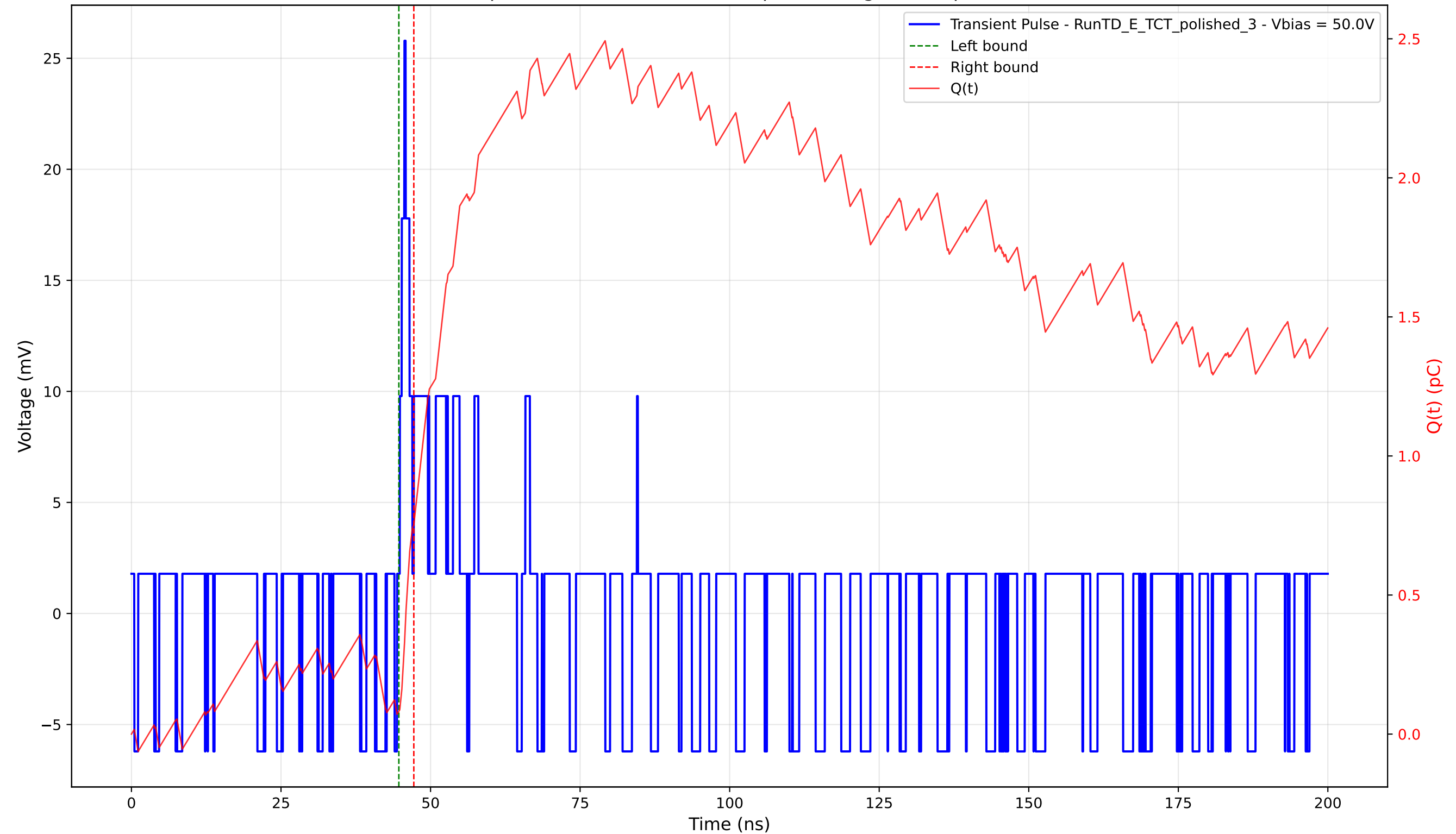
Transient Pulse - Sample: 4003 - Position: 700.0 \mu\text{m} - Charge: 0.67 pC - Rise Time: 0.78 ns
