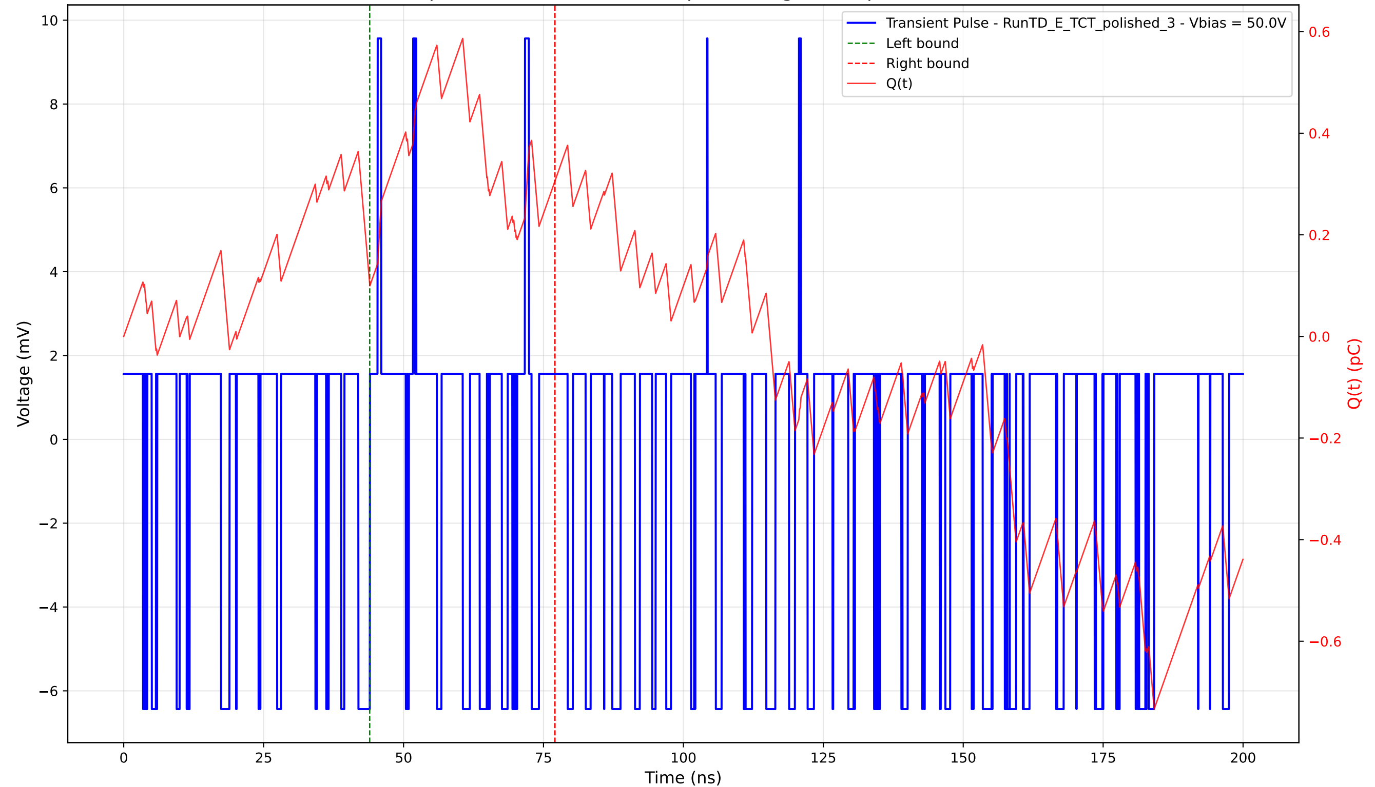
Transient Pulse - Sample: 4003 - Position: 770.0 \mu\text{m} - Charge: 0.20 pC - Rise Time: 0.00 ns (N/A)
