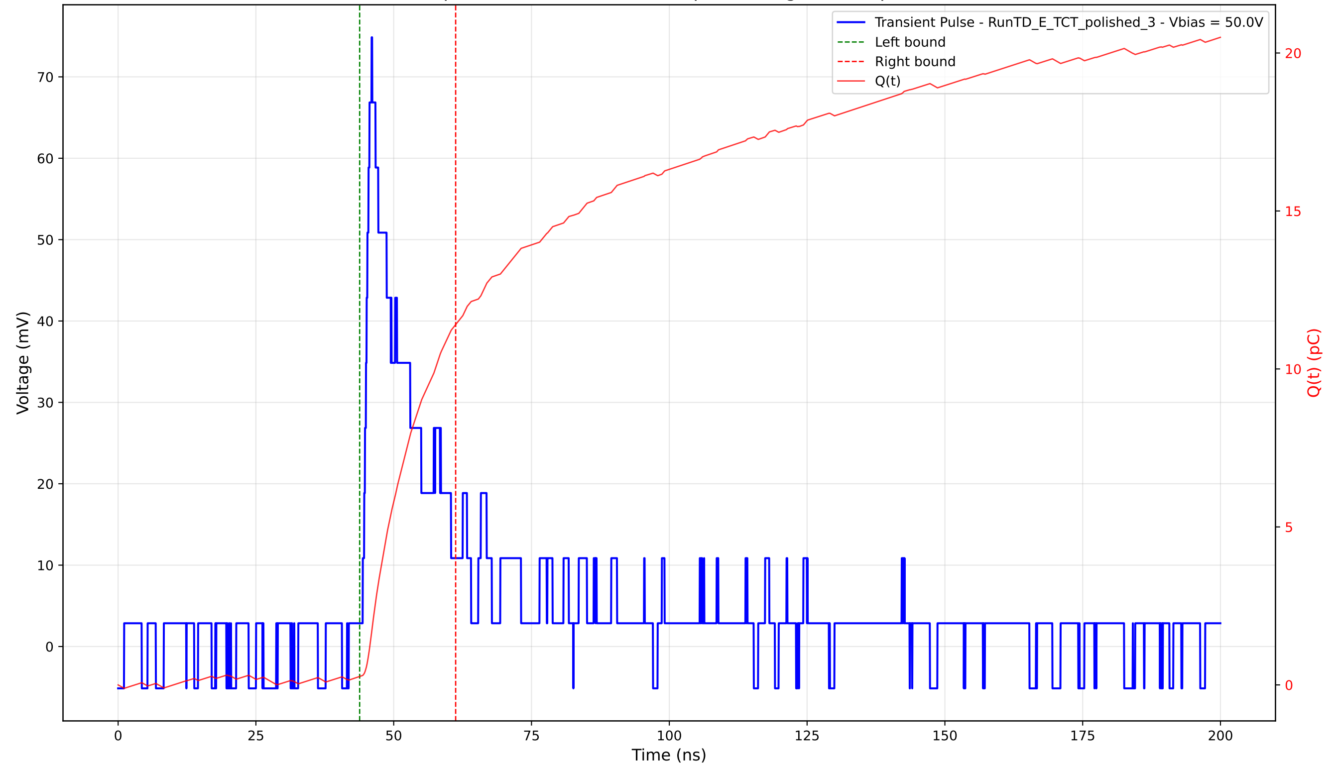
Transient Pulse - Sample: 4003 - Position: 350.0 \mu\text{m} - Charge: 11.14 pC - Rise Time: 1.61 ns
