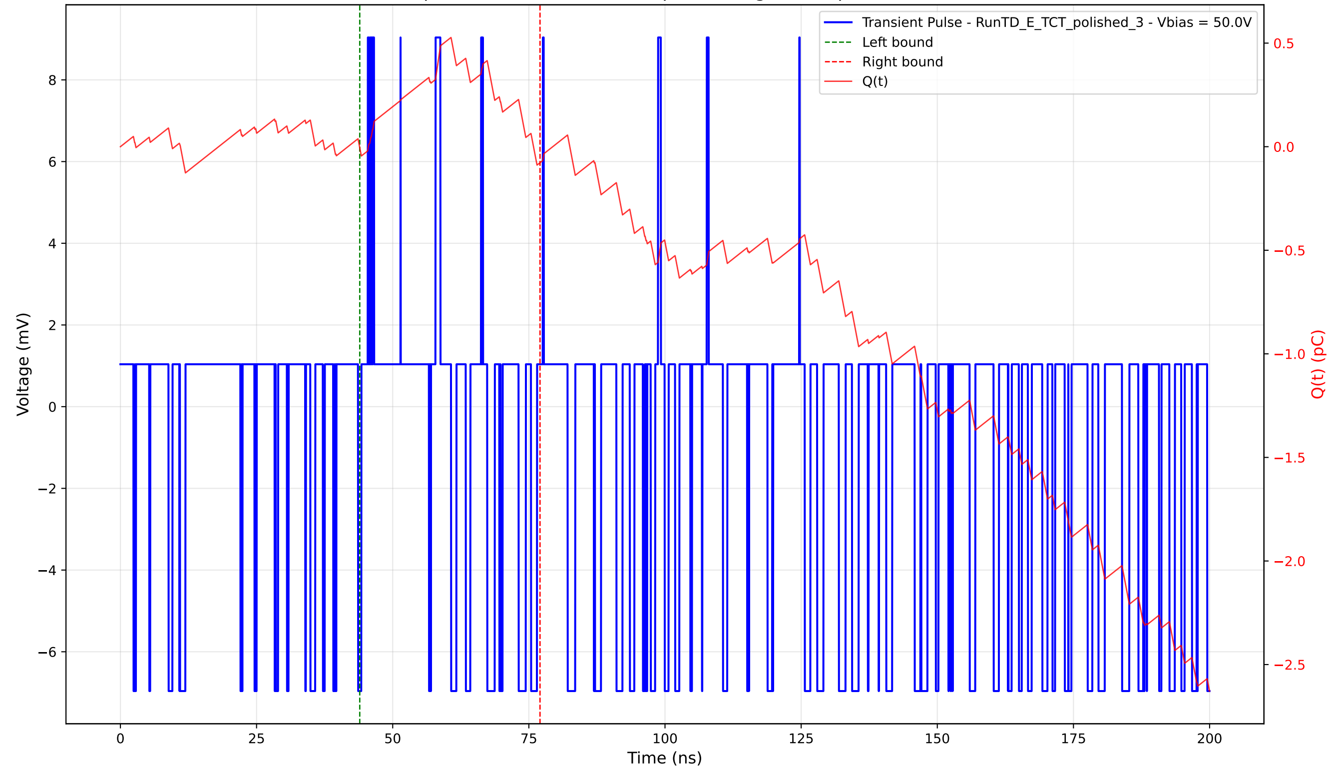
Transient Pulse - Sample: 4003 - Position: 30.0 \mu\text{m} - Charge: 0.07 pC - Rise Time: 0.00 ns (N/A)
