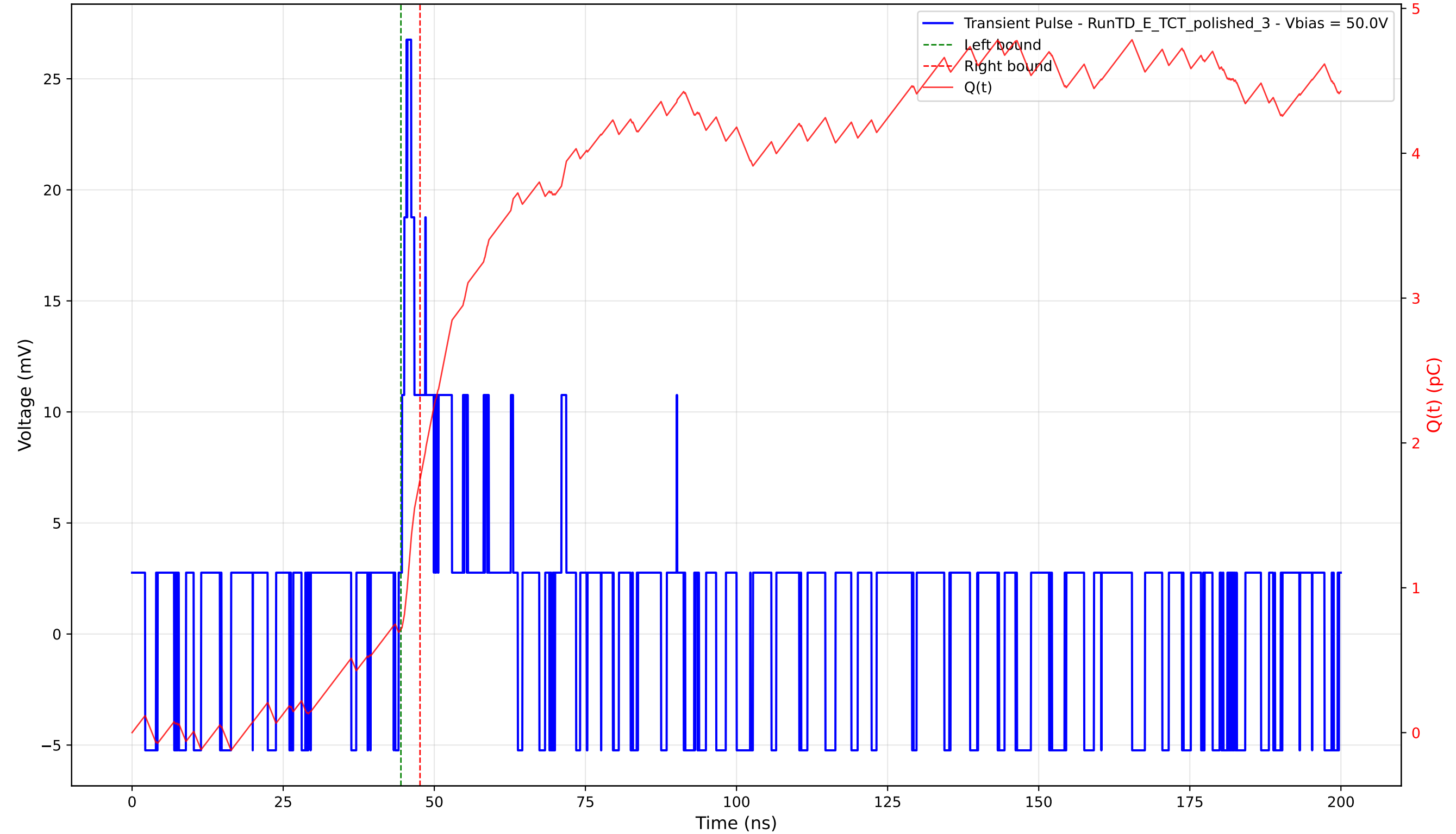
Transient Pulse - Sample: 4003 - Position: 635.0 \mu\text{m} - Charge: 1.03 pC - Rise Time: 0.00 ns (N/A)
