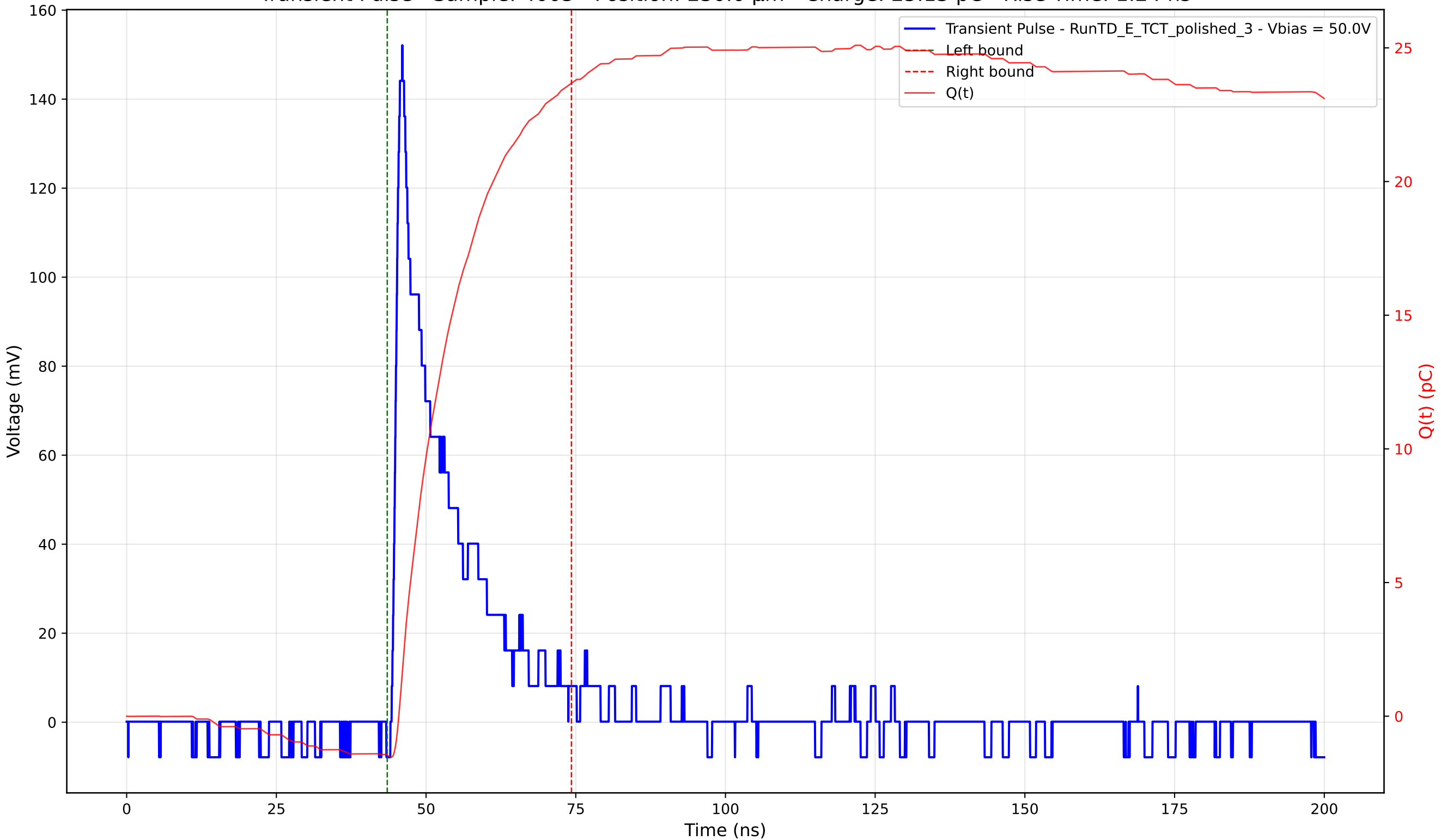
Transient Pulse - Sample: 4003 - Position: 230.0 \mu\text{m} - Charge: 25.13 pC - Rise Time: 1.24 ns
