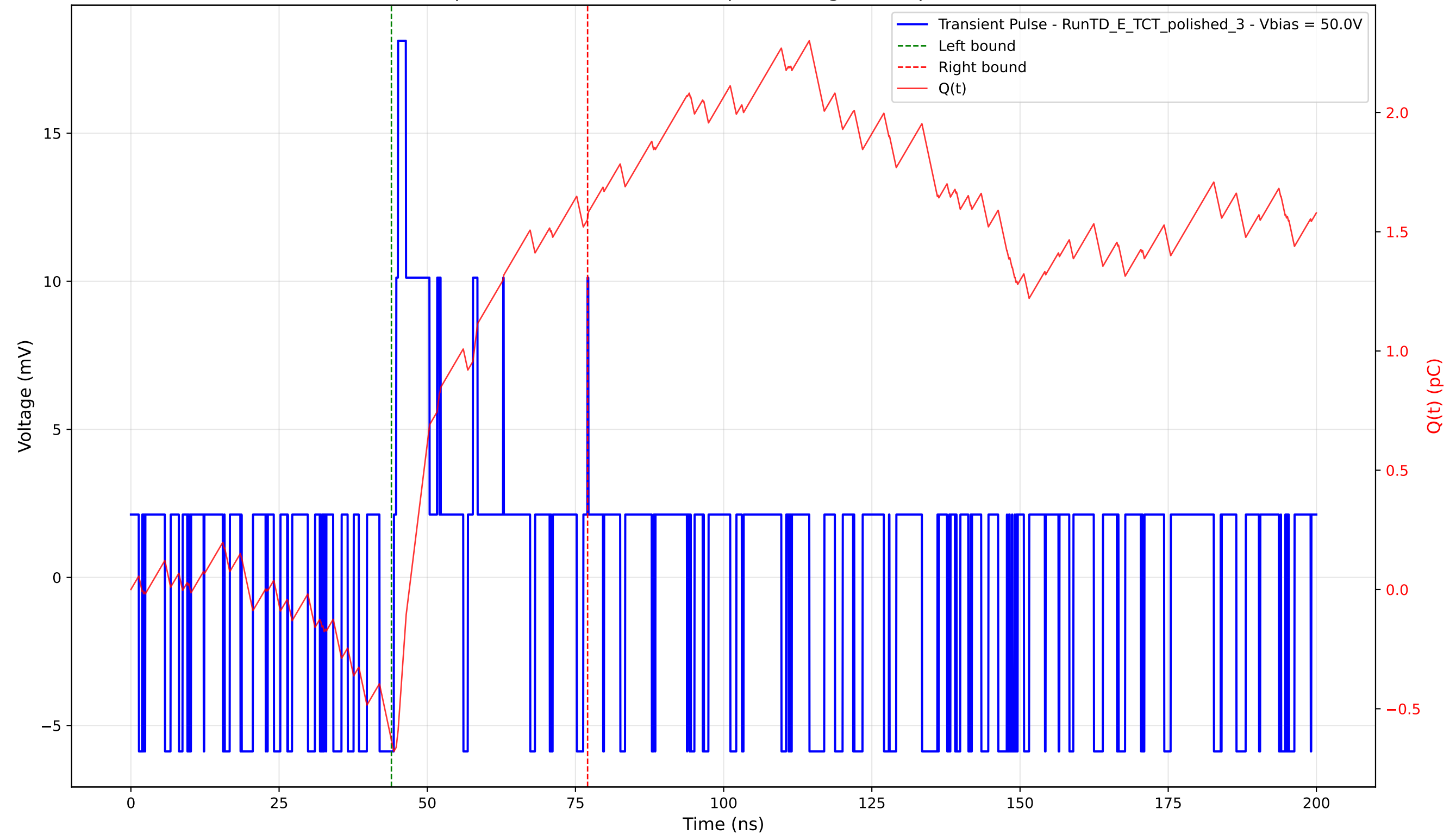
Transient Pulse - Sample: 4003 - Position: 510.0 \mu\text{m} - Charge: 2.19 pC - Rise Time: 0.00 ns (N/A)
