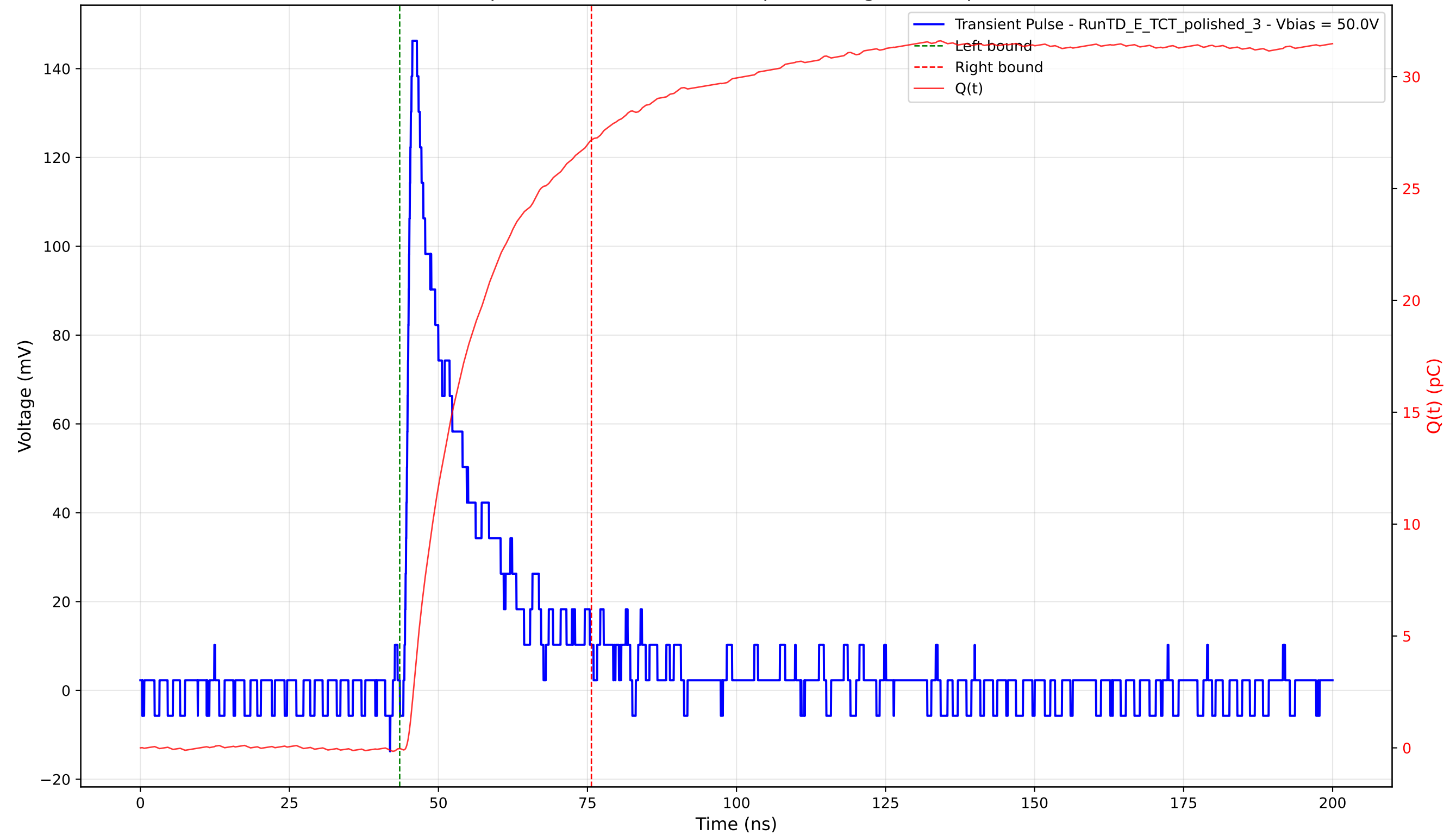
Transient Pulse - Sample: 4003 - Position: 245.0 \mu\text{m} - Charge: 27.19 pC - Rise Time: 1.09 ns
