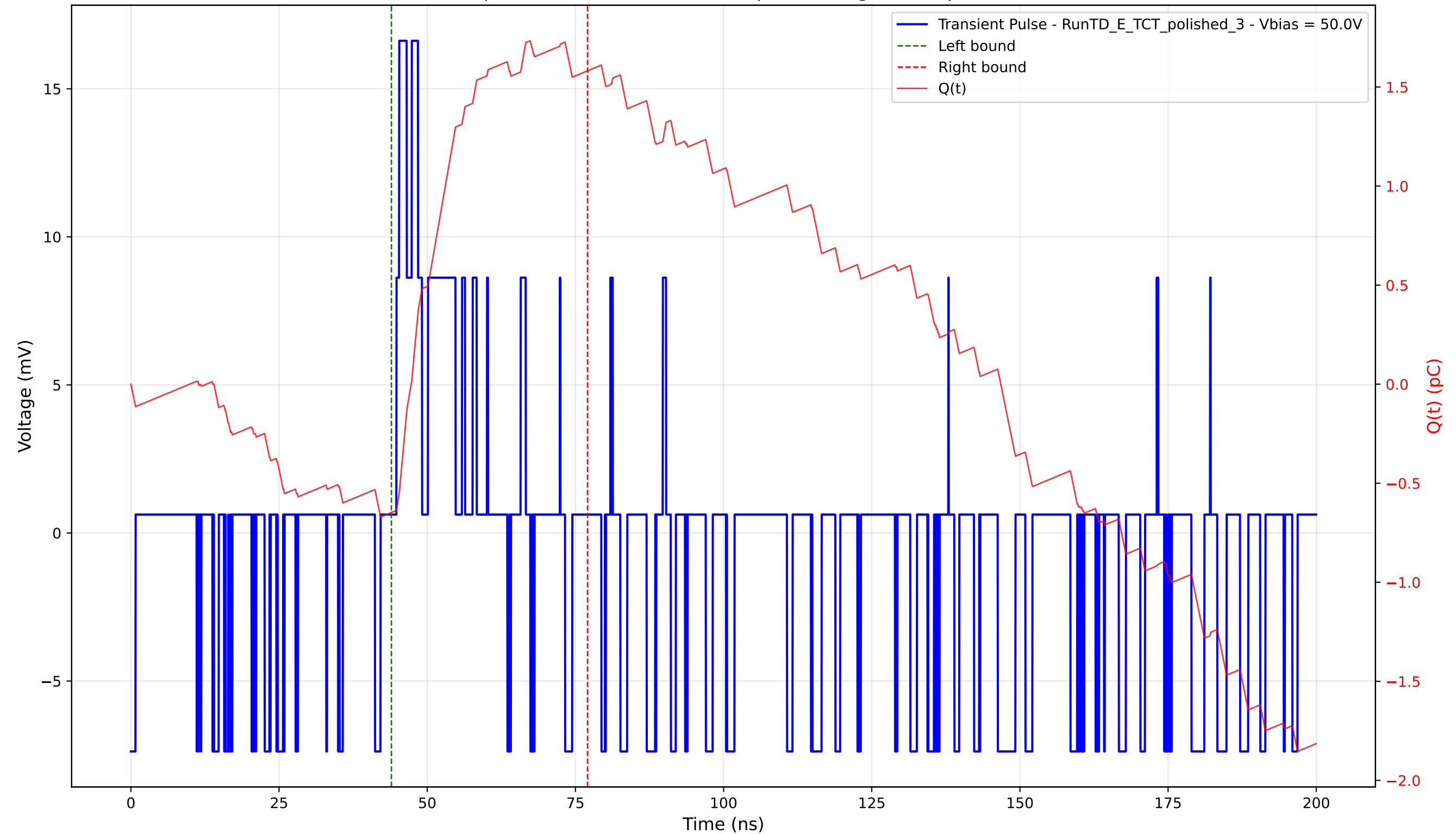
Transient Pulse - Sample: 4003 - Position: 430.0 \mu\text{m} - Charge: 2.23 pC - Rise Time: 0.48 ns
