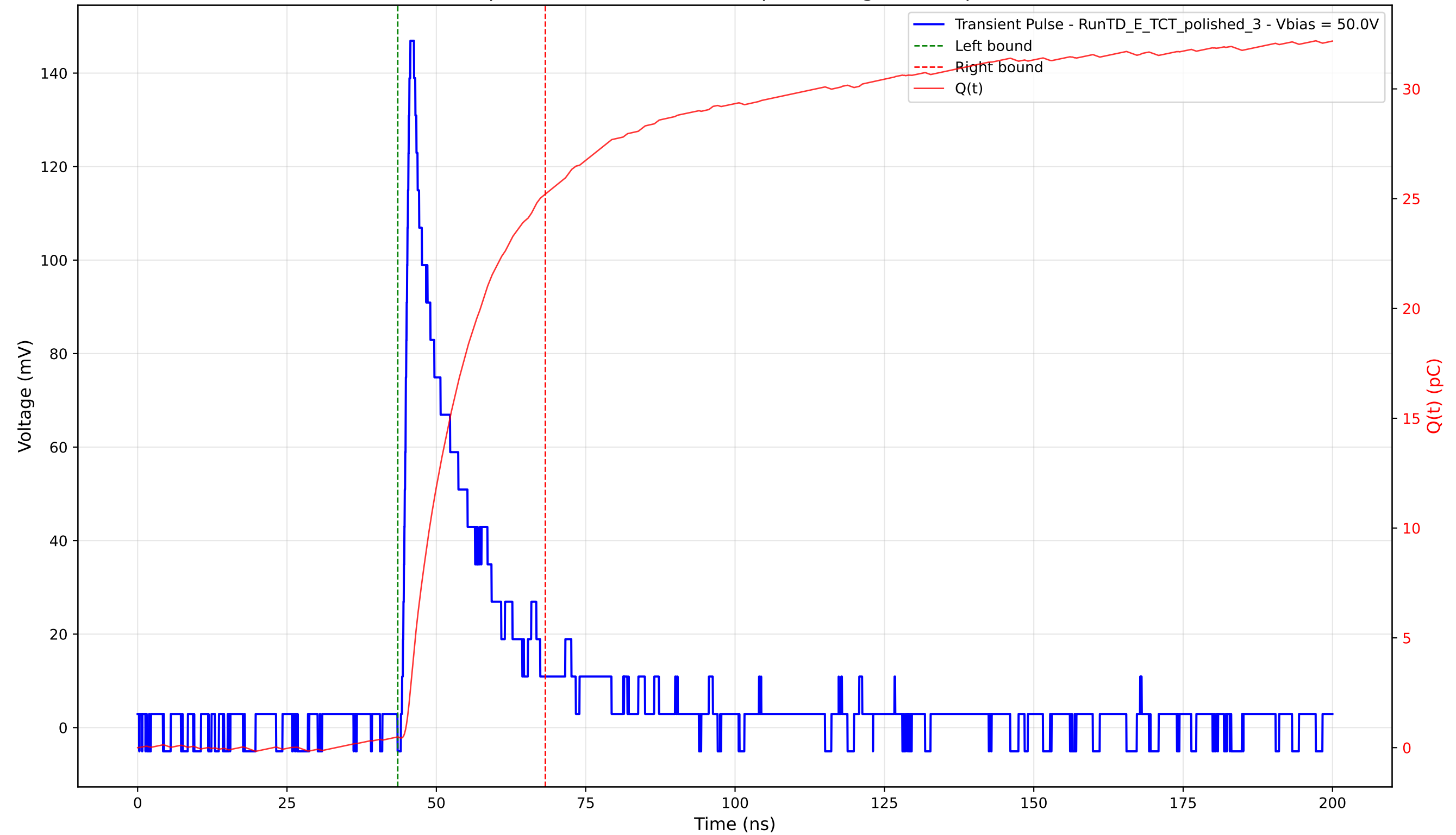
Transient Pulse - Sample: 4003 - Position: 225.0 \mu\text{m} - Charge: 24.72 pC - Rise Time: 1.09 ns
