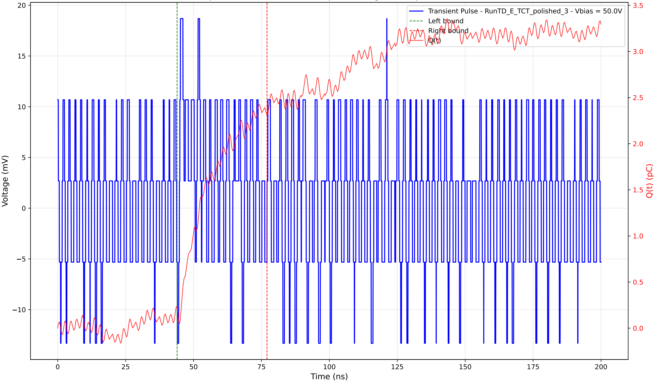
Transient Pulse - Sample: 4003 - Position: 90.0 \mu\text{m} - Charge: 2.09 pC - Rise Time: 0.00 ns (N/A)
