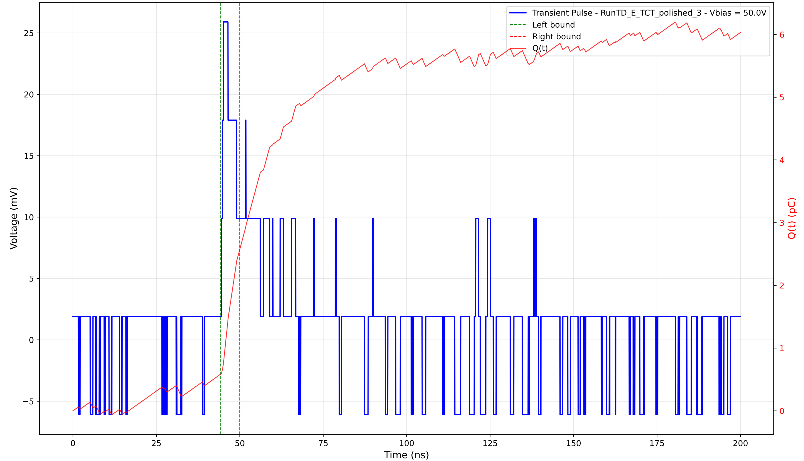
Transient Pulse - Sample: 4003 - Position: 680.0 \mu\text{m} - Charge: 1.99 pC - Rise Time: 0.62 ns
