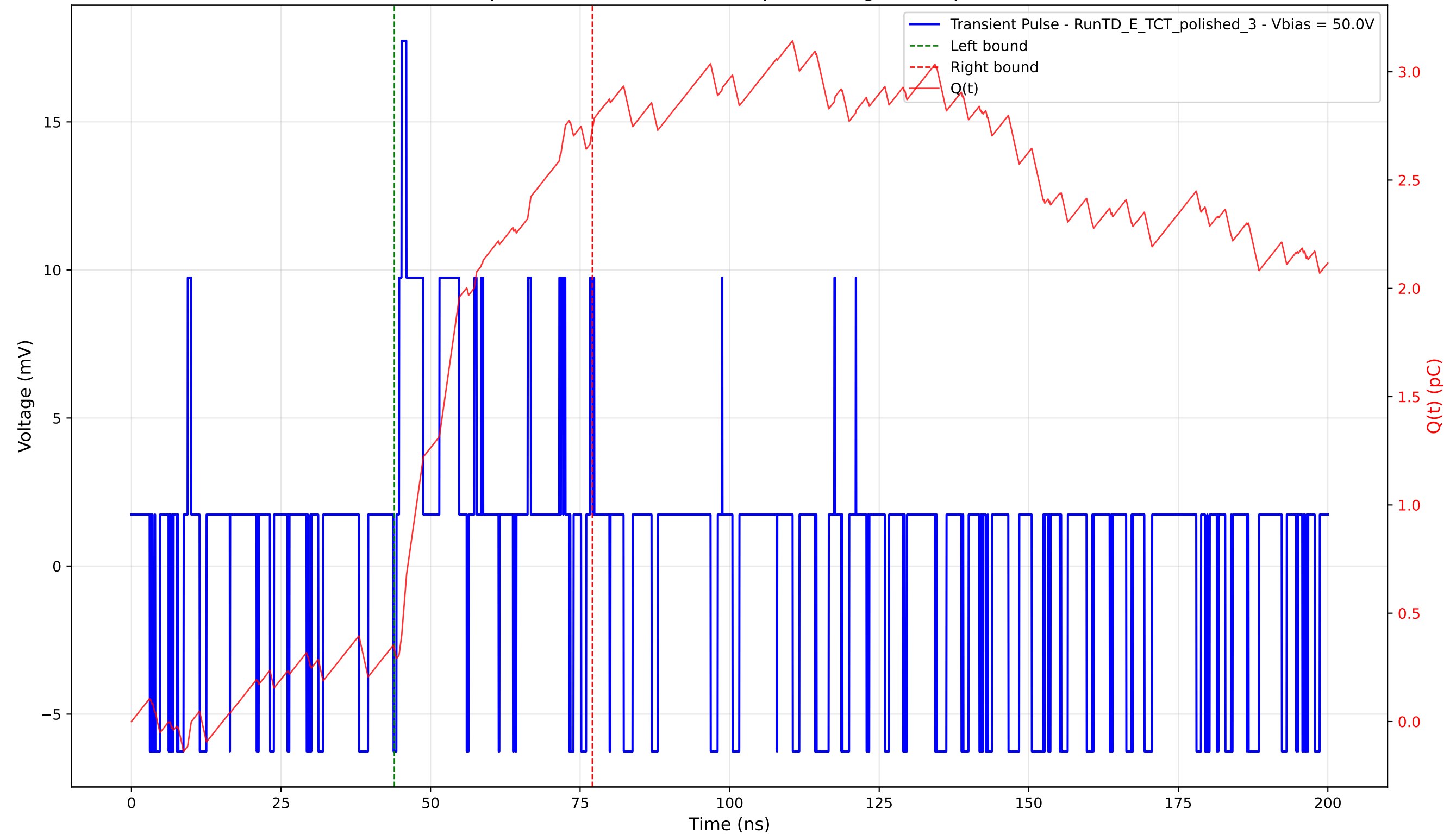
Transient Pulse - Sample: 4003 - Position: 630.0 \mu\text{m} - Charge: 2.41 pC - Rise Time: 0.44 ns
