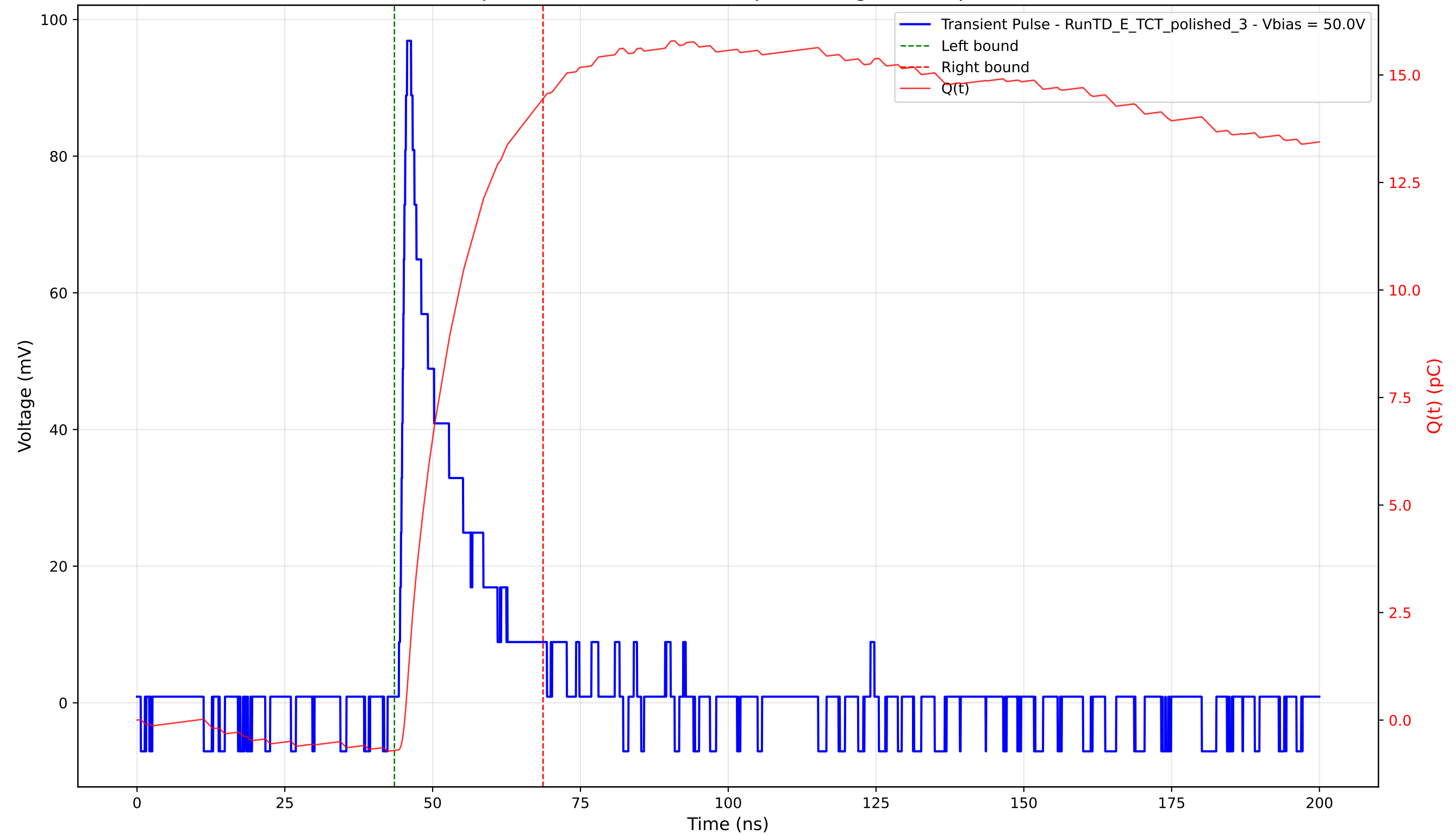
Transient Pulse - Sample: 4003 - Position: 175.0 \mu\text{m} - Charge: 15.16 pC - Rise Time: 1.00 ns
