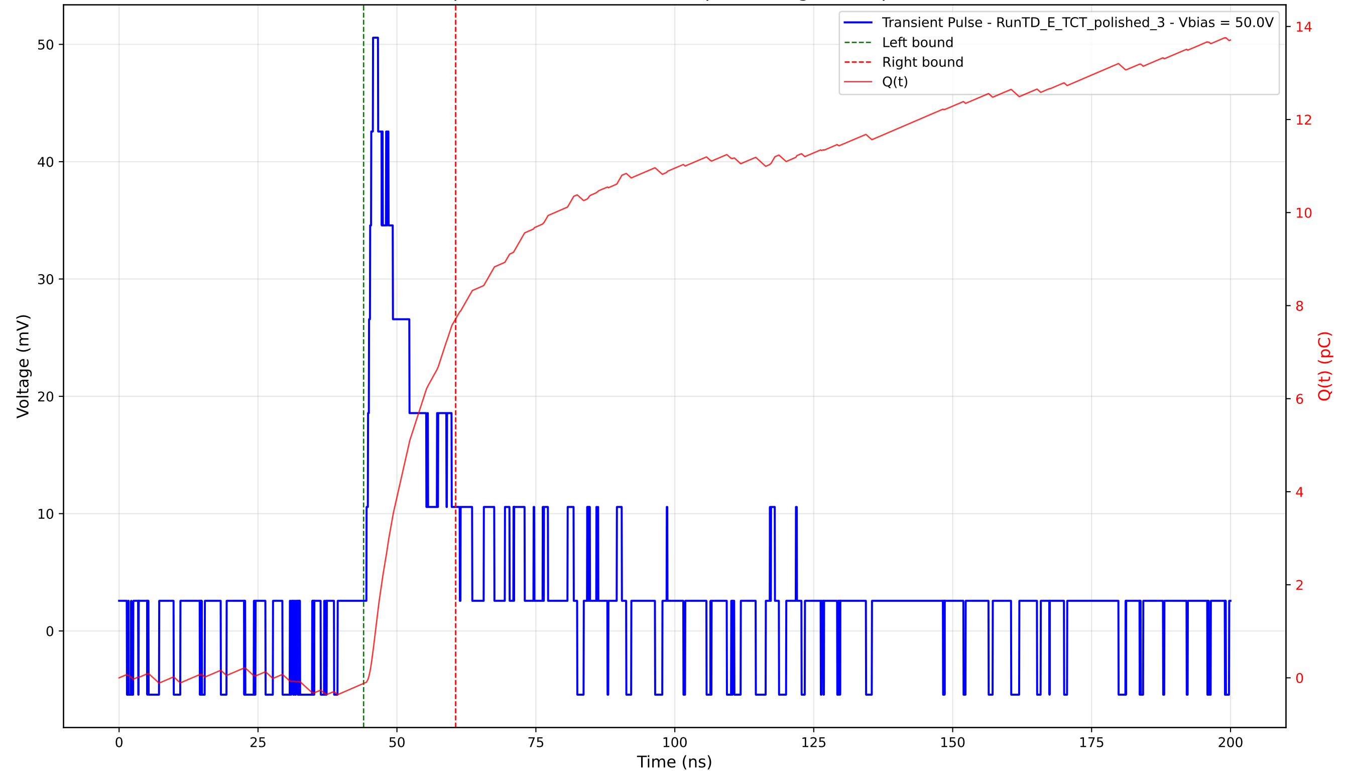
Transient Pulse - Sample: 4003 - Position: 370.0 \mu\text{m} - Charge: 7.84 pC - Rise Time: 1.17 ns
