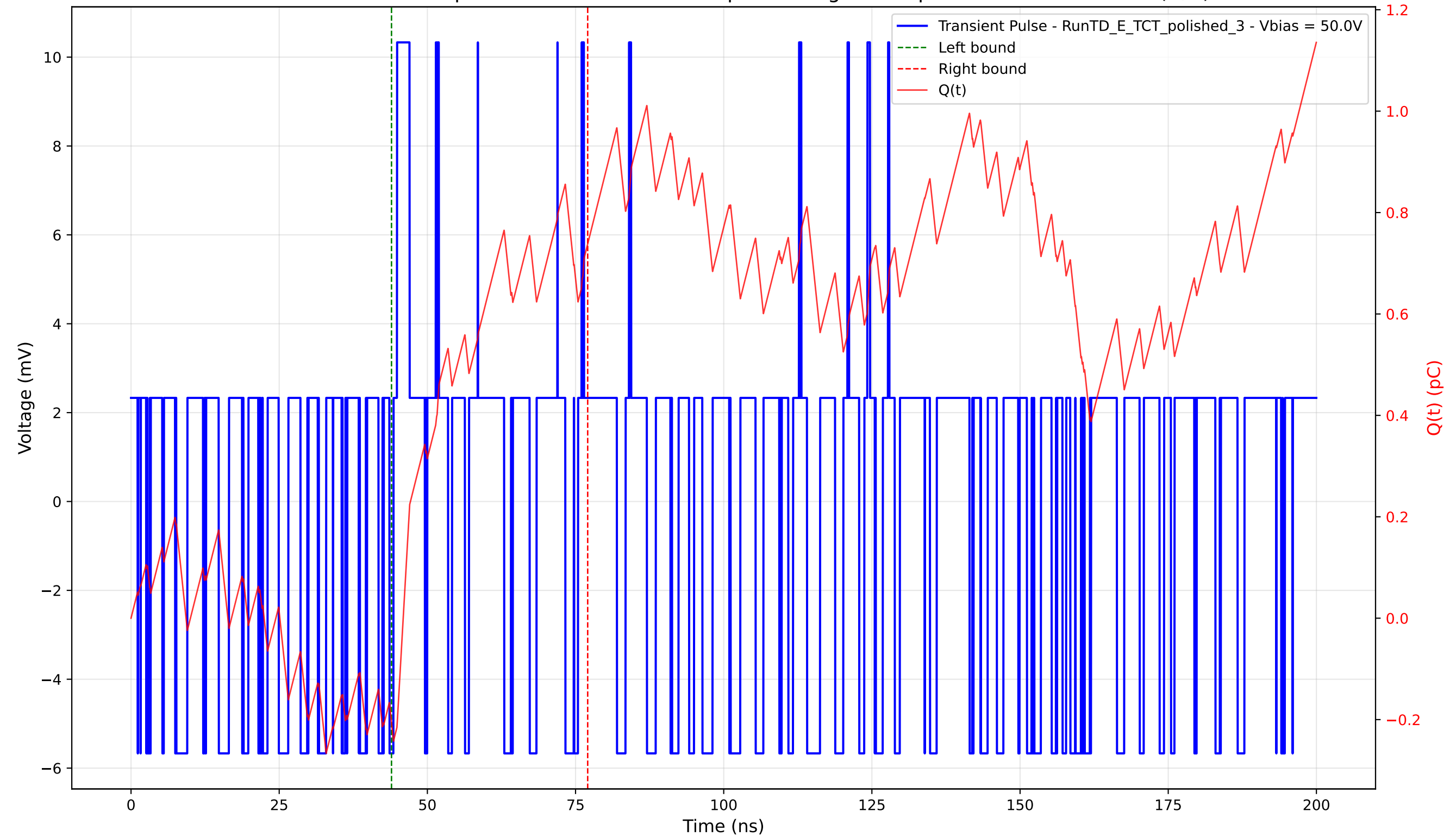
Transient Pulse - Sample: 4003 - Position: 710.0 \mu\text{m} - Charge: 0.95 pC - Rise Time: 0.00 ns (N/A)
