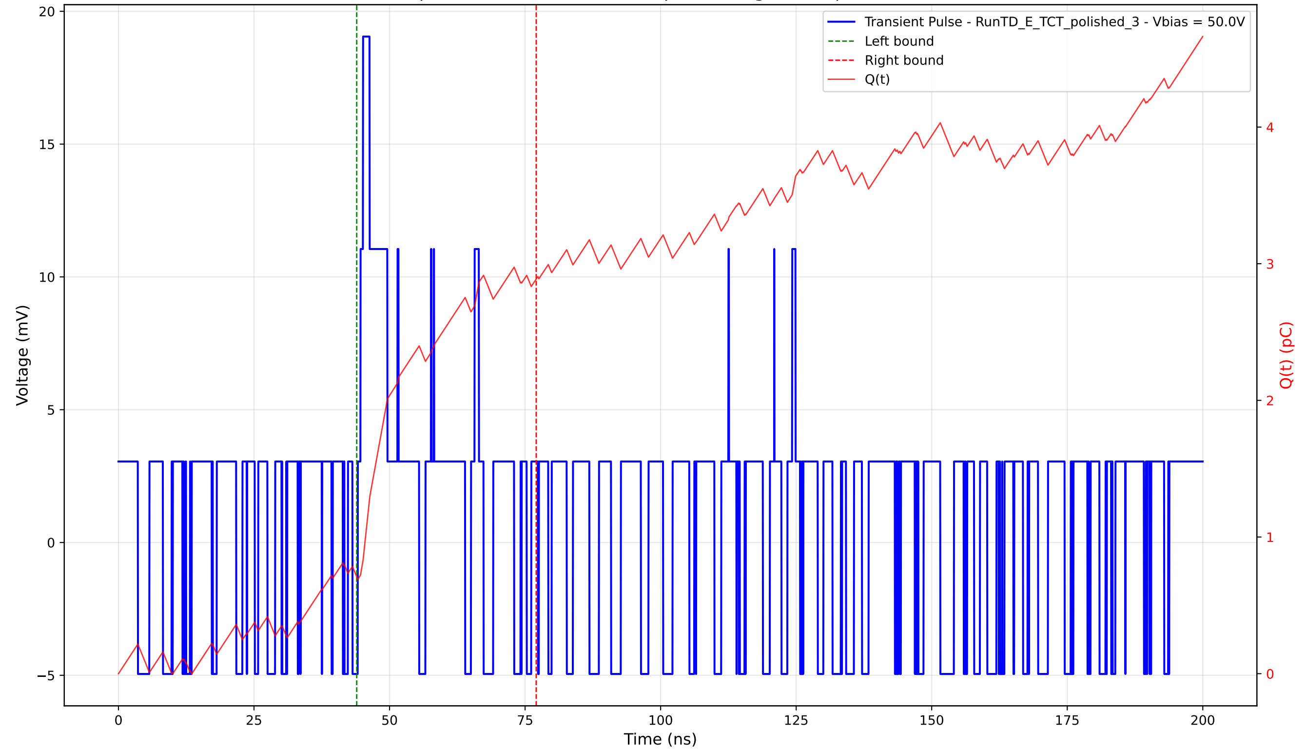
Transient Pulse - Sample: 4003 - Position: 445.0 \mu\text{m} - Charge: 2.18 pC - Rise Time: 0.00 ns (N/A)
