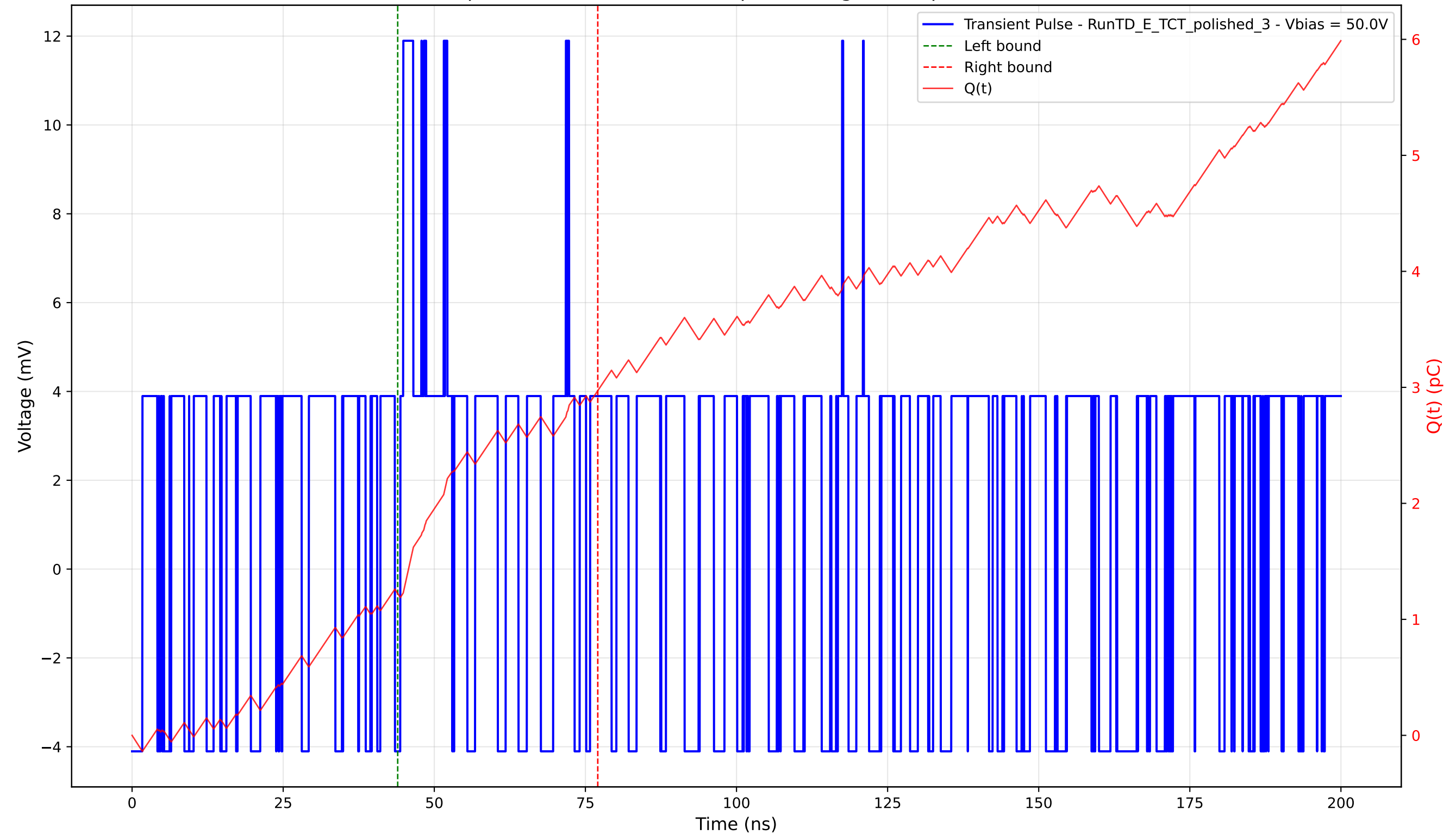
Transient Pulse - Sample: 4003 - Position: 600.0 \mu\text{m} - Charge: 1.75 pC - Rise Time: 0.00 ns (N/A)
