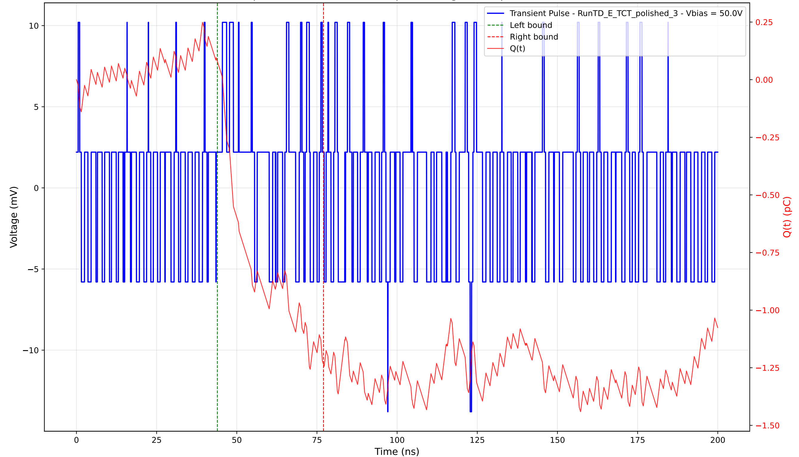
Transient Pulse - Sample: 4003 - Position: 55.0 \mu\text{m} - Charge: 1.31 pC - Rise Time: 0.00 ns (N/A)
