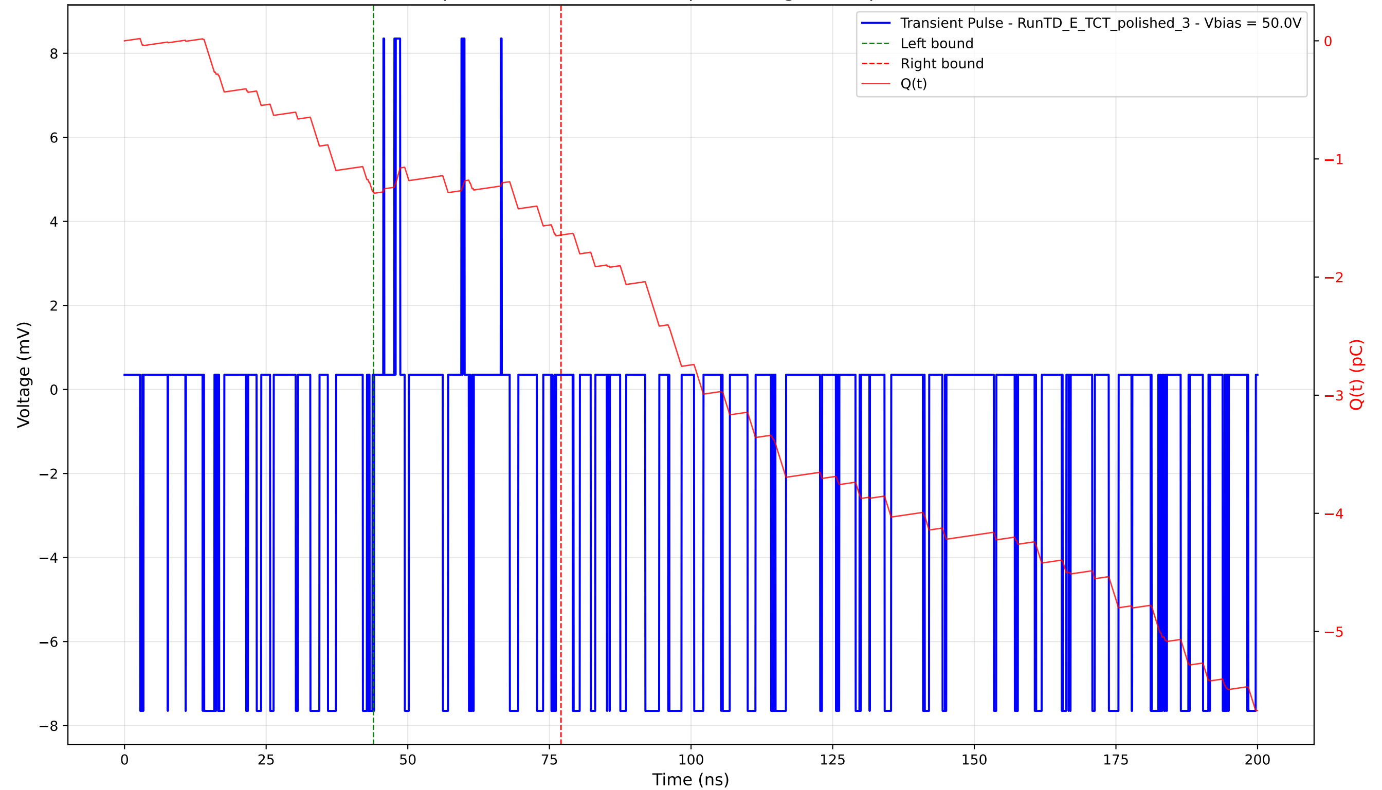
Transient Pulse - Sample: 4003 - Position: 20.0 \mu\text{m} - Charge: 0.37 pC - Rise Time: 0.00 ns (N/A)
