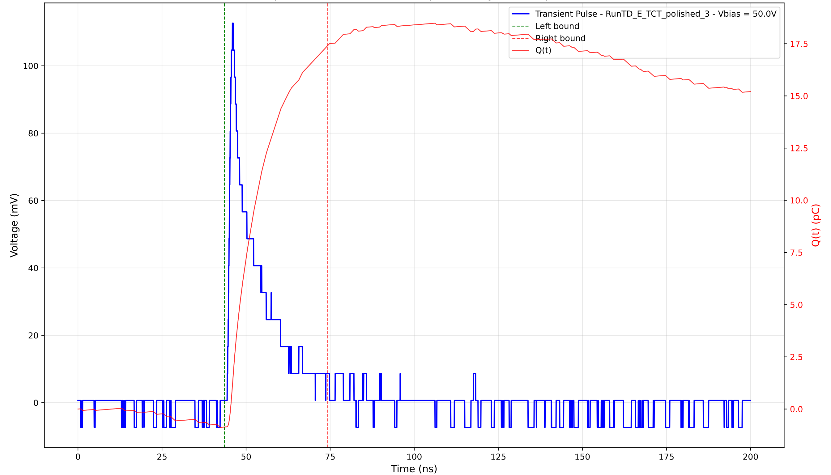
Transient Pulse - Sample: 4003 - Position: 185.0 \mu\text{m} - Charge: 18.28 pC - Rise Time: 1.09 ns
