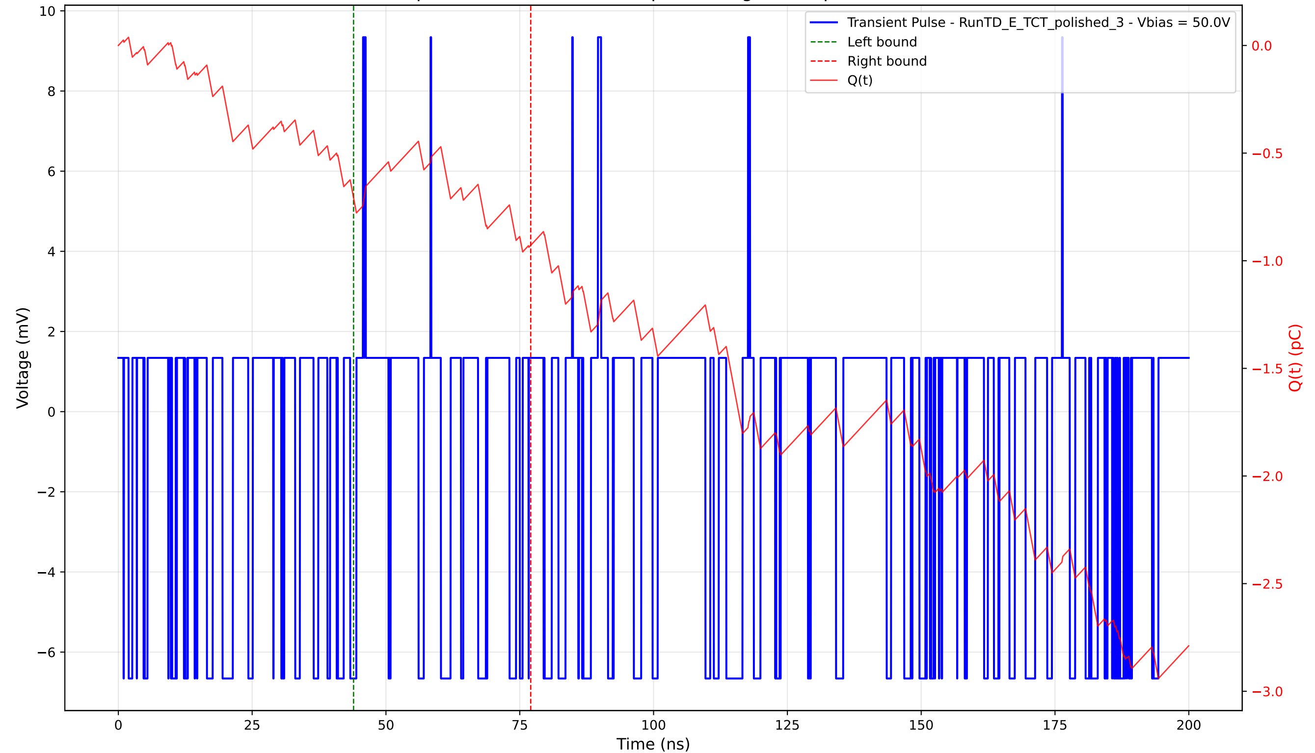
Transient Pulse - Sample: 4003 - Position: 10.0 \mu\text{m} - Charge: 0.22 pC - Rise Time: 0.00 ns (N/A)
