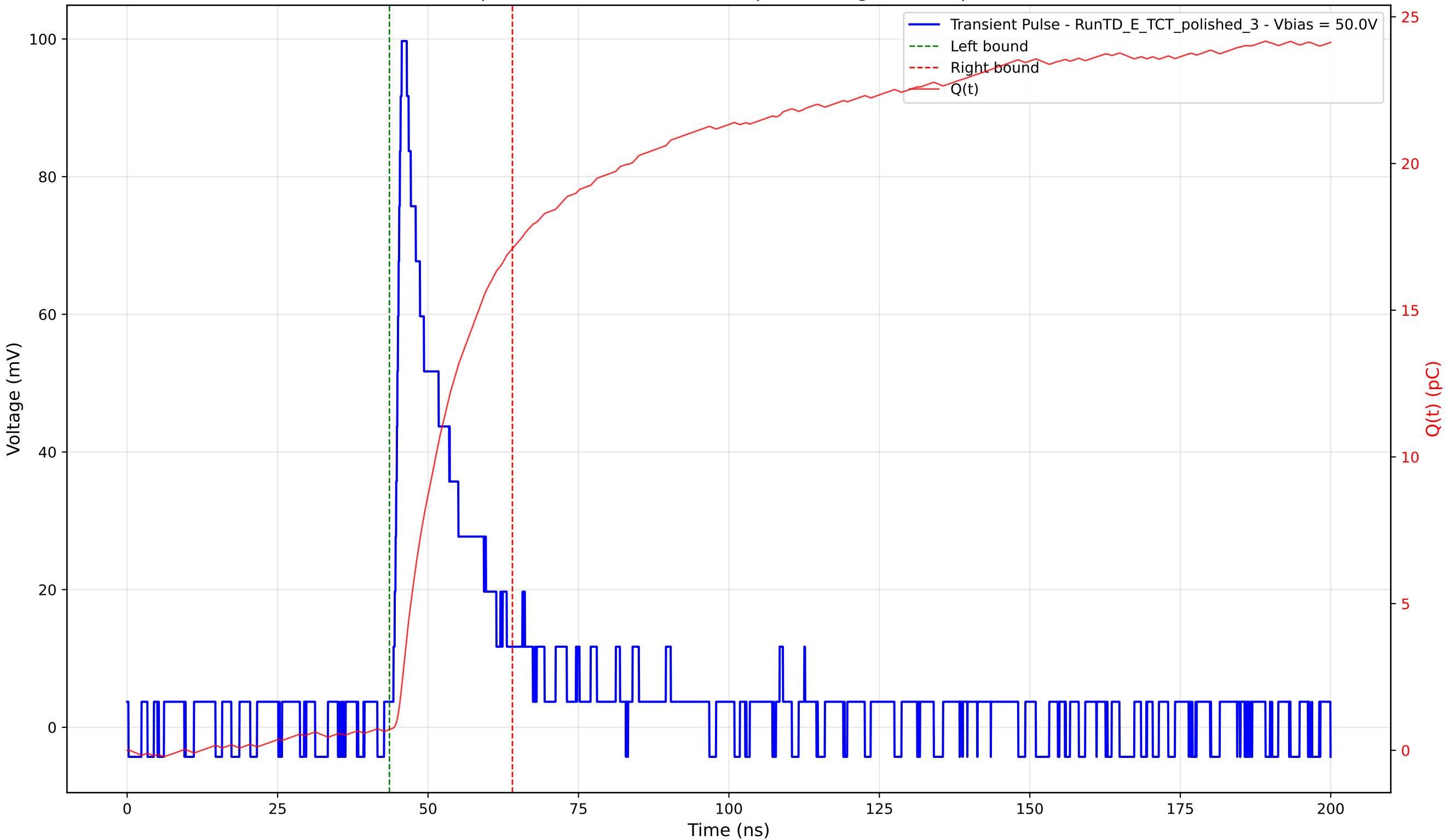
Transient Pulse - Sample: 4003 - Position: 180.0 \mu\text{m} - Charge: 16.39 pC - Rise Time: 1.18 ns
