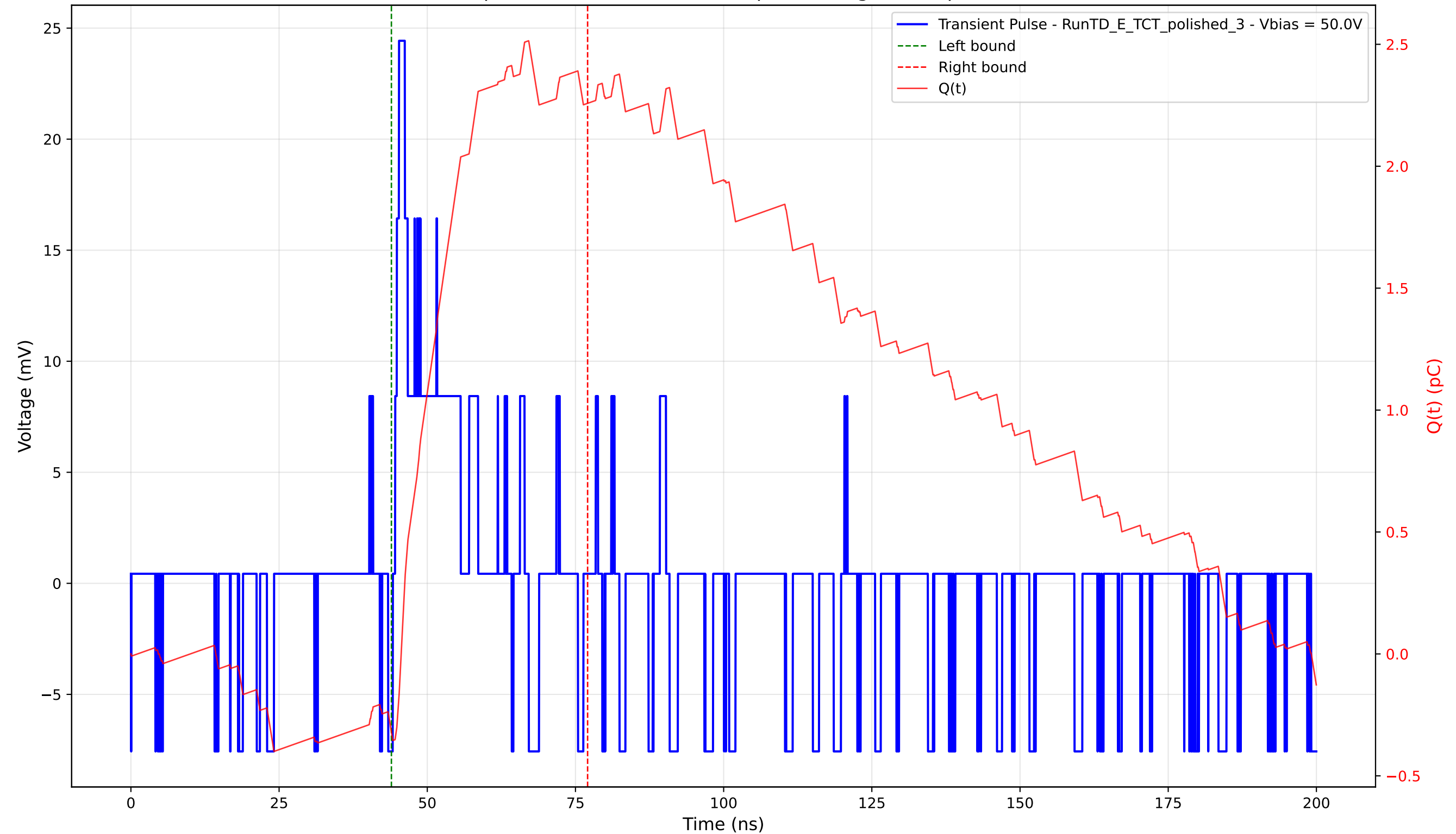
Transient Pulse - Sample: 4003 - Position: 675.0 \mu\text{m} - Charge: 2.58 pC - Rise Time: 0.65 ns
