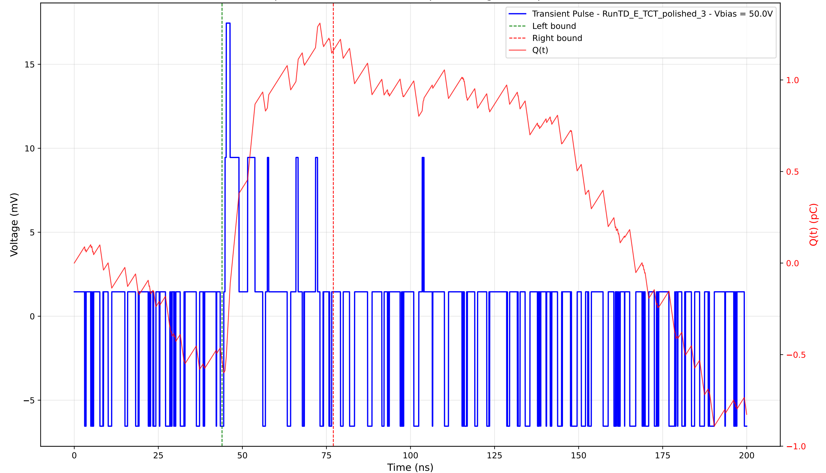
Transient Pulse - Sample: 4003 - Position: 460.0 \mu\text{m} - Charge: 1.70 pC - Rise Time: 0.38 ns
