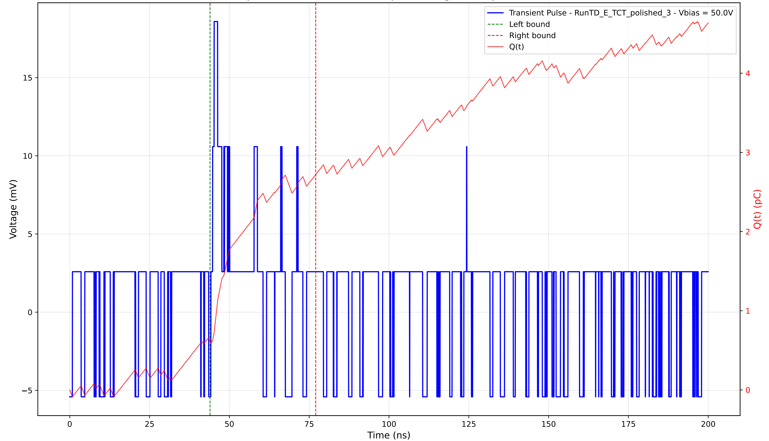
Transient Pulse - Sample: 4003 - Position: 540.0 \mu\text{m} - Charge: 2.11 pC - Rise Time: 0.00 ns (N/A)
