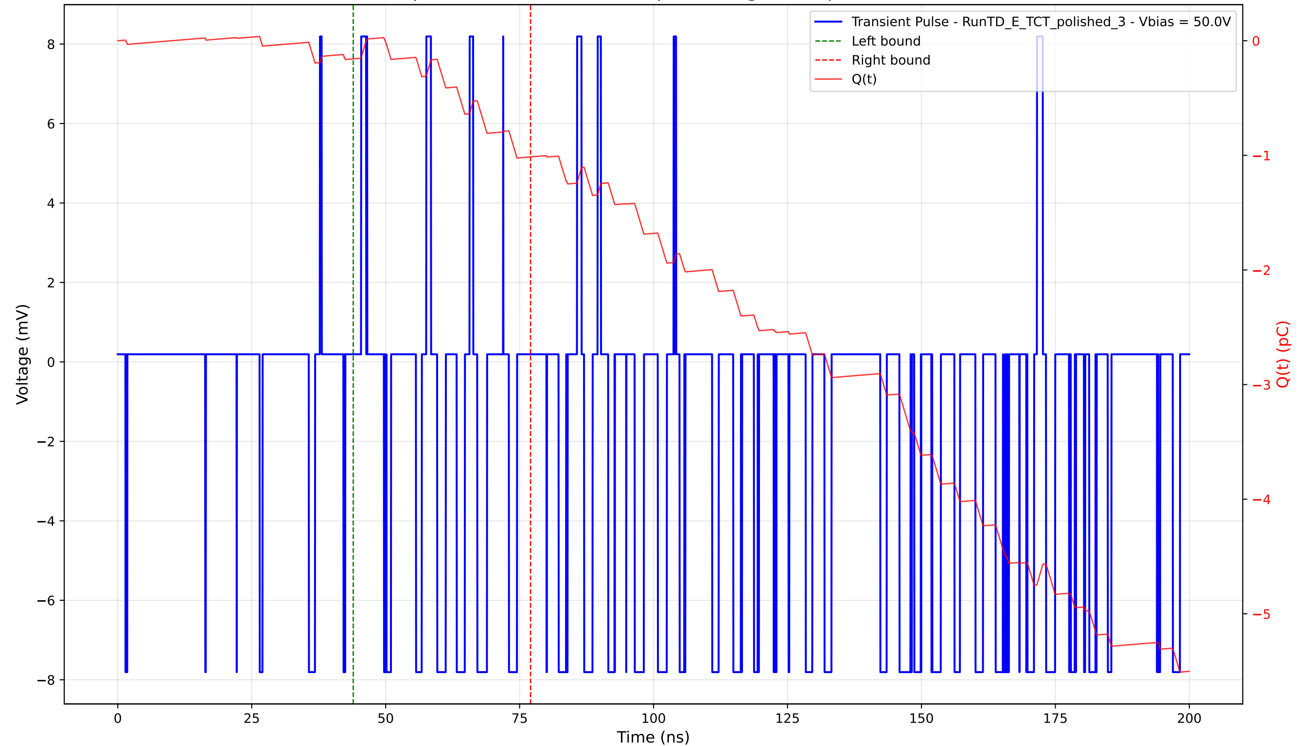
Transient Pulse - Sample: 4003 - Position: 720.0 \mu\text{m} - Charge: 0.86 pC - Rise Time: 0.00 ns (N/A)
