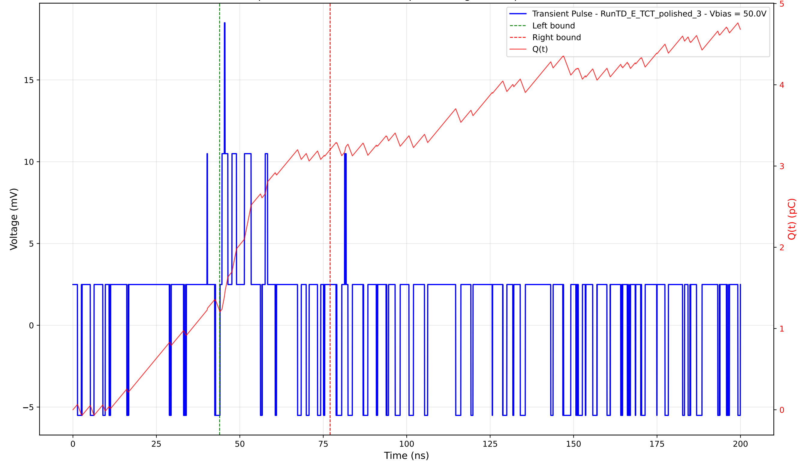
Transient Pulse - Sample: 4003 - Position: 655.0 \mu\text{m} - Charge: 1.99 pC - Rise Time: 0.00 ns (N/A)
