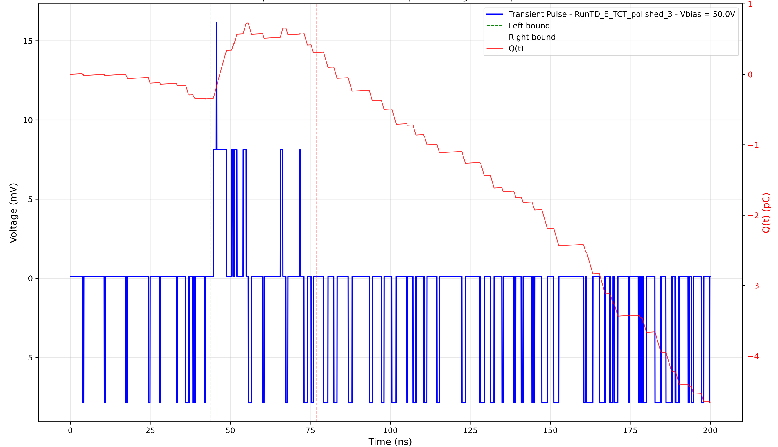
Transient Pulse - Sample: 4003 - Position: 620.0 \mu\text{m} - Charge: 0.66 pC - Rise Time: 0.96 ns
