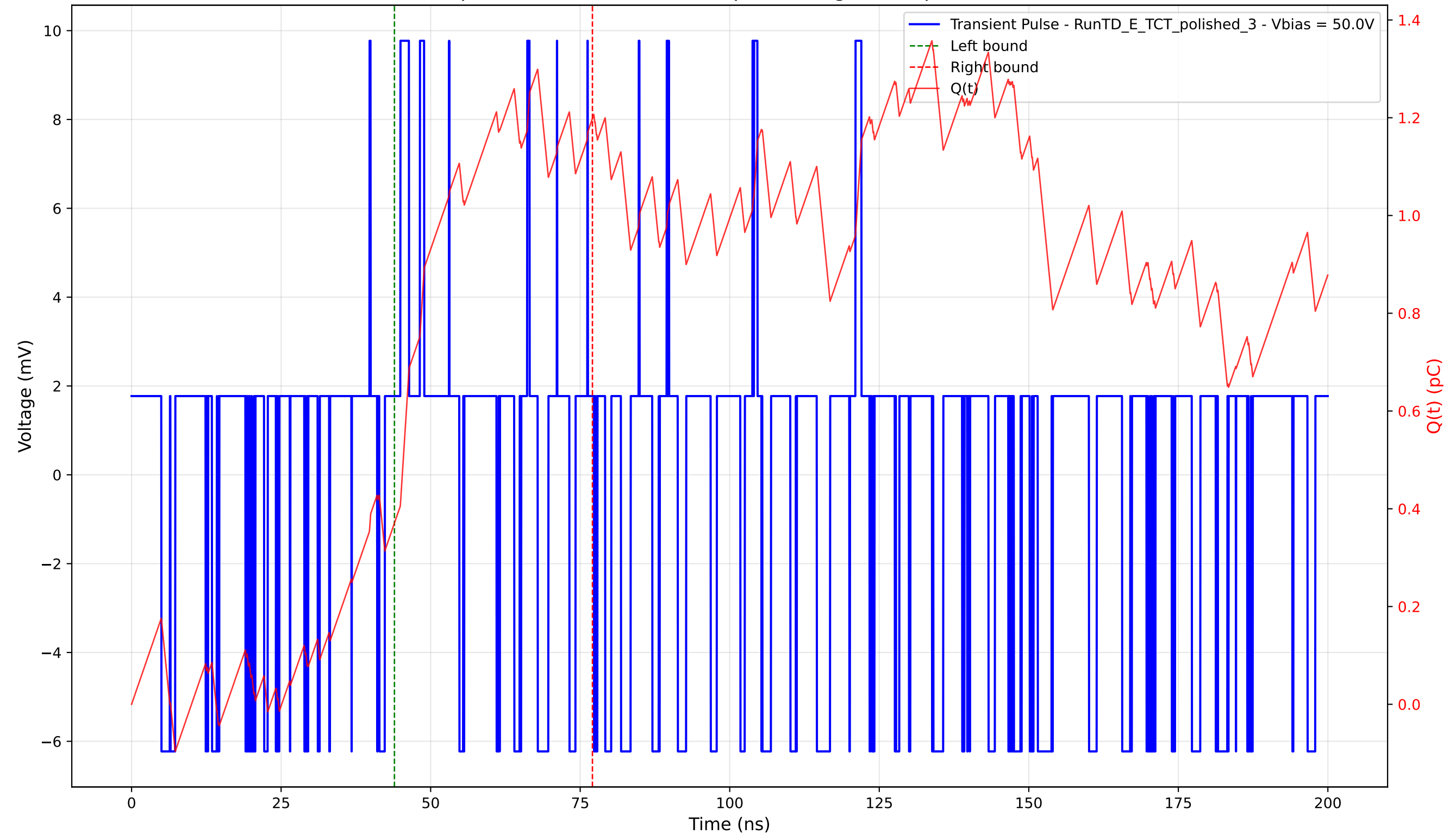
Transient Pulse - Sample: 4003 - Position: 715.0 \mu\text{m} - Charge: 0.83 pC - Rise Time: 0.00 ns (N/A)
