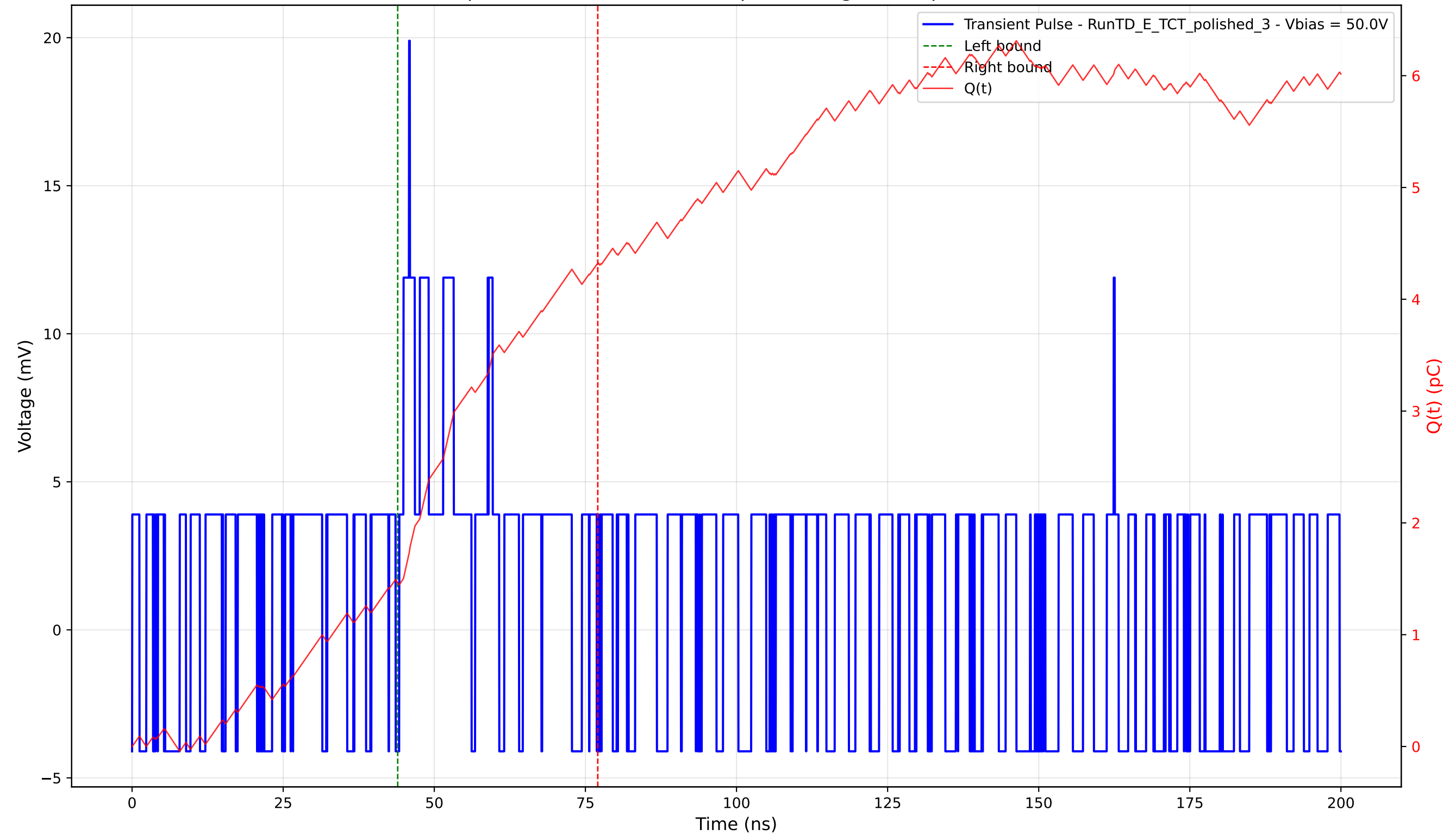
Transient Pulse - Sample: 4003 - Position: 610.0 \mu\text{m} - Charge: 2.85 pC - Rise Time: 0.00 ns (N/A)
