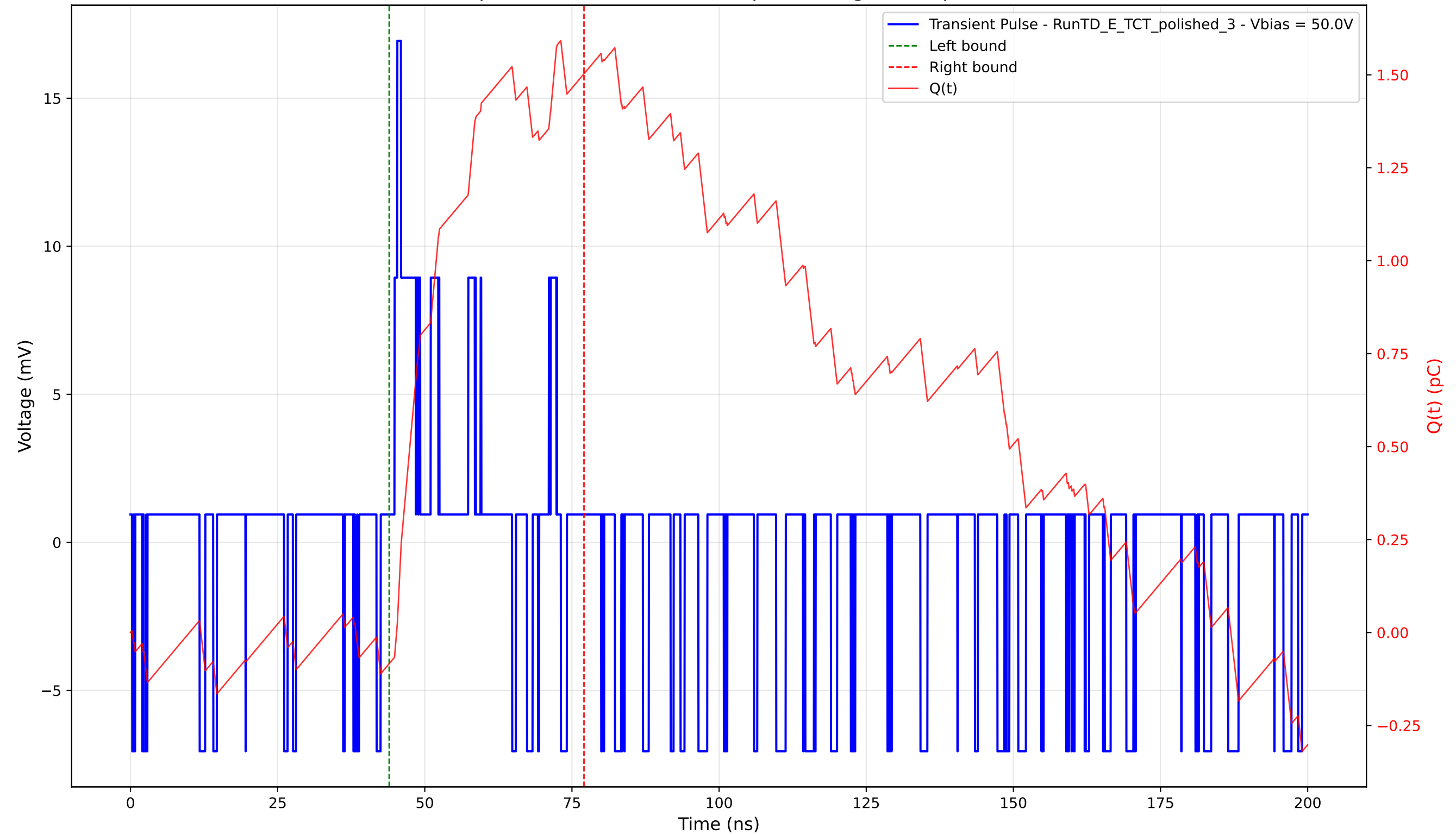
Transient Pulse - Sample: 4003 - Position: 470.0 \mu\text{m} - Charge: 1.59 pC - Rise Time: 0.48 ns
