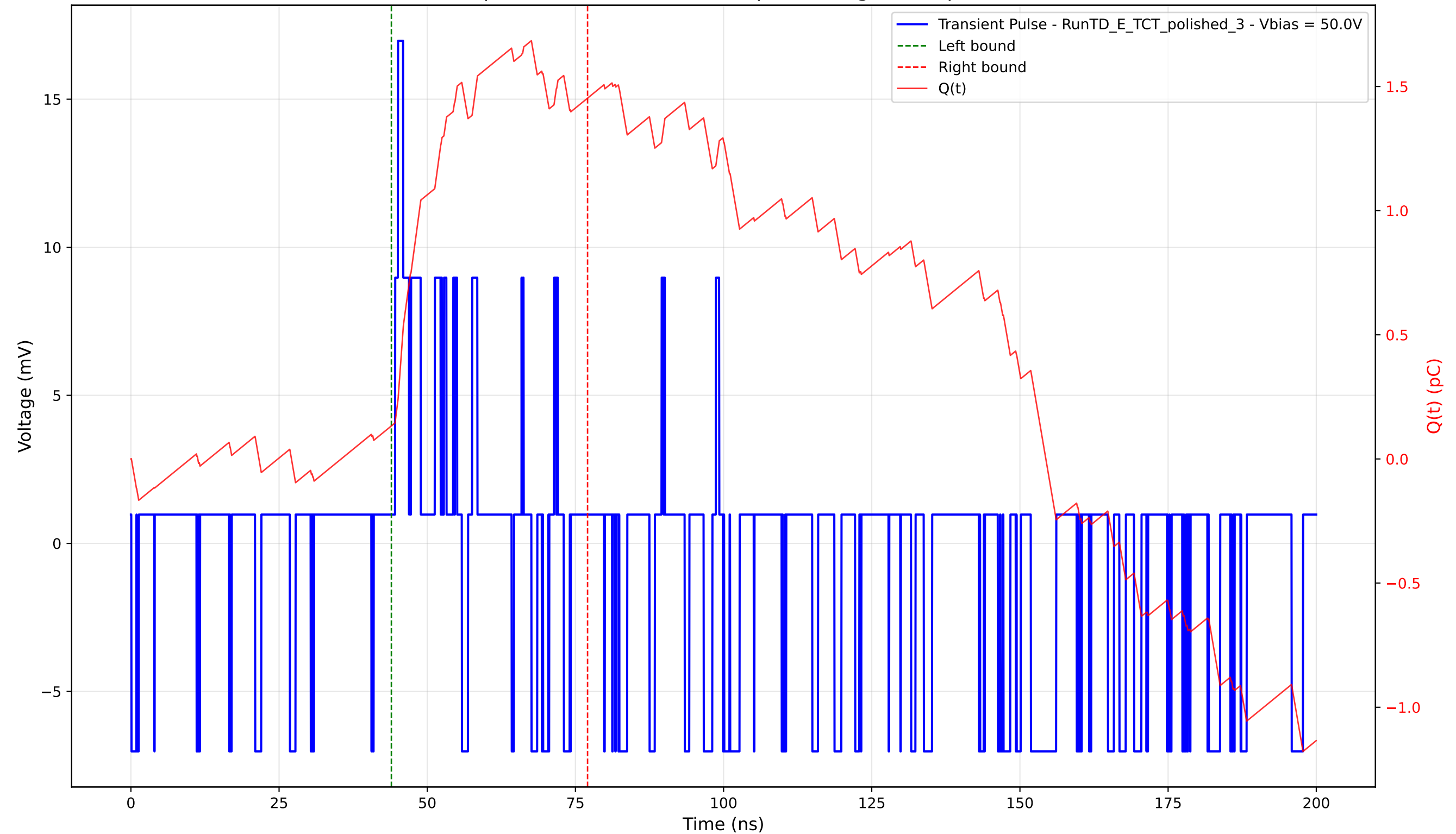
Transient Pulse - Sample: 4003 - Position: 485.0 \mu\text{m} - Charge: 1.32 pC - Rise Time: 0.50 ns
