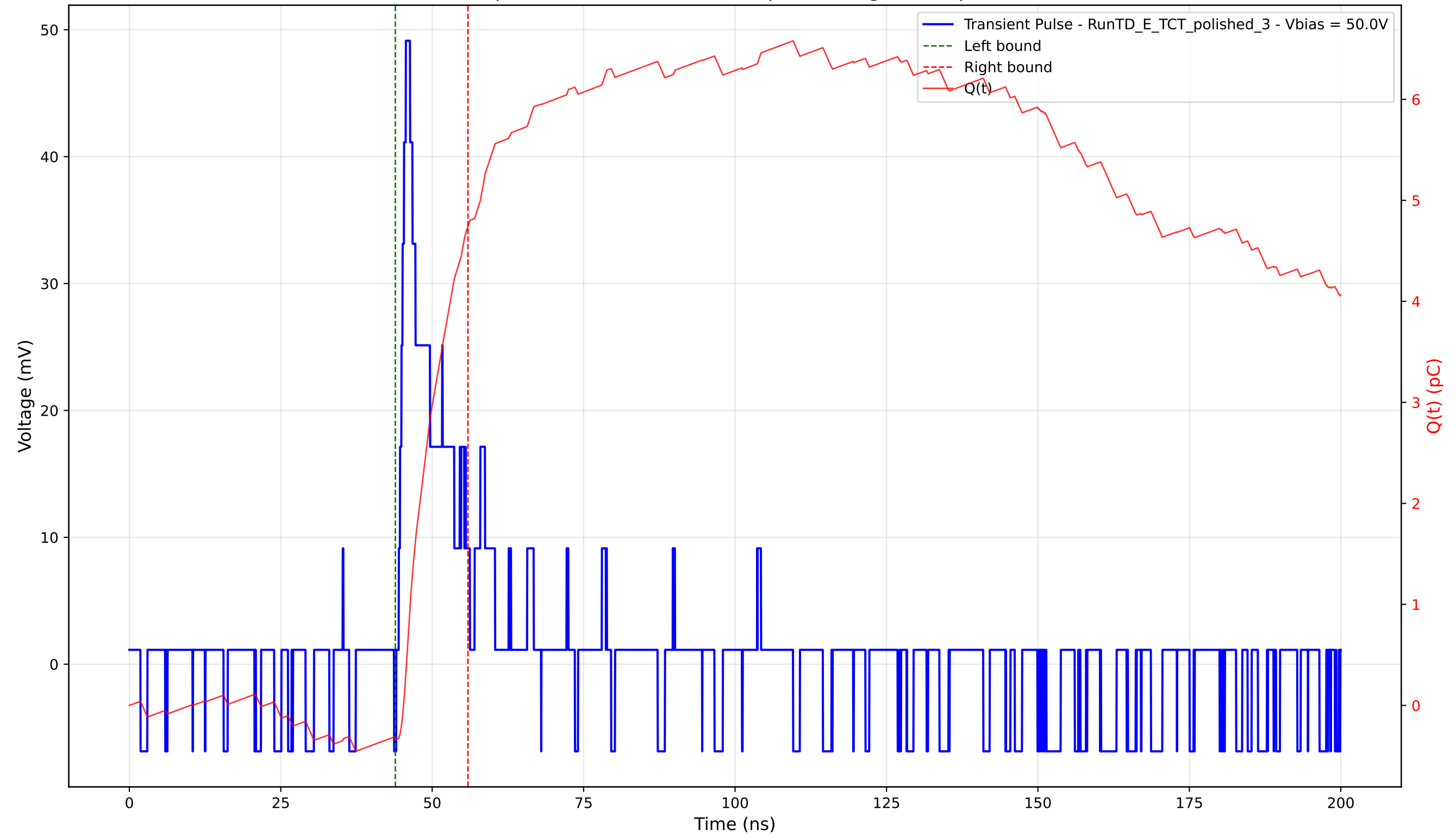
Transient Pulse - Sample: 4003 - Position: 135.0 \mu\text{m} - Charge: 5.08 pC - Rise Time: 1.17 ns
