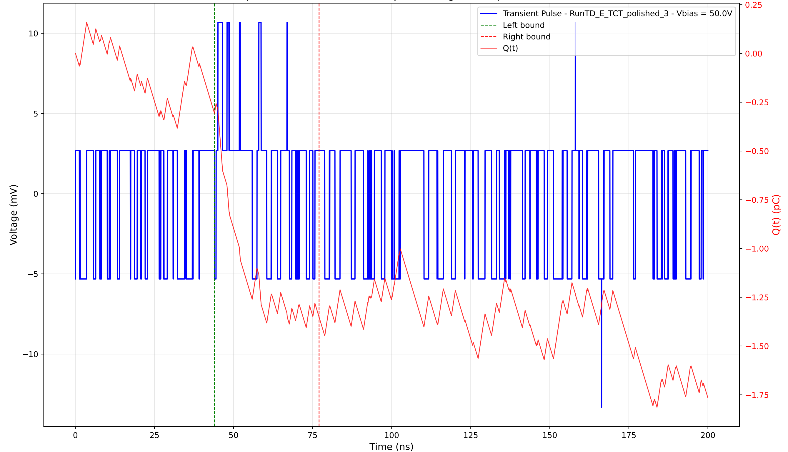
Transient Pulse - Sample: 4003 - Position: 765.0 \mu\text{m} - Charge: 1.05 pC - Rise Time: 0.00 ns (N/A)
