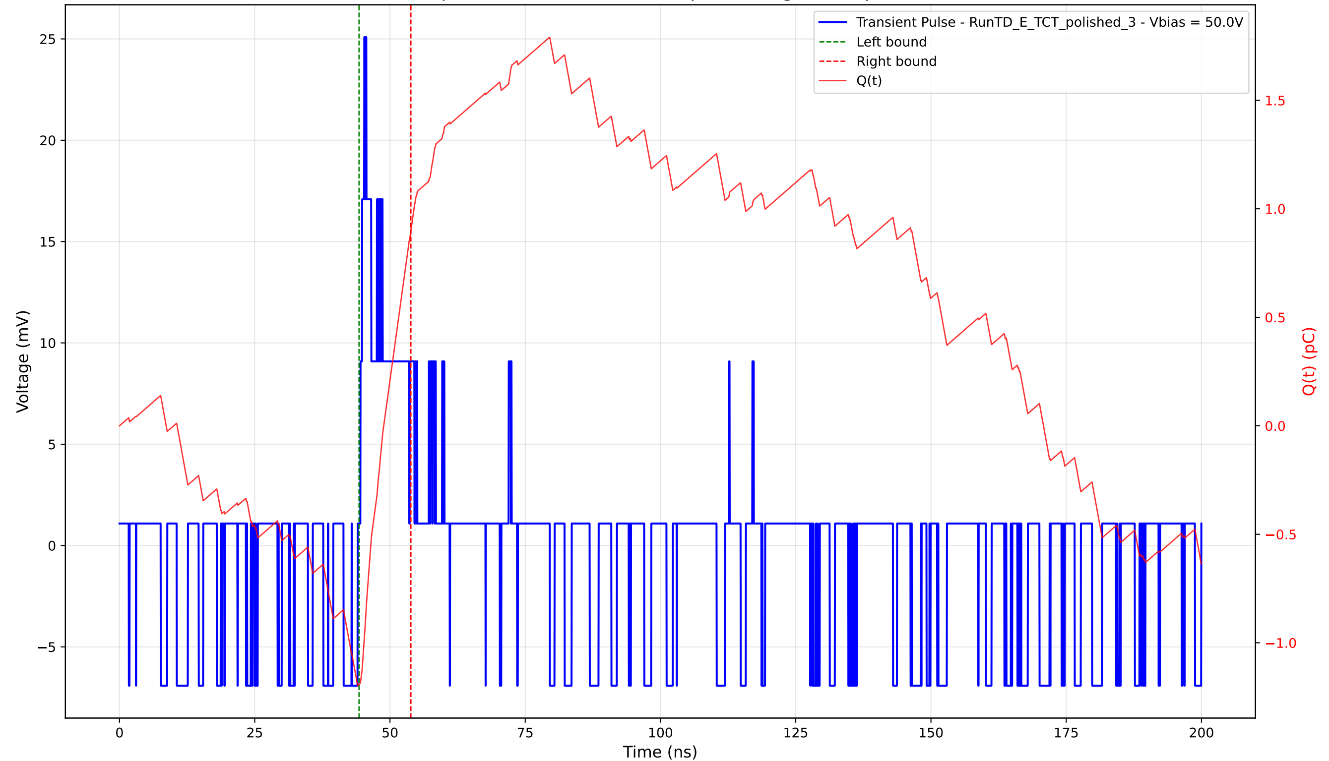
Transient Pulse - Sample: 4003 - Position: 685.0 \mu\text{m} - Charge: 2.09 pC - Rise Time: 0.72 ns
