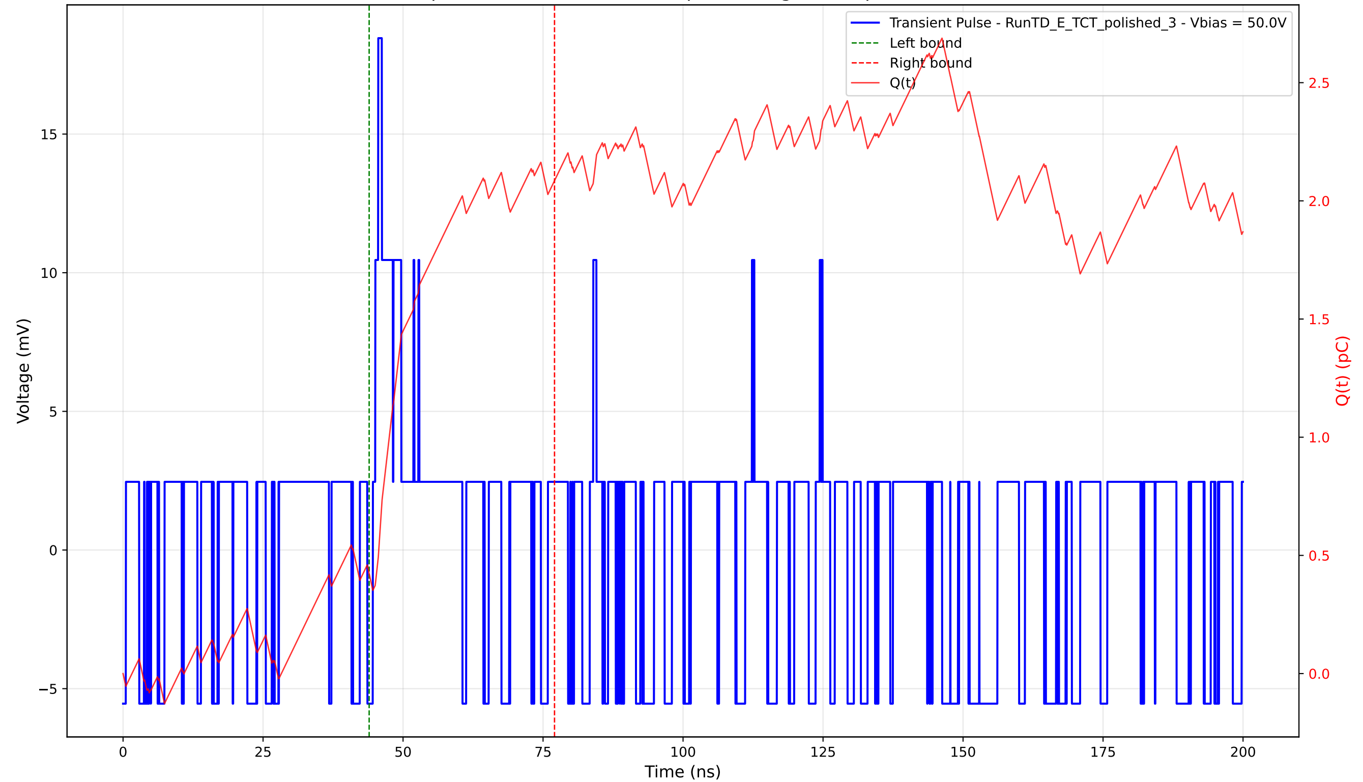
Transient Pulse - Sample: 4003 - Position: 615.0 \mu\text{m} - Charge: 1.66 pC - Rise Time: 0.00 ns (N/A)
