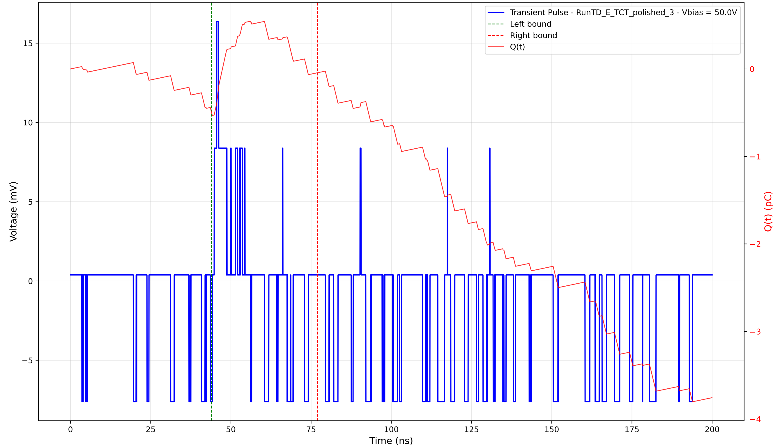
Transient Pulse - Sample: 4003 - Position: 595.0 \mu\text{m} - Charge: 0.45 pC - Rise Time: 0.82 ns
