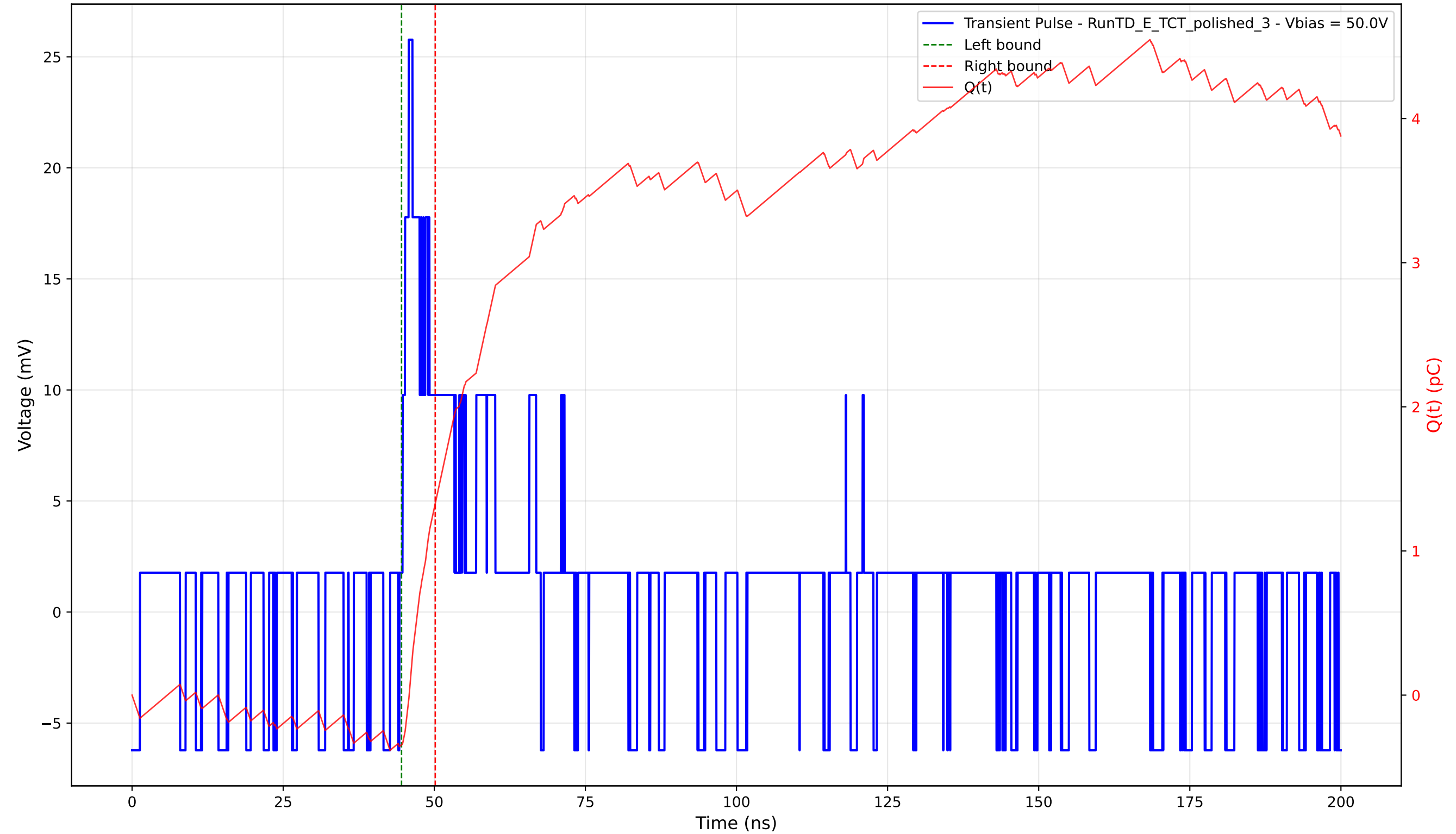
Transient Pulse - Sample: 4003 - Position: 420.0 \mu\text{m} - Charge: 1.67 pC - Rise Time: 1.02 ns
