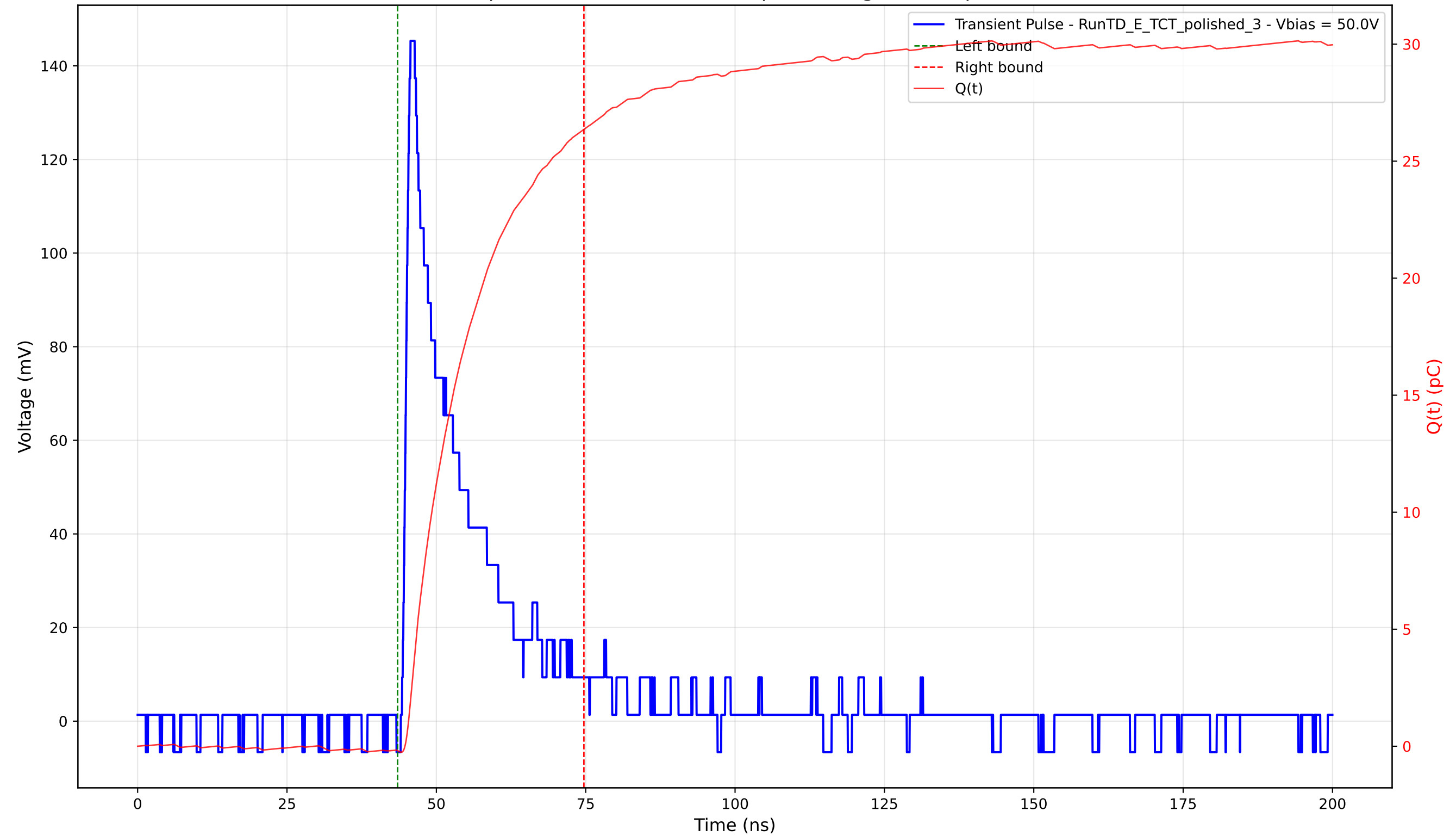
Transient Pulse - Sample: 4003 - Position: 235.0 \mu\text{m} - Charge: 26.55 pC - Rise Time: 1.13 ns
