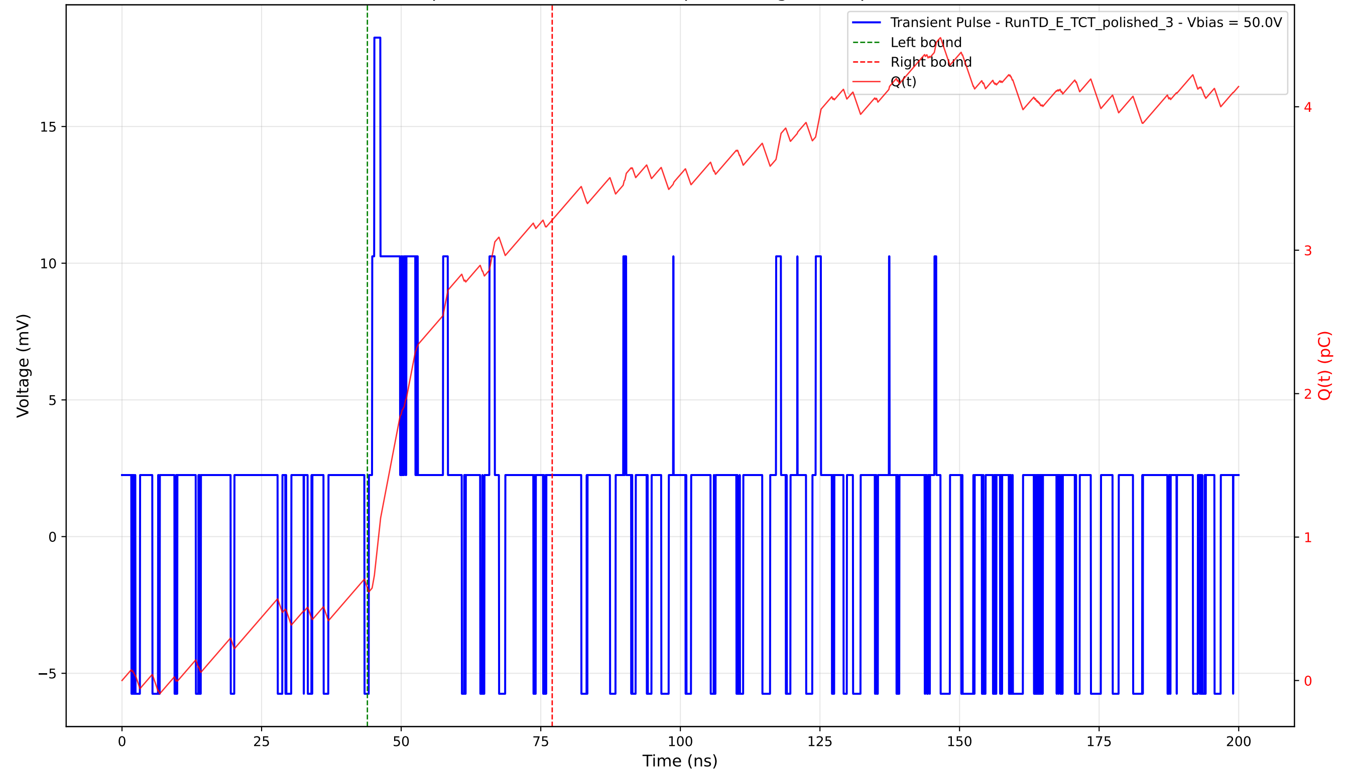
Transient Pulse - Sample: 4003 - Position: 530.0 \mu\text{m} - Charge: 2.57 pC - Rise Time: 0.00 ns (N/A)
