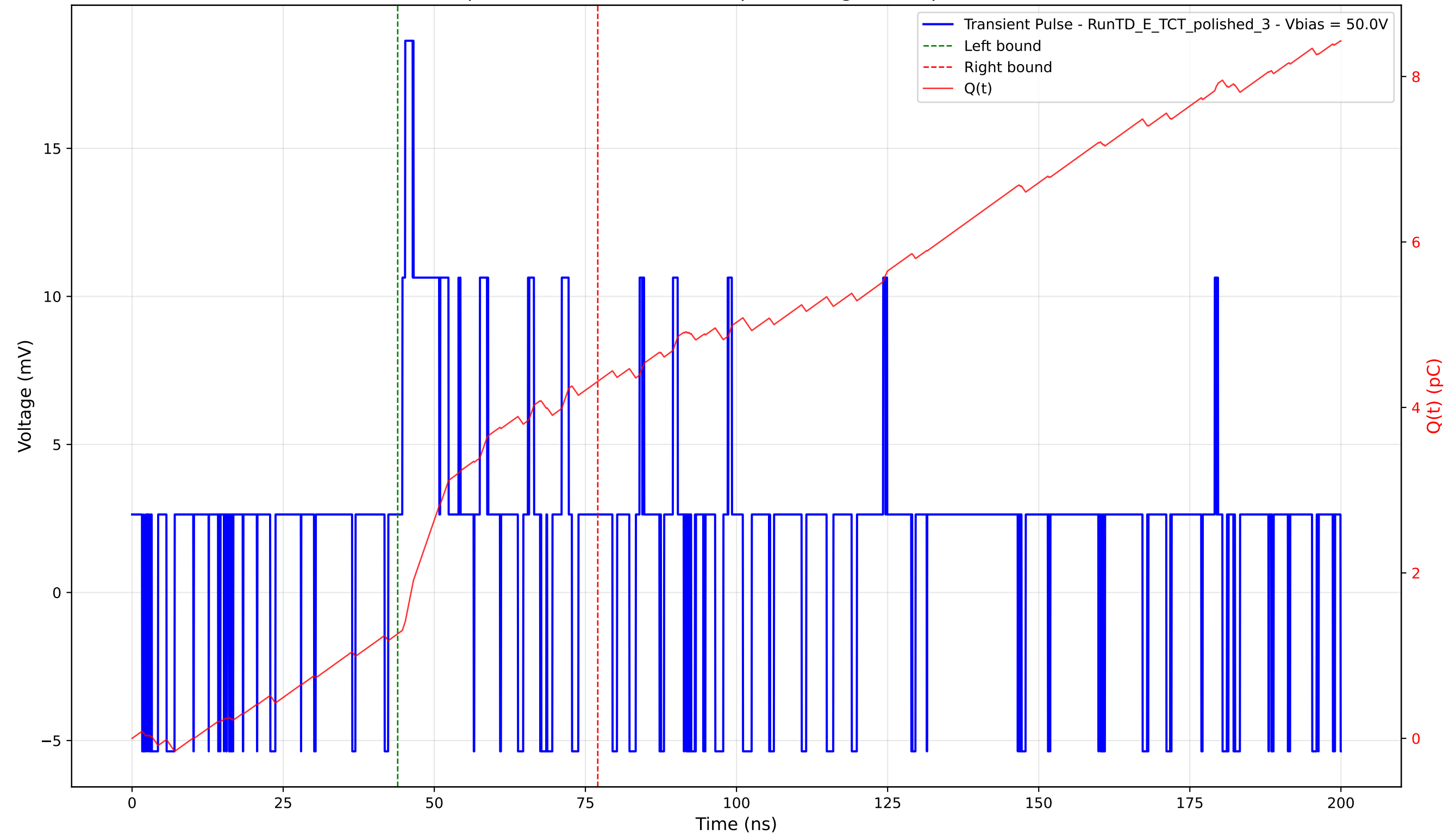
Transient Pulse - Sample: 4003 - Position: 440.0 \mu\text{m} - Charge: 3.05 pC - Rise Time: 0.00 ns (N/A)
