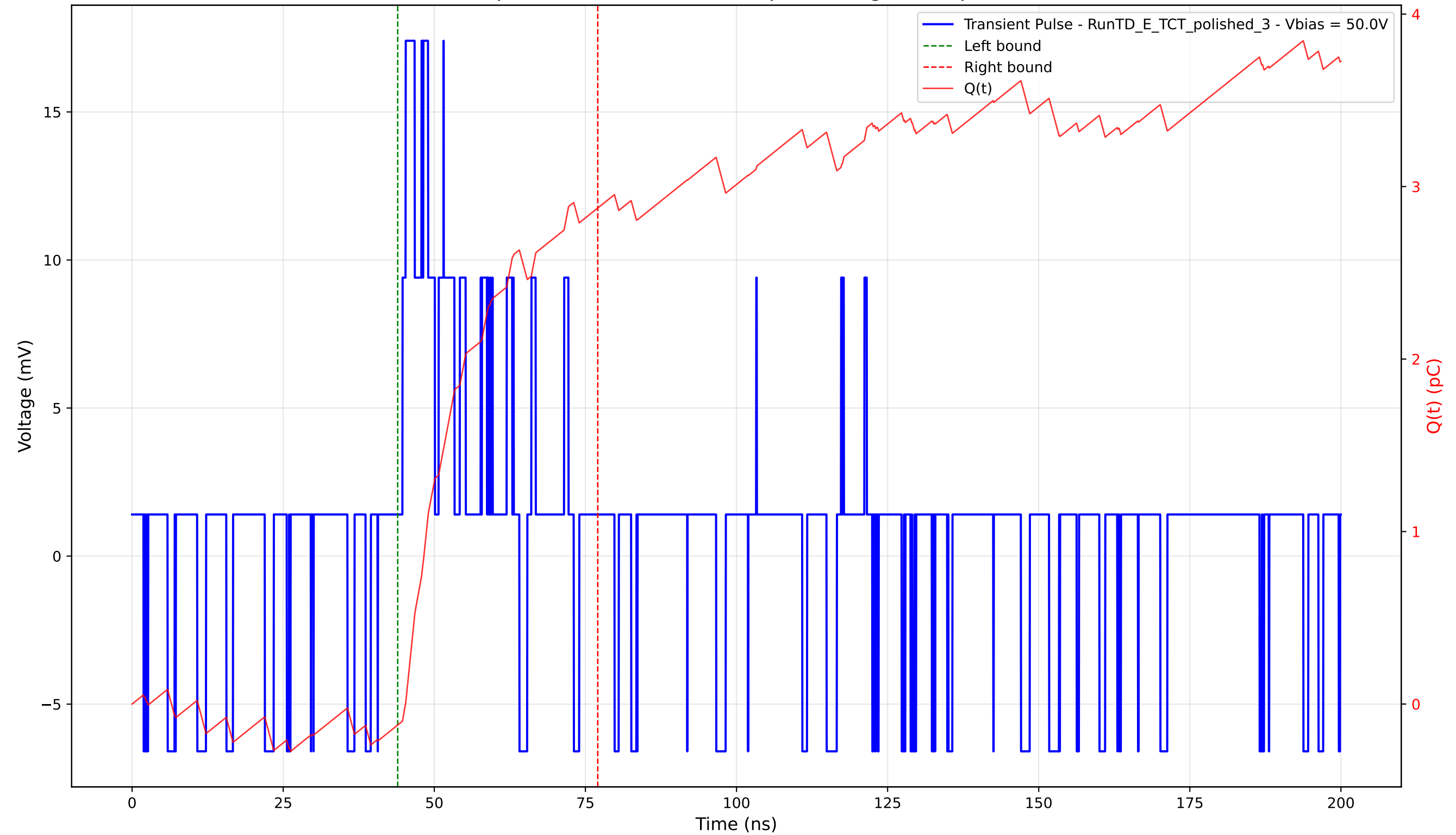
Transient Pulse - Sample: 4003 - Position: 425.0 \mu\text{m} - Charge: 3.00 pC - Rise Time: 0.54 ns
