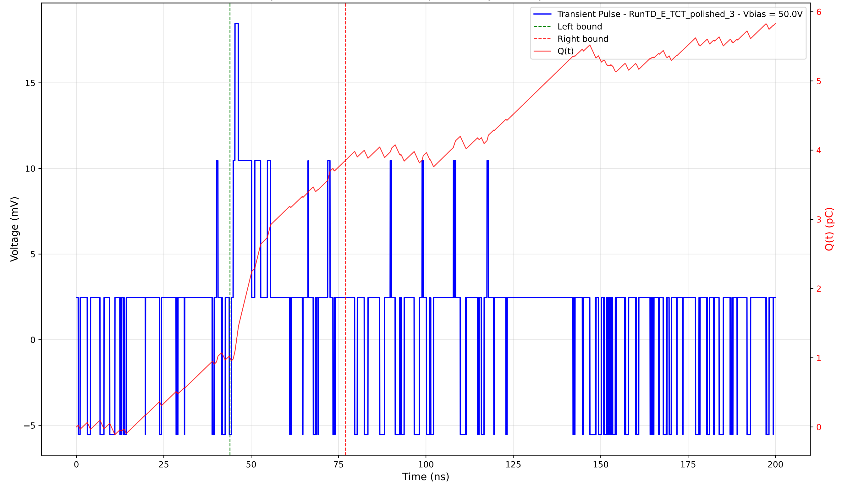
Transient Pulse - Sample: 4003 - Position: 550.0 \mu\text{m} - Charge: 2.86 pC - Rise Time: 0.00 ns (N/A)
