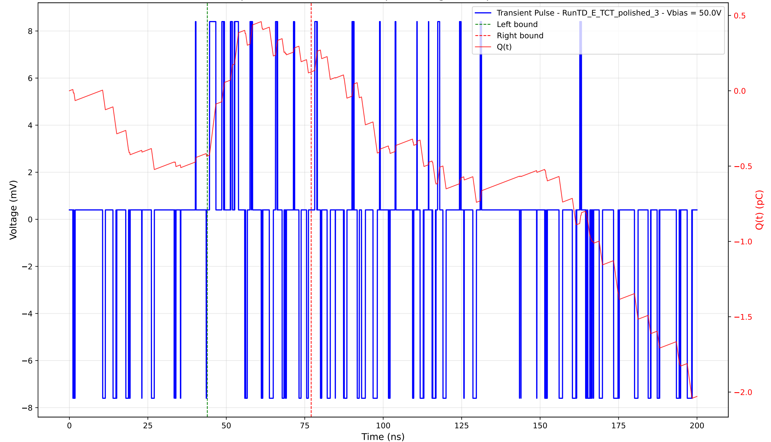
Transient Pulse - Sample: 4003 - Position: 745.0 \mu\text{m} - Charge: 0.56 pC - Rise Time: 0.00 ns (N/A)
