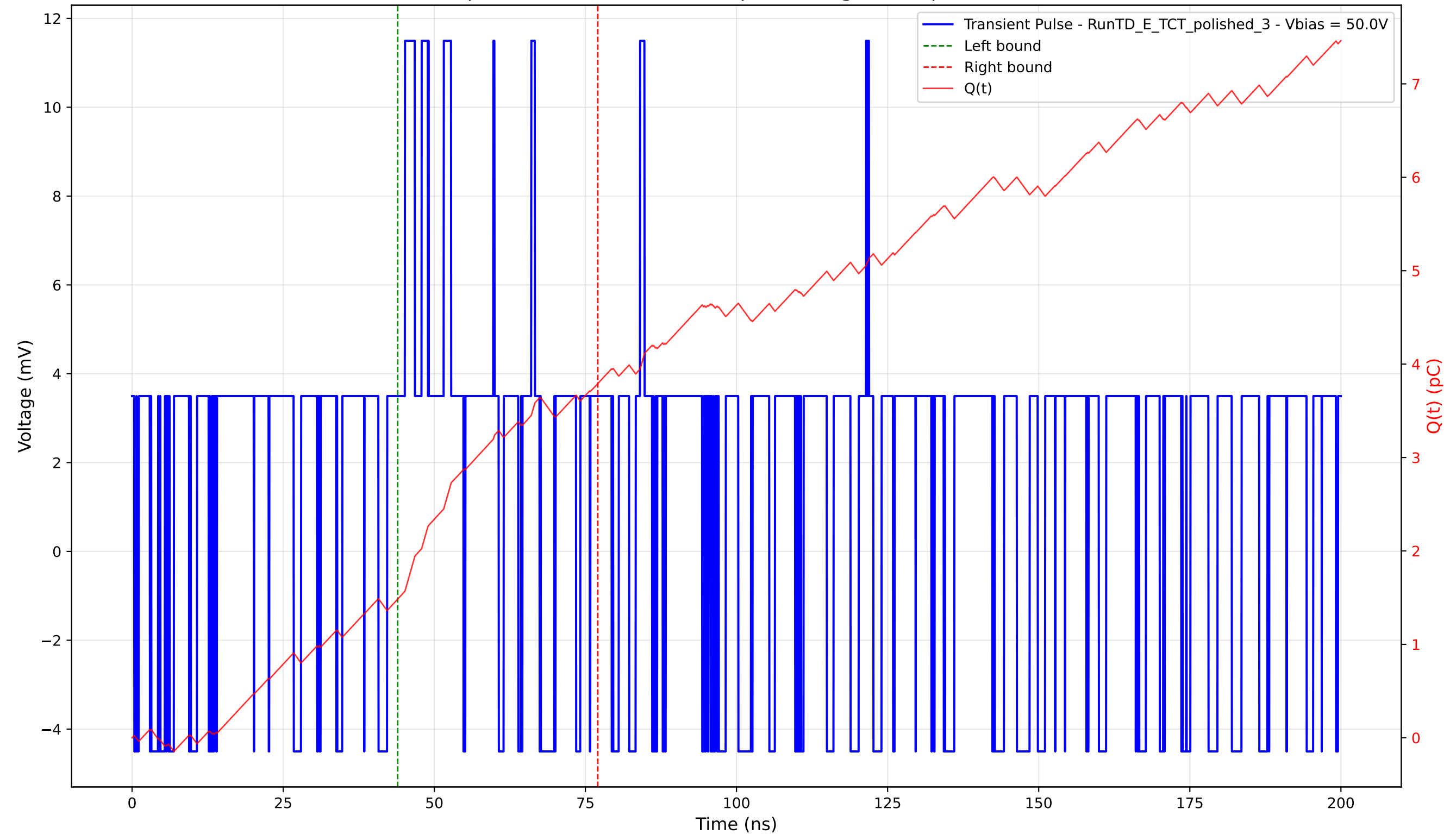
Transient Pulse - Sample: 4003 - Position: 740.0 \mu\text{m} - Charge: 2.31 pC - Rise Time: 0.00 ns (N/A)
