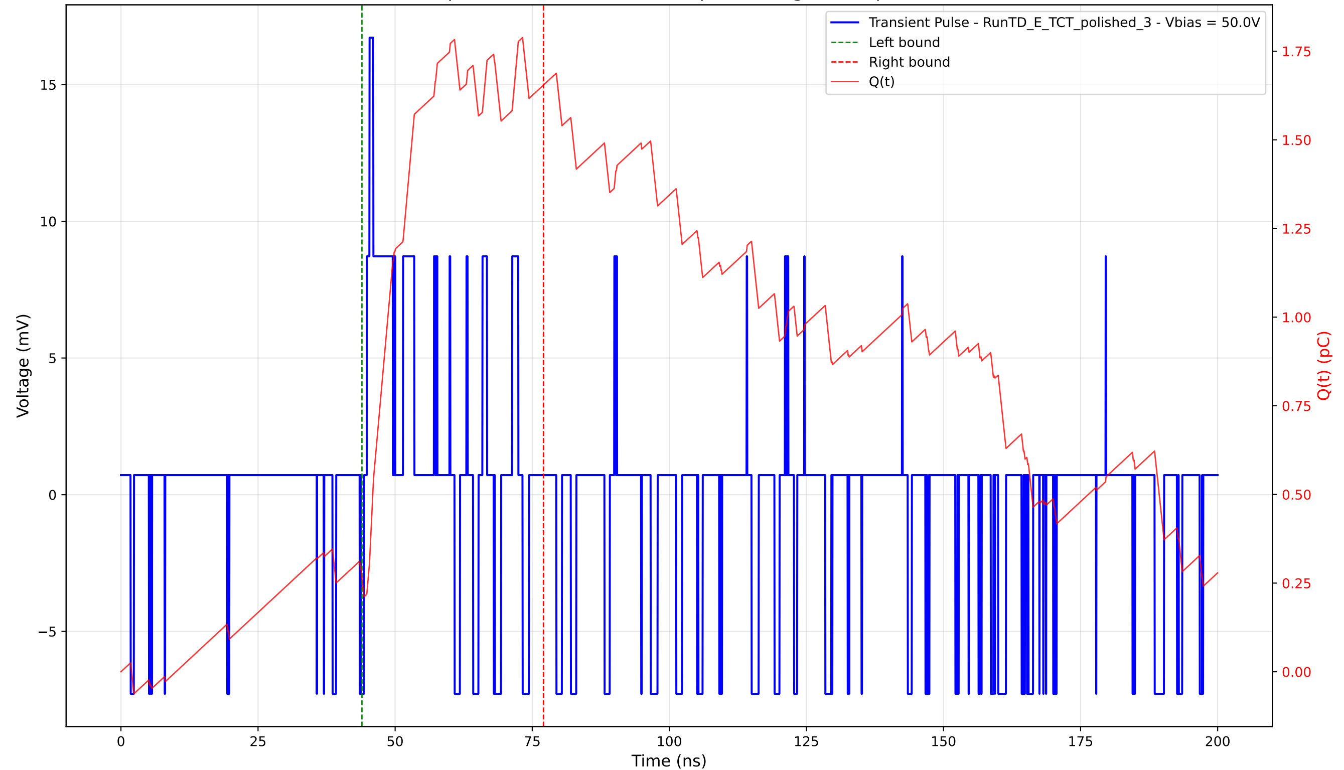
Transient Pulse - Sample: 4003 - Position: 650.0 \mu\text{m} - Charge: 1.39 pC - Rise Time: 0.50 ns
