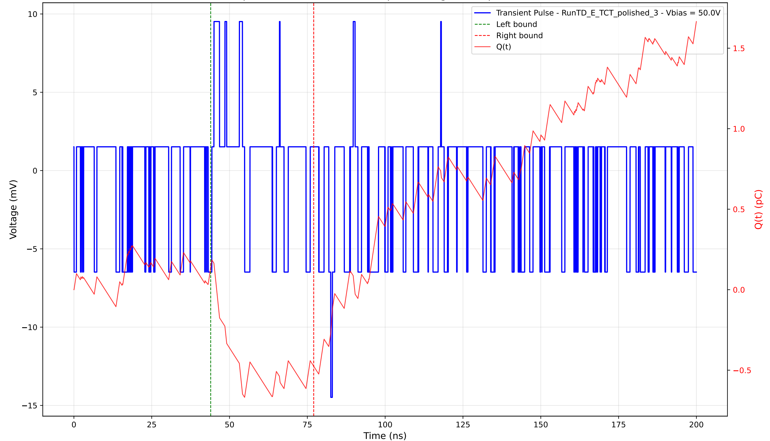
Transient Pulse - Sample: 4003 - Position: 660.0 \mu\text{m} - Charge: 0.61 pC - Rise Time: 0.00 ns (N/A)
