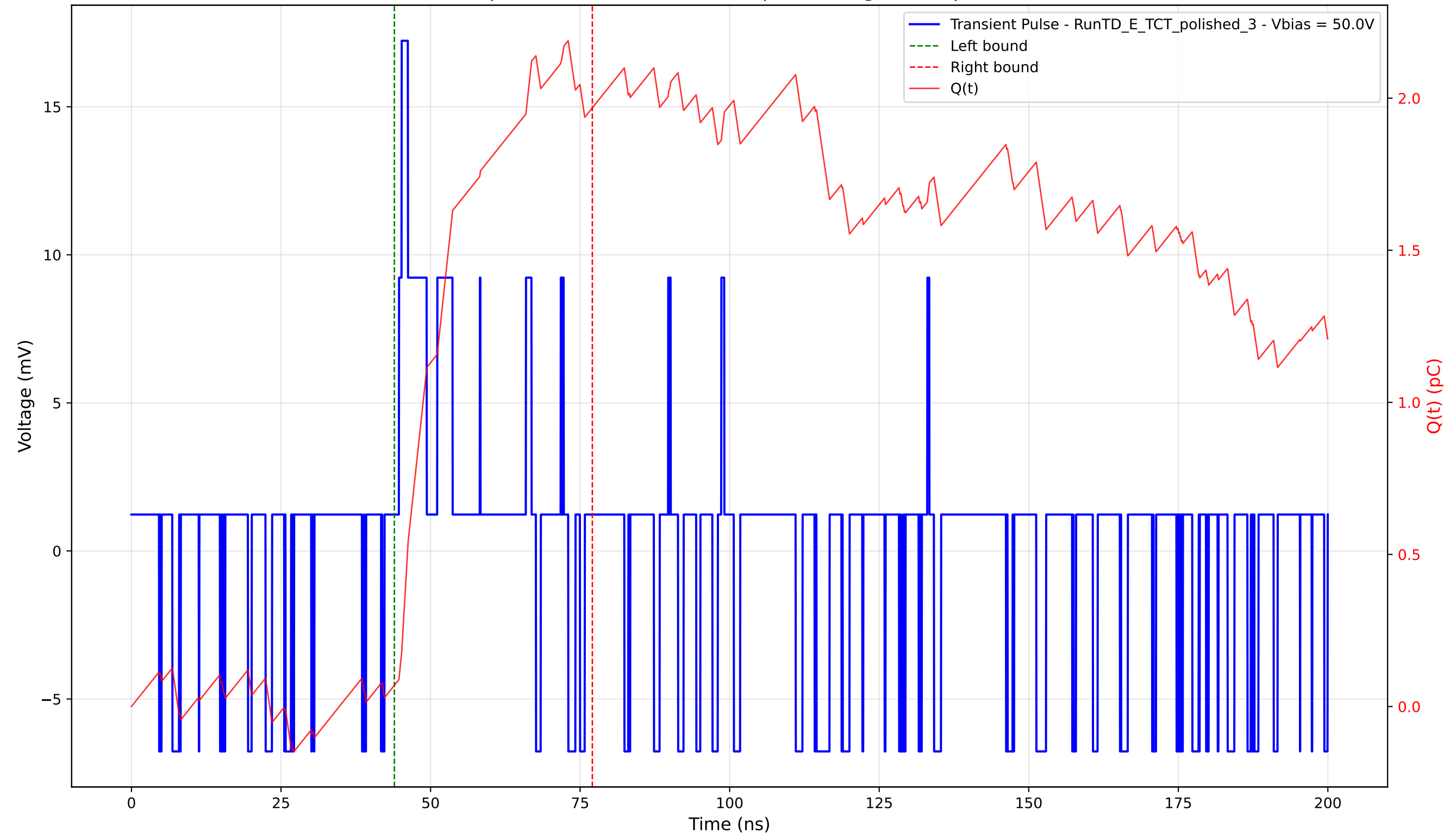
Transient Pulse - Sample: 4003 - Position: 455.0 \mu\text{m} - Charge: 1.90 pC - Rise Time: 0.46 ns
