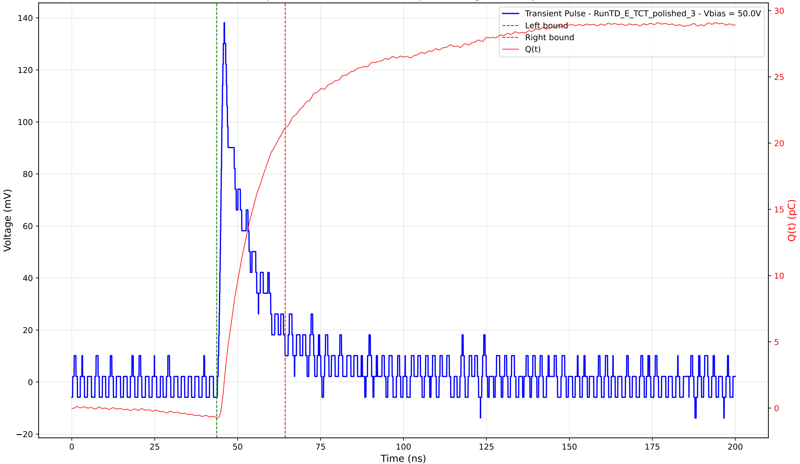
Transient Pulse - Sample: 4003 - Position: 290.0 \mu\text{m} - Charge: 21.88 pC - Rise Time: 1.39 ns
