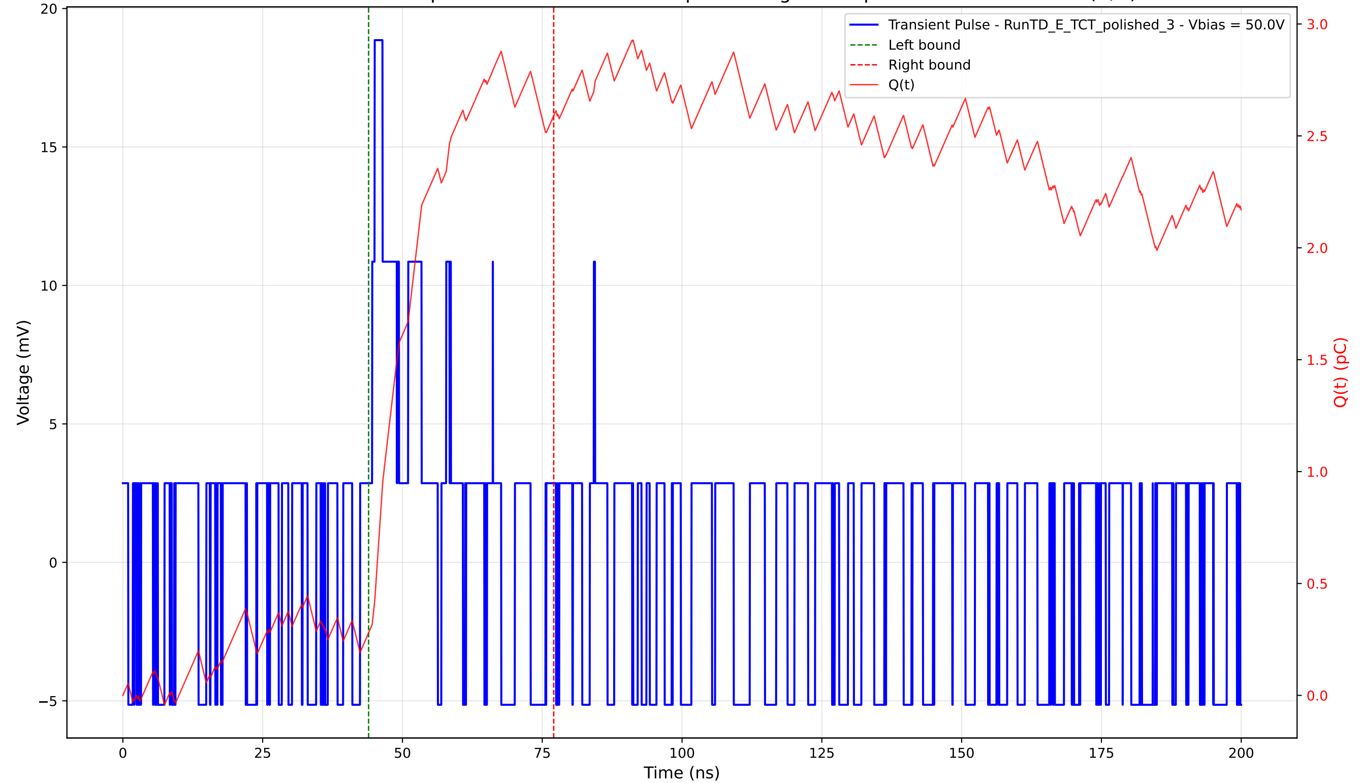
Transient Pulse - Sample: 4003 - Position: 555.0 \mu\text{m} - Charge: 2.31 pC - Rise Time: 0.00 ns (N/A)
