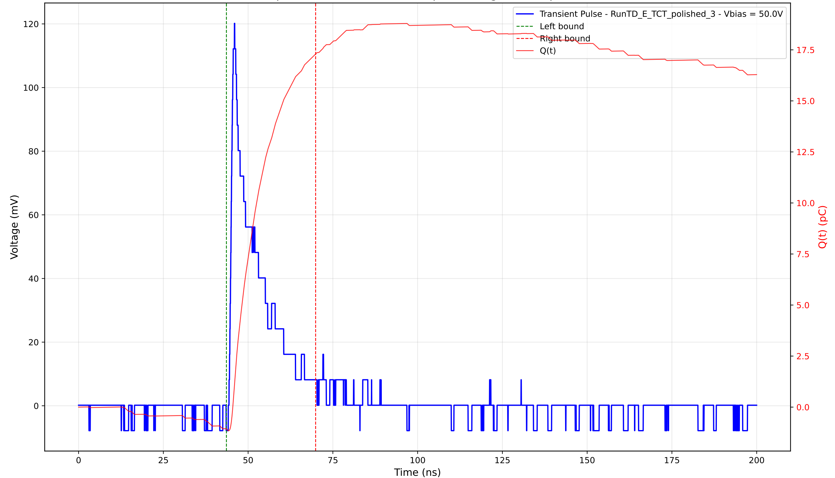
Transient Pulse - Sample: 4003 - Position: 190.0 \mu\text{m} - Charge: 18.37 pC - Rise Time: 1.09 ns
