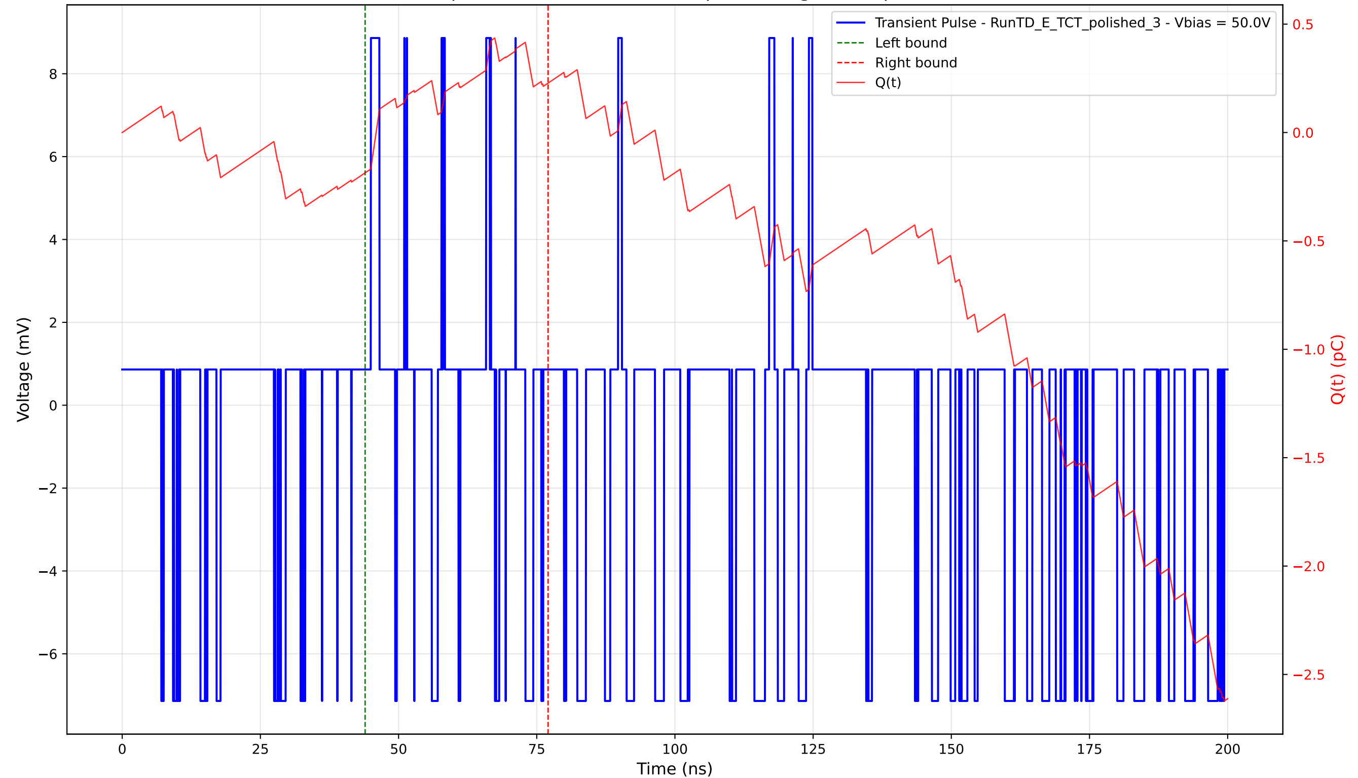
Transient Pulse - Sample: 4003 - Position: 785.0 \mu\text{m} - Charge: 0.41 pC - Rise Time: 0.02 ns
