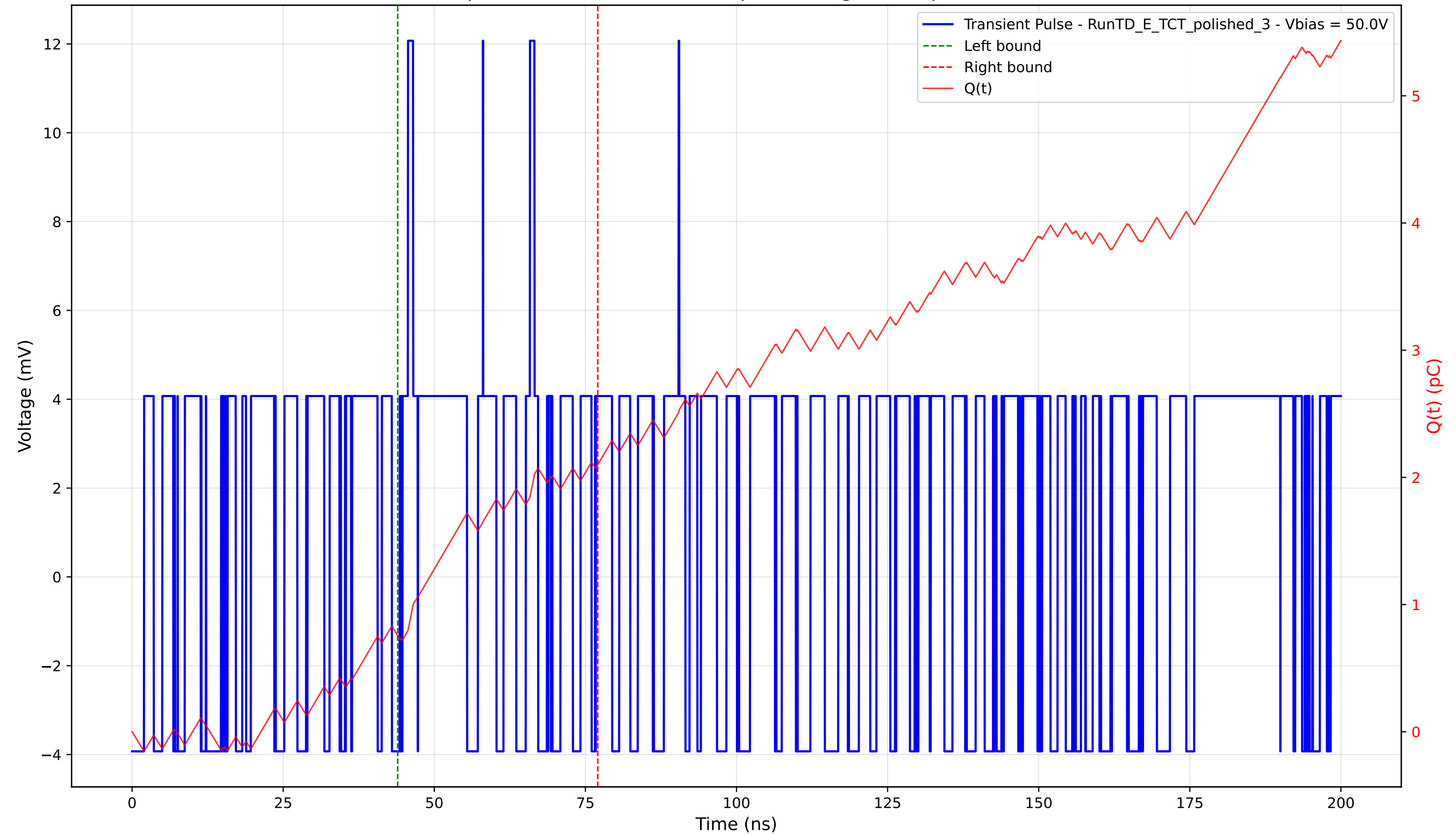
Transient Pulse - Sample: 4003 - Position: 725.0 \mu\text{m} - Charge: 1.35 pC - Rise Time: 0.00 ns (N/A)
