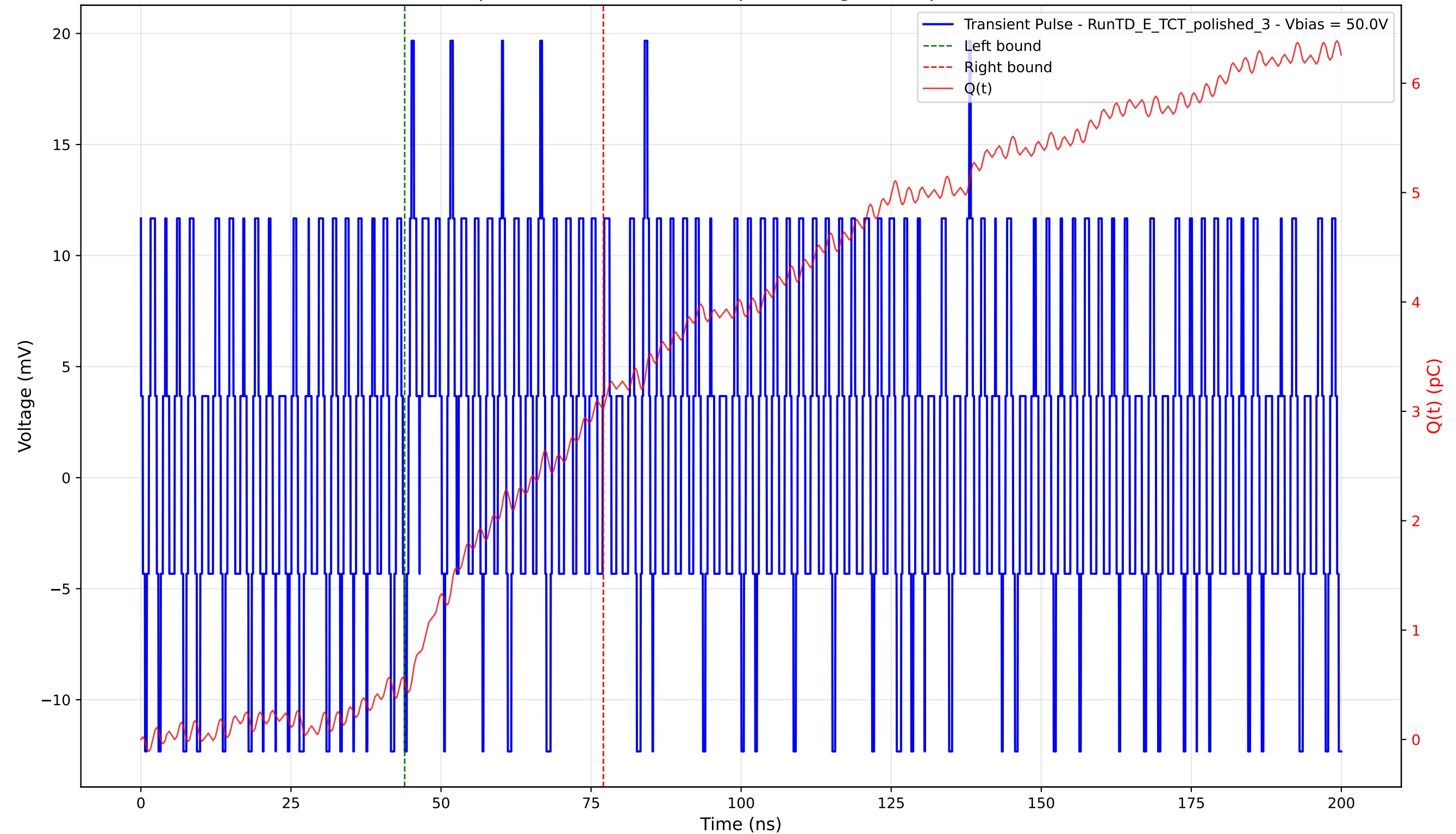
Transient Pulse - Sample: 4003 - Position: 75.0 \mu\text{m} - Charge: 2.50 pC - Rise Time: 0.00 ns (N/A)
