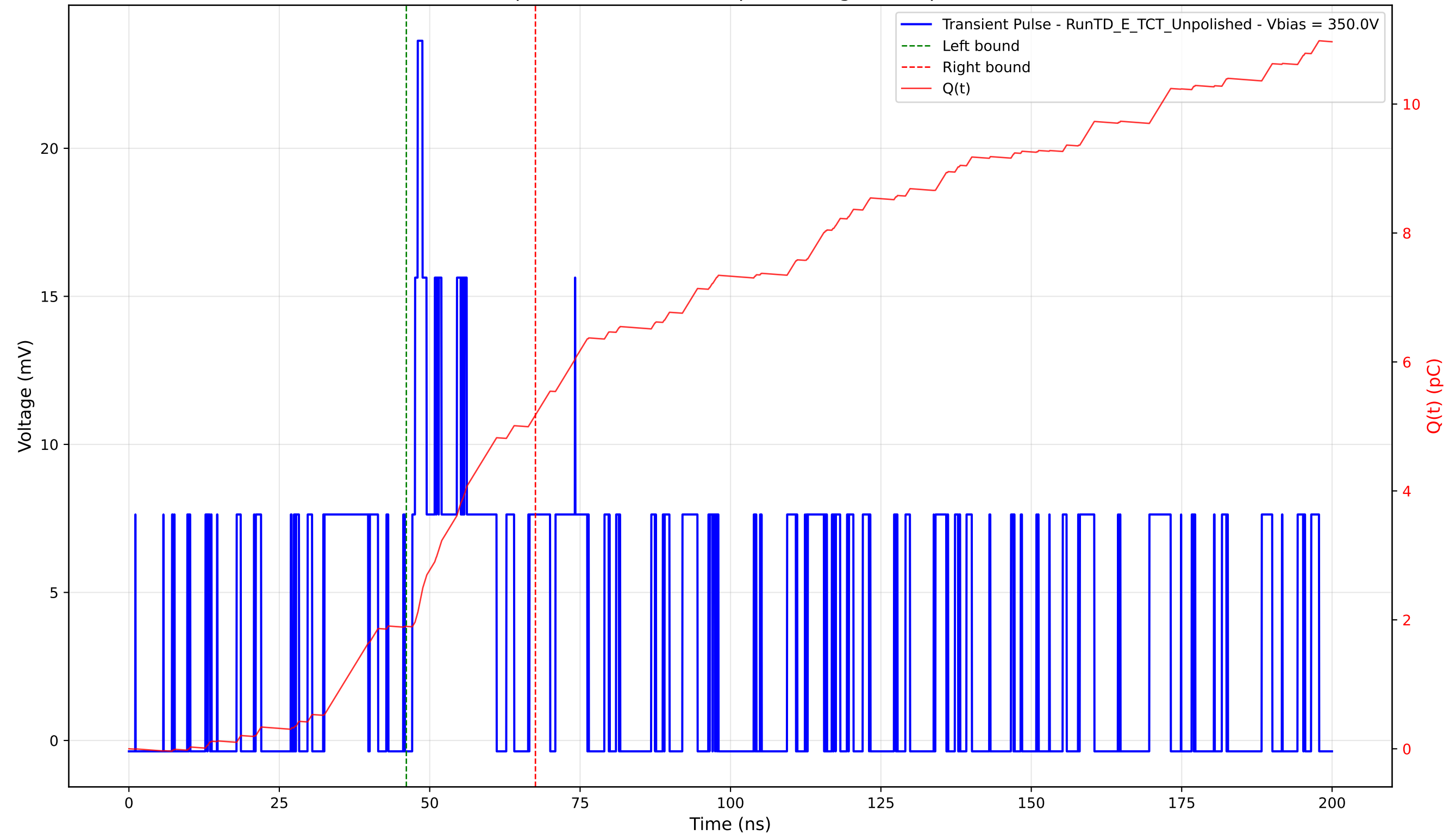
Transient Pulse - Sample: TD - Position: 5.0 \mu\text{m} - Charge: 3.27 pC - Rise Time: 0.91 ns
