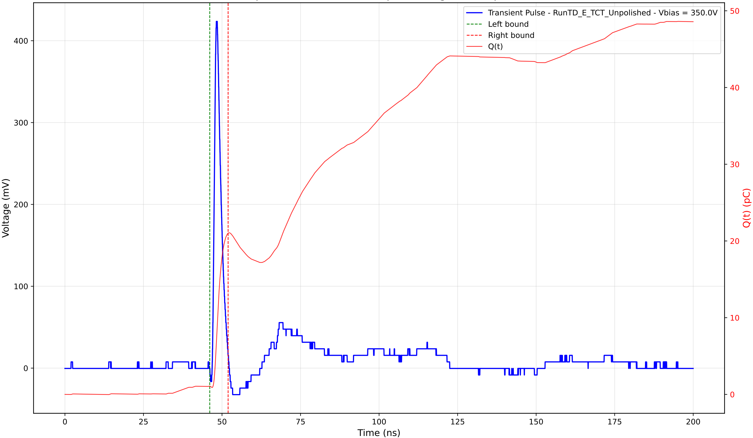
Transient Pulse - Sample: TD - Position: 180.0 \mu\text{m} - Charge: 19.94 pC - Rise Time: 0.89 ns
