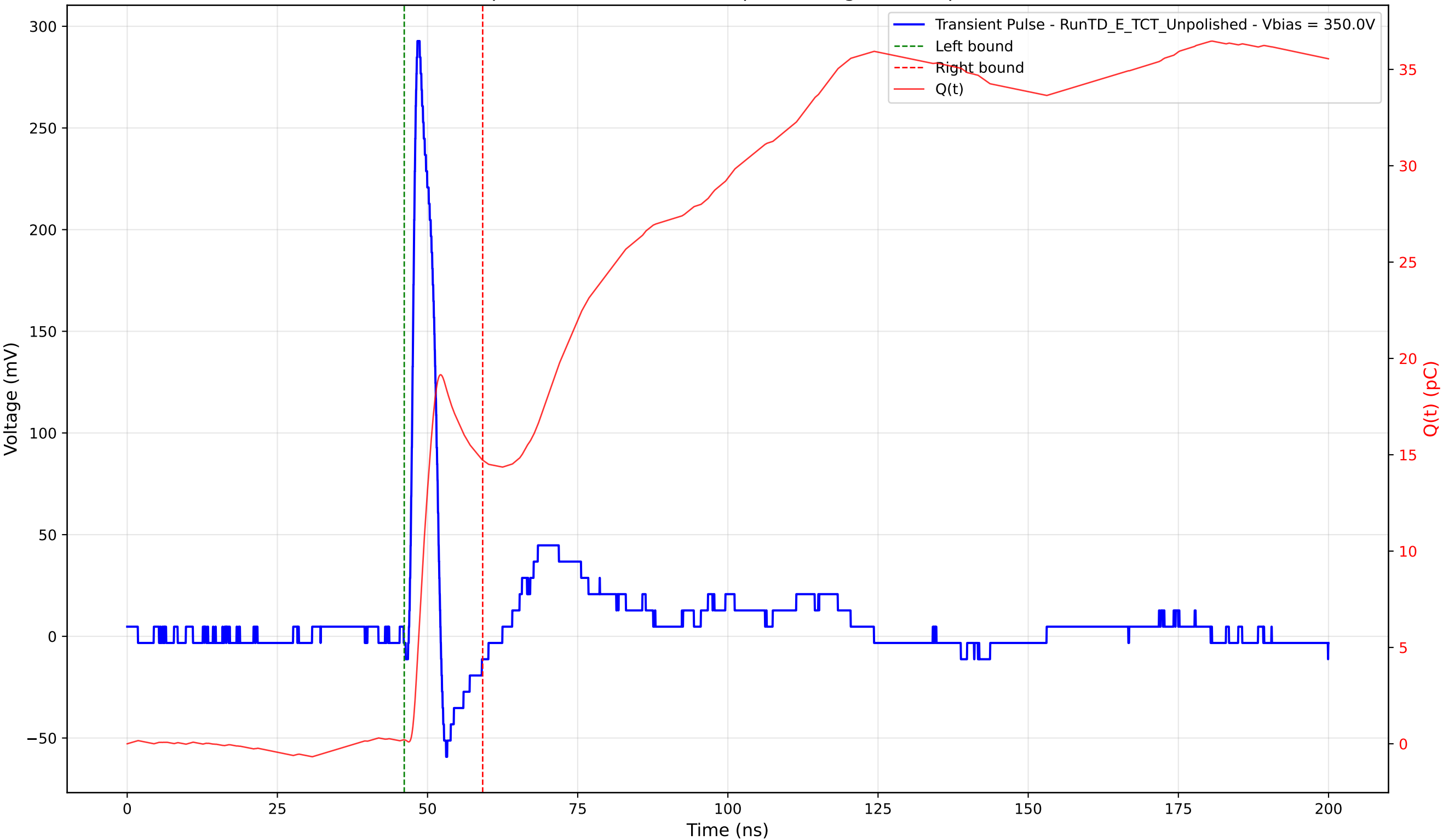
Transient Pulse - Sample: TD - Position: 290.0 \mu\text{m} - Charge: 14.51 pC - Rise Time: 0.96 ns
