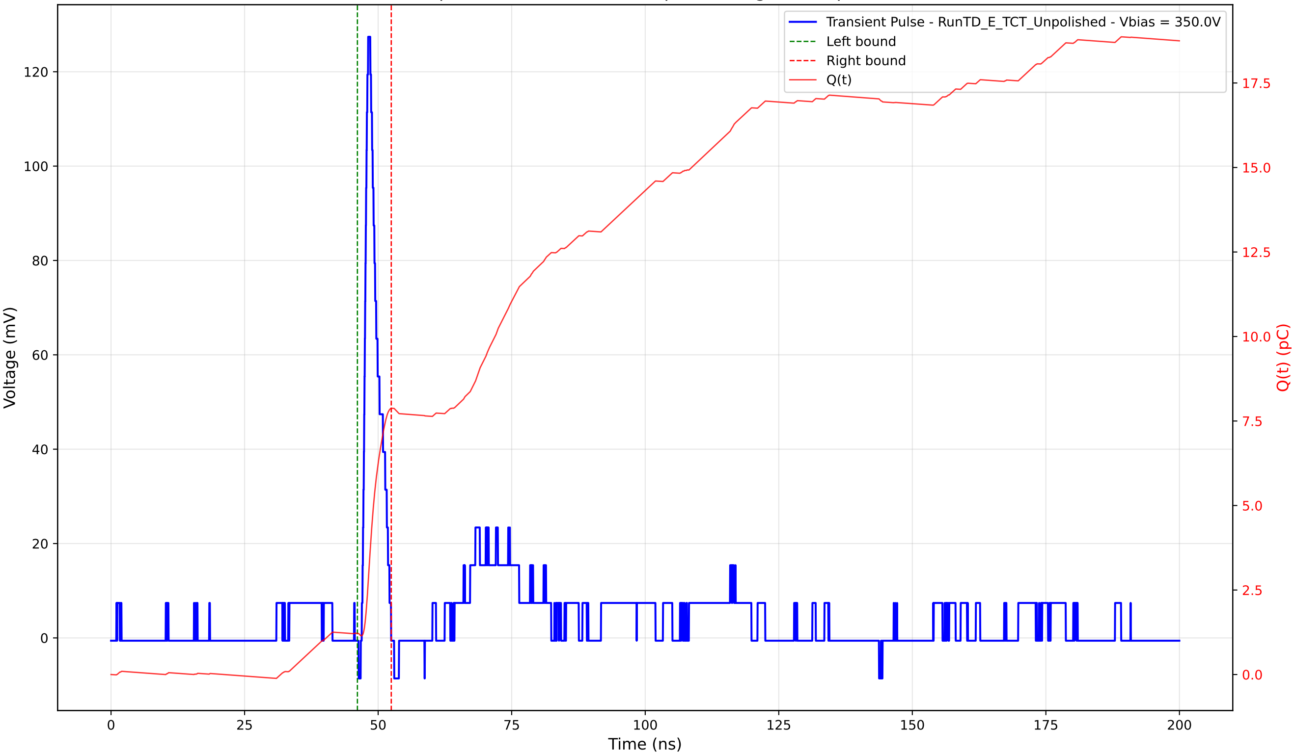
Transient Pulse - Sample: TD - Position: 340.0 \mu\text{m} - Charge: 6.66 pC - Rise Time: 0.91 ns
