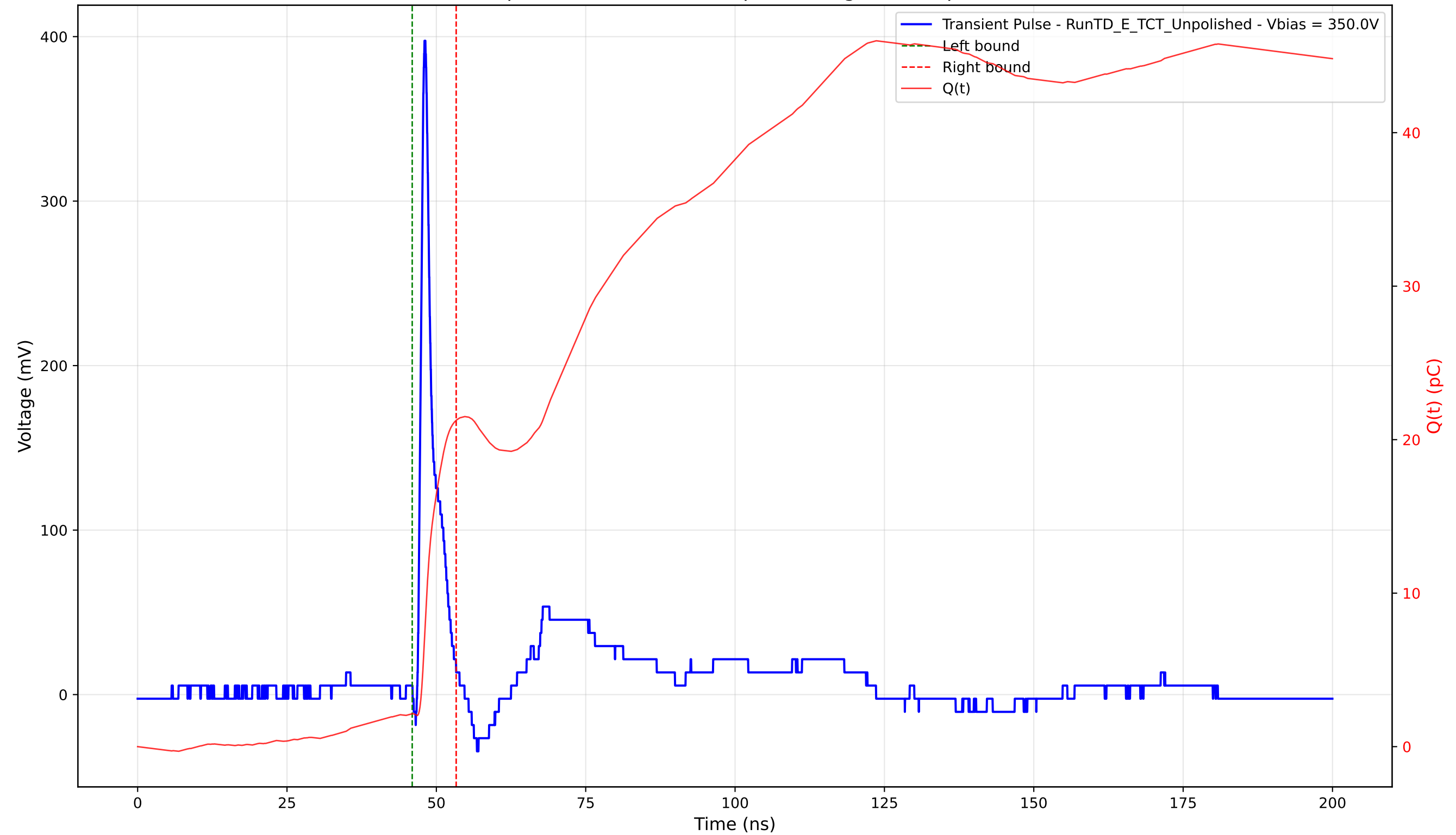
Transient Pulse - Sample: TD - Position: 40.0 \mu\text{m} - Charge: 19.12 pC - Rise Time: 0.83 ns
