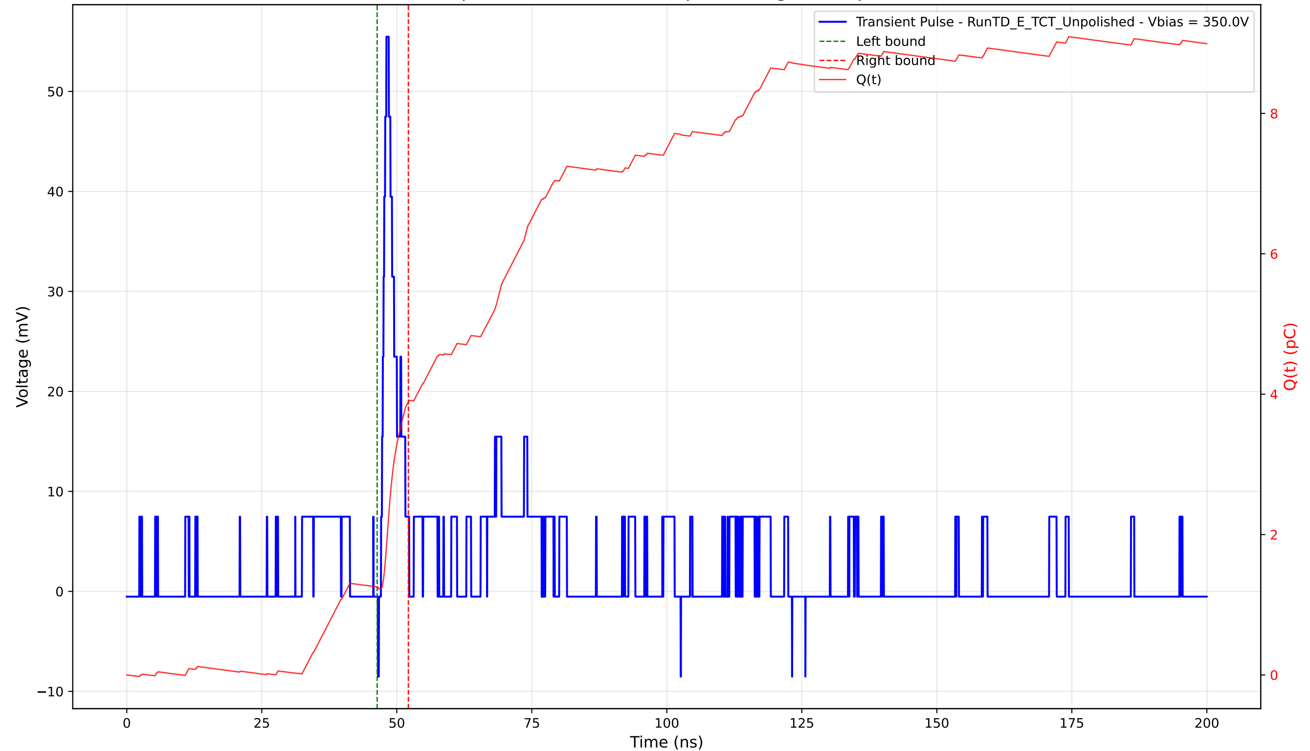
Transient Pulse - Sample: TD - Position: 365.0 \mu\text{m} - Charge: 2.64 pC - Rise Time: 0.99 ns
