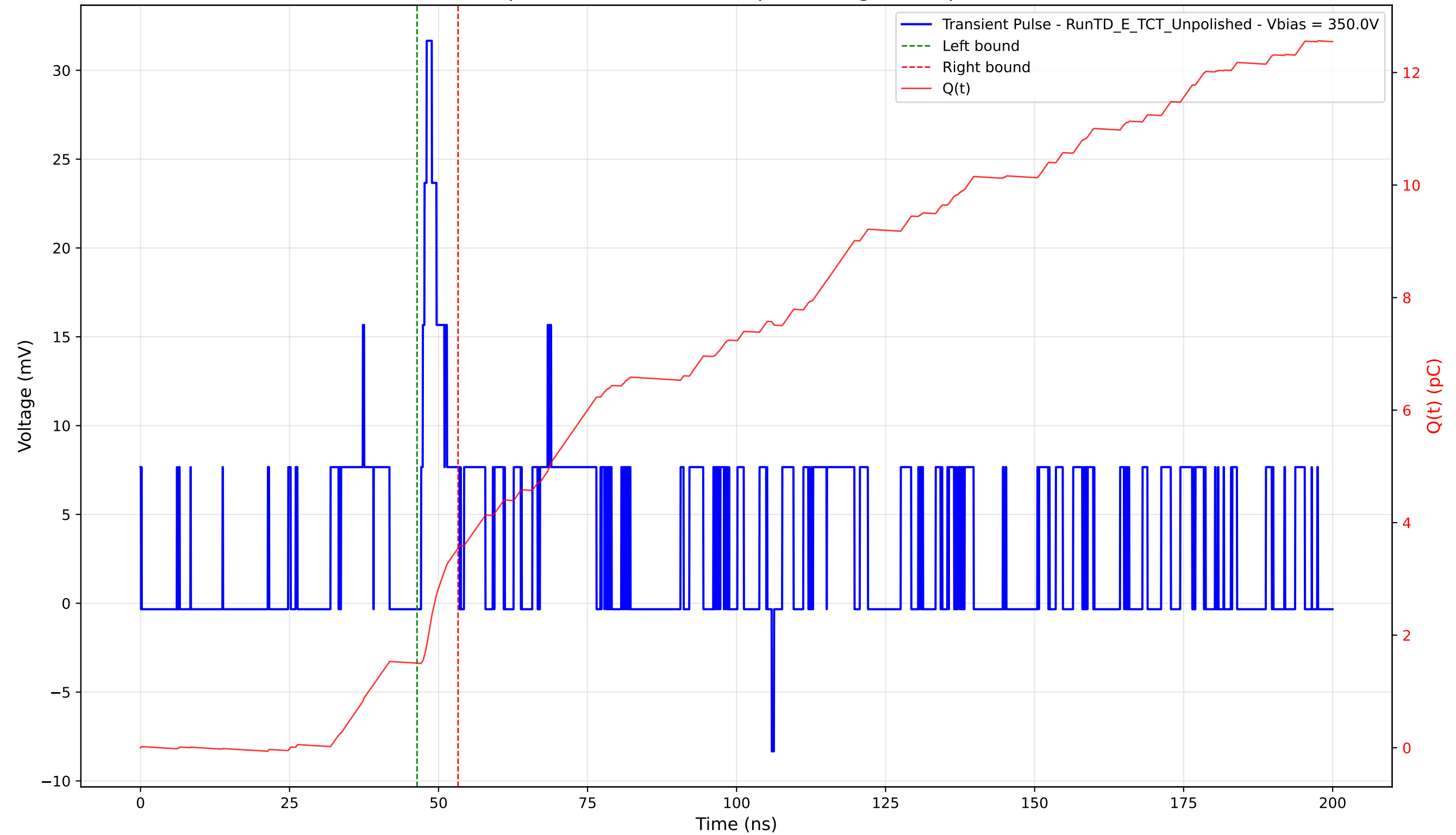
Transient Pulse - Sample: TD - Position: 355.0 \mu\text{m} - Charge: 2.05 pC - Rise Time: 0.93 ns
