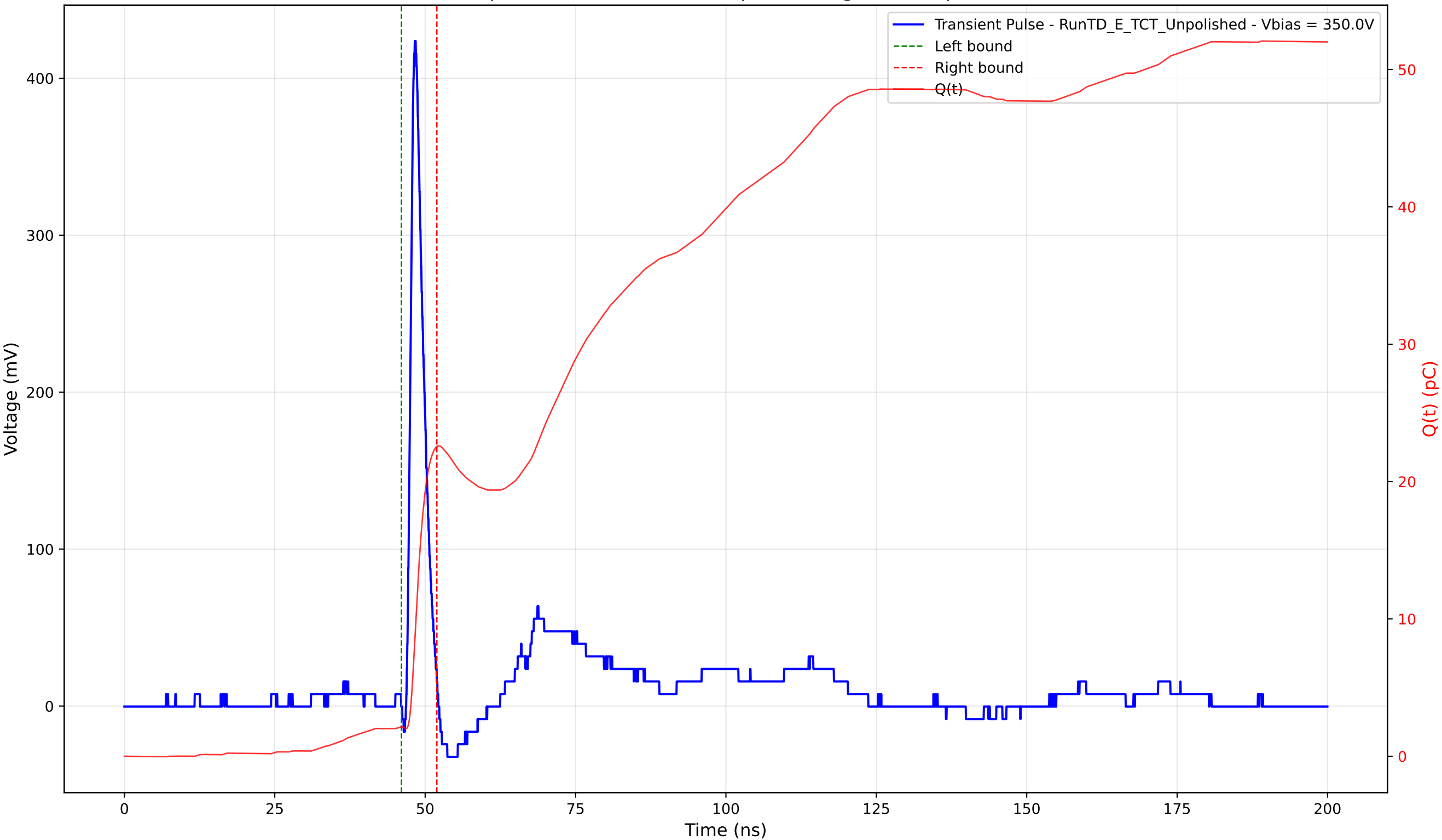
Transient Pulse - Sample: TD - Position: 185.0 \mu\text{m} - Charge: 20.41 pC - Rise Time: 0.91 ns
