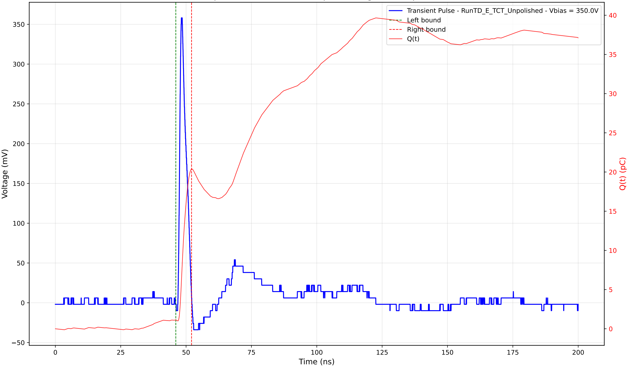
Transient Pulse - Sample: TD - Position: 250.0 \mu\text{m} - Charge: 19.26 pC - Rise Time: 0.93 ns
