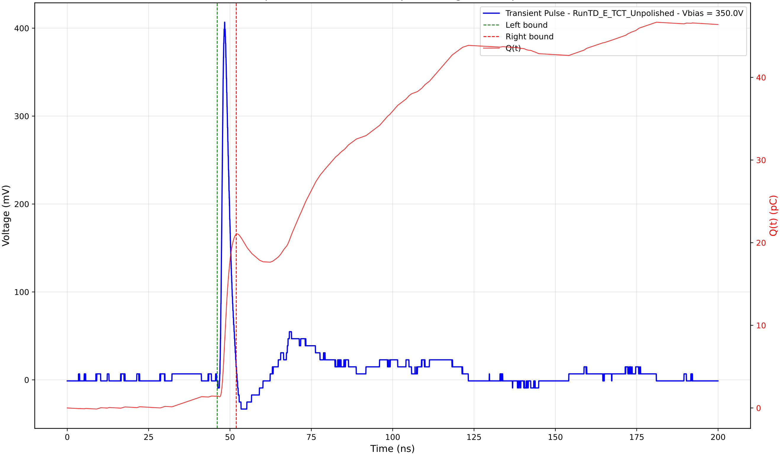
Transient Pulse - Sample: TD - Position: 220.0 \mu\text{m} - Charge: 19.58 pC - Rise Time: 0.94 ns
