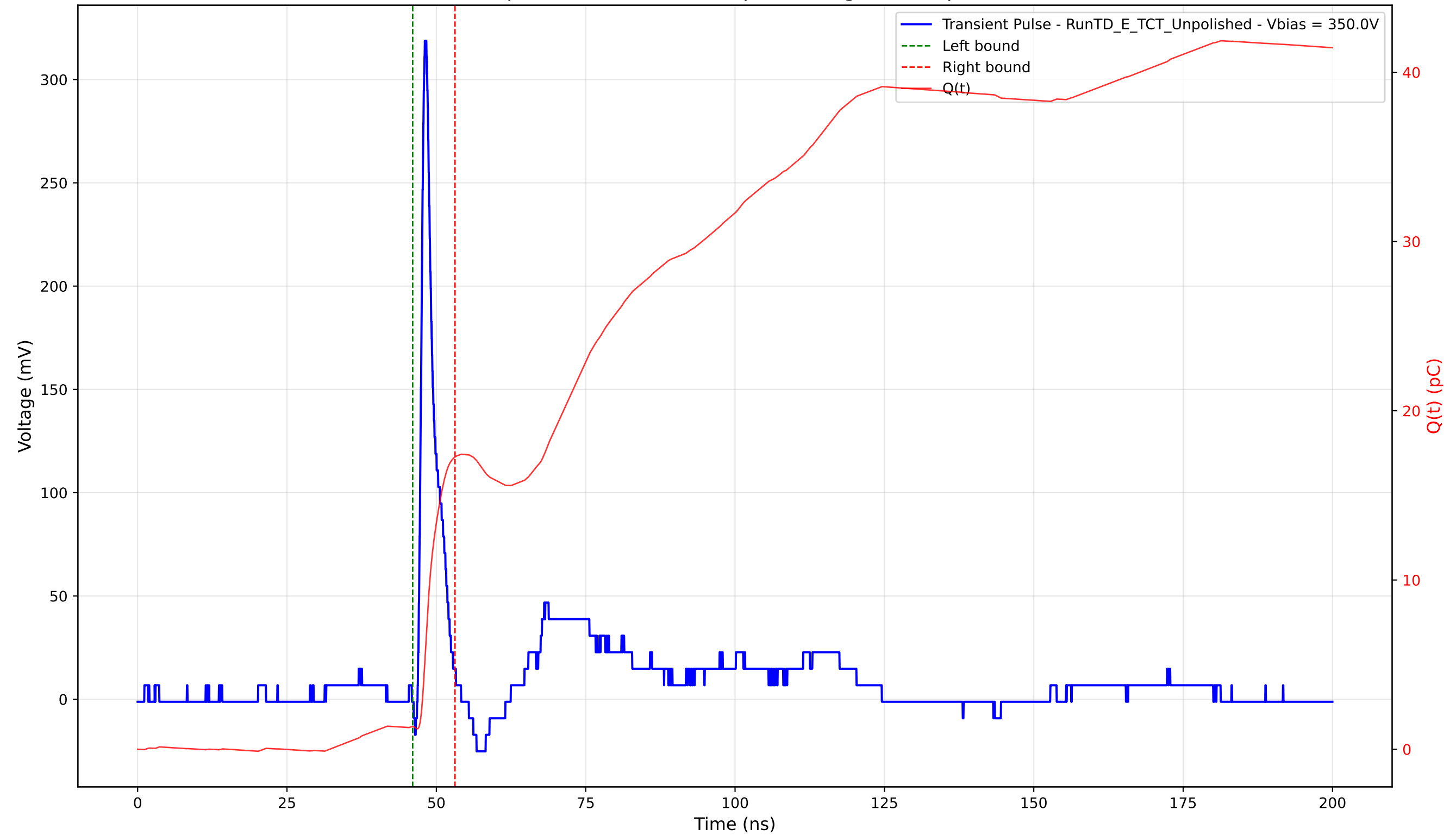
Transient Pulse - Sample: TD - Position: 80.0 \mu\text{m} - Charge: 15.93 pC - Rise Time: 0.88 ns
