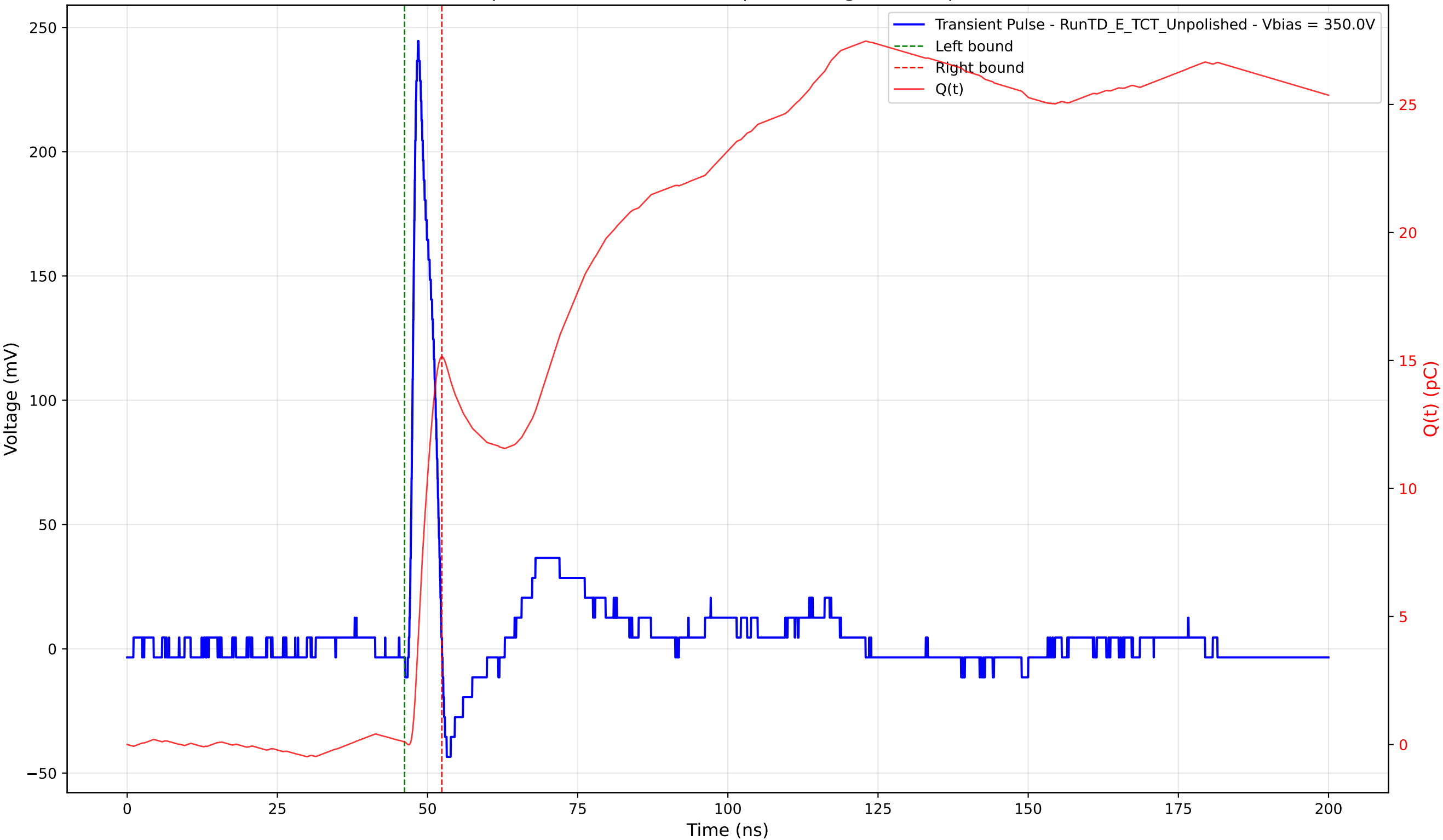
Transient Pulse - Sample: TD - Position: 325.0 \mu\text{m} - Charge: 15.04 pC - Rise Time: 0.95 ns
