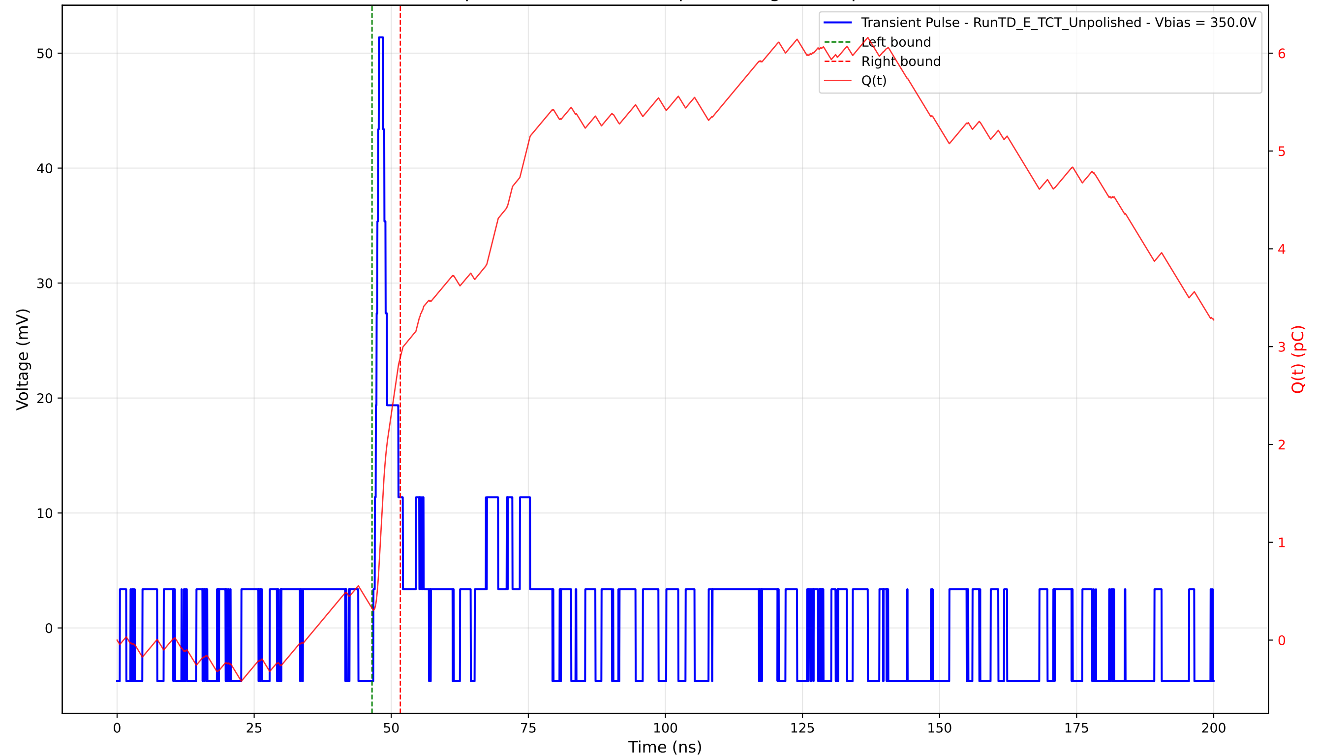
Transient Pulse - Sample: TD - Position: 25.0 \mu\text{m} - Charge: 2.57 pC - Rise Time: 0.76 ns
