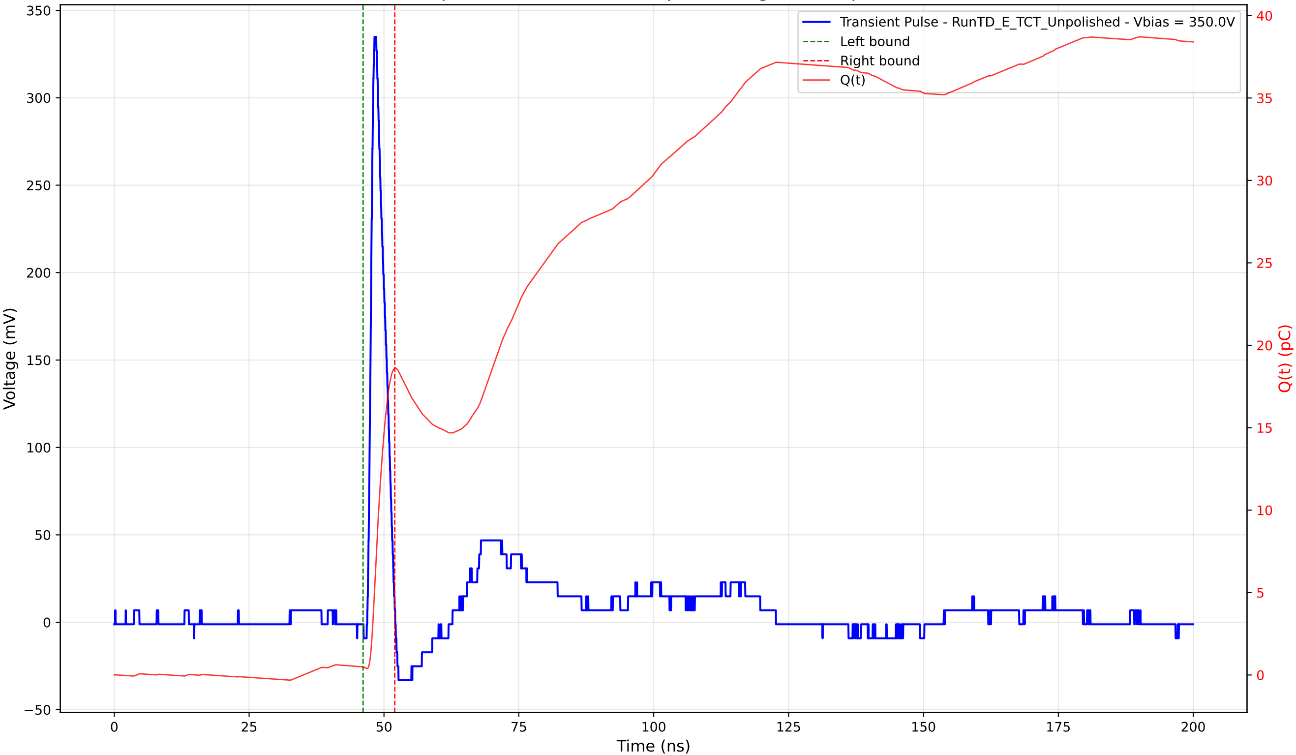
Transient Pulse - Sample: TD - Position: 275.0 \mu\text{m} - Charge: 18.12 pC - Rise Time: 0.91 ns
