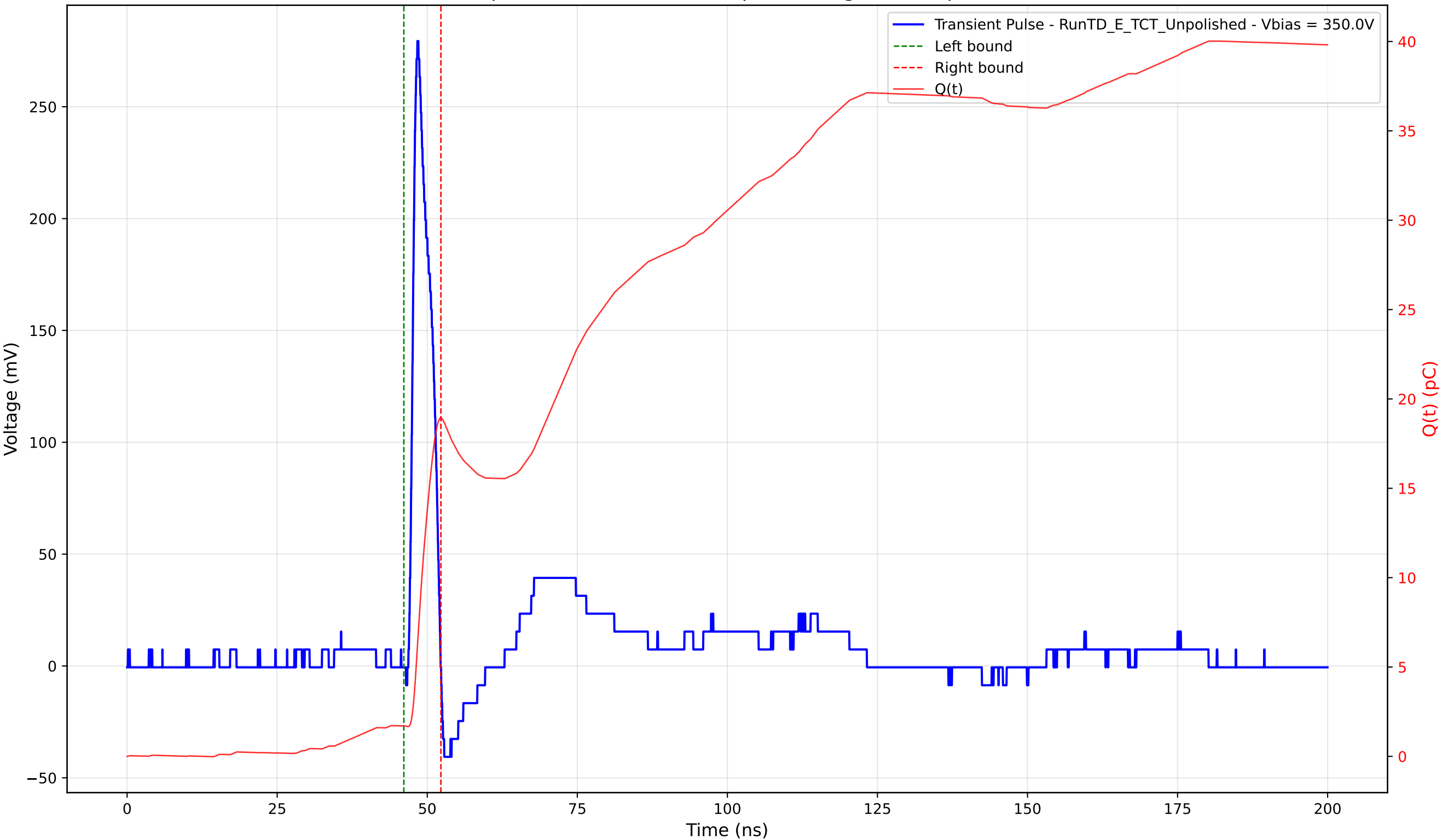
Transient Pulse - Sample: TD - Position: 295.0 \mu\text{m} - Charge: 17.23 pC - Rise Time: 0.99 ns
