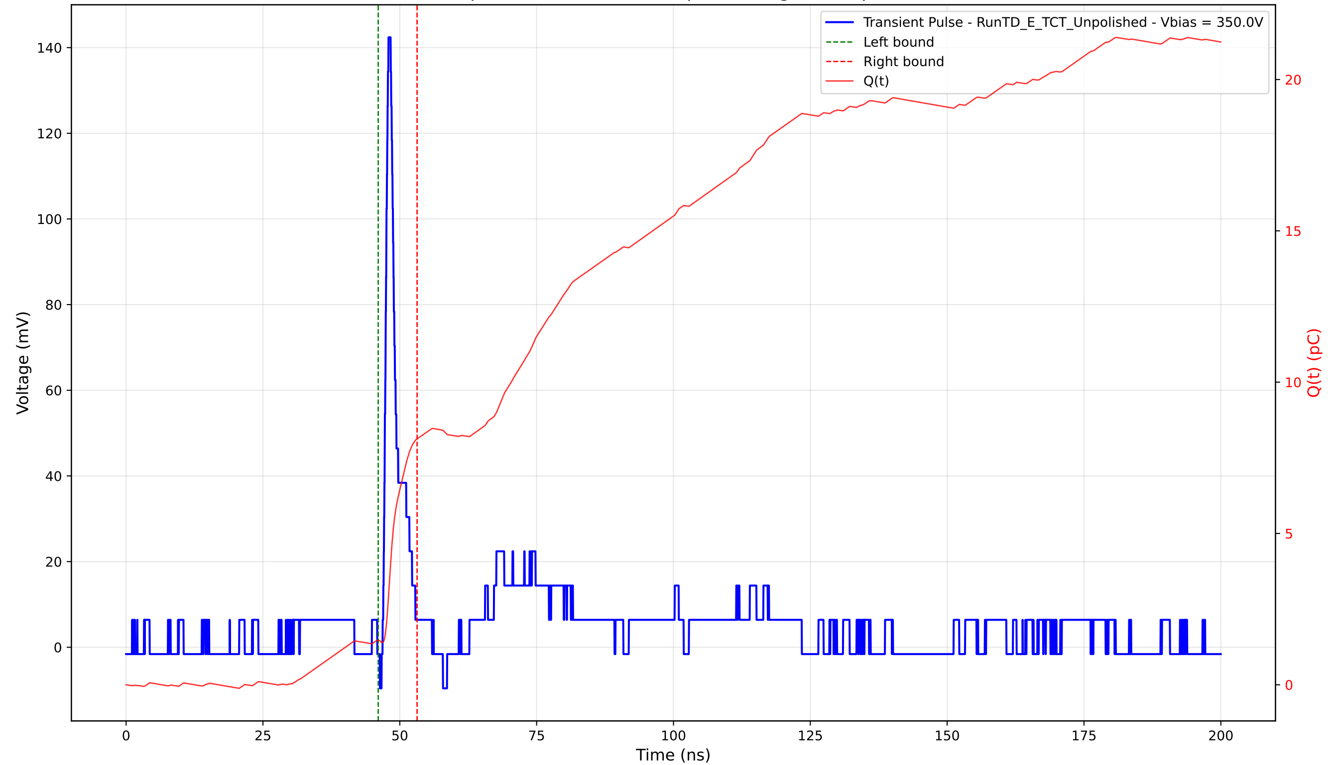
Transient Pulse - Sample: TD - Position: 30.0 \mu\text{m} - Charge: 6.65 pC - Rise Time: 0.84 ns
