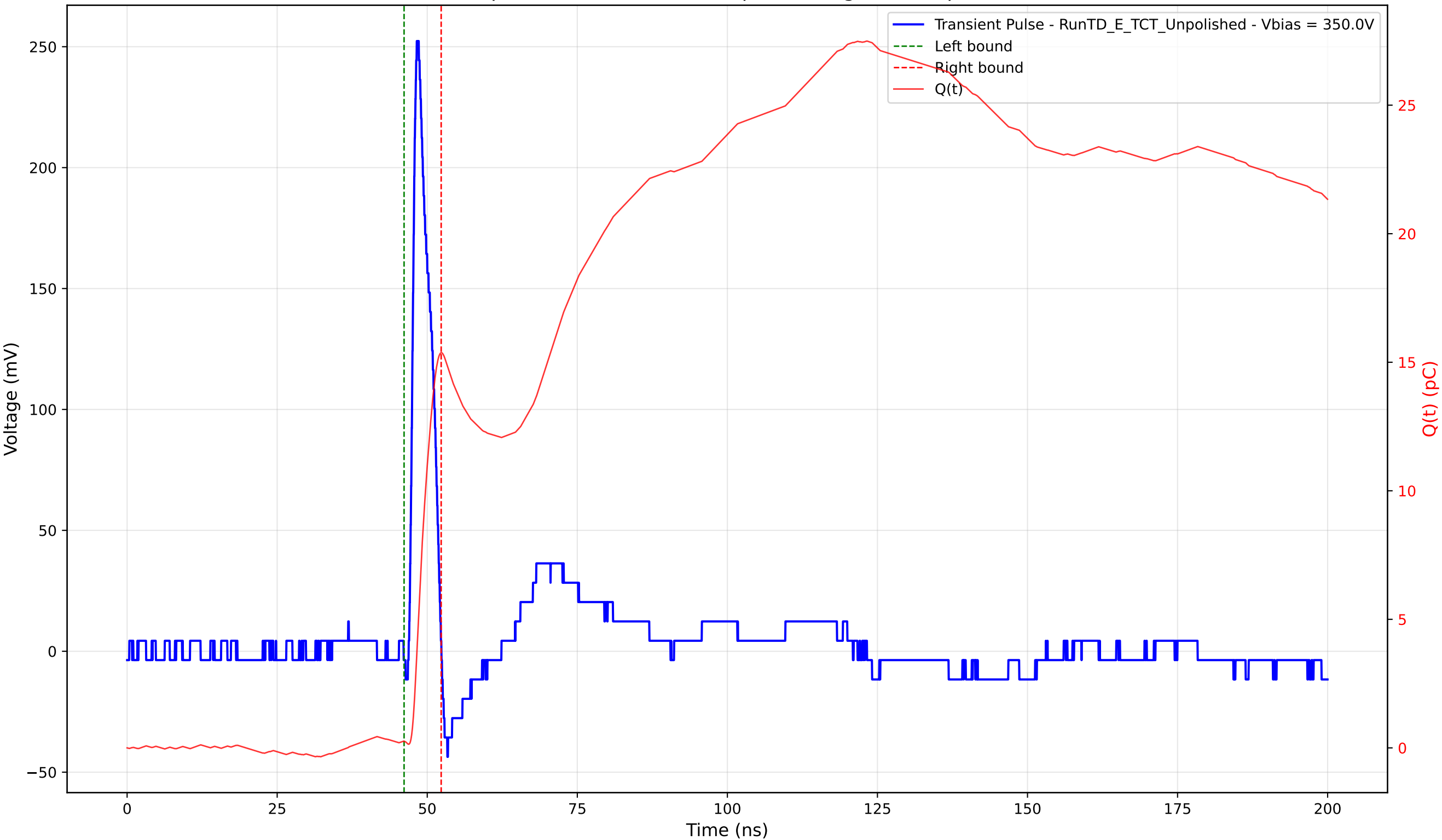
Transient Pulse - Sample: TD - Position: 320.0 \mu\text{m} - Charge: 15.11 pC - Rise Time: 0.91 ns
