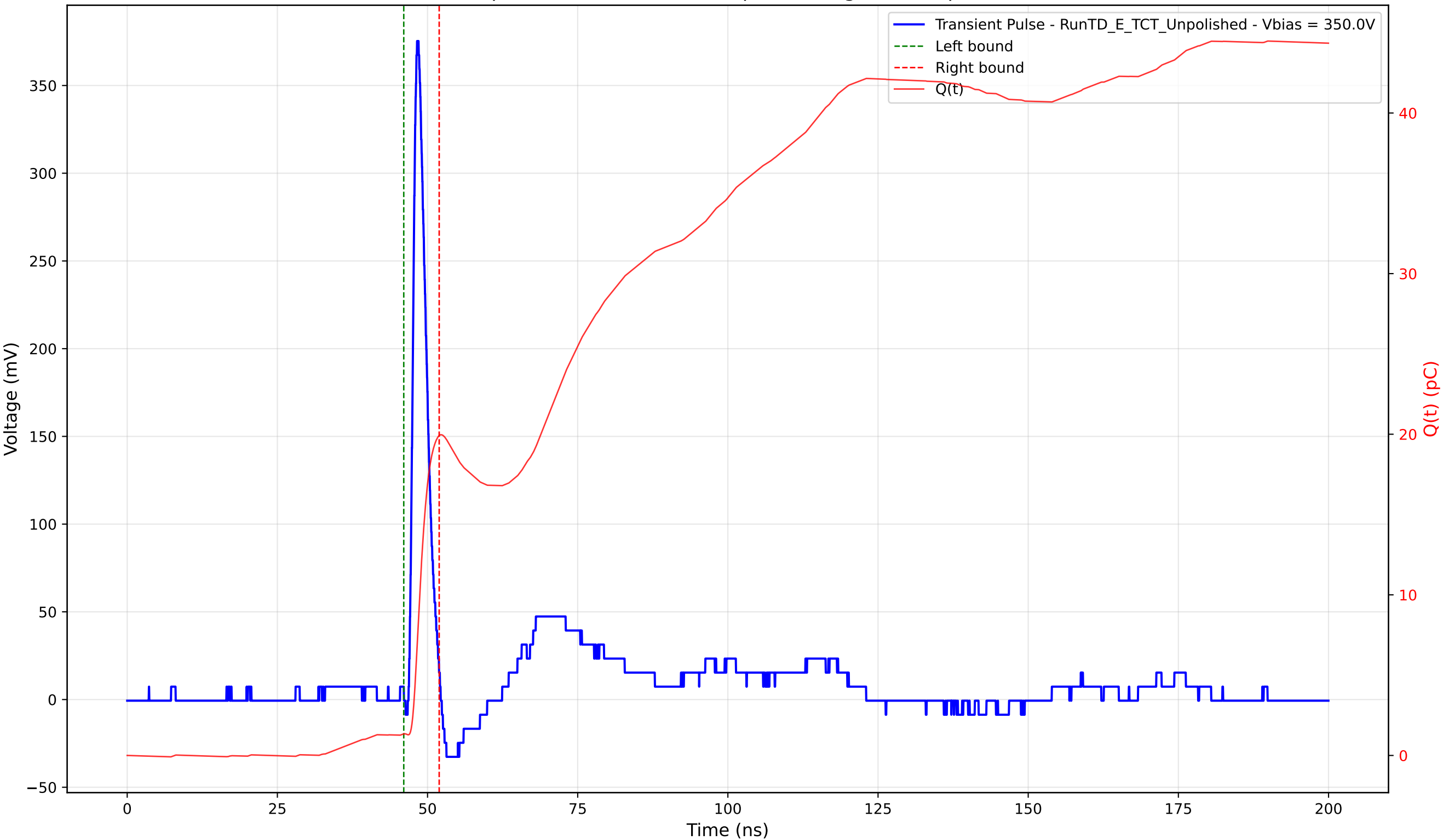
Transient Pulse - Sample: TD - Position: 215.0 \mu\text{m} - Charge: 18.57 pC - Rise Time: 0.96 ns
