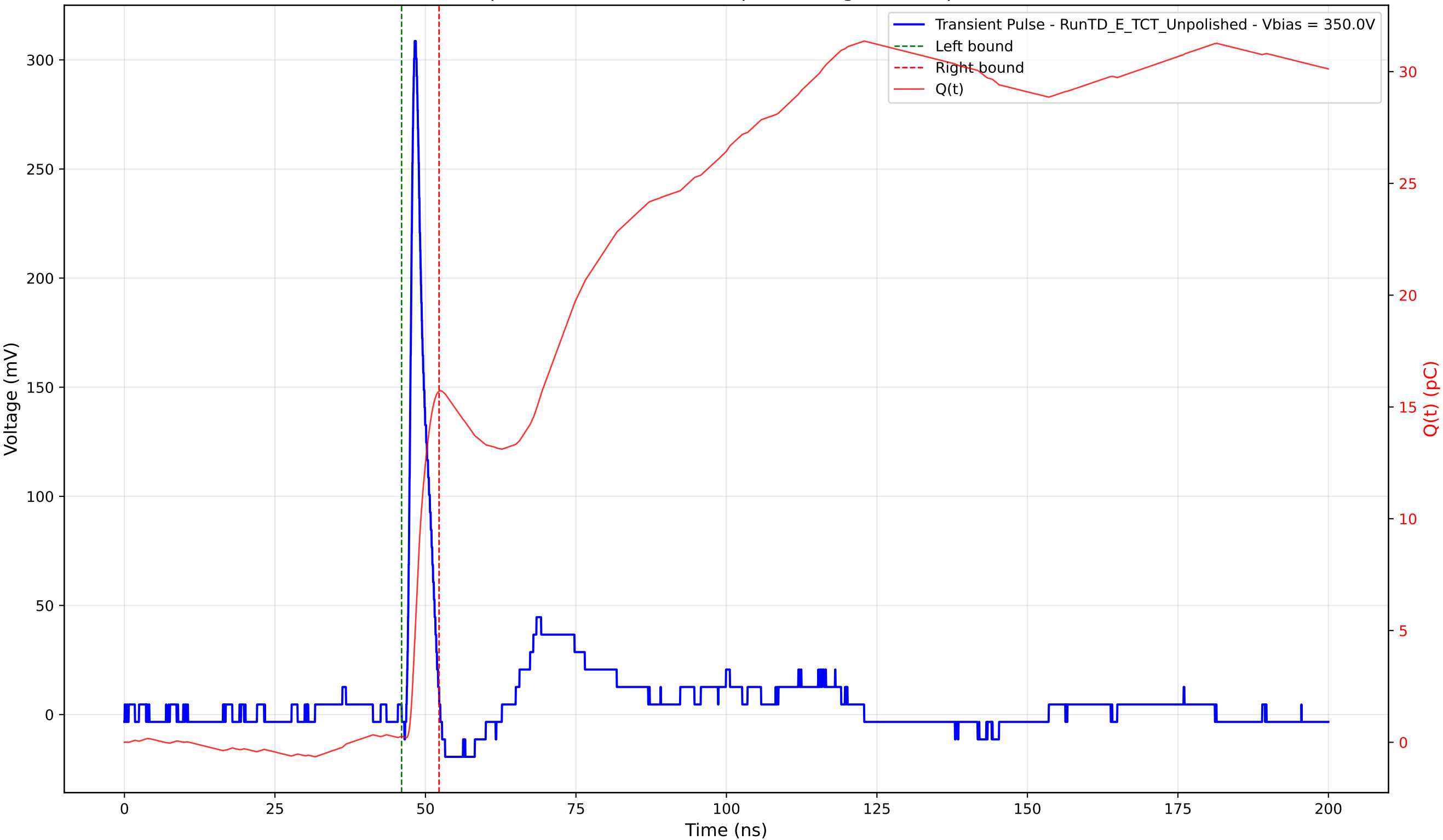
Transient Pulse - Sample: TD - Position: 145.0 \mu\text{m} - Charge: 15.44 pC - Rise Time: 0.93 ns
