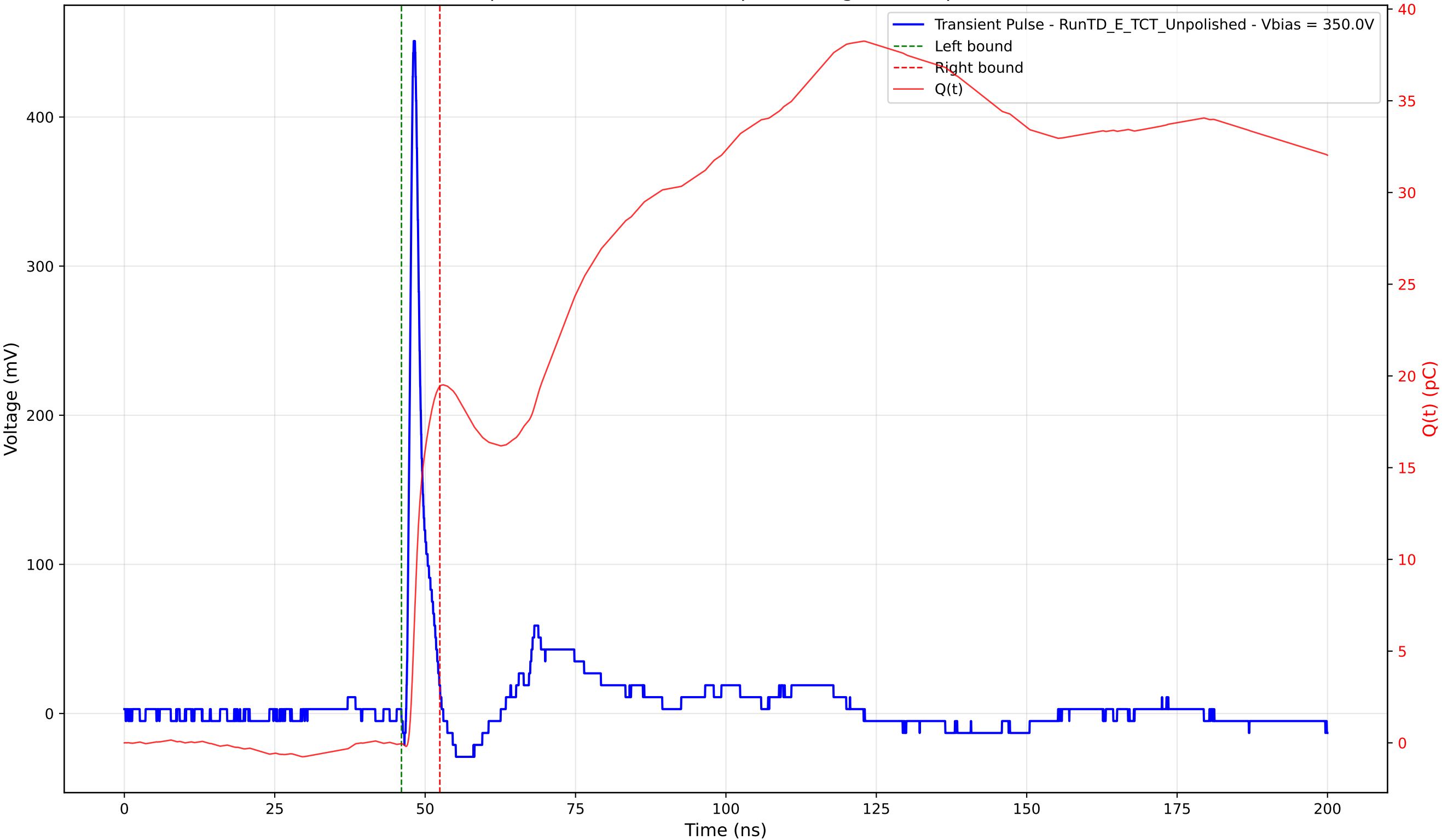
Transient Pulse - Sample: TD - Position: 115.0 \mu\text{m} - Charge: 19.47 pC - Rise Time: 0.84 ns
