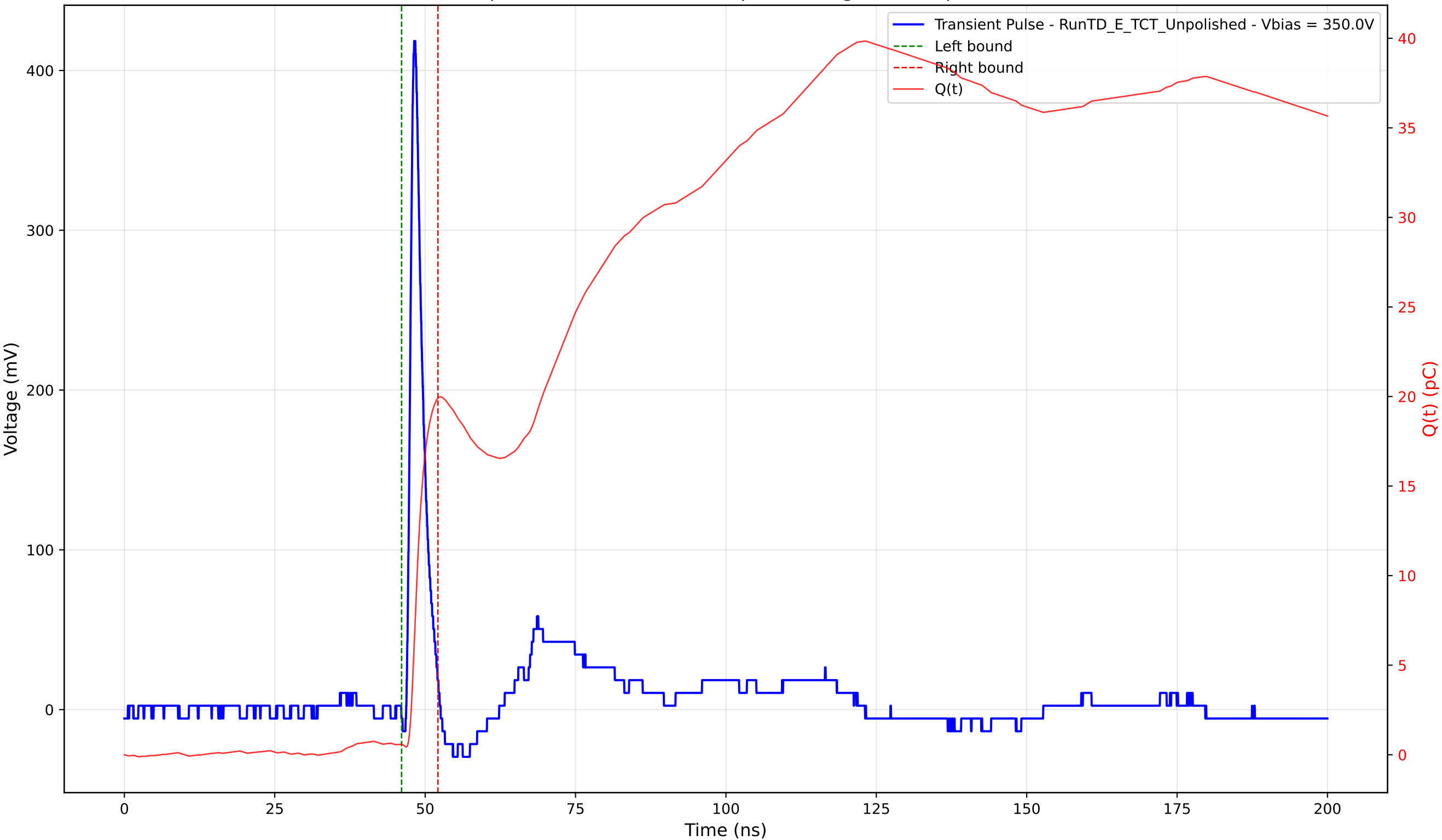
Transient Pulse - Sample: TD - Position: 200.0 \mu\text{m} - Charge: 19.32 pC - Rise Time: 0.88 ns
