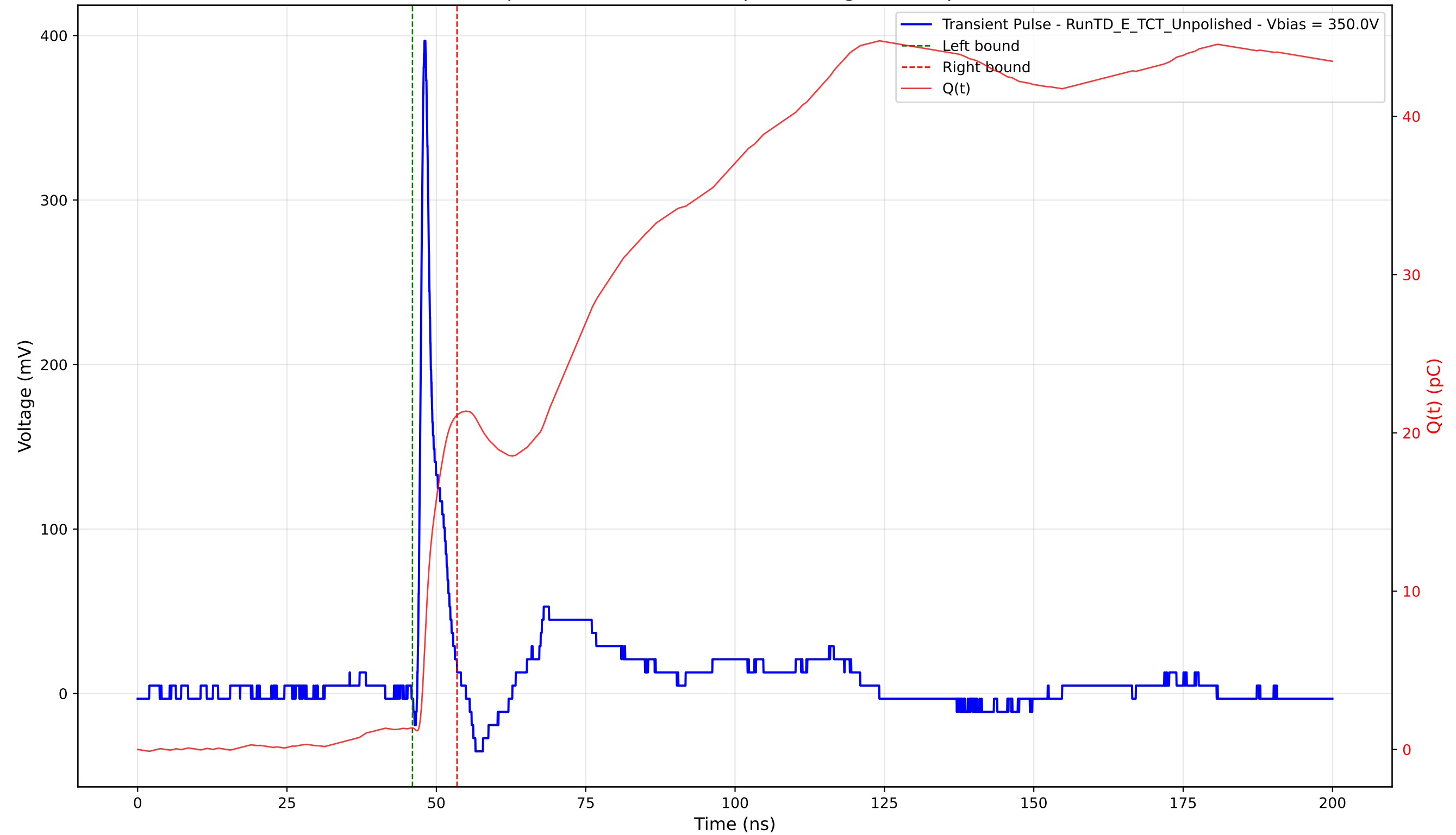
Transient Pulse - Sample: TD - Position: 45.0 \mu\text{m} - Charge: 19.77 pC - Rise Time: 0.81 ns
