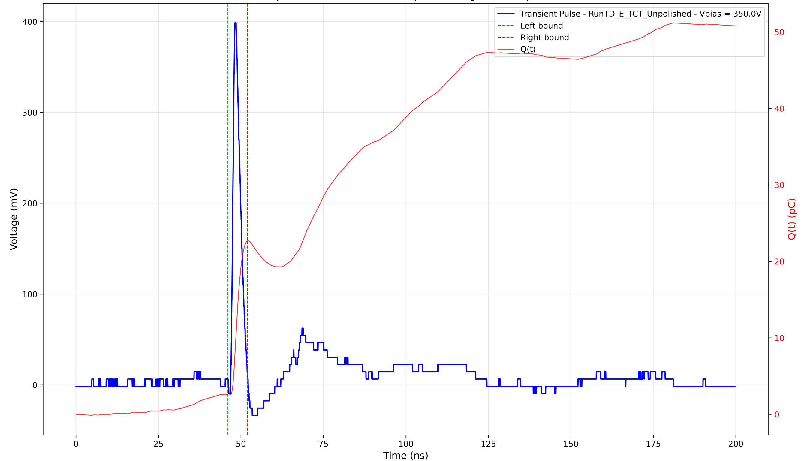
Transient Pulse - Sample: TD - Position: 205.0 \mu\text{m} - Charge: 20.01 pC - Rise Time: 0.94 ns
