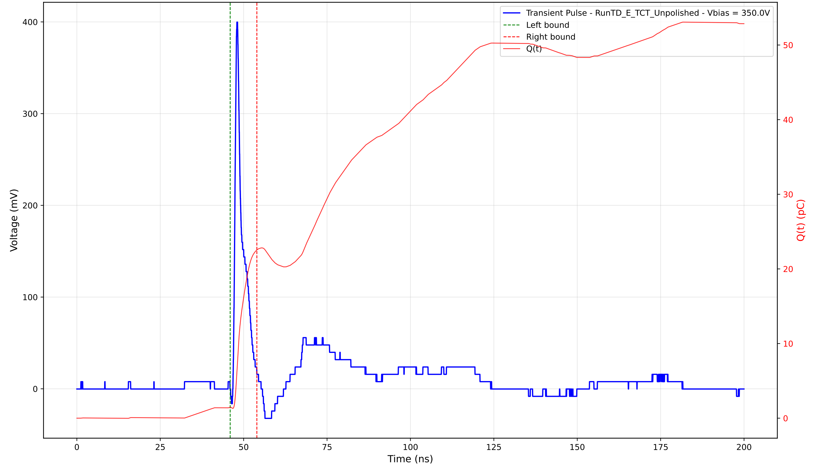
Transient Pulse - Sample: TD - Position: 60.0 \mu\text{m} - Charge: 21.08 pC - Rise Time: 0.82 ns
