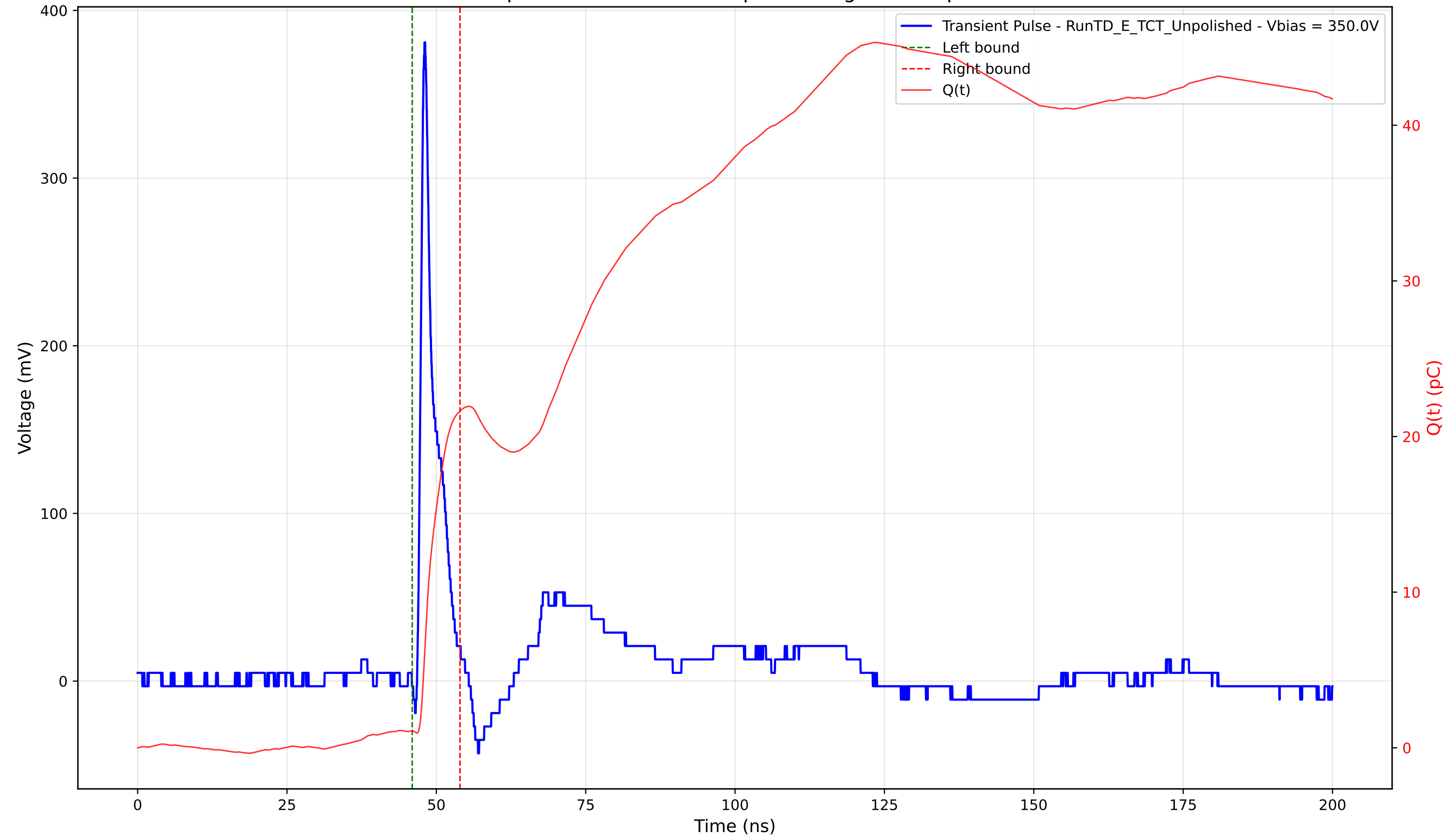
Transient Pulse - Sample: TD - Position: 65.0 \mu\text{m} - Charge: 20.55 pC - Rise Time: 0.82 ns
