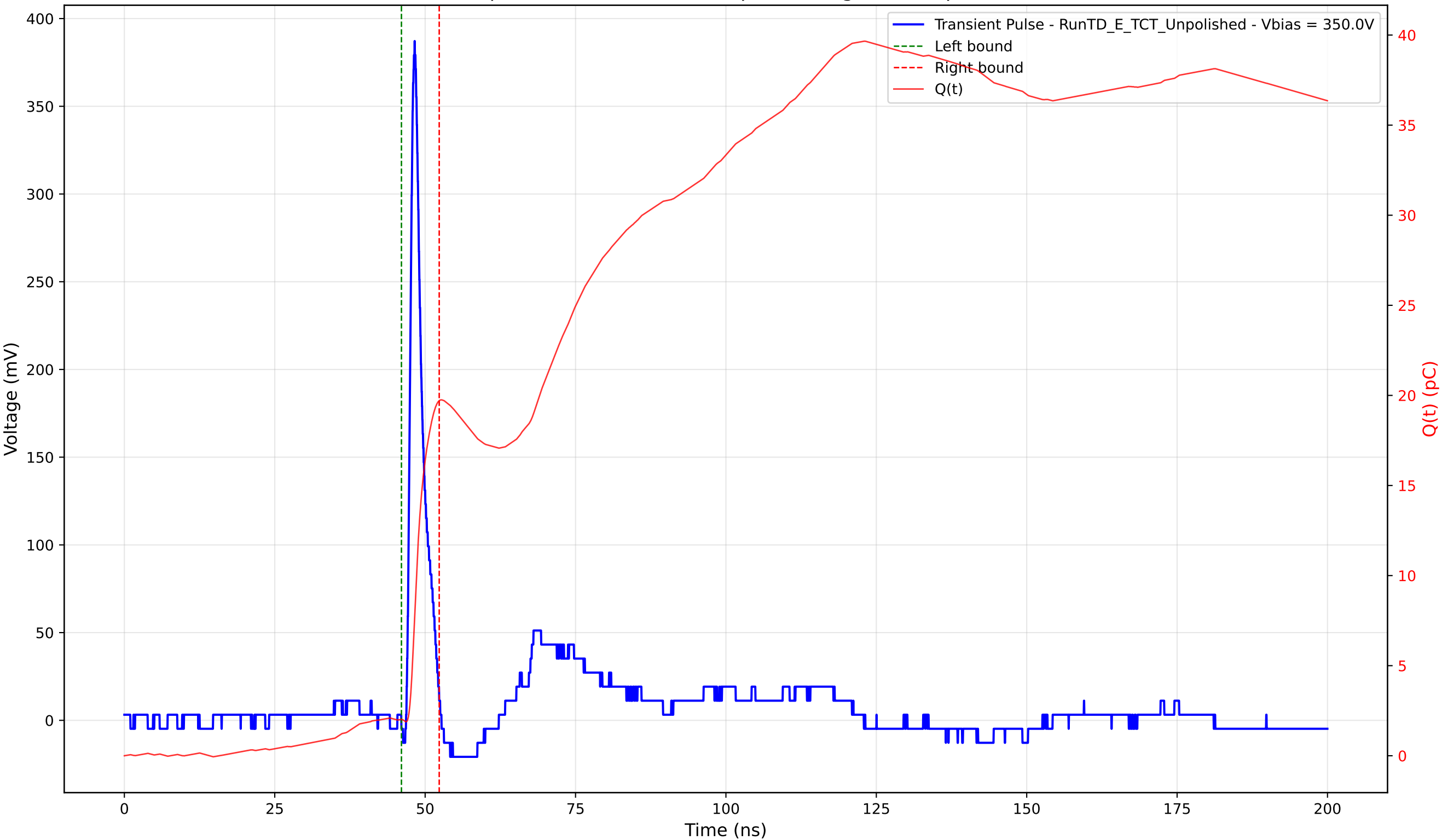
Transient Pulse - Sample: TD - Position: 135.0 \mu\text{m} - Charge: 17.69 pC - Rise Time: 0.91 ns
