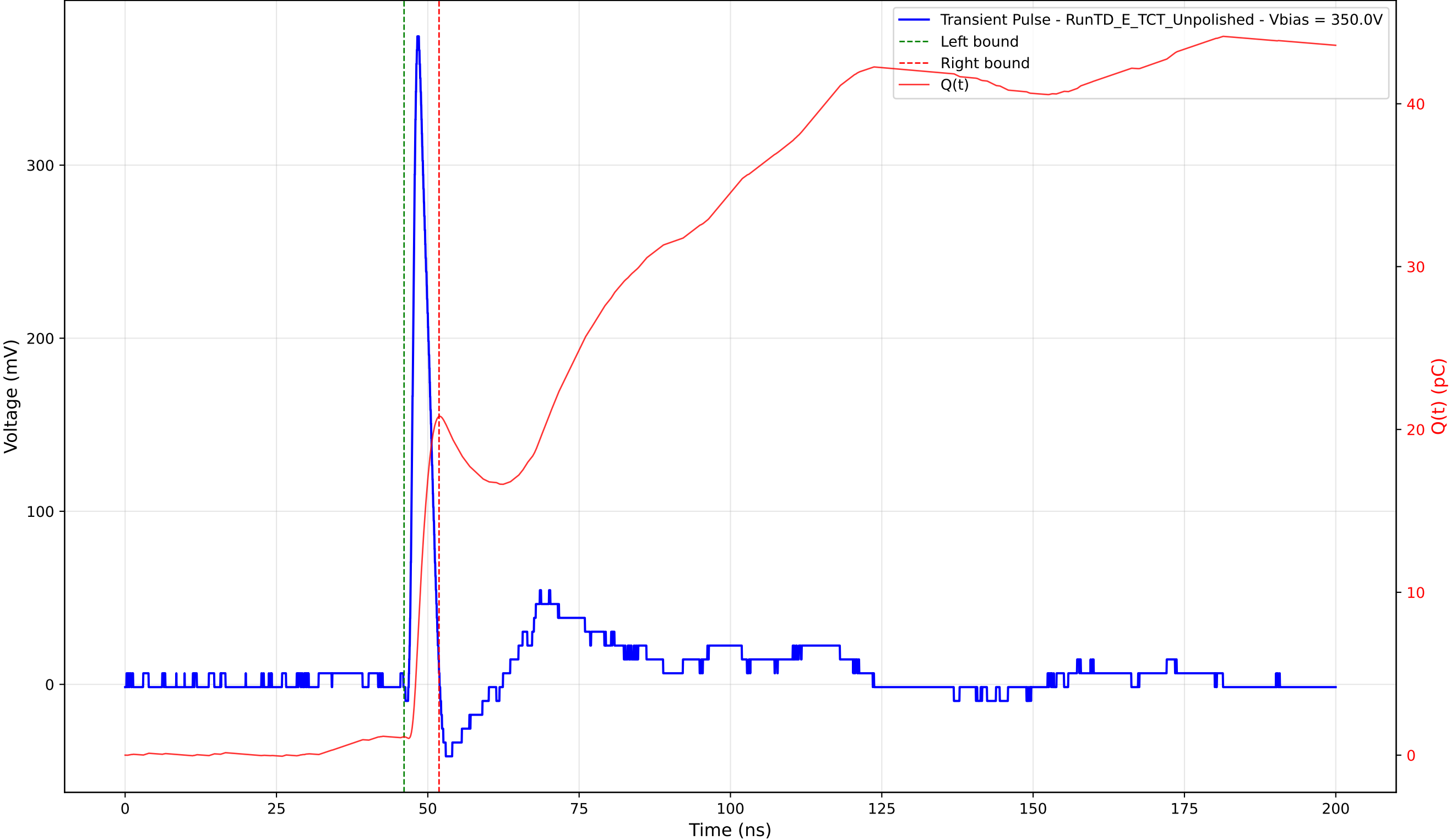
Transient Pulse - Sample: TD - Position: 265.0 \mu\text{m} - Charge: 19.68 pC - Rise Time: 0.96 ns
