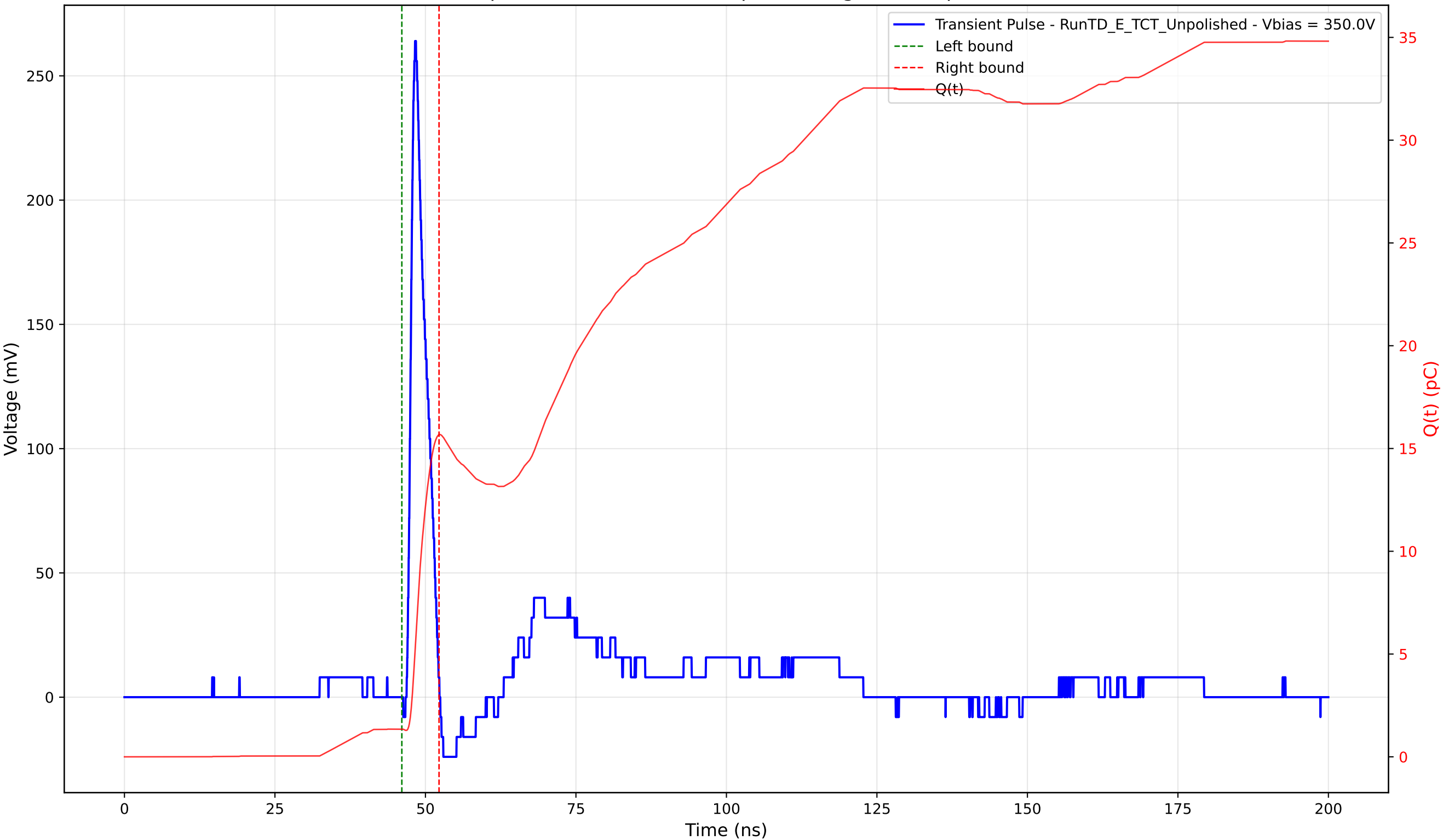
Transient Pulse - Sample: TD - Position: 315.0 \mu\text{m} - Charge: 14.32 pC - Rise Time: 0.93 ns
