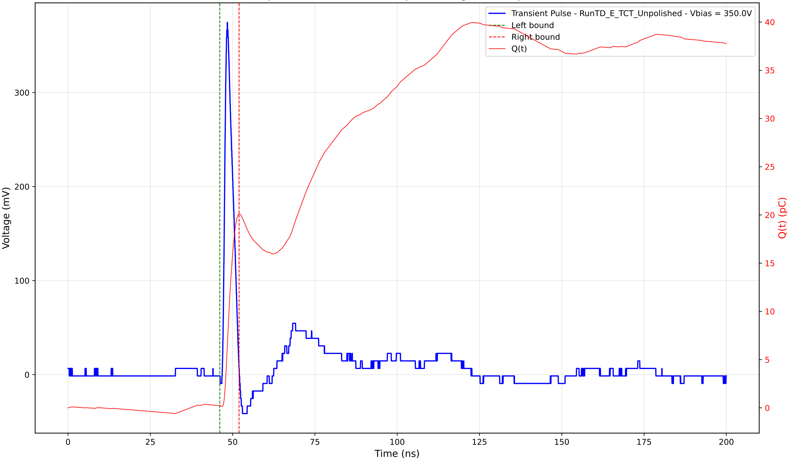
Transient Pulse - Sample: TD - Position: 155.0 \mu\text{m} - Charge: 19.87 pC - Rise Time: 1.00 ns
