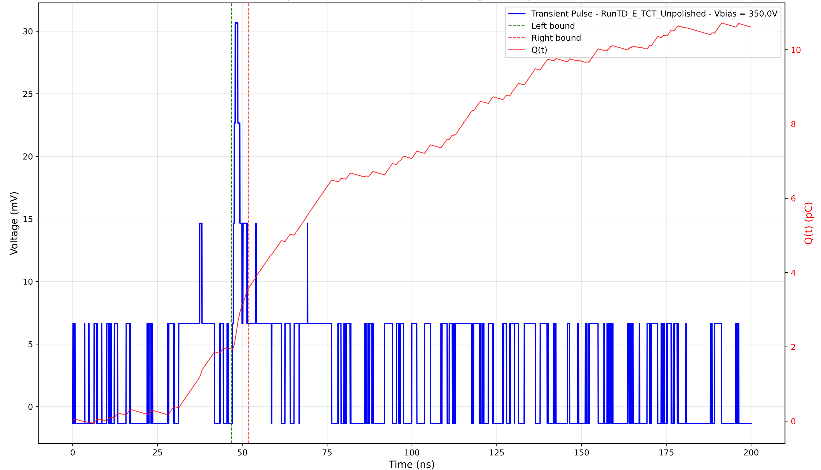
Transient Pulse - Sample: TD - Position: 15.0 \mu\text{m} - Charge: 1.65 pC - Rise Time: 0.87 ns
