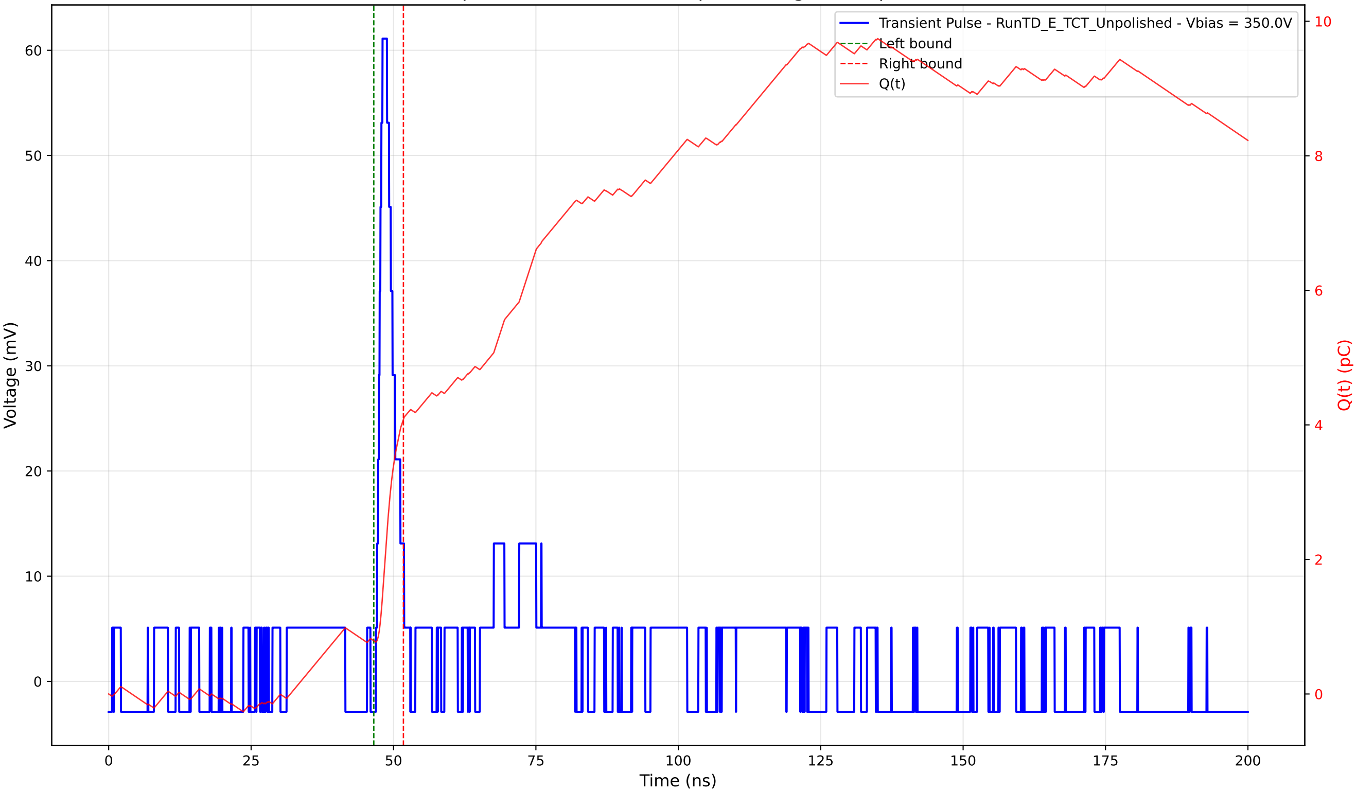
Transient Pulse - Sample: TD - Position: 345.0 \mu\text{m} - Charge: 3.29 pC - Rise Time: 0.96 ns
