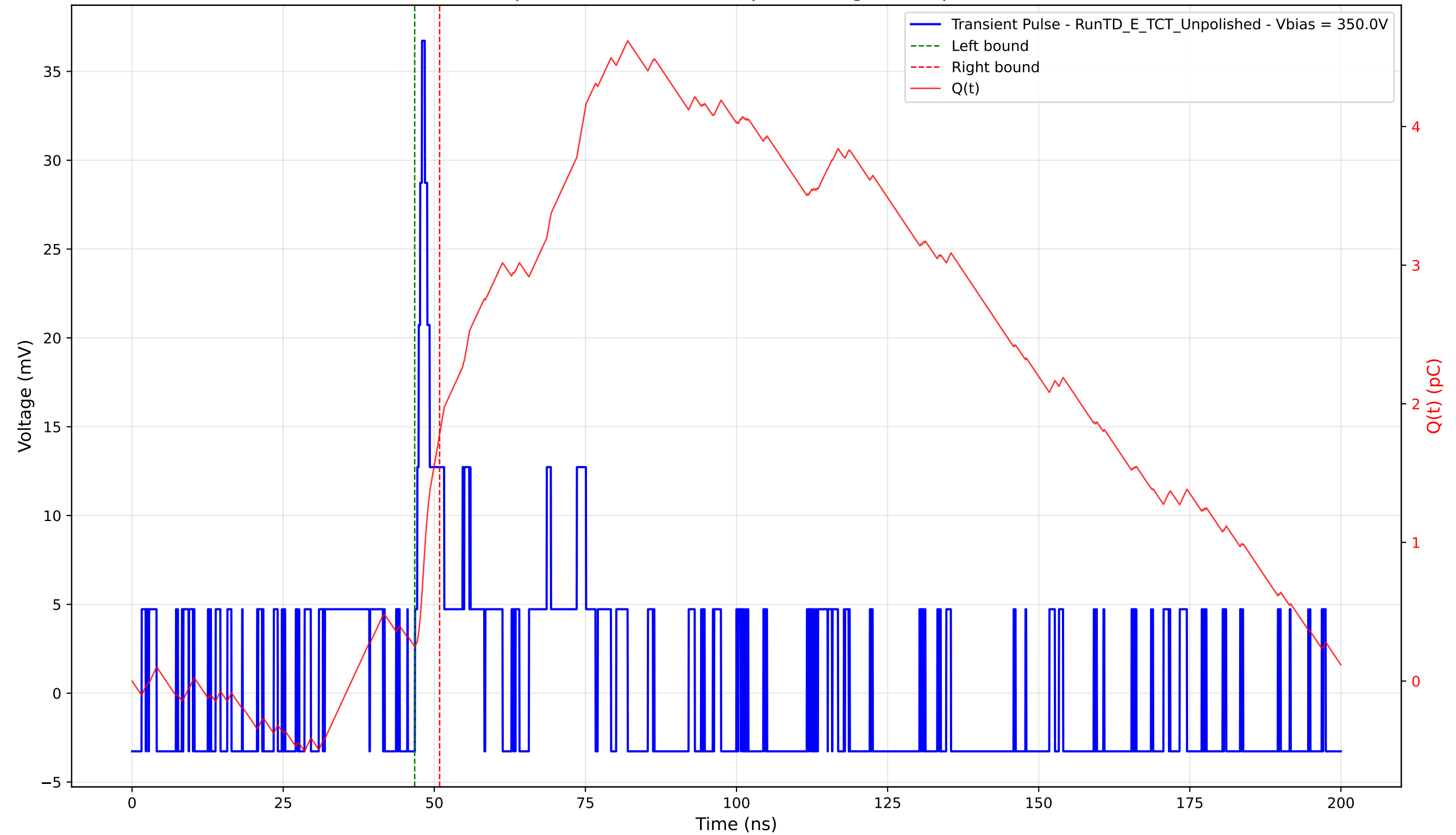
Transient Pulse - Sample: TD - Position: 20.0 \mu\text{m} - Charge: 1.54 pC - Rise Time: 1.17 ns
