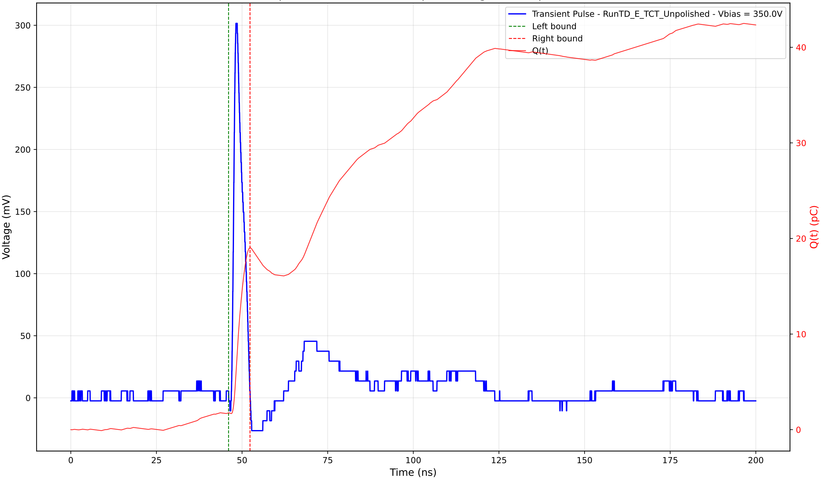
Transient Pulse - Sample: TD - Position: 235.0 \mu\text{m} - Charge: 17.27 pC - Rise Time: 0.94 ns
