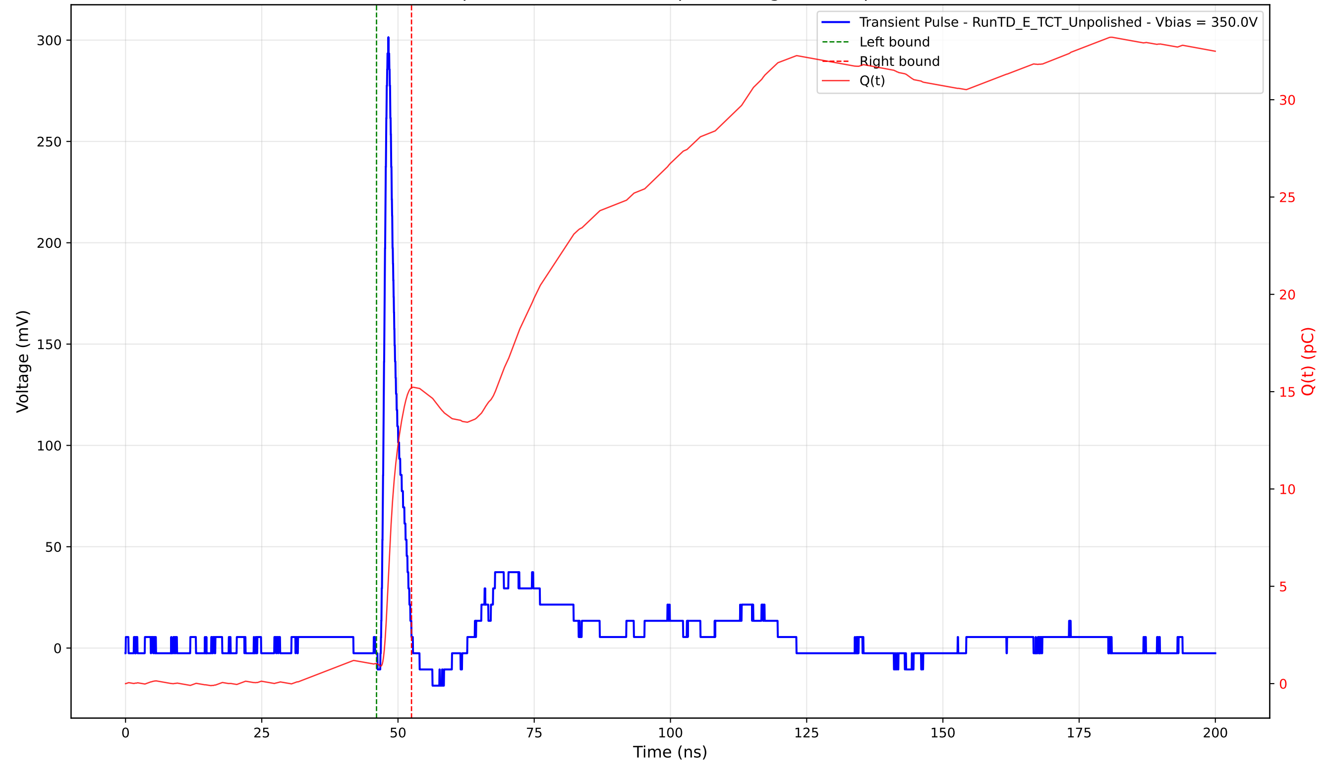
Transient Pulse - Sample: TD - Position: 90.0 \mu\text{m} - Charge: 14.18 pC - Rise Time: 0.88 ns
