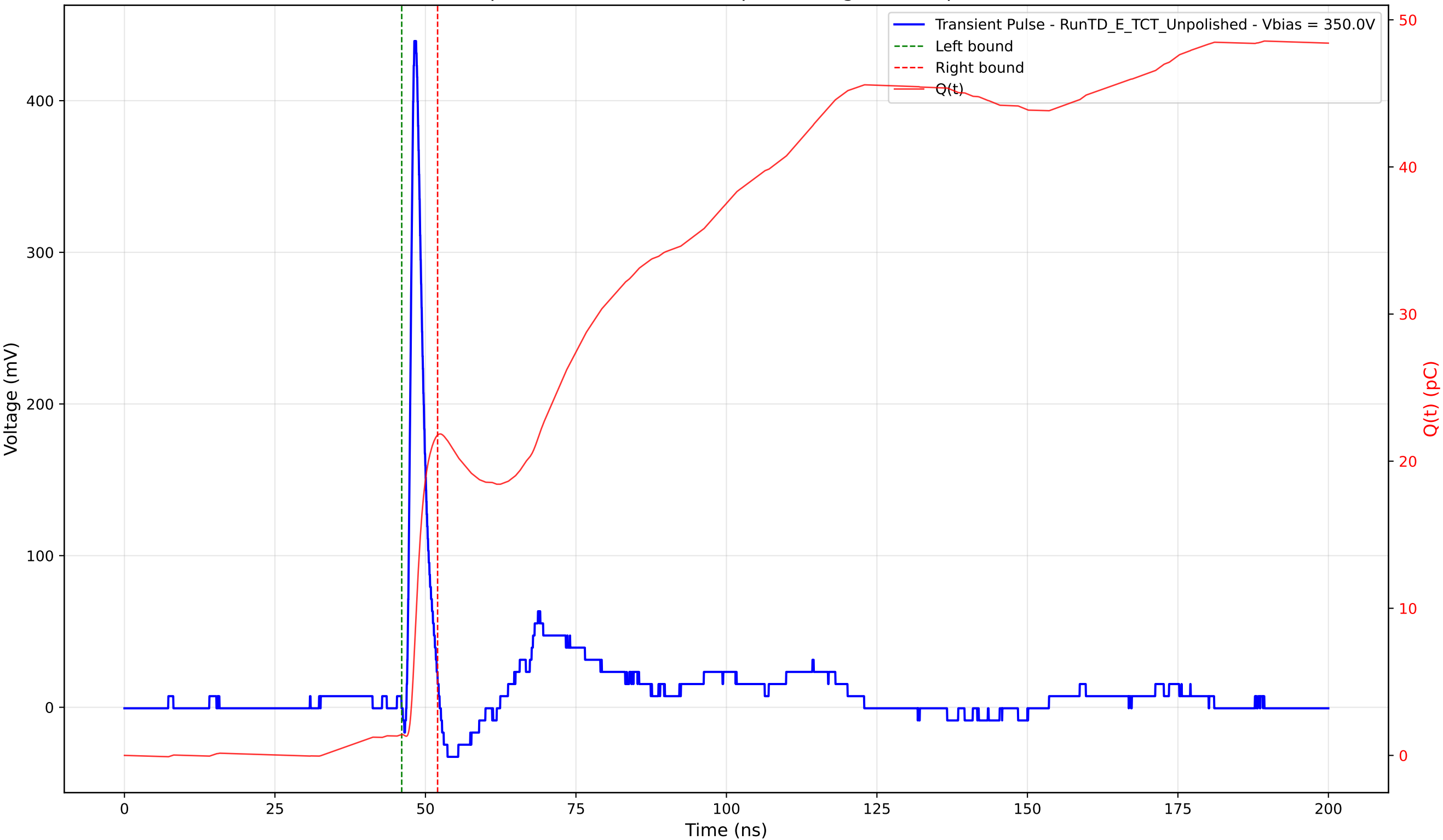
Transient Pulse - Sample: TD - Position: 165.0 \mu\text{m} - Charge: 20.36 pC - Rise Time: 0.91 ns
