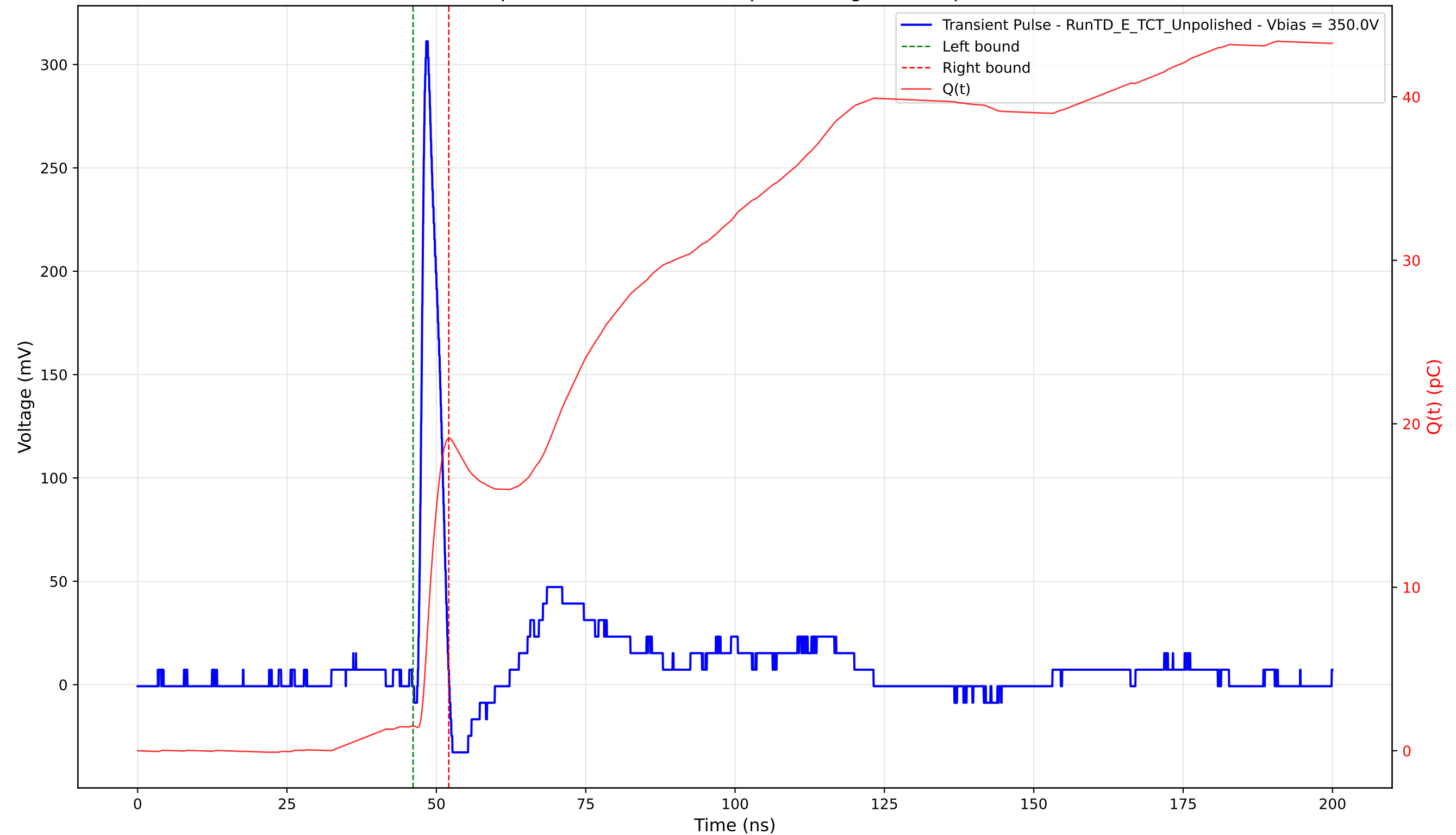
Transient Pulse - Sample: TD - Position: 280.0 \mu\text{m} - Charge: 17.59 pC - Rise Time: 0.98 ns
