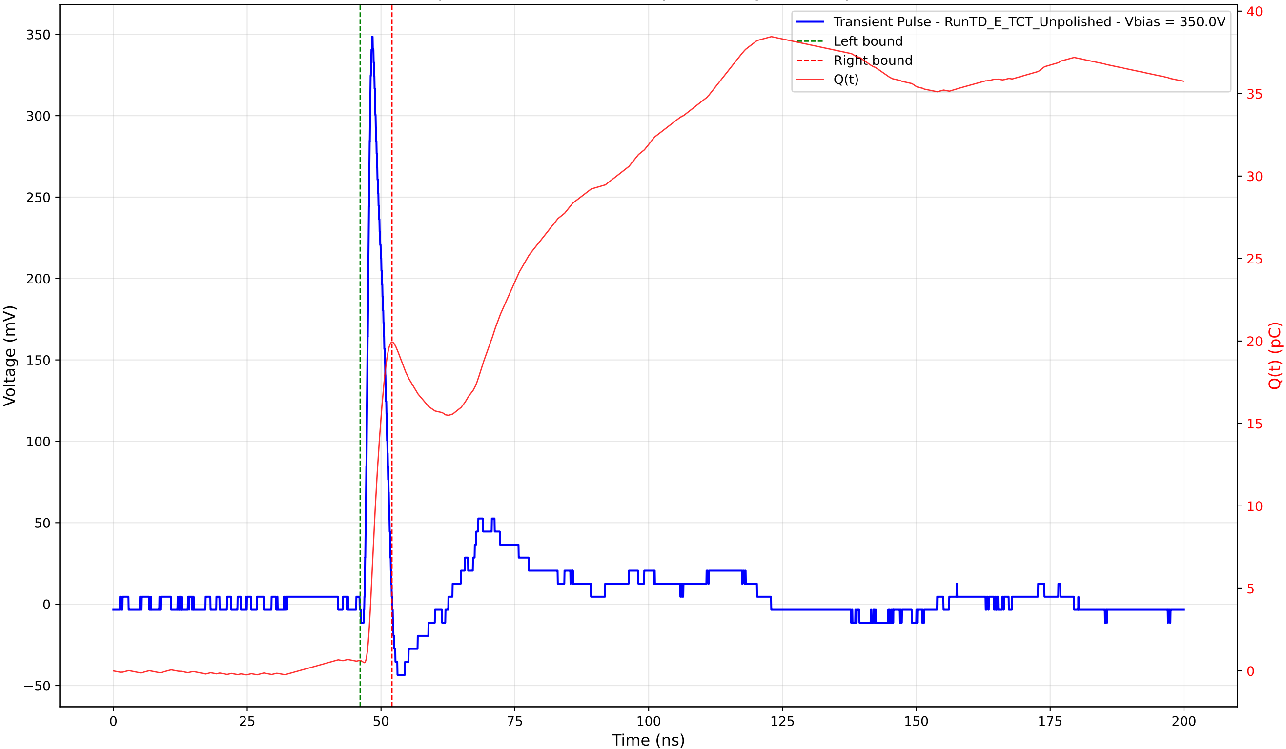
Transient Pulse - Sample: TD - Position: 255.0 \mu\text{m} - Charge: 19.30 pC - Rise Time: 0.94 ns
