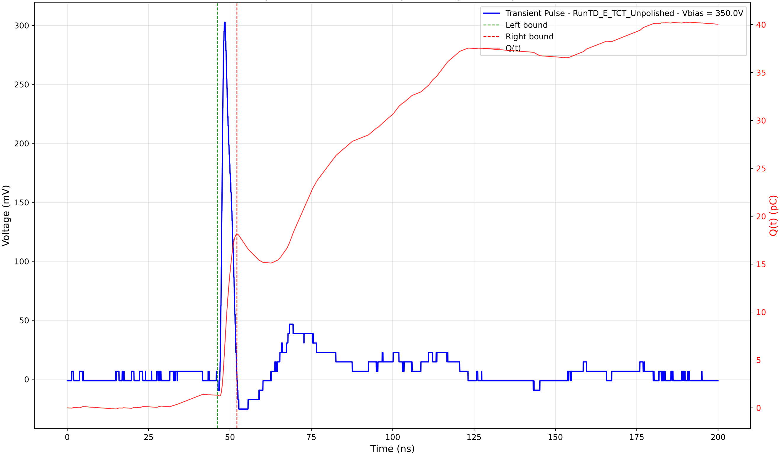
Transient Pulse - Sample: TD - Position: 150.0 \mu\text{m} - Charge: 16.81 pC - Rise Time: 0.98 ns
