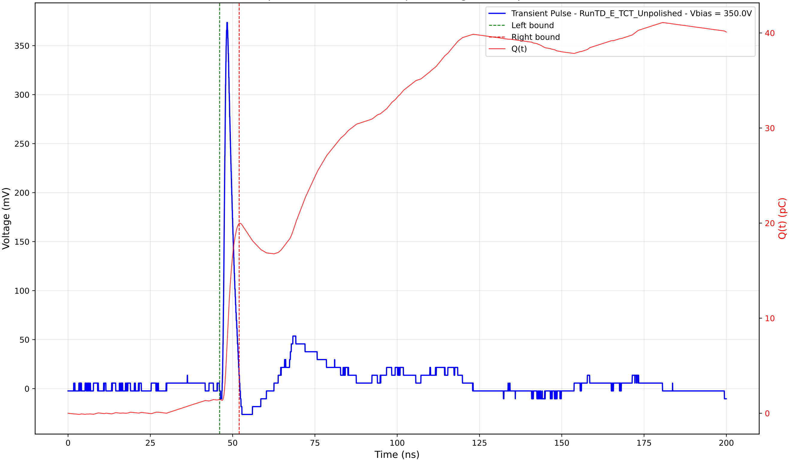
Transient Pulse - Sample: TD - Position: 190.0 \mu\text{m} - Charge: 18.51 pC - Rise Time: 0.96 ns
