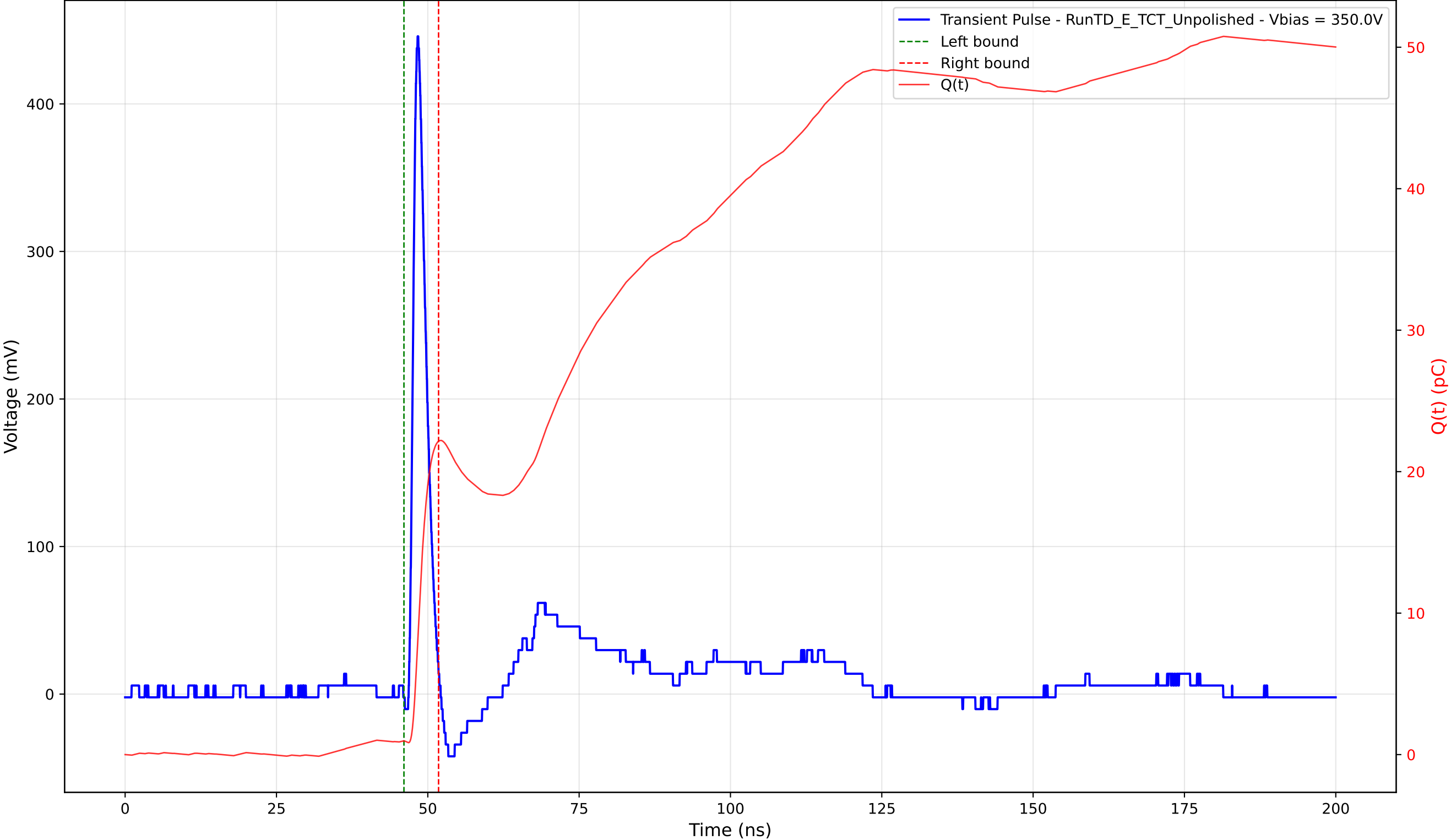
Transient Pulse - Sample: TD - Position: 160.0 \mu\text{m} - Charge: 21.19 pC - Rise Time: 0.95 ns
