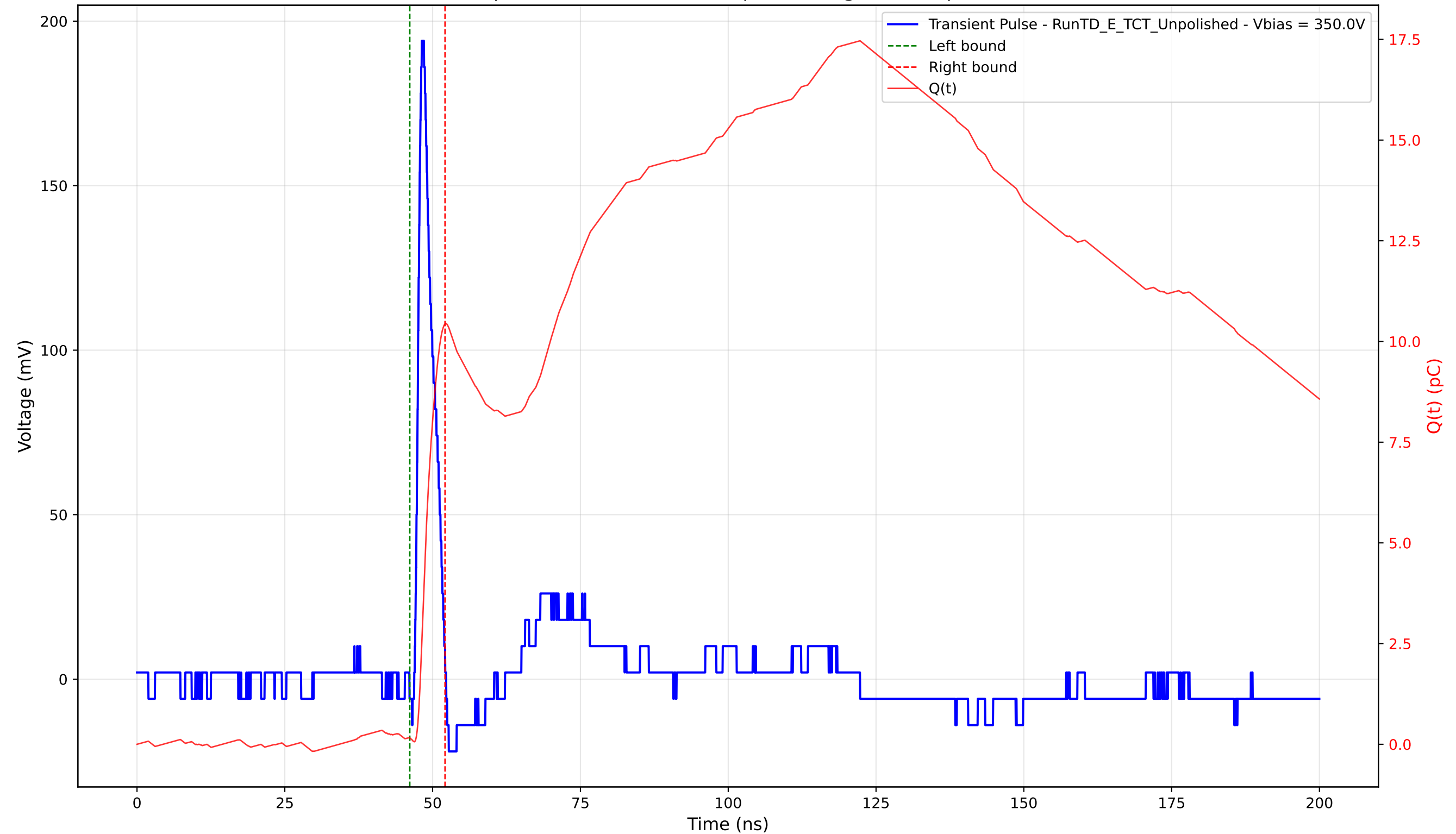
Transient Pulse - Sample: TD - Position: 335.0 \mu\text{m} - Charge: 10.28 pC - Rise Time: 0.88 ns
