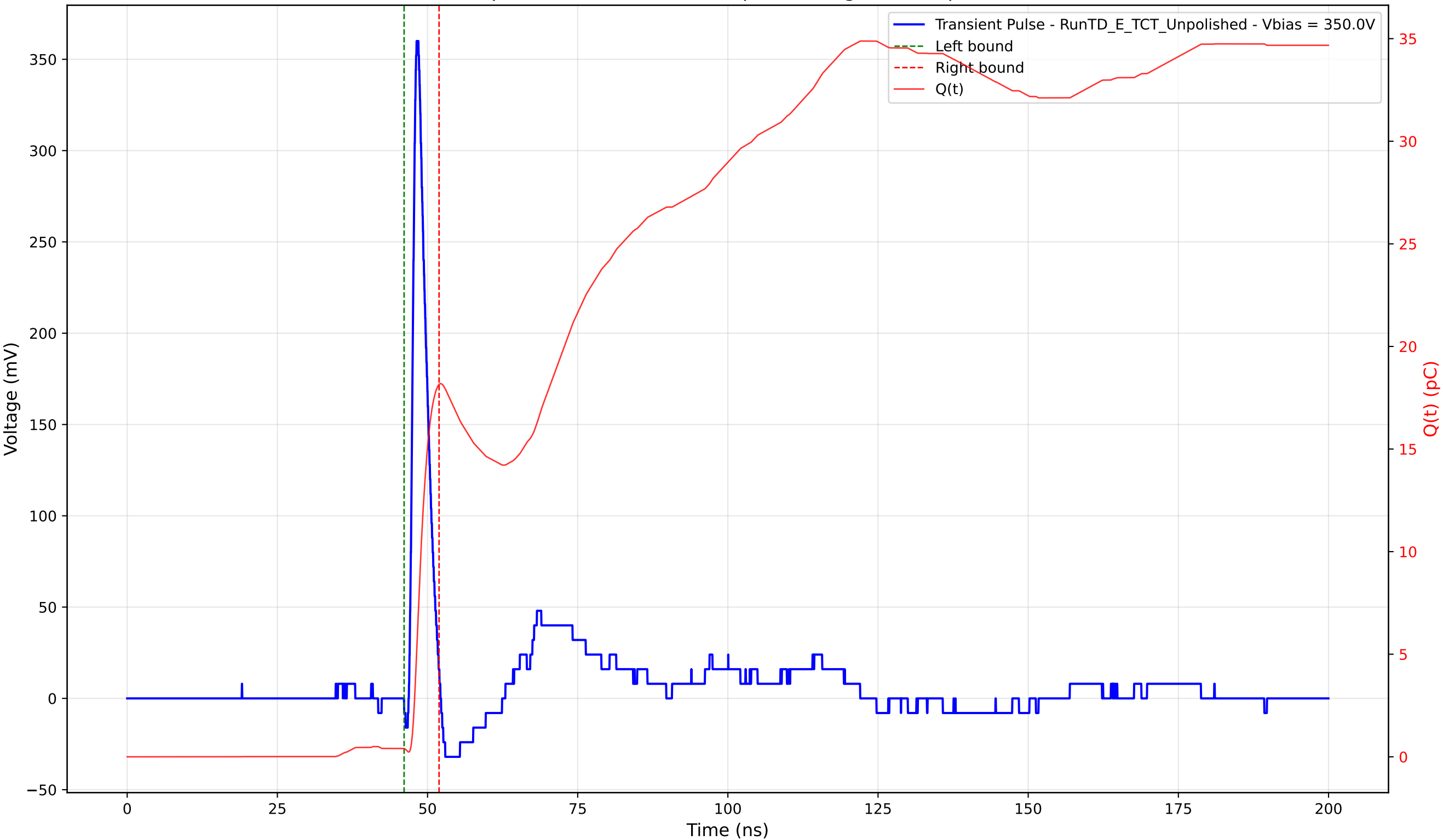
Transient Pulse - Sample: TD - Position: 225.0 \mu\text{m} - Charge: 17.74 pC - Rise Time: 0.89 ns
