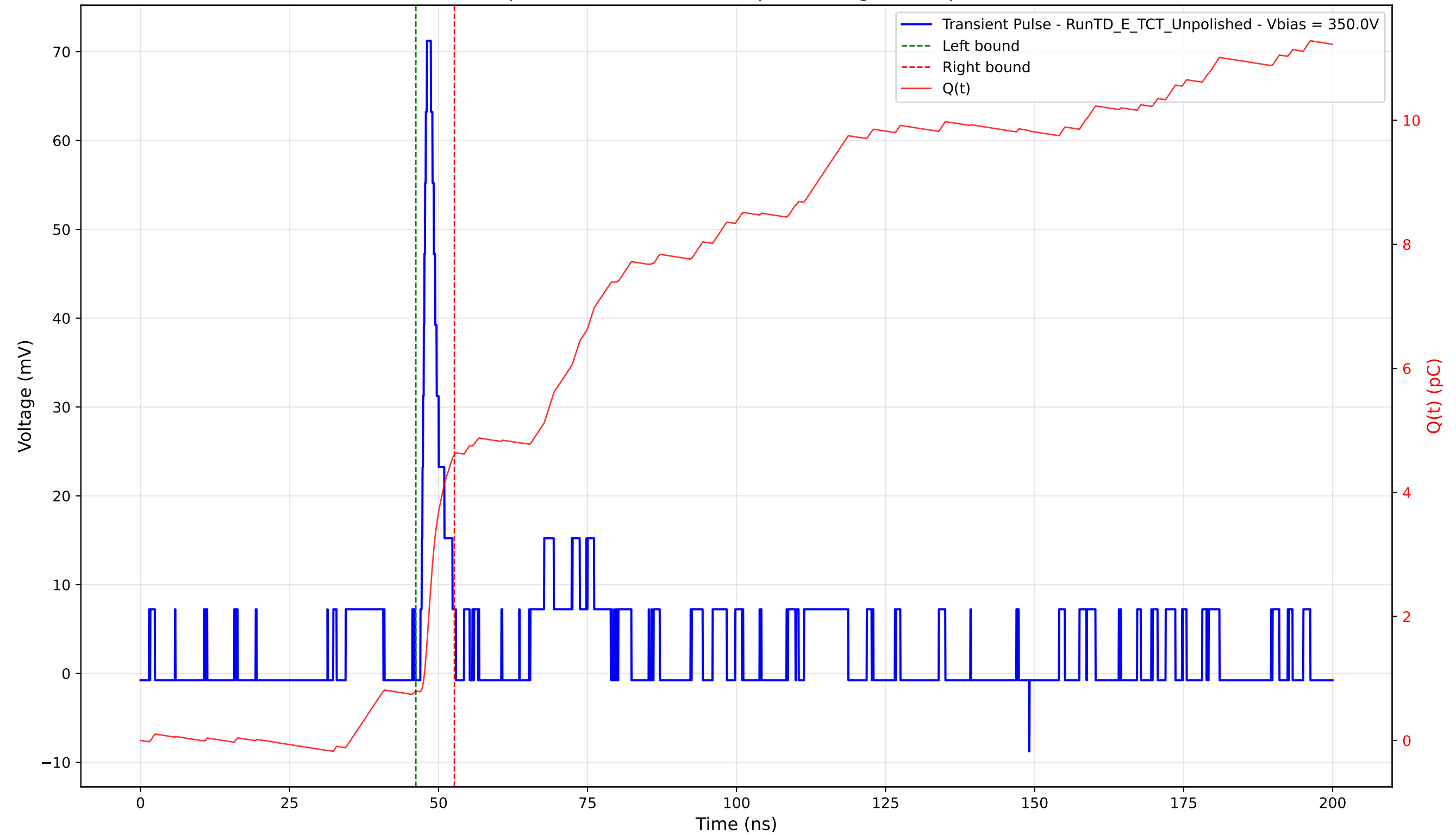
Transient Pulse - Sample: TD - Position: 370.0 \mu\text{m} - Charge: 3.81 pC - Rise Time: 1.08 ns
