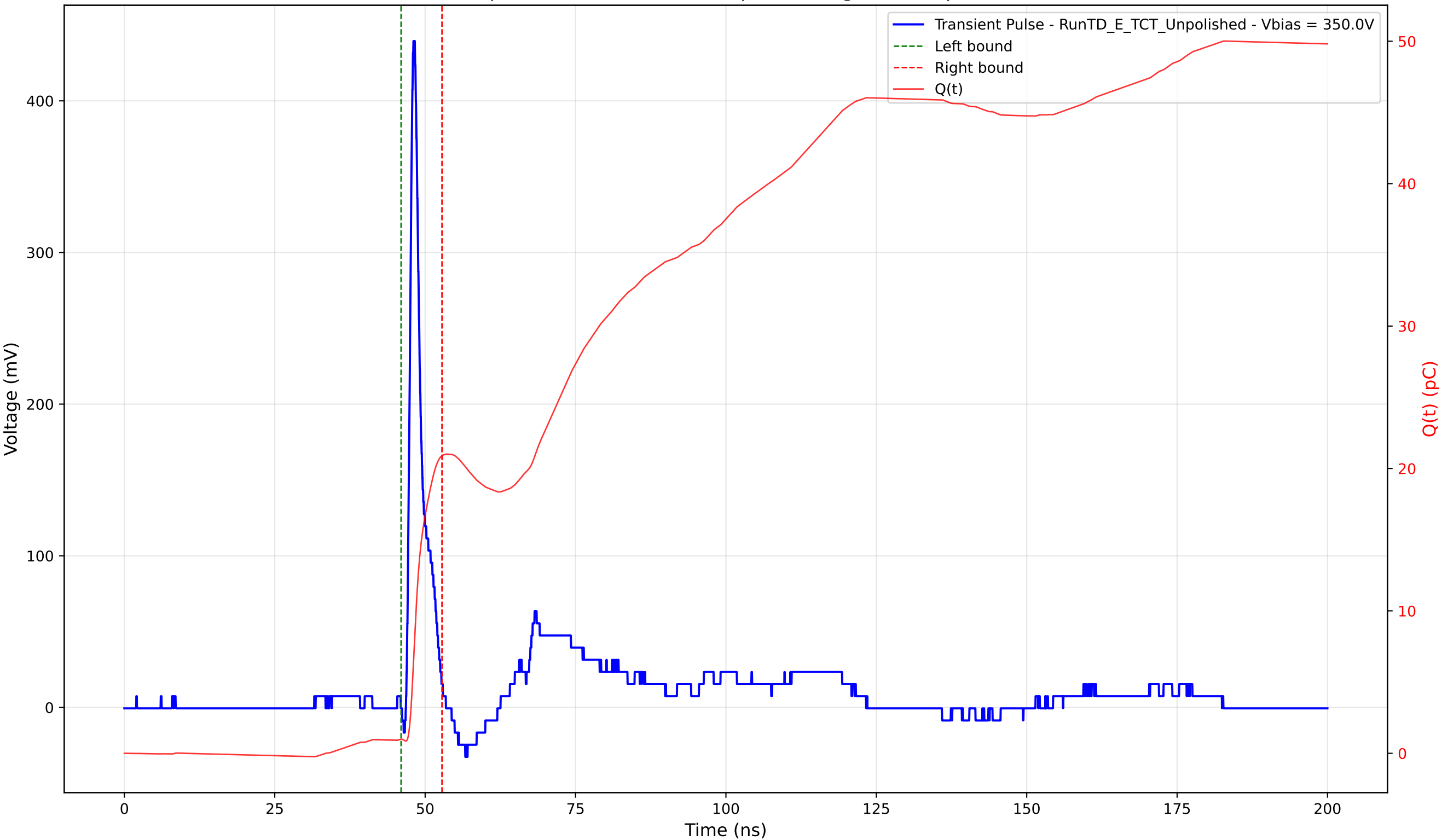
Transient Pulse - Sample: TD - Position: 105.0 \mu\text{m} - Charge: 19.90 pC - Rise Time: 0.84 ns
