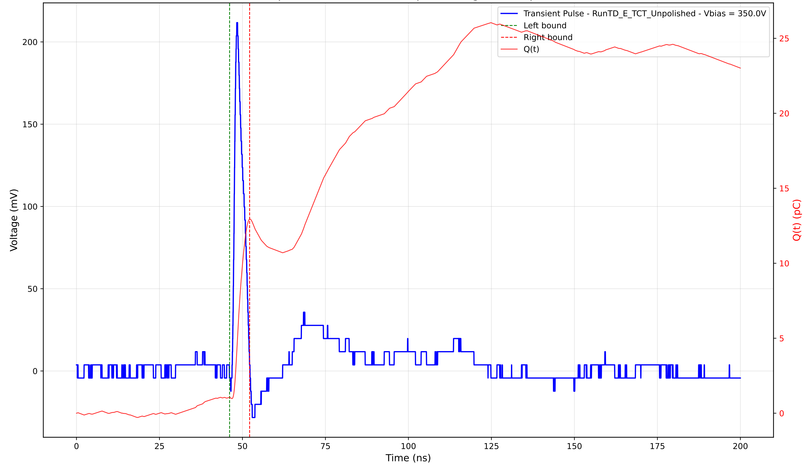
Transient Pulse - Sample: TD - Position: 300.0 \mu\text{m} - Charge: 11.88 pC - Rise Time: 0.98 ns
