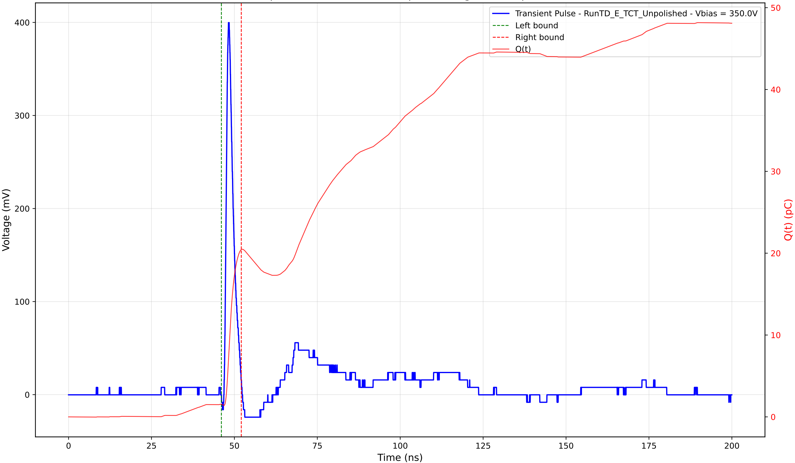
Transient Pulse - Sample: TD - Position: 175.0 \mu\text{m} - Charge: 18.89 pC - Rise Time: 0.92 ns
