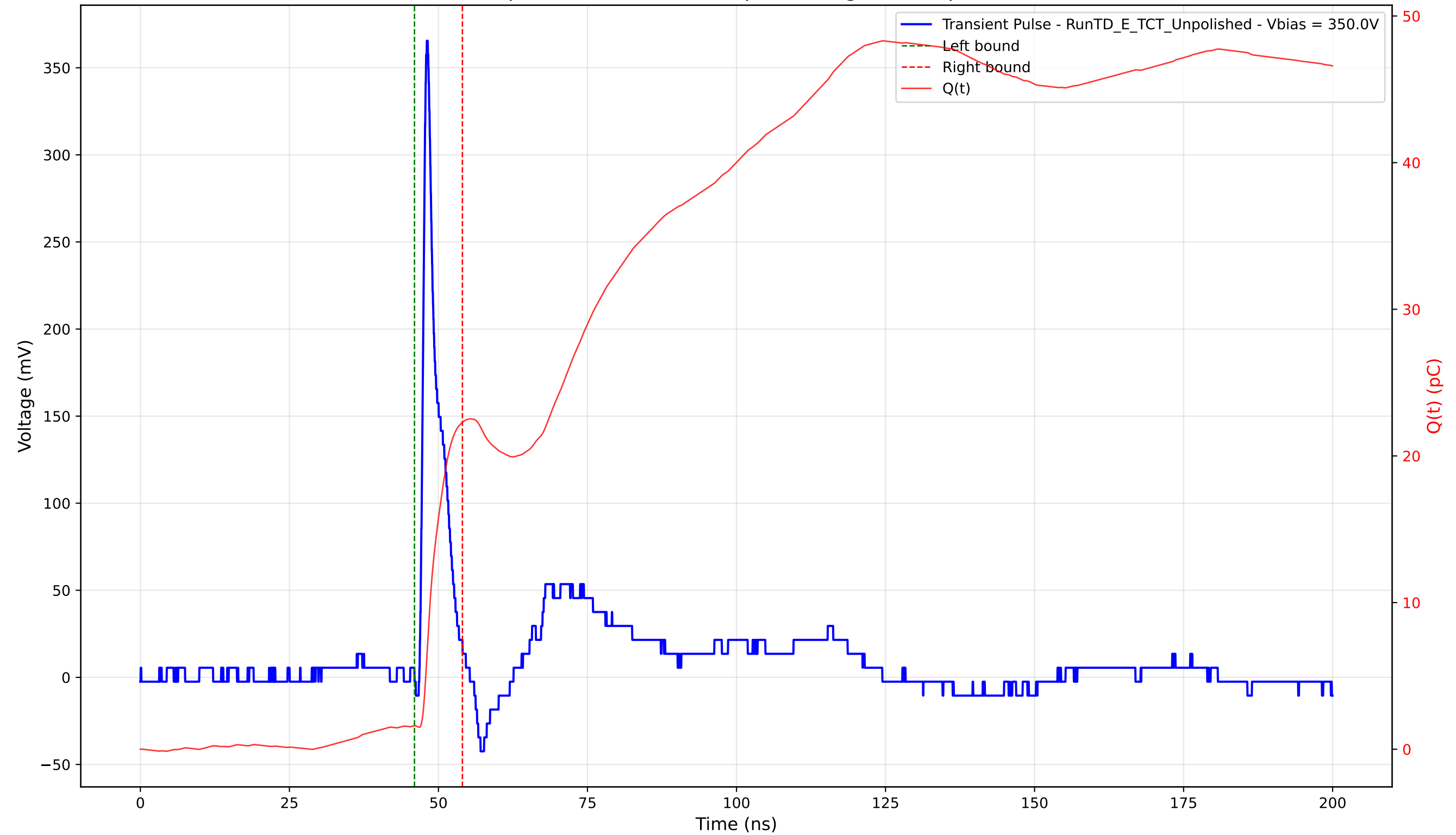
Transient Pulse - Sample: TD - Position: 70.0 \mu\text{m} - Charge: 20.70 pC - Rise Time: 0.84 ns
