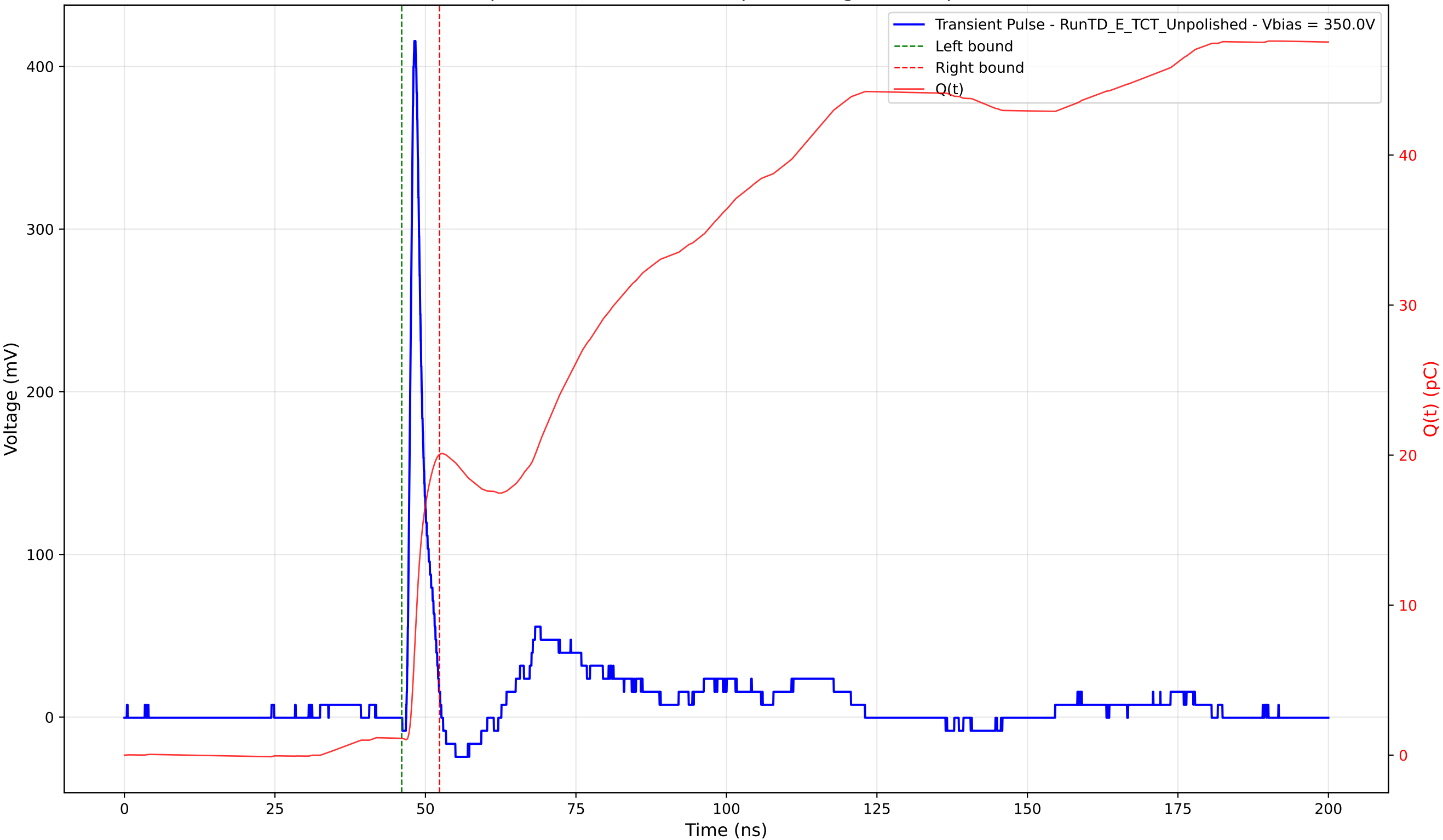
Transient Pulse - Sample: TD - Position: 125.0 \mu\text{m} - Charge: 18.92 pC - Rise Time: 0.88 ns
