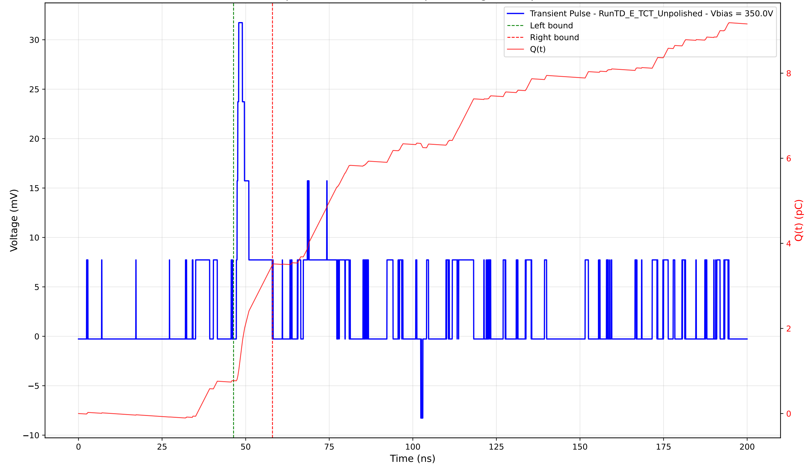
Transient Pulse - Sample: TD - Position: 360.0 \mu\text{m} - Charge: 2.72 pC - Rise Time: 0.71 ns
