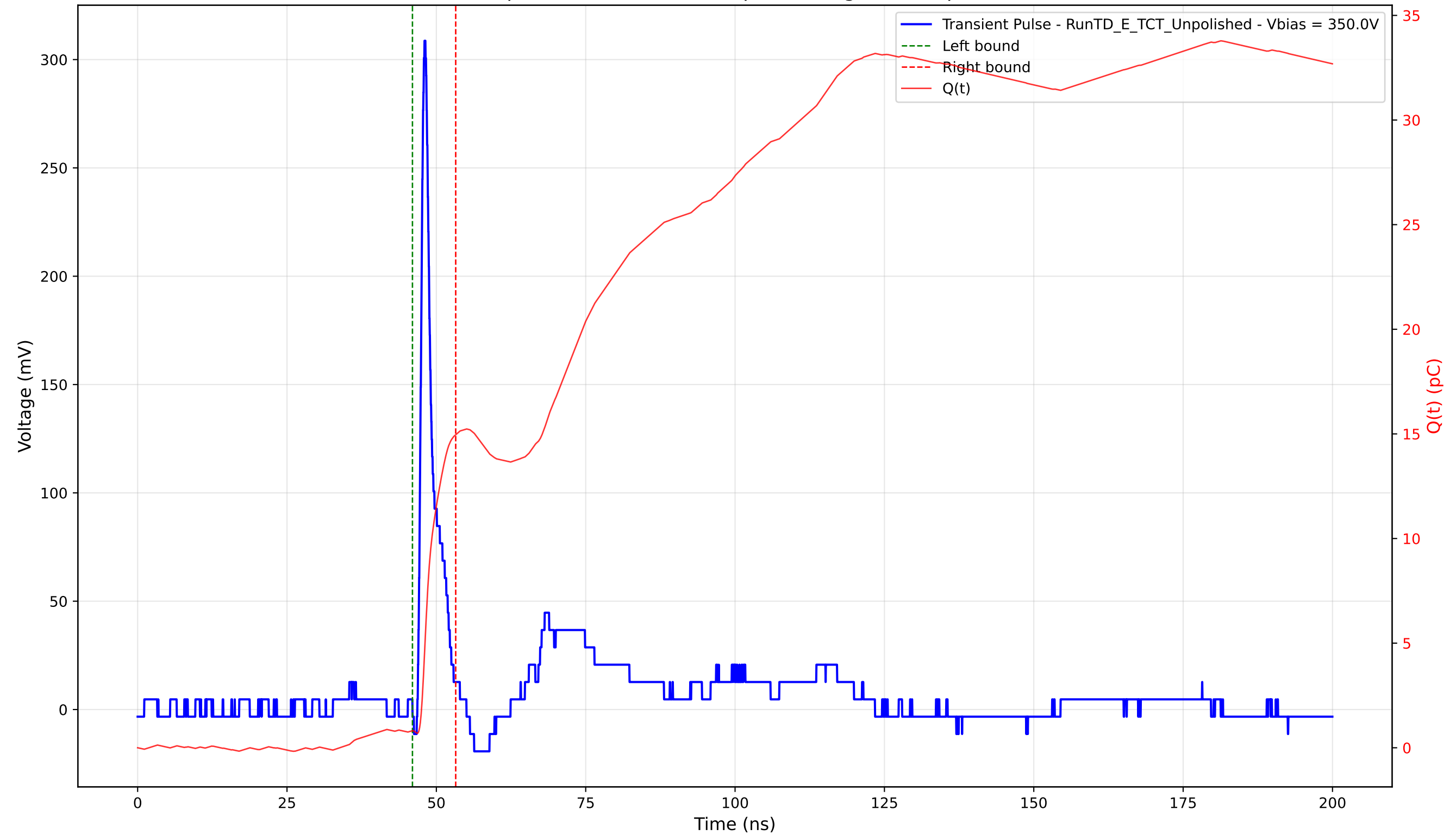
Transient Pulse - Sample: TD - Position: 35.0 \mu\text{m} - Charge: 14.14 pC - Rise Time: 0.81 ns
