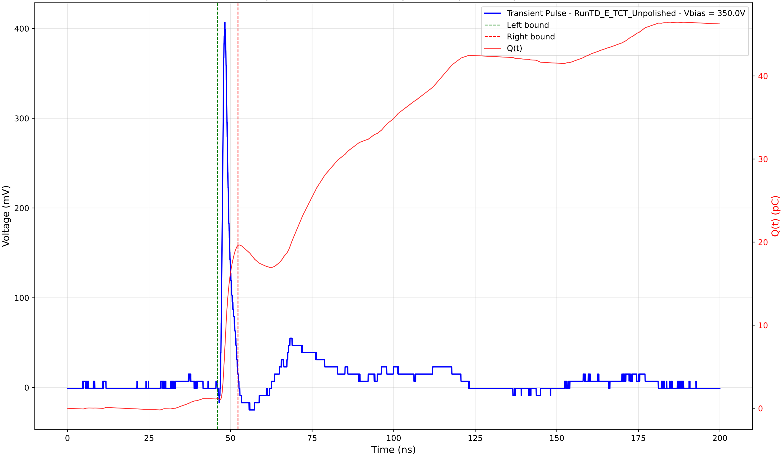
Transient Pulse - Sample: TD - Position: 130.0 \mu\text{m} - Charge: 18.44 pC - Rise Time: 0.88 ns
