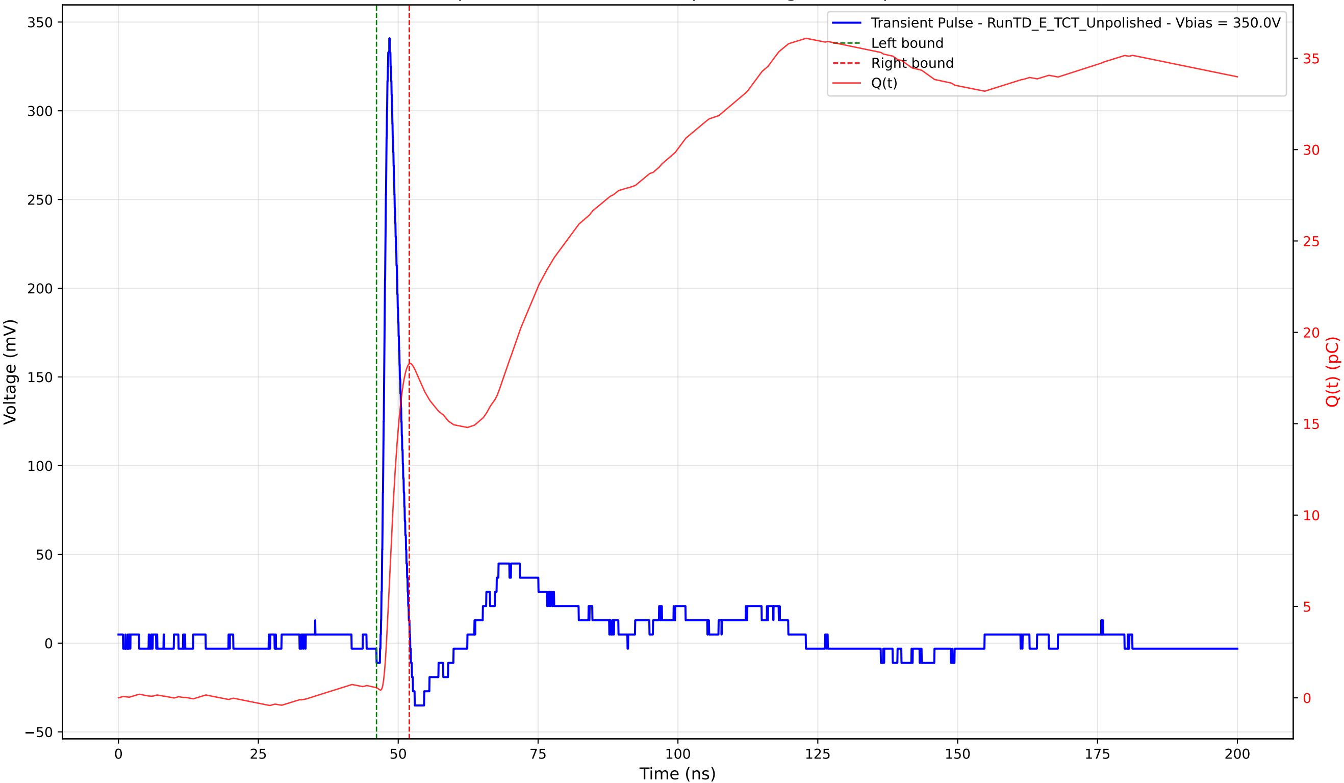
Transient Pulse - Sample: TD - Position: 210.0 \mu\text{m} - Charge: 17.71 pC - Rise Time: 0.97 ns
