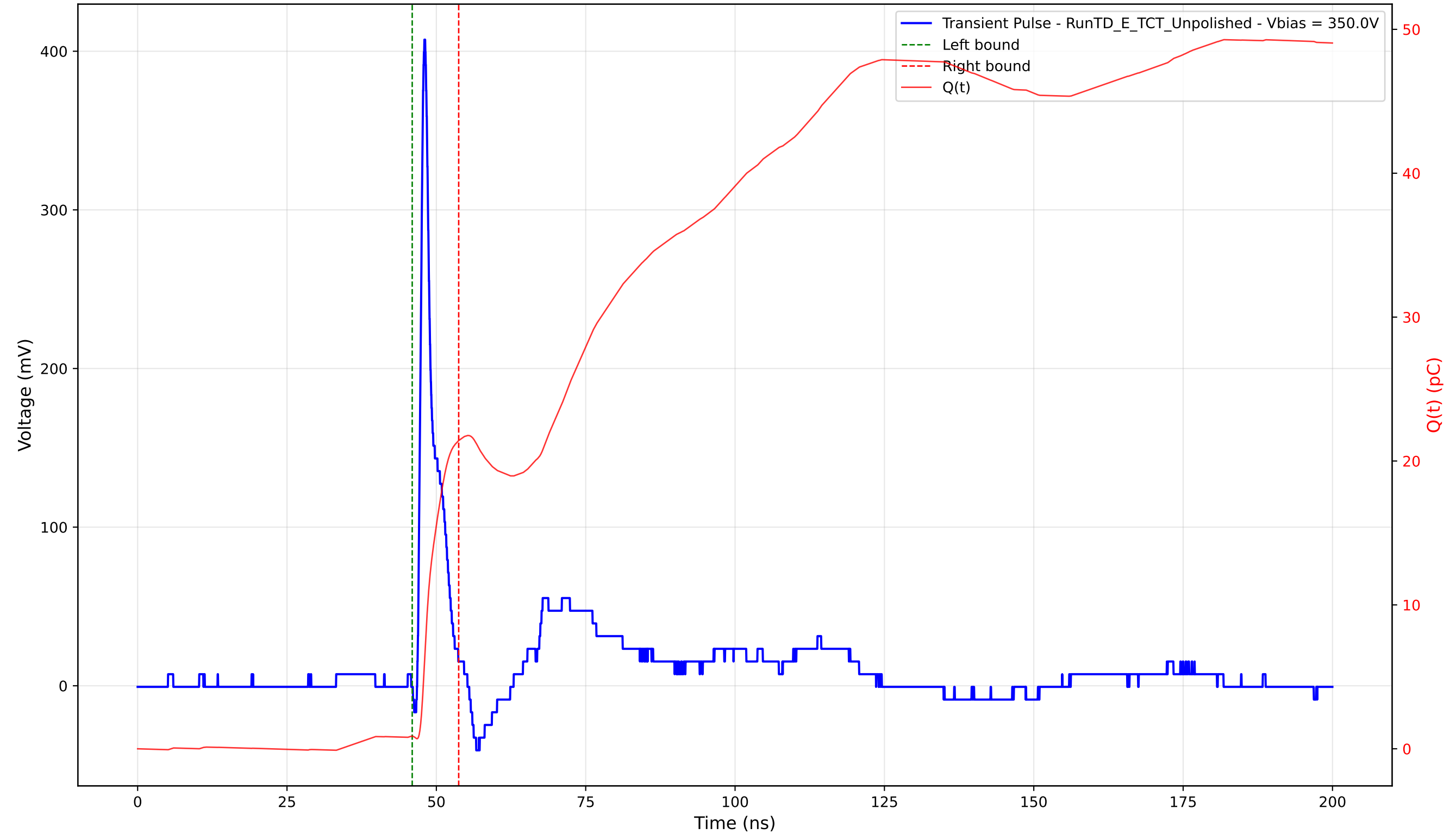
Transient Pulse - Sample: TD - Position: 55.0 \mu\text{m} - Charge: 20.55 pC - Rise Time: 0.79 ns
