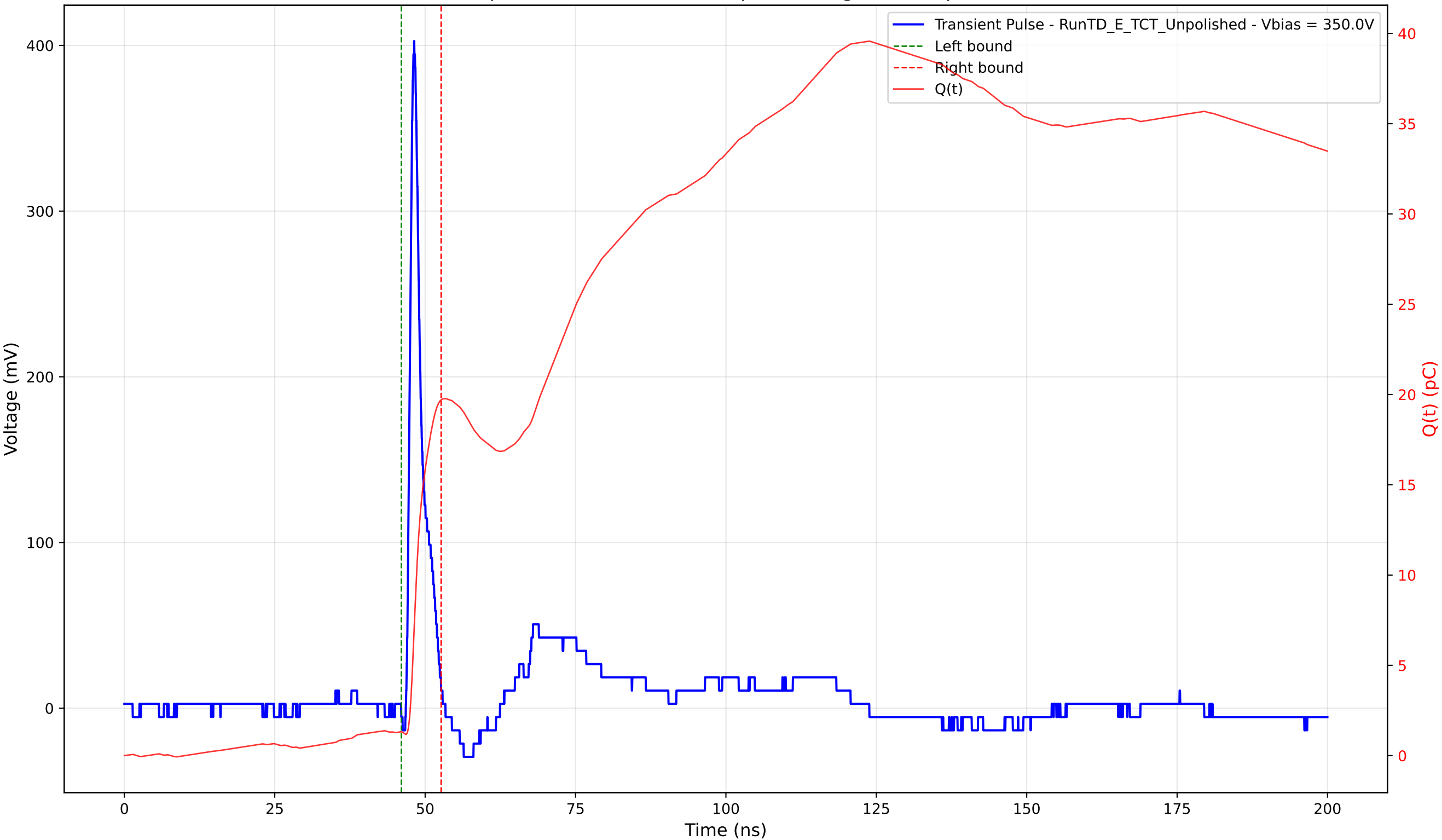
Transient Pulse - Sample: TD - Position: 100.0 \mu\text{m} - Charge: 18.38 pC - Rise Time: 0.87 ns
