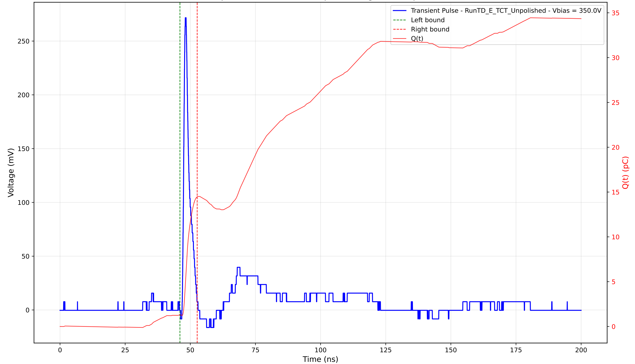
Transient Pulse - Sample: TD - Position: 85.0 \mu\text{m} - Charge: 13.16 pC - Rise Time: 0.85 ns
