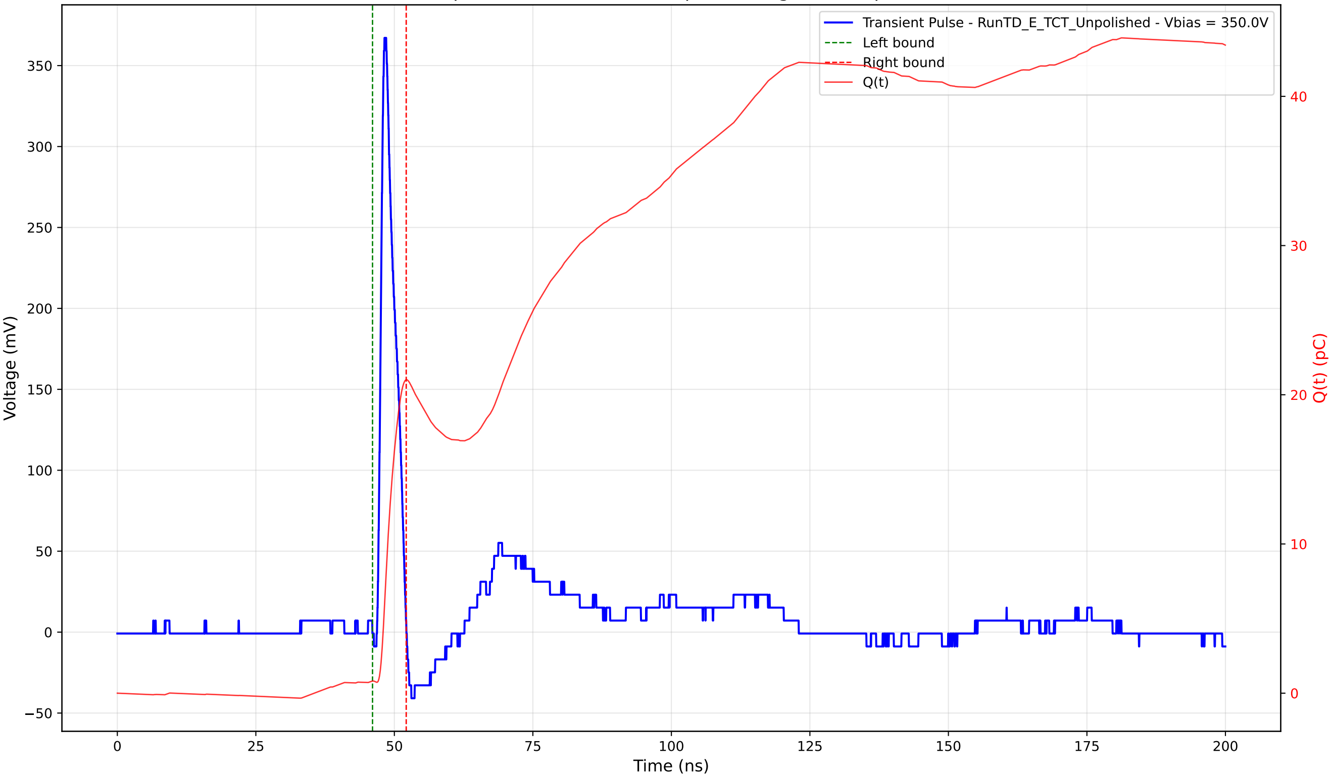
Transient Pulse - Sample: TD - Position: 245.0 \mu\text{m} - Charge: 20.19 pC - Rise Time: 0.91 ns
