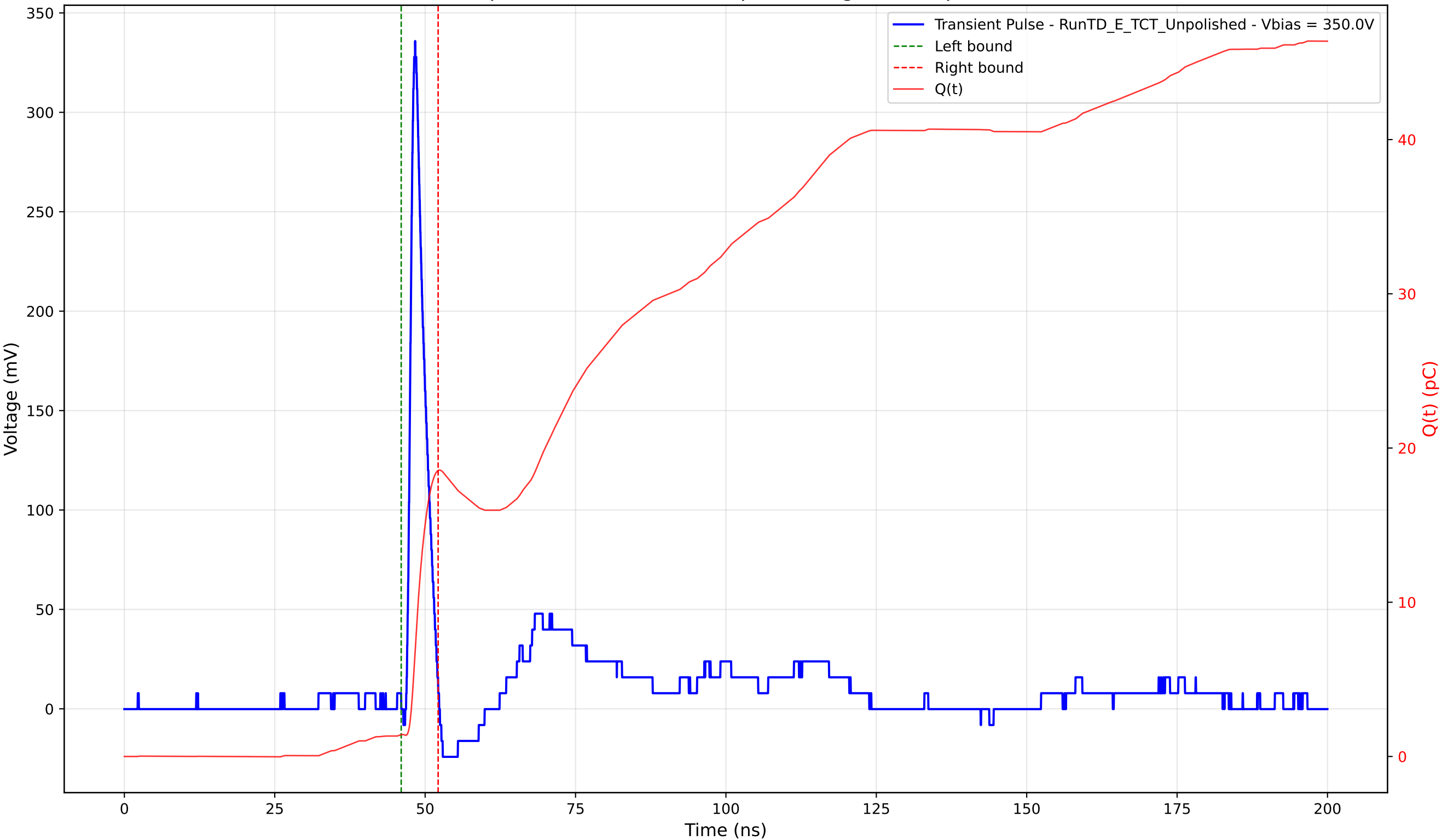
Transient Pulse - Sample: TD - Position: 230.0 \mu\text{m} - Charge: 17.12 pC - Rise Time: 0.96 ns
