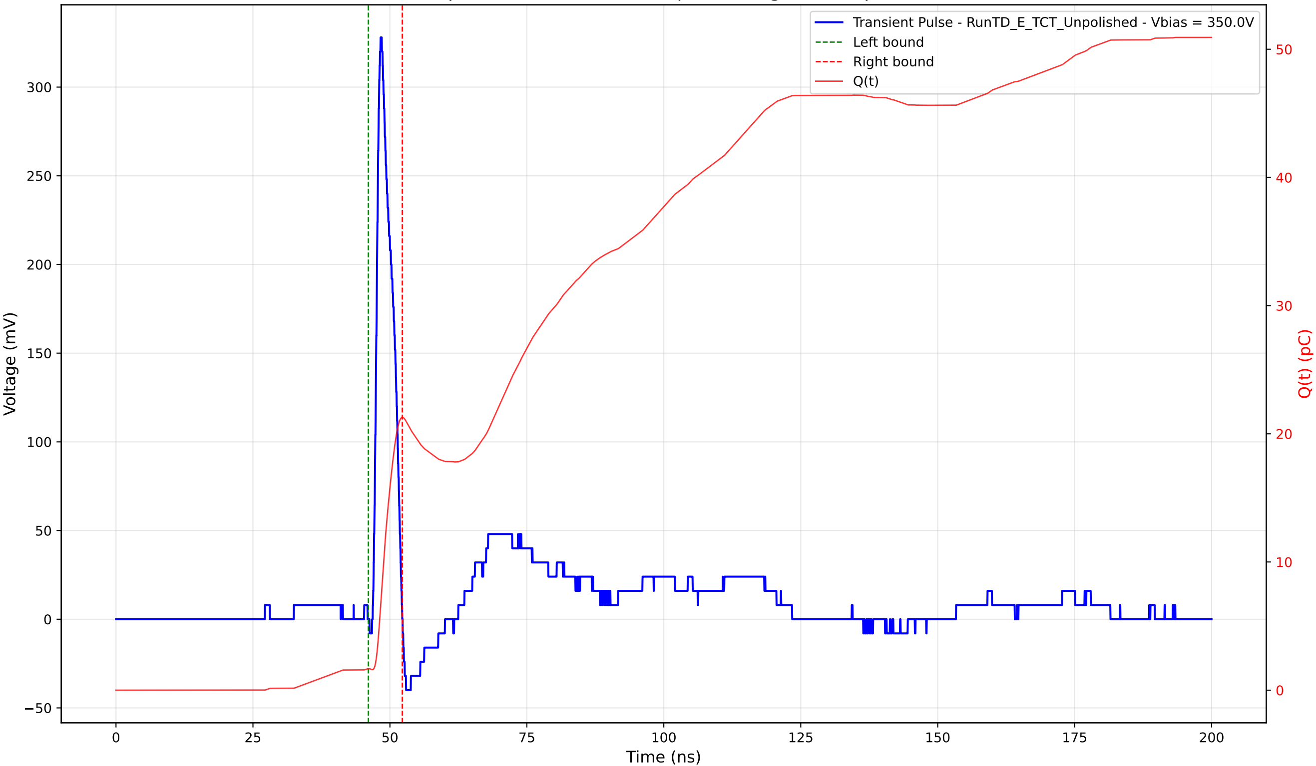
Transient Pulse - Sample: TD - Position: 240.0 \mu\text{m} - Charge: 19.61 pC - Rise Time: 0.96 ns
