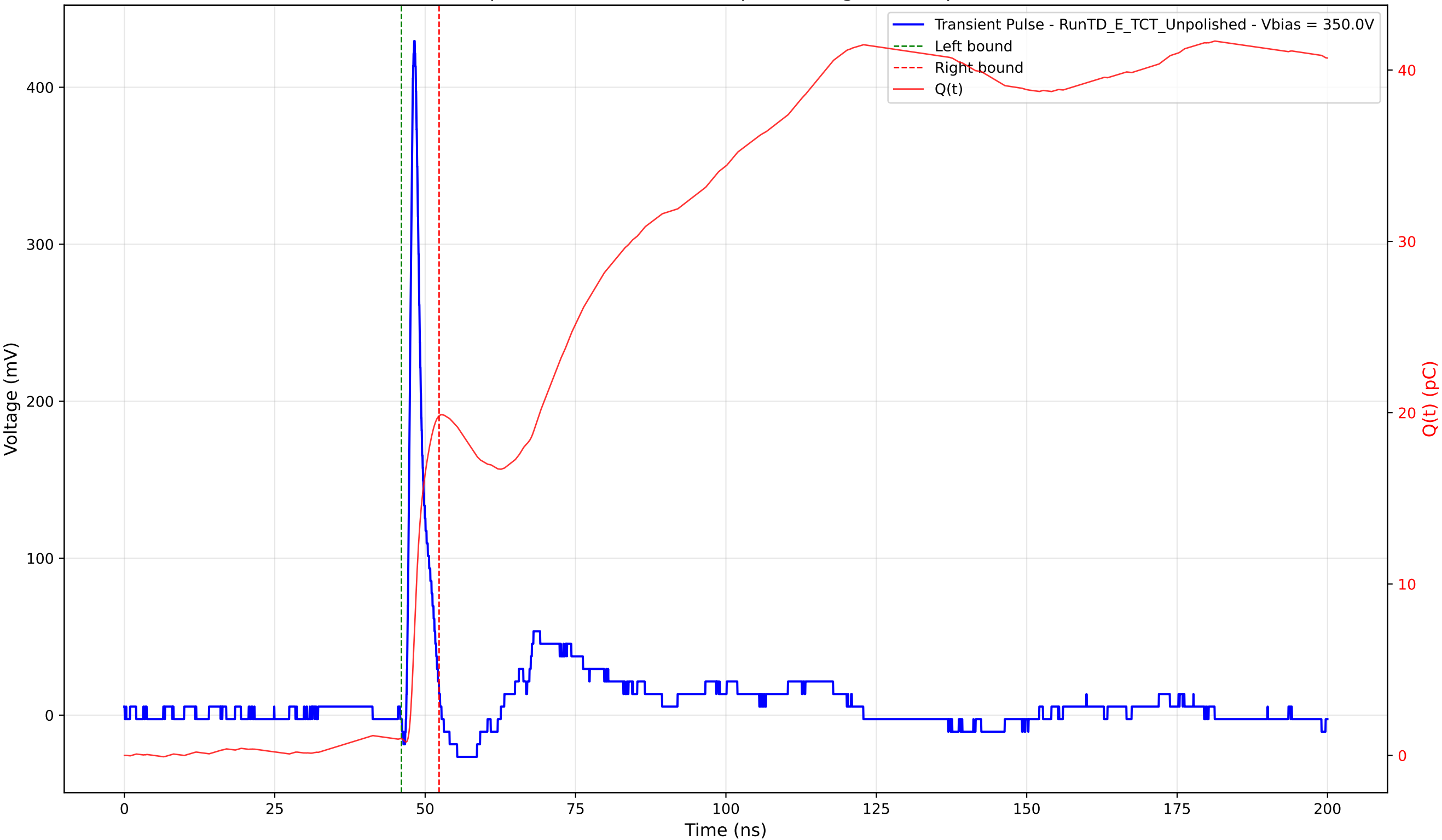
Transient Pulse - Sample: TD - Position: 120.0 \mu\text{m} - Charge: 18.85 pC - Rise Time: 0.87 ns
