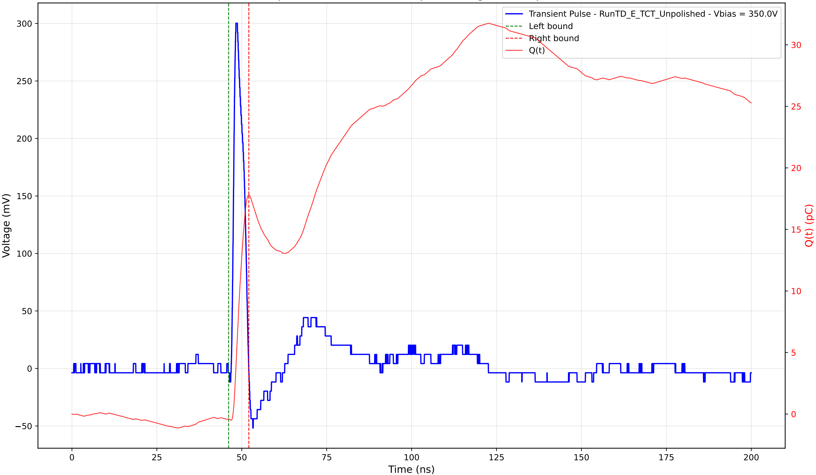
Transient Pulse - Sample: TD - Position: 285.0 \mu\text{m} - Charge: 18.20 pC - Rise Time: 0.96 ns
