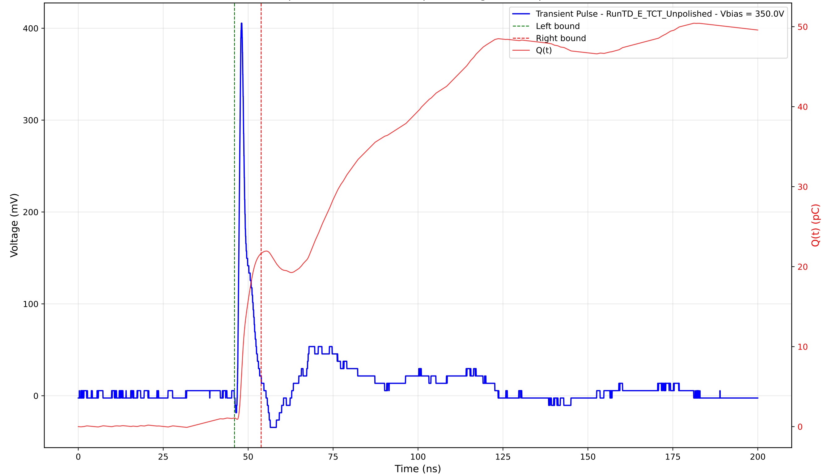
Transient Pulse - Sample: TD - Position: 50.0 \mu\text{m} - Charge: 20.58 pC - Rise Time: 0.79 ns
