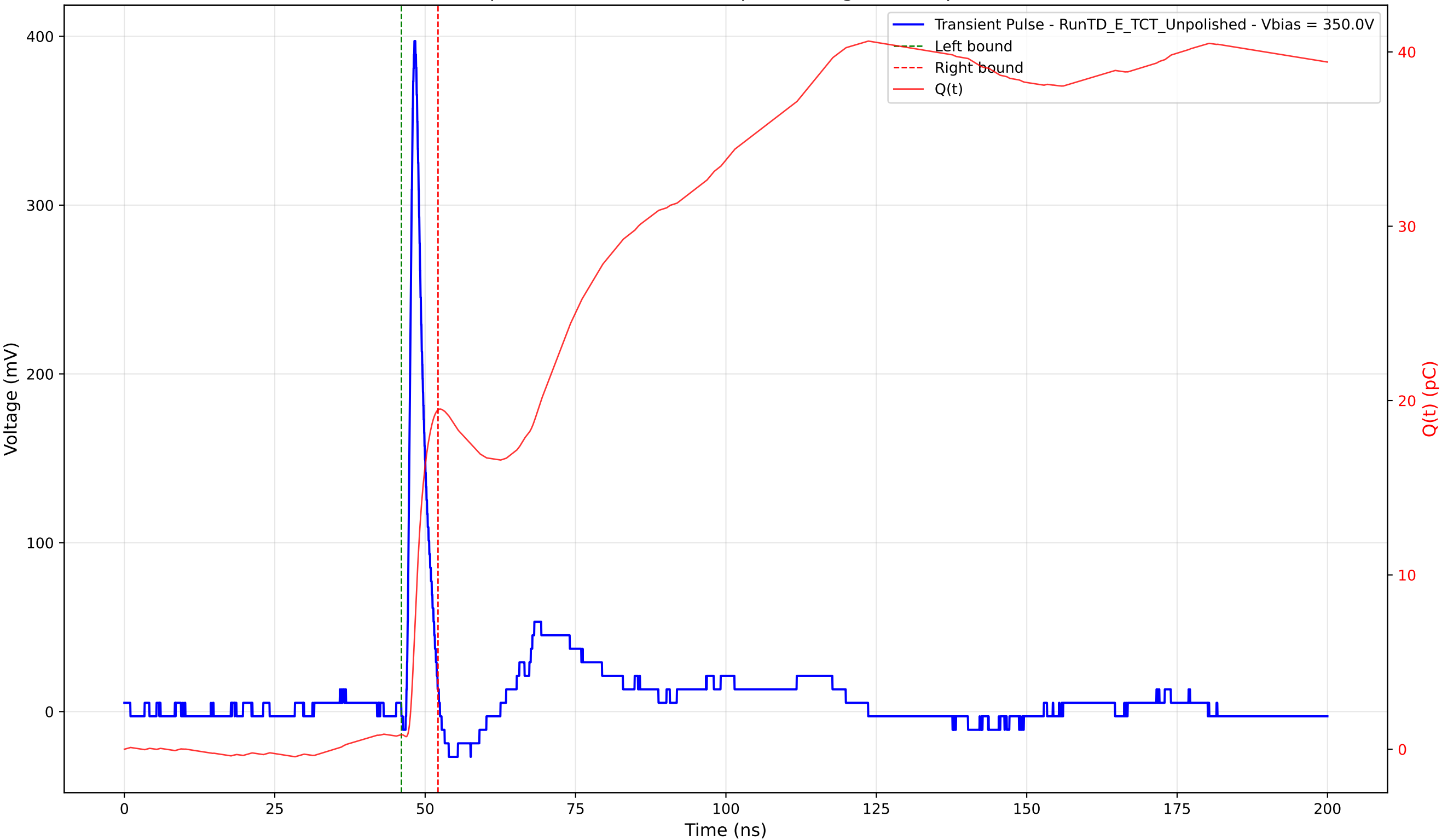
Transient Pulse - Sample: TD - Position: 170.0 \mu\text{m} - Charge: 18.63 pC - Rise Time: 0.91 ns
