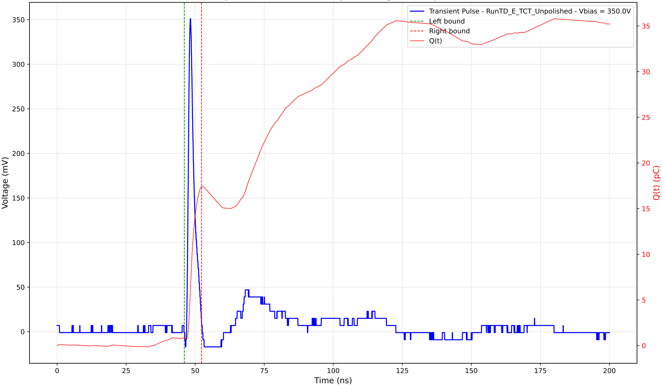
Transient Pulse - Sample: TD - Position: 140.0 \mu\text{m} - Charge: 16.54 pC - Rise Time: 0.89 ns
