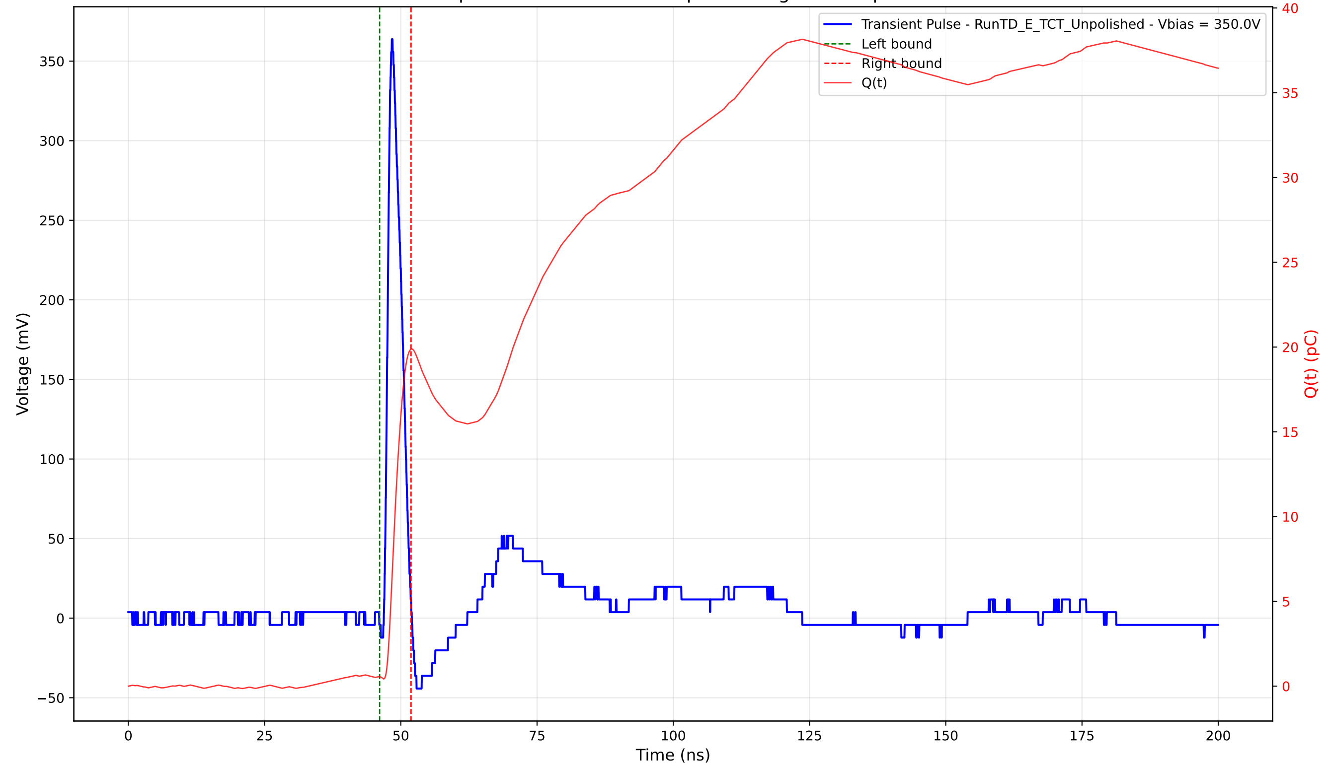
Transient Pulse - Sample: TD - Position: 260.0 \mu\text{m} - Charge: 19.32 pC - Rise Time: 0.94 ns
