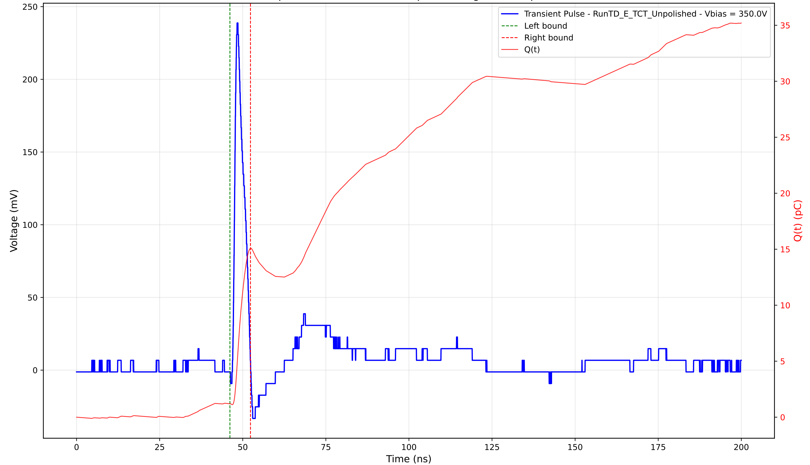
Transient Pulse - Sample: TD - Position: 330.0 \mu\text{m} - Charge: 13.88 pC - Rise Time: 0.98 ns
