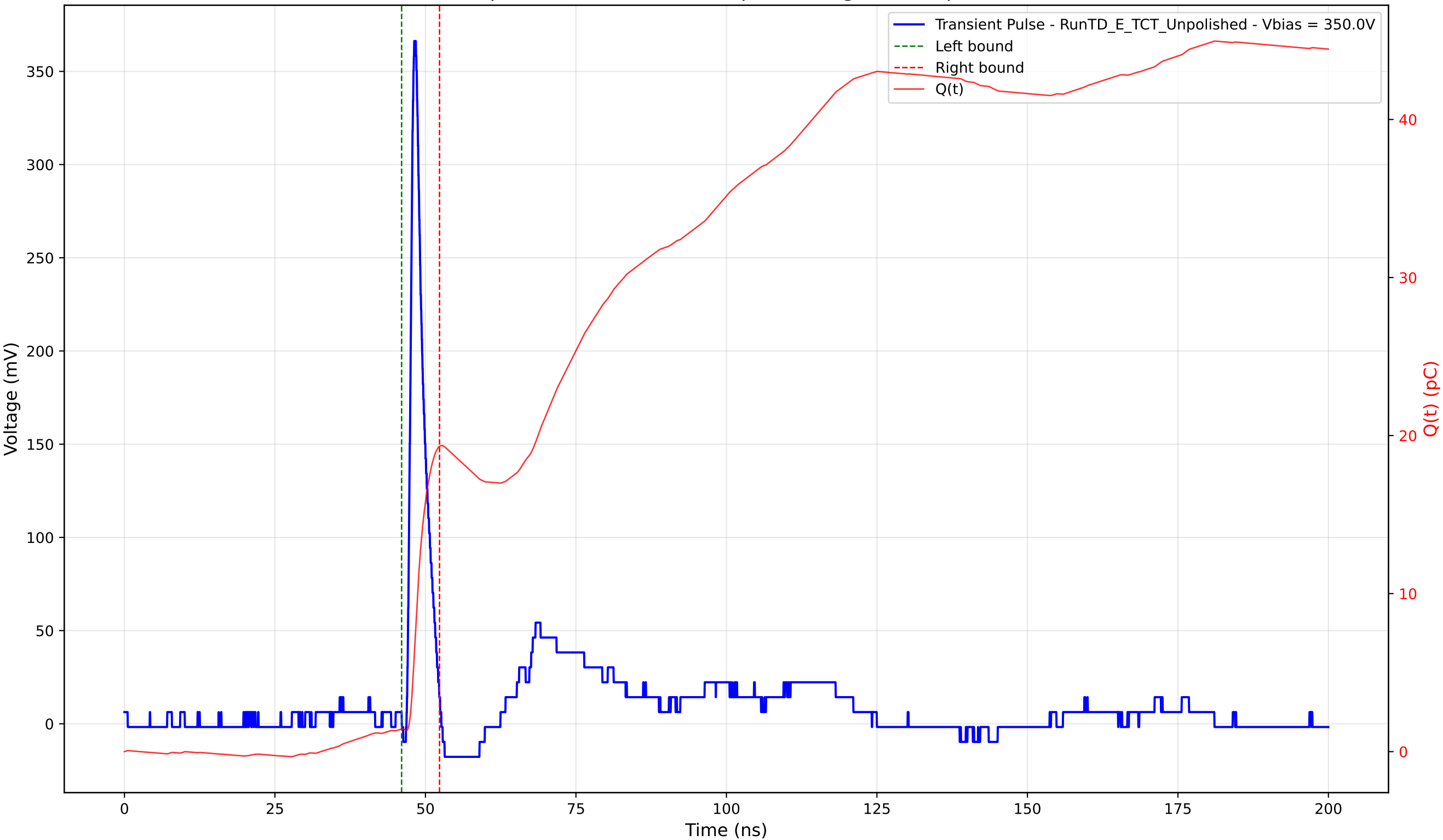
Transient Pulse - Sample: TD - Position: 195.0 \mu\text{m} - Charge: 17.88 pC - Rise Time: 0.88 ns
