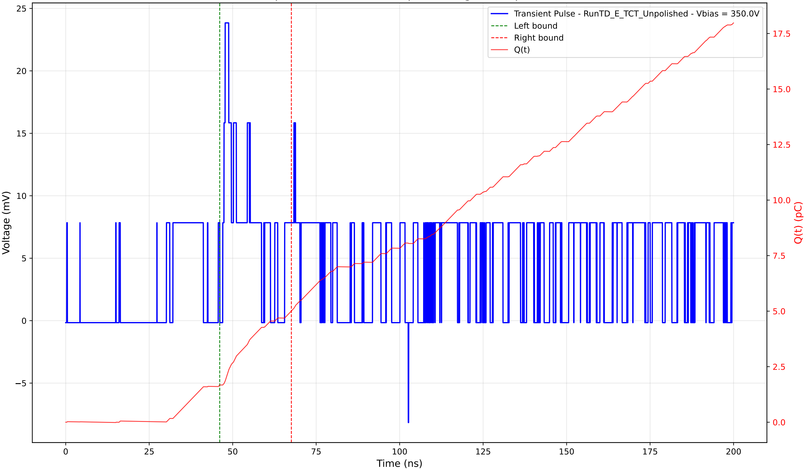
Transient Pulse - Sample: TD - Position: 10.0 \mu\text{m} - Charge: 3.33 pC - Rise Time: 0.73 ns
