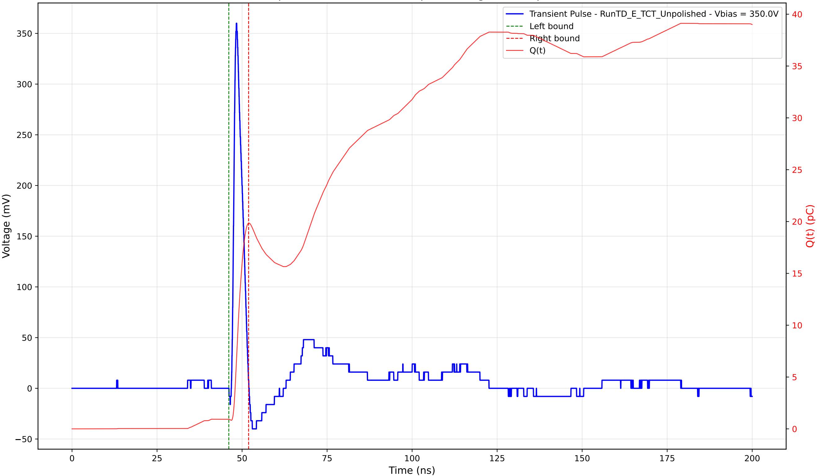
Transient Pulse - Sample: TD - Position: 270.0 \mu\text{m} - Charge: 18.91 pC - Rise Time: 0.95 ns
