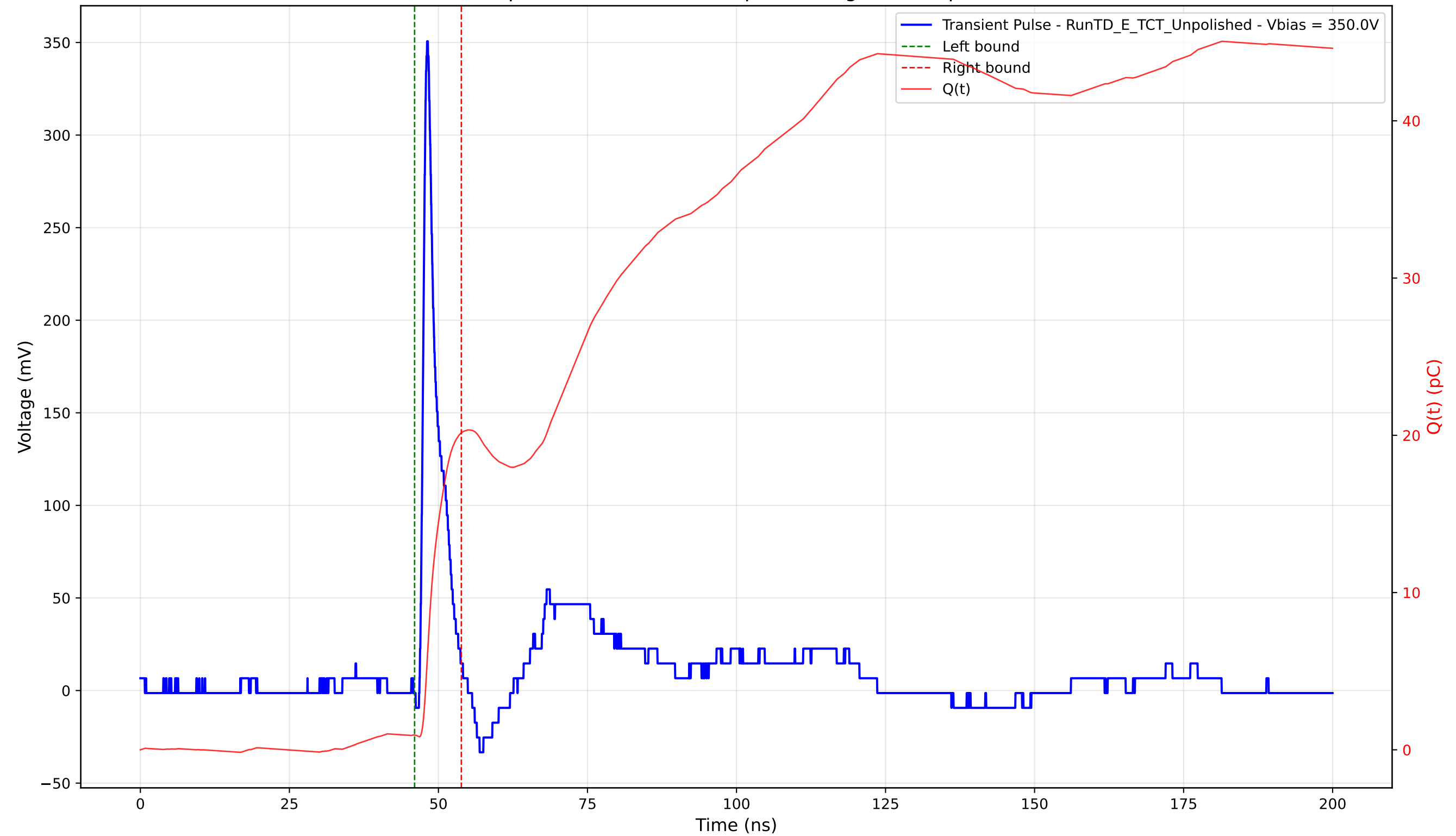
Transient Pulse - Sample: TD - Position: 75.0 \mu\text{m} - Charge: 19.22 pC - Rise Time: 0.85 ns
