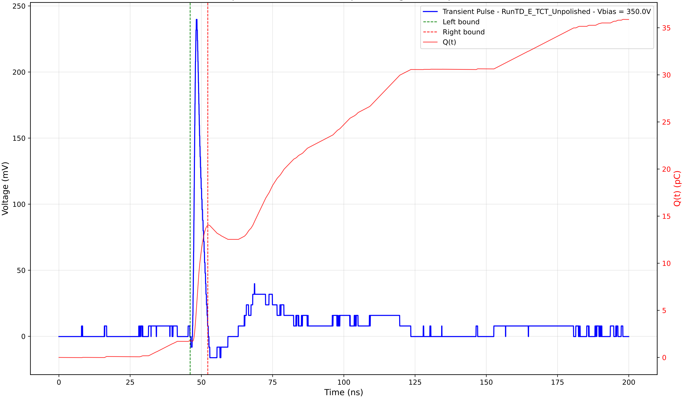
Transient Pulse - Sample: TD - Position: 310.0 \mu\text{m} - Charge: 12.25 pC - Rise Time: 0.96 ns
