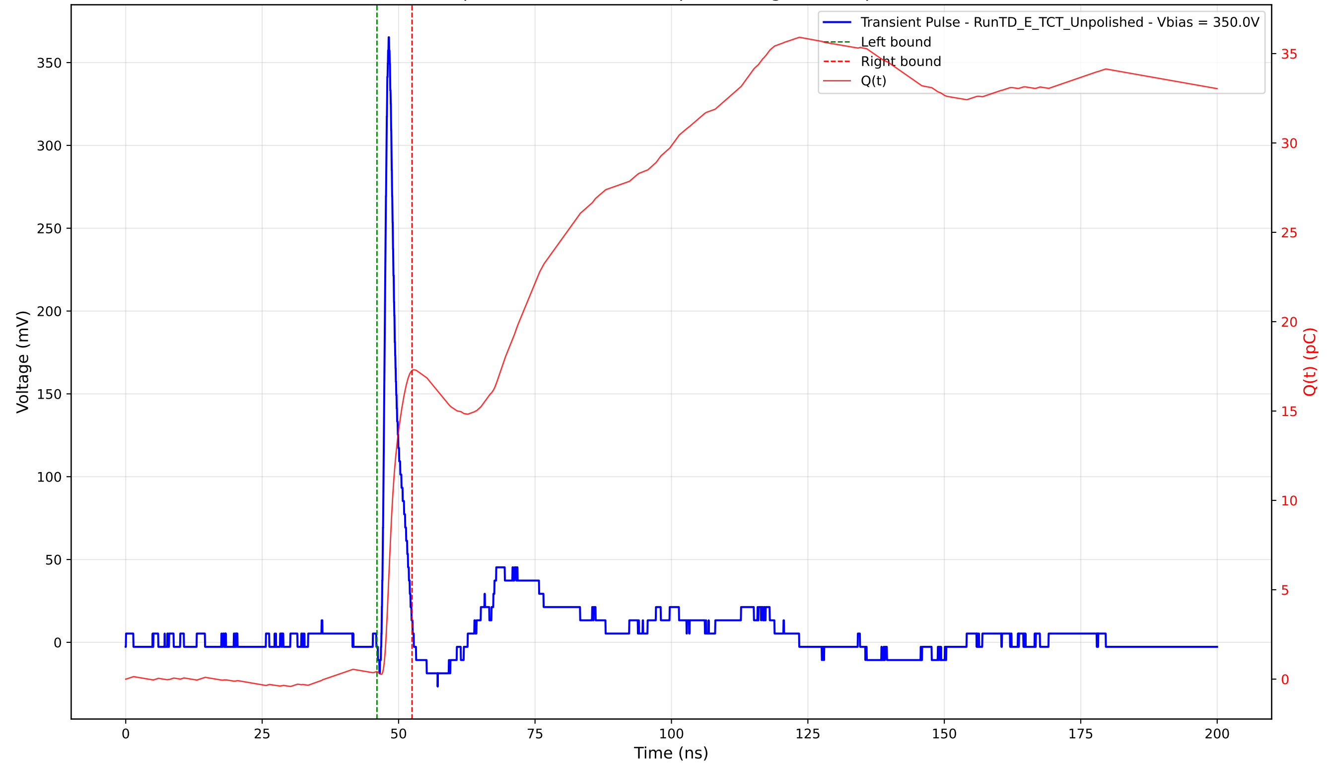
Transient Pulse - Sample: TD - Position: 95.0 \mu\text{m} - Charge: 16.85 pC - Rise Time: 0.88 ns
