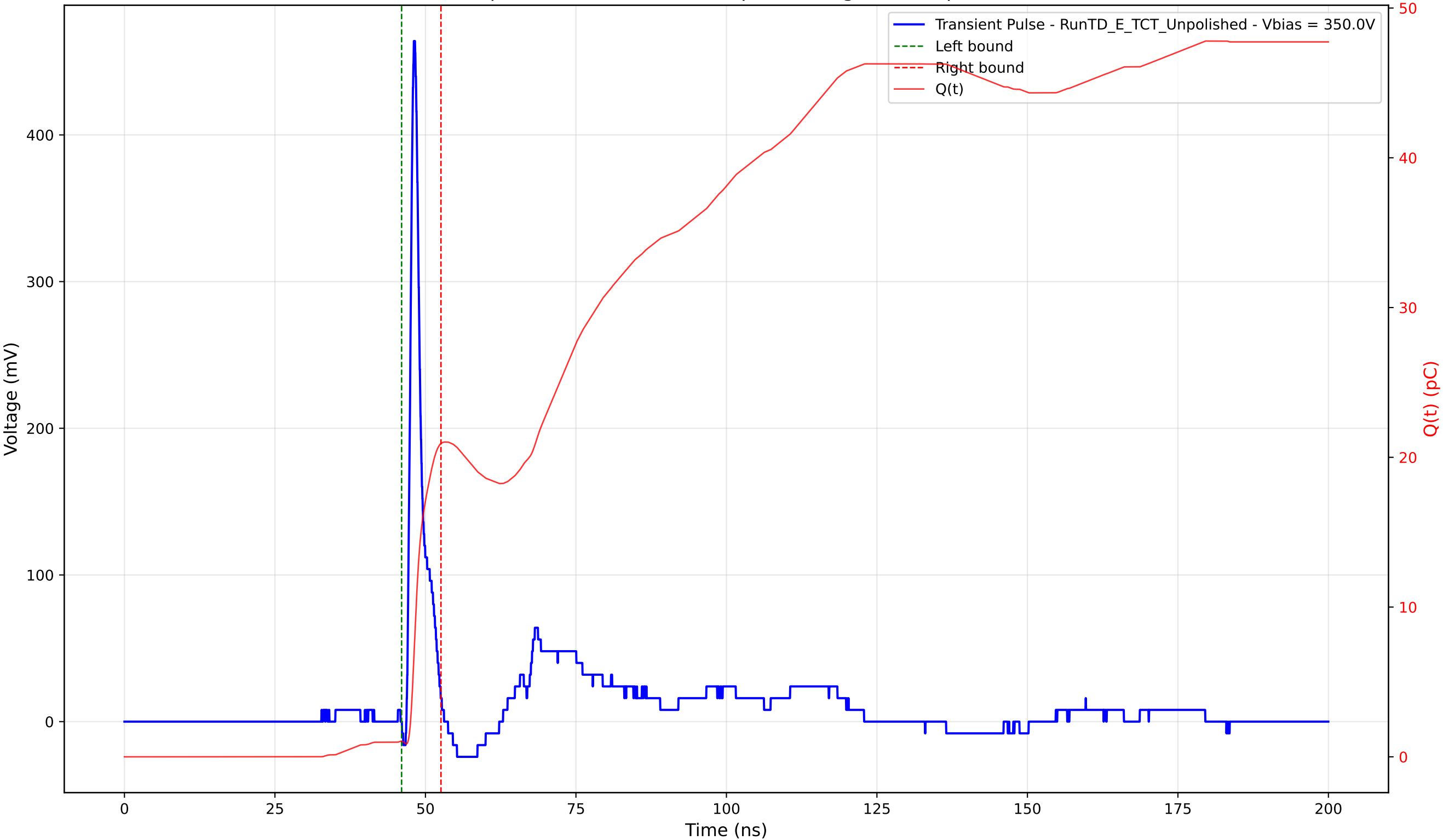
Transient Pulse - Sample: TD - Position: 110.0 \mu\text{m} - Charge: 19.88 pC - Rise Time: 0.85 ns
