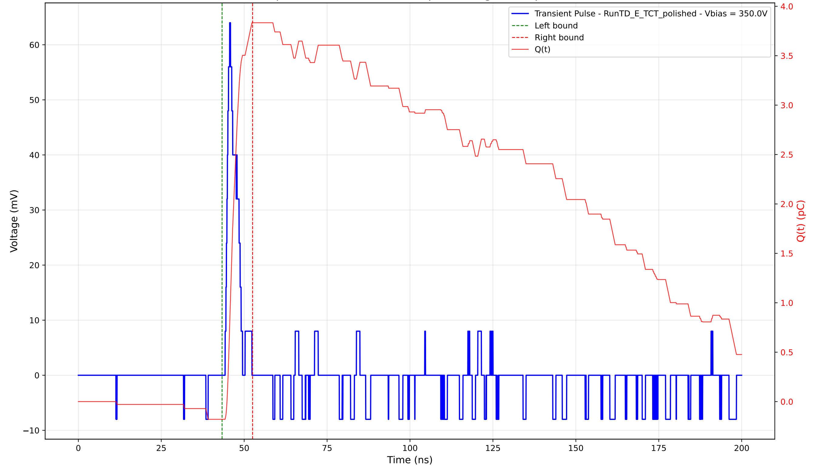
Transient Pulse - Sample: 4003 - Position: 585.0 \mu\text{m} - Charge: 4.01 pC - Rise Time: 1.36 ns
