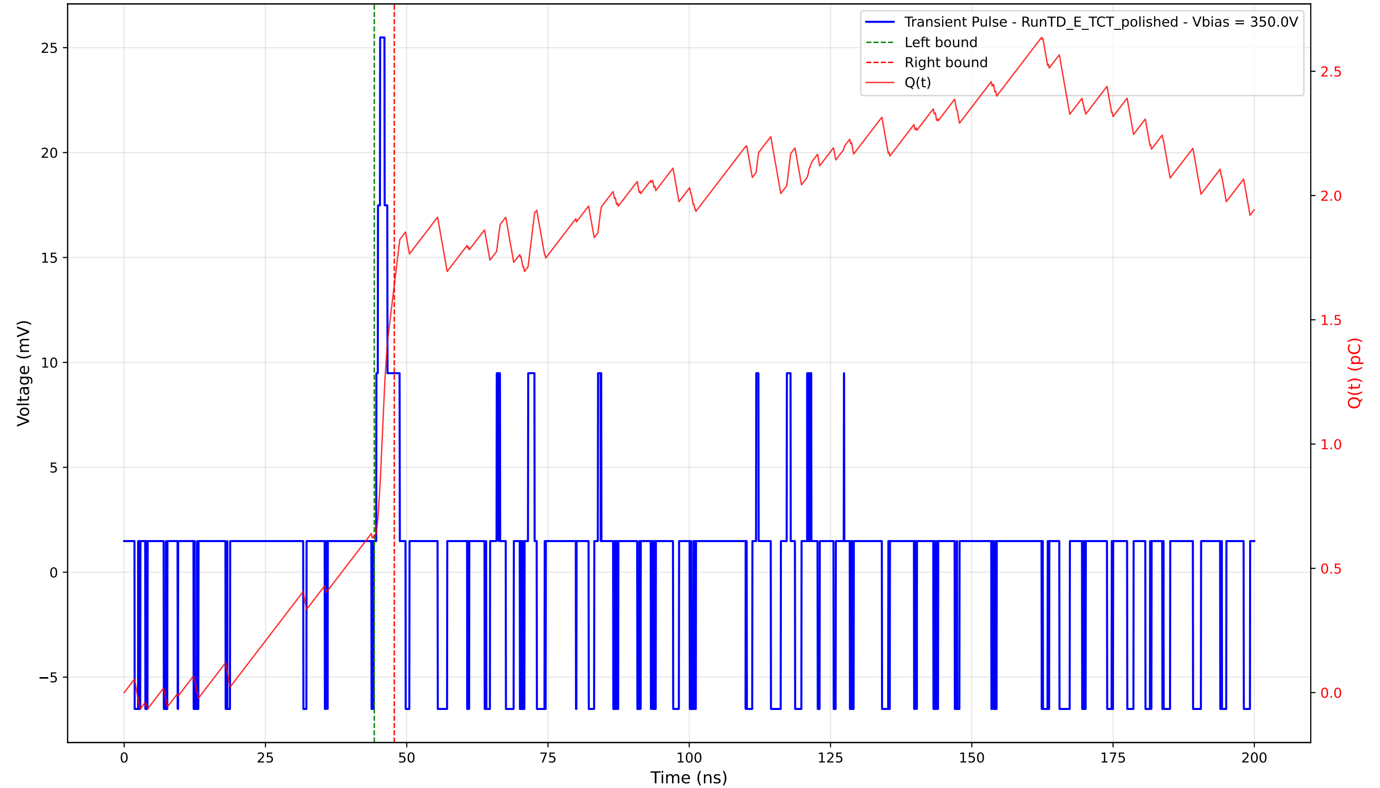
Transient Pulse - Sample: 4003 - Position: 70.0 \mu\text{m} - Charge: 1.01 pC - Rise Time: 0.68 ns
