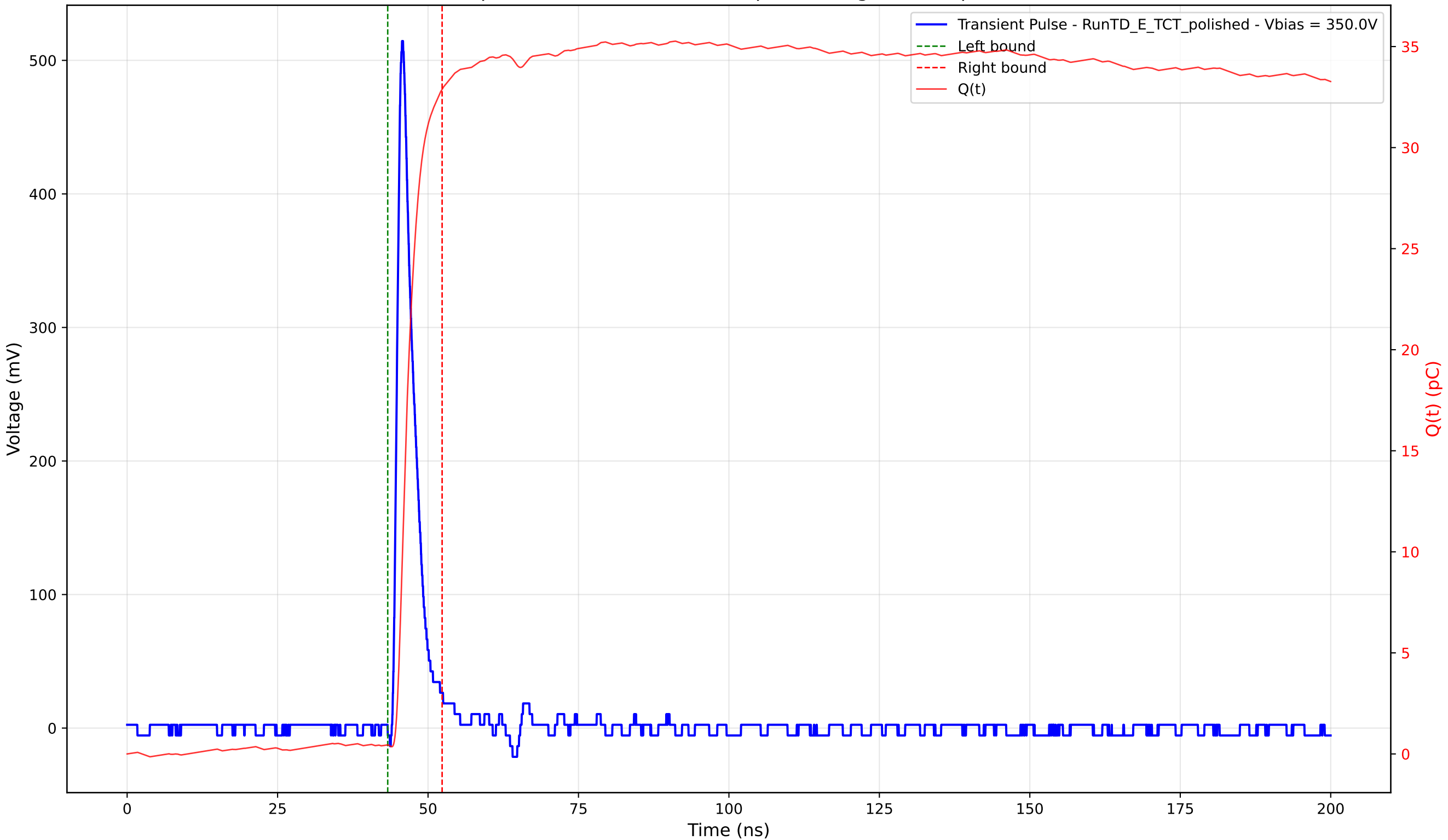
Transient Pulse - Sample: 4003 - Position: 355.0 \mu\text{m} - Charge: 32.44 pC - Rise Time: 1.06 ns
