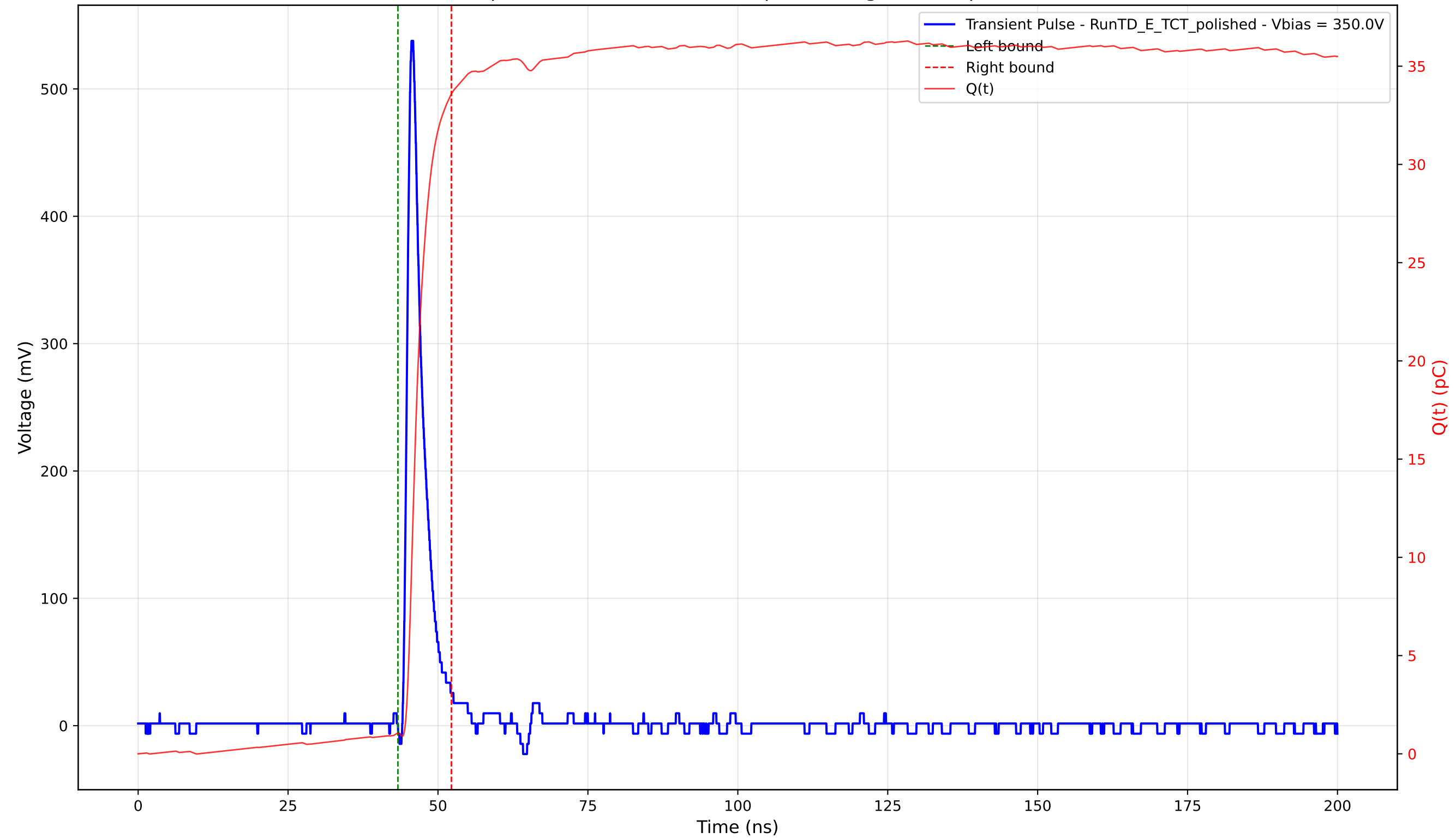
Transient Pulse - Sample: 4003 - Position: 330.0 \mu\text{m} - Charge: 32.55 pC - Rise Time: 1.00 ns
