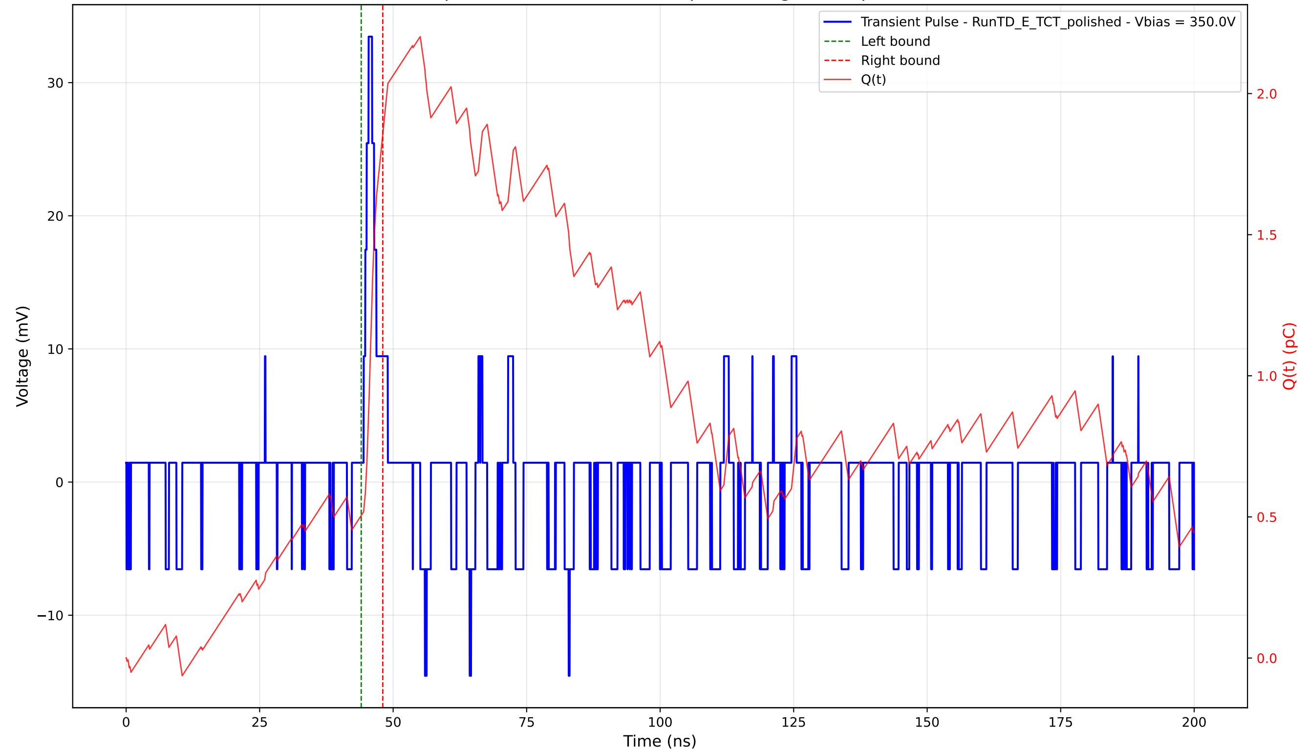
Transient Pulse - Sample: 4003 - Position: 745.0 \mu\text{m} - Charge: 1.35 pC - Rise Time: 0.94 ns
