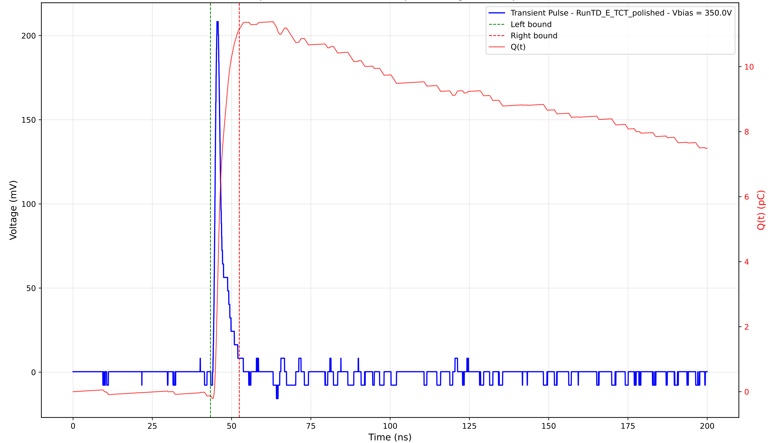
Transient Pulse - Sample: 4003 - Position: 165.0 \mu\text{m} - Charge: 11.28 pC - Rise Time: 0.93 ns
