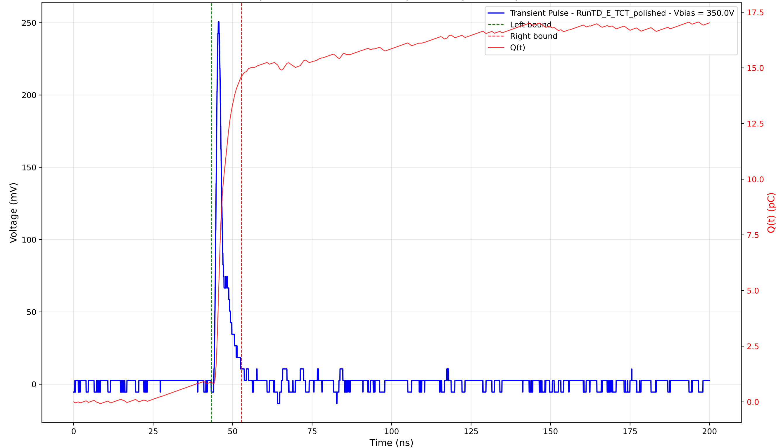
Transient Pulse - Sample: 4003 - Position: 175.0 \mu\text{m} - Charge: 13.74 pC - Rise Time: 0.96 ns
