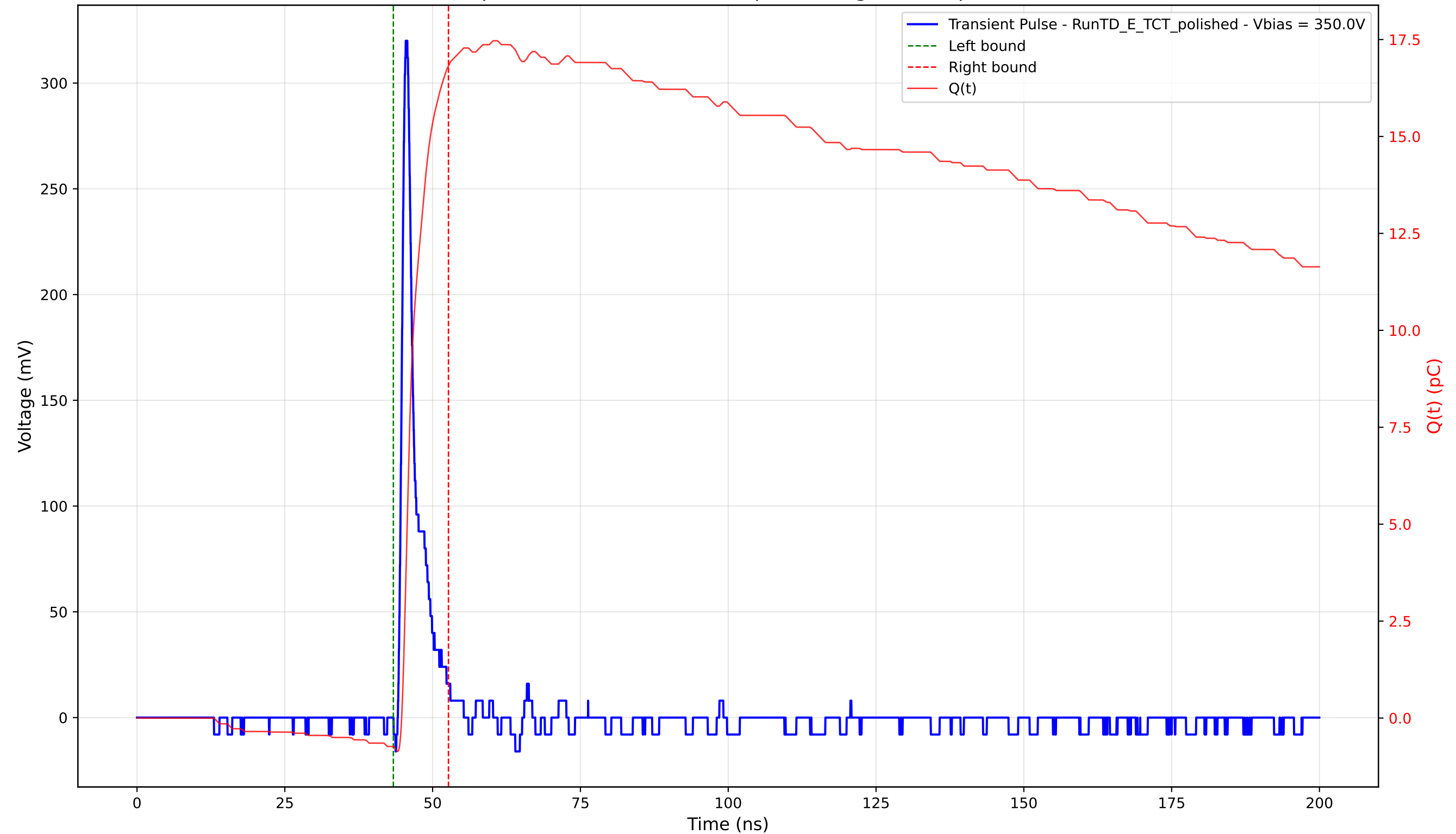
Transient Pulse - Sample: 4003 - Position: 195.0 \mu\text{m} - Charge: 17.56 pC - Rise Time: 0.90 ns
