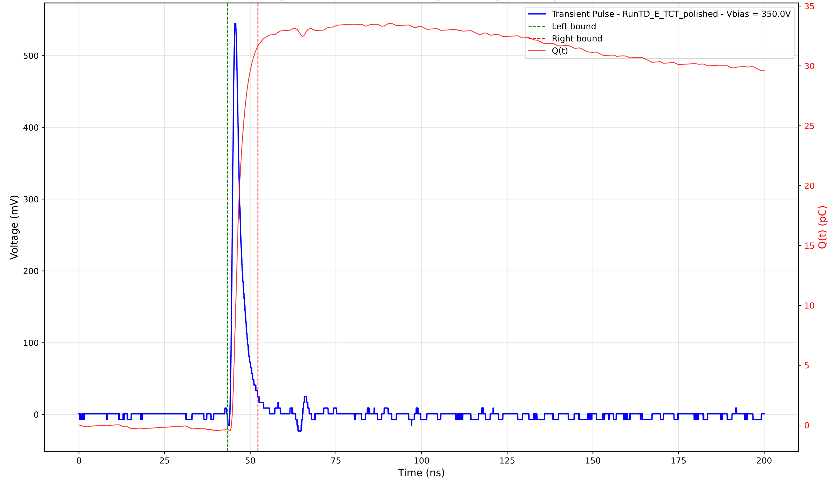
Transient Pulse - Sample: 4003 - Position: 300.0 \mu\text{m} - Charge: 32.02 pC - Rise Time: 0.99 ns
