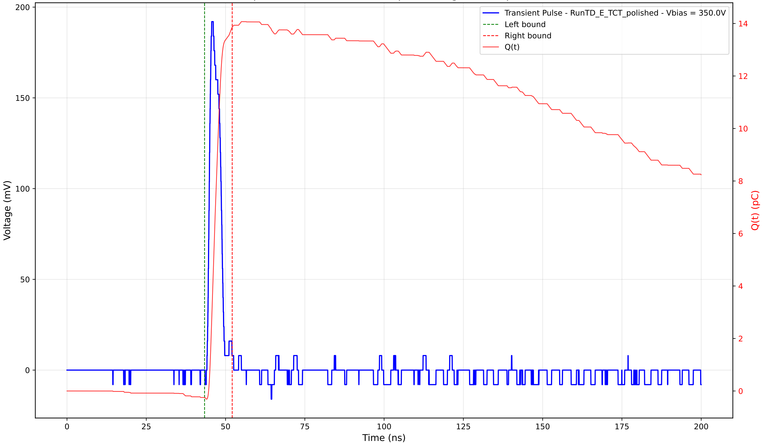
Transient Pulse - Sample: 4003 - Position: 510.0 \mu\text{m} - Charge: 14.11 pC - Rise Time: 1.05 ns
