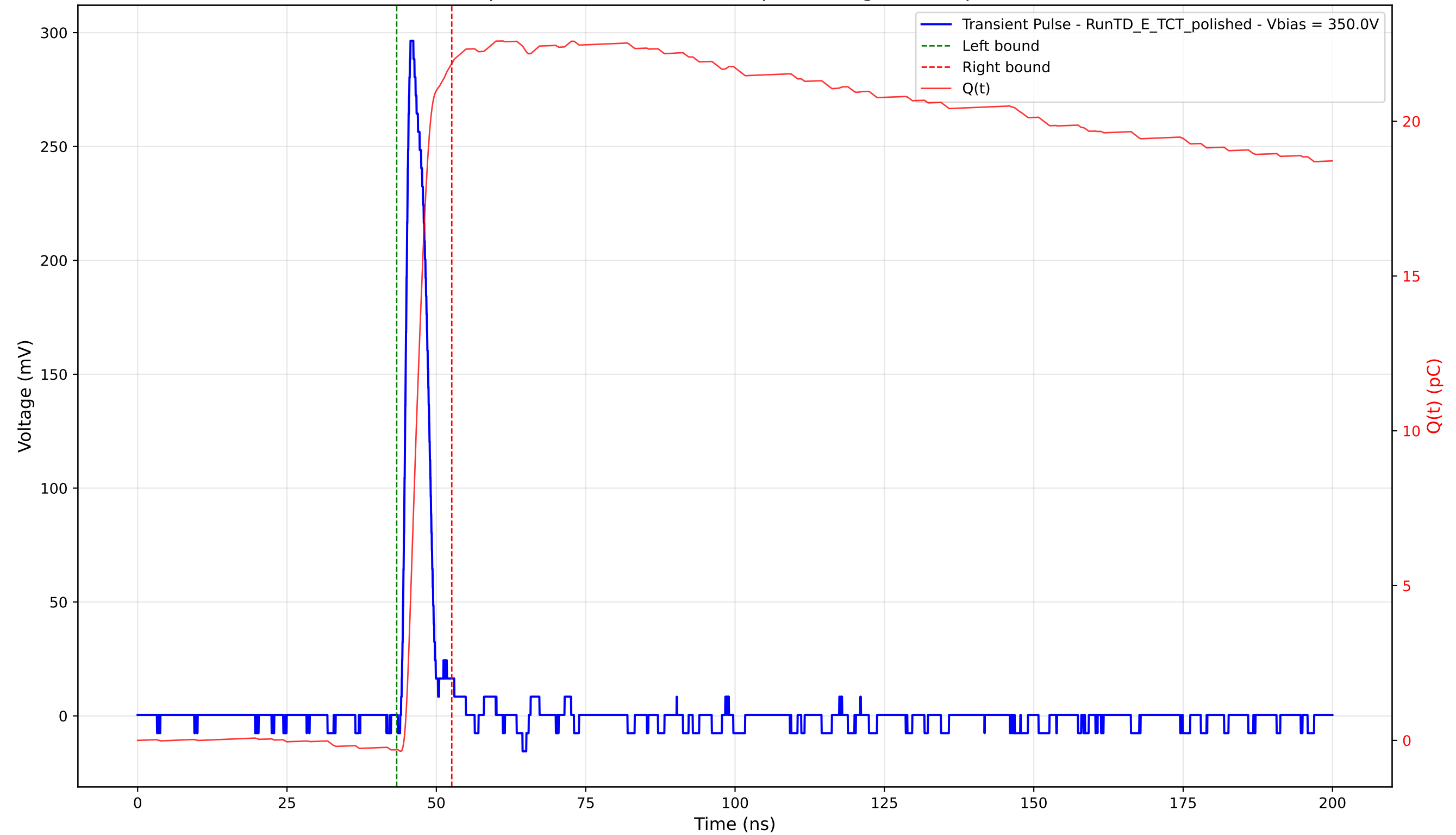
Transient Pulse - Sample: 4003 - Position: 465.0 \mu\text{m} - Charge: 22.17 pC - Rise Time: 1.11 ns
