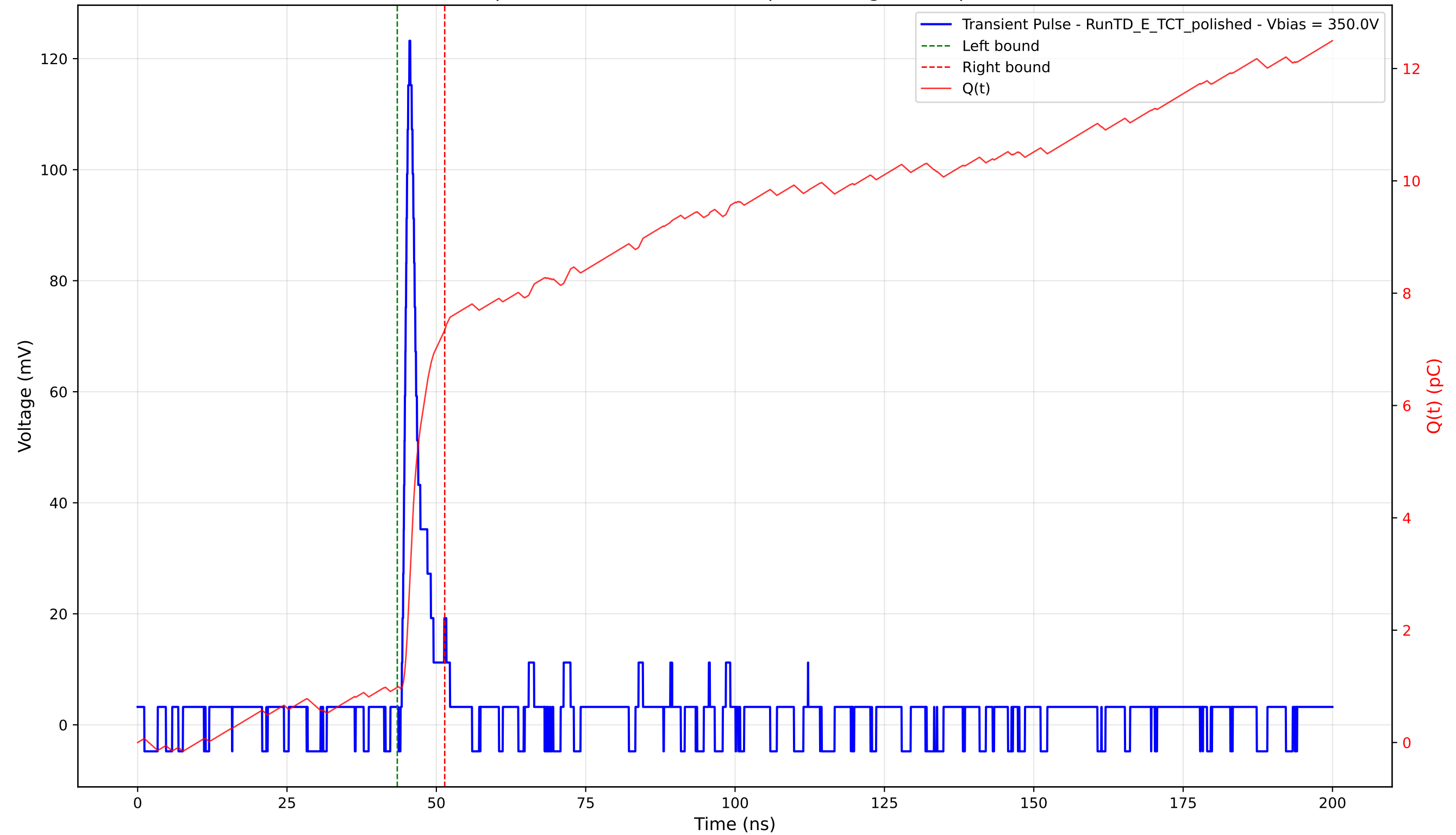
Transient Pulse - Sample: 4003 - Position: 135.0 \mu\text{m} - Charge: 6.37 pC - Rise Time: 0.98 ns
