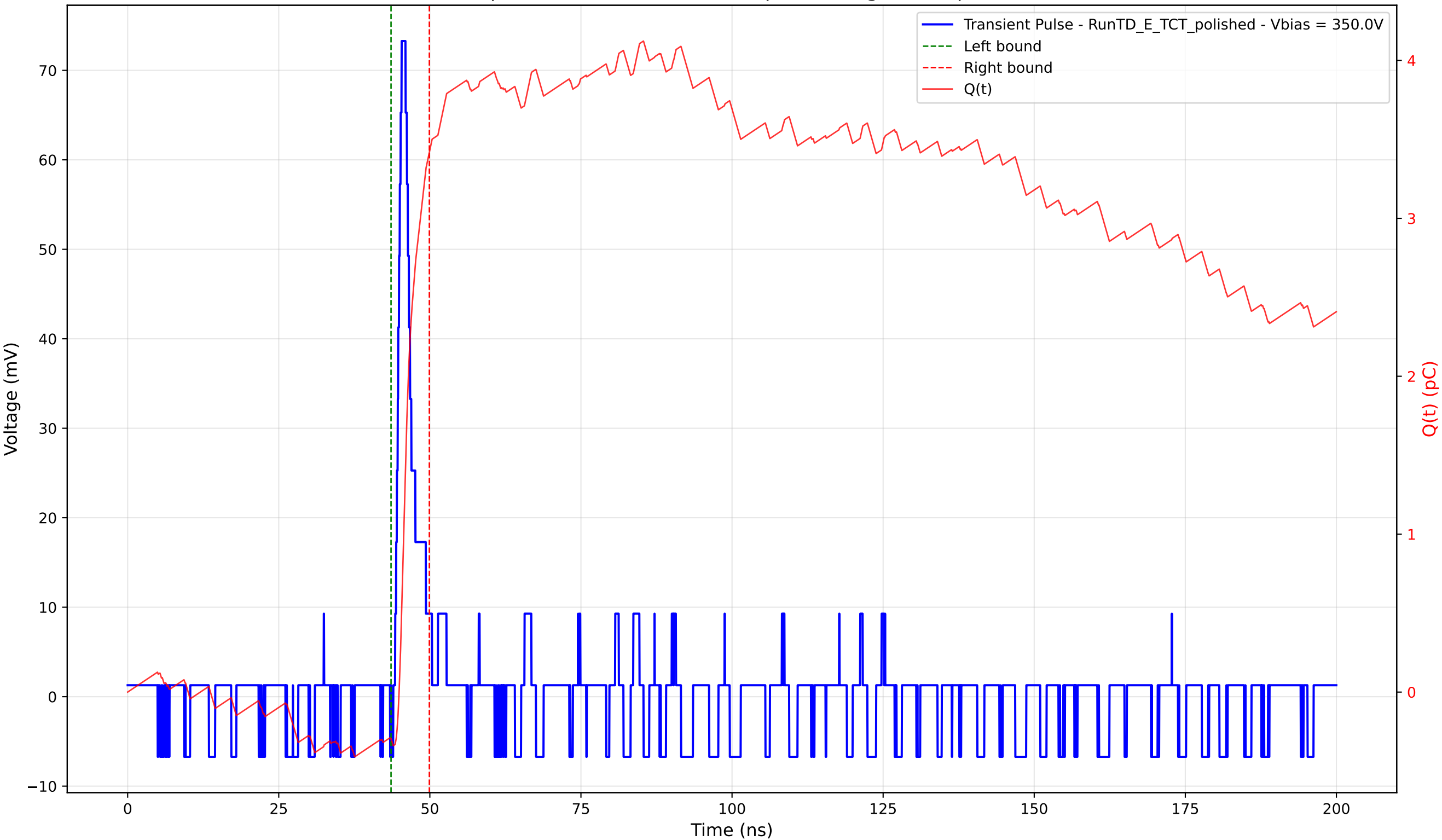
Transient Pulse - Sample: 4003 - Position: 120.0 \mu\text{m} - Charge: 3.72 pC - Rise Time: 1.06 ns
