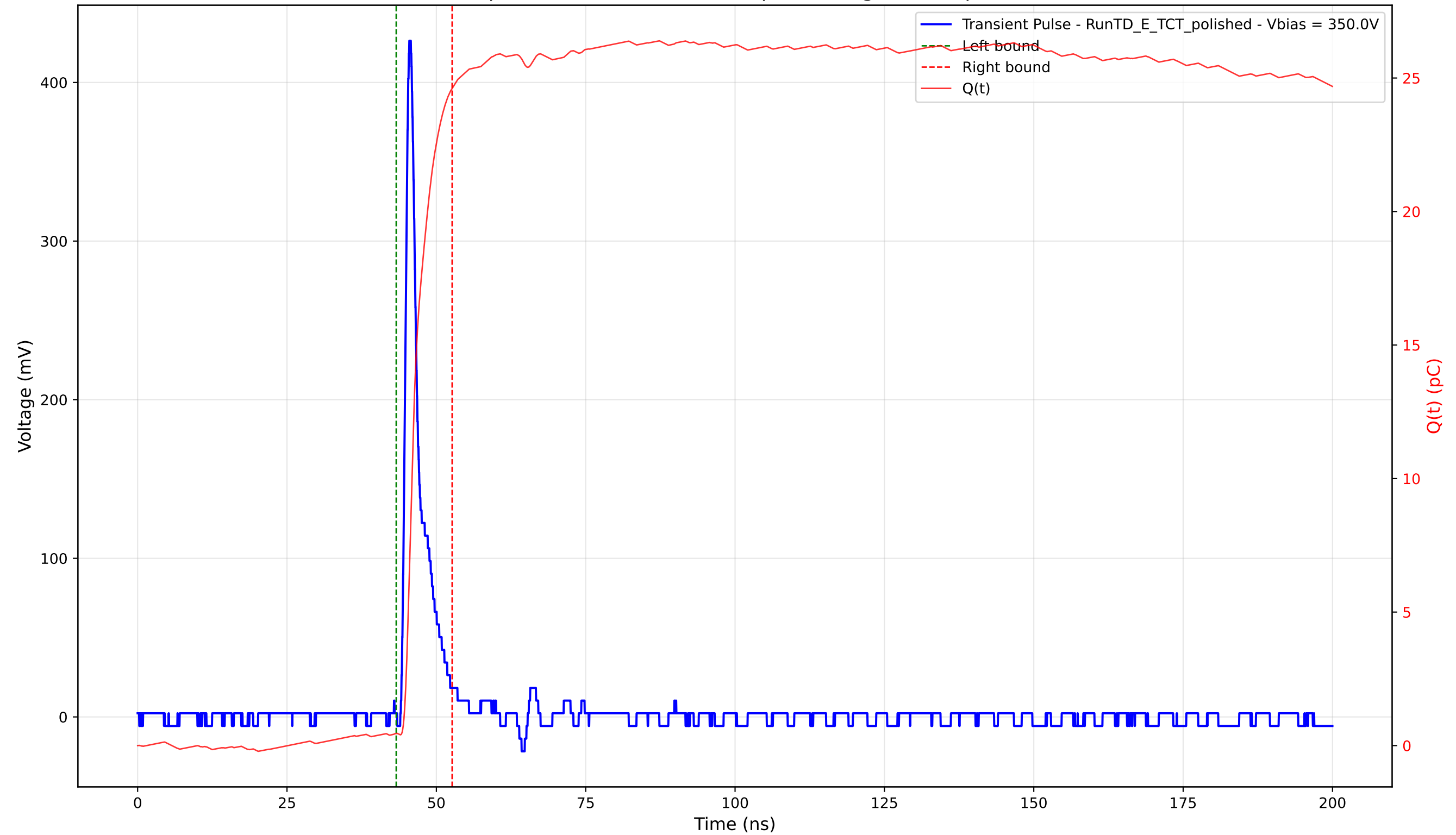
Transient Pulse - Sample: 4003 - Position: 225.0 \mu\text{m} - Charge: 24.16 pC - Rise Time: 0.96 ns
