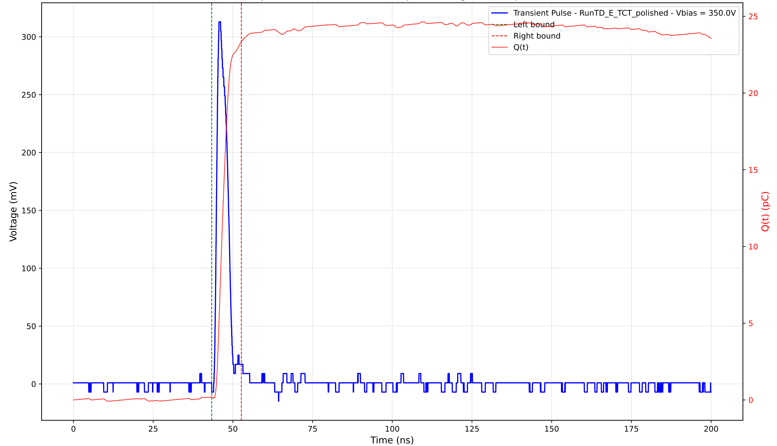
Transient Pulse - Sample: 4003 - Position: 460.0 \mu\text{m} - Charge: 23.15 pC - Rise Time: 1.12 ns
