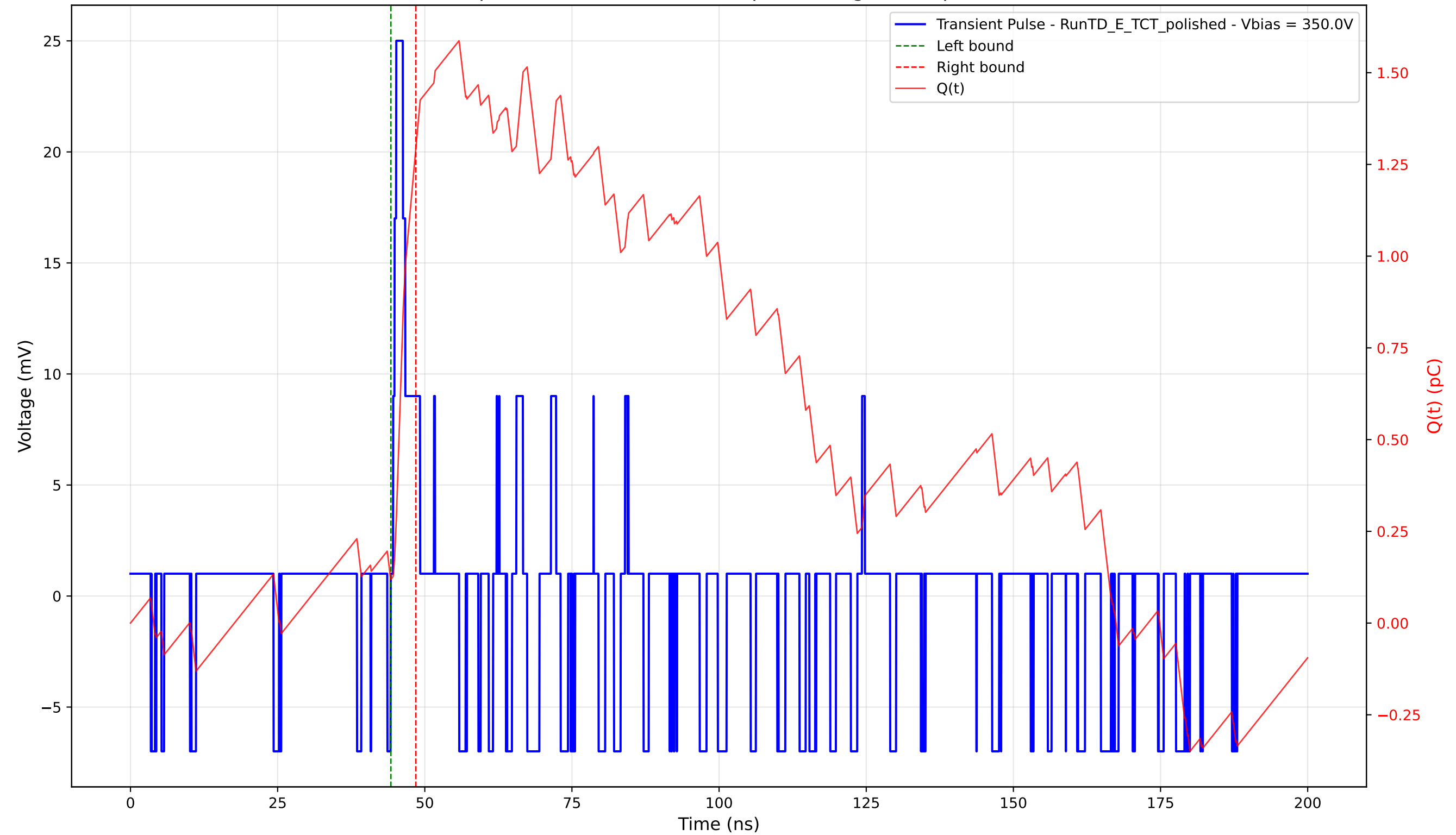
Transient Pulse - Sample: 4003 - Position: 765.0 \mu\text{m} - Charge: 1.18 pC - Rise Time: 0.54 ns
