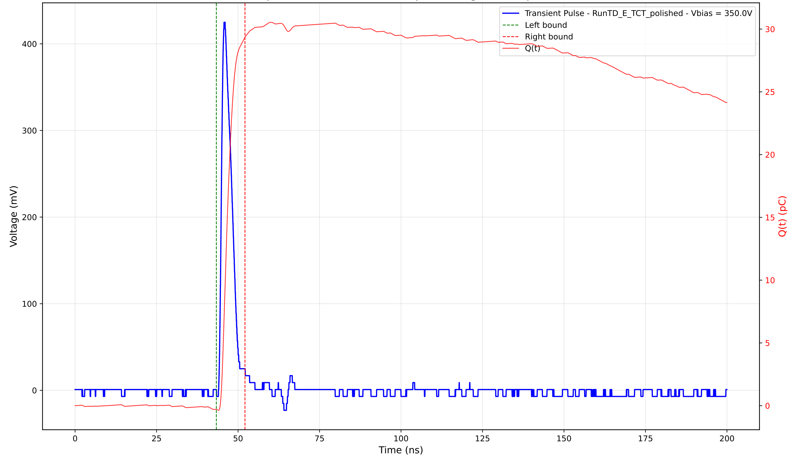
Transient Pulse - Sample: 4003 - Position: 410.0 \mu\text{m} - Charge: 29.64 pC - Rise Time: 1.06 ns
