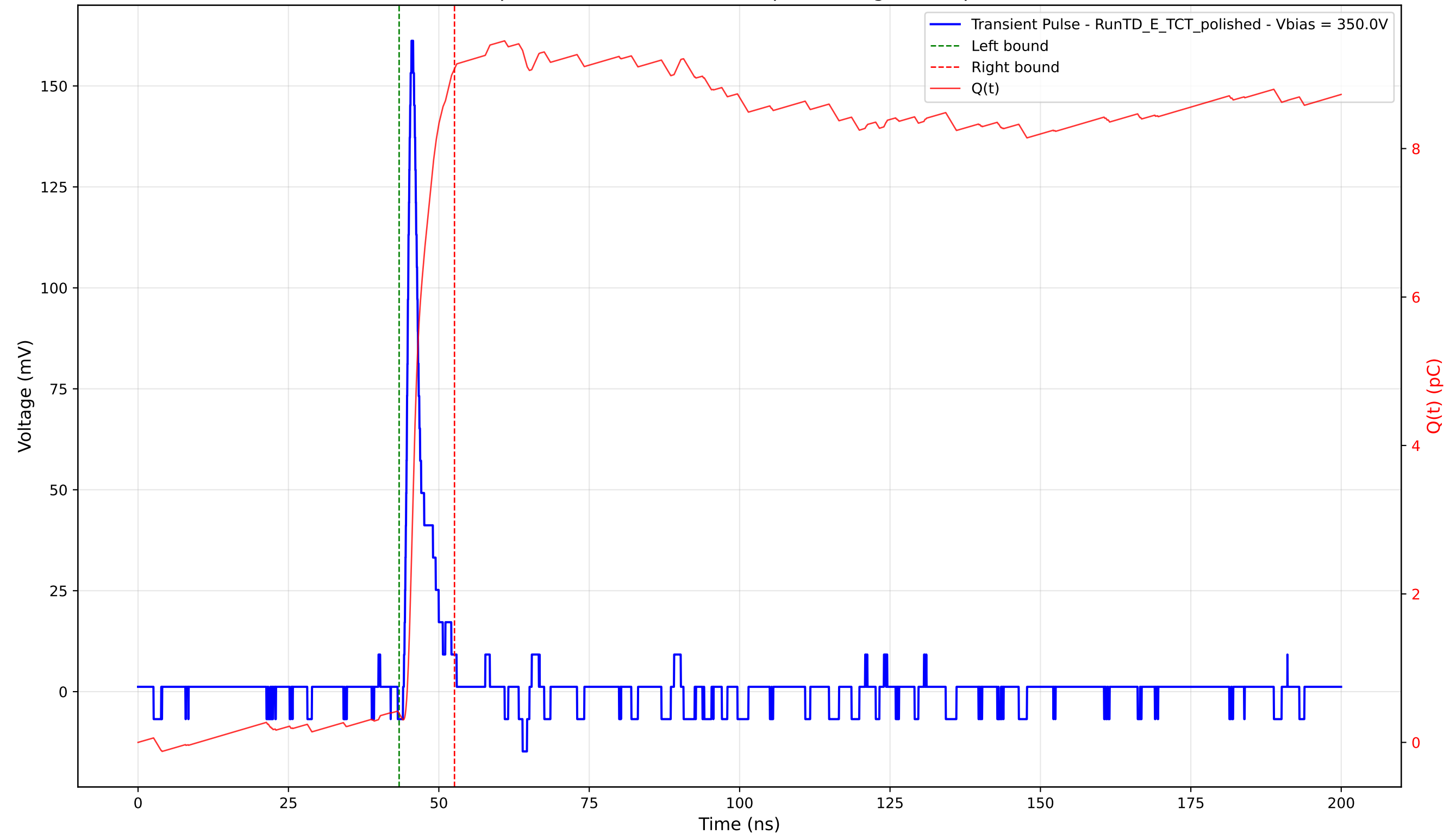
Transient Pulse - Sample: 4003 - Position: 150.0 \mu\text{m} - Charge: 8.69 pC - Rise Time: 0.92 ns
