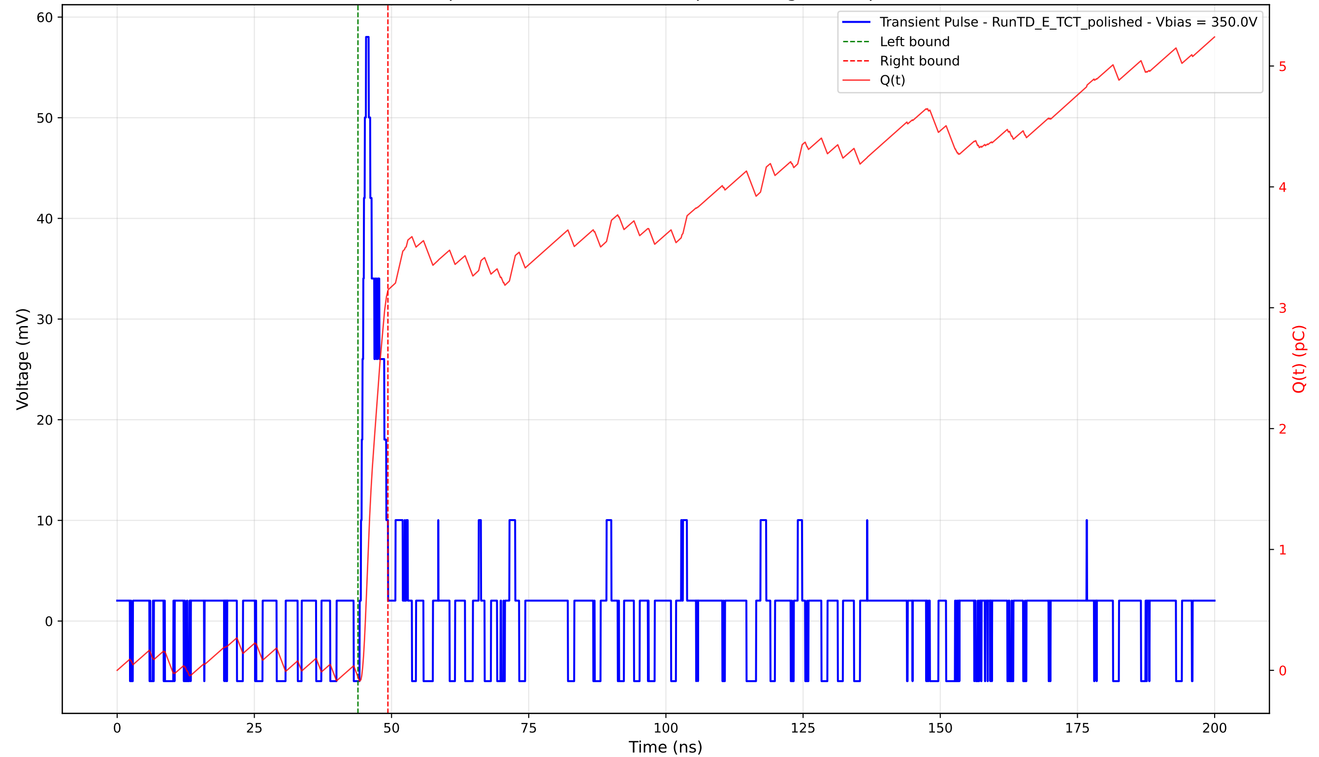
Transient Pulse - Sample: 4003 - Position: 590.0 \mu\text{m} - Charge: 3.20 pC - Rise Time: 0.93 ns
