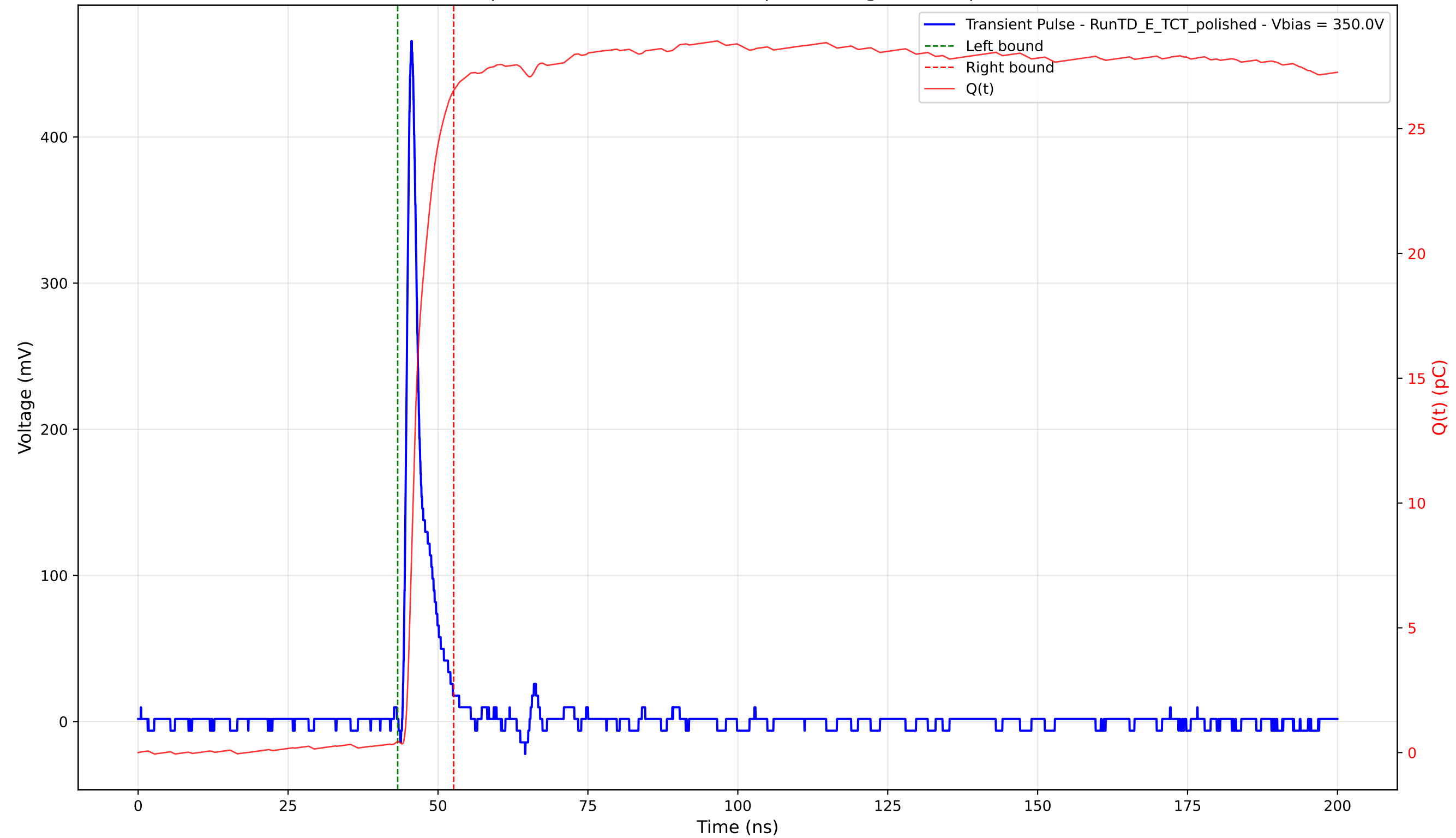
Transient Pulse - Sample: 4003 - Position: 235.0 \mu\text{m} - Charge: 26.10 pC - Rise Time: 0.97 ns
