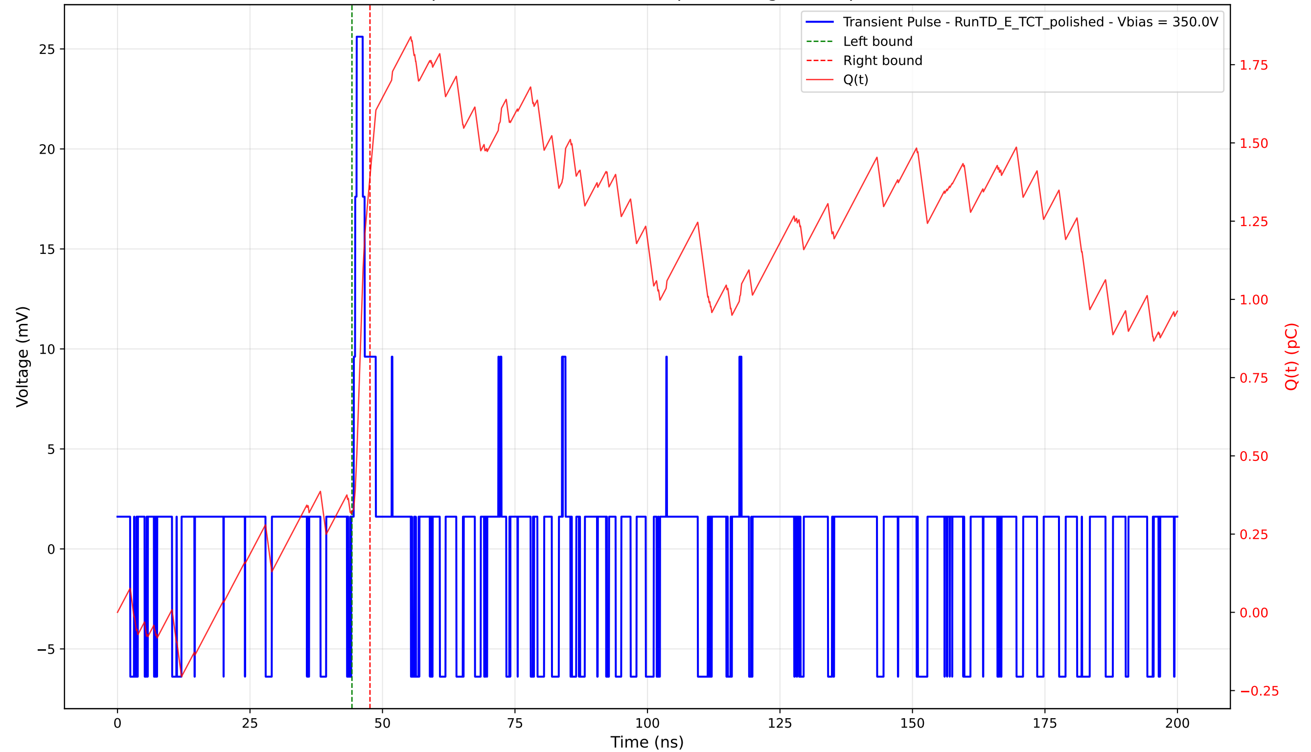
Transient Pulse - Sample: 4003 - Position: 770.0 \mu\text{m} - Charge: 1.07 pC - Rise Time: 0.56 ns
