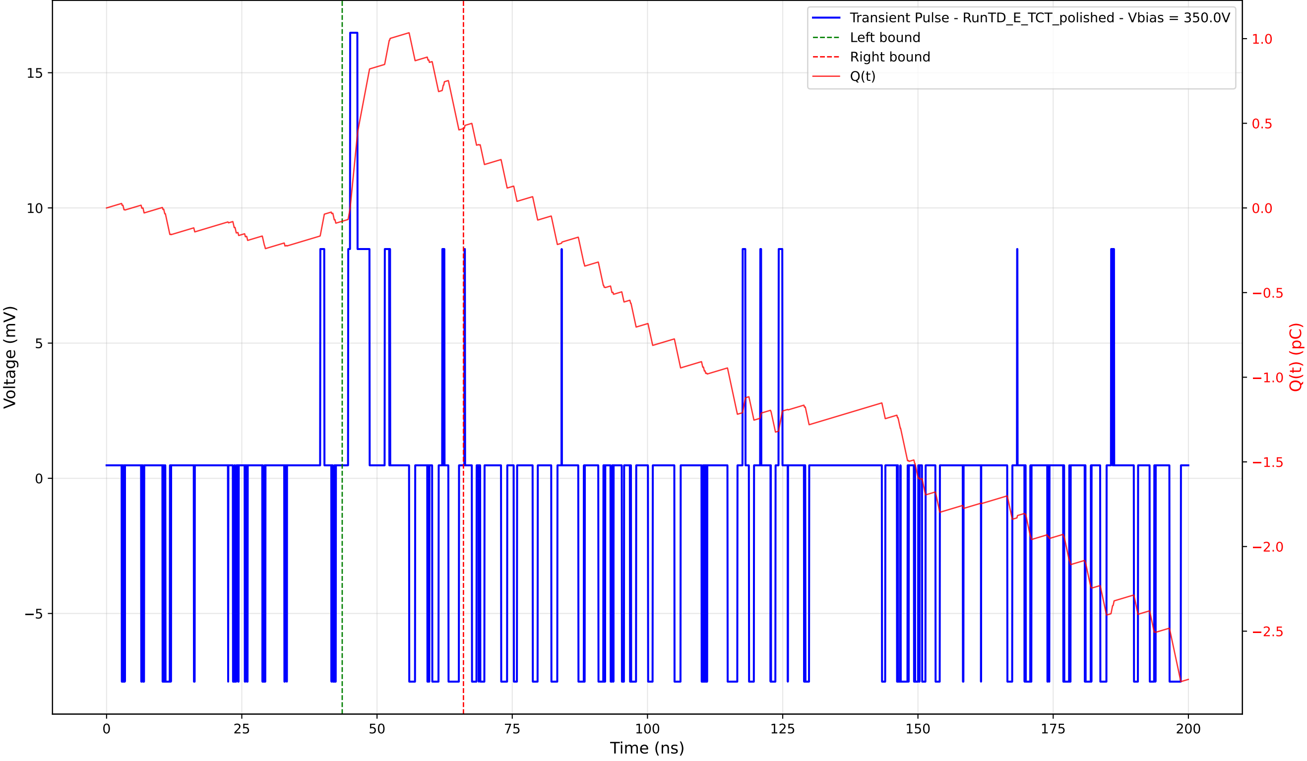
Transient Pulse - Sample: 4003 - Position: 40.0 \mu\text{m} - Charge: 0.55 pC - Rise Time: 0.38 ns
