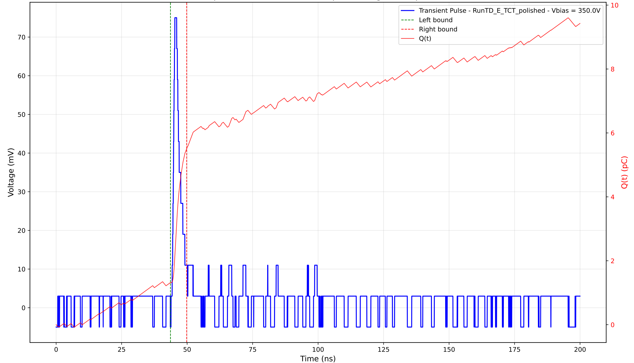
Transient Pulse - Sample: 4003 - Position: 685.0 \mu\text{m} - Charge: 4.19 pC - Rise Time: 1.01 ns
