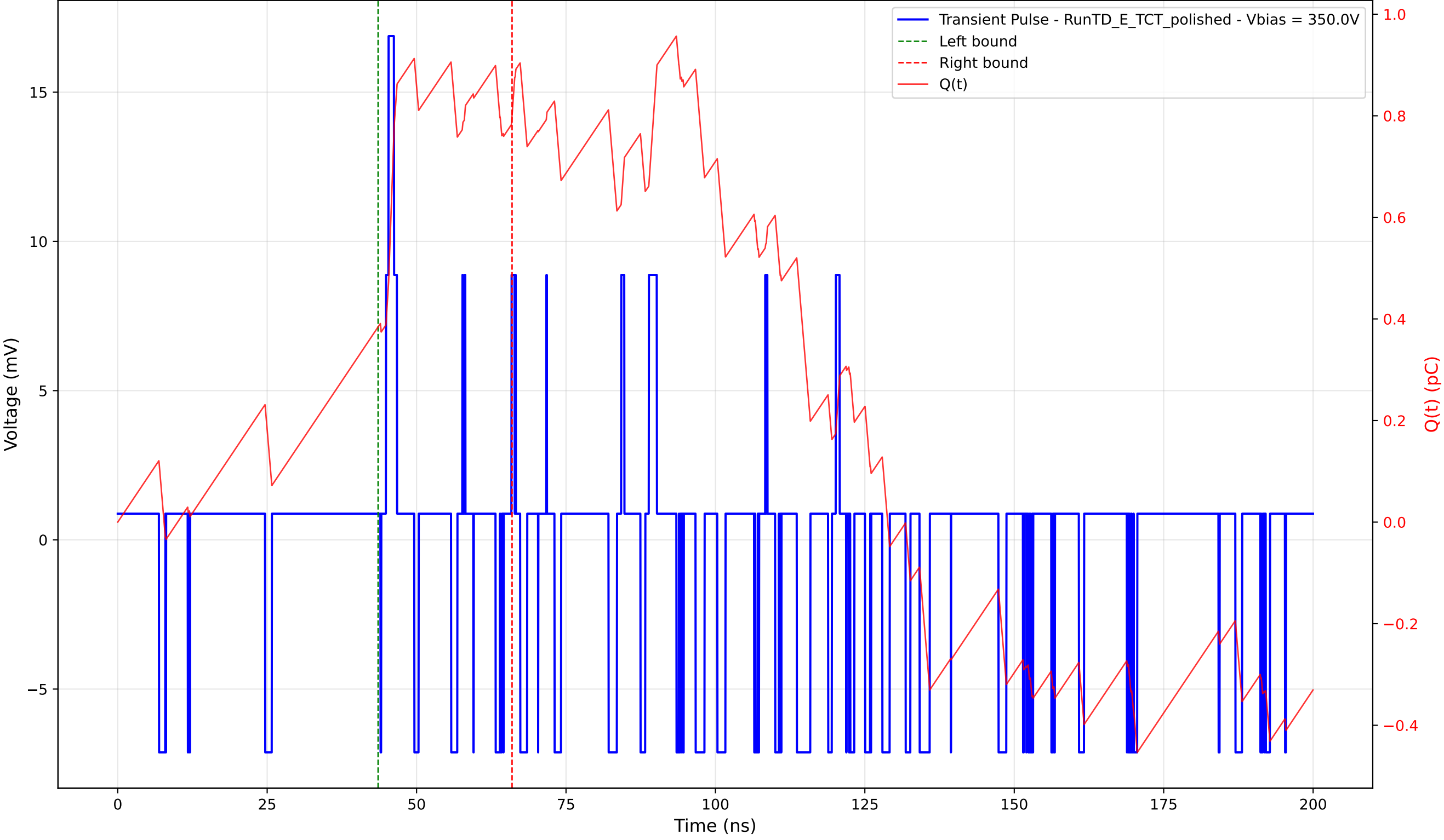
Transient Pulse - Sample: 4003 - Position: 10.0 \mu\text{m} - Charge: 0.41 pC - Rise Time: 0.44 ns
