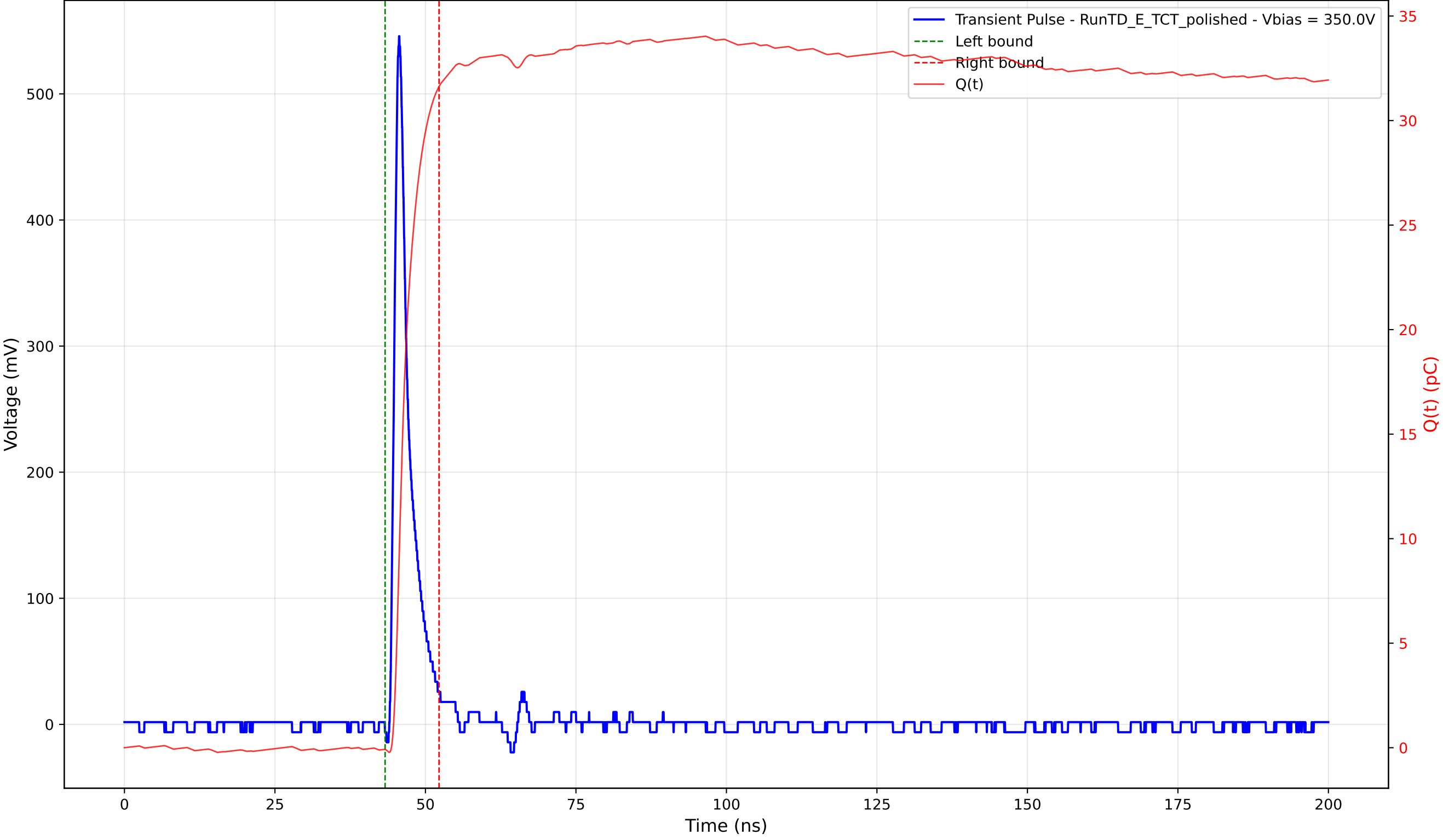
Transient Pulse - Sample: 4003 - Position: 290.0 \mu\text{m} - Charge: 31.71 pC - Rise Time: 1.01 ns
