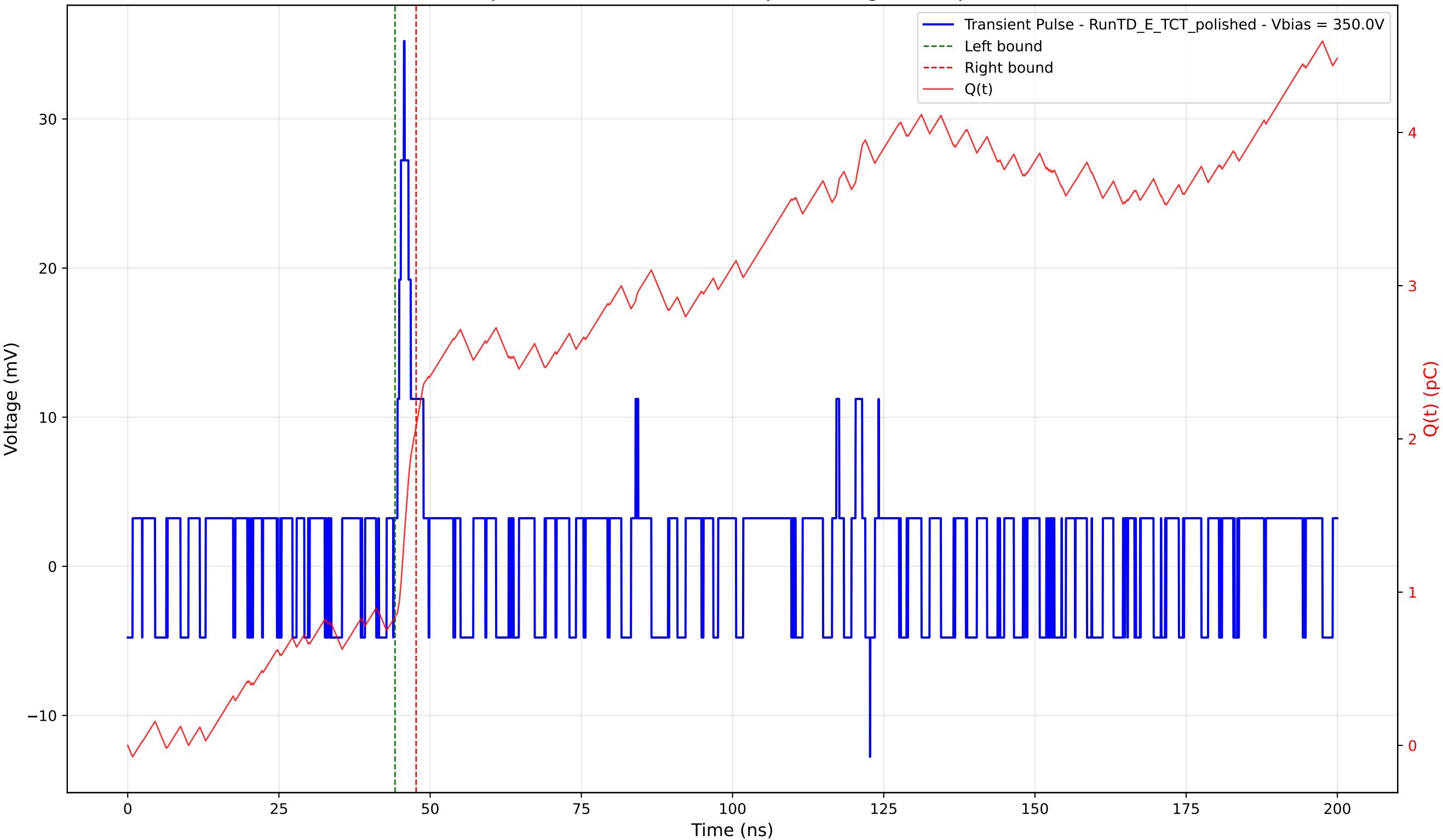
Transient Pulse - Sample: 4003 - Position: 790.0 \mu\text{m} - Charge: 1.25 pC - Rise Time: 1.08 ns
