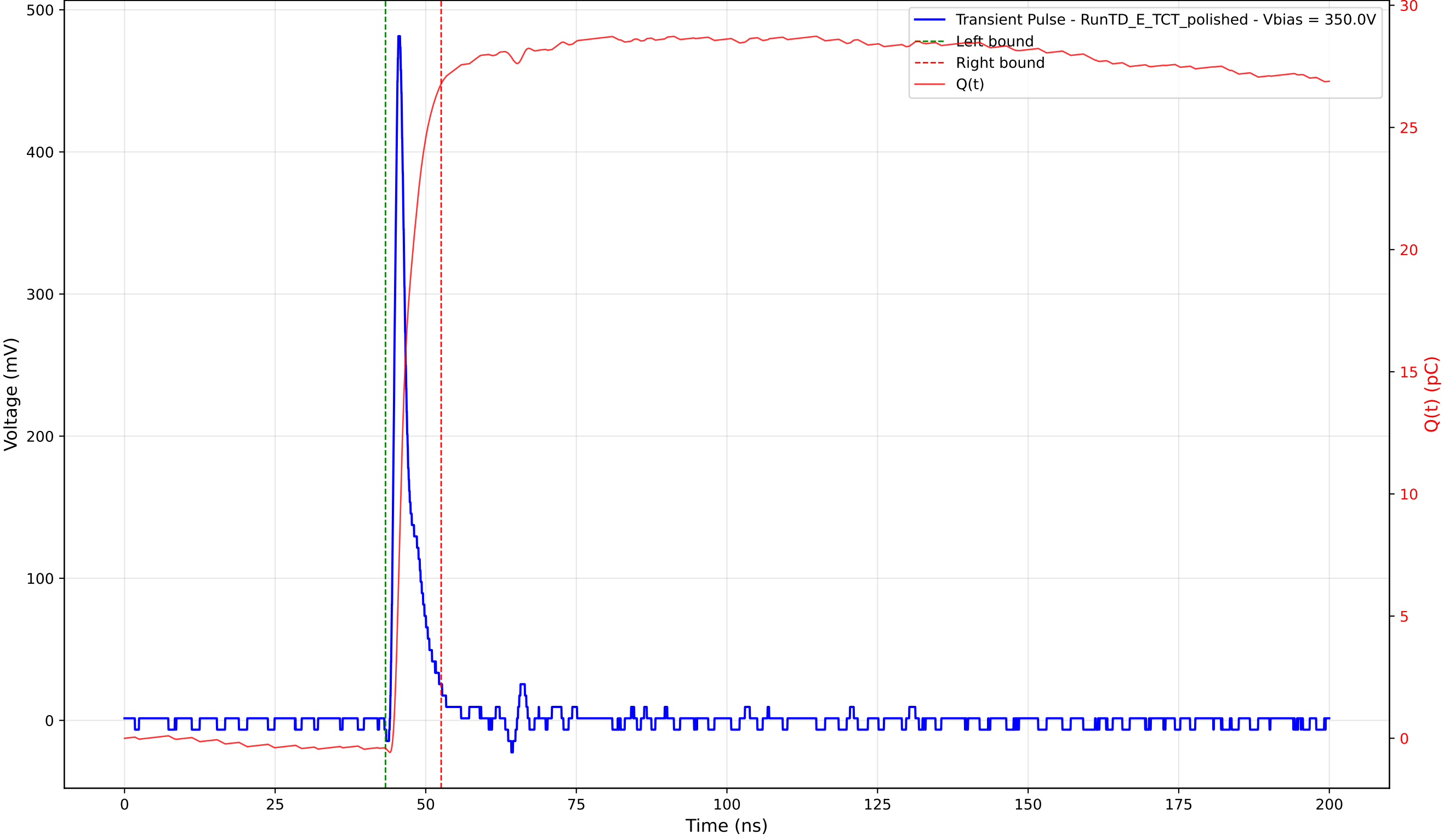
Transient Pulse - Sample: 4003 - Position: 245.0 \mu\text{m} - Charge: 27.20 pC - Rise Time: 0.96 ns
