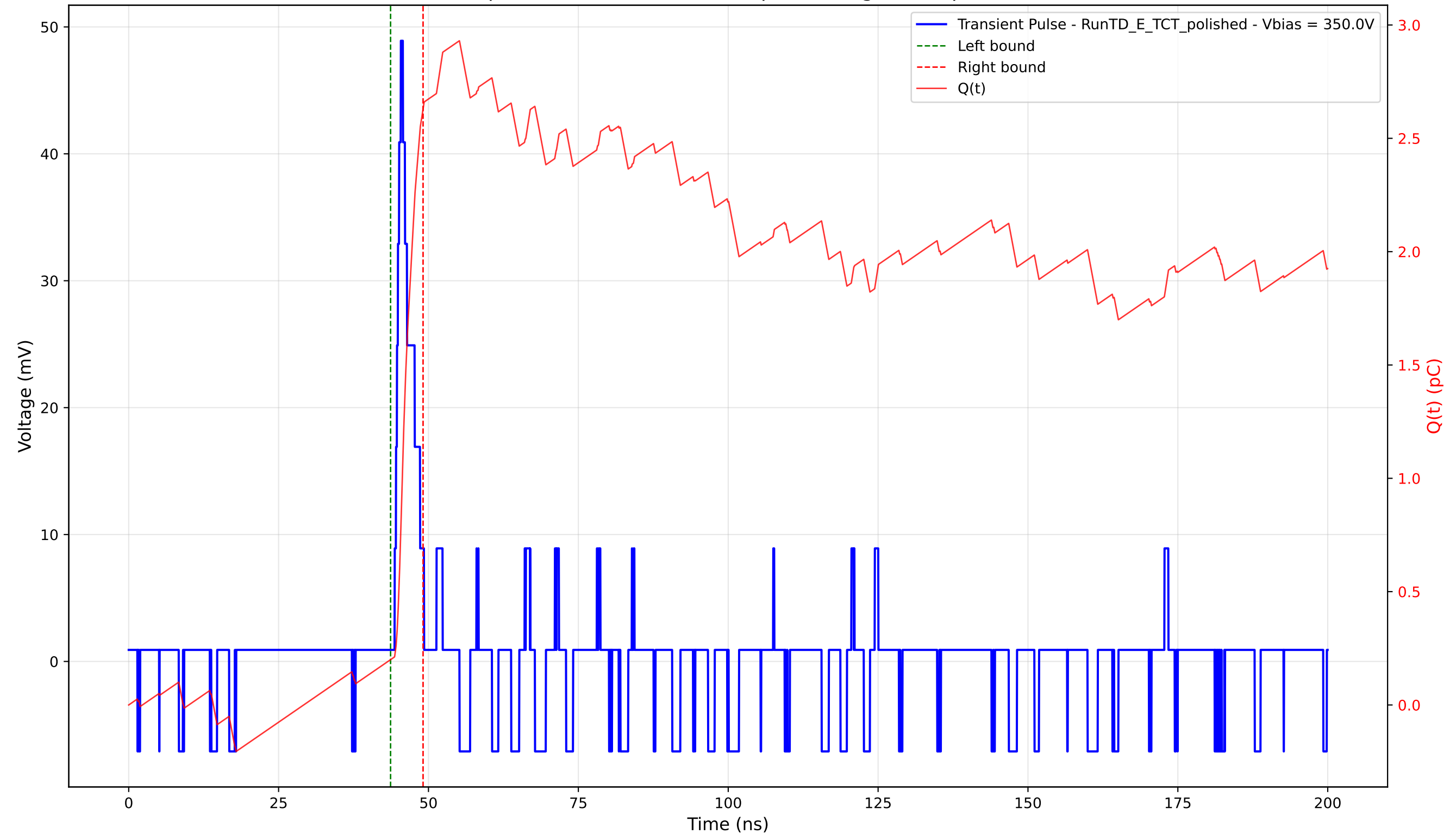
Transient Pulse - Sample: 4003 - Position: 700.0 \mu\text{m} - Charge: 2.43 pC - Rise Time: 1.03 ns
