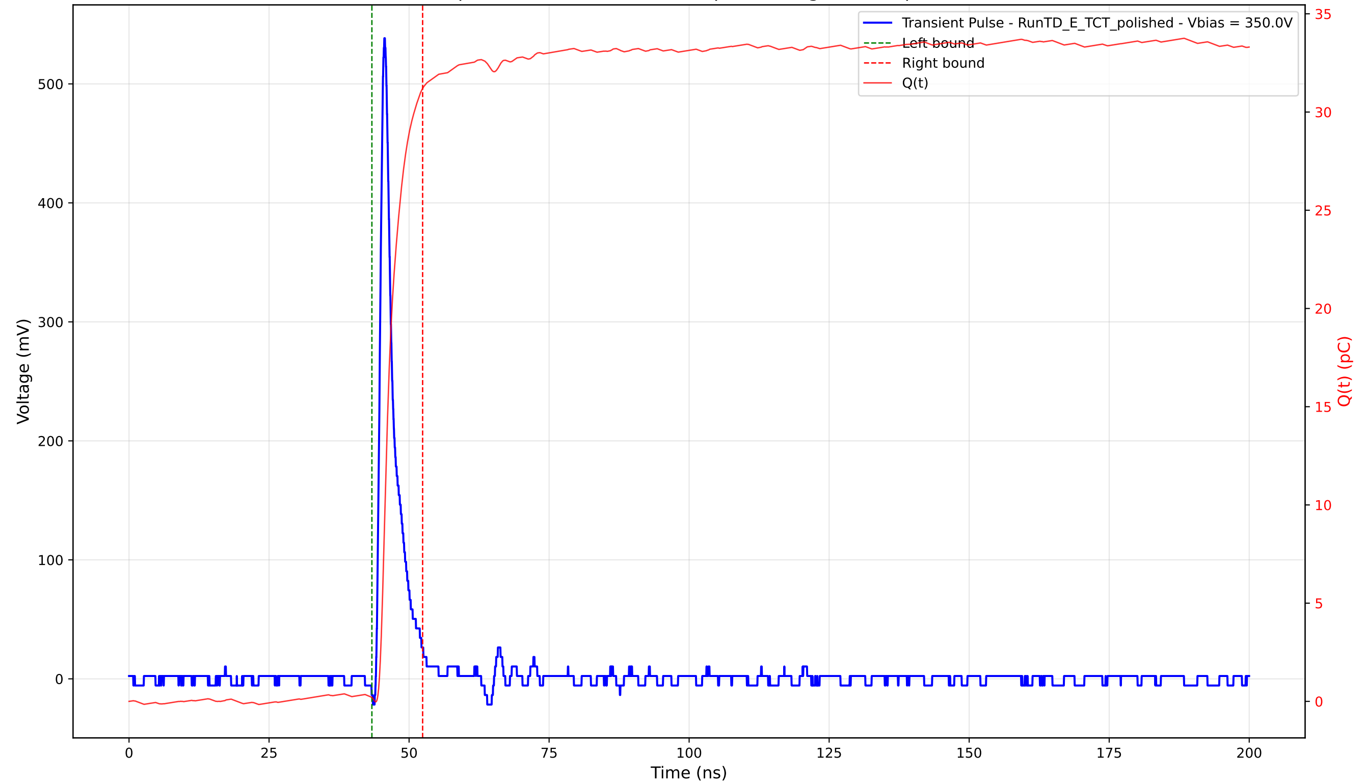
Transient Pulse - Sample: 4003 - Position: 280.0 \mu\text{m} - Charge: 31.00 pC - Rise Time: 0.99 ns
