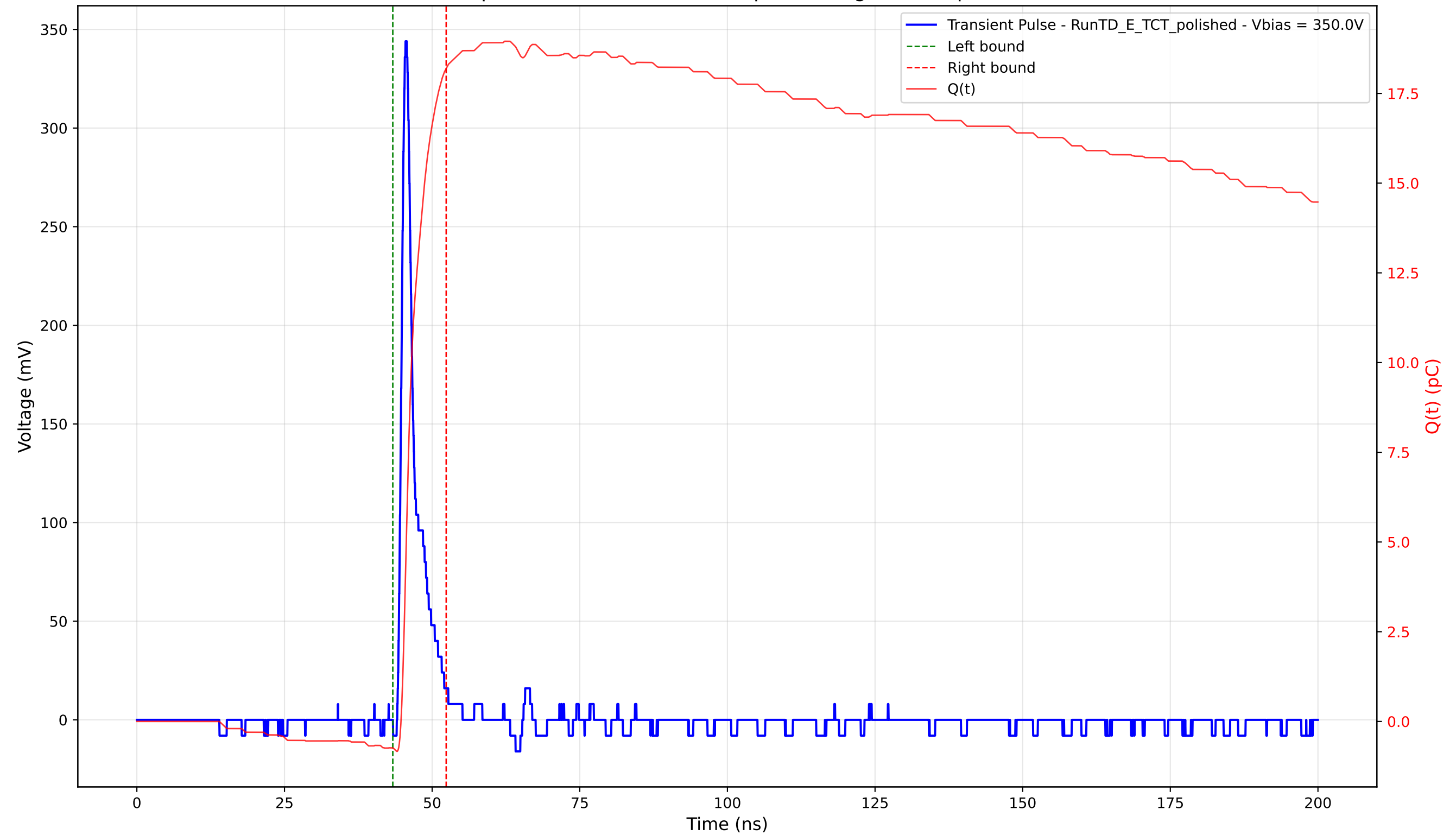
Transient Pulse - Sample: 4003 - Position: 200.0 \mu\text{m} - Charge: 18.93 pC - Rise Time: 0.95 ns
