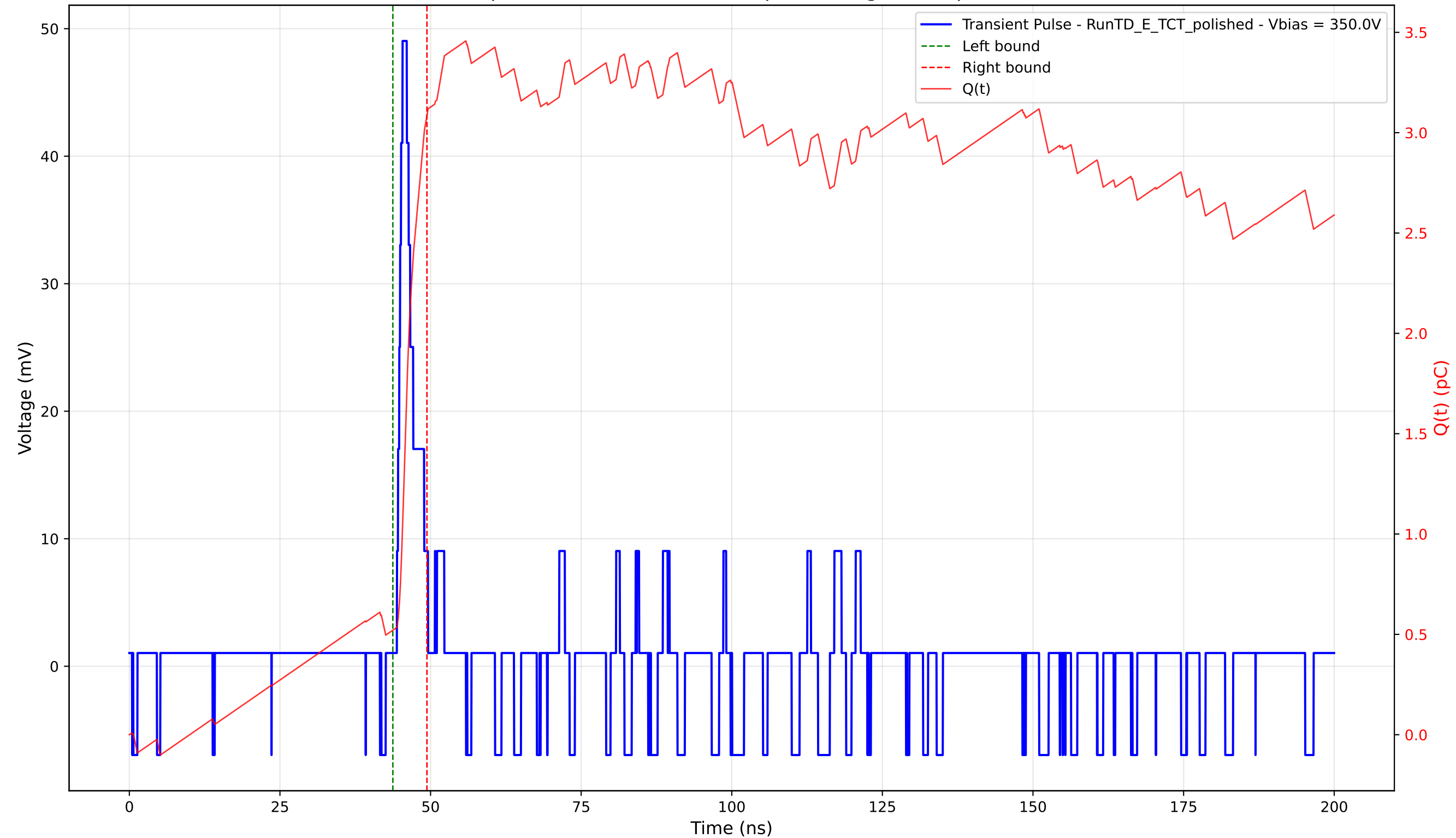
Transient Pulse - Sample: 4003 - Position: 610.0 \mu\text{m} - Charge: 2.57 pC - Rise Time: 0.93 ns
