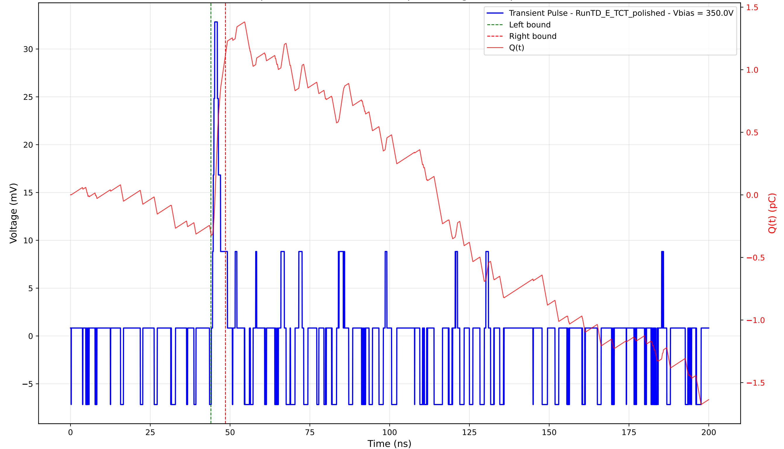
Transient Pulse - Sample: 4003 - Position: 750.0 \mu\text{m} - Charge: 1.43 pC - Rise Time: 0.67 ns
