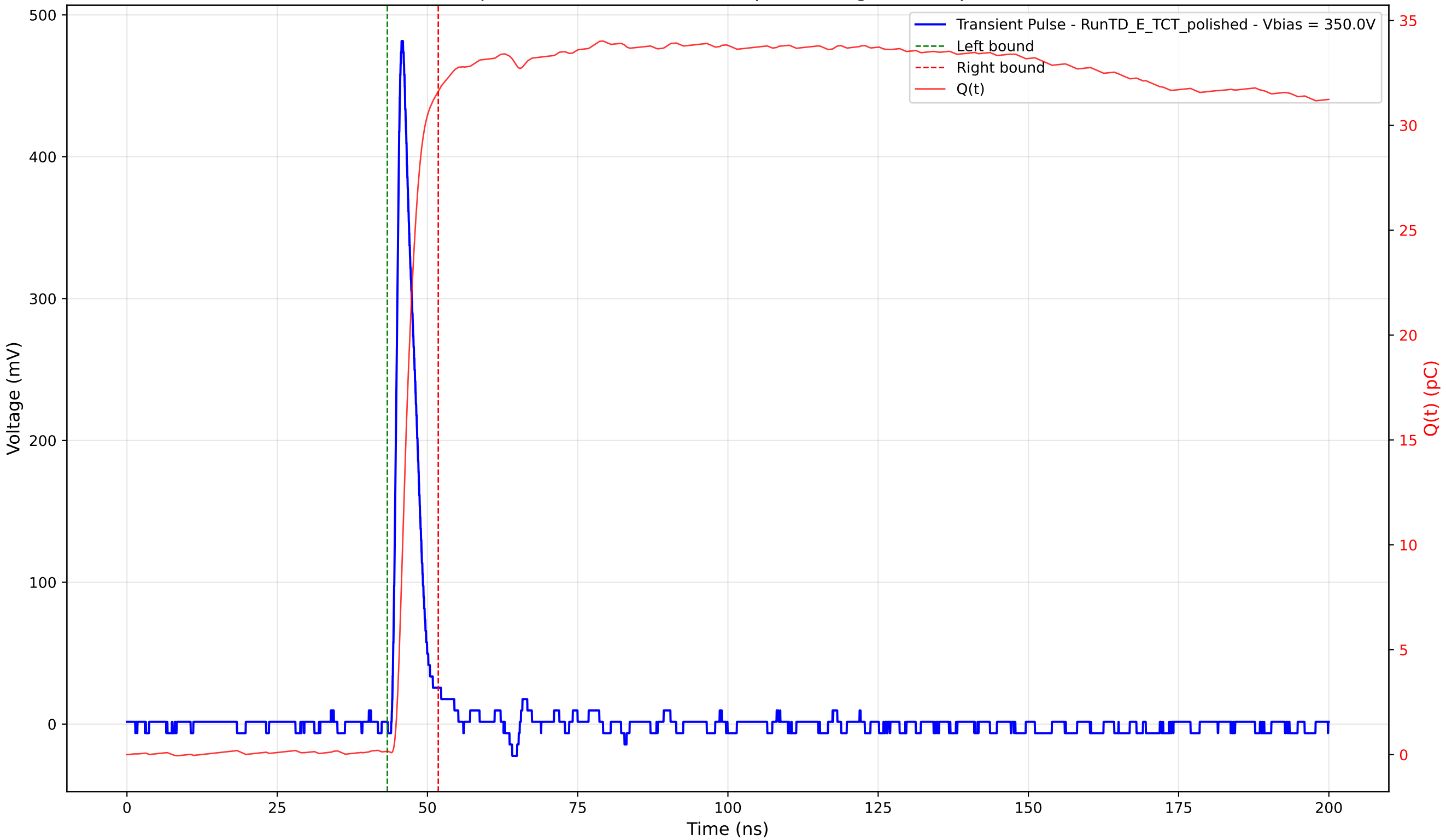
Transient Pulse - Sample: 4003 - Position: 380.0 \mu\text{m} - Charge: 31.46 pC - Rise Time: 1.06 ns
