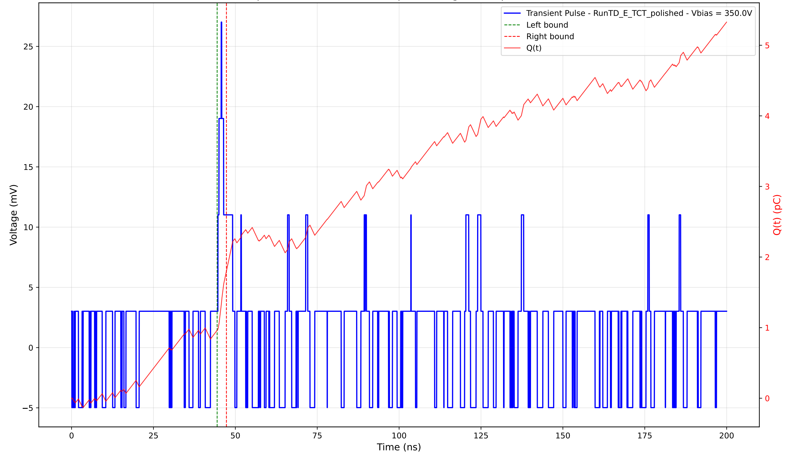
Transient Pulse - Sample: 4003 - Position: 50.0 \mu\text{m} - Charge: 0.84 pC - Rise Time: 0.00 ns (N/A)
