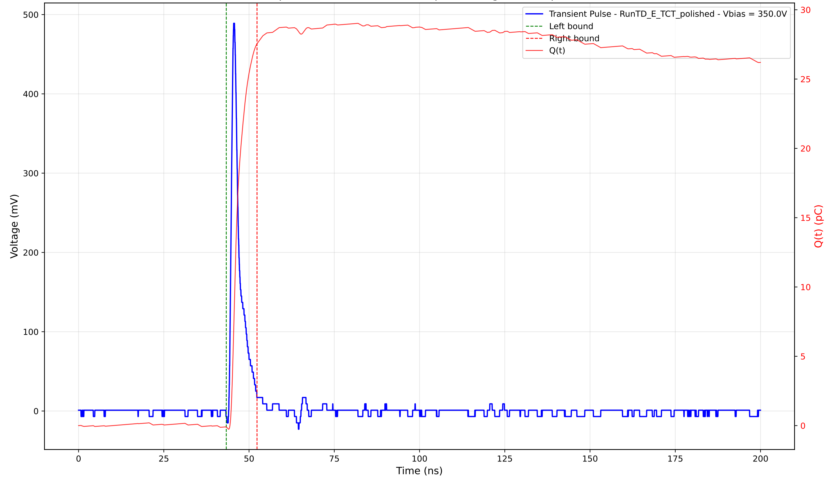
Transient Pulse - Sample: 4003 - Position: 250.0 \mu\text{m} - Charge: 27.65 pC - Rise Time: 0.96 ns
