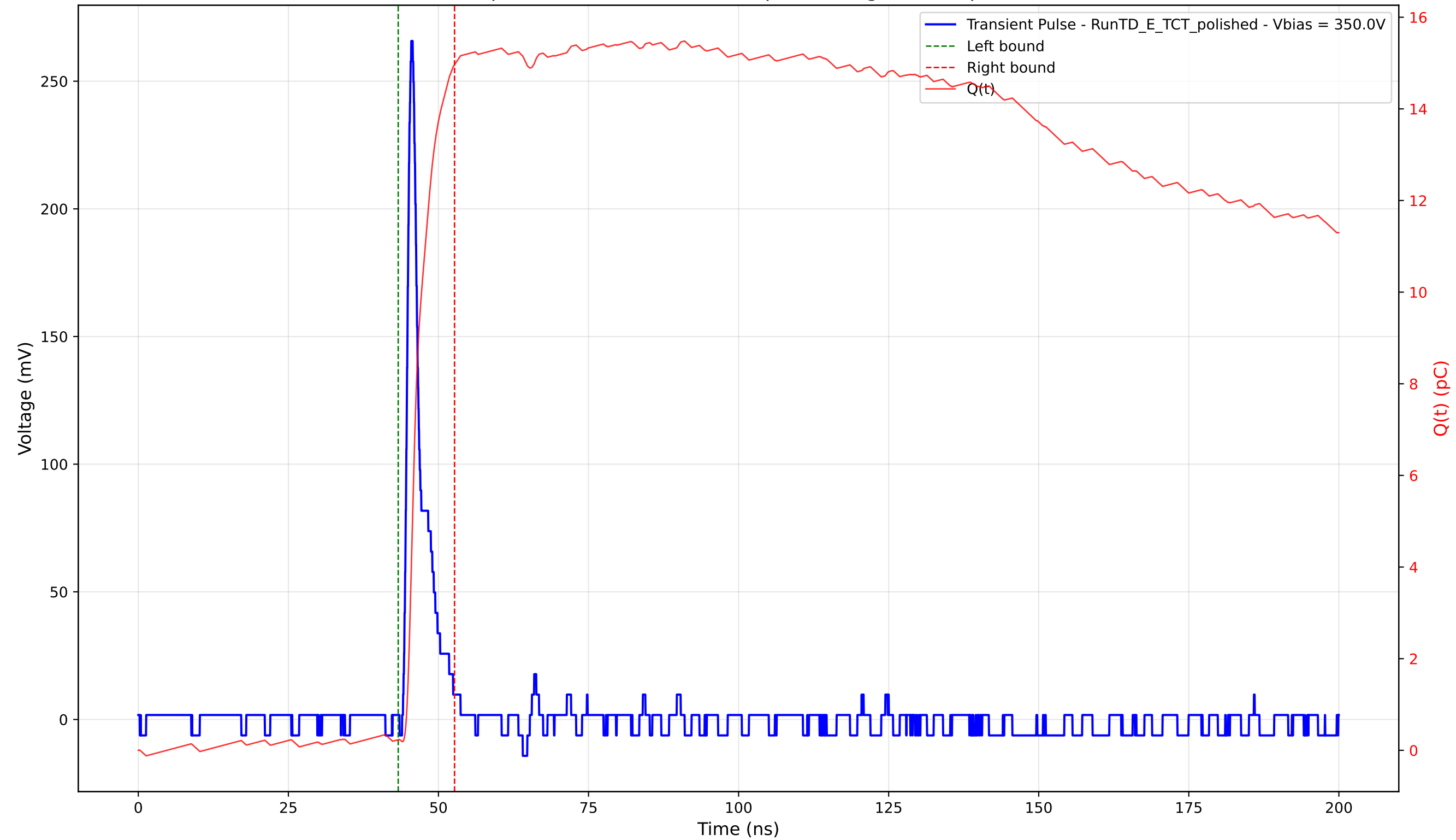
Transient Pulse - Sample: 4003 - Position: 180.0 \mu\text{m} - Charge: 14.73 pC - Rise Time: 0.94 ns
