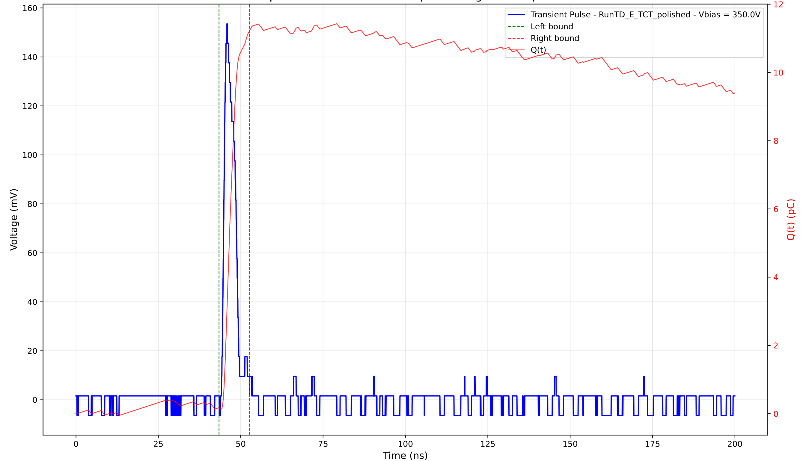
Transient Pulse - Sample: 4003 - Position: 530.0 \mu\text{m} - Charge: 11.05 pC - Rise Time: 1.23 ns
