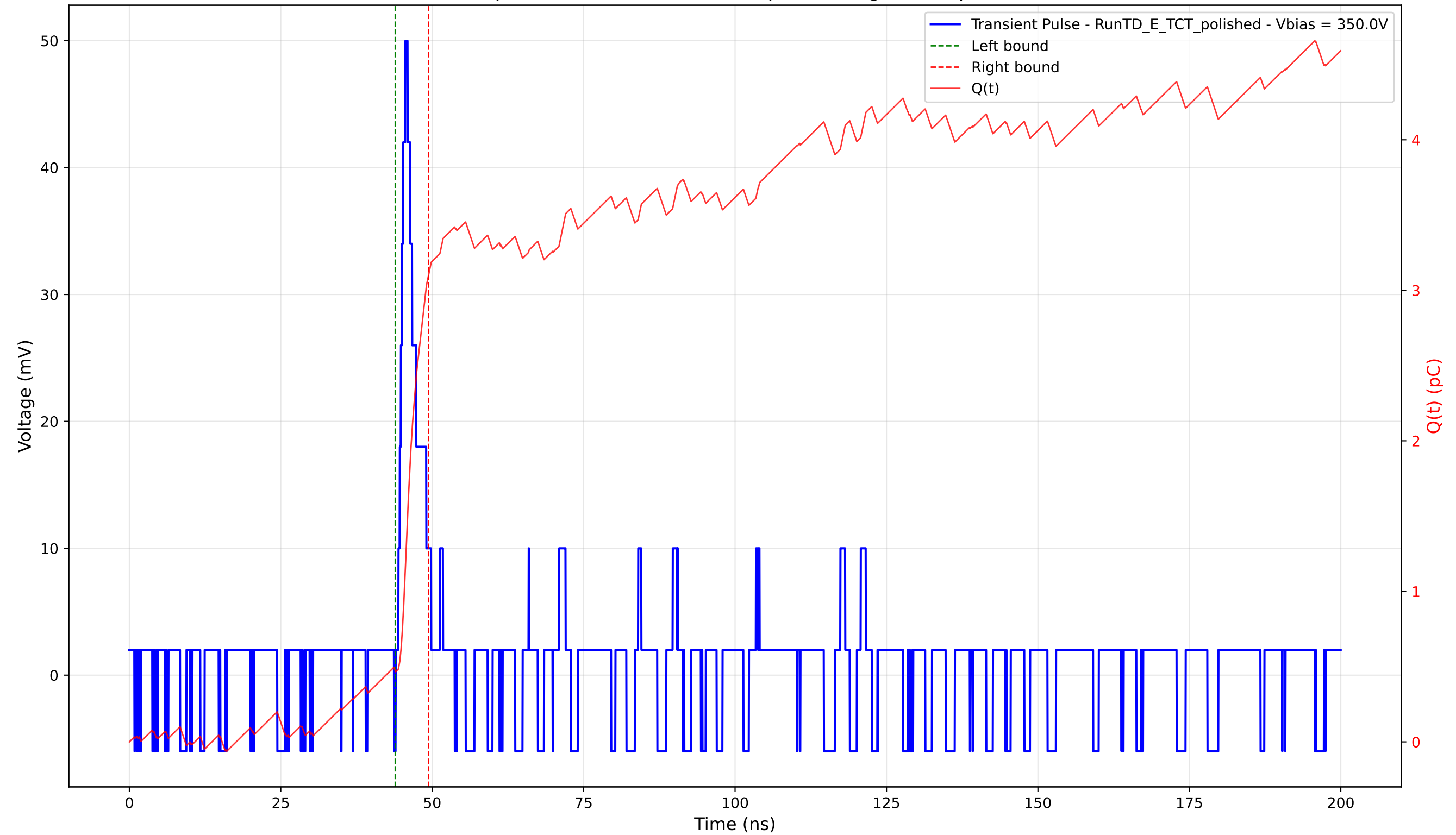
Transient Pulse - Sample: 4003 - Position: 600.0 \mu\text{m} - Charge: 2.63 pC - Rise Time: 1.15 ns
