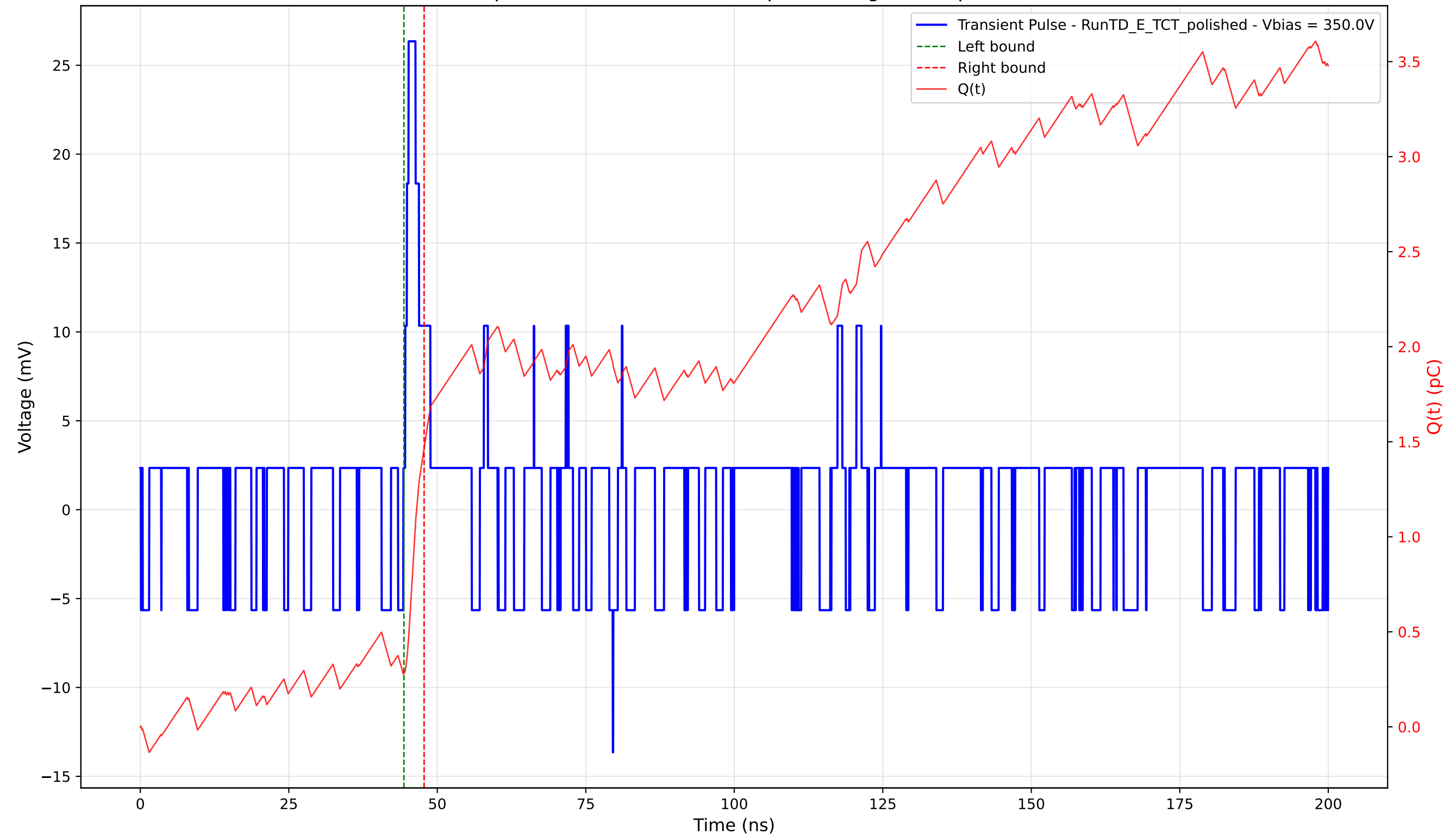
Transient Pulse - Sample: 4003 - Position: 775.0 \mu\text{m} - Charge: 1.19 pC - Rise Time: 0.58 ns
