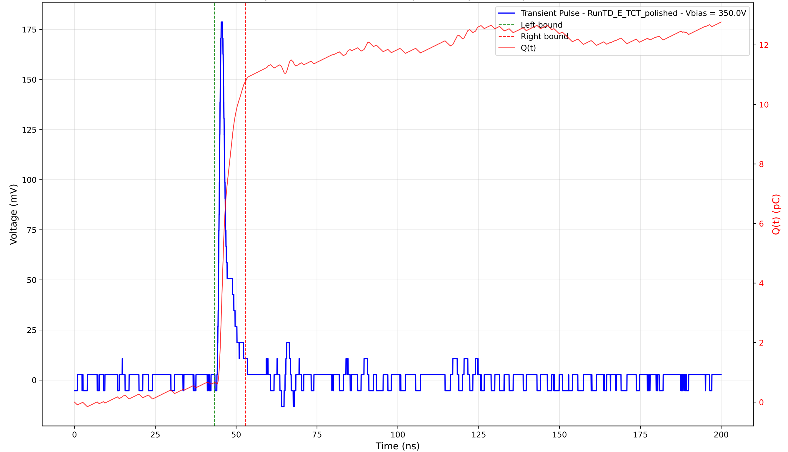
Transient Pulse - Sample: 4003 - Position: 155.0 \mu\text{m} - Charge: 10.11 pC - Rise Time: 0.92 ns
