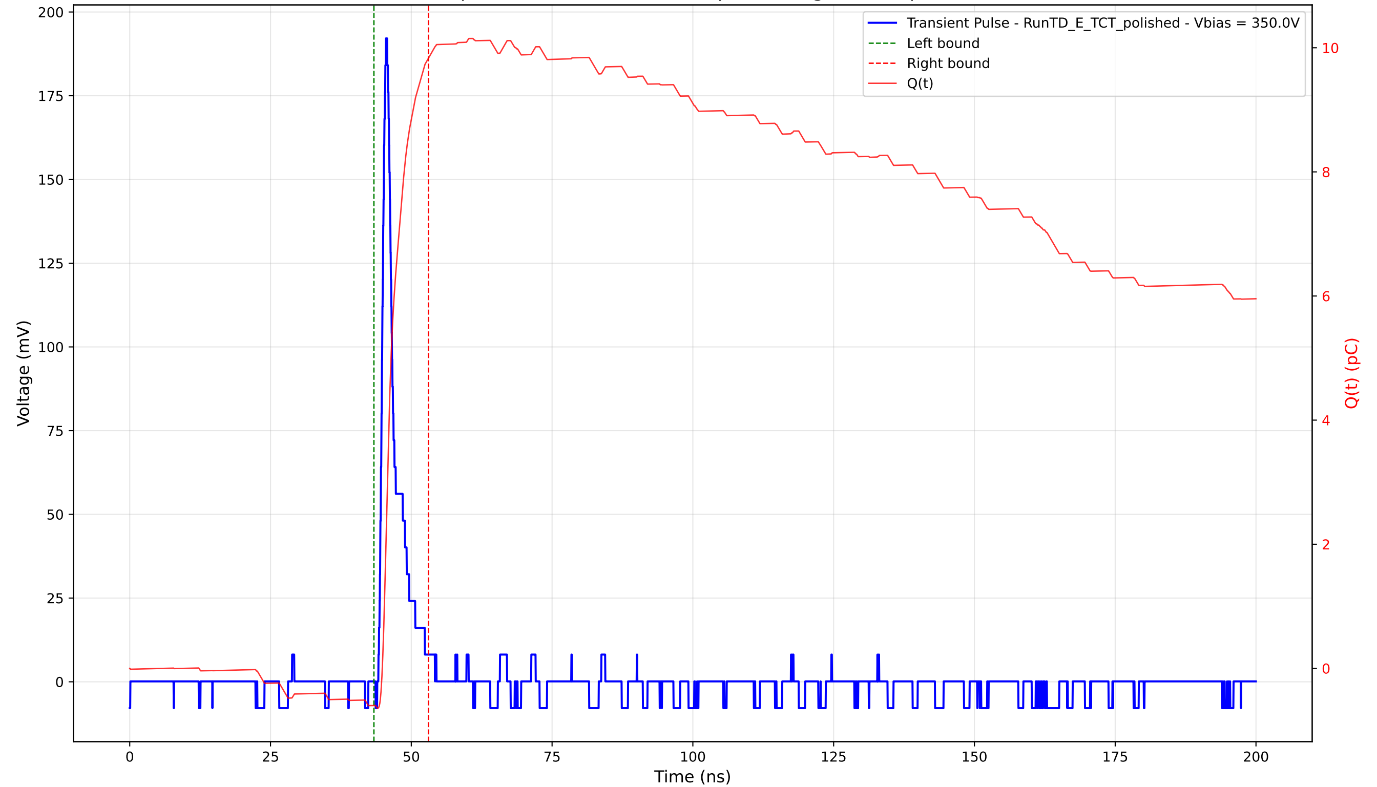
Transient Pulse - Sample: 4003 - Position: 160.0 \mu\text{m} - Charge: 10.43 pC - Rise Time: 0.95 ns
