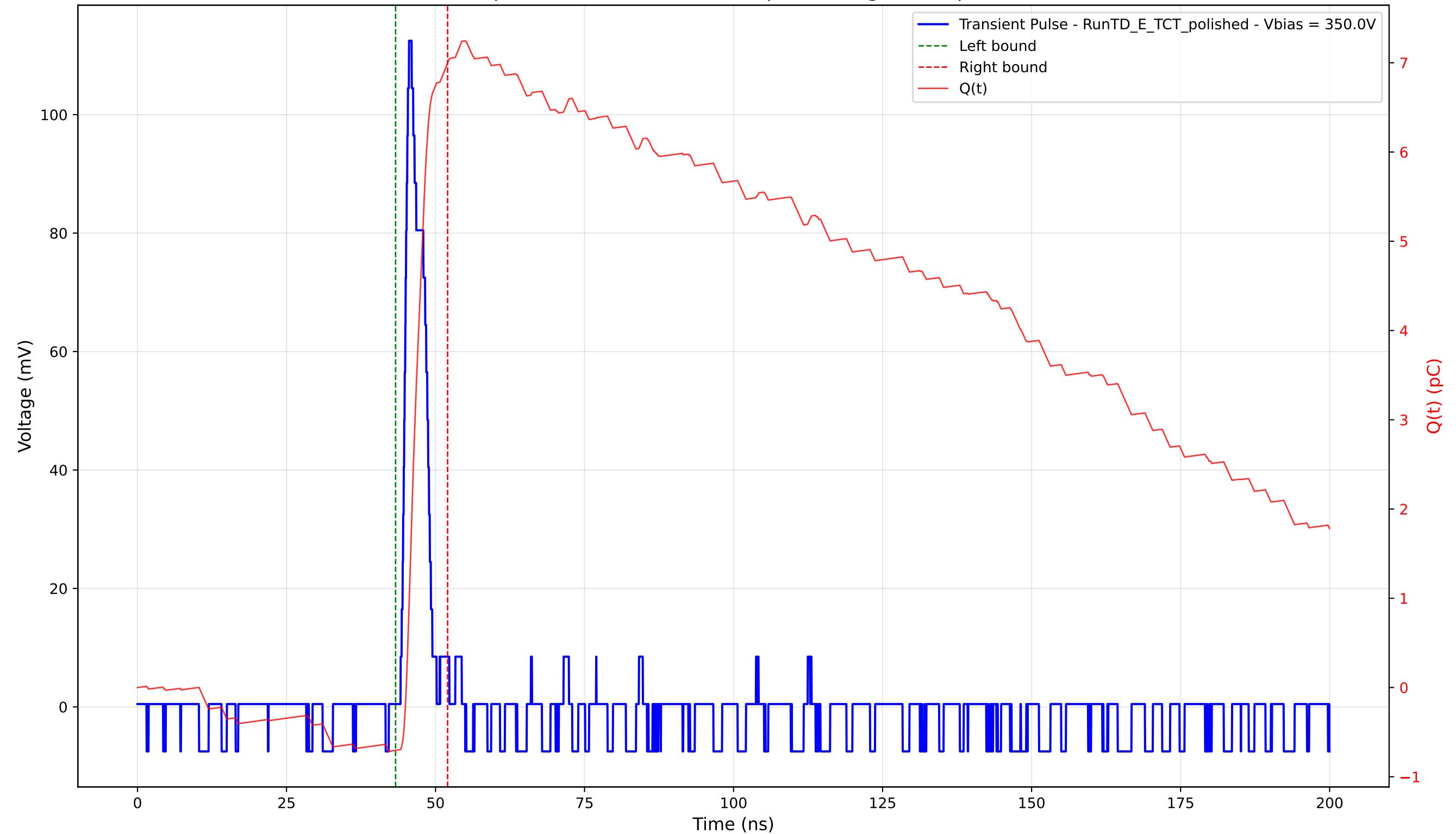
Transient Pulse - Sample: 4003 - Position: 550.0 \mu\text{m} - Charge: 7.70 pC - Rise Time: 1.05 ns
