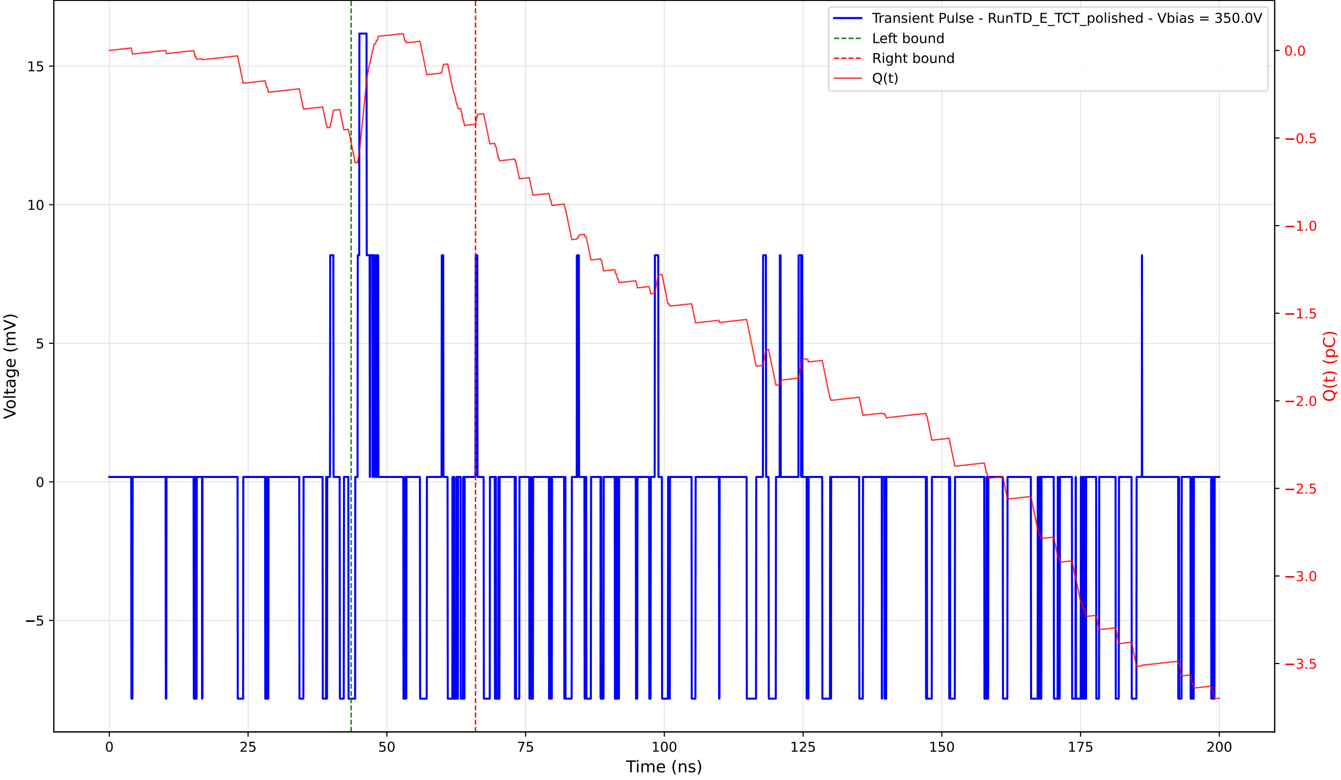
Transient Pulse - Sample: 4003 - Position: 20.0 \mu\text{m} - Charge: 0.11 pC - Rise Time: 0.32 ns
