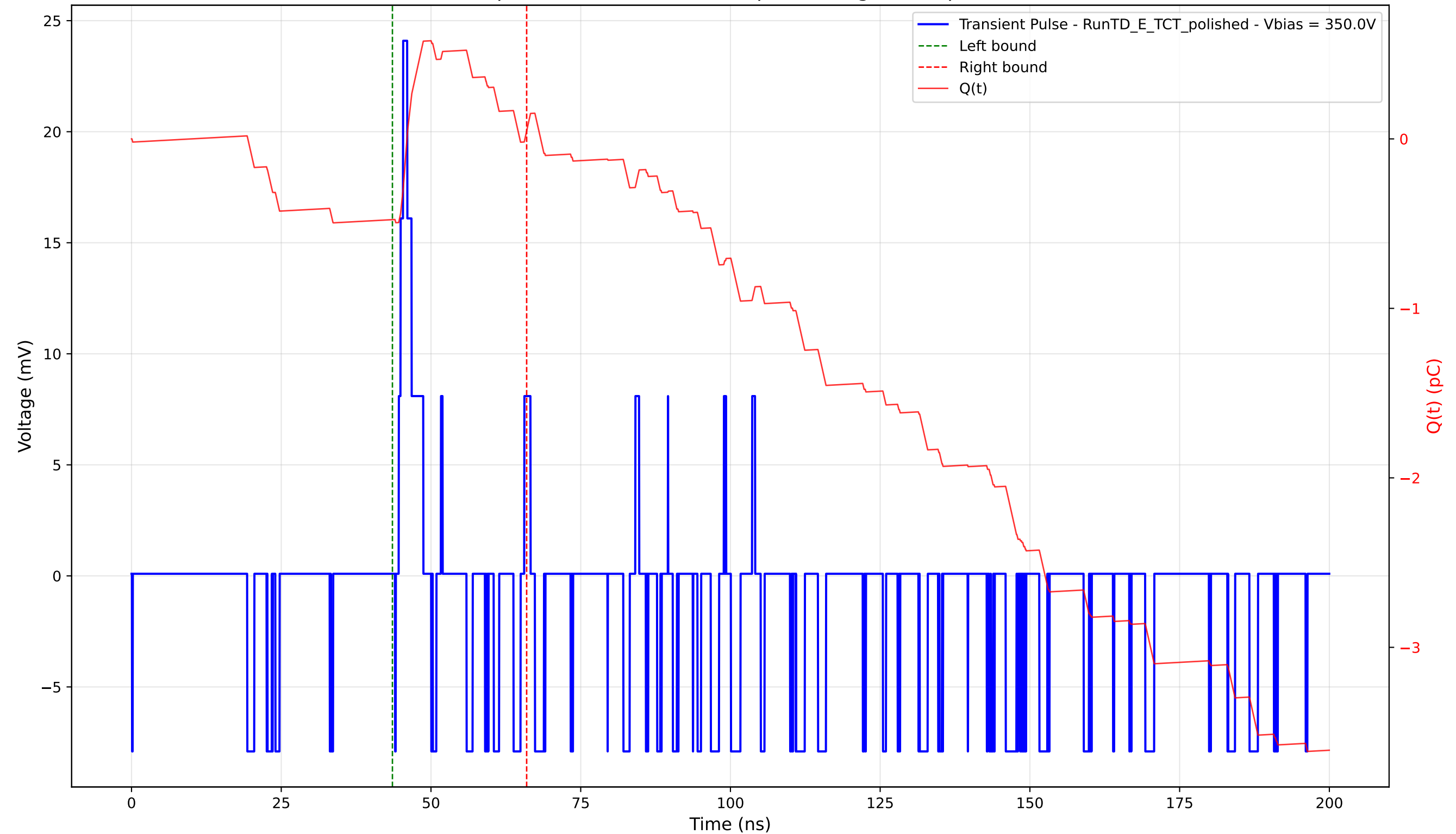
Transient Pulse - Sample: 4003 - Position: 60.0 \mu\text{m} - Charge: 0.52 pC - Rise Time: 0.73 ns
