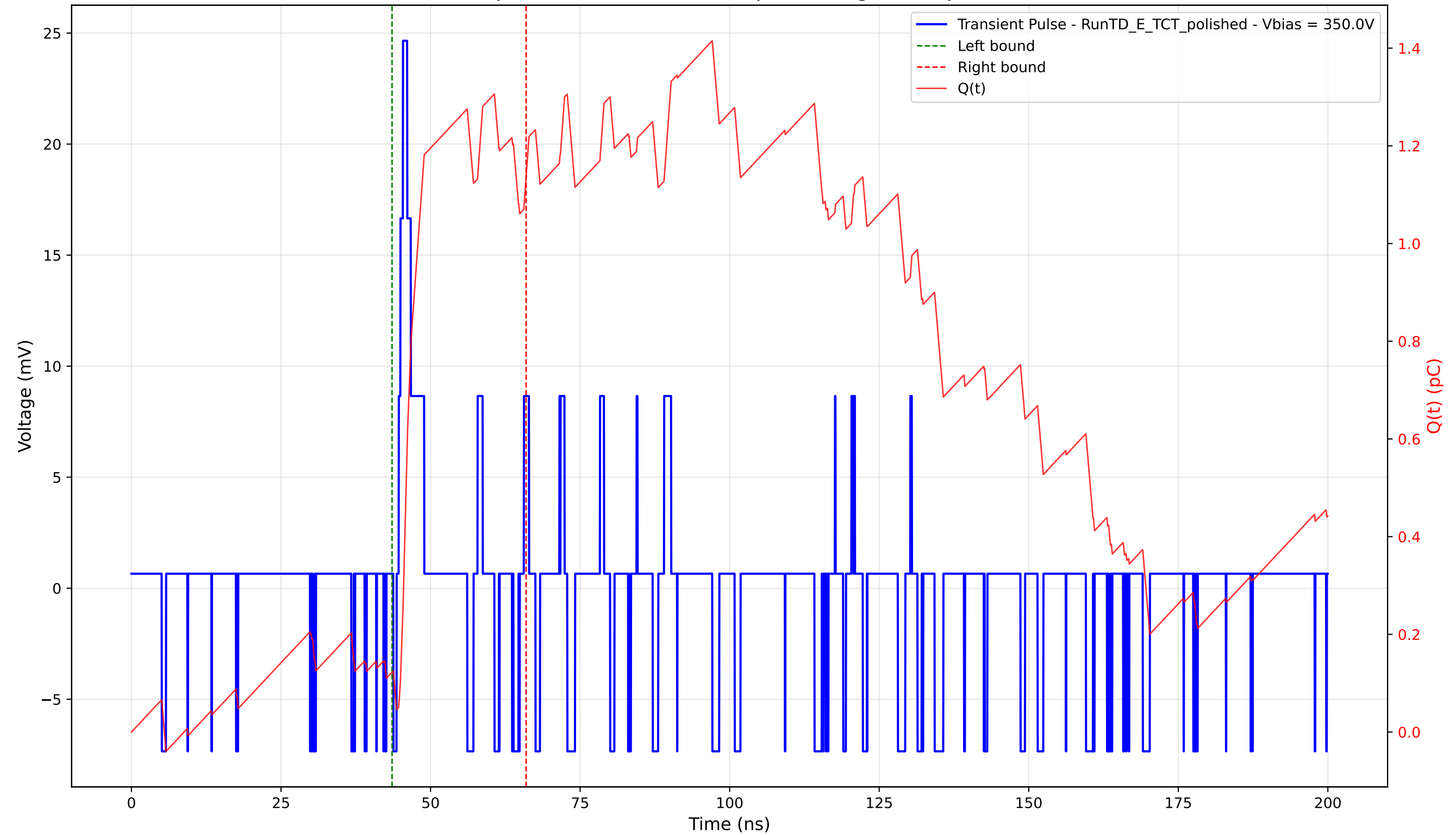
Transient Pulse - Sample: 4003 - Position: 55.0 \mu\text{m} - Charge: 1.01 pC - Rise Time: 0.72 ns
