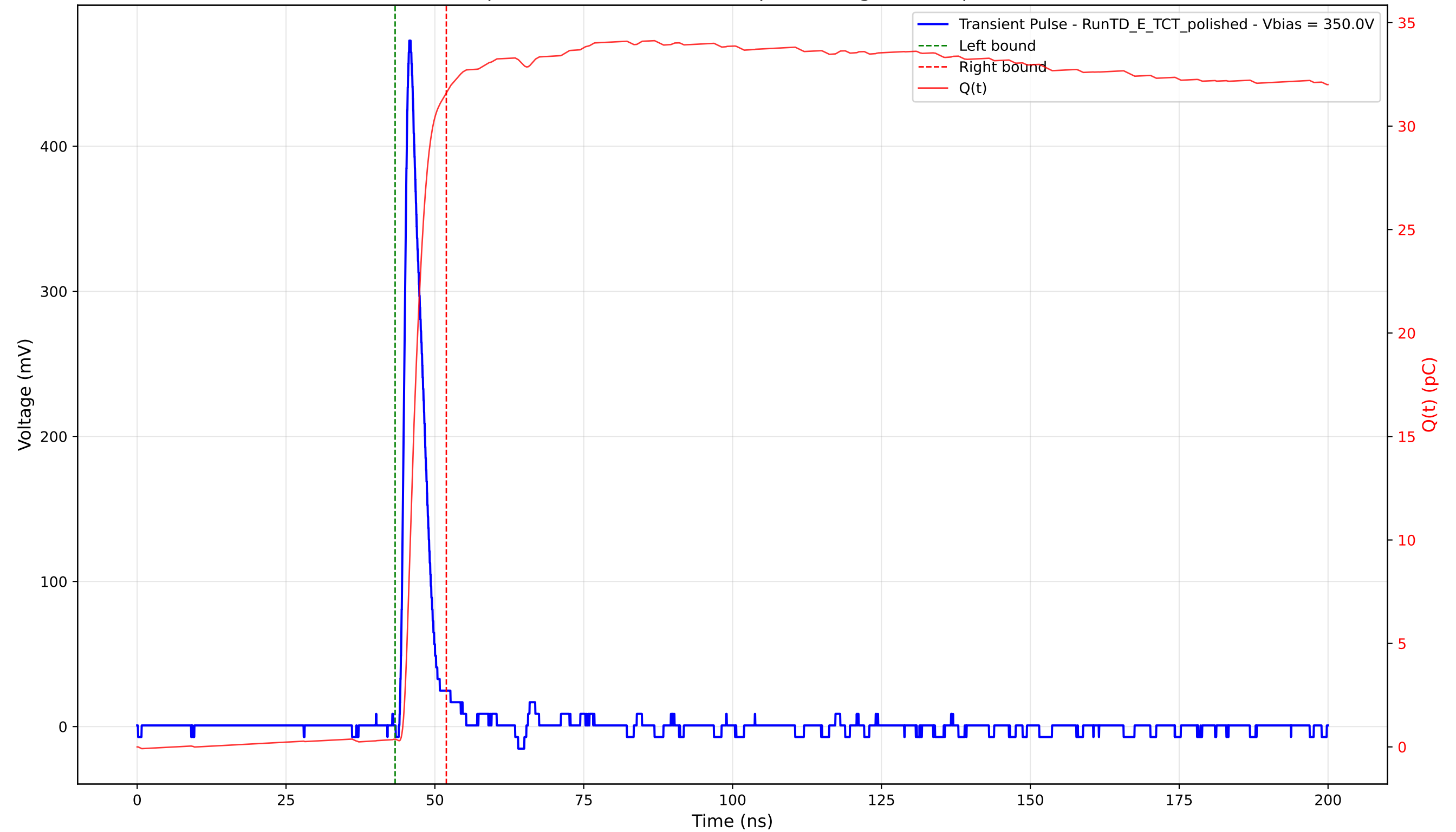
Transient Pulse - Sample: 4003 - Position: 385.0 \mu\text{m} - Charge: 31.24 pC - Rise Time: 1.10 ns
