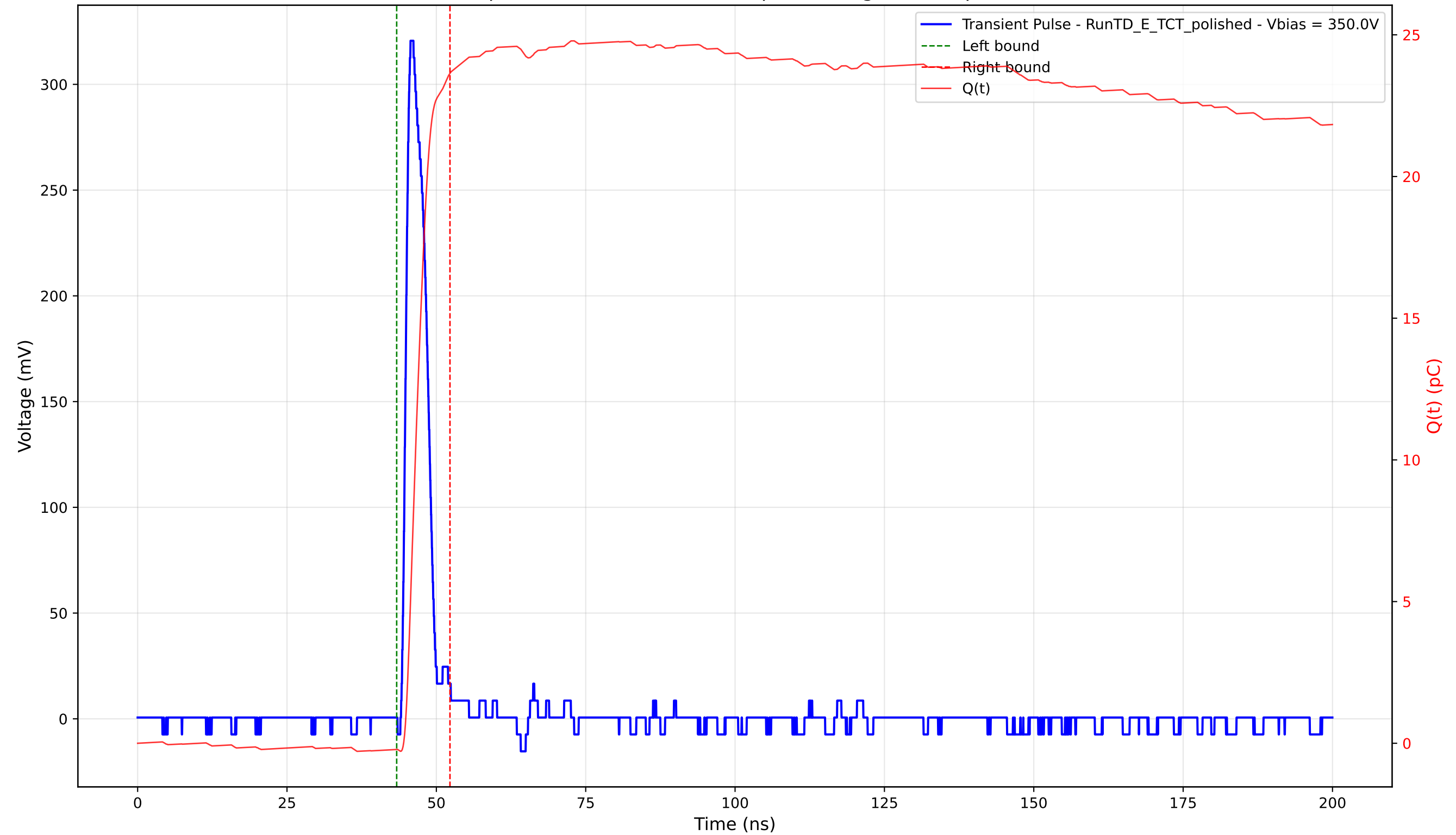
Transient Pulse - Sample: 4003 - Position: 455.0 \mu\text{m} - Charge: 23.86 pC - Rise Time: 1.08 ns
