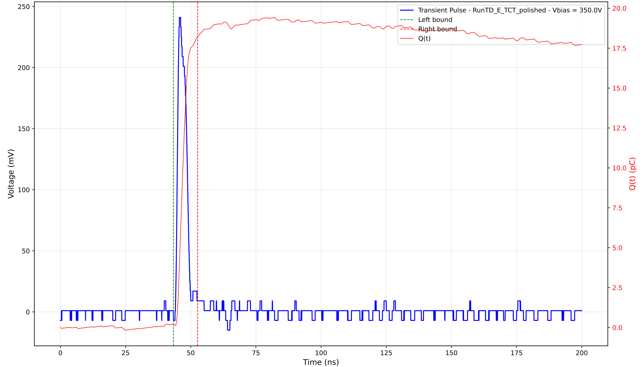
Transient Pulse - Sample: 4003 - Position: 490.0 \mu\text{m} - Charge: 18.03 pC - Rise Time: 1.06 ns
