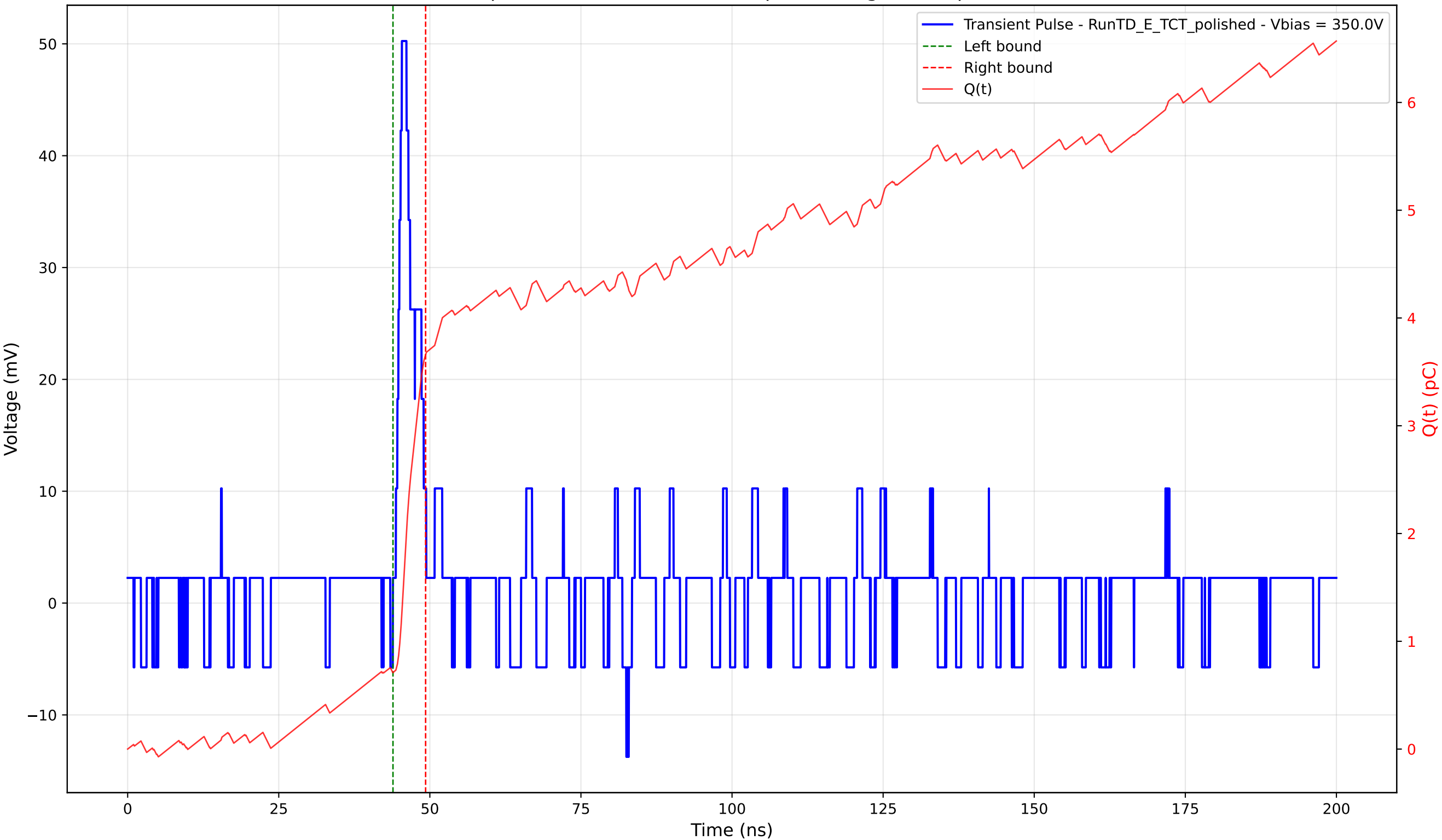
Transient Pulse - Sample: 4003 - Position: 595.0 \mu\text{m} - Charge: 2.95 pC - Rise Time: 0.99 ns
