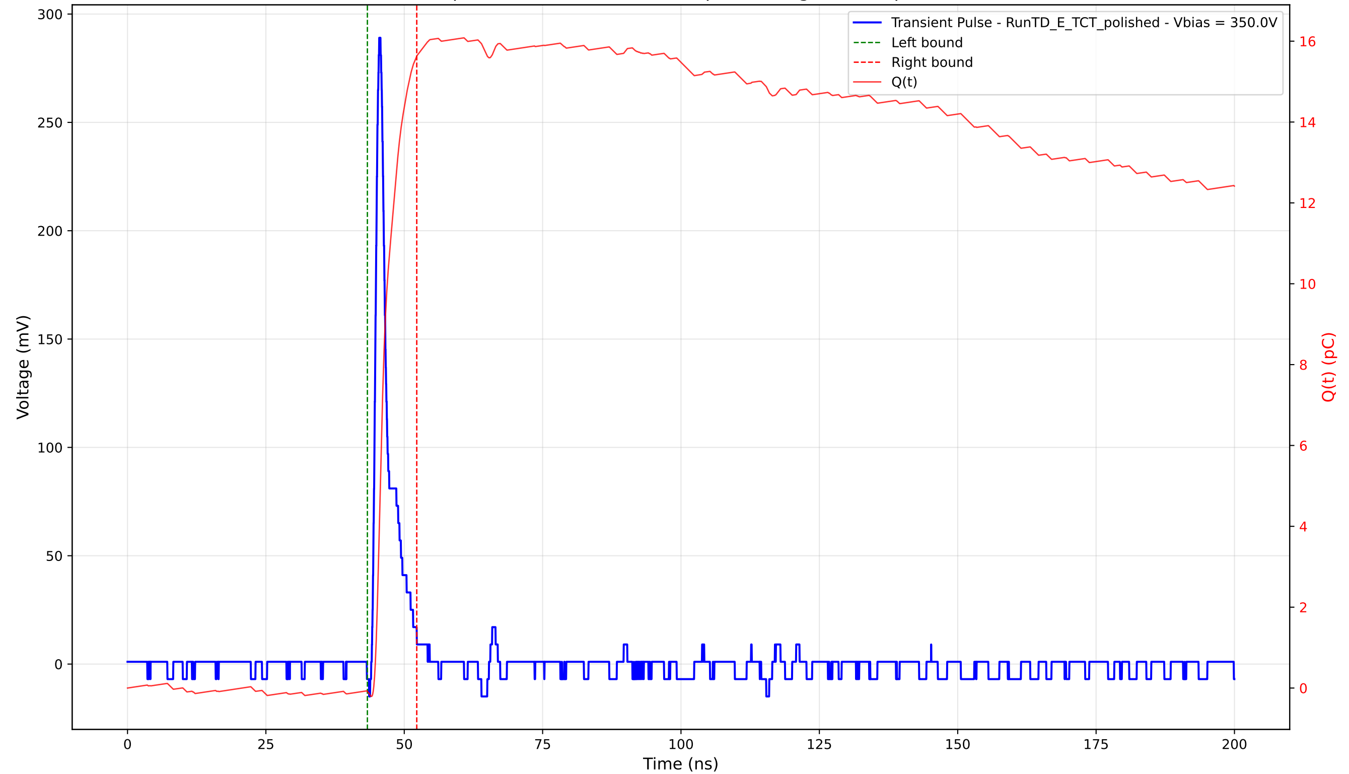
Transient Pulse - Sample: 4003 - Position: 185.0 \mu\text{m} - Charge: 15.72 pC - Rise Time: 0.95 ns
