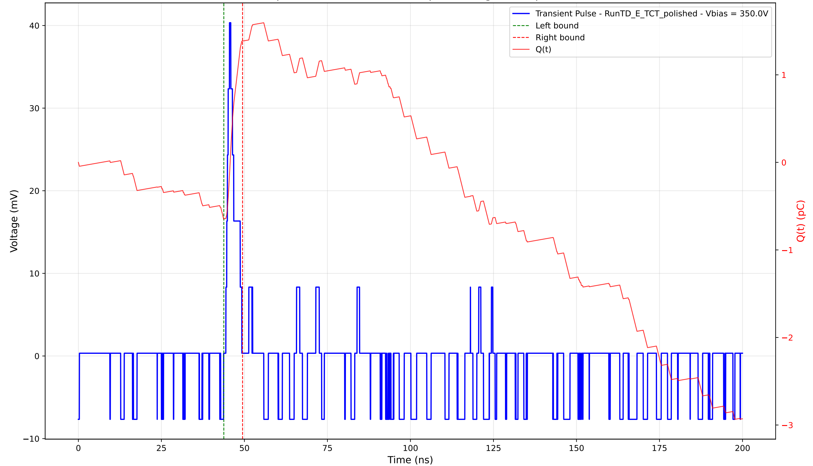
Transient Pulse - Sample: 4003 - Position: 695.0 \mu\text{m} - Charge: 2.03 pC - Rise Time: 1.09 ns
