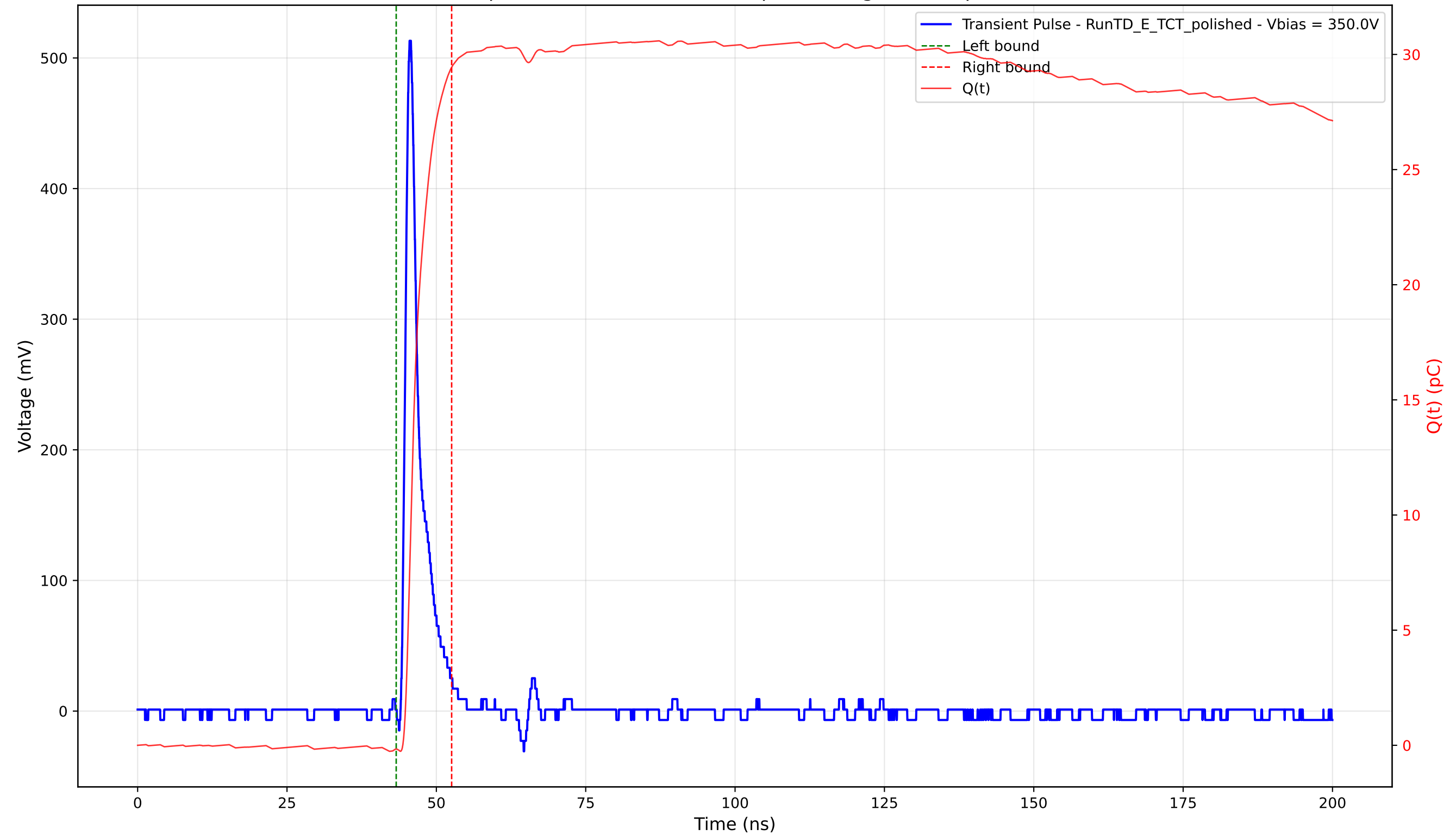
Transient Pulse - Sample: 4003 - Position: 265.0 \mu\text{m} - Charge: 29.61 pC - Rise Time: 0.97 ns
