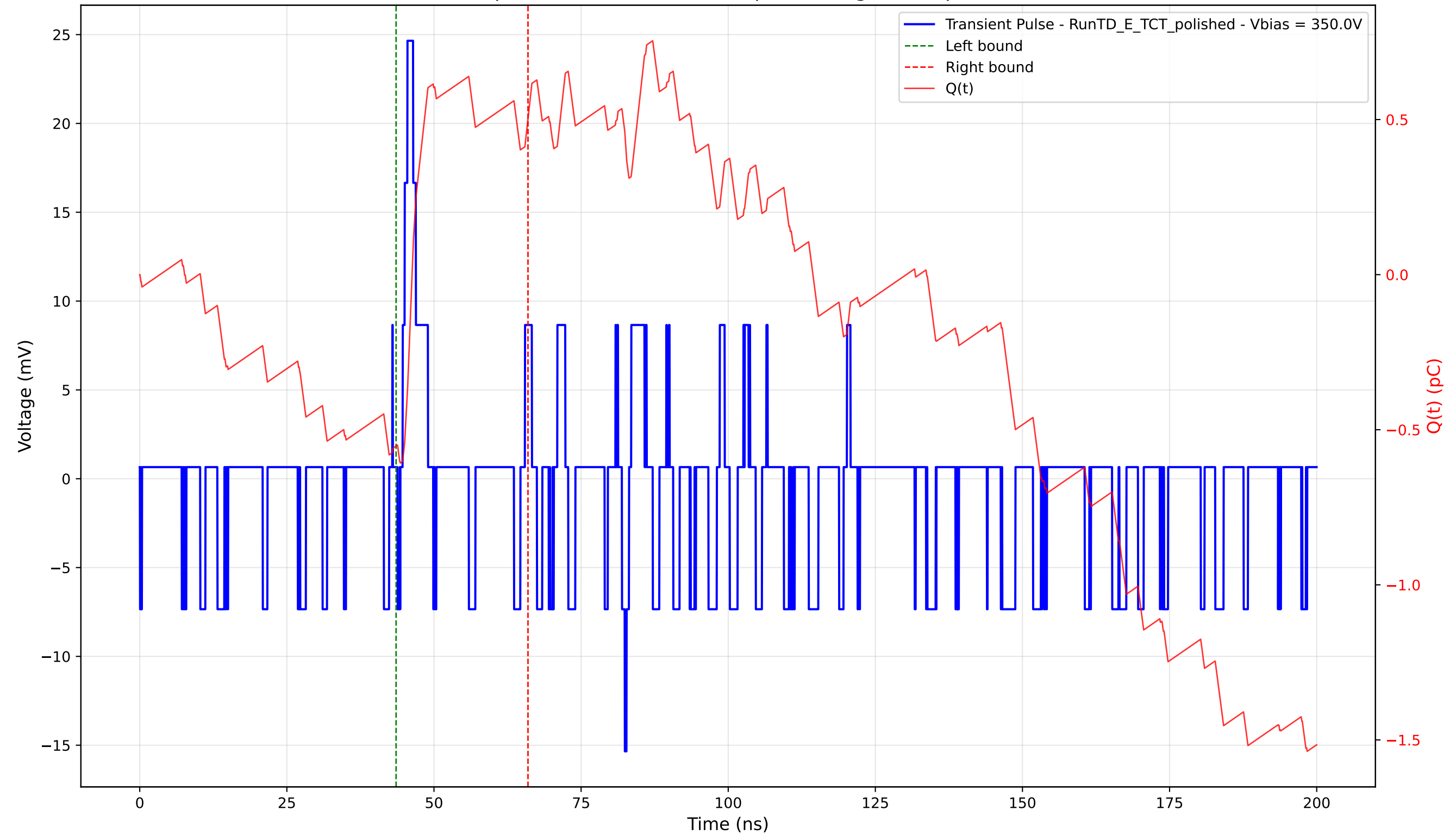
Transient Pulse - Sample: 4003 - Position: 65.0 \mu\text{m} - Charge: 1.05 pC - Rise Time: 0.82 ns
