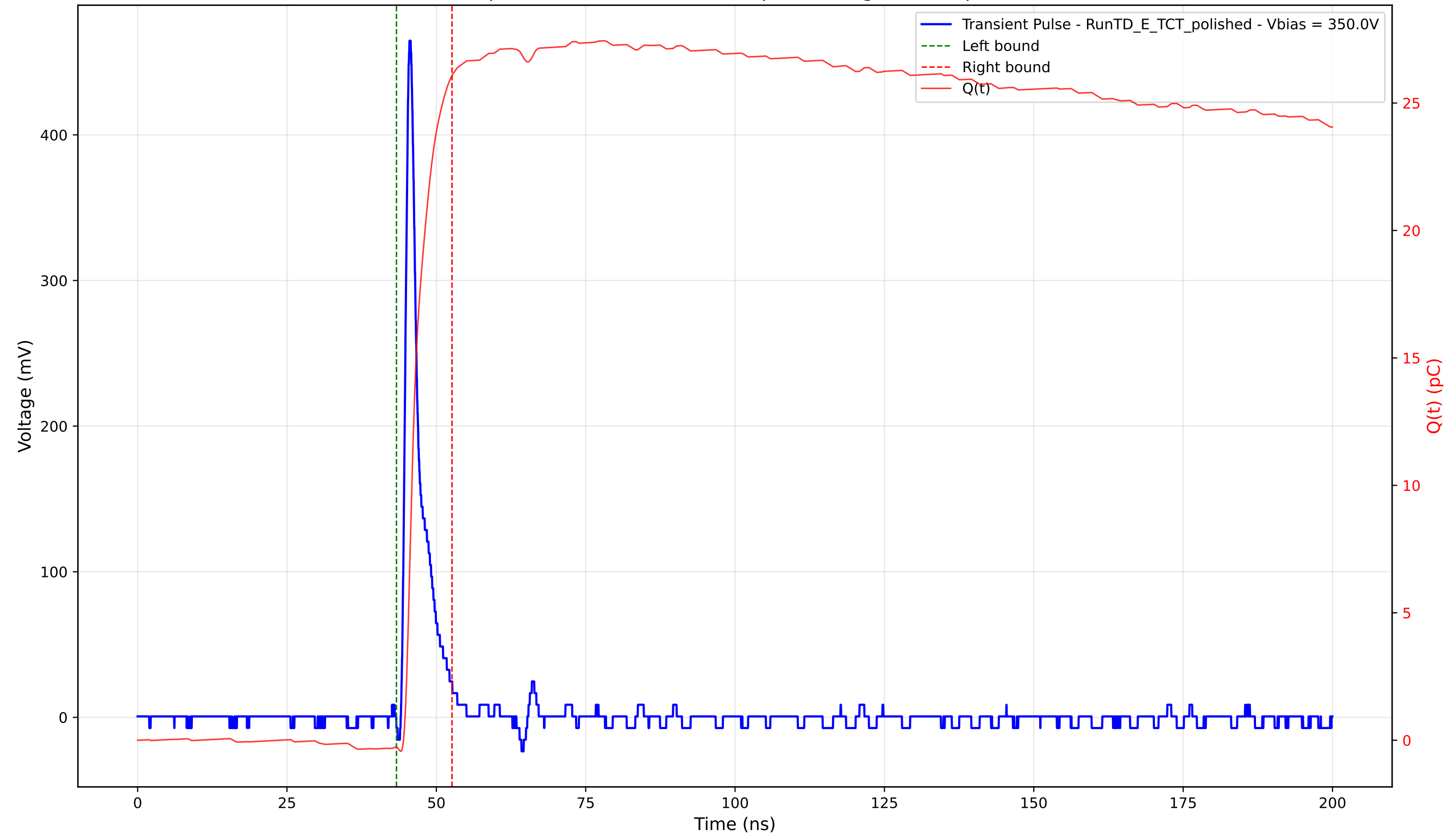
Transient Pulse - Sample: 4003 - Position: 240.0 \mu\text{m} - Charge: 26.36 pC - Rise Time: 0.97 ns
