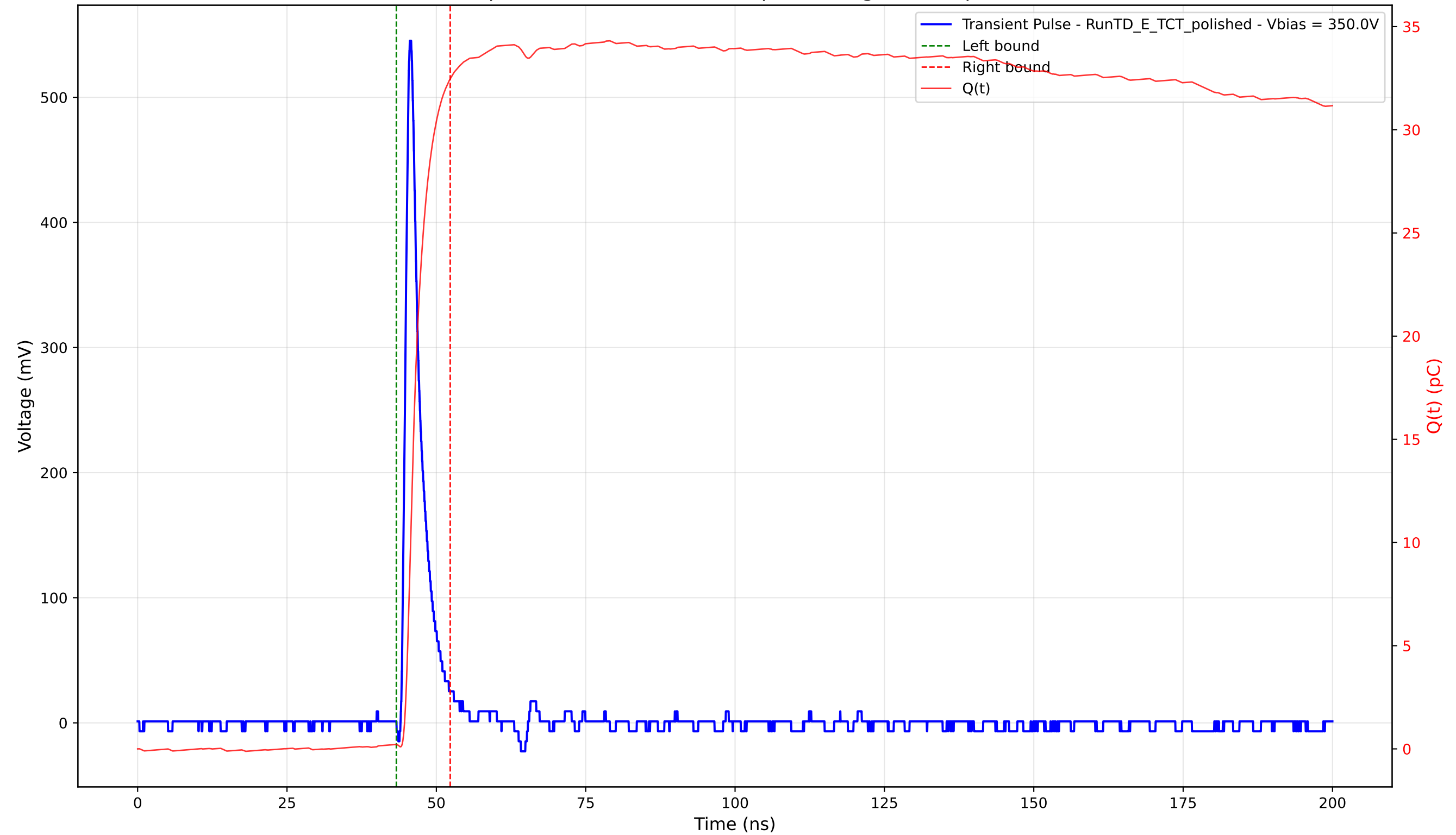
Transient Pulse - Sample: 4003 - Position: 305.0 \mu\text{m} - Charge: 32.25 pC - Rise Time: 1.01 ns
