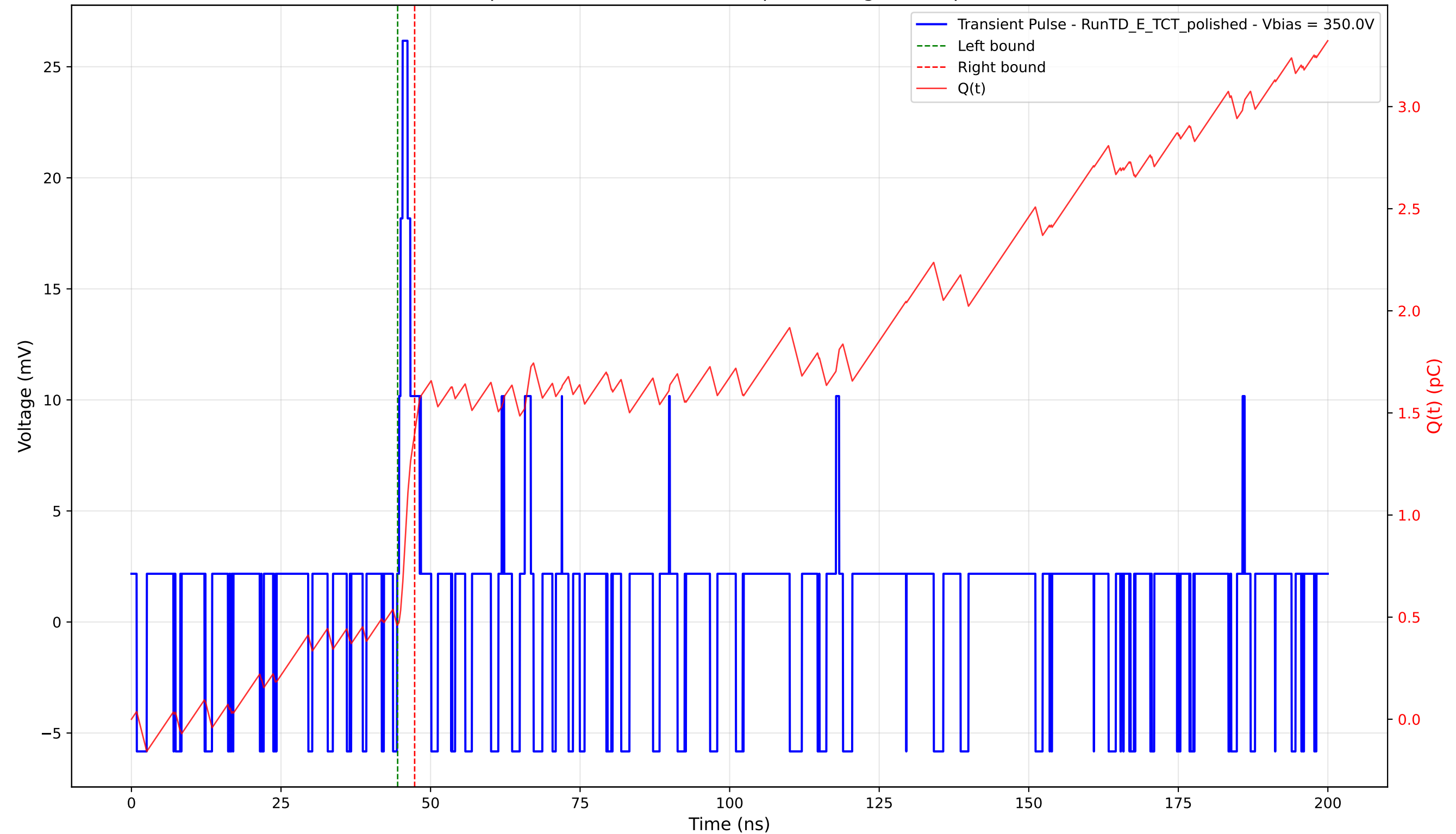
Transient Pulse - Sample: 4003 - Position: 725.0 \mu\text{m} - Charge: 0.94 pC - Rise Time: 0.60 ns
