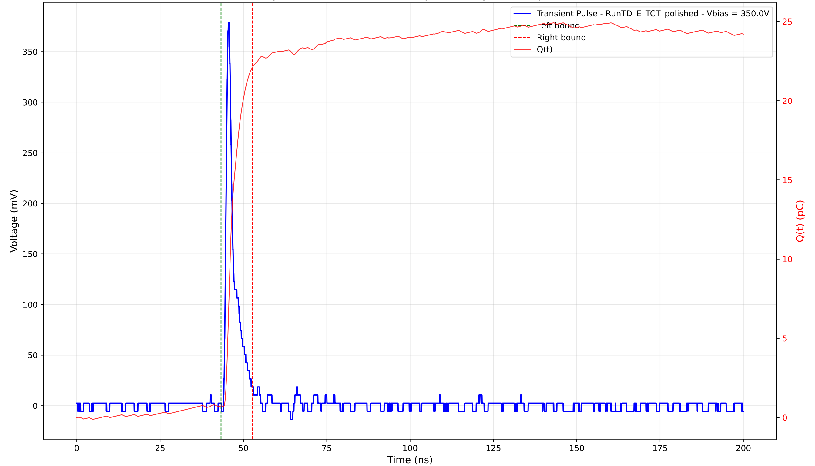
Transient Pulse - Sample: 4003 - Position: 210.0 \mu\text{m} - Charge: 21.36 pC - Rise Time: 0.97 ns
