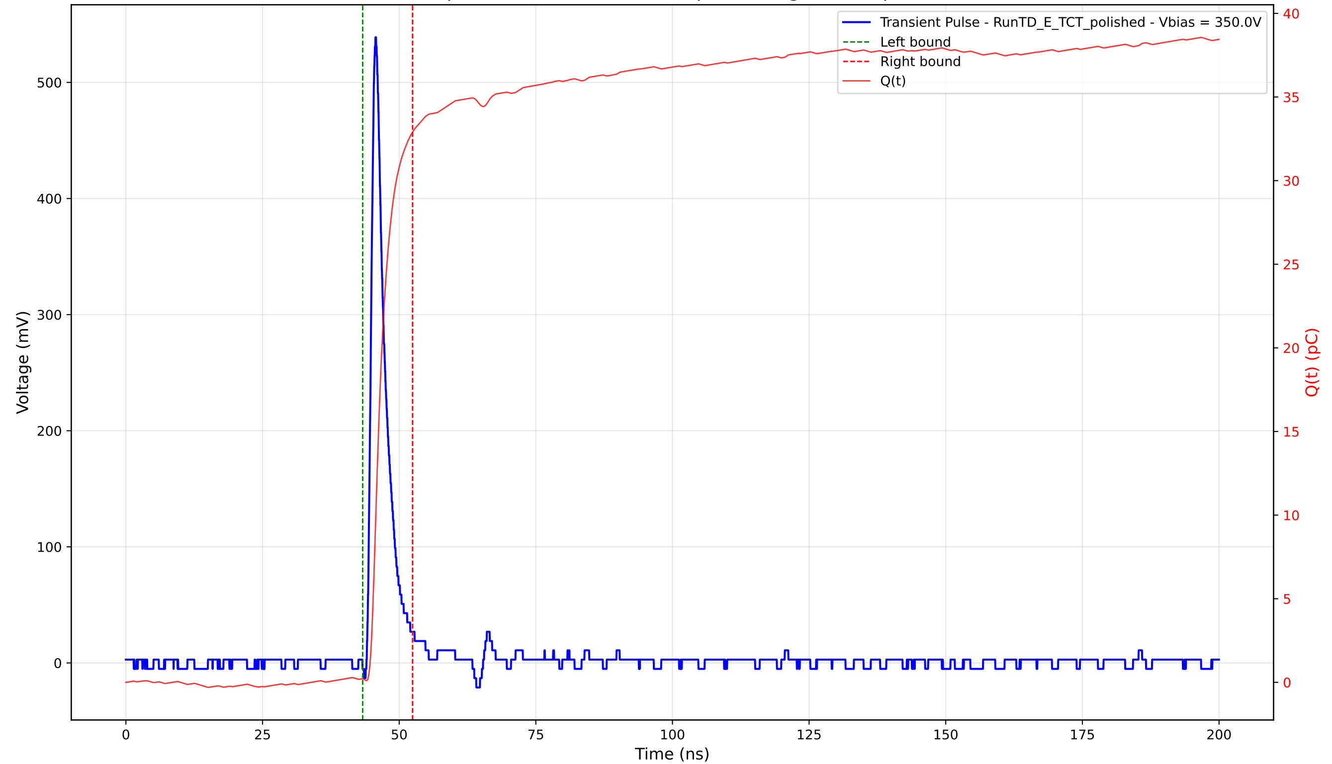
Transient Pulse - Sample: 4003 - Position: 325.0 \mu\text{m} - Charge: 32.68 pC - Rise Time: 1.03 ns
