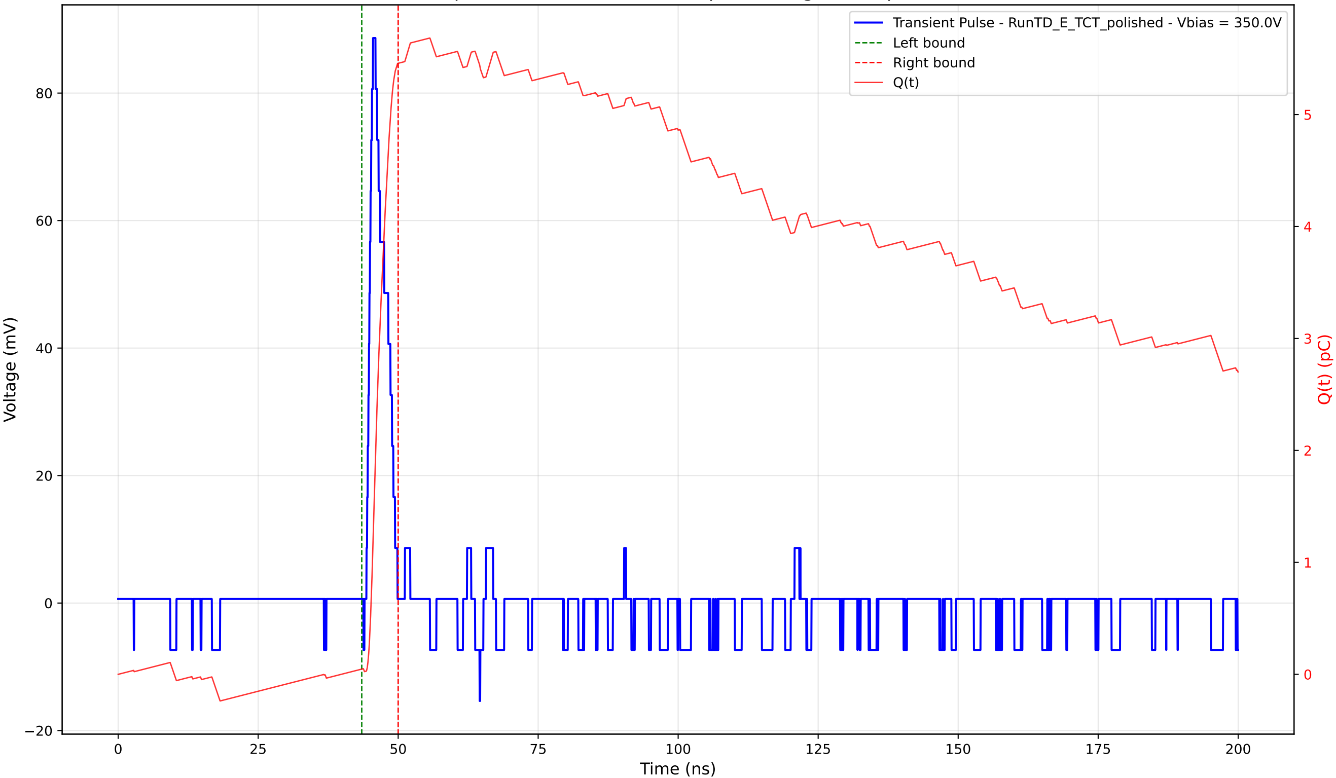
Transient Pulse - Sample: 4003 - Position: 570.0 \mu\text{m} - Charge: 5.41 pC - Rise Time: 0.88 ns
