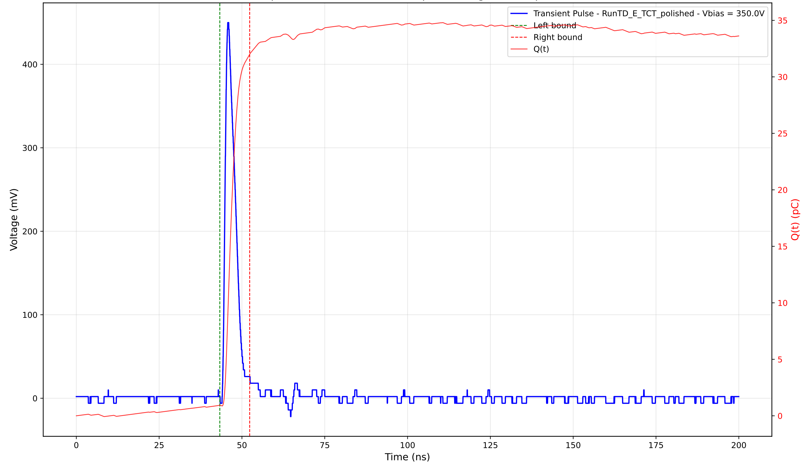
Transient Pulse - Sample: 4003 - Position: 400.0 \mu\text{m} - Charge: 31.07 pC - Rise Time: 1.09 ns
