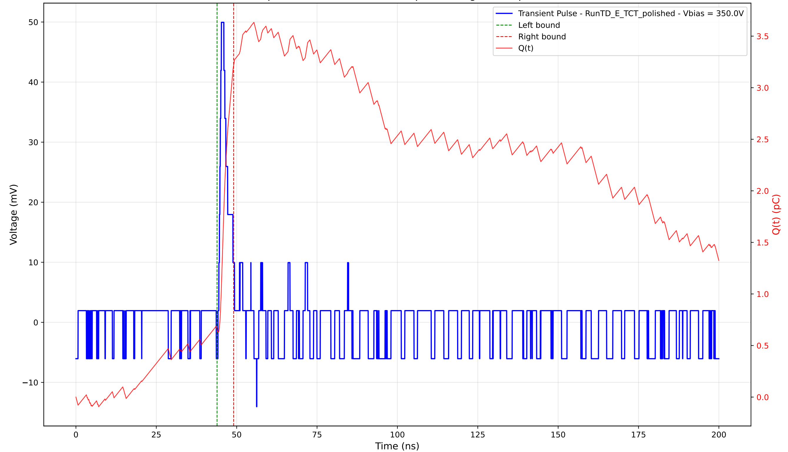
Transient Pulse - Sample: 4003 - Position: 645.0 \mu\text{m} - Charge: 2.56 pC - Rise Time: 0.79 ns
