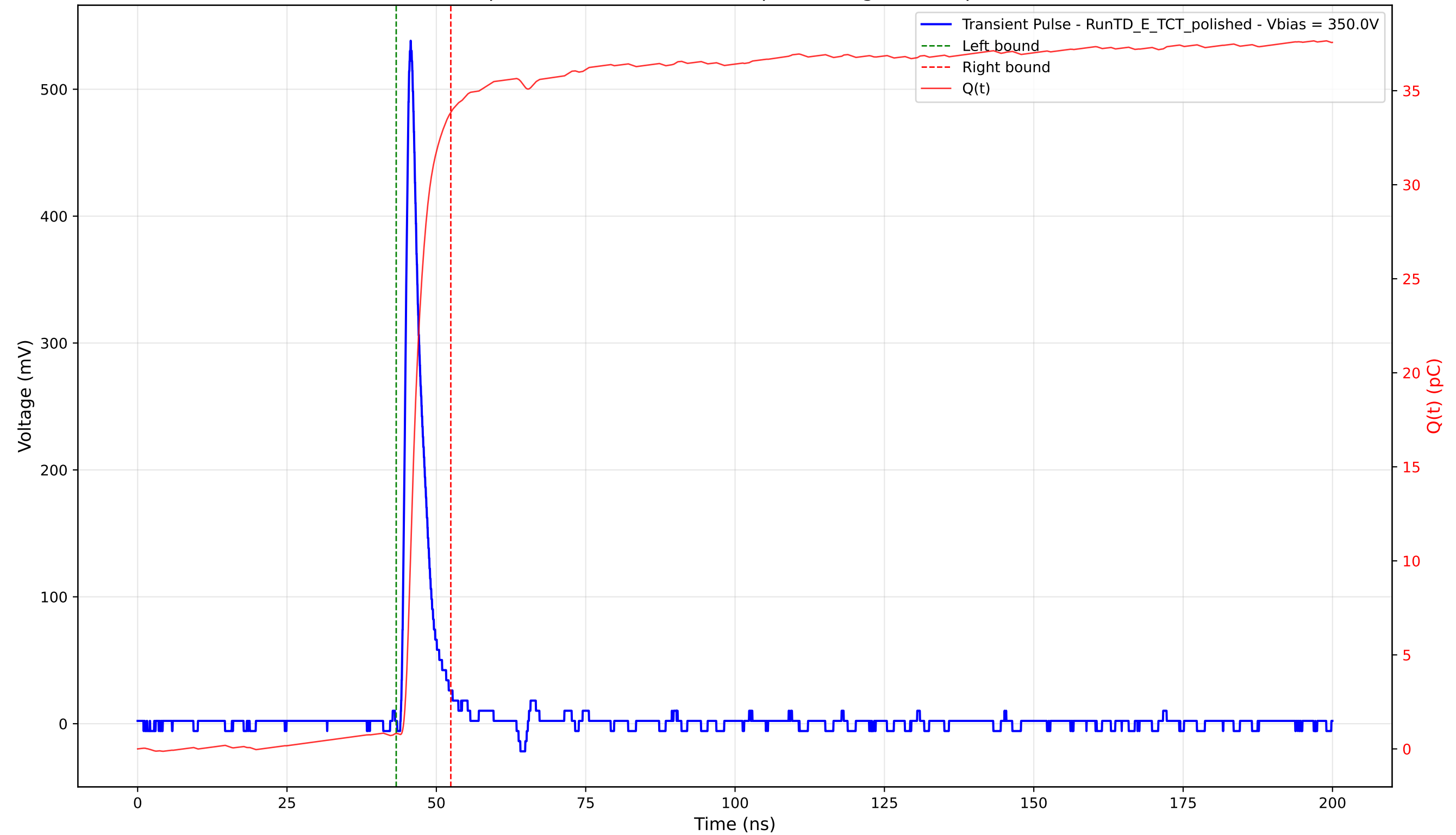
Transient Pulse - Sample: 4003 - Position: 335.0 \mu\text{m} - Charge: 33.03 pC - Rise Time: 1.05 ns
