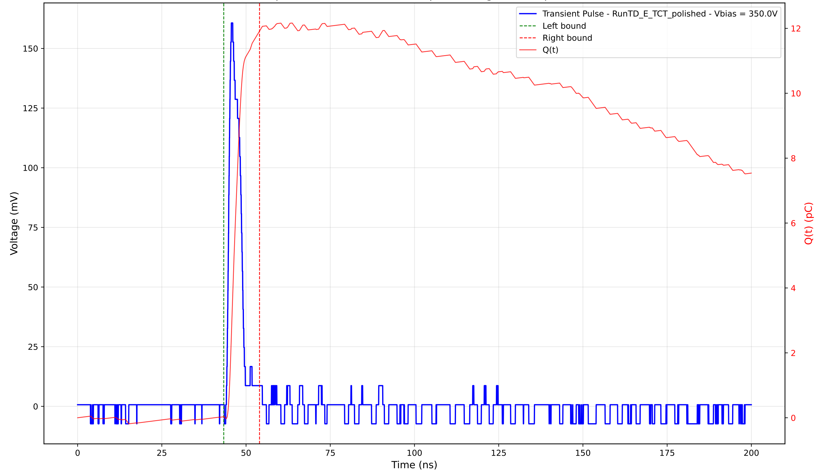
Transient Pulse - Sample: 4003 - Position: 525.0 \mu\text{m} - Charge: 11.89 pC - Rise Time: 1.04 ns
