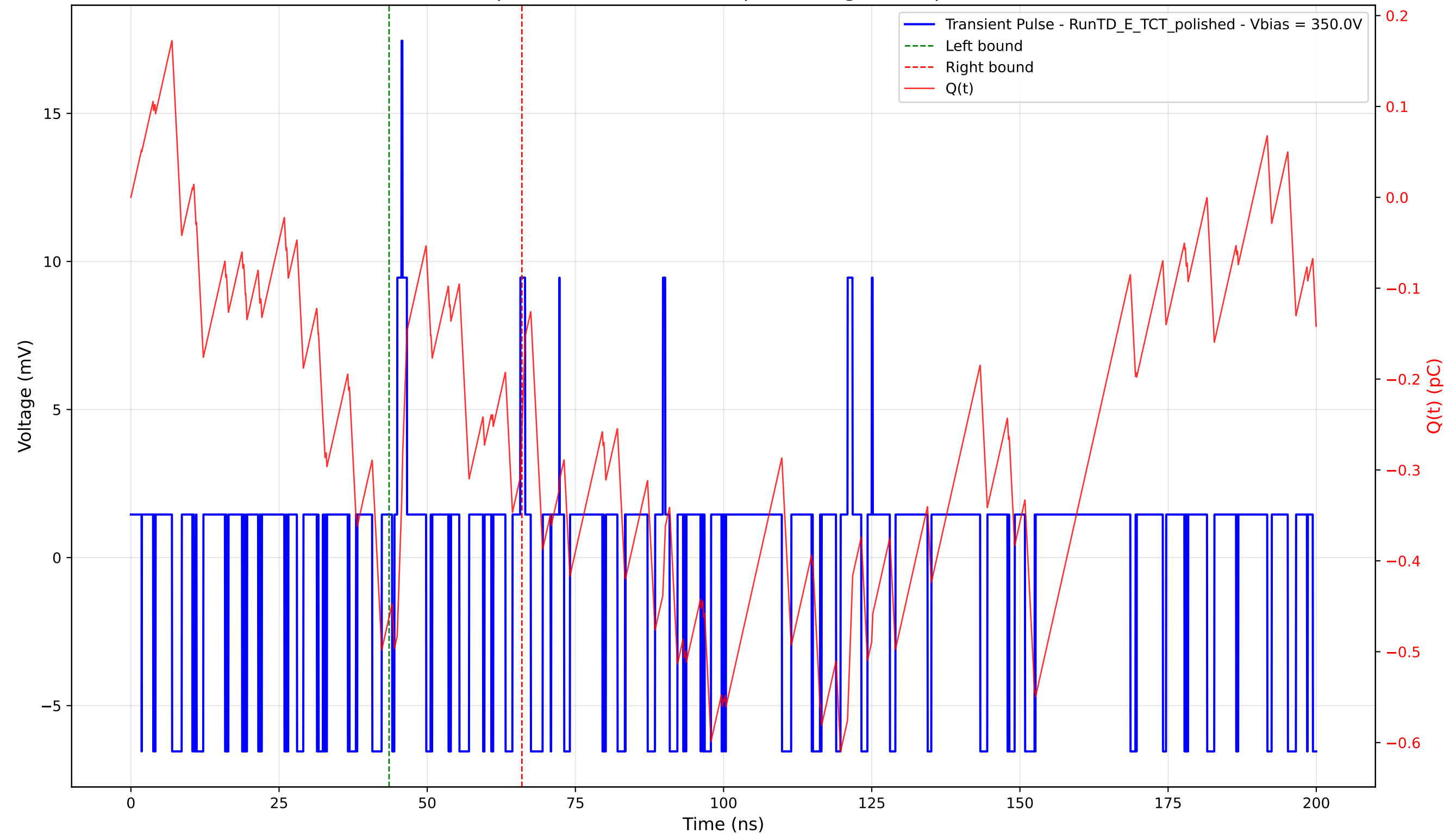
Transient Pulse - Sample: 4003 - Position: 0.0 \mu\text{m} - Charge: 0.20 pC - Rise Time: 0.74 ns
