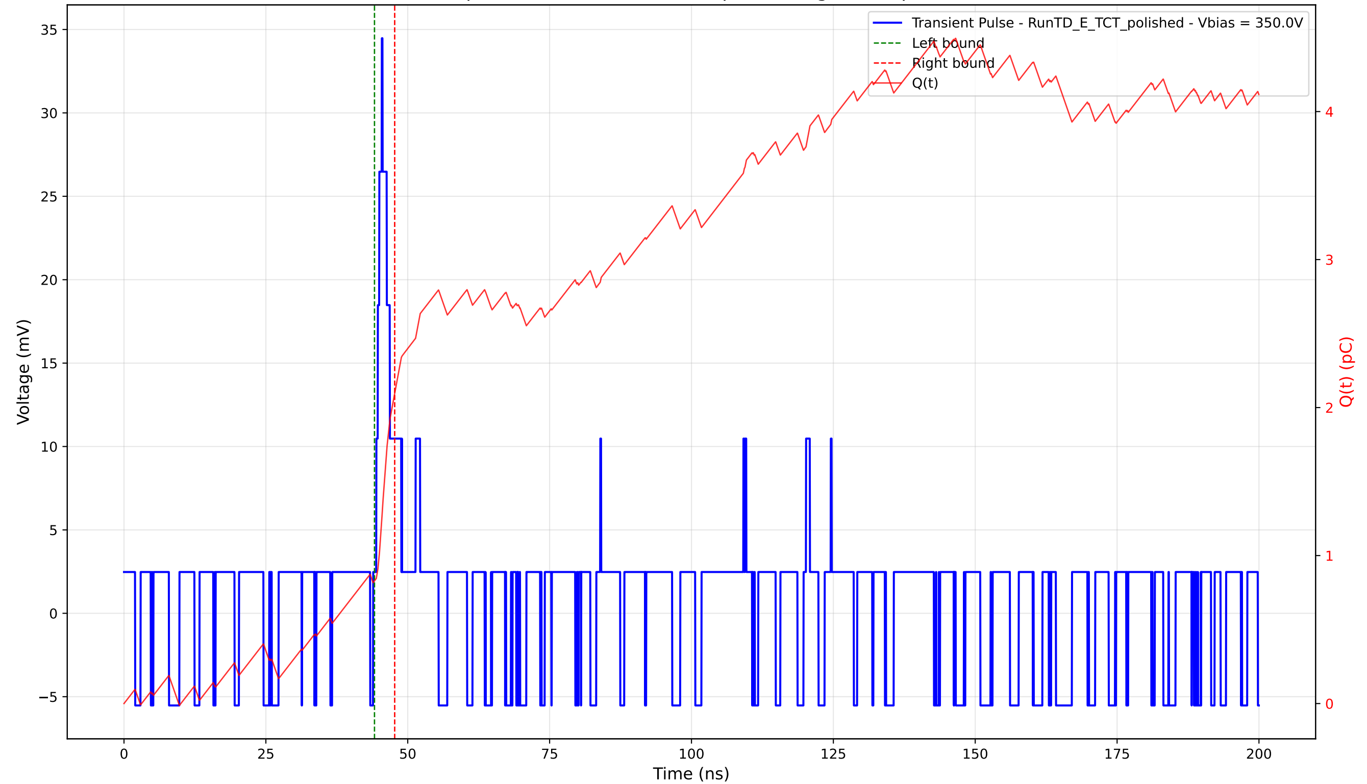
Transient Pulse - Sample: 4003 - Position: 785.0 \mu\text{m} - Charge: 1.27 pC - Rise Time: 0.98 ns
