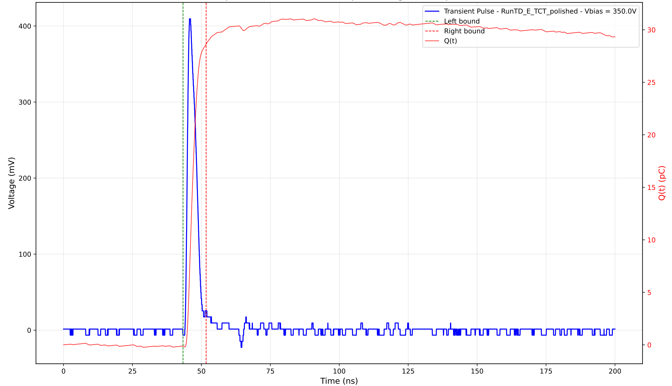
Transient Pulse - Sample: 4003 - Position: 420.0 \mu\text{m} - Charge: 28.76 pC - Rise Time: 1.08 ns
