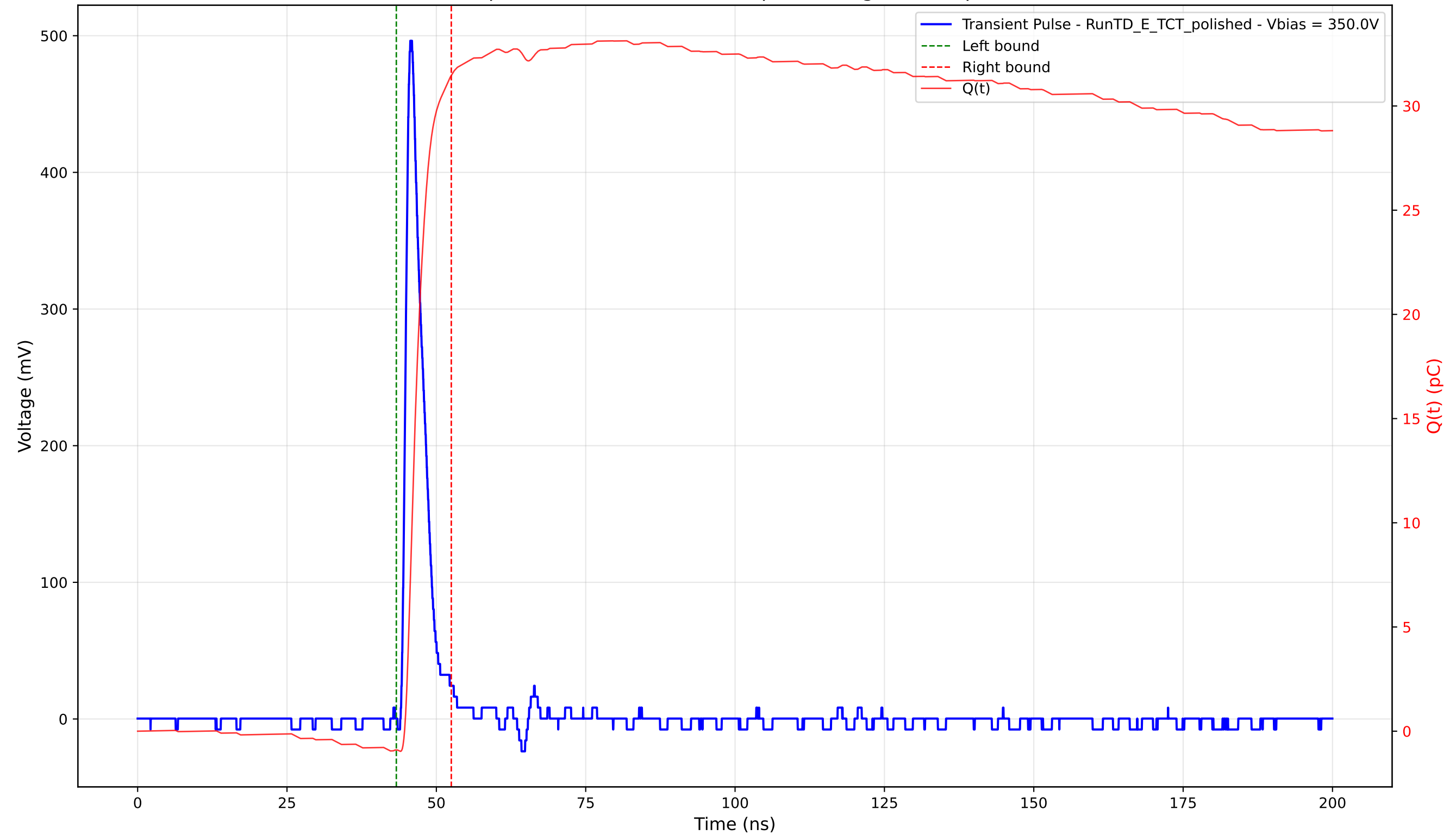
Transient Pulse - Sample: 4003 - Position: 365.0 \mu\text{m} - Charge: 32.37 pC - Rise Time: 1.03 ns
