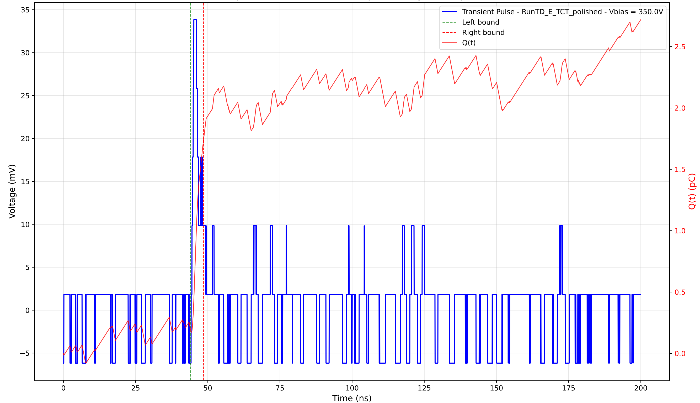
Transient Pulse - Sample: 4003 - Position: 665.0 \mu\text{m} - Charge: 1.57 pC - Rise Time: 0.66 ns
