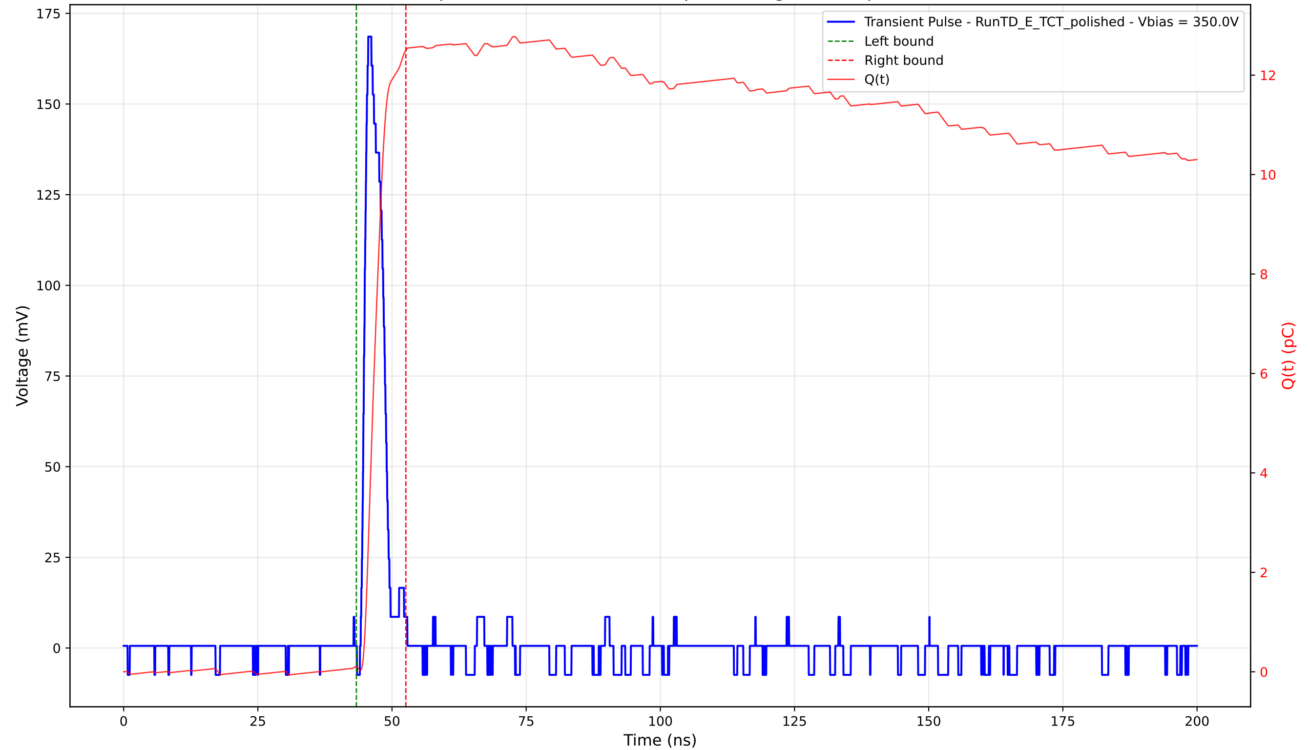
Transient Pulse - Sample: 4003 - Position: 520.0 \mu\text{m} - Charge: 12.40 pC - Rise Time: 0.96 ns
