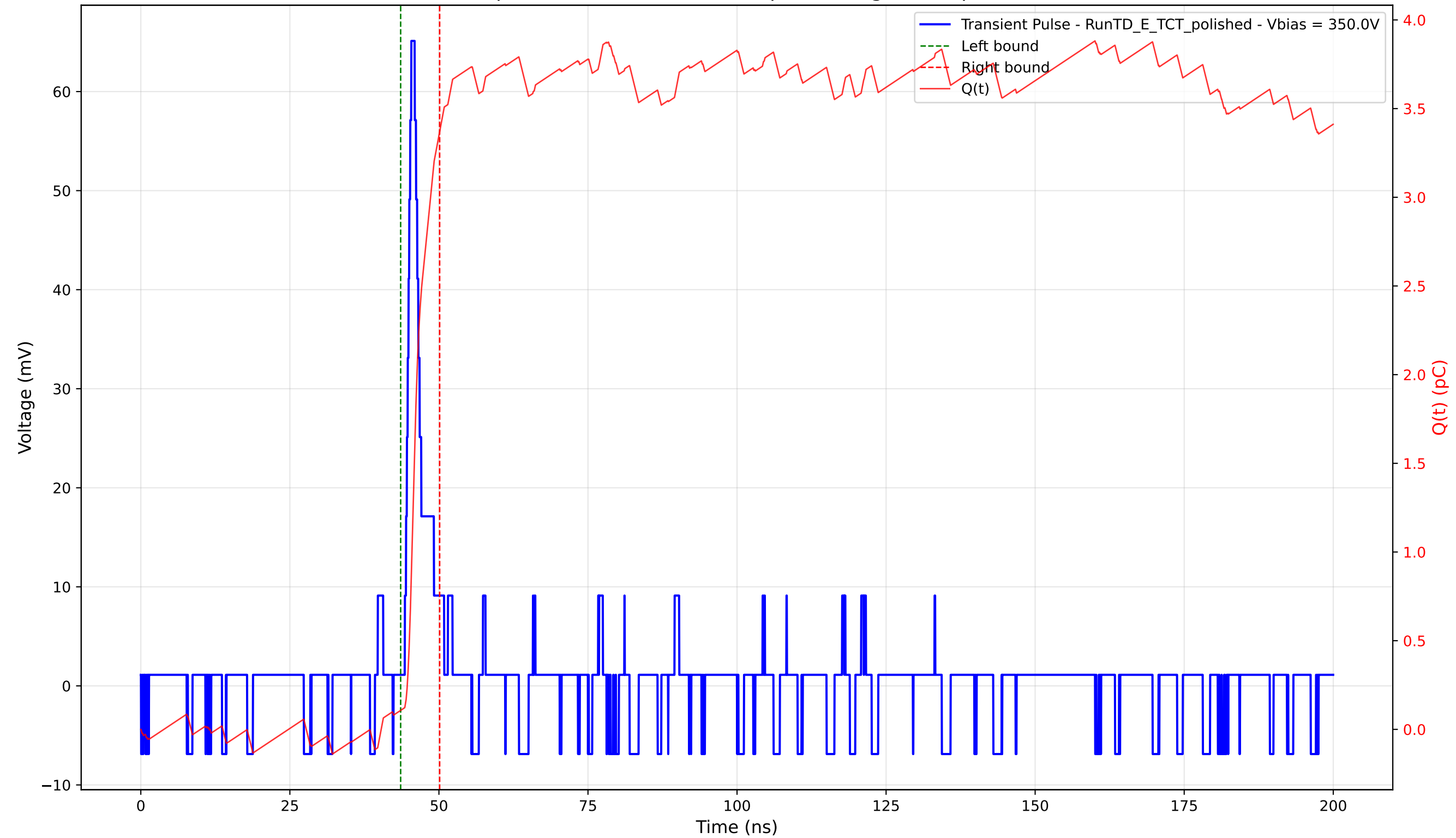
Transient Pulse - Sample: 4003 - Position: 115.0 \mu\text{m} - Charge: 3.26 pC - Rise Time: 1.09 ns
