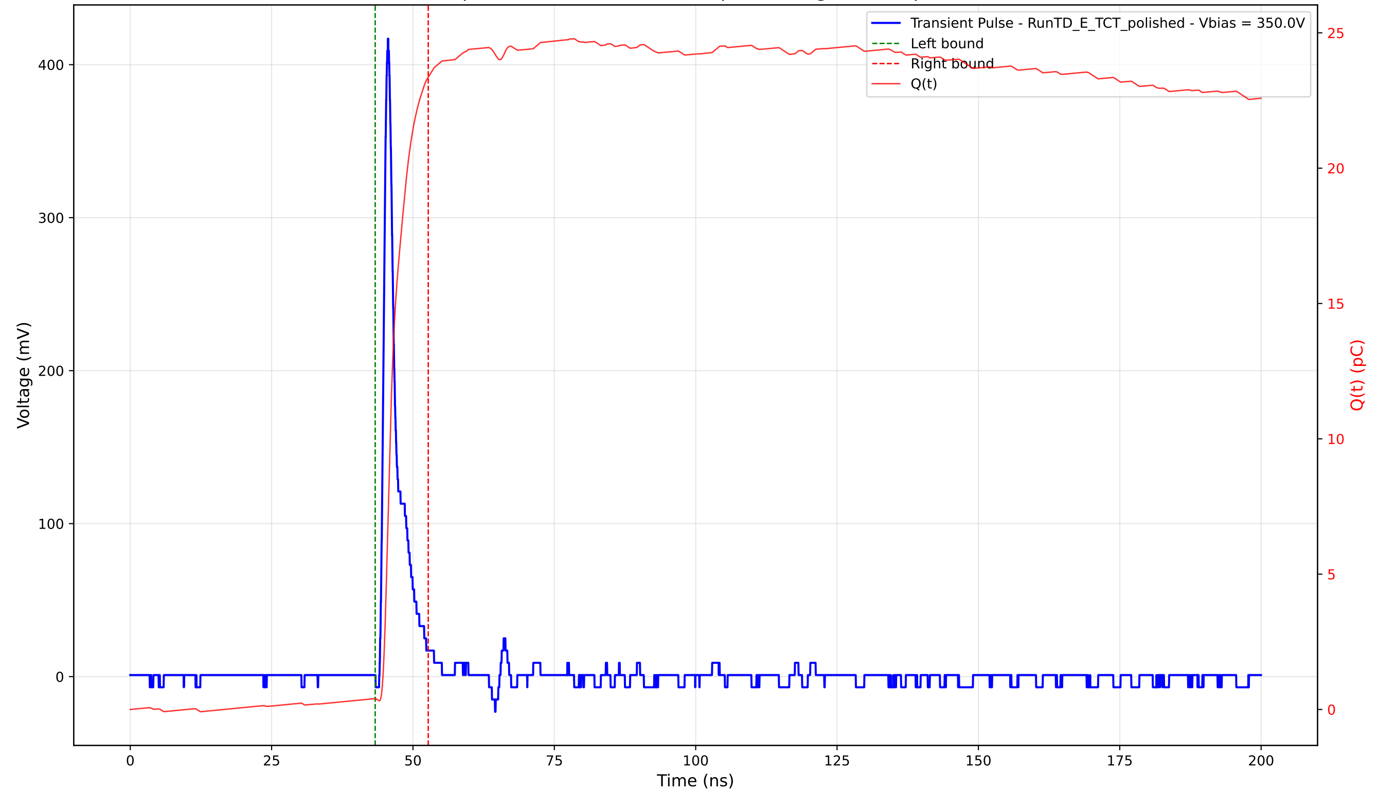
Transient Pulse - Sample: 4003 - Position: 220.0 \mu\text{m} - Charge: 22.96 pC - Rise Time: 0.96 ns
