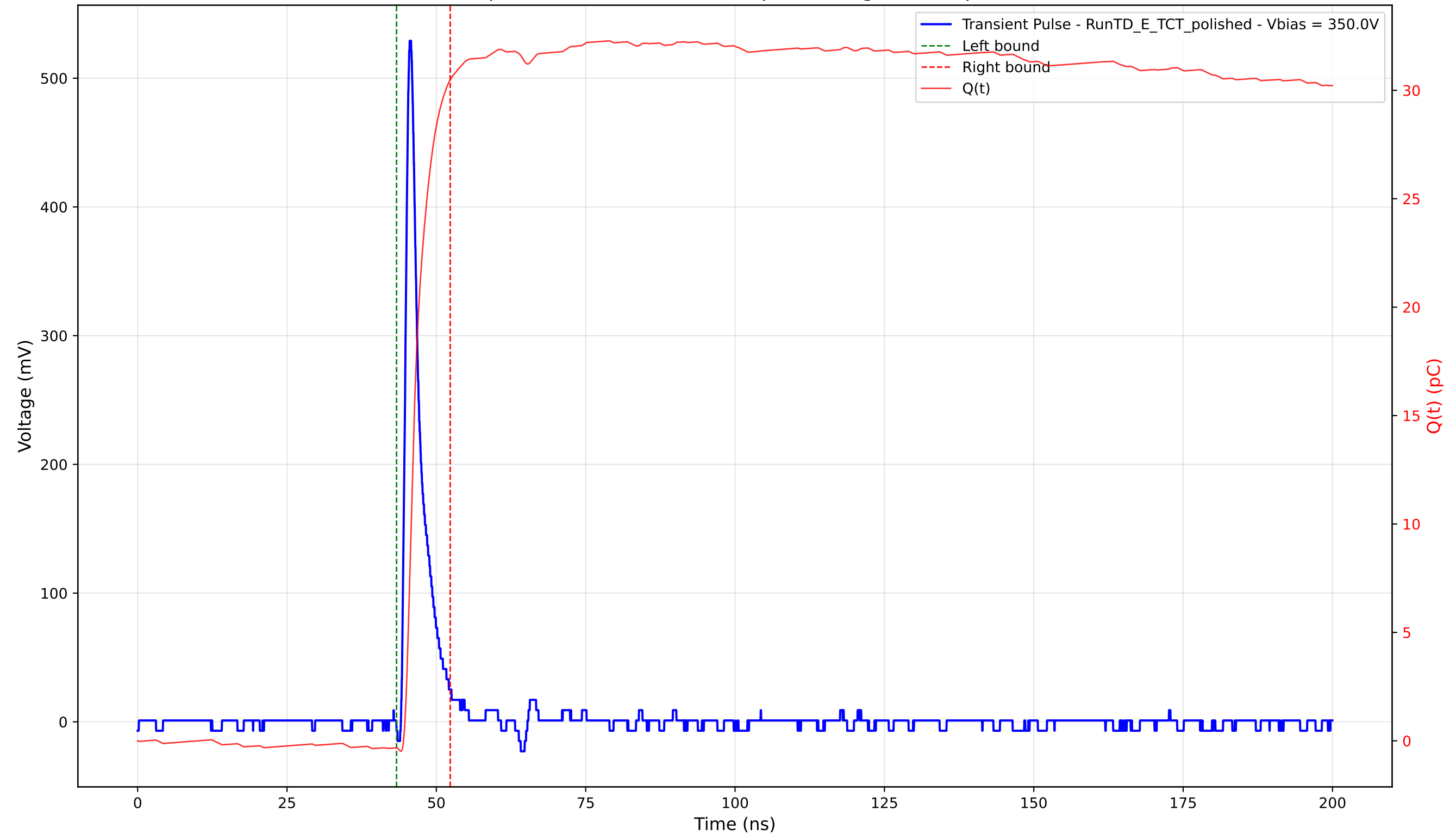
Transient Pulse - Sample: 4003 - Position: 285.0 \mu\text{m} - Charge: 30.81 pC - Rise Time: 0.96 ns
