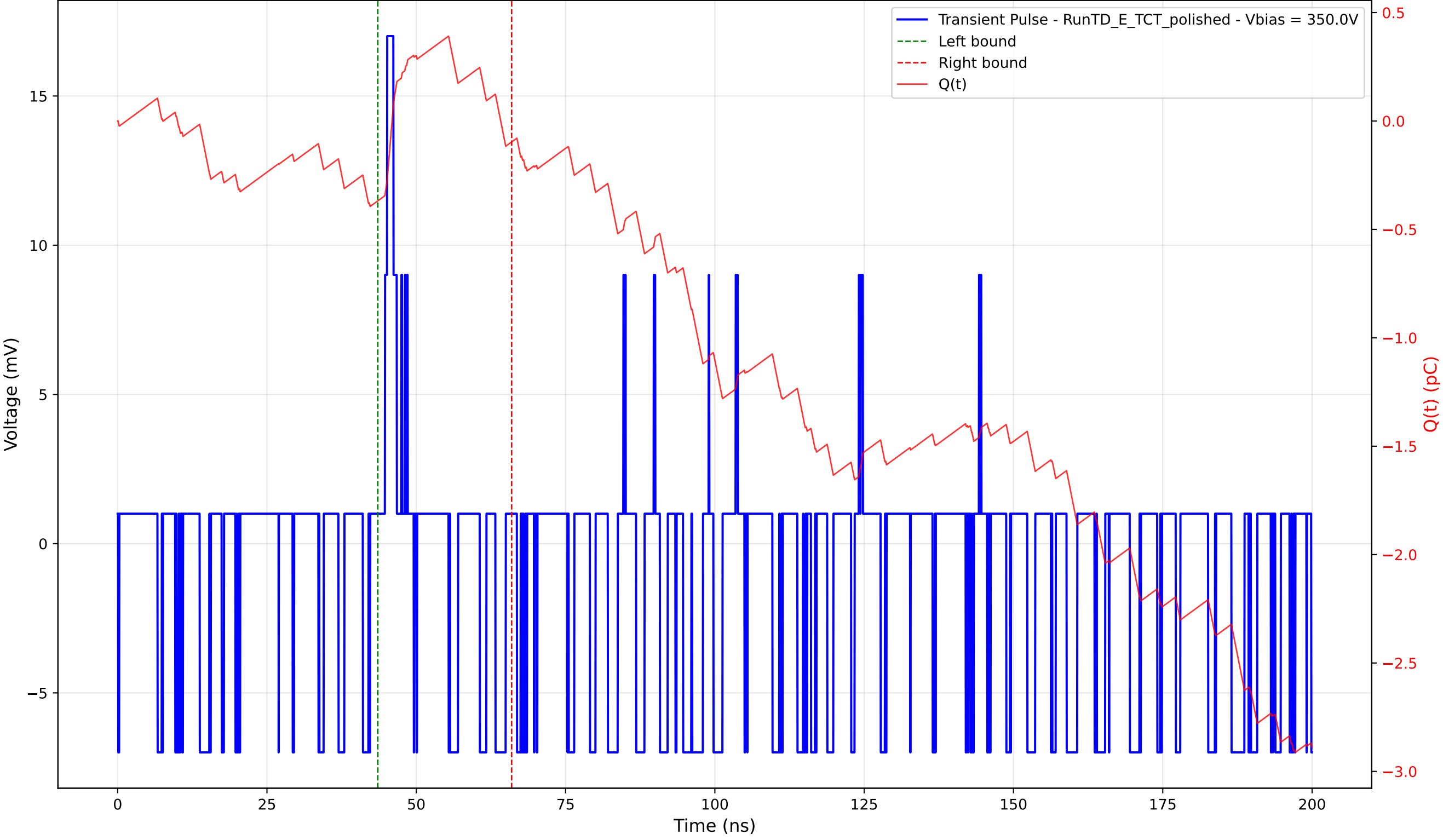
Transient Pulse - Sample: 4003 - Position: 25.0 \mu\text{m} - Charge: 0.27 pC - Rise Time: 0.38 ns
