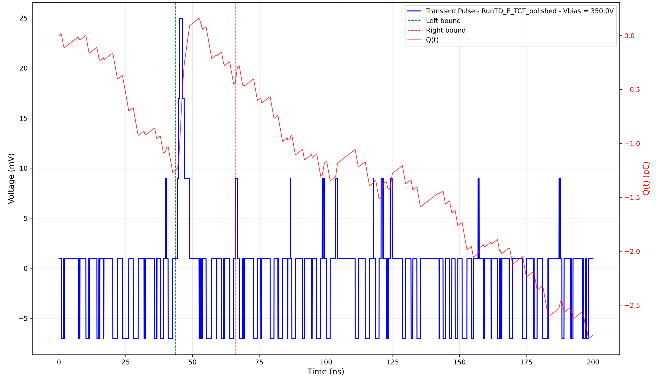
Transient Pulse - Sample: 4003 - Position: 715.0 \mu\text{m} - Charge: 0.81 pC - Rise Time: 0.74 ns
