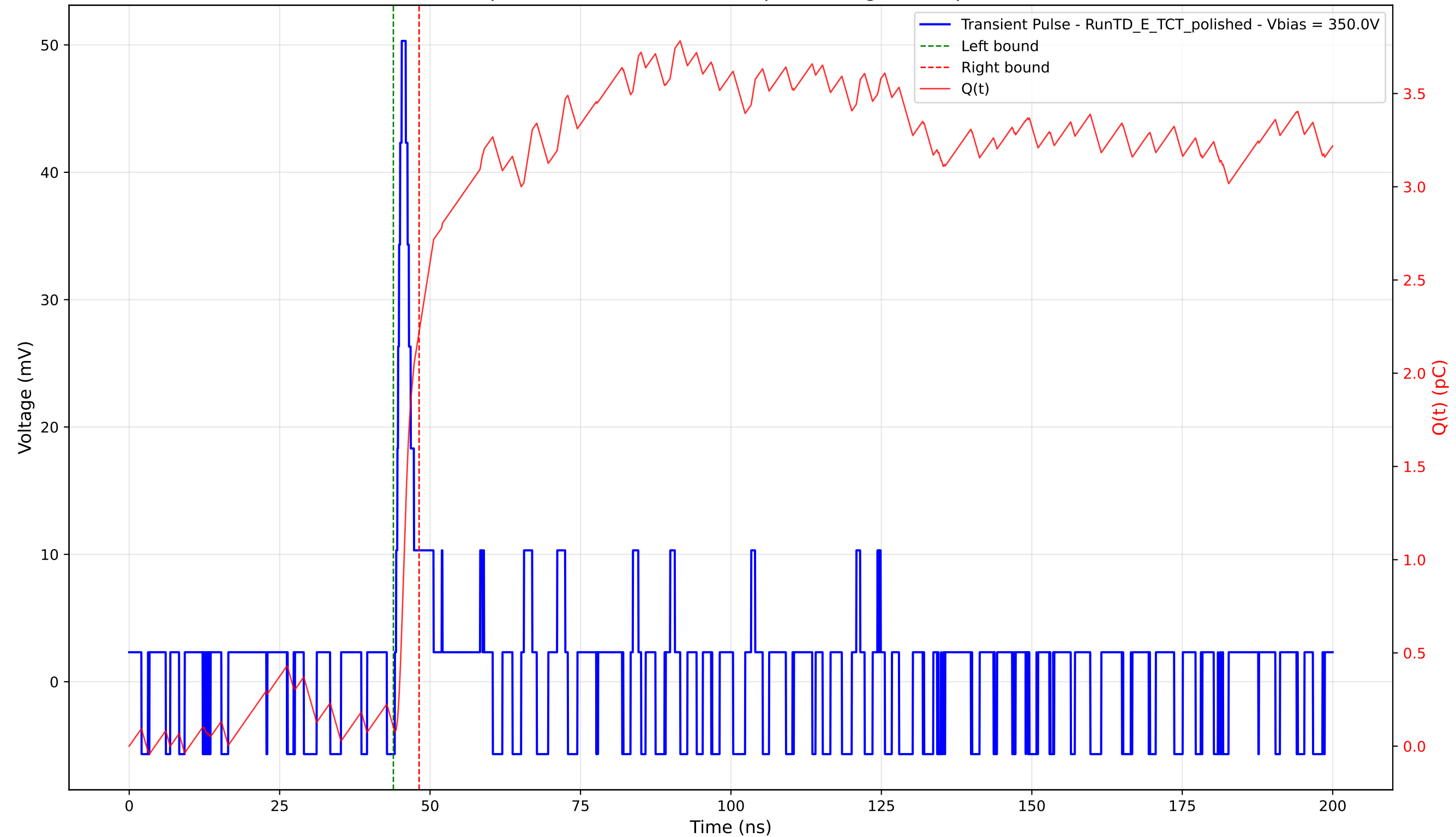
Transient Pulse - Sample: 4003 - Position: 670.0 \mu\text{m} - Charge: 2.12 pC - Rise Time: 0.93 ns
