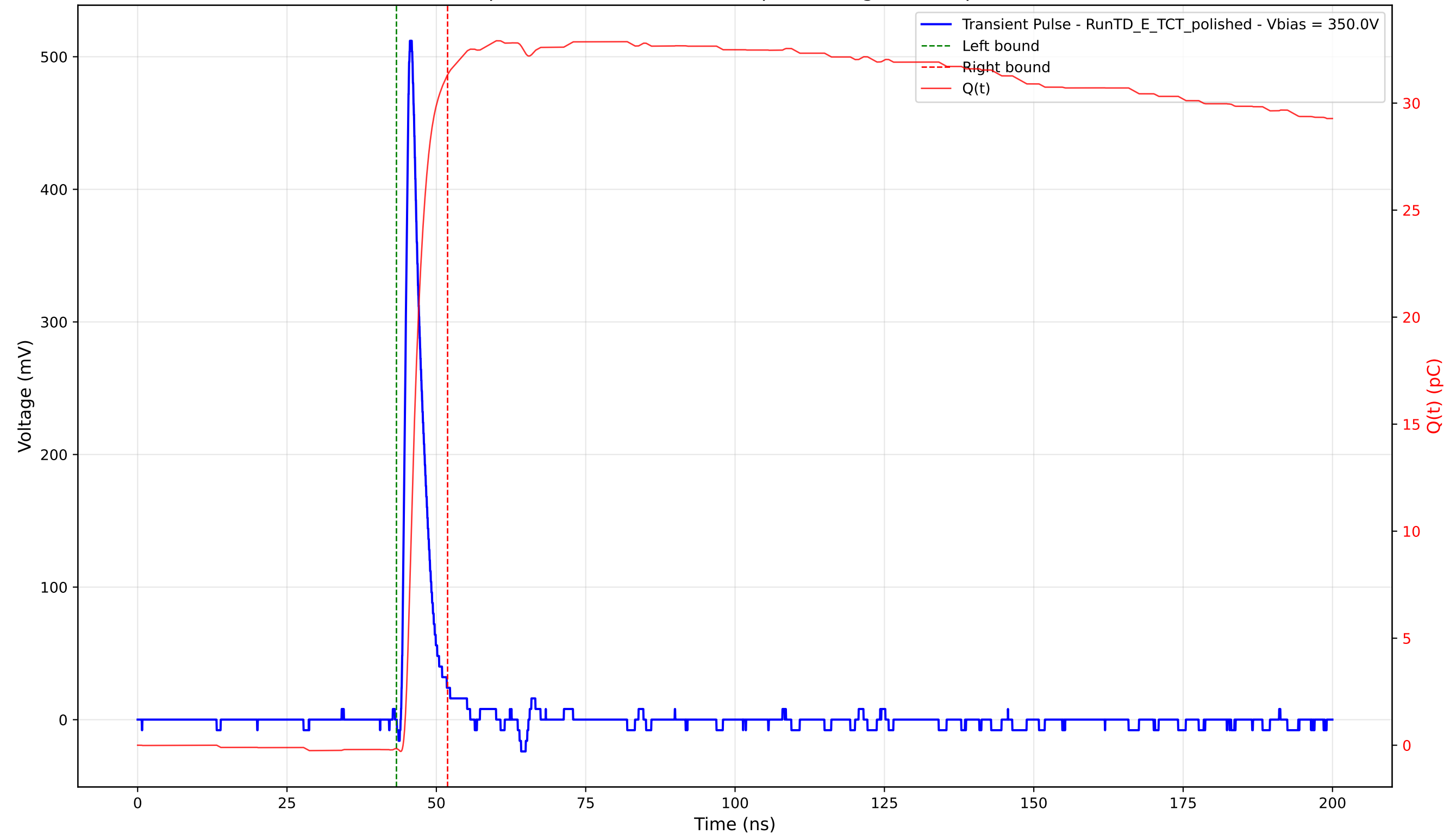
Transient Pulse - Sample: 4003 - Position: 345.0 \mu\text{m} - Charge: 31.48 pC - Rise Time: 0.99 ns
