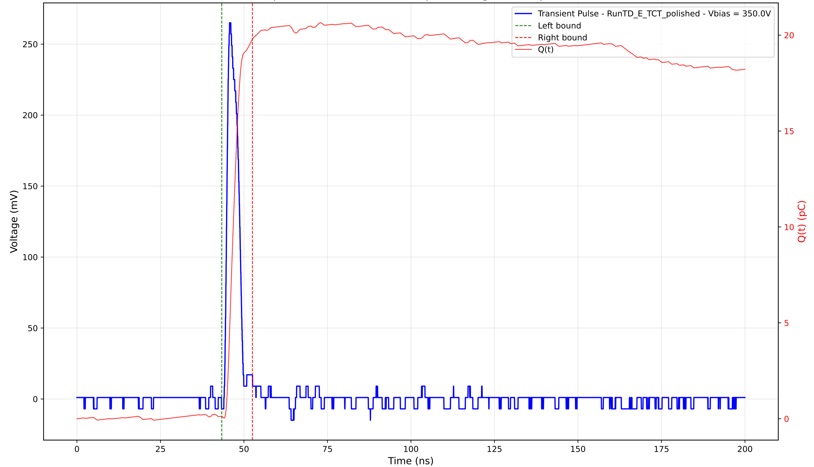
Transient Pulse - Sample: 4003 - Position: 480.0 \mu\text{m} - Charge: 19.69 pC - Rise Time: 1.08 ns
