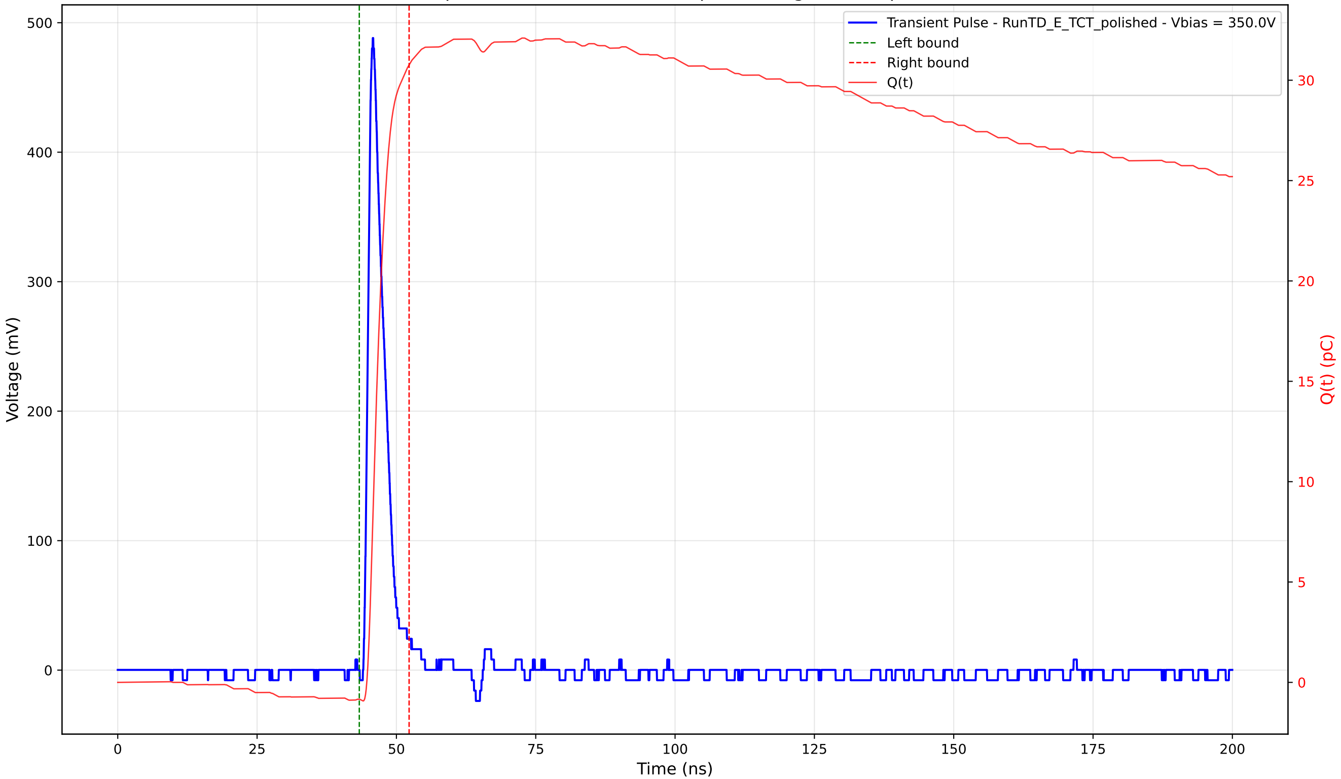
Transient Pulse - Sample: 4003 - Position: 375.0 \mu\text{m} - Charge: 31.60 pC - Rise Time: 1.04 ns
