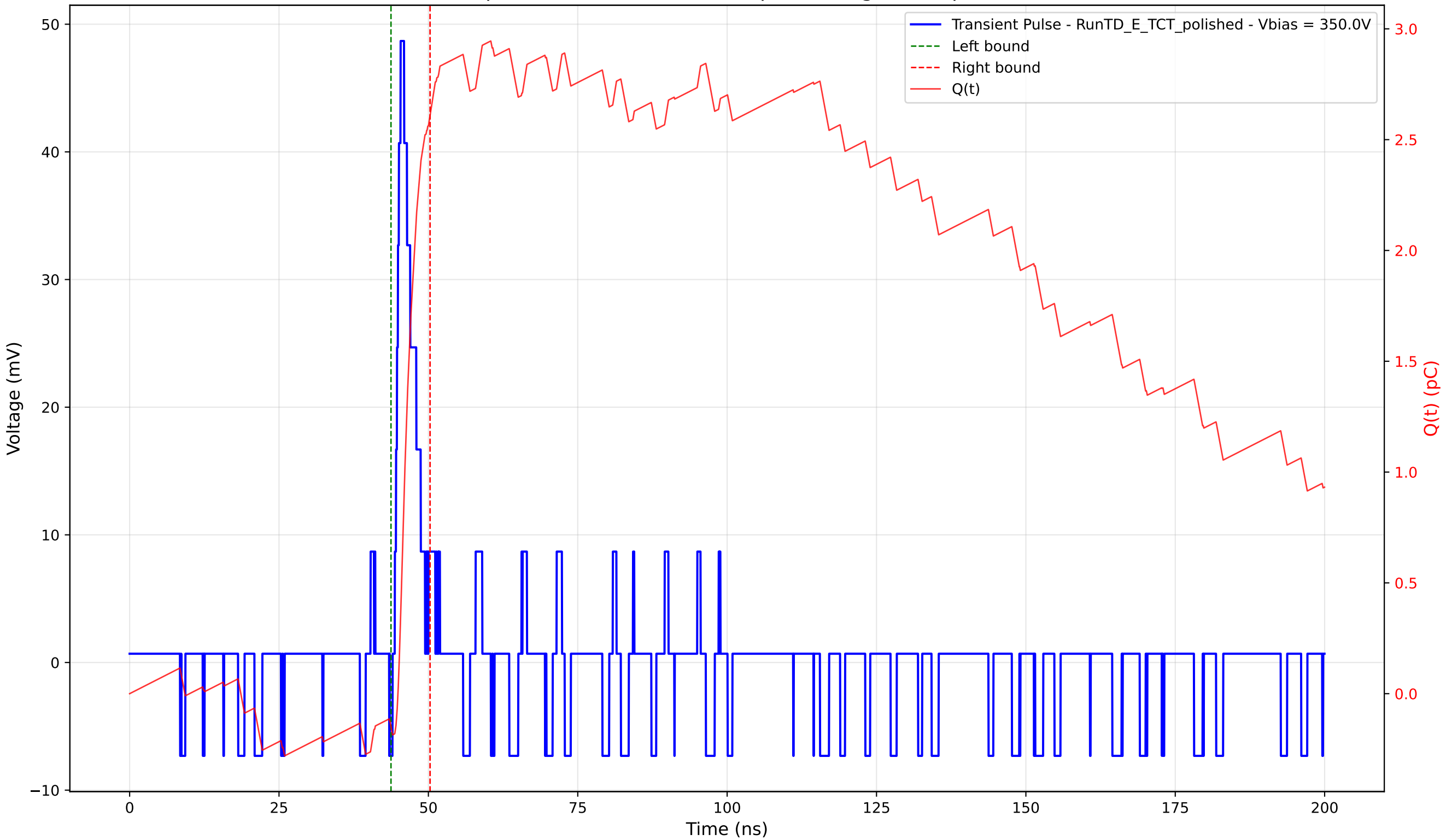
Transient Pulse - Sample: 4003 - Position: 705.0 \mu\text{m} - Charge: 2.76 pC - Rise Time: 0.97 ns
