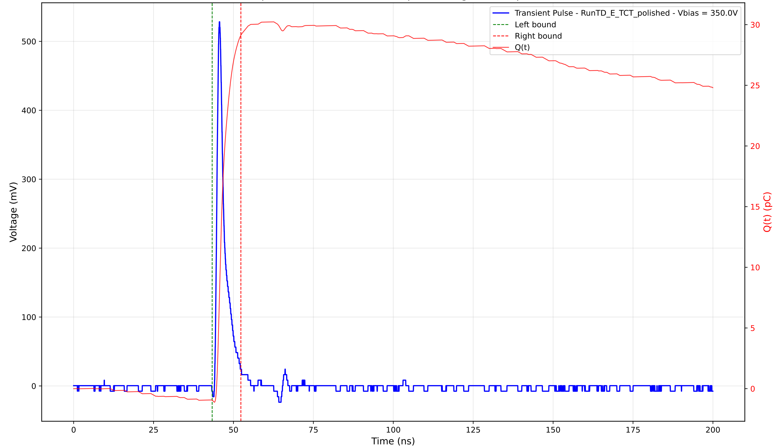
Transient Pulse - Sample: 4003 - Position: 270.0 \mu\text{m} - Charge: 30.08 pC - Rise Time: 0.99 ns
