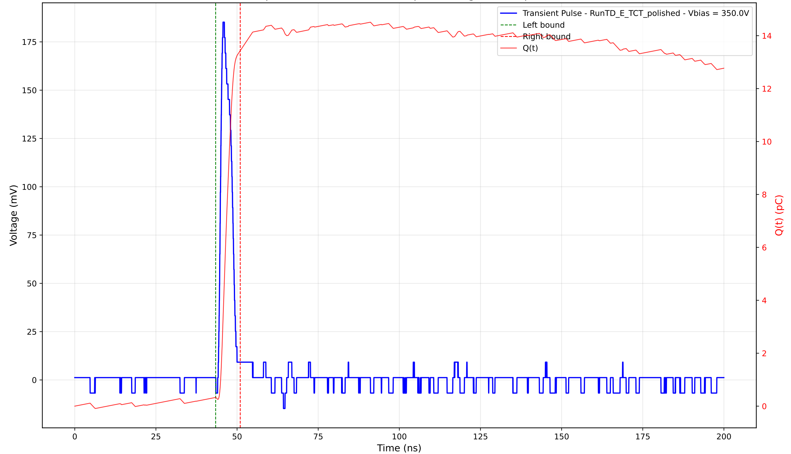
Transient Pulse - Sample: 4003 - Position: 515.0 \mu\text{m} - Charge: 13.10 pC - Rise Time: 1.02 ns
