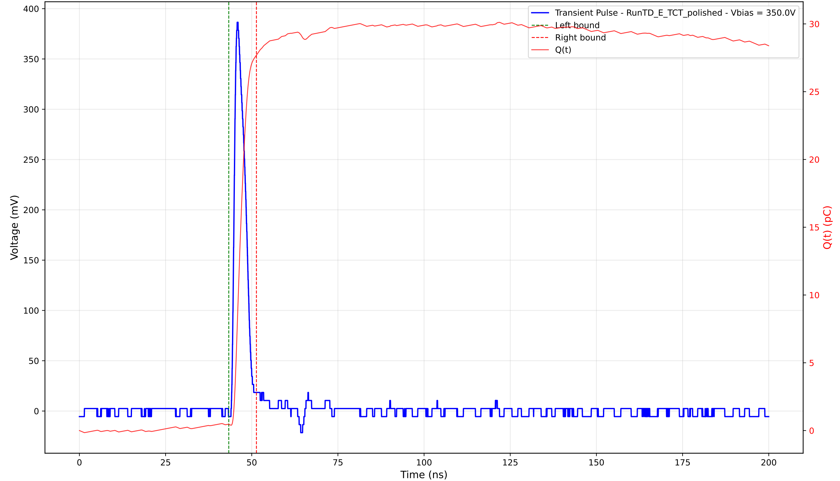
Transient Pulse - Sample: 4003 - Position: 430.0 \mu\text{m} - Charge: 27.24 pC - Rise Time: 1.13 ns
