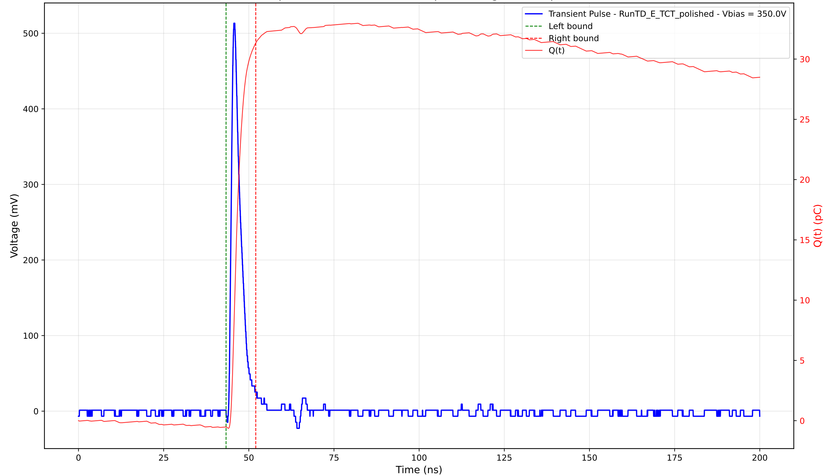
Transient Pulse - Sample: 4003 - Position: 350.0 \mu\text{m} - Charge: 31.85 pC - Rise Time: 1.03 ns
