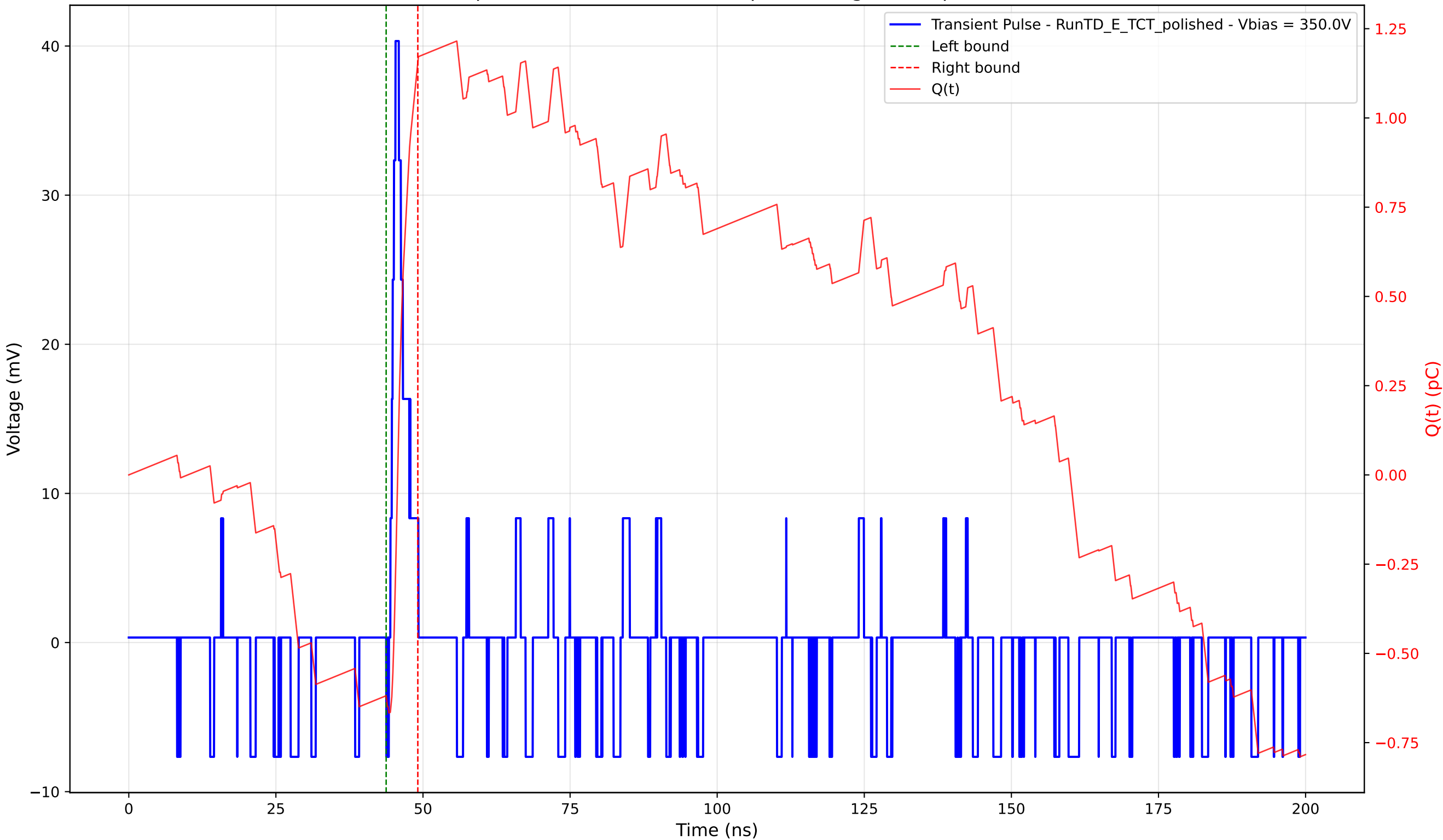
Transient Pulse - Sample: 4003 - Position: 100.0 \mu\text{m} - Charge: 1.78 pC - Rise Time: 0.87 ns
