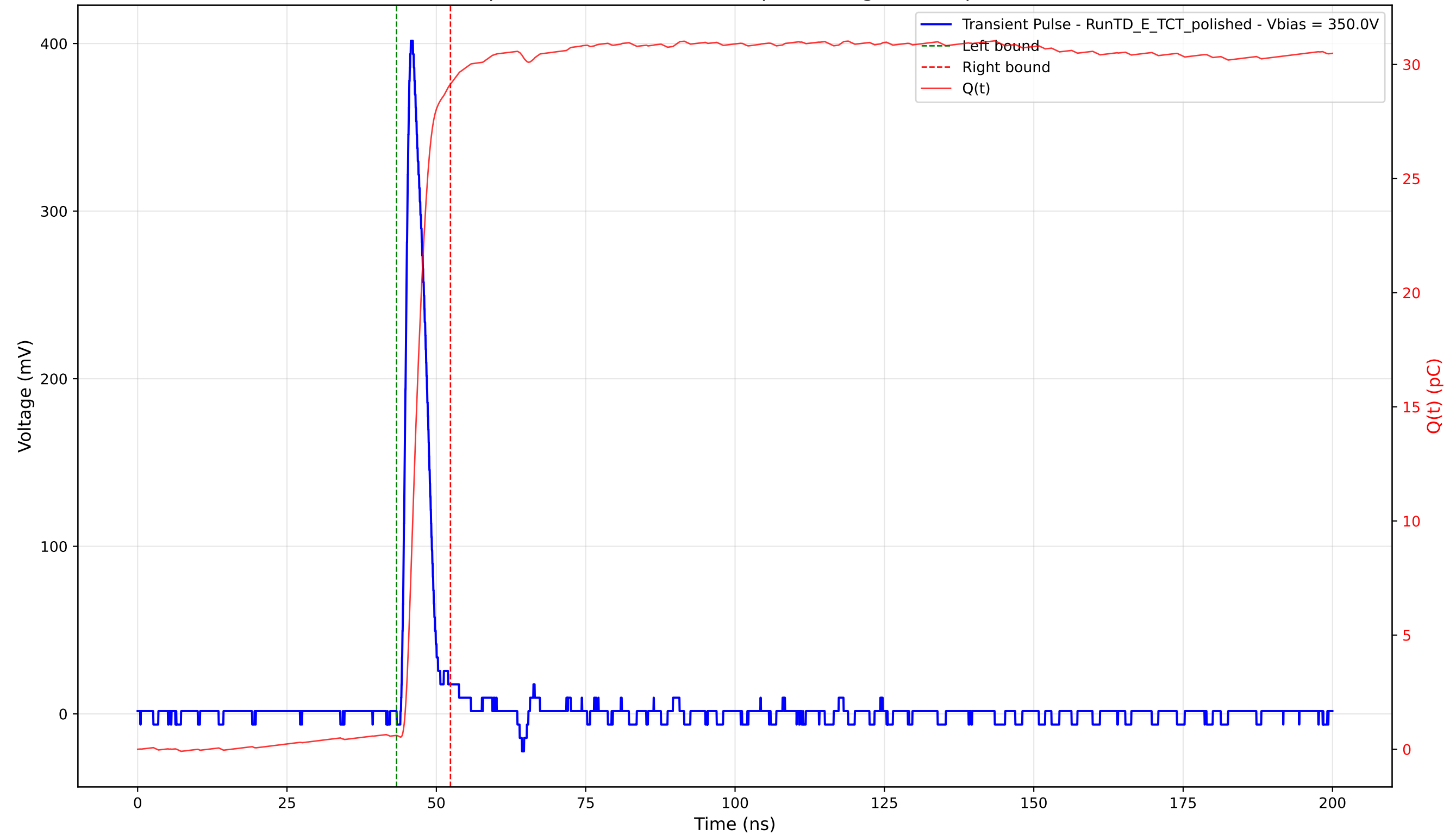
Transient Pulse - Sample: 4003 - Position: 425.0 \mu\text{m} - Charge: 28.53 pC - Rise Time: 1.10 ns
