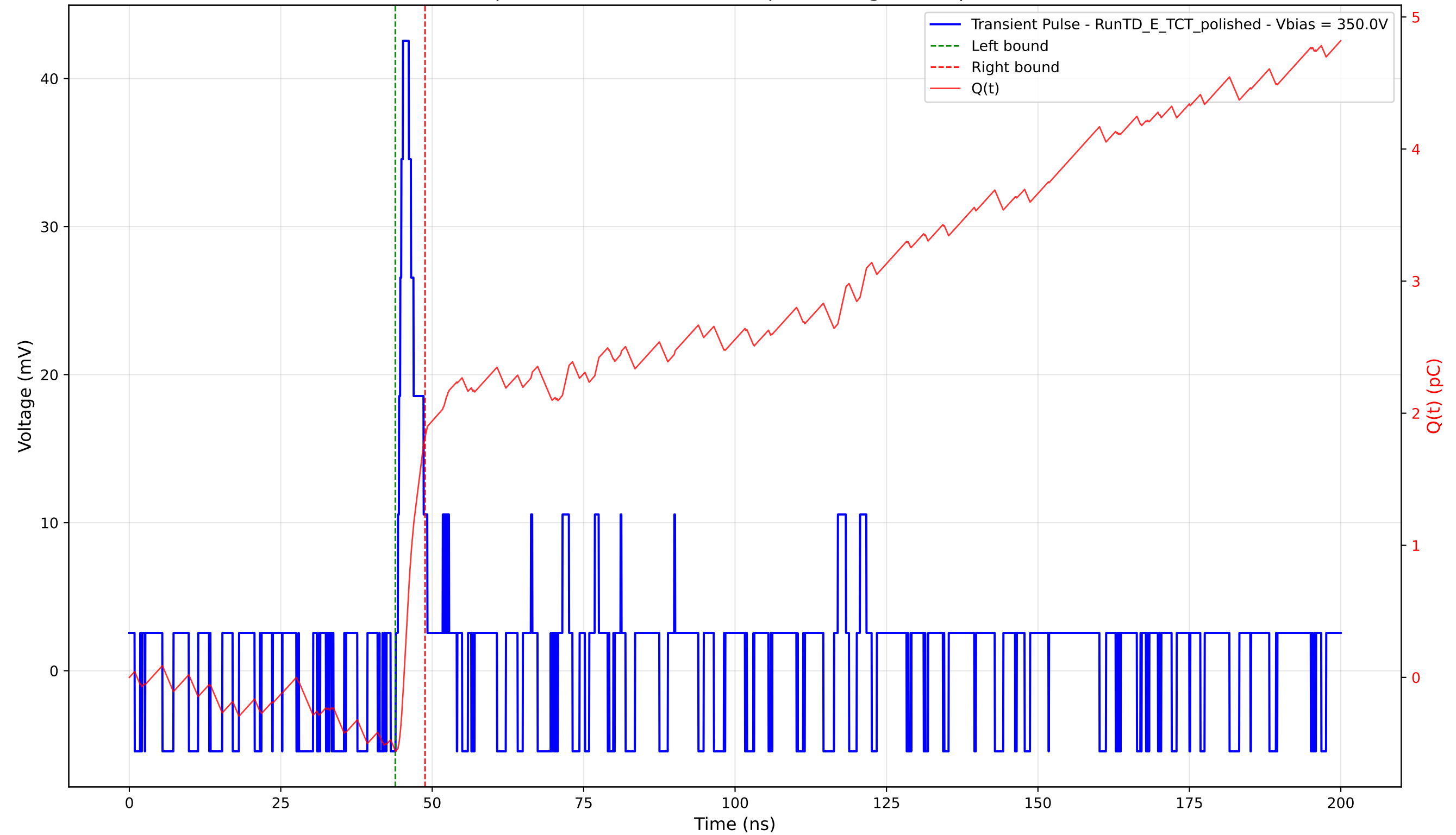
Transient Pulse - Sample: 4003 - Position: 710.0 \mu\text{m} - Charge: 2.38 pC - Rise Time: 0.84 ns
