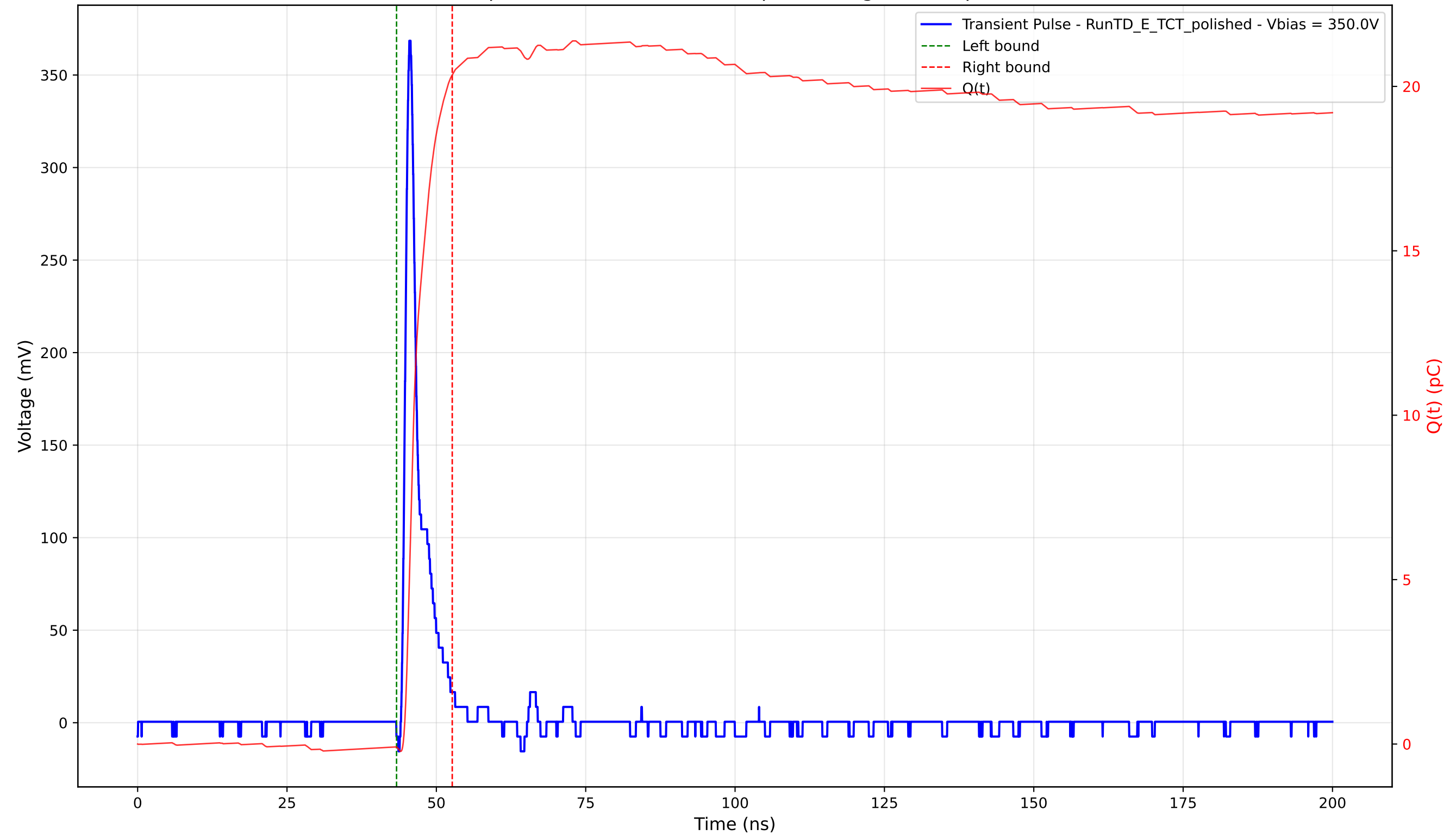
Transient Pulse - Sample: 4003 - Position: 205.0 \mu\text{m} - Charge: 20.44 pC - Rise Time: 0.97 ns
