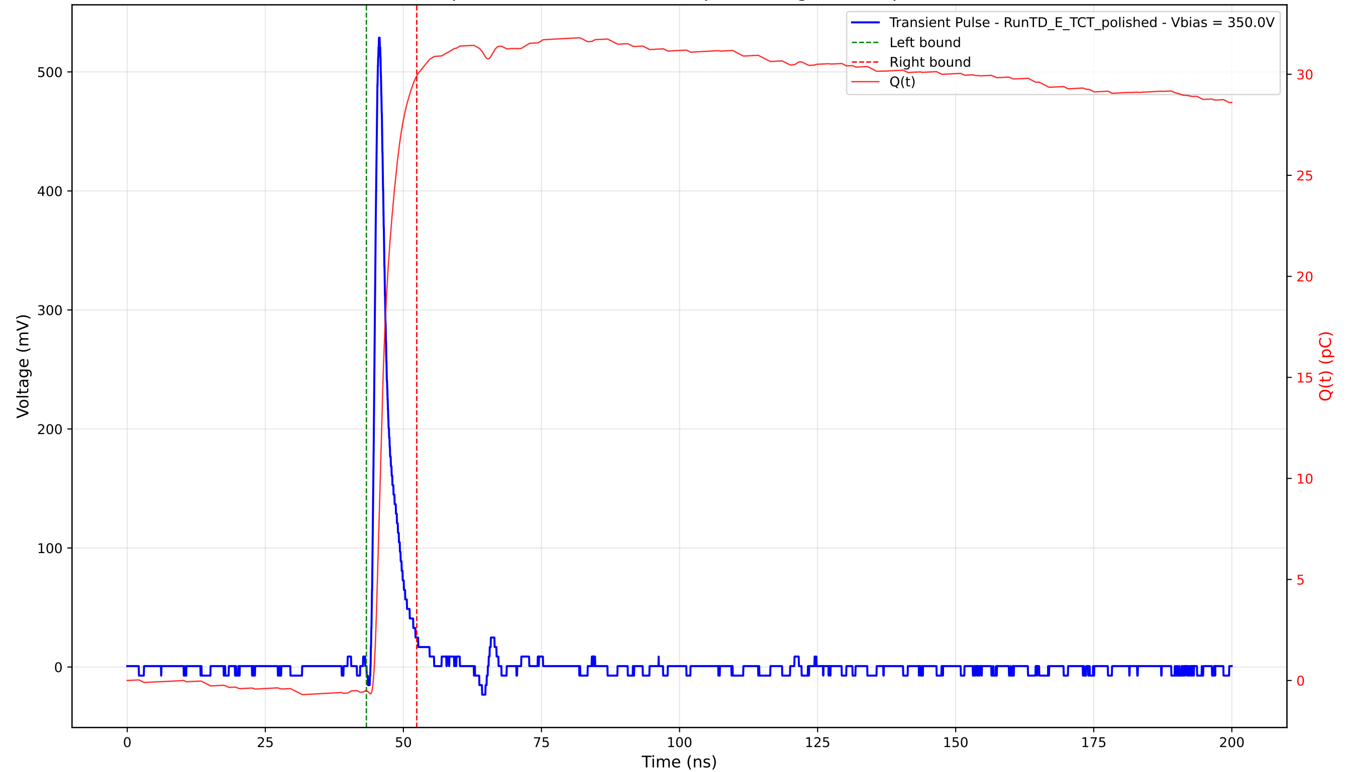
Transient Pulse - Sample: 4003 - Position: 275.0 \mu\text{m} - Charge: 30.43 pC - Rise Time: 0.98 ns
