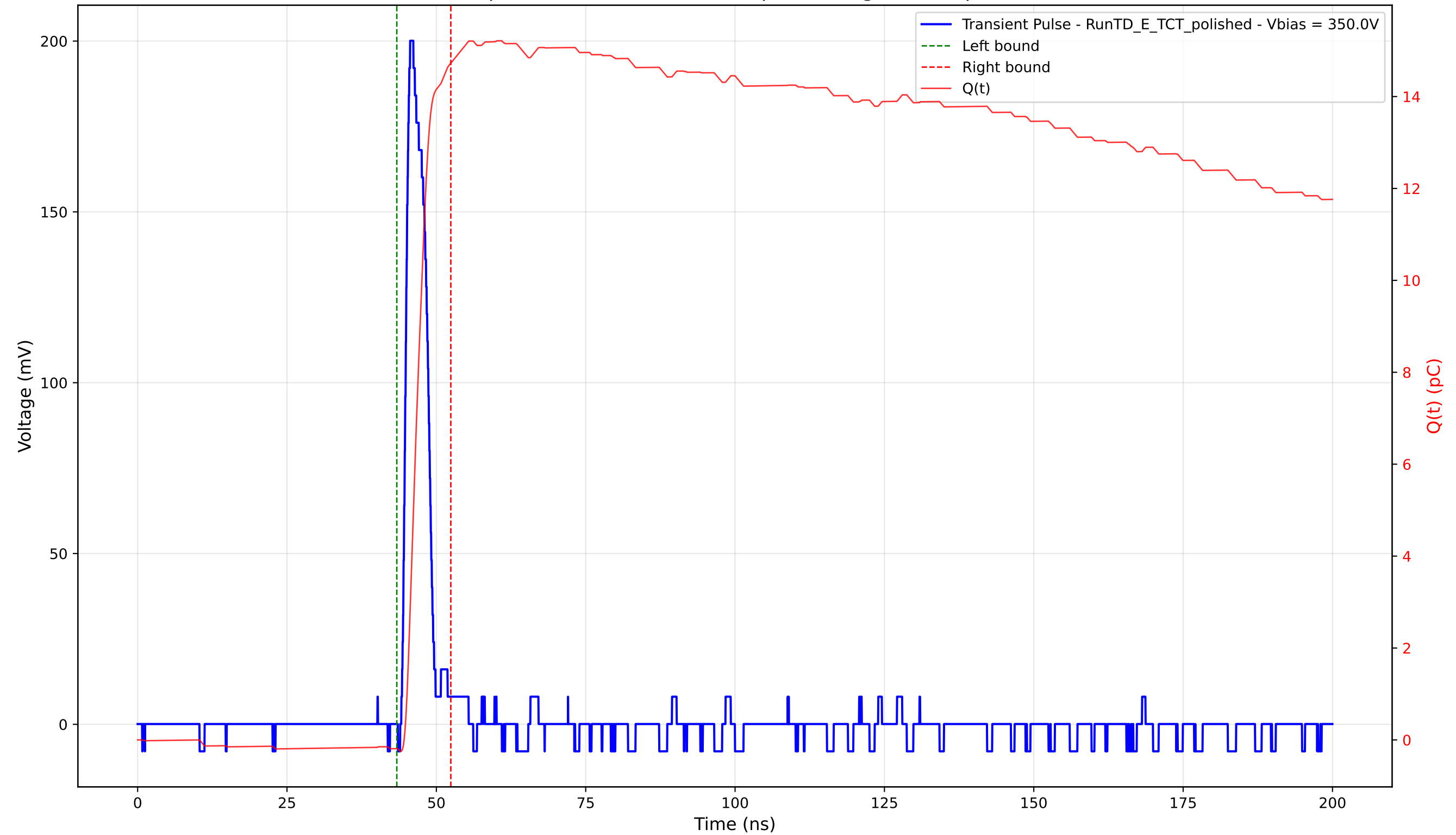
Transient Pulse - Sample: 4003 - Position: 505.0 \mu\text{m} - Charge: 14.91 pC - Rise Time: 1.05 ns
