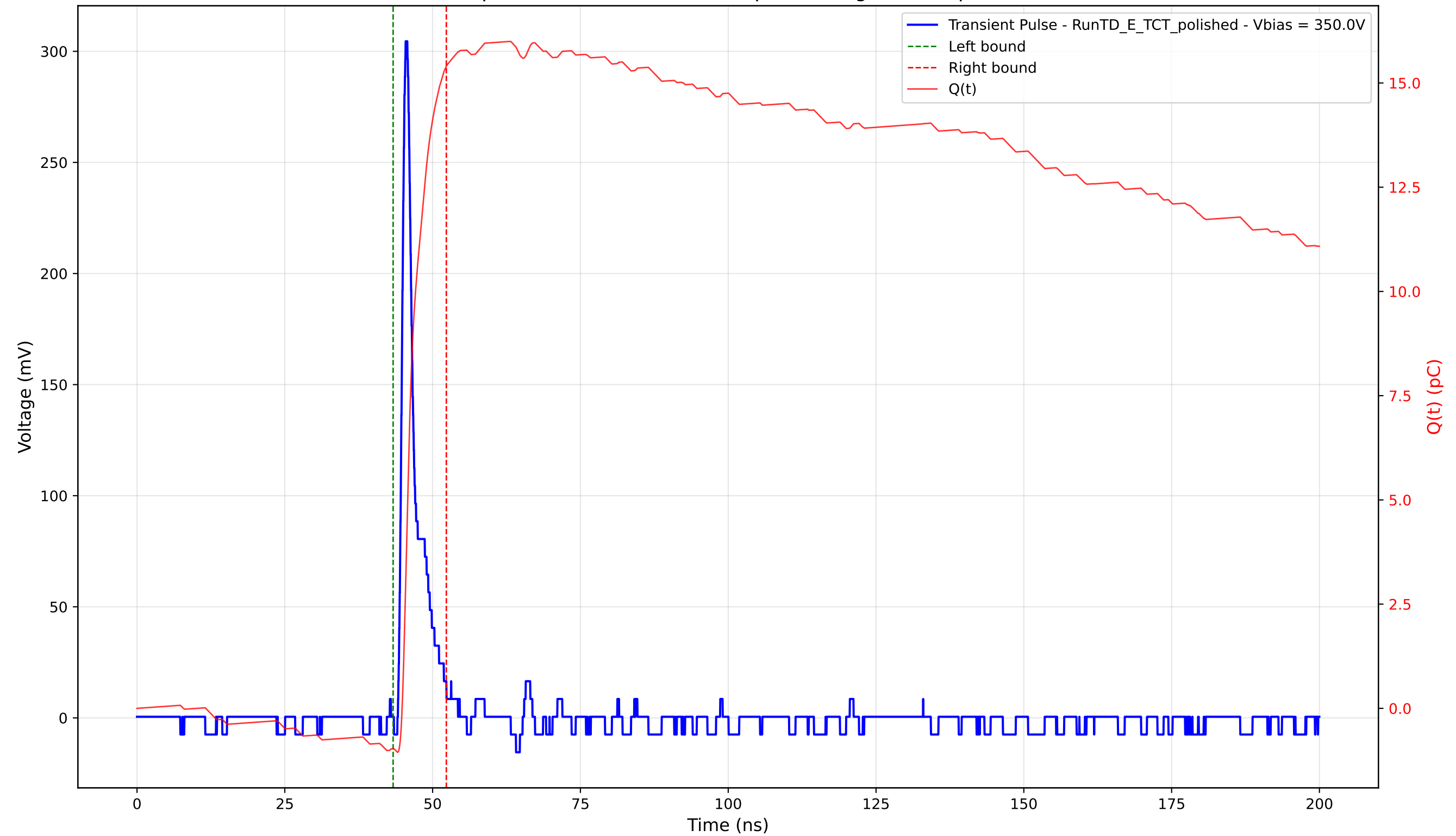
Transient Pulse - Sample: 4003 - Position: 190.0 \mu\text{m} - Charge: 16.38 pC - Rise Time: 0.93 ns
