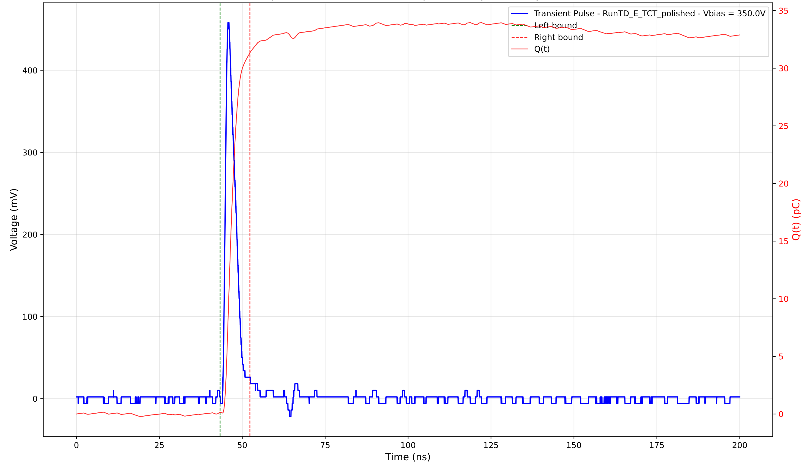
Transient Pulse - Sample: 4003 - Position: 395.0 \mu\text{m} - Charge: 31.20 pC - Rise Time: 1.09 ns
