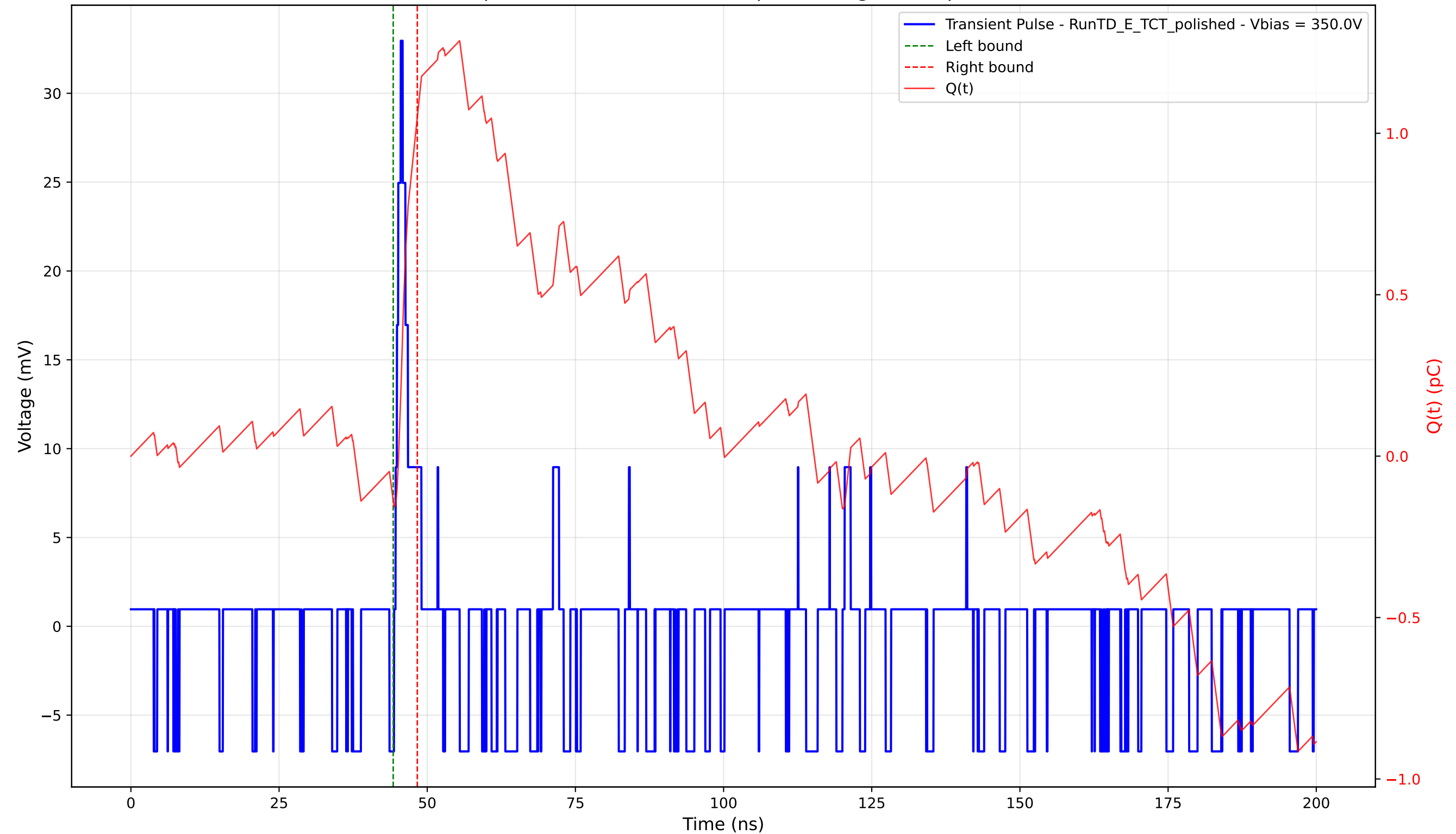
Transient Pulse - Sample: 4003 - Position: 780.0 \mu\text{m} - Charge: 1.19 pC - Rise Time: 0.87 ns
