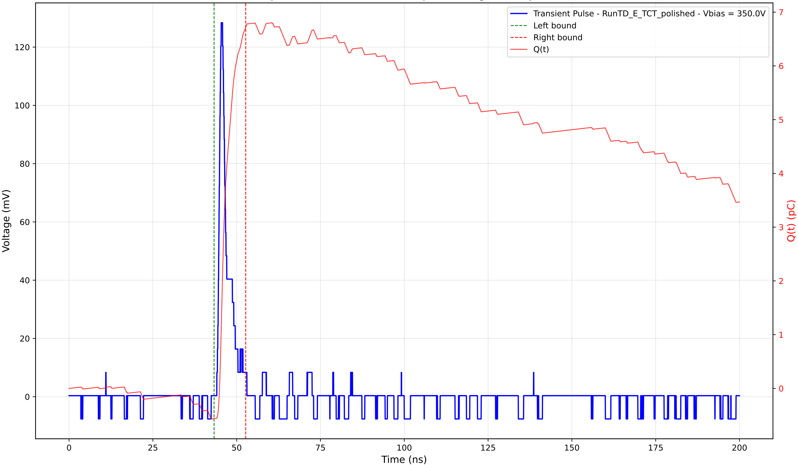
Transient Pulse - Sample: 4003 - Position: 140.0 \mu\text{m} - Charge: 7.28 pC - Rise Time: 0.99 ns
