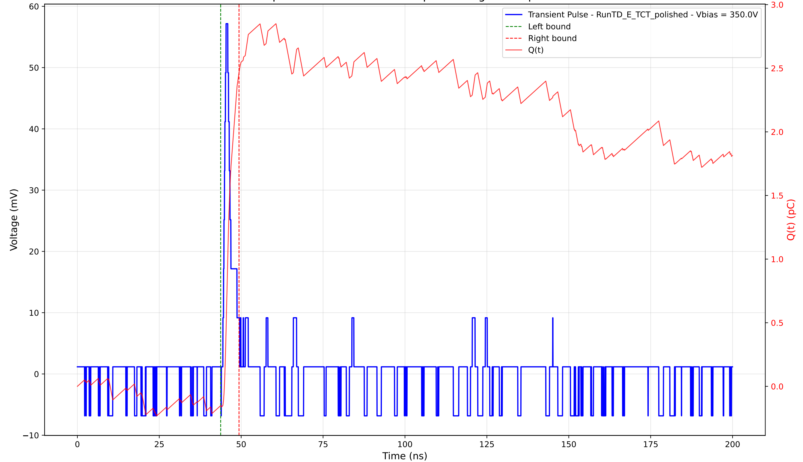
Transient Pulse - Sample: 4003 - Position: 110.0 \mu\text{m} - Charge: 2.62 pC - Rise Time: 0.97 ns
