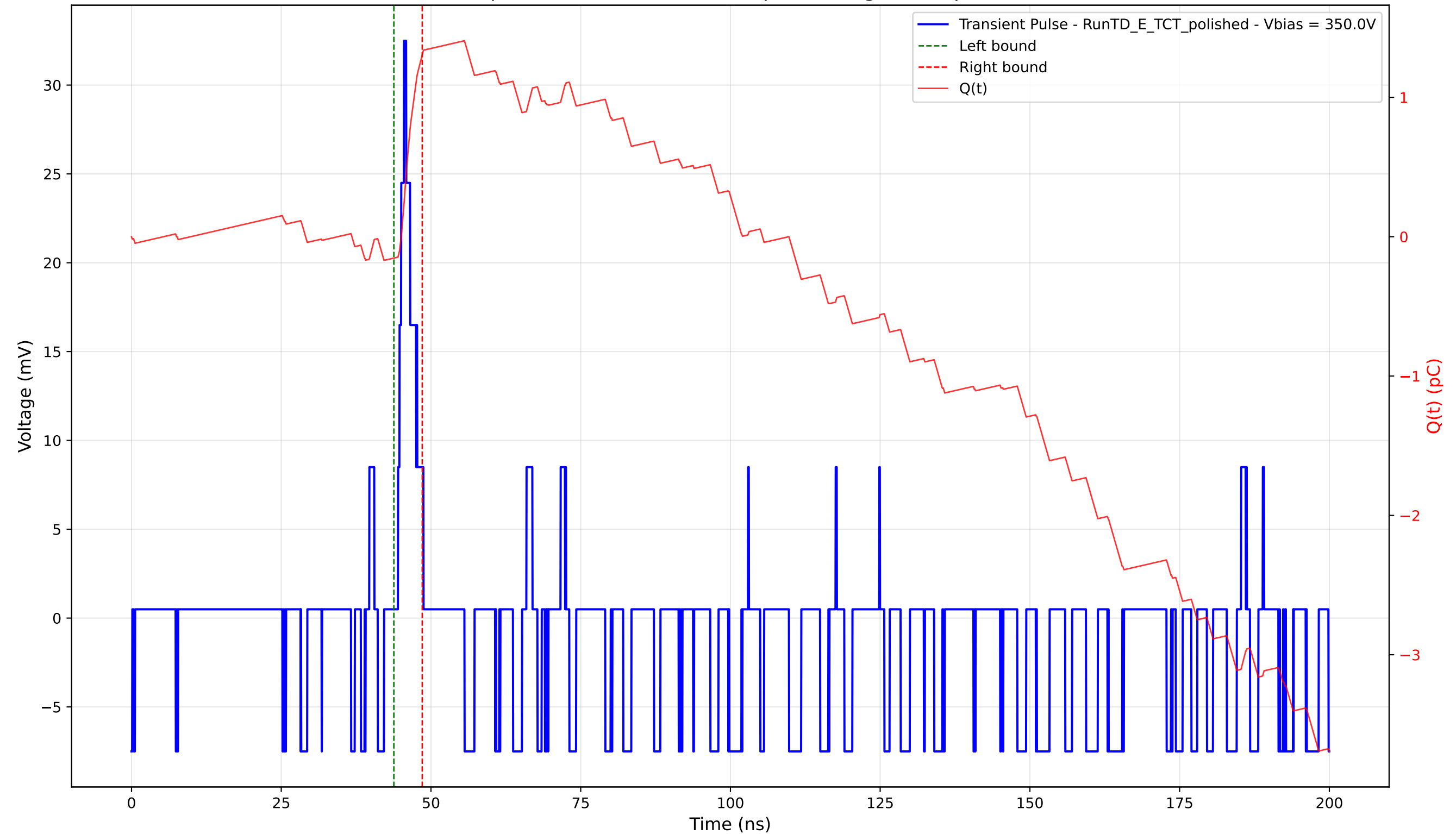
Transient Pulse - Sample: 4003 - Position: 735.0 \mu\text{m} - Charge: 1.46 pC - Rise Time: 0.99 ns
