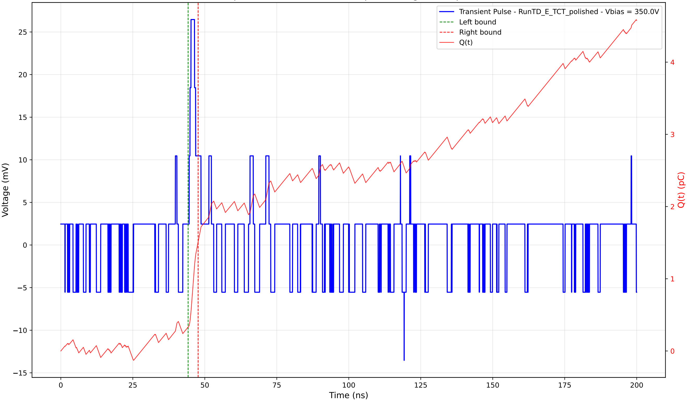
Transient Pulse - Sample: 4003 - Position: 755.0 \mu\text{m} - Charge: 1.18 pC - Rise Time: 0.64 ns
