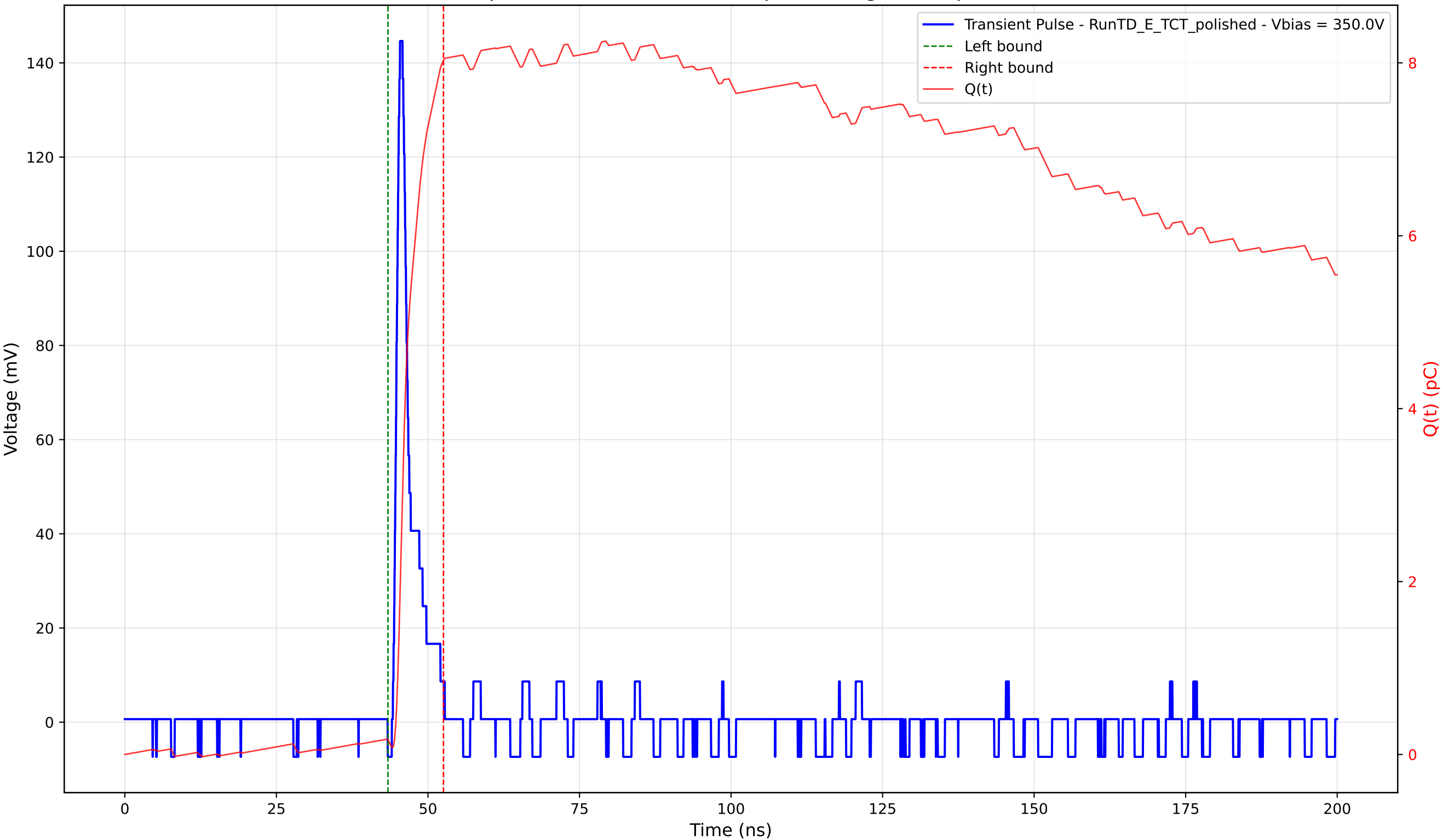
Transient Pulse - Sample: 4003 - Position: 145.0 \mu\text{m} - Charge: 7.86 pC - Rise Time: 0.97 ns
