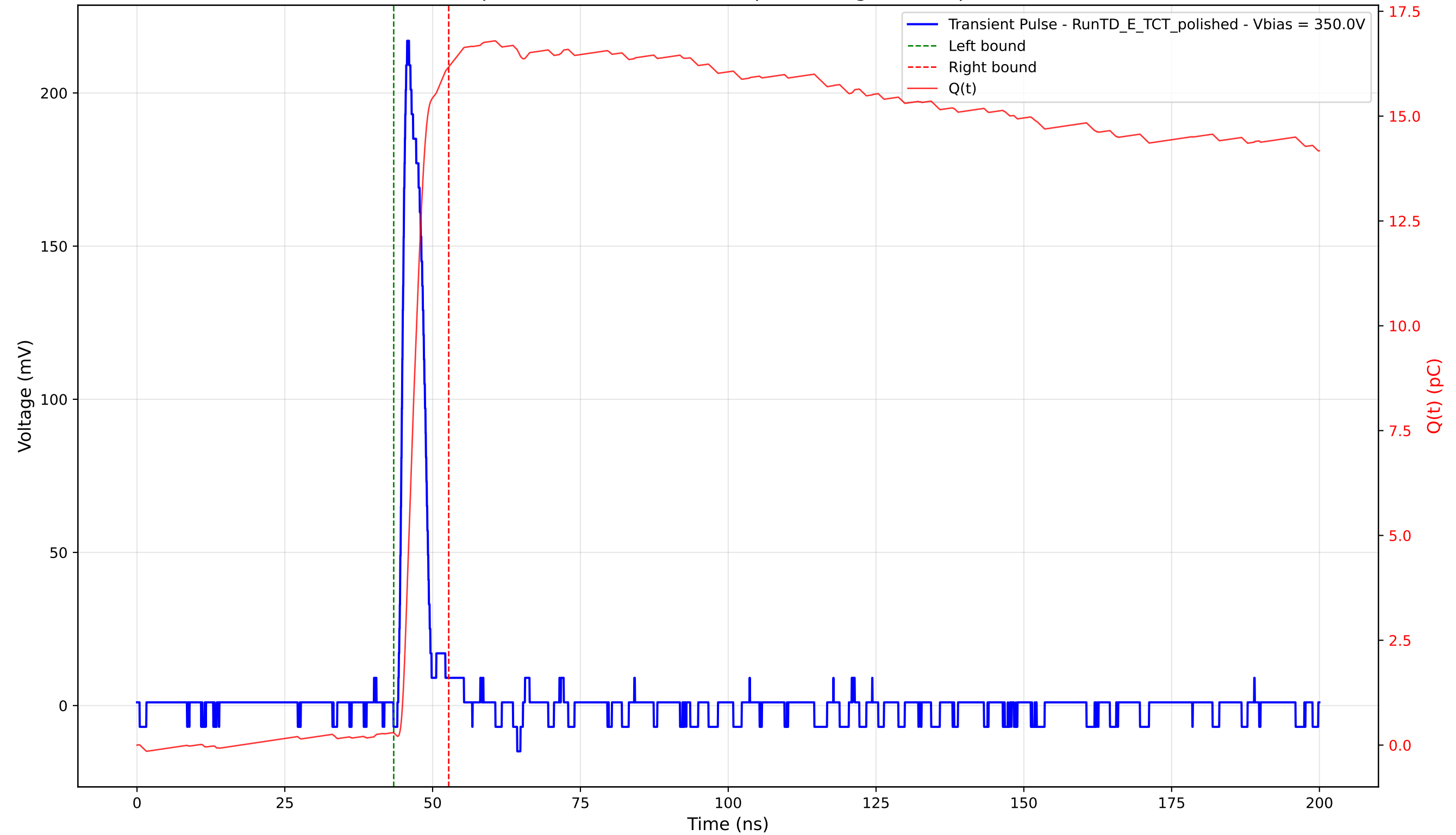
Transient Pulse - Sample: 4003 - Position: 500.0 \mu\text{m} - Charge: 15.88 pC - Rise Time: 1.09 ns
