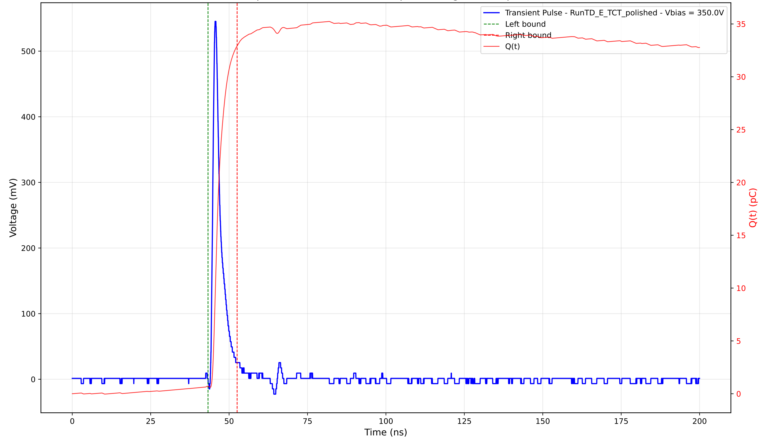
Transient Pulse - Sample: 4003 - Position: 295.0 \mu\text{m} - Charge: 32.20 pC - Rise Time: 1.01 ns
