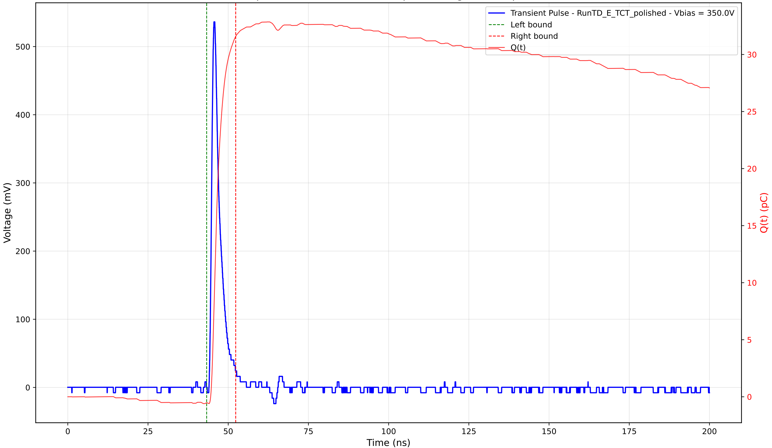
Transient Pulse - Sample: 4003 - Position: 315.0 \mu\text{m} - Charge: 32.12 pC - Rise Time: 1.01 ns
