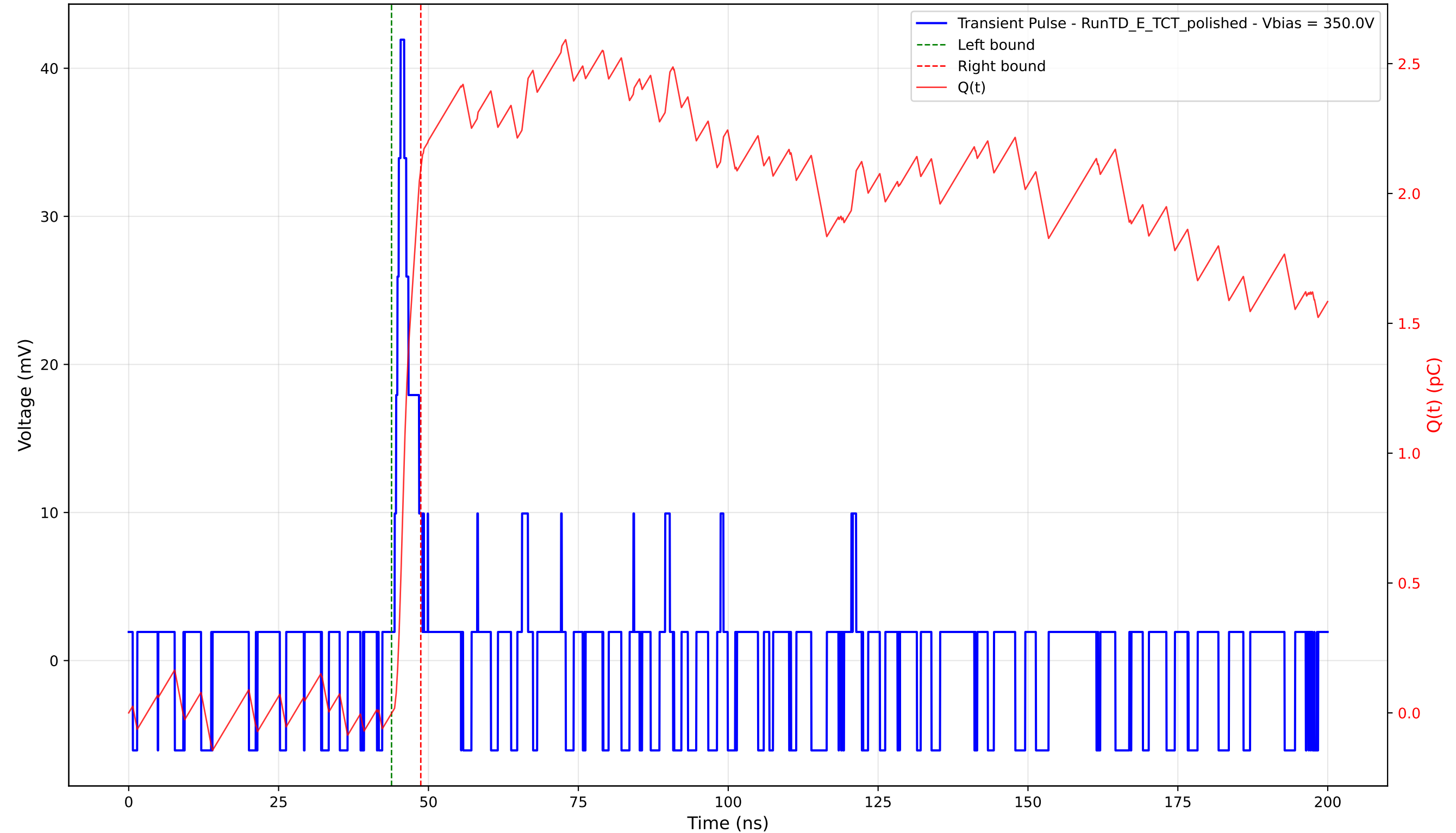
Transient Pulse - Sample: 4003 - Position: 650.0 \mu\text{m} - Charge: 2.10 pC - Rise Time: 0.99 ns
