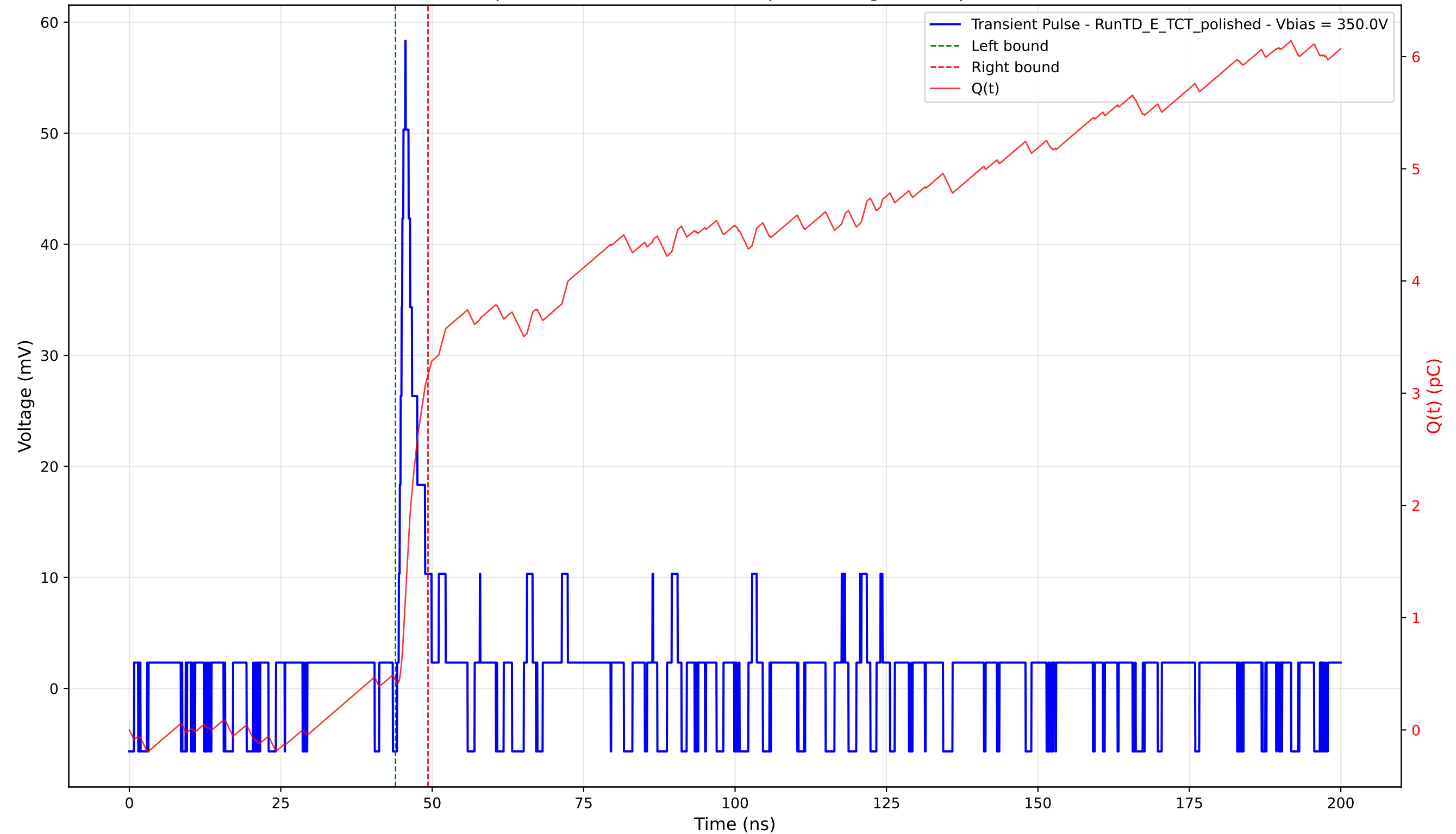
Transient Pulse - Sample: 4003 - Position: 605.0 \mu\text{m} - Charge: 2.72 pC - Rise Time: 1.09 ns
