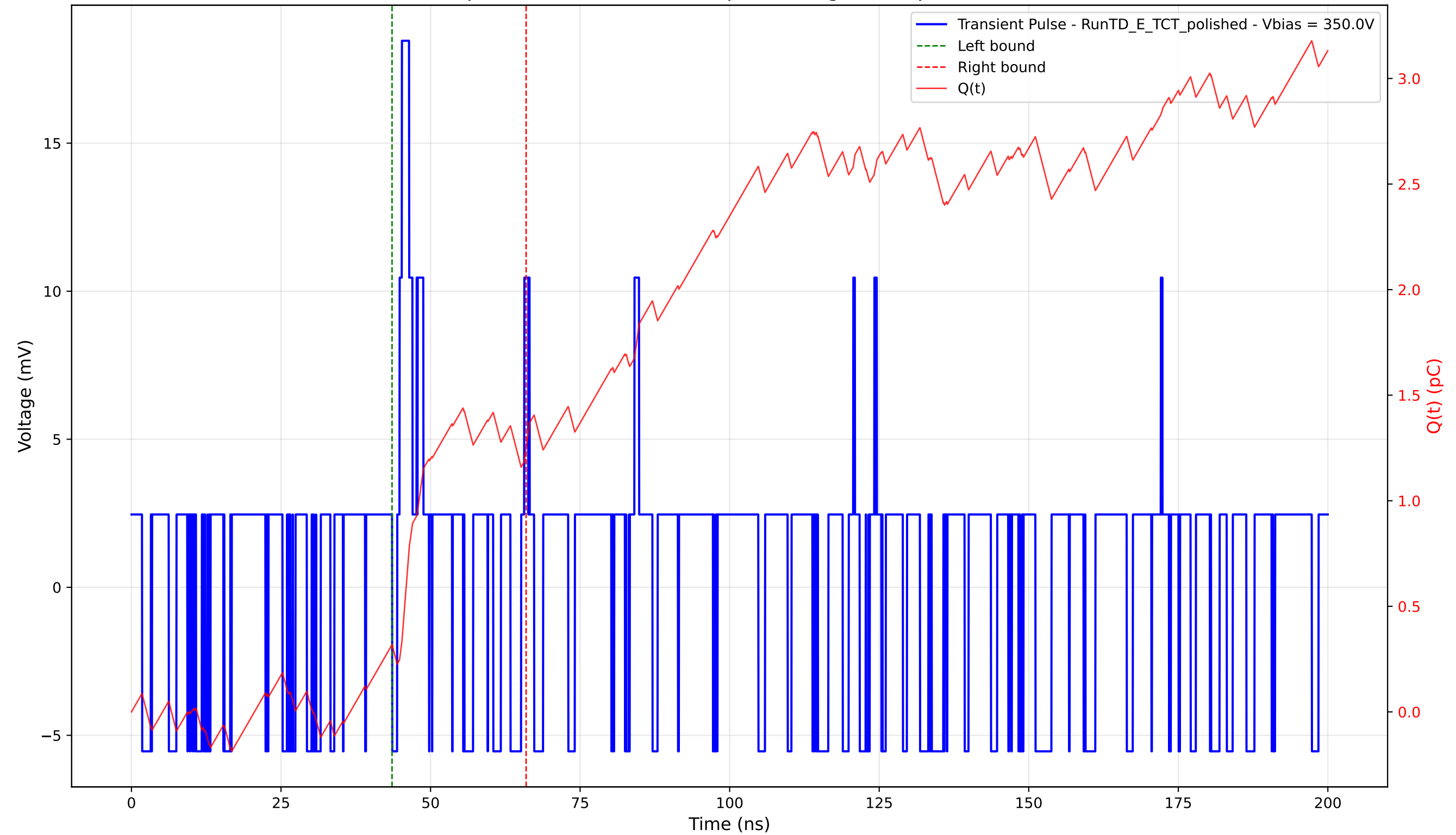
Transient Pulse - Sample: 4003 - Position: 30.0 \mu\text{m} - Charge: 0.93 pC - Rise Time: 0.00 ns (N/A)
