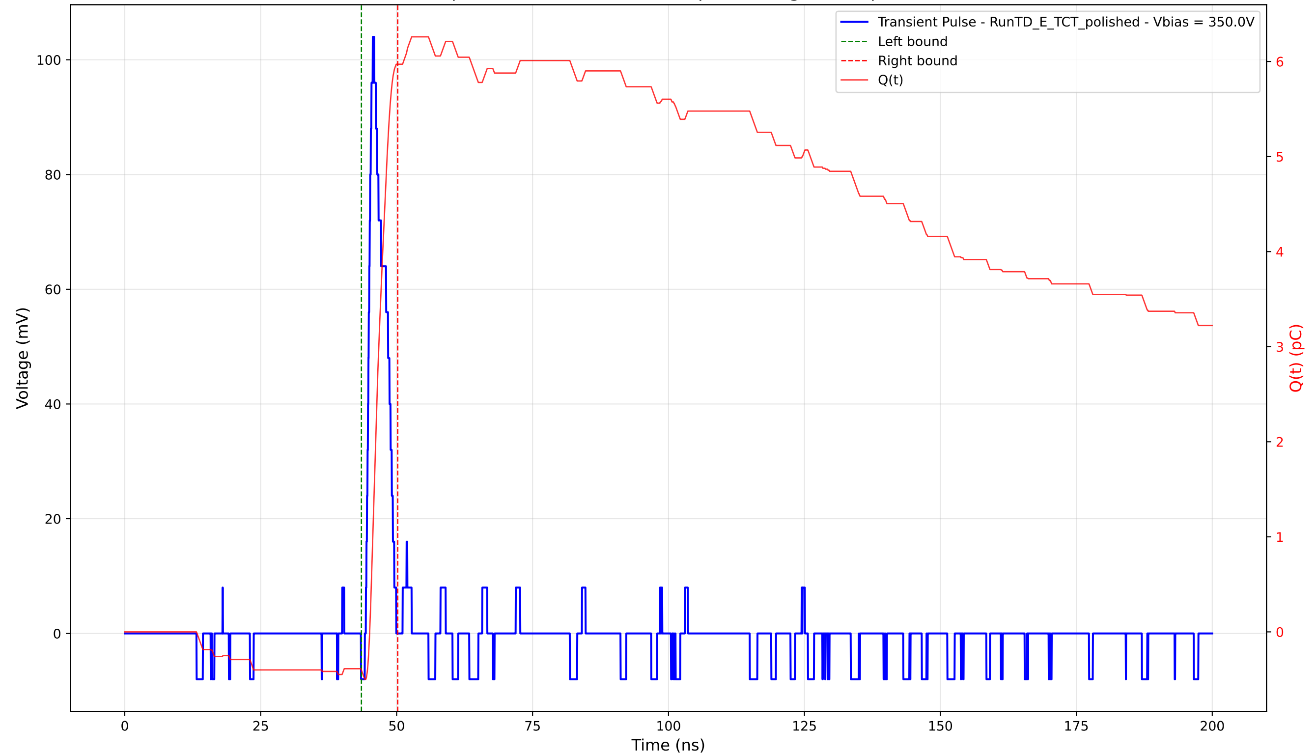
Transient Pulse - Sample: 4003 - Position: 560.0 \mu\text{m} - Charge: 6.37 pC - Rise Time: 0.93 ns
