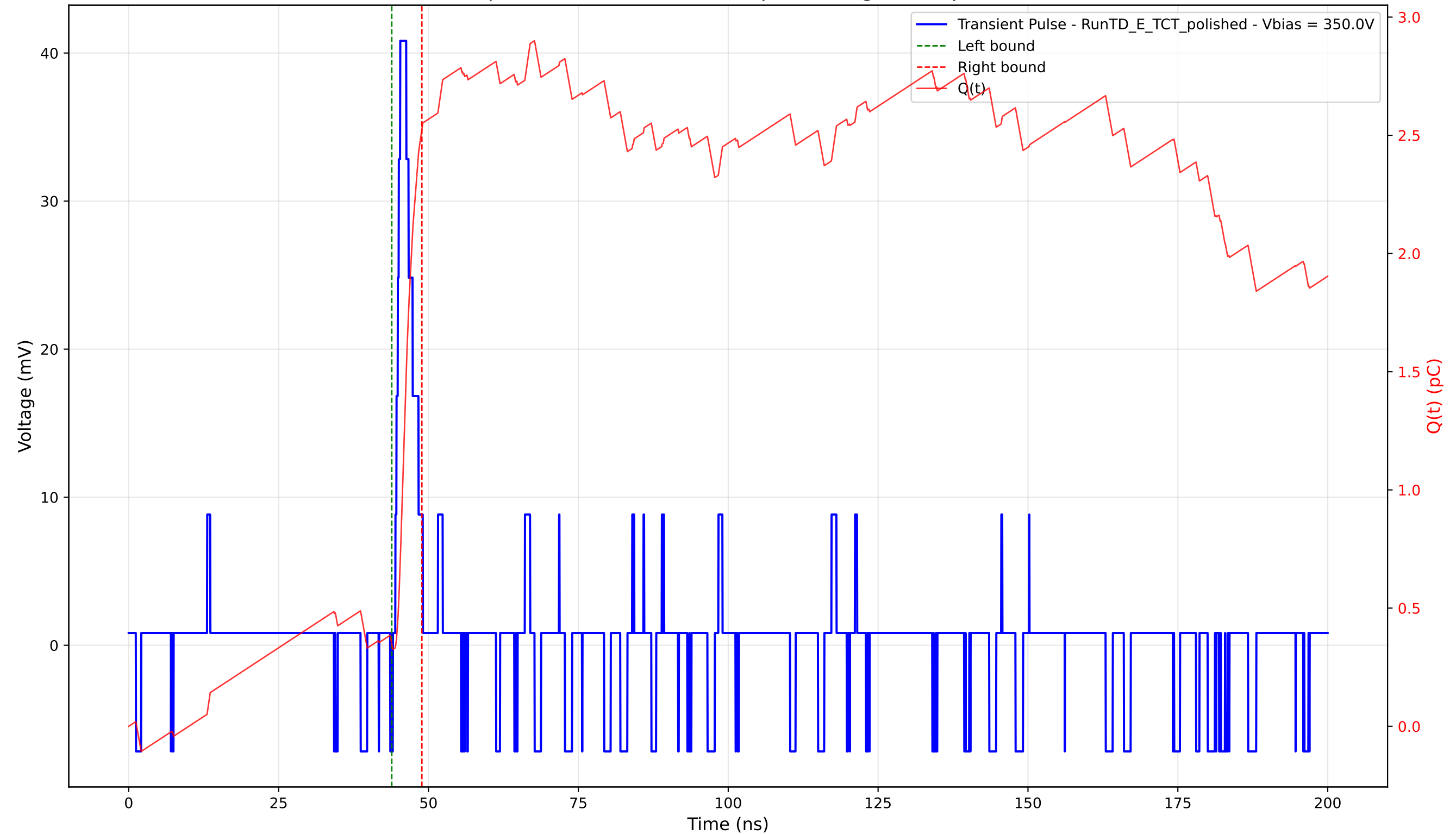
Transient Pulse - Sample: 4003 - Position: 620.0 \mu\text{m} - Charge: 2.18 pC - Rise Time: 0.81 ns
