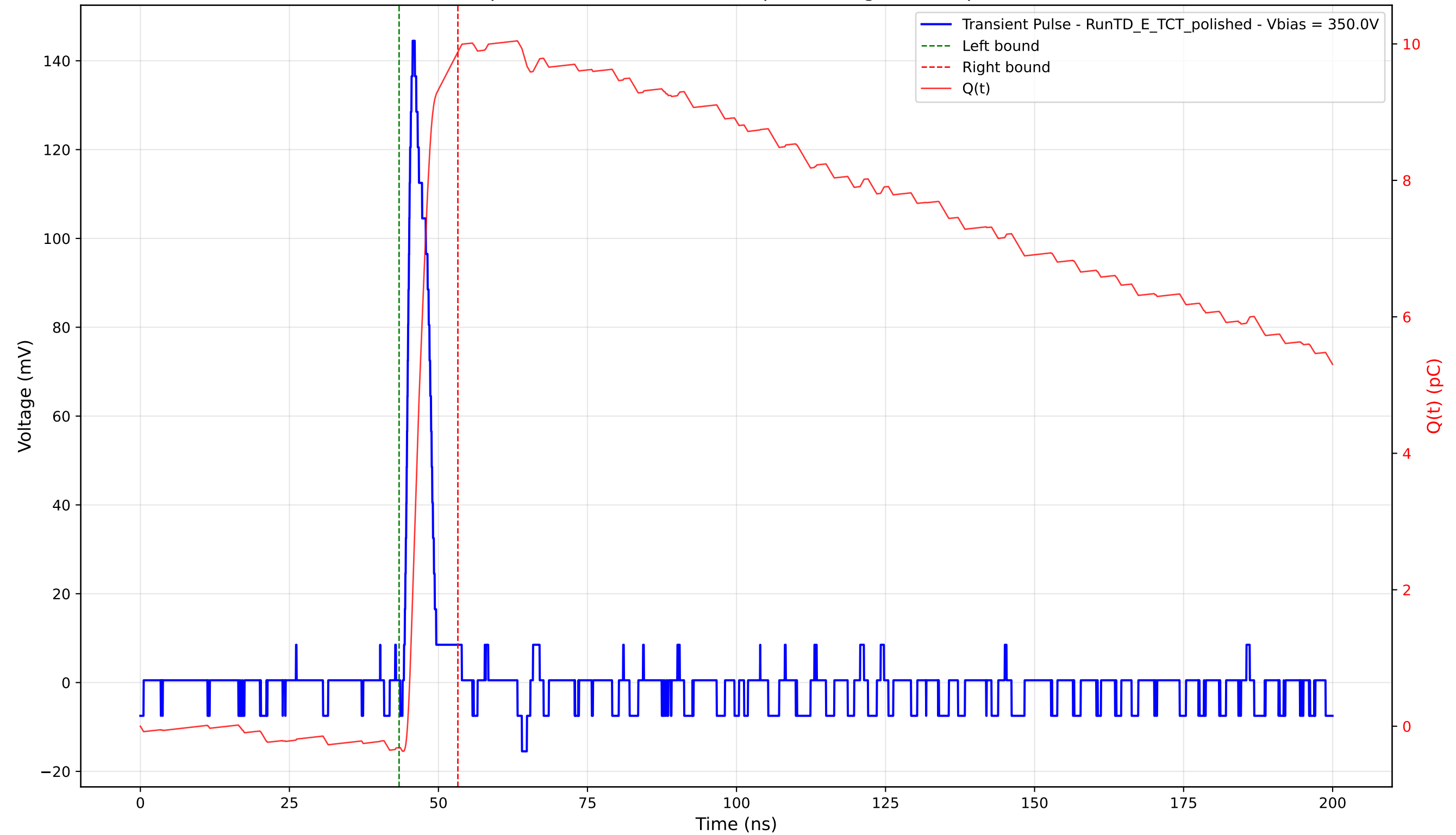
Transient Pulse - Sample: 4003 - Position: 535.0 \mu\text{m} - Charge: 10.20 pC - Rise Time: 1.13 ns
