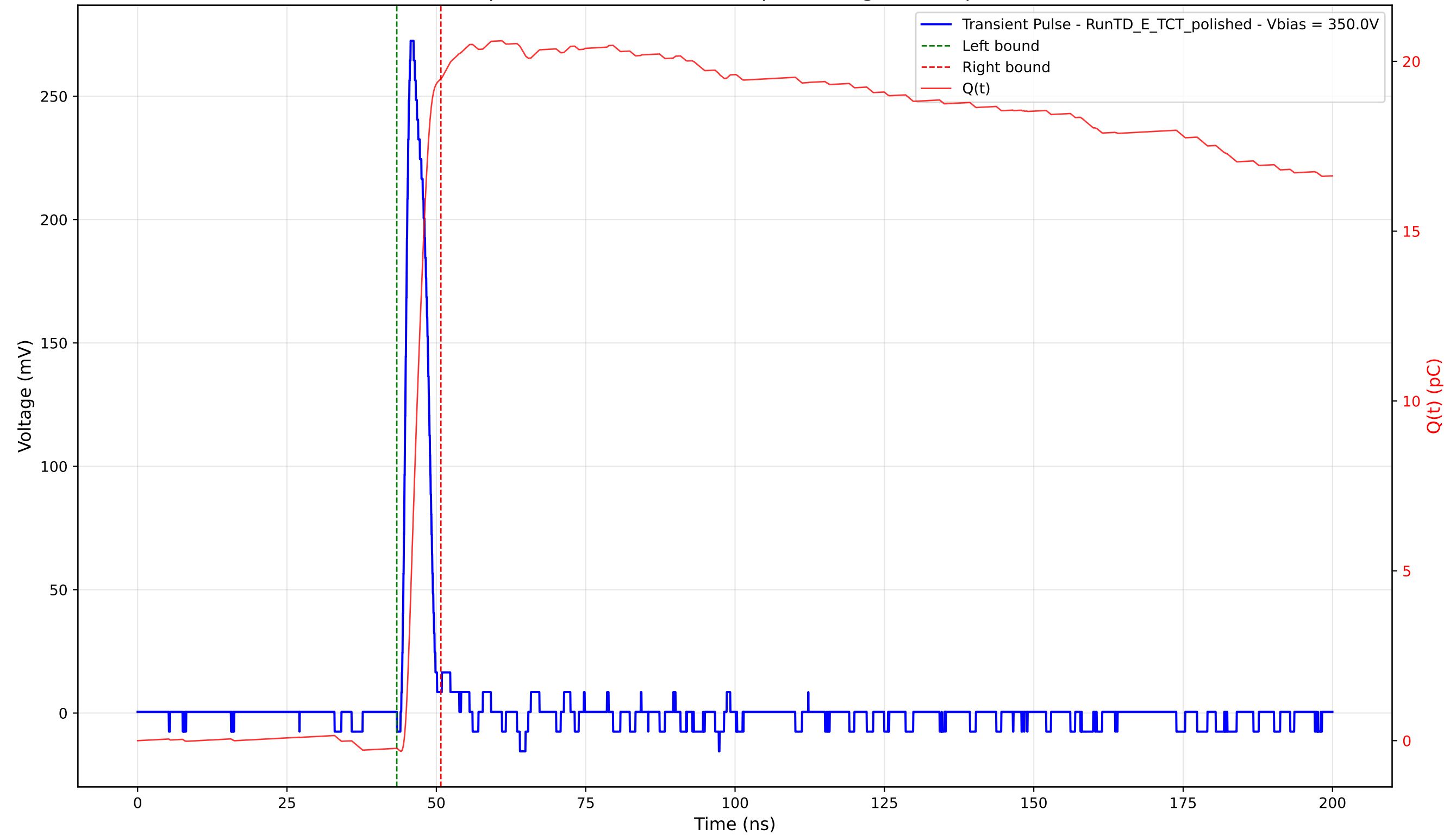
Transient Pulse - Sample: 4003 - Position: 475.0 \mu\text{m} - Charge: 19.71 pC - Rise Time: 1.05 ns
