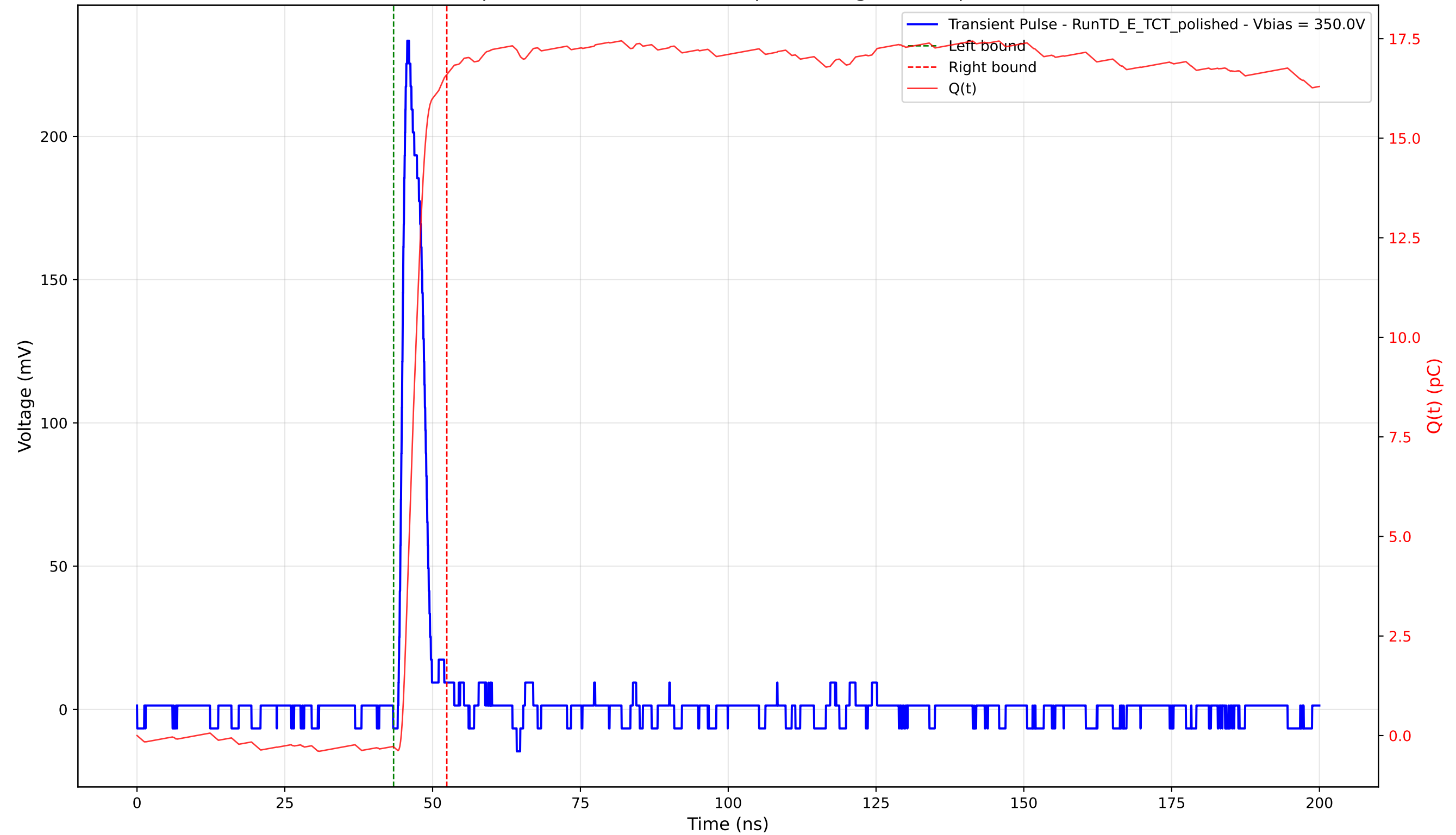
Transient Pulse - Sample: 4003 - Position: 495.0 \mu\text{m} - Charge: 16.88 pC - Rise Time: 1.11 ns
