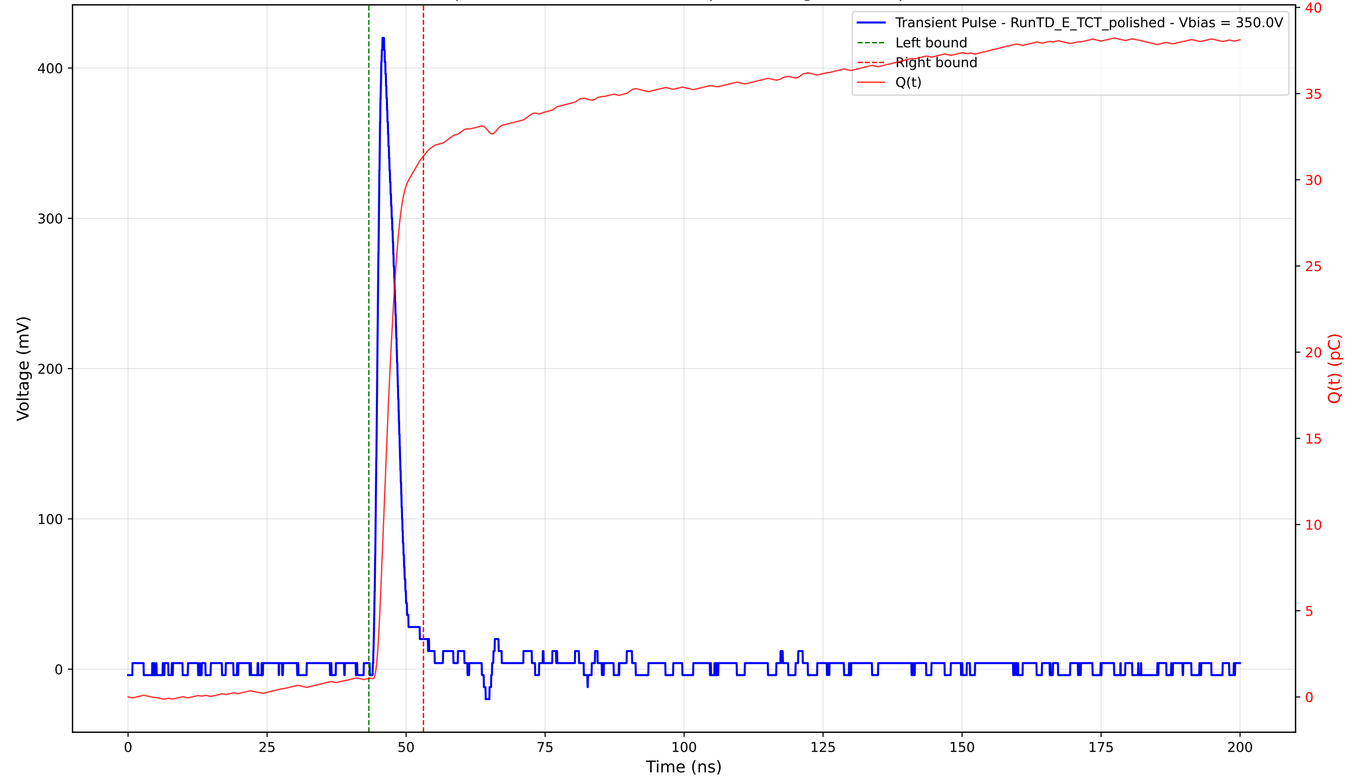
Transient Pulse - Sample: 4003 - Position: 415.0 \mu\text{m} - Charge: 30.29 pC - Rise Time: 1.11 ns
