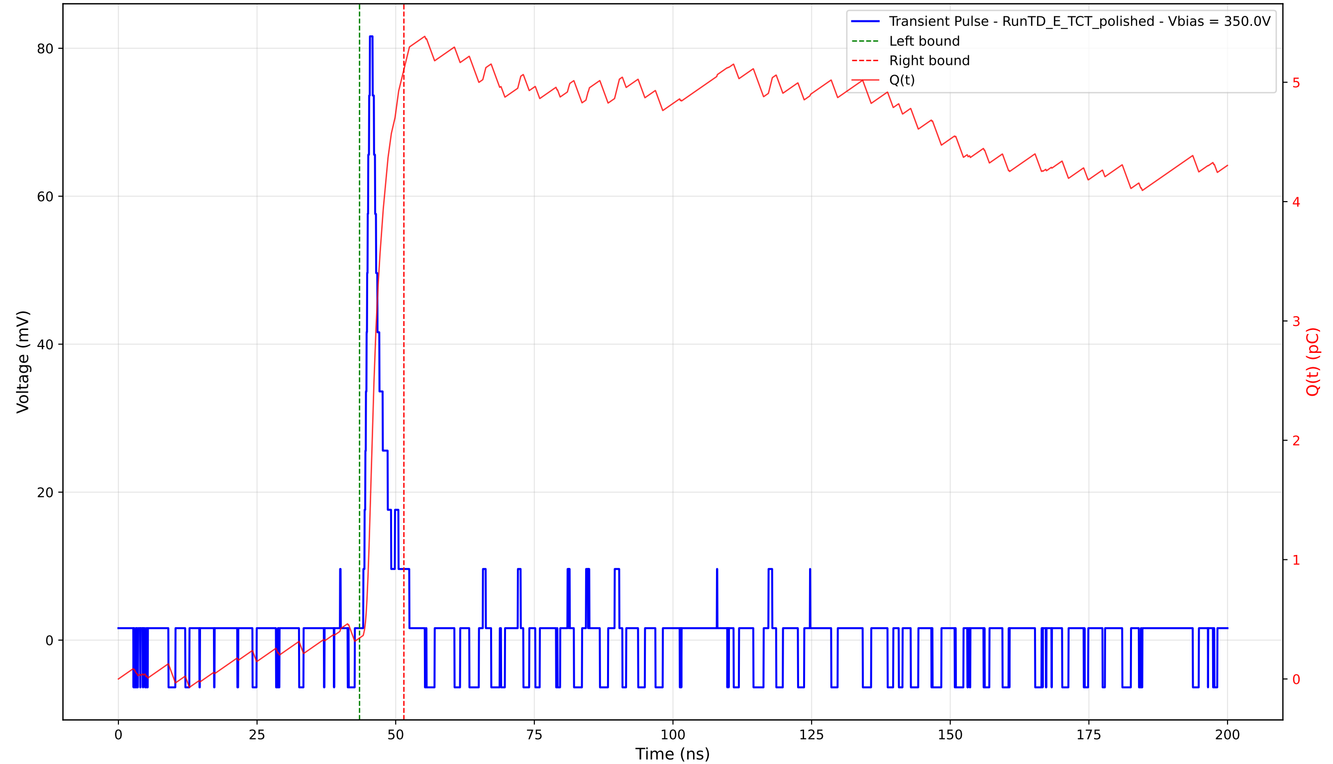
Transient Pulse - Sample: 4003 - Position: 680.0 \mu\text{m} - Charge: 4.77 pC - Rise Time: 1.04 ns
