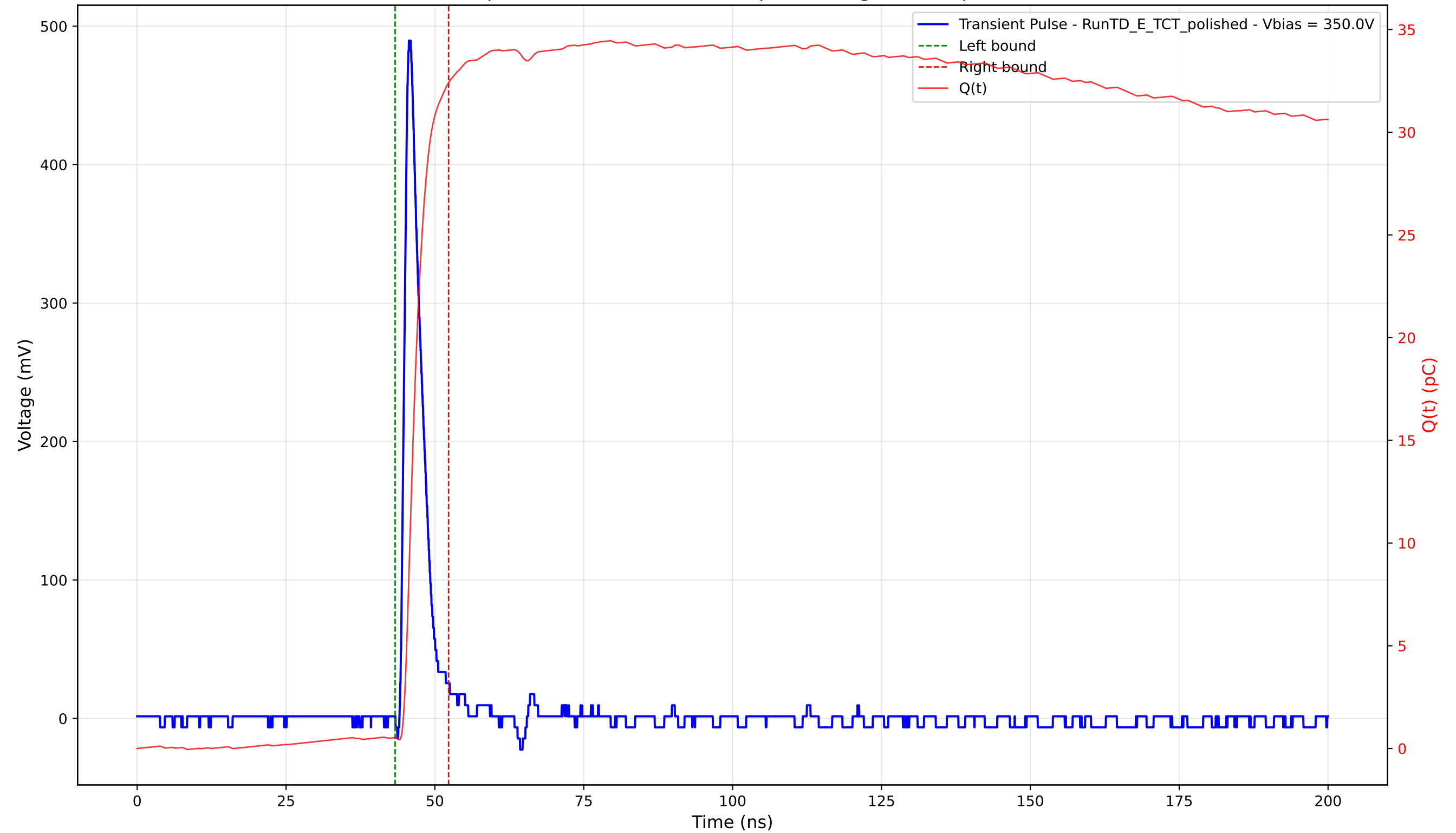
Transient Pulse - Sample: 4003 - Position: 370.0 \mu\text{m} - Charge: 31.88 pC - Rise Time: 1.04 ns
