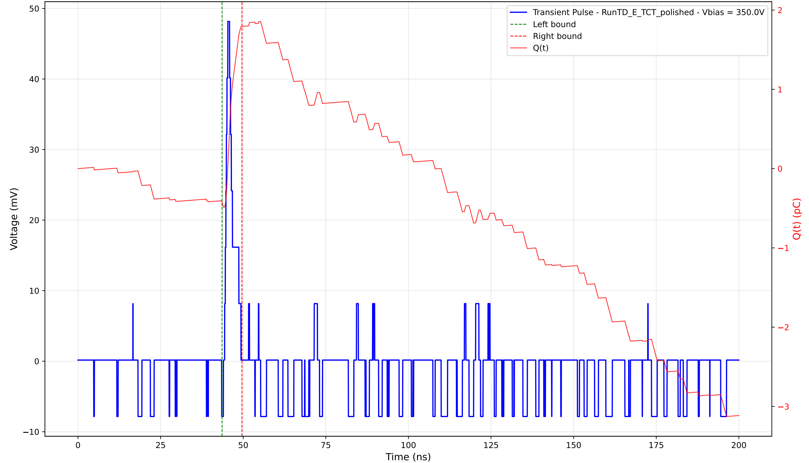
Transient Pulse - Sample: 4003 - Position: 105.0 \mu\text{m} - Charge: 2.22 pC - Rise Time: 0.97 ns
