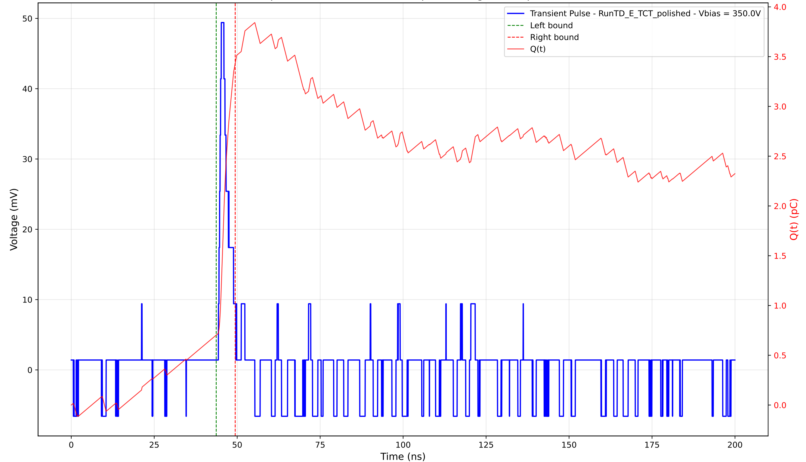
Transient Pulse - Sample: 4003 - Position: 635.0 \mu\text{m} - Charge: 2.73 pC - Rise Time: 0.87 ns
