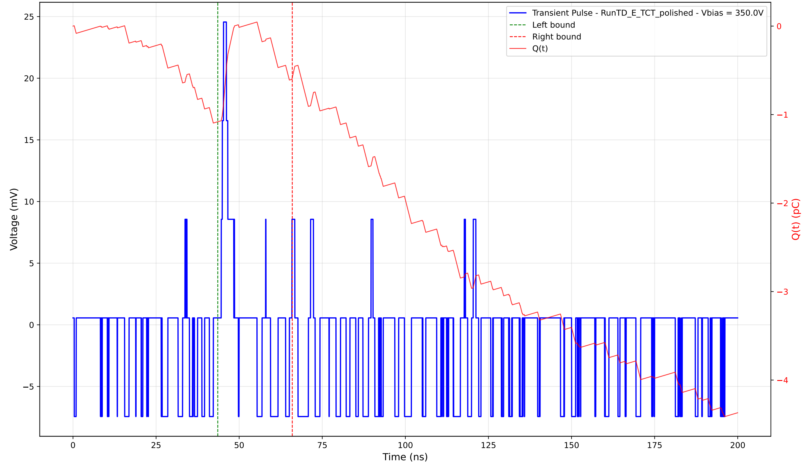
Transient Pulse - Sample: 4003 - Position: 75.0 \mu\text{m} - Charge: 0.49 pC - Rise Time: 0.70 ns
