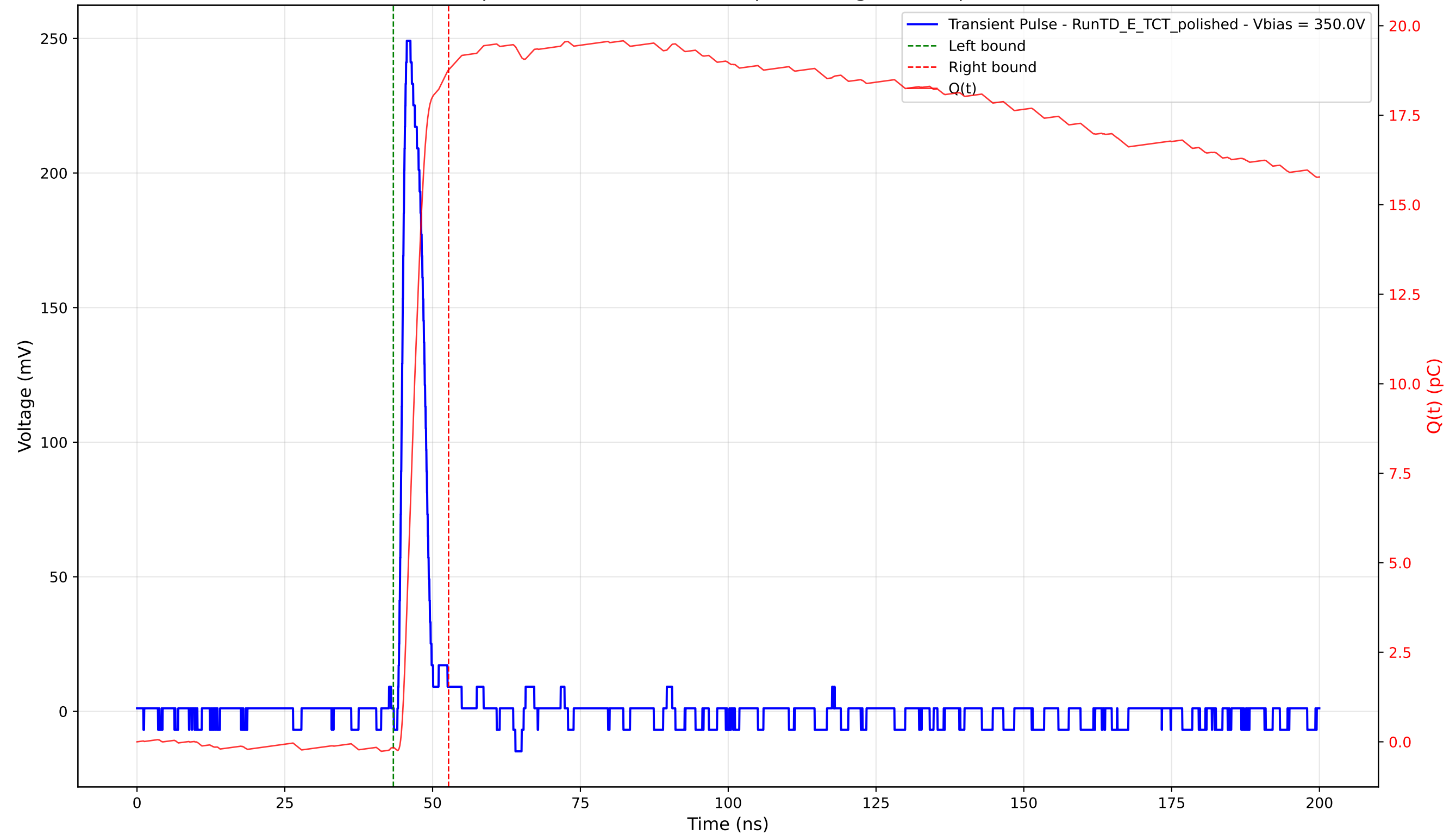
Transient Pulse - Sample: 4003 - Position: 485.0 \mu\text{m} - Charge: 18.93 pC - Rise Time: 1.04 ns
