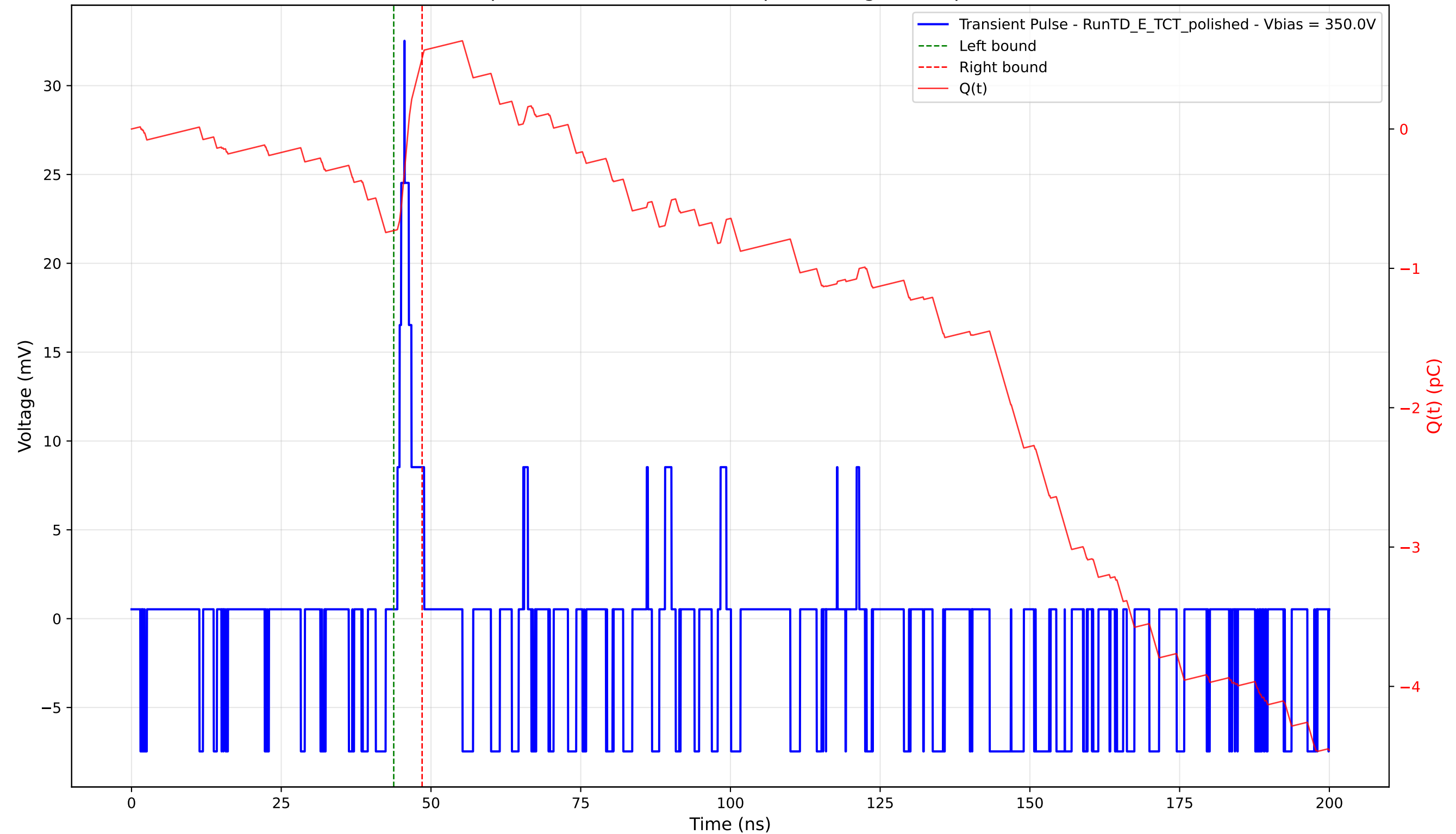
Transient Pulse - Sample: 4003 - Position: 660.0 \mu\text{m} - Charge: 1.24 pC - Rise Time: 1.17 ns
