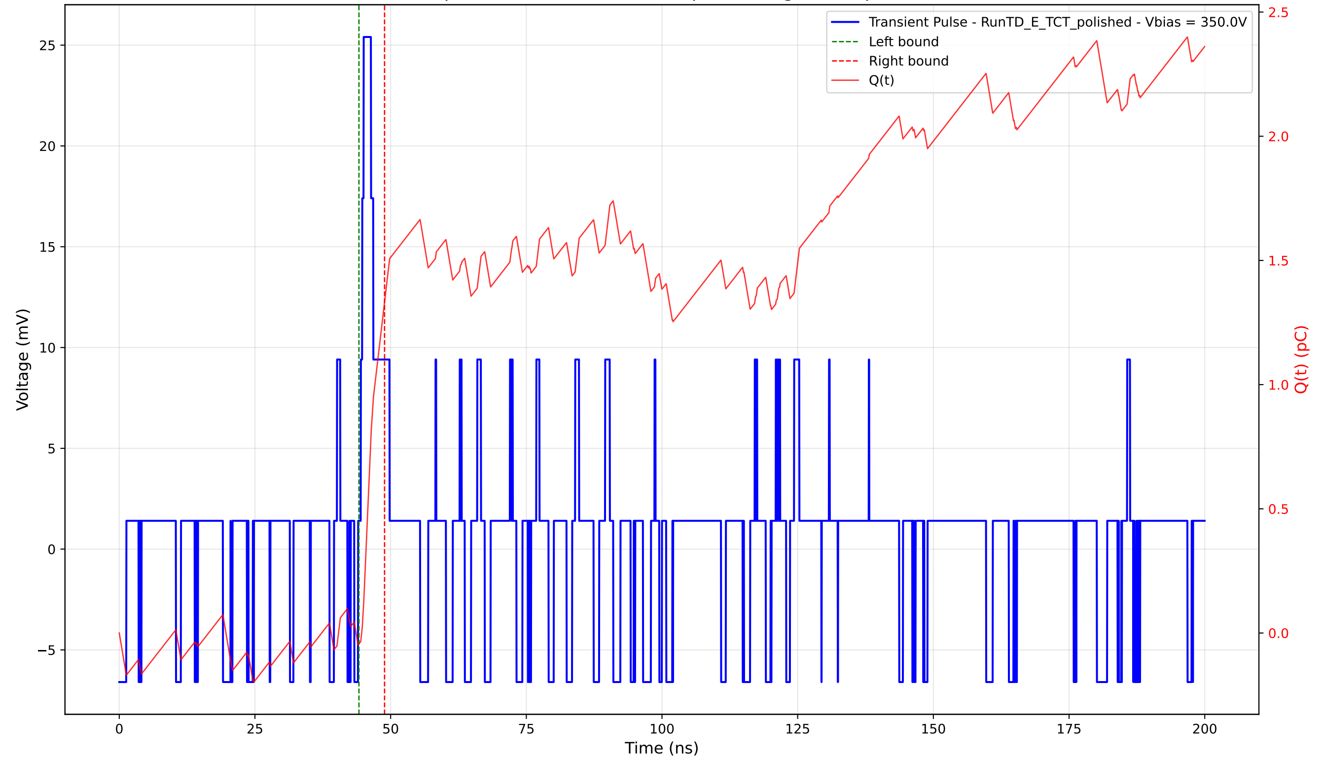
Transient Pulse - Sample: 4003 - Position: 730.0 \mu\text{m} - Charge: 1.38 pC - Rise Time: 0.54 ns
