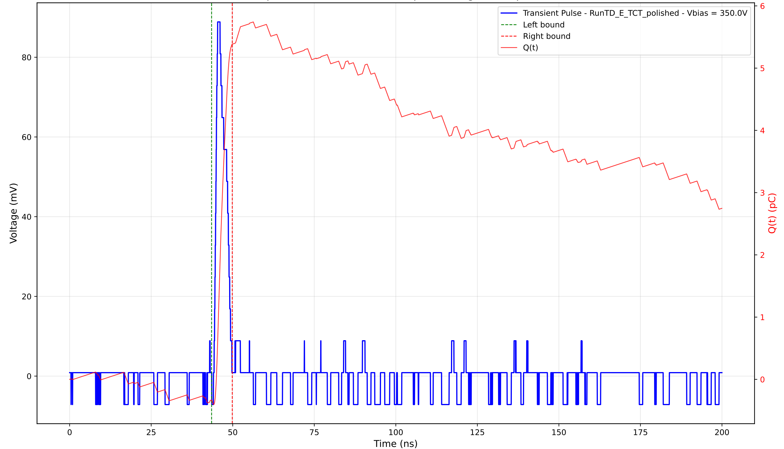
Transient Pulse - Sample: 4003 - Position: 565.0 \mu\text{m} - Charge: 5.72 pC - Rise Time: 0.82 ns
