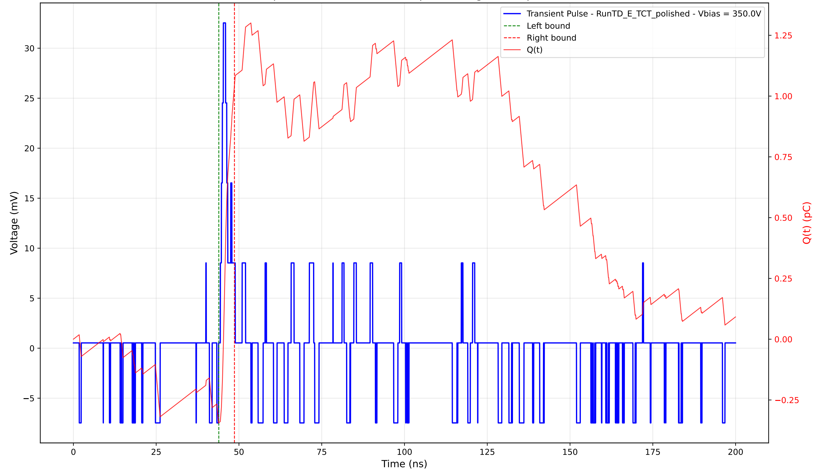
Transient Pulse - Sample: 4003 - Position: 90.0 \mu\text{m} - Charge: 1.39 pC - Rise Time: 0.91 ns
