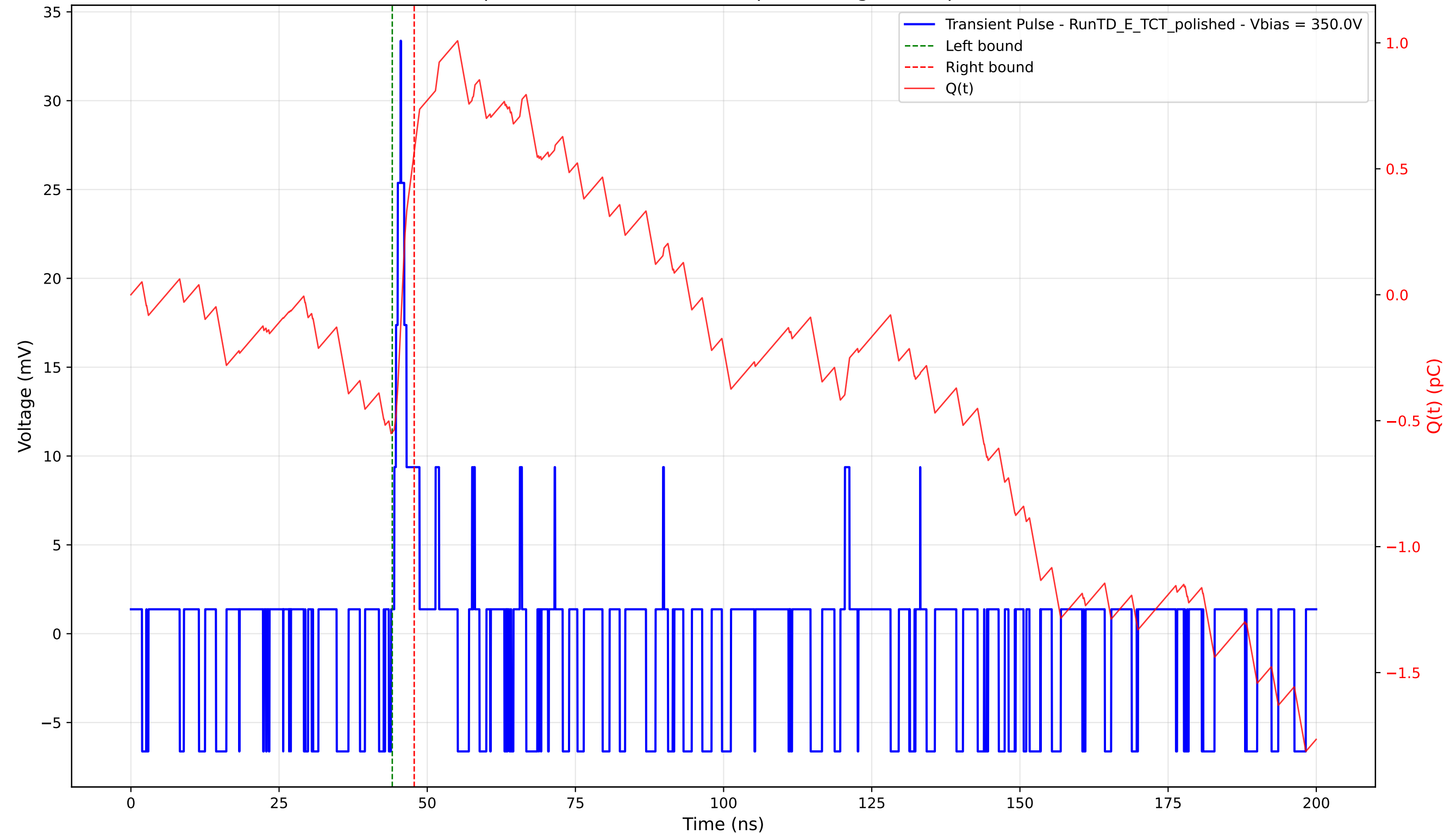
Transient Pulse - Sample: 4003 - Position: 800.0 \mu\text{m} - Charge: 1.11 pC - Rise Time: 1.08 ns
