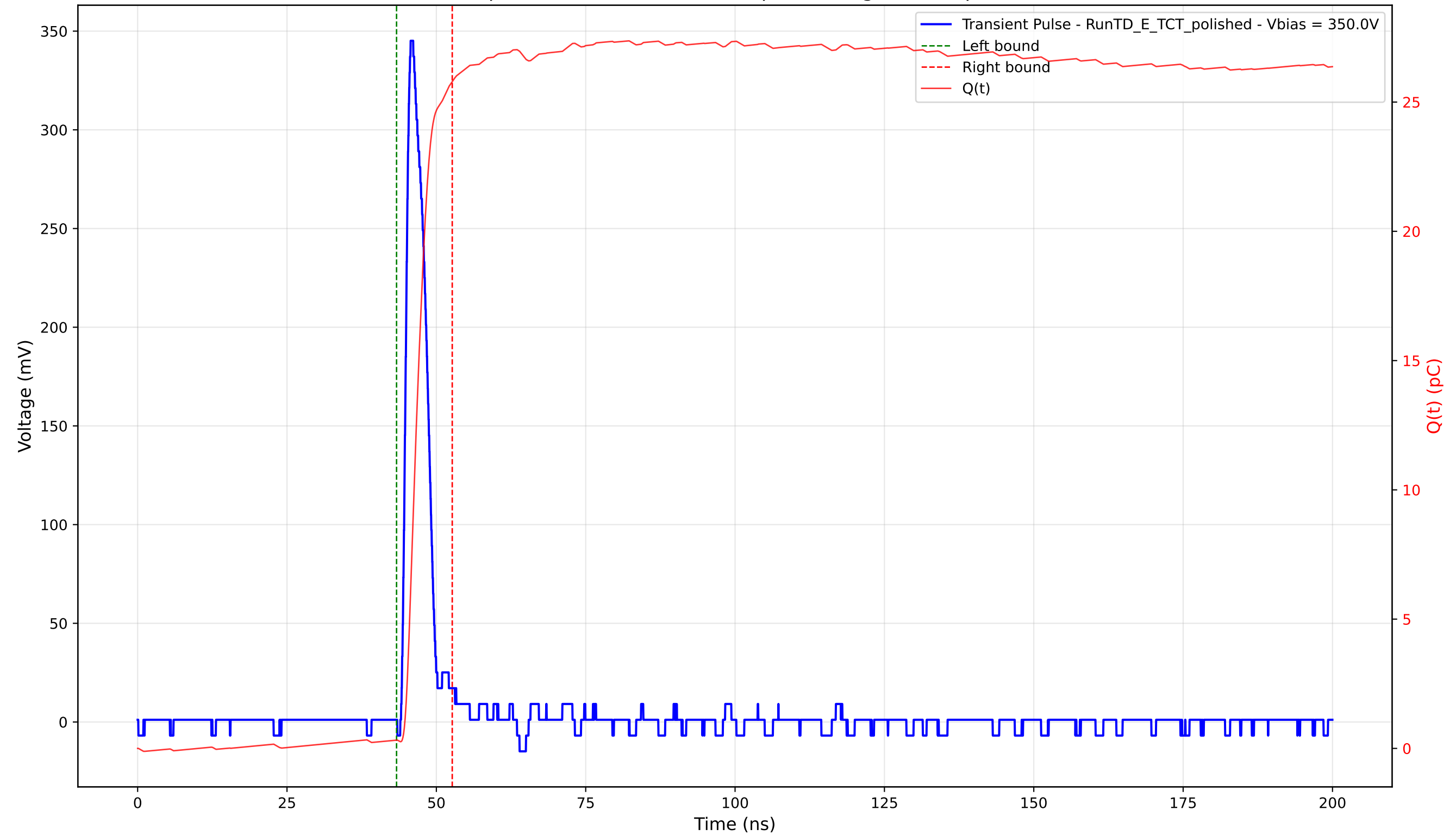
Transient Pulse - Sample: 4003 - Position: 445.0 \mu\text{m} - Charge: 25.47 pC - Rise Time: 1.08 ns
