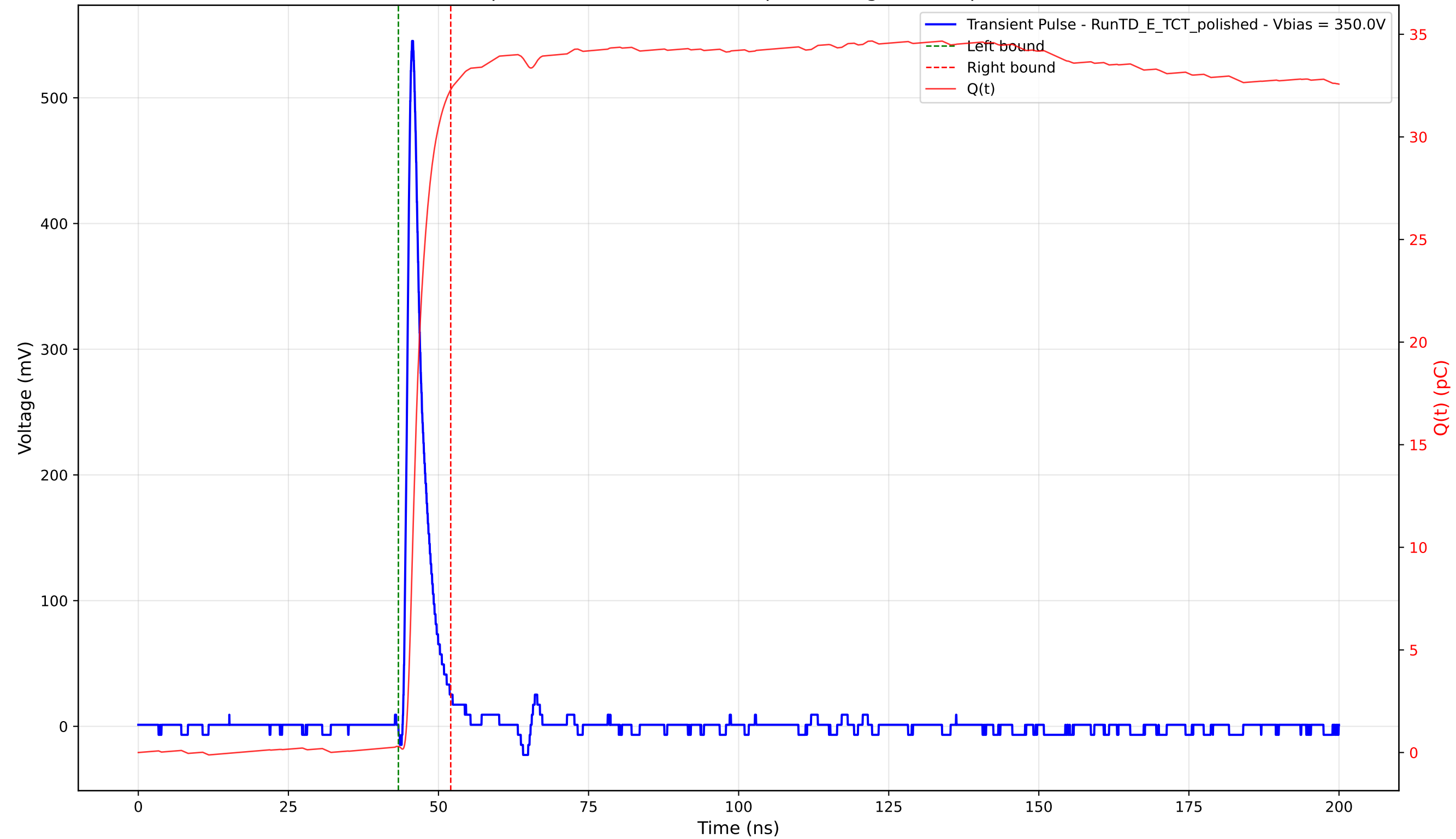
Transient Pulse - Sample: 4003 - Position: 310.0 \mu\text{m} - Charge: 32.00 pC - Rise Time: 1.01 ns
