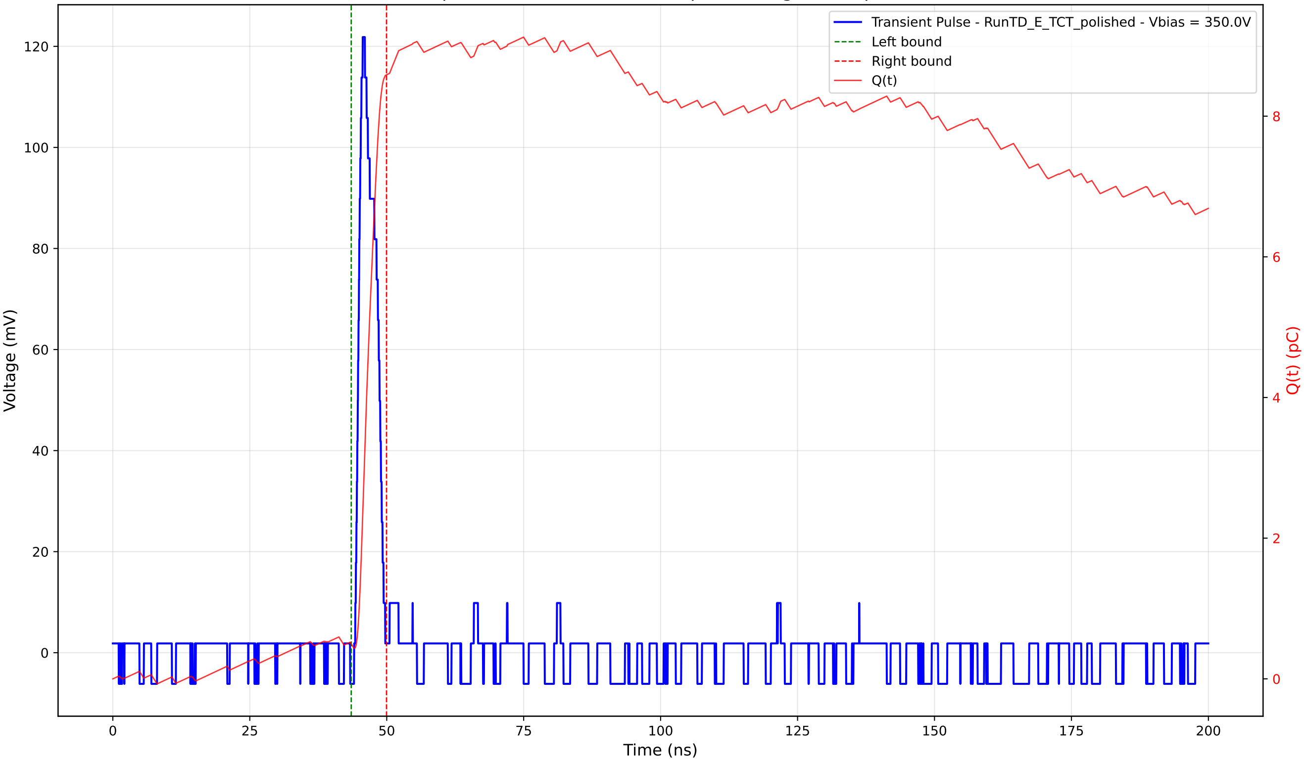
Transient Pulse - Sample: 4003 - Position: 545.0 \mu\text{m} - Charge: 8.09 pC - Rise Time: 1.03 ns
