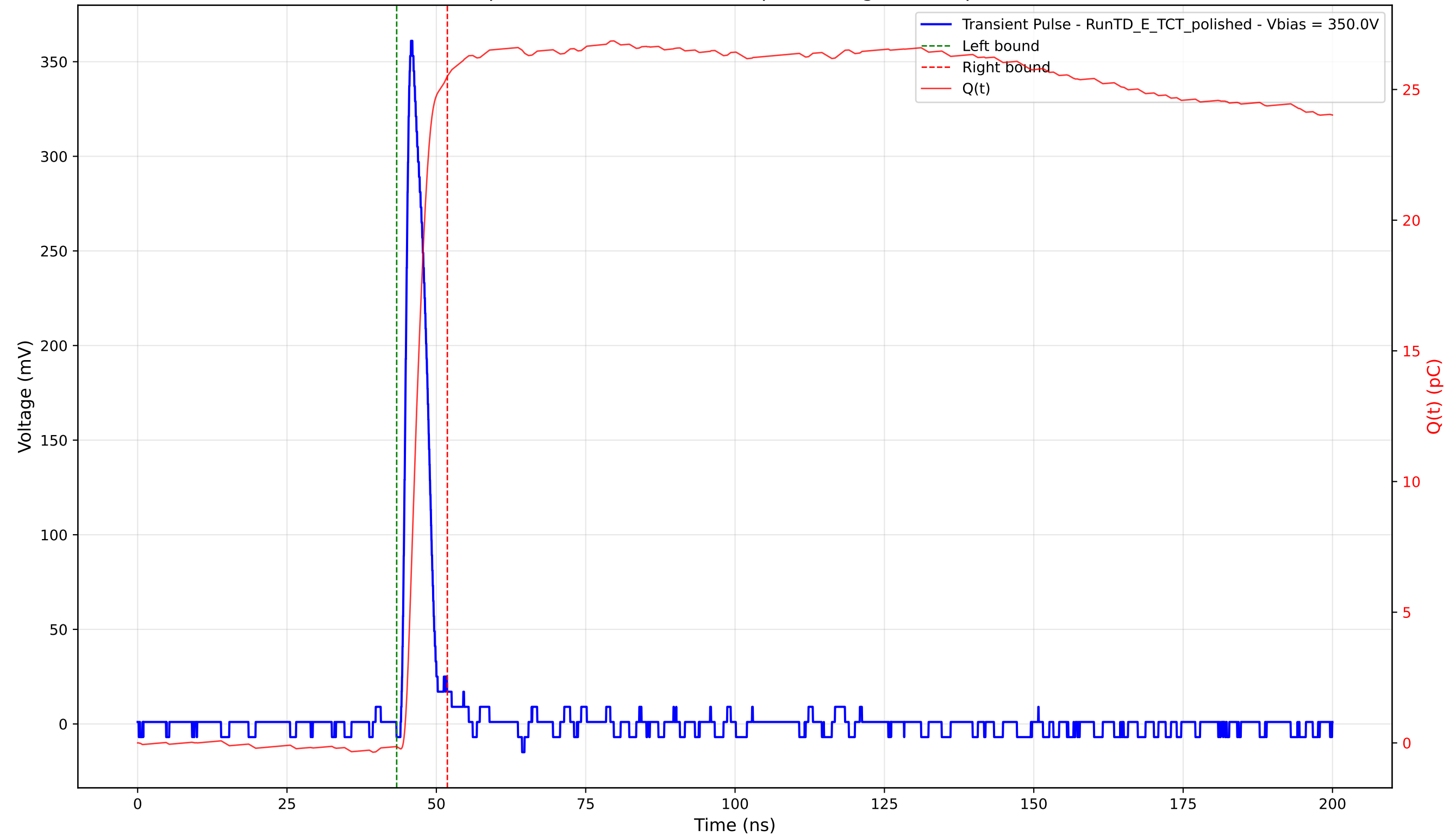
Transient Pulse - Sample: 4003 - Position: 440.0 \mu\text{m} - Charge: 25.65 pC - Rise Time: 1.09 ns
