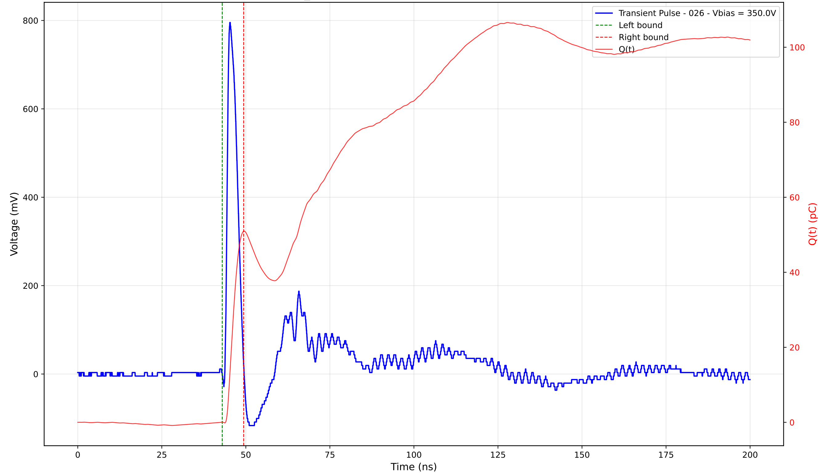
Transient Pulse - Sample: TD_4004 - Position: 240.0 \mu\text{m} - Charge: 50.90 pC - Rise Time: 0.91 ns
