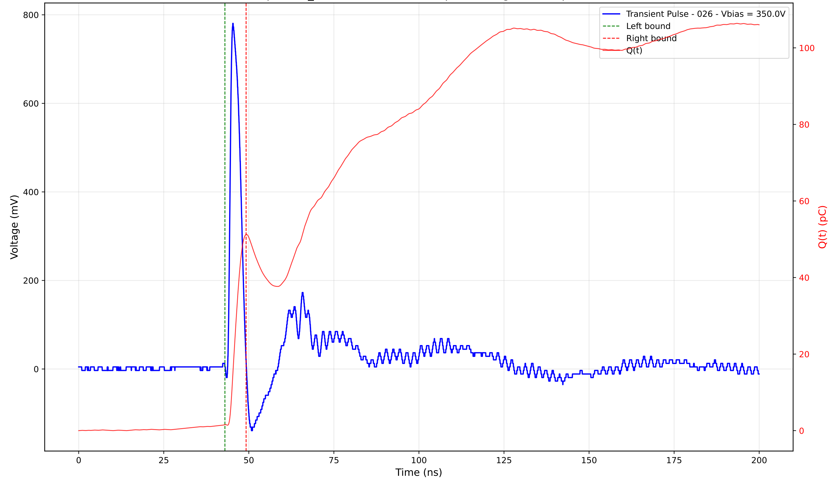
Transient Pulse - Sample: TD_4004 - Position: 305.0 \mu\text{m} - Charge: 49.68 pC - Rise Time: 0.92 ns
