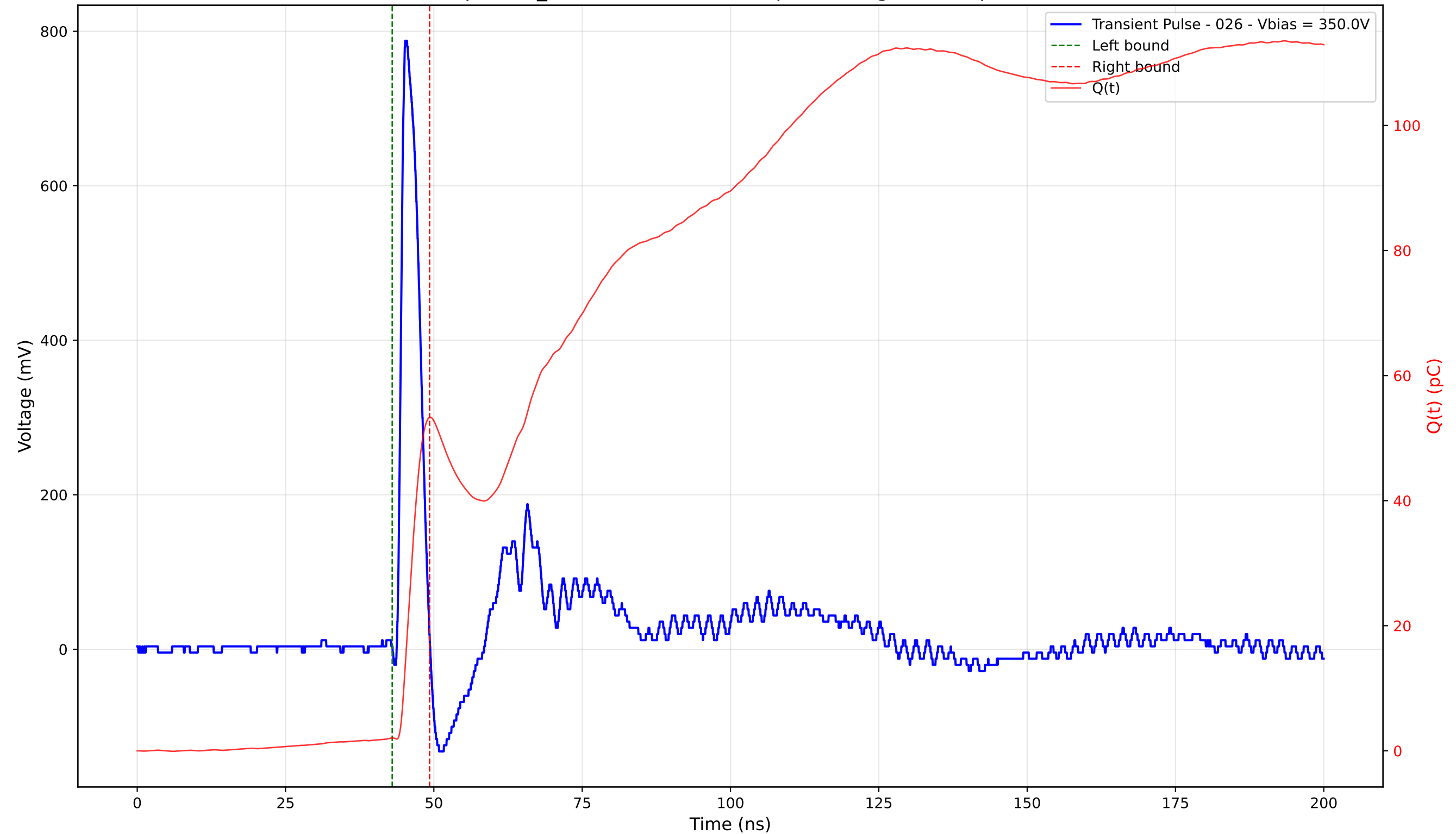
Transient Pulse - Sample: TD_4004 - Position: 265.0 \mu\text{m} - Charge: 51.25 pC - Rise Time: 0.91 ns
