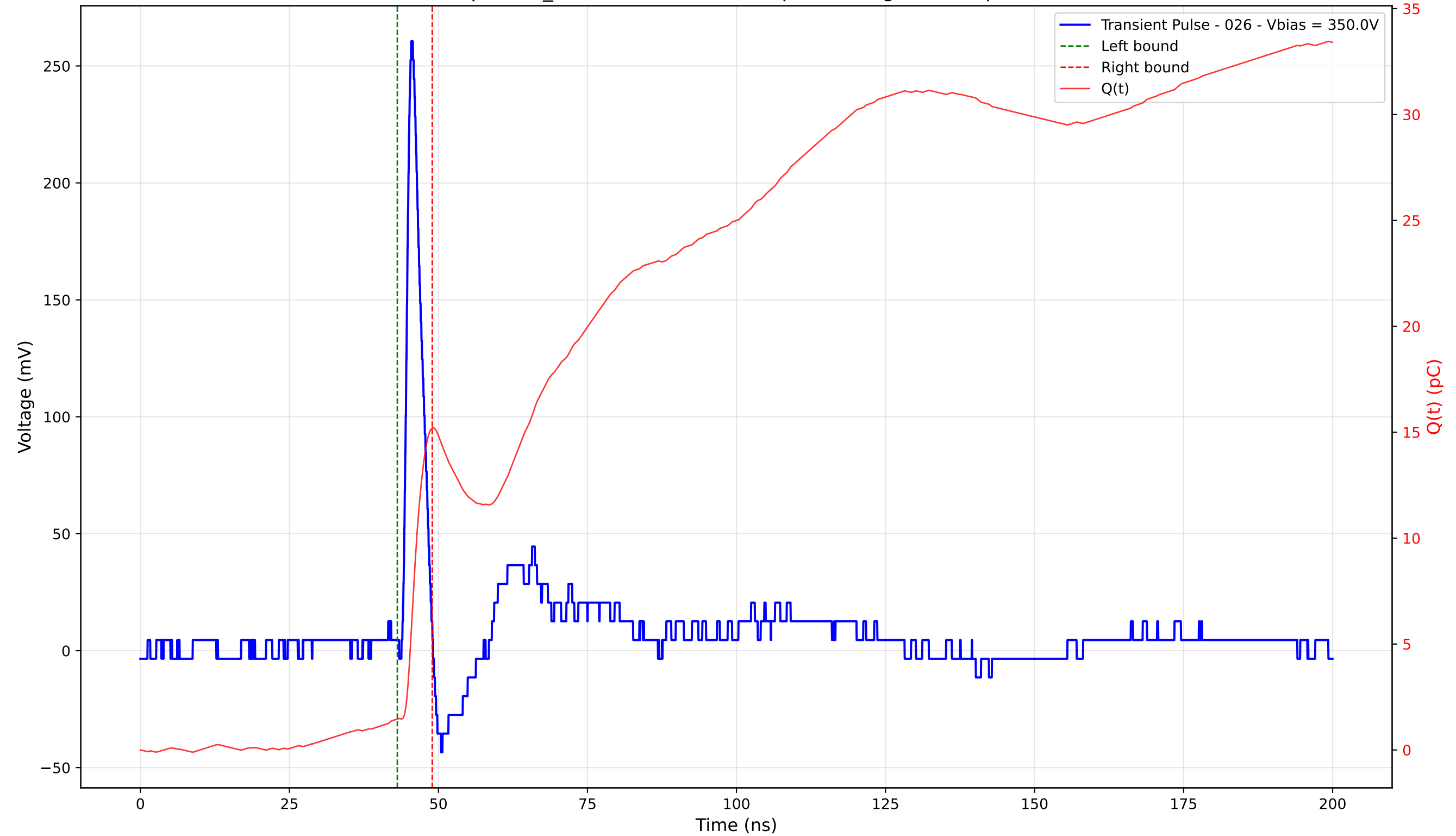
Transient Pulse - Sample: TD_4004 - Position: 410.0 \mu\text{m} - Charge: 13.74 pC - Rise Time: 1.05 ns
