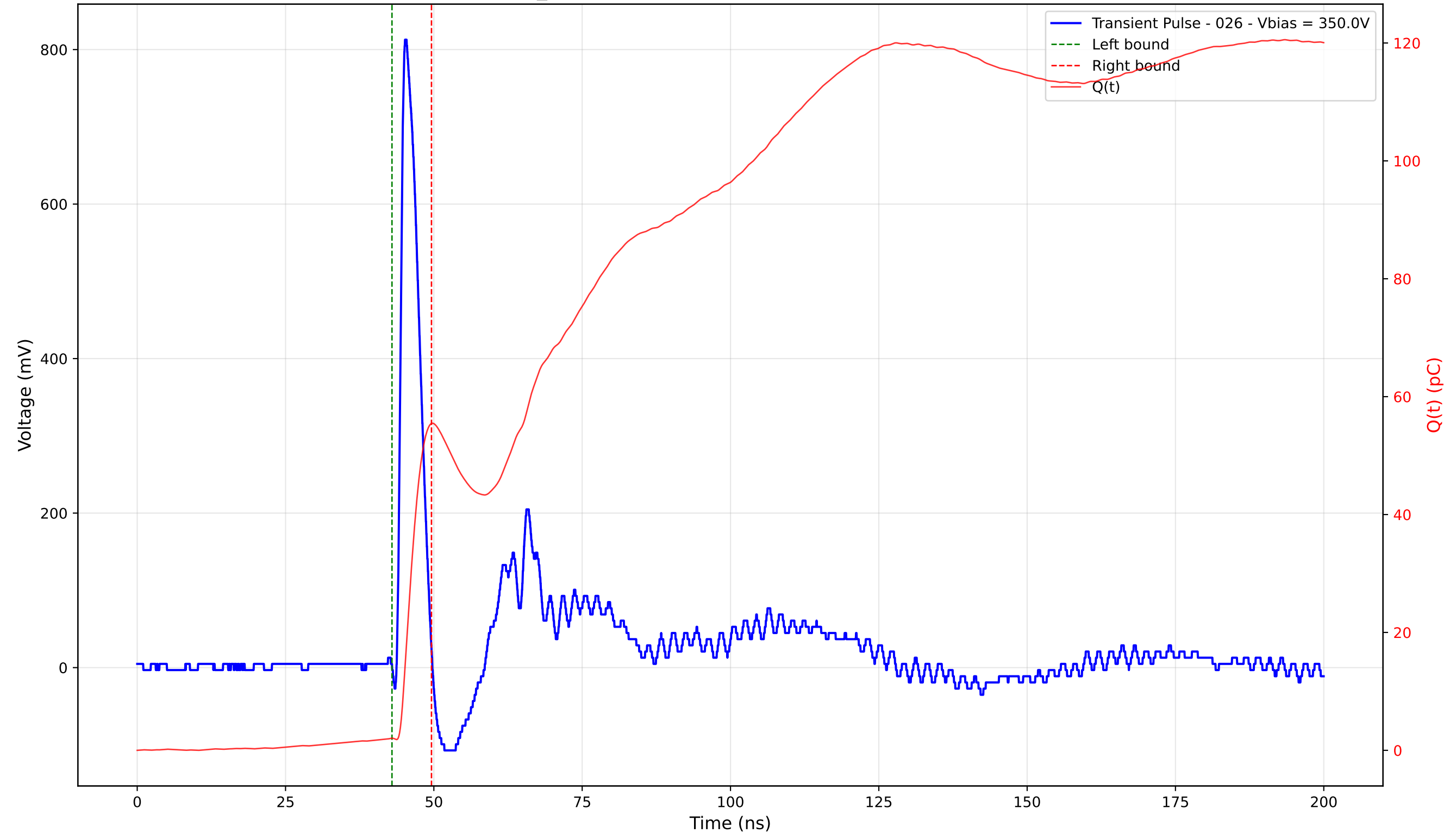
Transient Pulse - Sample: TD_4004 - Position: 170.0 \mu\text{m} - Charge: 53.40 pC - Rise Time: 0.89 ns
