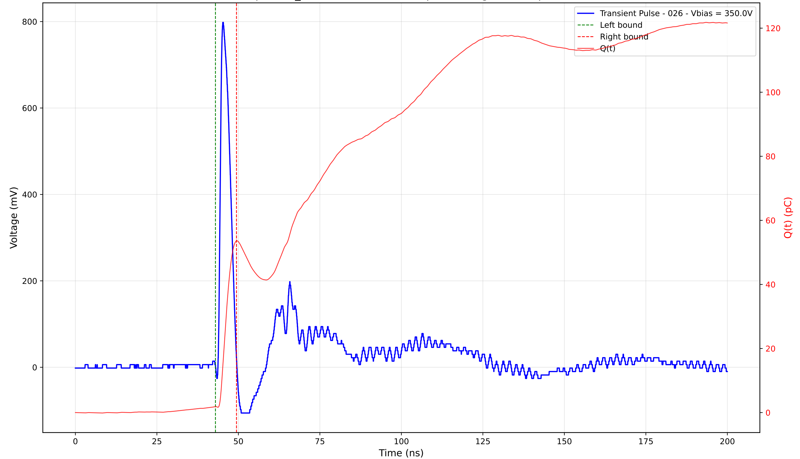
Transient Pulse - Sample: TD_4004 - Position: 145.0 \mu\text{m} - Charge: 51.71 pC - Rise Time: 0.90 ns
