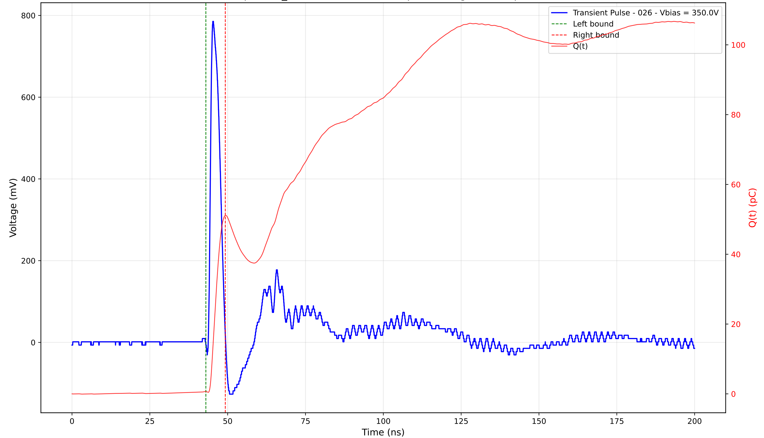
Transient Pulse - Sample: TD_4004 - Position: 260.0 \mu\text{m} - Charge: 50.45 pC - Rise Time: 0.90 ns
