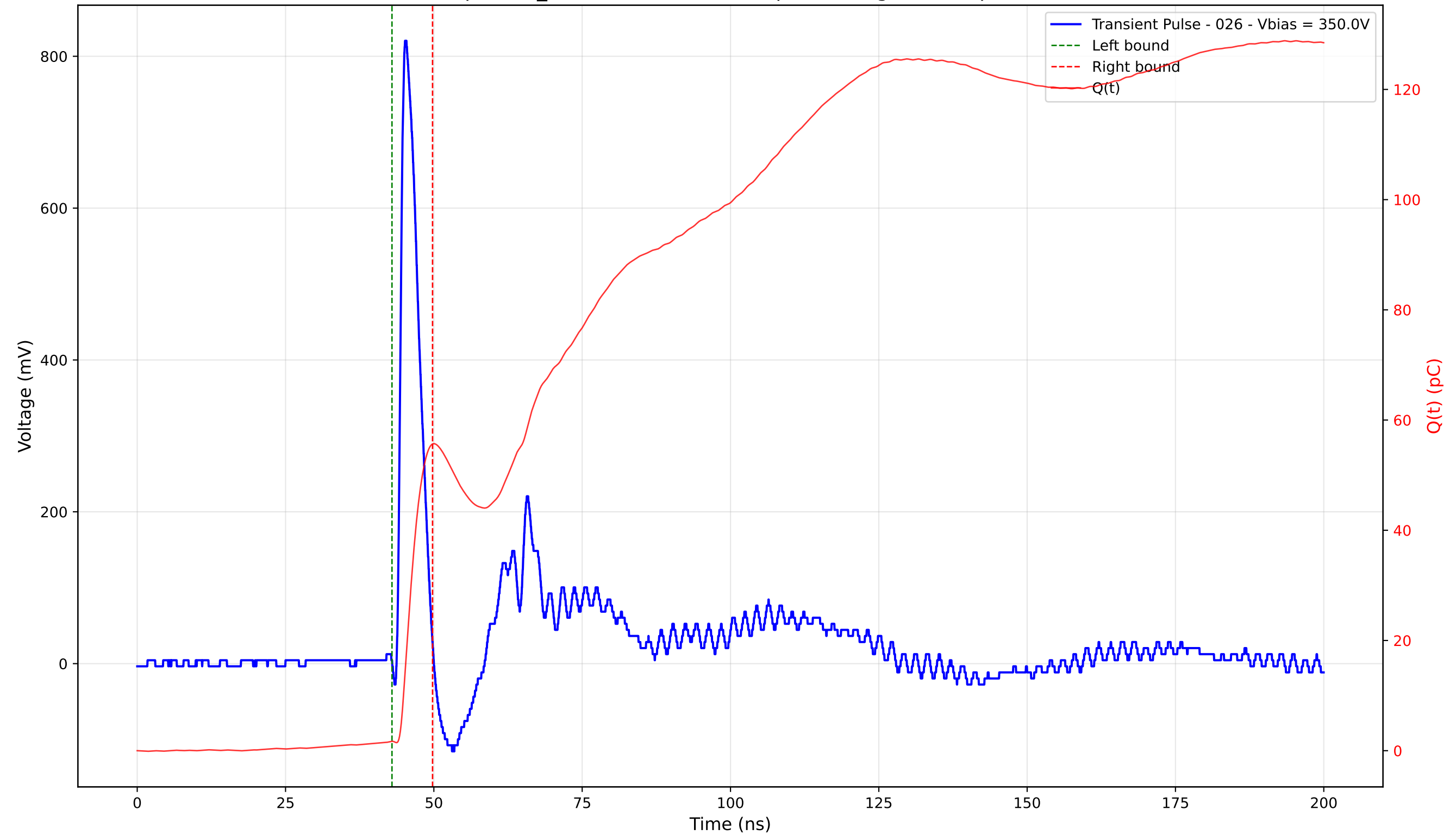
Transient Pulse - Sample: TD_4004 - Position: 185.0 \mu\text{m} - Charge: 53.95 pC - Rise Time: 0.88 ns
