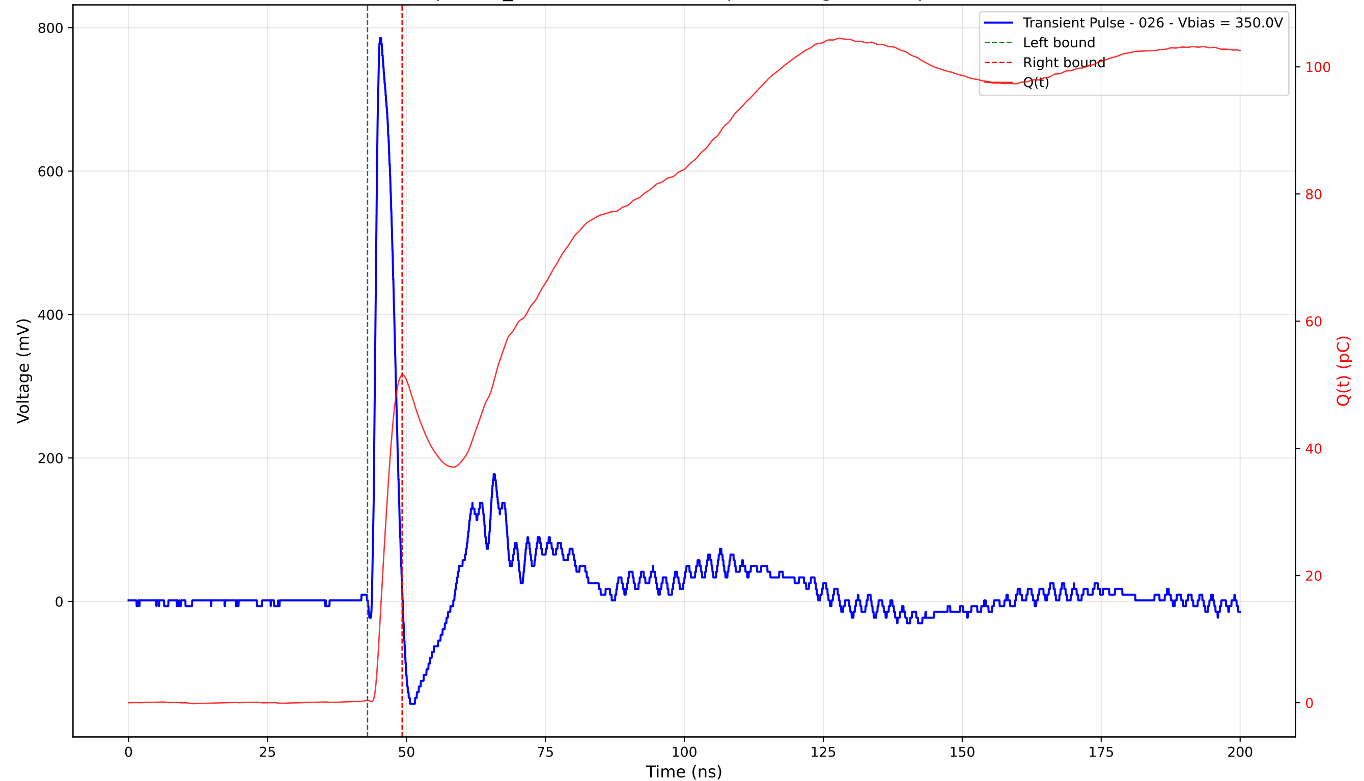
Transient Pulse - Sample: TD_4004 - Position: 290.0 \mu\text{m} - Charge: 51.15 pC - Rise Time: 0.89 ns
