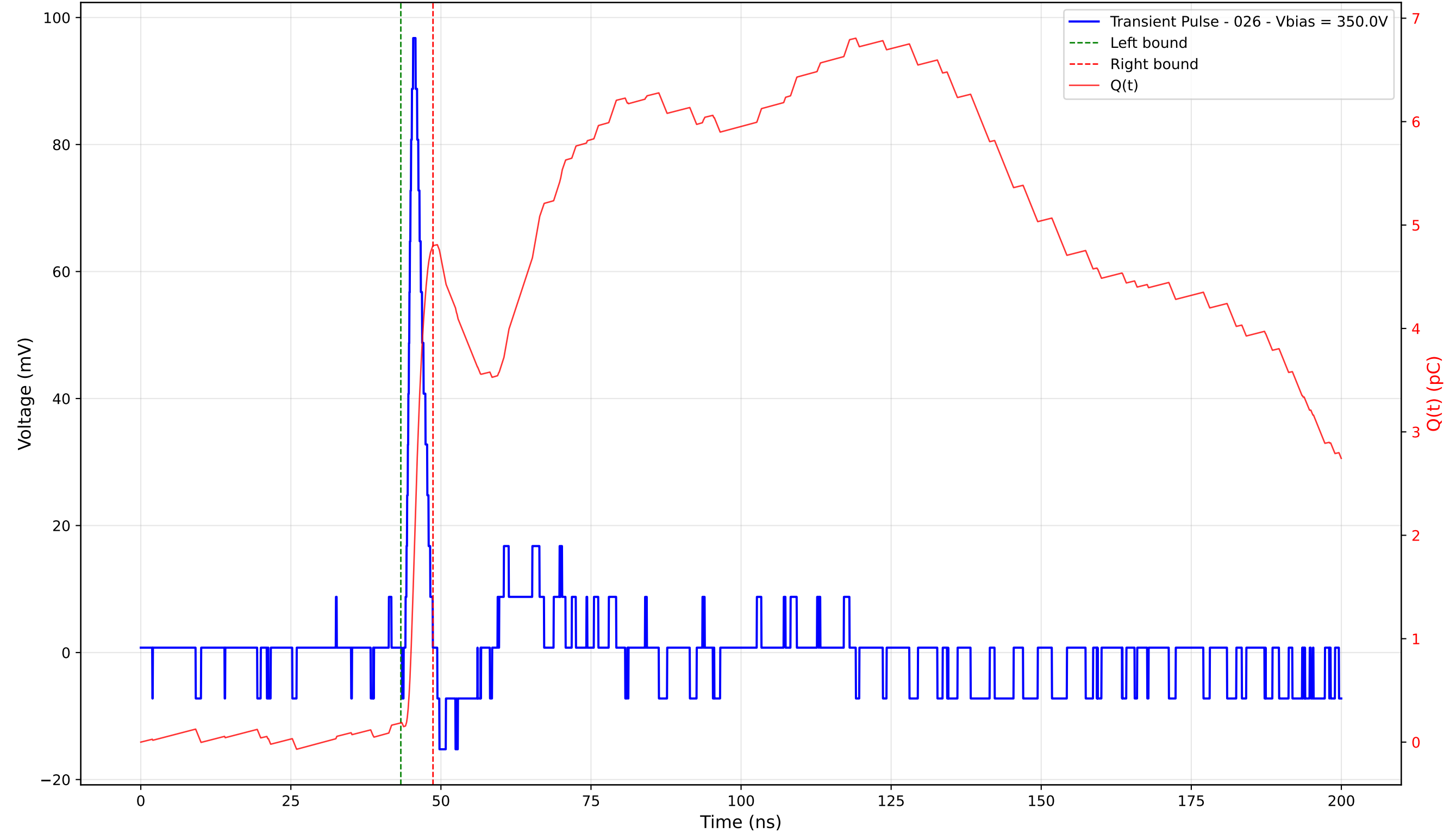
Transient Pulse - Sample: TD_4004 - Position: 425.0 \mu\text{m} - Charge: 4.61 pC - Rise Time: 0.92 ns
