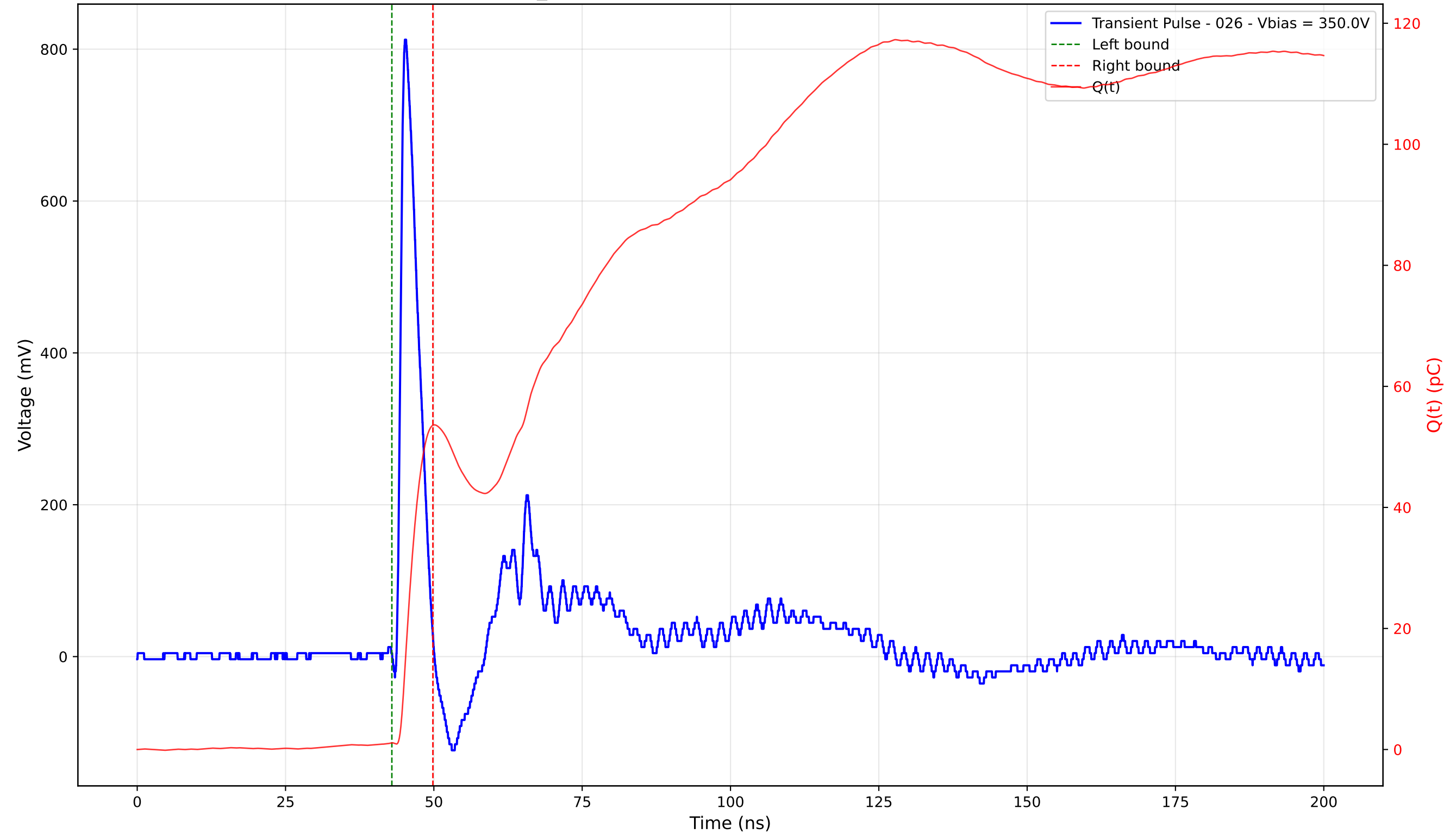
Transient Pulse - Sample: TD_4004 - Position: 105.0 \mu\text{m} - Charge: 52.49 pC - Rise Time: 0.88 ns
