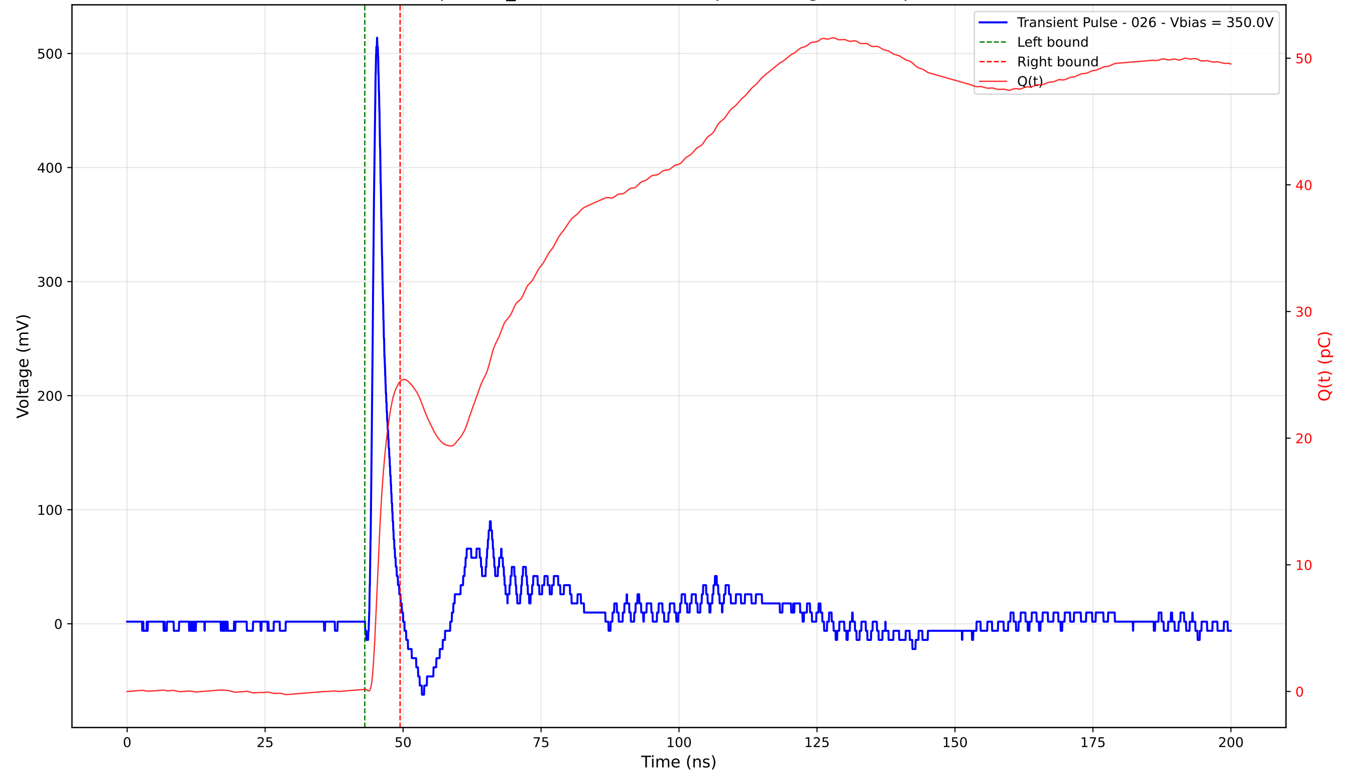
Transient Pulse - Sample: TD_4004 - Position: 65.0 \mu\text{m} - Charge: 24.29 pC - Rise Time: 0.92 ns
