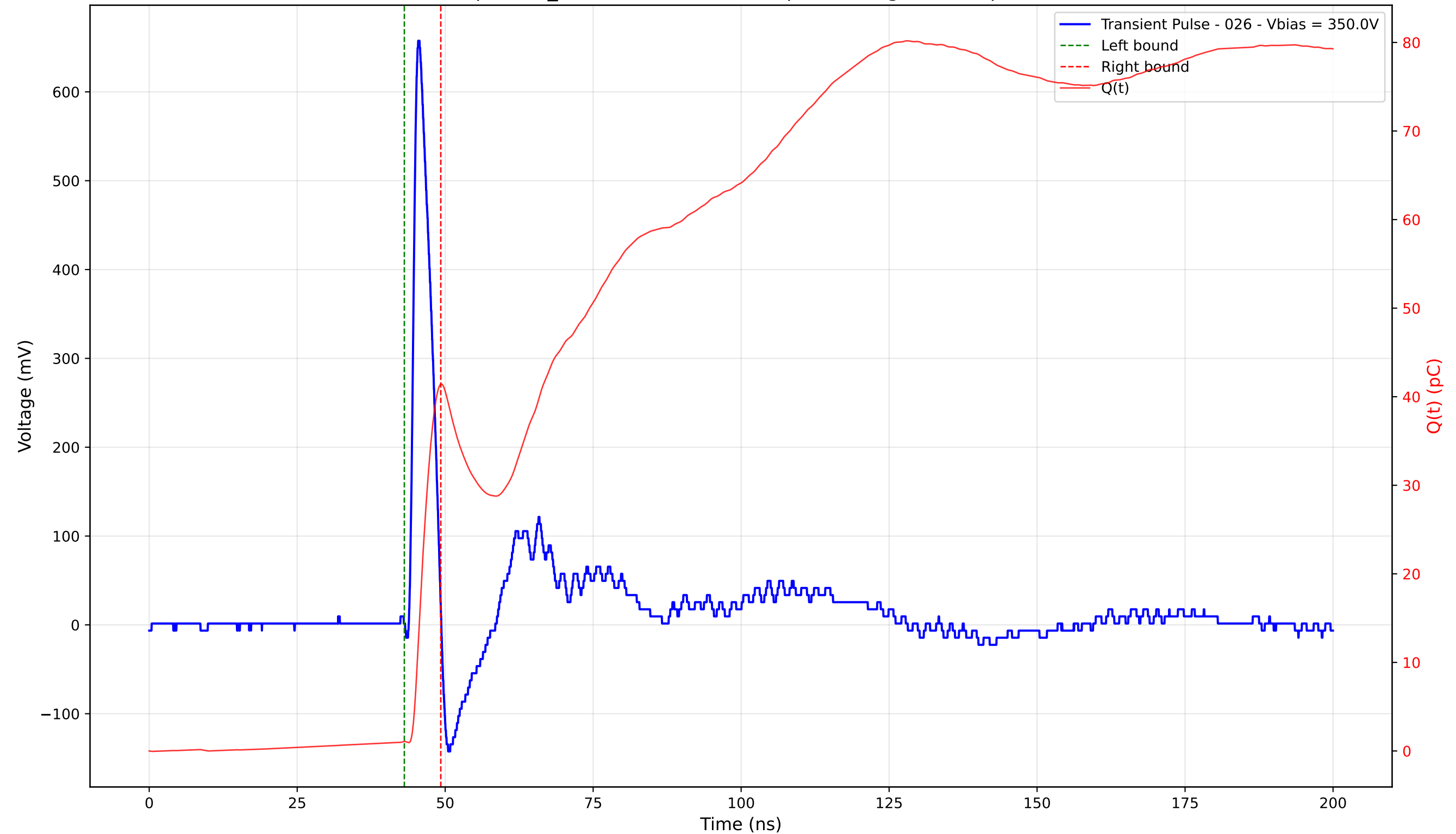
Transient Pulse - Sample: TD_4004 - Position: 385.0 \mu\text{m} - Charge: 40.35 pC - Rise Time: 1.00 ns
