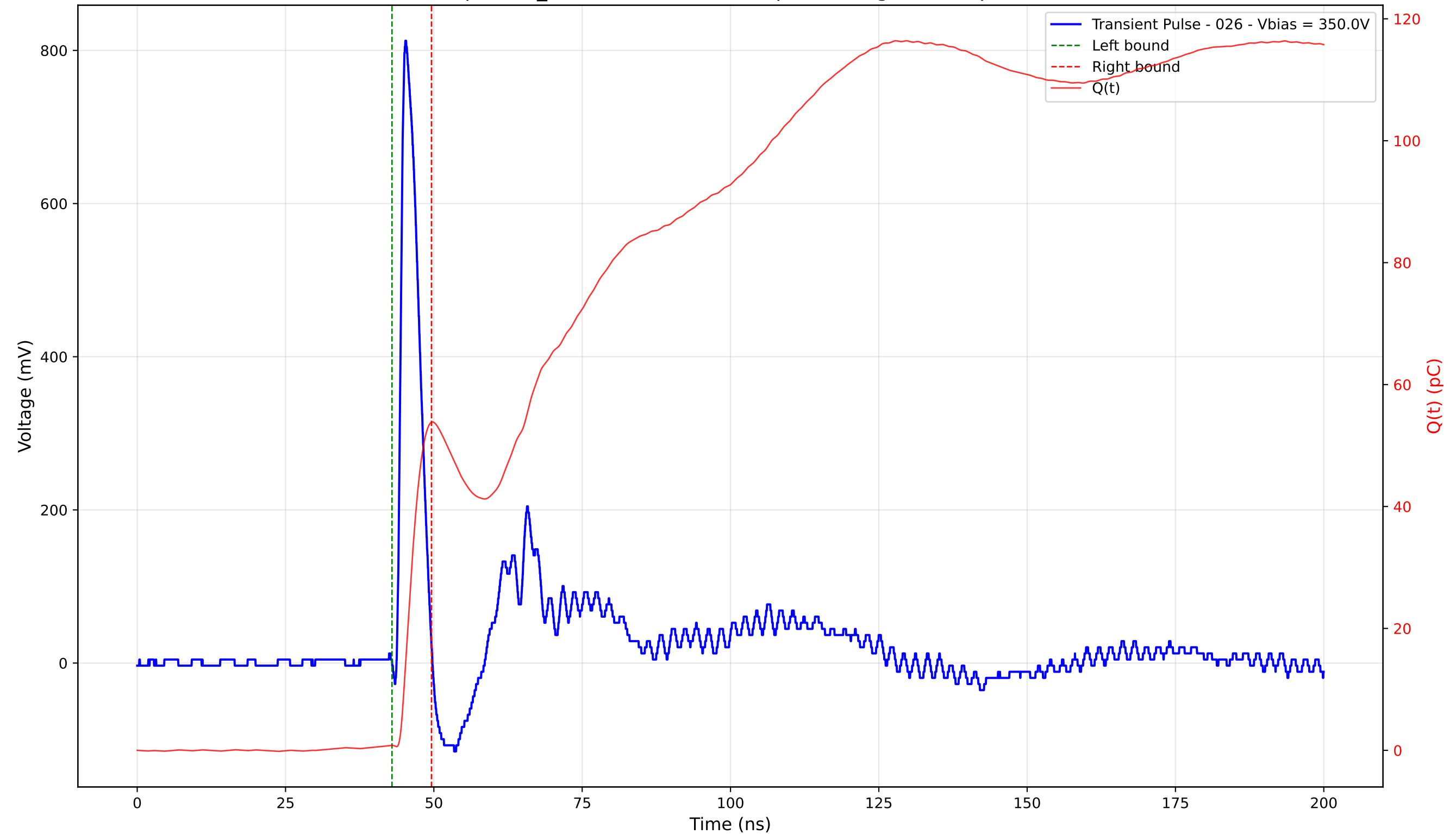
Transient Pulse - Sample: TD_4004 - Position: 220.0 \mu\text{m} - Charge: 53.01 pC - Rise Time: 0.90 ns
