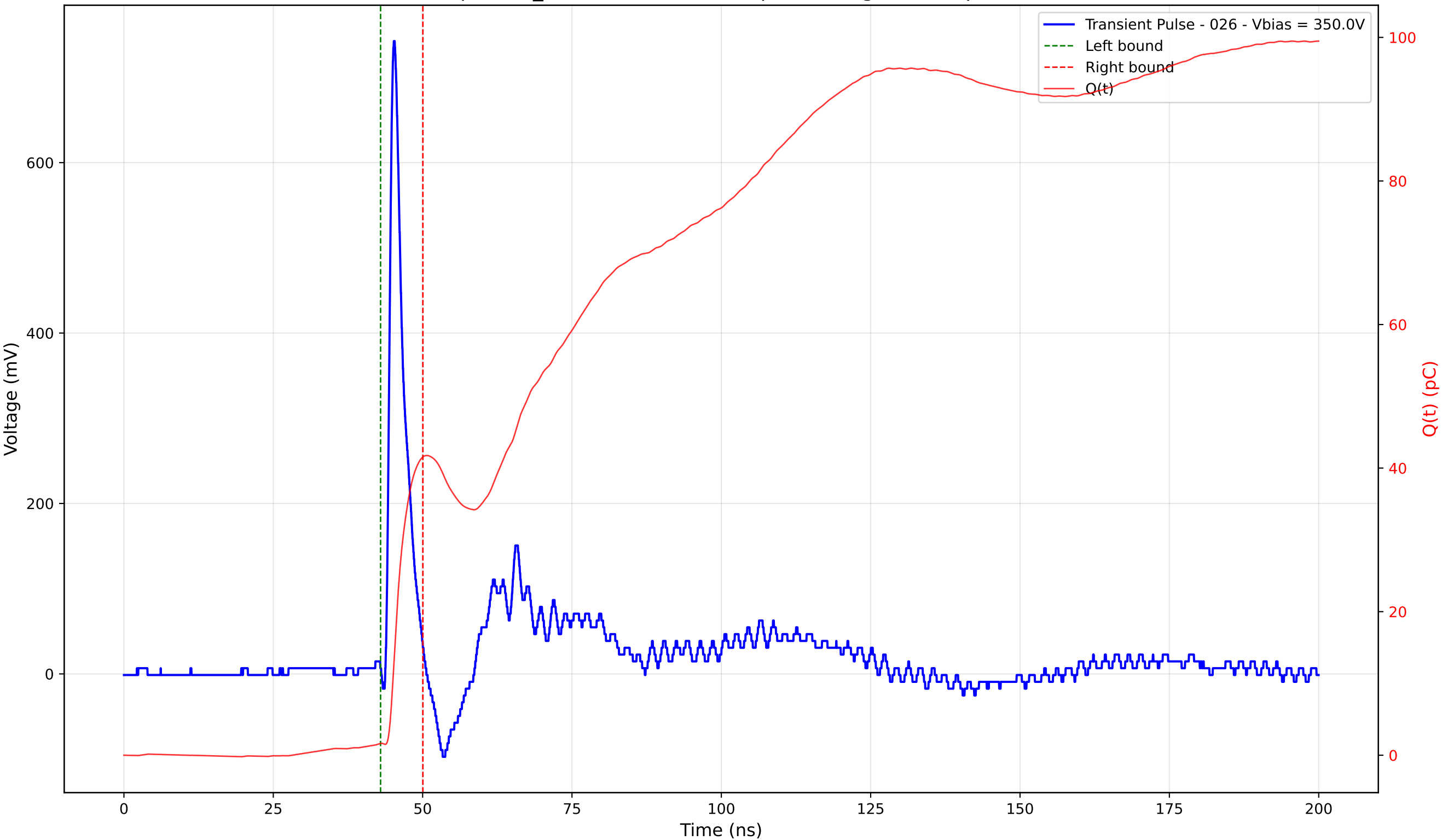
Transient Pulse - Sample: TD_4004 - Position: 80.0 \mu\text{m} - Charge: 39.90 pC - Rise Time: 0.89 ns
