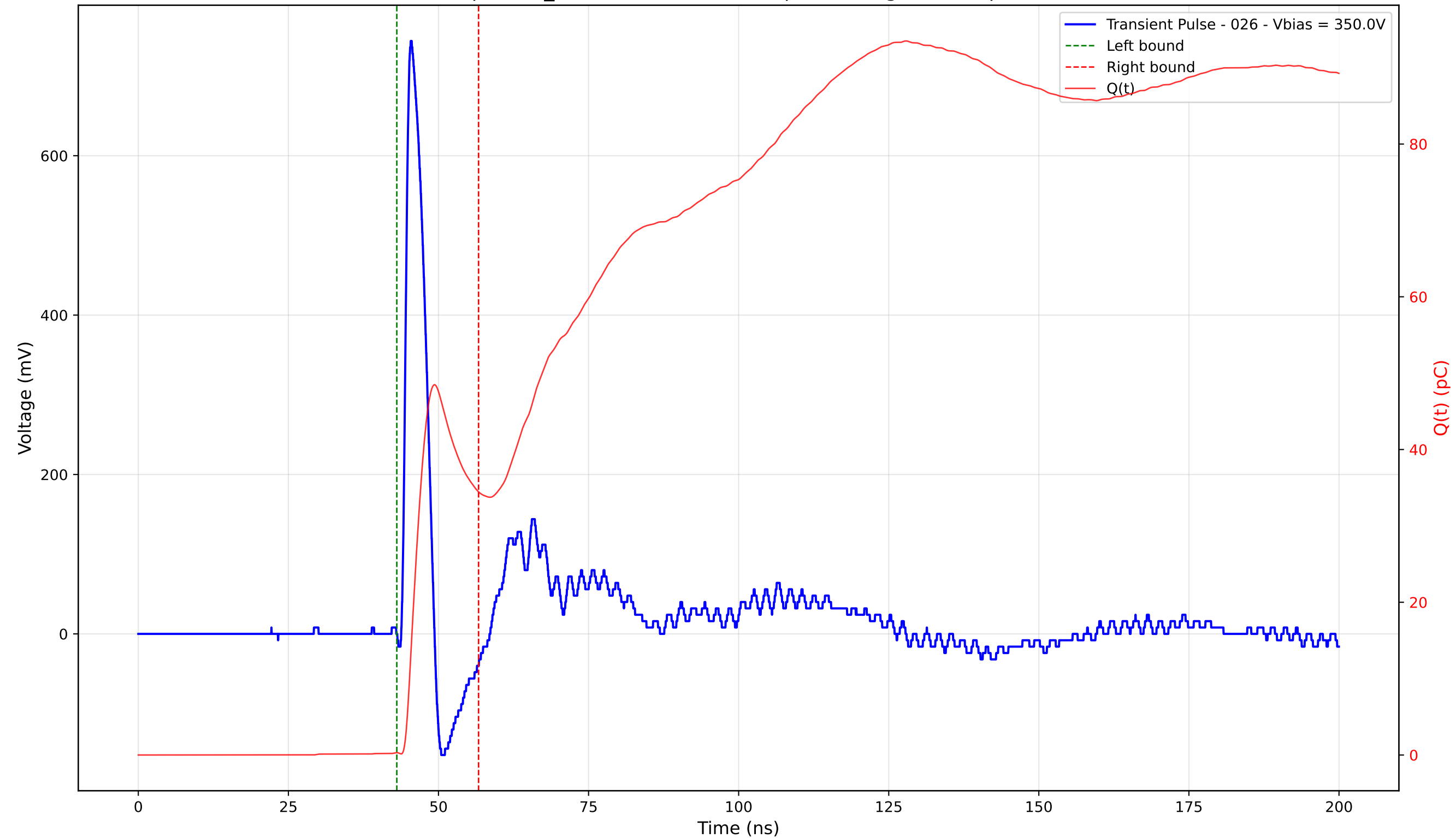
Transient Pulse - Sample: TD_4004 - Position: 330.0 \mu\text{m} - Charge: 34.14 pC - Rise Time: 0.95 ns
