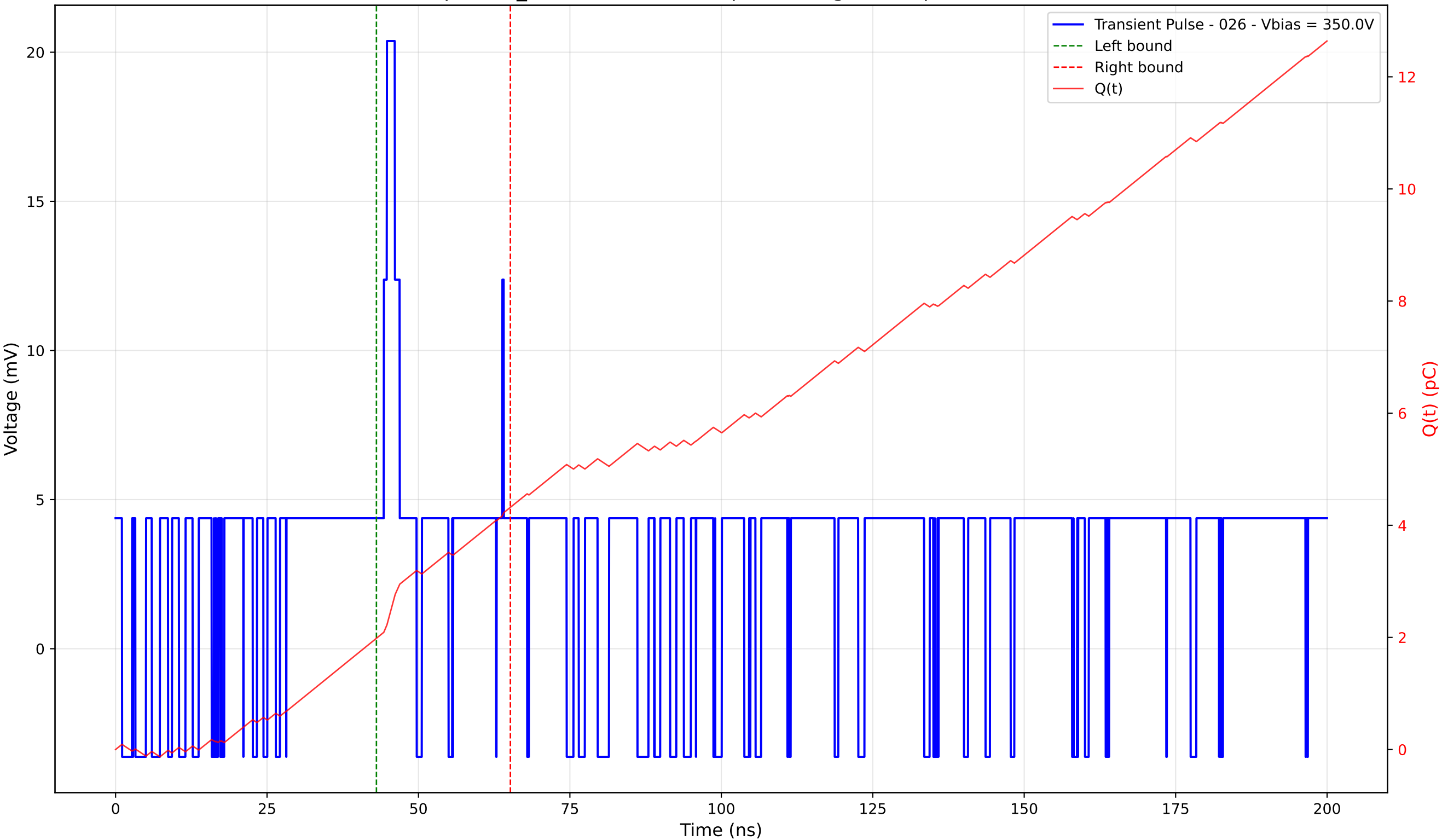
Transient Pulse - Sample: TD_4004 - Position: 5.0 \mu\text{m} - Charge: 2.34 pC - Rise Time: 0.00 ns (N/A)
