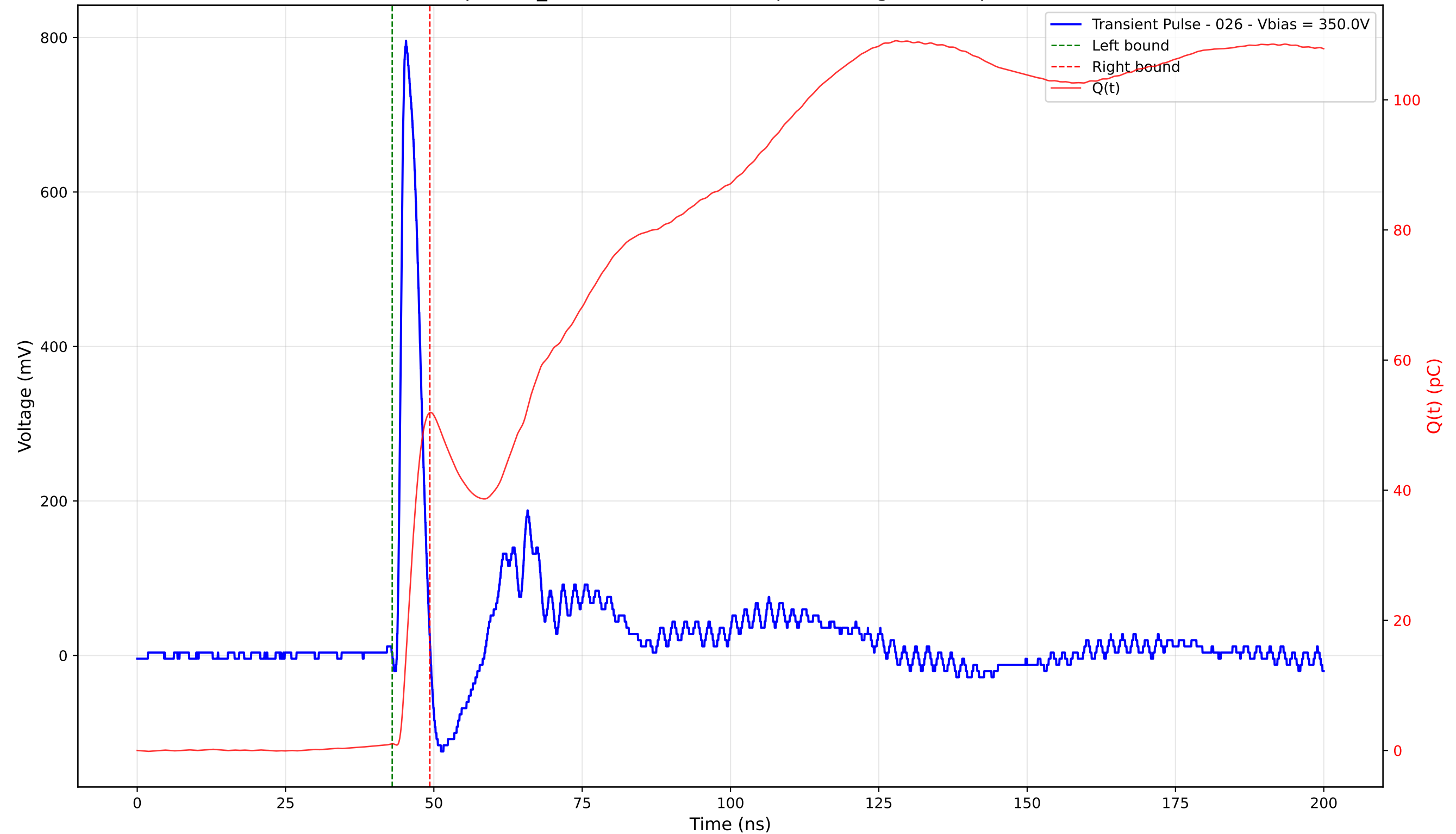
Transient Pulse - Sample: TD_4004 - Position: 245.0 \mu\text{m} - Charge: 50.91 pC - Rise Time: 0.91 ns
