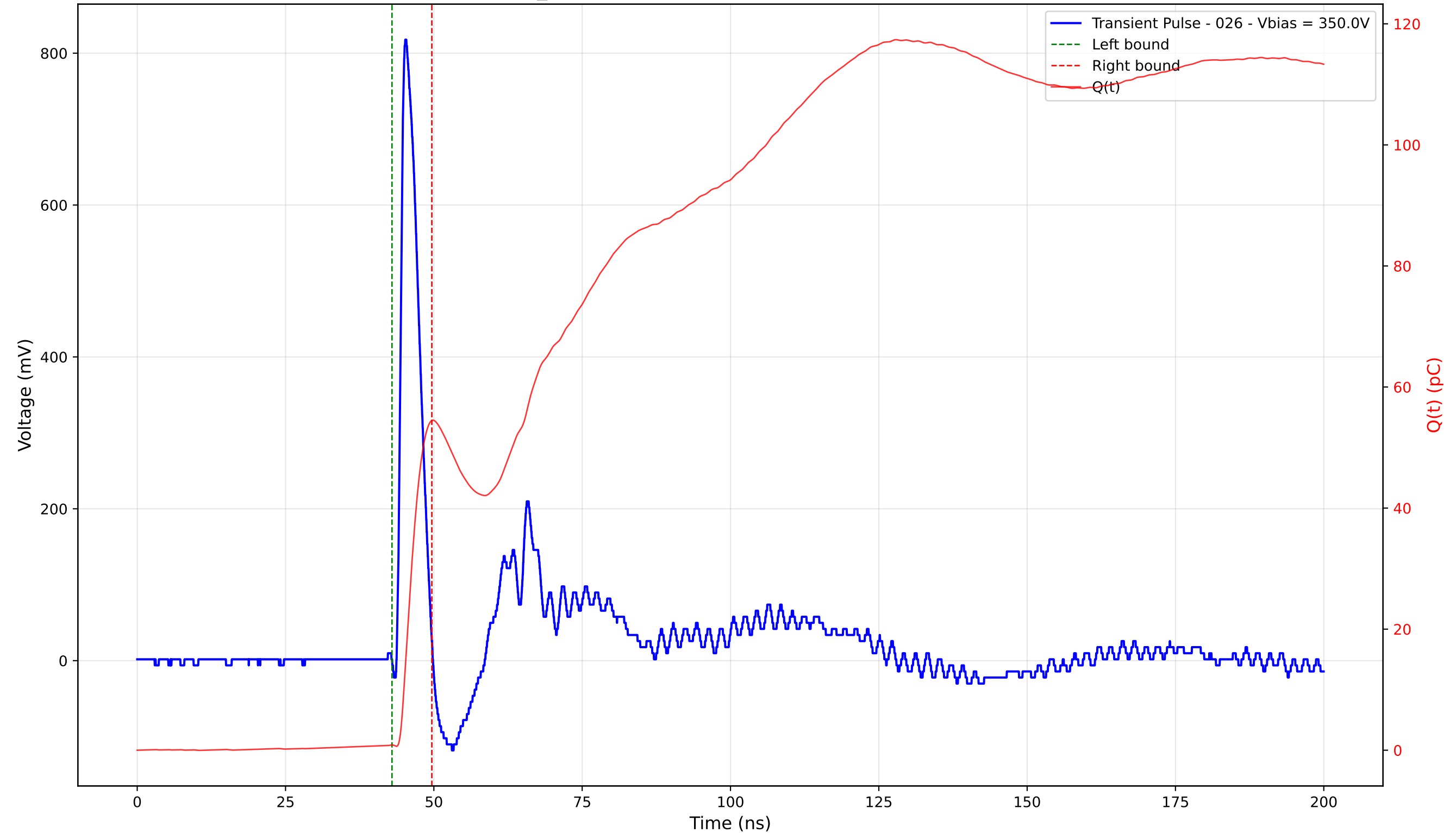
Transient Pulse - Sample: TD_4004 - Position: 175.0 \mu\text{m} - Charge: 53.60 pC - Rise Time: 0.90 ns
