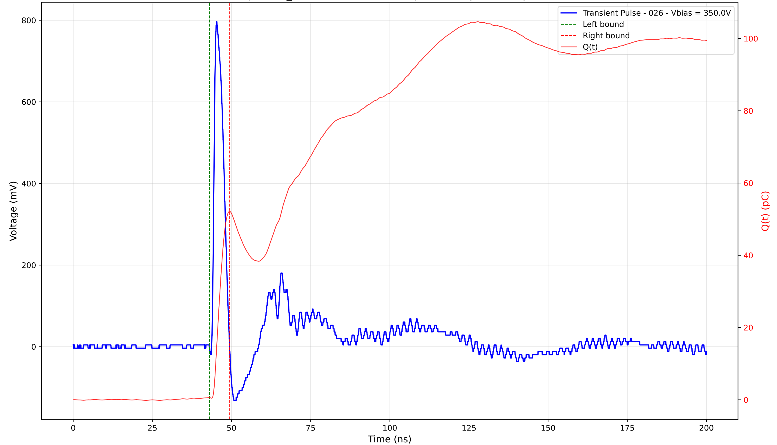
Transient Pulse - Sample: TD_4004 - Position: 270.0 \mu\text{m} - Charge: 51.51 pC - Rise Time: 0.92 ns
