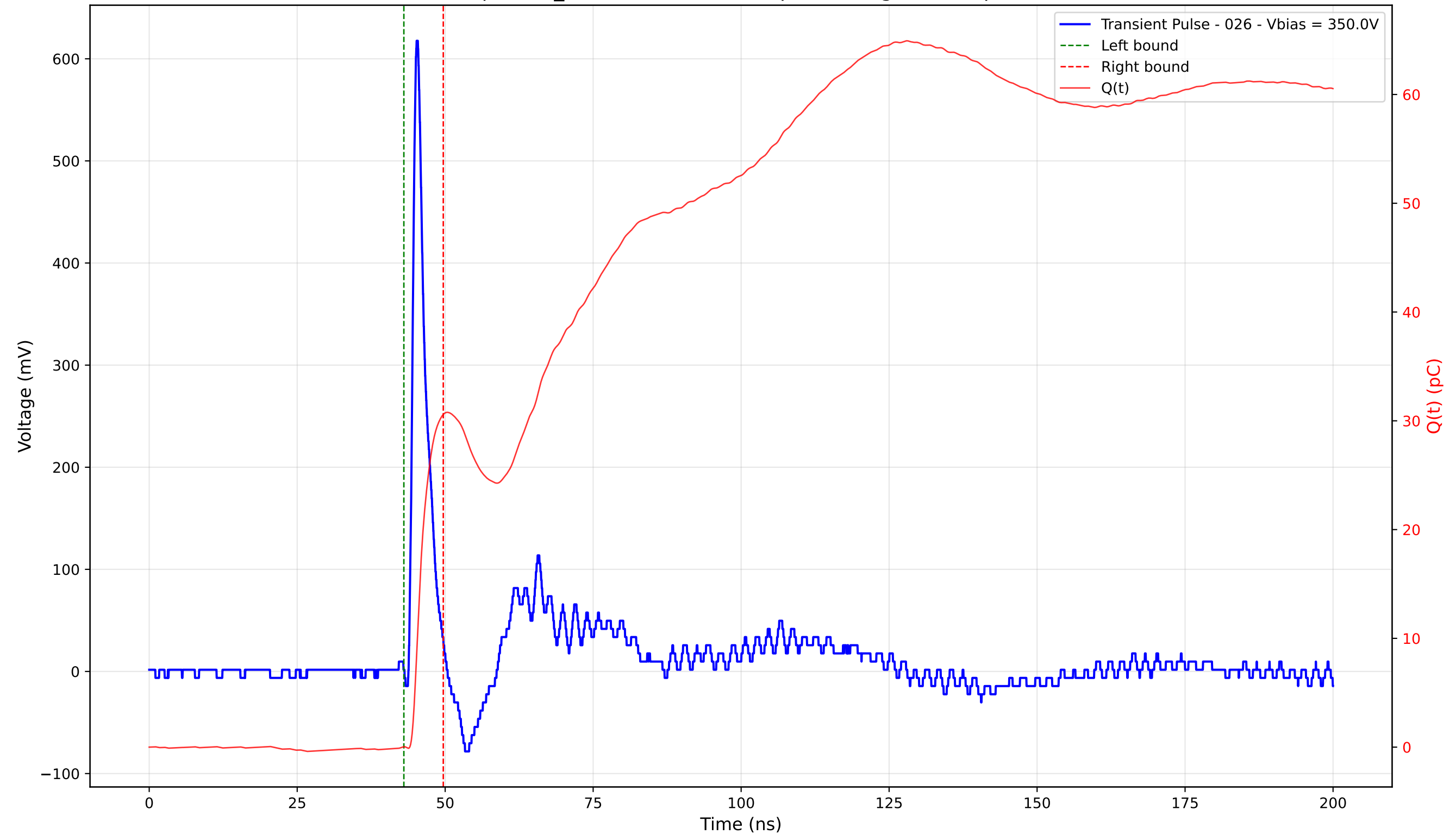
Transient Pulse - Sample: TD_4004 - Position: 70.0 \mu\text{m} - Charge: 30.55 pC - Rise Time: 0.90 ns
