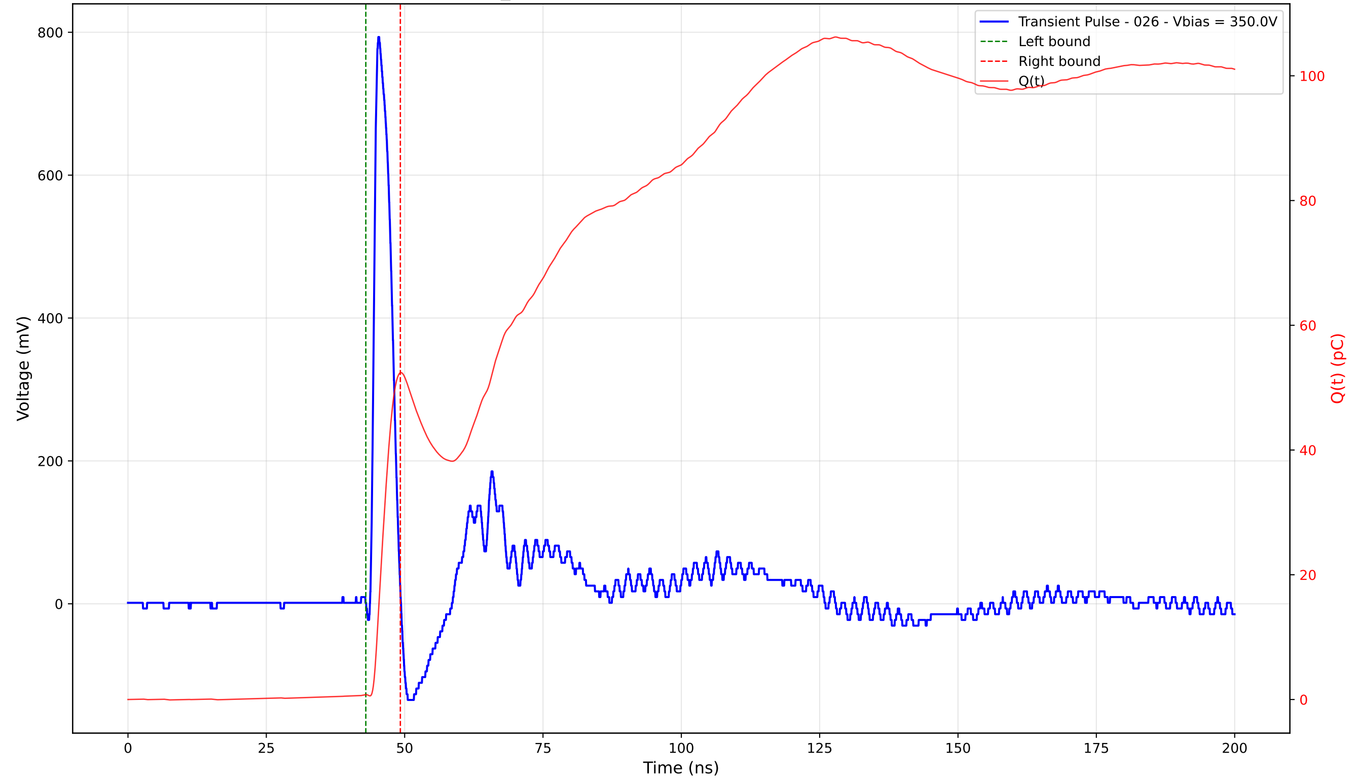
Transient Pulse - Sample: TD_4004 - Position: 285.0 \mu\text{m} - Charge: 51.62 pC - Rise Time: 0.91 ns
