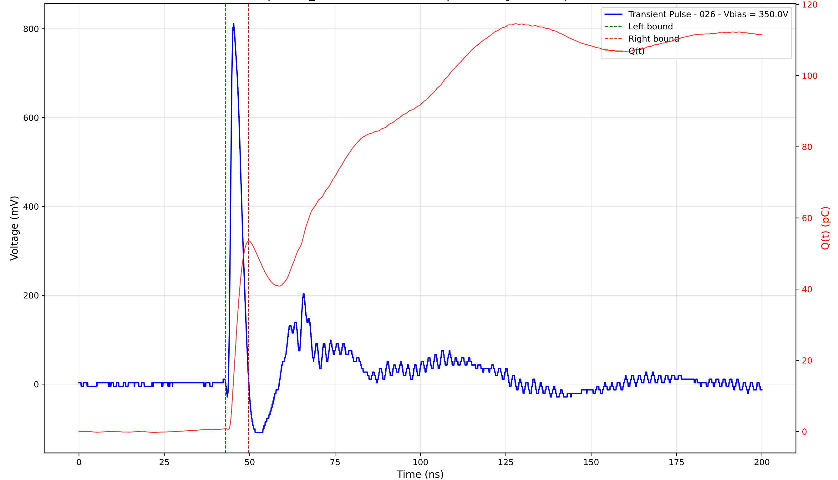
Transient Pulse - Sample: TD_4004 - Position: 210.0 \mu\text{m} - Charge: 52.68 pC - Rise Time: 0.88 ns
