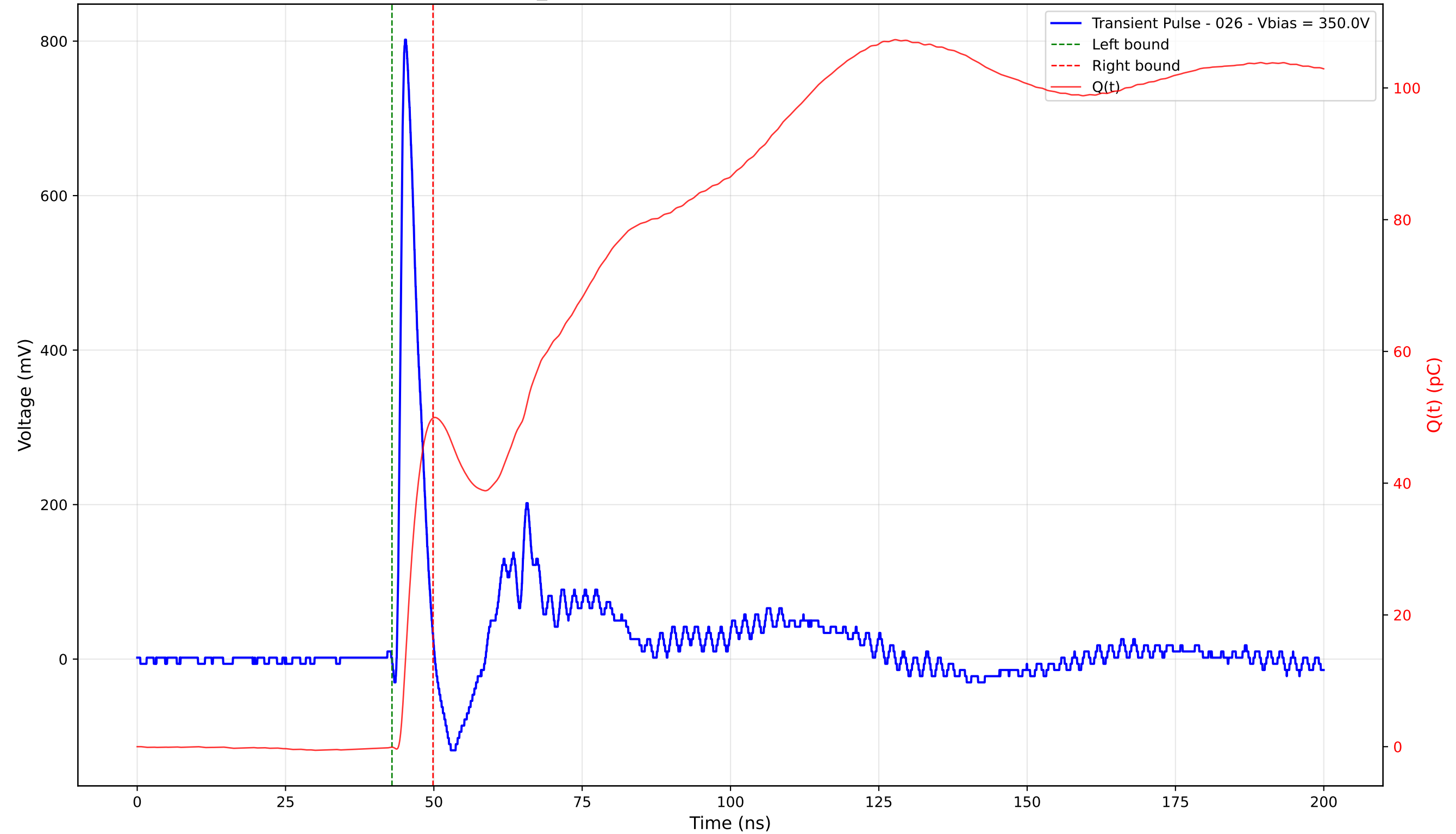
Transient Pulse - Sample: TD_4004 - Position: 100.0 \mu\text{m} - Charge: 49.96 pC - Rise Time: 0.86 ns
