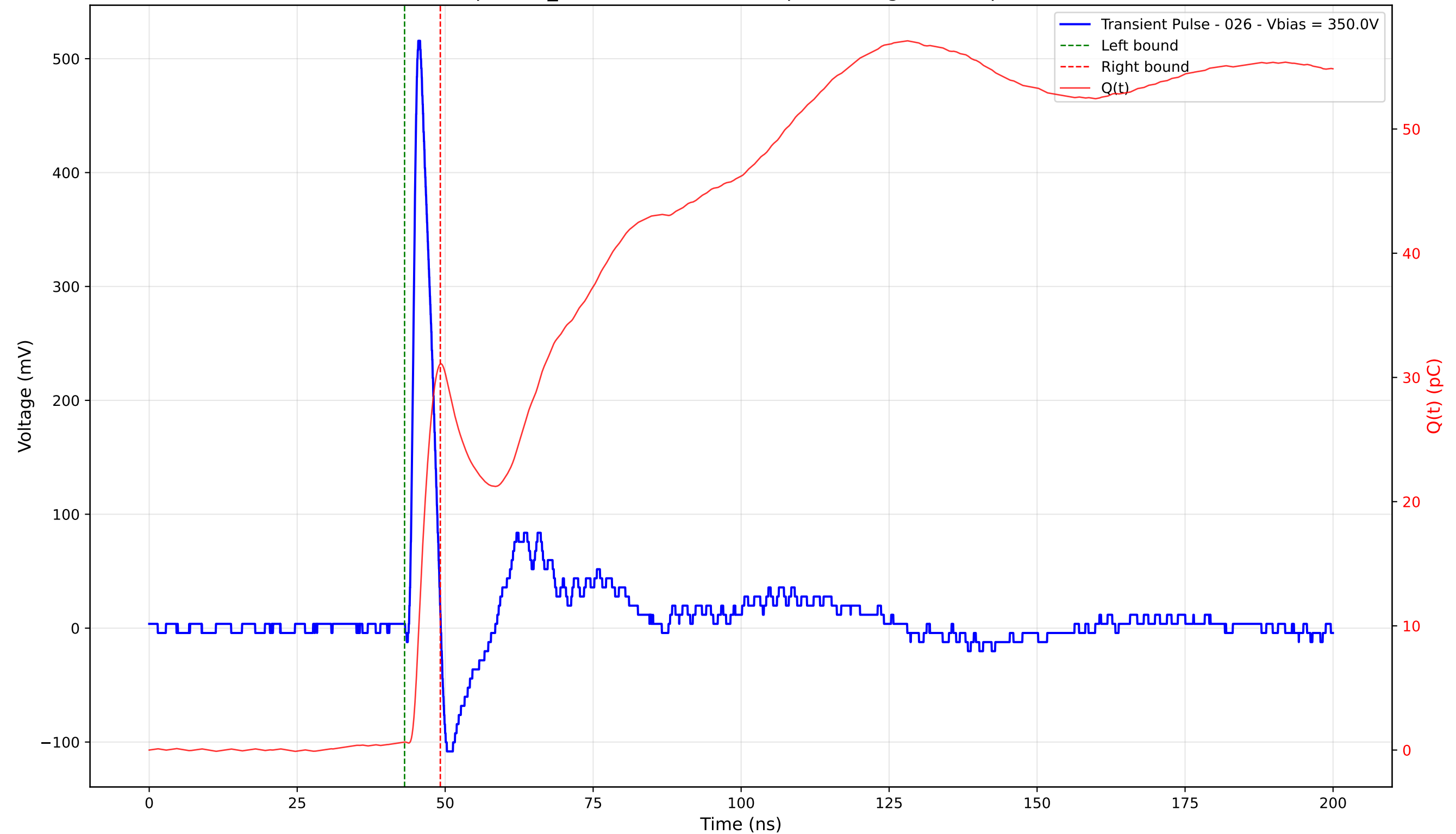
Transient Pulse - Sample: TD_4004 - Position: 395.0 \mu\text{m} - Charge: 30.45 pC - Rise Time: 1.04 ns
