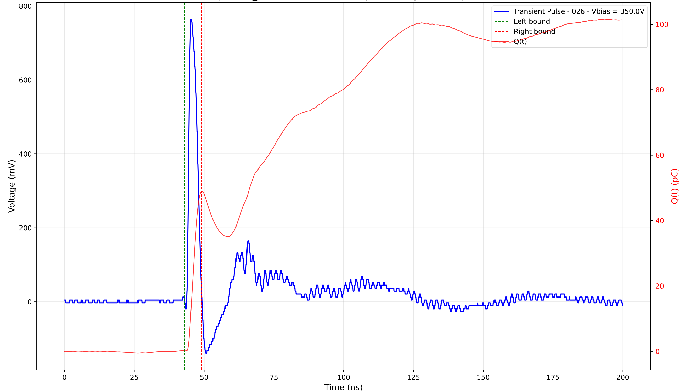
Transient Pulse - Sample: TD_4004 - Position: 310.0 \mu\text{m} - Charge: 48.61 pC - Rise Time: 0.94 ns
