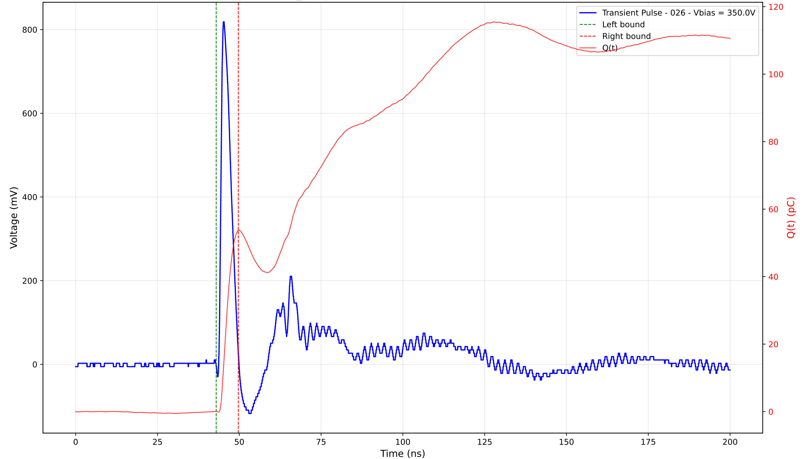
Transient Pulse - Sample: TD_4004 - Position: 180.0 \mu\text{m} - Charge: 53.58 pC - Rise Time: 0.89 ns
