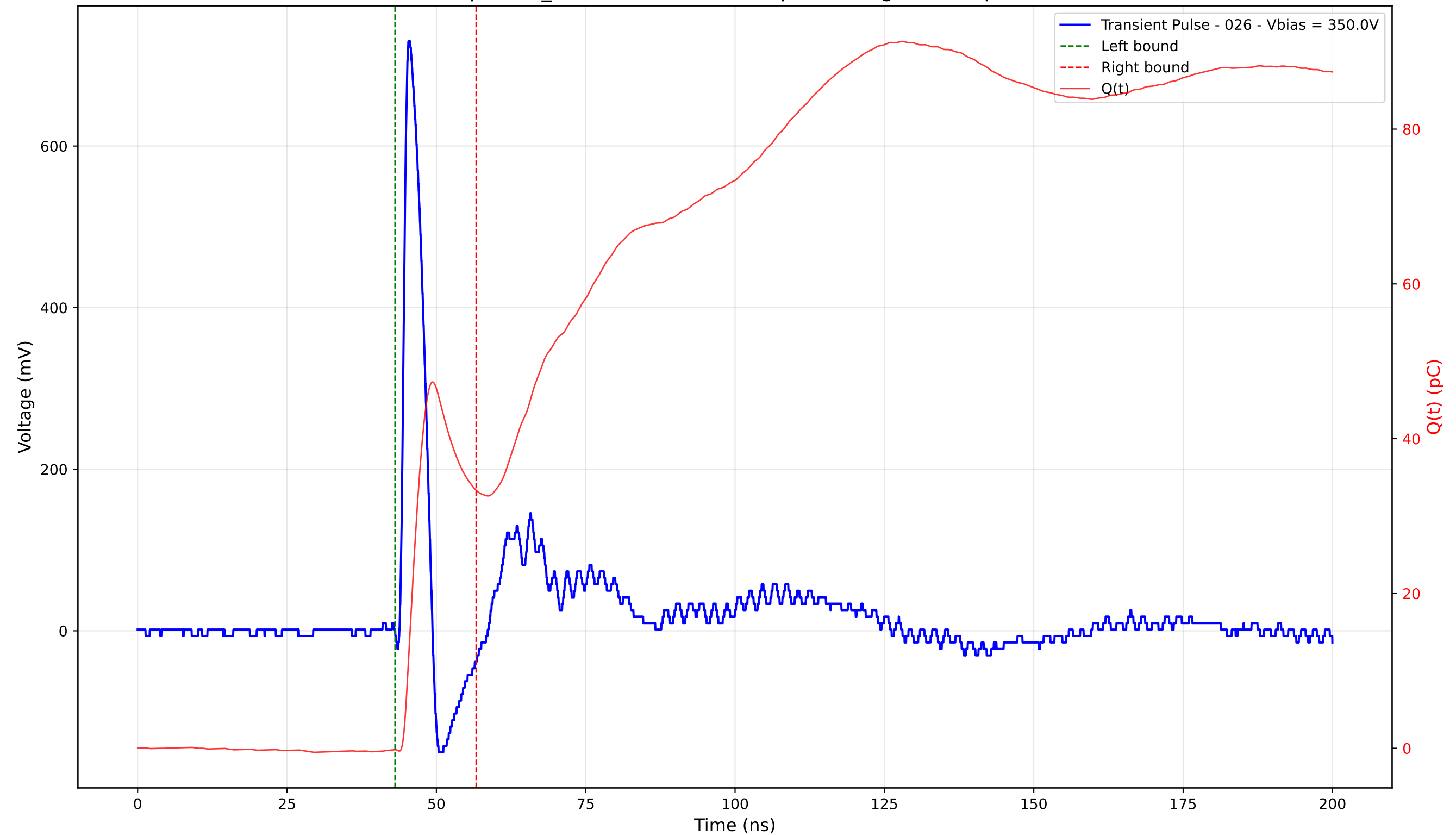
Transient Pulse - Sample: TD_4004 - Position: 335.0 \mu\text{m} - Charge: 33.51 pC - Rise Time: 0.94 ns
