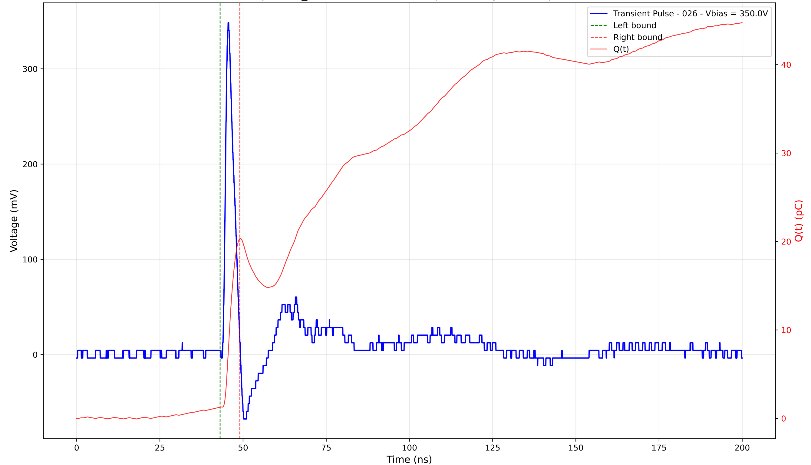
Transient Pulse - Sample: TD_4004 - Position: 405.0 \mu\text{m} - Charge: 19.05 pC - Rise Time: 1.10 ns
