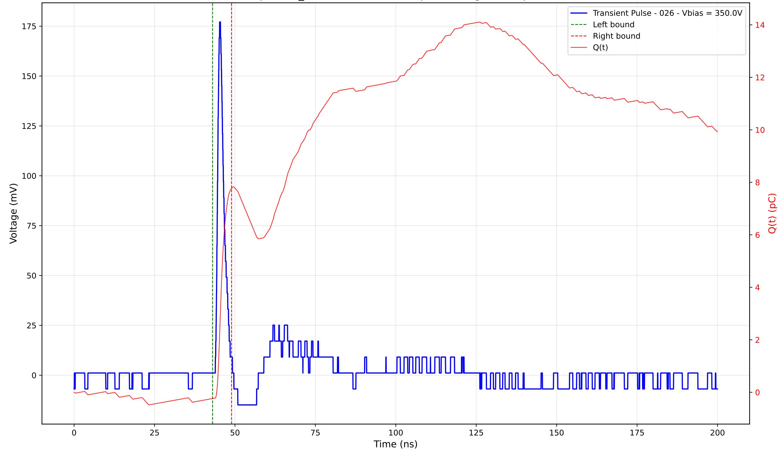
Transient Pulse - Sample: TD_4004 - Position: 50.0 \mu\text{m} - Charge: 8.01 pC - Rise Time: 0.90 ns
