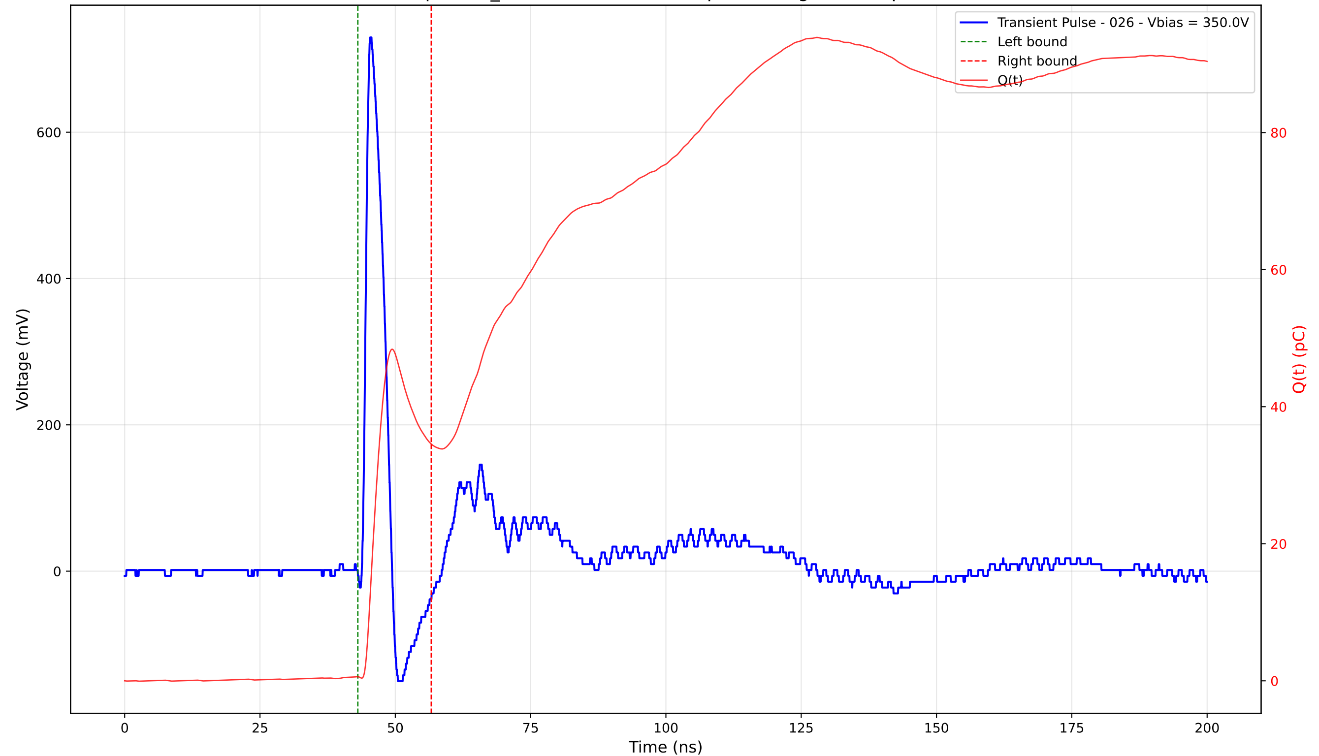
Transient Pulse - Sample: TD_4004 - Position: 350.0 \mu\text{m} - Charge: 33.95 pC - Rise Time: 0.96 ns
