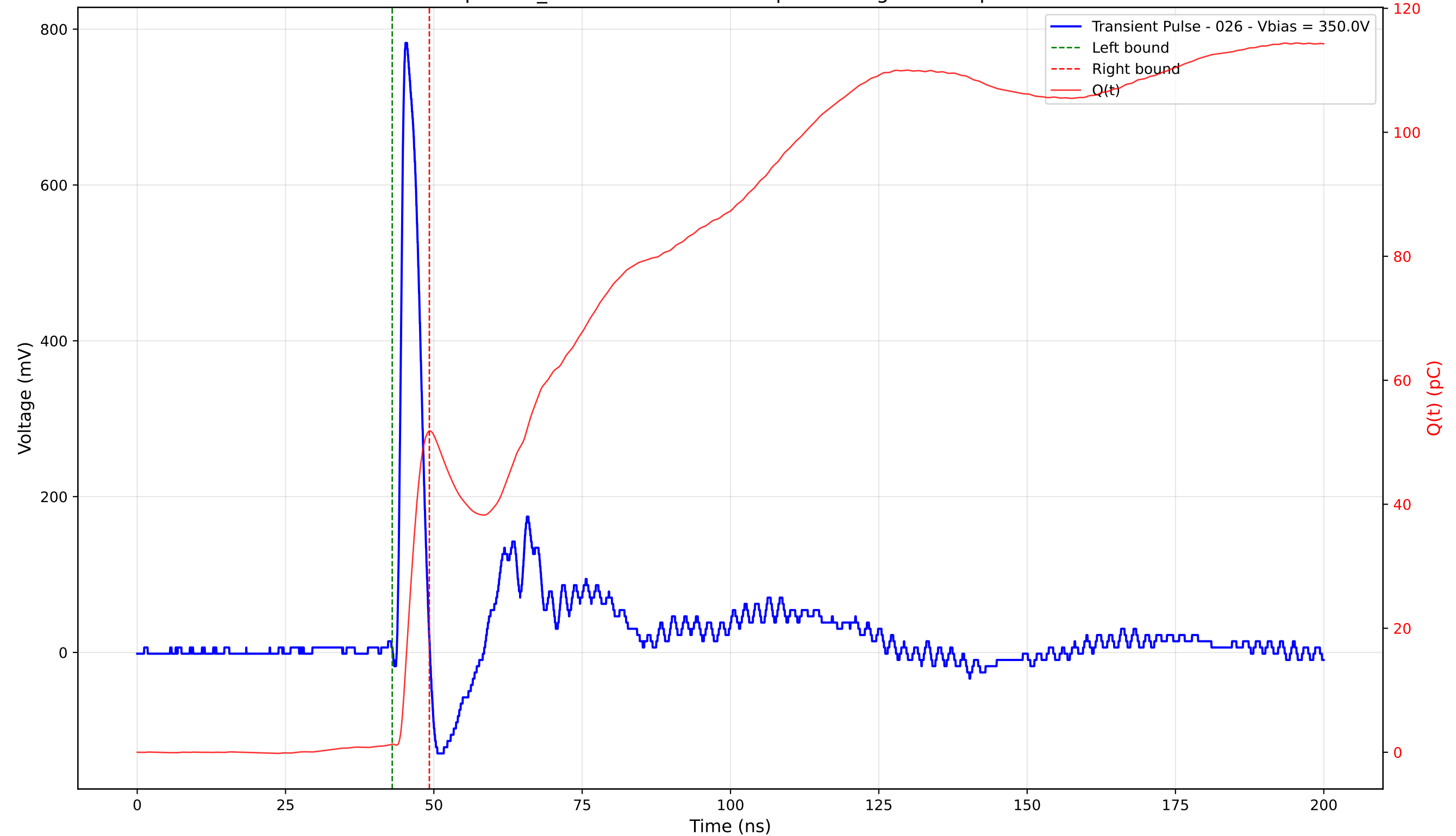
Transient Pulse - Sample: TD_4004 - Position: 300.0 \mu\text{m} - Charge: 50.51 pC - Rise Time: 0.94 ns
