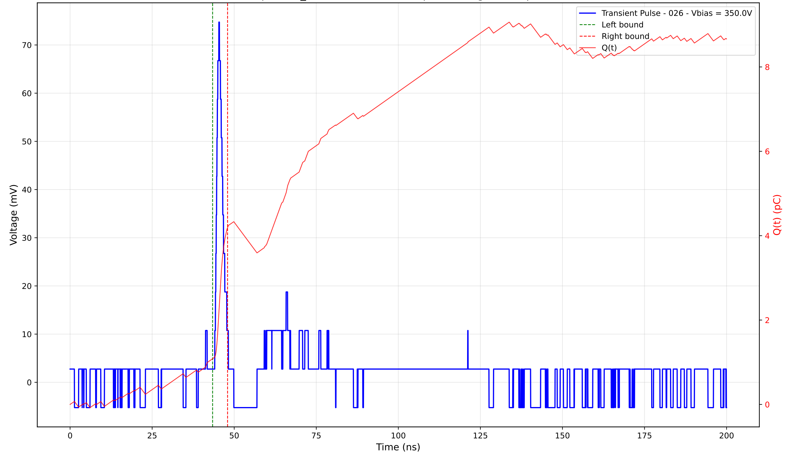
Transient Pulse - Sample: TD_4004 - Position: 40.0 \mu\text{m} - Charge: 3.11 pC - Rise Time: 1.25 ns
