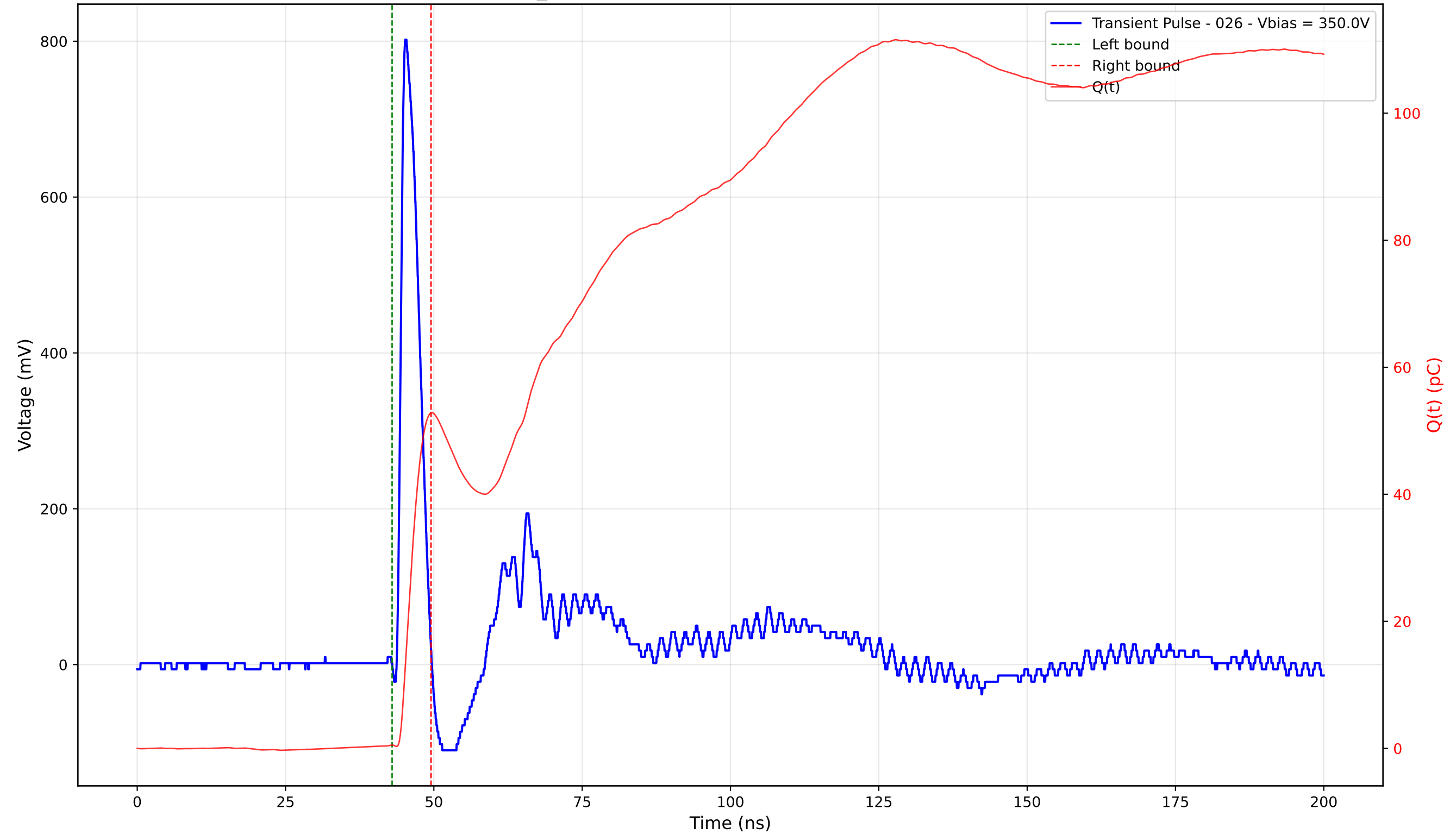
Transient Pulse - Sample: TD_4004 - Position: 225.0 \mu\text{m} - Charge: 52.30 pC - Rise Time: 0.88 ns
