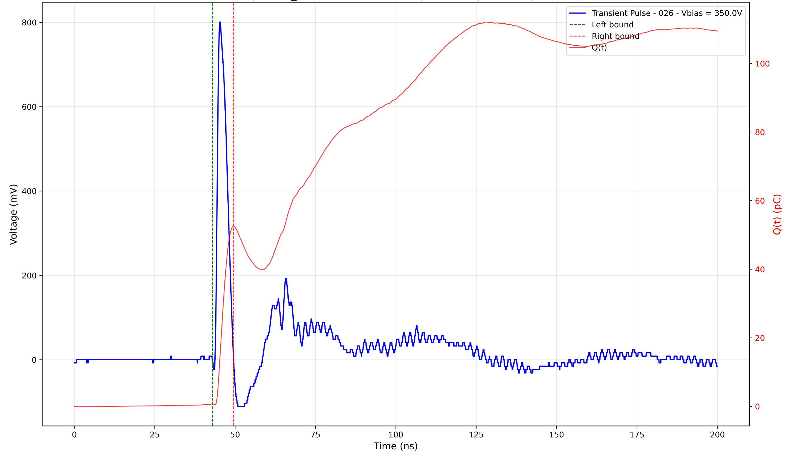
Transient Pulse - Sample: TD_4004 - Position: 140.0 \mu\text{m} - Charge: 51.80 pC - Rise Time: 0.90 ns
