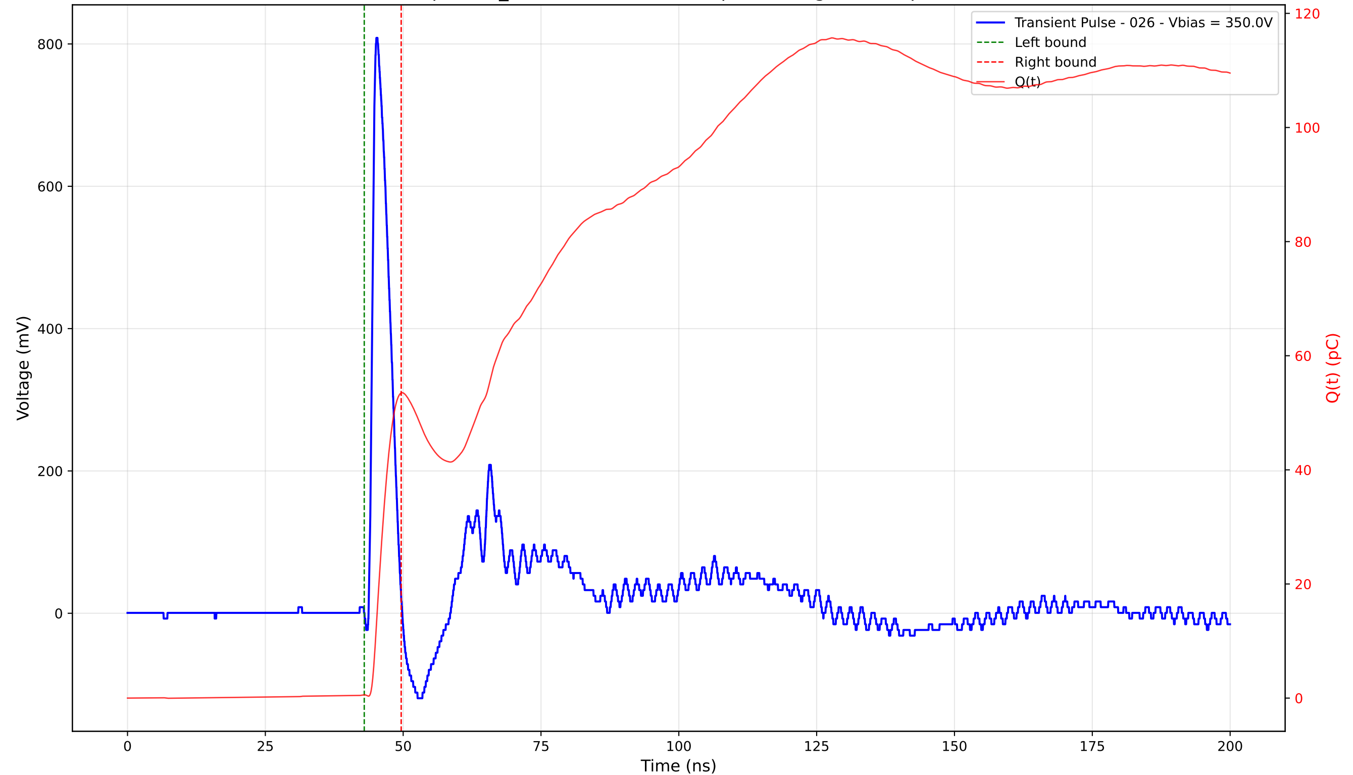
Transient Pulse - Sample: TD_4004 - Position: 120.0 \mu\text{m} - Charge: 52.90 pC - Rise Time: 0.88 ns
