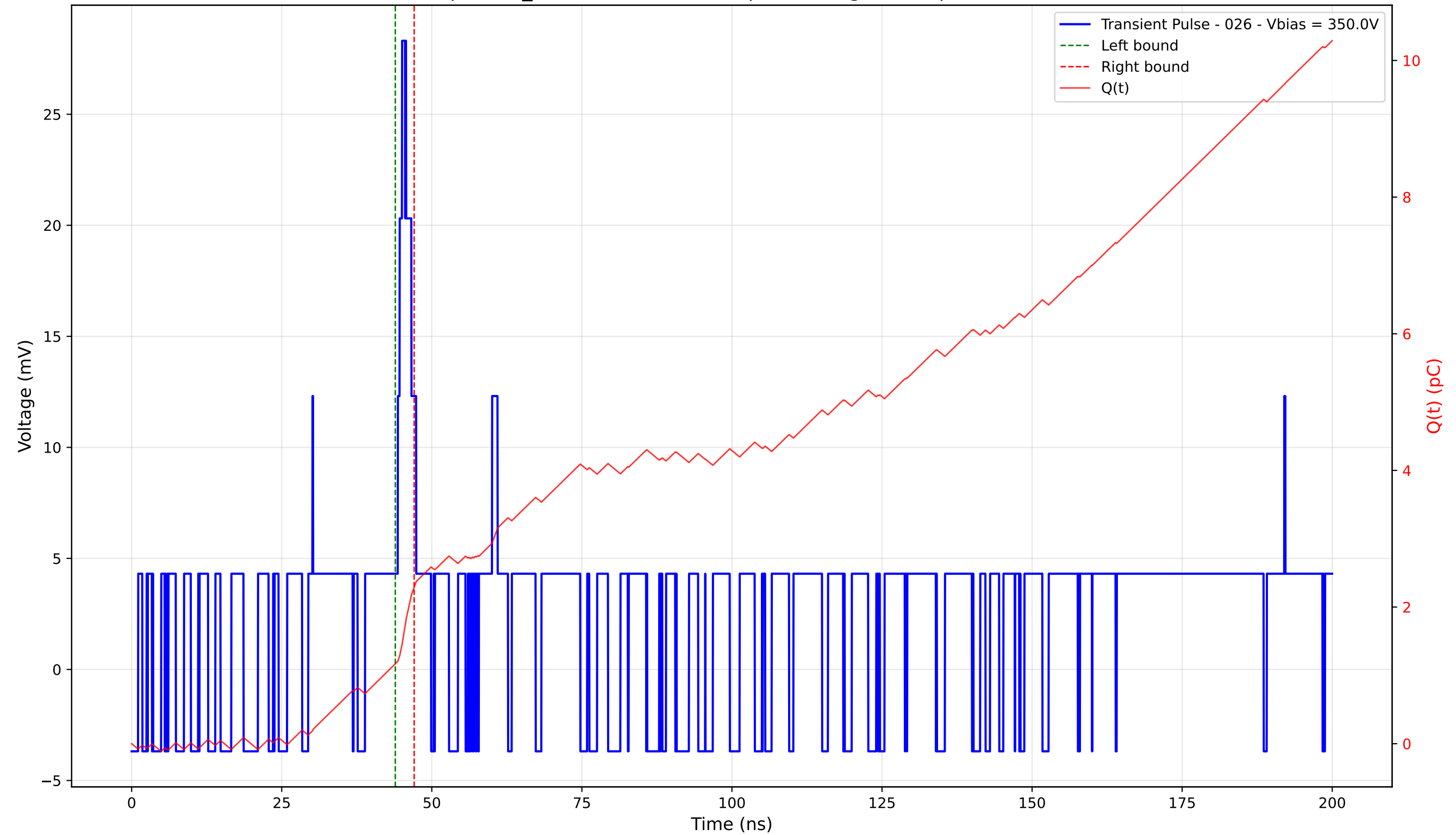
Transient Pulse - Sample: TD_4004 - Position: 20.0 \mu\text{m} - Charge: 1.12 pC - Rise Time: 0.00 ns (N/A)
