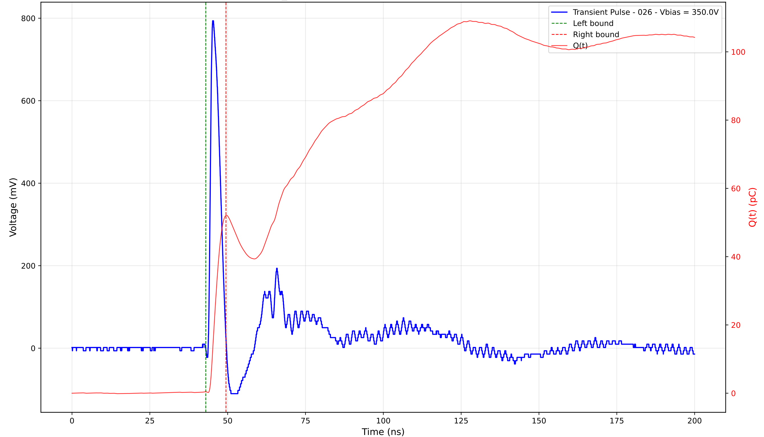
Transient Pulse - Sample: TD_4004 - Position: 155.0 \mu\text{m} - Charge: 51.65 pC - Rise Time: 0.90 ns
