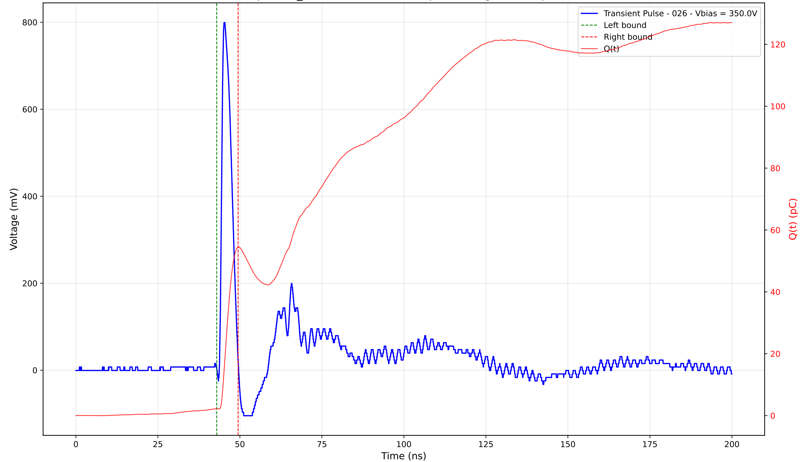
Transient Pulse - Sample: TD_4004 - Position: 230.0 \mu\text{m} - Charge: 52.20 pC - Rise Time: 0.90 ns
