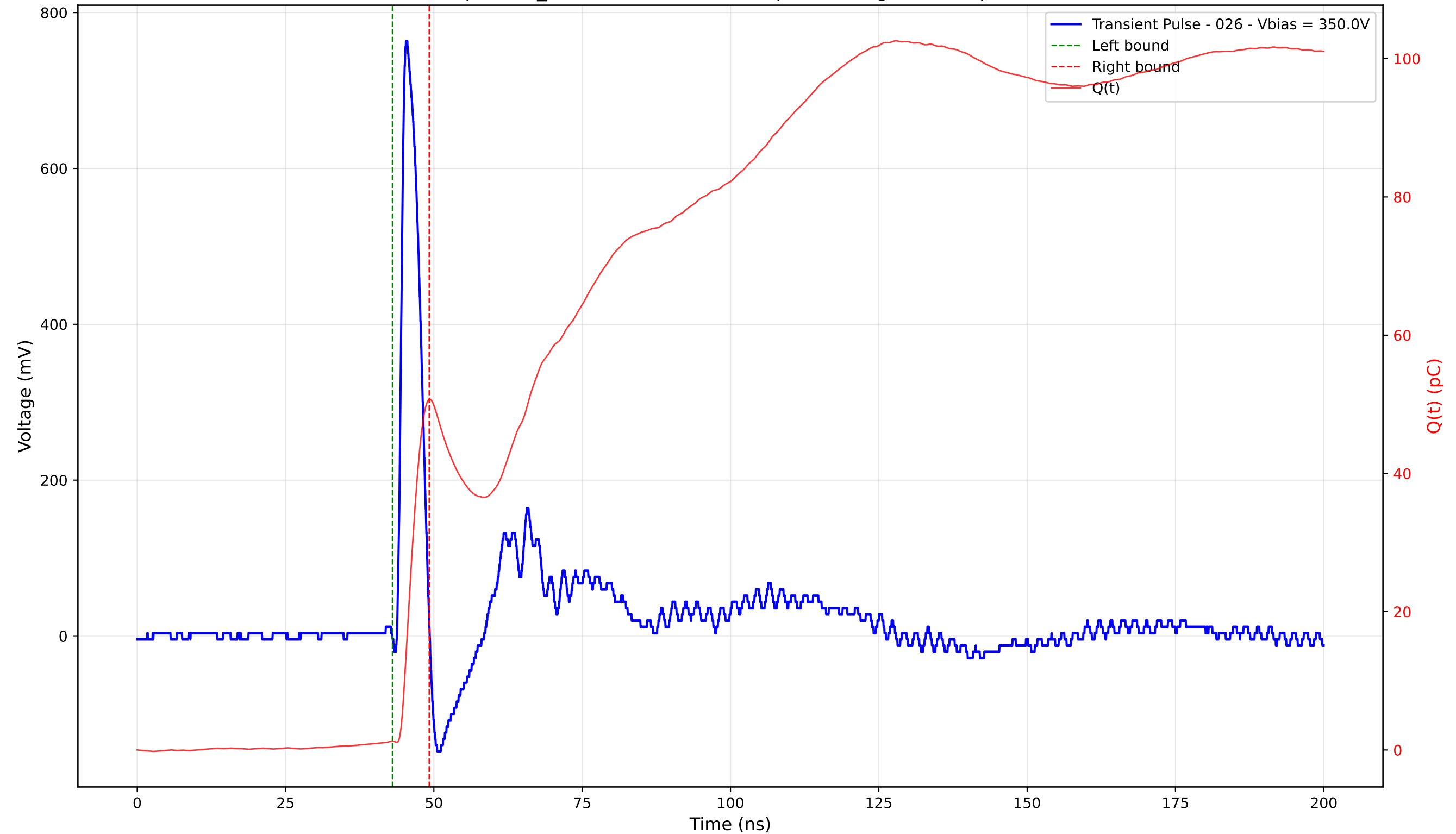
Transient Pulse - Sample: TD_4004 - Position: 320.0 \mu\text{m} - Charge: 49.44 pC - Rise Time: 0.95 ns
