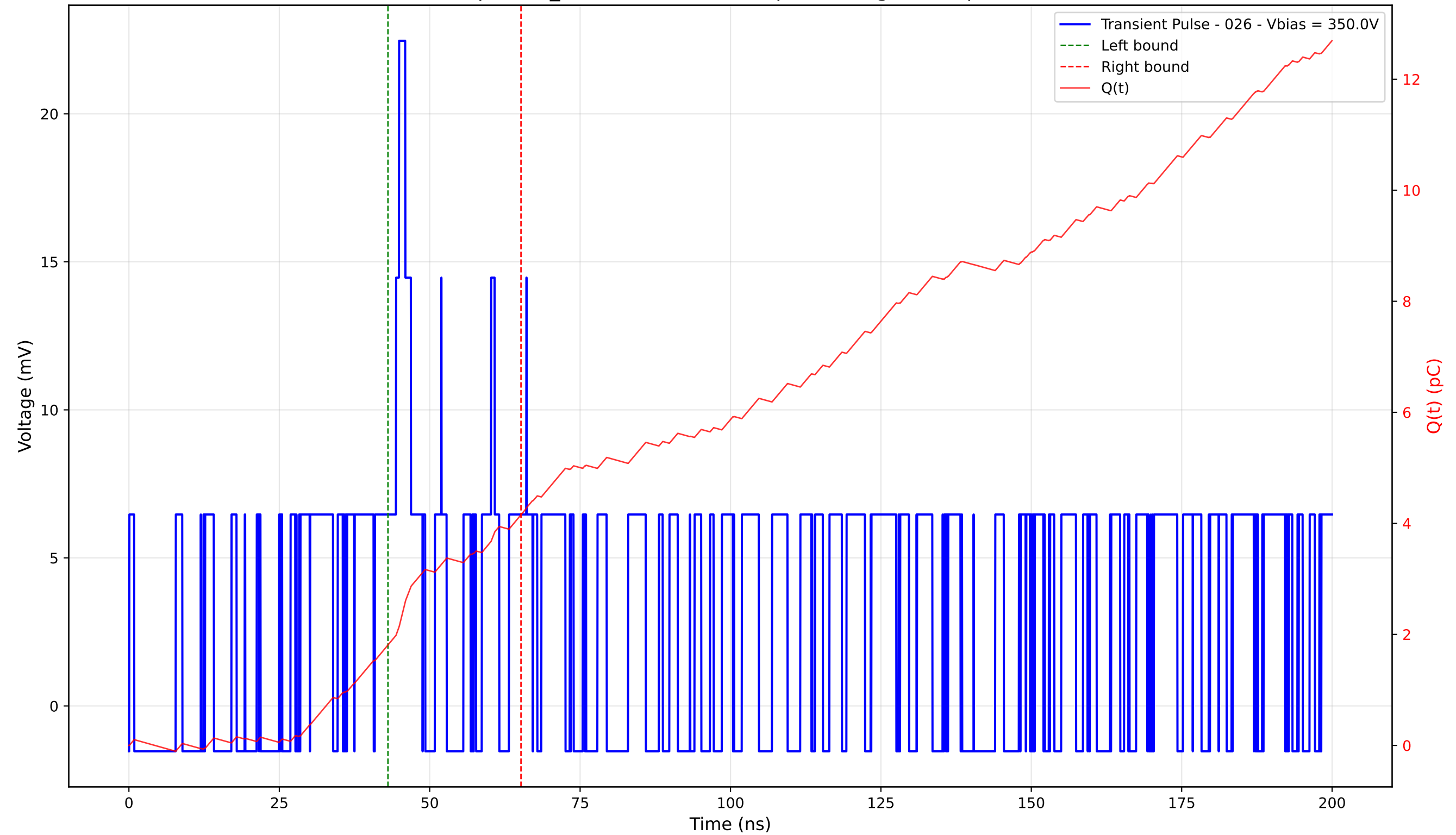
Transient Pulse - Sample: TD_4004 - Position: 10.0 \mu\text{m} - Charge: 2.34 pC - Rise Time: 4.04 ns
