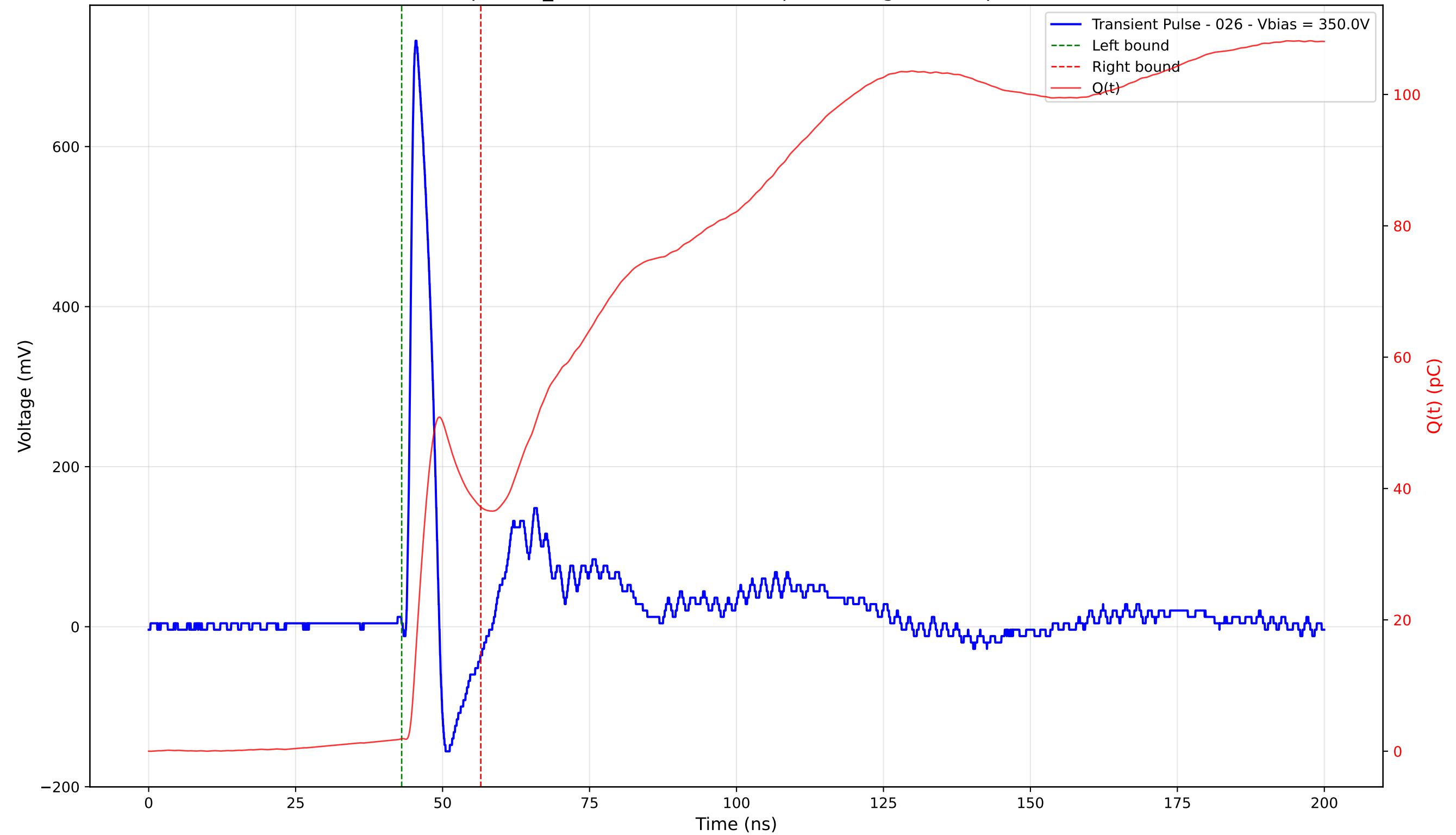
Transient Pulse - Sample: TD_4004 - Position: 360.0 \mu\text{m} - Charge: 35.28 pC - Rise Time: 0.98 ns
