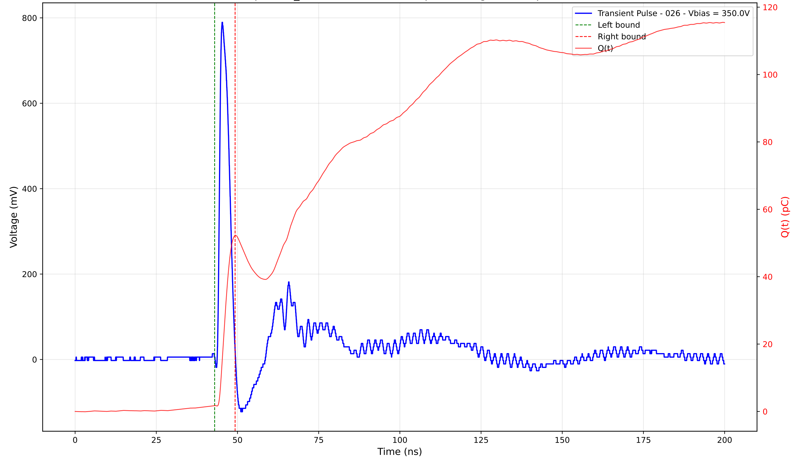
Transient Pulse - Sample: TD_4004 - Position: 255.0 \mu\text{m} - Charge: 50.48 pC - Rise Time: 0.90 ns
