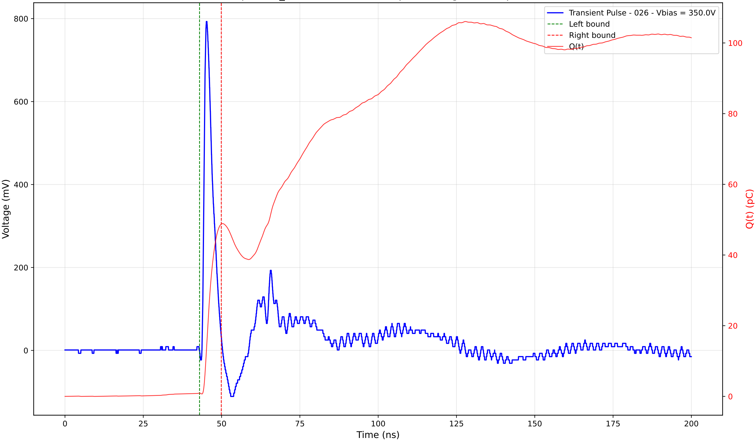
Transient Pulse - Sample: TD_4004 - Position: 95.0 \mu\text{m} - Charge: 47.84 pC - Rise Time: 0.88 ns
