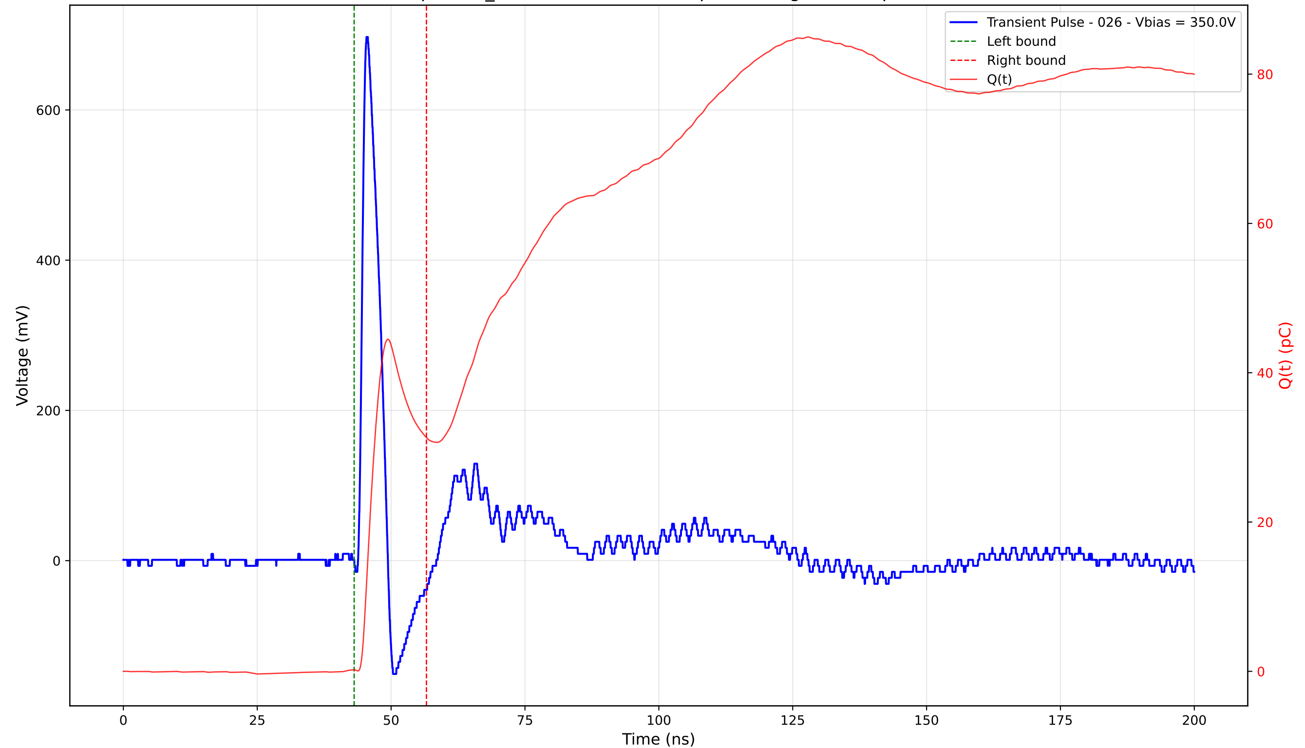
Transient Pulse - Sample: TD_4004 - Position: 380.0 \mu\text{m} - Charge: 31.10 pC - Rise Time: 0.97 ns
