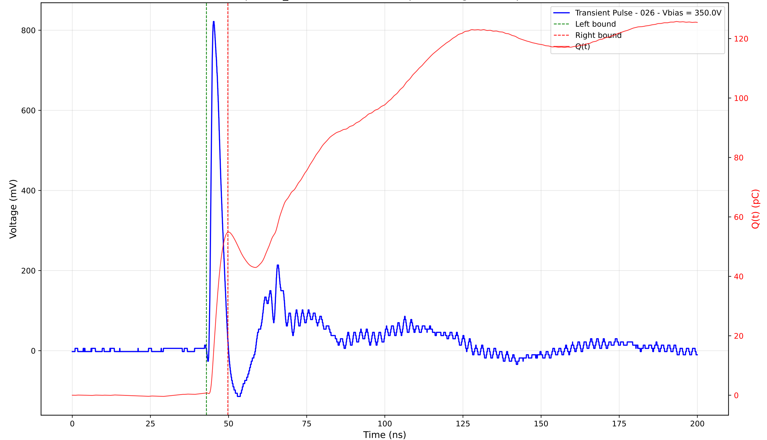
Transient Pulse - Sample: TD_4004 - Position: 190.0 \mu\text{m} - Charge: 54.07 pC - Rise Time: 0.88 ns
