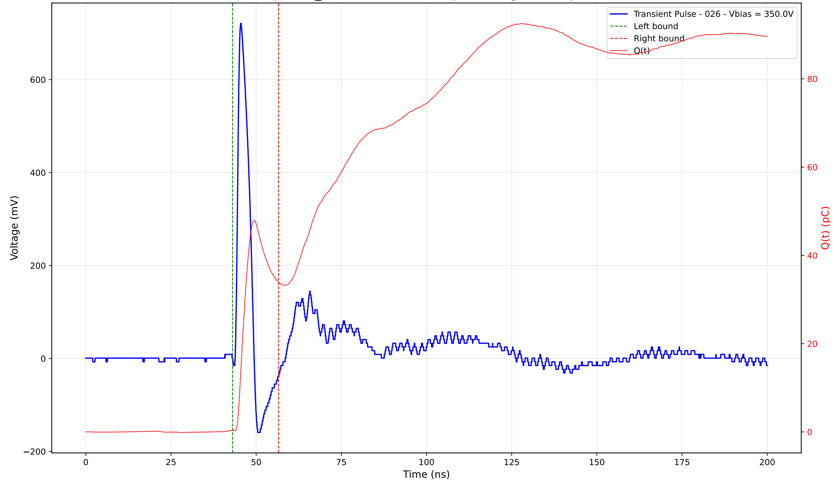
Transient Pulse - Sample: TD_4004 - Position: 365.0 \mu\text{m} - Charge: 33.42 pC - Rise Time: 0.96 ns
