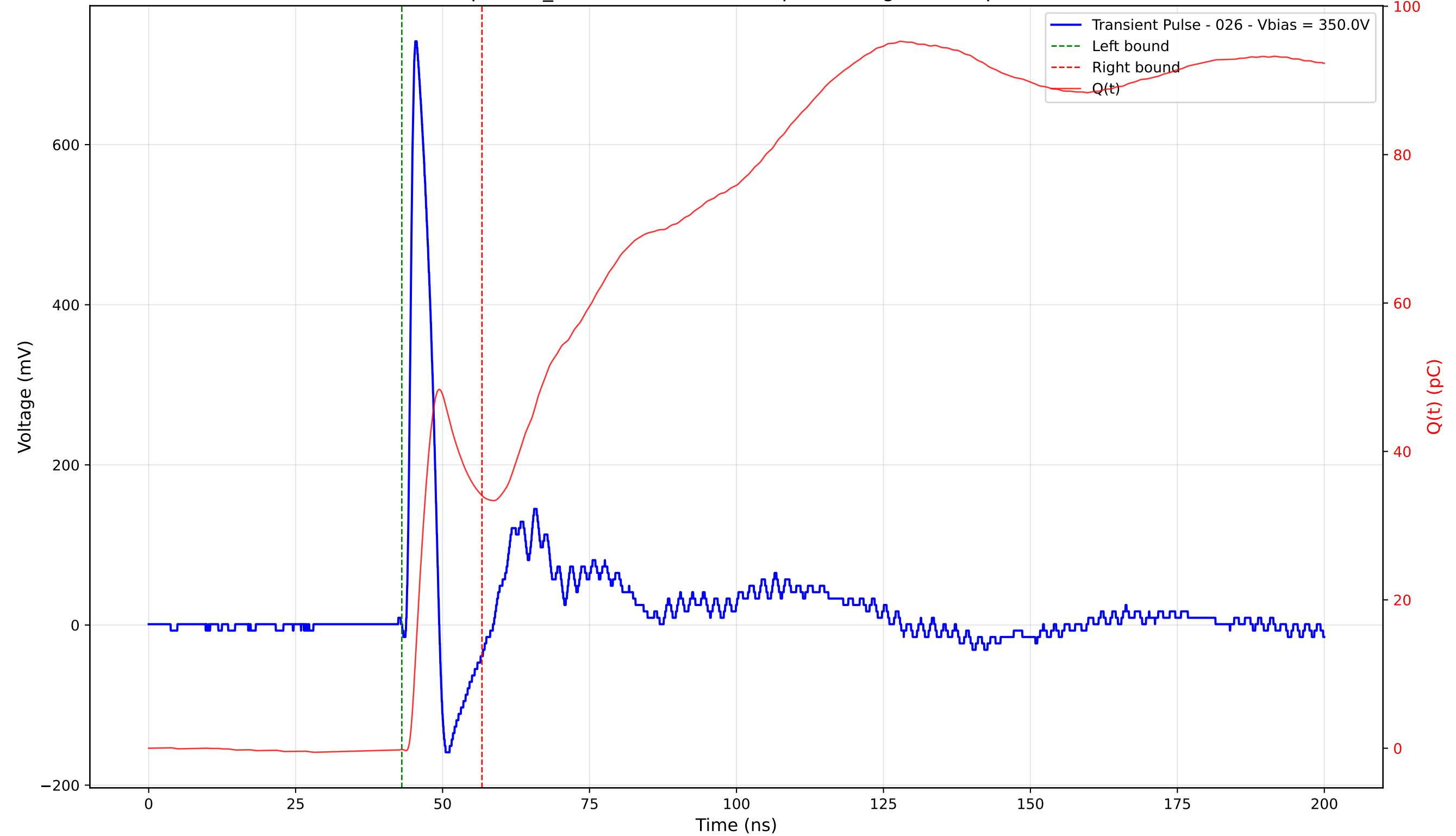
Transient Pulse - Sample: TD_4004 - Position: 355.0 \mu\text{m} - Charge: 34.22 pC - Rise Time: 0.96 ns
