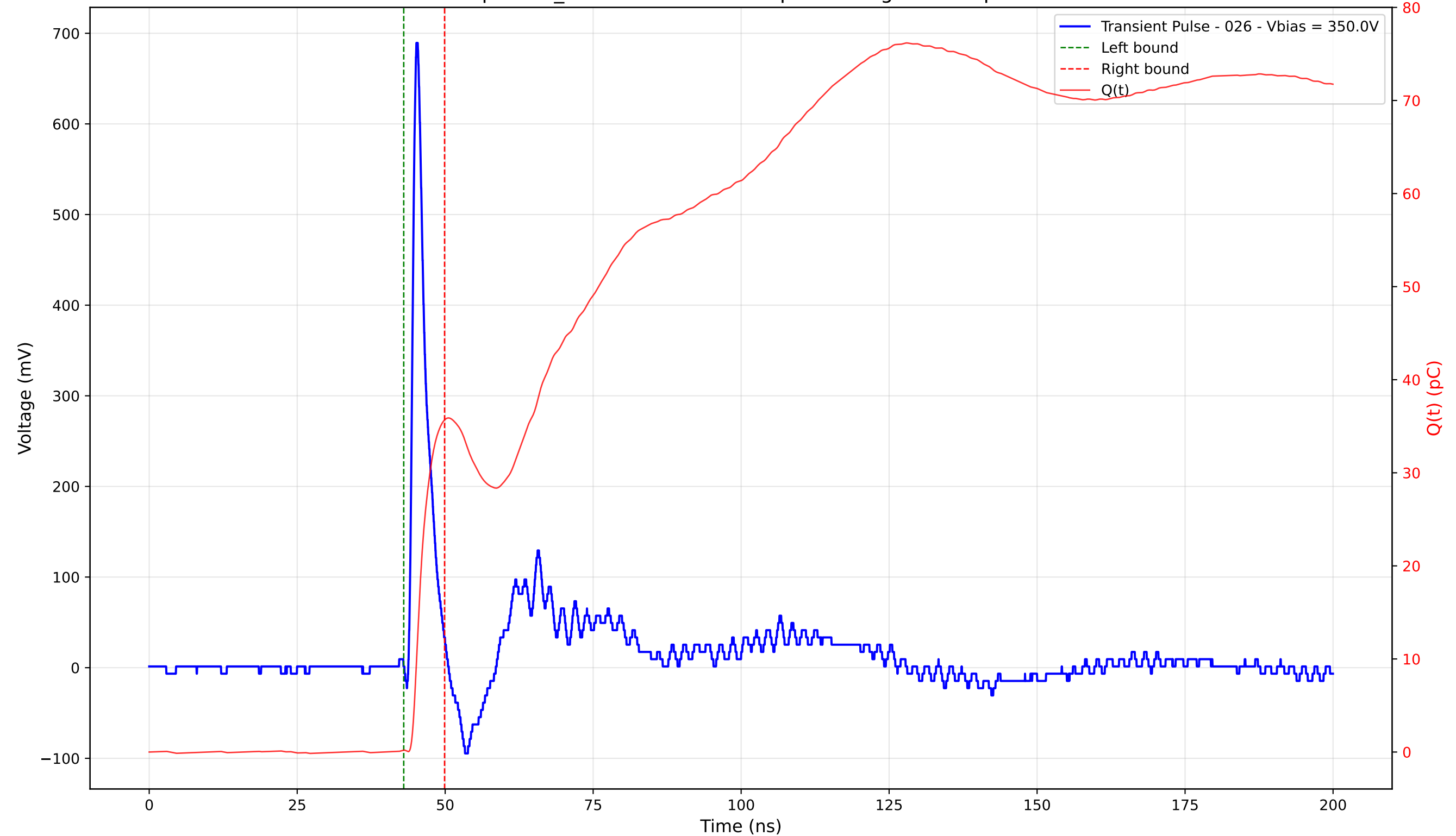
Transient Pulse - Sample: TD_4004 - Position: 75.0 \mu\text{m} - Charge: 35.48 pC - Rise Time: 0.88 ns
