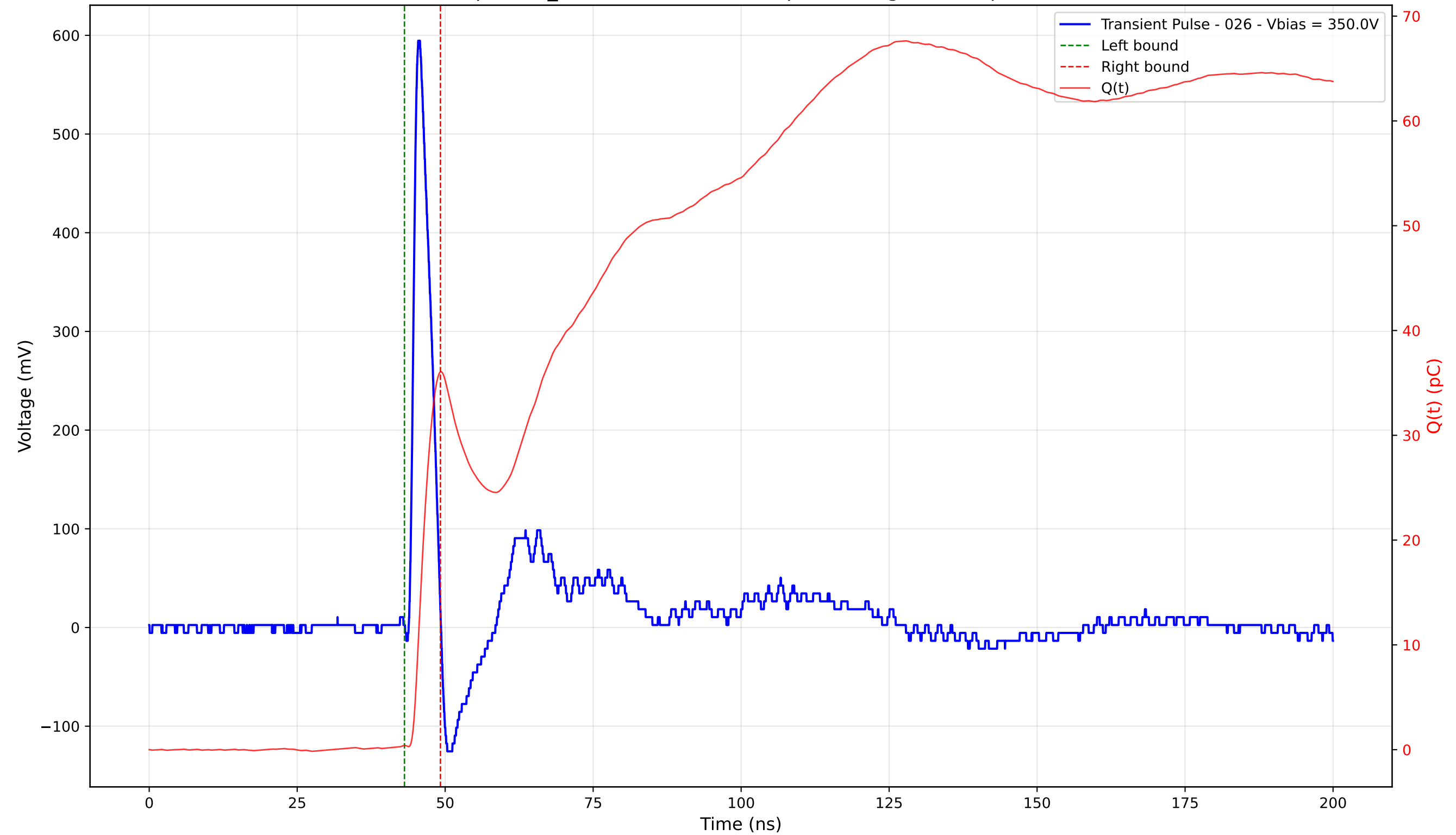
Transient Pulse - Sample: TD_4004 - Position: 390.0 \mu\text{m} - Charge: 35.66 pC - Rise Time: 1.03 ns
