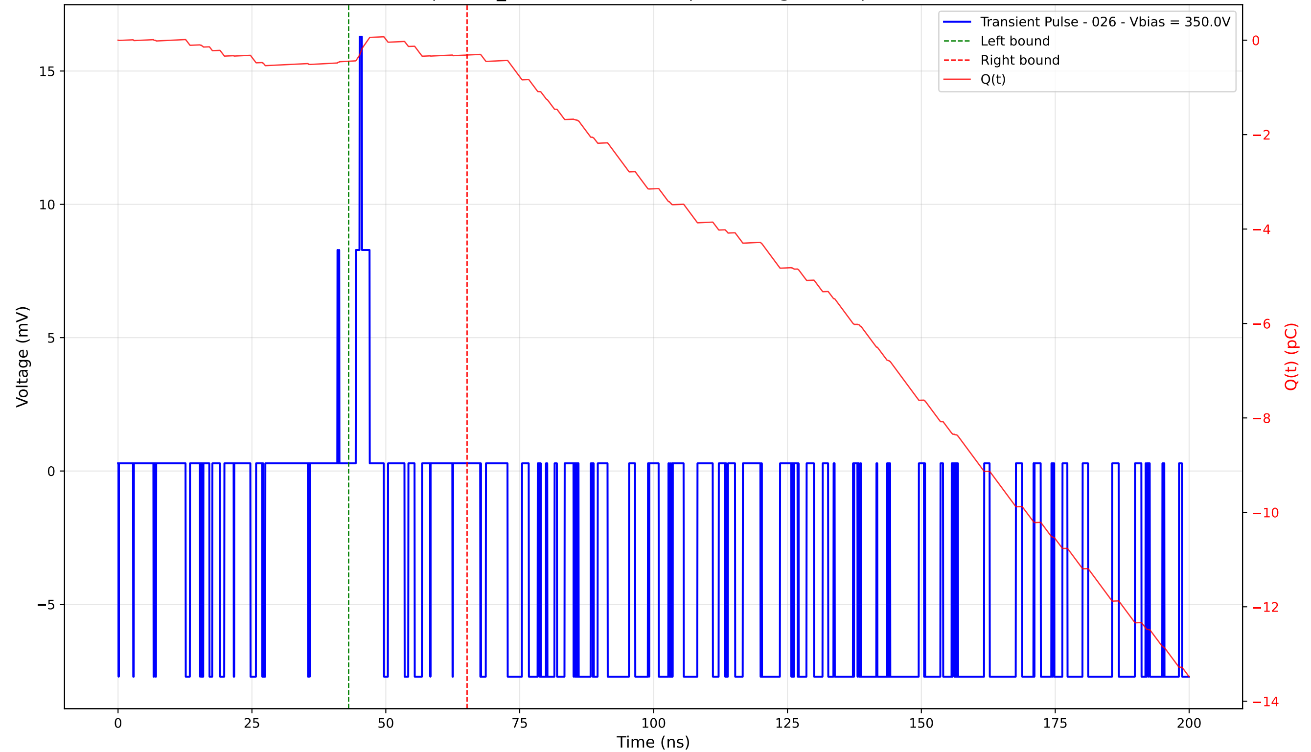
Transient Pulse - Sample: TD_4004 - Position: 0.0 \mu\text{m} - Charge: 0.13 pC - Rise Time: 0.72 ns
