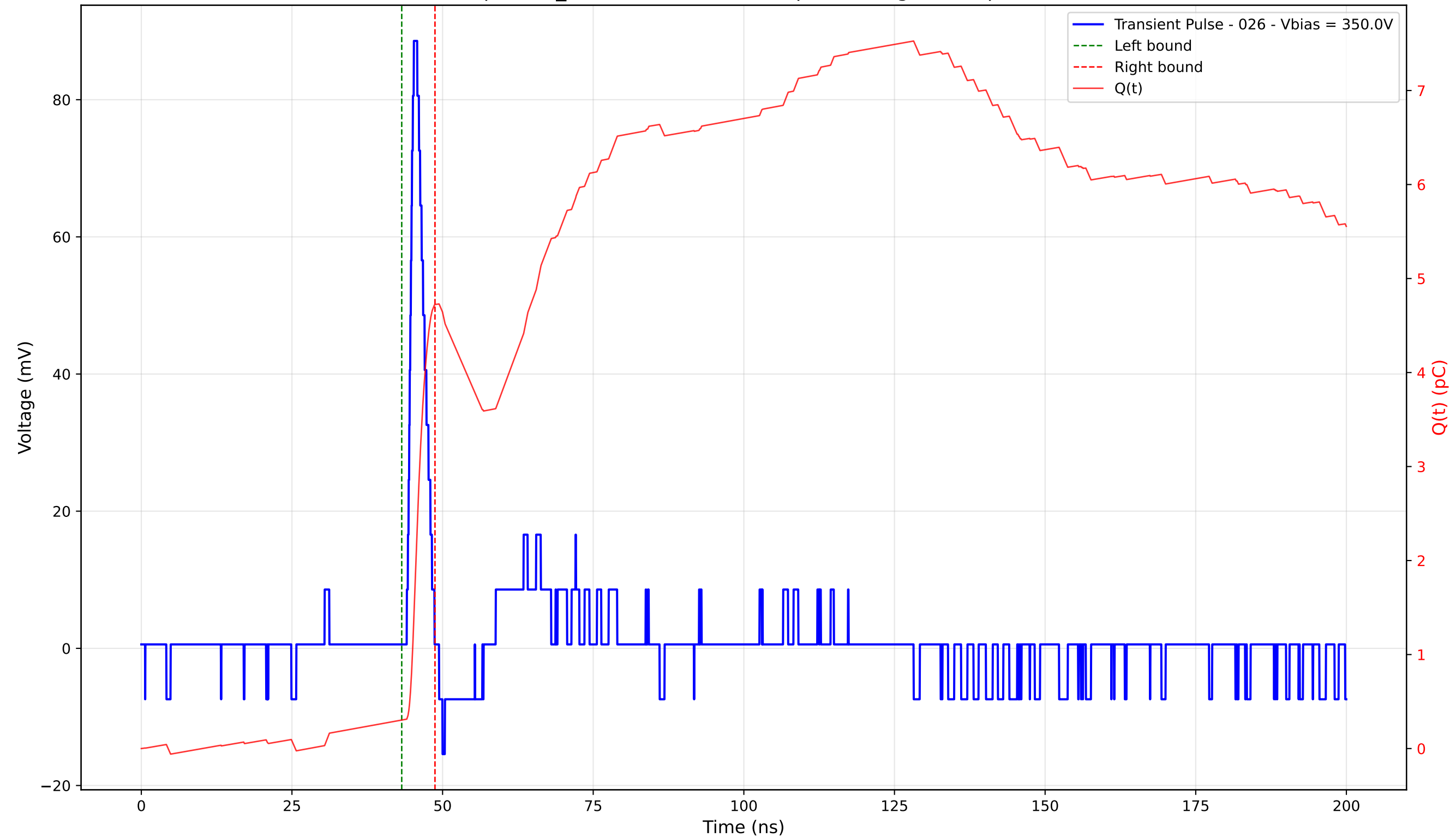
Transient Pulse - Sample: TD_4004 - Position: 435.0 \mu\text{m} - Charge: 4.42 pC - Rise Time: 0.84 ns
