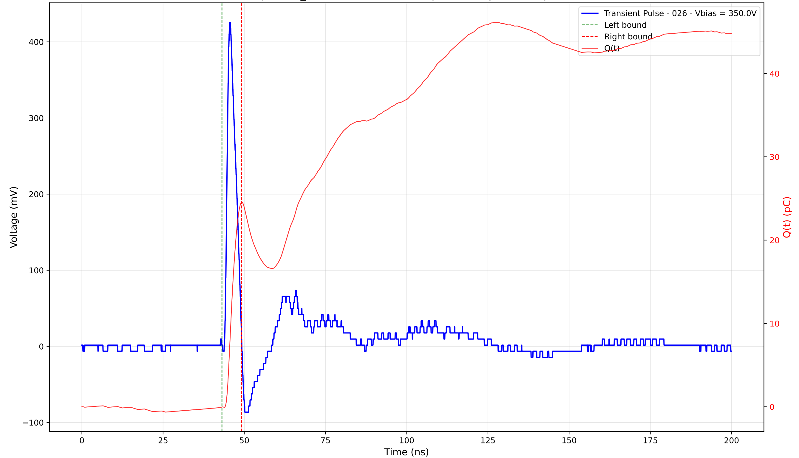
Transient Pulse - Sample: TD_4004 - Position: 400.0 \mu\text{m} - Charge: 24.57 pC - Rise Time: 1.04 ns
