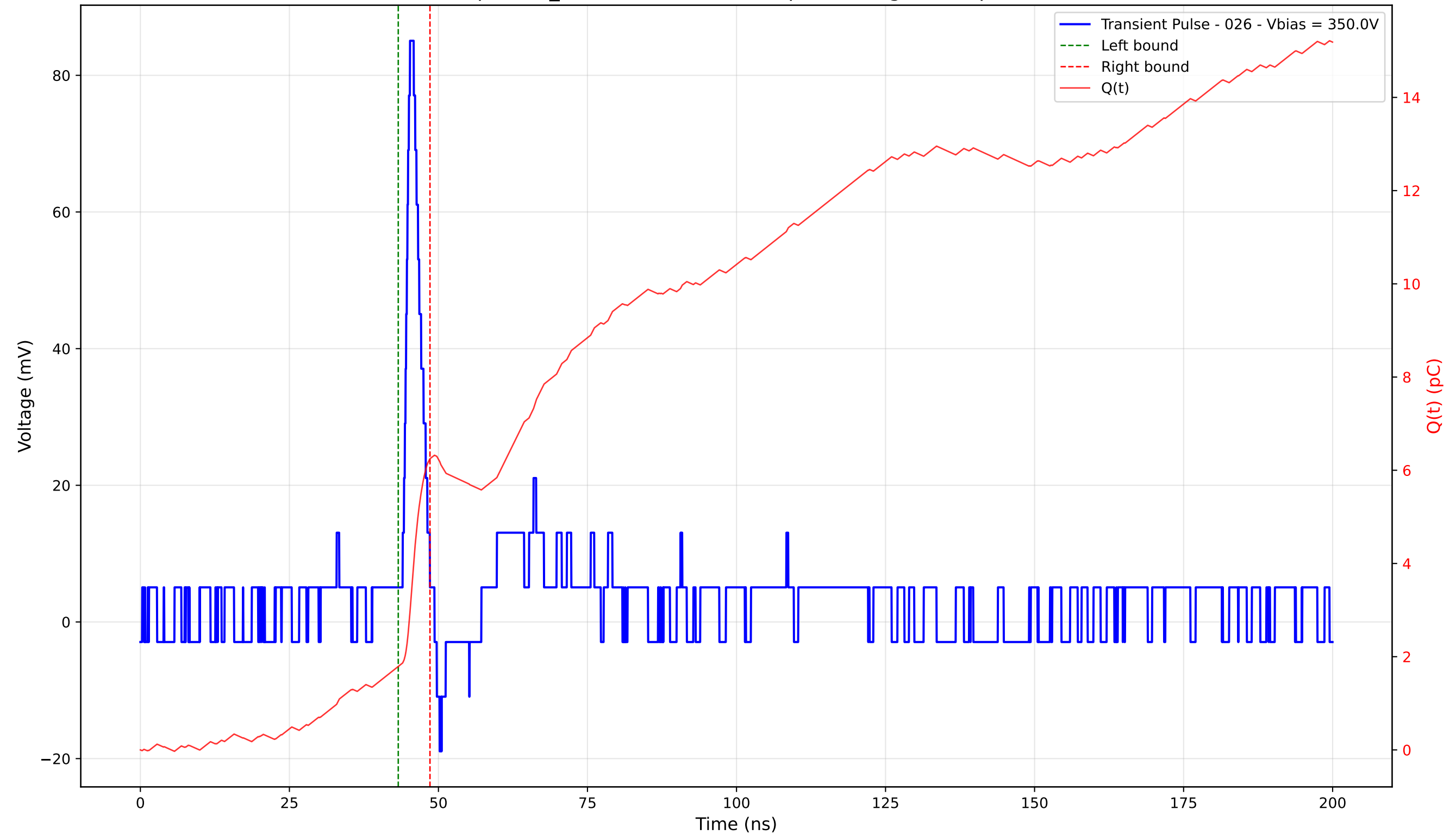
Transient Pulse - Sample: TD_4004 - Position: 430.0 \mu\text{m} - Charge: 4.46 pC - Rise Time: 1.05 ns
