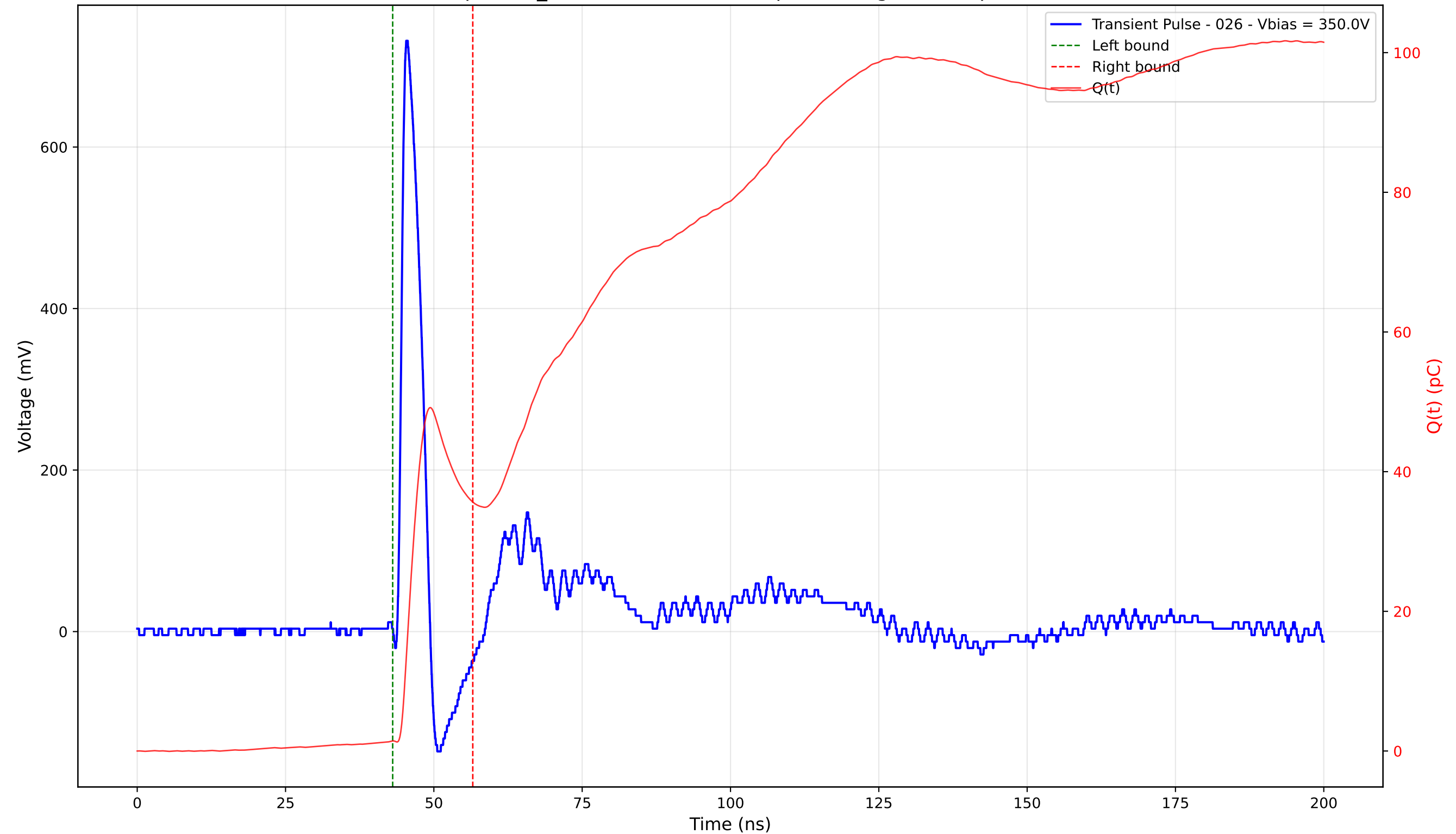
Transient Pulse - Sample: TD_4004 - Position: 345.0 \mu\text{m} - Charge: 34.20 pC - Rise Time: 0.96 ns
