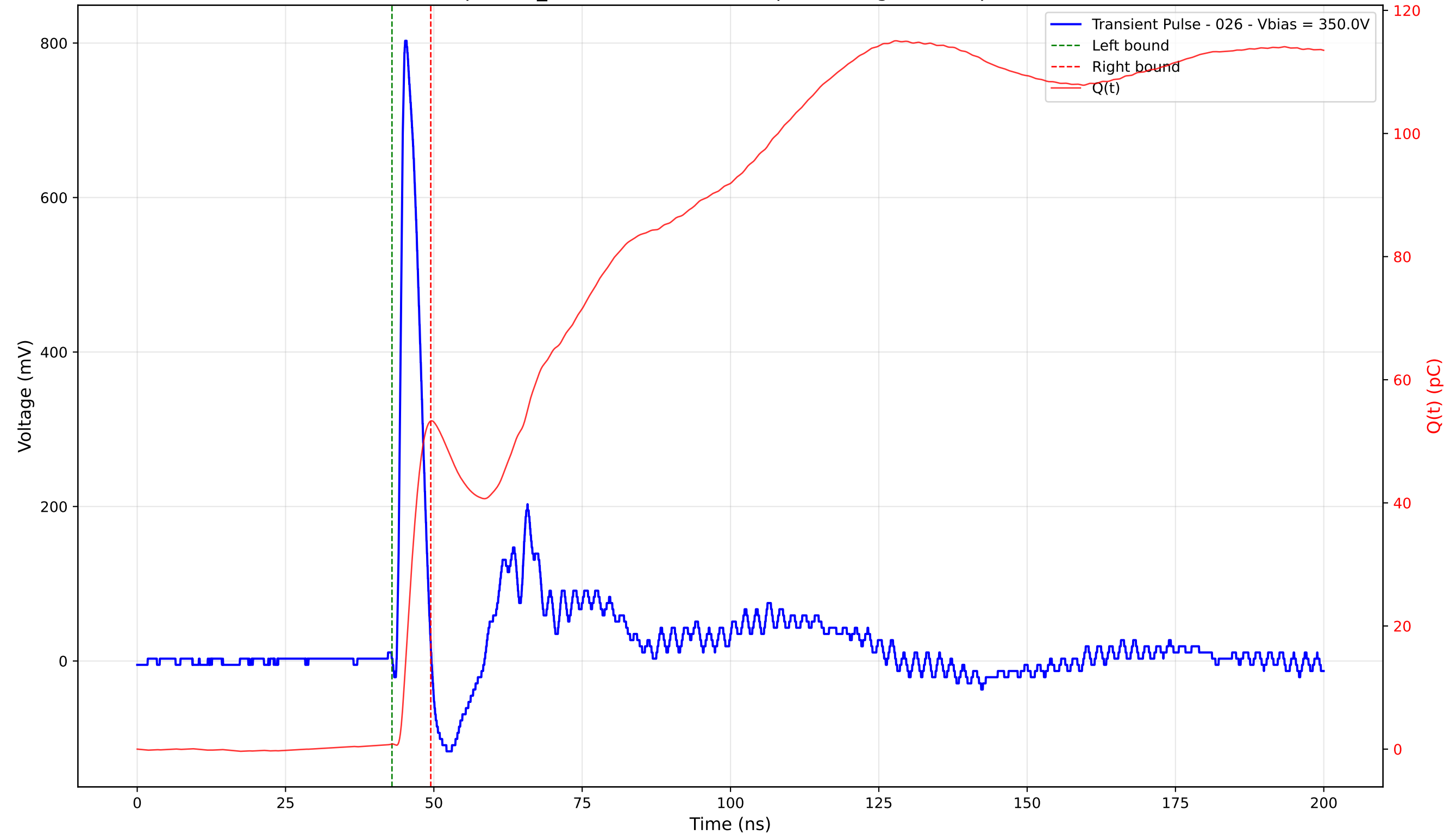
Transient Pulse - Sample: TD_4004 - Position: 130.0 \mu\text{m} - Charge: 52.48 pC - Rise Time: 0.89 ns
