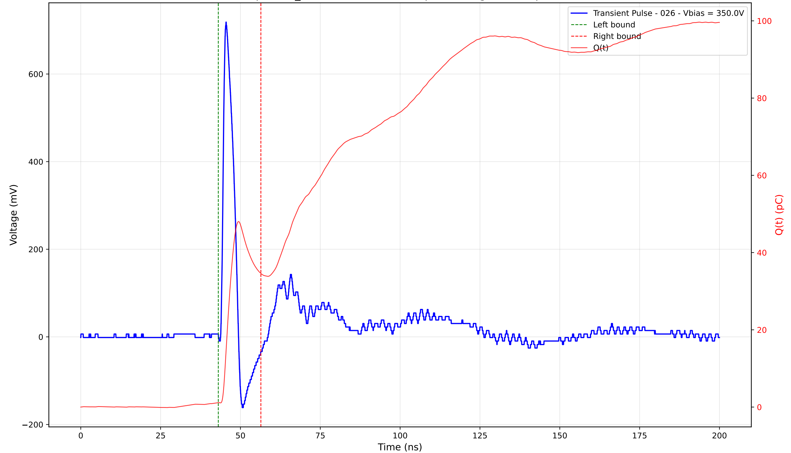
Transient Pulse - Sample: TD_4004 - Position: 370.0 \mu\text{m} - Charge: 33.43 pC - Rise Time: 1.00 ns
