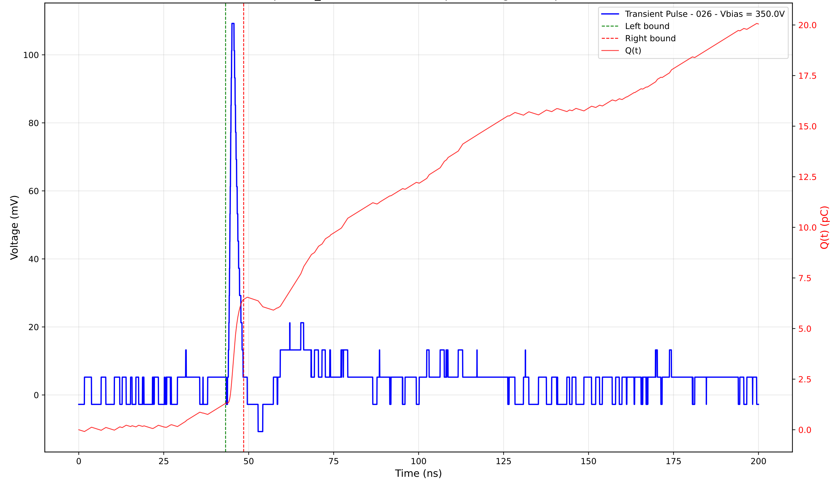
Transient Pulse - Sample: TD_4004 - Position: 45.0 \mu\text{m} - Charge: 5.13 pC - Rise Time: 0.95 ns
