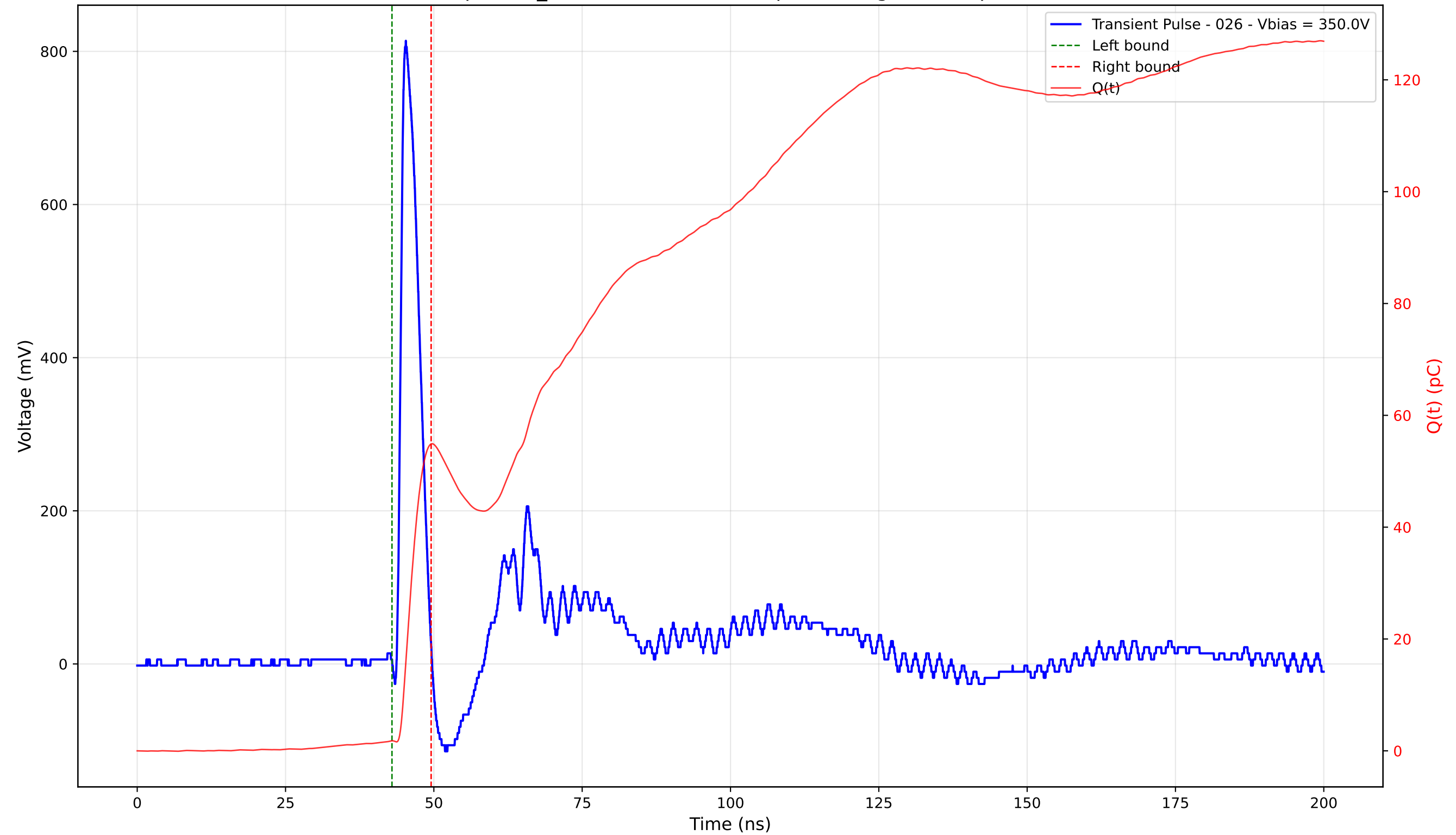
Transient Pulse - Sample: TD_4004 - Position: 165.0 \mu\text{m} - Charge: 53.08 pC - Rise Time: 0.89 ns
