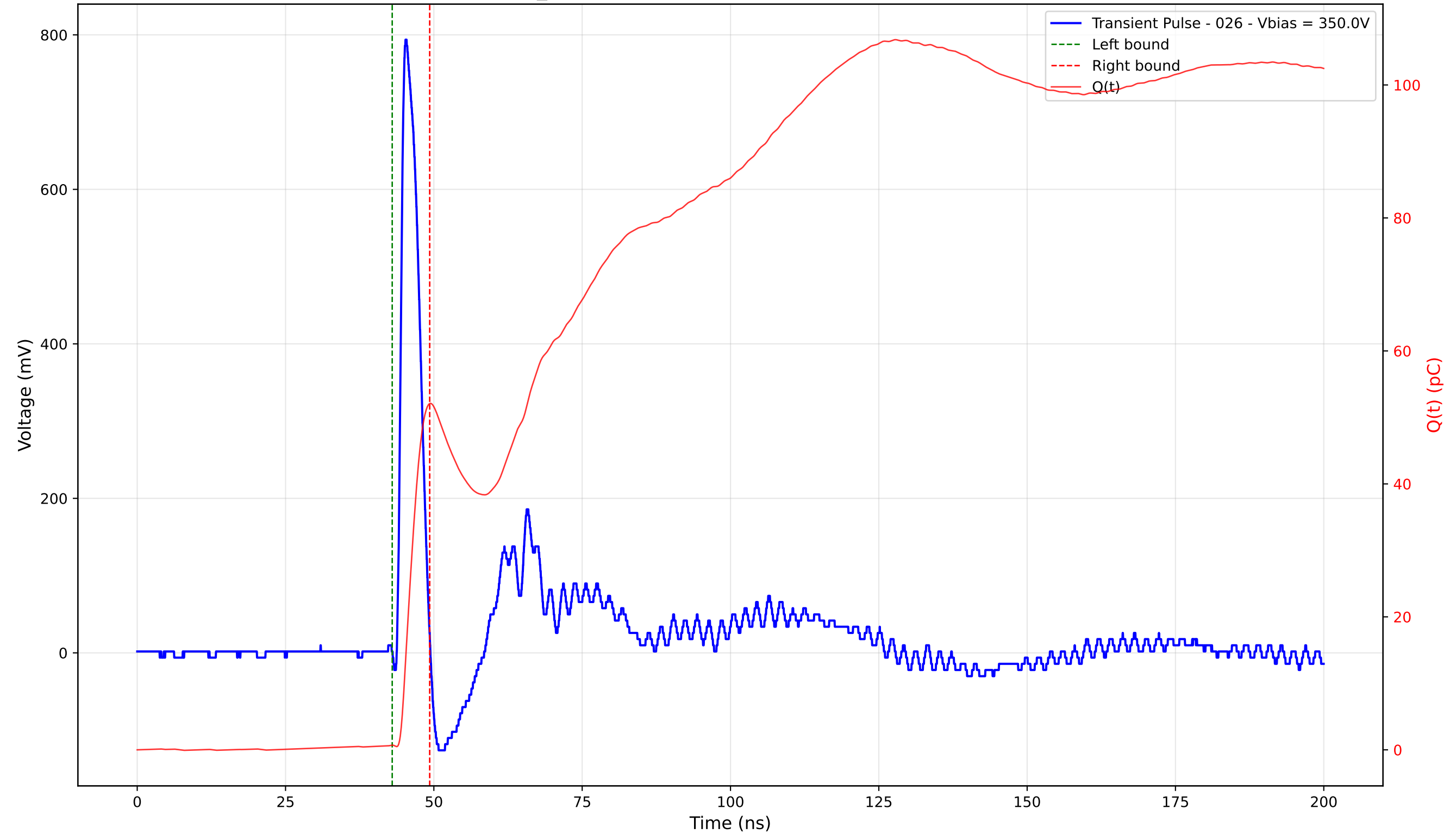
Transient Pulse - Sample: TD_4004 - Position: 275.0 \mu\text{m} - Charge: 51.38 pC - Rise Time: 0.91 ns
