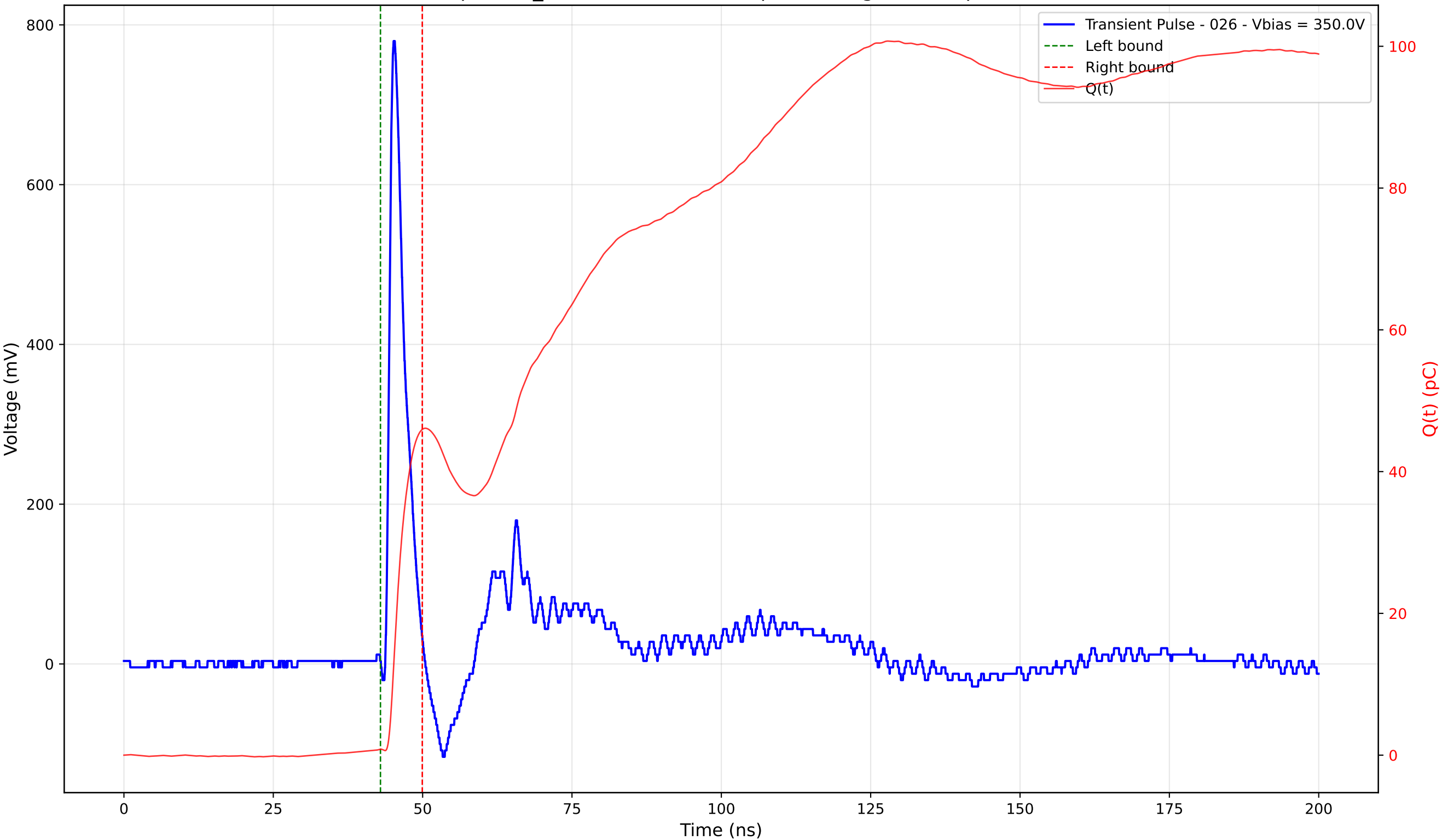
Transient Pulse - Sample: TD_4004 - Position: 90.0 \mu\text{m} - Charge: 45.12 pC - Rise Time: 0.88 ns
