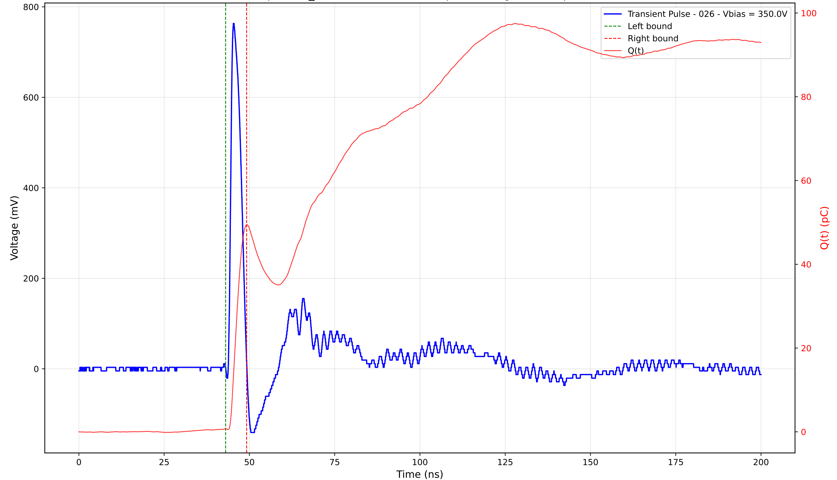
Transient Pulse - Sample: TD_4004 - Position: 315.0 \mu\text{m} - Charge: 48.73 pC - Rise Time: 0.93 ns
