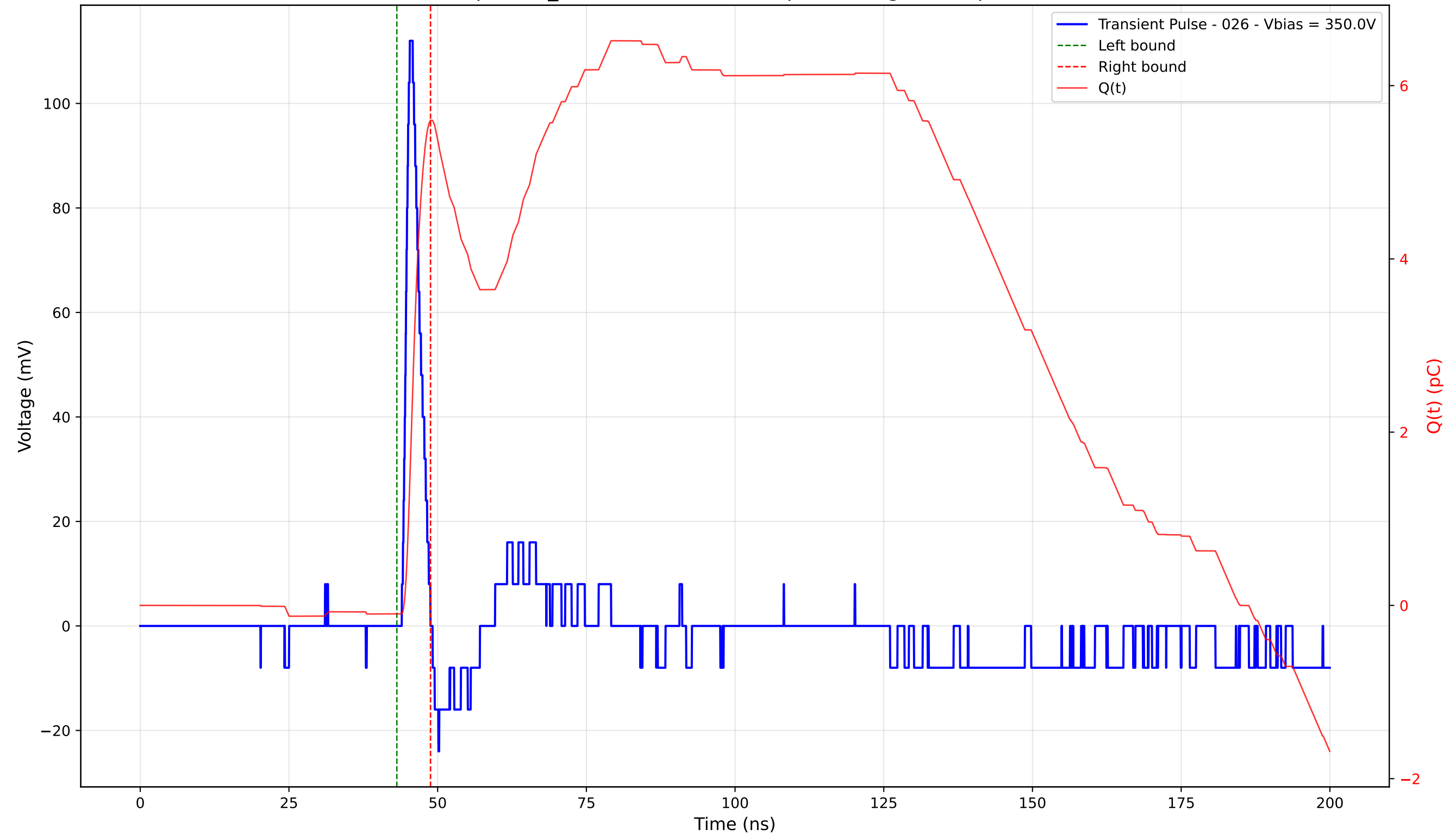
Transient Pulse - Sample: TD_4004 - Position: 420.0 \mu\text{m} - Charge: 5.70 pC - Rise Time: 0.99 ns
