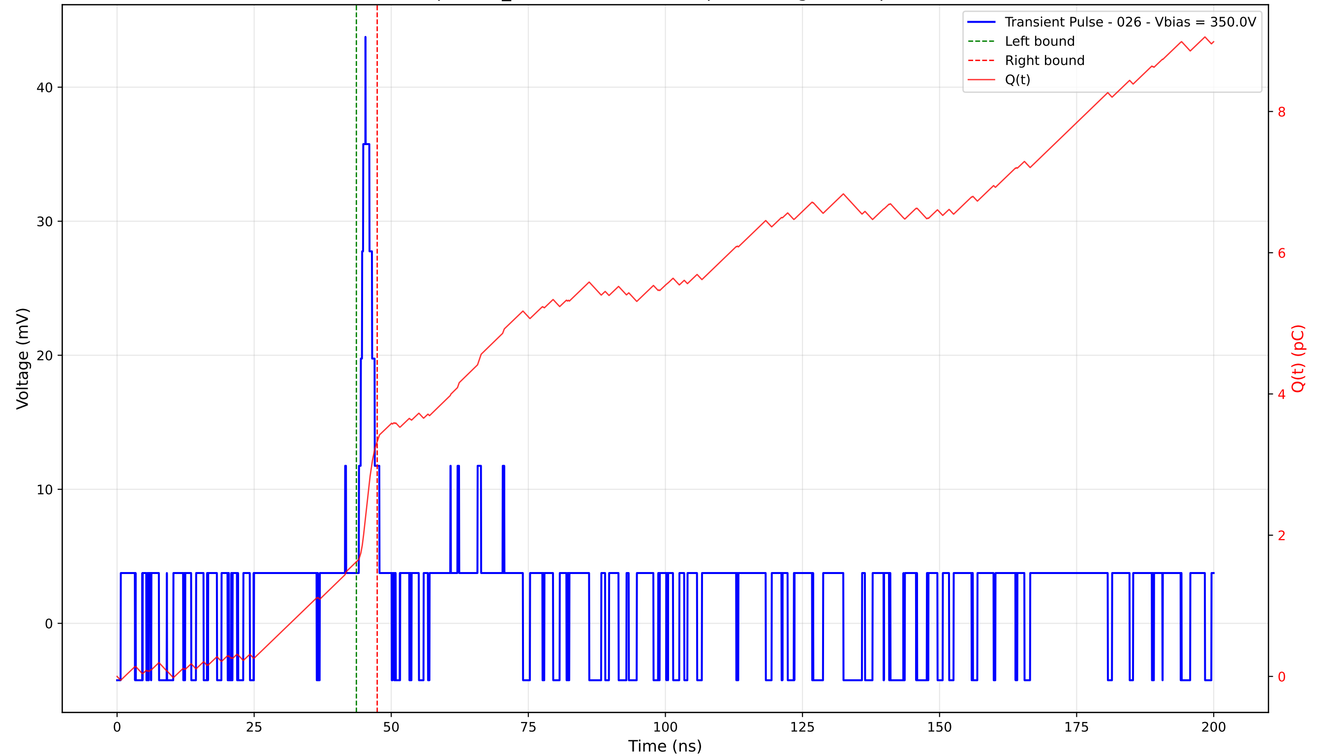
Transient Pulse - Sample: TD_4004 - Position: 30.0 \mu\text{m} - Charge: 1.70 pC - Rise Time: 1.22 ns
