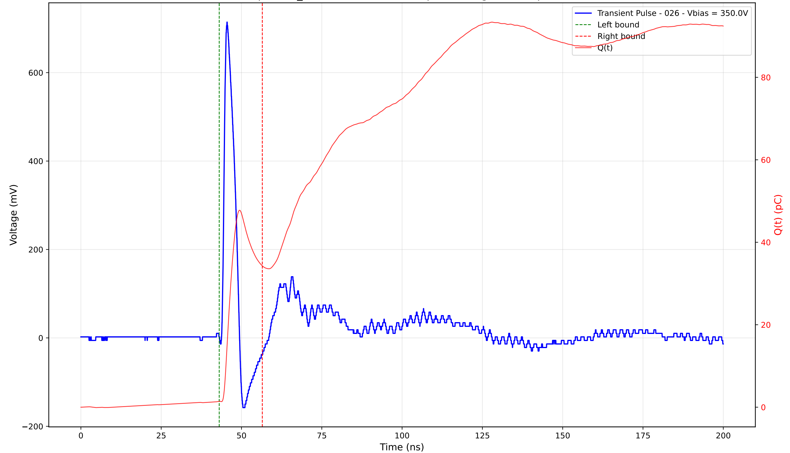
Transient Pulse - Sample: TD_4004 - Position: 375.0 \mu\text{m} - Charge: 32.83 pC - Rise Time: 1.01 ns
