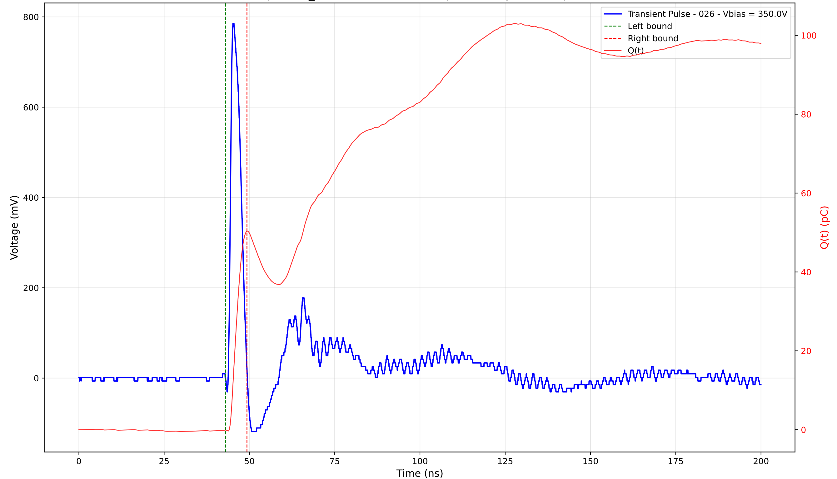
Transient Pulse - Sample: TD_4004 - Position: 250.0 \mu\text{m} - Charge: 50.42 pC - Rise Time: 0.89 ns
