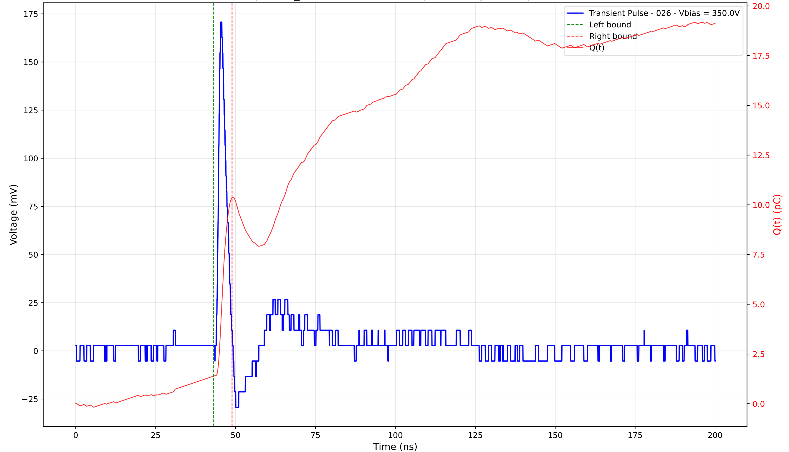
Transient Pulse - Sample: TD_4004 - Position: 415.0 \mu\text{m} - Charge: 8.97 pC - Rise Time: 1.04 ns
