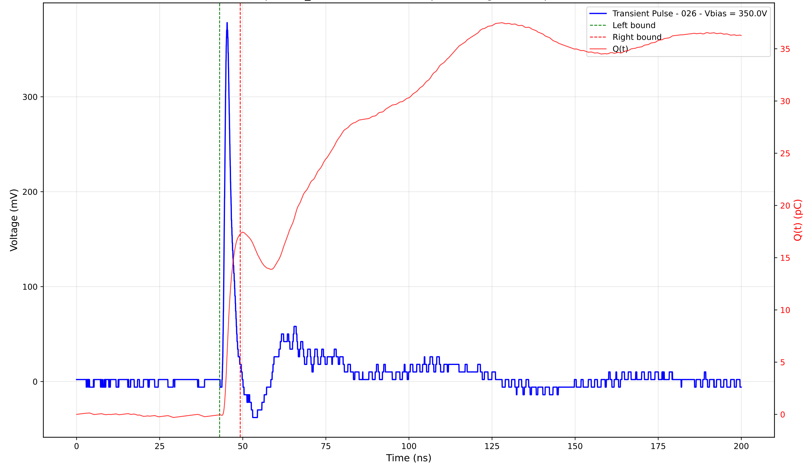
Transient Pulse - Sample: TD_4004 - Position: 60.0 \mu\text{m} - Charge: 17.30 pC - Rise Time: 0.95 ns
