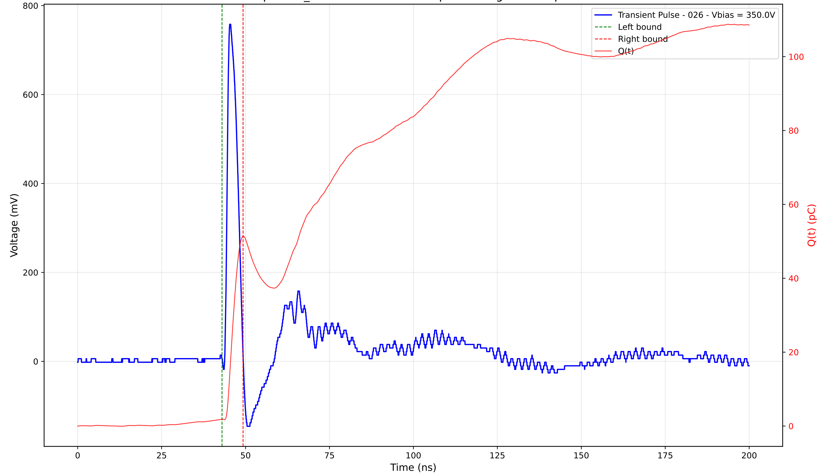
Transient Pulse - Sample: TD_4004 - Position: 325.0 \mu\text{m} - Charge: 49.55 pC - Rise Time: 0.94 ns
