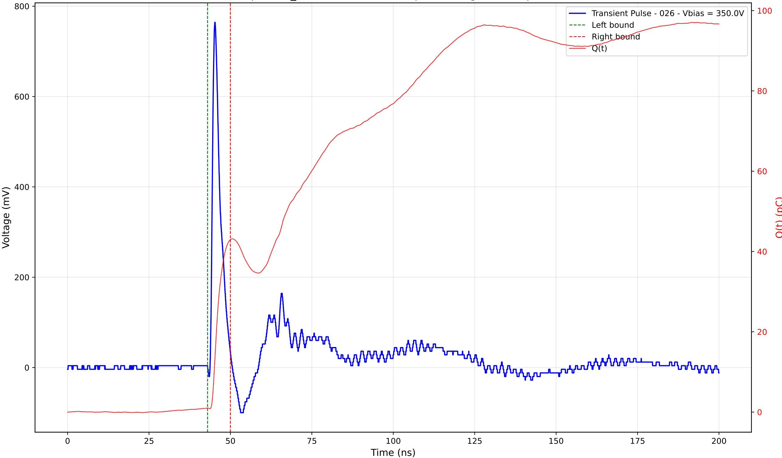
Transient Pulse - Sample: TD_4004 - Position: 85.0 \mu\text{m} - Charge: 41.95 pC - Rise Time: 0.91 ns
