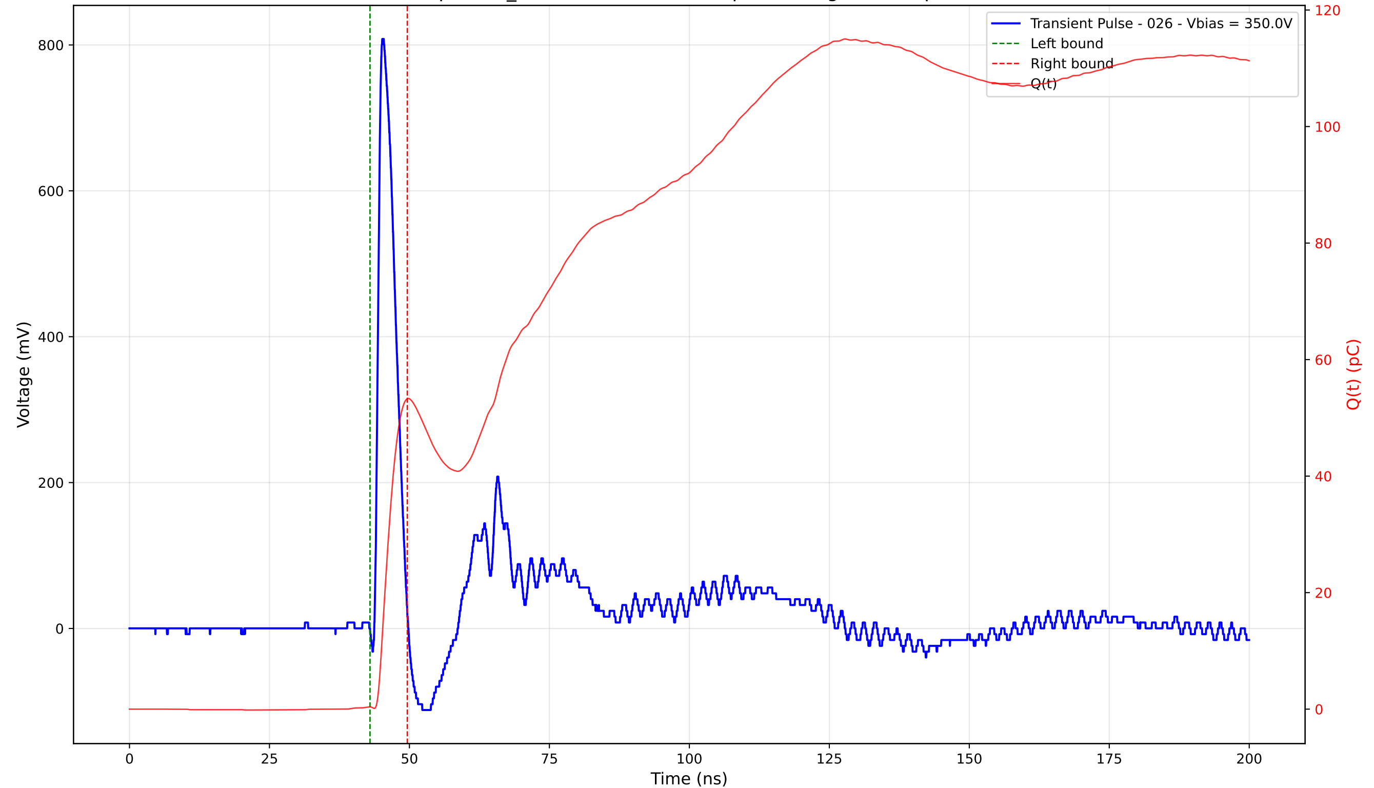
Transient Pulse - Sample: TD_4004 - Position: 205.0 \mu\text{m} - Charge: 52.88 pC - Rise Time: 0.88 ns
