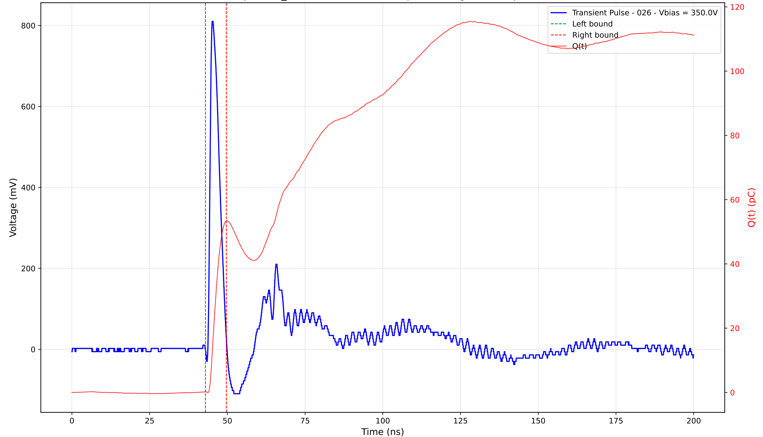
Transient Pulse - Sample: TD_4004 - Position: 200.0 \mu\text{m} - Charge: 53.19 pC - Rise Time: 0.88 ns
