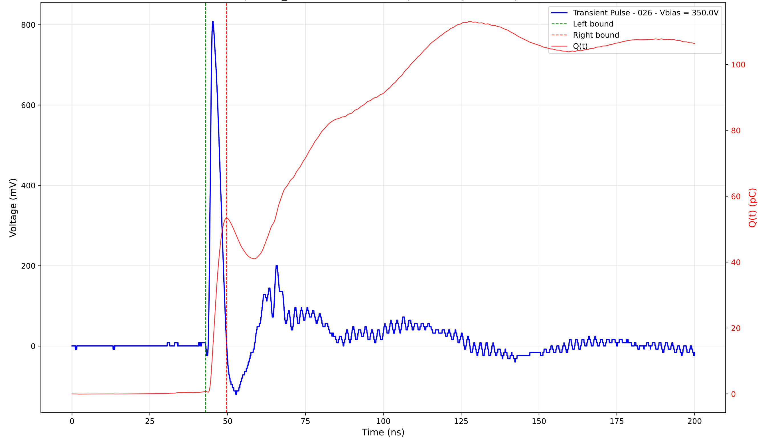
Transient Pulse - Sample: TD_4004 - Position: 125.0 \mu\text{m} - Charge: 52.61 pC - Rise Time: 0.90 ns
