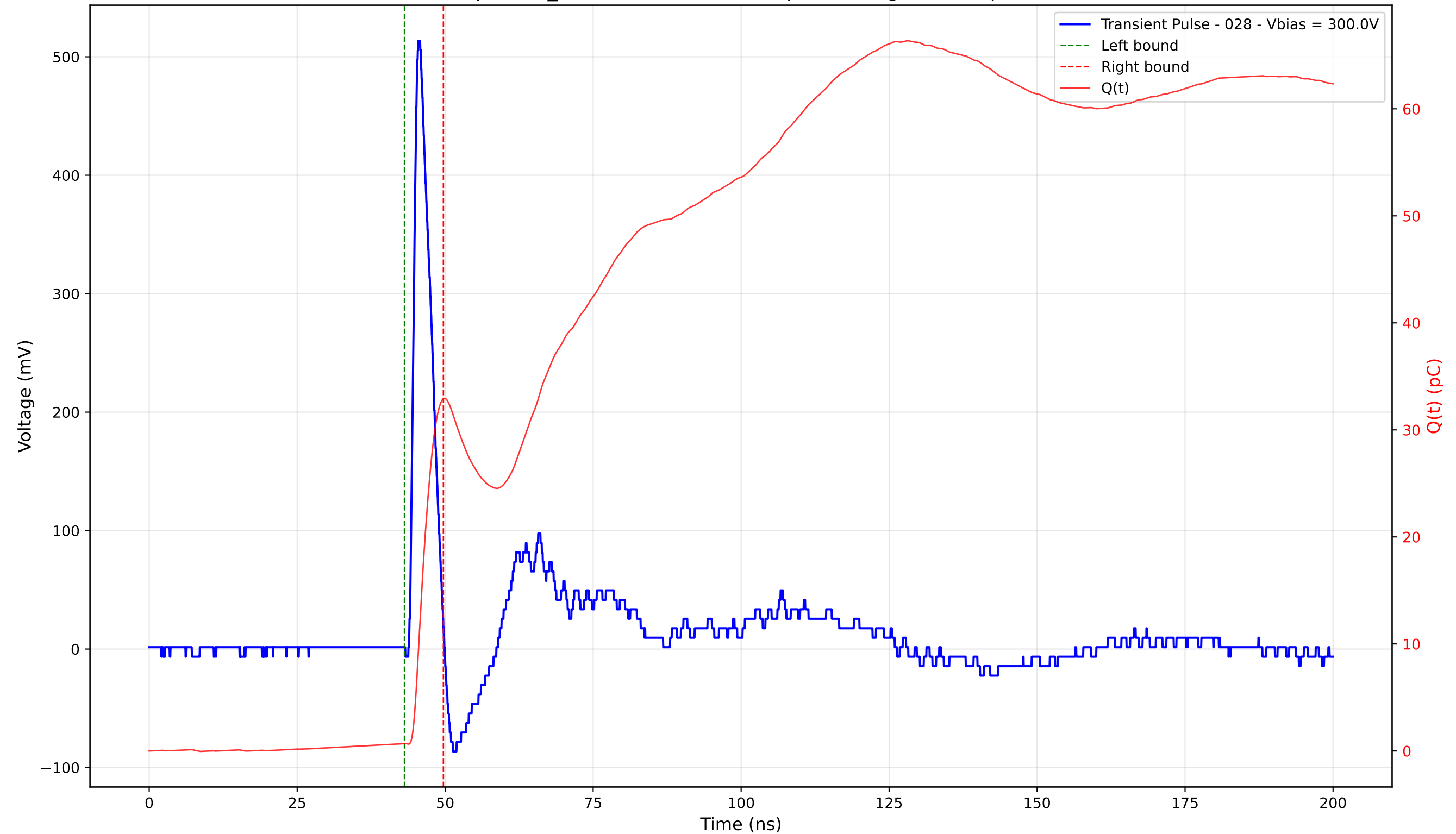
Transient Pulse - Sample: TD_4004 - Position: 390.0 \mu\text{m} - Charge: 32.22 pC - Rise Time: 1.03 ns
