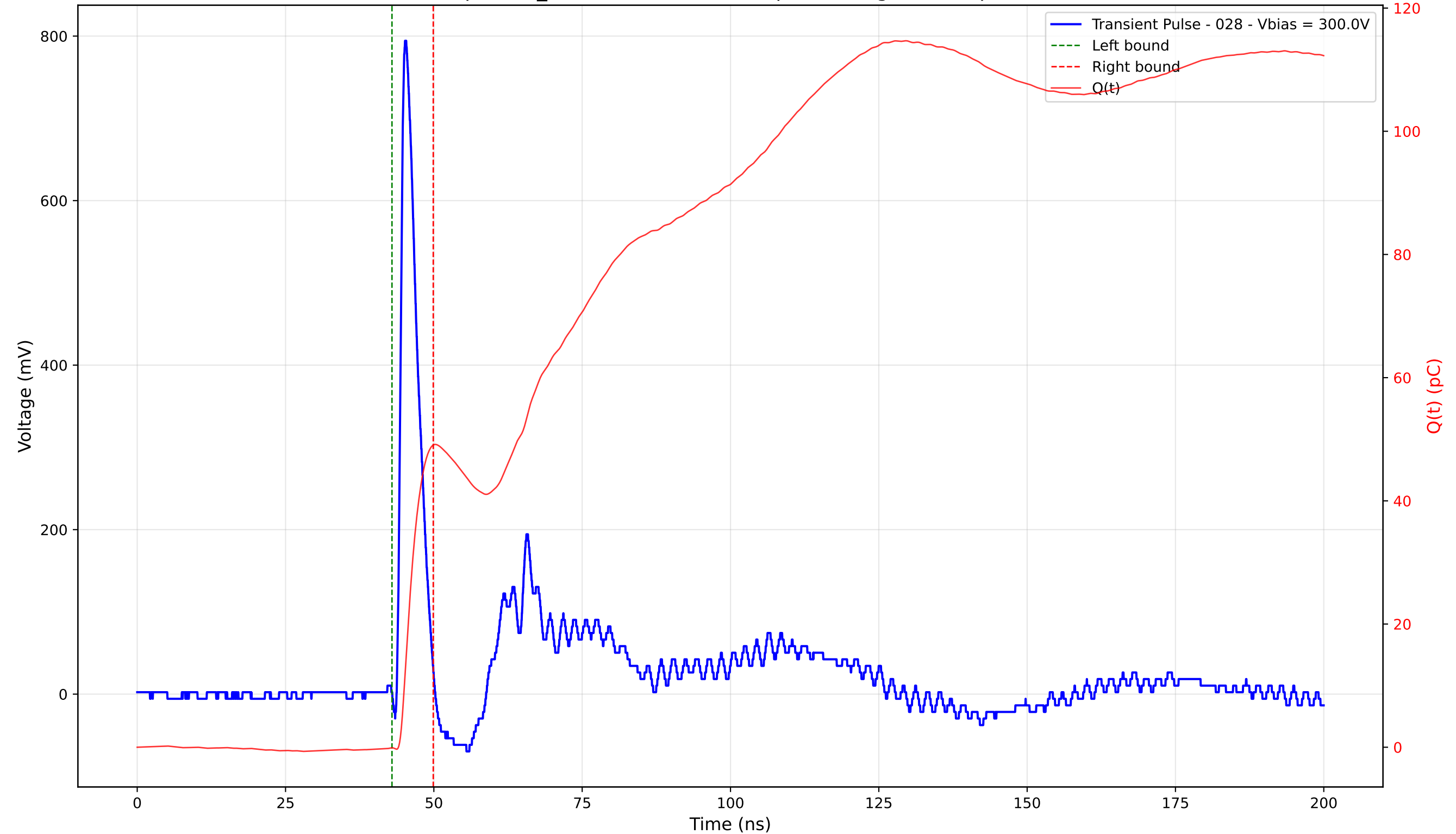
Transient Pulse - Sample: TD_4004 - Position: 105.0 \mu\text{m} - Charge: 49.16 pC - Rise Time: 0.88 ns
