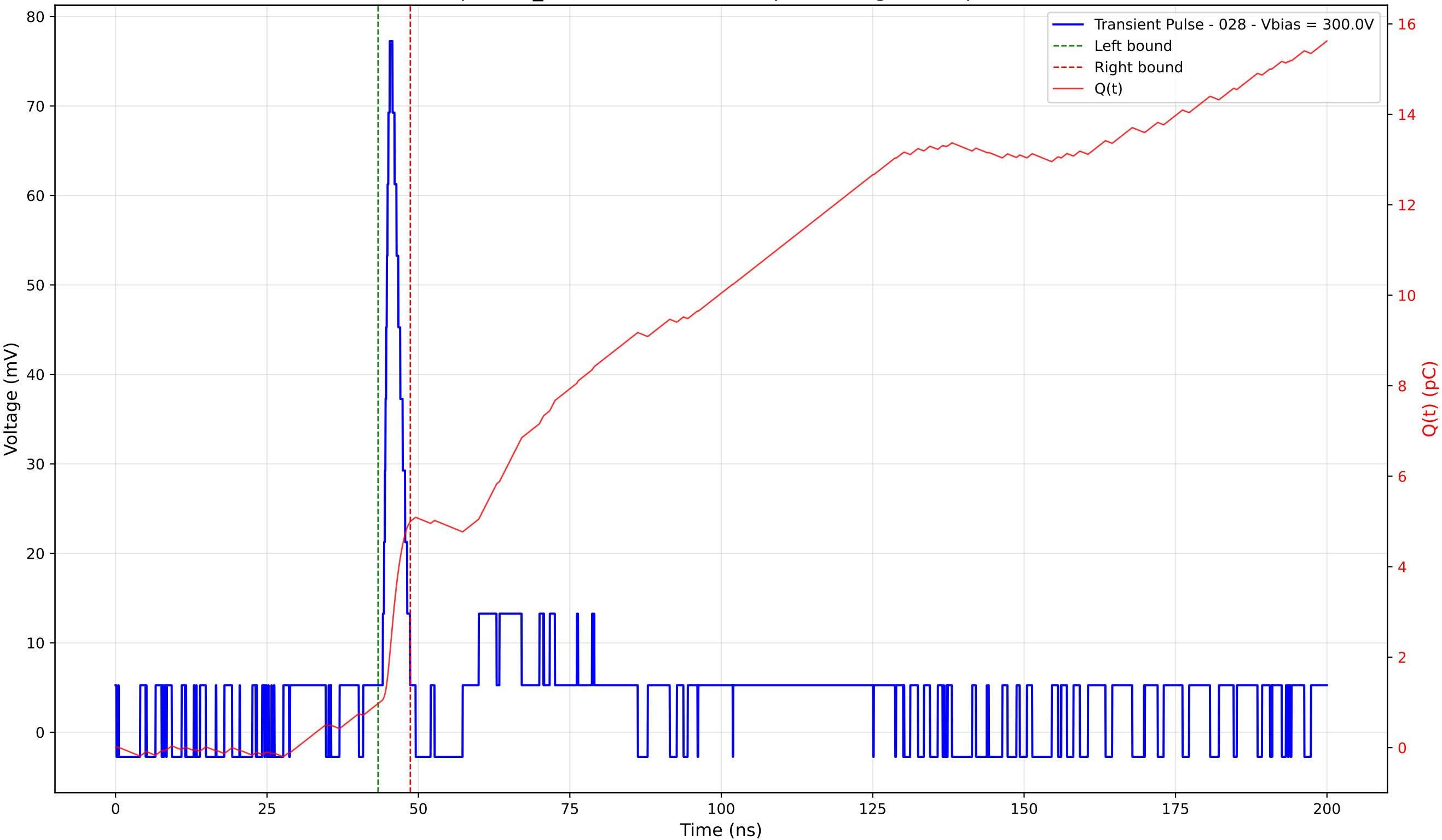
Transient Pulse - Sample: TD_4004 - Position: 430.0 \mu\text{m} - Charge: 4.03 pC - Rise Time: 1.15 ns
