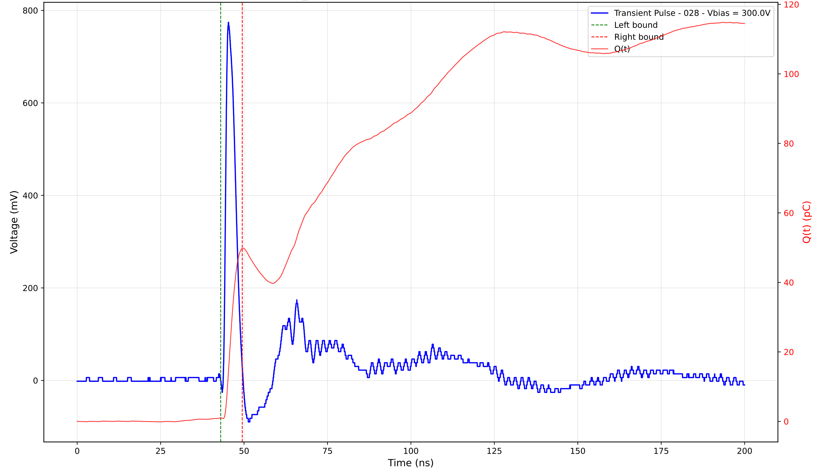
Transient Pulse - Sample: TD_4004 - Position: 245.0 \mu\text{m} - Charge: 48.77 pC - Rise Time: 0.94 ns
