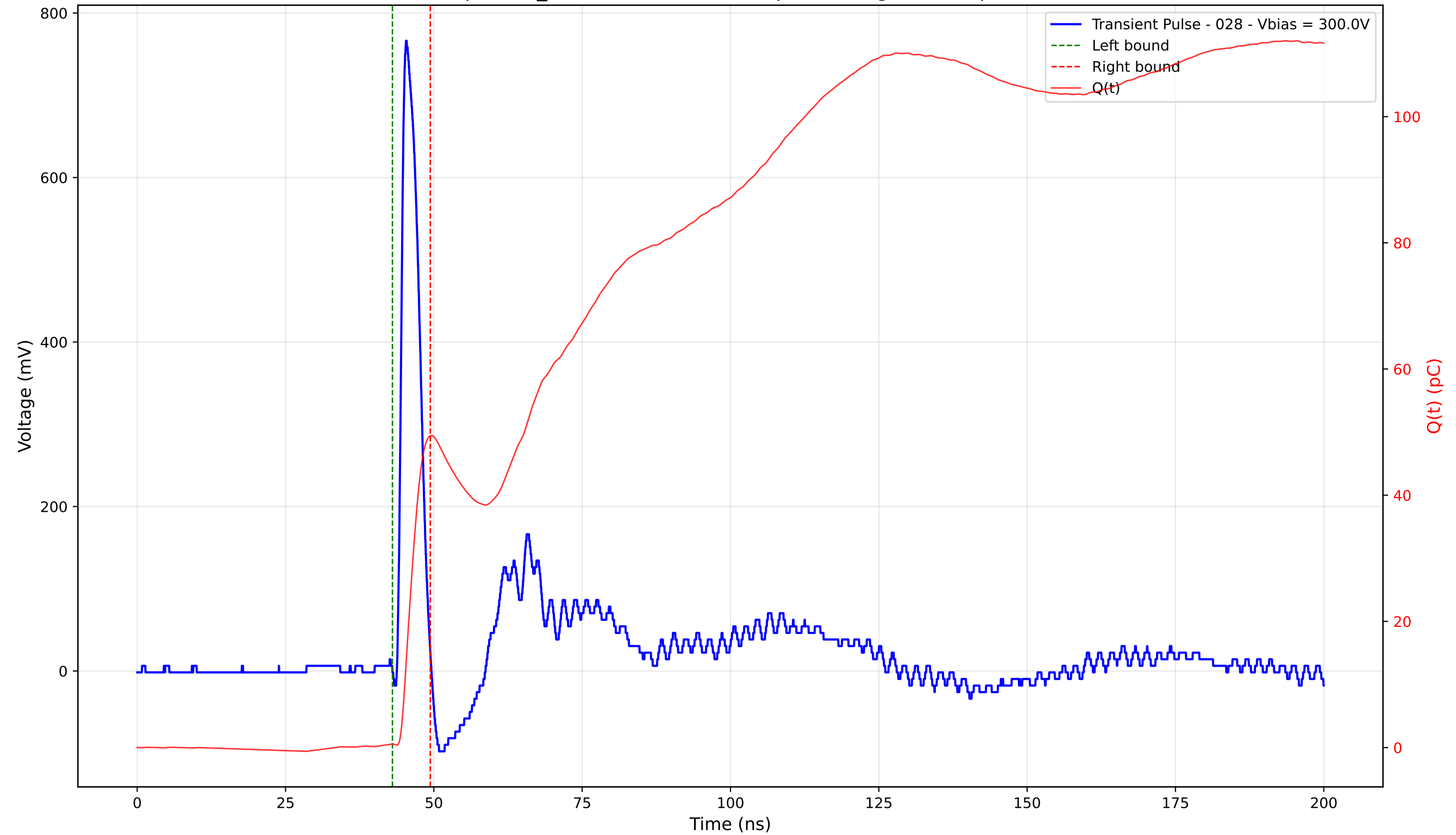
Transient Pulse - Sample: TD_4004 - Position: 295.0 \mu\text{m} - Charge: 48.87 pC - Rise Time: 0.94 ns
