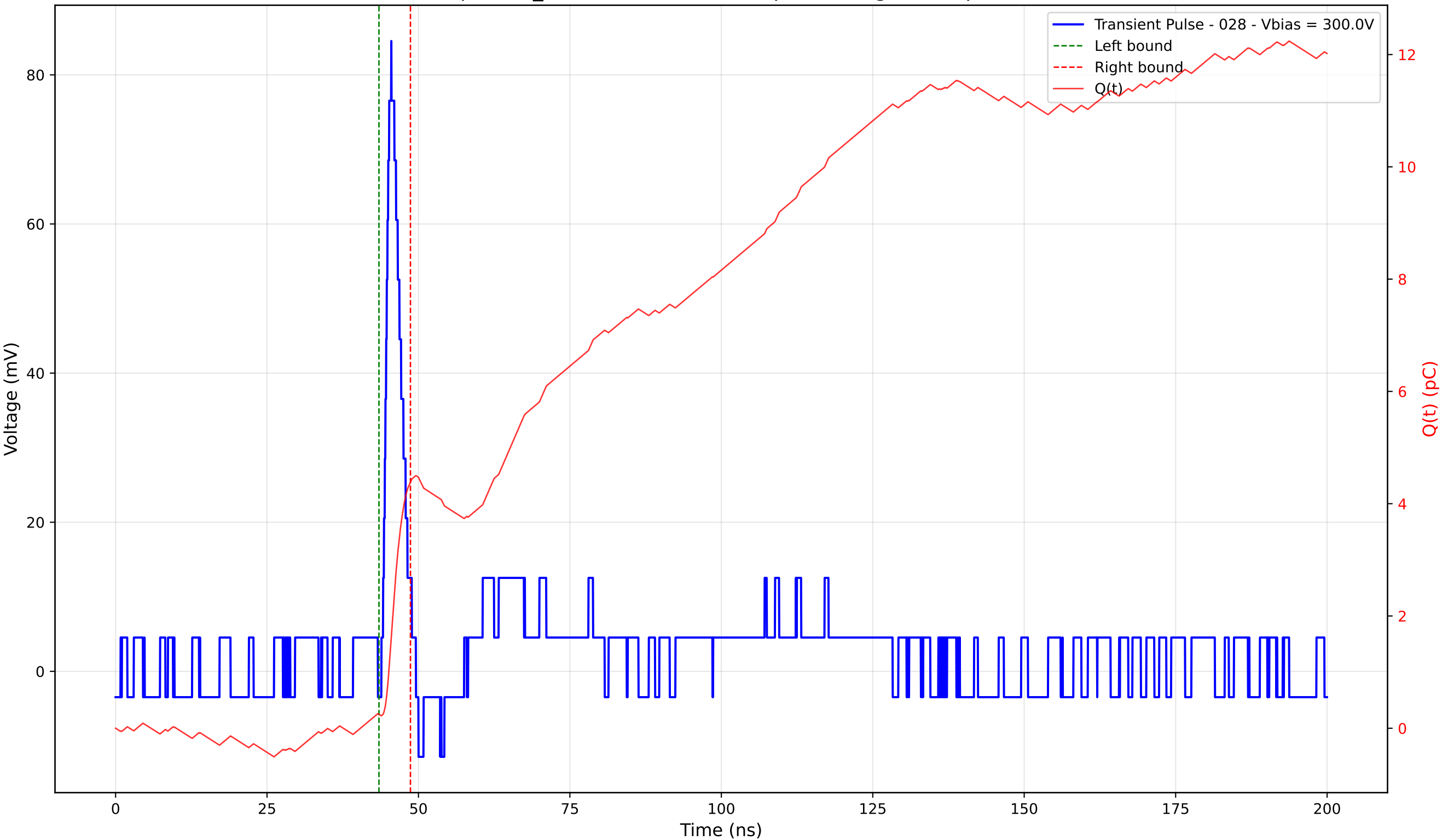
Transient Pulse - Sample: TD_4004 - Position: 425.0 \mu\text{m} - Charge: 4.14 pC - Rise Time: 1.01 ns
