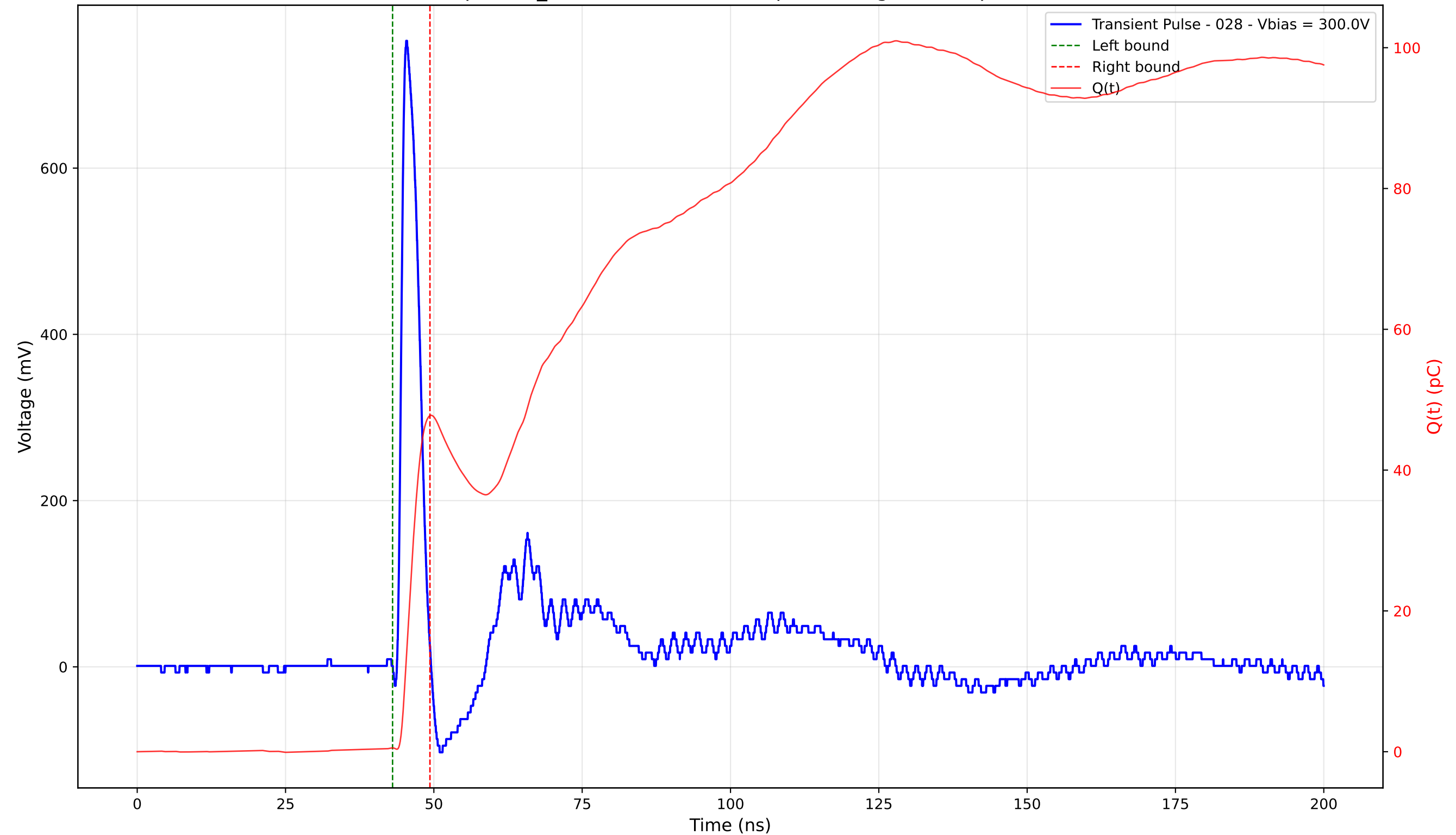
Transient Pulse - Sample: TD_4004 - Position: 305.0 \mu\text{m} - Charge: 47.19 pC - Rise Time: 0.95 ns
