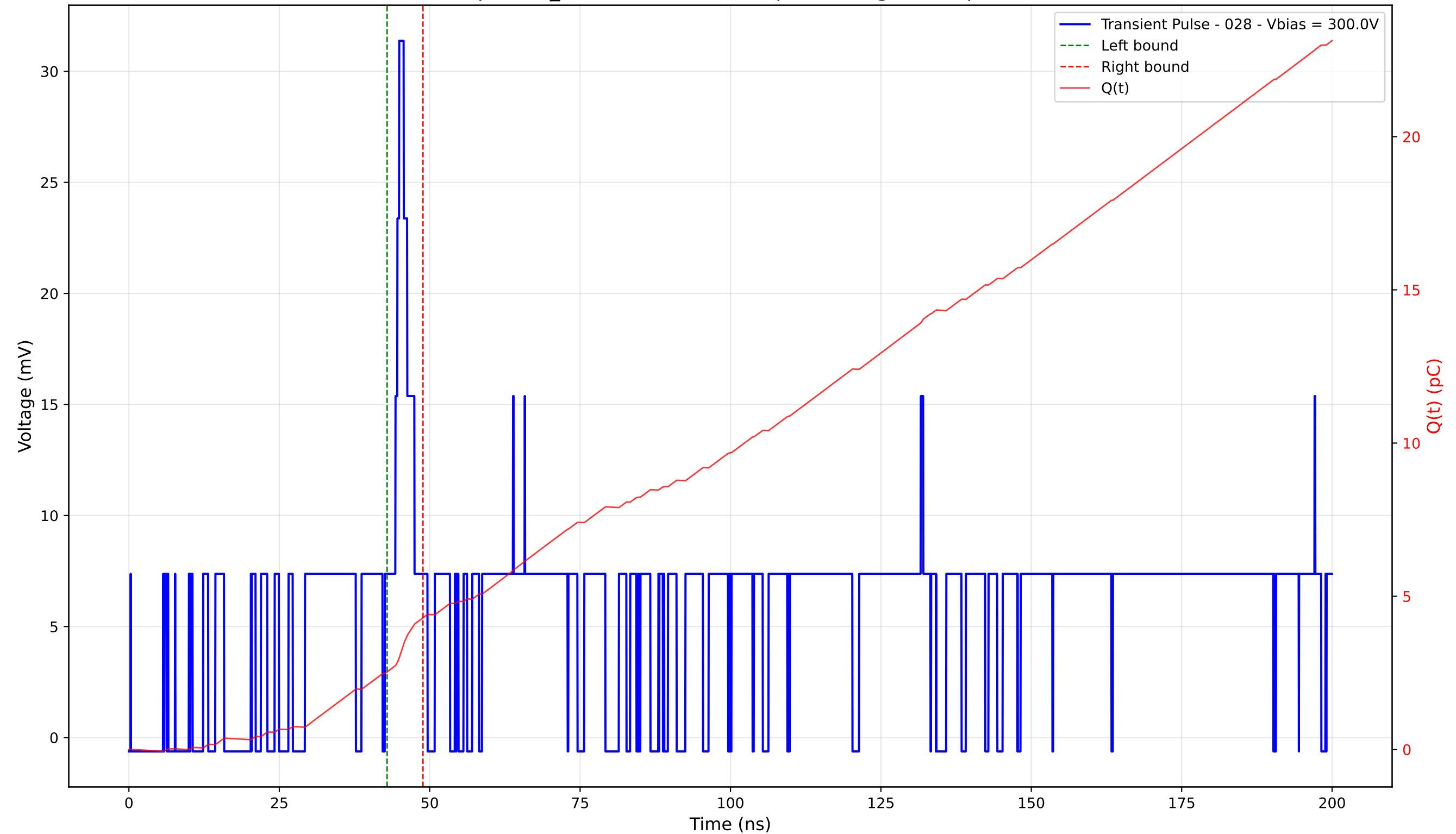
Transient Pulse - Sample: TD_4004 - Position: 25.0 \mu\text{m} - Charge: 1.77 pC - Rise Time: 2.39 ns
