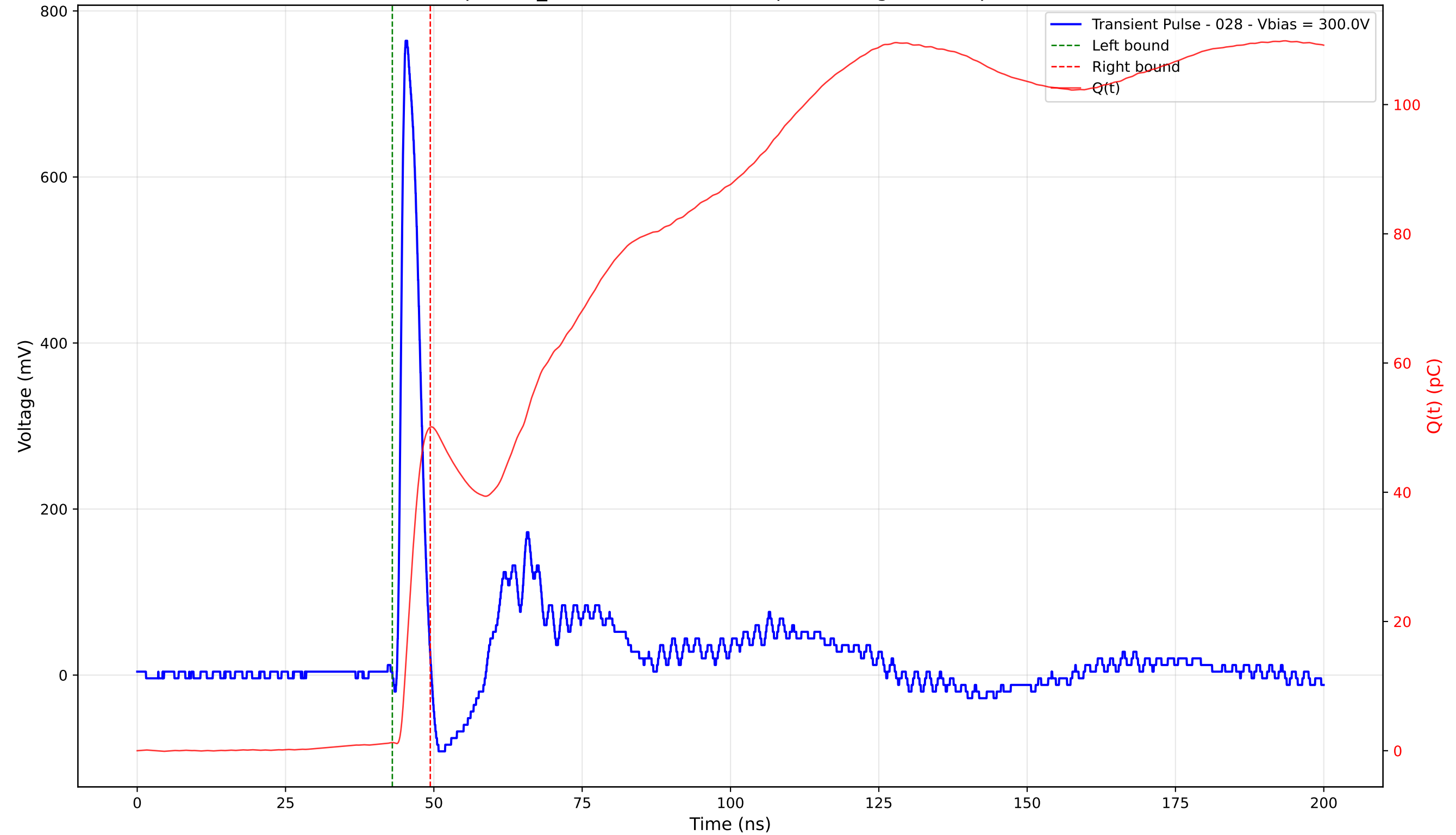
Transient Pulse - Sample: TD_4004 - Position: 265.0 \mu\text{m} - Charge: 48.81 pC - Rise Time: 0.93 ns
