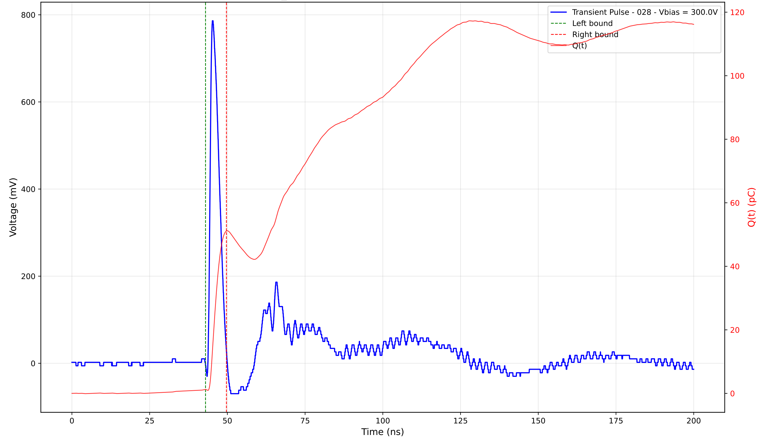
Transient Pulse - Sample: TD_4004 - Position: 125.0 \mu\text{m} - Charge: 49.91 pC - Rise Time: 0.89 ns
