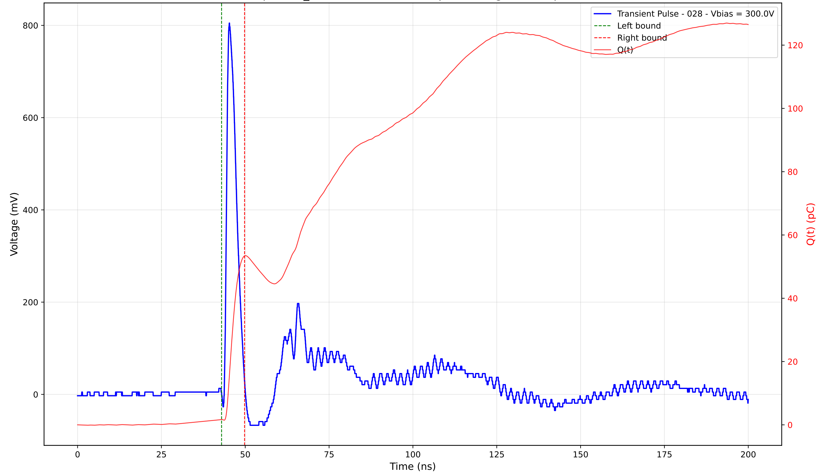
Transient Pulse - Sample: TD_4004 - Position: 175.0 \mu\text{m} - Charge: 51.70 pC - Rise Time: 0.91 ns
