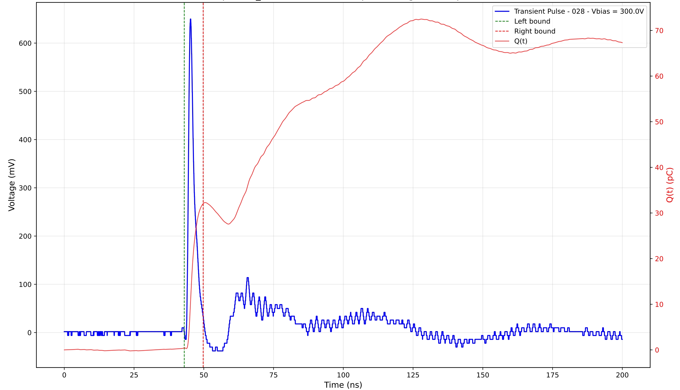
Transient Pulse - Sample: TD_4004 - Position: 75.0 \mu\text{m} - Charge: 31.63 pC - Rise Time: 0.88 ns
