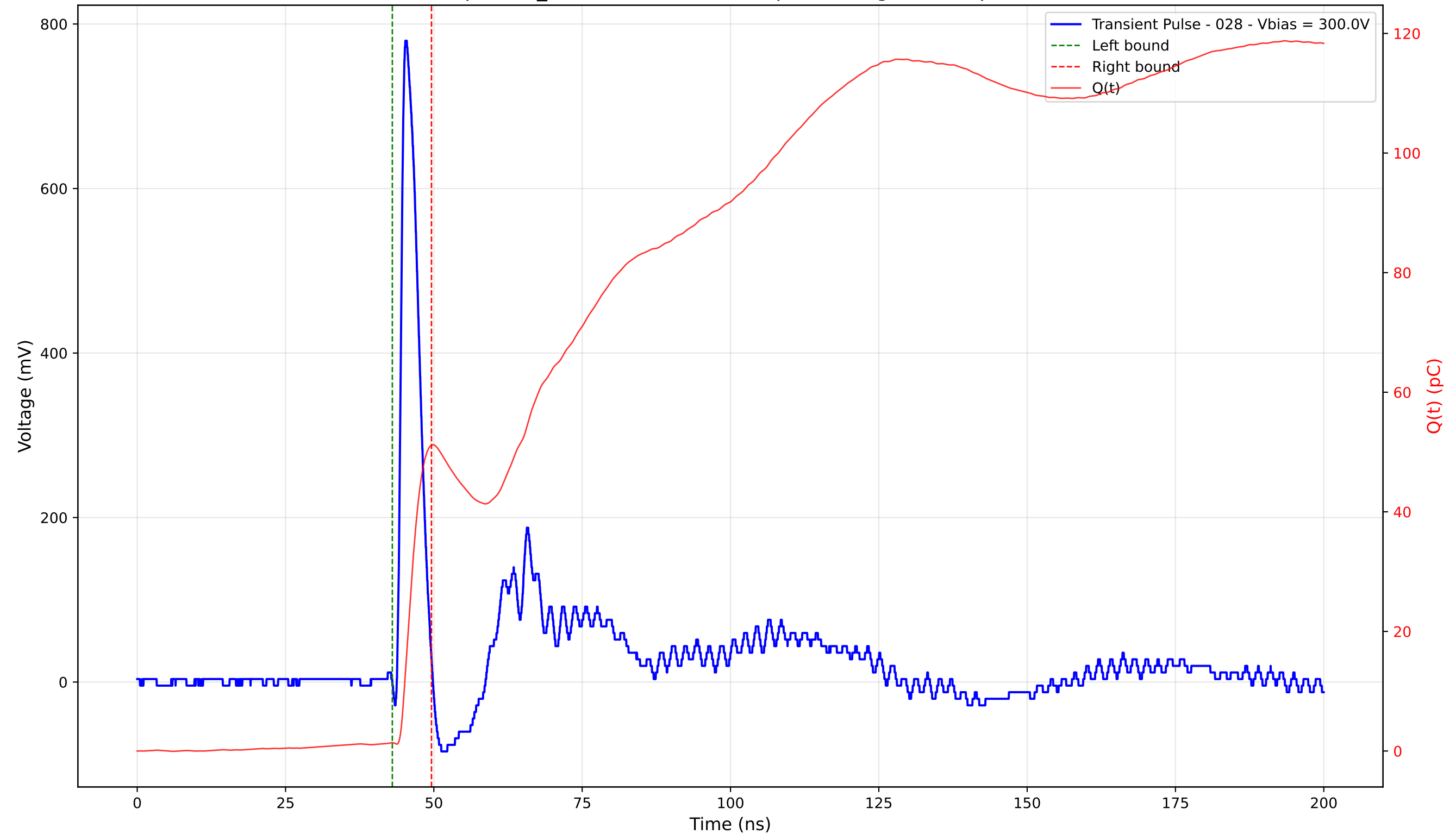
Transient Pulse - Sample: TD_4004 - Position: 135.0 \mu\text{m} - Charge: 49.76 pC - Rise Time: 0.90 ns
