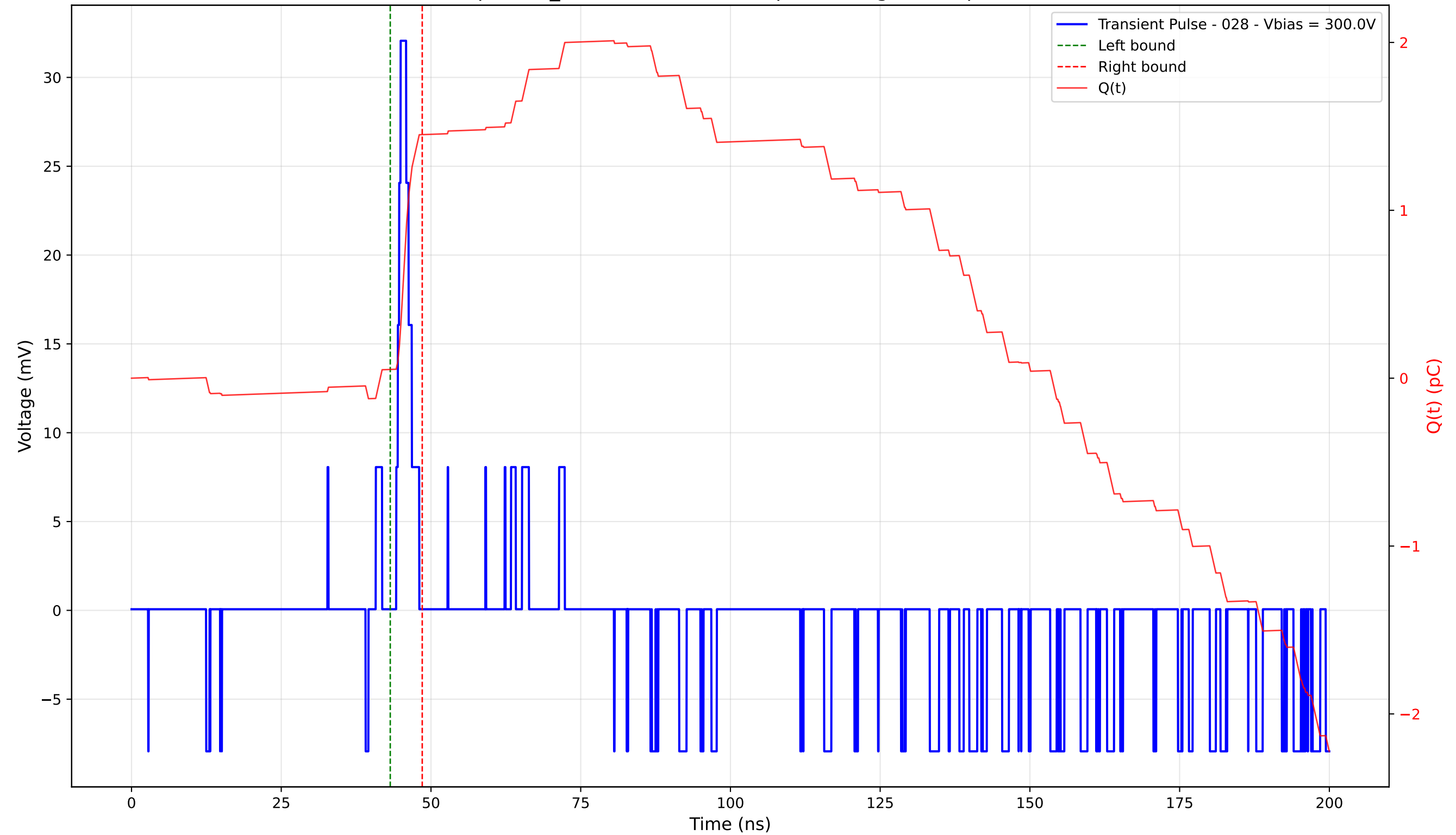
Transient Pulse - Sample: TD_4004 - Position: 30.0 \mu\text{m} - Charge: 1.40 pC - Rise Time: 0.73 ns
