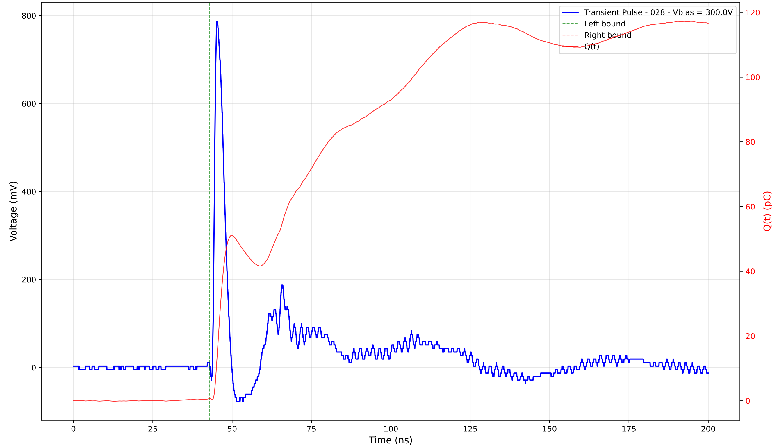
Transient Pulse - Sample: TD_4004 - Position: 165.0 \mu\text{m} - Charge: 50.42 pC - Rise Time: 0.89 ns
