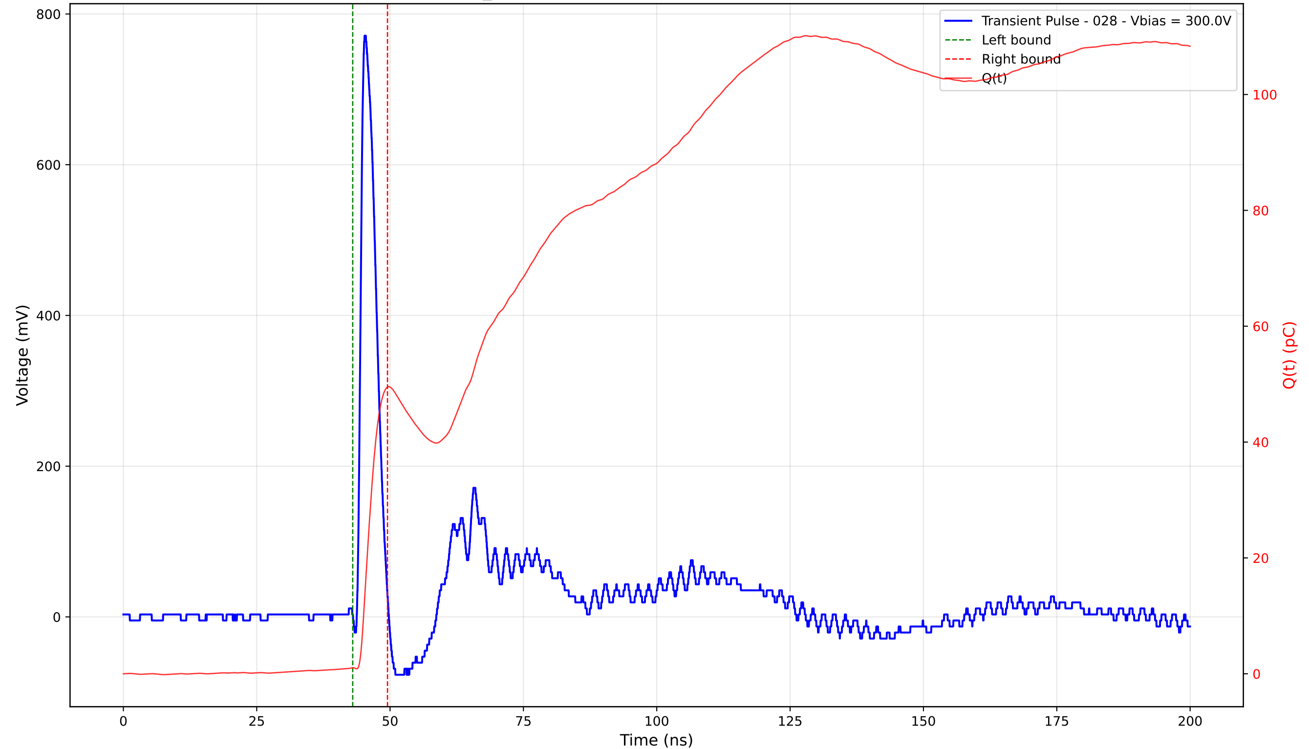
Transient Pulse - Sample: TD_4004 - Position: 235.0 \mu\text{m} - Charge: 48.44 pC - Rise Time: 0.90 ns
