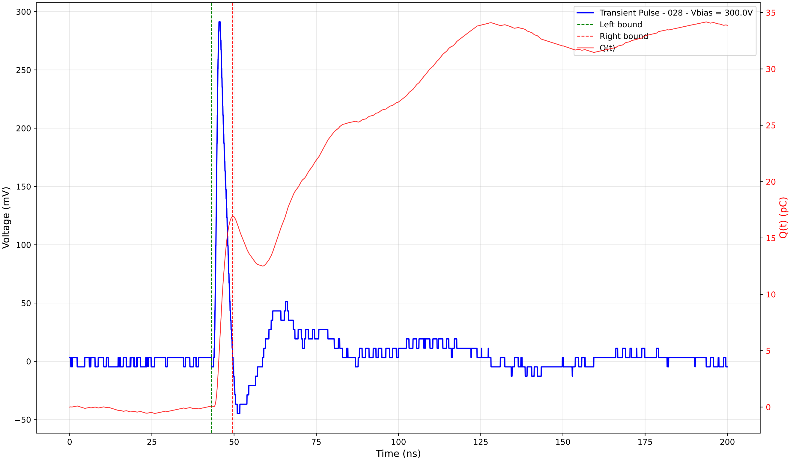
Transient Pulse - Sample: TD_4004 - Position: 405.0 \mu\text{m} - Charge: 16.81 pC - Rise Time: 1.04 ns
