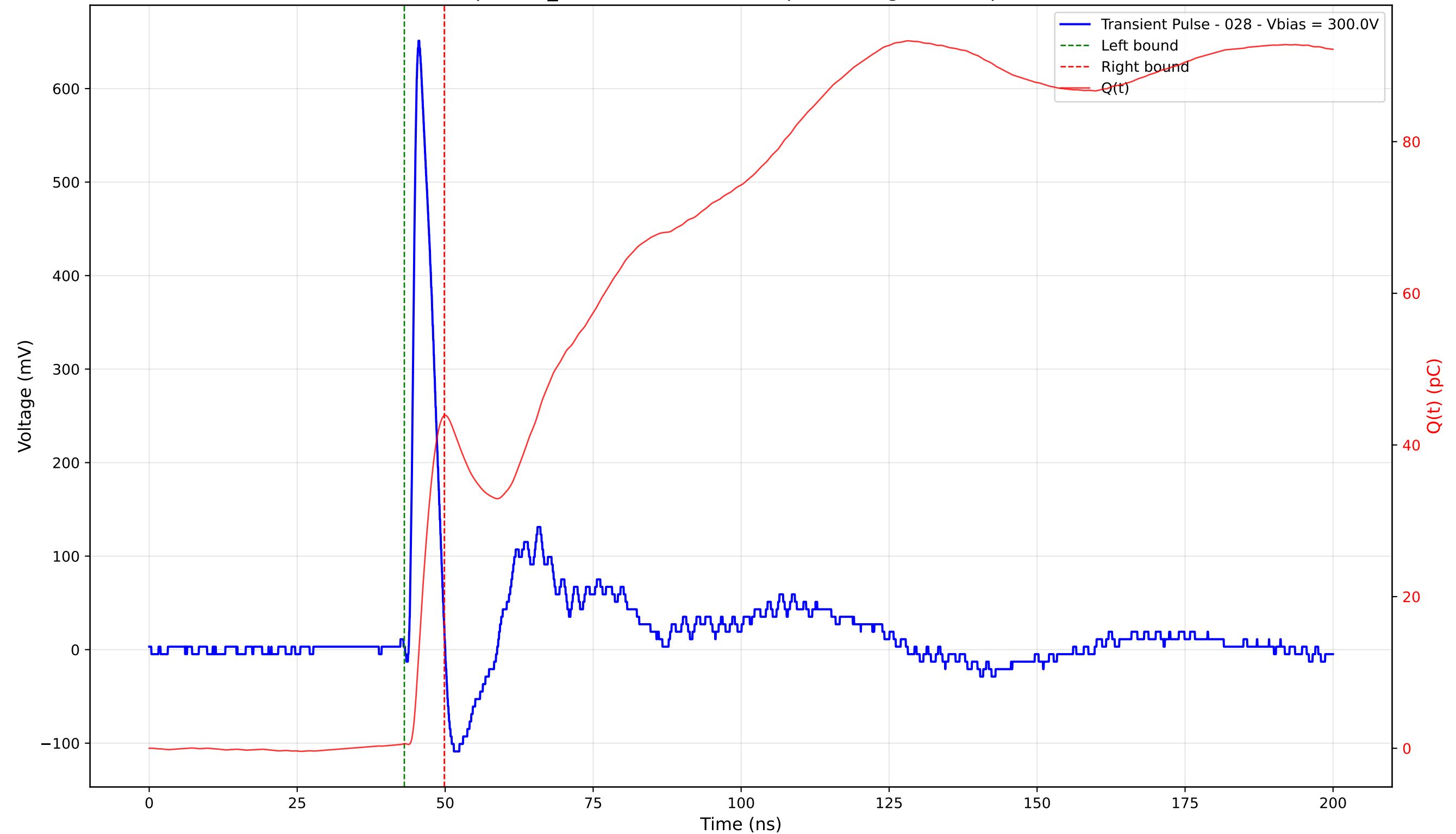
Transient Pulse - Sample: TD_4004 - Position: 370.0 \mu\text{m} - Charge: 43.30 pC - Rise Time: 1.00 ns
