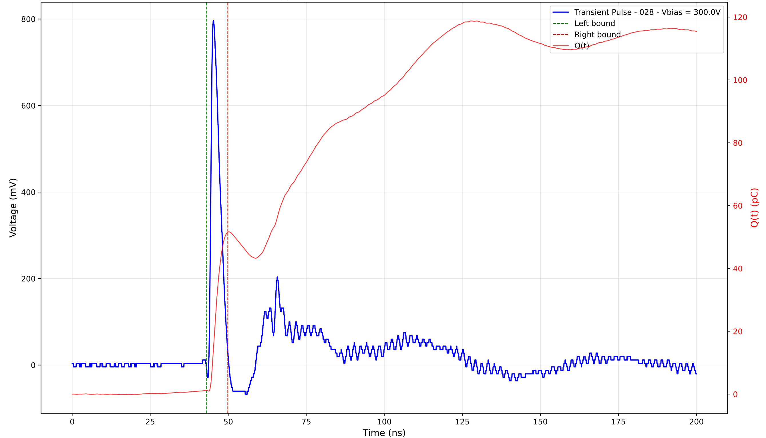
Transient Pulse - Sample: TD_4004 - Position: 115.0 \mu\text{m} - Charge: 50.32 pC - Rise Time: 0.89 ns
