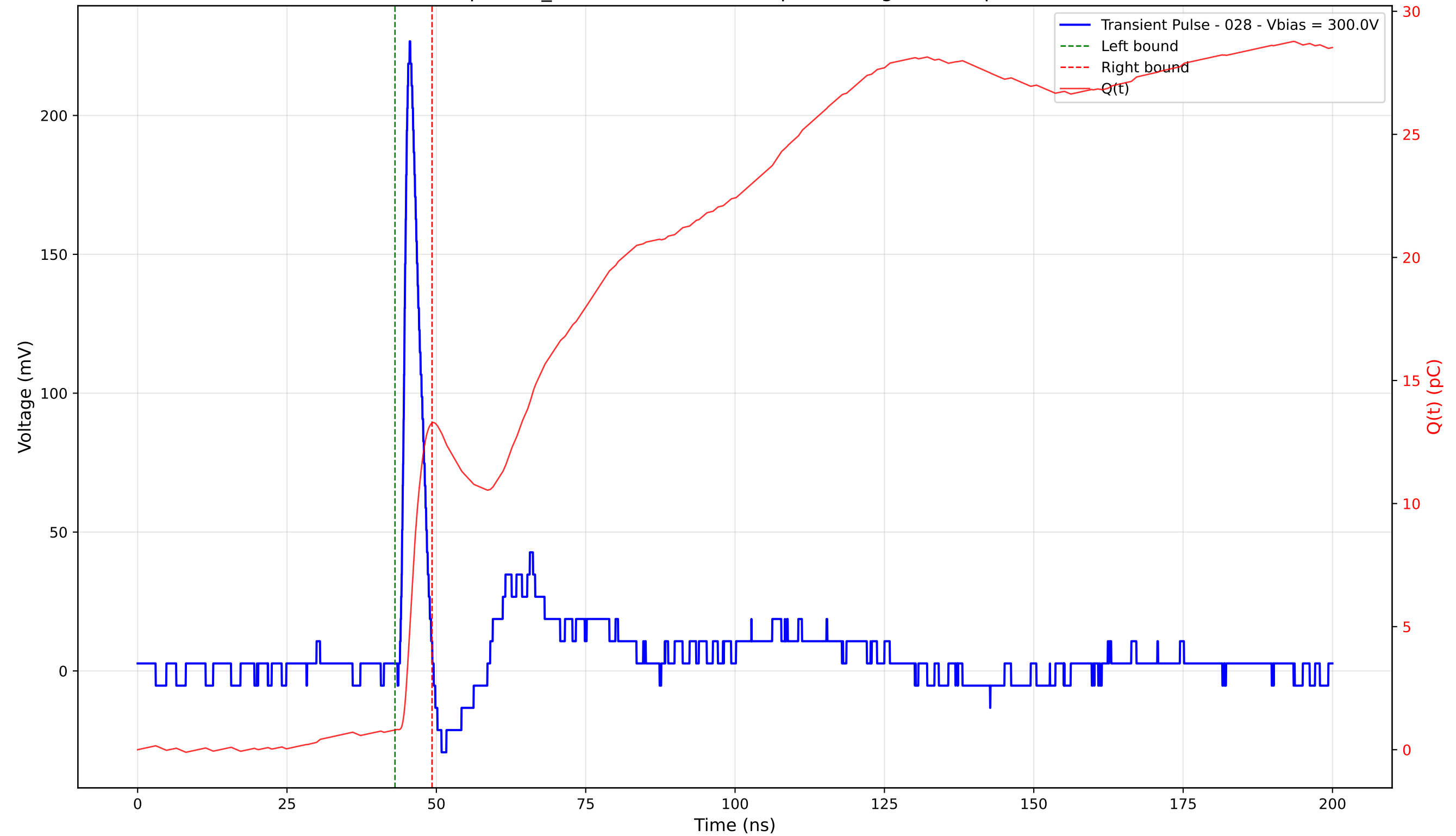
Transient Pulse - Sample: TD_4004 - Position: 410.0 \mu\text{m} - Charge: 12.47 pC - Rise Time: 1.11 ns
