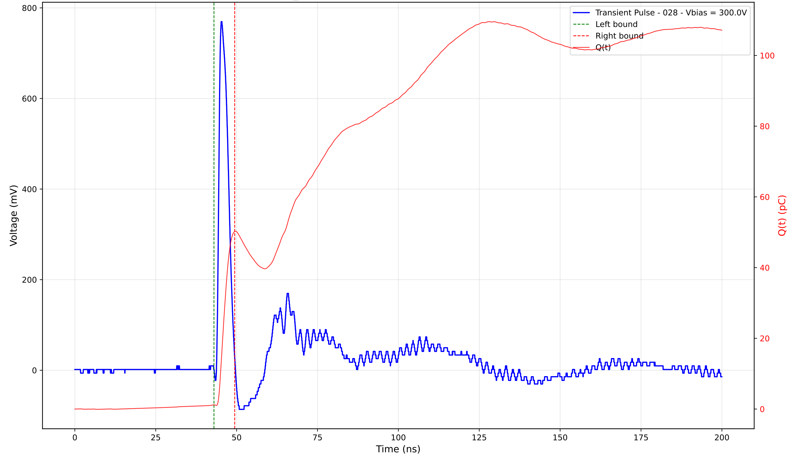
Transient Pulse - Sample: TD_4004 - Position: 270.0 \mu\text{m} - Charge: 49.04 pC - Rise Time: 0.91 ns
