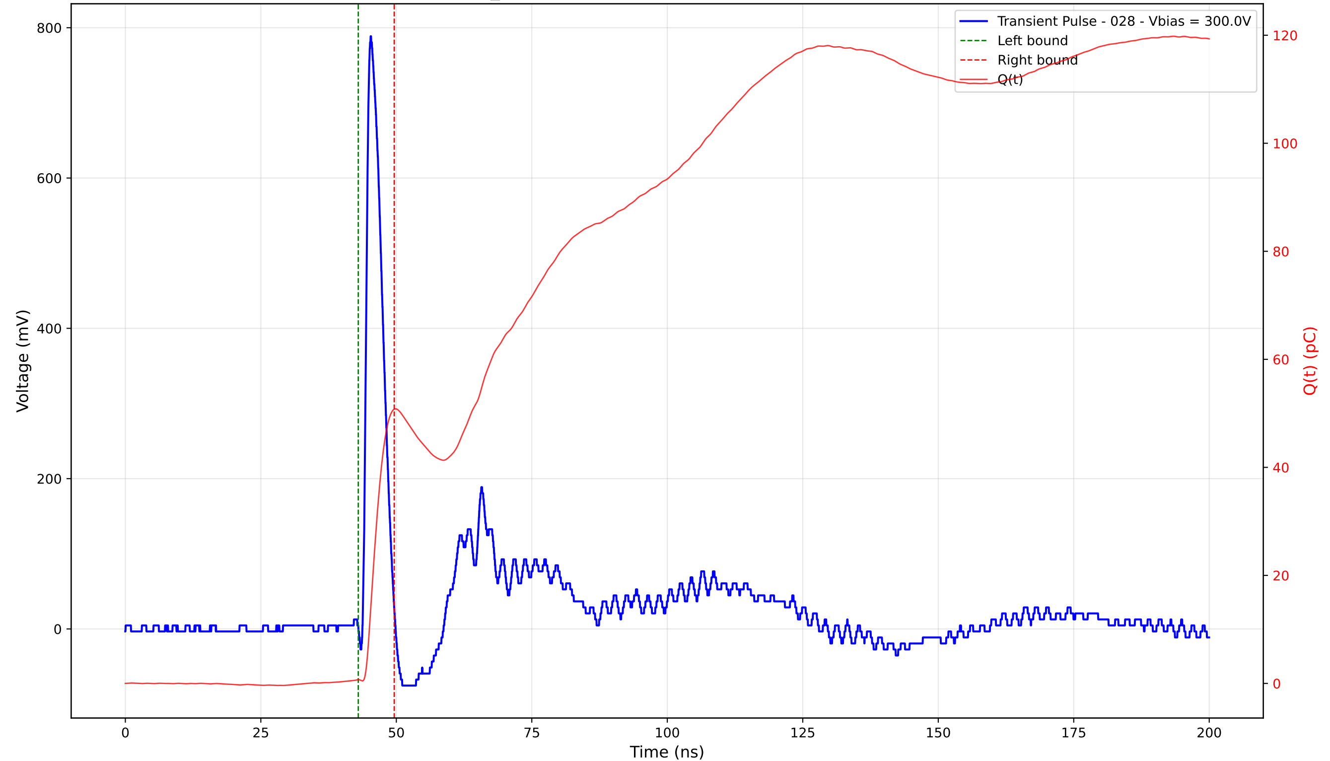
Transient Pulse - Sample: TD_4004 - Position: 130.0 \mu\text{m} - Charge: 50.08 pC - Rise Time: 0.90 ns
