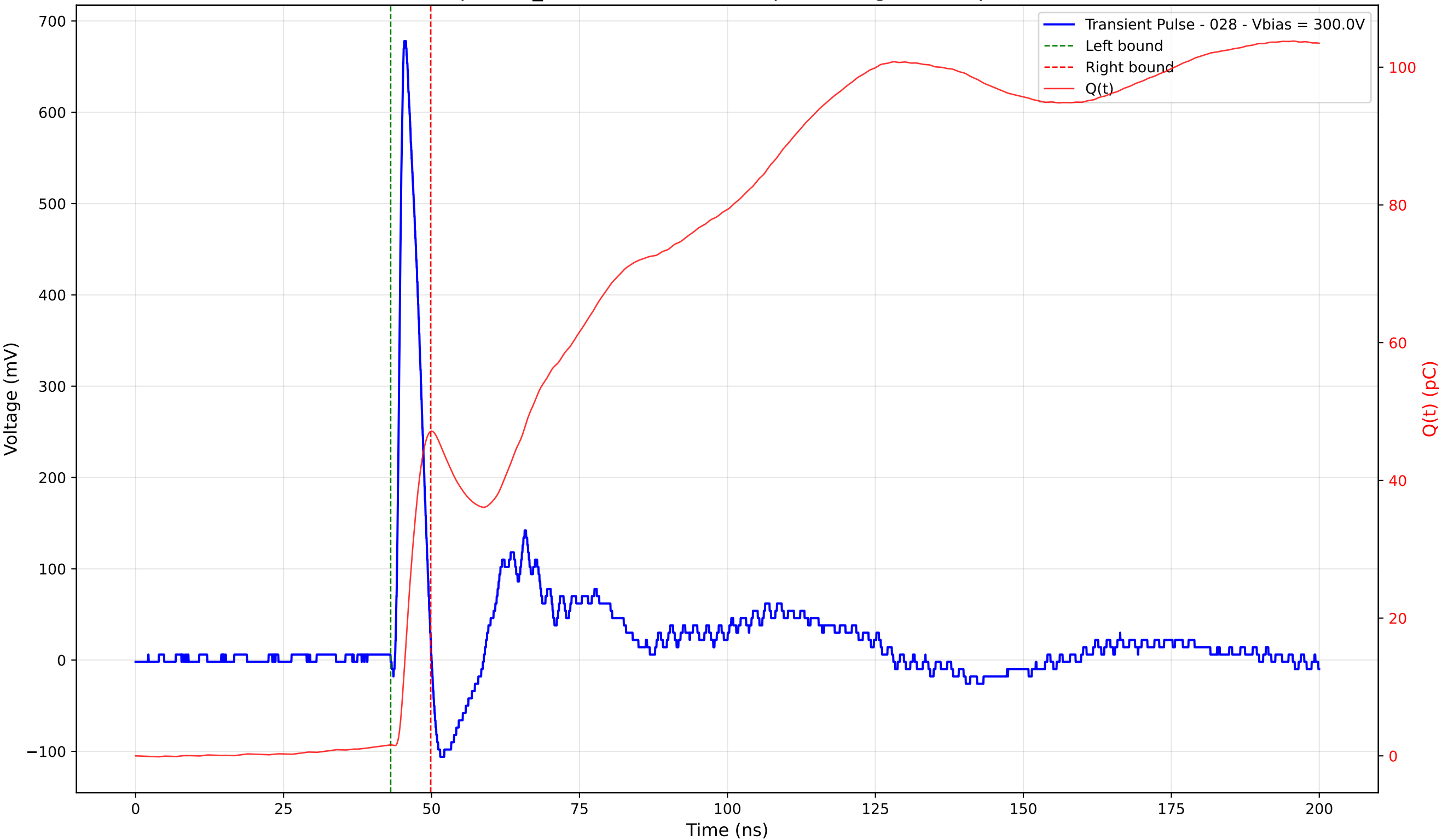
Transient Pulse - Sample: TD_4004 - Position: 355.0 \mu\text{m} - Charge: 45.52 pC - Rise Time: 1.01 ns
