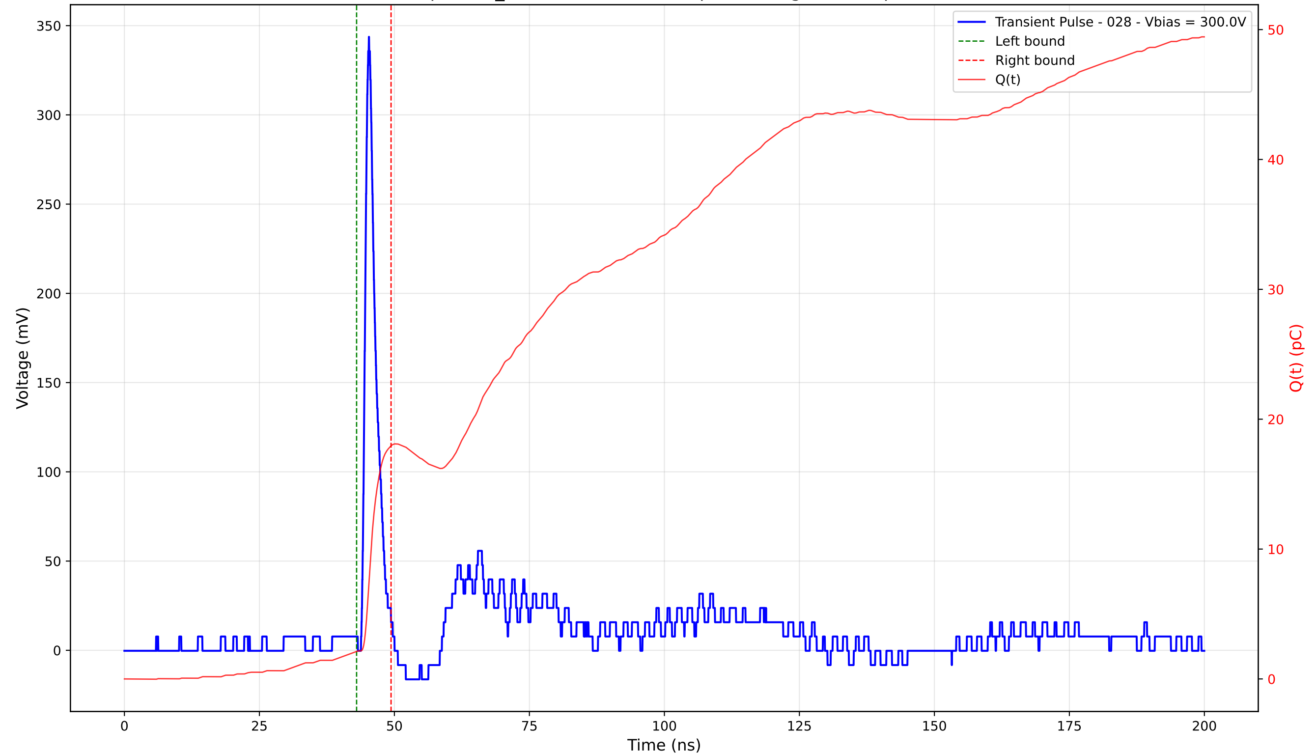
Transient Pulse - Sample: TD_4004 - Position: 60.0 \mu\text{m} - Charge: 15.83 pC - Rise Time: 0.93 ns
