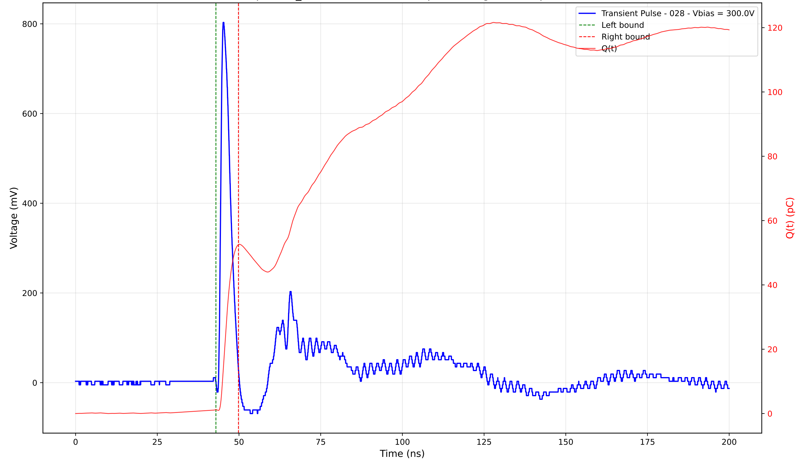
Transient Pulse - Sample: TD_4004 - Position: 185.0 \mu\text{m} - Charge: 51.35 pC - Rise Time: 0.89 ns
