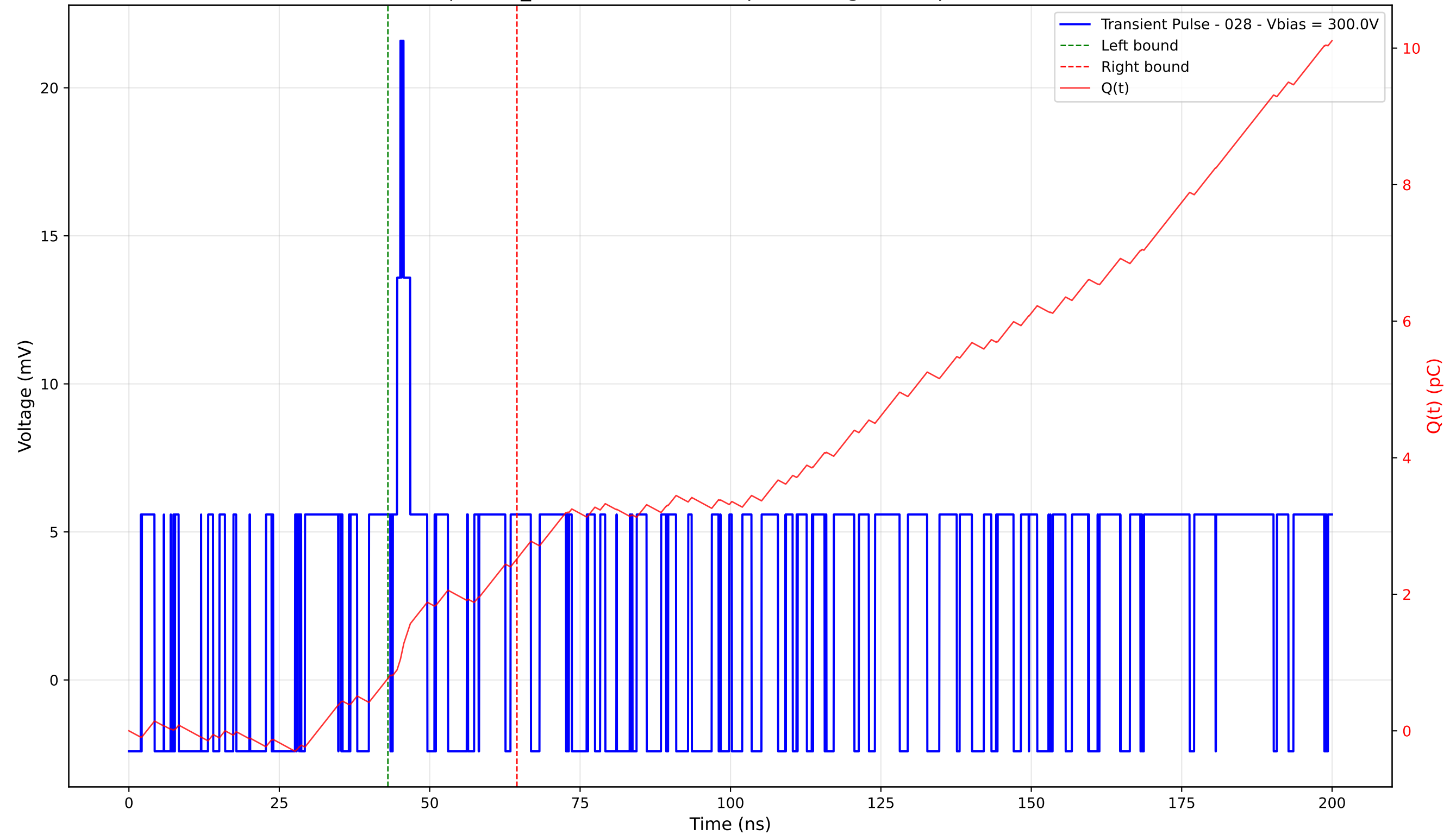
Transient Pulse - Sample: TD_4004 - Position: 15.0 \mu m - Charge: 1.75 pC - Rise Time: 0.00 ns (N/A)
