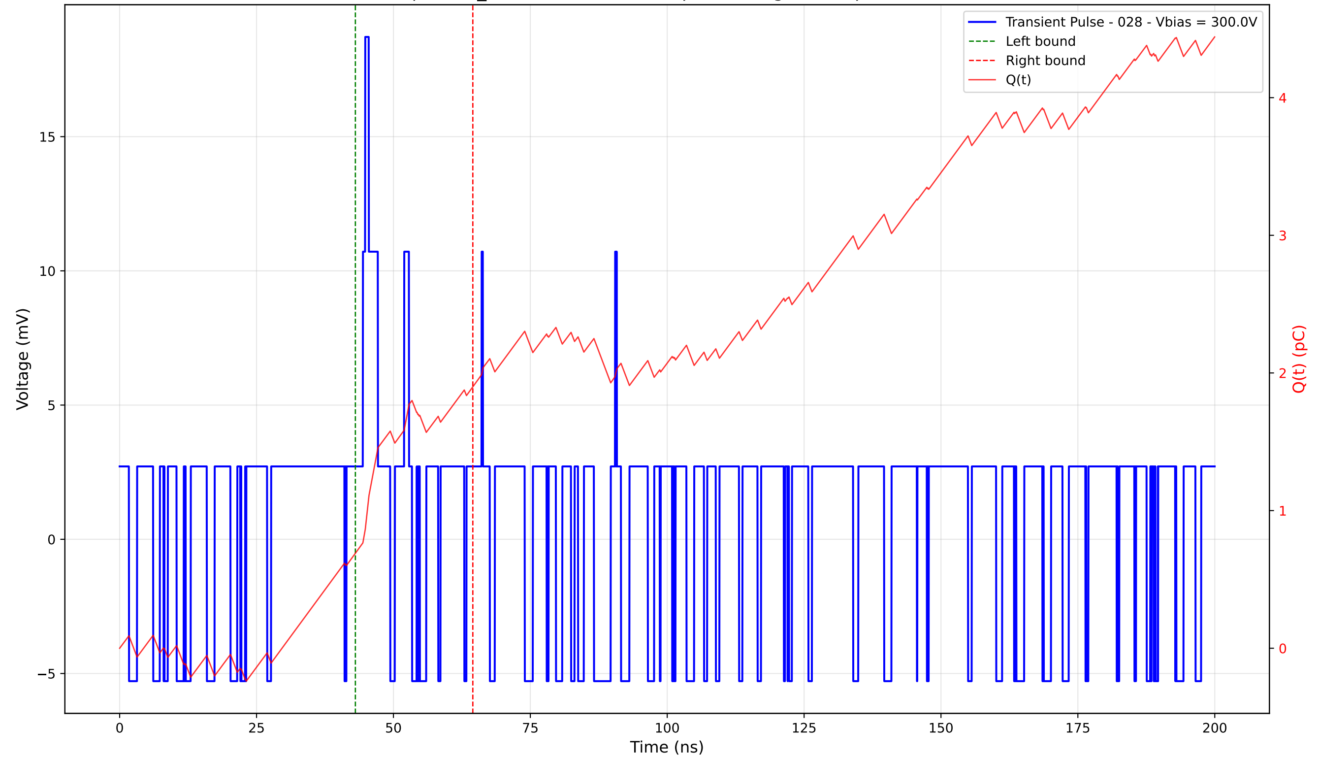
Transient Pulse - Sample: TD_4004 - Position: 10.0 \mu\text{m} - Charge: 1.21 pC - Rise Time: 0.00 ns (N/A)
