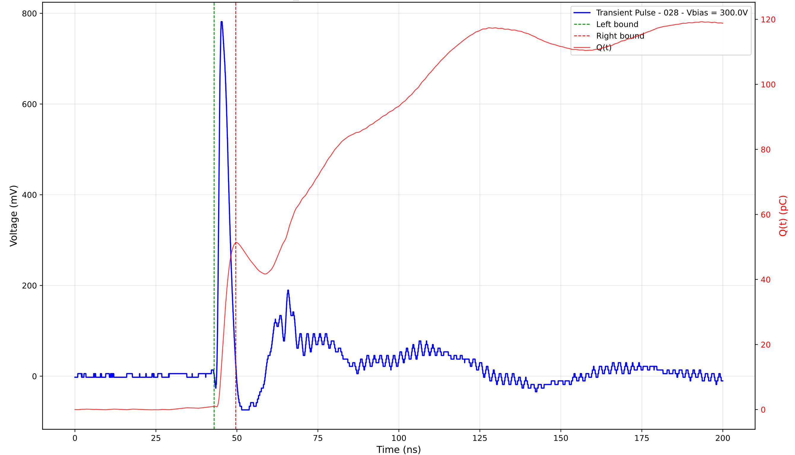
Transient Pulse - Sample: TD_4004 - Position: 225.0 \mu\text{m} - Charge: 50.24 pC - Rise Time: 0.90 ns
