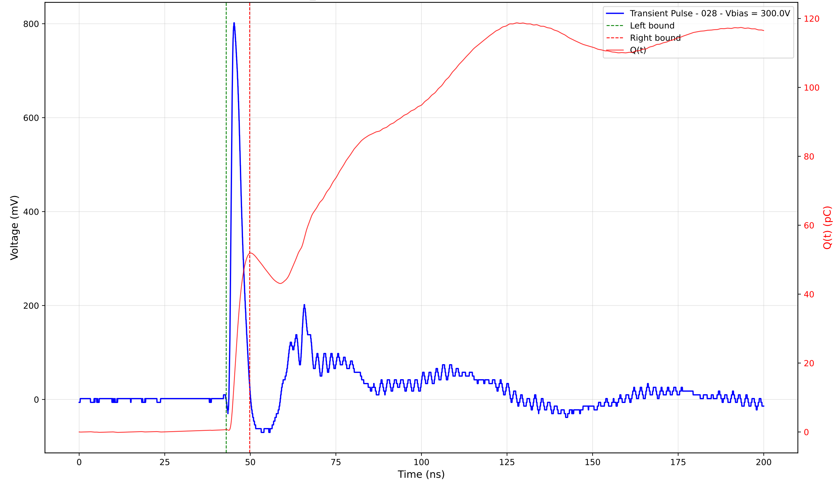
Transient Pulse - Sample: TD_4004 - Position: 195.0 \mu\text{m} - Charge: 51.14 pC - Rise Time: 0.88 ns
