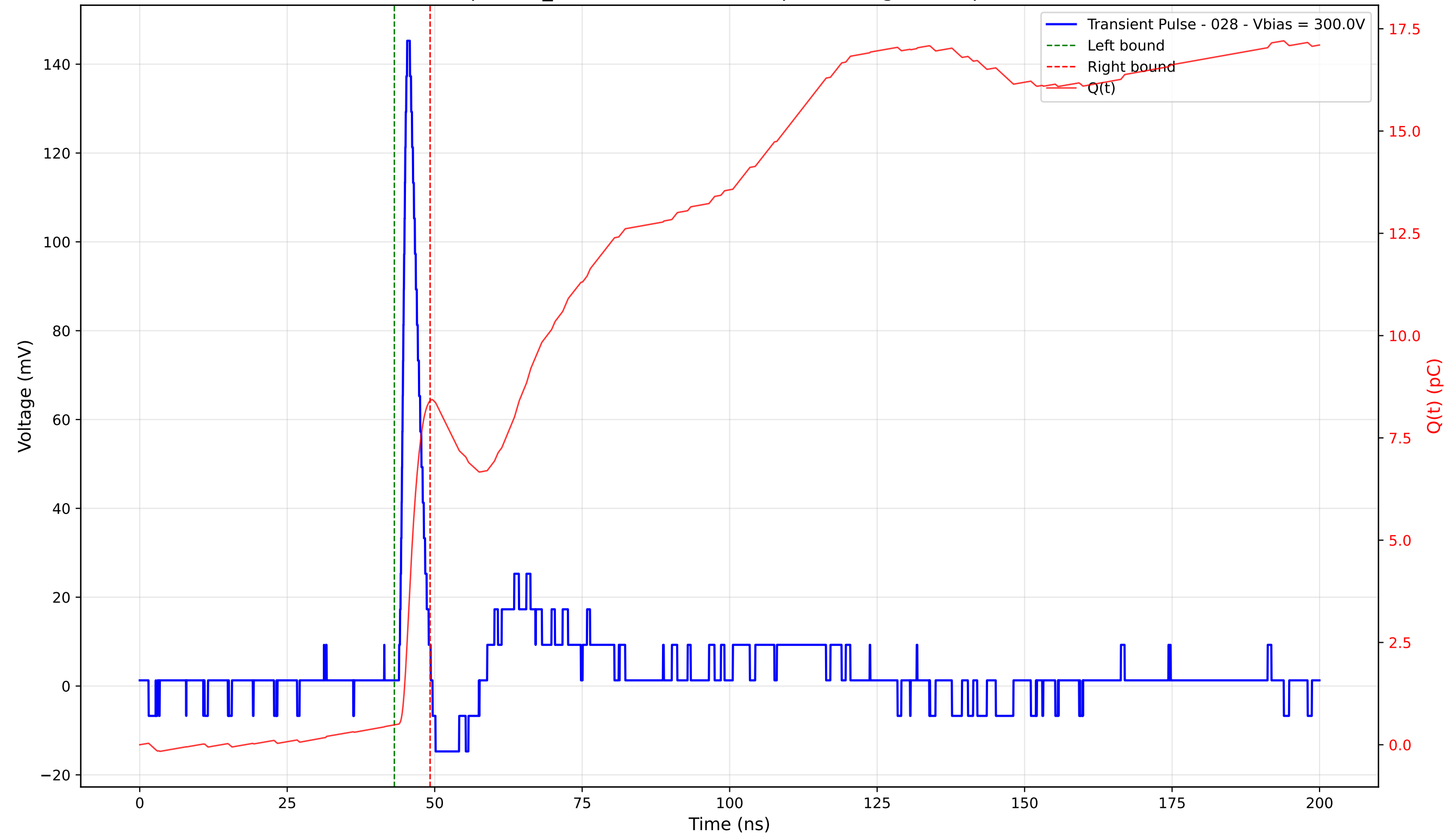
Transient Pulse - Sample: TD_4004 - Position: 415.0 \mu\text{m} - Charge: 7.93 pC - Rise Time: 1.07 ns
