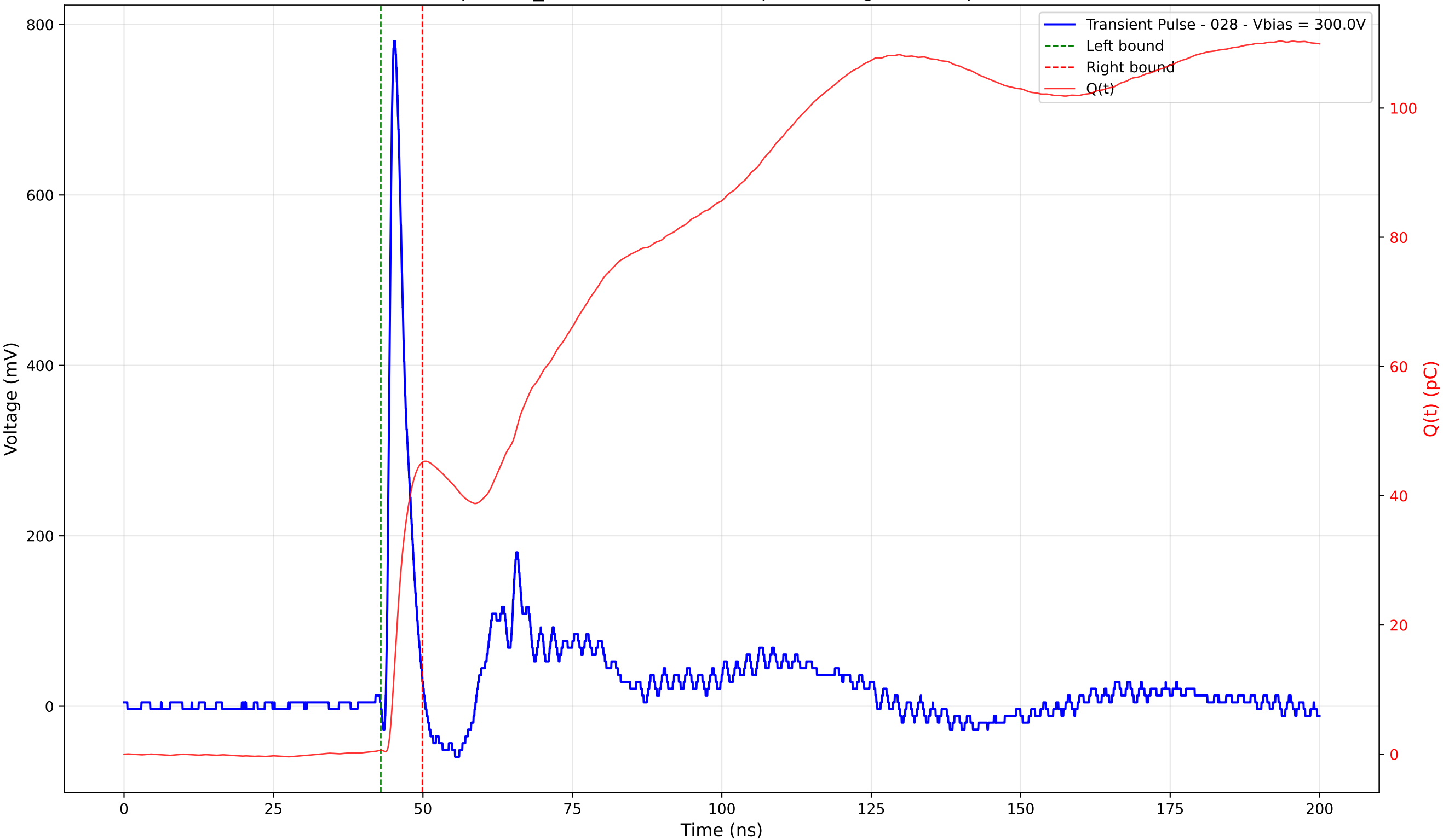
Transient Pulse - Sample: TD_4004 - Position: 95.0 \mu\text{m} - Charge: 44.55 pC - Rise Time: 0.88 ns
