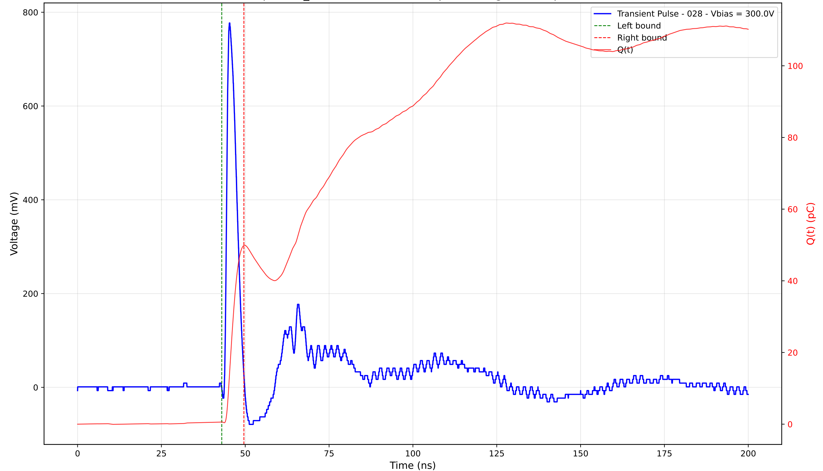
Transient Pulse - Sample: TD_4004 - Position: 155.0 \mu\text{m} - Charge: 49.25 pC - Rise Time: 0.91 ns
