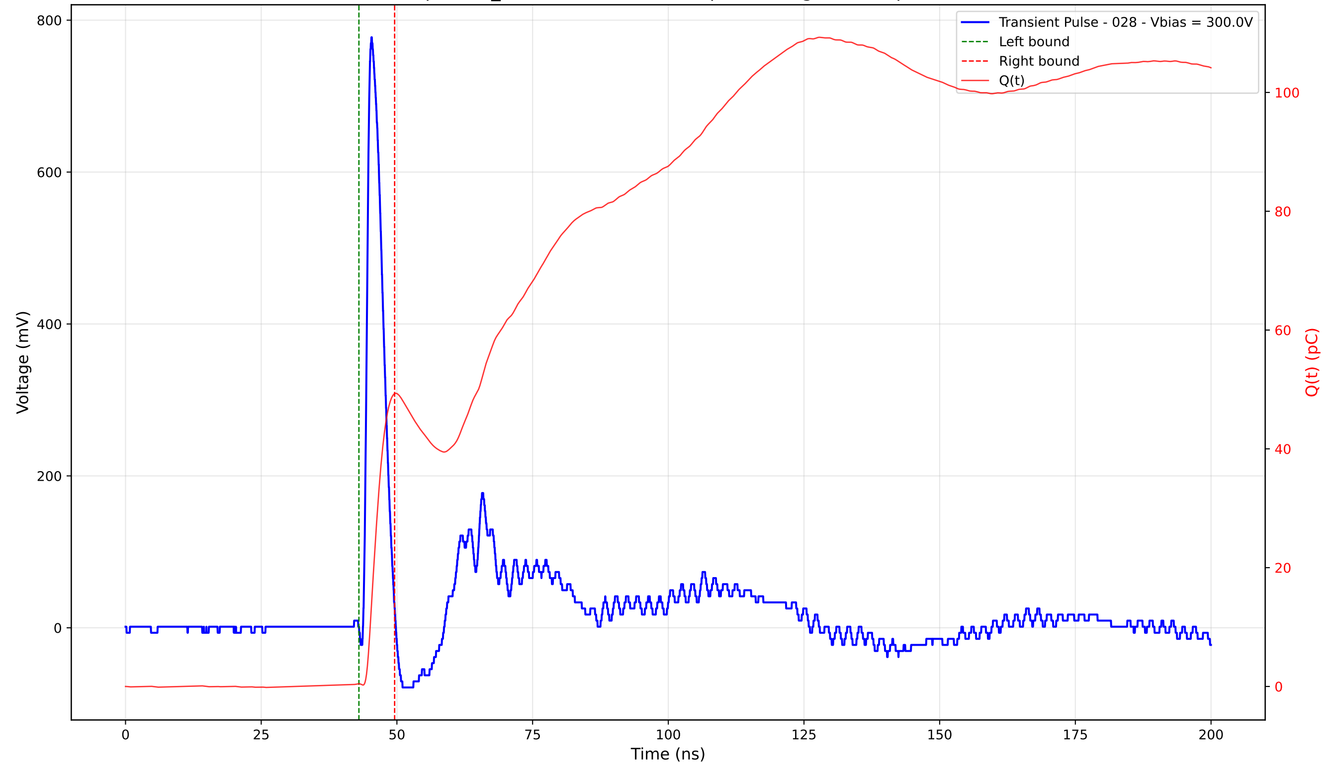
Transient Pulse - Sample: TD_4004 - Position: 150.0 \mu\text{m} - Charge: 48.84 pC - Rise Time: 0.91 ns
