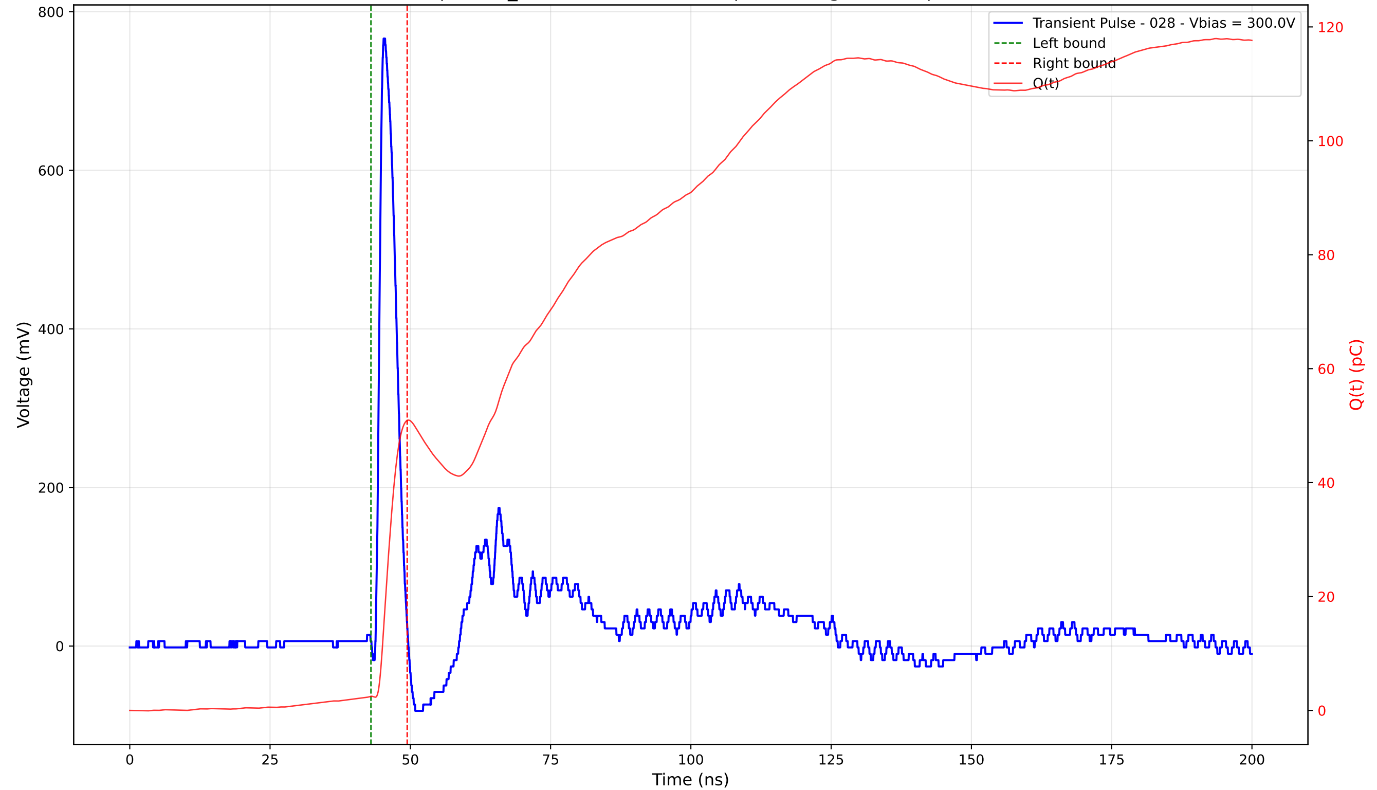
Transient Pulse - Sample: TD_4004 - Position: 255.0 \mu\text{m} - Charge: 48.44 pC - Rise Time: 0.91 ns
