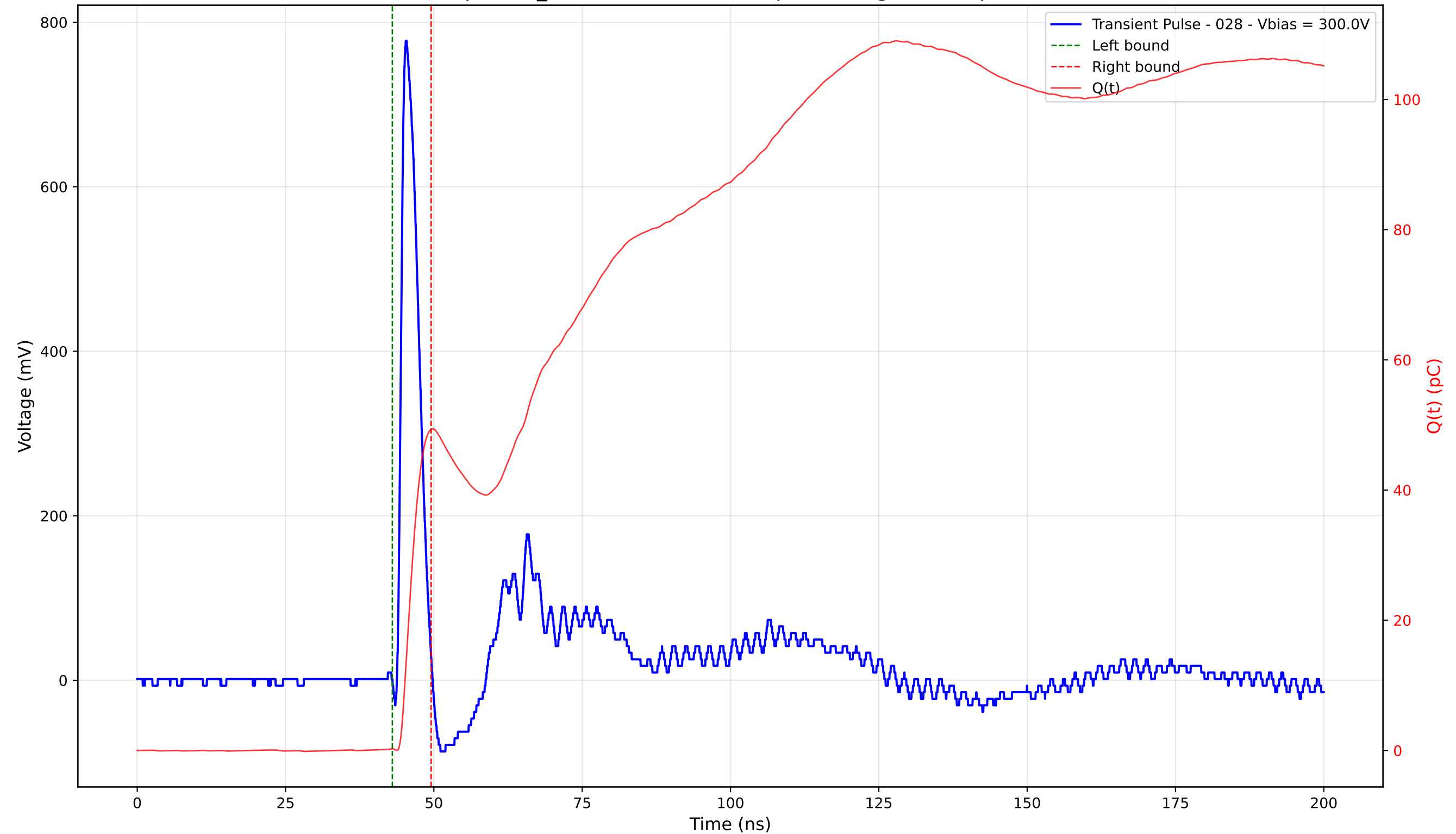
Transient Pulse - Sample: TD_4004 - Position: 140.0 \mu\text{m} - Charge: 49.09 pC - Rise Time: 0.91 ns
