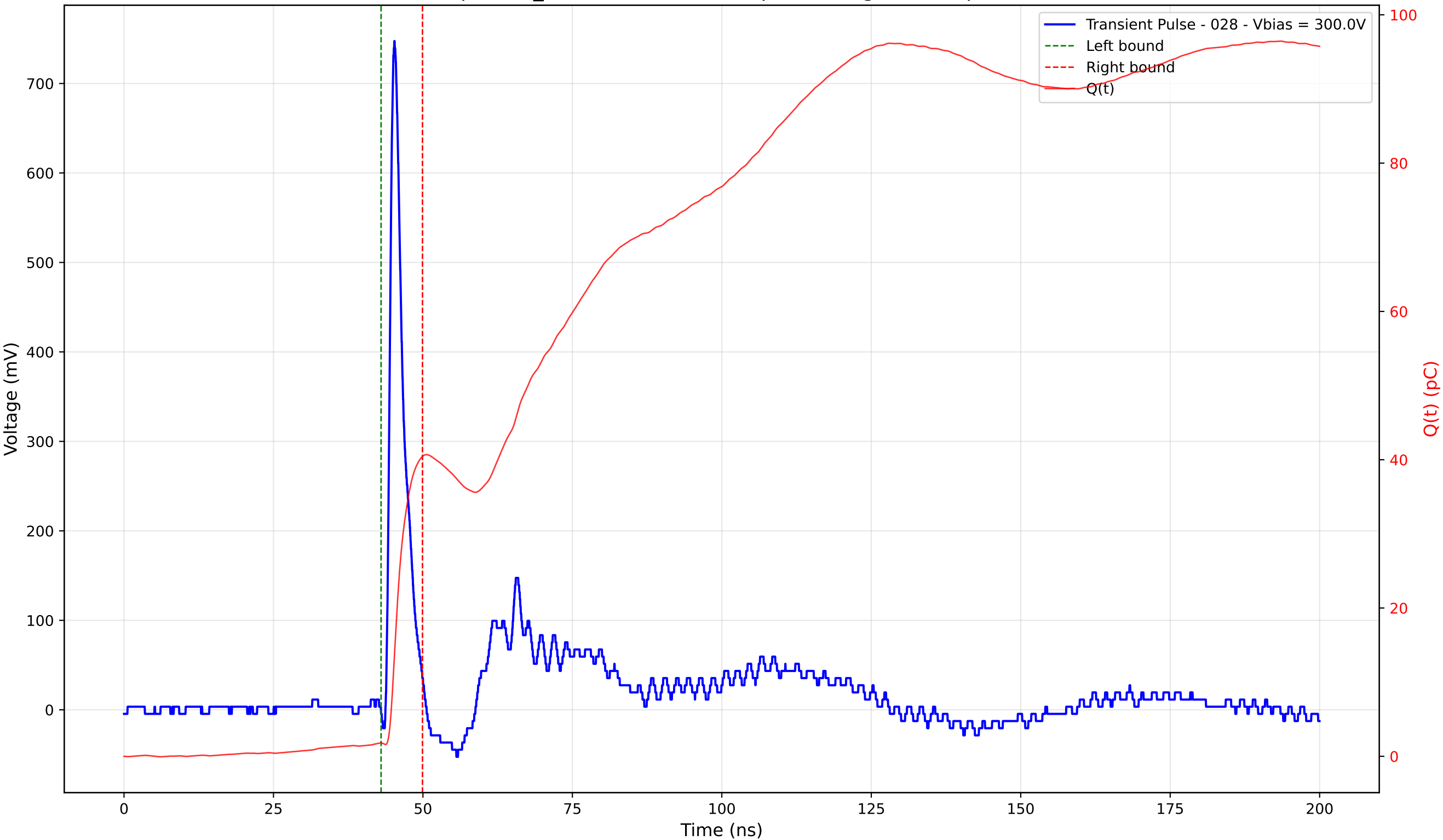
Transient Pulse - Sample: TD_4004 - Position: 85.0 \mu\text{m} - Charge: 38.64 pC - Rise Time: 0.89 ns
