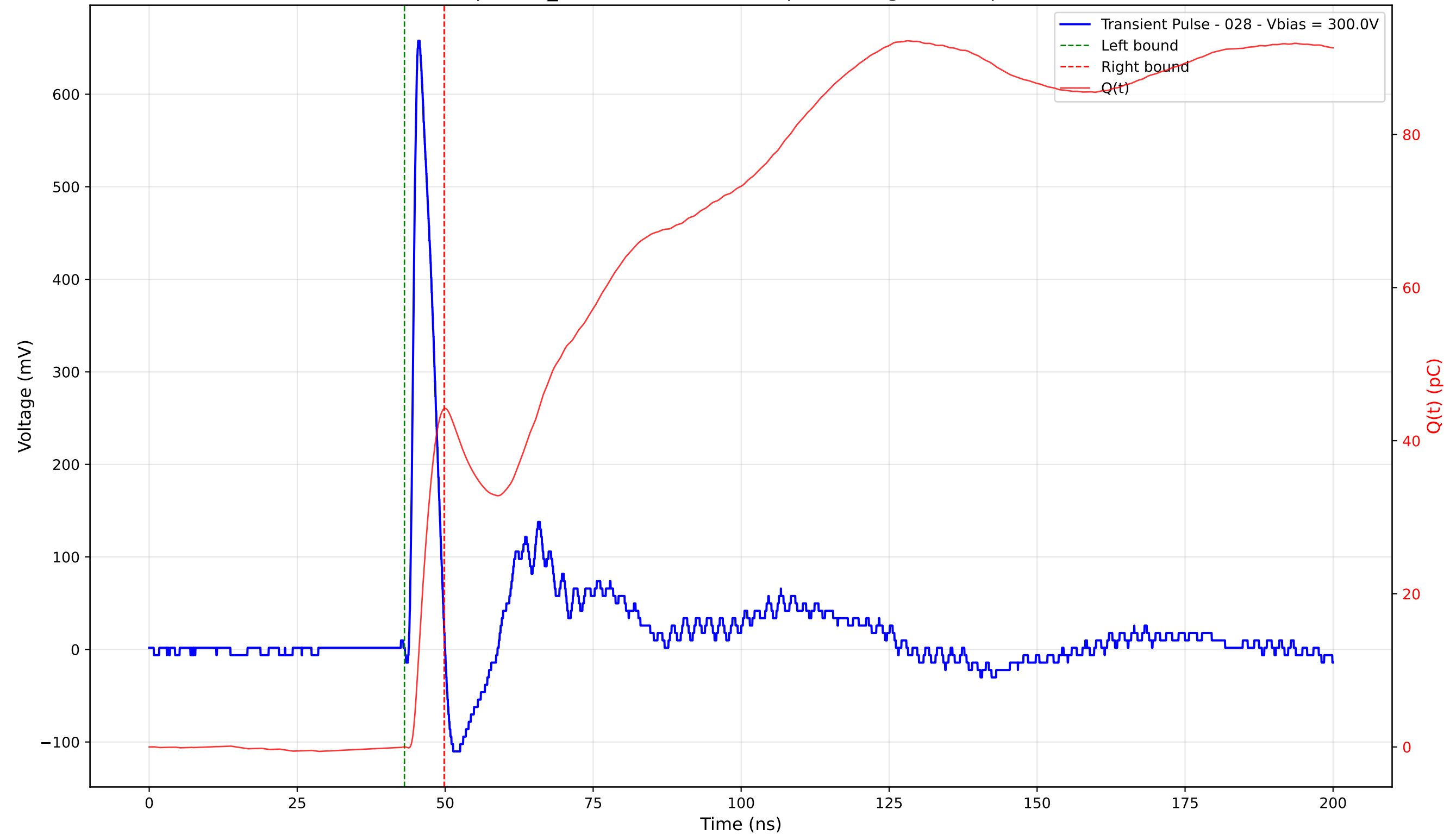
Transient Pulse - Sample: TD_4004 - Position: 365.0 \mu\text{m} - Charge: 44.19 pC - Rise Time: 1.00 ns
