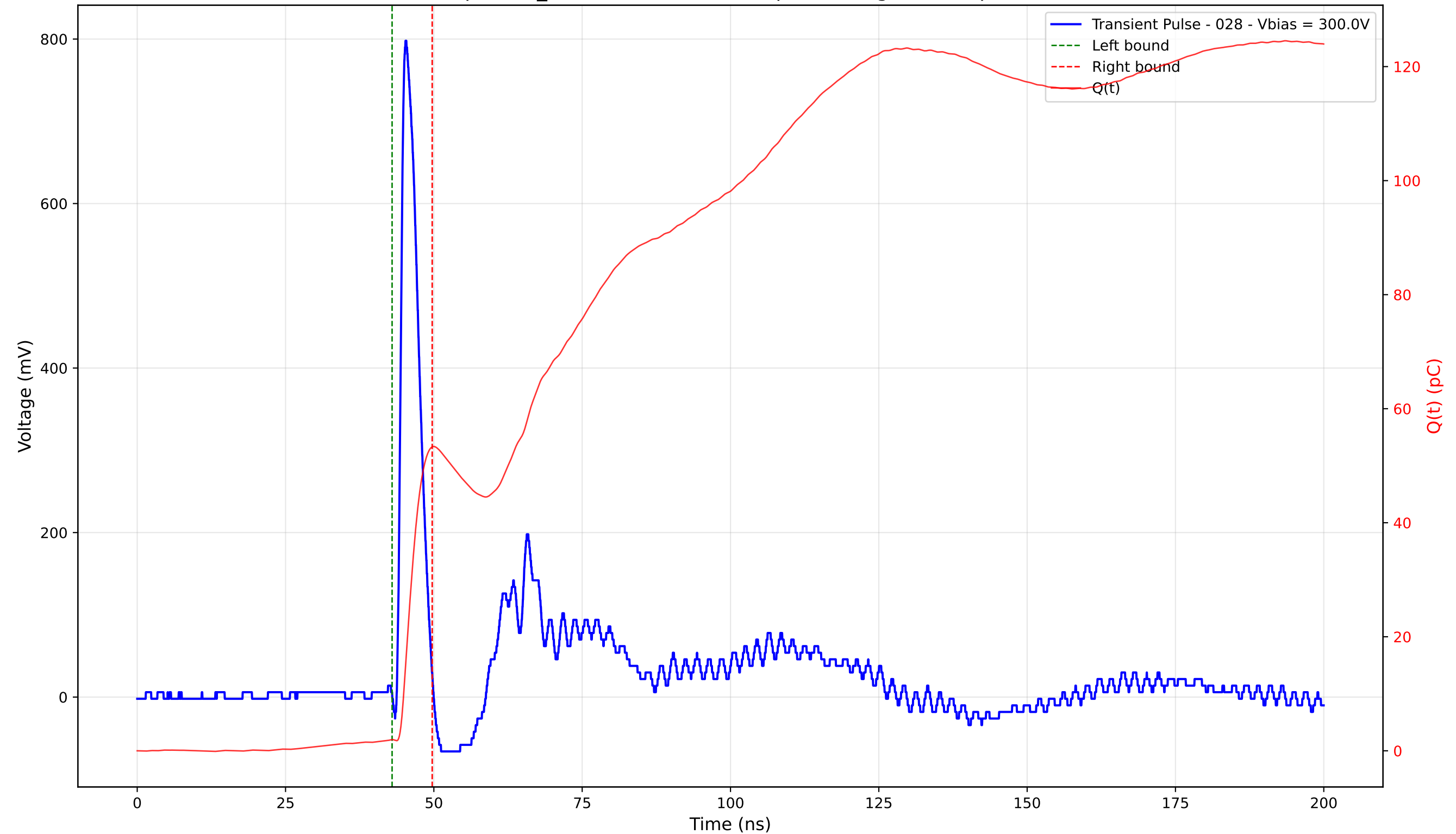
Transient Pulse - Sample: TD_4004 - Position: 170.0 \mu\text{m} - Charge: 51.35 pC - Rise Time: 0.90 ns
