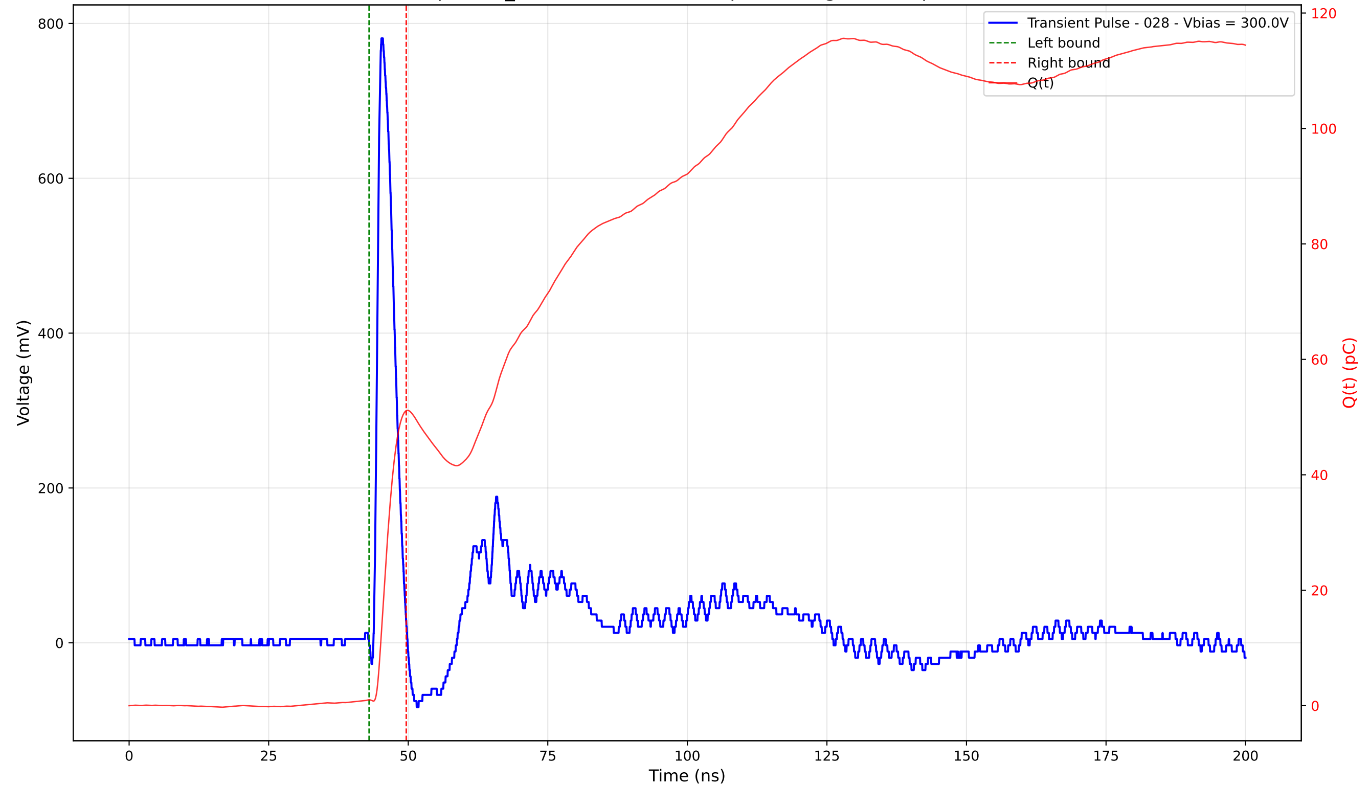
Transient Pulse - Sample: TD_4004 - Position: 160.0 \mu\text{m} - Charge: 50.09 pC - Rise Time: 0.90 ns
