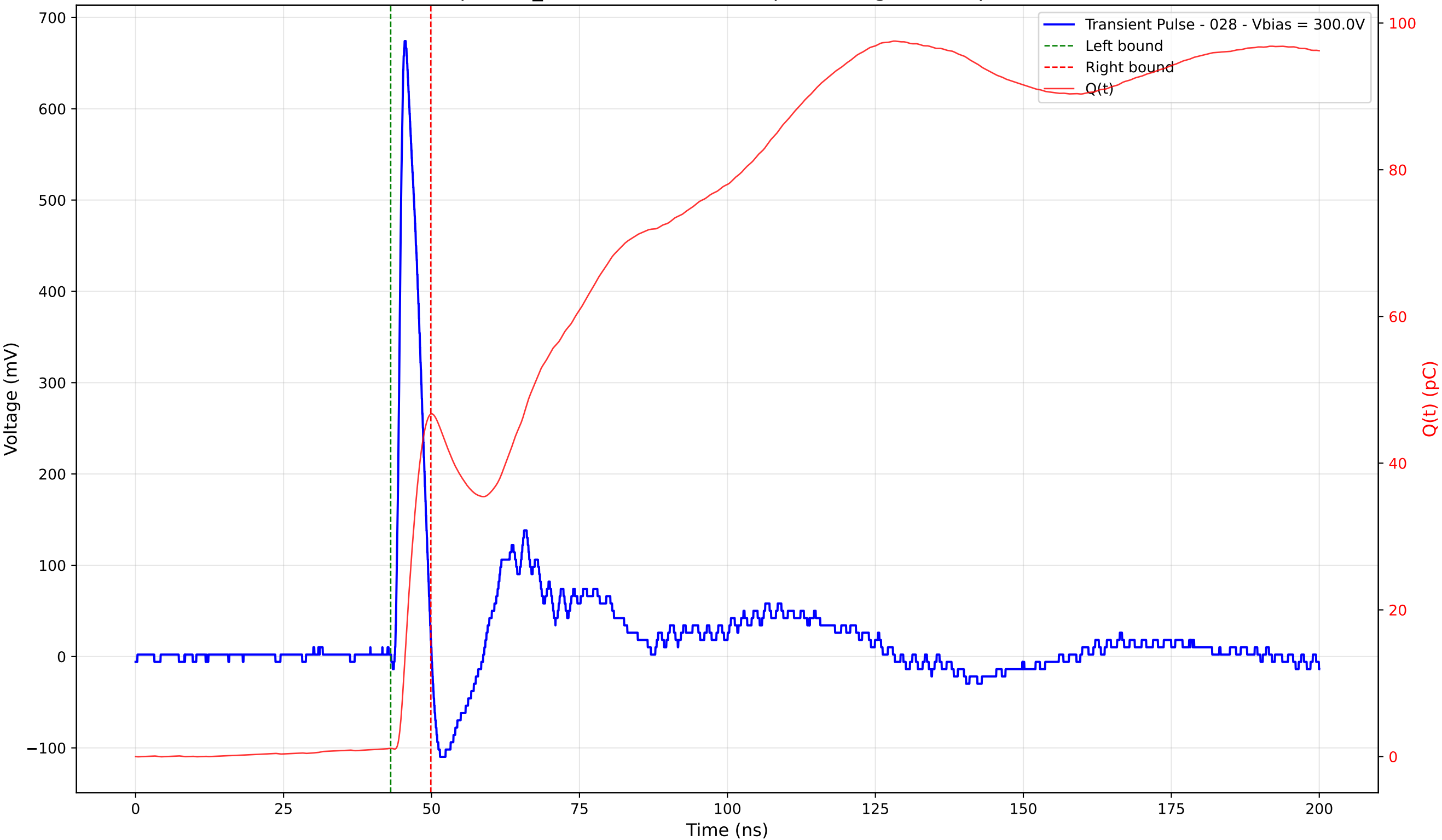
Transient Pulse - Sample: TD_4004 - Position: 360.0 \mu\text{m} - Charge: 45.58 pC - Rise Time: 1.02 ns
