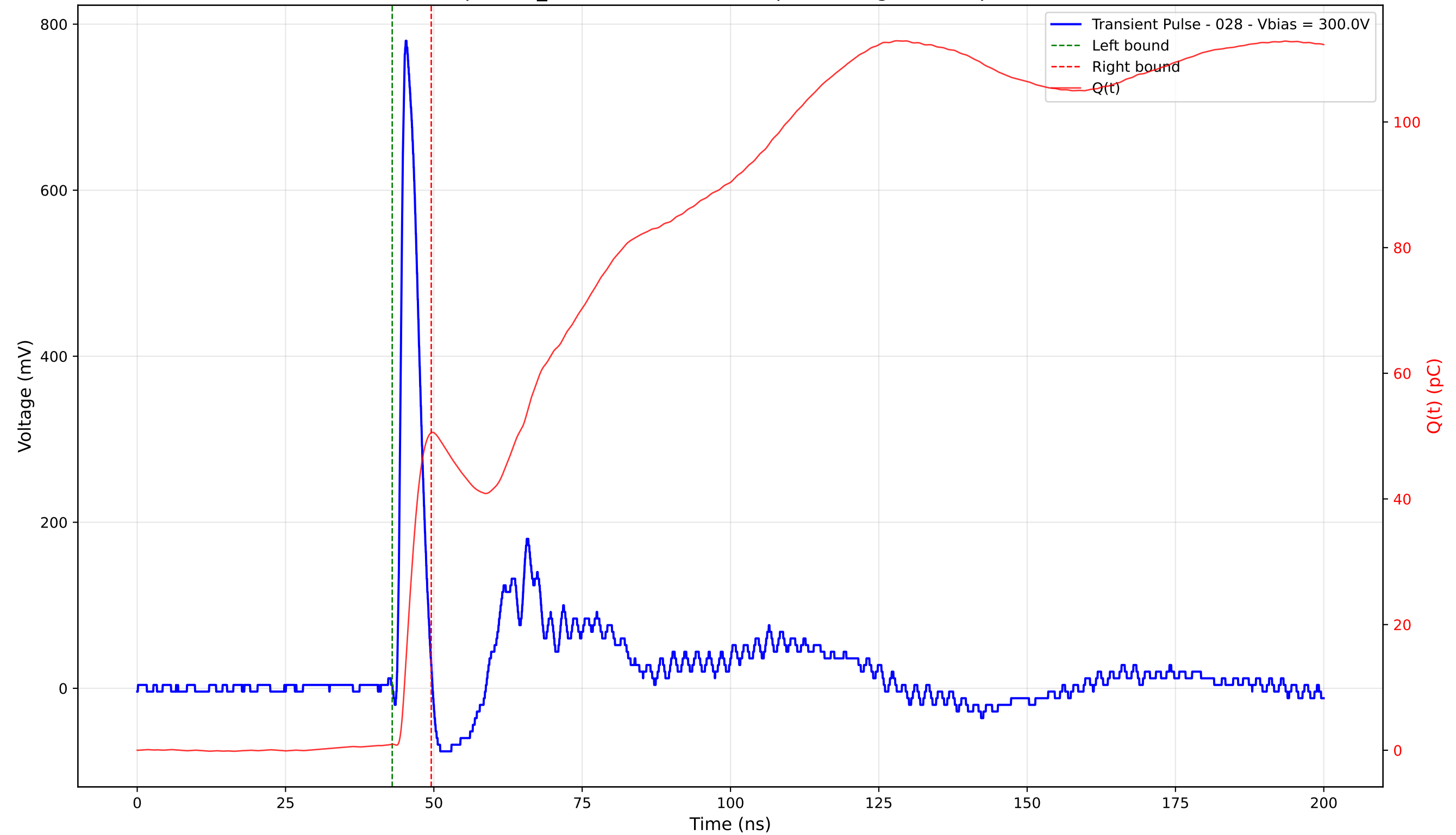
Transient Pulse - Sample: TD_4004 - Position: 230.0 \mu\text{m} - Charge: 49.58 pC - Rise Time: 0.92 ns
