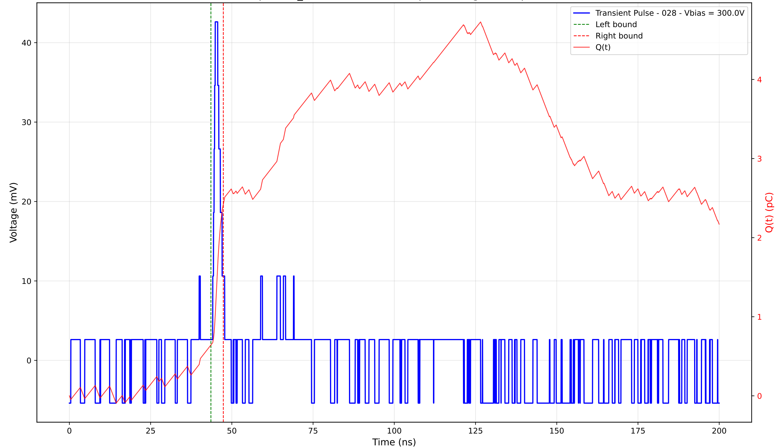
Transient Pulse - Sample: TD_4004 - Position: 35.0 \mu\text{m} - Charge: 1.78 pC - Rise Time: 0.78 ns
