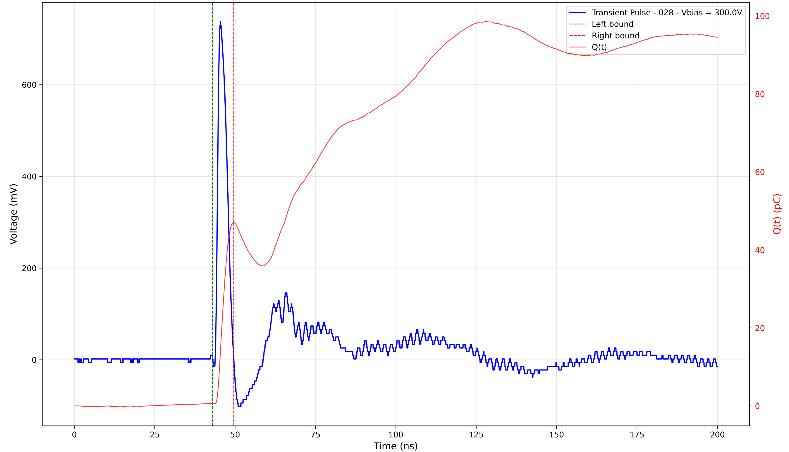
Transient Pulse - Sample: TD_4004 - Position: 315.0 \mu\text{m} - Charge: 46.28 pC - Rise Time: 0.98 ns
