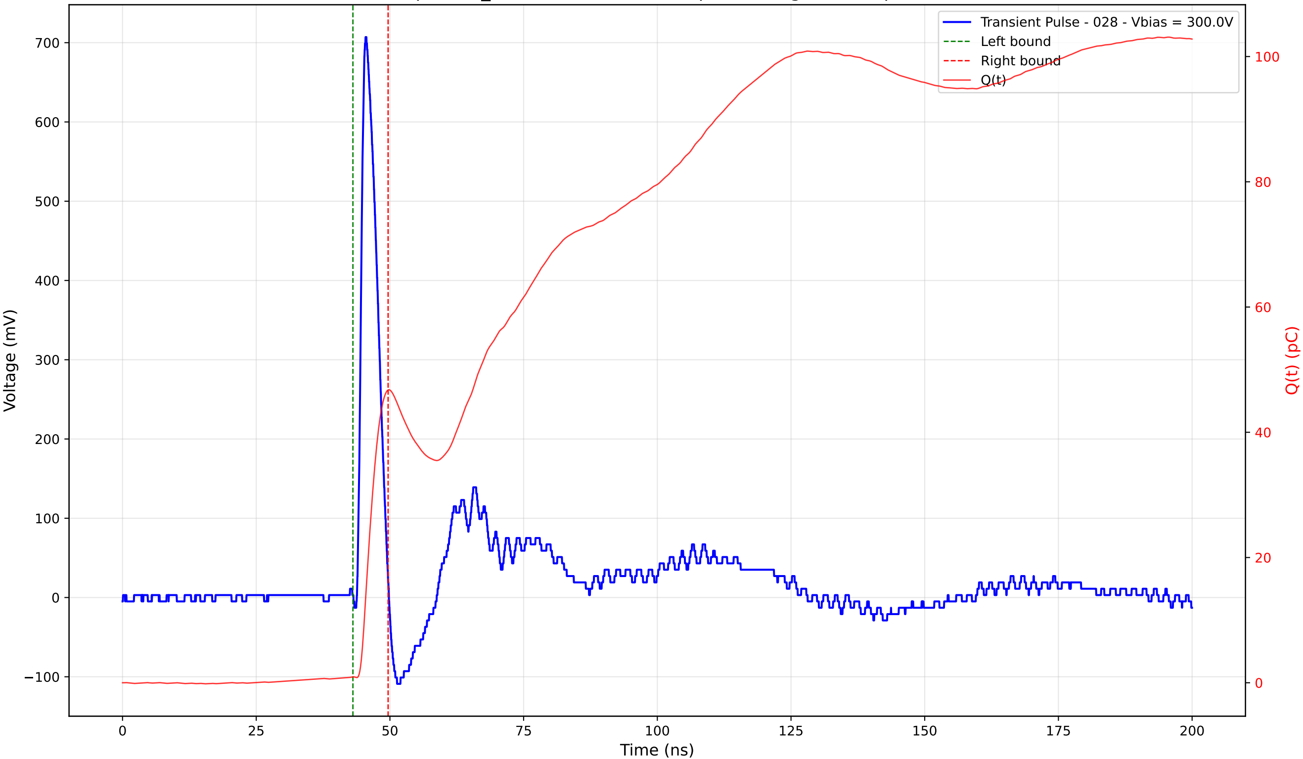
Transient Pulse - Sample: TD_4004 - Position: 330.0 \mu\text{m} - Charge: 45.81 pC - Rise Time: 0.99 ns
