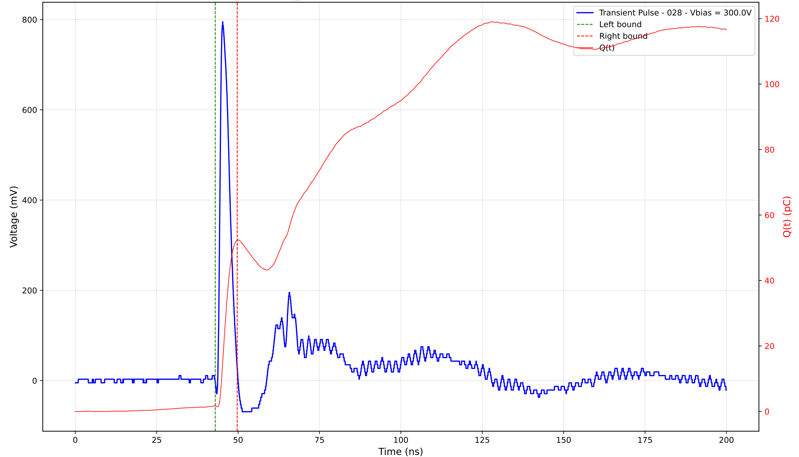
Transient Pulse - Sample: TD_4004 - Position: 220.0 \mu\text{m} - Charge: 50.64 pC - Rise Time: 0.90 ns
