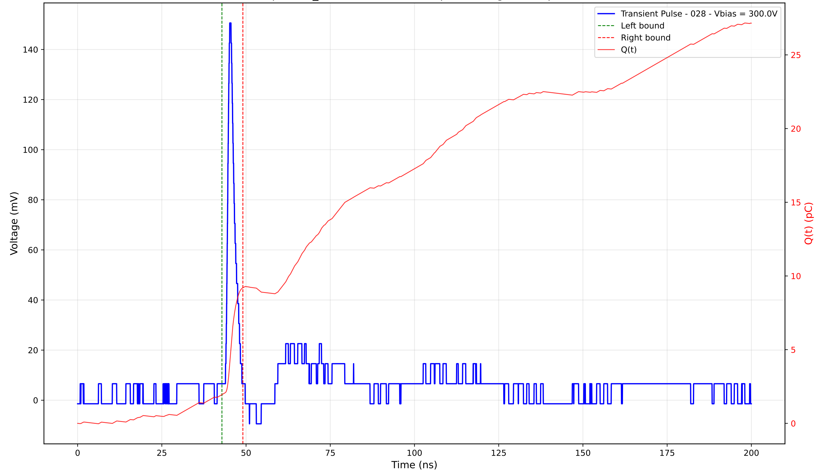
Transient Pulse - Sample: TD_4004 - Position: 50.0 \mu\text{m} - Charge: 7.25 pC - Rise Time: 1.00 ns
