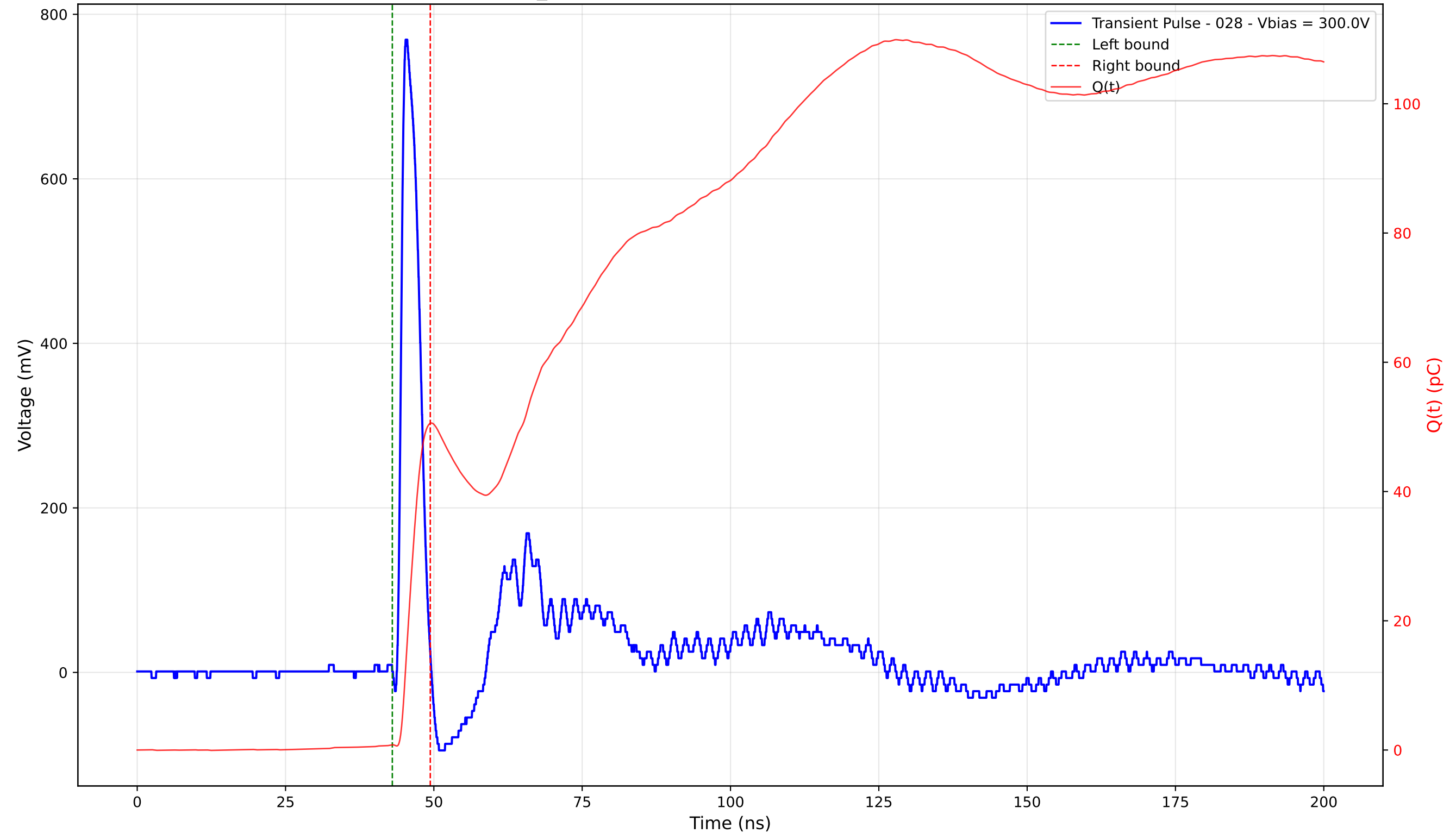
Transient Pulse - Sample: TD_4004 - Position: 285.0 \mu\text{m} - Charge: 49.75 pC - Rise Time: 0.92 ns
