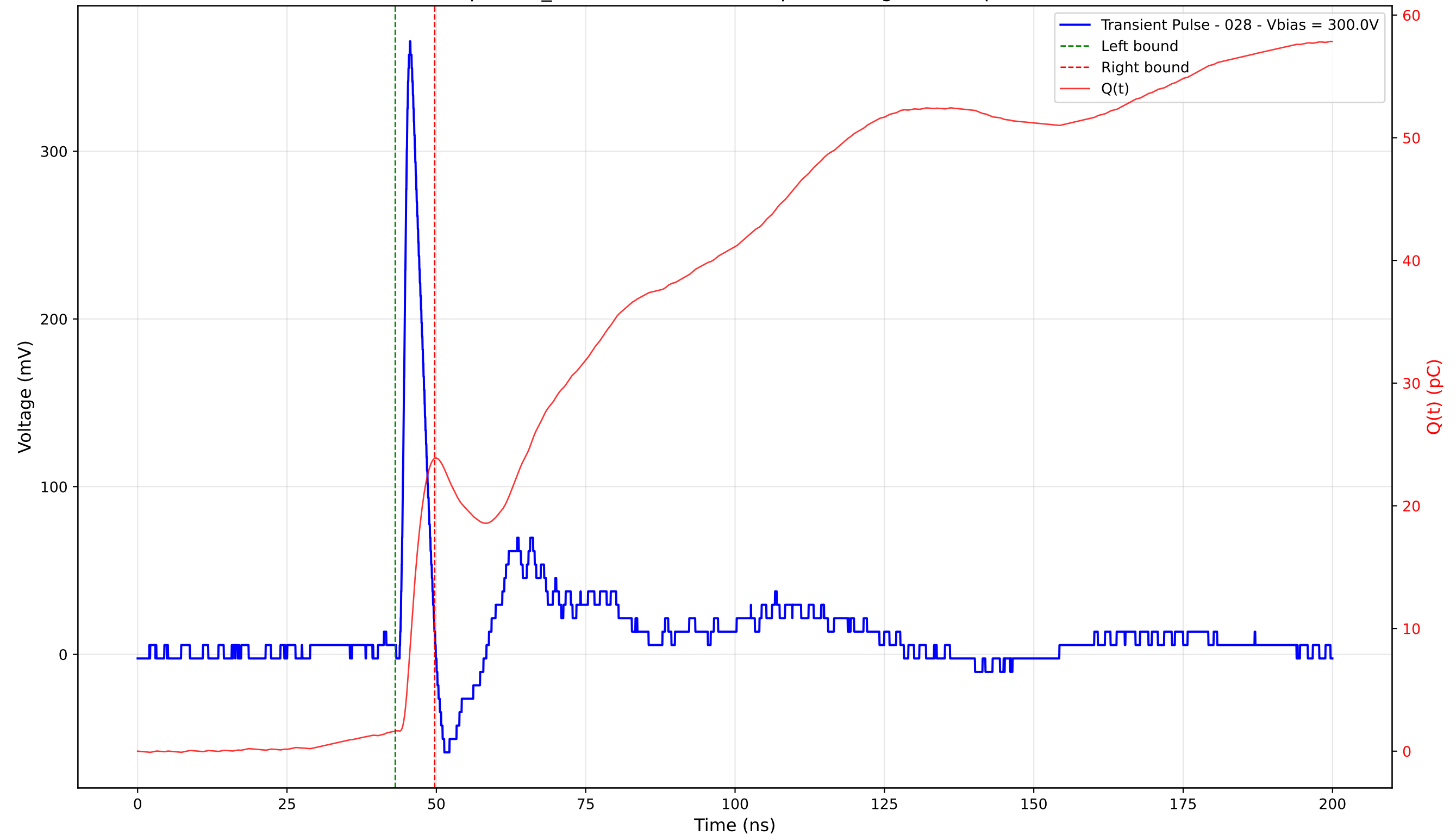
Transient Pulse - Sample: TD_4004 - Position: 400.0 \mu\text{m} - Charge: 22.23 pC - Rise Time: 1.10 ns
