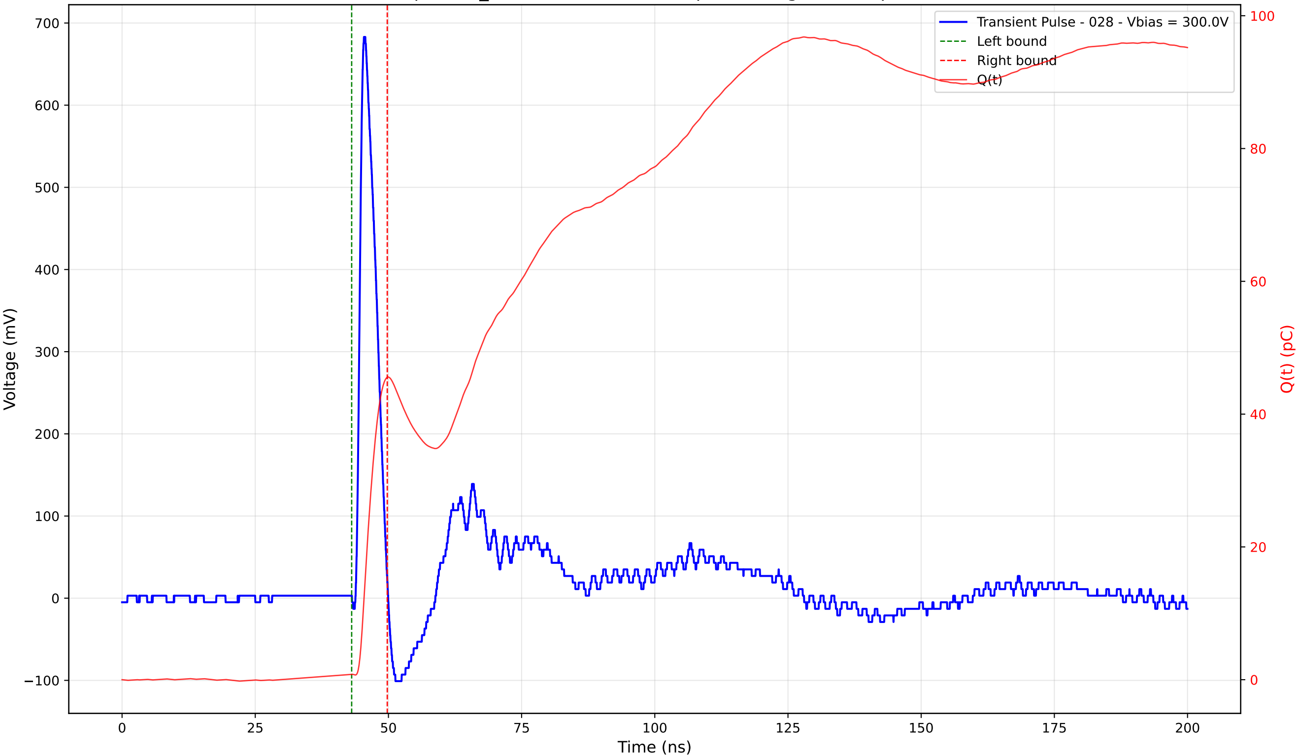
Transient Pulse - Sample: TD_4004 - Position: 345.0 \mu\text{m} - Charge: 44.73 pC - Rise Time: 0.99 ns
