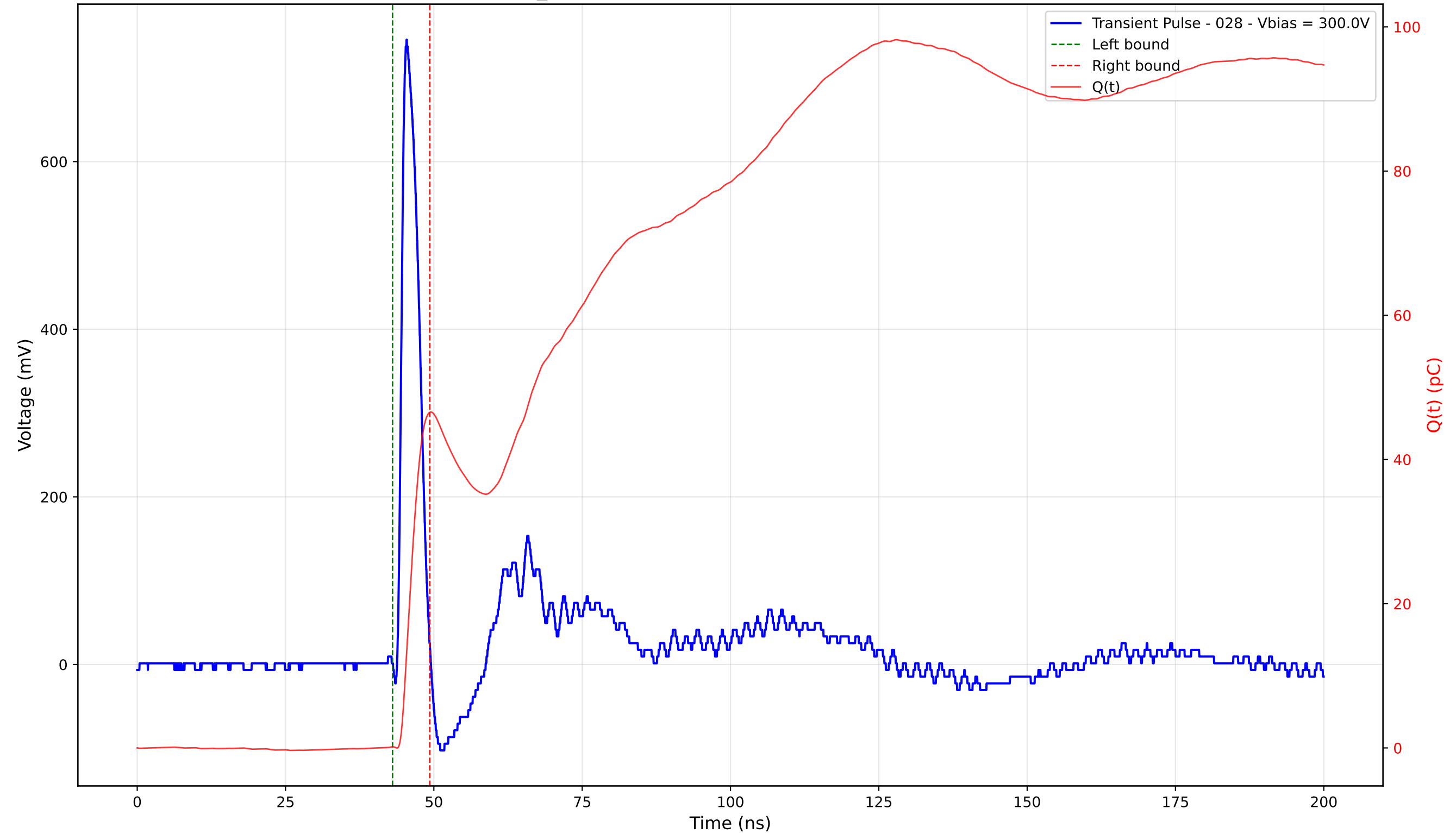
Transient Pulse - Sample: TD_4004 - Position: 310.0 \mu\text{m} - Charge: 46.39 pC - Rise Time: 0.95 ns
