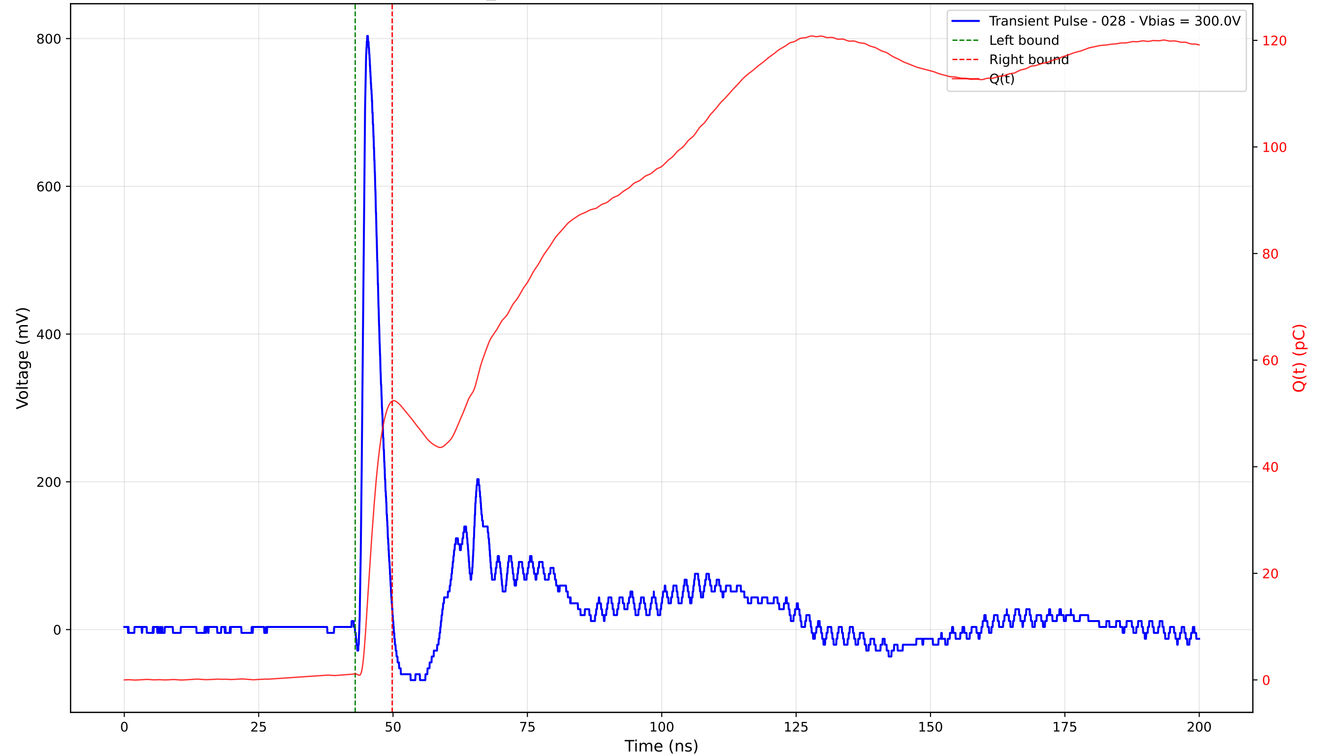
Transient Pulse - Sample: TD_4004 - Position: 190.0 \mu\text{m} - Charge: 51.18 pC - Rise Time: 0.89 ns
