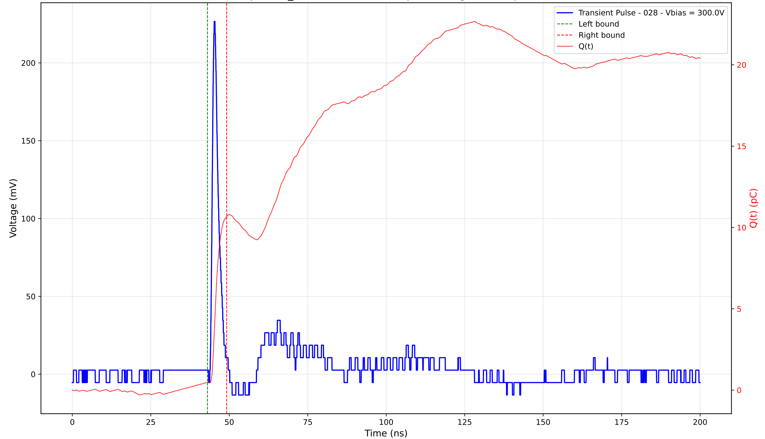
Transient Pulse - Sample: TD_4004 - Position: 55.0 \mu\text{m} - Charge: 10.19 pC - Rise Time: 0.93 ns
