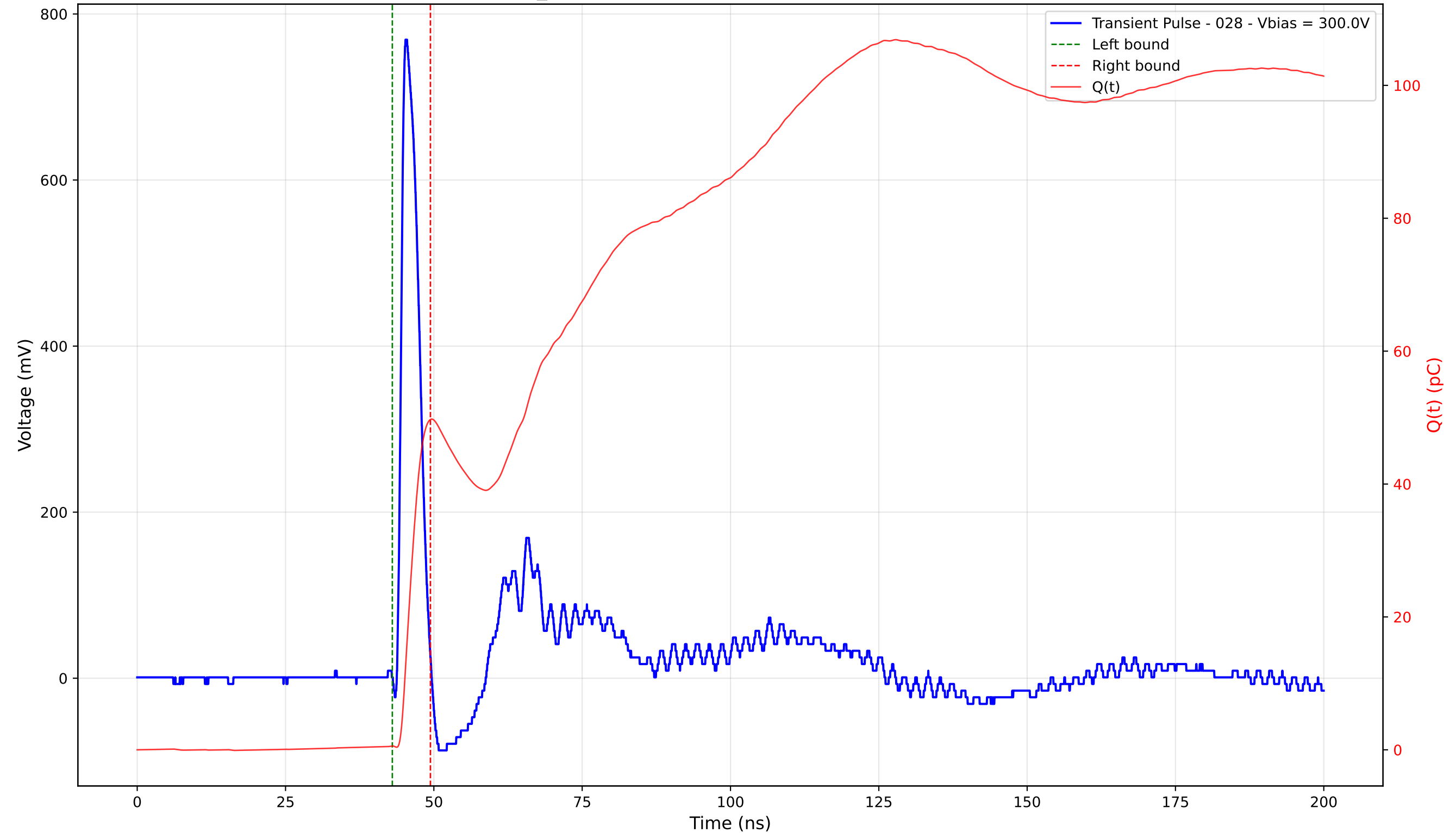
Transient Pulse - Sample: TD_4004 - Position: 275.0 \mu\text{m} - Charge: 49.14 pC - Rise Time: 0.92 ns
