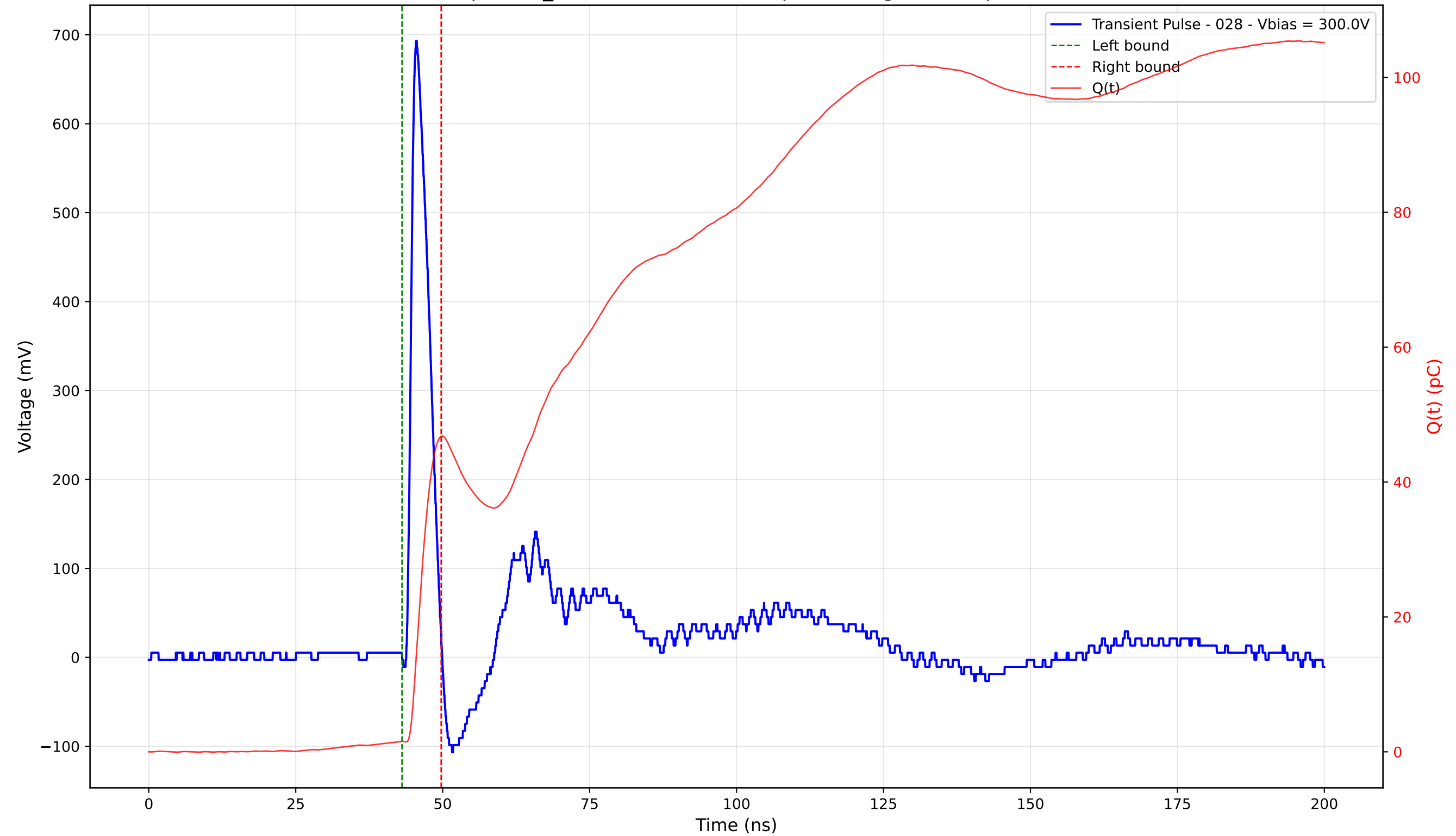
Transient Pulse - Sample: TD_4004 - Position: 335.0 \mu\text{m} - Charge: 45.22 pC - Rise Time: 1.01 ns
