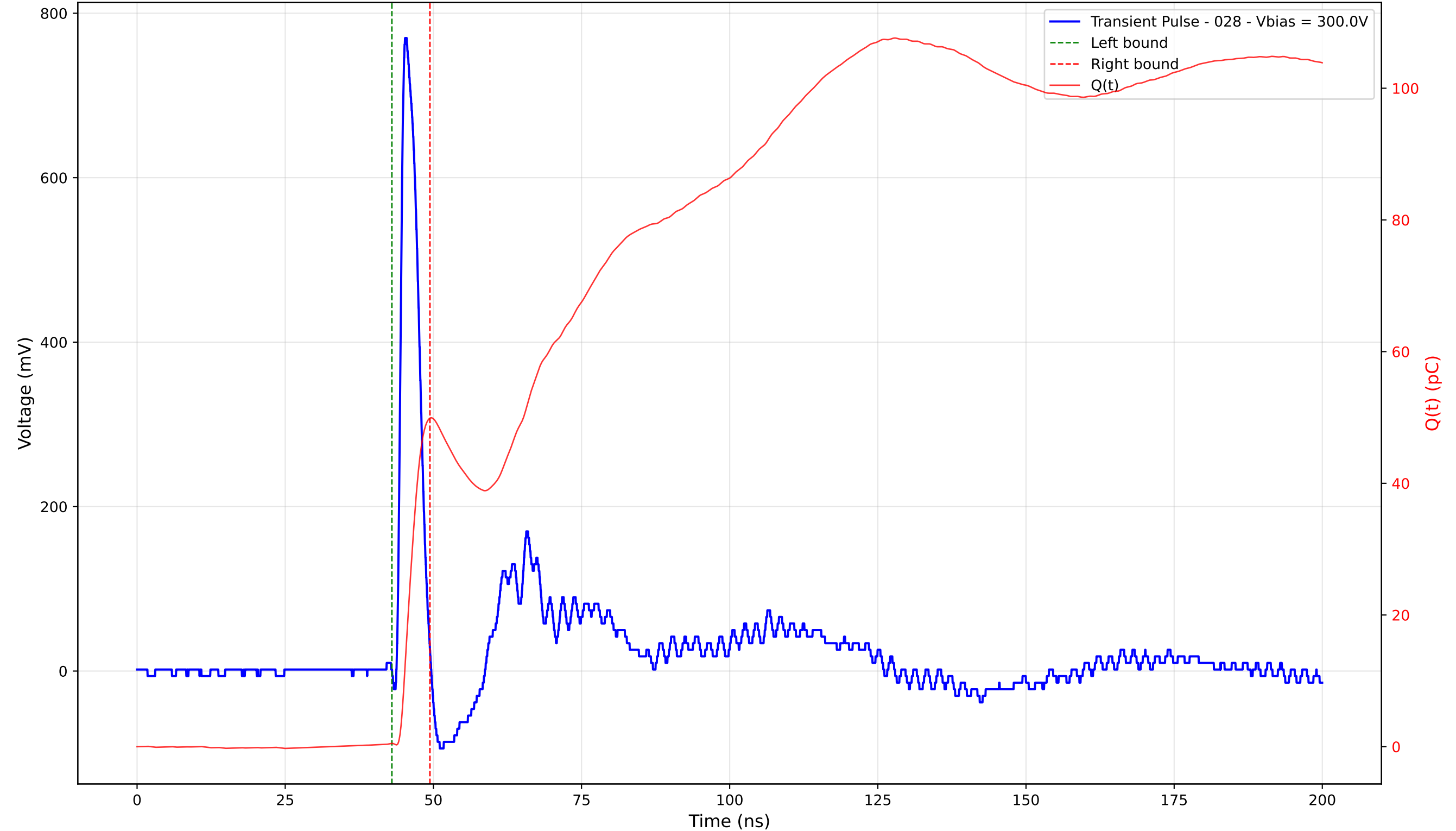
Transient Pulse - Sample: TD_4004 - Position: 280.0 \mu\text{m} - Charge: 49.40 pC - Rise Time: 0.91 ns
