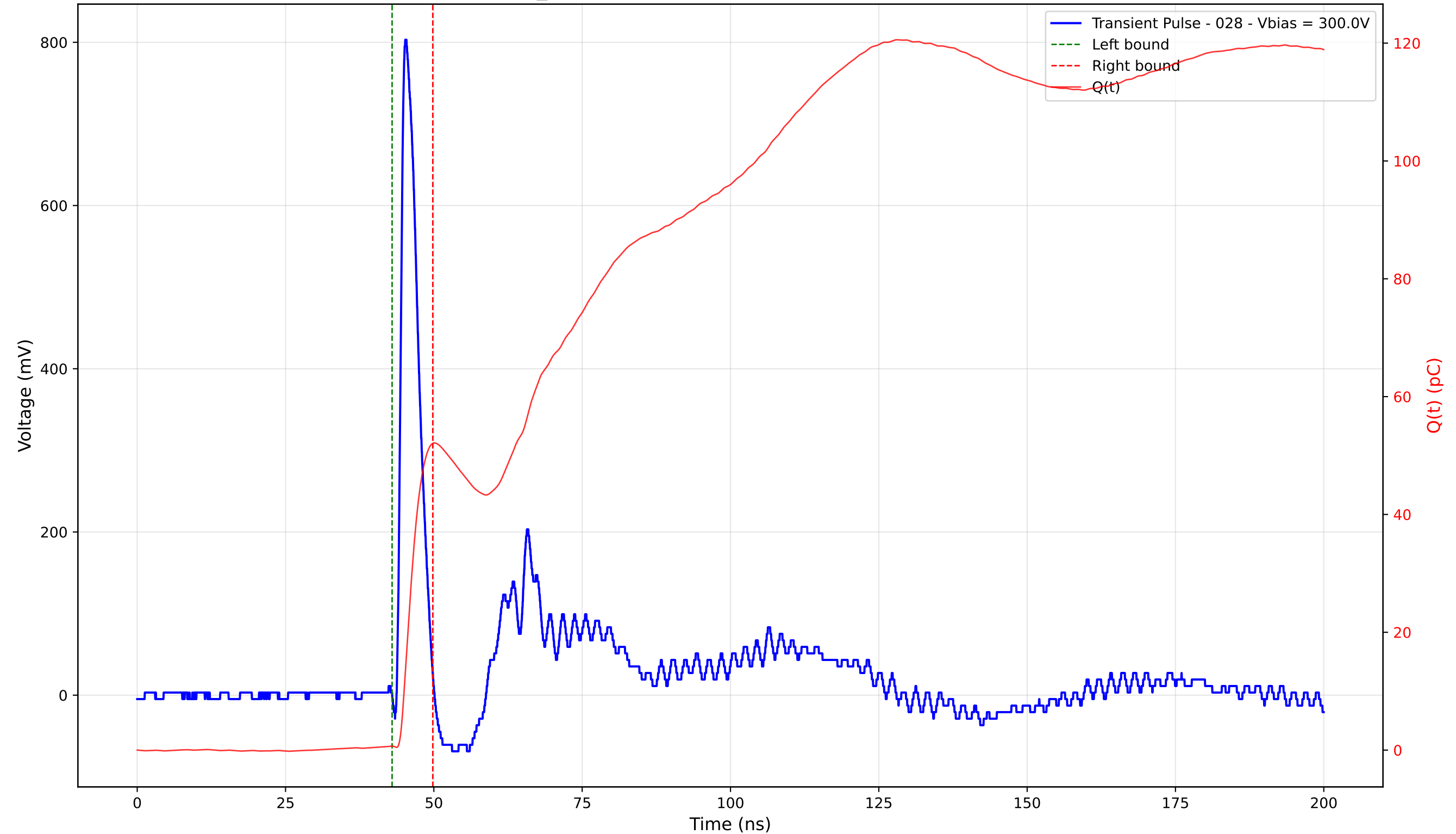
Transient Pulse - Sample: TD_4004 - Position: 180.0 \mu\text{m} - Charge: 51.39 pC - Rise Time: 0.89 ns
