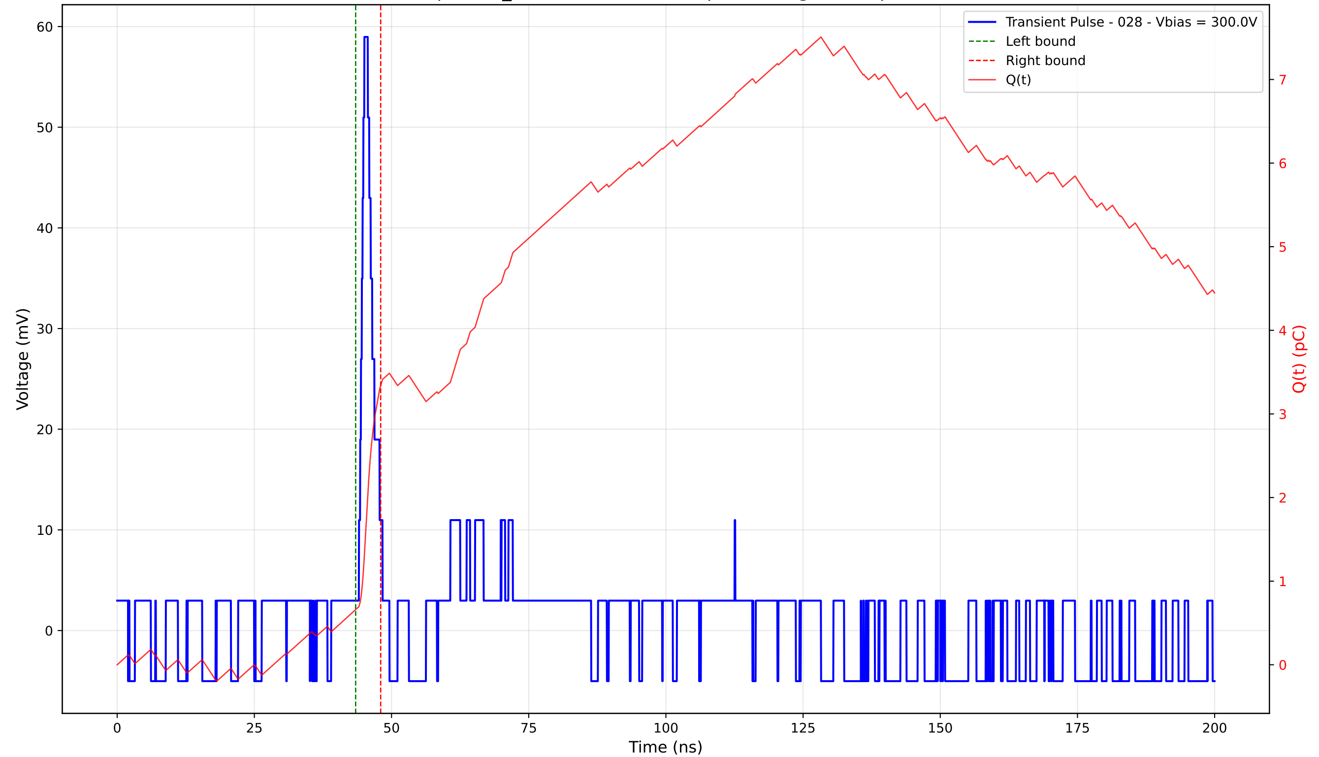
Transient Pulse - Sample: TD_4004 - Position: 40.0 \mu\text{m} - Charge: 2.68 pC - Rise Time: 0.99 ns
