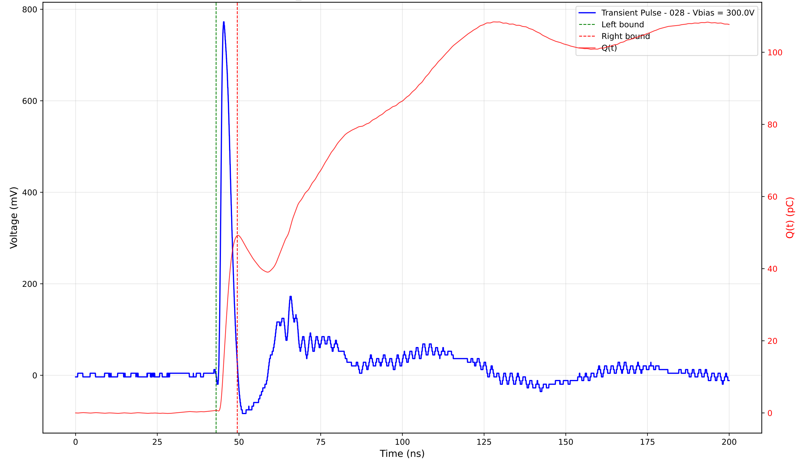
Transient Pulse - Sample: TD_4004 - Position: 240.0 \mu\text{m} - Charge: 48.46 pC - Rise Time: 0.93 ns
