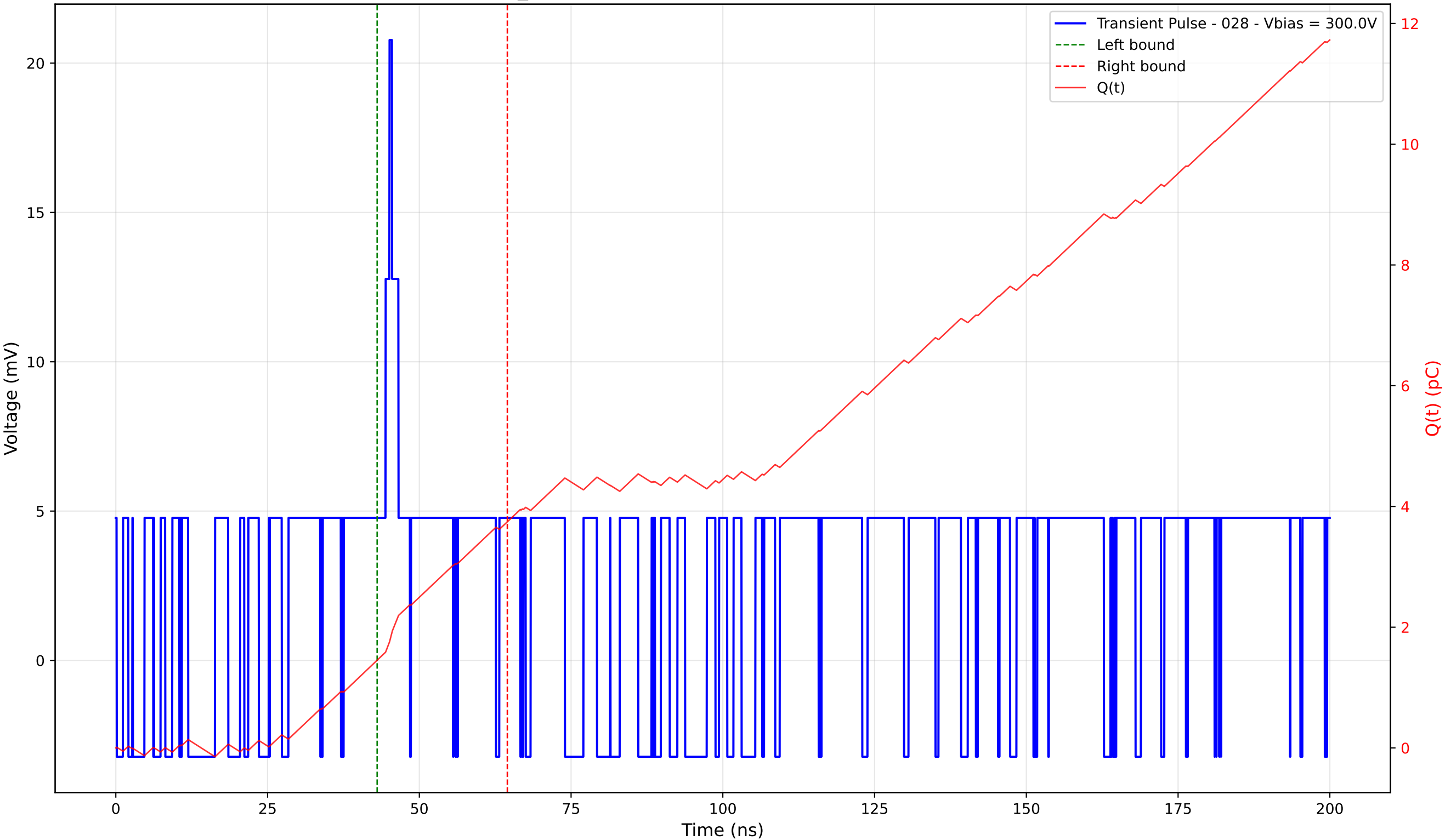
Transient Pulse - Sample: TD_4004 - Position: 0.0 \mu\text{m} - Charge: 2.29 pC - Rise Time: 0.00 ns (N/A)
