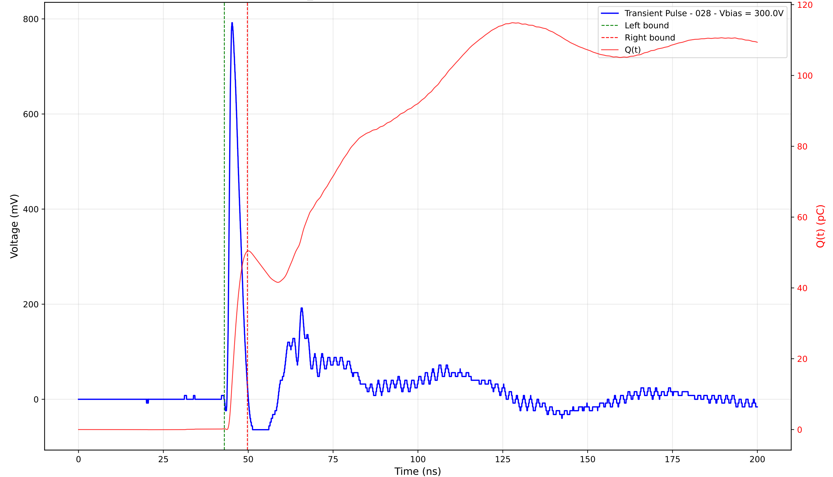
Transient Pulse - Sample: TD_4004 - Position: 120.0 \mu\text{m} - Charge: 50.15 pC - Rise Time: 0.90 ns
