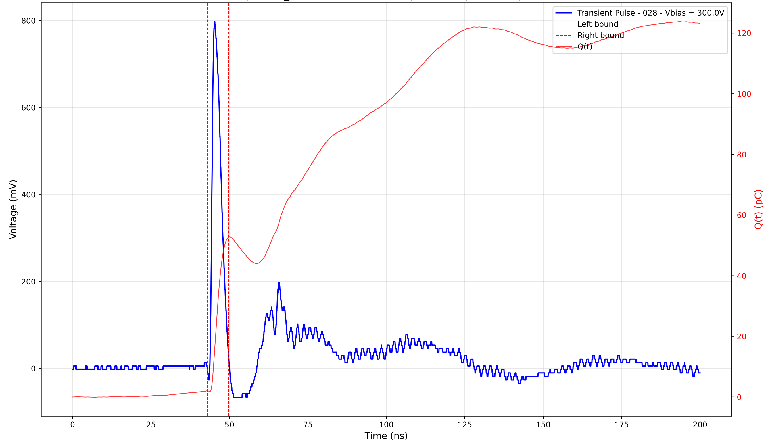
Transient Pulse - Sample: TD_4004 - Position: 205.0 \mu\text{m} - Charge: 50.68 pC - Rise Time: 0.91 ns
