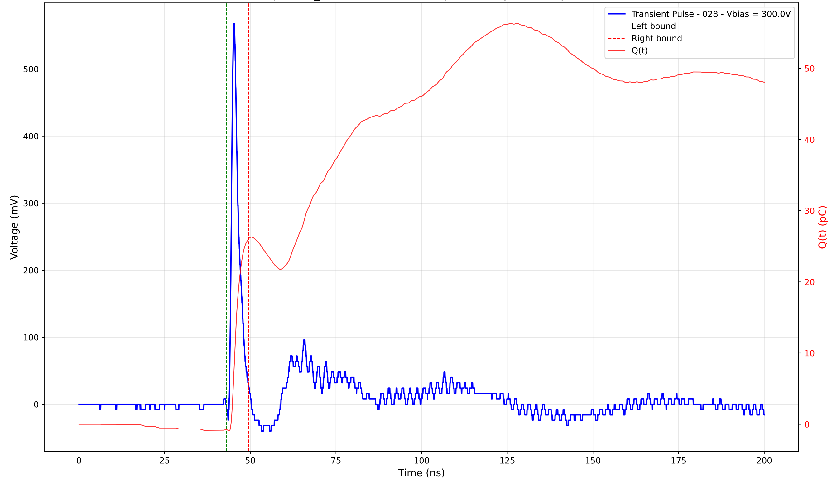
Transient Pulse - Sample: TD_4004 - Position: 70.0 \mu\text{m} - Charge: 26.82 pC - Rise Time: 0.88 ns
