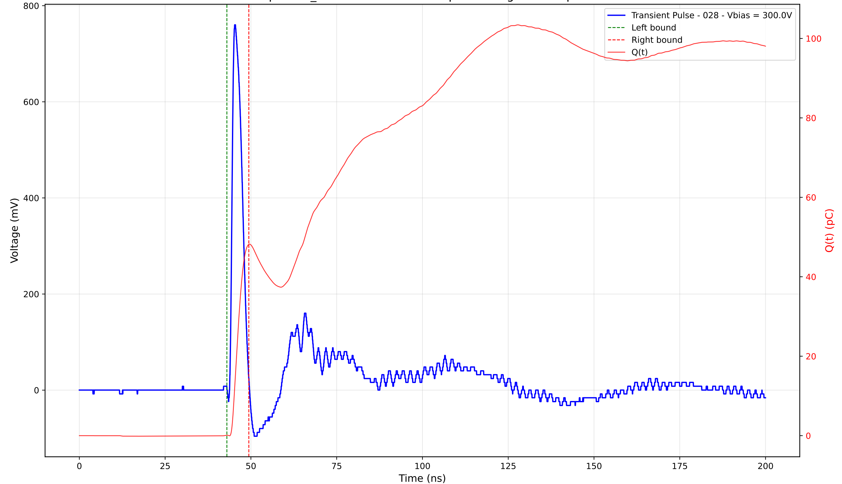
Transient Pulse - Sample: TD_4004 - Position: 260.0 \mu\text{m} - Charge: 48.04 pC - Rise Time: 0.92 ns
