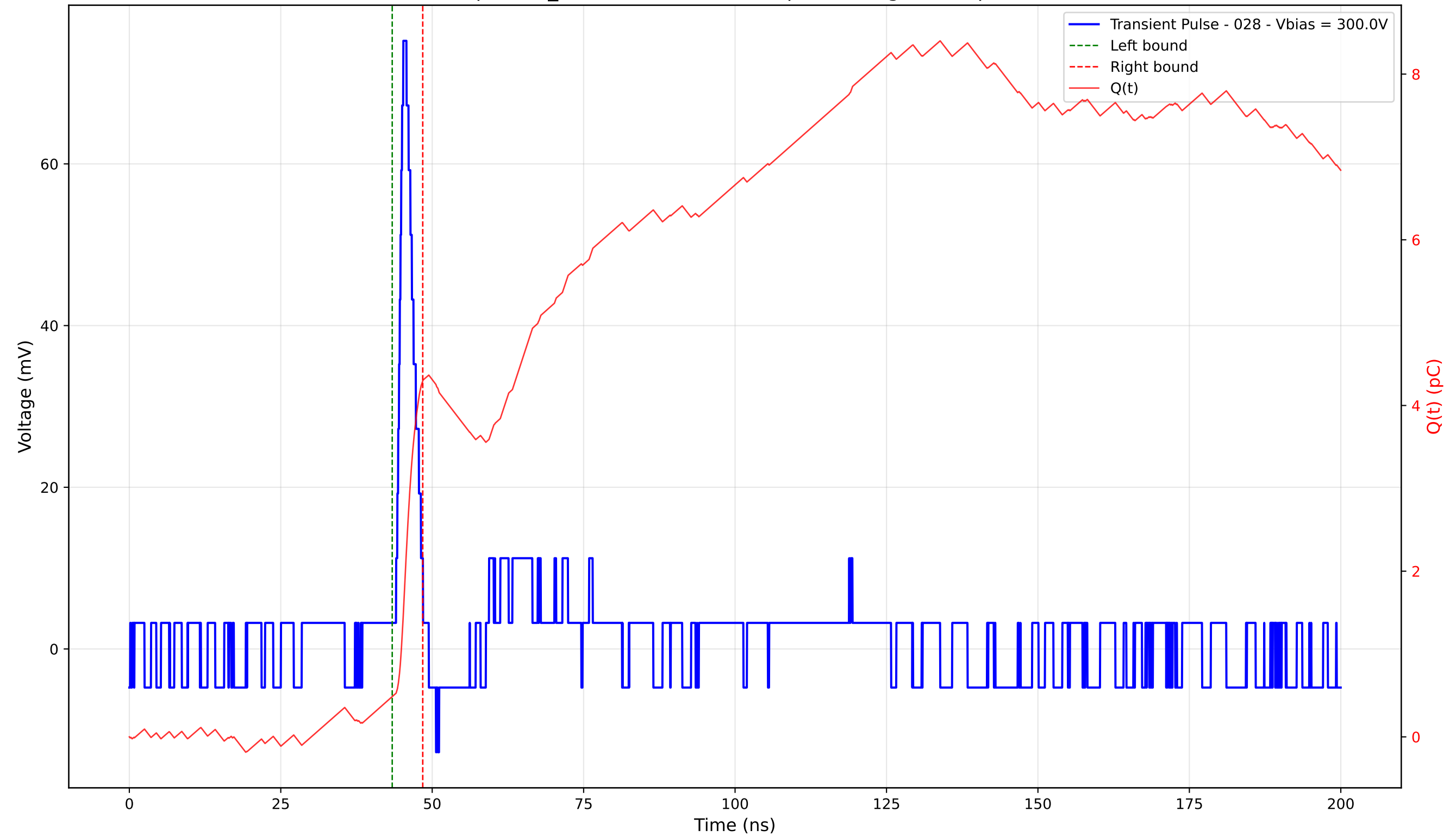
Transient Pulse - Sample: TD_4004 - Position: 435.0 \mu\text{m} - Charge: 3.81 pC - Rise Time: 1.19 ns
