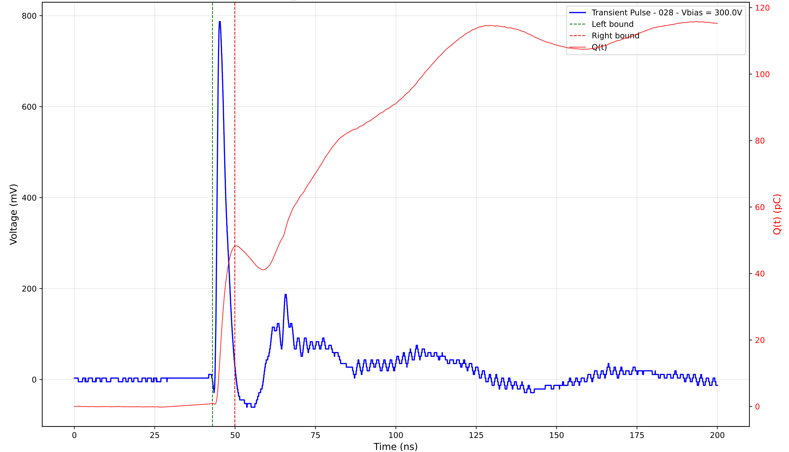
Transient Pulse - Sample: TD_4004 - Position: 100.0 \mu\text{m} - Charge: 47.27 pC - Rise Time: 0.88 ns
