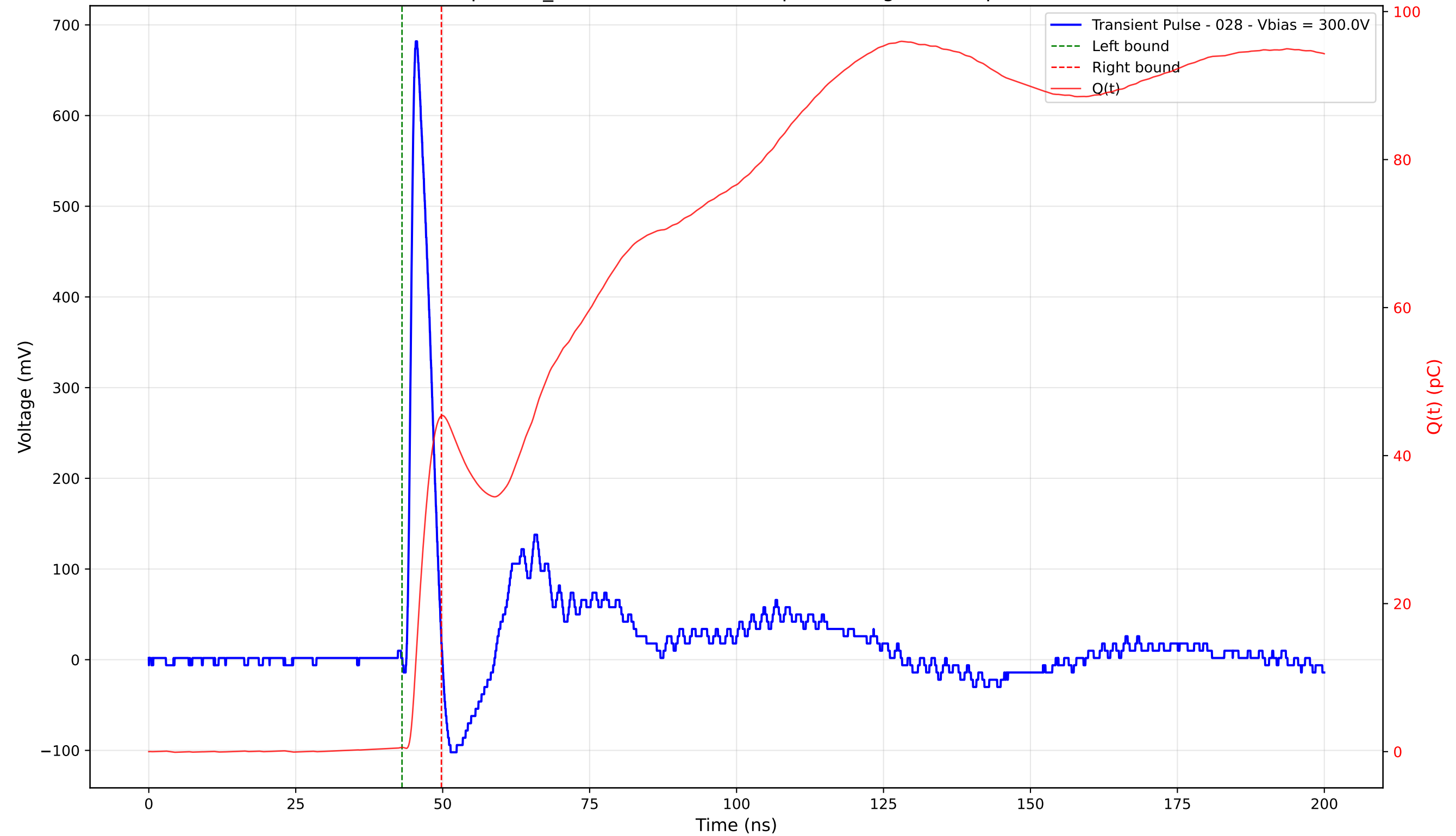
Transient Pulse - Sample: TD_4004 - Position: 350.0 \mu\text{m} - Charge: 44.81 pC - Rise Time: 0.99 ns
