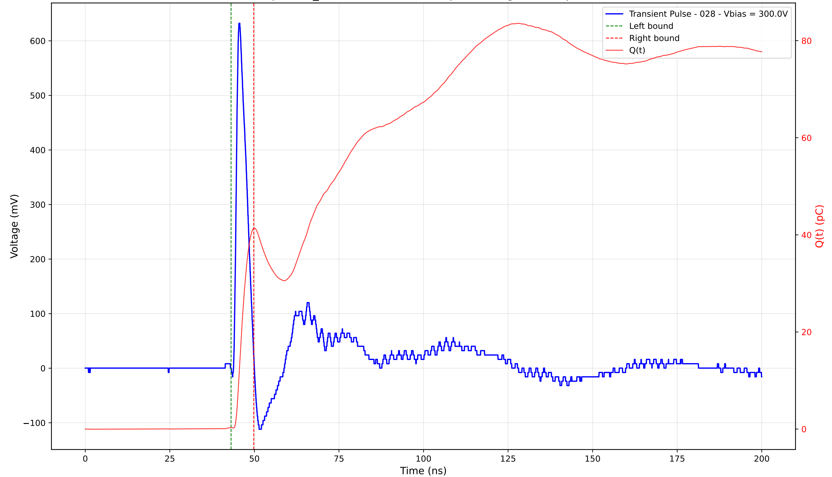
Transient Pulse - Sample: TD_4004 - Position: 380.0 \mu\text{m} - Charge: 41.05 pC - Rise Time: 1.02 ns
