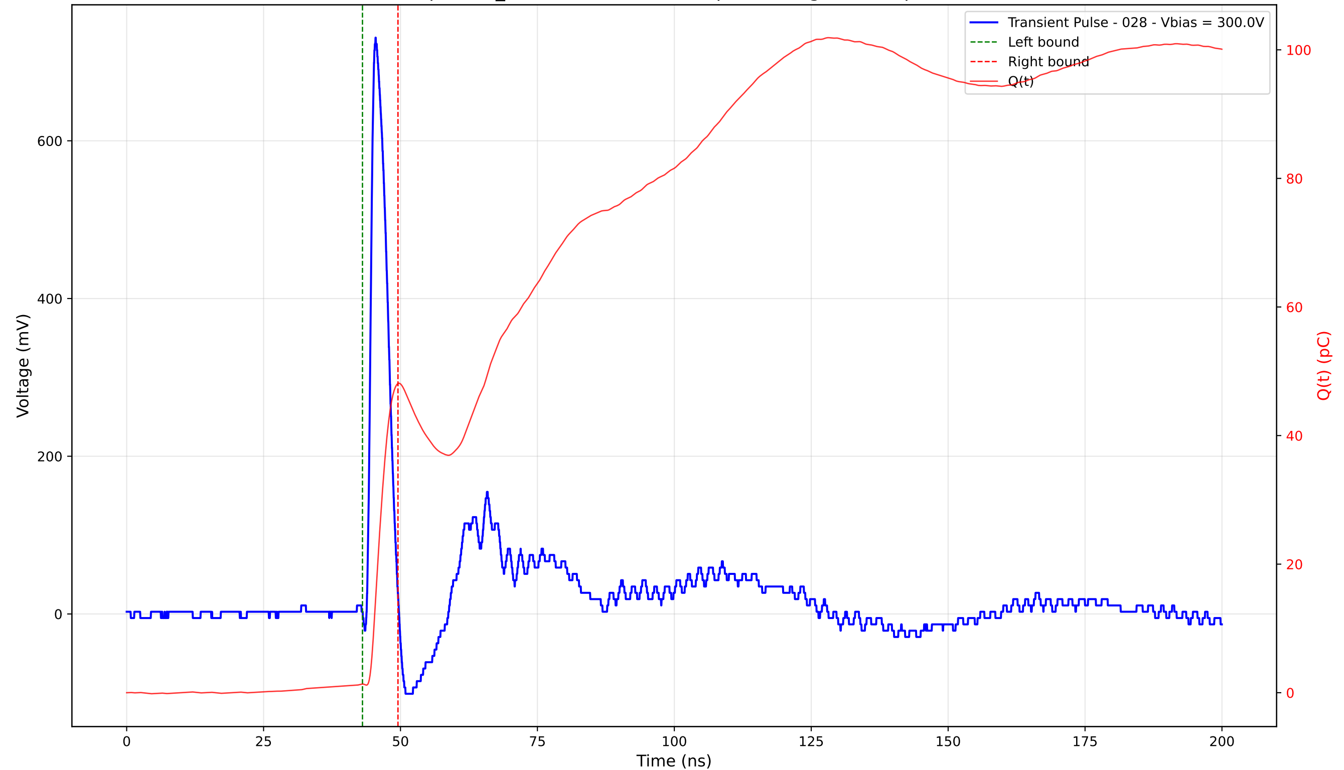
Transient Pulse - Sample: TD_4004 - Position: 325.0 \mu\text{m} - Charge: 46.75 pC - Rise Time: 0.98 ns
