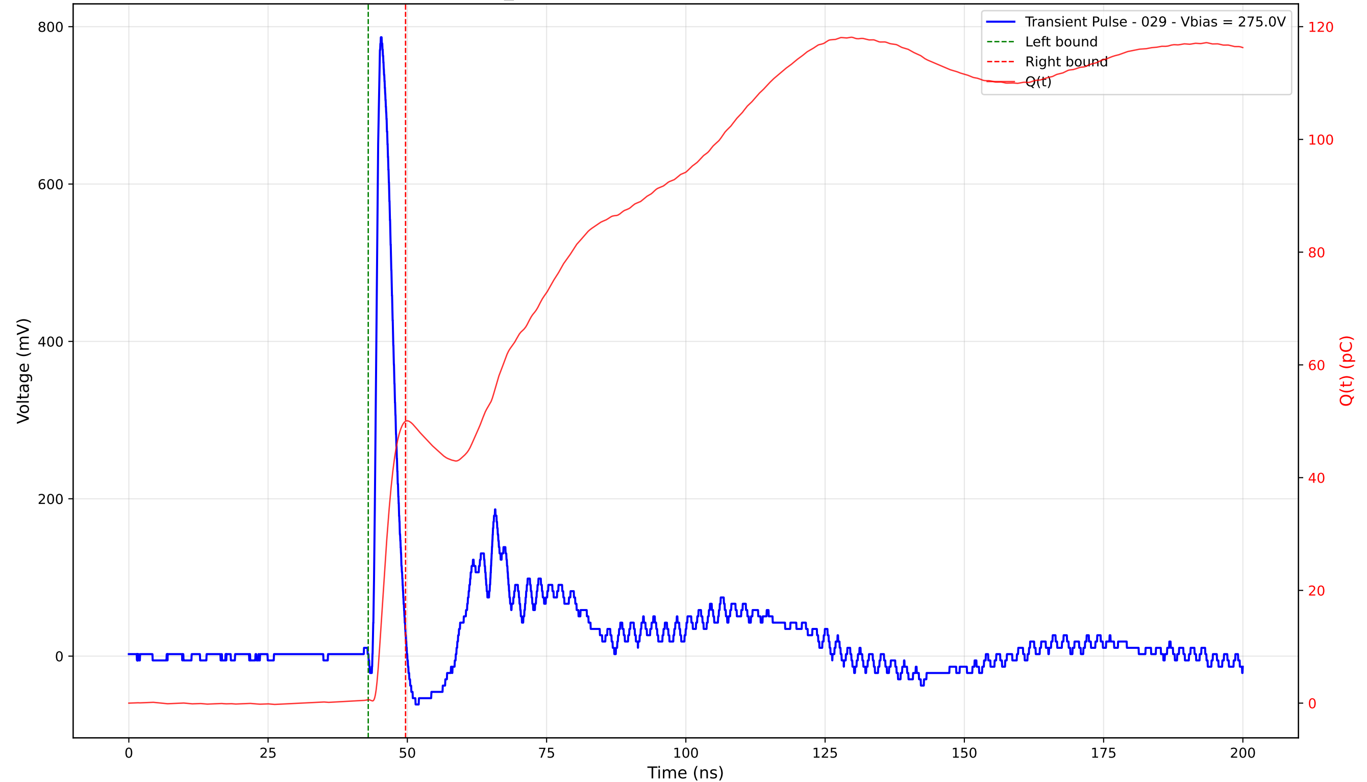
Transient Pulse - Sample: TD_4004 - Position: 210.0 \mu\text{m} - Charge: 49.40 pC - Rise Time: 0.91 ns
