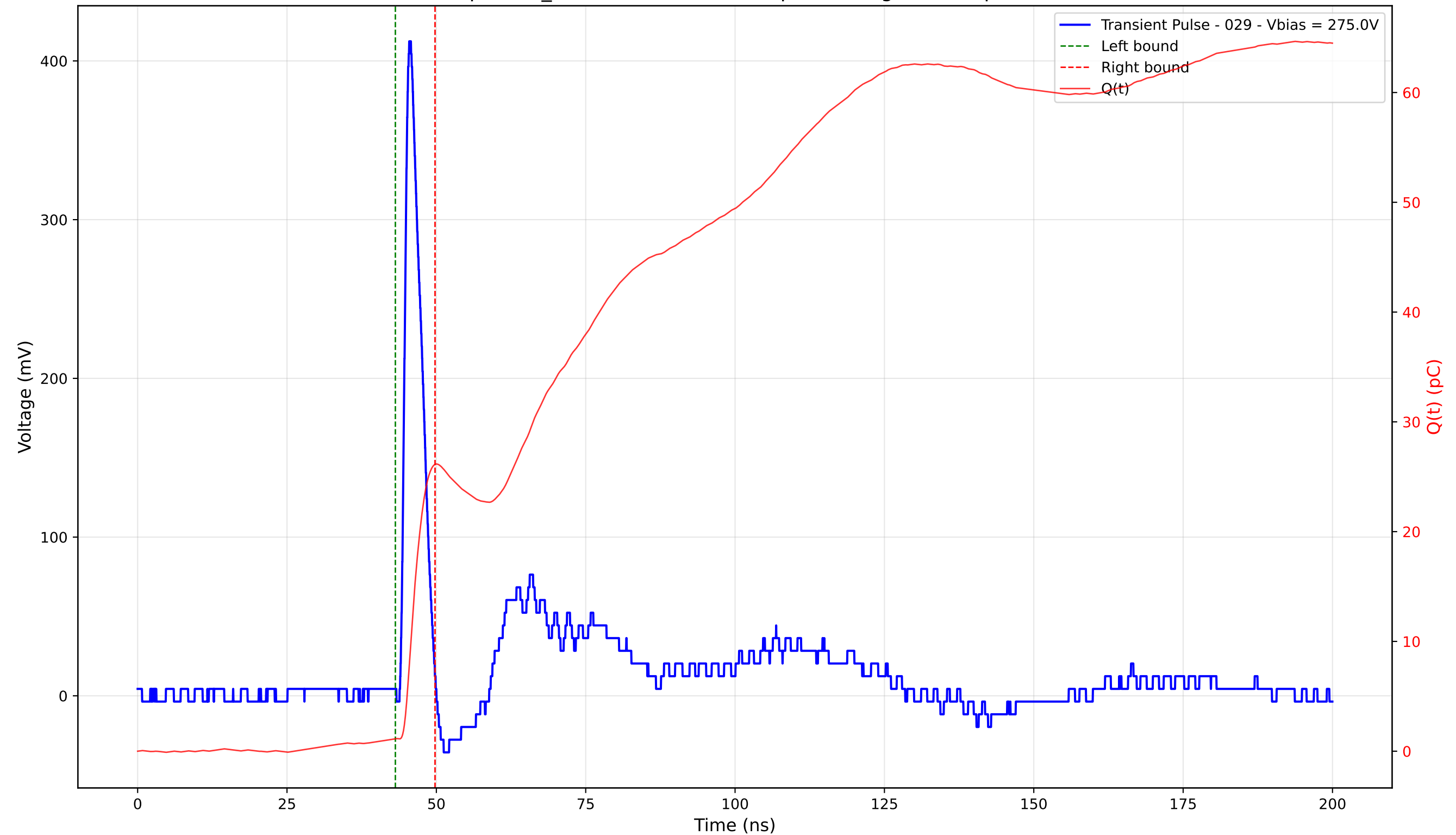
Transient Pulse - Sample: TD_4004 - Position: 395.0 \mu\text{m} - Charge: 24.99 pC - Rise Time: 1.03 ns
