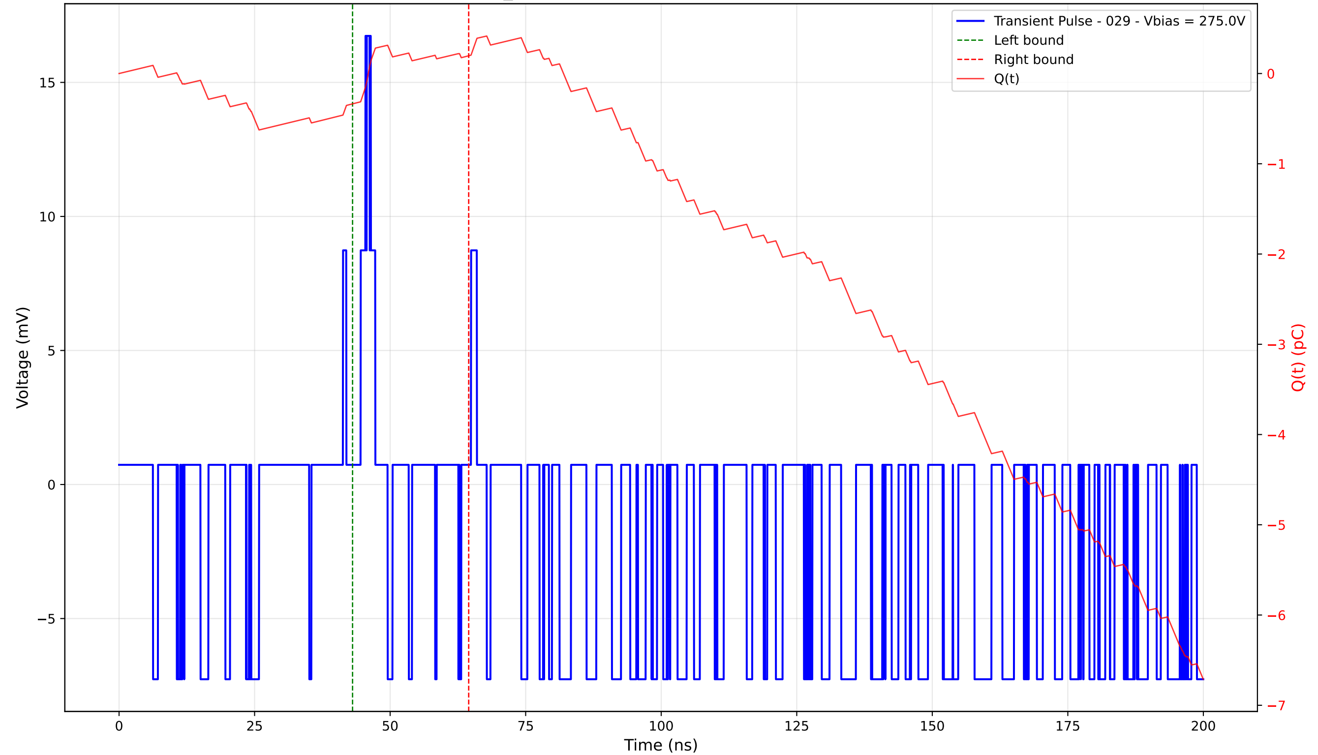
Transient Pulse - Sample: TD_4004 - Position: 5.0 \mu\text{m} - Charge: 0.53 pC - Rise Time: 0.90 ns
