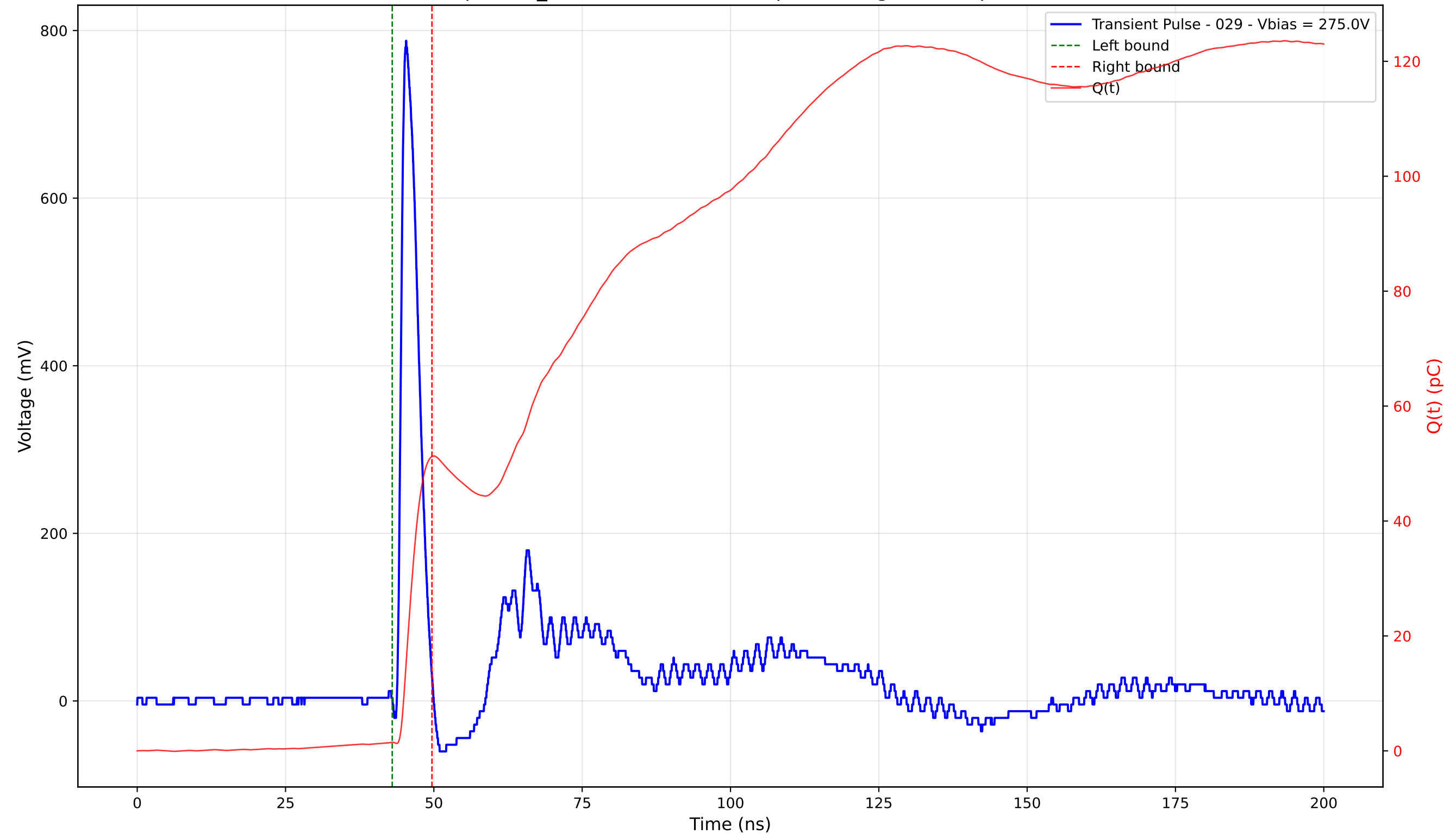
Transient Pulse - Sample: TD_4004 - Position: 165.0 \mu\text{m} - Charge: 49.74 pC - Rise Time: 0.92 ns
