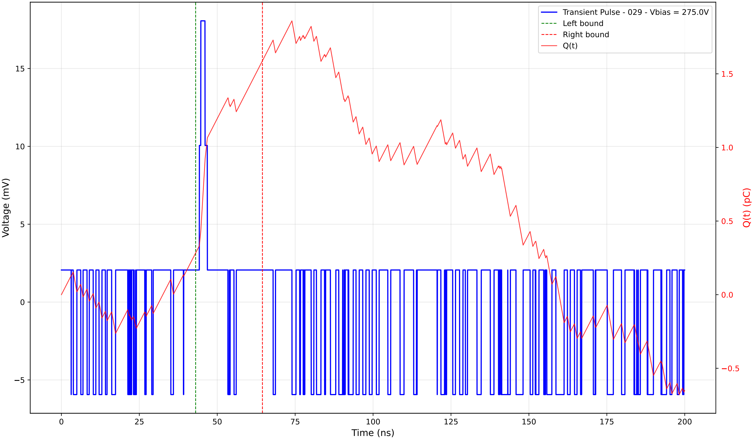
Transient Pulse - Sample: TD_4004 - Position: 15.0 \mu\text{m} - Charge: 1.30 pC - Rise Time: 0.00 ns (N/A)
