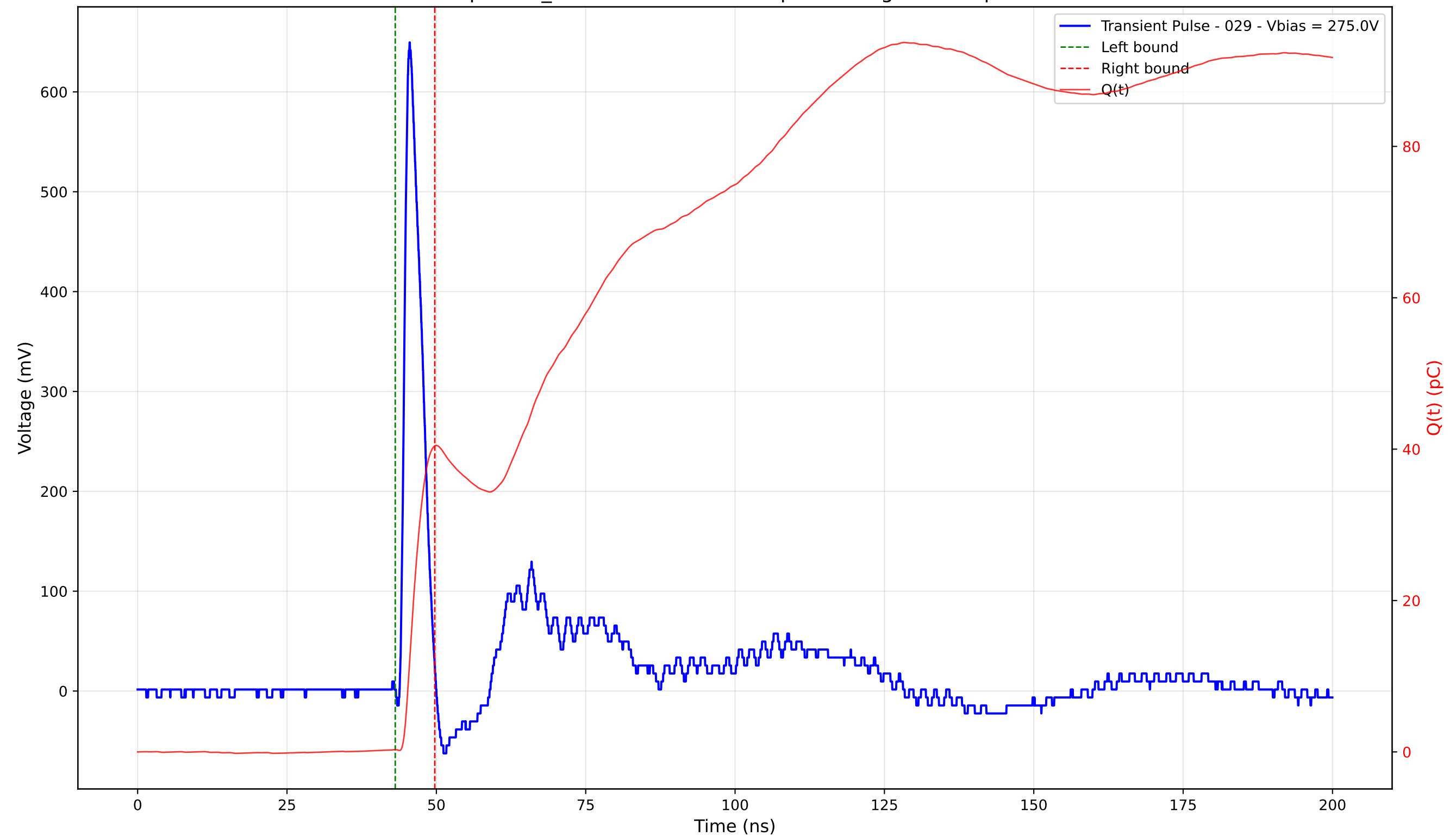
Transient Pulse - Sample: TD_4004 - Position: 345.0 \mu\text{m} - Charge: 40.13 pC - Rise Time: 1.00 ns
