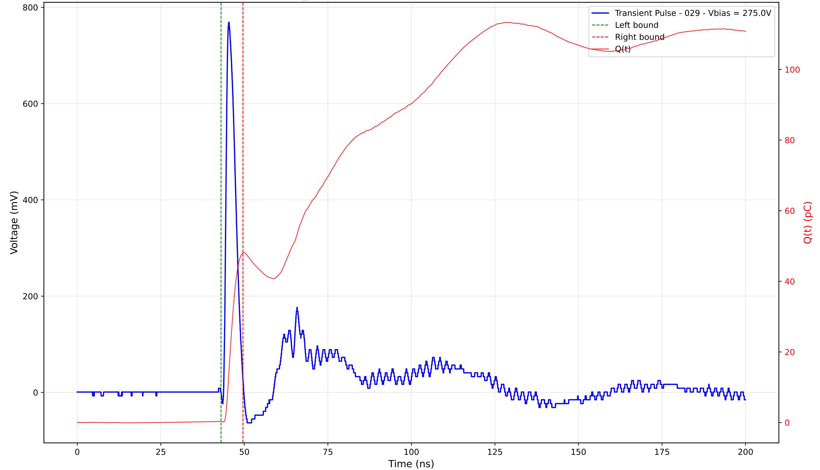
Transient Pulse - Sample: TD_4004 - Position: 145.0 \mu\text{m} - Charge: 47.67 pC - Rise Time: 0.92 ns
