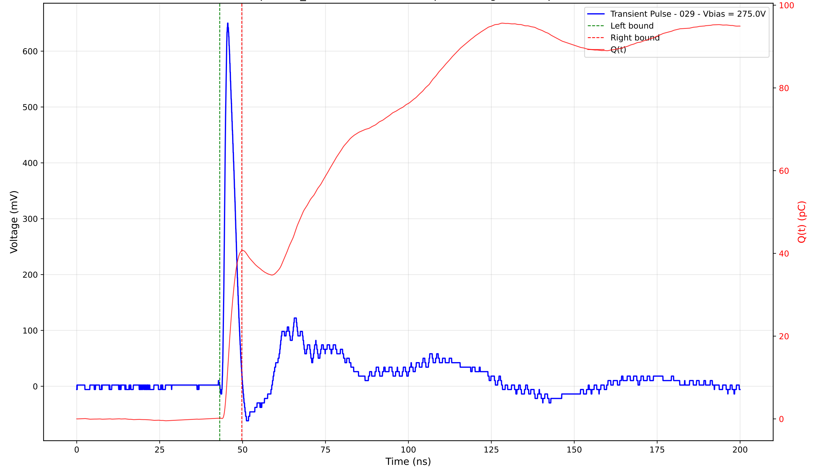
Transient Pulse - Sample: TD_4004 - Position: 340.0 \mu\text{m} - Charge: 40.47 pC - Rise Time: 1.02 ns
