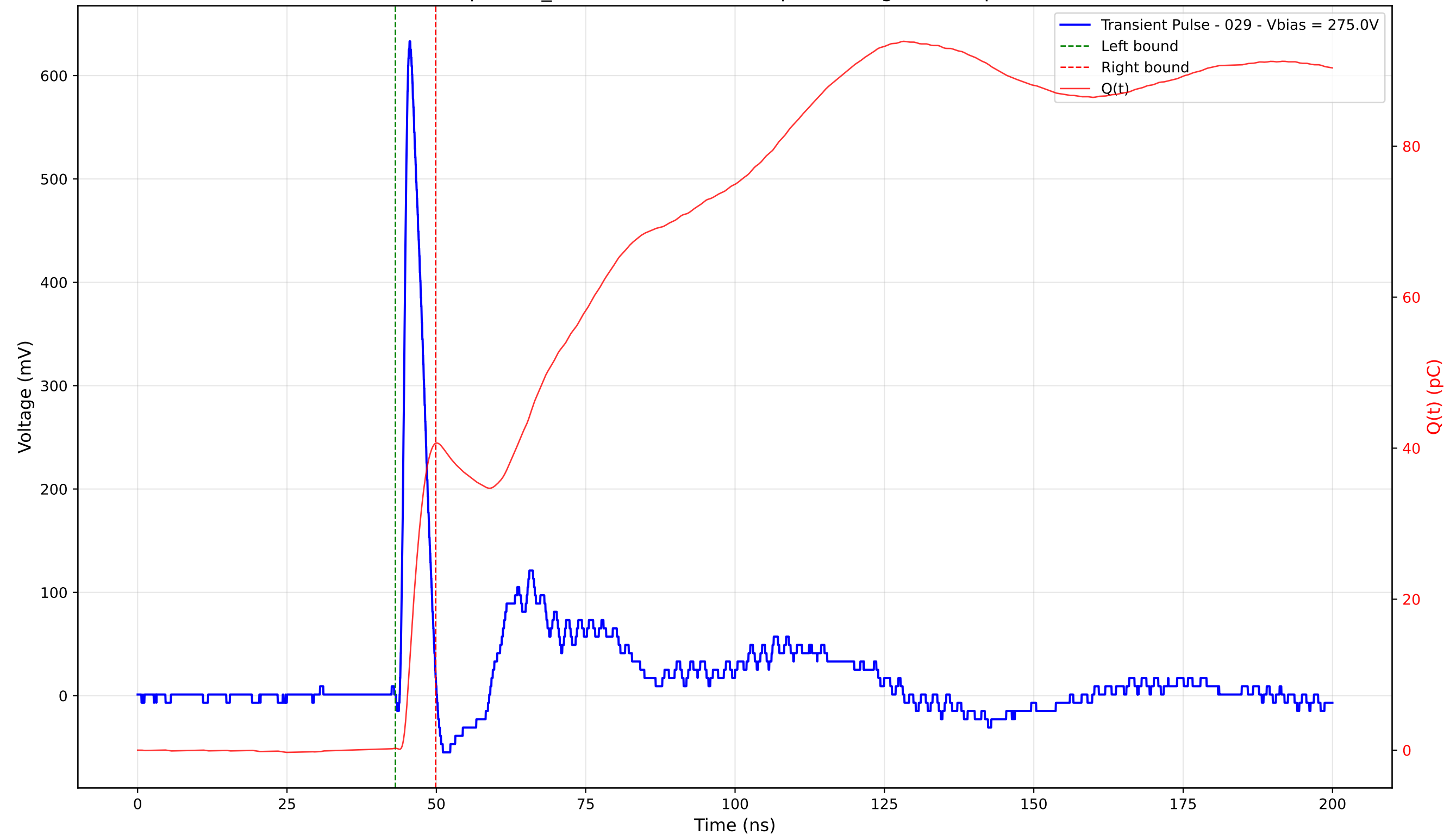
Transient Pulse - Sample: TD_4004 - Position: 360.0 \mu\text{m} - Charge: 40.40 pC - Rise Time: 1.03 ns
