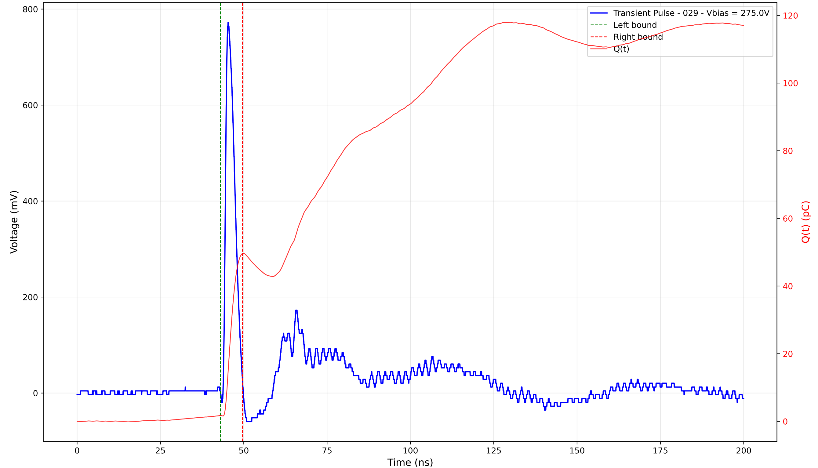
Transient Pulse - Sample: TD_4004 - Position: 150.0 \mu\text{m} - Charge: 47.86 pC - Rise Time: 0.93 ns
