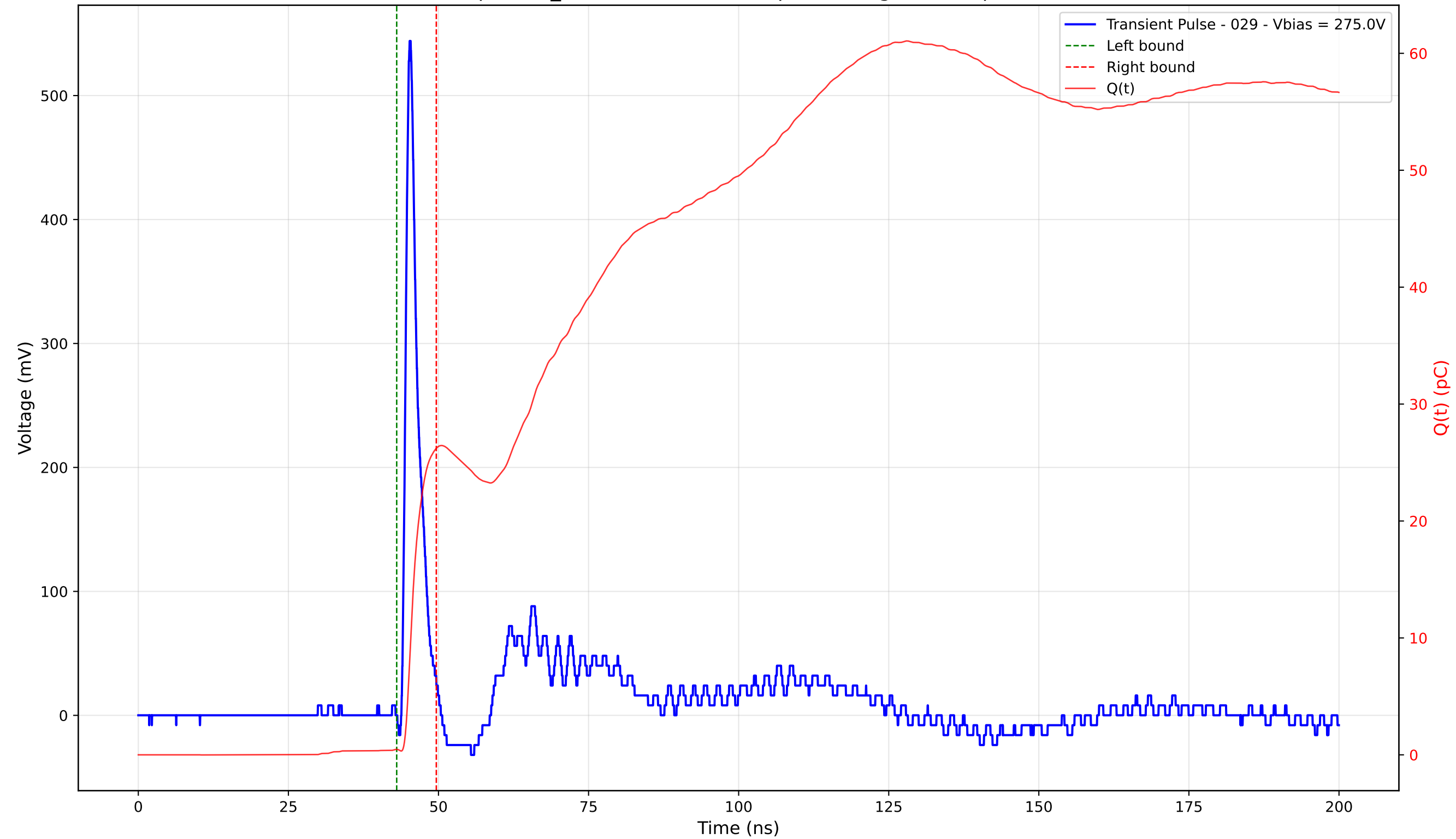
Transient Pulse - Sample: TD_4004 - Position: 70.0 \mu\text{m} - Charge: 25.76 pC - Rise Time: 0.91 ns
