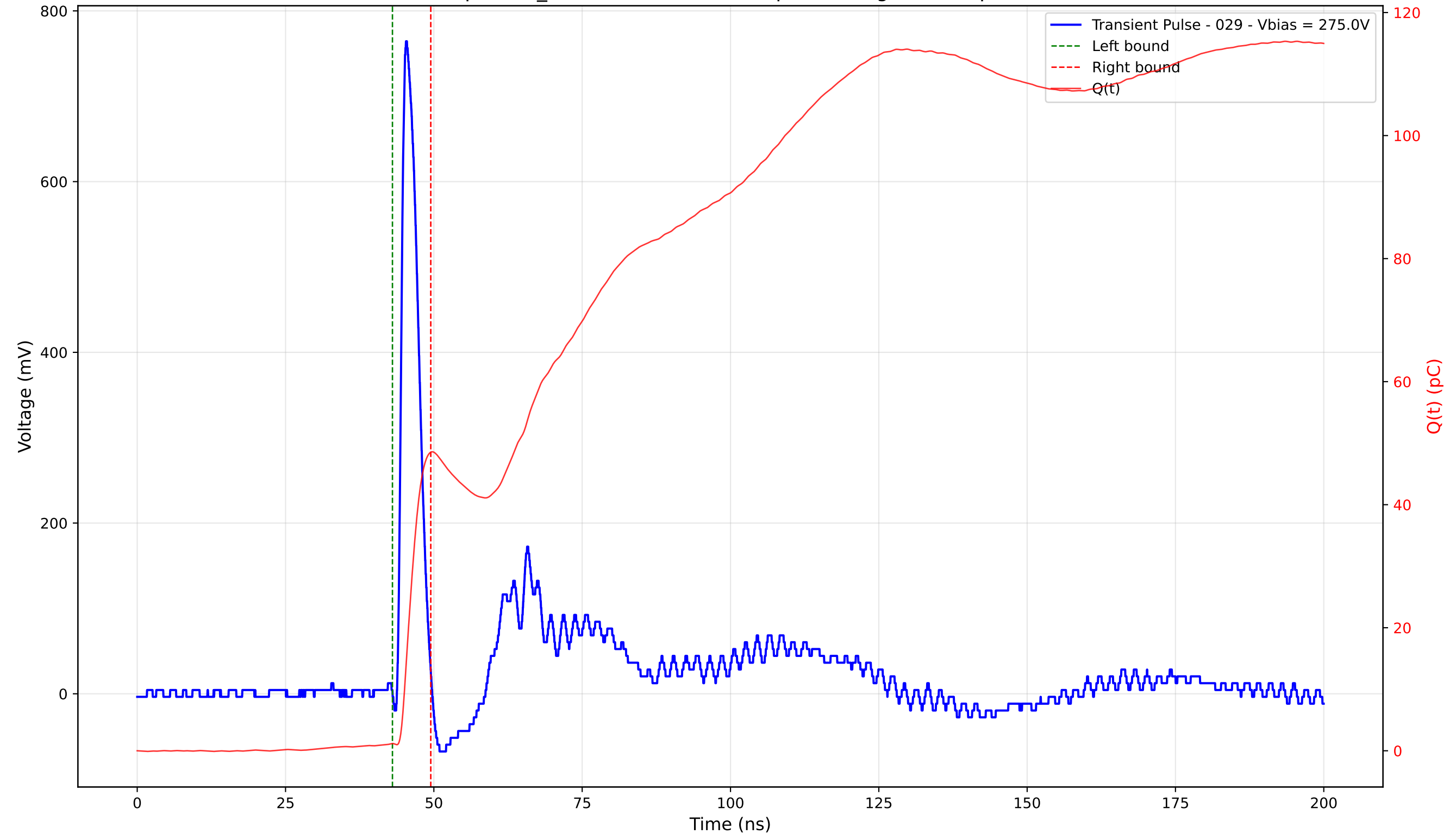
Transient Pulse - Sample: TD_4004 - Position: 245.0 \mu\text{m} - Charge: 47.36 pC - Rise Time: 0.93 ns
