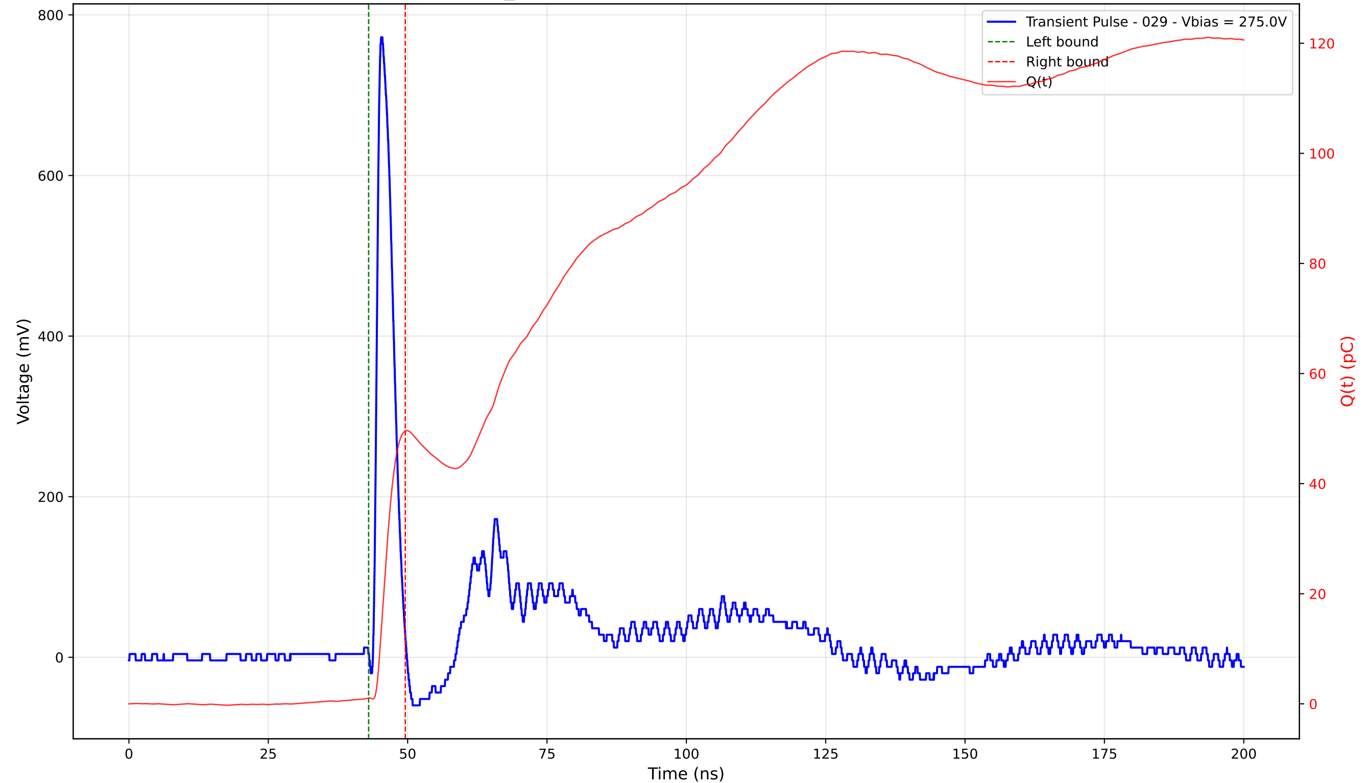
Transient Pulse - Sample: TD_4004 - Position: 230.0 \mu\text{m} - Charge: 48.52 pC - Rise Time: 0.90 ns
