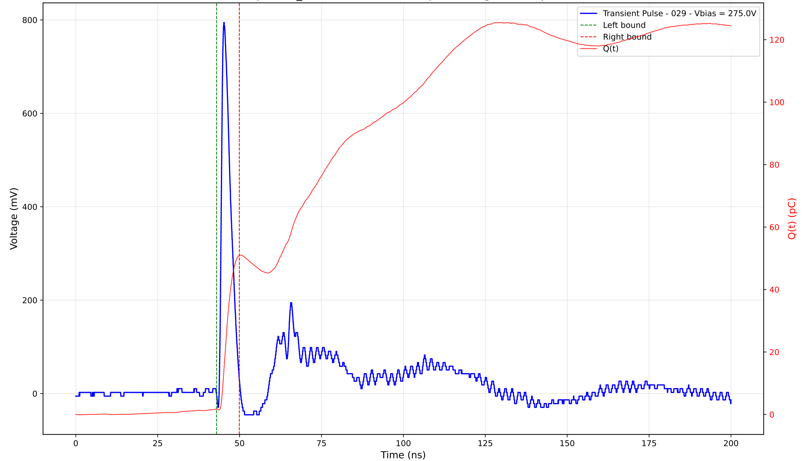
Transient Pulse - Sample: TD_4004 - Position: 115.0 \mu\text{m} - Charge: 49.19 pC - Rise Time: 0.87 ns
