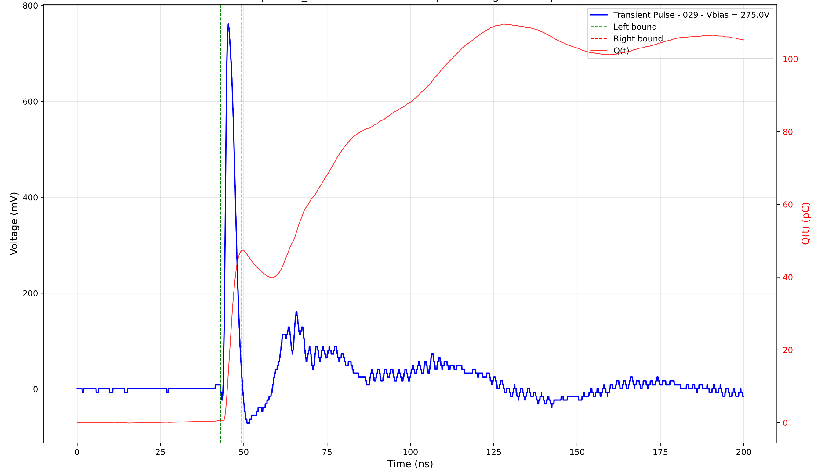
Transient Pulse - Sample: TD_4004 - Position: 255.0 \mu\text{m} - Charge: 46.67 pC - Rise Time: 0.92 ns
