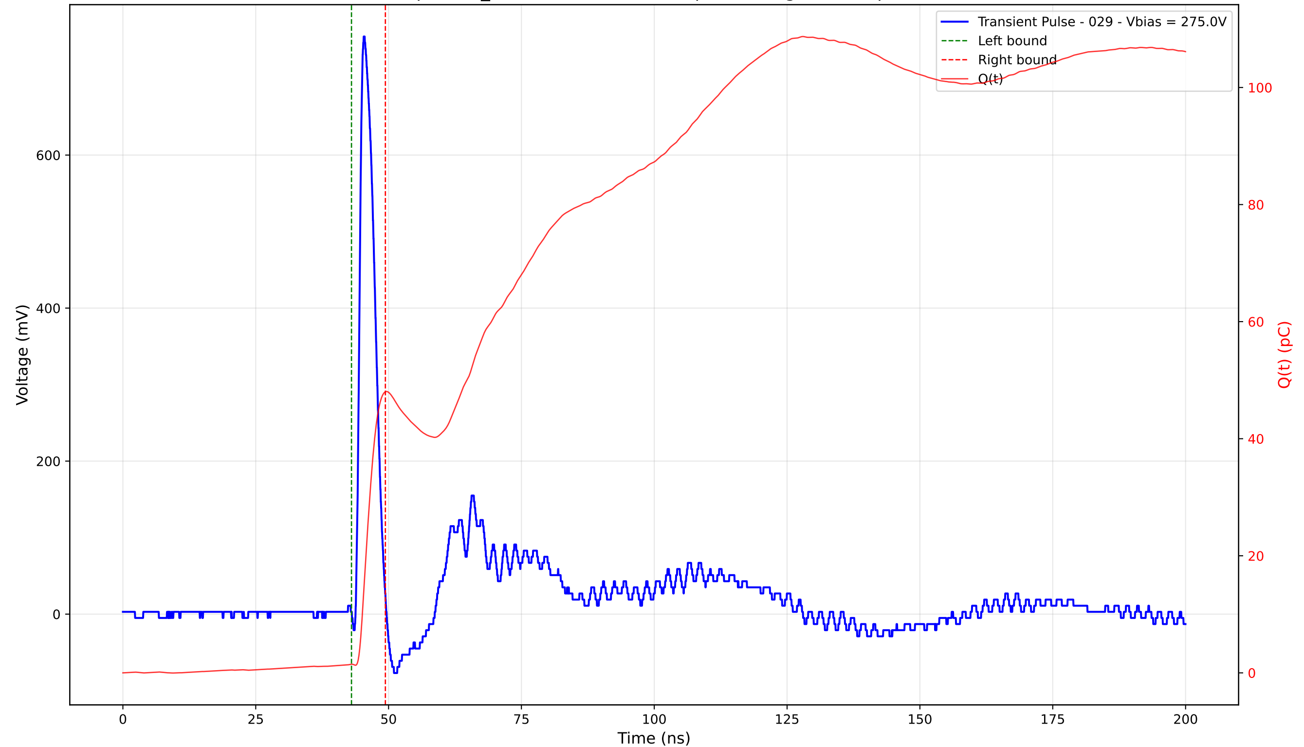
Transient Pulse - Sample: TD_4004 - Position: 260.0 \mu\text{m} - Charge: 46.54 pC - Rise Time: 0.95 ns
