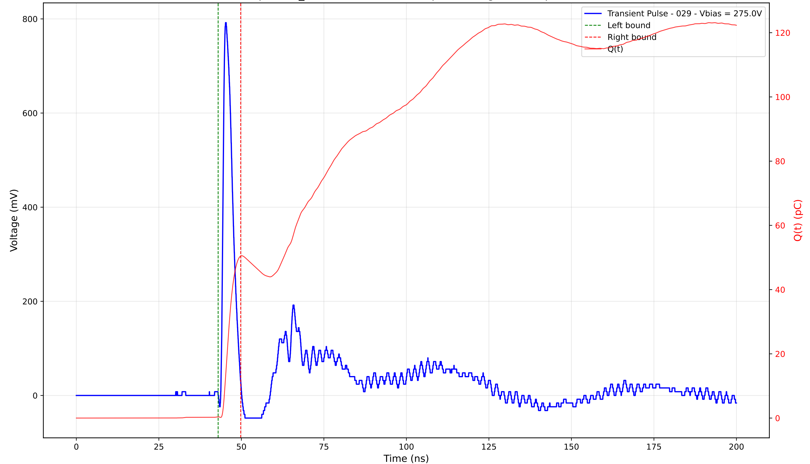
Transient Pulse - Sample: TD_4004 - Position: 200.0 \mu\text{m} - Charge: 50.07 pC - Rise Time: 0.90 ns
