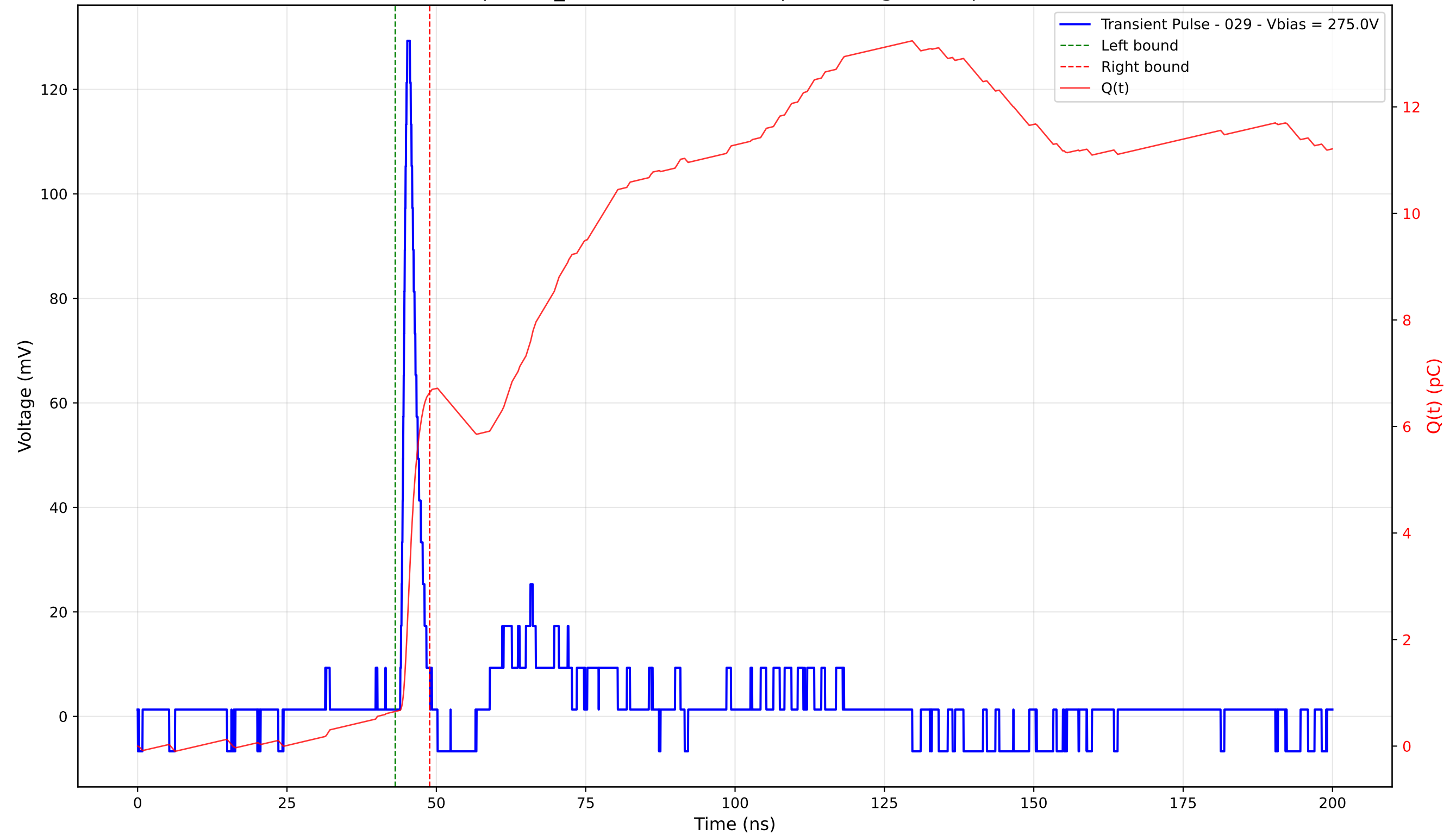
Transient Pulse - Sample: TD_4004 - Position: 50.0 \mu\text{m} - Charge: 5.99 pC - Rise Time: 0.93 ns
