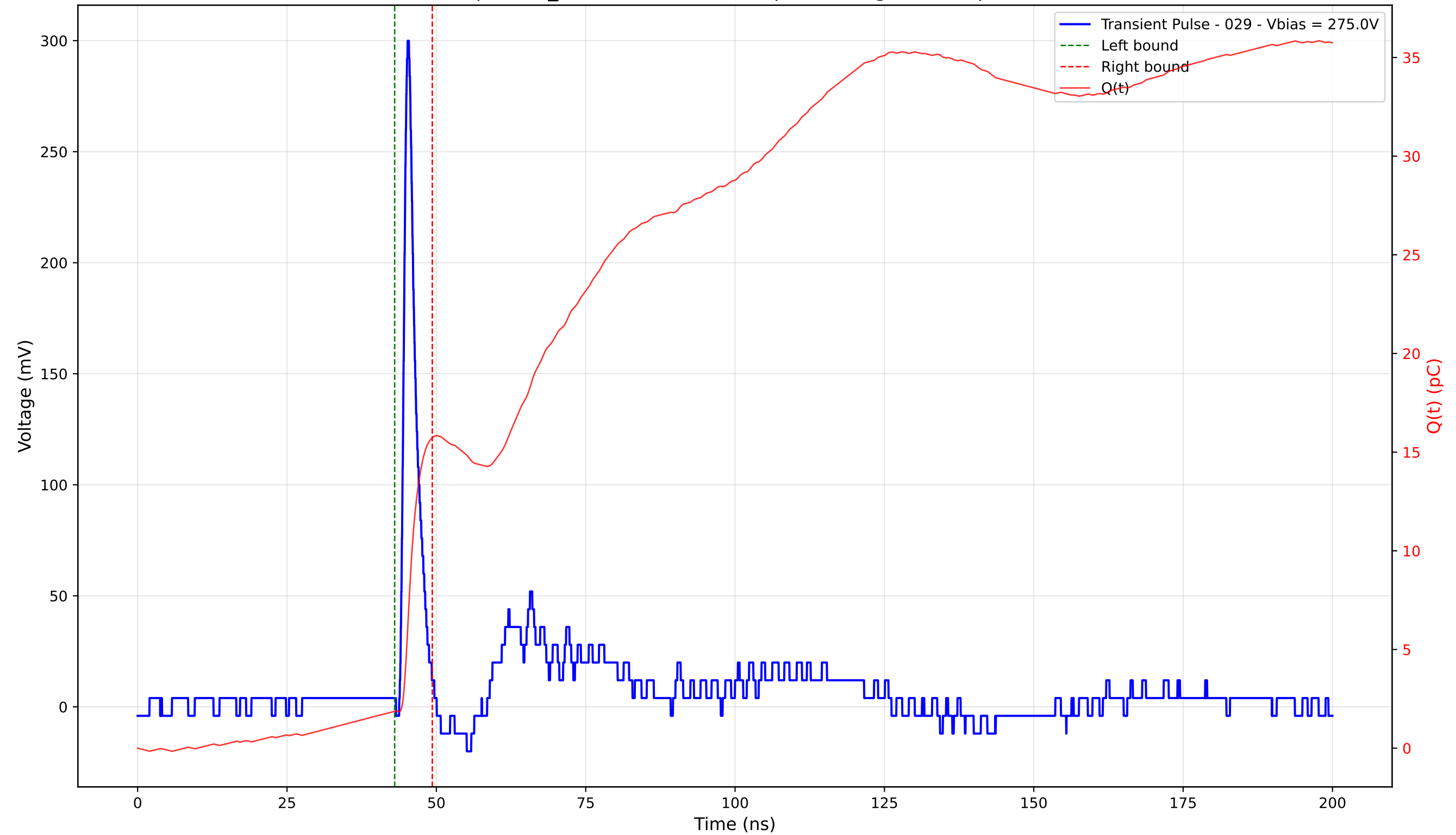
Transient Pulse - Sample: TD_4004 - Position: 60.0 \mu\text{m} - Charge: 13.86 pC - Rise Time: 0.93 ns
