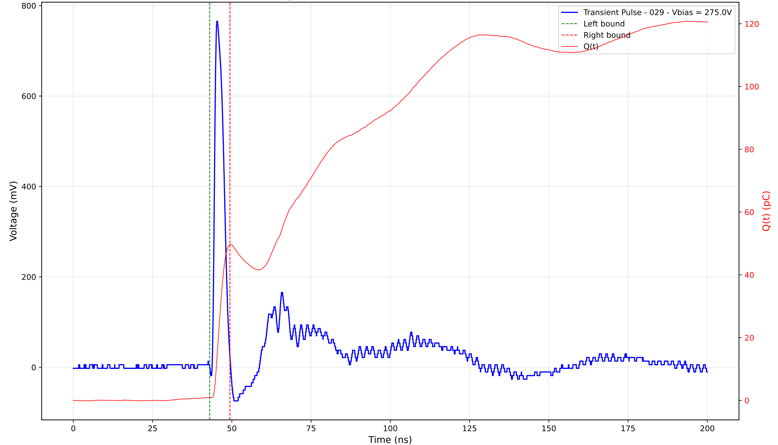
Transient Pulse - Sample: TD_4004 - Position: 285.0 \mu\text{m} - Charge: 48.59 pC - Rise Time: 0.93 ns
