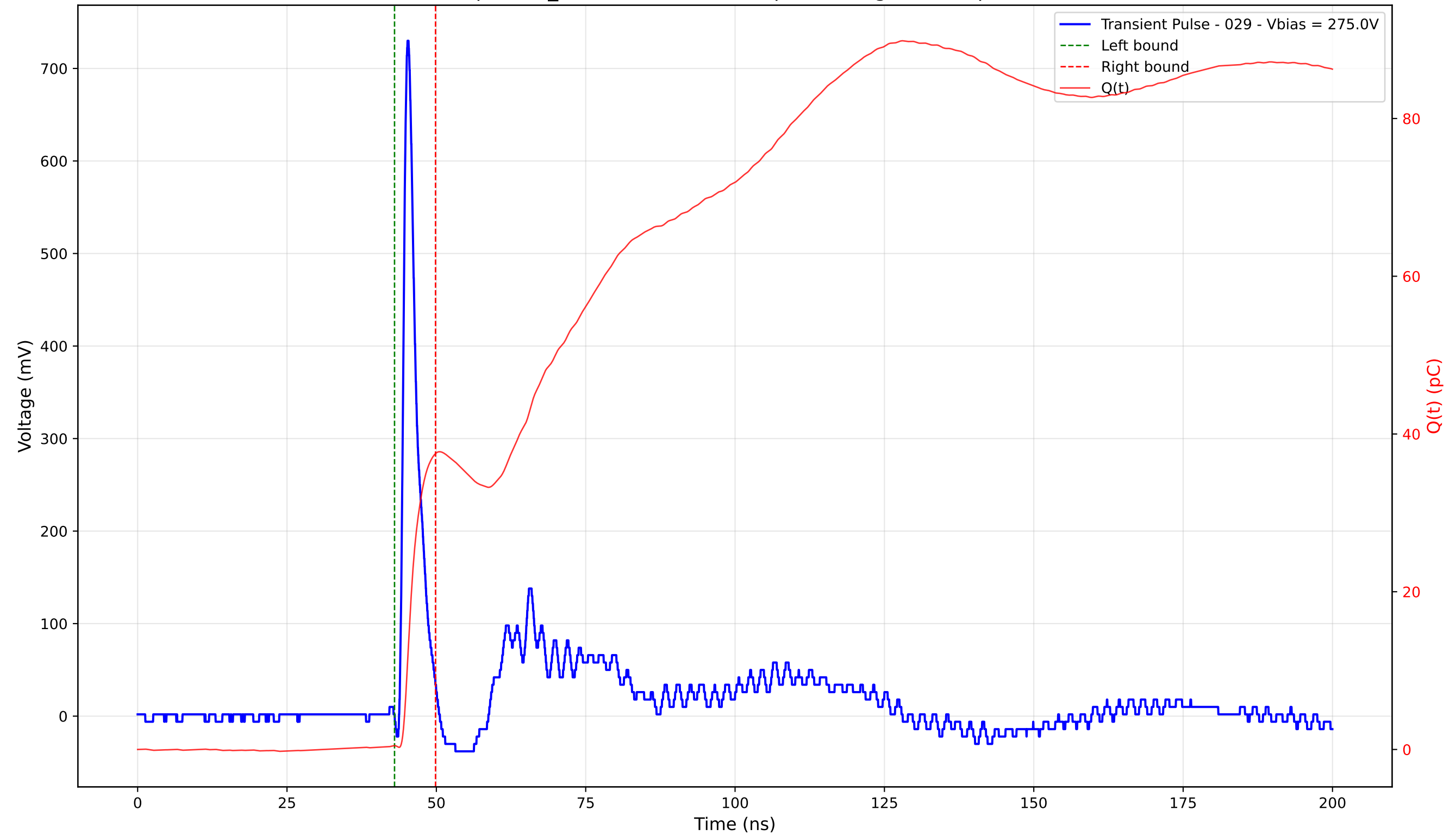
Transient Pulse - Sample: TD_4004 - Position: 85.0 \mu\text{m} - Charge: 37.04 pC - Rise Time: 0.90 ns
