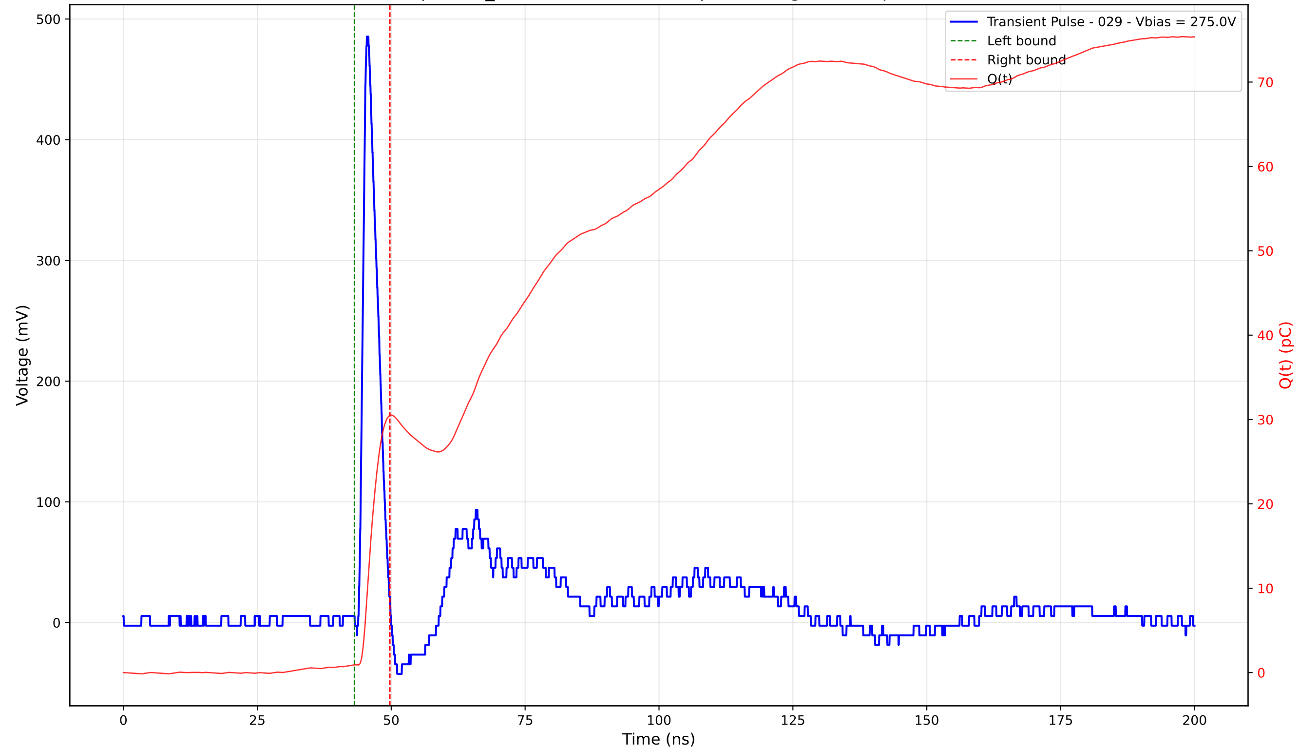
Transient Pulse - Sample: TD_4004 - Position: 390.0 \mu\text{m} - Charge: 29.56 pC - Rise Time: 1.03 ns
