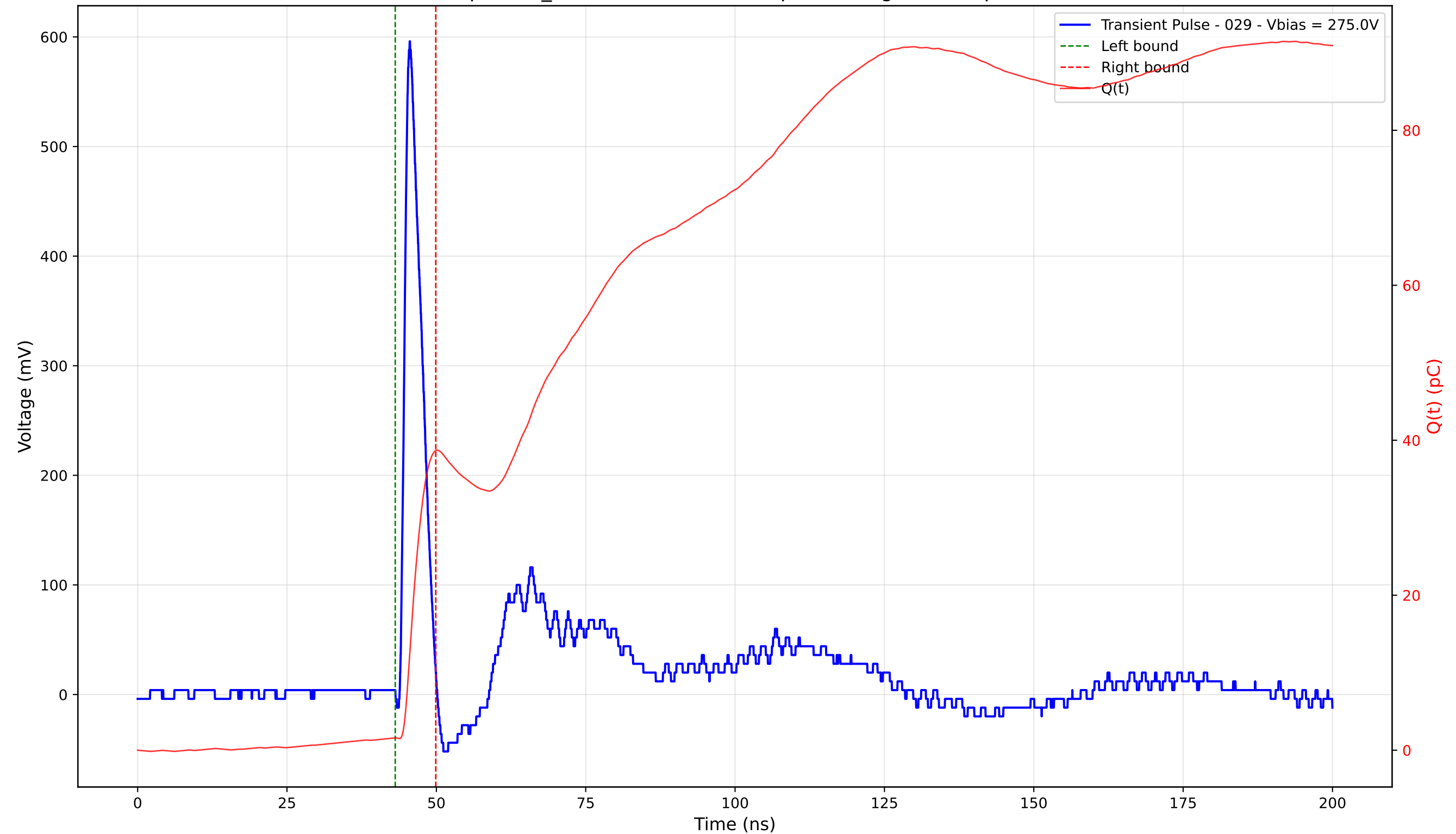
Transient Pulse - Sample: TD_4004 - Position: 380.0 \mu\text{m} - Charge: 37.07 pC - Rise Time: 1.03 ns
