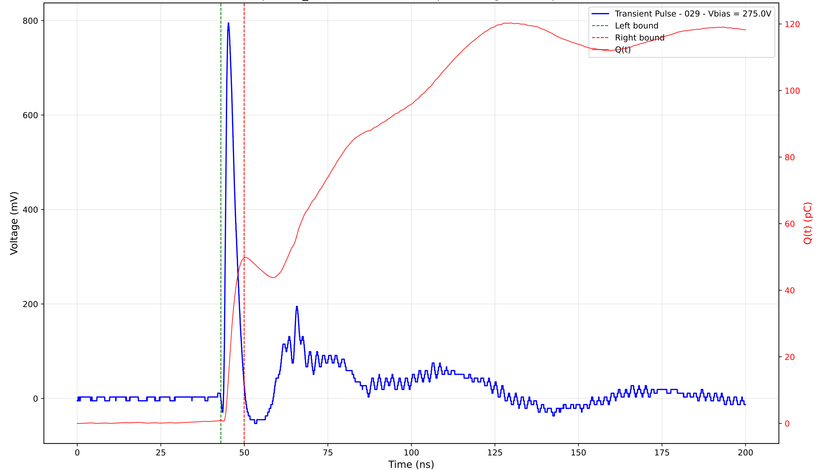
Transient Pulse - Sample: TD_4004 - Position: 110.0 \mu\text{m} - Charge: 48.86 pC - Rise Time: 0.88 ns
