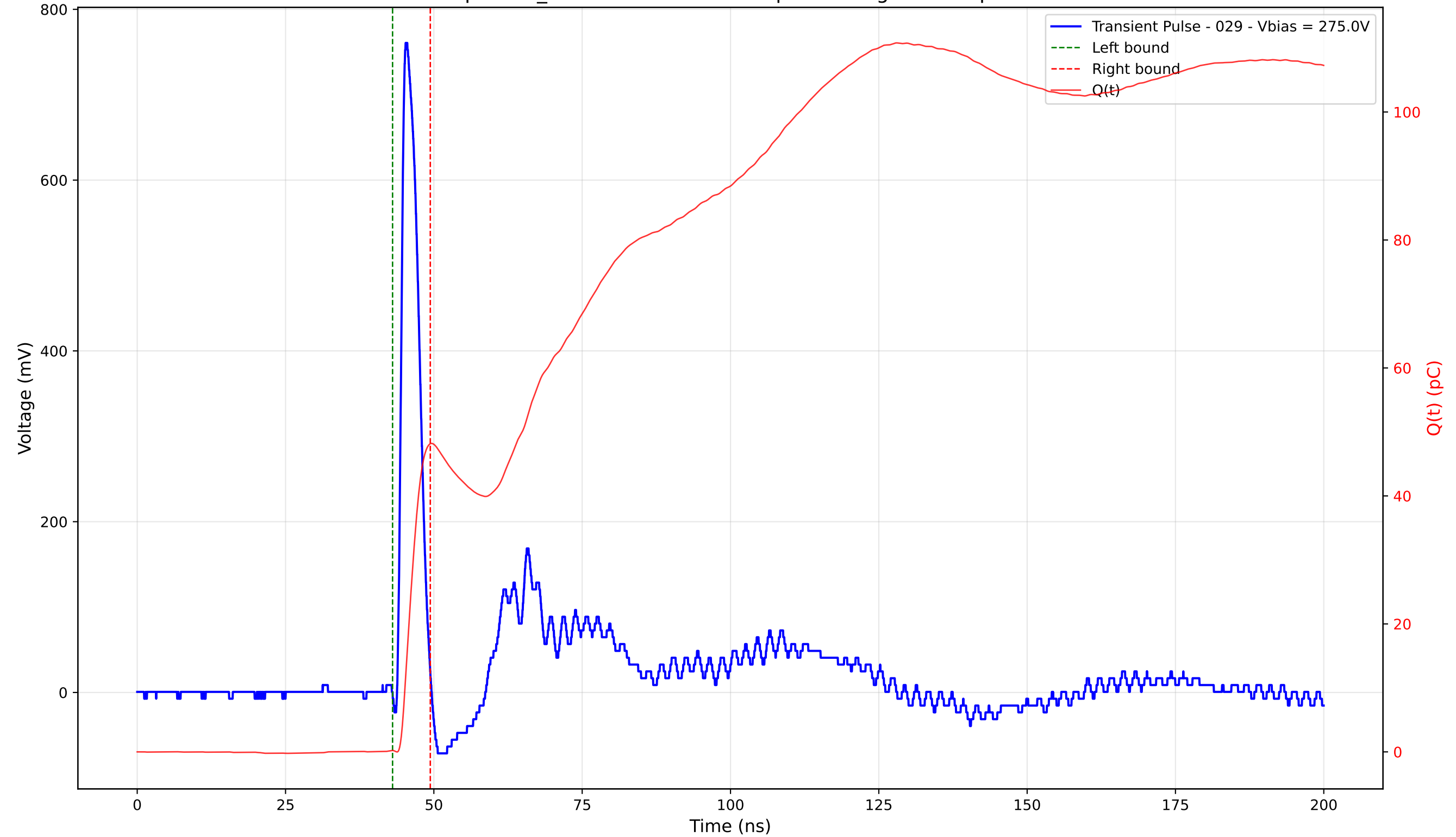
Transient Pulse - Sample: TD_4004 - Position: 280.0 \mu\text{m} - Charge: 47.94 pC - Rise Time: 0.92 ns
