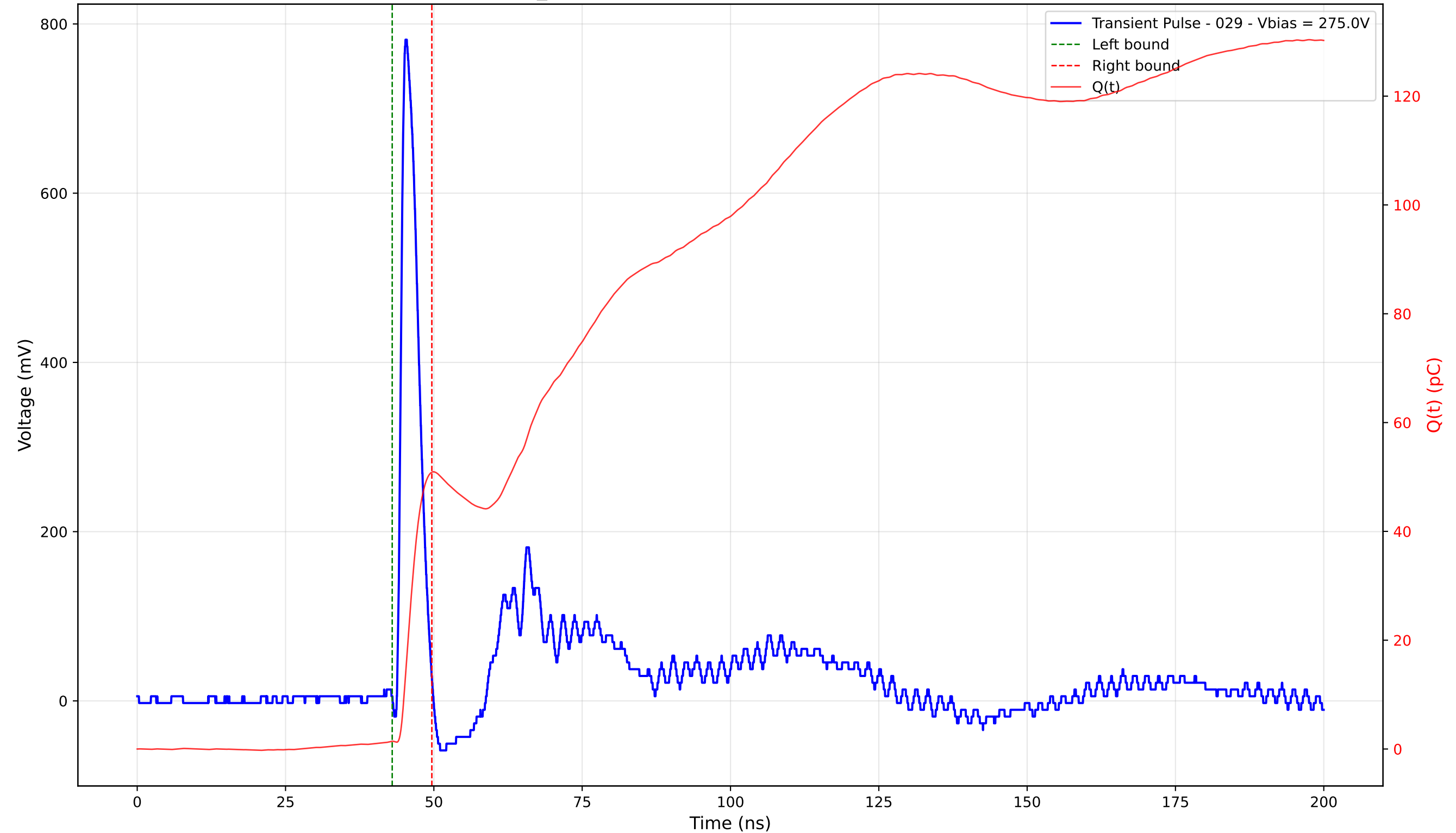
Transient Pulse - Sample: TD_4004 - Position: 225.0 \mu\text{m} - Charge: 49.45 pC - Rise Time: 0.90 ns
