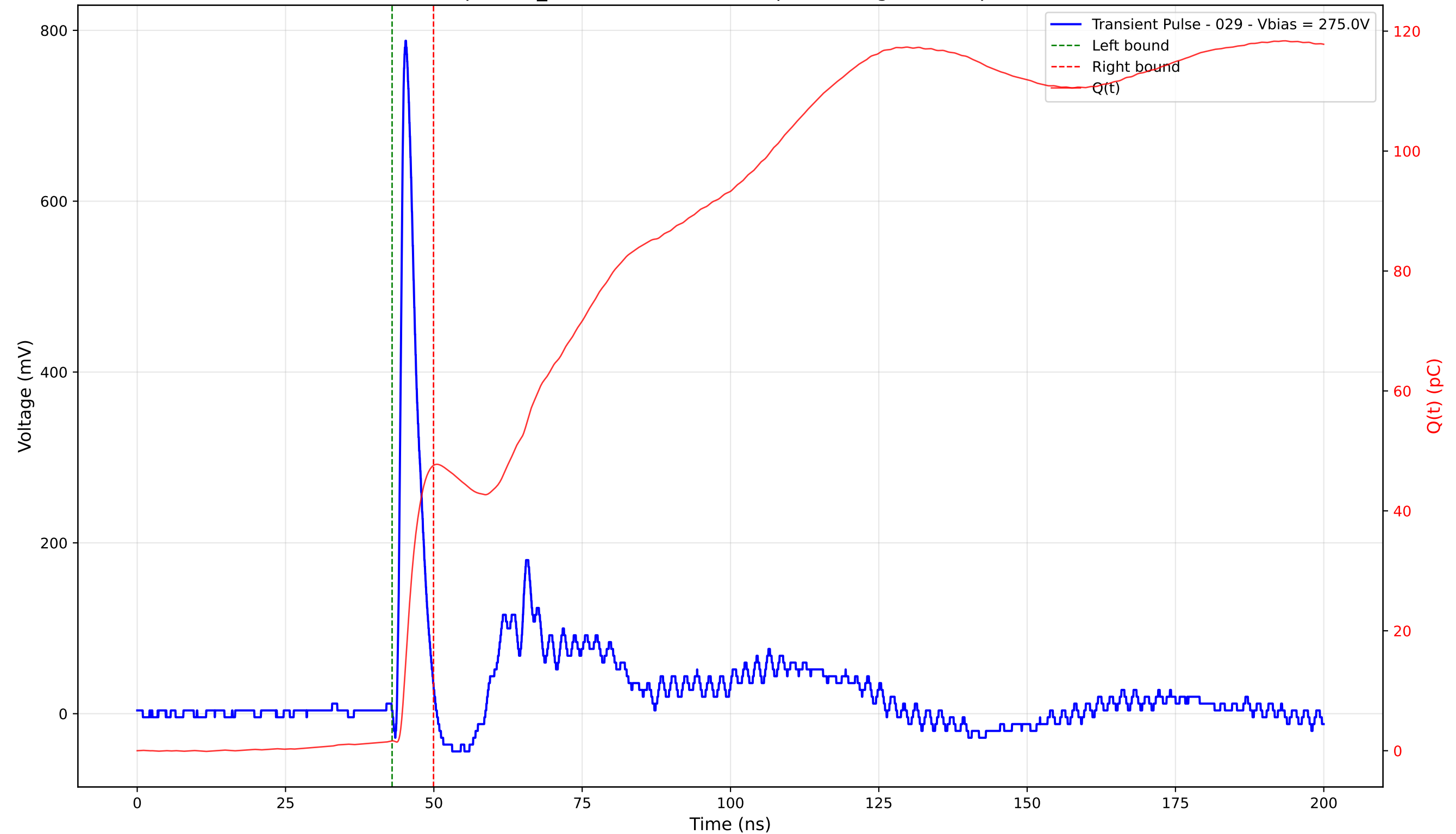
Transient Pulse - Sample: TD_4004 - Position: 100.0 \mu\text{m} - Charge: 45.95 pC - Rise Time: 0.88 ns
