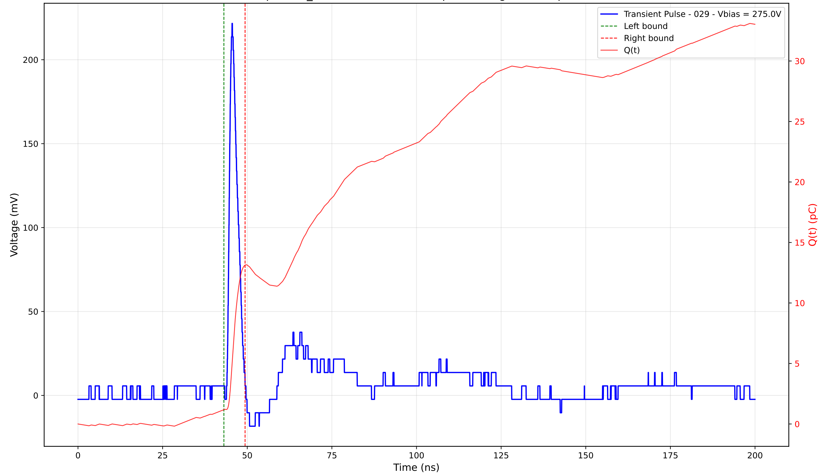
Transient Pulse - Sample: TD_4004 - Position: 410.0 \mu\text{m} - Charge: 11.95 pC - Rise Time: 1.06 ns
