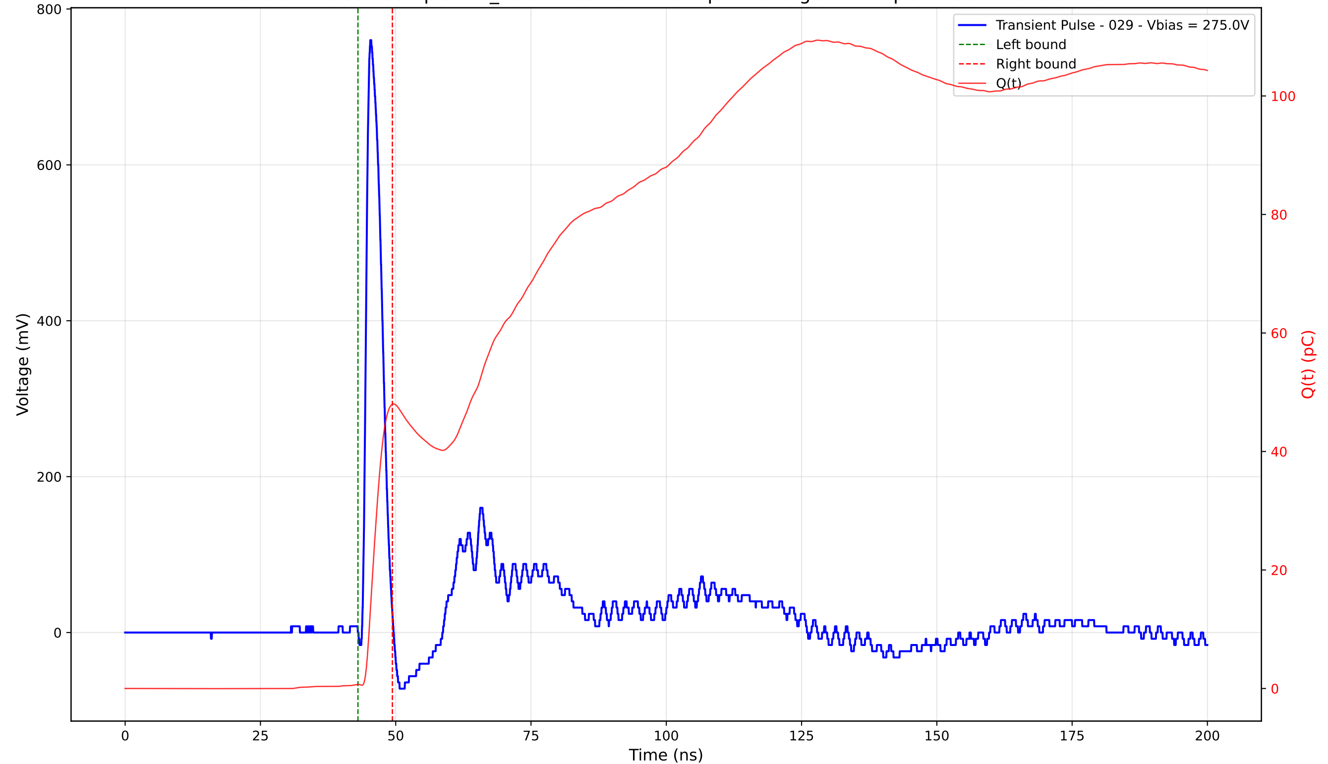
Transient Pulse - Sample: TD_4004 - Position: 270.0 \mu\text{m} - Charge: 47.27 pC - Rise Time: 0.94 ns
