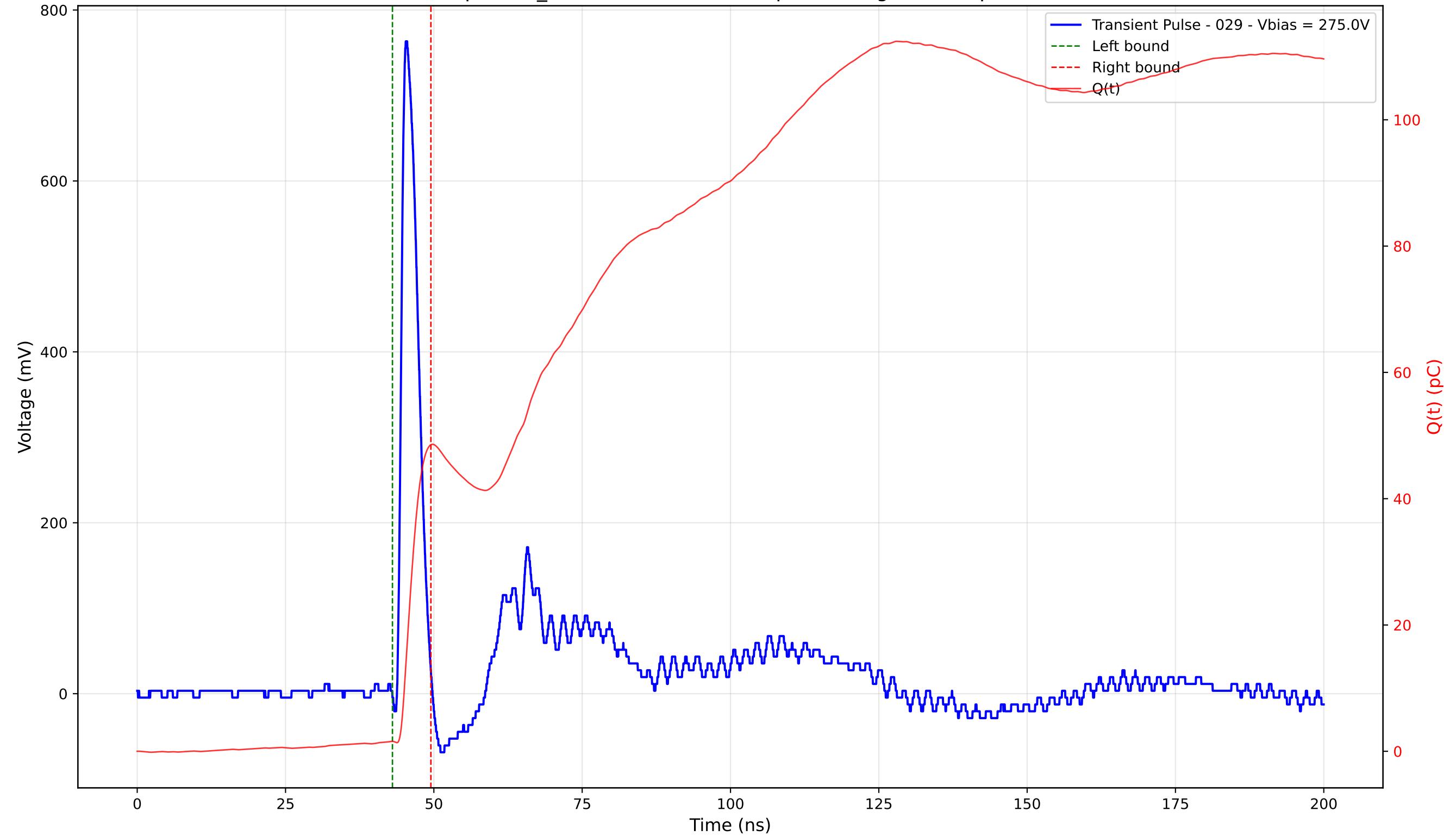
Transient Pulse - Sample: TD_4004 - Position: 240.0 \mu\text{m} - Charge: 46.97 pC - Rise Time: 0.92 ns
