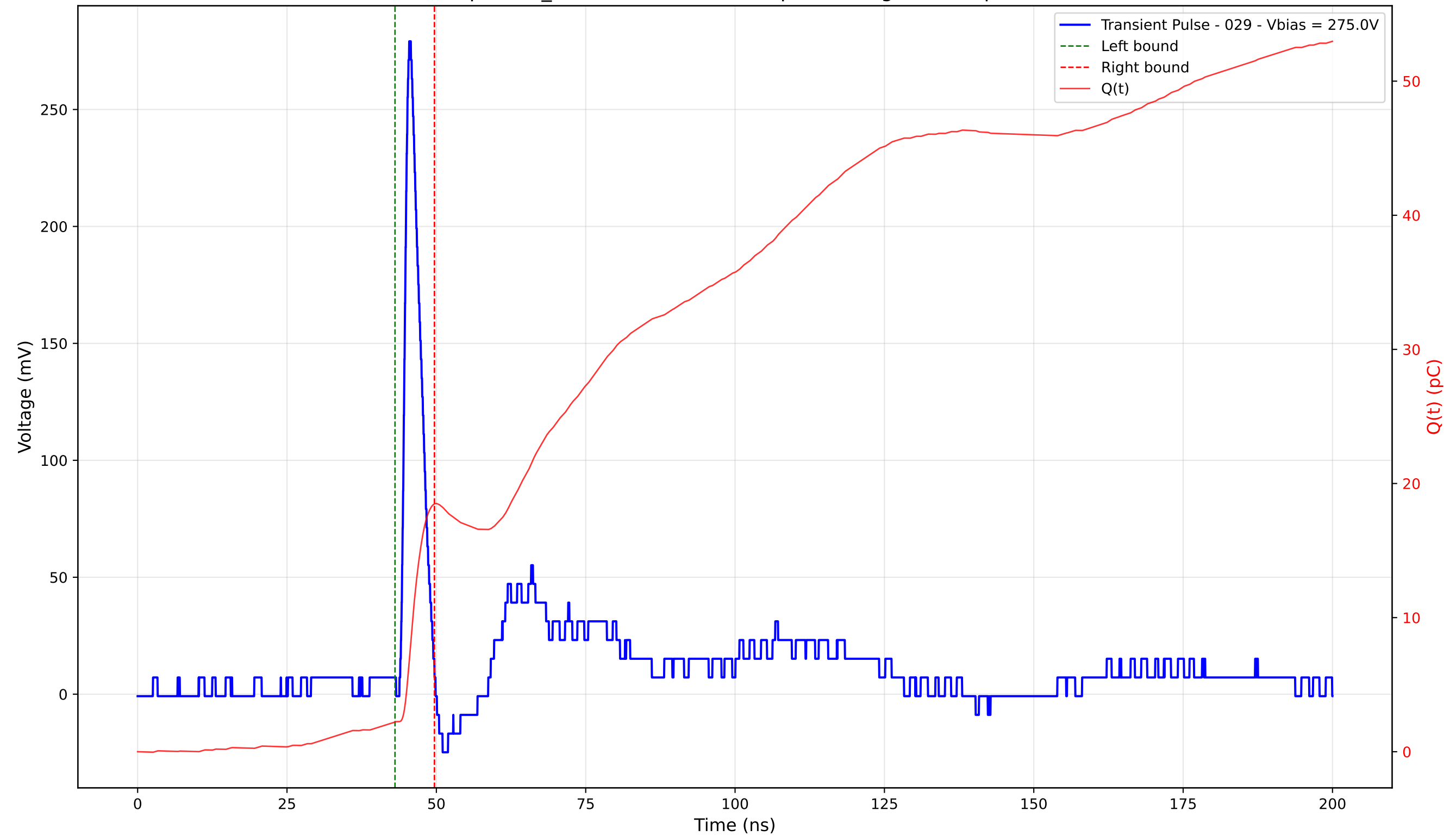
Transient Pulse - Sample: TD_4004 - Position: 405.0 \mu\text{m} - Charge: 16.26 pC - Rise Time: 1.07 ns
