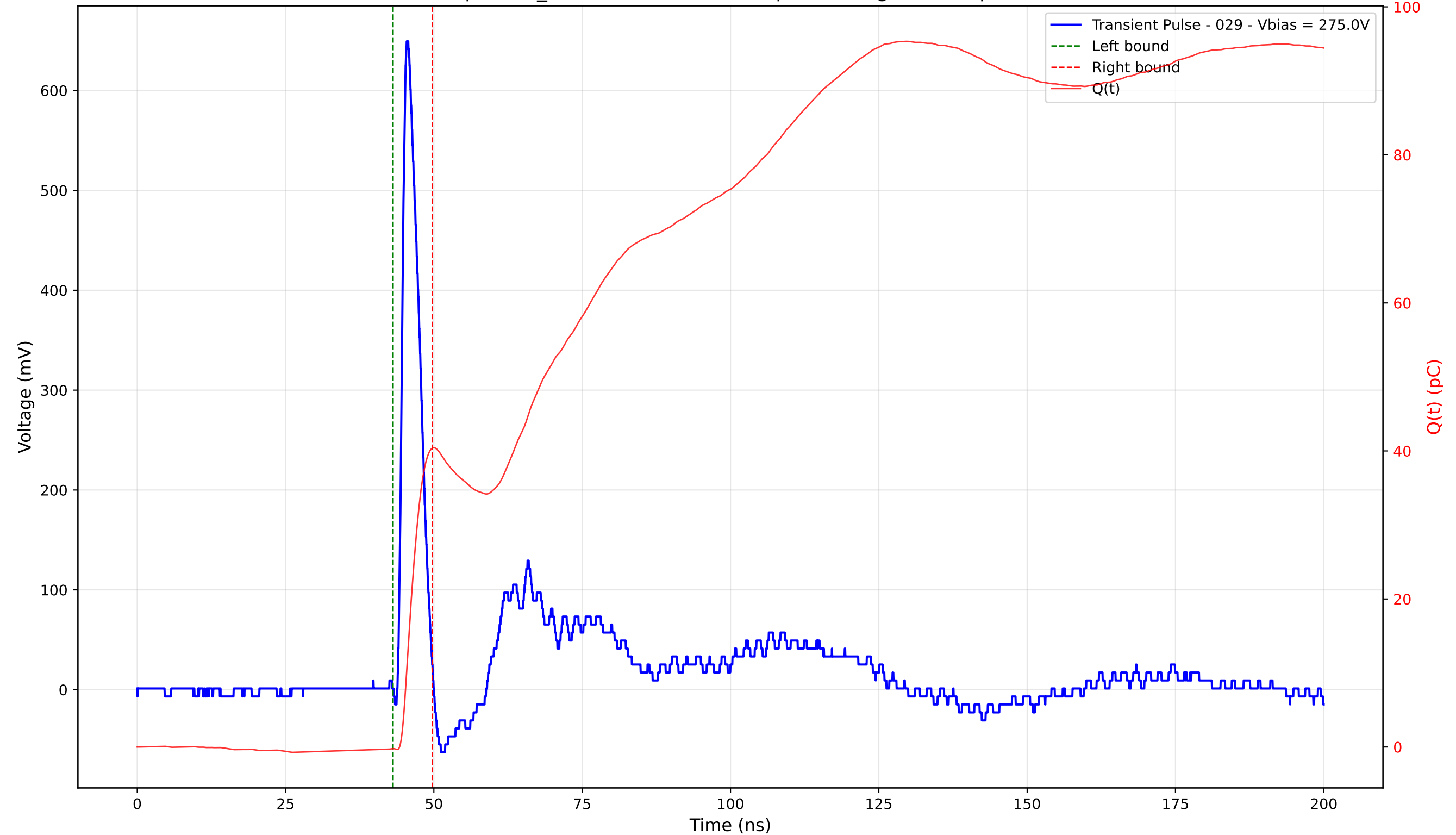
Transient Pulse - Sample: TD_4004 - Position: 335.0 \mu\text{m} - Charge: 40.60 pC - Rise Time: 1.00 ns
