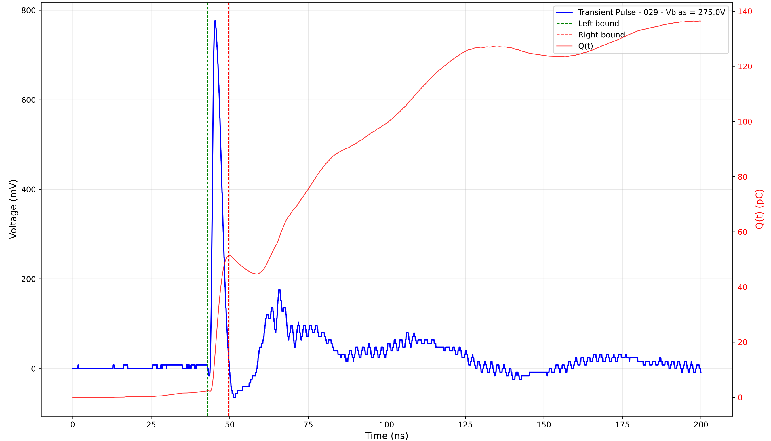
Transient Pulse - Sample: TD_4004 - Position: 135.0 \mu\text{m} - Charge: 48.96 pC - Rise Time: 0.91 ns
