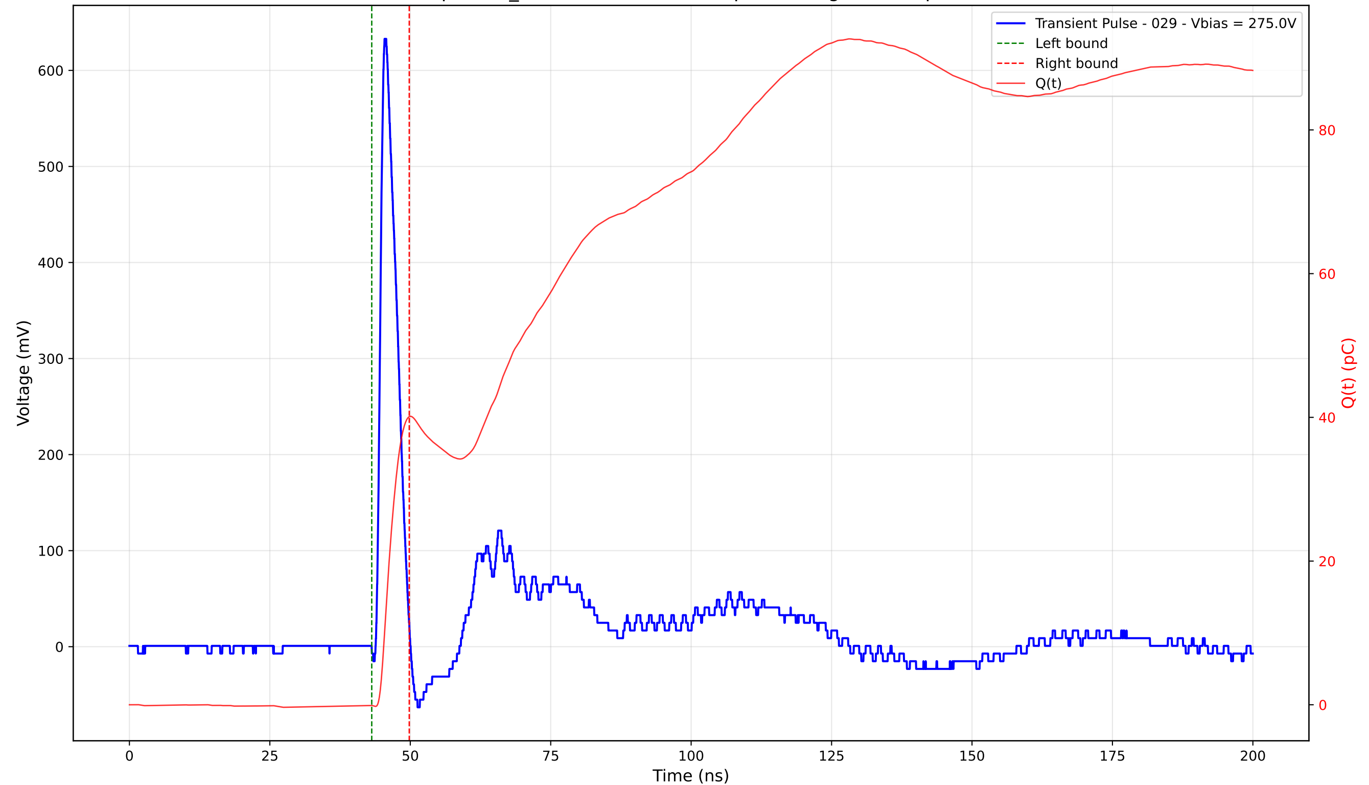
Transient Pulse - Sample: TD_4004 - Position: 355.0 \mu\text{m} - Charge: 40.20 pC - Rise Time: 1.03 ns
