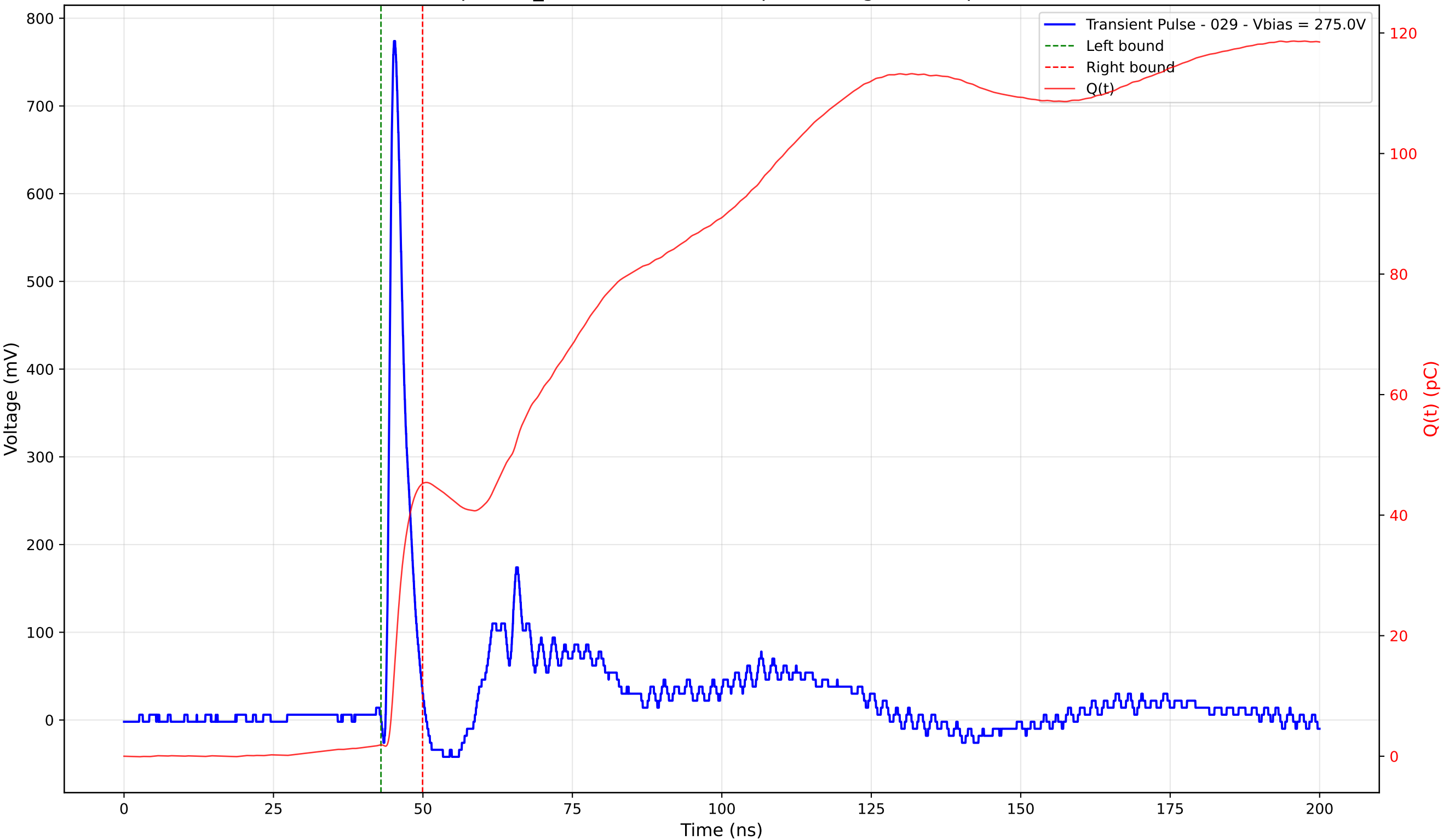
Transient Pulse - Sample: TD_4004 - Position: 95.0 \mu\text{m} - Charge: 43.35 pC - Rise Time: 0.89 ns
