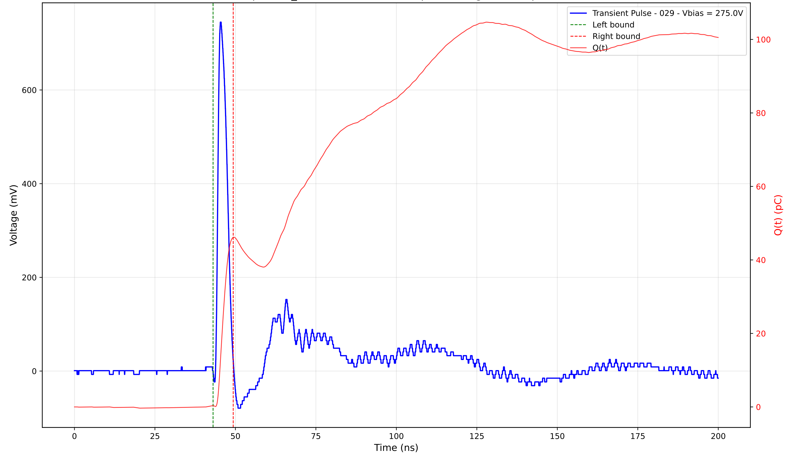
Transient Pulse - Sample: TD_4004 - Position: 305.0 \mu\text{m} - Charge: 45.78 pC - Rise Time: 0.95 ns
