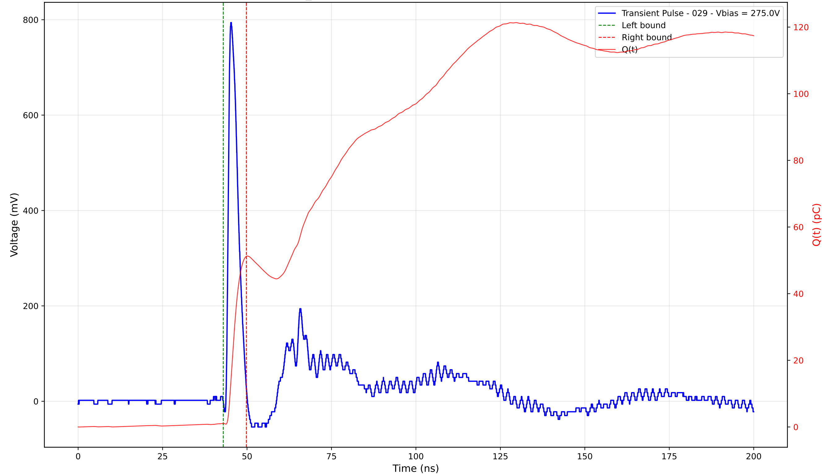
Transient Pulse - Sample: TD_4004 - Position: 195.0 \mu\text{m} - Charge: 50.12 pC - Rise Time: 0.89 ns
