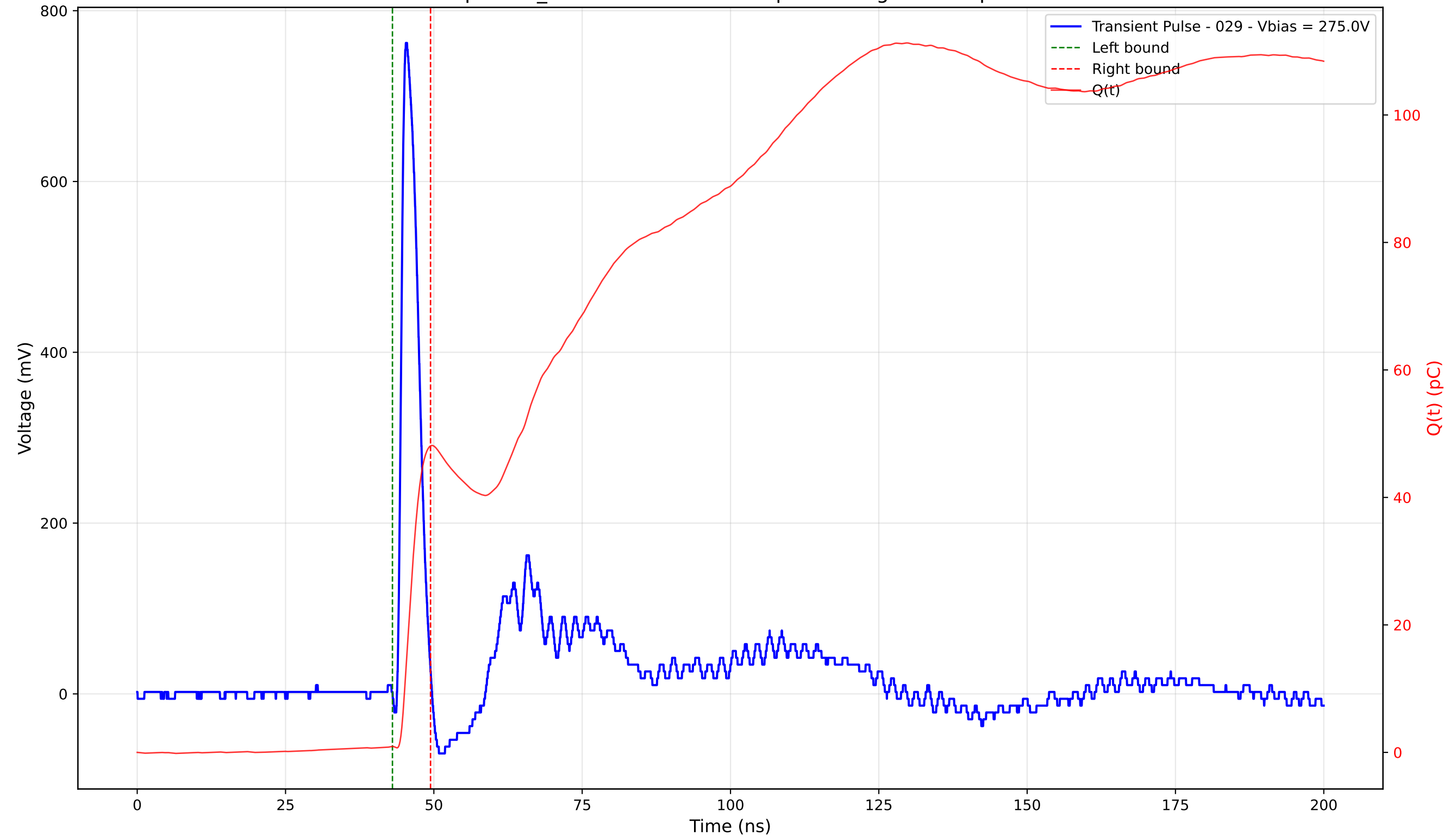
Transient Pulse - Sample: TD_4004 - Position: 250.0 \mu\text{m} - Charge: 47.15 pC - Rise Time: 0.90 ns
