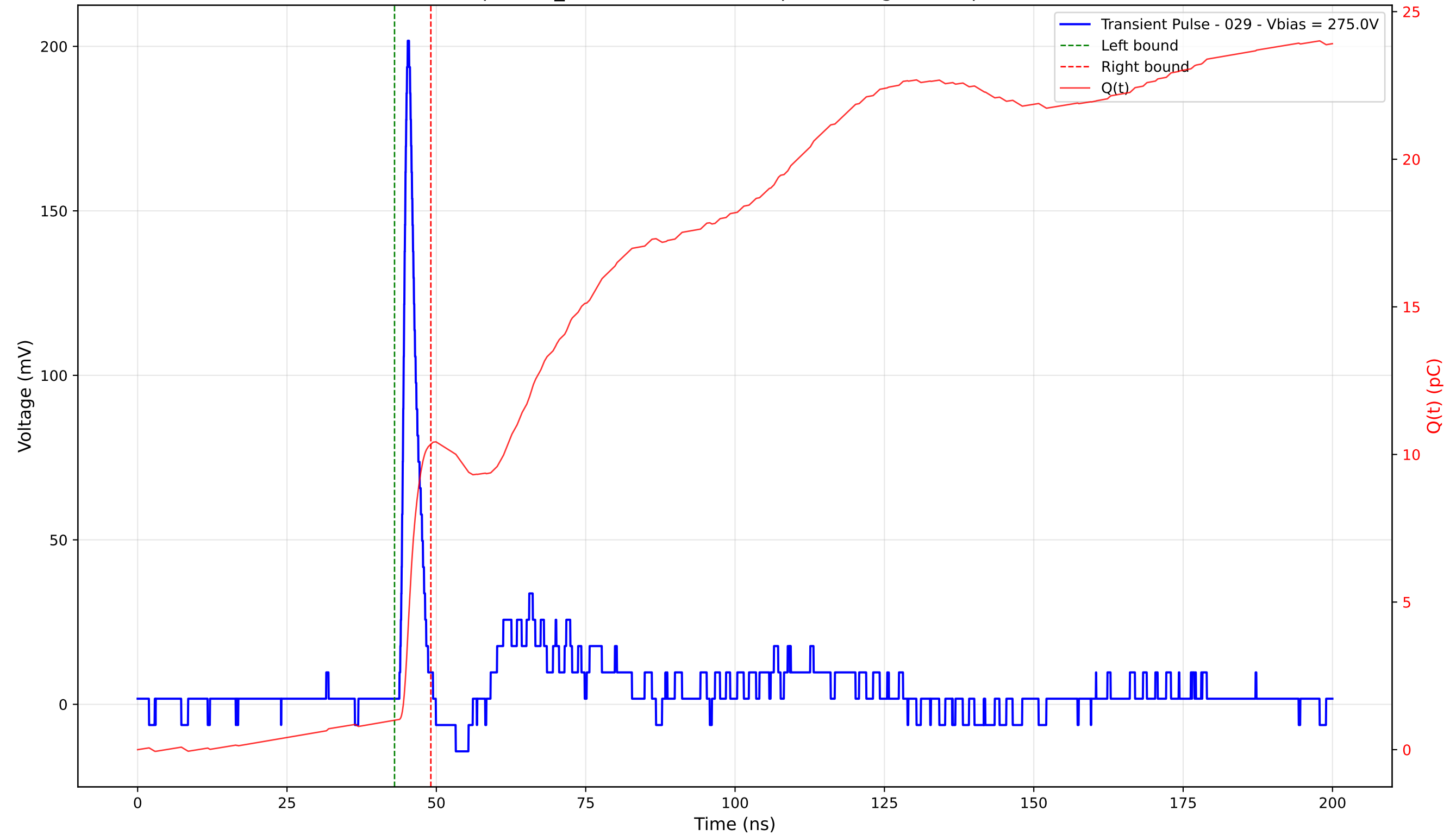
Transient Pulse - Sample: TD_4004 - Position: 55.0 \mu\text{m} - Charge: 9.35 pC - Rise Time: 0.97 ns
