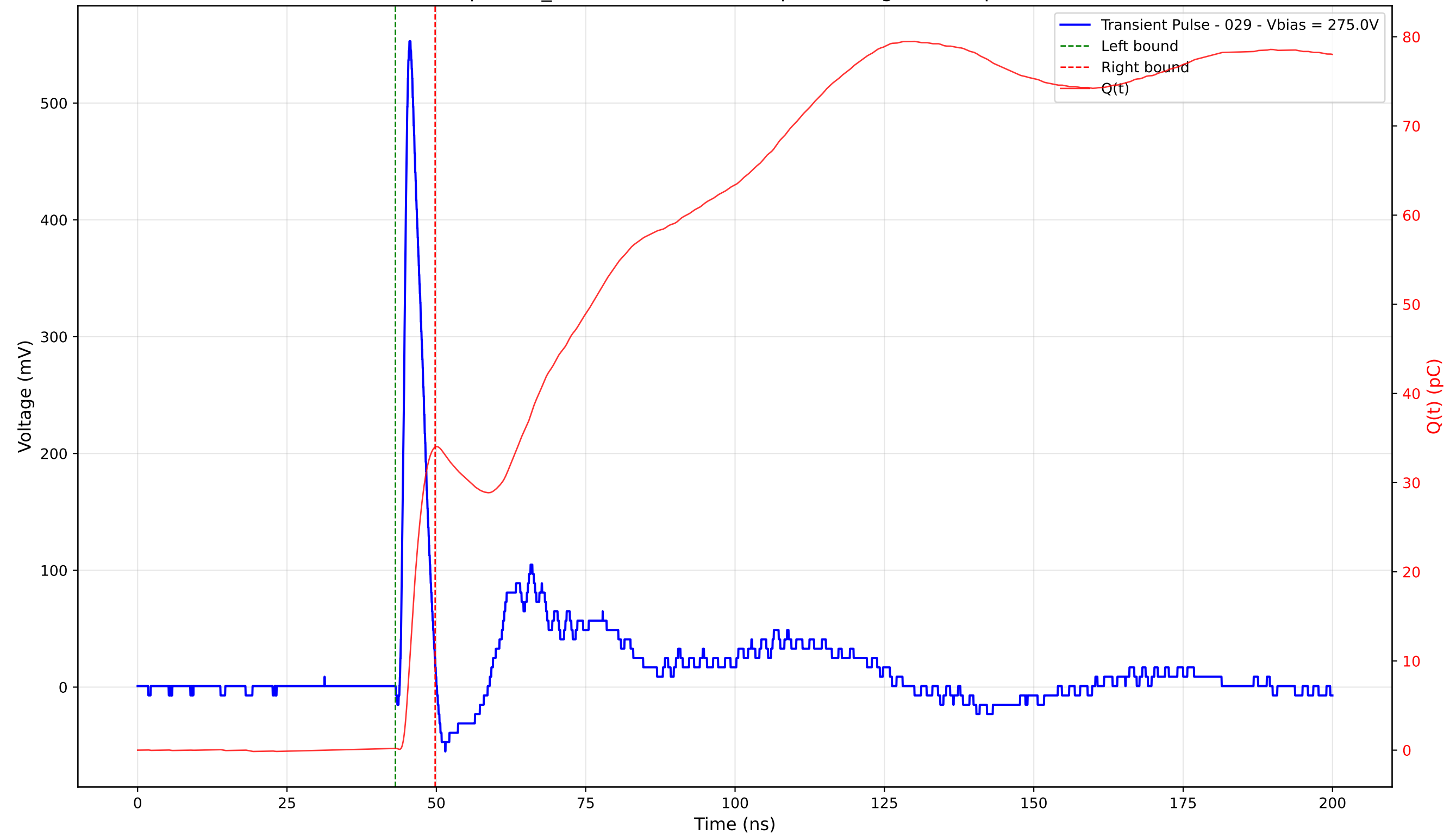
Transient Pulse - Sample: TD_4004 - Position: 385.0 \mu\text{m} - Charge: 33.78 pC - Rise Time: 1.05 ns
