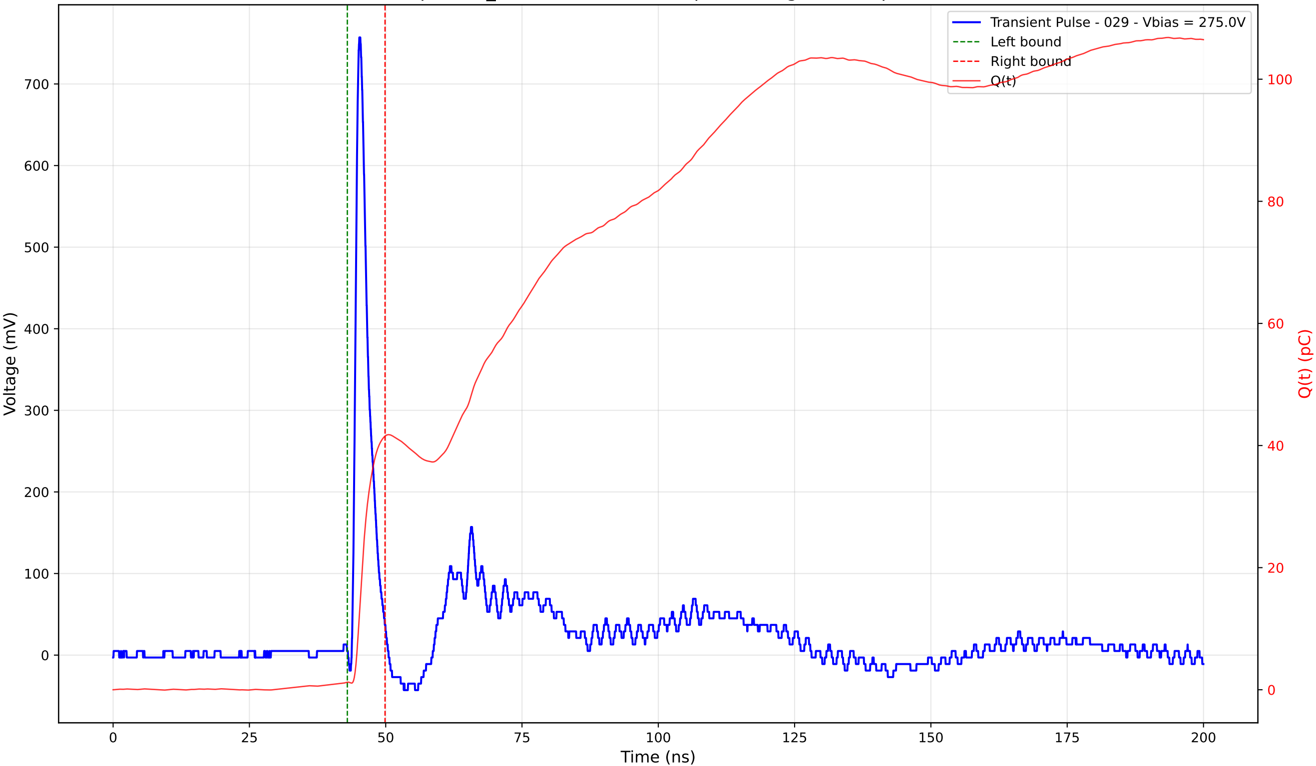
Transient Pulse - Sample: TD_4004 - Position: 90.0 \mu\text{m} - Charge: 40.31 pC - Rise Time: 0.89 ns
