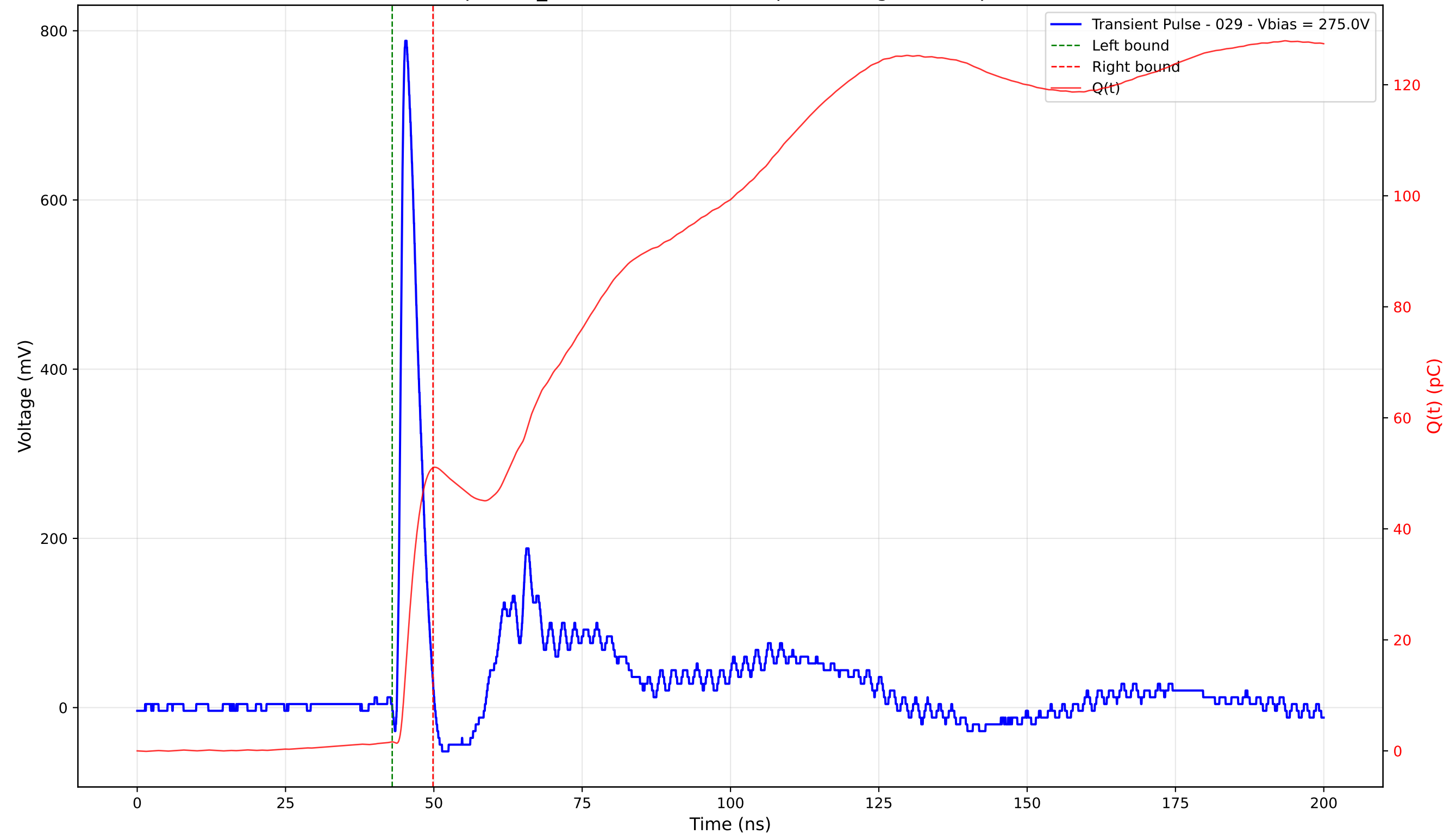
Transient Pulse - Sample: TD_4004 - Position: 120.0 \mu\text{m} - Charge: 49.39 pC - Rise Time: 0.90 ns
