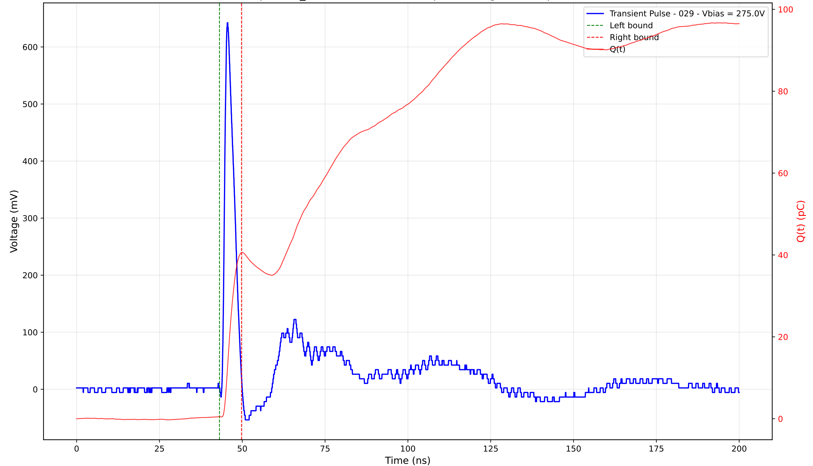
Transient Pulse - Sample: TD_4004 - Position: 350.0 \mu\text{m} - Charge: 40.07 pC - Rise Time: 1.02 ns
