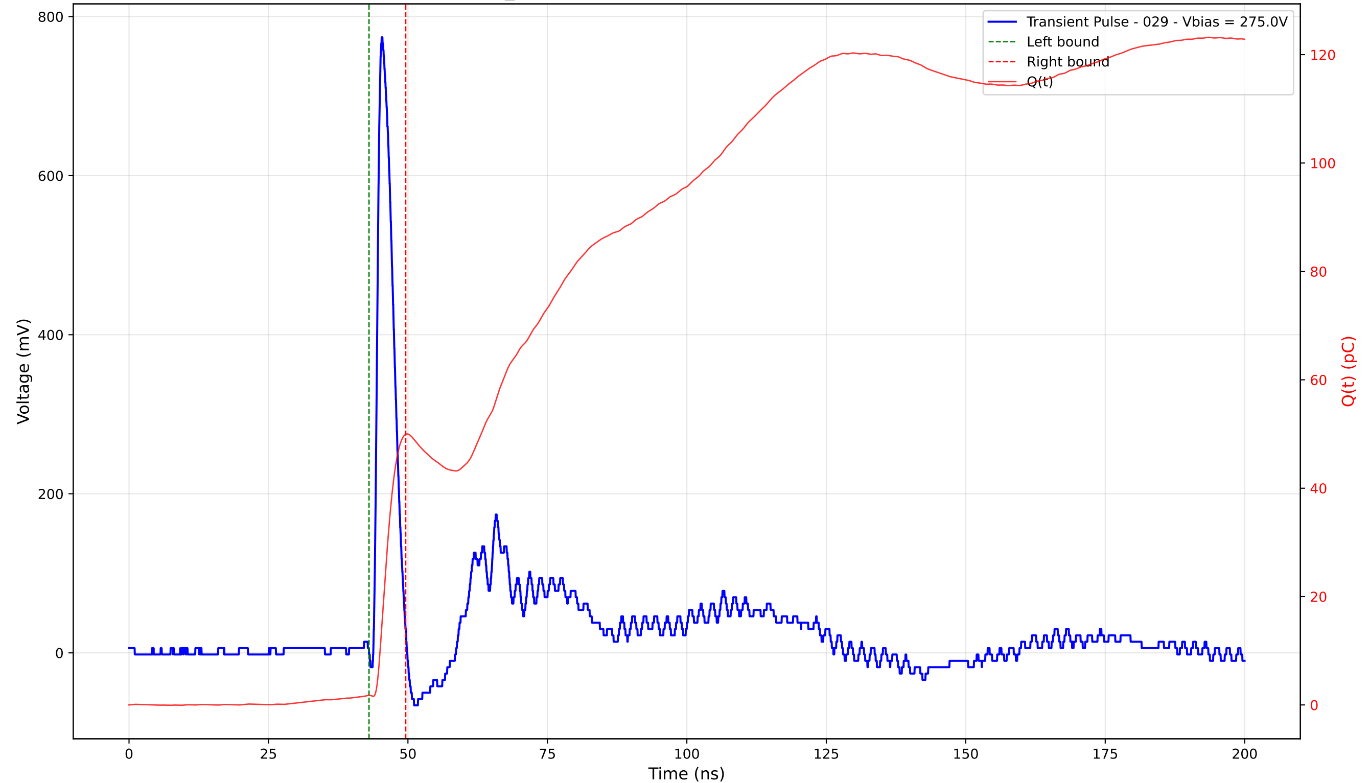
Transient Pulse - Sample: TD_4004 - Position: 140.0 \mu\text{m} - Charge: 48.16 pC - Rise Time: 0.91 ns
