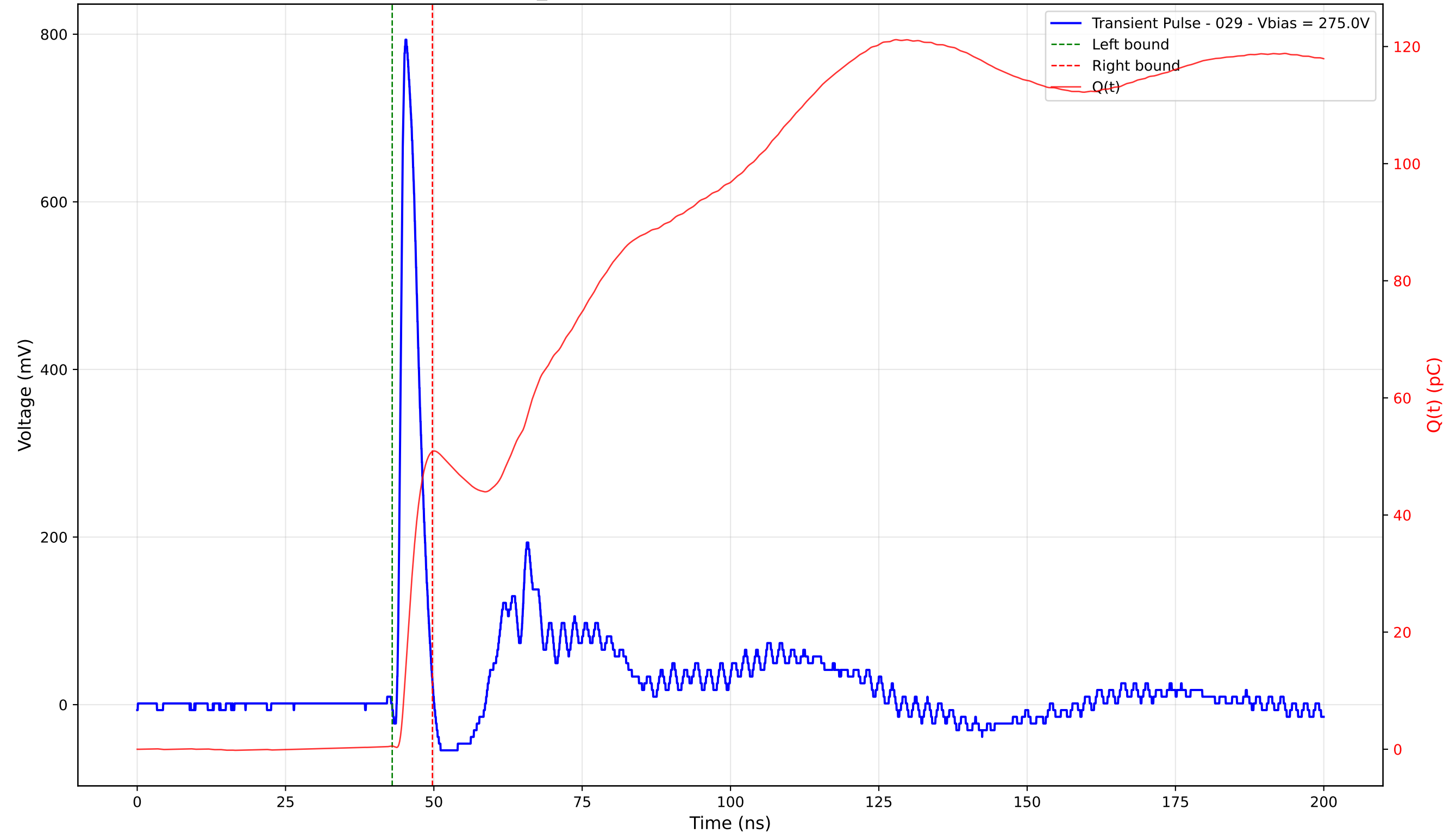
Transient Pulse - Sample: TD_4004 - Position: 175.0 \mu\text{m} - Charge: 50.31 pC - Rise Time: 0.91 ns
