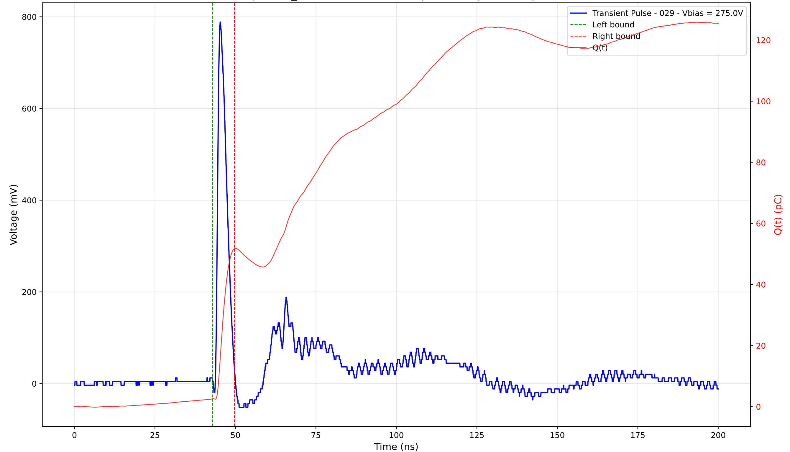
Transient Pulse - Sample: TD_4004 - Position: 125.0 \mu\text{m} - Charge: 49.13 pC - Rise Time: 0.90 ns
