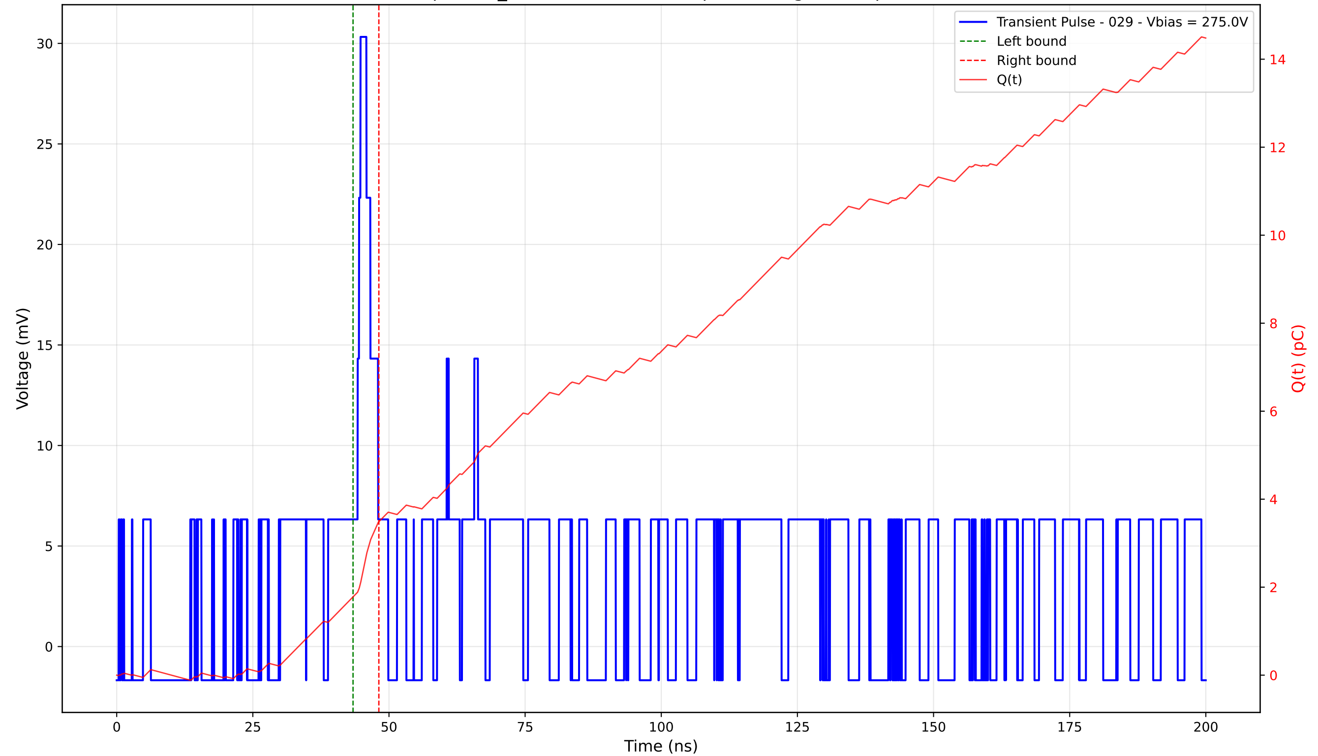
Transient Pulse - Sample: TD_4004 - Position: 30.0 \mu\text{m} - Charge: 1.71 pC - Rise Time: 5.95 ns
