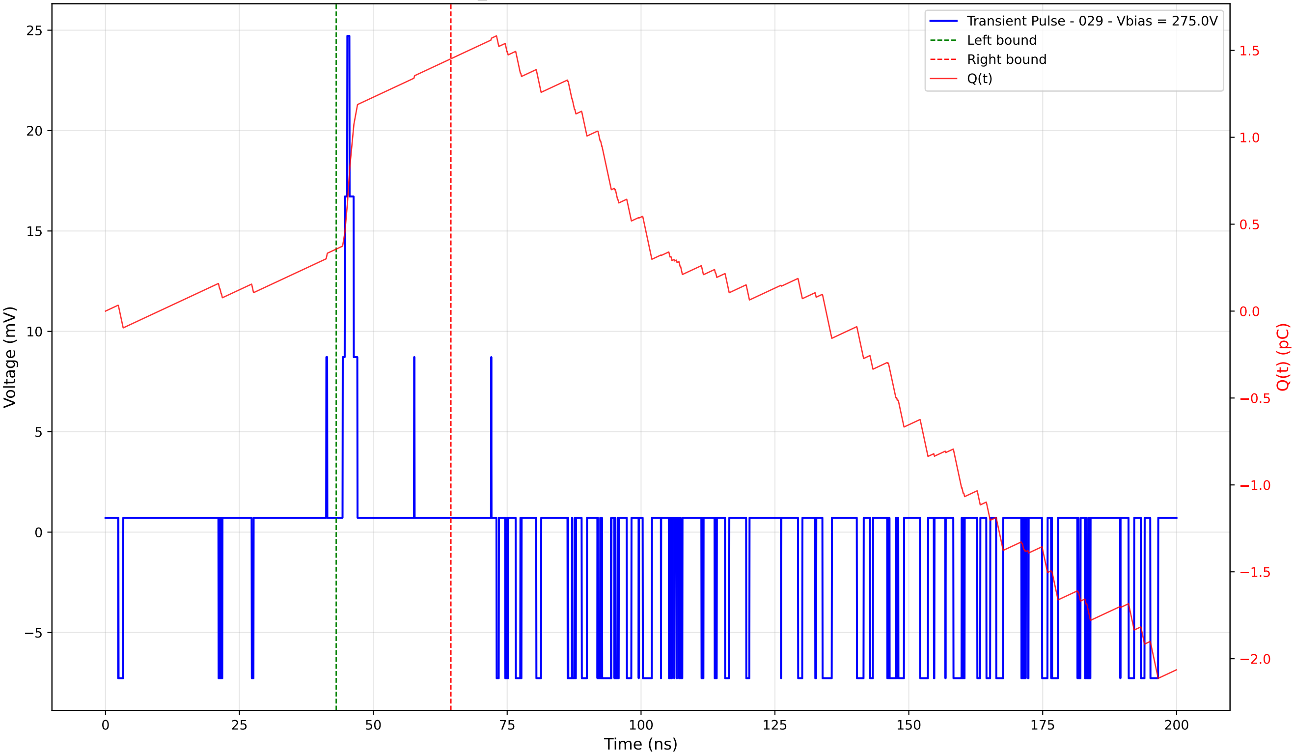
Transient Pulse - Sample: TD_4004 - Position: 20.0 \mu\text{m} - Charge: 1.09 pC - Rise Time: 0.88 ns
