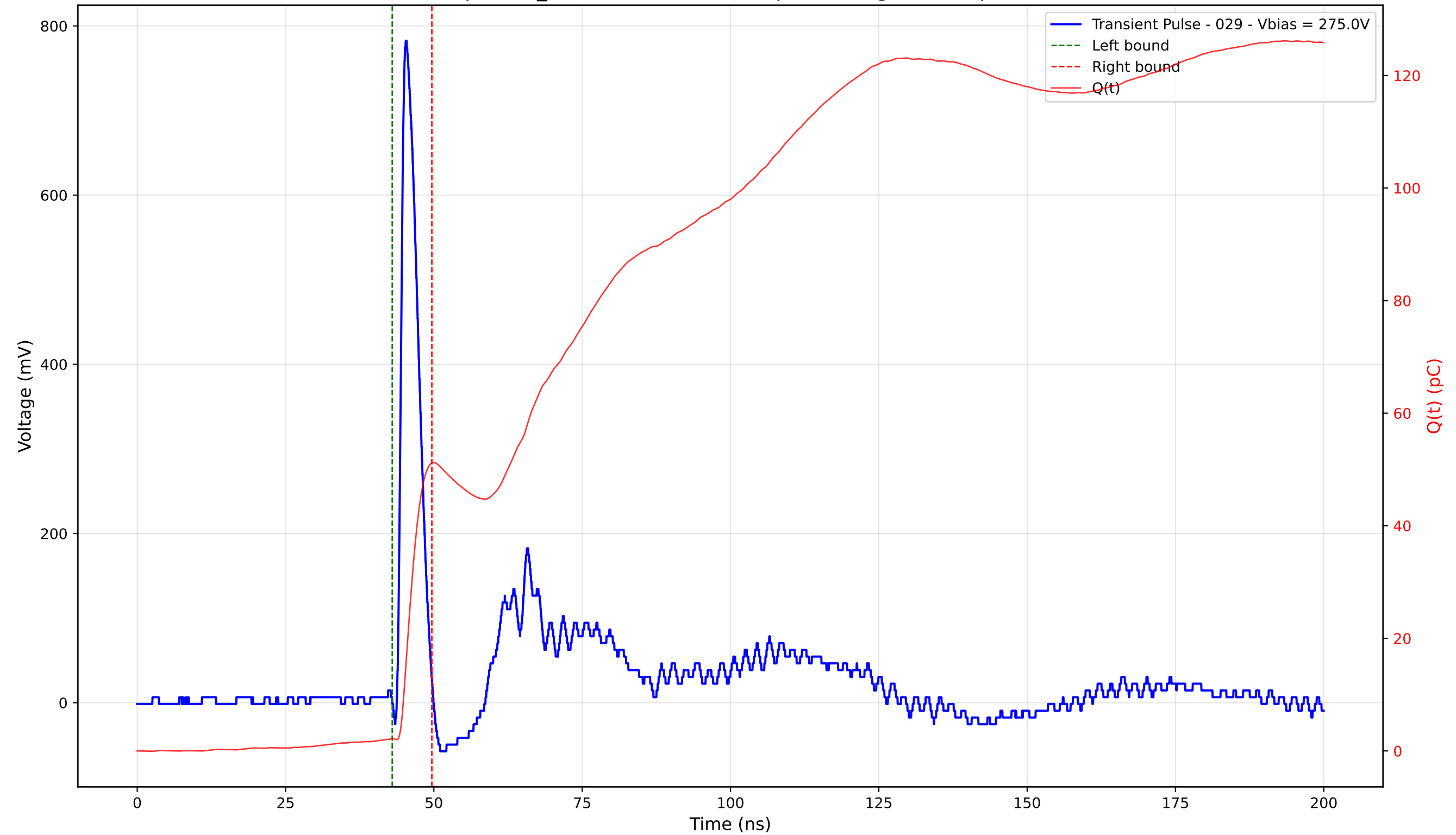
Transient Pulse - Sample: TD_4004 - Position: 130.0 \mu\text{m} - Charge: 48.97 pC - Rise Time: 0.92 ns
