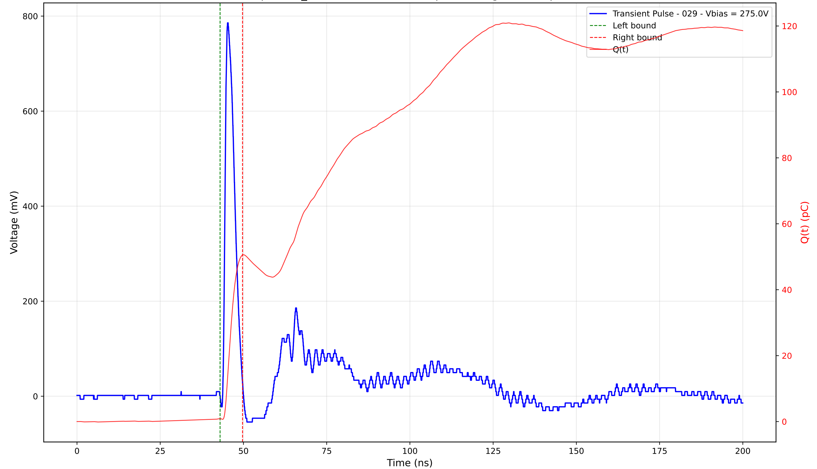
Transient Pulse - Sample: TD_4004 - Position: 220.0 \mu\text{m} - Charge: 49.62 pC - Rise Time: 0.91 ns
