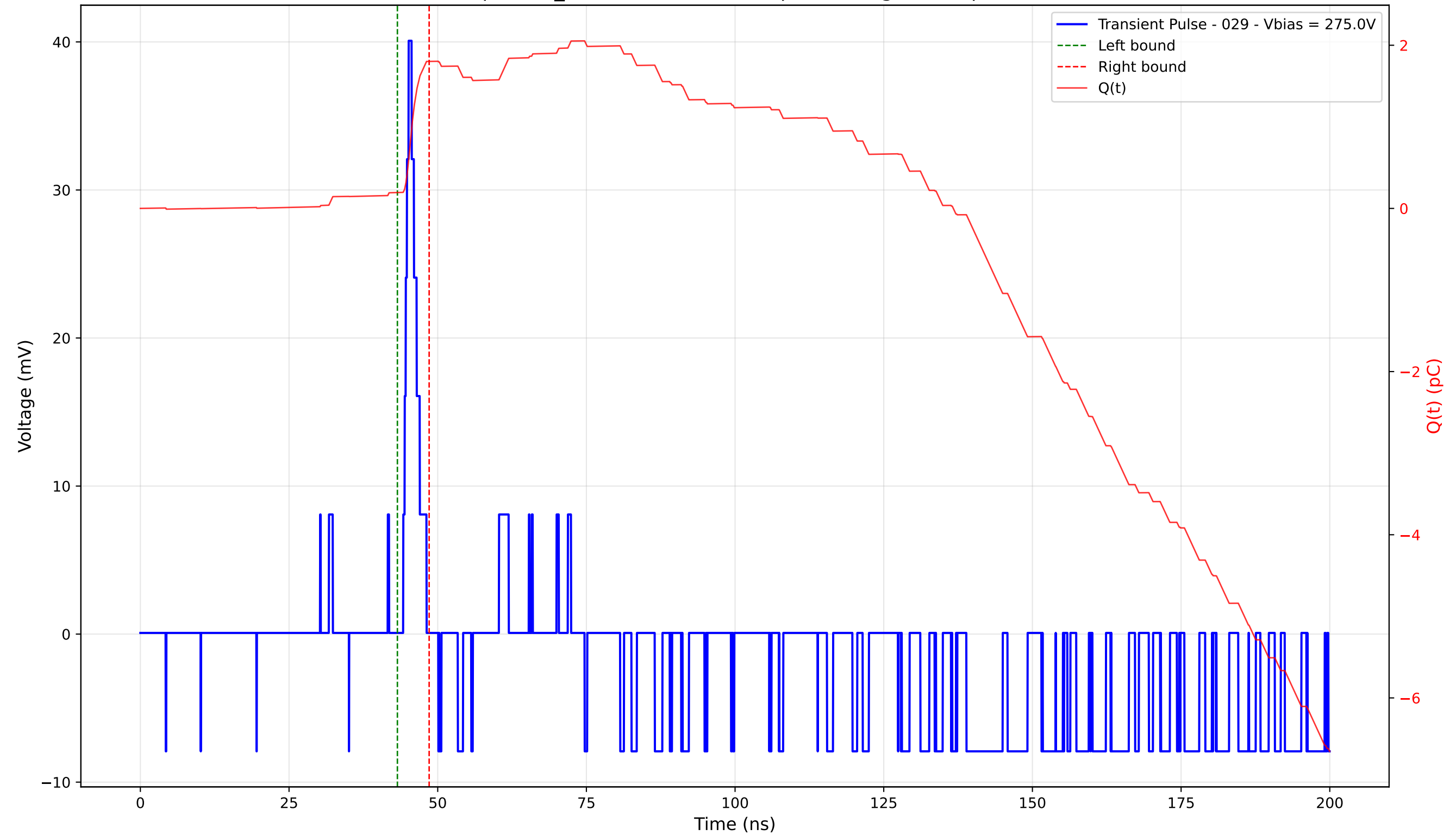
Transient Pulse - Sample: TD_4004 - Position: 35.0 \mu\text{m} - Charge: 1.61 pC - Rise Time: 0.91 ns
