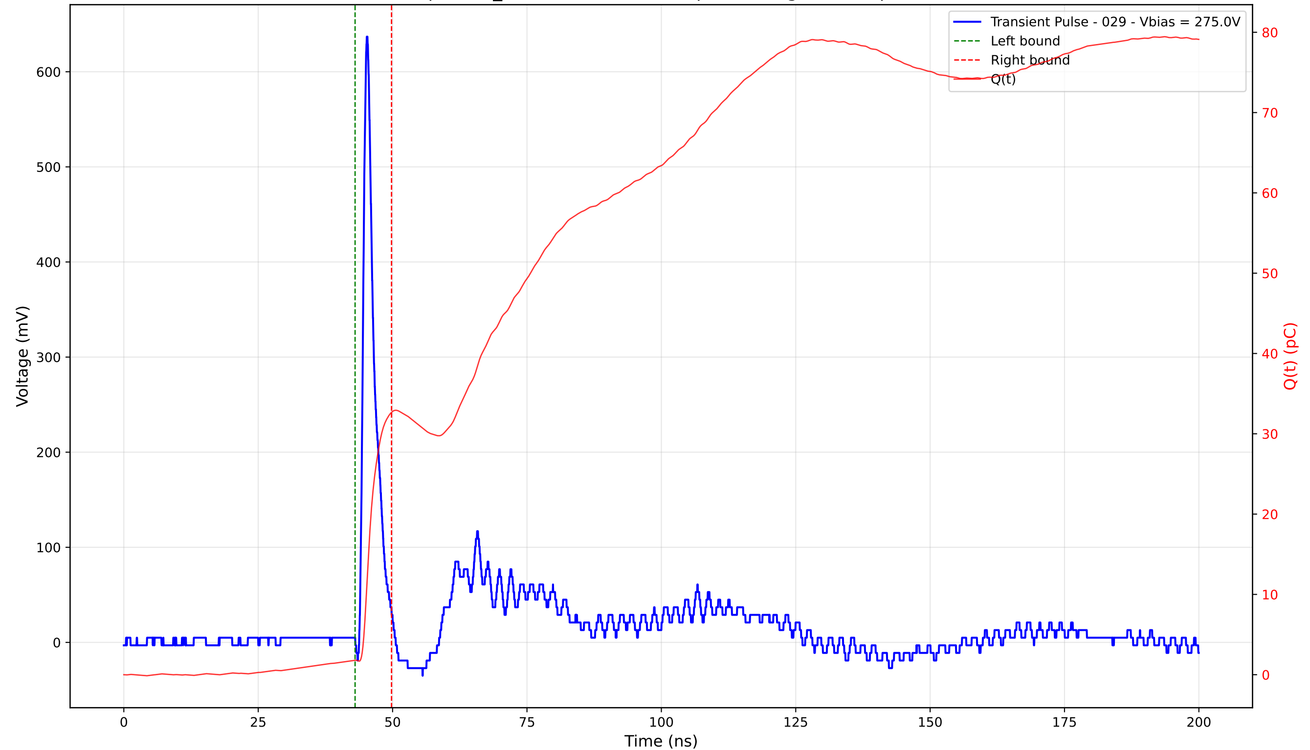
Transient Pulse - Sample: TD_4004 - Position: 75.0 \mu\text{m} - Charge: 30.87 pC - Rise Time: 0.91 ns
