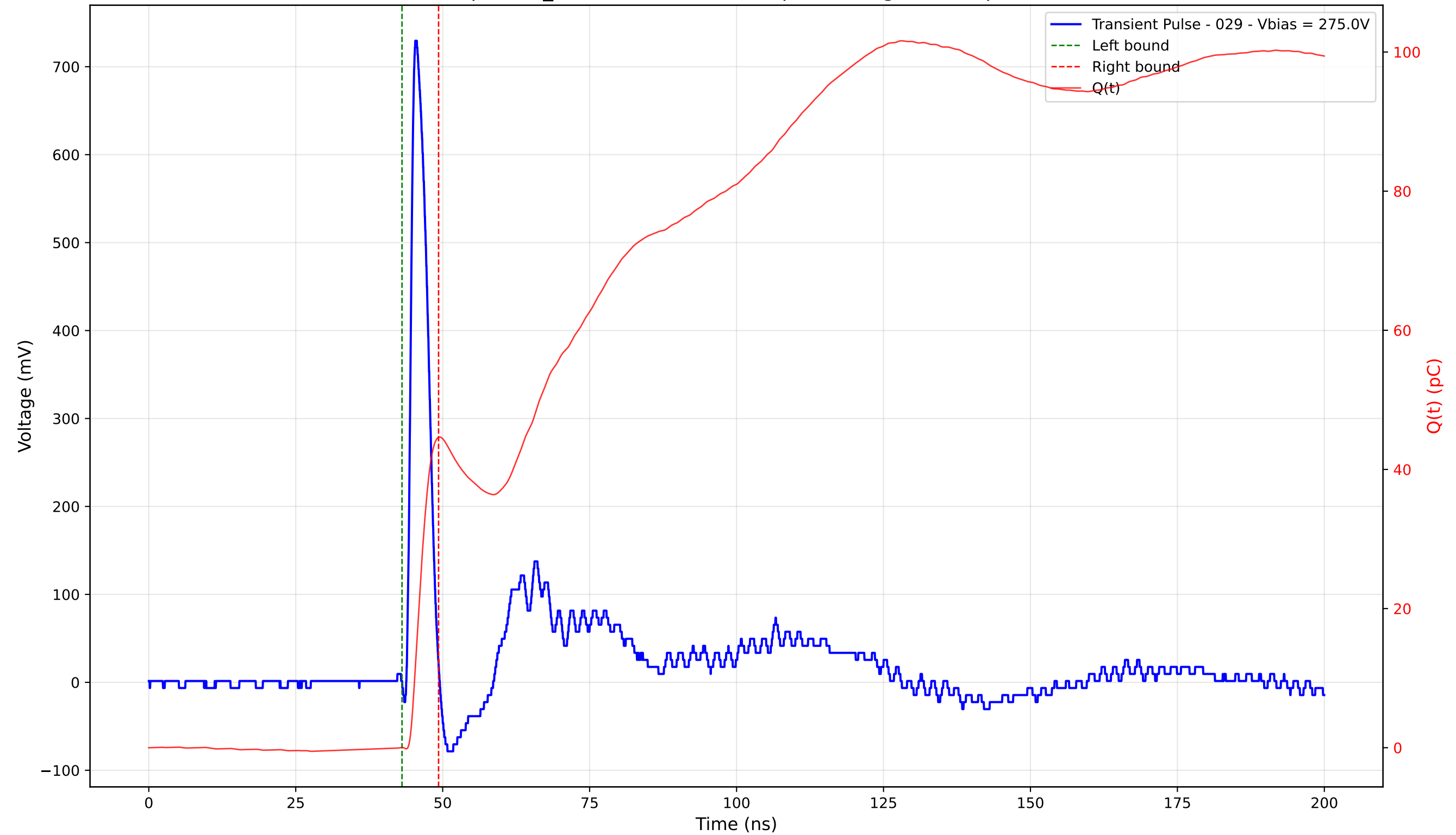
Transient Pulse - Sample: TD_4004 - Position: 310.0 \mu\text{m} - Charge: 44.58 pC - Rise Time: 0.96 ns
