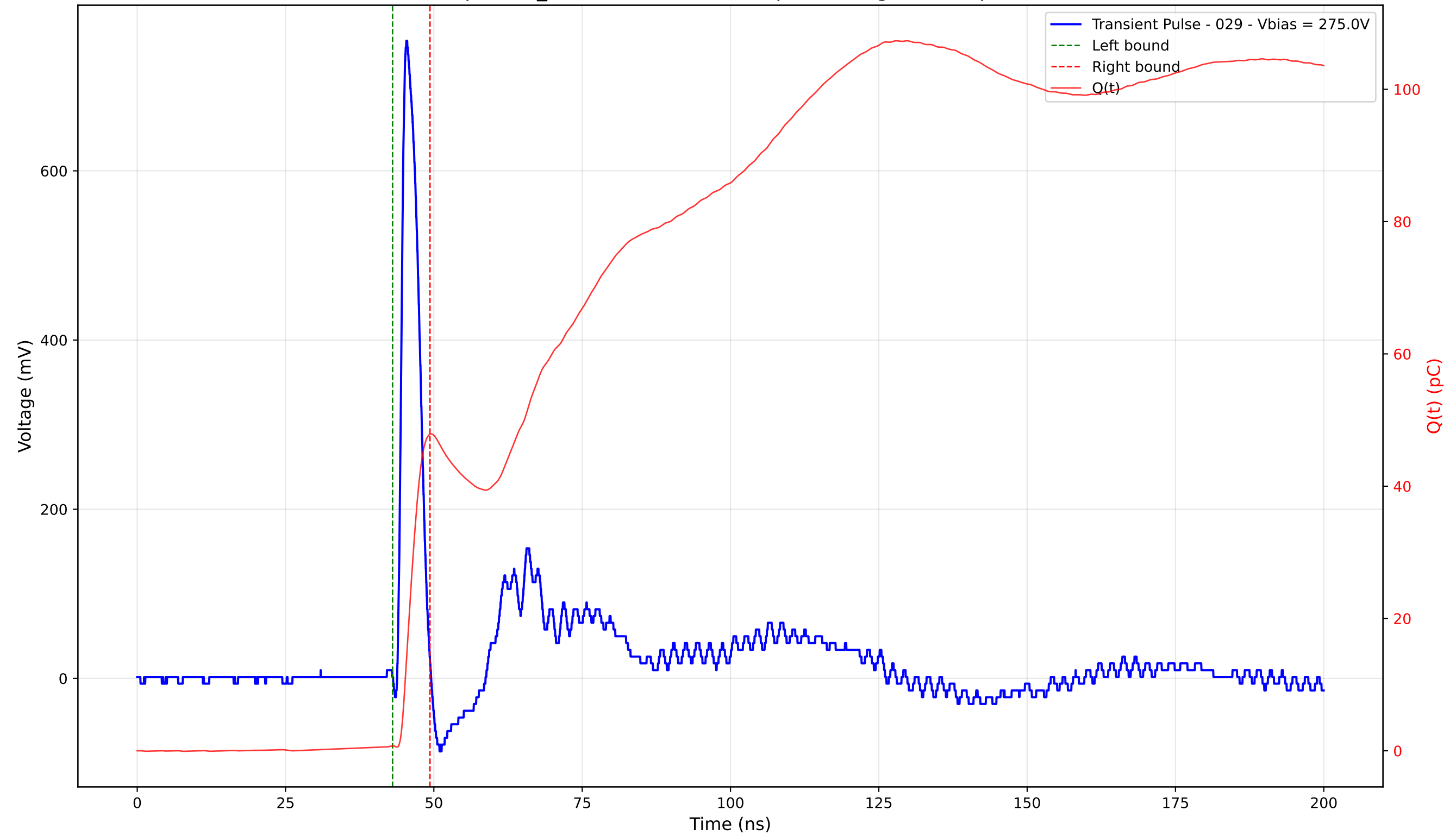
Transient Pulse - Sample: TD_4004 - Position: 295.0 \mu\text{m} - Charge: 47.10 pC - Rise Time: 0.95 ns
