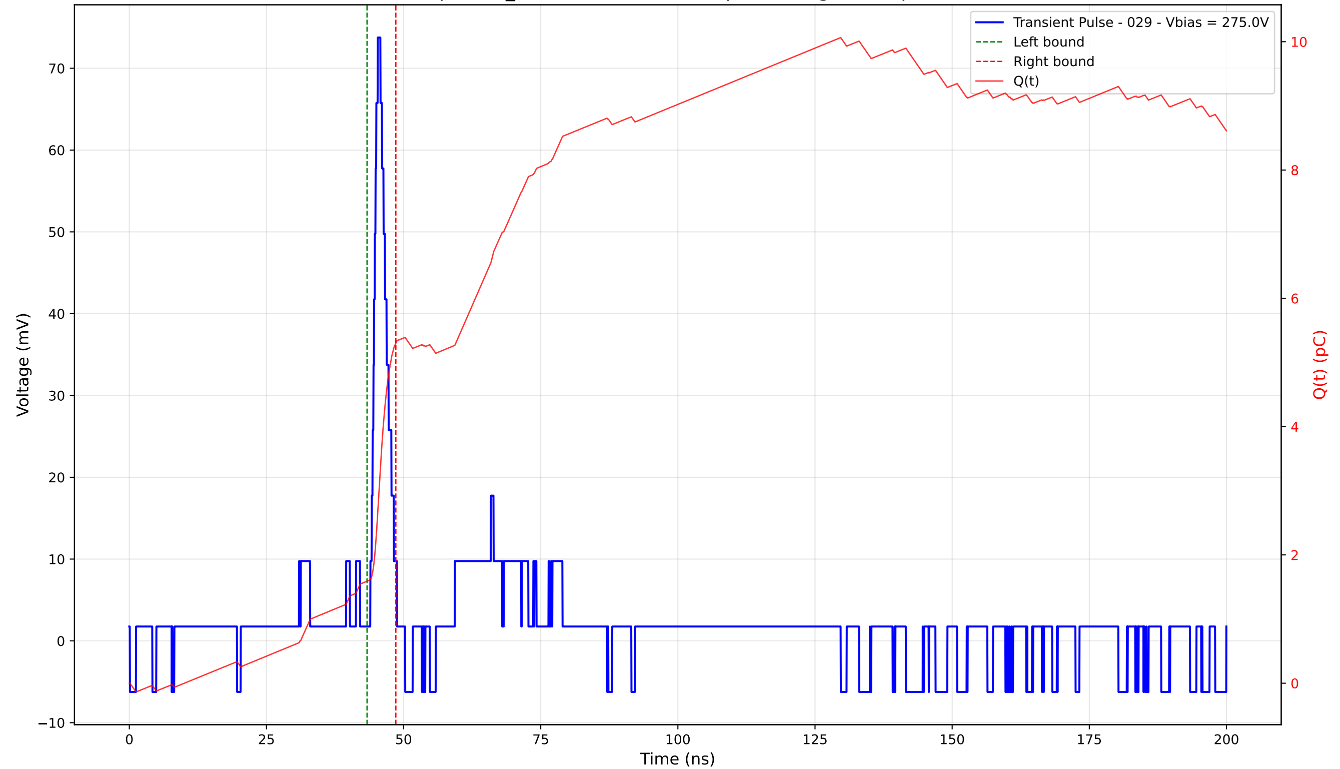
Transient Pulse - Sample: TD_4004 - Position: 435.0 \mu\text{m} - Charge: 3.71 pC - Rise Time: 1.35 ns
