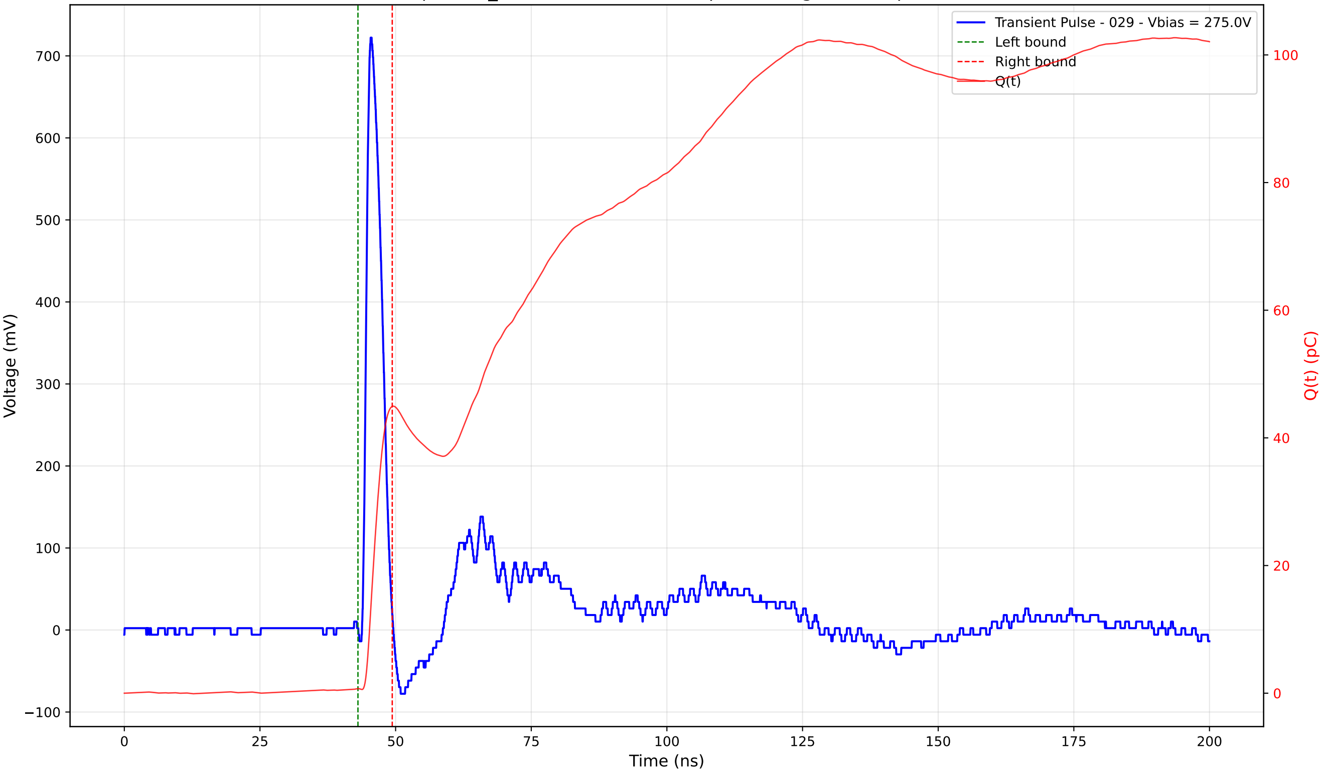
Transient Pulse - Sample: TD_4004 - Position: 315.0 \mu\text{m} - Charge: 44.22 pC - Rise Time: 0.98 ns
