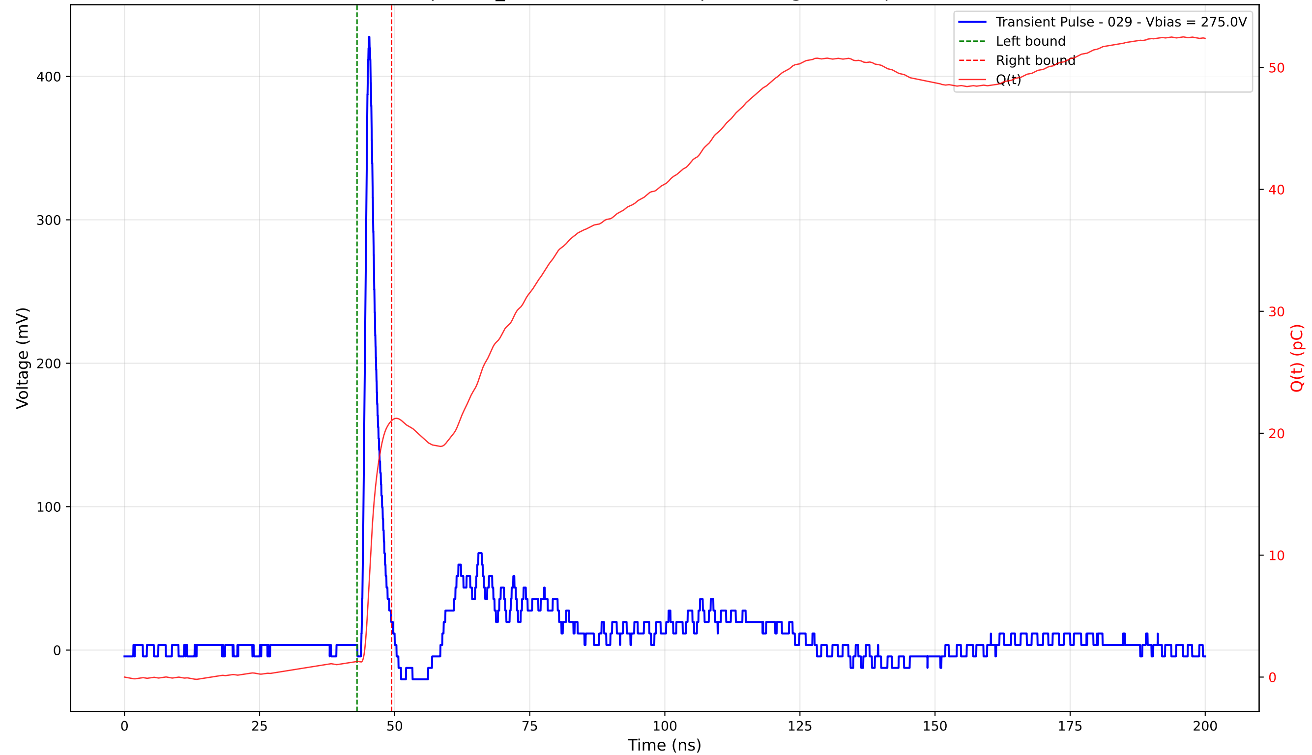
Transient Pulse - Sample: TD_4004 - Position: 65.0 \mu\text{m} - Charge: 19.75 pC - Rise Time: 0.92 ns
