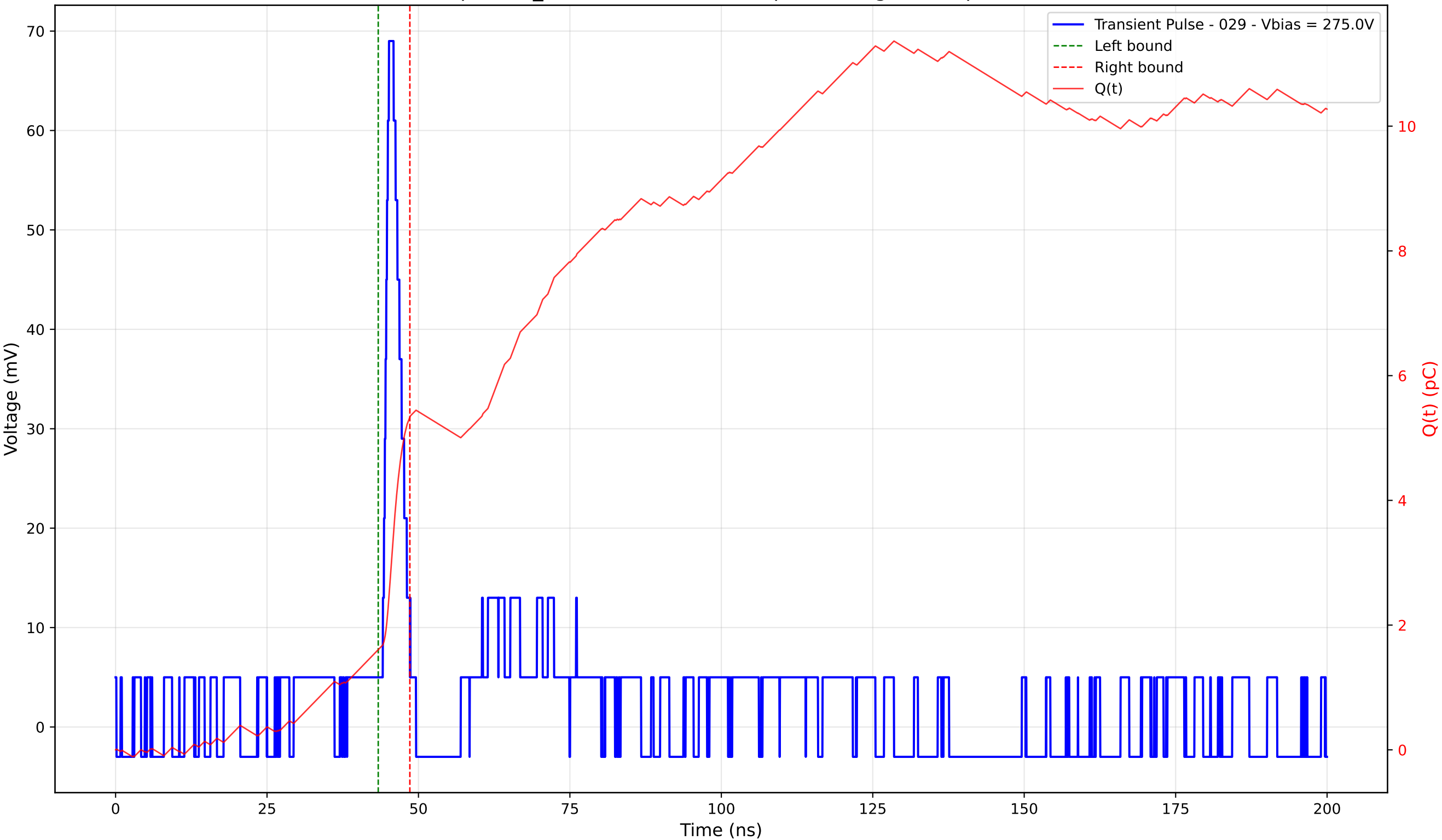
Transient Pulse - Sample: TD_4004 - Position: 430.0 \mu\text{m} - Charge: 3.73 pC - Rise Time: 1.02 ns
