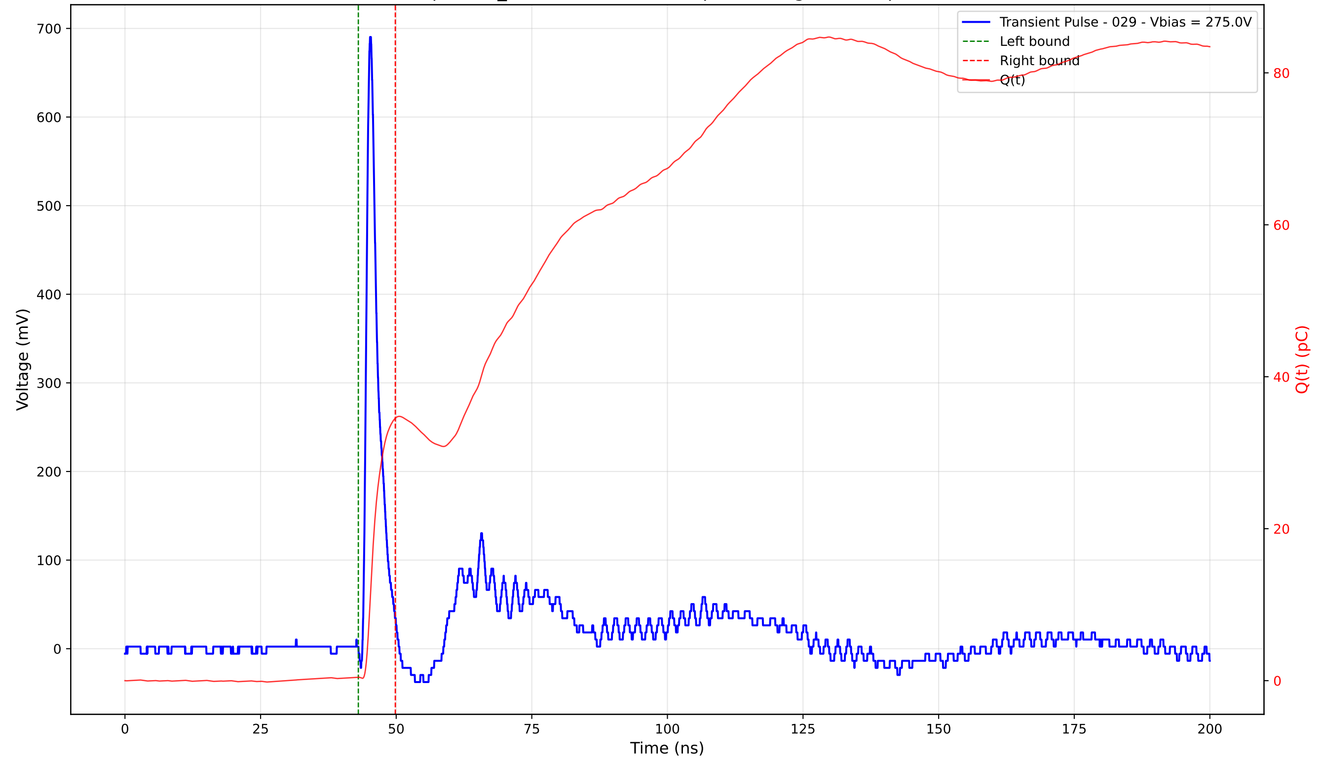
Transient Pulse - Sample: TD_4004 - Position: 80.0 \mu\text{m} - Charge: 34.08 pC - Rise Time: 0.90 ns
