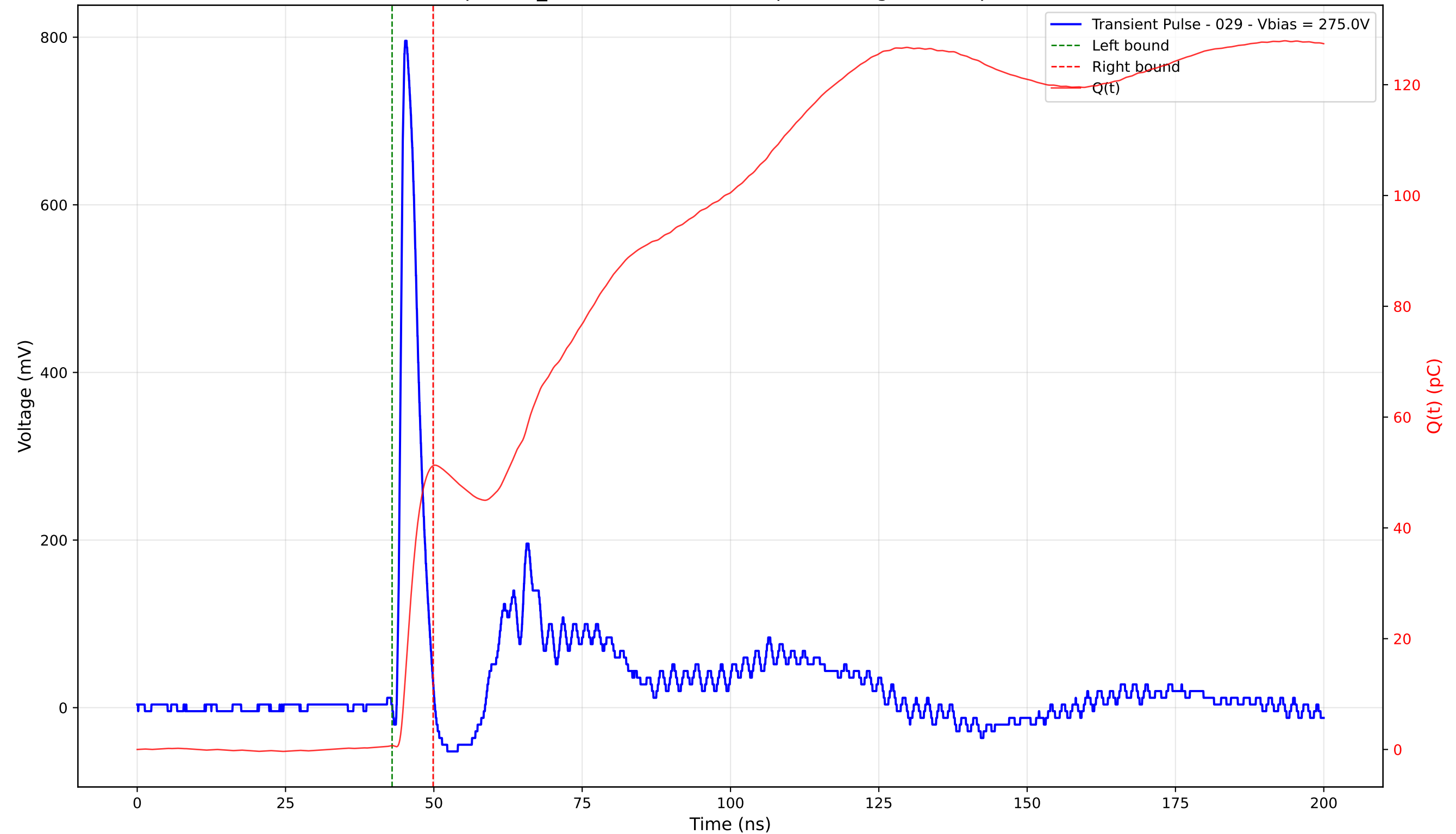
Transient Pulse - Sample: TD_4004 - Position: 190.0 \mu\text{m} - Charge: 50.54 pC - Rise Time: 0.89 ns
