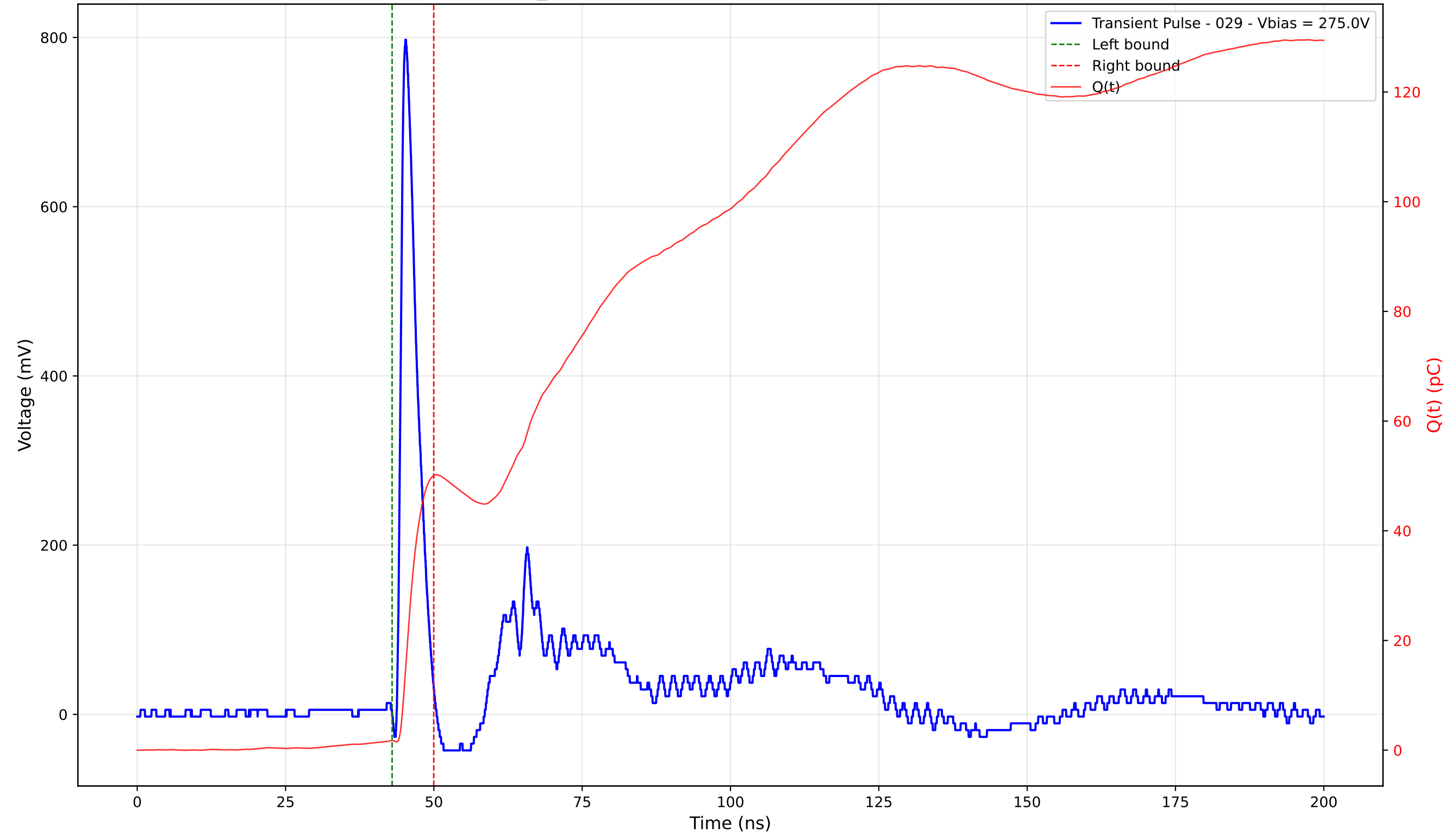
Transient Pulse - Sample: TD_4004 - Position: 105.0 \mu\text{m} - Charge: 48.30 pC - Rise Time: 0.89 ns
