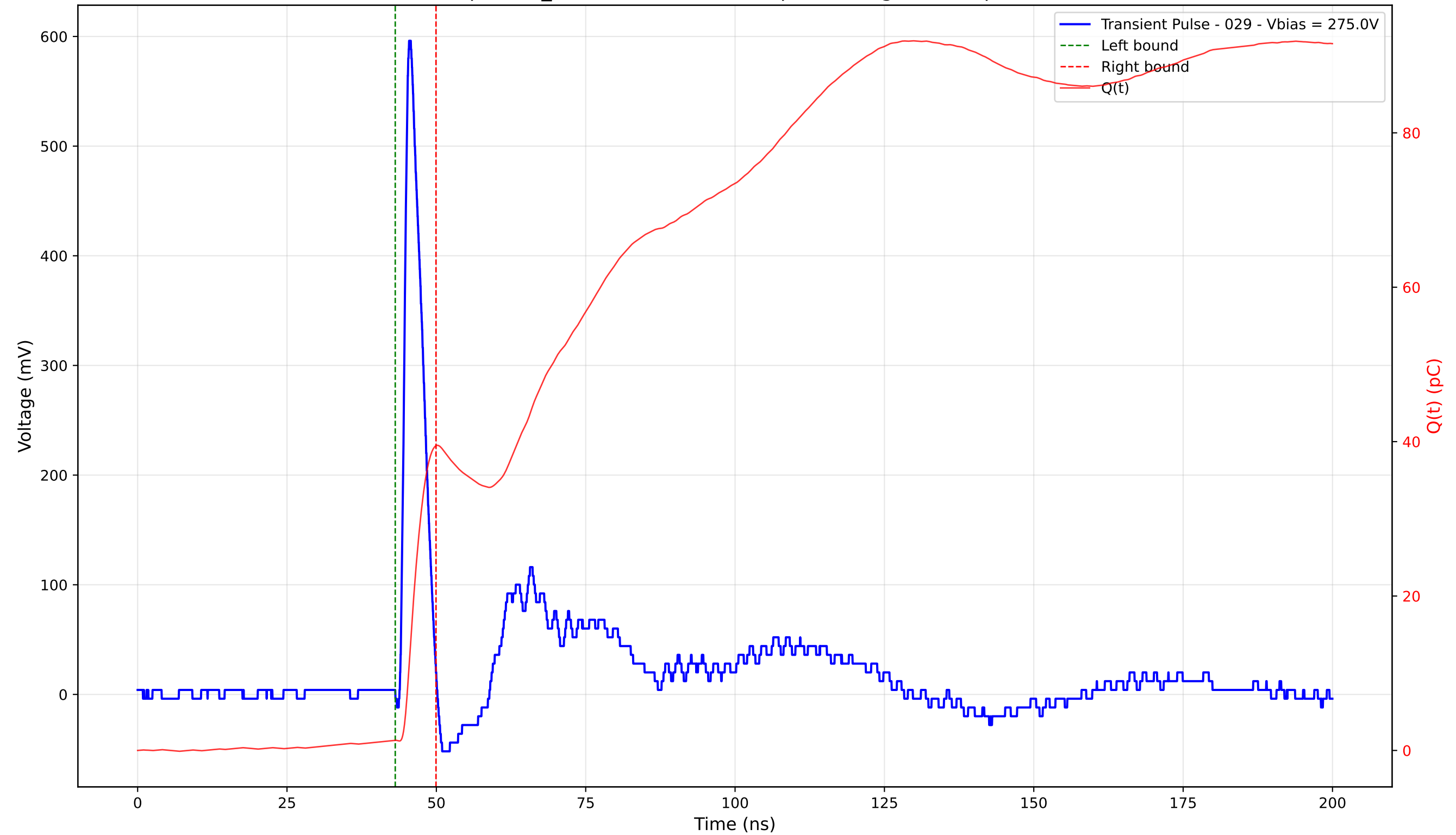
Transient Pulse - Sample: TD_4004 - Position: 375.0 \mu\text{m} - Charge: 38.15 pC - Rise Time: 1.01 ns
