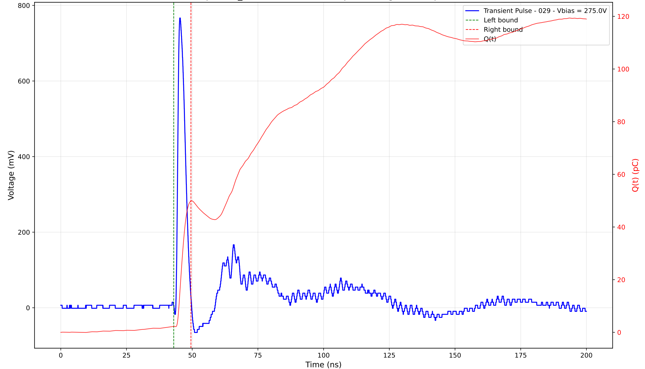
Transient Pulse - Sample: TD_4004 - Position: 235.0 \mu\text{m} - Charge: 47.59 pC - Rise Time: 0.93 ns
