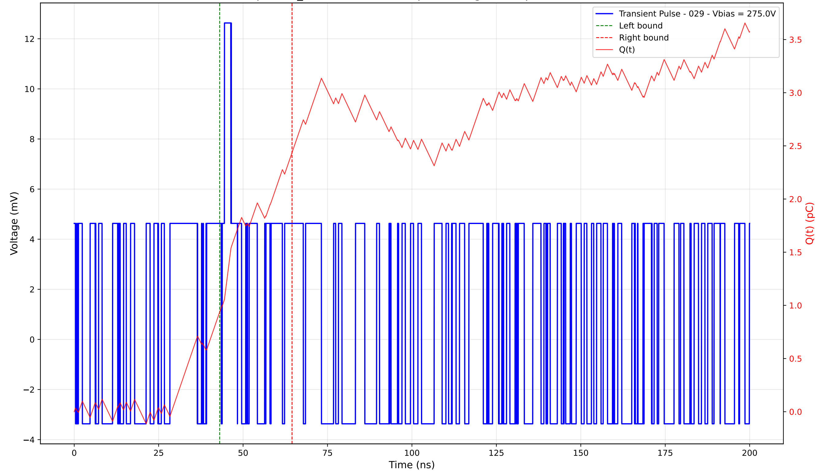
Transient Pulse - Sample: TD_4004 - Position: 0.0 \mu\text{m} - Charge: 1.50 pC - Rise Time: 0.00 ns (N/A)
