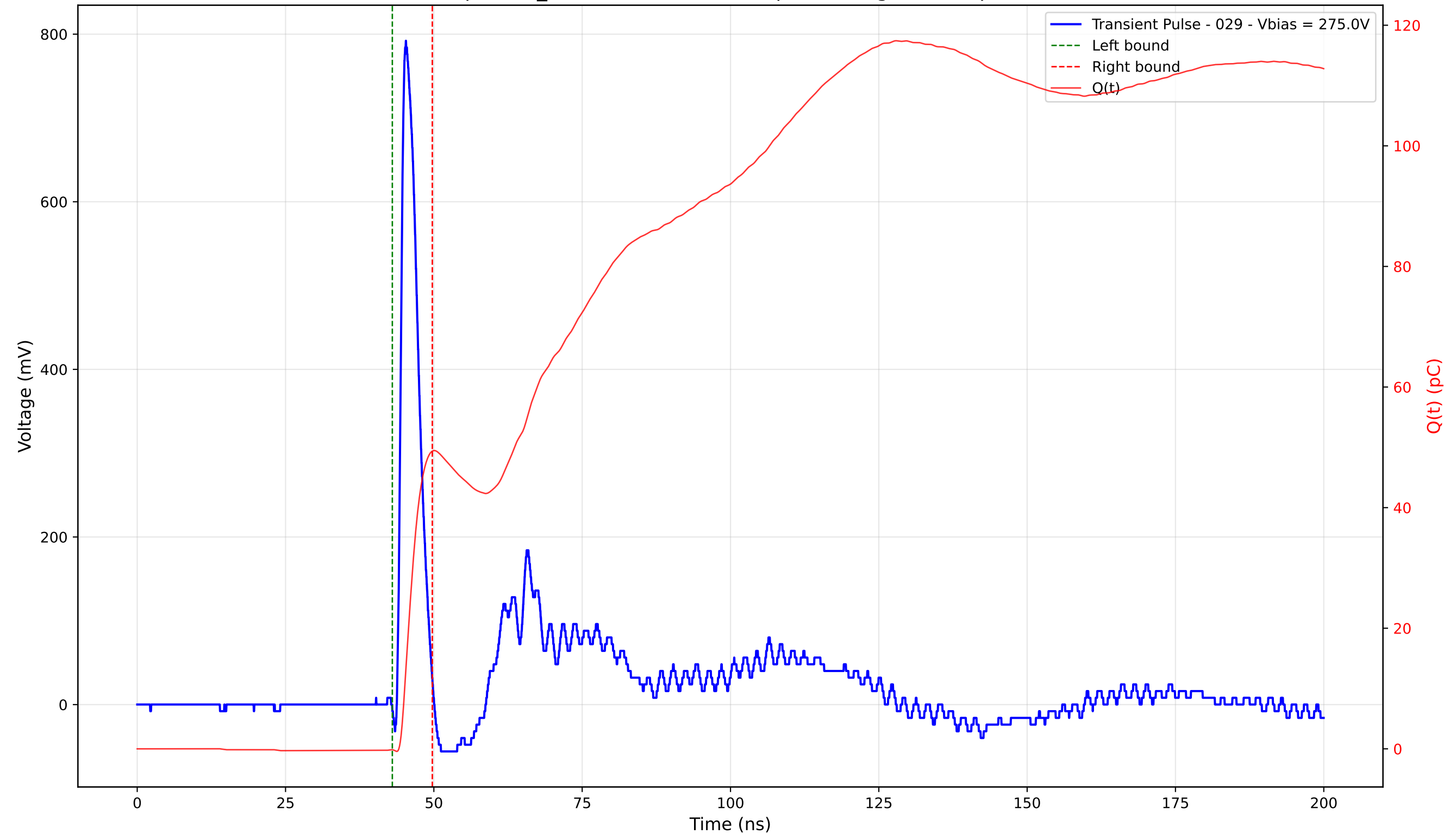
Transient Pulse - Sample: TD_4004 - Position: 205.0 \mu\text{m} - Charge: 49.53 pC - Rise Time: 0.90 ns
