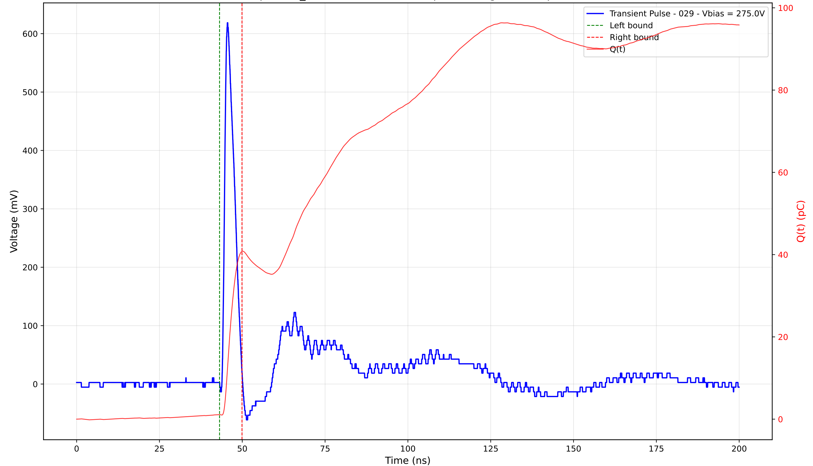
Transient Pulse - Sample: TD_4004 - Position: 365.0 \mu\text{m} - Charge: 39.69 pC - Rise Time: 1.02 ns
