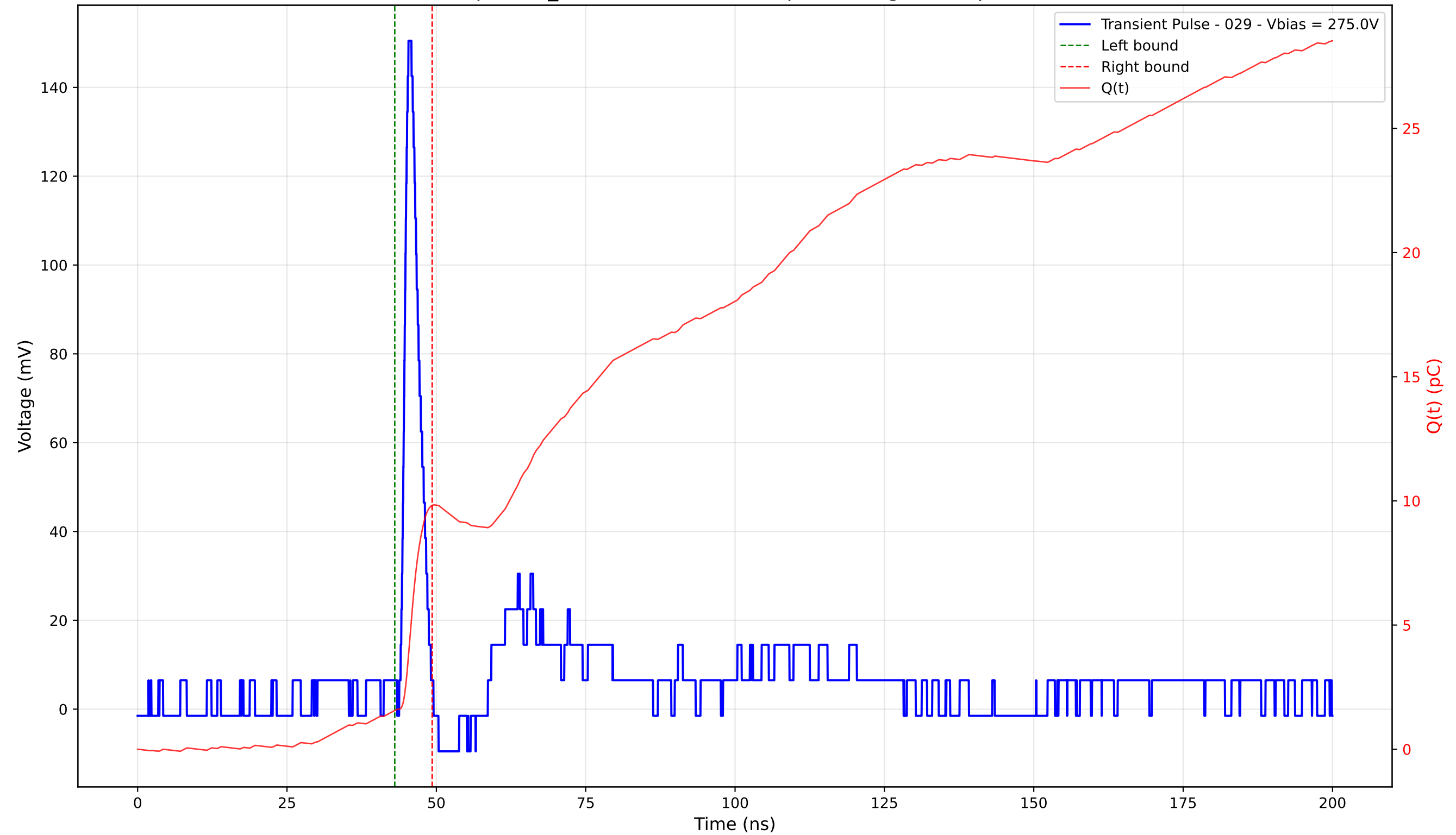
Transient Pulse - Sample: TD_4004 - Position: 415.0 \mu\text{m} - Charge: 8.25 pC - Rise Time: 1.08 ns
