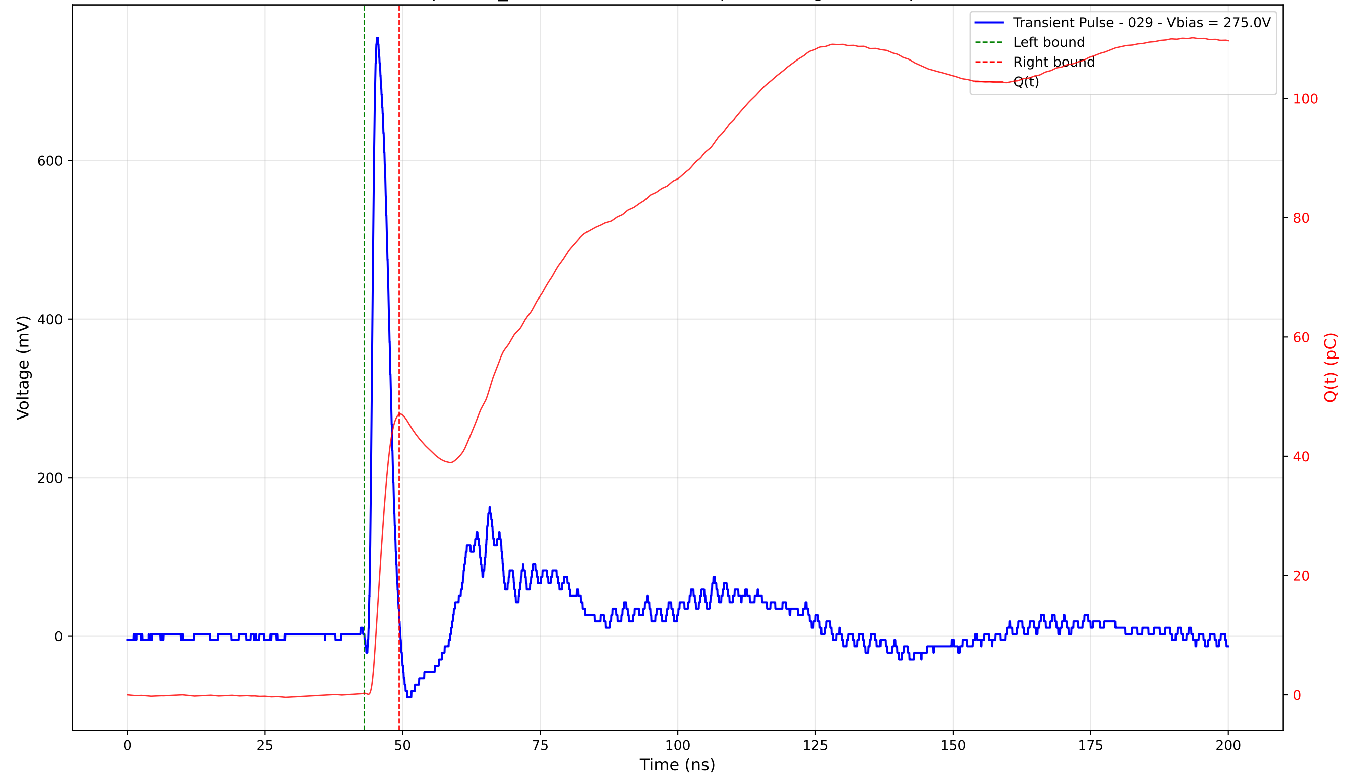
Transient Pulse - Sample: TD_4004 - Position: 265.0 \mu\text{m} - Charge: 46.76 pC - Rise Time: 0.94 ns
