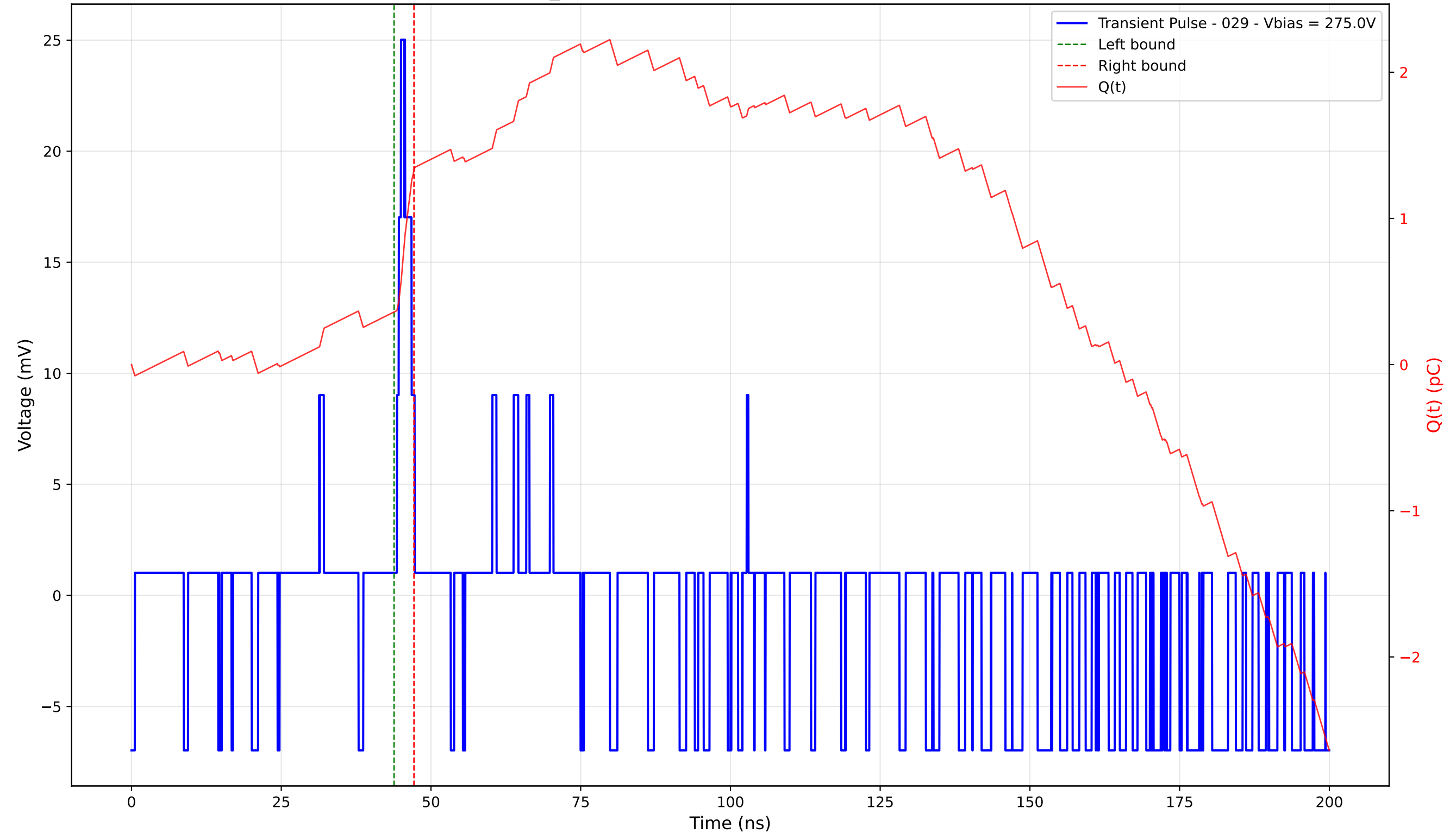
Transient Pulse - Sample: TD_4004 - Position: 25.0 \mu\text{m} - Charge: 0.97 pC - Rise Time: 0.68 ns
