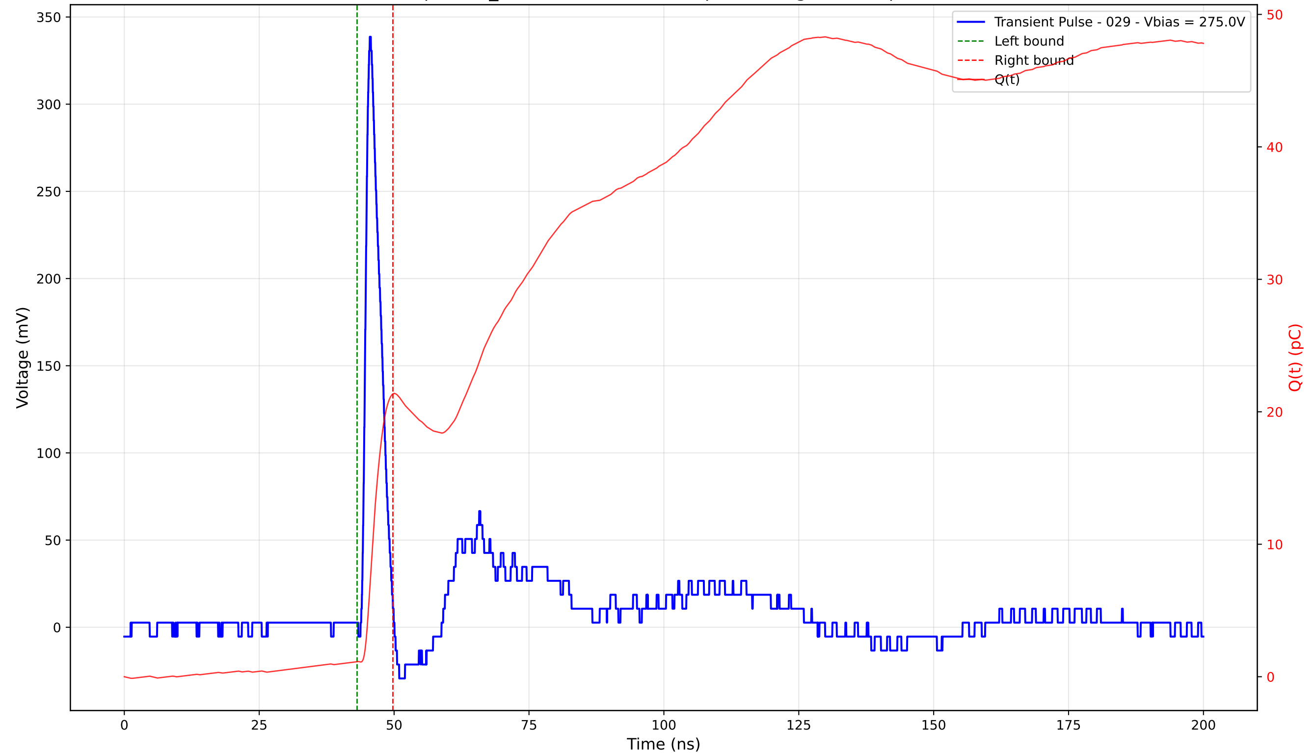
Transient Pulse - Sample: TD_4004 - Position: 400.0 \mu\text{m} - Charge: 20.21 pC - Rise Time: 1.04 ns
