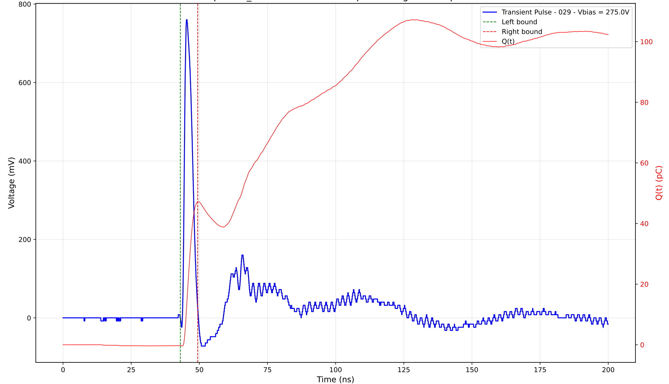
Transient Pulse - Sample: TD_4004 - Position: 275.0 \mu\text{m} - Charge: 47.40 pC - Rise Time: 0.94 ns
