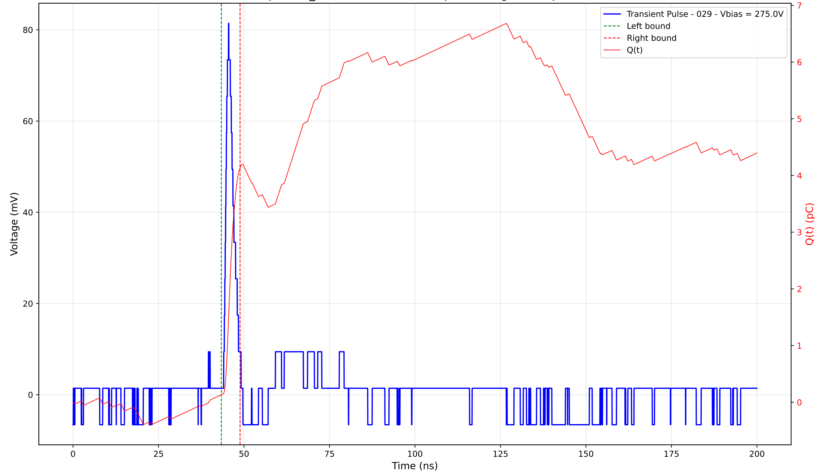
Transient Pulse - Sample: TD_4004 - Position: 425.0 \mu\text{m} - Charge: 4.00 pC - Rise Time: 1.08 ns
