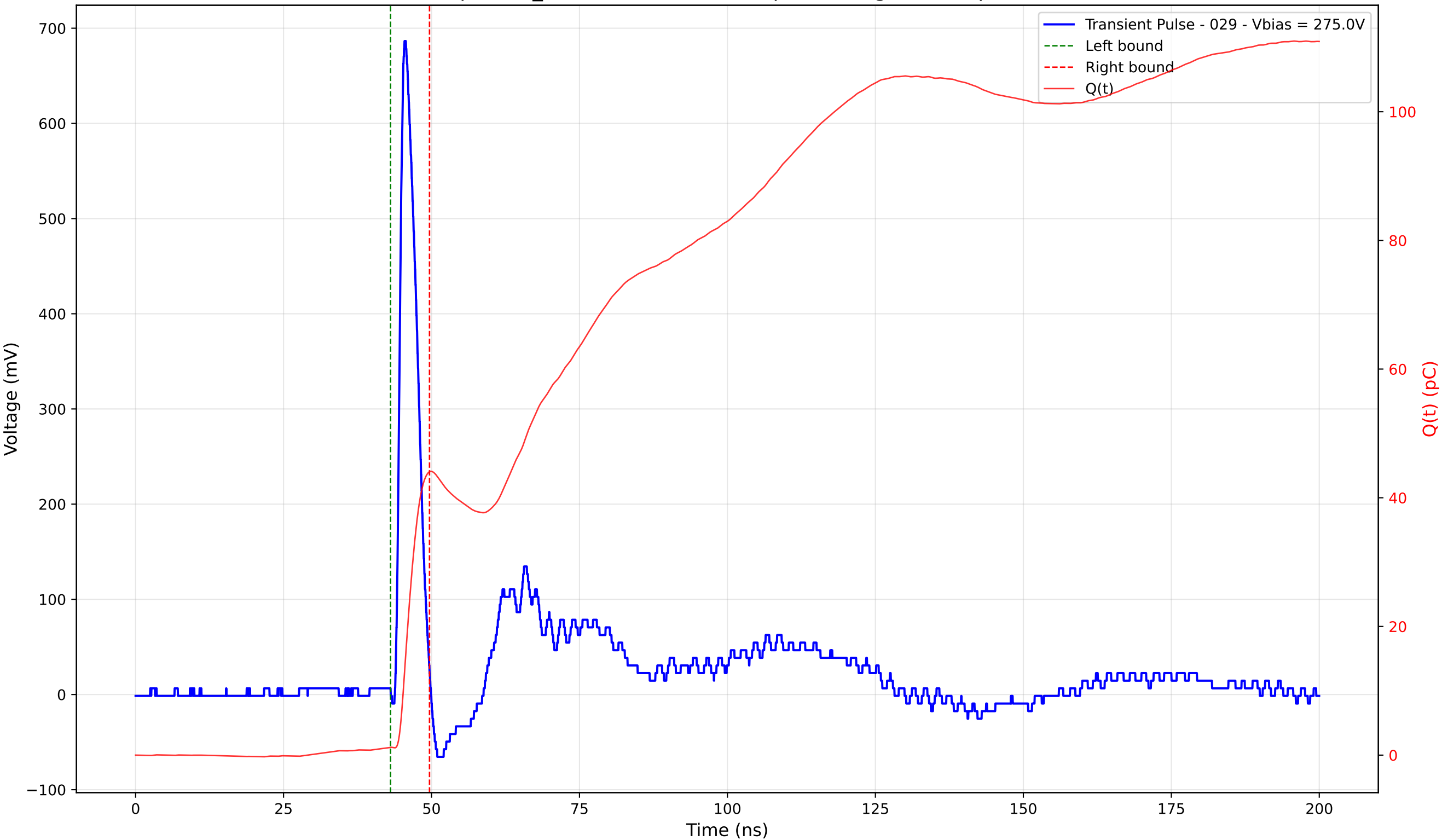
Transient Pulse - Sample: TD_4004 - Position: 330.0 \mu\text{m} - Charge: 42.83 pC - Rise Time: 1.01 ns
