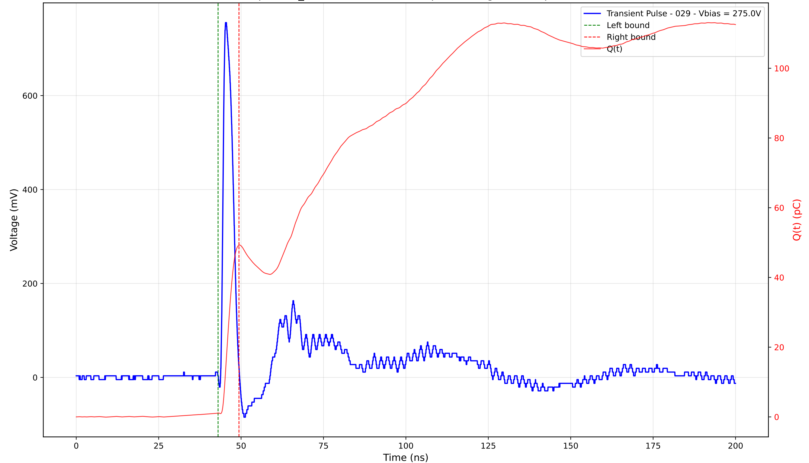
Transient Pulse - Sample: TD_4004 - Position: 290.0 \mu\text{m} - Charge: 48.13 pC - Rise Time: 0.93 ns
