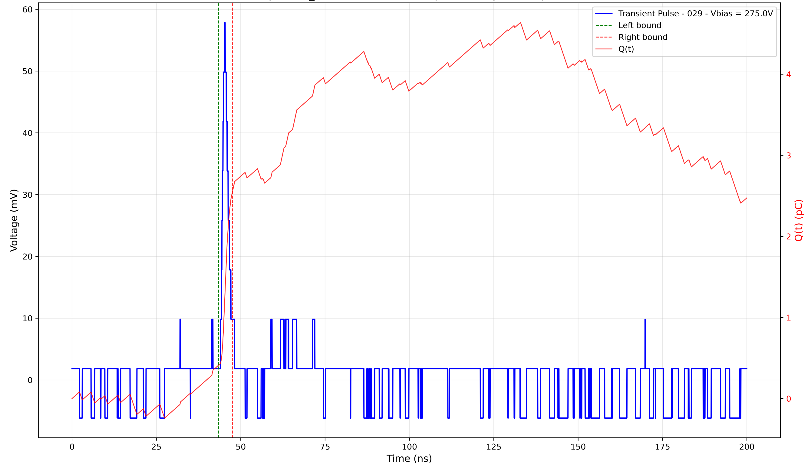
Transient Pulse - Sample: TD_4004 - Position: 40.0 \mu\text{m} - Charge: 2.16 pC - Rise Time: 1.25 ns
