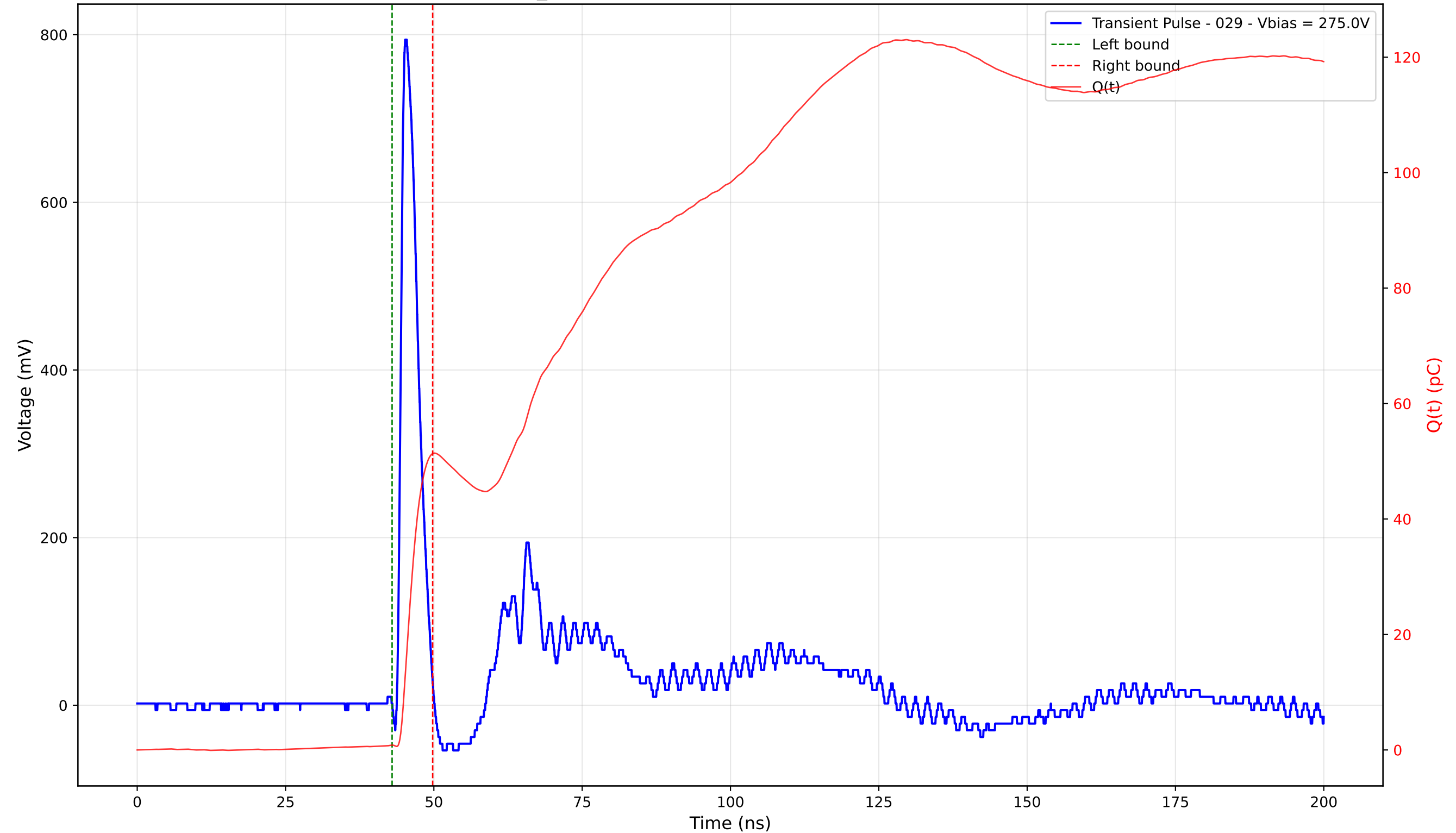
Transient Pulse - Sample: TD_4004 - Position: 180.0 \mu\text{m} - Charge: 50.50 pC - Rise Time: 0.88 ns
