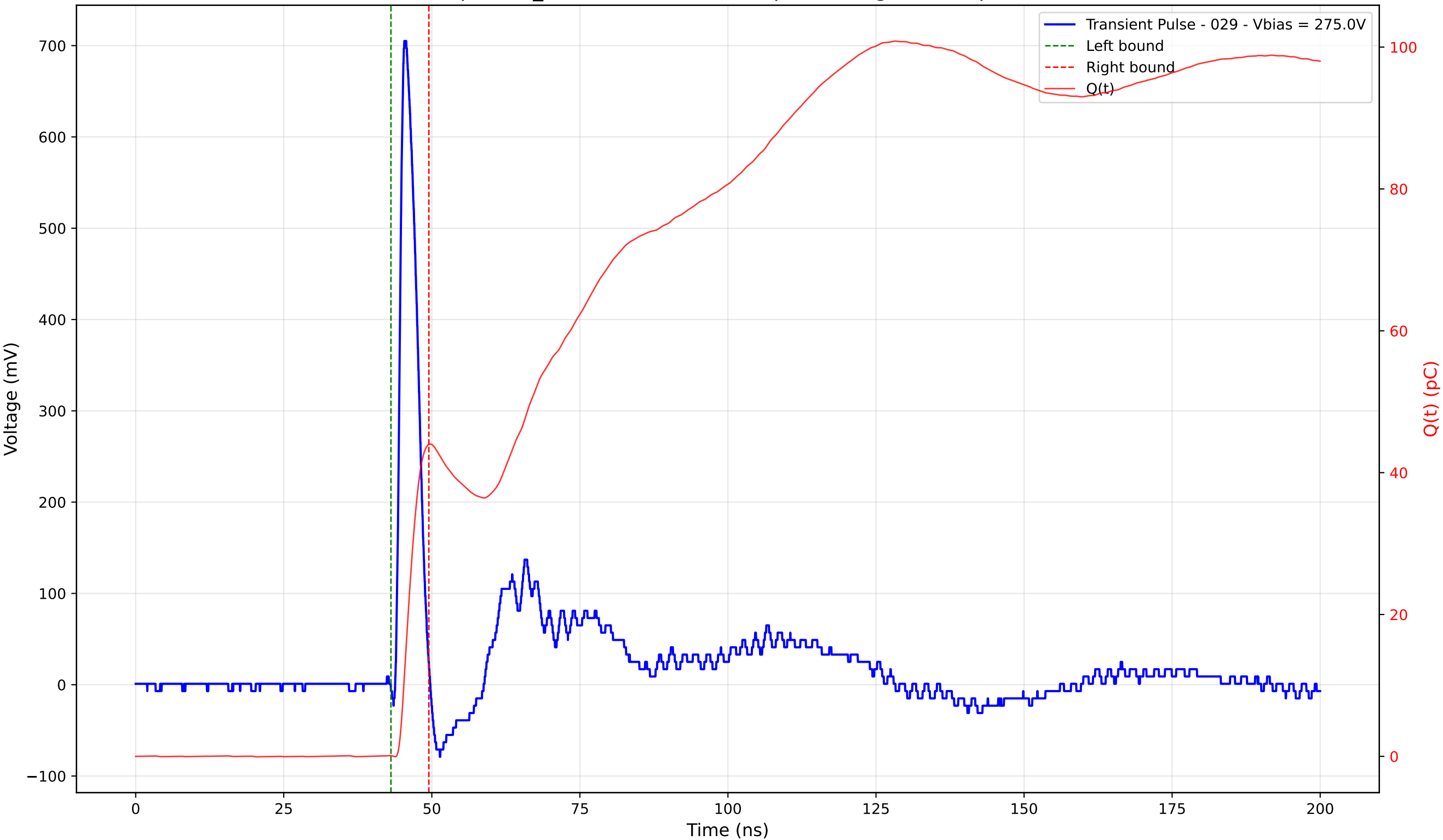
Transient Pulse - Sample: TD_4004 - Position: 325.0 \mu\text{m} - Charge: 43.88 pC - Rise Time: 0.99 ns
