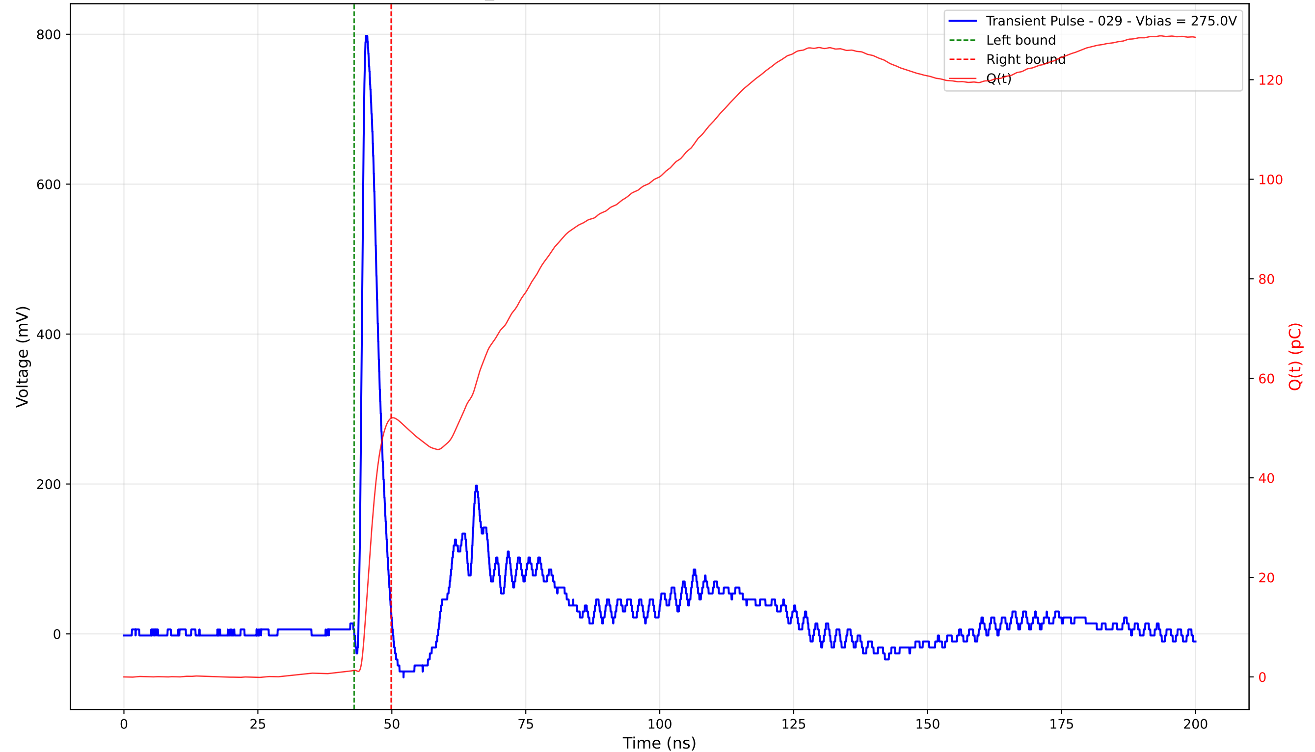
Transient Pulse - Sample: TD_4004 - Position: 185.0 \mu\text{m} - Charge: 50.66 pC - Rise Time: 0.88 ns
