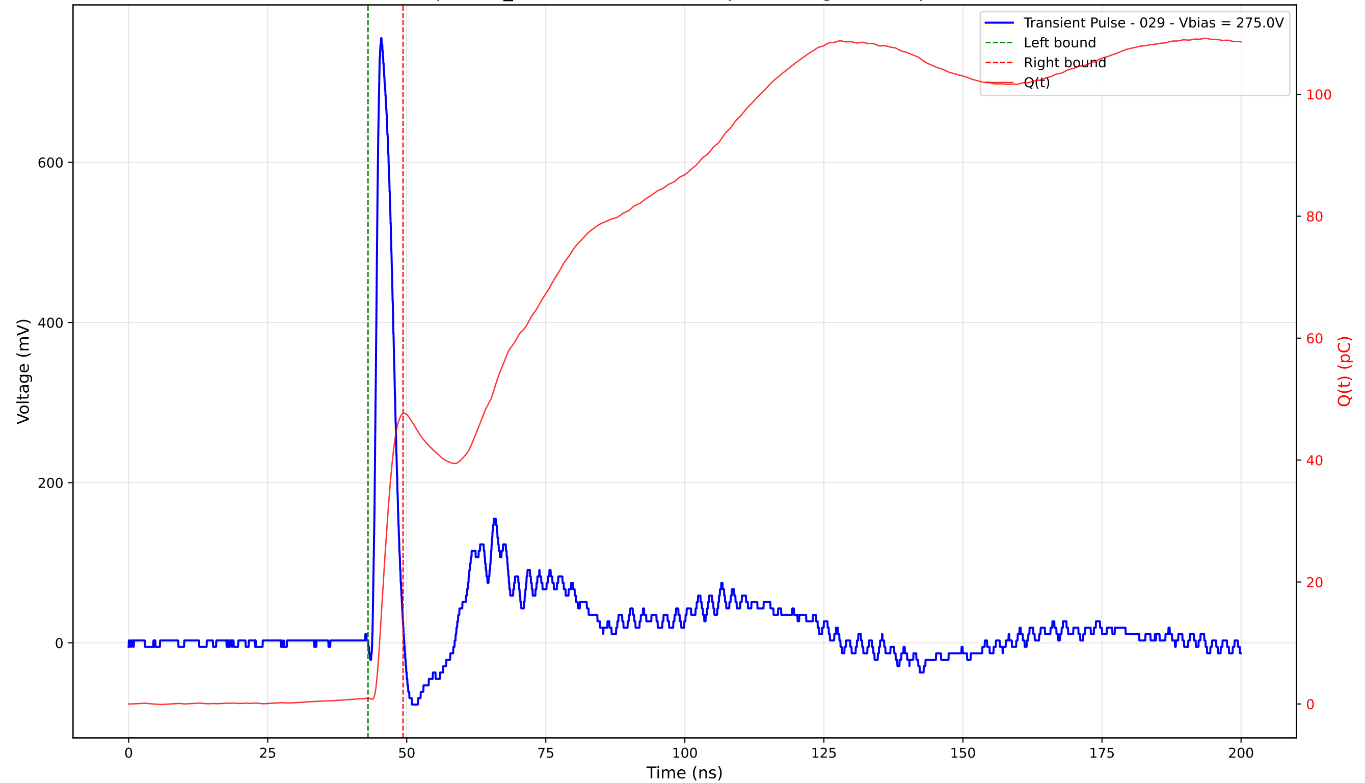
Transient Pulse - Sample: TD_4004 - Position: 300.0 \mu\text{m} - Charge: 46.69 pC - Rise Time: 0.96 ns
