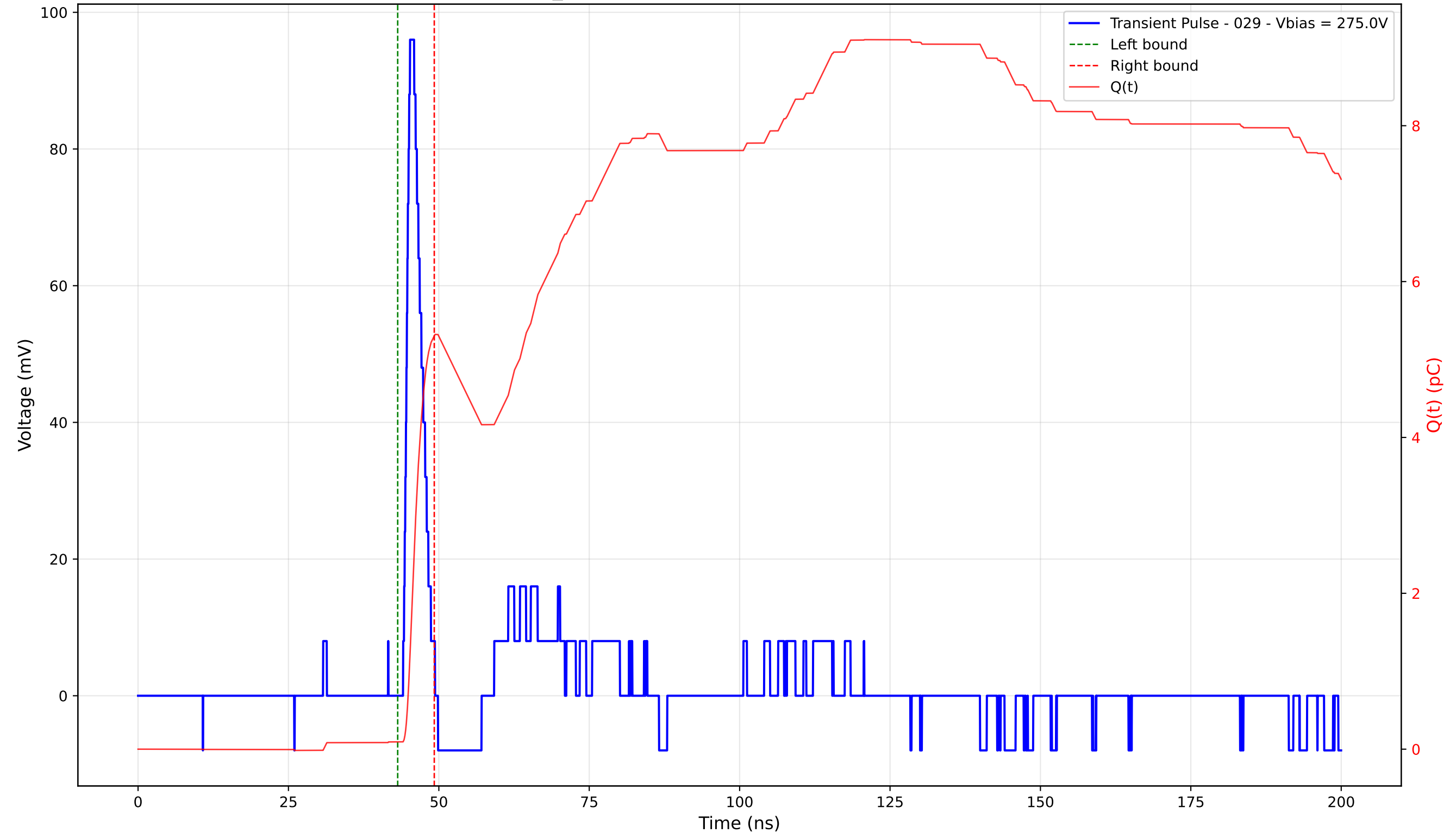
Transient Pulse - Sample: TD_4004 - Position: 420.0 \mu\text{m} - Charge: 5.21 pC - Rise Time: 0.86 ns
