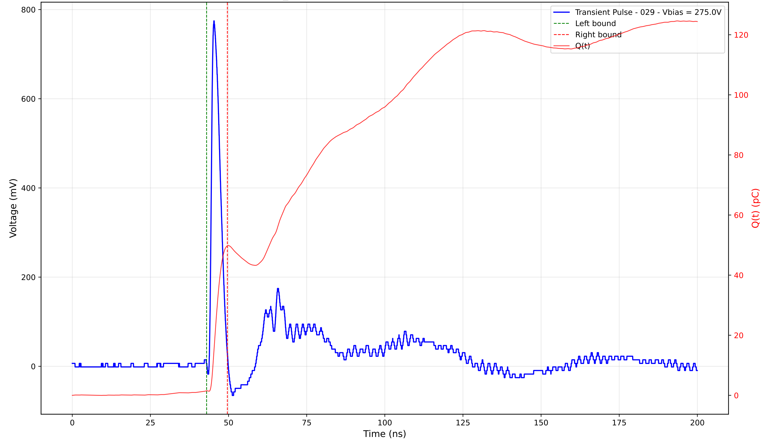
Transient Pulse - Sample: TD_4004 - Position: 155.0 \mu\text{m} - Charge: 48.26 pC - Rise Time: 0.93 ns
