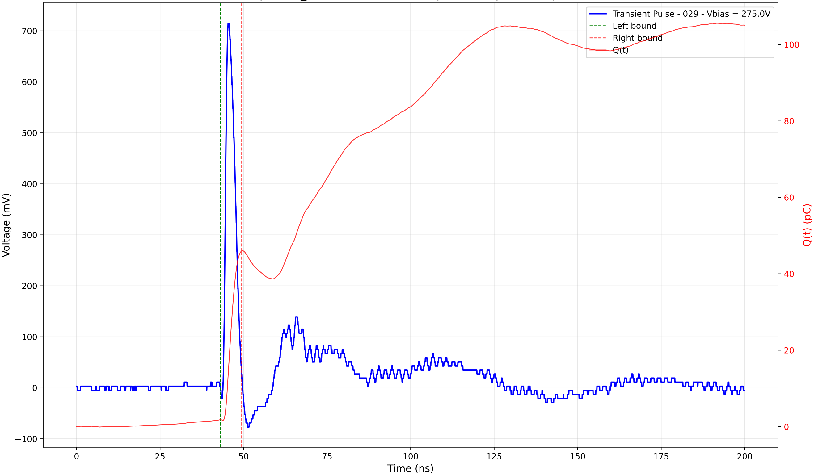
Transient Pulse - Sample: TD_4004 - Position: 320.0 \mu\text{m} - Charge: 44.17 pC - Rise Time: 0.97 ns
