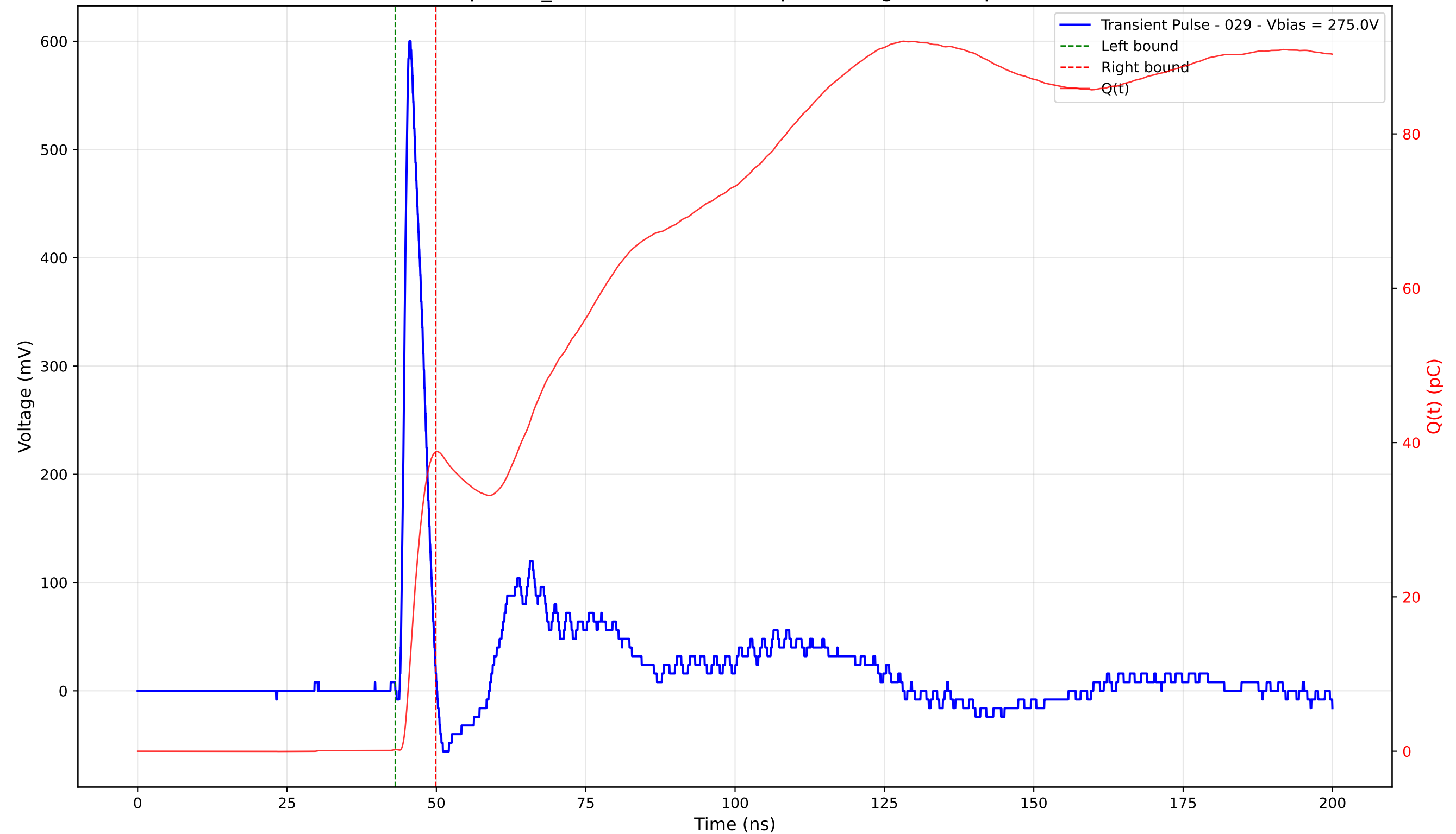
Transient Pulse - Sample: TD_4004 - Position: 370.0 \mu\text{m} - Charge: 38.59 pC - Rise Time: 1.03 ns
