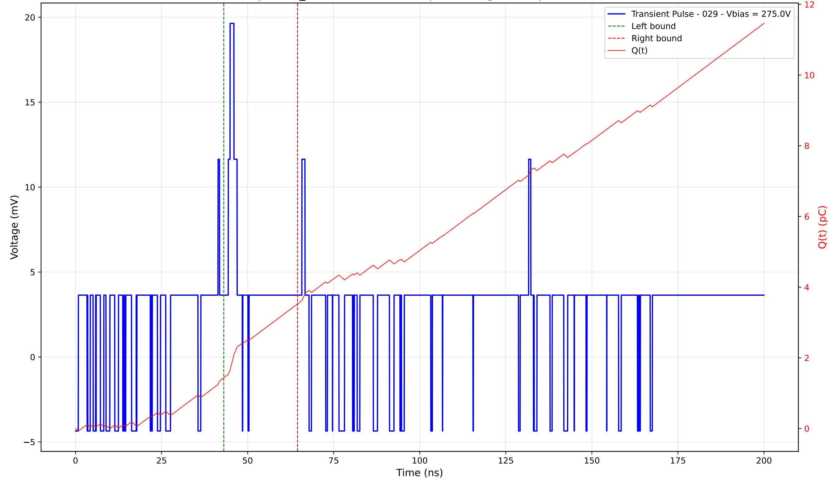
Transient Pulse - Sample: TD_4004 - Position: 10.0 \mu\text{m} - Charge: 2.09 pC - Rise Time: 0.00 ns (N/A)
