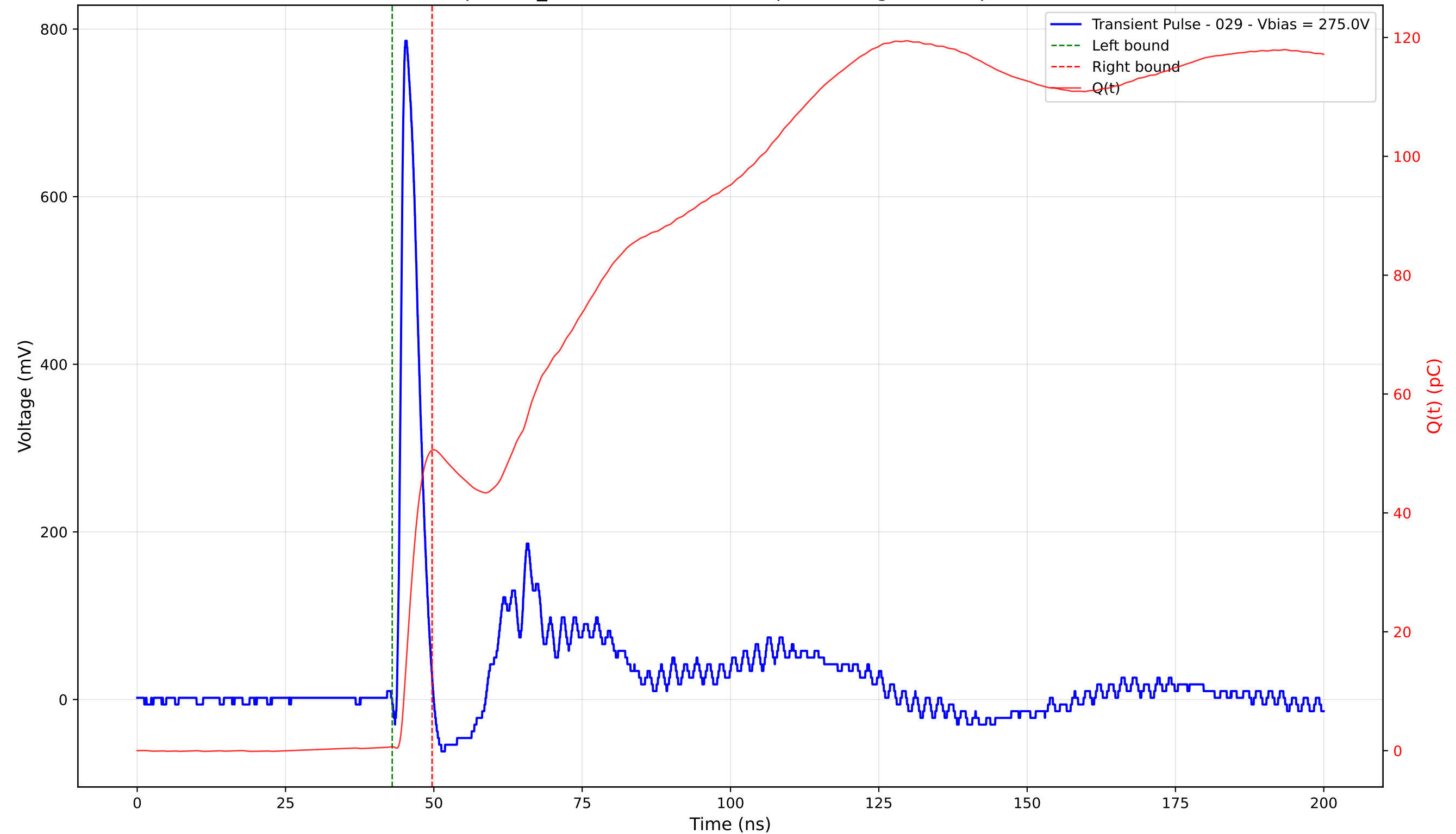
Transient Pulse - Sample: TD_4004 - Position: 170.0 \mu\text{m} - Charge: 49.88 pC - Rise Time: 0.91 ns
