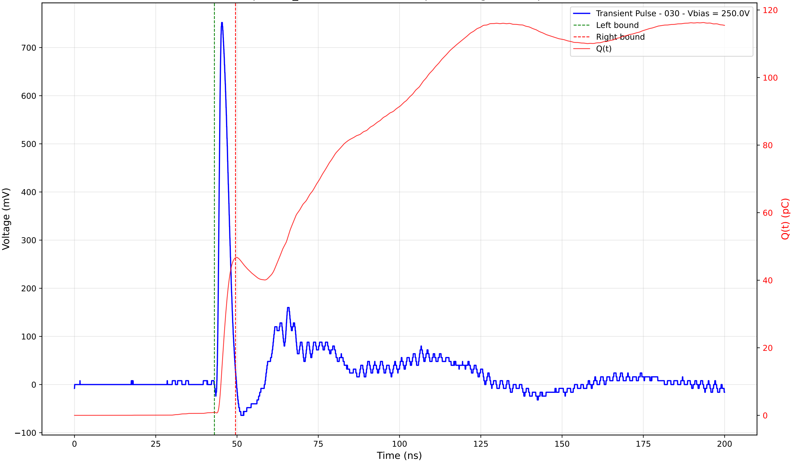
Transient Pulse - Sample: TD_4004 - Position: 140.0 \mu\text{m} - Charge: 45.77 pC - Rise Time: 0.93 ns
