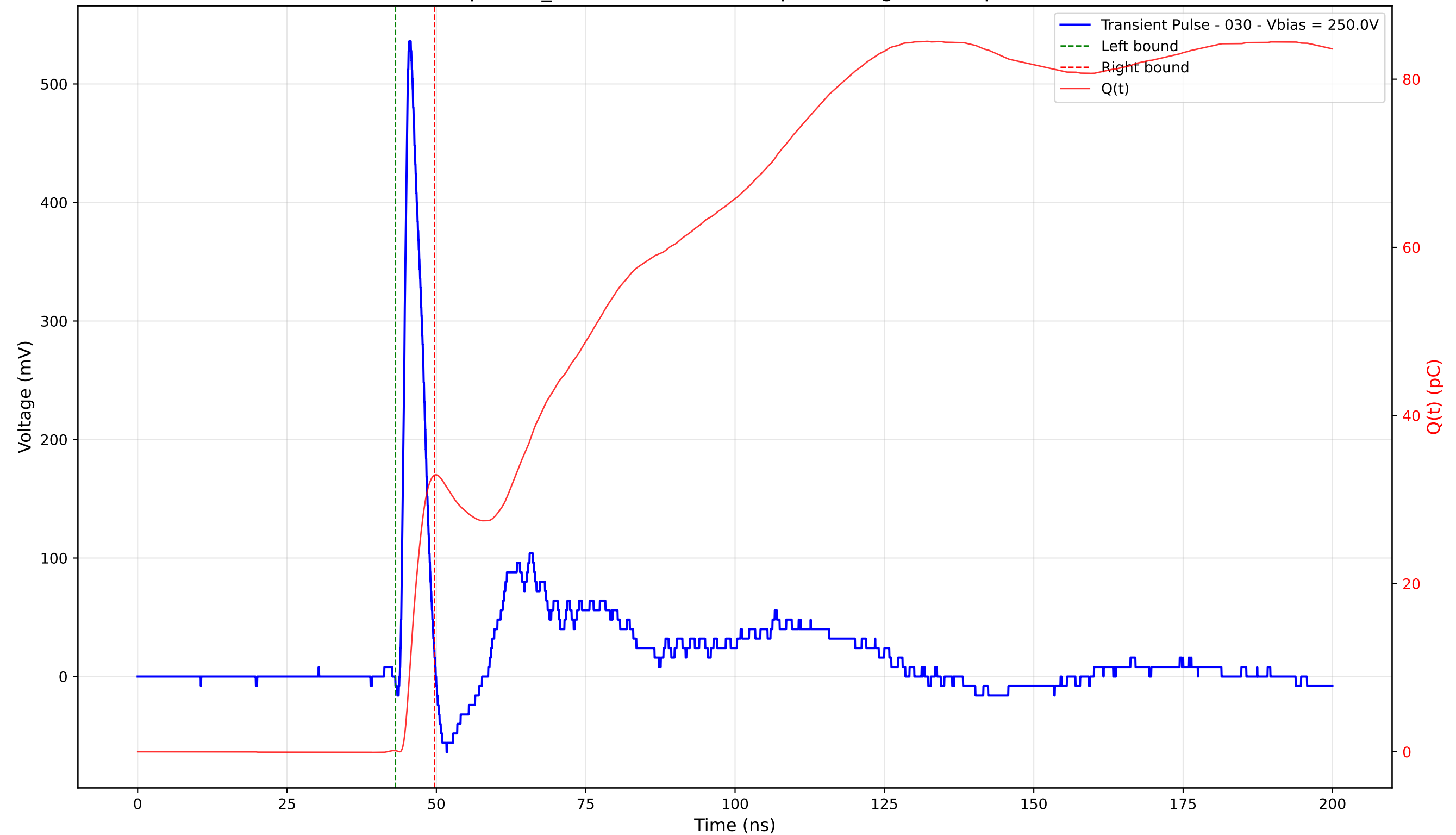
Transient Pulse - Sample: TD_4004 - Position: 365.0 \mu\text{m} - Charge: 32.76 pC - Rise Time: 1.03 ns
