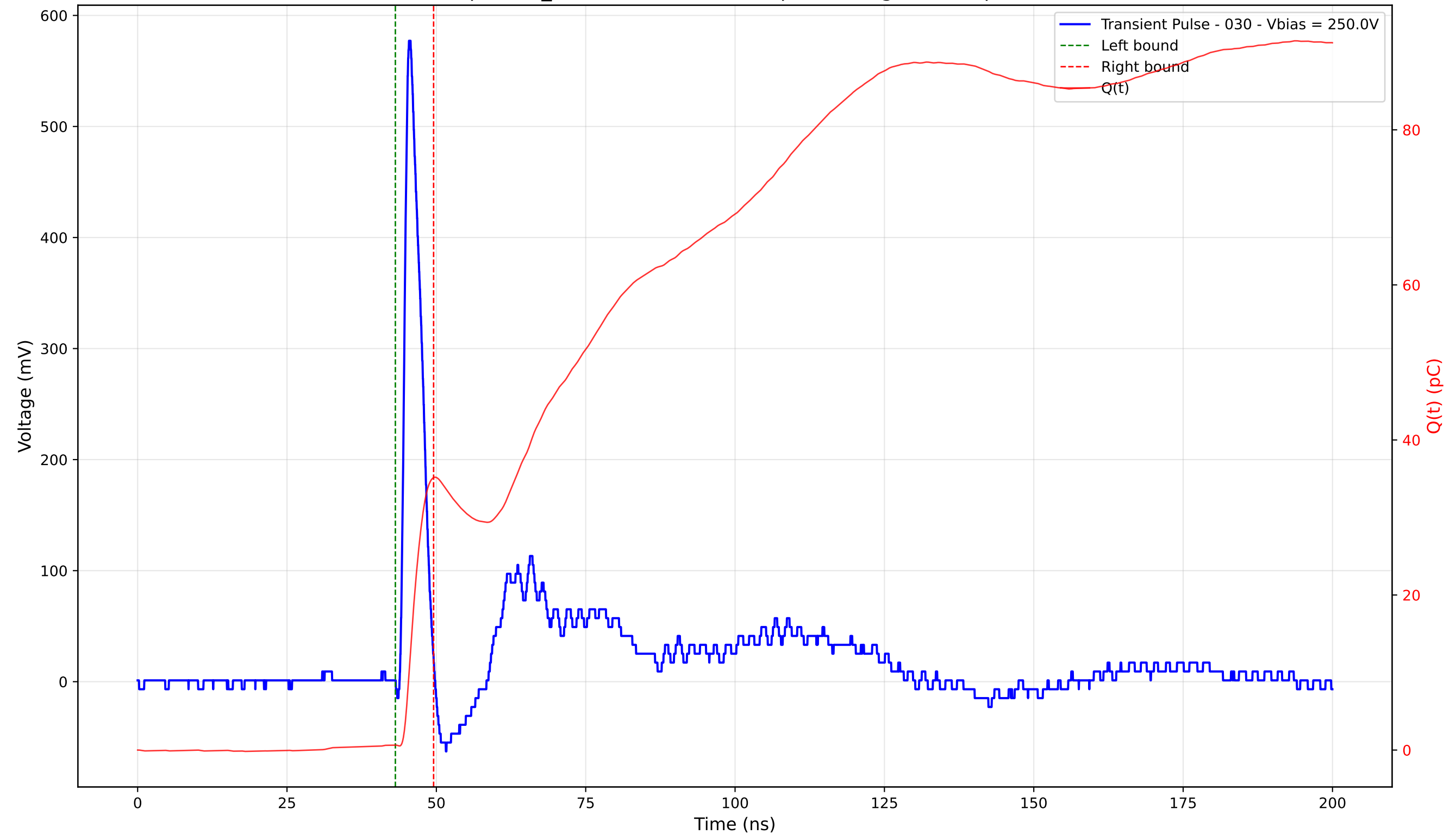
Transient Pulse - Sample: TD_4004 - Position: 345.0 \mu\text{m} - Charge: 34.50 pC - Rise Time: 0.99 ns
