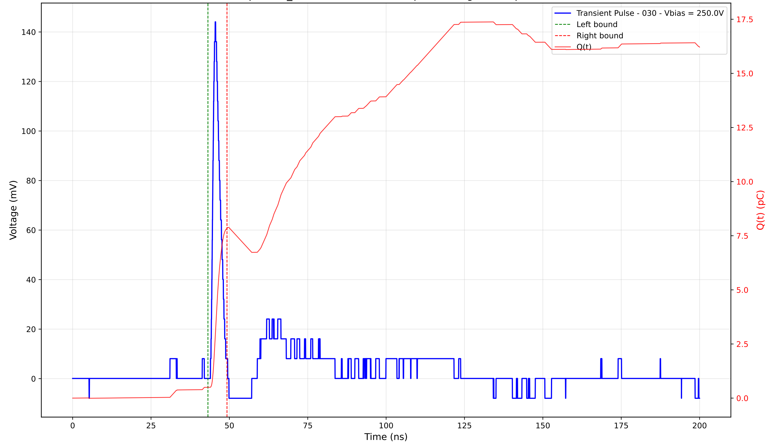
Transient Pulse - Sample: TD_4004 - Position: 415.0 \mu\text{m} - Charge: 7.35 pC - Rise Time: 1.10 ns
