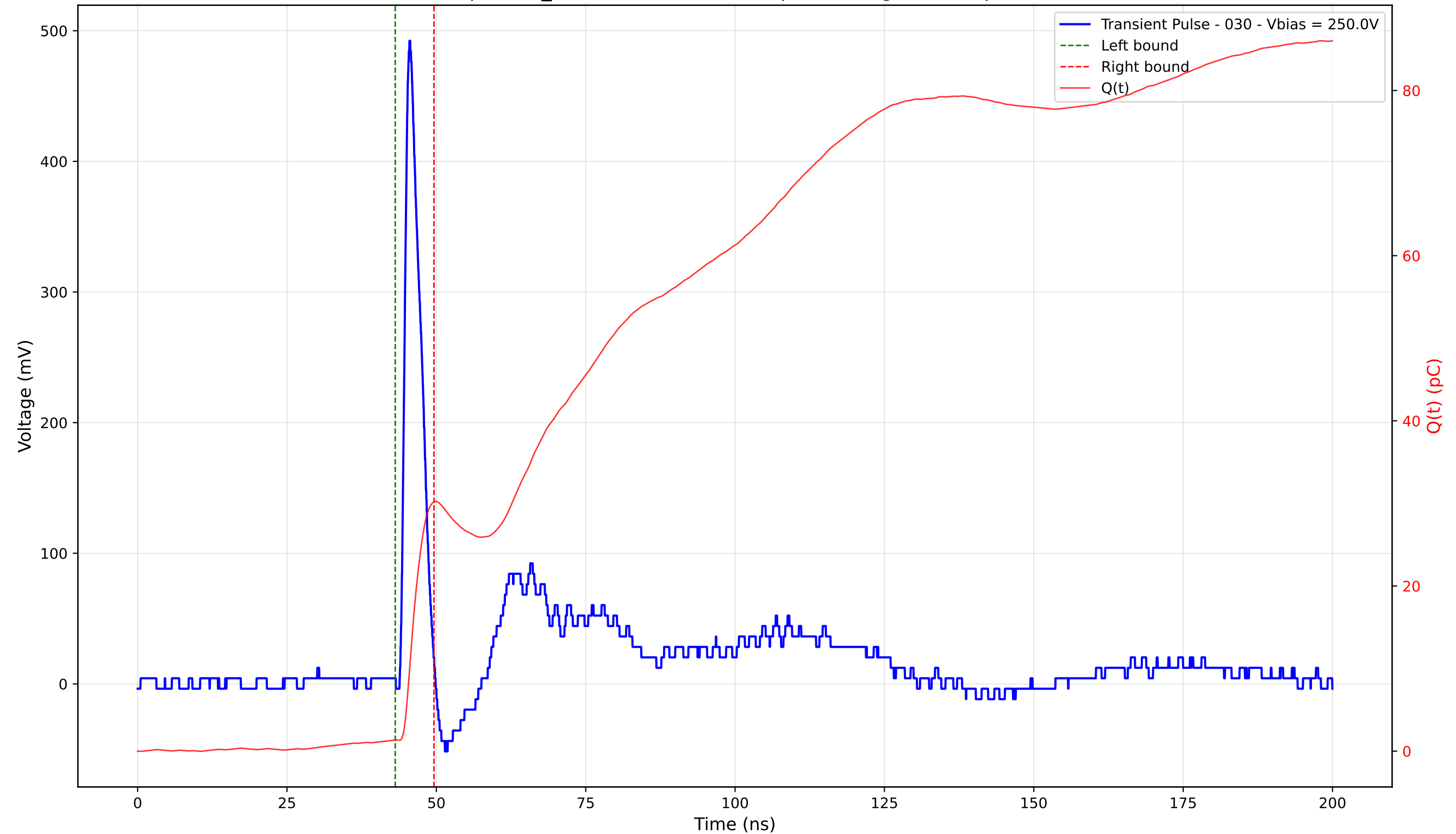
Transient Pulse - Sample: TD_4004 - Position: 385.0 \mu\text{m} - Charge: 28.83 pC - Rise Time: 1.03 ns
