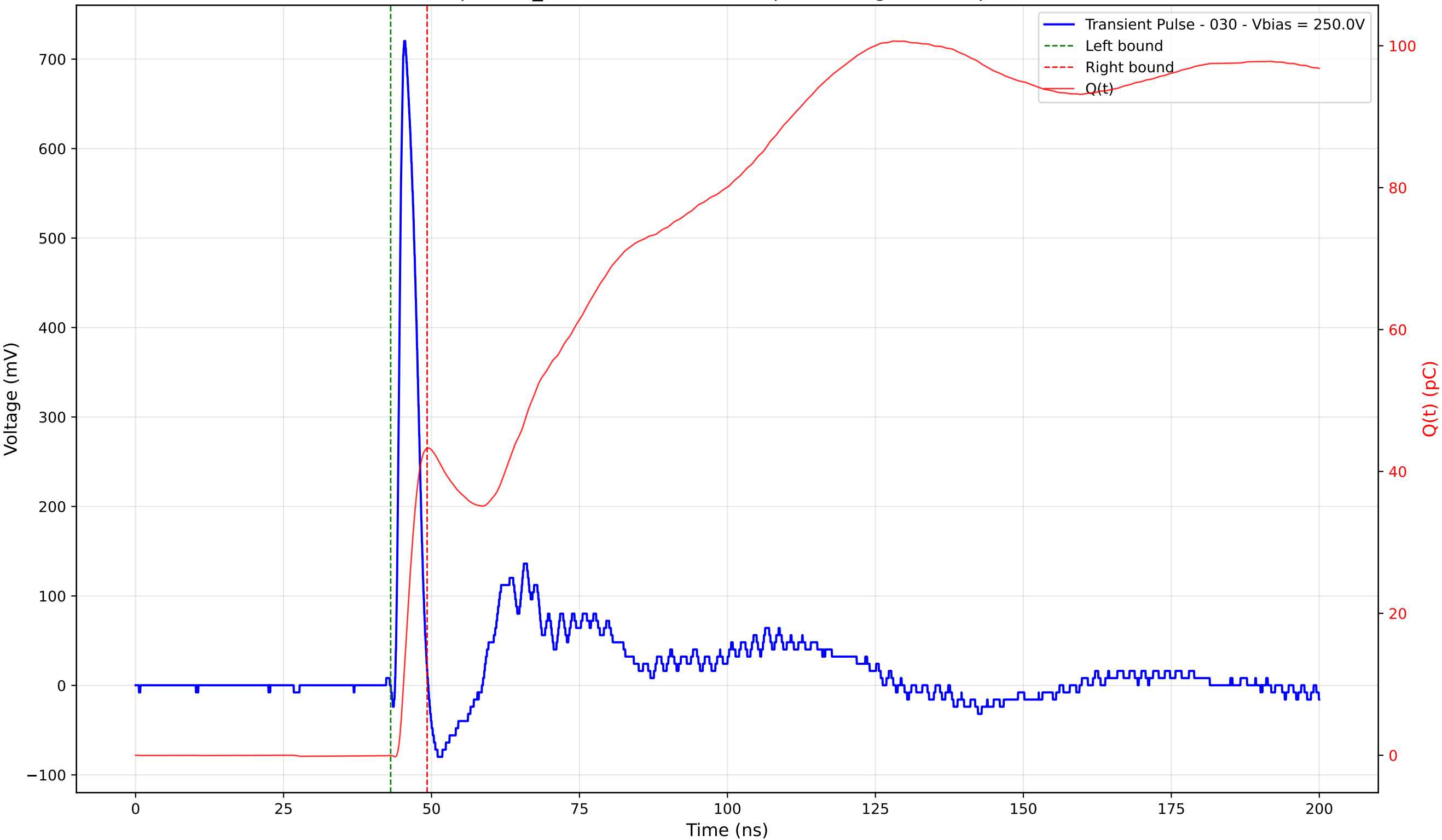
Transient Pulse - Sample: TD_4004 - Position: 305.0 \mu\text{m} - Charge: 43.30 pC - Rise Time: 0.96 ns
