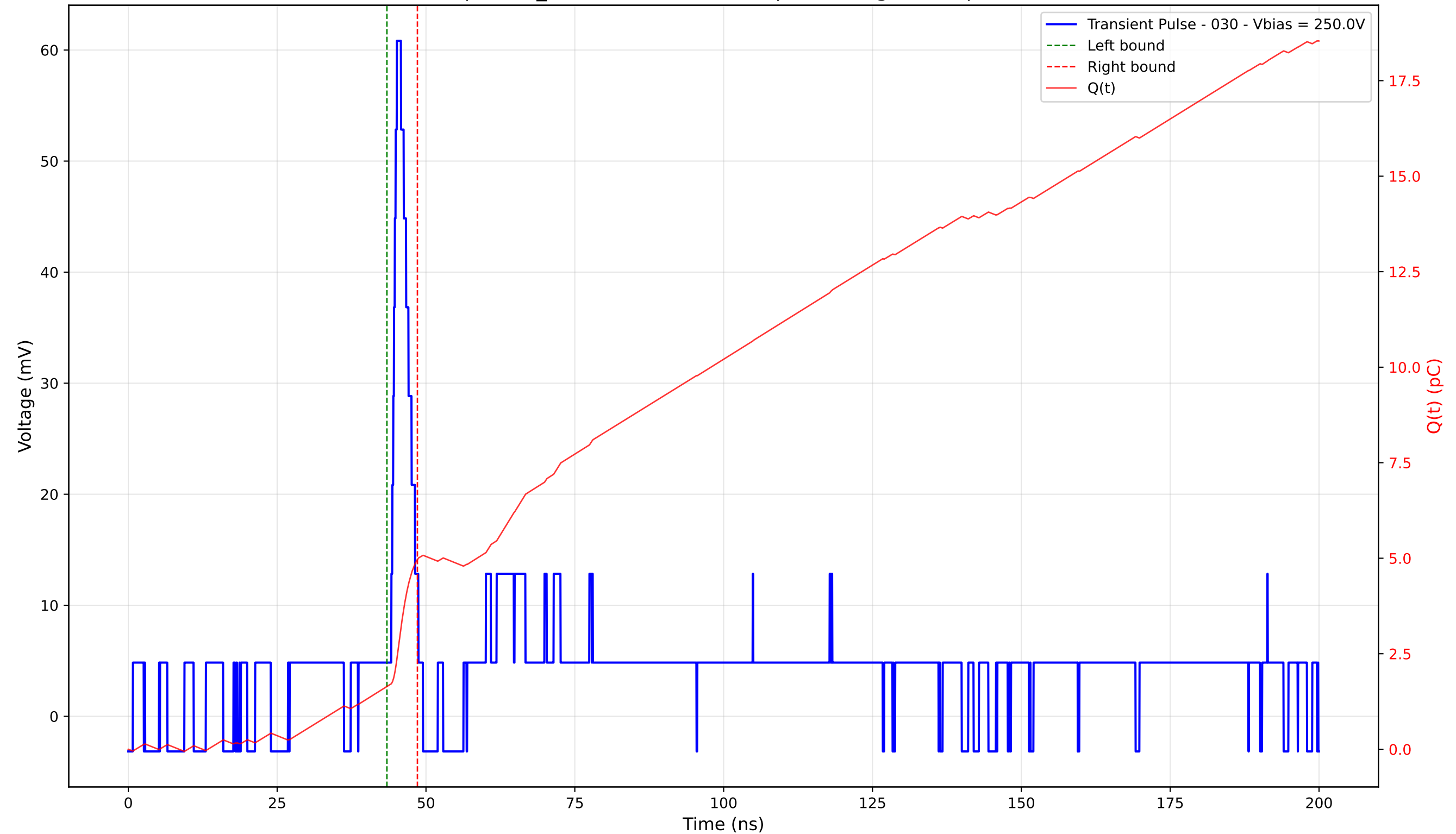
Transient Pulse - Sample: TD_4004 - Position: 430.0 \mu\text{m} - Charge: 3.33 pC - Rise Time: 0.94 ns
