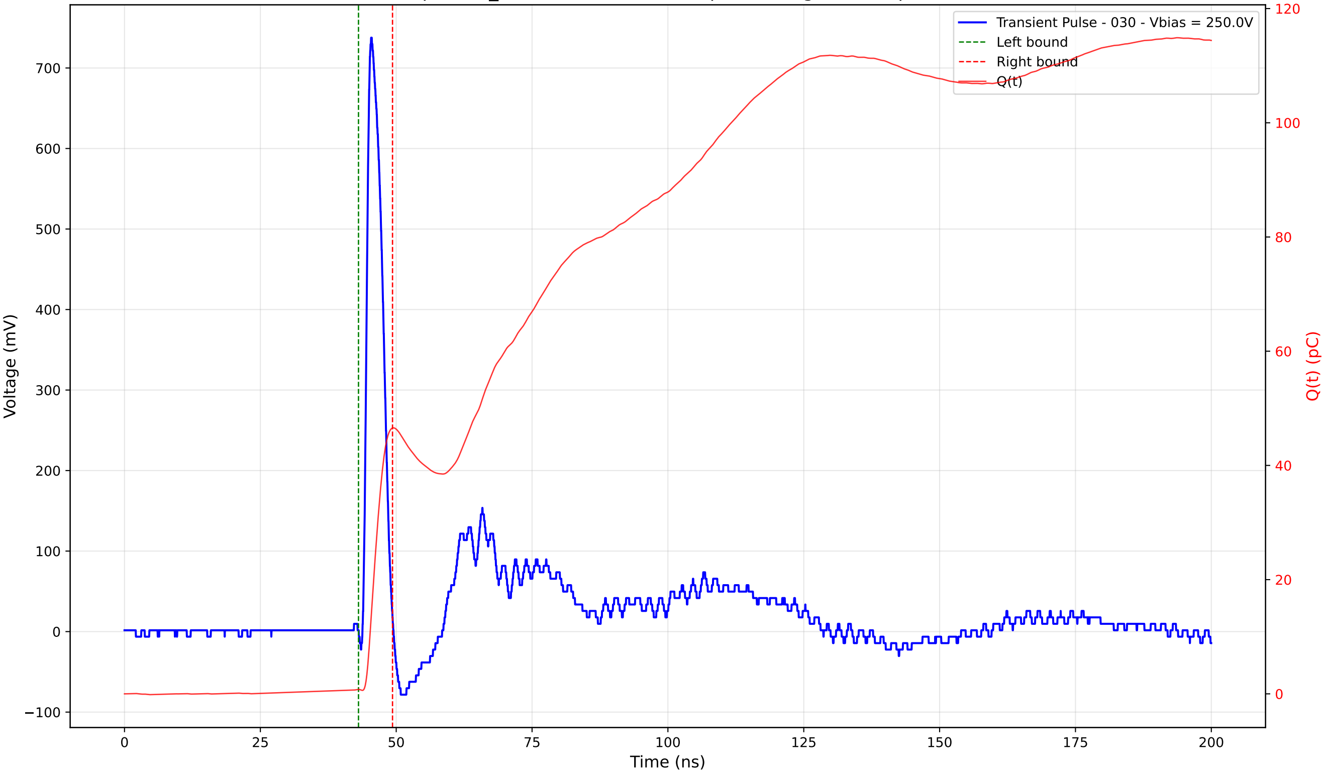
Transient Pulse - Sample: TD_4004 - Position: 290.0 \mu\text{m} - Charge: 45.78 pC - Rise Time: 0.96 ns
