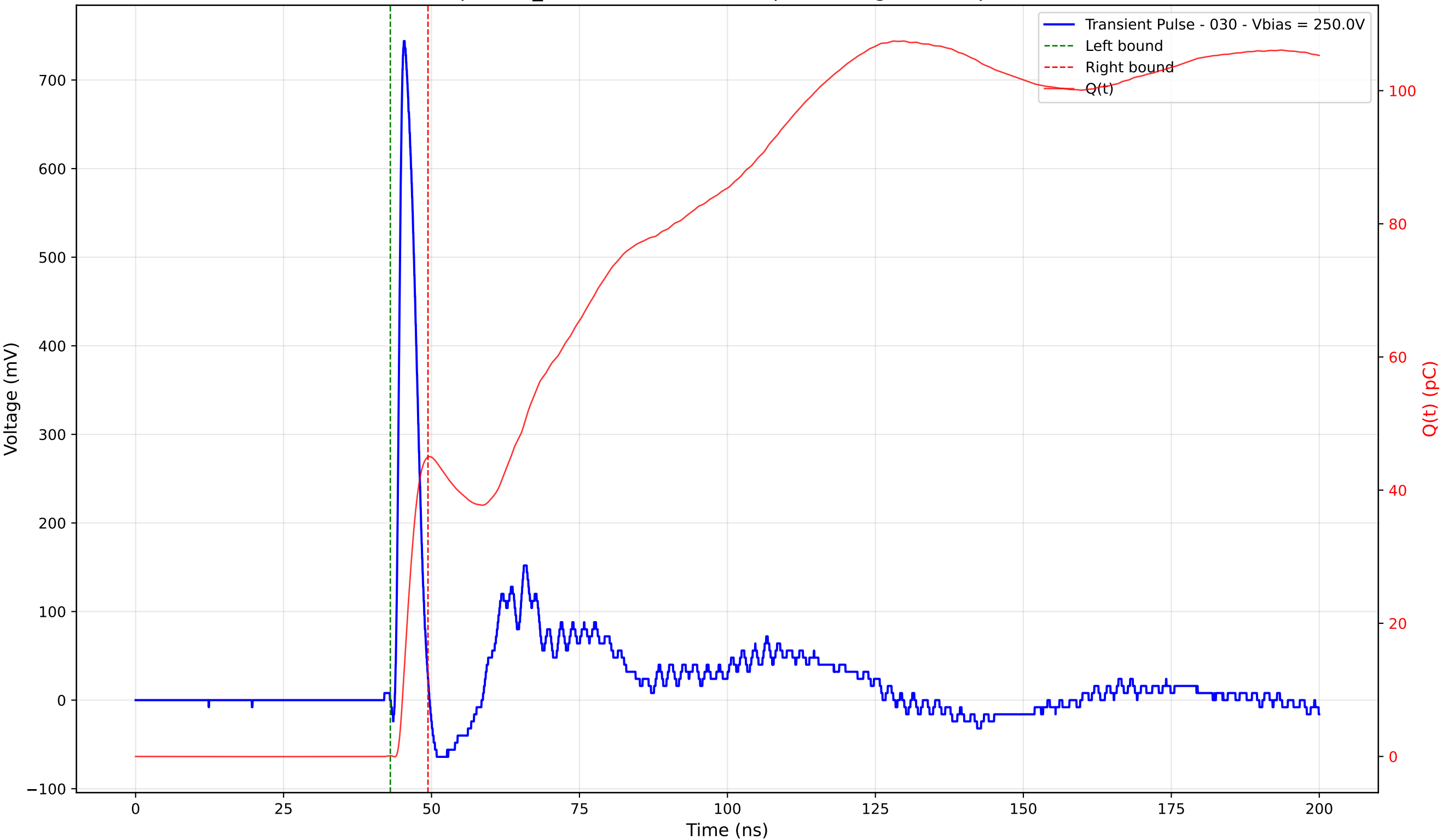
Transient Pulse - Sample: TD_4004 - Position: 250.0 \mu\text{m} - Charge: 44.86 pC - Rise Time: 0.93 ns
