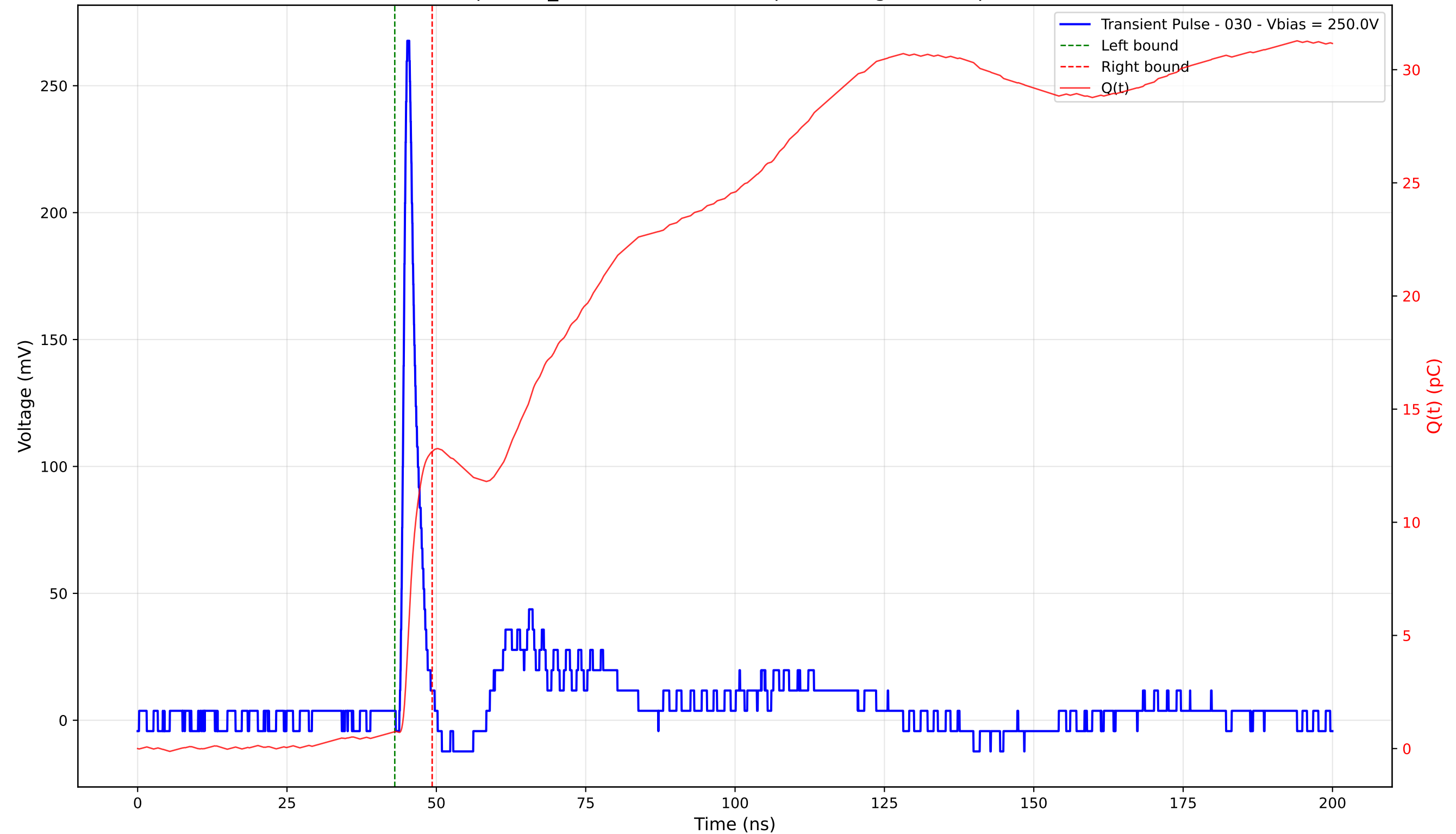
Transient Pulse - Sample: TD_4004 - Position: 60.0 \mu\text{m} - Charge: 12.38 pC - Rise Time: 0.90 ns
