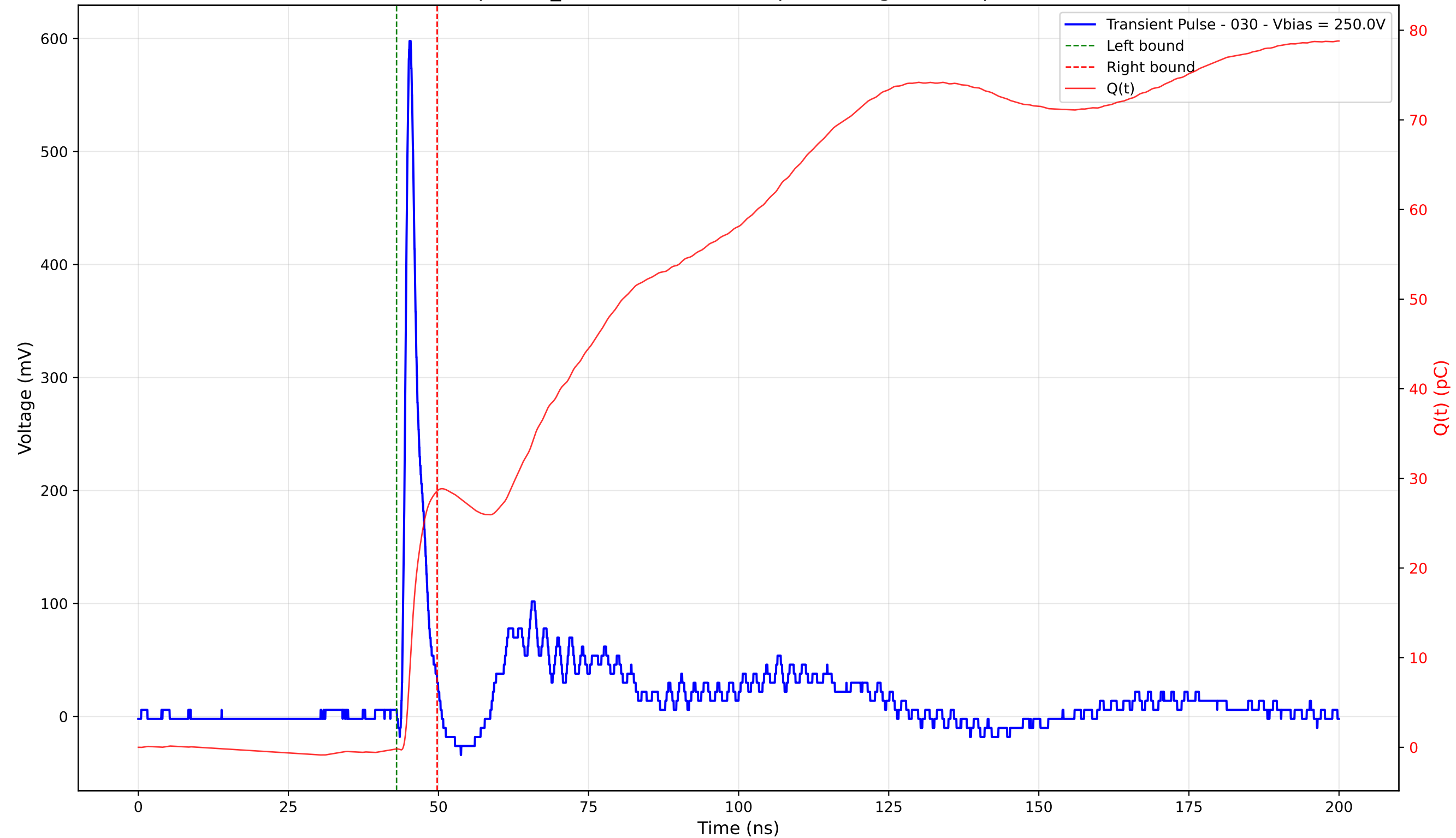
Transient Pulse - Sample: TD_4004 - Position: 75.0 \mu\text{m} - Charge: 28.78 pC - Rise Time: 0.90 ns
