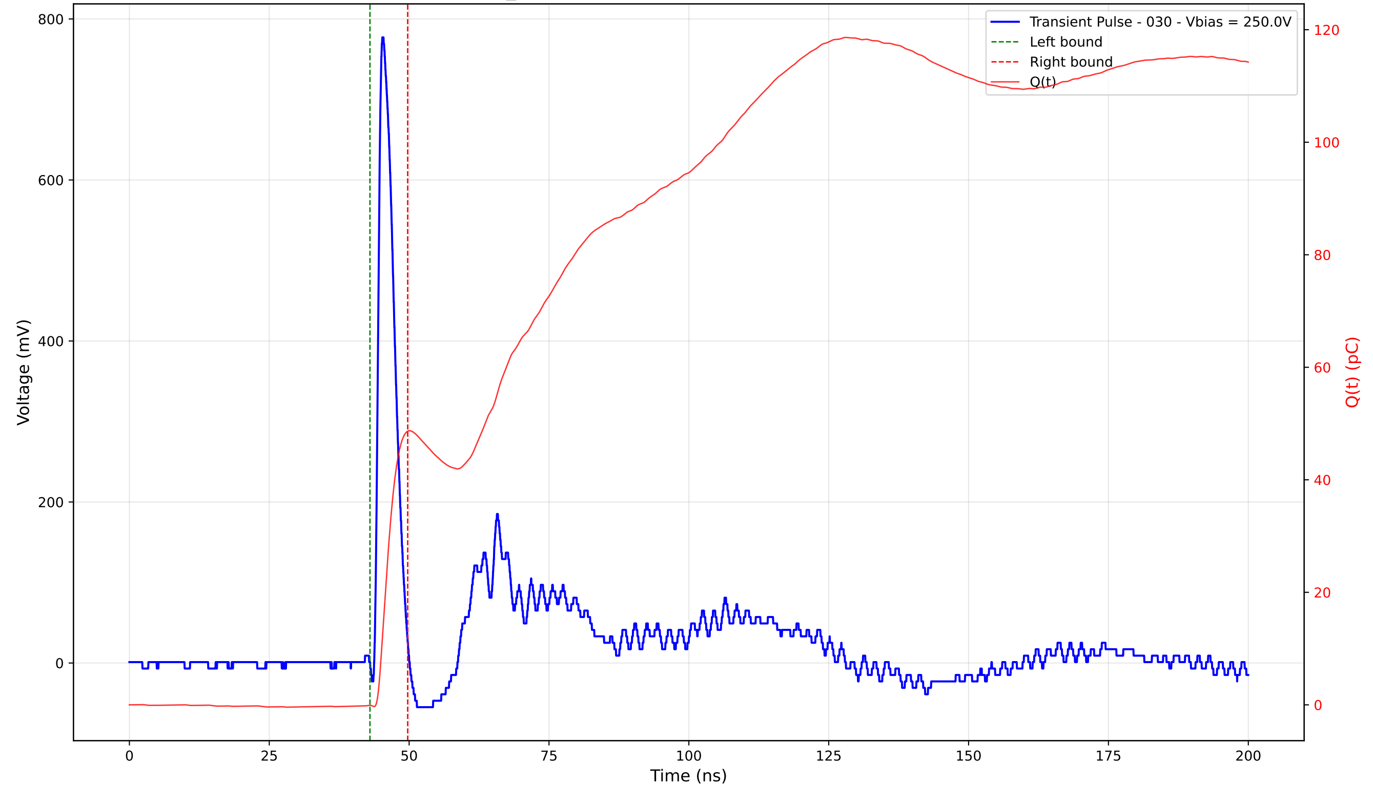
Transient Pulse - Sample: TD_4004 - Position: 175.0 \mu\text{m} - Charge: 48.72 pC - Rise Time: 0.90 ns
