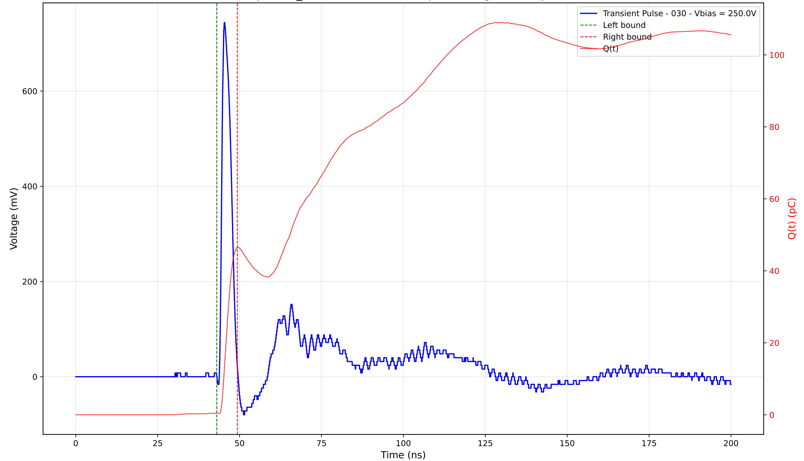
Transient Pulse - Sample: TD_4004 - Position: 285.0 \mu\text{m} - Charge: 45.95 pC - Rise Time: 0.95 ns
