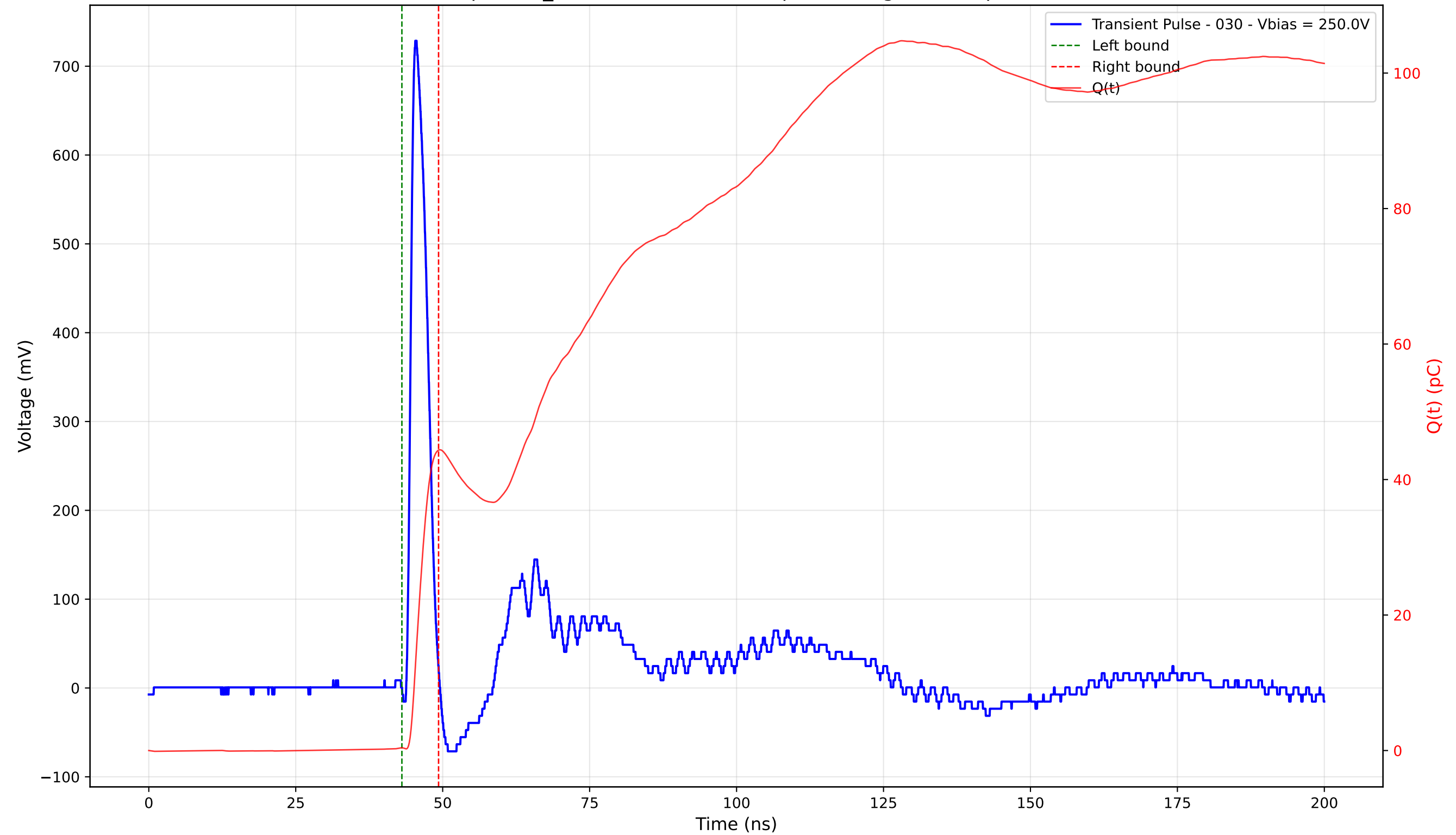
Transient Pulse - Sample: TD_4004 - Position: 265.0 \mu\text{m} - Charge: 43.93 pC - Rise Time: 0.96 ns
