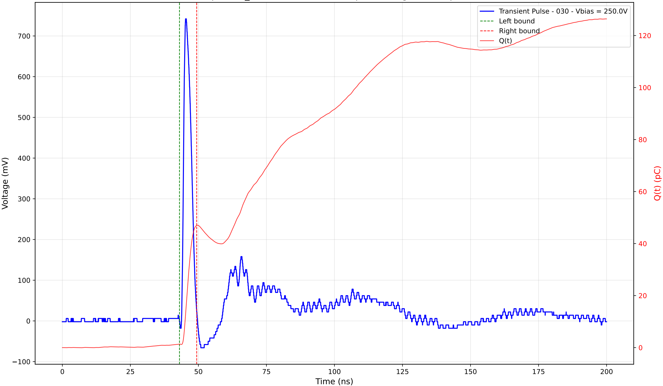
Transient Pulse - Sample: TD_4004 - Position: 275.0 \mu\text{m} - Charge: 45.62 pC - Rise Time: 0.94 ns
