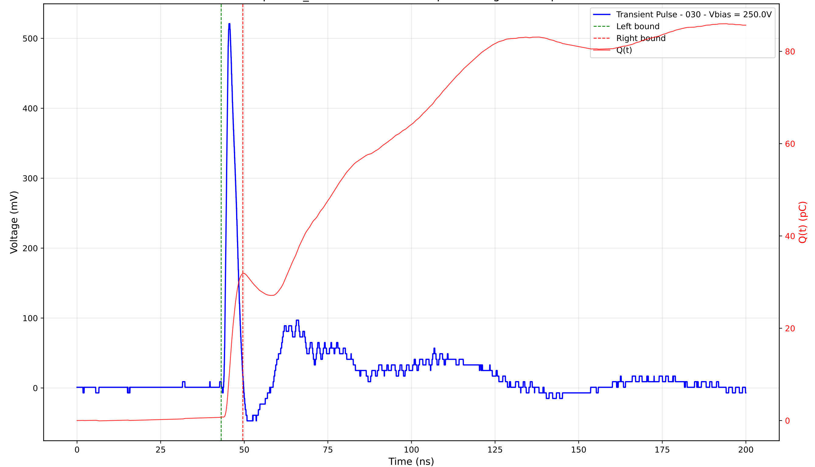
Transient Pulse - Sample: TD_4004 - Position: 380.0 \mu\text{m} - Charge: 31.09 pC - Rise Time: 1.03 ns
