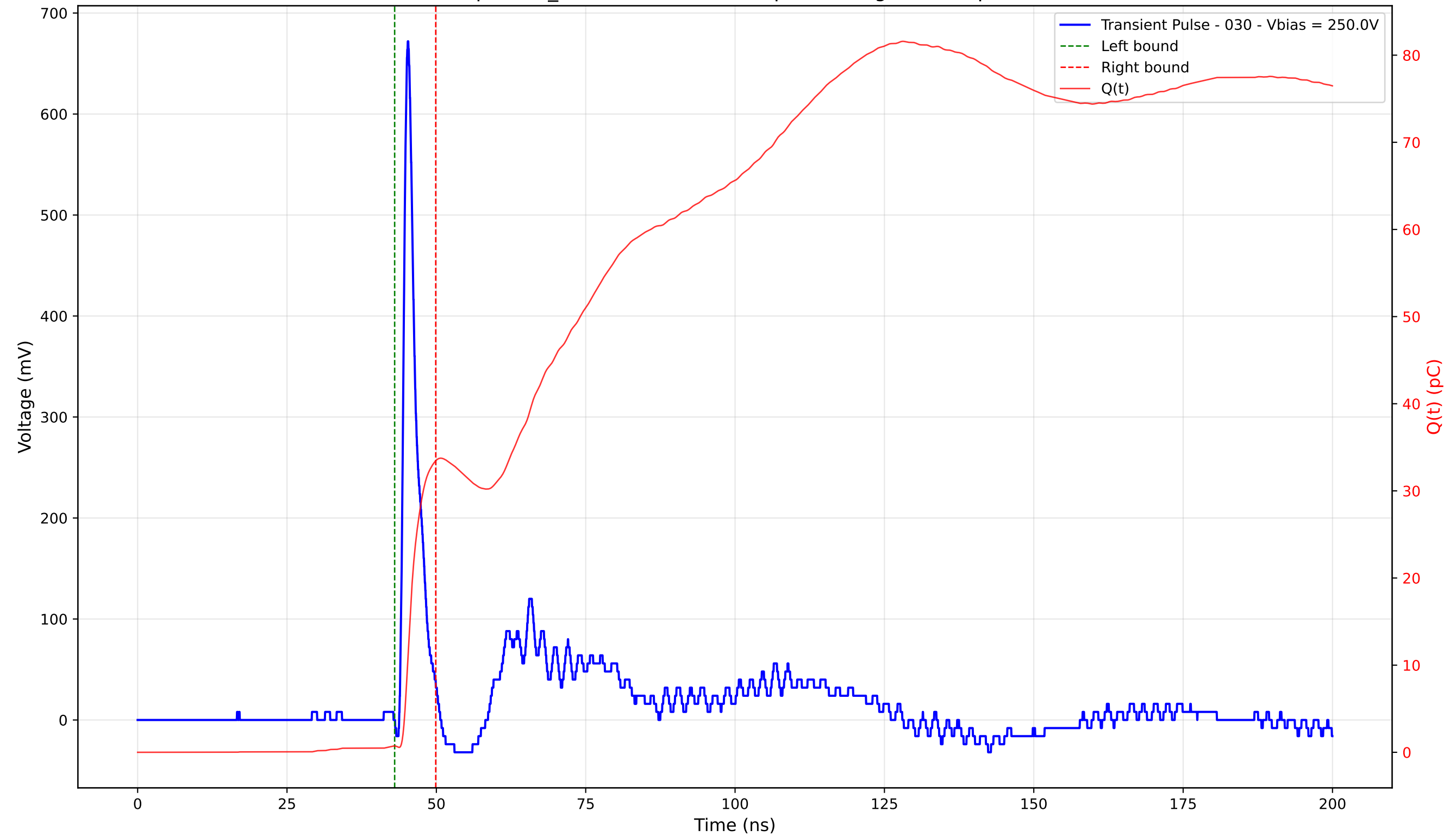
Transient Pulse - Sample: TD_4004 - Position: 80.0 \mu\text{m} - Charge: 32.73 pC - Rise Time: 0.88 ns
