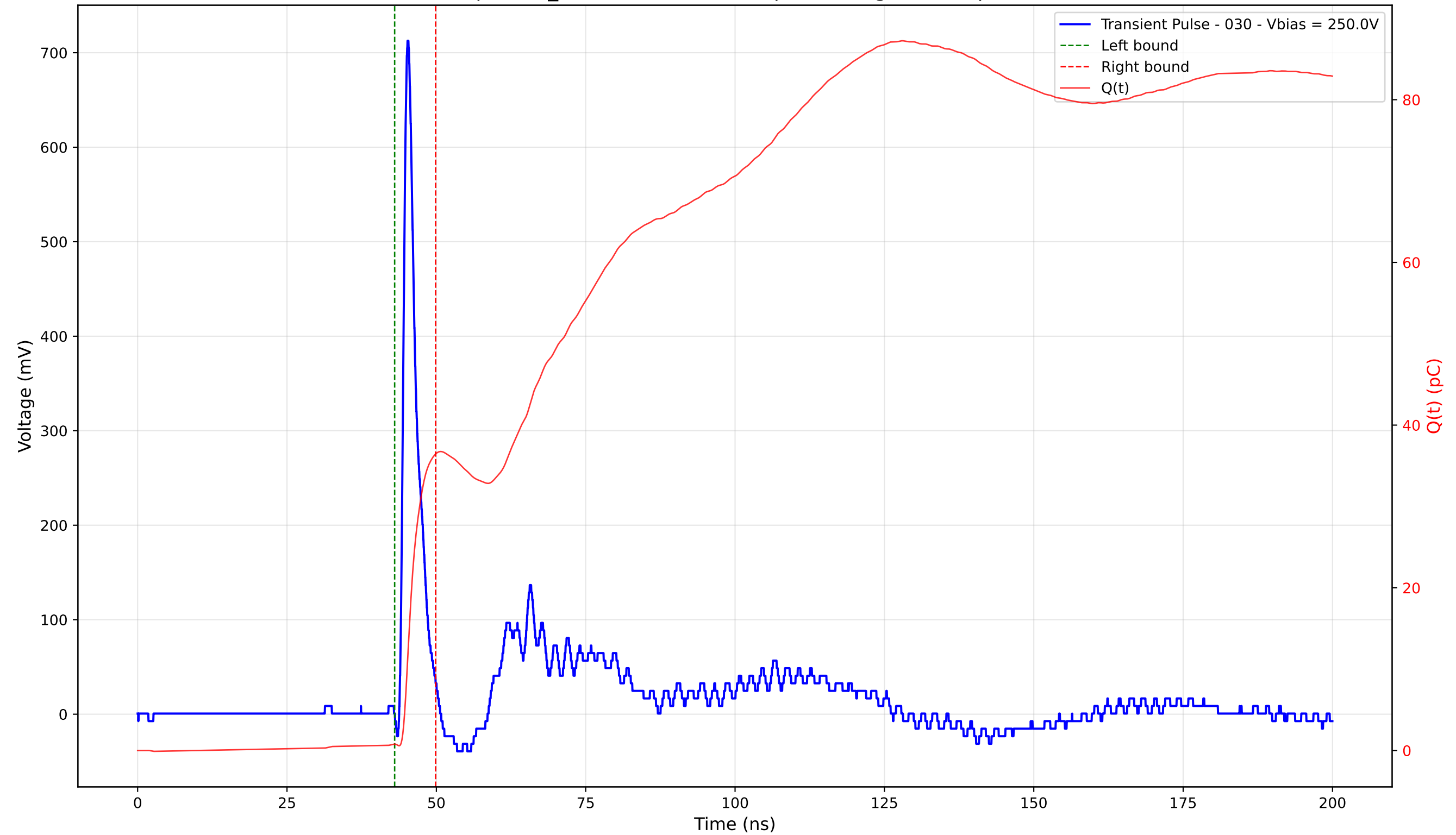
Transient Pulse - Sample: TD_4004 - Position: 85.0 \mu\text{m} - Charge: 35.67 pC - Rise Time: 0.89 ns
