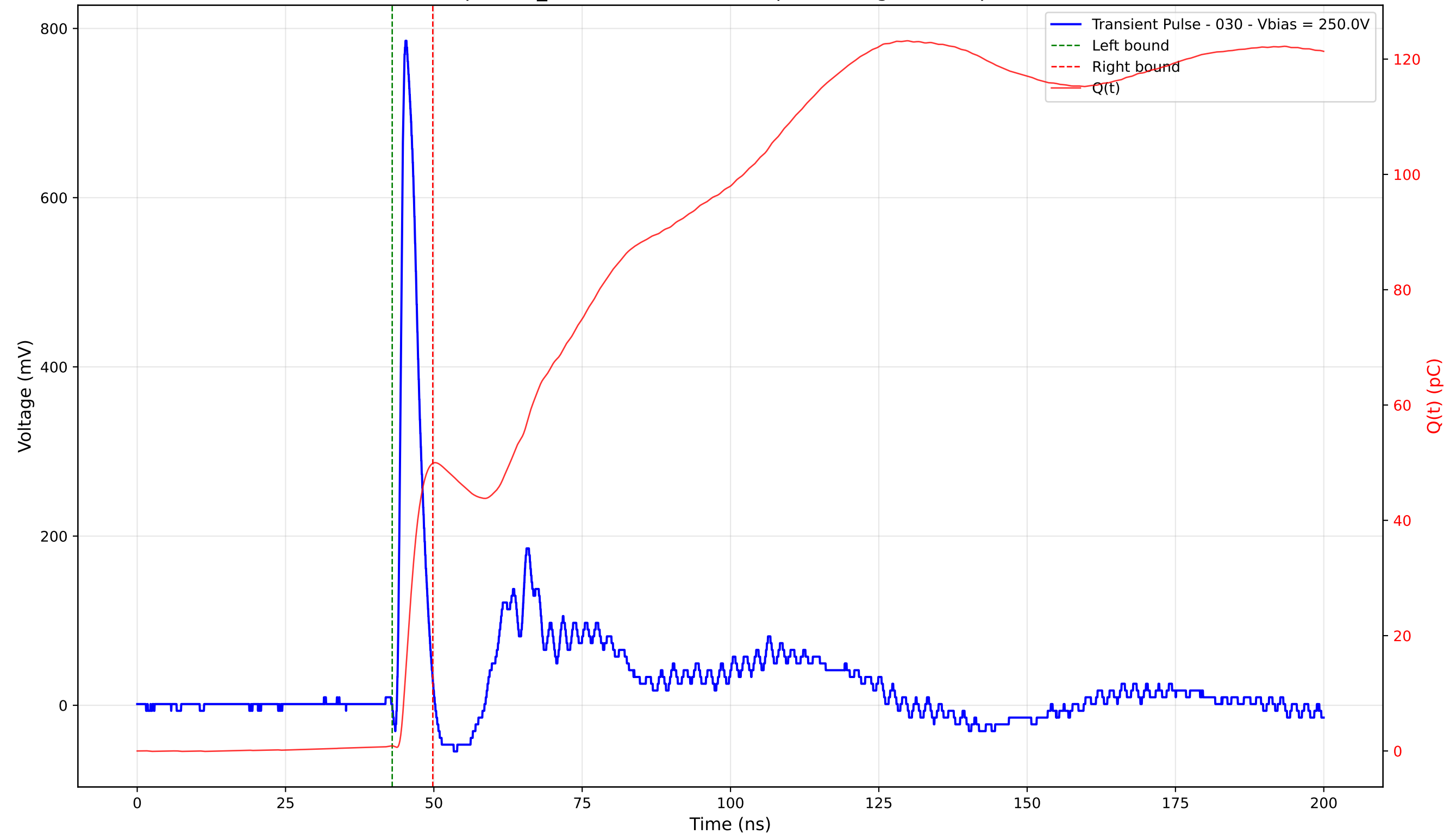
Transient Pulse - Sample: TD_4004 - Position: 185.0 \mu\text{m} - Charge: 49.01 pC - Rise Time: 0.89 ns
