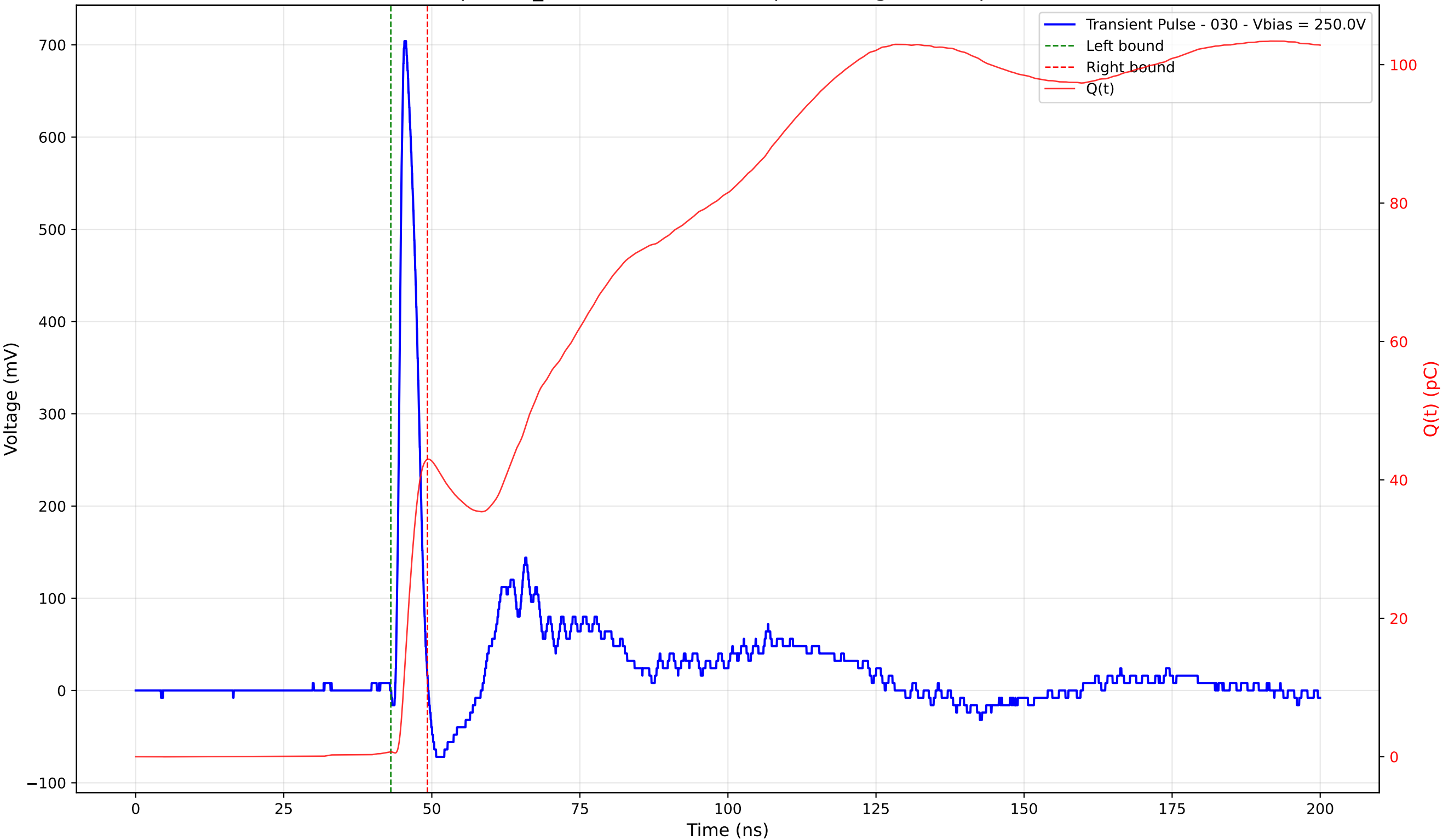
Transient Pulse - Sample: TD_4004 - Position: 310.0 \mu\text{m} - Charge: 42.27 pC - Rise Time: 0.97 ns
