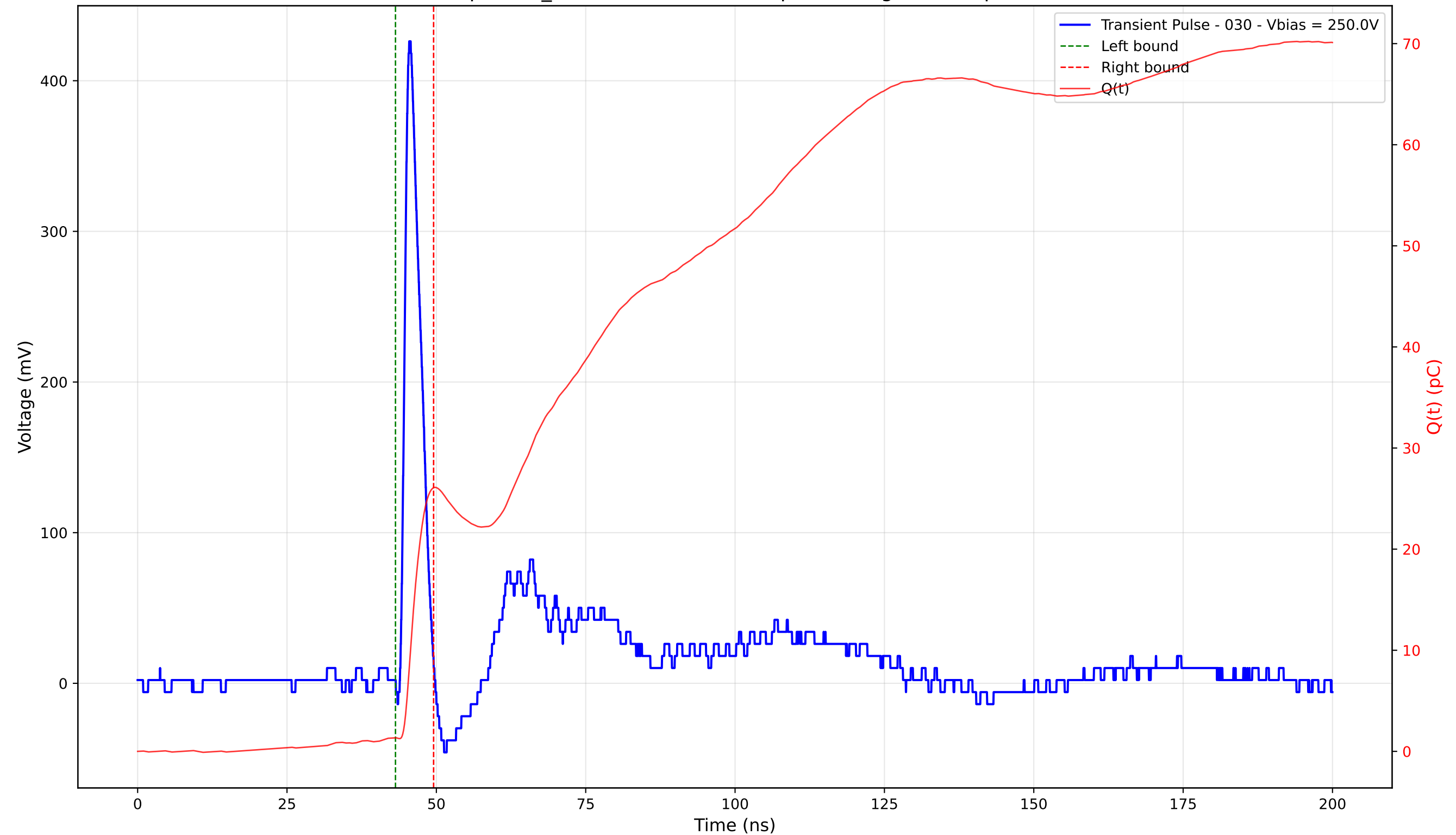
Transient Pulse - Sample: TD_4004 - Position: 390.0 \mu\text{m} - Charge: 24.73 pC - Rise Time: 1.02 ns
