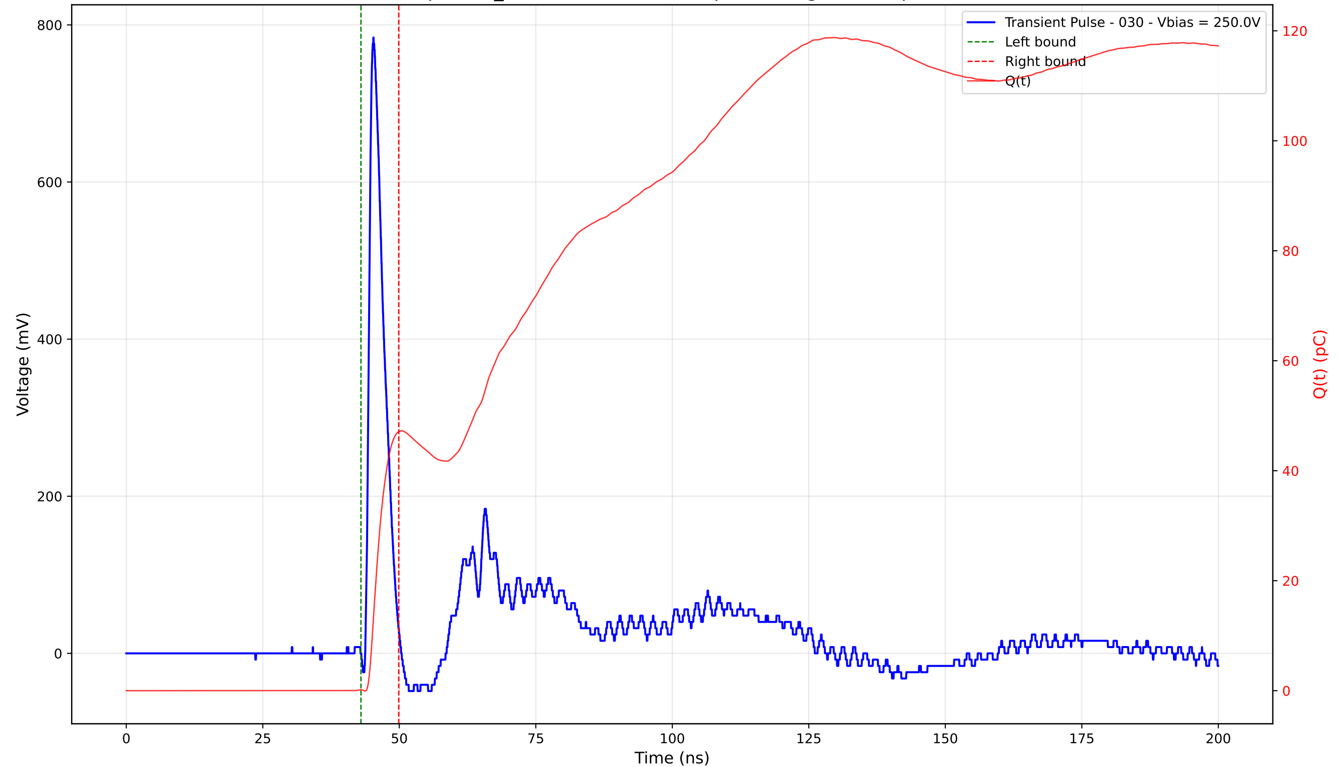
Transient Pulse - Sample: TD_4004 - Position: 115.0 \mu\text{m} - Charge: 46.95 pC - Rise Time: 0.89 ns
