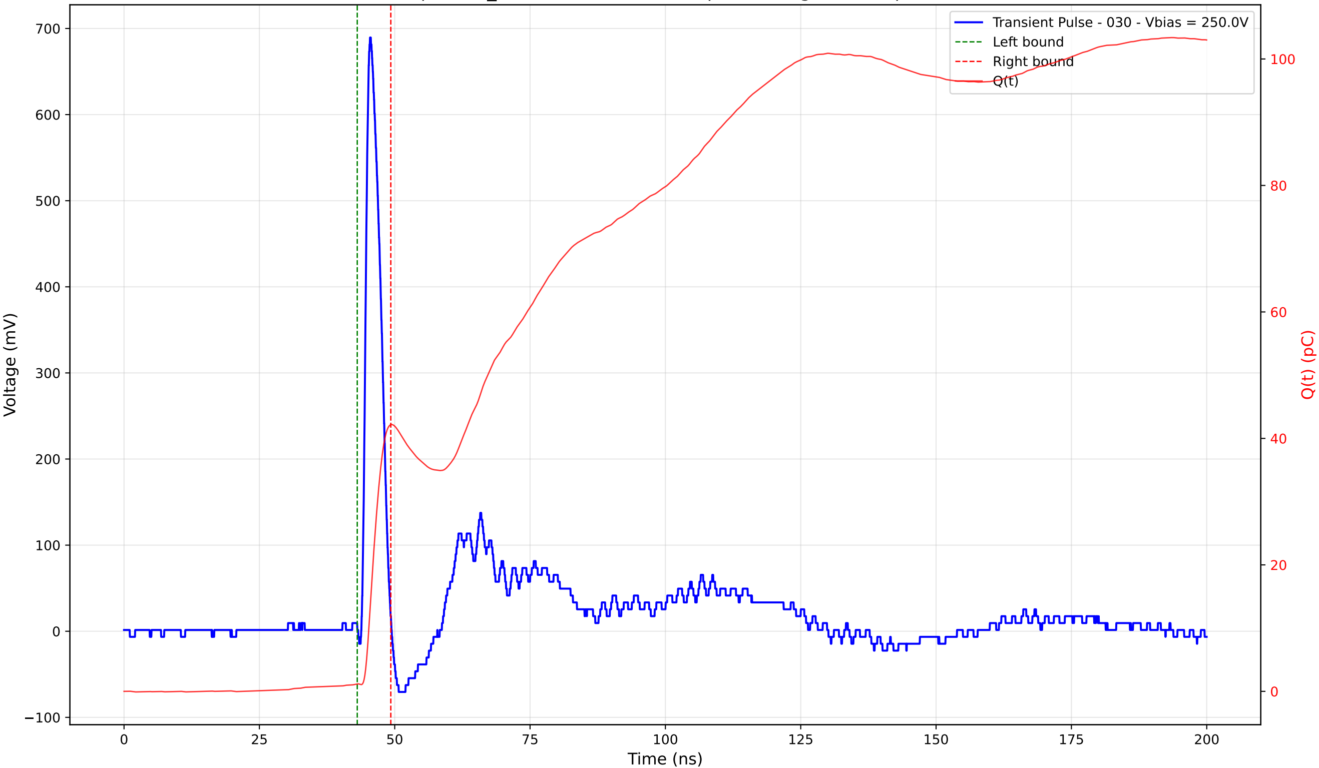
Transient Pulse - Sample: TD_4004 - Position: 315.0 \mu\text{m} - Charge: 40.99 pC - Rise Time: 1.00 ns
