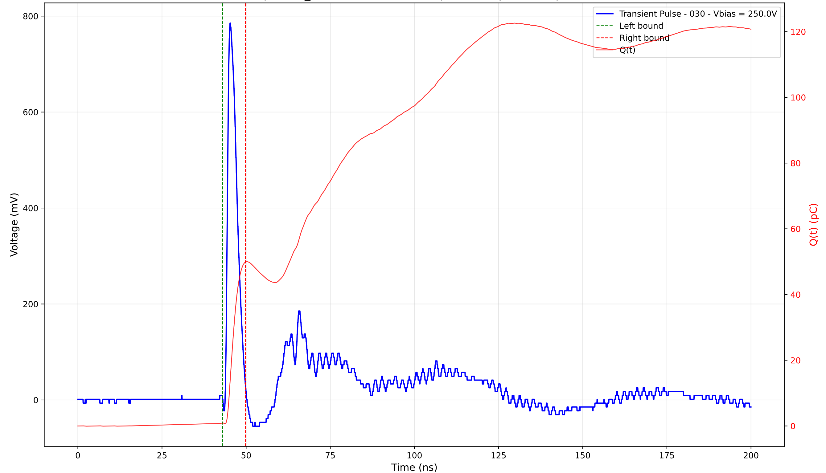
Transient Pulse - Sample: TD_4004 - Position: 190.0 \mu\text{m} - Charge: 49.00 pC - Rise Time: 0.89 ns
