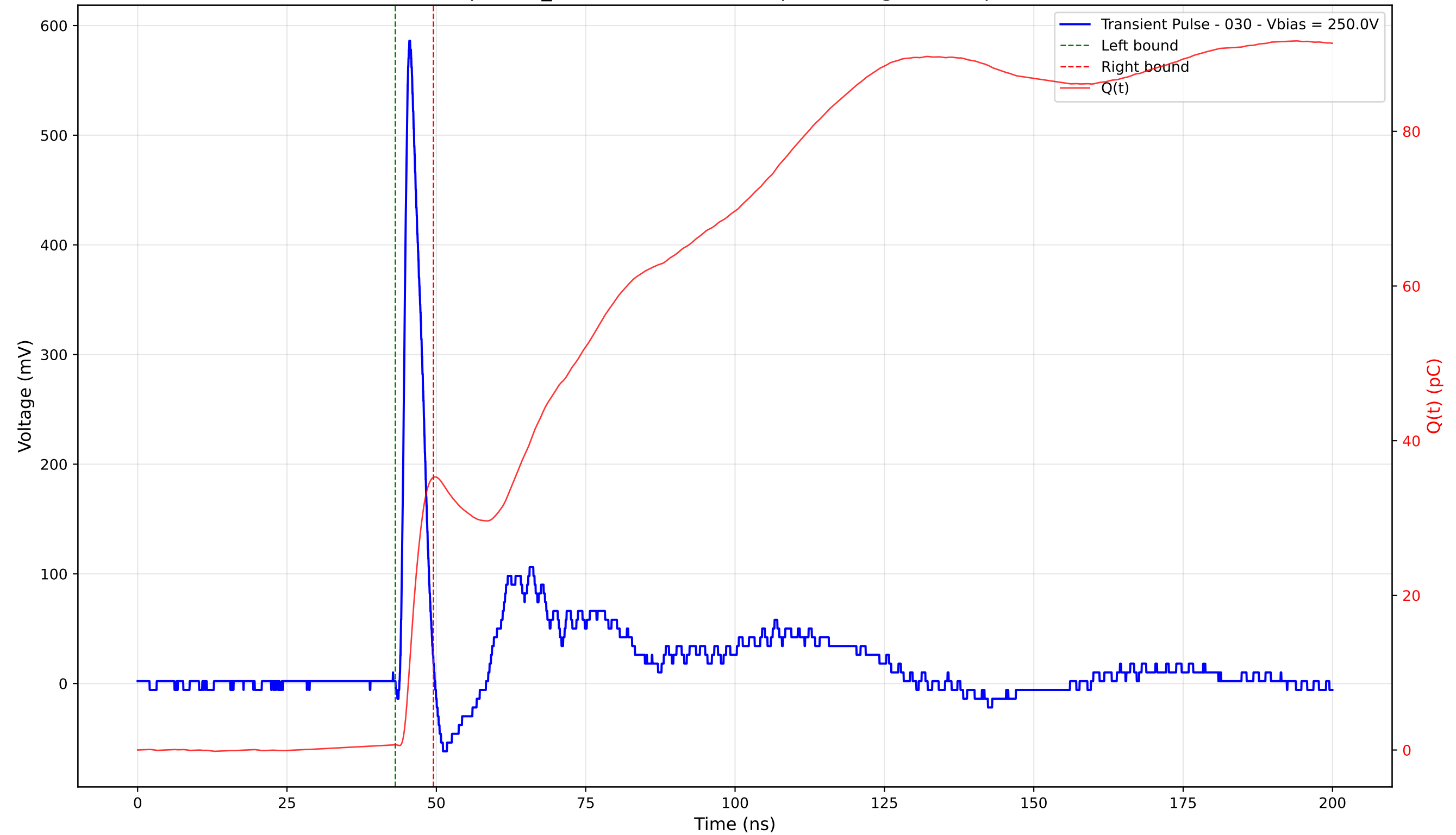
Transient Pulse - Sample: TD_4004 - Position: 340.0 \mu\text{m} - Charge: 34.58 pC - Rise Time: 1.02 ns
