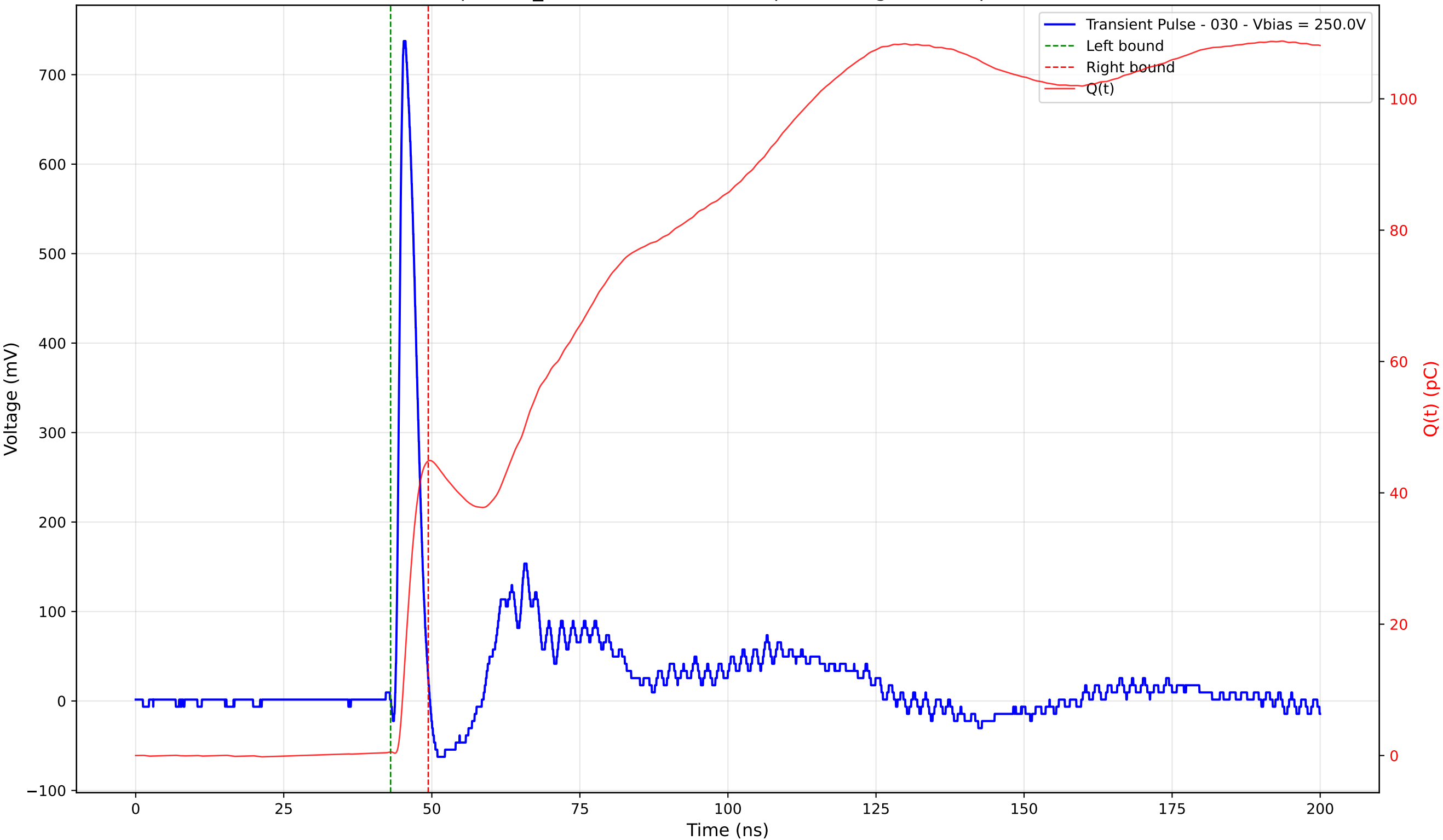
Transient Pulse - Sample: TD_4004 - Position: 240.0 \mu\text{m} - Charge: 44.32 pC - Rise Time: 0.92 ns
