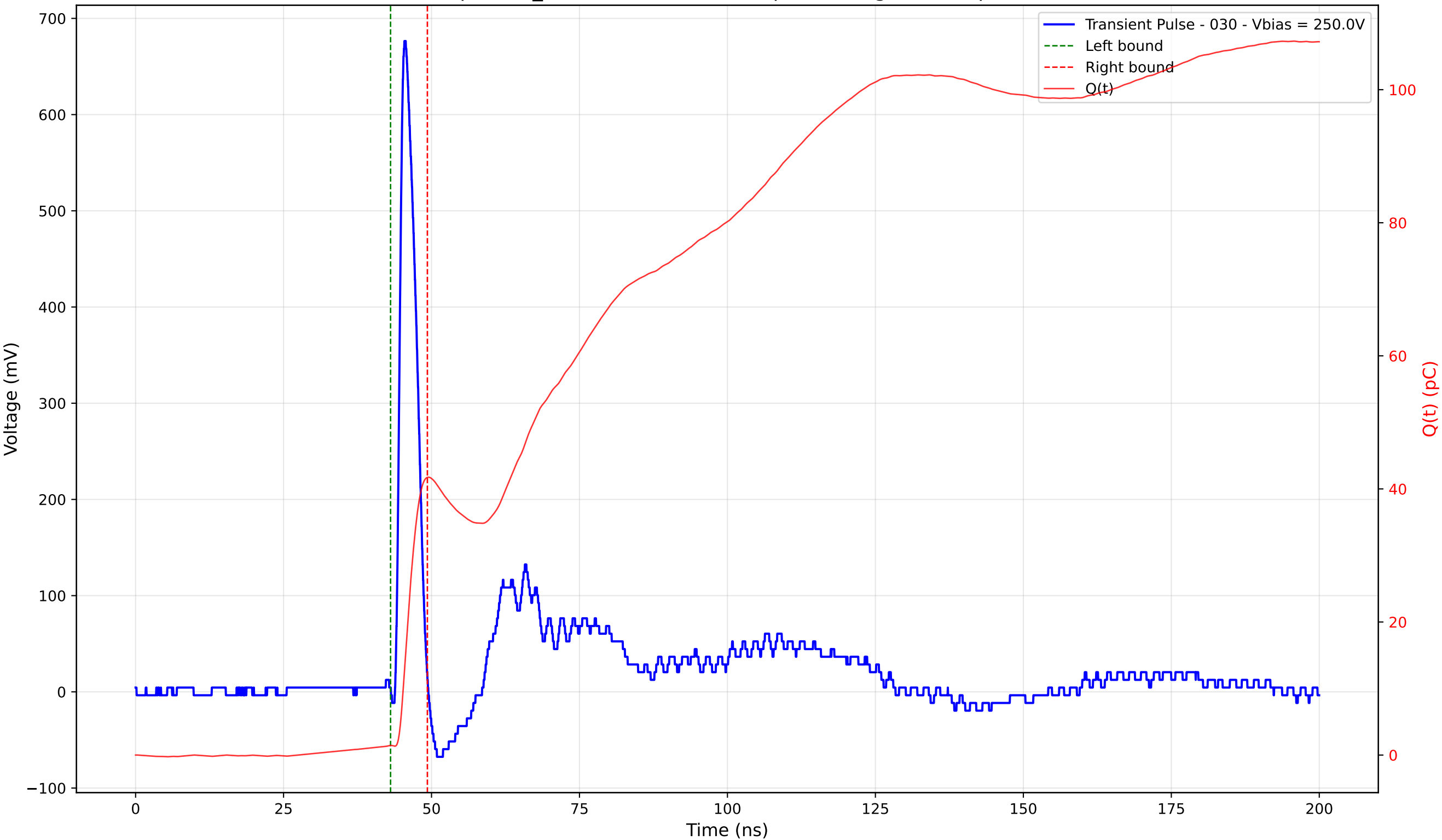
Transient Pulse - Sample: TD_4004 - Position: 320.0 \mu\text{m} - Charge: 40.29 pC - Rise Time: 1.01 ns
