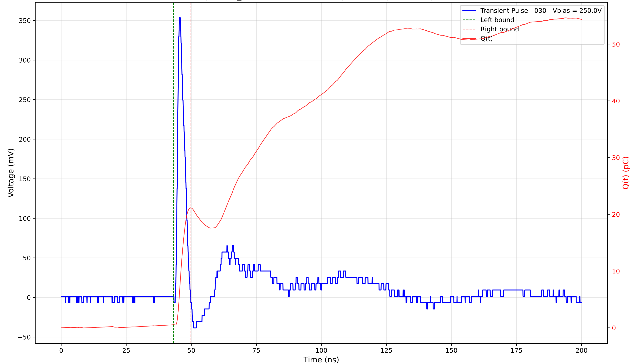
Transient Pulse - Sample: TD_4004 - Position: 395.0 \mu\text{m} - Charge: 20.56 pC - Rise Time: 1.02 ns
