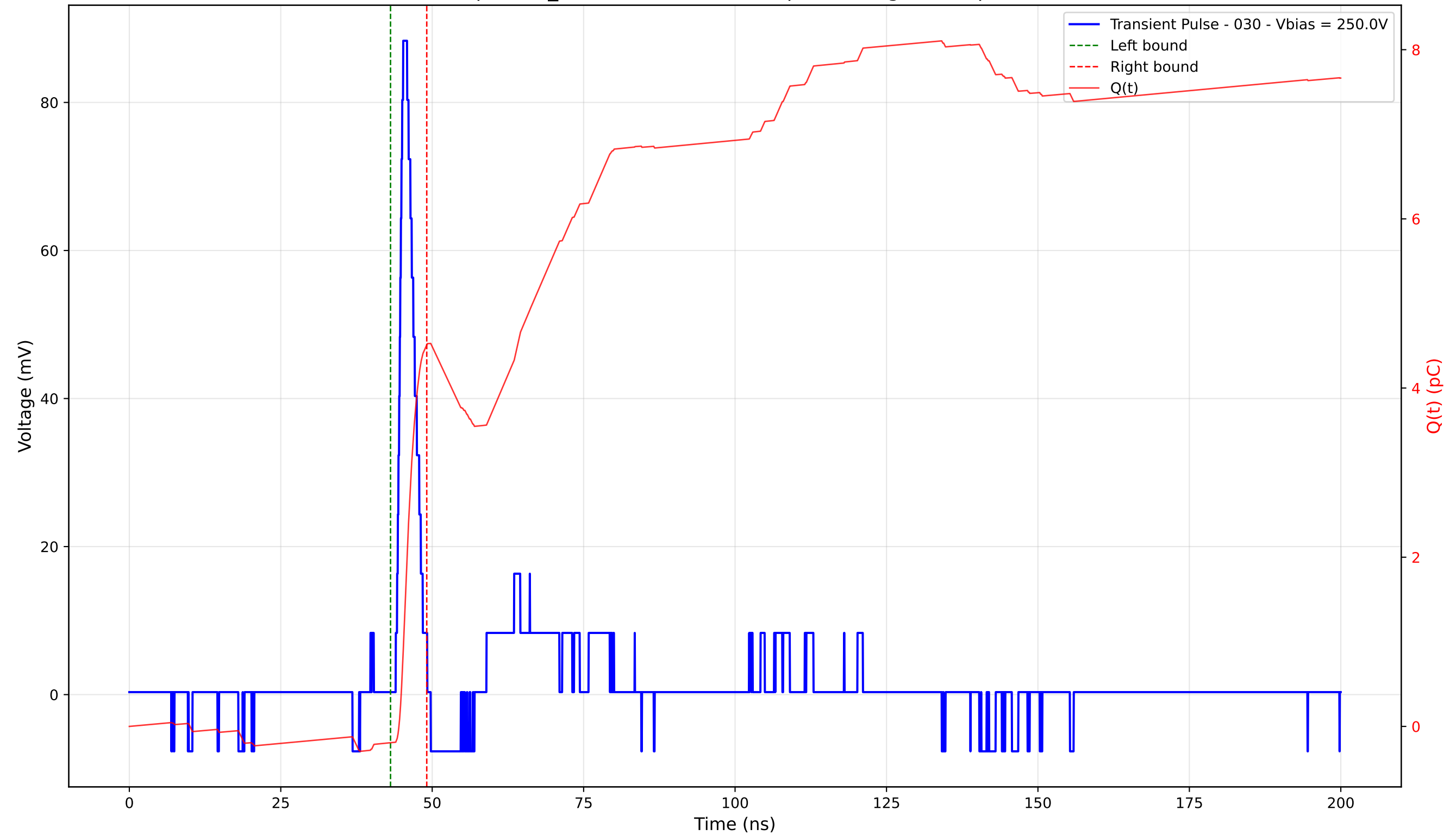
Transient Pulse - Sample: TD_4004 - Position: 420.0 \mu\text{m} - Charge: 4.71 pC - Rise Time: 0.86 ns
