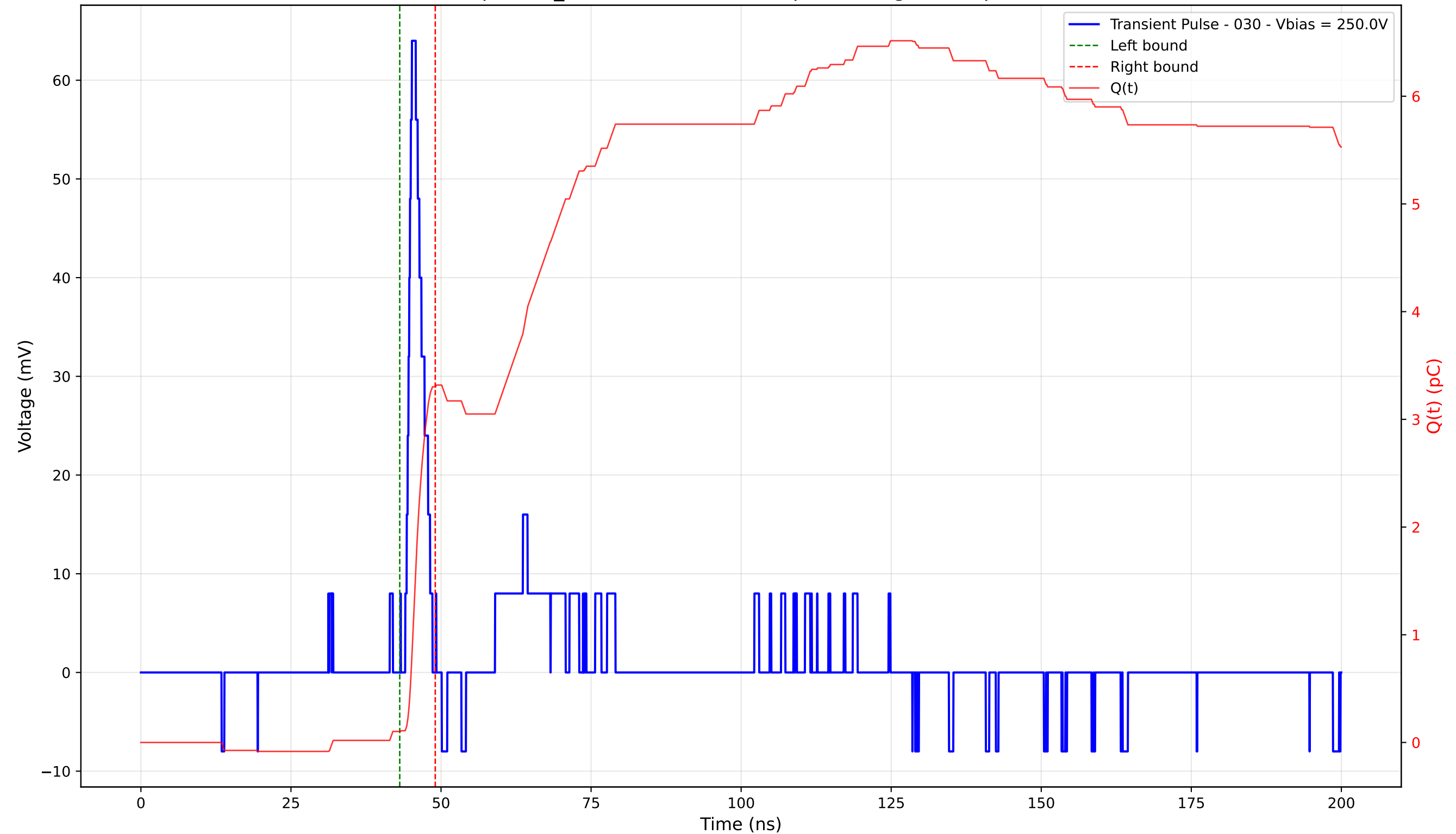
Transient Pulse - Sample: TD_4004 - Position: 435.0 \mu\text{m} - Charge: 3.20 pC - Rise Time: 1.10 ns
