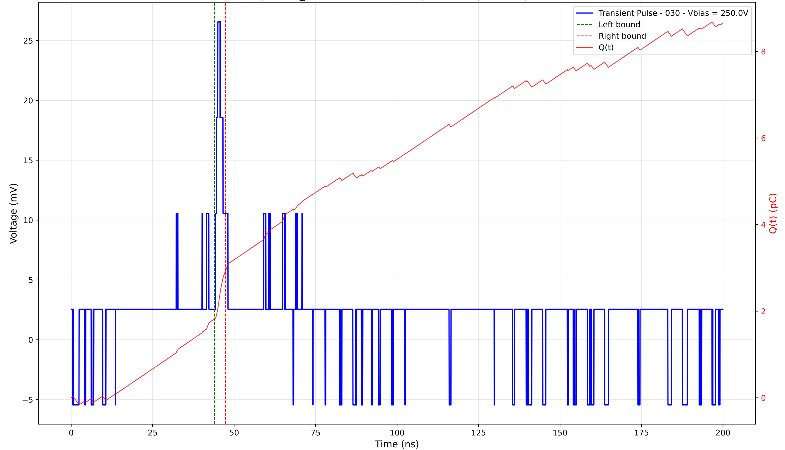
Transient Pulse - Sample: TD_4004 - Position: 25.0 \mu\text{m} - Charge: 1.10 pC - Rise Time: 0.70 ns
