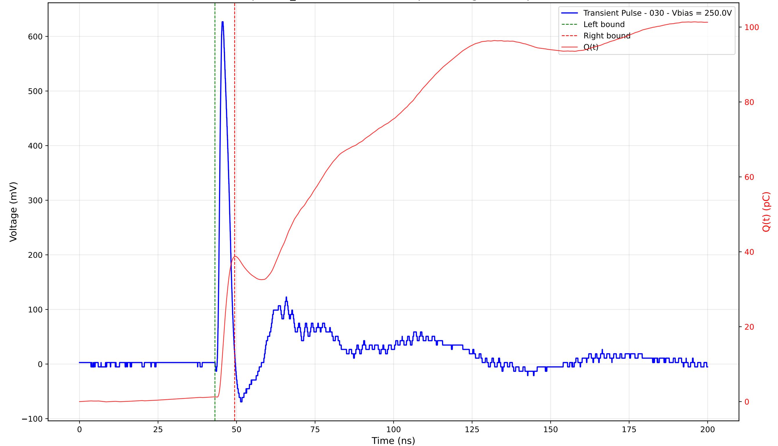
Transient Pulse - Sample: TD_4004 - Position: 330.0 \mu\text{m} - Charge: 37.45 pC - Rise Time: 1.03 ns
