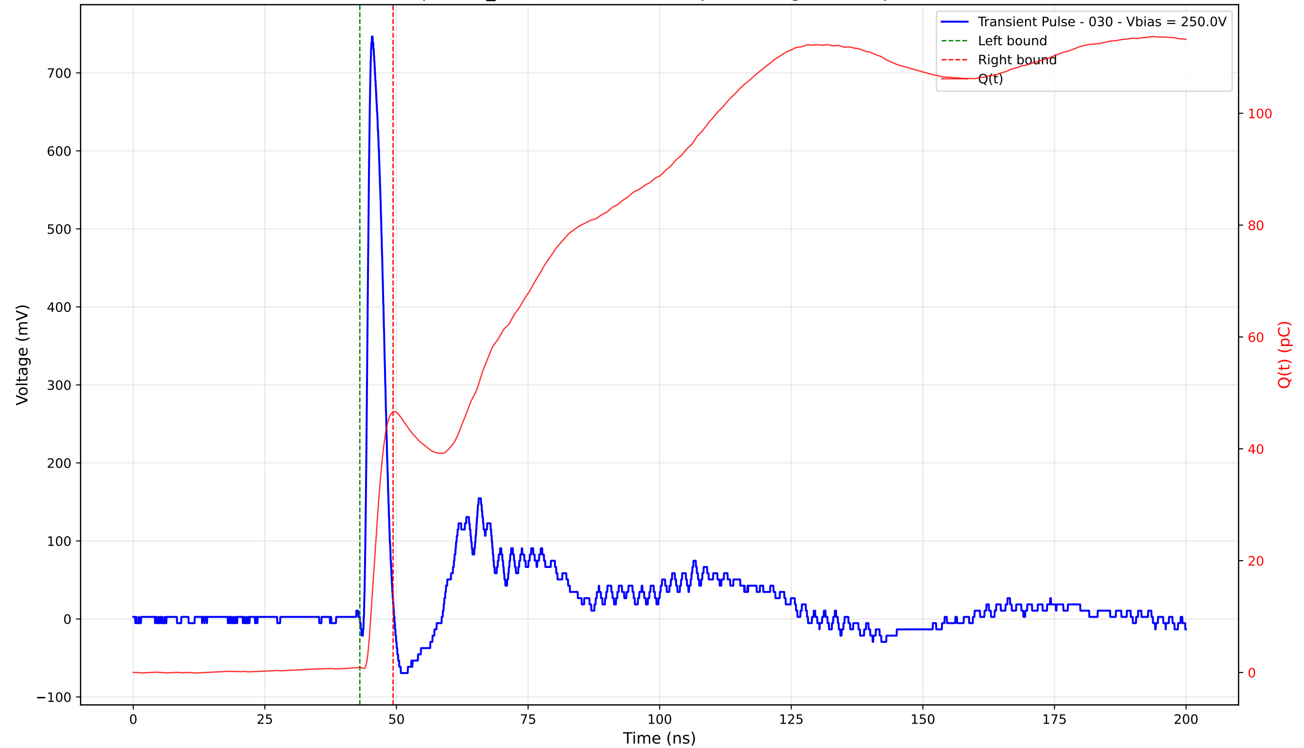
Transient Pulse - Sample: TD_4004 - Position: 280.0 \mu\text{m} - Charge: 45.68 pC - Rise Time: 0.93 ns
