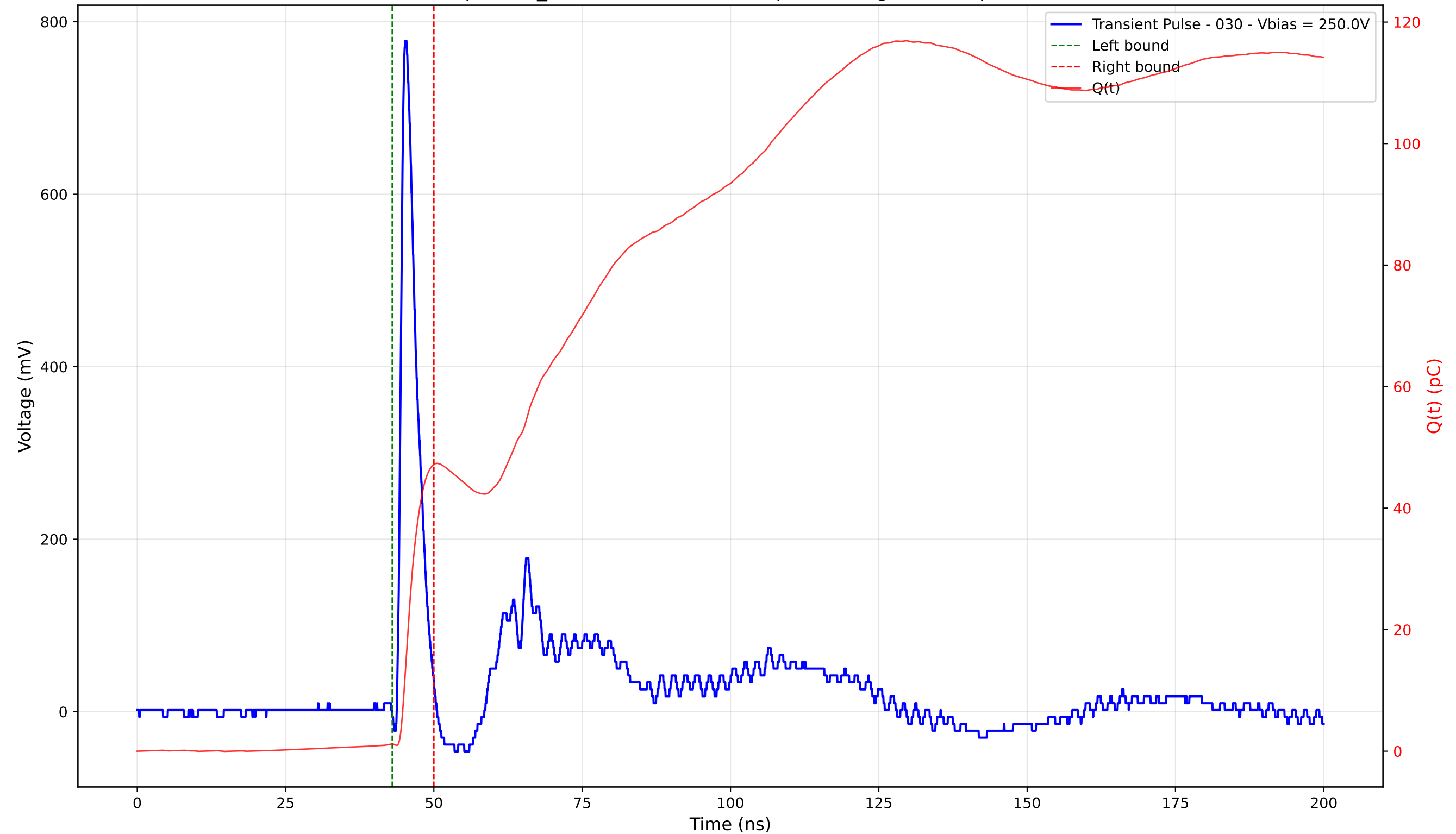
Transient Pulse - Sample: TD_4004 - Position: 105.0 \mu\text{m} - Charge: 46.01 pC - Rise Time: 0.88 ns
