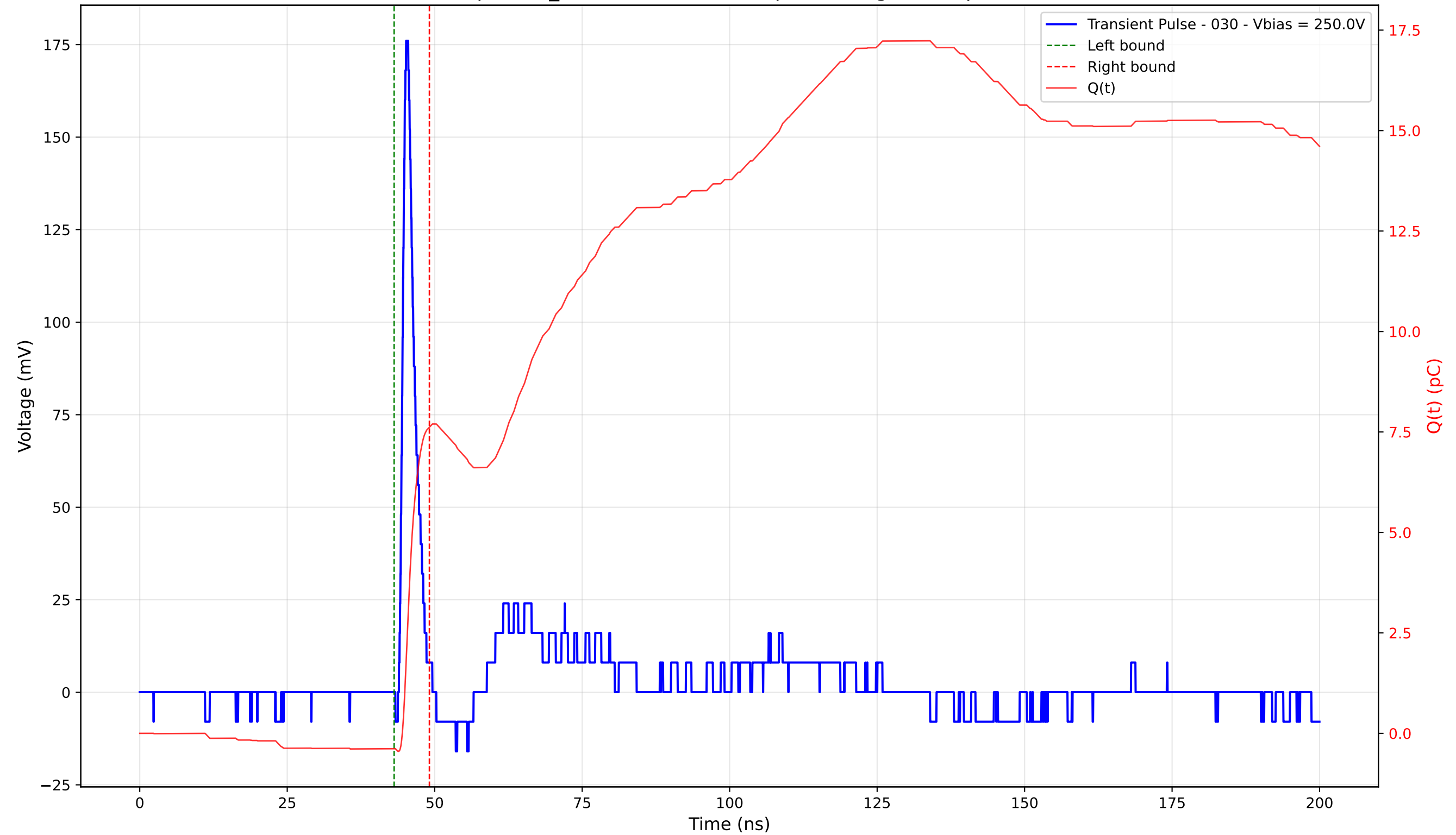
Transient Pulse - Sample: TD_4004 - Position: 55.0 \mu\text{m} - Charge: 8.00 pC - Rise Time: 0.84 ns
