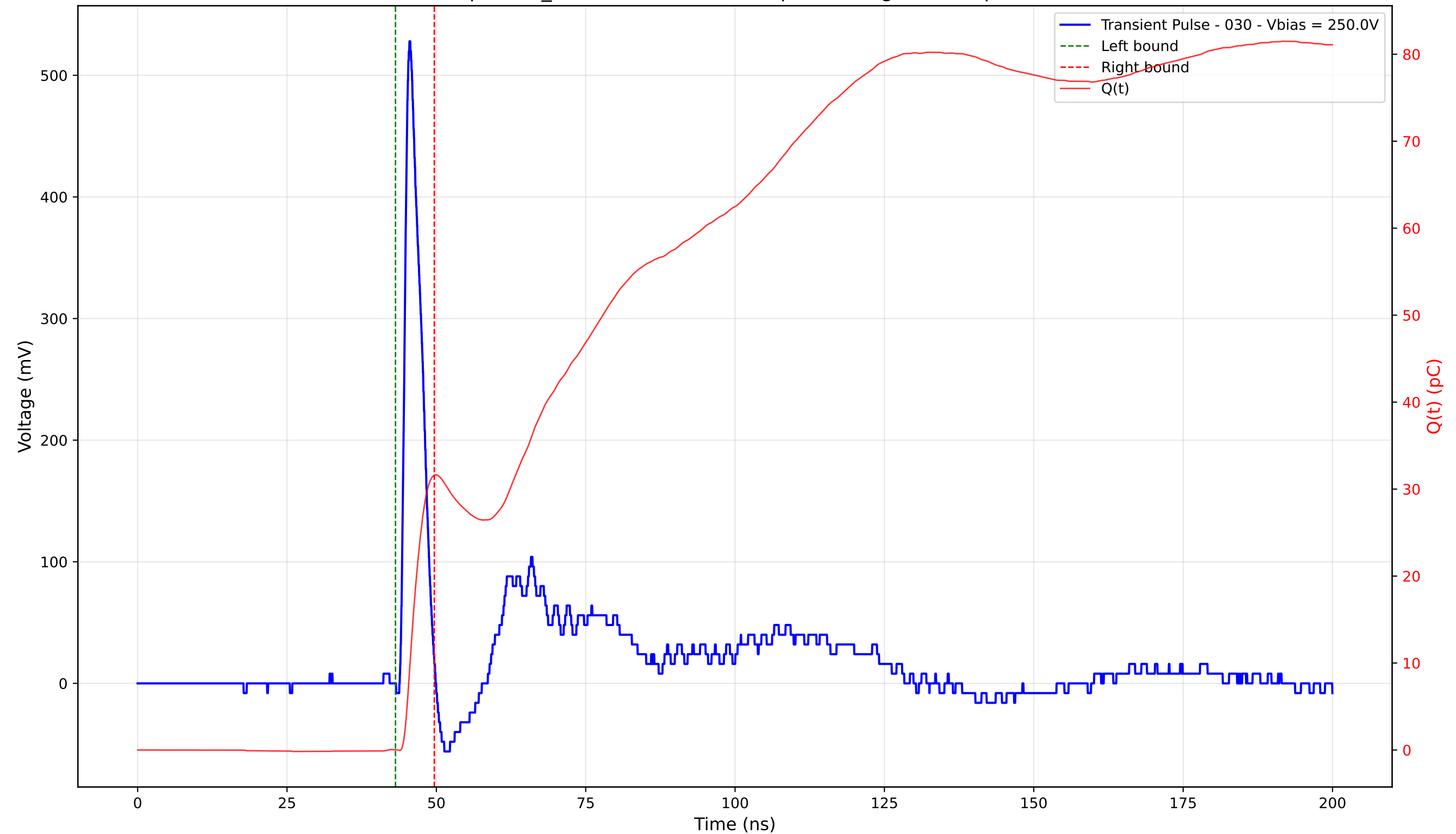
Transient Pulse - Sample: TD_4004 - Position: 375.0 \mu\text{m} - Charge: 31.56 pC - Rise Time: 1.03 ns
