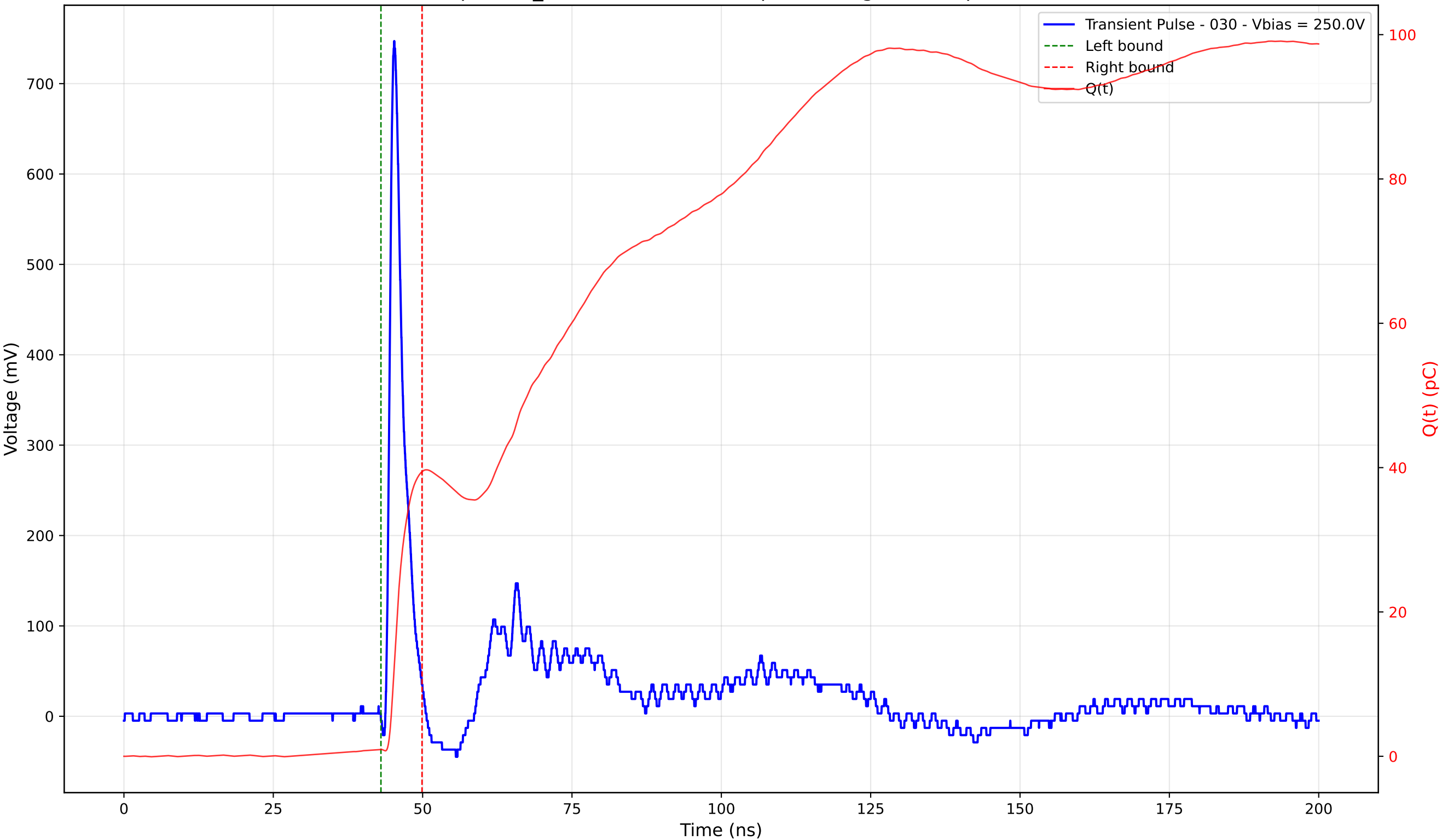
Transient Pulse - Sample: TD_4004 - Position: 90.0 \mu\text{m} - Charge: 38.49 pC - Rise Time: 0.89 ns
