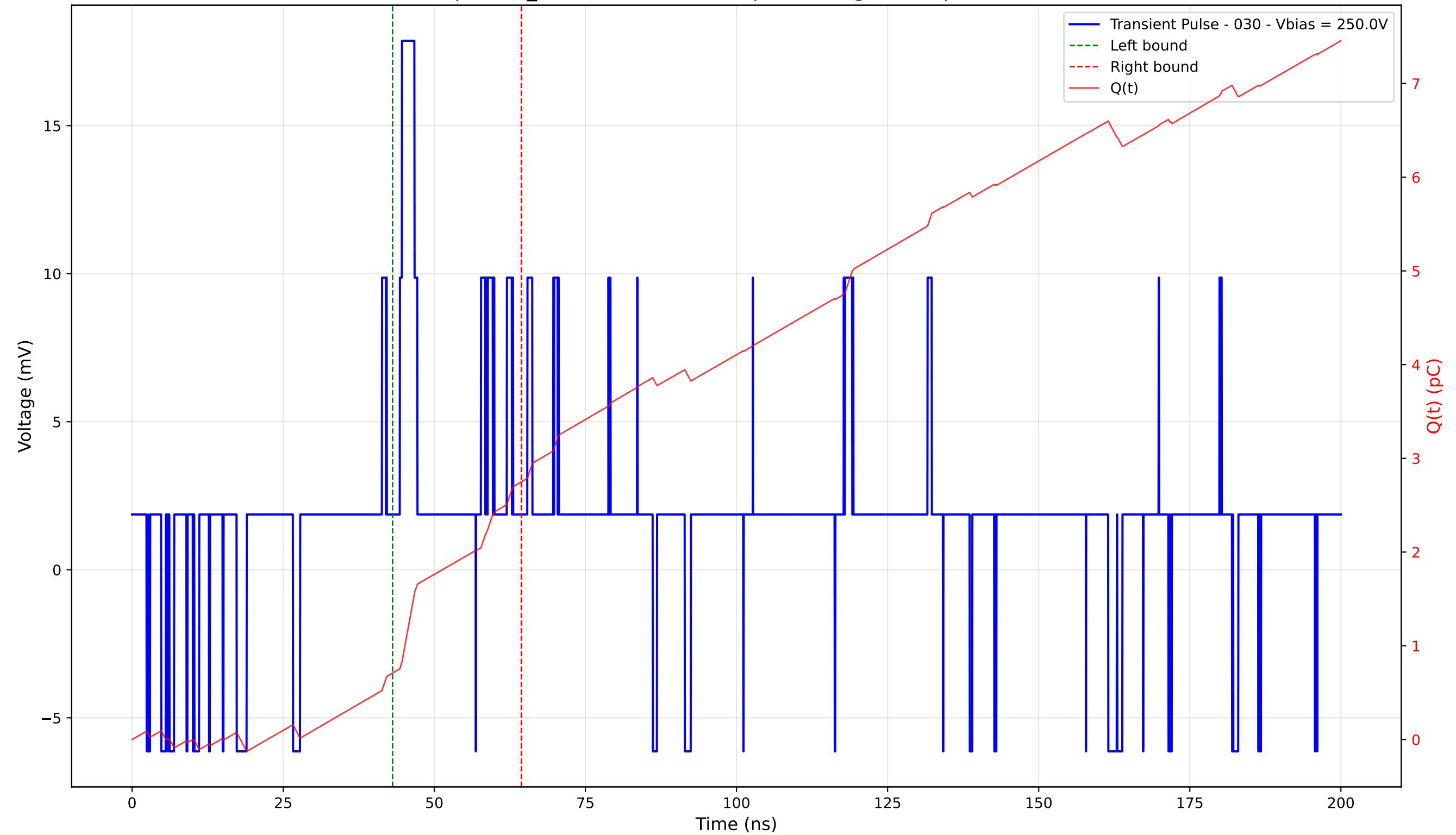
Transient Pulse - Sample: TD_4004 - Position: 20.0 \mu\text{m} - Charge: 2.04 pC - Rise Time: 0.00 ns (N/A)
