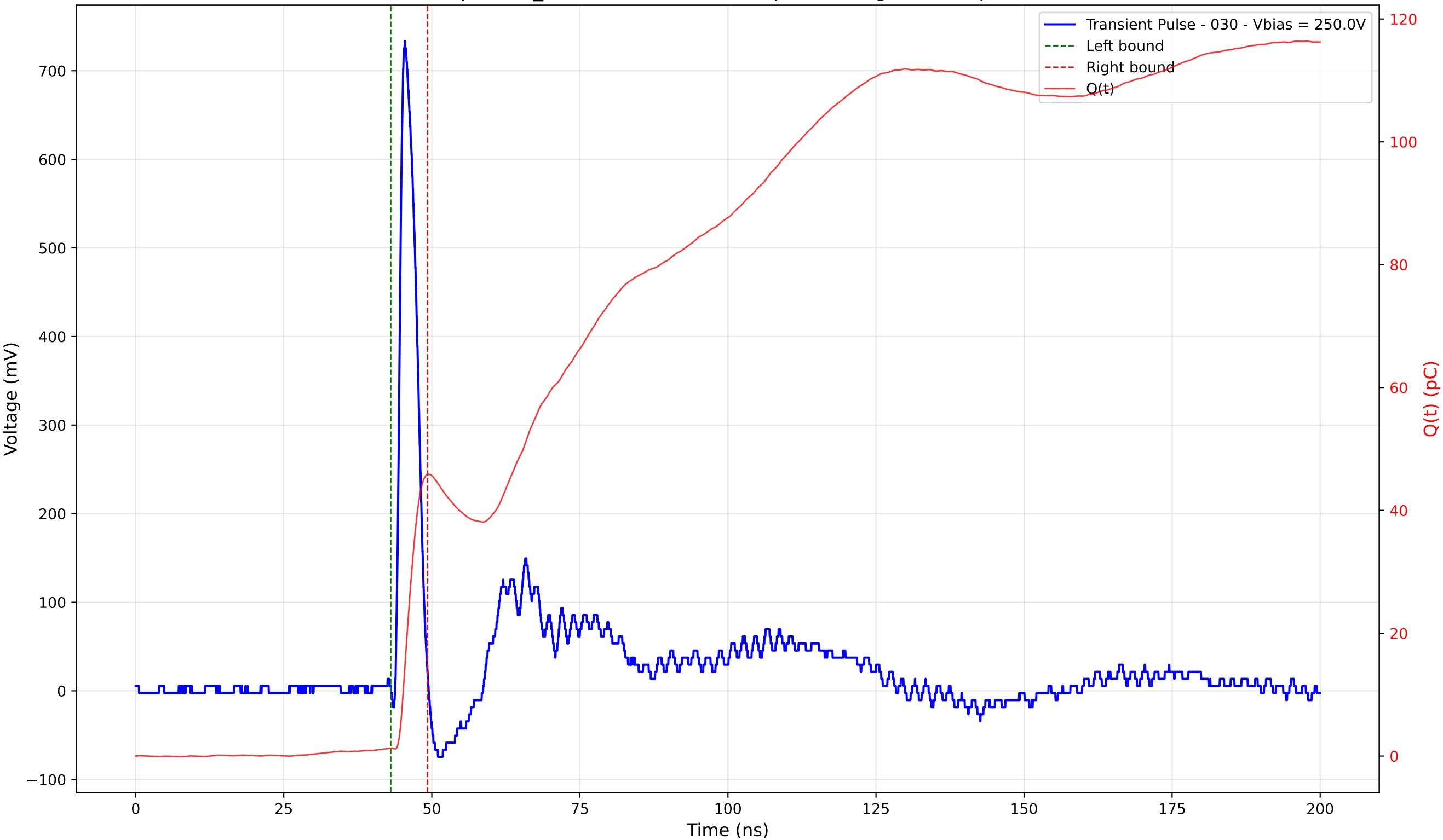
Transient Pulse - Sample: TD_4004 - Position: 300.0 \mu\text{m} - Charge: 44.56 pC - Rise Time: 0.97 ns
