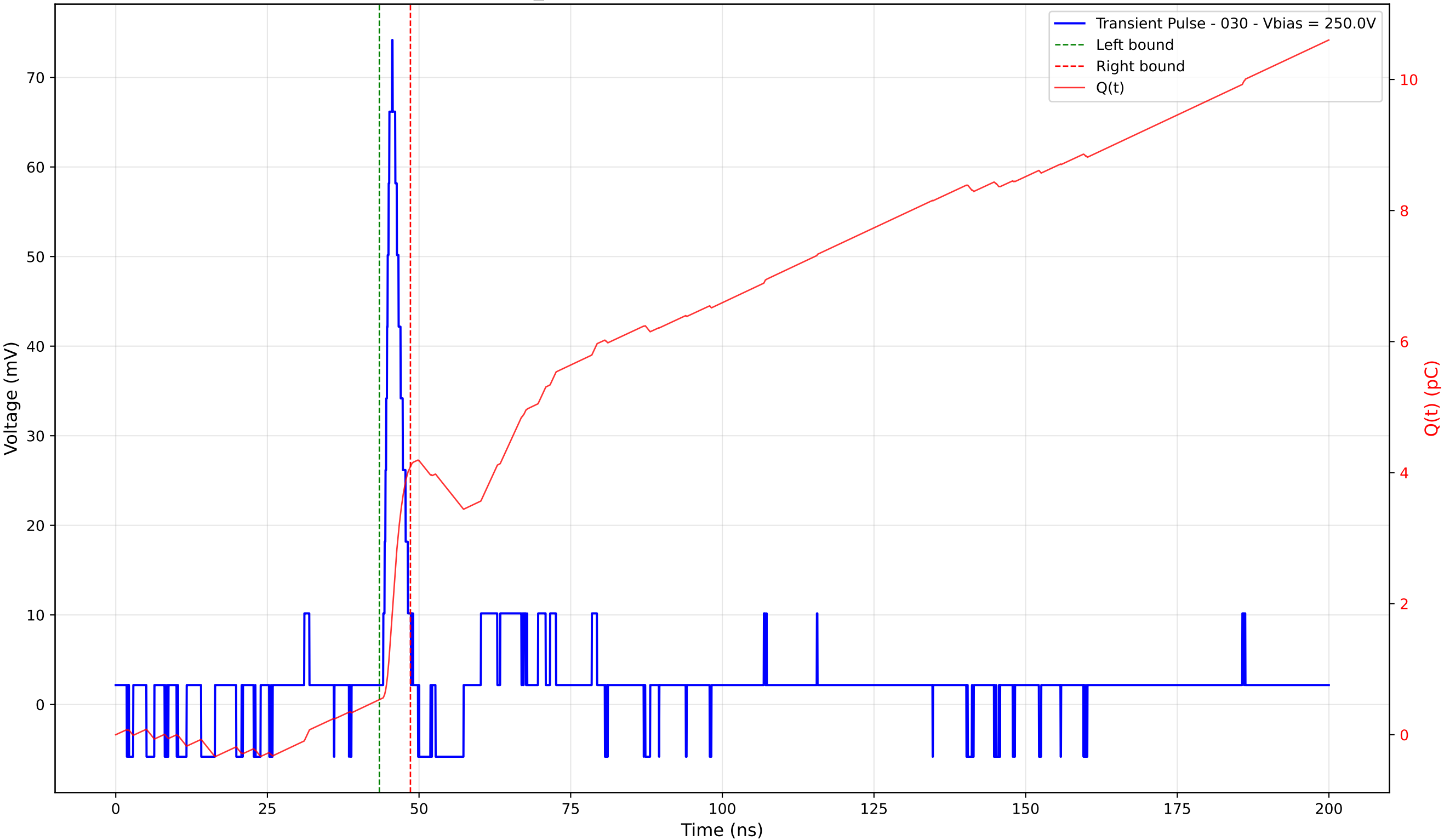
Transient Pulse - Sample: TD_4004 - Position: 425.0 \mu\text{m} - Charge: 3.56 pC - Rise Time: 1.47 ns
