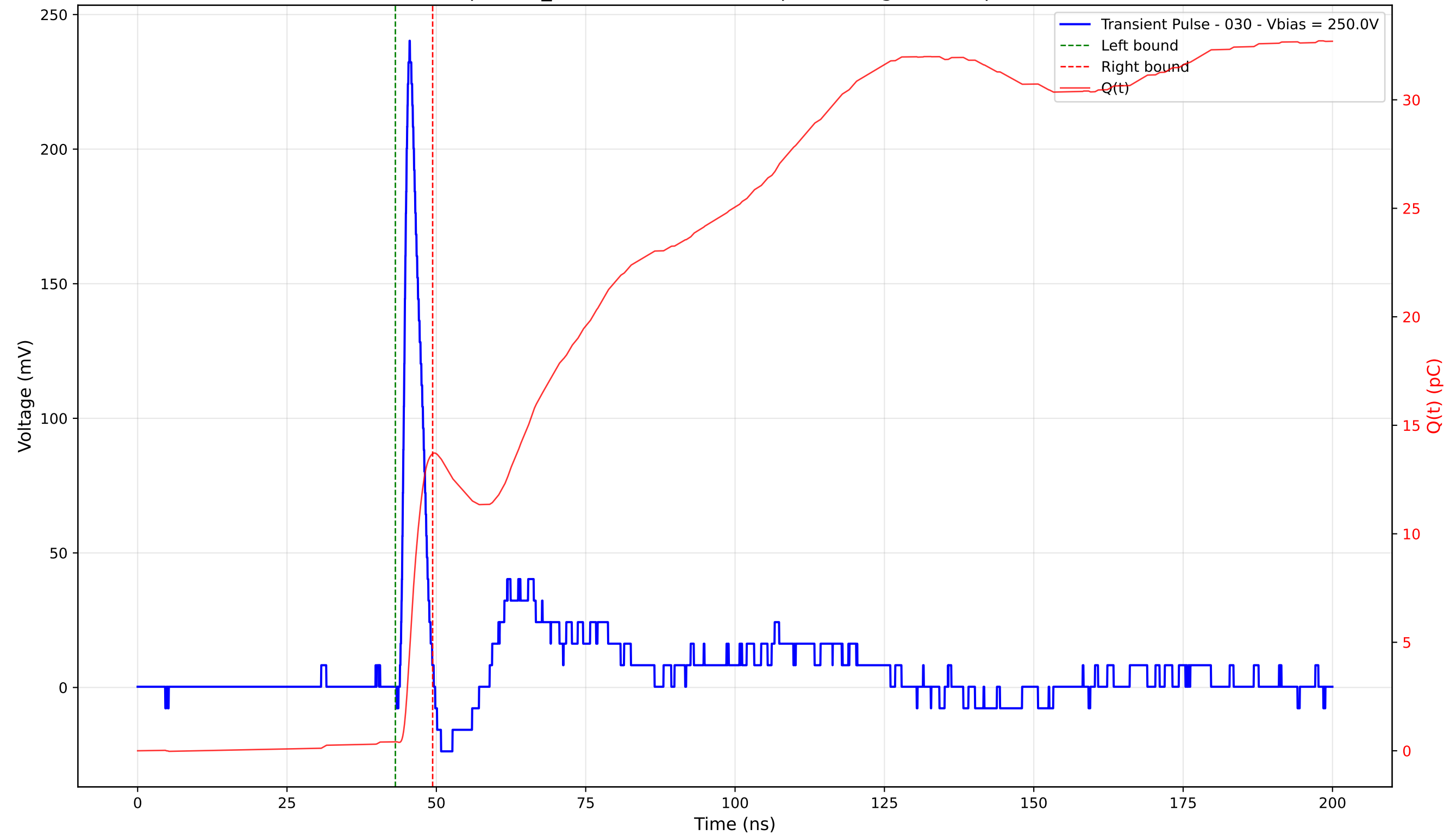
Transient Pulse - Sample: TD_4004 - Position: 405.0 \mu\text{m} - Charge: 13.28 pC - Rise Time: 1.06 ns
