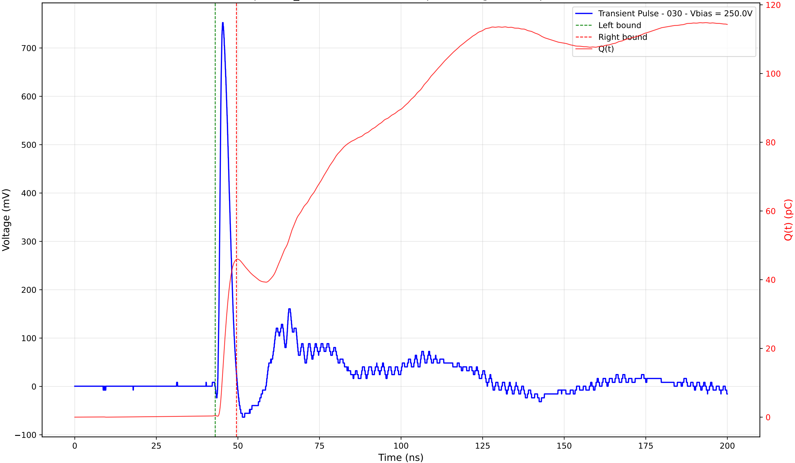
Transient Pulse - Sample: TD_4004 - Position: 150.0 \mu\text{m} - Charge: 45.45 pC - Rise Time: 0.92 ns
