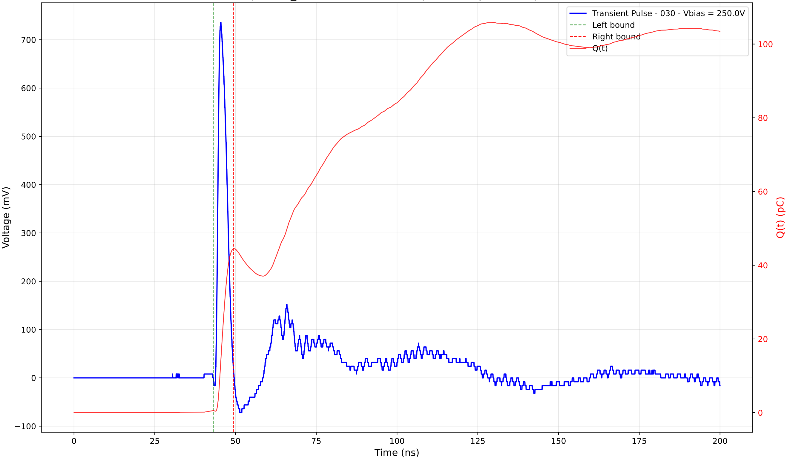
Transient Pulse - Sample: TD_4004 - Position: 260.0 \mu\text{m} - Charge: 43.89 pC - Rise Time: 0.95 ns
