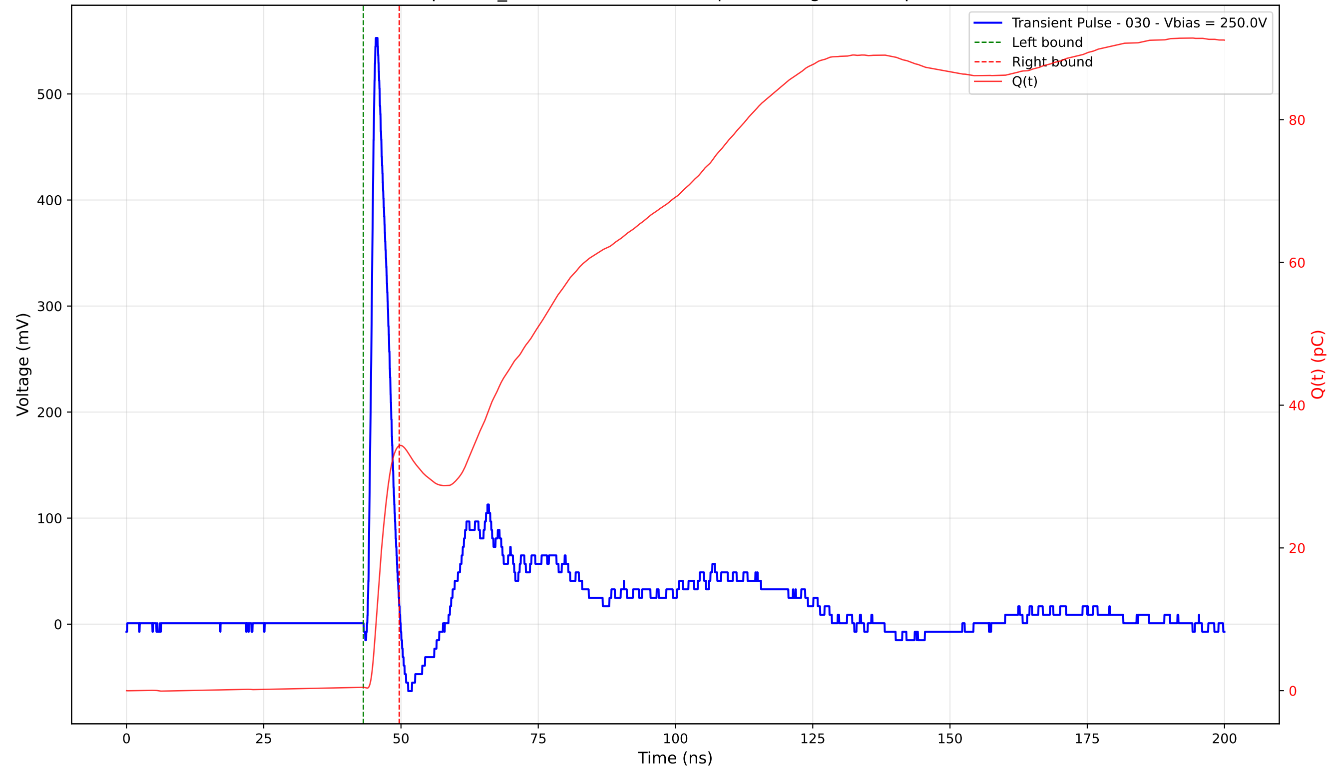
Transient Pulse - Sample: TD_4004 - Position: 360.0 \mu\text{m} - Charge: 33.86 pC - Rise Time: 1.03 ns
