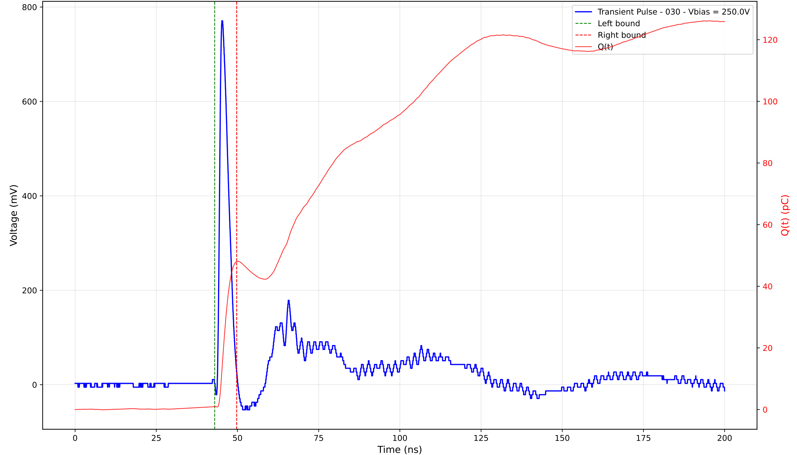
Transient Pulse - Sample: TD_4004 - Position: 125.0 \mu\text{m} - Charge: 47.01 pC - Rise Time: 0.90 ns
