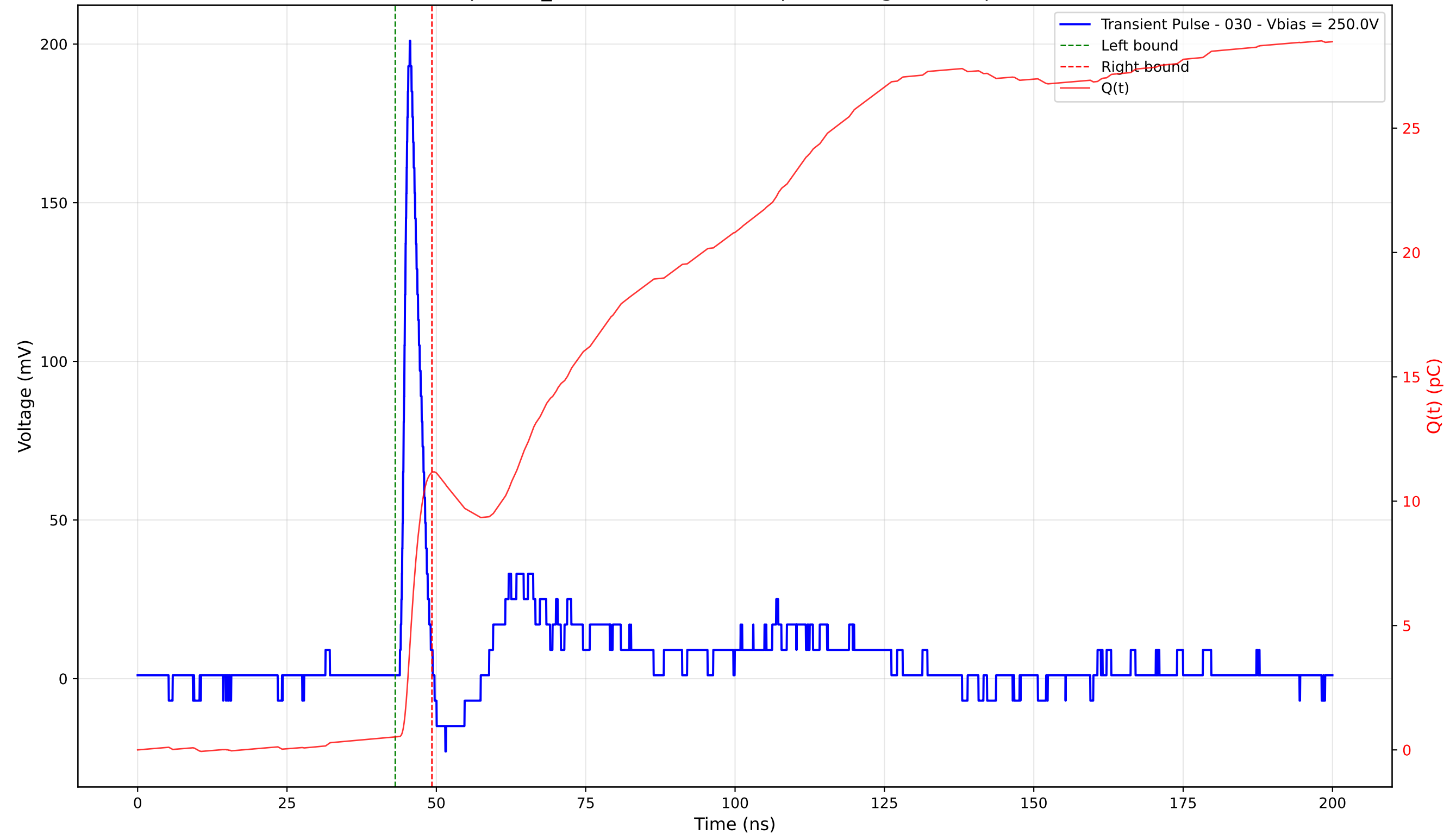
Transient Pulse - Sample: TD_4004 - Position: 410.0 \mu\text{m} - Charge: 10.64 pC - Rise Time: 1.09 ns
