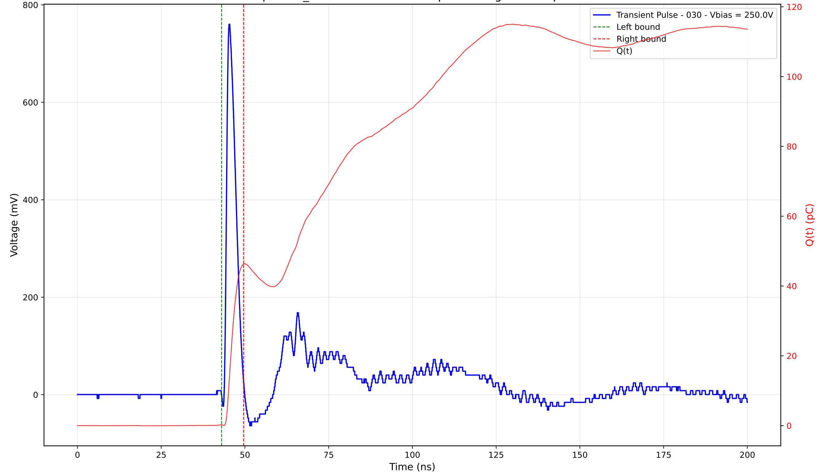
Transient Pulse - Sample: TD_4004 - Position: 130.0 \mu\text{m} - Charge: 46.02 pC - Rise Time: 0.90 ns
