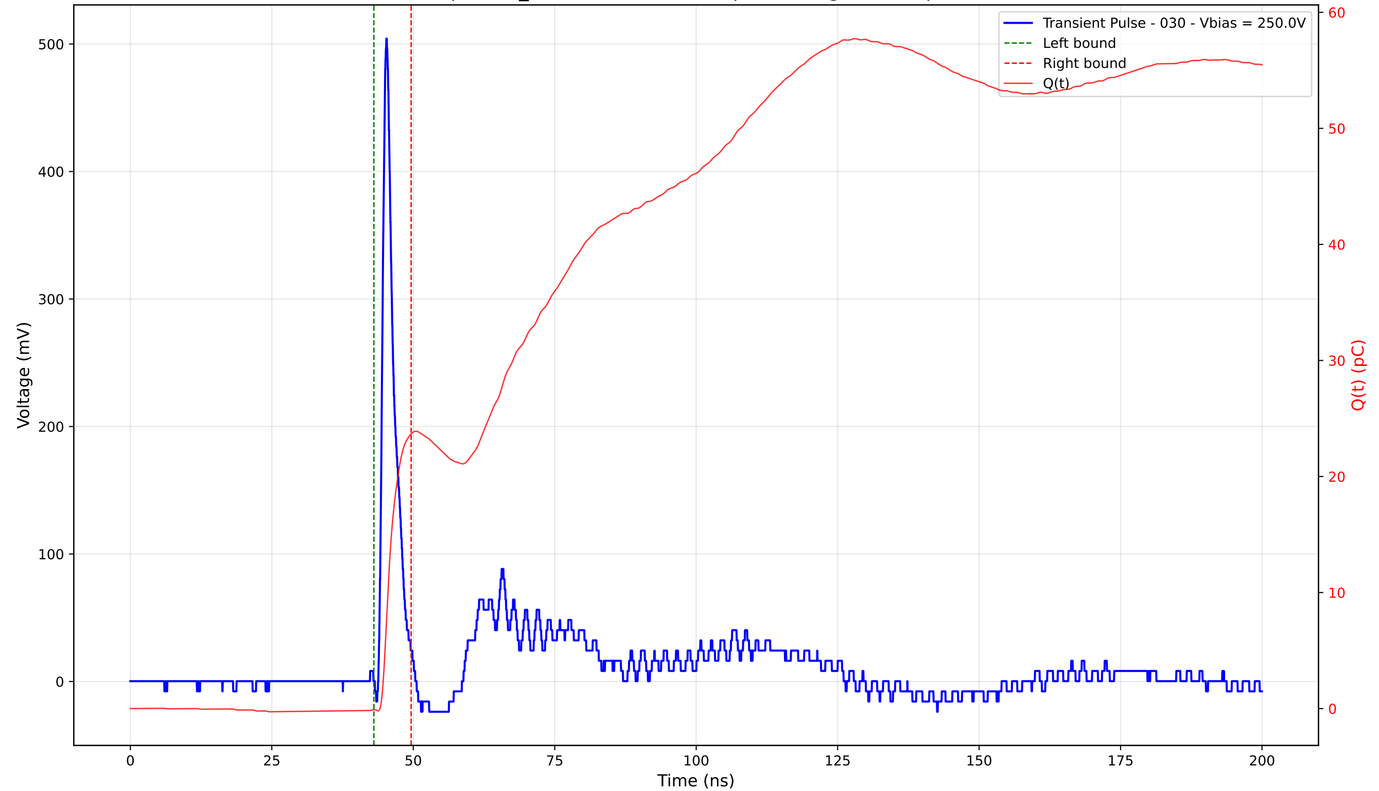
Transient Pulse - Sample: TD_4004 - Position: 70.0 \mu\text{m} - Charge: 23.76 pC - Rise Time: 0.91 ns
