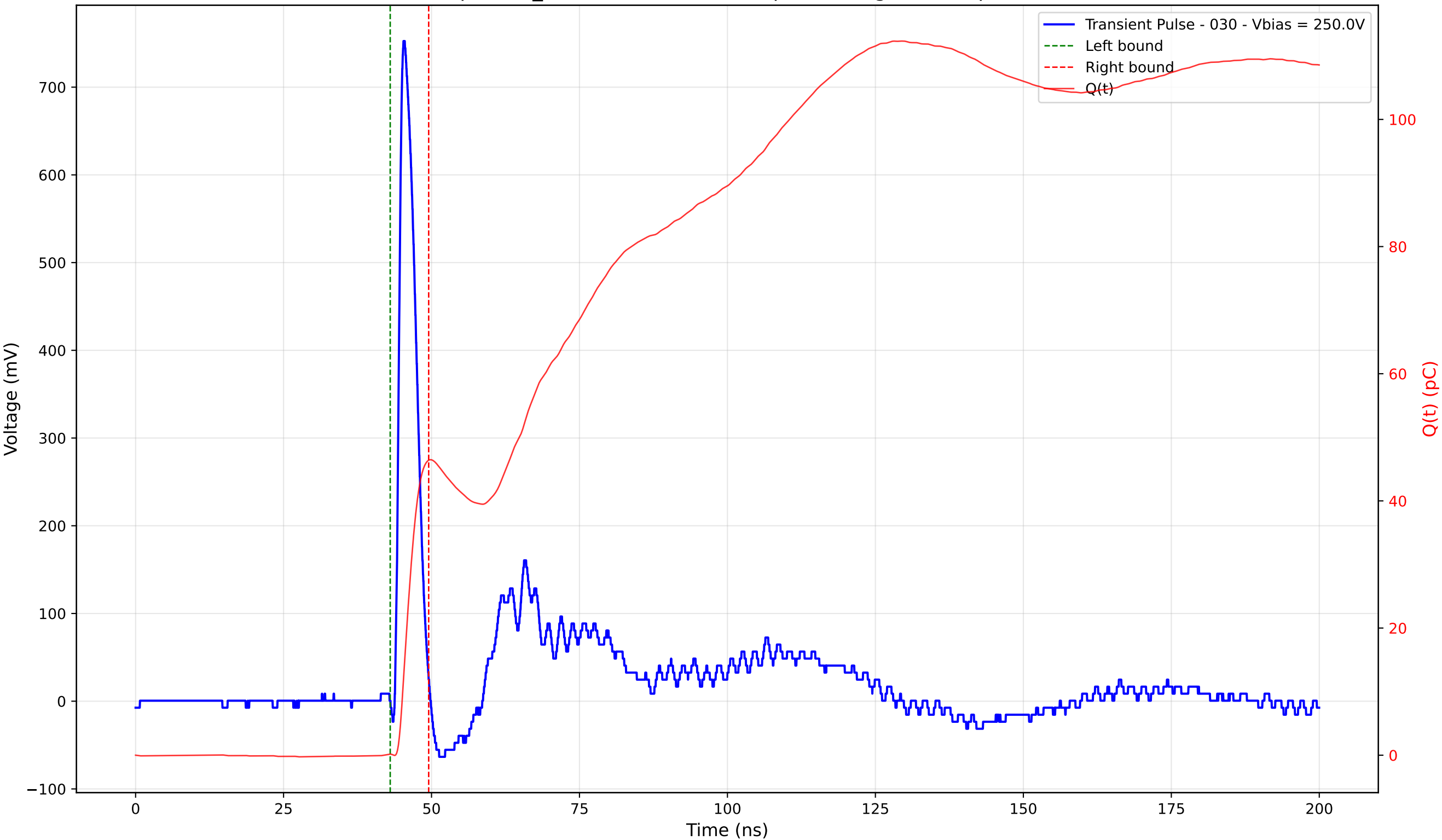
Transient Pulse - Sample: TD_4004 - Position: 230.0 \mu\text{m} - Charge: 46.23 pC - Rise Time: 0.93 ns
