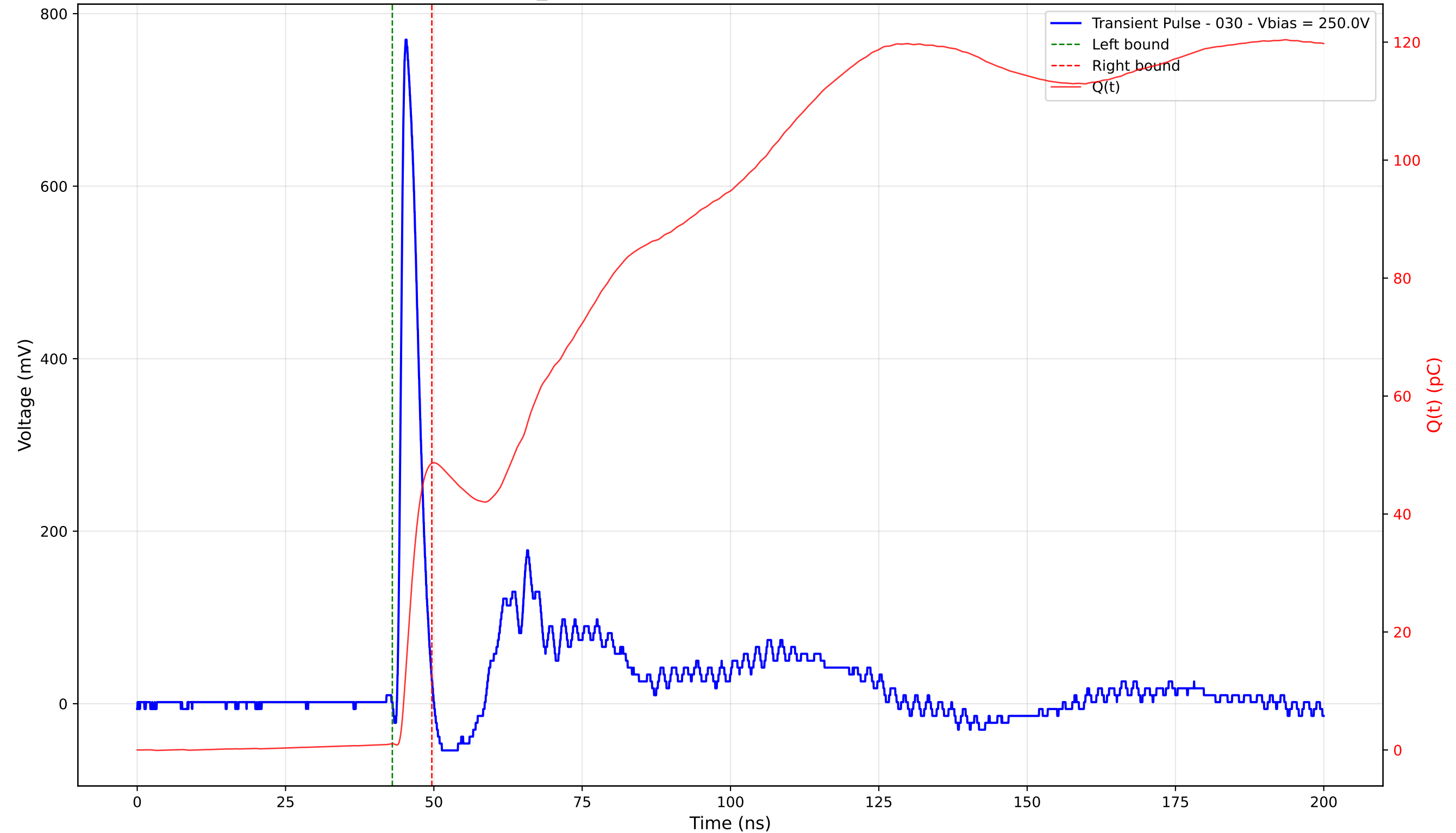
Transient Pulse - Sample: TD_4004 - Position: 210.0 \mu\text{m} - Charge: 47.54 pC - Rise Time: 0.90 ns
