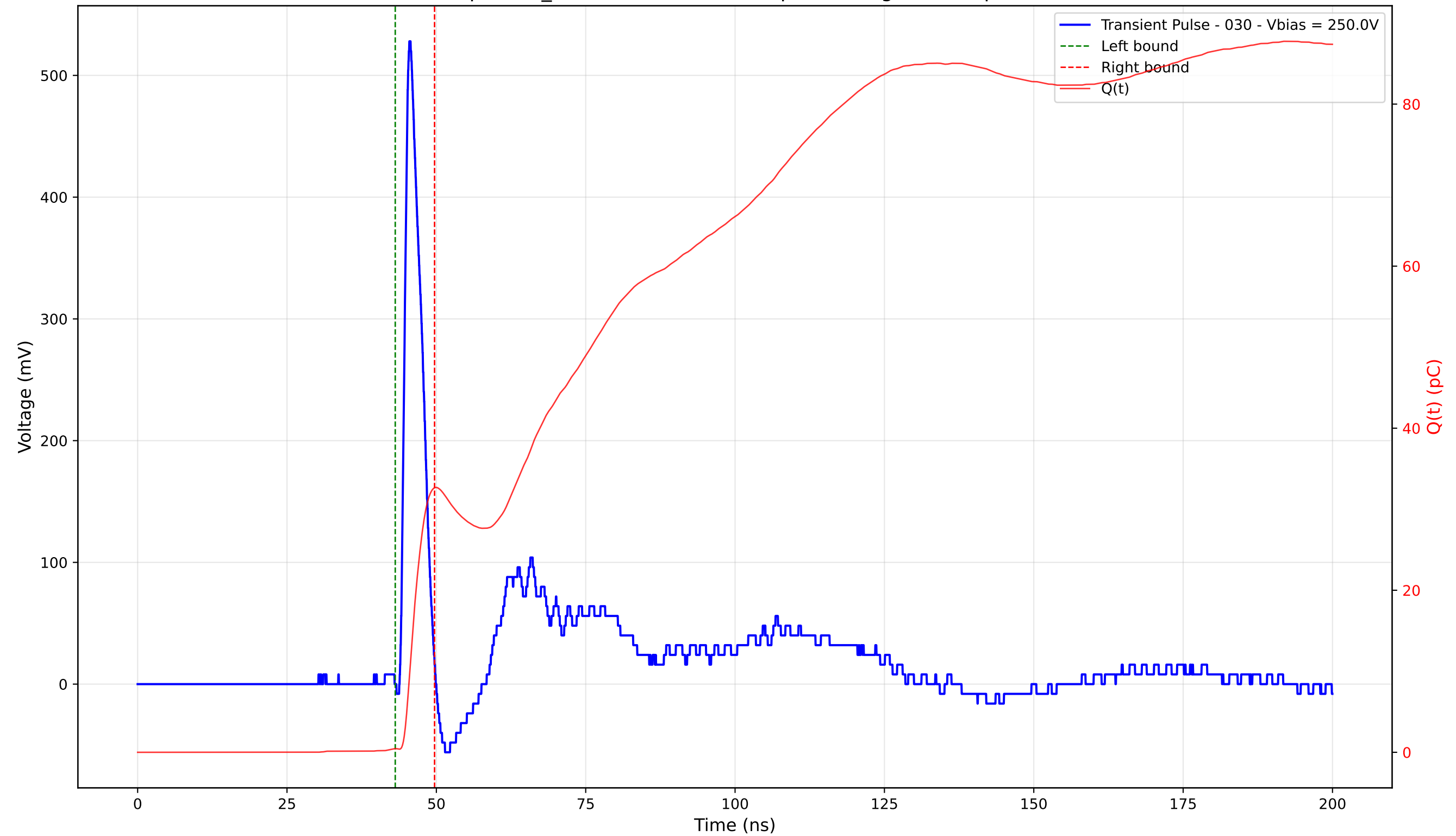
Transient Pulse - Sample: TD_4004 - Position: 370.0 \mu\text{m} - Charge: 32.20 pC - Rise Time: 1.05 ns
