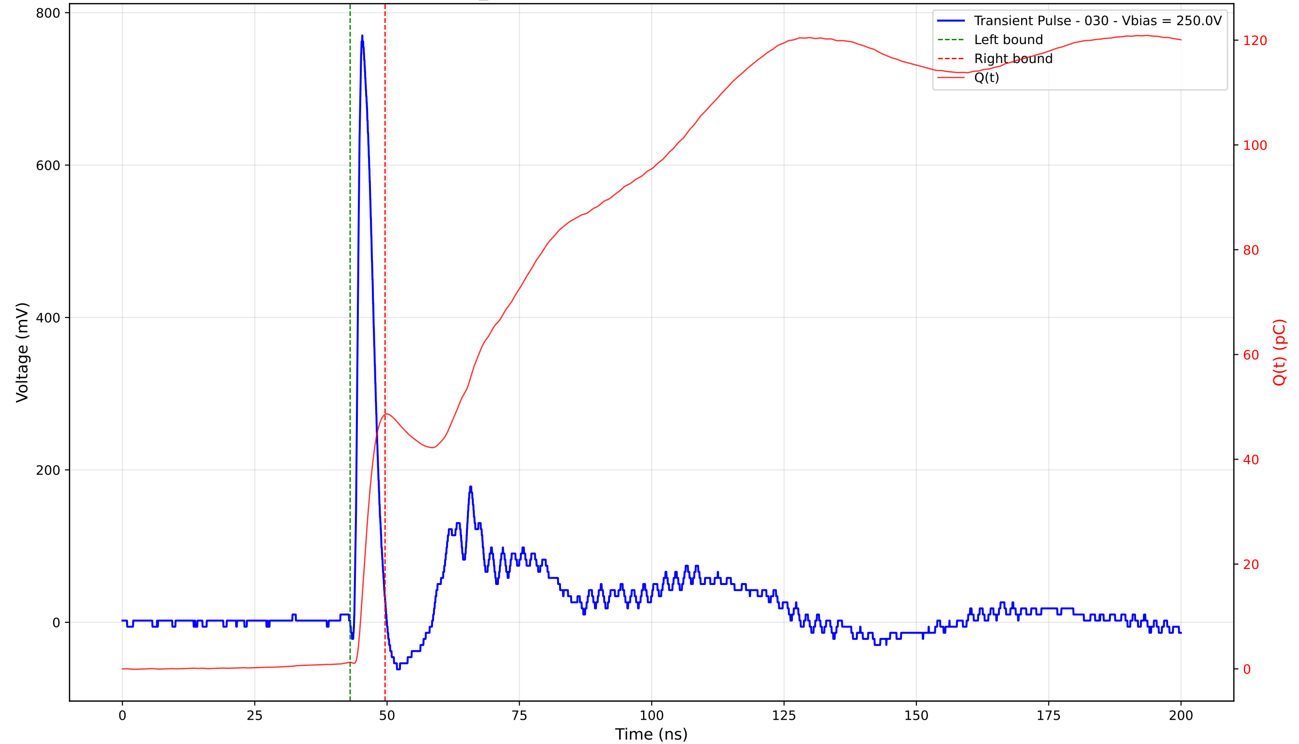
Transient Pulse - Sample: TD_4004 - Position: 225.0 \mu\text{m} - Charge: 47.32 pC - Rise Time: 0.92 ns
