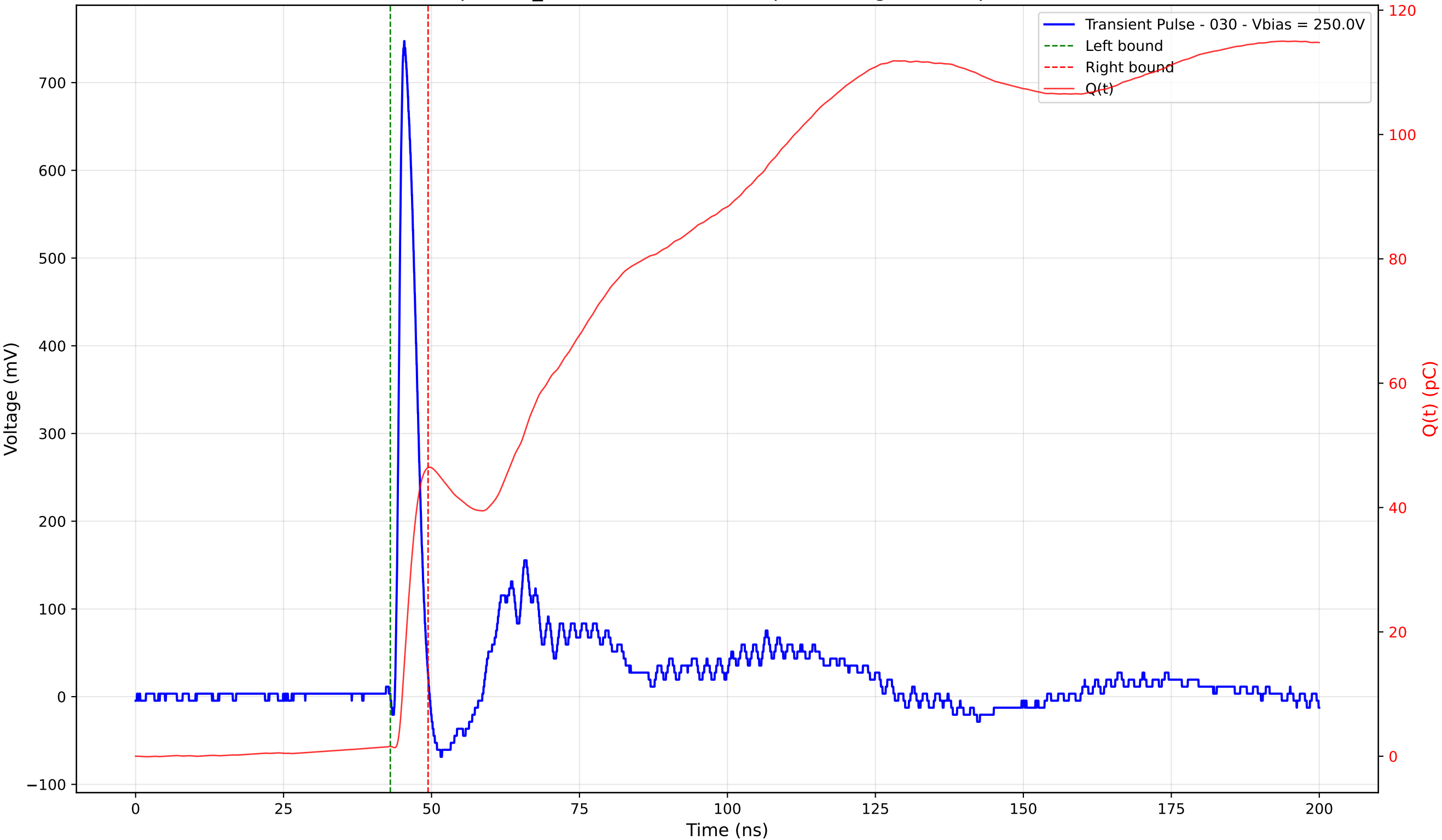
Transient Pulse - Sample: TD_4004 - Position: 245.0 \mu\text{m} - Charge: 44.85 pC - Rise Time: 0.93 ns
