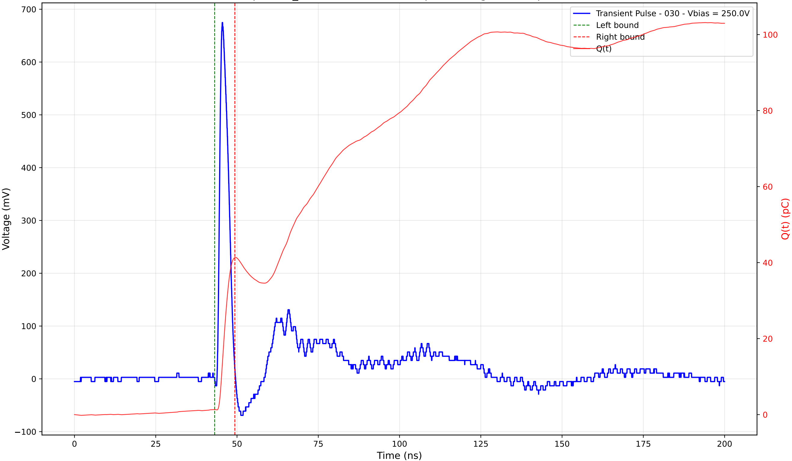
Transient Pulse - Sample: TD_4004 - Position: 325.0 \mu\text{m} - Charge: 39.96 pC - Rise Time: 0.99 ns
