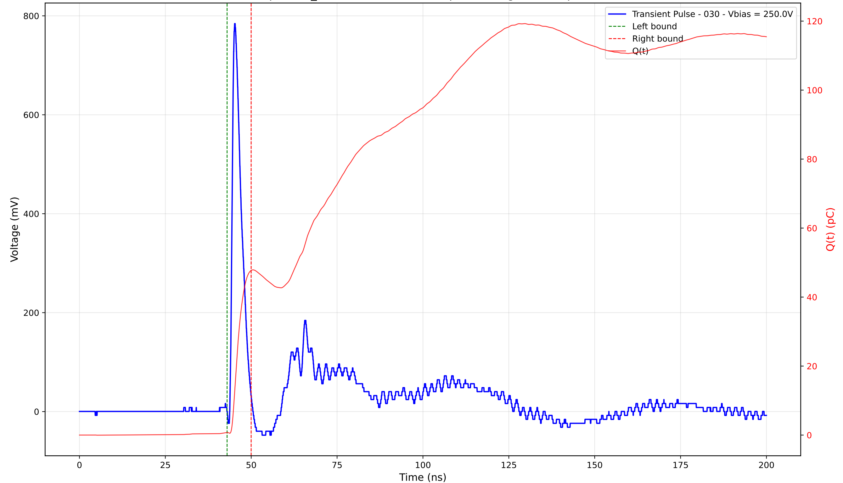
Transient Pulse - Sample: TD_4004 - Position: 110.0 \mu\text{m} - Charge: 46.96 pC - Rise Time: 0.87 ns
