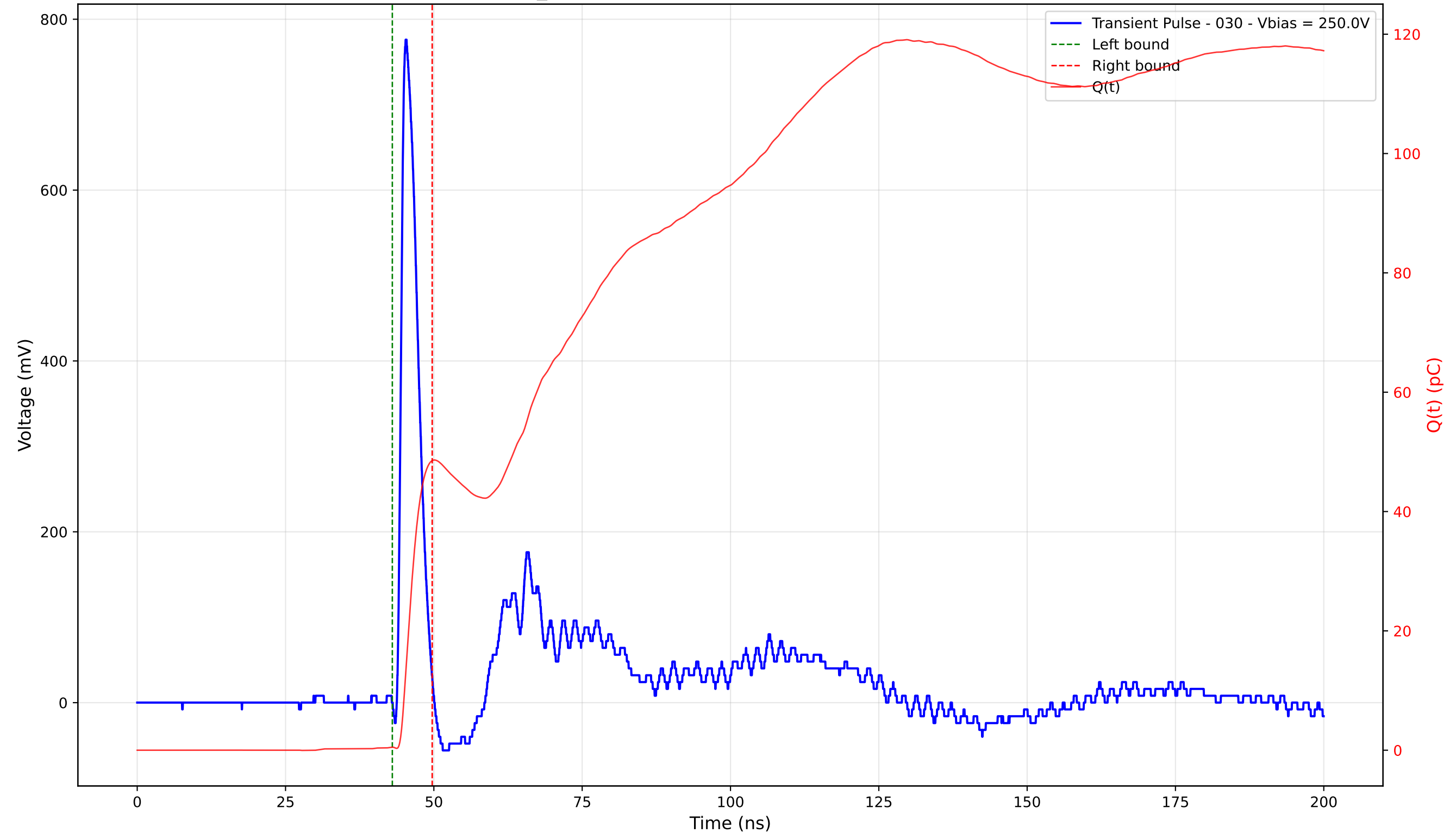
Transient Pulse - Sample: TD_4004 - Position: 205.0 \mu\text{m} - Charge: 48.03 pC - Rise Time: 0.90 ns
