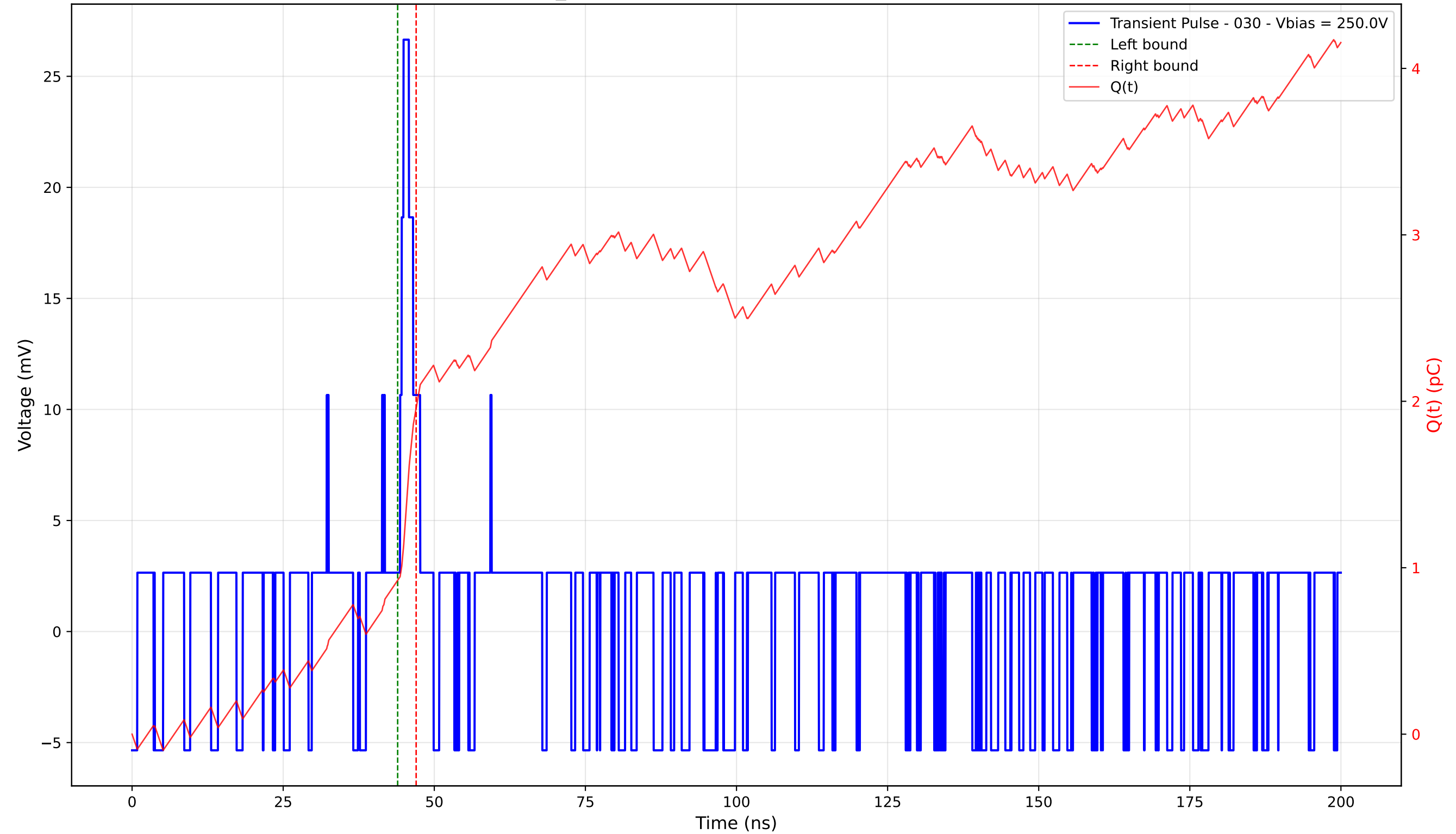
Transient Pulse - Sample: TD_4004 - Position: 30.0 \mu\text{m} - Charge: 1.04 pC - Rise Time: 0.58 ns
