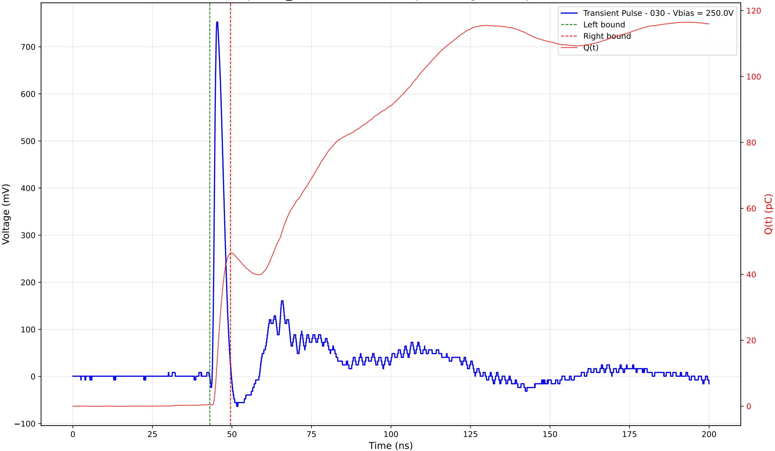
Transient Pulse - Sample: TD_4004 - Position: 135.0 \mu\text{m} - Charge: 45.86 pC - Rise Time: 0.91 ns
