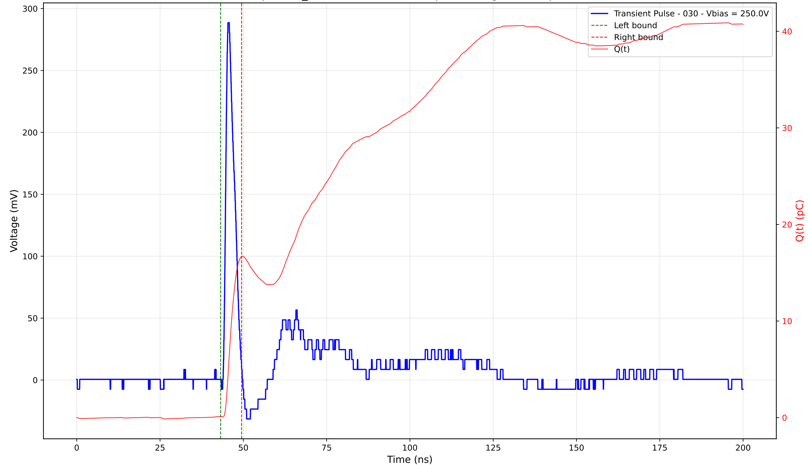
Transient Pulse - Sample: TD_4004 - Position: 400.0 \mu\text{m} - Charge: 16.58 pC - Rise Time: 1.01 ns
