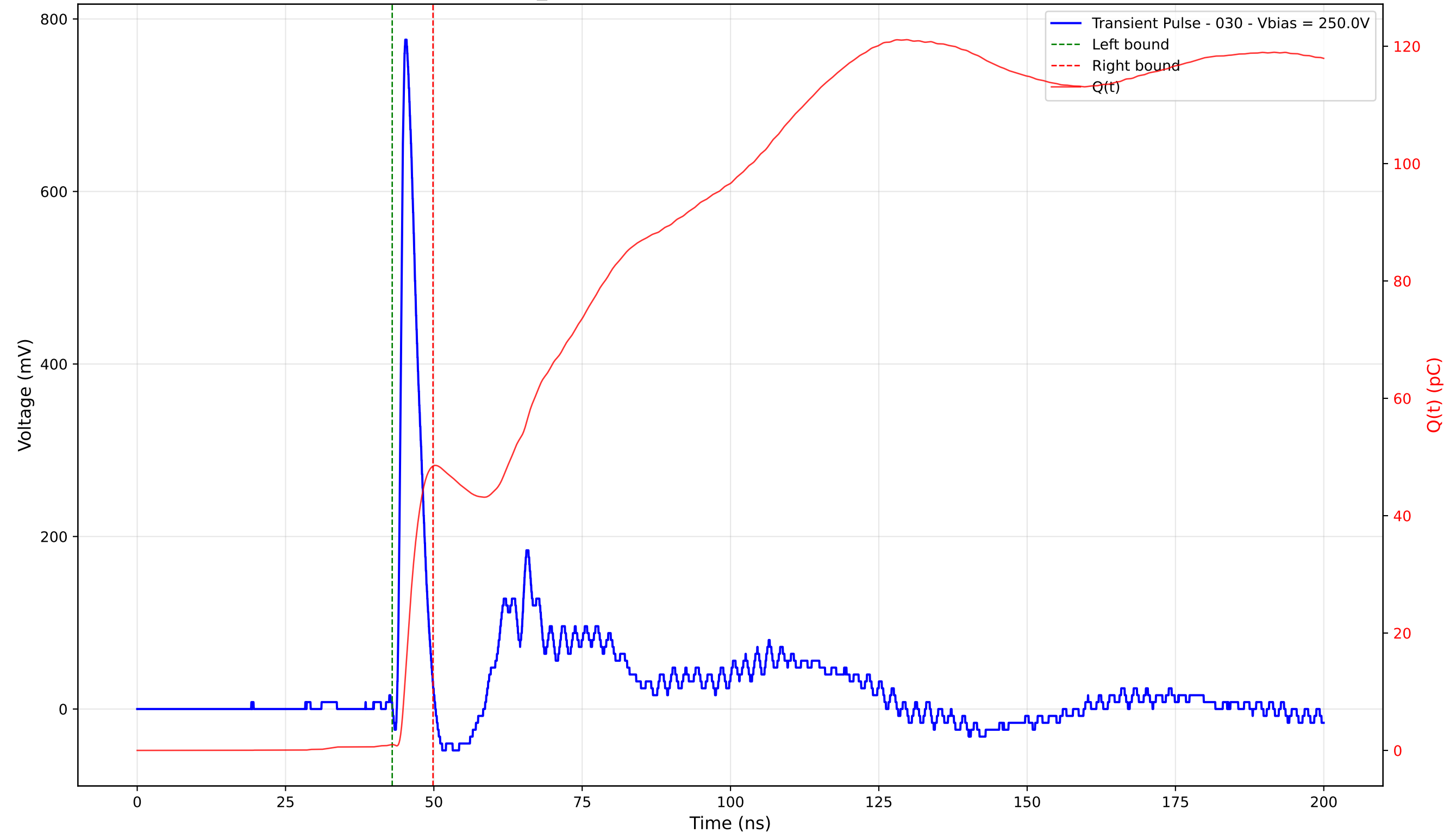
Transient Pulse - Sample: TD_4004 - Position: 120.0 \mu\text{m} - Charge: 47.46 pC - Rise Time: 0.88 ns
