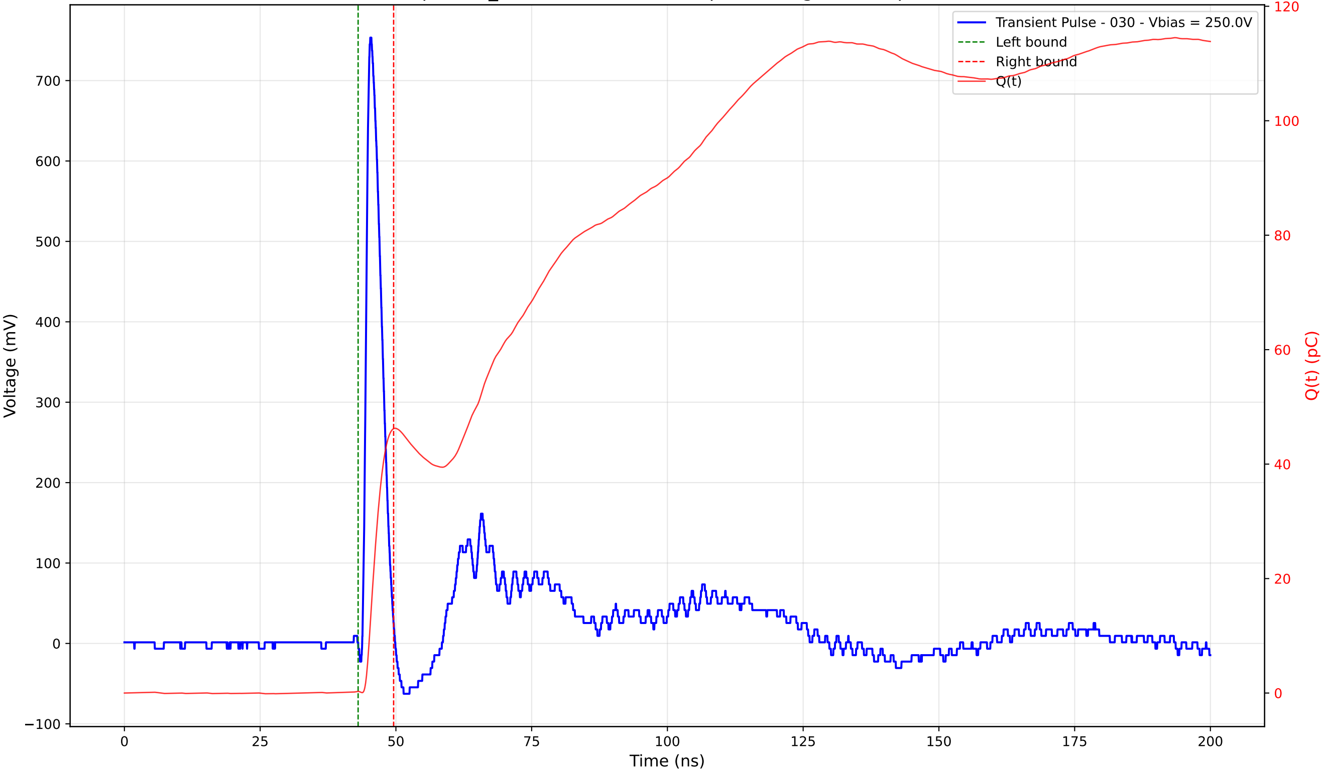
Transient Pulse - Sample: TD_4004 - Position: 155.0 \mu\text{m} - Charge: 45.92 pC - Rise Time: 0.93 ns
