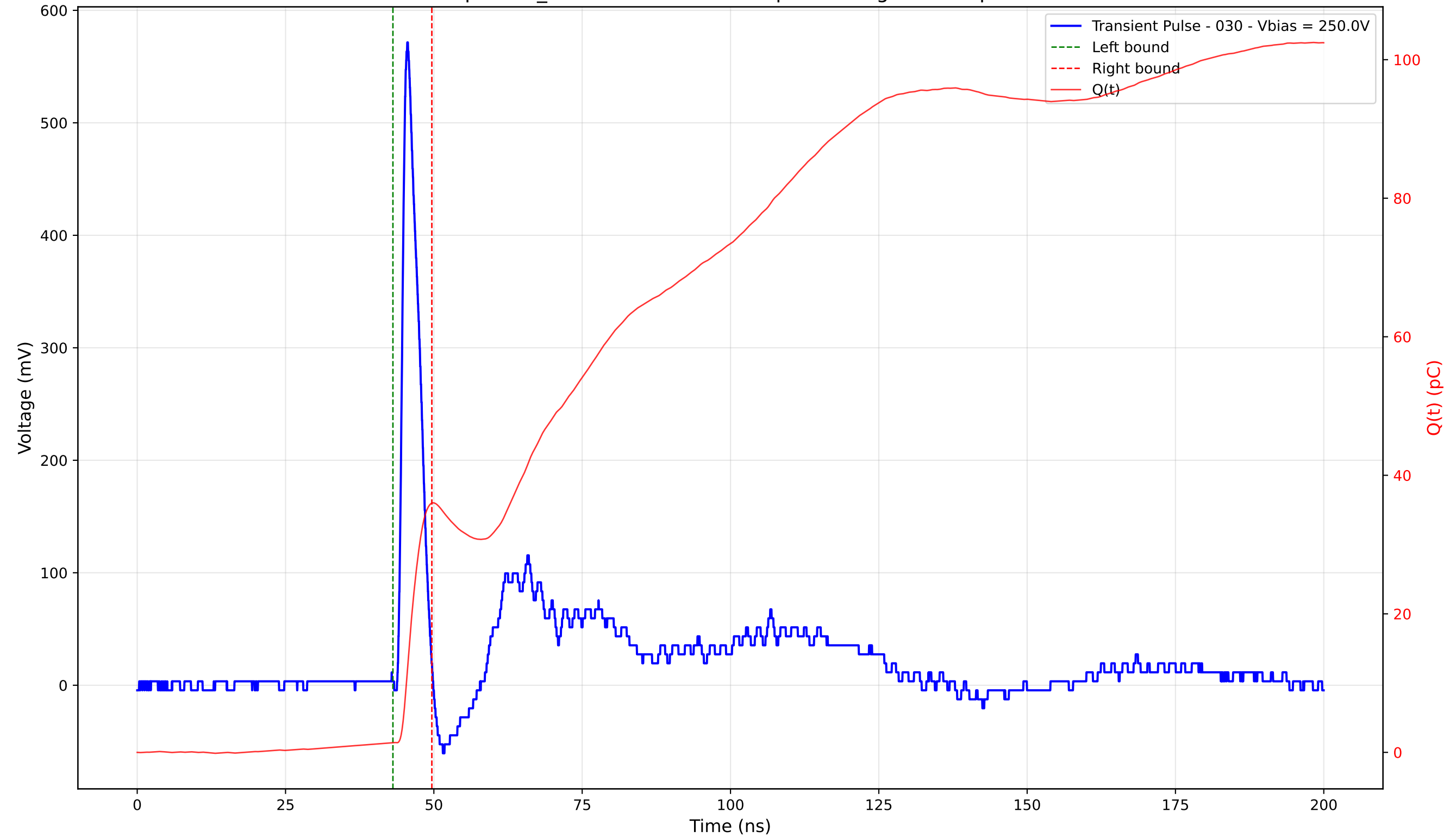
Transient Pulse - Sample: TD_4004 - Position: 355.0 \mu\text{m} - Charge: 34.57 pC - Rise Time: 1.04 ns
