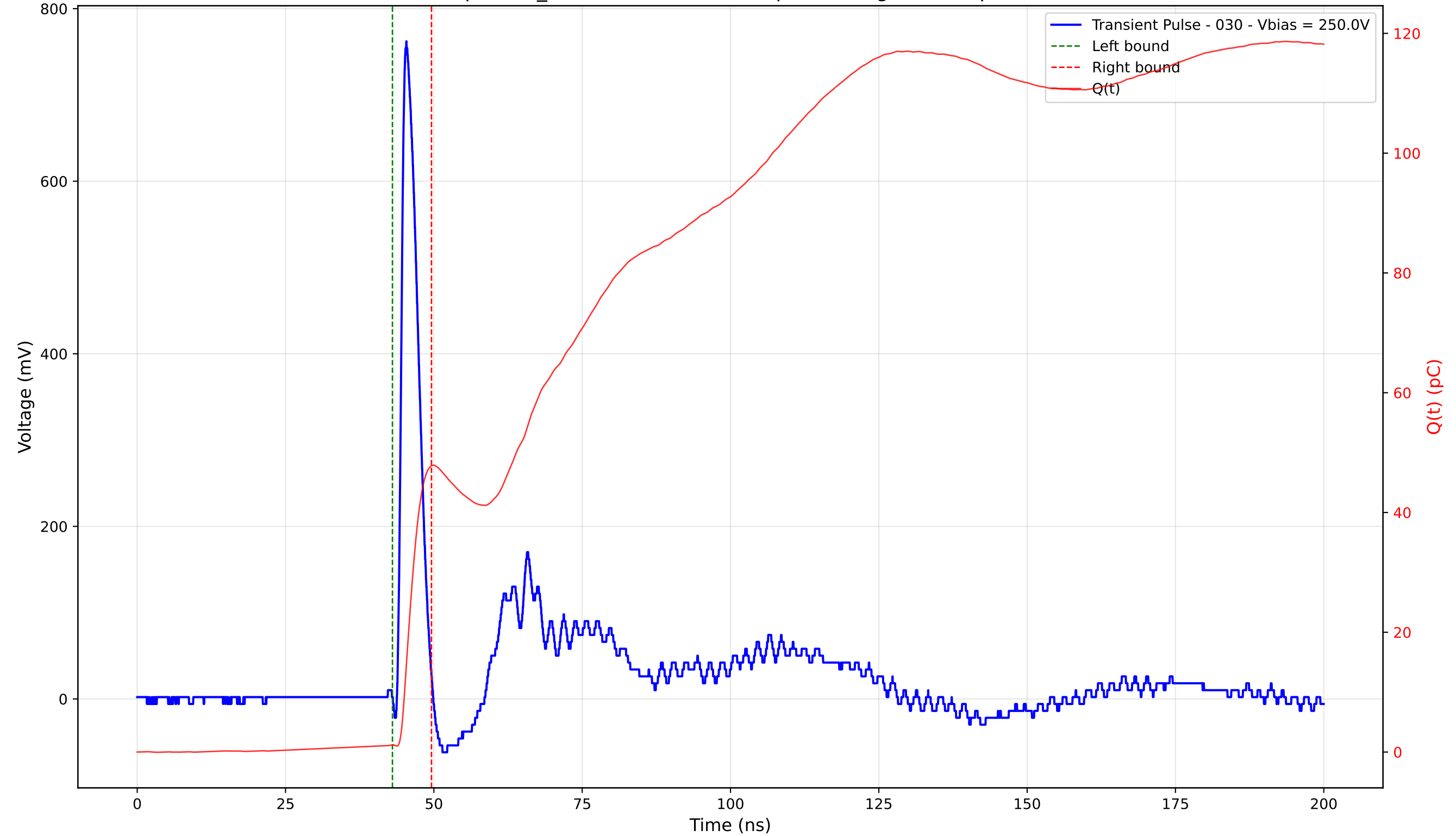
Transient Pulse - Sample: TD_4004 - Position: 160.0 \mu\text{m} - Charge: 46.62 pC - Rise Time: 0.93 ns
