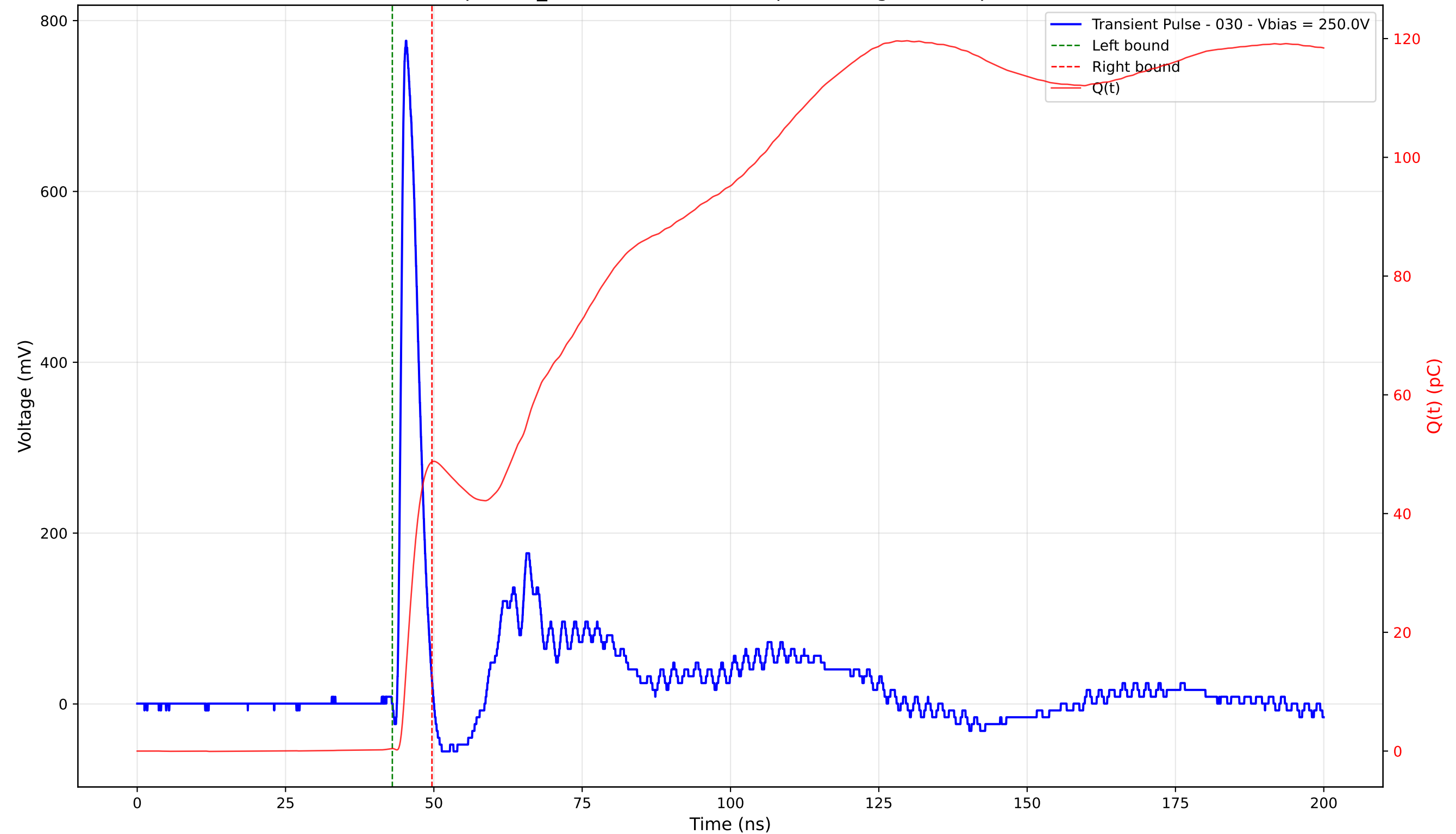
Transient Pulse - Sample: TD_4004 - Position: 170.0 \mu\text{m} - Charge: 48.29 pC - Rise Time: 0.91 ns
