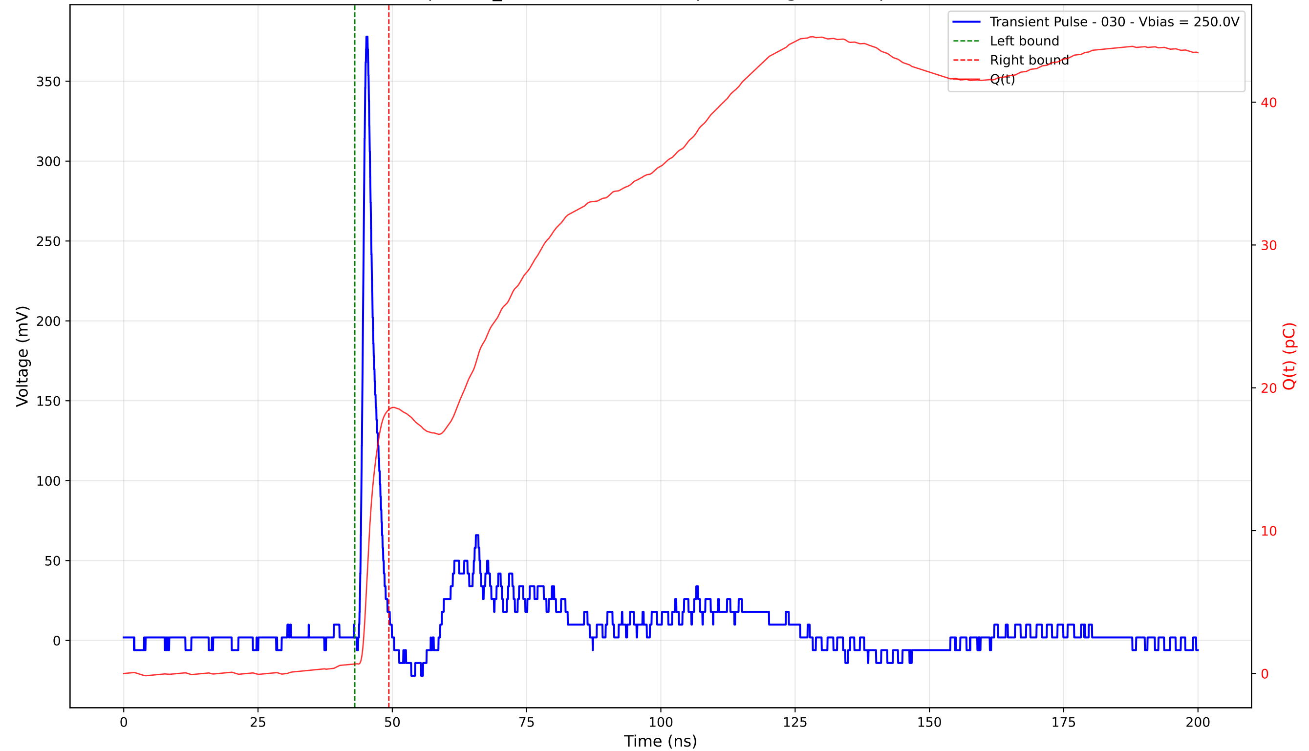
Transient Pulse - Sample: TD_4004 - Position: 65.0 \mu\text{m} - Charge: 17.81 pC - Rise Time: 0.93 ns
