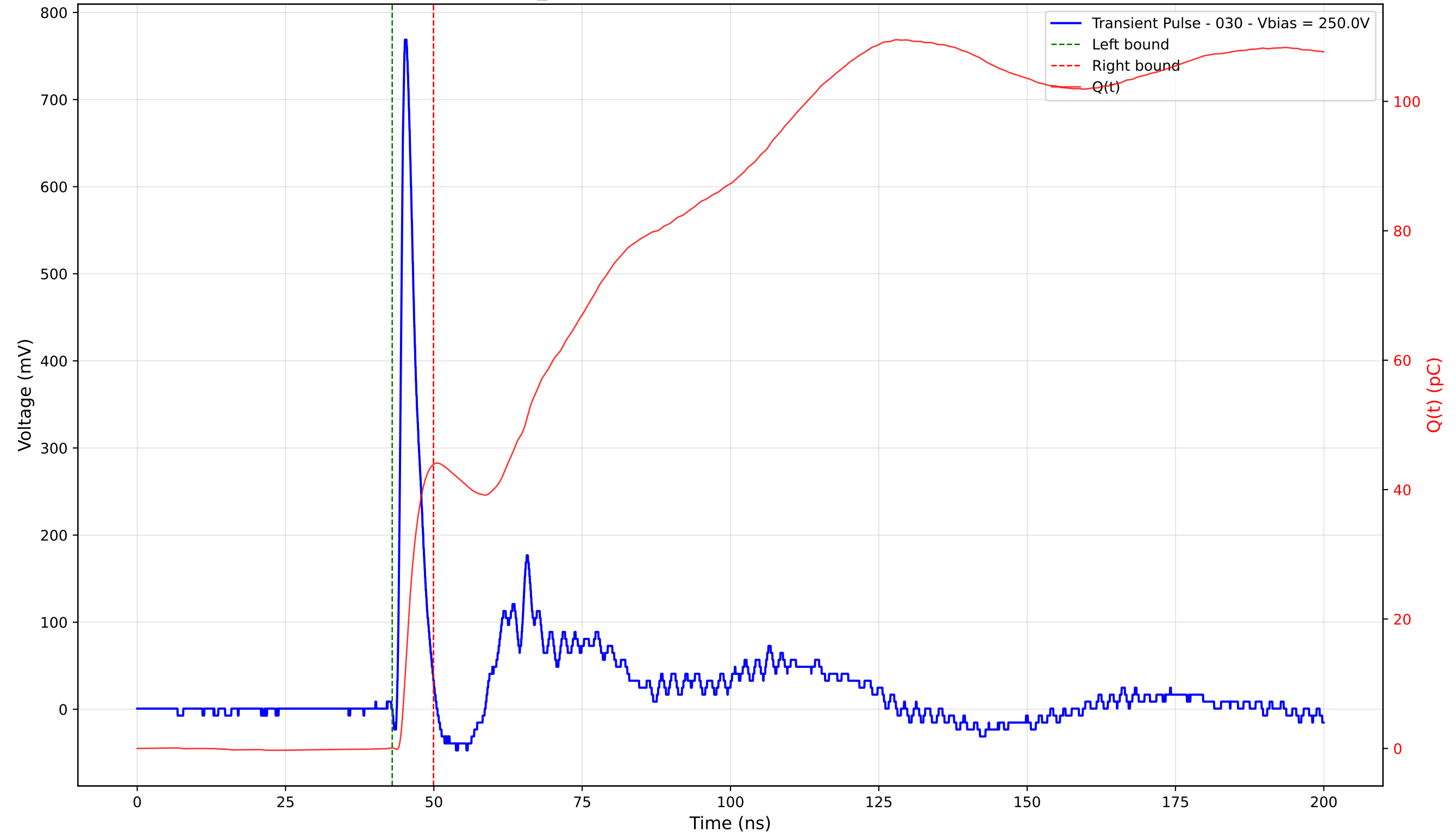
Transient Pulse - Sample: TD_4004 - Position: 100.0 \mu\text{m} - Charge: 43.83 pC - Rise Time: 0.87 ns
