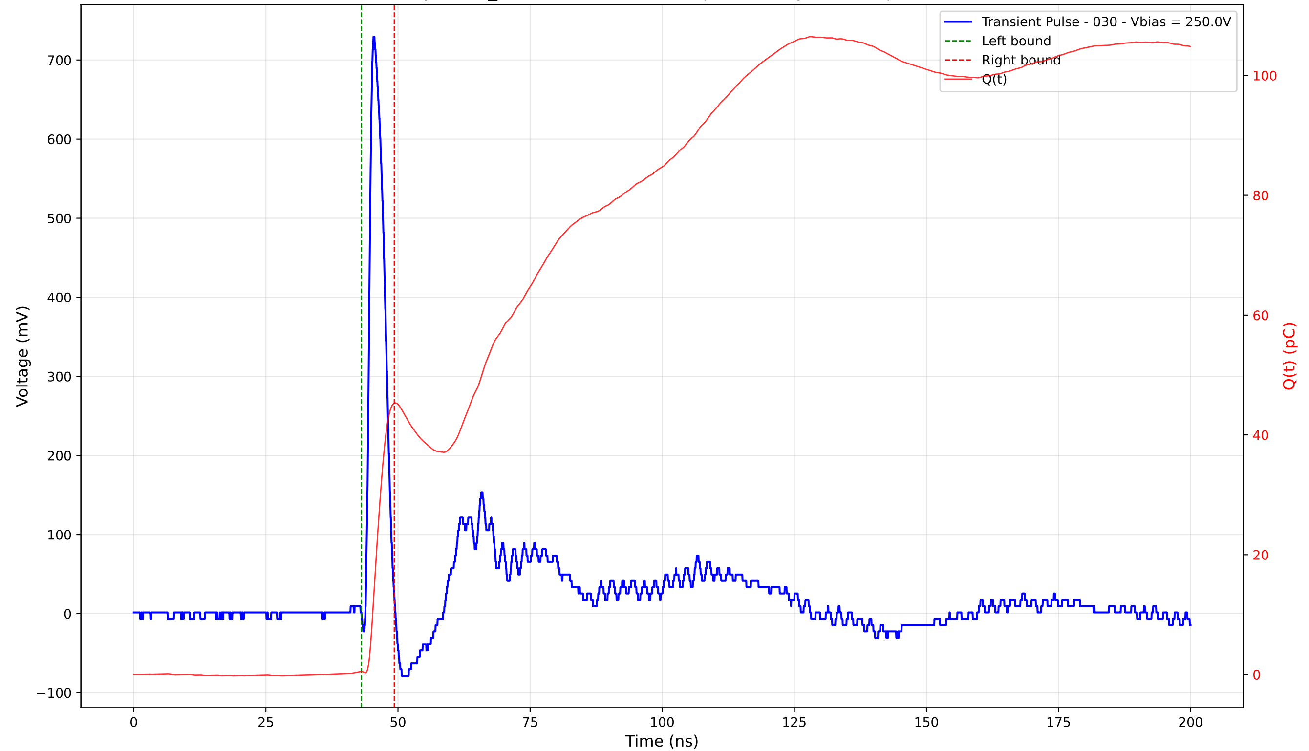
Transient Pulse - Sample: TD_4004 - Position: 295.0 \mu\text{m} - Charge: 44.82 pC - Rise Time: 0.96 ns
