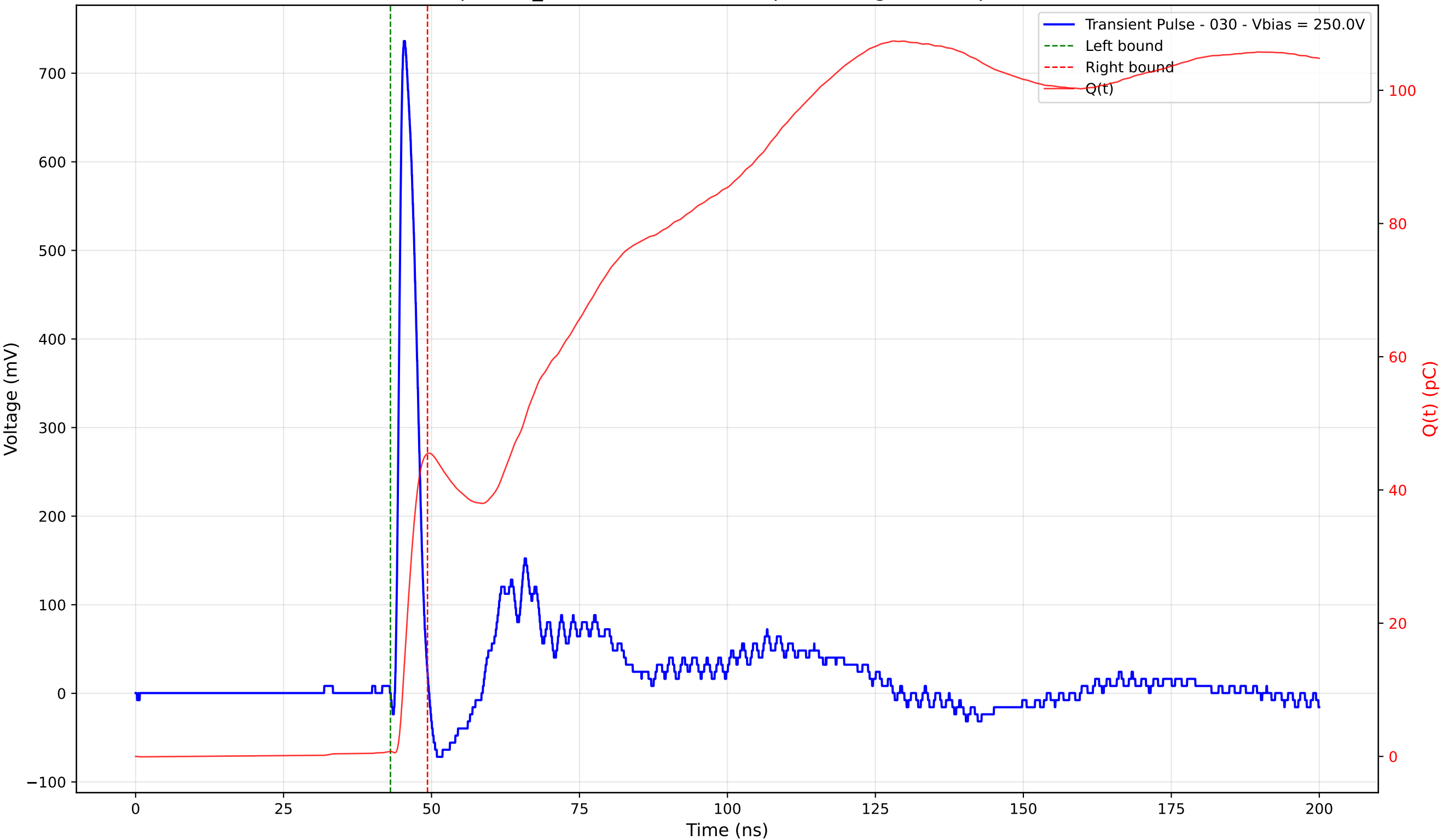
Transient Pulse - Sample: TD_4004 - Position: 270.0 \mu\text{m} - Charge: 44.72 pC - Rise Time: 0.93 ns
