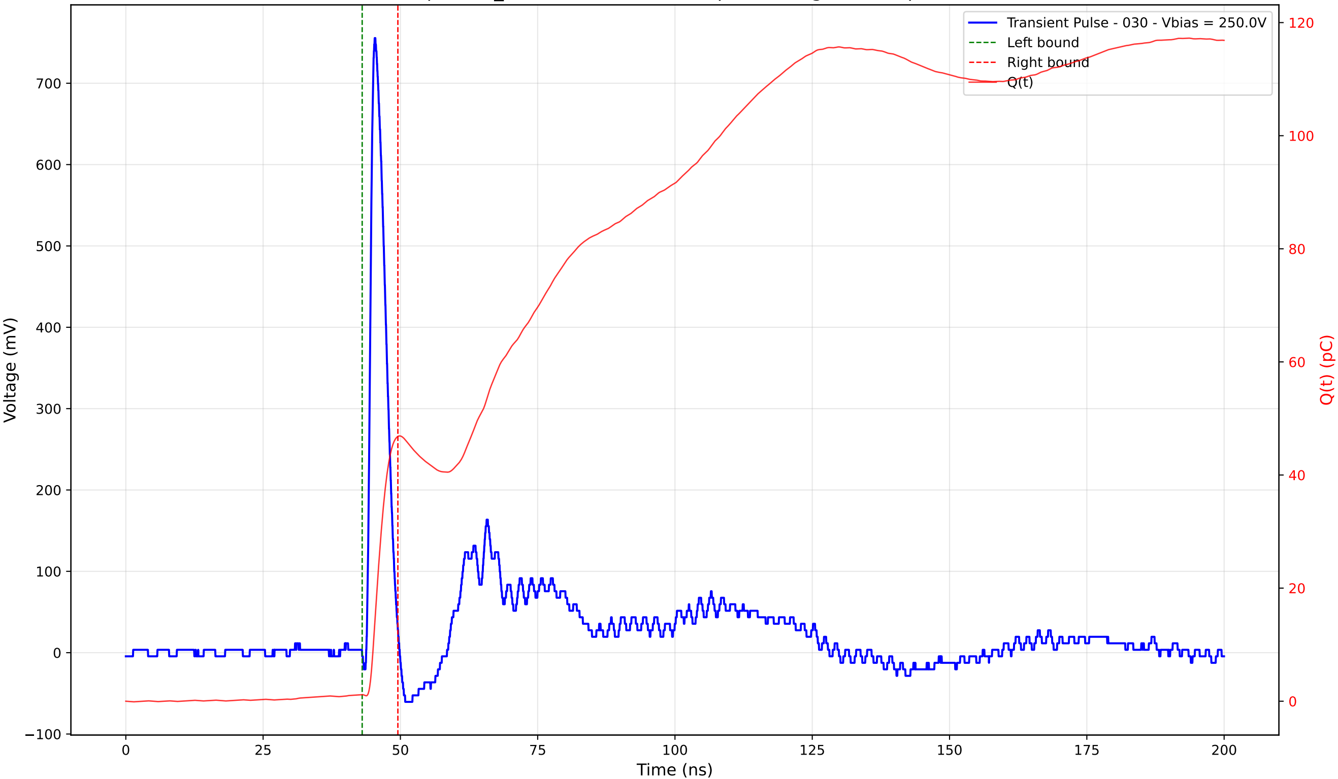
Transient Pulse - Sample: TD_4004 - Position: 145.0 \mu\text{m} - Charge: 45.66 pC - Rise Time: 0.93 ns
