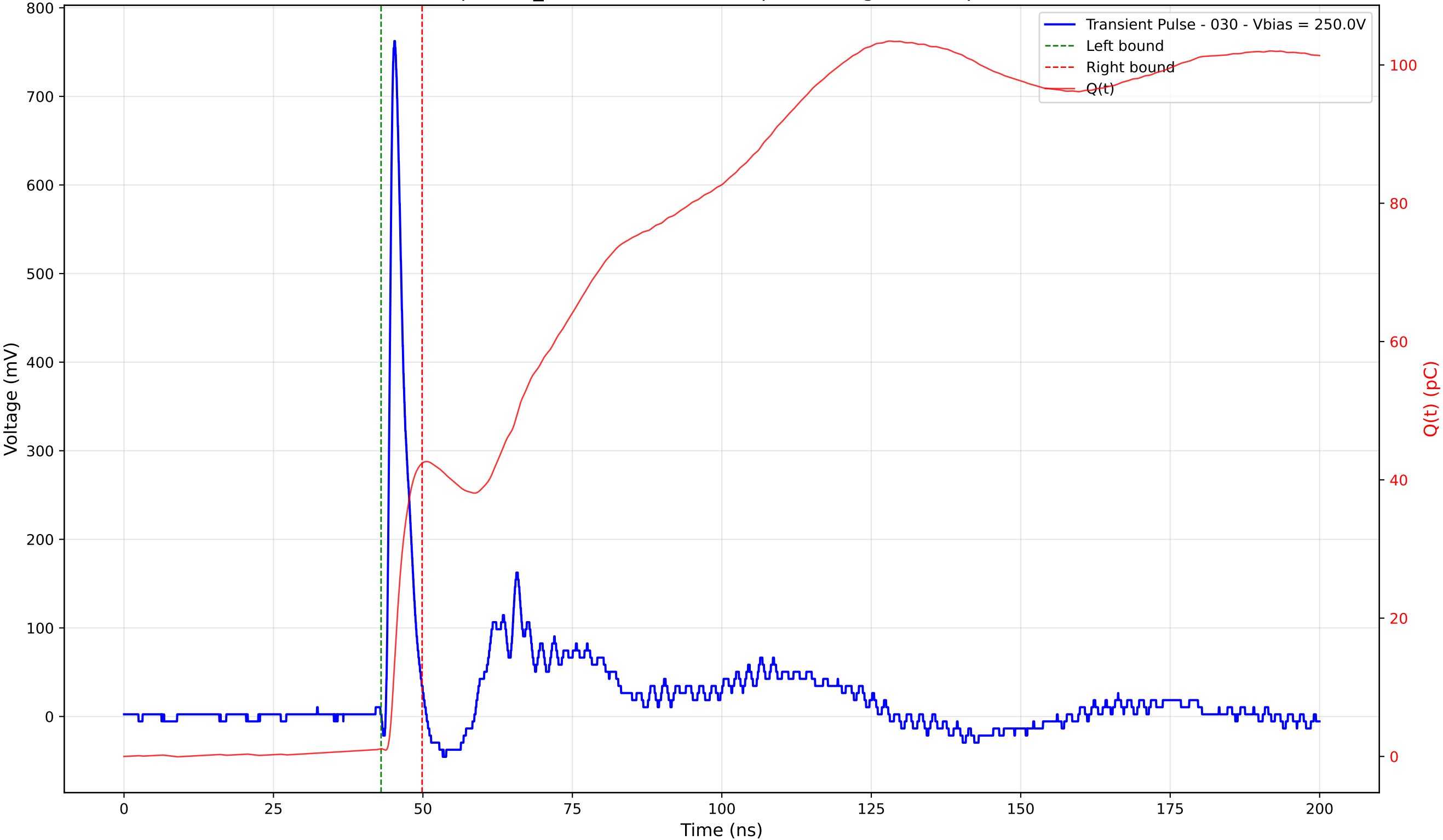
Transient Pulse - Sample: TD_4004 - Position: 95.0 \mu\text{m} - Charge: 41.29 pC - Rise Time: 0.88 ns
