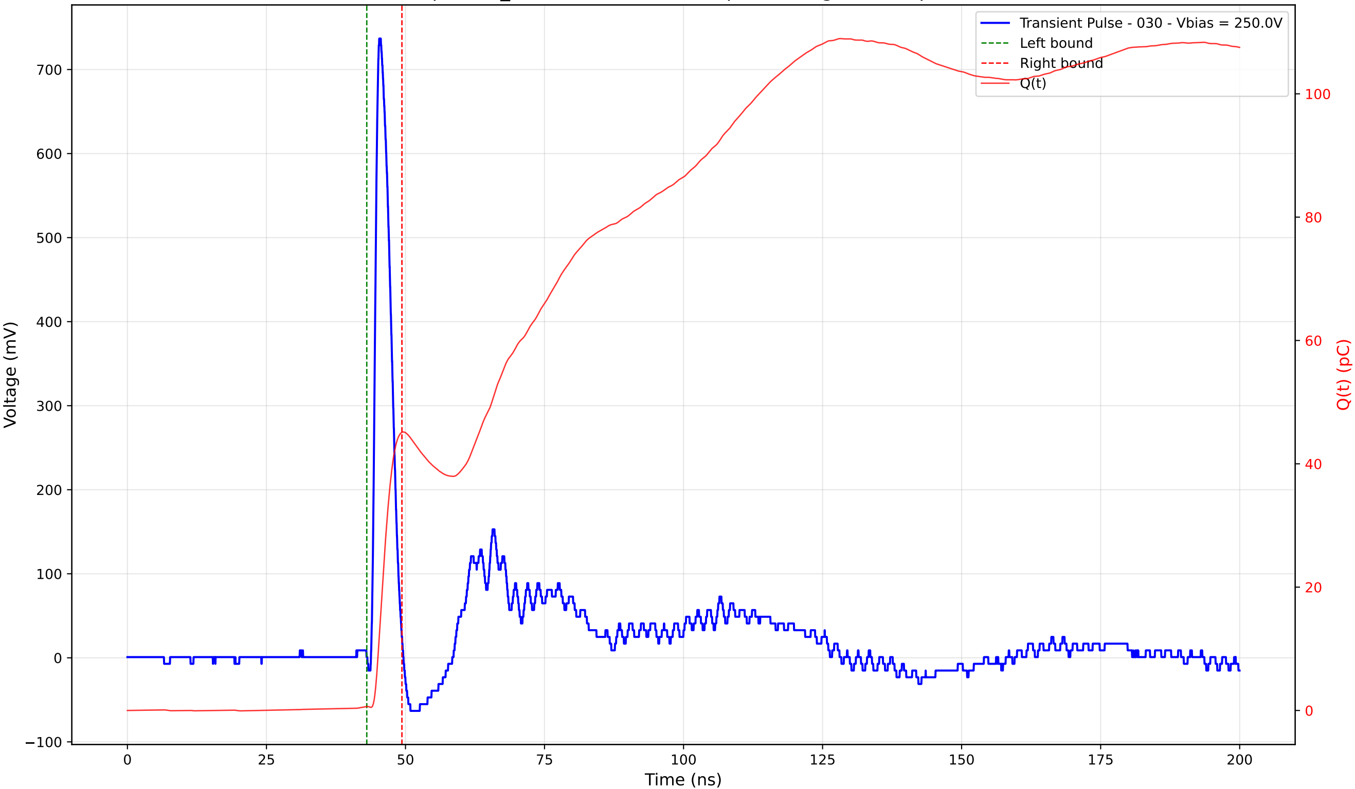
Transient Pulse - Sample: TD_4004 - Position: 255.0 \mu\text{m} - Charge: 44.45 pC - Rise Time: 0.93 ns
