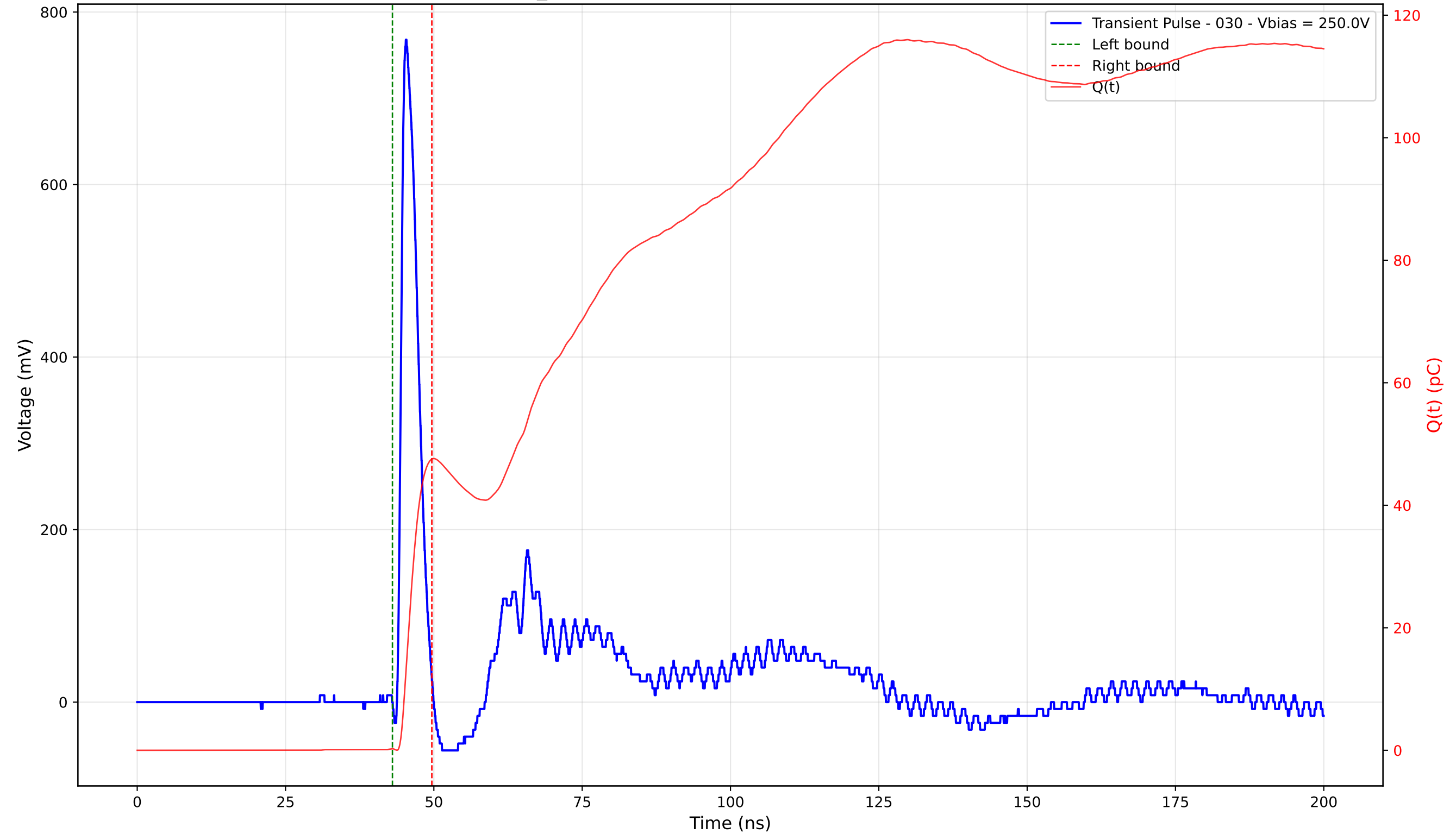
Transient Pulse - Sample: TD_4004 - Position: 220.0 \mu\text{m} - Charge: 47.30 pC - Rise Time: 0.90 ns
