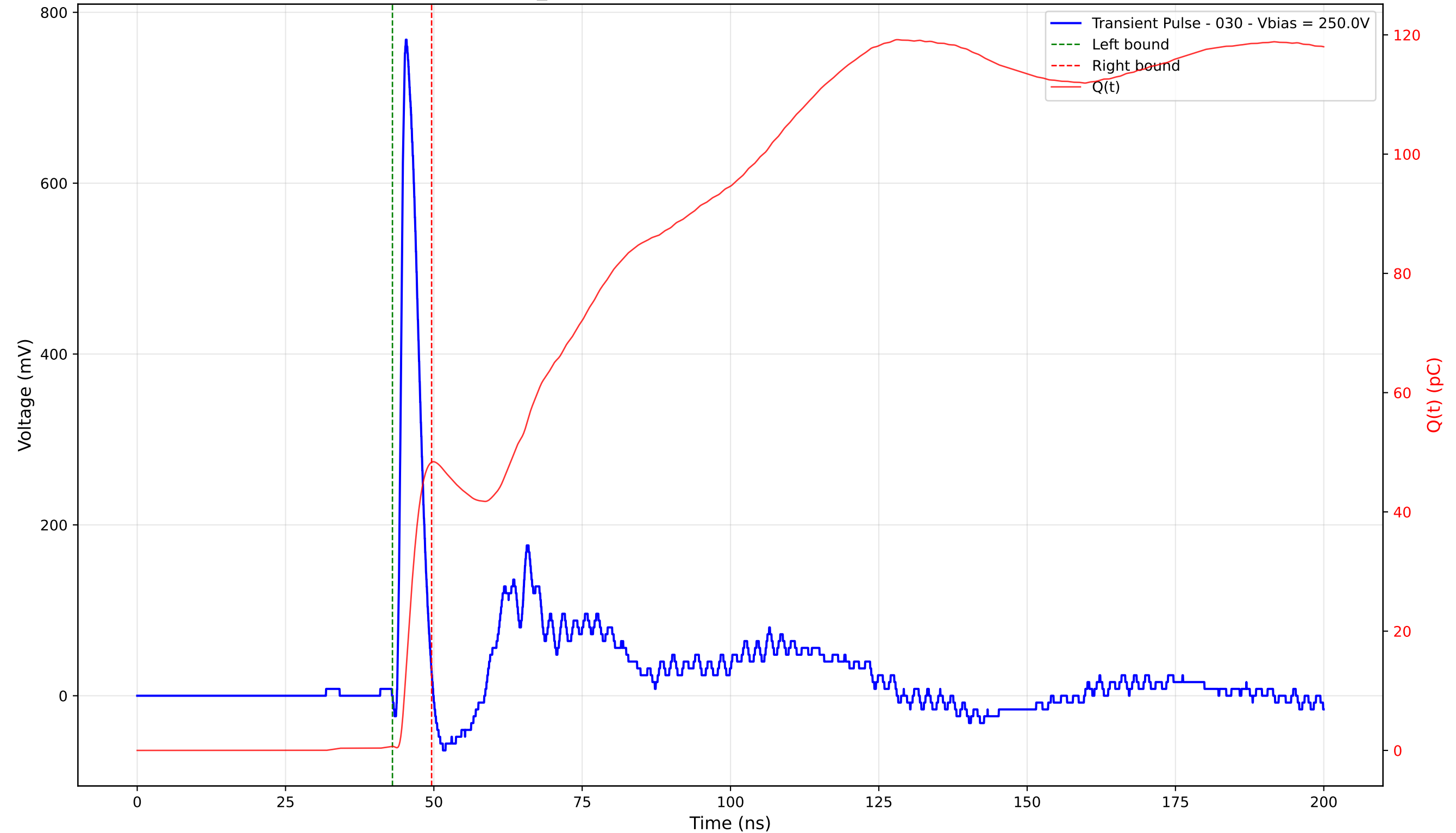
Transient Pulse - Sample: TD_4004 - Position: 165.0 \mu\text{m} - Charge: 47.66 pC - Rise Time: 0.92 ns
