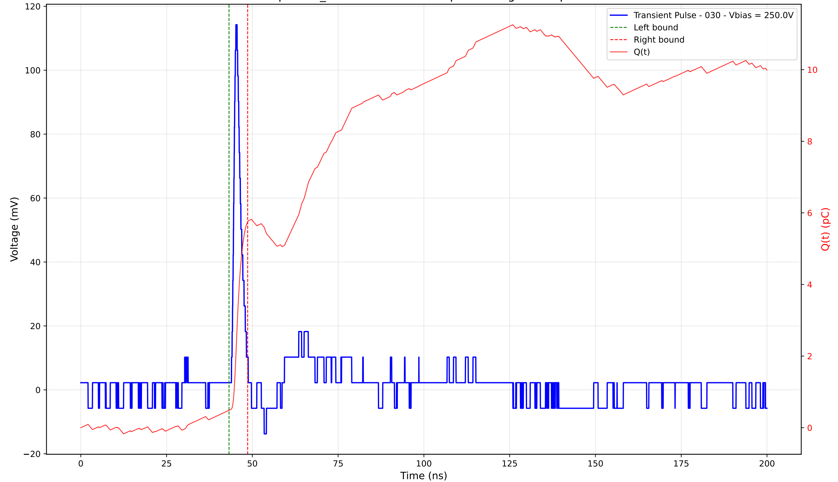
Transient Pulse - Sample: TD_4004 - Position: 50.0 \mu\text{m} - Charge: 5.26 pC - Rise Time: 0.96 ns
