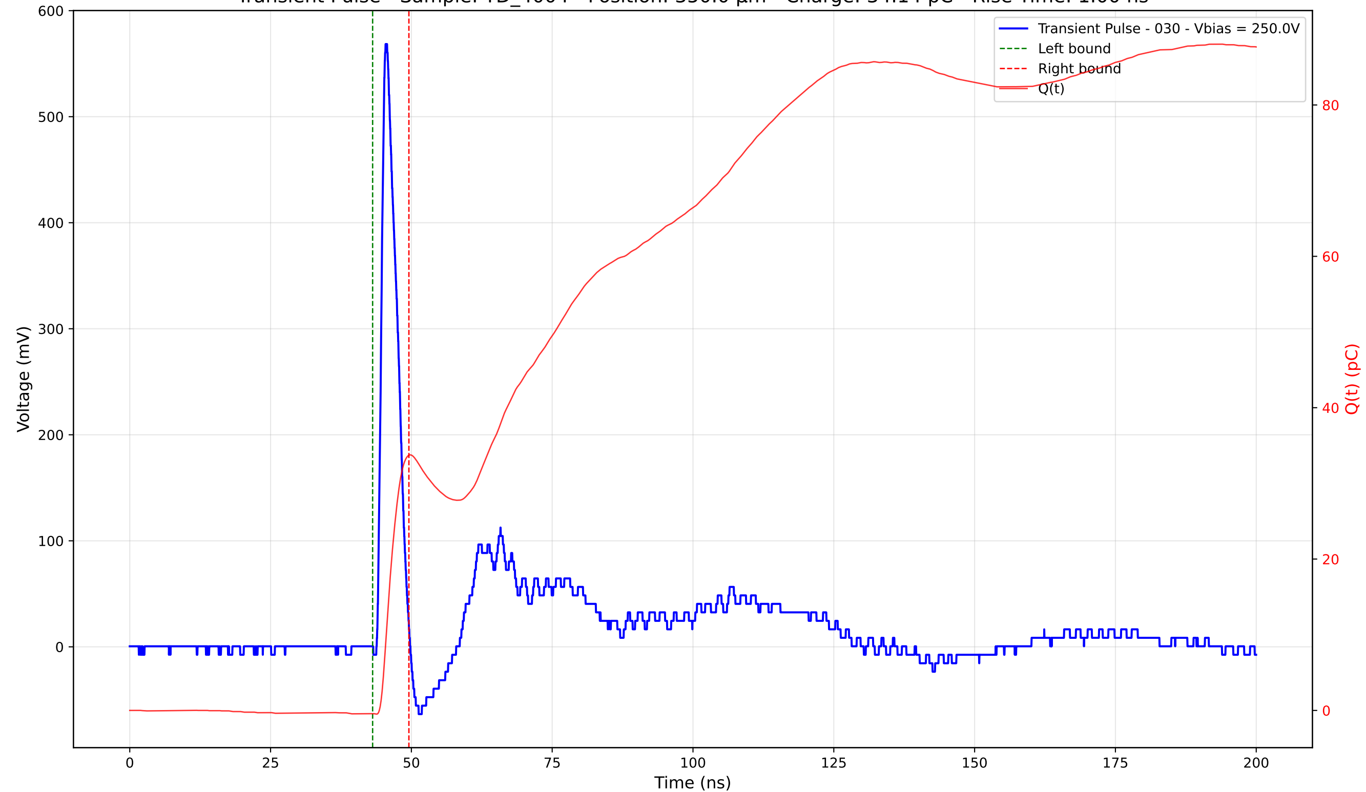
Transient Pulse - Sample: TD_4004 - Position: 350.0 \mu\text{m} - Charge: 34.14 pC - Rise Time: 1.00 ns
