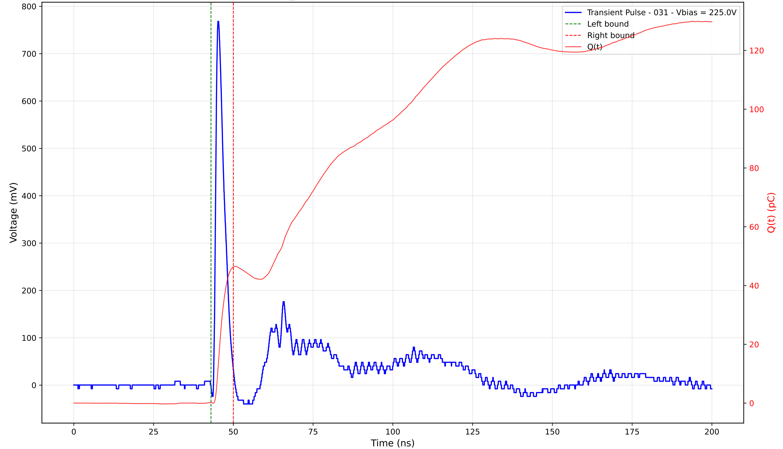
Transient Pulse - Sample: TD_4004 - Position: 115.0 \mu\text{m} - Charge: 46.11 pC - Rise Time: 0.88 ns
