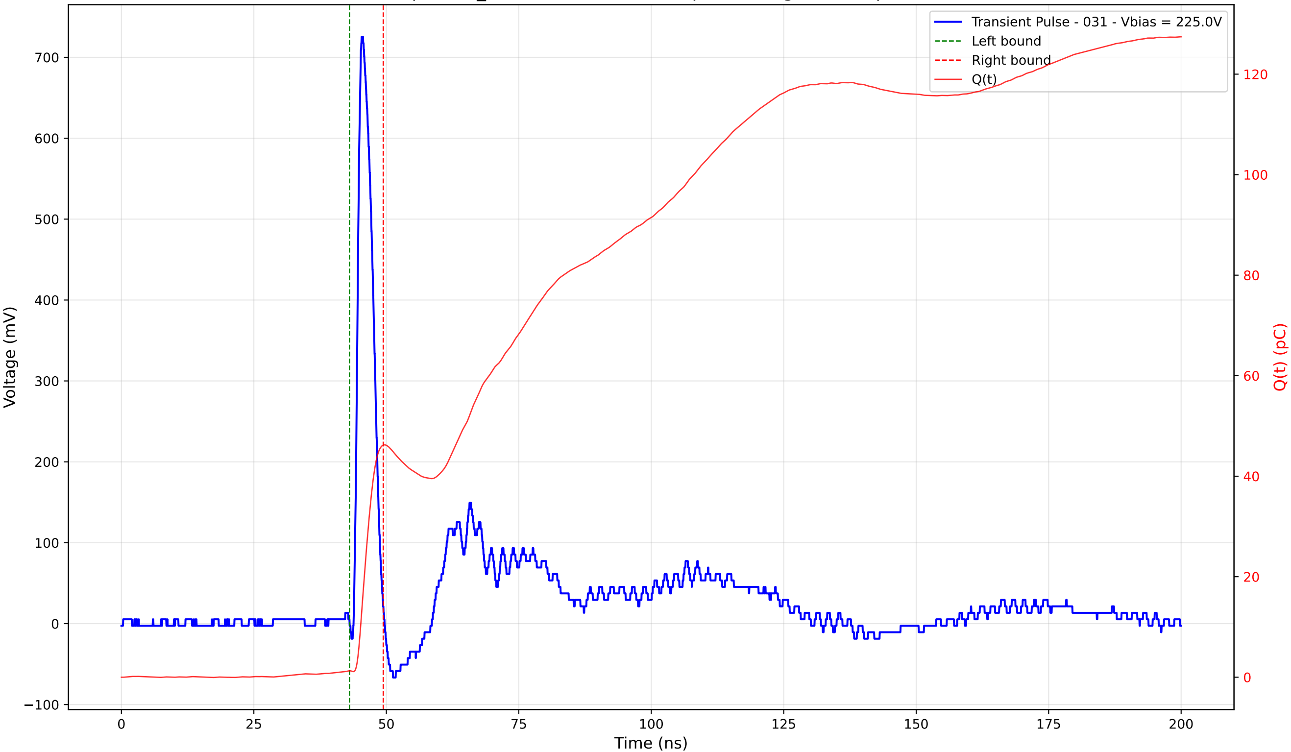
Transient Pulse - Sample: TD_4004 - Position: 285.0 \mu\text{m} - Charge: 44.91 pC - Rise Time: 0.97 ns
