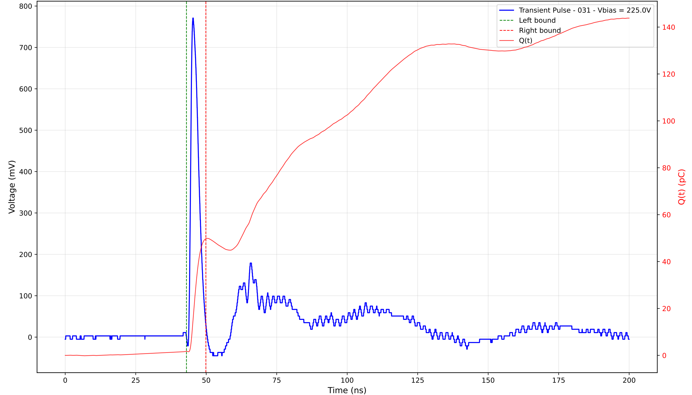
Transient Pulse - Sample: TD_4004 - Position: 200.0 \mu\text{m} - Charge: 48.03 pC - Rise Time: 0.92 ns
