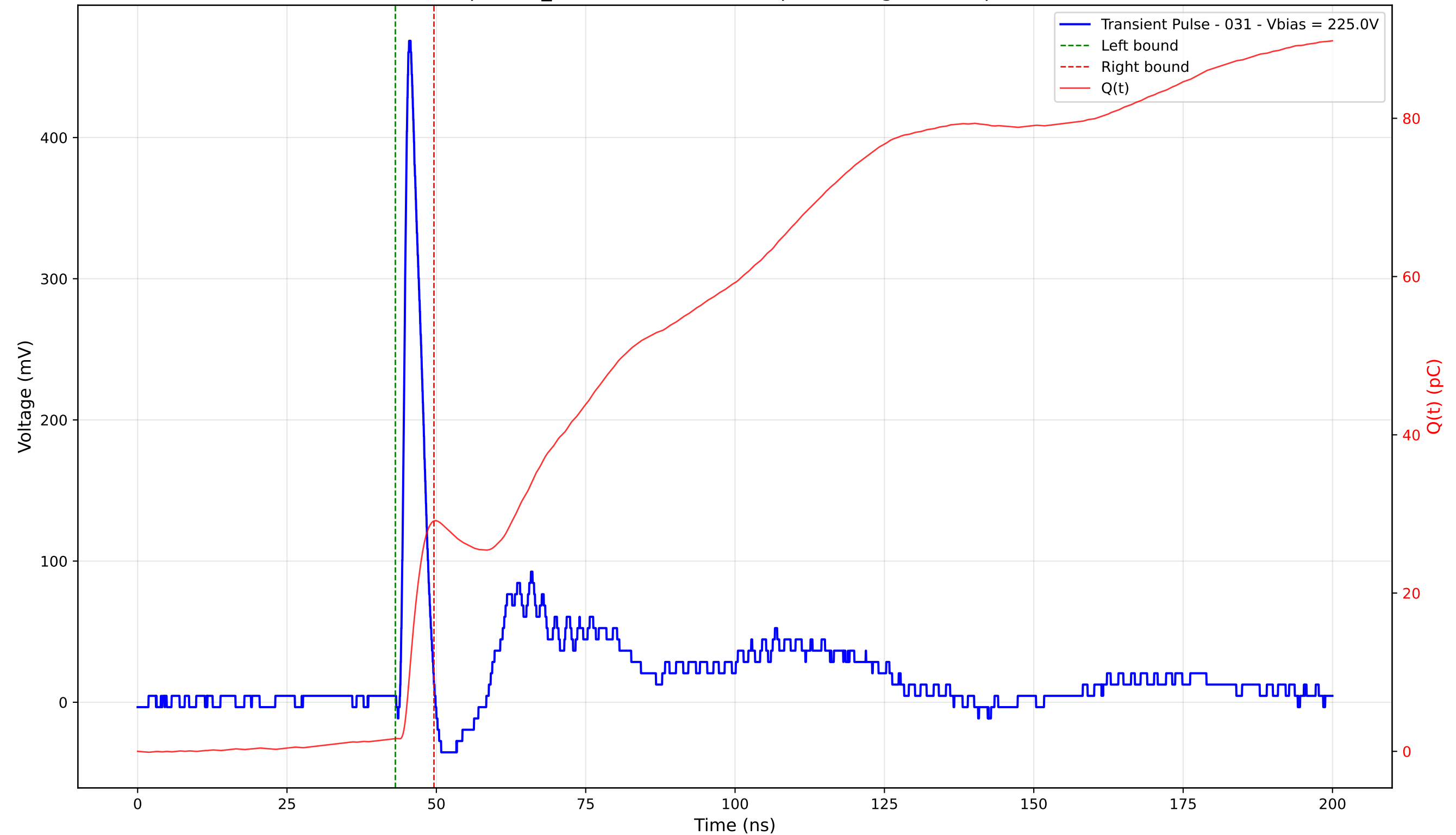
Transient Pulse - Sample: TD_4004 - Position: 375.0 \mu\text{m} - Charge: 27.50 pC - Rise Time: 1.03 ns
