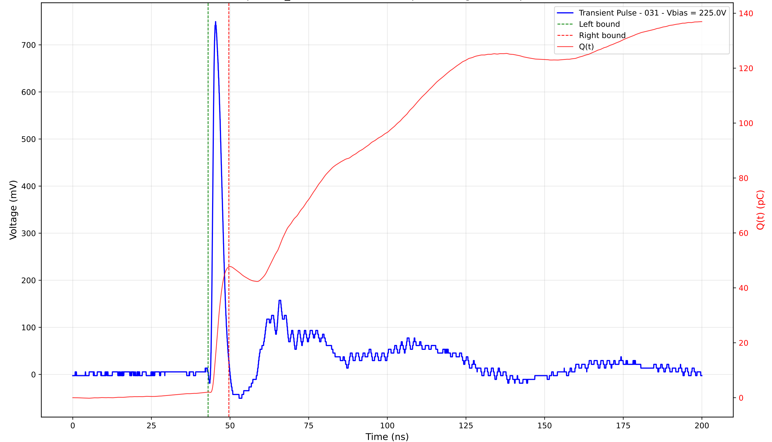
Transient Pulse - Sample: TD_4004 - Position: 230.0 \mu\text{m} - Charge: 45.59 pC - Rise Time: 0.94 ns
