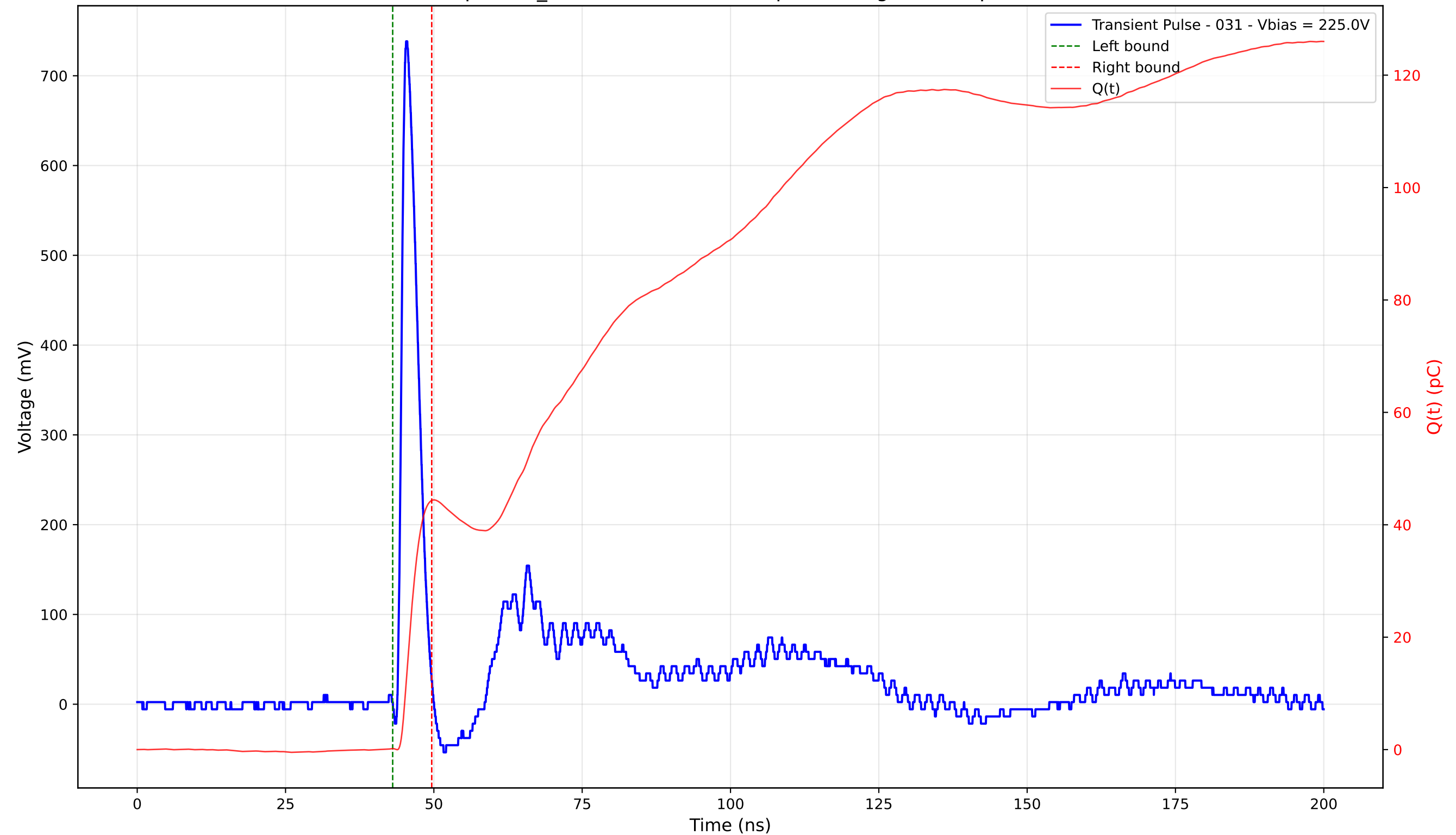
Transient Pulse - Sample: TD_4004 - Position: 150.0 \mu\text{m} - Charge: 44.16 pC - Rise Time: 0.94 ns
