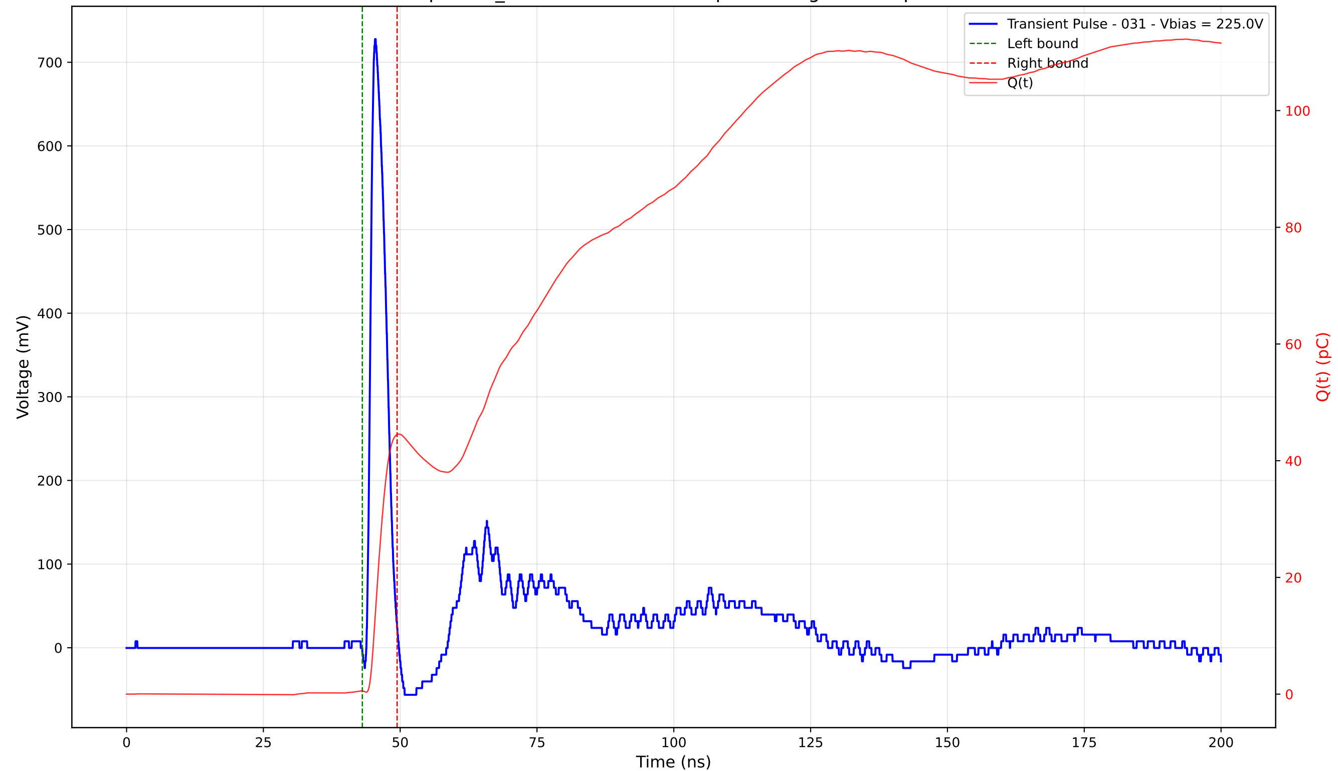
Transient Pulse - Sample: TD_4004 - Position: 275.0 \mu\text{m} - Charge: 43.95 pC - Rise Time: 0.96 ns
