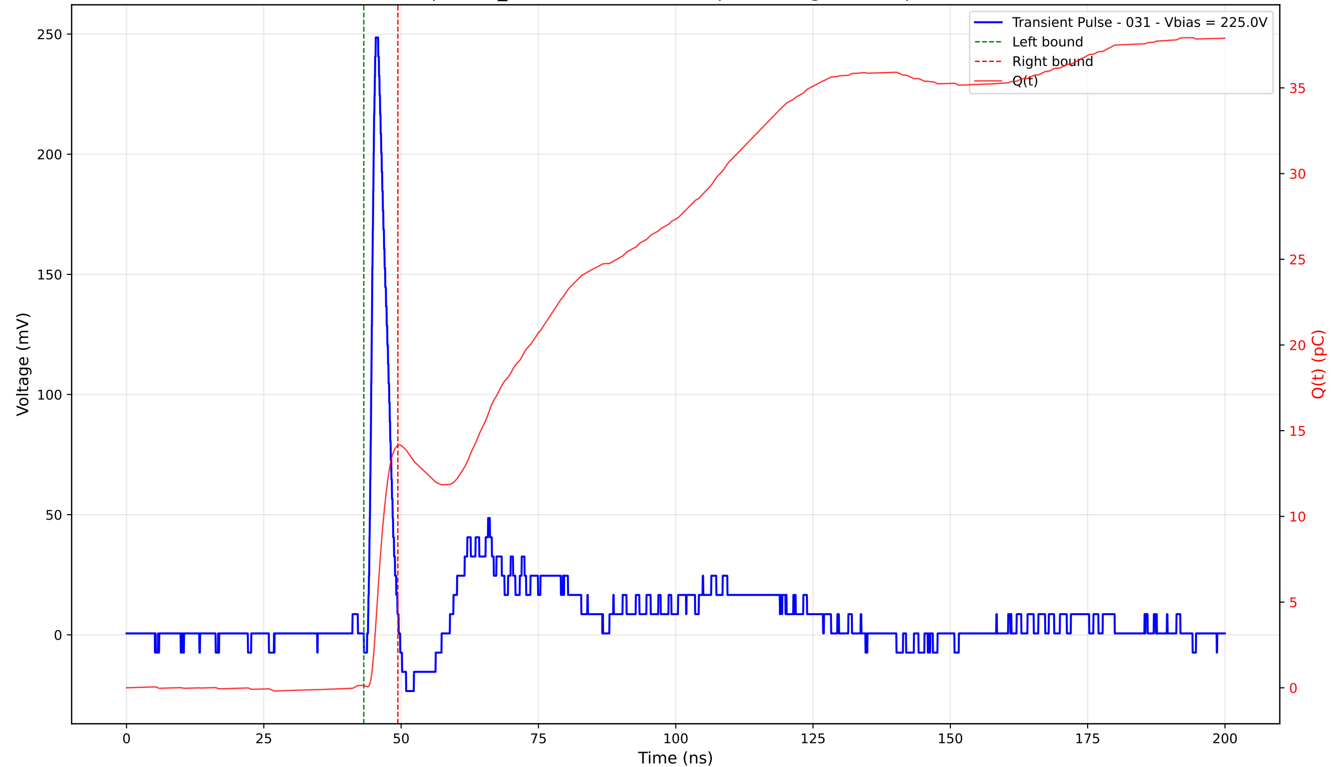
Transient Pulse - Sample: TD_4004 - Position: 400.0 \mu\text{m} - Charge: 13.99 pC - Rise Time: 0.96 ns
