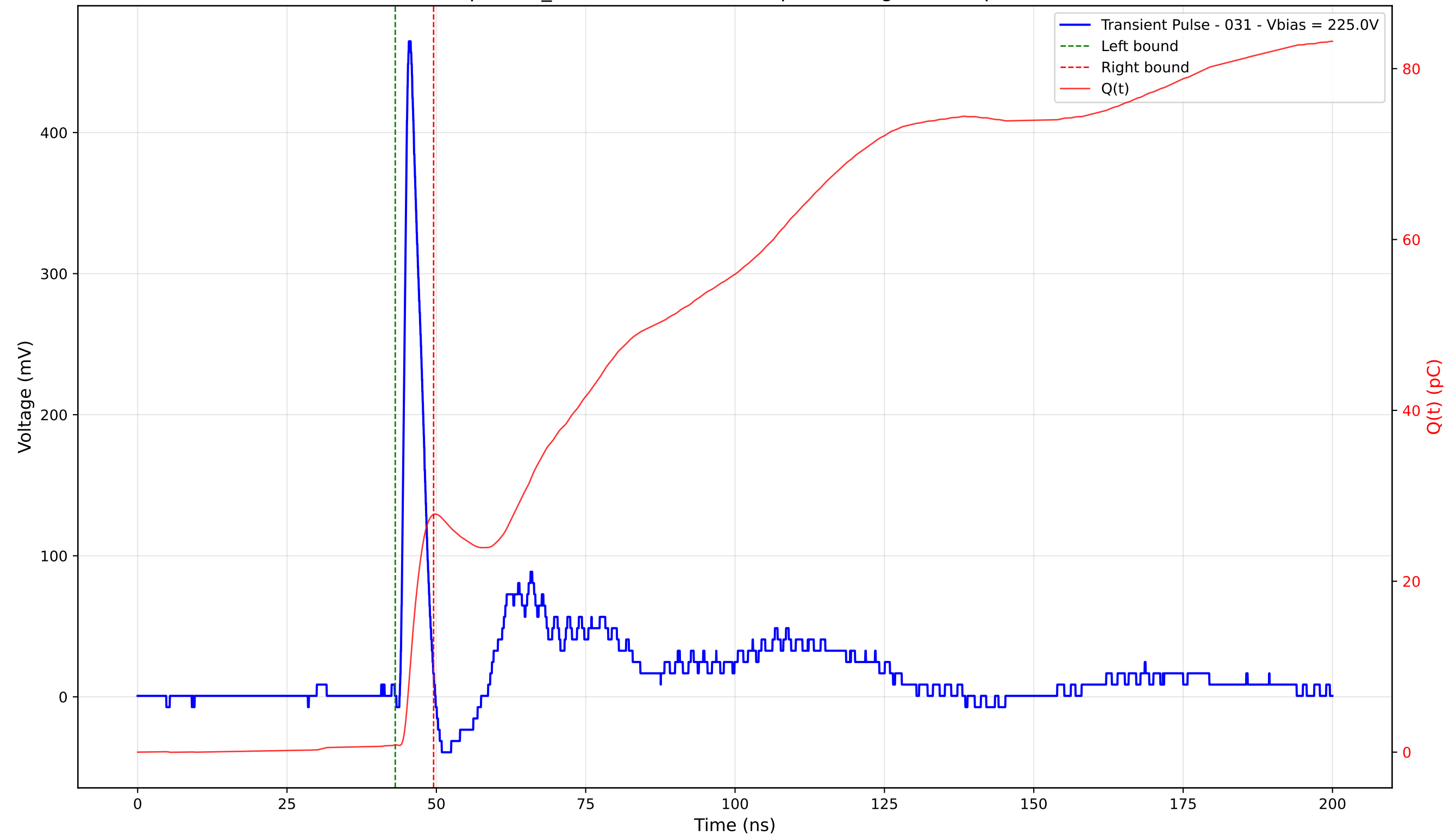
Transient Pulse - Sample: TD_4004 - Position: 380.0 \mu\text{m} - Charge: 26.97 pC - Rise Time: 1.03 ns
