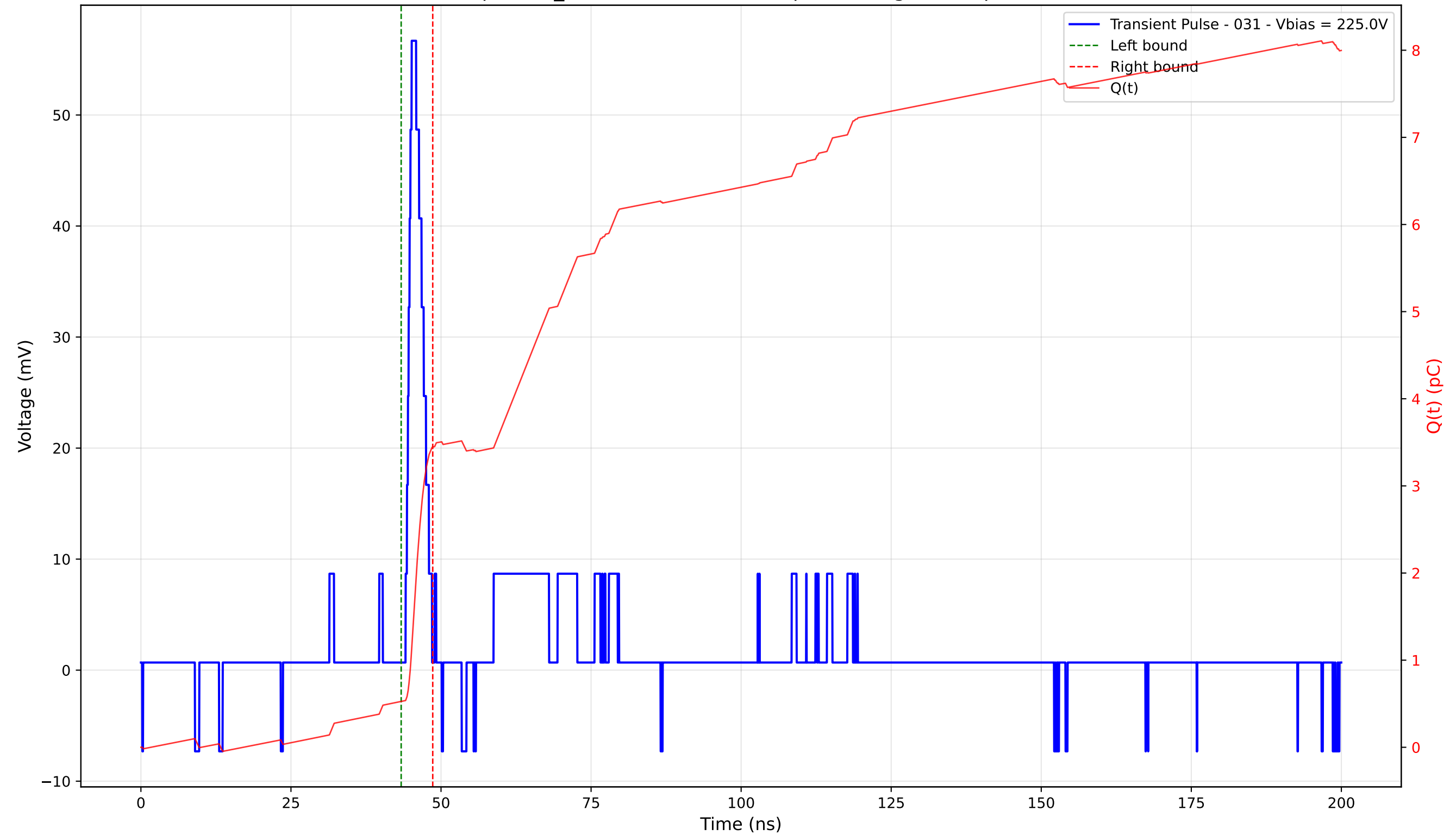
Transient Pulse - Sample: TD_4004 - Position: 430.0 \mu\text{m} - Charge: 2.92 pC - Rise Time: 1.01 ns
