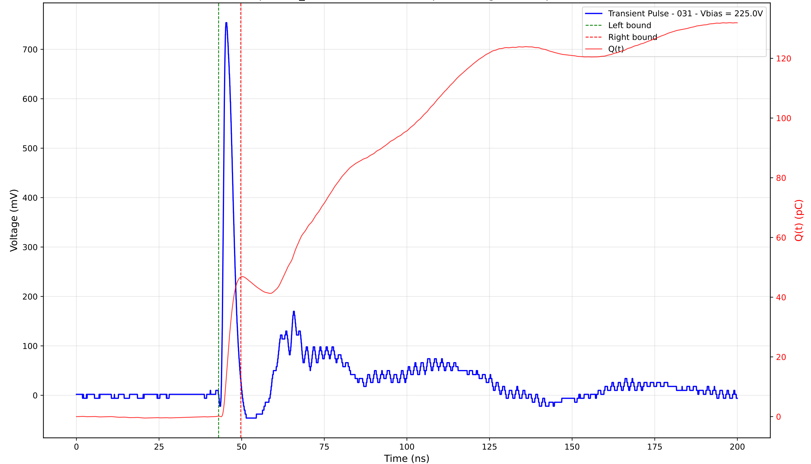
Transient Pulse - Sample: TD_4004 - Position: 220.0 \mu\text{m} - Charge: 46.59 pC - Rise Time: 0.92 ns
