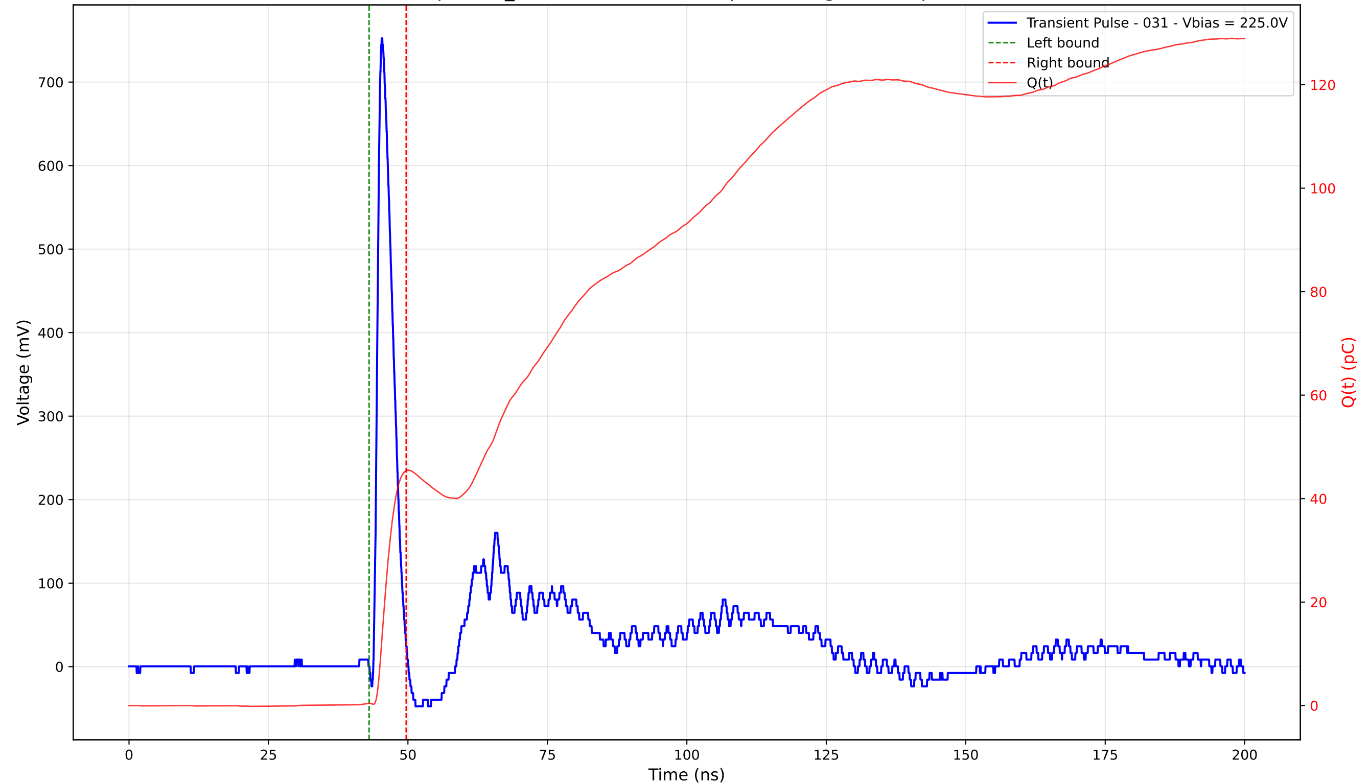
Transient Pulse - Sample: TD_4004 - Position: 130.0 \mu\text{m} - Charge: 44.97 pC - Rise Time: 0.92 ns
