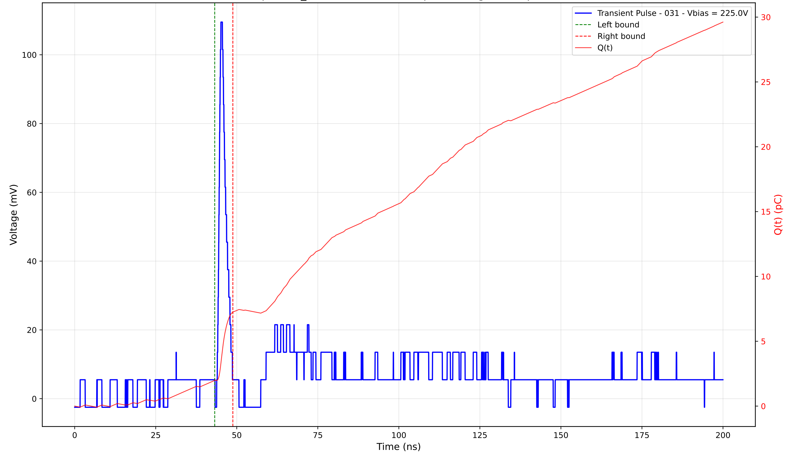
Transient Pulse - Sample: TD_4004 - Position: 50.0 \mu\text{m} - Charge: 5.26 pC - Rise Time: 0.97 ns
