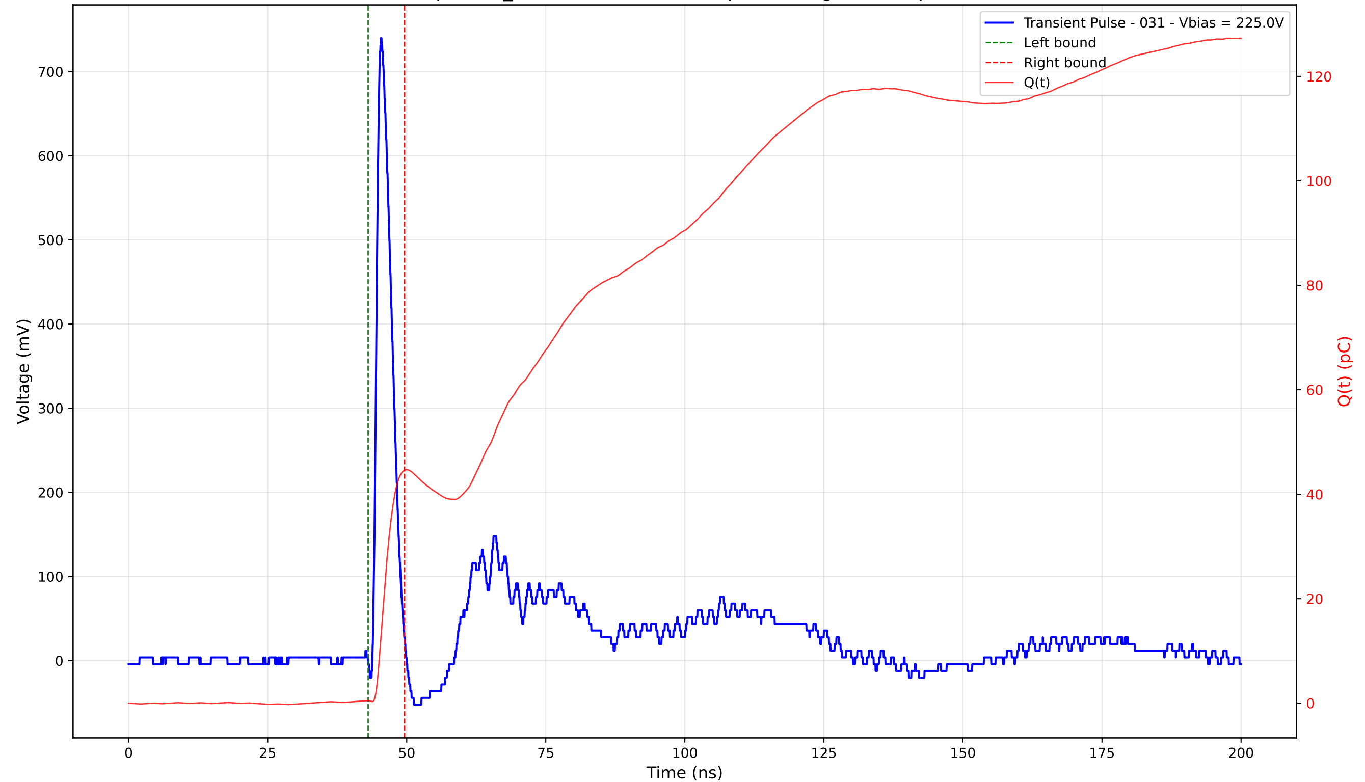
Transient Pulse - Sample: TD_4004 - Position: 140.0 \mu\text{m} - Charge: 44.12 pC - Rise Time: 0.94 ns
