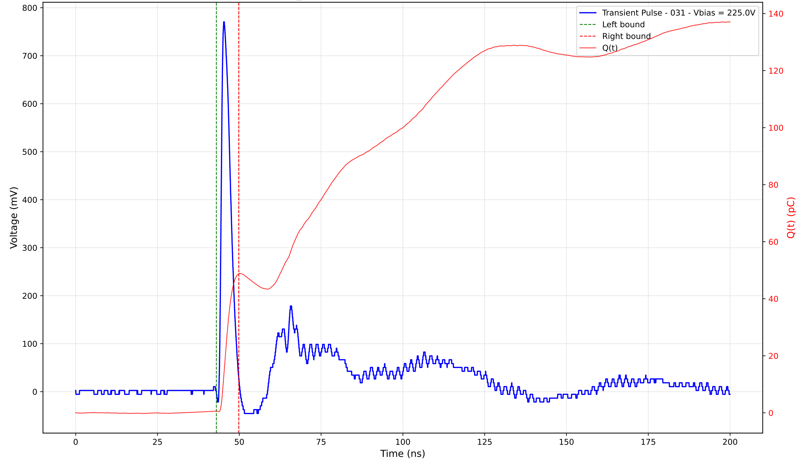
Transient Pulse - Sample: TD_4004 - Position: 175.0 \mu\text{m} - Charge: 48.14 pC - Rise Time: 0.91 ns
