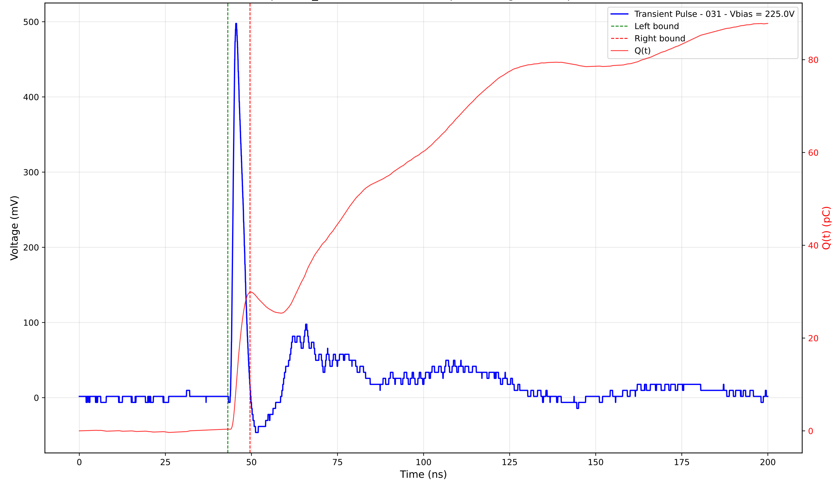
Transient Pulse - Sample: TD_4004 - Position: 360.0 \mu\text{m} - Charge: 29.49 pC - Rise Time: 1.02 ns
