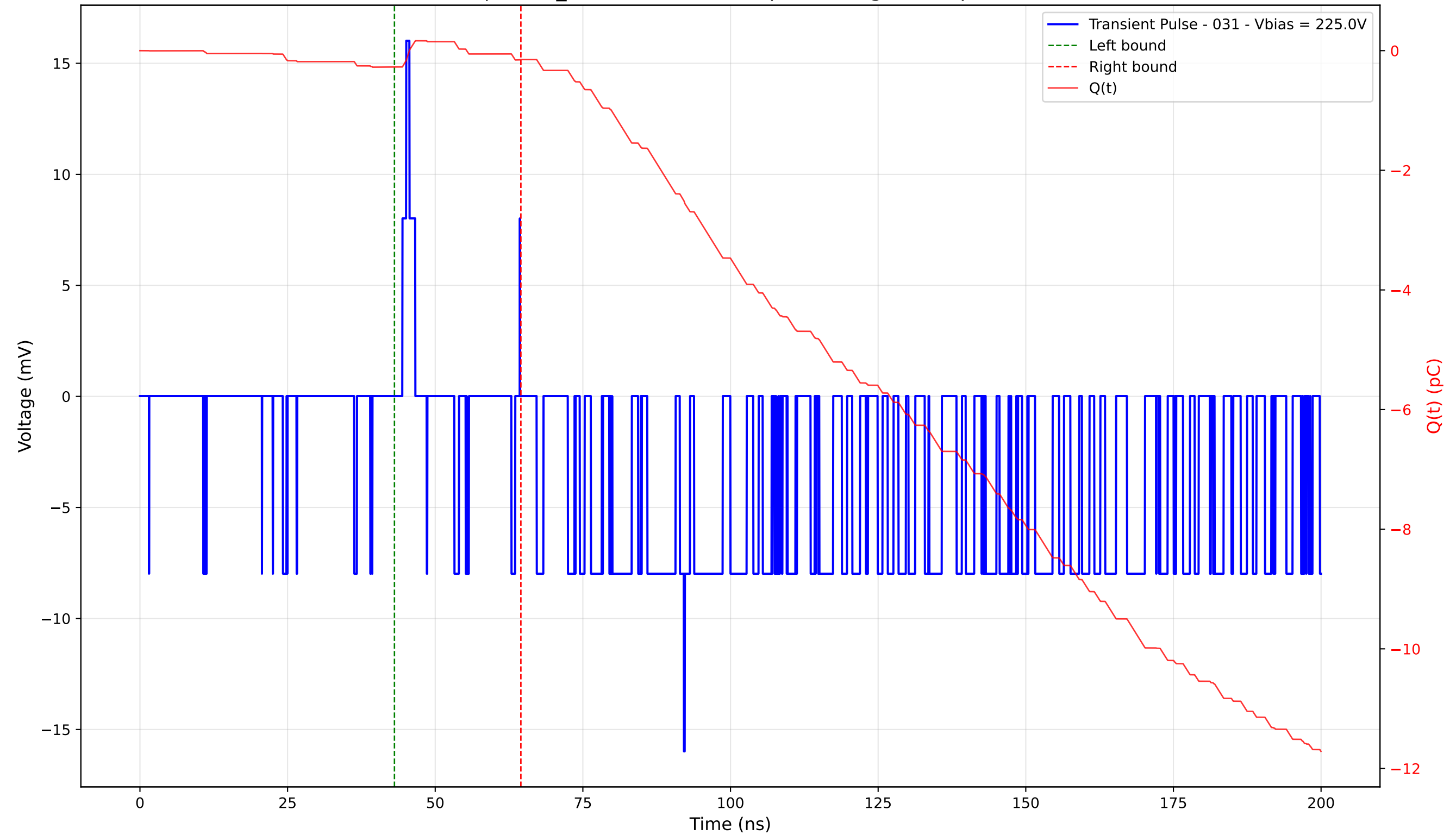
Transient Pulse - Sample: TD_4004 - Position: 5.0 \mu\text{m} - Charge: 0.13 pC - Rise Time: 0.66 ns
