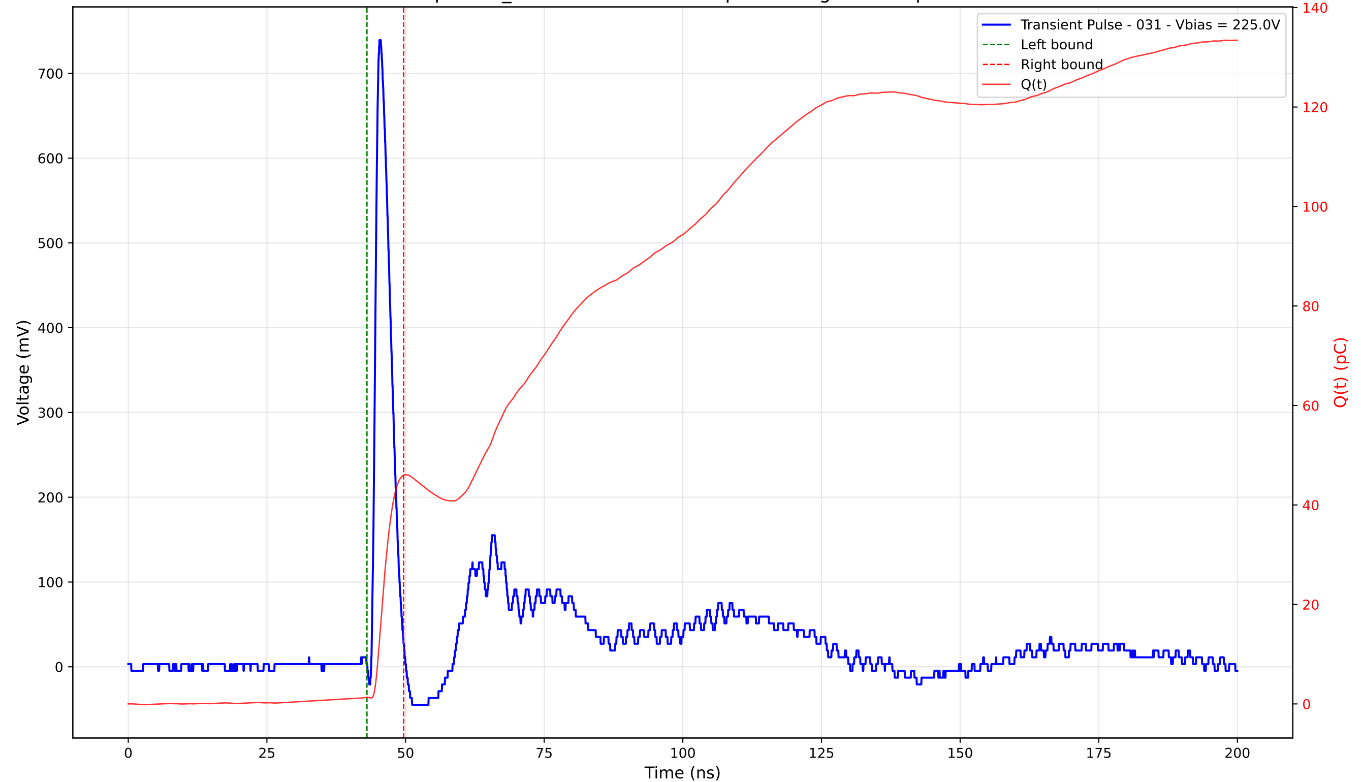
Transient Pulse - Sample: TD_4004 - Position: 155.0 \mu\text{m} - Charge: 44.64 pC - Rise Time: 0.94 ns
