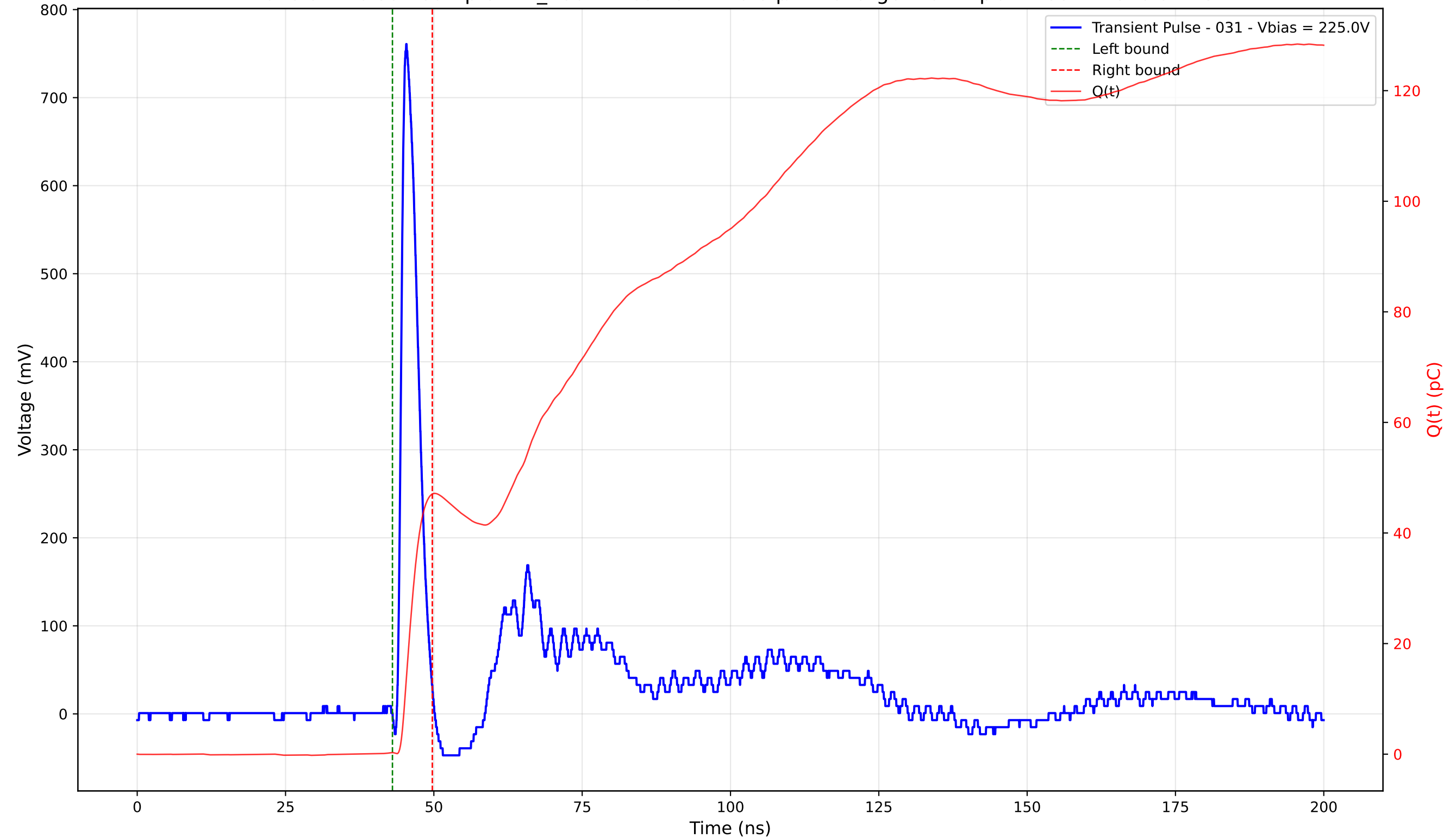
Transient Pulse - Sample: TD_4004 - Position: 210.0 \mu\text{m} - Charge: 46.77 pC - Rise Time: 0.92 ns
