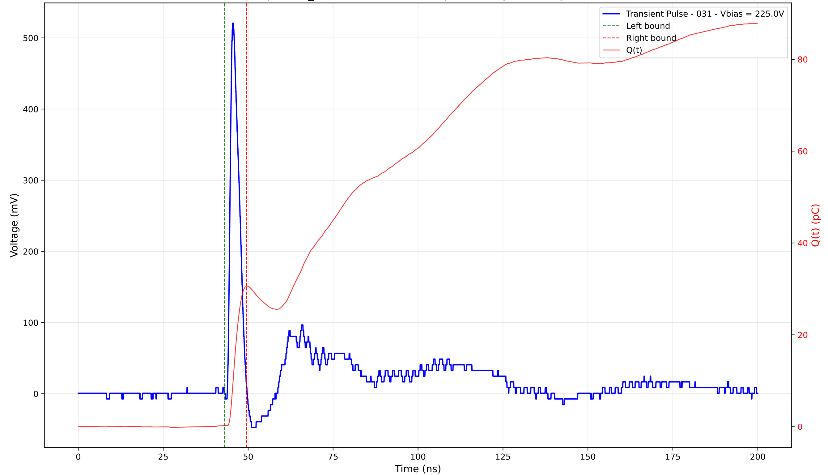
Transient Pulse - Sample: TD_4004 - Position: 340.0 \mu\text{m} - Charge: 30.32 pC - Rise Time: 1.01 ns
