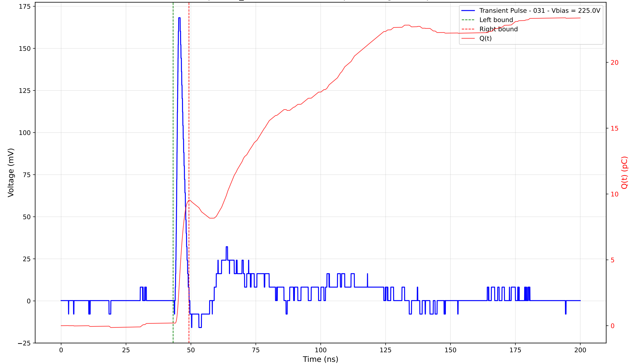
Transient Pulse - Sample: TD_4004 - Position: 410.0 \mu\text{m} - Charge: 9.32 pC - Rise Time: 0.92 ns
