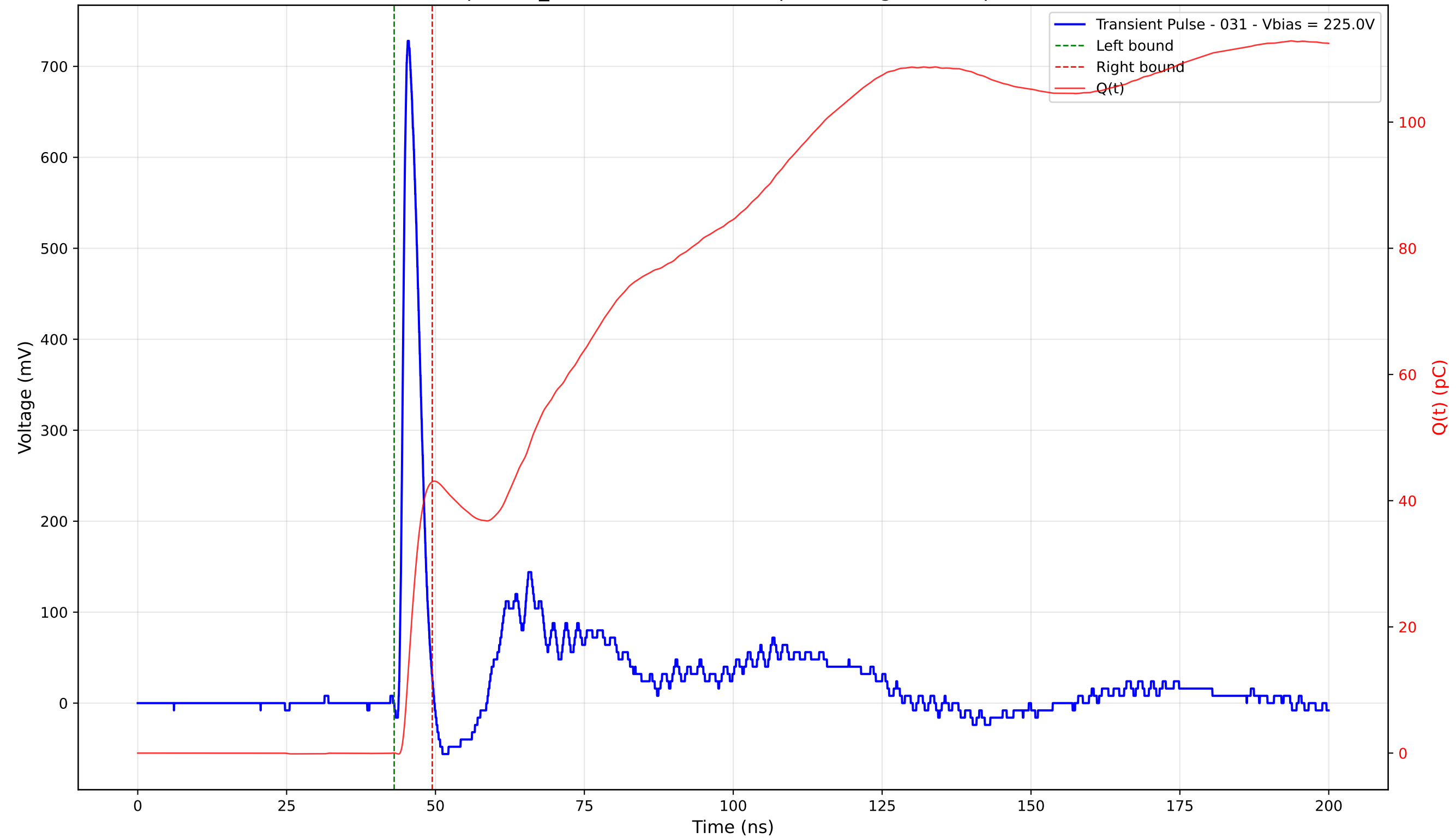
Transient Pulse - Sample: TD_4004 - Position: 240.0 \mu\text{m} - Charge: 42.99 pC - Rise Time: 0.96 ns
