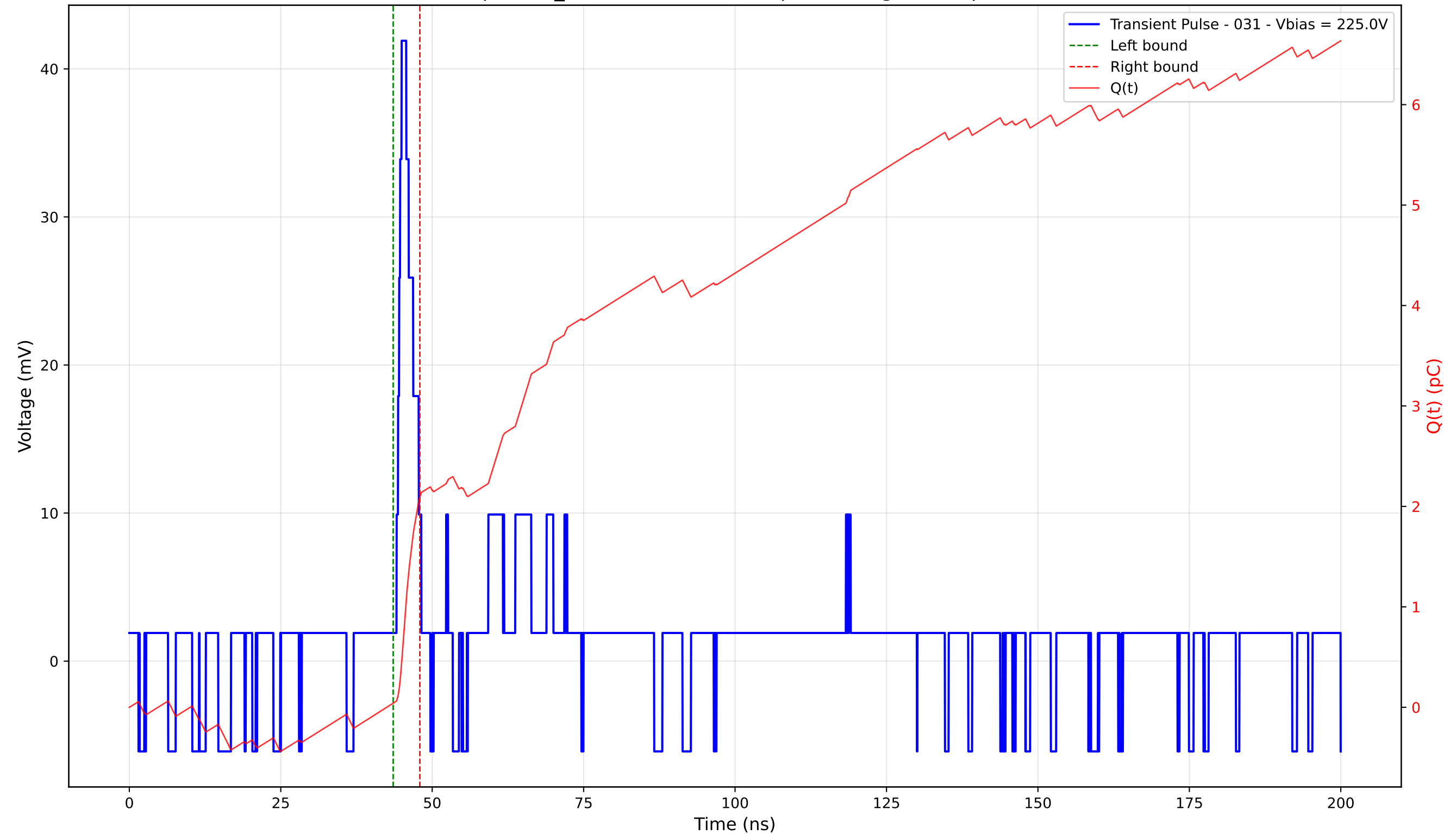
Transient Pulse - Sample: TD_4004 - Position: 40.0 \mu\text{m} - Charge: 2.05 pC - Rise Time: 0.83 ns
