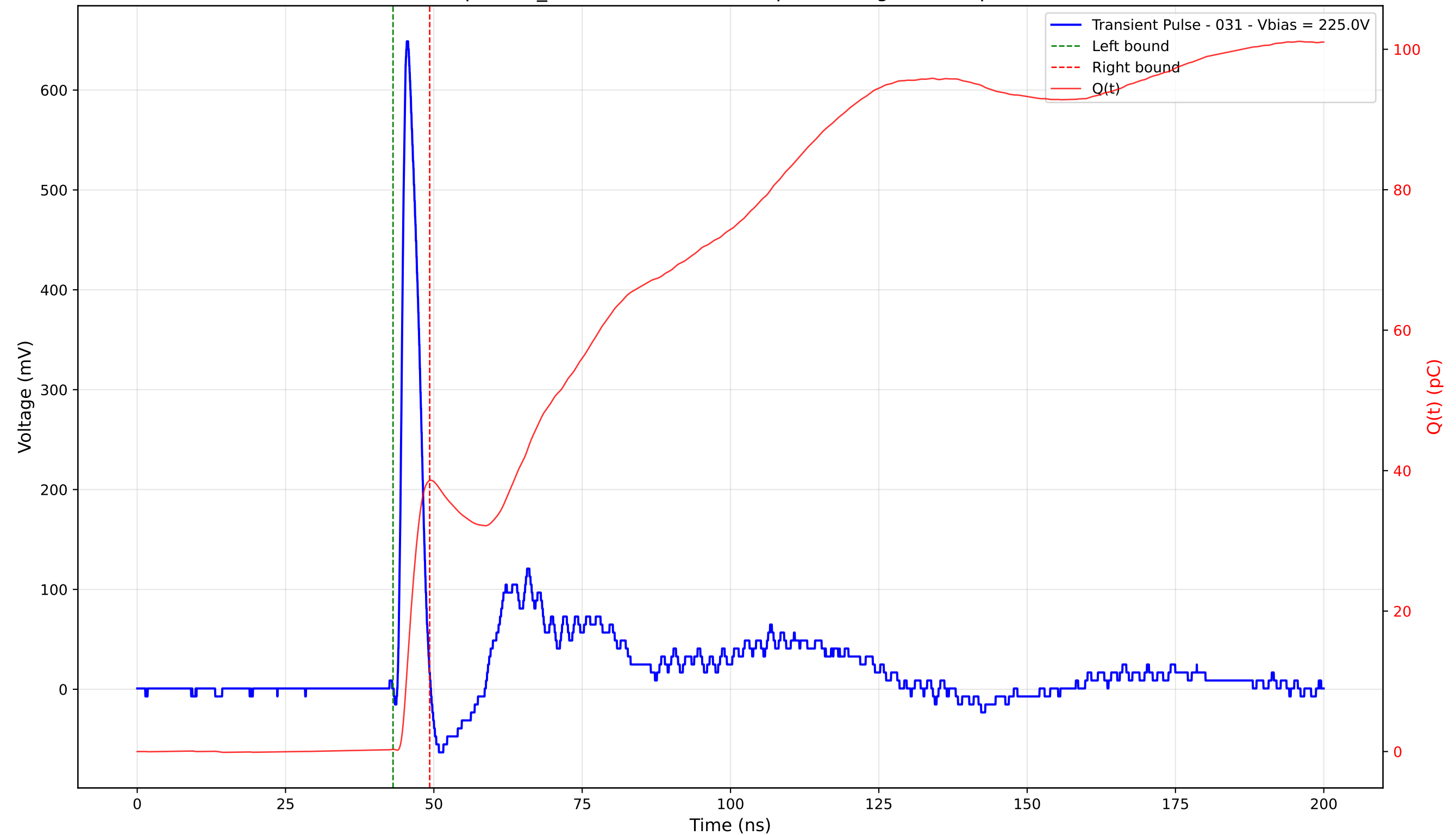
Transient Pulse - Sample: TD_4004 - Position: 315.0 \mu\text{m} - Charge: 38.29 pC - Rise Time: 1.00 ns
