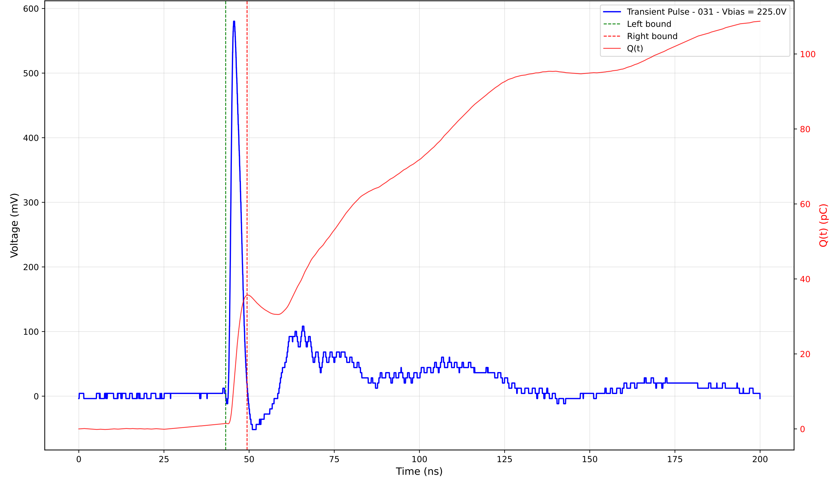
Transient Pulse - Sample: TD_4004 - Position: 330.0 \mu\text{m} - Charge: 34.17 pC - Rise Time: 1.02 ns
