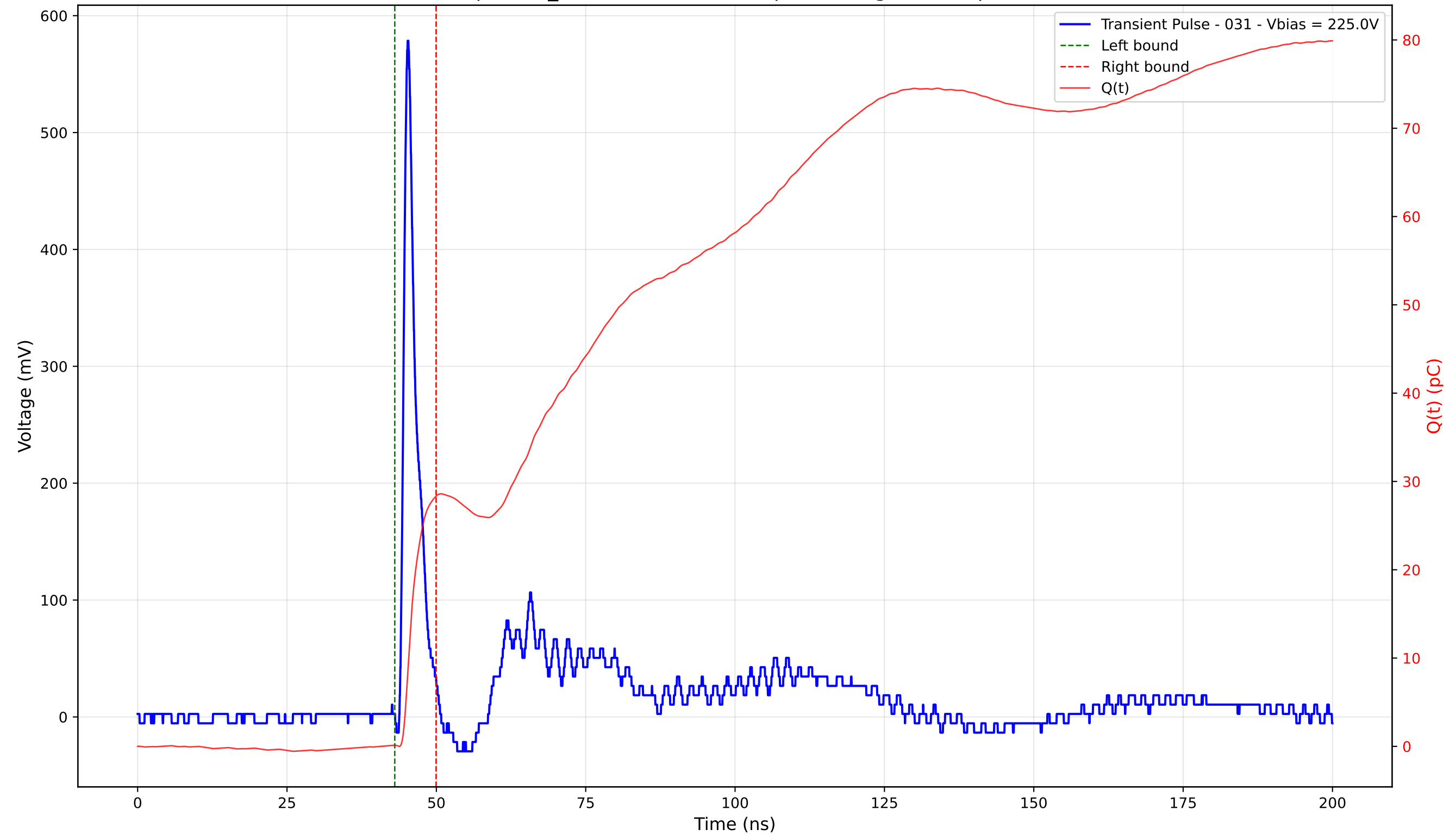
Transient Pulse - Sample: TD_4004 - Position: 75.0 \mu\text{m} - Charge: 28.22 pC - Rise Time: 0.90 ns
