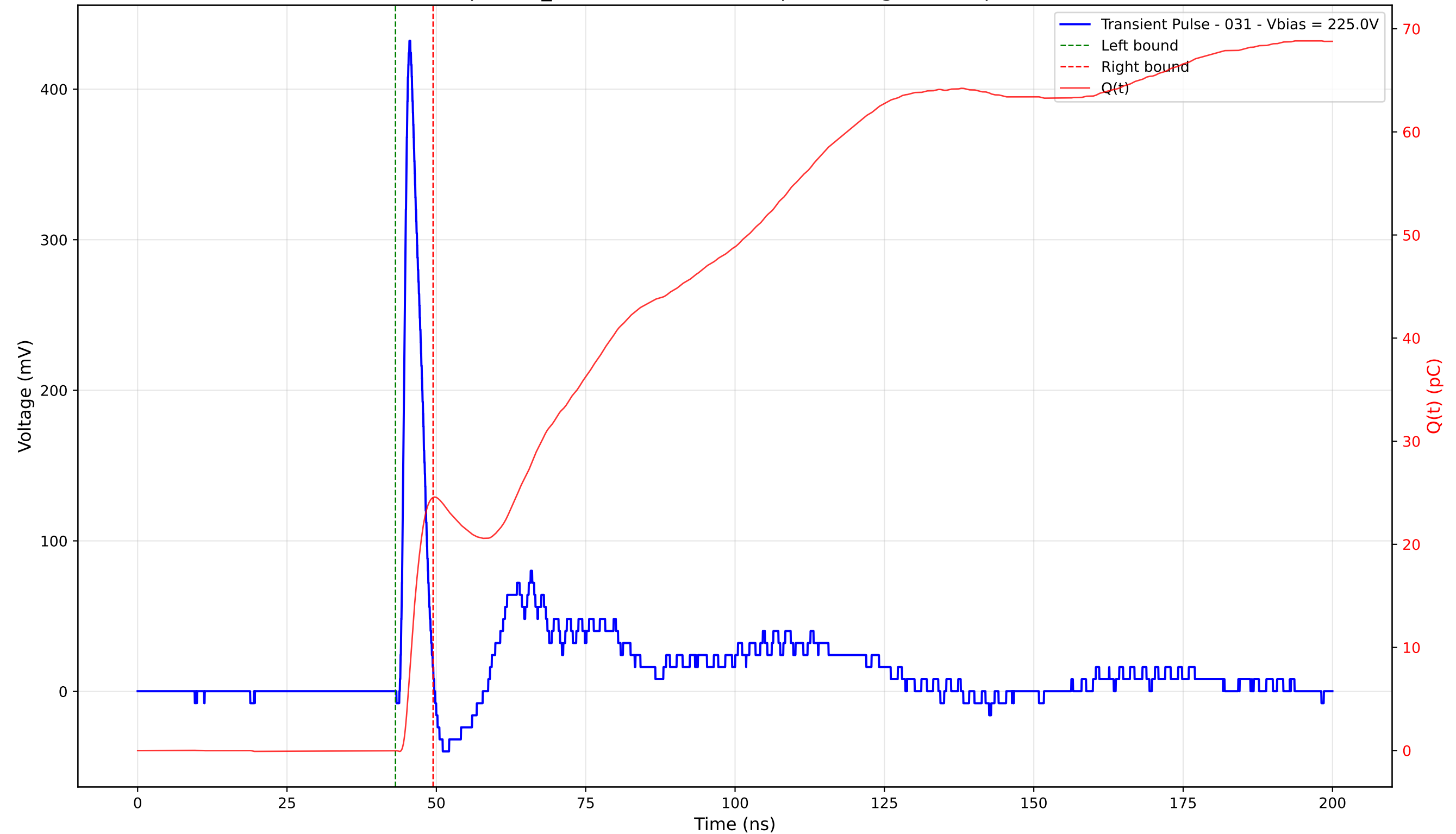
Transient Pulse - Sample: TD_4004 - Position: 385.0 \mu\text{m} - Charge: 24.56 pC - Rise Time: 1.03 ns
