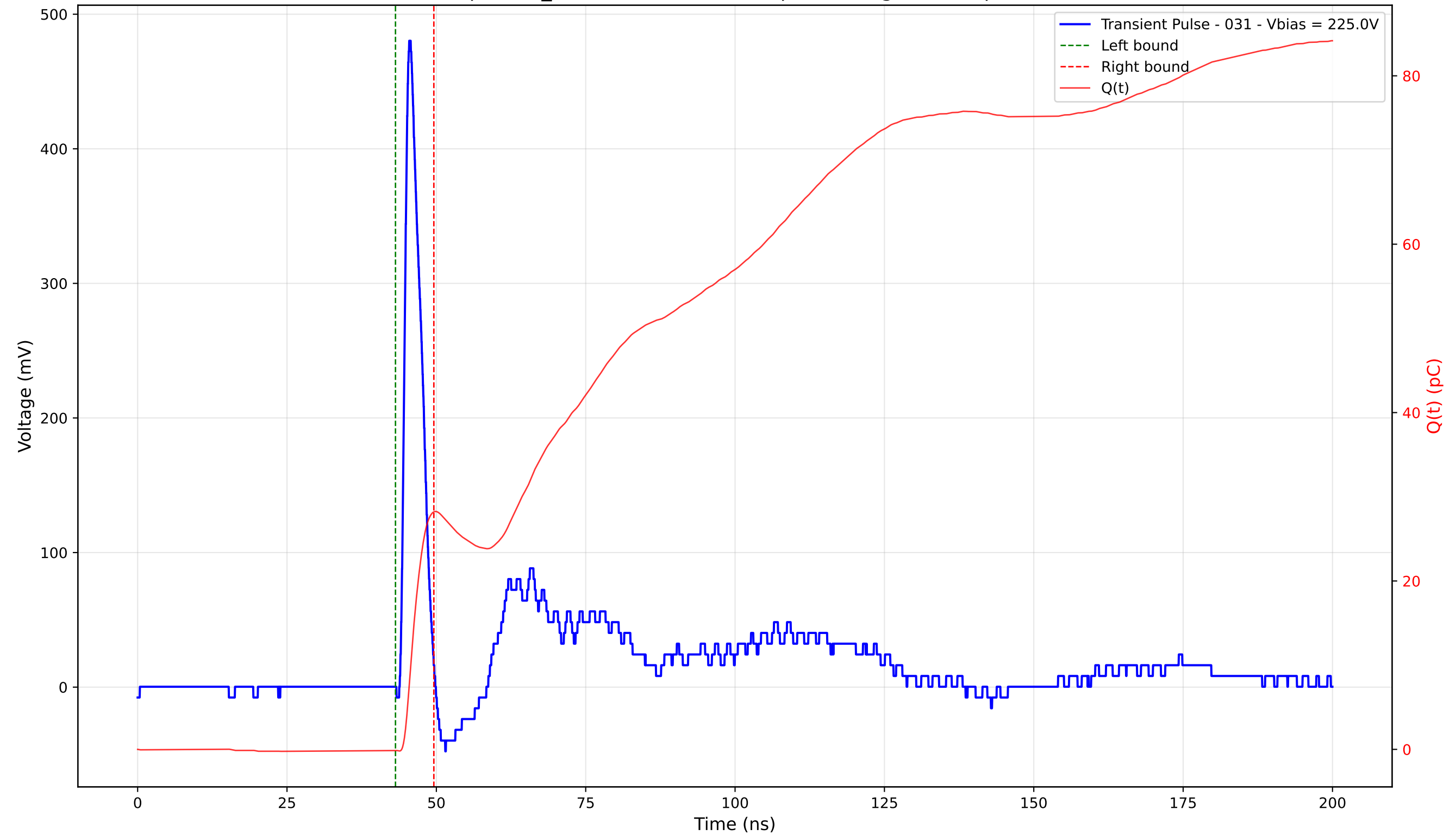
Transient Pulse - Sample: TD_4004 - Position: 365.0 \mu\text{m} - Charge: 28.33 pC - Rise Time: 1.04 ns
