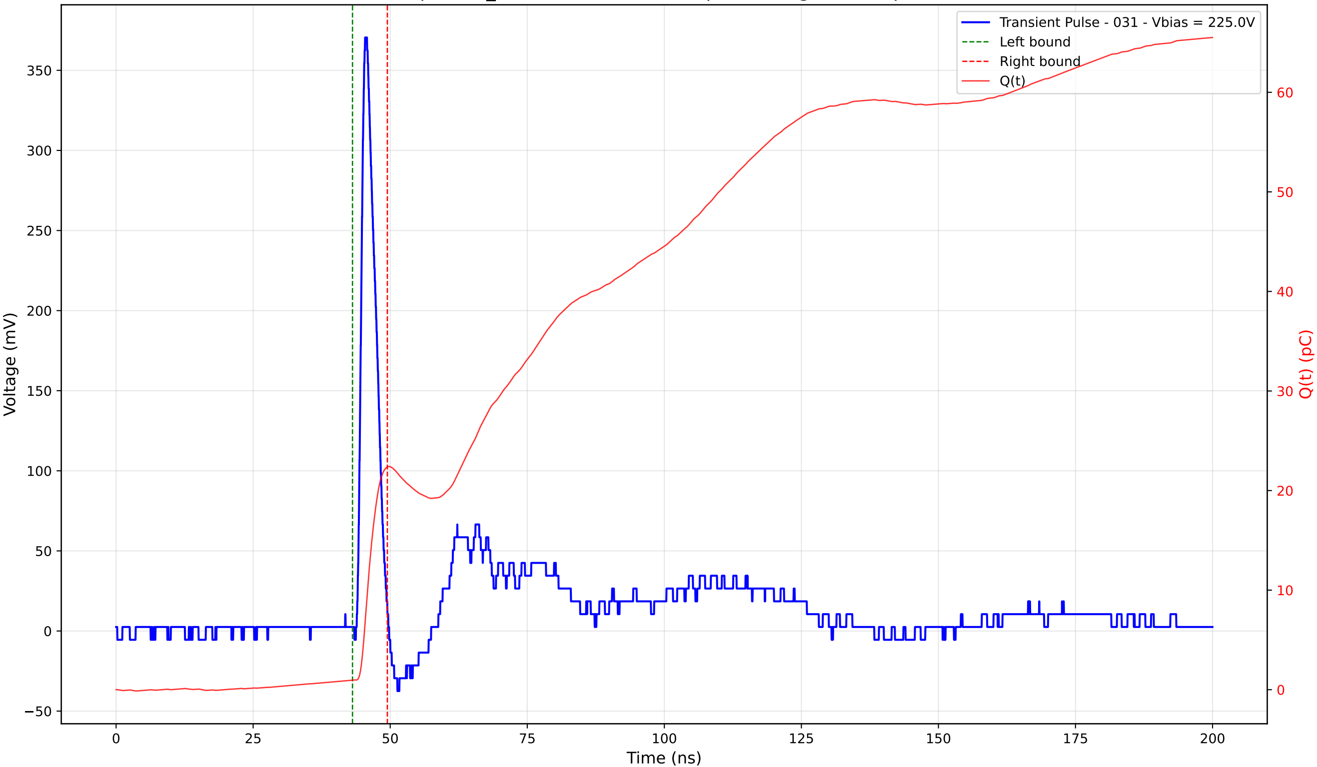
Transient Pulse - Sample: TD_4004 - Position: 390.0 \mu\text{m} - Charge: 21.40 pC - Rise Time: 1.05 ns
