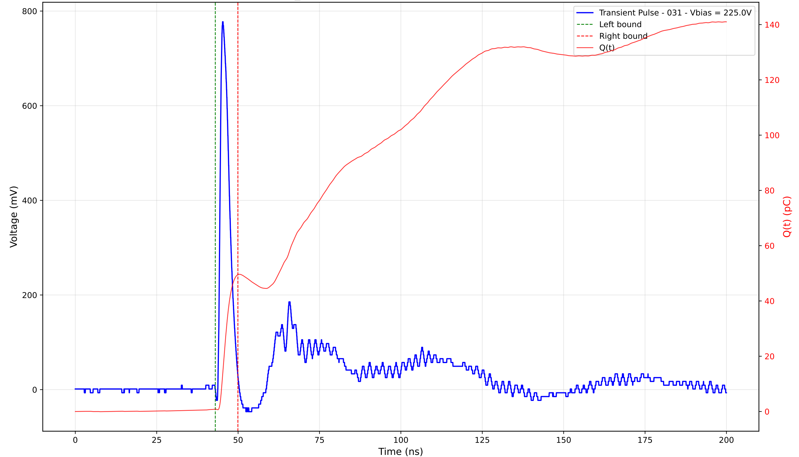
Transient Pulse - Sample: TD_4004 - Position: 185.0 \mu\text{m} - Charge: 48.66 pC - Rise Time: 0.89 ns
