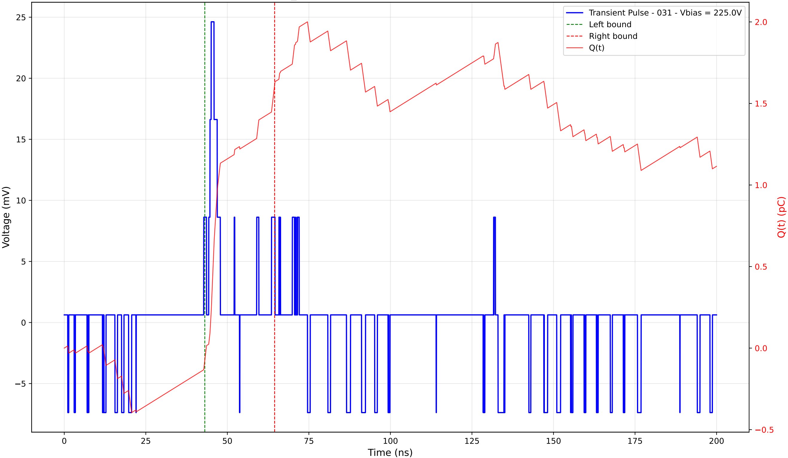
Transient Pulse - Sample: TD_4004 - Position: 30.0 \mu\text{m} - Charge: 1.69 pC - Rise Time: 0.76 ns
