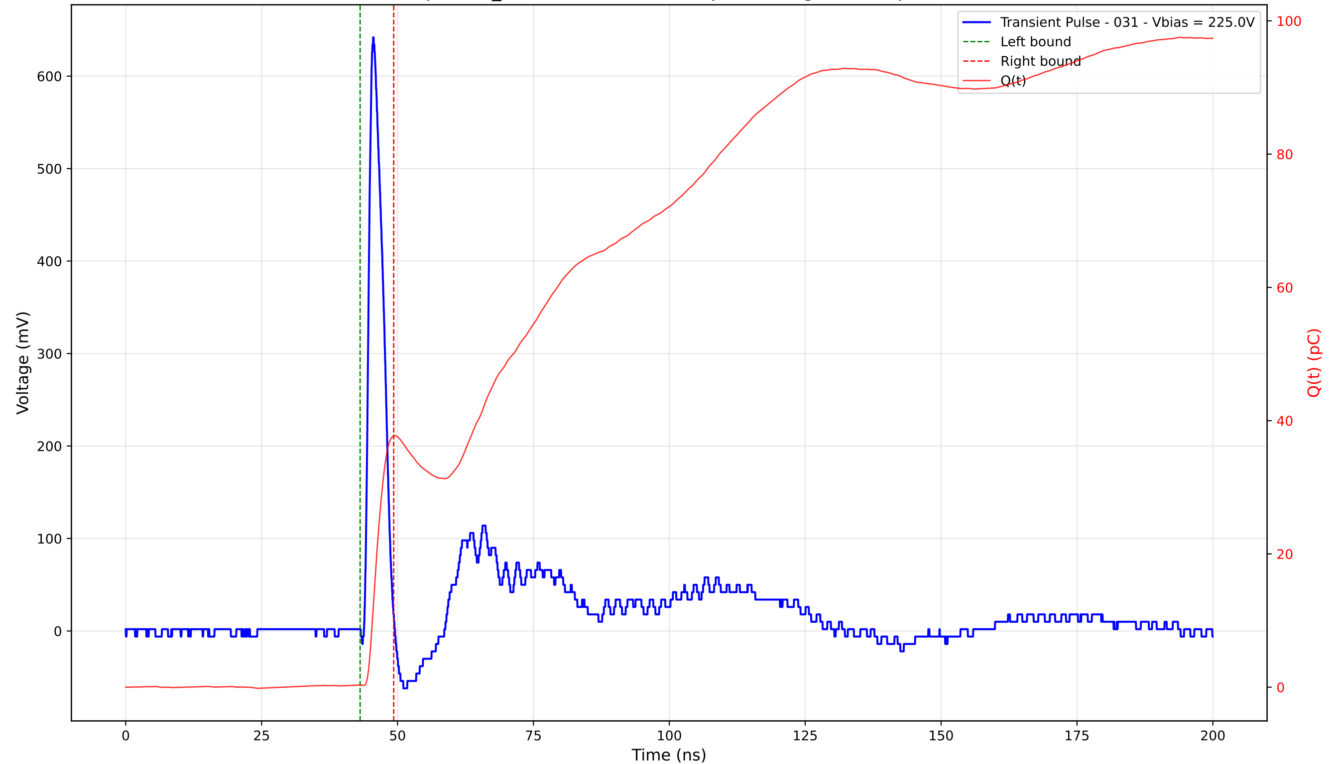
Transient Pulse - Sample: TD_4004 - Position: 320.0 \mu\text{m} - Charge: 37.37 pC - Rise Time: 1.04 ns
