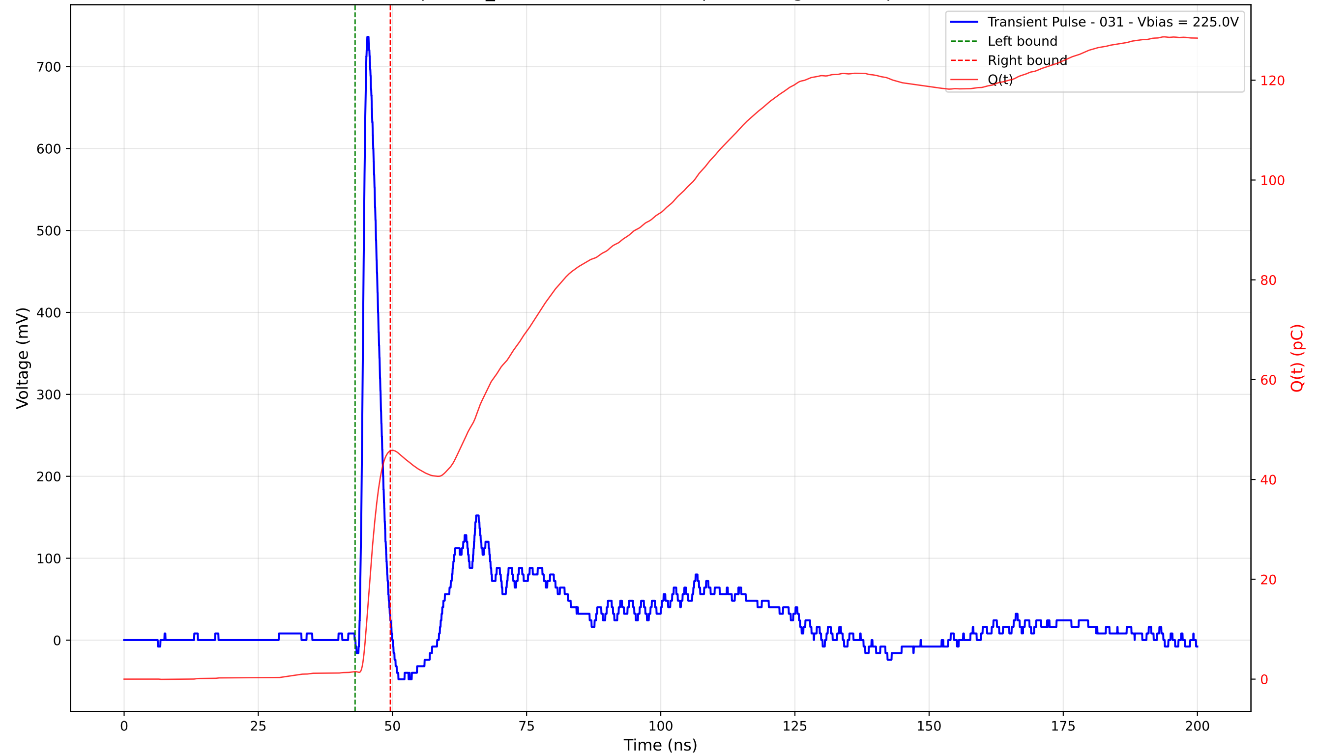
Transient Pulse - Sample: TD_4004 - Position: 145.0 \mu\text{m} - Charge: 44.23 pC - Rise Time: 0.95 ns
