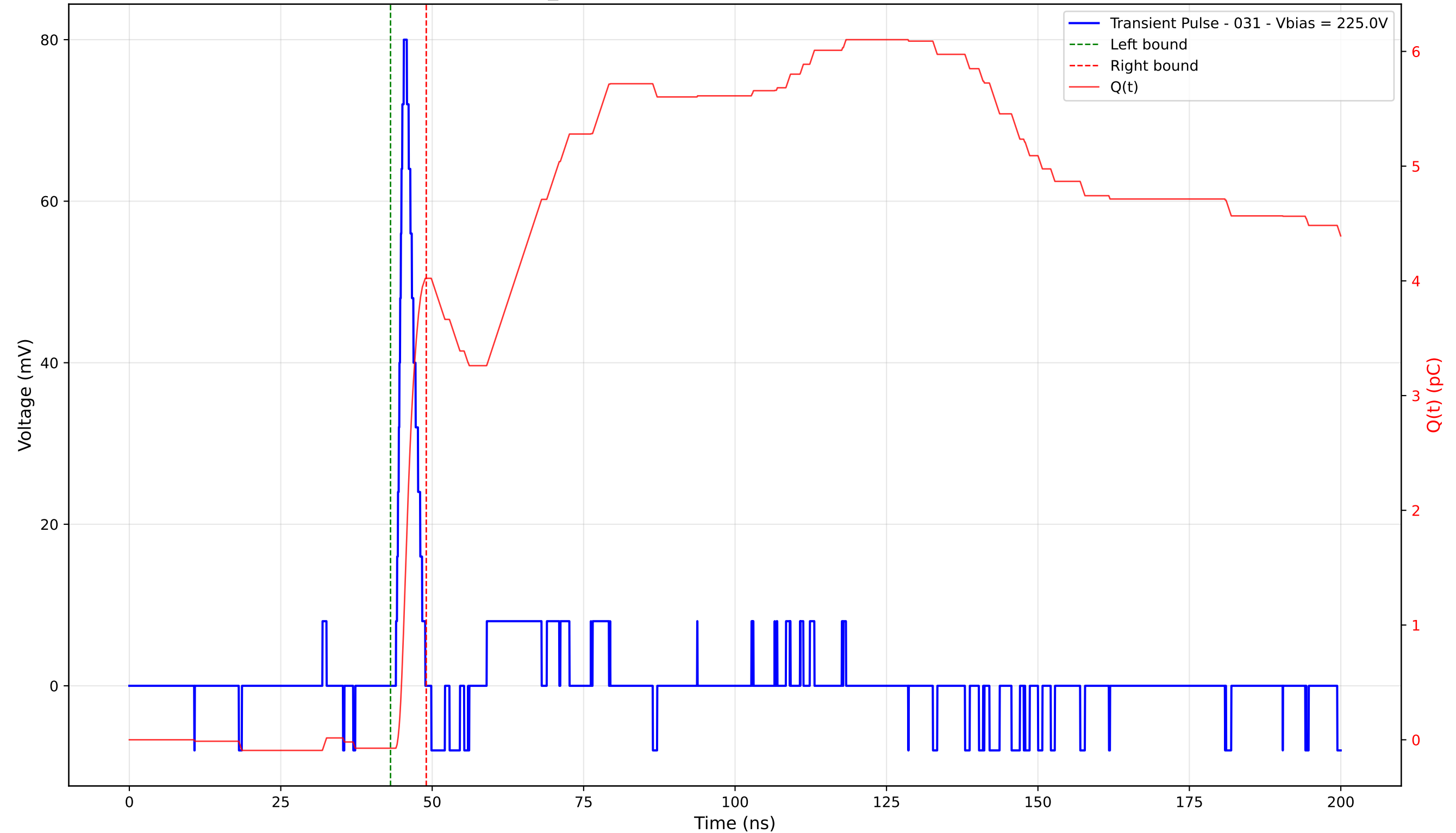
Transient Pulse - Sample: TD_4004 - Position: 420.0 \mu\text{m} - Charge: 4.10 pC - Rise Time: 0.88 ns
