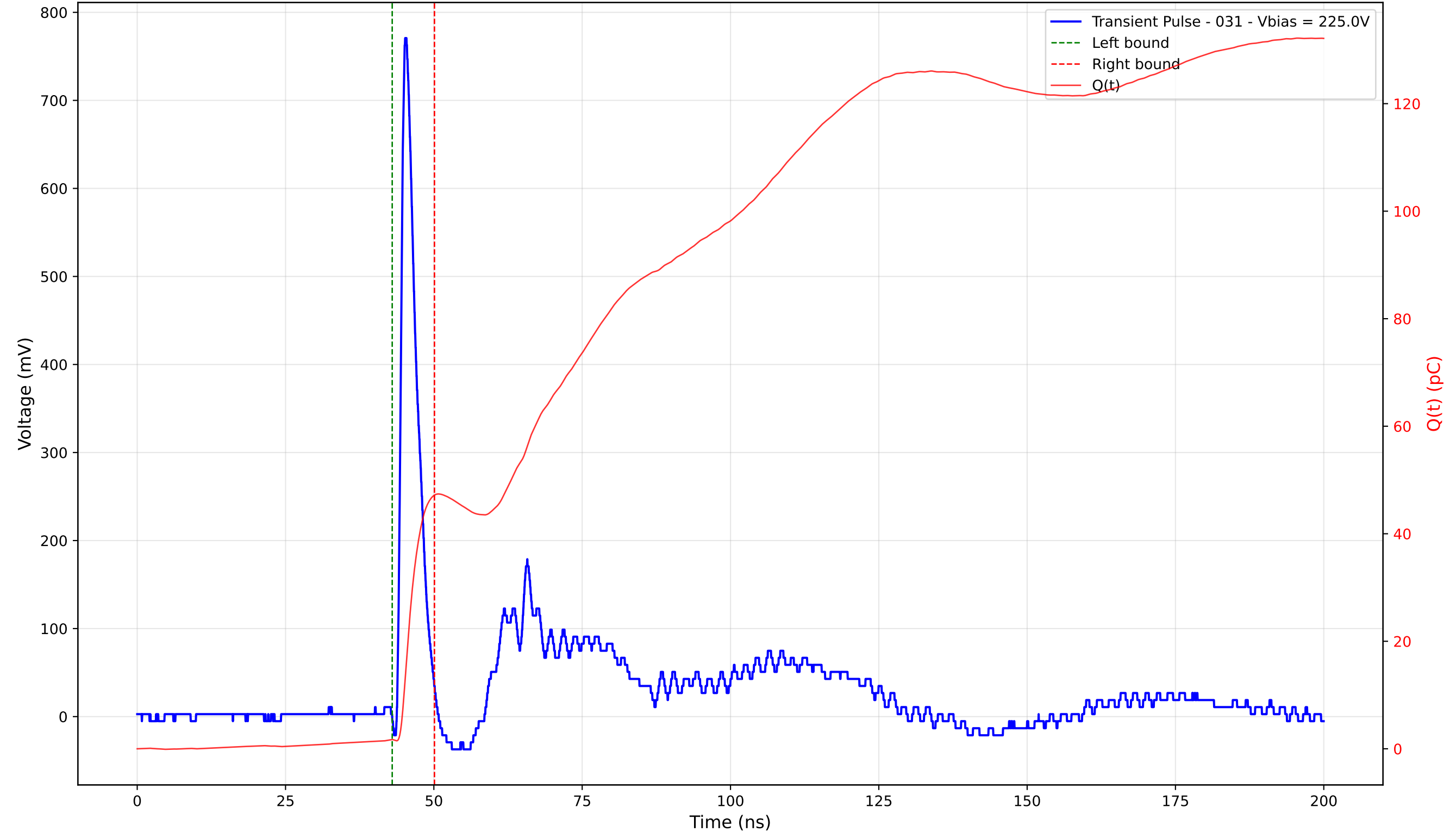
Transient Pulse - Sample: TD_4004 - Position: 105.0 \mu\text{m} - Charge: 45.48 pC - Rise Time: 0.90 ns
