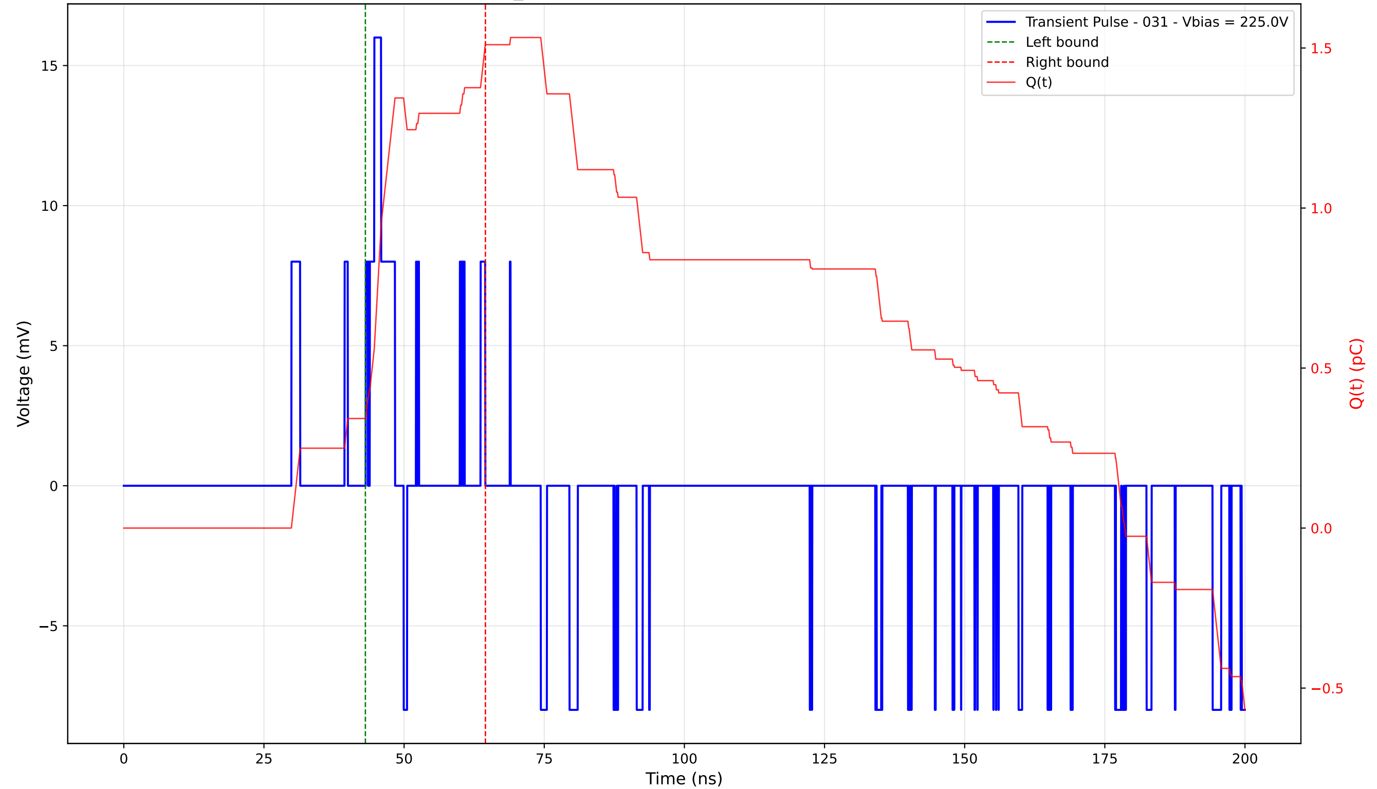
Transient Pulse - Sample: TD_4004 - Position: 20.0 \mu\text{m} - Charge: 1.17 pC - Rise Time: 0.82 ns
