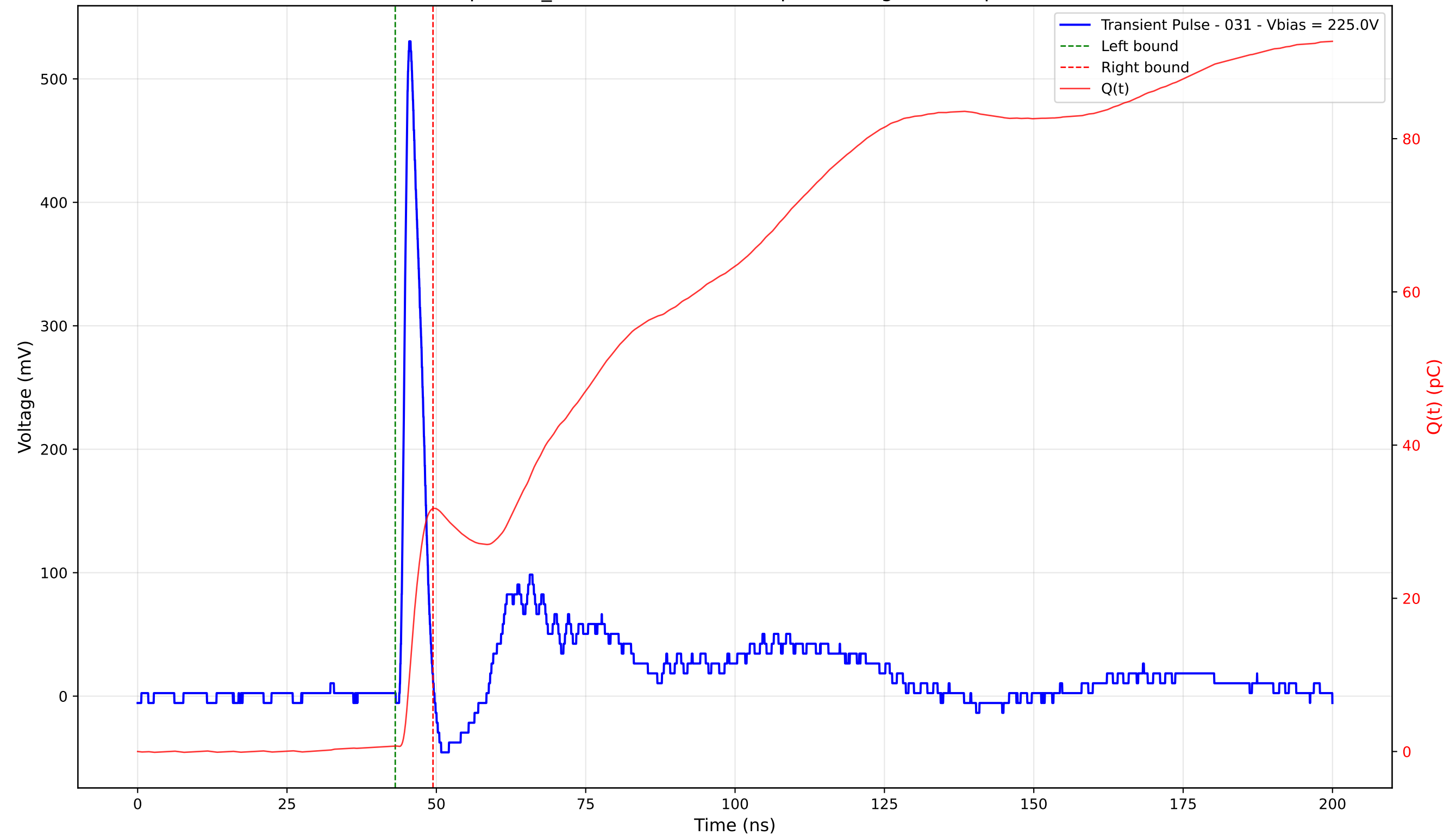
Transient Pulse - Sample: TD_4004 - Position: 335.0 \mu\text{m} - Charge: 31.00 pC - Rise Time: 1.04 ns
