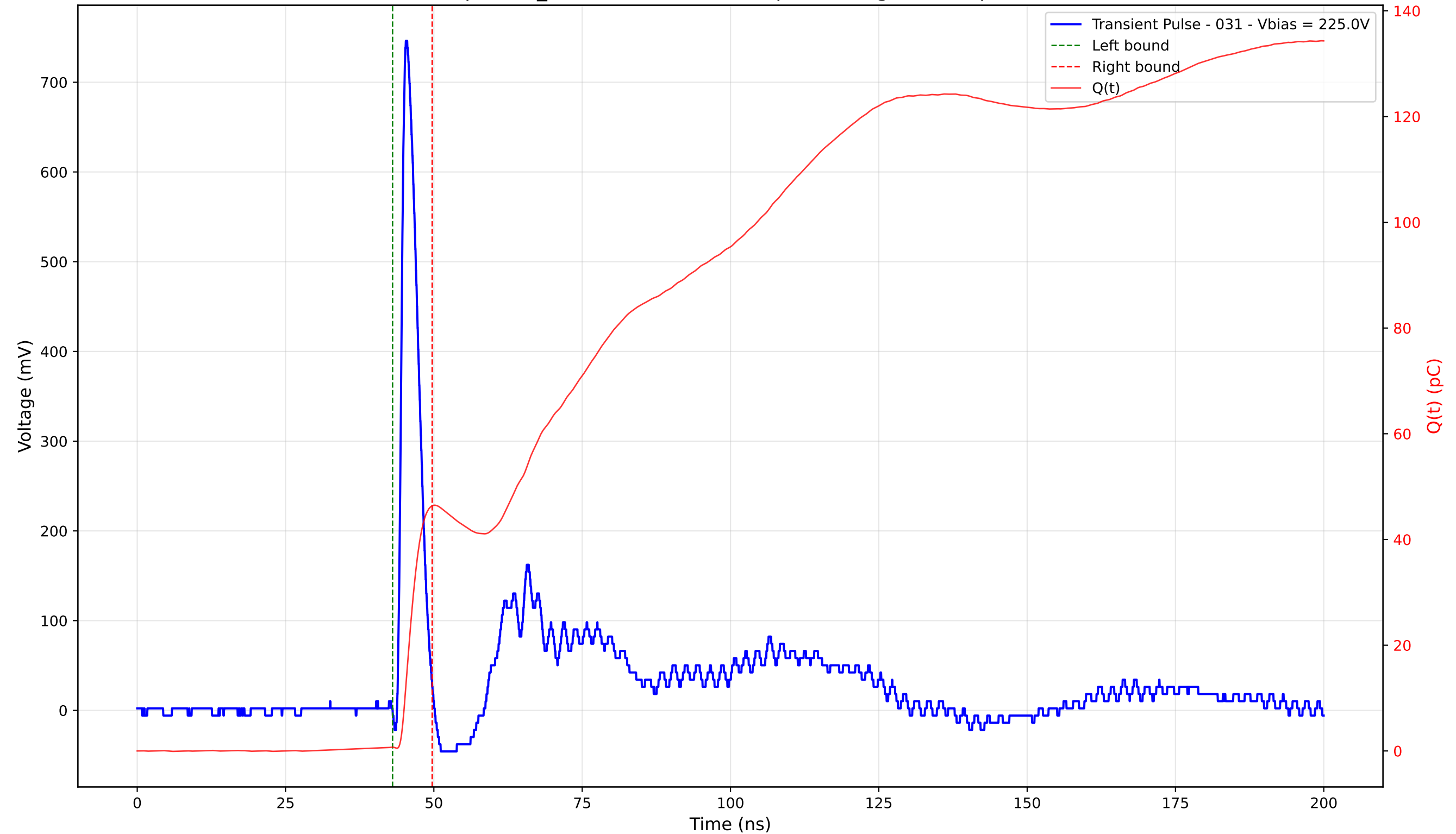
Transient Pulse - Sample: TD_4004 - Position: 160.0 \mu\text{m} - Charge: 45.66 pC - Rise Time: 0.93 ns
