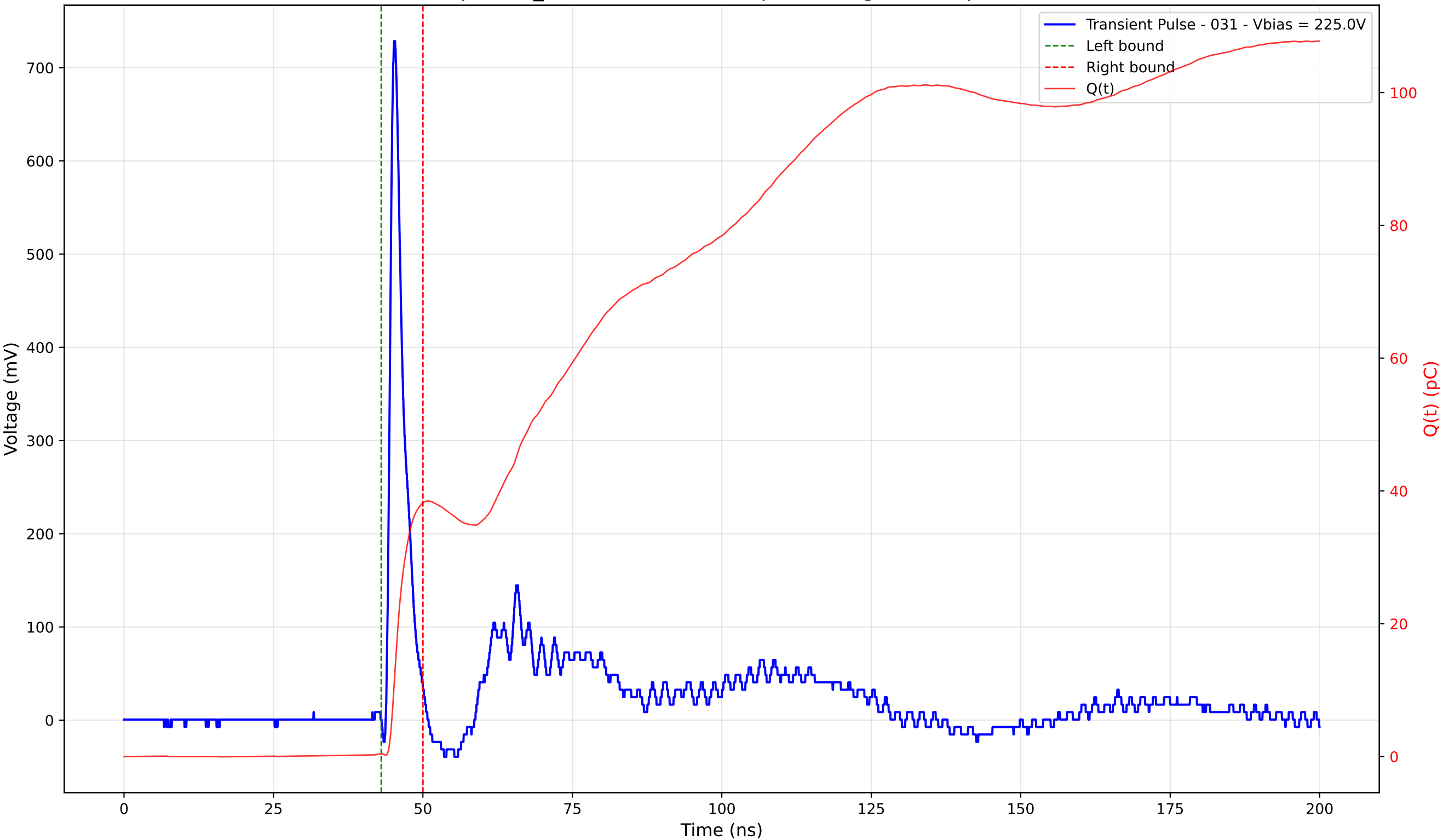
Transient Pulse - Sample: TD_4004 - Position: 90.0 \mu\text{m} - Charge: 37.80 pC - Rise Time: 0.90 ns
