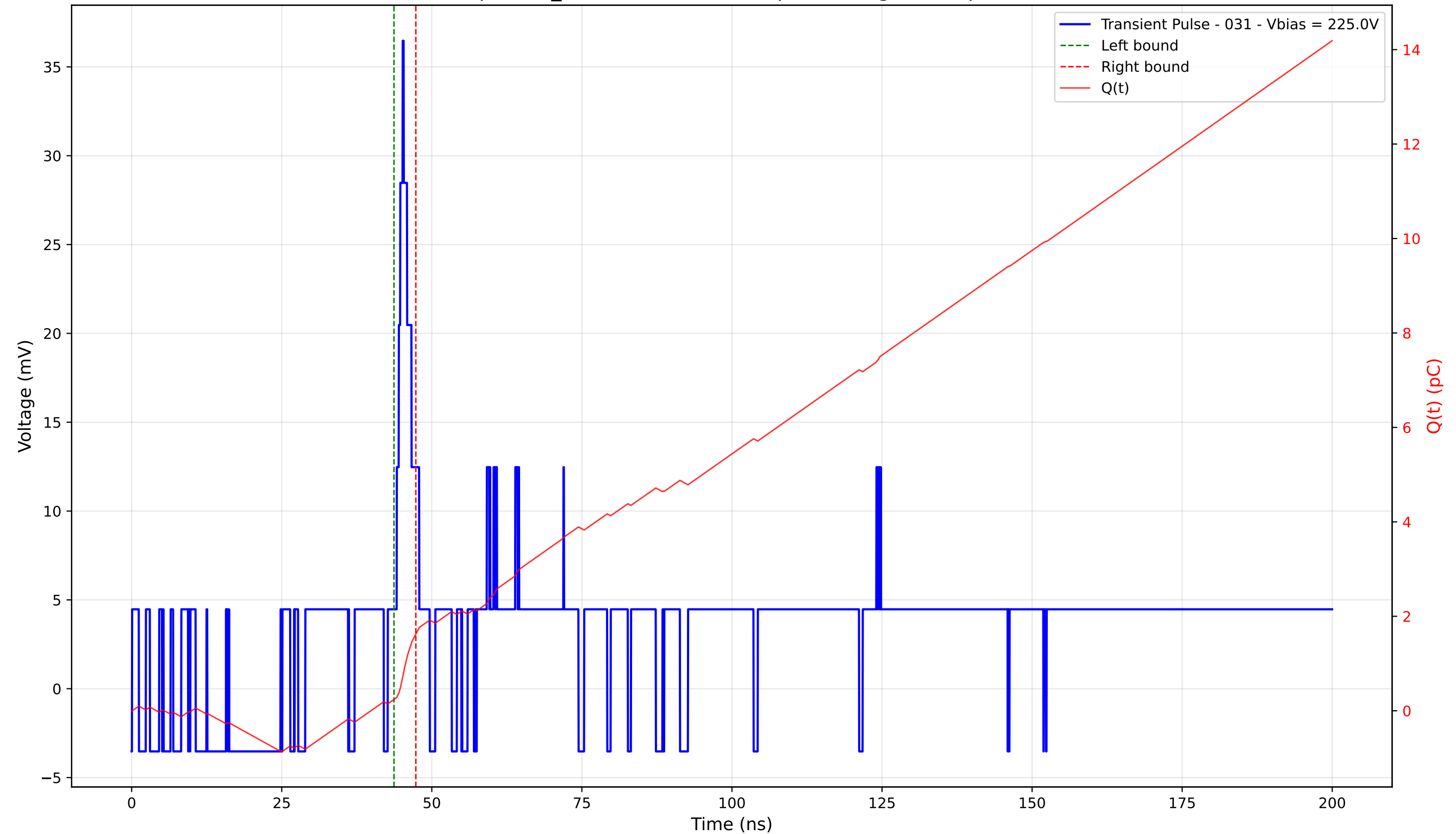
Transient Pulse - Sample: TD_4004 - Position: 35.0 \mu\text{m} - Charge: 1.39 pC - Rise Time: 2.50 ns
