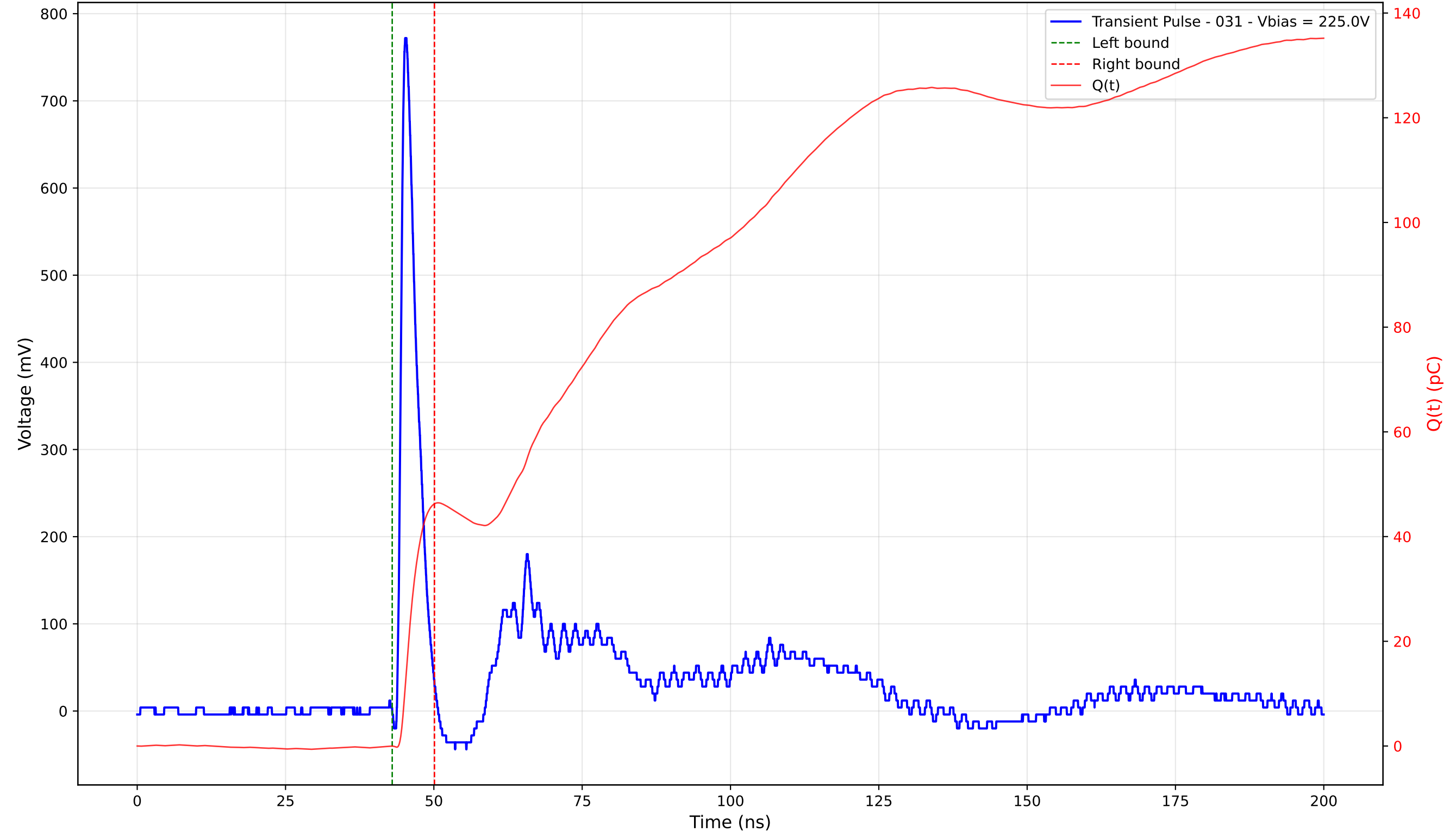
Transient Pulse - Sample: TD_4004 - Position: 110.0 \mu\text{m} - Charge: 46.28 pC - Rise Time: 0.88 ns
