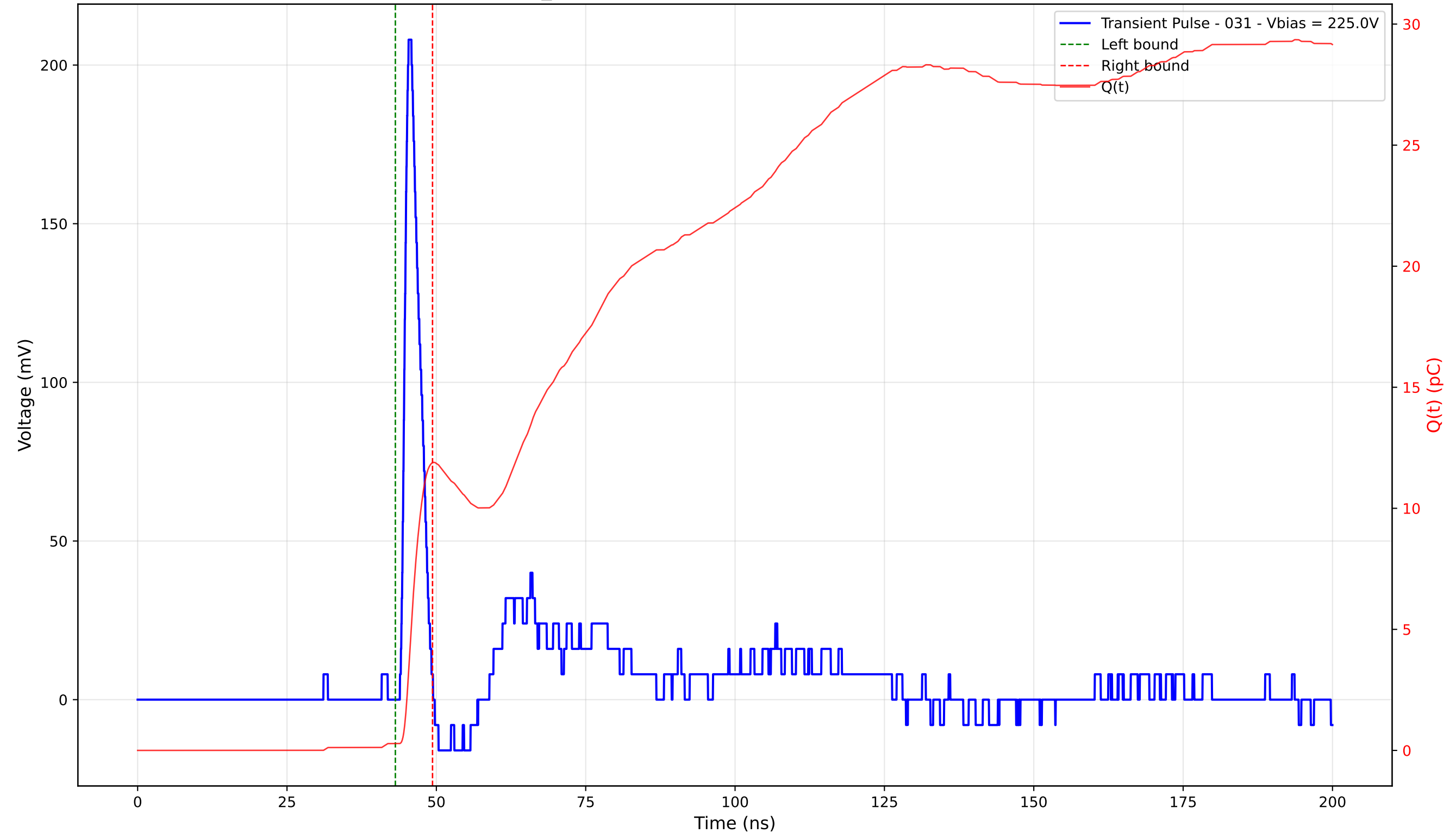
Transient Pulse - Sample: TD_4004 - Position: 405.0 \mu\text{m} - Charge: 11.60 pC - Rise Time: 1.03 ns
