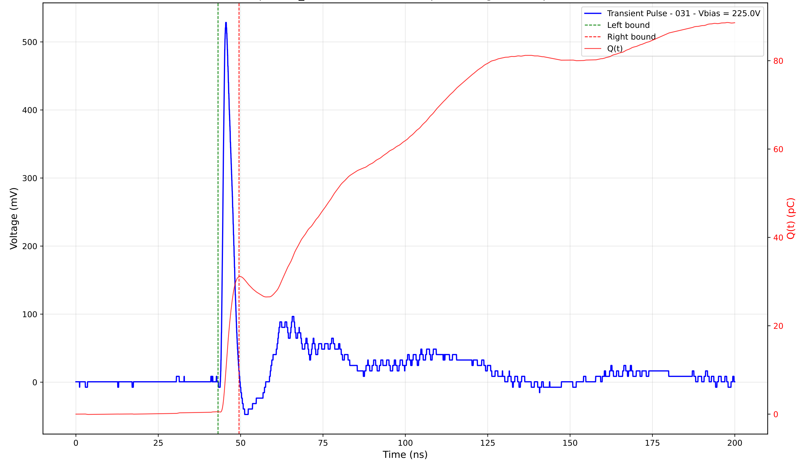
Transient Pulse - Sample: TD_4004 - Position: 345.0 \mu\text{m} - Charge: 30.57 pC - Rise Time: 1.02 ns
