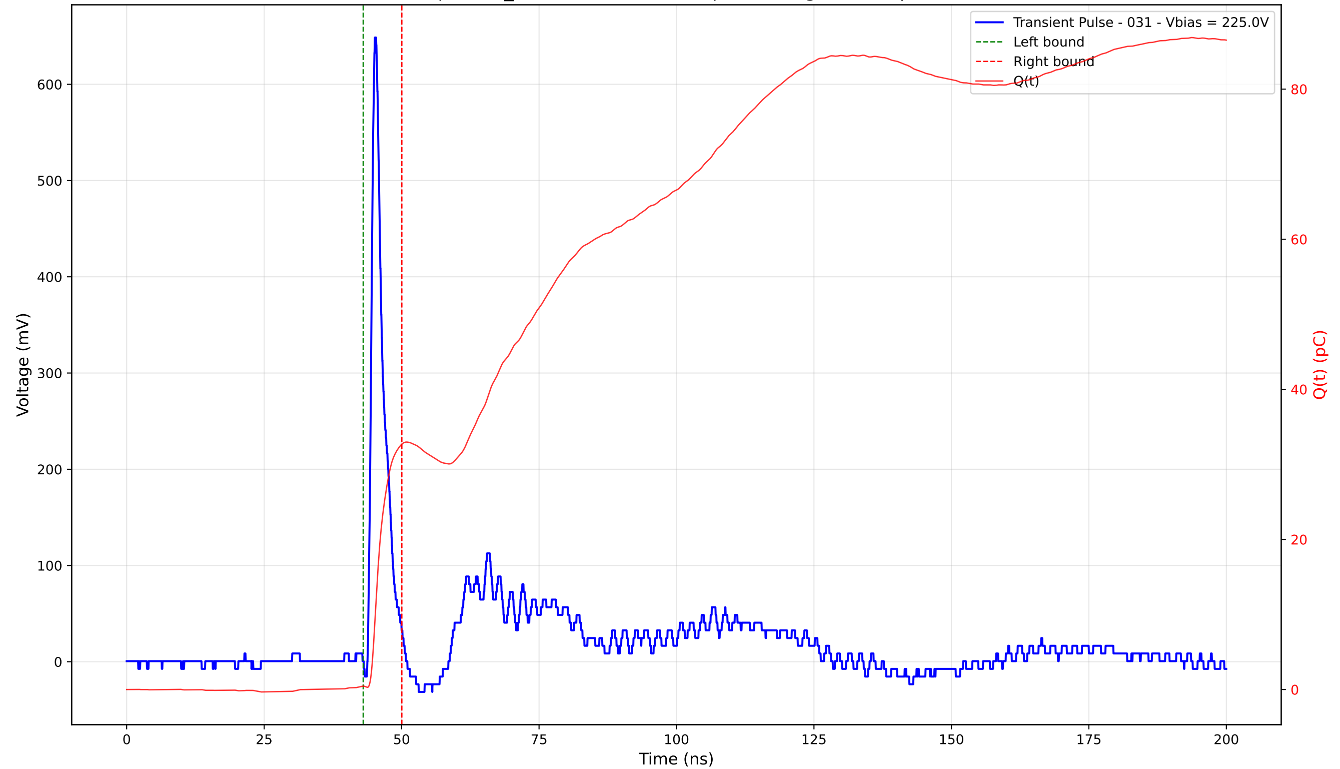
Transient Pulse - Sample: TD_4004 - Position: 80.0 \mu\text{m} - Charge: 32.25 pC - Rise Time: 0.90 ns
