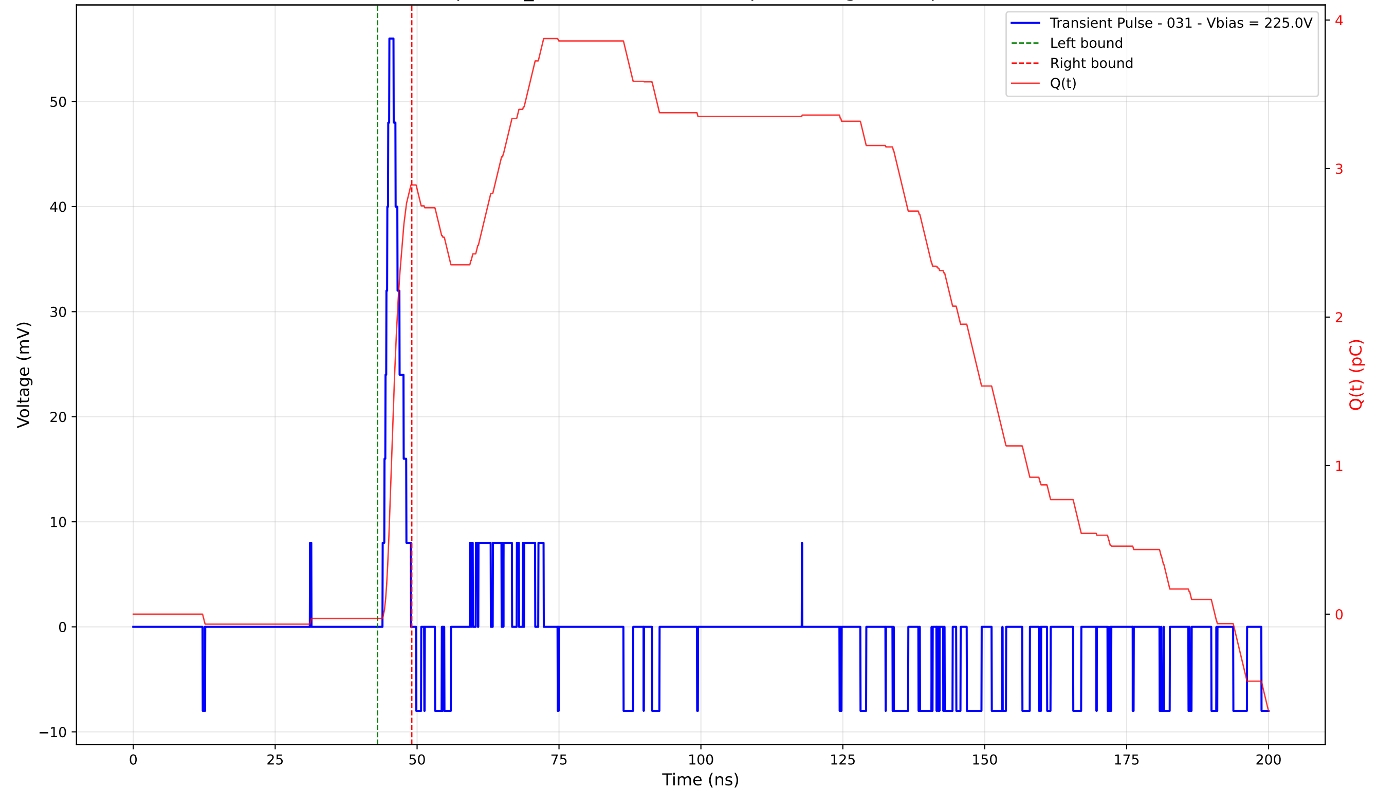
Transient Pulse - Sample: TD_4004 - Position: 435.0 \mu\text{m} - Charge: 2.92 pC - Rise Time: 1.19 ns
