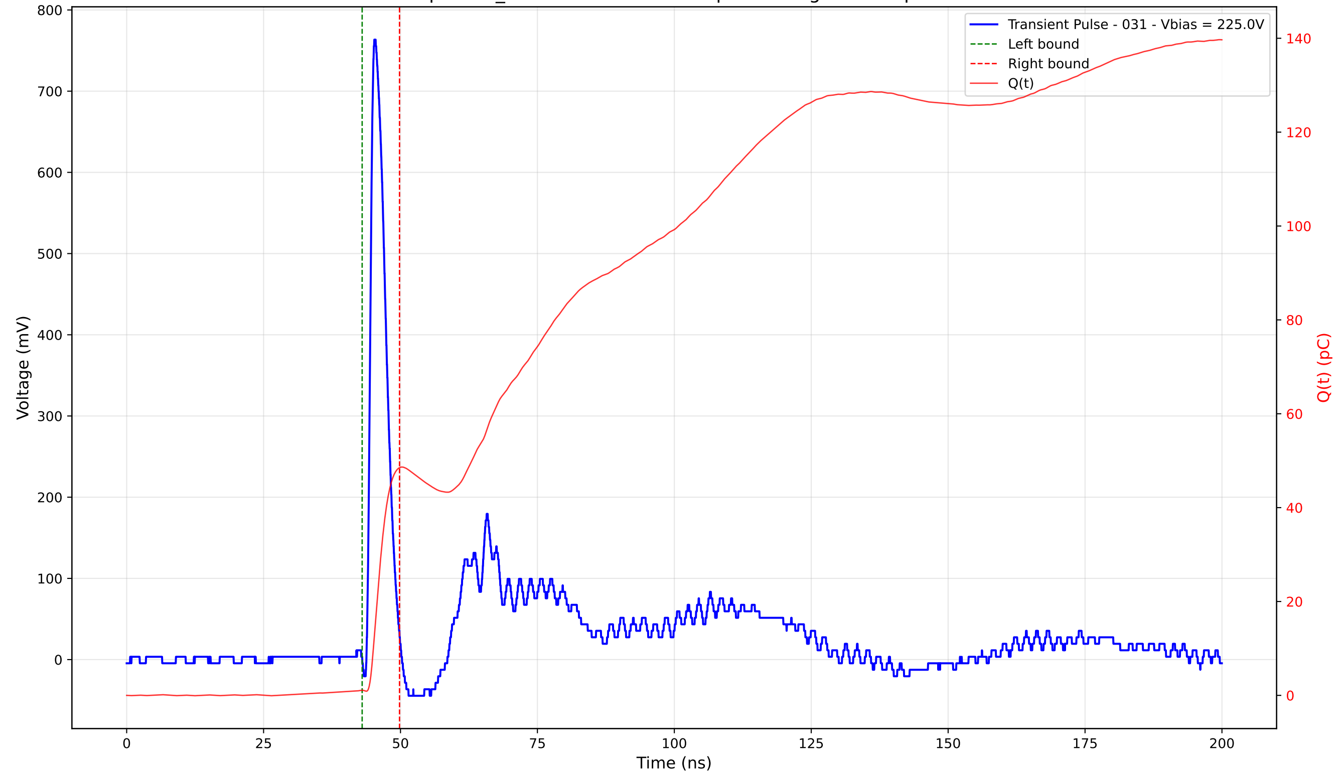
Transient Pulse - Sample: TD_4004 - Position: 205.0 \mu\text{m} - Charge: 47.42 pC - Rise Time: 0.91 ns
