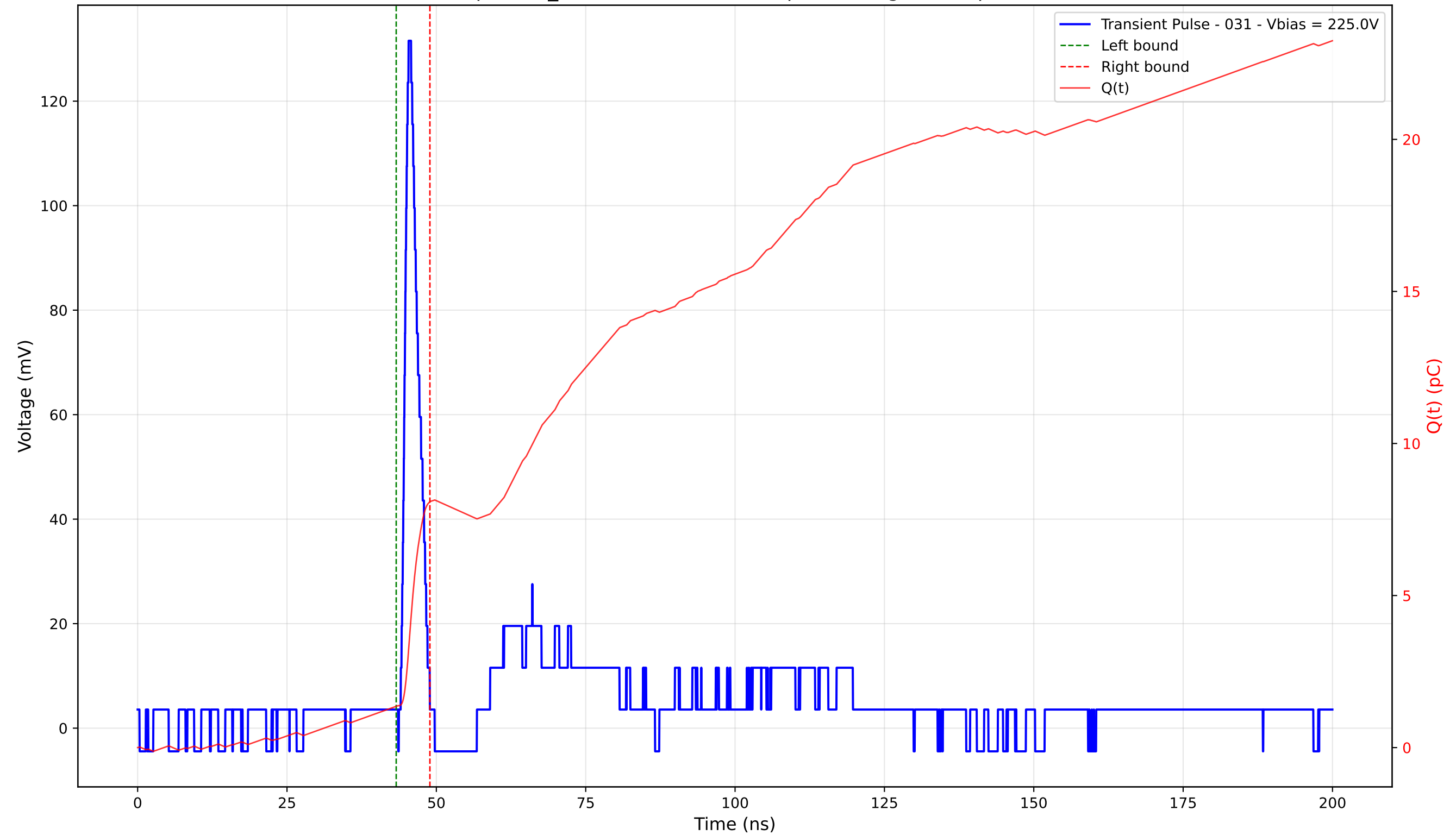
Transient Pulse - Sample: TD_4004 - Position: 415.0 \mu\text{m} - Charge: 6.73 pC - Rise Time: 1.04 ns
