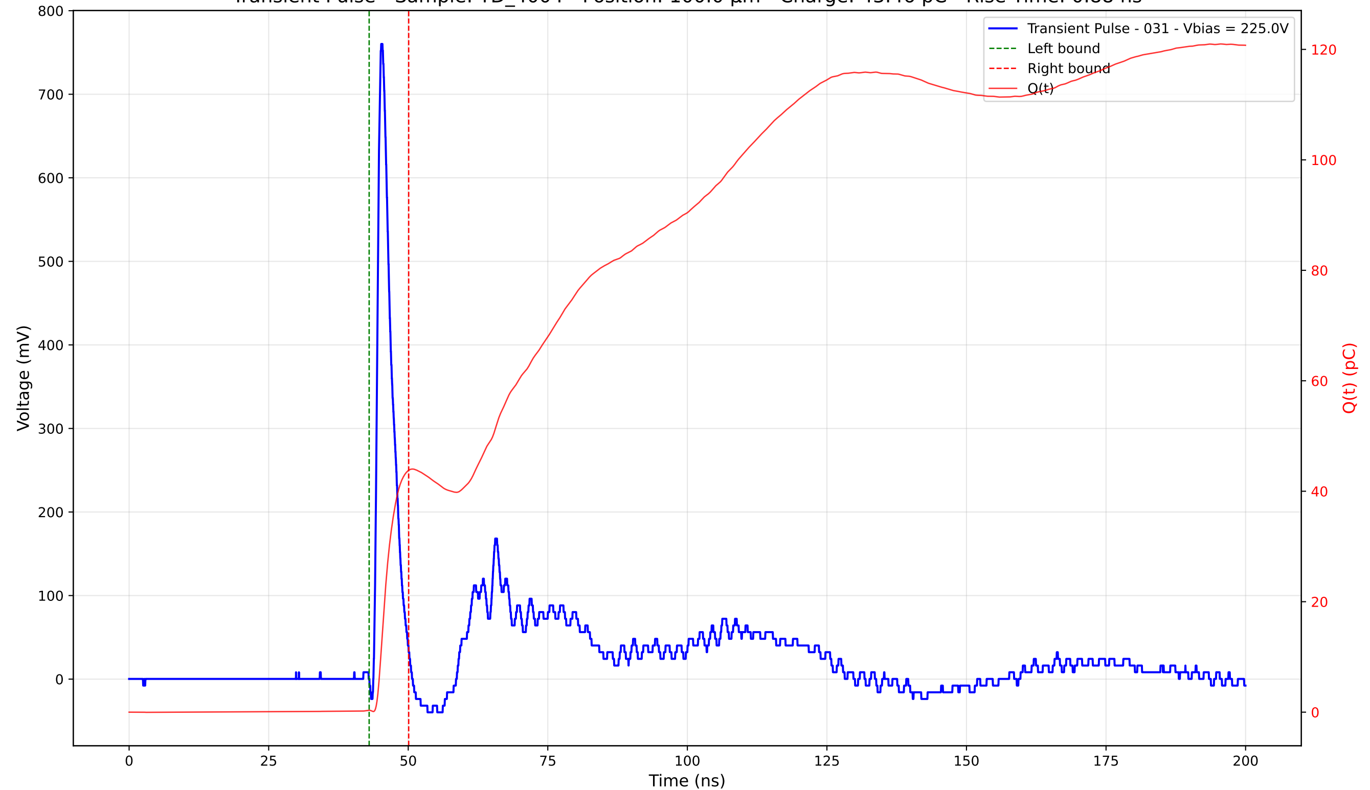
Transient Pulse - Sample: TD_4004 - Position: 100.0 \mu\text{m} - Charge: 43.46 pC - Rise Time: 0.88 ns
