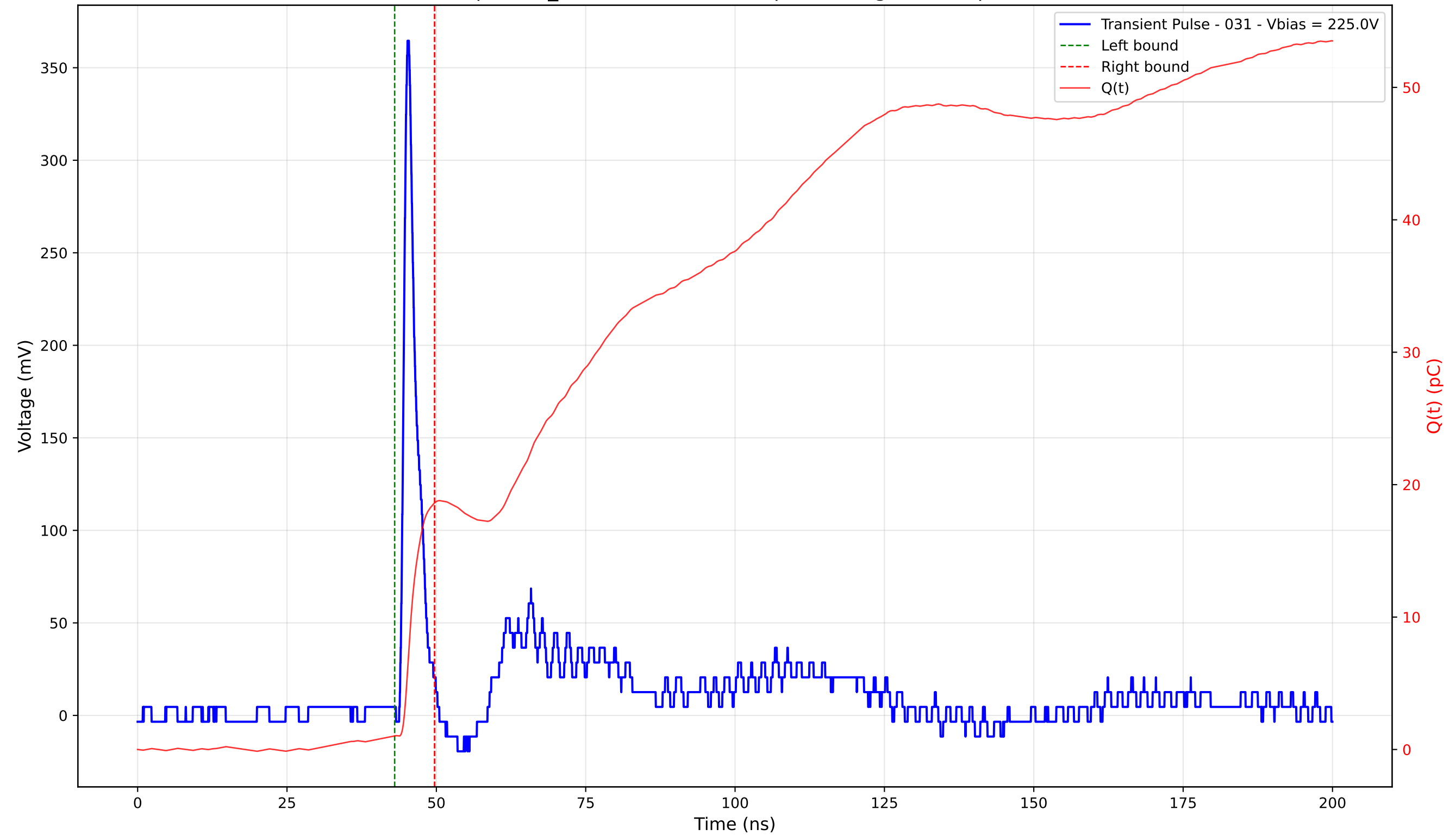
Transient Pulse - Sample: TD_4004 - Position: 65.0 \mu\text{m} - Charge: 17.59 pC - Rise Time: 0.94 ns
