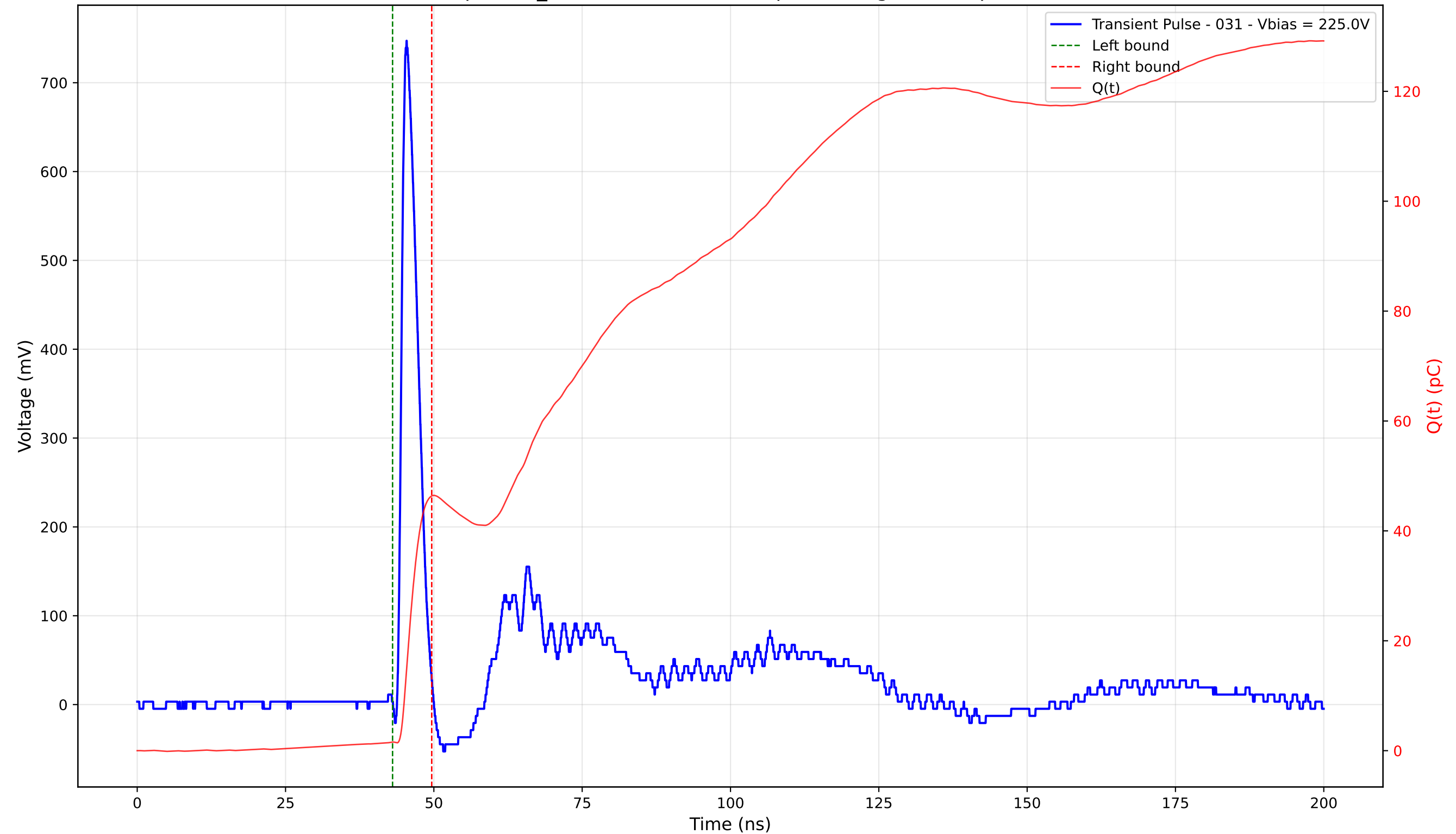
Transient Pulse - Sample: TD_4004 - Position: 135.0 \mu\text{m} - Charge: 44.79 pC - Rise Time: 0.95 ns
