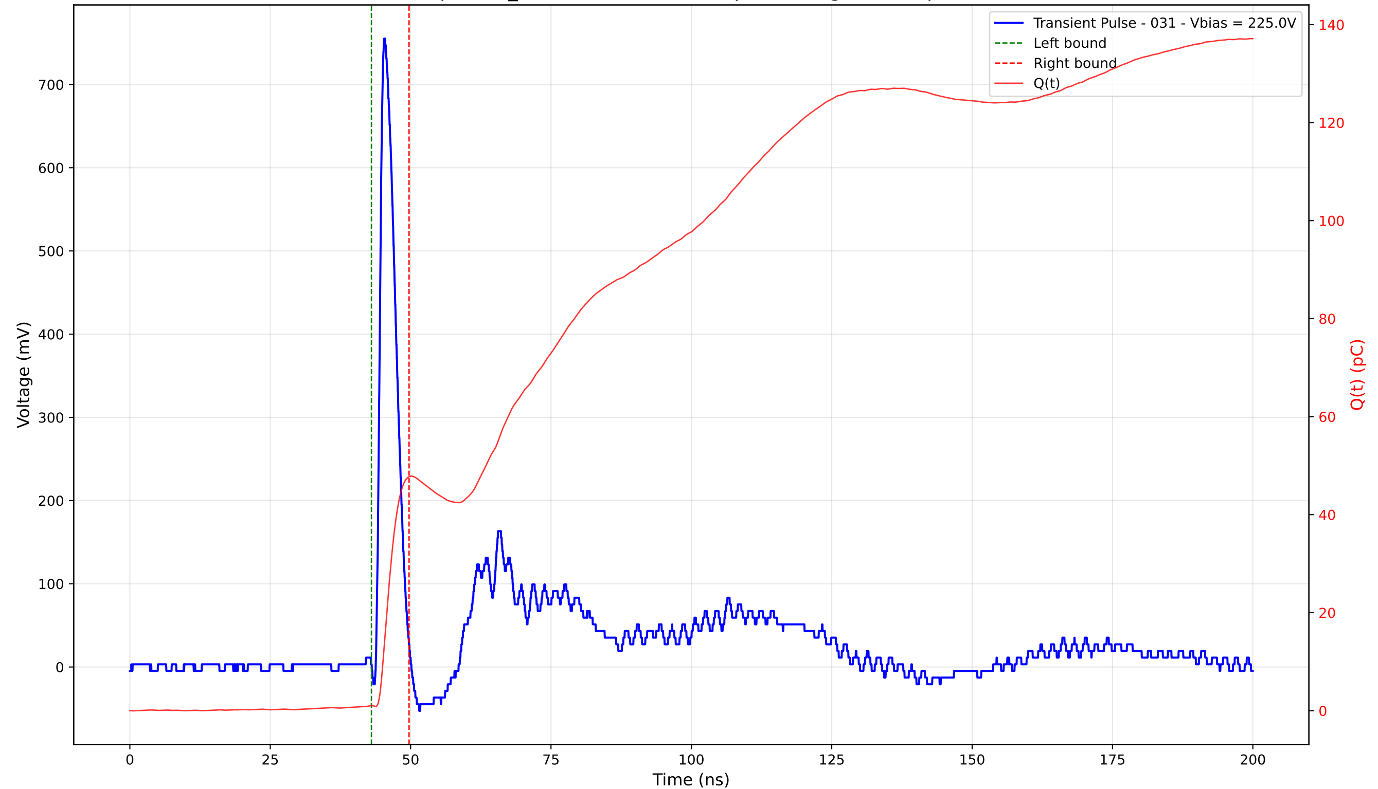
Transient Pulse - Sample: TD_4004 - Position: 165.0 \mu\text{m} - Charge: 46.71 pC - Rise Time: 0.93 ns
