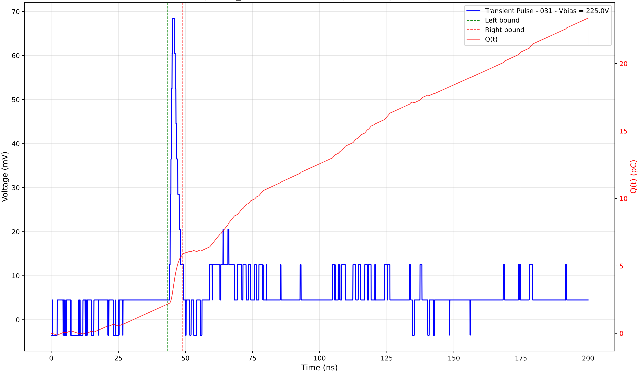
Transient Pulse - Sample: TD_4004 - Position: 425.0 \mu\text{m} - Charge: 3.62 pC - Rise Time: 1.15 ns
