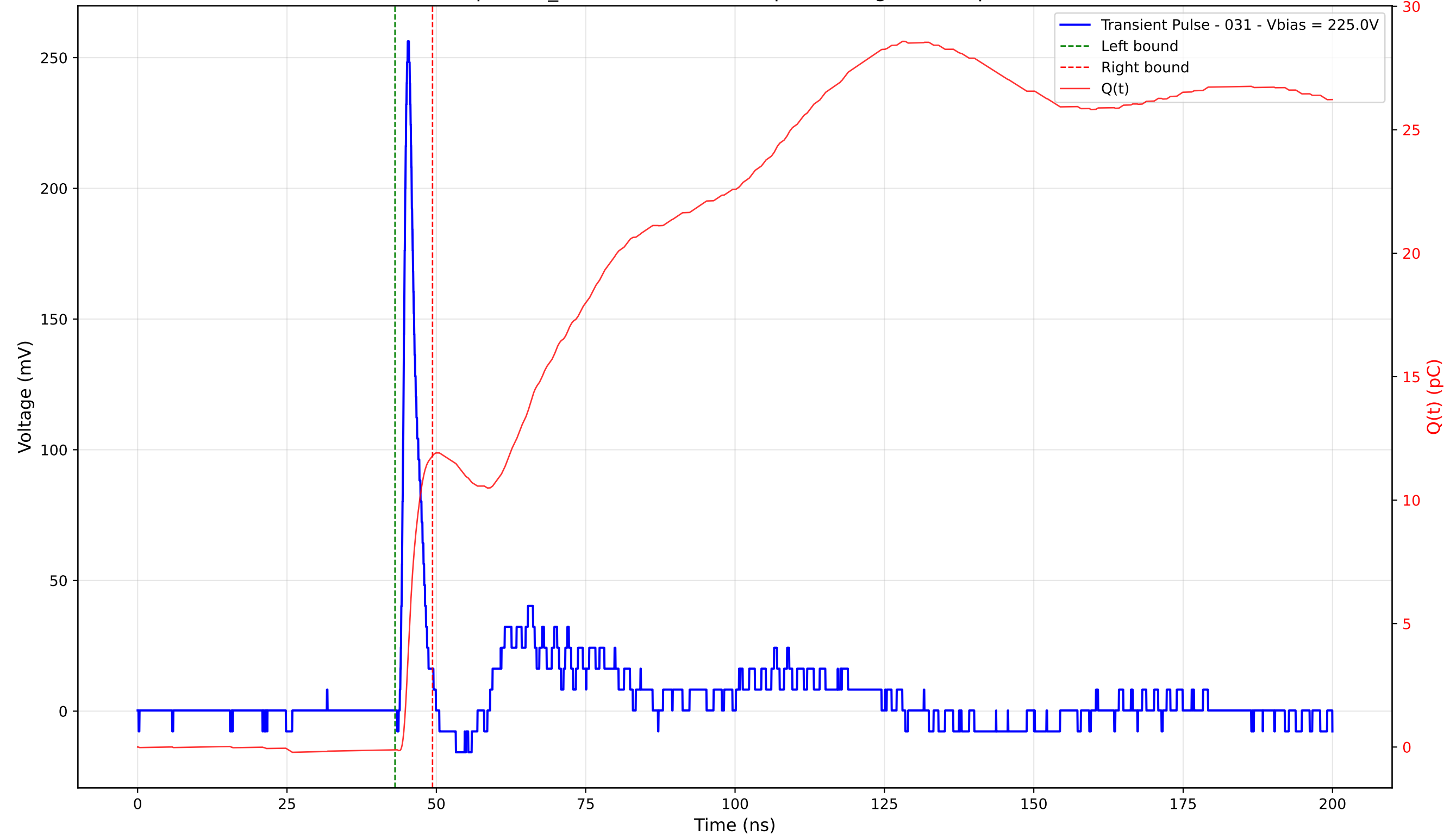
Transient Pulse - Sample: TD_4004 - Position: 60.0 \mu\text{m} - Charge: 11.91 pC - Rise Time: 0.88 ns
