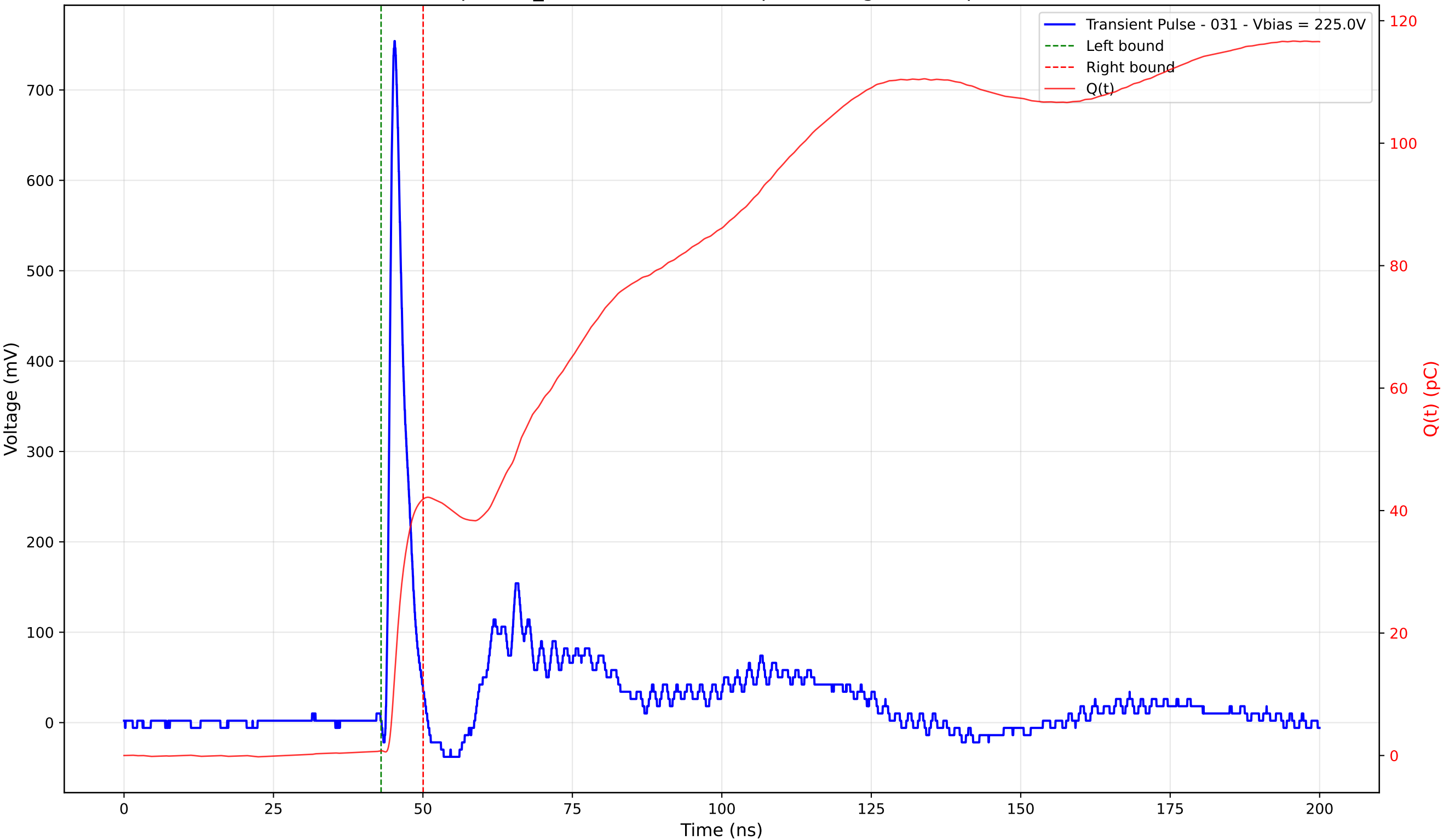
Transient Pulse - Sample: TD_4004 - Position: 95.0 \mu\text{m} - Charge: 41.11 pC - Rise Time: 0.89 ns
