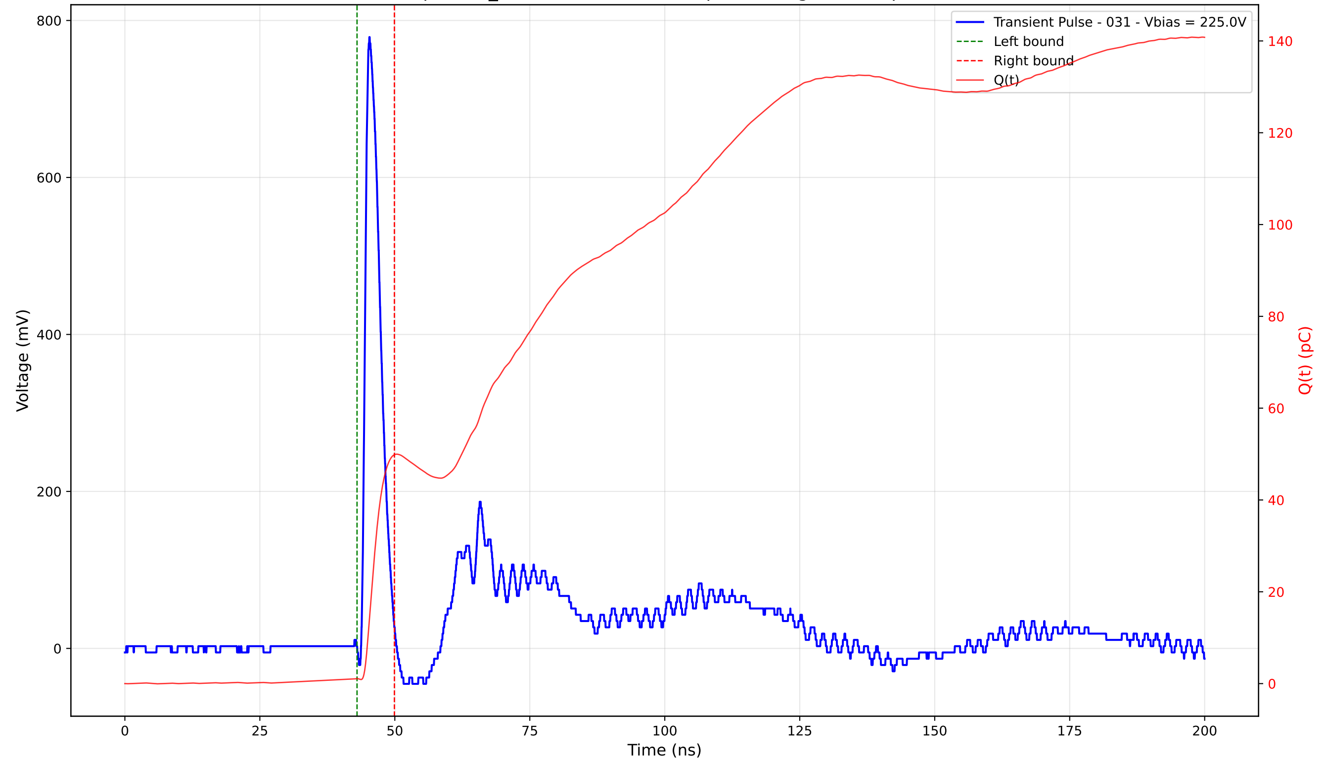
Transient Pulse - Sample: TD_4004 - Position: 180.0 \mu\text{m} - Charge: 48.79 pC - Rise Time: 0.92 ns
