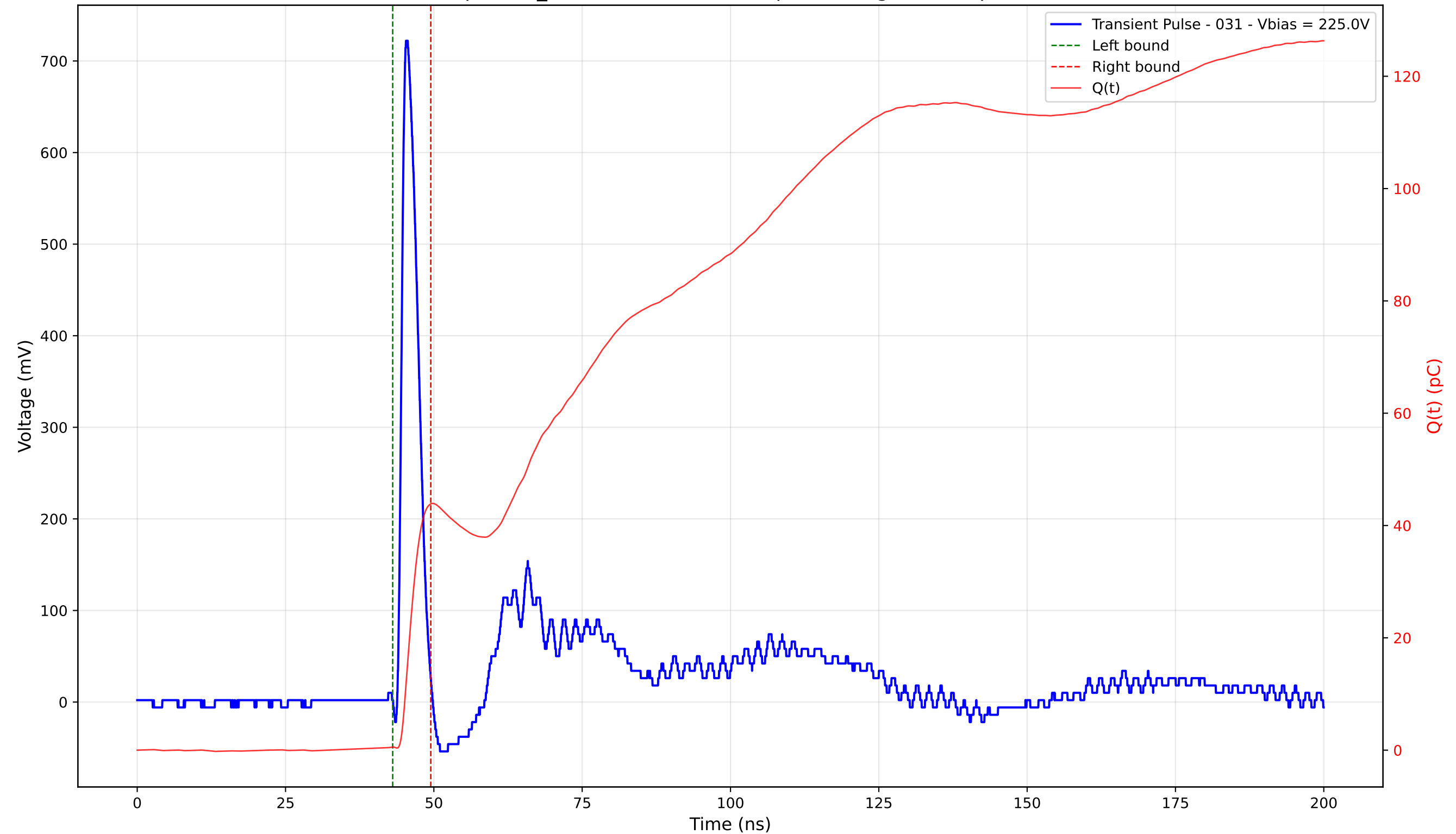
Transient Pulse - Sample: TD_4004 - Position: 245.0 \mu\text{m} - Charge: 43.30 pC - Rise Time: 0.94 ns
