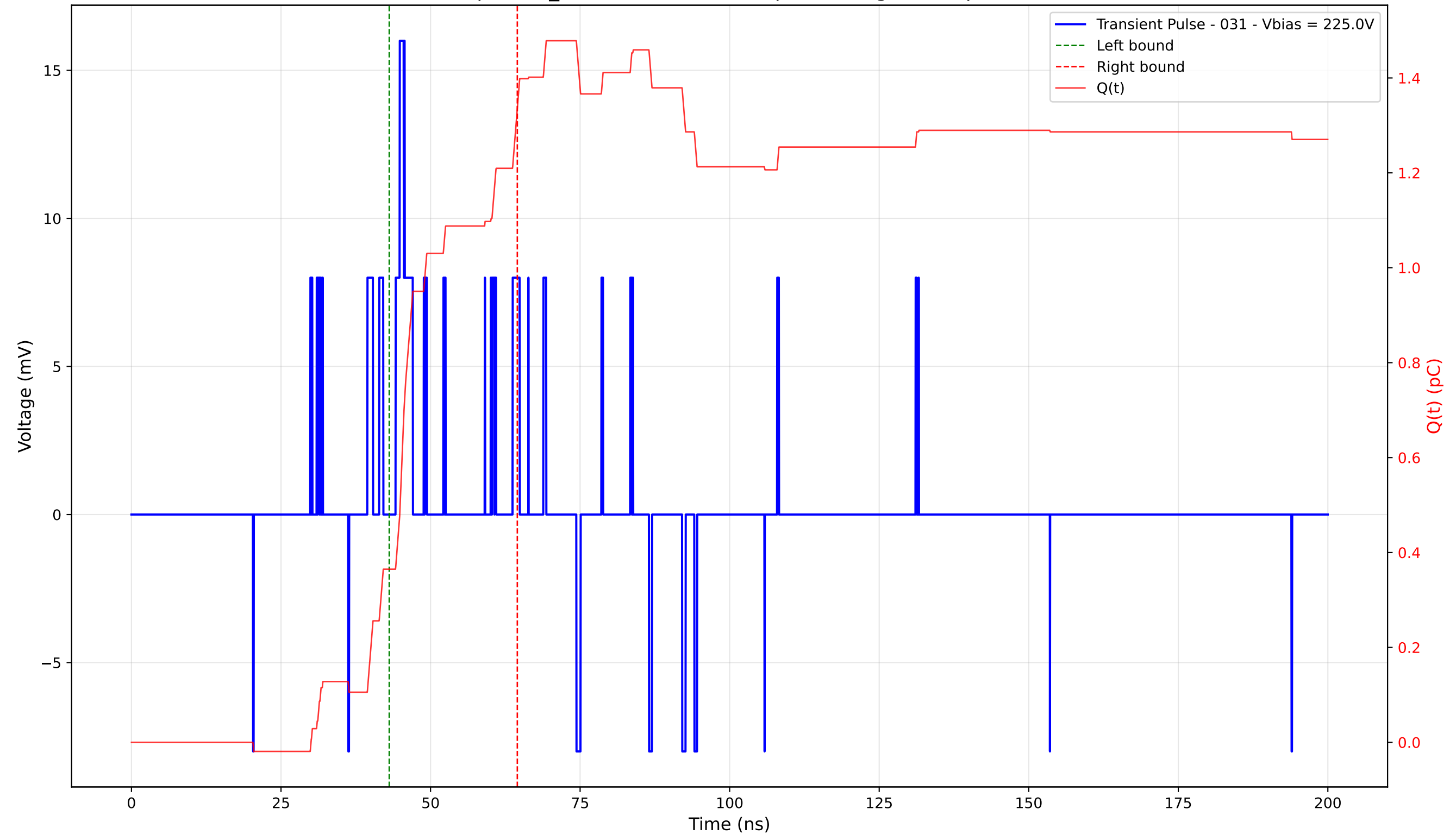
Transient Pulse - Sample: TD_4004 - Position: 10.0 \mu\text{m} - Charge: 0.97 pC - Rise Time: 0.70 ns
