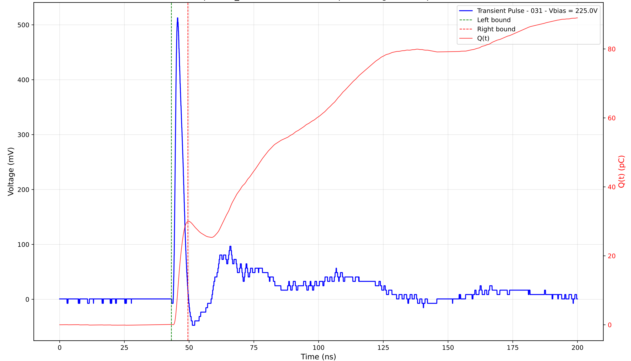
Transient Pulse - Sample: TD_4004 - Position: 355.0 \mu\text{m} - Charge: 29.89 pC - Rise Time: 1.03 ns
