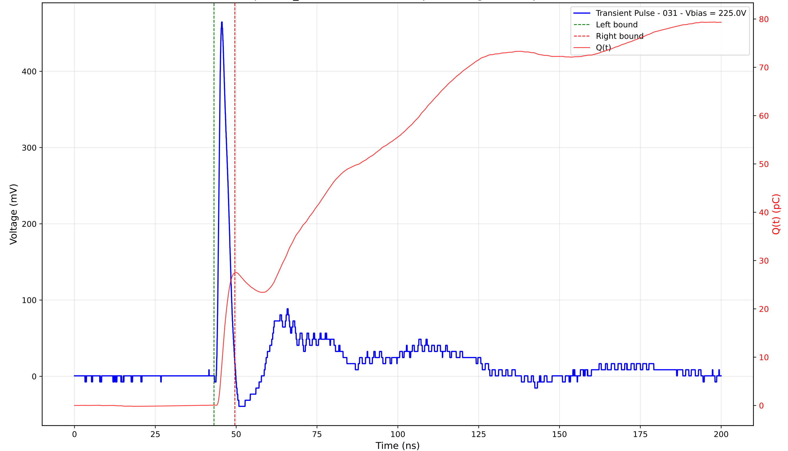
Transient Pulse - Sample: TD_4004 - Position: 370.0 \mu\text{m} - Charge: 27.41 pC - Rise Time: 1.07 ns
