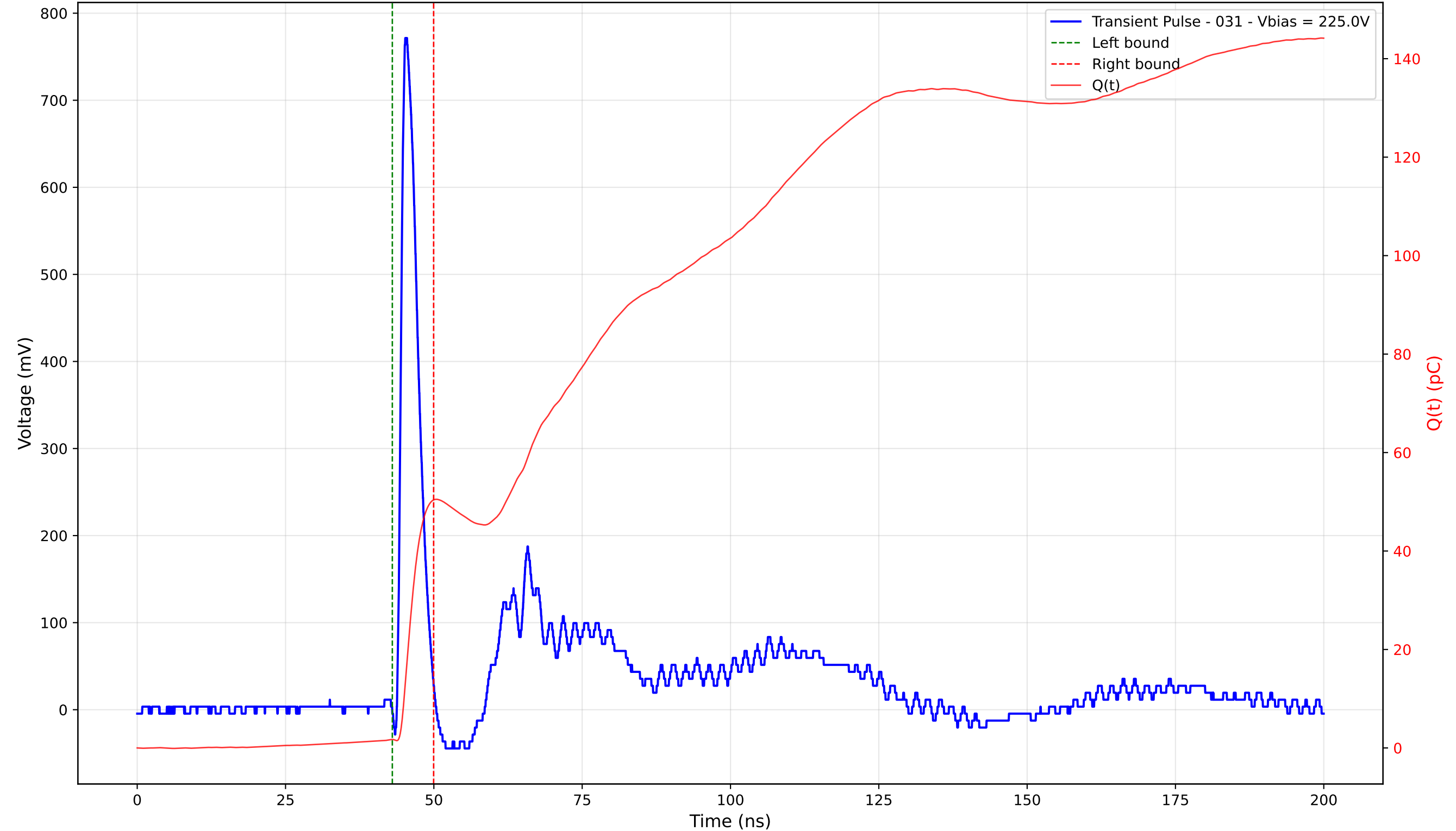
Transient Pulse - Sample: TD_4004 - Position: 190.0 \mu\text{m} - Charge: 48.66 pC - Rise Time: 0.90 ns
