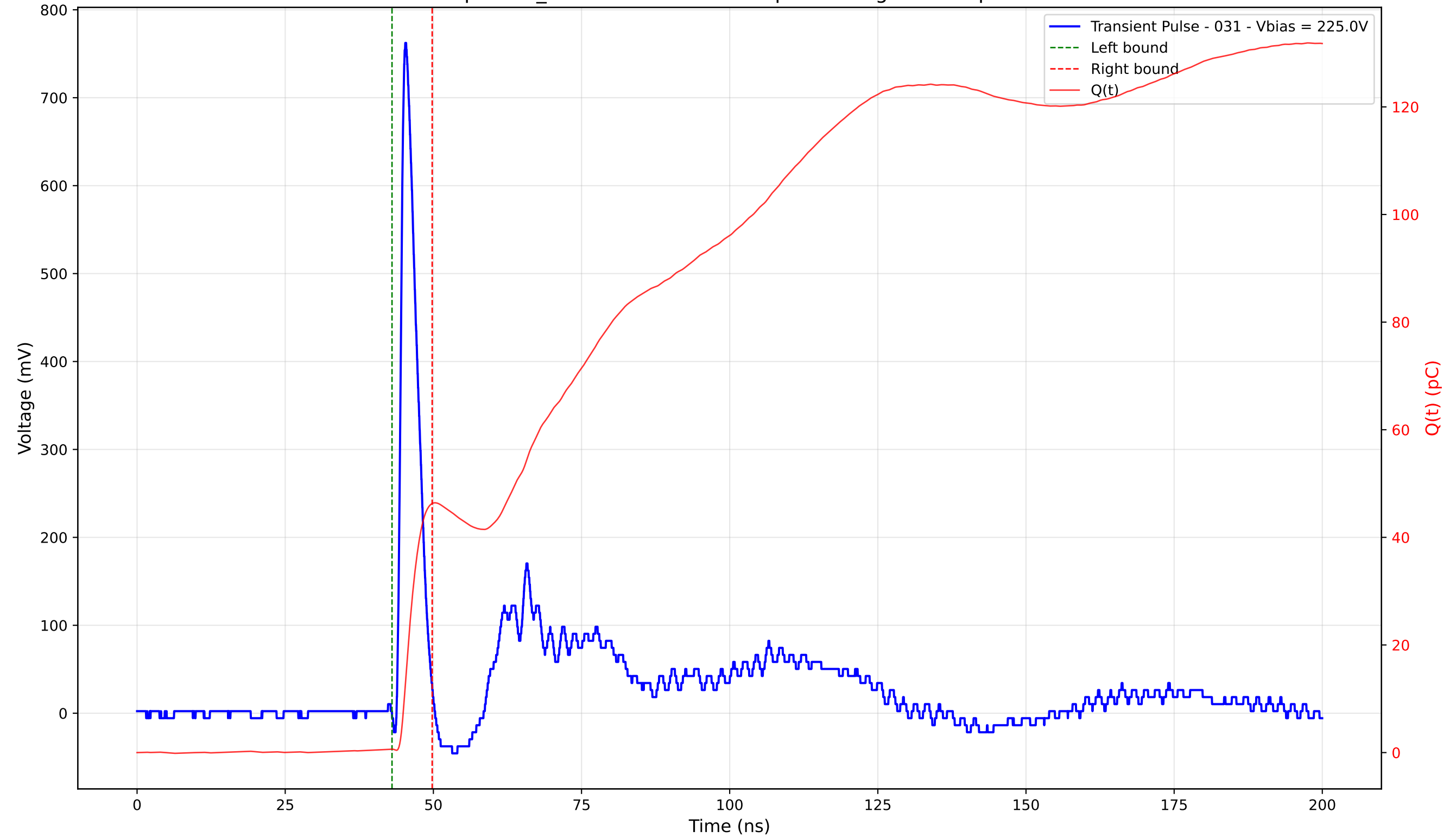
Transient Pulse - Sample: TD_4004 - Position: 125.0 \mu\text{m} - Charge: 45.66 pC - Rise Time: 0.92 ns
