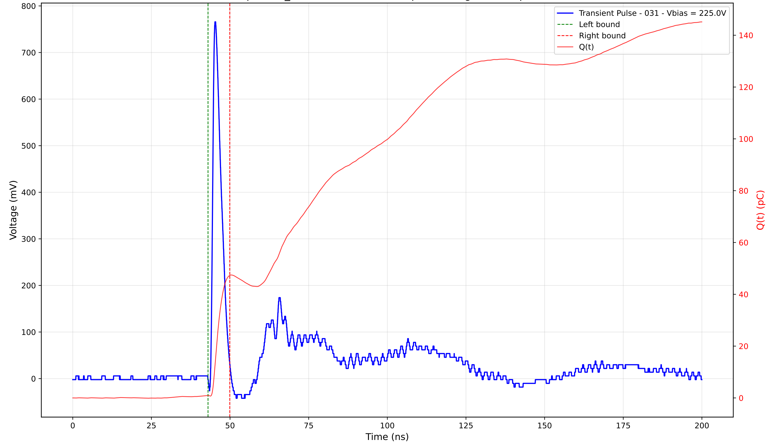
Transient Pulse - Sample: TD_4004 - Position: 120.0 \mu\text{m} - Charge: 46.36 pC - Rise Time: 0.89 ns
