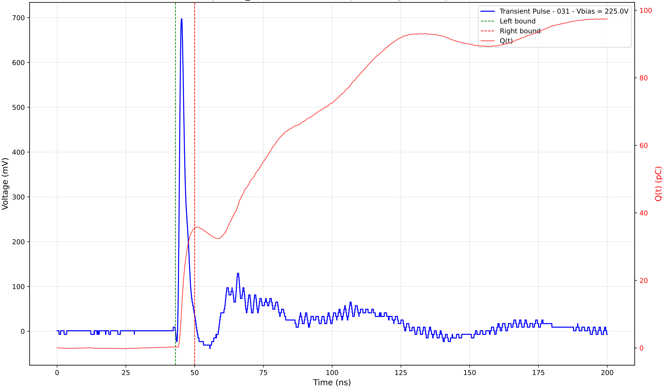
Transient Pulse - Sample: TD_4004 - Position: 85.0 \mu\text{m} - Charge: 35.14 pC - Rise Time: 0.87 ns
