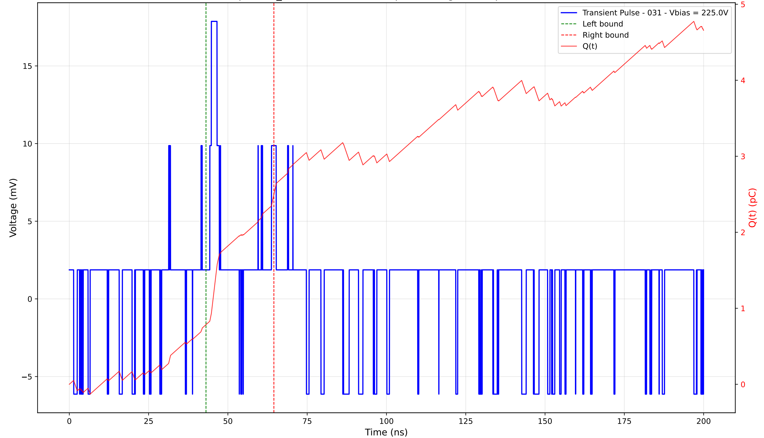
Transient Pulse - Sample: TD_4004 - Position: 25.0 \mu\text{m} - Charge: 1.71 pC - Rise Time: 0.00 ns (N/A)
