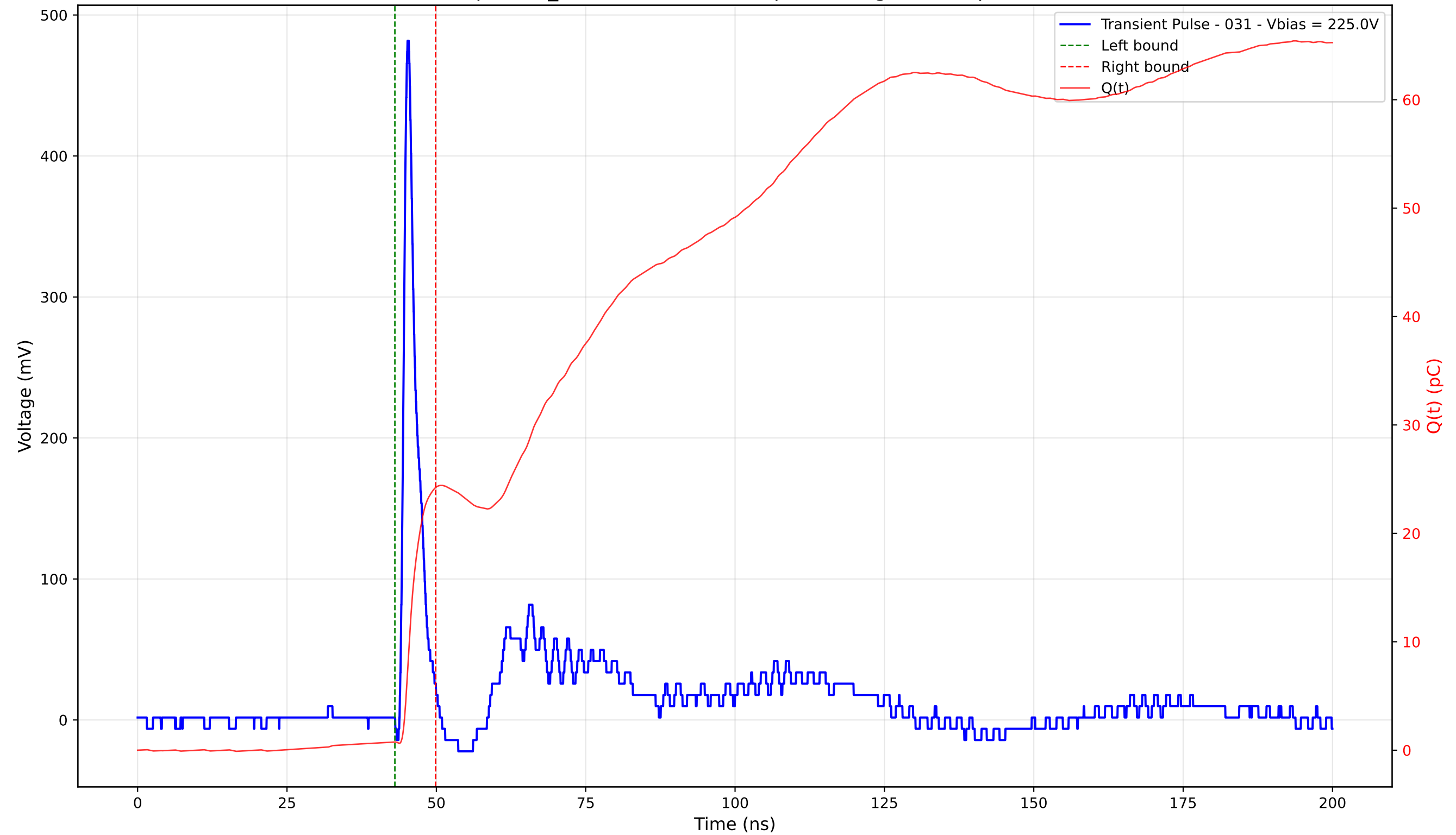
Transient Pulse - Sample: TD_4004 - Position: 70.0 \mu\text{m} - Charge: 23.46 pC - Rise Time: 0.90 ns
