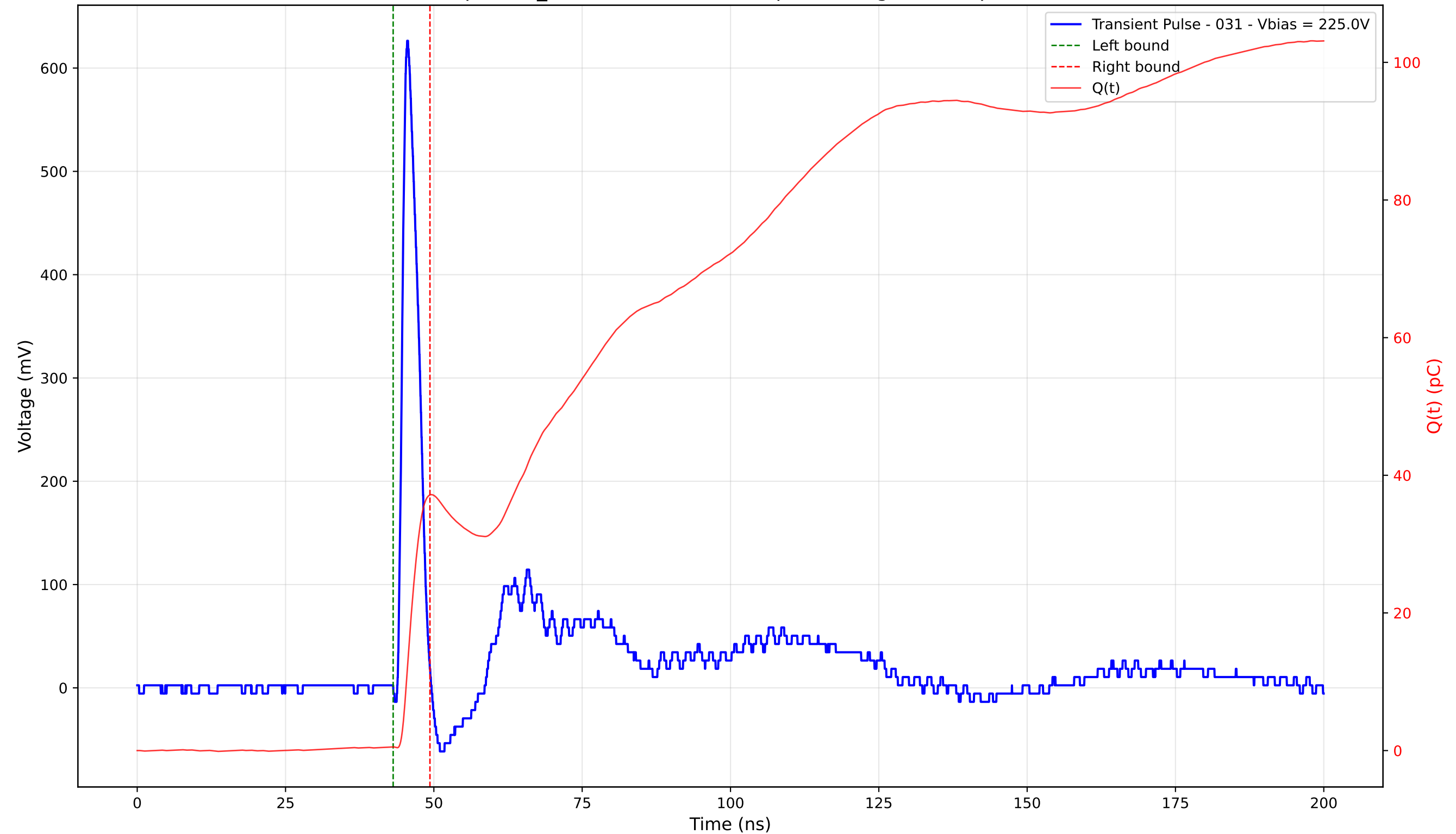
Transient Pulse - Sample: TD_4004 - Position: 325.0 \mu\text{m} - Charge: 36.60 pC - Rise Time: 1.03 ns
