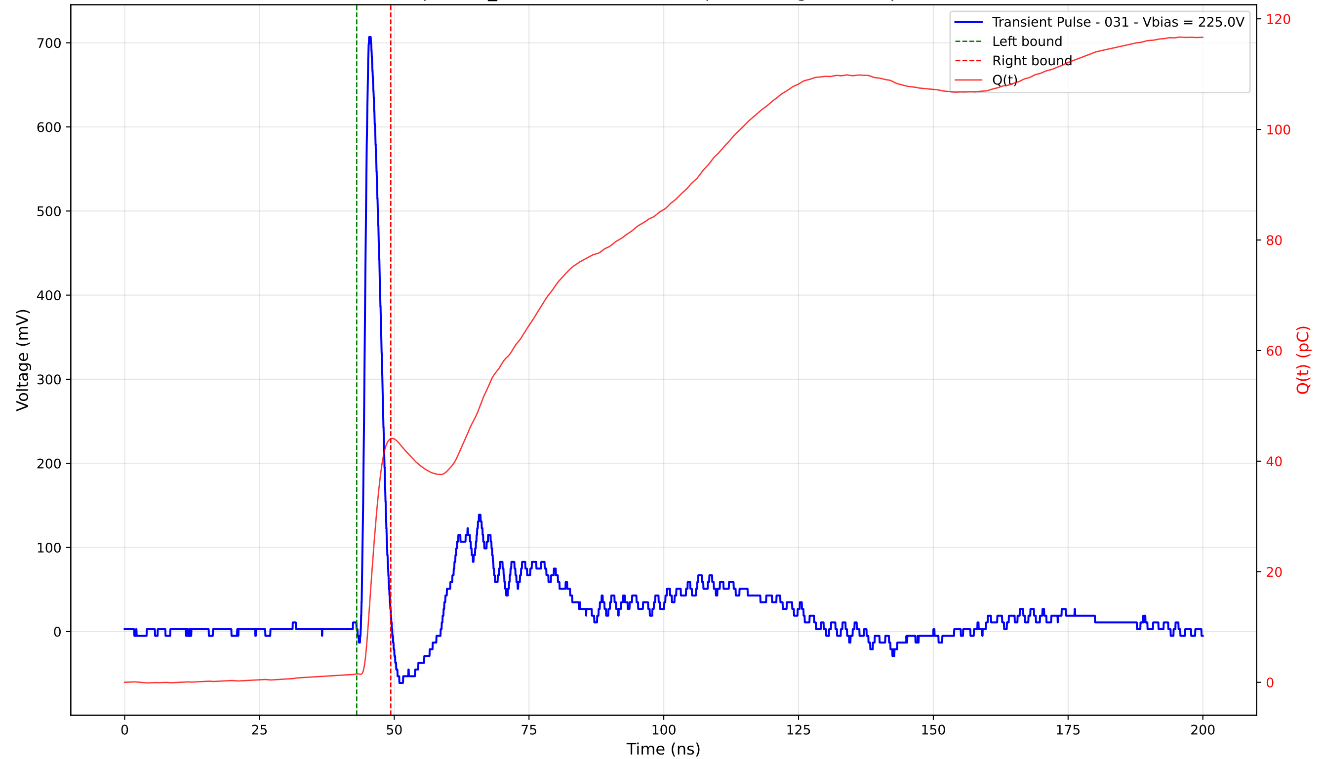
Transient Pulse - Sample: TD_4004 - Position: 265.0 \mu\text{m} - Charge: 42.54 pC - Rise Time: 0.99 ns
