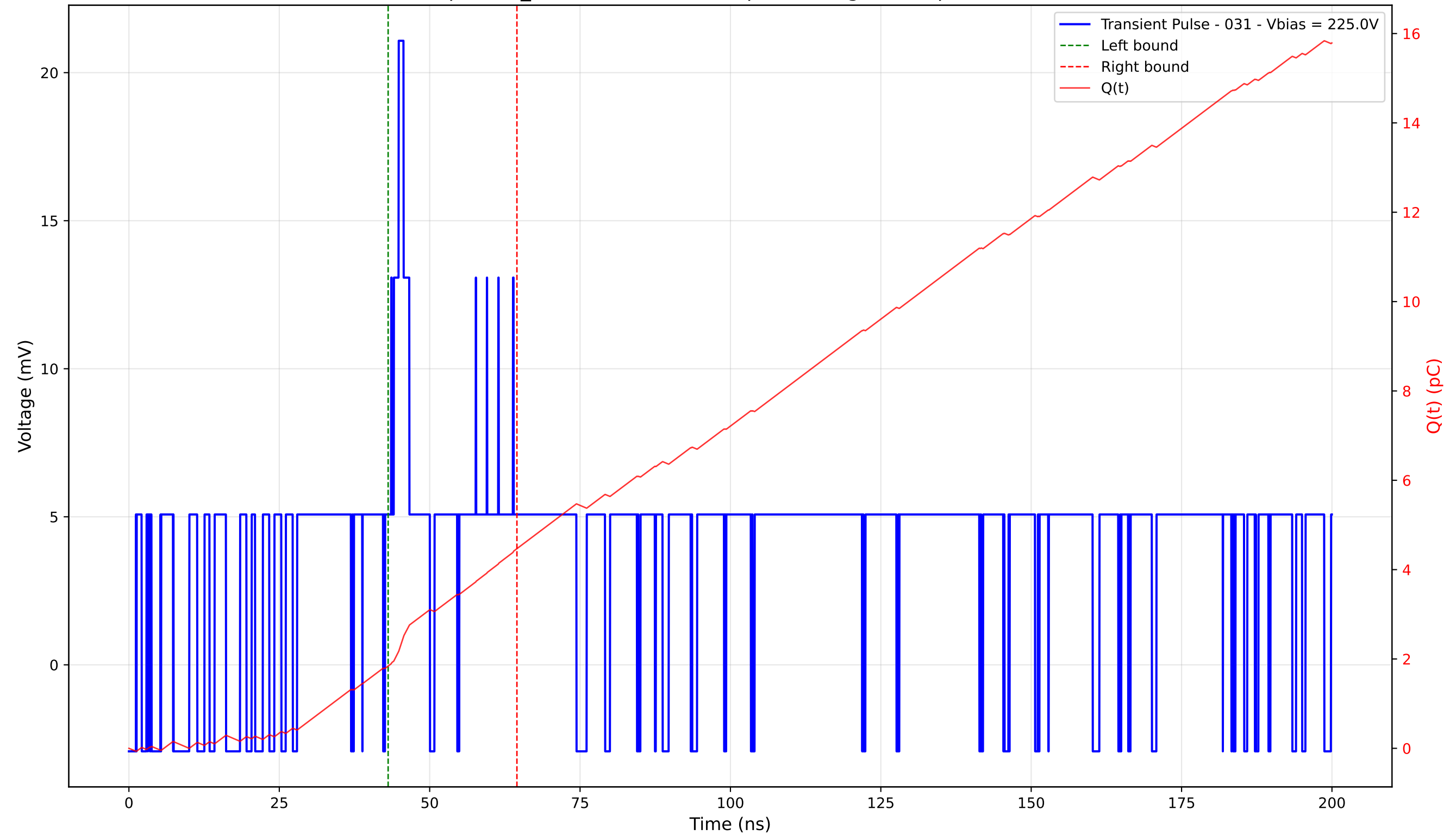
Transient Pulse - Sample: TD_4004 - Position: 15.0 \mu m - Charge: 2.63 pC - Rise Time: 0.00 ns (N/A)
