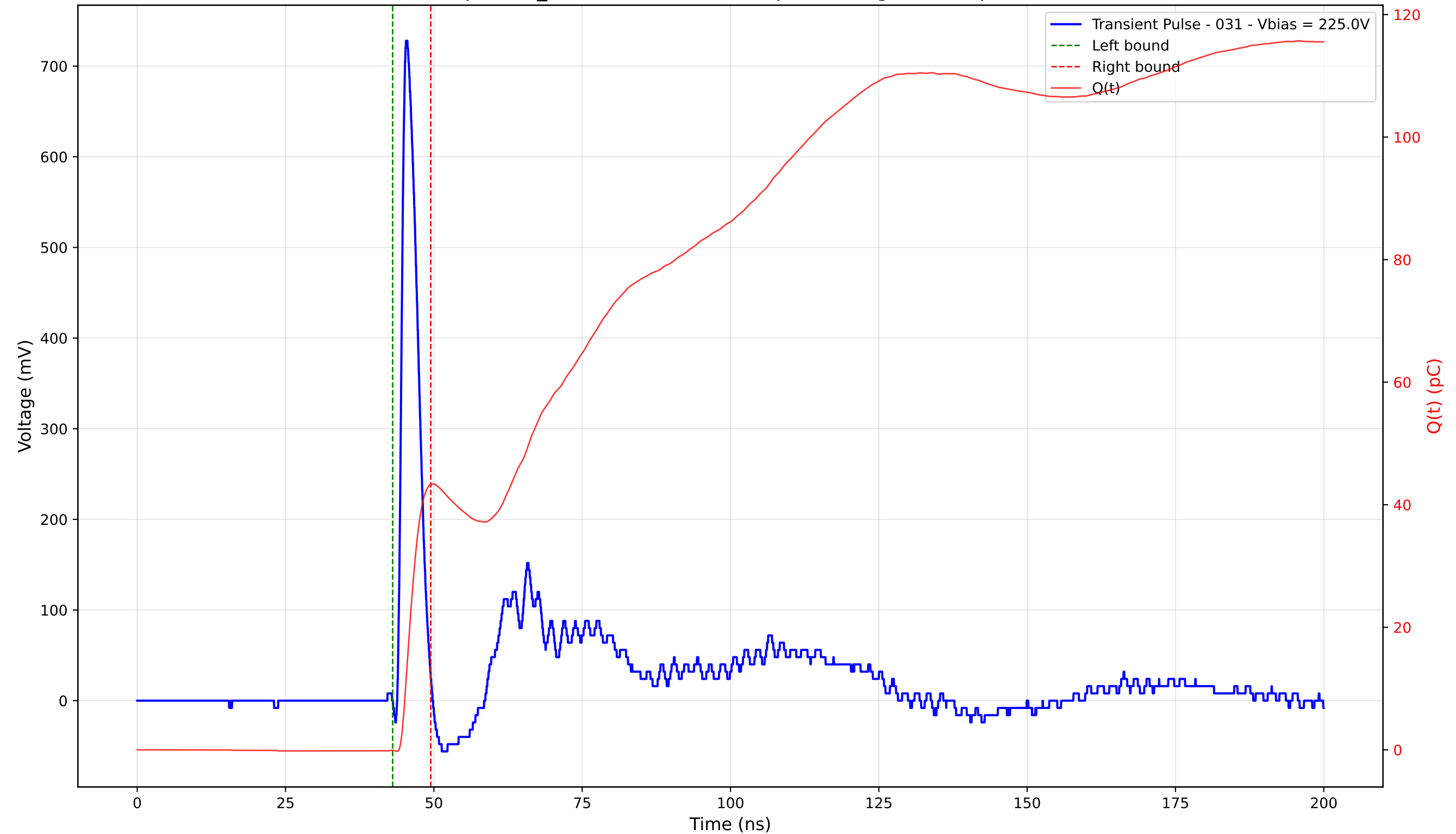
Transient Pulse - Sample: TD_4004 - Position: 235.0 \mu\text{m} - Charge: 43.39 pC - Rise Time: 0.96 ns
