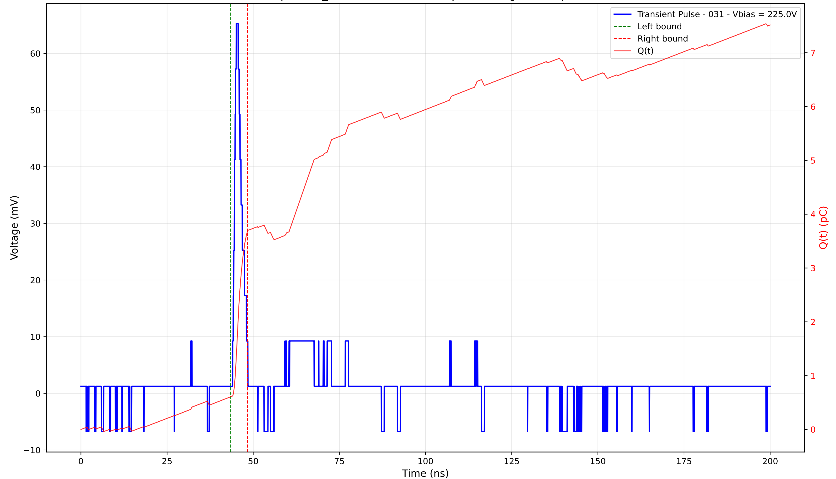
Transient Pulse - Sample: TD_4004 - Position: 45.0 \mu\text{m} - Charge: 3.08 pC - Rise Time: 1.03 ns
