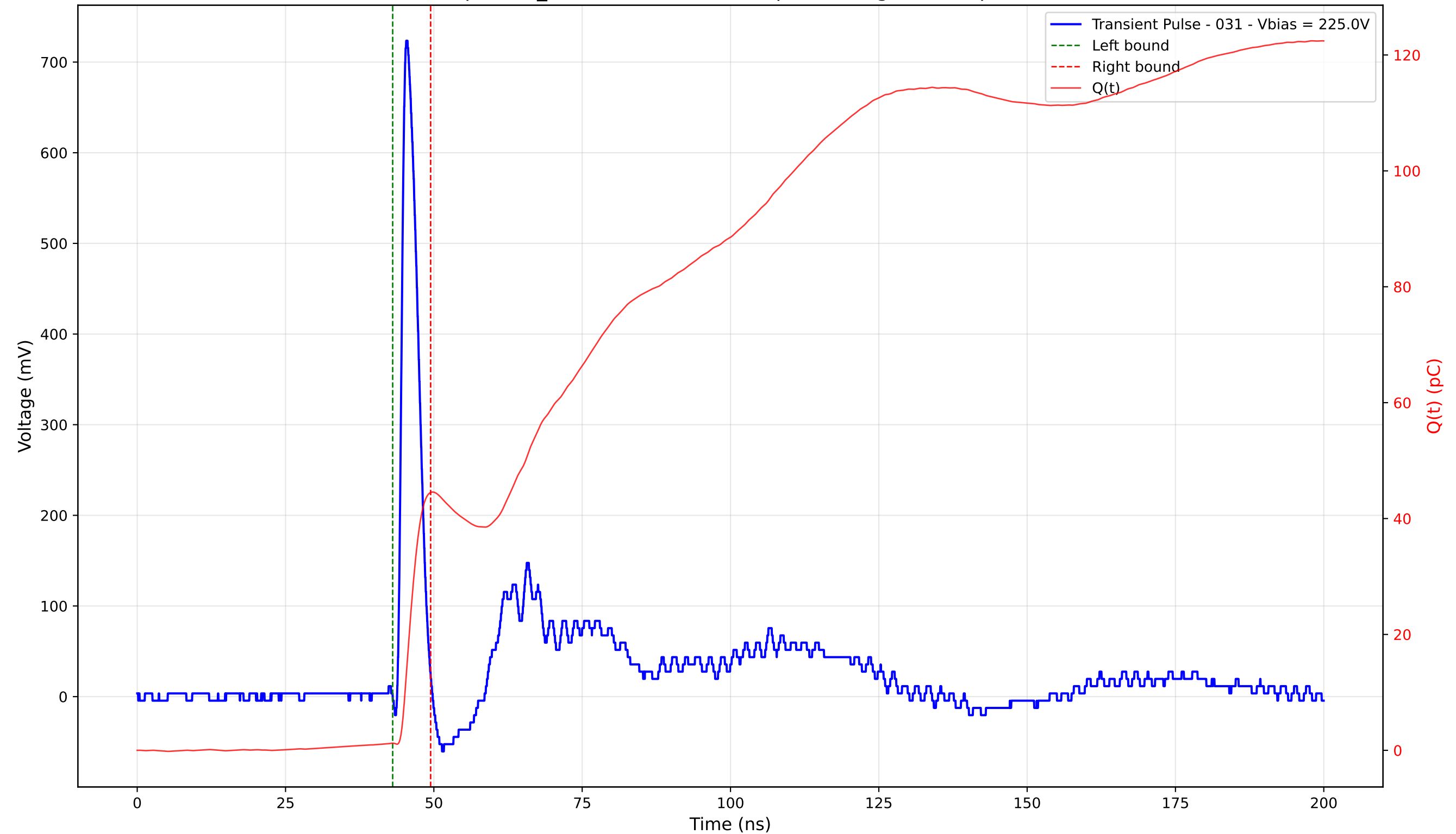
Transient Pulse - Sample: TD_4004 - Position: 255.0 \mu\text{m} - Charge: 43.27 pC - Rise Time: 0.95 ns
