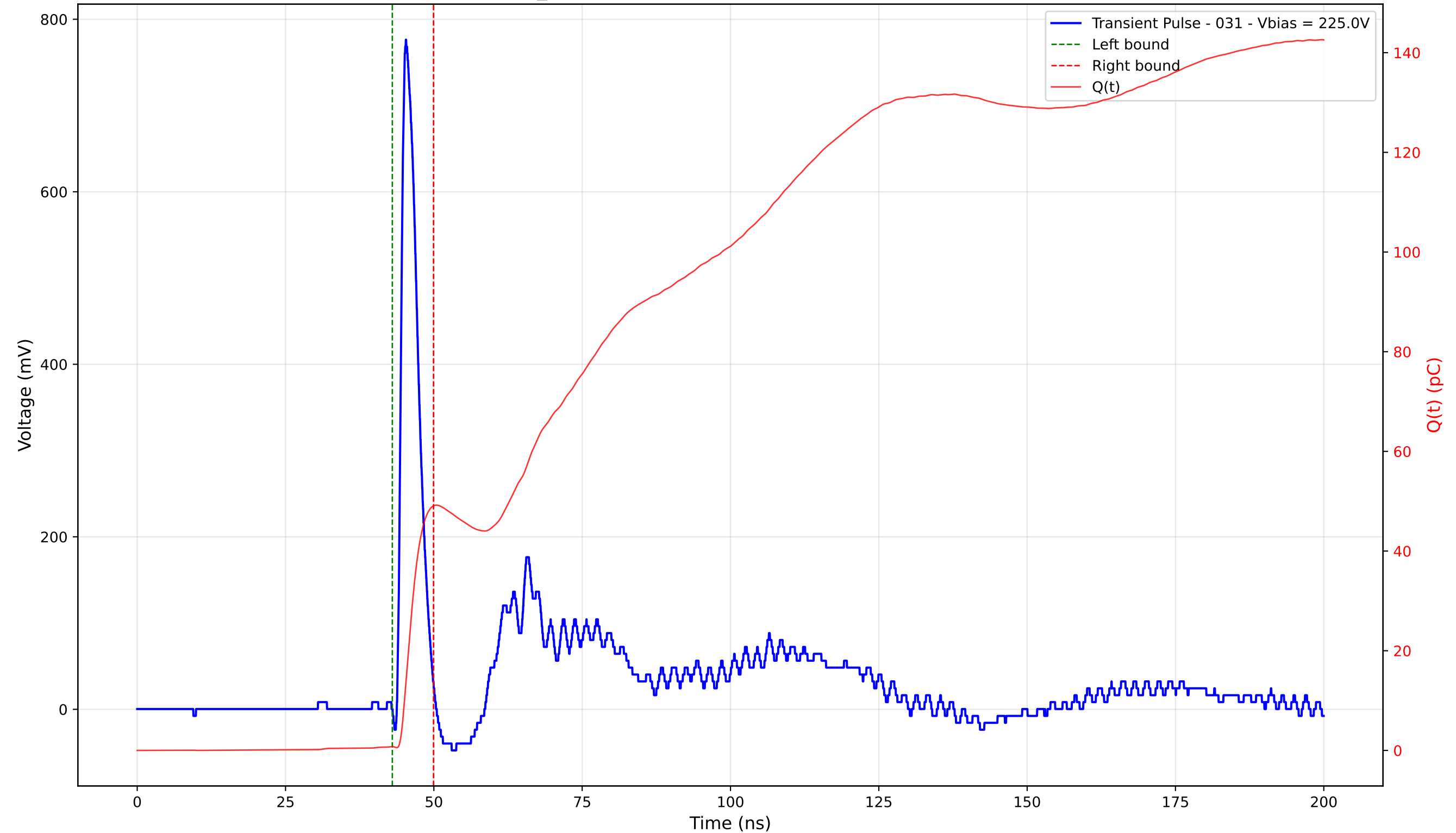
Transient Pulse - Sample: TD_4004 - Position: 195.0 \mu\text{m} - Charge: 48.31 pC - Rise Time: 0.91 ns
