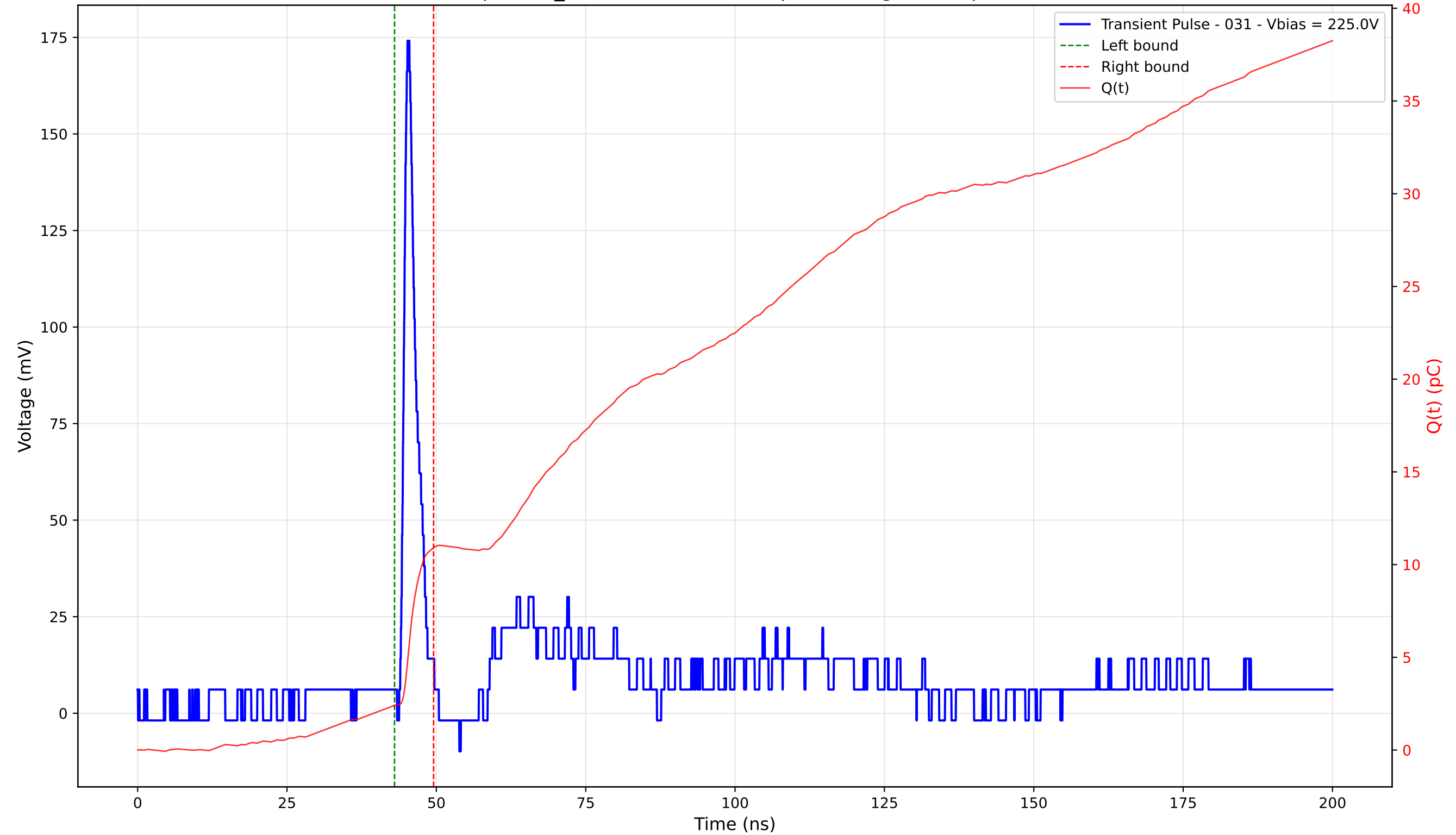
Transient Pulse - Sample: TD_4004 - Position: 55.0 \mu\text{m} - Charge: 8.51 pC - Rise Time: 0.91 ns
