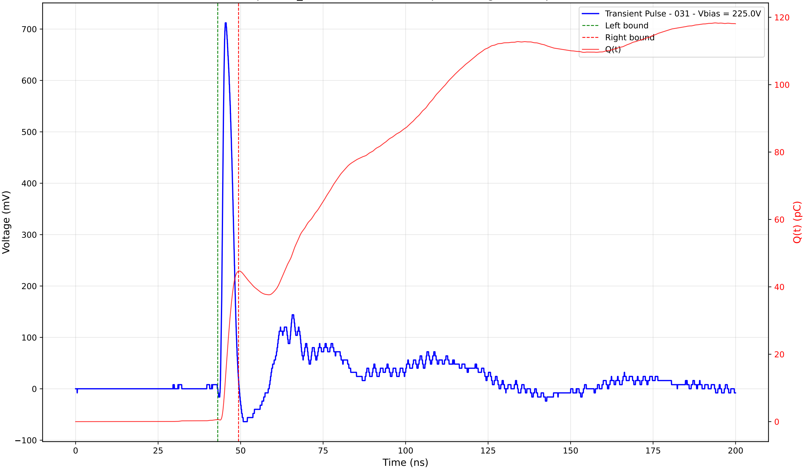
Transient Pulse - Sample: TD_4004 - Position: 290.0 \mu\text{m} - Charge: 44.02 pC - Rise Time: 0.98 ns
