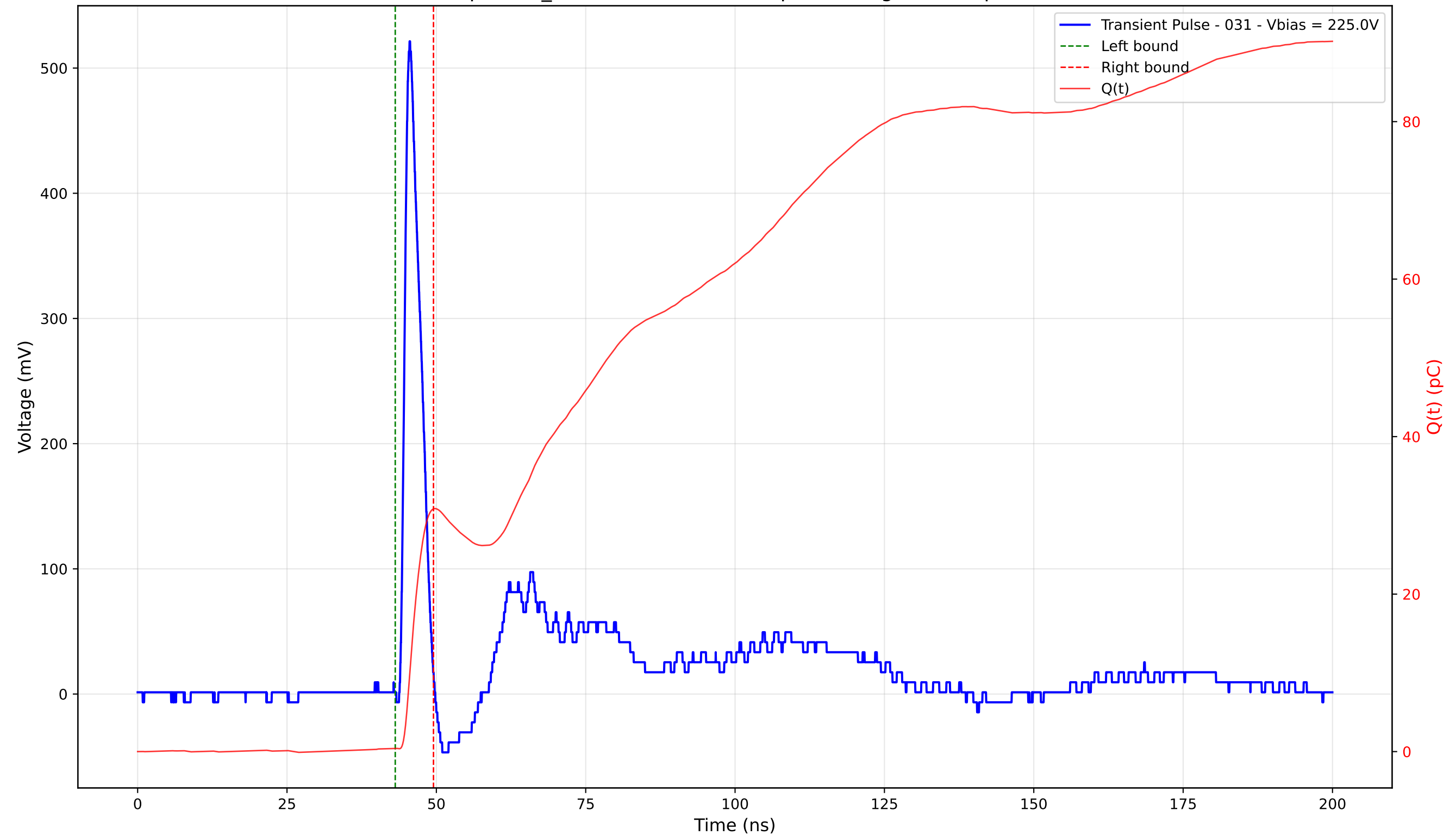
Transient Pulse - Sample: TD_4004 - Position: 350.0 \mu\text{m} - Charge: 30.41 pC - Rise Time: 1.05 ns
