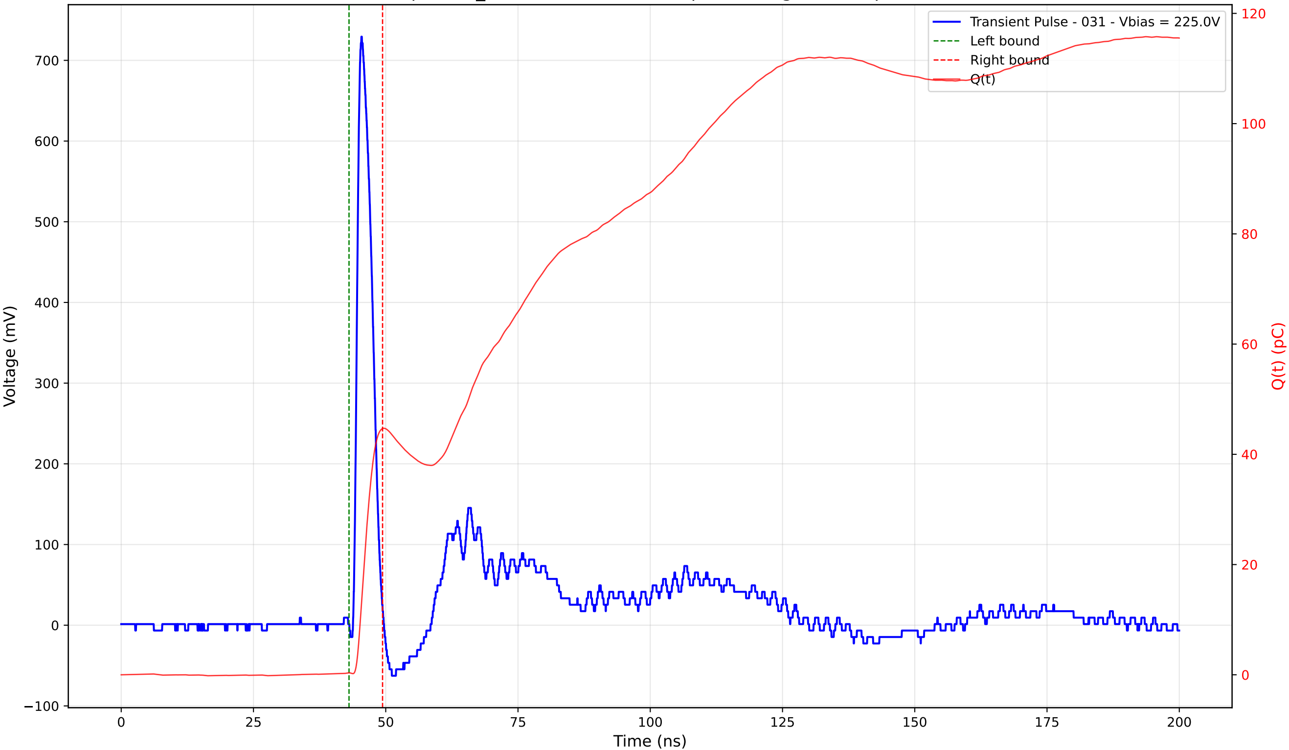
Transient Pulse - Sample: TD_4004 - Position: 280.0 \mu\text{m} - Charge: 44.32 pC - Rise Time: 0.96 ns
