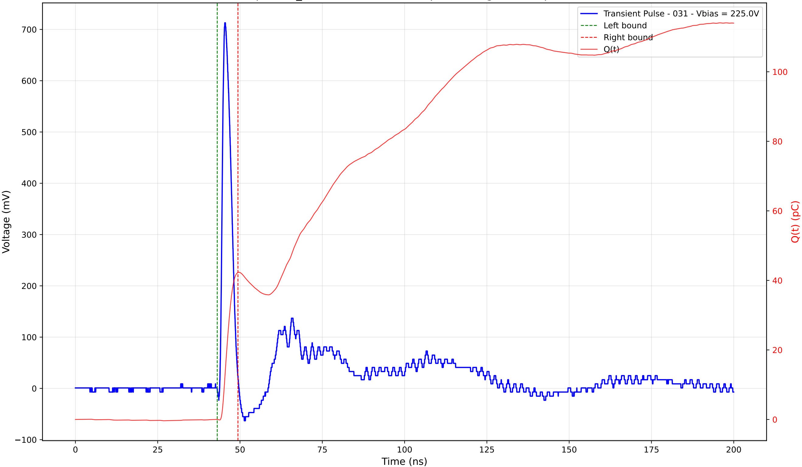
Transient Pulse - Sample: TD_4004 - Position: 260.0 \mu\text{m} - Charge: 42.26 pC - Rise Time: 0.97 ns
