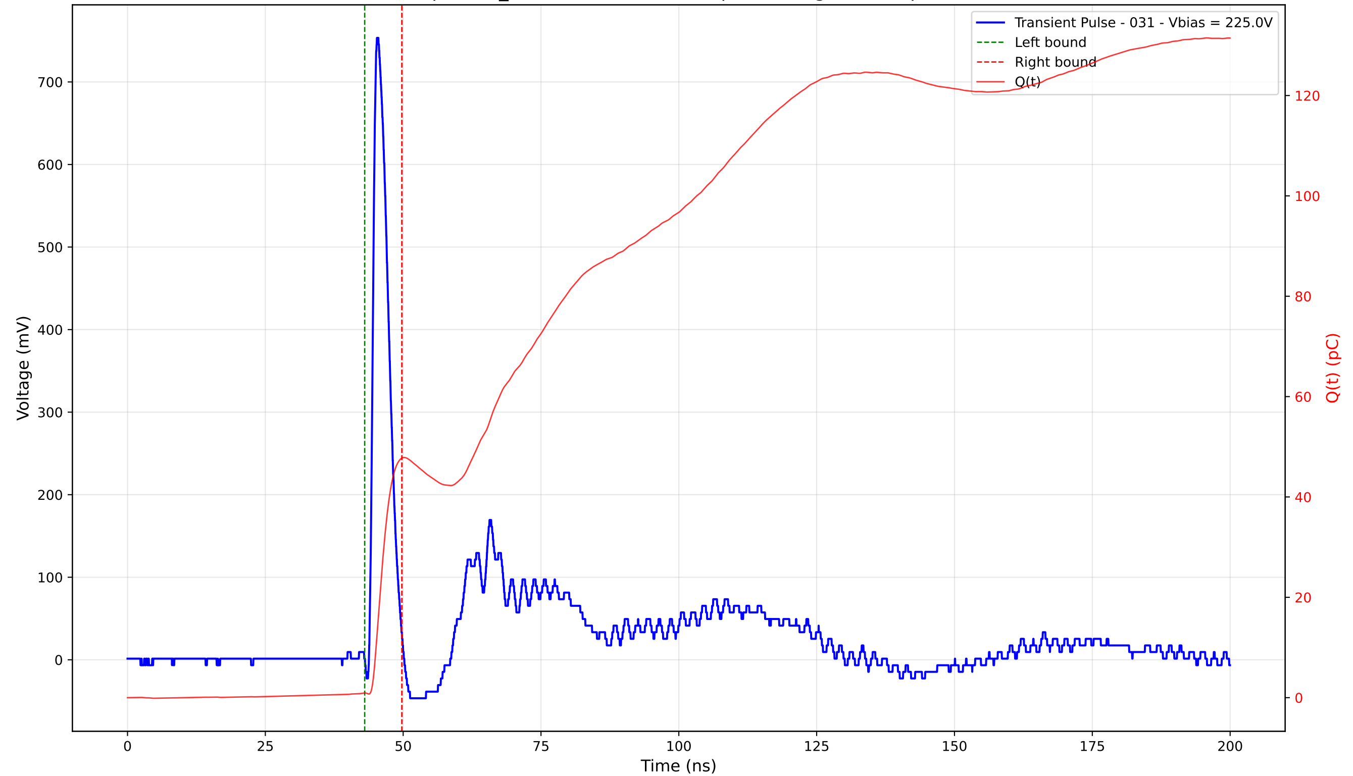
Transient Pulse - Sample: TD_4004 - Position: 215.0 \mu\text{m} - Charge: 46.80 pC - Rise Time: 0.93 ns
