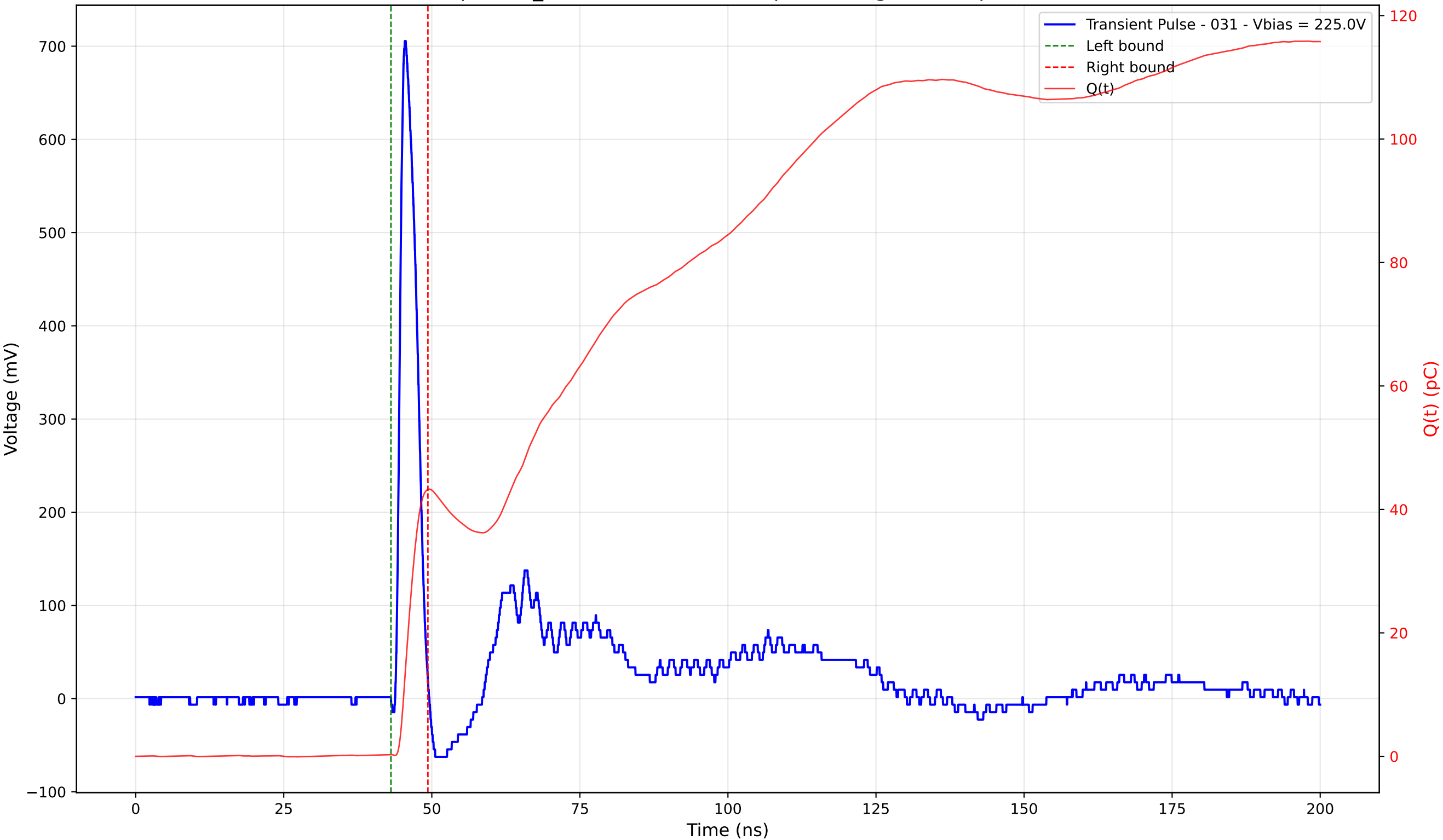
Transient Pulse - Sample: TD_4004 - Position: 295.0 \mu\text{m} - Charge: 42.96 pC - Rise Time: 0.99 ns
