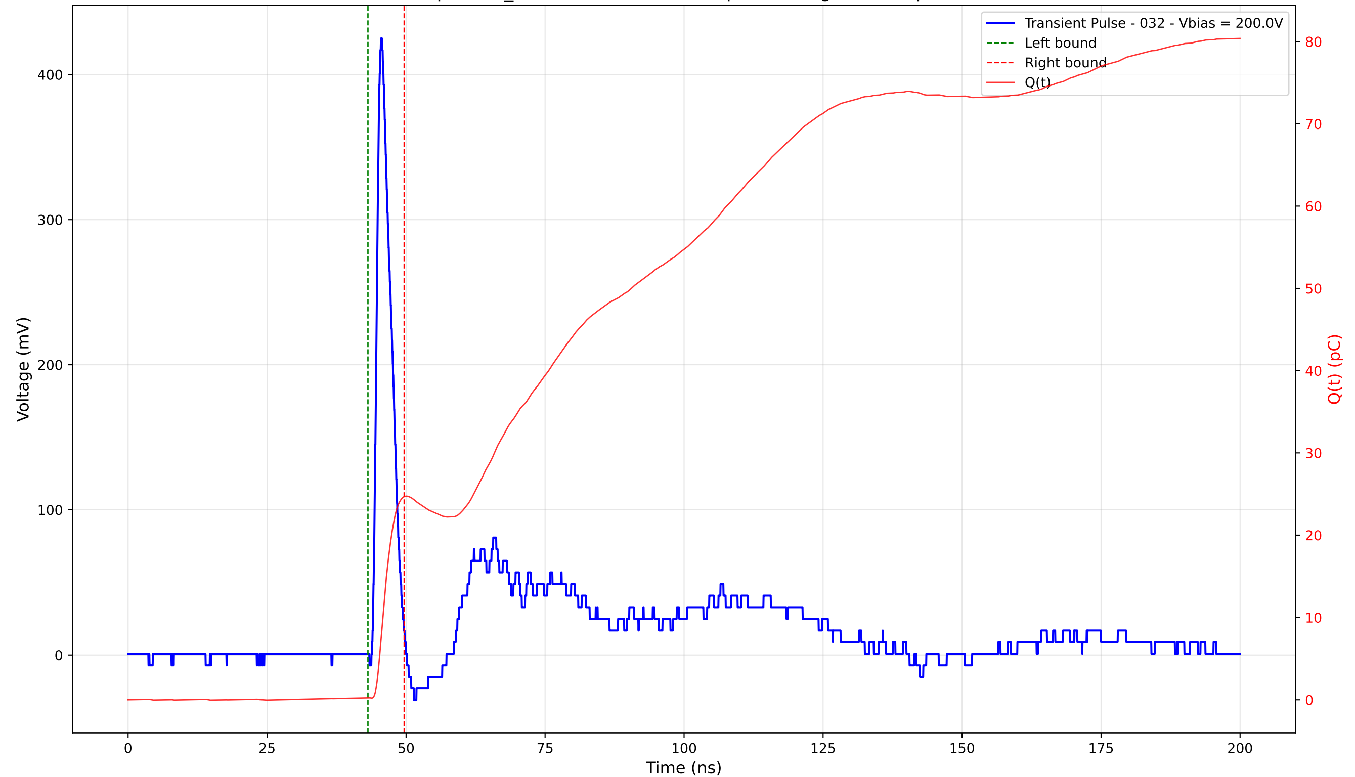
Transient Pulse - Sample: TD_4004 - Position: 375.0 \mu\text{m} - Charge: 24.42 pC - Rise Time: 1.04 ns
