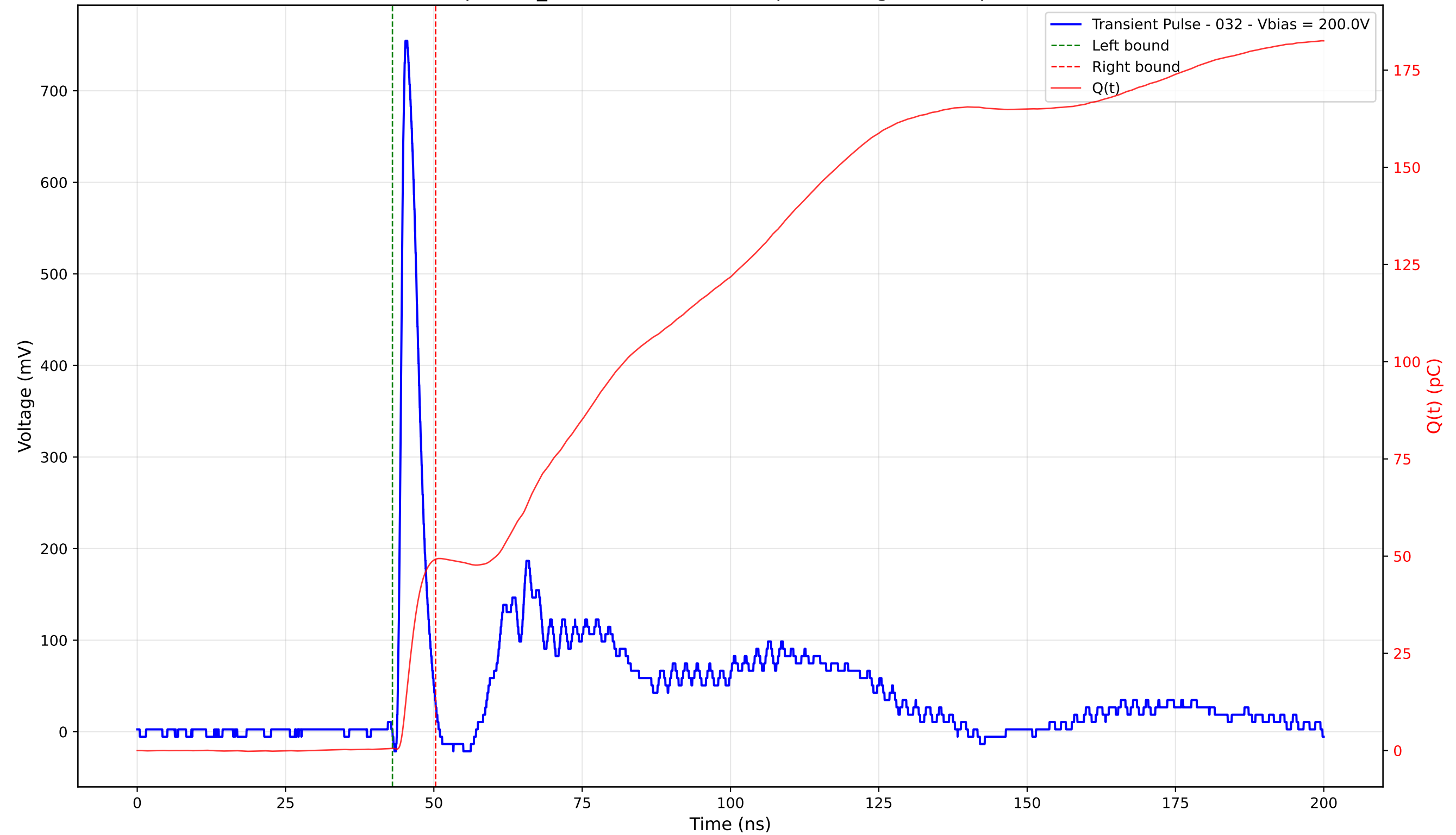
Transient Pulse - Sample: TD_4004 - Position: 205.0 \mu\text{m} - Charge: 48.65 pC - Rise Time: 0.91 ns
