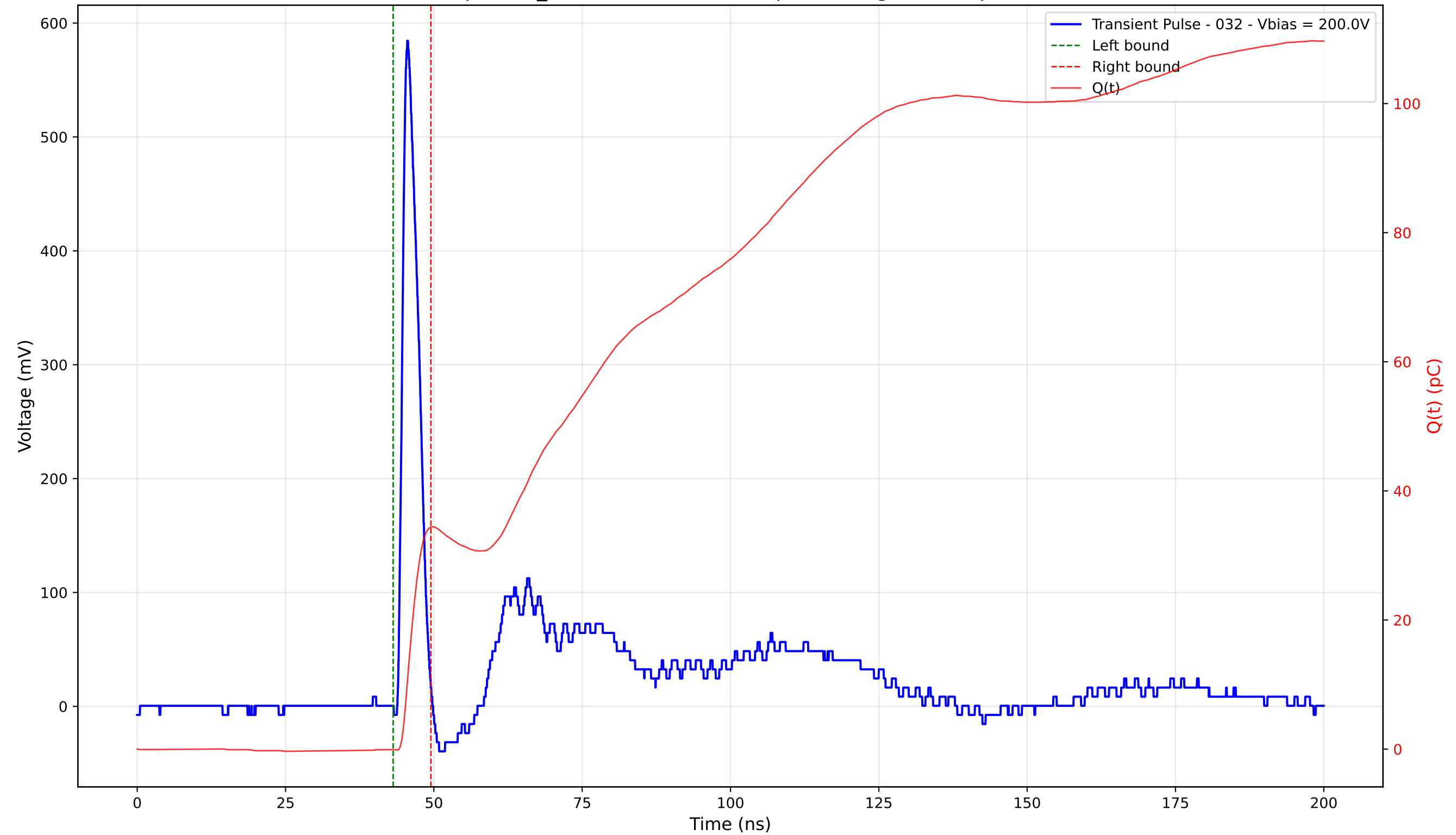
Transient Pulse - Sample: TD_4004 - Position: 325.0 \mu\text{m} - Charge: 34.46 pC - Rise Time: 1.03 ns
