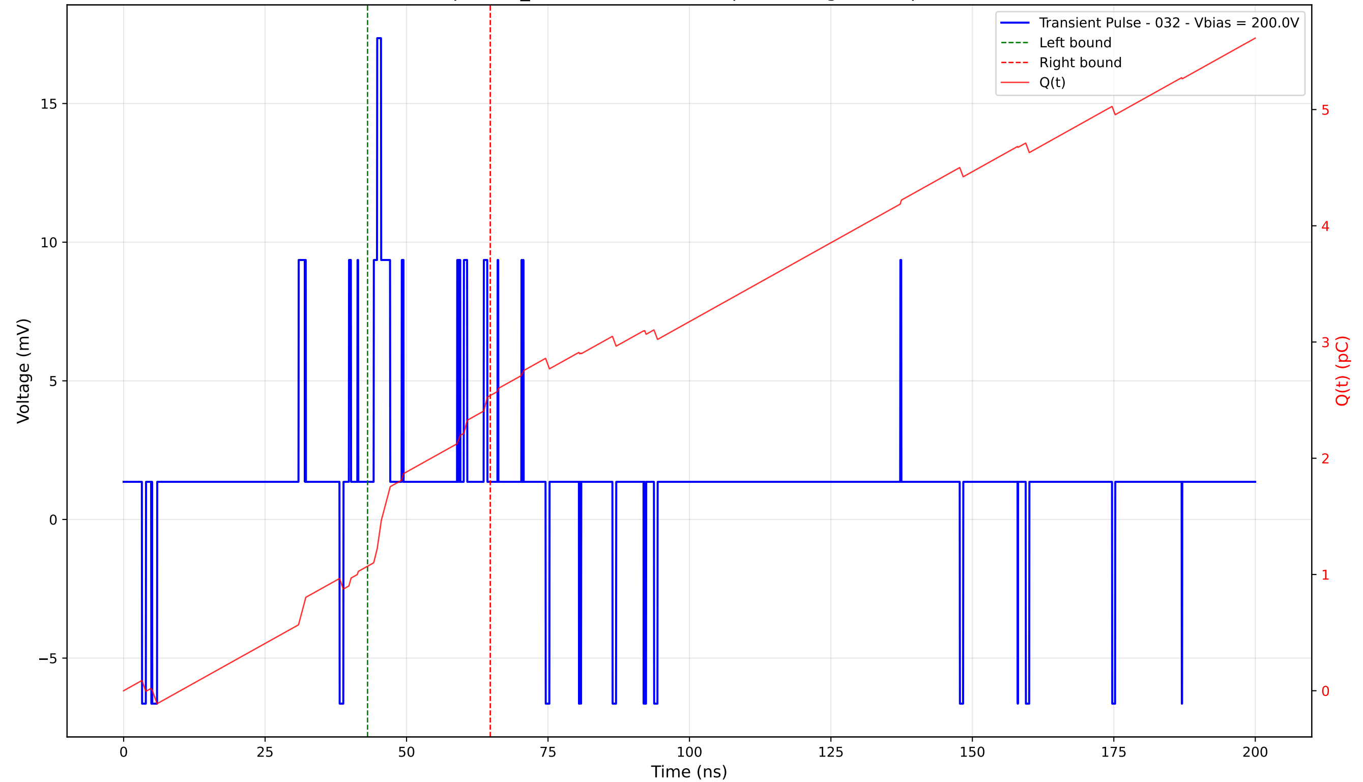
Transient Pulse - Sample: TD_4004 - Position: 10.0 \mu\text{m} - Charge: 1.47 pC - Rise Time: 0.62 ns
