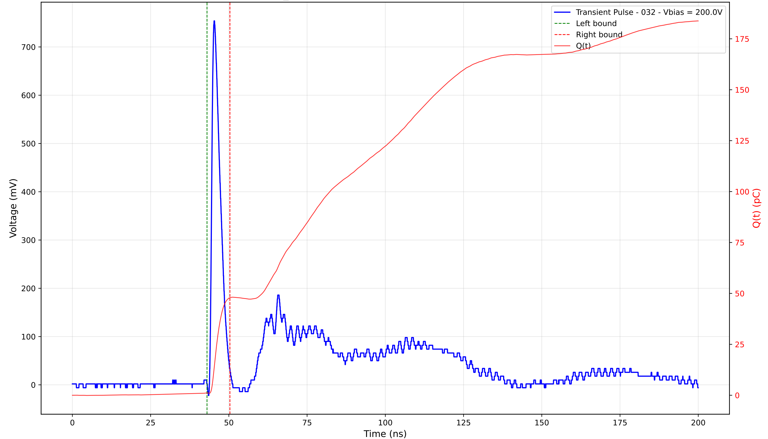
Transient Pulse - Sample: TD_4004 - Position: 125.0 \mu\text{m} - Charge: 46.73 pC - Rise Time: 0.91 ns
