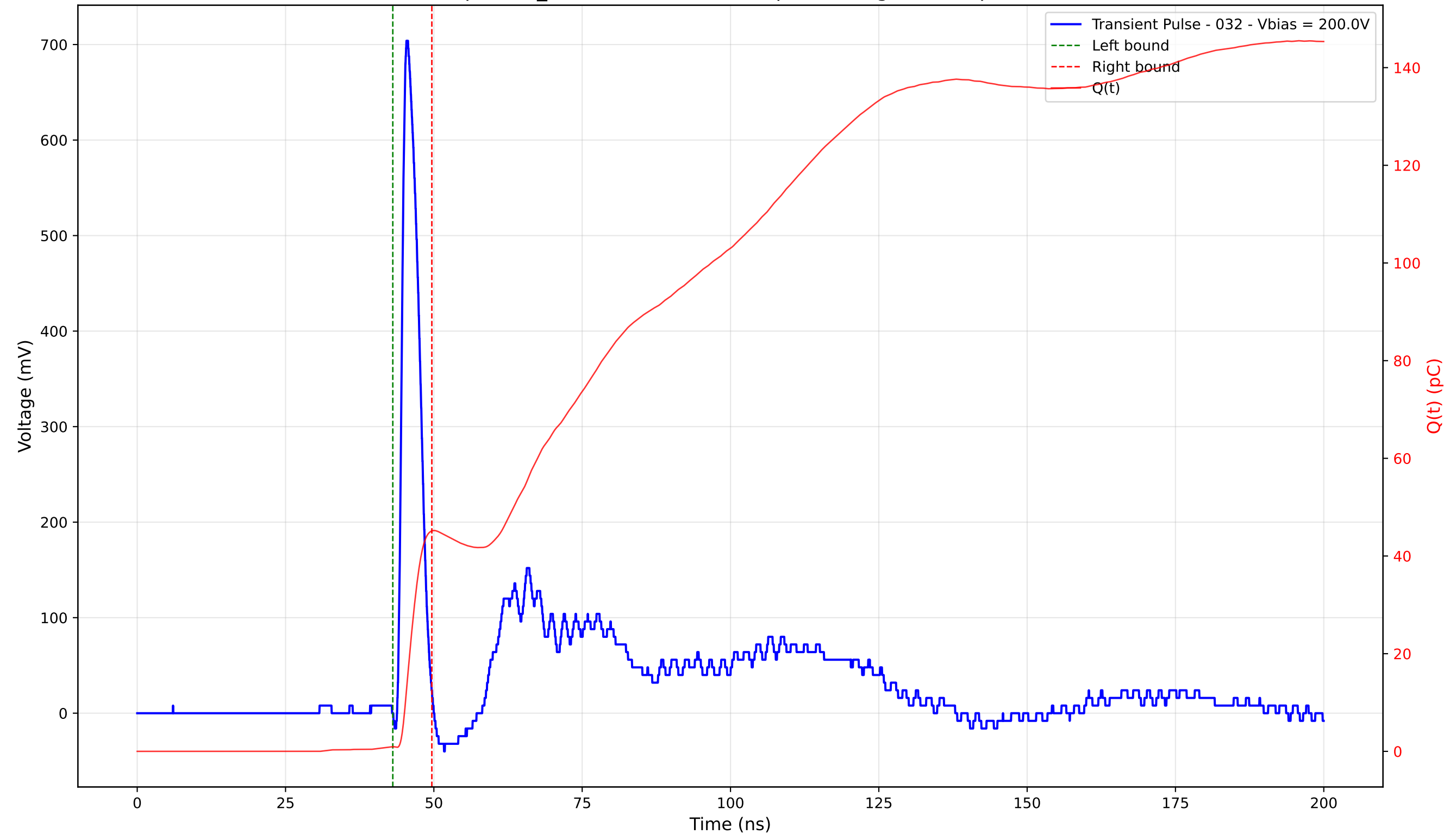
Transient Pulse - Sample: TD_4004 - Position: 285.0 \mu\text{m} - Charge: 44.19 pC - Rise Time: 1.00 ns
