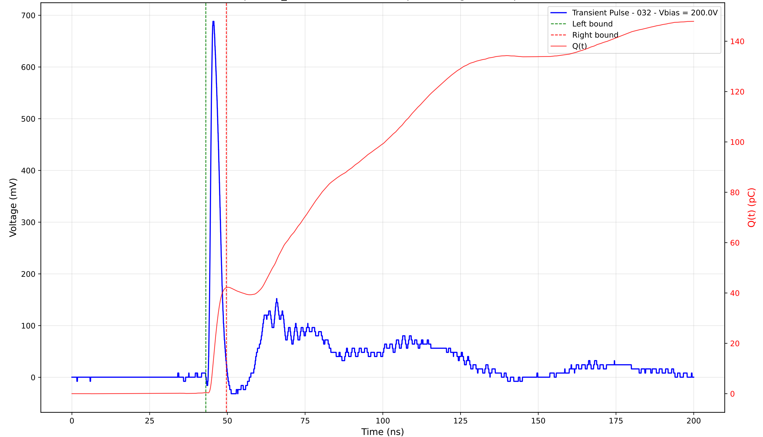
Transient Pulse - Sample: TD_4004 - Position: 260.0 \mu\text{m} - Charge: 41.72 pC - Rise Time: 0.99 ns
