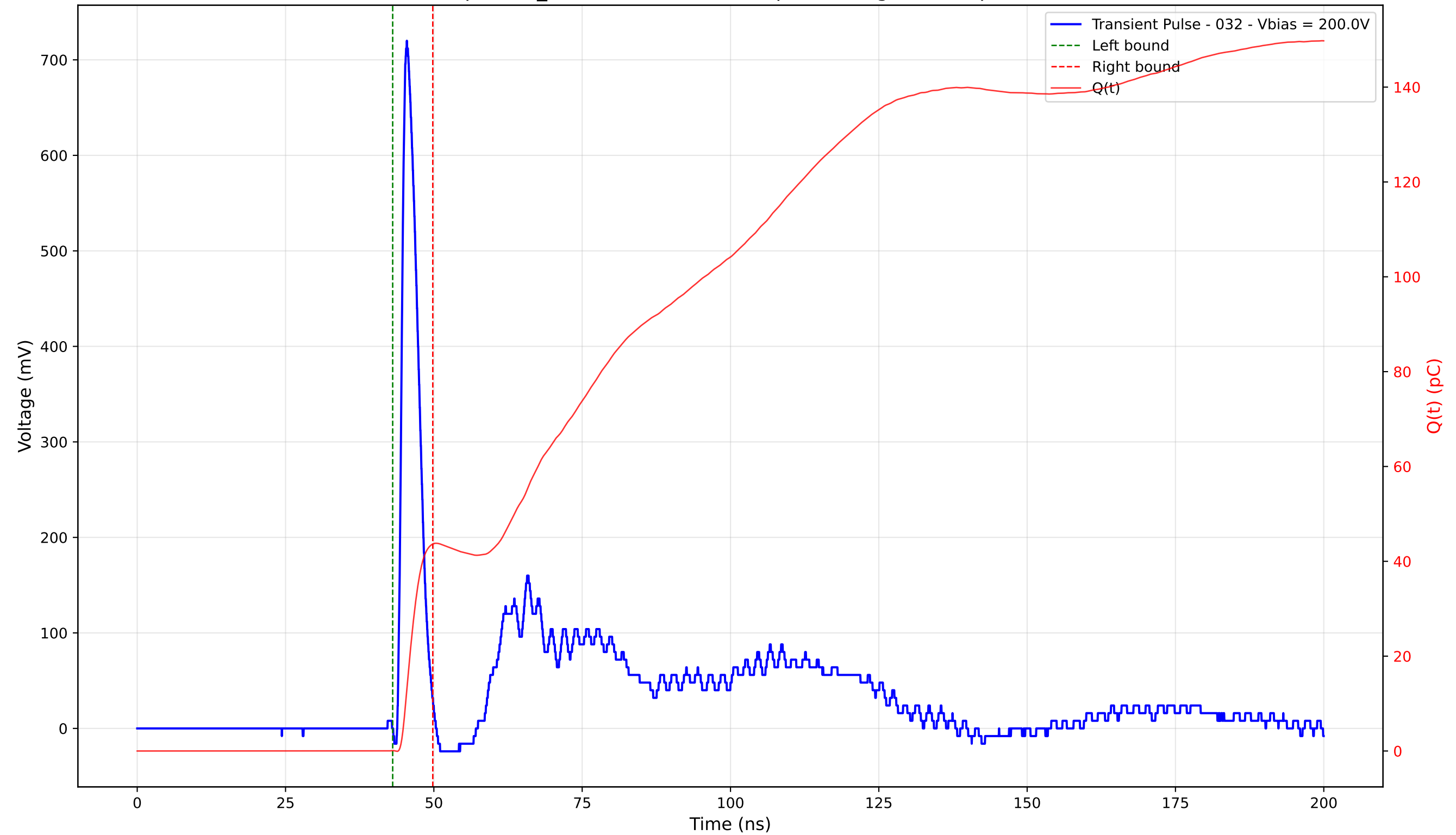
Transient Pulse - Sample: TD_4004 - Position: 235.0 \mu\text{m} - Charge: 43.56 pC - Rise Time: 0.96 ns
