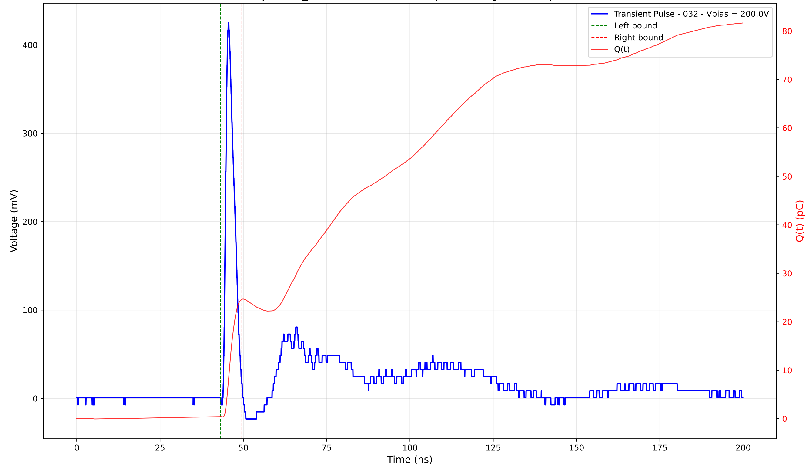
Transient Pulse - Sample: TD_4004 - Position: 380.0 \mu\text{m} - Charge: 24.22 pC - Rise Time: 1.04 ns
