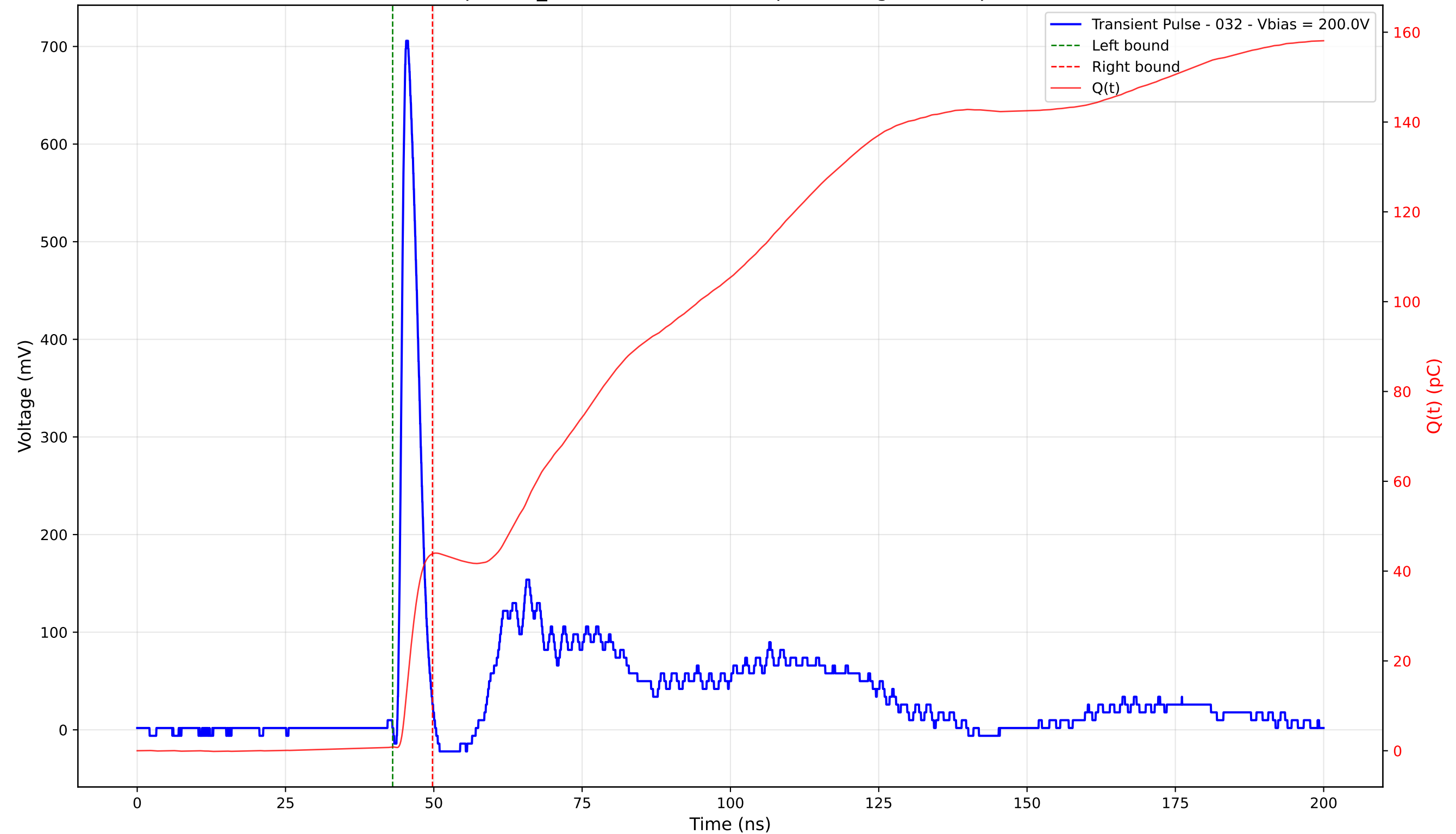
Transient Pulse - Sample: TD_4004 - Position: 245.0 \mu\text{m} - Charge: 43.03 pC - Rise Time: 0.97 ns
