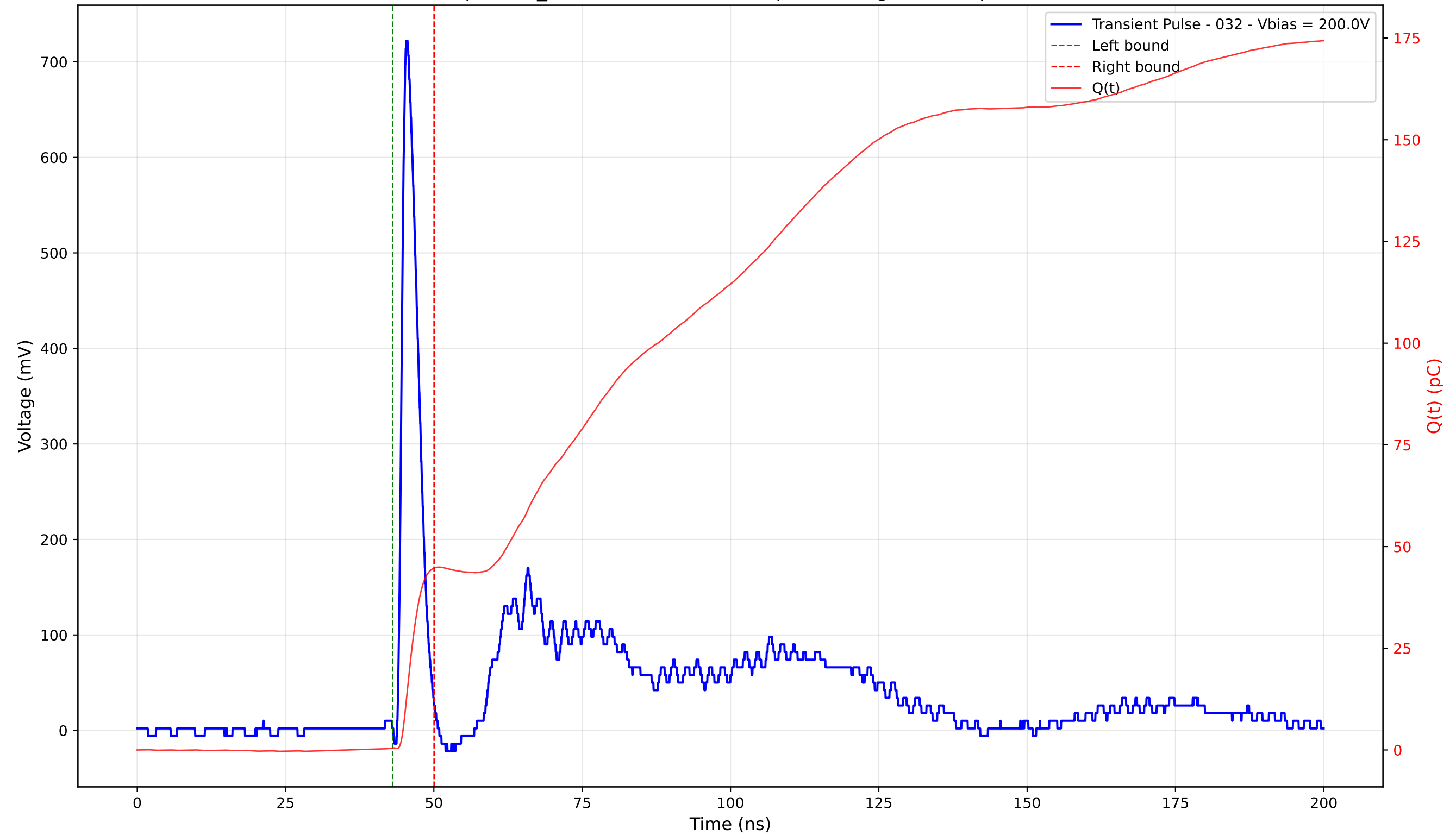
Transient Pulse - Sample: TD_4004 - Position: 145.0 \mu\text{m} - Charge: 44.23 pC - Rise Time: 0.96 ns
