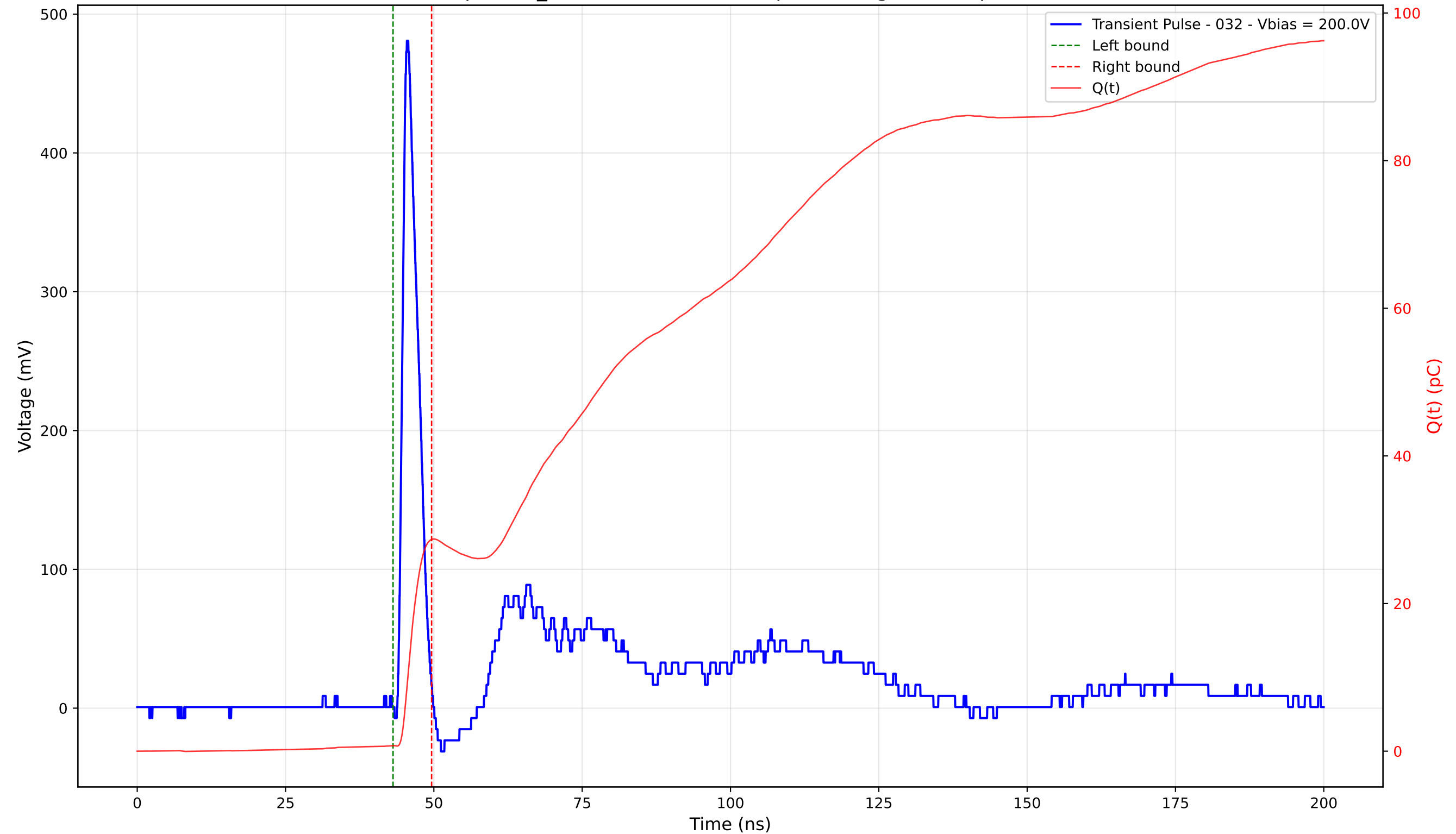
Transient Pulse - Sample: TD_4004 - Position: 345.0 \mu\text{m} - Charge: 27.94 pC - Rise Time: 1.04 ns
