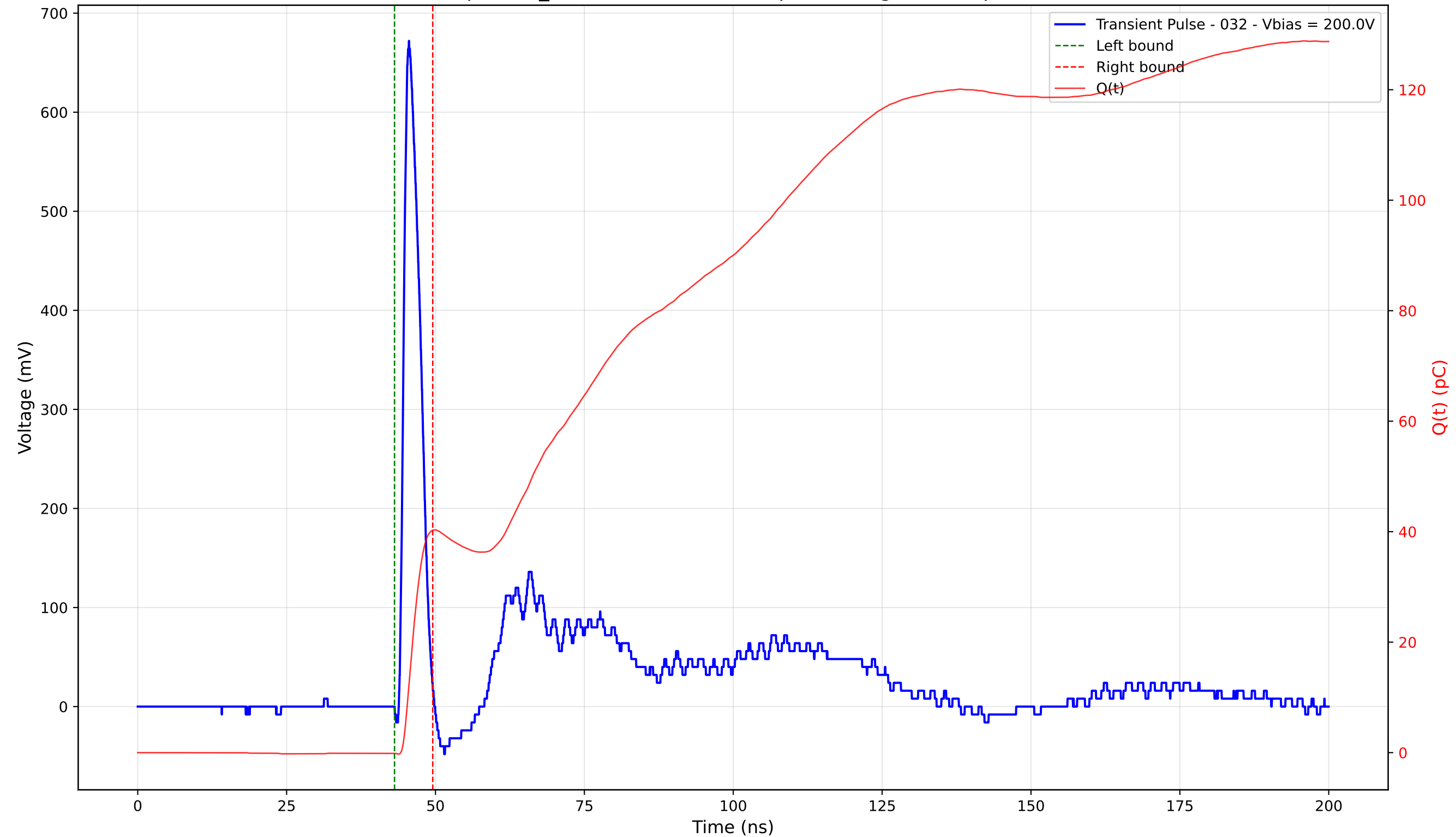
Transient Pulse - Sample: TD_4004 - Position: 305.0 \mu\text{m} - Charge: 40.37 pC - Rise Time: 1.00 ns
