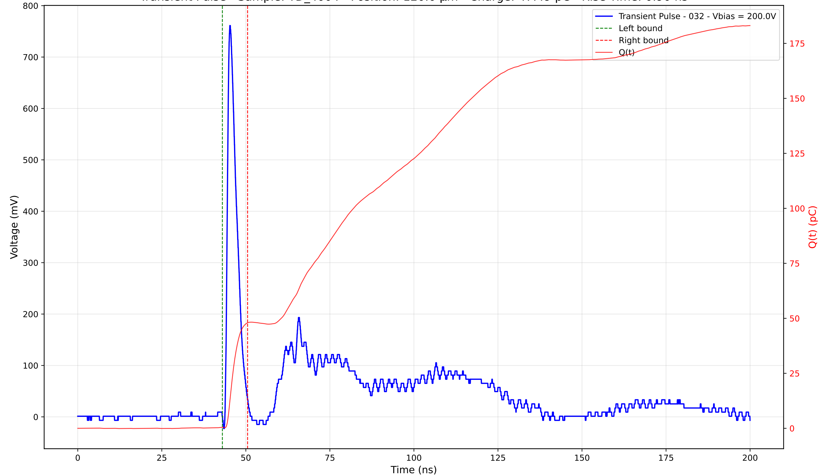
Transient Pulse - Sample: TD_4004 - Position: 120.0 \mu\text{m} - Charge: 47.49 pC - Rise Time: 0.90 ns
