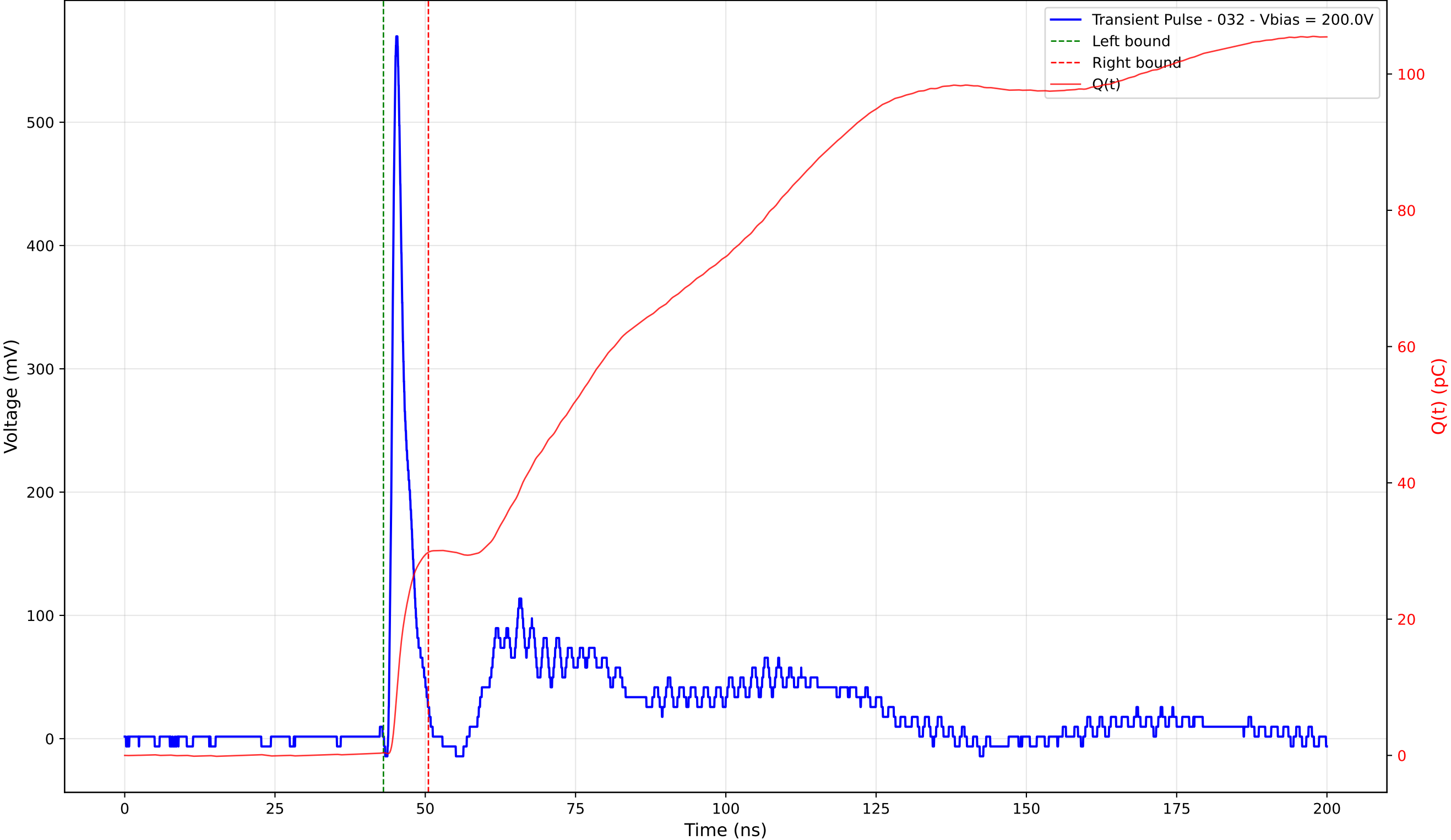
Transient Pulse - Sample: TD_4004 - Position: 75.0 \mu\text{m} - Charge: 29.42 pC - Rise Time: 0.88 ns
