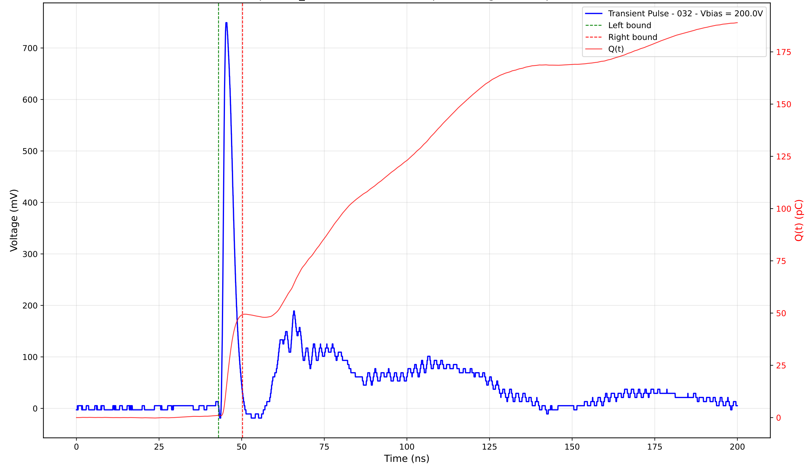
Transient Pulse - Sample: TD_4004 - Position: 210.0 \mu\text{m} - Charge: 48.17 pC - Rise Time: 0.92 ns
