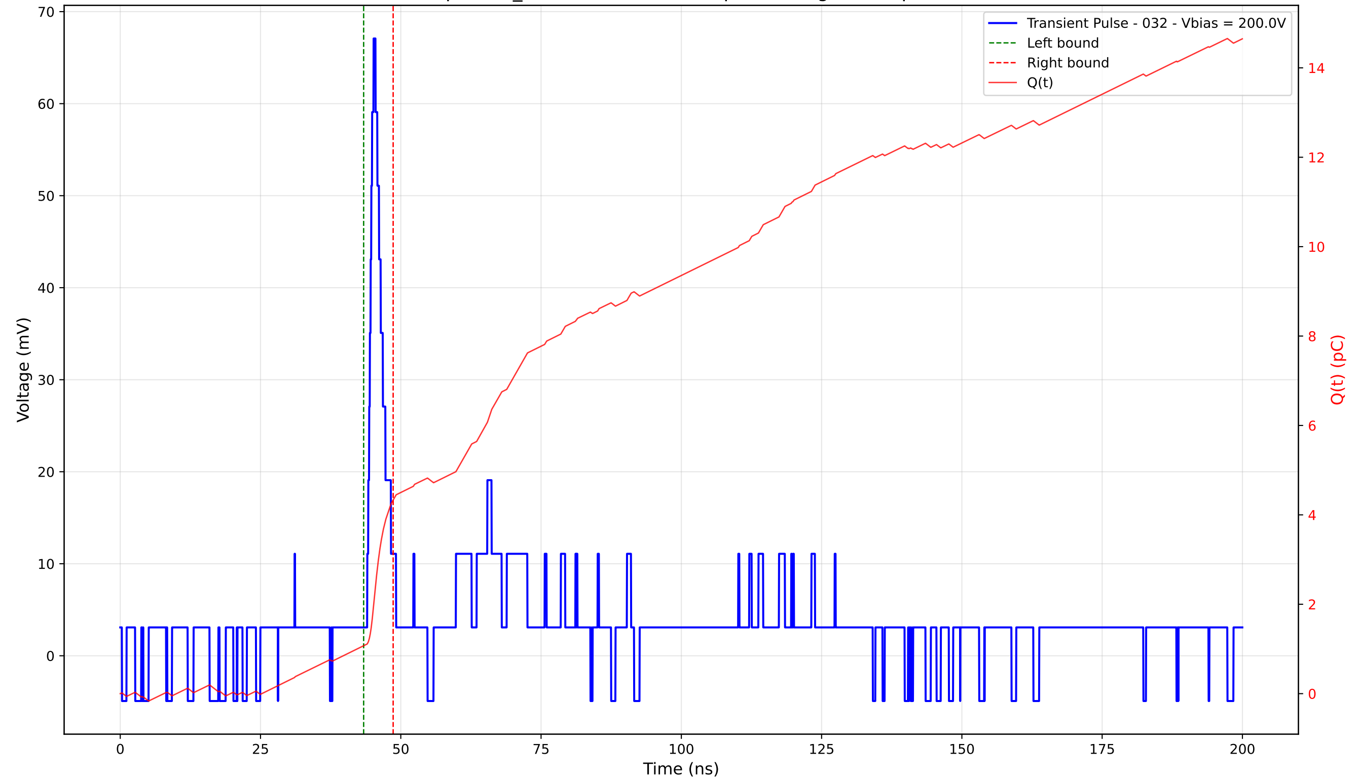
Transient Pulse - Sample: TD_4004 - Position: 45.0 \mu\text{m} - Charge: 3.26 pC - Rise Time: 1.13 ns
