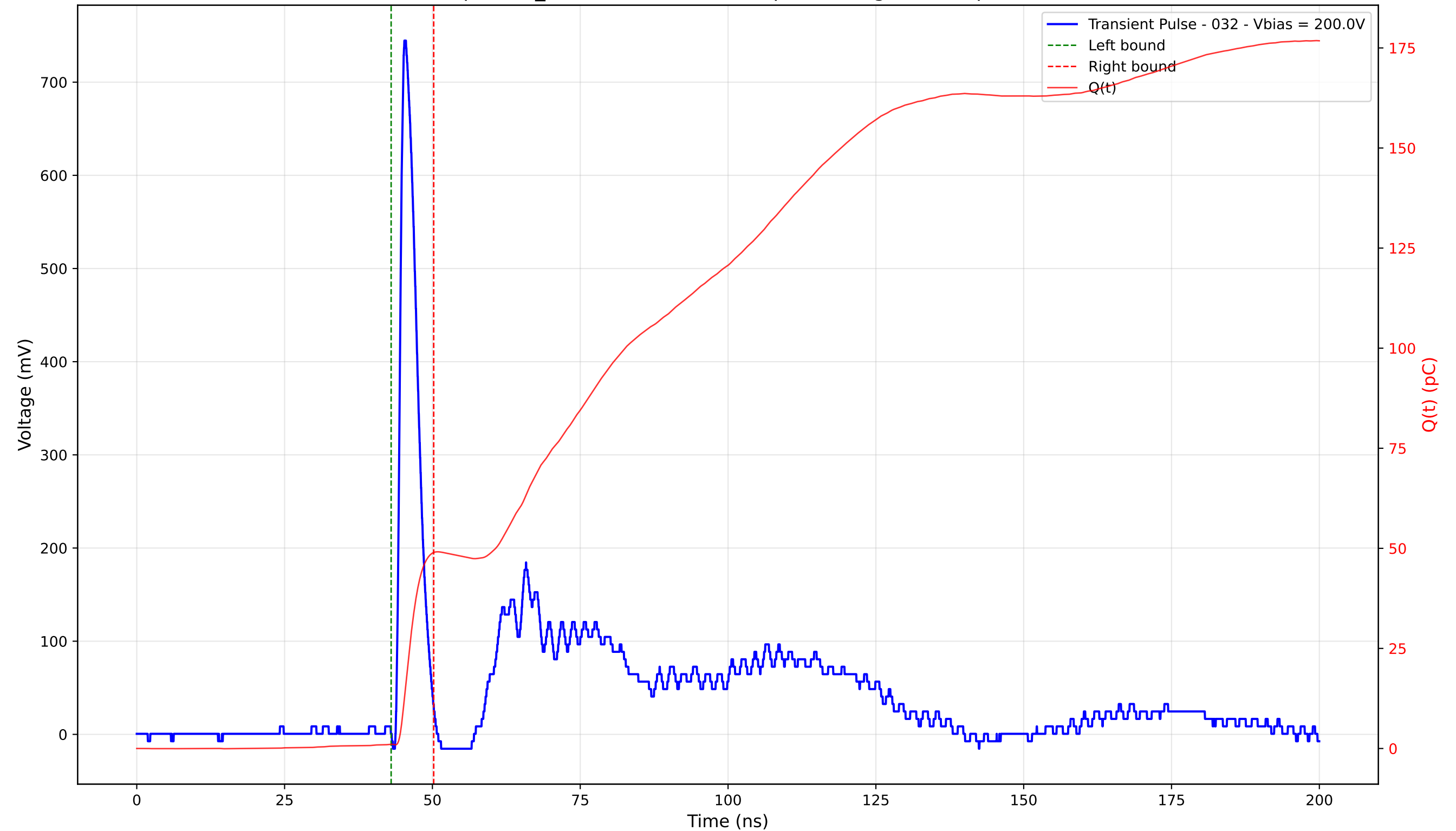
Transient Pulse - Sample: TD_4004 - Position: 215.0 \mu\text{m} - Charge: 47.90 pC - Rise Time: 0.95 ns
