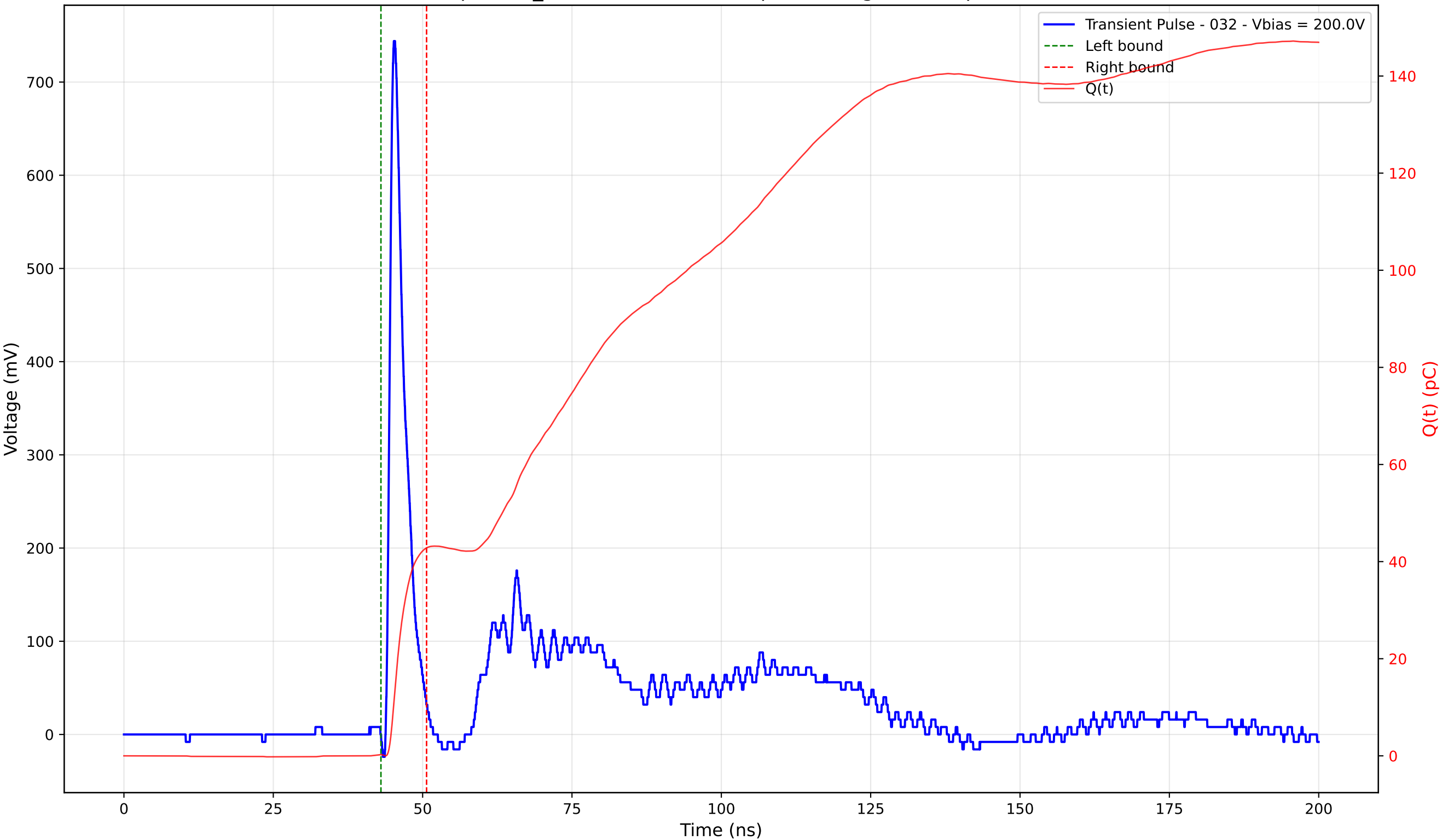
Transient Pulse - Sample: TD_4004 - Position: 95.0 \mu\text{m} - Charge: 42.57 pC - Rise Time: 0.88 ns
