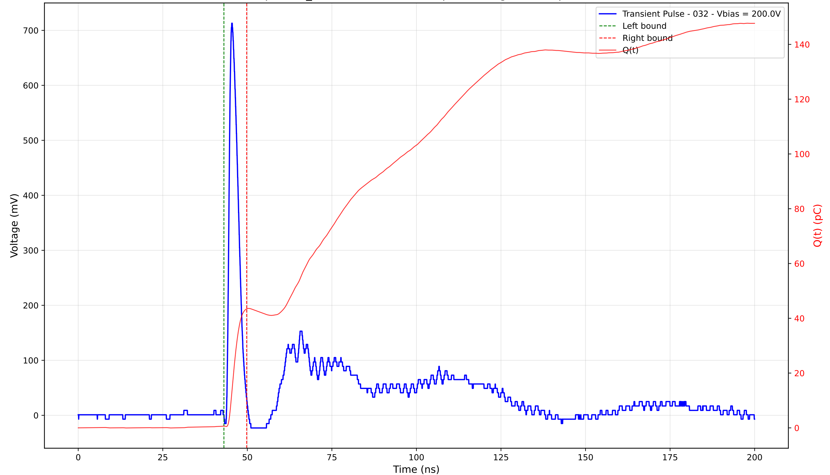
Transient Pulse - Sample: TD_4004 - Position: 240.0 \mu\text{m} - Charge: 42.81 pC - Rise Time: 0.99 ns
