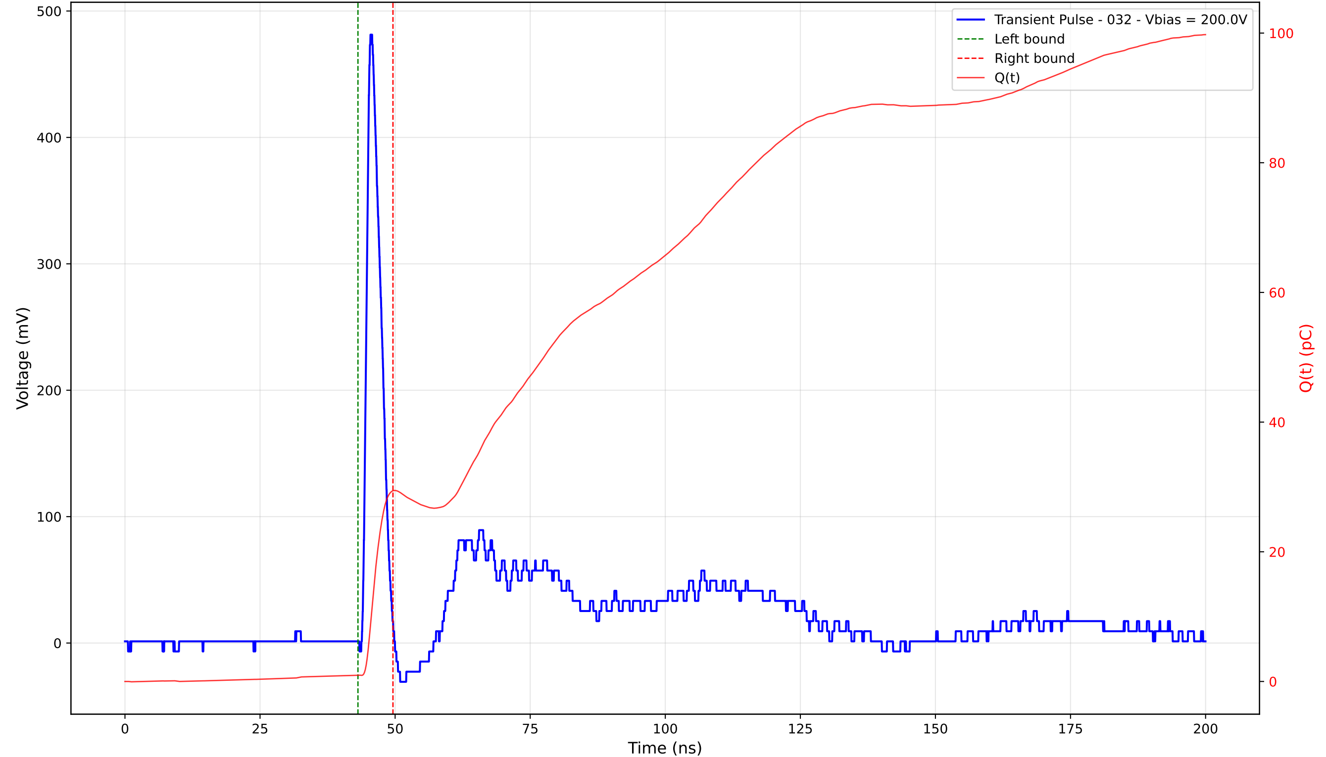
Transient Pulse - Sample: TD_4004 - Position: 335.0 \mu\text{m} - Charge: 28.44 pC - Rise Time: 1.04 ns
