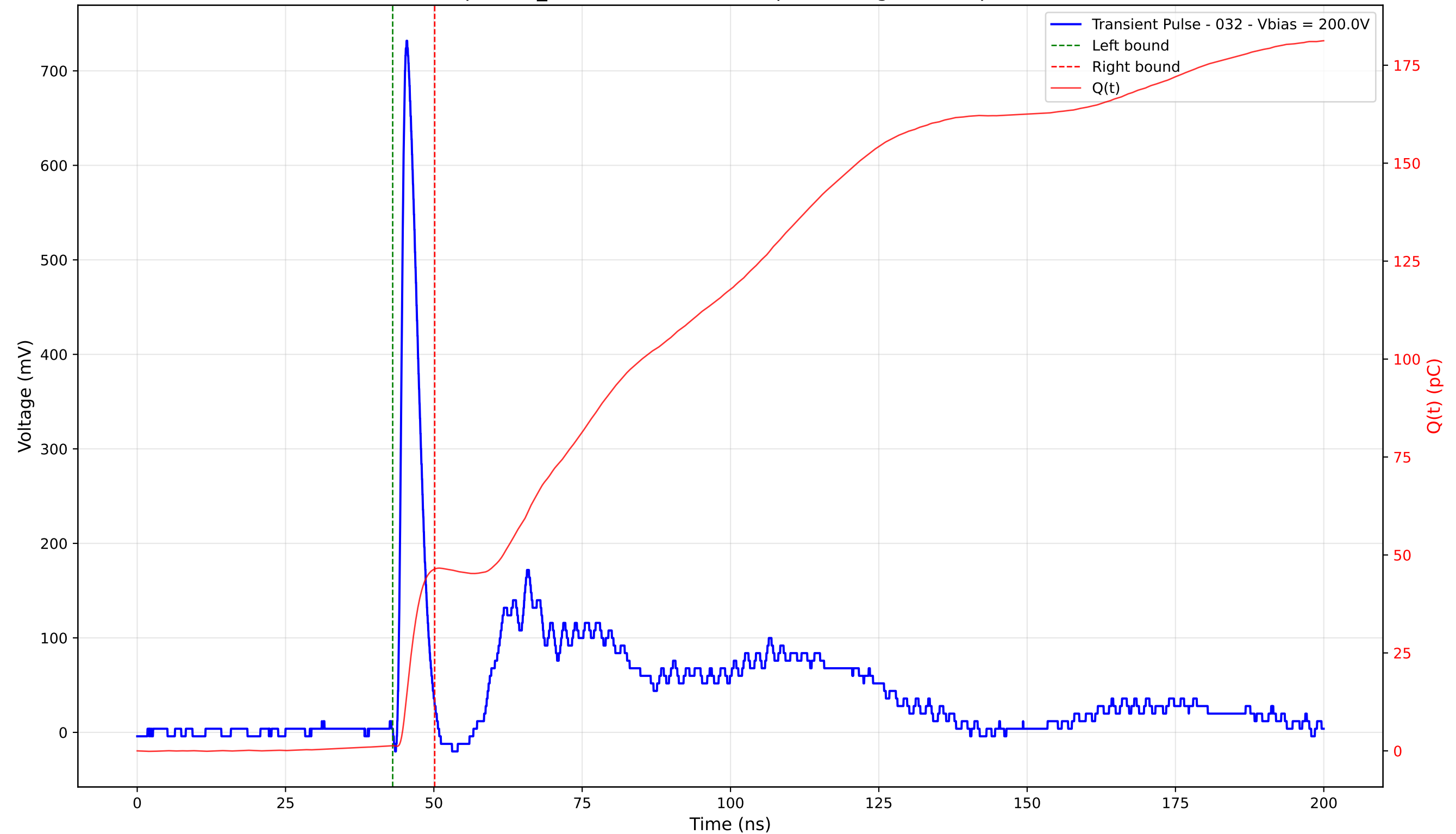
Transient Pulse - Sample: TD_4004 - Position: 155.0 \mu\text{m} - Charge: 45.11 pC - Rise Time: 0.96 ns
