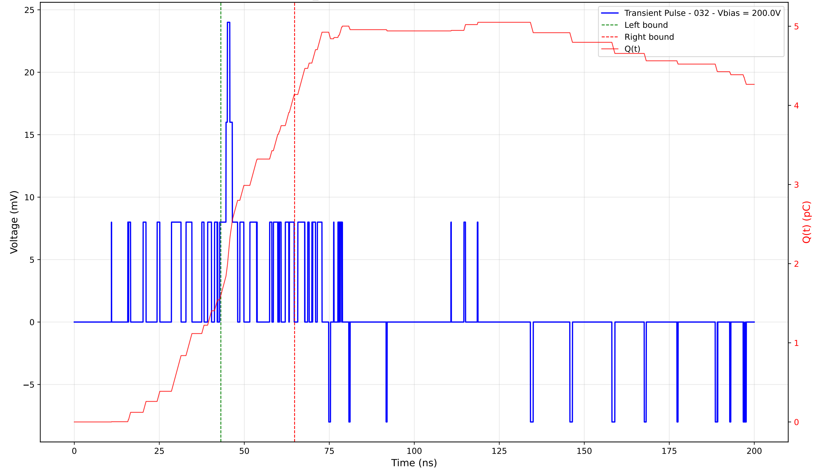
Transient Pulse - Sample: TD_4004 - Position: 25.0 \mu\text{m} - Charge: 2.54 pC - Rise Time: 2.27 ns
