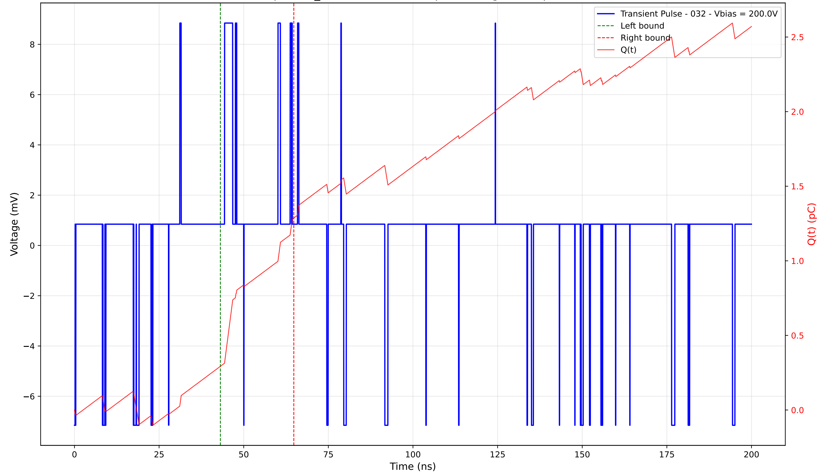
Transient Pulse - Sample: TD_4004 - Position: 5.0 \mu\text{m} - Charge: 0.99 pC - Rise Time: 0.02 ns
