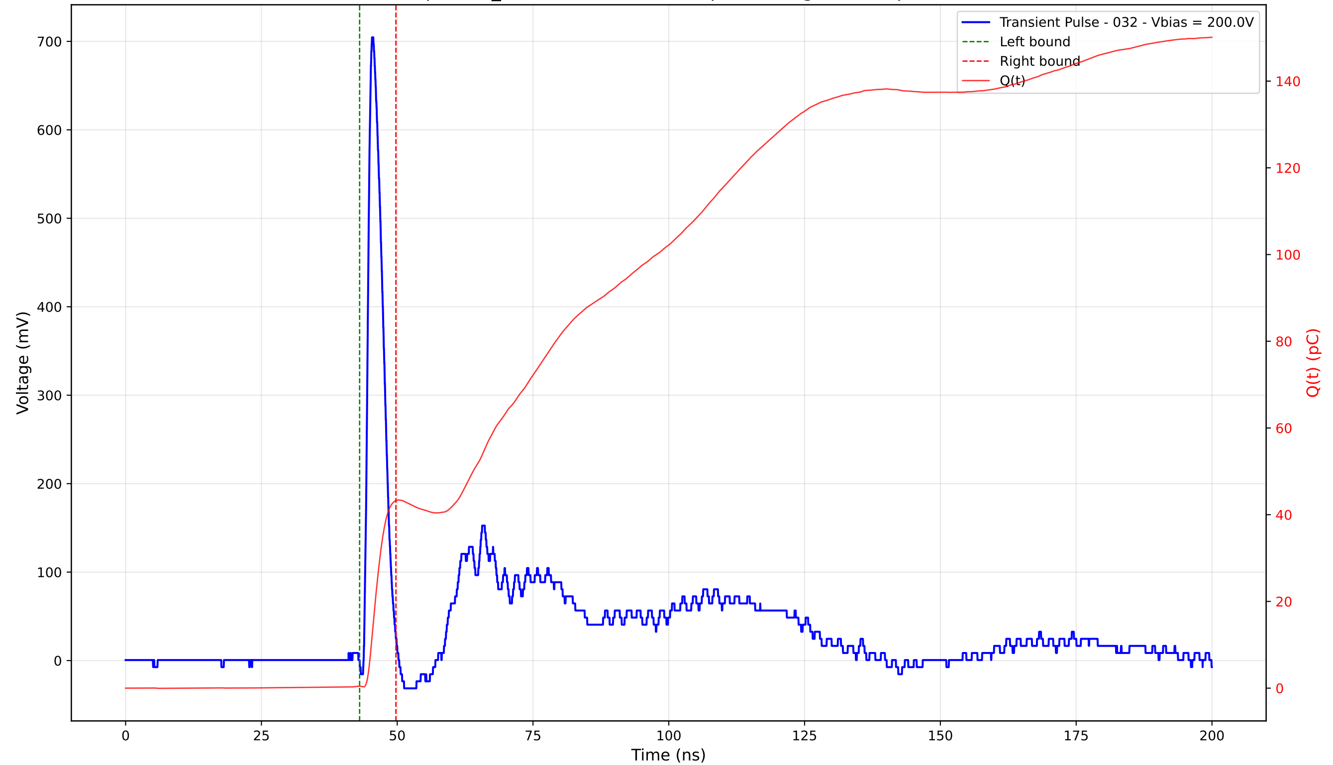
Transient Pulse - Sample: TD_4004 - Position: 255.0 \mu\text{m} - Charge: 42.79 pC - Rise Time: 0.99 ns
