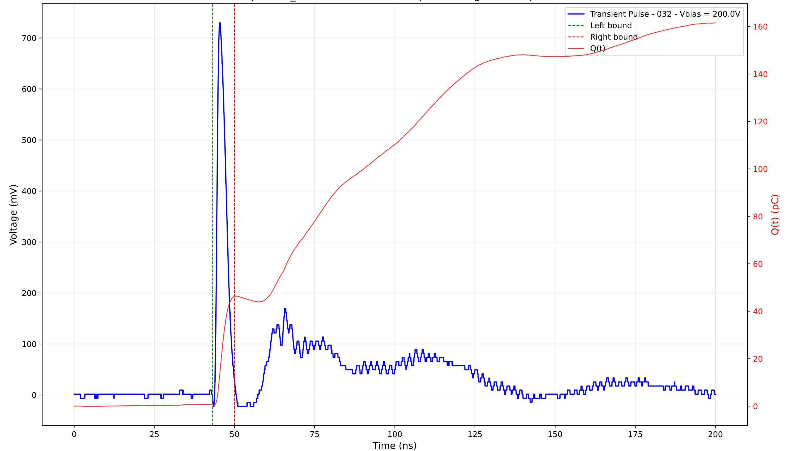
Transient Pulse - Sample: TD_4004 - Position: 230.0 \mu\text{m} - Charge: 45.38 pC - Rise Time: 0.96 ns
