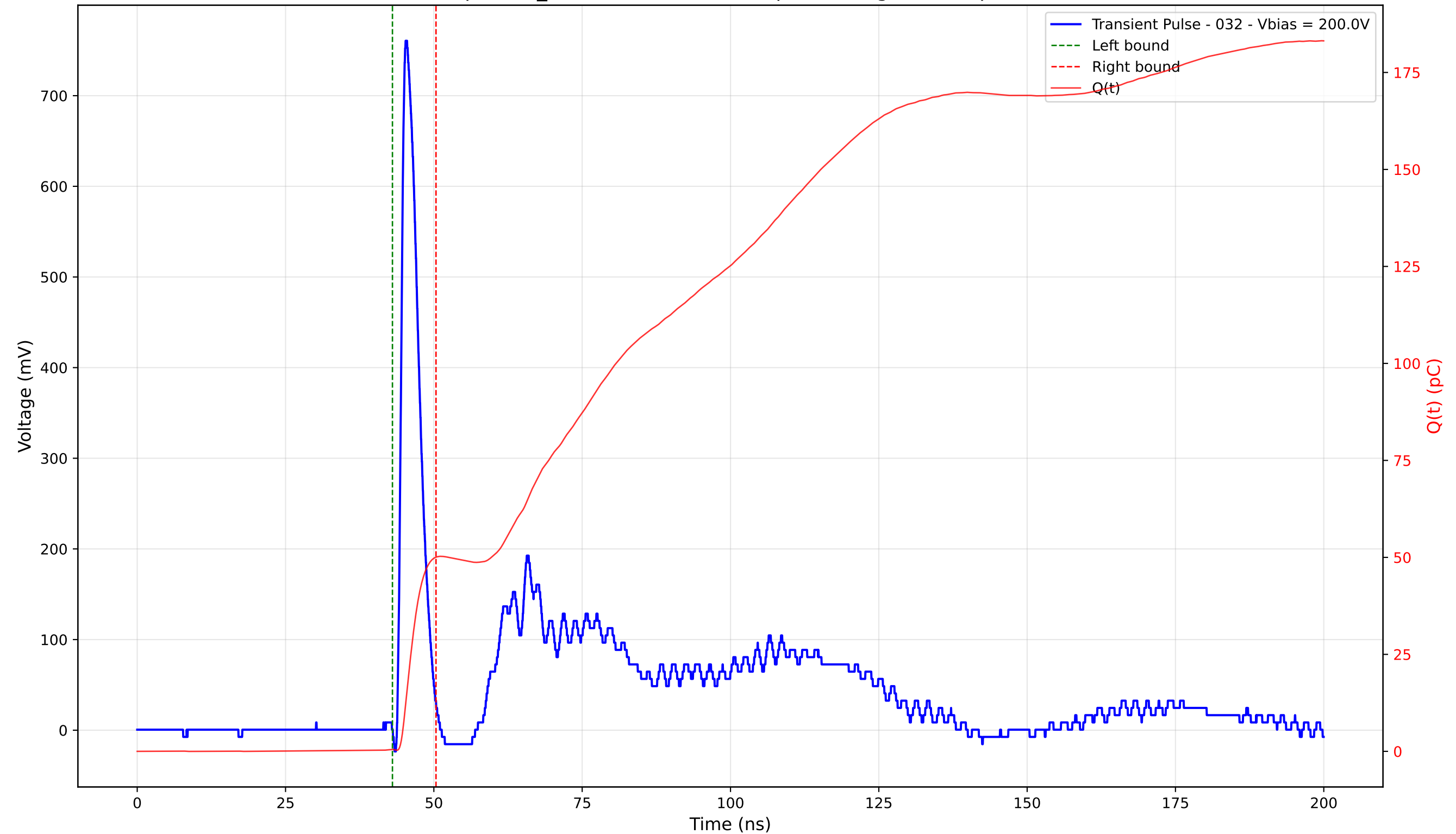
Transient Pulse - Sample: TD_4004 - Position: 175.0 \mu\text{m} - Charge: 49.57 pC - Rise Time: 0.92 ns
