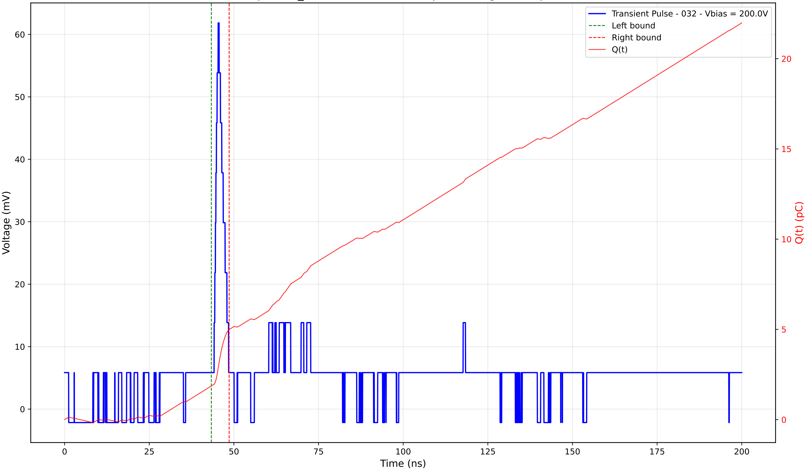
Transient Pulse - Sample: TD_4004 - Position: 435.0 \mu\text{m} - Charge: 3.13 pC - Rise Time: 1.20 ns
