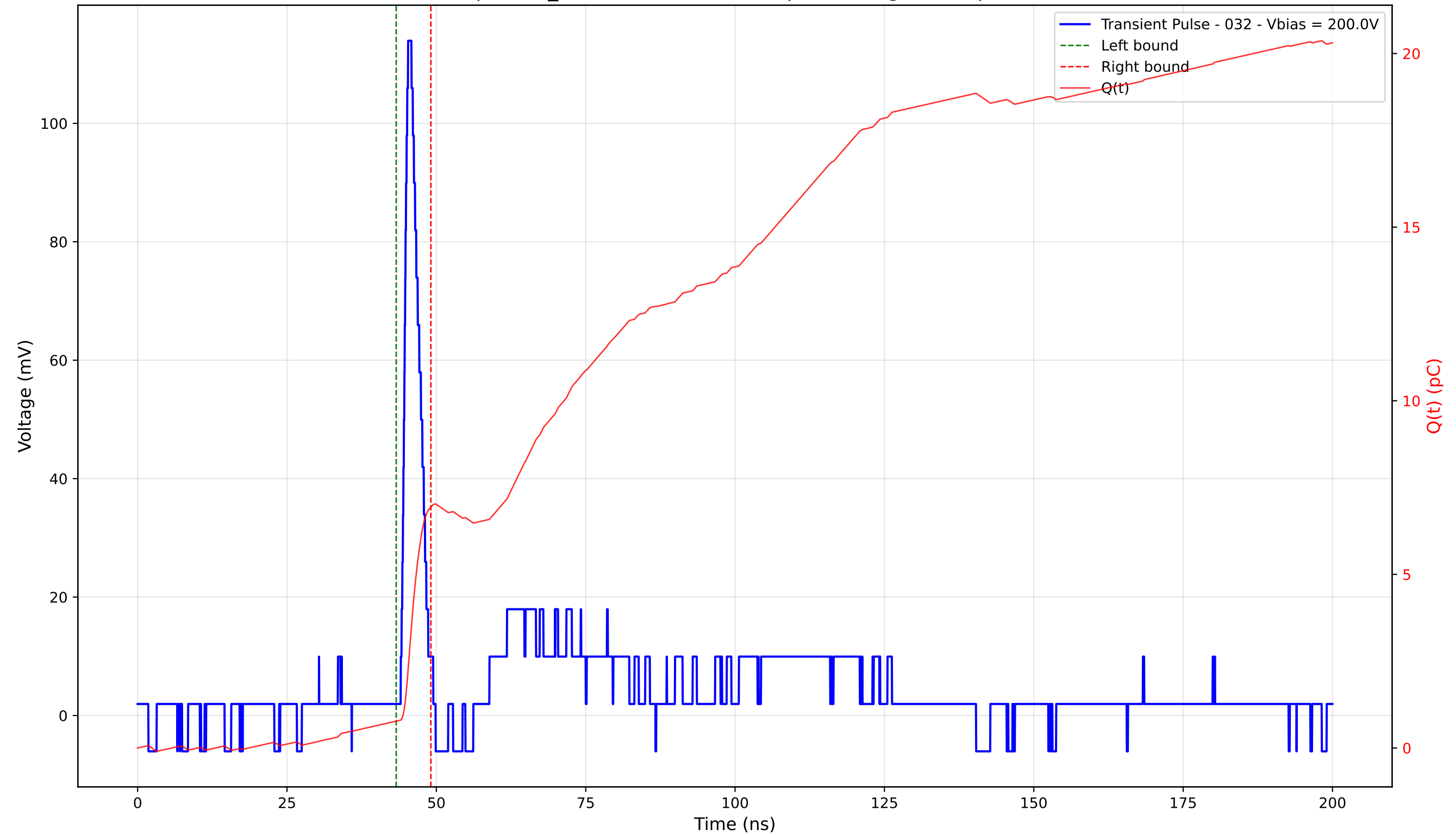
Transient Pulse - Sample: TD_4004 - Position: 415.0 \mu\text{m} - Charge: 6.17 pC - Rise Time: 0.96 ns
