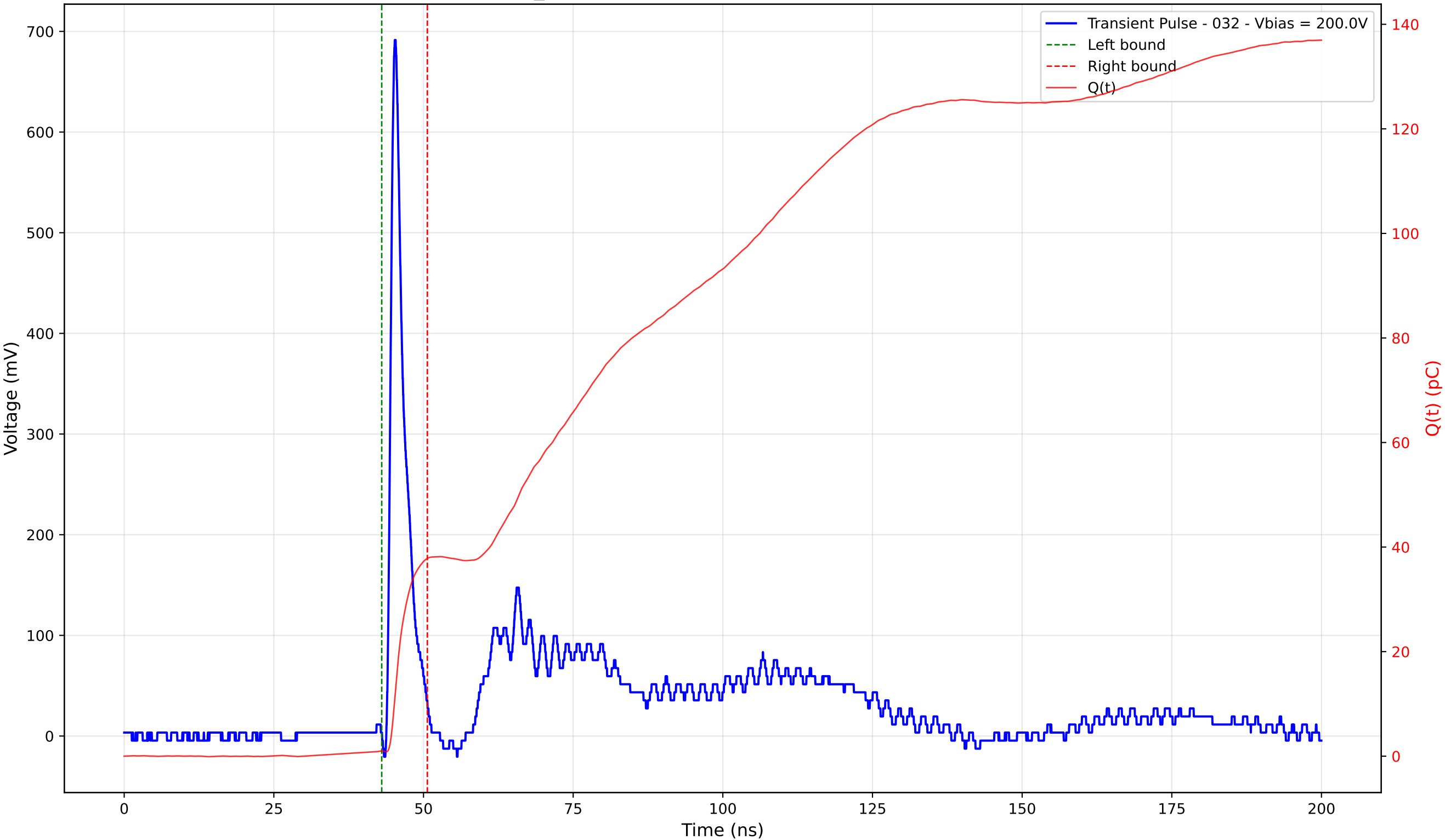
Transient Pulse - Sample: TD_4004 - Position: 85.0 \mu\text{m} - Charge: 36.83 pC - Rise Time: 0.88 ns
