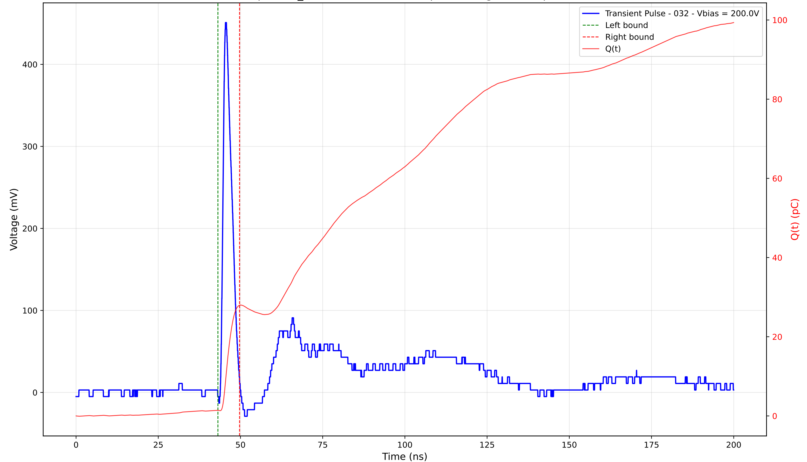
Transient Pulse - Sample: TD_4004 - Position: 360.0 \mu\text{m} - Charge: 26.53 pC - Rise Time: 1.03 ns
