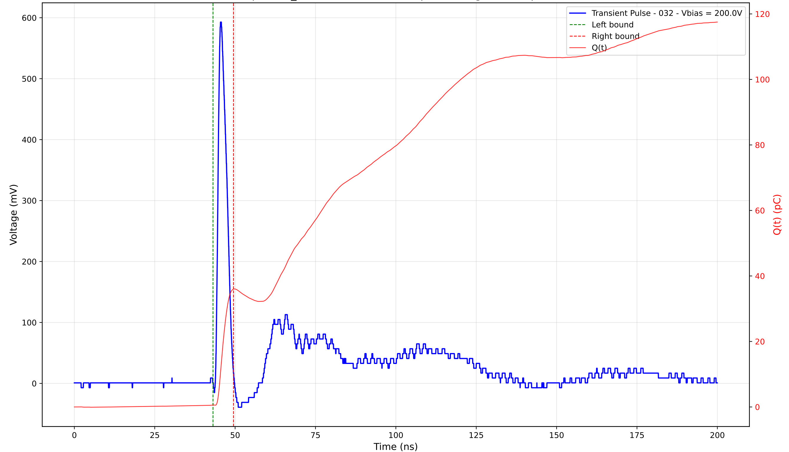
Transient Pulse - Sample: TD_4004 - Position: 320.0 \mu\text{m} - Charge: 35.37 pC - Rise Time: 1.03 ns
