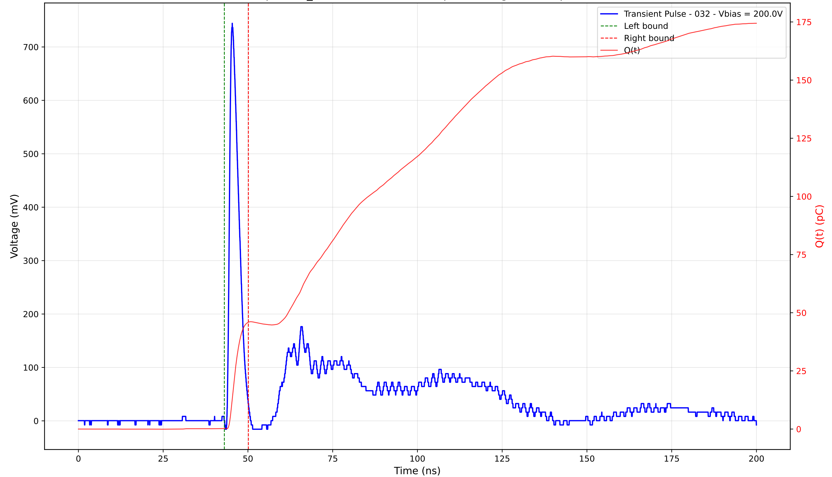
Transient Pulse - Sample: TD_4004 - Position: 130.0 \mu\text{m} - Charge: 45.67 pC - Rise Time: 0.93 ns
