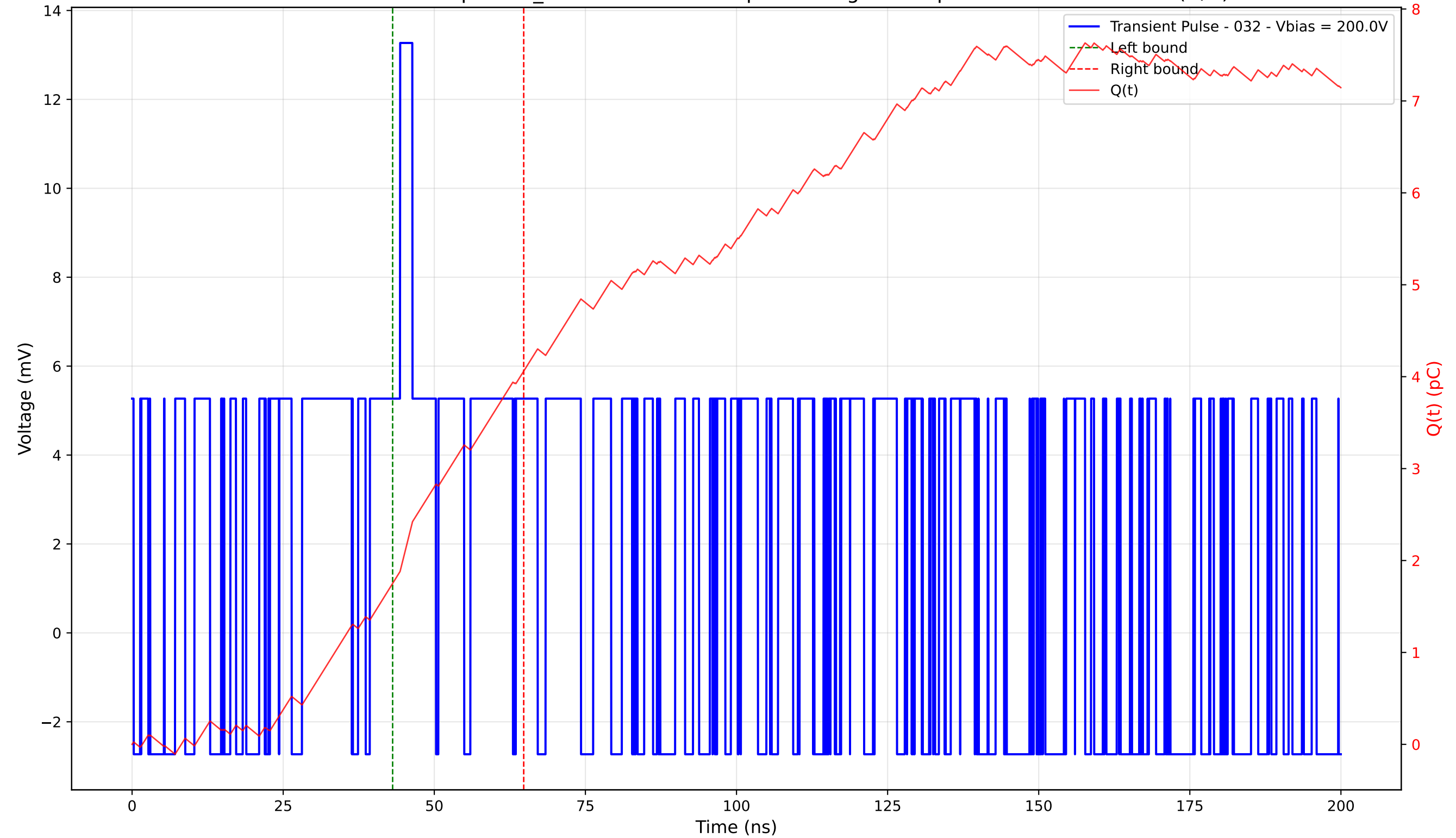
Transient Pulse - Sample: TD_4004 - Position: 0.0 \mu m - Charge: 2.31 pC - Rise Time: 0.00 ns (N/A)
