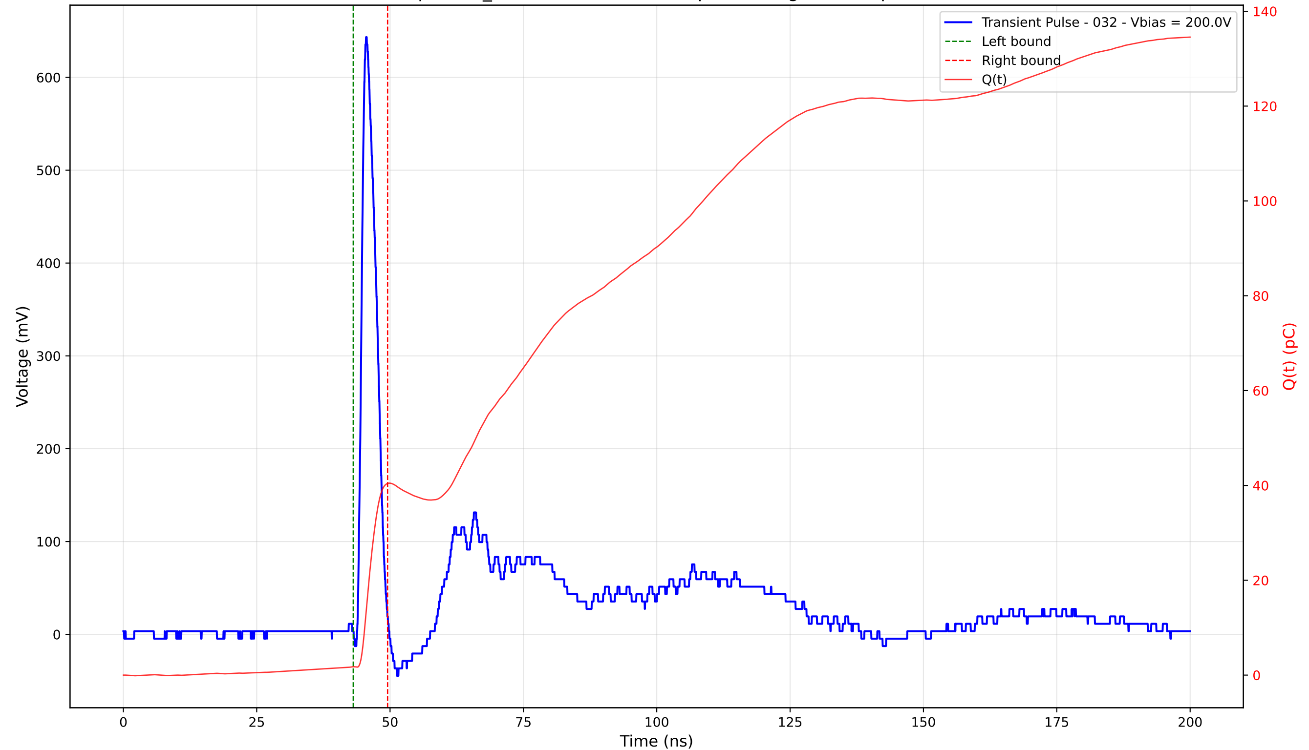
Transient Pulse - Sample: TD_4004 - Position: 310.0 \mu\text{m} - Charge: 38.66 pC - Rise Time: 1.03 ns
