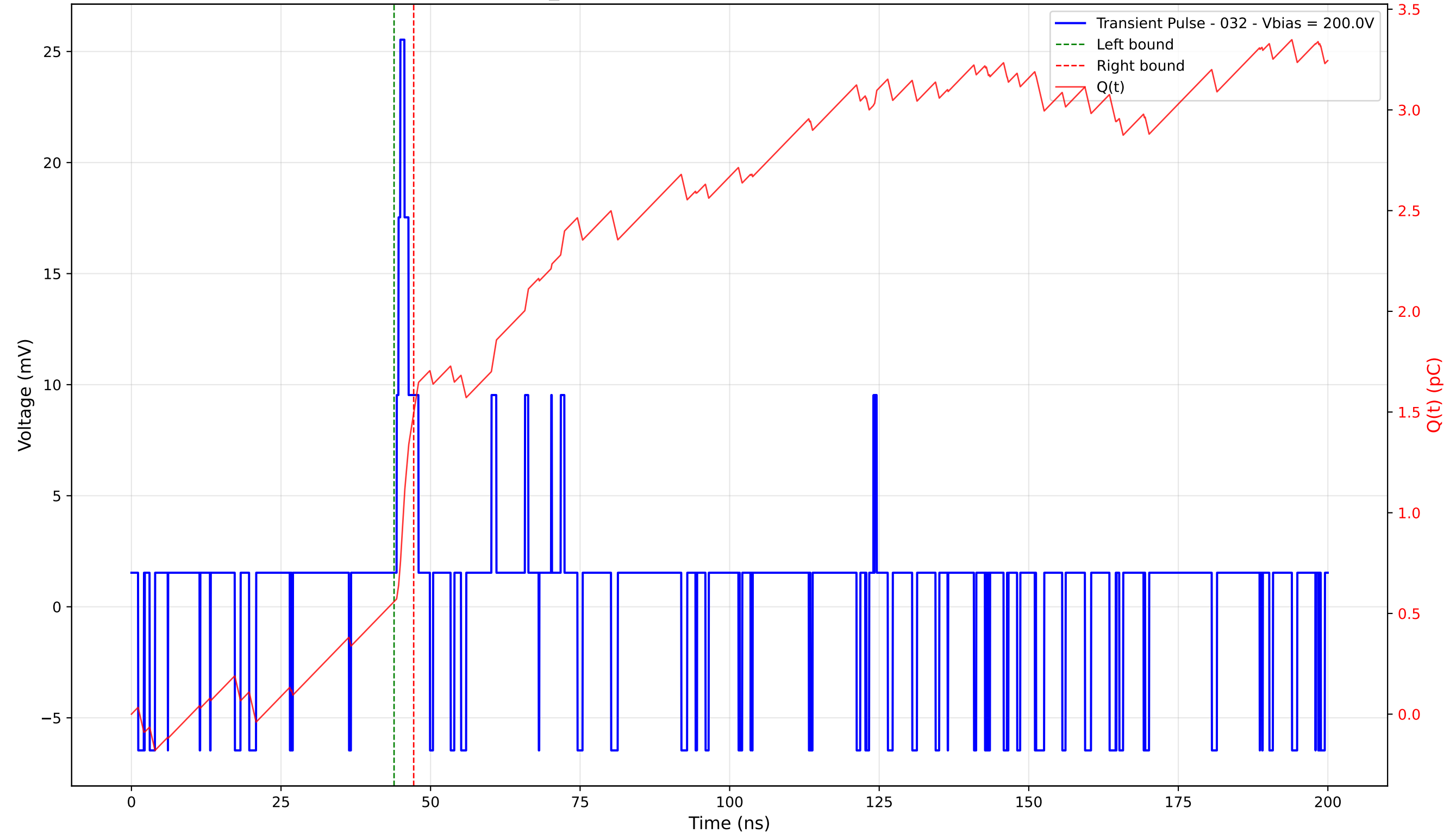
Transient Pulse - Sample: TD_4004 - Position: 30.0 \mu\text{m} - Charge: 0.94 pC - Rise Time: 0.62 ns
