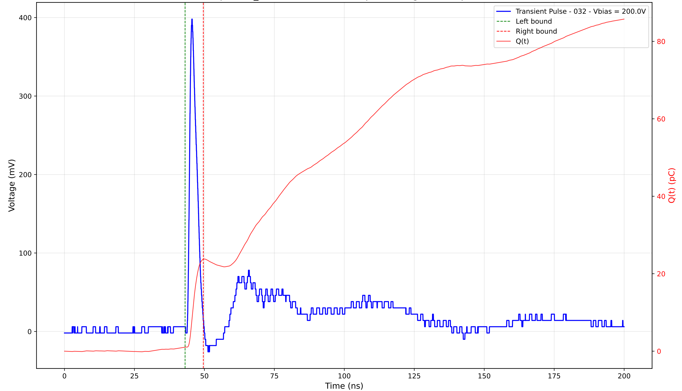
Transient Pulse - Sample: TD_4004 - Position: 385.0 \mu\text{m} - Charge: 22.70 pC - Rise Time: 1.08 ns
