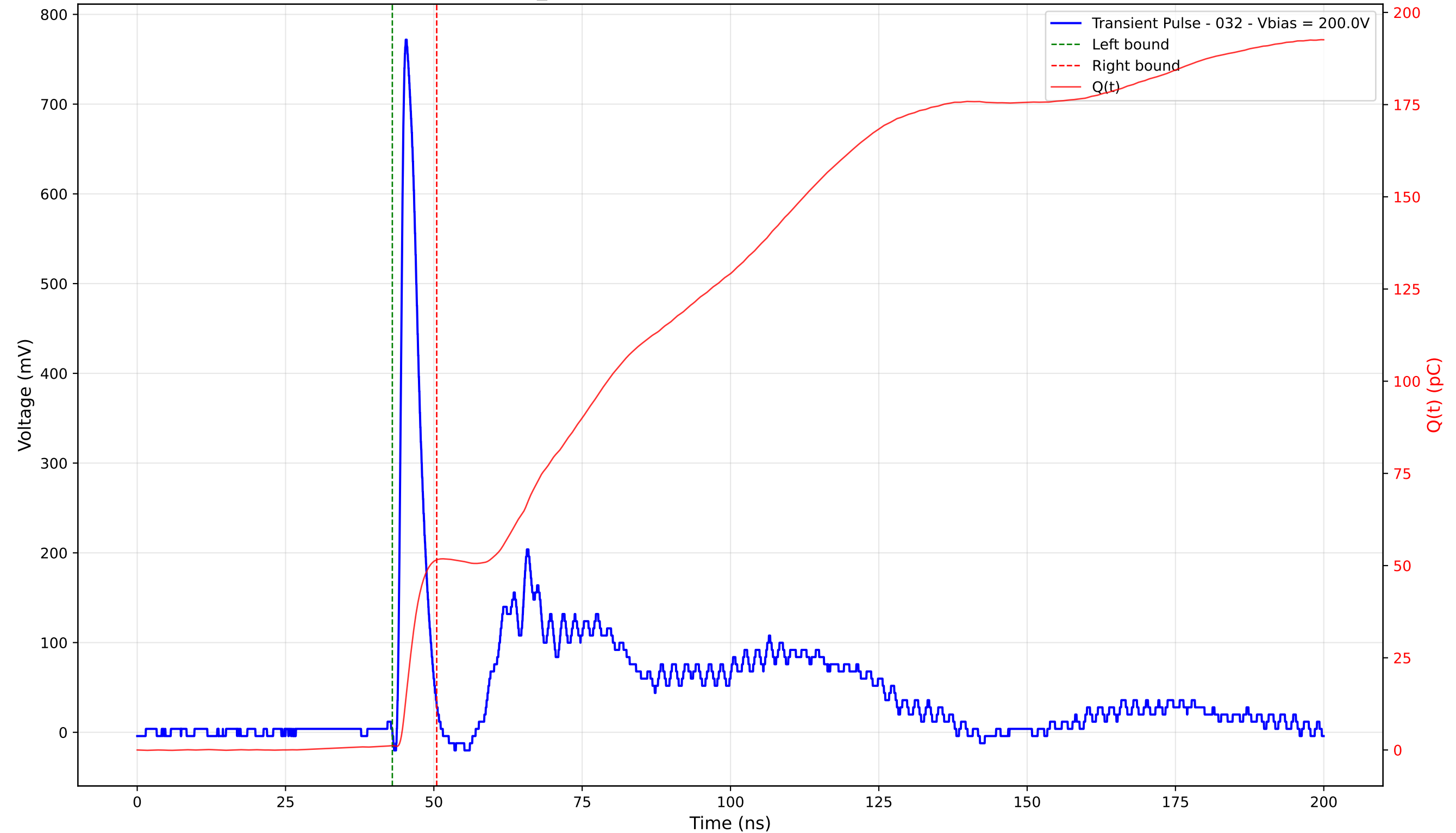
Transient Pulse - Sample: TD_4004 - Position: 185.0 \mu\text{m} - Charge: 50.39 pC - Rise Time: 0.92 ns
