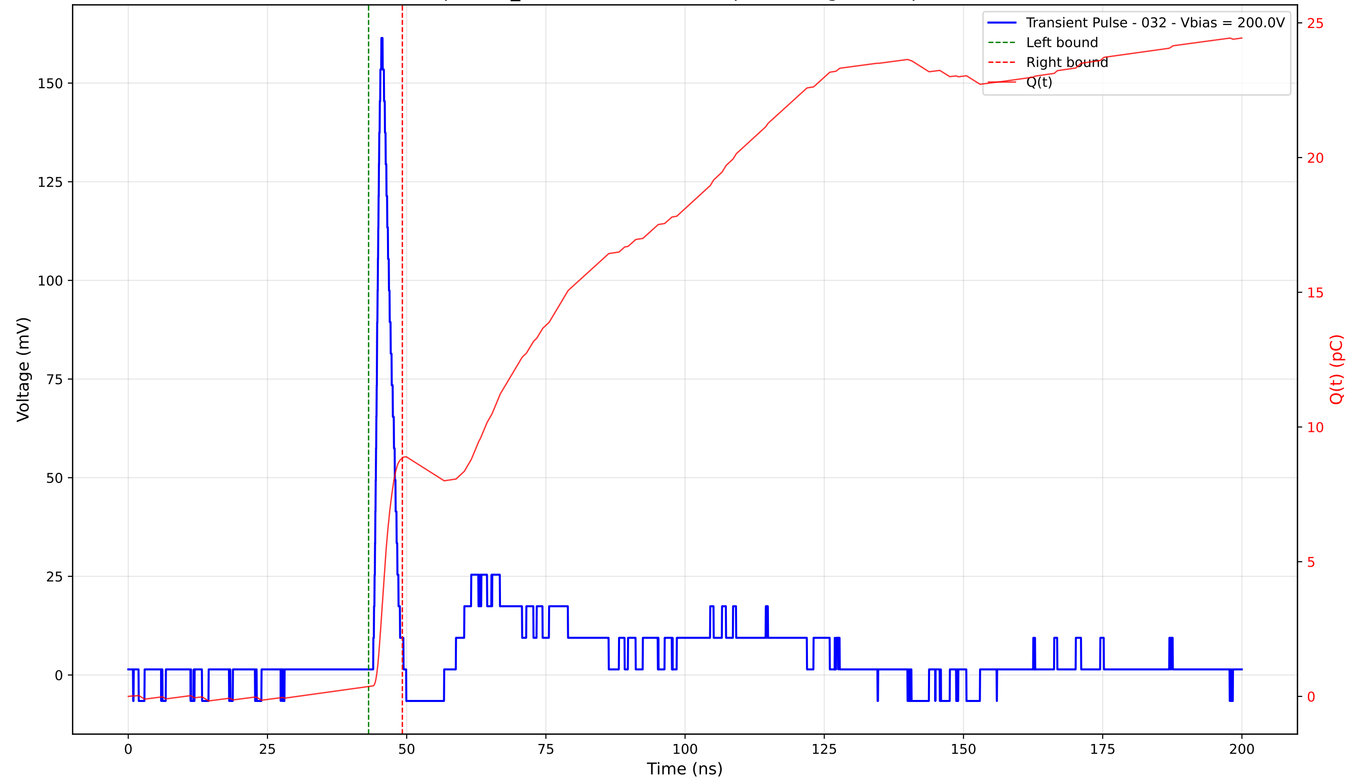
Transient Pulse - Sample: TD_4004 - Position: 410.0 \mu\text{m} - Charge: 8.48 pC - Rise Time: 1.04 ns
