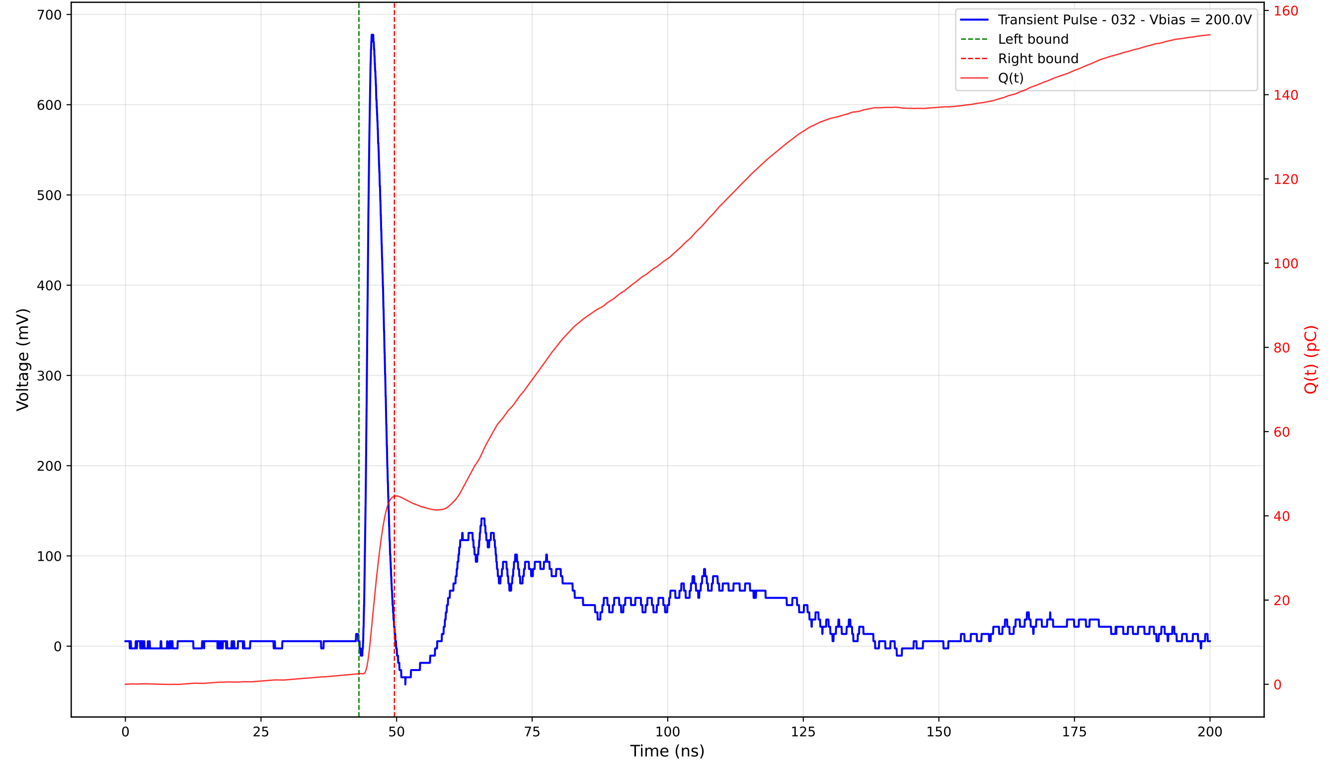
Transient Pulse - Sample: TD_4004 - Position: 295.0 \mu\text{m} - Charge: 42.13 pC - Rise Time: 1.02 ns
