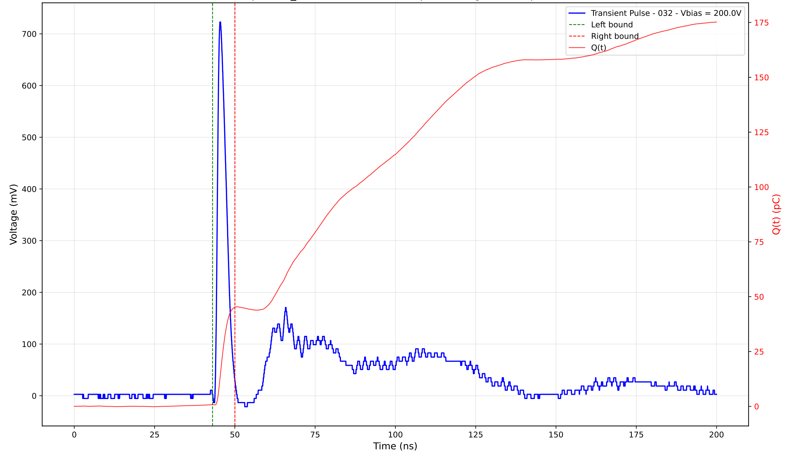
Transient Pulse - Sample: TD_4004 - Position: 140.0 \mu\text{m} - Charge: 44.42 pC - Rise Time: 0.97 ns
