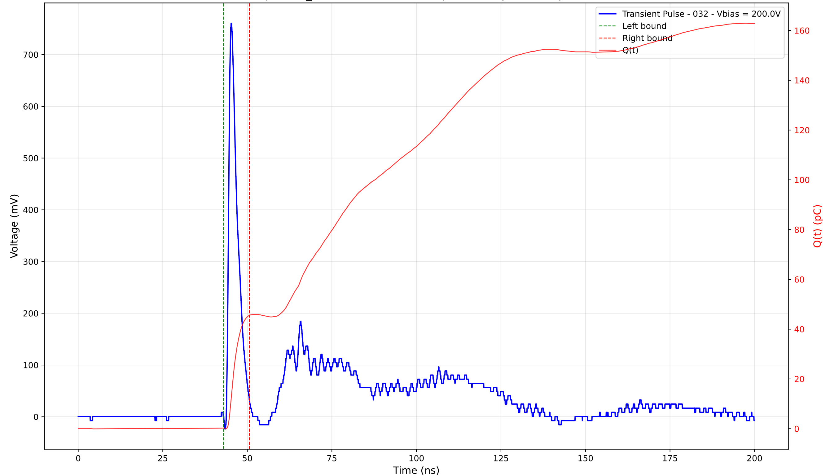
Transient Pulse - Sample: TD_4004 - Position: 100.0 \mu\text{m} - Charge: 45.25 pC - Rise Time: 0.90 ns
