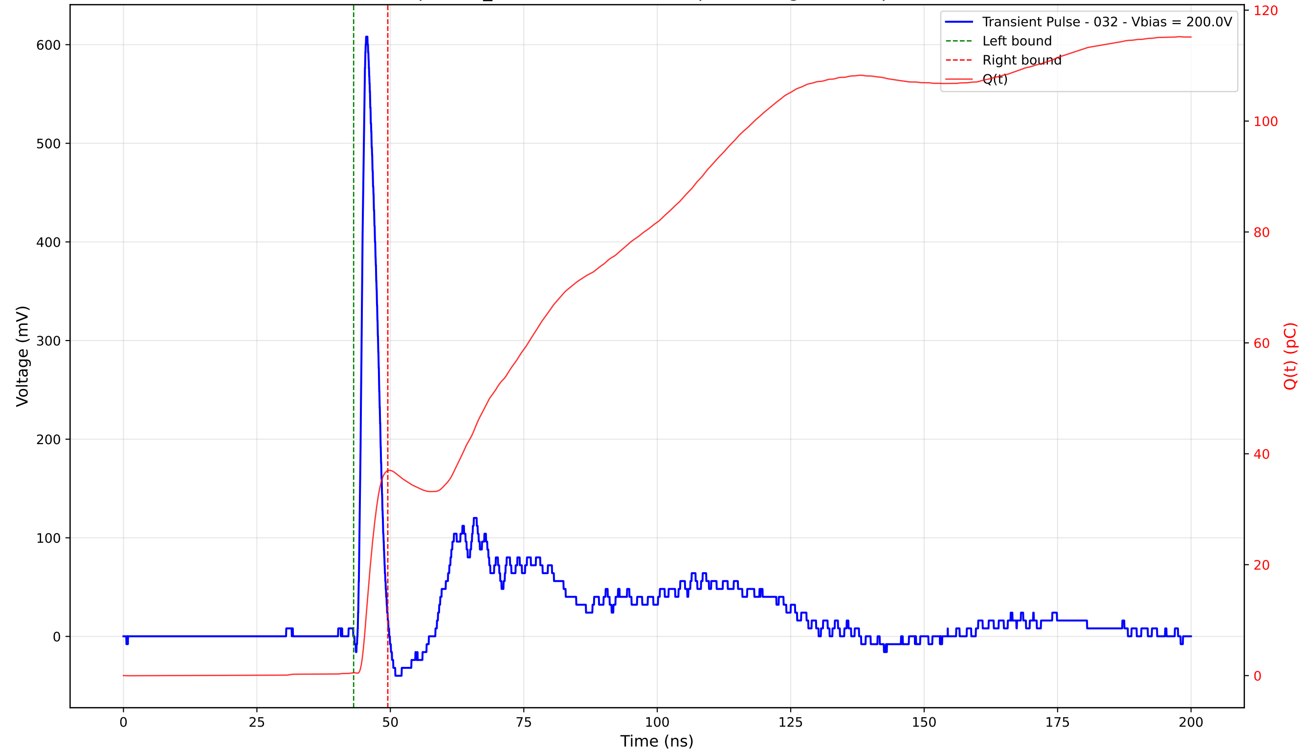
Transient Pulse - Sample: TD_4004 - Position: 315.0 \mu\text{m} - Charge: 36.44 pC - Rise Time: 1.02 ns
