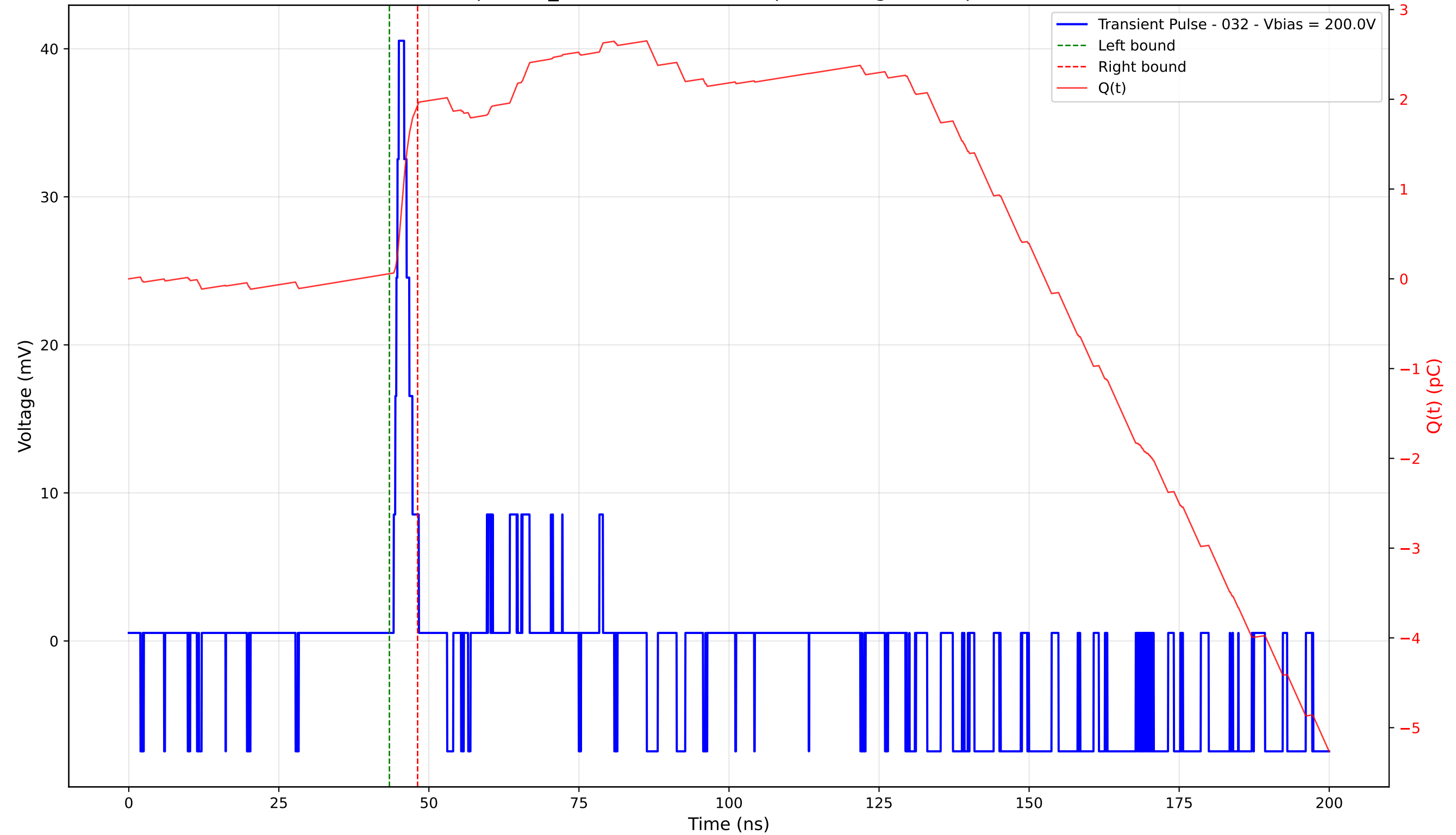
Transient Pulse - Sample: TD_4004 - Position: 40.0 \mu\text{m} - Charge: 1.88 pC - Rise Time: 0.85 ns
