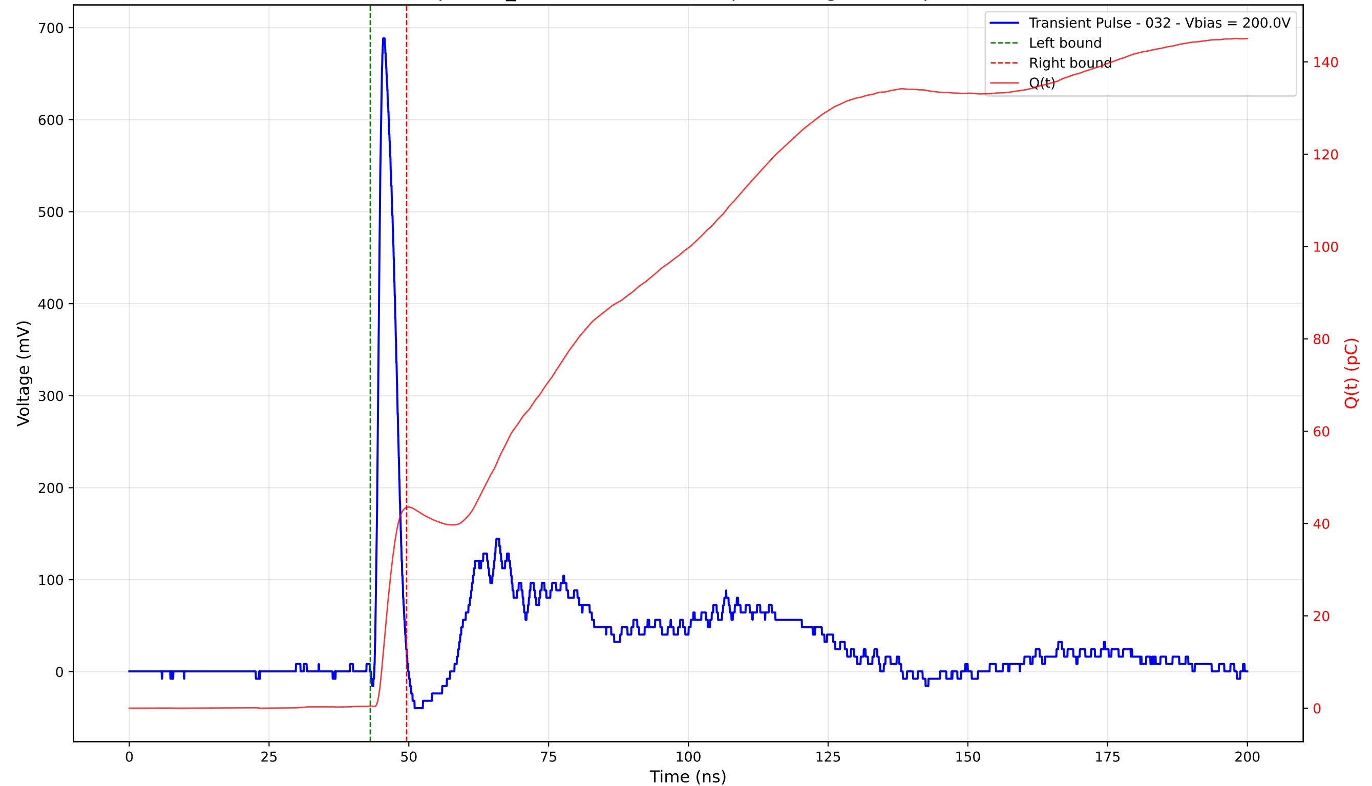
Transient Pulse - Sample: TD_4004 - Position: 290.0 \mu\text{m} - Charge: 43.03 pC - Rise Time: 1.00 ns
