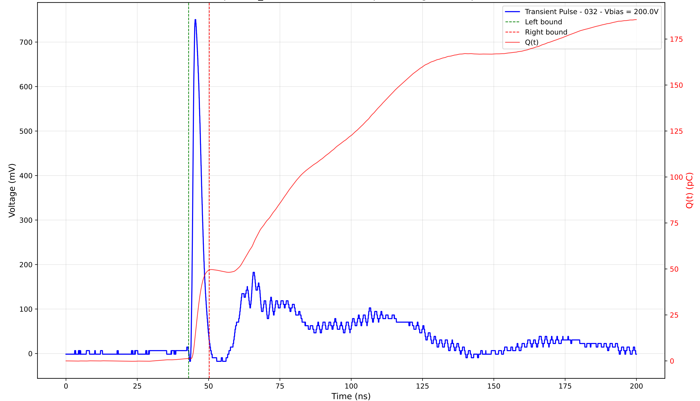
Transient Pulse - Sample: TD_4004 - Position: 220.0 \mu\text{m} - Charge: 48.11 pC - Rise Time: 0.94 ns
