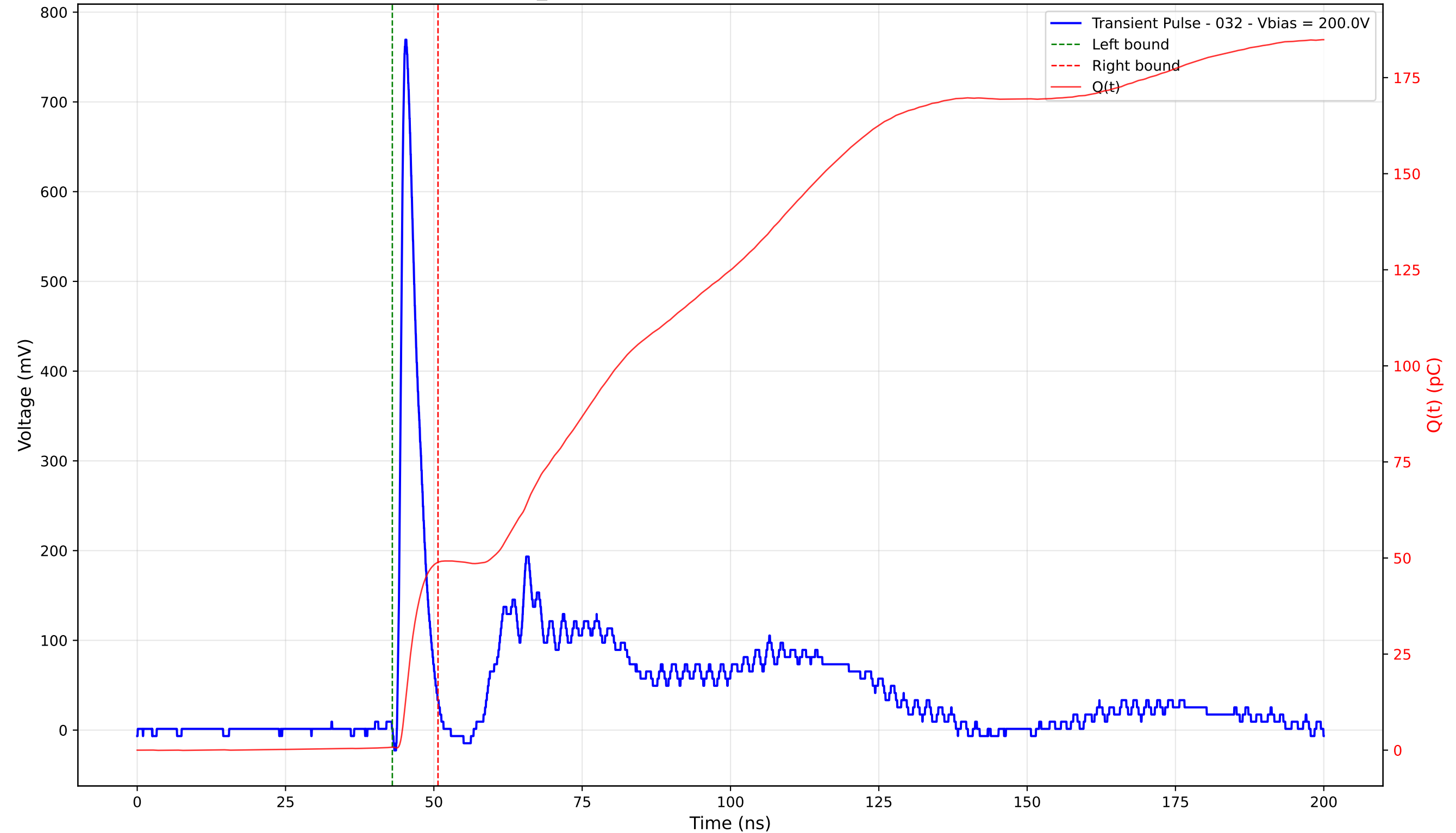
Transient Pulse - Sample: TD_4004 - Position: 110.0 \mu\text{m} - Charge: 48.09 pC - Rise Time: 0.88 ns
