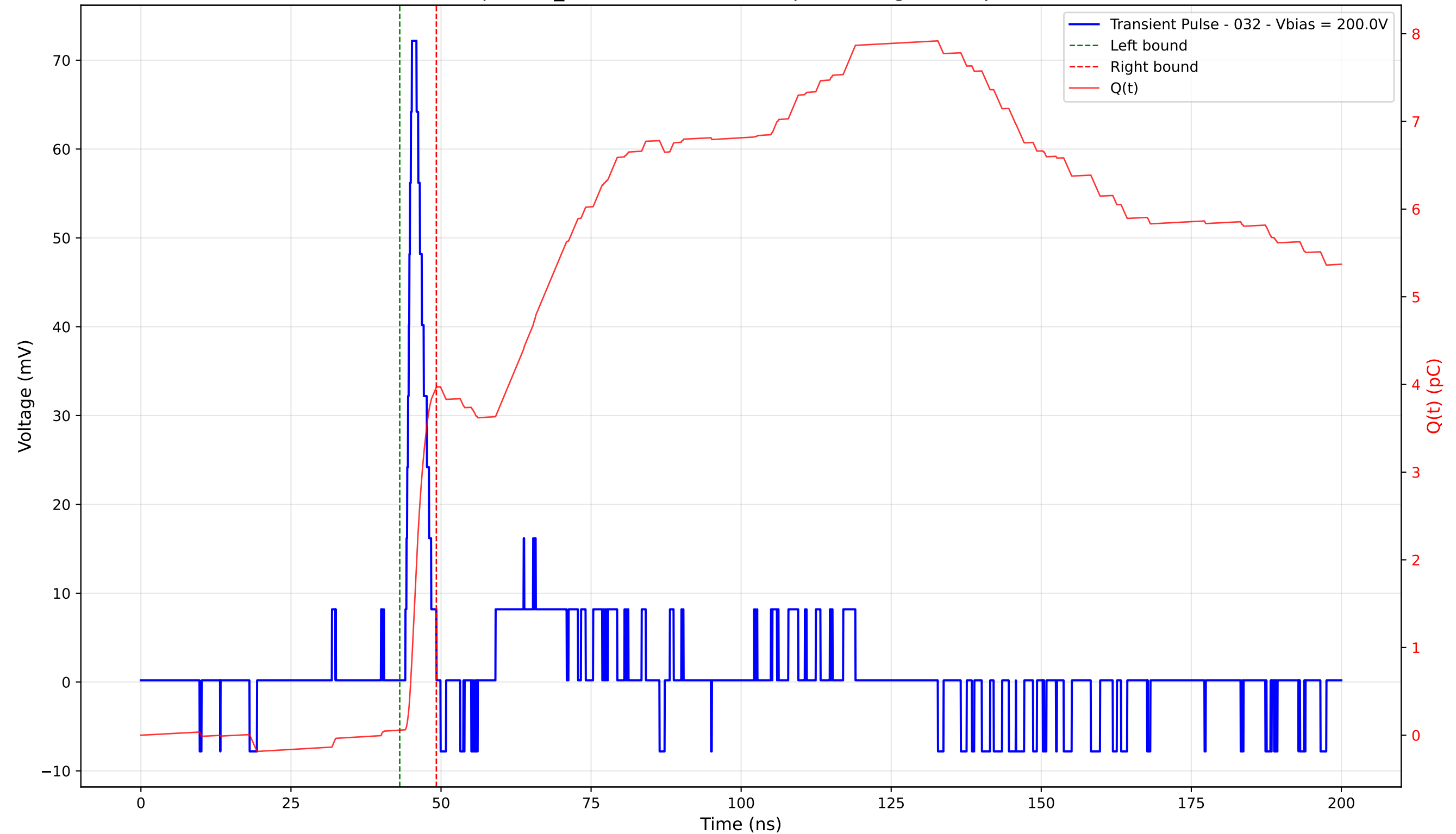
Transient Pulse - Sample: TD_4004 - Position: 420.0 \mu\text{m} - Charge: 3.91 pC - Rise Time: 1.08 ns
