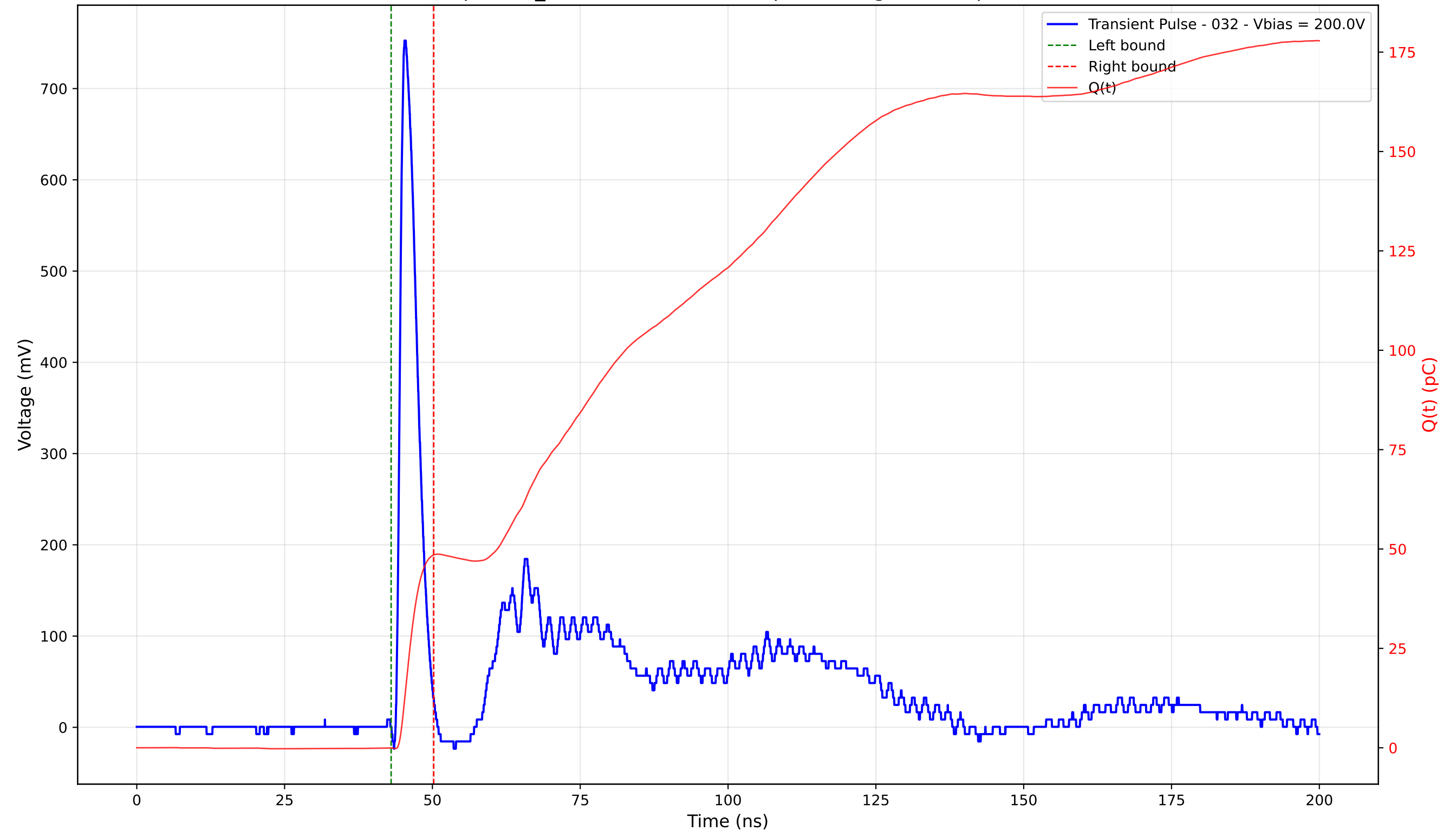
Transient Pulse - Sample: TD_4004 - Position: 170.0 \mu\text{m} - Charge: 48.53 pC - Rise Time: 0.95 ns
