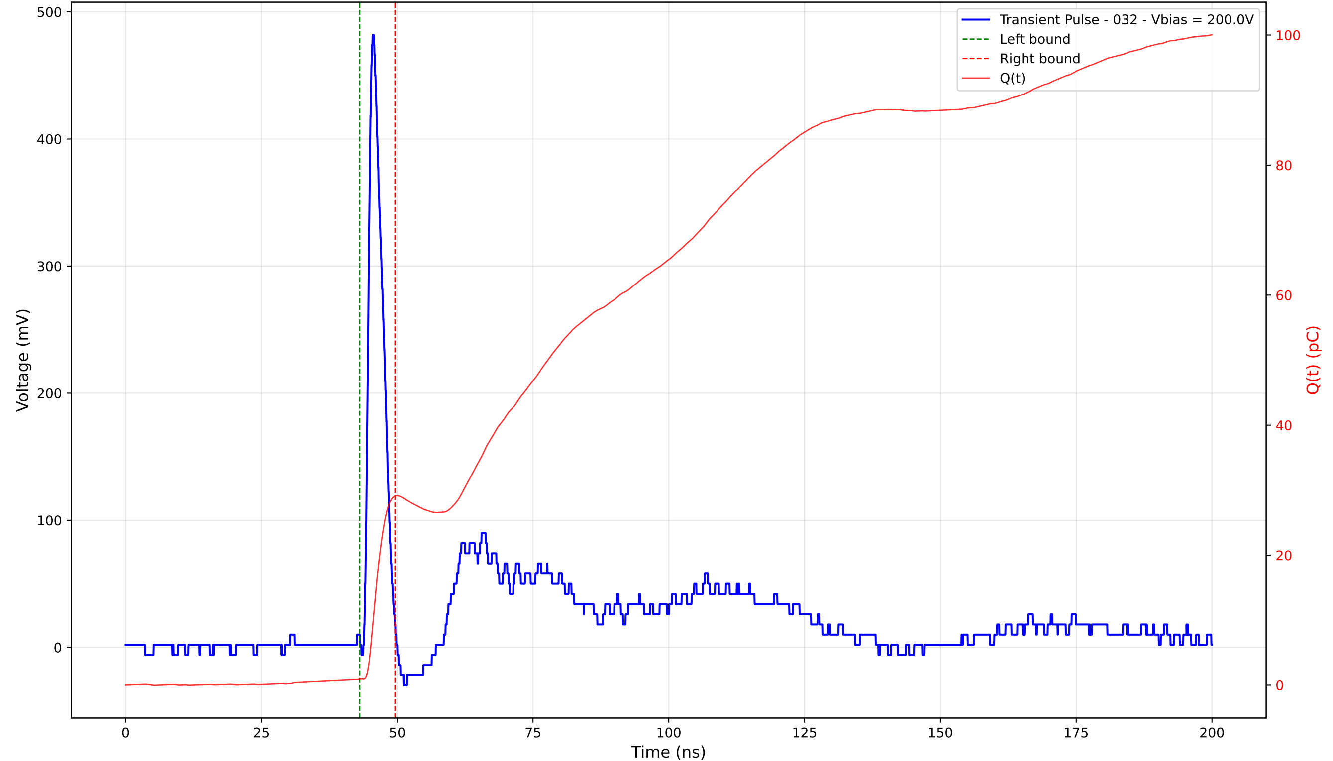
Transient Pulse - Sample: TD_4004 - Position: 340.0 \mu\text{m} - Charge: 28.15 pC - Rise Time: 1.02 ns
