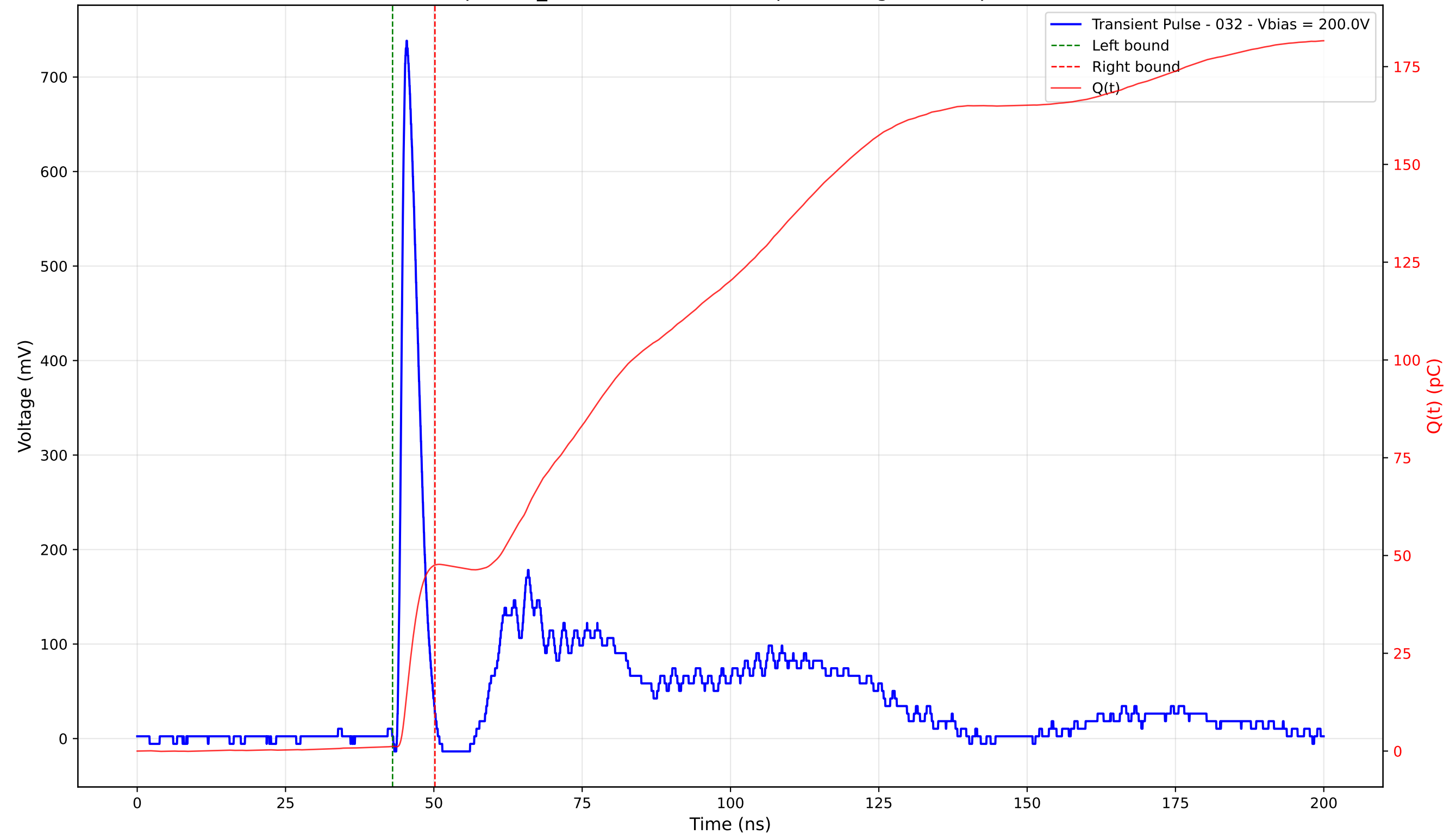
Transient Pulse - Sample: TD_4004 - Position: 160.0 \mu\text{m} - Charge: 46.35 pC - Rise Time: 0.96 ns
