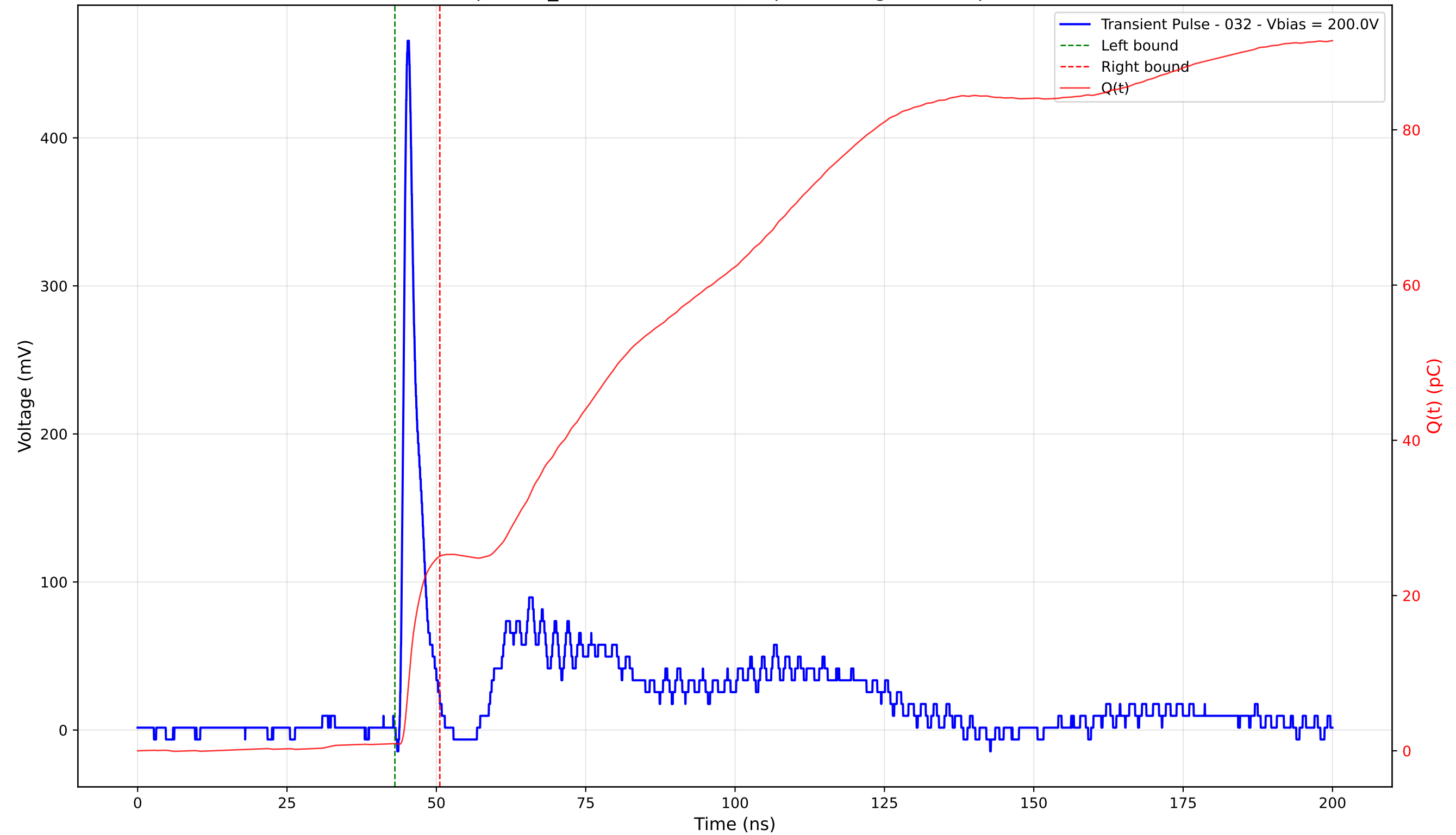
Transient Pulse - Sample: TD_4004 - Position: 70.0 \mu\text{m} - Charge: 24.12 pC - Rise Time: 0.91 ns
