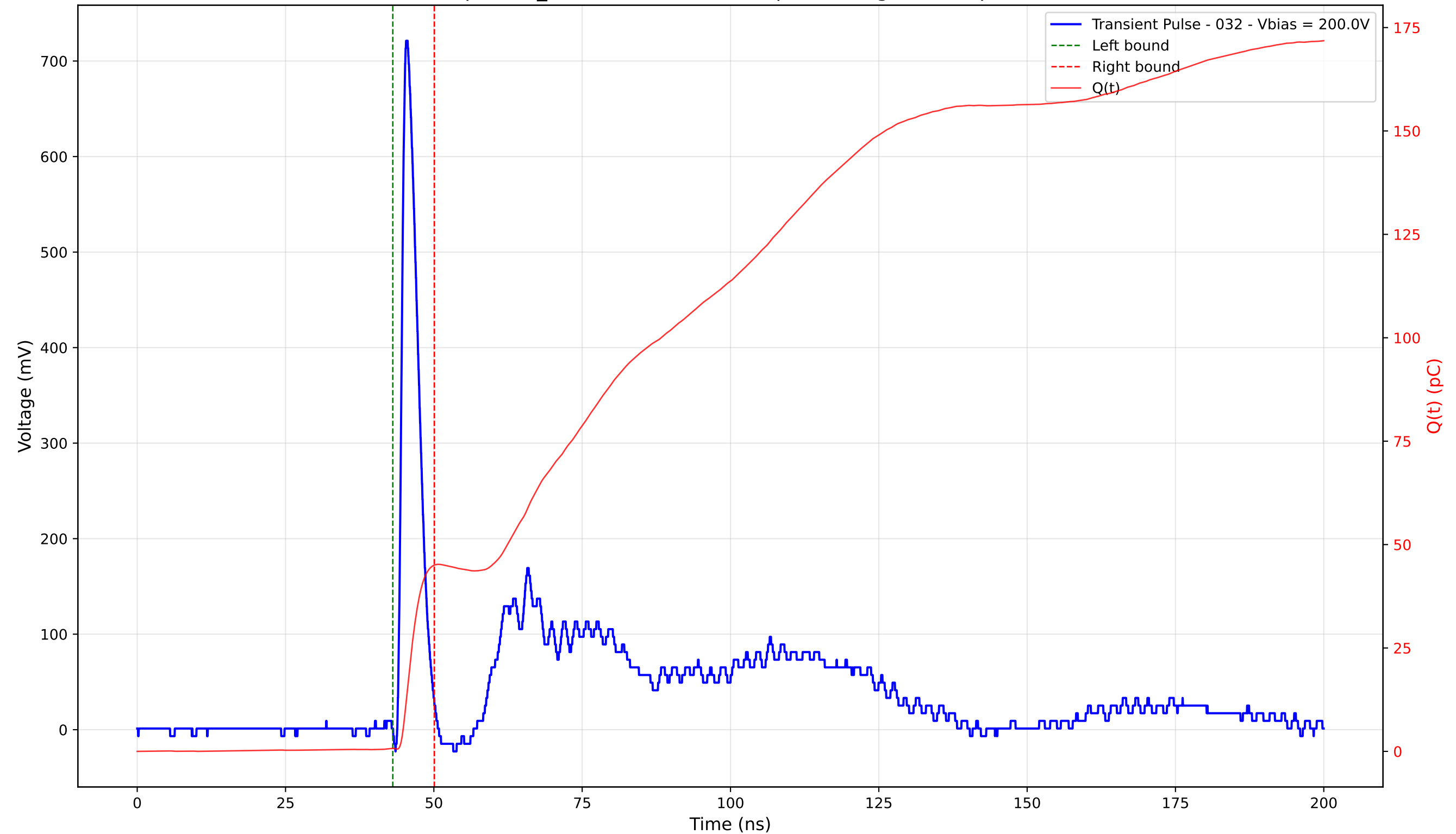
Transient Pulse - Sample: TD_4004 - Position: 150.0 \mu\text{m} - Charge: 44.31 pC - Rise Time: 0.96 ns
