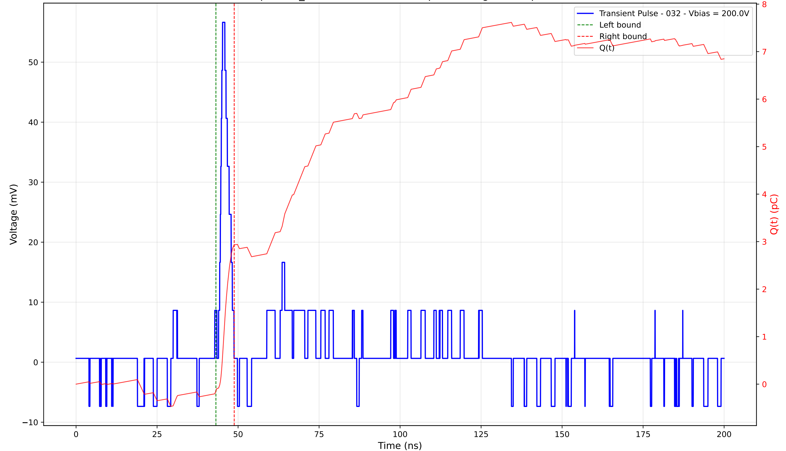
Transient Pulse - Sample: TD_4004 - Position: 425.0 \mu\text{m} - Charge: 3.07 pC - Rise Time: 1.23 ns
