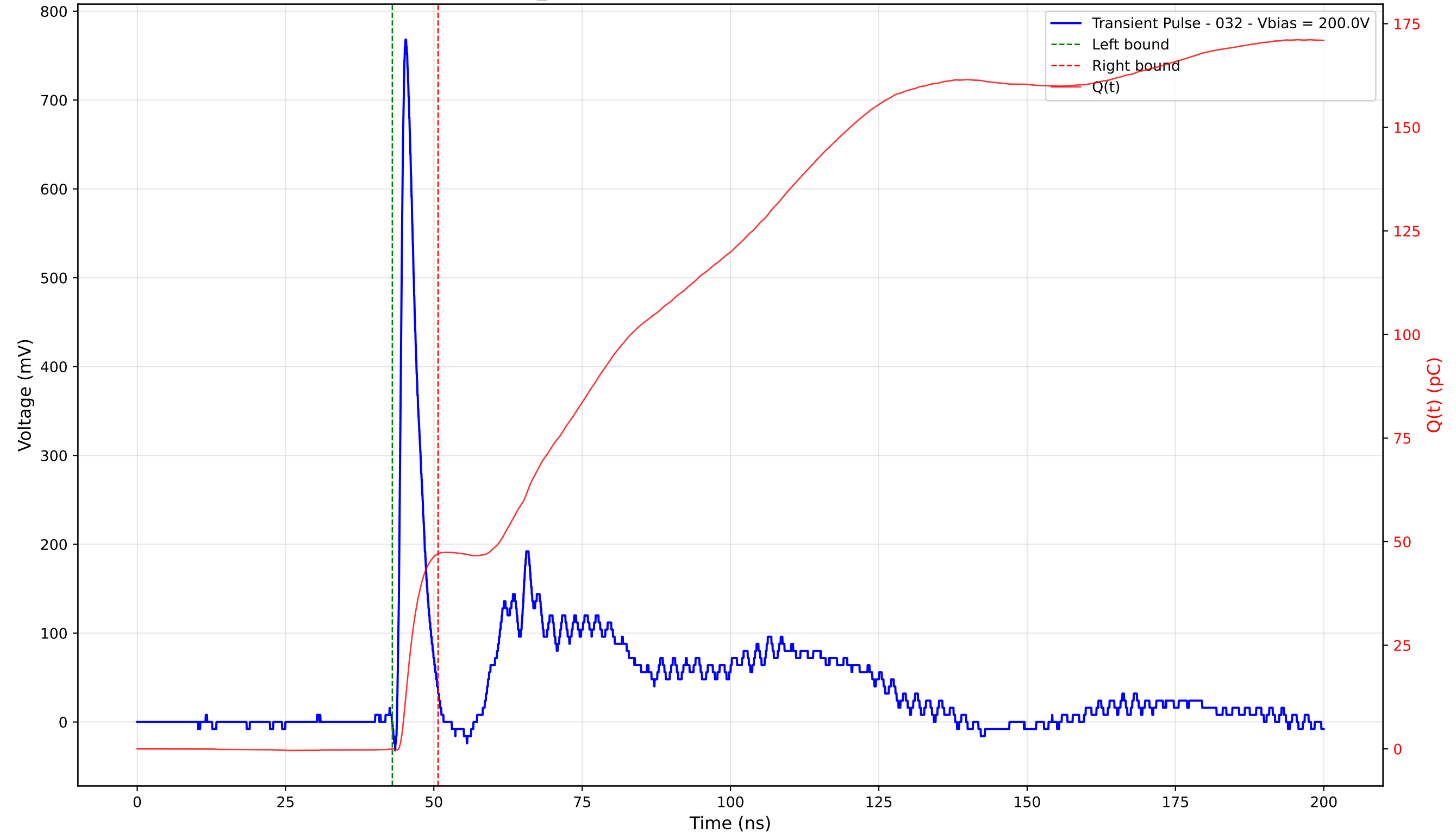
Transient Pulse - Sample: TD_4004 - Position: 105.0 \mu\text{m} - Charge: 47.11 pC - Rise Time: 0.90 ns
