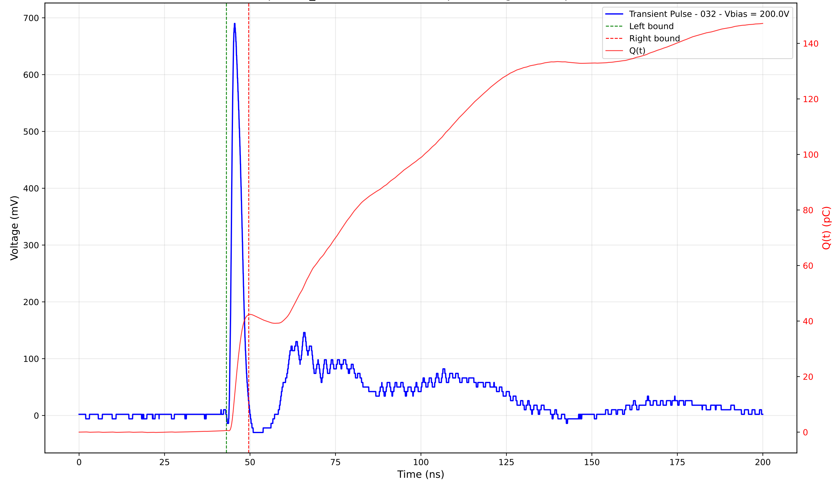
Transient Pulse - Sample: TD_4004 - Position: 265.0 \mu\text{m} - Charge: 41.66 pC - Rise Time: 1.00 ns
