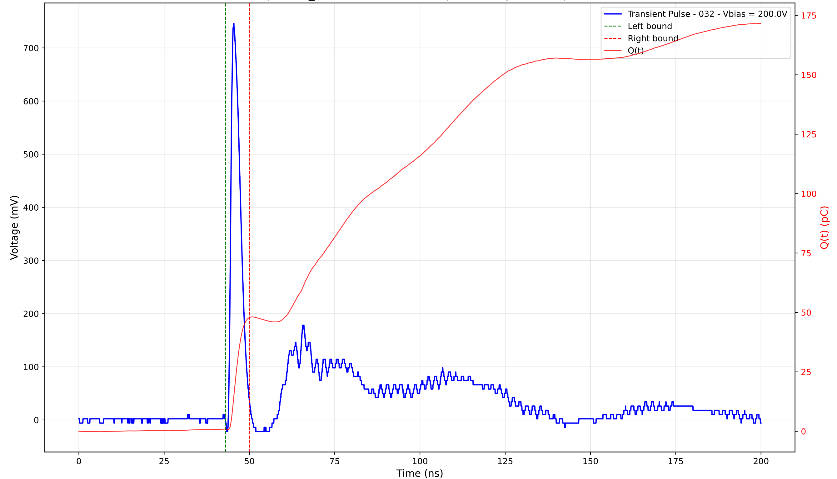
Transient Pulse - Sample: TD_4004 - Position: 225.0 \mu\text{m} - Charge: 46.98 pC - Rise Time: 0.95 ns
