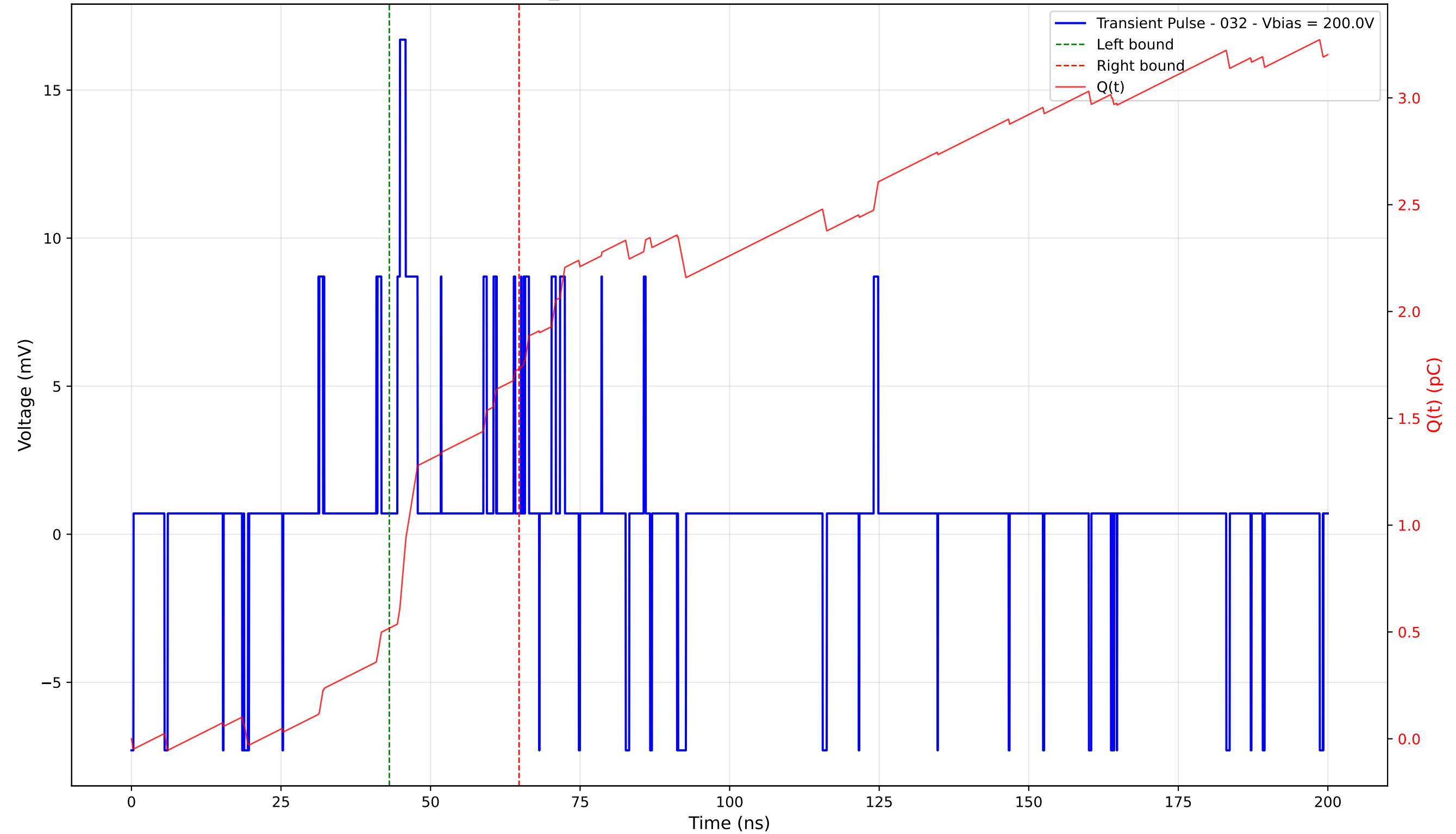
Transient Pulse - Sample: TD_4004 - Position: 15.0 \mu\text{m} - Charge: 1.21 pC - Rise Time: 0.44 ns
