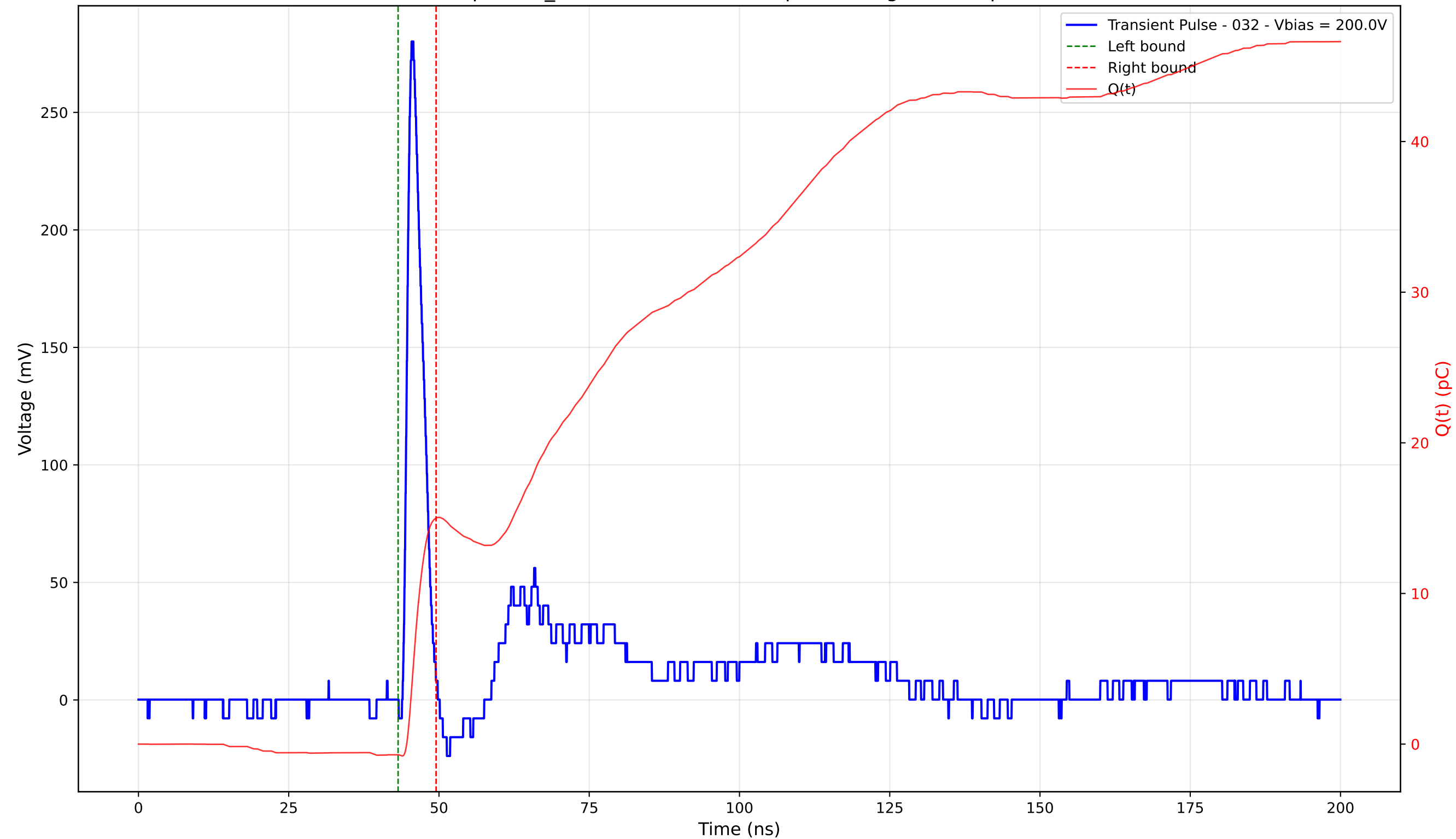
Transient Pulse - Sample: TD_4004 - Position: 395.0 \mu\text{m} - Charge: 15.71 pC - Rise Time: 1.03 ns
