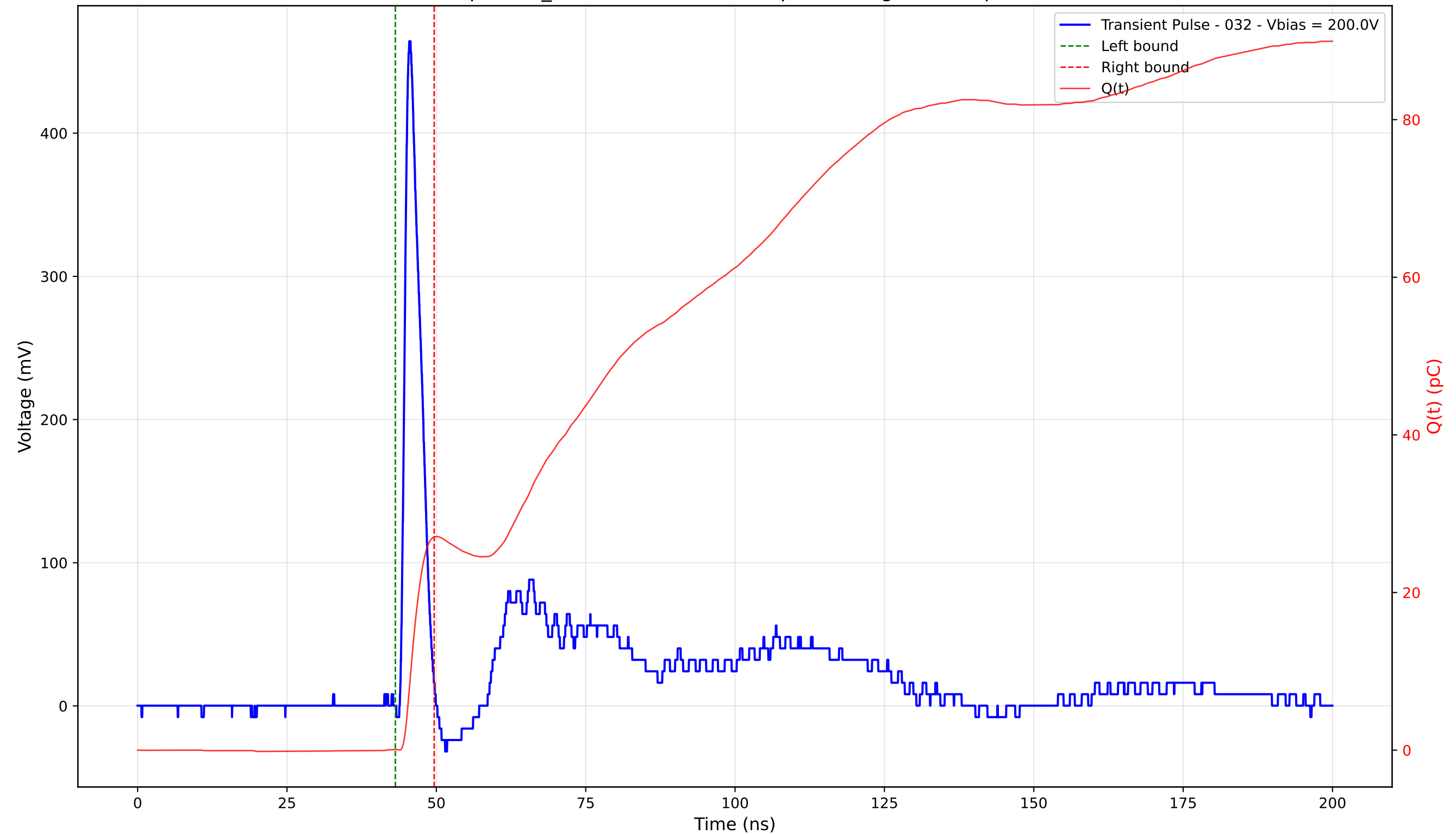
Transient Pulse - Sample: TD_4004 - Position: 355.0 \mu\text{m} - Charge: 26.97 pC - Rise Time: 1.02 ns
