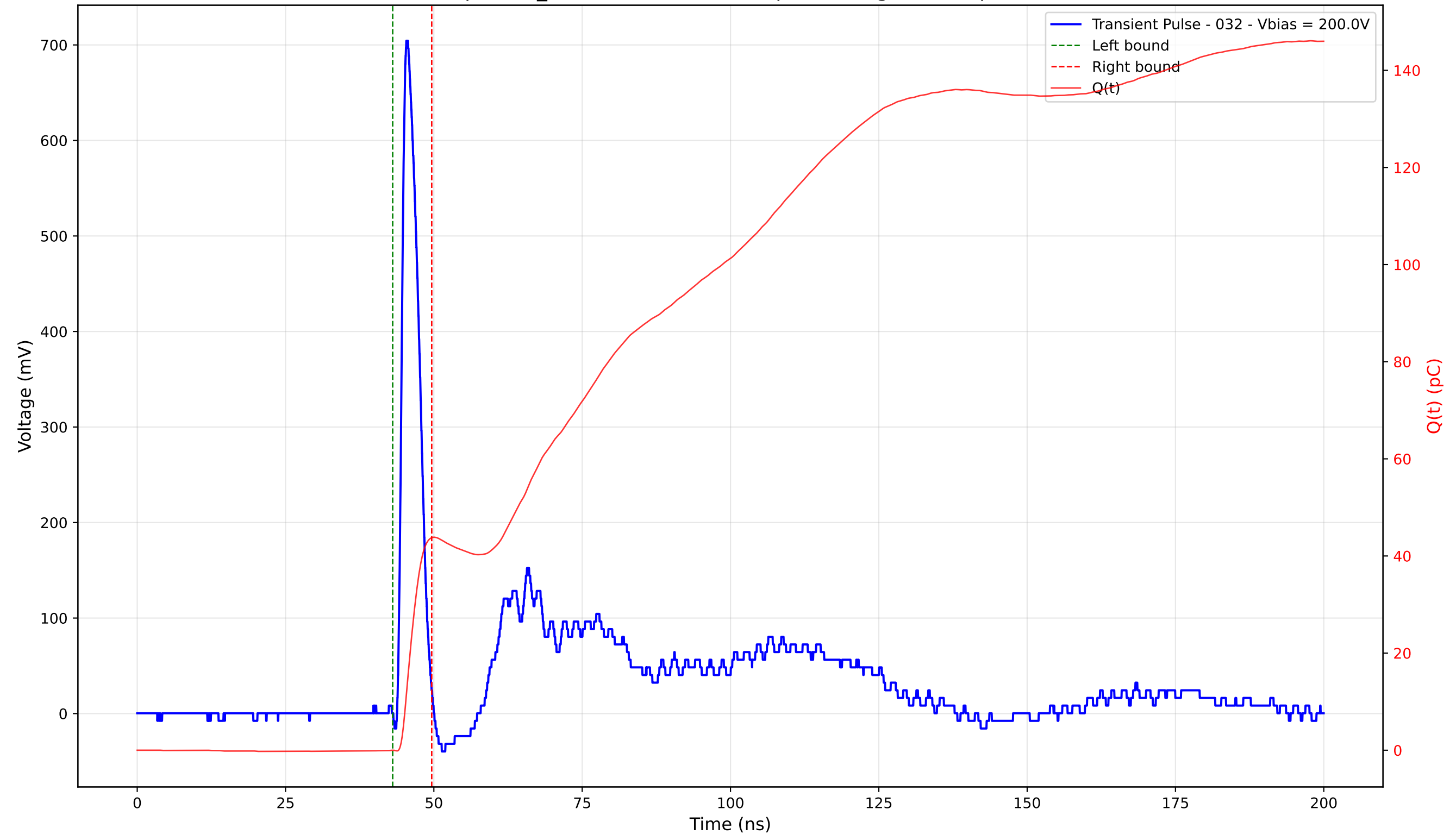
Transient Pulse - Sample: TD_4004 - Position: 280.0 \mu\text{m} - Charge: 43.77 pC - Rise Time: 0.99 ns
