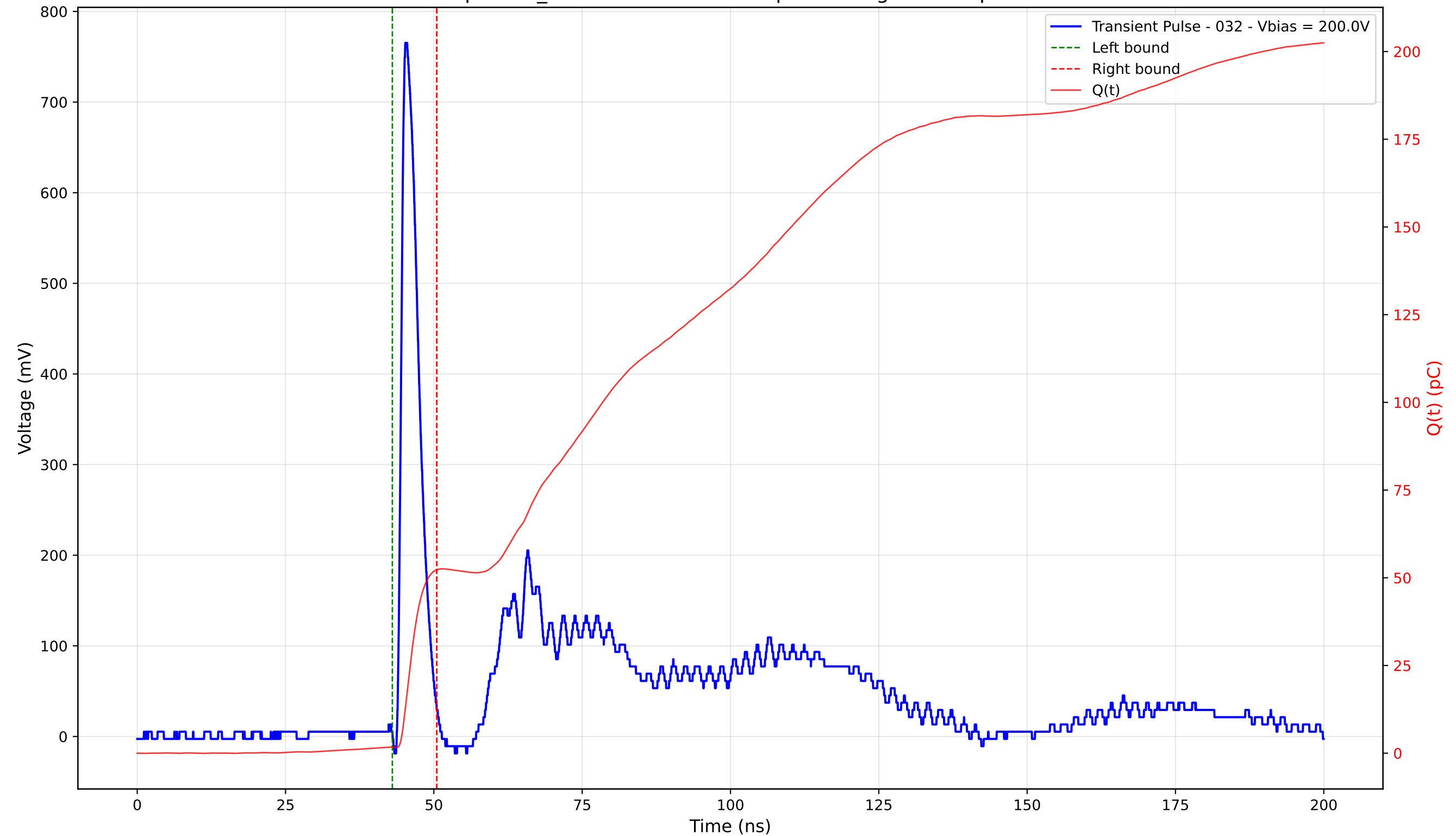
Transient Pulse - Sample: TD_4004 - Position: 180.0 \mu\text{m} - Charge: 50.49 pC - Rise Time: 0.91 ns
