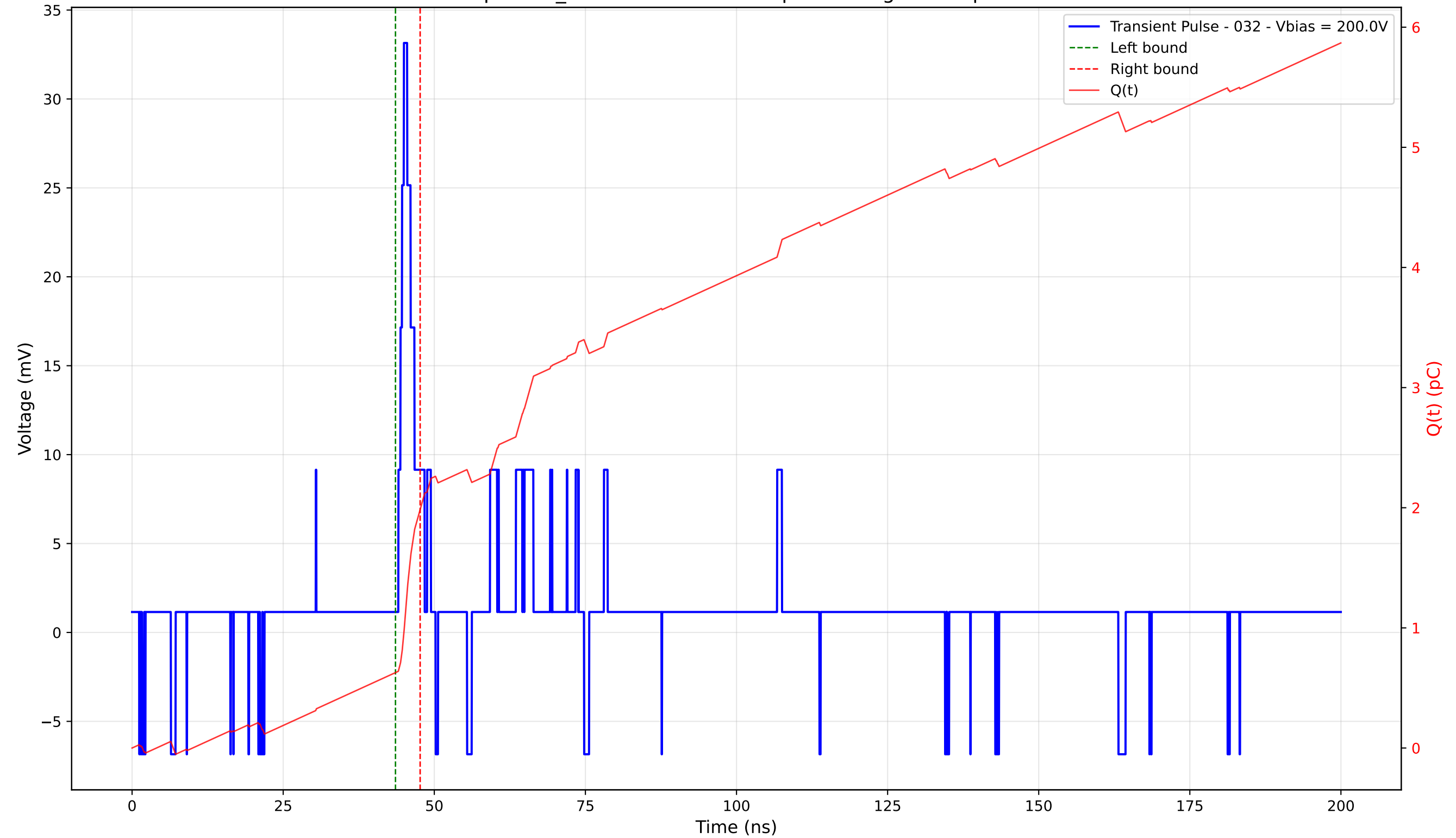
Transient Pulse - Sample: TD_4004 - Position: 35.0 \mu\text{m} - Charge: 1.36 pC - Rise Time: 0.91 ns
