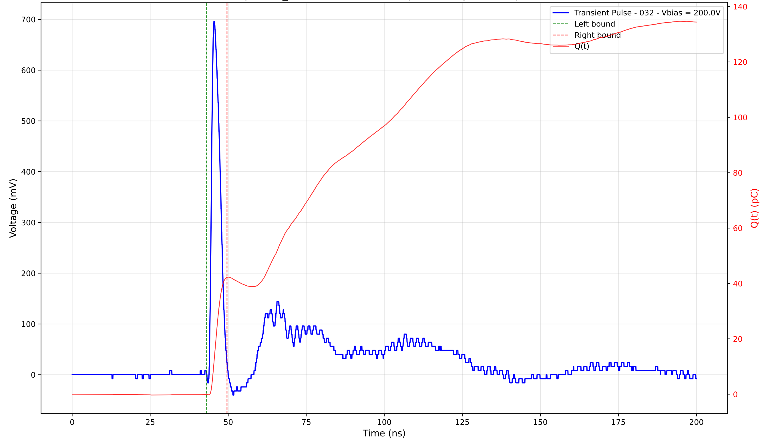
Transient Pulse - Sample: TD_4004 - Position: 270.0 \mu\text{m} - Charge: 42.28 pC - Rise Time: 0.99 ns
