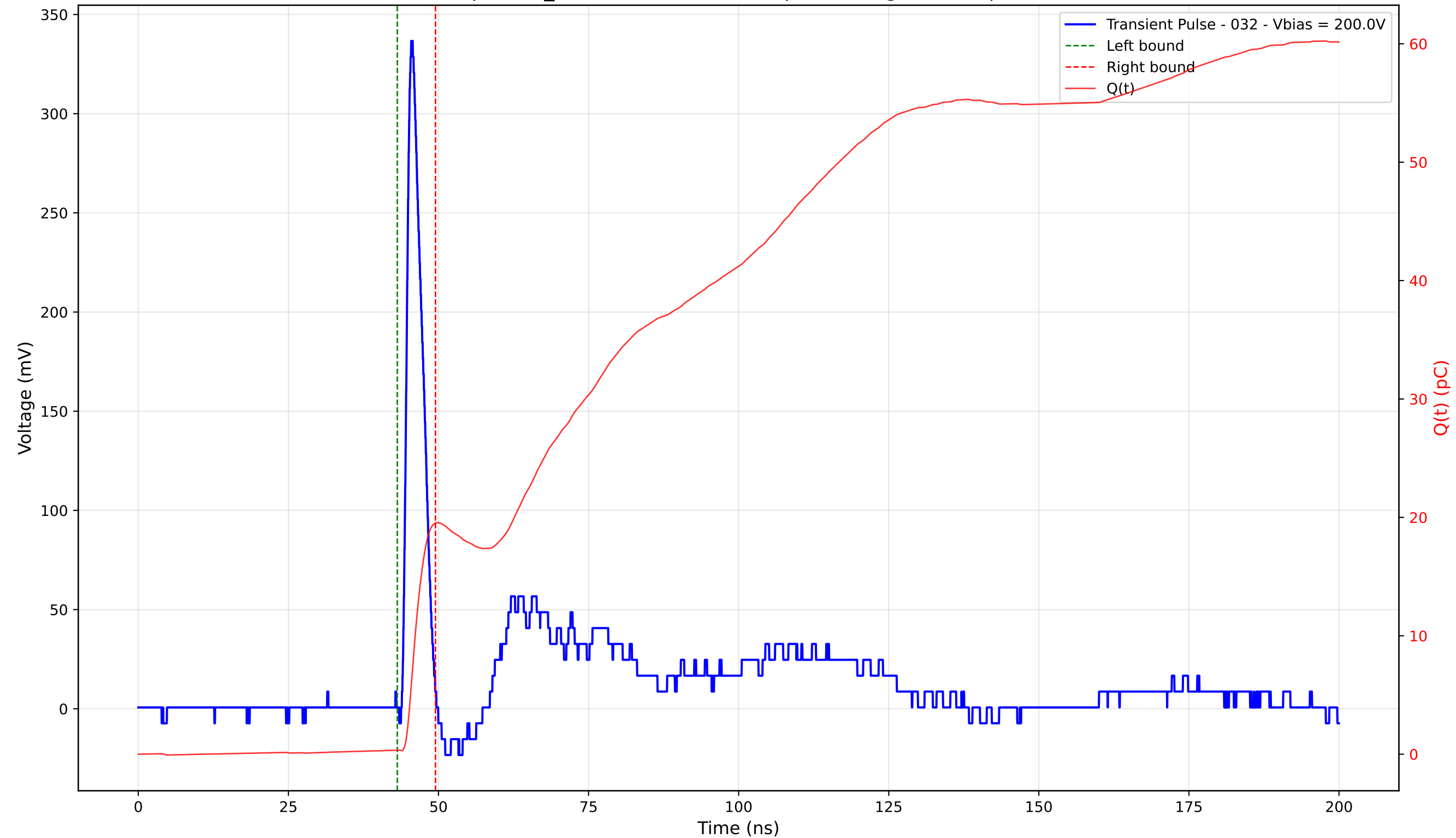
Transient Pulse - Sample: TD_4004 - Position: 390.0 \mu\text{m} - Charge: 19.18 pC - Rise Time: 1.02 ns
