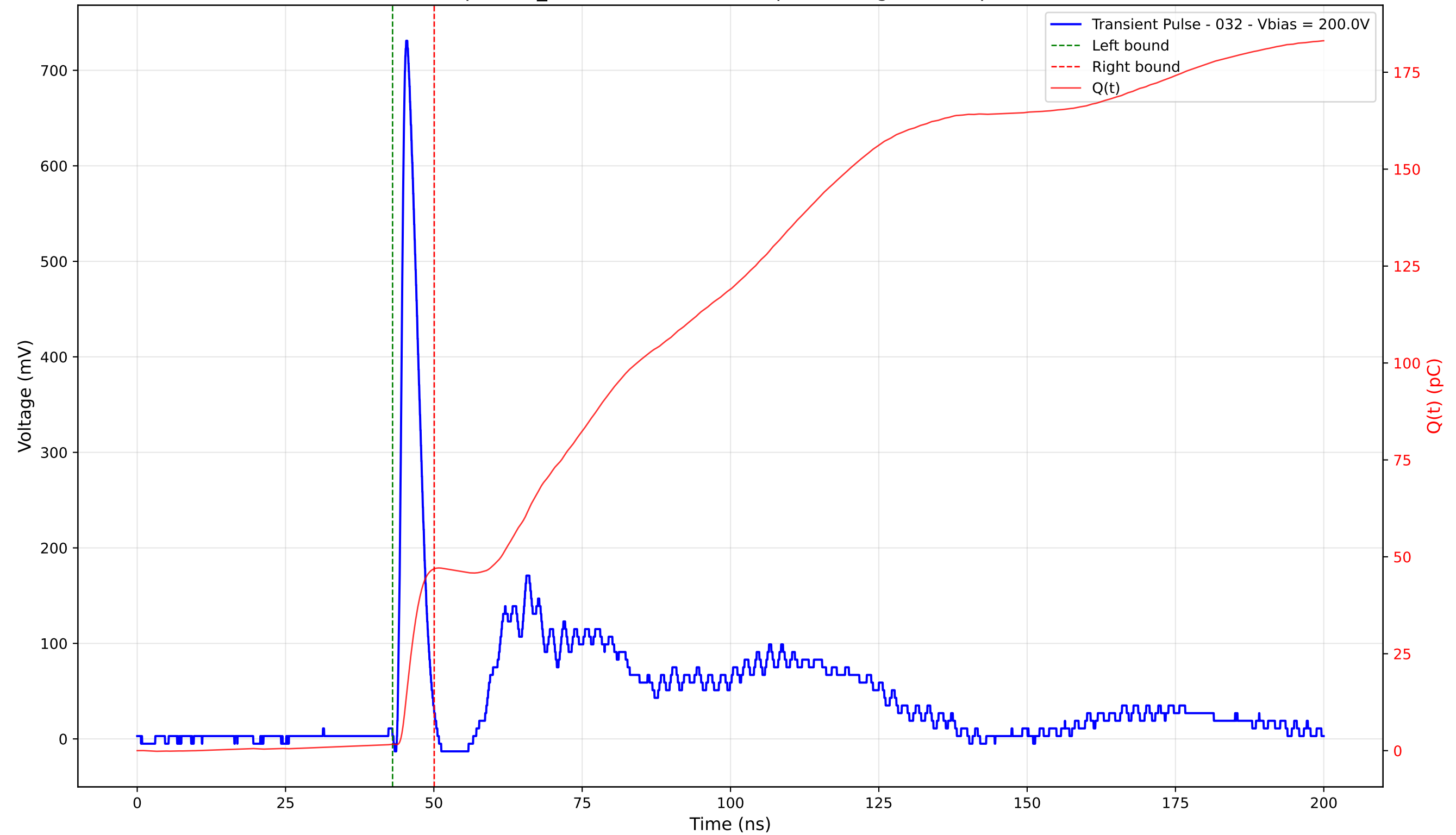
Transient Pulse - Sample: TD_4004 - Position: 135.0 \mu\text{m} - Charge: 45.25 pC - Rise Time: 0.96 ns
