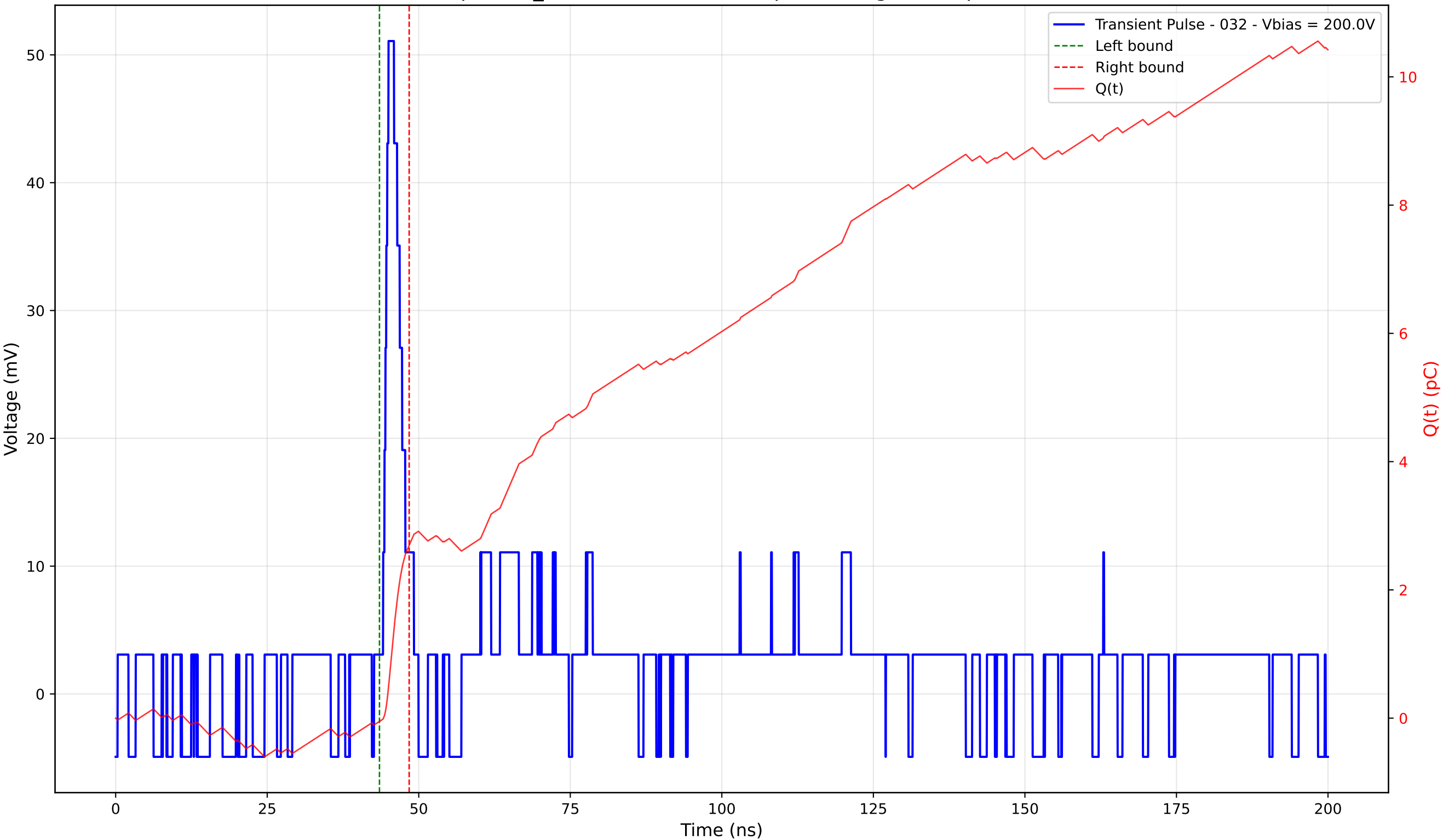
Transient Pulse - Sample: TD_4004 - Position: 430.0 \mu\text{m} - Charge: 2.75 pC - Rise Time: 0.89 ns
