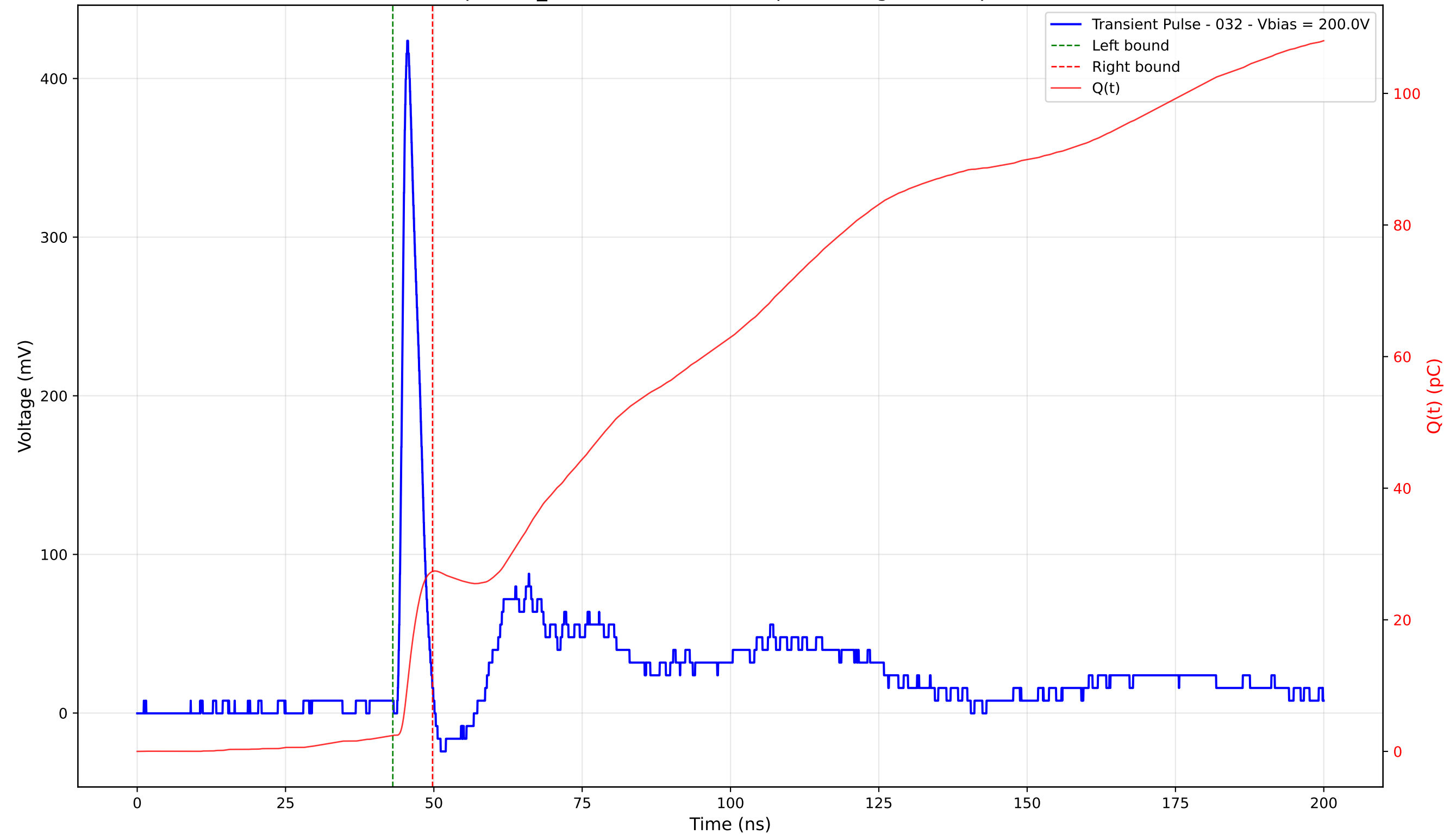
Transient Pulse - Sample: TD_4004 - Position: 370.0 \mu\text{m} - Charge: 24.91 pC - Rise Time: 1.07 ns
