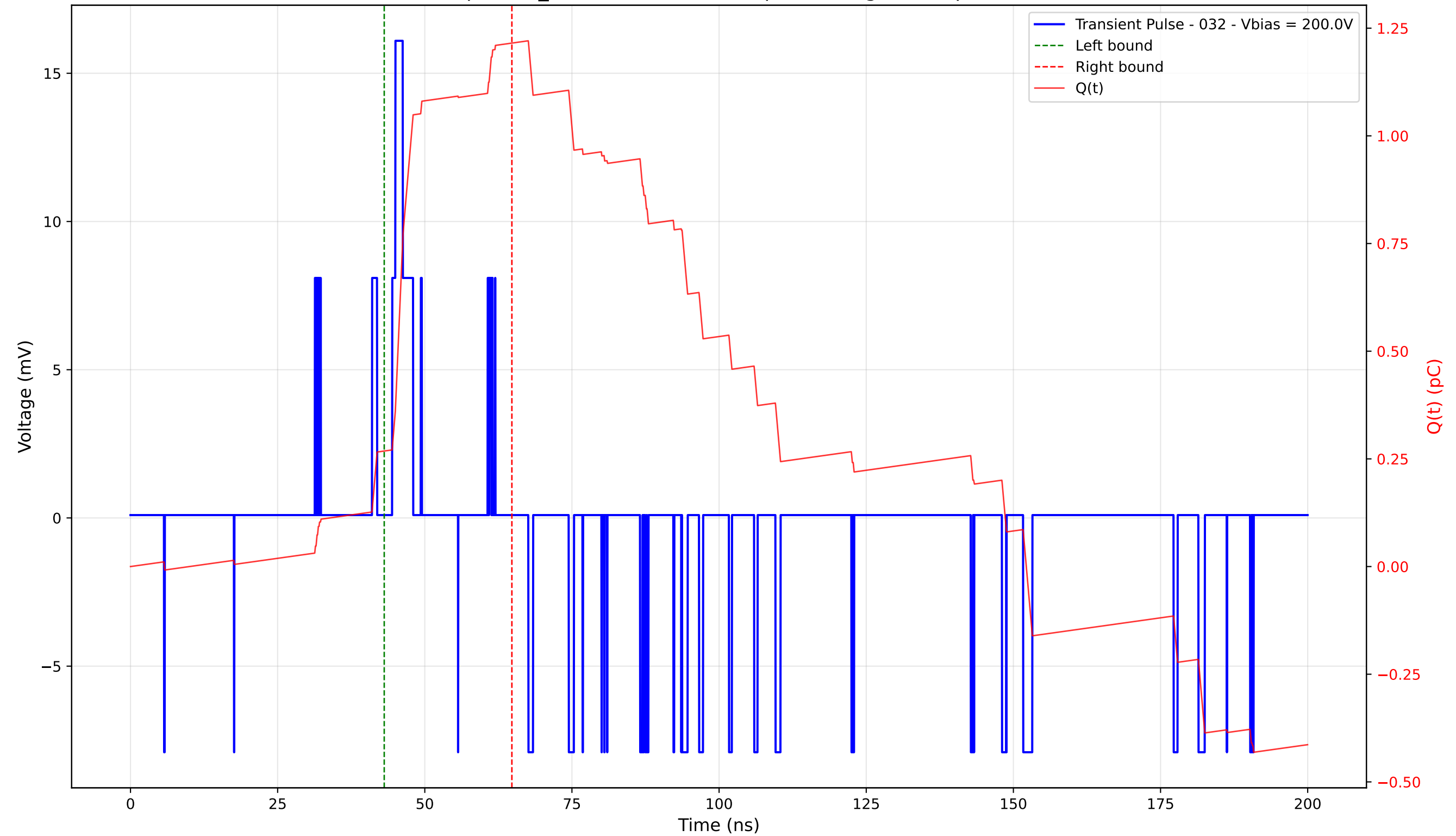
Transient Pulse - Sample: TD_4004 - Position: 20.0 \mu\text{m} - Charge: 0.95 pC - Rise Time: 0.56 ns
