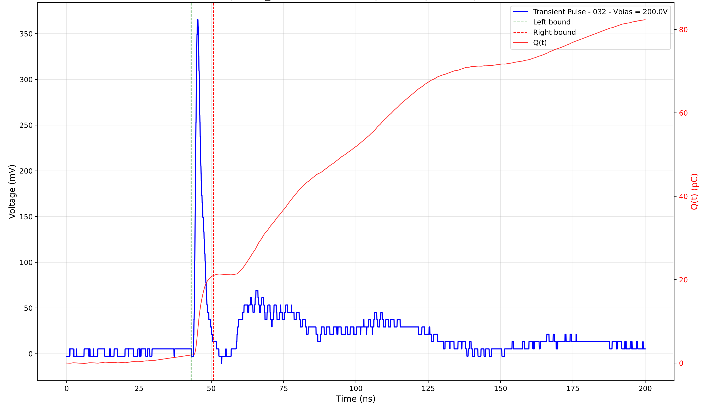
Transient Pulse - Sample: TD_4004 - Position: 65.0 \mu\text{m} - Charge: 19.04 pC - Rise Time: 0.94 ns
