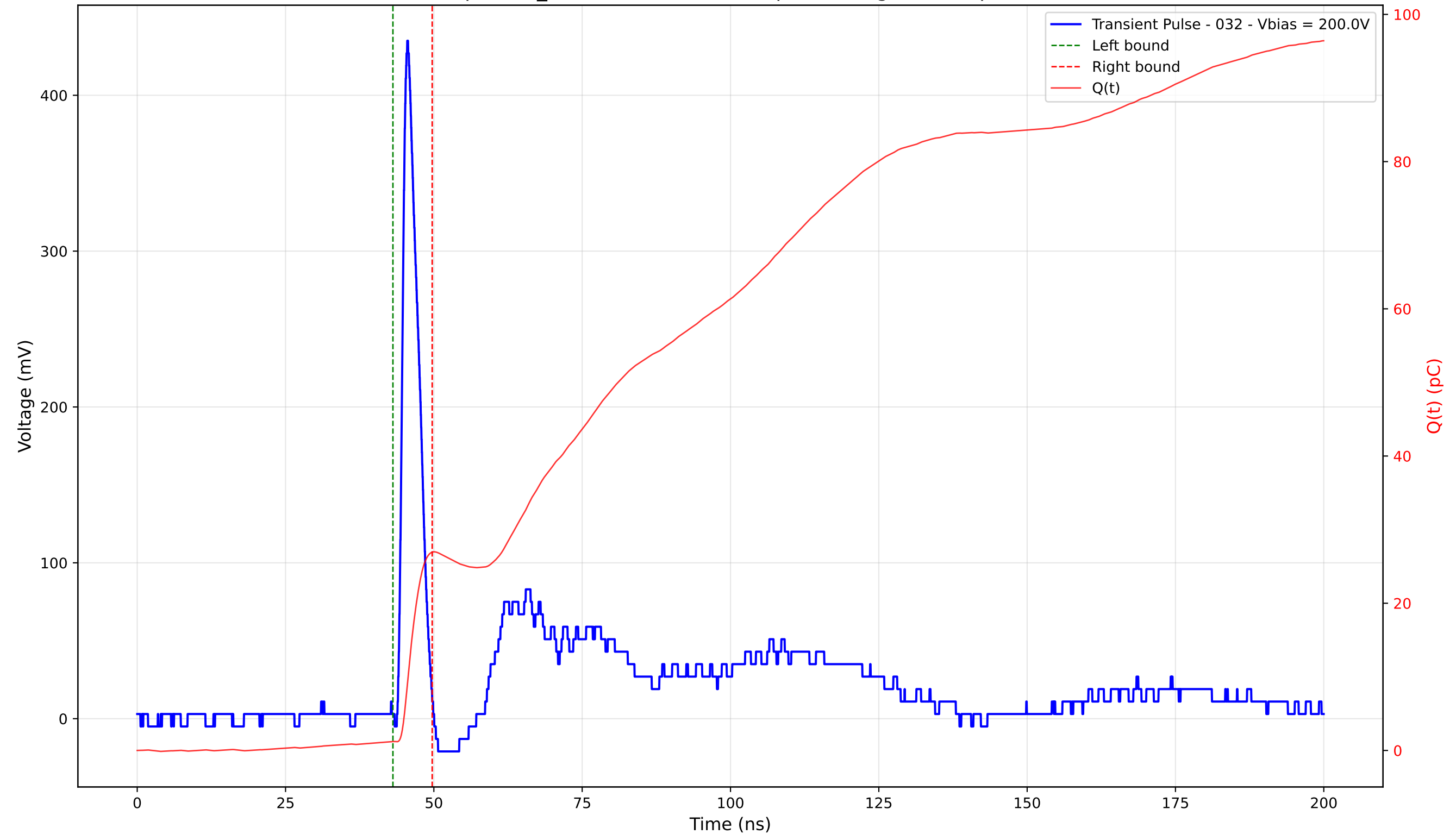
Transient Pulse - Sample: TD_4004 - Position: 365.0 \mu\text{m} - Charge: 25.74 pC - Rise Time: 1.06 ns
