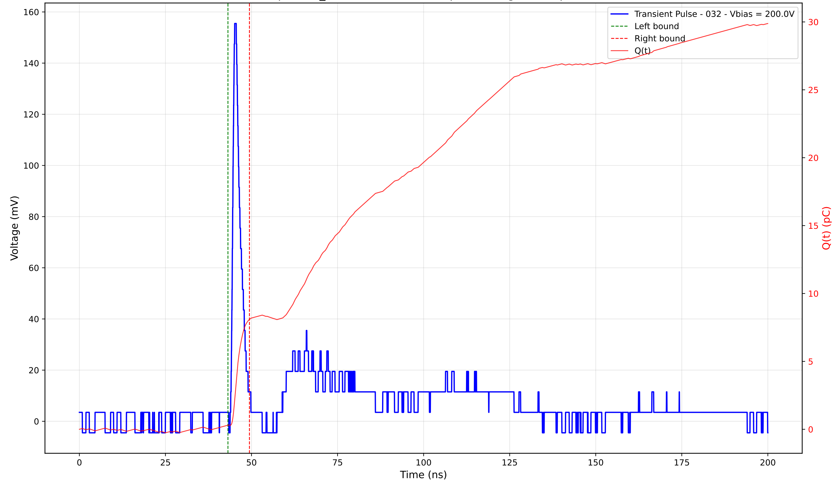
Transient Pulse - Sample: TD_4004 - Position: 55.0 \mu\text{m} - Charge: 7.78 pC - Rise Time: 0.91 ns
