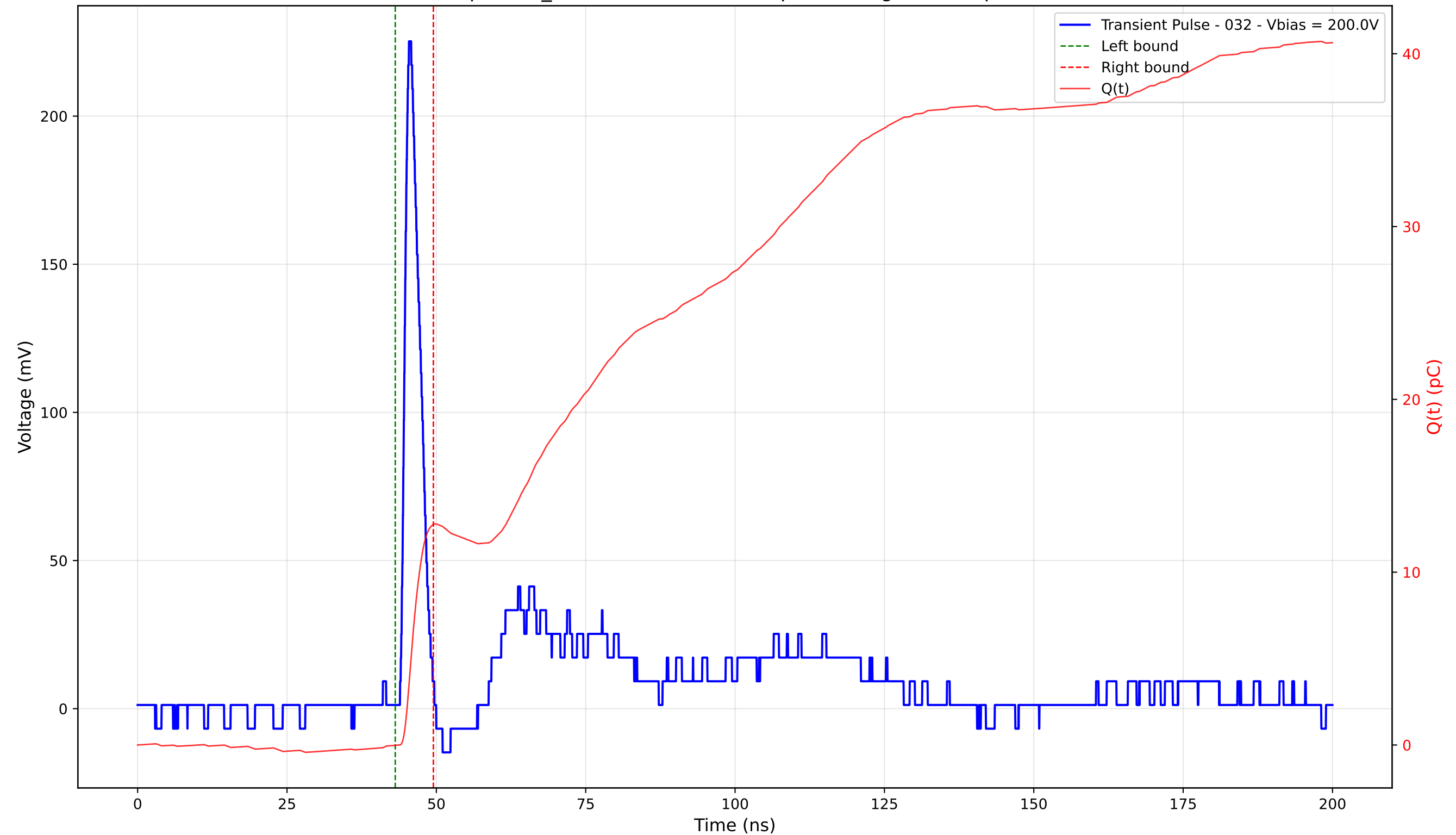
Transient Pulse - Sample: TD_4004 - Position: 400.0 \mu\text{m} - Charge: 12.78 pC - Rise Time: 1.09 ns
