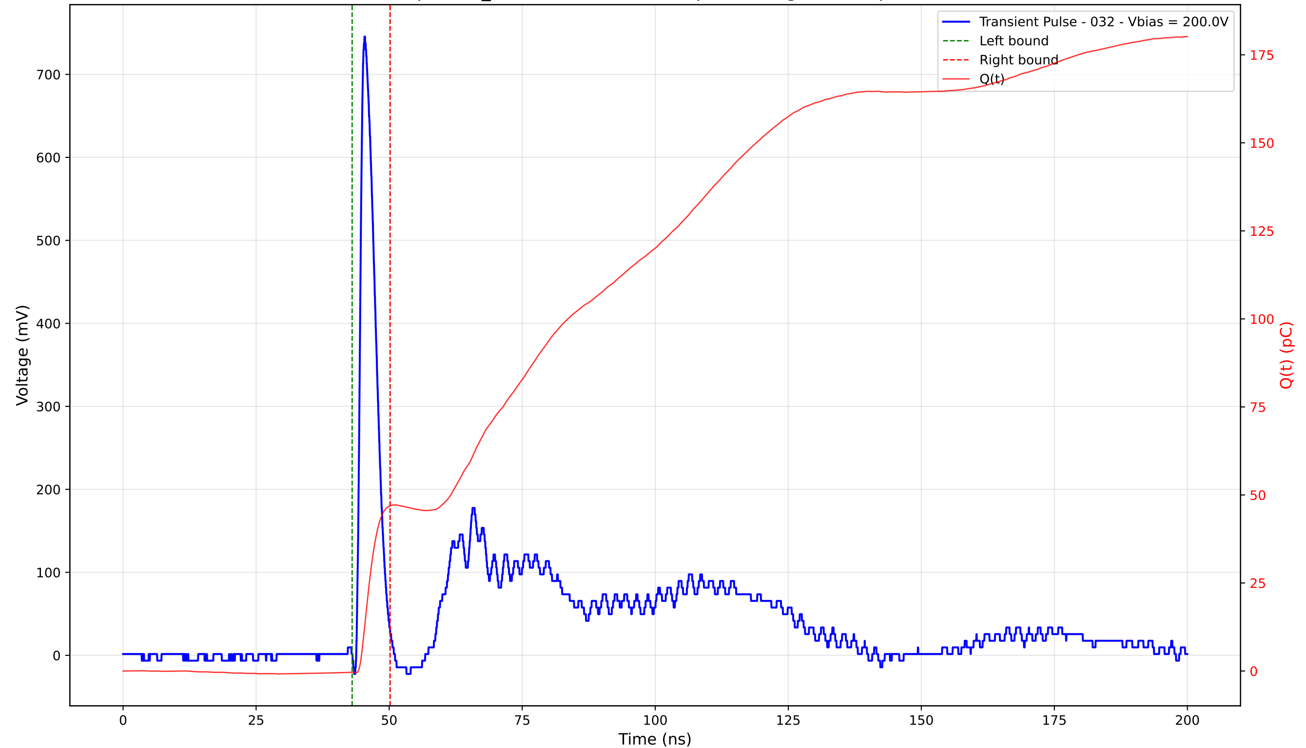
Transient Pulse - Sample: TD_4004 - Position: 165.0 \mu\text{m} - Charge: 47.26 pC - Rise Time: 0.93 ns
