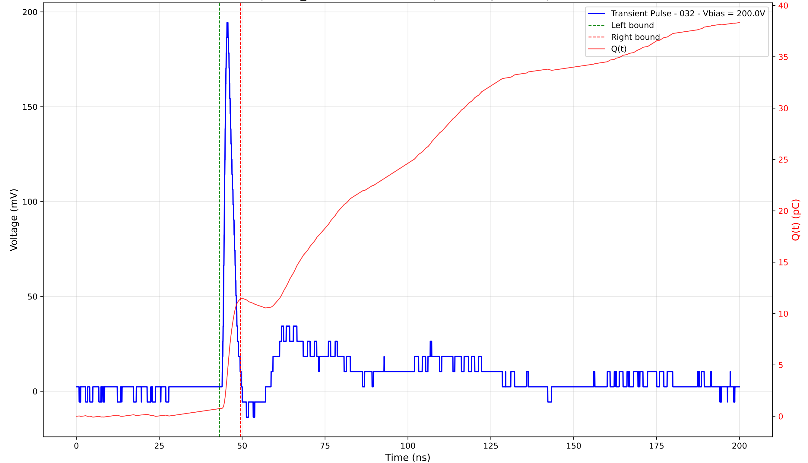
Transient Pulse - Sample: TD_4004 - Position: 405.0 \mu\text{m} - Charge: 10.69 pC - Rise Time: 1.02 ns
