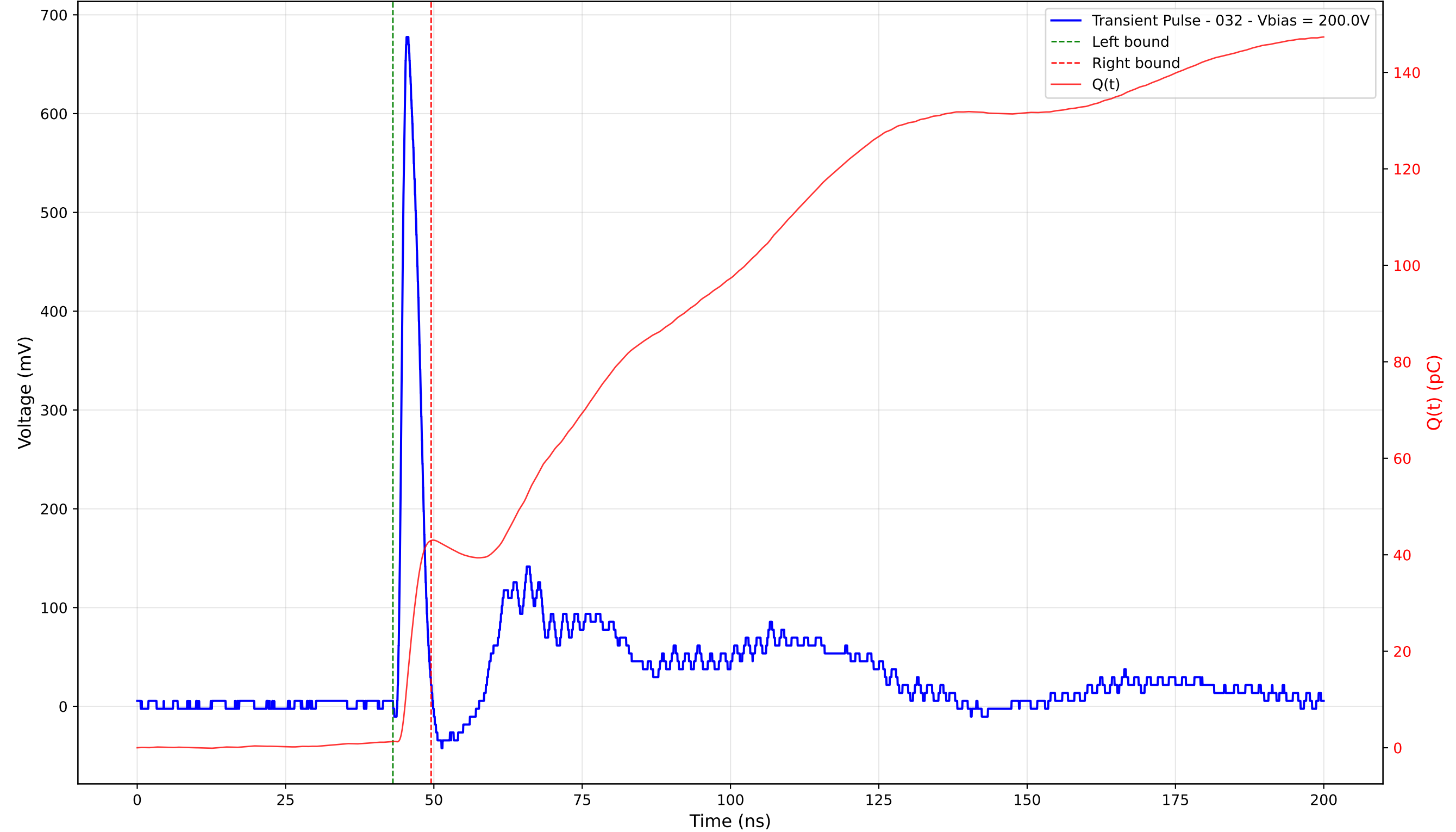
Transient Pulse - Sample: TD_4004 - Position: 300.0 \mu\text{m} - Charge: 41.64 pC - Rise Time: 1.00 ns
