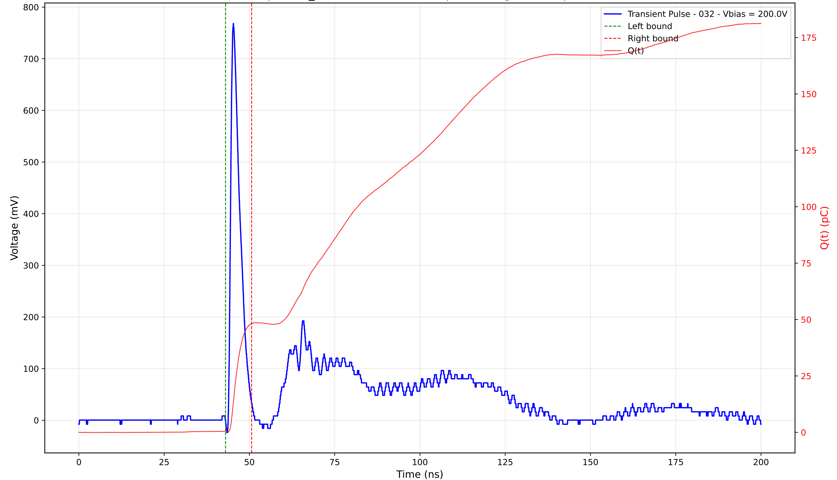
Transient Pulse - Sample: TD_4004 - Position: 115.0 \mu\text{m} - Charge: 47.70 pC - Rise Time: 0.92 ns
