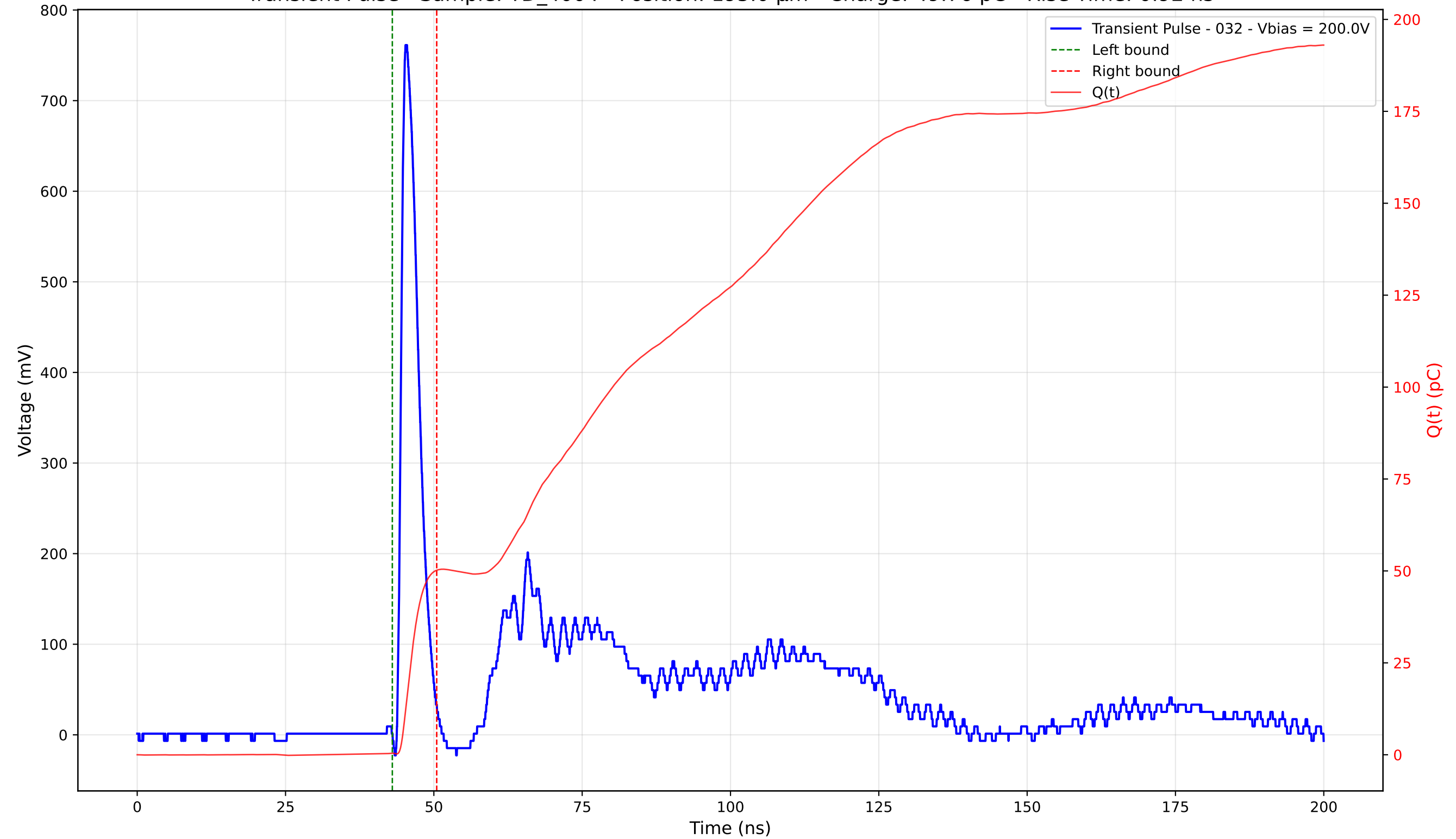
Transient Pulse - Sample: TD_4004 - Position: 195.0 \mu\text{m} - Charge: 49.76 pC - Rise Time: 0.92 ns
