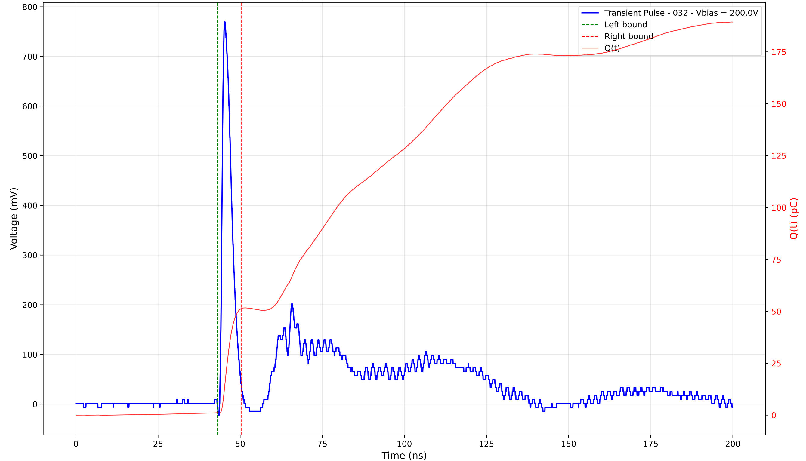
Transient Pulse - Sample: TD_4004 - Position: 190.0 \mu\text{m} - Charge: 50.24 pC - Rise Time: 0.92 ns
