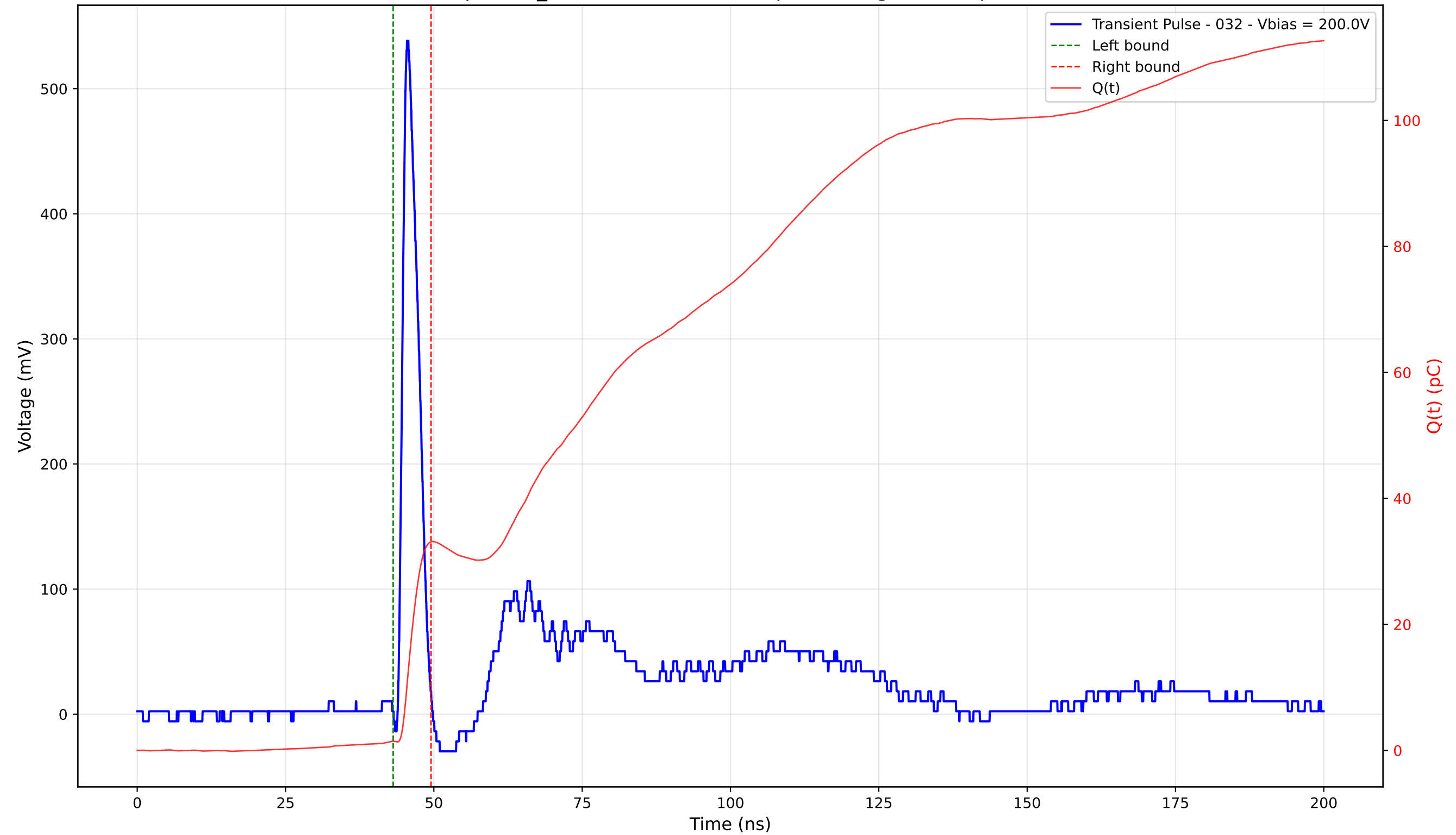
Transient Pulse - Sample: TD_4004 - Position: 330.0 \mu\text{m} - Charge: 31.65 pC - Rise Time: 1.04 ns
