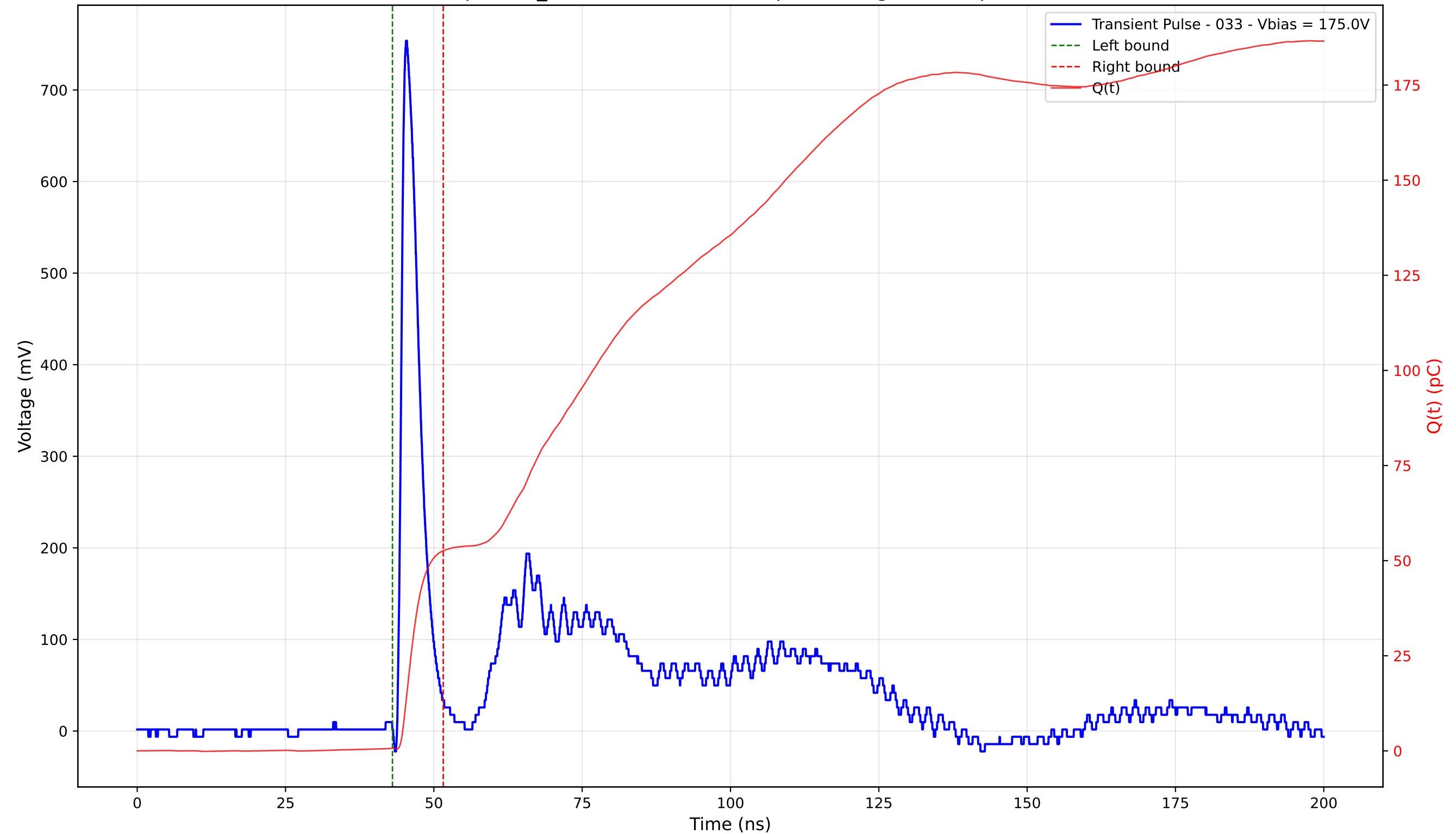
Transient Pulse - Sample: TD_4004 - Position: 200.0 \mu\text{m} - Charge: 51.88 pC - Rise Time: 0.93 ns
