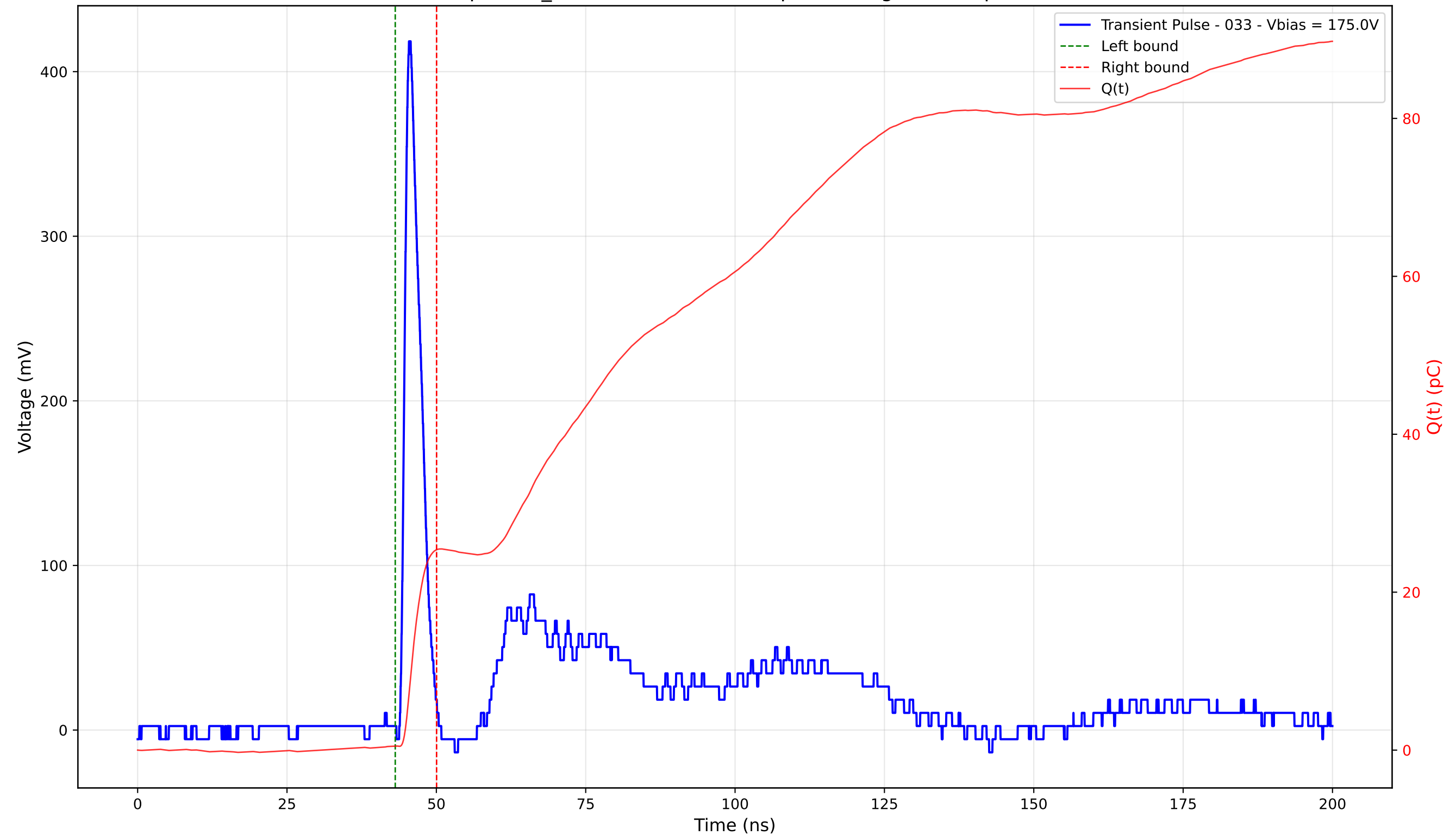
Transient Pulse - Sample: TD_4004 - Position: 350.0 \mu\text{m} - Charge: 24.87 pC - Rise Time: 1.02 ns
