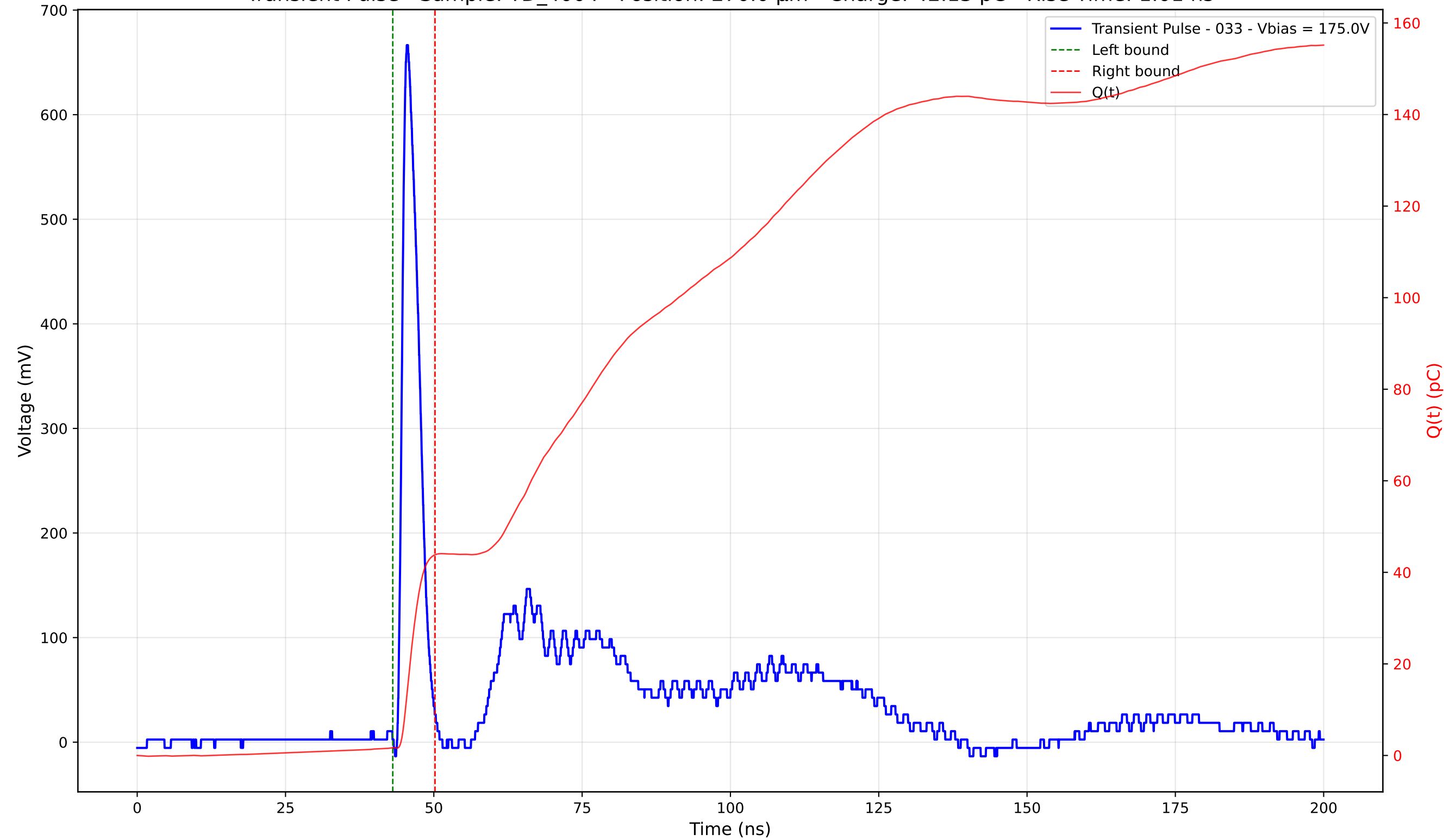
Transient Pulse - Sample: TD_4004 - Position: 270.0 \mu\text{m} - Charge: 42.13 pC - Rise Time: 1.01 ns
