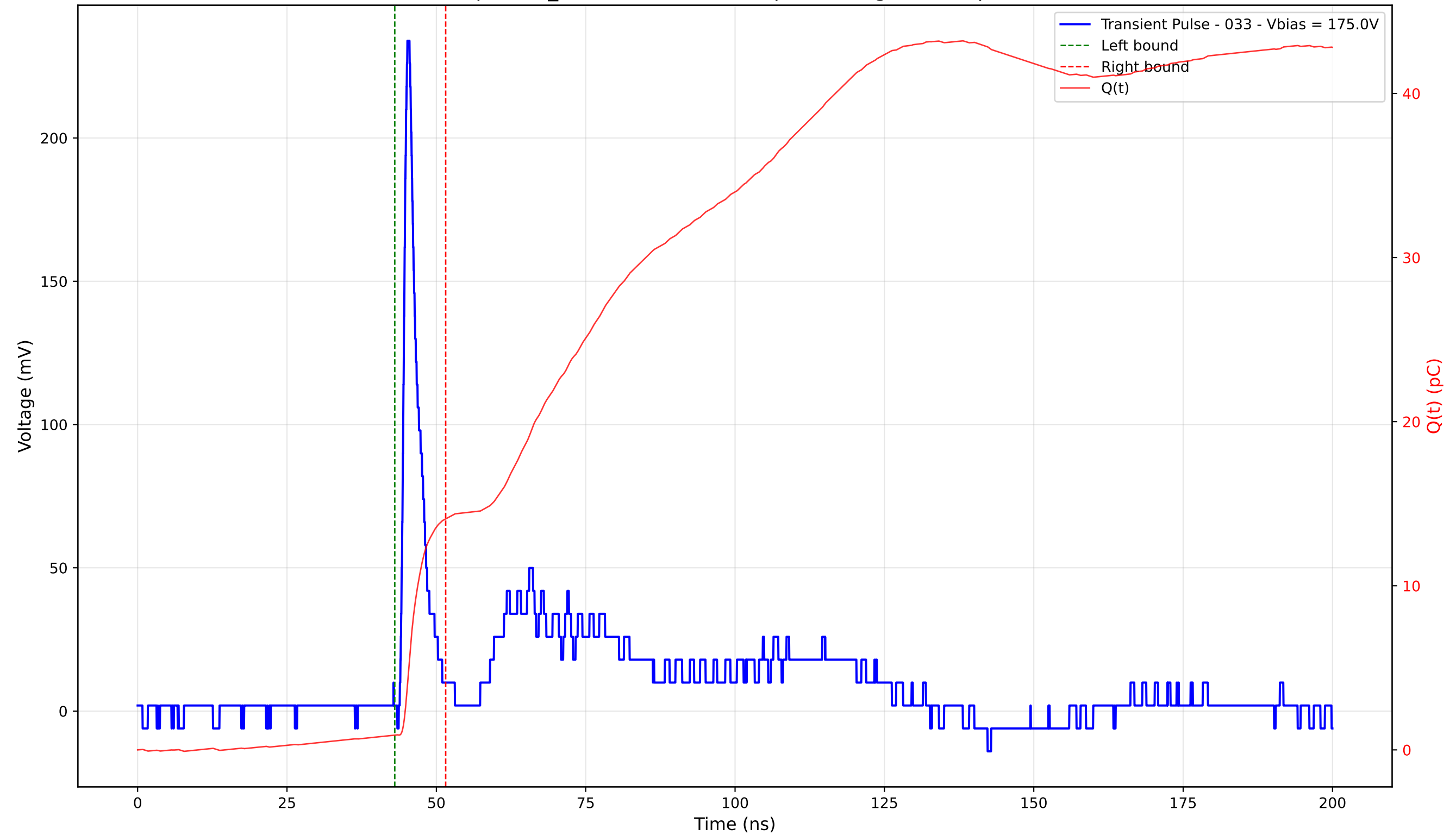
Transient Pulse - Sample: TD_4004 - Position: 60.0 \mu\text{m} - Charge: 13.17 pC - Rise Time: 0.97 ns
