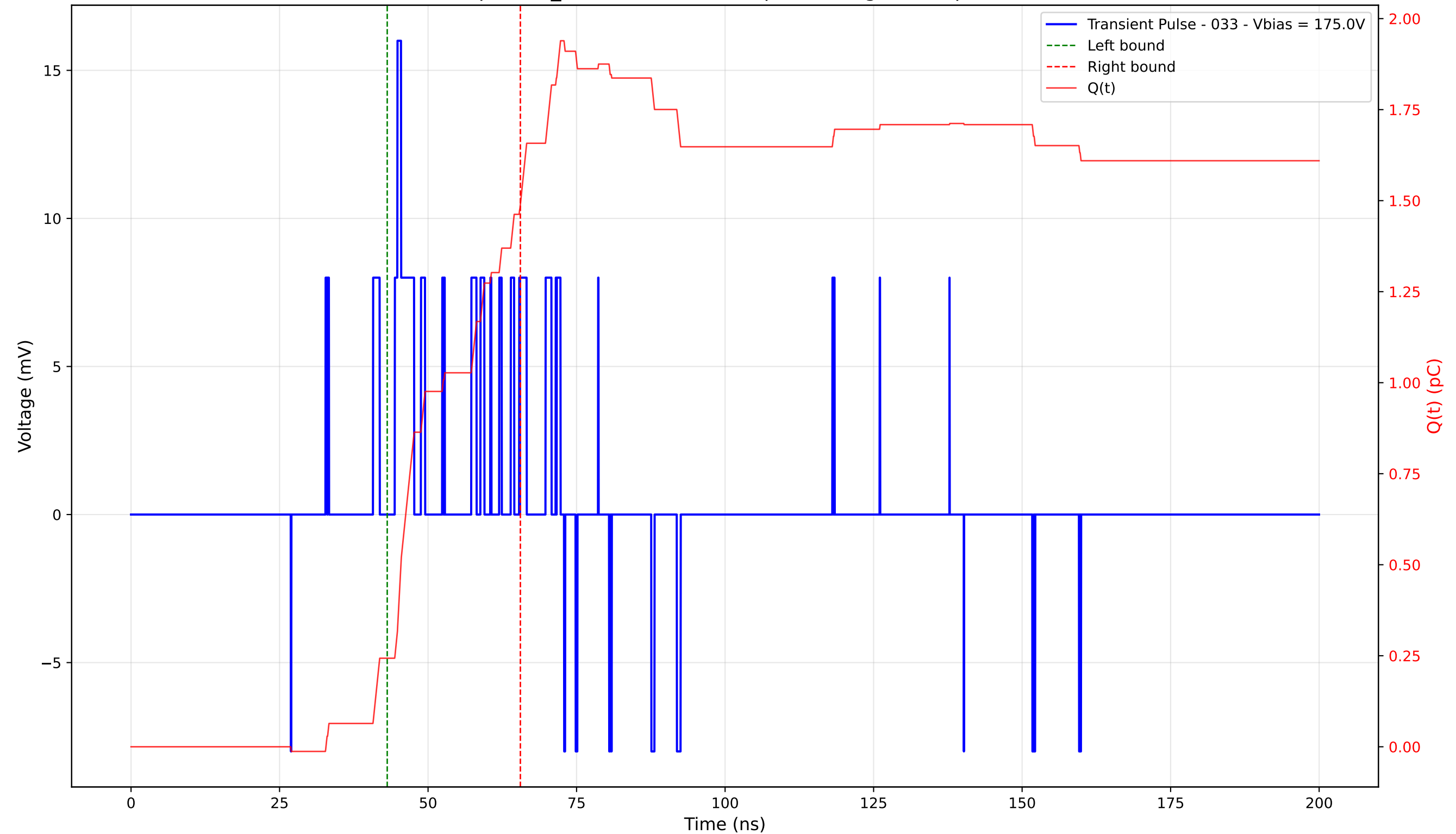
Transient Pulse - Sample: TD_4004 - Position: 0.0 \mu\text{m} - Charge: 1.24 pC - Rise Time: 0.46 ns
