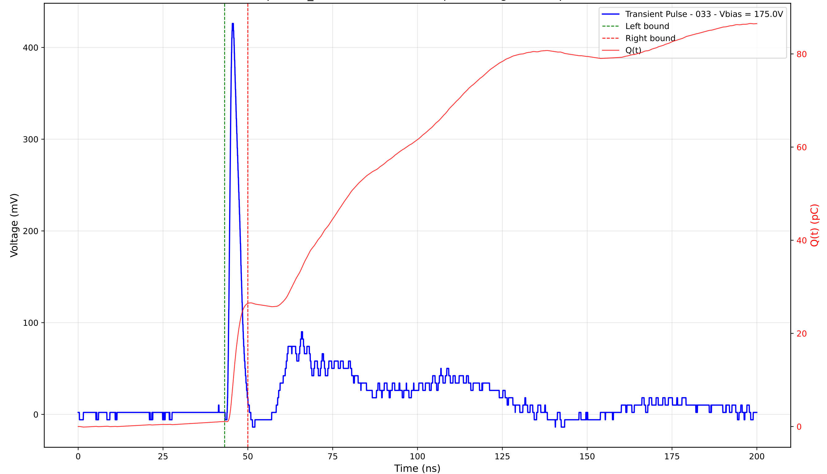
Transient Pulse - Sample: TD_4004 - Position: 340.0 \mu\text{m} - Charge: 25.35 pC - Rise Time: 1.02 ns
