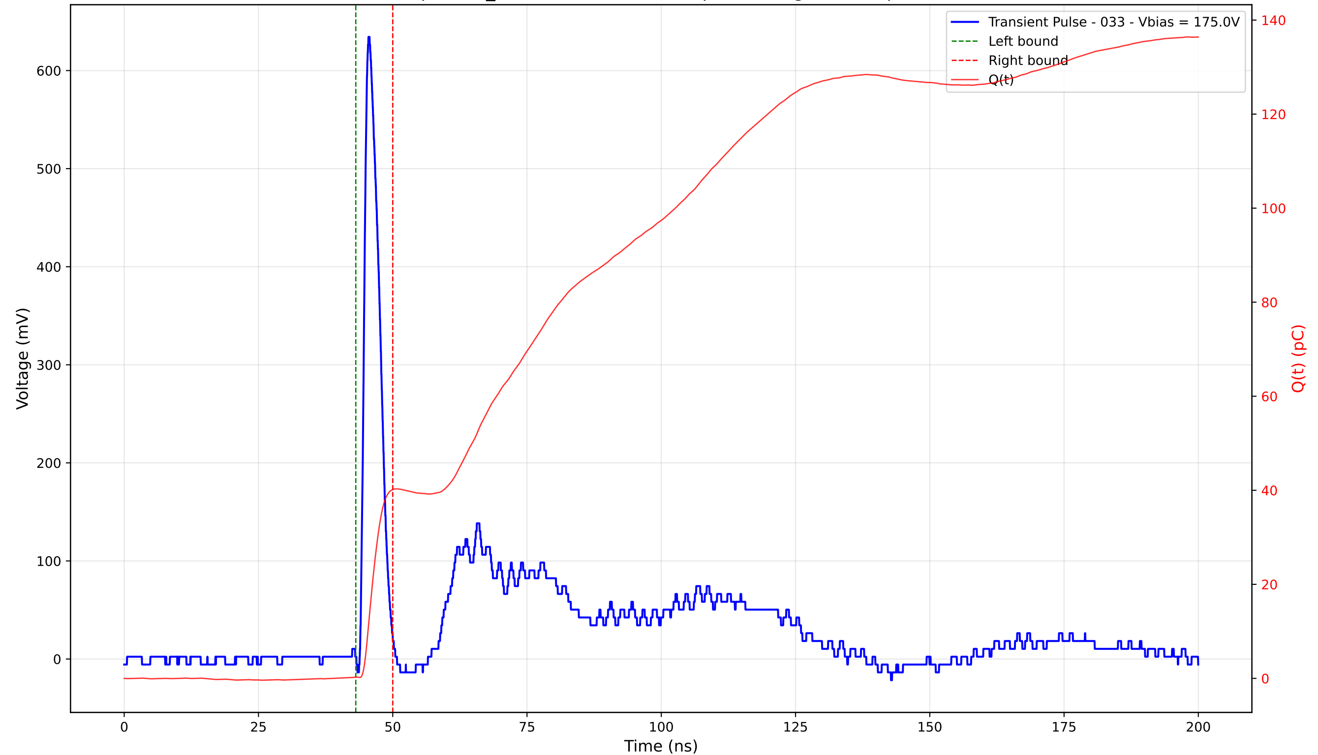
Transient Pulse - Sample: TD_4004 - Position: 300.0 \mu\text{m} - Charge: 39.89 pC - Rise Time: 1.03 ns
