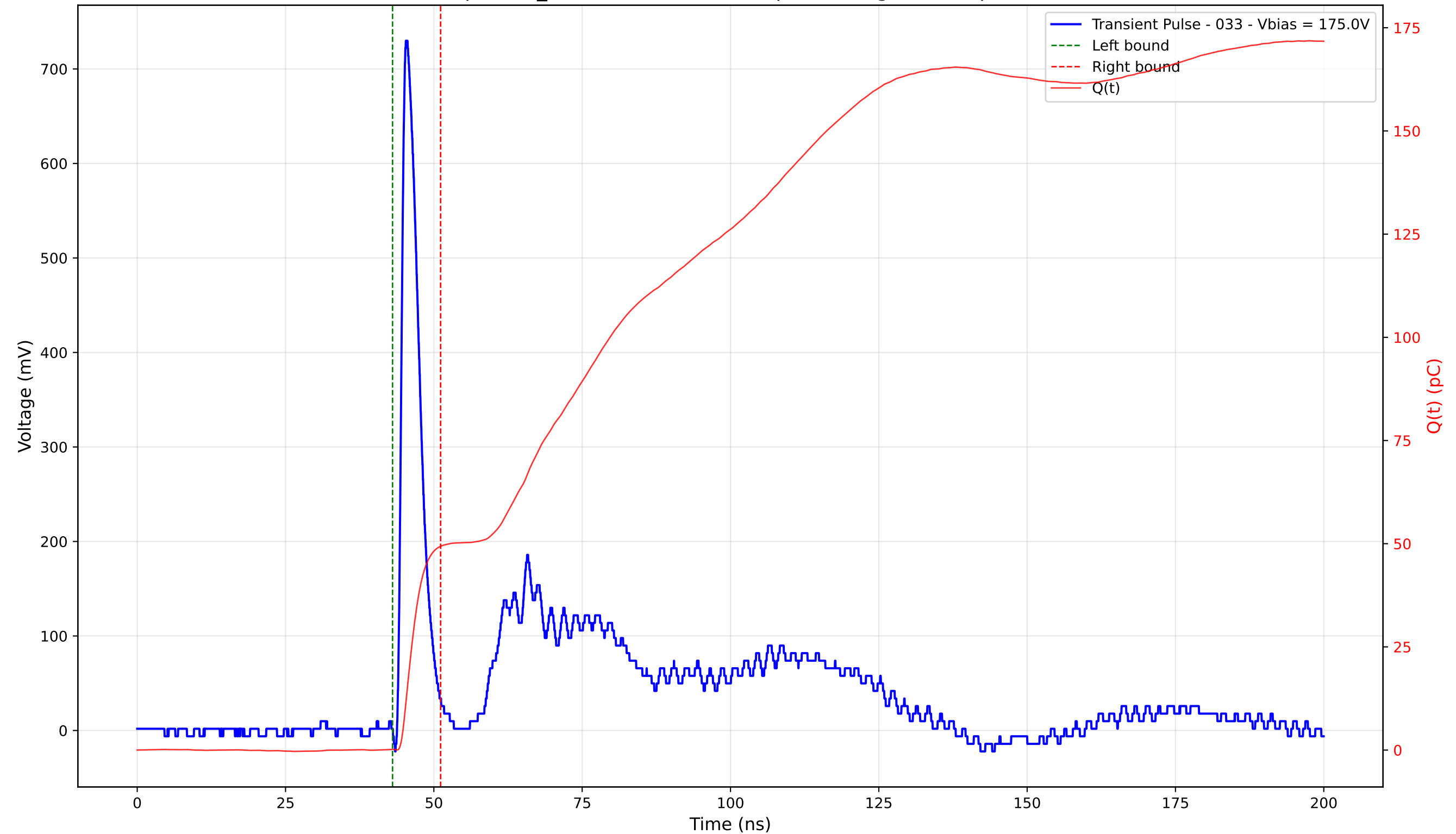
Transient Pulse - Sample: TD_4004 - Position: 215.0 \mu\text{m} - Charge: 49.20 pC - Rise Time: 0.94 ns
