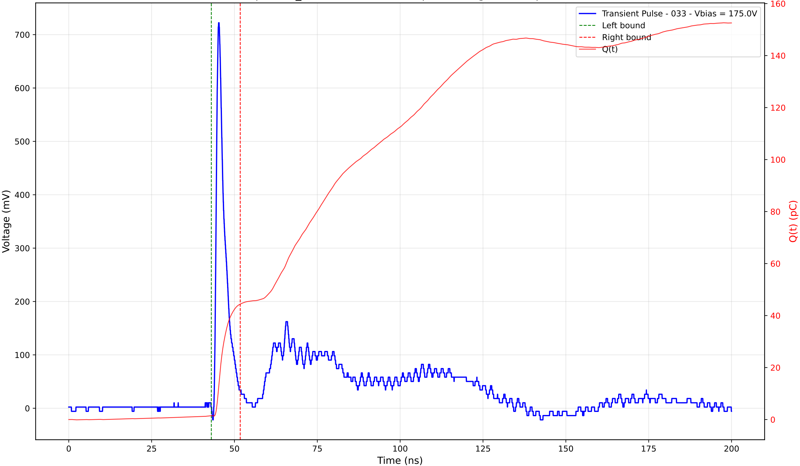
Transient Pulse - Sample: TD_4004 - Position: 90.0 \mu\text{m} - Charge: 42.91 pC - Rise Time: 0.90 ns
