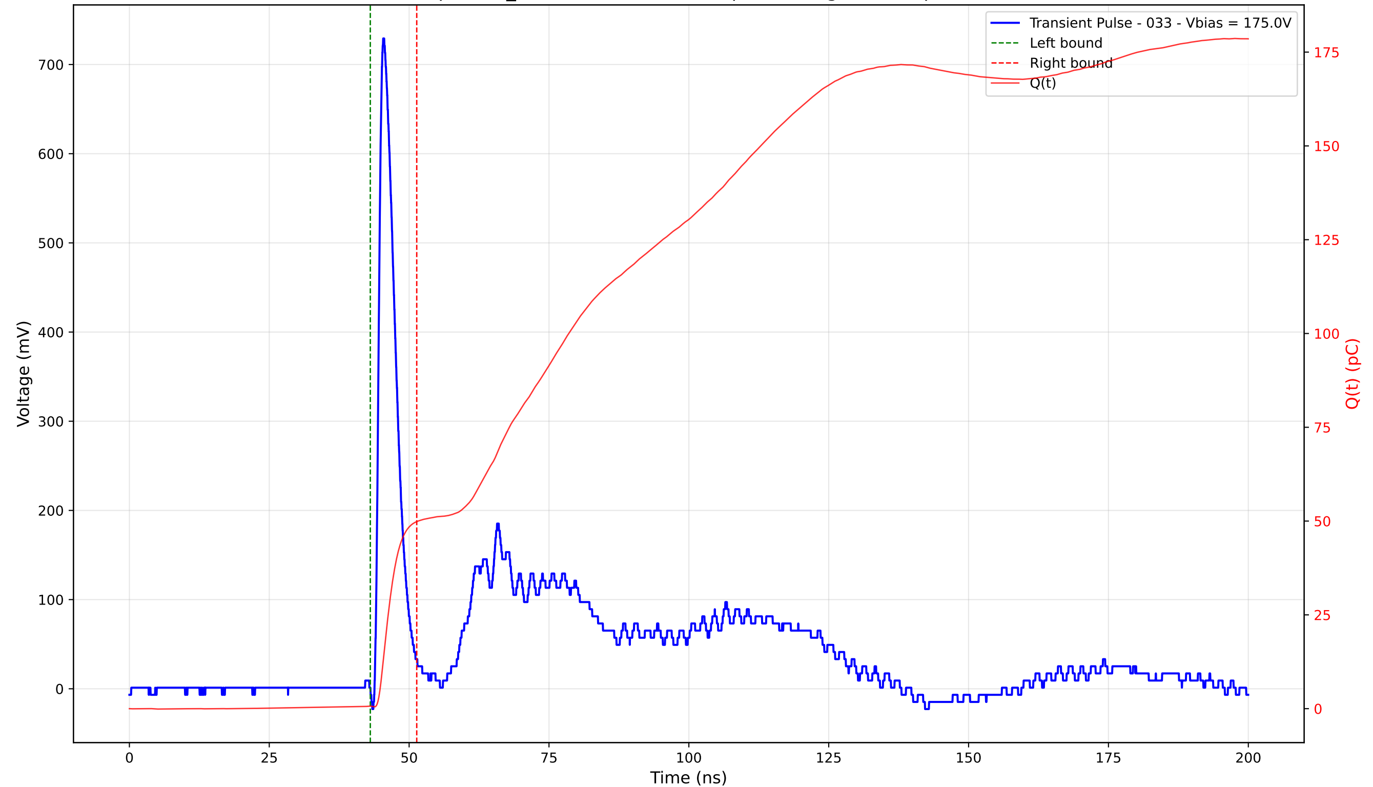
Transient Pulse - Sample: TD_4004 - Position: 165.0 \mu\text{m} - Charge: 49.18 pC - Rise Time: 0.97 ns
