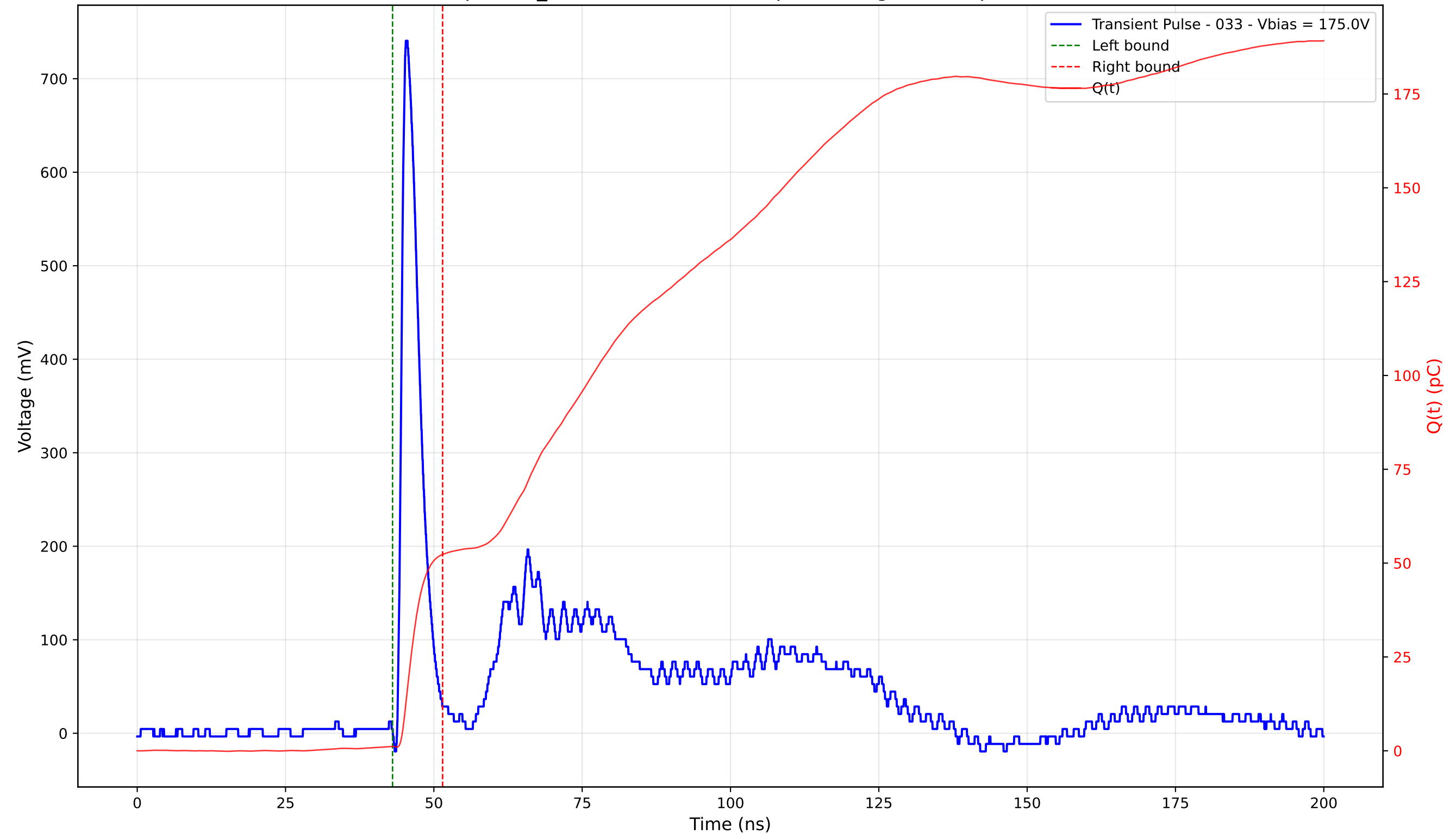
Transient Pulse - Sample: TD_4004 - Position: 170.0 \mu\text{m} - Charge: 51.14 pC - Rise Time: 0.94 ns
