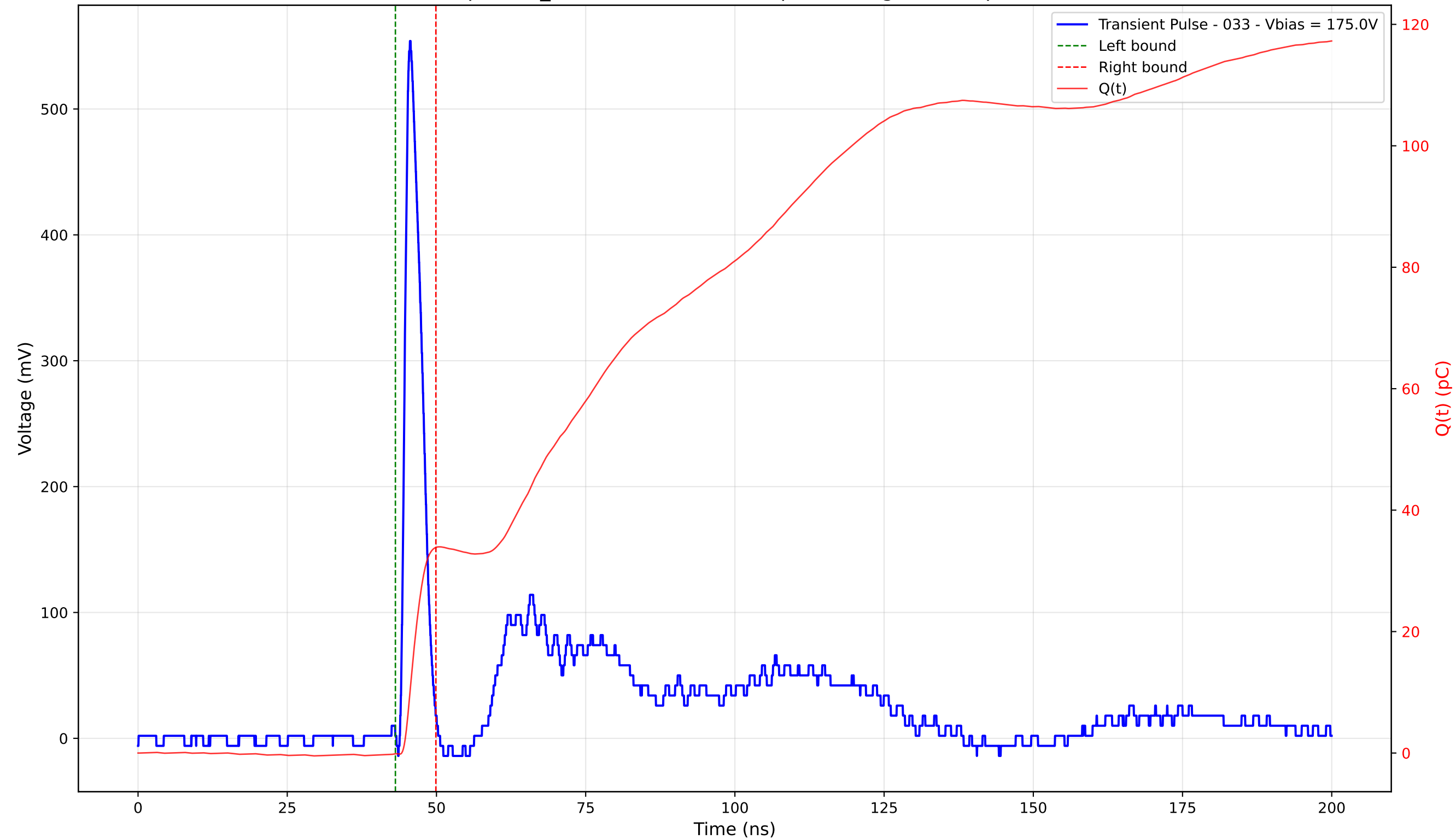
Transient Pulse - Sample: TD_4004 - Position: 315.0 \mu\text{m} - Charge: 33.98 pC - Rise Time: 1.05 ns
