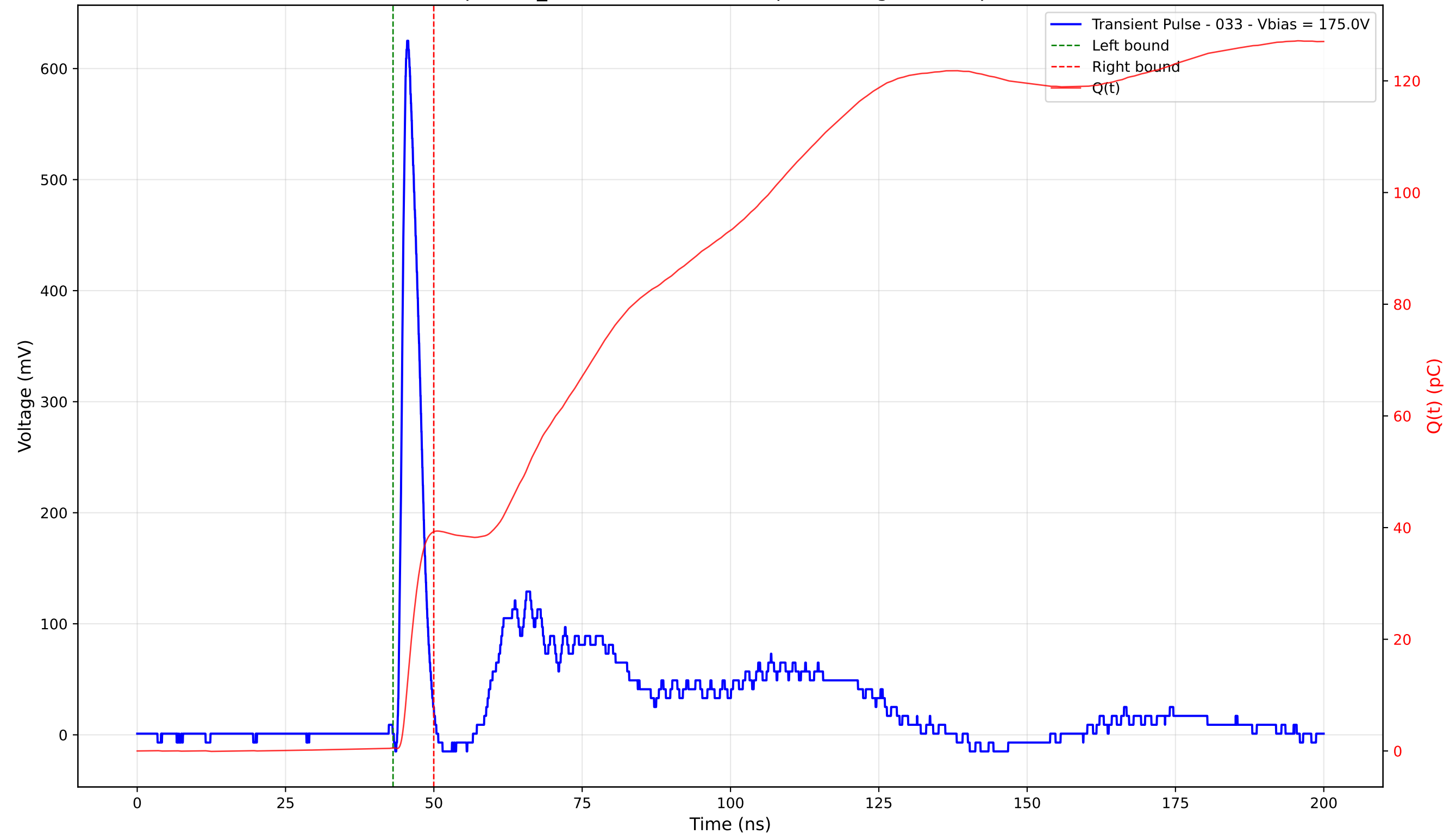
Transient Pulse - Sample: TD_4004 - Position: 305.0 \mu\text{m} - Charge: 38.71 pC - Rise Time: 1.03 ns
