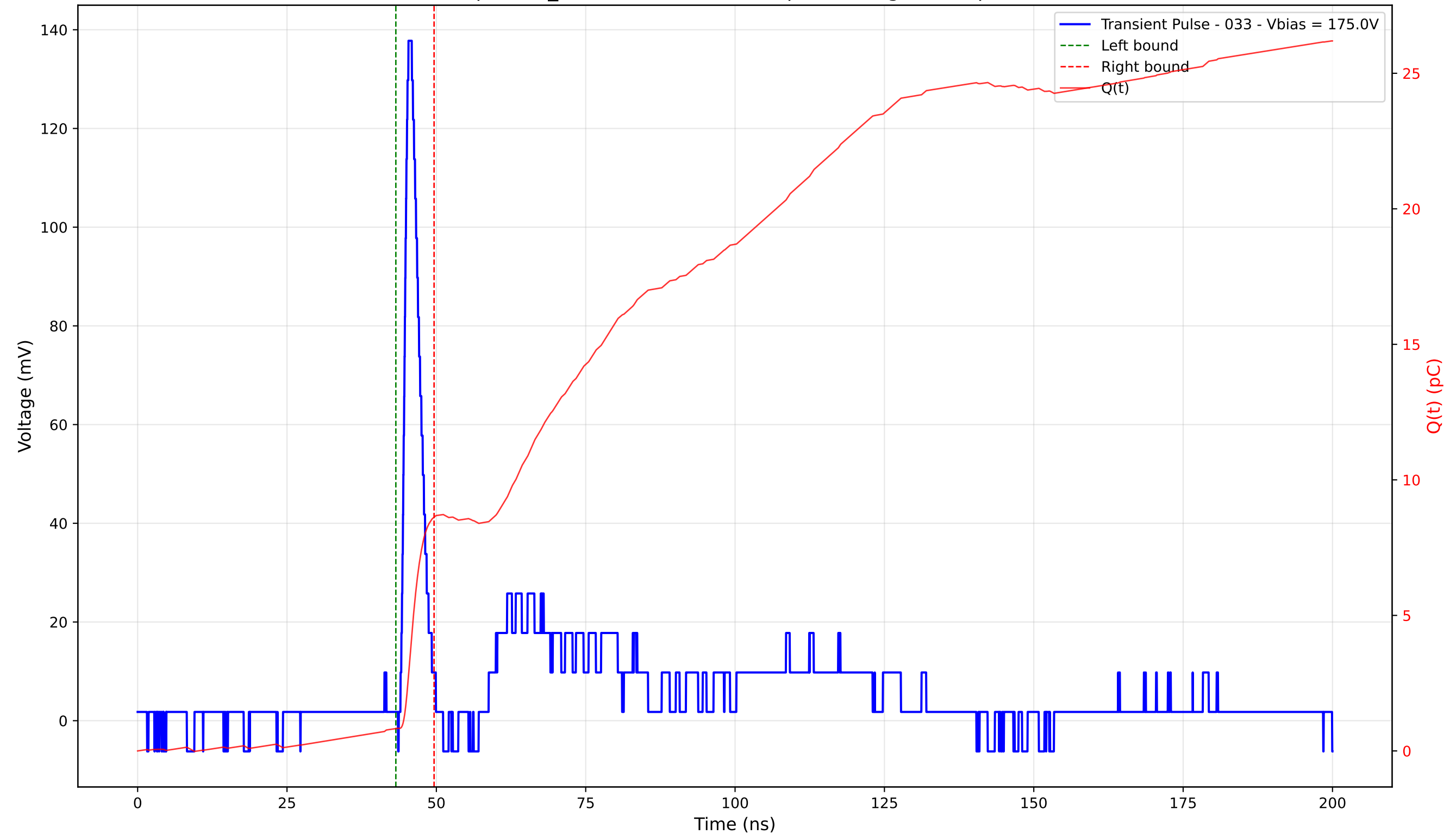
Transient Pulse - Sample: TD_4004 - Position: 410.0 \mu\text{m} - Charge: 7.80 pC - Rise Time: 1.03 ns
