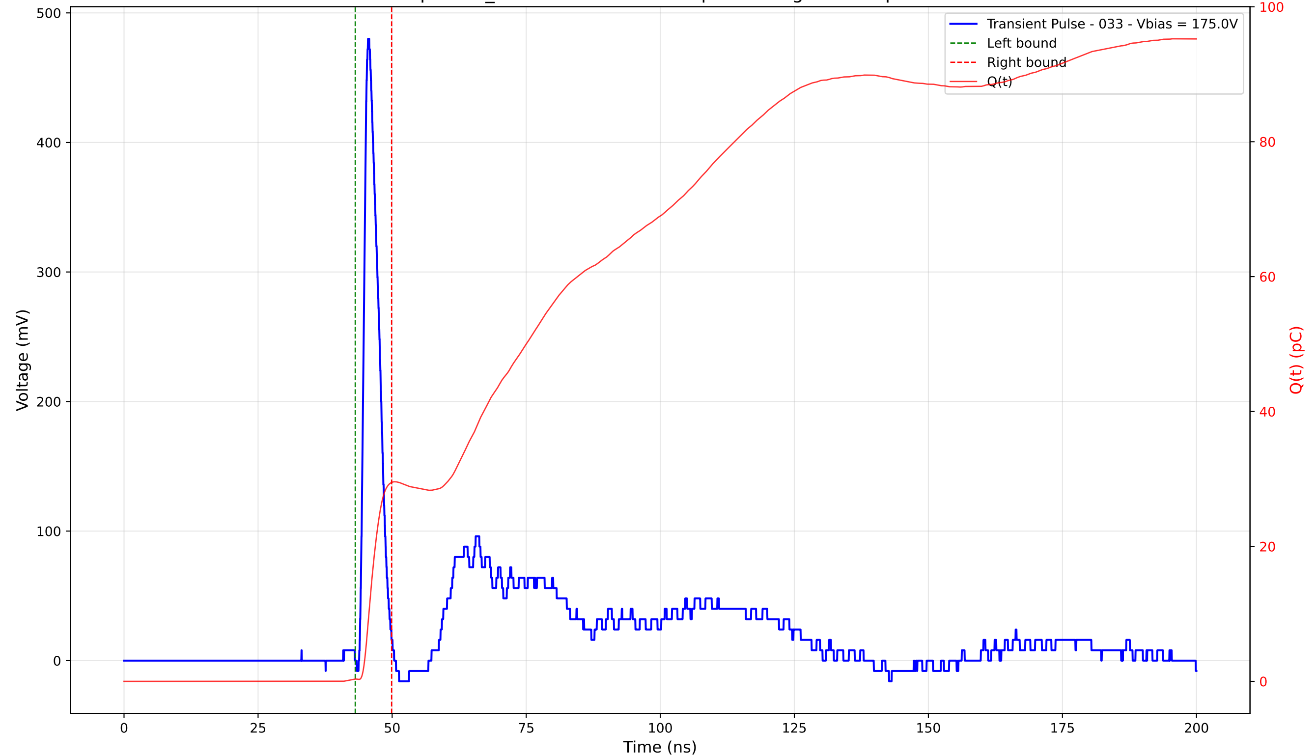
Transient Pulse - Sample: TD_4004 - Position: 330.0 \mu\text{m} - Charge: 29.15 pC - Rise Time: 1.04 ns
