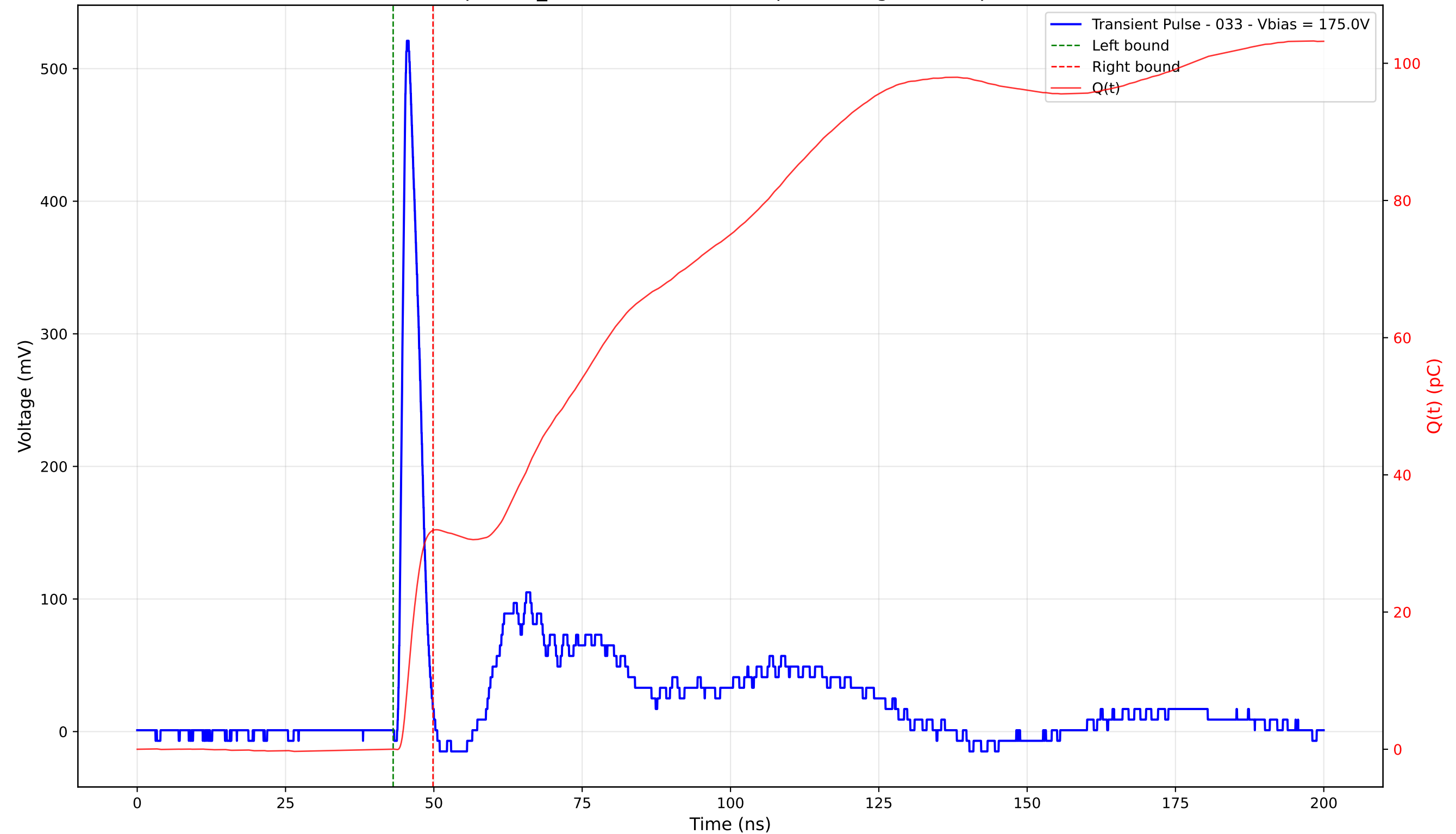
Transient Pulse - Sample: TD_4004 - Position: 325.0 \mu\text{m} - Charge: 31.90 pC - Rise Time: 1.03 ns
