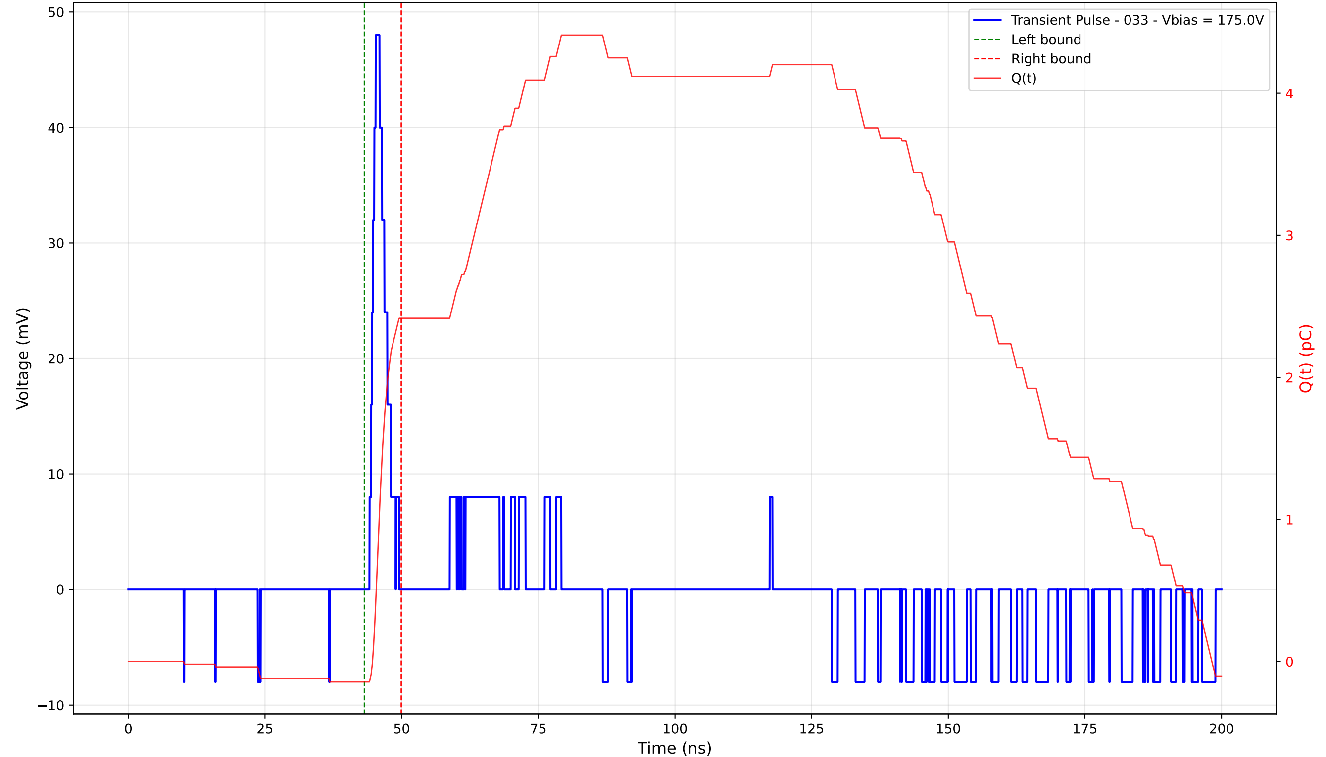
Transient Pulse - Sample: TD_4004 - Position: 435.0 \mu\text{m} - Charge: 2.56 pC - Rise Time: 1.13 ns
