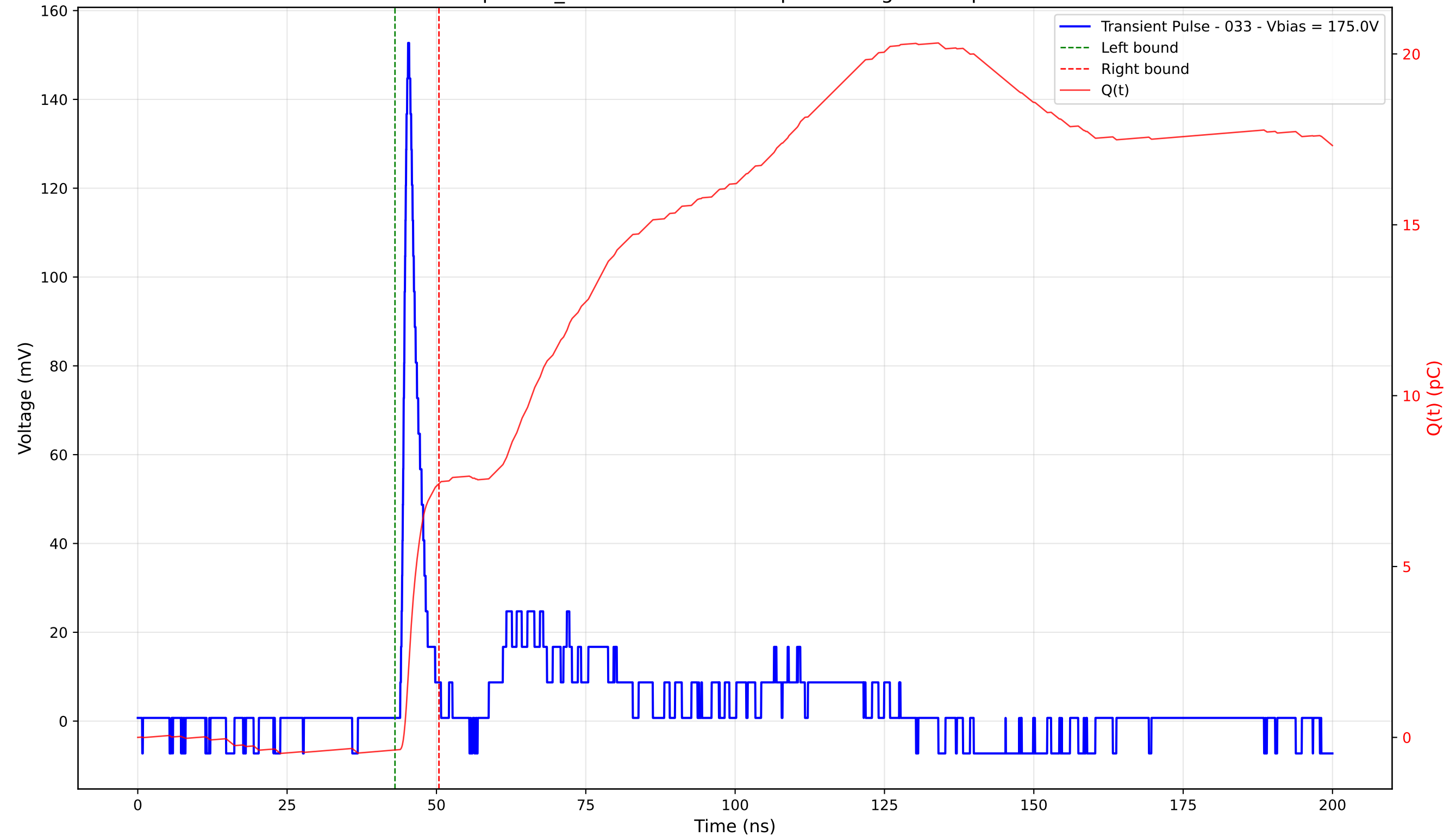
Transient Pulse - Sample: TD_4004 - Position: 55.0 \mu\text{m} - Charge: 7.80 pC - Rise Time: 1.04 ns
