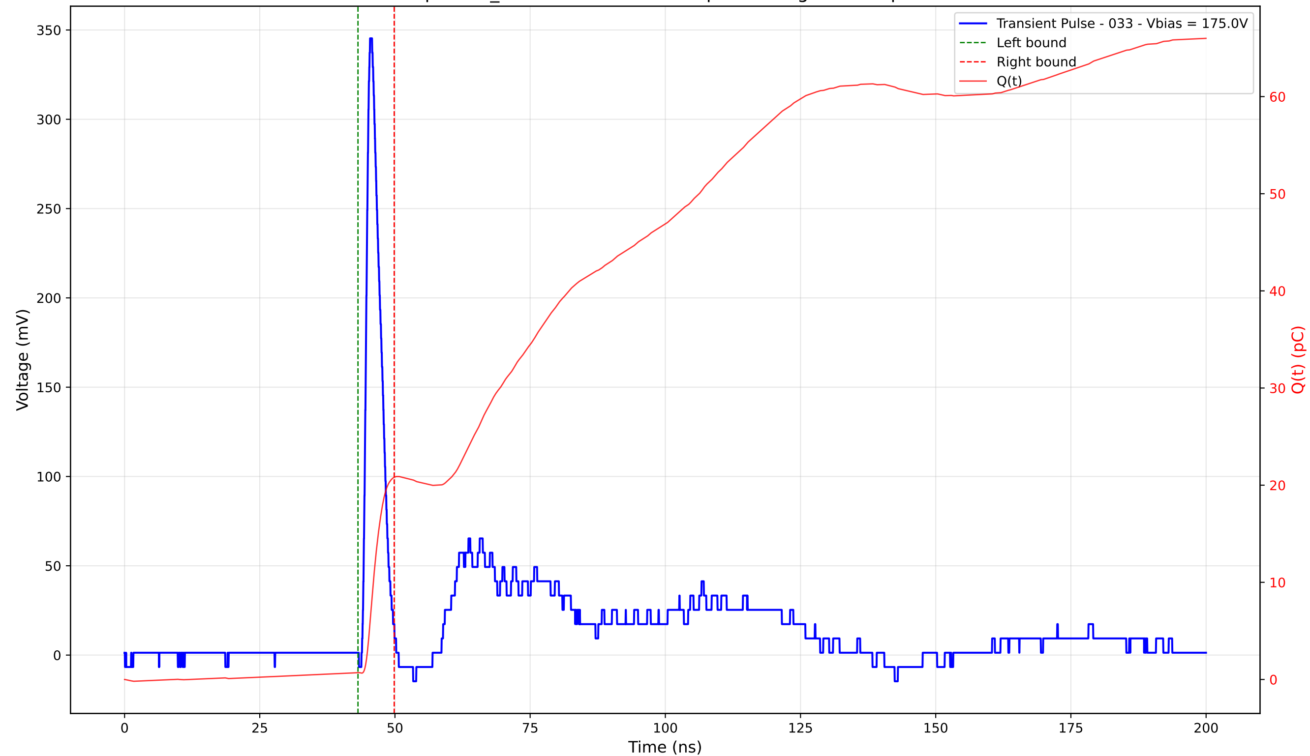
Transient Pulse - Sample: TD_4004 - Position: 385.0 \mu\text{m} - Charge: 20.11 pC - Rise Time: 1.00 ns
