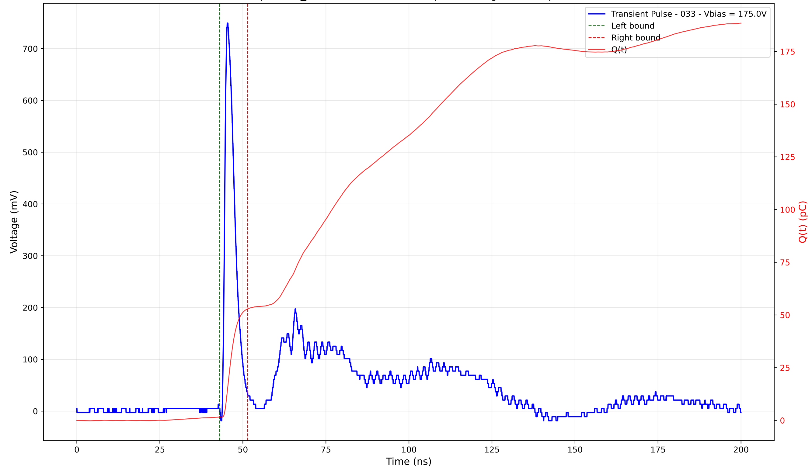
Transient Pulse - Sample: TD_4004 - Position: 205.0 \mu\text{m} - Charge: 51.26 pC - Rise Time: 0.94 ns
