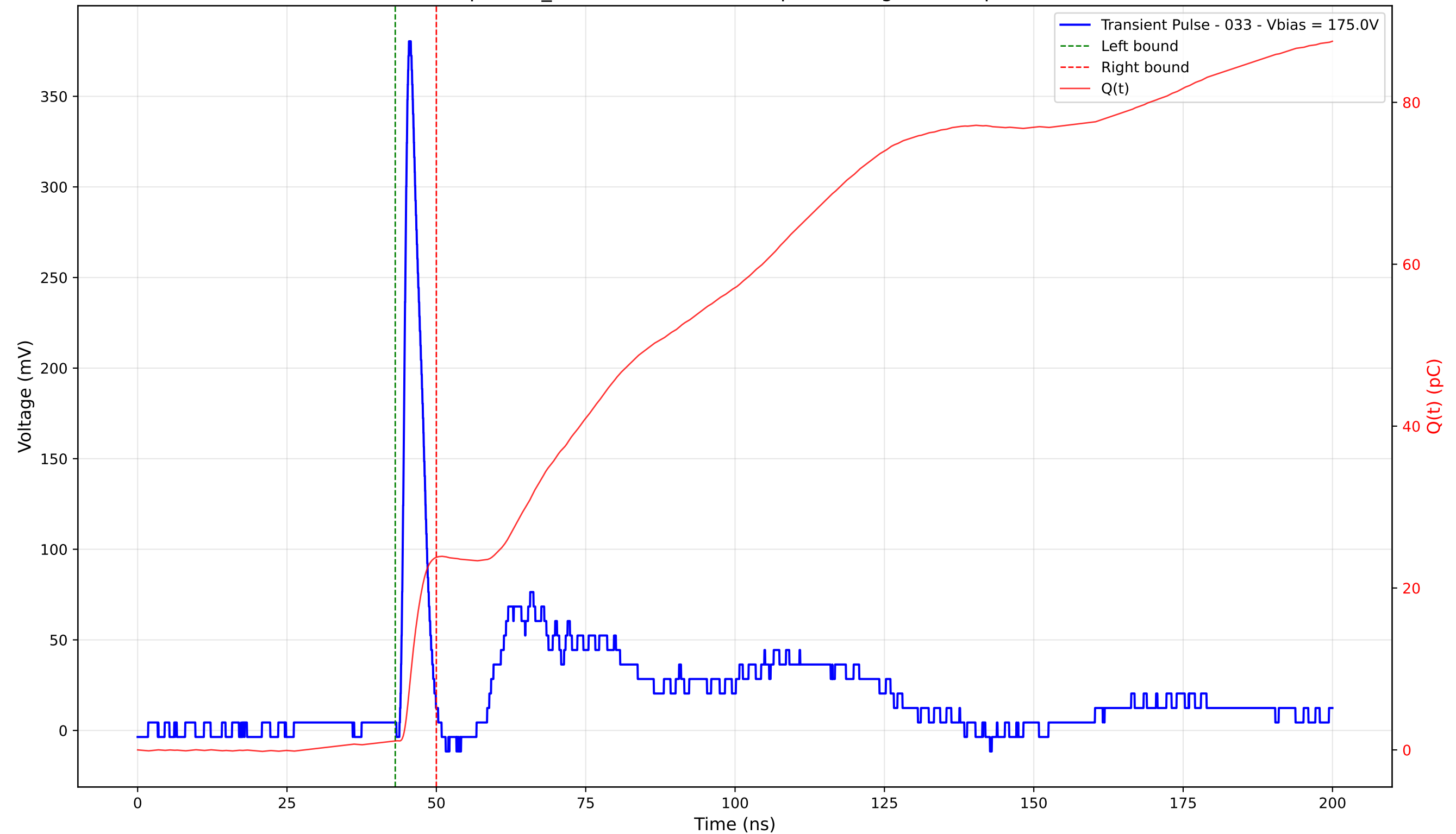
Transient Pulse - Sample: TD_4004 - Position: 365.0 \mu\text{m} - Charge: 22.68 pC - Rise Time: 1.04 ns
