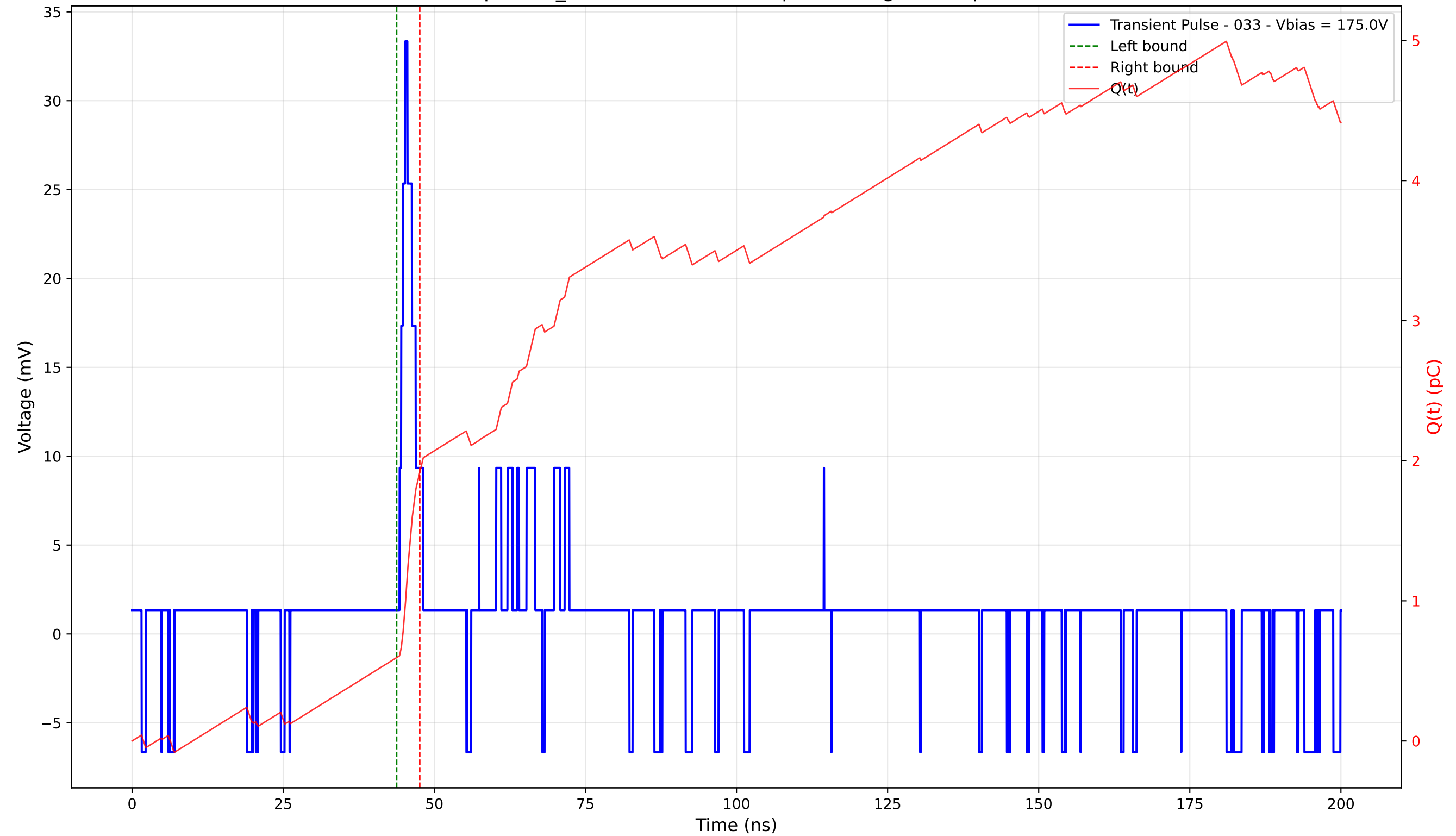
Transient Pulse - Sample: TD_4004 - Position: 35.0 \mu\text{m} - Charge: 1.32 pC - Rise Time: 0.94 ns
