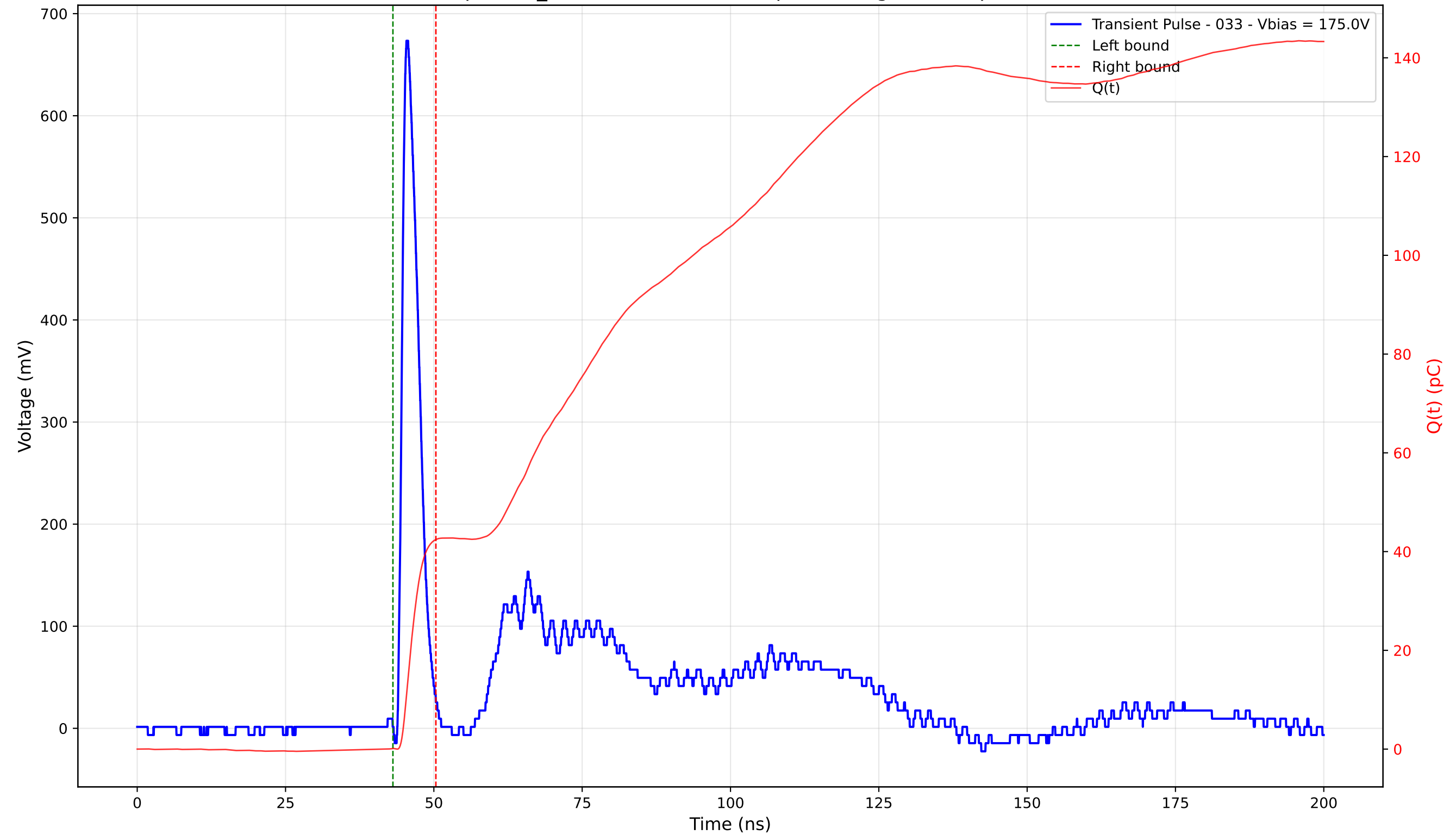
Transient Pulse - Sample: TD_4004 - Position: 255.0 \mu\text{m} - Charge: 42.32 pC - Rise Time: 0.99 ns
