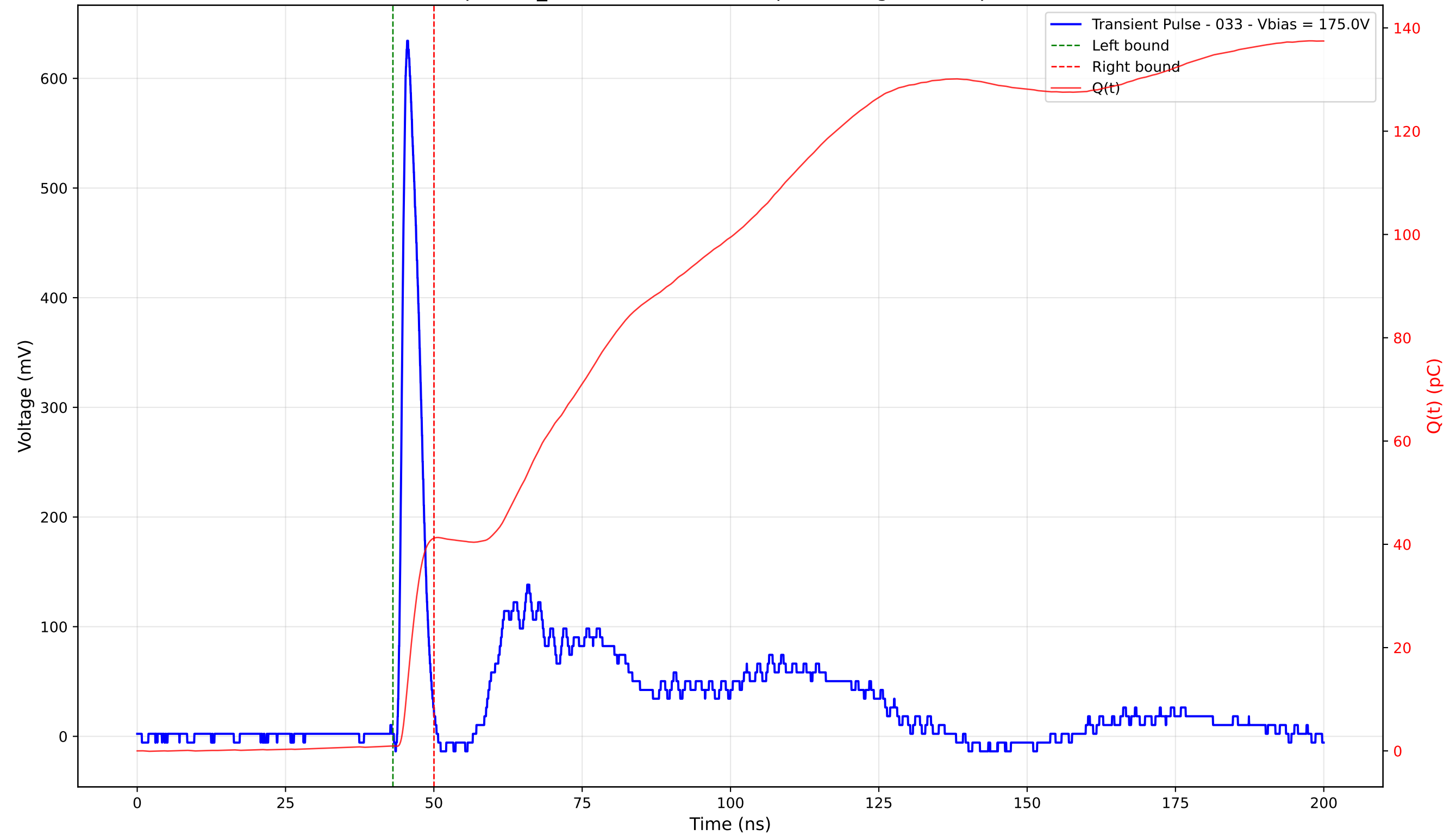
Transient Pulse - Sample: TD_4004 - Position: 295.0 \mu\text{m} - Charge: 40.24 pC - Rise Time: 1.05 ns
