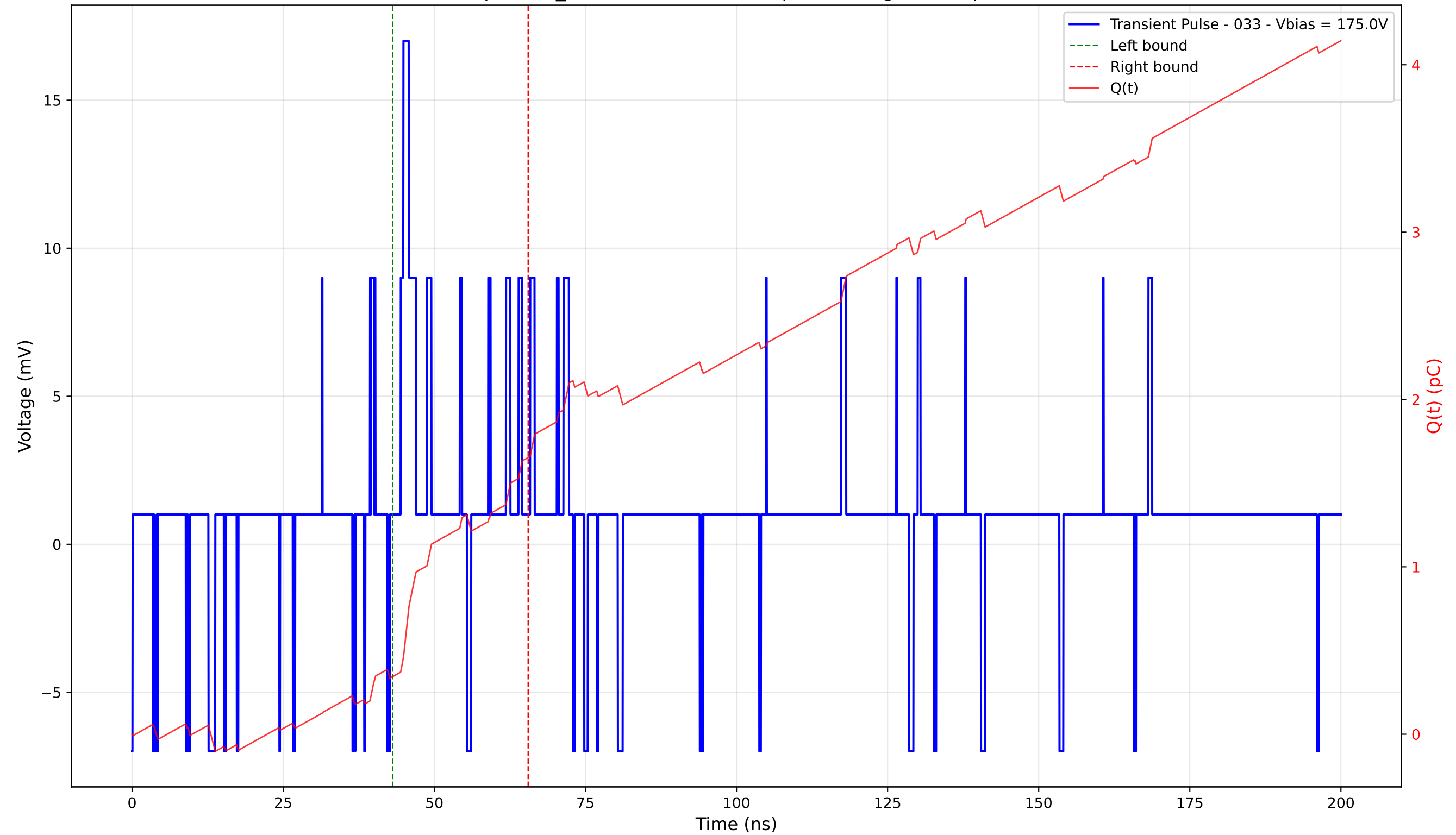
Transient Pulse - Sample: TD_4004 - Position: 15.0 \mu\text{m} - Charge: 1.31 pC - Rise Time: 0.46 ns
