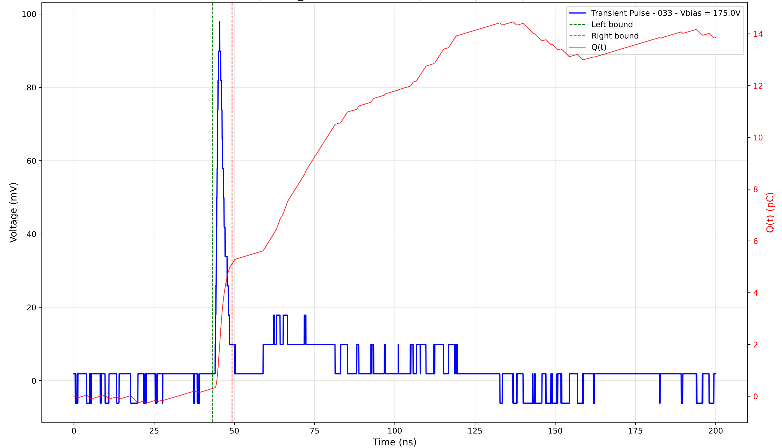
Transient Pulse - Sample: TD_4004 - Position: 50.0 \mu\text{m} - Charge: 4.82 pC - Rise Time: 1.04 ns
