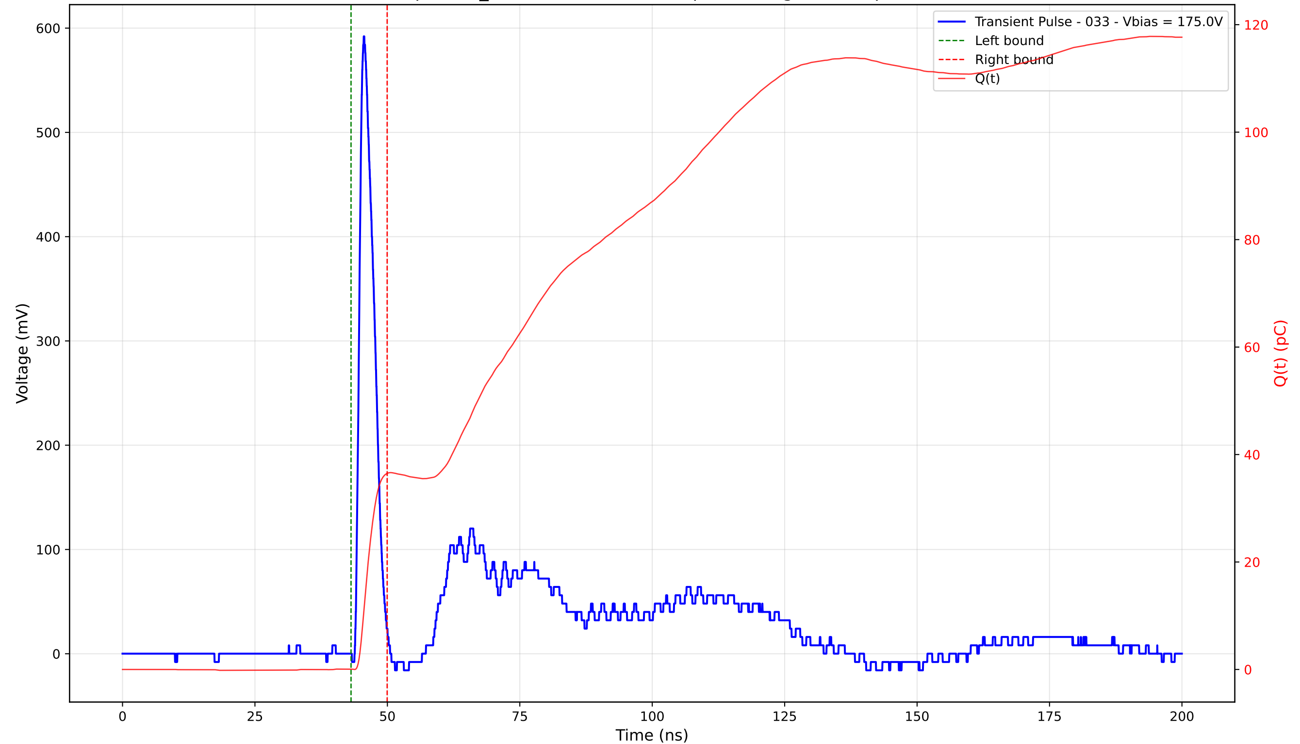
Transient Pulse - Sample: TD_4004 - Position: 310.0 \mu\text{m} - Charge: 36.43 pC - Rise Time: 1.03 ns
