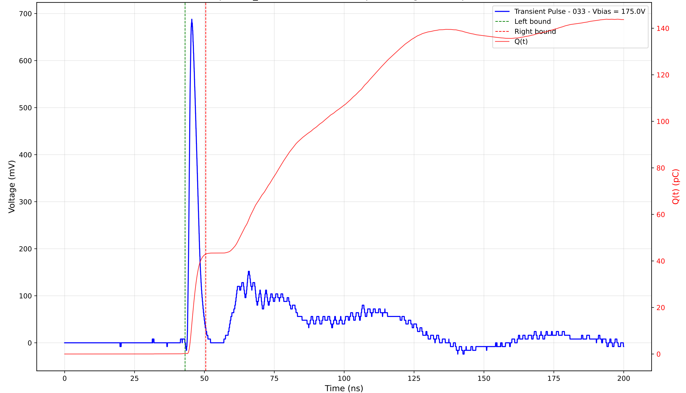
Transient Pulse - Sample: TD_4004 - Position: 240.0 \mu\text{m} - Charge: 42.67 pC - Rise Time: 1.01 ns
