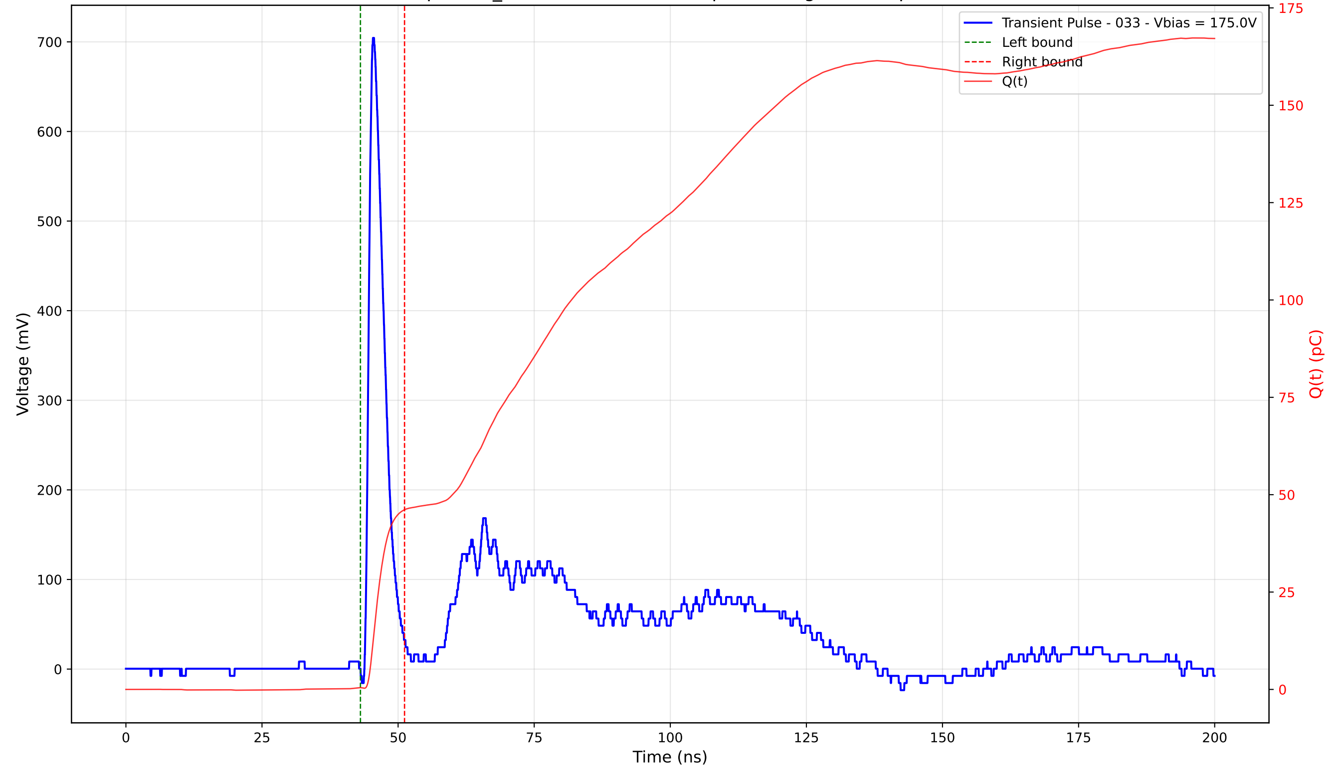
Transient Pulse - Sample: TD_4004 - Position: 150.0 \mu\text{m} - Charge: 45.69 pC - Rise Time: 0.97 ns
