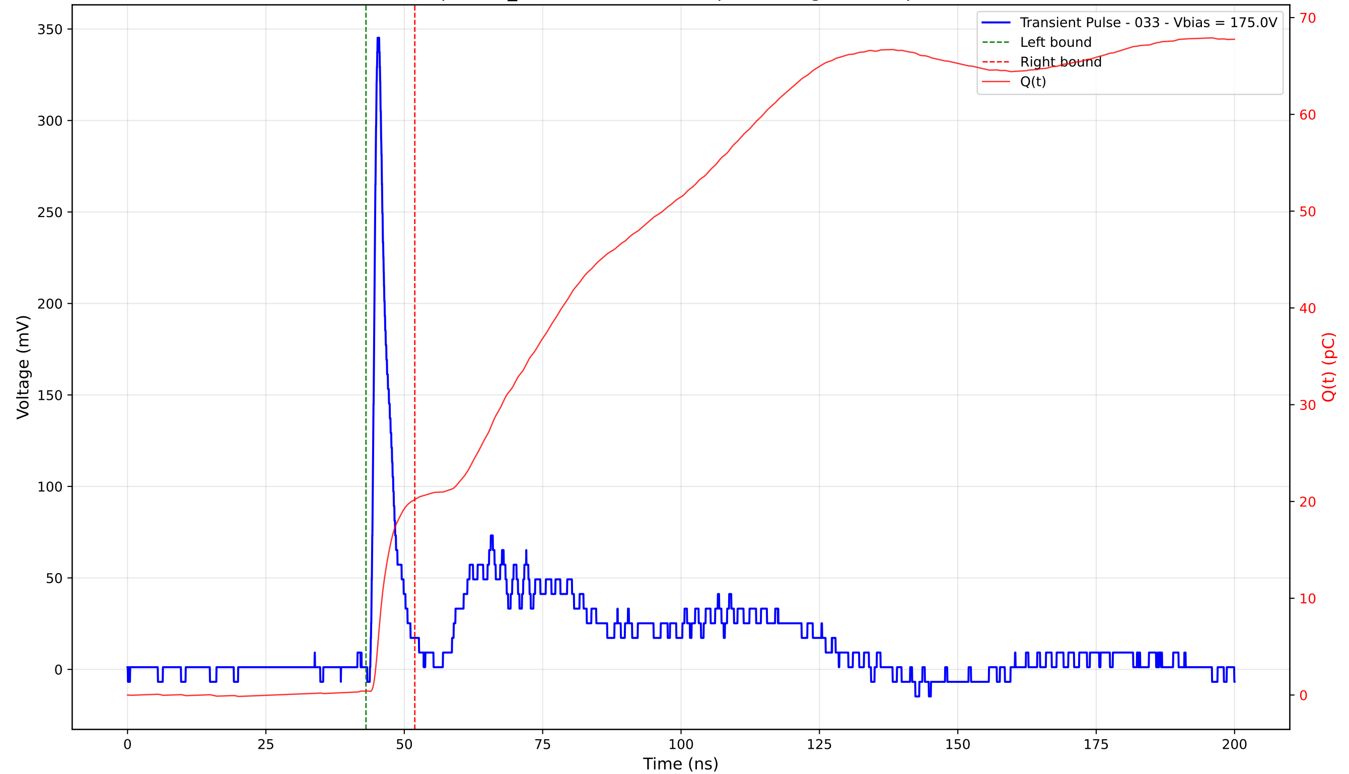
Transient Pulse - Sample: TD_4004 - Position: 65.0 \mu\text{m} - Charge: 19.78 pC - Rise Time: 0.88 ns
