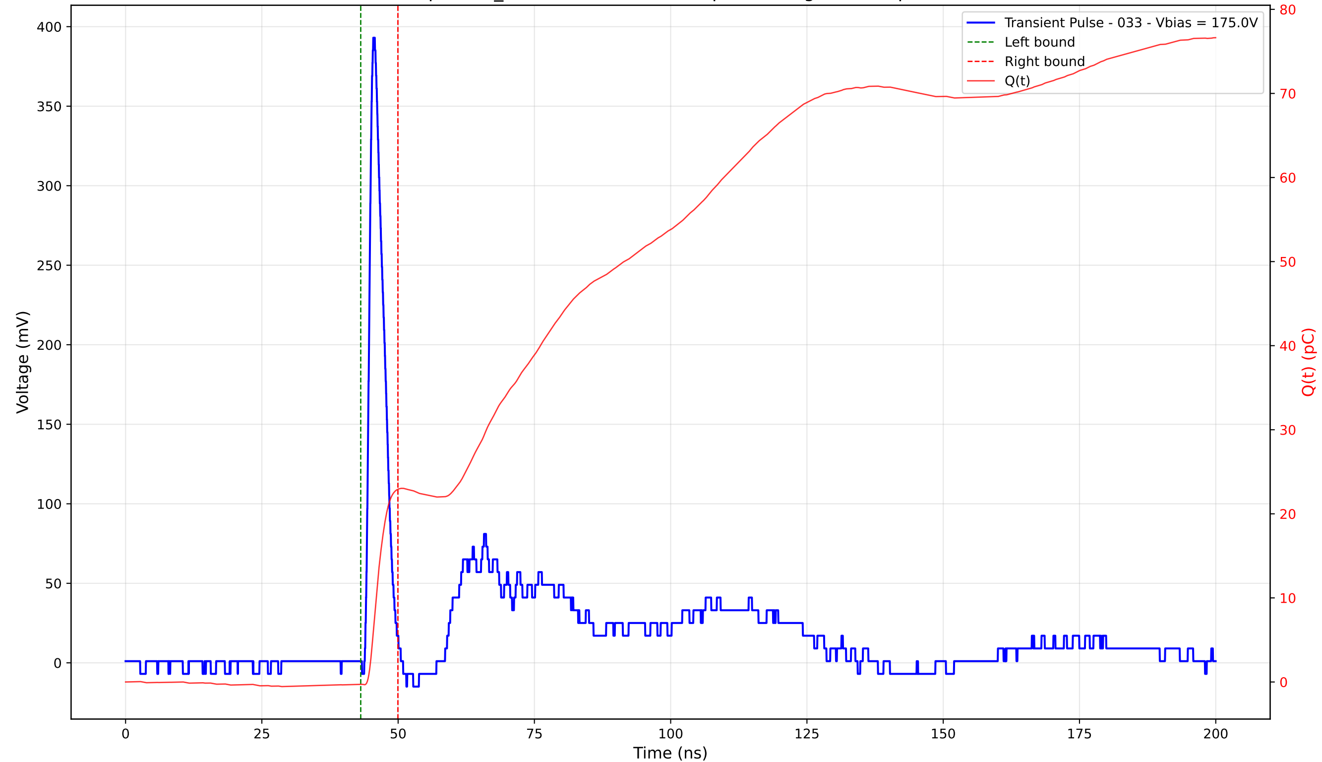
Transient Pulse - Sample: TD_4004 - Position: 360.0 \mu\text{m} - Charge: 23.19 pC - Rise Time: 1.06 ns
