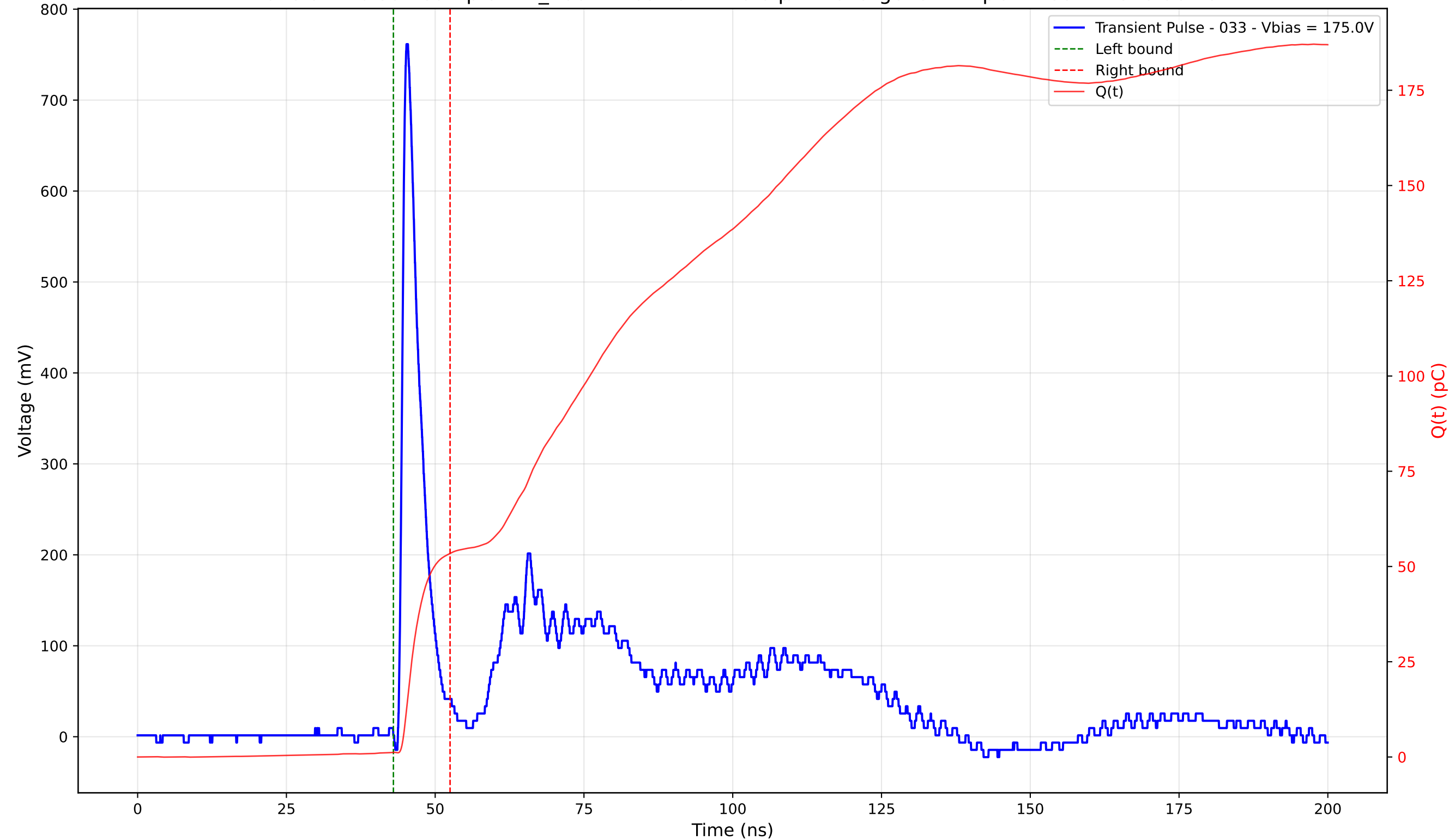
Transient Pulse - Sample: TD_4004 - Position: 110.0 \mu\text{m} - Charge: 52.21 pC - Rise Time: 0.90 ns
