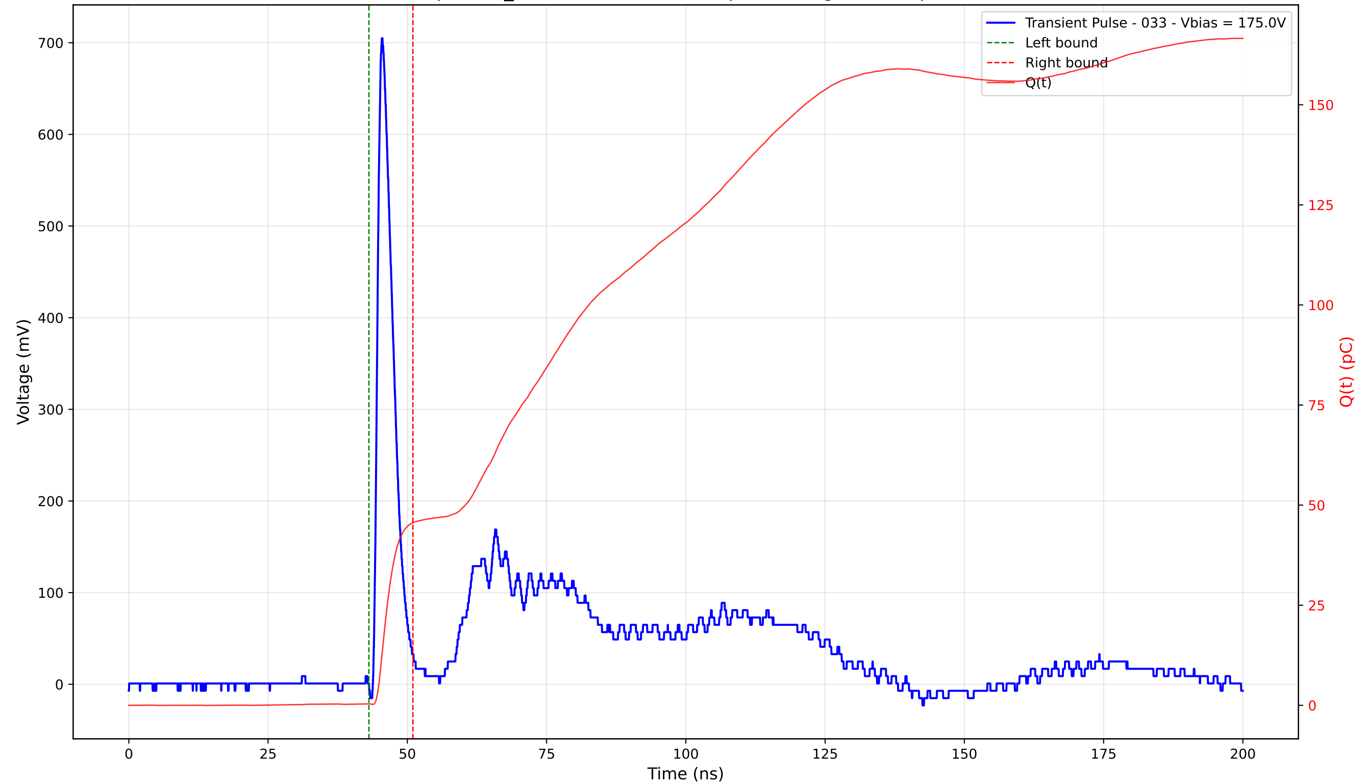
Transient Pulse - Sample: TD_4004 - Position: 145.0 \mu\text{m} - Charge: 45.25 pC - Rise Time: 0.99 ns
