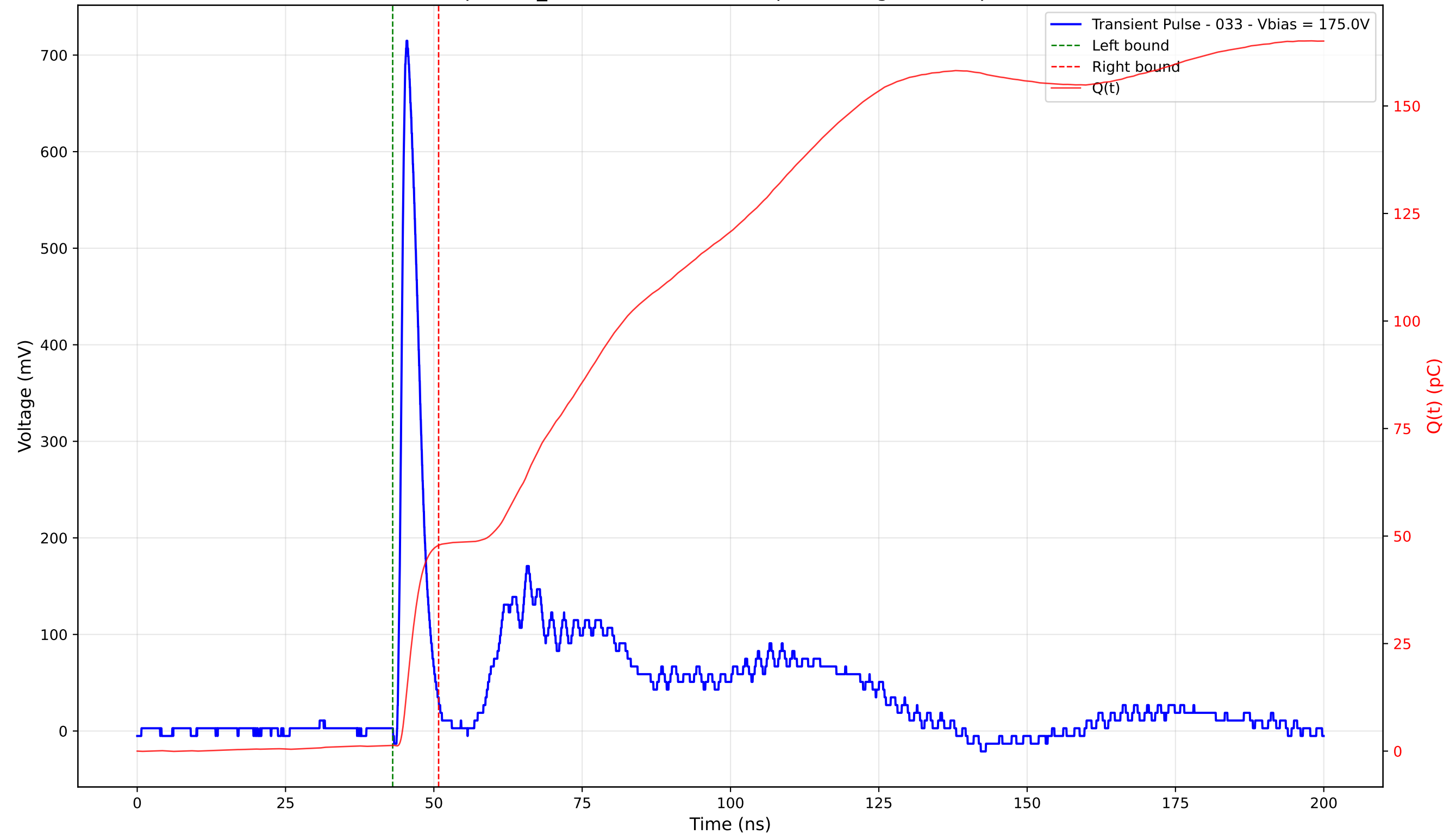
Transient Pulse - Sample: TD_4004 - Position: 230.0 \mu\text{m} - Charge: 46.52 pC - Rise Time: 0.99 ns
