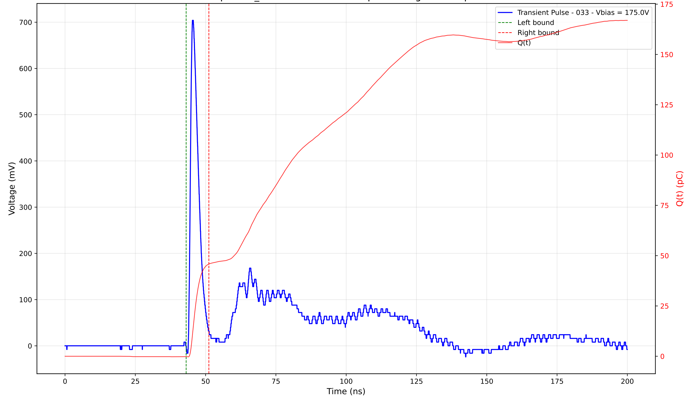
Transient Pulse - Sample: TD_4004 - Position: 155.0 \mu\text{m} - Charge: 45.99 pC - Rise Time: 0.95 ns
