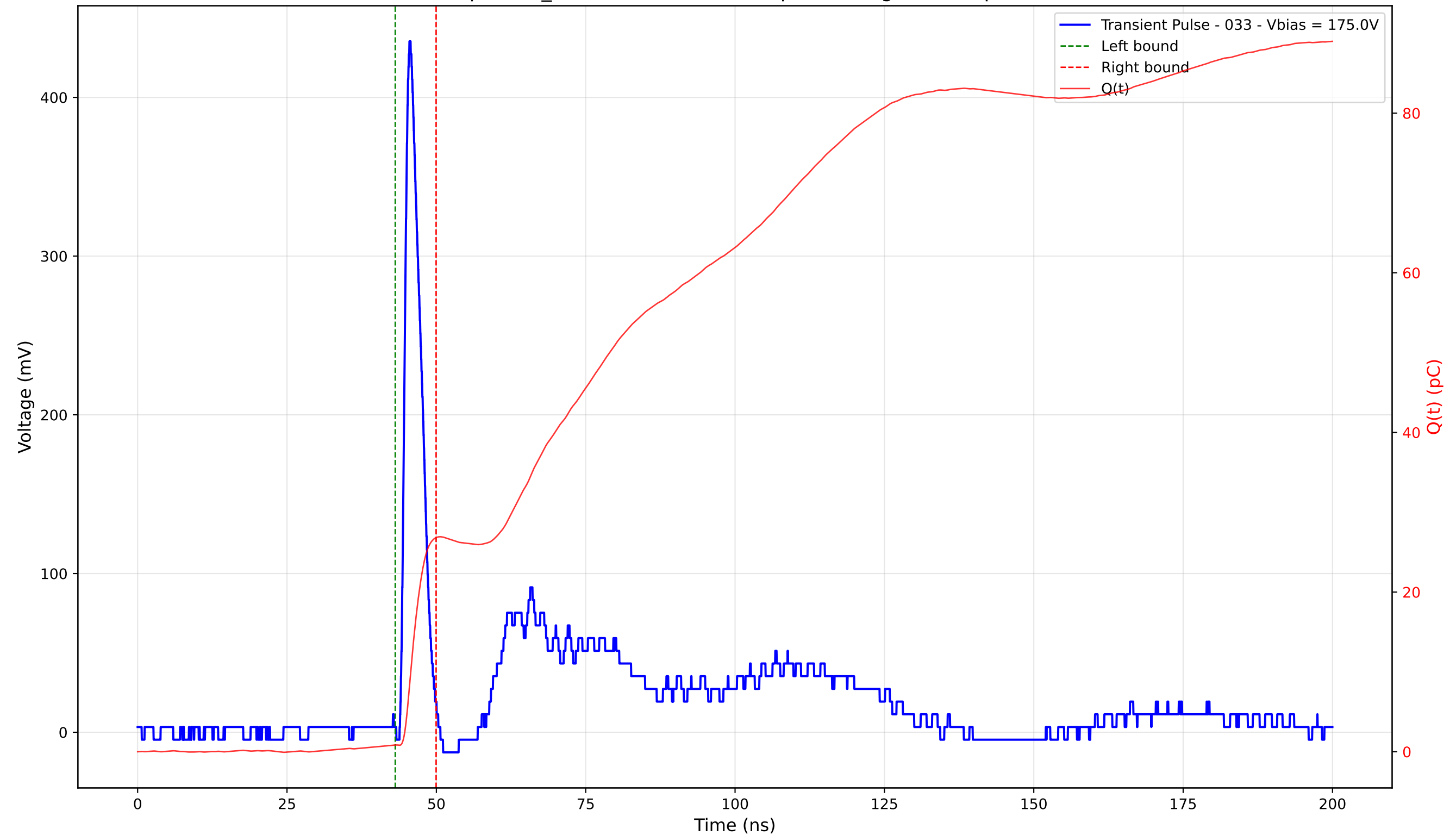
Transient Pulse - Sample: TD_4004 - Position: 335.0 \mu\text{m} - Charge: 25.98 pC - Rise Time: 1.04 ns
