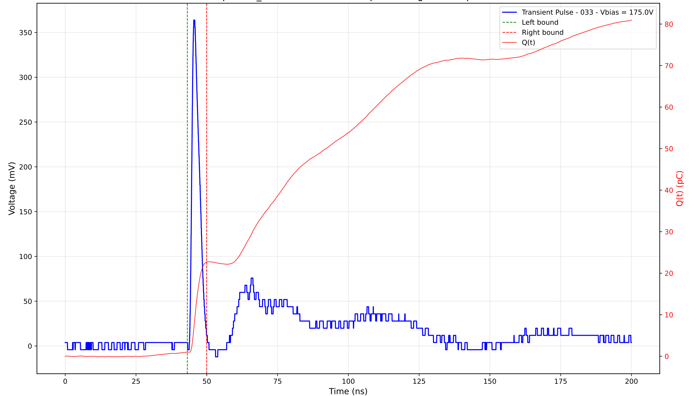
Transient Pulse - Sample: TD_4004 - Position: 370.0 \mu\text{m} - Charge: 21.68 pC - Rise Time: 1.02 ns
