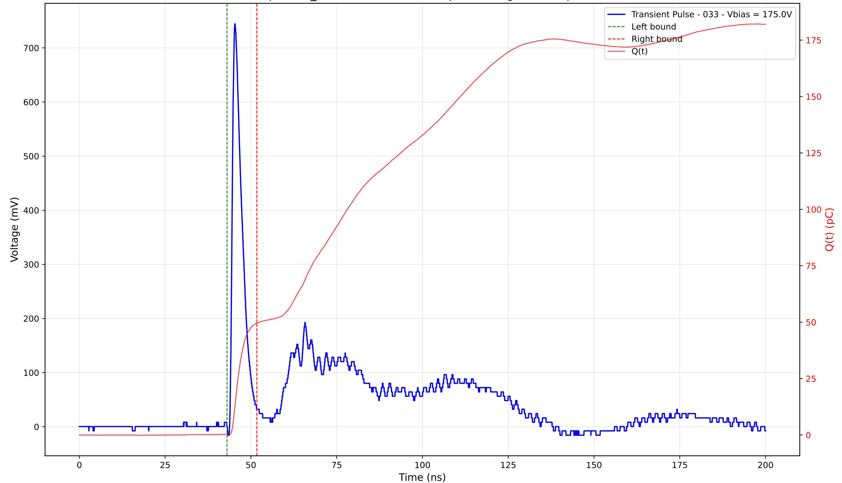
Transient Pulse - Sample: TD_4004 - Position: 125.0 \mu\text{m} - Charge: 49.18 pC - Rise Time: 0.95 ns
