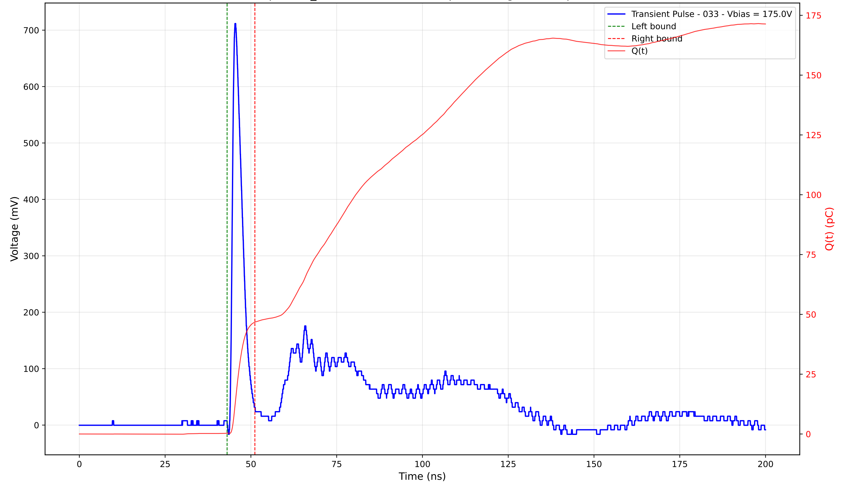
Transient Pulse - Sample: TD_4004 - Position: 135.0 \mu\text{m} - Charge: 46.37 pC - Rise Time: 0.98 ns
