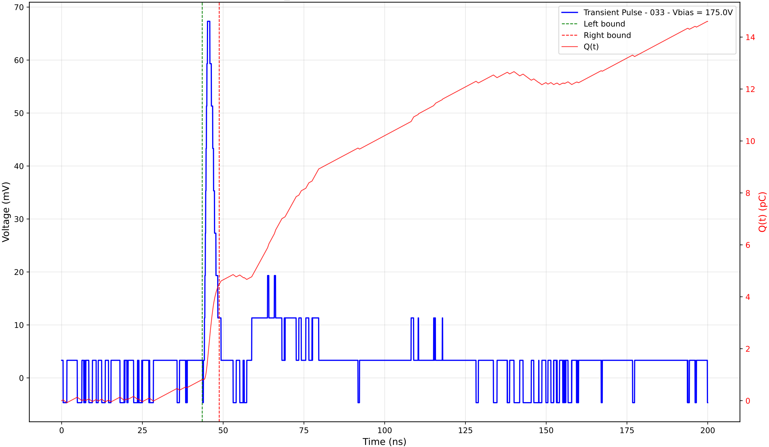
Transient Pulse - Sample: TD_4004 - Position: 420.0 \mu\text{m} - Charge: 3.67 pC - Rise Time: 0.95 ns
