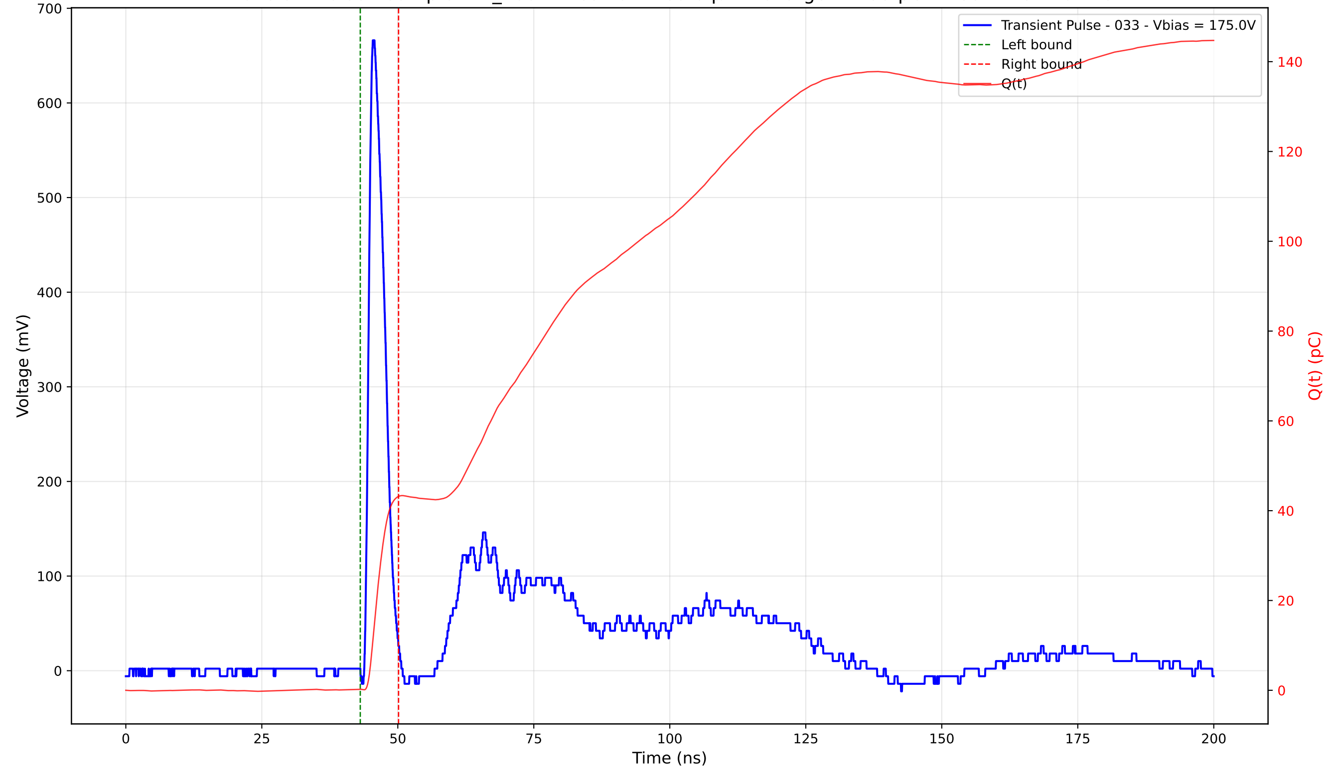
Transient Pulse - Sample: TD_4004 - Position: 285.0 \mu\text{m} - Charge: 42.95 pC - Rise Time: 1.01 ns
