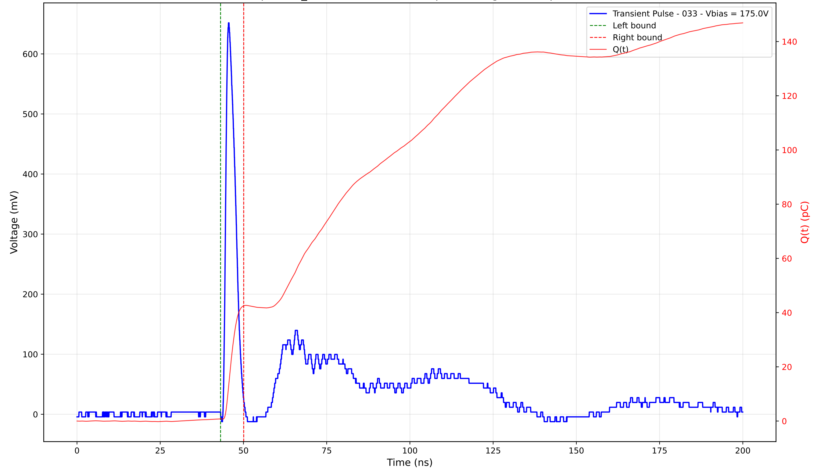
Transient Pulse - Sample: TD_4004 - Position: 290.0 \mu\text{m} - Charge: 41.71 pC - Rise Time: 1.03 ns
