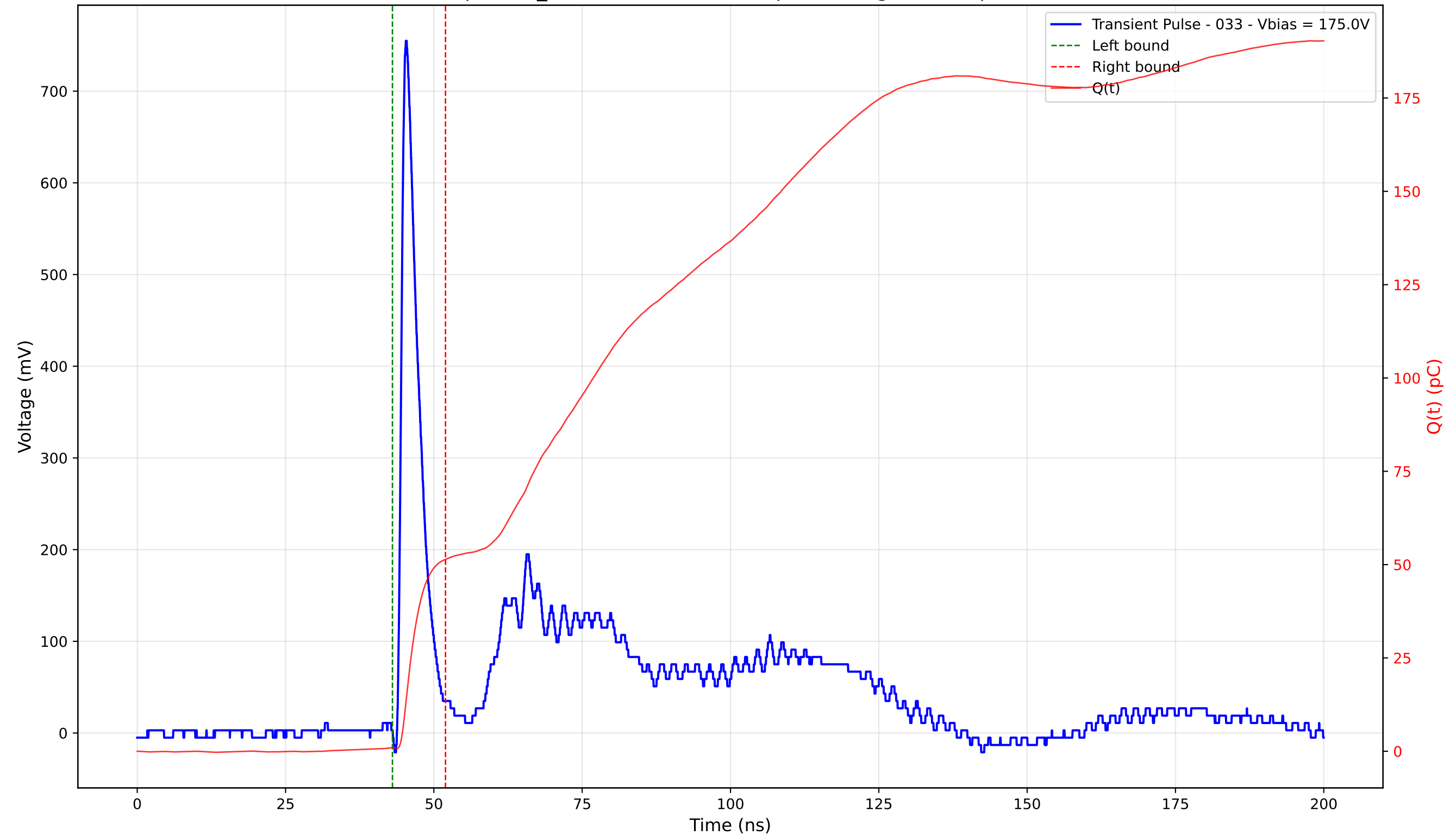
Transient Pulse - Sample: TD_4004 - Position: 120.0 \mu\text{m} - Charge: 50.43 pC - Rise Time: 0.91 ns
