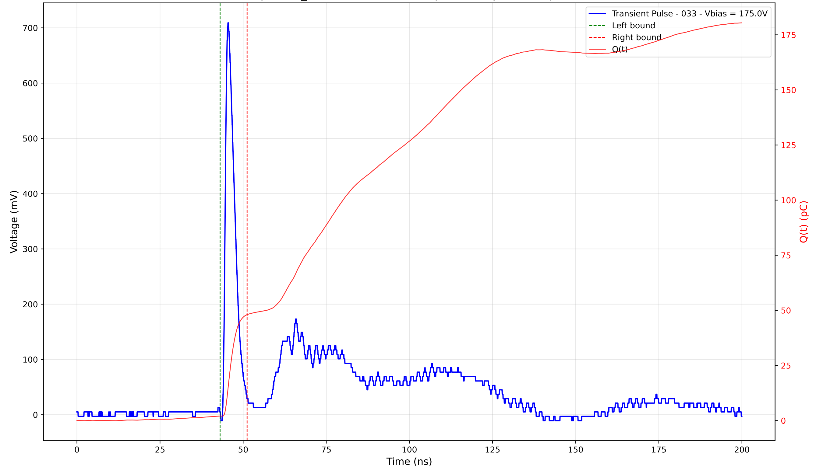
Transient Pulse - Sample: TD_4004 - Position: 140.0 \mu\text{m} - Charge: 45.97 pC - Rise Time: 0.98 ns
