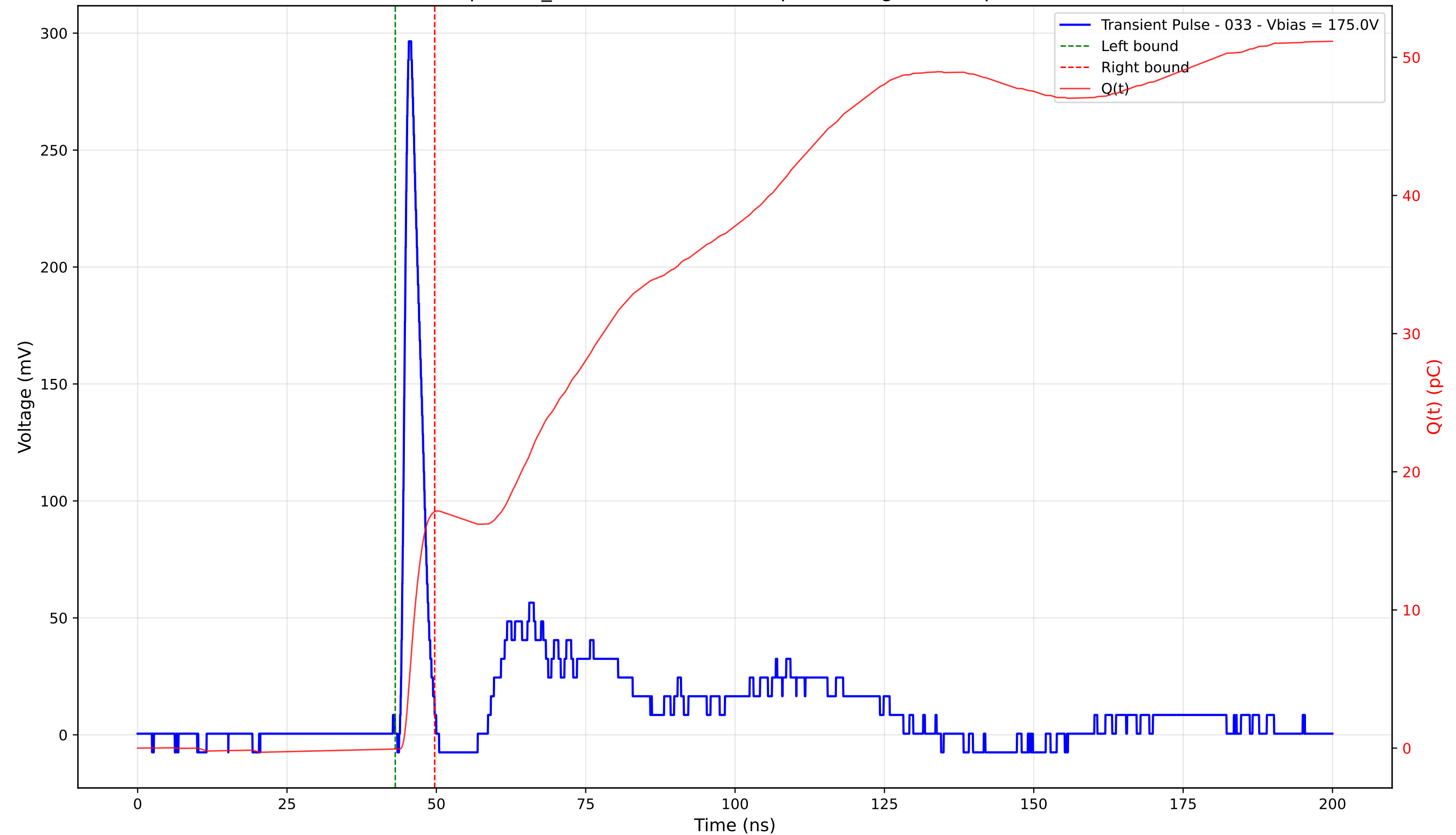
Transient Pulse - Sample: TD_4004 - Position: 390.0 \mu\text{m} - Charge: 17.15 pC - Rise Time: 1.03 ns
