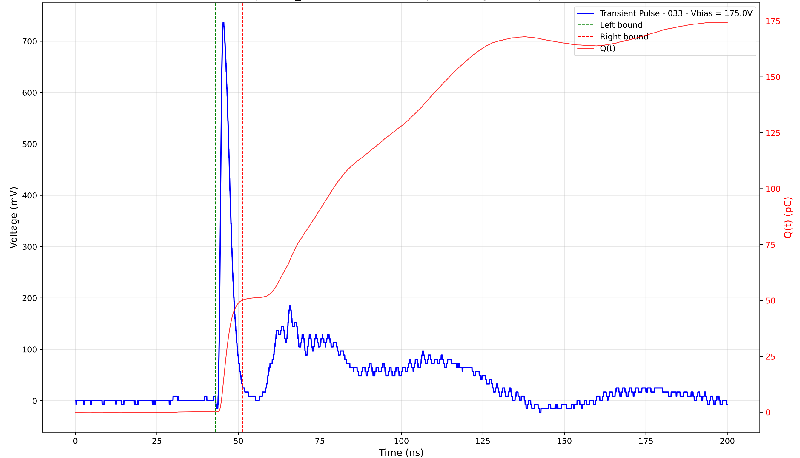
Transient Pulse - Sample: TD_4004 - Position: 210.0 \mu\text{m} - Charge: 49.66 pC - Rise Time: 0.95 ns
