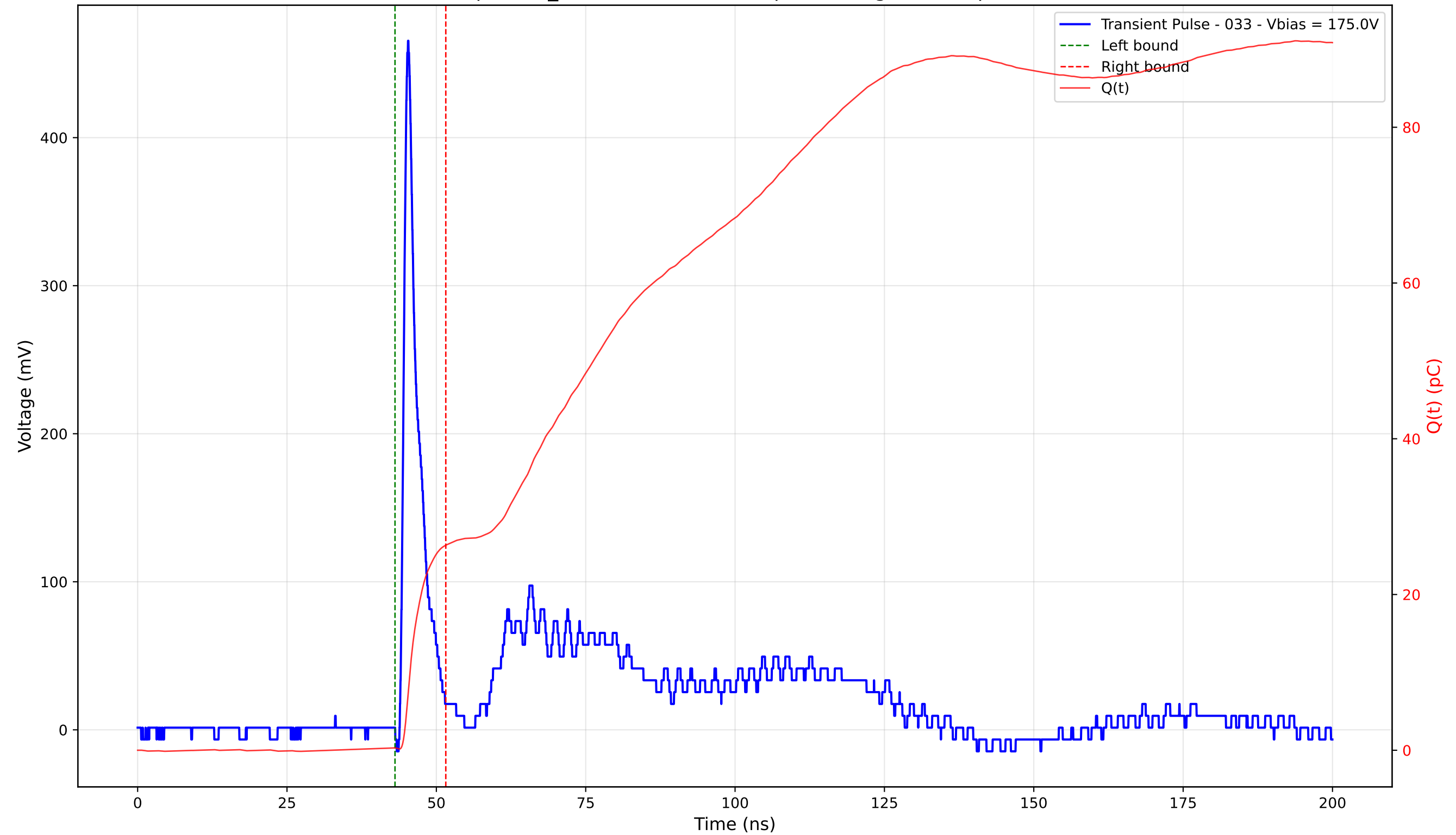
Transient Pulse - Sample: TD_4004 - Position: 70.0 \mu\text{m} - Charge: 26.03 pC - Rise Time: 0.93 ns
