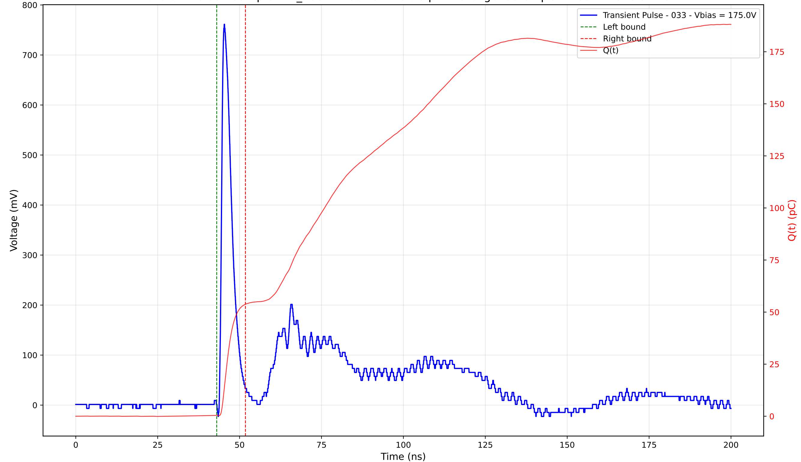
Transient Pulse - Sample: TD_4004 - Position: 190.0 \mu\text{m} - Charge: 53.31 pC - Rise Time: 0.92 ns
