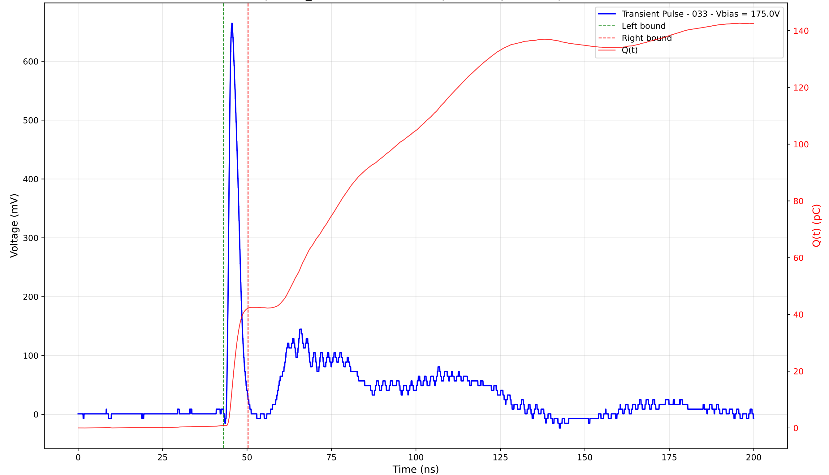
Transient Pulse - Sample: TD_4004 - Position: 260.0 \mu\text{m} - Charge: 41.28 pC - Rise Time: 1.01 ns
