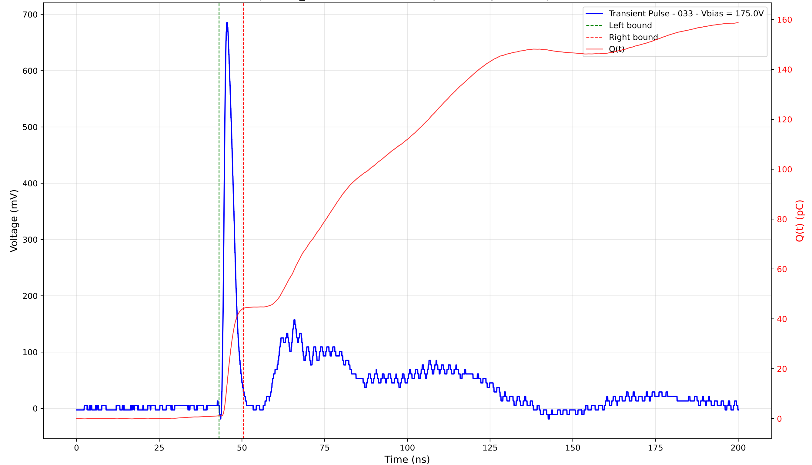
Transient Pulse - Sample: TD_4004 - Position: 245.0 \mu\text{m} - Charge: 43.02 pC - Rise Time: 0.99 ns
