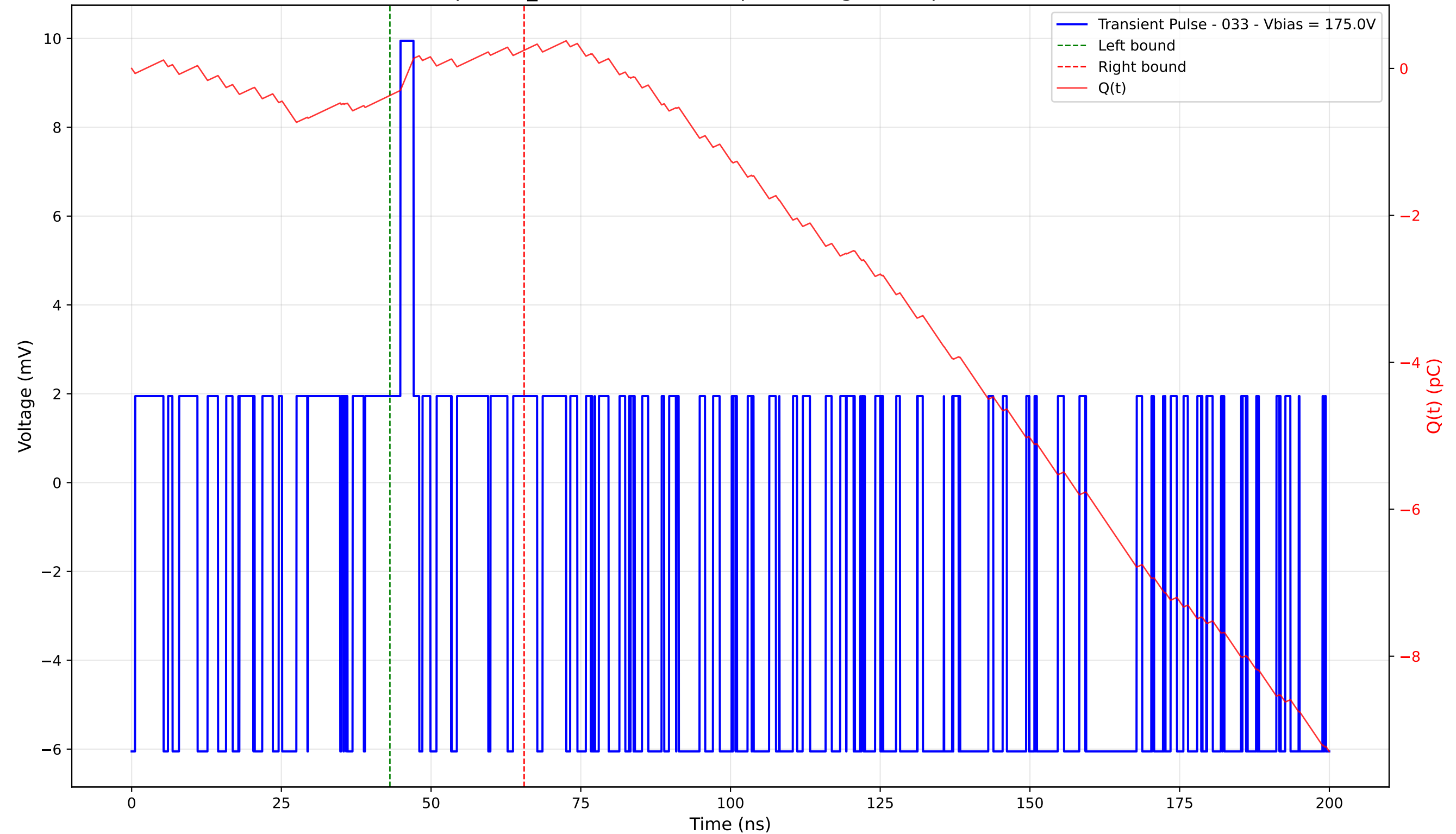
Transient Pulse - Sample: TD_4004 - Position: 5.0 \mu\text{m} - Charge: 0.62 pC - Rise Time: 0.00 ns (N/A)
