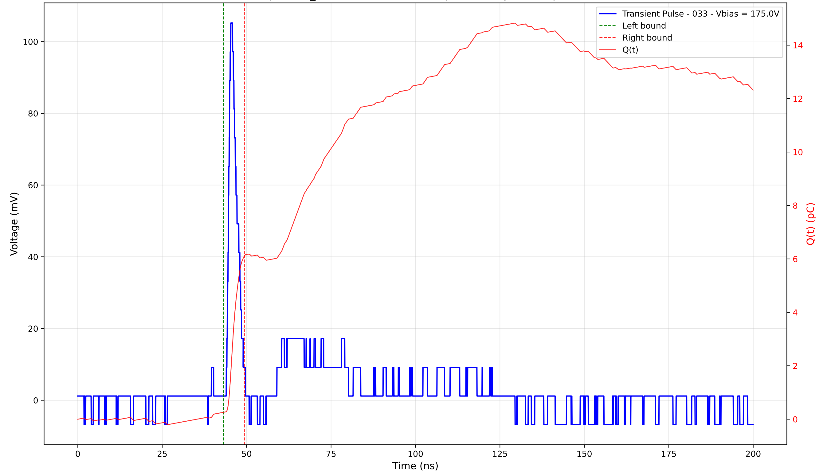
Transient Pulse - Sample: TD_4004 - Position: 415.0 \mu\text{m} - Charge: 5.87 pC - Rise Time: 0.98 ns
