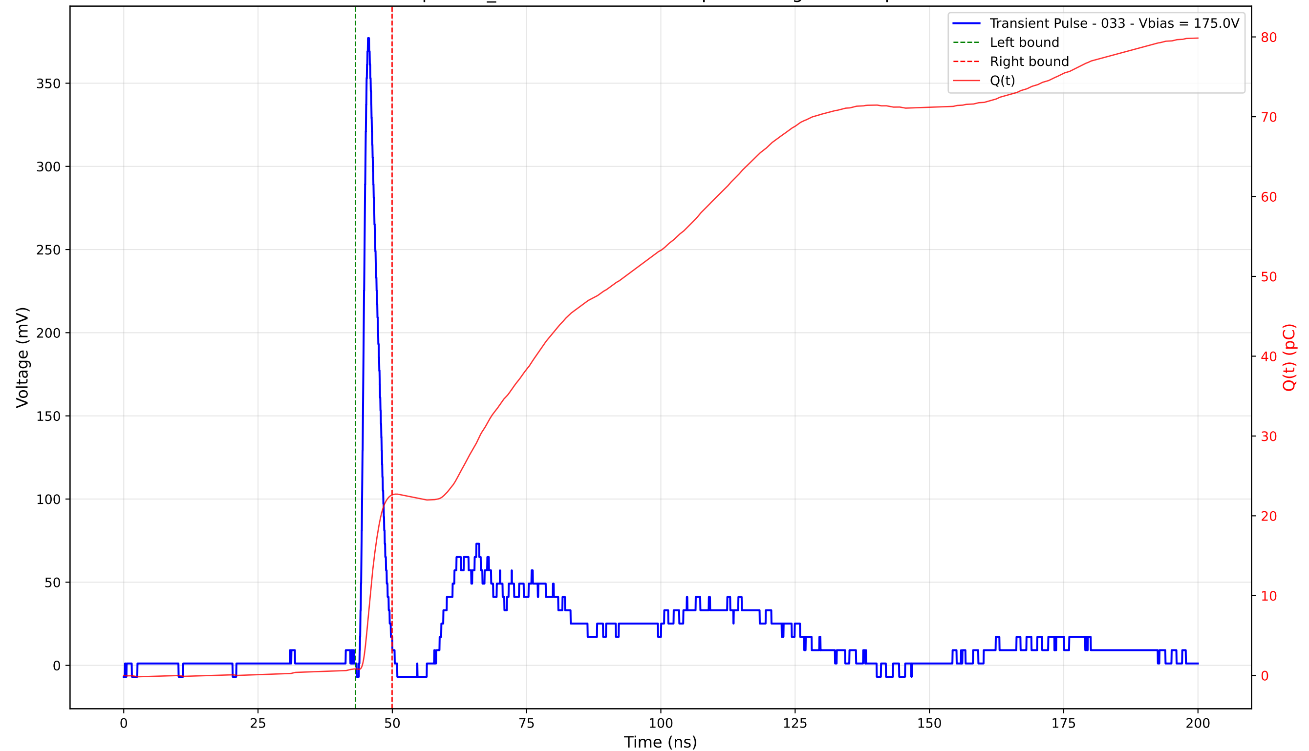
Transient Pulse - Sample: TD_4004 - Position: 380.0 \mu\text{m} - Charge: 21.81 pC - Rise Time: 1.05 ns
