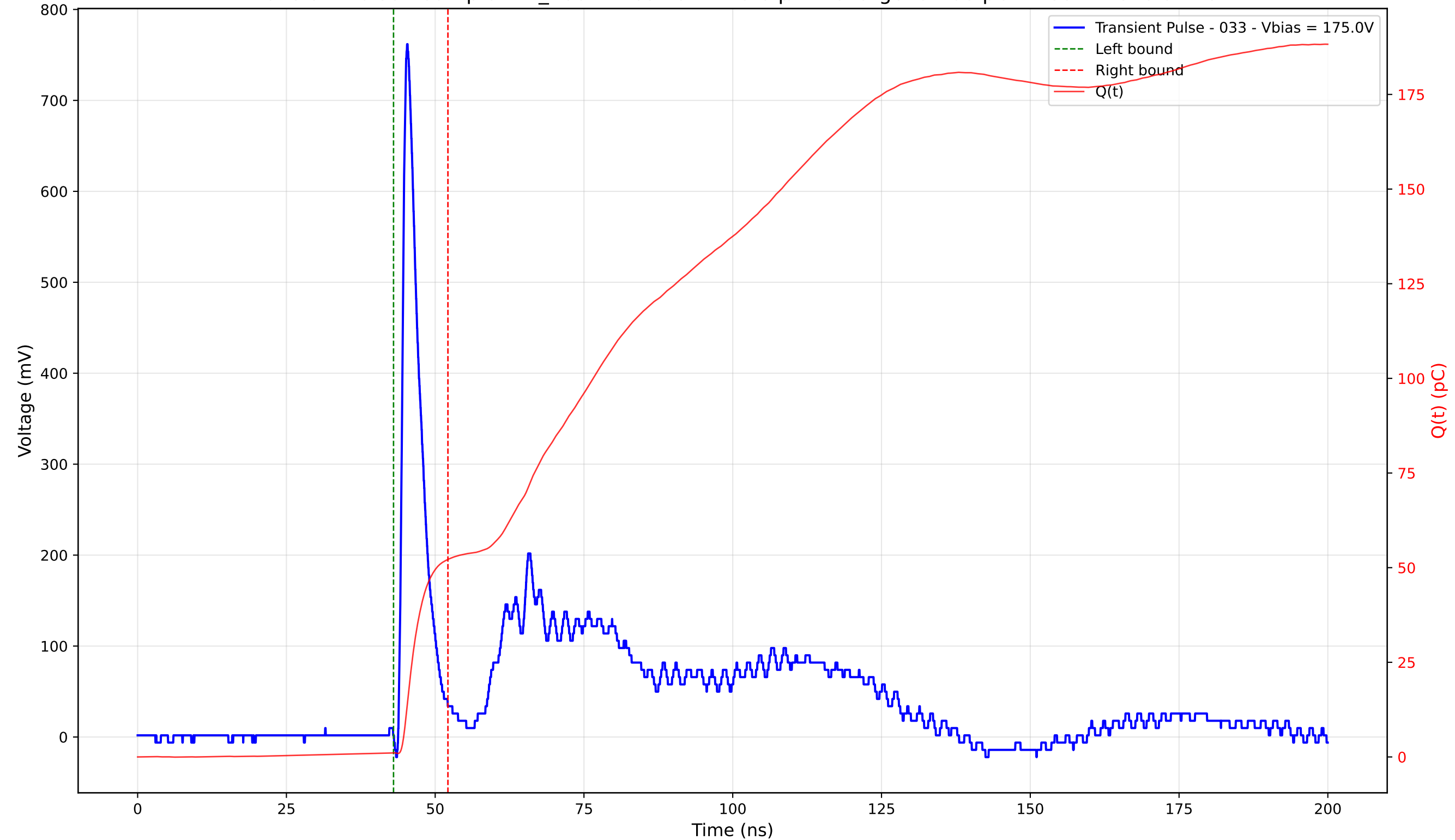
Transient Pulse - Sample: TD_4004 - Position: 115.0 \mu\text{m} - Charge: 51.08 pC - Rise Time: 0.92 ns
