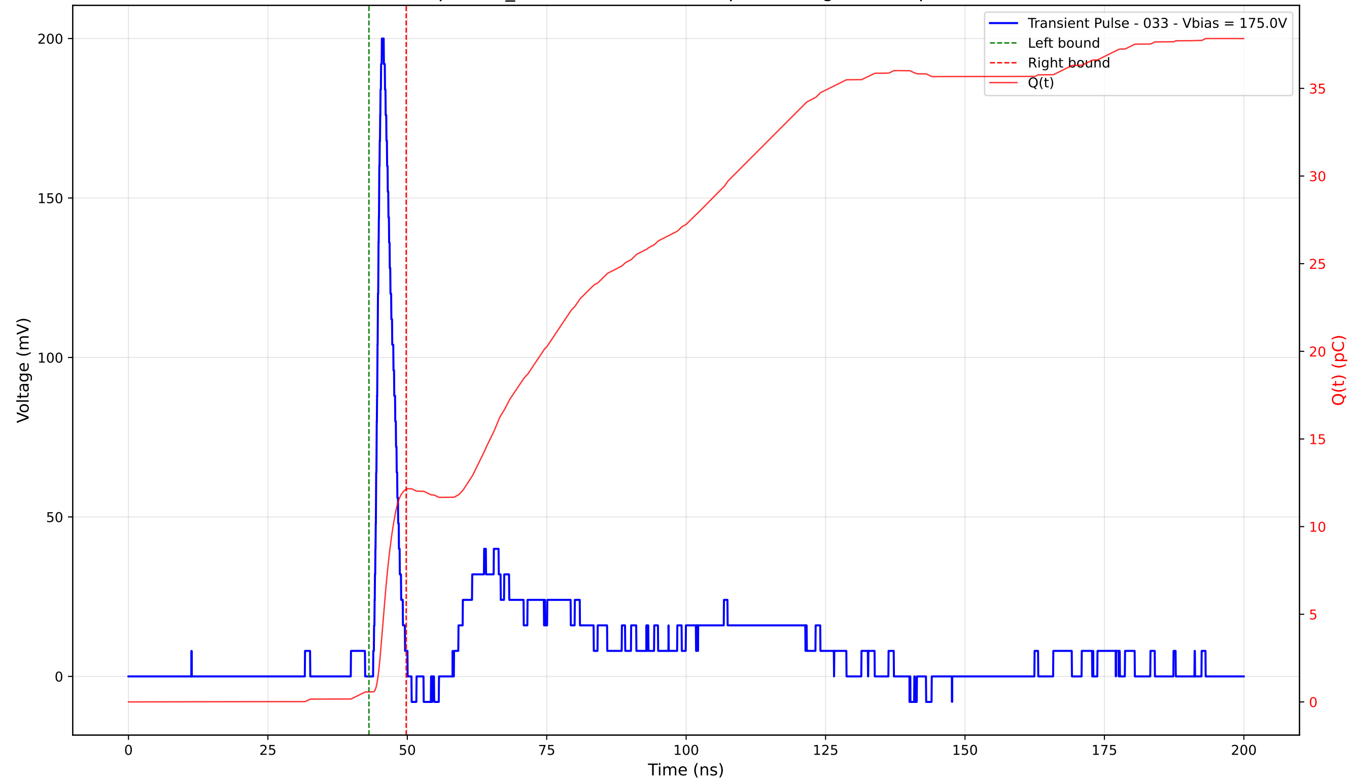
Transient Pulse - Sample: TD_4004 - Position: 400.0 \mu\text{m} - Charge: 11.56 pC - Rise Time: 1.07 ns
