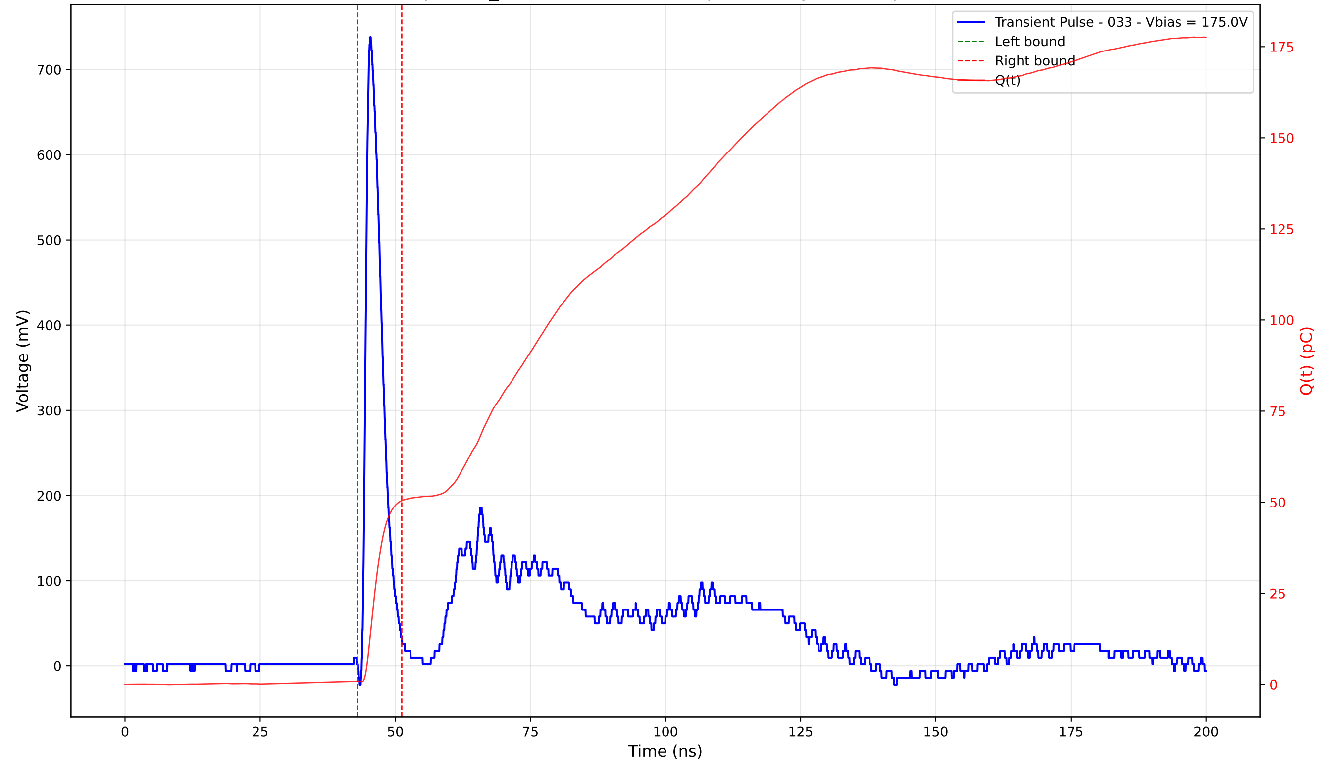
Transient Pulse - Sample: TD_4004 - Position: 220.0 \mu\text{m} - Charge: 49.57 pC - Rise Time: 0.94 ns
