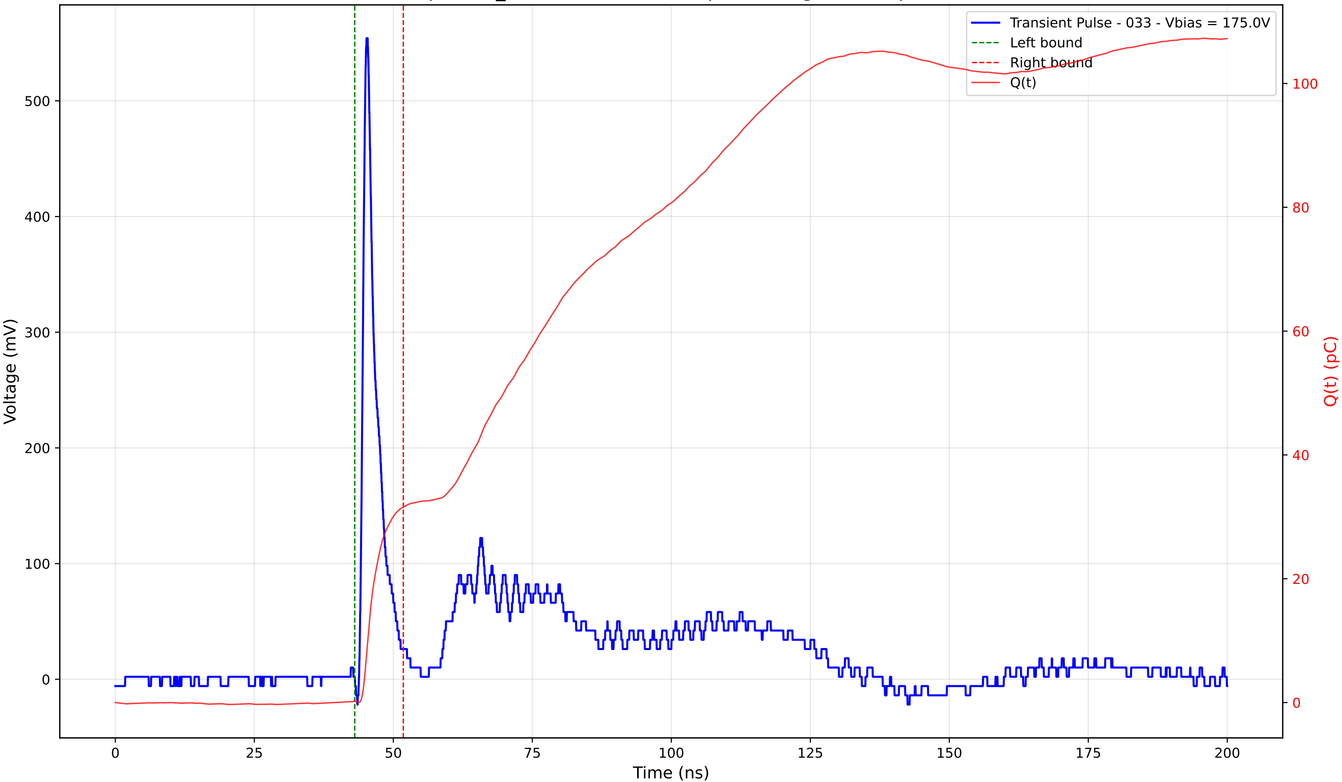
Transient Pulse - Sample: TD_4004 - Position: 75.0 \mu\text{m} - Charge: 31.37 pC - Rise Time: 0.91 ns
