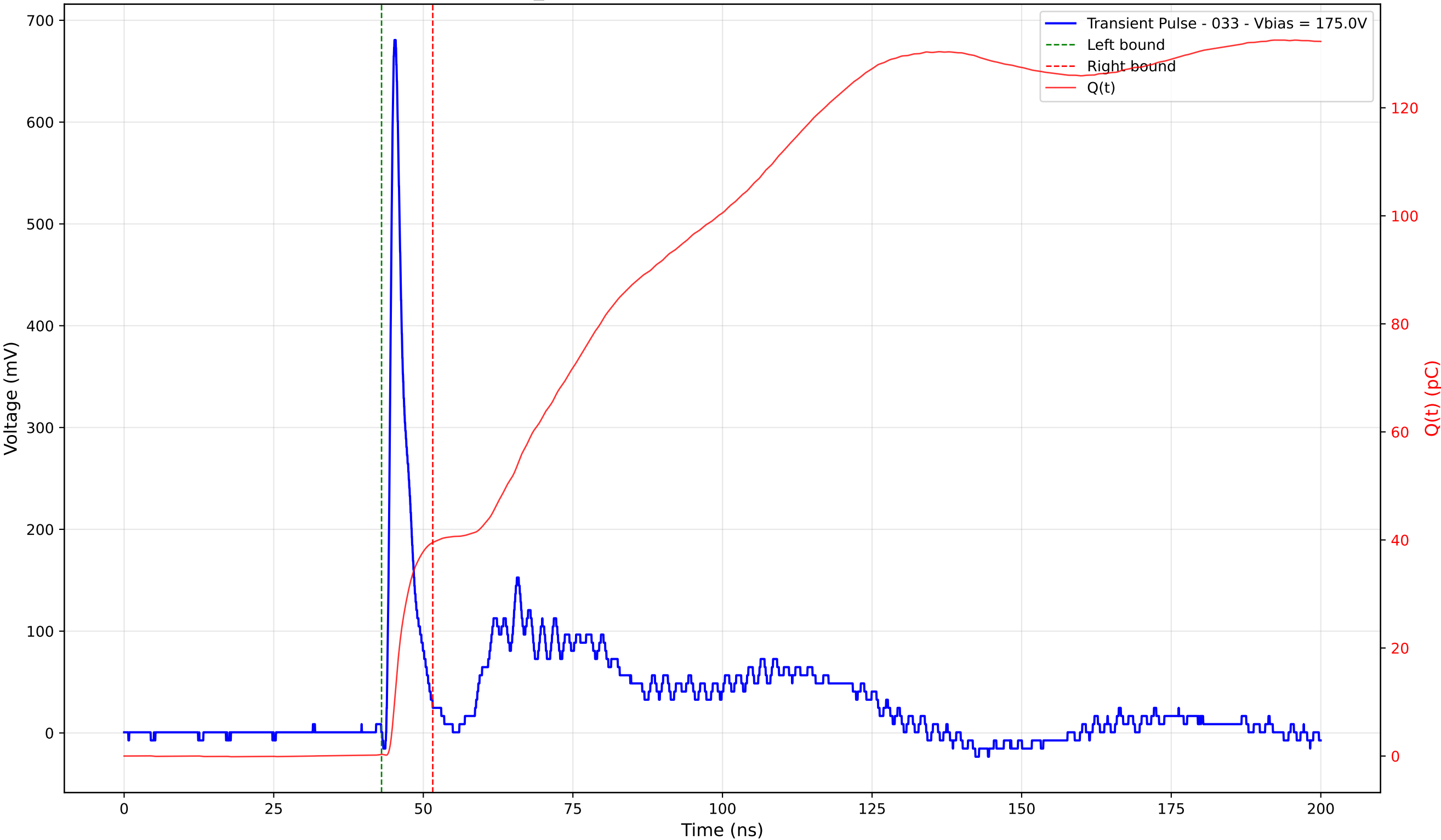
Transient Pulse - Sample: TD_4004 - Position: 85.0 \mu\text{m} - Charge: 39.23 pC - Rise Time: 0.88 ns
