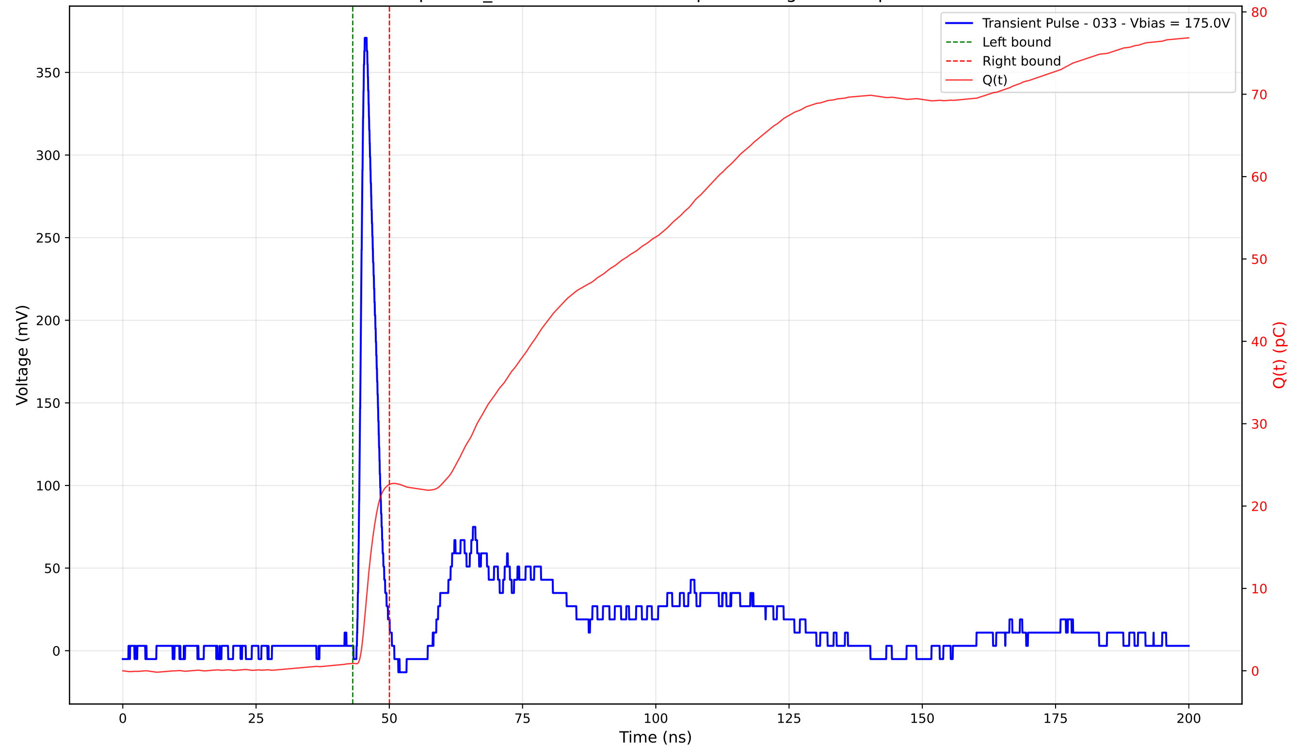
Transient Pulse - Sample: TD_4004 - Position: 375.0 \mu\text{m} - Charge: 21.73 pC - Rise Time: 1.01 ns
