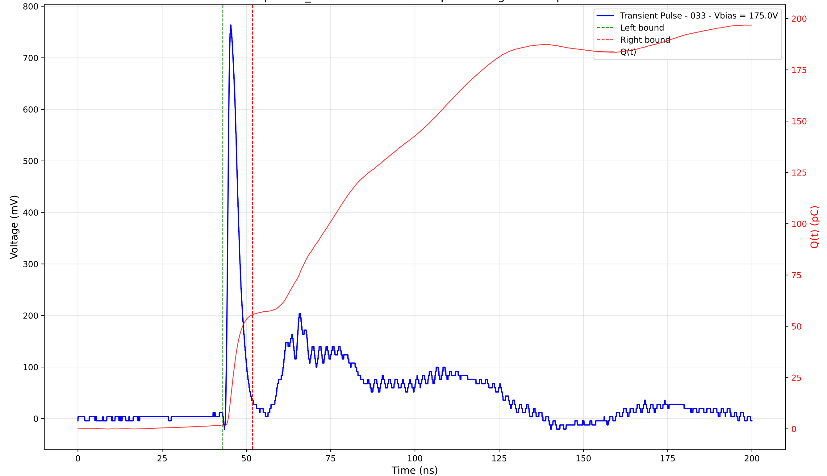
Transient Pulse - Sample: TD_4004 - Position: 180.0 \mu\text{m} - Charge: 53.70 pC - Rise Time: 0.95 ns
