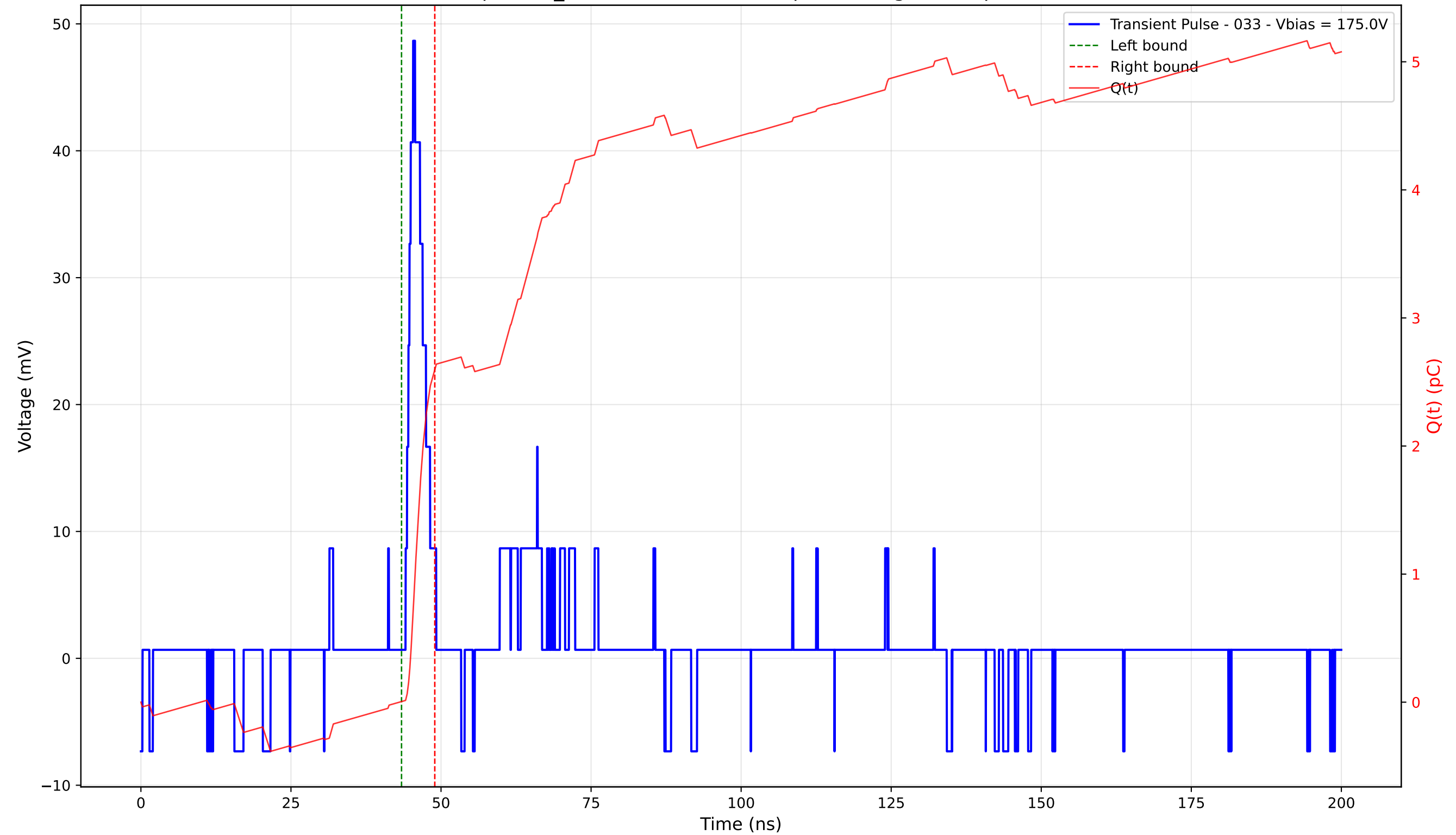
Transient Pulse - Sample: TD_4004 - Position: 430.0 \mu\text{m} - Charge: 2.59 pC - Rise Time: 1.25 ns
