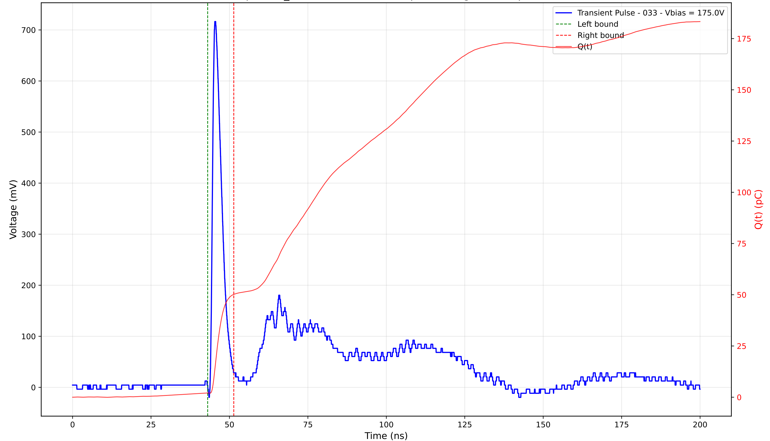
Transient Pulse - Sample: TD_4004 - Position: 160.0 \mu\text{m} - Charge: 48.07 pC - Rise Time: 0.97 ns
