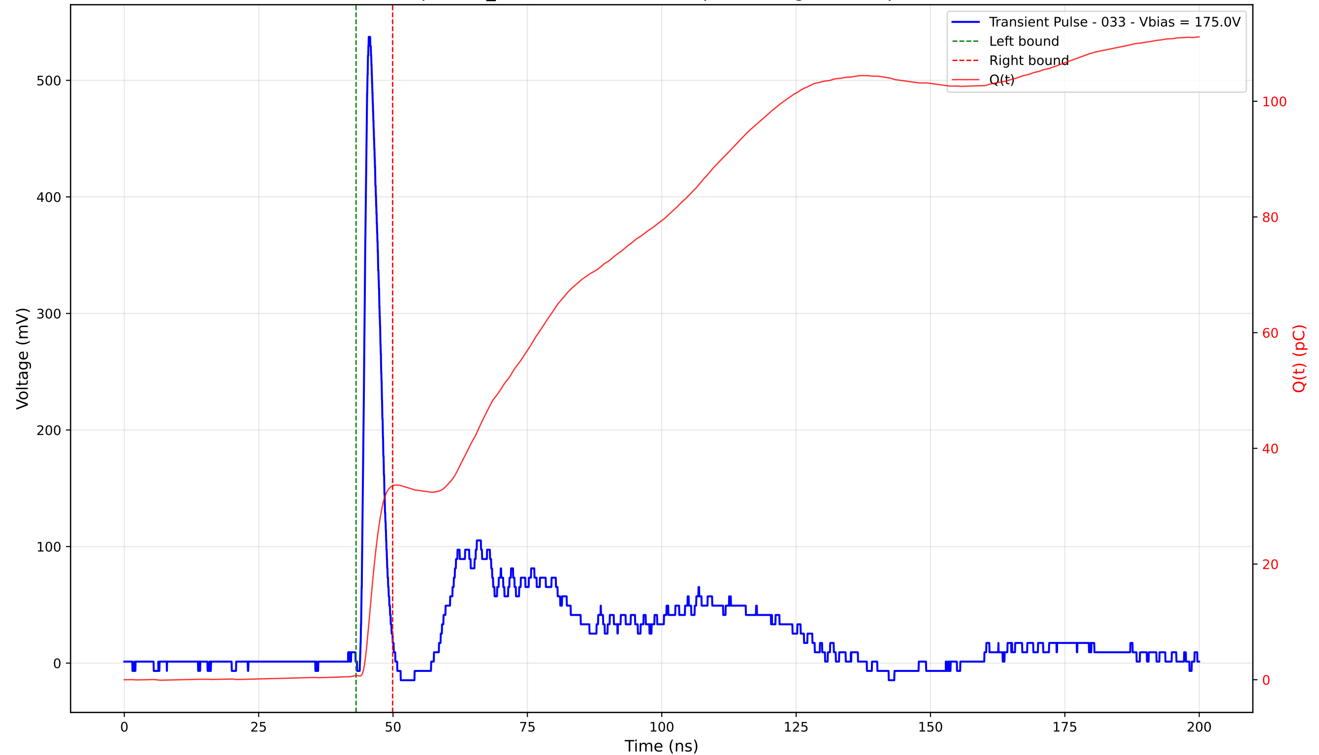
Transient Pulse - Sample: TD_4004 - Position: 320.0 \mu\text{m} - Charge: 32.83 pC - Rise Time: 1.05 ns
