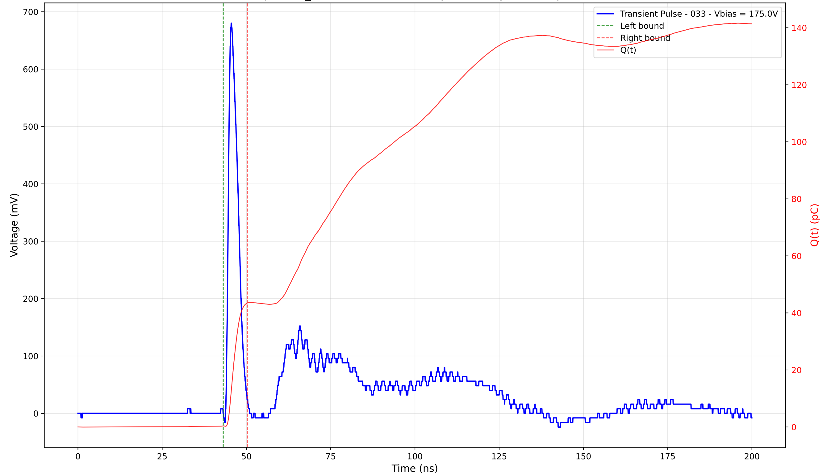
Transient Pulse - Sample: TD_4004 - Position: 280.0 \mu\text{m} - Charge: 43.08 pC - Rise Time: 1.00 ns
