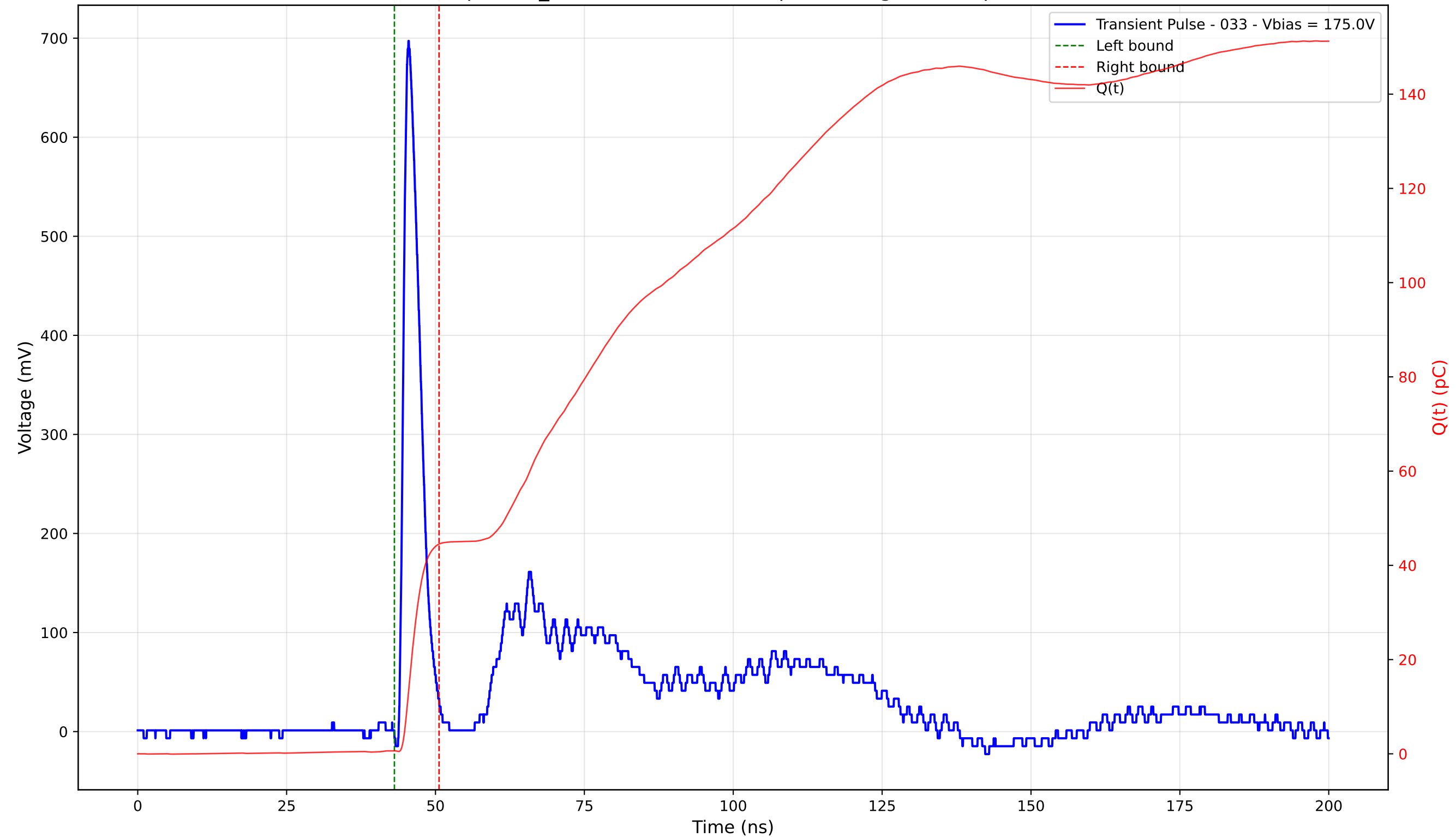
Transient Pulse - Sample: TD_4004 - Position: 235.0 \mu\text{m} - Charge: 43.87 pC - Rise Time: 0.99 ns
