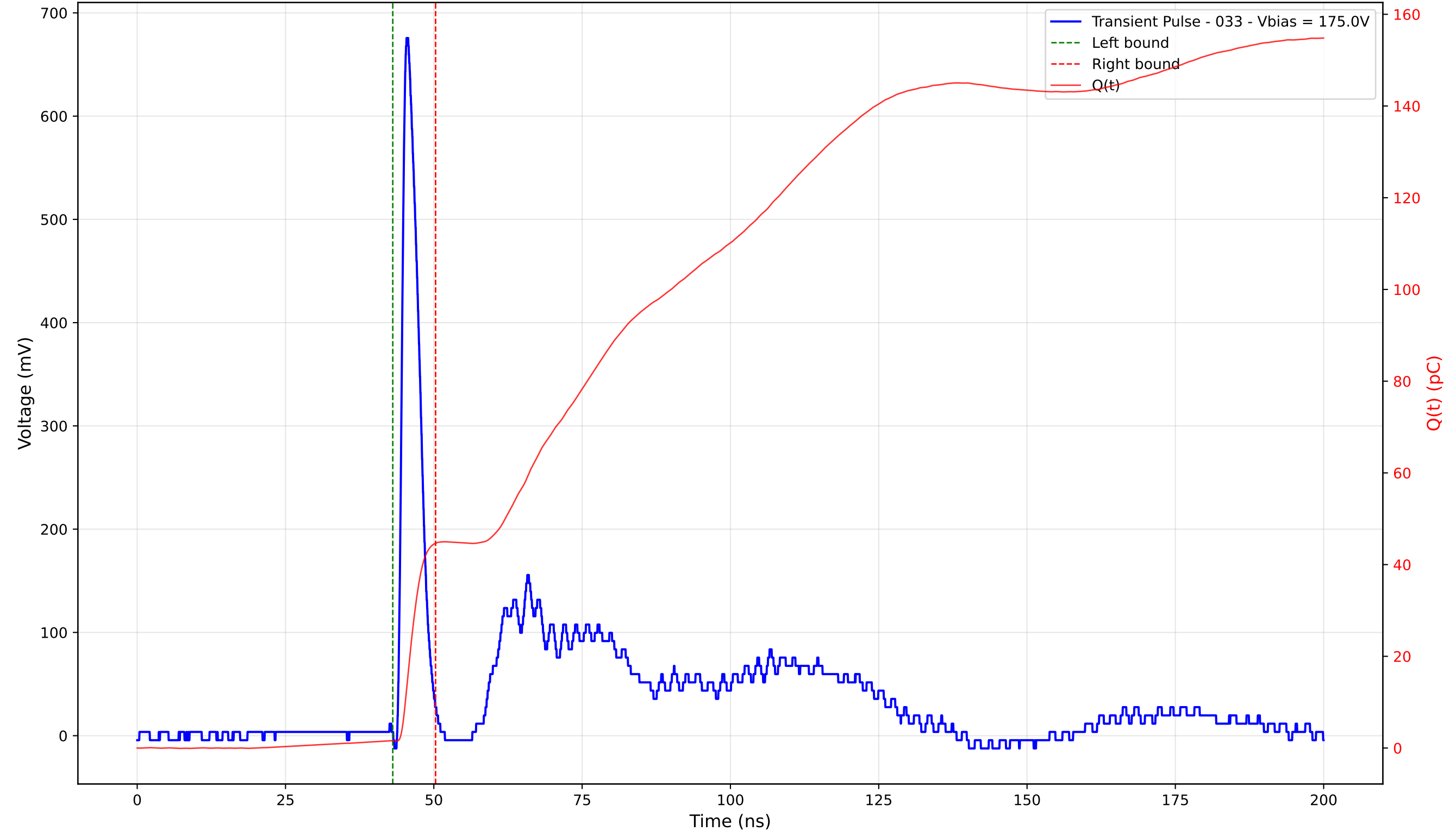
Transient Pulse - Sample: TD_4004 - Position: 275.0 \mu\text{m} - Charge: 43.04 pC - Rise Time: 0.99 ns
