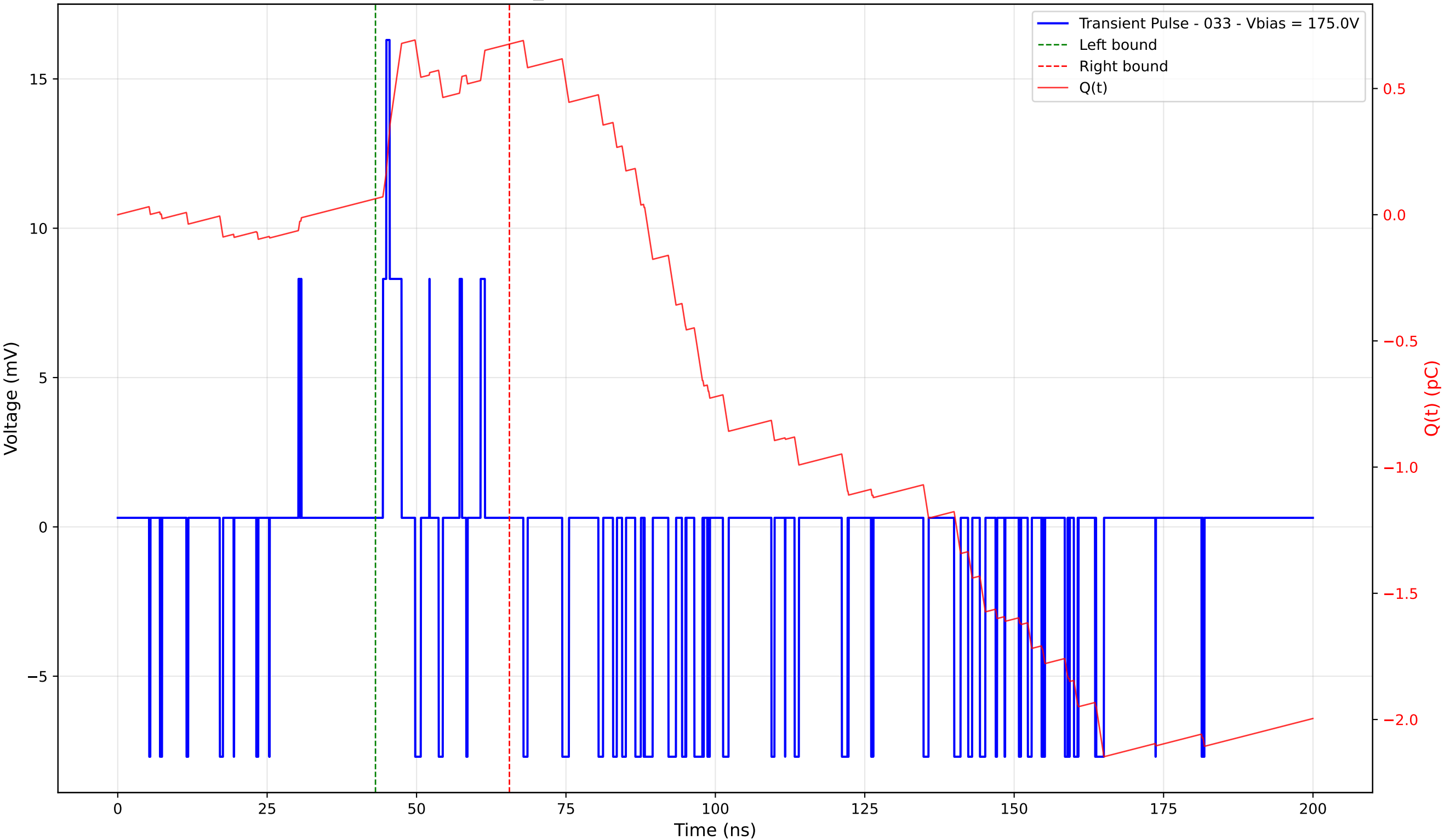
Transient Pulse - Sample: TD_4004 - Position: 20.0 \mu\text{m} - Charge: 0.61 pC - Rise Time: 0.58 ns
