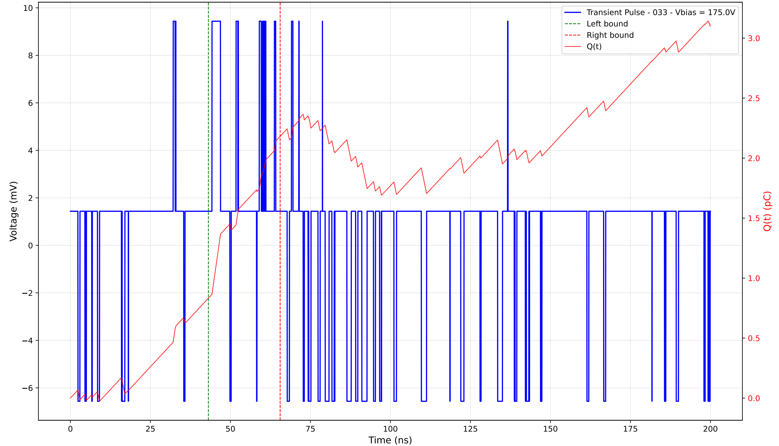
Transient Pulse - Sample: TD_4004 - Position: 10.0 \mu\text{m} - Charge: 1.35 pC - Rise Time: 0.00 ns (N/A)
