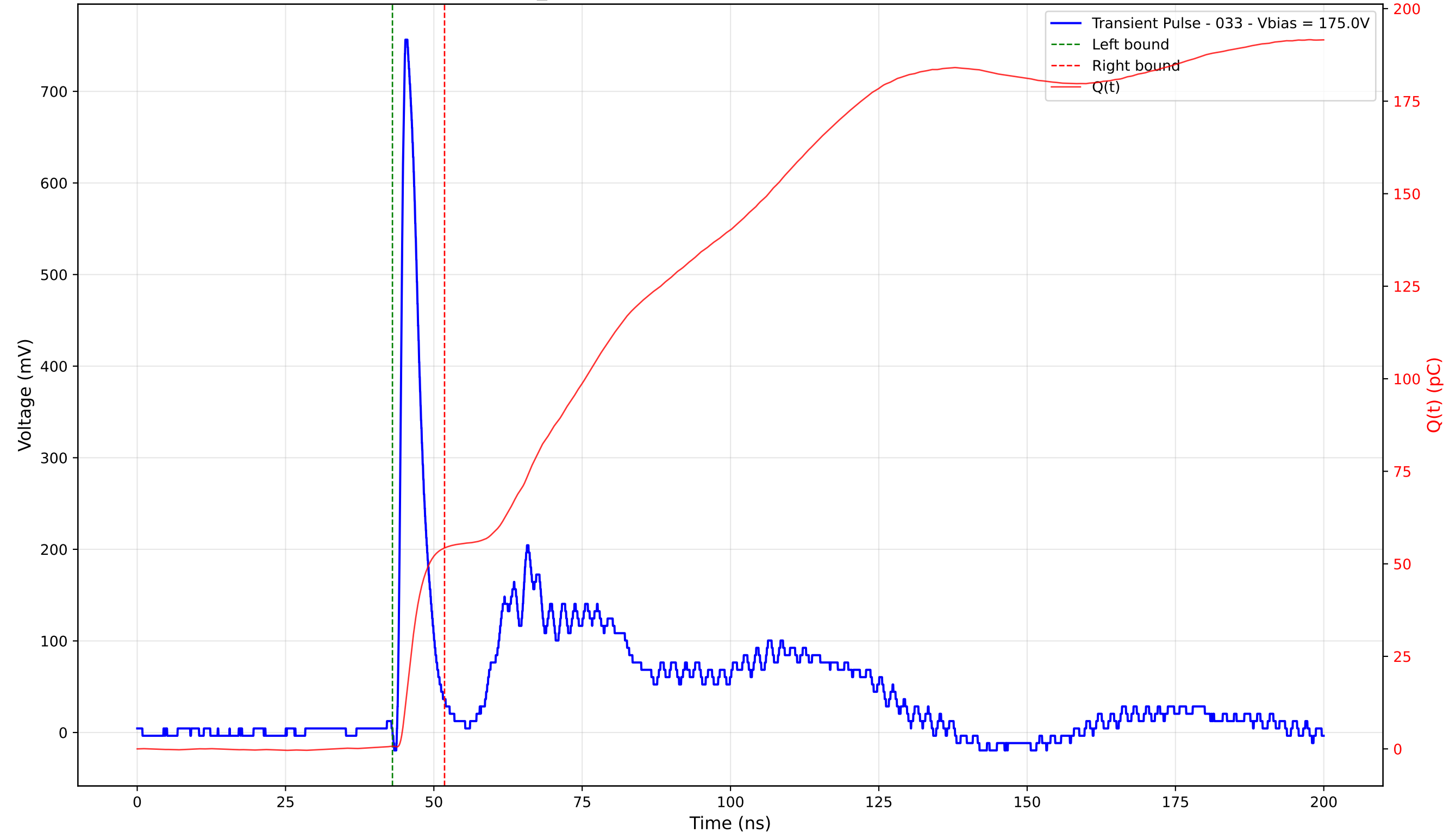
Transient Pulse - Sample: TD_4004 - Position: 185.0 \mu\text{m} - Charge: 53.55 pC - Rise Time: 0.92 ns
