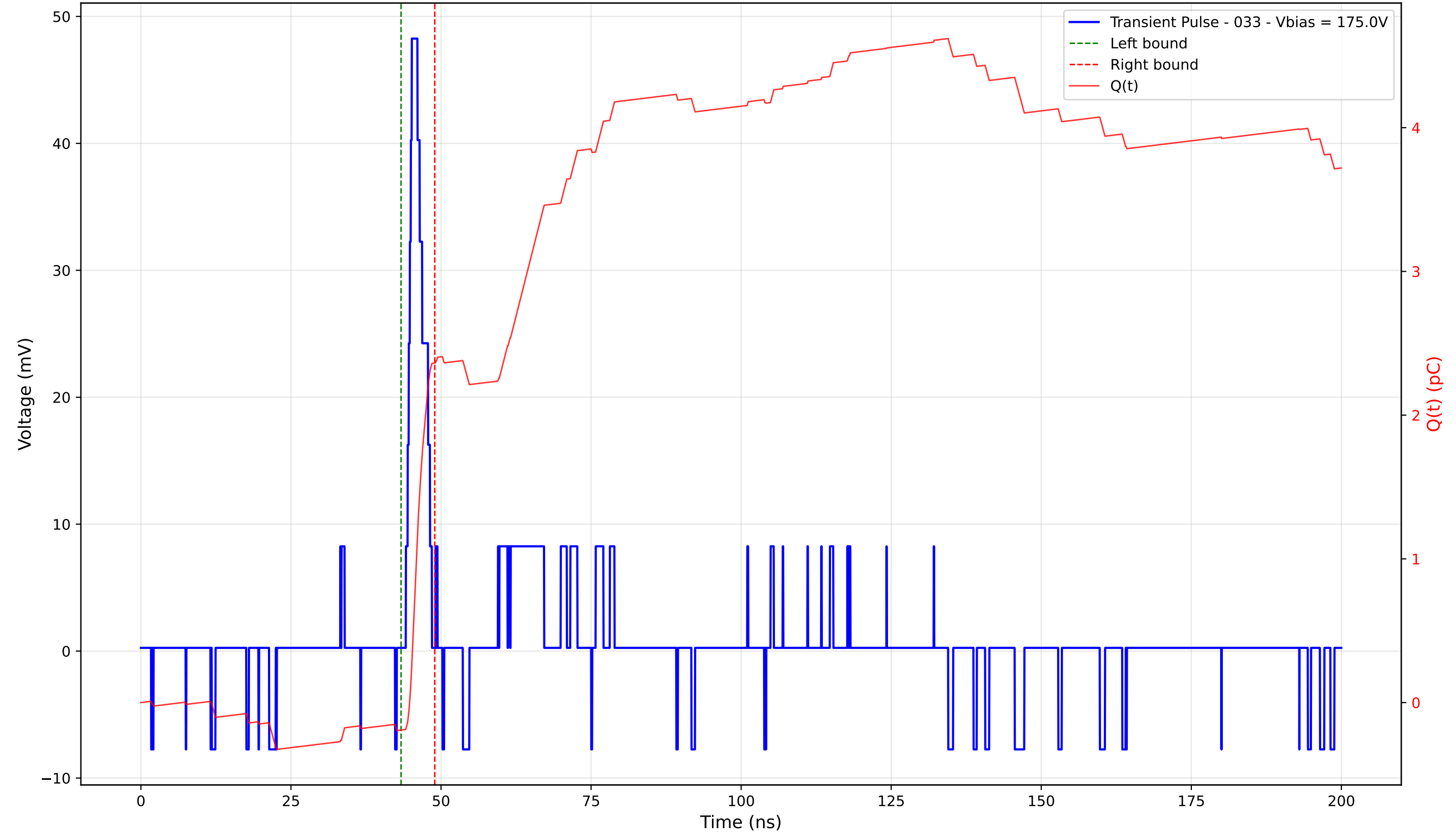
Transient Pulse - Sample: TD_4004 - Position: 425.0 \mu\text{m} - Charge: 2.55 pC - Rise Time: 0.99 ns
