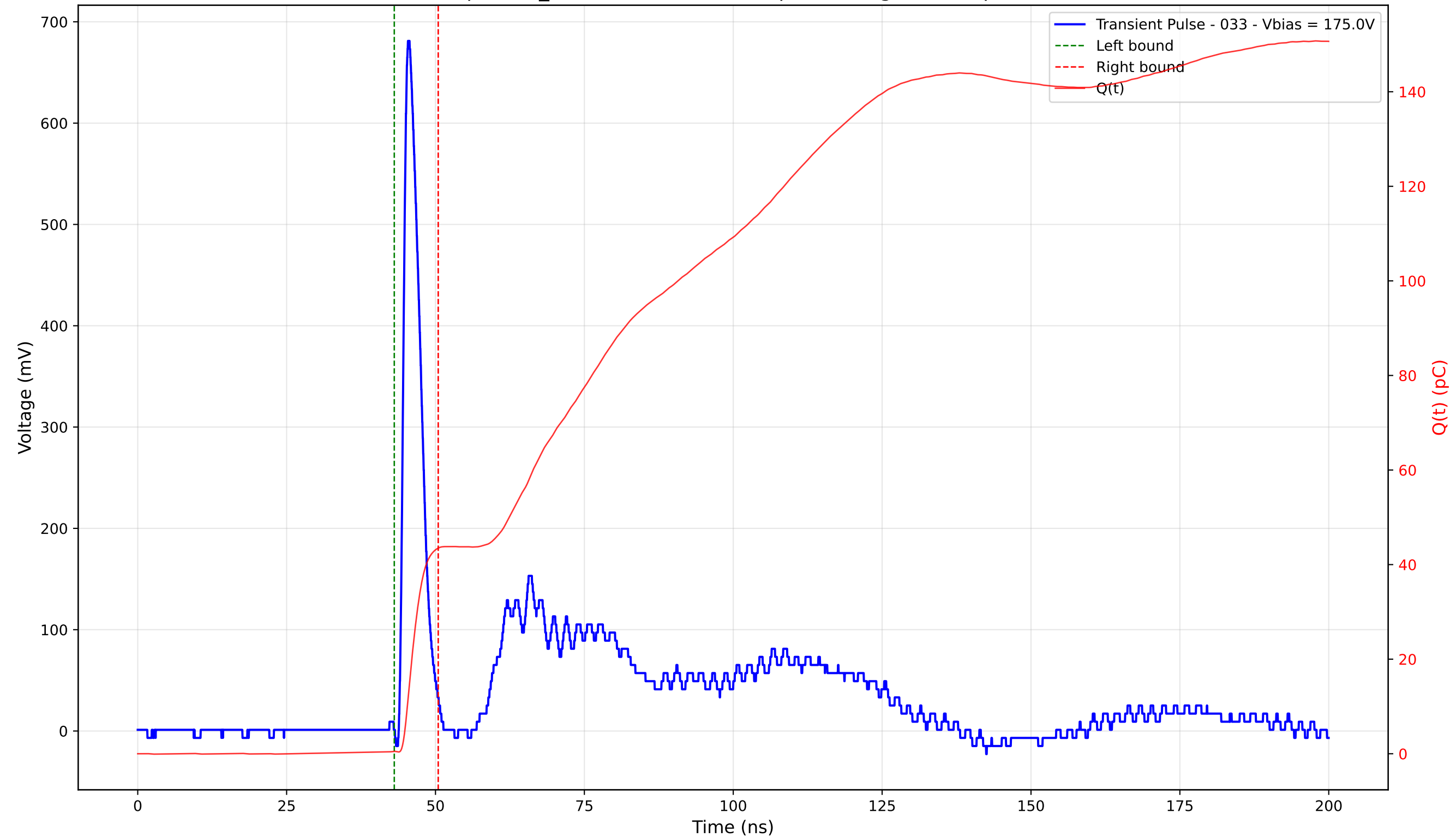
Transient Pulse - Sample: TD_4004 - Position: 250.0 \mu\text{m} - Charge: 42.99 pC - Rise Time: 0.98 ns
