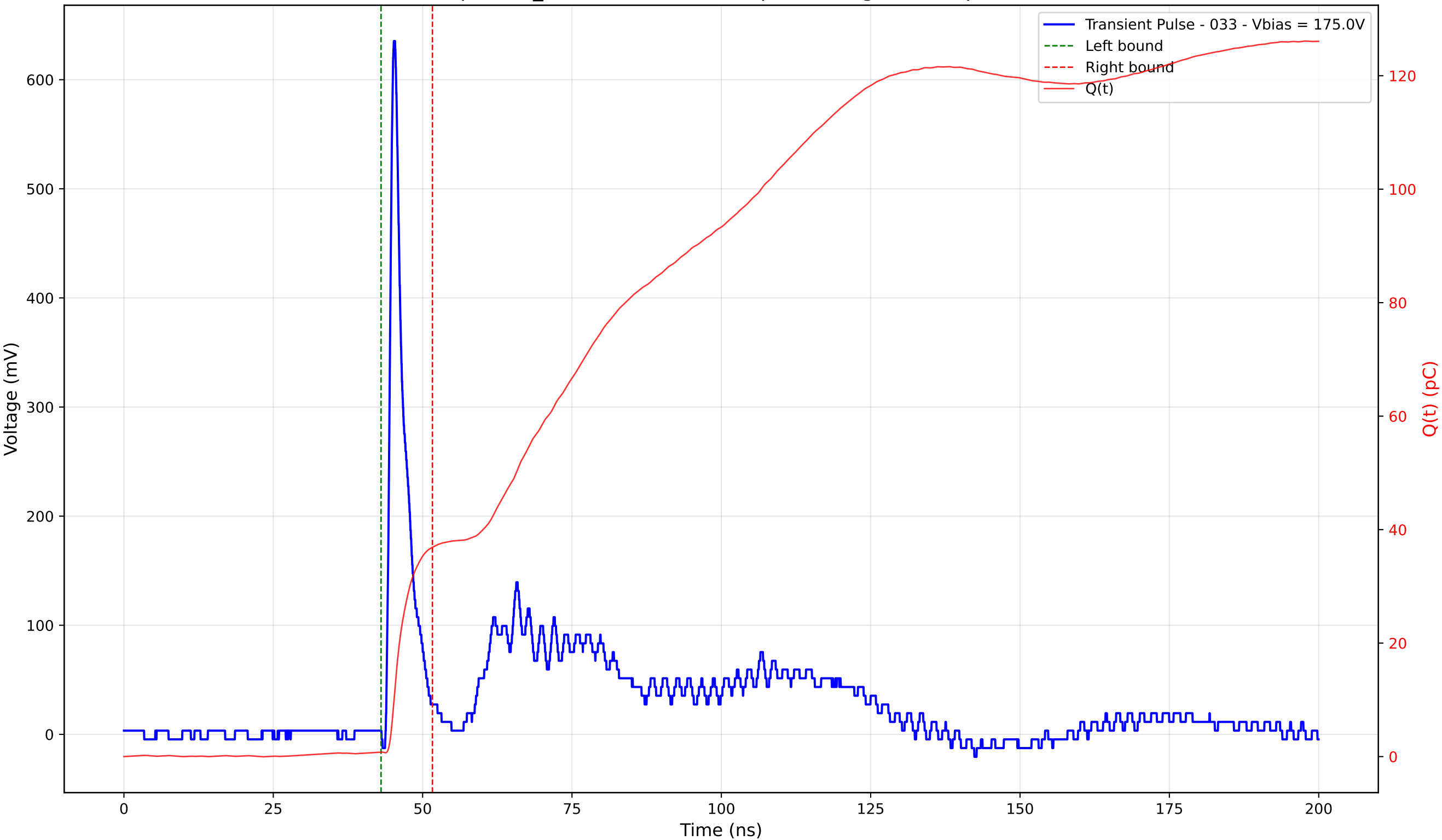
Transient Pulse - Sample: TD_4004 - Position: 80.0 \mu\text{m} - Charge: 36.09 pC - Rise Time: 0.89 ns
