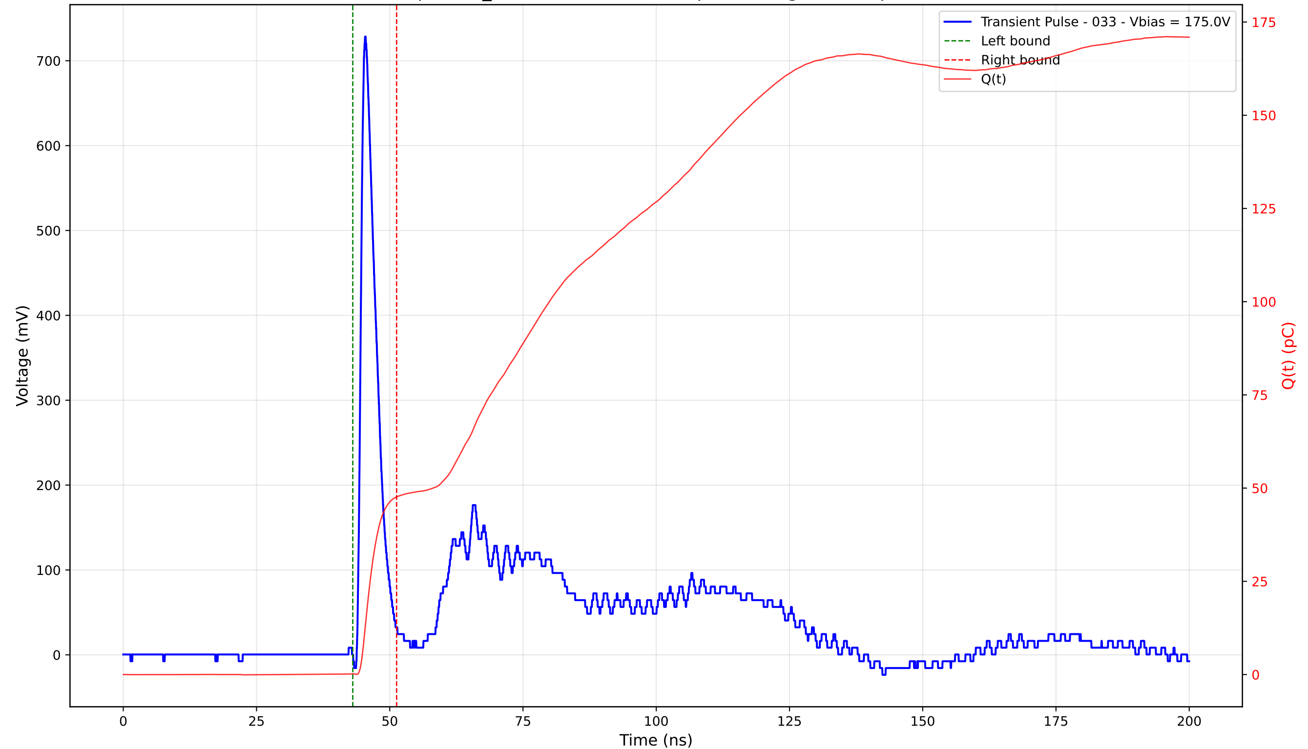
Transient Pulse - Sample: TD_4004 - Position: 130.0 \mu\text{m} - Charge: 47.45 pC - Rise Time: 0.96 ns
