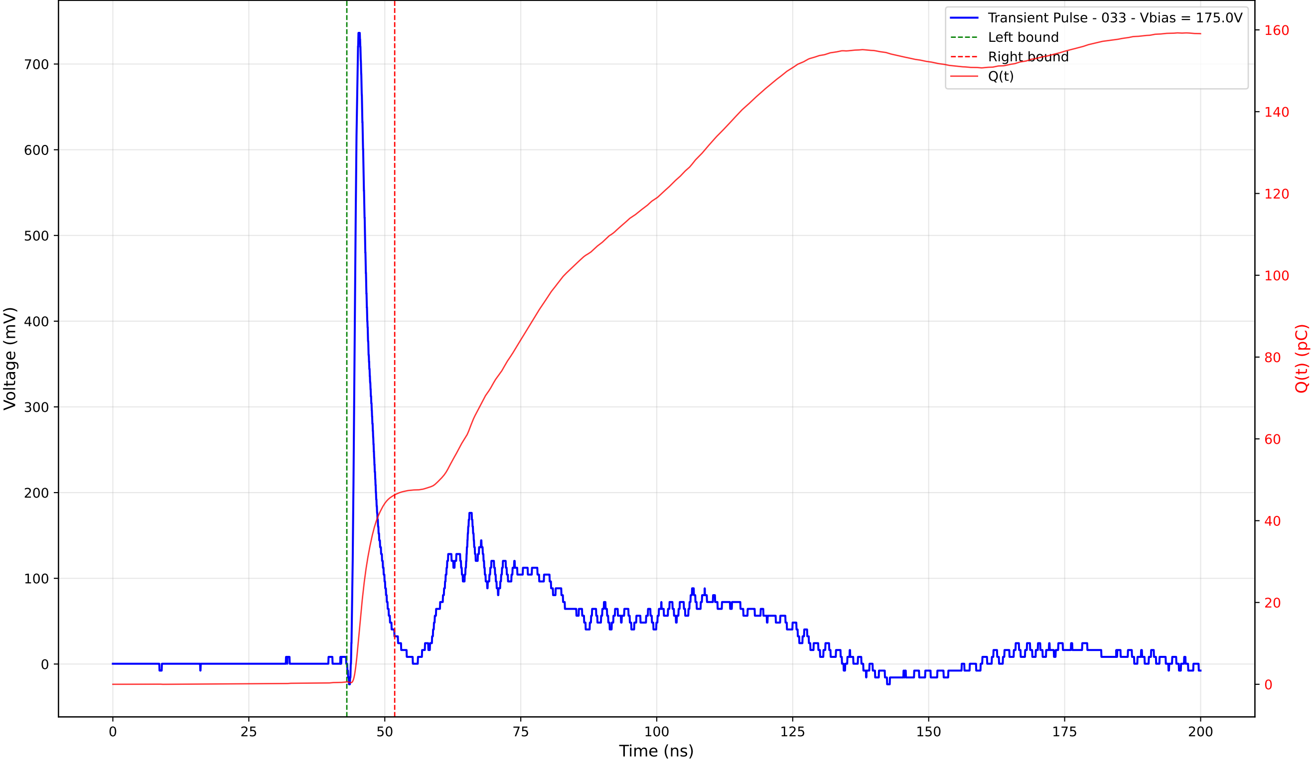
Transient Pulse - Sample: TD_4004 - Position: 95.0 \mu\text{m} - Charge: 45.73 pC - Rise Time: 0.89 ns
