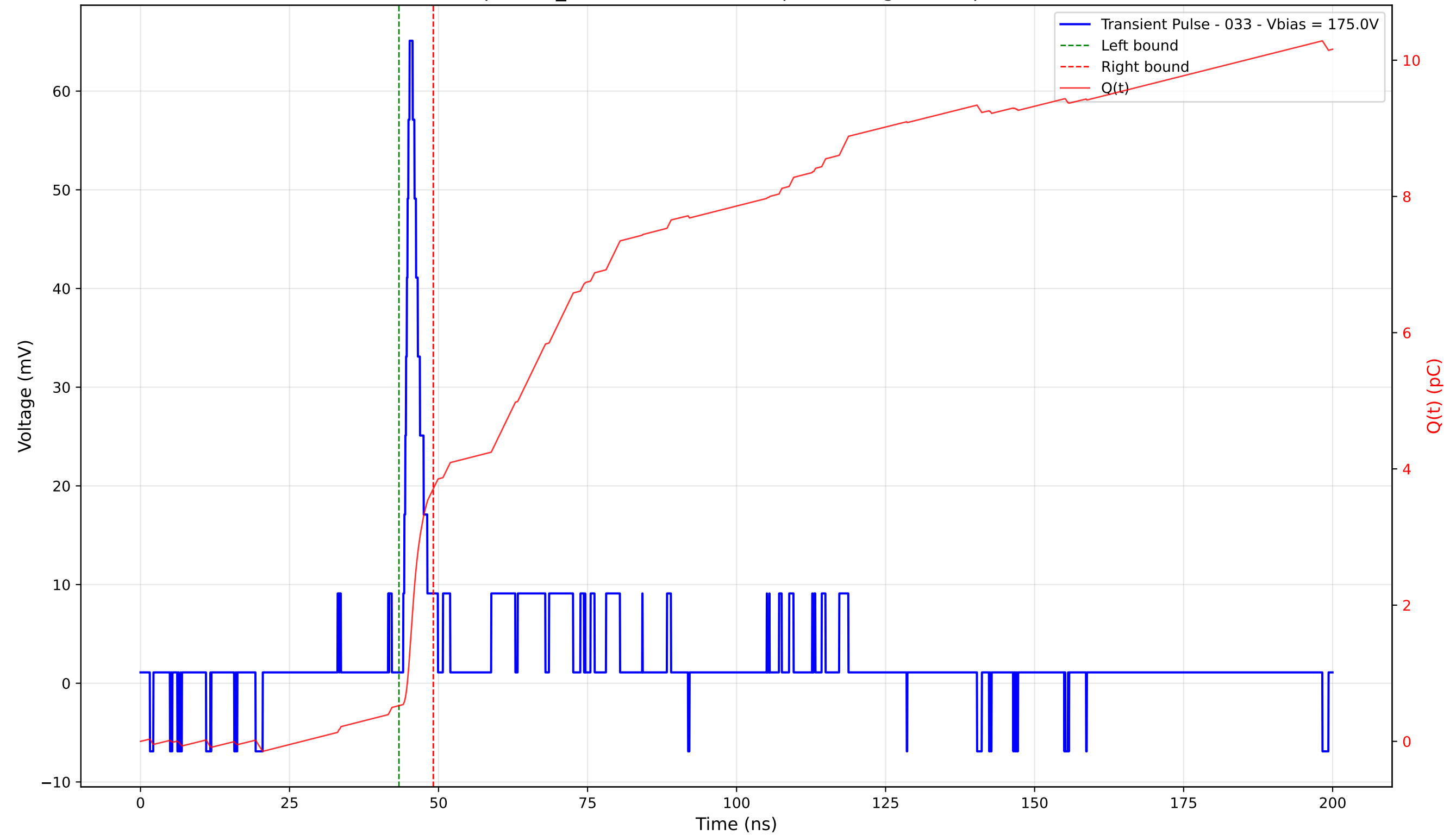
Transient Pulse - Sample: TD_4004 - Position: 45.0 \mu\text{m} - Charge: 3.19 pC - Rise Time: 1.07 ns
