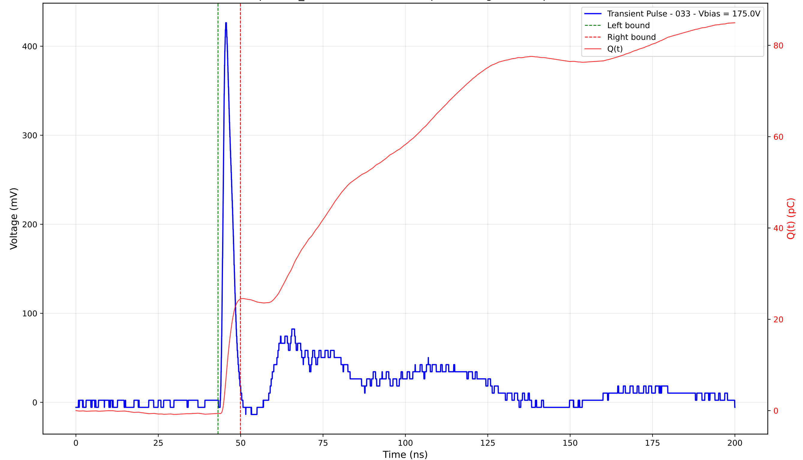
Transient Pulse - Sample: TD_4004 - Position: 345.0 \mu\text{m} - Charge: 25.05 pC - Rise Time: 1.04 ns
