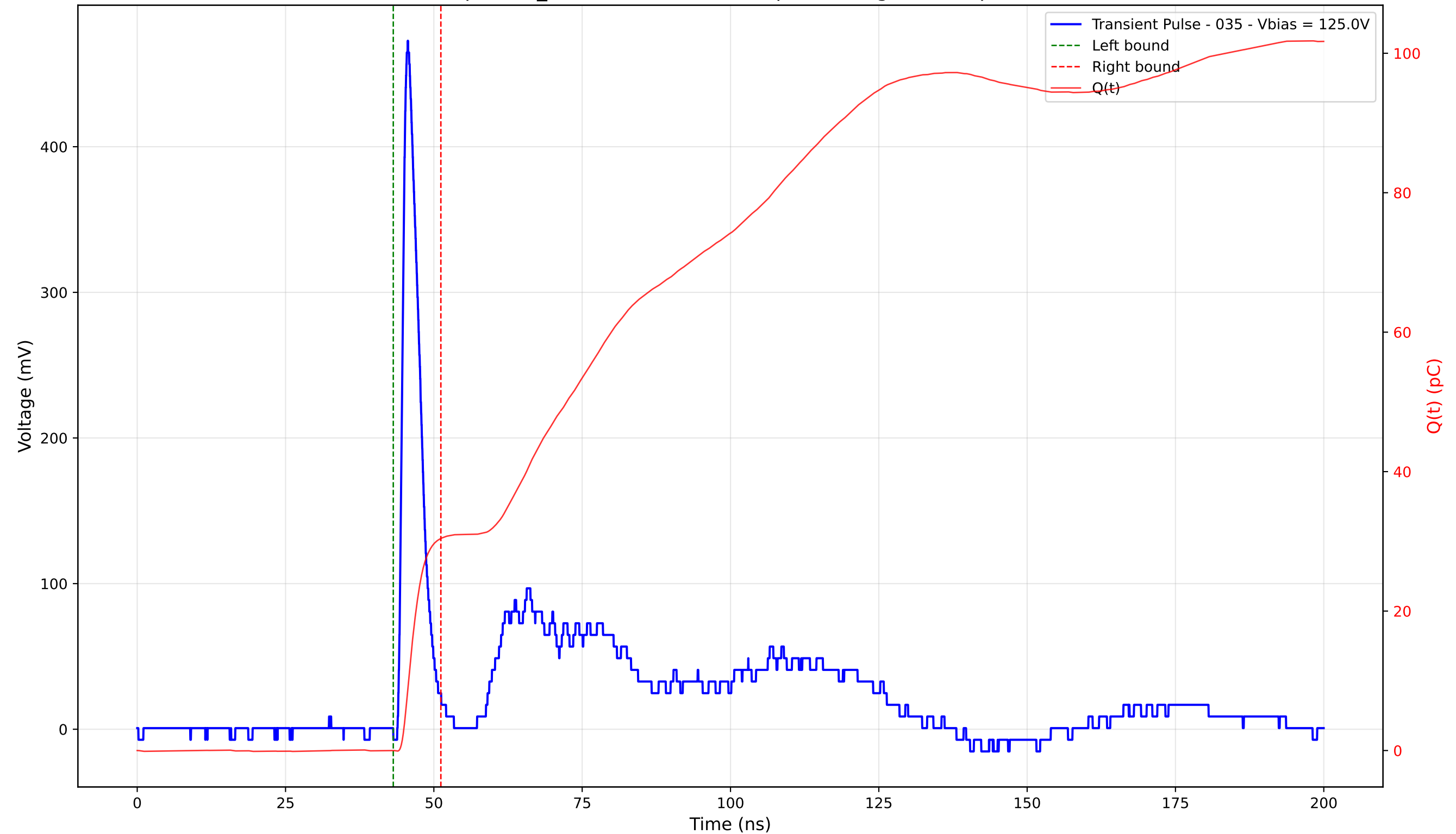
Transient Pulse - Sample: TD_4004 - Position: 300.0 \mu\text{m} - Charge: 30.40 pC - Rise Time: 1.08 ns
