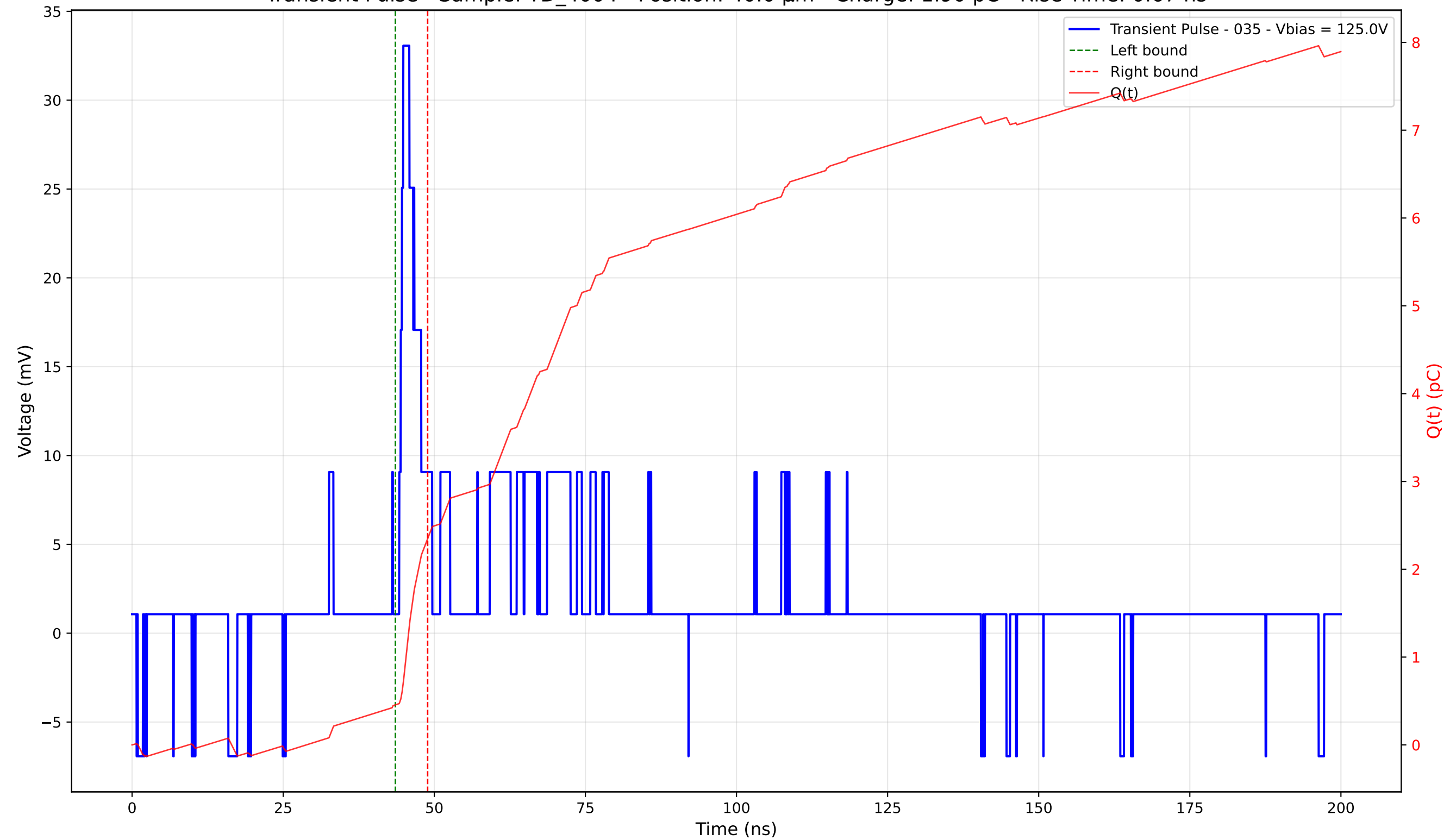
Transient Pulse - Sample: TD_4004 - Position: 40.0 \mu\text{m} - Charge: 1.90 pC - Rise Time: 0.67 ns
