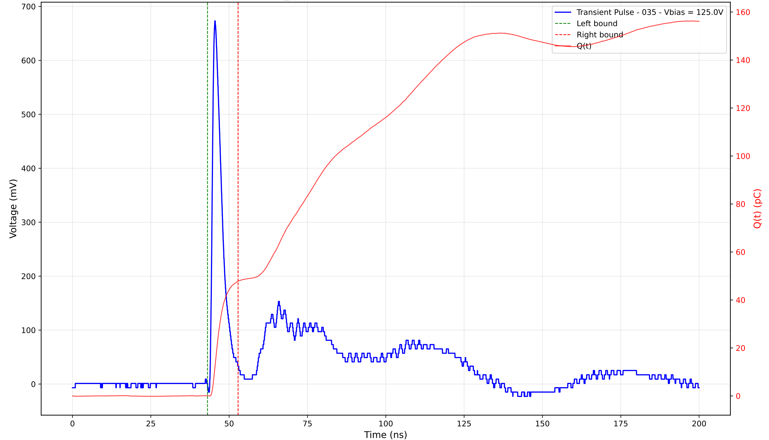
Transient Pulse - Sample: TD_4004 - Position: 215.0 \mu\text{m} - Charge: 47.69 pC - Rise Time: 0.99 ns
