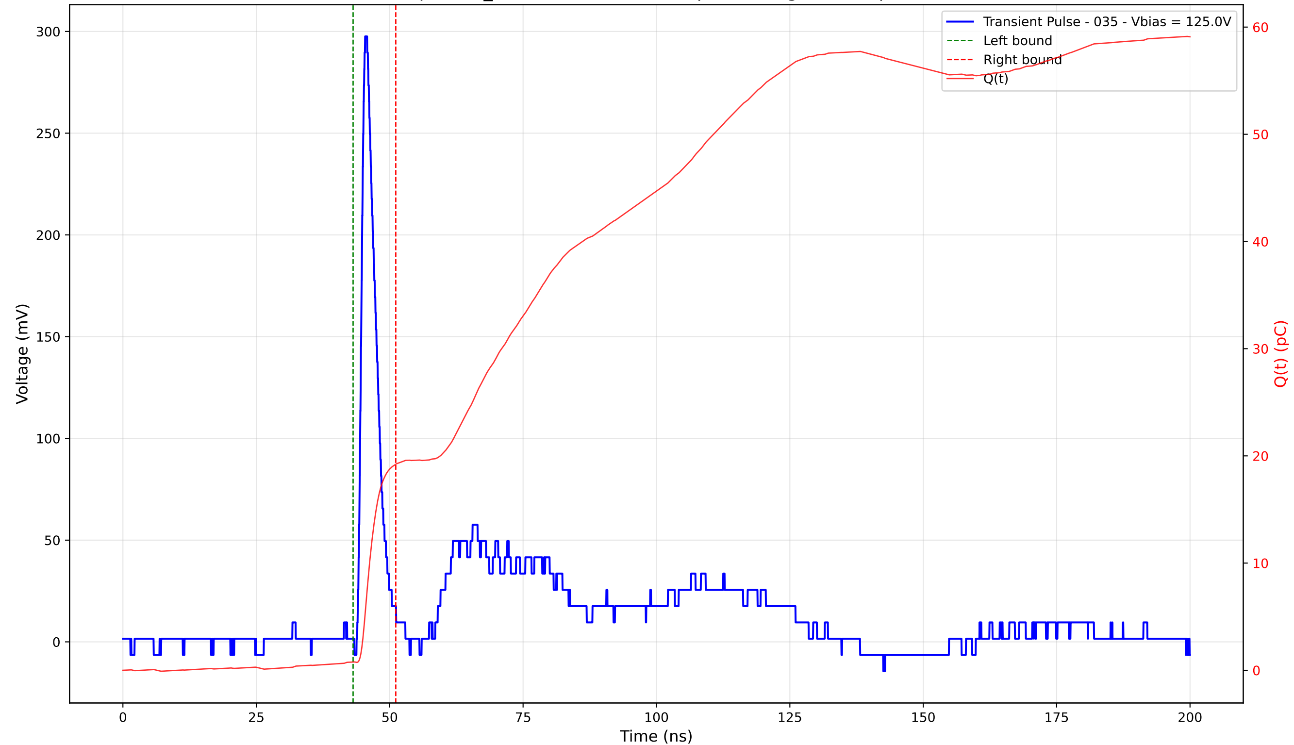
Transient Pulse - Sample: TD_4004 - Position: 355.0 \mu\text{m} - Charge: 18.45 pC - Rise Time: 1.03 ns
