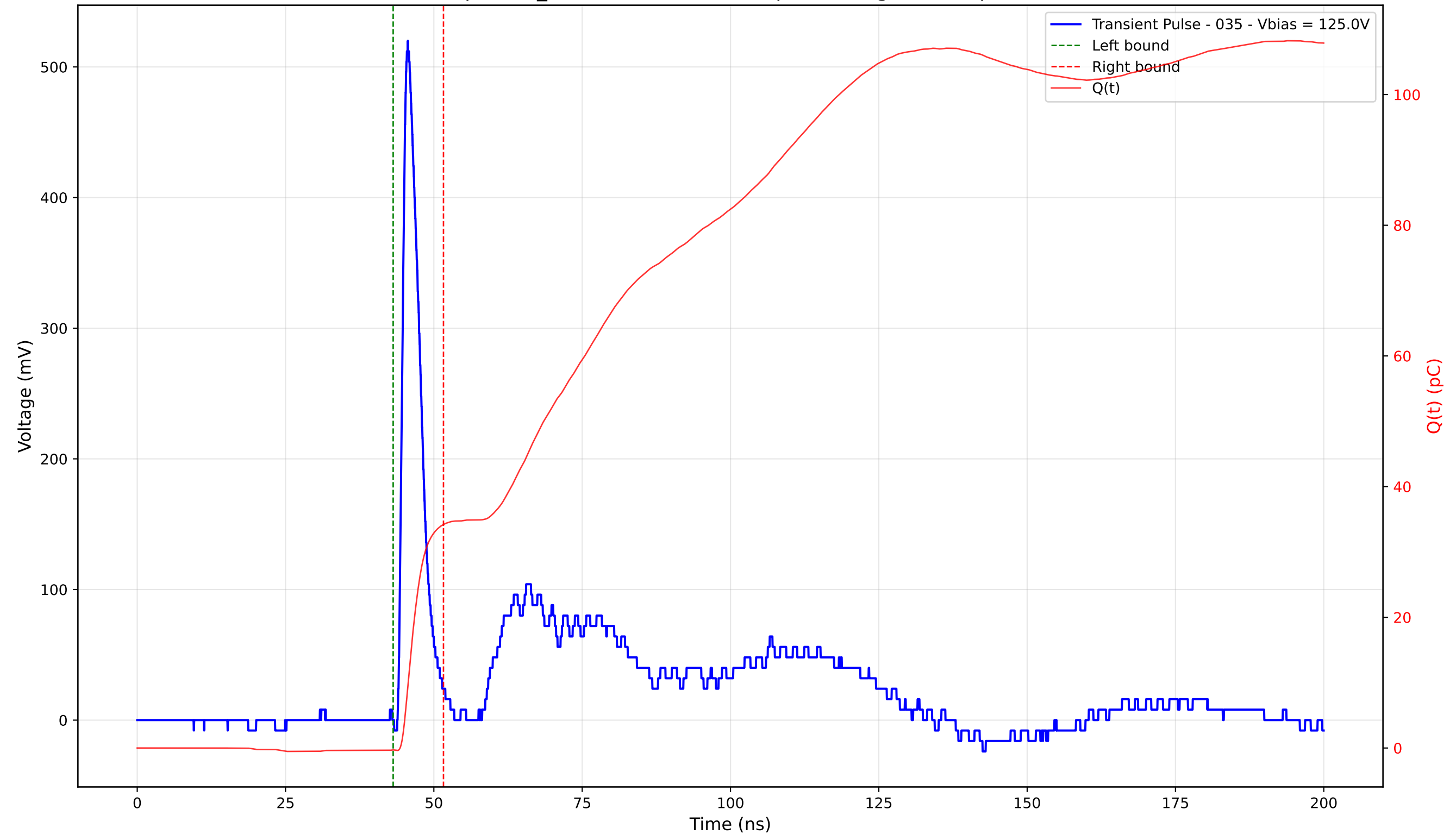
Transient Pulse - Sample: TD_4004 - Position: 270.0 \mu\text{m} - Charge: 34.50 pC - Rise Time: 1.05 ns
