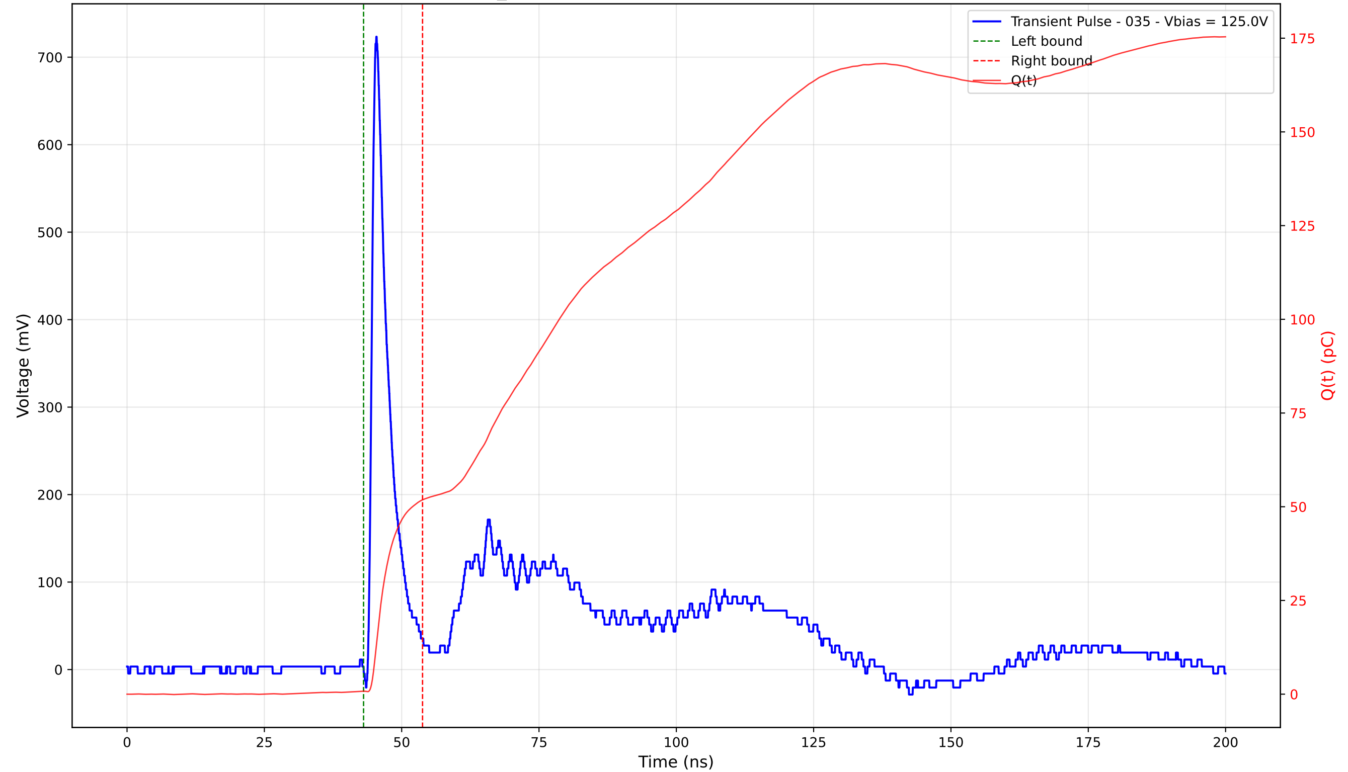
Transient Pulse - Sample: TD_4004 - Position: 120.0 \mu\text{m} - Charge: 51.03 pC - Rise Time: 0.95 ns
