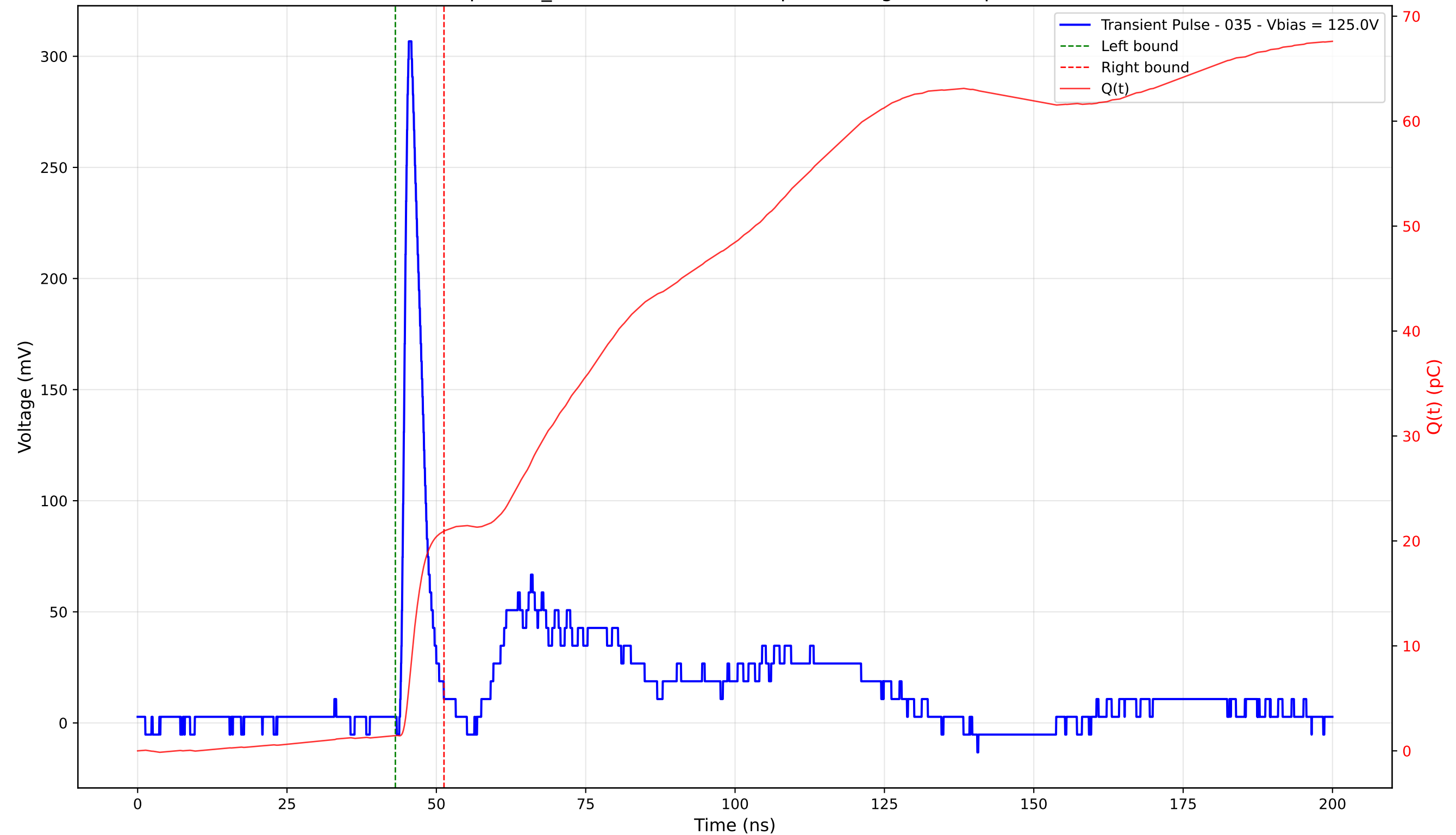
Transient Pulse - Sample: TD_4004 - Position: 335.0 \mu\text{m} - Charge: 19.49 pC - Rise Time: 1.05 ns
