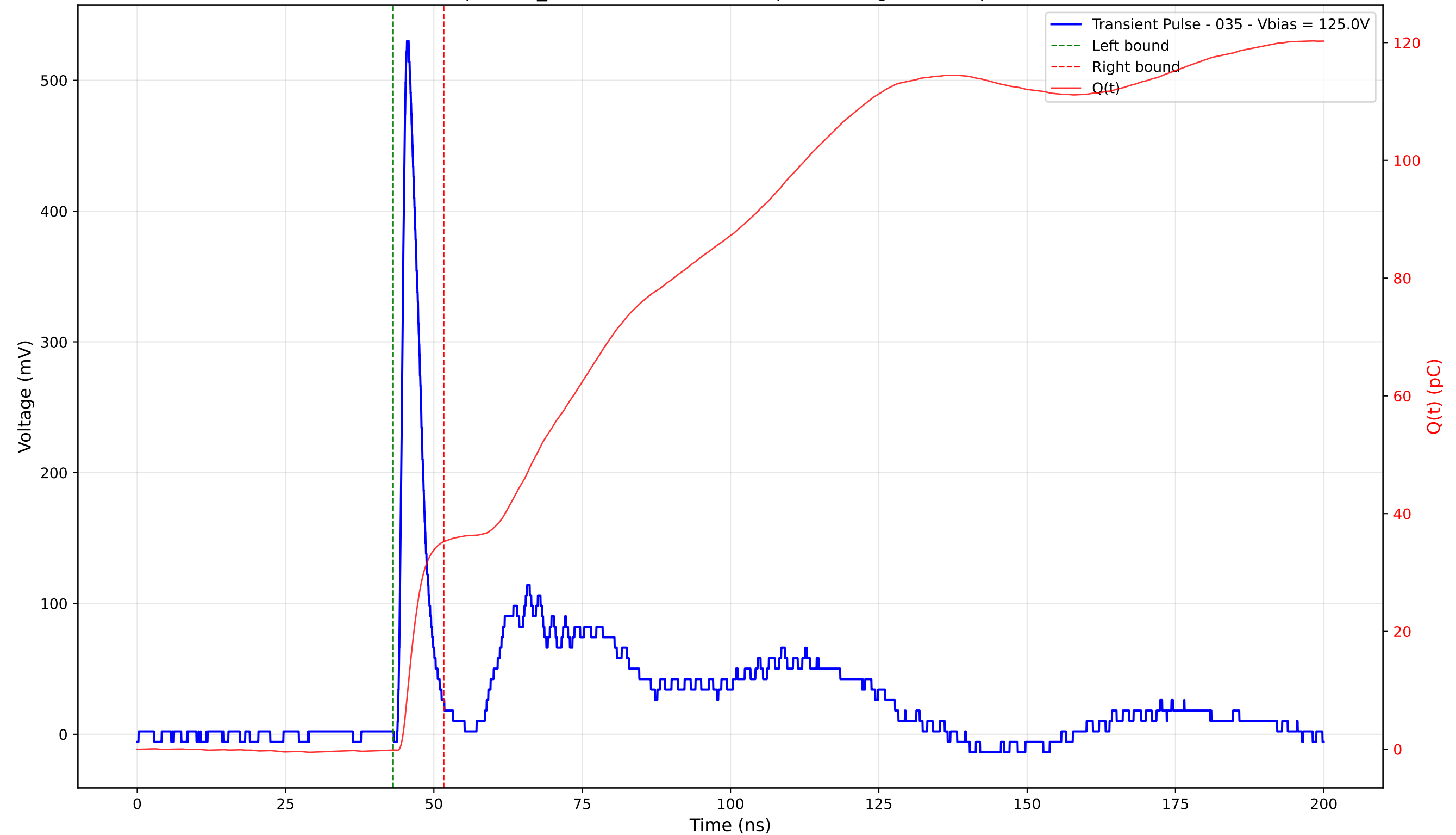
Transient Pulse - Sample: TD_4004 - Position: 260.0 \mu\text{m} - Charge: 35.37 pC - Rise Time: 1.04 ns
