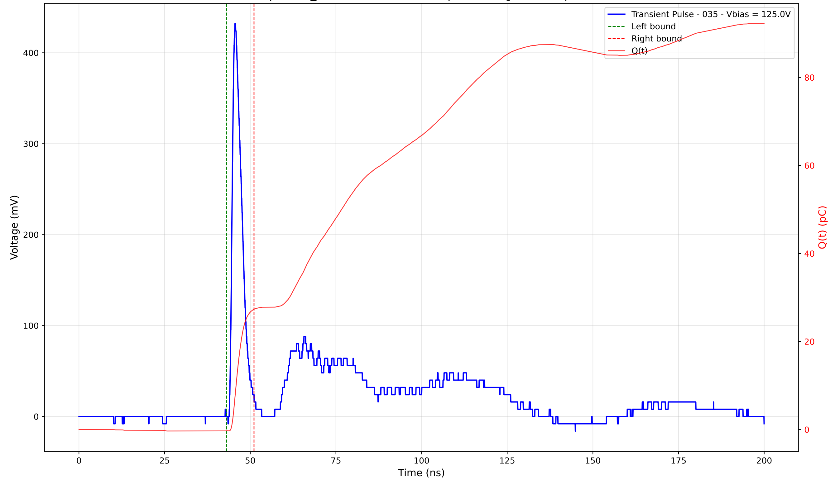
Transient Pulse - Sample: TD_4004 - Position: 310.0 \mu\text{m} - Charge: 27.63 pC - Rise Time: 1.07 ns
