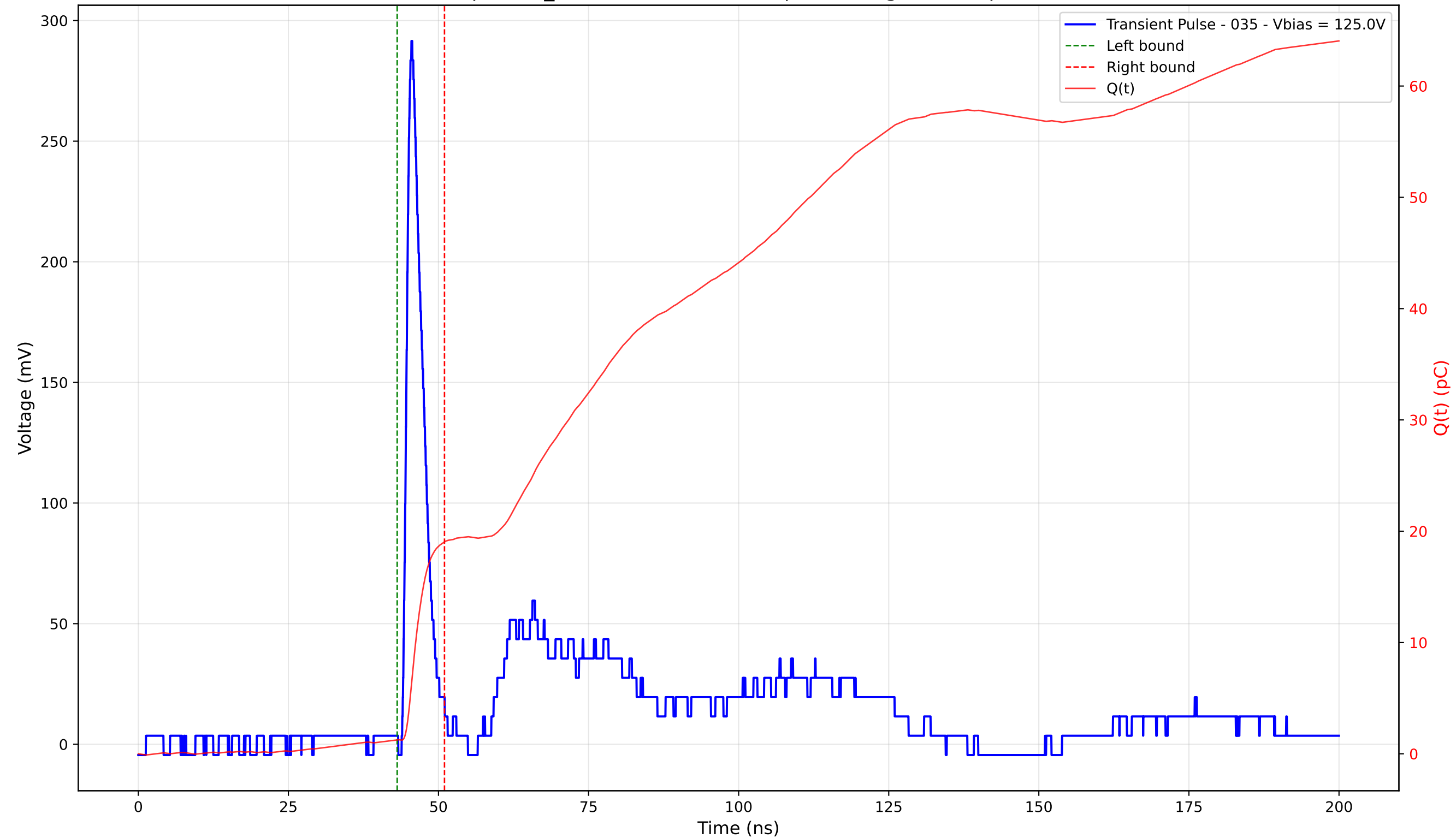
Transient Pulse - Sample: TD_4004 - Position: 360.0 \mu\text{m} - Charge: 17.79 pC - Rise Time: 1.04 ns
