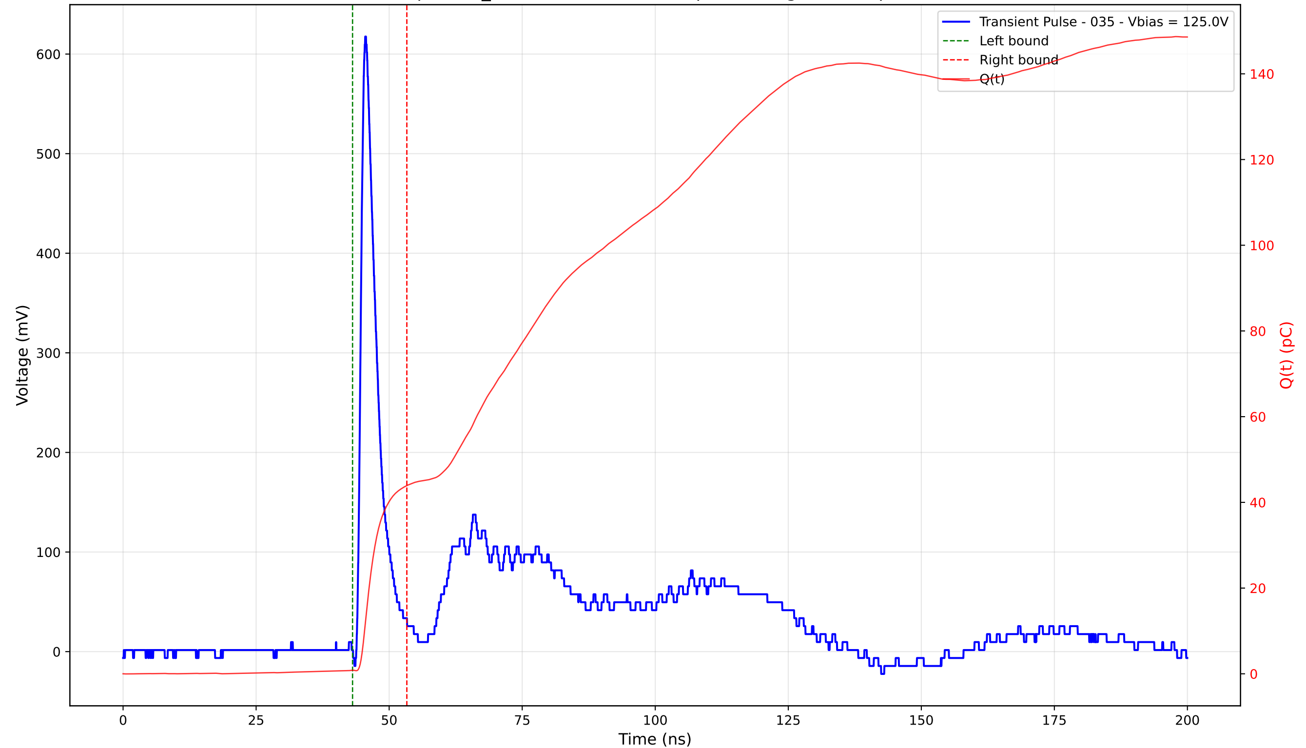
Transient Pulse - Sample: TD_4004 - Position: 150.0 \mu\text{m} - Charge: 43.10 pC - Rise Time: 1.04 ns
