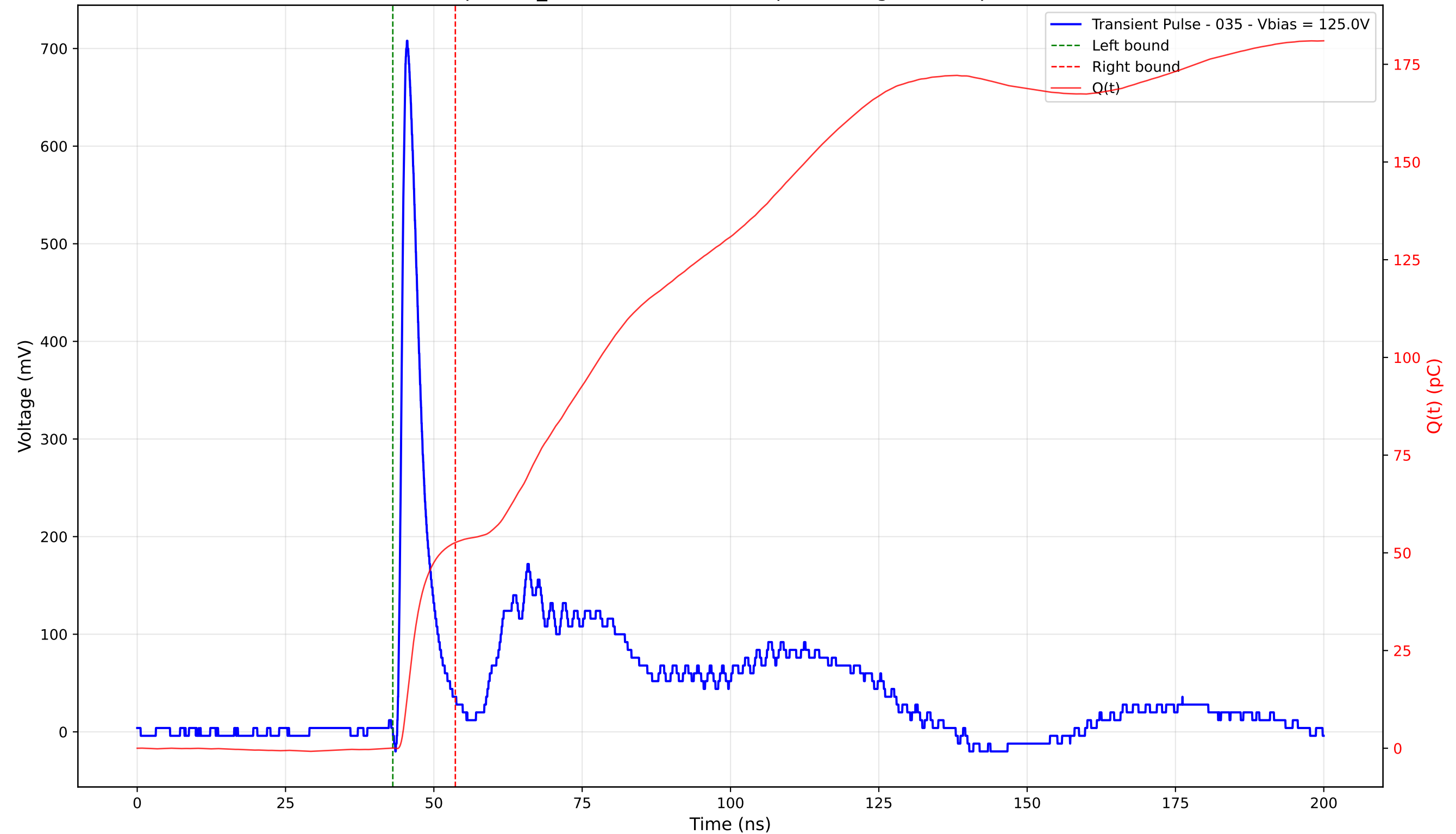
Transient Pulse - Sample: TD_4004 - Position: 175.0 \mu\text{m} - Charge: 52.58 pC - Rise Time: 1.00 ns
