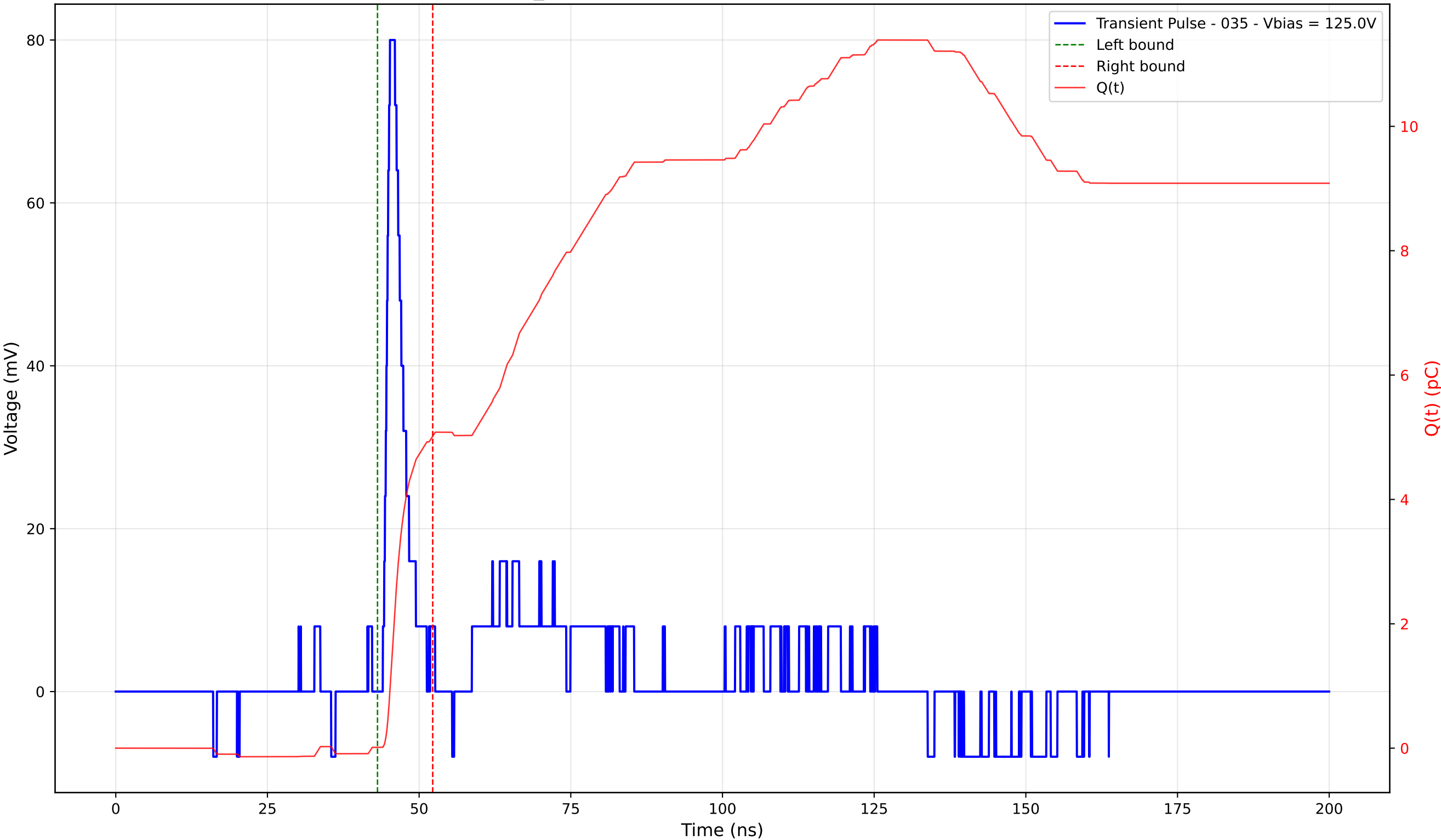
Transient Pulse - Sample: TD_4004 - Position: 415.0 \mu\text{m} - Charge: 5.01 pC - Rise Time: 0.82 ns
