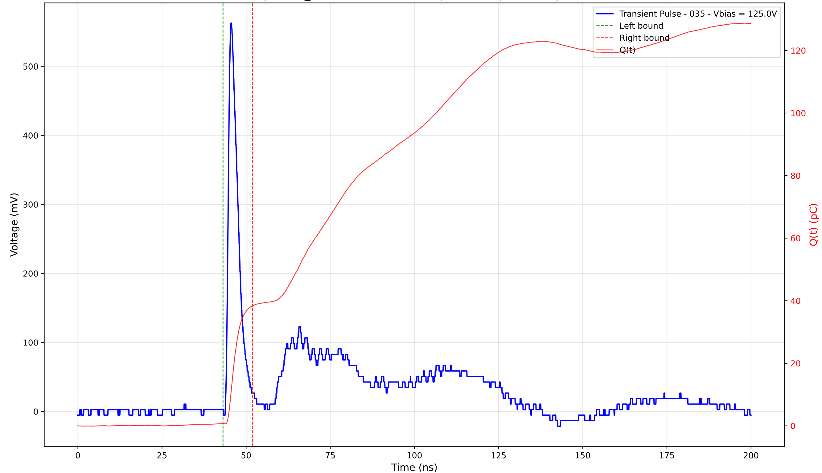
Transient Pulse - Sample: TD_4004 - Position: 255.0 \mu\text{m} - Charge: 37.67 pC - Rise Time: 1.05 ns
