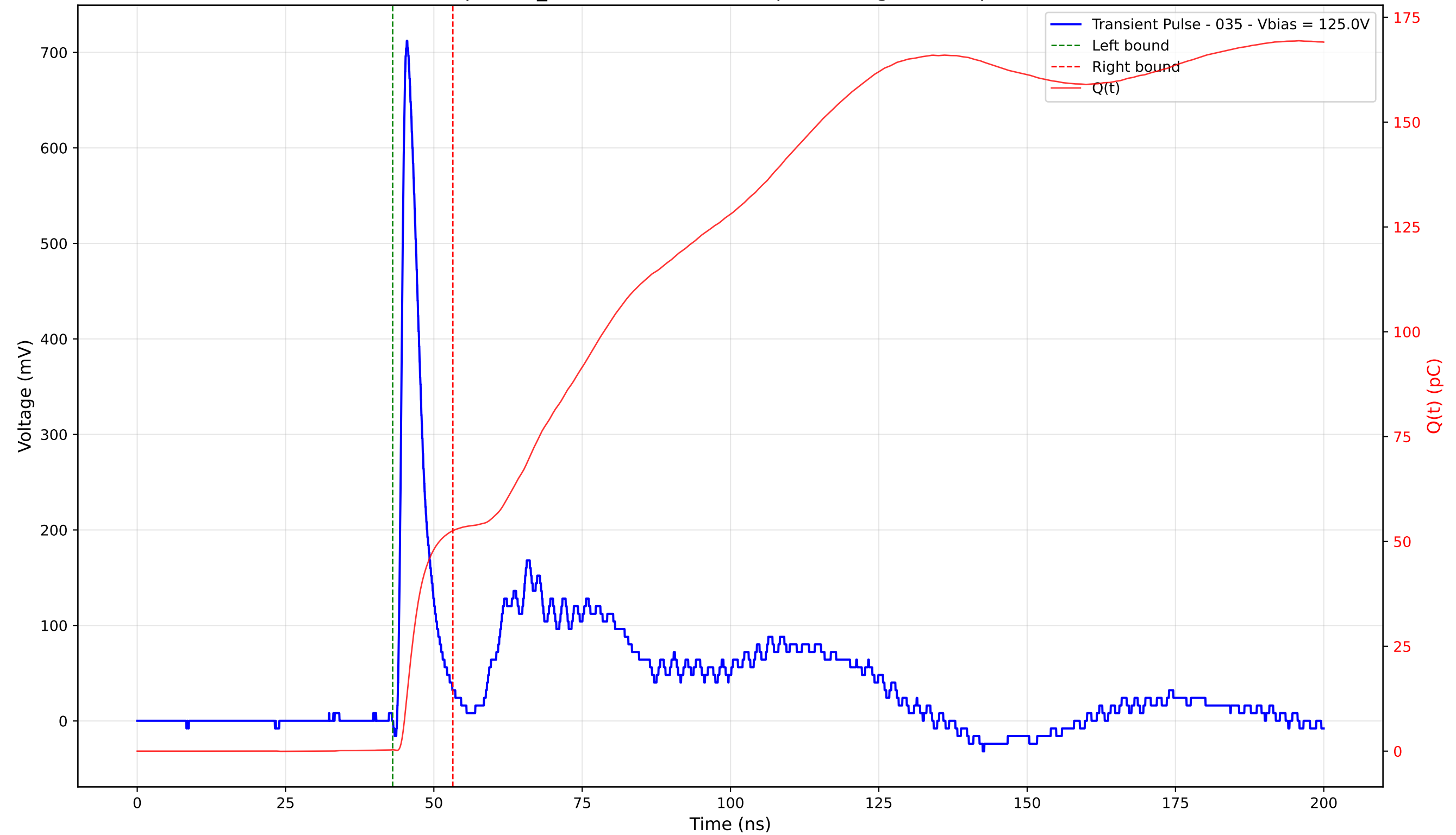
Transient Pulse - Sample: TD_4004 - Position: 200.0 \mu\text{m} - Charge: 52.26 pC - Rise Time: 0.98 ns
