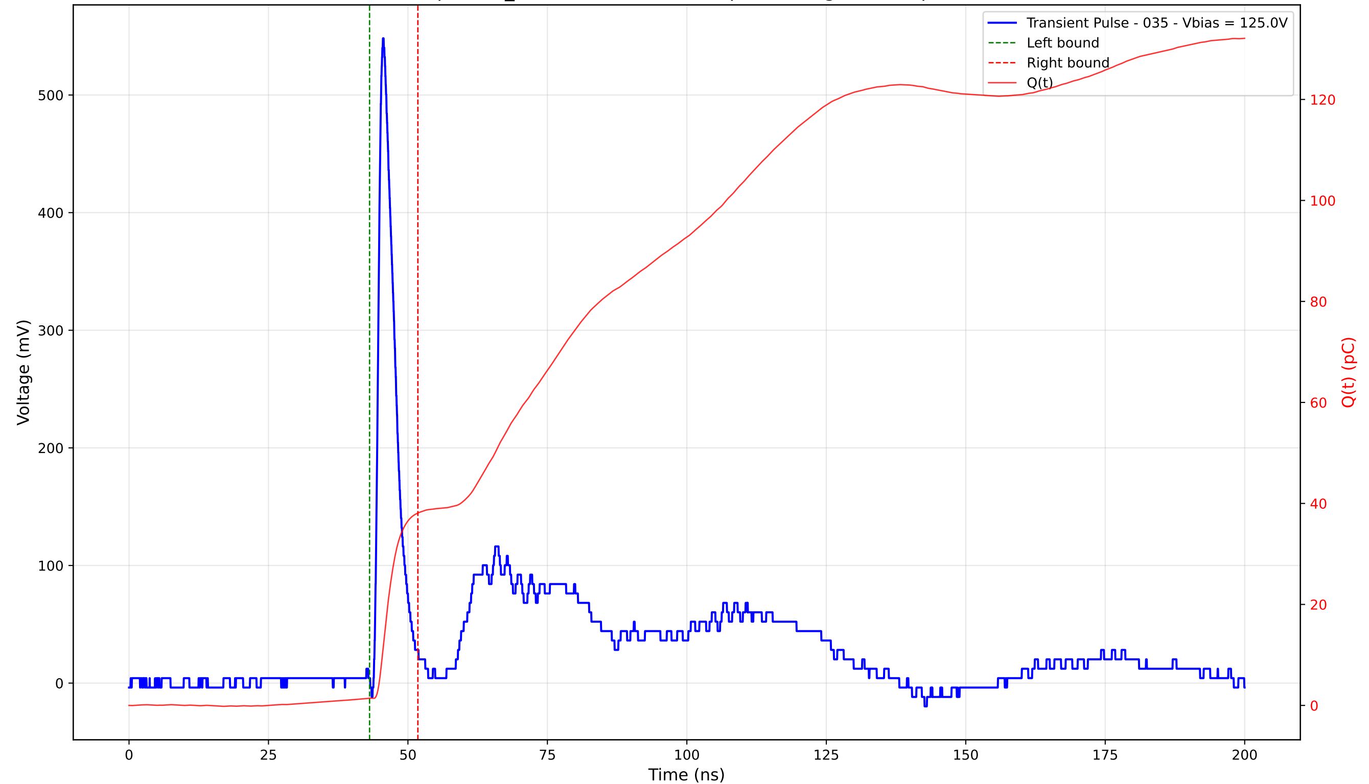
Transient Pulse - Sample: TD_4004 - Position: 280.0 \mu\text{m} - Charge: 36.66 pC - Rise Time: 1.04 ns
