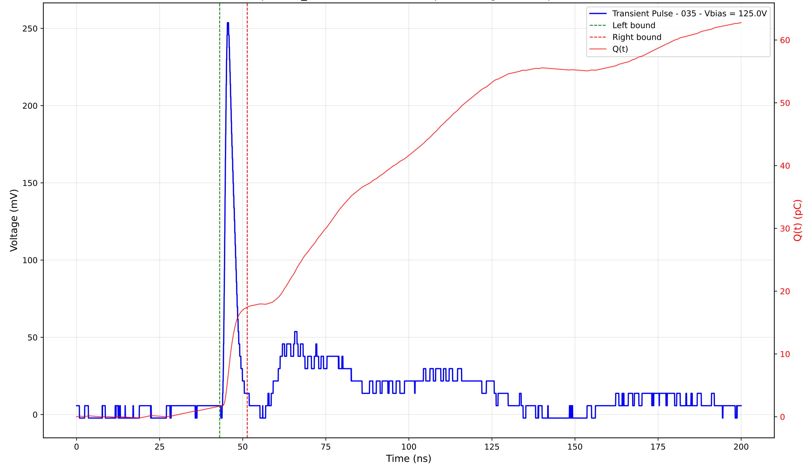
Transient Pulse - Sample: TD_4004 - Position: 385.0 \mu\text{m} - Charge: 15.75 pC - Rise Time: 1.01 ns
