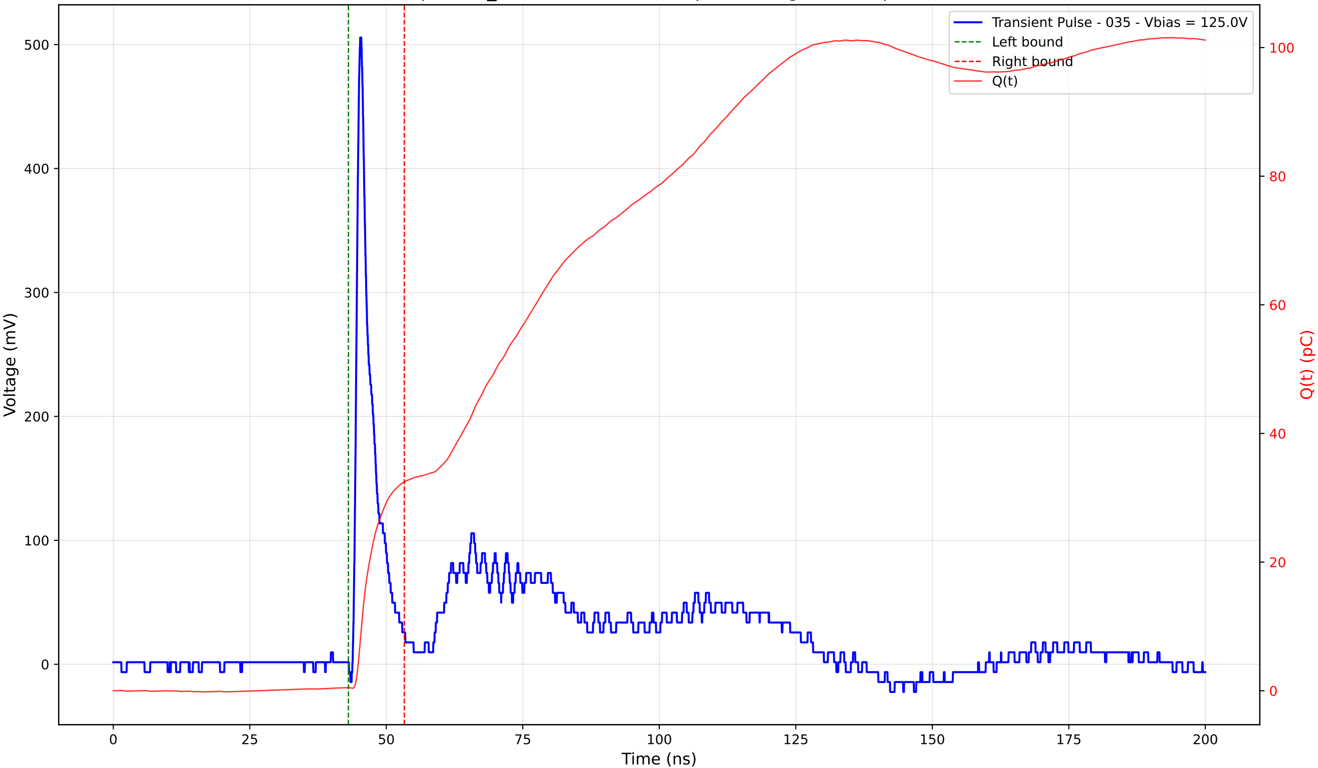
Transient Pulse - Sample: TD_4004 - Position: 75.0 \mu\text{m} - Charge: 32.00 pC - Rise Time: 0.89 ns
