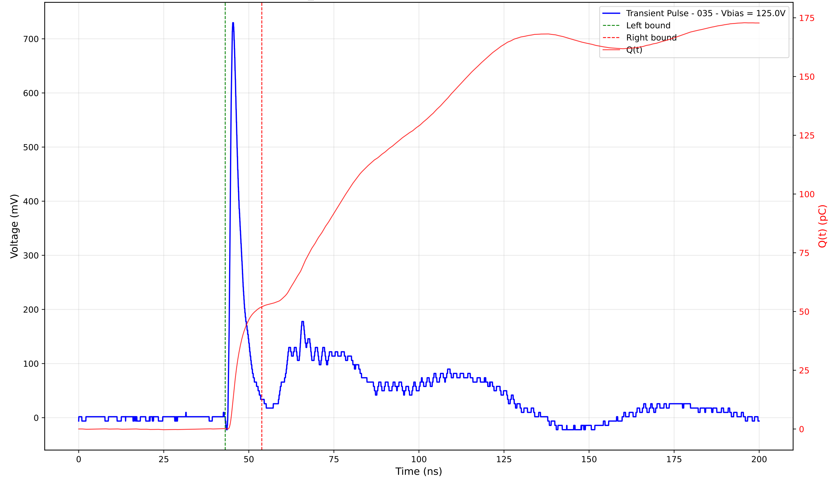
Transient Pulse - Sample: TD_4004 - Position: 115.0 \mu\text{m} - Charge: 51.84 pC - Rise Time: 0.94 ns
