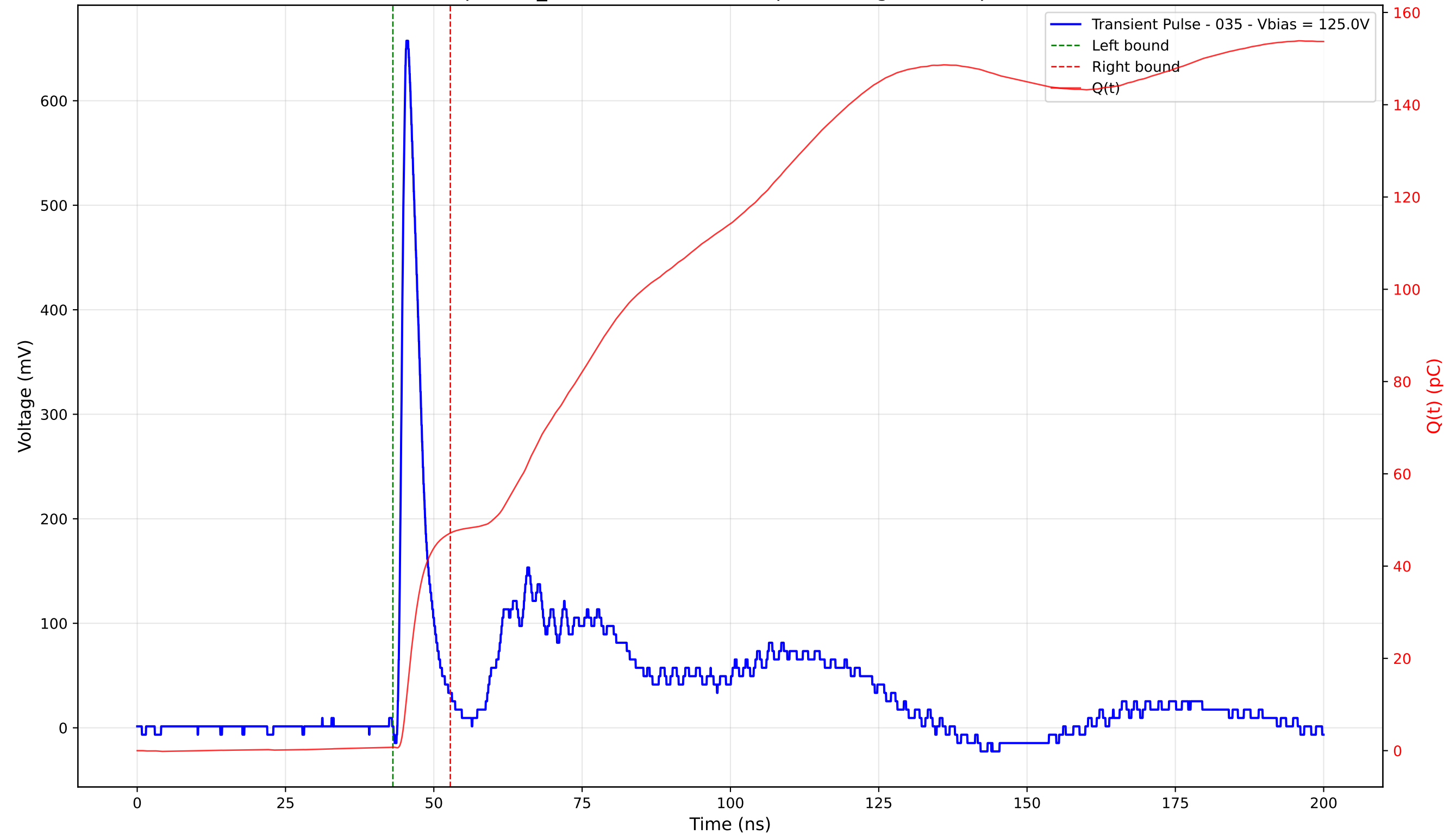
Transient Pulse - Sample: TD_4004 - Position: 225.0 \mu\text{m} - Charge: 46.41 pC - Rise Time: 0.97 ns
