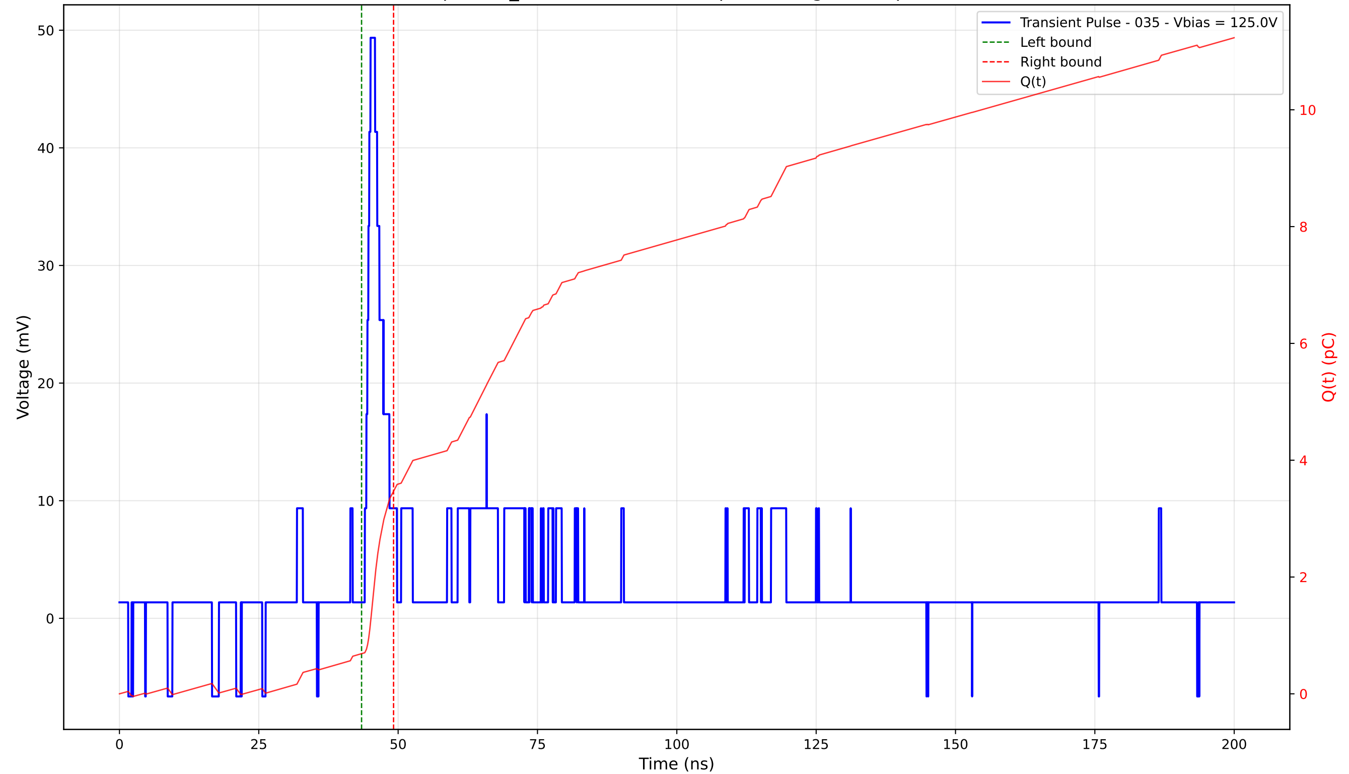
Transient Pulse - Sample: TD_4004 - Position: 45.0 \mu\text{m} - Charge: 2.78 pC - Rise Time: 1.03 ns
