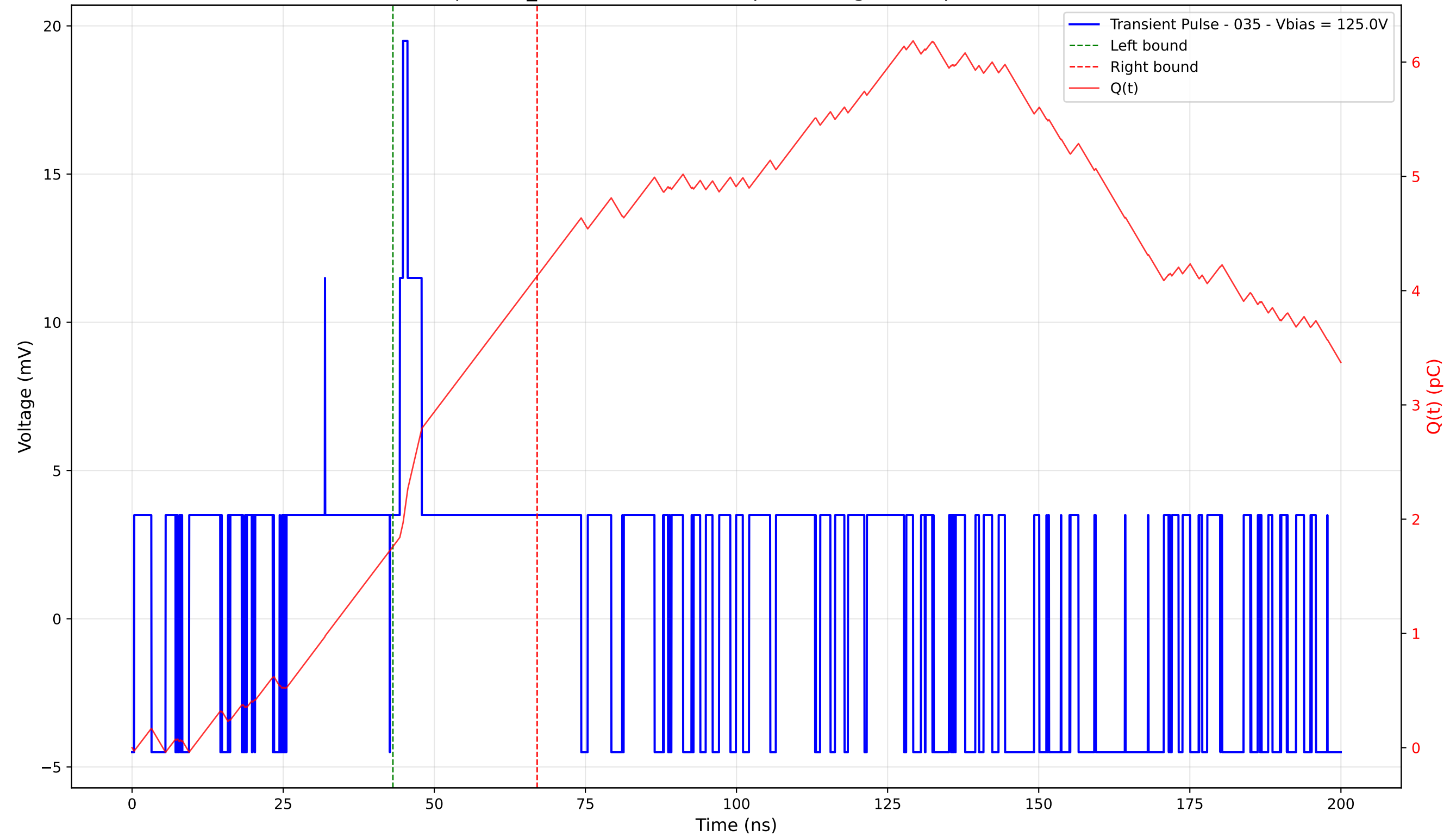
Transient Pulse - Sample: TD_4004 - Position: 25.0 \mu\text{m} - Charge: 2.37 pC - Rise Time: 0.00 ns (N/A)
