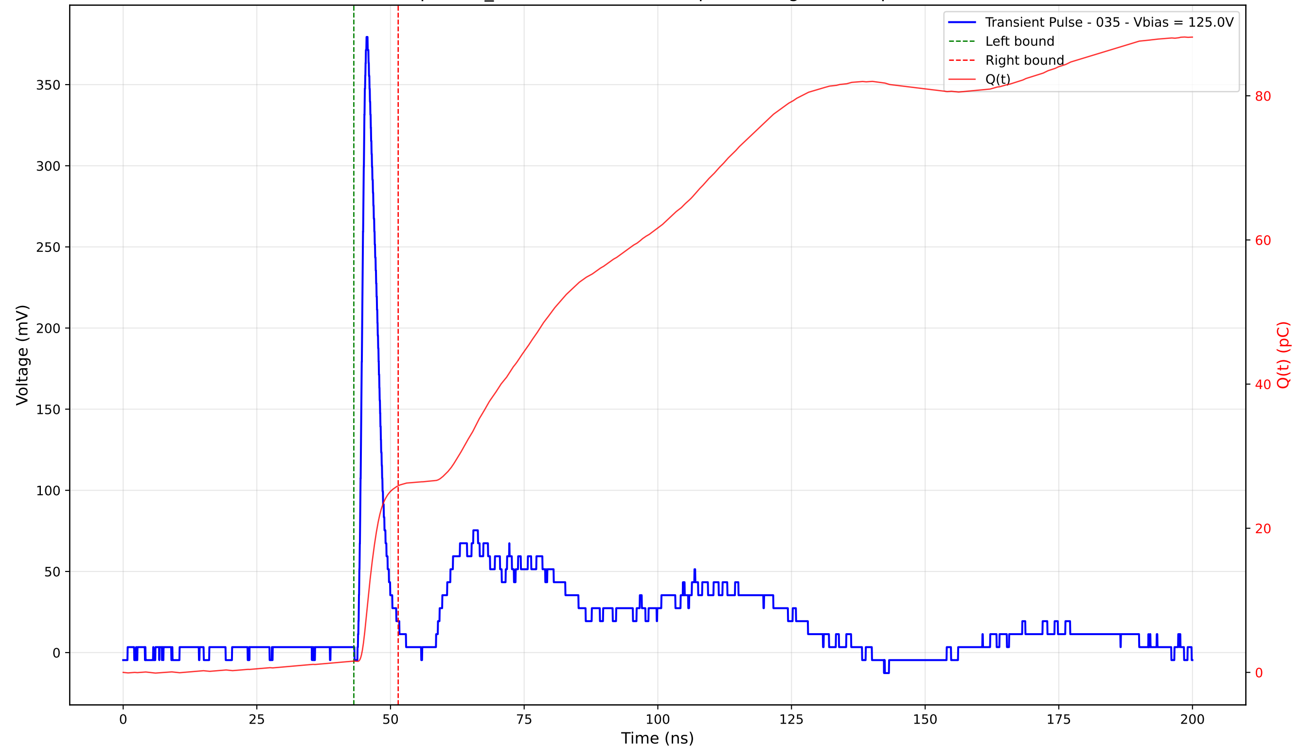
Transient Pulse - Sample: TD_4004 - Position: 325.0 \mu\text{m} - Charge: 24.33 pC - Rise Time: 1.07 ns
