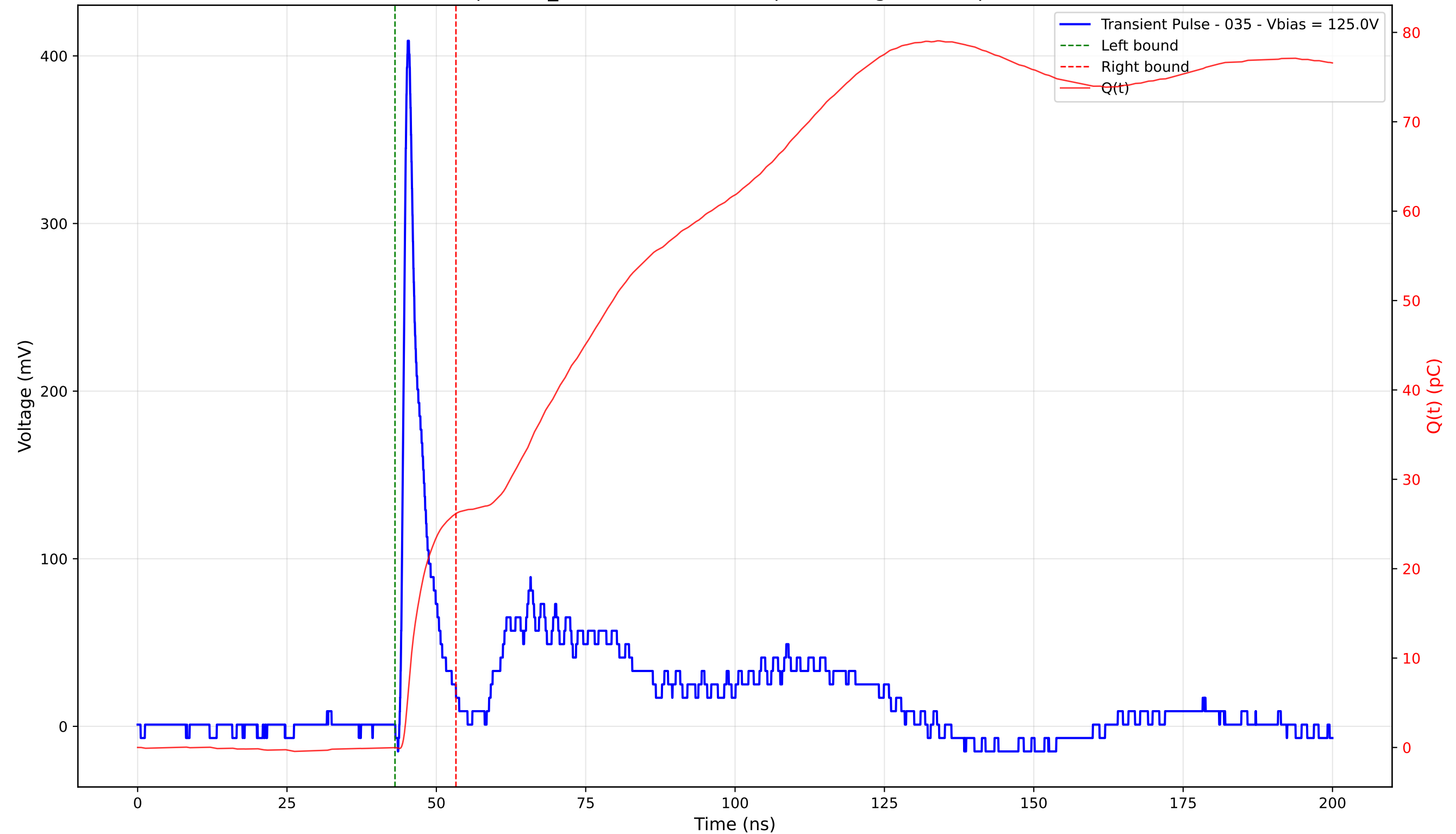
Transient Pulse - Sample: TD_4004 - Position: 70.0 \mu\text{m} - Charge: 26.20 pC - Rise Time: 0.92 ns
