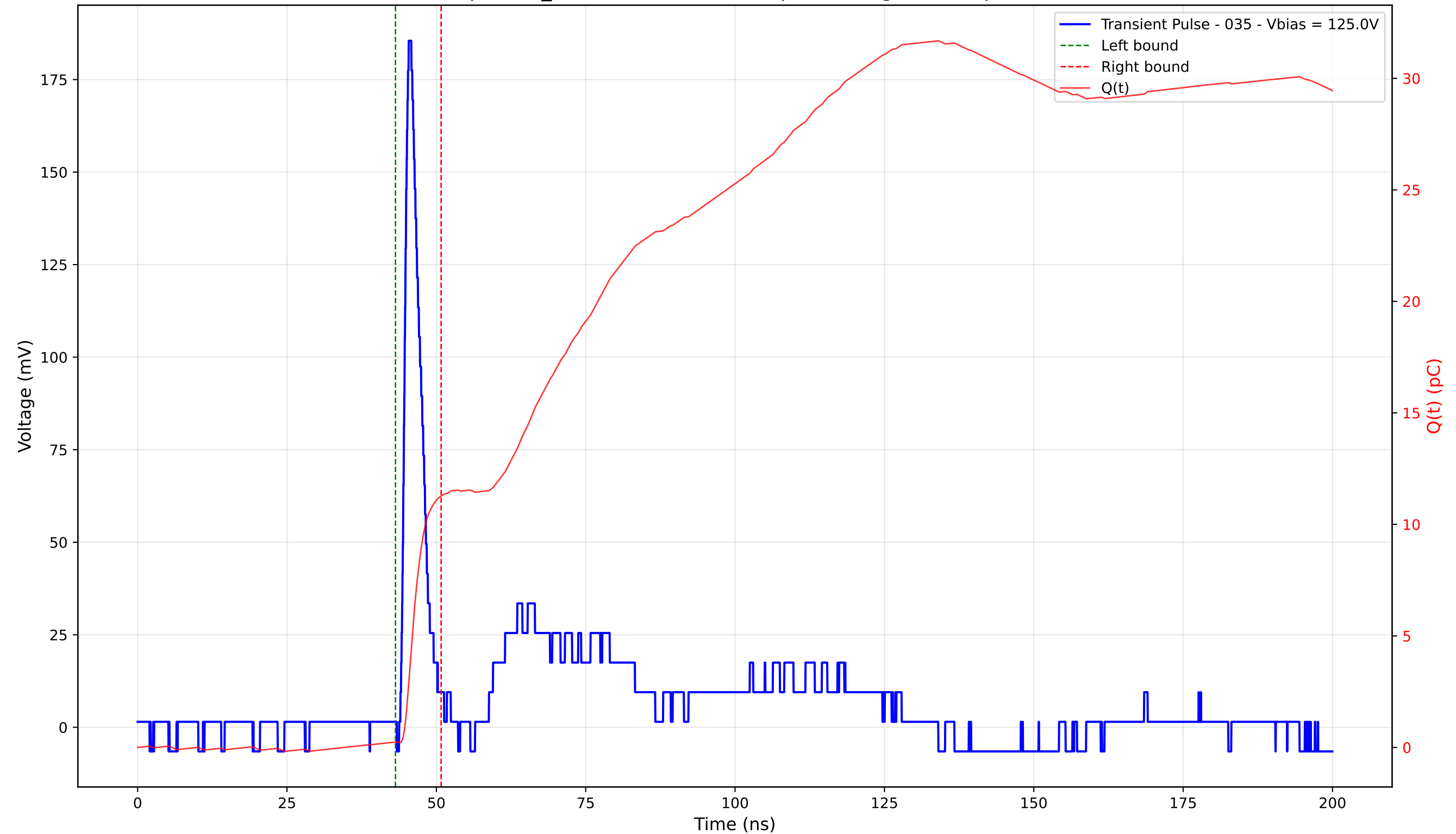
Transient Pulse - Sample: TD_4004 - Position: 395.0 \mu\text{m} - Charge: 11.03 pC - Rise Time: 1.00 ns
