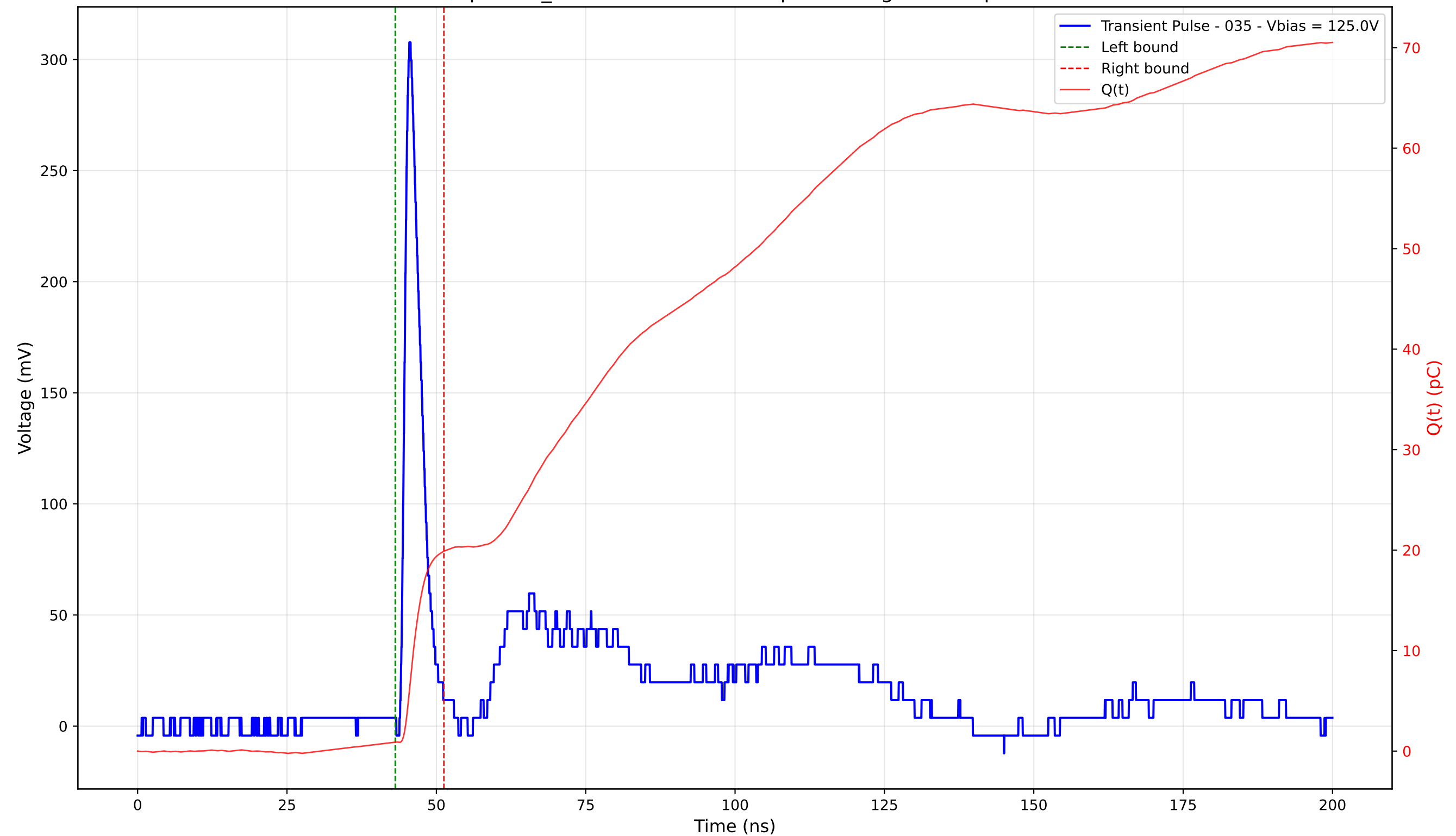
Transient Pulse - Sample: TD_4004 - Position: 350.0 \mu\text{m} - Charge: 19.00 pC - Rise Time: 1.07 ns
