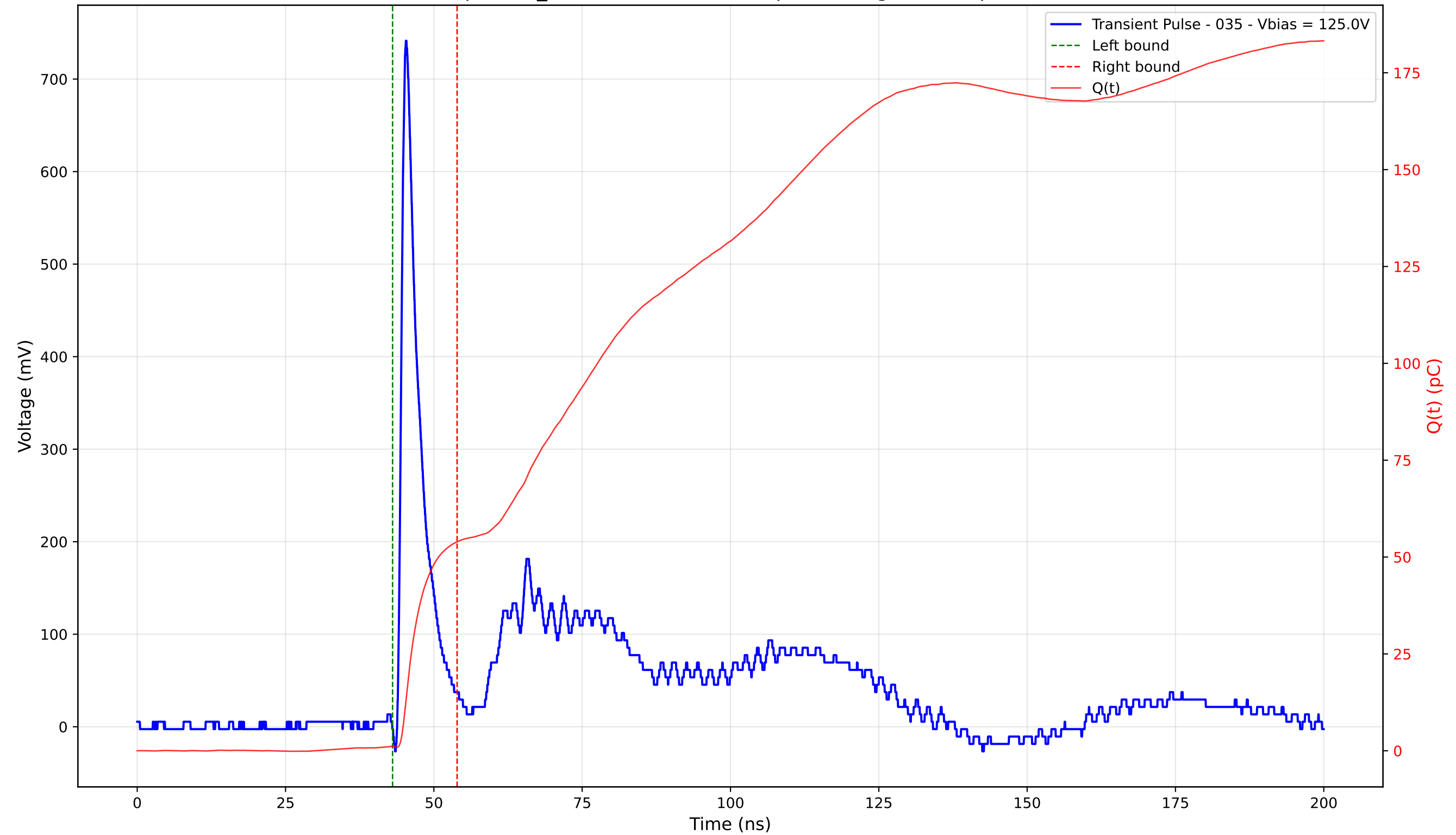
Transient Pulse - Sample: TD_4004 - Position: 105.0 \mu\text{m} - Charge: 52.79 pC - Rise Time: 0.92 ns
