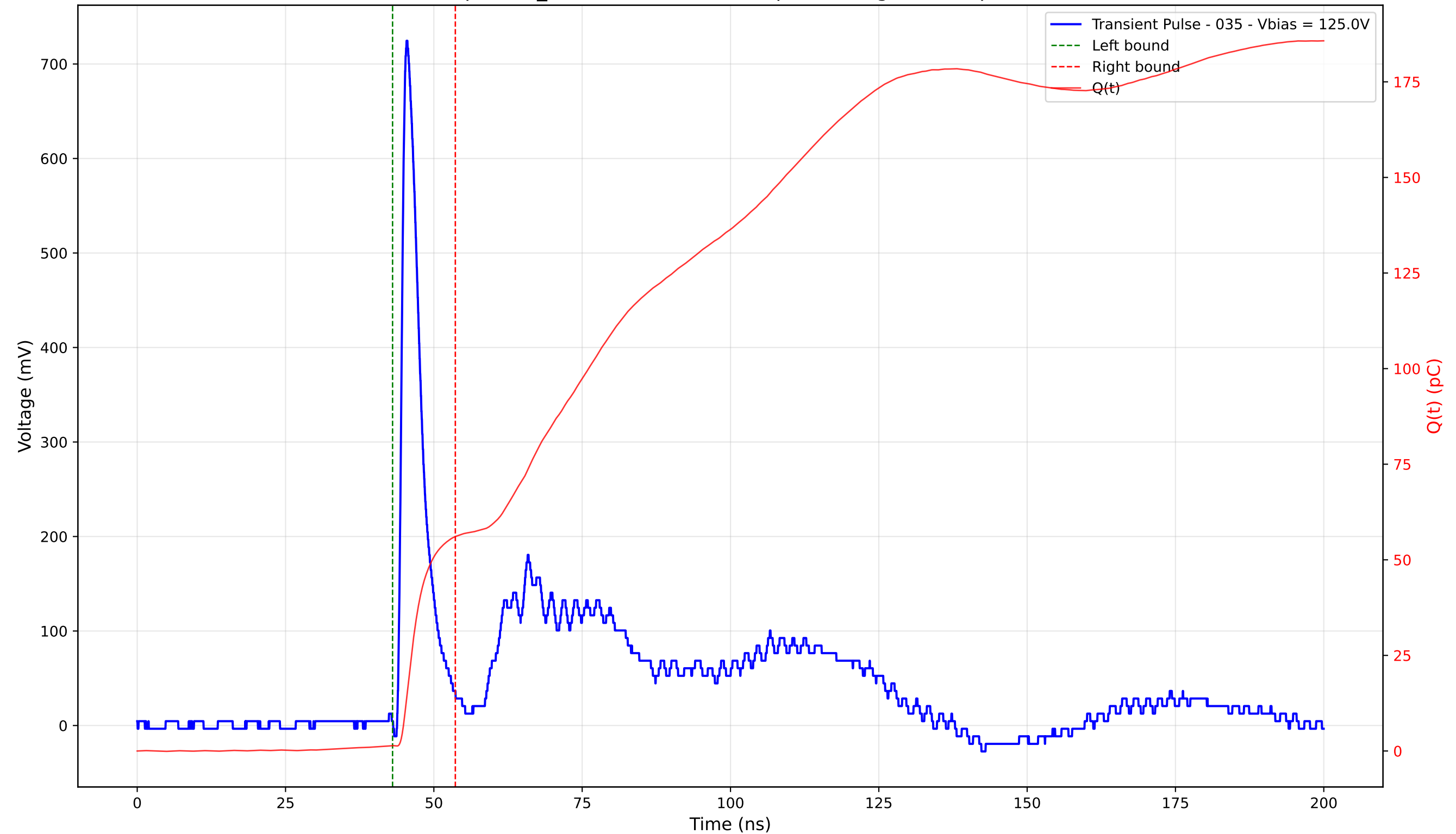
Transient Pulse - Sample: TD_4004 - Position: 185.0 \mu\text{m} - Charge: 54.67 pC - Rise Time: 0.99 ns
