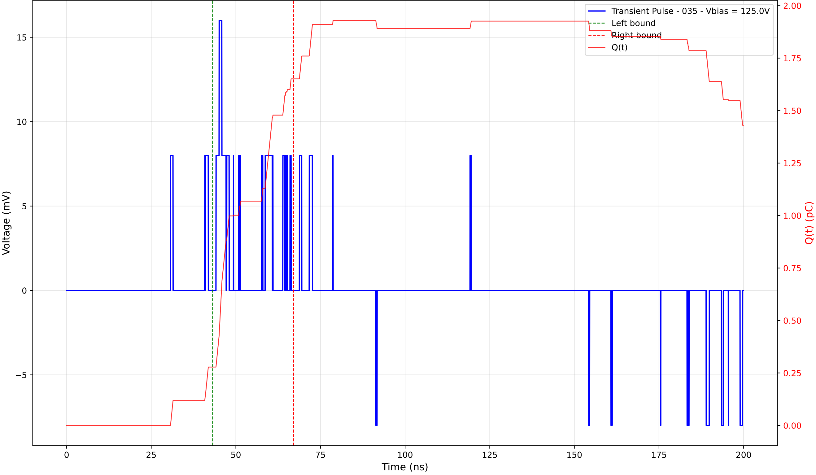
Transient Pulse - Sample: TD_4004 - Position: 10.0 \mu\text{m} - Charge: 1.37 pC - Rise Time: 0.94 ns
