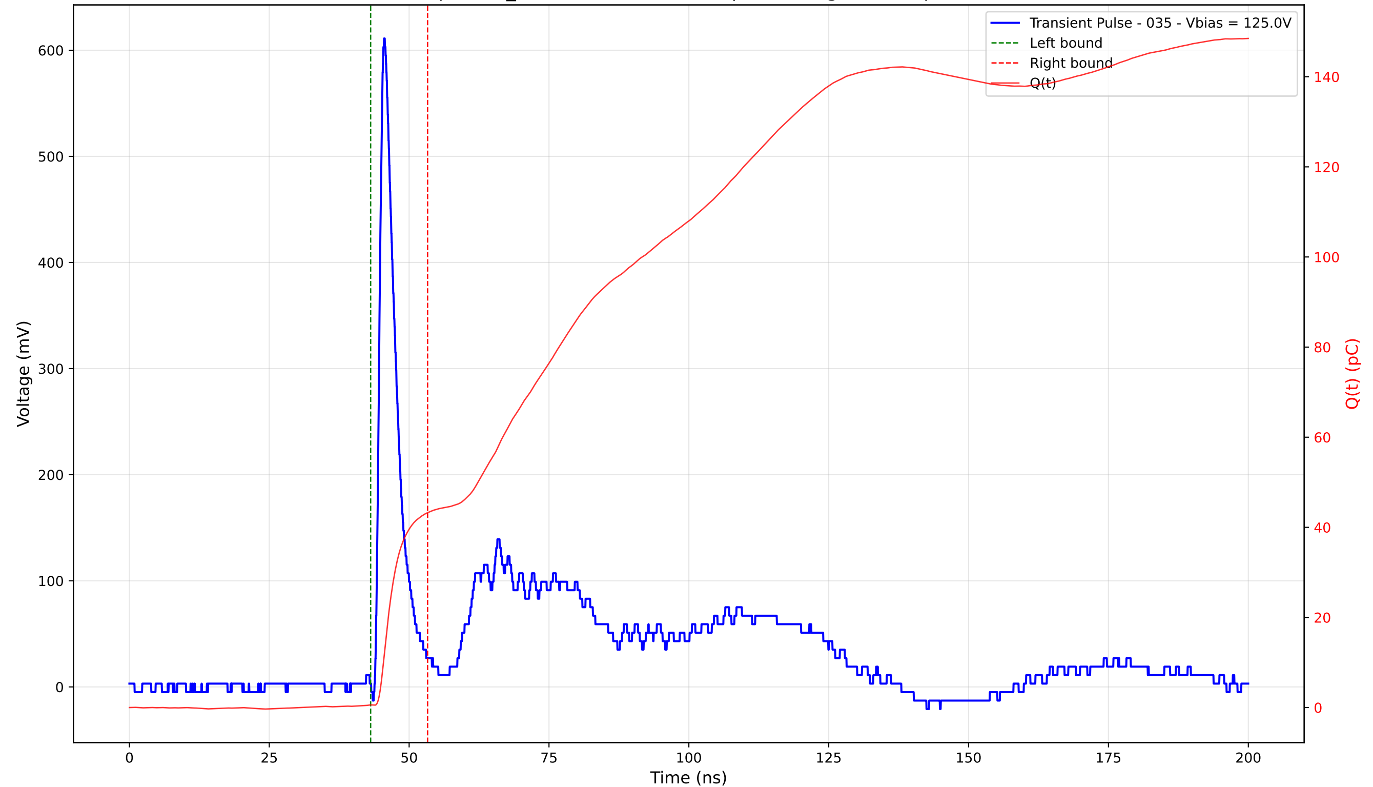
Transient Pulse - Sample: TD_4004 - Position: 145.0 \mu\text{m} - Charge: 42.66 pC - Rise Time: 1.06 ns
