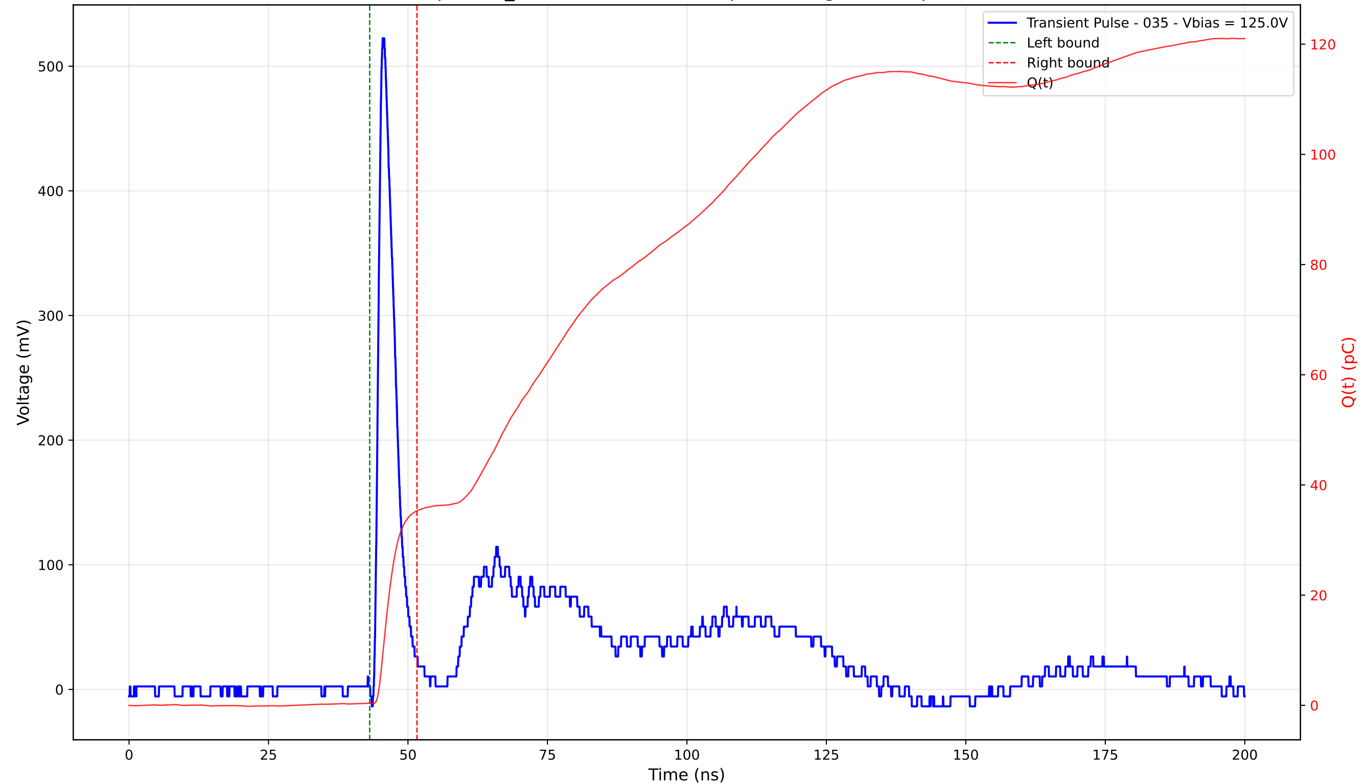
Transient Pulse - Sample: TD_4004 - Position: 285.0 \mu\text{m} - Charge: 34.89 pC - Rise Time: 1.04 ns
