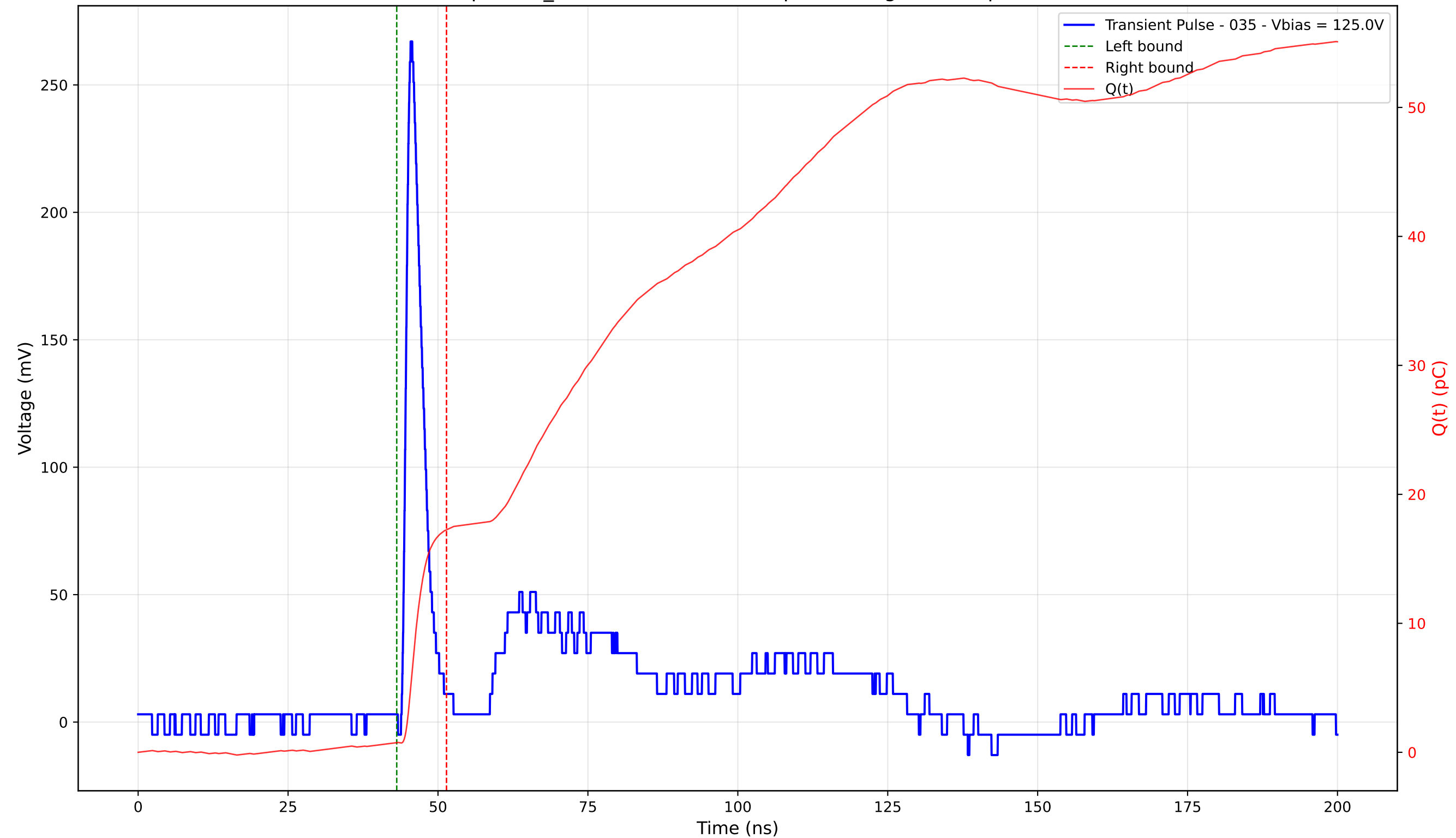
Transient Pulse - Sample: TD_4004 - Position: 375.0 \mu\text{m} - Charge: 16.50 pC - Rise Time: 1.06 ns
