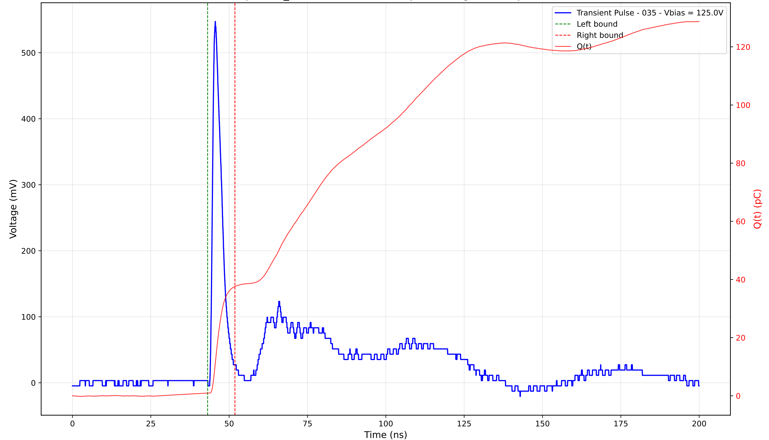
Transient Pulse - Sample: TD_4004 - Position: 275.0 \mu\text{m} - Charge: 36.60 pC - Rise Time: 1.07 ns
