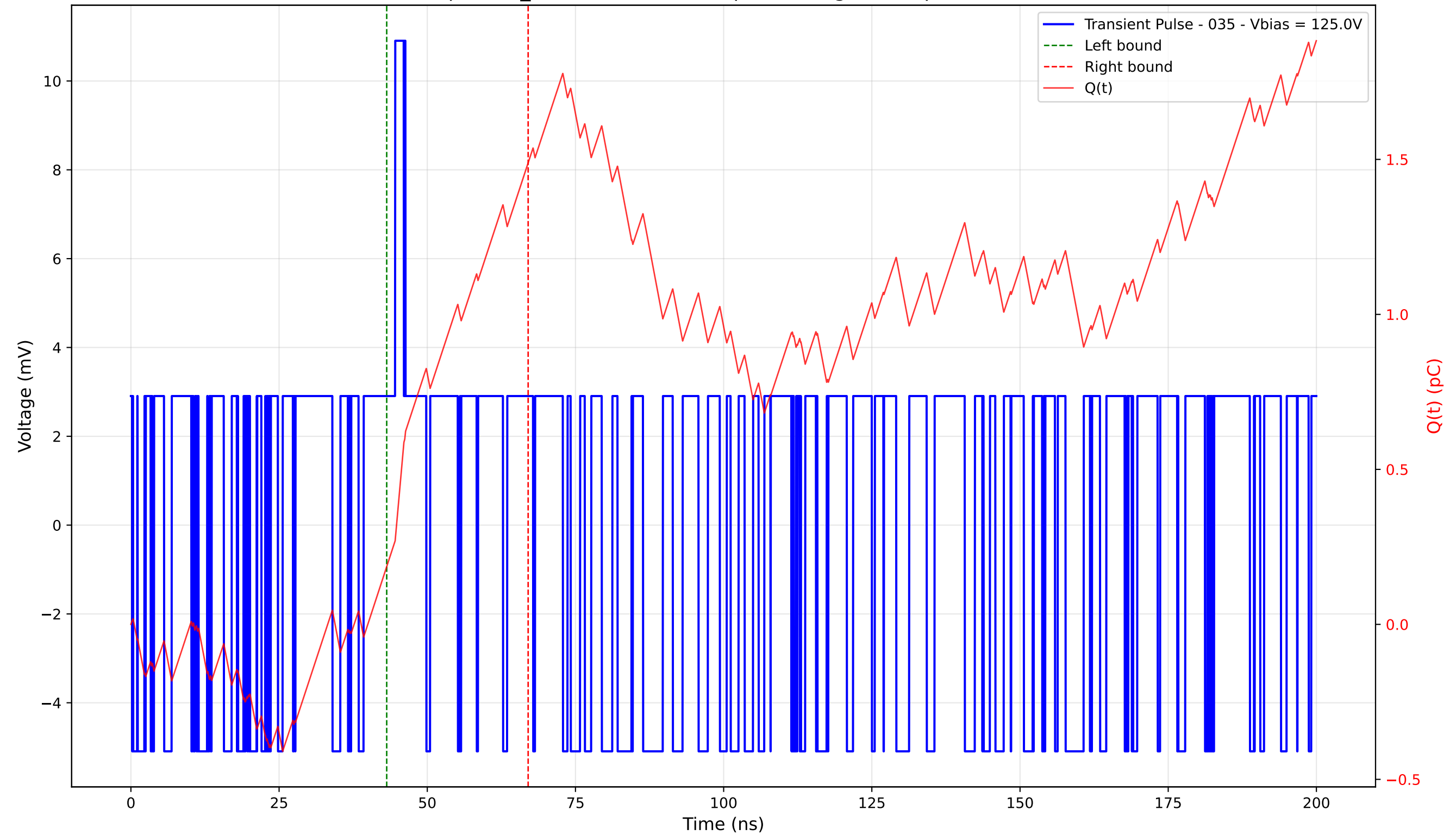
Transient Pulse - Sample: TD_4004 - Position: 5.0 \mu\text{m} - Charge: 1.30 pC - Rise Time: 0.00 ns (N/A)
