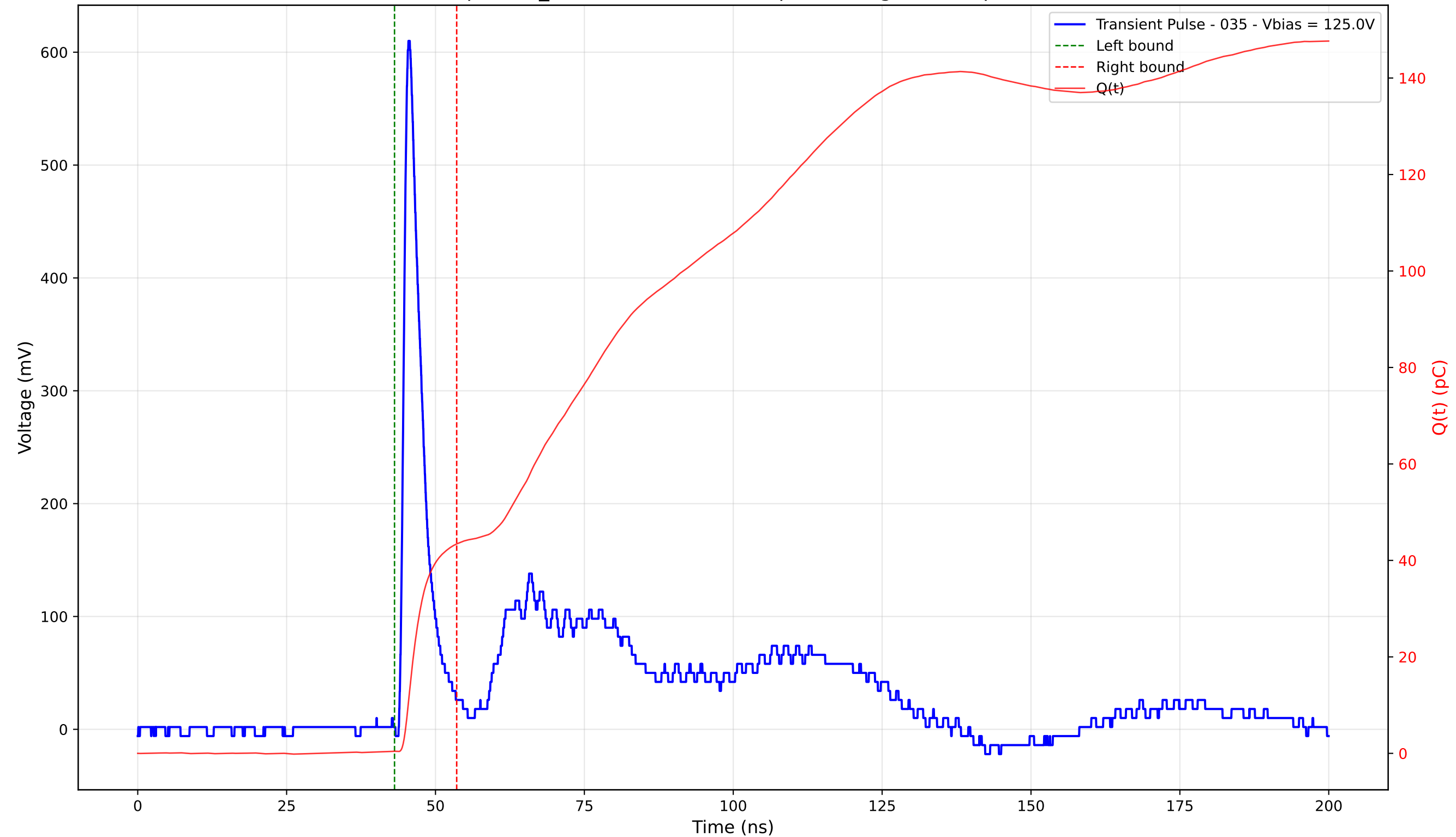
Transient Pulse - Sample: TD_4004 - Position: 140.0 \mu\text{m} - Charge: 42.99 pC - Rise Time: 1.04 ns
