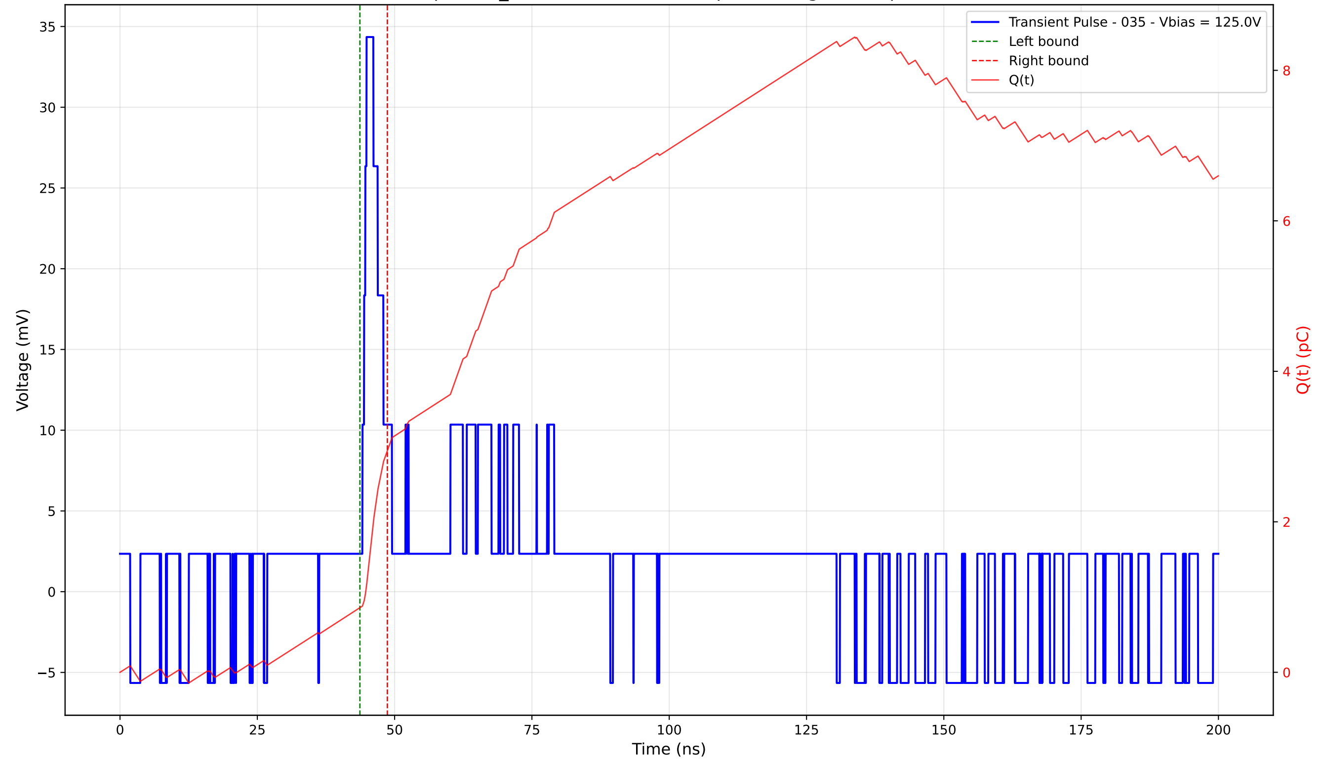
Transient Pulse - Sample: TD_4004 - Position: 430.0 \mu\text{m} - Charge: 2.09 pC - Rise Time: 0.76 ns
