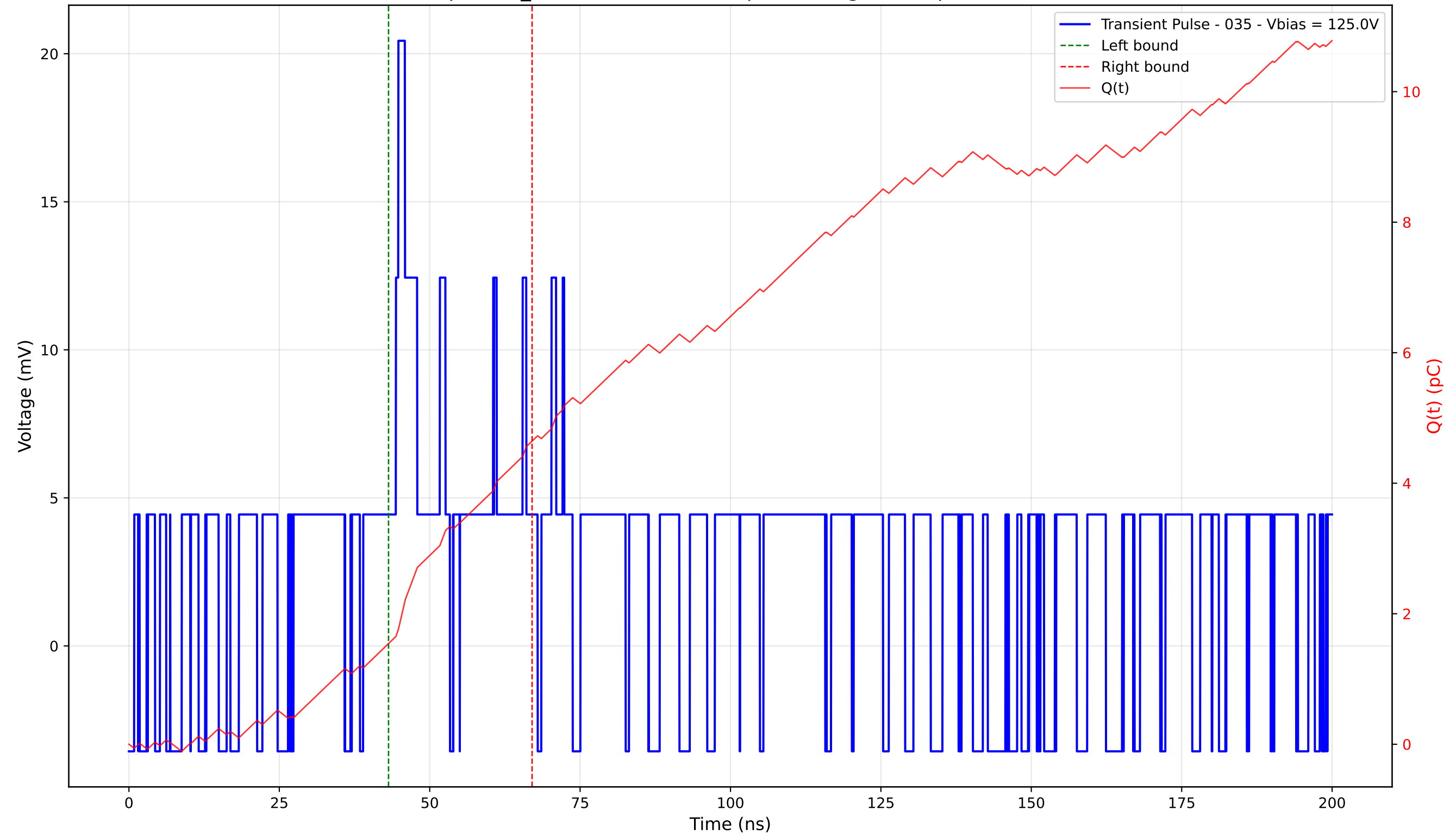
Transient Pulse - Sample: TD_4004 - Position: 30.0 \mu m - Charge: 3.10 pC - Rise Time: 0.00 ns (N/A)
