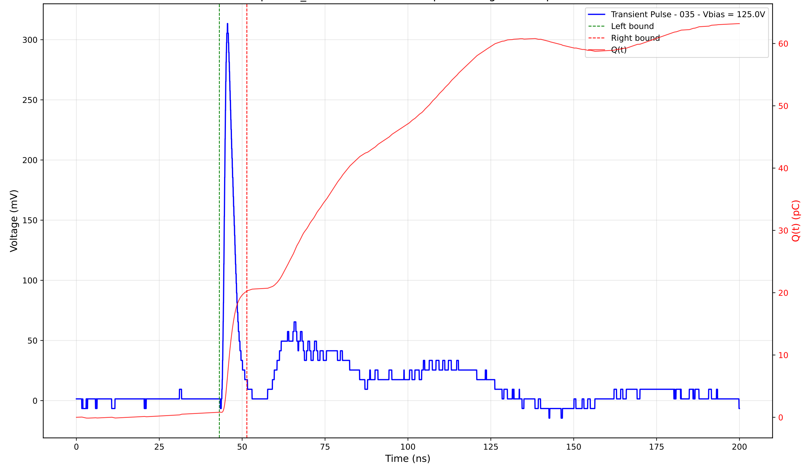
Transient Pulse - Sample: TD_4004 - Position: 345.0 \mu\text{m} - Charge: 19.43 pC - Rise Time: 1.13 ns
