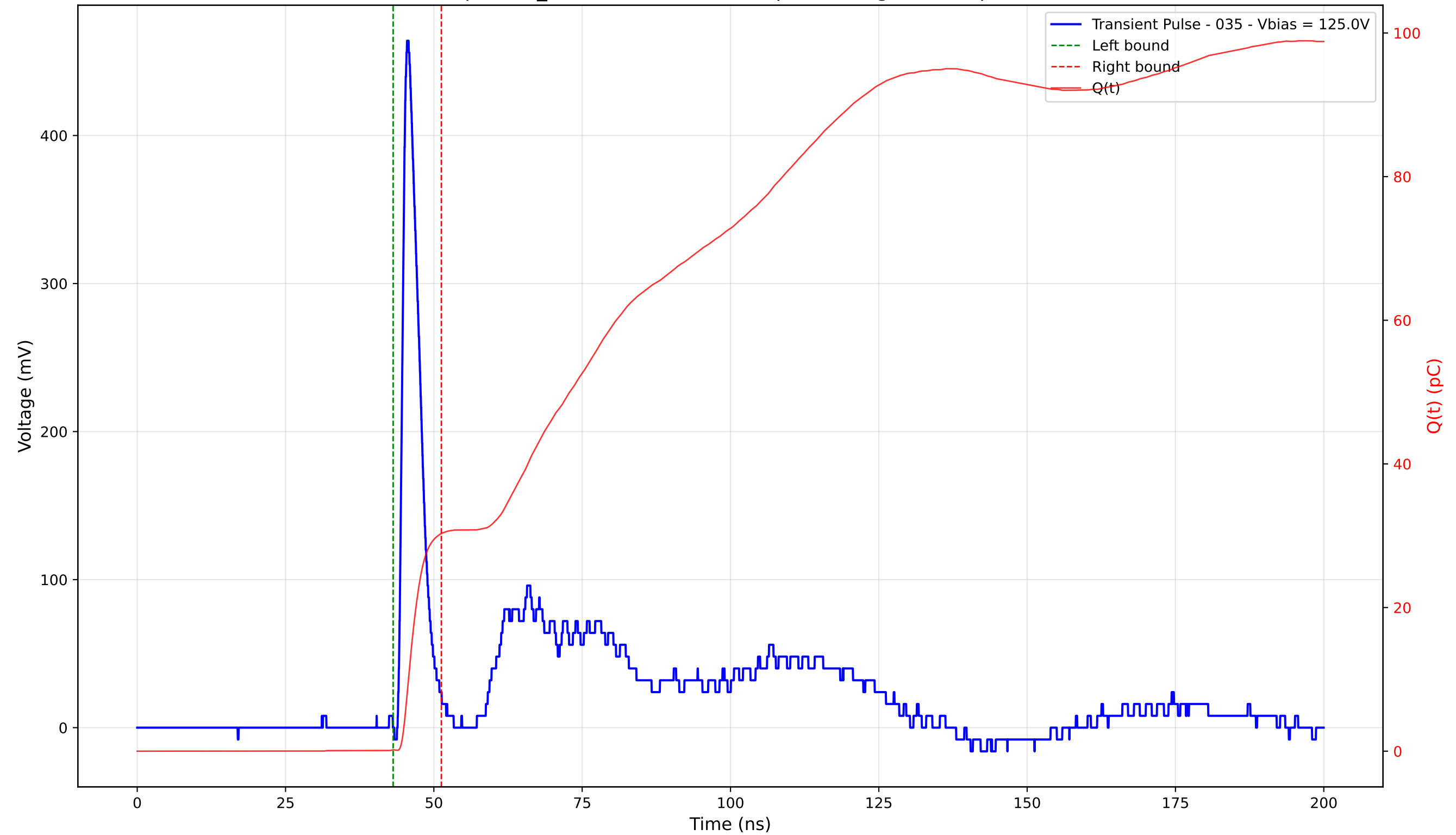
Transient Pulse - Sample: TD_4004 - Position: 305.0 \mu\text{m} - Charge: 30.13 pC - Rise Time: 1.04 ns
