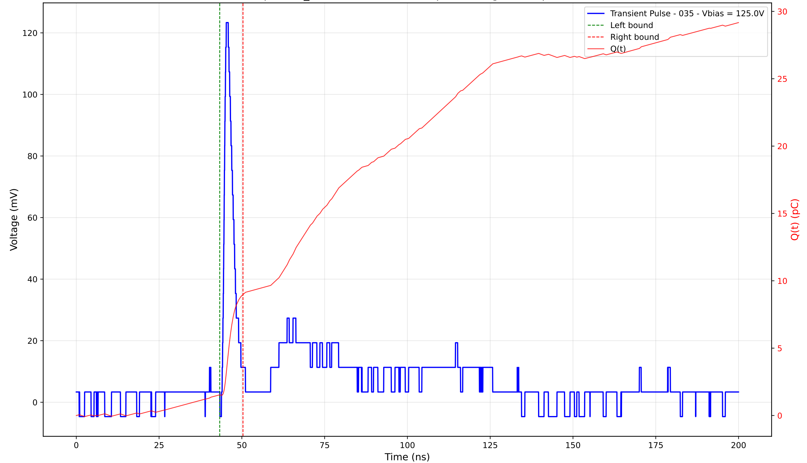
Transient Pulse - Sample: TD_4004 - Position: 405.0 \mu\text{m} - Charge: 7.44 pC - Rise Time: 0.96 ns
