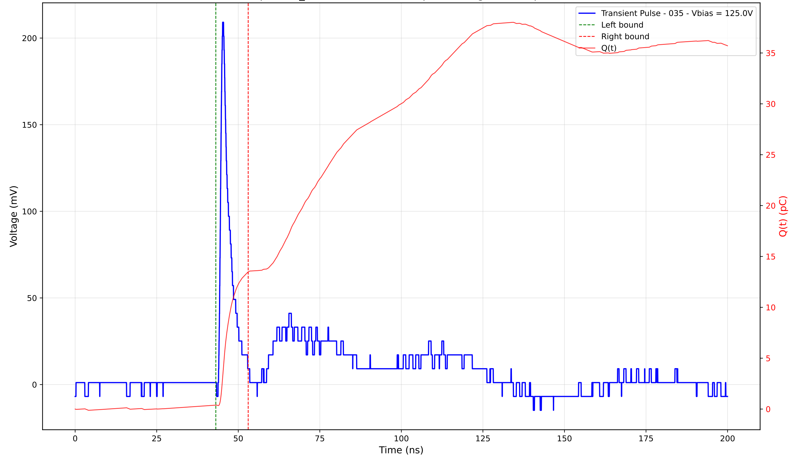
Transient Pulse - Sample: TD_4004 - Position: 60.0 \mu\text{m} - Charge: 13.08 pC - Rise Time: 0.93 ns
