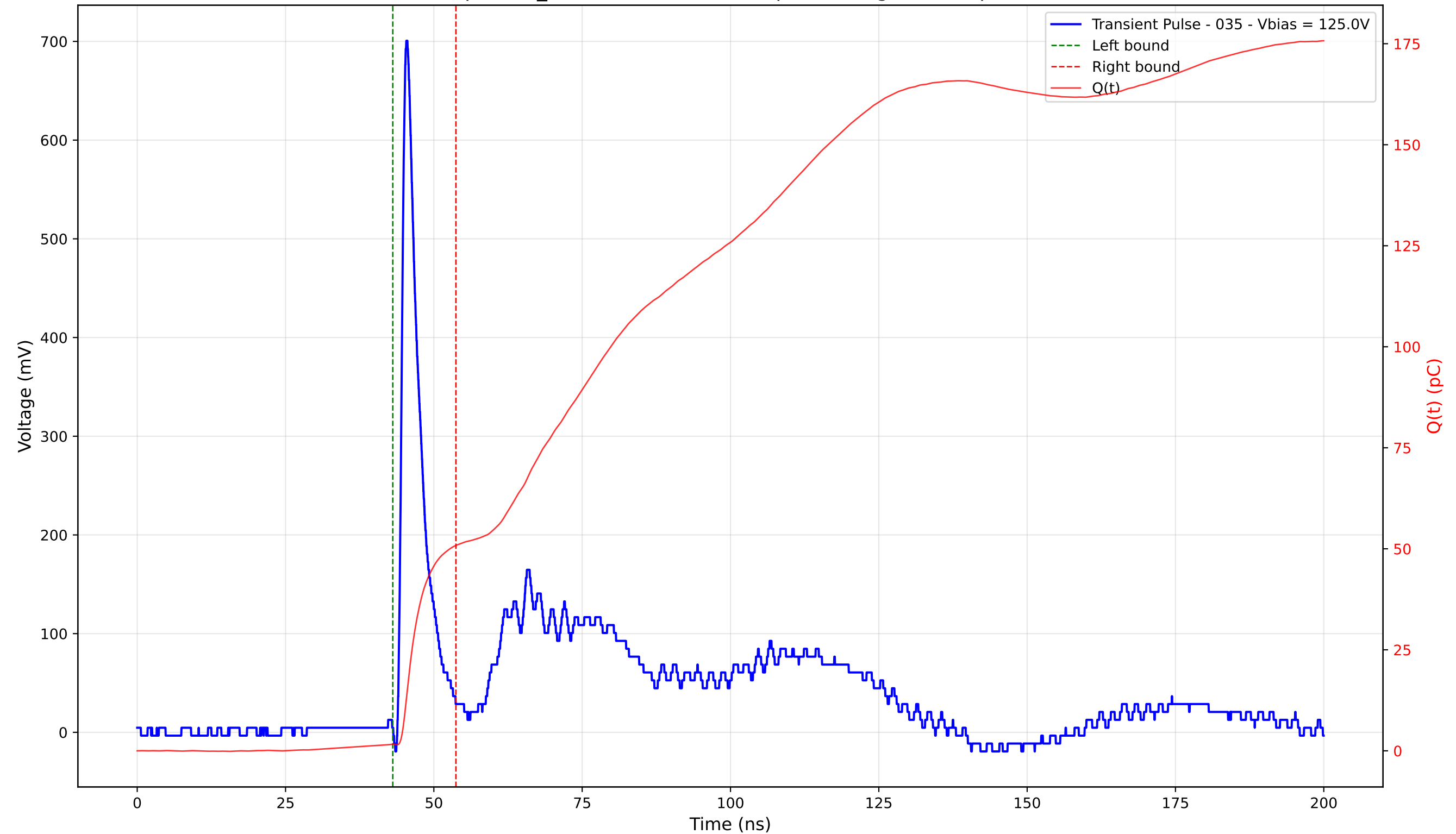
Transient Pulse - Sample: TD_4004 - Position: 125.0 \mu\text{m} - Charge: 49.19 pC - Rise Time: 0.96 ns
