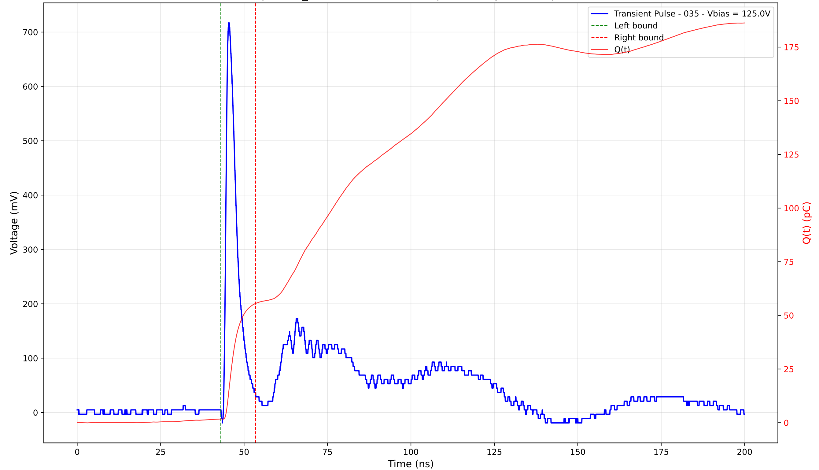
Transient Pulse - Sample: TD_4004 - Position: 195.0 \mu\text{m} - Charge: 53.81 pC - Rise Time: 0.97 ns
