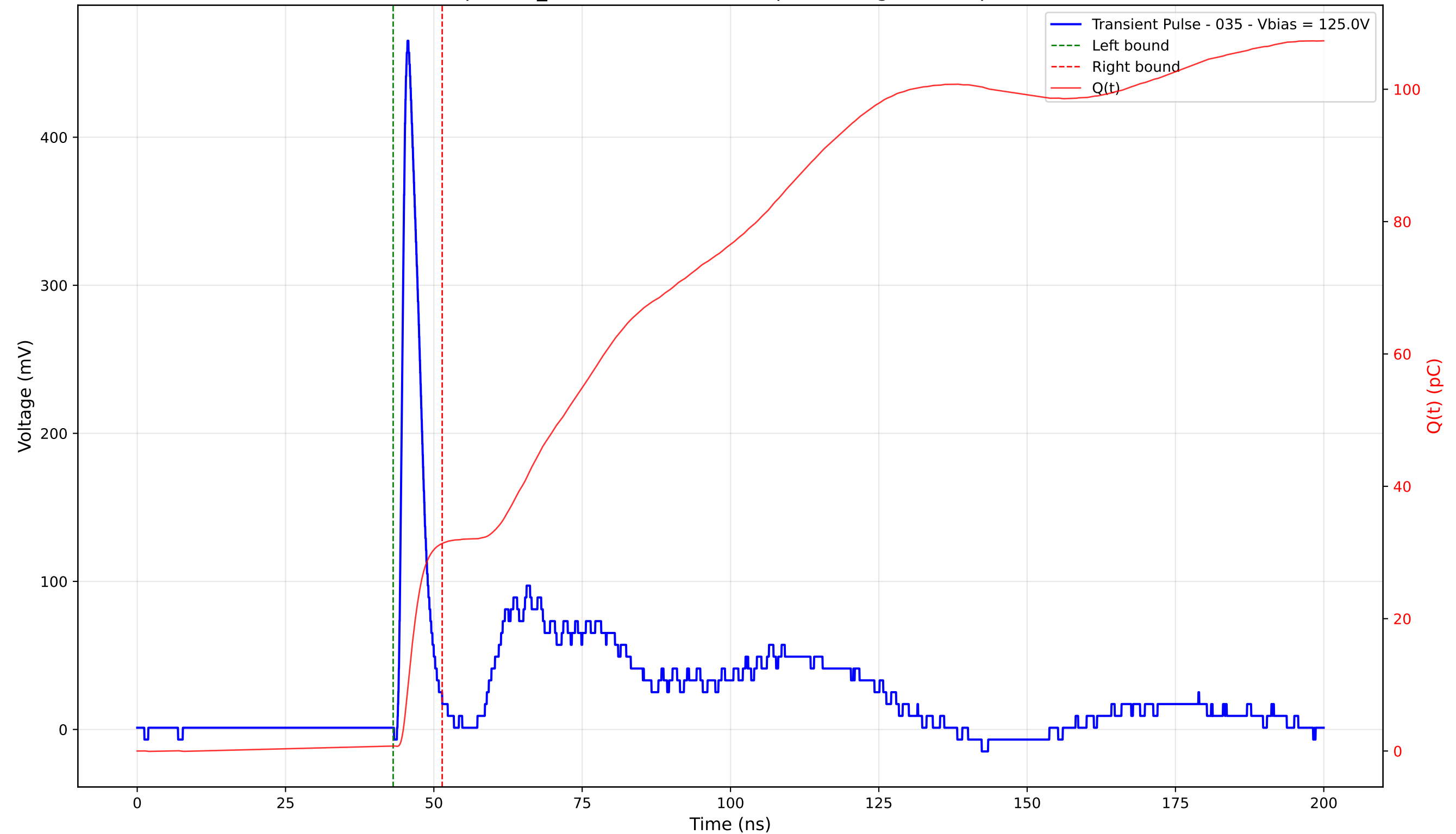
Transient Pulse - Sample: TD_4004 - Position: 295.0 \mu\text{m} - Charge: 30.60 pC - Rise Time: 1.09 ns
