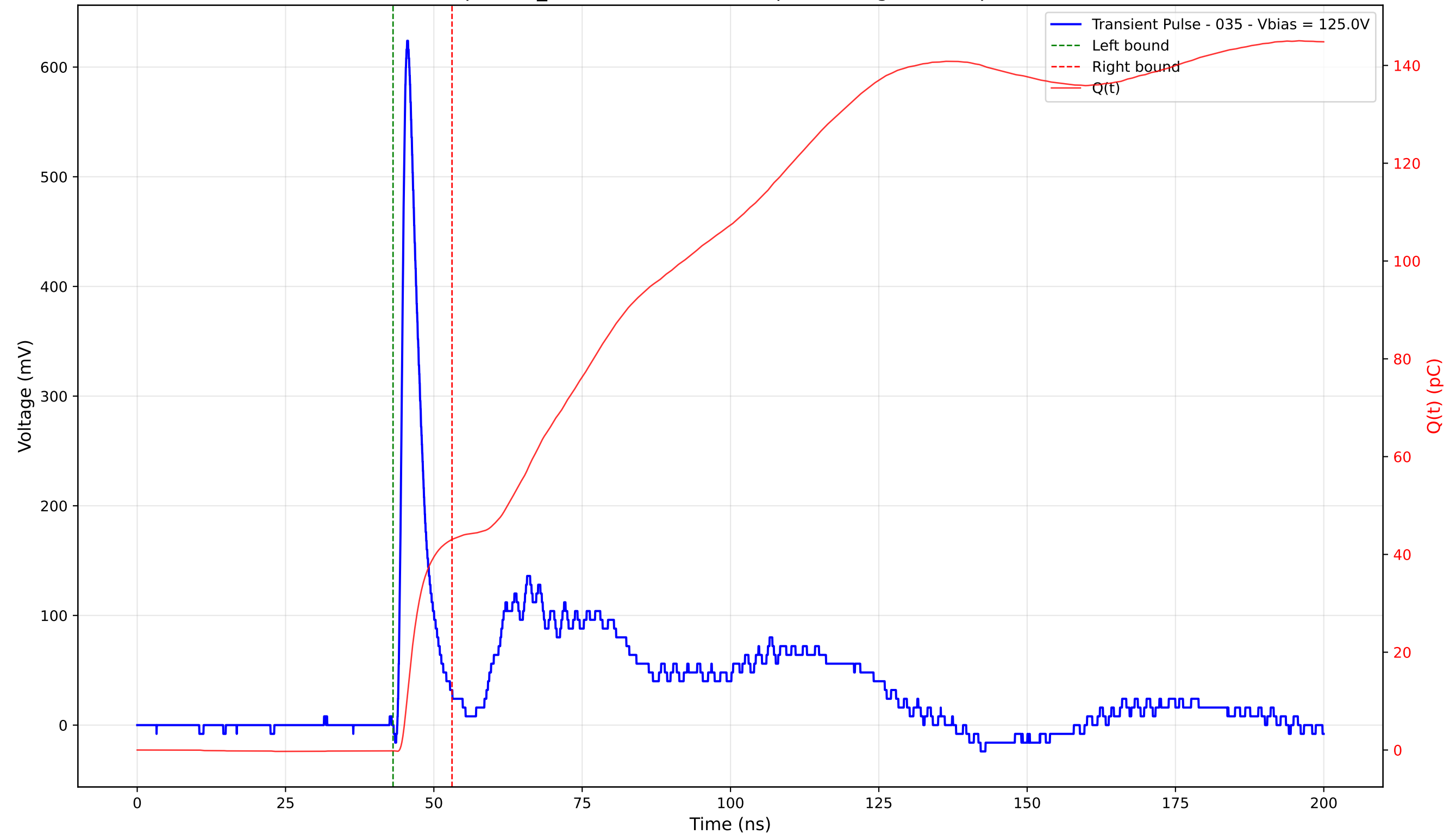
Transient Pulse - Sample: TD_4004 - Position: 155.0 \mu\text{m} - Charge: 43.23 pC - Rise Time: 1.03 ns
