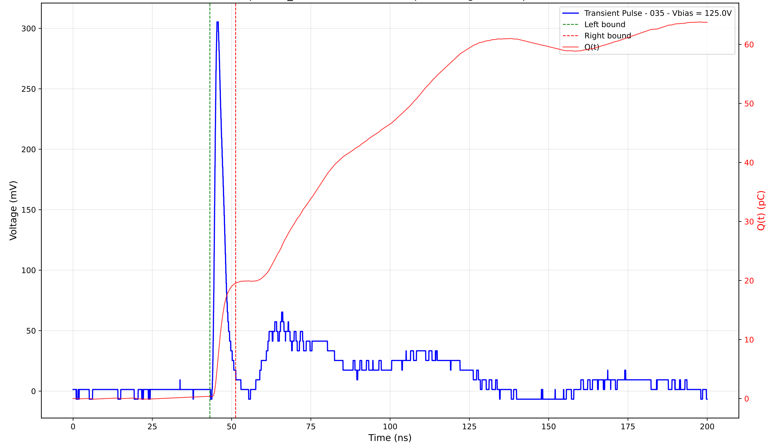
Transient Pulse - Sample: TD_4004 - Position: 340.0 \mu\text{m} - Charge: 19.17 pC - Rise Time: 1.05 ns
