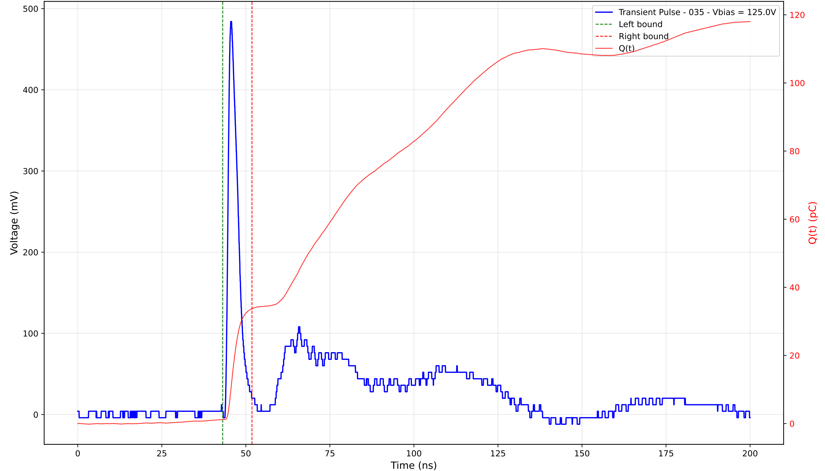
Transient Pulse - Sample: TD_4004 - Position: 290.0 \mu\text{m} - Charge: 32.49 pC - Rise Time: 1.05 ns
