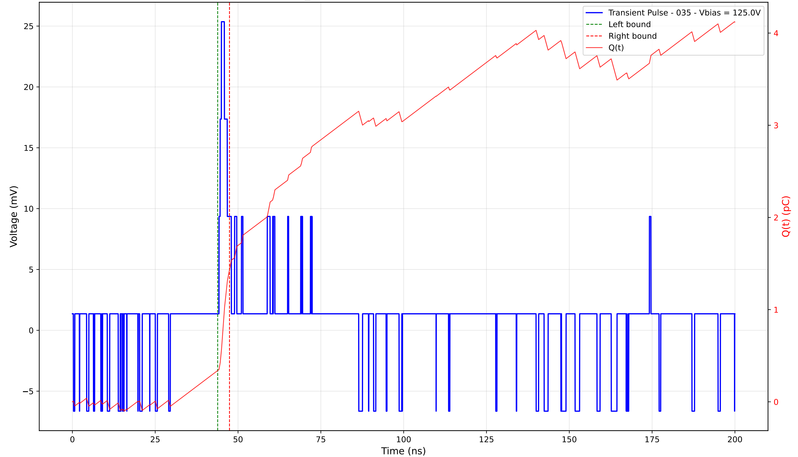
Transient Pulse - Sample: TD_4004 - Position: 35.0 \mu\text{m} - Charge: 1.09 pC - Rise Time: 0.74 ns
