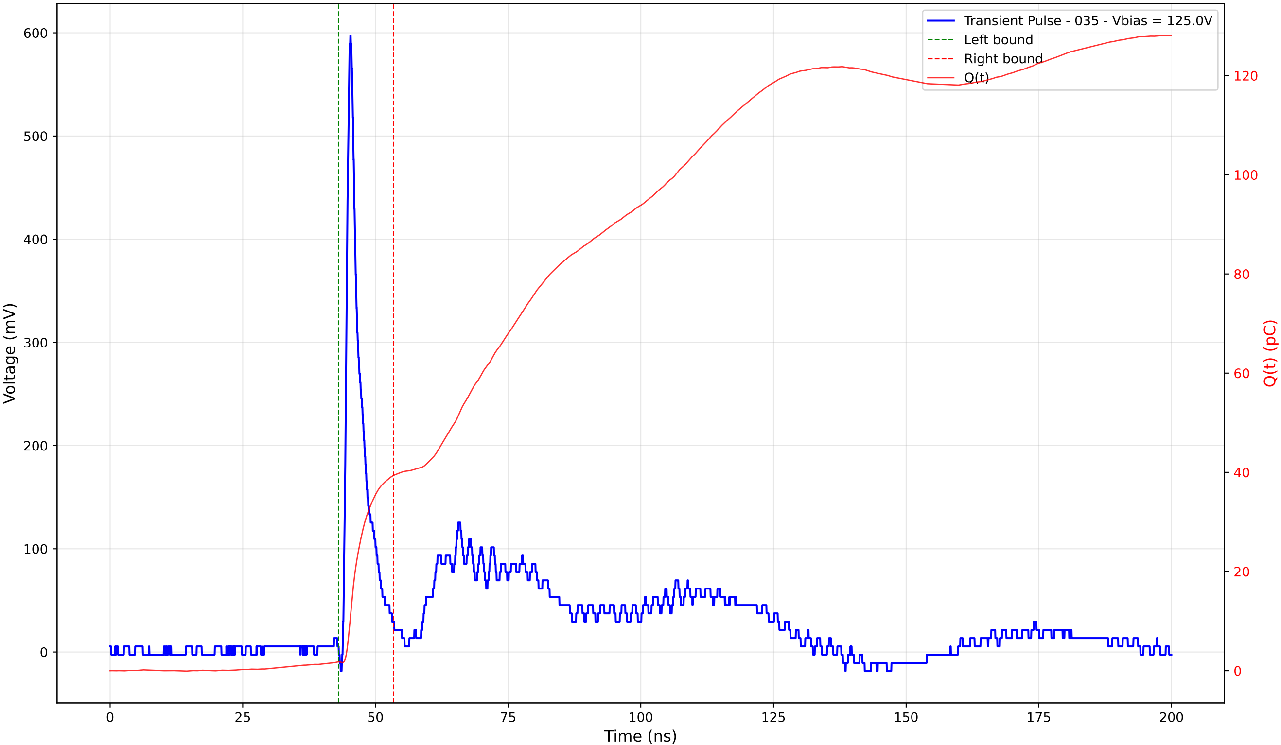
Transient Pulse - Sample: TD_4004 - Position: 80.0 \mu\text{m} - Charge: 37.60 pC - Rise Time: 0.91 ns
