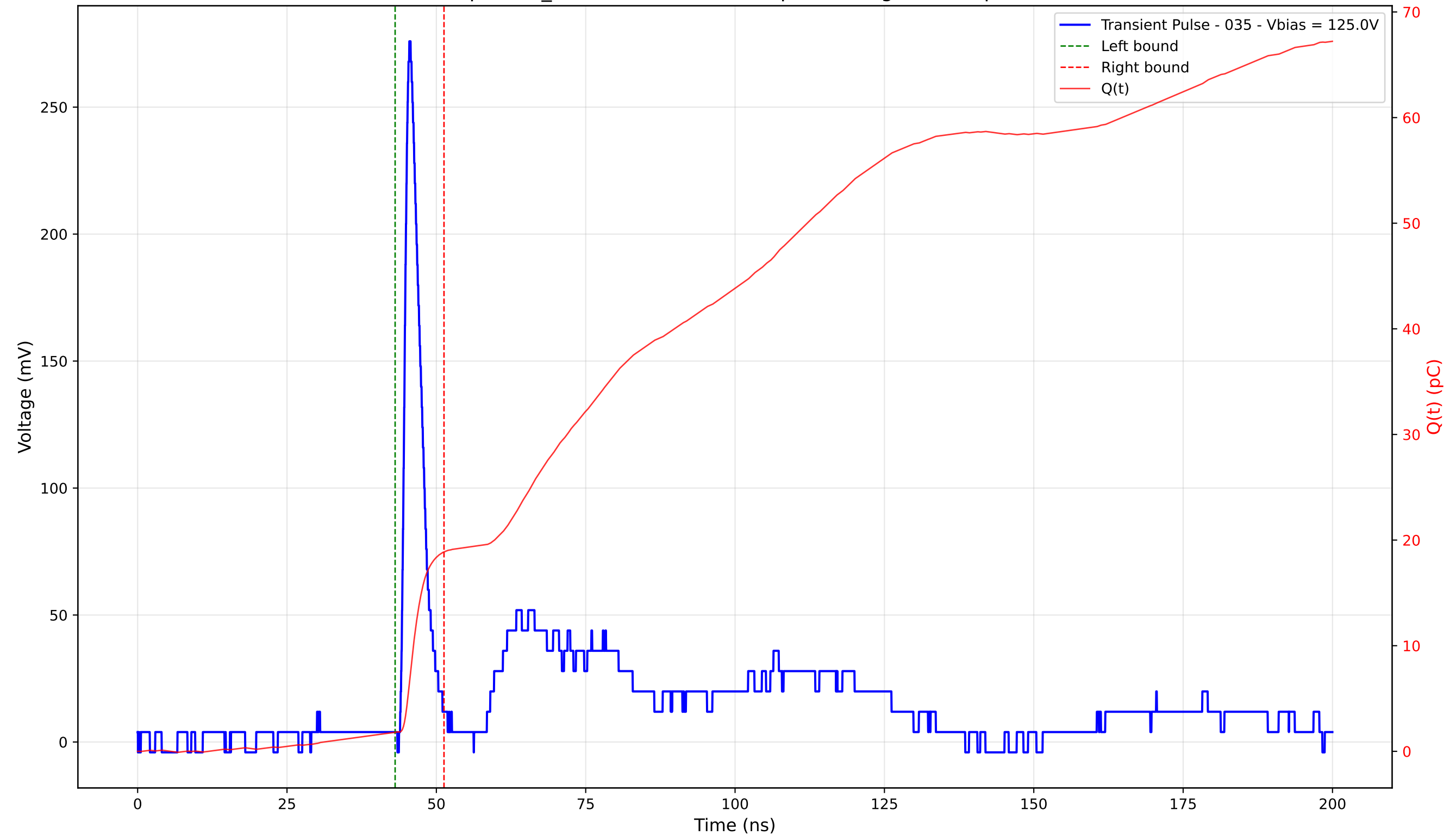
Transient Pulse - Sample: TD_4004 - Position: 365.0 \mu\text{m} - Charge: 17.06 pC - Rise Time: 1.08 ns
