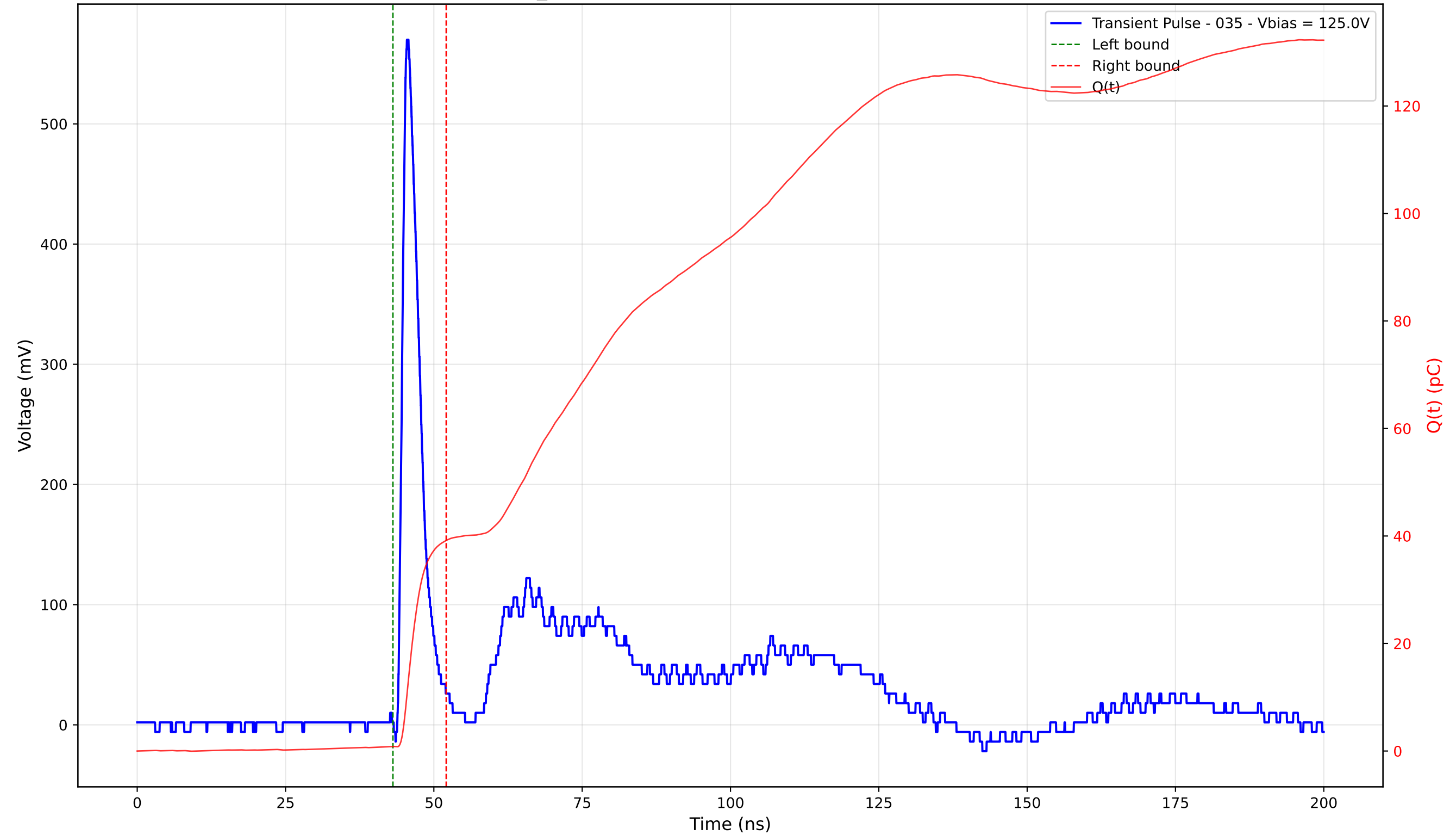
Transient Pulse - Sample: TD_4004 - Position: 245.0 \mu\text{m} - Charge: 38.33 pC - Rise Time: 1.04 ns
