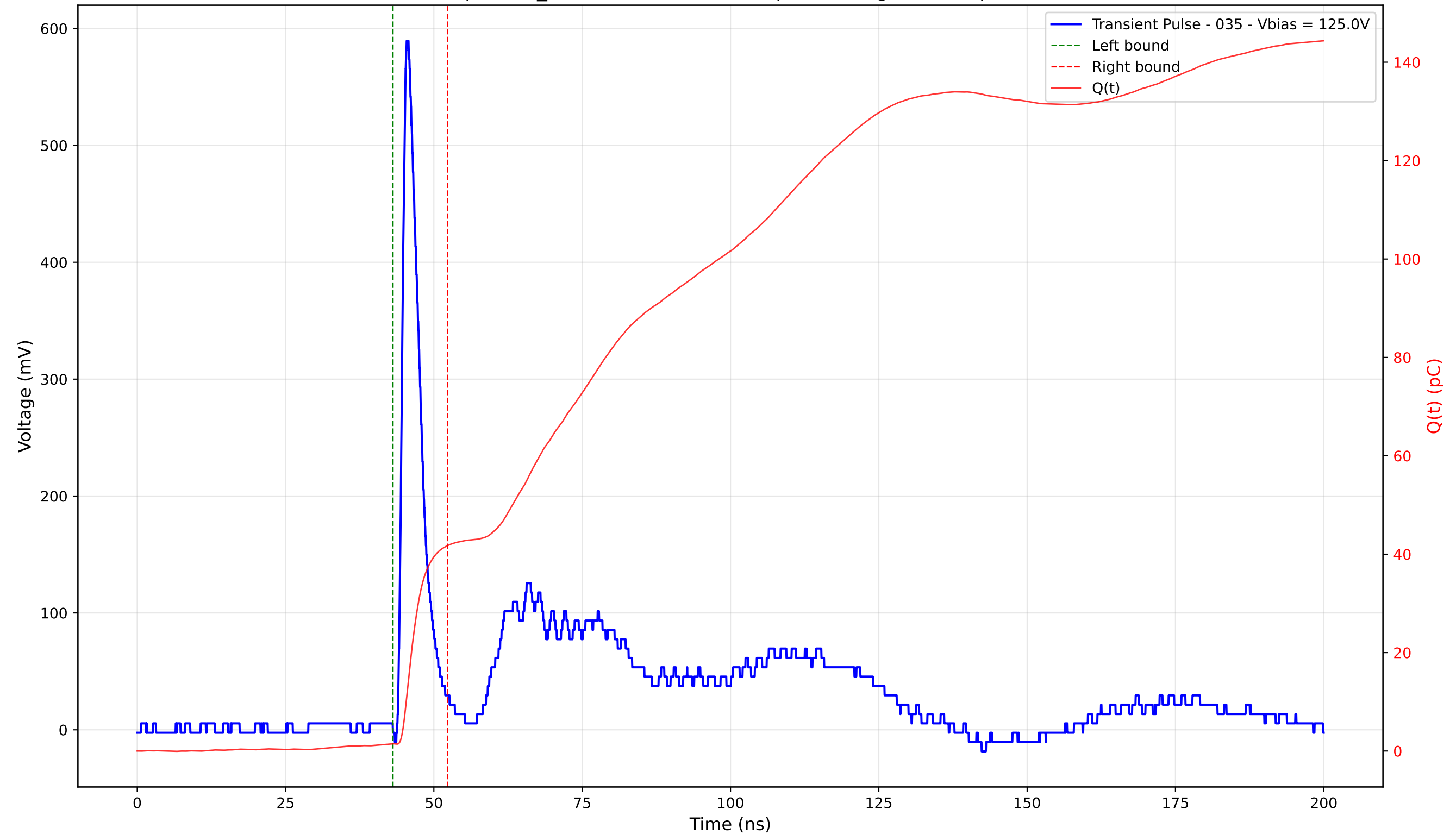
Transient Pulse - Sample: TD_4004 - Position: 235.0 \mu\text{m} - Charge: 40.27 pC - Rise Time: 1.03 ns
