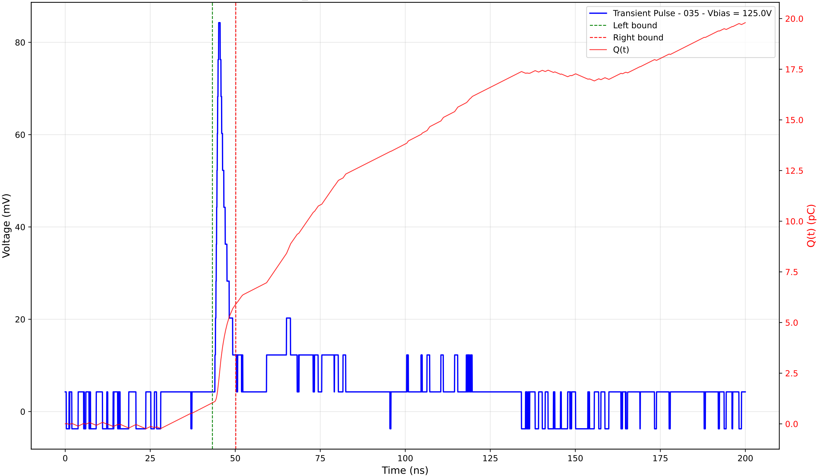
Transient Pulse - Sample: TD_4004 - Position: 50.0 \mu\text{m} - Charge: 4.88 pC - Rise Time: 0.93 ns
