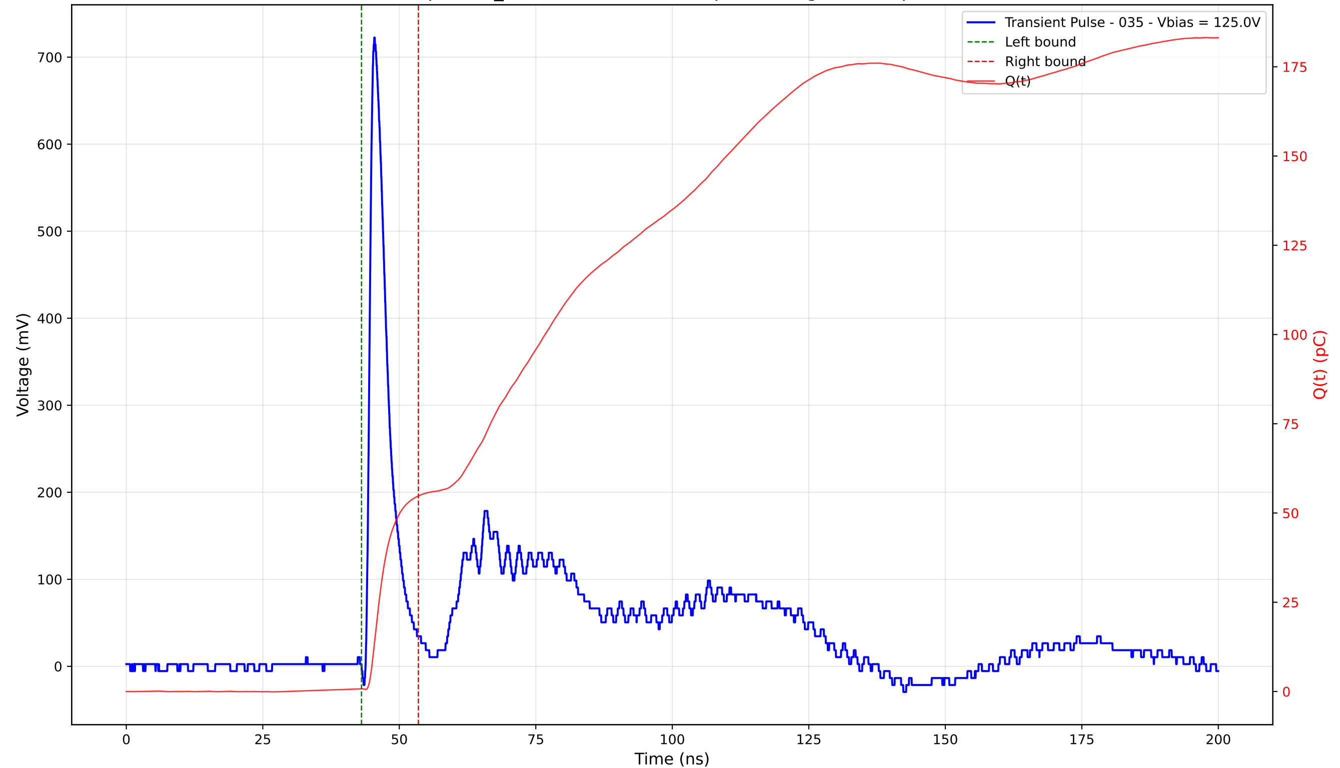
Transient Pulse - Sample: TD_4004 - Position: 190.0 \mu\text{m} - Charge: 54.02 pC - Rise Time: 0.99 ns
