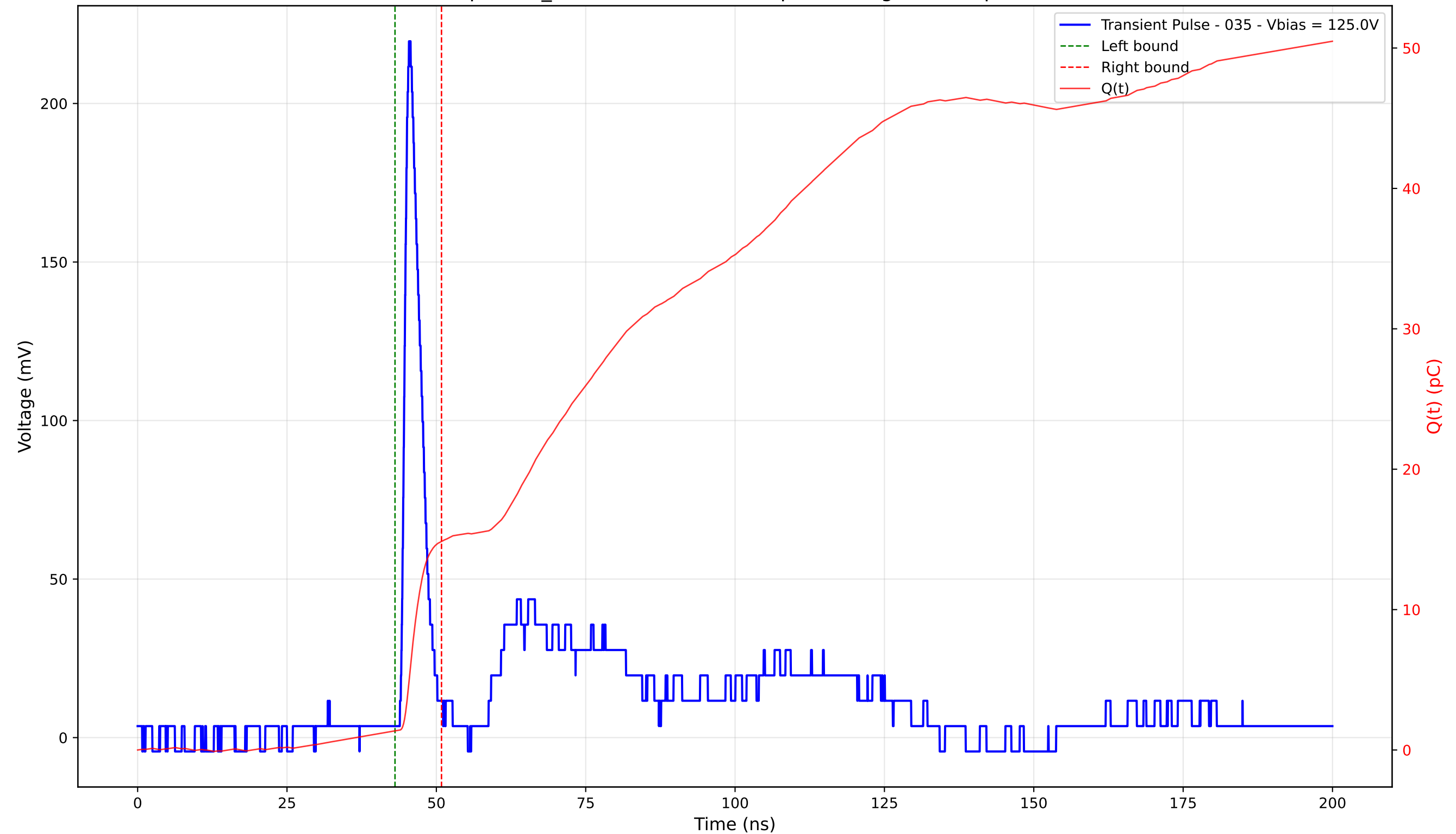
Transient Pulse - Sample: TD_4004 - Position: 390.0 \mu\text{m} - Charge: 13.51 pC - Rise Time: 1.05 ns
