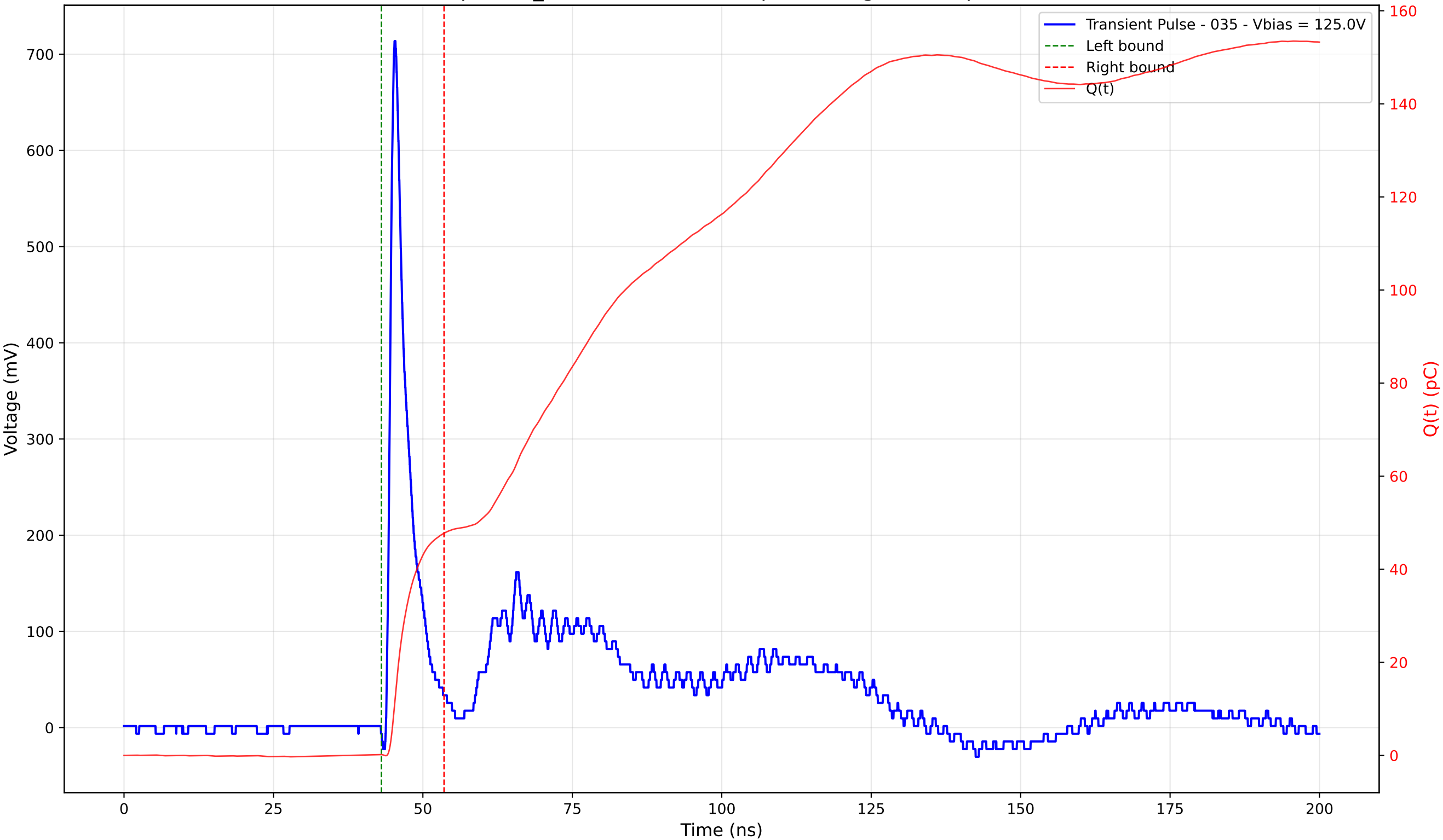
Transient Pulse - Sample: TD_4004 - Position: 95.0 \mu\text{m} - Charge: 47.58 pC - Rise Time: 0.93 ns
