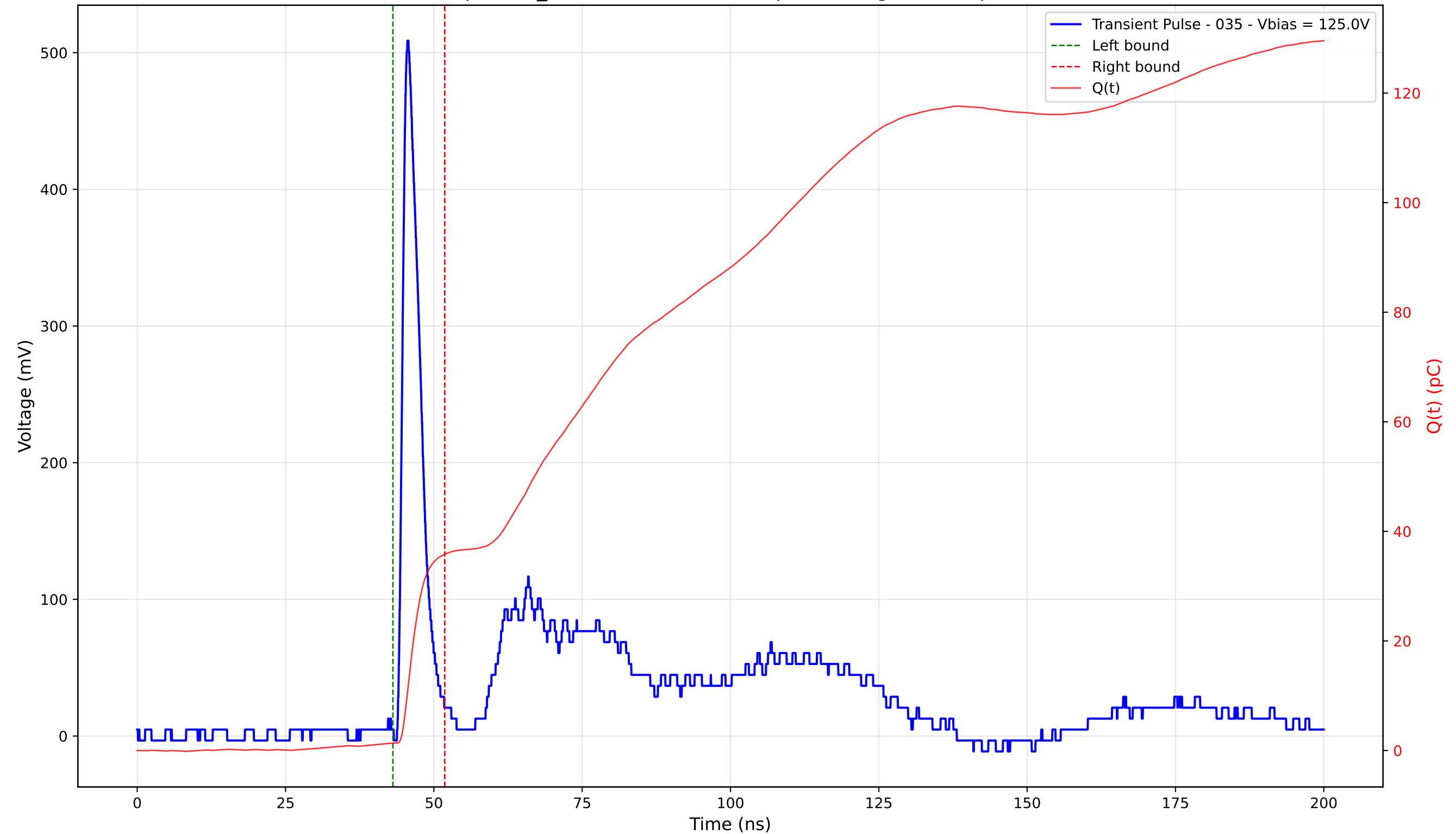
Transient Pulse - Sample: TD_4004 - Position: 265.0 \mu\text{m} - Charge: 34.47 pC - Rise Time: 1.08 ns
