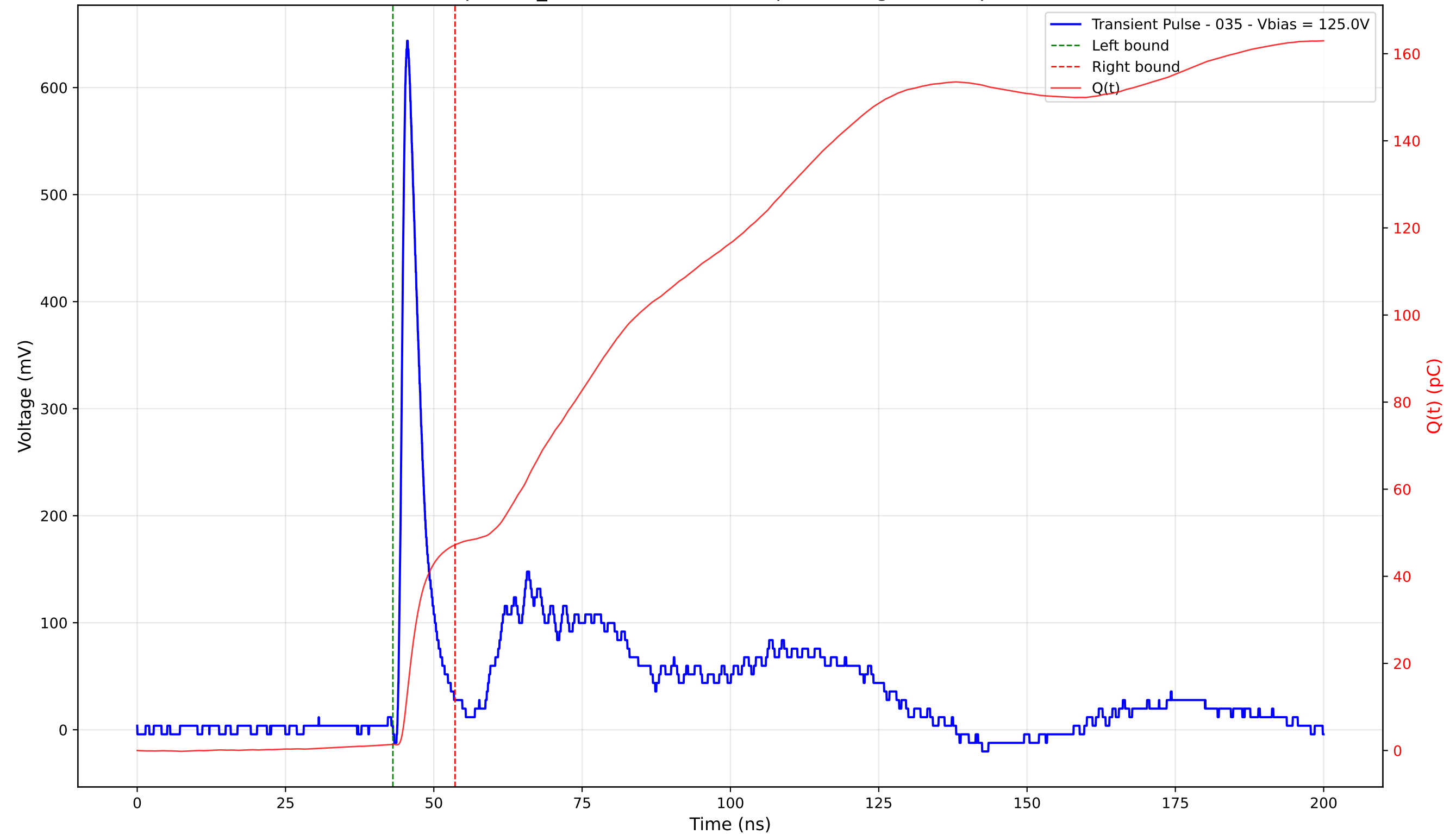
Transient Pulse - Sample: TD_4004 - Position: 160.0 \mu\text{m} - Charge: 45.82 pC - Rise Time: 1.03 ns
