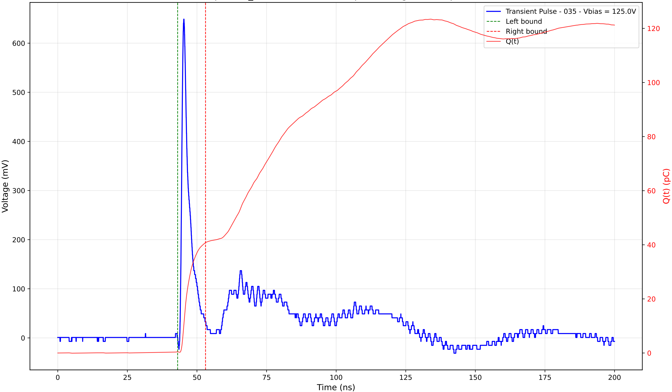
Transient Pulse - Sample: TD_4004 - Position: 85.0 \mu\text{m} - Charge: 40.35 pC - Rise Time: 0.92 ns
