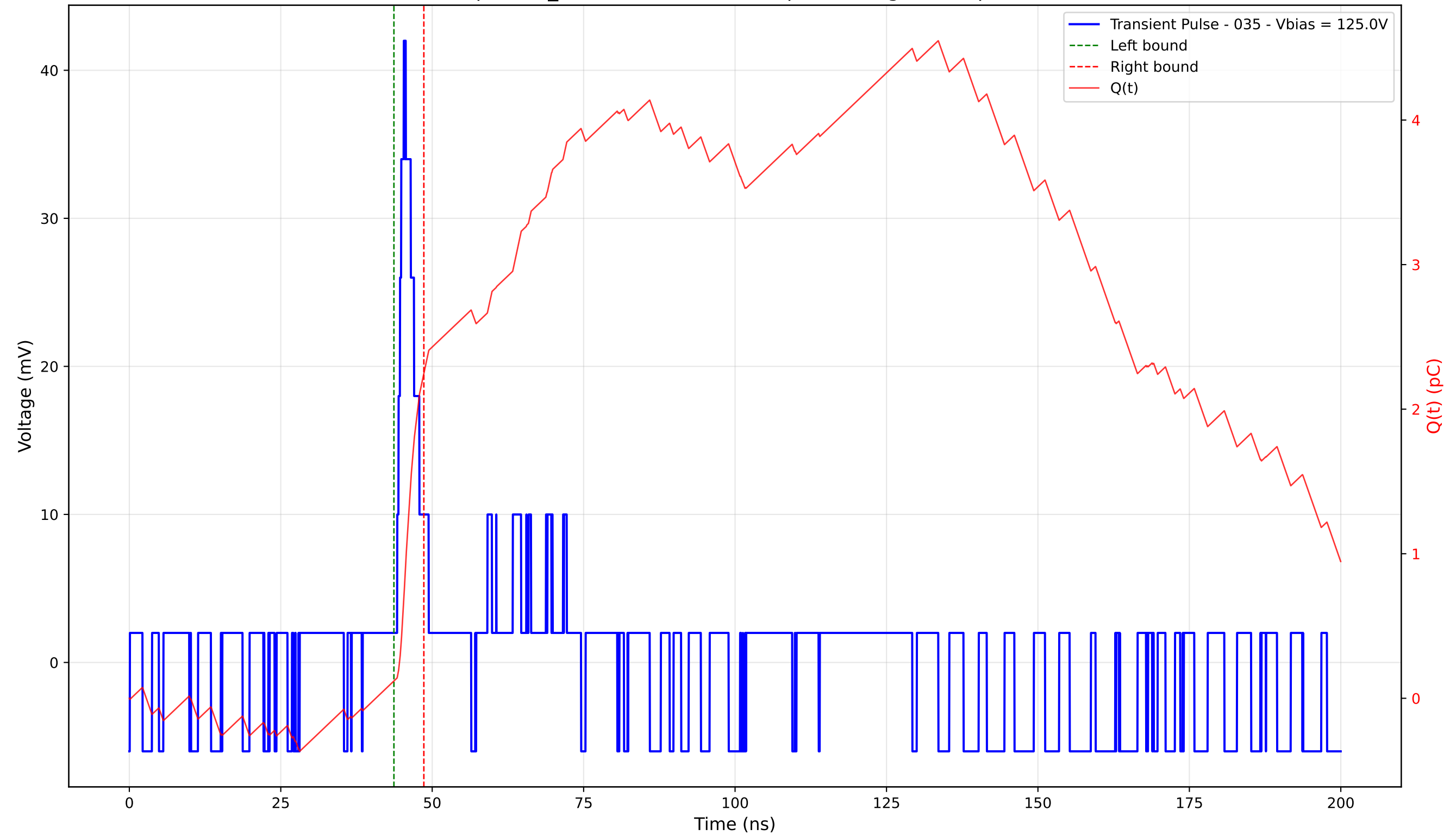
Transient Pulse - Sample: TD_4004 - Position: 425.0 \mu\text{m} - Charge: 2.13 pC - Rise Time: 1.09 ns
