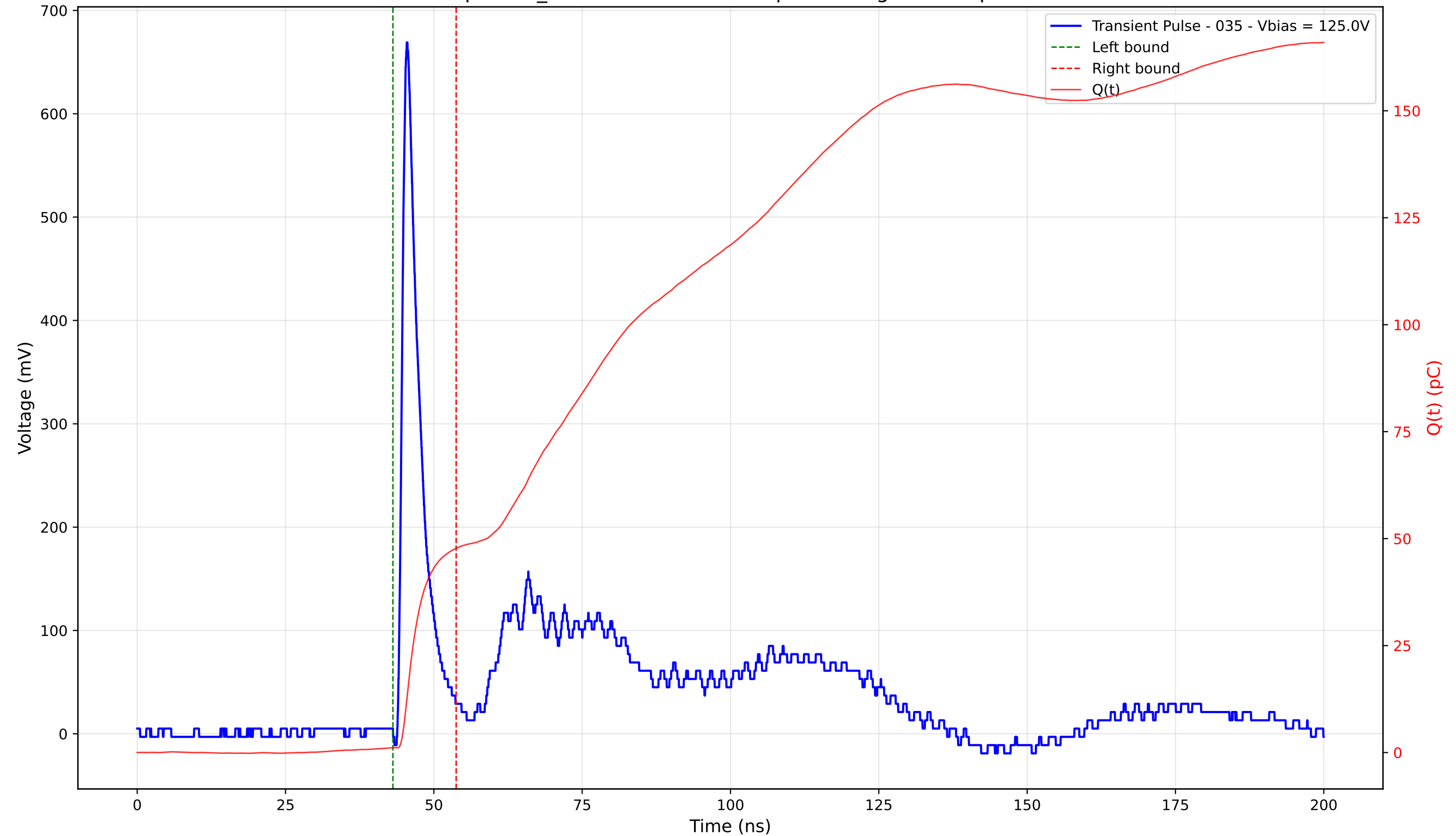
Transient Pulse - Sample: TD_4004 - Position: 130.0 \mu\text{m} - Charge: 46.60 pC - Rise Time: 1.00 ns
