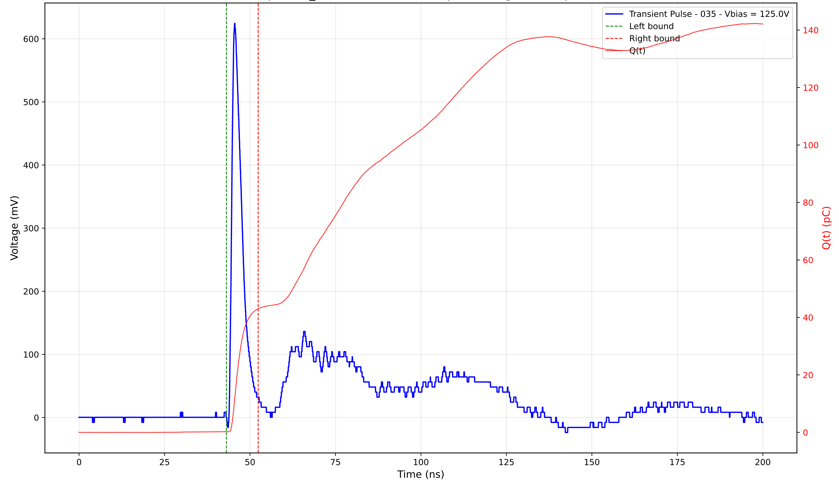
Transient Pulse - Sample: TD_4004 - Position: 230.0 \mu\text{m} - Charge: 42.69 pC - Rise Time: 1.03 ns
