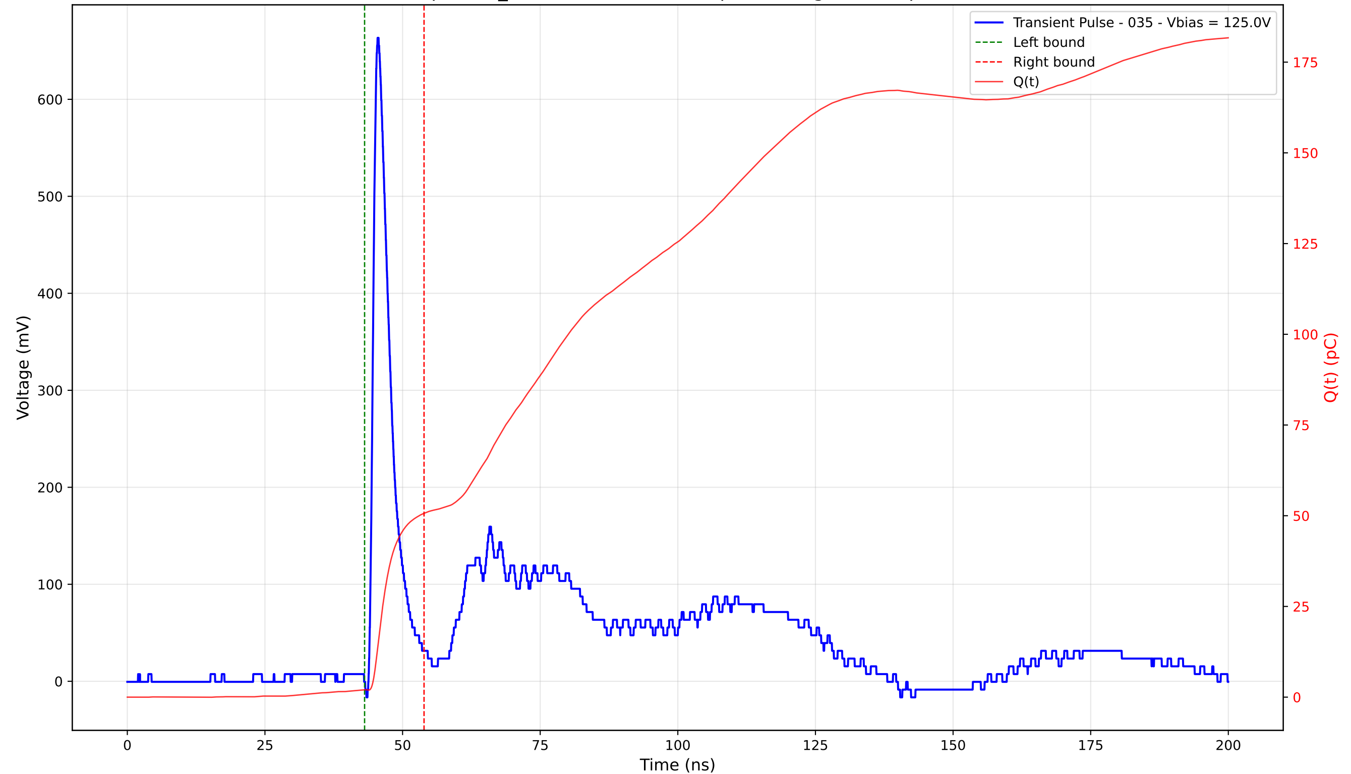
Transient Pulse - Sample: TD_4004 - Position: 165.0 \mu\text{m} - Charge: 48.61 pC - Rise Time: 1.01 ns
