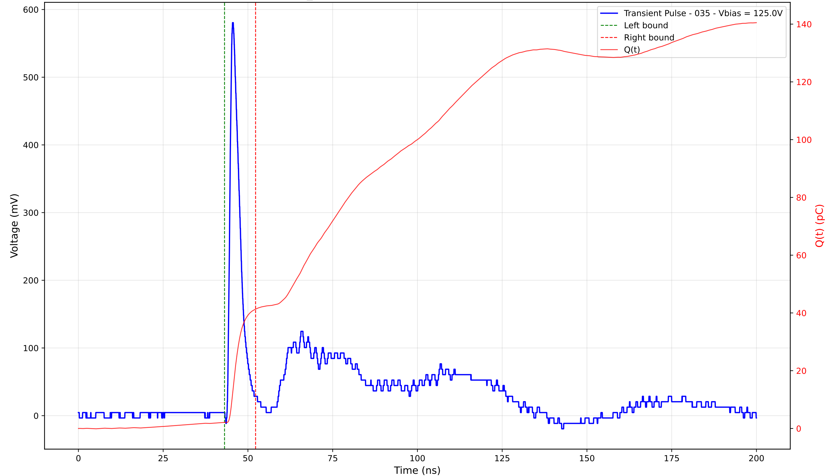
Transient Pulse - Sample: TD_4004 - Position: 240.0 \mu\text{m} - Charge: 39.18 pC - Rise Time: 1.04 ns
