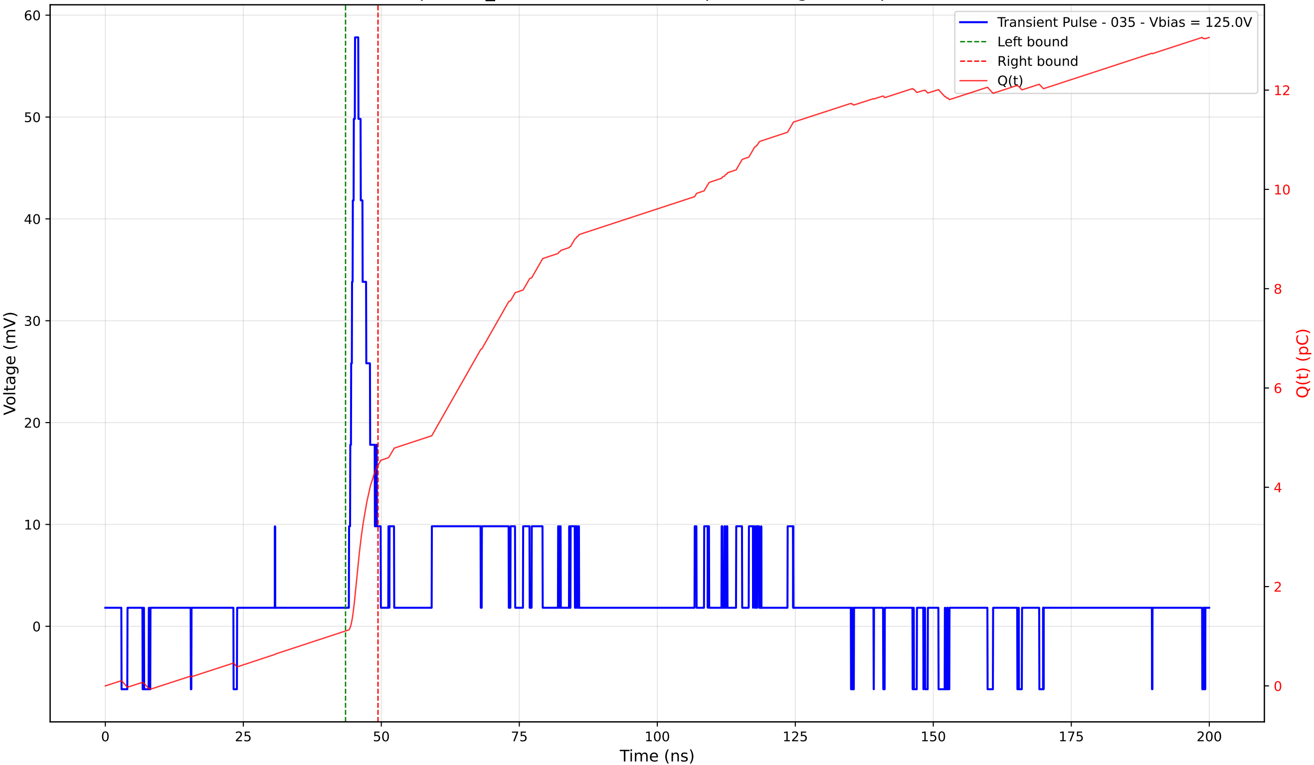
Transient Pulse - Sample: TD_4004 - Position: 420.0 \mu\text{m} - Charge: 3.34 pC - Rise Time: 1.09 ns
