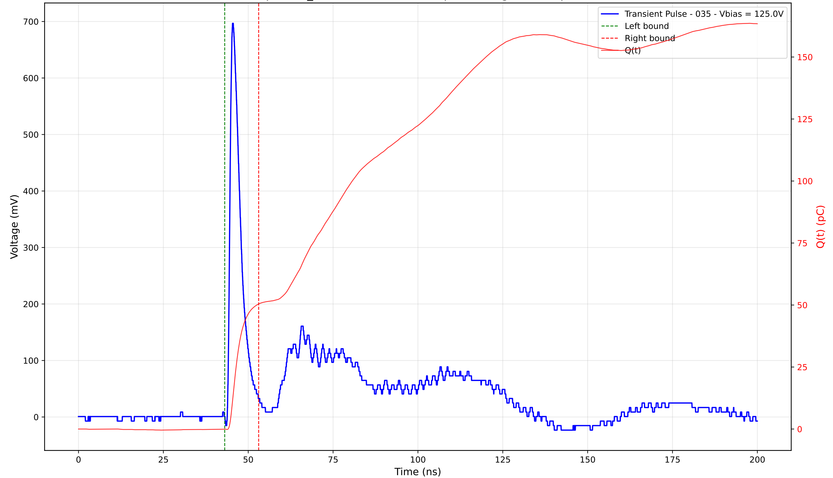
Transient Pulse - Sample: TD_4004 - Position: 205.0 \mu\text{m} - Charge: 50.47 pC - Rise Time: 0.97 ns
