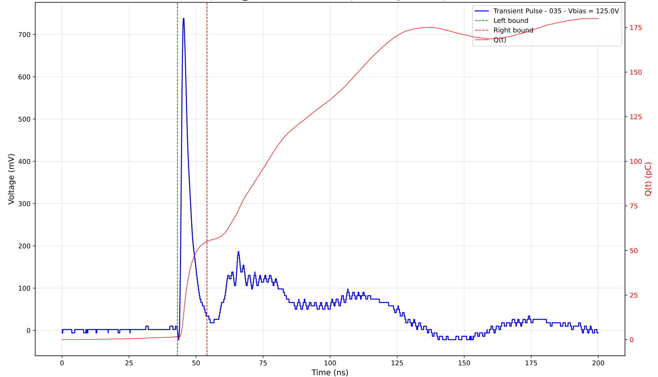
Transient Pulse - Sample: TD_4004 - Position: 110.0 \mu\text{m} - Charge: 53.36 pC - Rise Time: 0.94 ns
