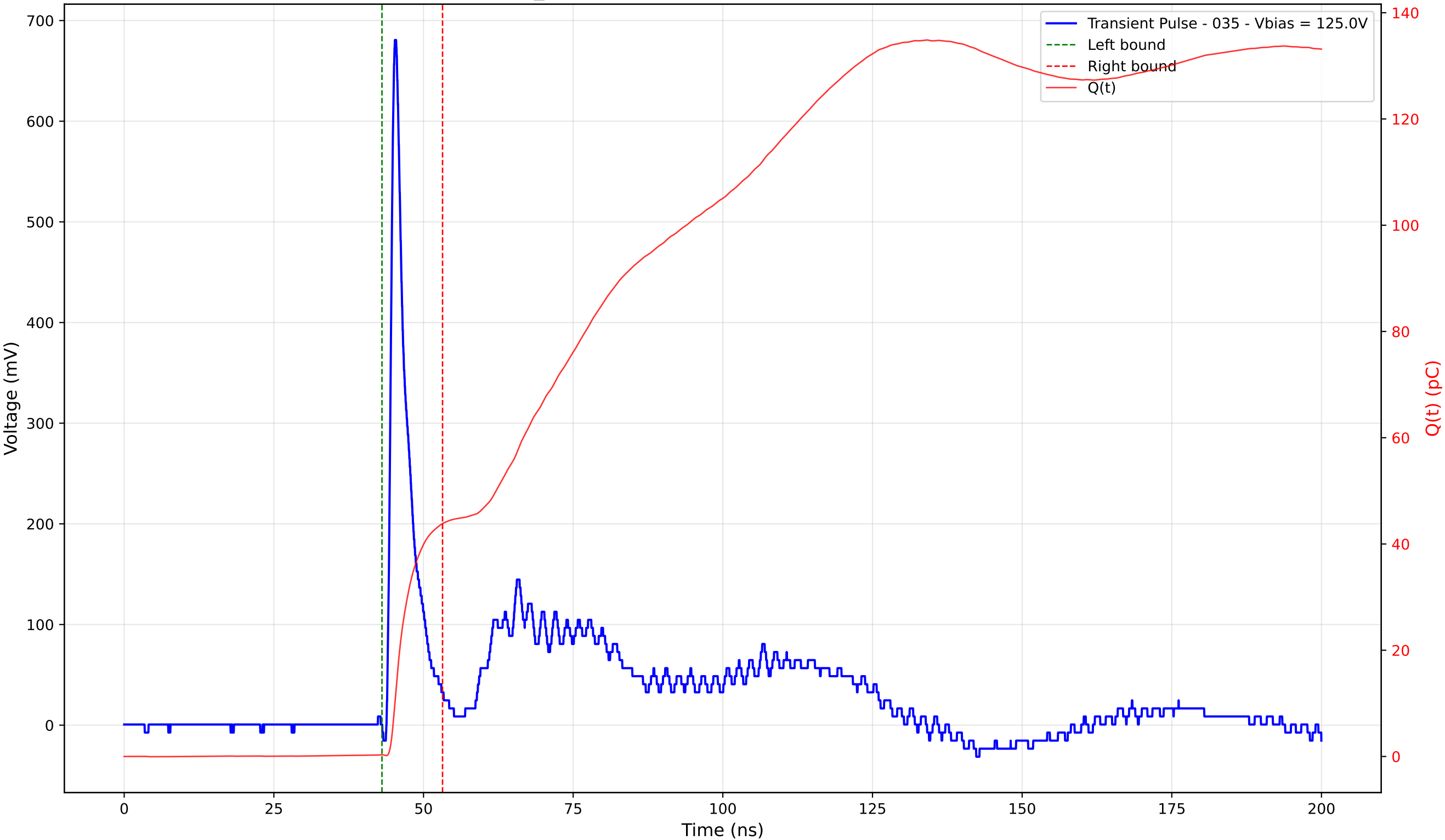
Transient Pulse - Sample: TD_4004 - Position: 90.0 \mu\text{m} - Charge: 43.52 pC - Rise Time: 0.90 ns
