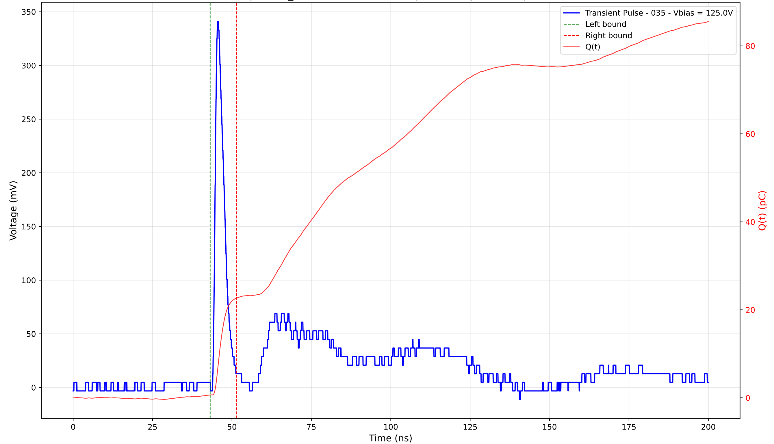
Transient Pulse - Sample: TD_4004 - Position: 330.0 \mu\text{m} - Charge: 22.01 pC - Rise Time: 1.03 ns
