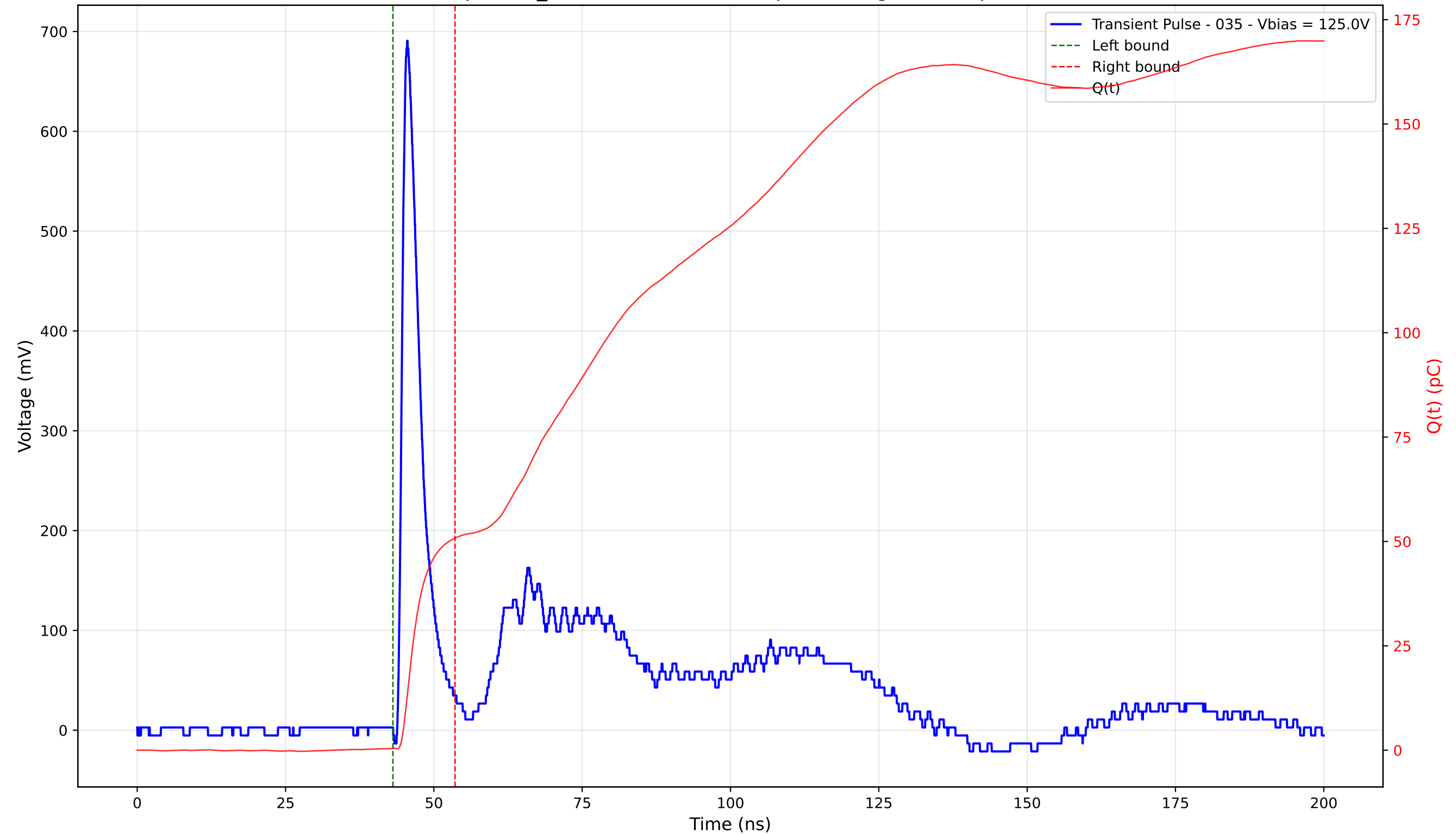
Transient Pulse - Sample: TD_4004 - Position: 170.0 \mu\text{m} - Charge: 50.37 pC - Rise Time: 1.00 ns
