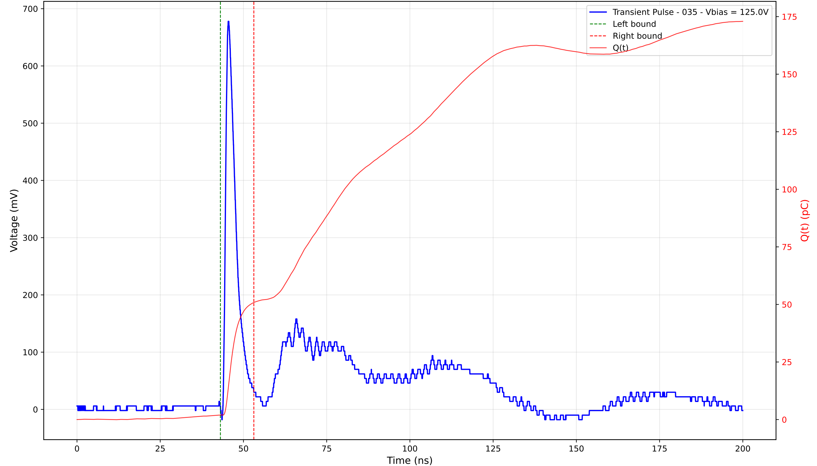
Transient Pulse - Sample: TD_4004 - Position: 220.0 \mu\text{m} - Charge: 48.81 pC - Rise Time: 1.00 ns
