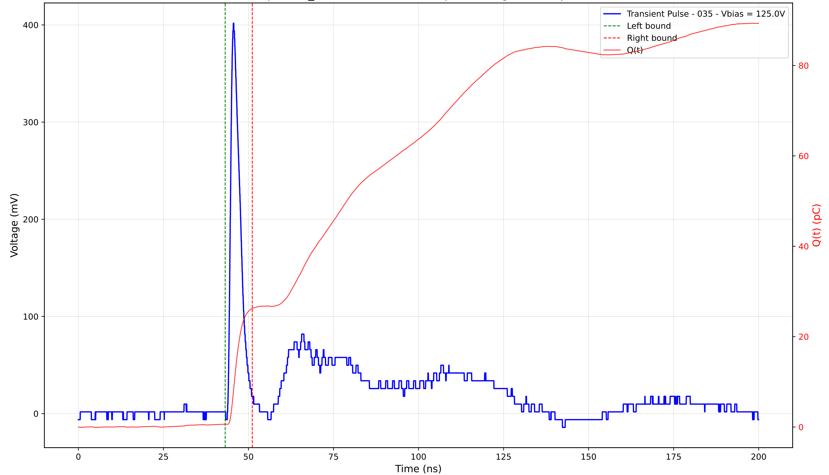
Transient Pulse - Sample: TD_4004 - Position: 315.0 \mu\text{m} - Charge: 25.59 pC - Rise Time: 1.06 ns
