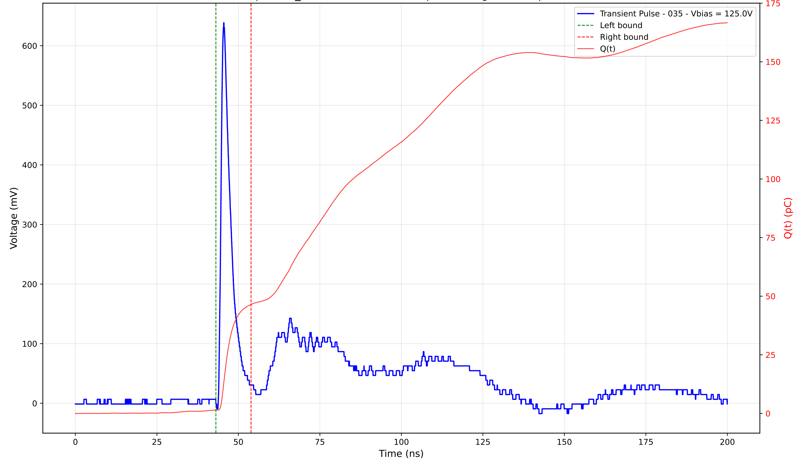
Transient Pulse - Sample: TD_4004 - Position: 135.0 \mu\text{m} - Charge: 44.97 pC - Rise Time: 1.04 ns
