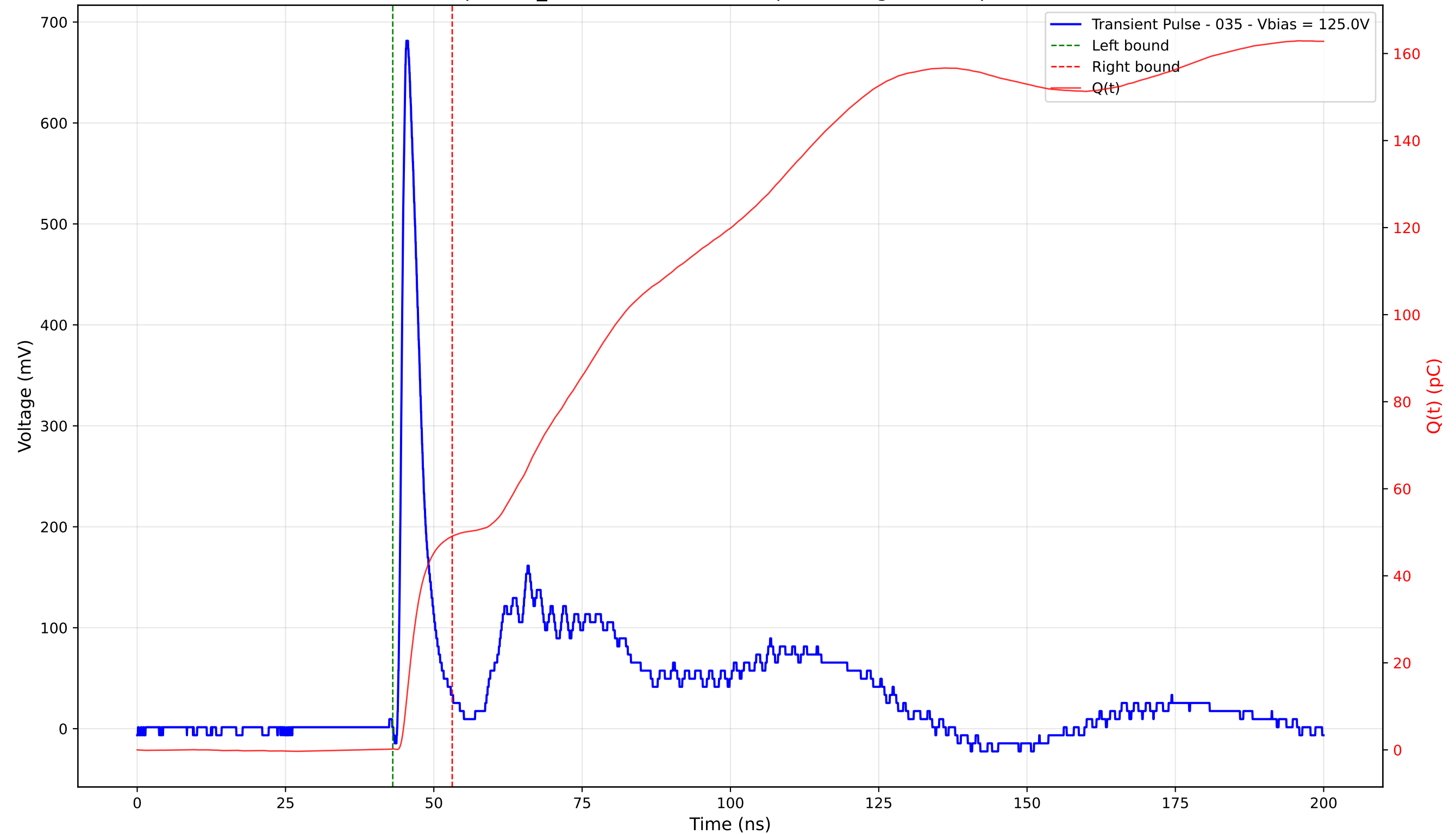
Transient Pulse - Sample: TD_4004 - Position: 210.0 \mu\text{m} - Charge: 48.88 pC - Rise Time: 0.98 ns
