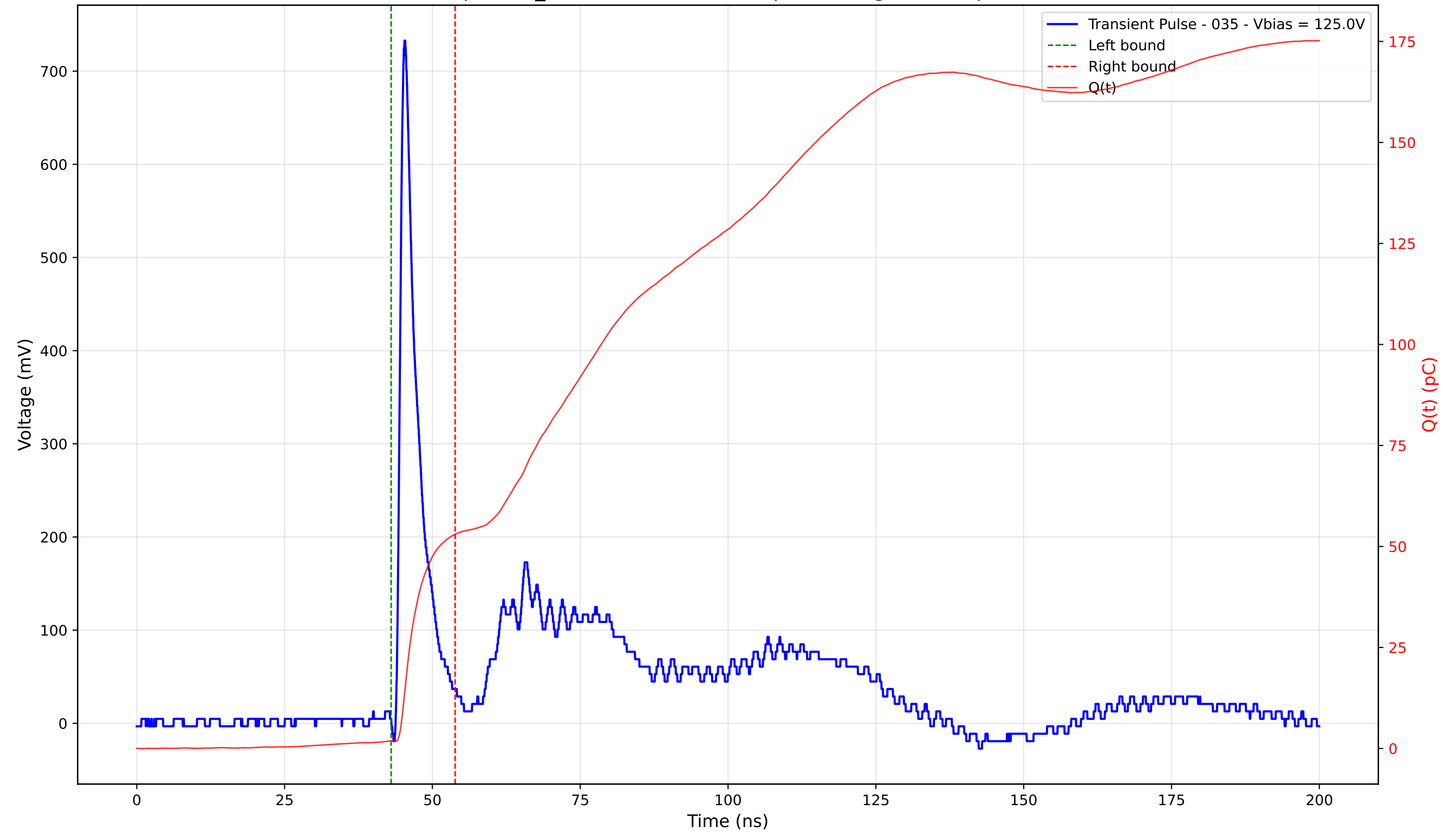
Transient Pulse - Sample: TD_4004 - Position: 100.0 \mu\text{m} - Charge: 51.10 pC - Rise Time: 0.93 ns
