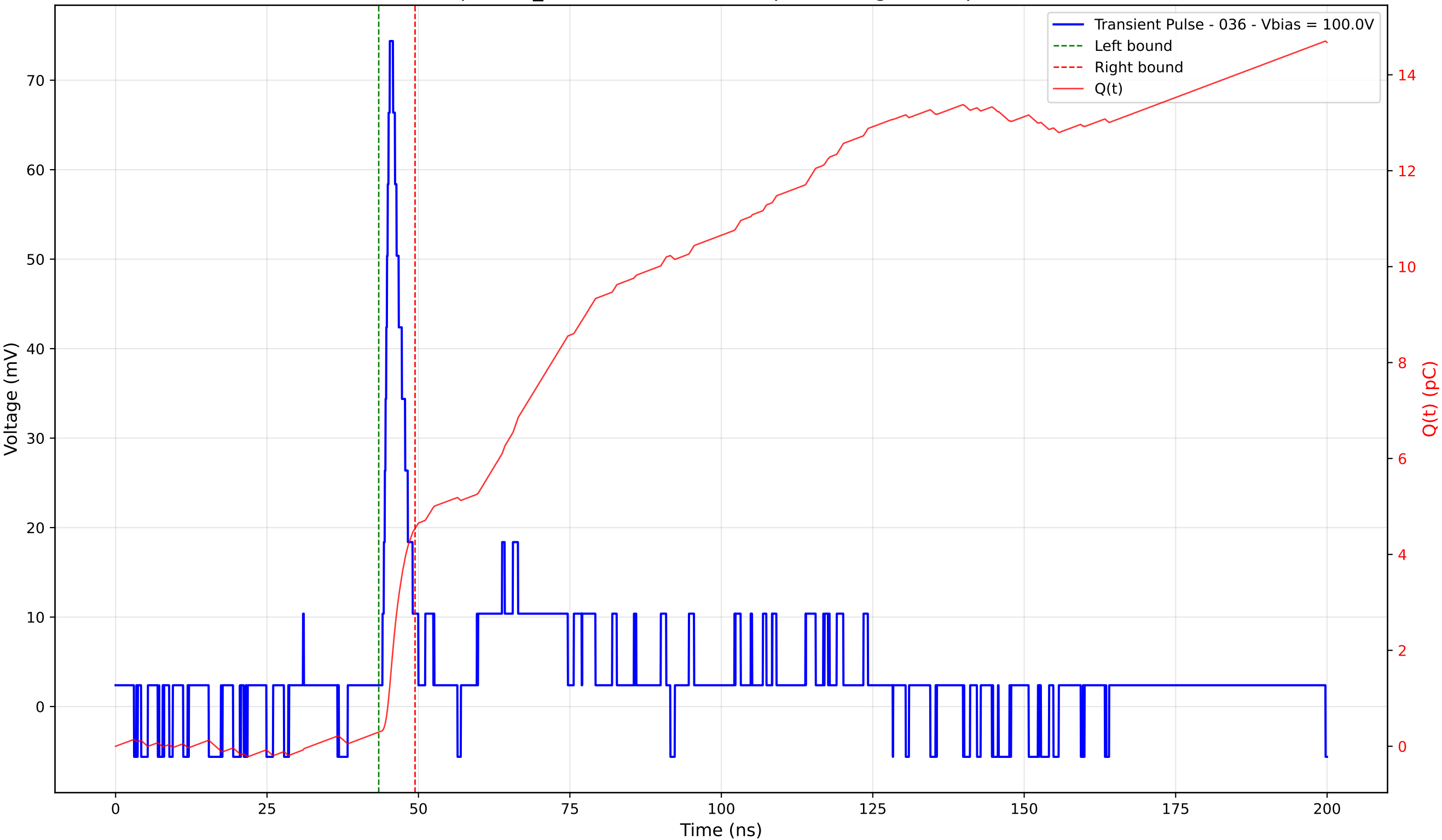
Transient Pulse - Sample: TD_4004 - Position: 415.0 \mu\text{m} - Charge: 4.25 pC - Rise Time: 1.21 ns
