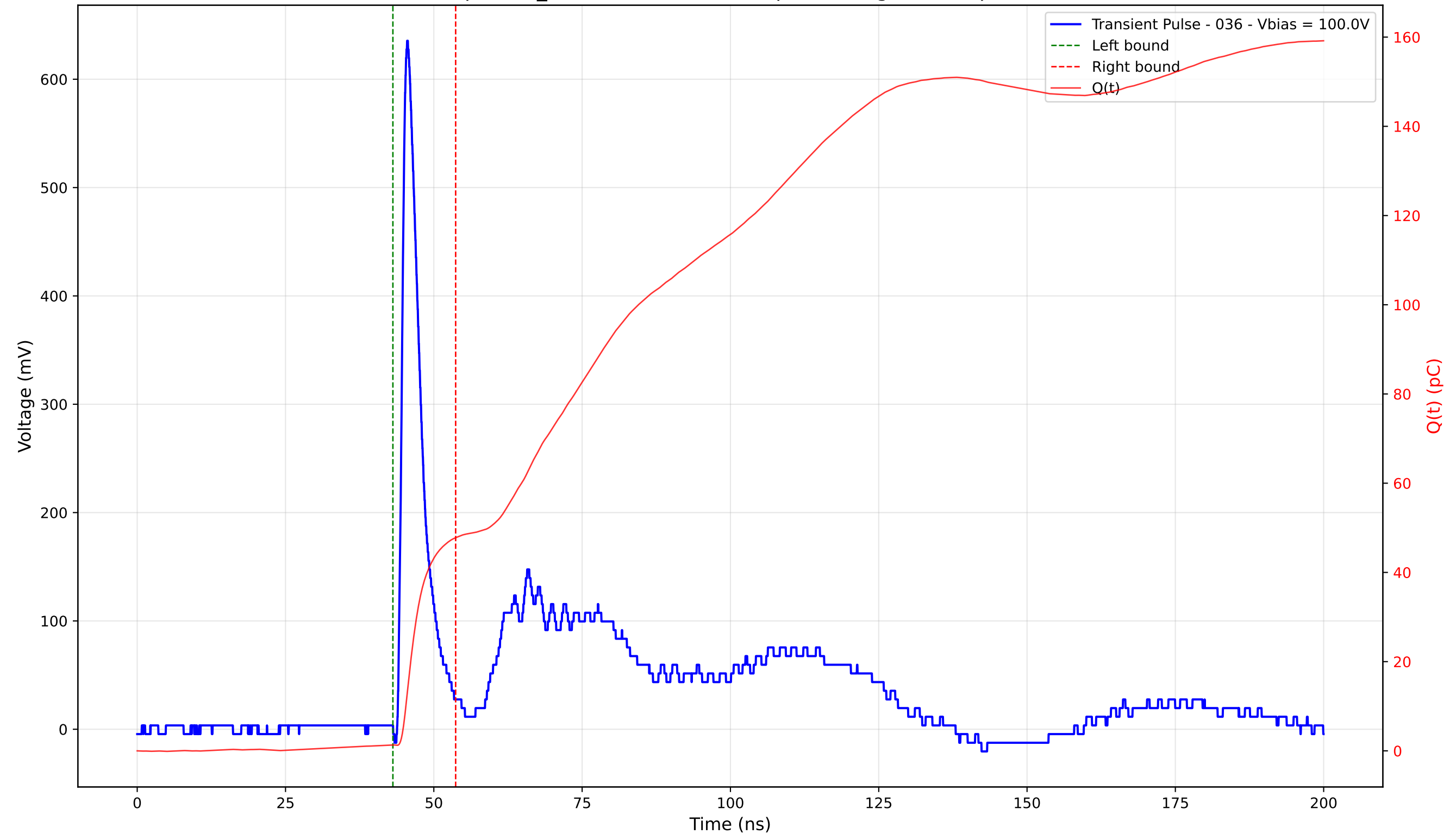
Transient Pulse - Sample: TD_4004 - Position: 210.0 \mu\text{m} - Charge: 46.44 pC - Rise Time: 1.03 ns
