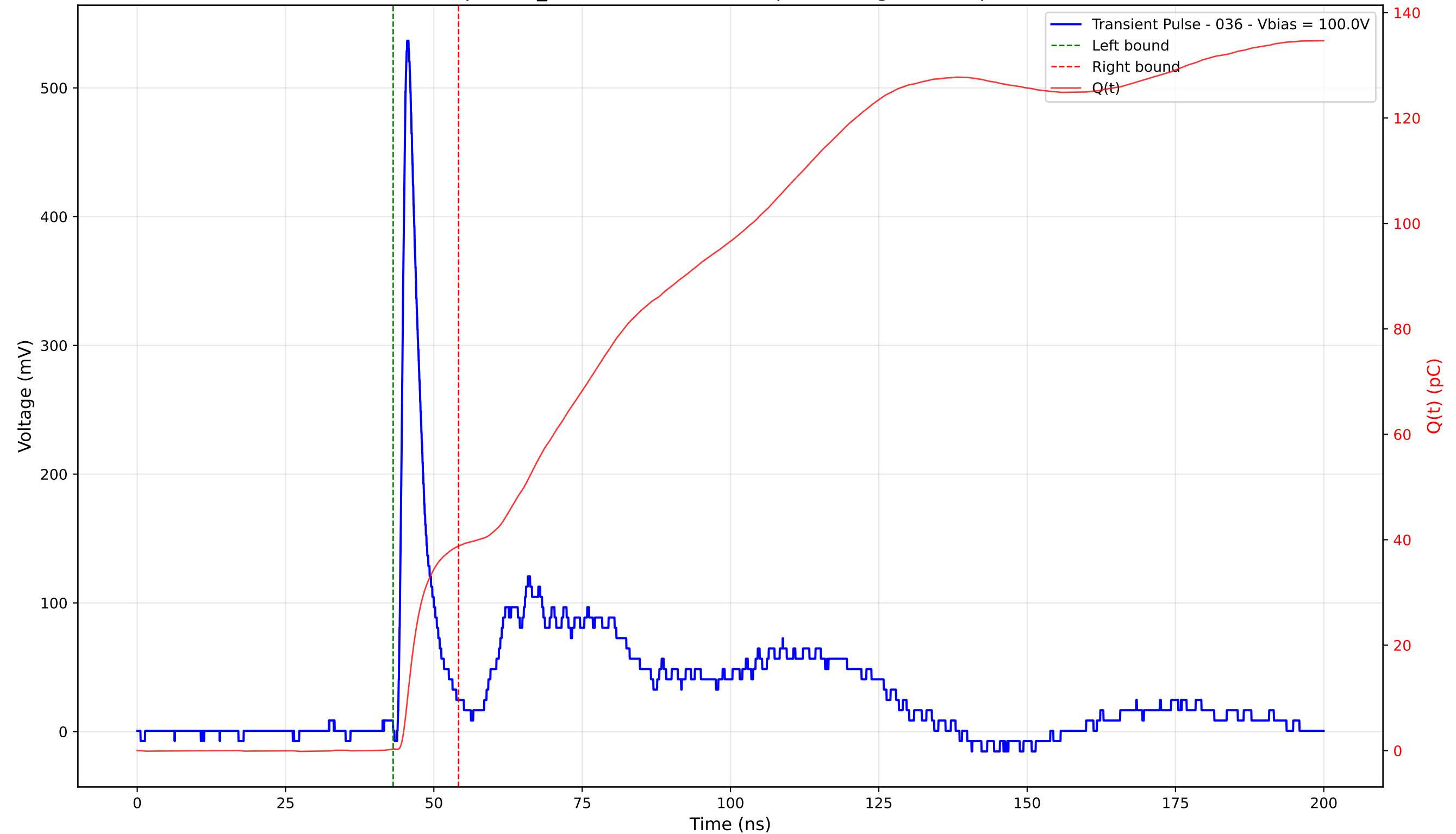
Transient Pulse - Sample: TD_4004 - Position: 140.0 \mu\text{m} - Charge: 38.50 pC - Rise Time: 1.05 ns
