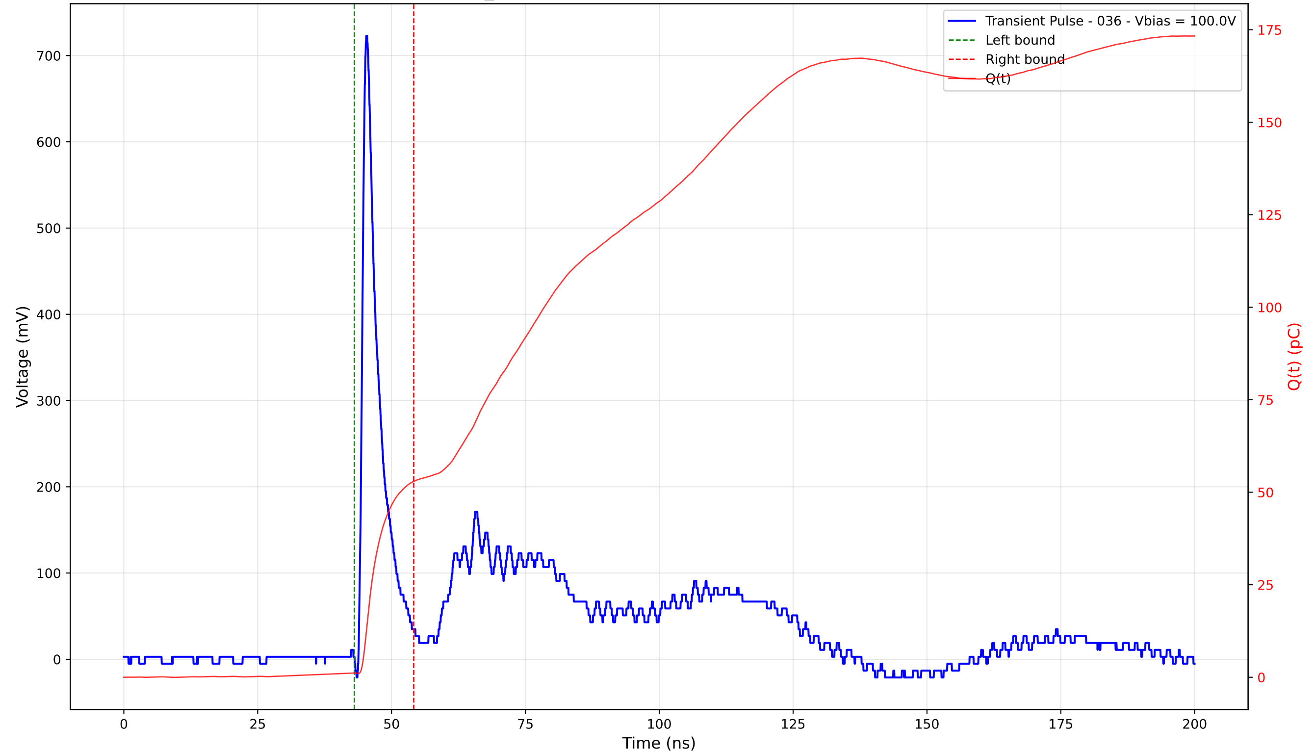
Transient Pulse - Sample: TD_4004 - Position: 105.0 \mu\text{m} - Charge: 51.77 pC - Rise Time: 0.93 ns
