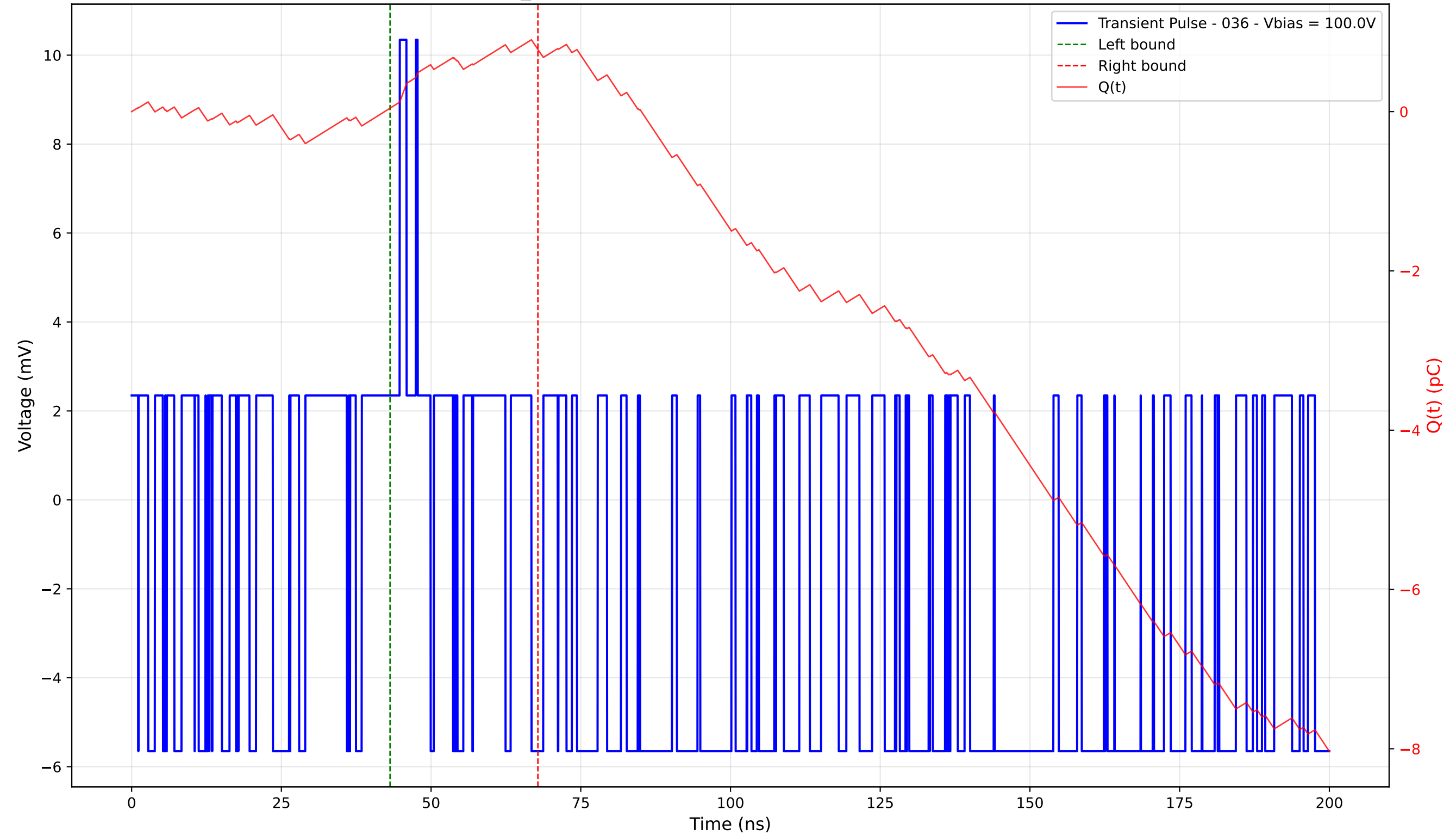
Transient Pulse - Sample: TD_4004 - Position: 15.0 \mu m - Charge: 0.74 pC - Rise Time: 0.00 ns (N/A)
