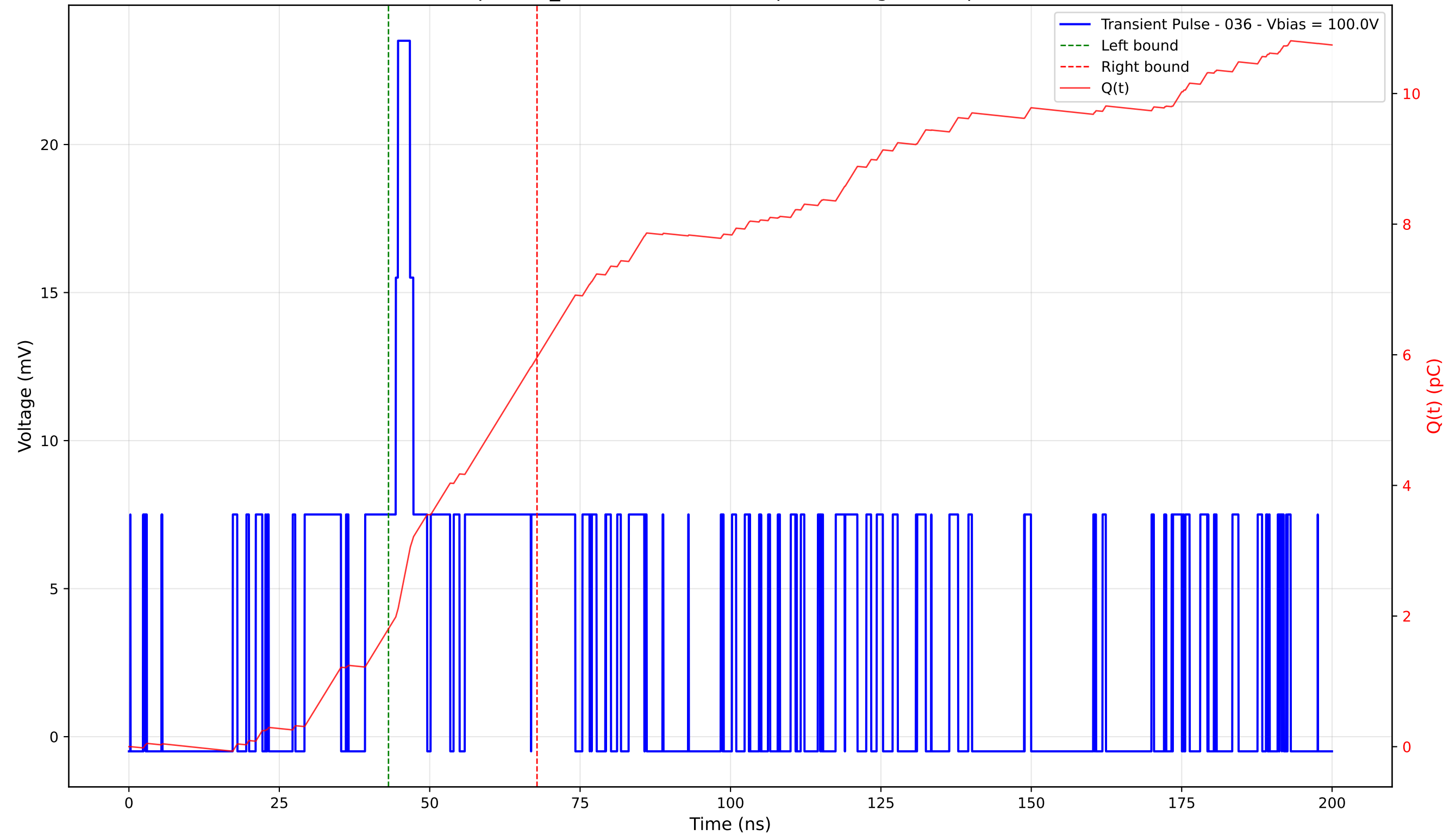
Transient Pulse - Sample: TD_4004 - Position: 35.0 \mu\text{m} - Charge: 4.15 pC - Rise Time: 5.47 ns
