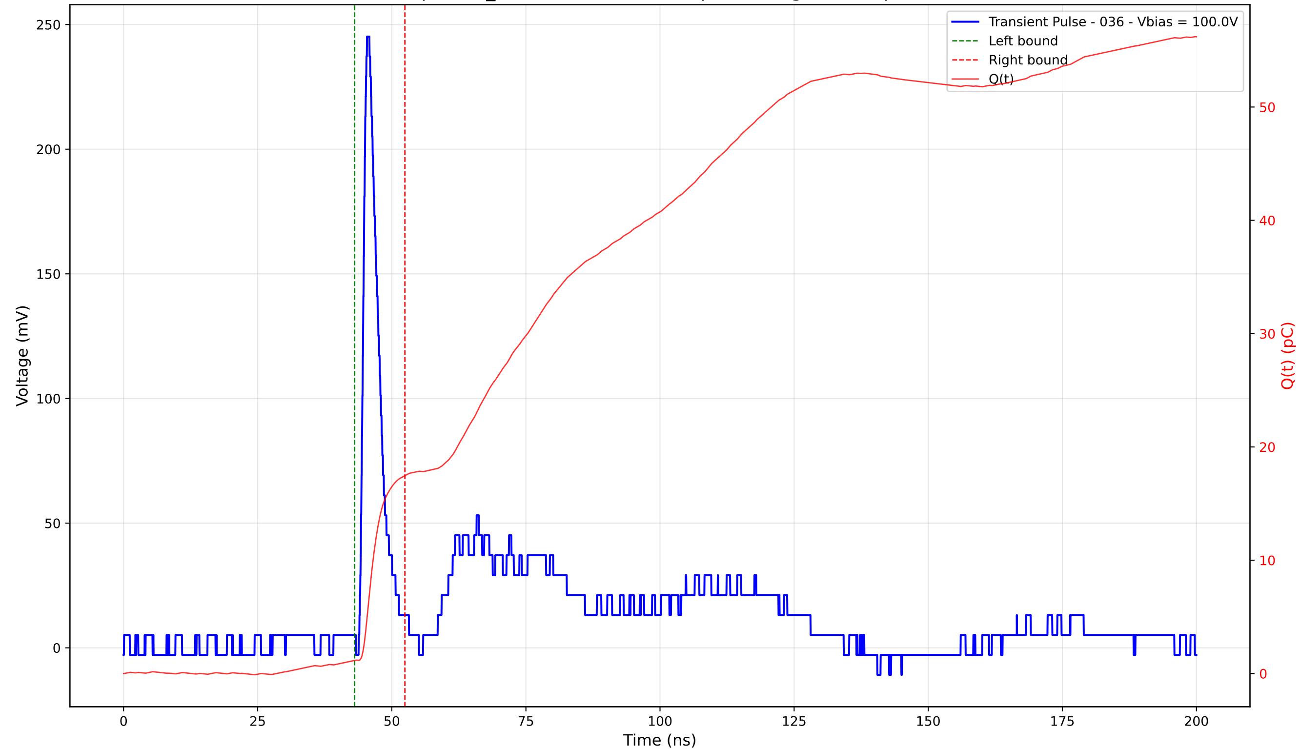
Transient Pulse - Sample: TD_4004 - Position: 355.0 \mu\text{m} - Charge: 16.30 pC - Rise Time: 1.01 ns
