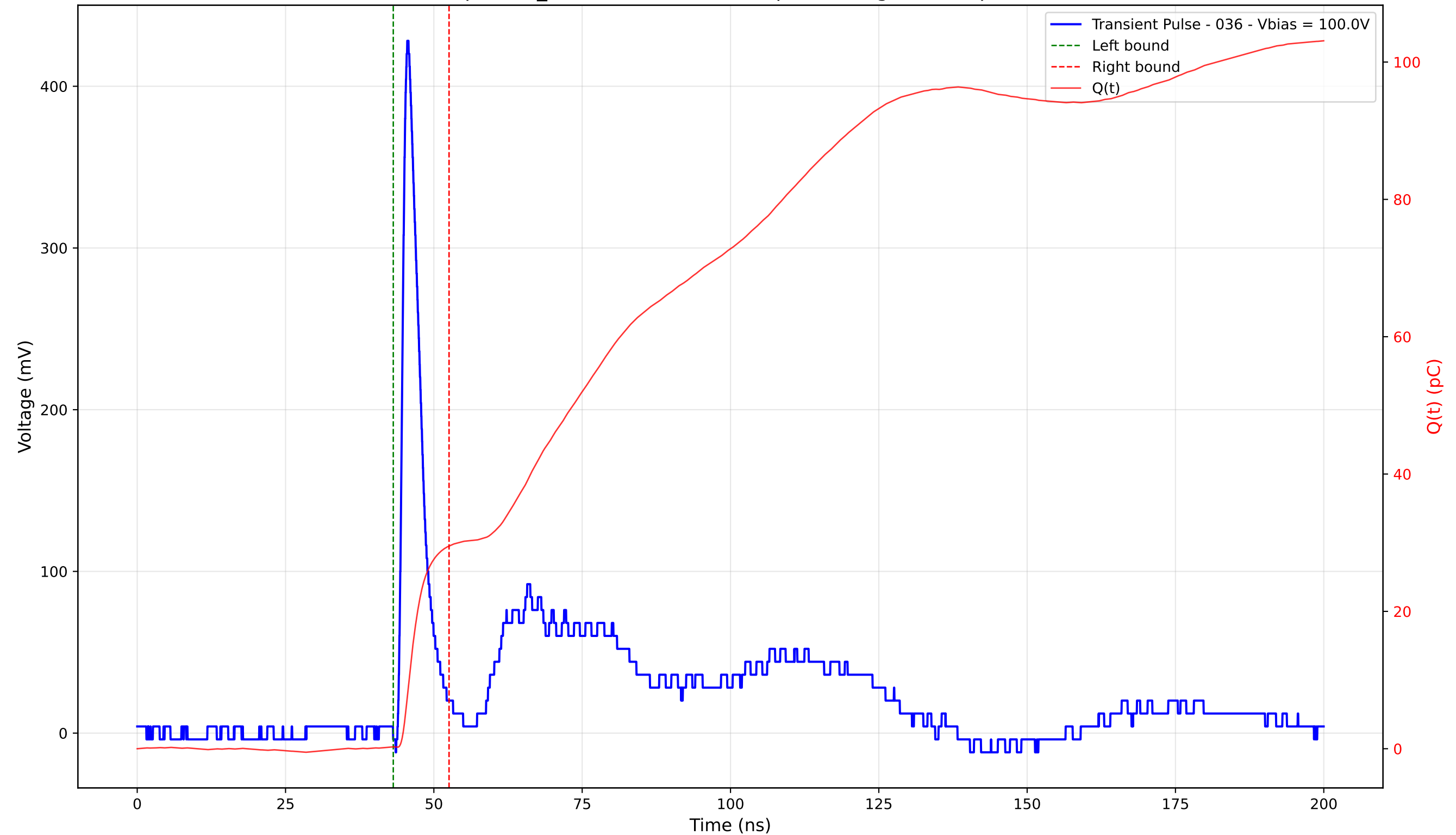
Transient Pulse - Sample: TD_4004 - Position: 270.0 \mu\text{m} - Charge: 29.23 pC - Rise Time: 1.06 ns
