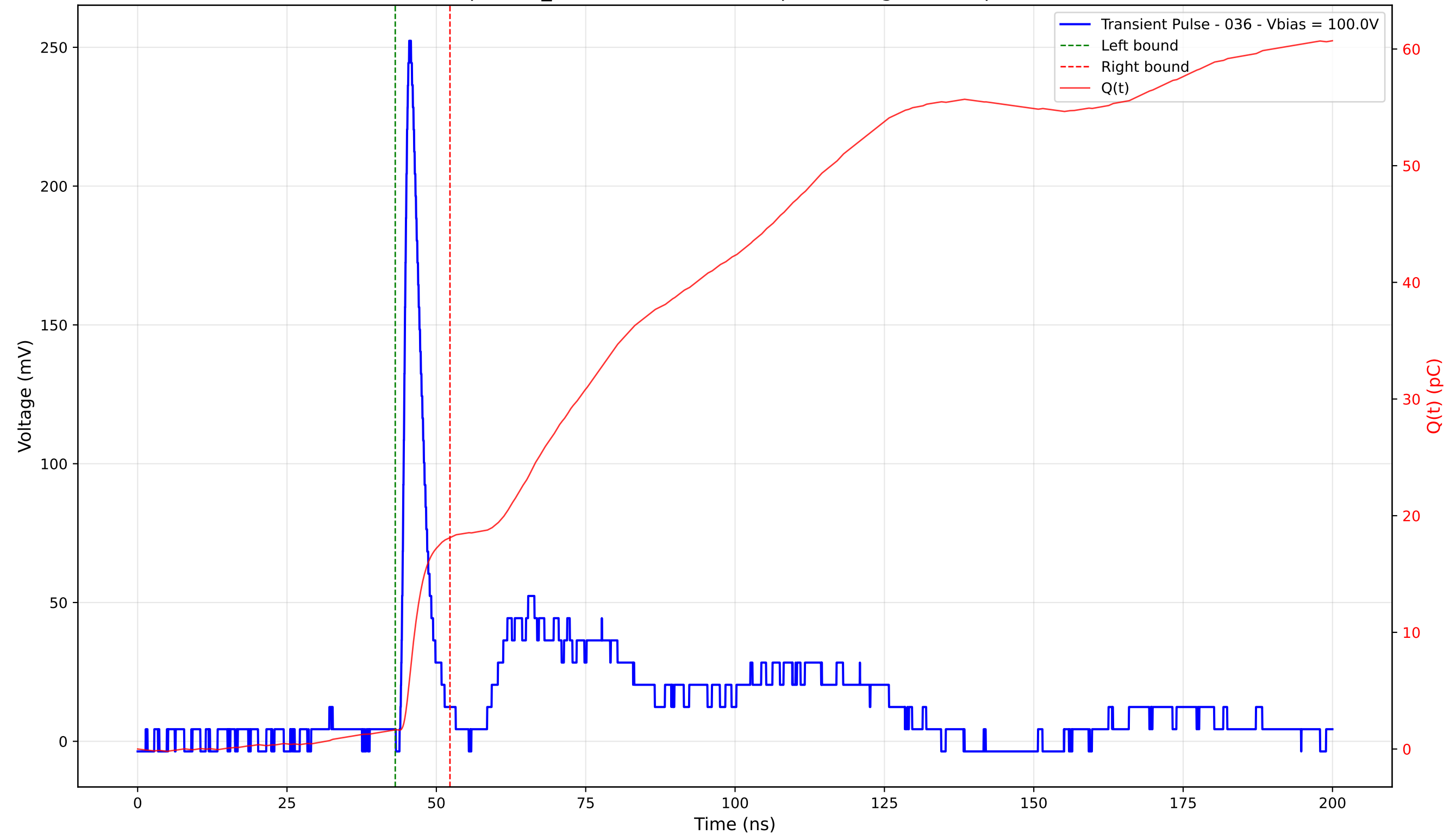
Transient Pulse - Sample: TD_4004 - Position: 335.0 \mu\text{m} - Charge: 16.47 pC - Rise Time: 1.05 ns
