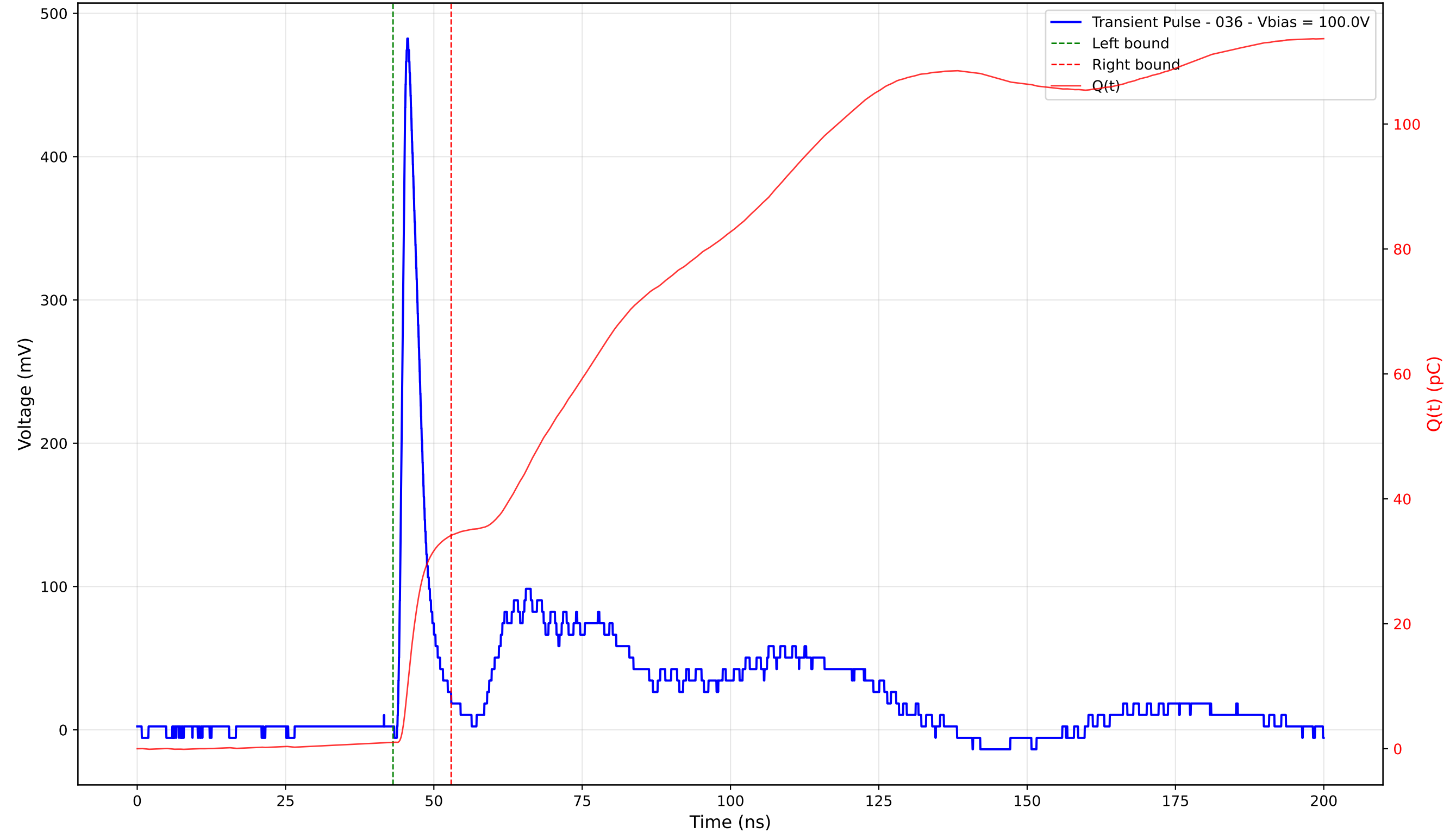
Transient Pulse - Sample: TD_4004 - Position: 255.0 \mu\text{m} - Charge: 33.12 pC - Rise Time: 1.05 ns
