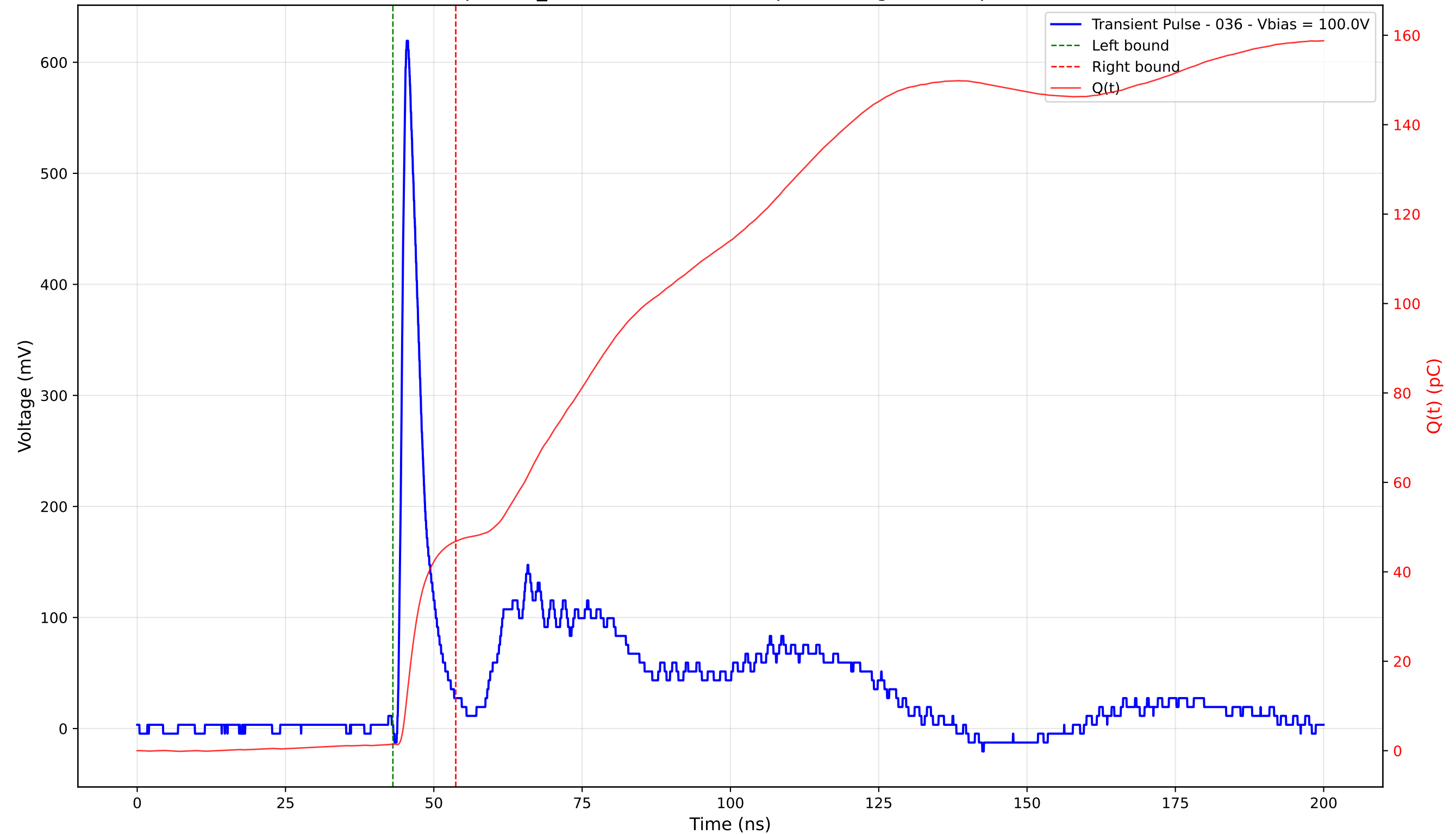
Transient Pulse - Sample: TD_4004 - Position: 220.0 \mu\text{m} - Charge: 45.35 pC - Rise Time: 1.00 ns
