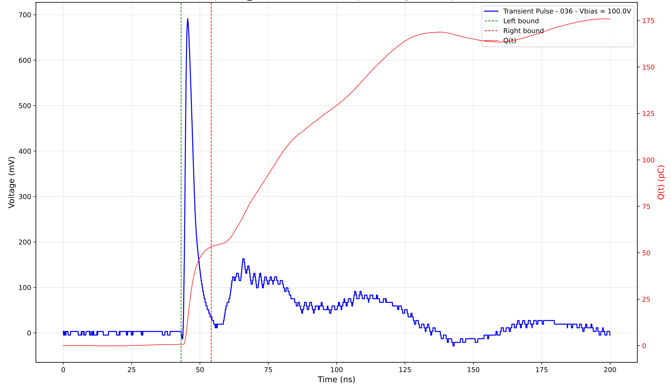
Transient Pulse - Sample: TD_4004 - Position: 190.0 \mu\text{m} - Charge: 52.50 pC - Rise Time: 1.00 ns
