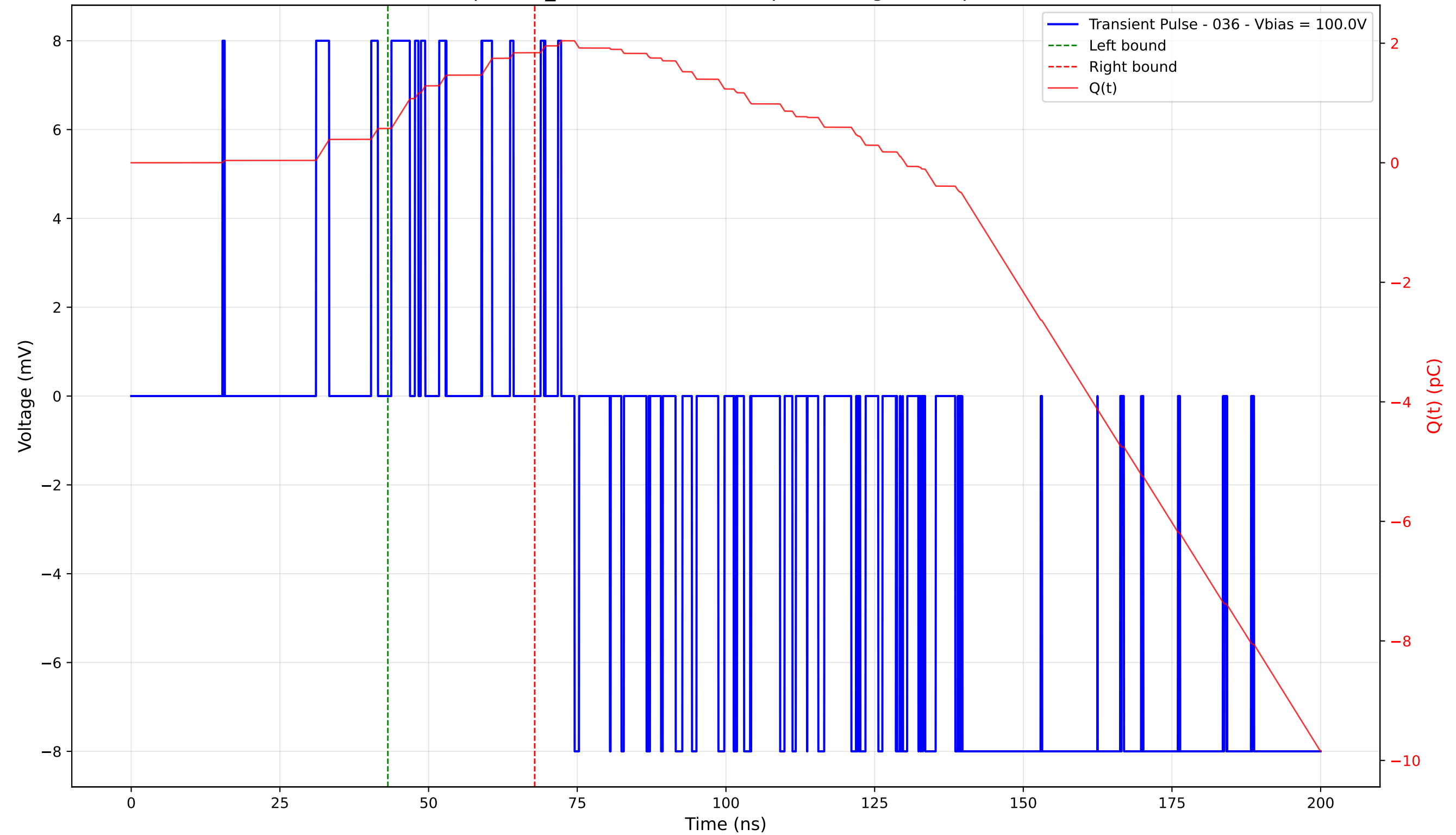
Transient Pulse - Sample: TD_4004 - Position: 20.0 \mu\text{m} - Charge: 1.27 pC - Rise Time: 0.02 ns
