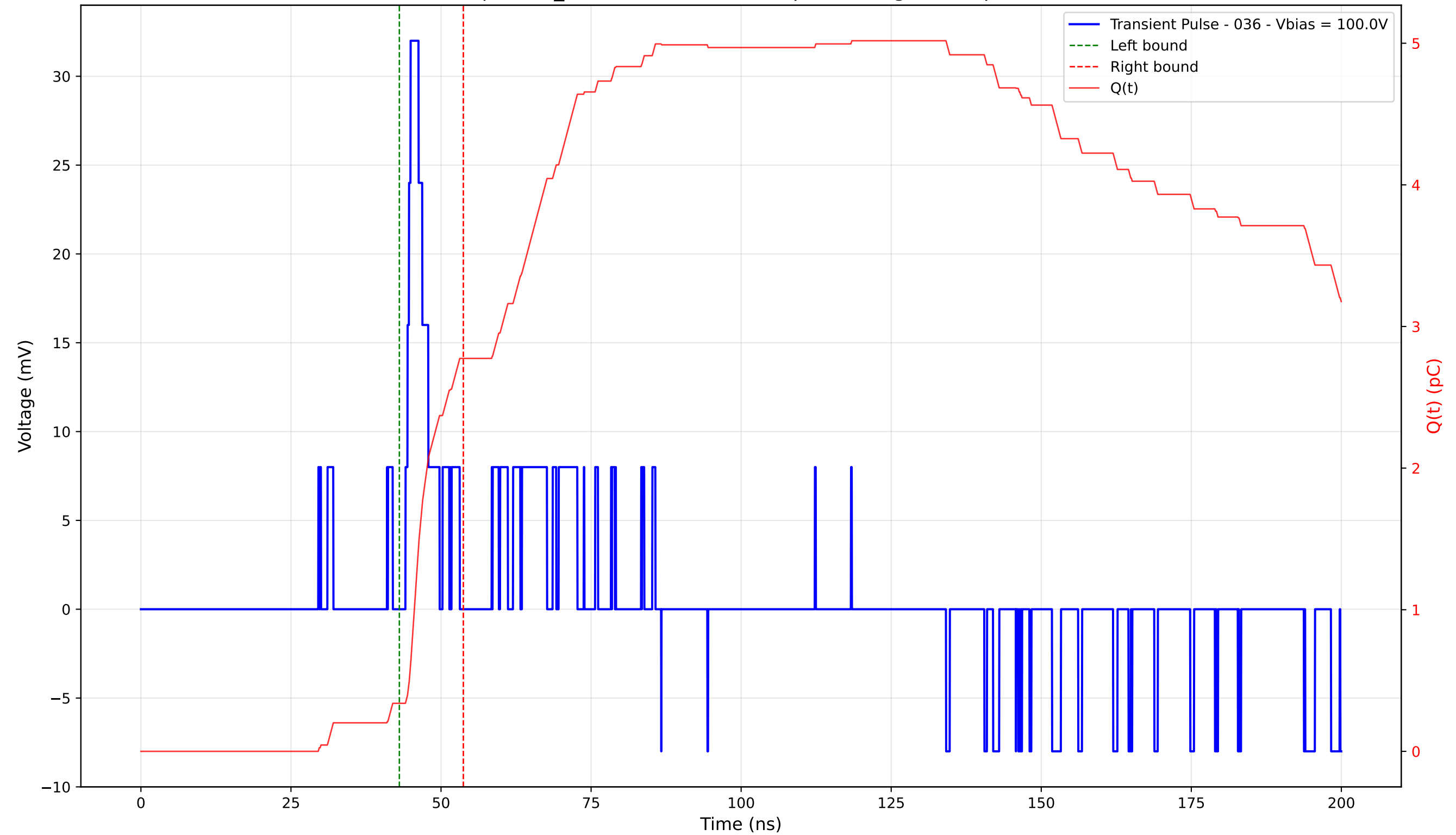
Transient Pulse - Sample: TD_4004 - Position: 435.0 \mu\text{m} - Charge: 2.44 pC - Rise Time: 0.85 ns
