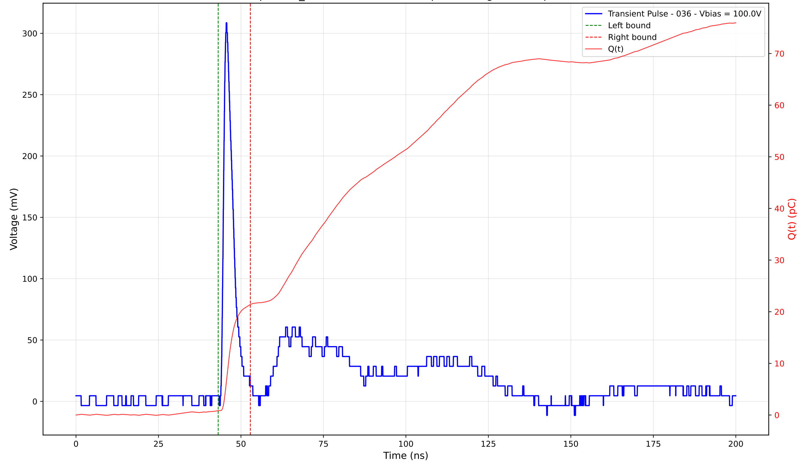
Transient Pulse - Sample: TD_4004 - Position: 325.0 \mu\text{m} - Charge: 20.56 pC - Rise Time: 1.11 ns
