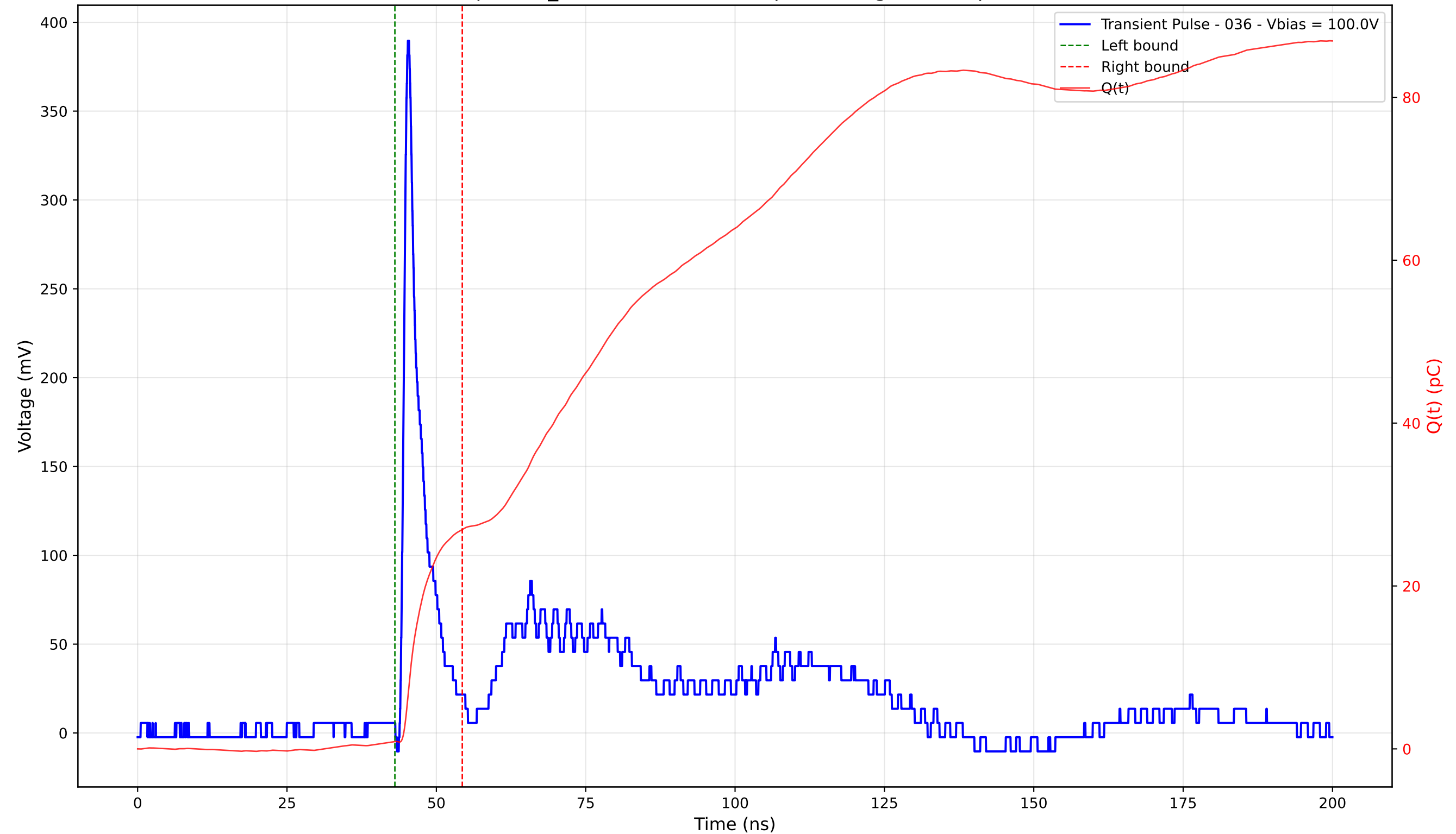
Transient Pulse - Sample: TD_4004 - Position: 70.0 \mu\text{m} - Charge: 26.03 pC - Rise Time: 0.92 ns
