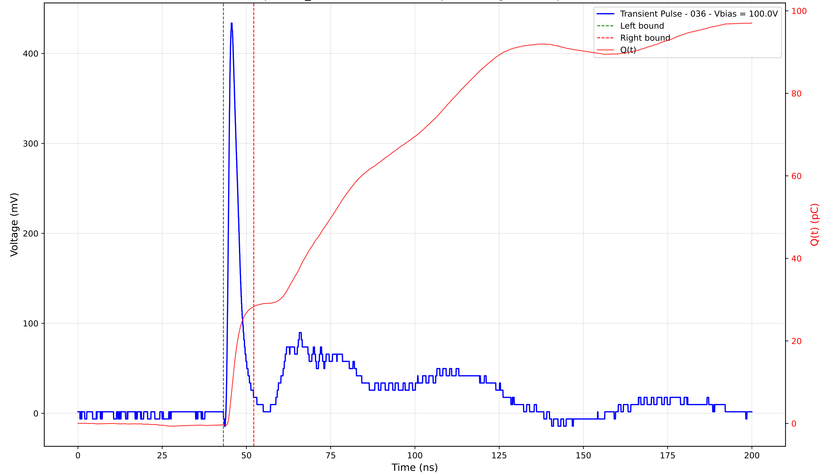
Transient Pulse - Sample: TD_4004 - Position: 285.0 \mu\text{m} - Charge: 28.68 pC - Rise Time: 1.04 ns
