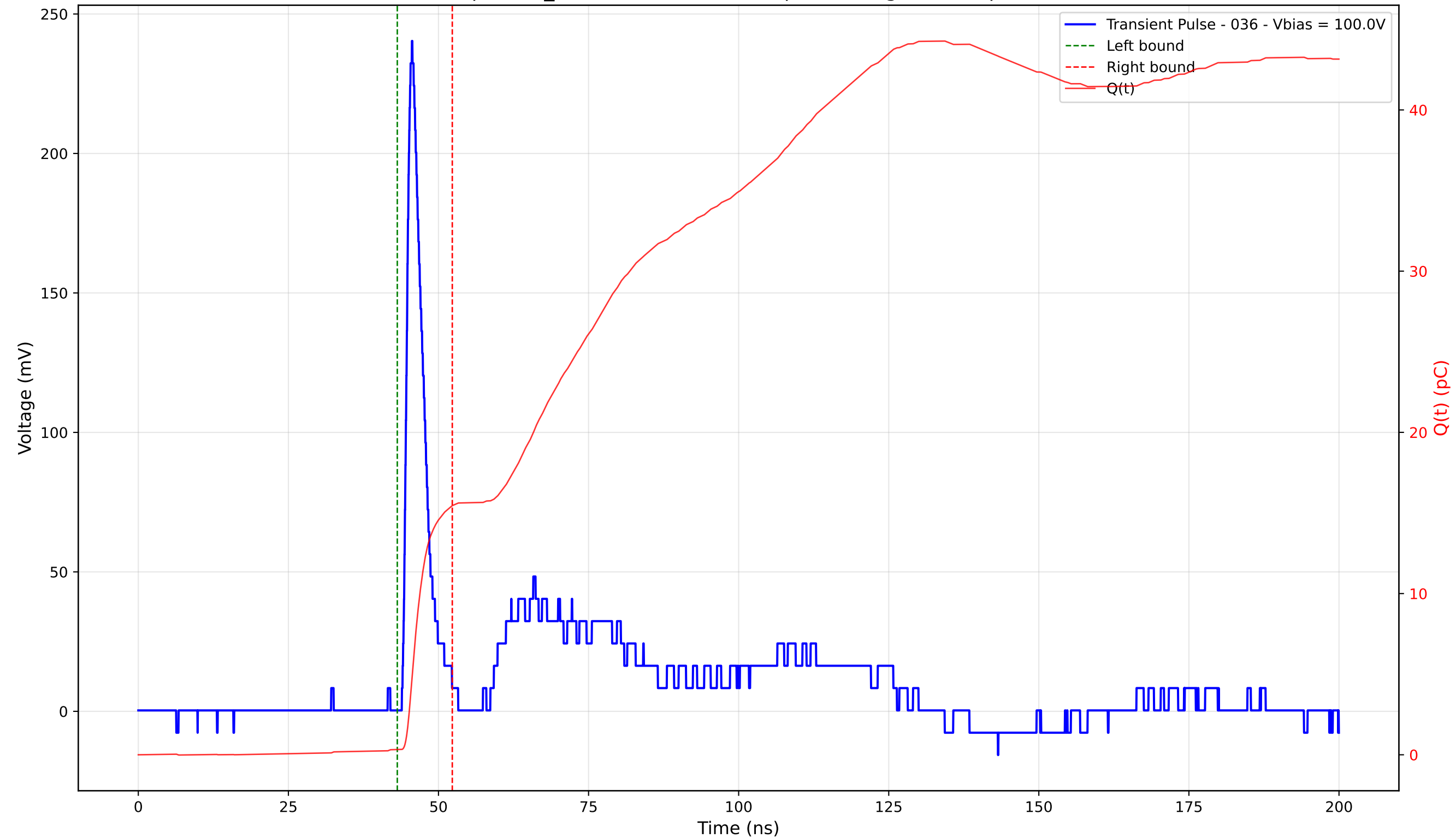
Transient Pulse - Sample: TD_4004 - Position: 360.0 \mu\text{m} - Charge: 15.14 pC - Rise Time: 1.08 ns
