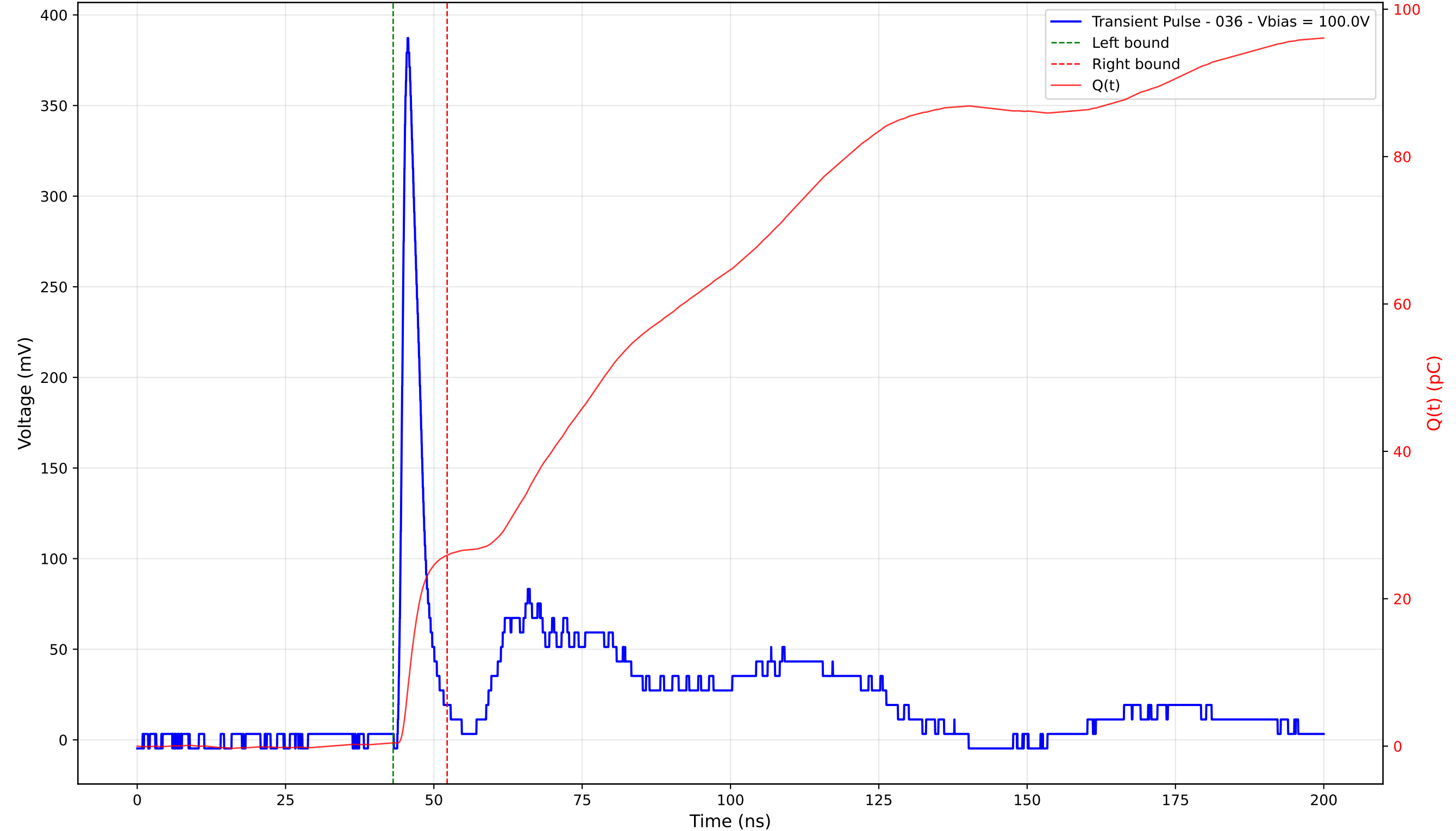
Transient Pulse - Sample: TD_4004 - Position: 305.0 \mu\text{m} - Charge: 25.46 pC - Rise Time: 1.09 ns
