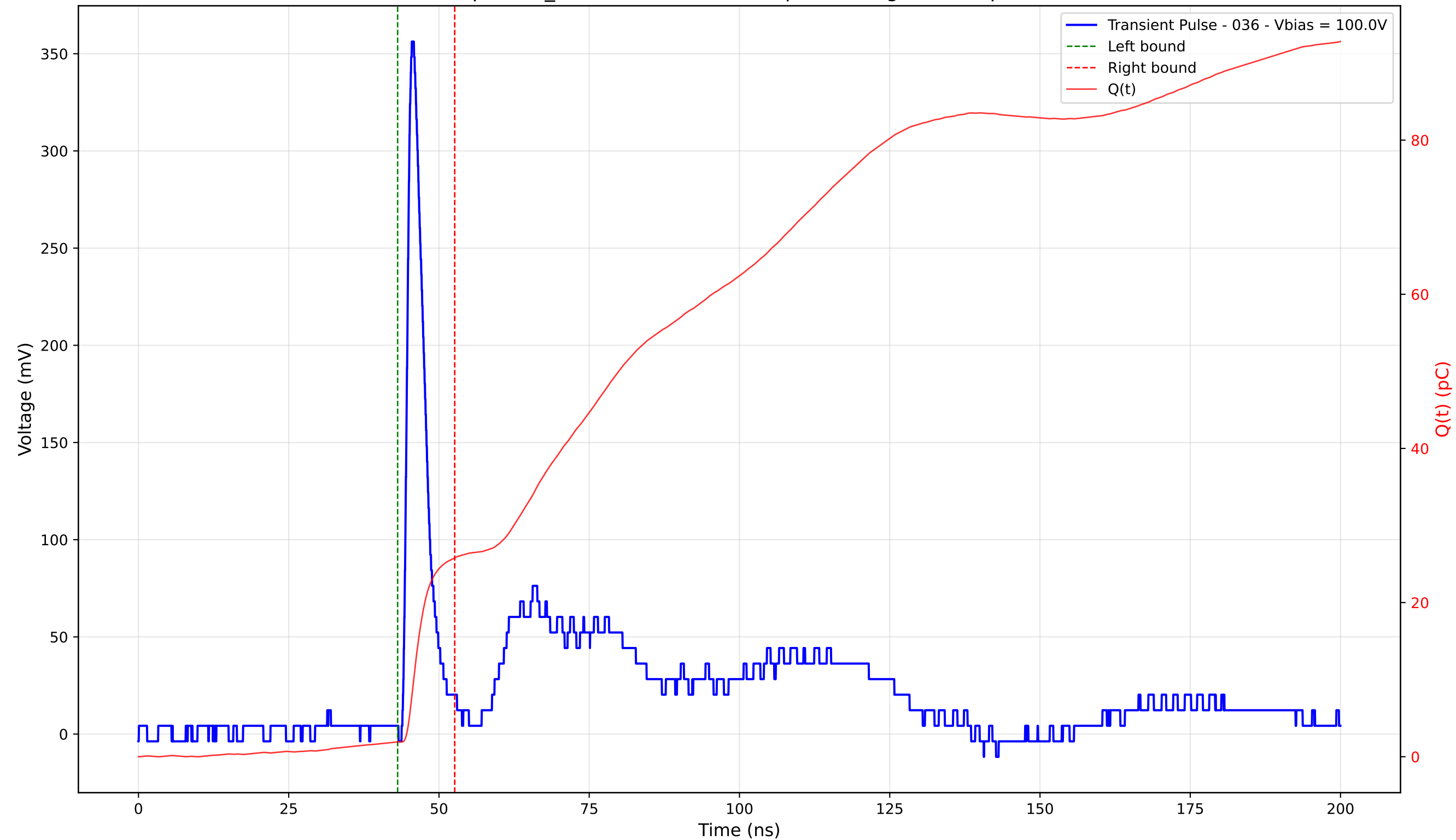
Transient Pulse - Sample: TD_4004 - Position: 310.0 \mu\text{m} - Charge: 23.87 pC - Rise Time: 1.06 ns
