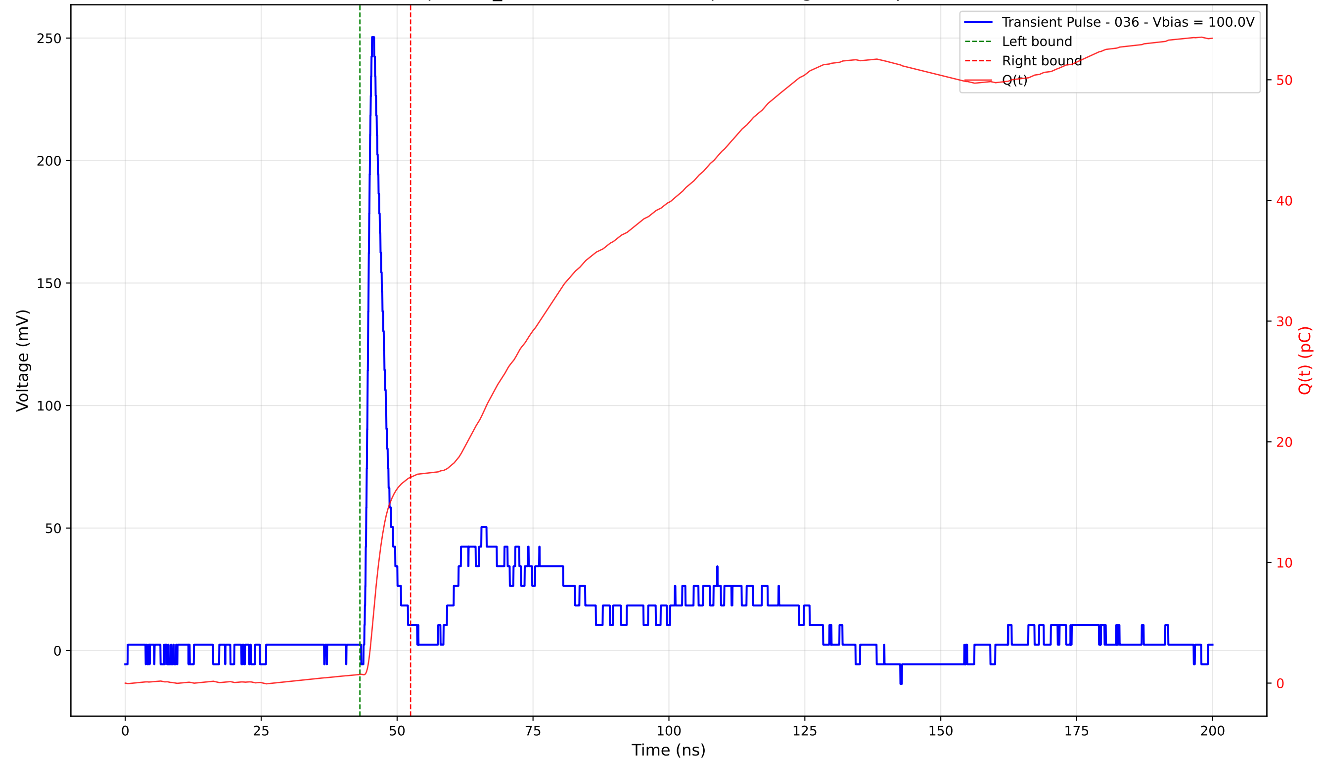
Transient Pulse - Sample: TD_4004 - Position: 340.0 \mu\text{m} - Charge: 16.33 pC - Rise Time: 1.00 ns
