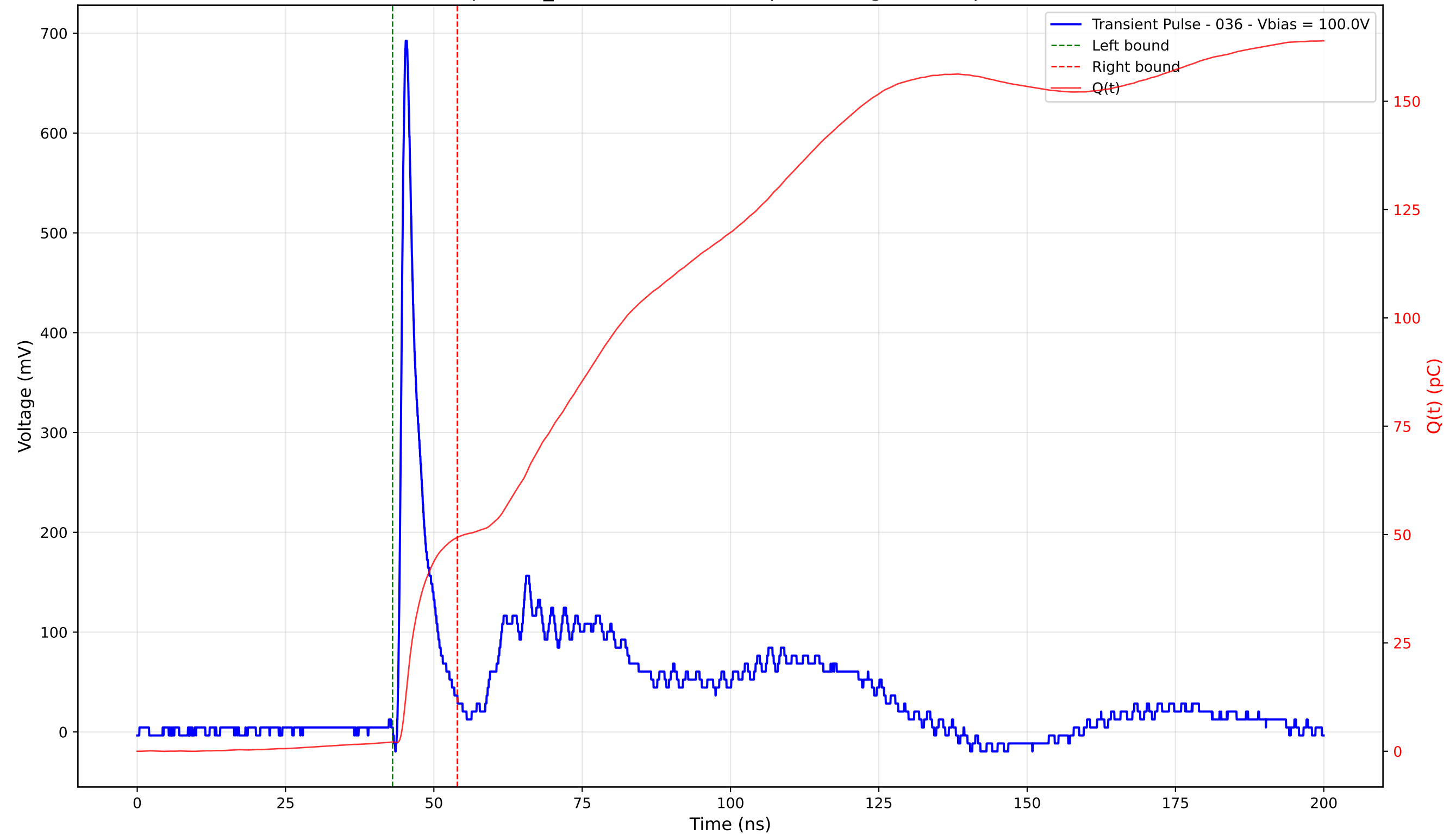
Transient Pulse - Sample: TD_4004 - Position: 95.0 \mu\text{m} - Charge: 47.23 pC - Rise Time: 0.92 ns
