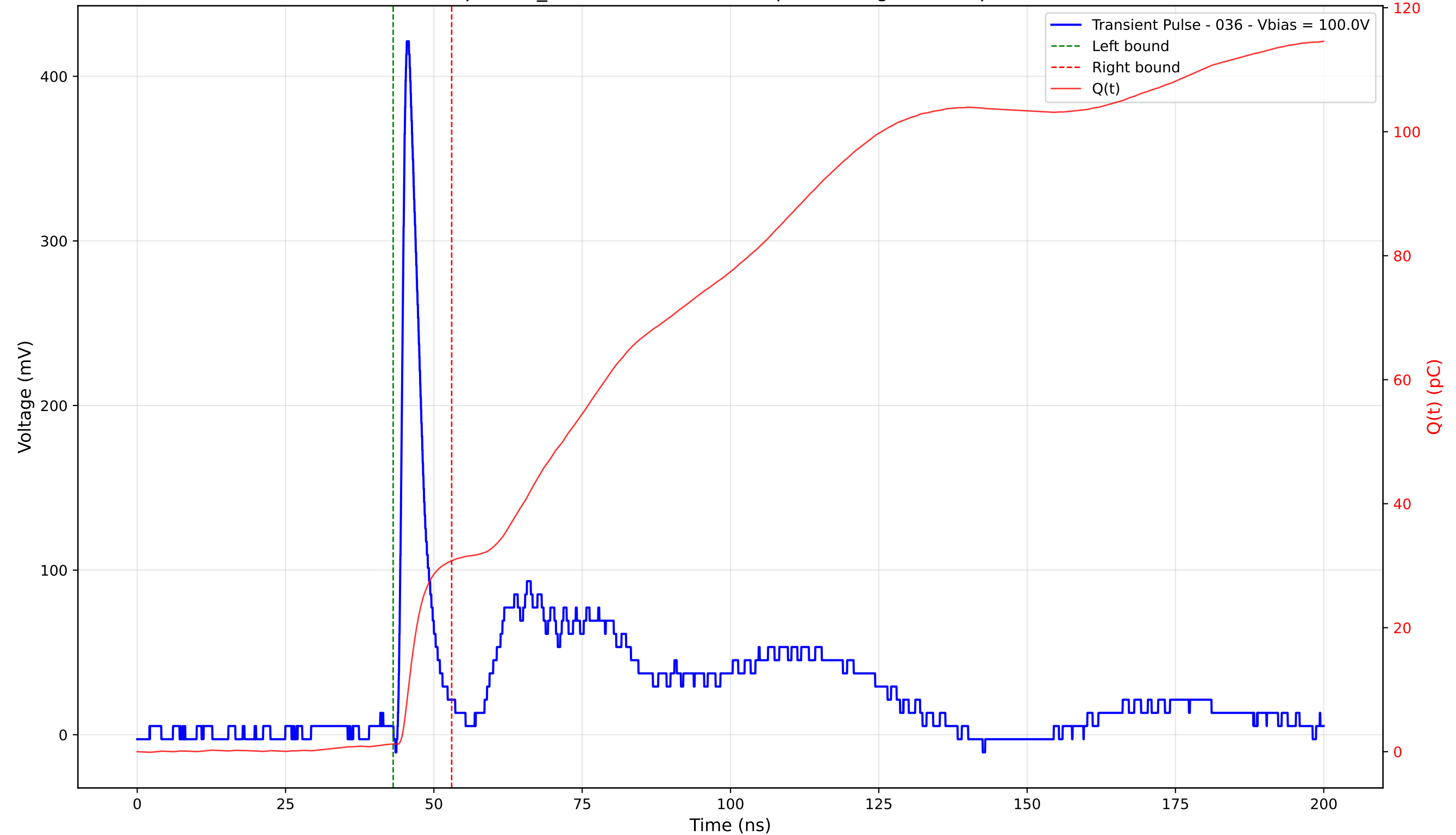
Transient Pulse - Sample: TD_4004 - Position: 265.0 \mu\text{m} - Charge: 29.53 pC - Rise Time: 1.03 ns
