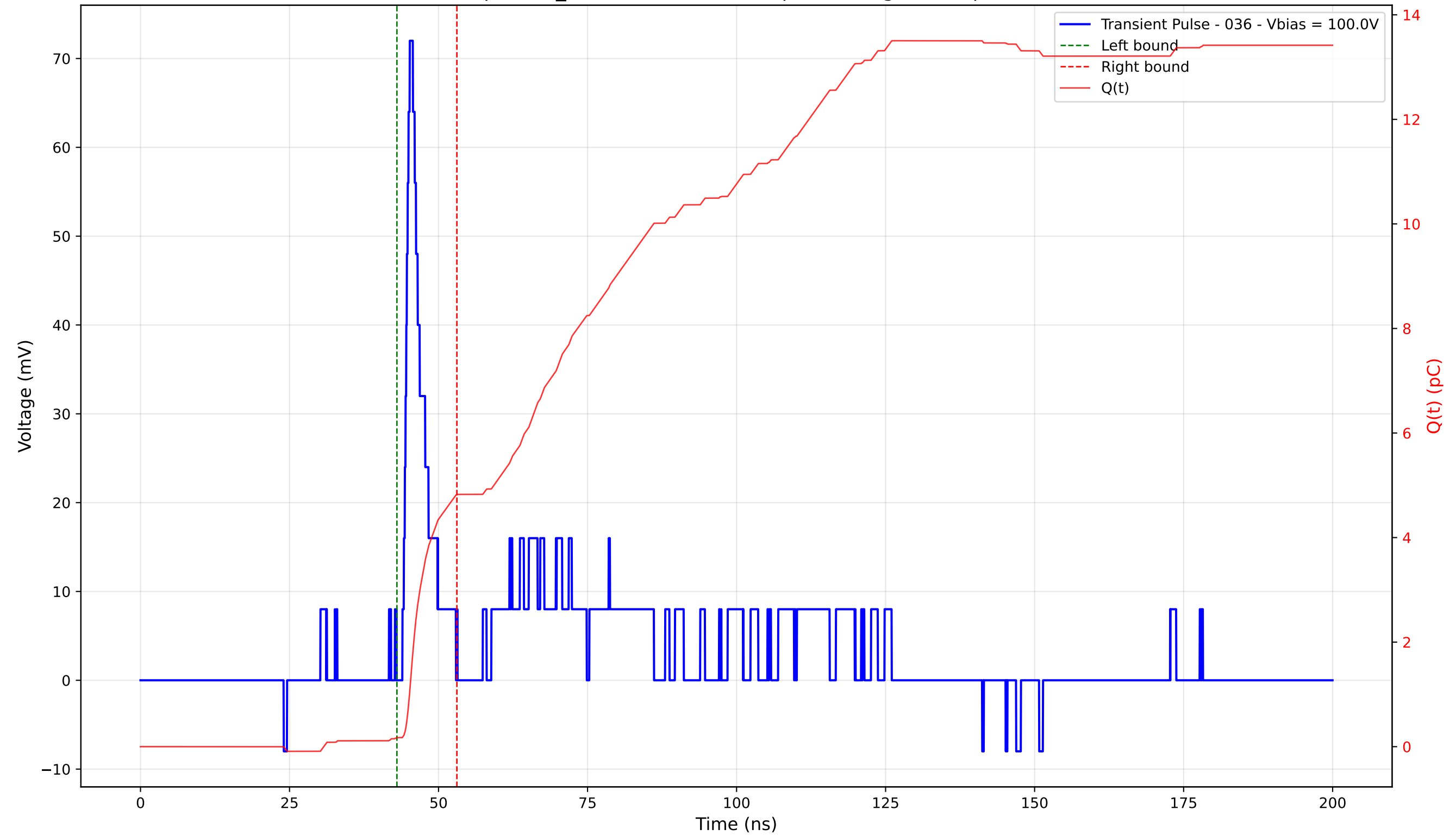
Transient Pulse - Sample: TD_4004 - Position: 50.0 \mu\text{m} - Charge: 4.64 pC - Rise Time: 1.22 ns
