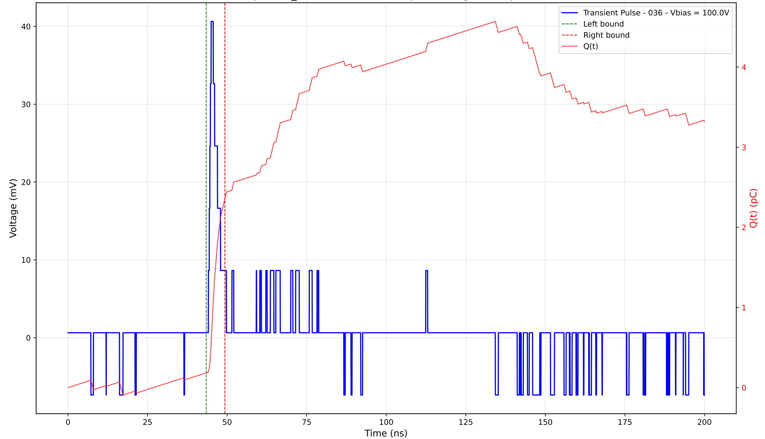
Transient Pulse - Sample: TD_4004 - Position: 45.0 \mu\text{m} - Charge: 2.18 pC - Rise Time: 0.87 ns
