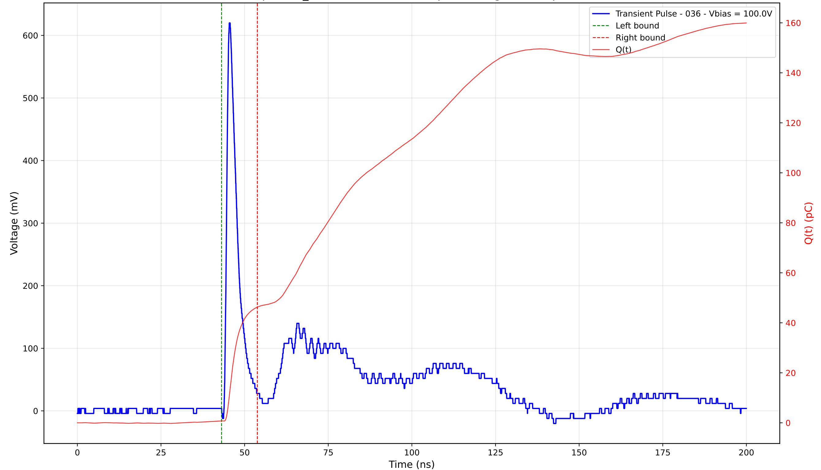
Transient Pulse - Sample: TD_4004 - Position: 215.0 \mu\text{m} - Charge: 45.51 pC - Rise Time: 1.02 ns
