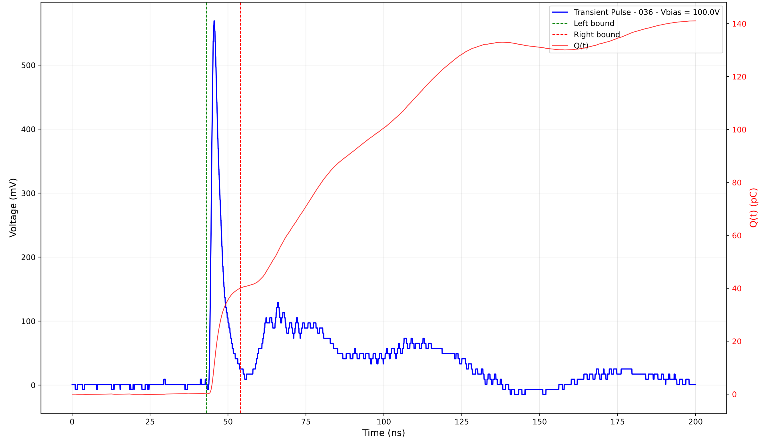
Transient Pulse - Sample: TD_4004 - Position: 135.0 \mu\text{m} - Charge: 39.70 pC - Rise Time: 1.02 ns
