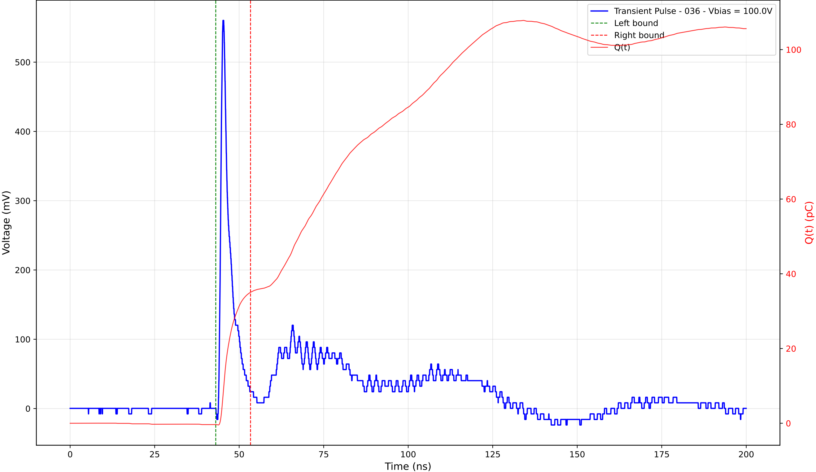
Transient Pulse - Sample: TD_4004 - Position: 80.0 \mu\text{m} - Charge: 35.36 pC - Rise Time: 0.90 ns
