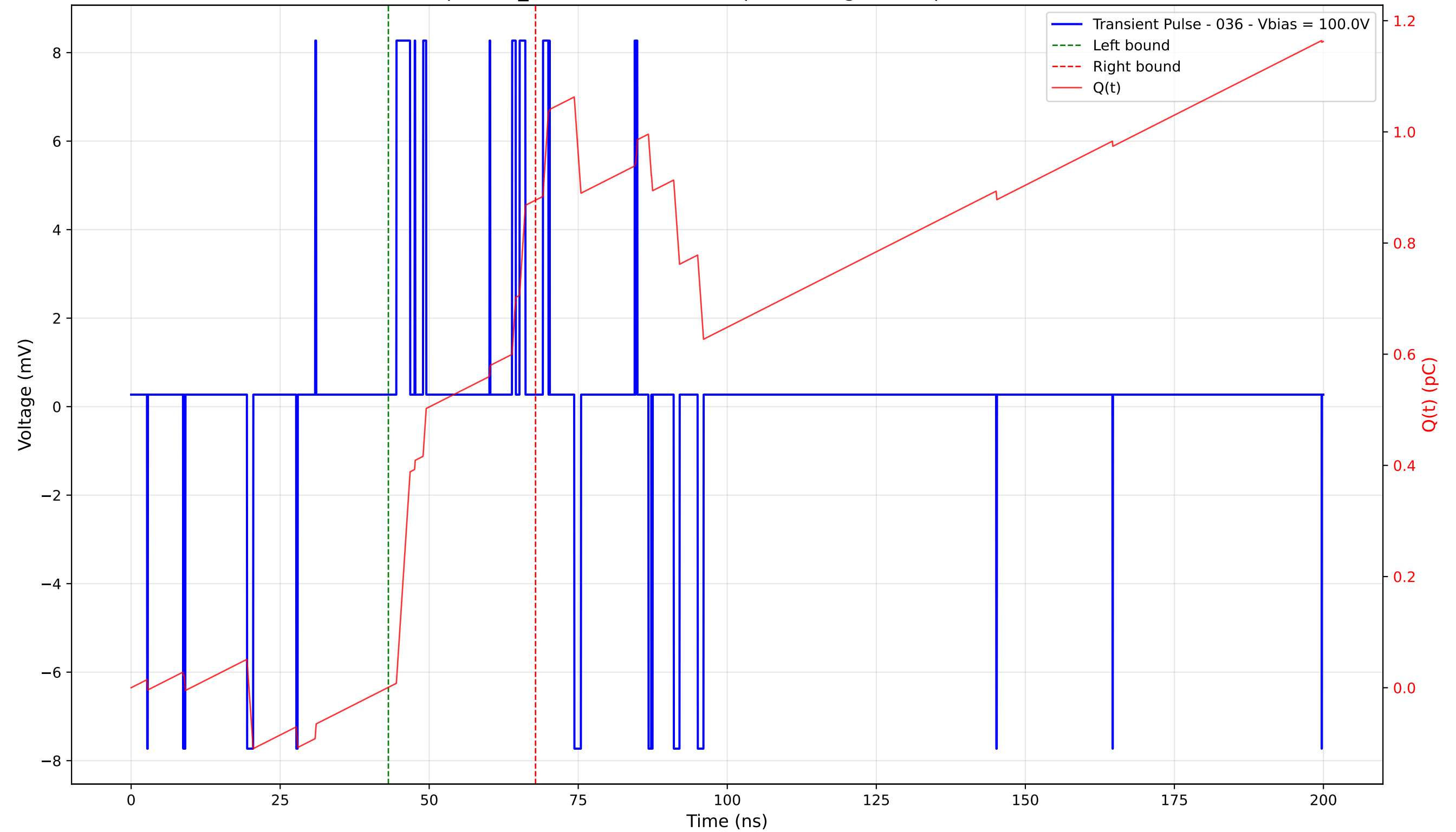
Transient Pulse - Sample: TD_4004 - Position: 10.0 \mu\text{m} - Charge: 0.88 pC - Rise Time: 0.00 ns (N/A)
