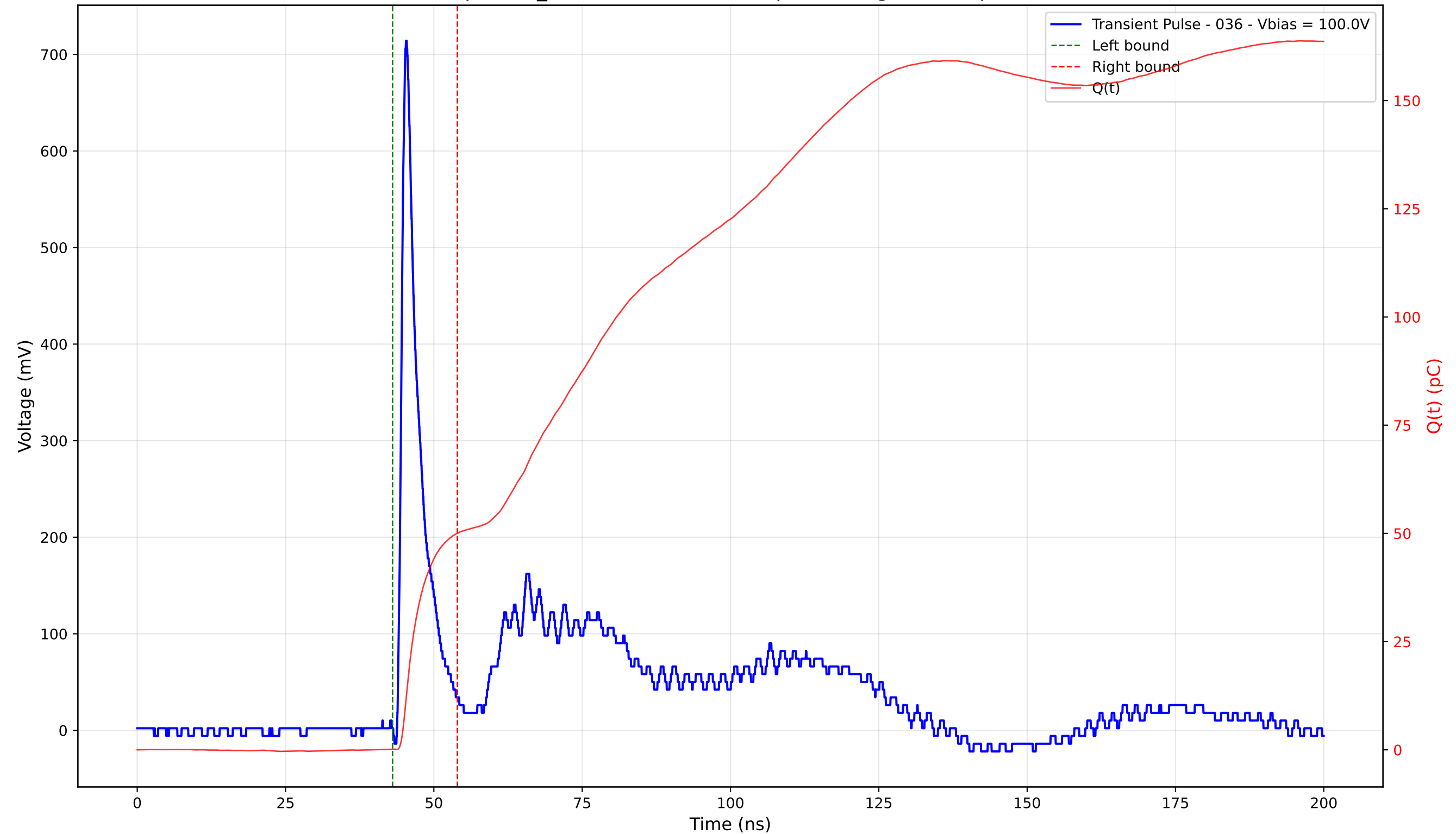
Transient Pulse - Sample: TD_4004 - Position: 100.0 \mu\text{m} - Charge: 49.85 pC - Rise Time: 0.95 ns
