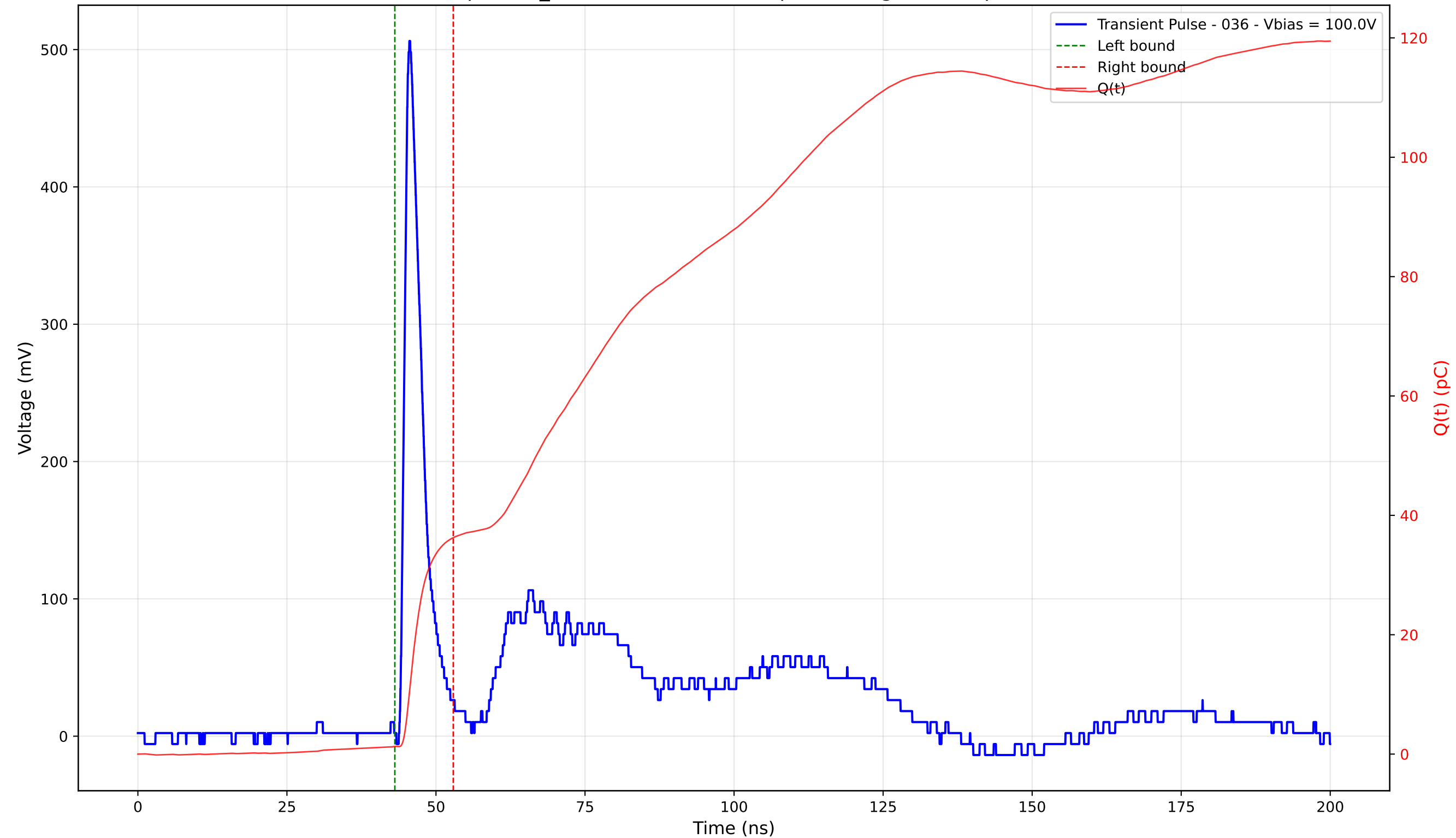
Transient Pulse - Sample: TD_4004 - Position: 240.0 \mu\text{m} - Charge: 34.98 pC - Rise Time: 1.06 ns
