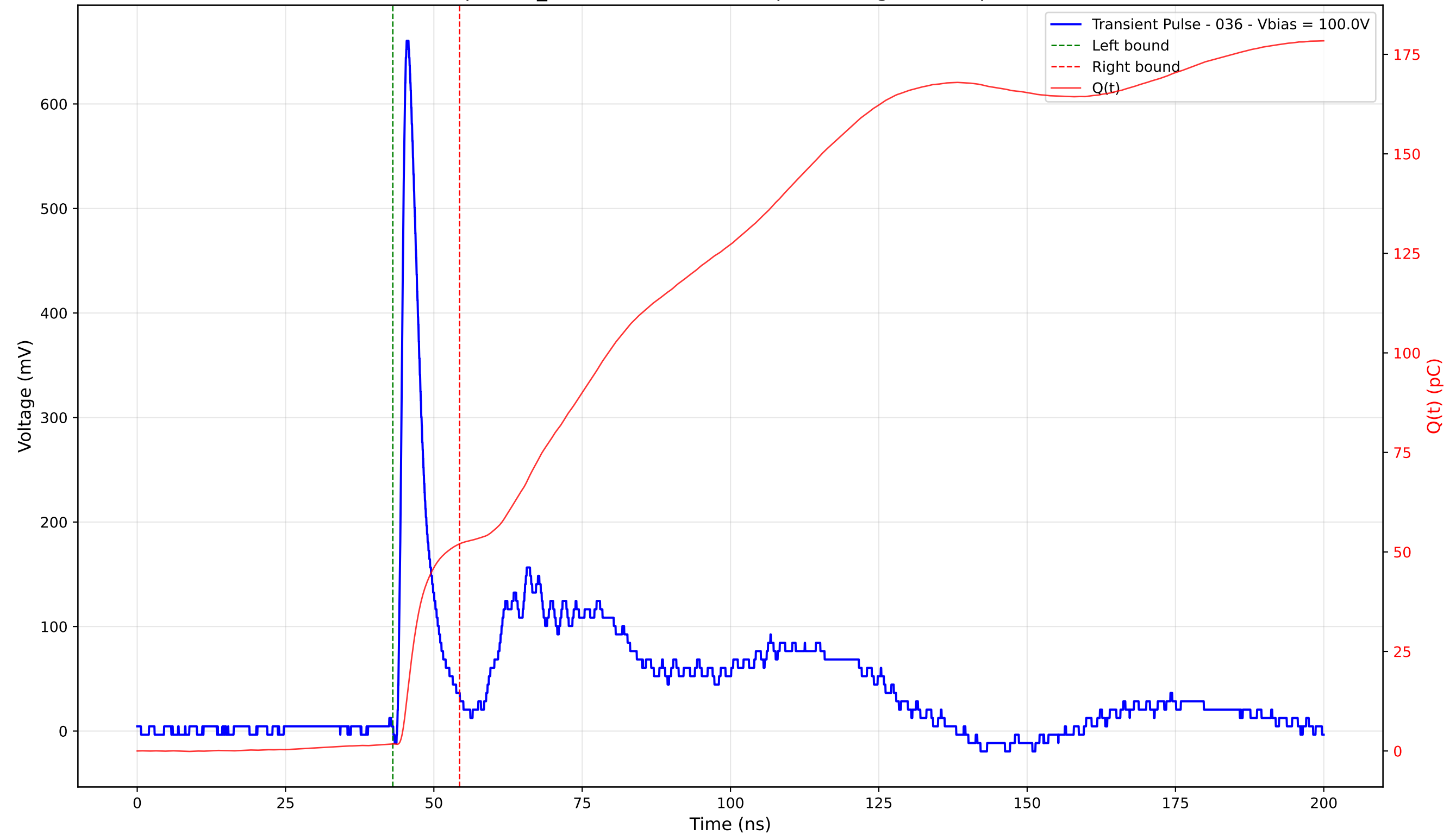
Transient Pulse - Sample: TD_4004 - Position: 175.0 \mu\text{m} - Charge: 50.28 pC - Rise Time: 1.02 ns
