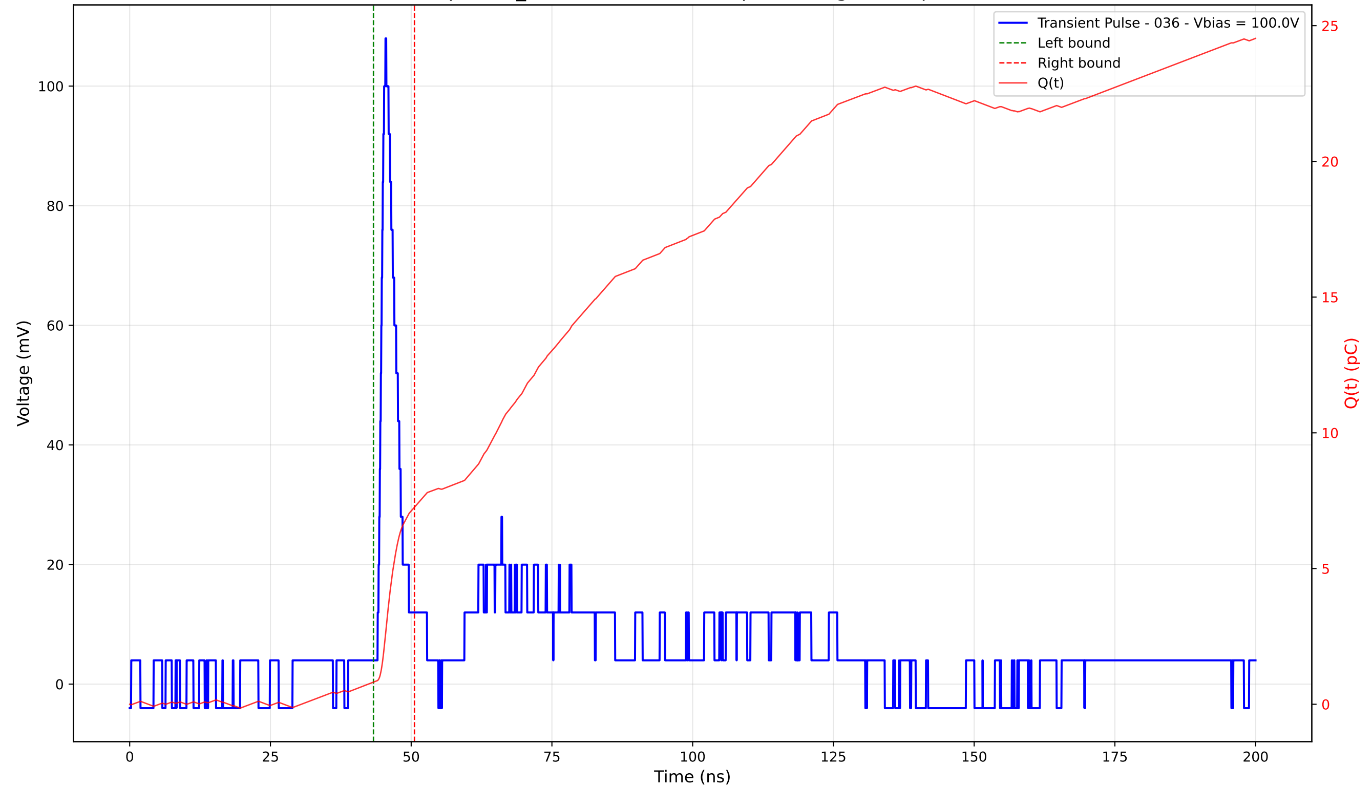
Transient Pulse - Sample: TD_4004 - Position: 405.0 \mu\text{m} - Charge: 6.45 pC - Rise Time: 1.14 ns
