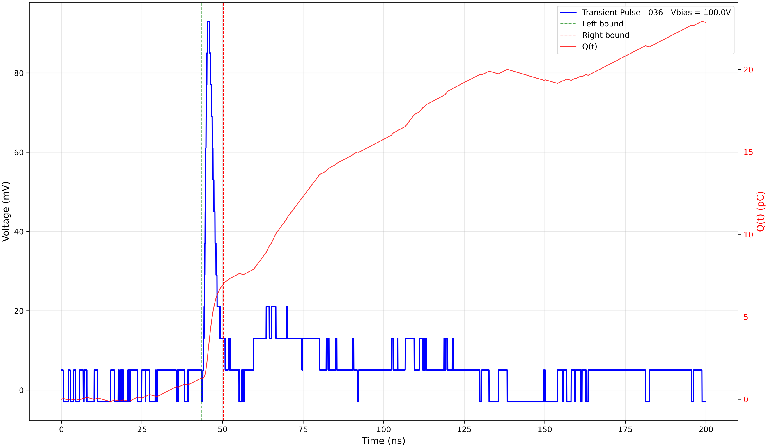
Transient Pulse - Sample: TD_4004 - Position: 410.0 \mu\text{m} - Charge: 5.69 pC - Rise Time: 1.01 ns
