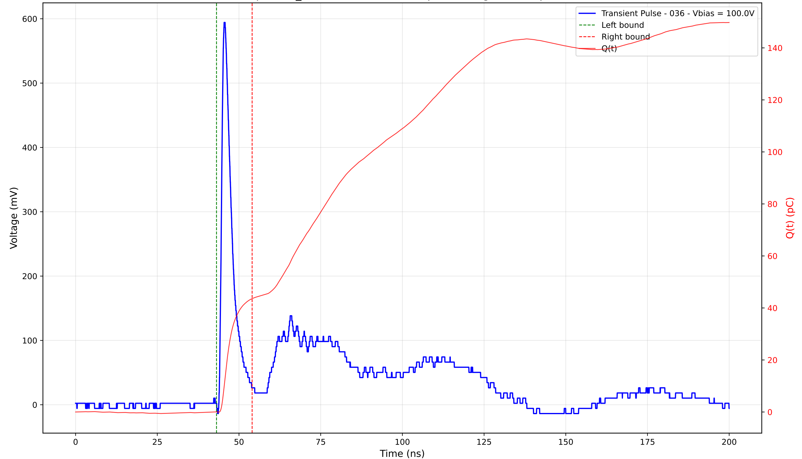
Transient Pulse - Sample: TD_4004 - Position: 165.0 \mu\text{m} - Charge: 43.56 pC - Rise Time: 1.02 ns
