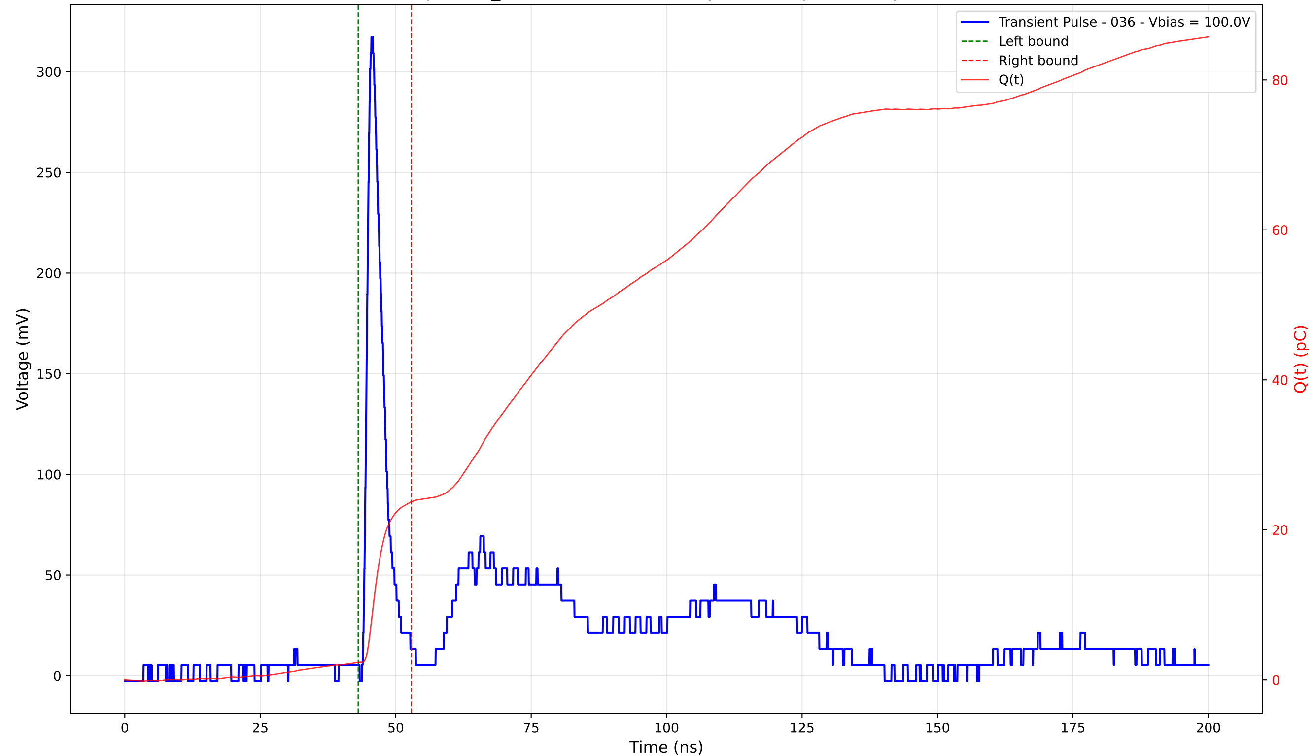
Transient Pulse - Sample: TD_4004 - Position: 320.0 \mu\text{m} - Charge: 21.43 pC - Rise Time: 1.13 ns
