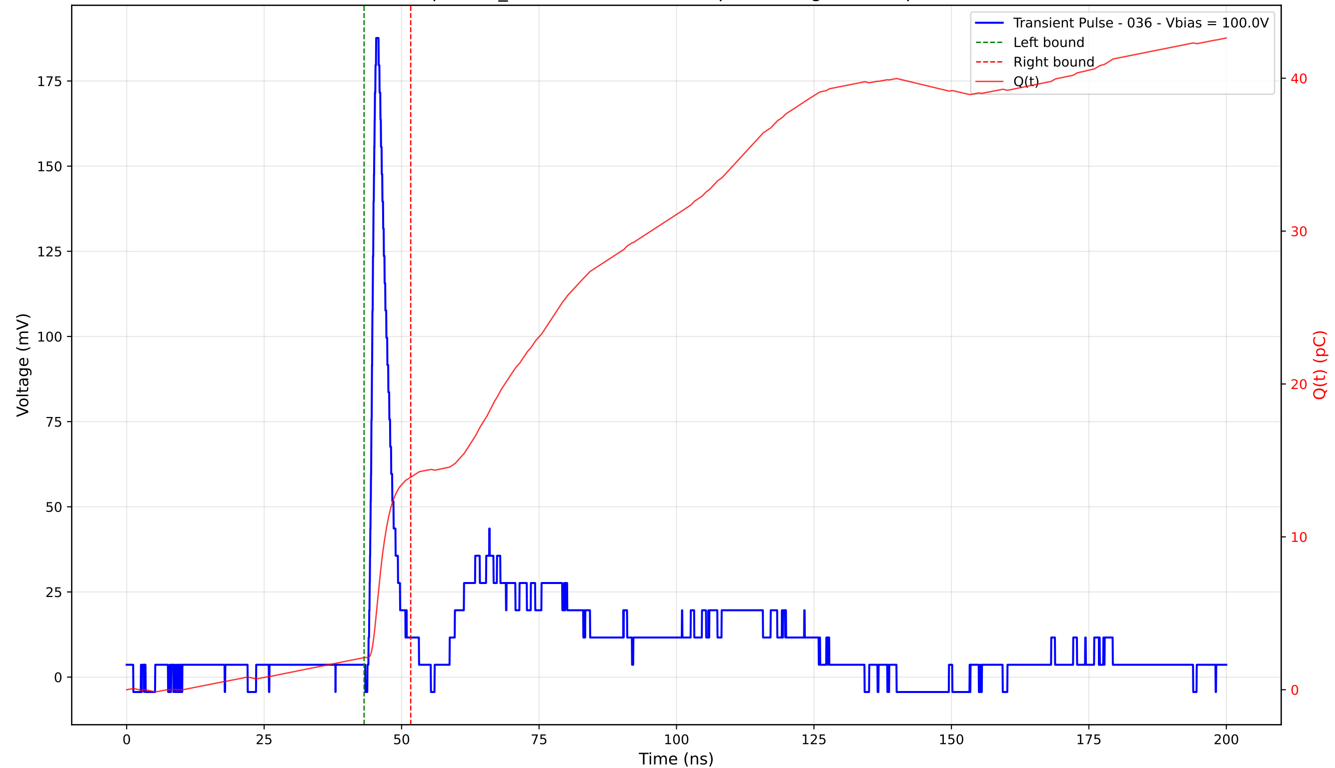
Transient Pulse - Sample: TD_4004 - Position: 390.0 \mu\text{m} - Charge: 11.81 pC - Rise Time: 1.04 ns
