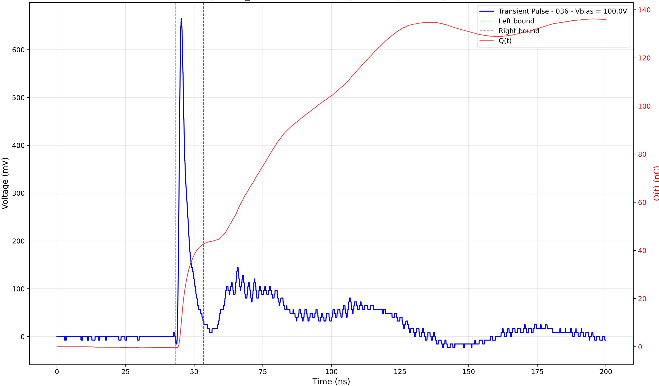
Transient Pulse - Sample: TD_4004 - Position: 90.0 \mu\text{m} - Charge: 42.99 pC - Rise Time: 0.91 ns
