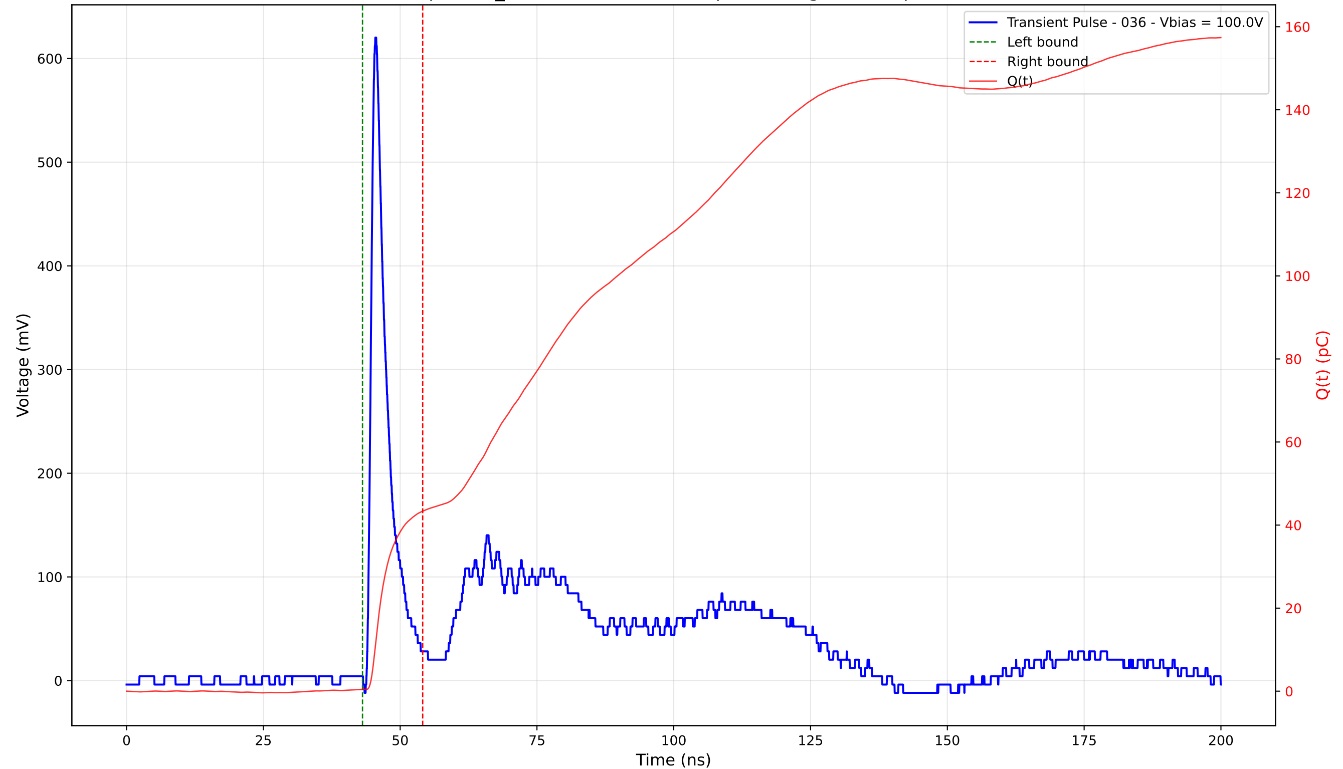
Transient Pulse - Sample: TD_4004 - Position: 130.0 \mu\text{m} - Charge: 42.88 pC - Rise Time: 1.02 ns
