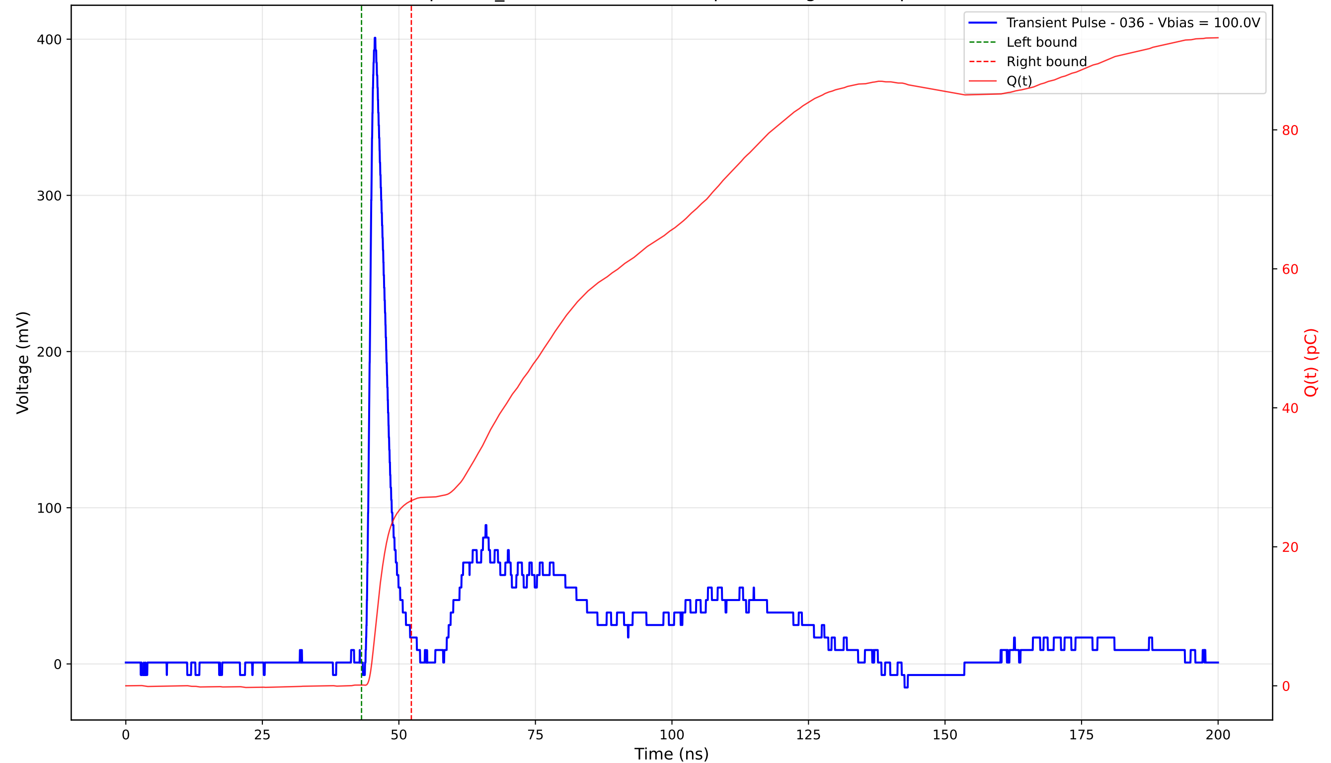
Transient Pulse - Sample: TD_4004 - Position: 290.0 \mu\text{m} - Charge: 26.52 pC - Rise Time: 1.06 ns
