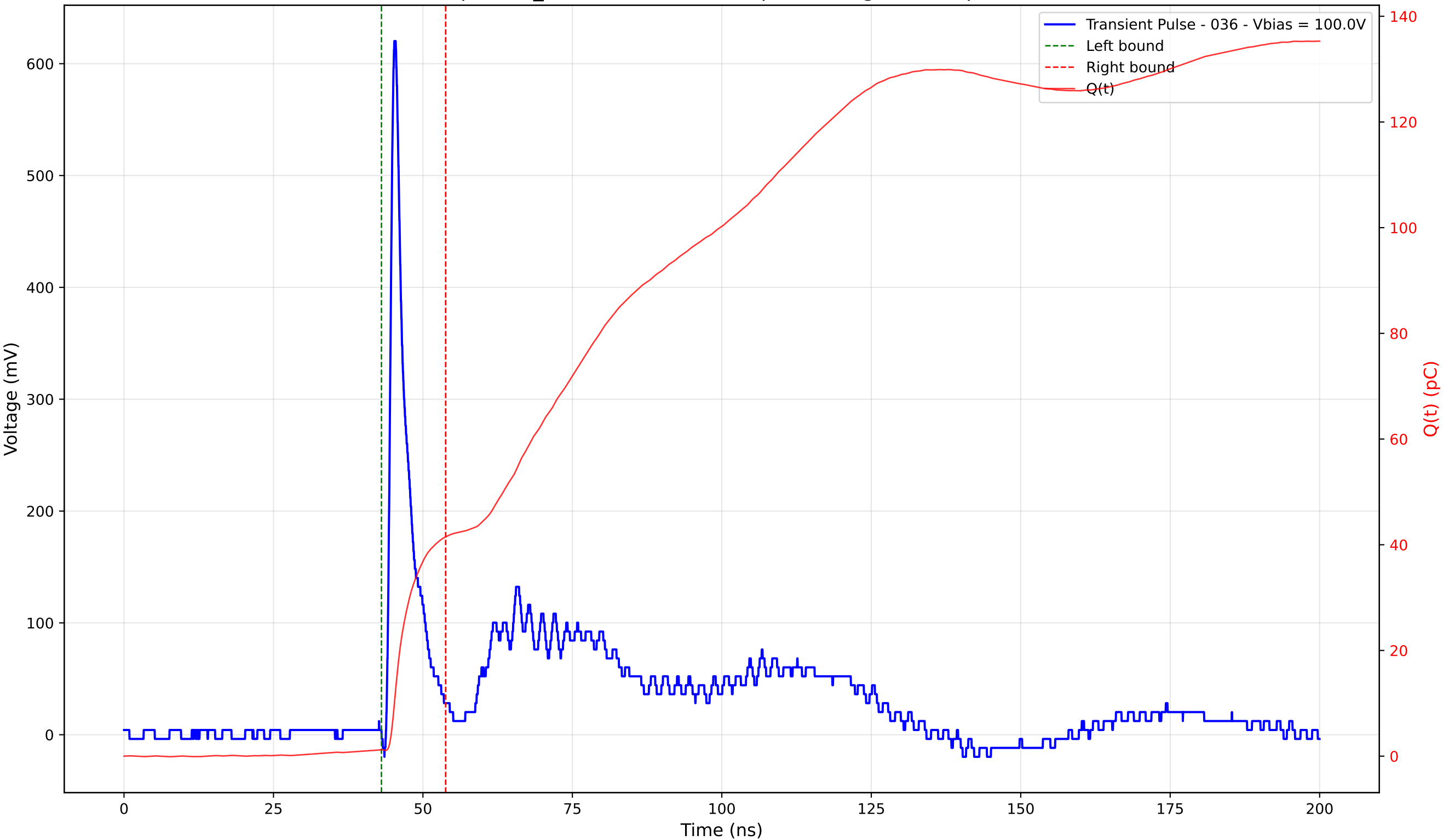
Transient Pulse - Sample: TD_4004 - Position: 85.0 \mu\text{m} - Charge: 40.27 pC - Rise Time: 0.92 ns
