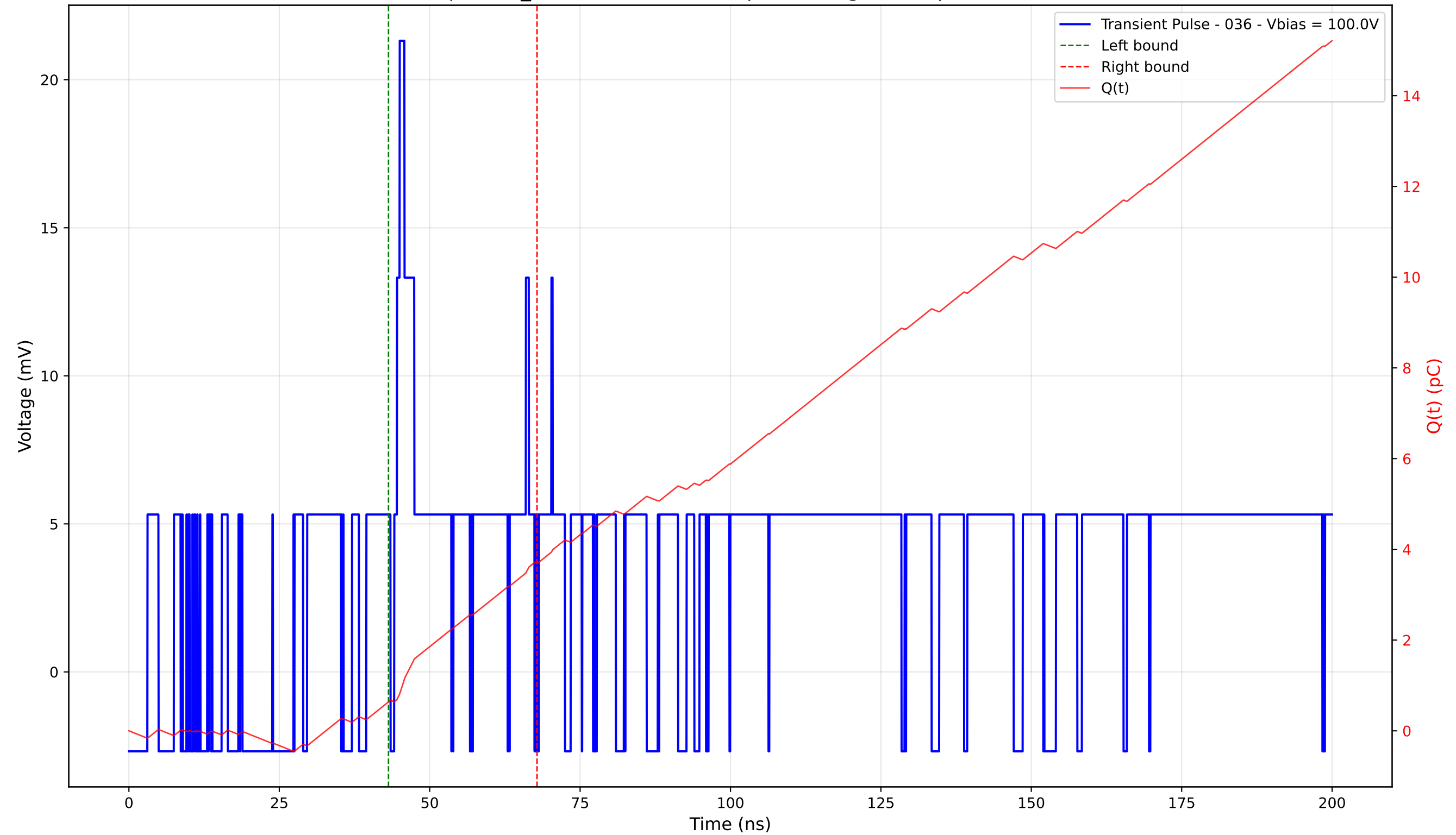
Transient Pulse - Sample: TD_4004 - Position: 30.0 \mu m - Charge: 3.07 pC - Rise Time: 0.00 ns (N/A)
