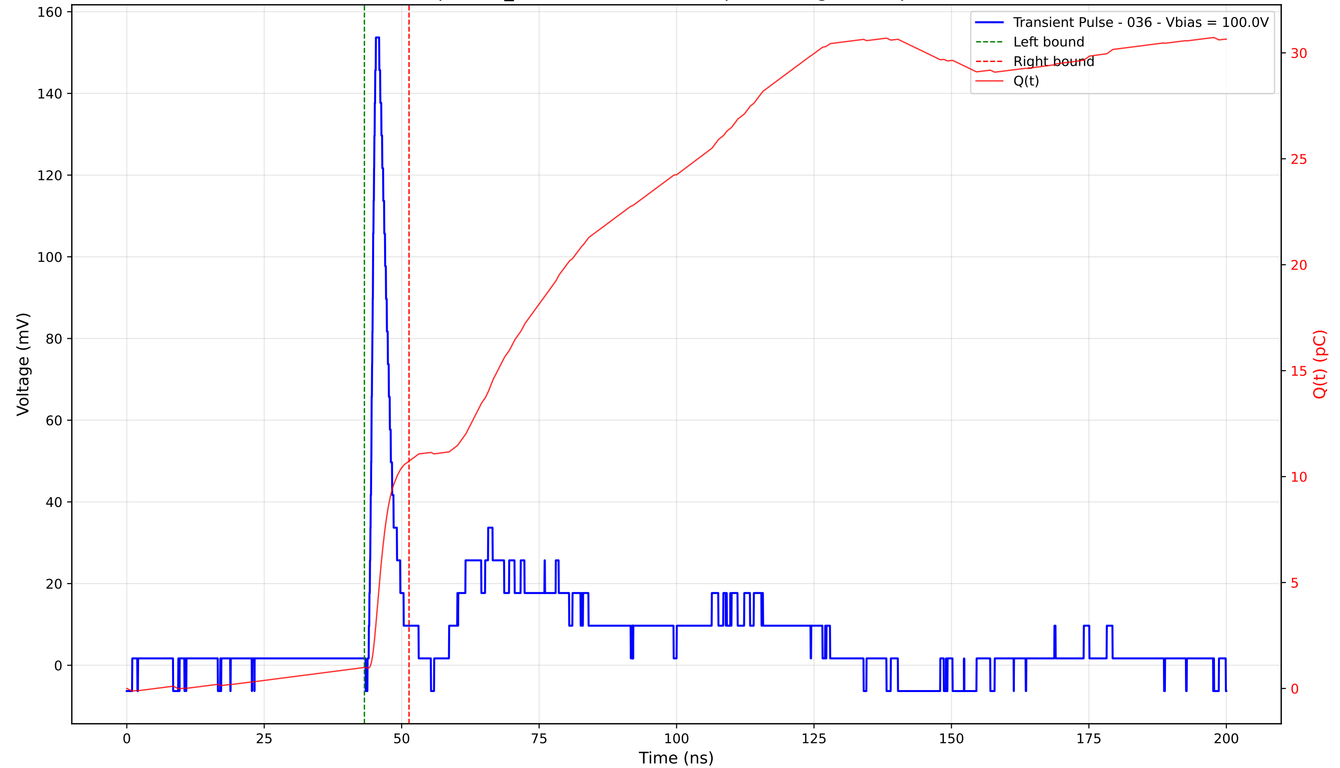
Transient Pulse - Sample: TD_4004 - Position: 395.0 \mu\text{m} - Charge: 9.74 pC - Rise Time: 1.07 ns
