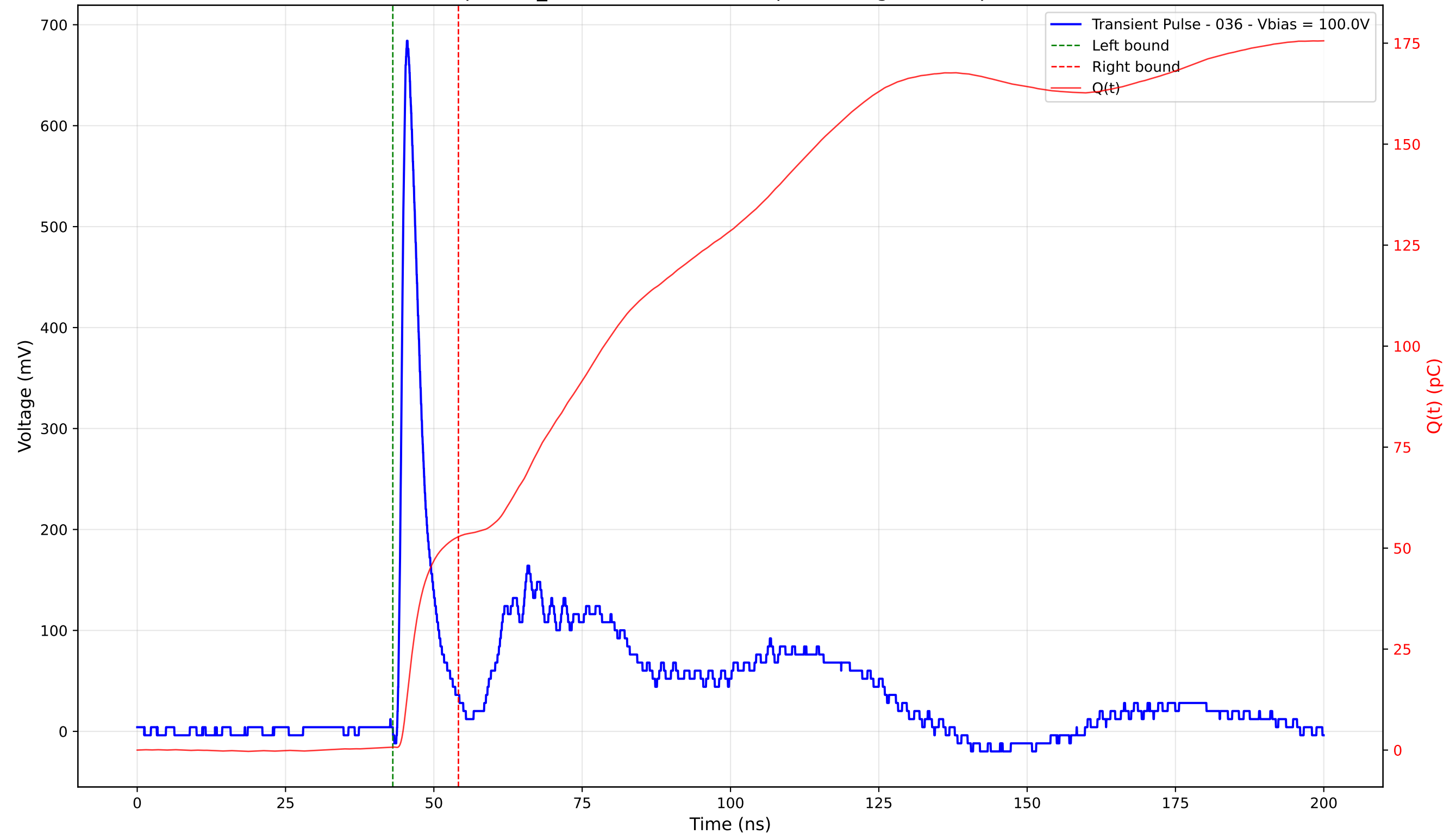
Transient Pulse - Sample: TD_4004 - Position: 195.0 \mu\text{m} - Charge: 52.06 pC - Rise Time: 1.03 ns
