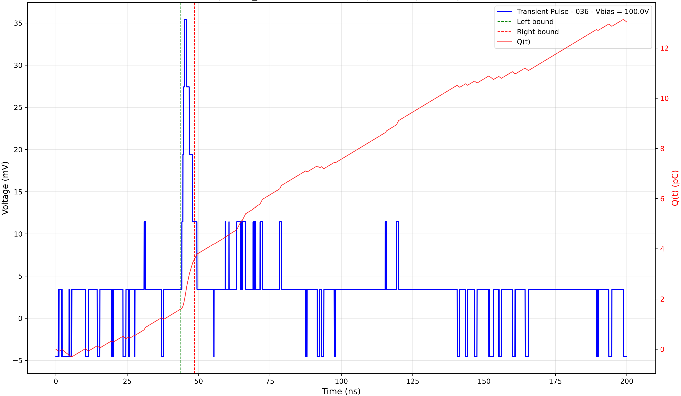
Transient Pulse - Sample: TD_4004 - Position: 430.0 \mu\text{m} - Charge: 2.00 pC - Rise Time: 1.02 ns
