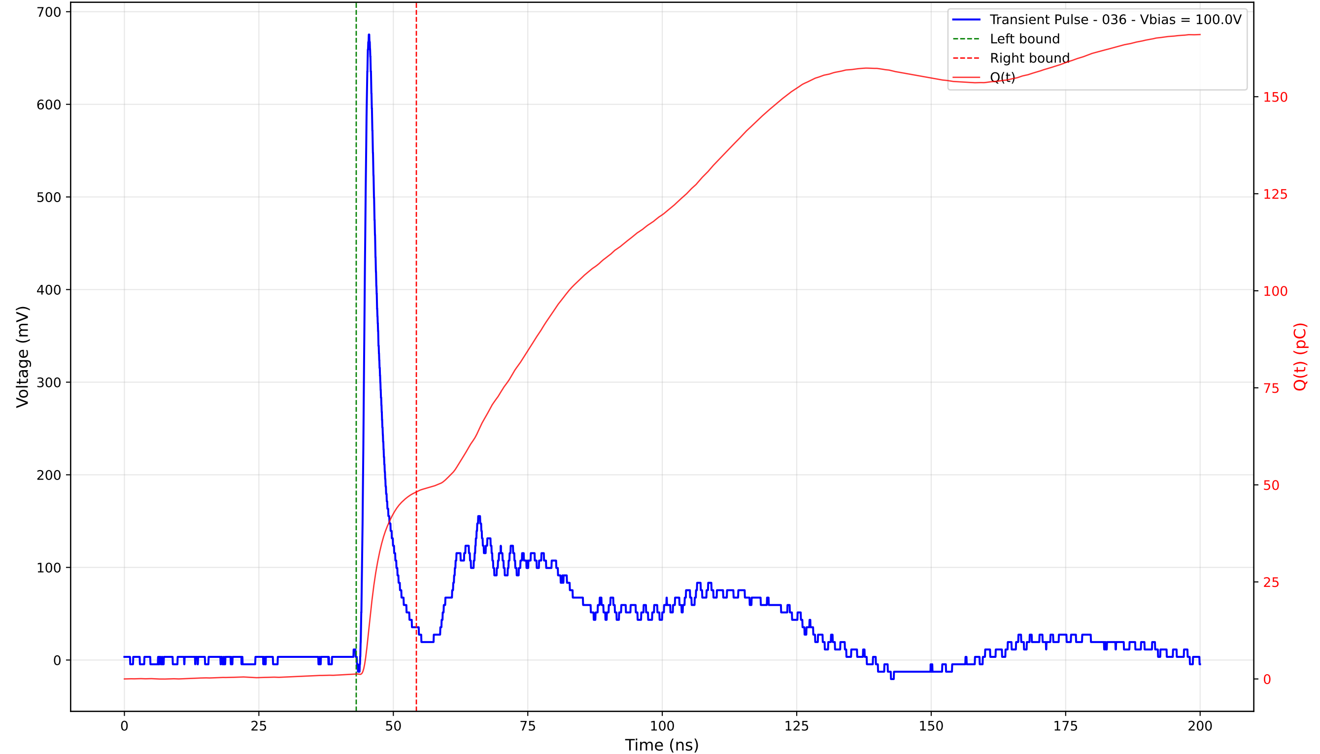
Transient Pulse - Sample: TD_4004 - Position: 125.0 \mu\text{m} - Charge: 46.90 pC - Rise Time: 0.98 ns
