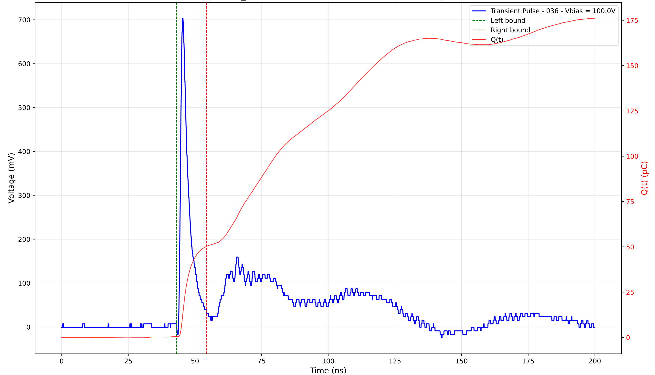
Transient Pulse - Sample: TD_4004 - Position: 120.0 \mu\text{m} - Charge: 49.64 pC - Rise Time: 0.97 ns
