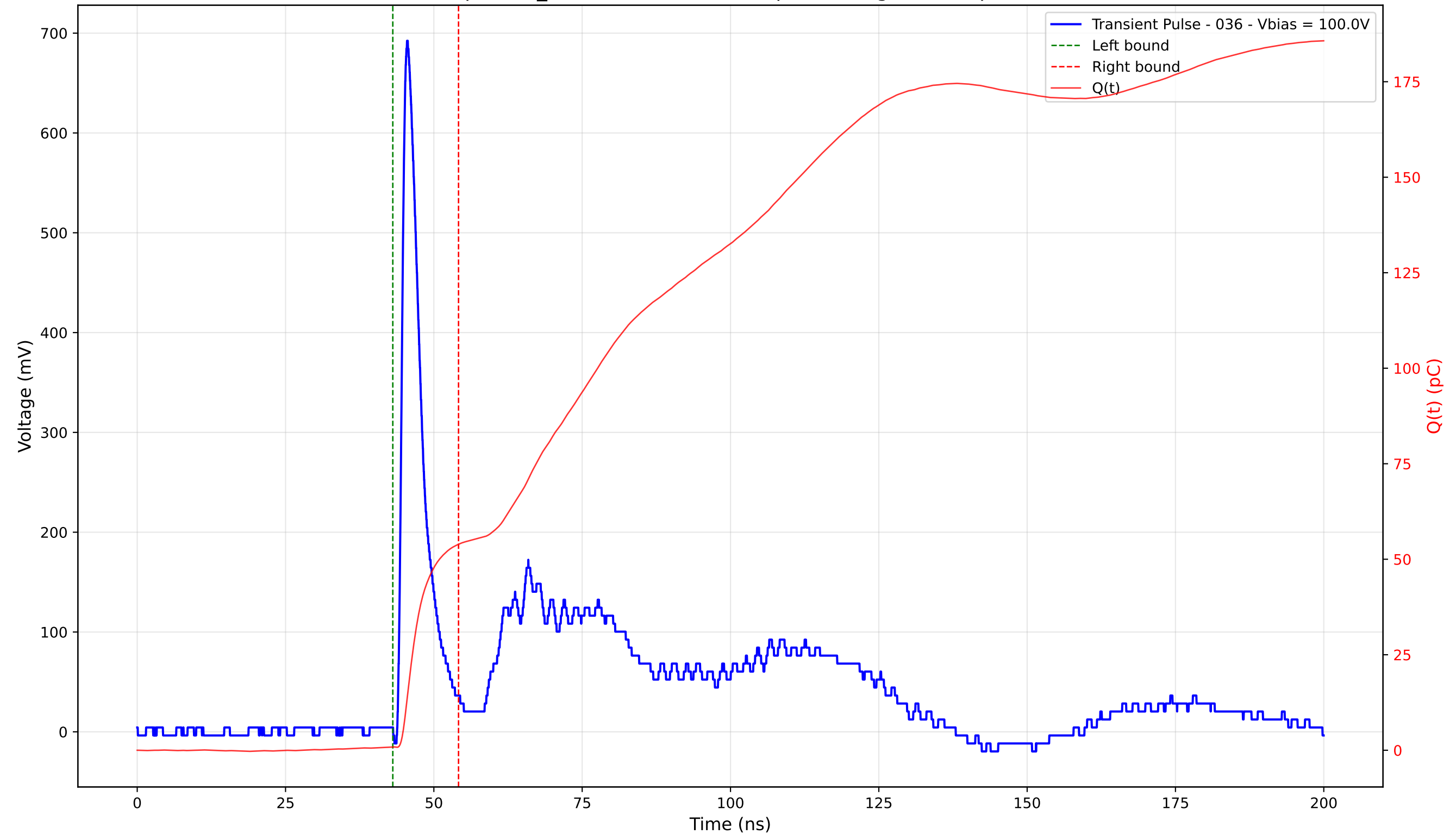
Transient Pulse - Sample: TD_4004 - Position: 185.0 \mu\text{m} - Charge: 53.04 pC - Rise Time: 1.00 ns
