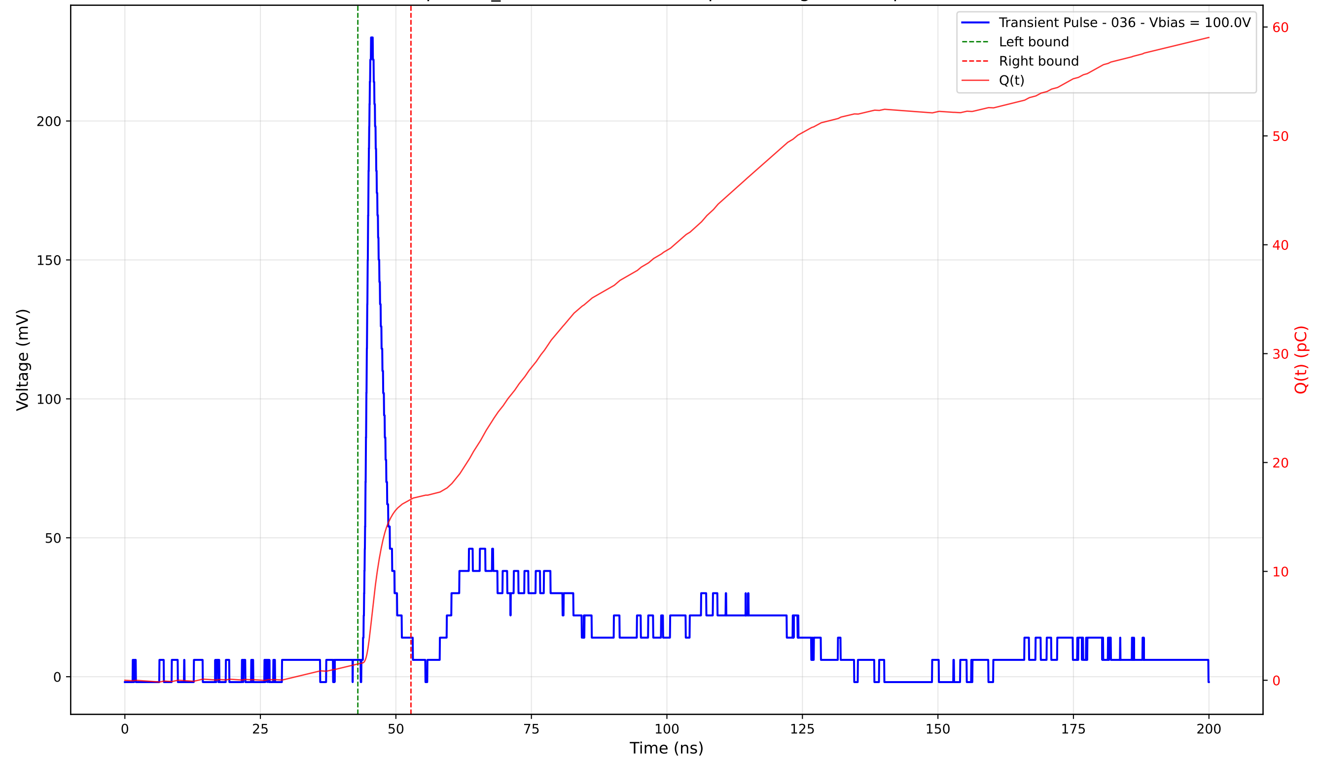
Transient Pulse - Sample: TD_4004 - Position: 380.0 \mu\text{m} - Charge: 15.13 pC - Rise Time: 1.08 ns
