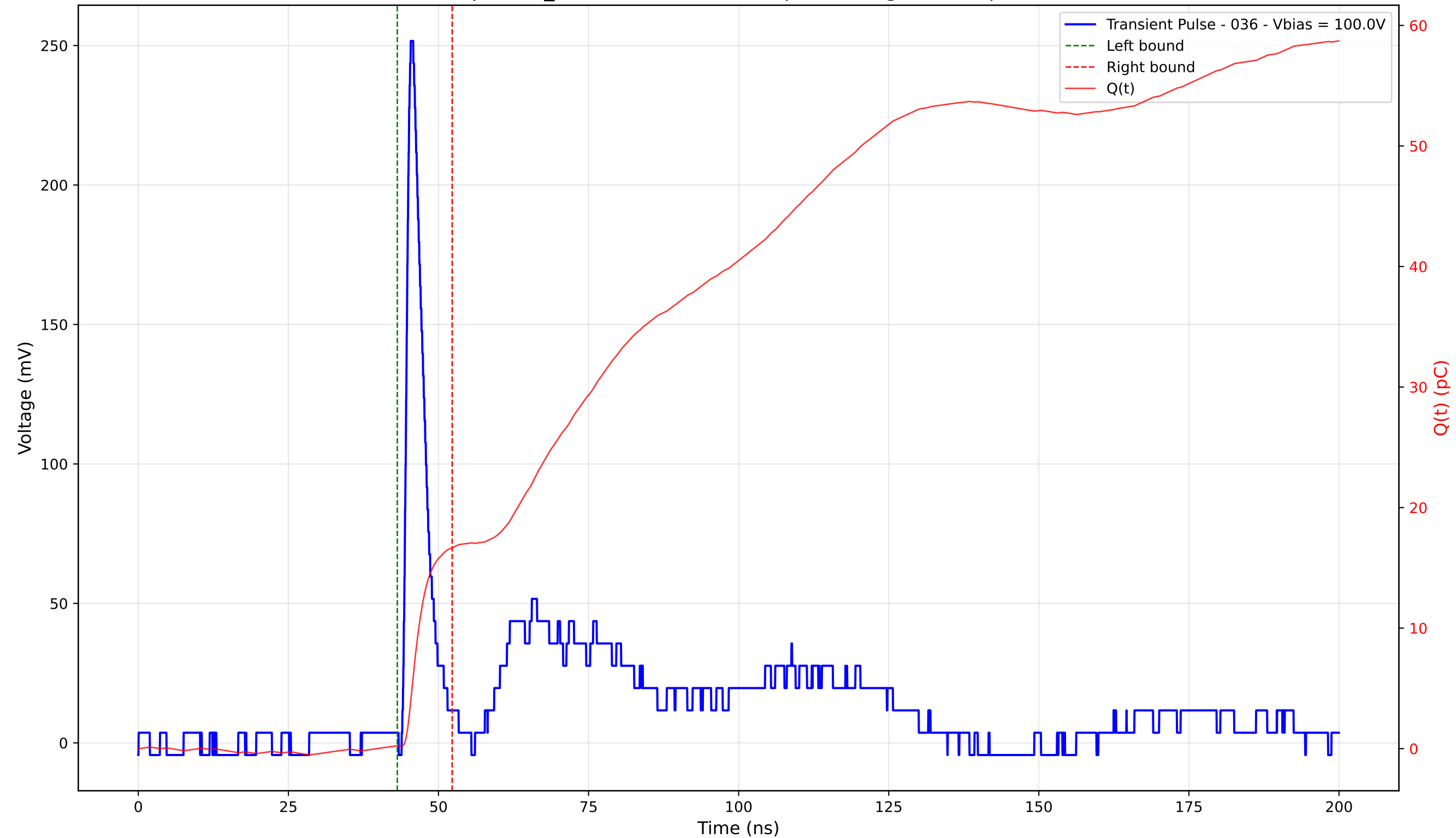
Transient Pulse - Sample: TD_4004 - Position: 350.0 \mu\text{m} - Charge: 16.43 pC - Rise Time: 0.99 ns
