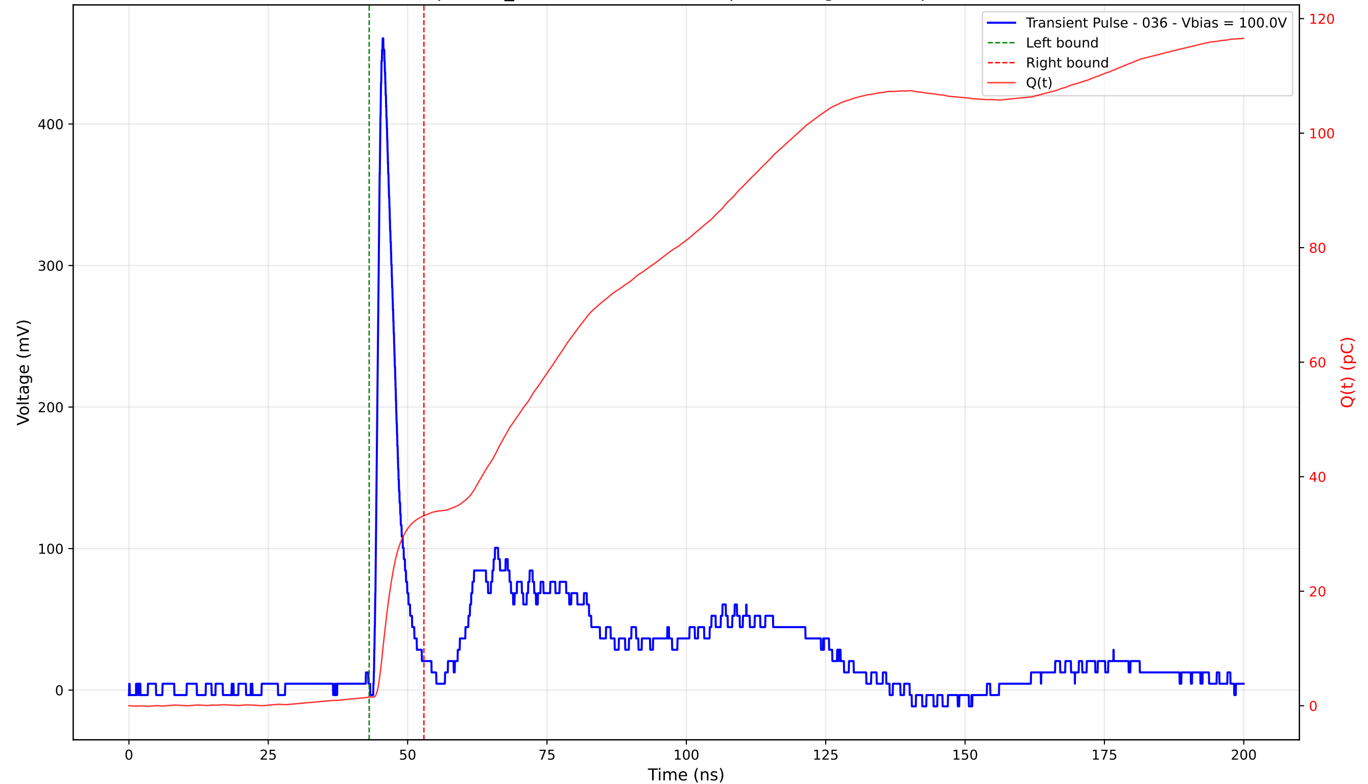
Transient Pulse - Sample: TD_4004 - Position: 275.0 \mu\text{m} - Charge: 31.67 pC - Rise Time: 1.06 ns
