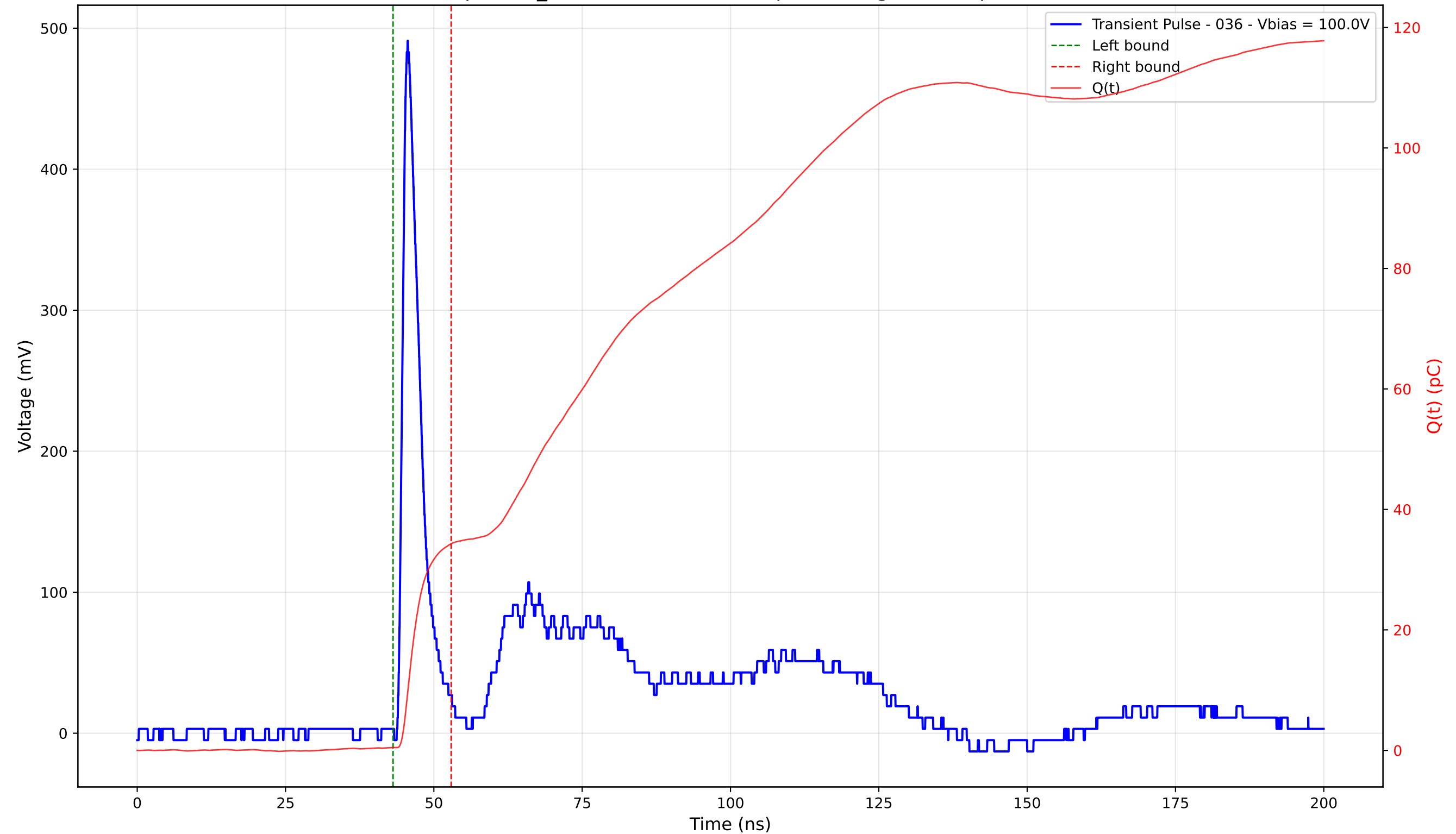
Transient Pulse - Sample: TD_4004 - Position: 250.0 \mu\text{m} - Charge: 33.82 pC - Rise Time: 1.06 ns
