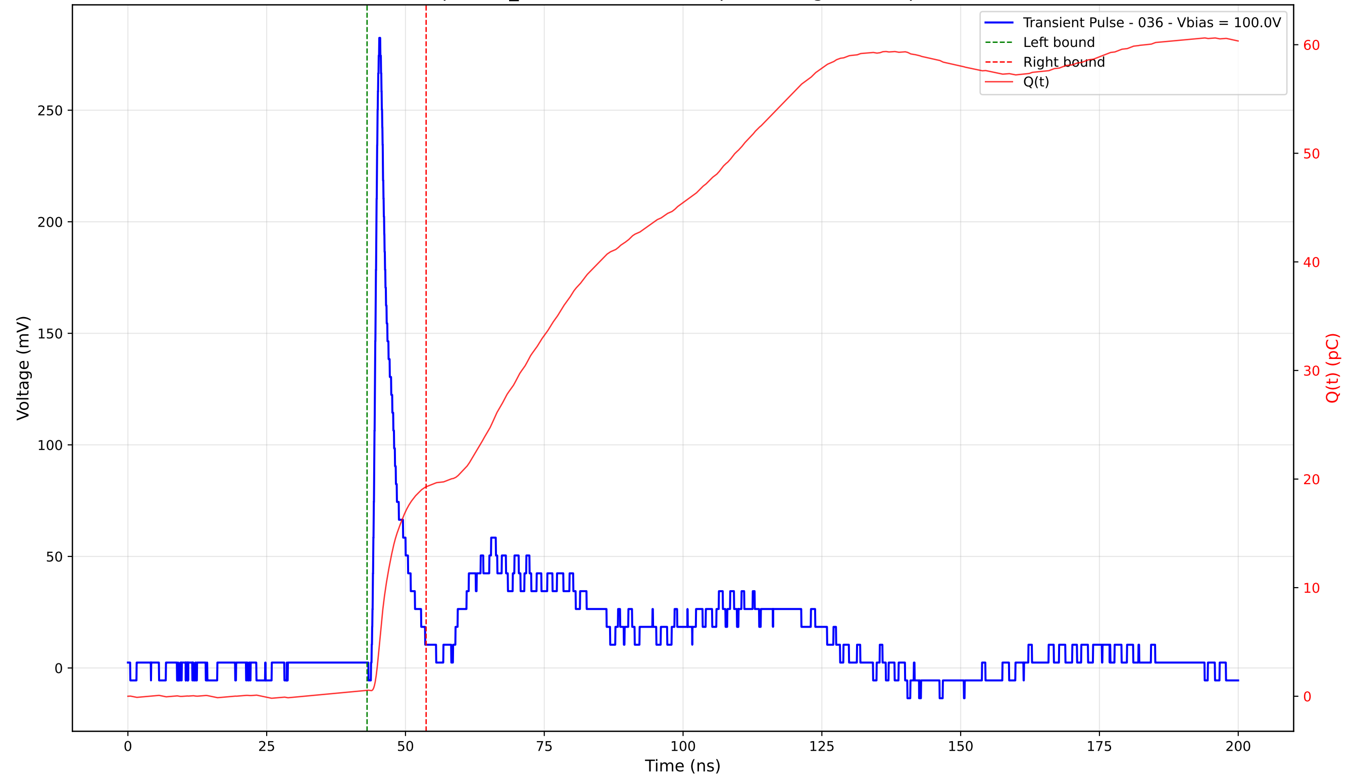
Transient Pulse - Sample: TD_4004 - Position: 65.0 \mu\text{m} - Charge: 18.74 pC - Rise Time: 0.94 ns
