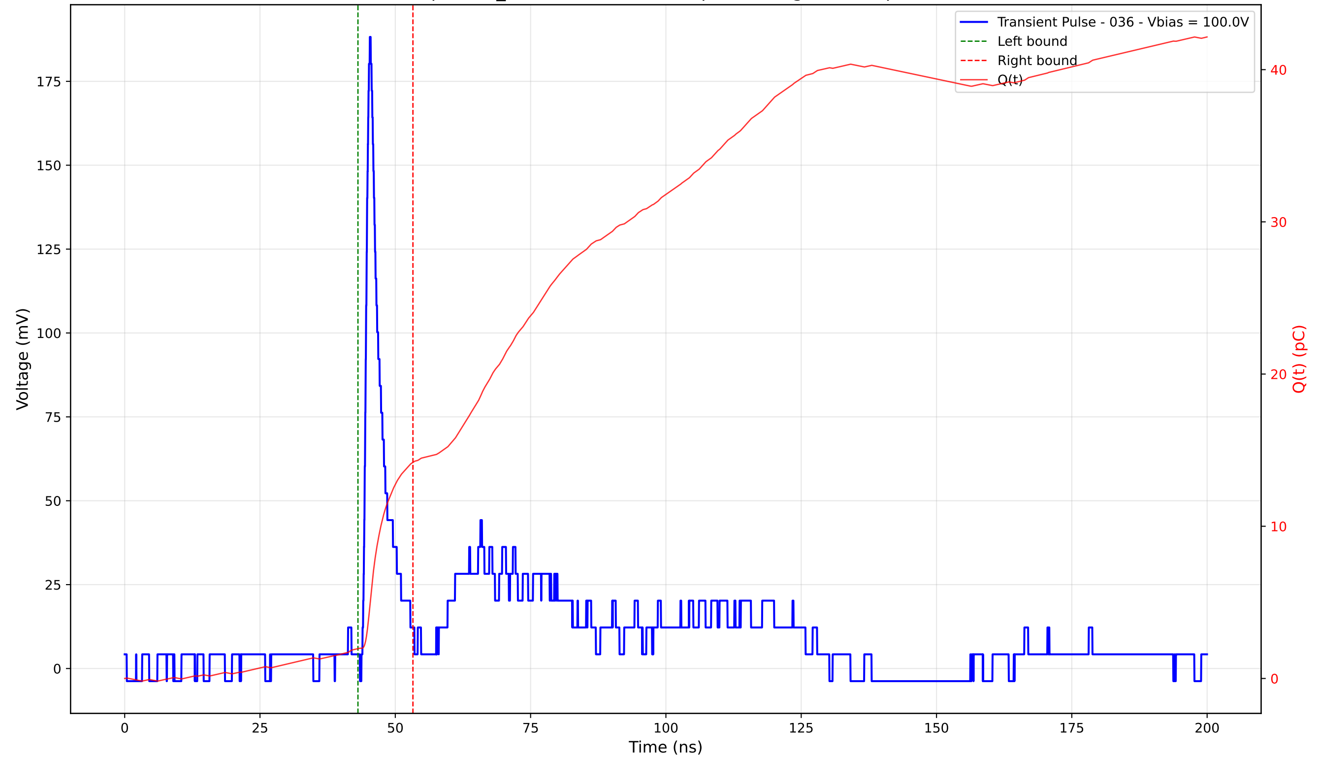
Transient Pulse - Sample: TD_4004 - Position: 60.0 \mu\text{m} - Charge: 12.24 pC - Rise Time: 0.98 ns
