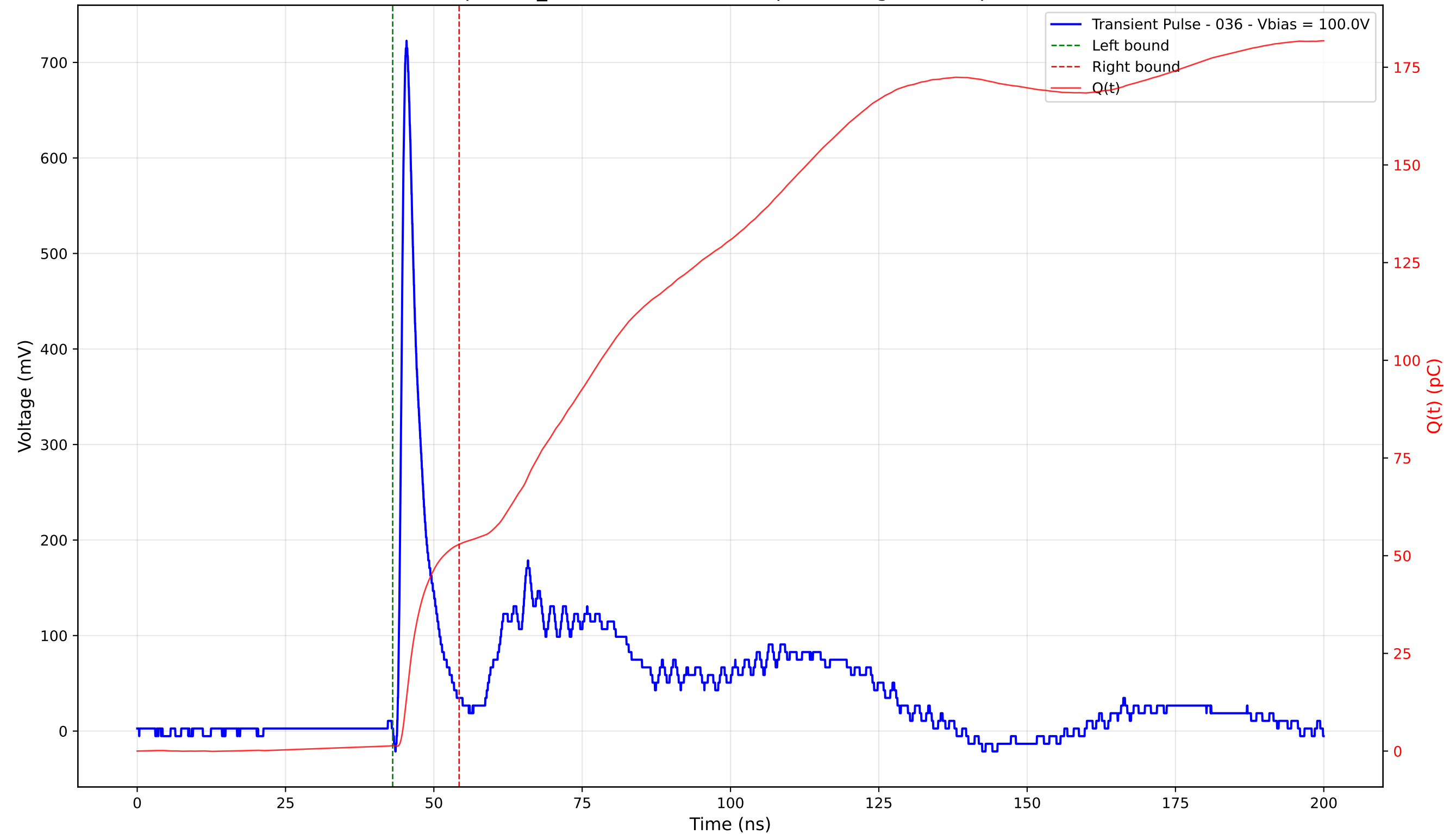
Transient Pulse - Sample: TD_4004 - Position: 115.0 \mu\text{m} - Charge: 51.52 pC - Rise Time: 0.95 ns
