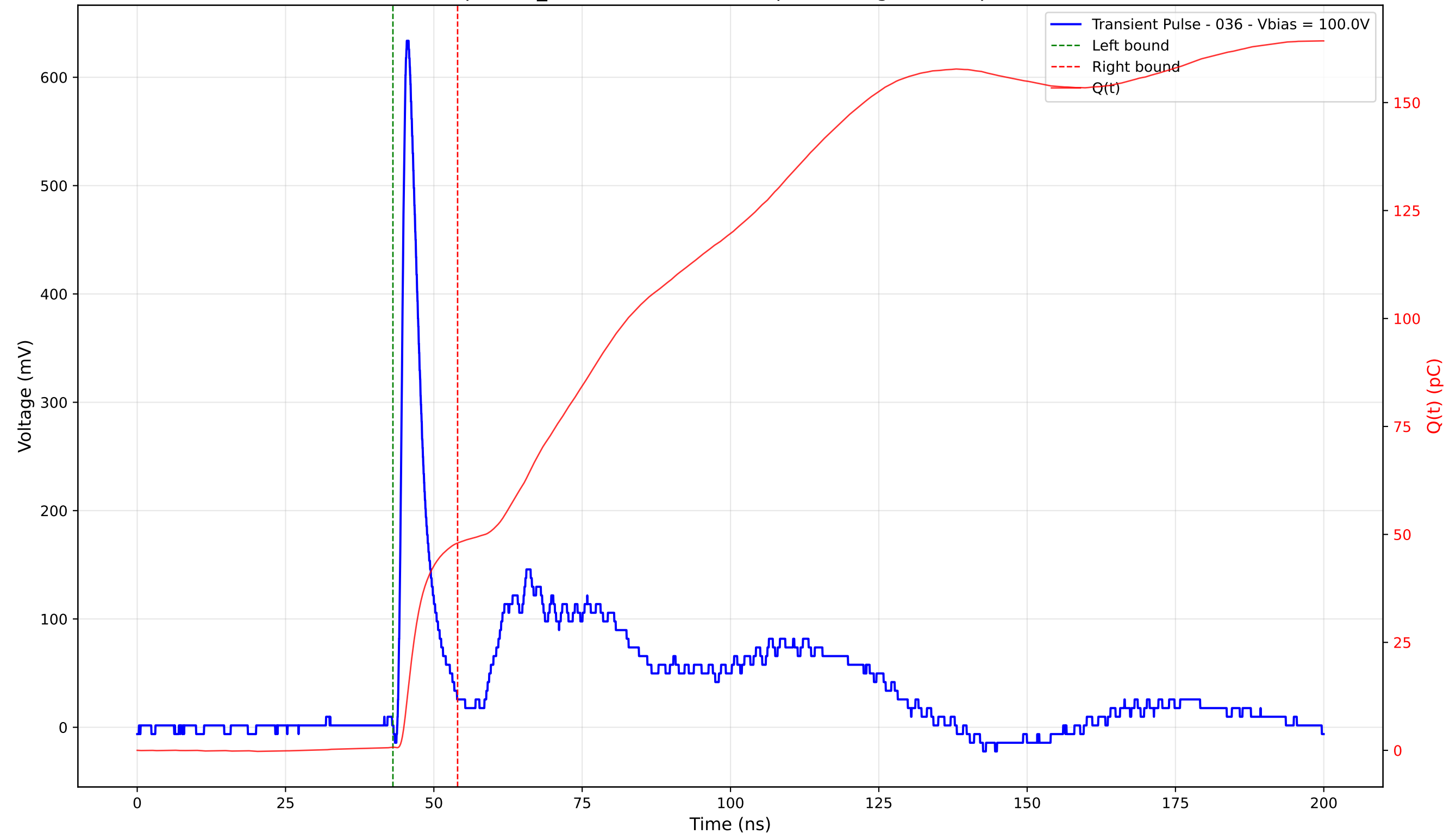
Transient Pulse - Sample: TD_4004 - Position: 170.0 \mu\text{m} - Charge: 47.28 pC - Rise Time: 1.03 ns
