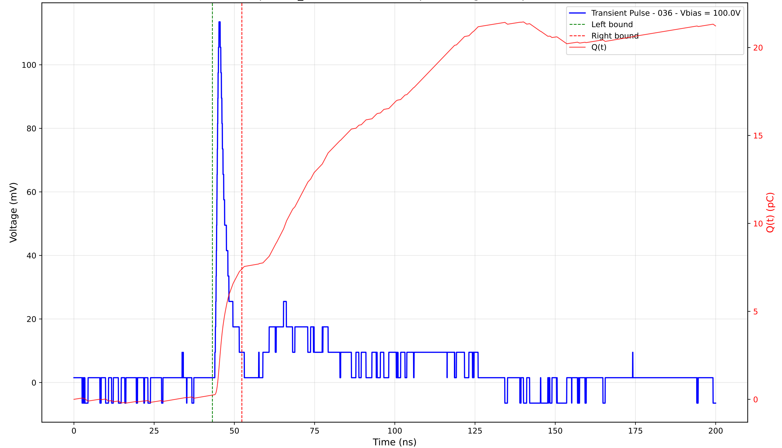
Transient Pulse - Sample: TD_4004 - Position: 55.0 \mu\text{m} - Charge: 7.17 pC - Rise Time: 0.98 ns
