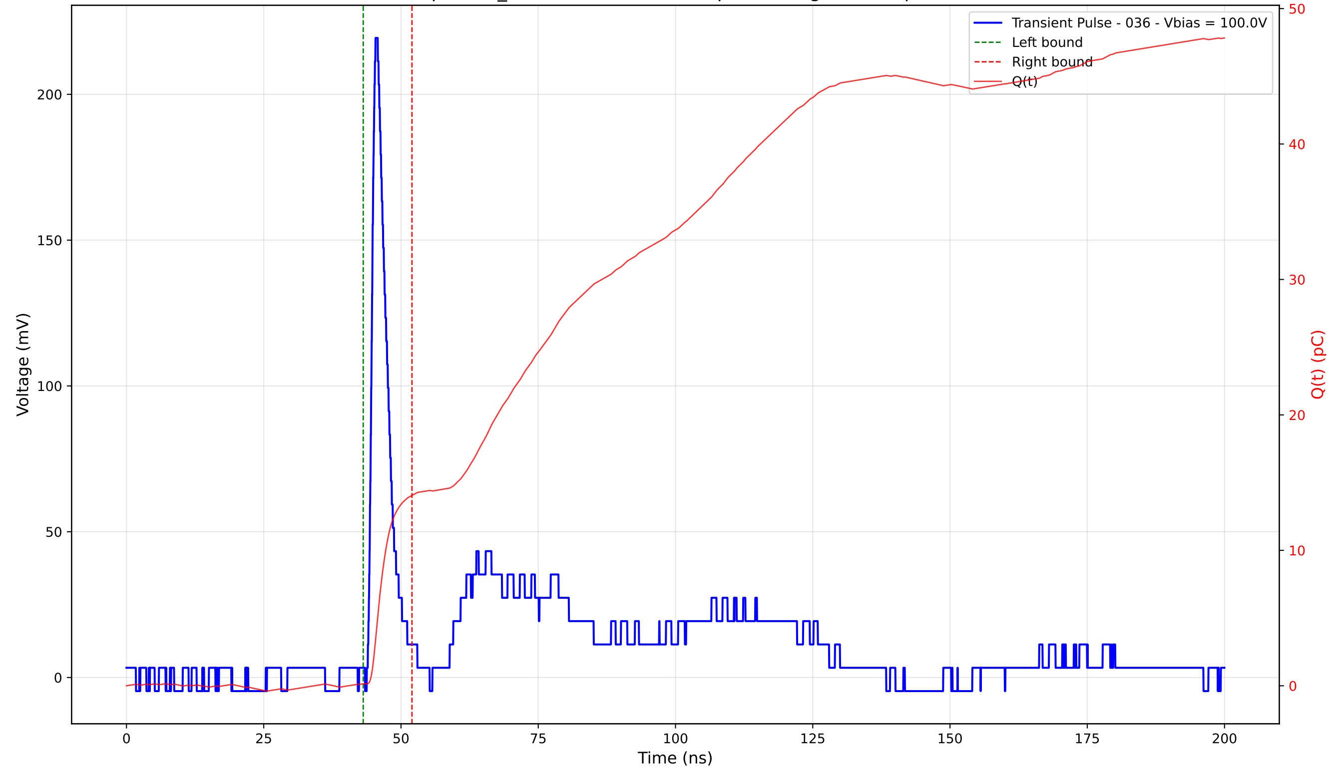
Transient Pulse - Sample: TD_4004 - Position: 375.0 \mu\text{m} - Charge: 13.91 pC - Rise Time: 1.03 ns
