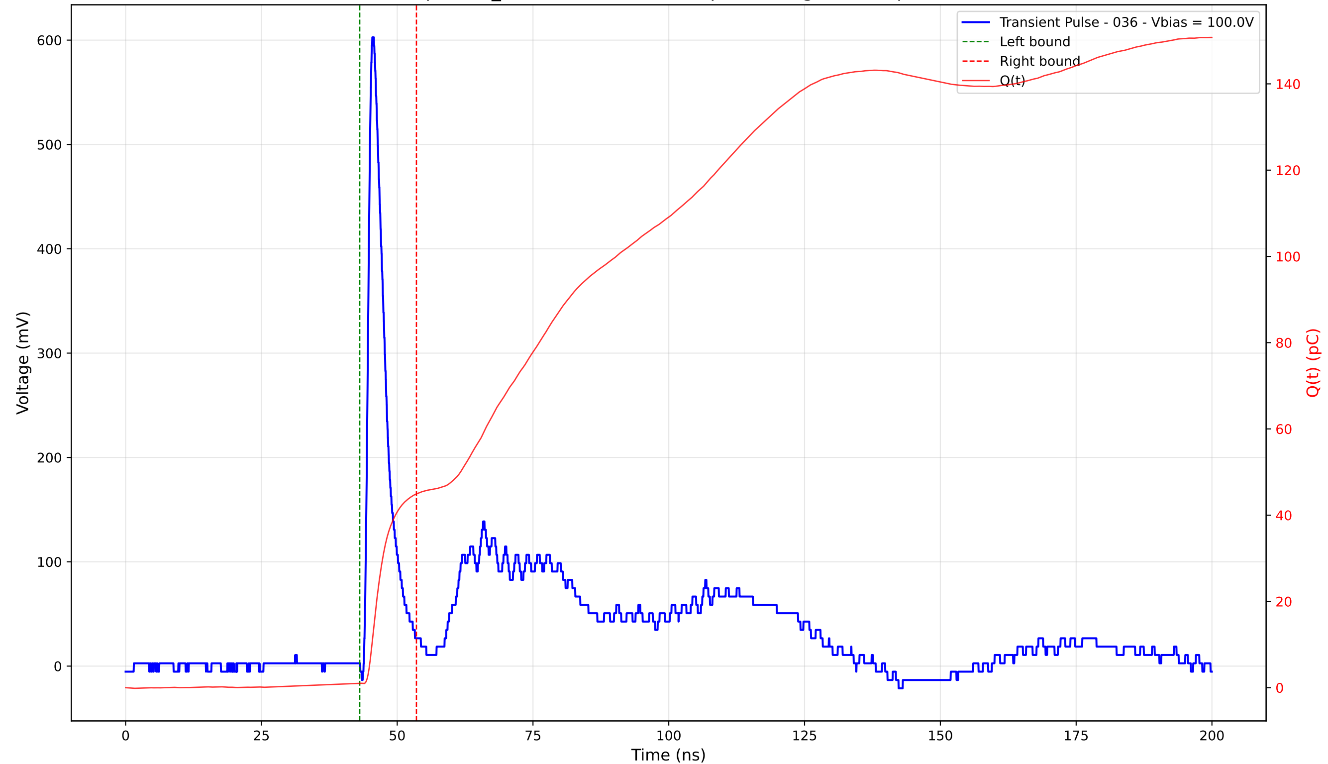
Transient Pulse - Sample: TD_4004 - Position: 225.0 \mu\text{m} - Charge: 43.89 pC - Rise Time: 1.01 ns
