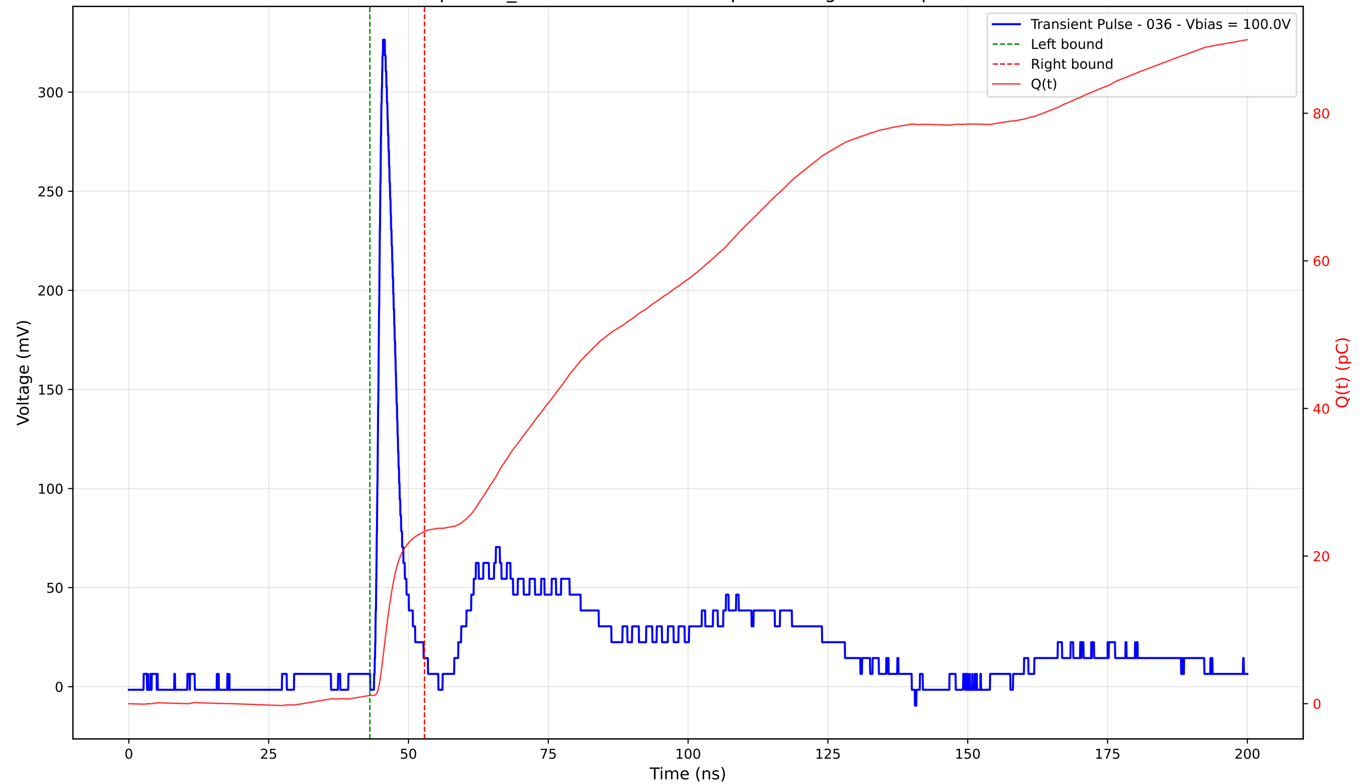
Transient Pulse - Sample: TD_4004 - Position: 315.0 \mu\text{m} - Charge: 22.22 pC - Rise Time: 1.03 ns
