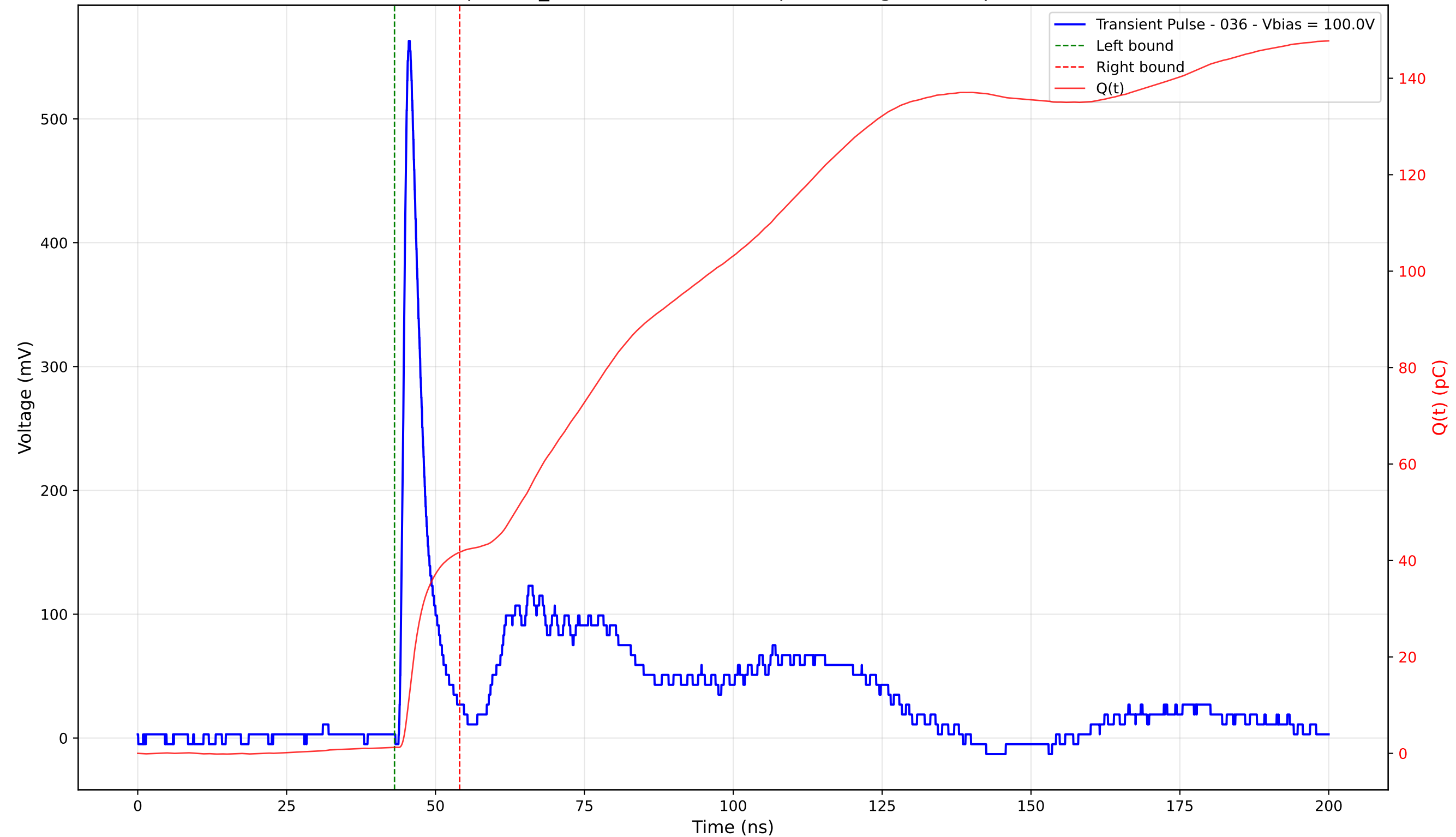
Transient Pulse - Sample: TD_4004 - Position: 155.0 \mu\text{m} - Charge: 40.44 pC - Rise Time: 1.05 ns
