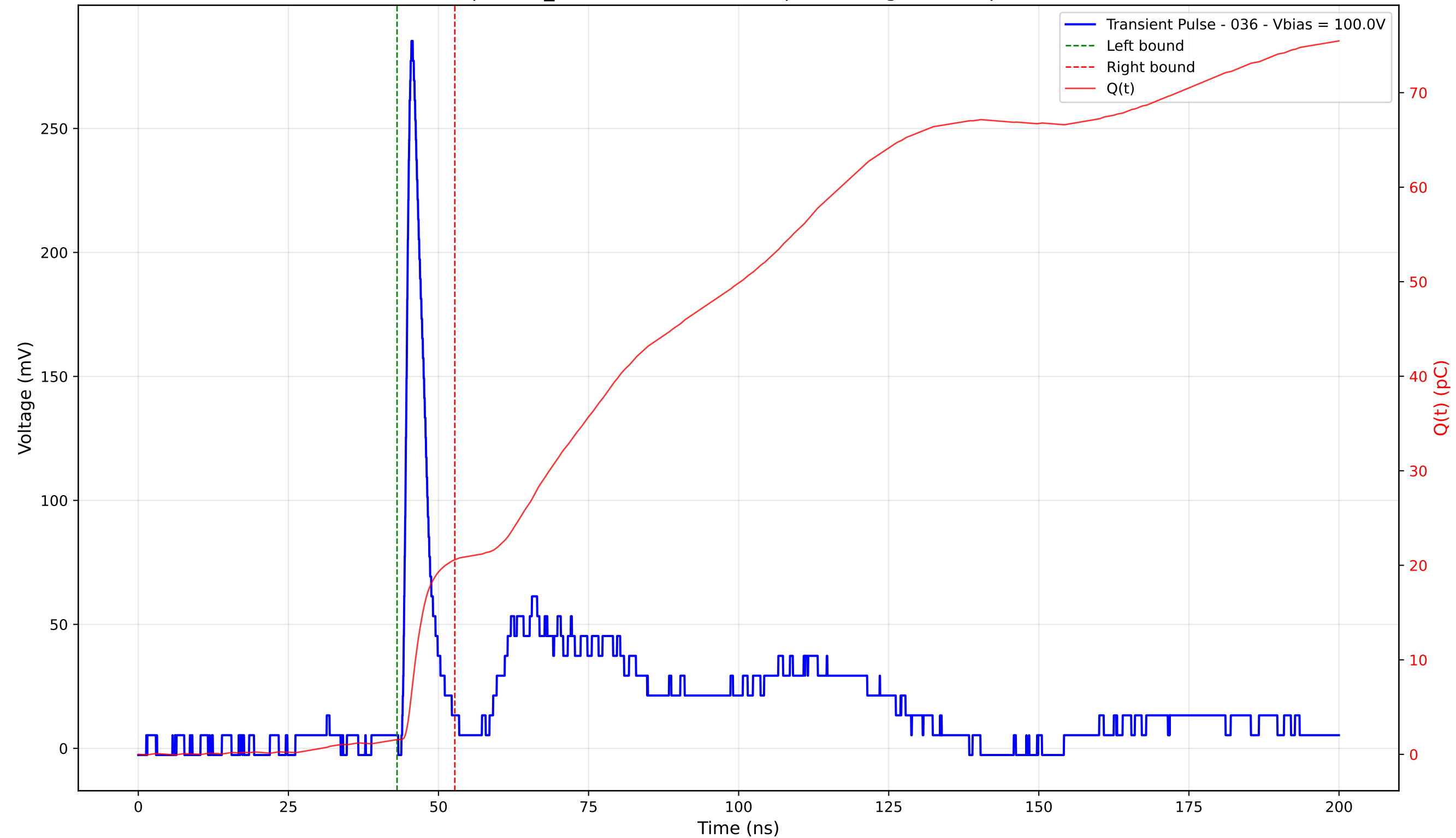
Transient Pulse - Sample: TD_4004 - Position: 330.0 \mu\text{m} - Charge: 19.02 pC - Rise Time: 1.08 ns
