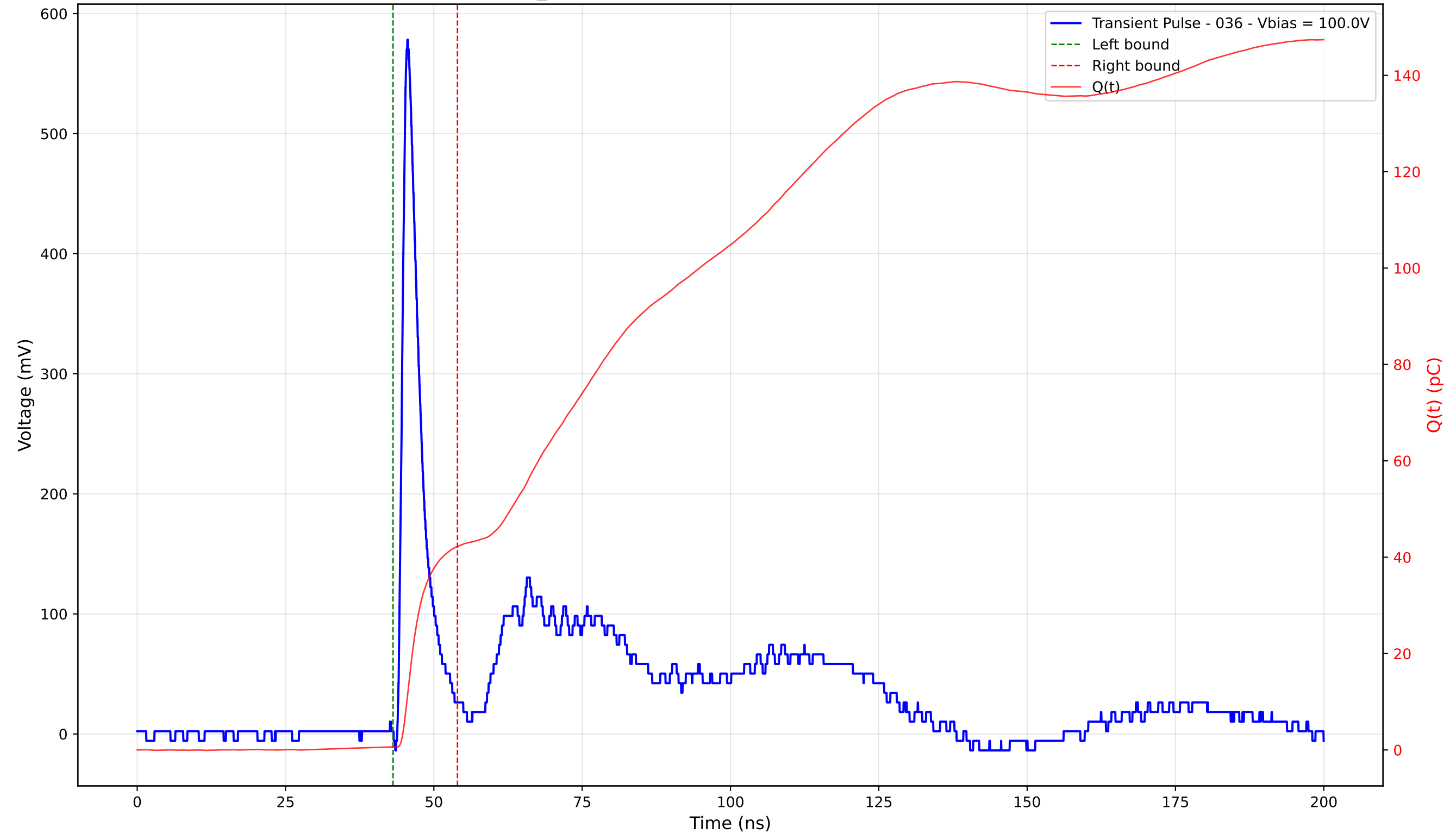
Transient Pulse - Sample: TD_4004 - Position: 160.0 \mu\text{m} - Charge: 41.55 pC - Rise Time: 1.06 ns
