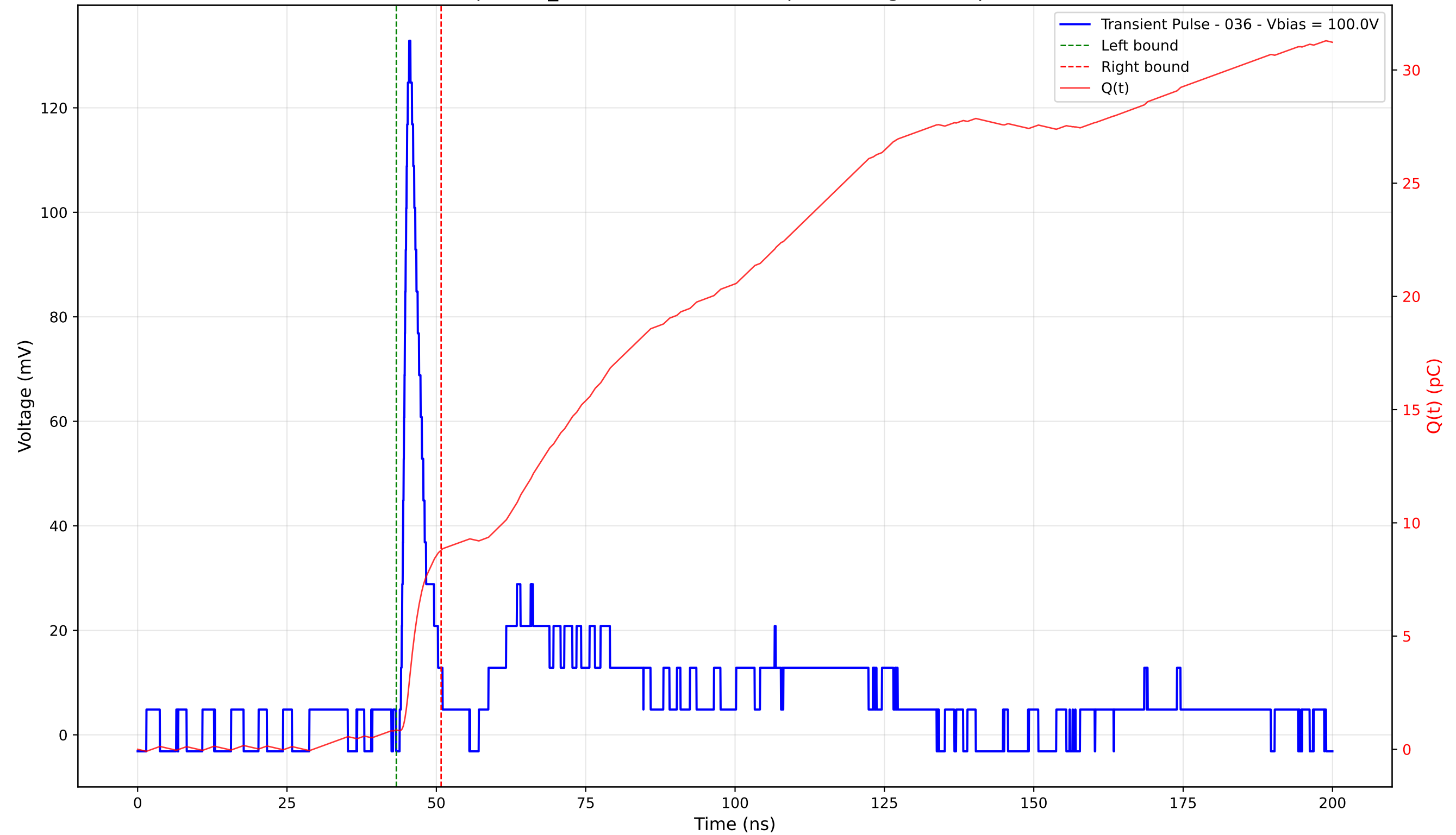
Transient Pulse - Sample: TD_4004 - Position: 400.0 \mu\text{m} - Charge: 7.95 pC - Rise Time: 1.04 ns
