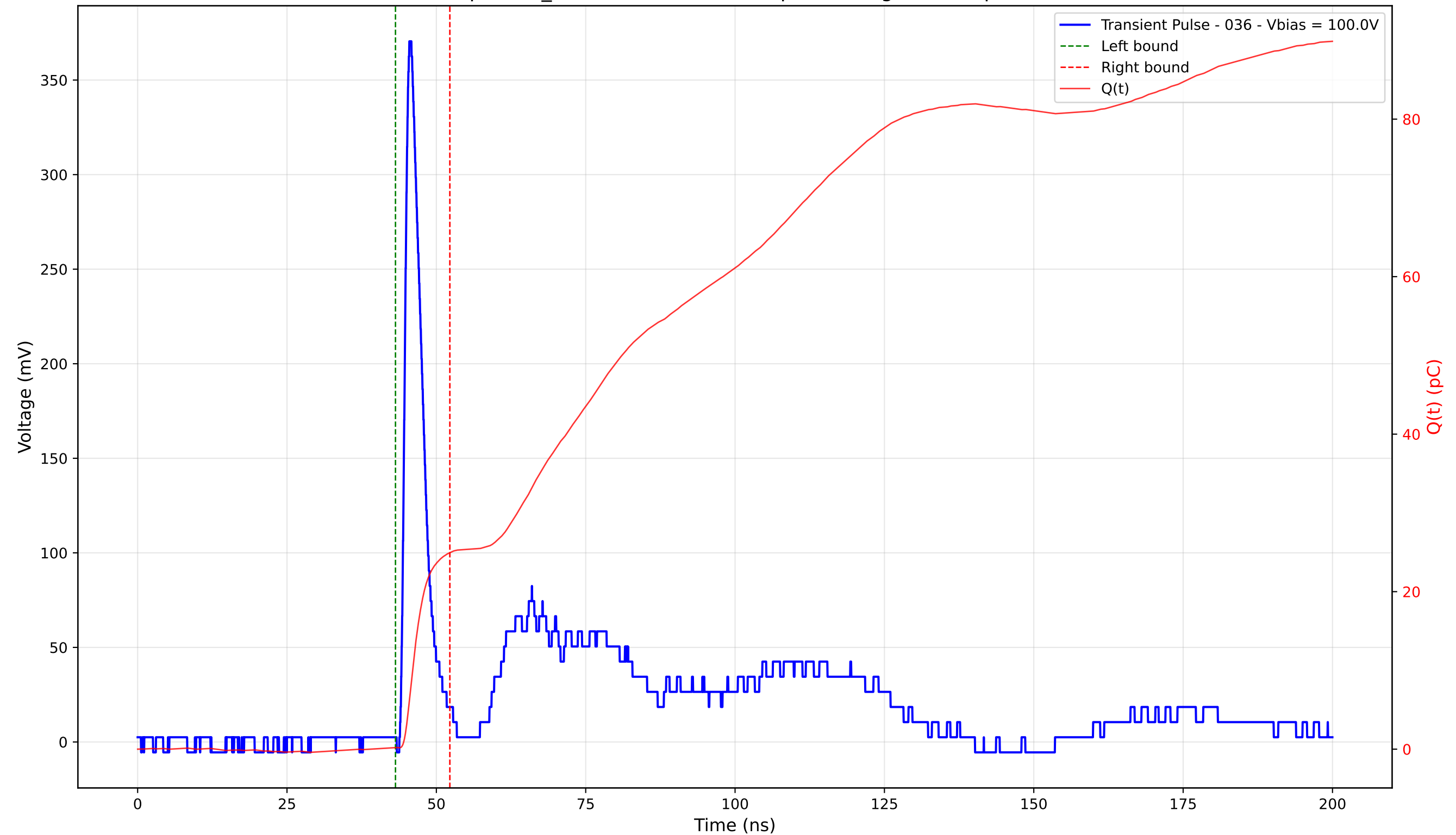
Transient Pulse - Sample: TD_4004 - Position: 295.0 \mu\text{m} - Charge: 24.74 pC - Rise Time: 1.07 ns
