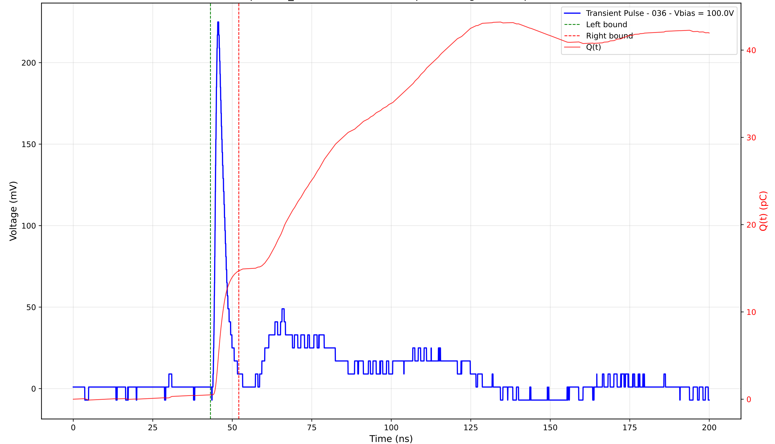
Transient Pulse - Sample: TD_4004 - Position: 365.0 \mu\text{m} - Charge: 14.20 pC - Rise Time: 1.09 ns
