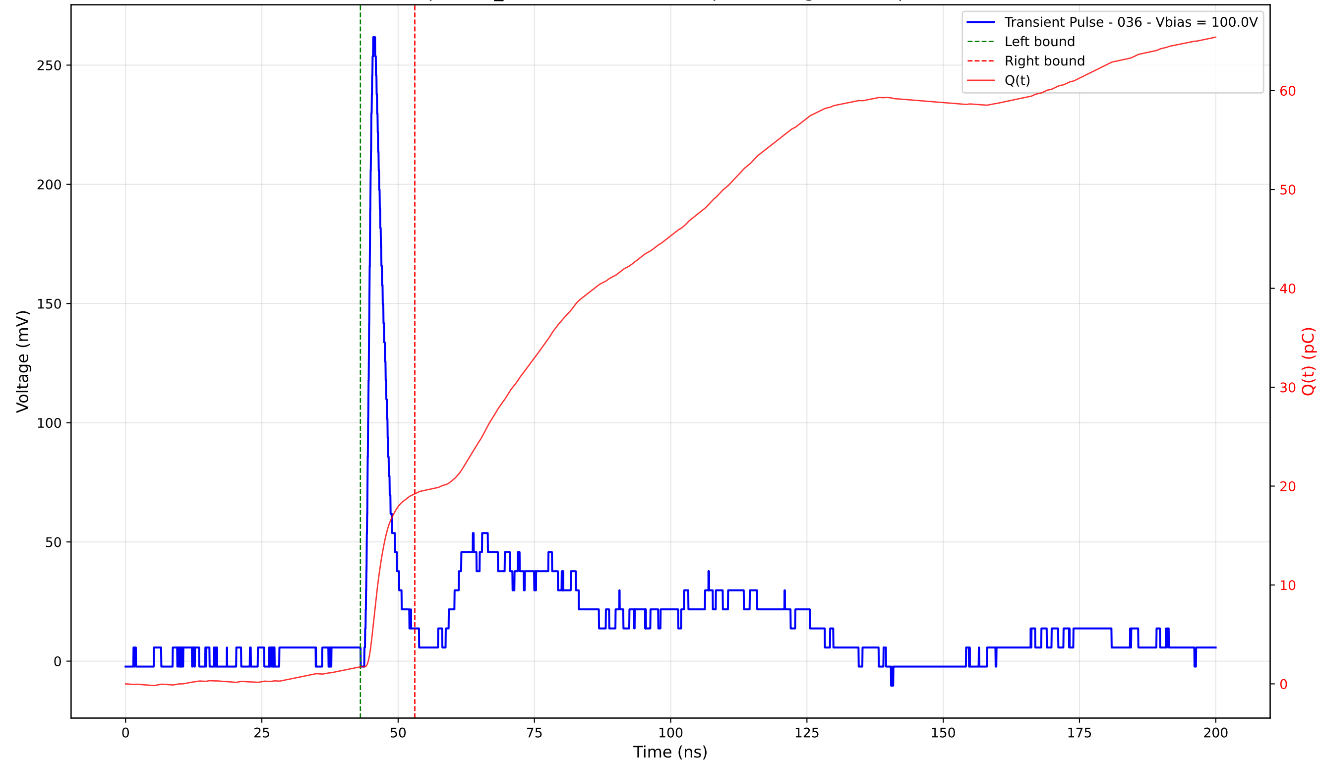
Transient Pulse - Sample: TD_4004 - Position: 345.0 \mu\text{m} - Charge: 17.50 pC - Rise Time: 1.07 ns
