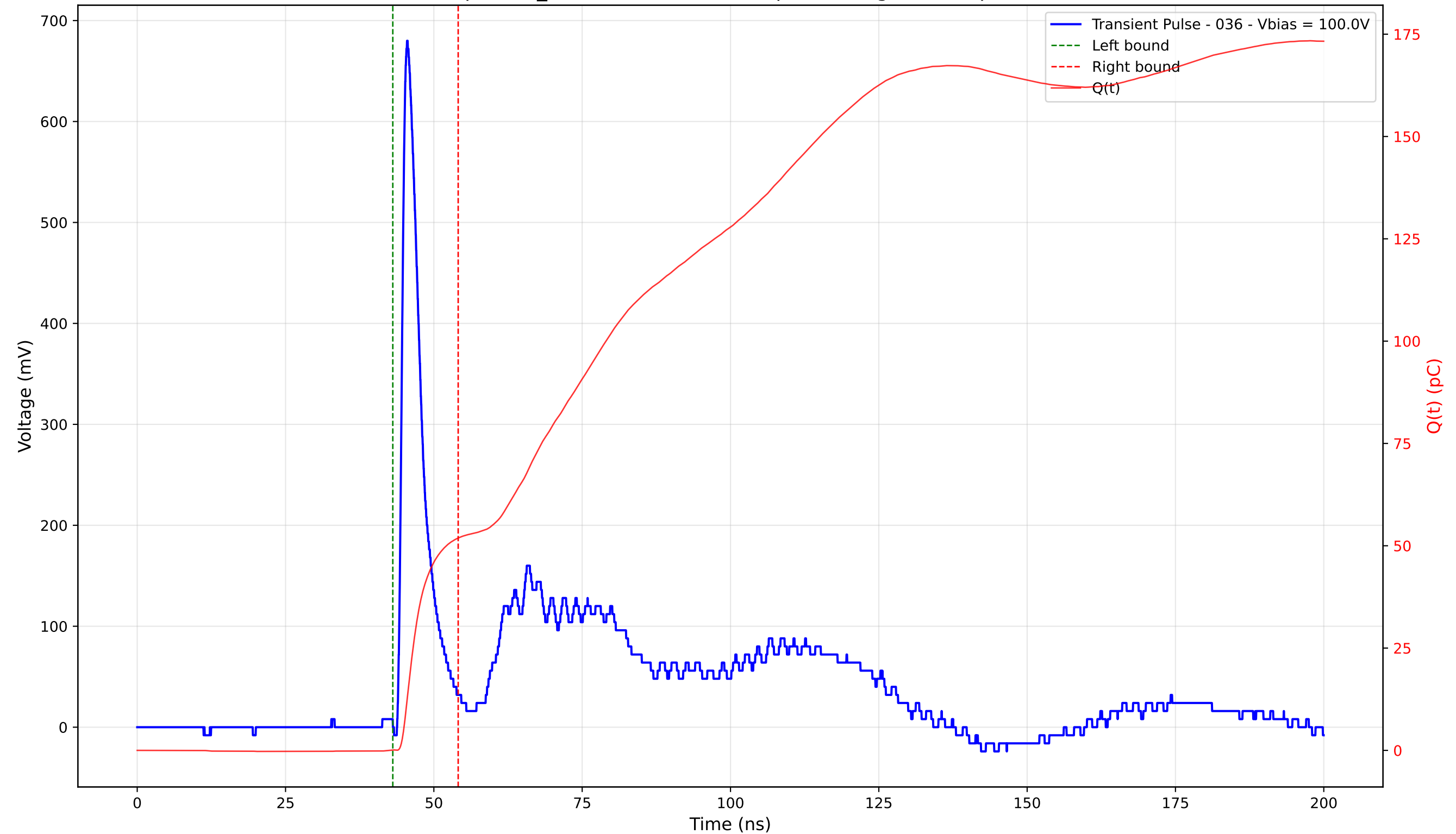
Transient Pulse - Sample: TD_4004 - Position: 180.0 \mu\text{m} - Charge: 51.78 pC - Rise Time: 1.03 ns
