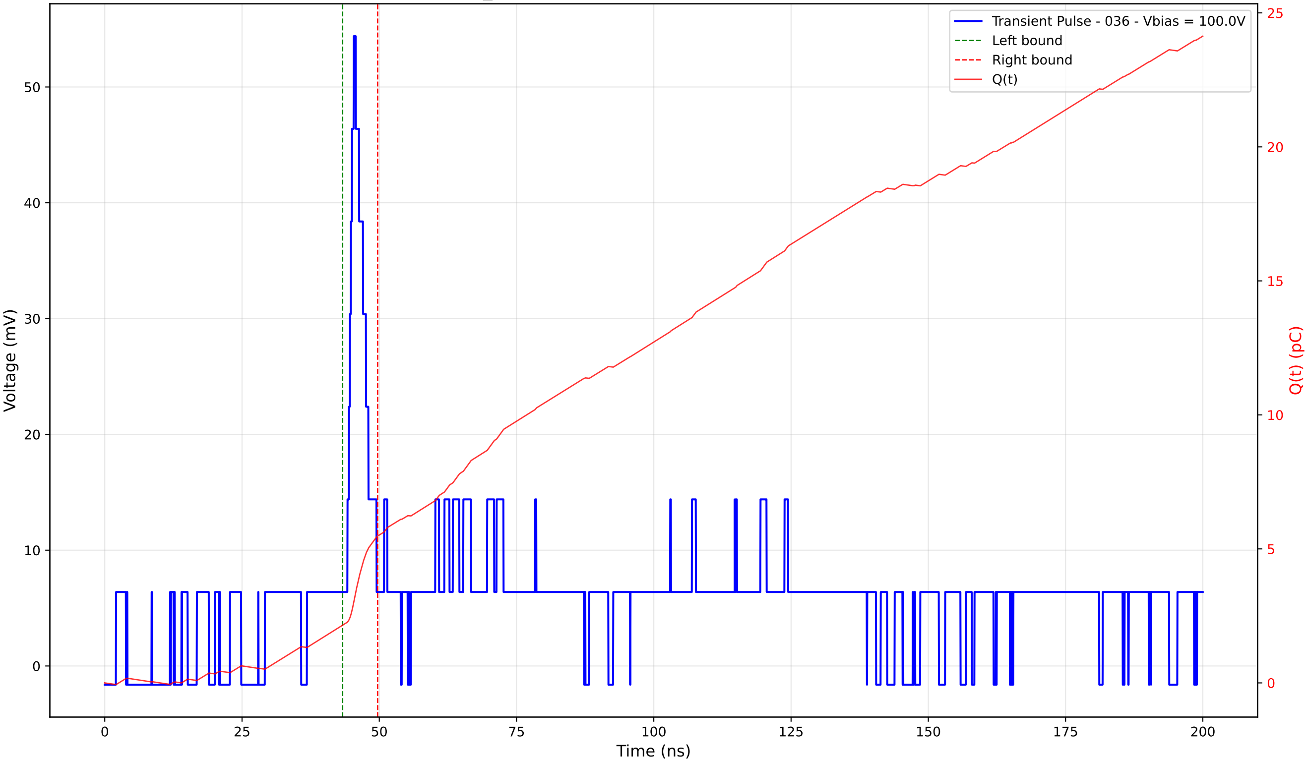
Transient Pulse - Sample: TD_4004 - Position: 420.0 \mu\text{m} - Charge: 3.33 pC - Rise Time: 8.52 ns
