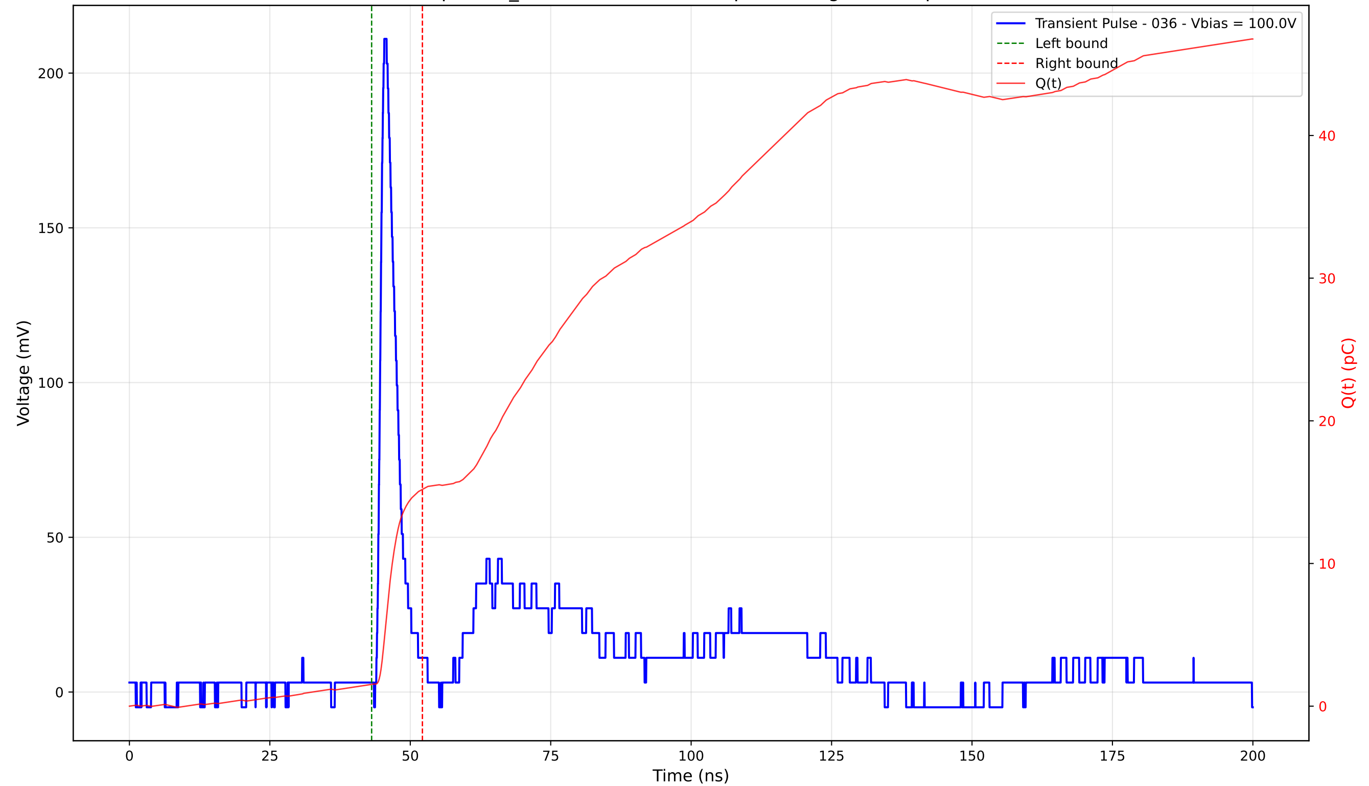
Transient Pulse - Sample: TD_4004 - Position: 385.0 \mu\text{m} - Charge: 13.66 pC - Rise Time: 1.03 ns
