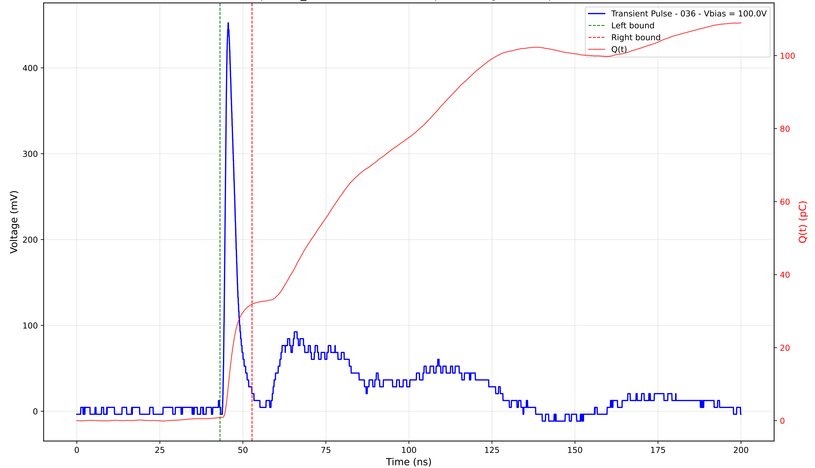
Transient Pulse - Sample: TD_4004 - Position: 260.0 \mu\text{m} - Charge: 31.03 pC - Rise Time: 1.06 ns
