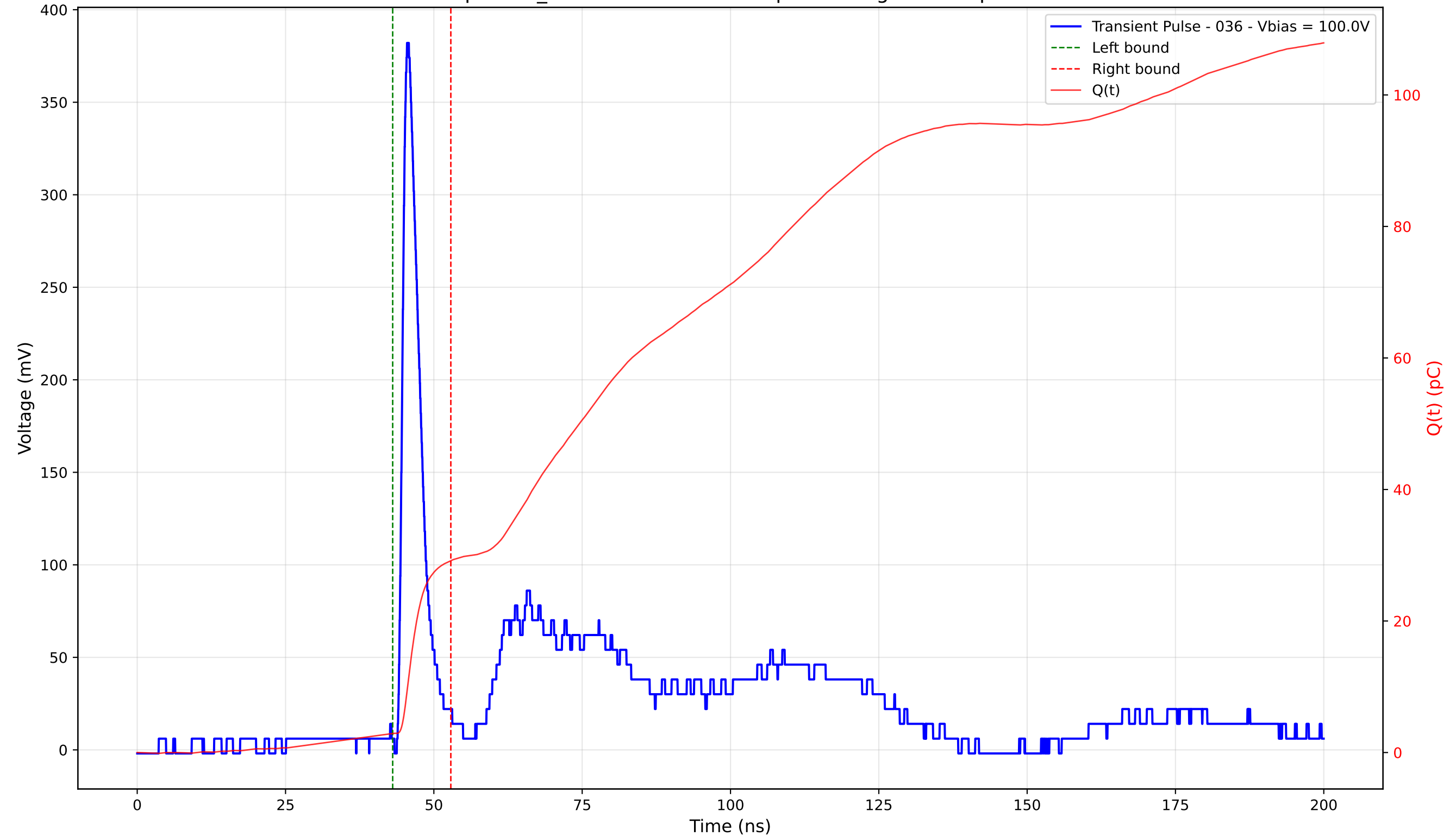
Transient Pulse - Sample: TD_4004 - Position: 300.0 \mu\text{m} - Charge: 26.29 pC - Rise Time: 1.08 ns
