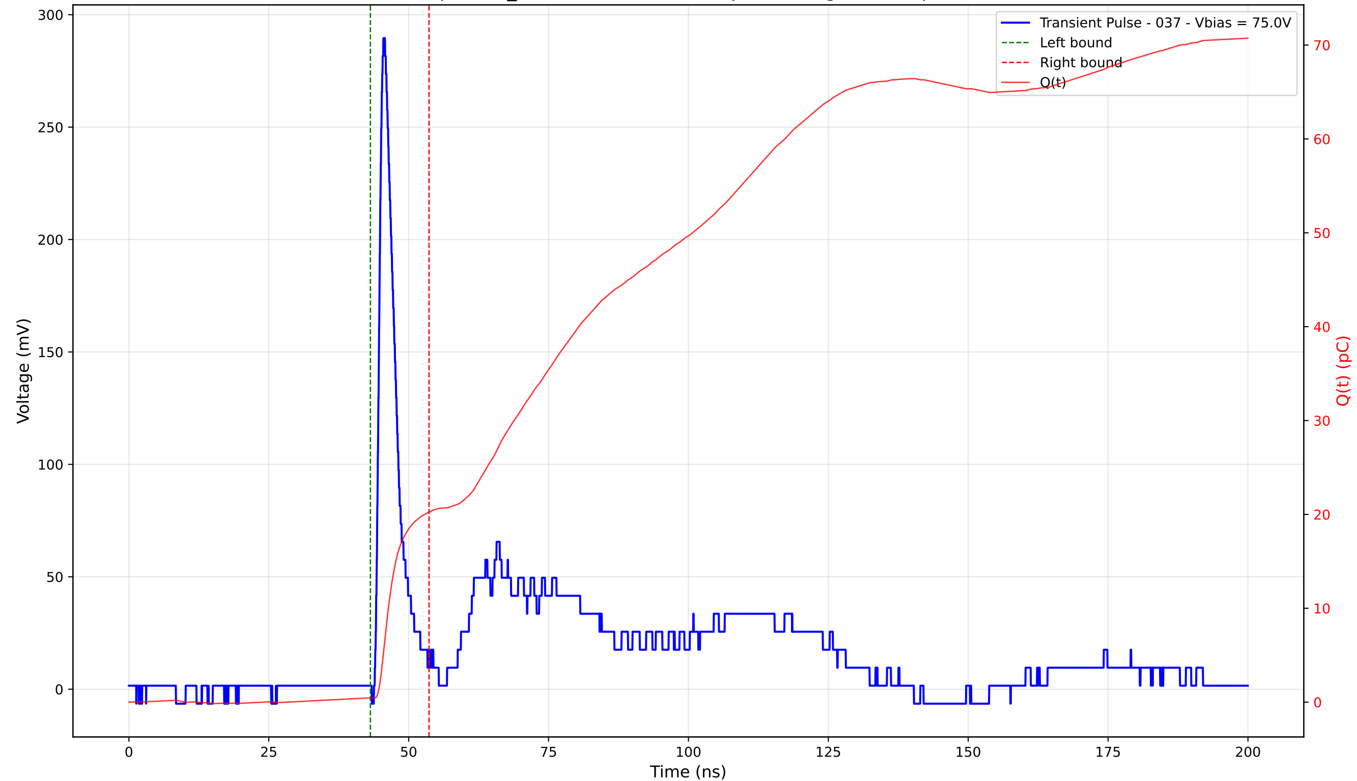
Transient Pulse - Sample: TD_4004 - Position: 305.0 \mu\text{m} - Charge: 19.78 pC - Rise Time: 1.05 ns
