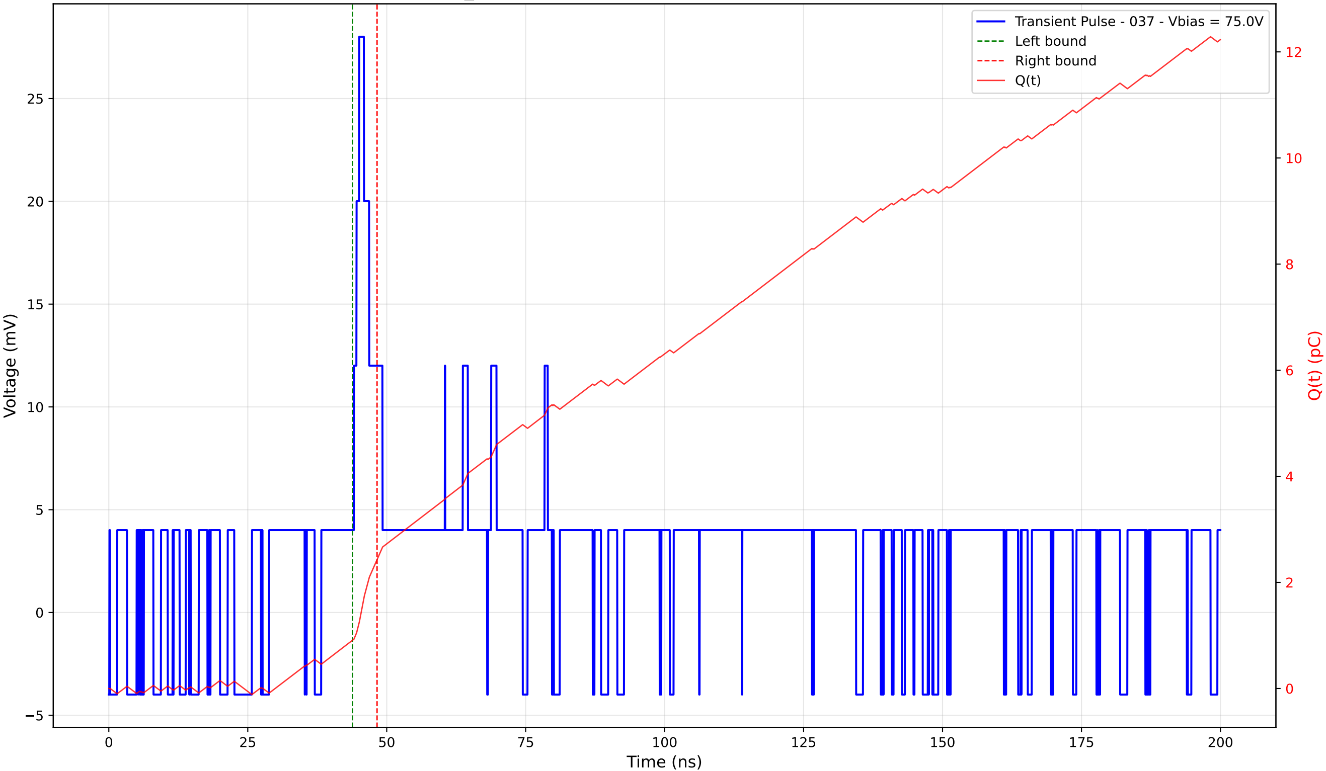
Transient Pulse - Sample: TD_4004 - Position: 430.0 \mu\text{m} - Charge: 1.52 pC - Rise Time: 0.00 ns (N/A)
