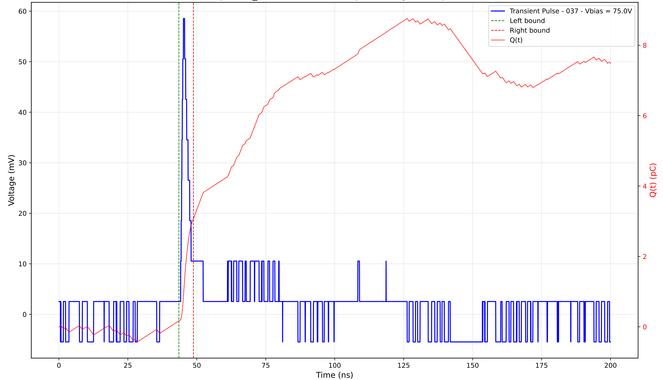
Transient Pulse - Sample: TD_4004 - Position: 50.0 \mu\text{m} - Charge: 2.91 pC - Rise Time: 1.01 ns
