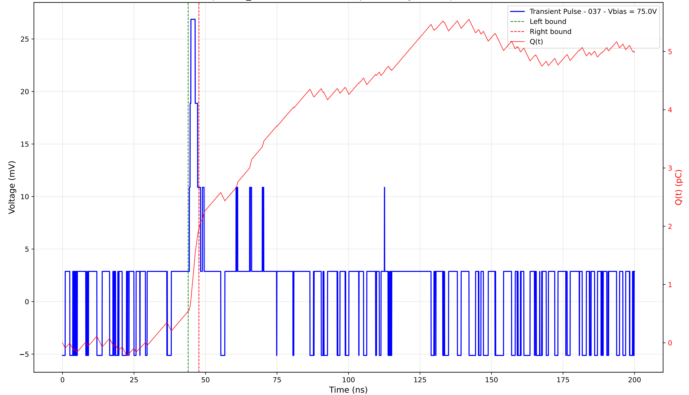
Transient Pulse - Sample: TD_4004 - Position: 425.0 \mu\text{m} - Charge: 1.41 pC - Rise Time: 0.00 ns (N/A)
