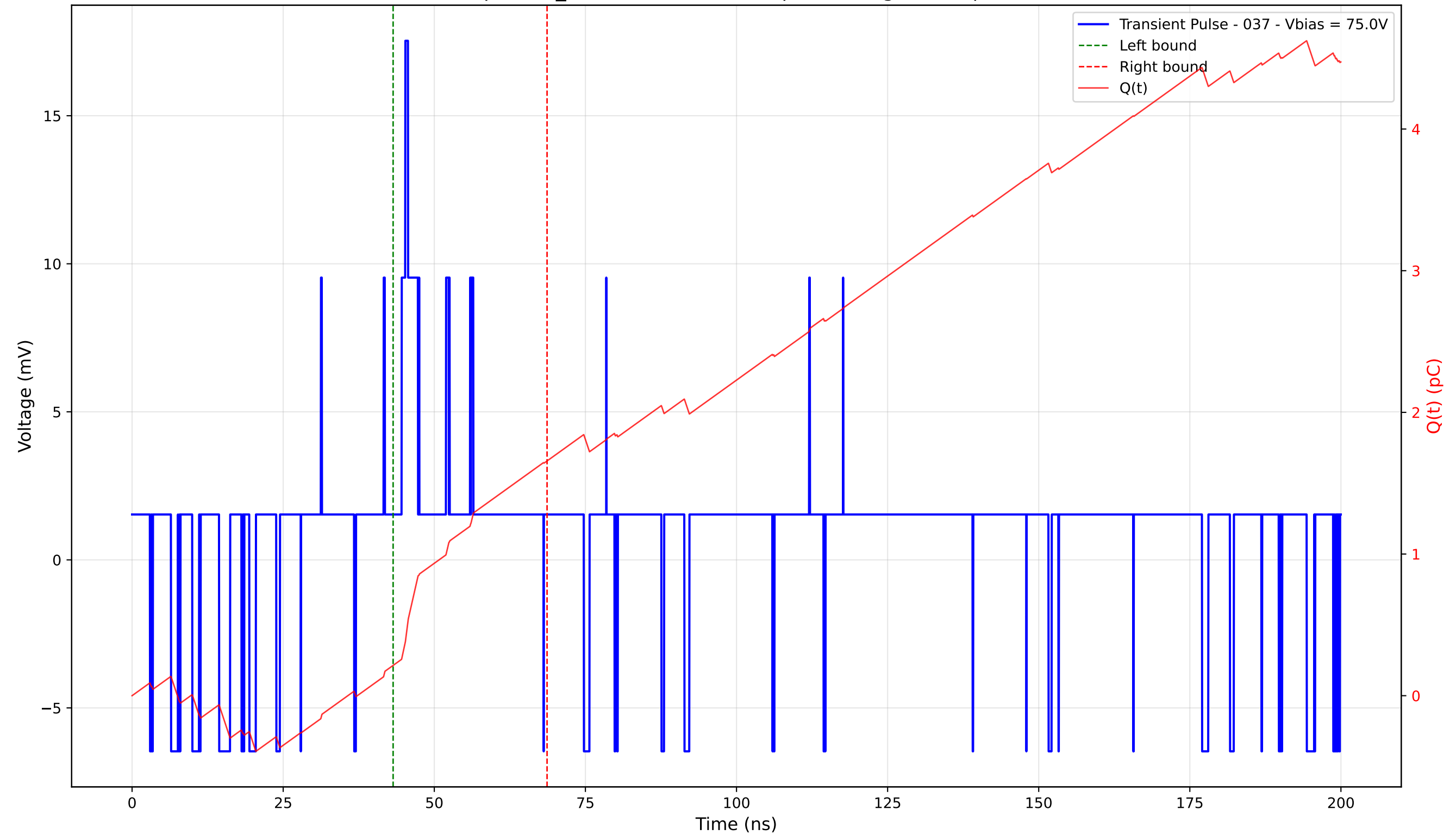
Transient Pulse - Sample: TD_4004 - Position: 30.0 \mu\text{m} - Charge: 1.44 pC - Rise Time: 0.62 ns
