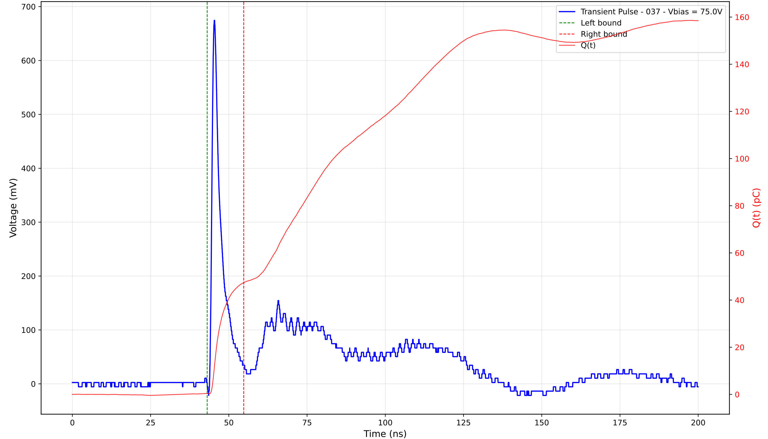
Transient Pulse - Sample: TD_4004 - Position: 100.0 \mu\text{m} - Charge: 46.99 pC - Rise Time: 0.96 ns
