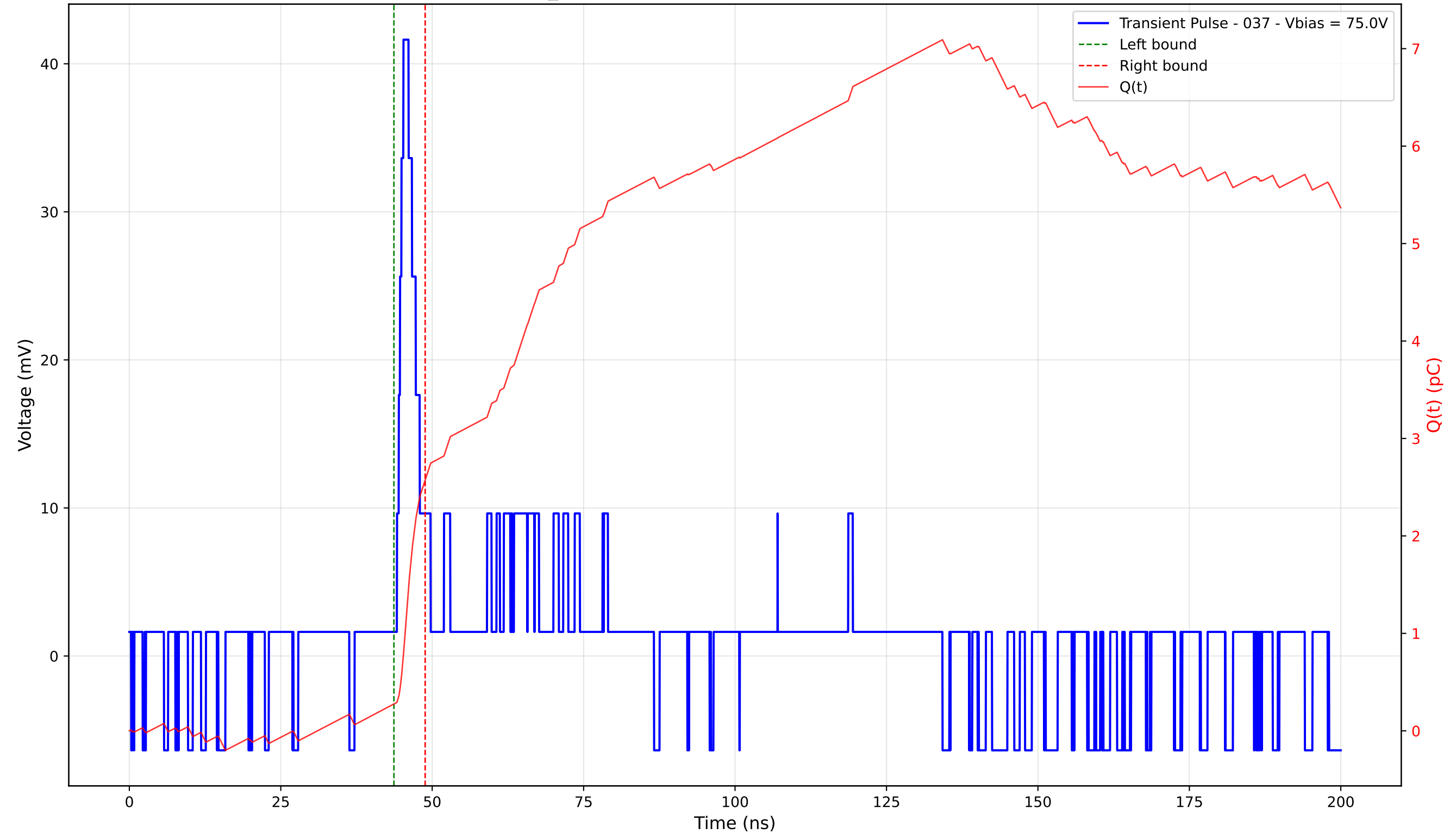
Transient Pulse - Sample: TD_4004 - Position: 420.0 \mu\text{m} - Charge: 2.30 pC - Rise Time: 1.07 ns
