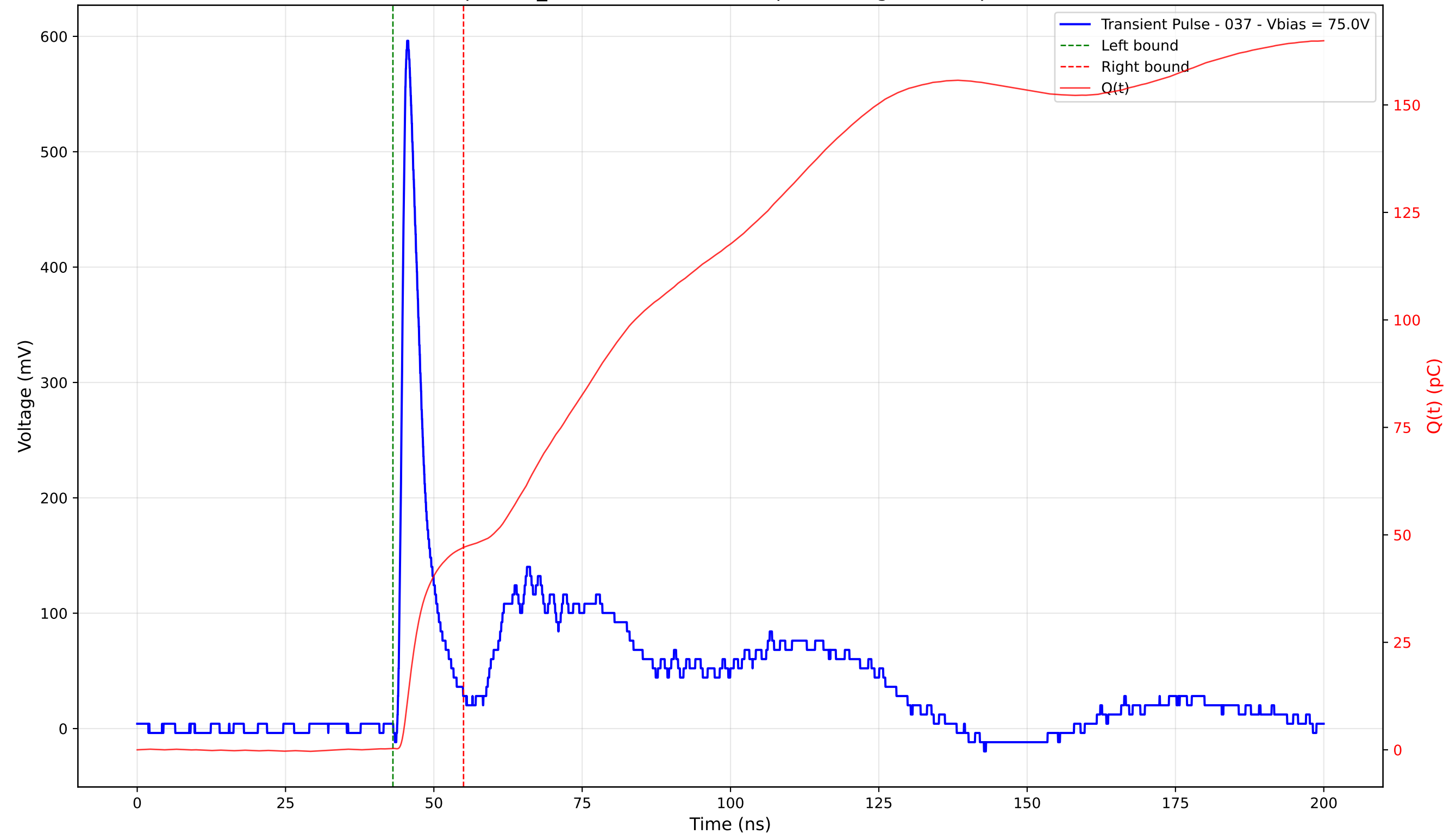
Transient Pulse - Sample: TD_4004 - Position: 195.0 \mu\text{m} - Charge: 46.75 pC - Rise Time: 1.04 ns
