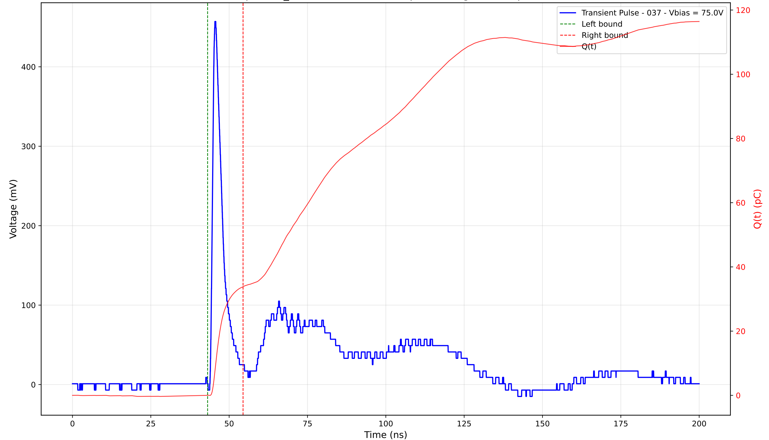
Transient Pulse - Sample: TD_4004 - Position: 230.0 \mu\text{m} - Charge: 33.81 pC - Rise Time: 1.03 ns
