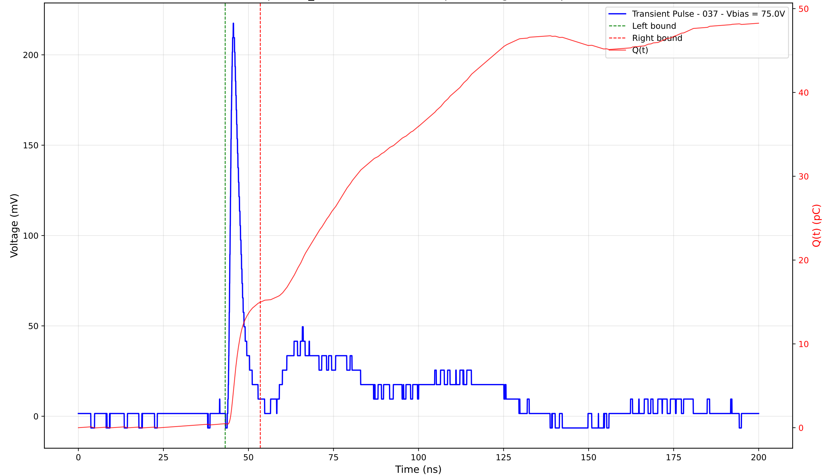
Transient Pulse - Sample: TD_4004 - Position: 330.0 \mu\text{m} - Charge: 14.49 pC - Rise Time: 1.11 ns
