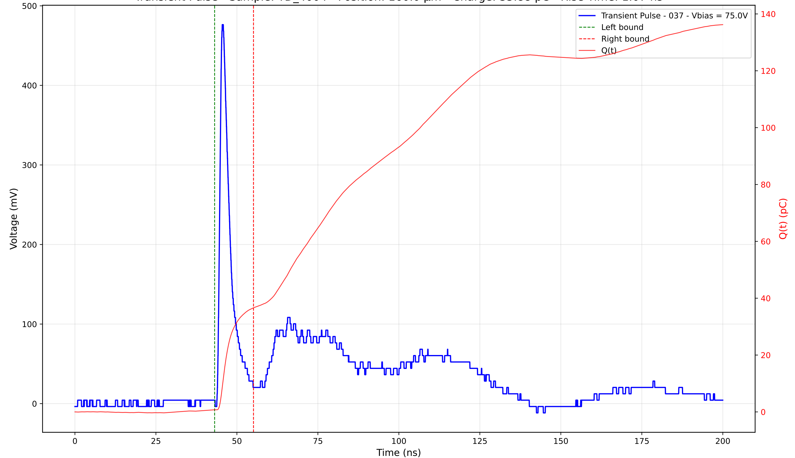
Transient Pulse - Sample: TD_4004 - Position: 160.0 \mu\text{m} - Charge: 35.88 pC - Rise Time: 1.07 ns
