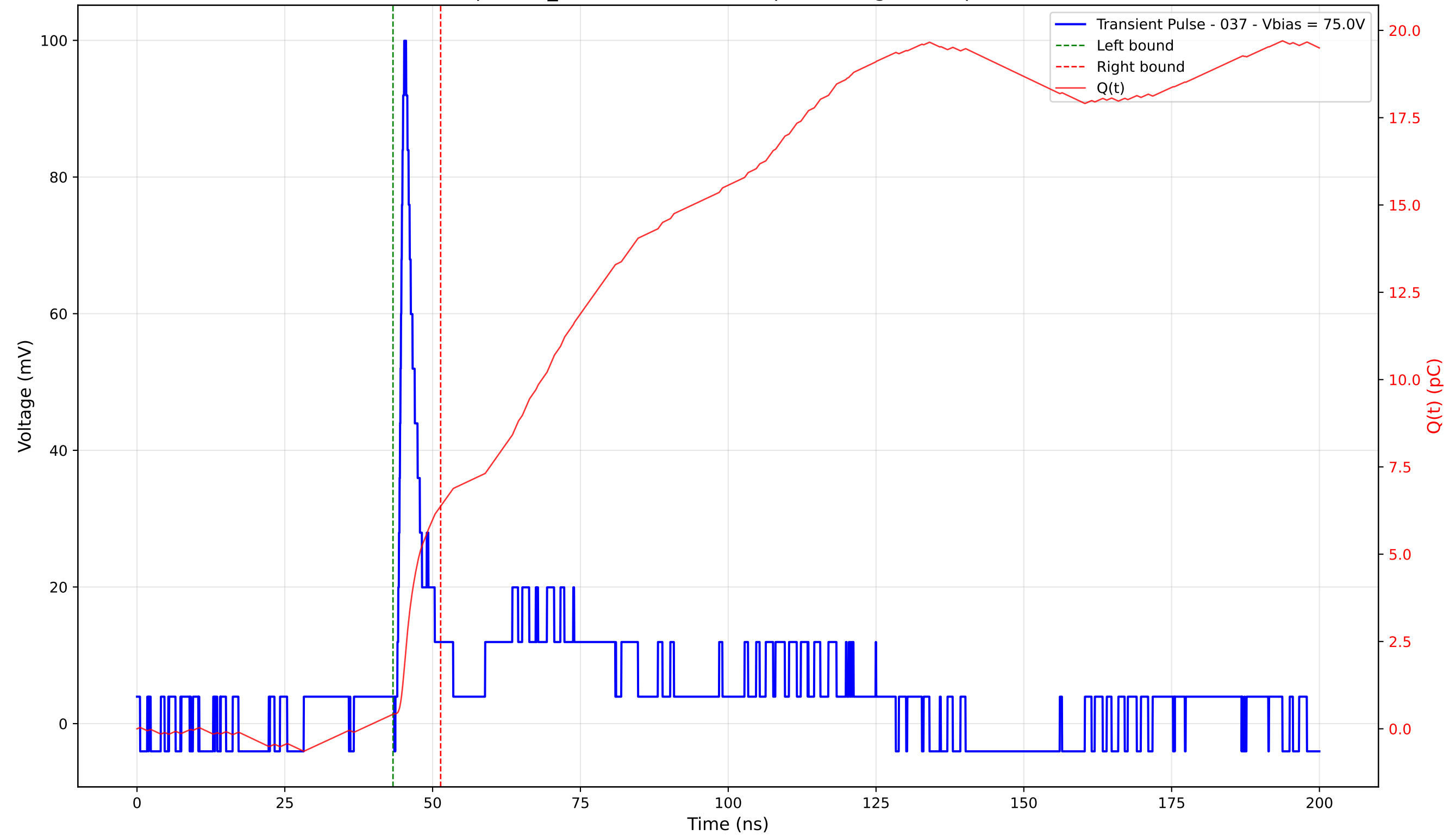
Transient Pulse - Sample: TD_4004 - Position: 55.0 \mu\text{m} - Charge: 5.96 pC - Rise Time: 0.96 ns
