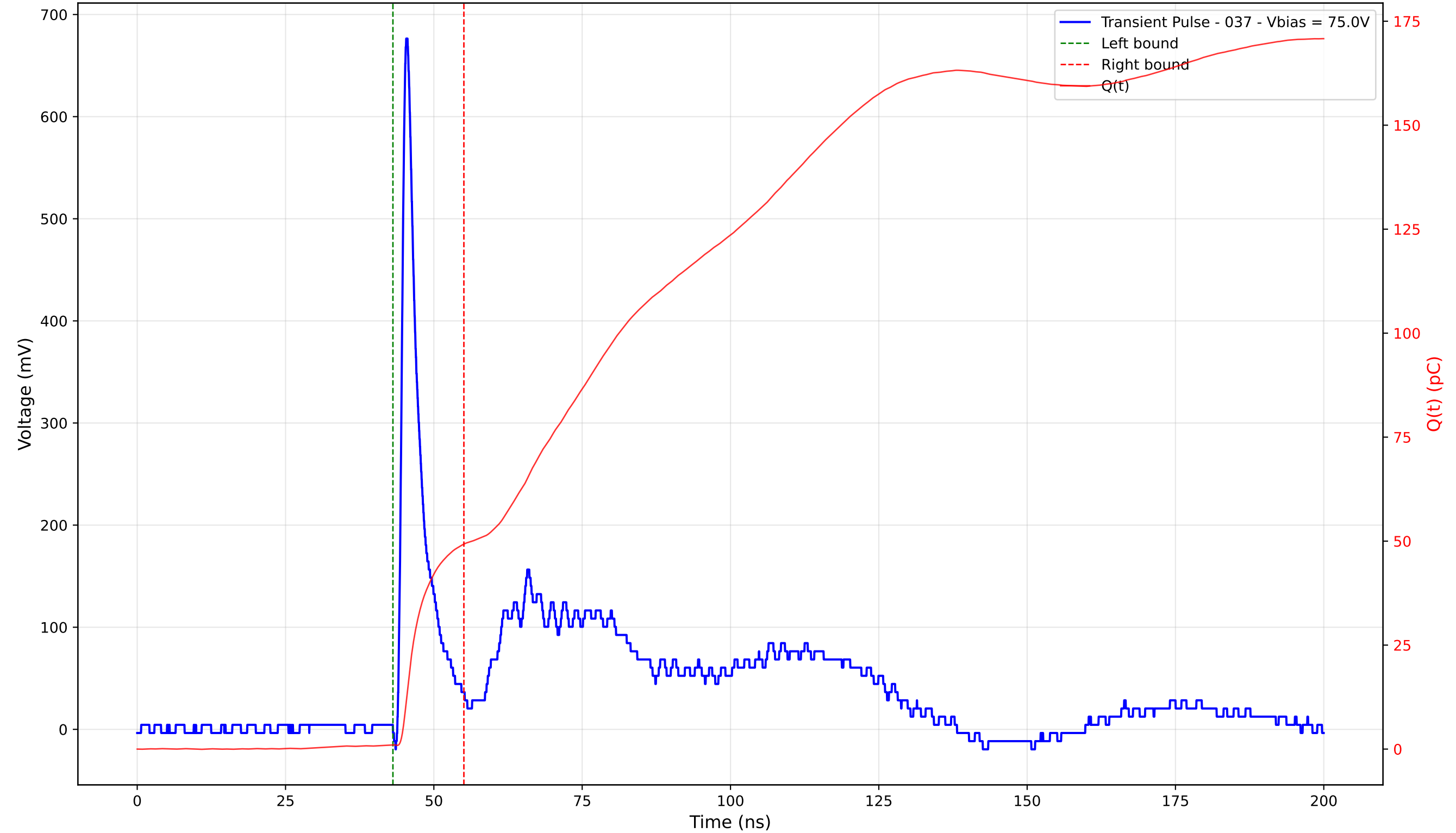
Transient Pulse - Sample: TD_4004 - Position: 115.0 \mu\text{m} - Charge: 48.27 pC - Rise Time: 0.97 ns
