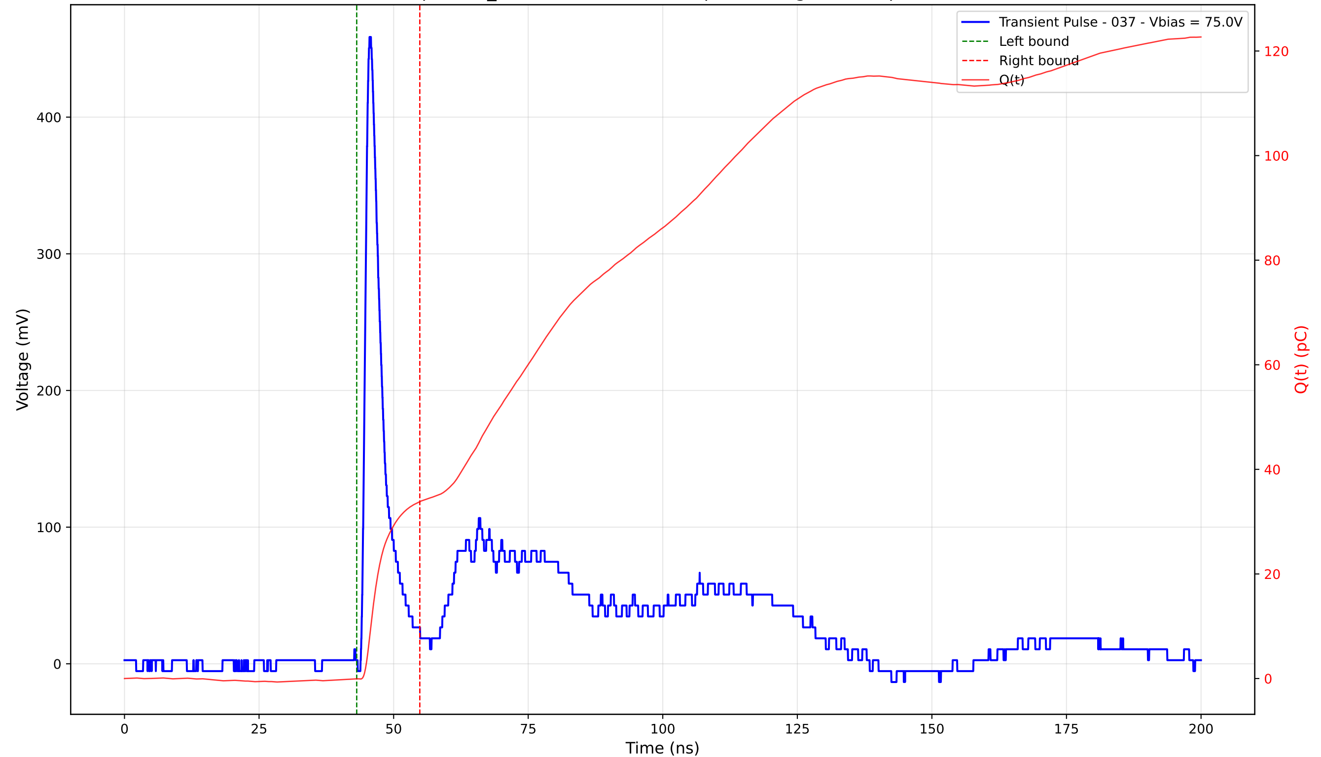
Transient Pulse - Sample: TD_4004 - Position: 155.0 \mu\text{m} - Charge: 33.89 pC - Rise Time: 1.07 ns
