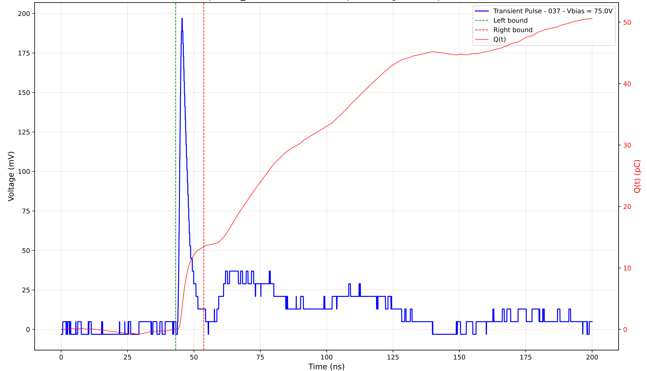
Transient Pulse - Sample: TD_4004 - Position: 335.0 \mu\text{m} - Charge: 13.41 pC - Rise Time: 1.10 ns
