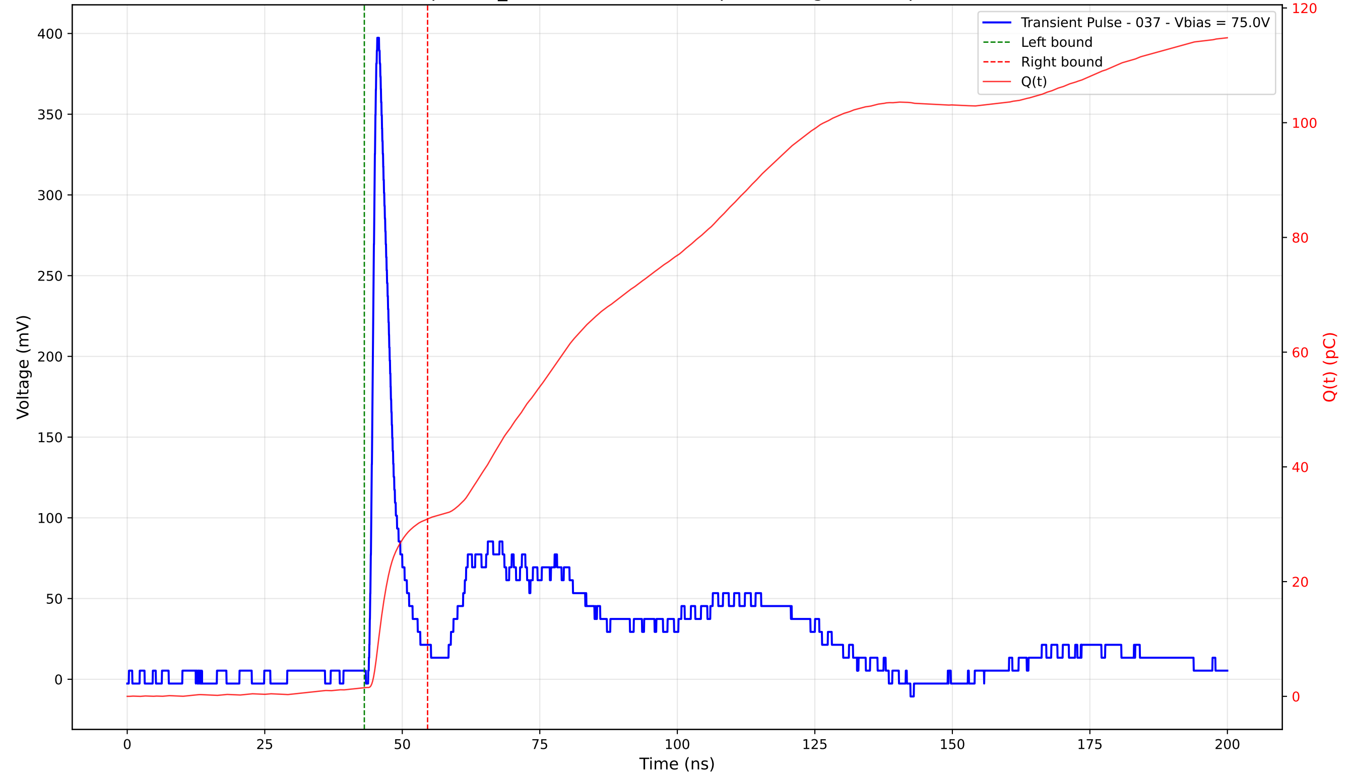
Transient Pulse - Sample: TD_4004 - Position: 240.0 \mu\text{m} - Charge: 29.41 pC - Rise Time: 1.07 ns
