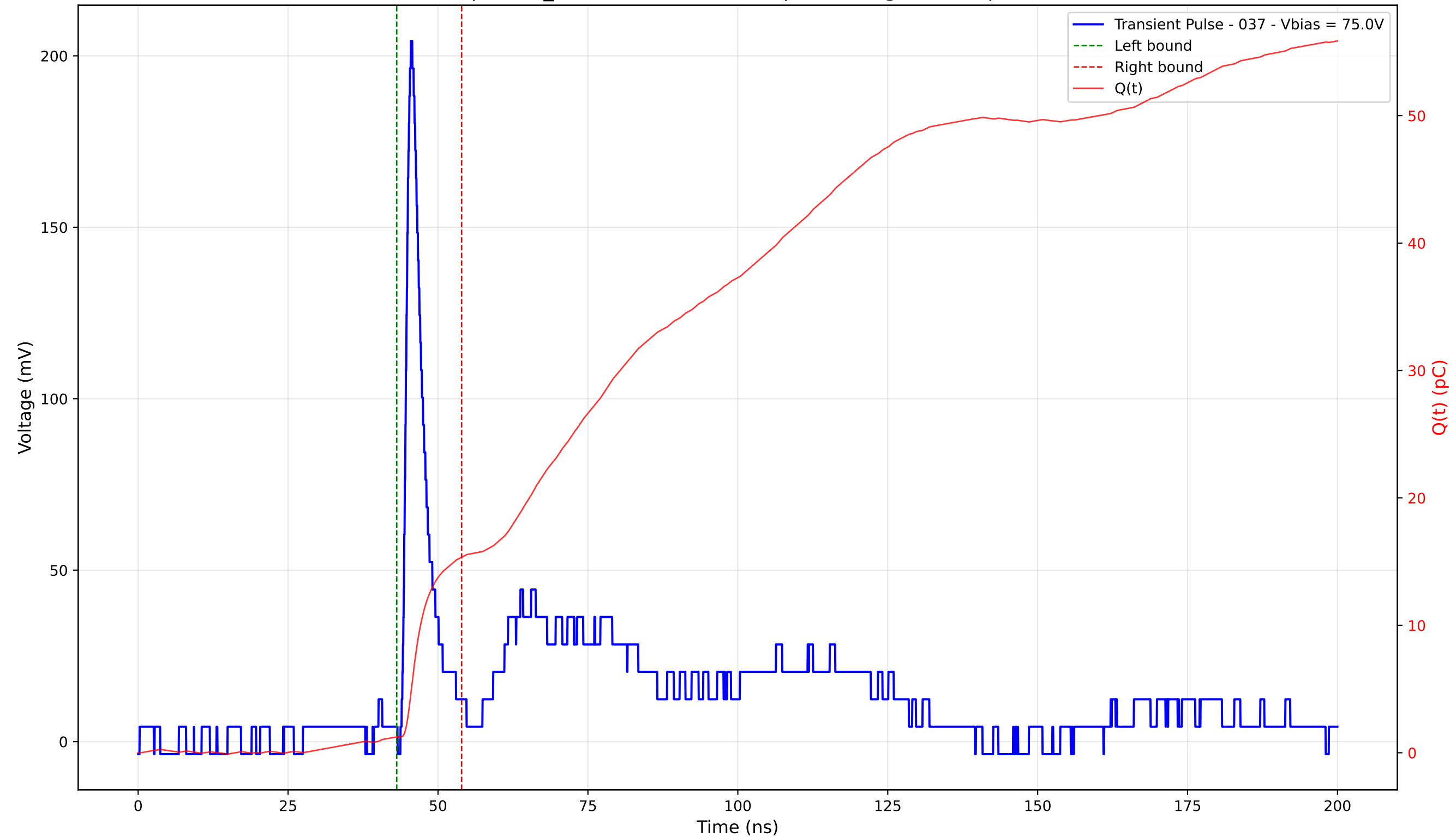
Transient Pulse - Sample: TD_4004 - Position: 350.0 \mu\text{m} - Charge: 14.10 pC - Rise Time: 1.10 ns
