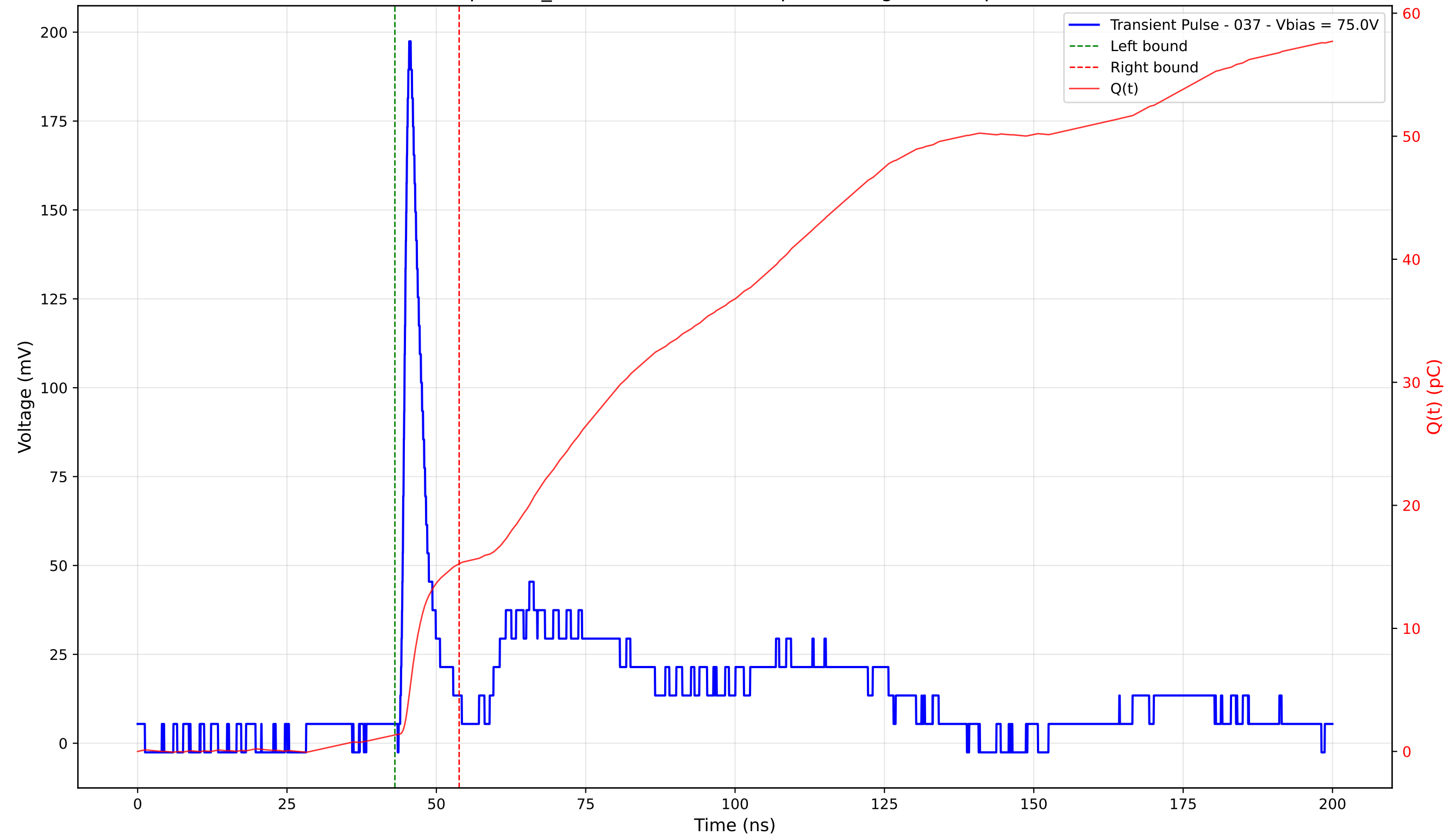
Transient Pulse - Sample: TD_4004 - Position: 340.0 \mu\text{m} - Charge: 13.91 pC - Rise Time: 1.12 ns
