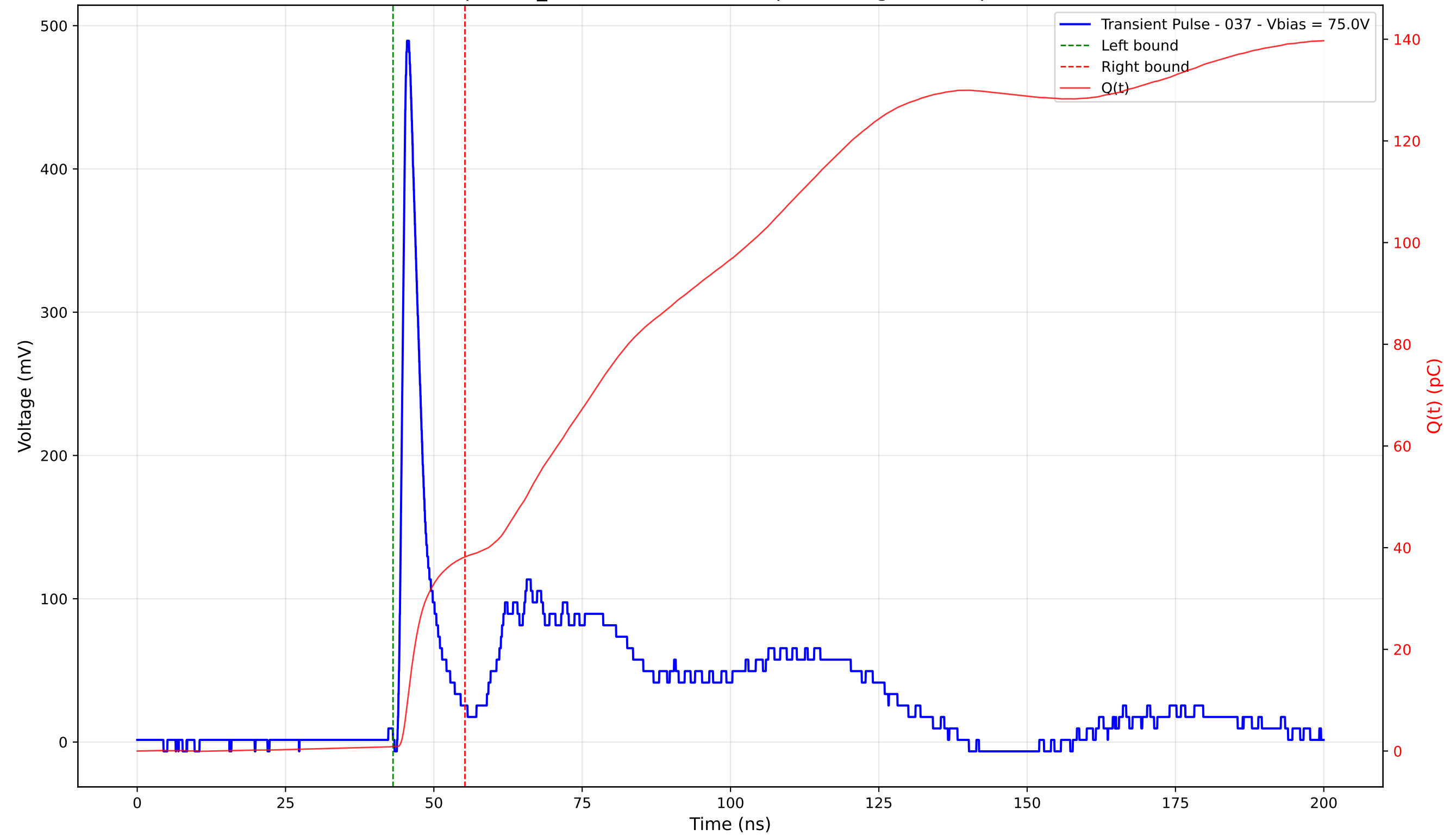
Transient Pulse - Sample: TD_4004 - Position: 165.0 \mu\text{m} - Charge: 37.26 pC - Rise Time: 1.06 ns
