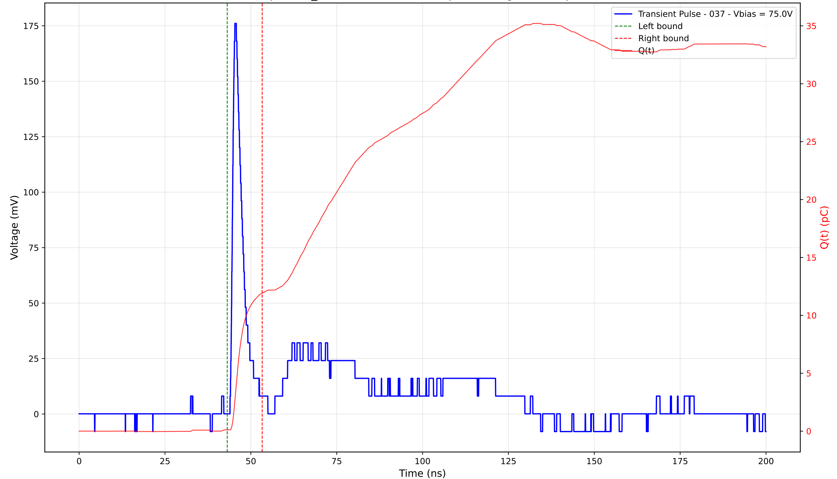
Transient Pulse - Sample: TD_4004 - Position: 380.0 \mu\text{m} - Charge: 11.80 pC - Rise Time: 0.98 ns
