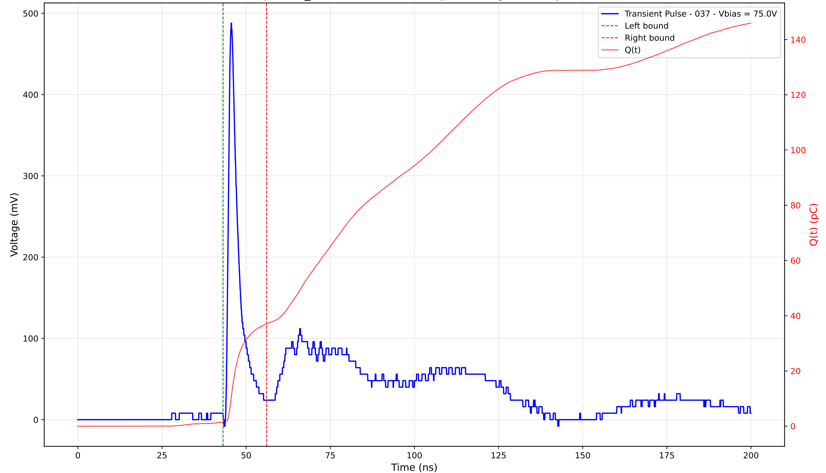
Transient Pulse - Sample: TD_4004 - Position: 135.0 \mu\text{m} - Charge: 35.49 pC - Rise Time: 1.06 ns
