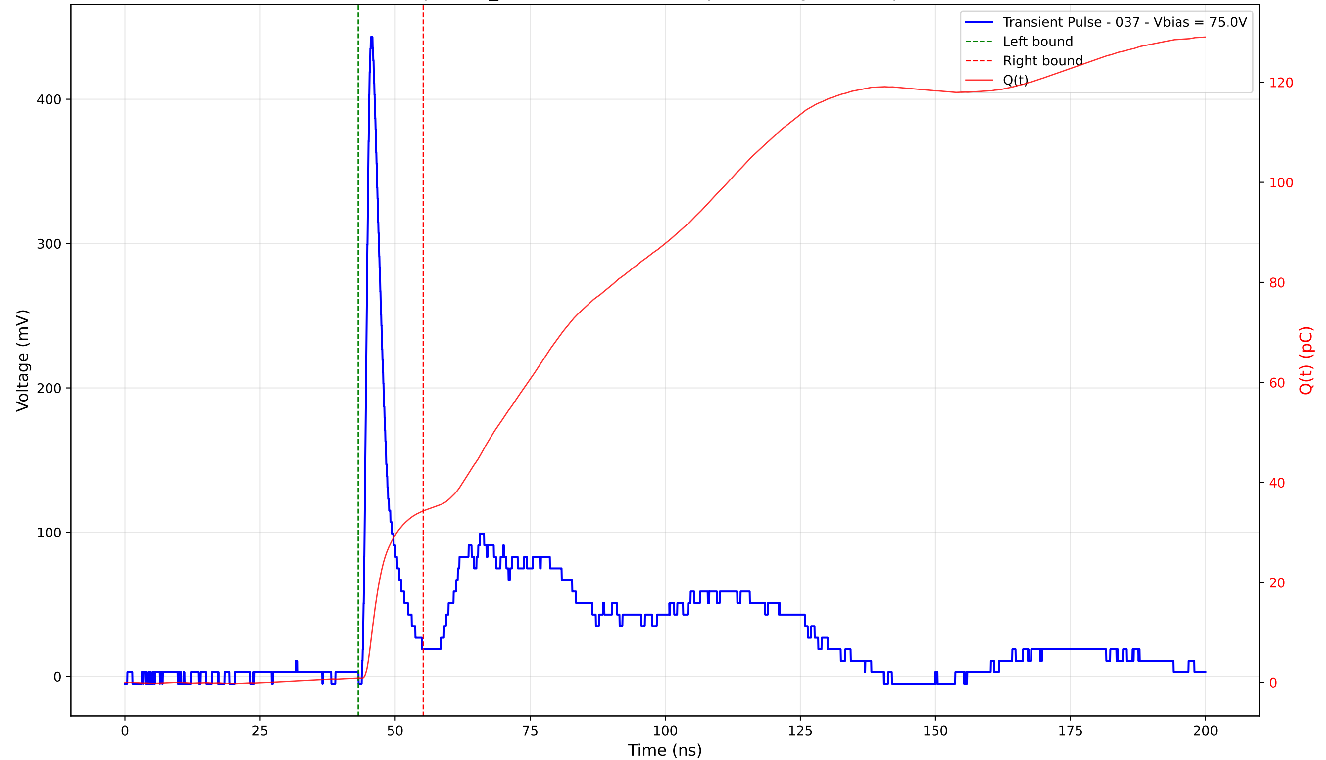
Transient Pulse - Sample: TD_4004 - Position: 150.0 \mu\text{m} - Charge: 33.45 pC - Rise Time: 1.06 ns
