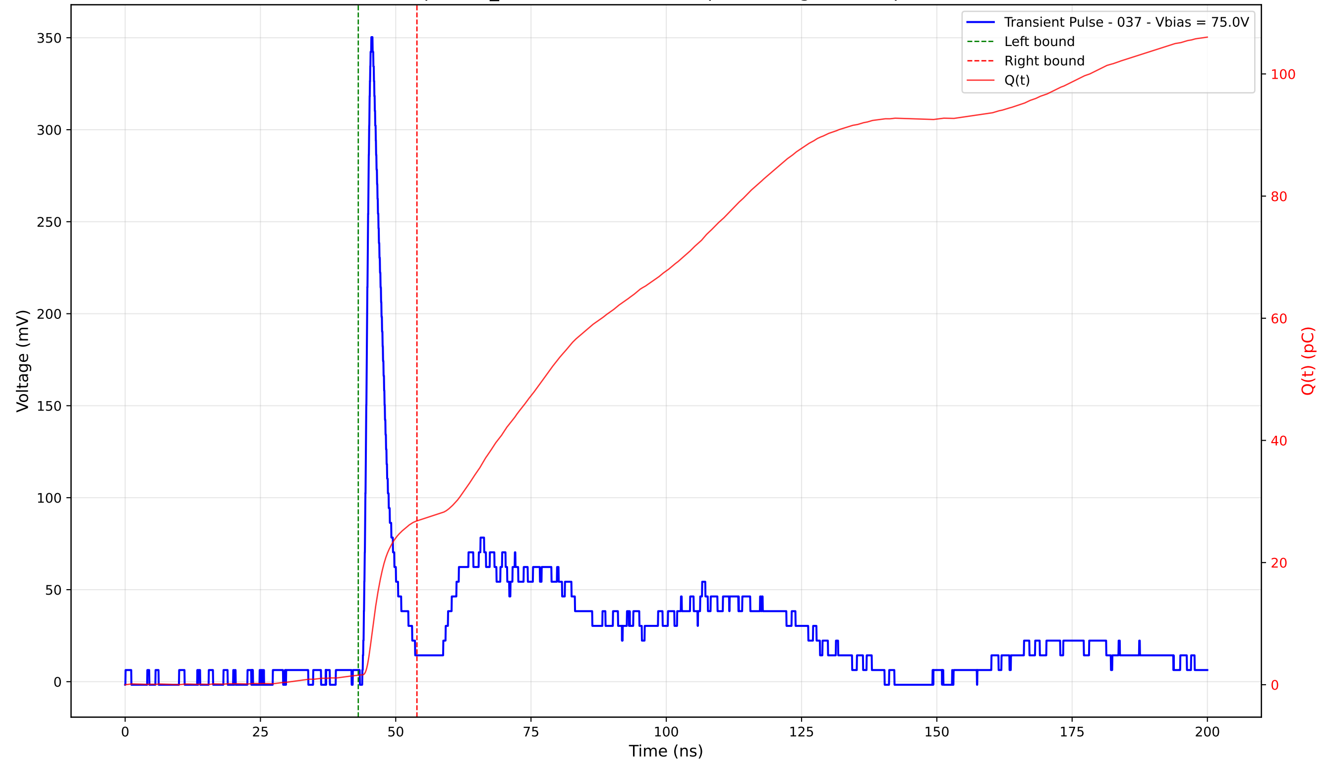
Transient Pulse - Sample: TD_4004 - Position: 275.0 \mu\text{m} - Charge: 25.24 pC - Rise Time: 1.07 ns
