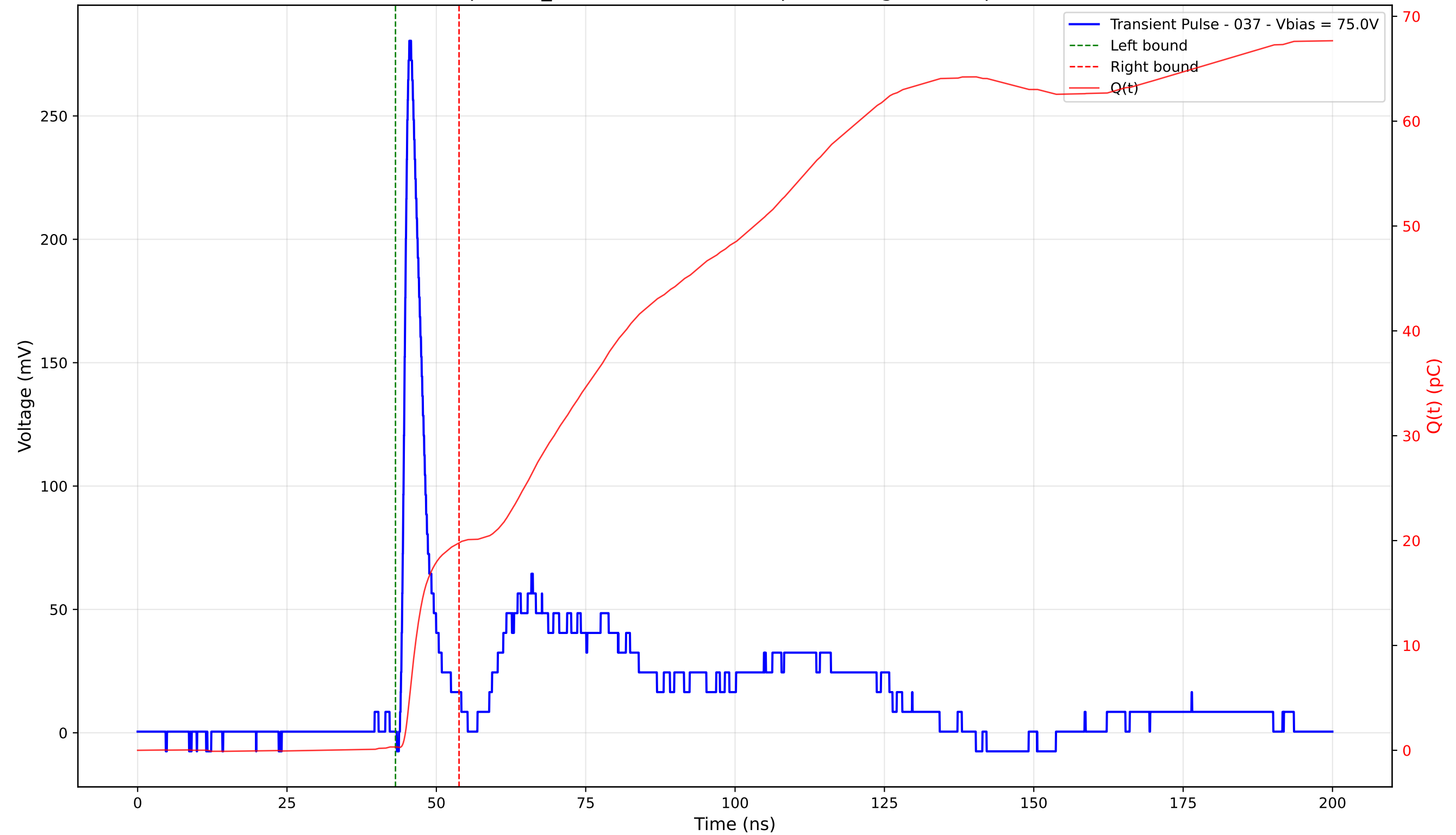
Transient Pulse - Sample: TD_4004 - Position: 300.0 \mu\text{m} - Charge: 19.47 pC - Rise Time: 1.05 ns
