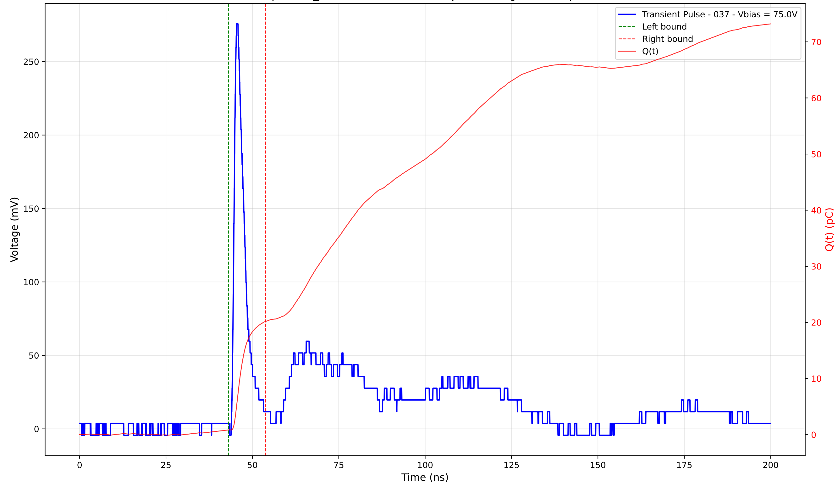
Transient Pulse - Sample: TD_4004 - Position: 295.0 \mu\text{m} - Charge: 19.30 pC - Rise Time: 1.06 ns
