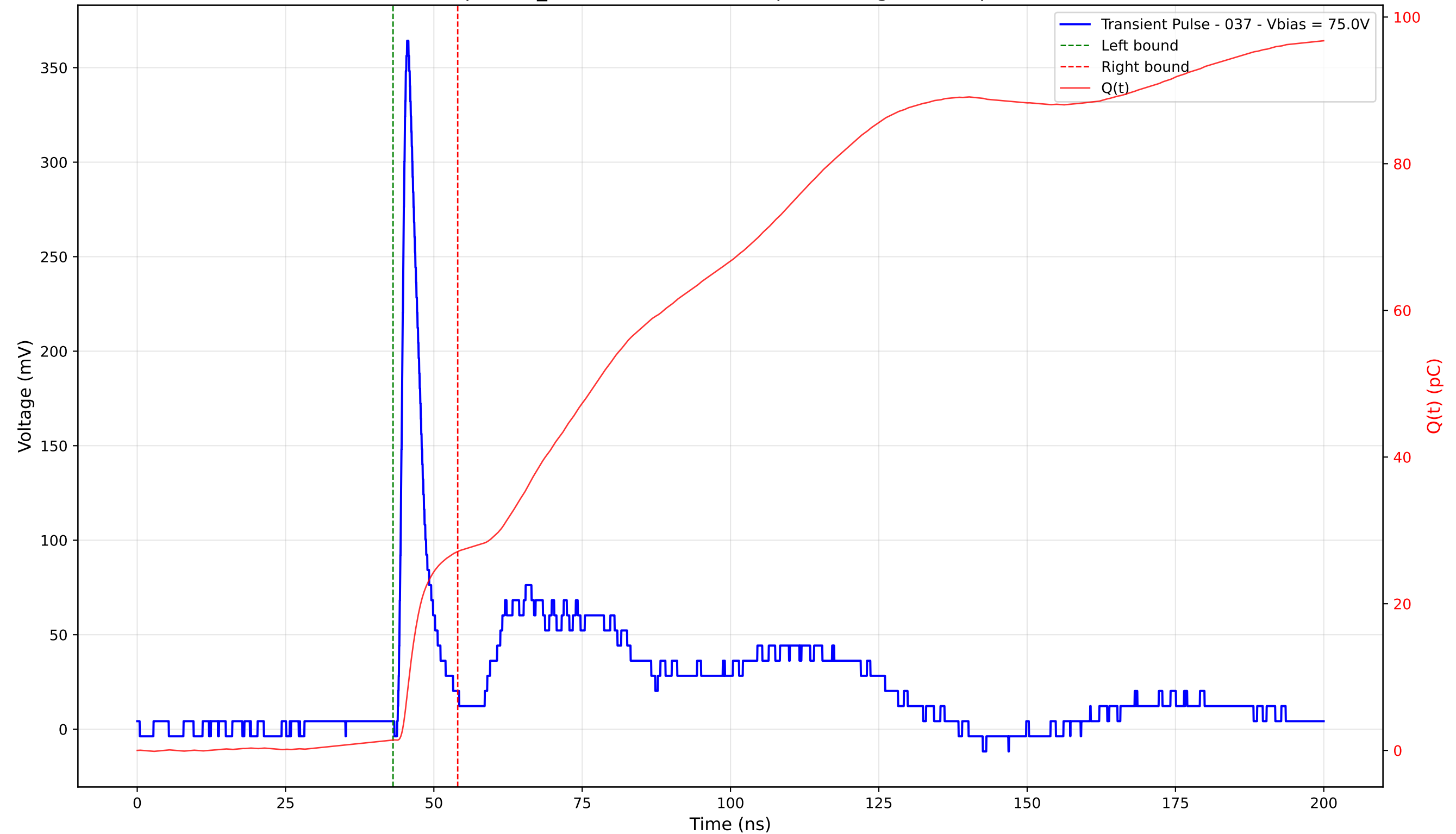
Transient Pulse - Sample: TD_4004 - Position: 280.0 \mu\text{m} - Charge: 25.71 pC - Rise Time: 1.04 ns
