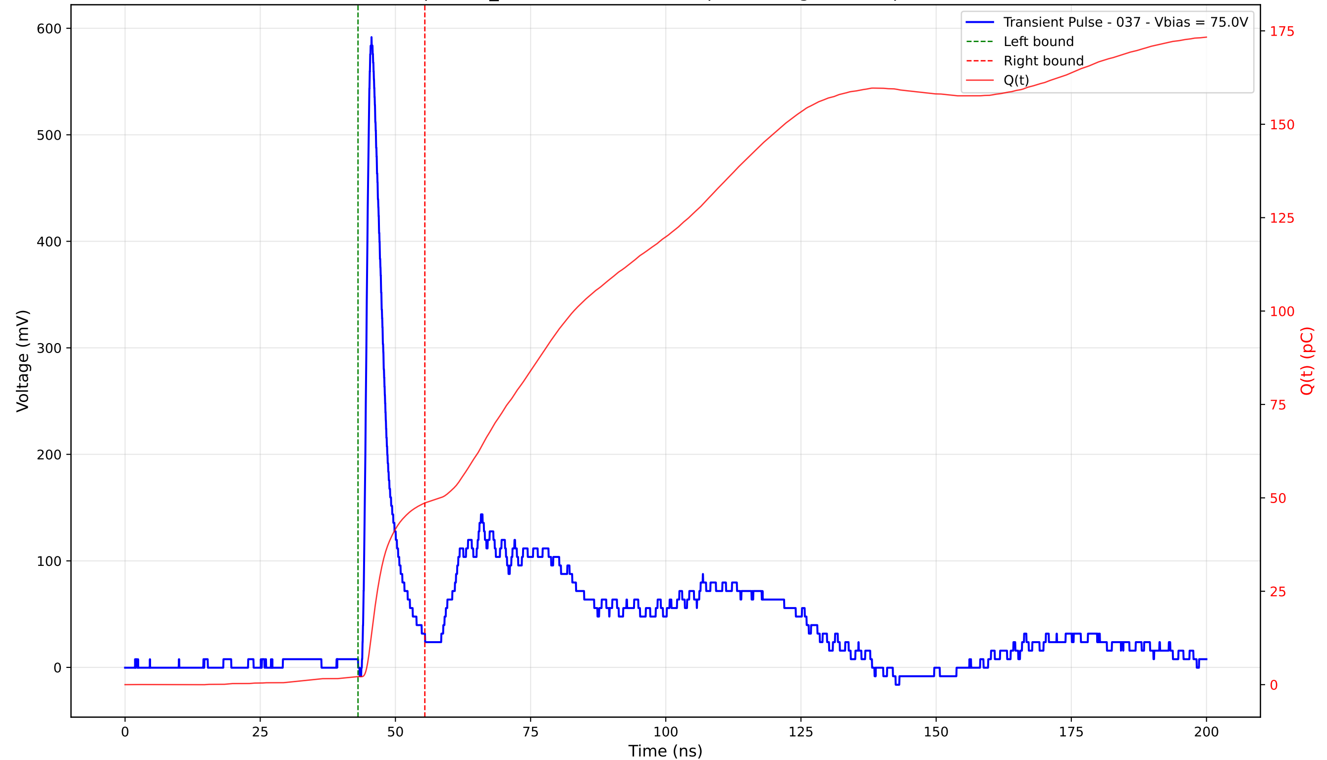
Transient Pulse - Sample: TD_4004 - Position: 200.0 \mu\text{m} - Charge: 46.44 pC - Rise Time: 1.06 ns
