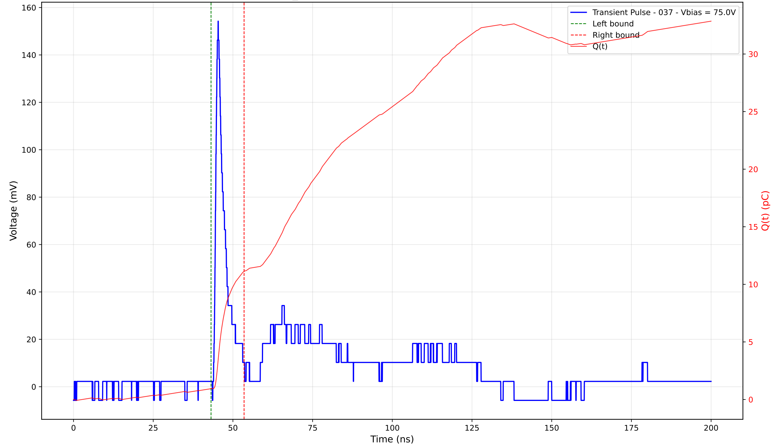
Transient Pulse - Sample: TD_4004 - Position: 60.0 \mu\text{m} - Charge: 10.18 pC - Rise Time: 1.05 ns
