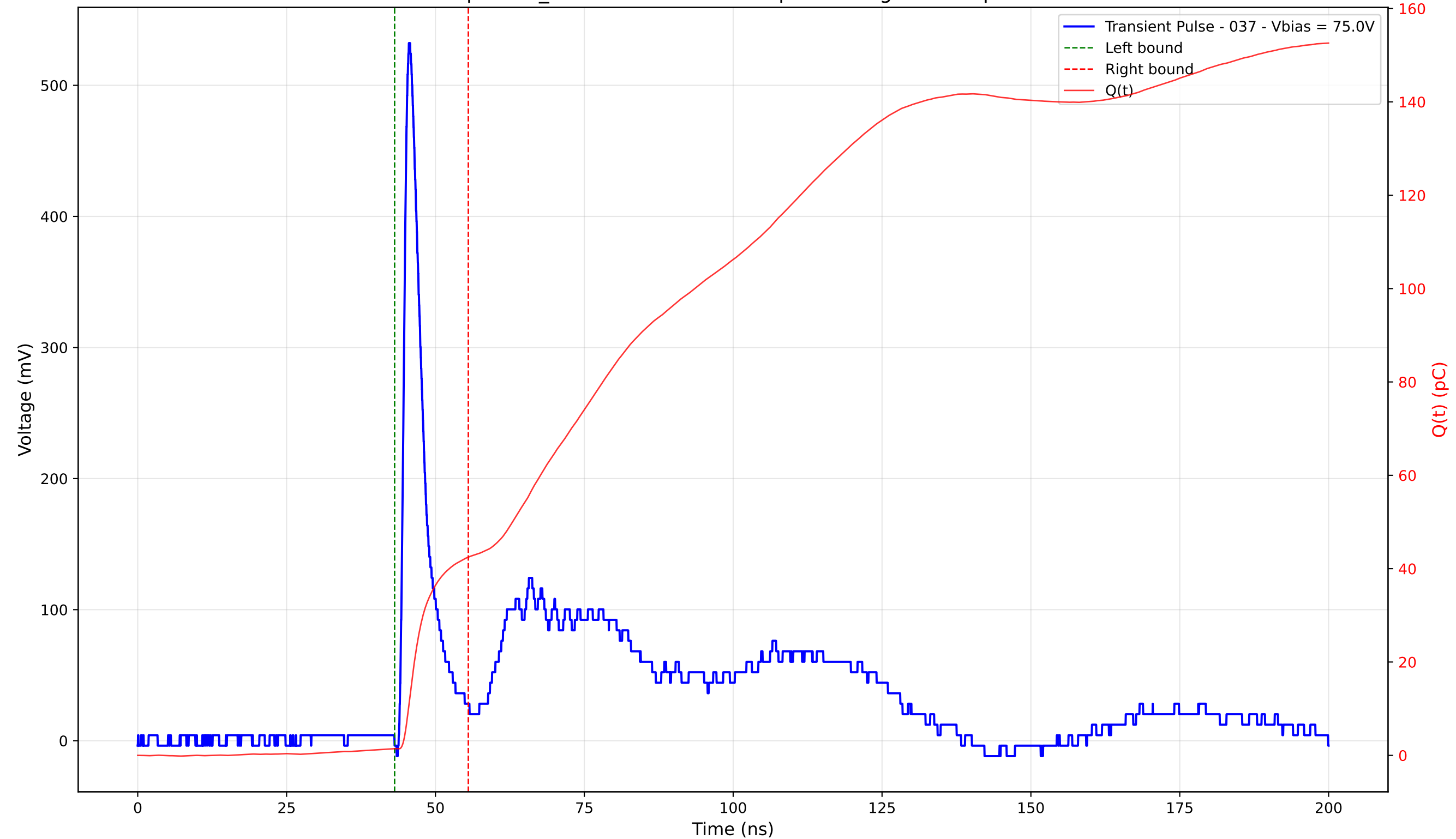
Transient Pulse - Sample: TD_4004 - Position: 170.0 \mu\text{m} - Charge: 41.02 pC - Rise Time: 1.08 ns
