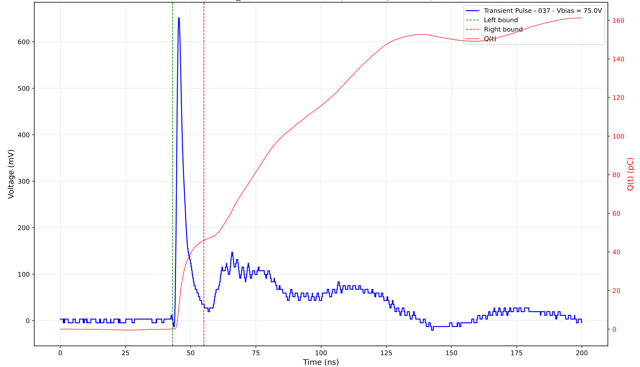
Transient Pulse - Sample: TD_4004 - Position: 120.0 \mu\text{m} - Charge: 45.84 pC - Rise Time: 0.98 ns
