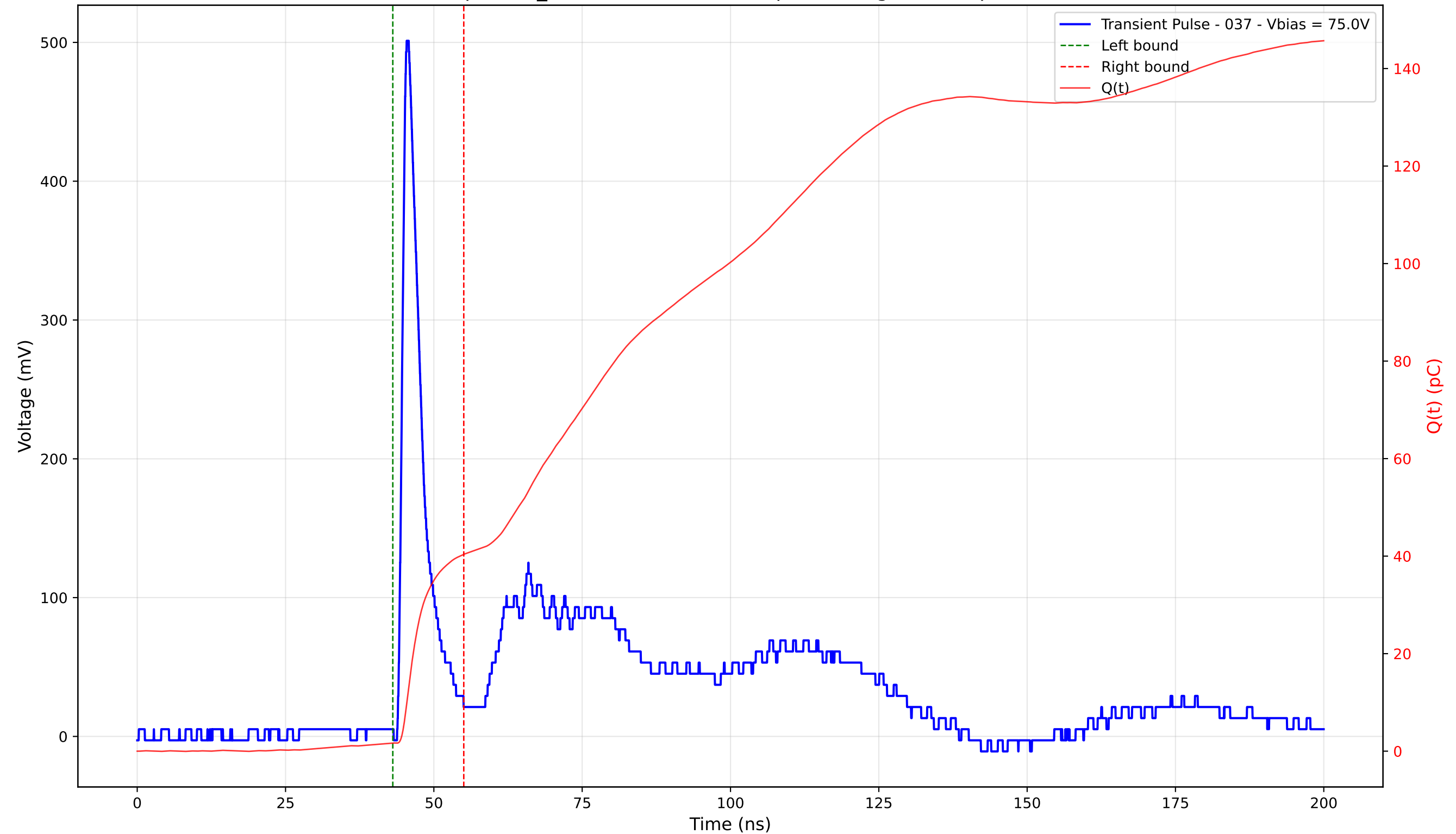
Transient Pulse - Sample: TD_4004 - Position: 225.0 \mu\text{m} - Charge: 38.71 pC - Rise Time: 1.04 ns
