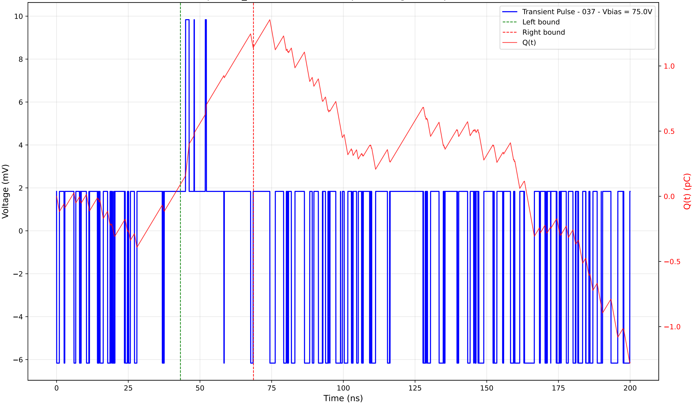
Transient Pulse - Sample: TD_4004 - Position: 10.0 \mu\text{m} - Charge: 1.05 pC - Rise Time: 0.00 ns (N/A)
