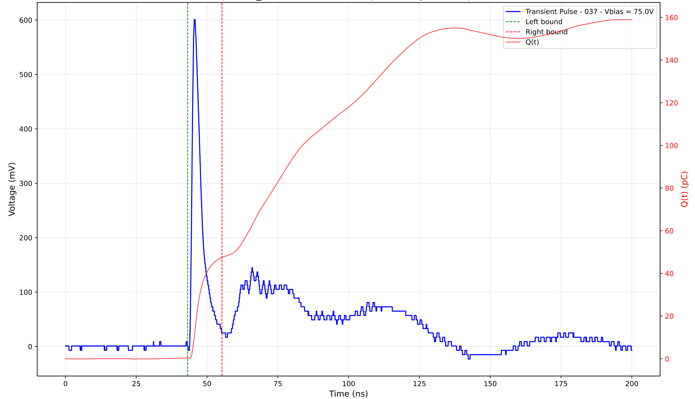
Transient Pulse - Sample: TD_4004 - Position: 185.0 \mu\text{m} - Charge: 47.19 pC - Rise Time: 1.04 ns
