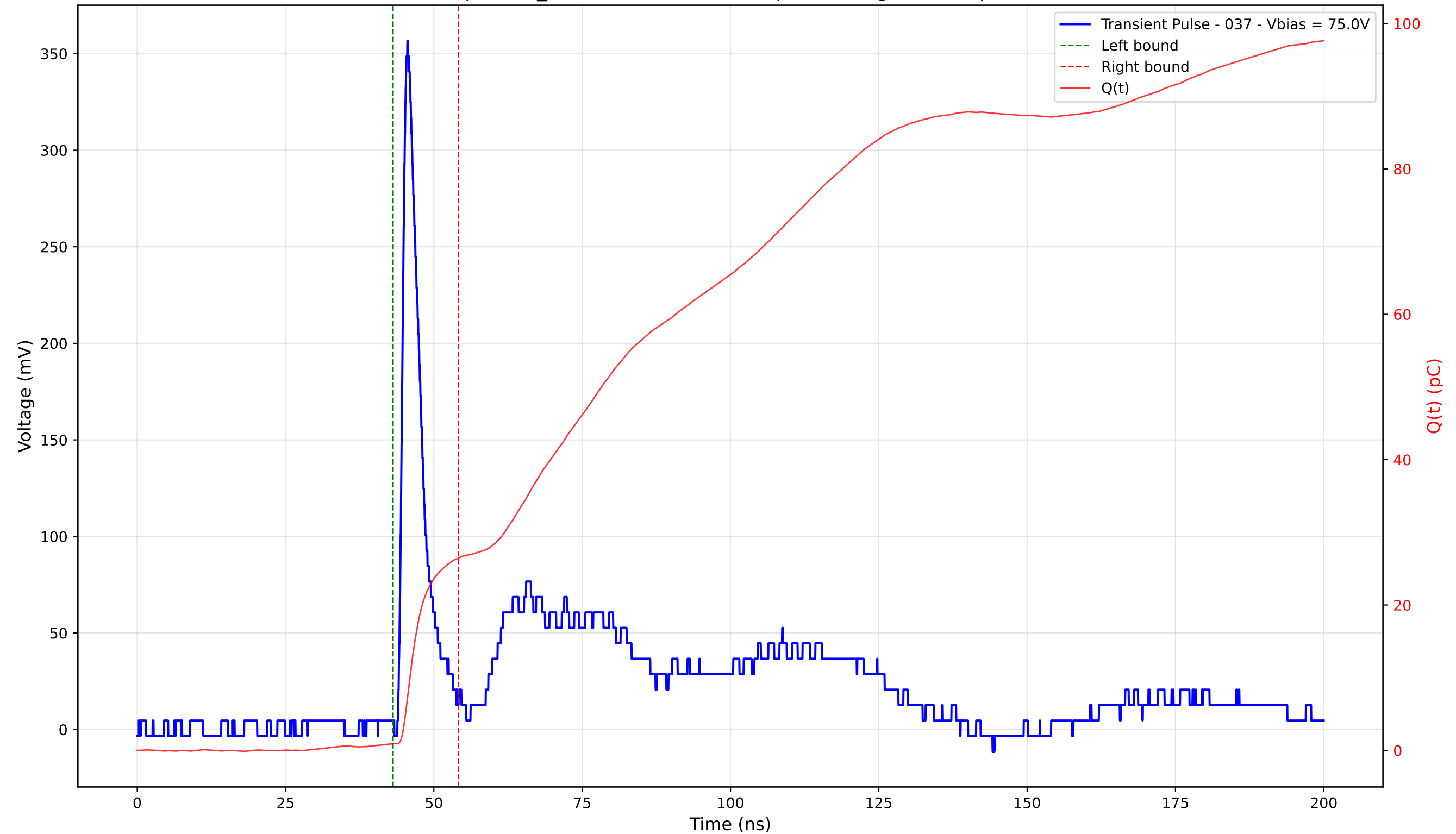
Transient Pulse - Sample: TD_4004 - Position: 260.0 \mu\text{m} - Charge: 25.52 pC - Rise Time: 1.08 ns
