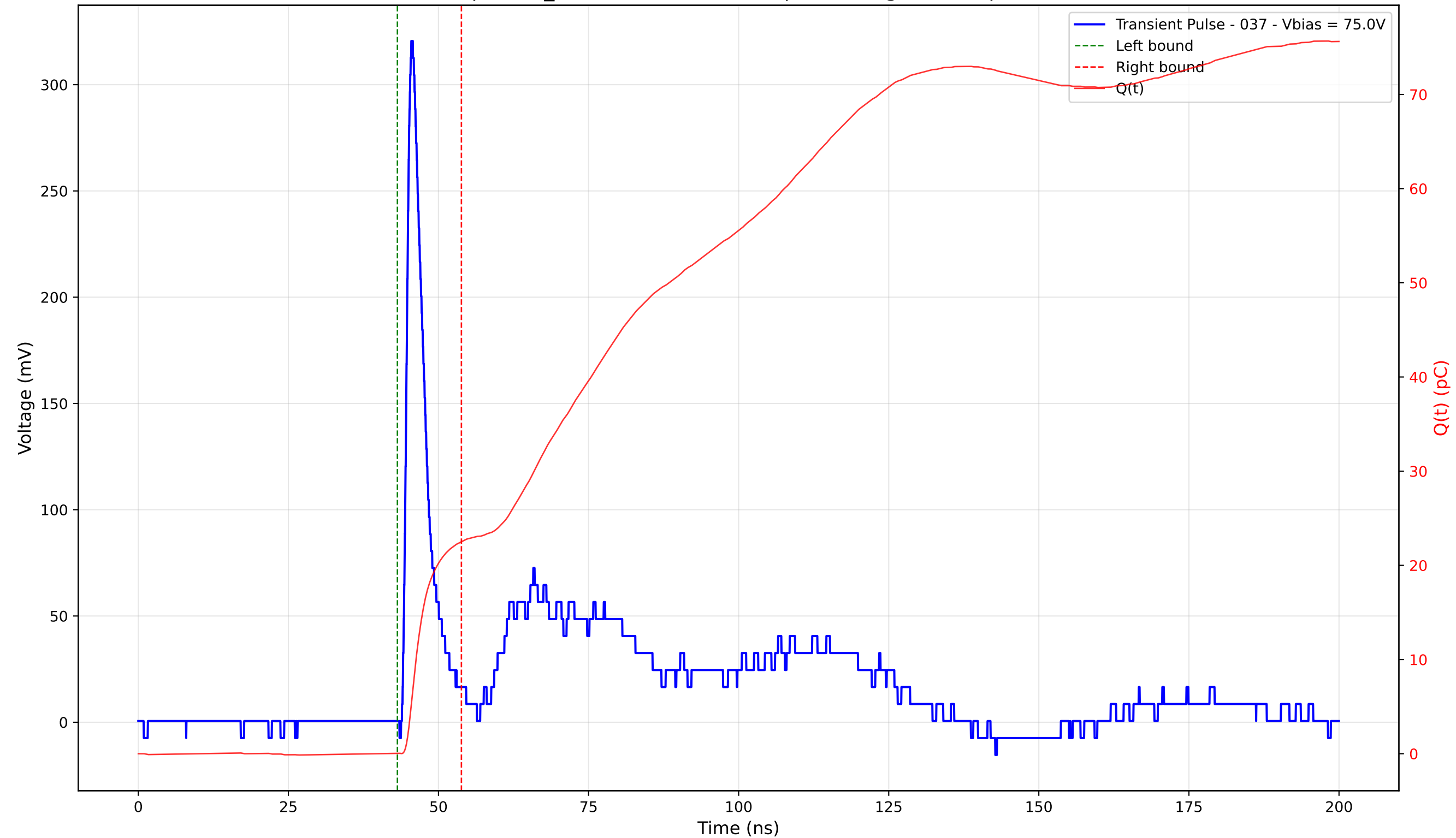
Transient Pulse - Sample: TD_4004 - Position: 270.0 \mu\text{m} - Charge: 22.46 pC - Rise Time: 1.04 ns
