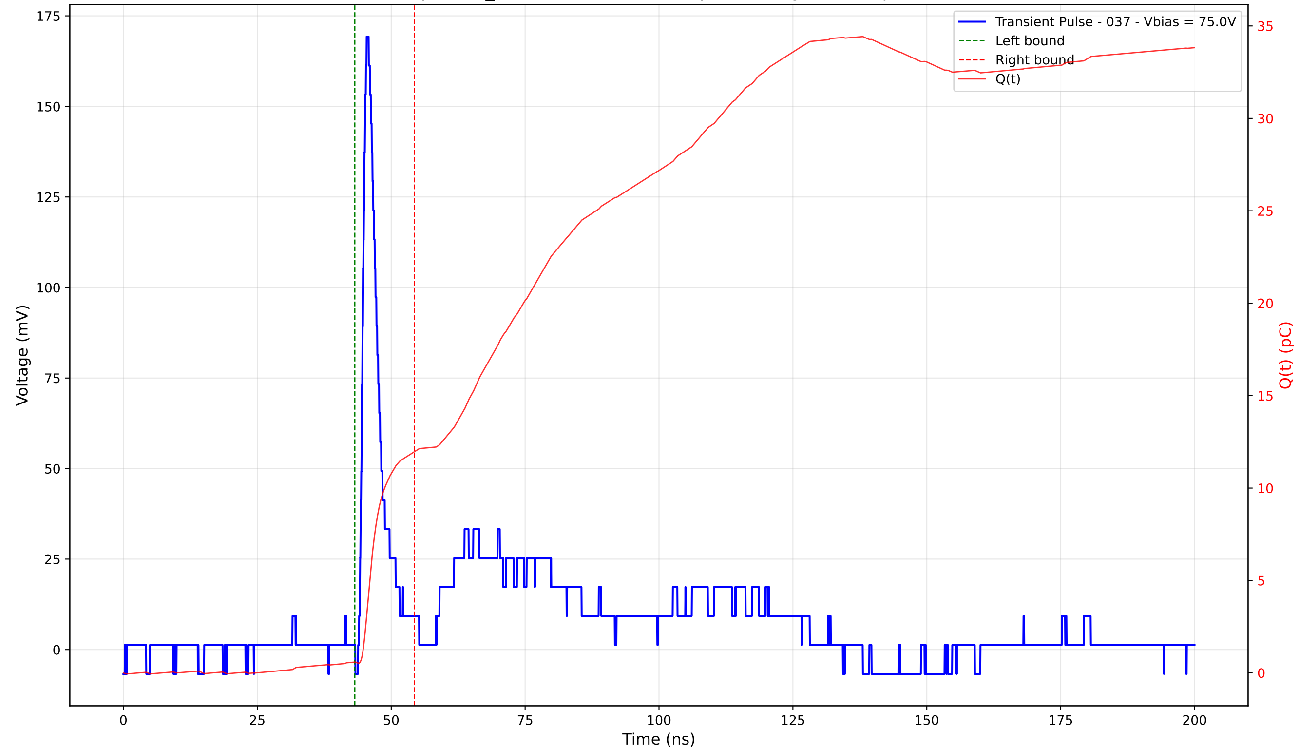
Transient Pulse - Sample: TD_4004 - Position: 375.0 \mu\text{m} - Charge: 11.38 pC - Rise Time: 1.02 ns
