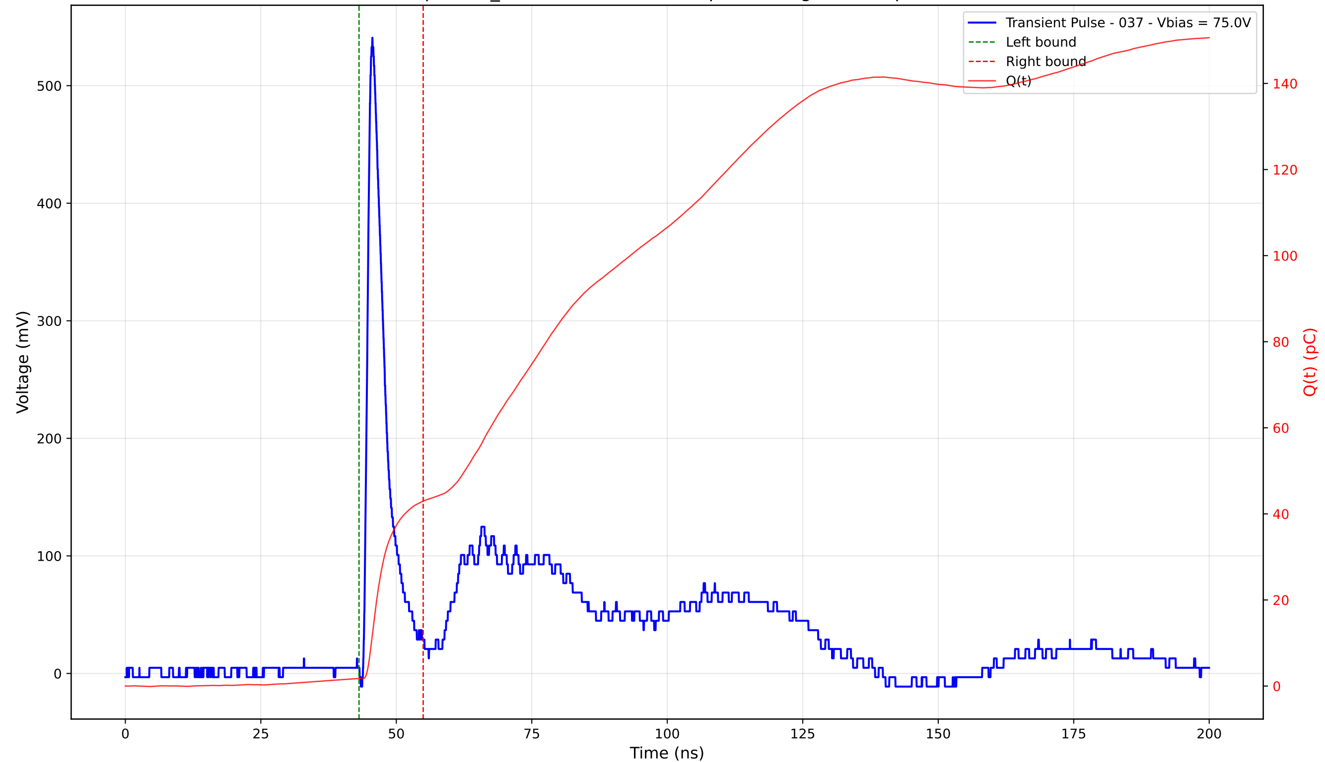
Transient Pulse - Sample: TD_4004 - Position: 210.0 \mu\text{m} - Charge: 41.17 pC - Rise Time: 1.06 ns
