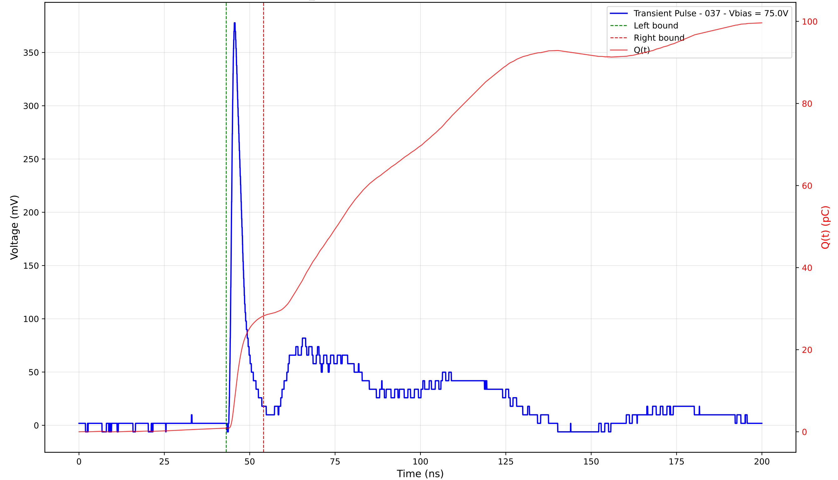
Transient Pulse - Sample: TD_4004 - Position: 255.0 \mu\text{m} - Charge: 27.33 pC - Rise Time: 1.09 ns
