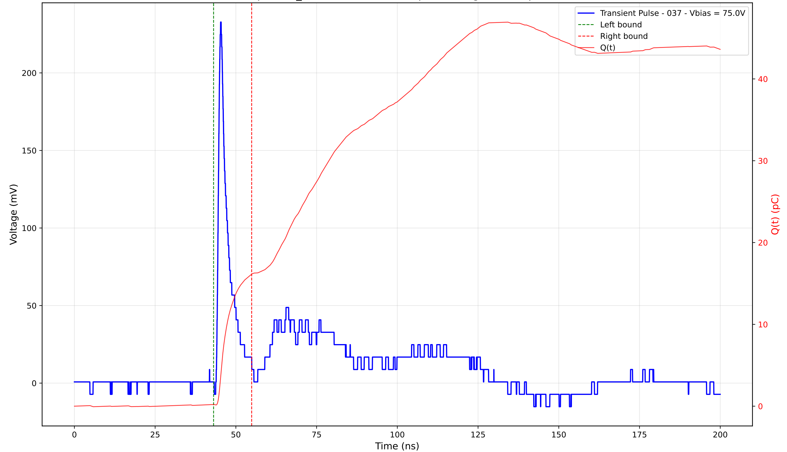
Transient Pulse - Sample: TD_4004 - Position: 65.0 \mu\text{m} - Charge: 15.94 pC - Rise Time: 0.98 ns
