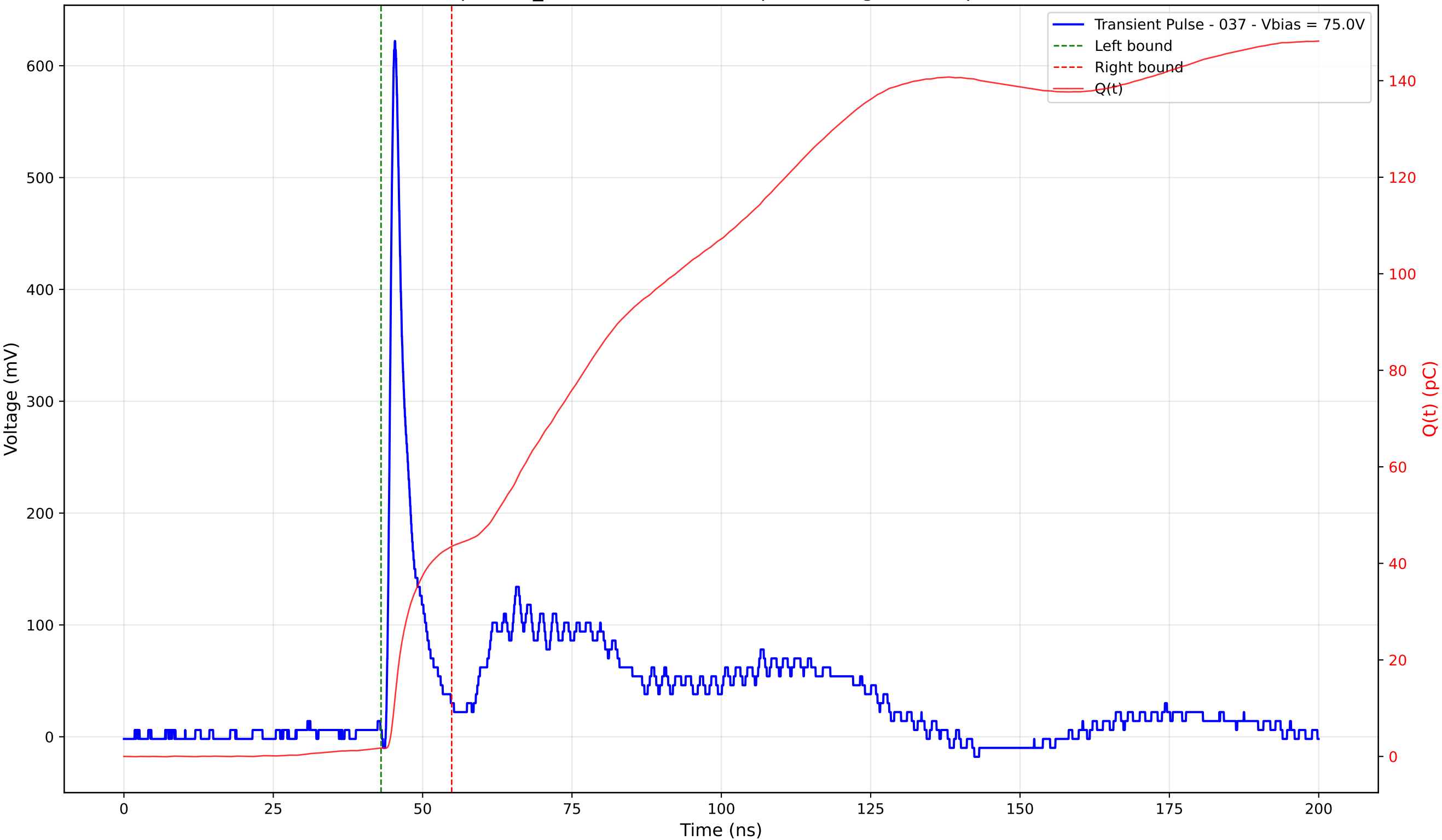
Transient Pulse - Sample: TD_4004 - Position: 90.0 \mu\text{m} - Charge: 41.76 pC - Rise Time: 0.96 ns
