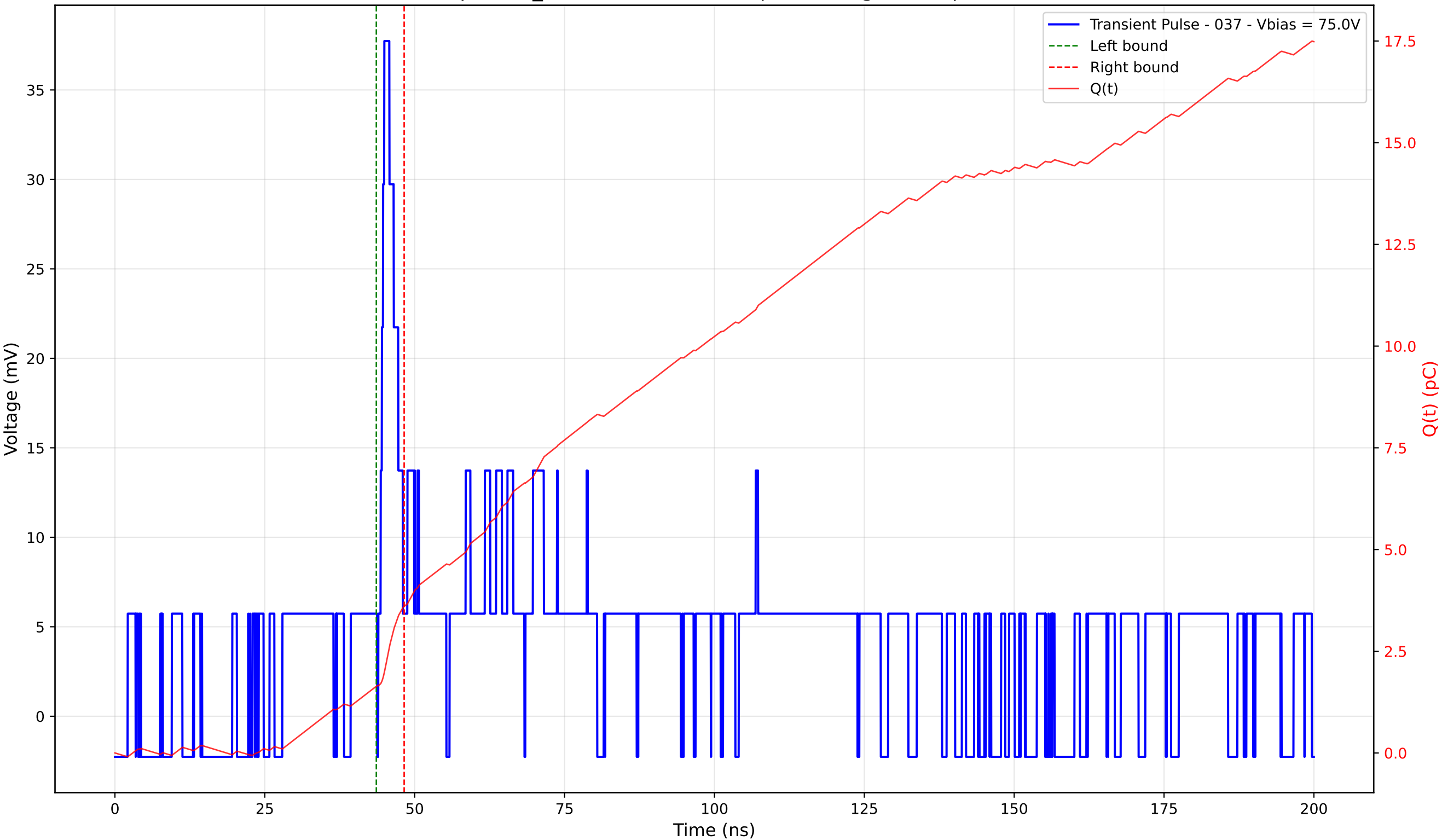
Transient Pulse - Sample: TD_4004 - Position: 45.0 \mu\text{m} - Charge: 1.96 pC - Rise Time: 1.01 ns
