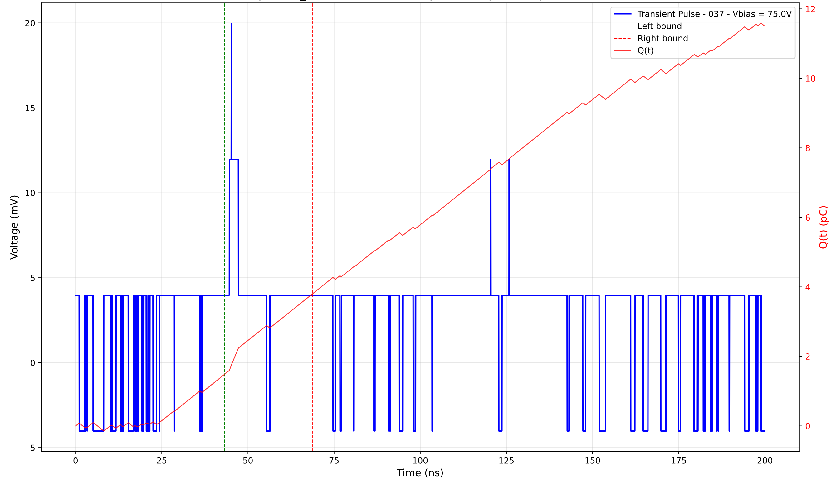
Transient Pulse - Sample: TD_4004 - Position: 25.0 \mu\text{m} - Charge: 2.31 pC - Rise Time: 0.00 ns (N/A)
