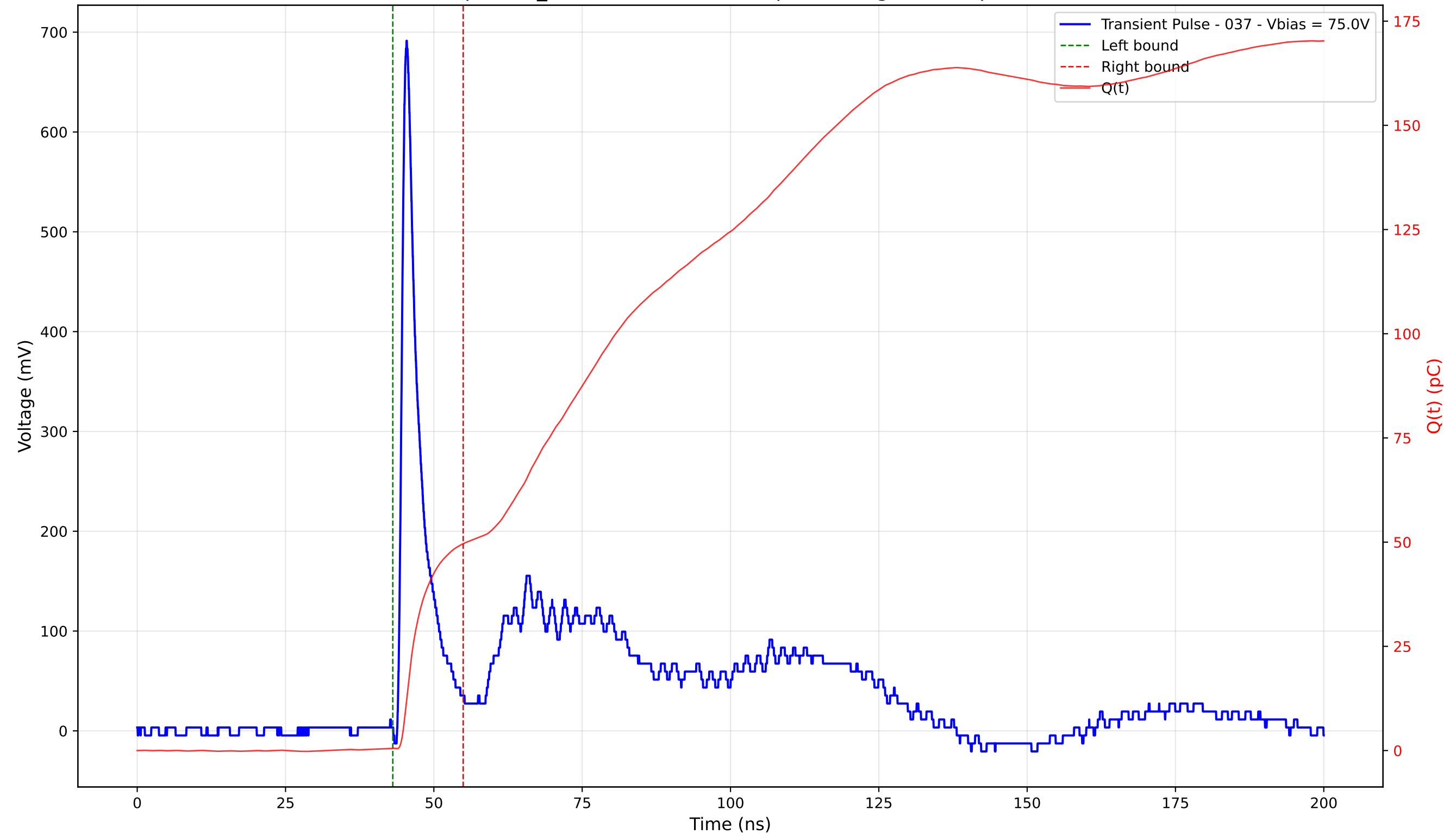
Transient Pulse - Sample: TD_4004 - Position: 110.0 \mu\text{m} - Charge: 49.06 pC - Rise Time: 0.96 ns
