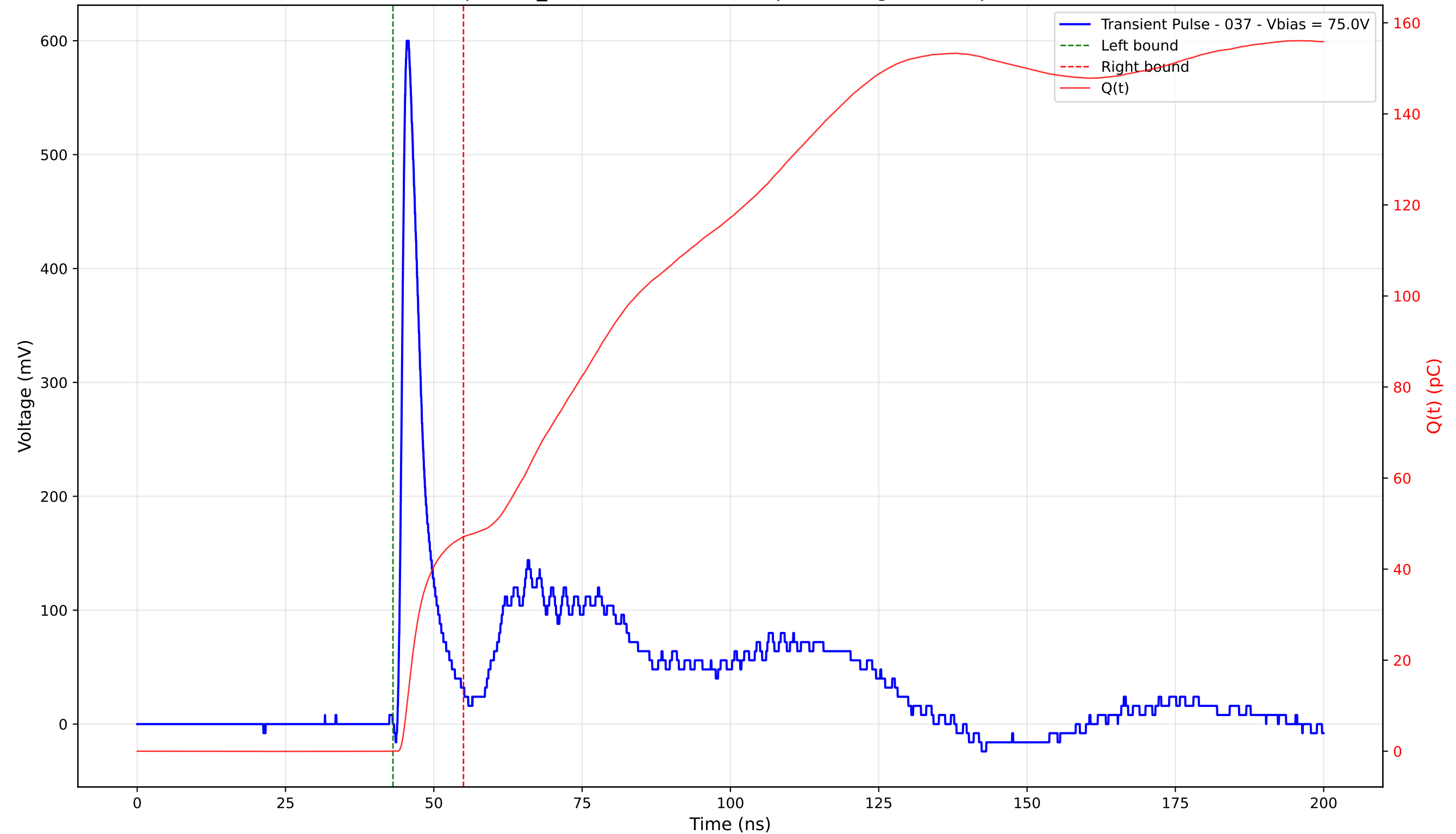
Transient Pulse - Sample: TD_4004 - Position: 190.0 \mu\text{m} - Charge: 47.02 pC - Rise Time: 1.02 ns
