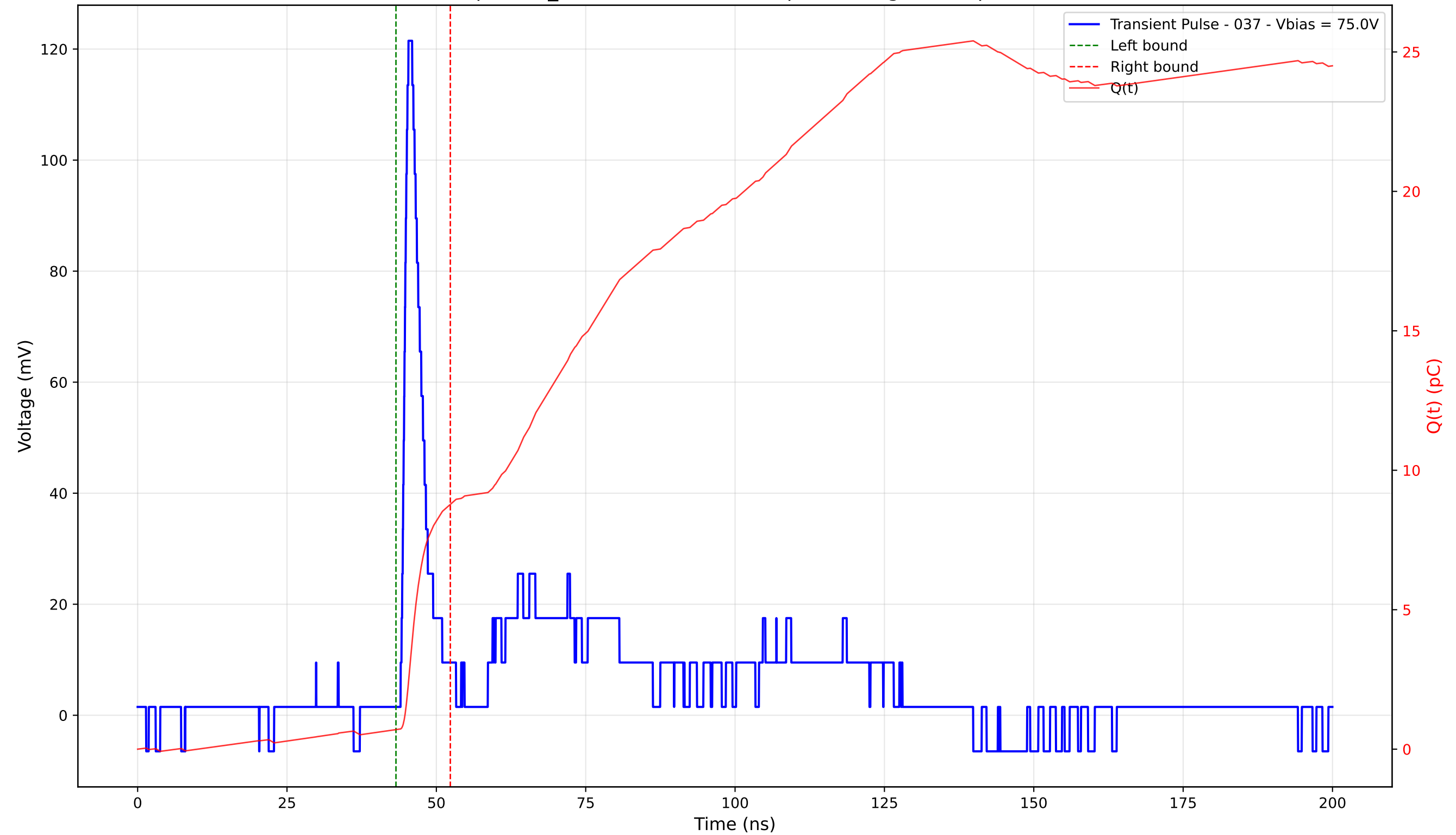
Transient Pulse - Sample: TD_4004 - Position: 395.0 \mu\text{m} - Charge: 8.08 pC - Rise Time: 0.99 ns
