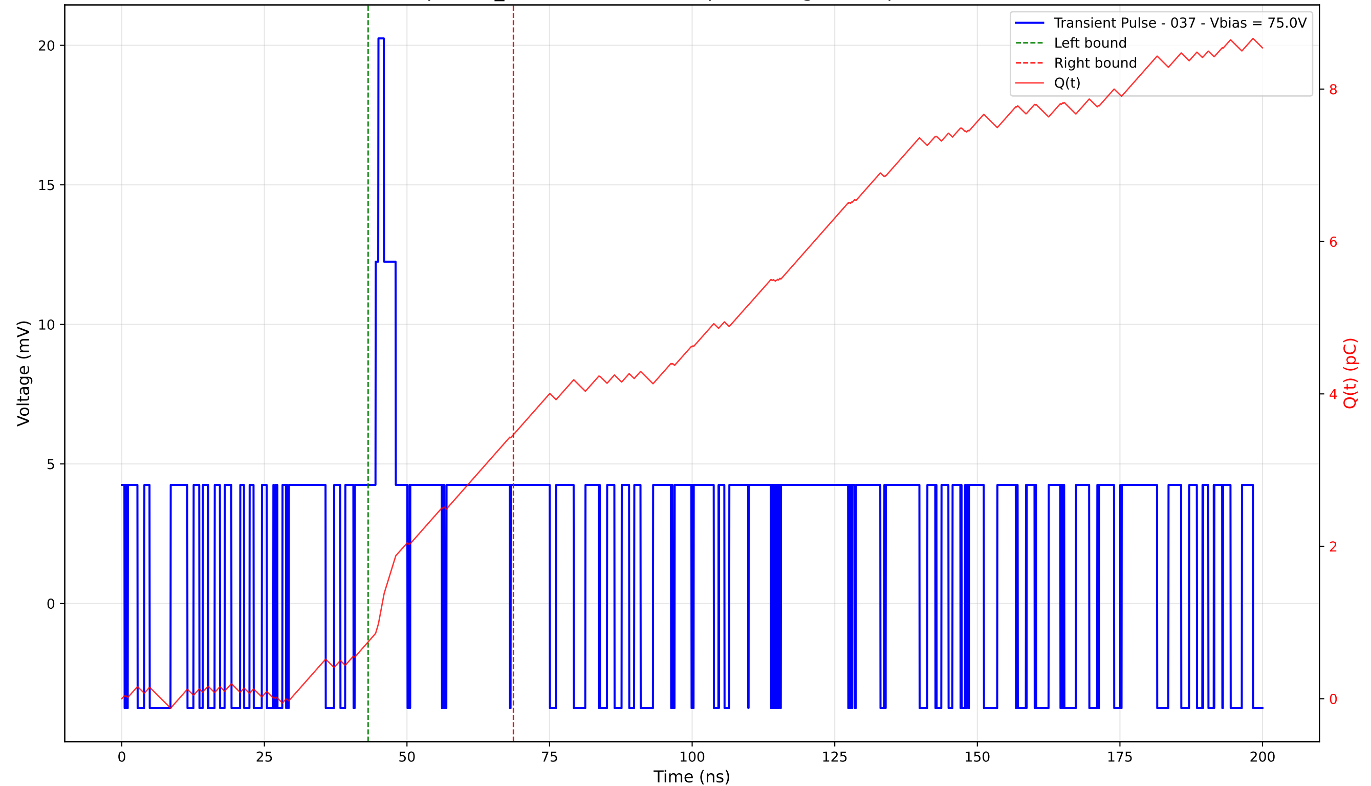
Transient Pulse - Sample: TD_4004 - Position: 35.0 \mu\text{m} - Charge: 2.72 pC - Rise Time: 0.00 ns (N/A)
