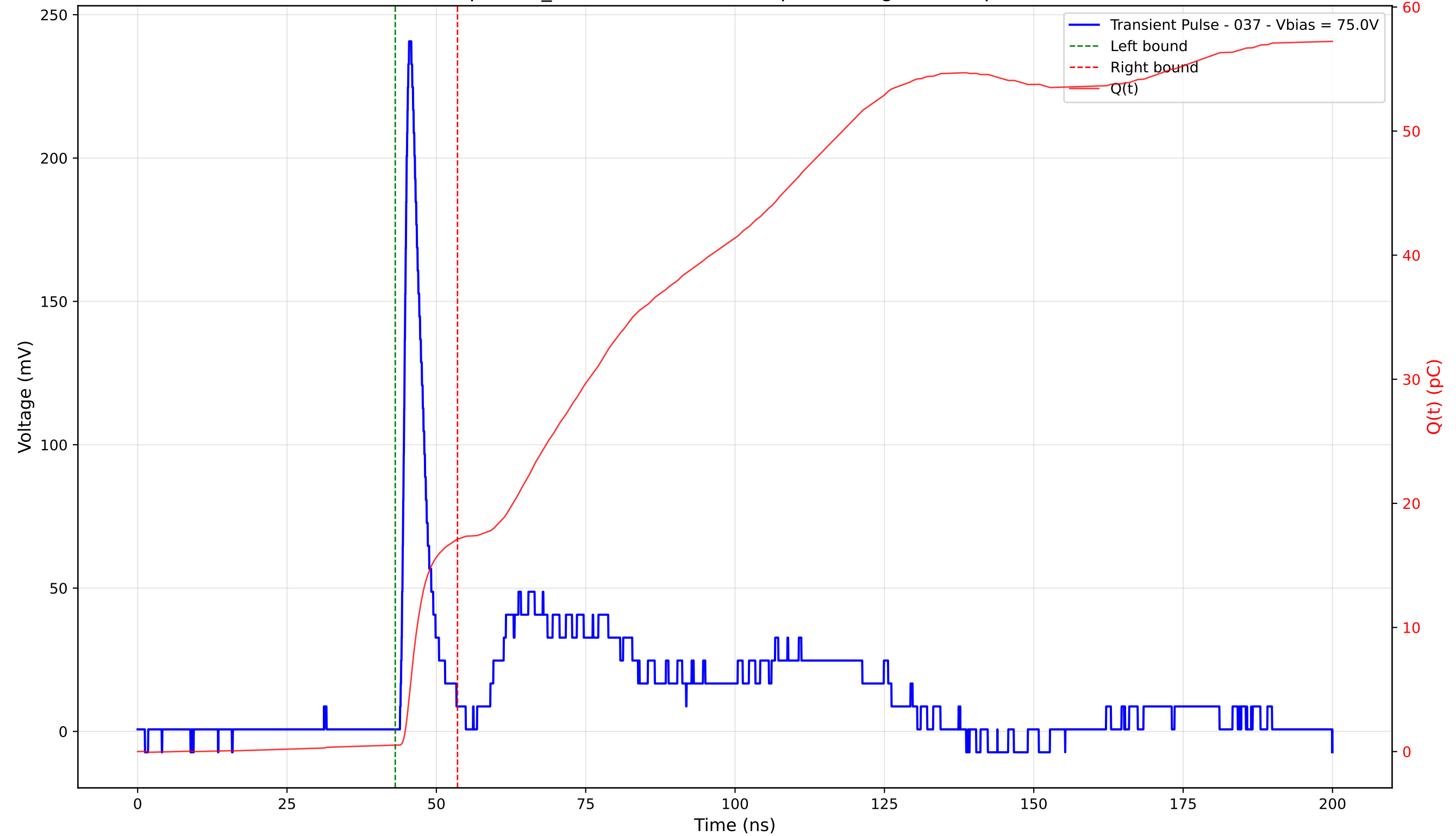
Transient Pulse - Sample: TD_4004 - Position: 315.0 \mu\text{m} - Charge: 16.61 pC - Rise Time: 1.06 ns
