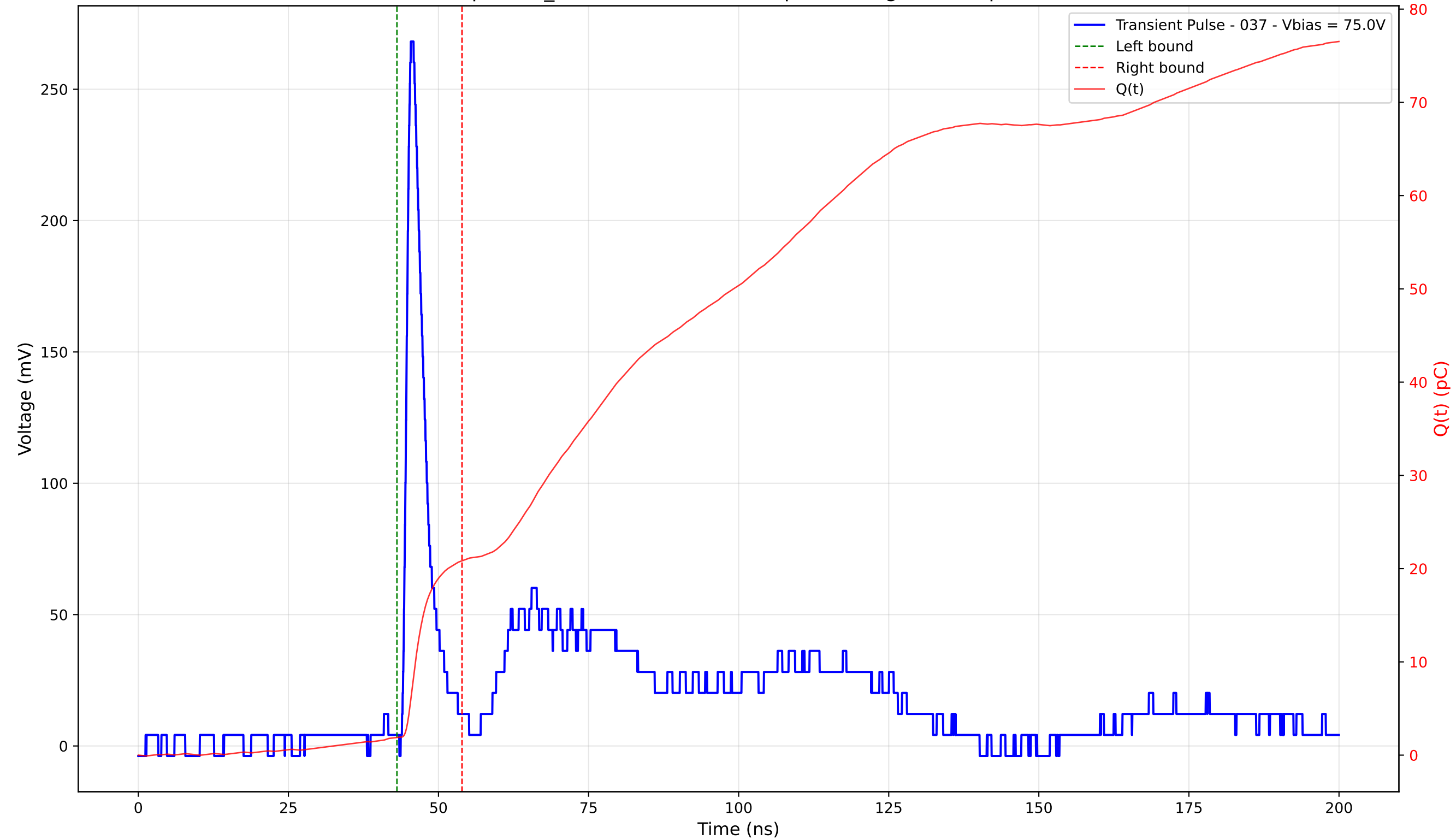
Transient Pulse - Sample: TD_4004 - Position: 310.0 \mu\text{m} - Charge: 18.94 pC - Rise Time: 1.06 ns
