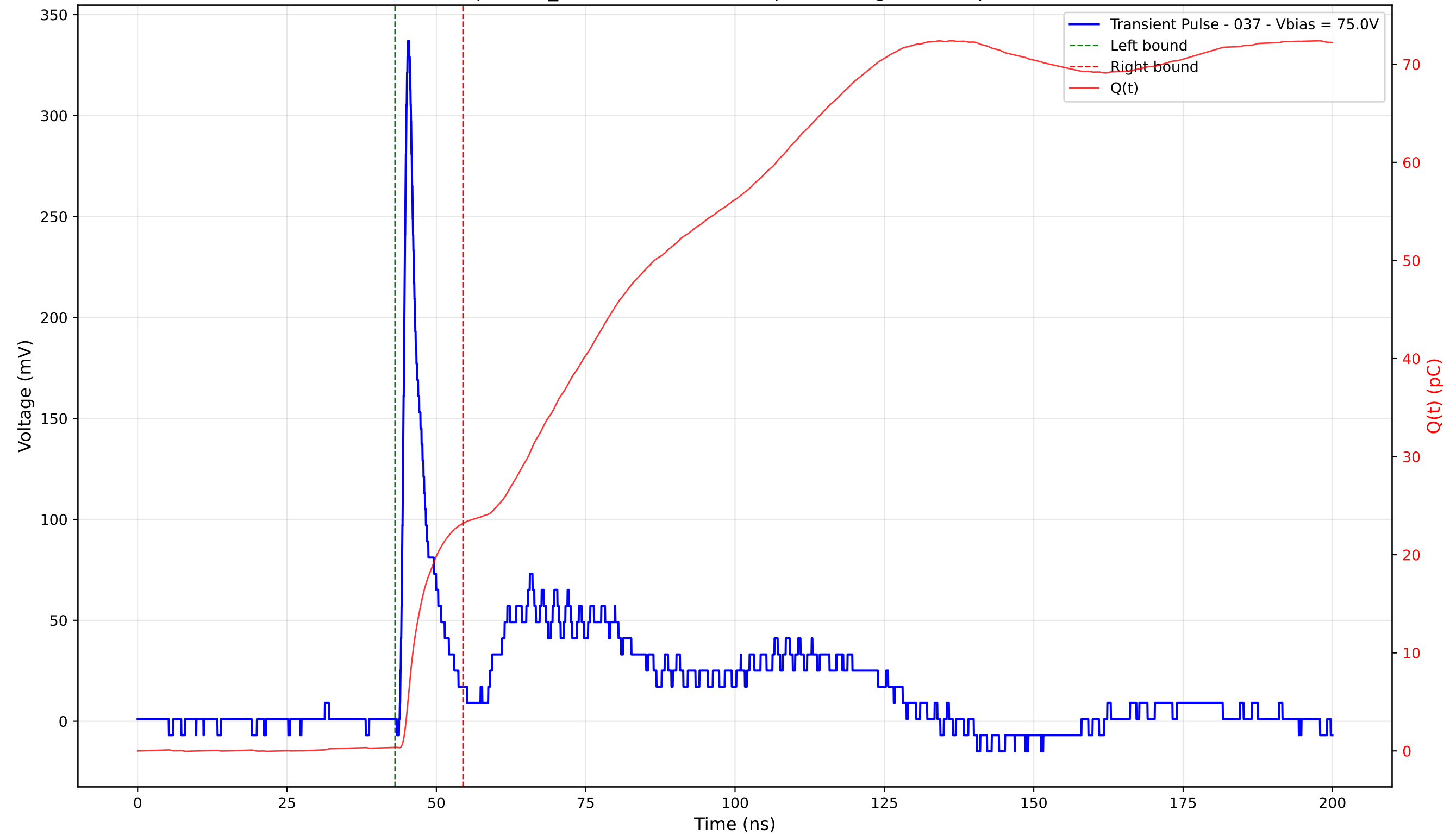
Transient Pulse - Sample: TD_4004 - Position: 70.0 \mu\text{m} - Charge: 22.82 pC - Rise Time: 0.92 ns
