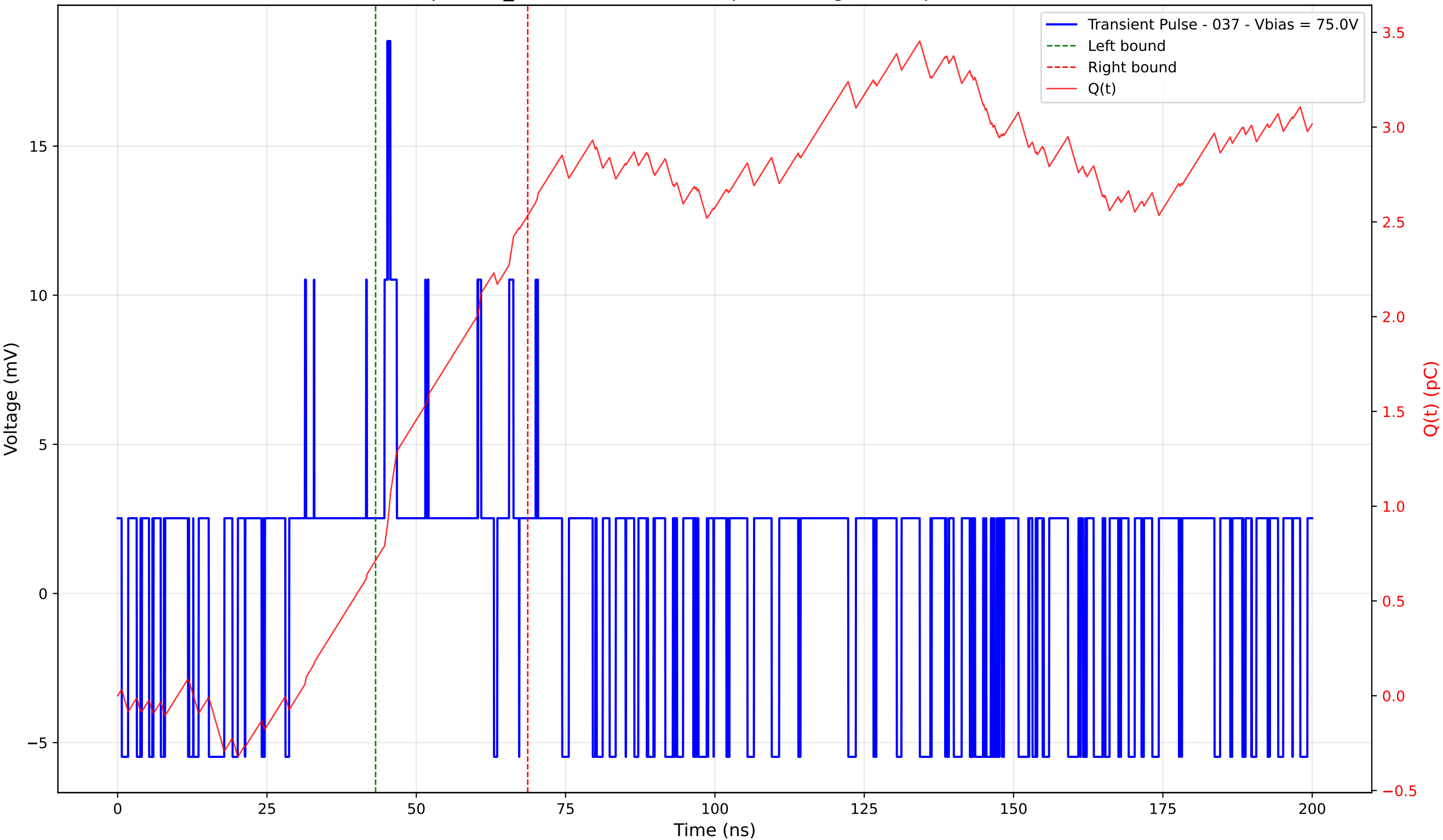
Transient Pulse - Sample: TD_4004 - Position: 20.0 \mu\text{m} - Charge: 1.82 pC - Rise Time: 0.00 ns (N/A)
