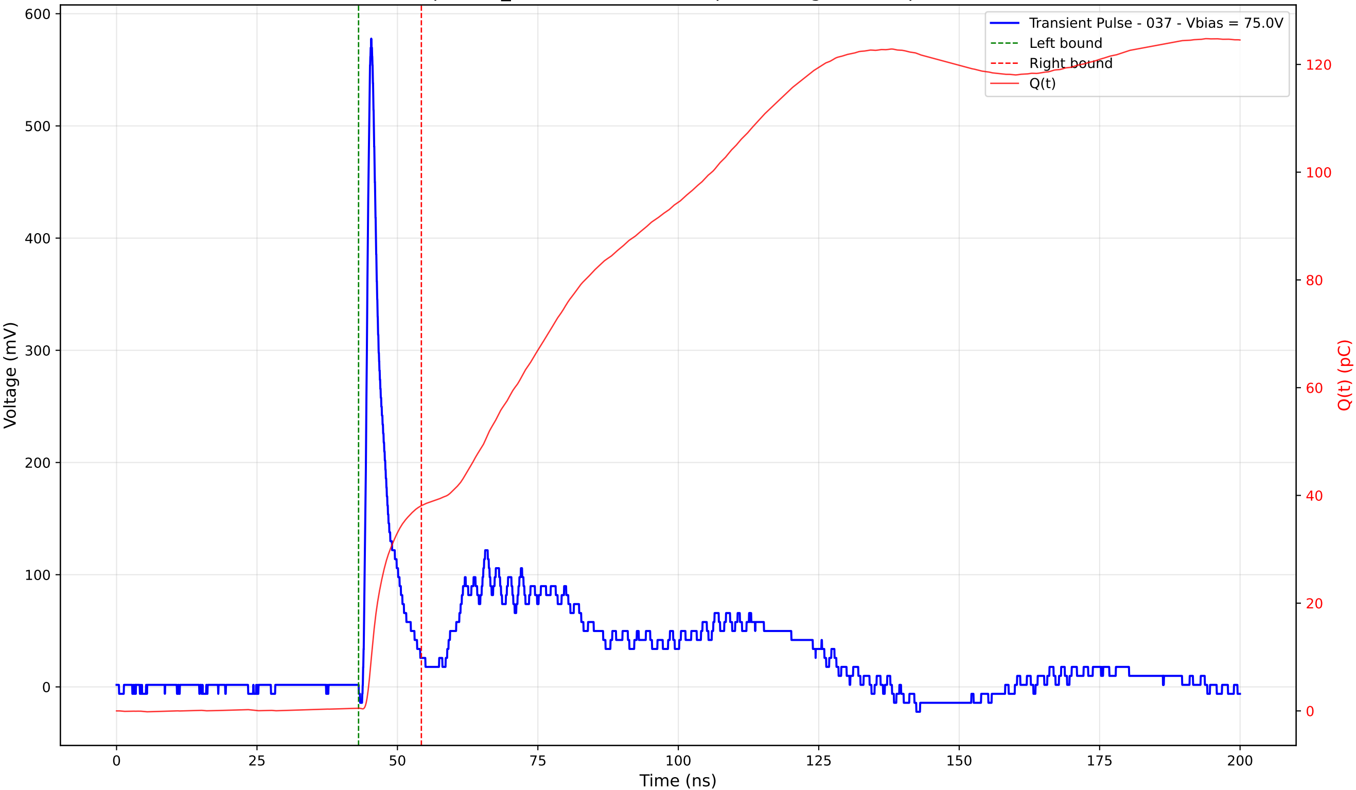
Transient Pulse - Sample: TD_4004 - Position: 85.0 \mu\text{m} - Charge: 37.58 pC - Rise Time: 0.94 ns
