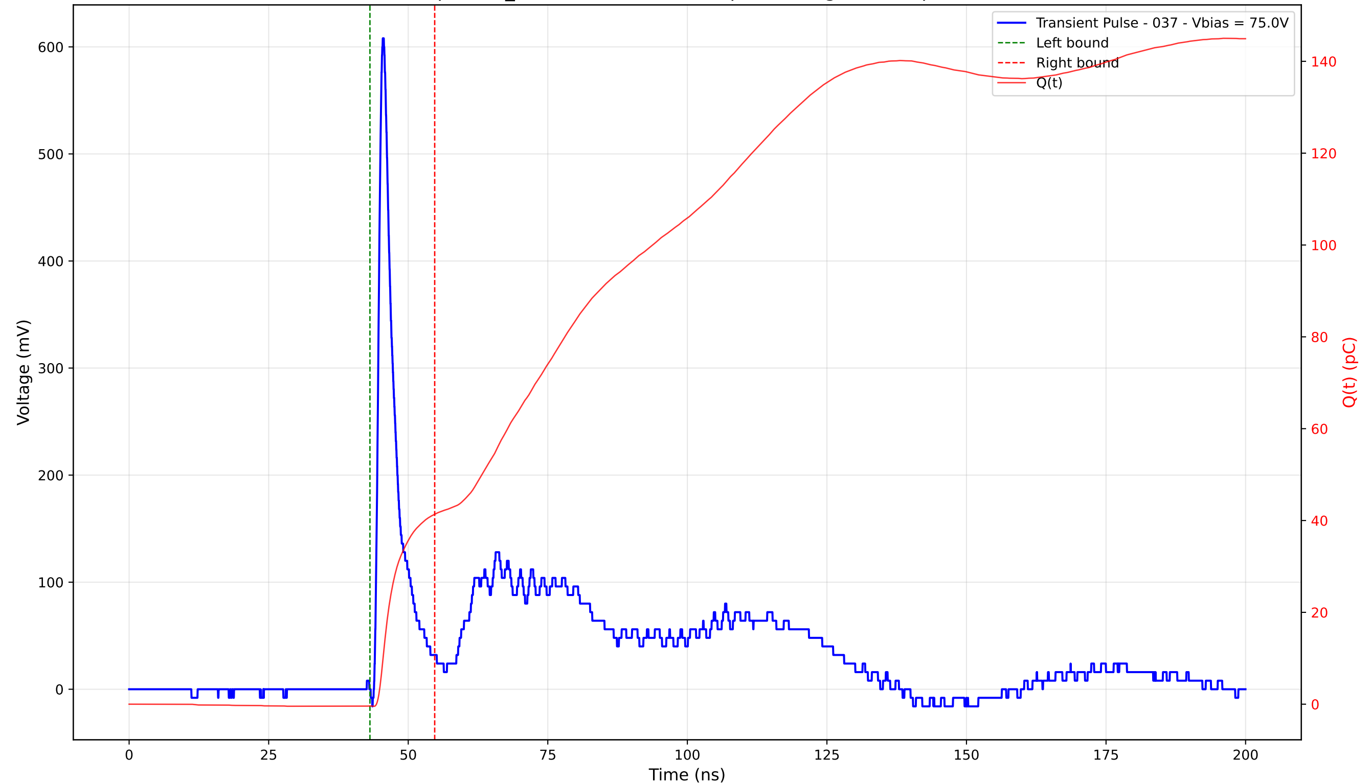
Transient Pulse - Sample: TD_4004 - Position: 125.0 \mu\text{m} - Charge: 41.75 pC - Rise Time: 1.00 ns
