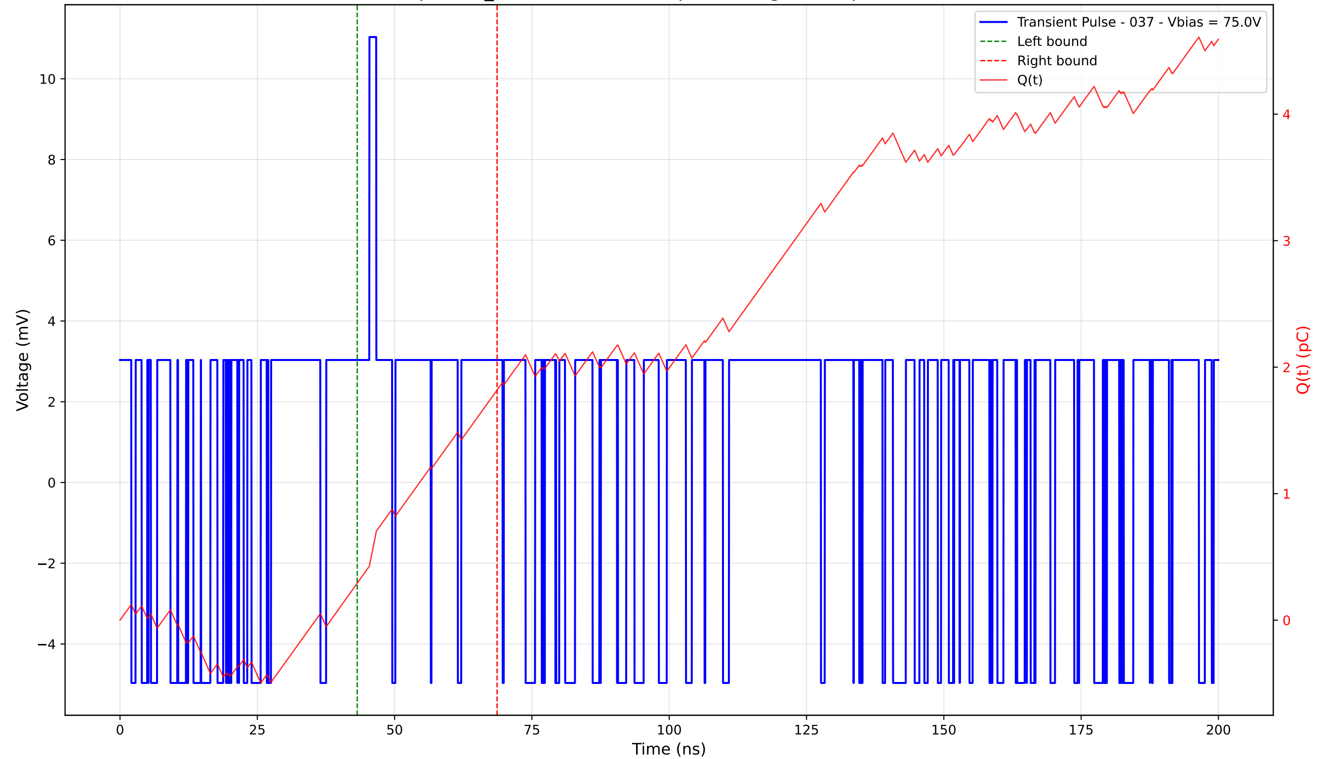
Transient Pulse - Sample: TD_4004 - Position: 0.0 \mu m - Charge: 1.53 pC - Rise Time: 0.00 ns (N/A)
