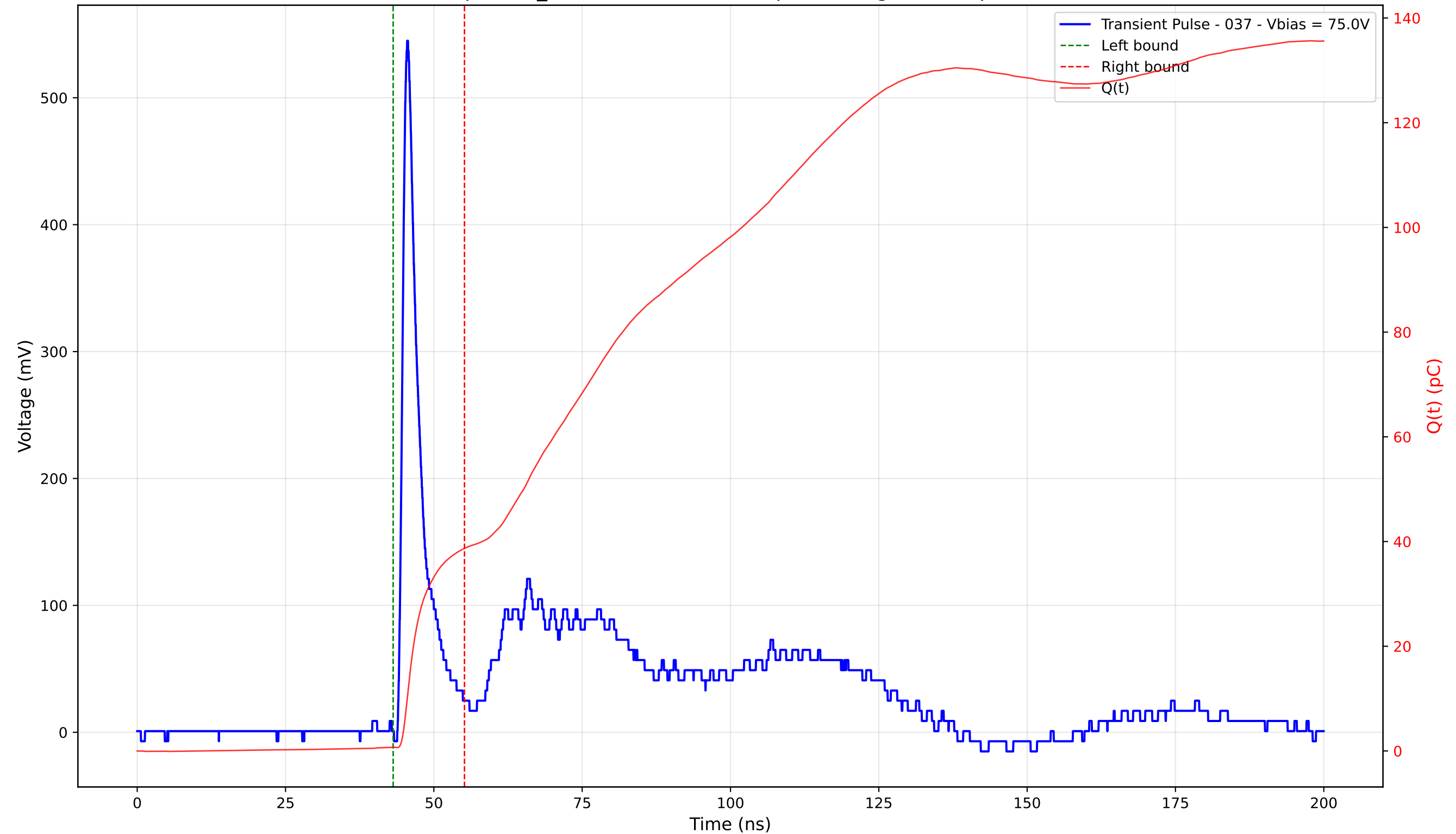
Transient Pulse - Sample: TD_4004 - Position: 130.0 \mu\text{m} - Charge: 38.00 pC - Rise Time: 1.05 ns
