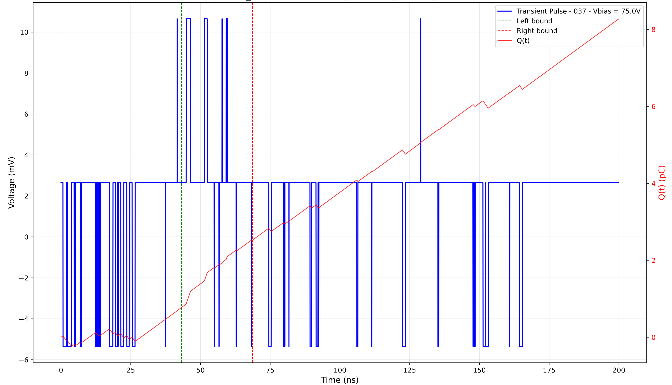
Transient Pulse - Sample: TD_4004 - Position: 5.0 \mu m - Charge: 1.75 pC - Rise Time: 0.00 ns (N/A)
