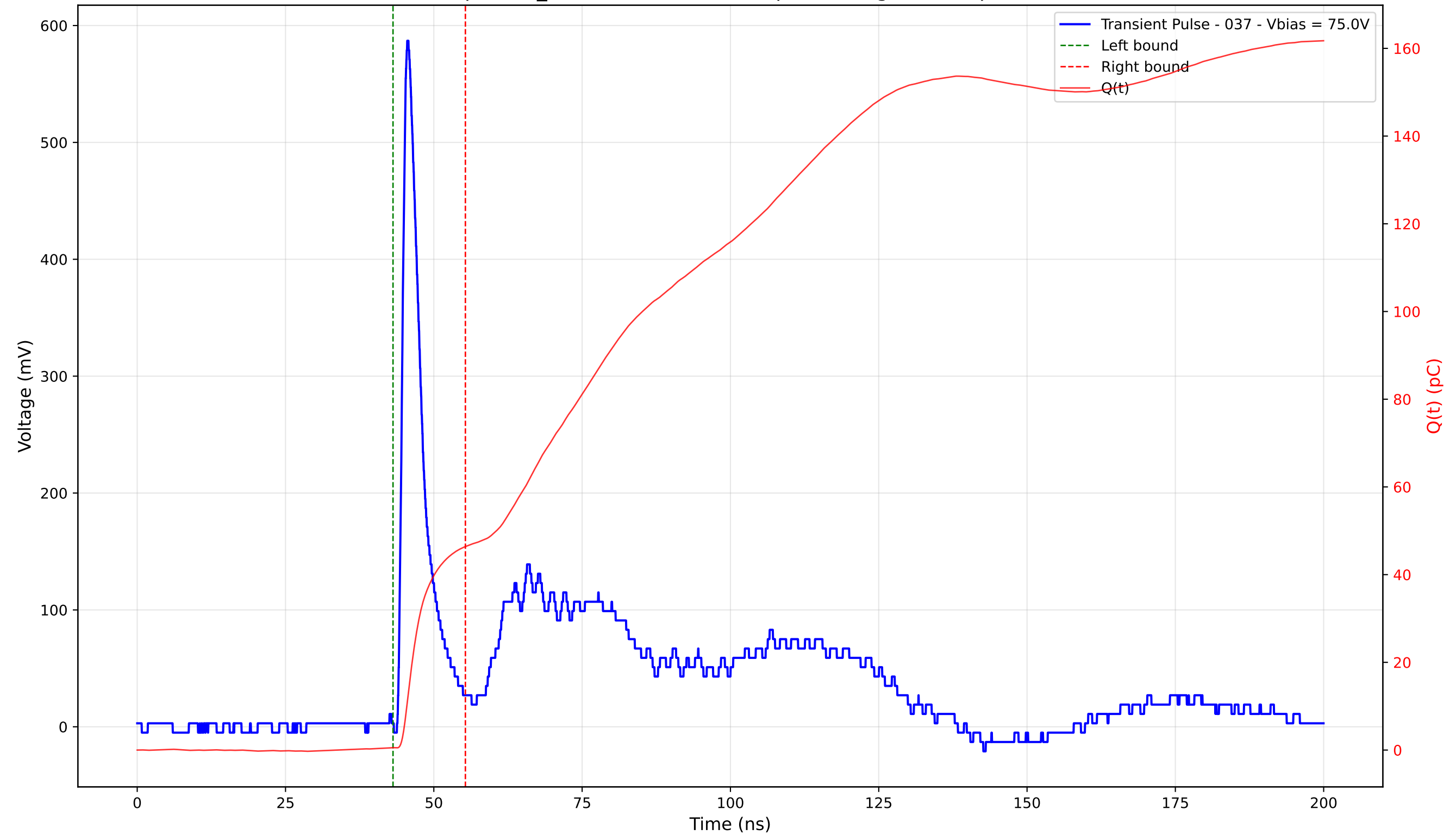
Transient Pulse - Sample: TD_4004 - Position: 180.0 \mu\text{m} - Charge: 45.85 pC - Rise Time: 1.05 ns
