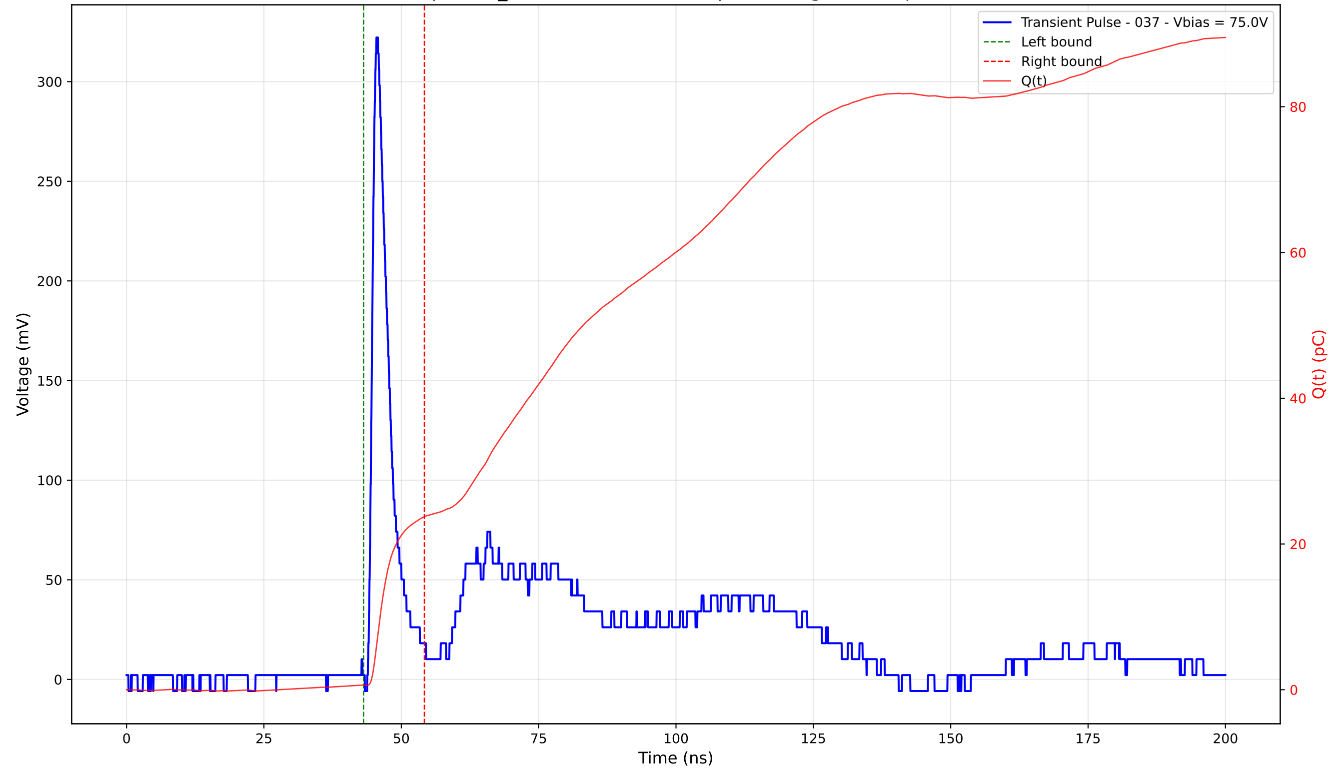
Transient Pulse - Sample: TD_4004 - Position: 265.0 \mu\text{m} - Charge: 23.09 pC - Rise Time: 1.04 ns
