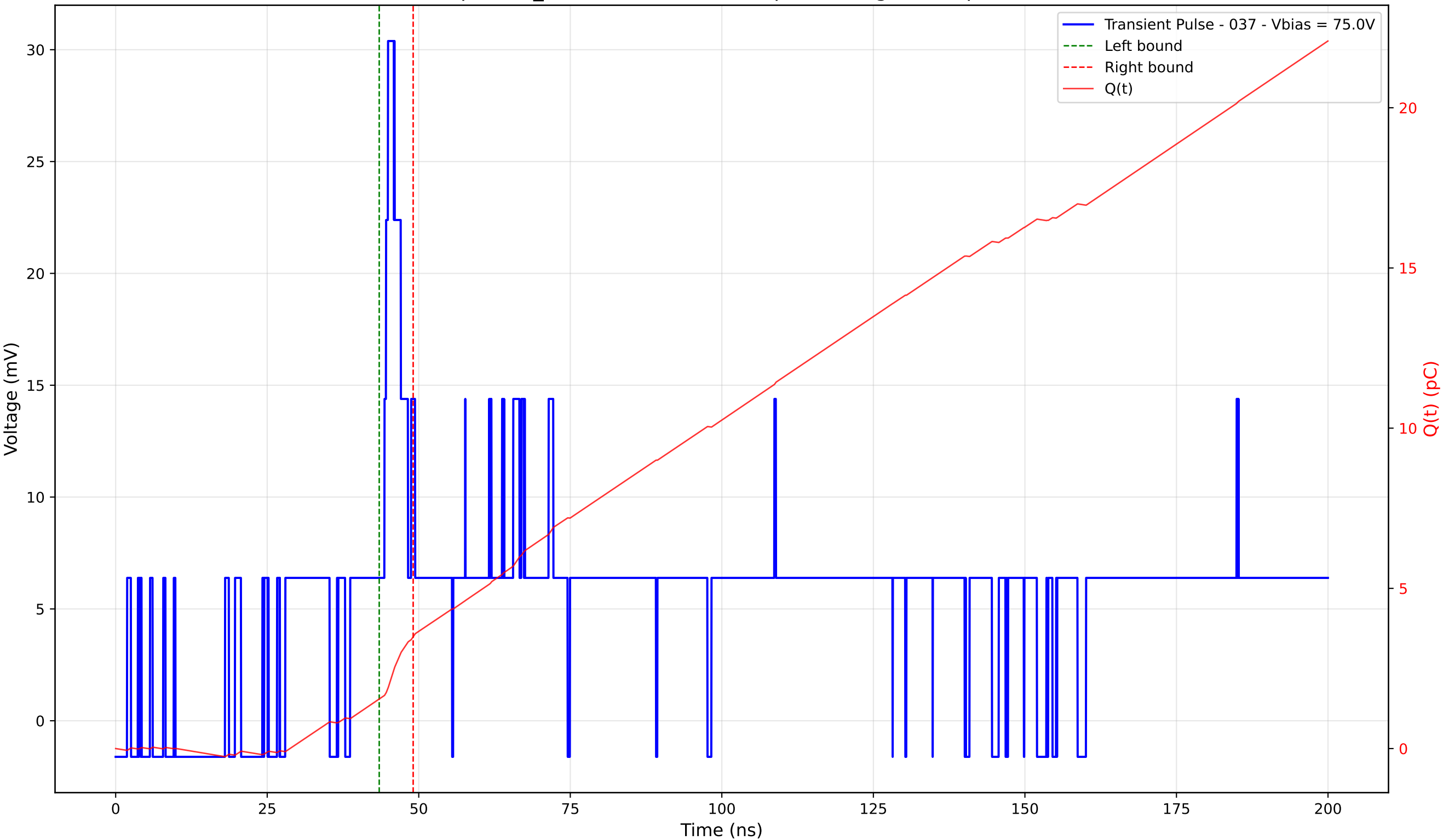
Transient Pulse - Sample: TD_4004 - Position: 435.0 \mu\text{m} - Charge: 1.95 pC - Rise Time: 6.25 ns
