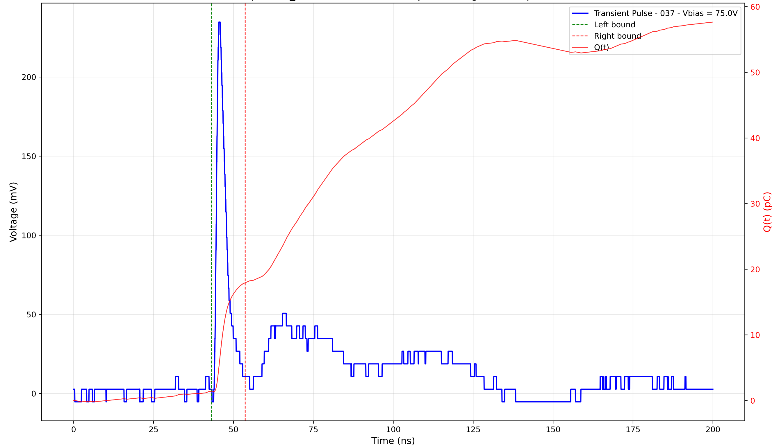
Transient Pulse - Sample: TD_4004 - Position: 320.0 \mu\text{m} - Charge: 16.51 pC - Rise Time: 1.07 ns
