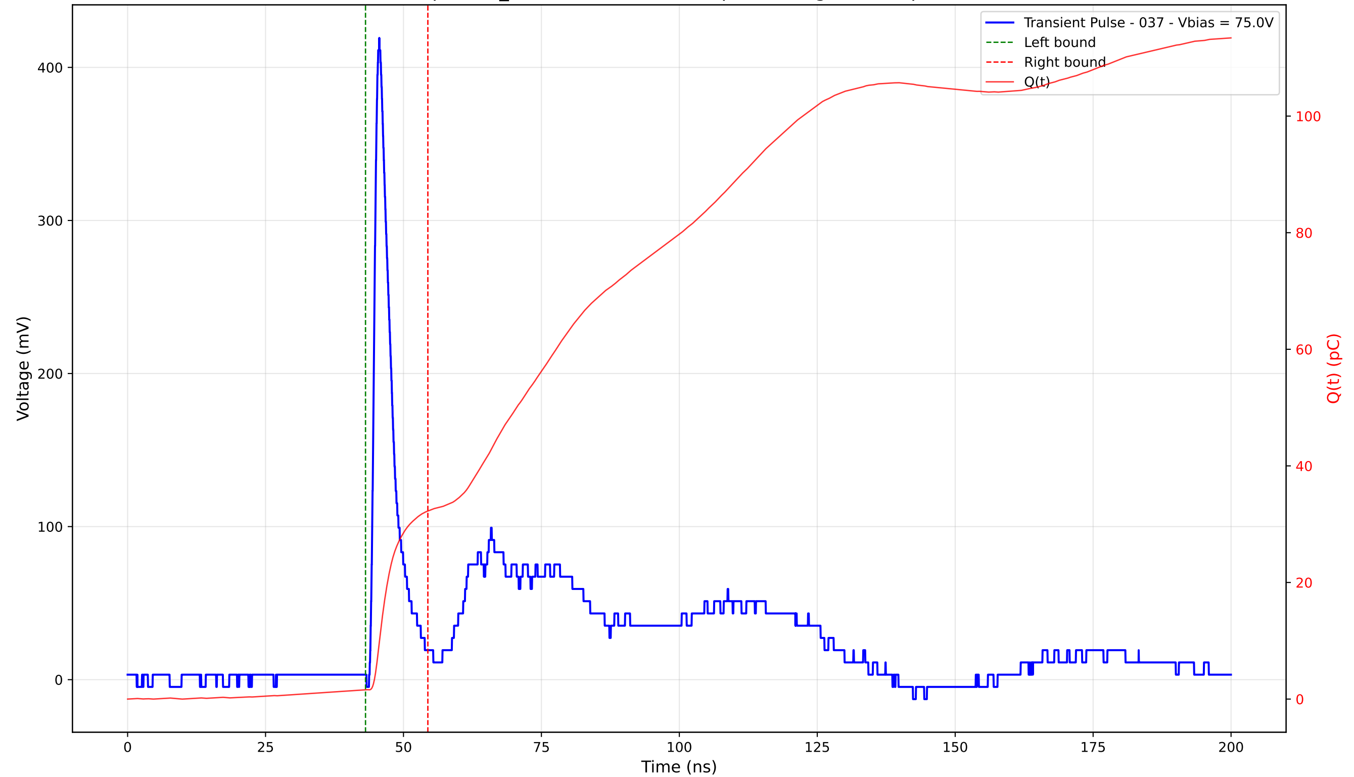
Transient Pulse - Sample: TD_4004 - Position: 235.0 \mu\text{m} - Charge: 30.65 pC - Rise Time: 1.08 ns
