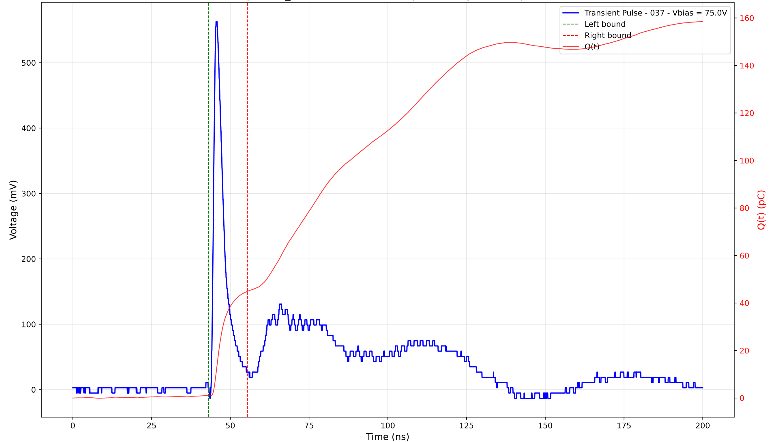
Transient Pulse - Sample: TD_4004 - Position: 175.0 \mu\text{m} - Charge: 43.81 pC - Rise Time: 1.05 ns
