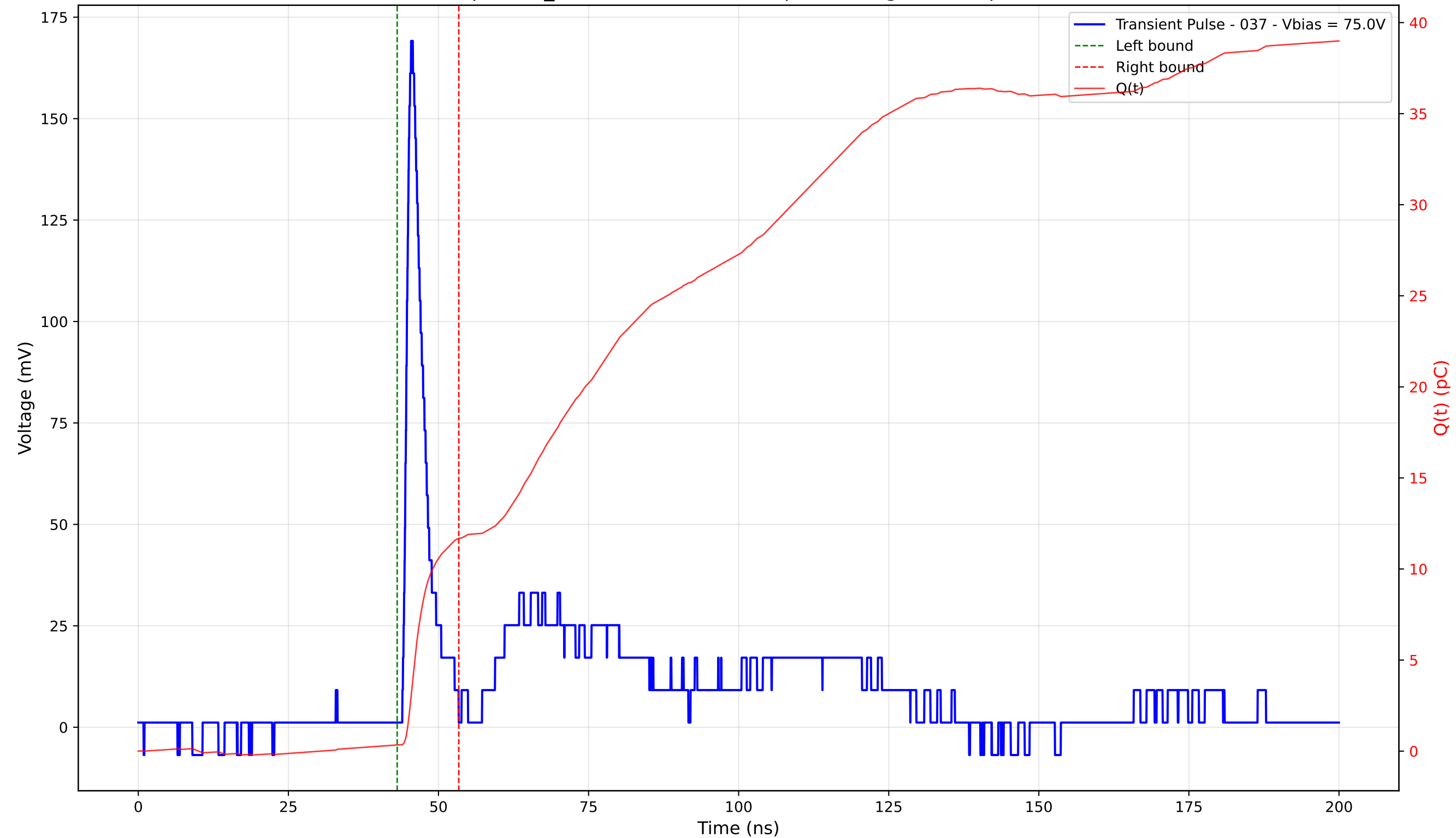
Transient Pulse - Sample: TD_4004 - Position: 385.0 \mu\text{m} - Charge: 11.36 pC - Rise Time: 1.06 ns
