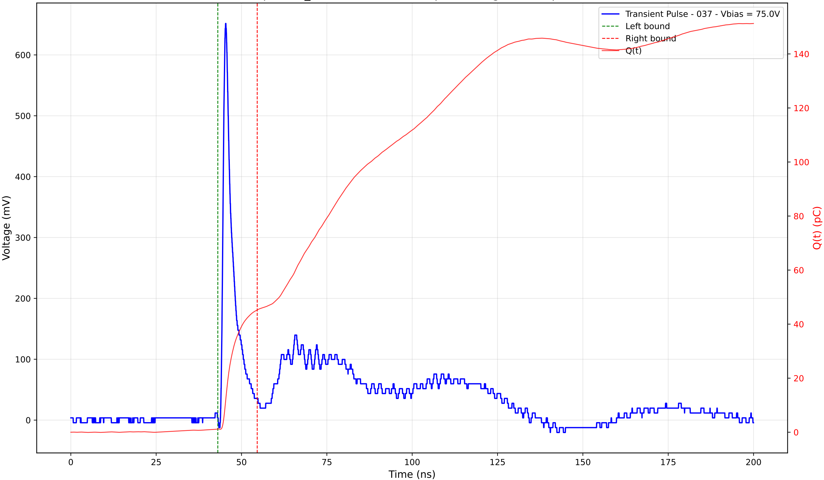
Transient Pulse - Sample: TD_4004 - Position: 95.0 \mu\text{m} - Charge: 44.06 pC - Rise Time: 0.94 ns
