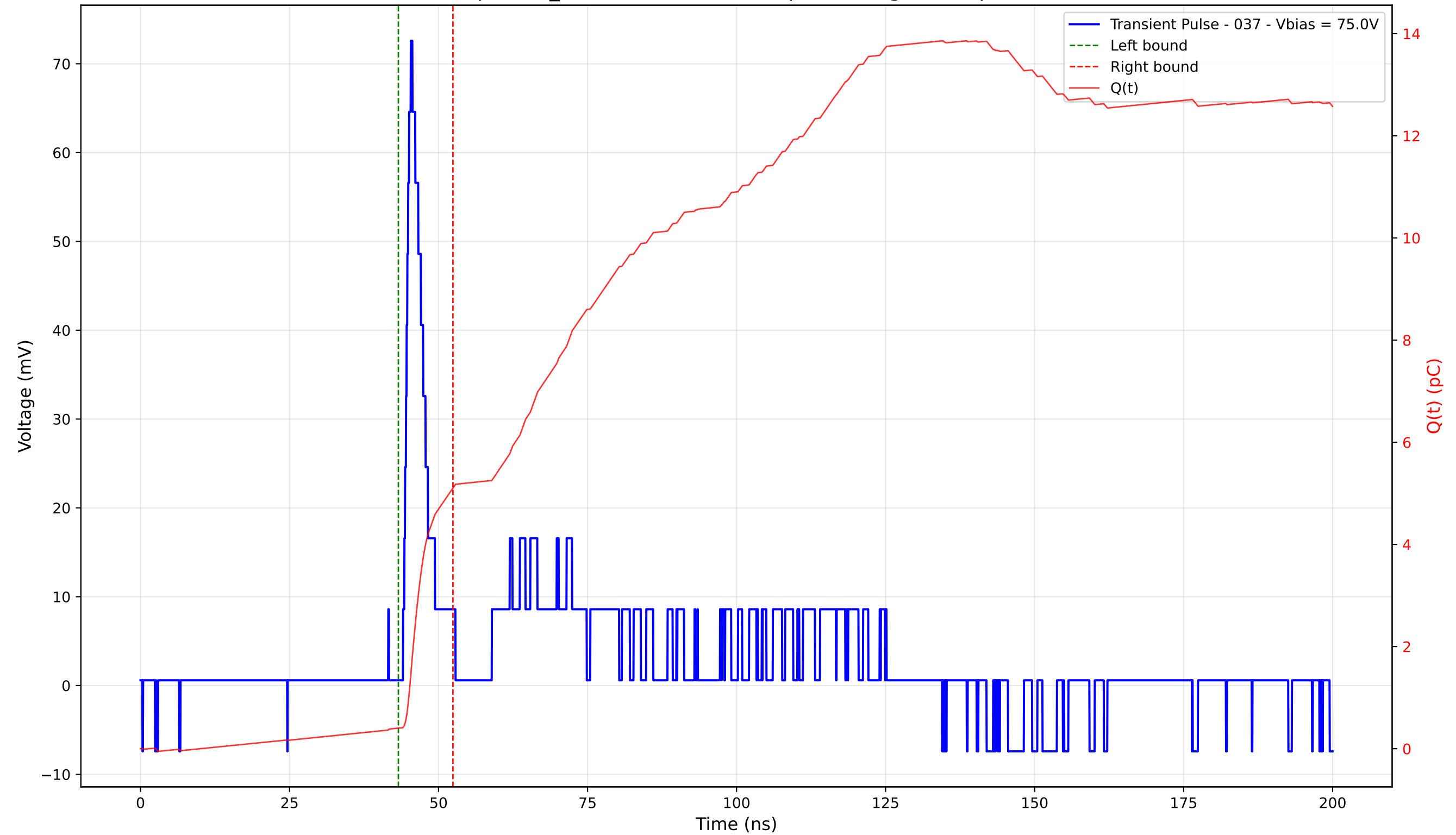
Transient Pulse - Sample: TD_4004 - Position: 410.0 \mu\text{m} - Charge: 4.71 pC - Rise Time: 1.30 ns
