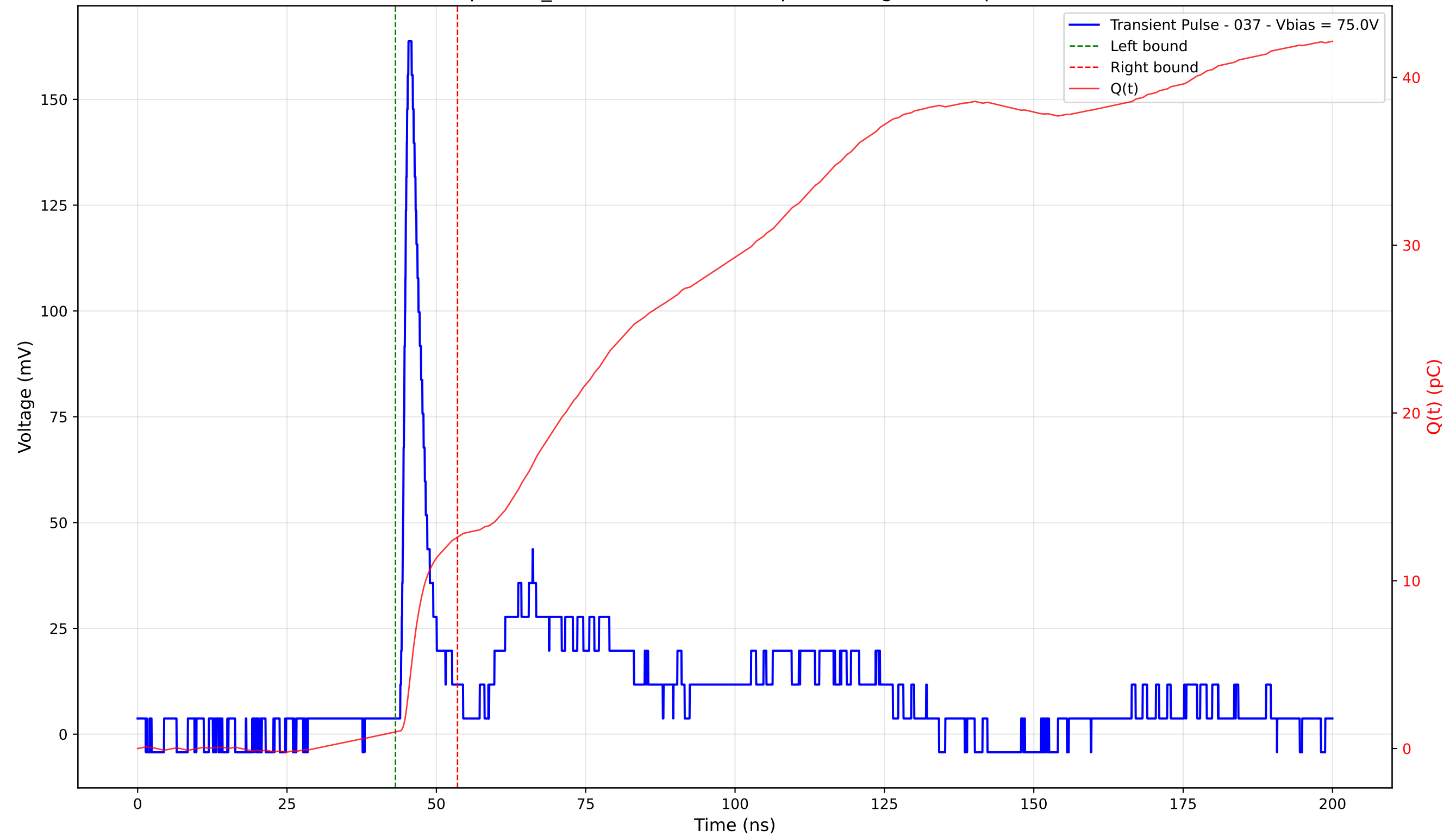
Transient Pulse - Sample: TD_4004 - Position: 370.0 \mu\text{m} - Charge: 11.63 pC - Rise Time: 1.01 ns
