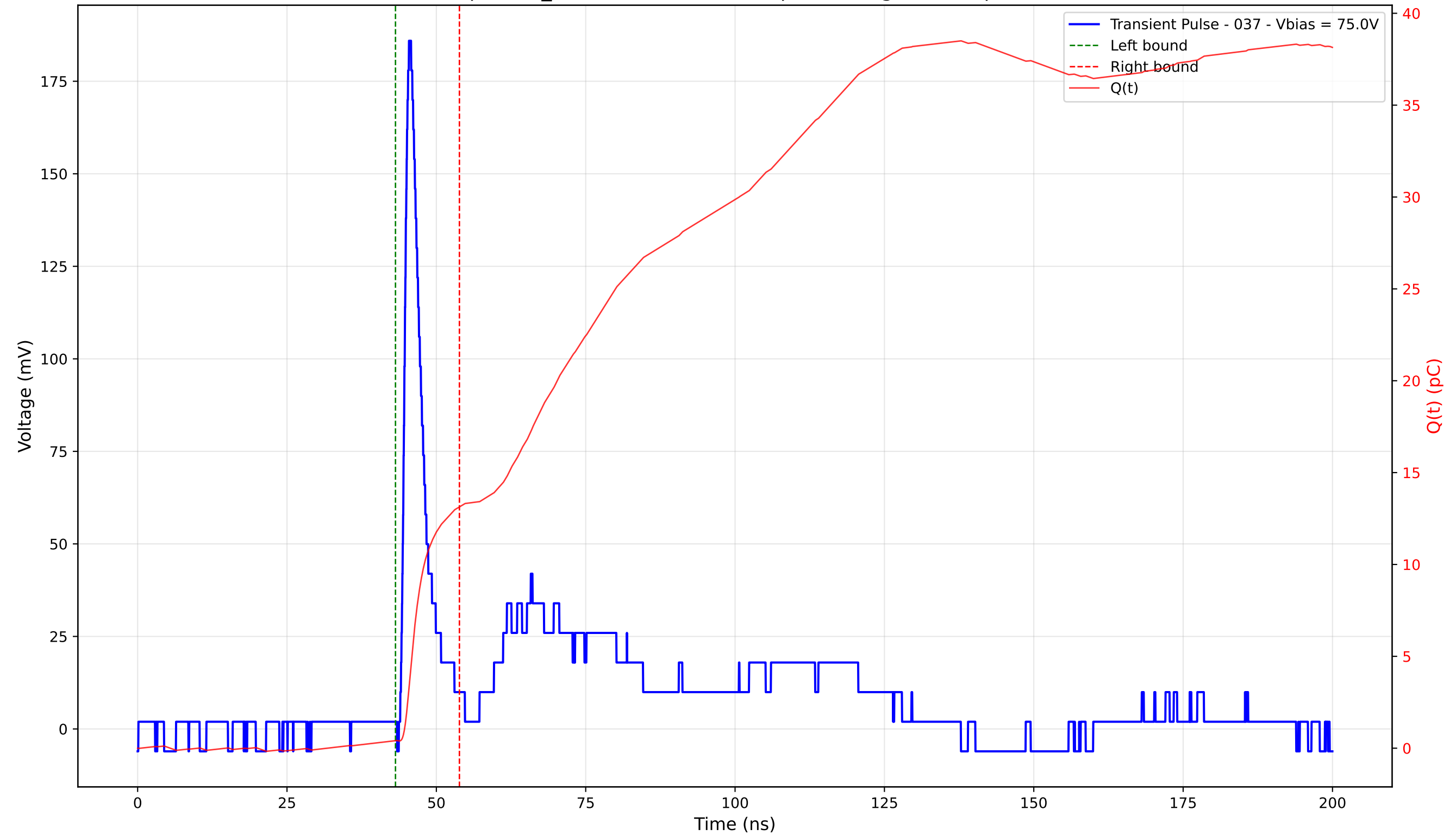
Transient Pulse - Sample: TD_4004 - Position: 360.0 \mu\text{m} - Charge: 12.72 pC - Rise Time: 1.02 ns
