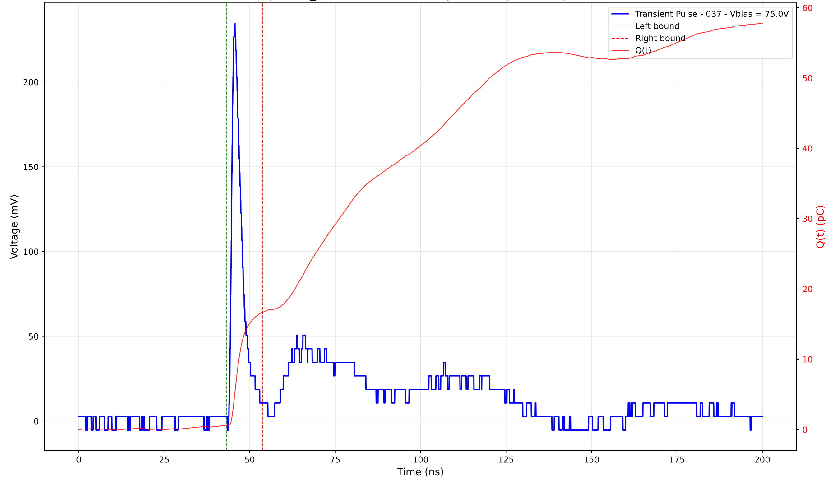
Transient Pulse - Sample: TD_4004 - Position: 325.0 \mu\text{m} - Charge: 16.06 pC - Rise Time: 1.13 ns
