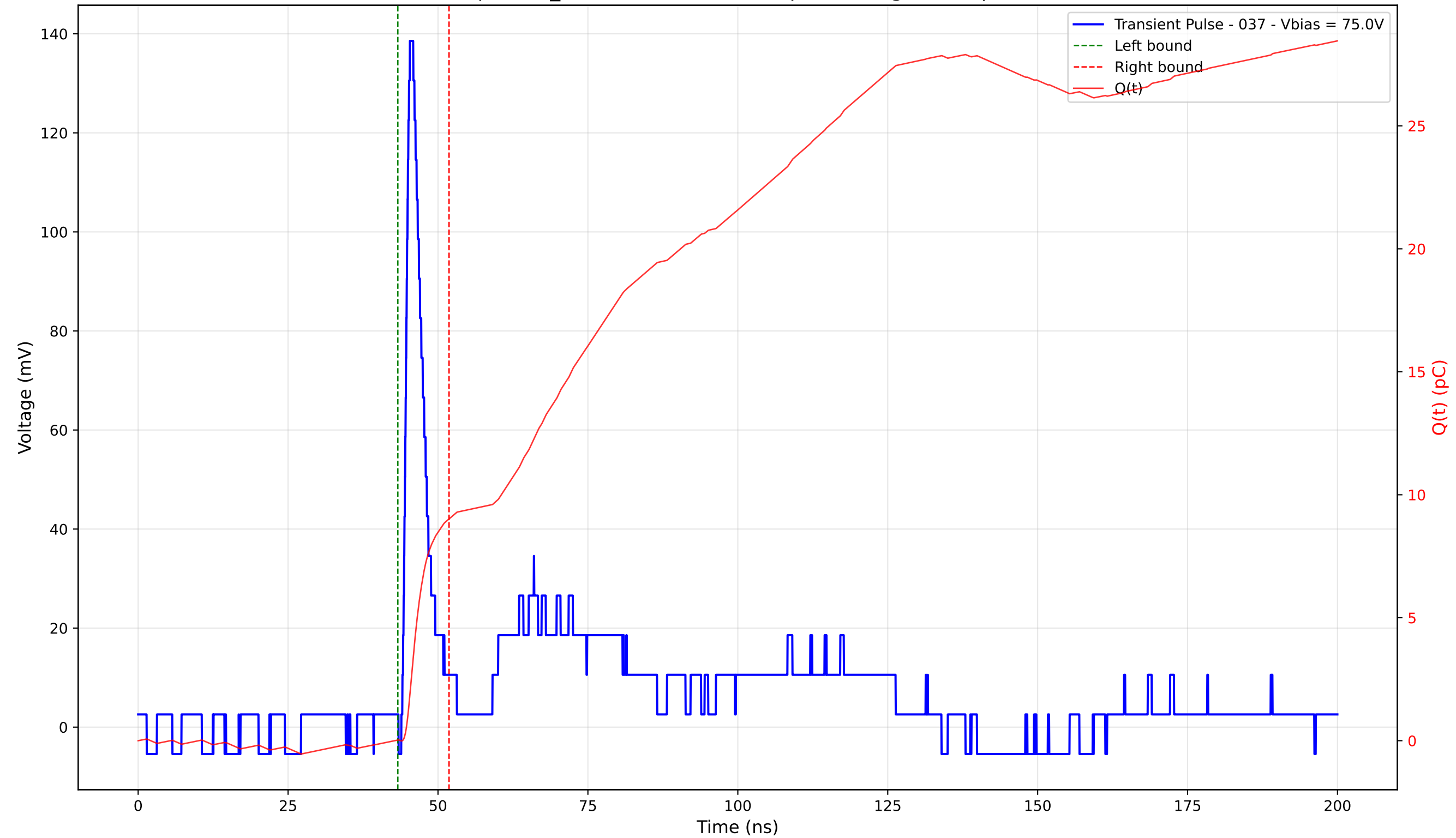
Transient Pulse - Sample: TD_4004 - Position: 390.0 \mu\text{m} - Charge: 8.99 pC - Rise Time: 0.99 ns
