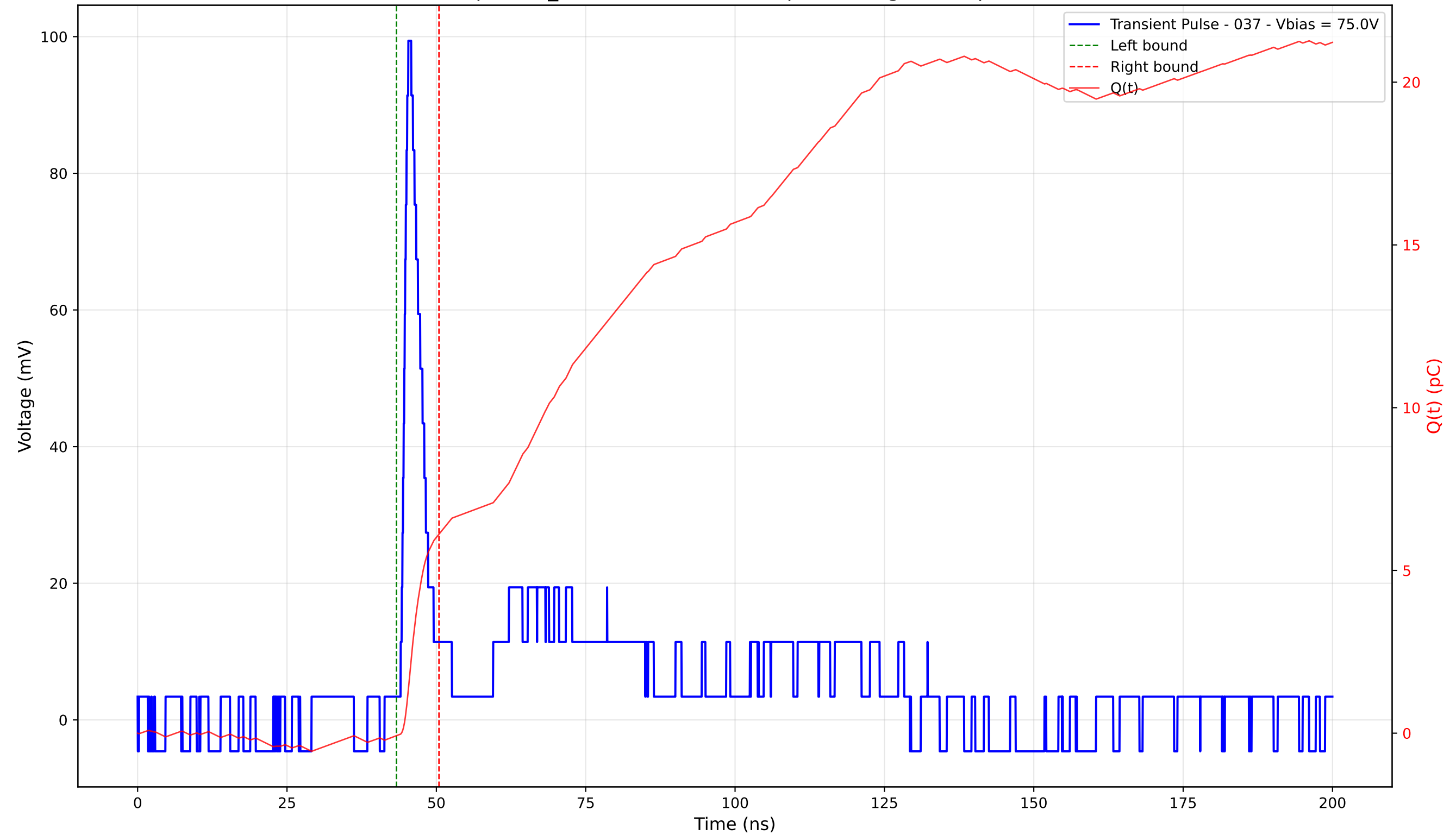
Transient Pulse - Sample: TD_4004 - Position: 400.0 \mu\text{m} - Charge: 6.19 pC - Rise Time: 1.10 ns
