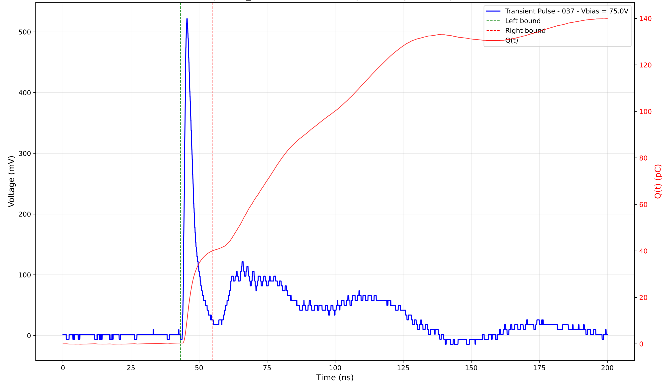
Transient Pulse - Sample: TD_4004 - Position: 215.0 \mu\text{m} - Charge: 39.57 pC - Rise Time: 1.05 ns
