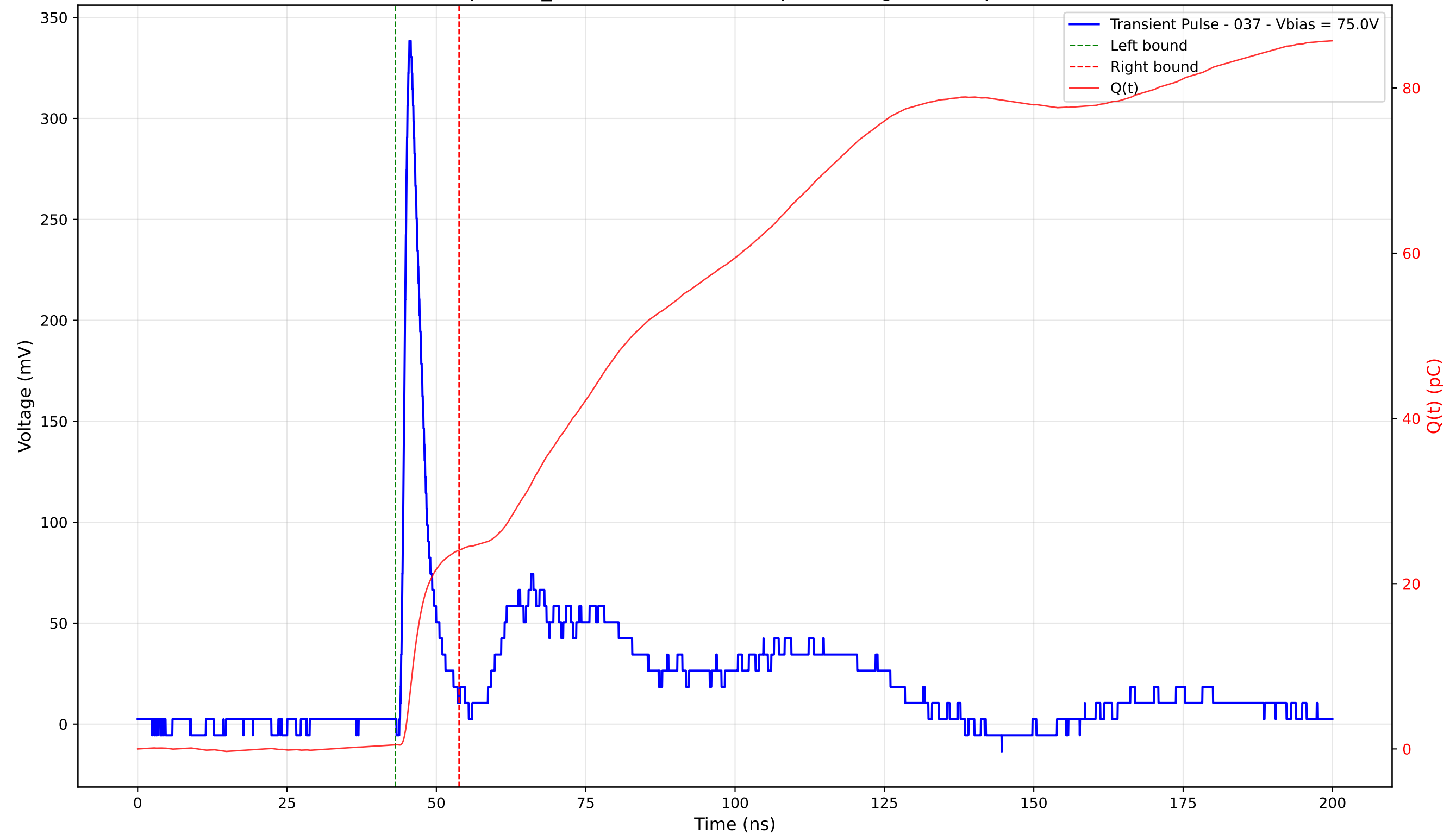
Transient Pulse - Sample: TD_4004 - Position: 285.0 \mu\text{m} - Charge: 23.54 pC - Rise Time: 1.06 ns
