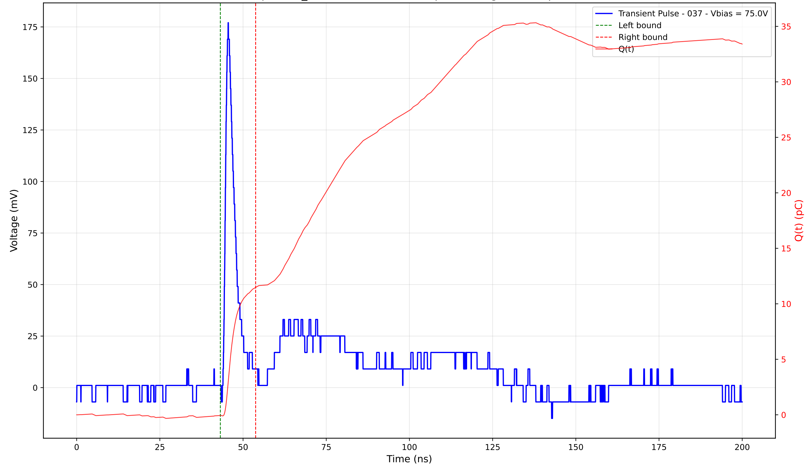
Transient Pulse - Sample: TD_4004 - Position: 365.0 \mu\text{m} - Charge: 11.54 pC - Rise Time: 1.02 ns
