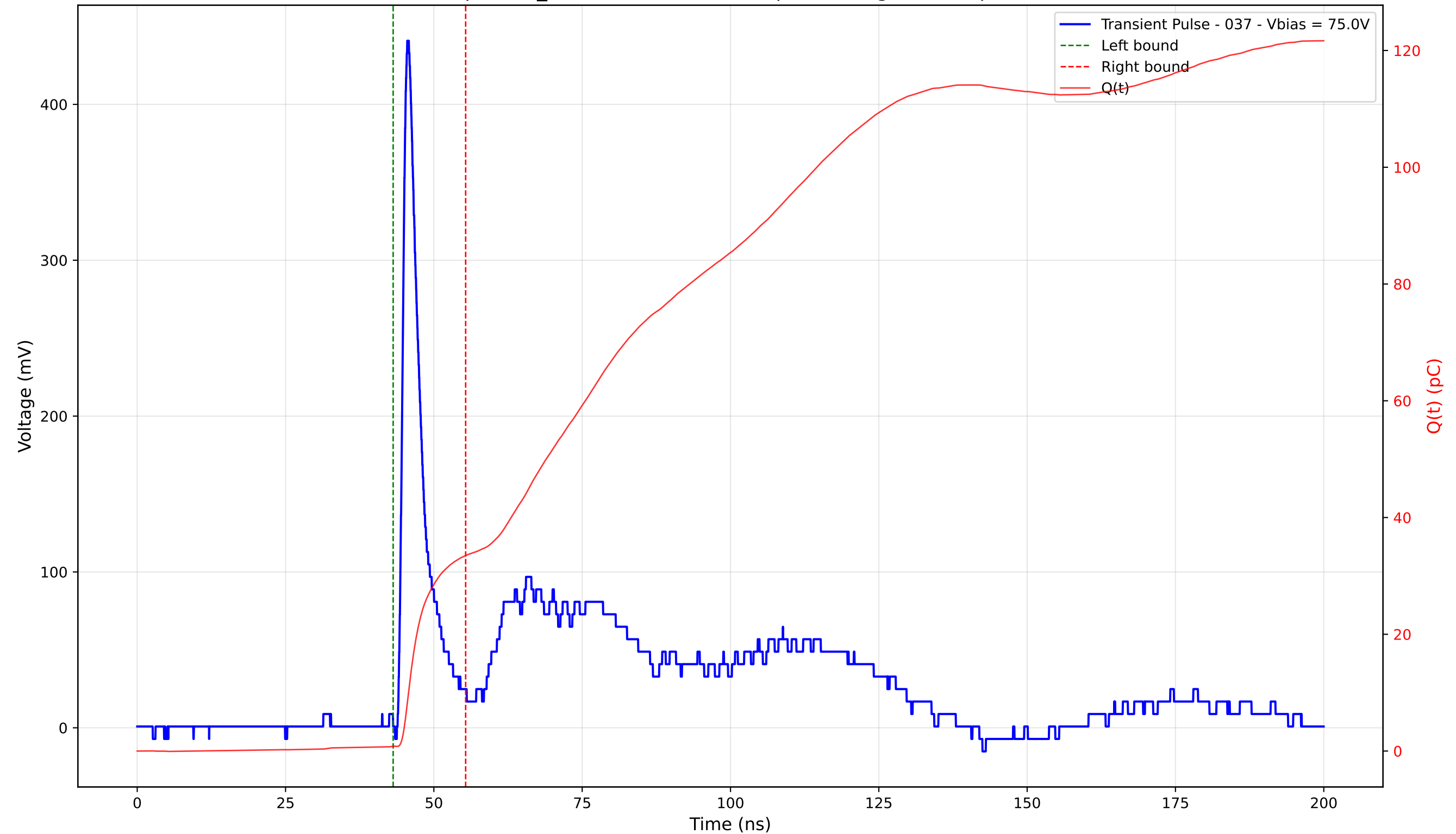
Transient Pulse - Sample: TD_4004 - Position: 140.0 \mu\text{m} - Charge: 32.67 pC - Rise Time: 1.07 ns
