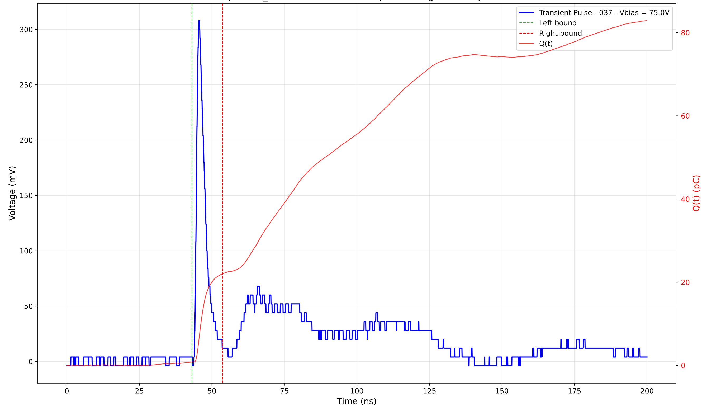
Transient Pulse - Sample: TD_4004 - Position: 290.0 \mu\text{m} - Charge: 21.24 pC - Rise Time: 1.07 ns
