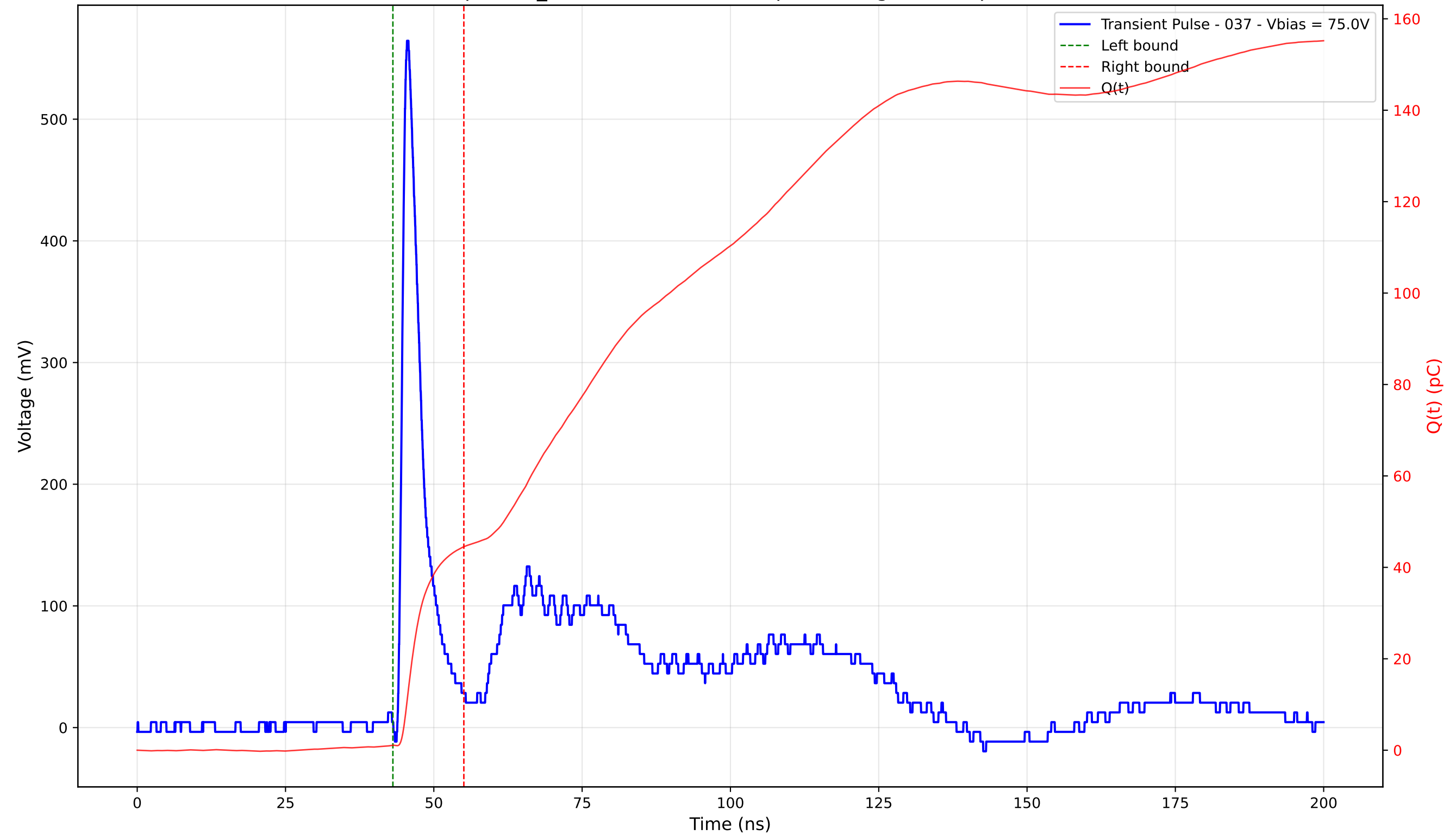
Transient Pulse - Sample: TD_4004 - Position: 205.0 \mu\text{m} - Charge: 43.43 pC - Rise Time: 1.03 ns
