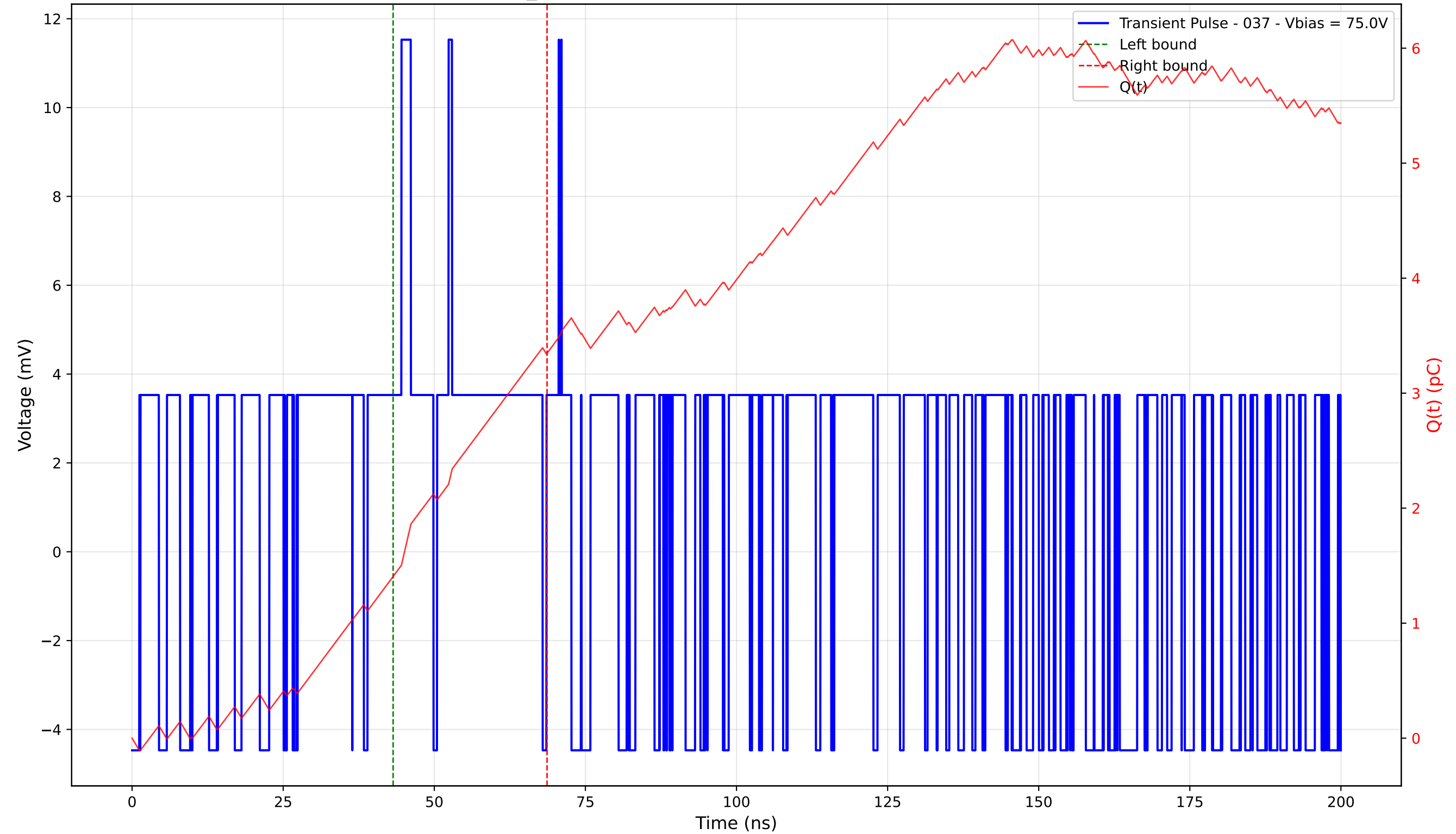
Transient Pulse - Sample: TD_4004 - Position: 15.0 \mu\text{m} - Charge: 1.94 pC - Rise Time: 0.00 ns (N/A)
