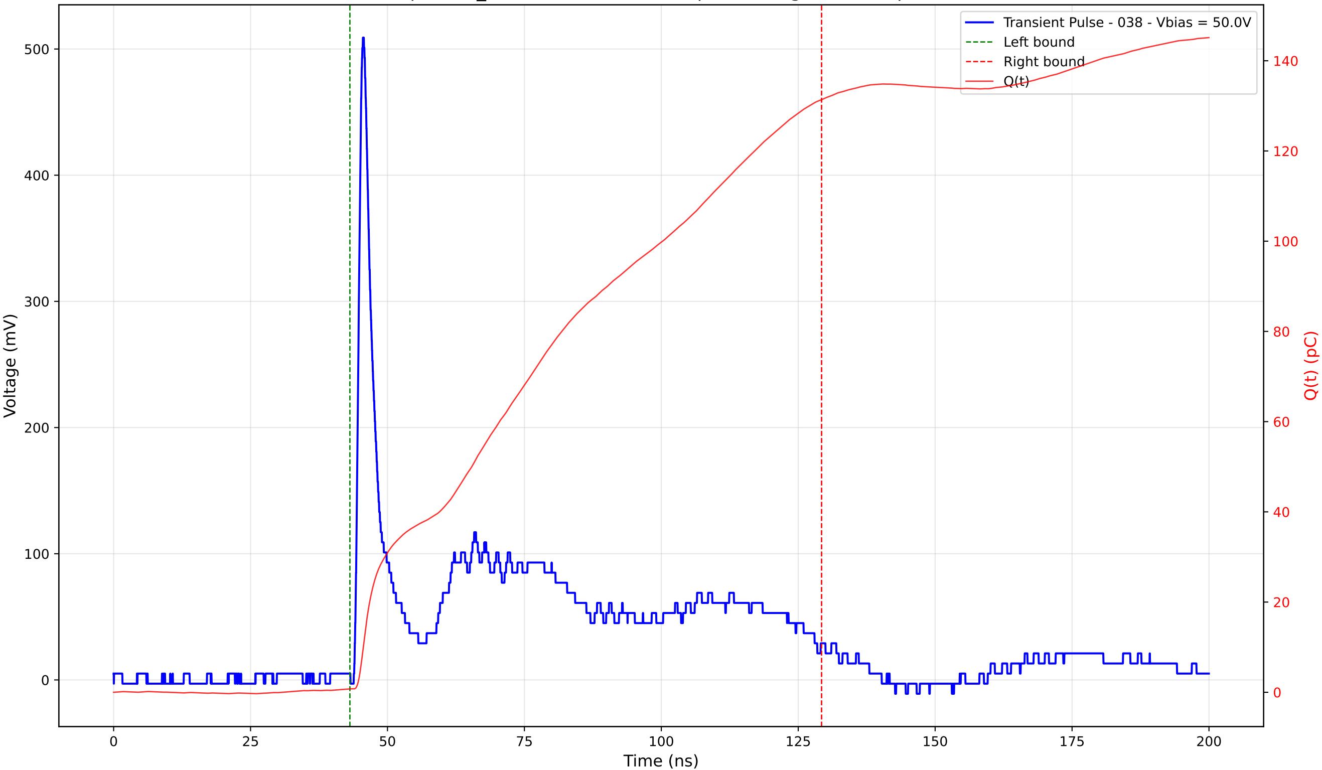
Transient Pulse - Sample: TD_4004 - Position: 125.0 \mu\text{m} - Charge: 130.59 pC - Rise Time: 1.05 ns
