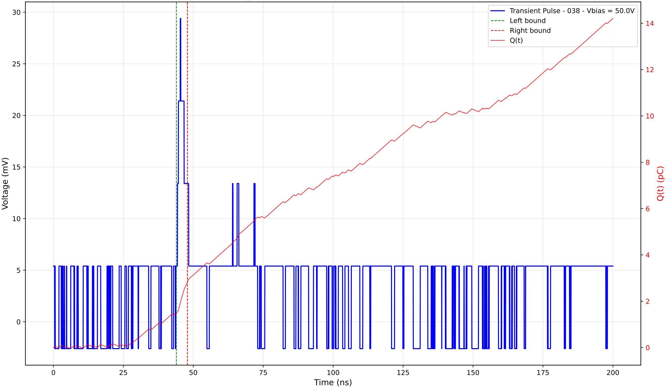
Transient Pulse - Sample: TD_4004 - Position: 425.0 \mu\text{m} - Charge: 1.35 pC - Rise Time: 1.60 ns
