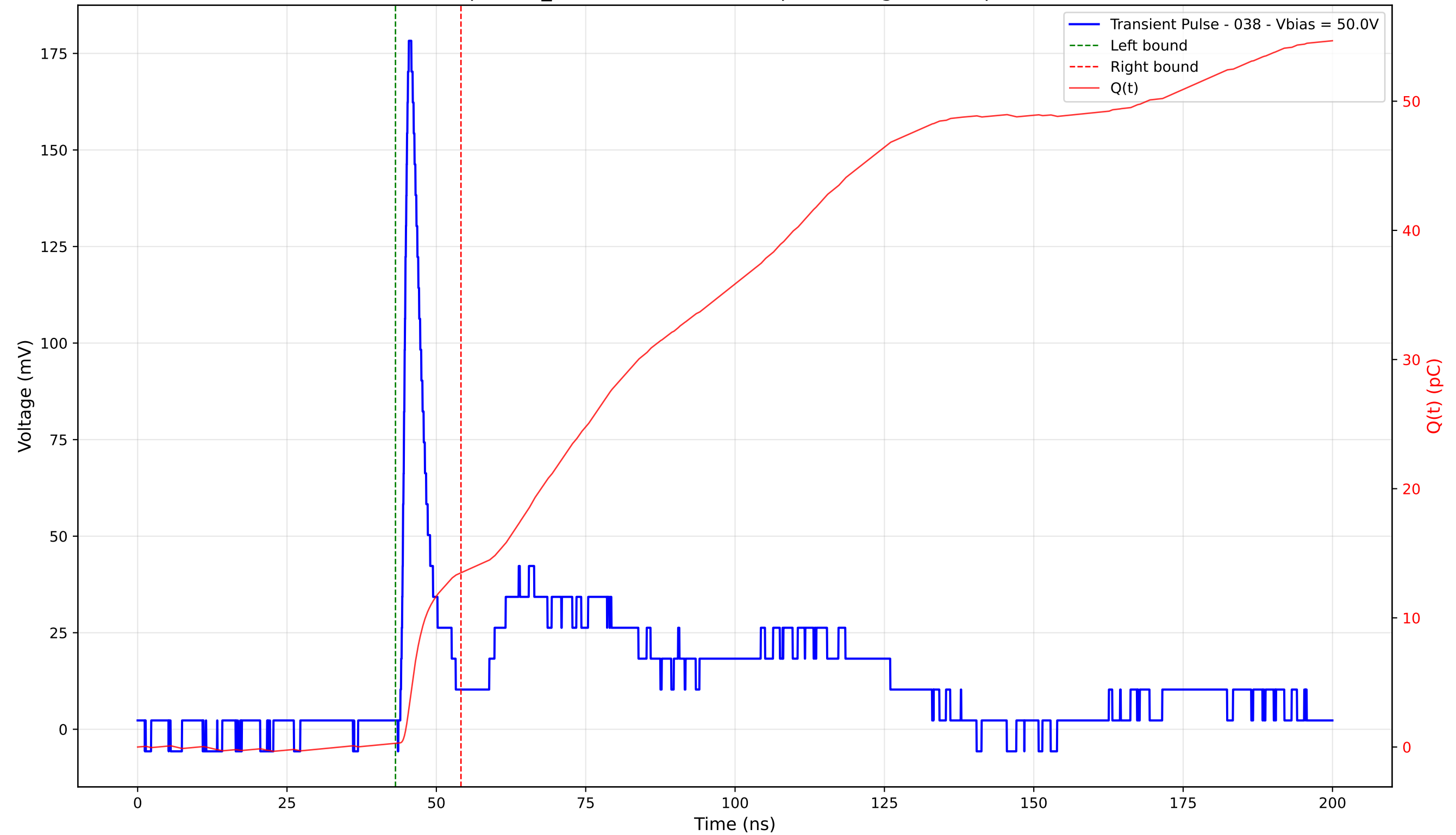
Transient Pulse - Sample: TD_4004 - Position: 310.0 \mu\text{m} - Charge: 13.19 pC - Rise Time: 1.06 ns
