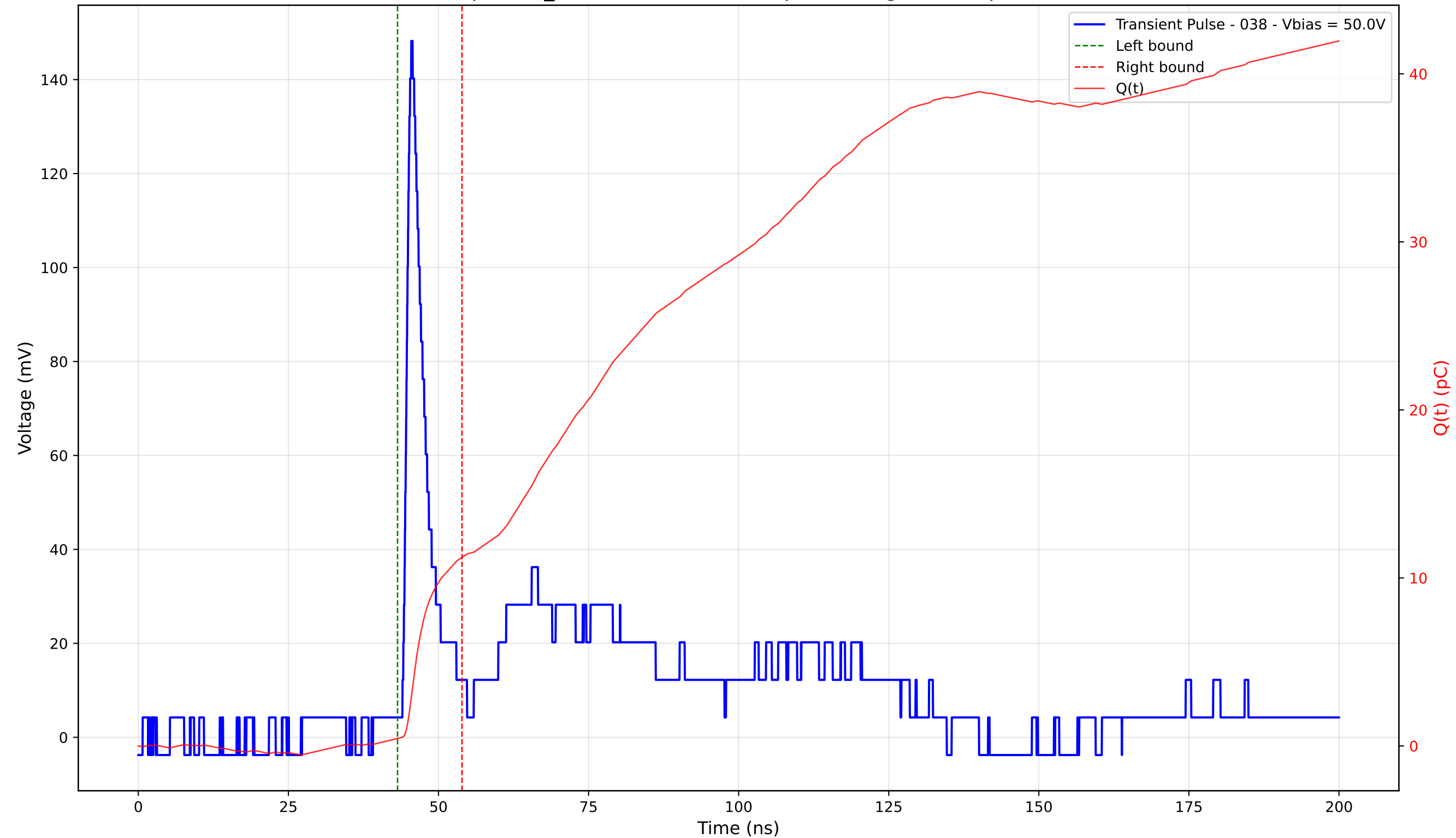
Transient Pulse - Sample: TD_4004 - Position: 330.0 \mu\text{m} - Charge: 10.79 pC - Rise Time: 1.13 ns
