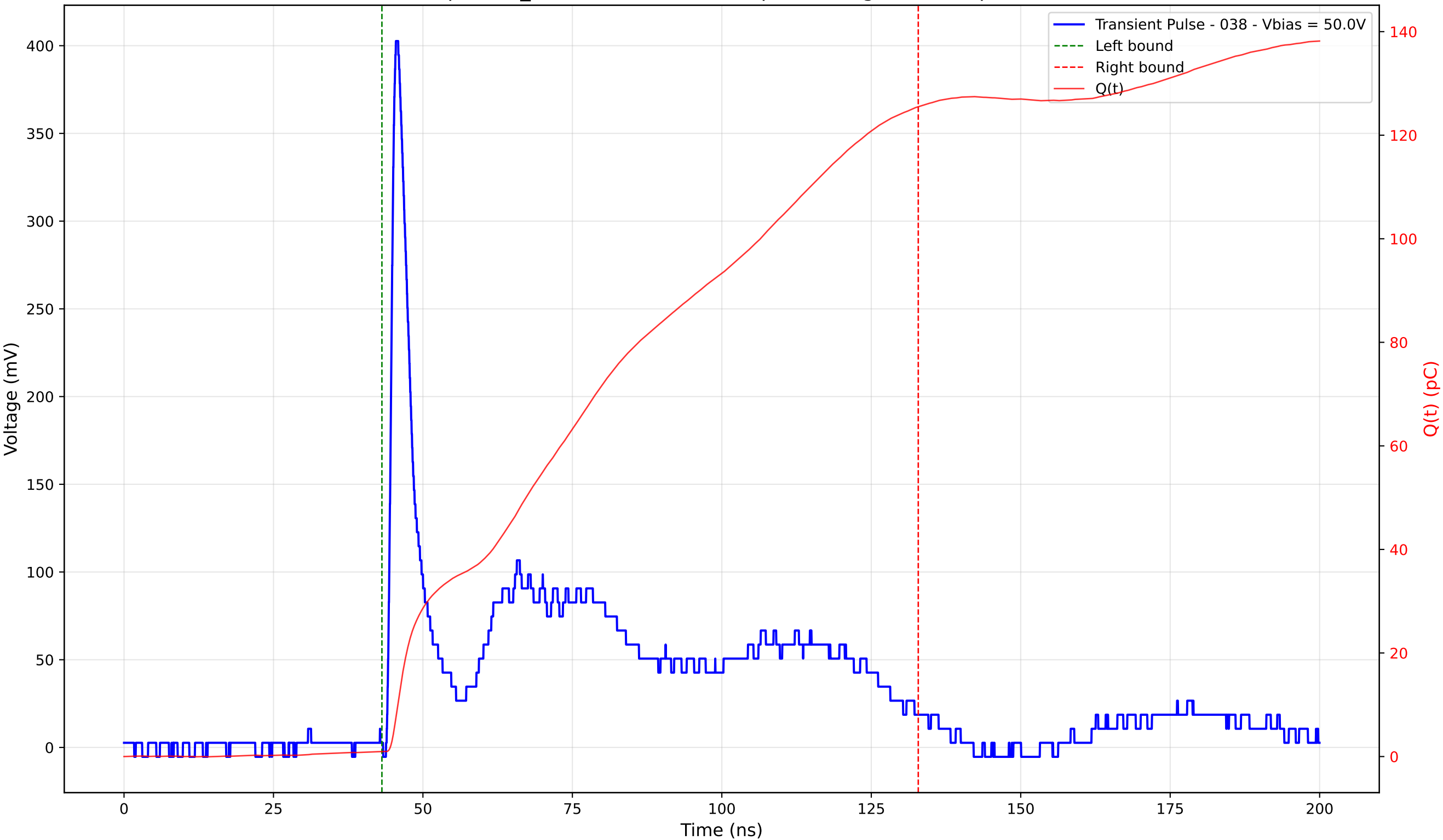
Transient Pulse - Sample: TD_4004 - Position: 175.0 \mu\text{m} - Charge: 124.50 pC - Rise Time: 1.05 ns
