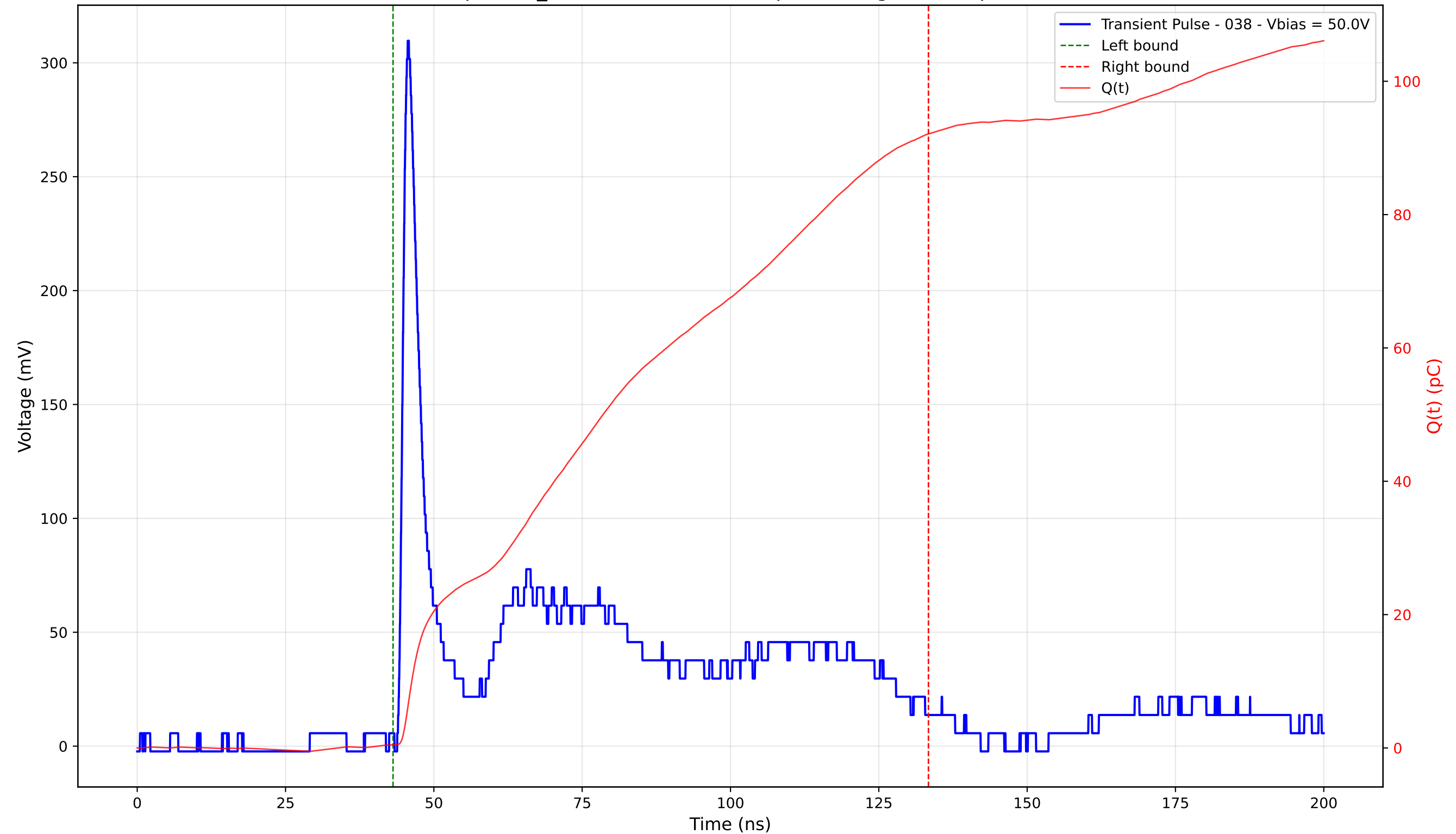
Transient Pulse - Sample: TD_4004 - Position: 145.0 \mu\text{m} - Charge: 91.61 pC - Rise Time: 1.14 ns
