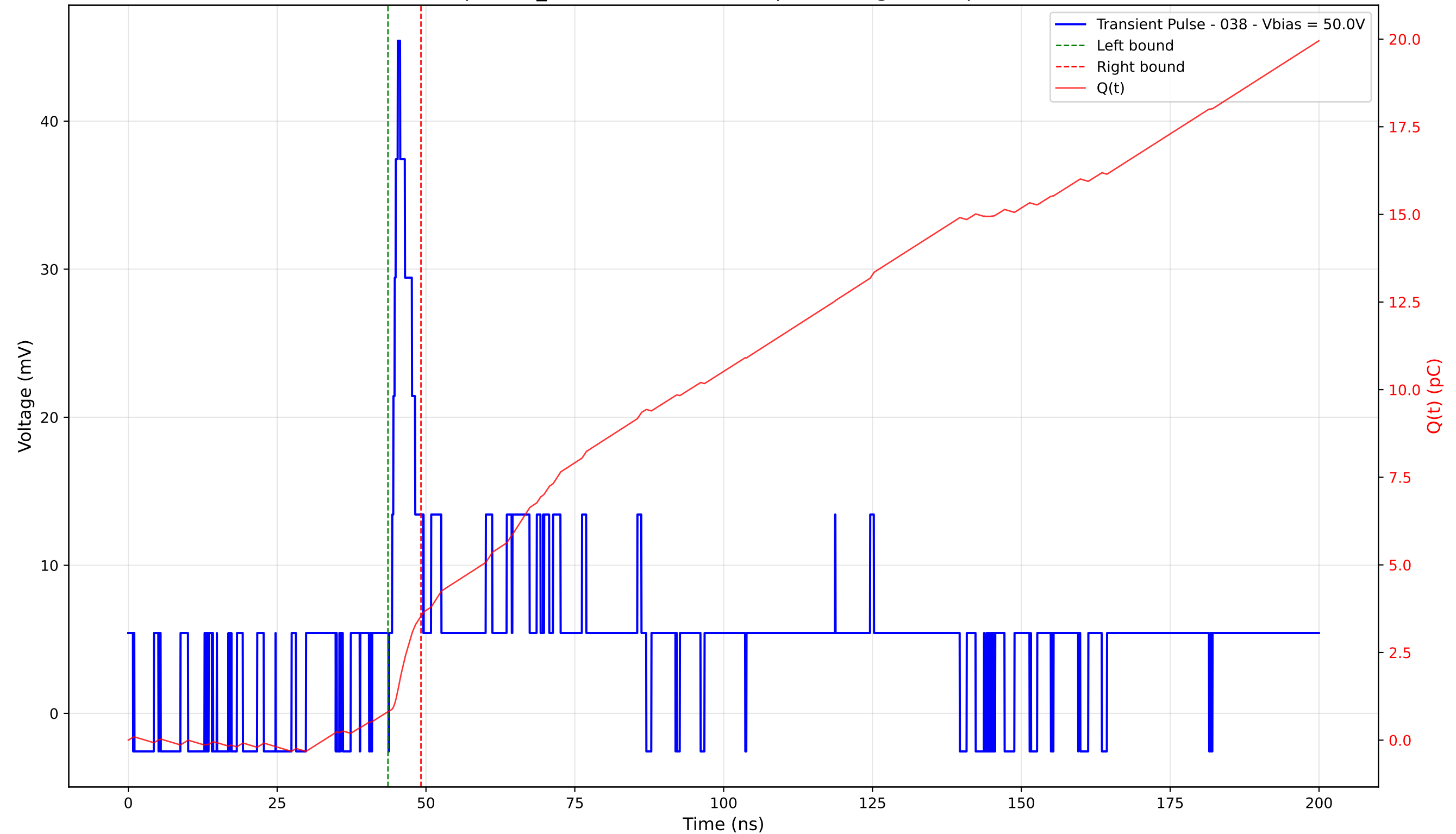
Transient Pulse - Sample: TD_4004 - Position: 415.0 \mu\text{m} - Charge: 2.72 pC - Rise Time: 1.47 ns
