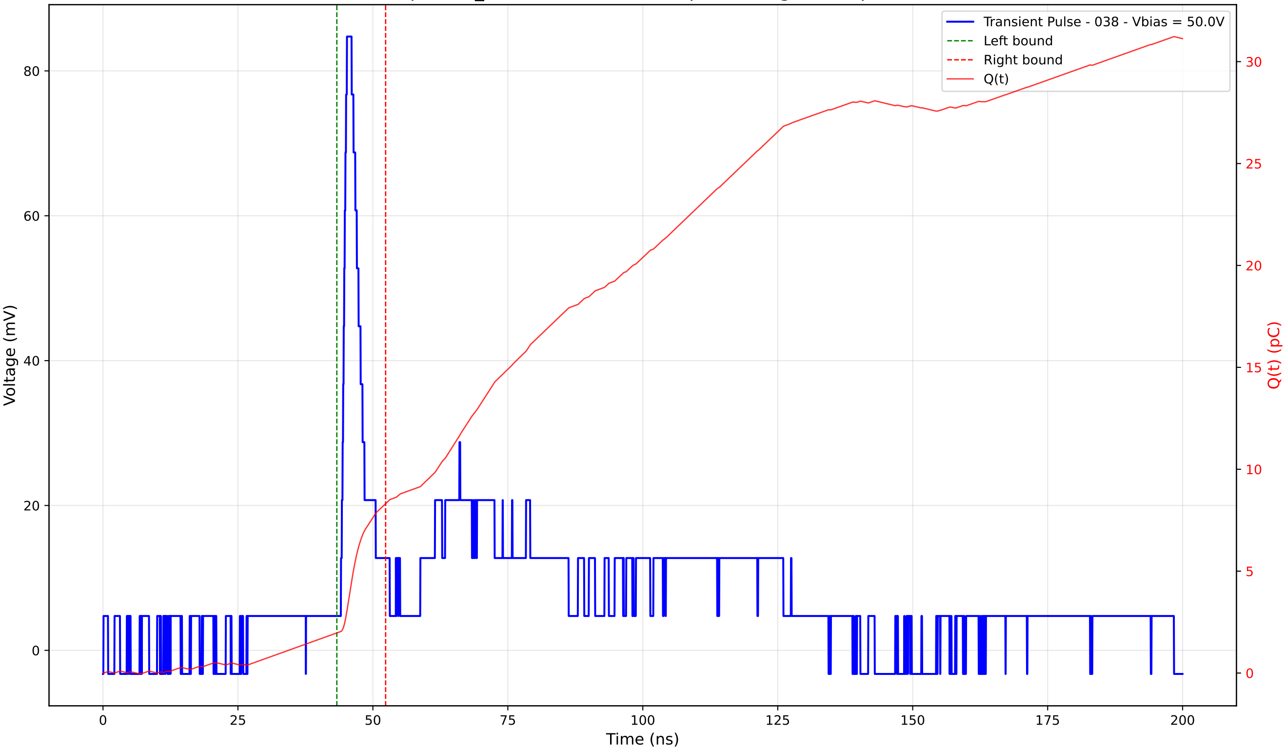
Transient Pulse - Sample: TD_4004 - Position: 395.0 \mu\text{m} - Charge: 6.36 pC - Rise Time: 0.95 ns
