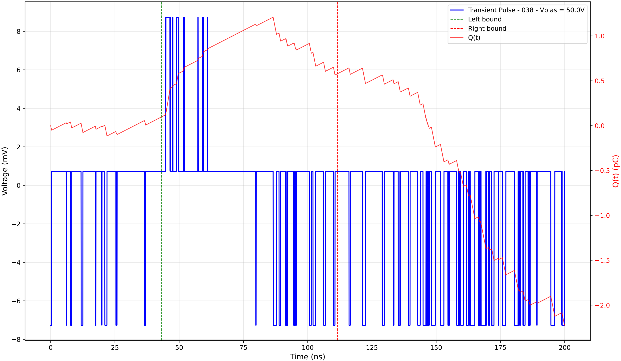
Transient Pulse - Sample: TD_4004 - Position: 10.0 \mu\text{m} - Charge: 0.48 pC - Rise Time: 0.02 ns
