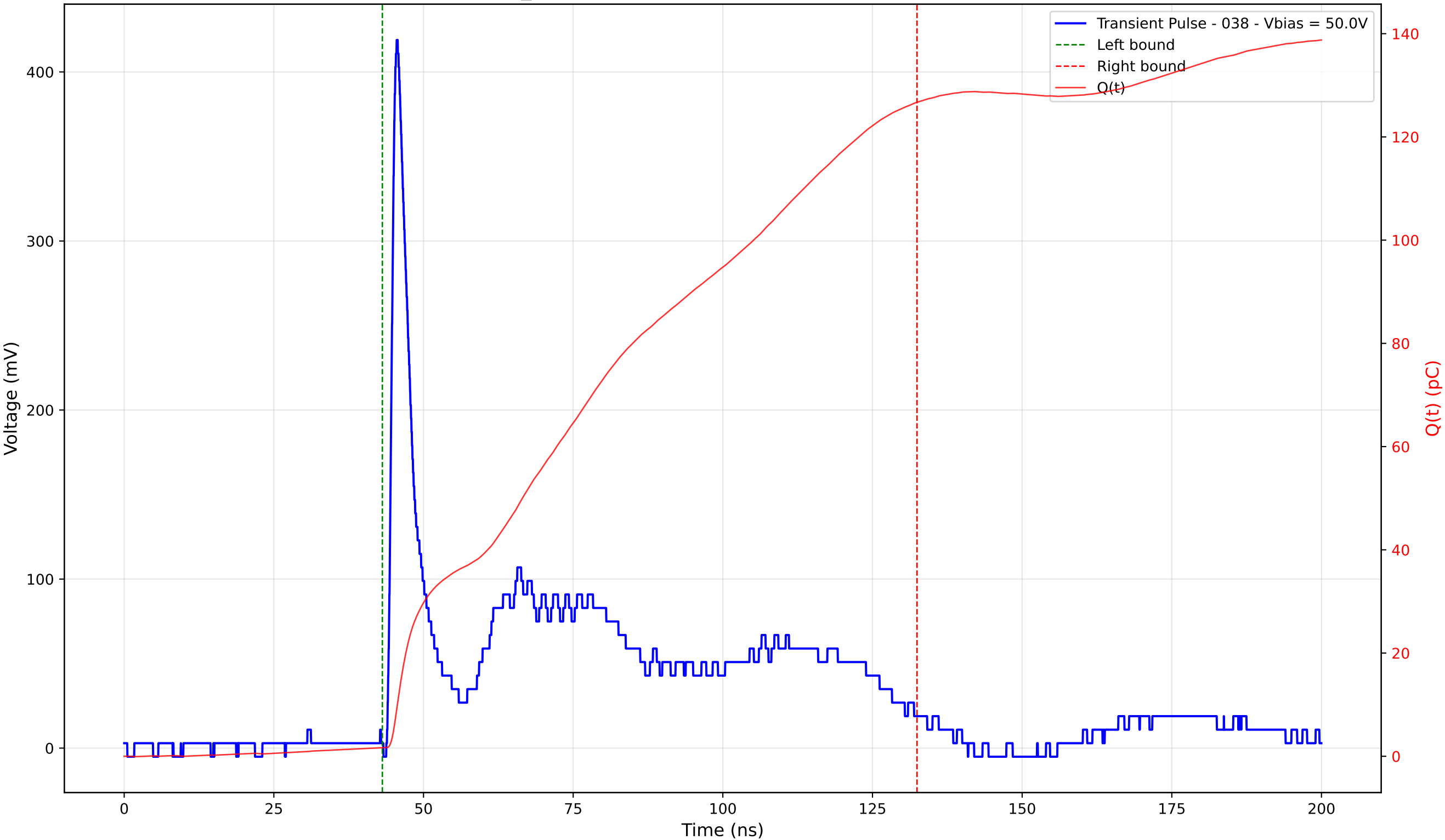
Transient Pulse - Sample: TD_4004 - Position: 205.0 \mu\text{m} - Charge: 124.99 pC - Rise Time: 1.06 ns
