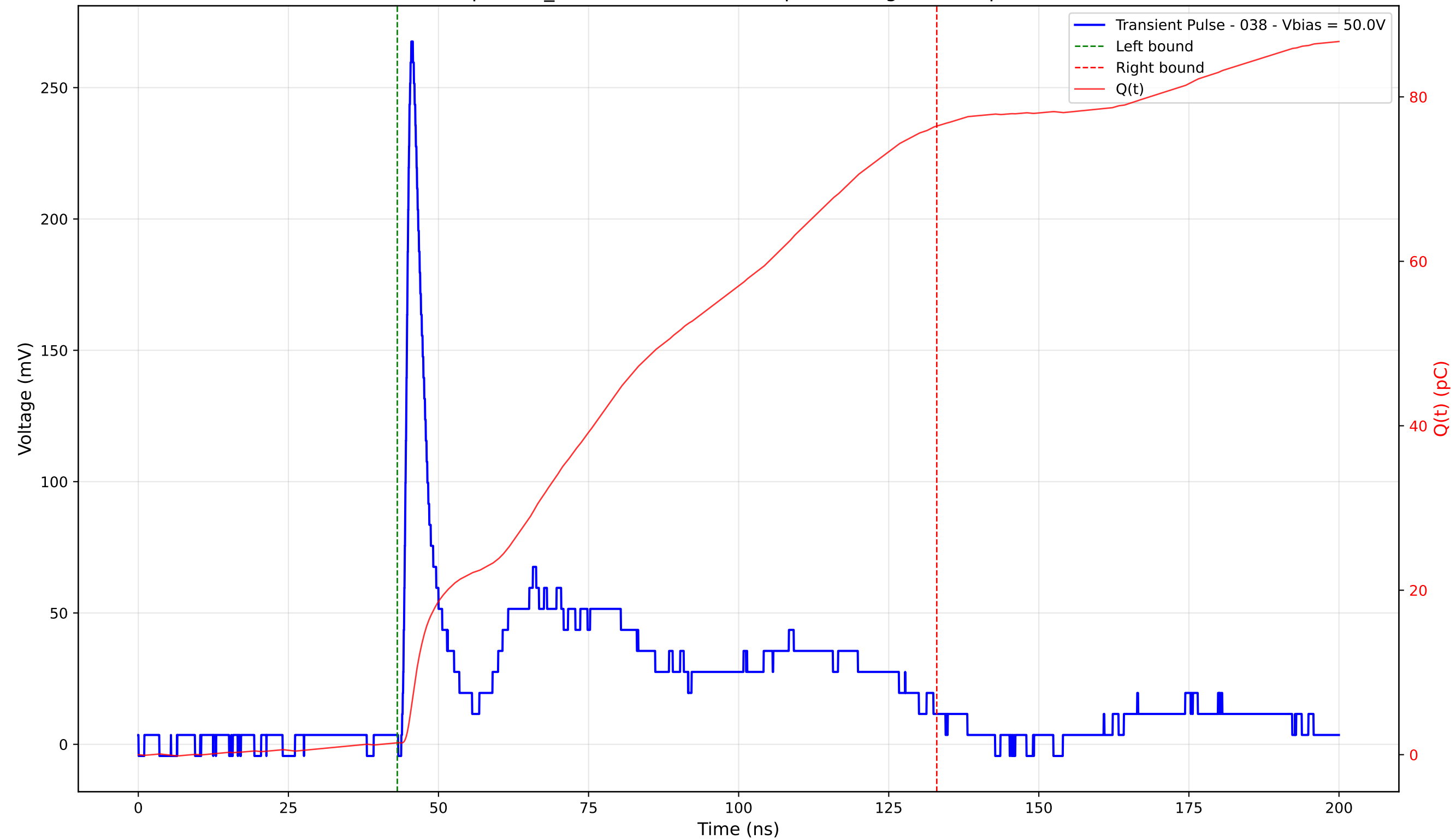
Transient Pulse - Sample: TD_4004 - Position: 245.0 \mu\text{m} - Charge: 74.99 pC - Rise Time: 1.06 ns
