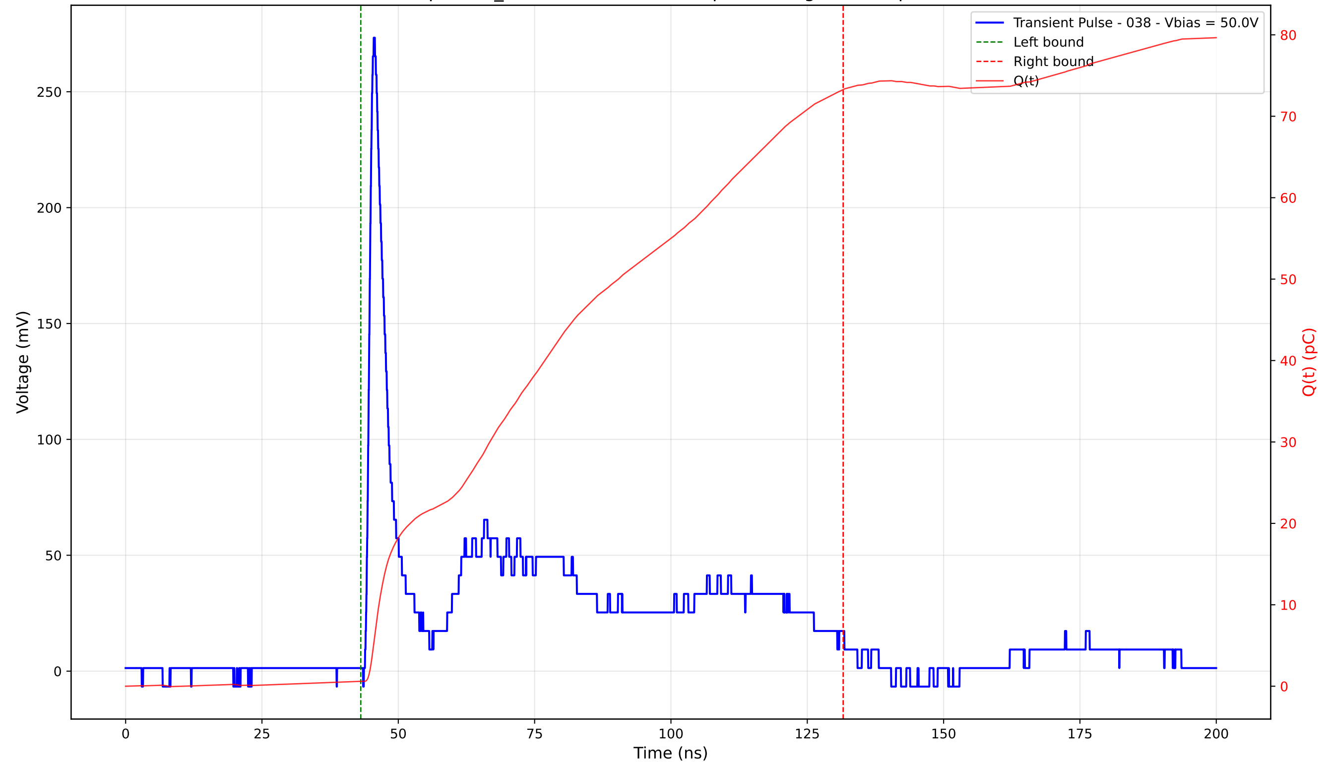
Transient Pulse - Sample: TD_4004 - Position: 240.0 \mu\text{m} - Charge: 72.68 pC - Rise Time: 1.05 ns
