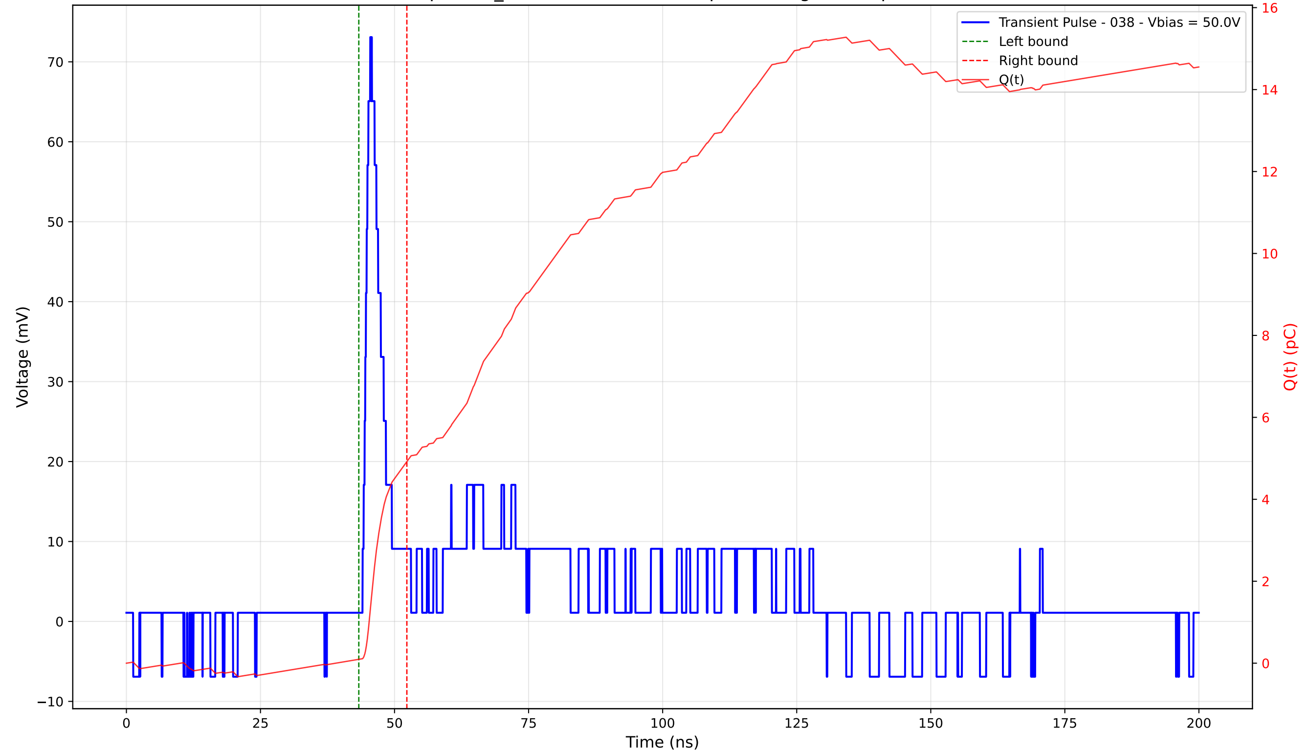
Transient Pulse - Sample: TD_4004 - Position: 400.0 \mu\text{m} - Charge: 4.83 pC - Rise Time: 1.42 ns
