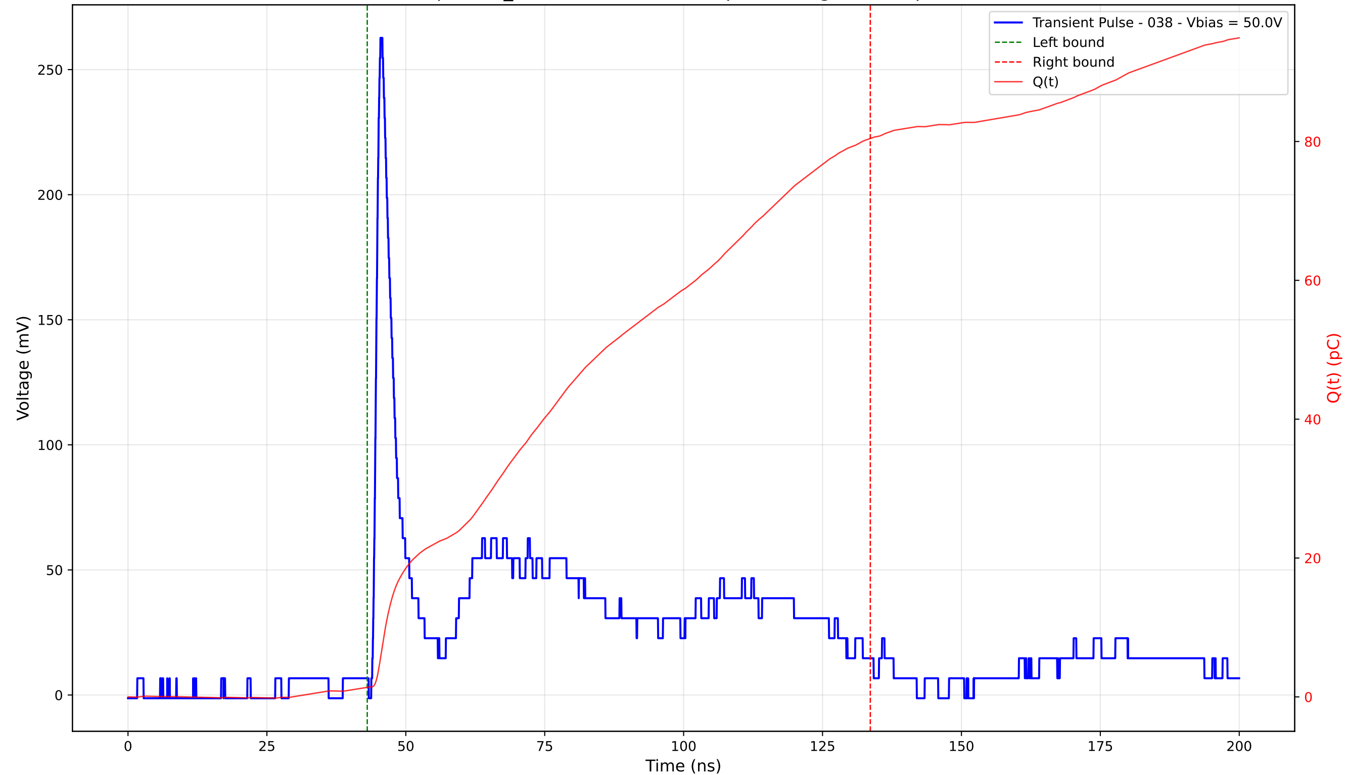
Transient Pulse - Sample: TD_4004 - Position: 250.0 \mu\text{m} - Charge: 79.05 pC - Rise Time: 1.07 ns
