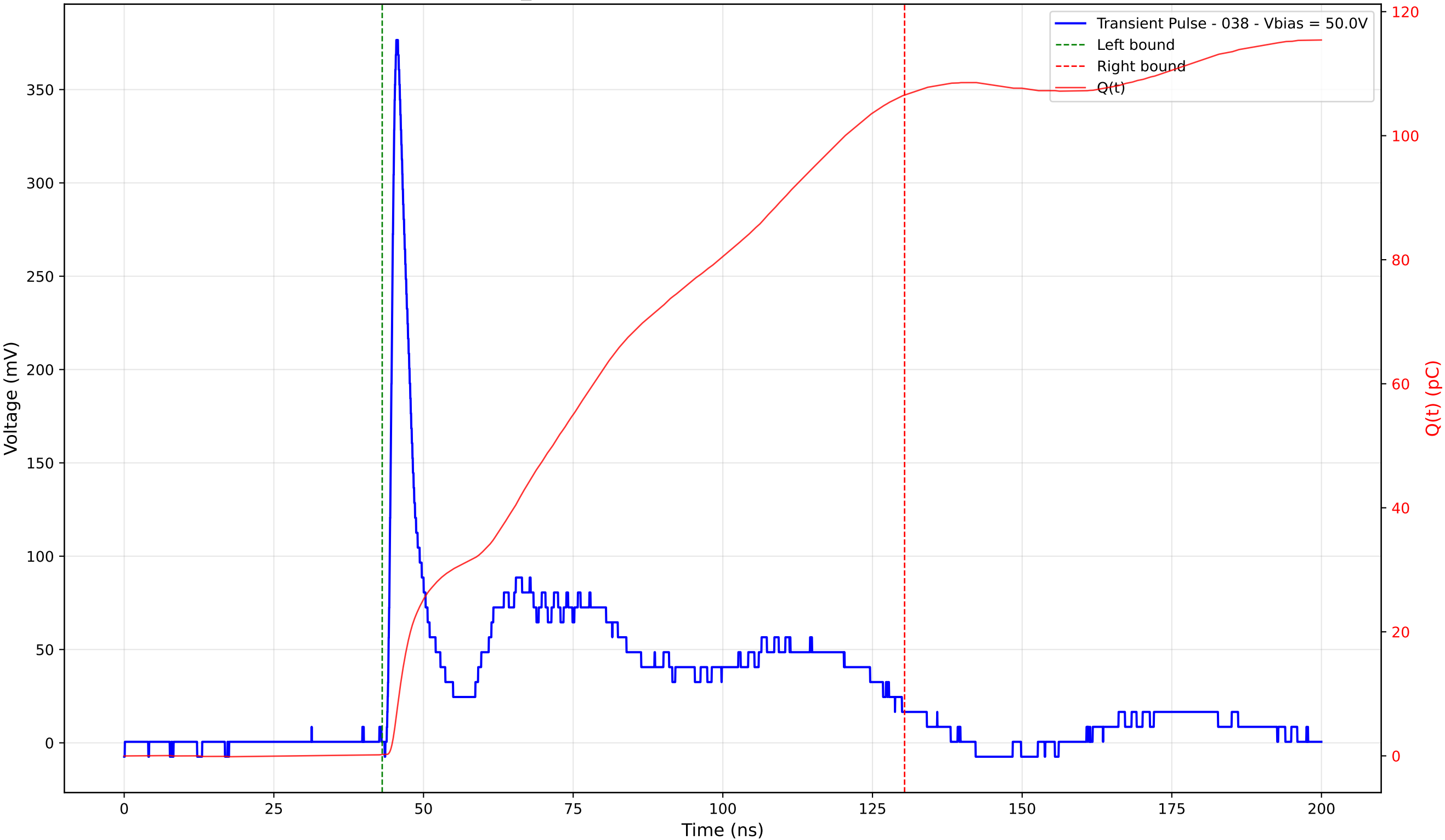
Transient Pulse - Sample: TD_4004 - Position: 215.0 \mu\text{m} - Charge: 106.33 pC - Rise Time: 1.07 ns
