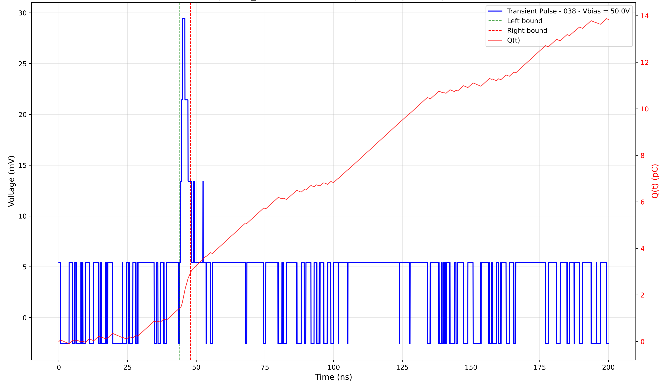
Transient Pulse - Sample: TD_4004 - Position: 45.0 \mu\text{m} - Charge: 1.54 pC - Rise Time: 1.04 ns
