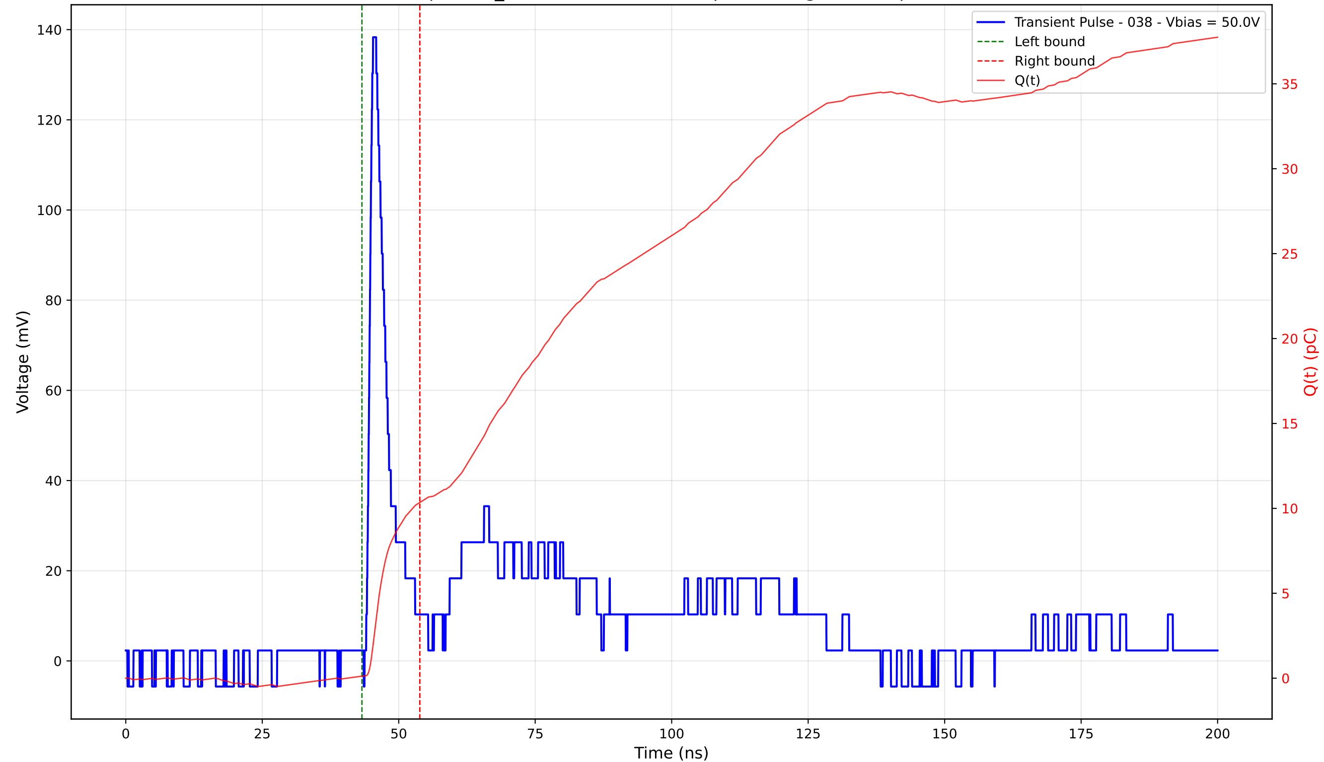
Transient Pulse - Sample: TD_4004 - Position: 350.0 \mu\text{m} - Charge: 10.22 pC - Rise Time: 0.97 ns
