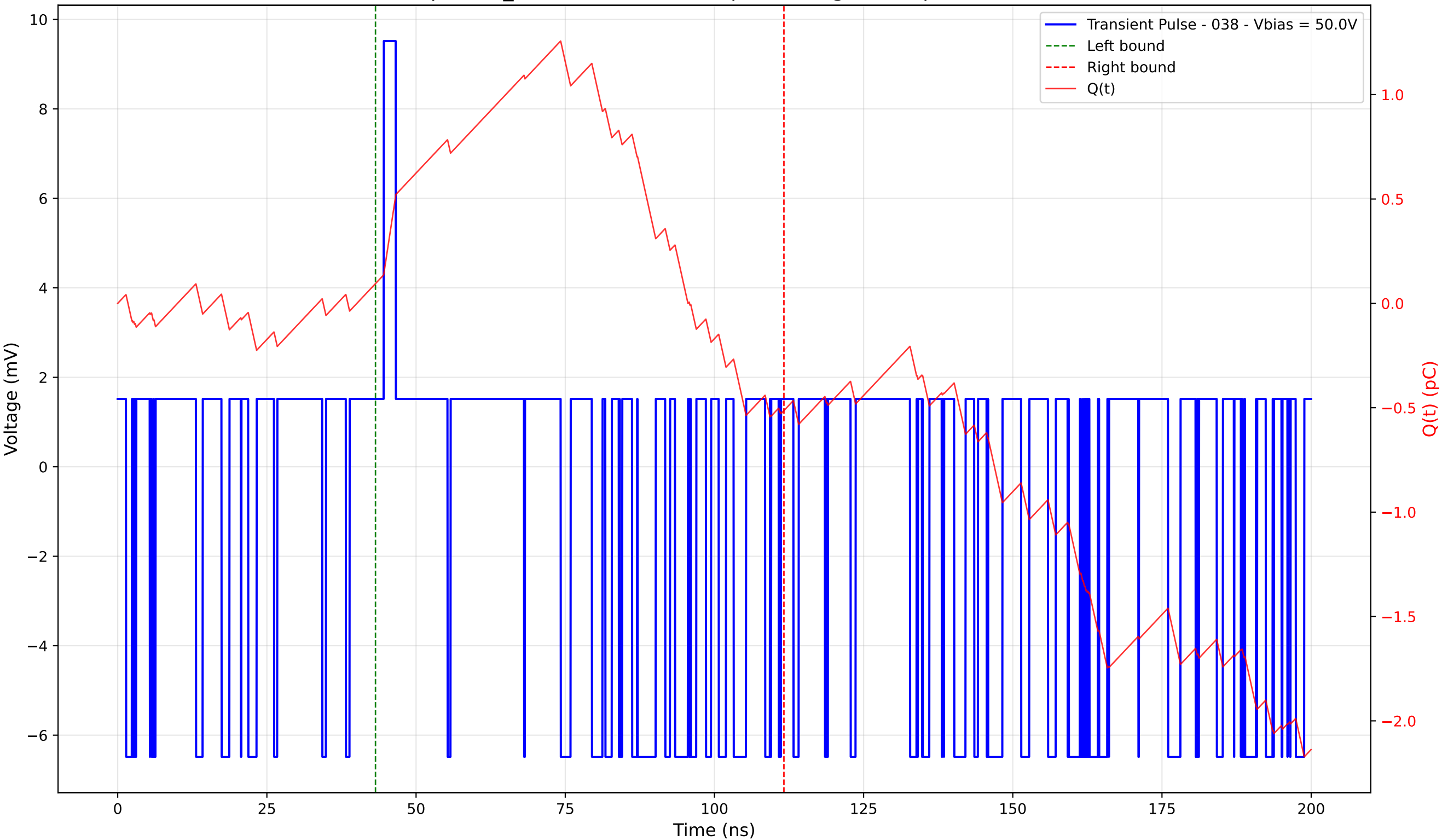
Transient Pulse - Sample: TD_4004 - Position: 30.0 \mu\text{m} - Charge: 0.61 pC - Rise Time: 0.00 ns (N/A)
