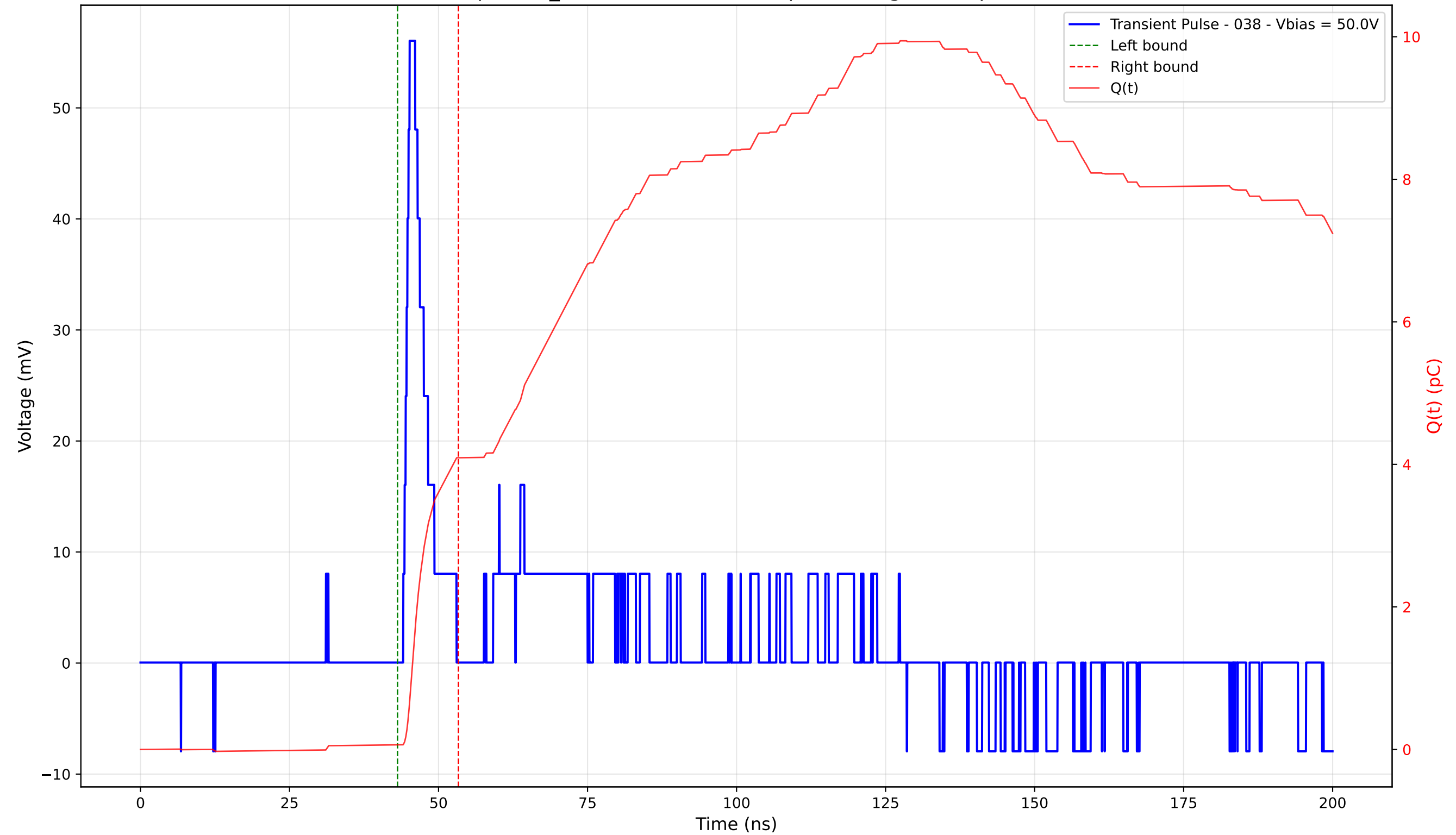
Transient Pulse - Sample: TD_4004 - Position: 405.0 \mu\text{m} - Charge: 4.03 pC - Rise Time: 1.07 ns
