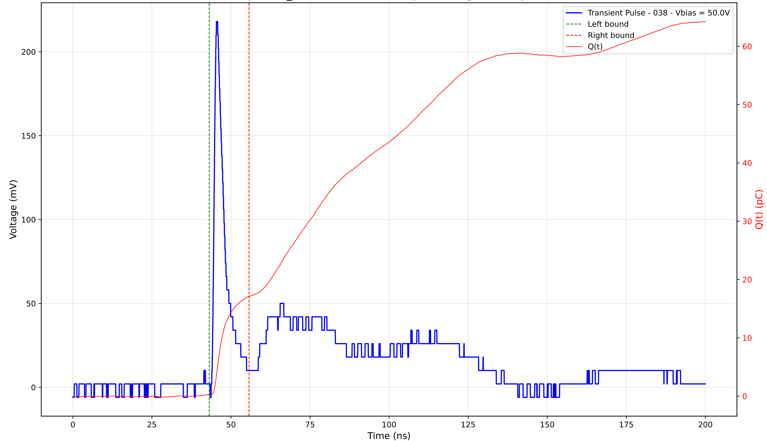
Transient Pulse - Sample: TD_4004 - Position: 265.0 \mu\text{m} - Charge: 16.83 pC - Rise Time: 1.05 ns
