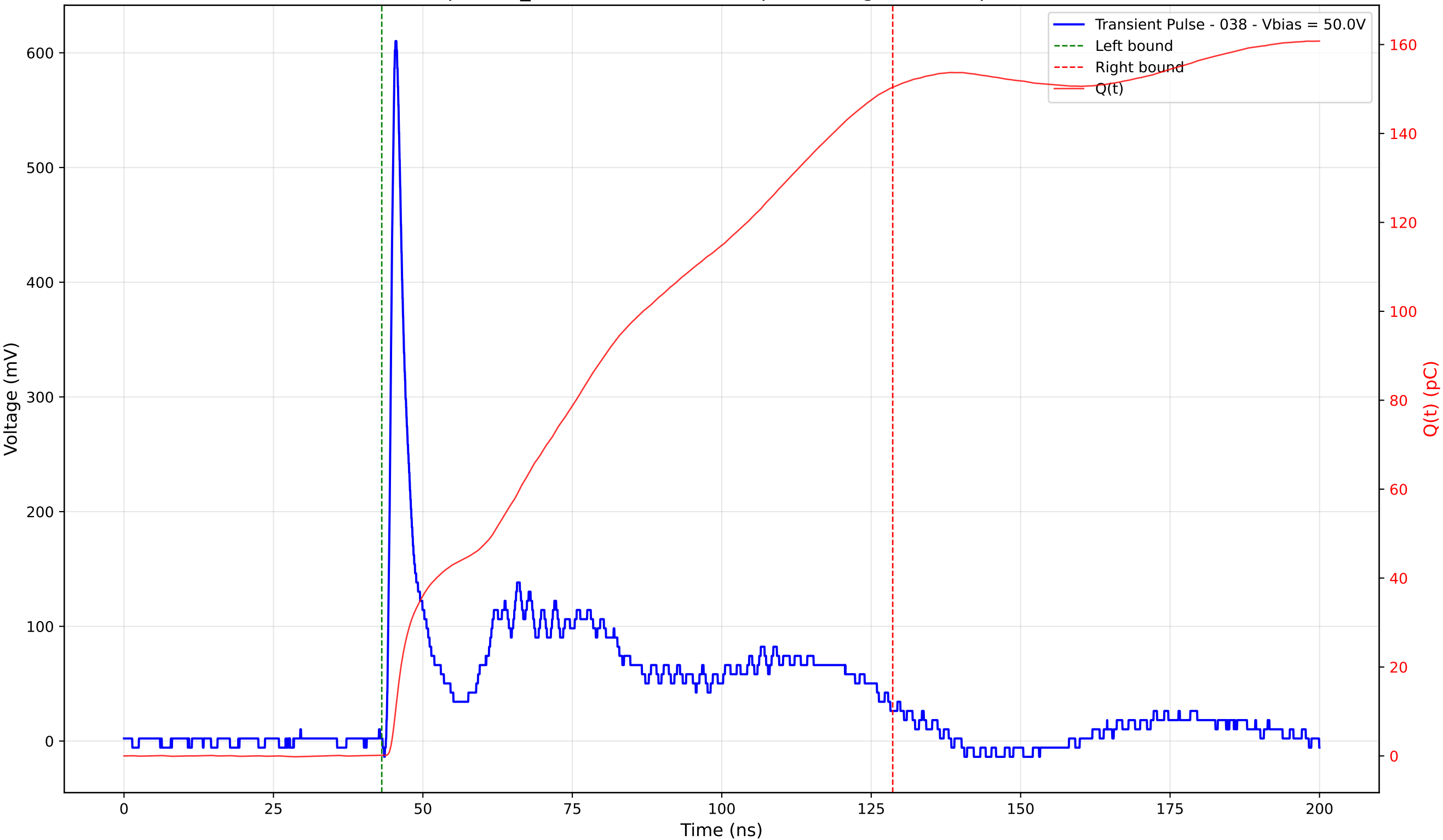
Transient Pulse - Sample: TD_4004 - Position: 110.0 \mu\text{m} - Charge: 150.16 pC - Rise Time: 1.00 ns
