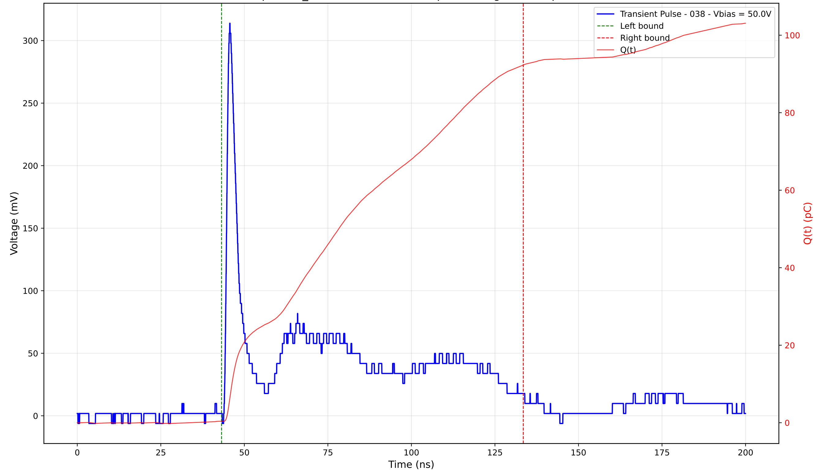
Transient Pulse - Sample: TD_4004 - Position: 150.0 \mu\text{m} - Charge: 91.93 pC - Rise Time: 1.15 ns
