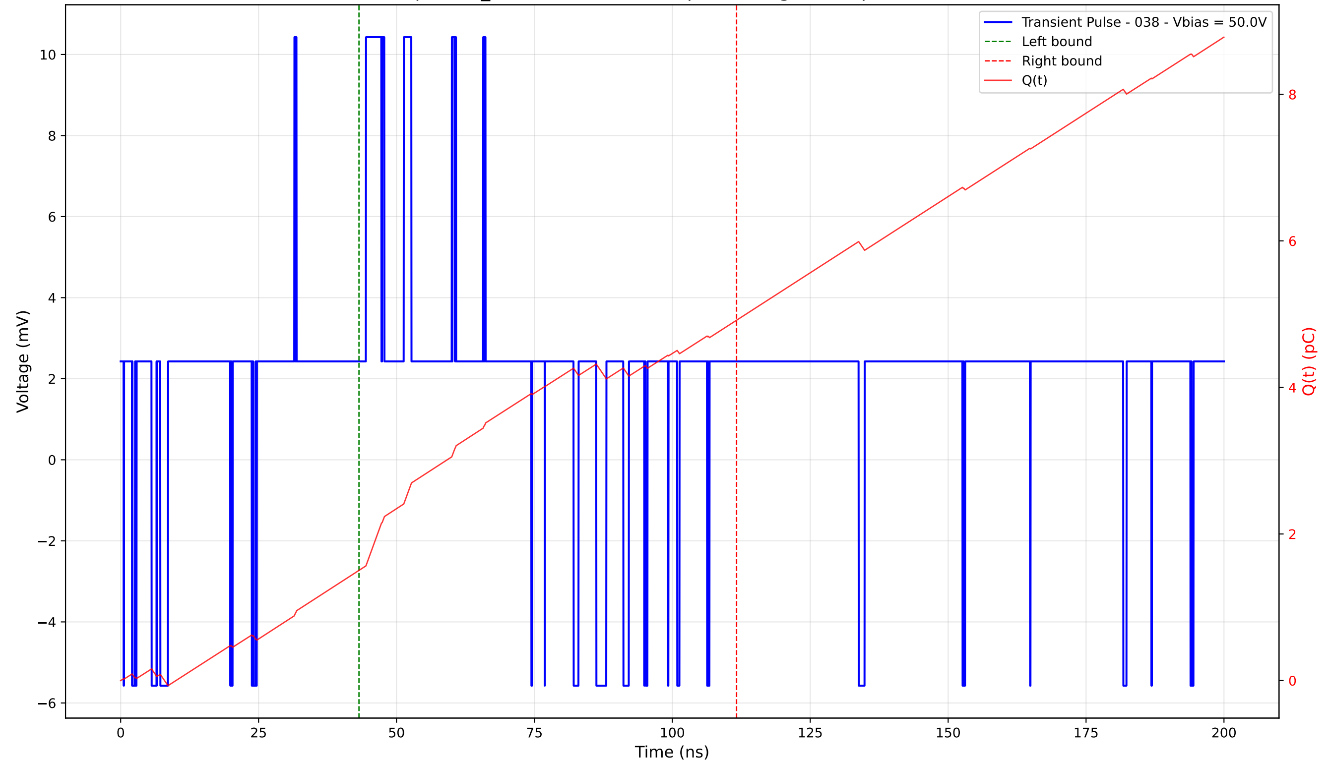
Transient Pulse - Sample: TD_4004 - Position: 25.0 \mu\text{m} - Charge: 3.42 pC - Rise Time: 0.00 ns (N/A)
