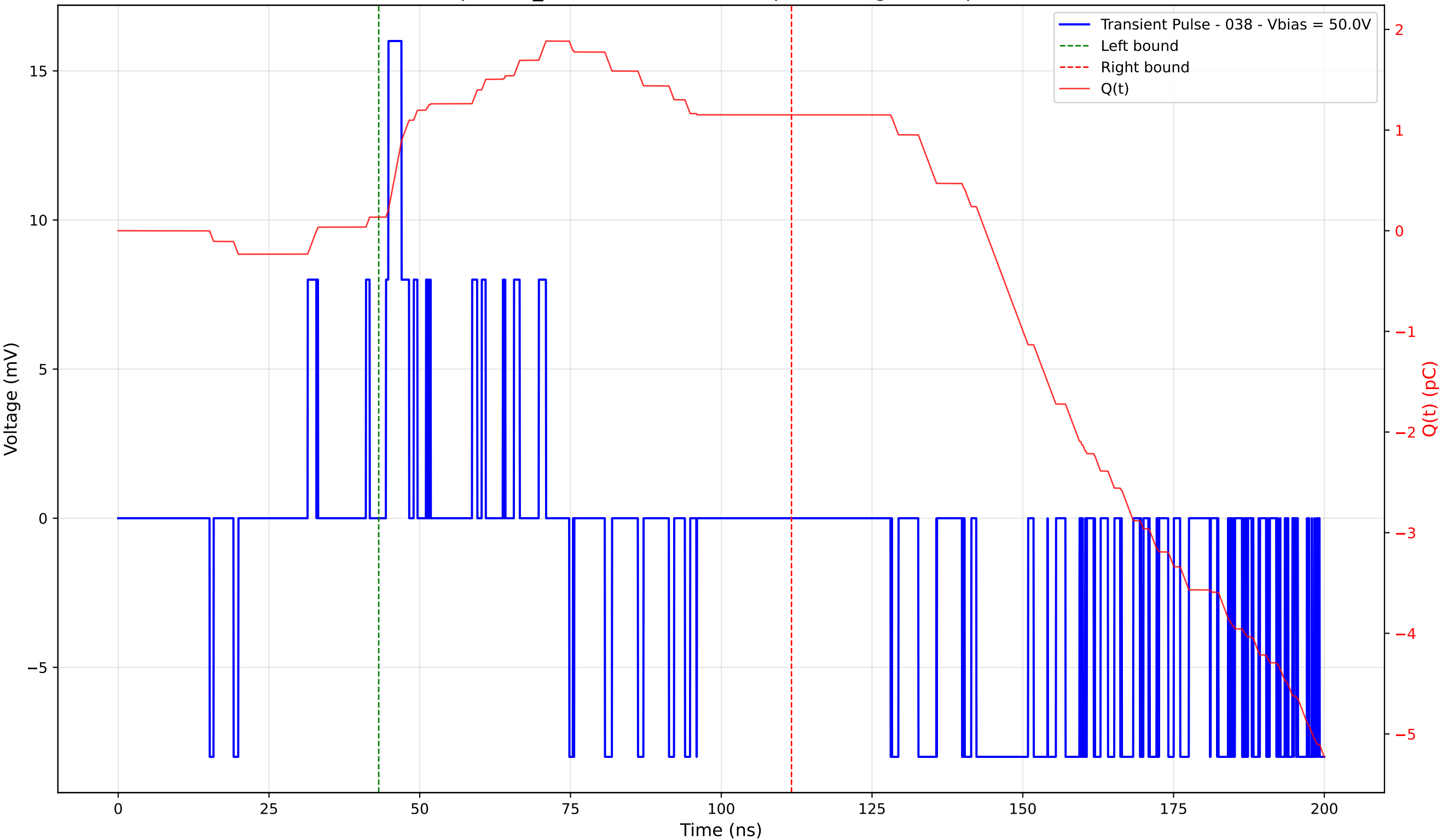
Transient Pulse - Sample: TD_4004 - Position: 435.0 \mu\text{m} - Charge: 1.02 pC - Rise Time: 0.42 ns
