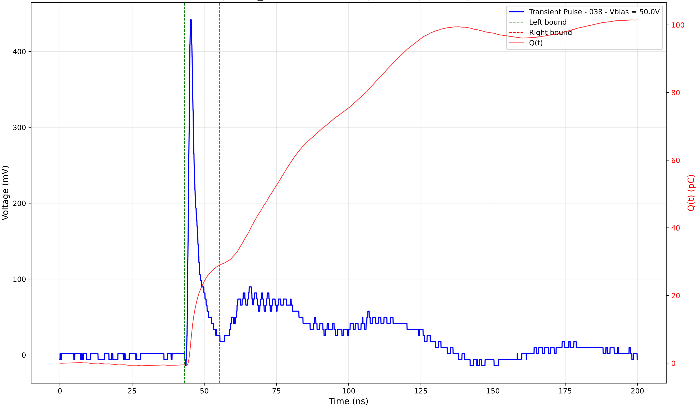
Transient Pulse - Sample: TD_4004 - Position: 80.0 \mu\text{m} - Charge: 29.49 pC - Rise Time: 0.92 ns
