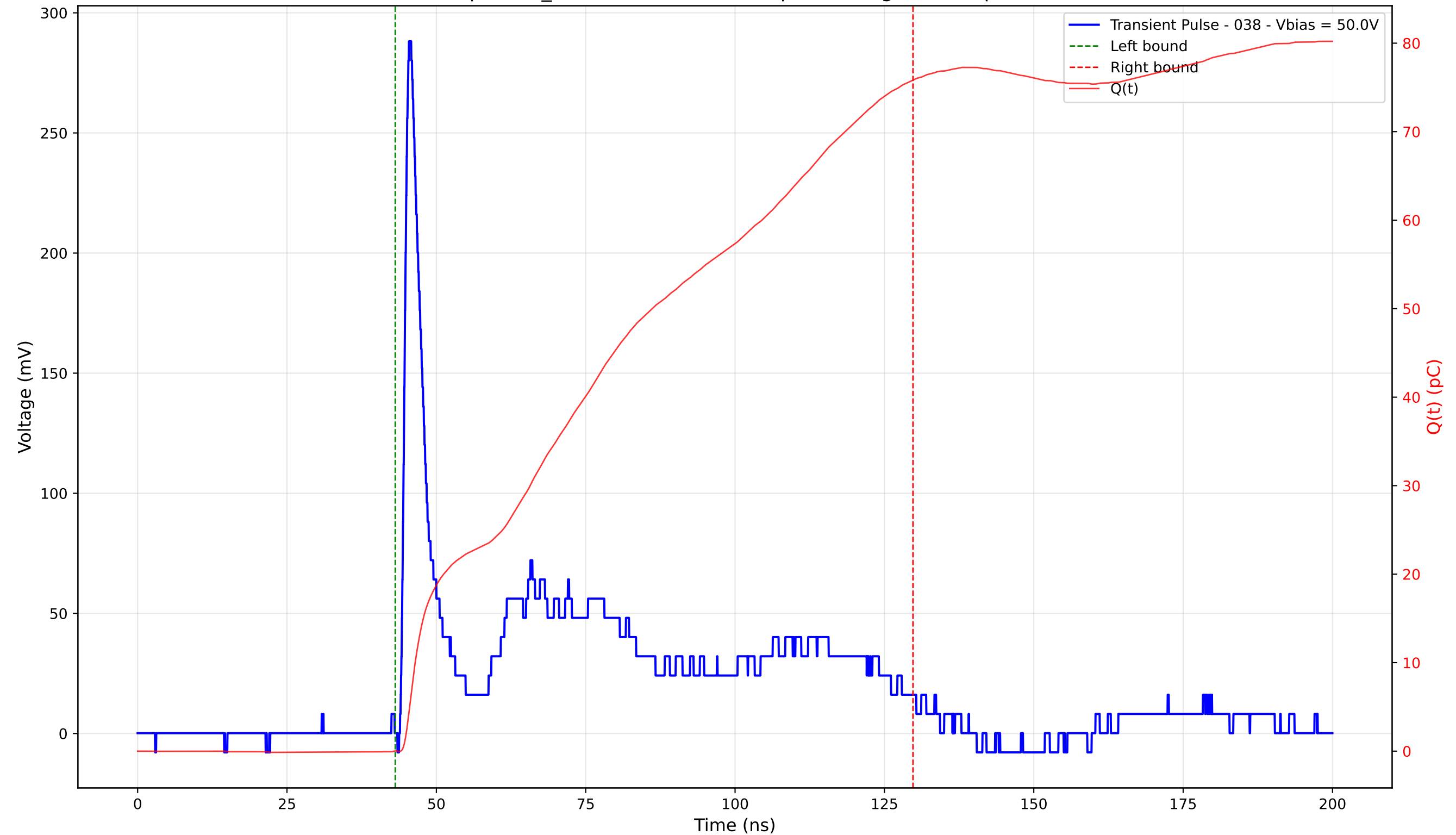
Transient Pulse - Sample: TD_4004 - Position: 235.0 \mu\text{m} - Charge: 75.81 pC - Rise Time: 1.05 ns
