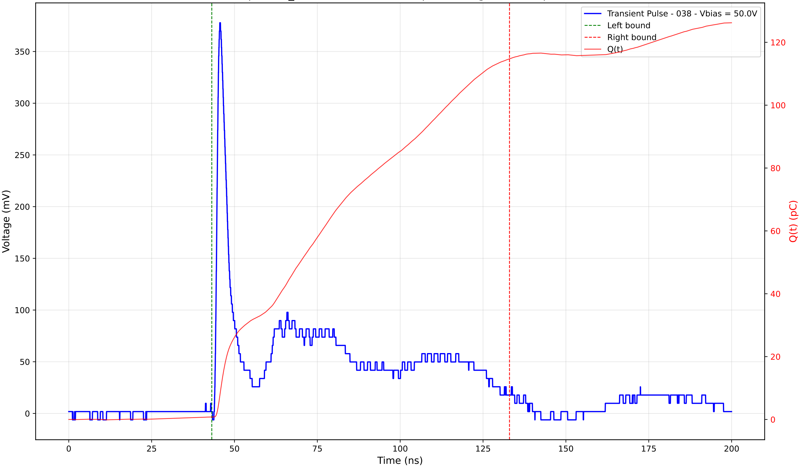
Transient Pulse - Sample: TD_4004 - Position: 170.0 \mu\text{m} - Charge: 113.90 pC - Rise Time: 1.09 ns
