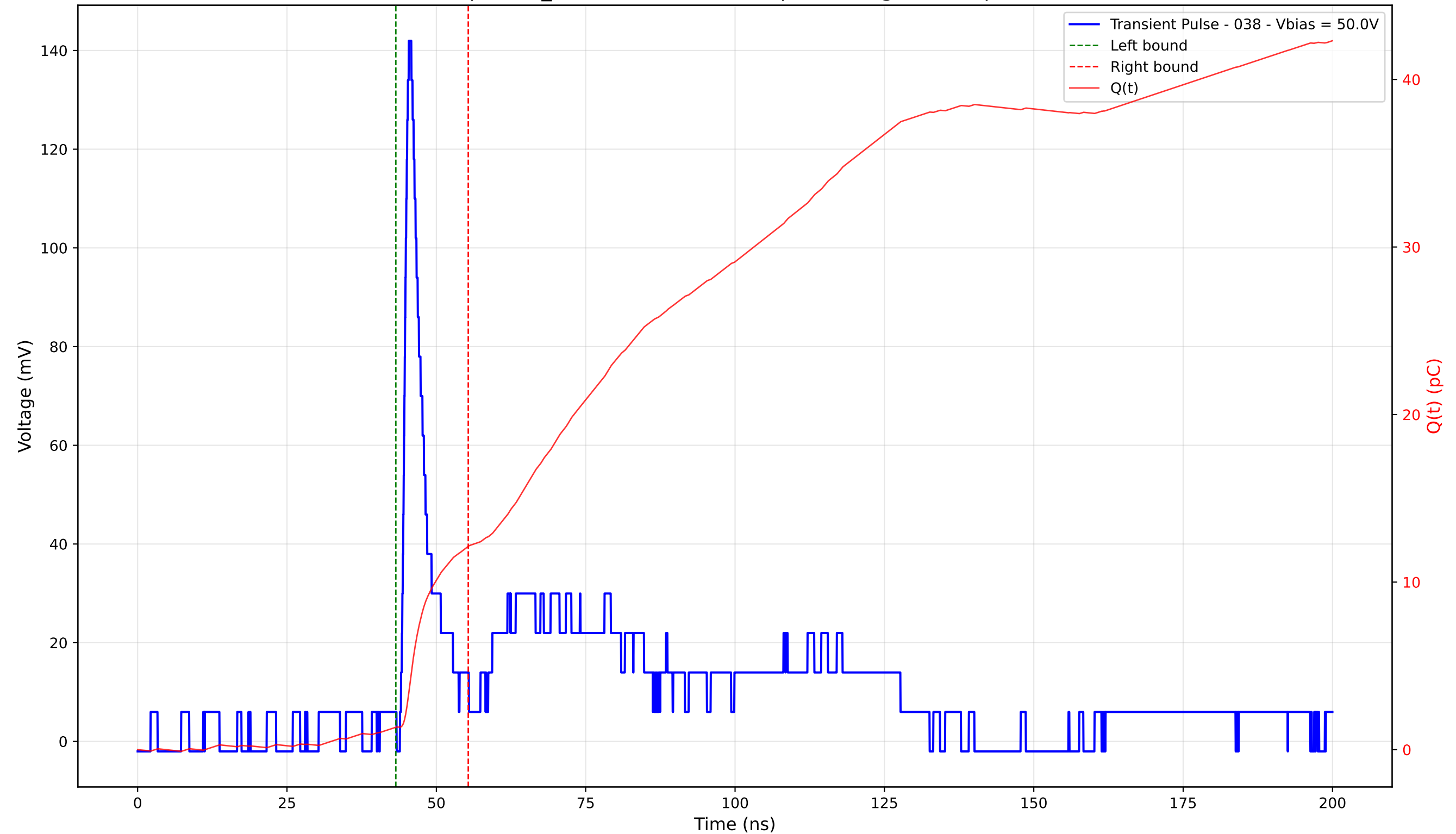
Transient Pulse - Sample: TD_4004 - Position: 355.0 \mu\text{m} - Charge: 10.80 pC - Rise Time: 1.02 ns
