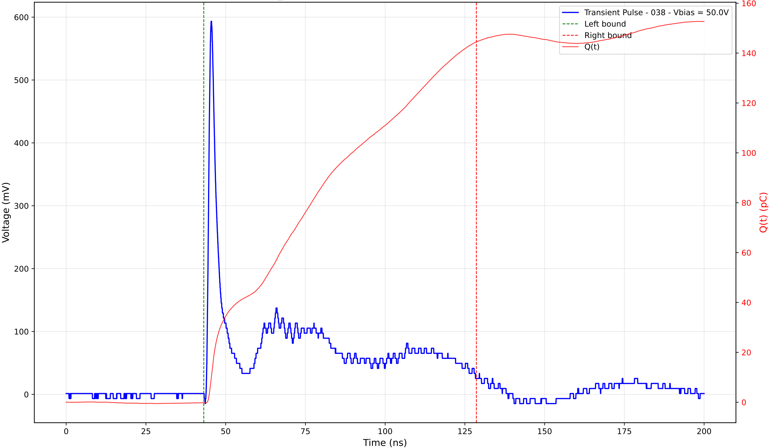
Transient Pulse - Sample: TD_4004 - Position: 115.0 \mu\text{m} - Charge: 144.71 pC - Rise Time: 1.01 ns
