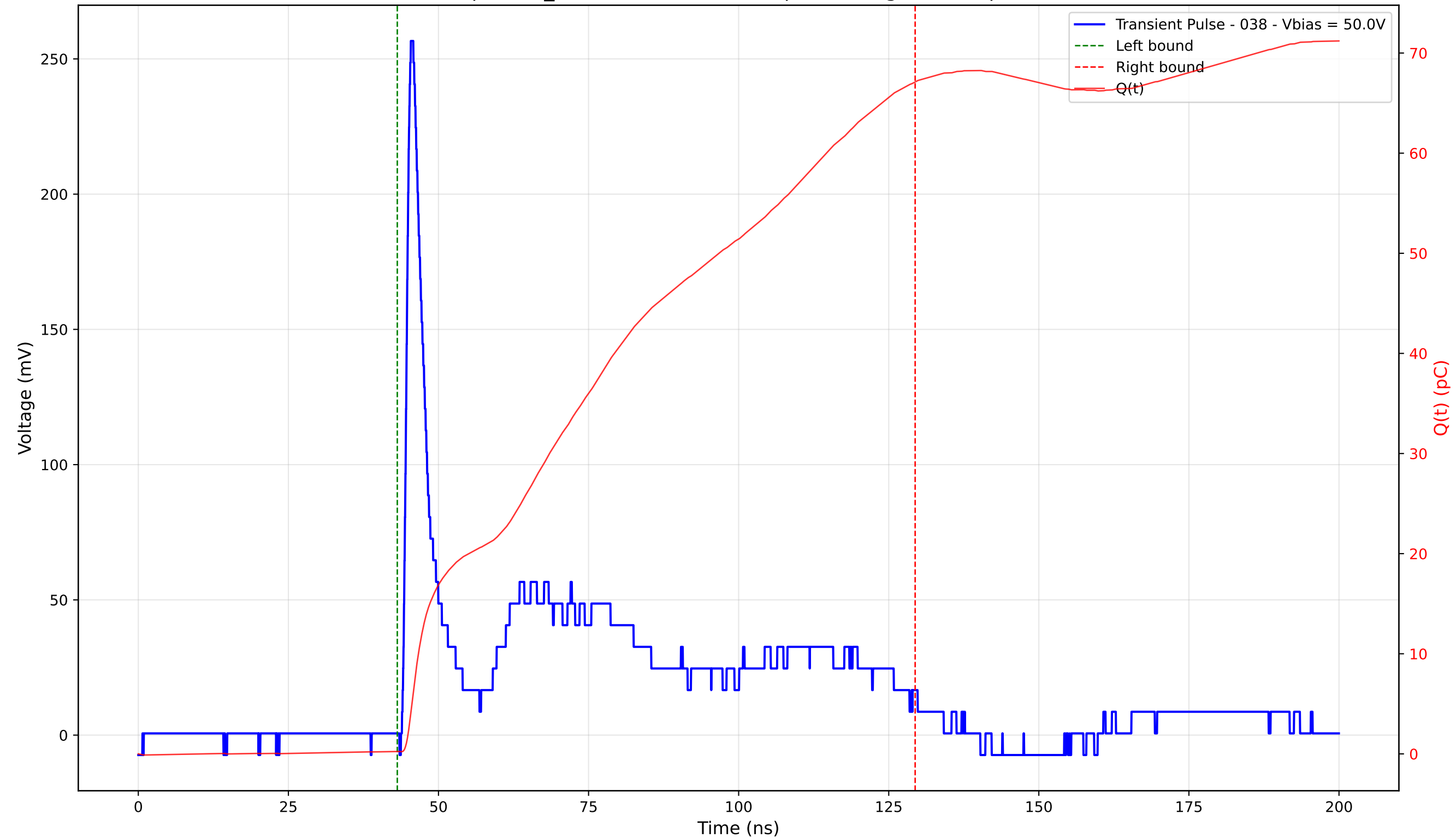
Transient Pulse - Sample: TD_4004 - Position: 255.0 \mu\text{m} - Charge: 66.87 pC - Rise Time: 1.00 ns
