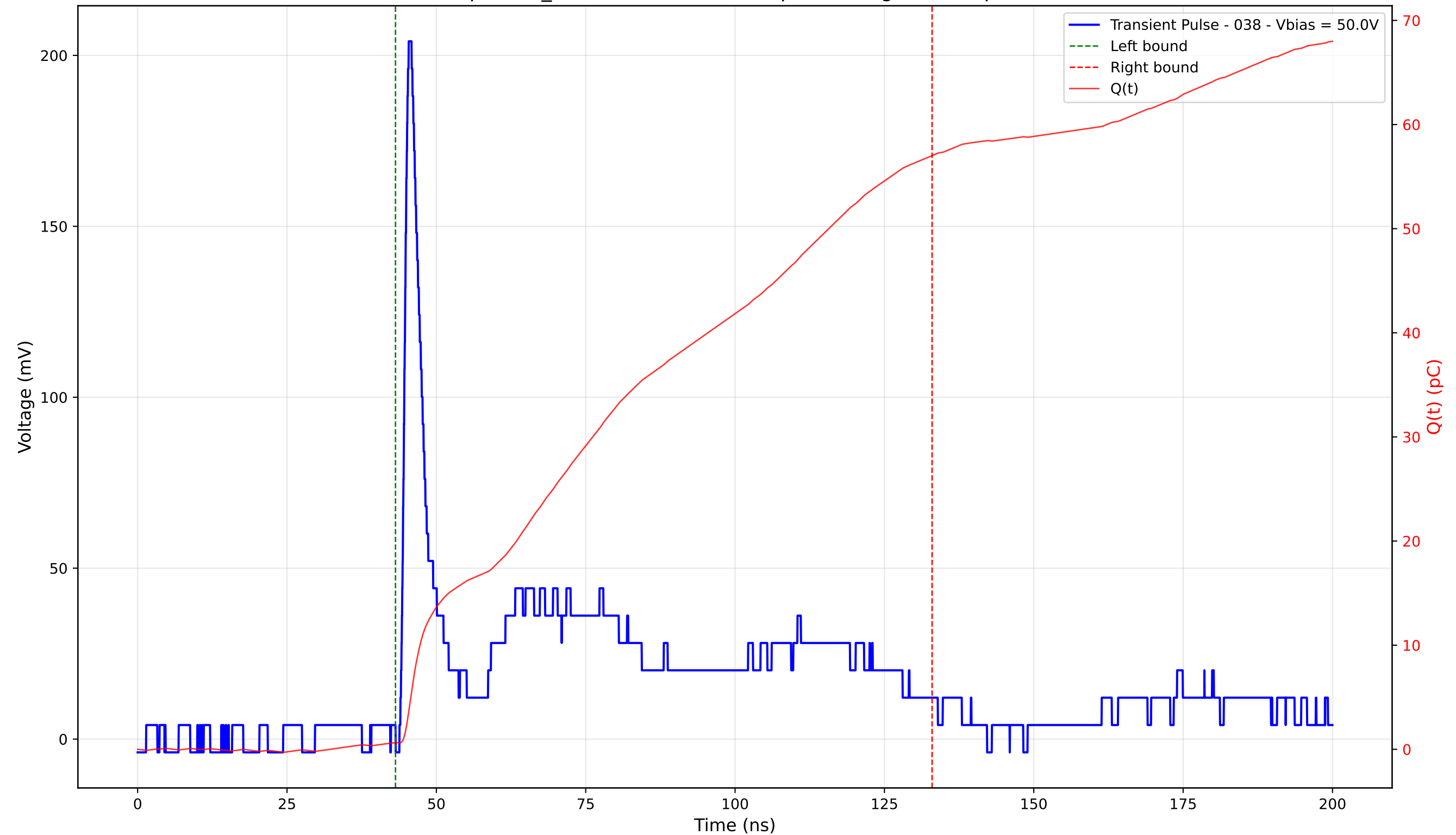
Transient Pulse - Sample: TD_4004 - Position: 290.0 \mu\text{m} - Charge: 56.38 pC - Rise Time: 1.02 ns
