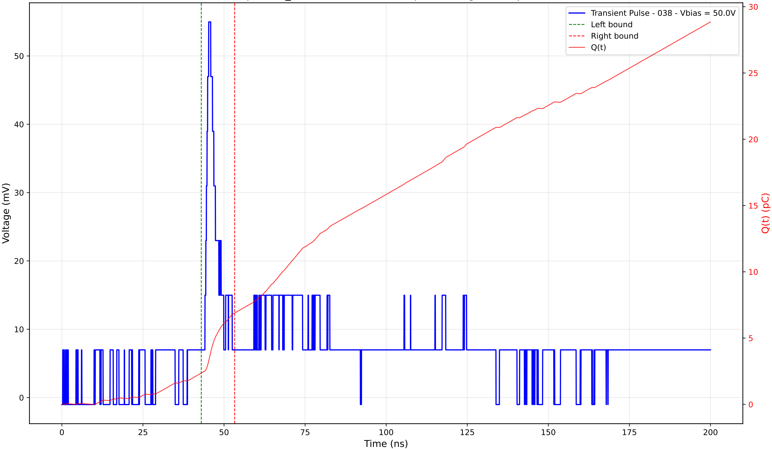
Transient Pulse - Sample: TD_4004 - Position: 410.0 \mu\text{m} - Charge: 4.54 pC - Rise Time: 6.54 ns
