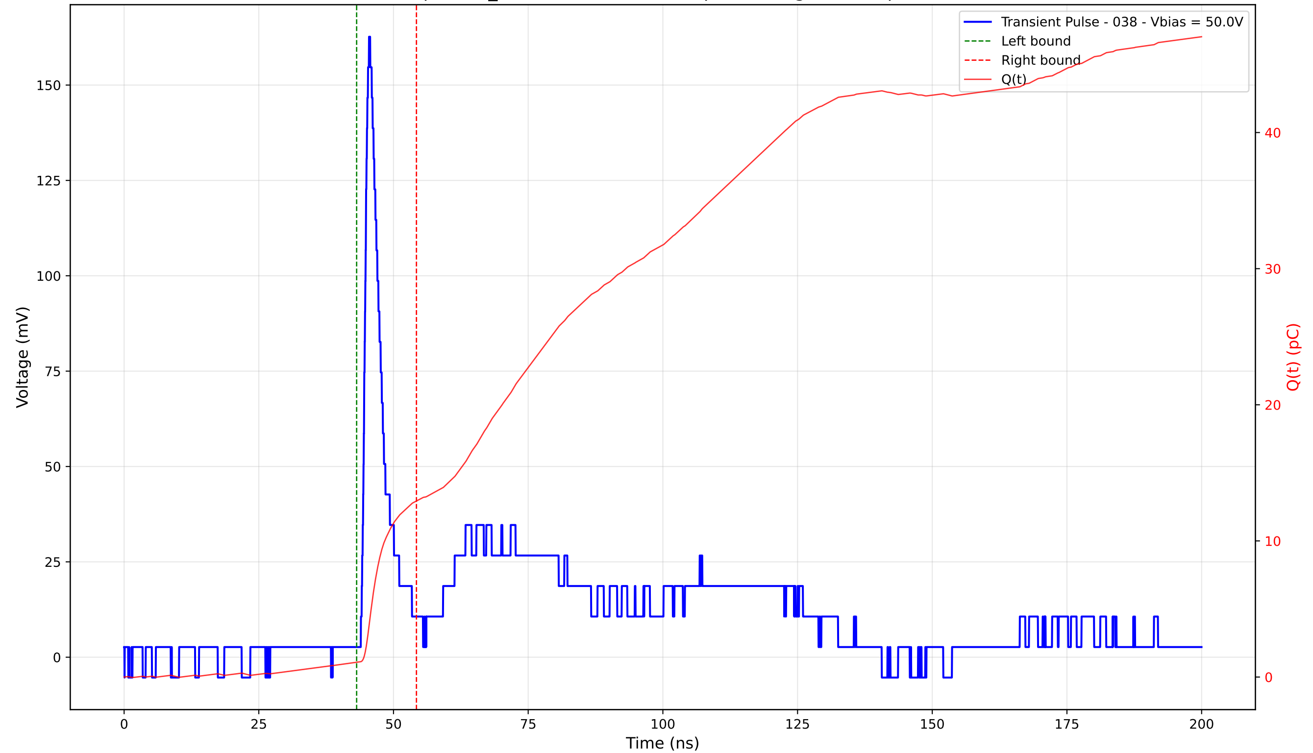
Transient Pulse - Sample: TD_4004 - Position: 320.0 \mu\text{m} - Charge: 11.86 pC - Rise Time: 1.05 ns
