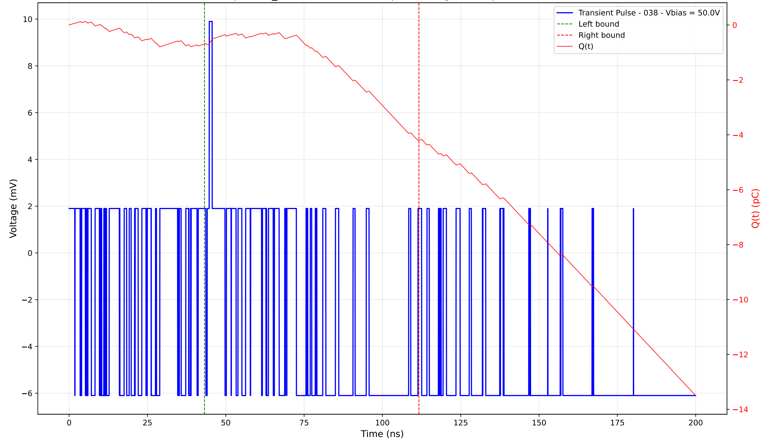
Transient Pulse - Sample: TD_4004 - Position: 20.0 \mu\text{m} - Charge: 3.51 pC - Rise Time: 0.00 ns (N/A)
