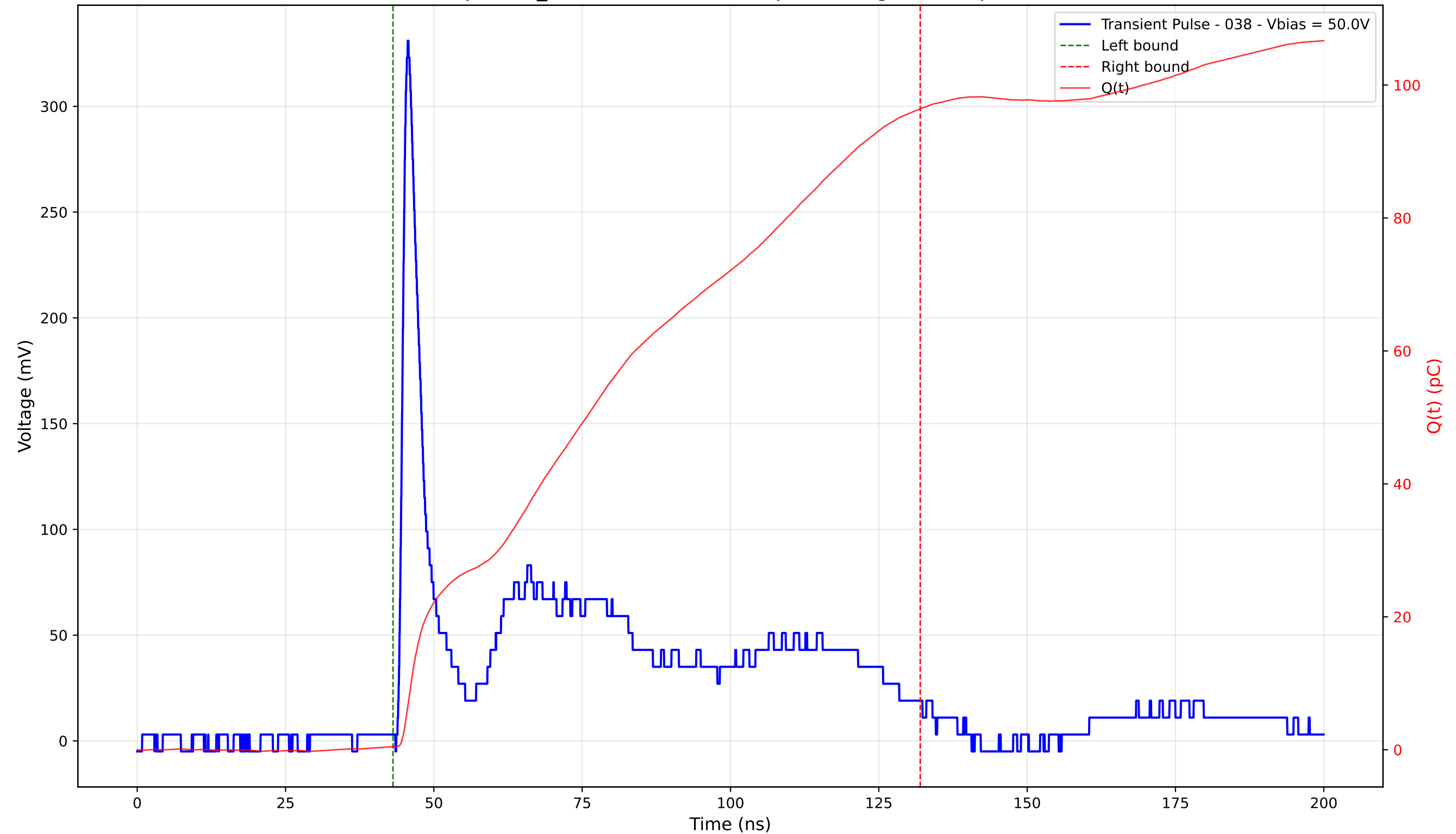
Transient Pulse - Sample: TD_4004 - Position: 155.0 \mu\text{m} - Charge: 96.00 pC - Rise Time: 1.12 ns
