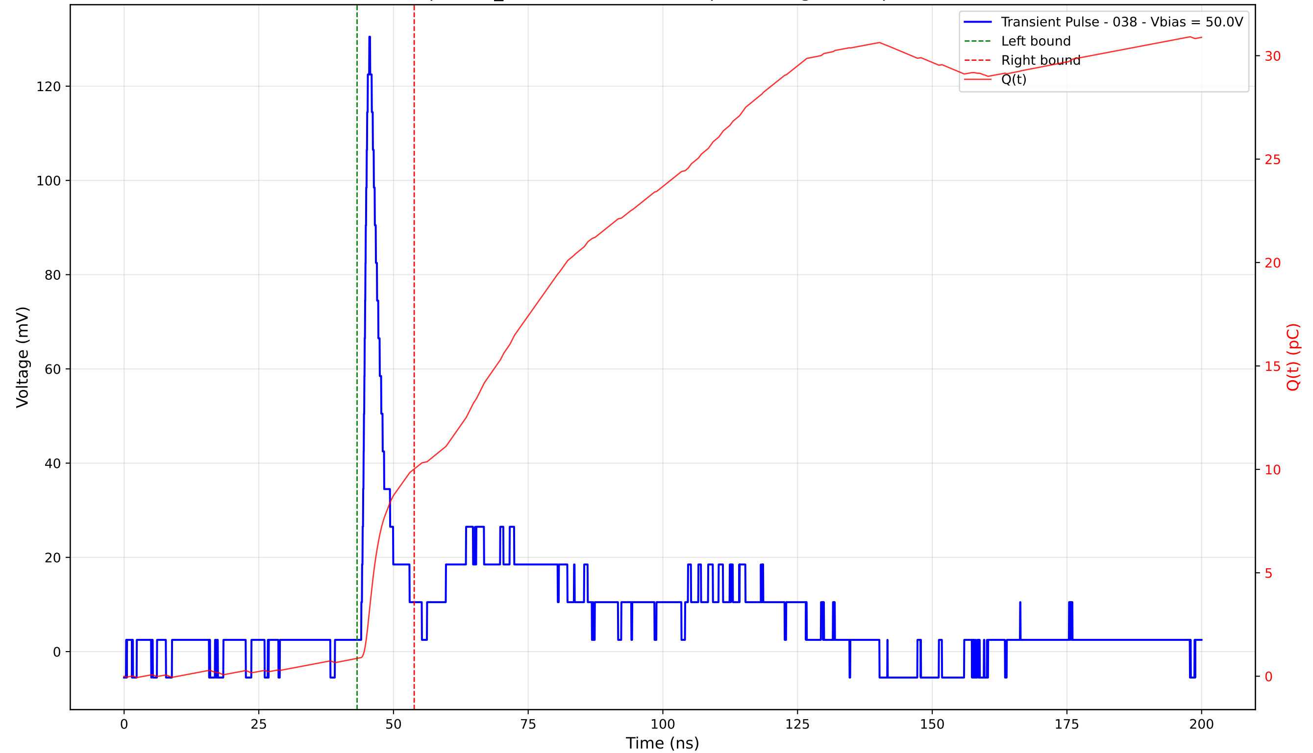
Transient Pulse - Sample: TD_4004 - Position: 380.0 \mu\text{m} - Charge: 9.16 pC - Rise Time: 1.07 ns
