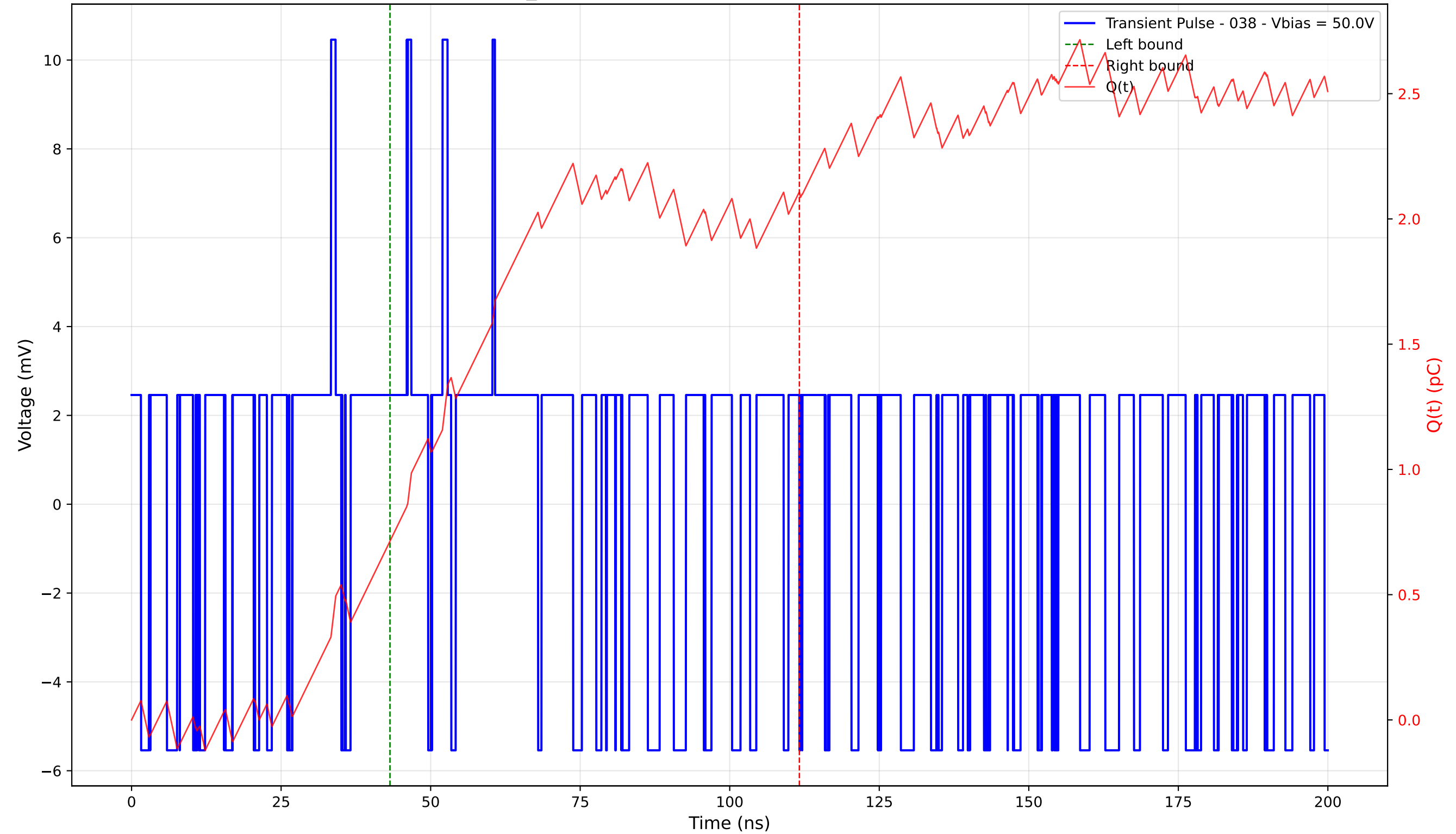
Transient Pulse - Sample: TD_4004 - Position: 0.0 \mu\text{m} - Charge: 1.39 pC - Rise Time: 0.00 ns (N/A)
