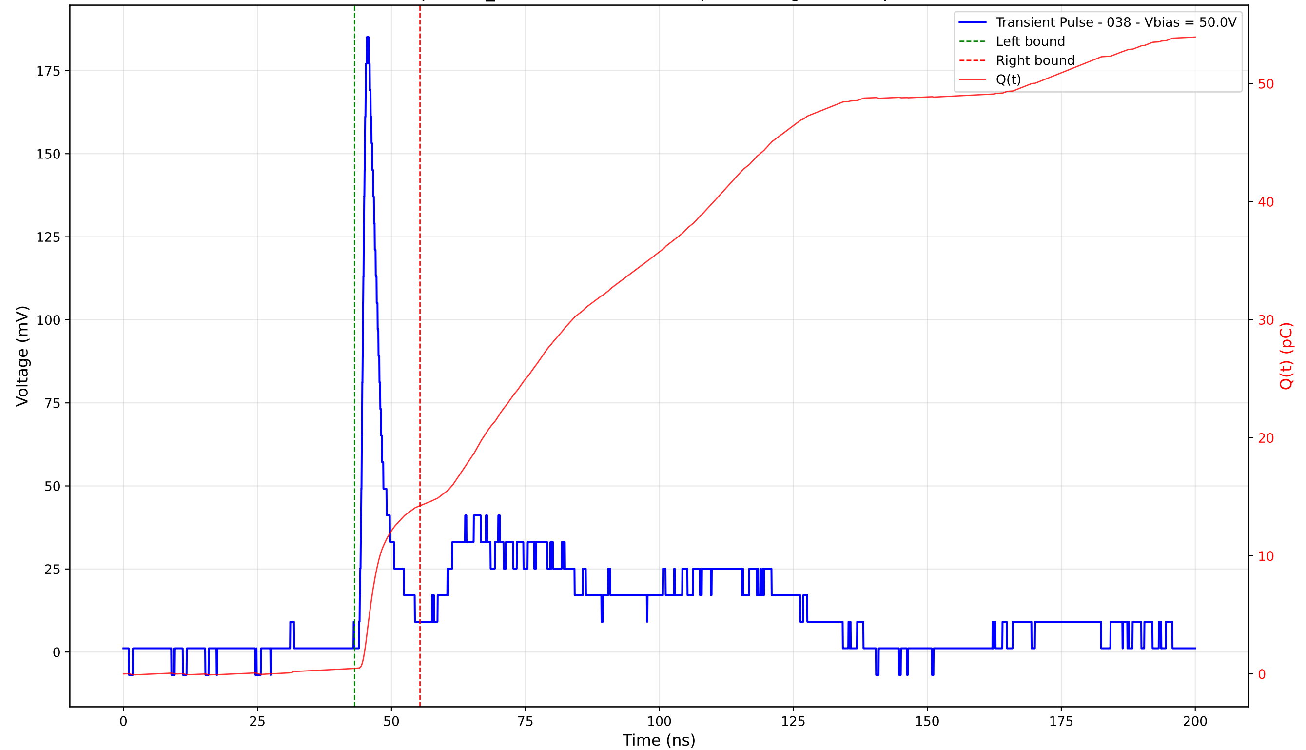
Transient Pulse - Sample: TD_4004 - Position: 295.0 \mu\text{m} - Charge: 13.77 pC - Rise Time: 1.02 ns
