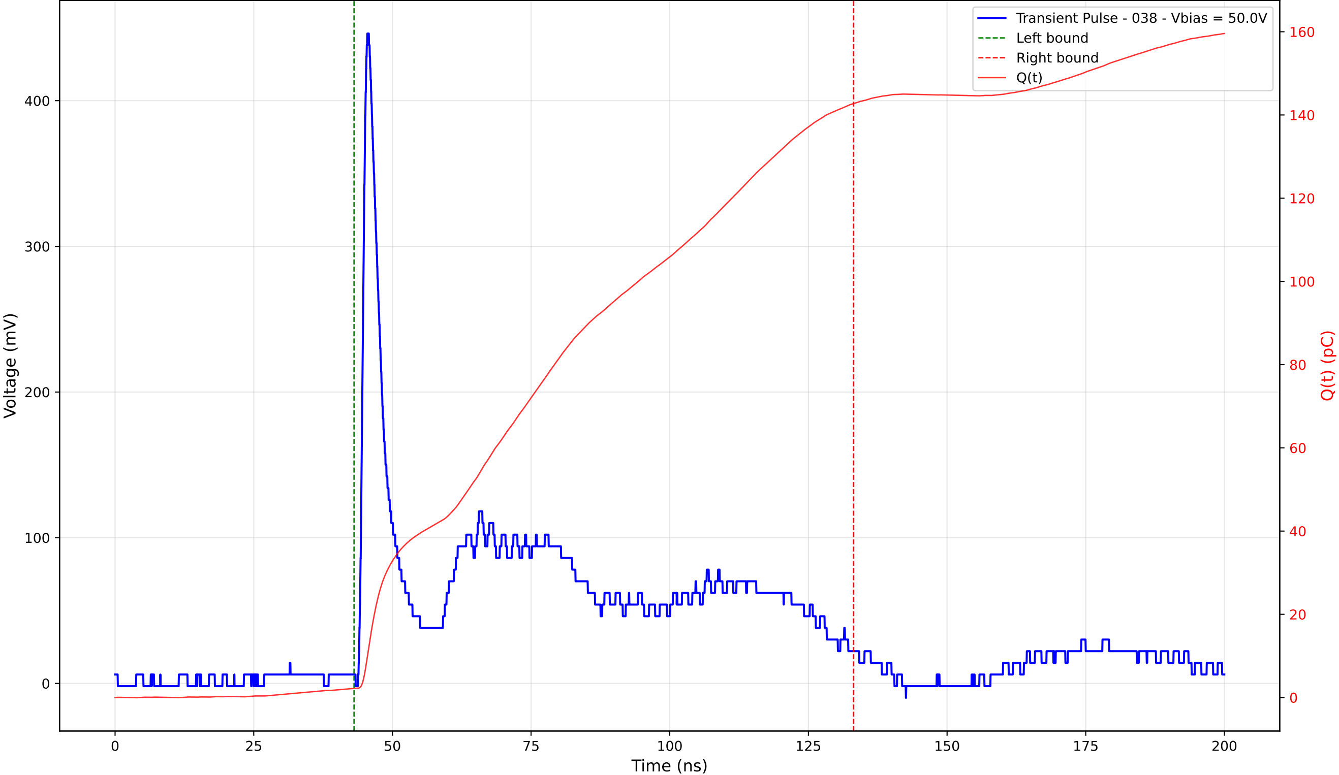
Transient Pulse - Sample: TD_4004 - Position: 195.0 \mu\text{m} - Charge: 140.53 pC - Rise Time: 1.08 ns
