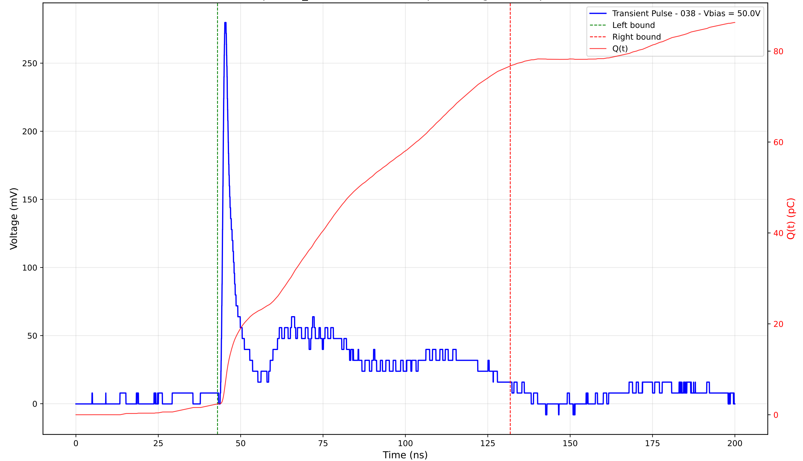
Transient Pulse - Sample: TD_4004 - Position: 70.0 \mu\text{m} - Charge: 74.34 pC - Rise Time: 0.97 ns
