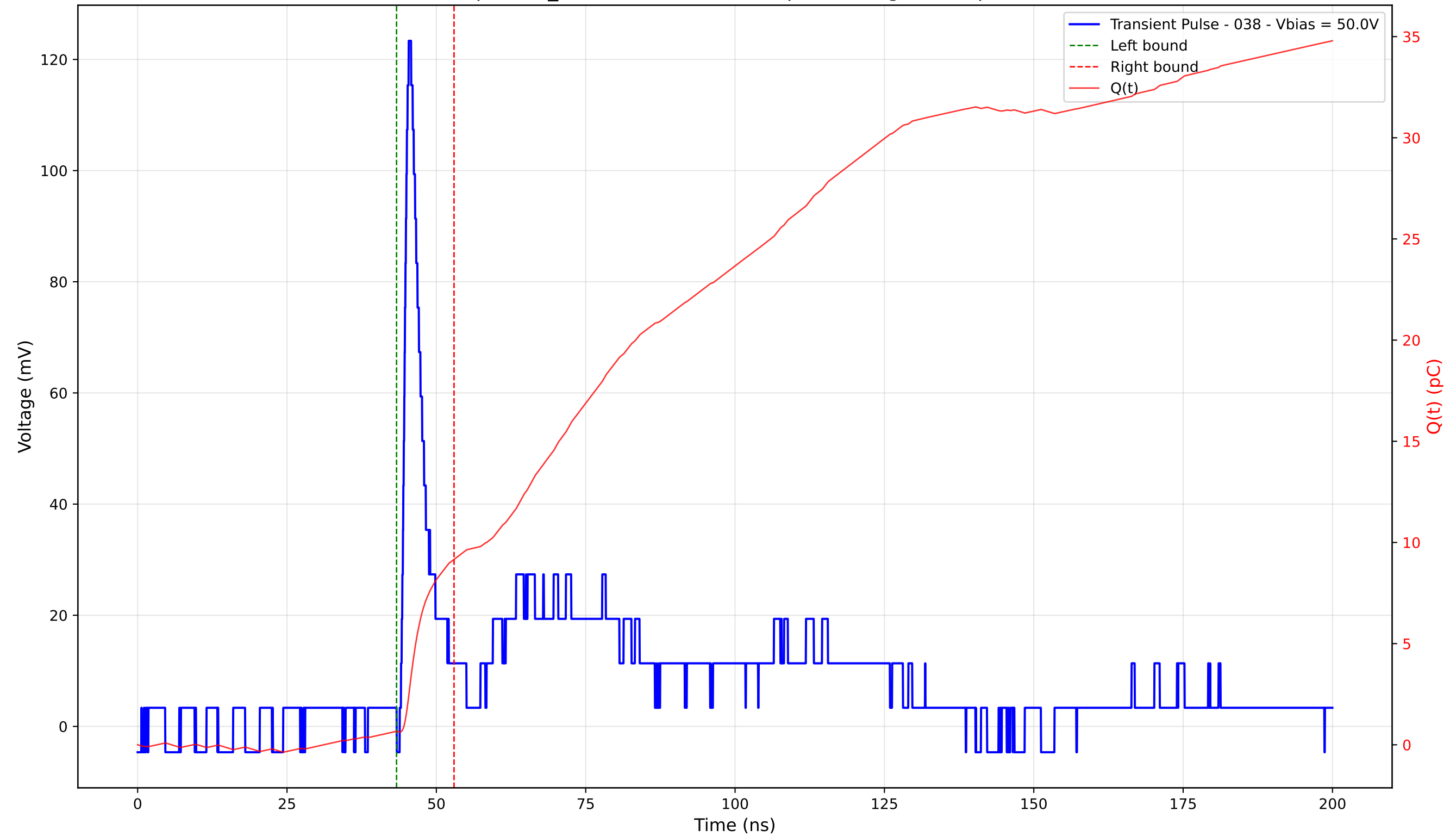
Transient Pulse - Sample: TD_4004 - Position: 385.0 \mu\text{m} - Charge: 8.49 pC - Rise Time: 1.00 ns
