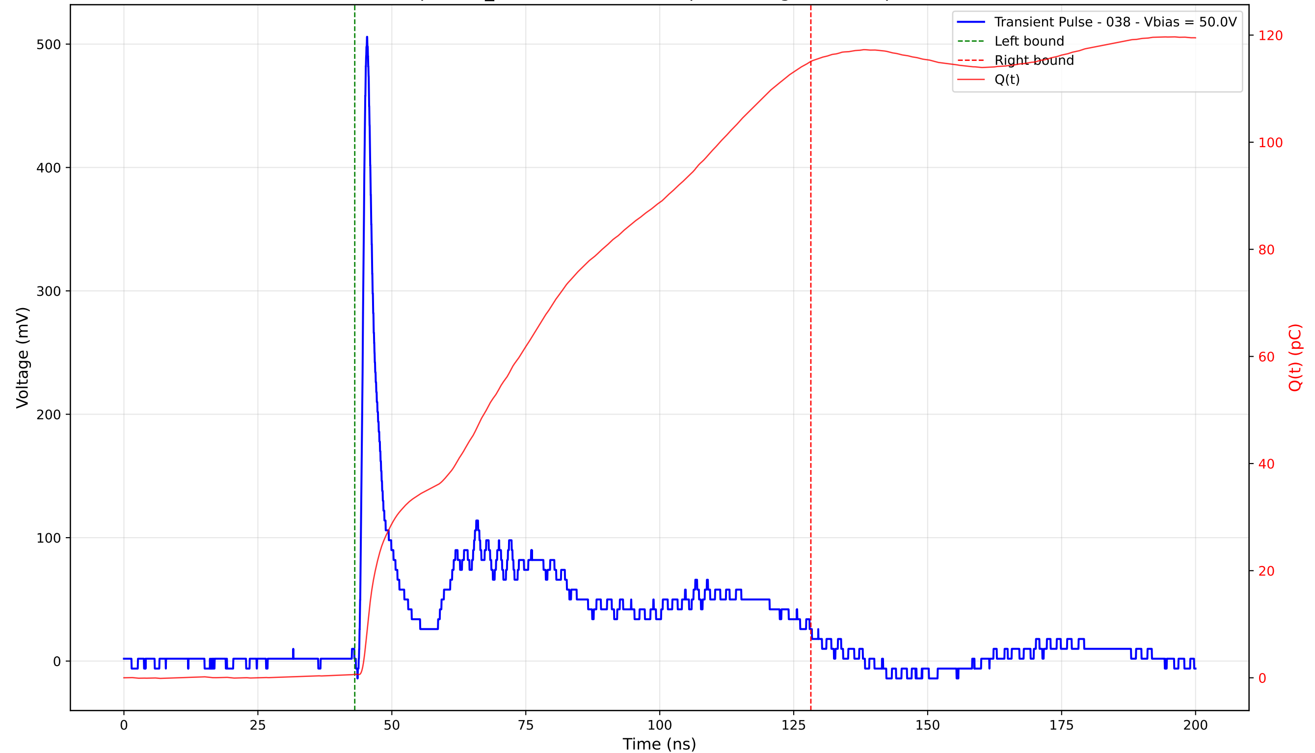
Transient Pulse - Sample: TD_4004 - Position: 85.0 \mu\text{m} - Charge: 114.43 pC - Rise Time: 0.94 ns
