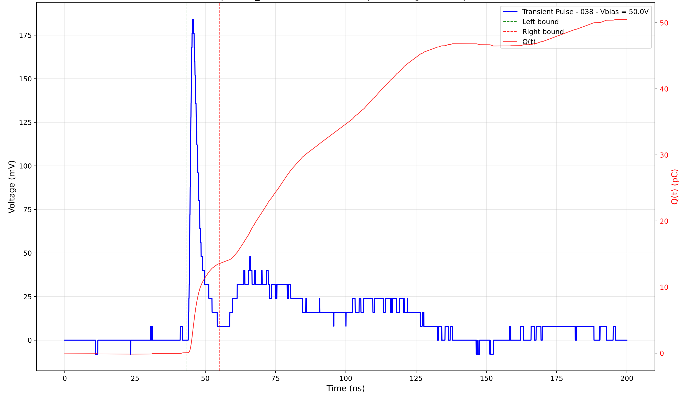
Transient Pulse - Sample: TD_4004 - Position: 300.0 \mu\text{m} - Charge: 13.49 pC - Rise Time: 1.03 ns
