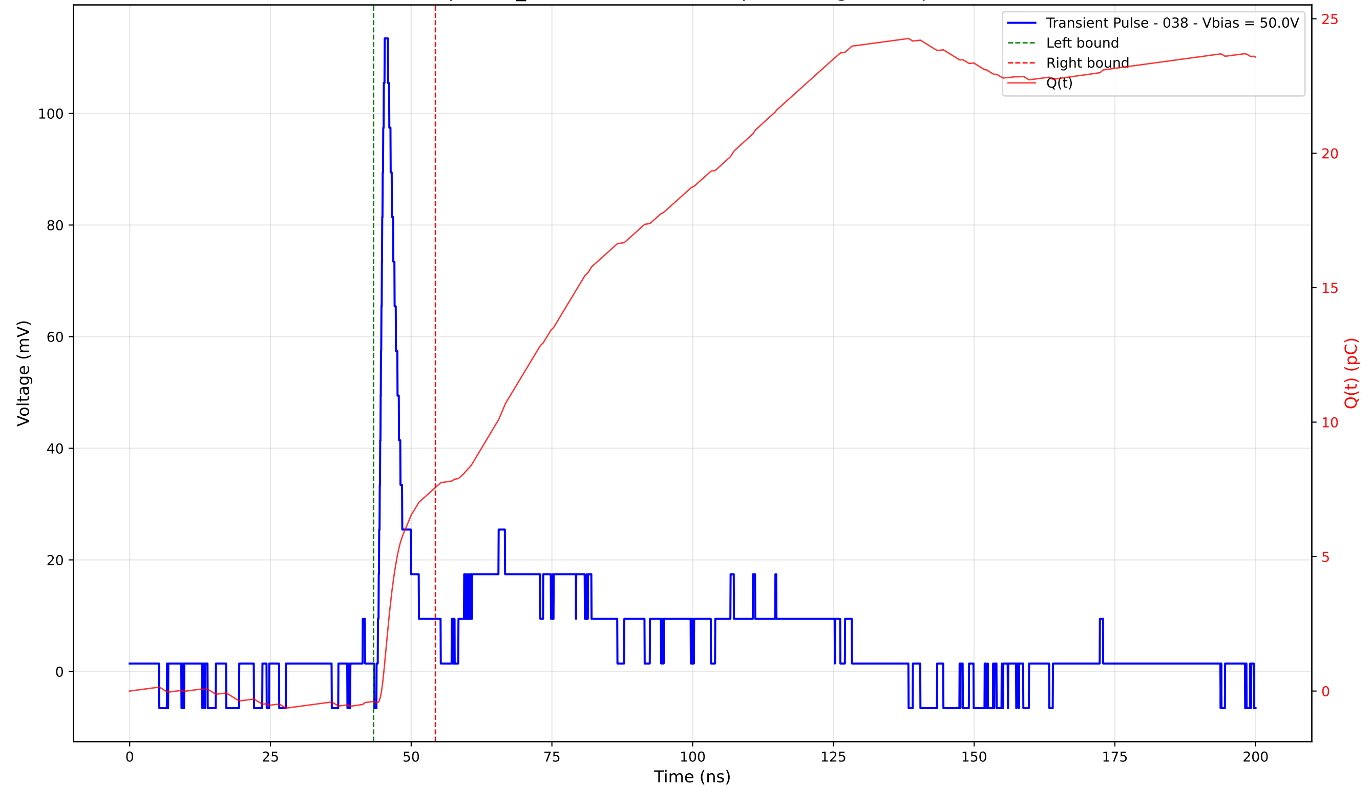
Transient Pulse - Sample: TD_4004 - Position: 370.0 \mu\text{m} - Charge: 7.96 pC - Rise Time: 0.92 ns
