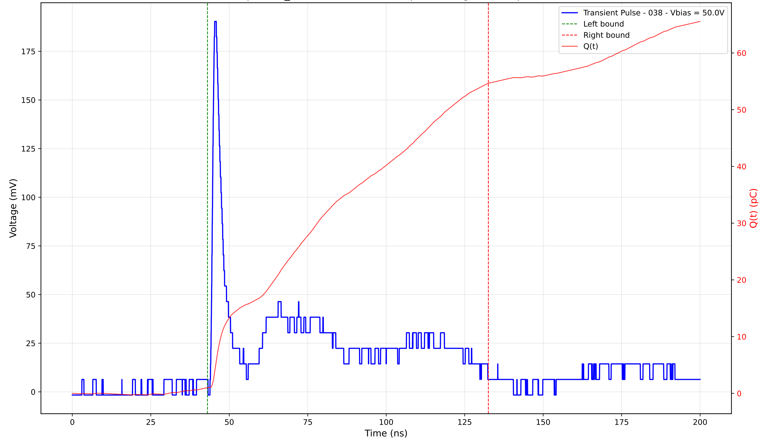
Transient Pulse - Sample: TD_4004 - Position: 305.0 \mu\text{m} - Charge: 53.64 pC - Rise Time: 1.03 ns
