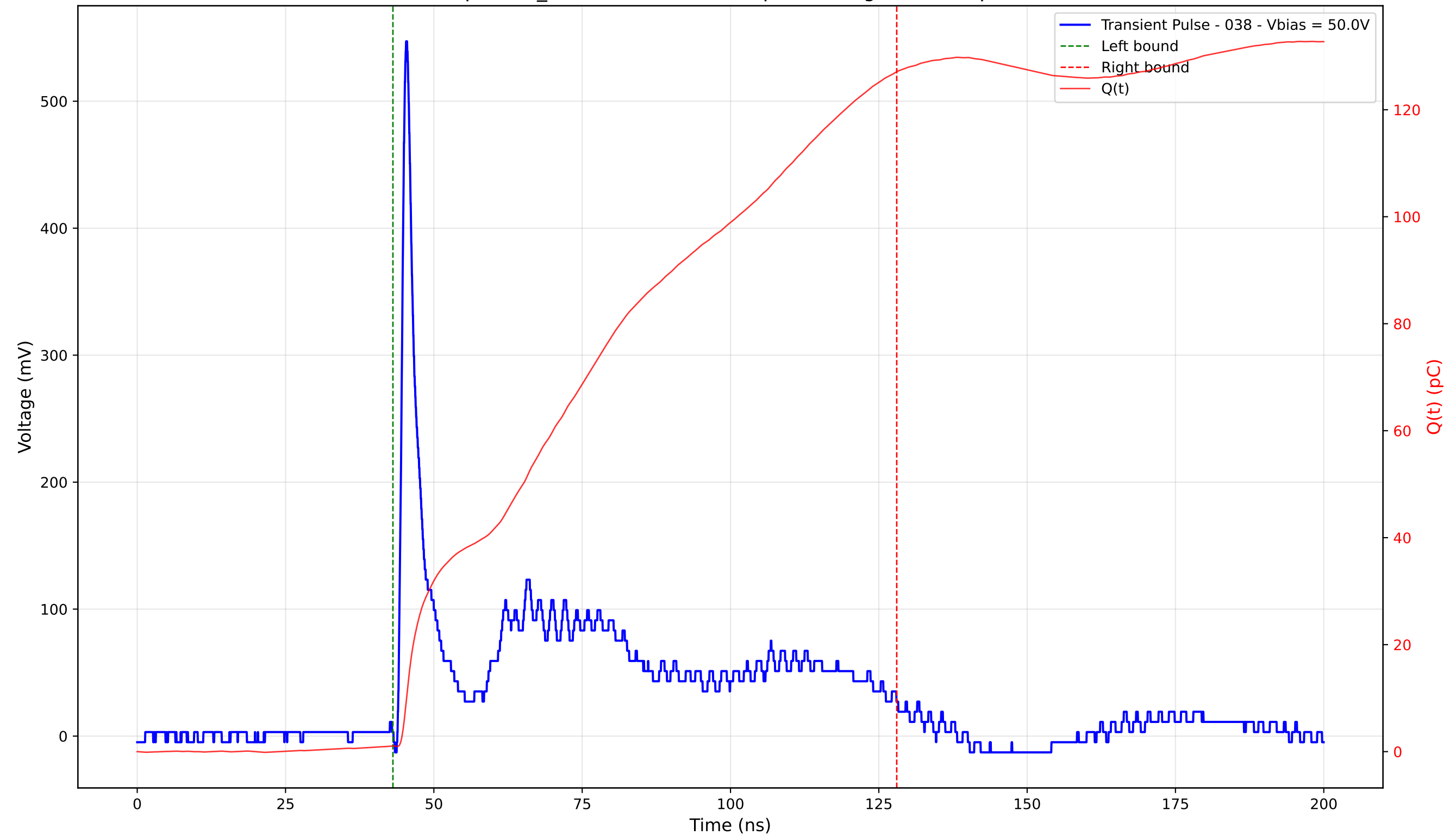
Transient Pulse - Sample: TD_4004 - Position: 90.0 \mu\text{m} - Charge: 126.06 pC - Rise Time: 0.93 ns
