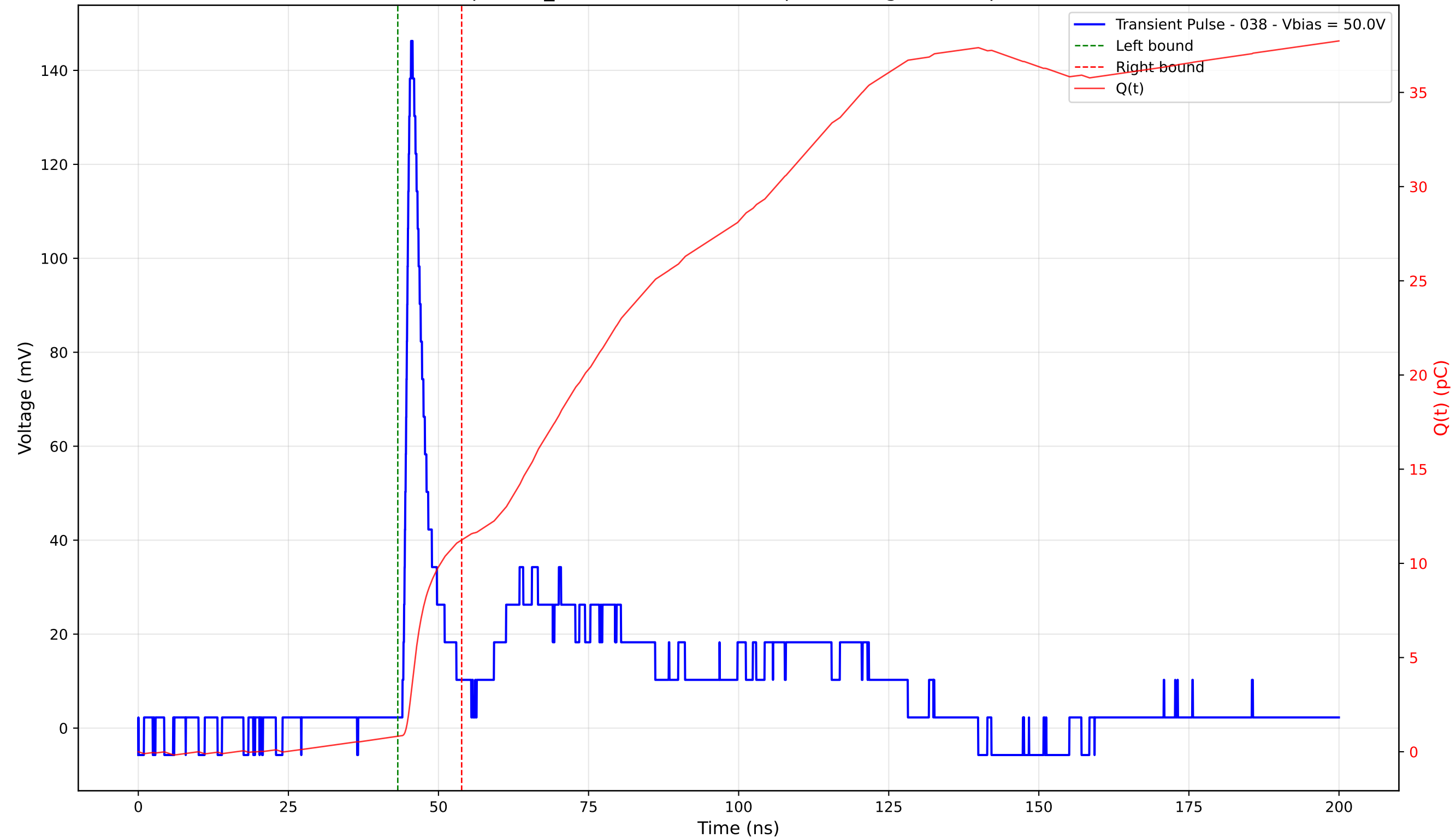
Transient Pulse - Sample: TD_4004 - Position: 345.0 \mu\text{m} - Charge: 10.43 pC - Rise Time: 1.07 ns
