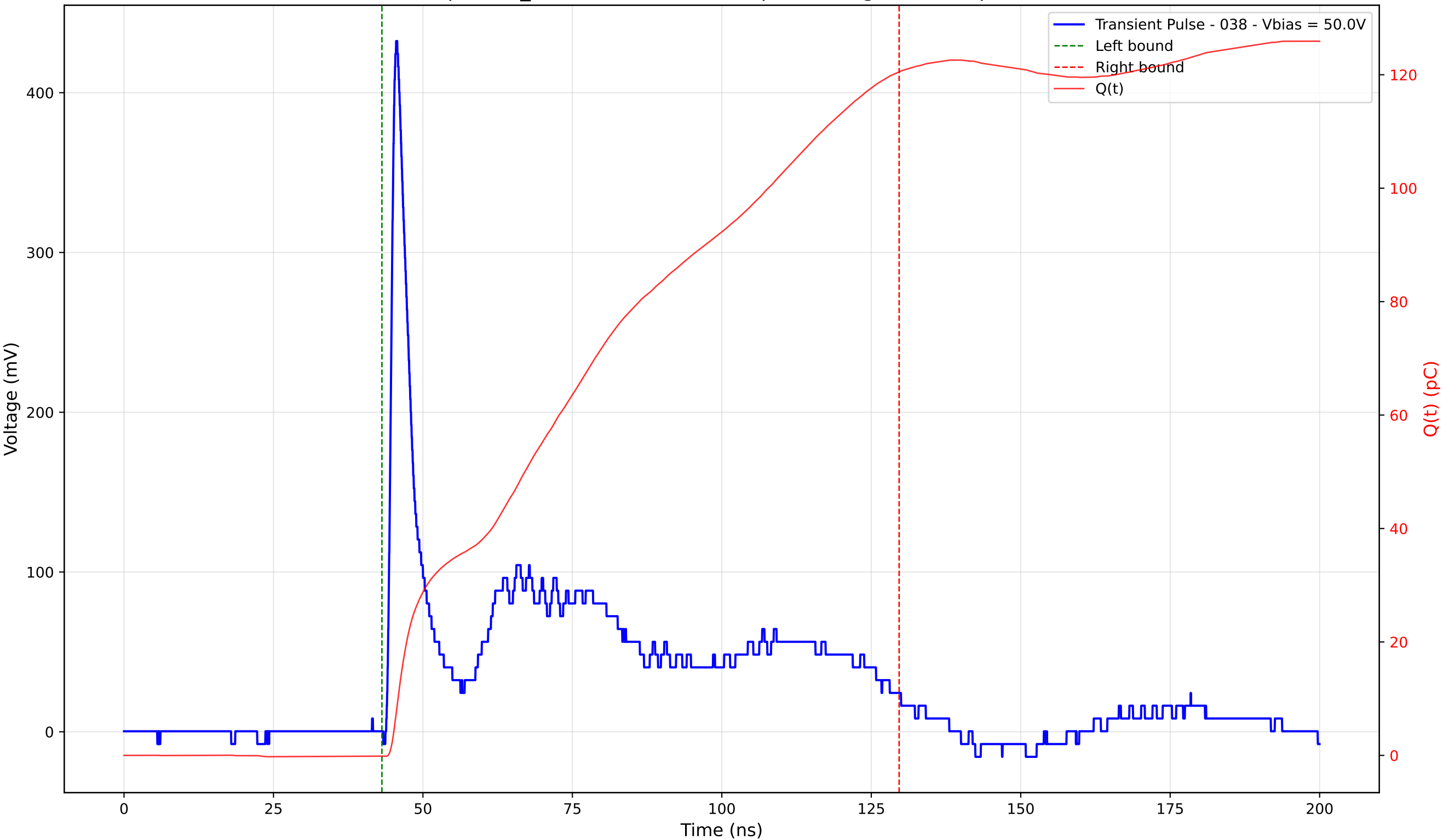
Transient Pulse - Sample: TD_4004 - Position: 200.0 \mu\text{m} - Charge: 120.63 pC - Rise Time: 1.05 ns
