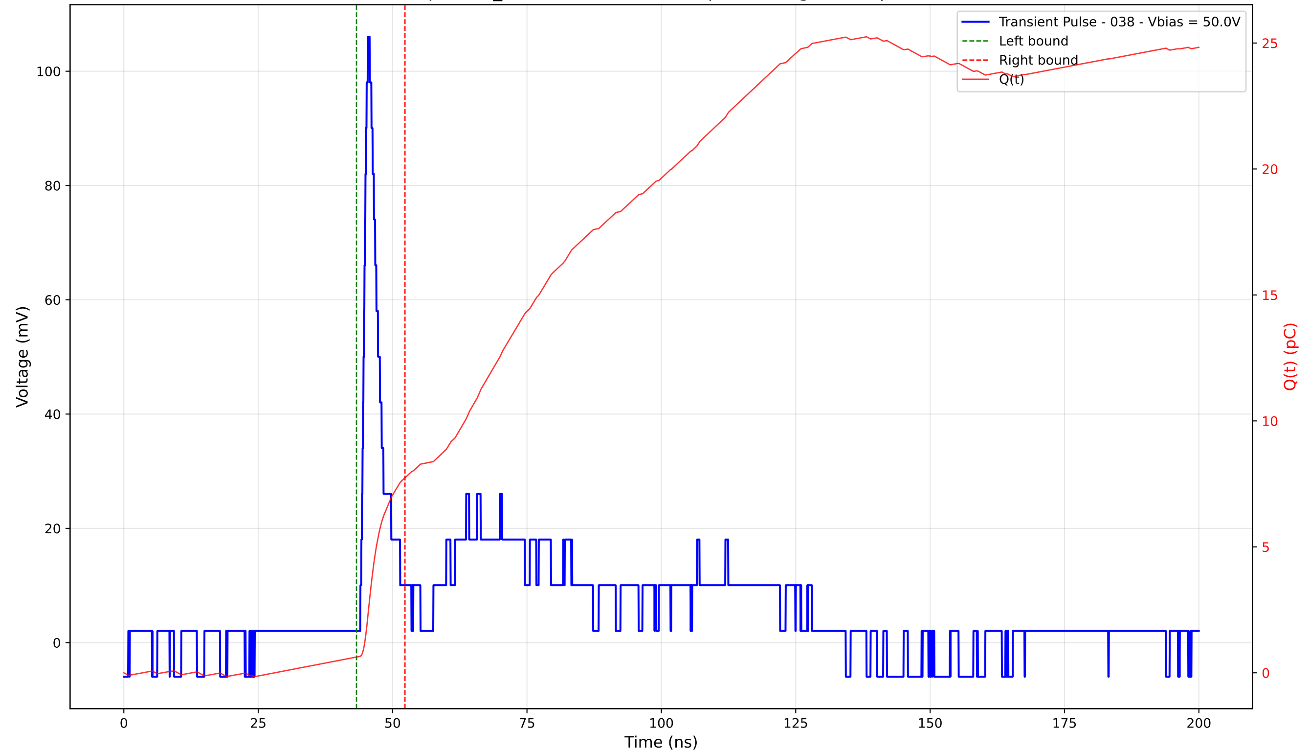
Transient Pulse - Sample: TD_4004 - Position: 390.0 \mu\text{m} - Charge: 7.12 pC - Rise Time: 1.00 ns
