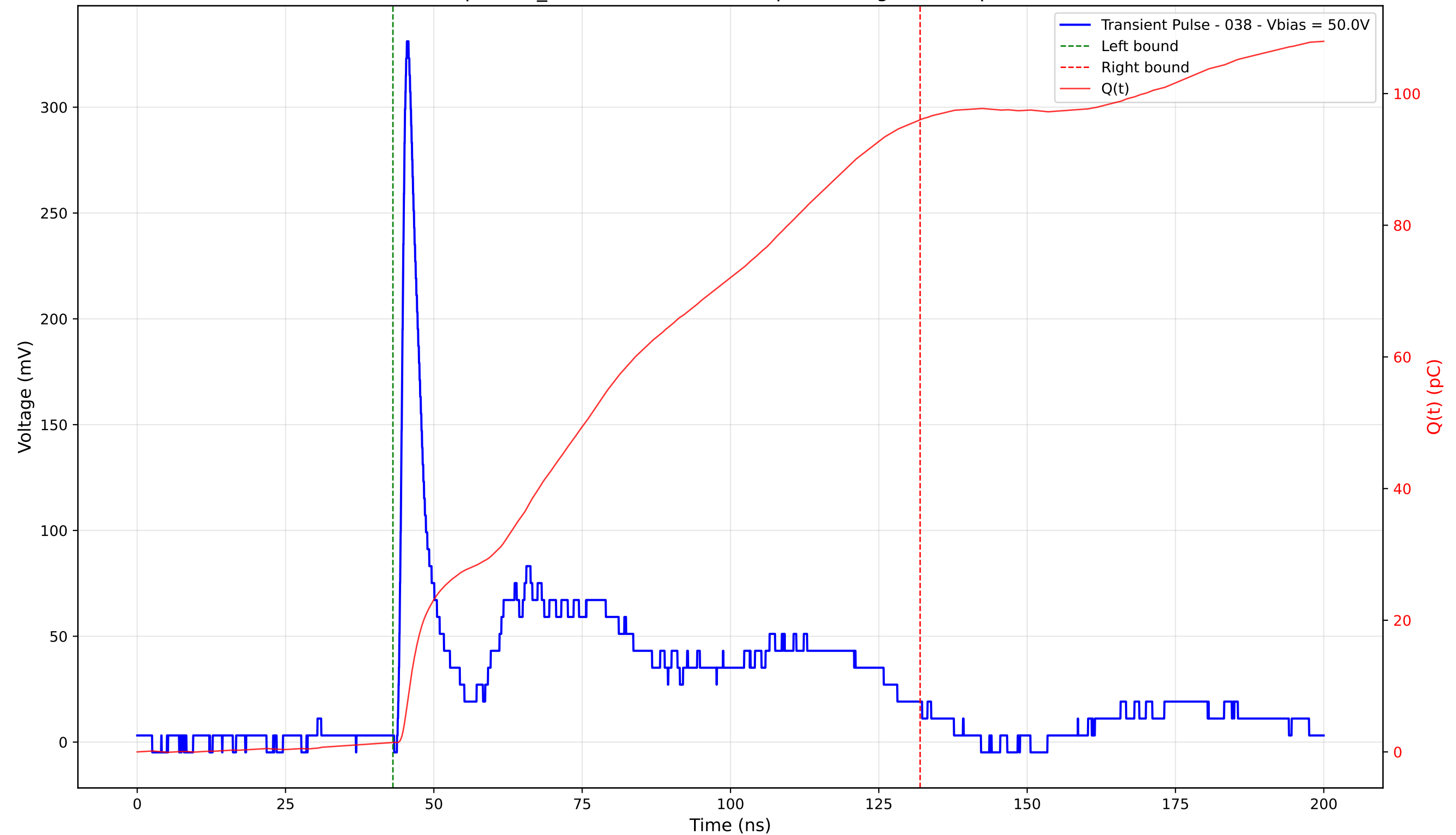
Transient Pulse - Sample: TD_4004 - Position: 230.0 \mu\text{m} - Charge: 94.60 pC - Rise Time: 1.05 ns
