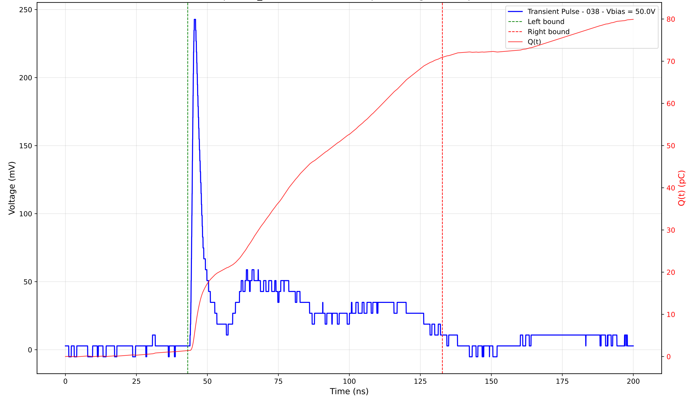
Transient Pulse - Sample: TD_4004 - Position: 260.0 \mu\text{m} - Charge: 69.53 pC - Rise Time: 1.03 ns
