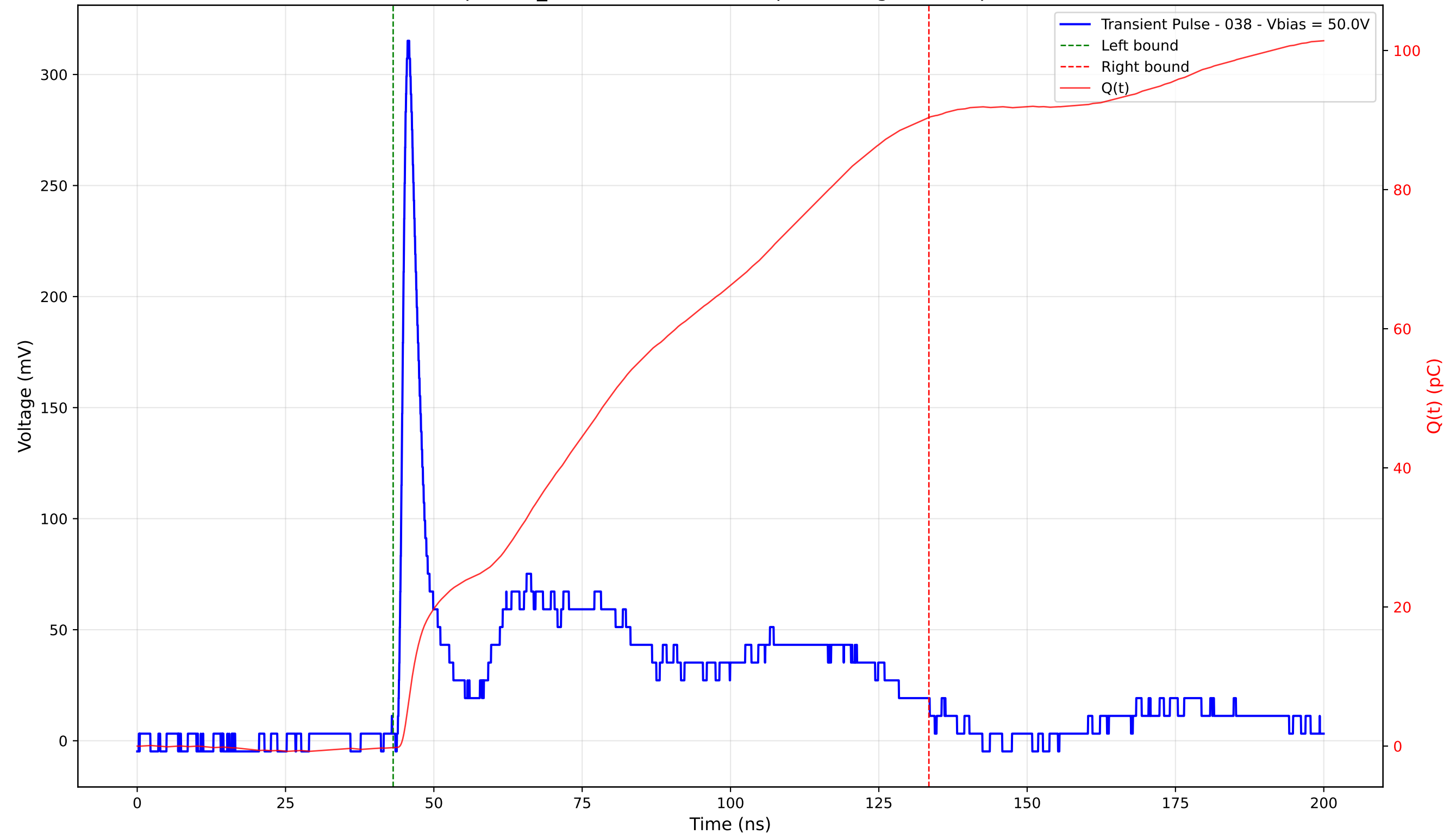
Transient Pulse - Sample: TD_4004 - Position: 140.0 \mu\text{m} - Charge: 90.58 pC - Rise Time: 1.15 ns
