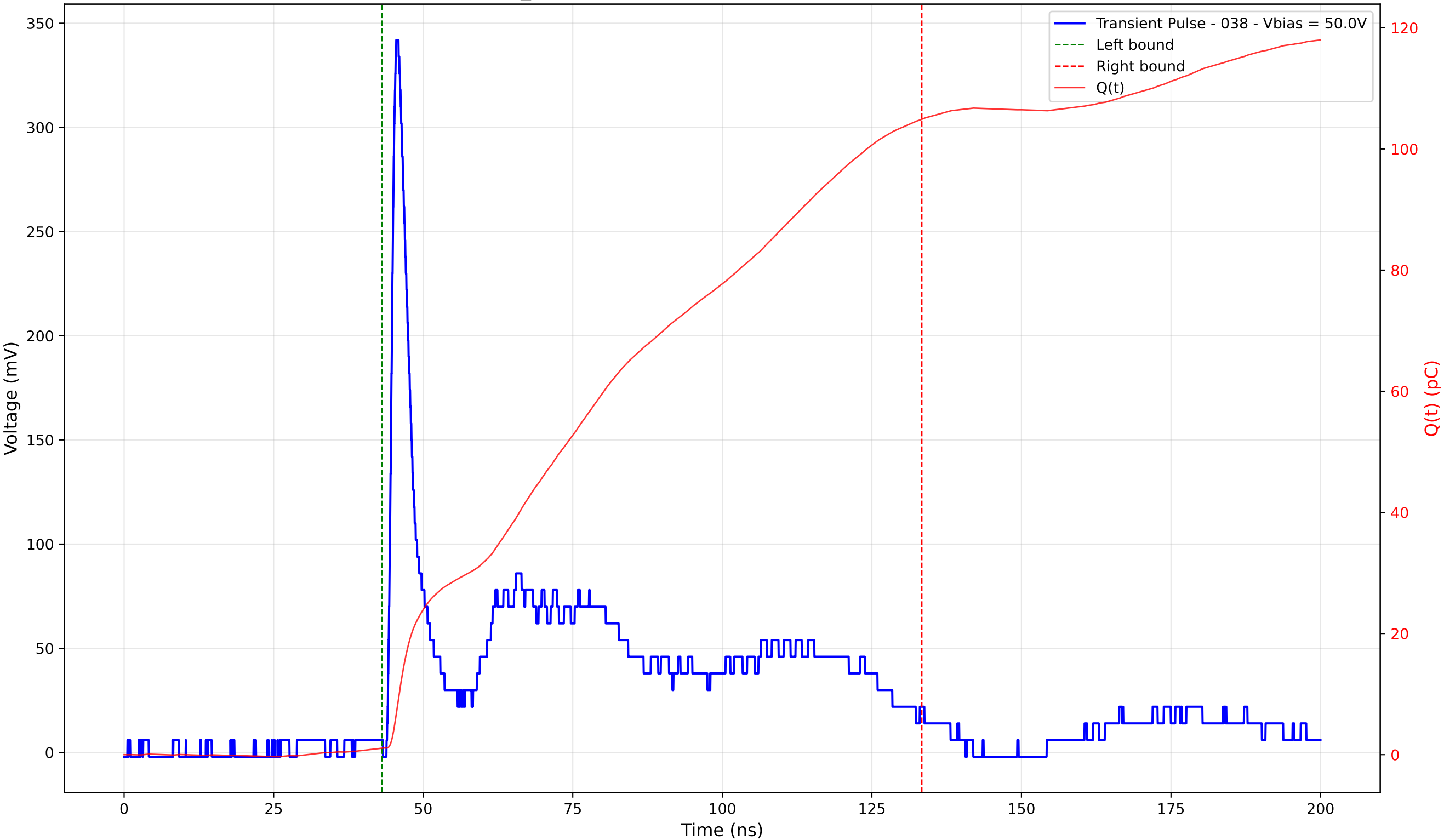
Transient Pulse - Sample: TD_4004 - Position: 160.0 \mu\text{m} - Charge: 103.82 pC - Rise Time: 1.07 ns
