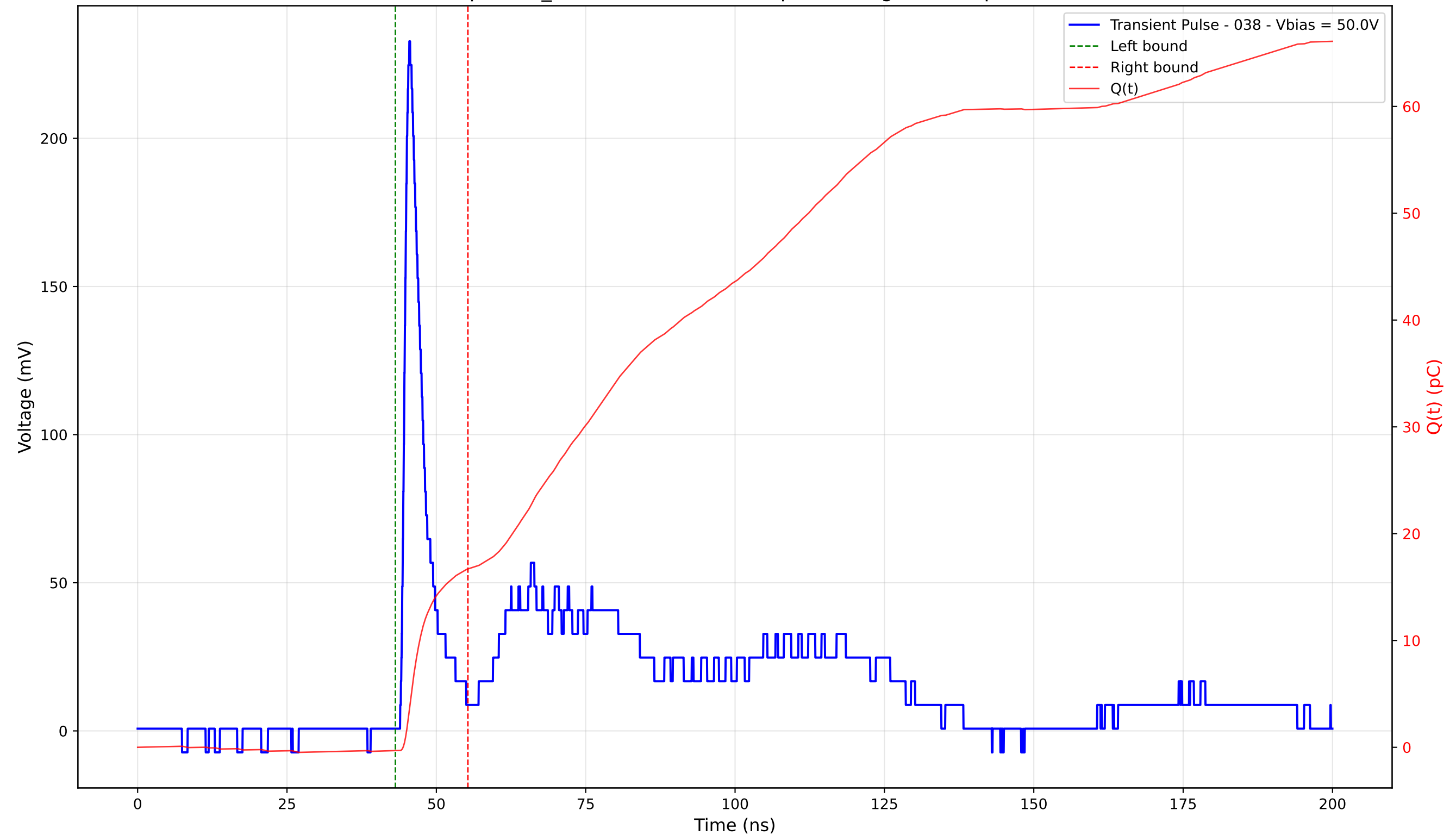
Transient Pulse - Sample: TD_4004 - Position: 285.0 \mu\text{m} - Charge: 17.02 pC - Rise Time: 1.08 ns
