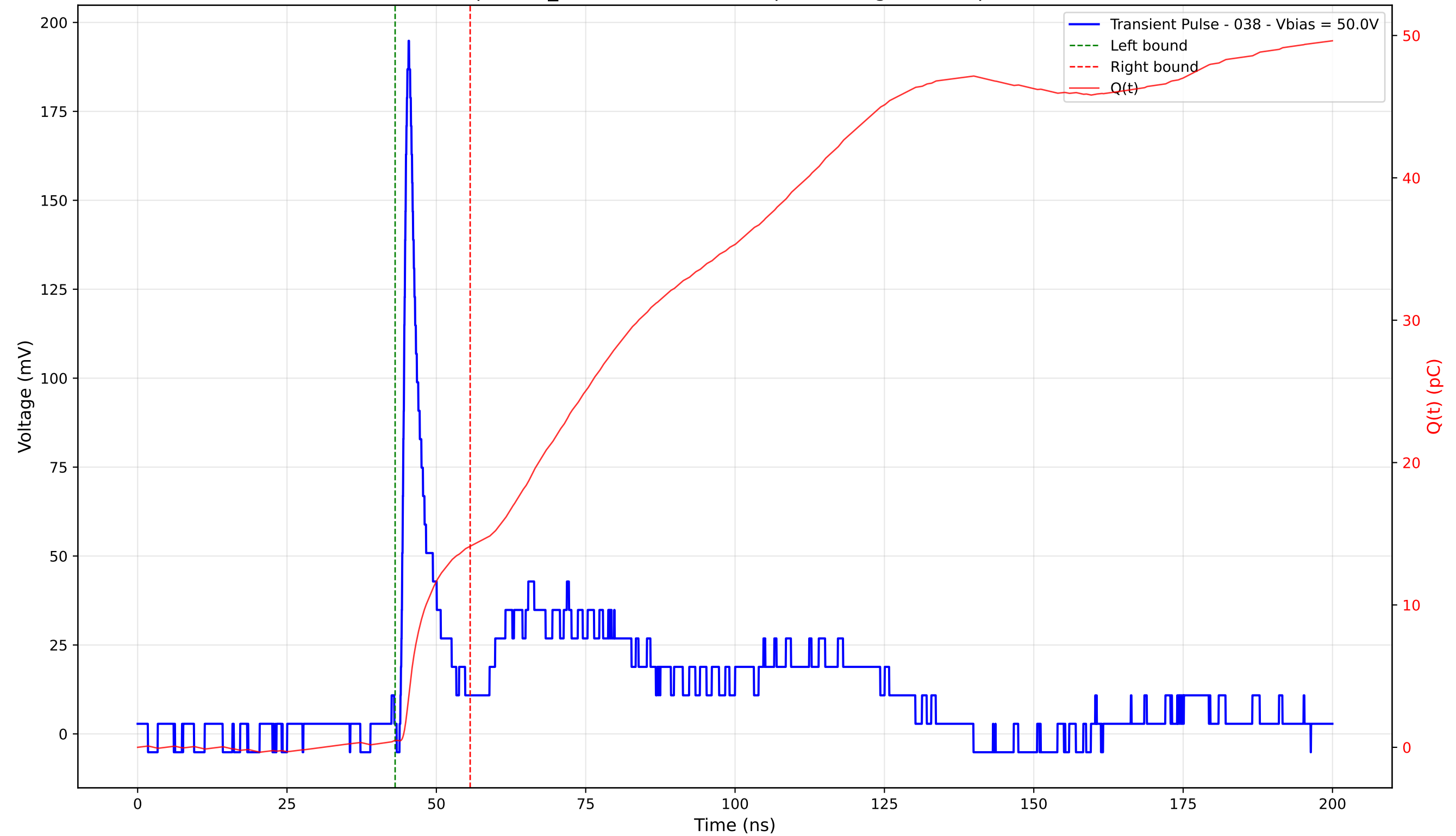
Transient Pulse - Sample: TD_4004 - Position: 65.0 \mu\text{m} - Charge: 13.64 pC - Rise Time: 0.94 ns
