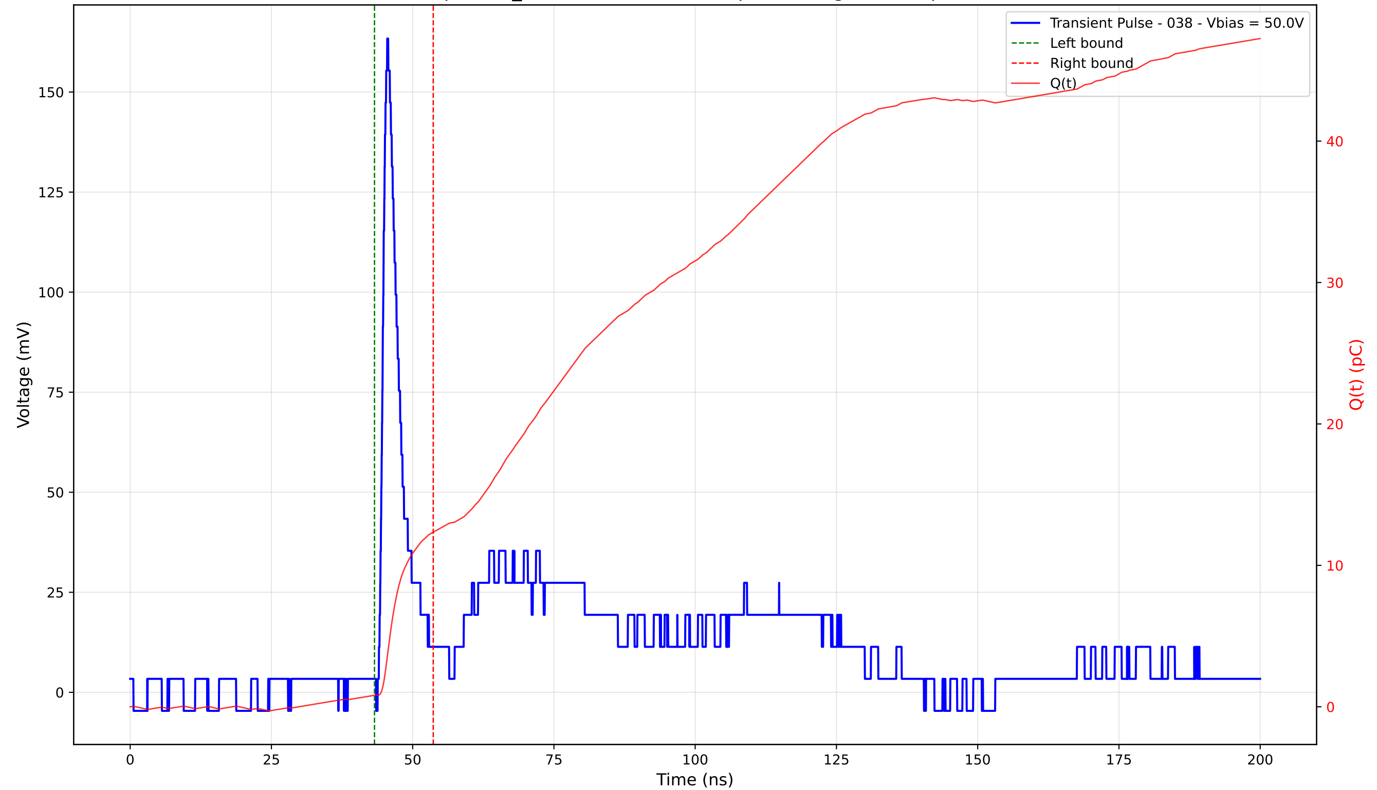
Transient Pulse - Sample: TD_4004 - Position: 325.0 \mu\text{m} - Charge: 11.53 pC - Rise Time: 1.05 ns
