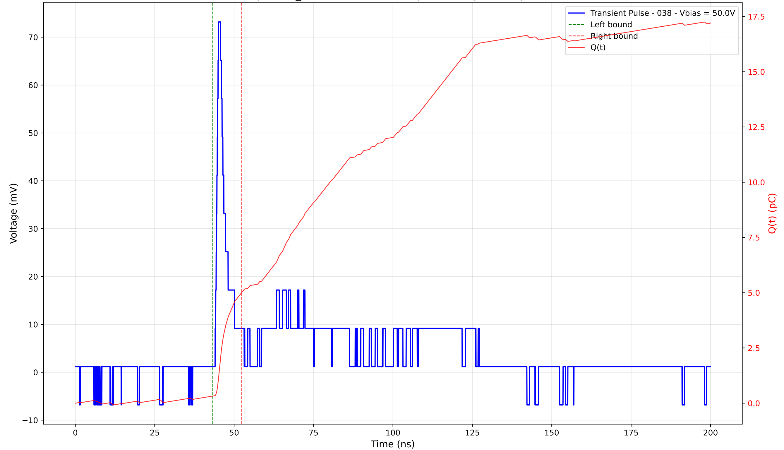
Transient Pulse - Sample: TD_4004 - Position: 55.0 \mu\text{m} - Charge: 4.70 pC - Rise Time: 1.08 ns
