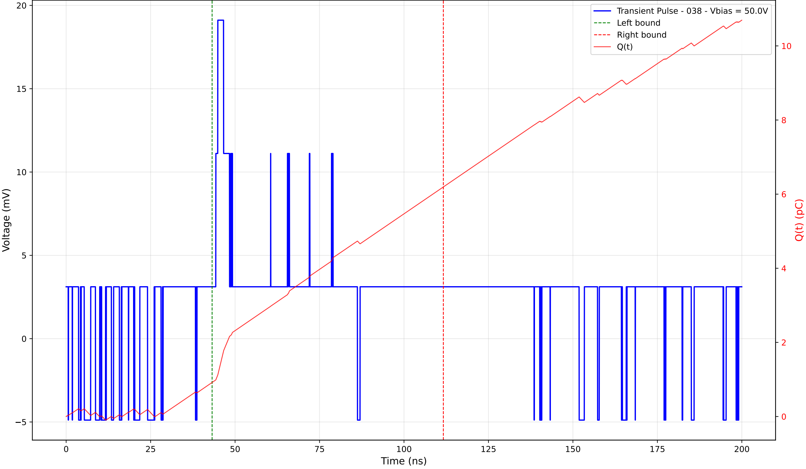
Transient Pulse - Sample: TD_4004 - Position: 430.0 \mu\text{m} - Charge: 5.28 pC - Rise Time: 0.00 ns (N/A)
