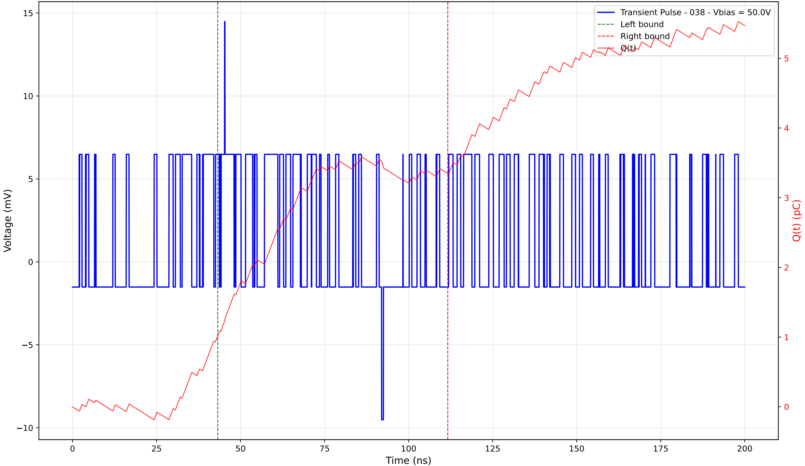
Transient Pulse - Sample: TD_4004 - Position: 15.0 \mu\text{m} - Charge: 2.33 pC - Rise Time: 0.00 ns (N/A)
