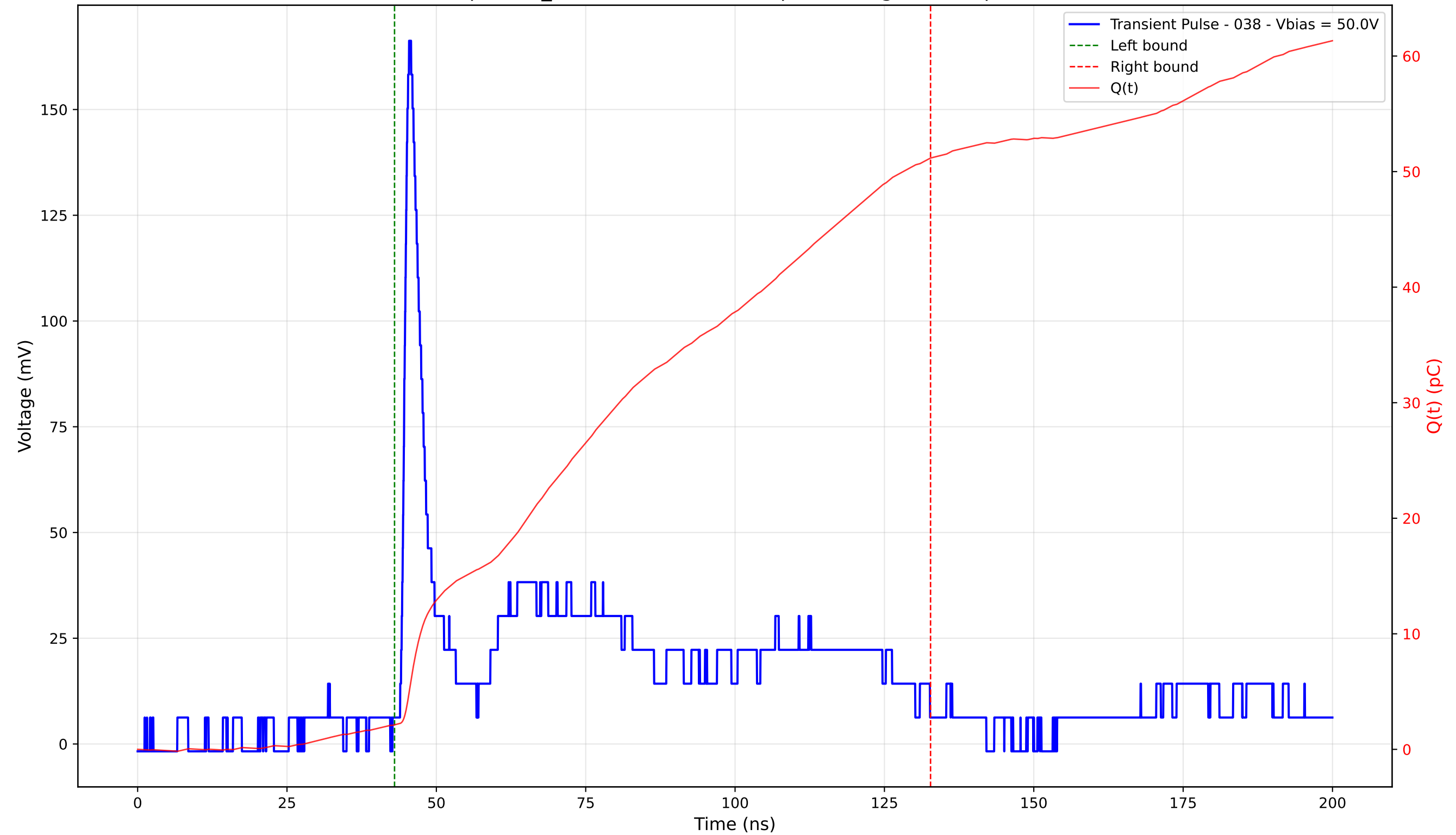
Transient Pulse - Sample: TD_4004 - Position: 315.0 \mu\text{m} - Charge: 49.05 pC - Rise Time: 1.05 ns
