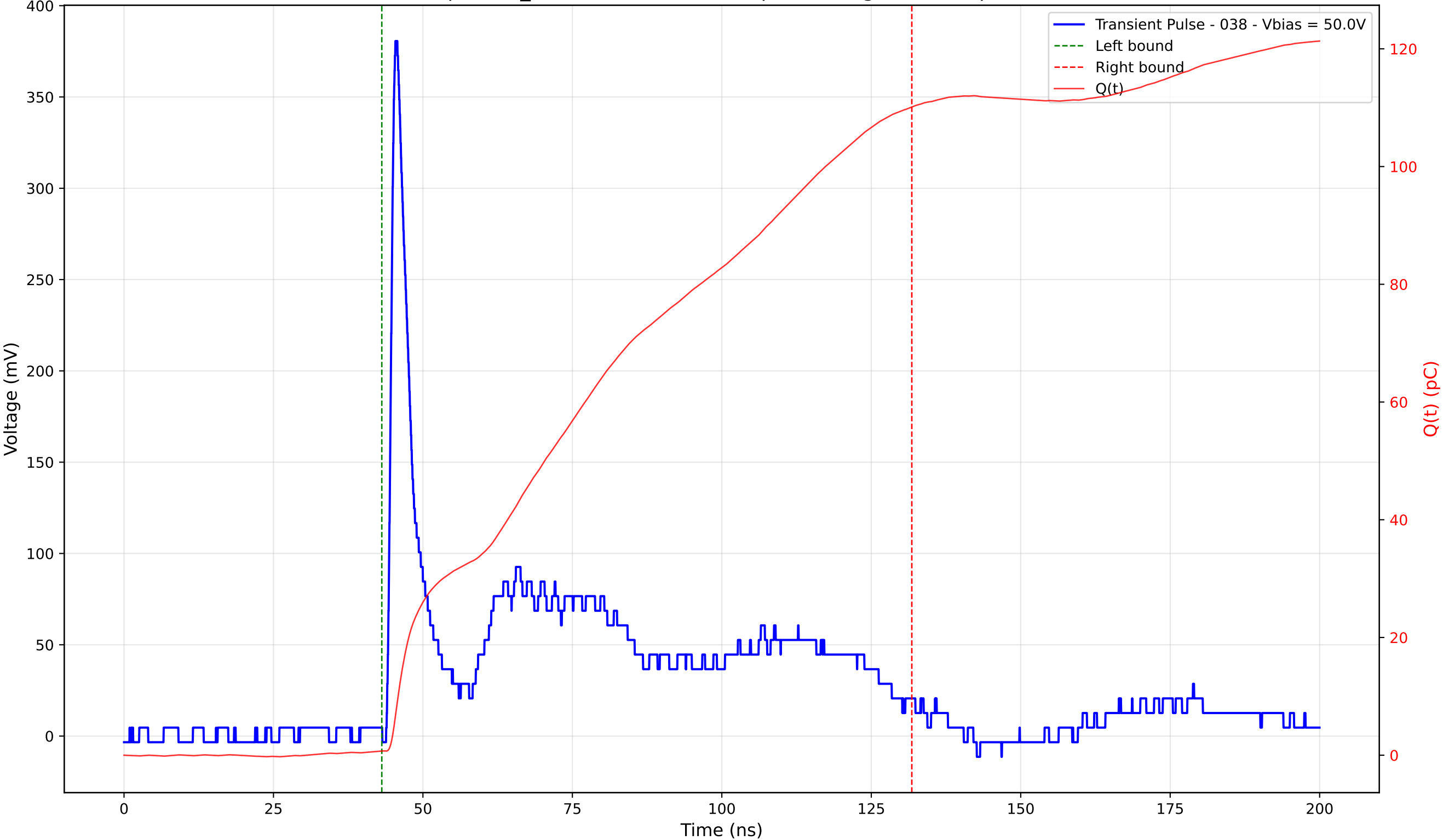
Transient Pulse - Sample: TD_4004 - Position: 220.0 \mu\text{m} - Charge: 109.40 pC - Rise Time: 1.02 ns
