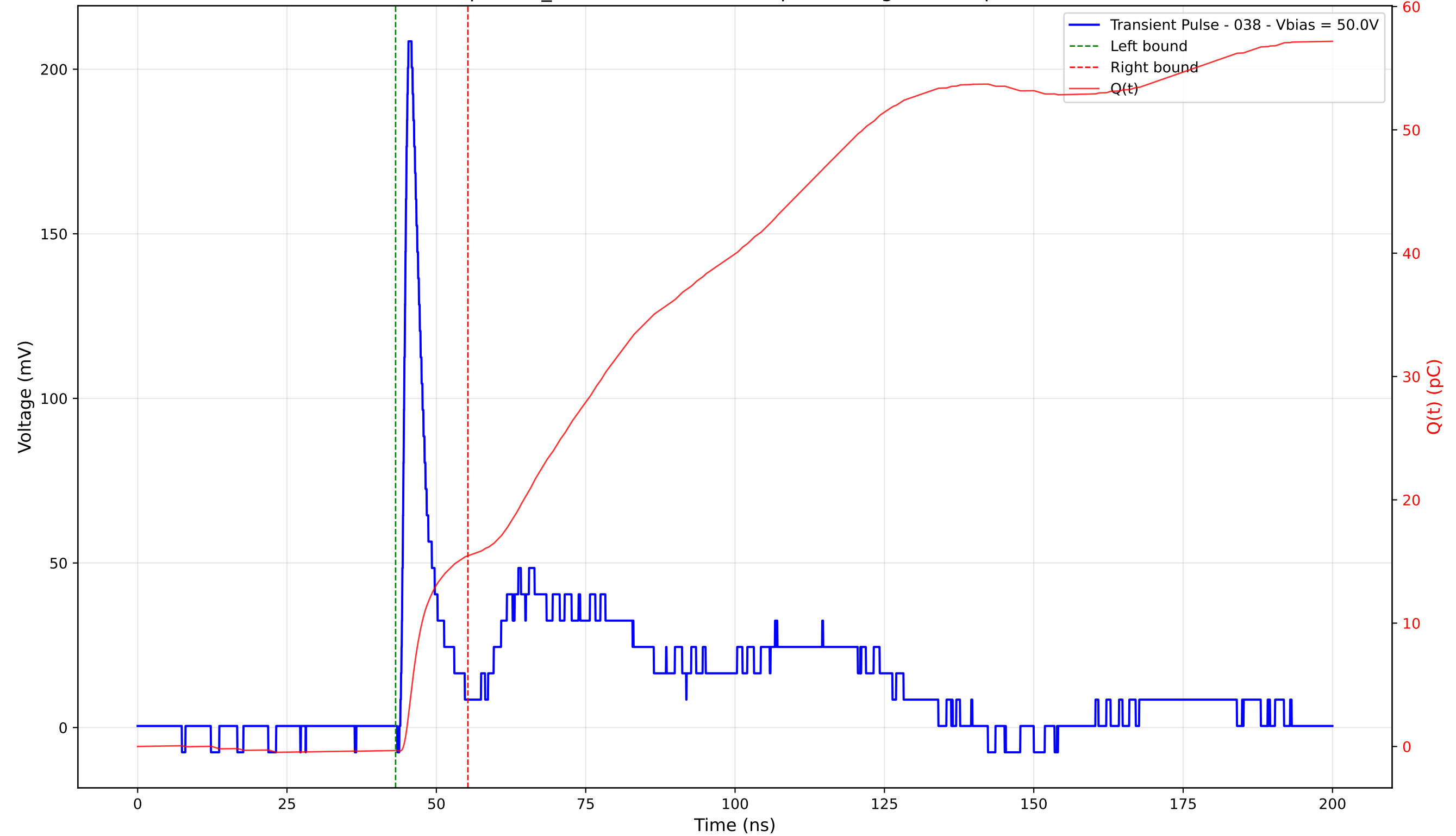
Transient Pulse - Sample: TD_4004 - Position: 270.0 \mu\text{m} - Charge: 15.78 pC - Rise Time: 0.99 ns
