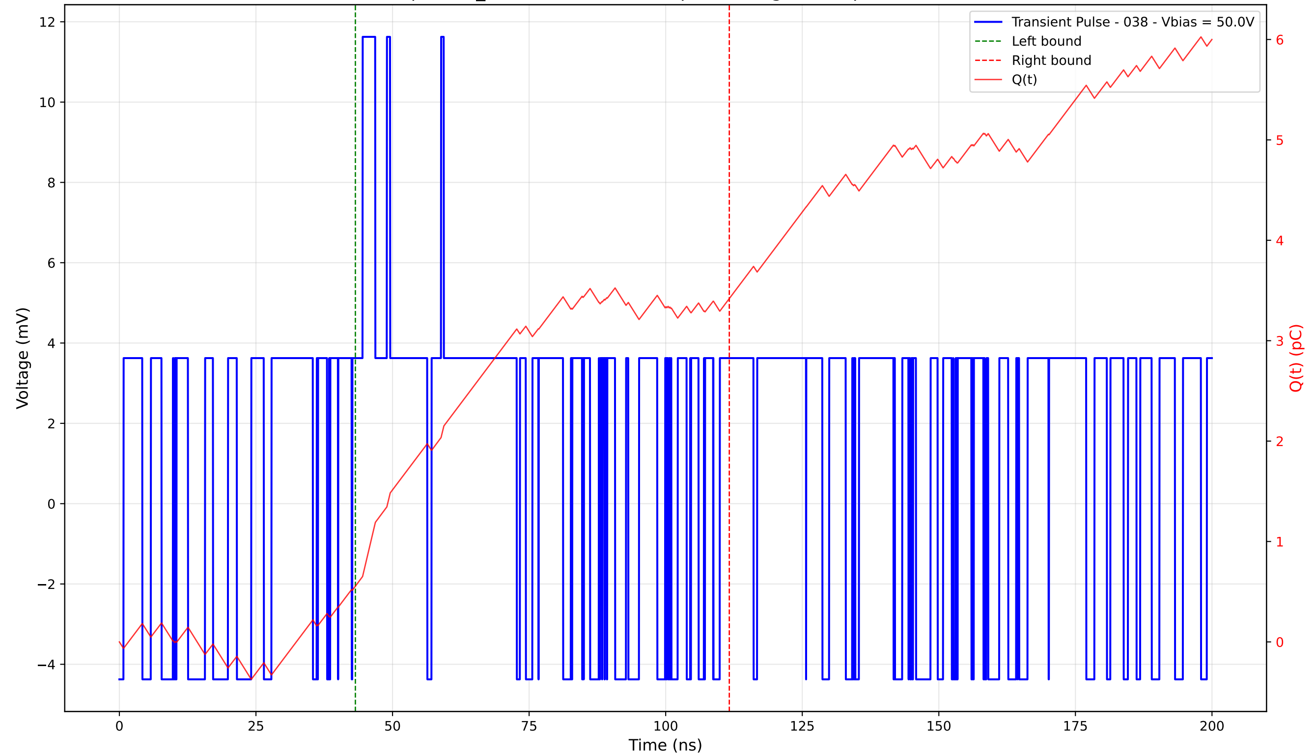
Transient Pulse - Sample: TD_4004 - Position: 35.0 \mu\text{m} - Charge: 2.87 pC - Rise Time: 0.00 ns (N/A)
