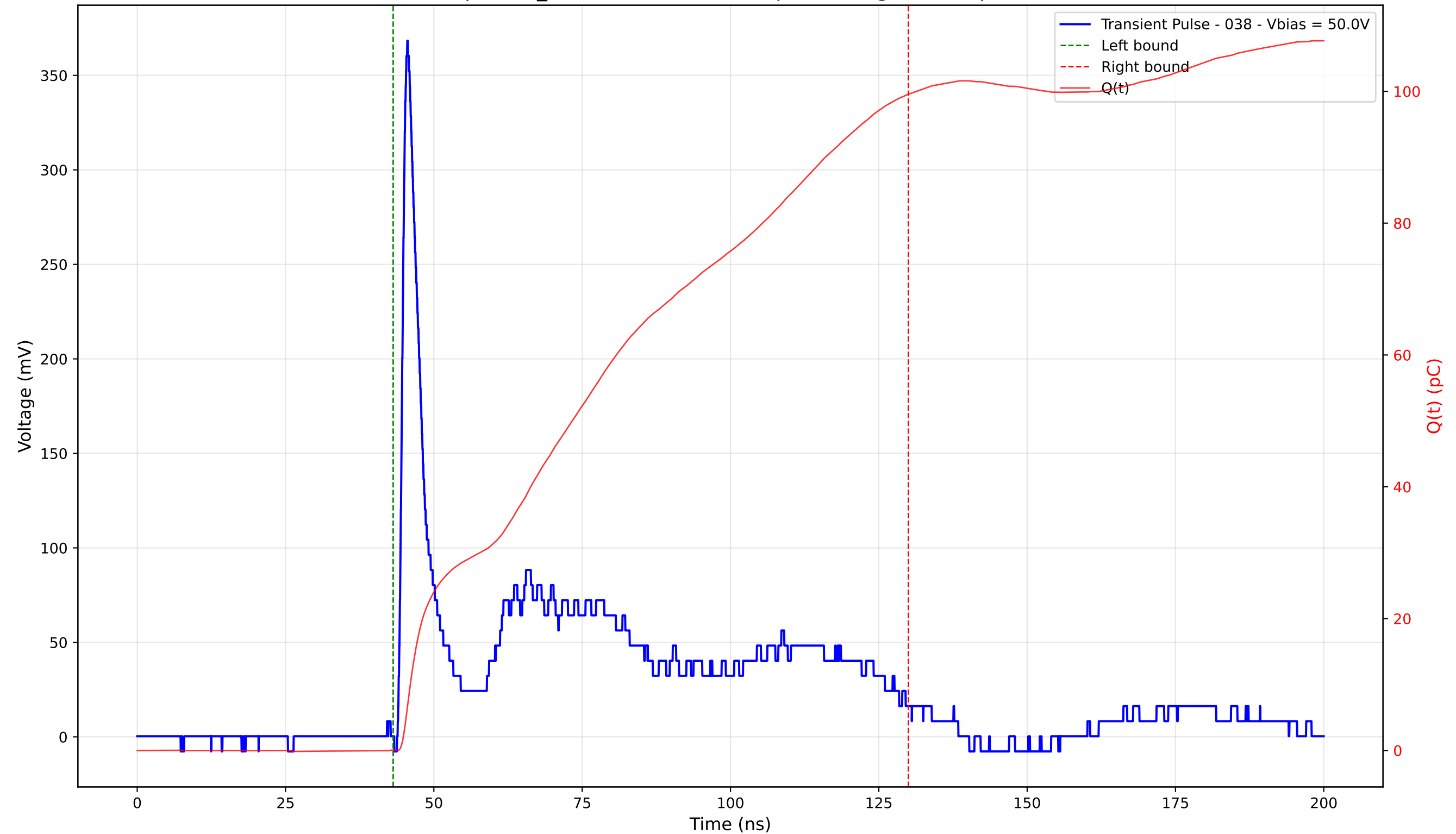
Transient Pulse - Sample: TD_4004 - Position: 225.0 \mu\text{m} - Charge: 99.51 pC - Rise Time: 1.05 ns
