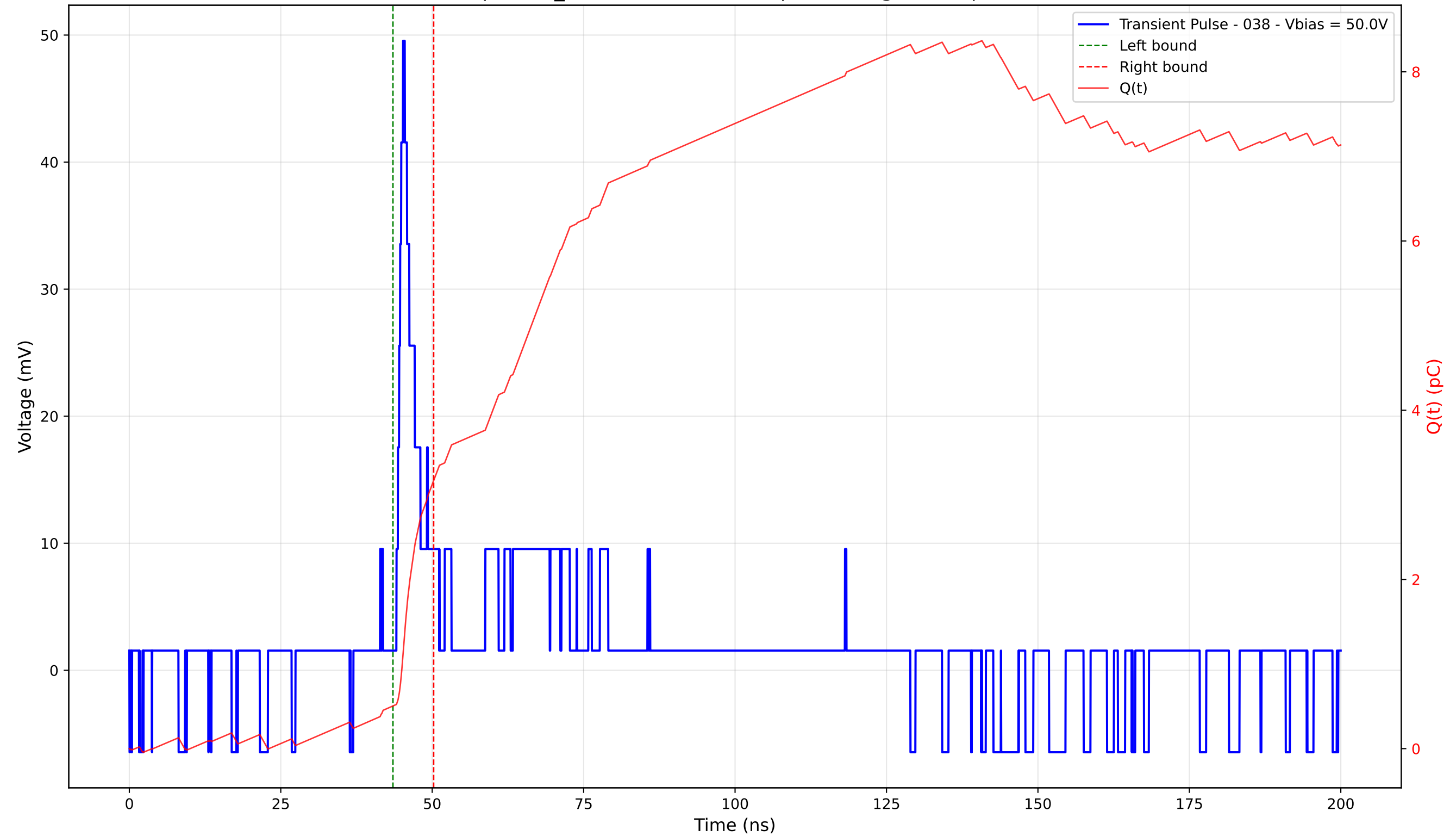
Transient Pulse - Sample: TD_4004 - Position: 50.0 \mu\text{m} - Charge: 2.67 pC - Rise Time: 1.09 ns
