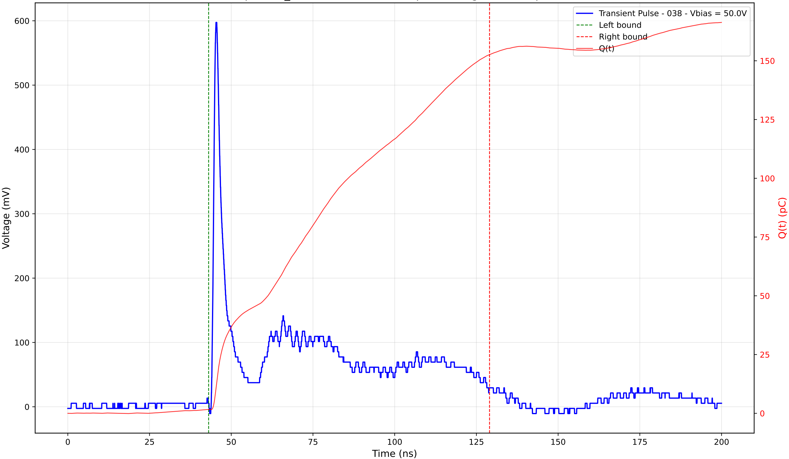
Transient Pulse - Sample: TD_4004 - Position: 100.0 \mu\text{m} - Charge: 150.95 pC - Rise Time: 0.96 ns
