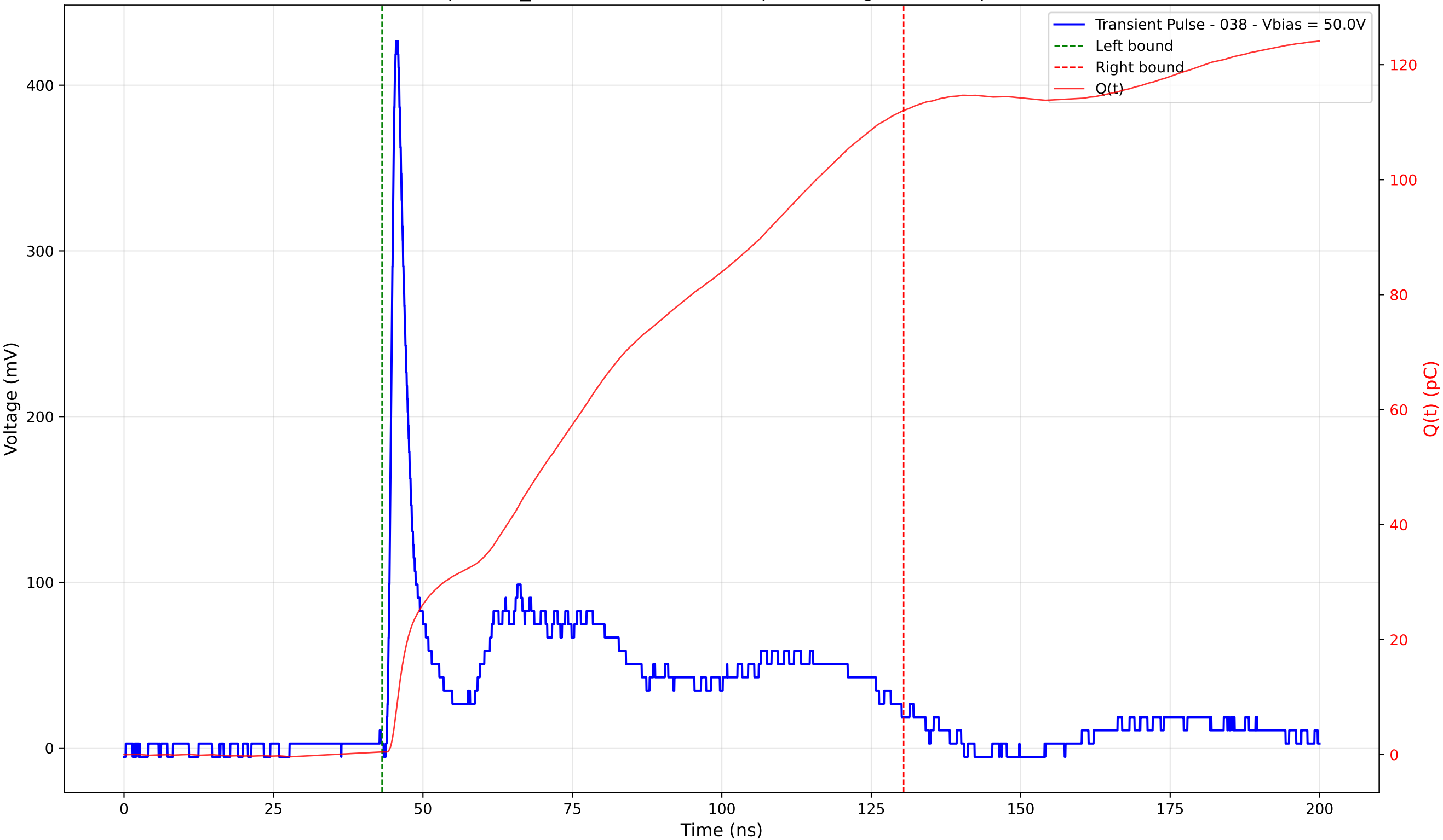
Transient Pulse - Sample: TD_4004 - Position: 130.0 \mu\text{m} - Charge: 111.57 pC - Rise Time: 1.04 ns
