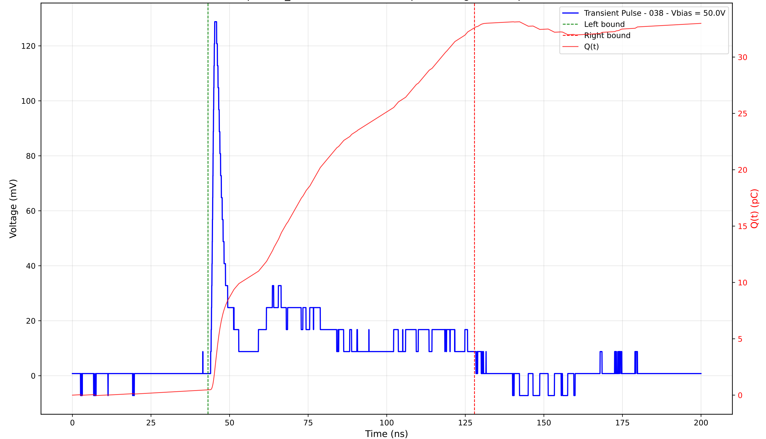
Transient Pulse - Sample: TD_4004 - Position: 335.0 \mu\text{m} - Charge: 32.14 pC - Rise Time: 1.01 ns
