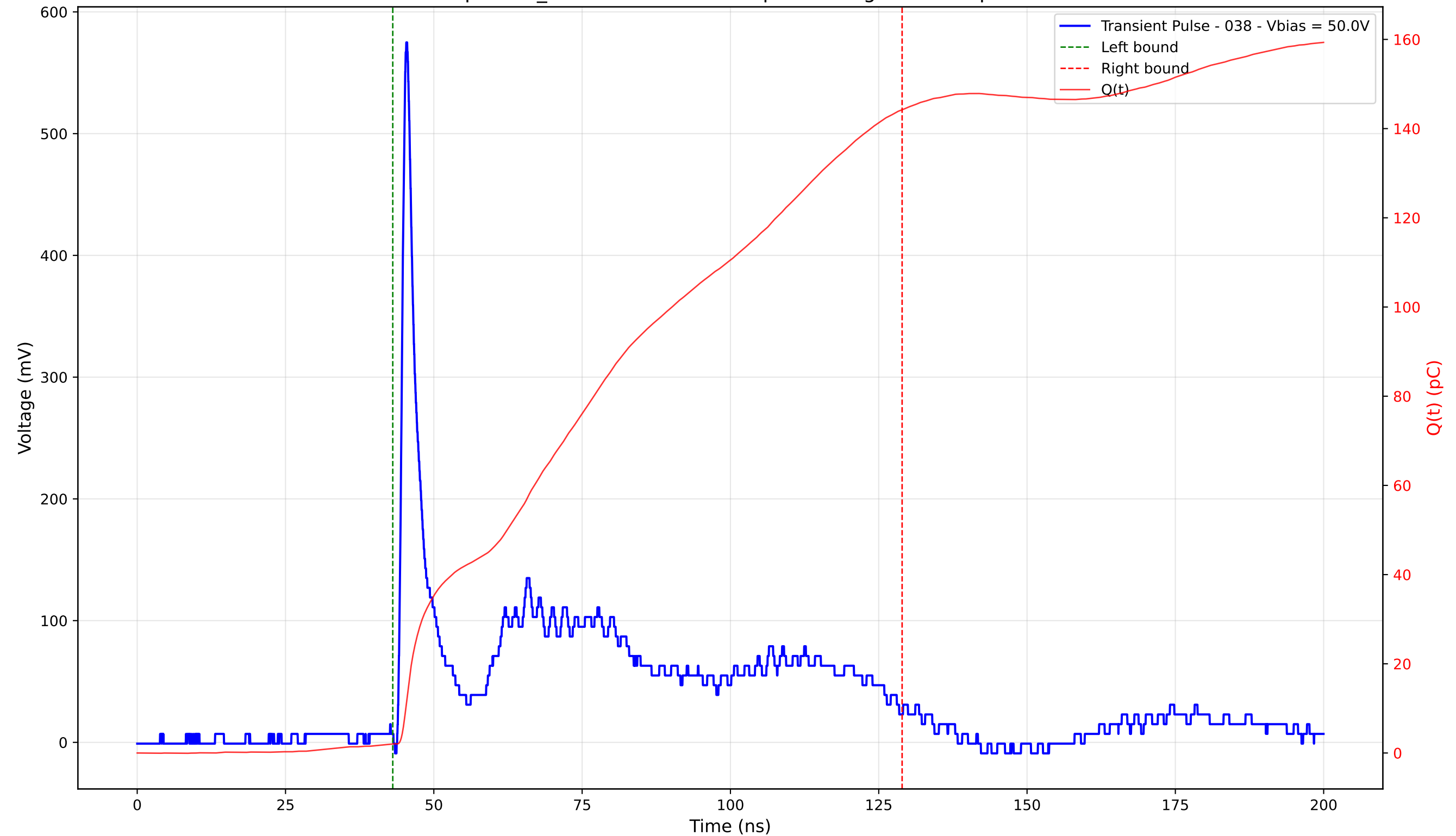
Transient Pulse - Sample: TD_4004 - Position: 95.0 \mu\text{m} - Charge: 142.14 pC - Rise Time: 0.97 ns
