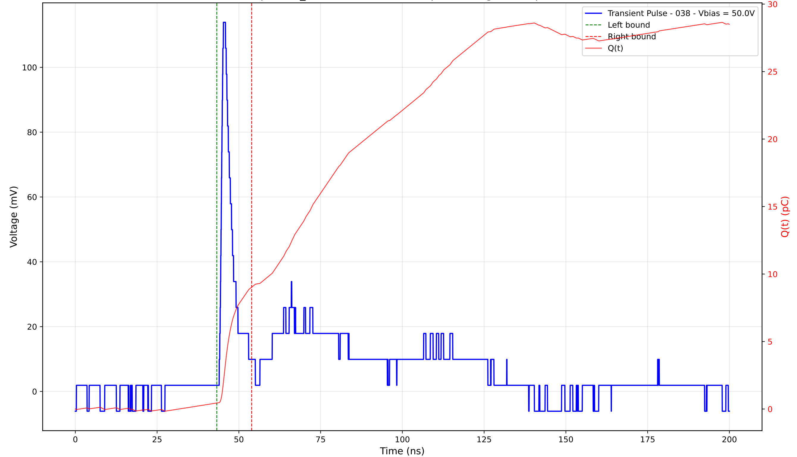
Transient Pulse - Sample: TD_4004 - Position: 375.0 \mu\text{m} - Charge: 8.59 pC - Rise Time: 0.96 ns
