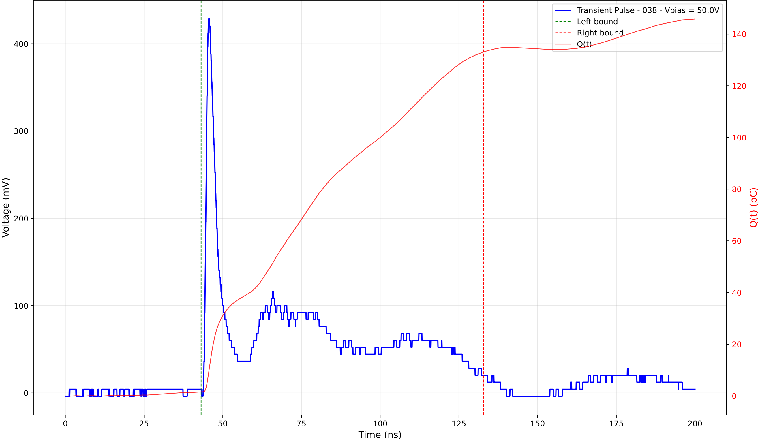
Transient Pulse - Sample: TD_4004 - Position: 180.0 \mu\text{m} - Charge: 131.47 pC - Rise Time: 1.08 ns
