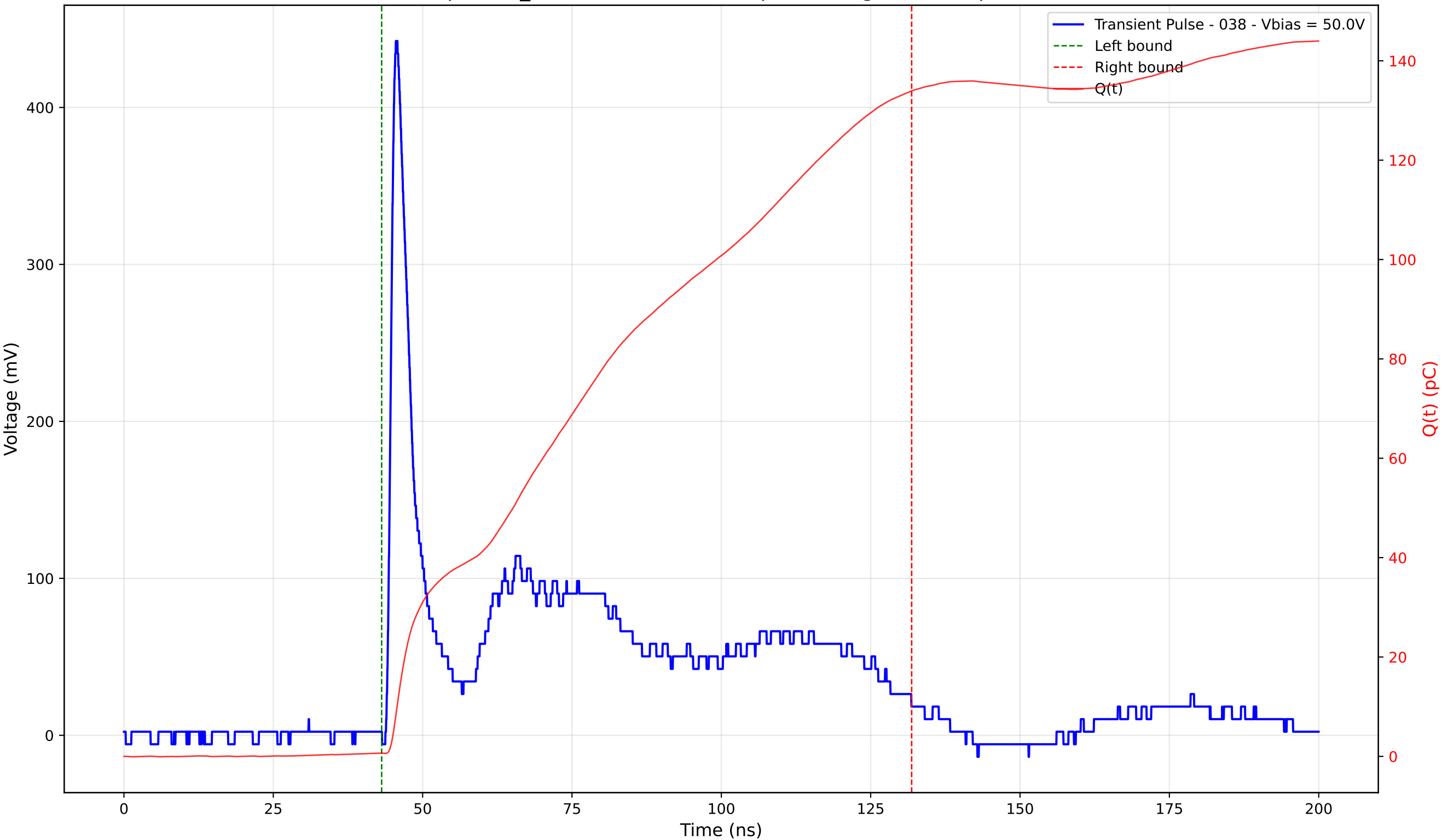
Transient Pulse - Sample: TD_4004 - Position: 185.0 \mu\text{m} - Charge: 133.31 pC - Rise Time: 1.08 ns
