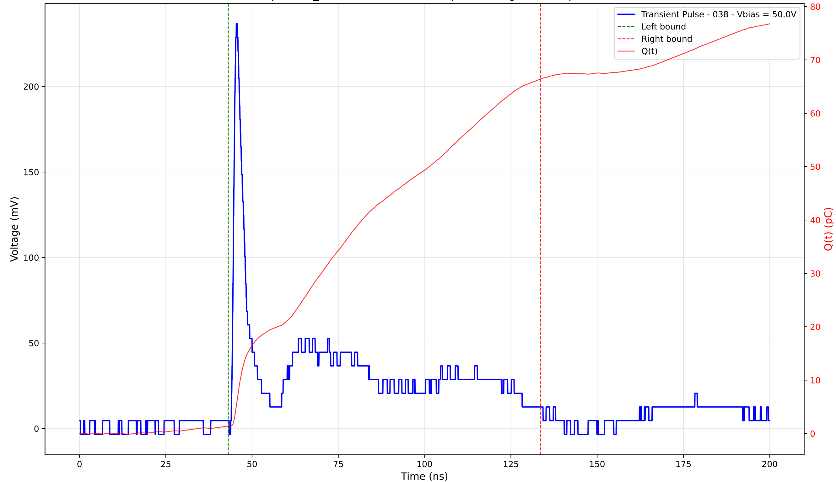
Transient Pulse - Sample: TD_4004 - Position: 275.0 \mu\text{m} - Charge: 64.99 pC - Rise Time: 1.07 ns
