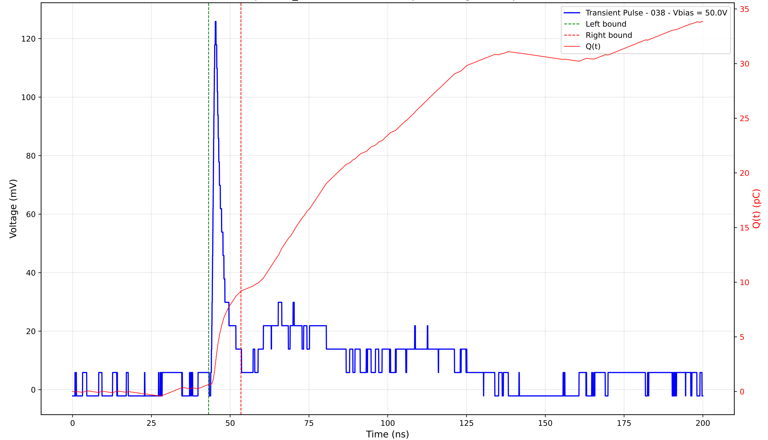
Transient Pulse - Sample: TD_4004 - Position: 60.0 \mu\text{m} - Charge: 8.51 pC - Rise Time: 1.04 ns
