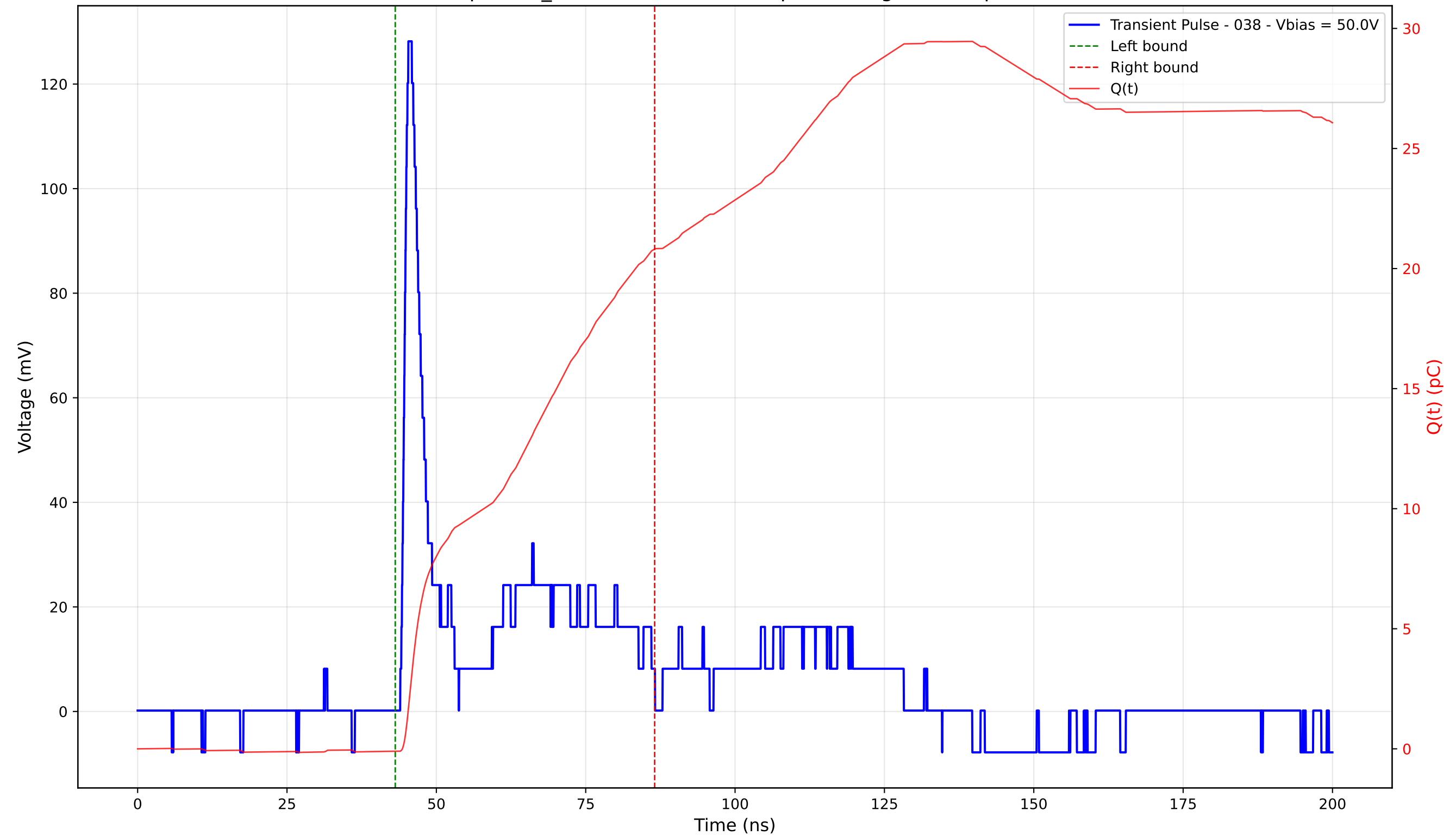
Transient Pulse - Sample: TD_4004 - Position: 360.0 \mu\text{m} - Charge: 20.93 pC - Rise Time: 1.03 ns
