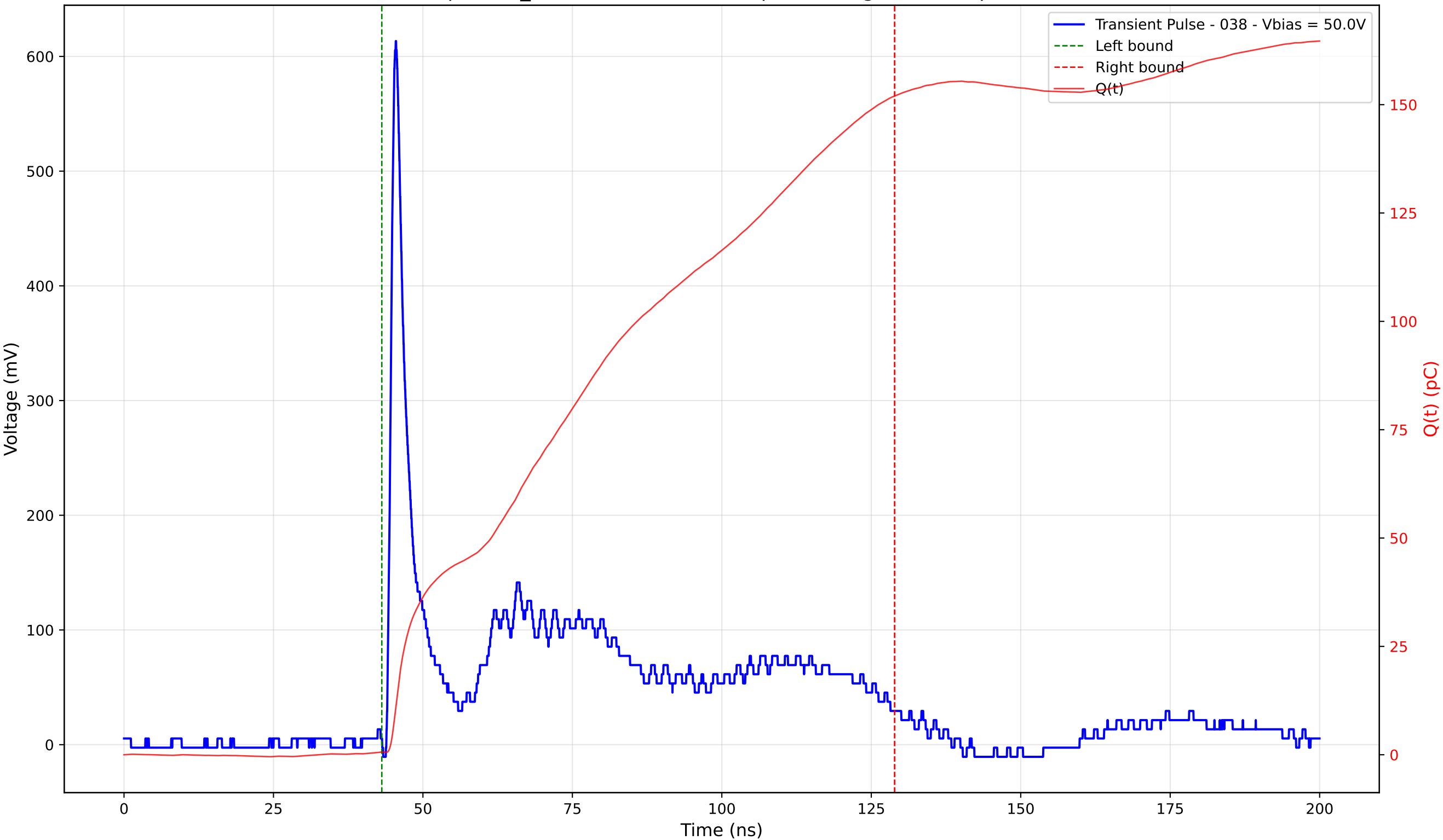
Transient Pulse - Sample: TD_4004 - Position: 105.0 \mu\text{m} - Charge: 151.36 pC - Rise Time: 0.99 ns
