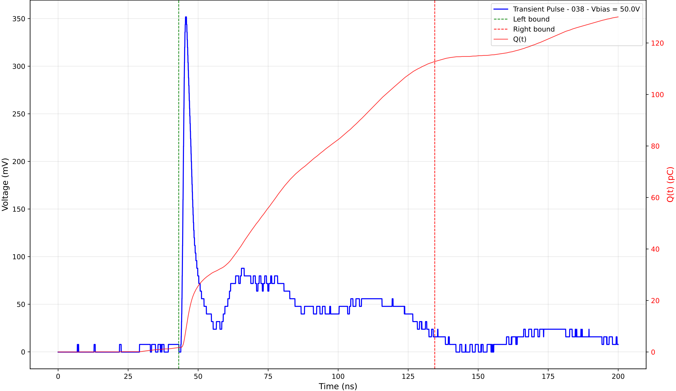
Transient Pulse - Sample: TD_4004 - Position: 165.0 \mu\text{m} - Charge: 111.05 pC - Rise Time: 1.09 ns
