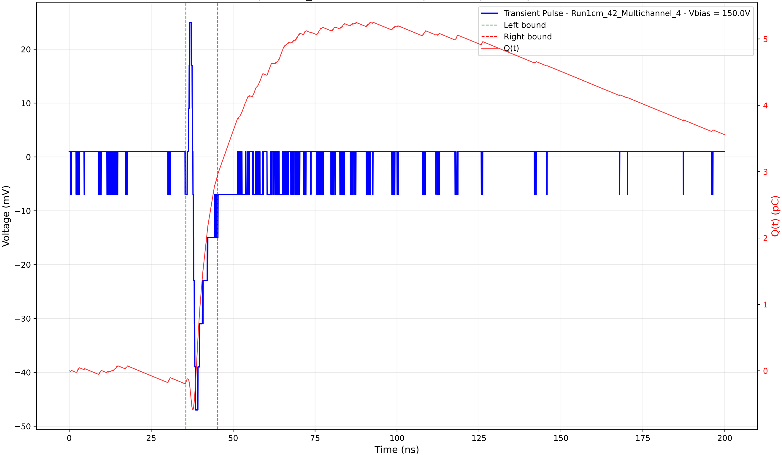
Transient Pulse - Sample: 1cm_42 - Position: 655.0 \mu\text{m} - Charge: 3.13 pC - Rise Time: 0.82 ns
