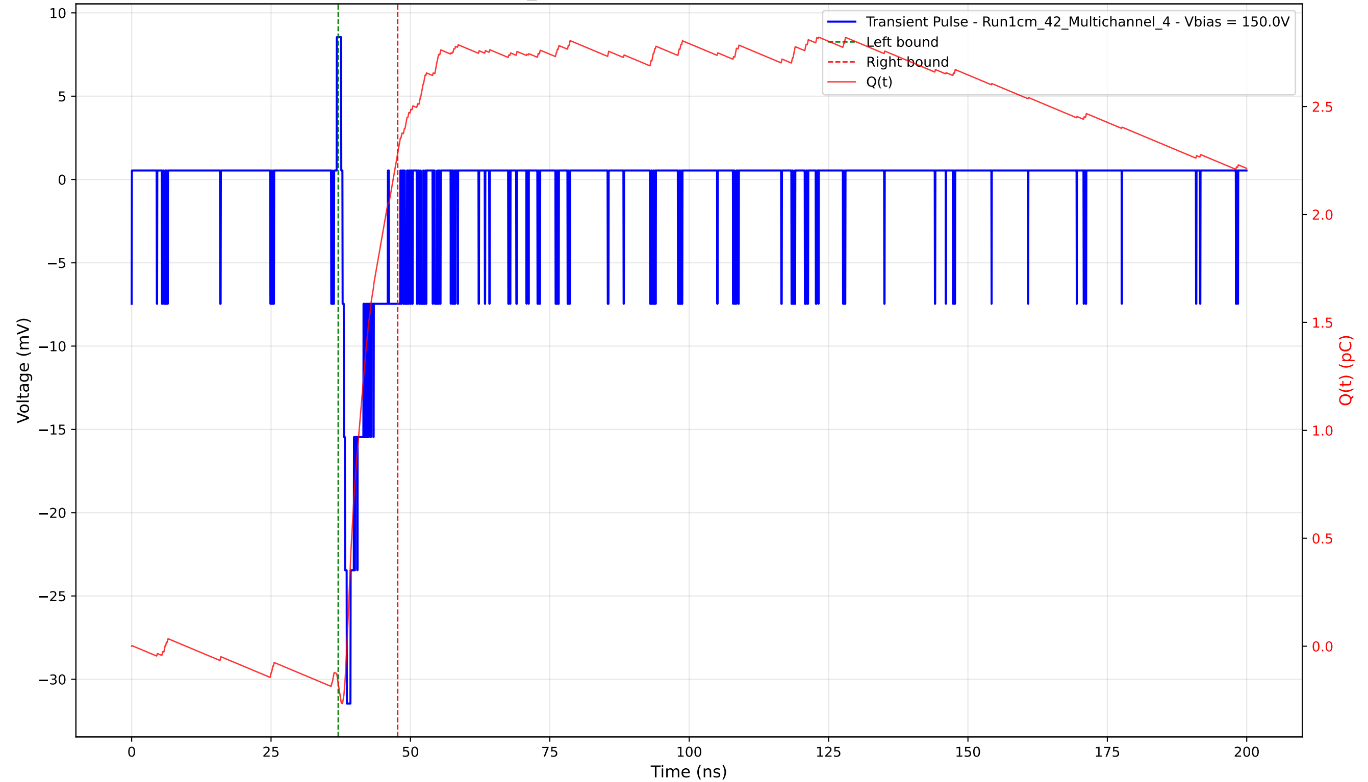
Transient Pulse - Sample: 1cm_42 - Position: 4900.0 \mu\text{m} - Charge: 2.46 pC - Rise Time: 0.78 ns
