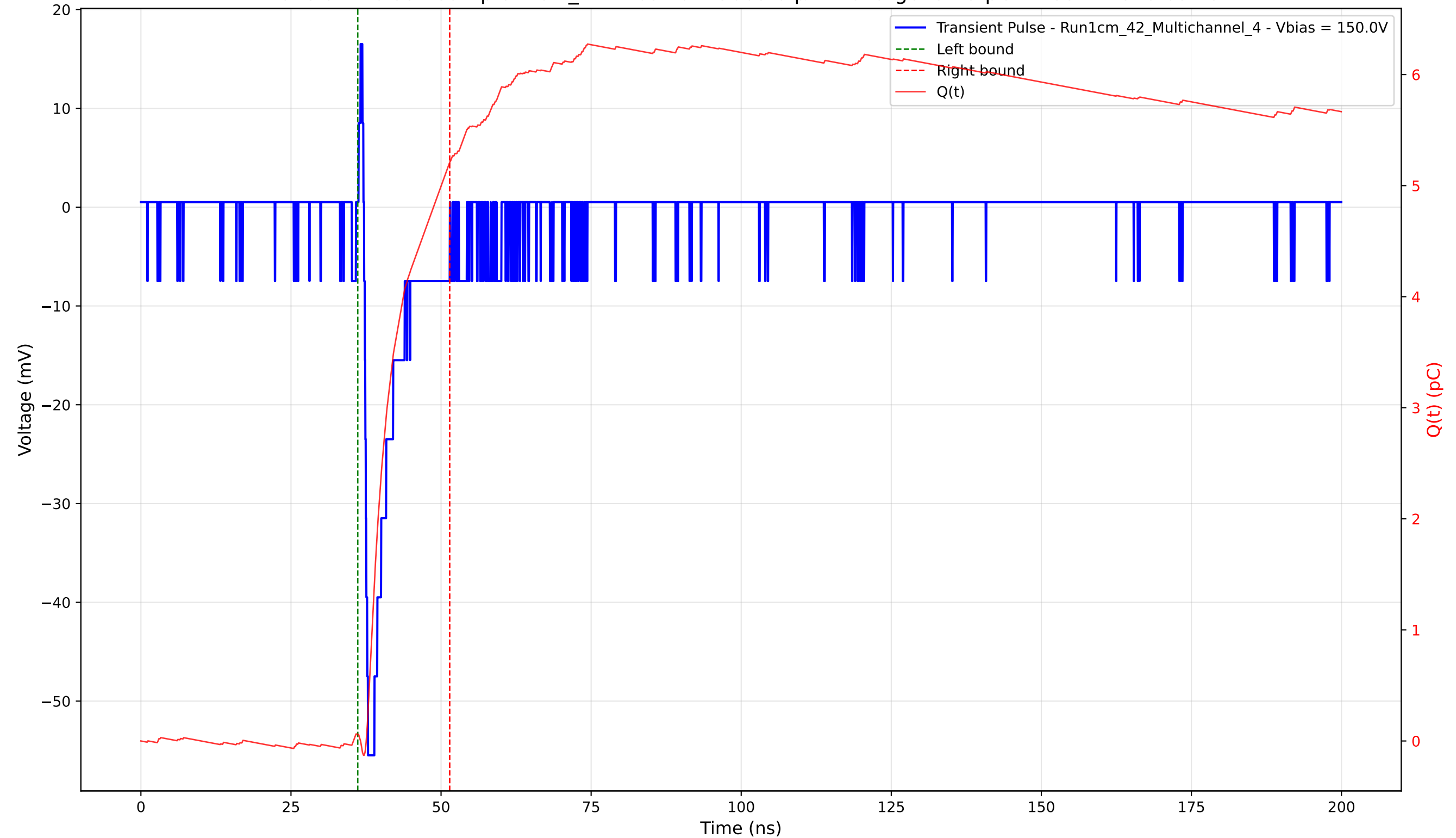
Transient Pulse - Sample: 1cm_42 - Position: 3665.0 \mu\text{m} - Charge: 5.15 pC - Rise Time: 0.65 ns
