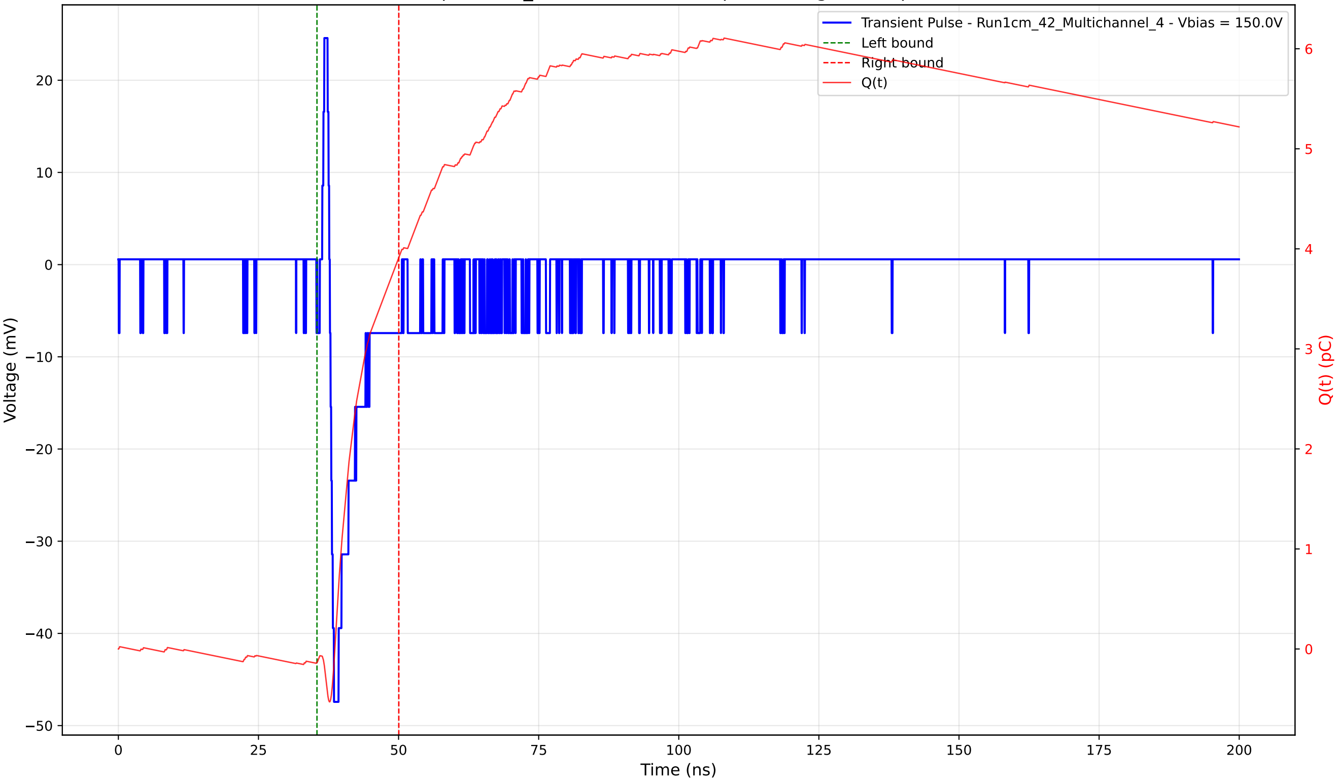
Transient Pulse - Sample: 1cm_42 - Position: 690.0 \mu\text{m} - Charge: 4.05 pC - Rise Time: 0.74 ns
