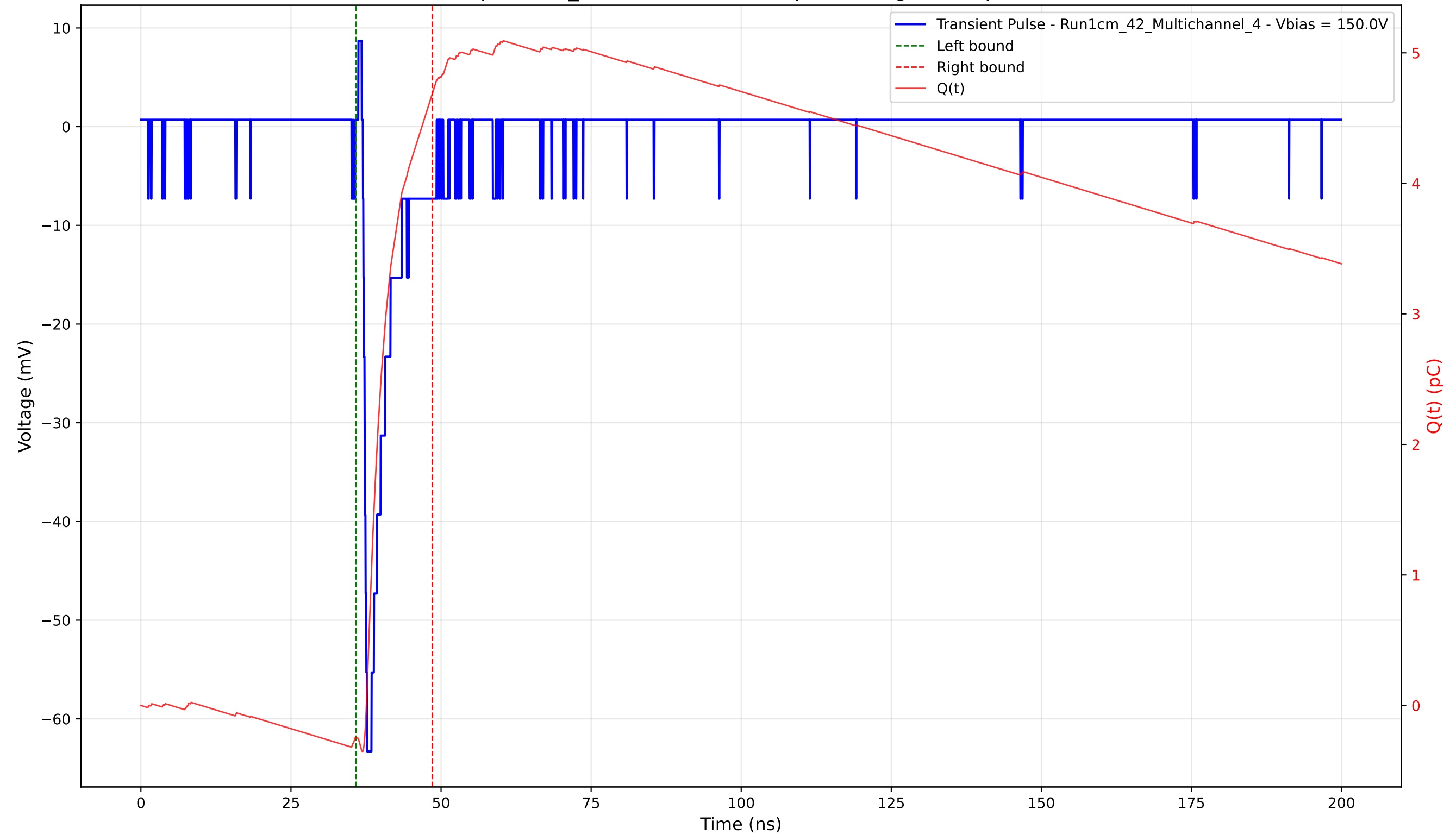
Transient Pulse - Sample: 1cm_42 - Position: 3550.0 \mu\text{m} - Charge: 4.94 pC - Rise Time: 0.69 ns
