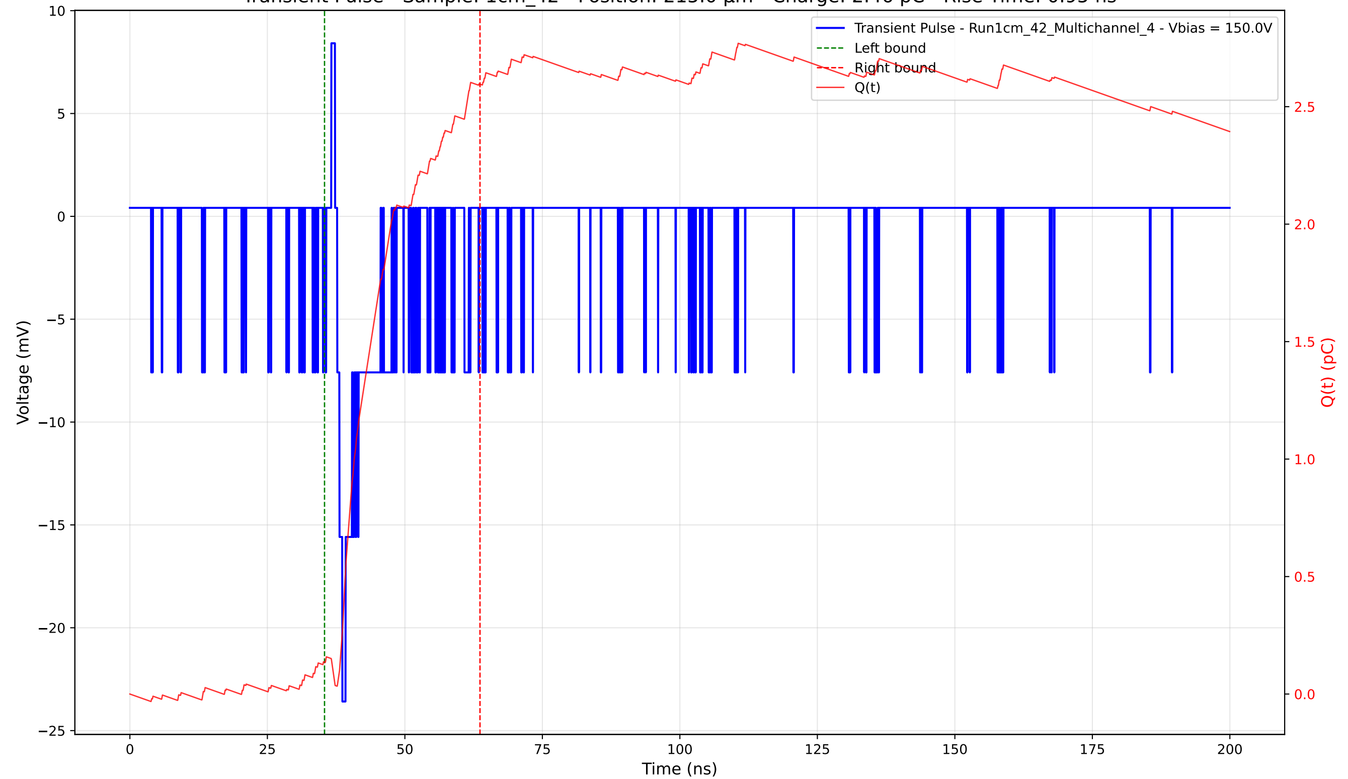
Transient Pulse - Sample: 1cm_42 - Position: 215.0 \mu\text{m} - Charge: 2.46 pC - Rise Time: 0.95 ns
