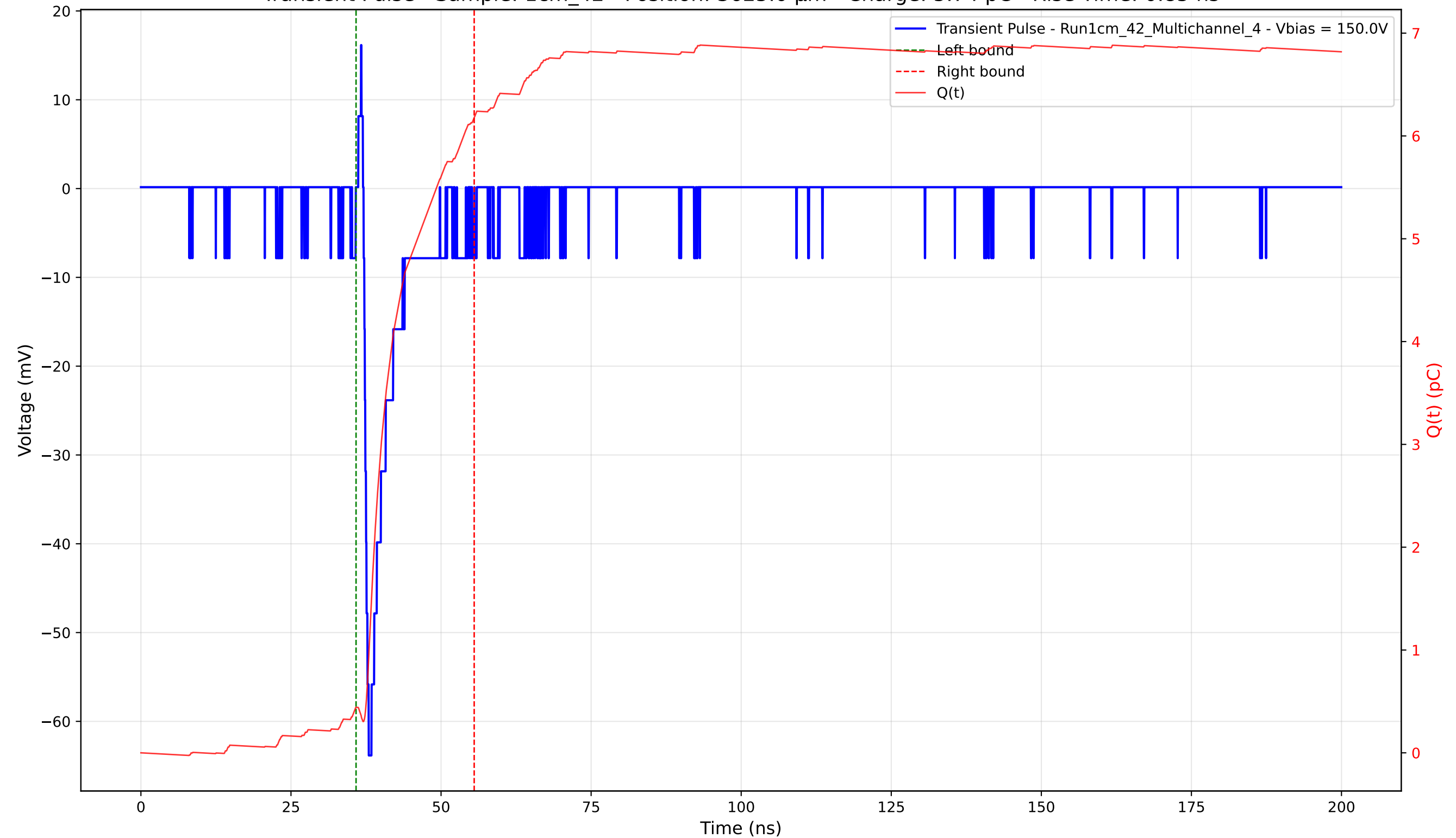
Transient Pulse - Sample: 1cm_42 - Position: 3625.0 \mu\text{m} - Charge: 5.74 pC - Rise Time: 0.85 ns
