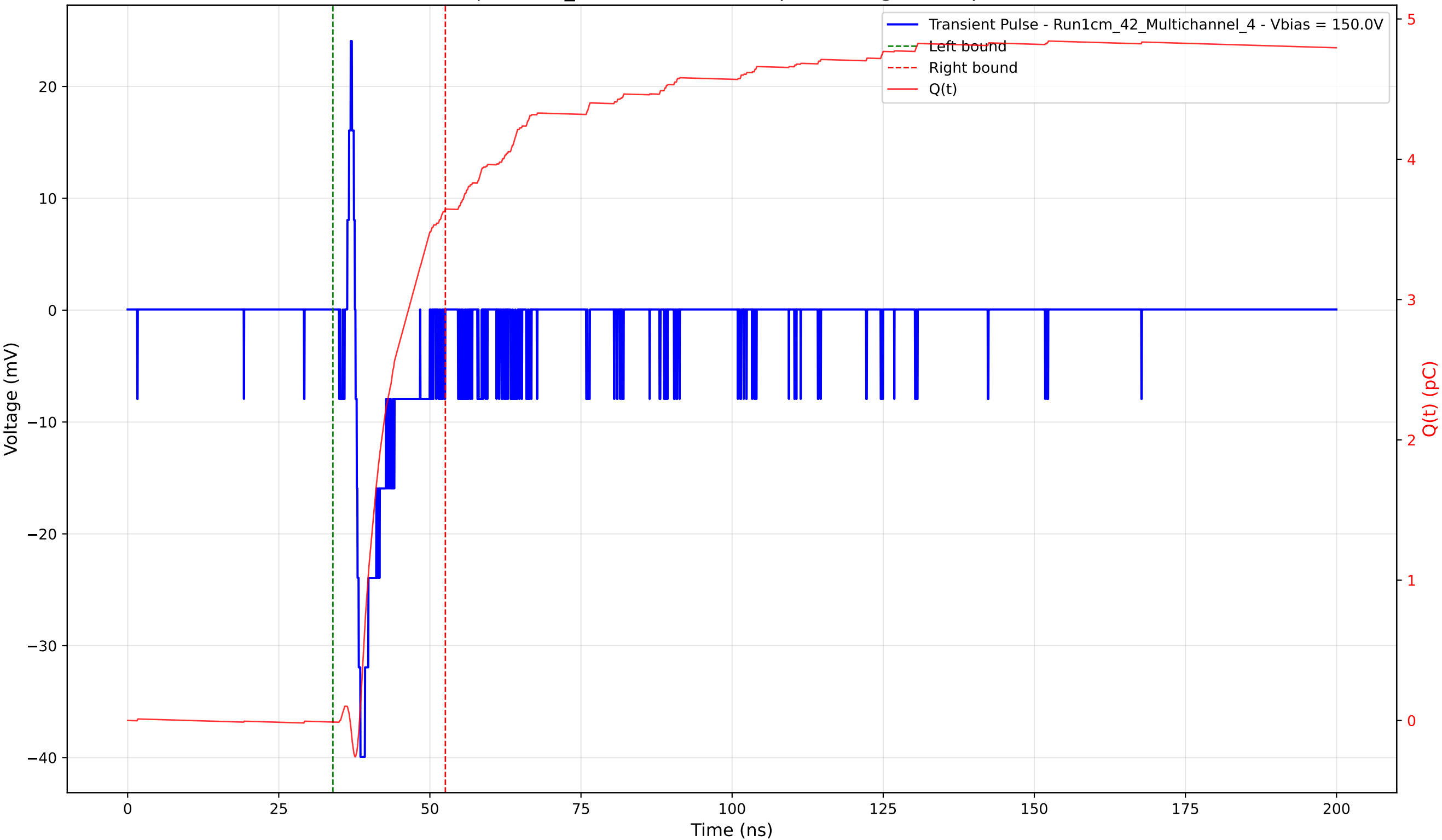
Transient Pulse - Sample: 1cm_42 - Position: 525.0 \mu\text{m} - Charge: 3.66 pC - Rise Time: 0.82 ns
