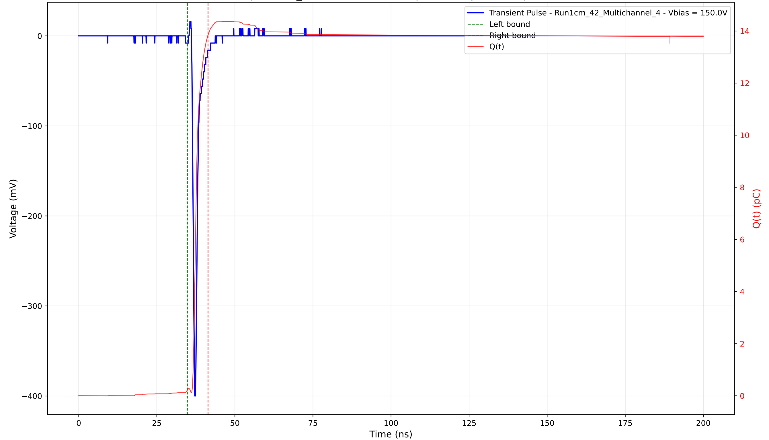
Transient Pulse - Sample: 1cm_42 - Position: 2855.0 \mu\text{m} - Charge: 13.61 pC - Rise Time: 0.70 ns
