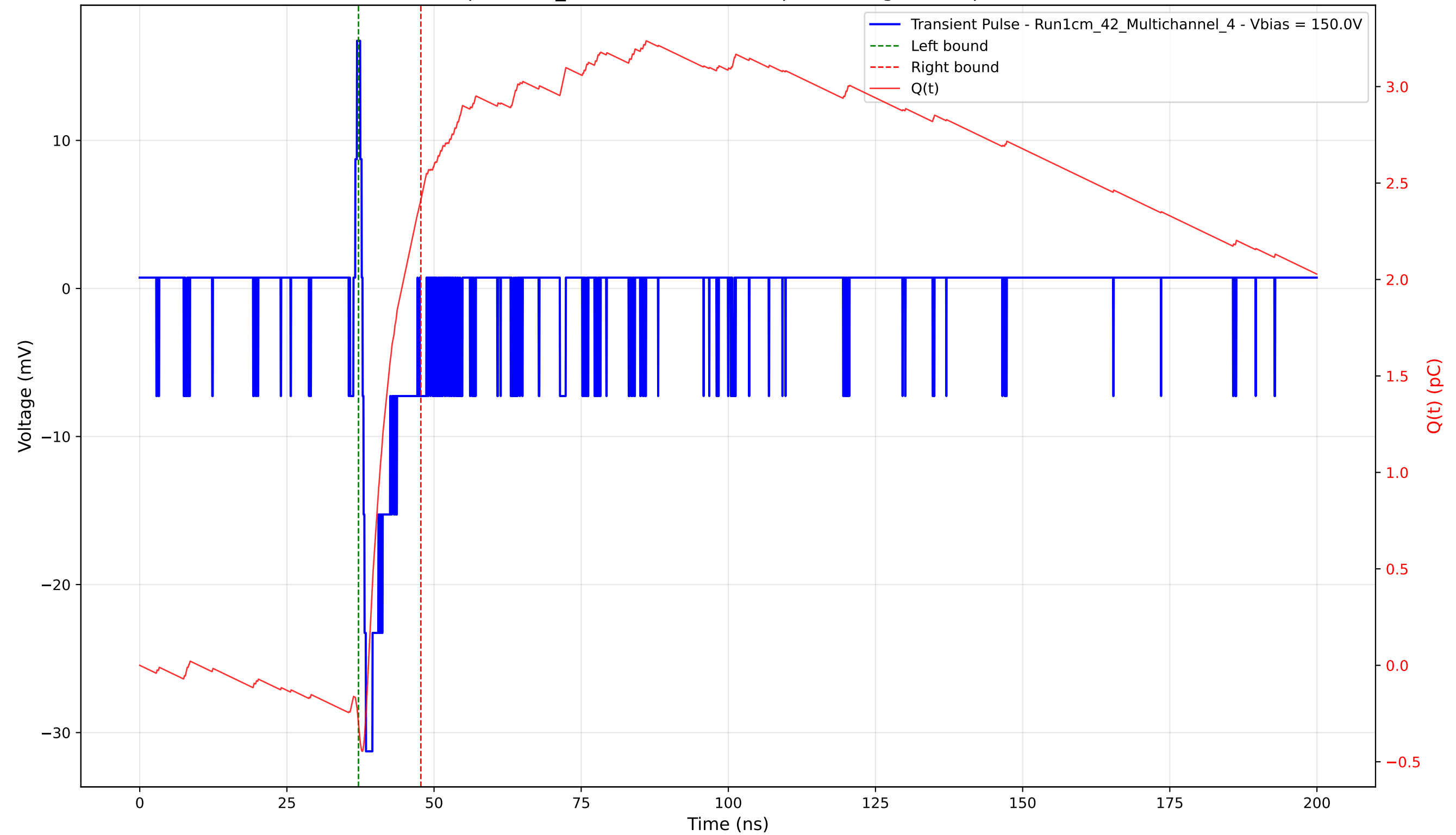
Transient Pulse - Sample: 1cm_42 - Position: 4745.0 \mu\text{m} - Charge: 2.71 pC - Rise Time: 0.59 ns
