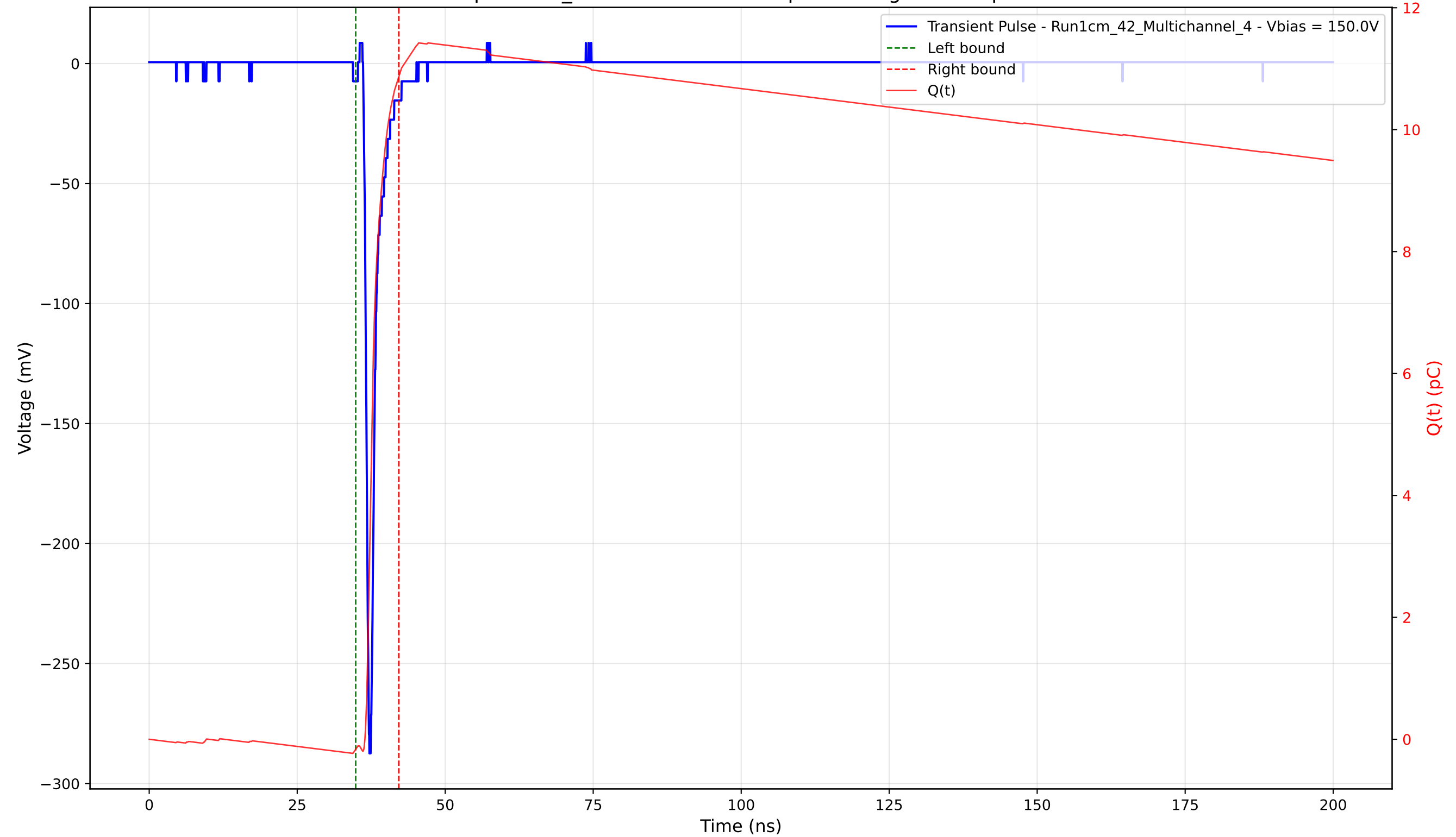
Transient Pulse - Sample: 1cm_42 - Position: 2070.0 \mu\text{m} - Charge: 11.03 pC - Rise Time: 0.75 ns
