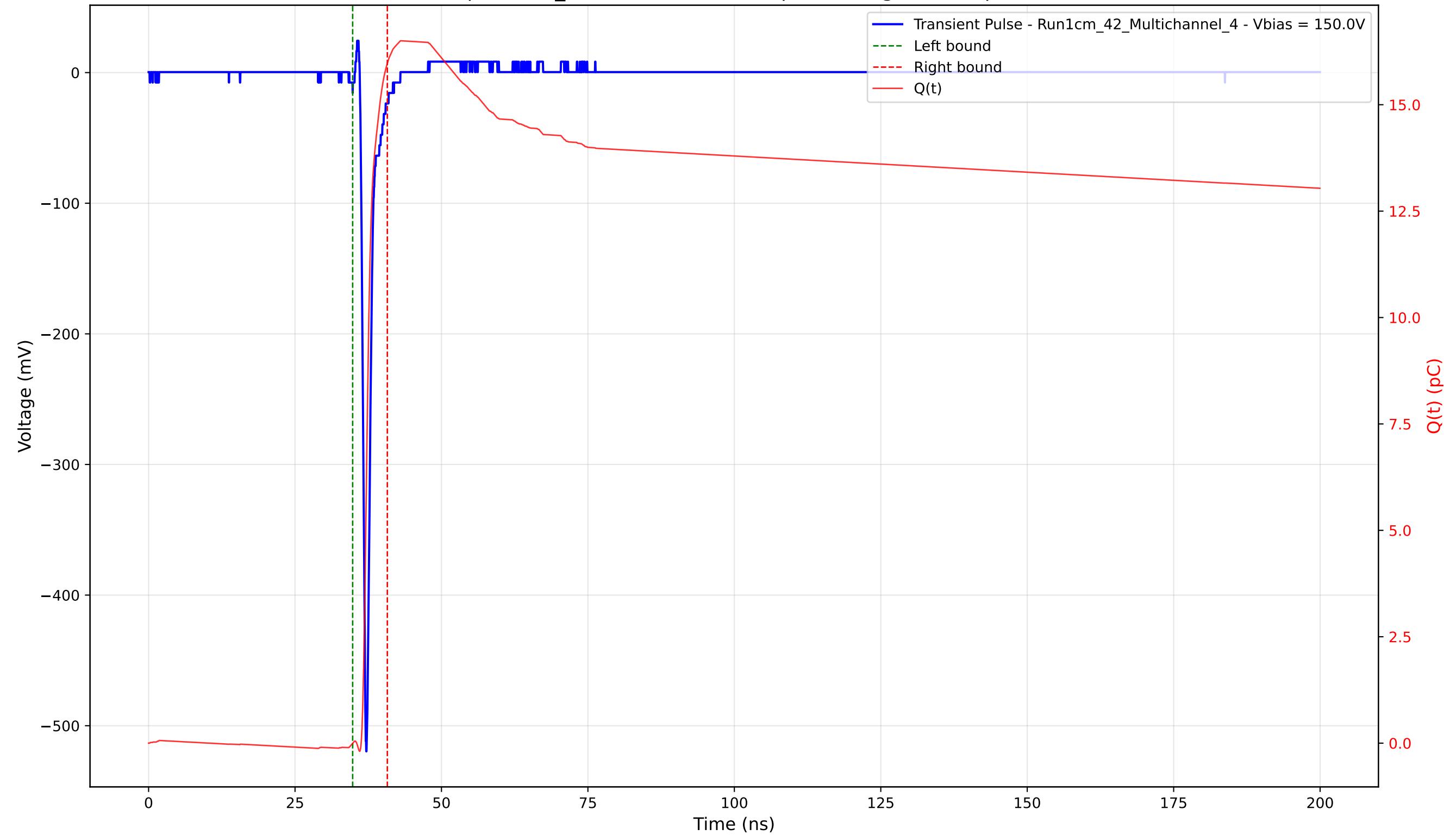
Transient Pulse - Sample: 1cm_42 - Position: 2650.0 \mu\text{m} - Charge: 15.98 pC - Rise Time: 0.69 ns
