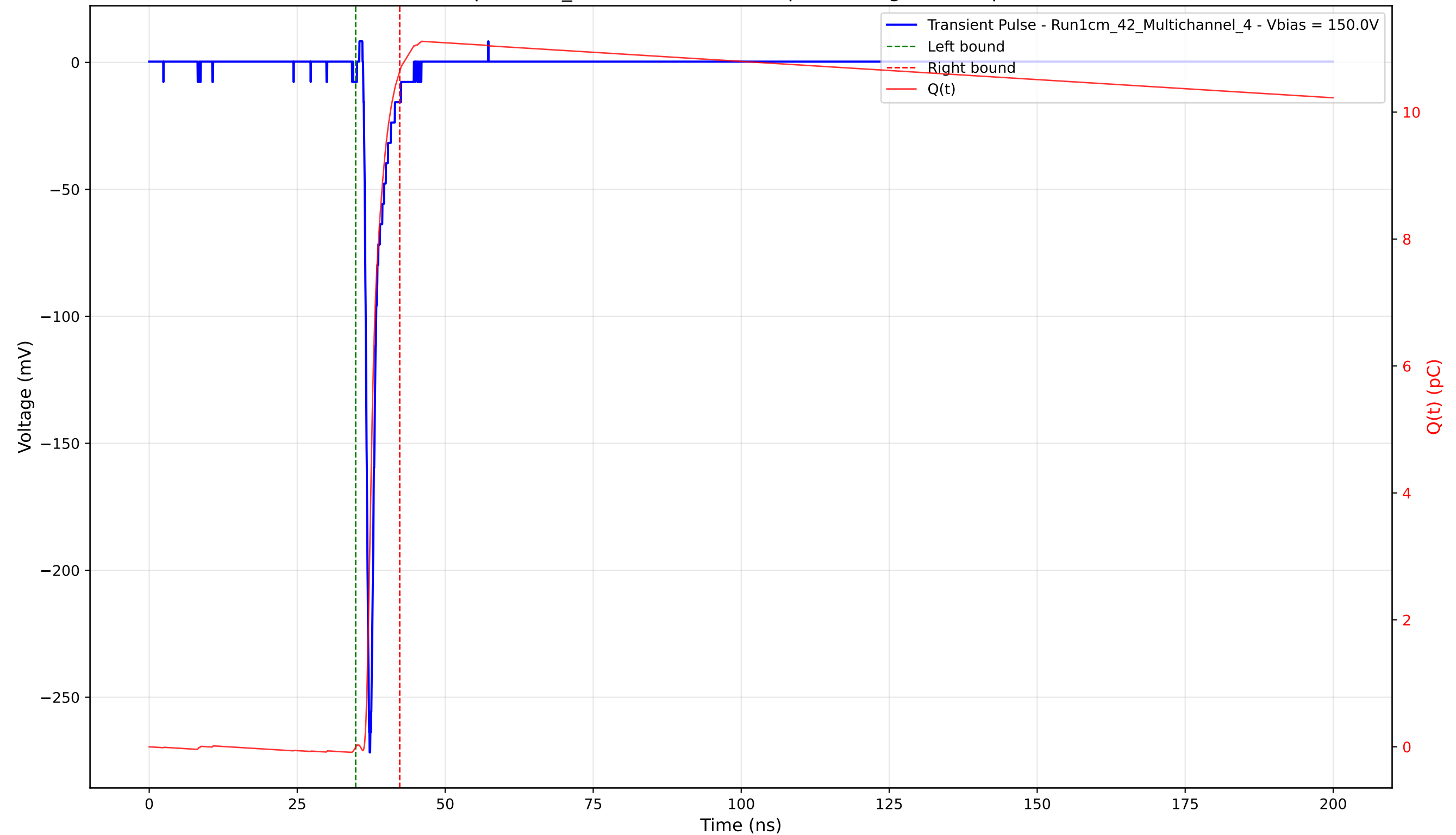
Transient Pulse - Sample: 1cm_42 - Position: 2050.0 \mu\text{m} - Charge: 10.65 pC - Rise Time: 0.77 ns
