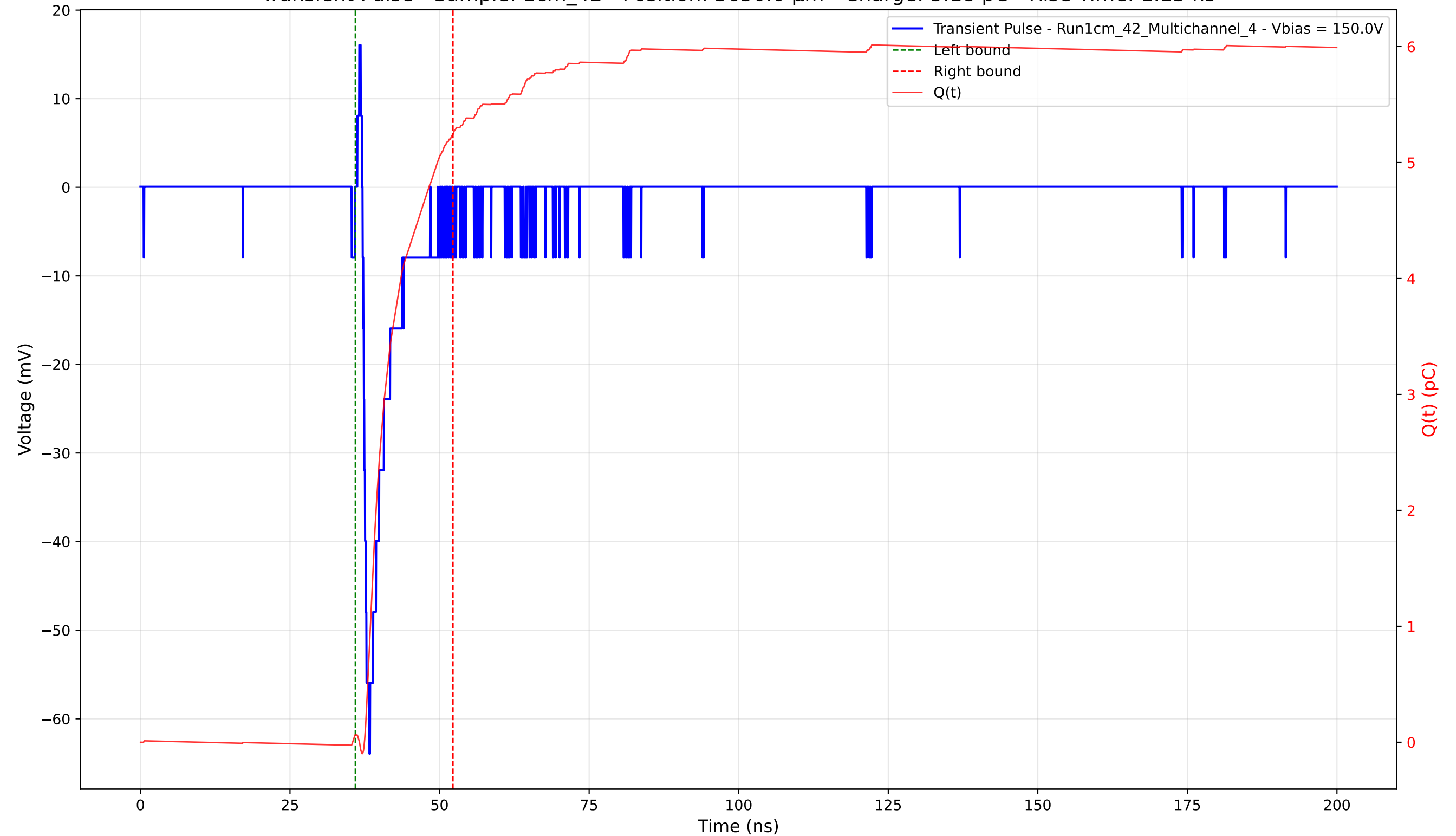
Transient Pulse - Sample: 1cm_42 - Position: 3650.0 \mu\text{m} - Charge: 5.18 pC - Rise Time: 1.13 ns
