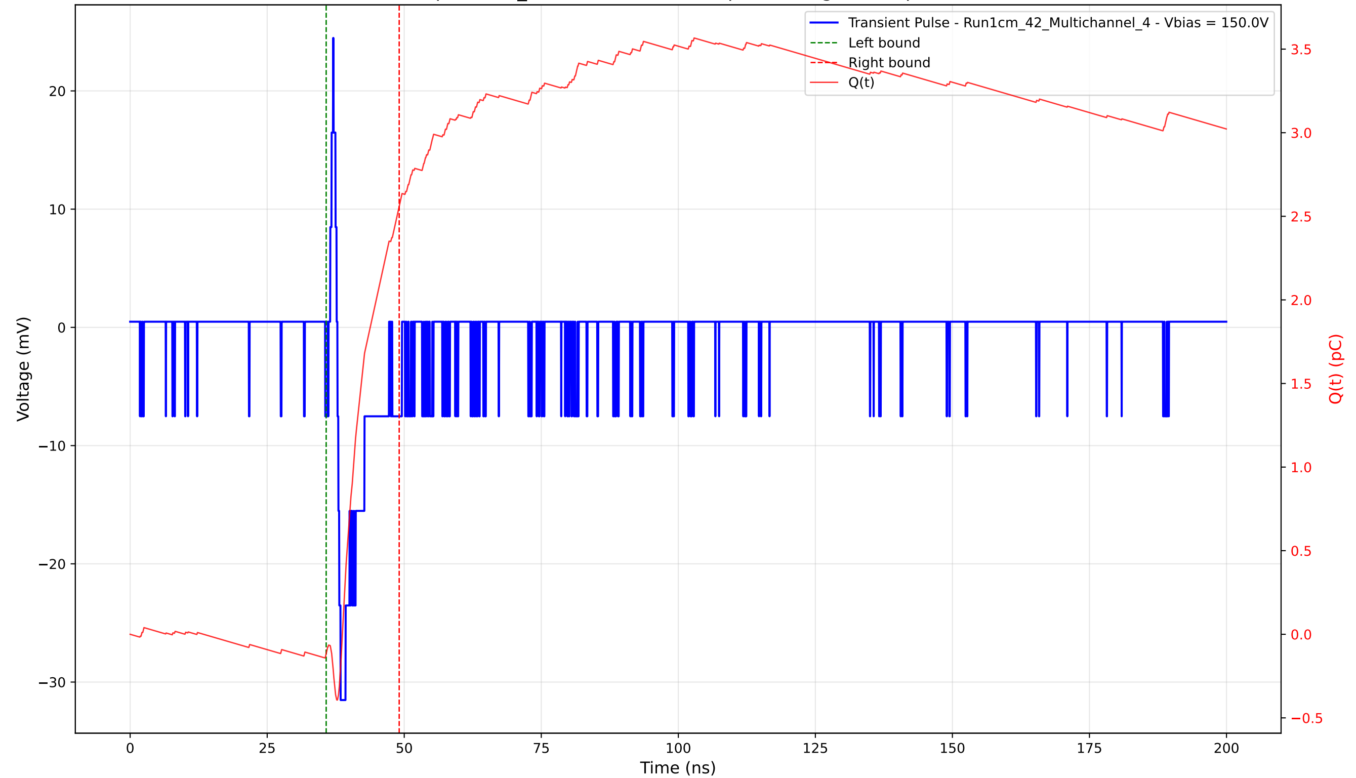
Transient Pulse - Sample: 1cm_42 - Position: 4470.0 \mu\text{m} - Charge: 2.68 pC - Rise Time: 0.58 ns
