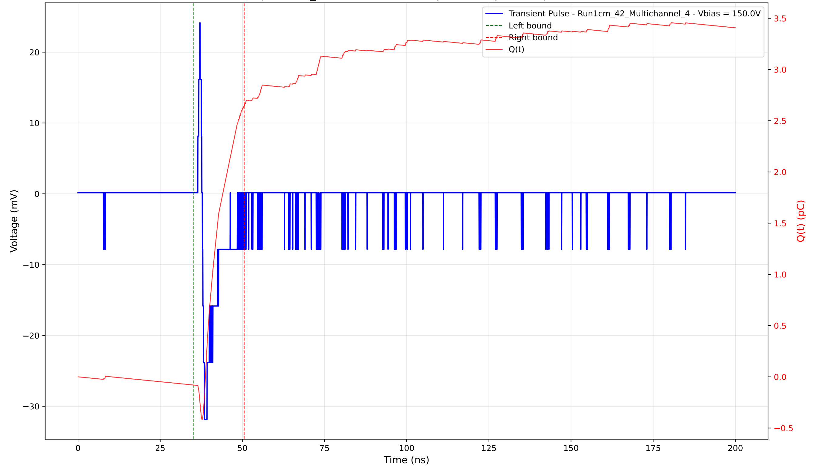
Transient Pulse - Sample: 1cm_42 - Position: 4500.0 \mu\text{m} - Charge: 2.72 pC - Rise Time: 0.62 ns
