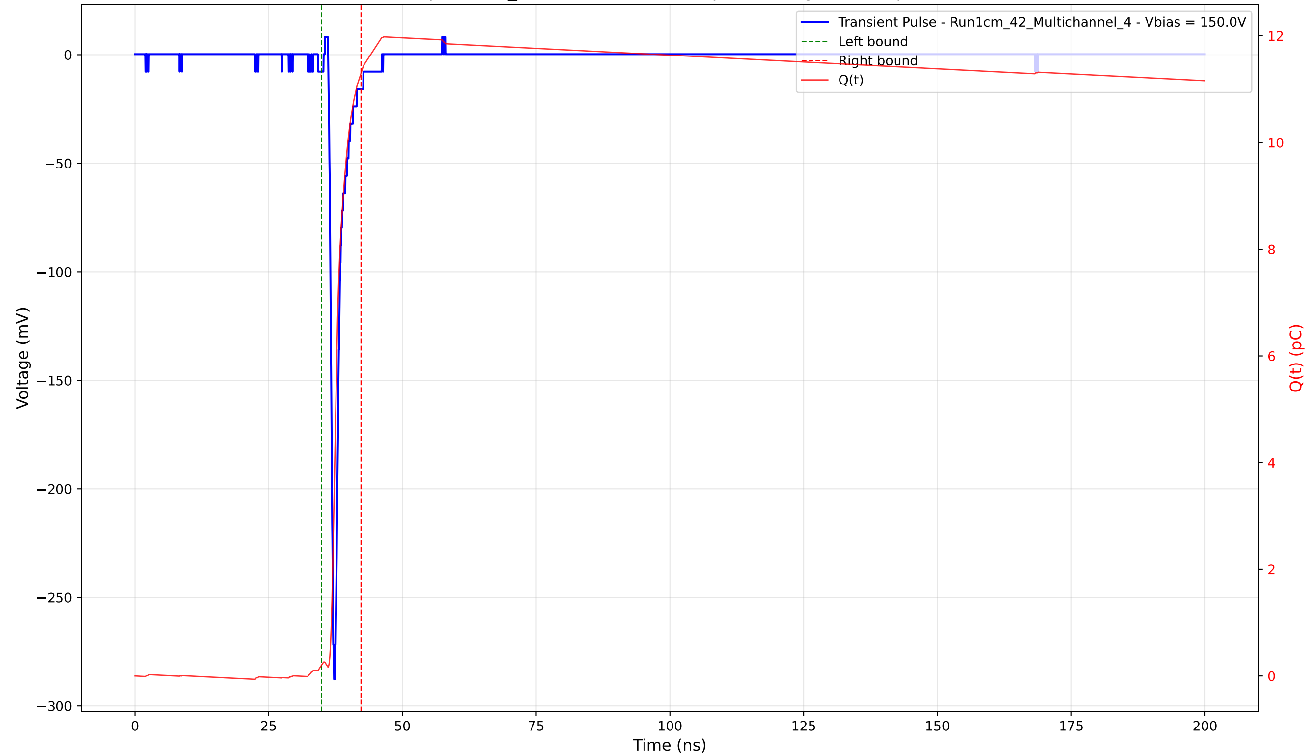
Transient Pulse - Sample: 1cm_42 - Position: 2065.0 \mu\text{m} - Charge: 11.10 pC - Rise Time: 0.72 ns
