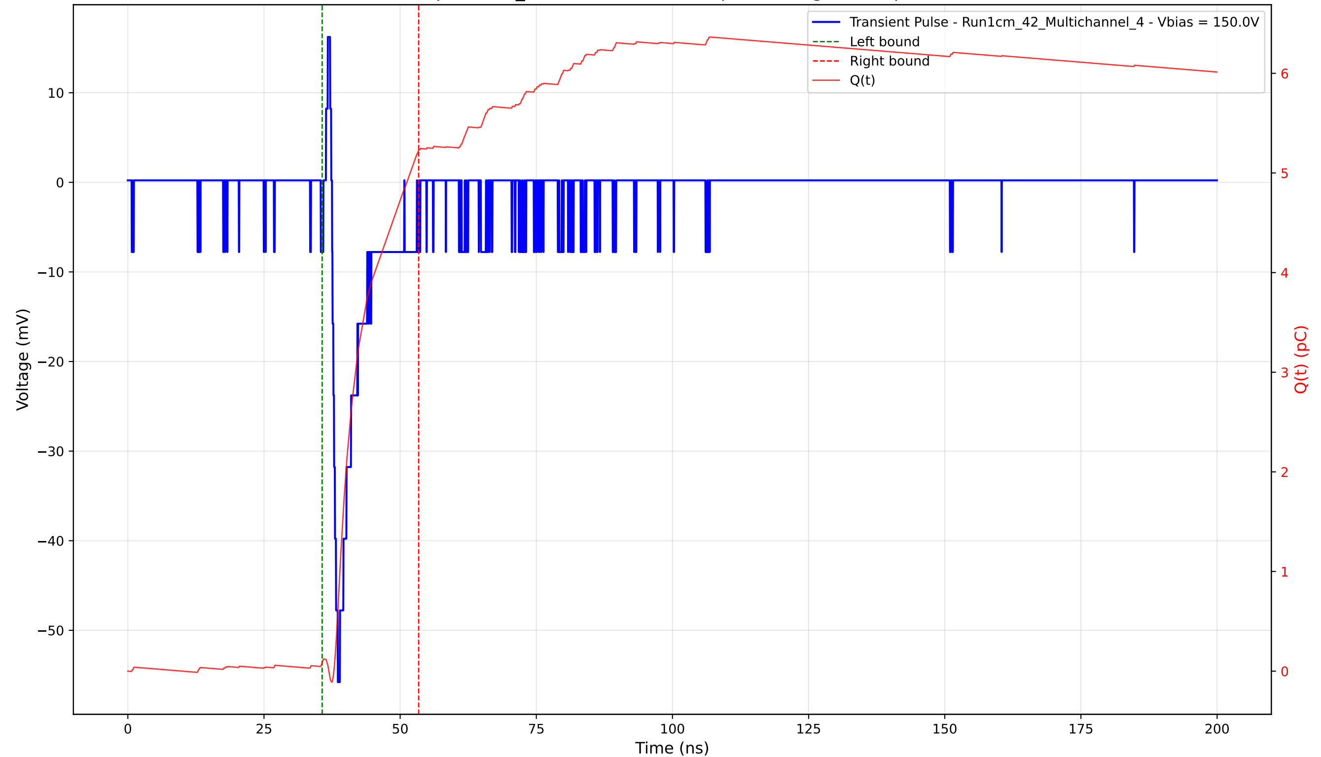
Transient Pulse - Sample: 1cm_42 - Position: 1070.0 \mu\text{m} - Charge: 5.14 pC - Rise Time: 1.05 ns
