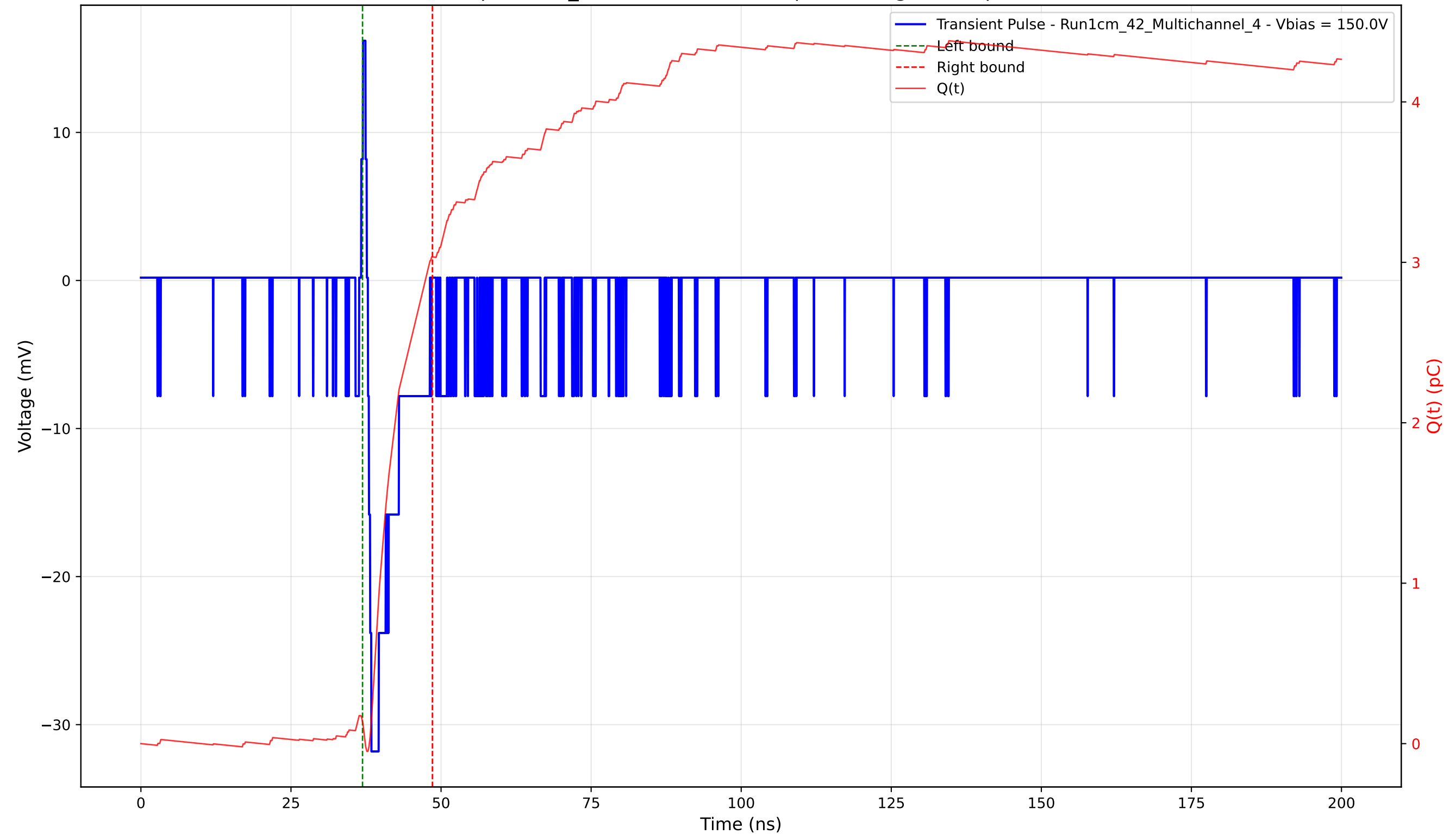
Transient Pulse - Sample: 1cm_42 - Position: 4795.0 \mu\text{m} - Charge: 2.90 pC - Rise Time: 0.58 ns
