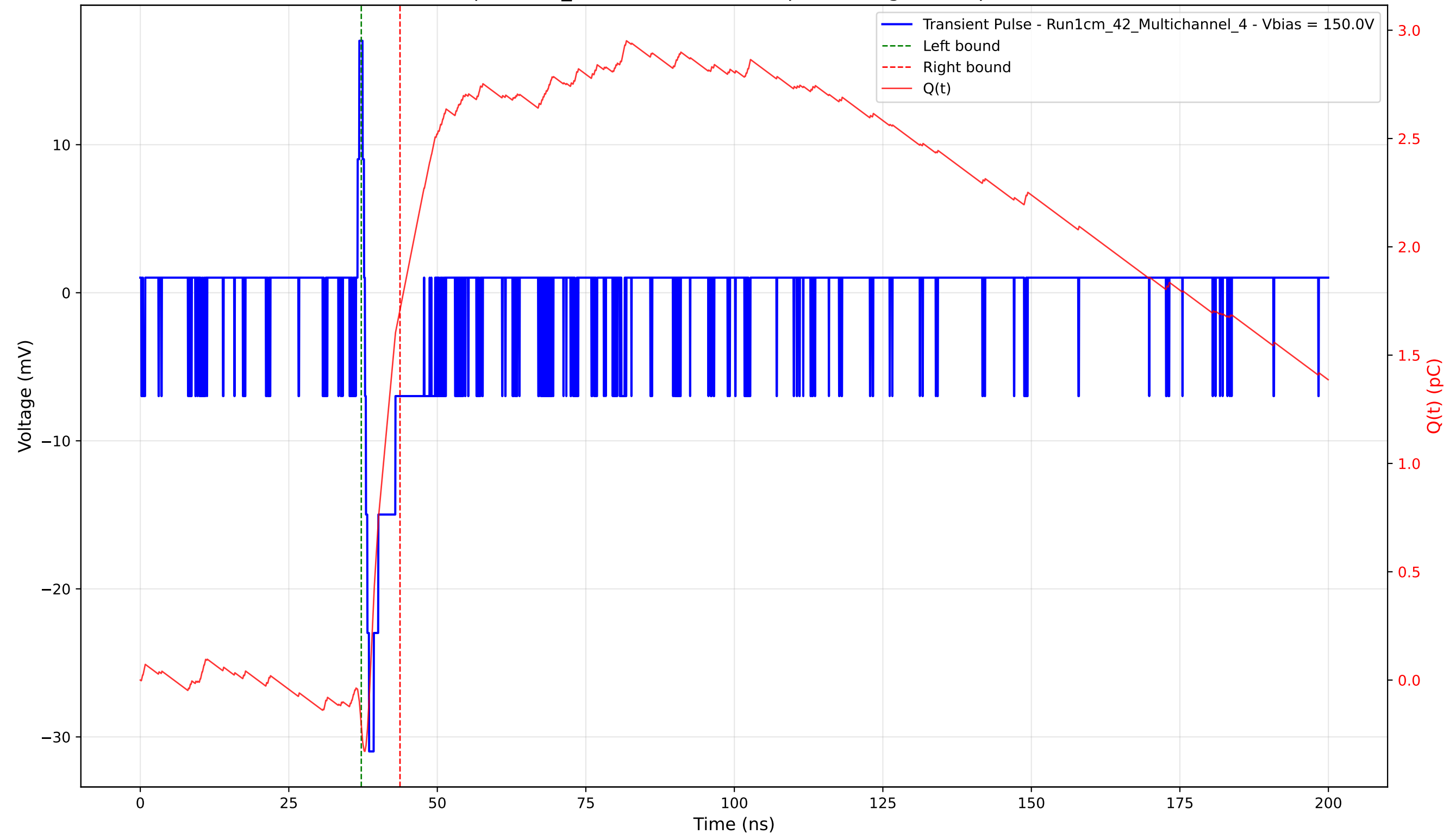
Transient Pulse - Sample: 1cm_42 - Position: 4620.0 \mu\text{m} - Charge: 1.92 pC - Rise Time: 0.71 ns
