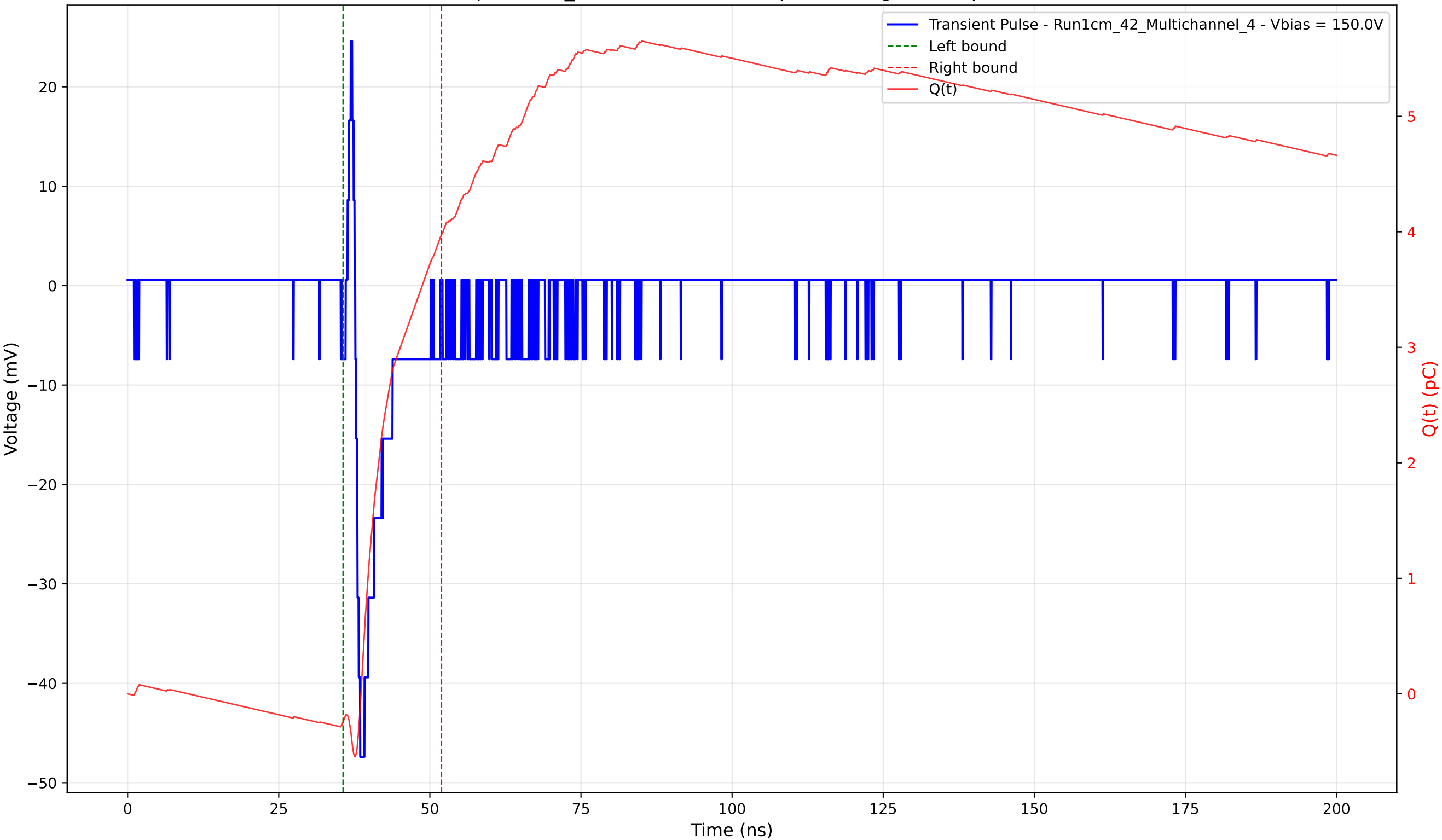
Transient Pulse - Sample: 1cm_42 - Position: 920.0 \mu\text{m} - Charge: 4.22 pC - Rise Time: 0.82 ns
