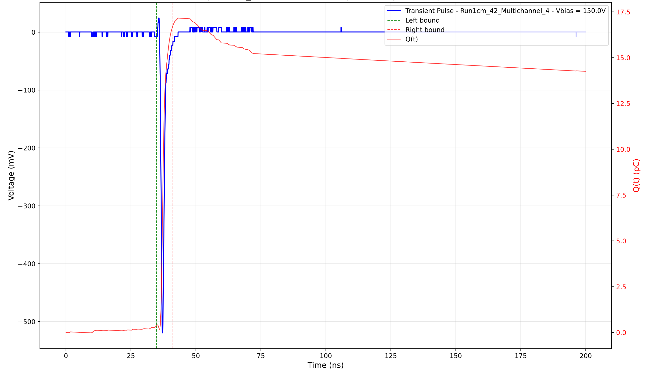
Transient Pulse - Sample: 1cm_42 - Position: 2380.0 \mu\text{m} - Charge: 16.24 pC - Rise Time: 0.72 ns
