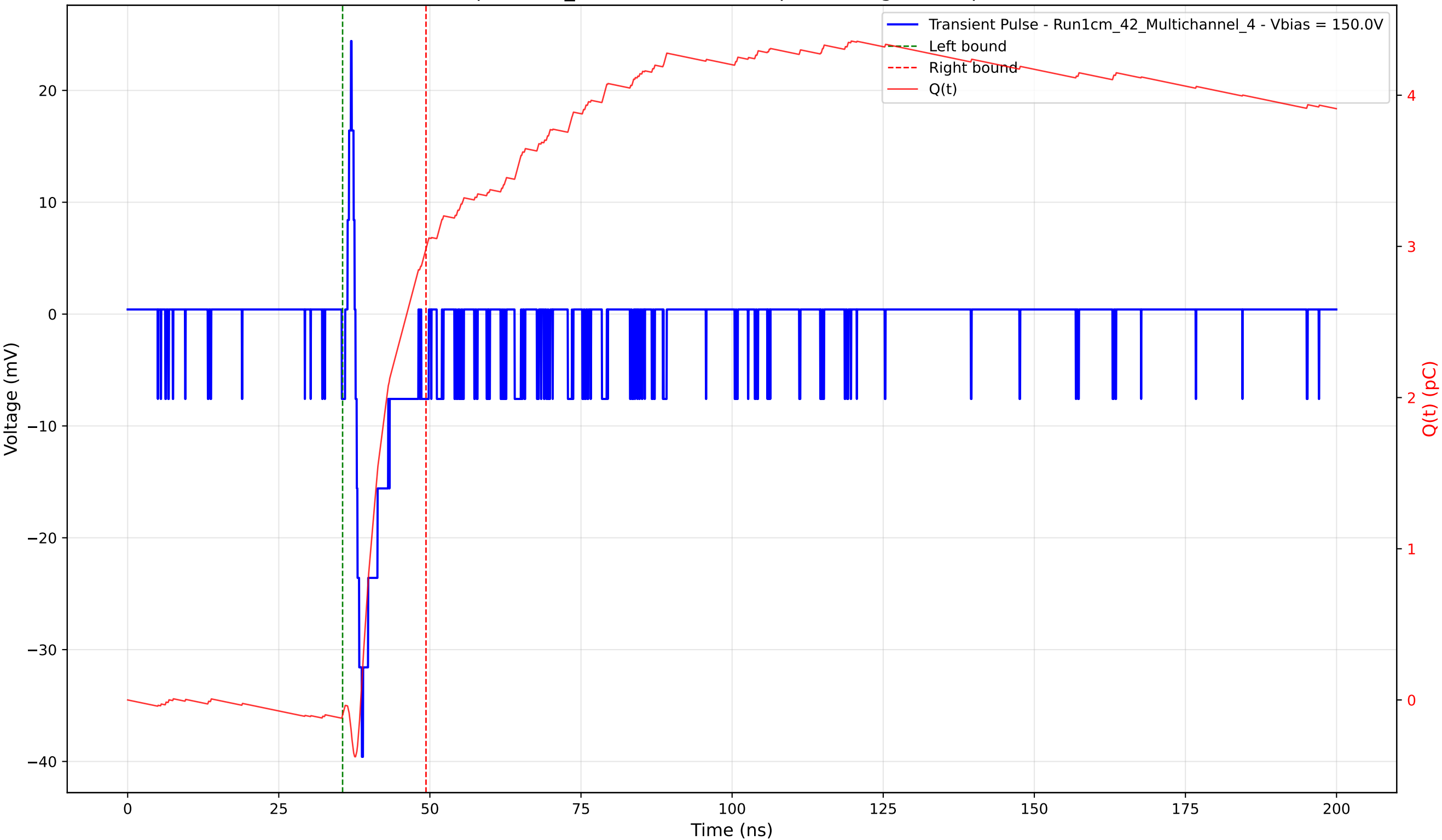
Transient Pulse - Sample: 1cm_42 - Position: 505.0 \mu\text{m} - Charge: 3.09 pC - Rise Time: 1.06 ns
