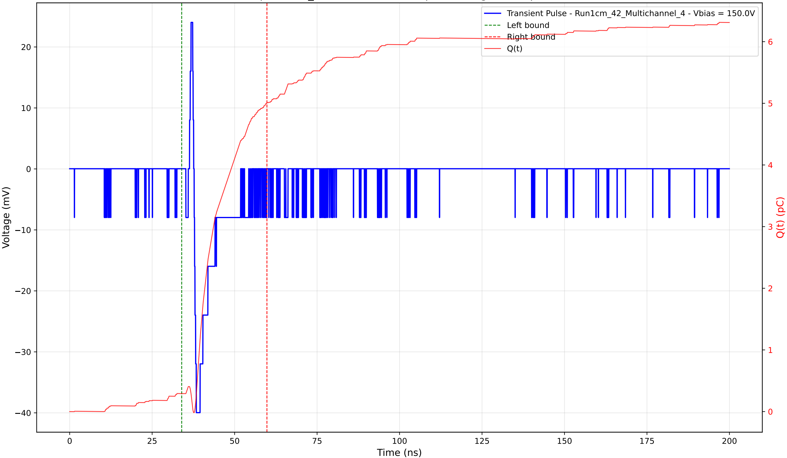
Transient Pulse - Sample: 1cm_42 - Position: 605.0 \mu\text{m} - Charge: 4.72 pC - Rise Time: 0.66 ns
