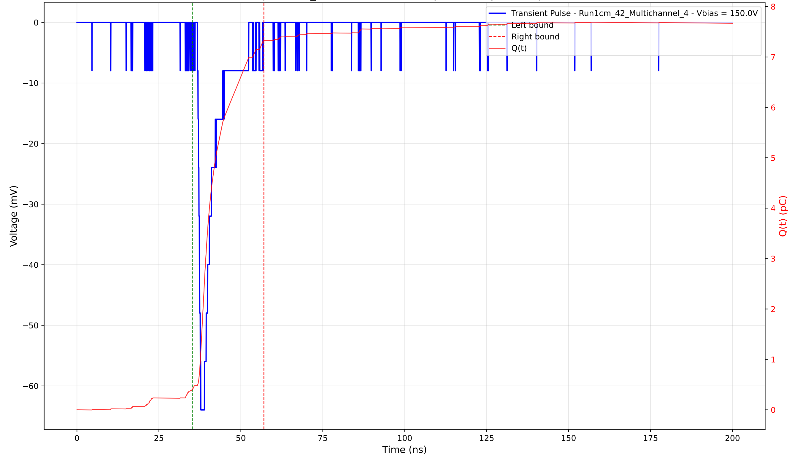
Transient Pulse - Sample: 1cm_42 - Position: 1455.0 \mu\text{m} - Charge: 6.92 pC - Rise Time: 1.05 ns
