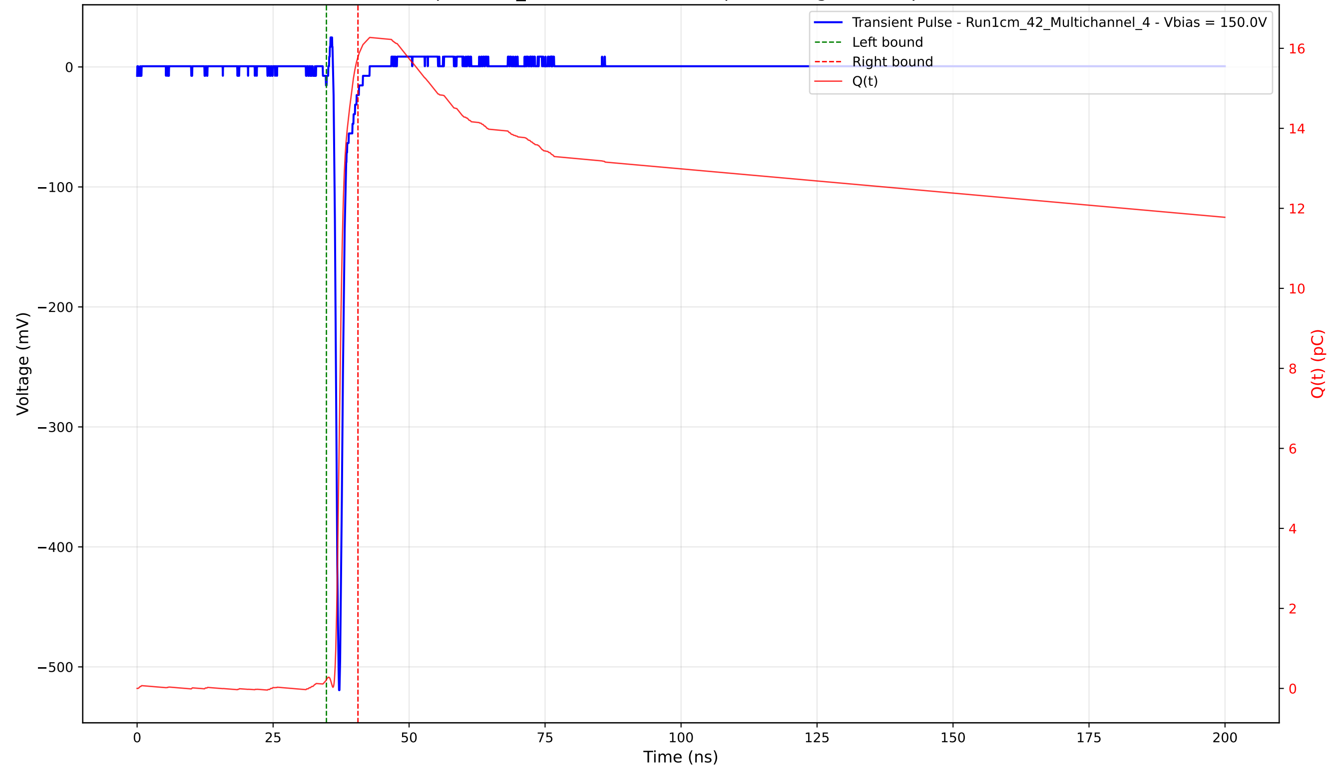
Transient Pulse - Sample: 1cm_42 - Position: 2520.0 \mu\text{m} - Charge: 15.56 pC - Rise Time: 0.72 ns
