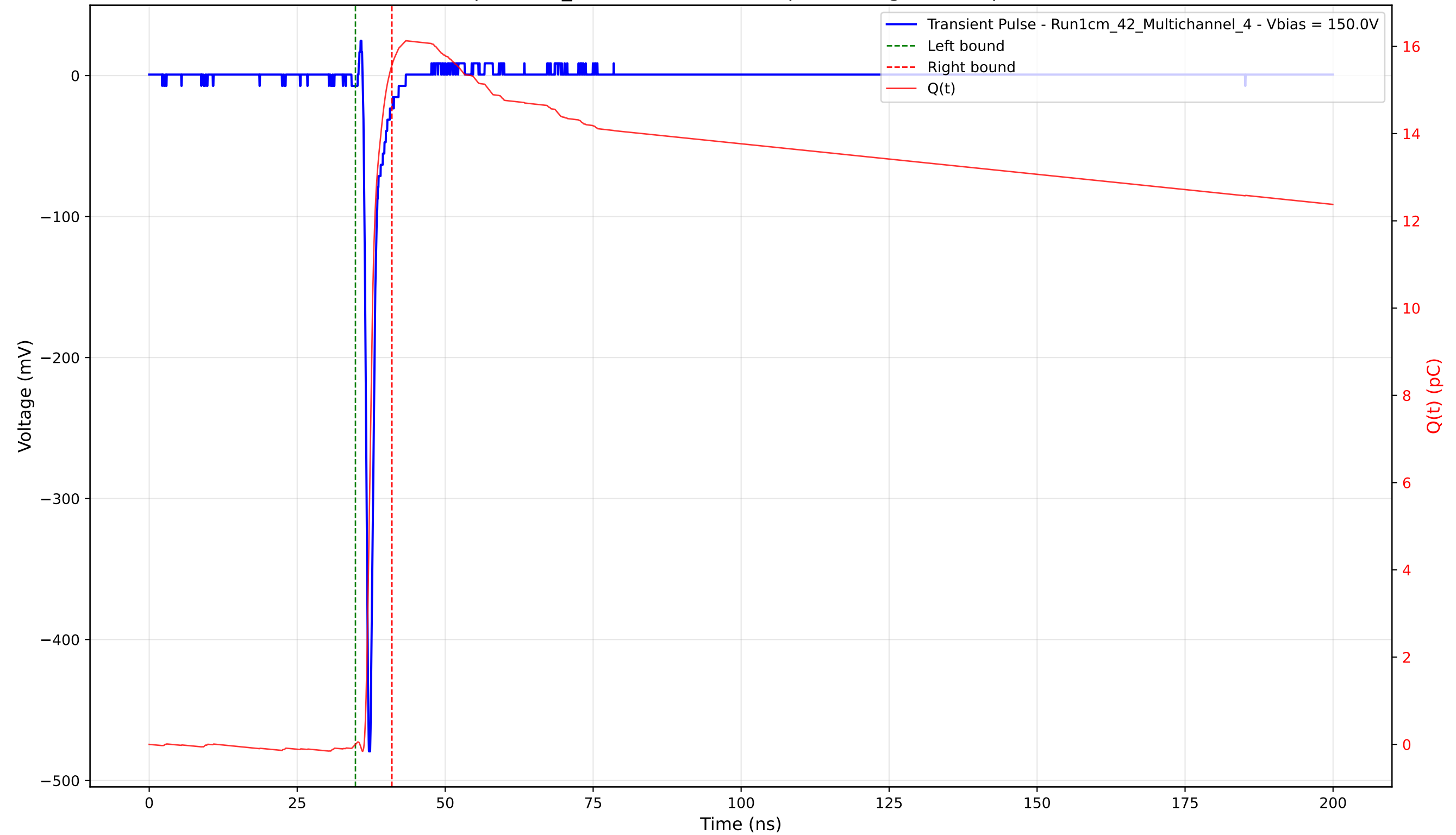
Transient Pulse - Sample: 1cm_42 - Position: 2750.0 \mu\text{m} - Charge: 15.57 pC - Rise Time: 0.68 ns
