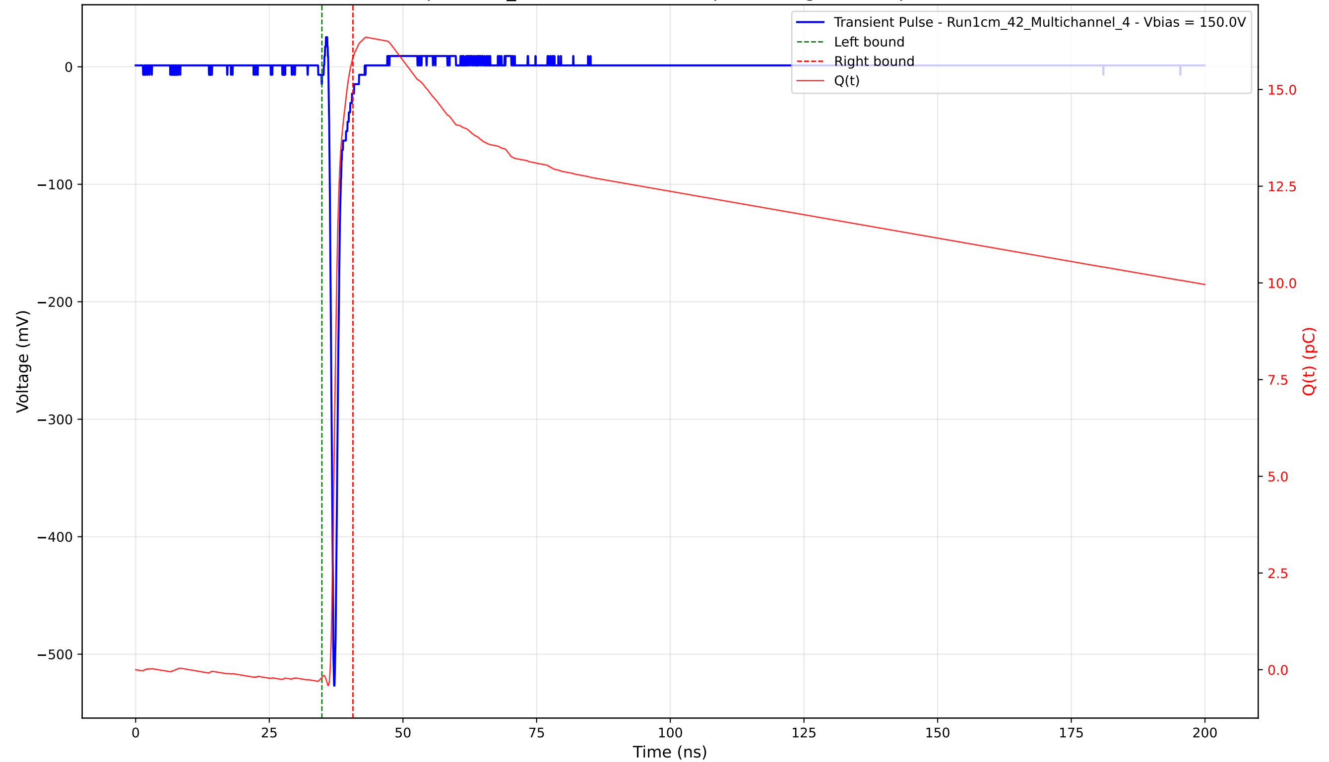
Transient Pulse - Sample: 1cm_42 - Position: 2630.0 \mu\text{m} - Charge: 16.02 pC - Rise Time: 0.71 ns
