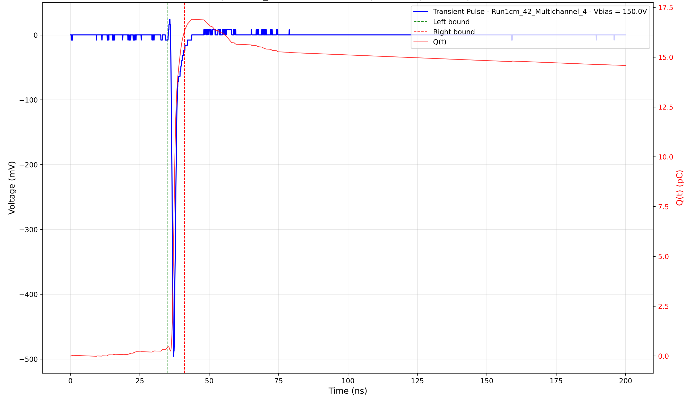
Transient Pulse - Sample: 1cm_42 - Position: 2730.0 \mu\text{m} - Charge: 15.86 pC - Rise Time: 0.71 ns
