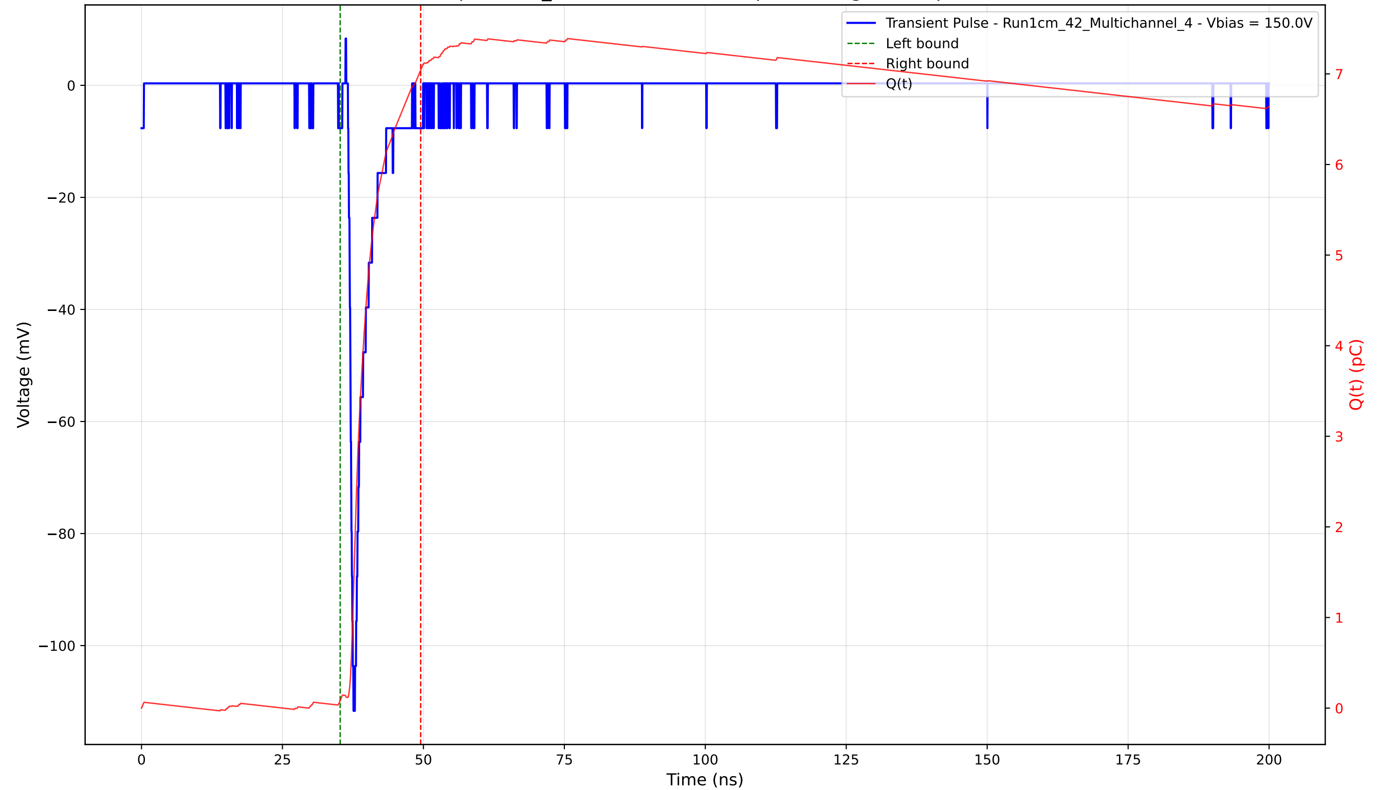
Transient Pulse - Sample: 1cm_42 - Position: 3385.0 \mu\text{m} - Charge: 6.96 pC - Rise Time: 0.78 ns
