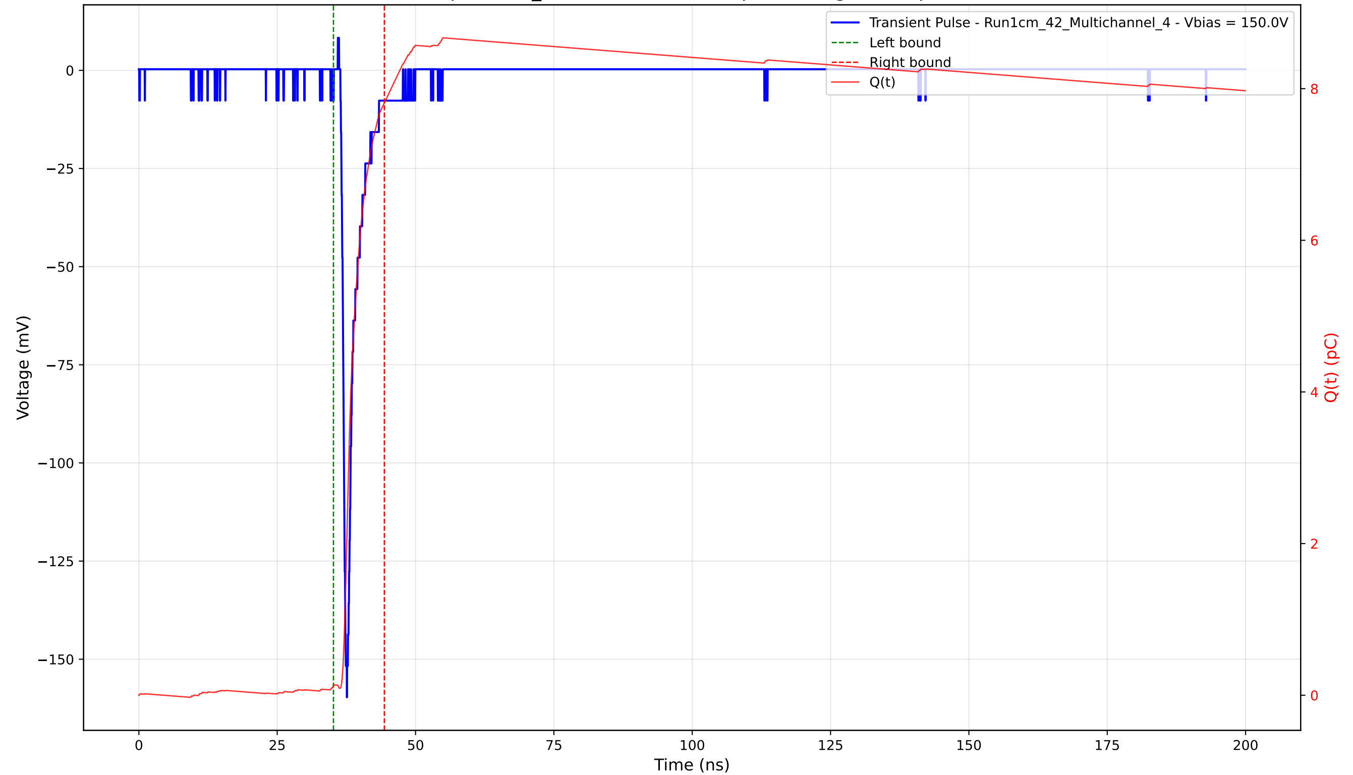
Transient Pulse - Sample: 1cm_42 - Position: 3180.0 \mu\text{m} - Charge: 7.68 pC - Rise Time: 0.84 ns
