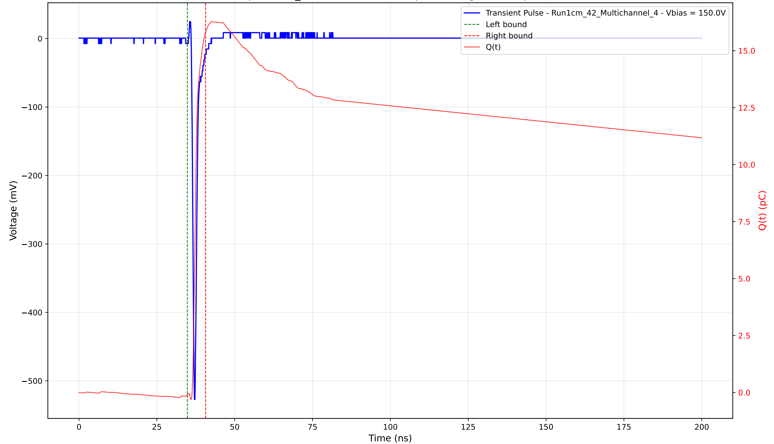
Transient Pulse - Sample: 1cm_42 - Position: 2565.0 \mu\text{m} - Charge: 15.89 pC - Rise Time: 0.71 ns
