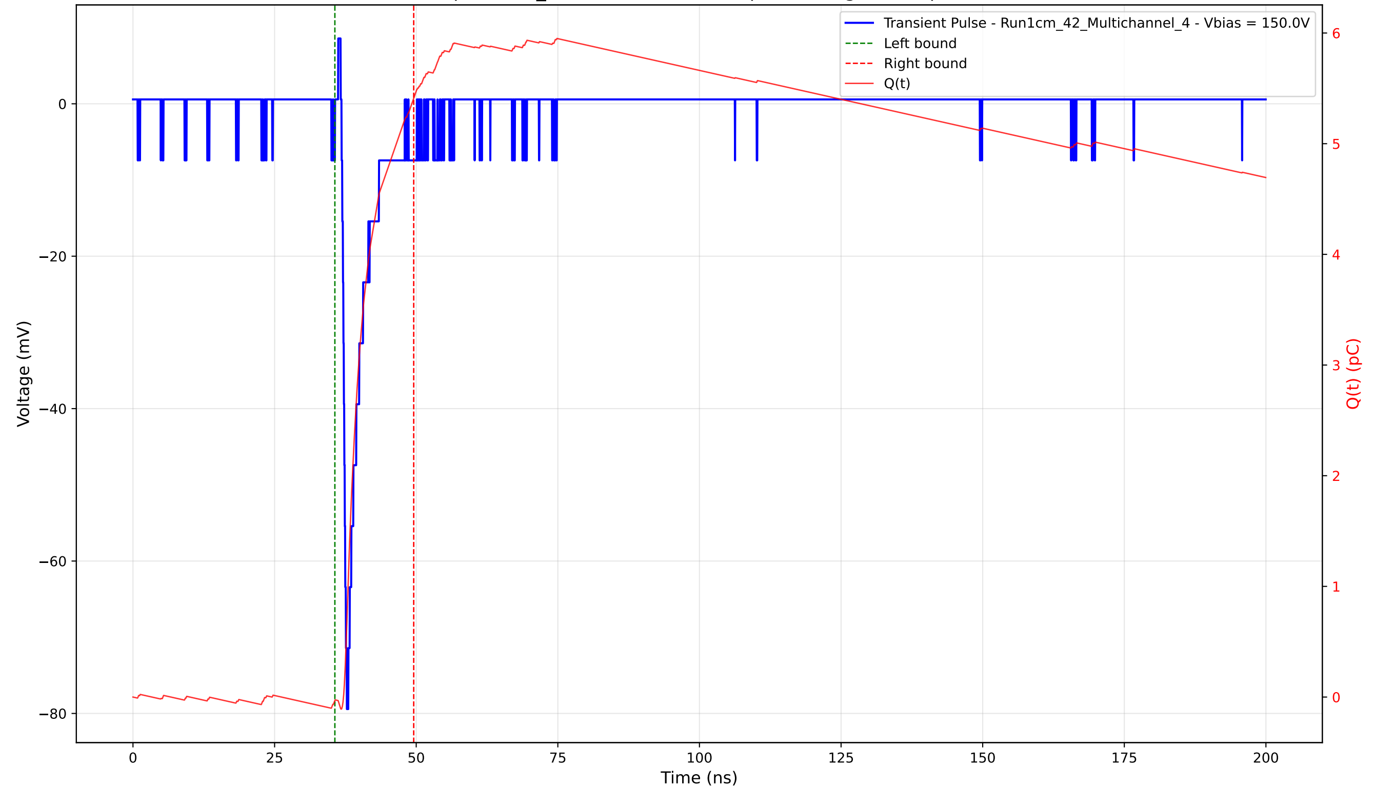
Transient Pulse - Sample: 1cm_42 - Position: 3500.0 \mu\text{m} - Charge: 5.44 pC - Rise Time: 0.84 ns
