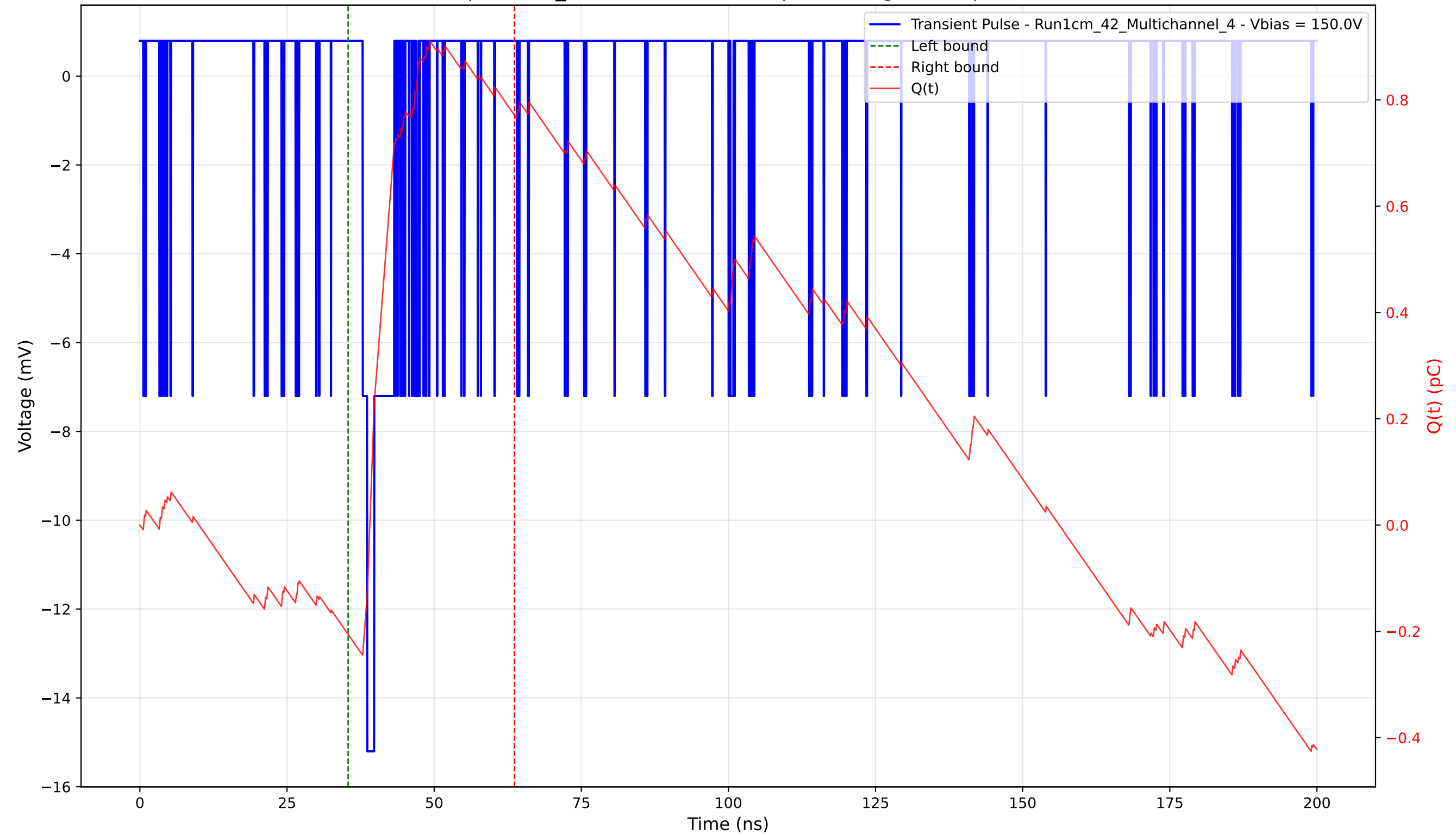
Transient Pulse - Sample: 1cm_42 - Position: 5065.0 \mu\text{m} - Charge: 0.98 pC - Rise Time: 0.80 ns
