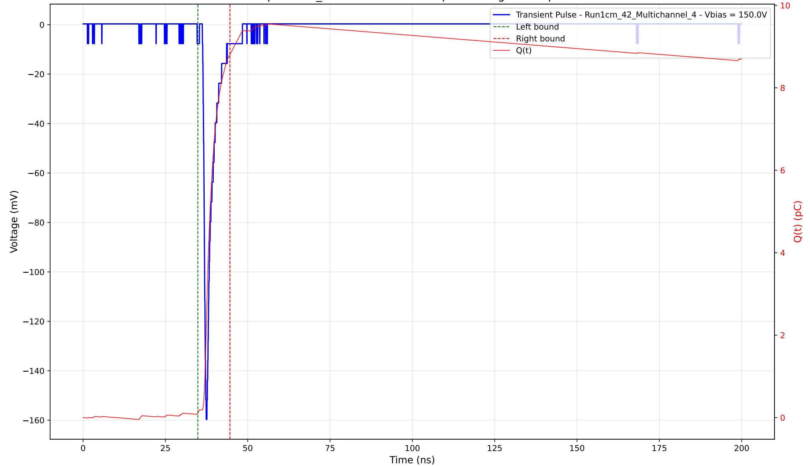
Transient Pulse - Sample: 1cm_42 - Position: 1865.0 \mu\text{m} - Charge: 8.69 pC - Rise Time: 0.88 ns
