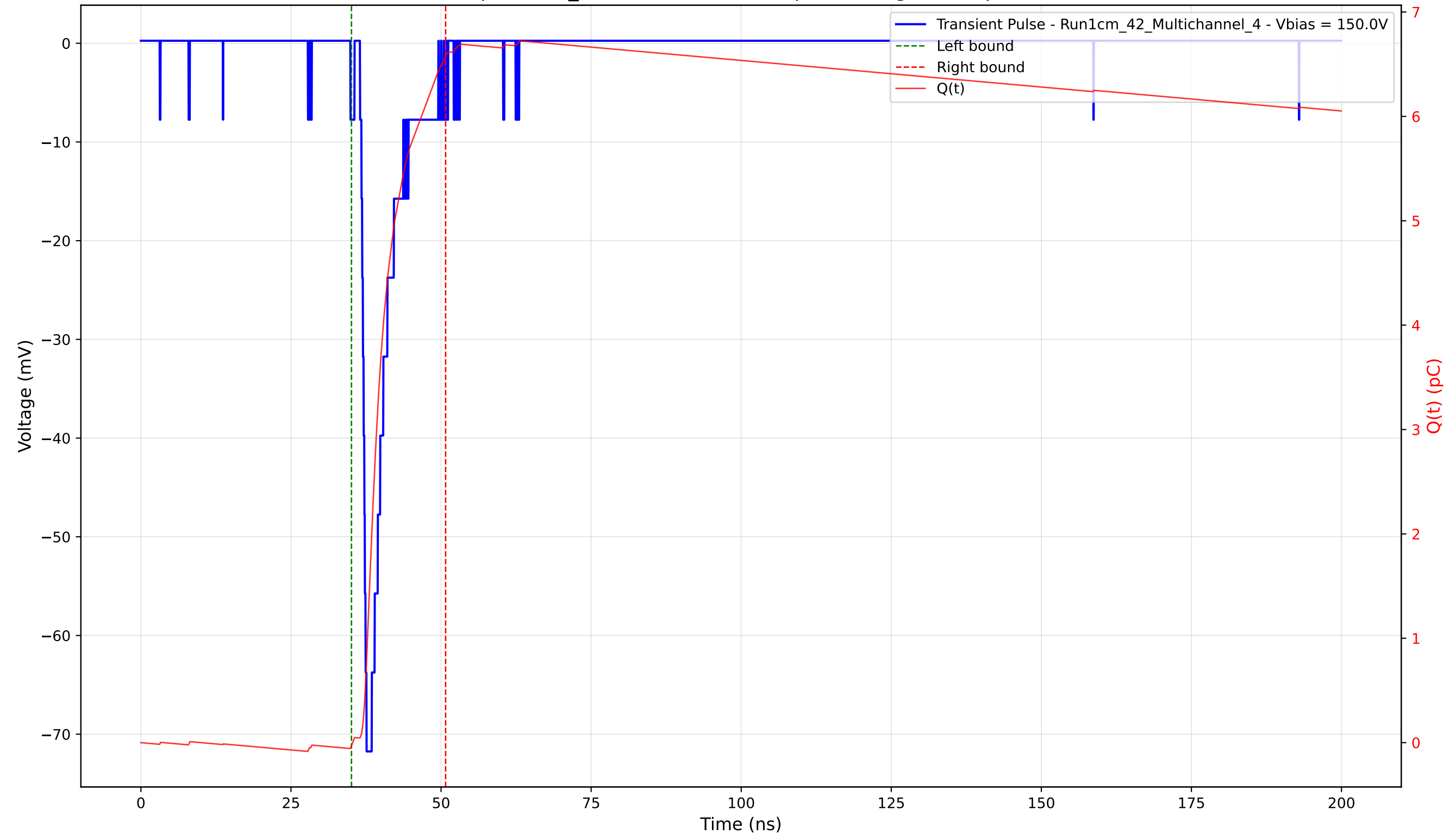
Transient Pulse - Sample: 1cm_42 - Position: 1530.0 \mu\text{m} - Charge: 6.61 pC - Rise Time: 1.08 ns
