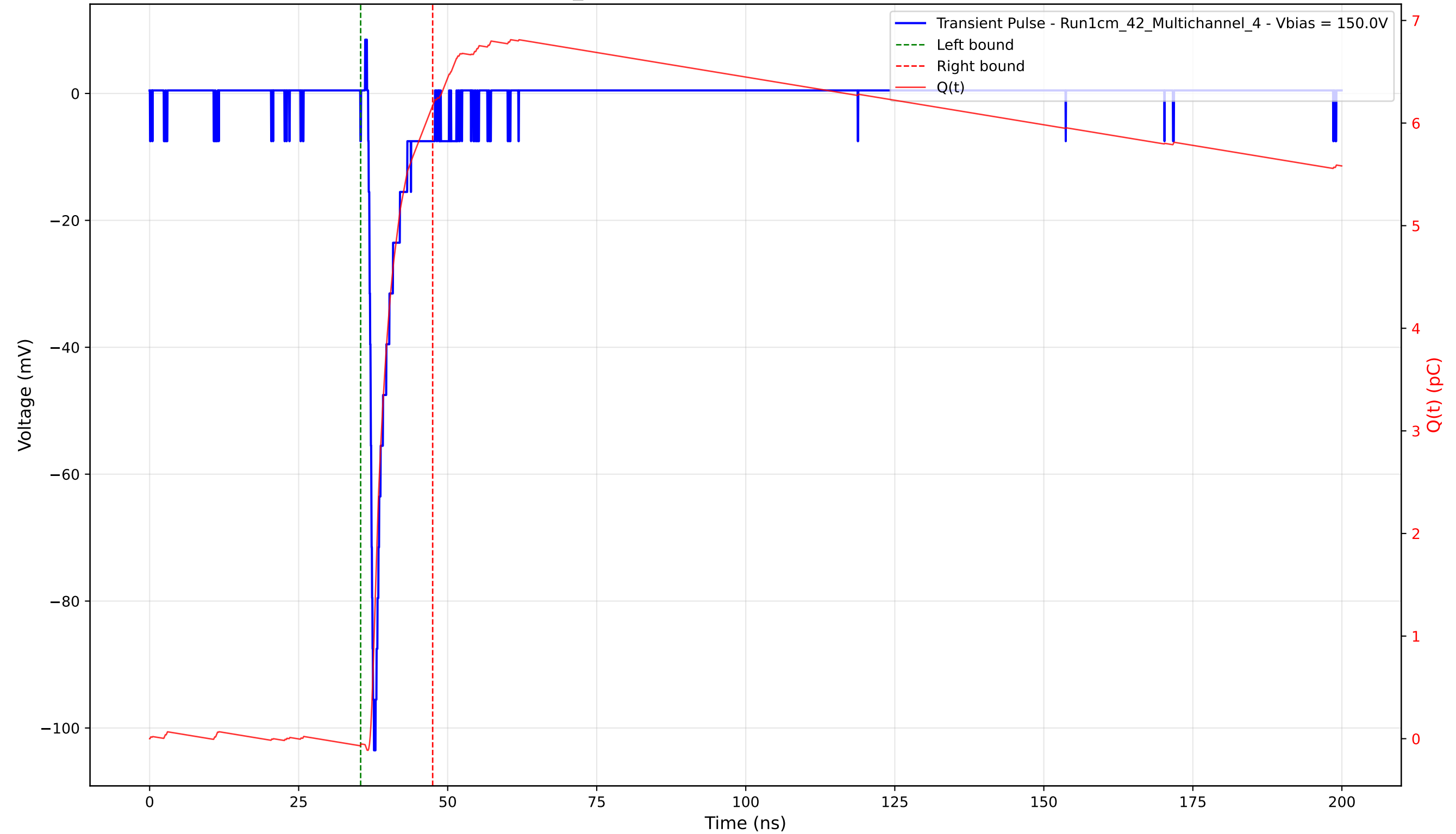
Transient Pulse - Sample: 1cm_42 - Position: 3410.0 \mu\text{m} - Charge: 6.23 pC - Rise Time: 0.75 ns
