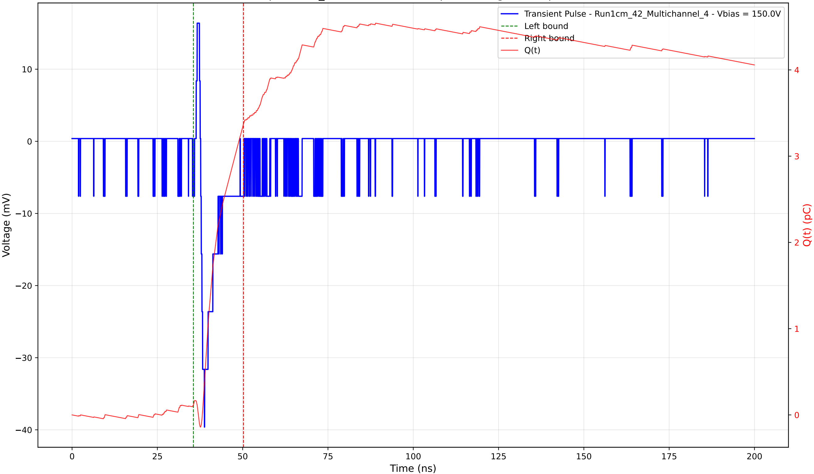
Transient Pulse - Sample: 1cm_42 - Position: 510.0 \mu\text{m} - Charge: 3.26 pC - Rise Time: 1.10 ns
