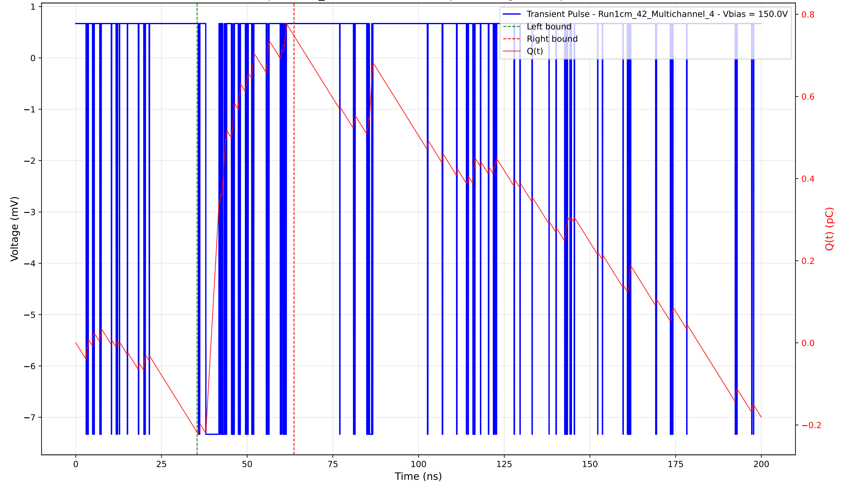
Transient Pulse - Sample: 1cm_42 - Position: 5125.0 \mu\text{m} - Charge: 0.97 pC - Rise Time: 0.04 ns
