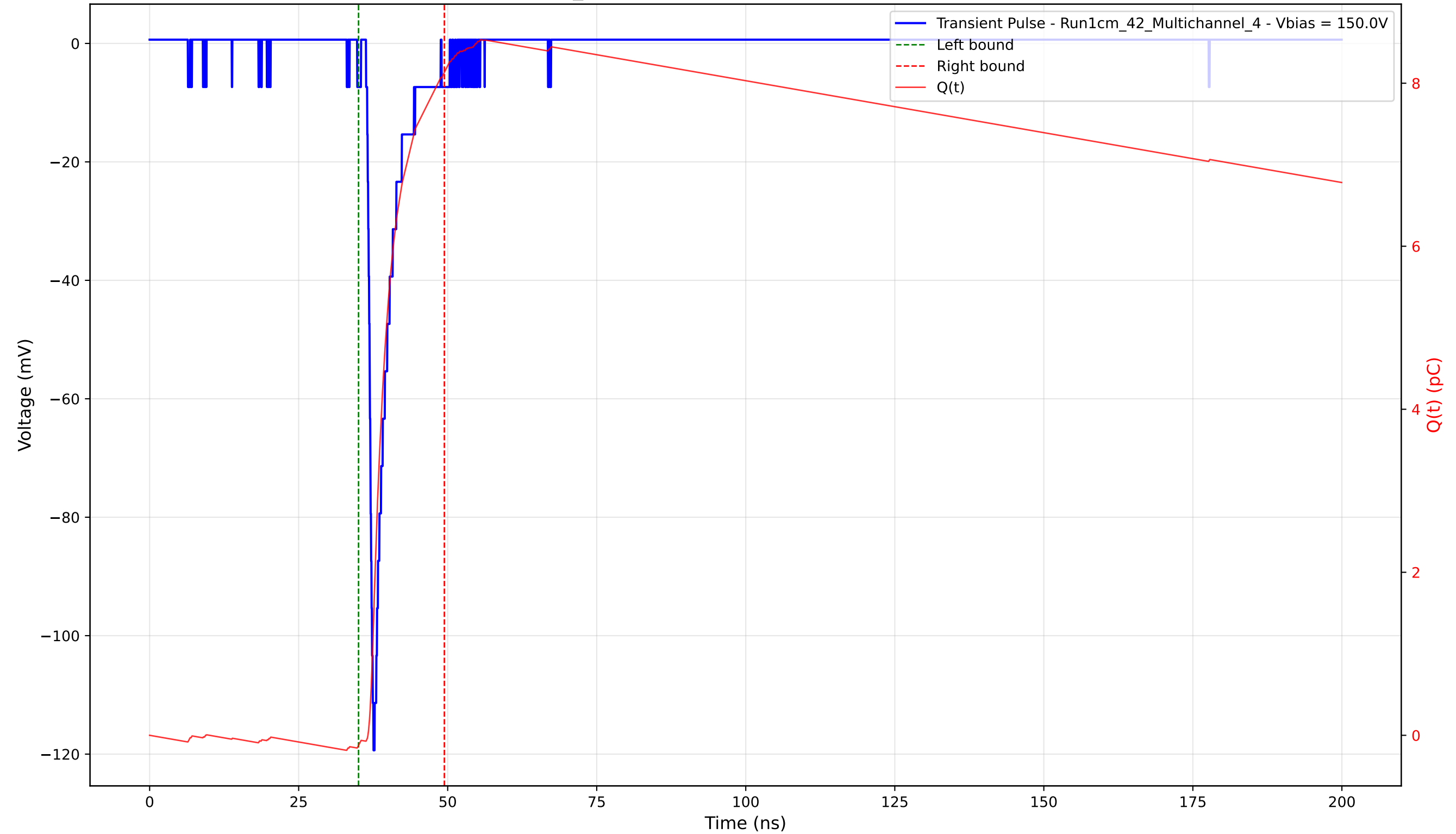
Transient Pulse - Sample: 1cm_42 - Position: 1655.0 \mu\text{m} - Charge: 8.26 pC - Rise Time: 0.94 ns
