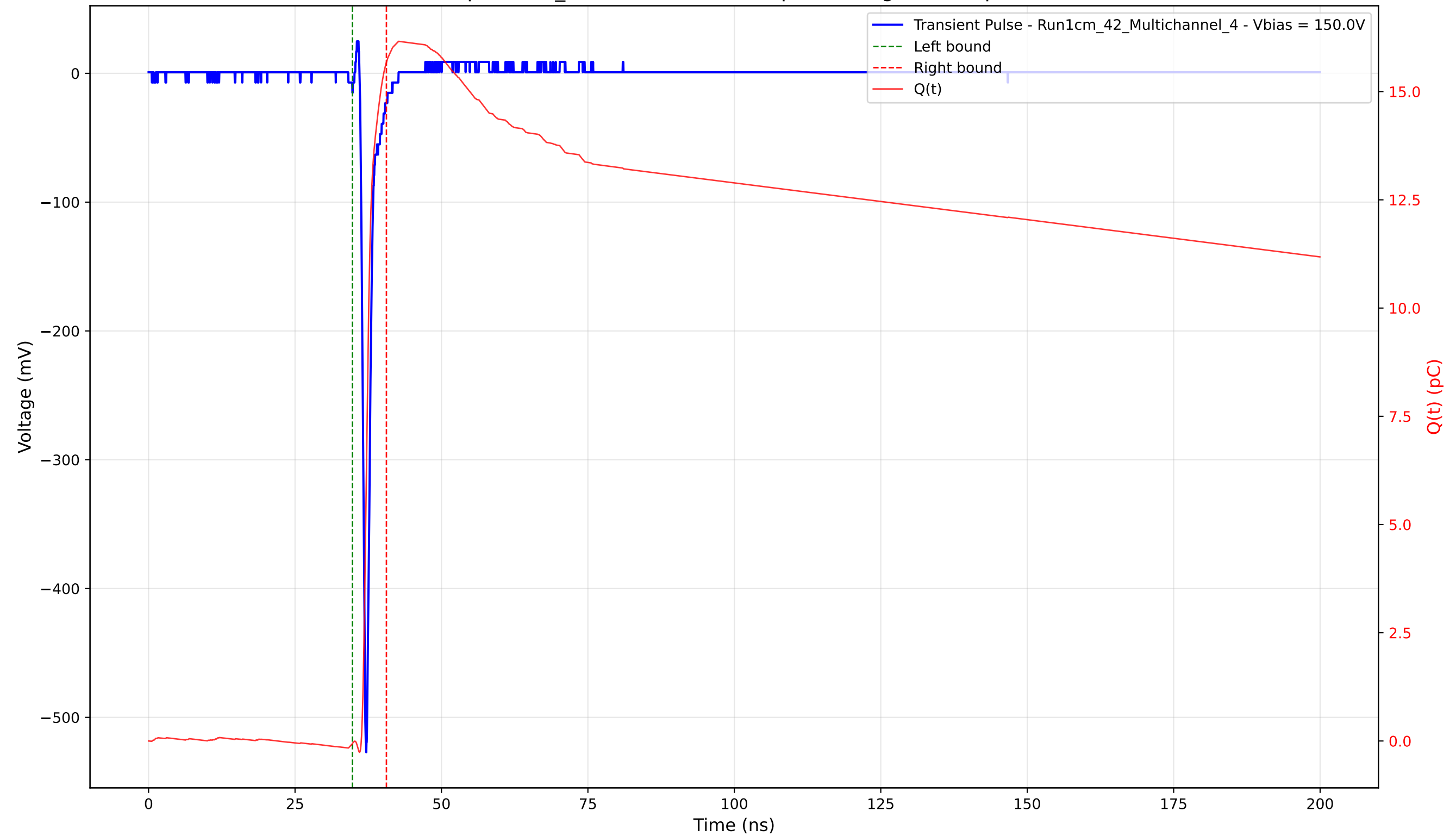
Transient Pulse - Sample: 1cm_42 - Position: 2475.0 \mu\text{m} - Charge: 15.74 pC - Rise Time: 0.71 ns
