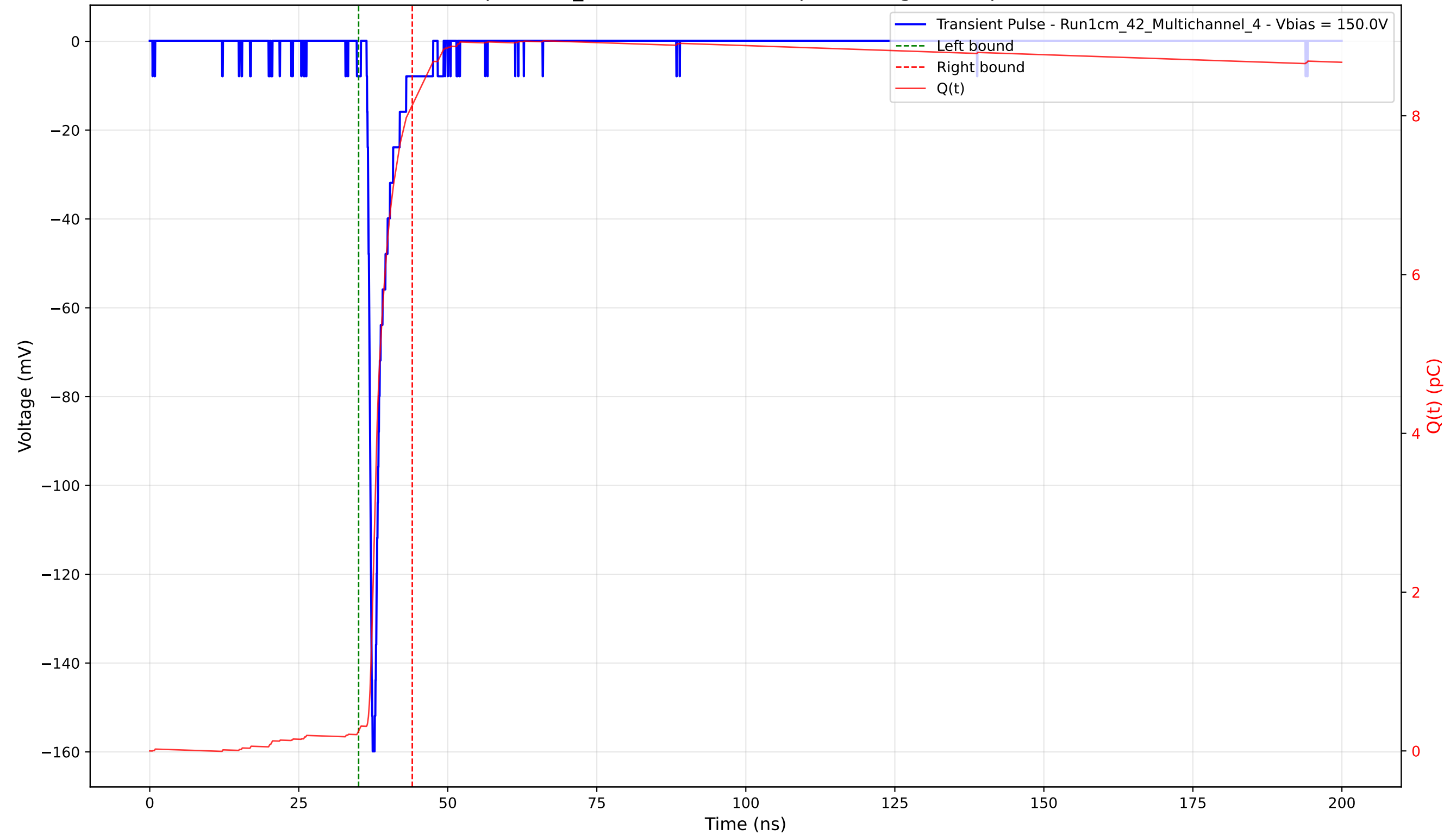
Transient Pulse - Sample: 1cm_42 - Position: 3160.0 \mu\text{m} - Charge: 7.88 pC - Rise Time: 0.80 ns
