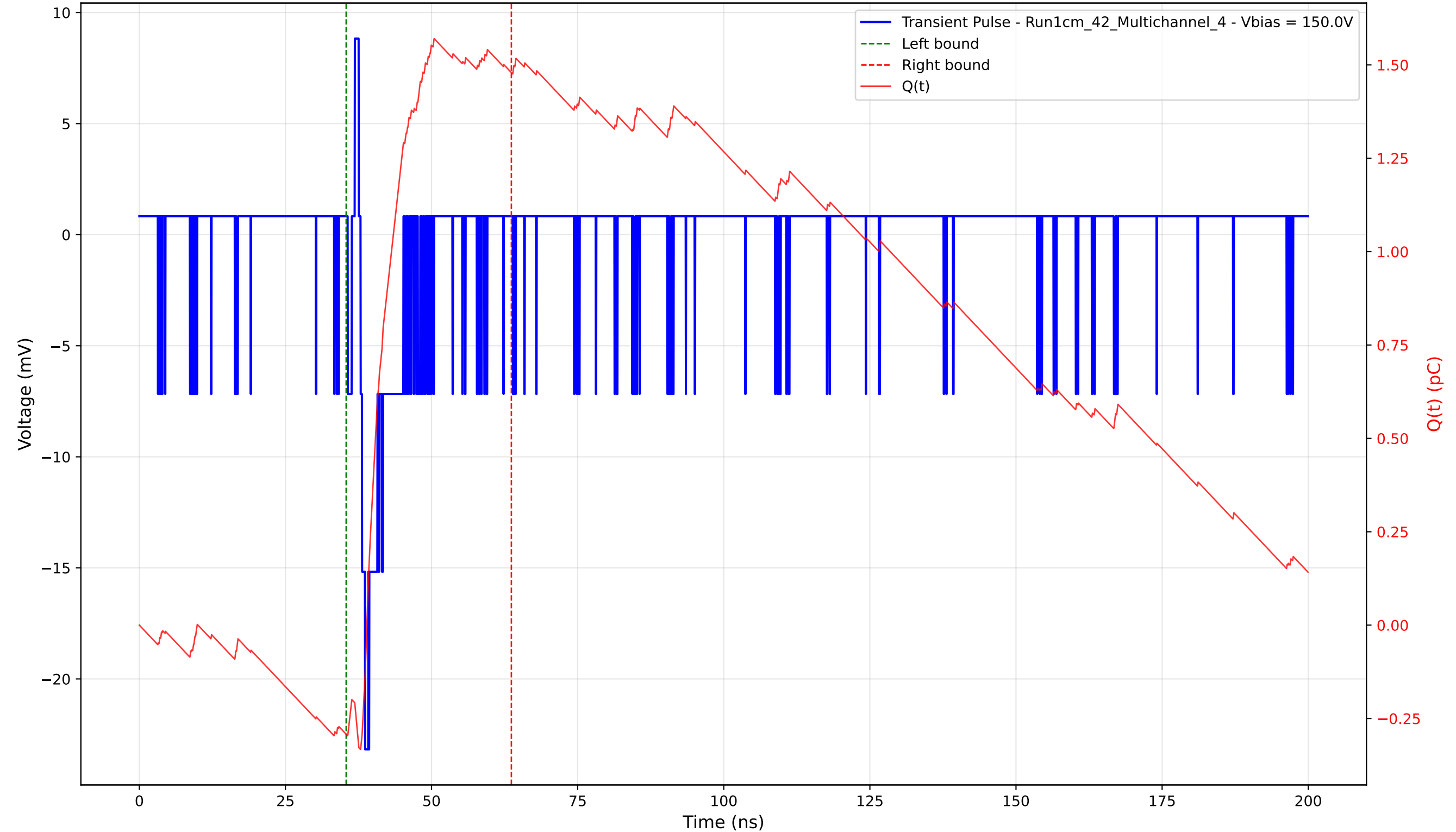
Transient Pulse - Sample: 1cm_42 - Position: 4985.0 \mu\text{m} - Charge: 1.77 pC - Rise Time: 0.79 ns
