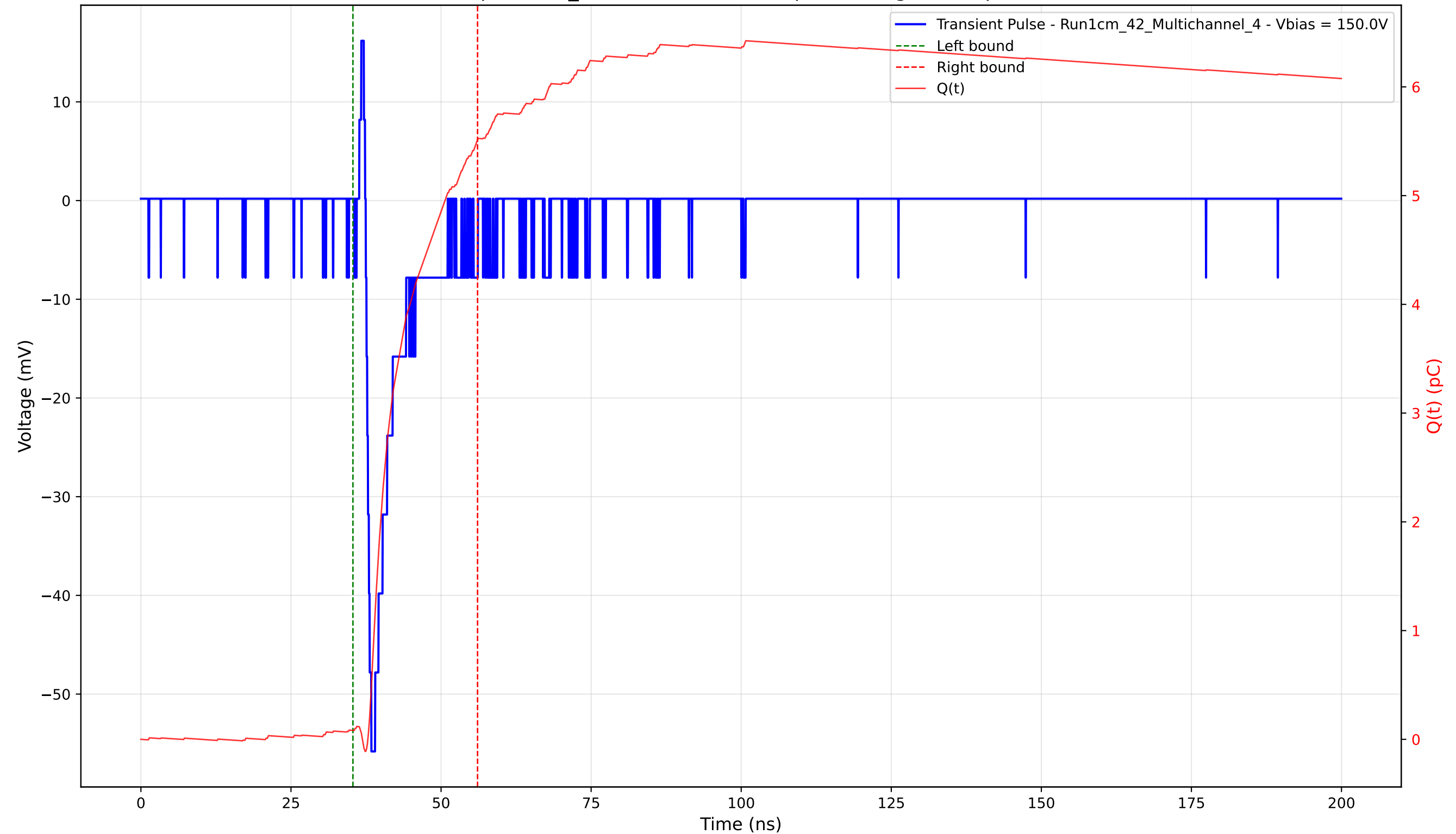
Transient Pulse - Sample: 1cm_42 - Position: 1090.0 \mu\text{m} - Charge: 5.43 pC - Rise Time: 0.93 ns
