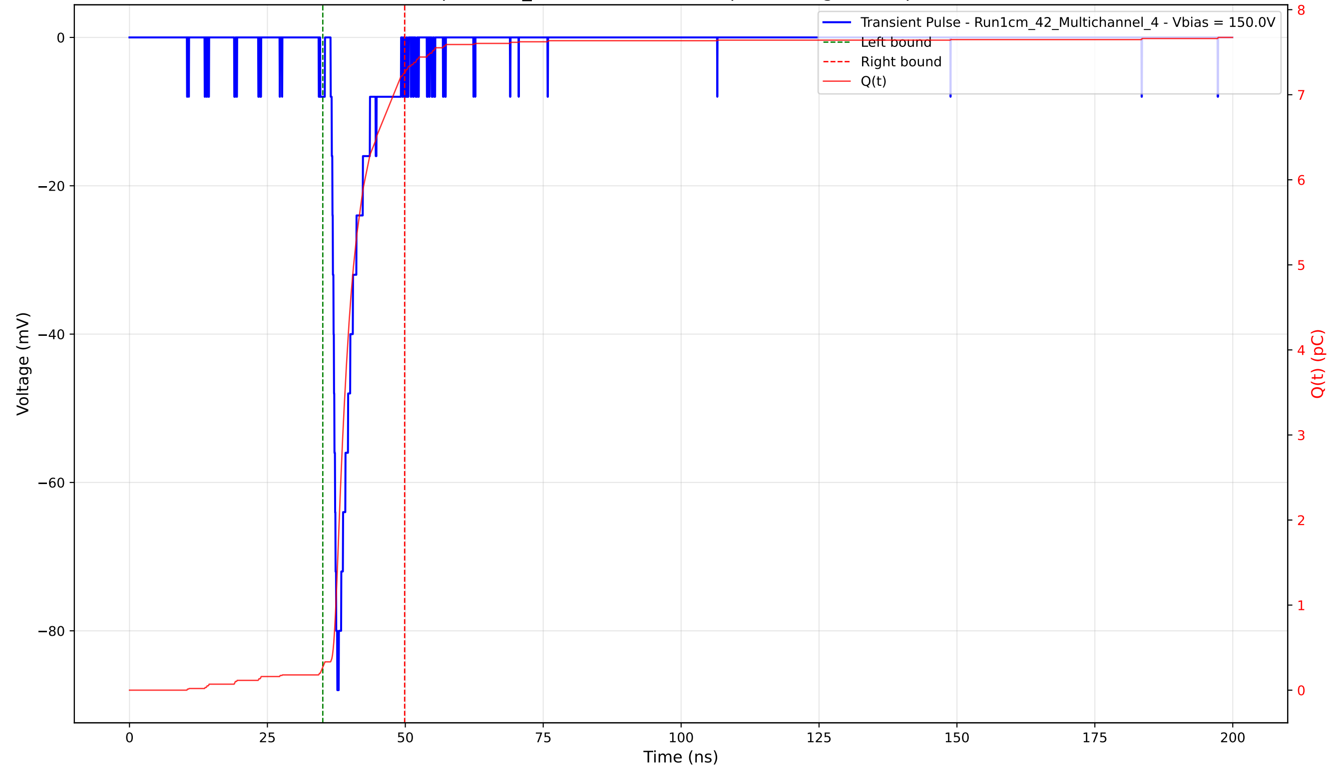
Transient Pulse - Sample: 1cm_42 - Position: 1565.0 \mu\text{m} - Charge: 6.98 pC - Rise Time: 0.84 ns
