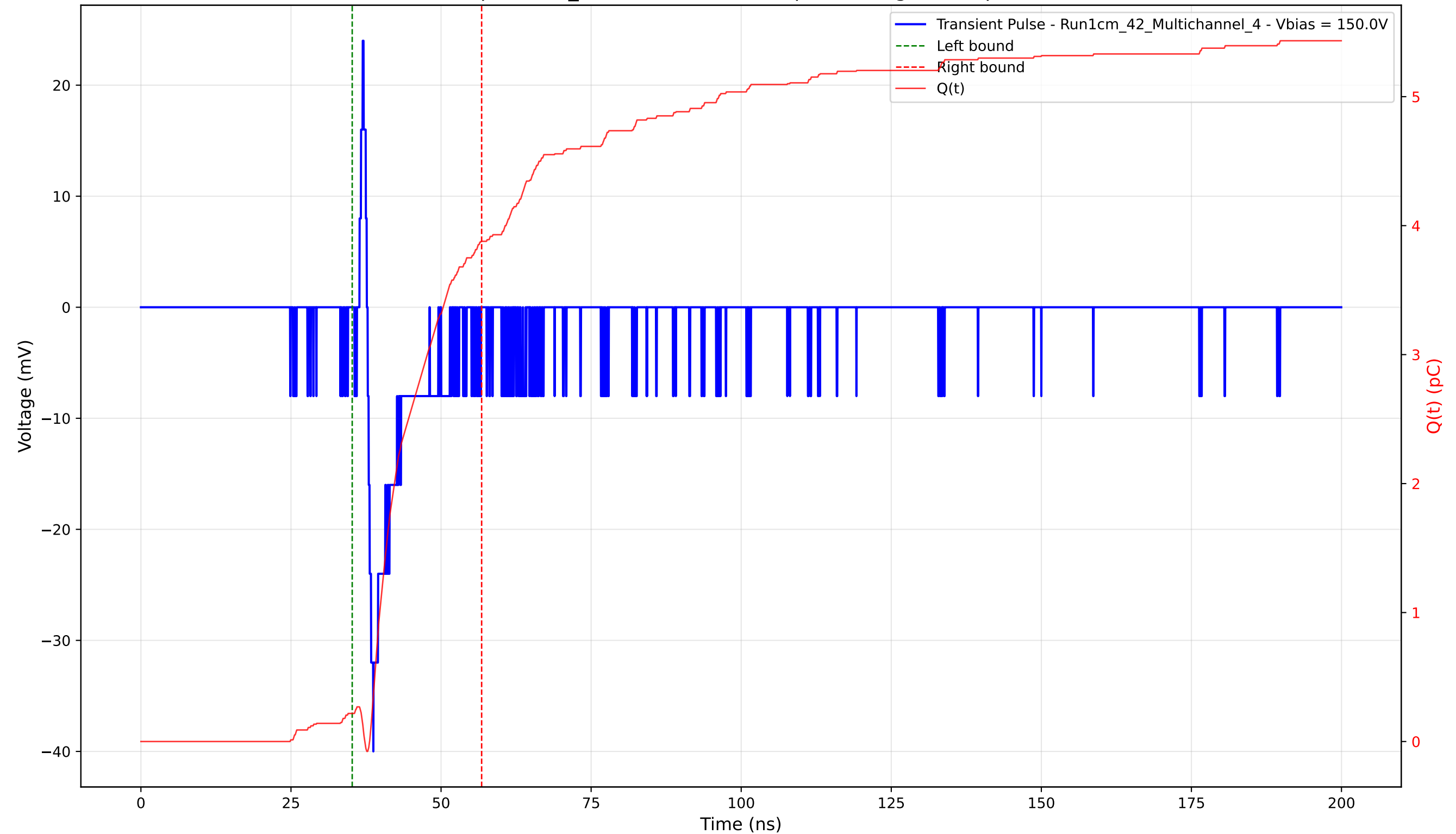
Transient Pulse - Sample: 1cm_42 - Position: 4425.0 \mu\text{m} - Charge: 3.66 pC - Rise Time: 0.94 ns
