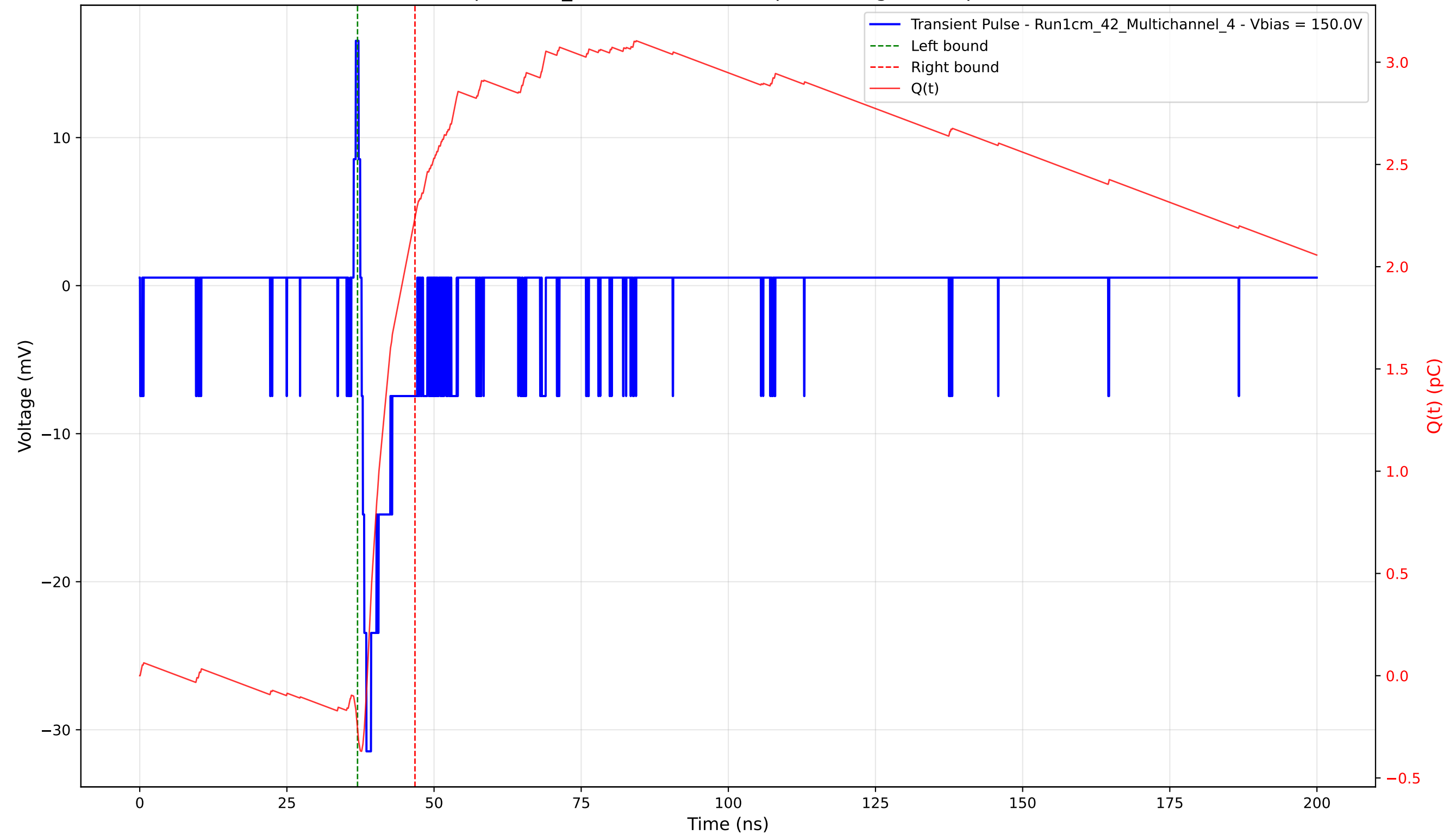
Transient Pulse - Sample: 1cm_42 - Position: 415.0 \mu\text{m} - Charge: 2.50 pC - Rise Time: 0.82 ns
