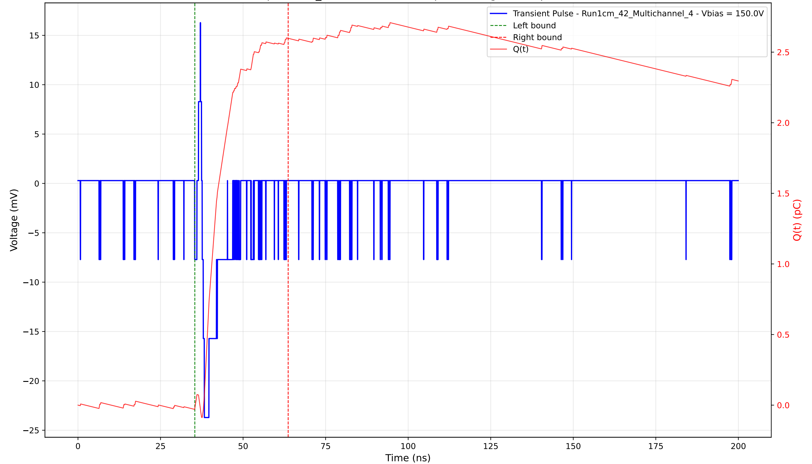
Transient Pulse - Sample: 1cm_42 - Position: 335.0 \mu\text{m} - Charge: 2.62 pC - Rise Time: 0.67 ns
