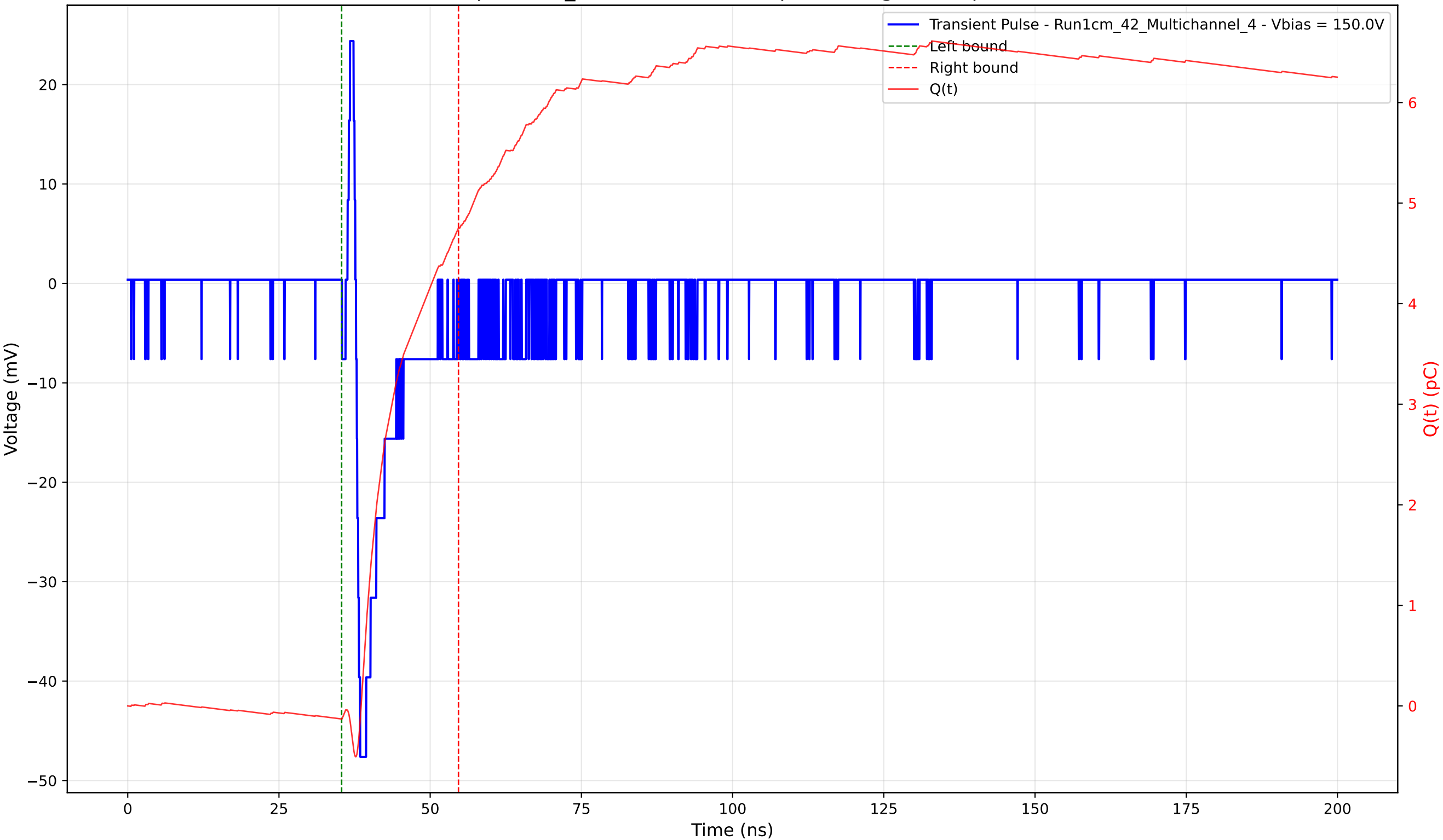
Transient Pulse - Sample: 1cm_42 - Position: 730.0 \mu\text{m} - Charge: 4.88 pC - Rise Time: 0.70 ns
