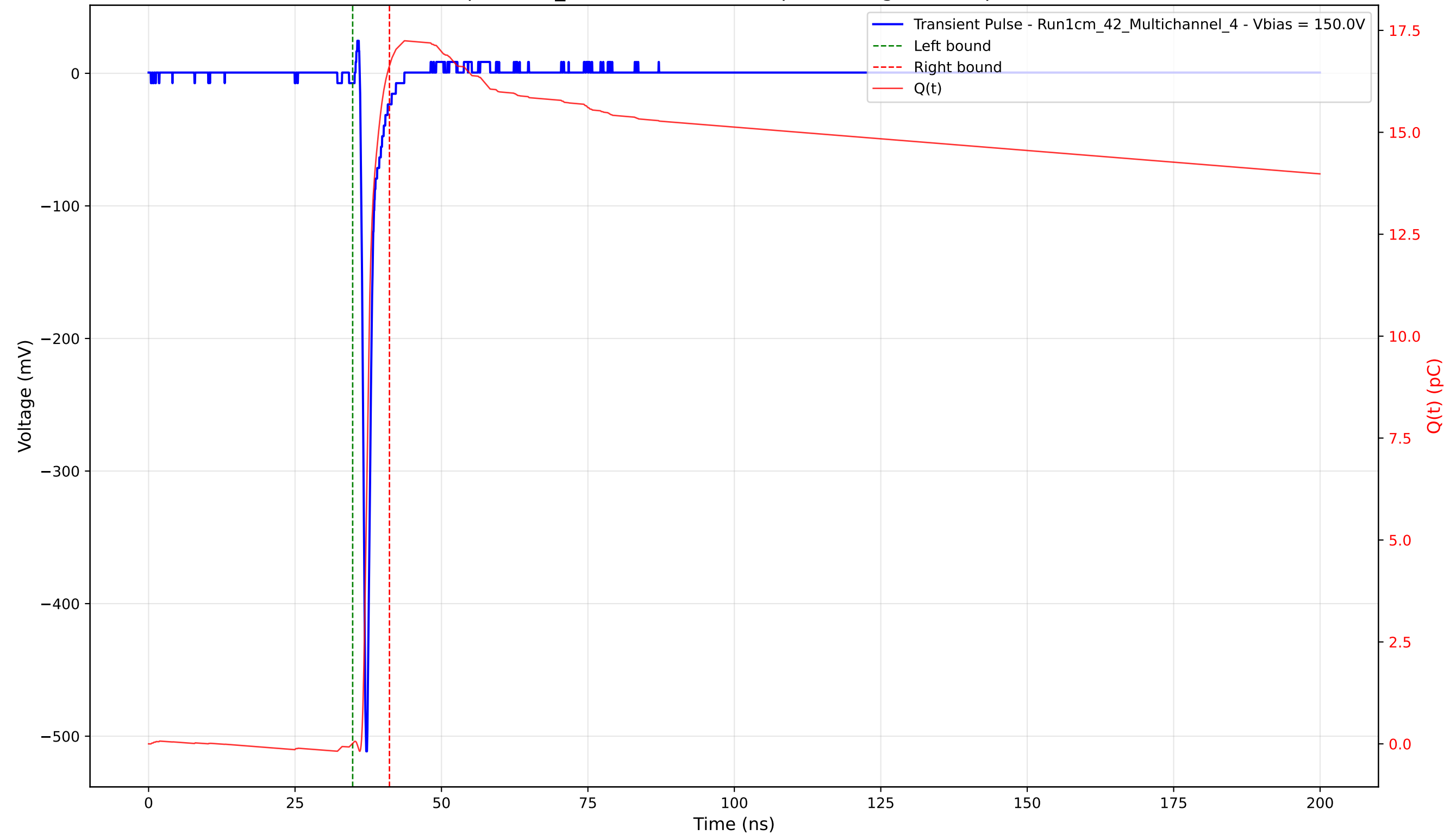
Transient Pulse - Sample: 1cm_42 - Position: 2255.0 \mu\text{m} - Charge: 16.62 pC - Rise Time: 0.72 ns
