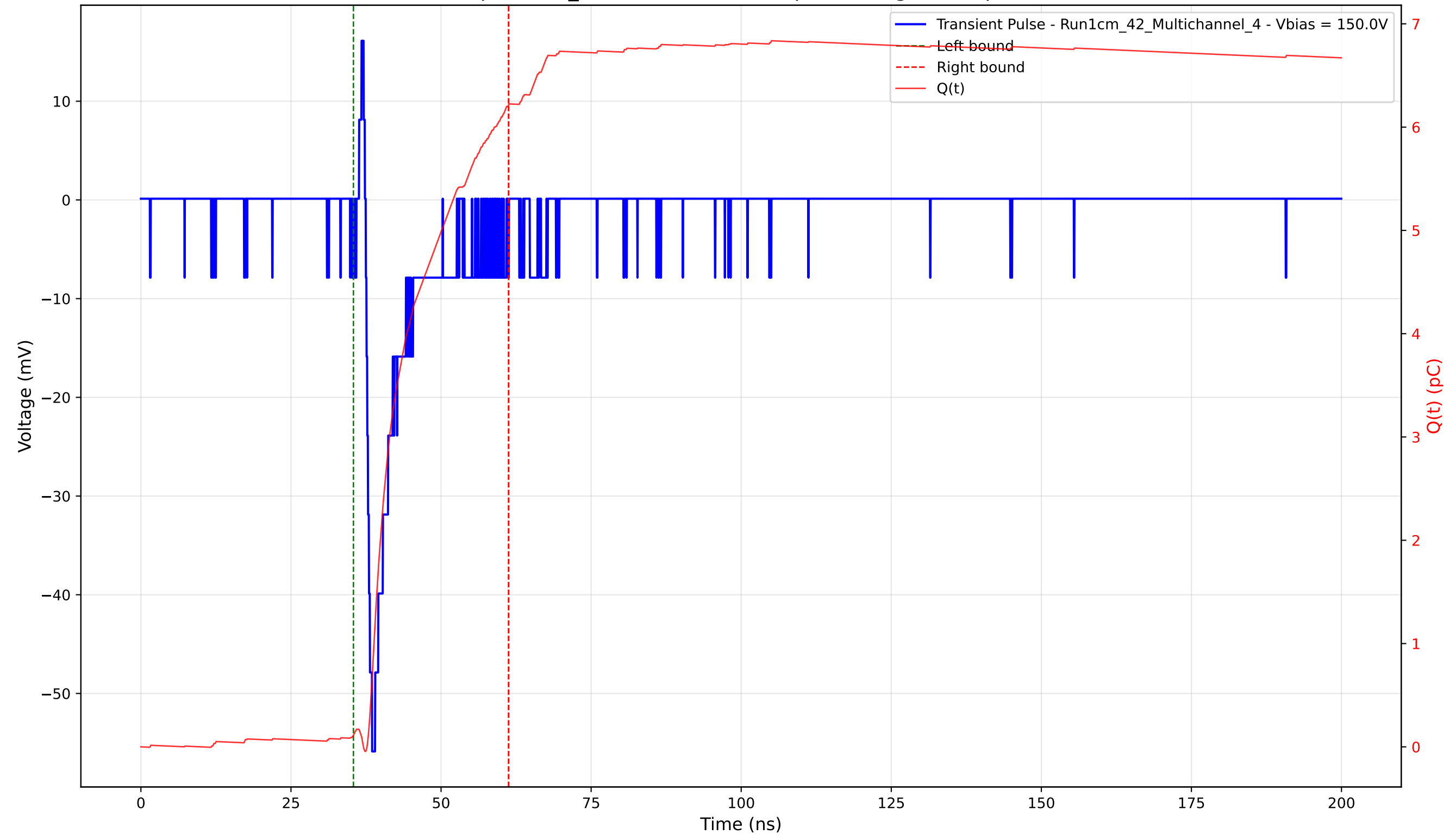
Transient Pulse - Sample: 1cm_42 - Position: 1085.0 \mu\text{m} - Charge: 6.10 pC - Rise Time: 1.05 ns
