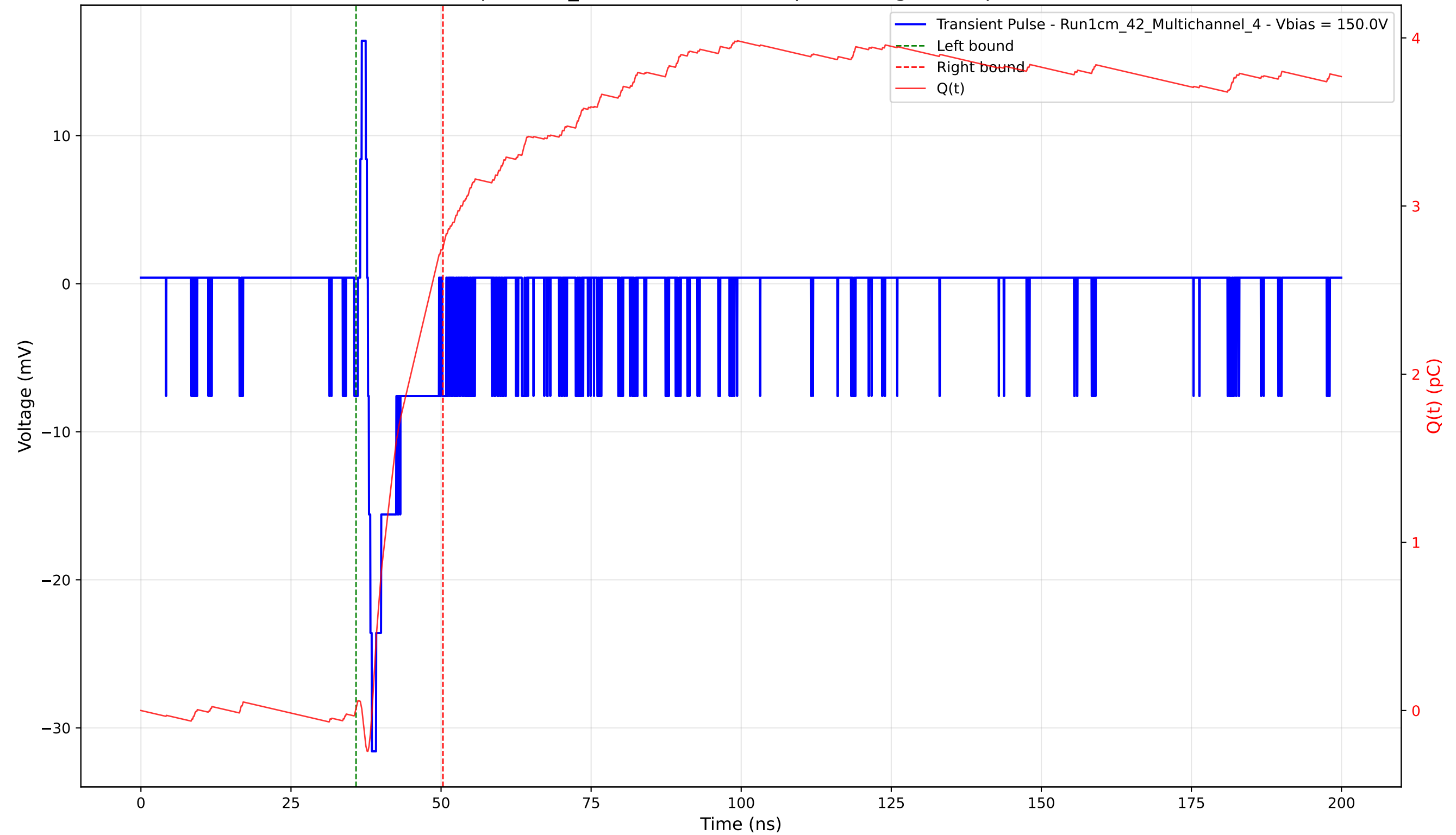
Transient Pulse - Sample: 1cm_42 - Position: 4515.0 \mu\text{m} - Charge: 2.74 pC - Rise Time: 0.66 ns
