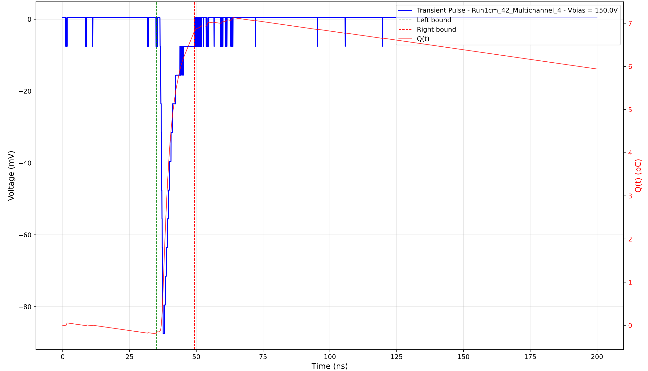
Transient Pulse - Sample: 1cm_42 - Position: 1570.0 \mu\text{m} - Charge: 6.98 pC - Rise Time: 0.83 ns
