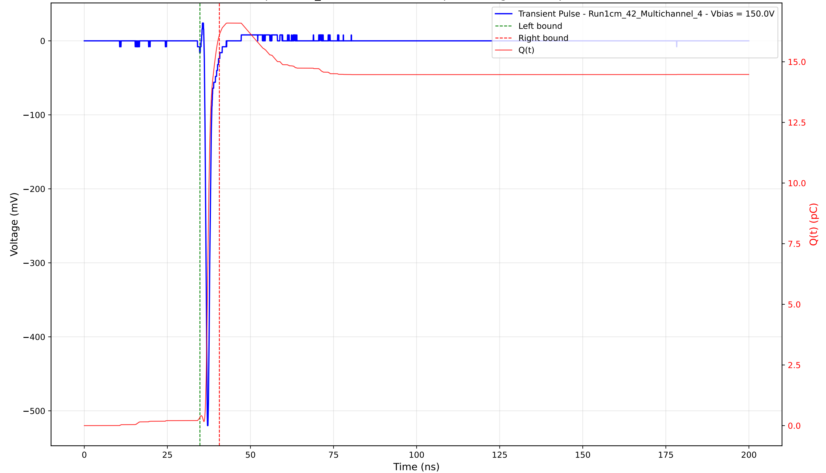
Transient Pulse - Sample: 1cm_42 - Position: 2490.0 \mu\text{m} - Charge: 15.76 pC - Rise Time: 0.72 ns
