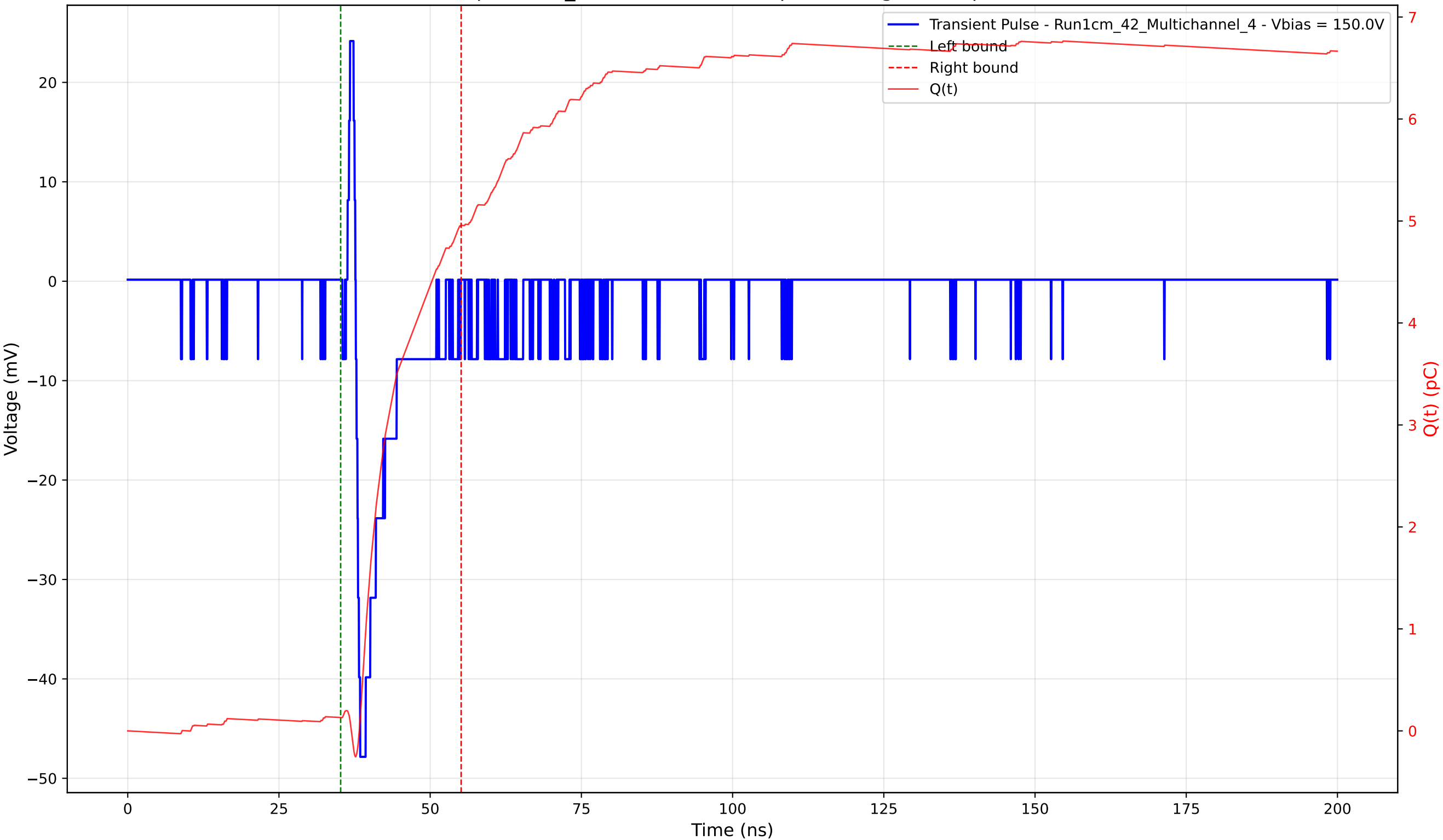
Transient Pulse - Sample: 1cm_42 - Position: 705.0 \mu\text{m} - Charge: 4.83 pC - Rise Time: 0.74 ns
