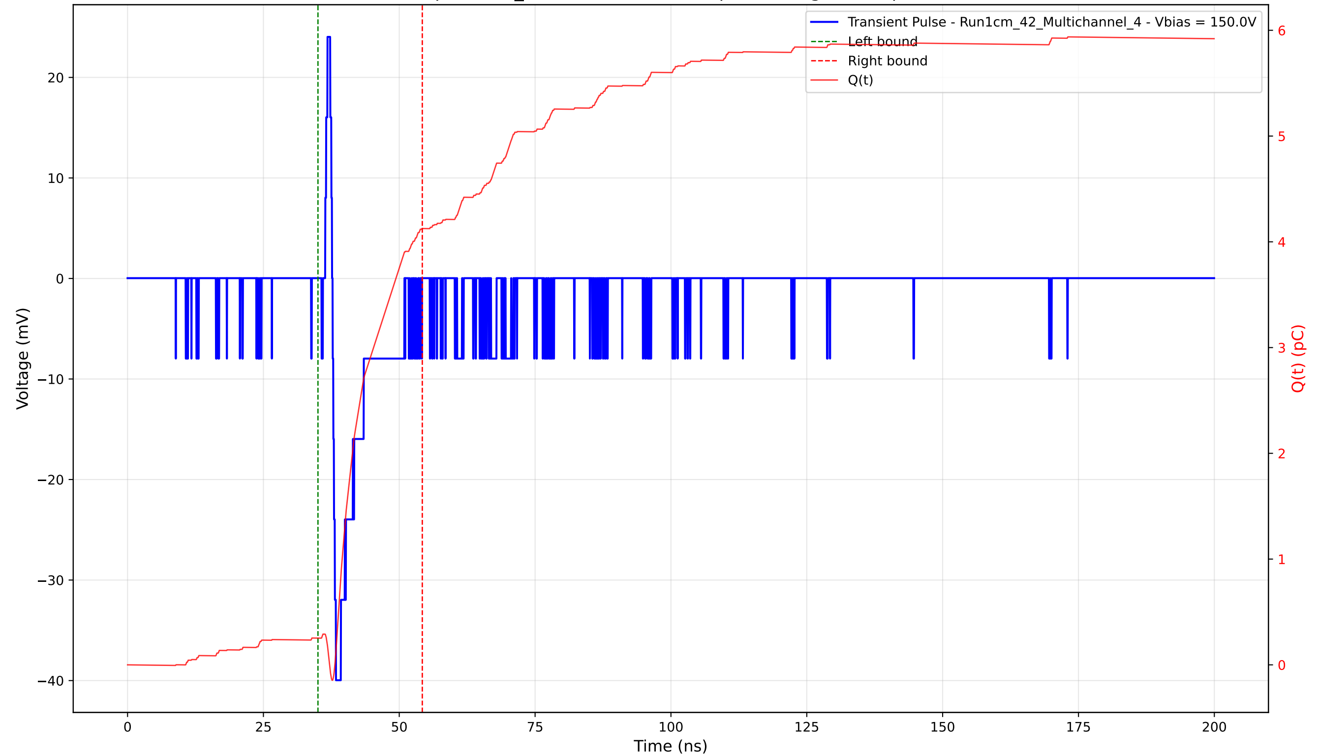
Transient Pulse - Sample: 1cm_42 - Position: 4220.0 \mu\text{m} - Charge: 3.87 pC - Rise Time: 0.62 ns
