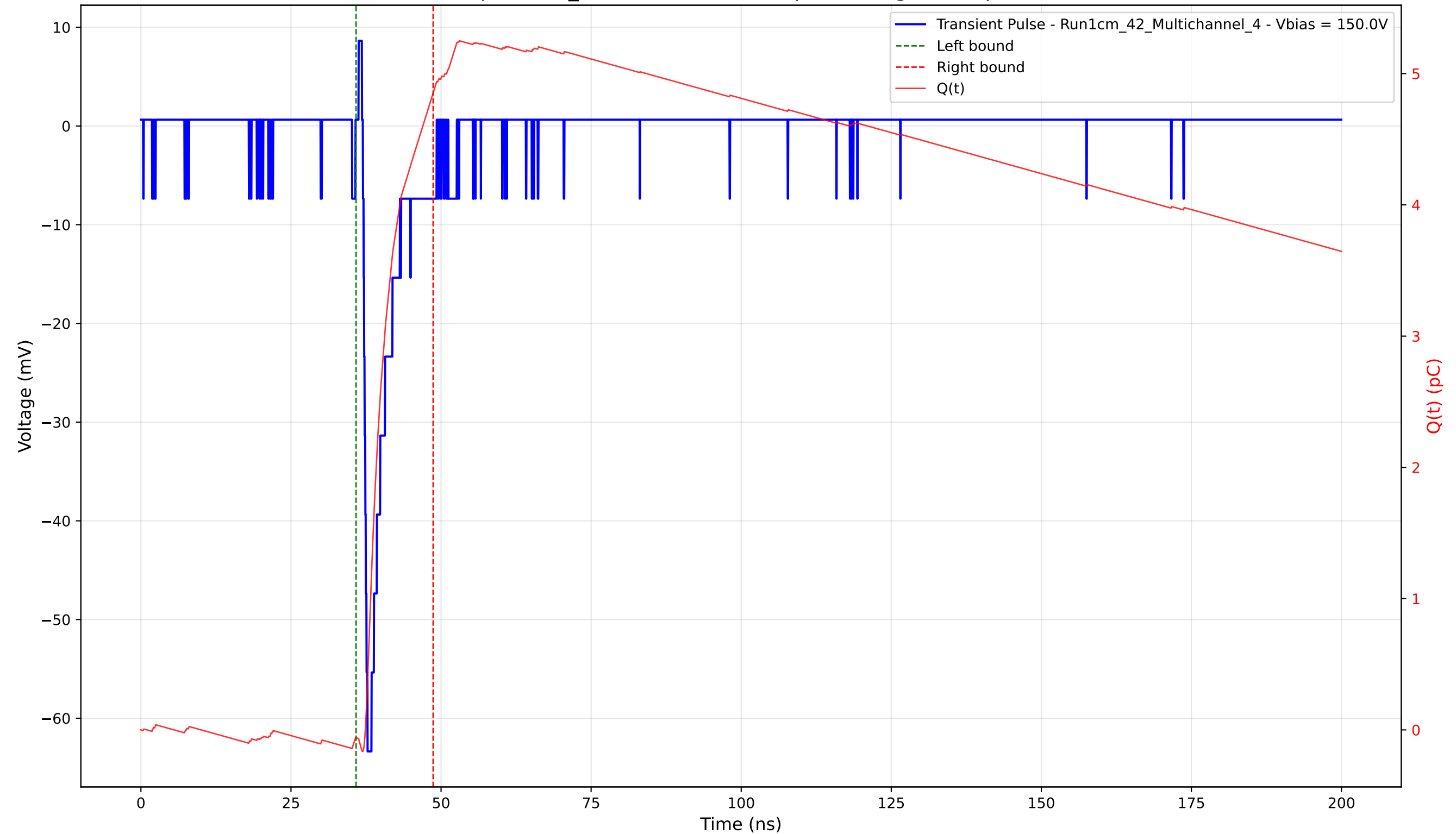
Transient Pulse - Sample: 1cm_42 - Position: 3565.0 \mu\text{m} - Charge: 4.91 pC - Rise Time: 0.77 ns
