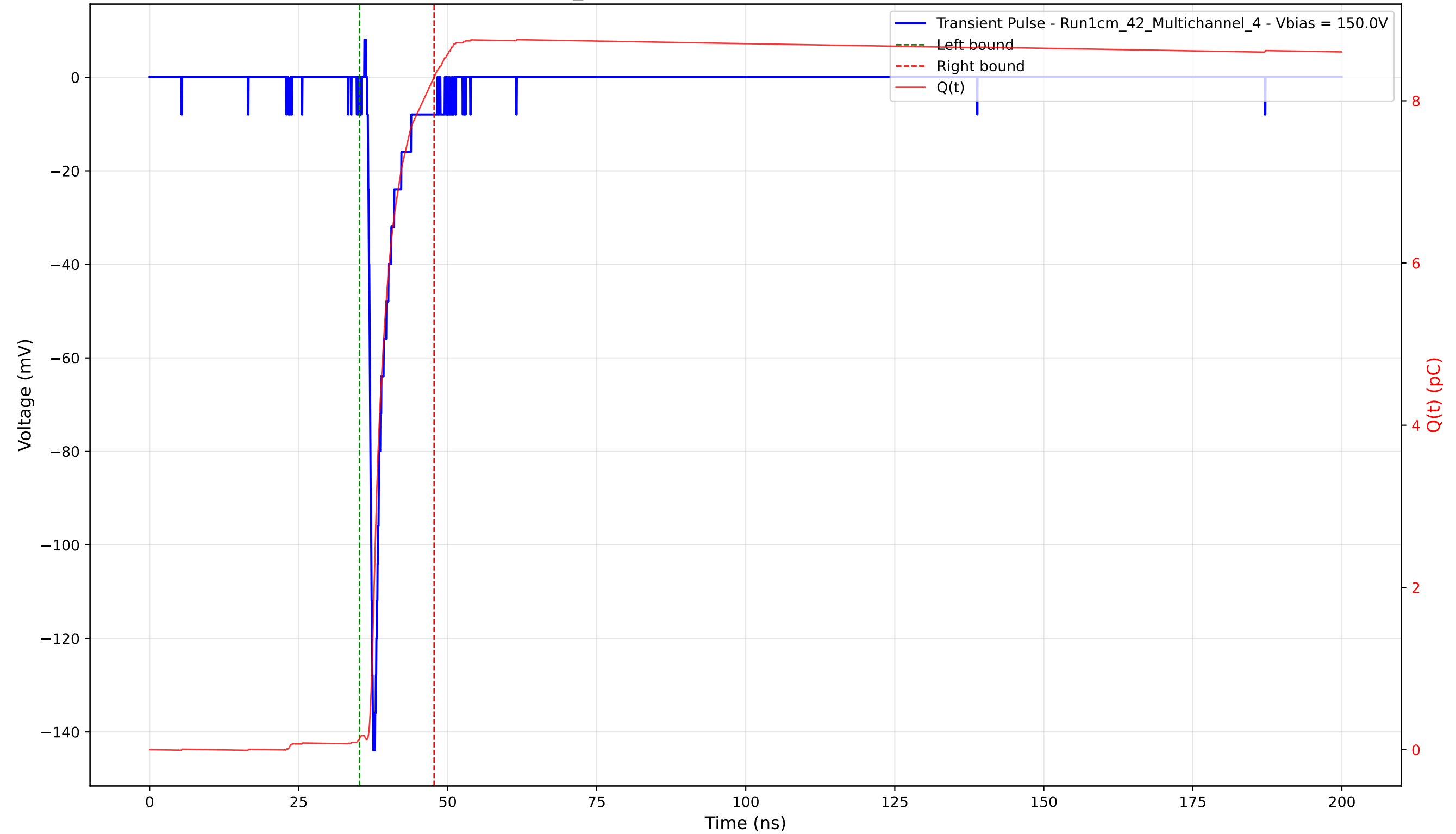
Transient Pulse - Sample: 1cm_42 - Position: 3275.0 \mu\text{m} - Charge: 8.16 pC - Rise Time: 0.81 ns
