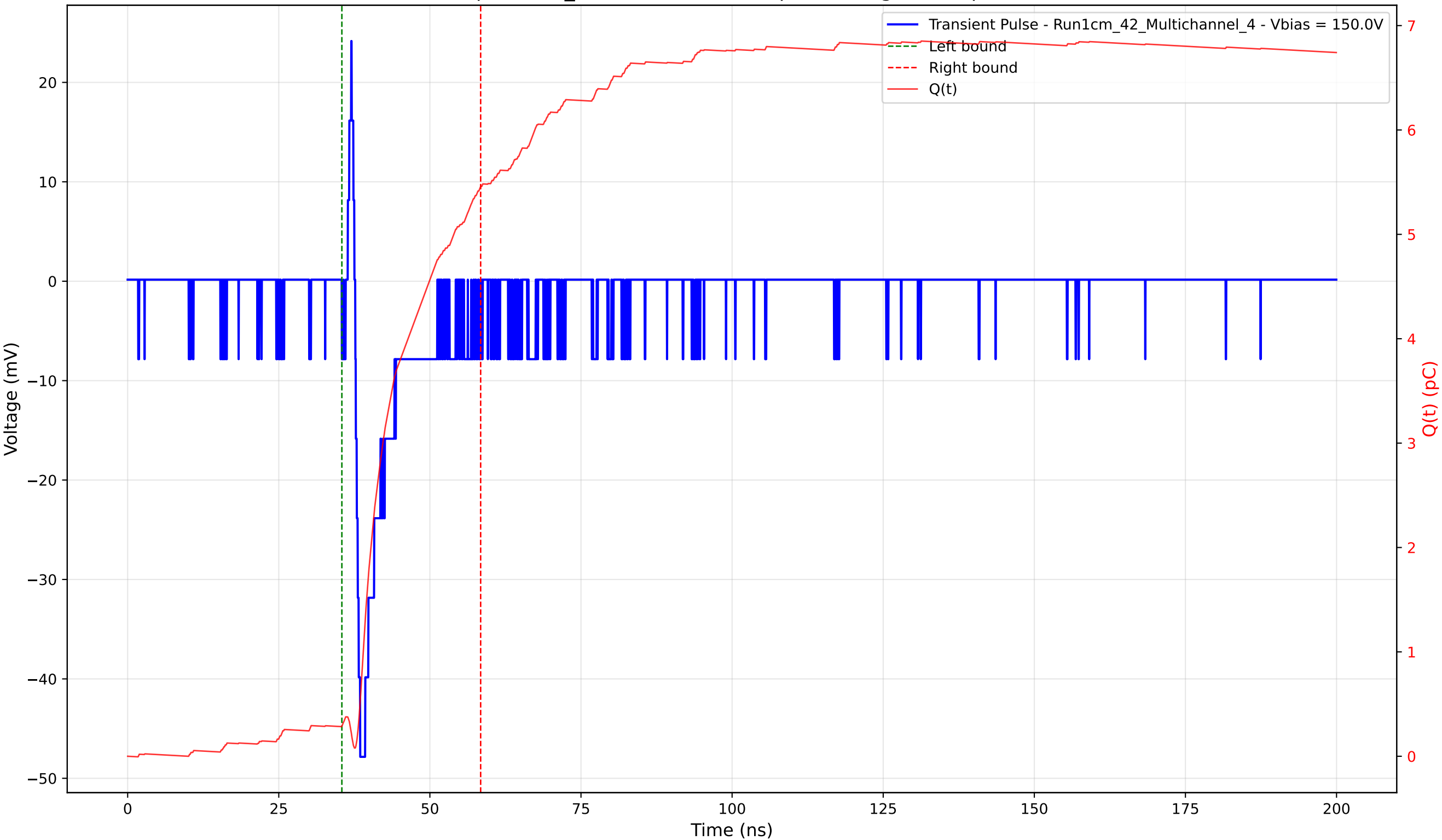
Transient Pulse - Sample: 1cm_42 - Position: 940.0 \mu\text{m} - Charge: 5.17 pC - Rise Time: 0.82 ns
