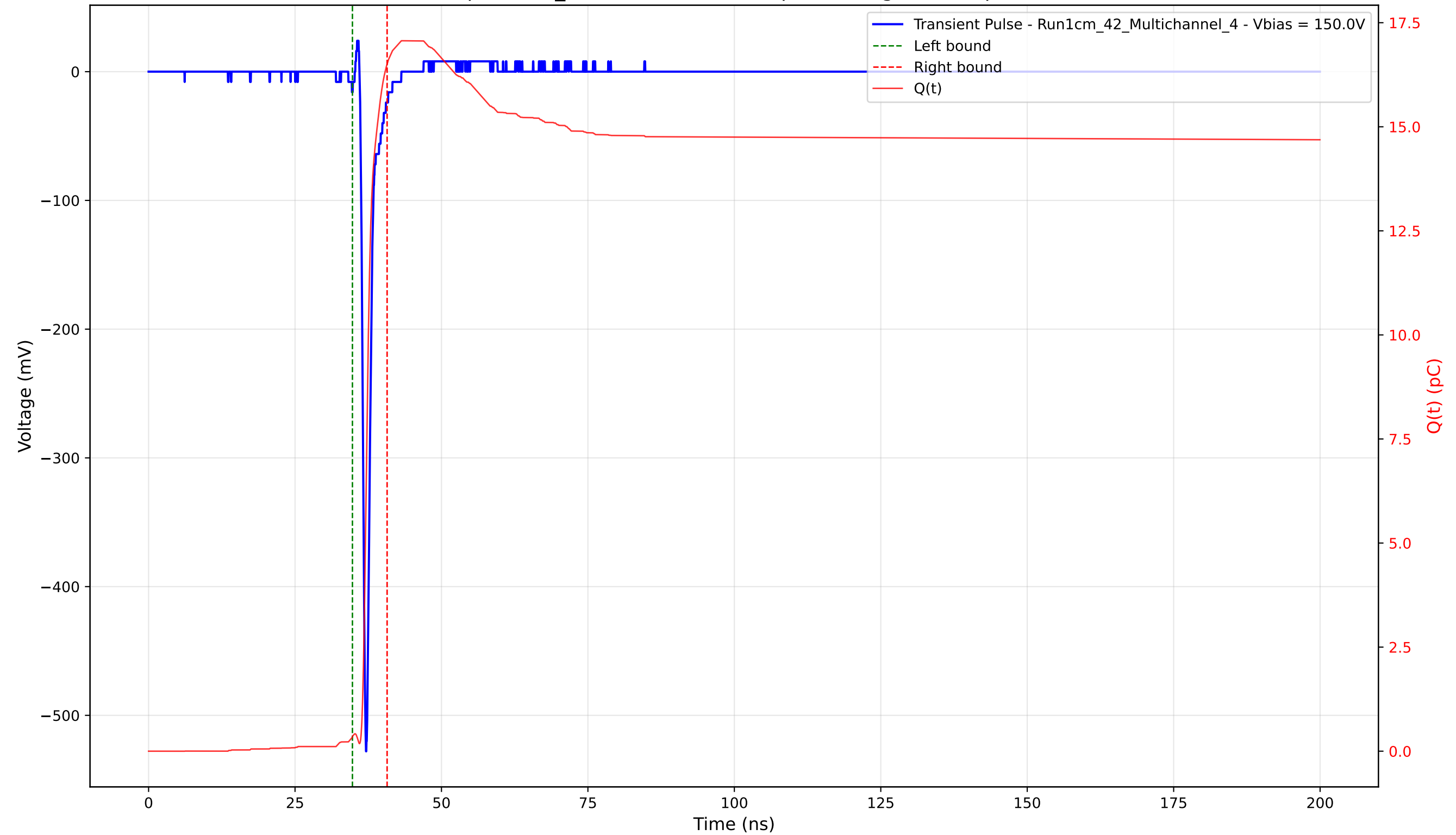
Transient Pulse - Sample: 1cm_42 - Position: 2410.0 \mu\text{m} - Charge: 16.16 pC - Rise Time: 0.74 ns
