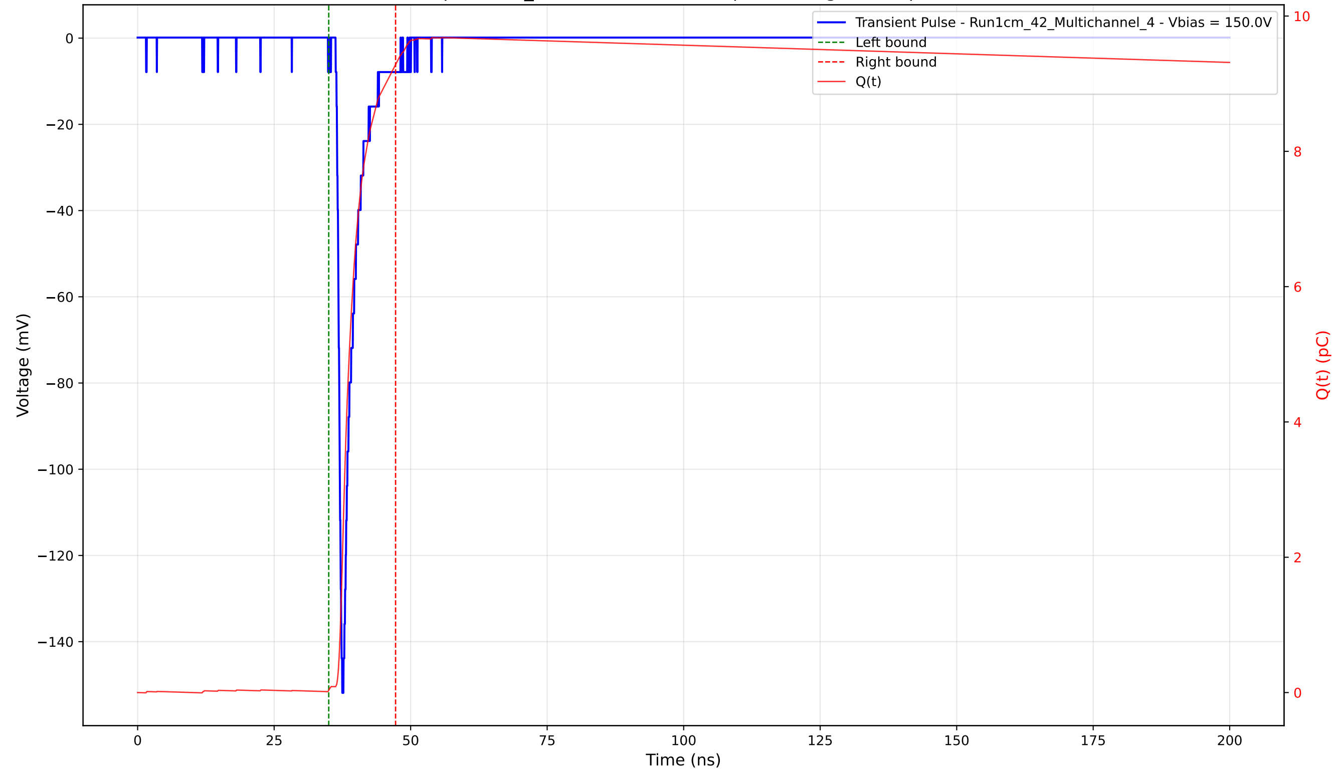
Transient Pulse - Sample: 1cm_42 - Position: 1770.0 \mu\text{m} - Charge: 9.25 pC - Rise Time: 0.92 ns
