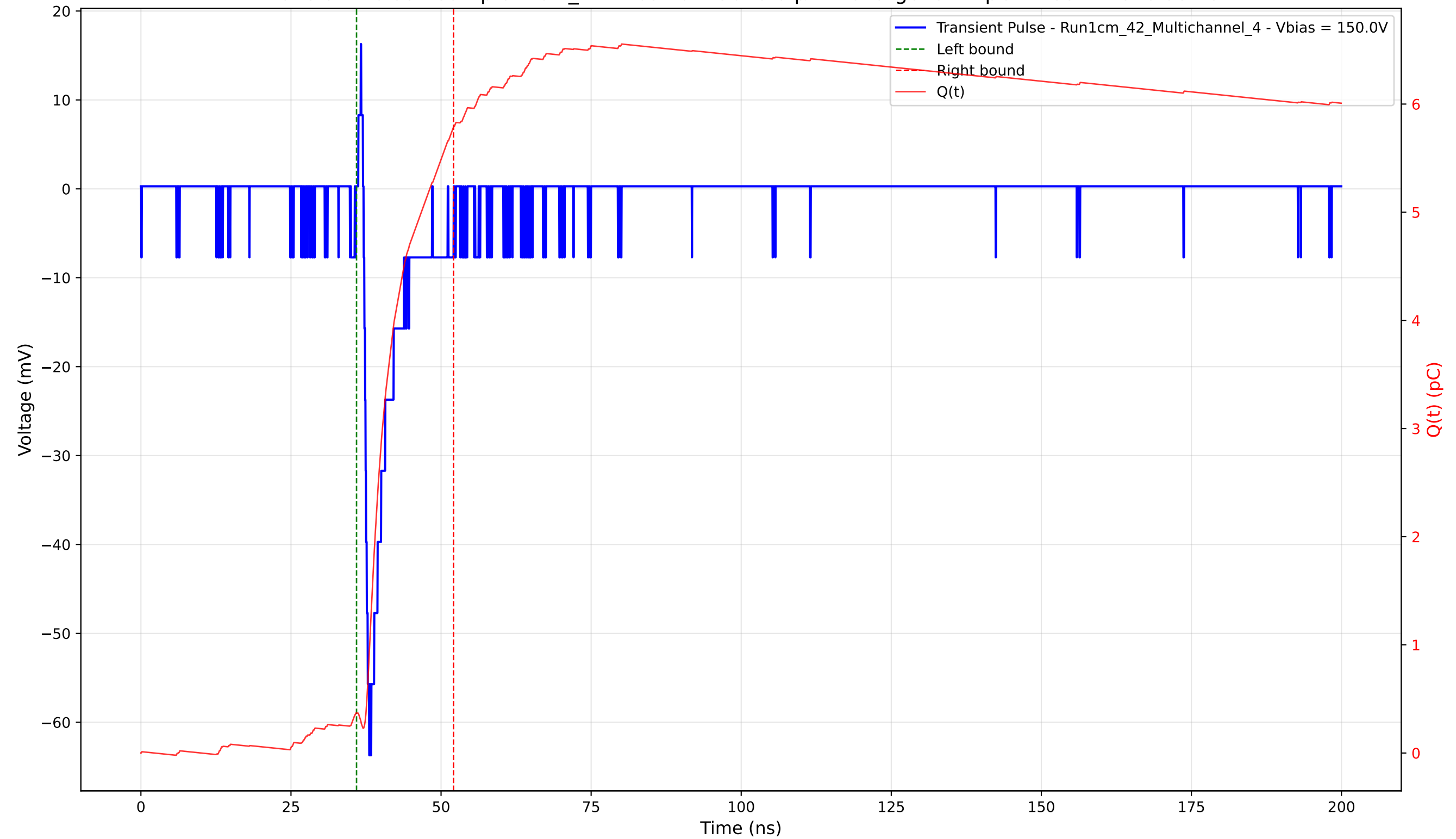
Transient Pulse - Sample: 1cm_42 - Position: 3640.0 \mu\text{m} - Charge: 5.42 pC - Rise Time: 0.93 ns
