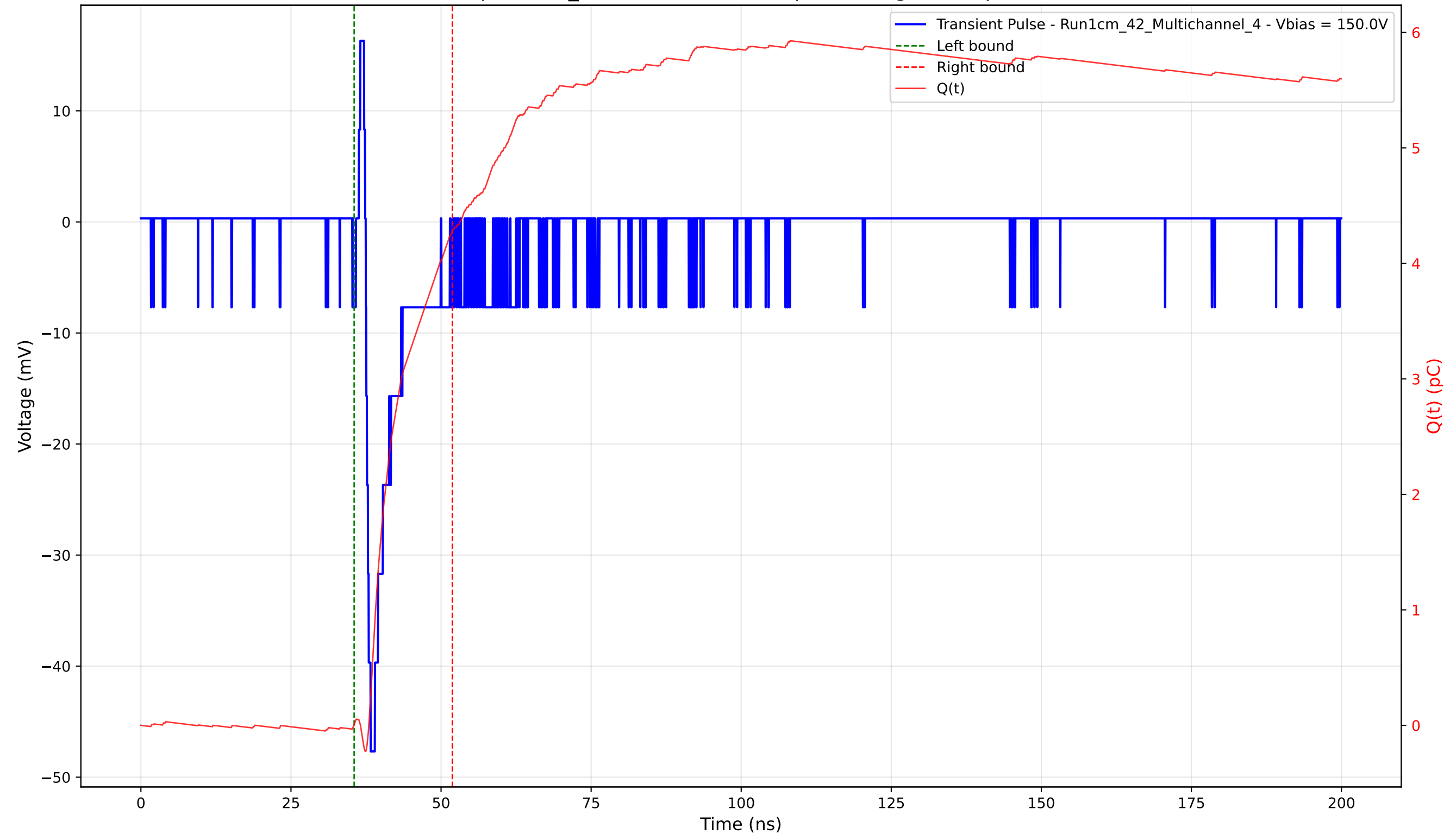
Transient Pulse - Sample: 1cm_42 - Position: 3925.0 \mu\text{m} - Charge: 4.28 pC - Rise Time: 0.82 ns
