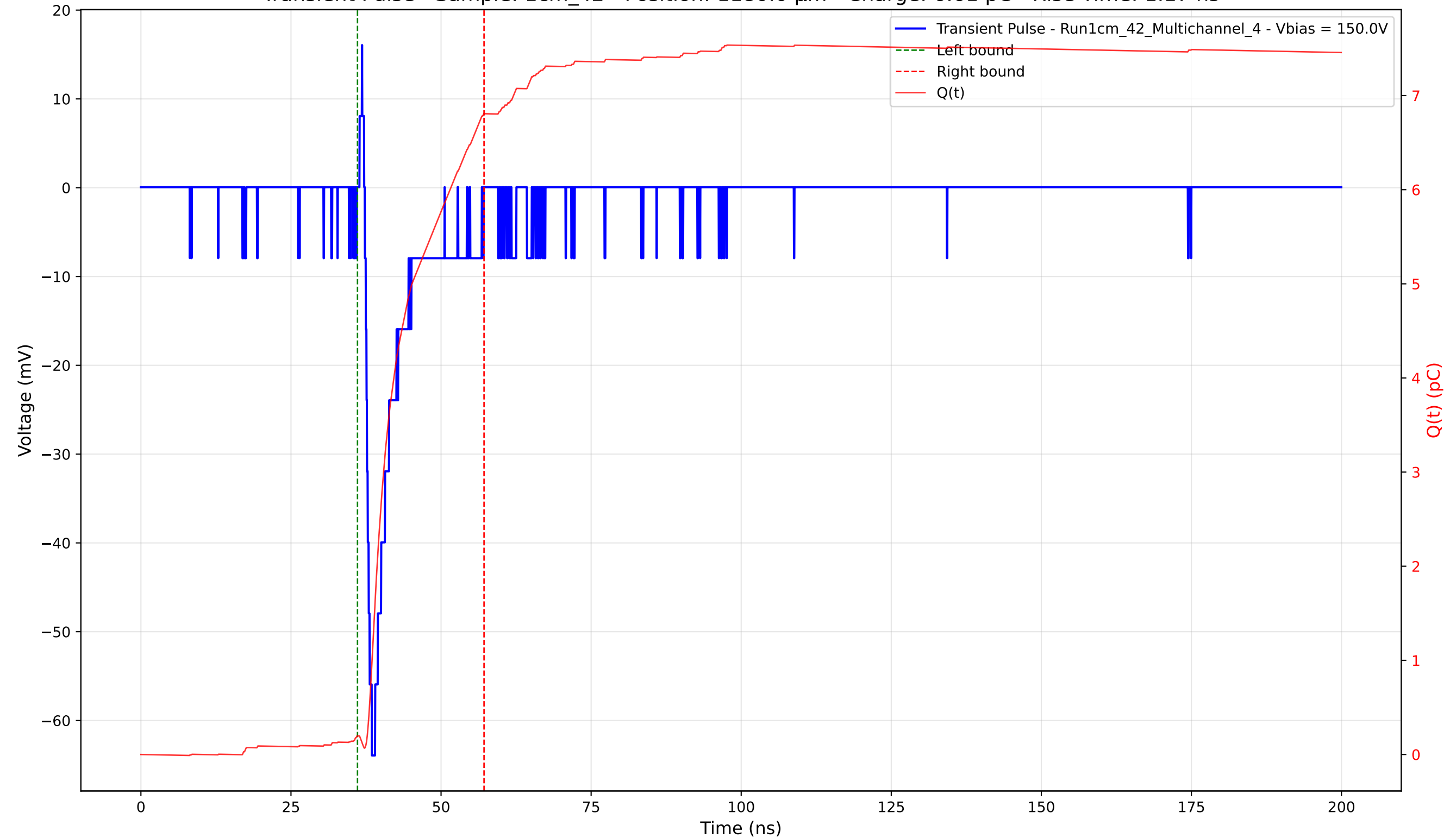
Transient Pulse - Sample: 1cm_42 - Position: 1180.0 \mu\text{m} - Charge: 6.61 pC - Rise Time: 1.17 ns
