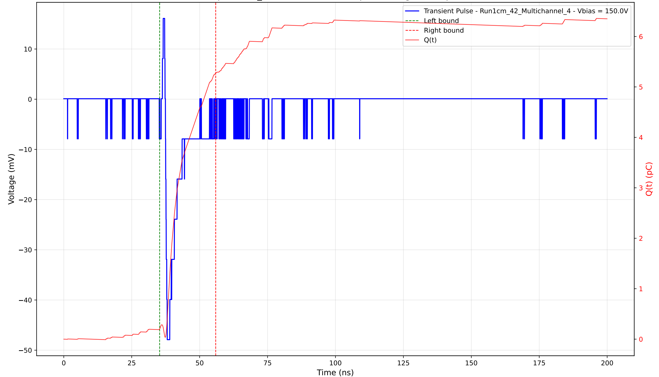
Transient Pulse - Sample: 1cm_42 - Position: 3900.0 \mu\text{m} - Charge: 5.07 pC - Rise Time: 0.66 ns
