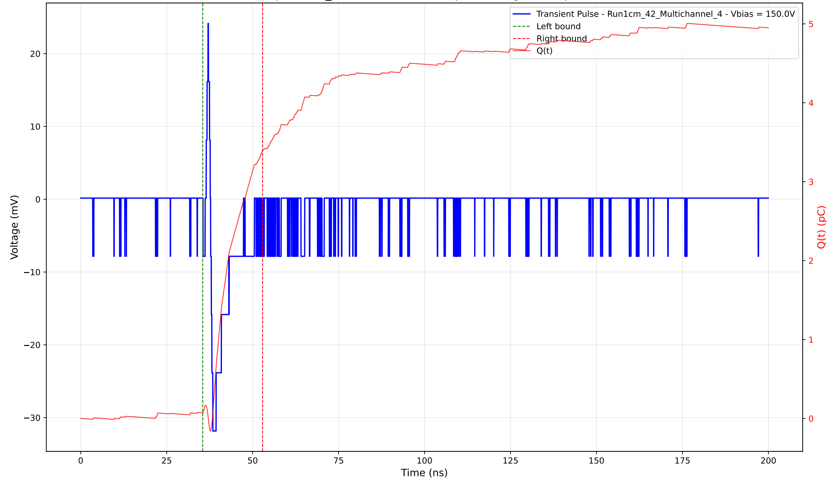
Transient Pulse - Sample: 1cm_42 - Position: 4465.0 \mu\text{m} - Charge: 3.31 pC - Rise Time: 0.66 ns
