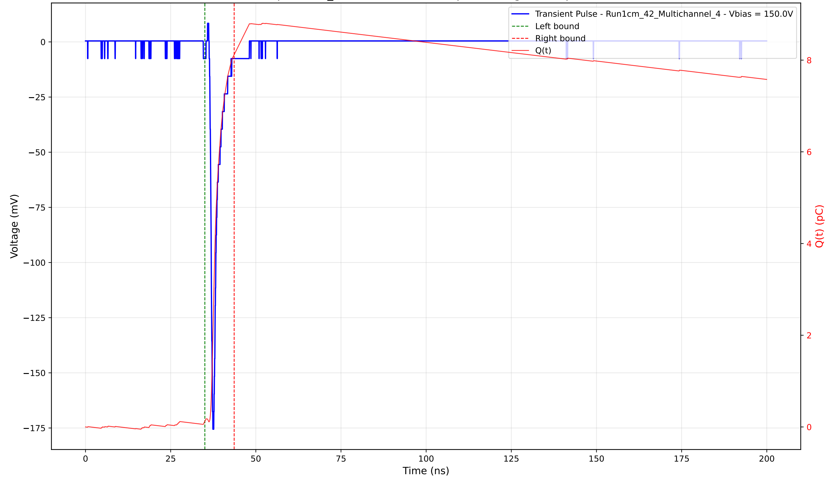
Transient Pulse - Sample: 1cm_42 - Position: 3115.0 \mu\text{m} - Charge: 7.99 pC - Rise Time: 0.74 ns
