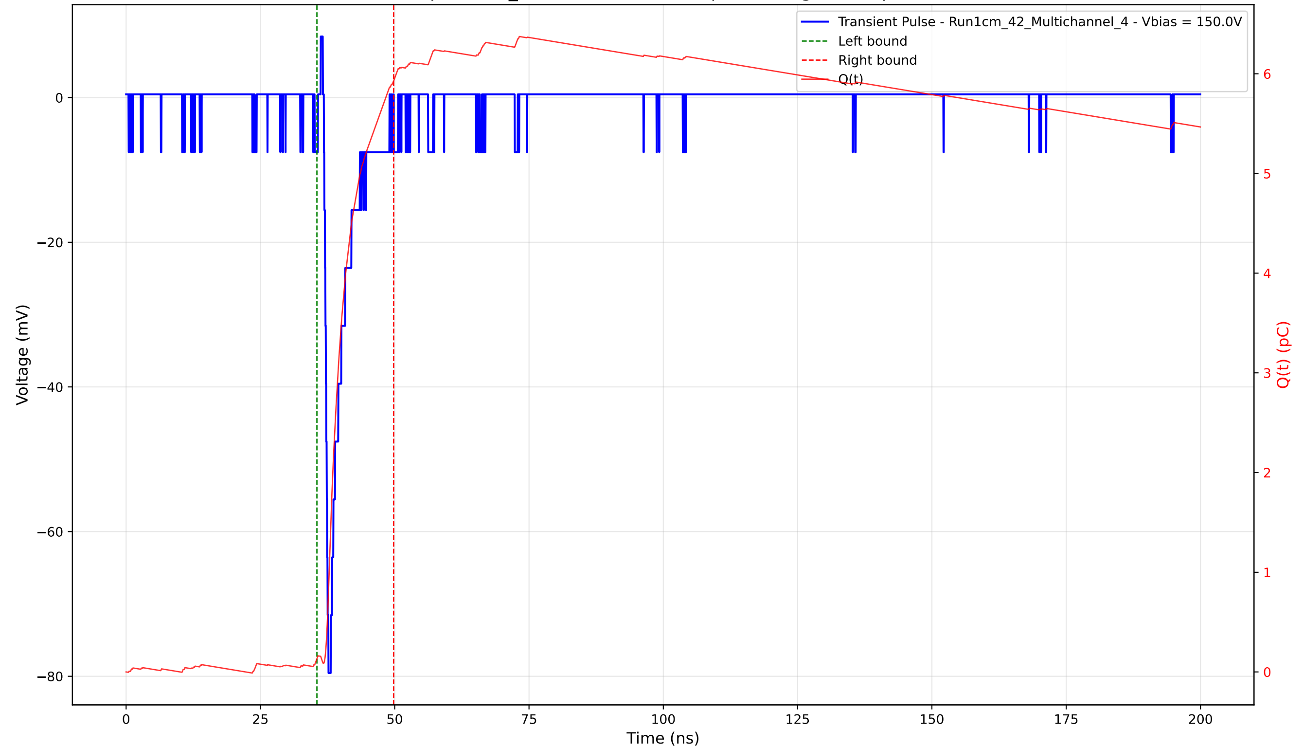
Transient Pulse - Sample: 1cm_42 - Position: 3490.0 \mu\text{m} - Charge: 5.80 pC - Rise Time: 0.80 ns
