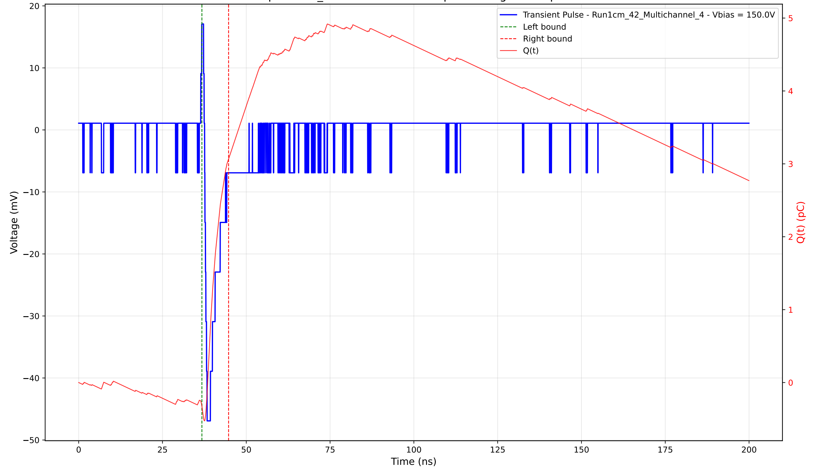
Transient Pulse - Sample: 1cm_42 - Position: 1015.0 \mu\text{m} - Charge: 3.39 pC - Rise Time: 0.74 ns
