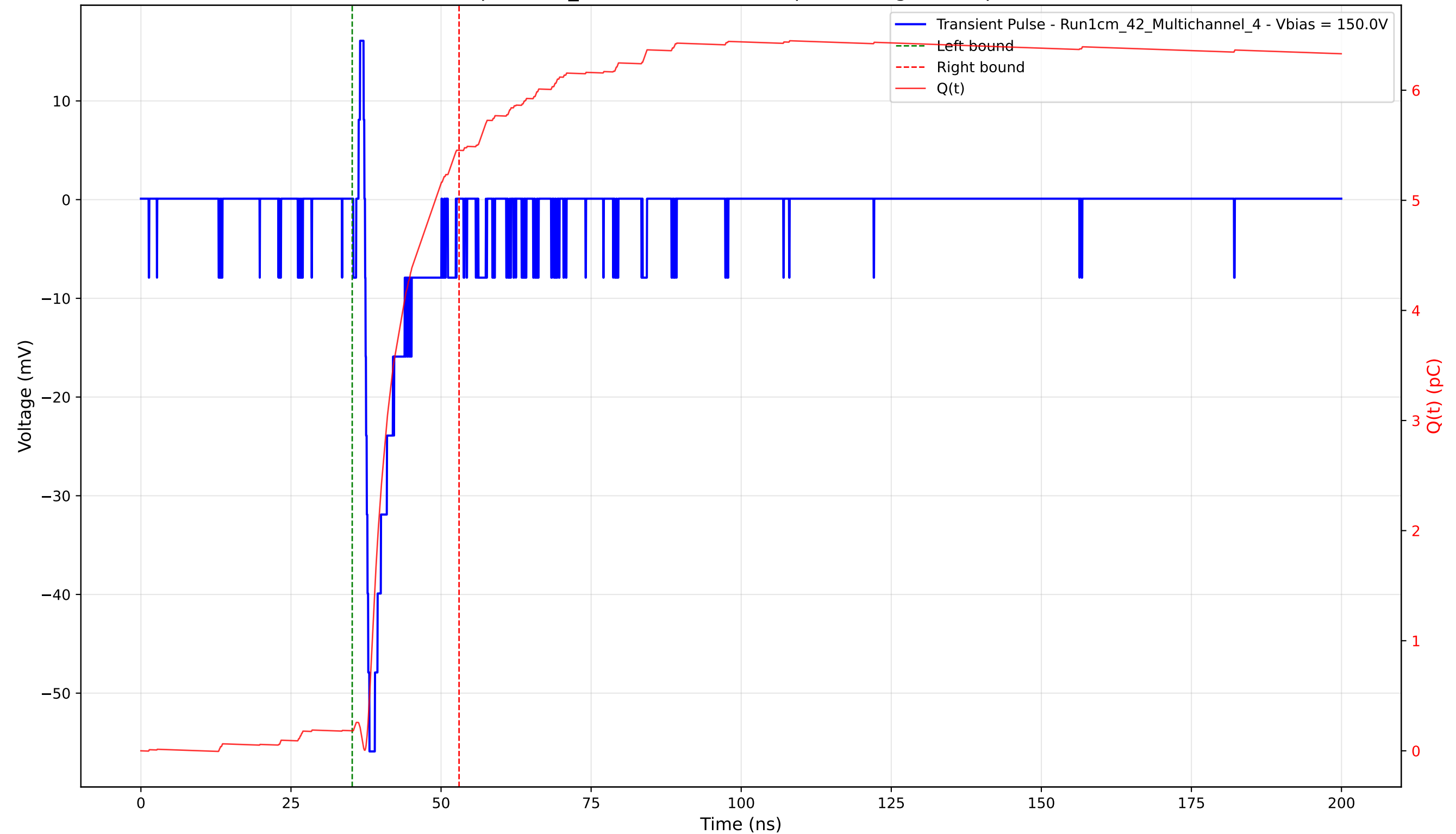
Transient Pulse - Sample: 1cm_42 - Position: 3805.0 \mu\text{m} - Charge: 5.27 pC - Rise Time: 0.73 ns
