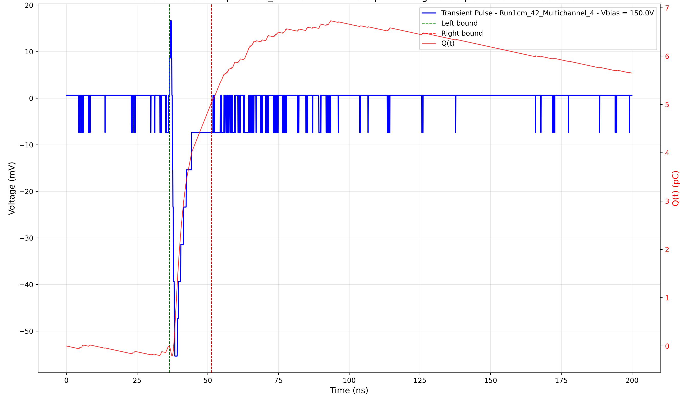
Transient Pulse - Sample: 1cm_42 - Position: 1115.0 \mu\text{m} - Charge: 5.06 pC - Rise Time: 0.93 ns
