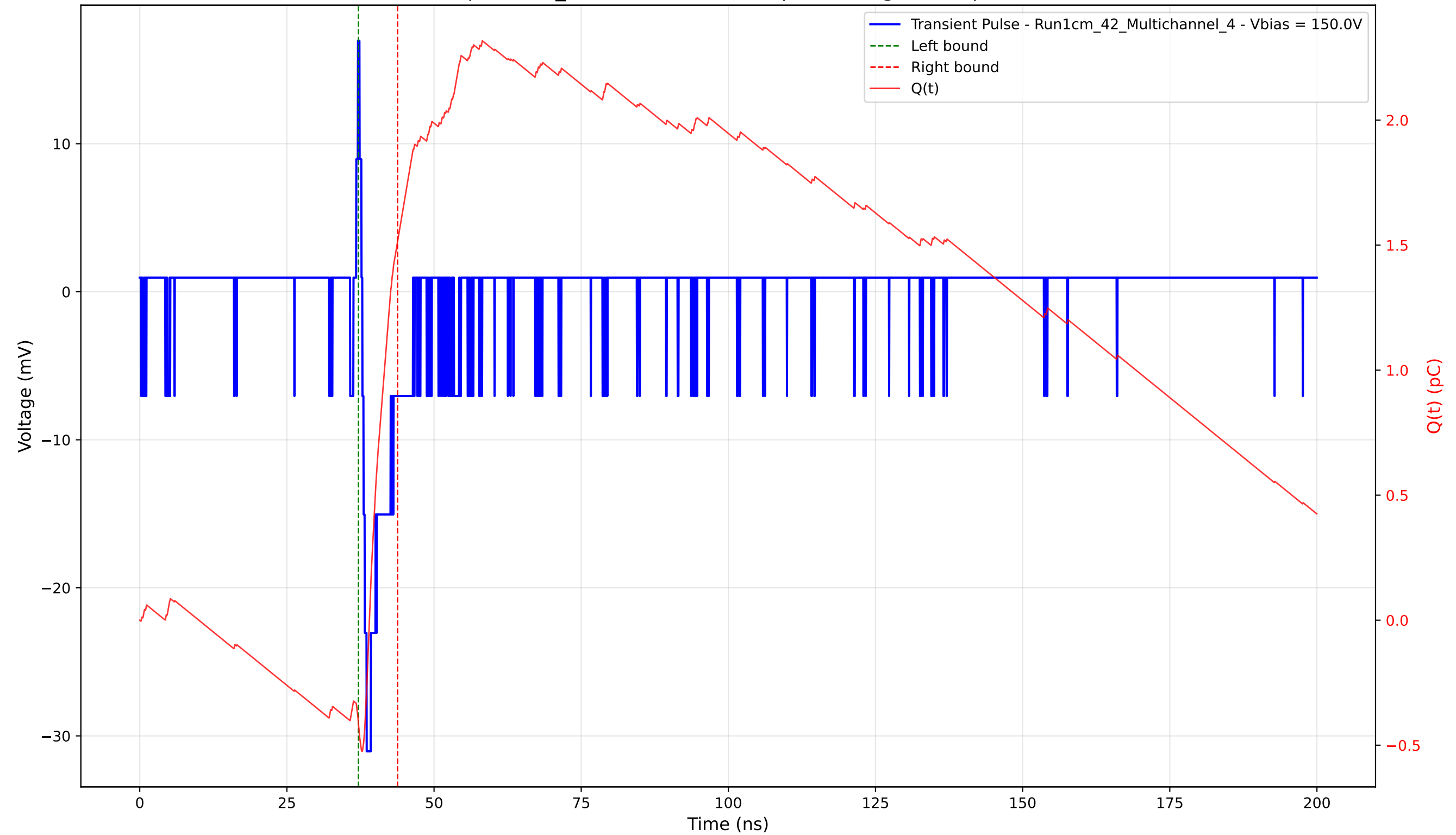
Transient Pulse - Sample: 1cm_42 - Position: 4875.0 \mu\text{m} - Charge: 1.93 pC - Rise Time: 0.75 ns
