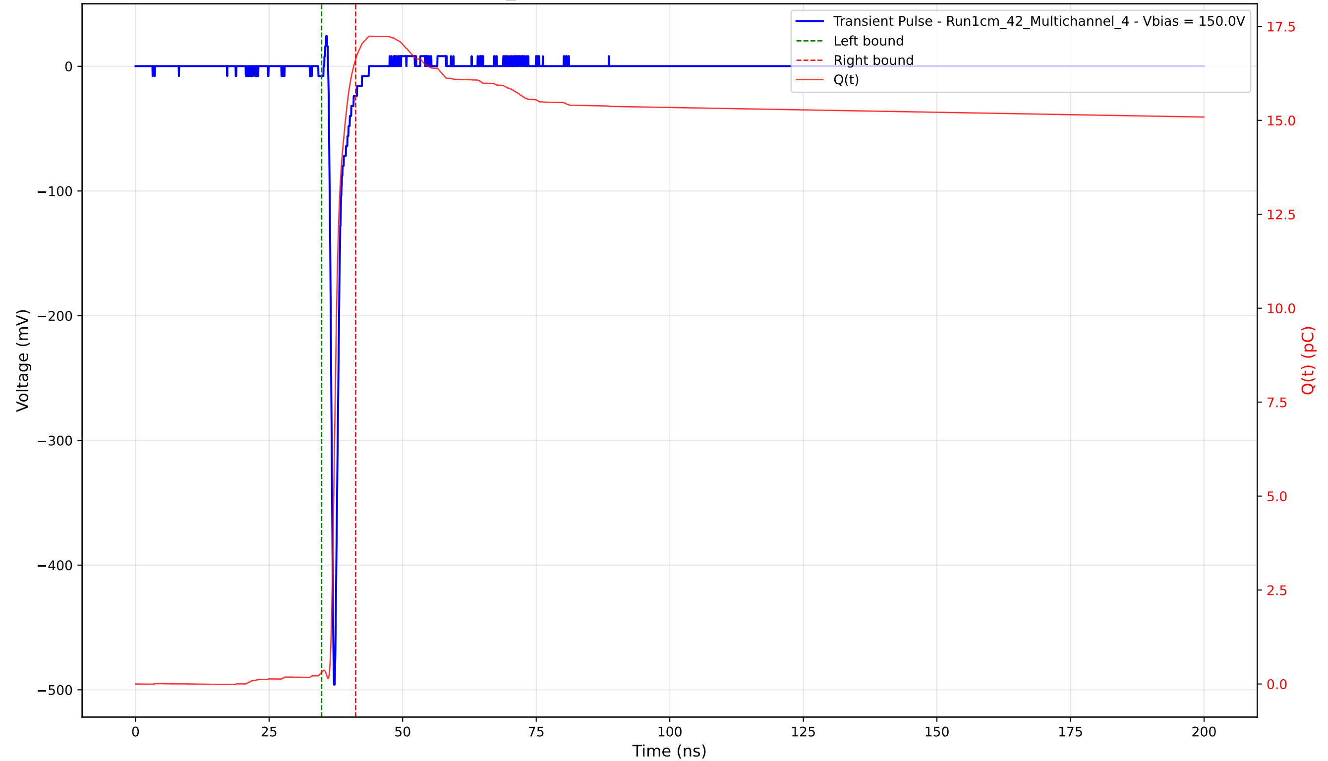
Transient Pulse - Sample: 1cm_42 - Position: 2235.0 \mu\text{m} - Charge: 16.31 pC - Rise Time: 0.73 ns
