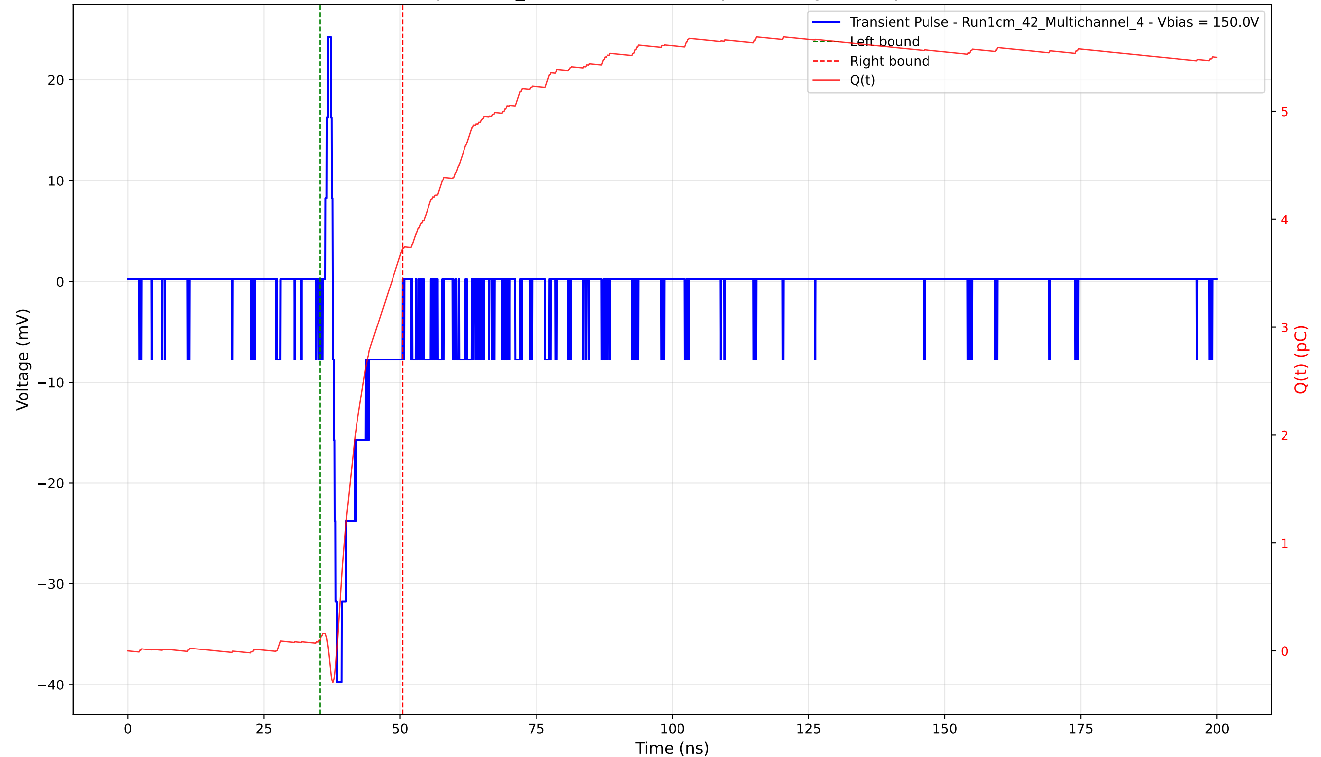
Transient Pulse - Sample: 1cm_42 - Position: 4225.0 \mu\text{m} - Charge: 3.63 pC - Rise Time: 0.70 ns
