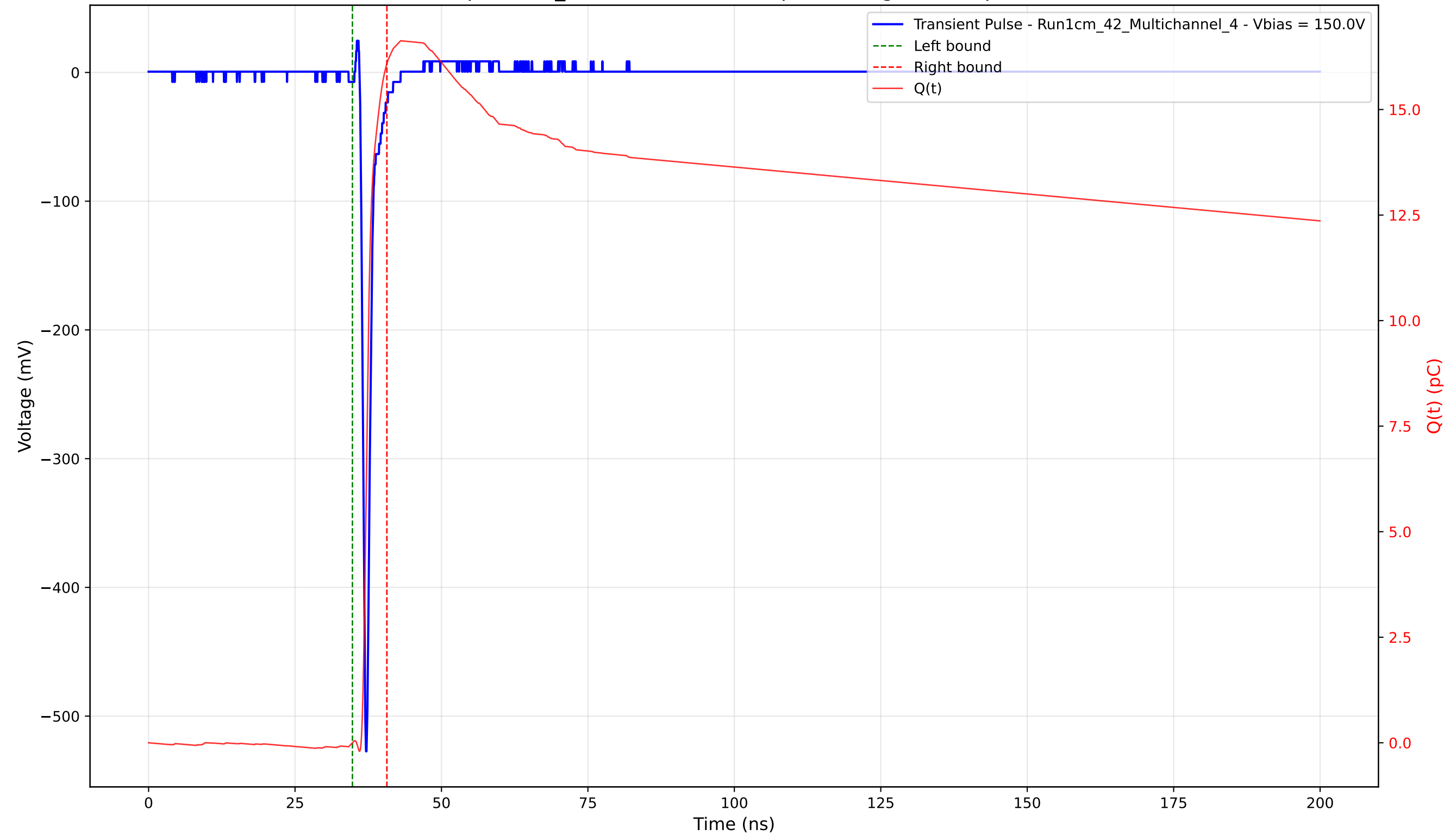
Transient Pulse - Sample: 1cm_42 - Position: 2430.0 \mu\text{m} - Charge: 16.09 pC - Rise Time: 0.71 ns
