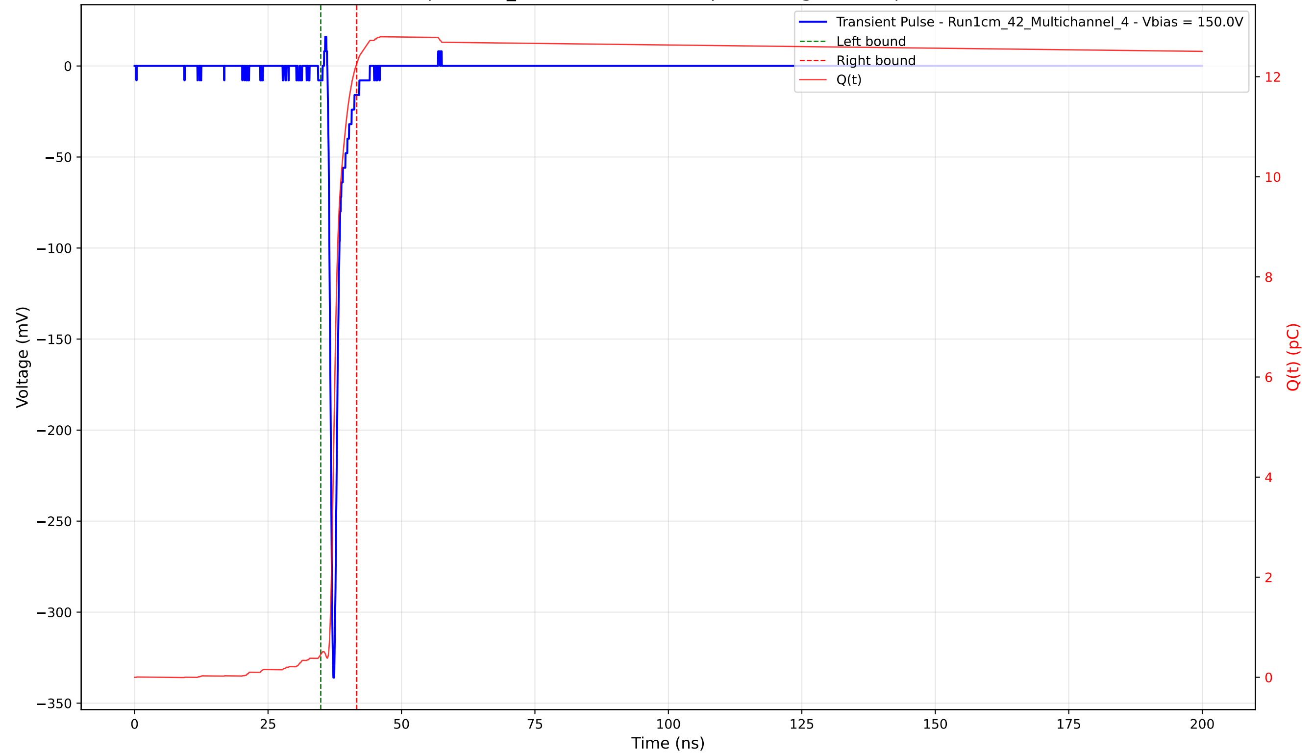
Transient Pulse - Sample: 1cm_42 - Position: 2905.0 \mu\text{m} - Charge: 11.80 pC - Rise Time: 0.74 ns
