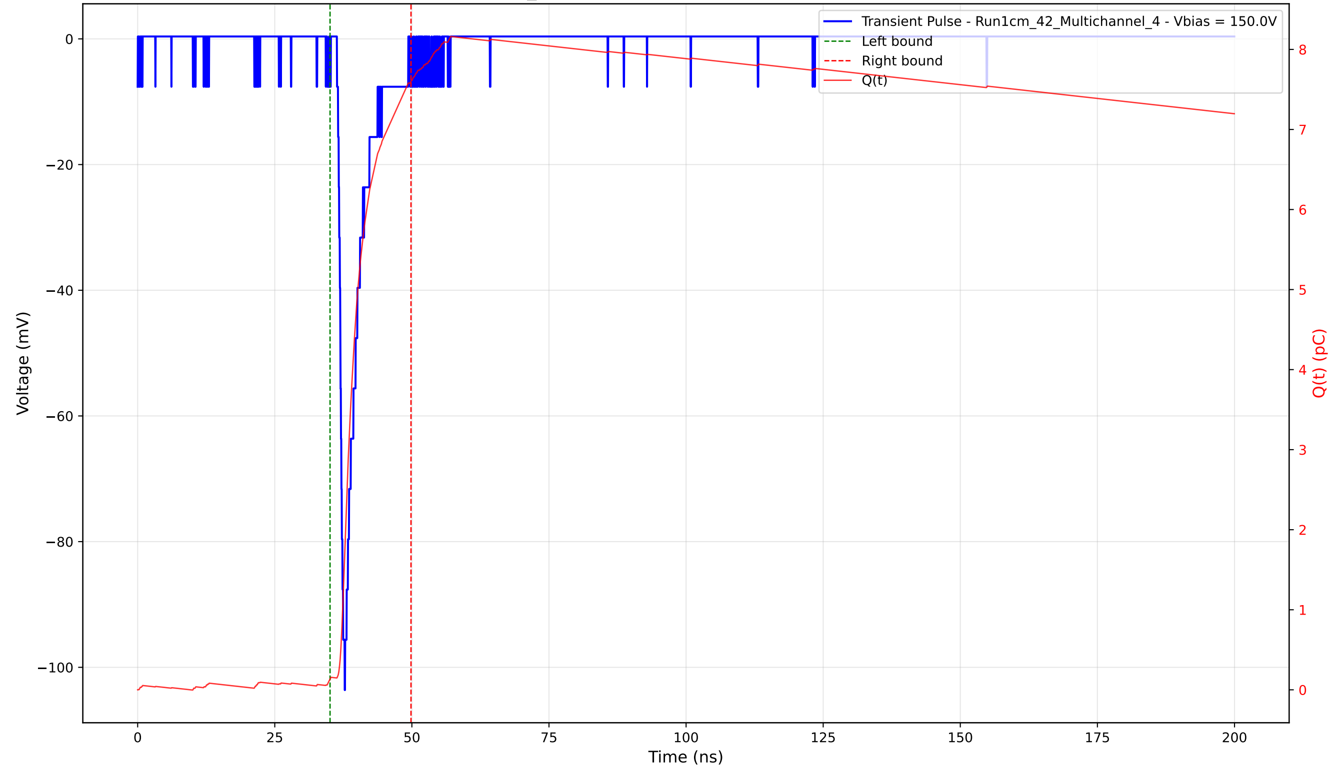
Transient Pulse - Sample: 1cm_42 - Position: 1615.0 \mu\text{m} - Charge: 7.47 pC - Rise Time: 0.95 ns
