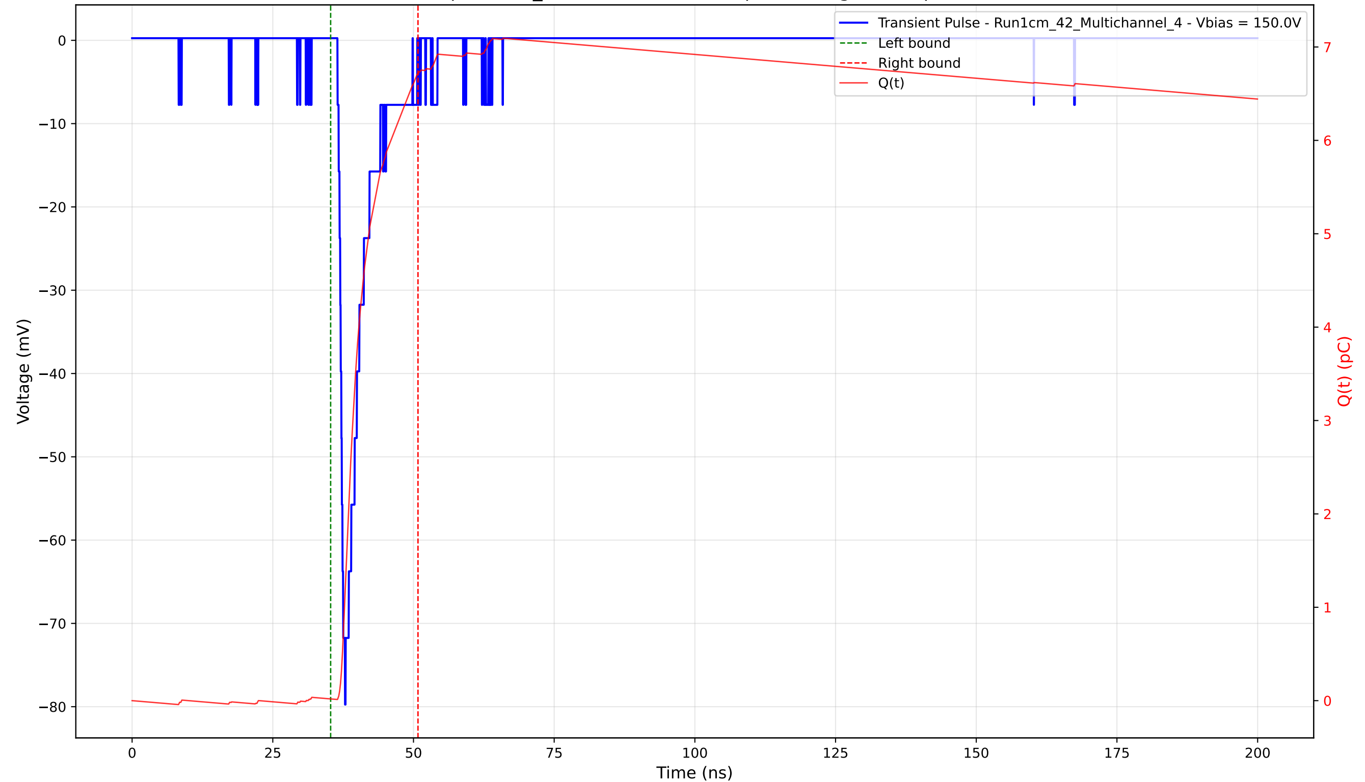
Transient Pulse - Sample: 1cm_42 - Position: 1535.0 \mu\text{m} - Charge: 6.69 pC - Rise Time: 1.16 ns
