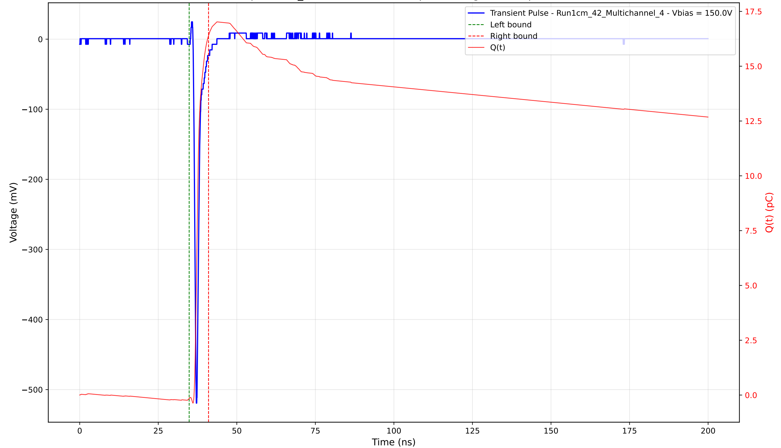
Transient Pulse - Sample: 1cm_42 - Position: 2305.0 \mu\text{m} - Charge: 16.55 pC - Rise Time: 0.72 ns
