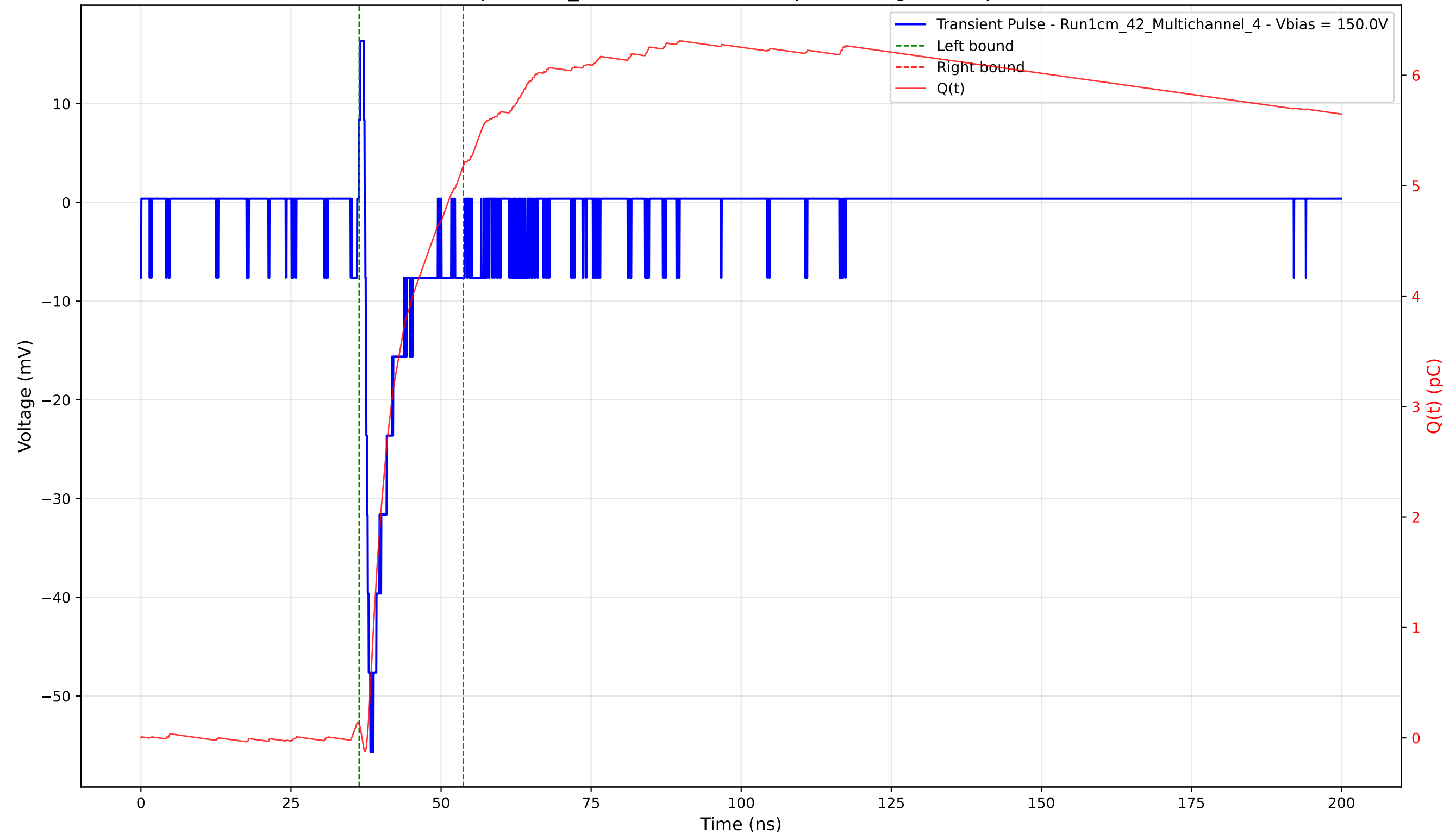
Transient Pulse - Sample: 1cm_42 - Position: 3860.0 \mu\text{m} - Charge: 5.06 pC - Rise Time: 0.85 ns
