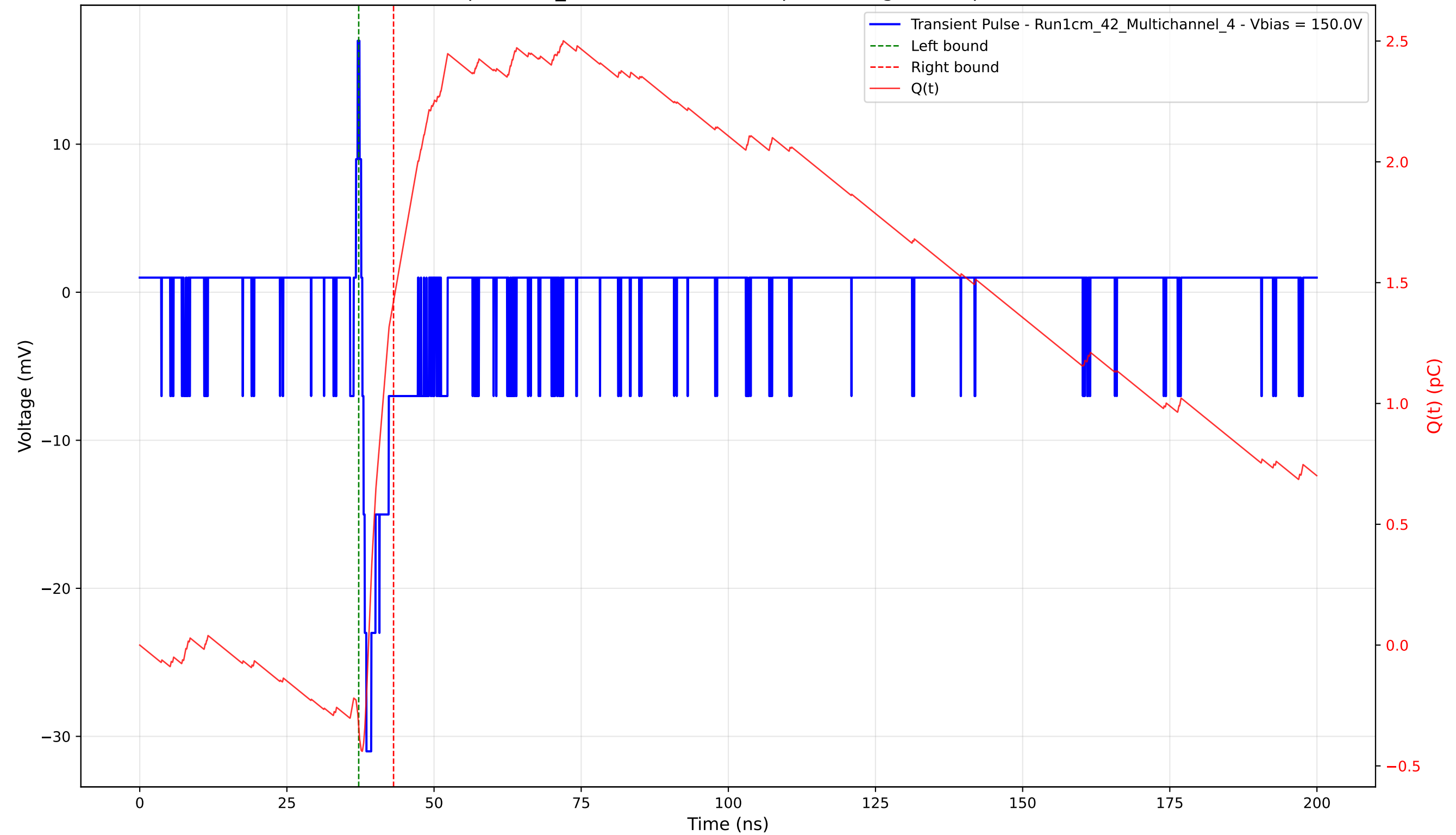
Transient Pulse - Sample: 1cm_42 - Position: 4860.0 \mu\text{m} - Charge: 1.76 pC - Rise Time: 0.71 ns
