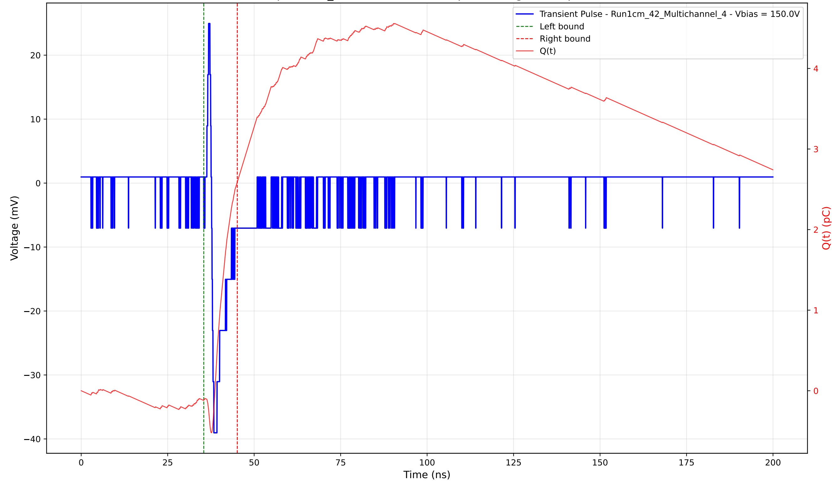
Transient Pulse - Sample: 1cm_42 - Position: 4165.0 \mu\text{m} - Charge: 2.71 pC - Rise Time: 0.66 ns
