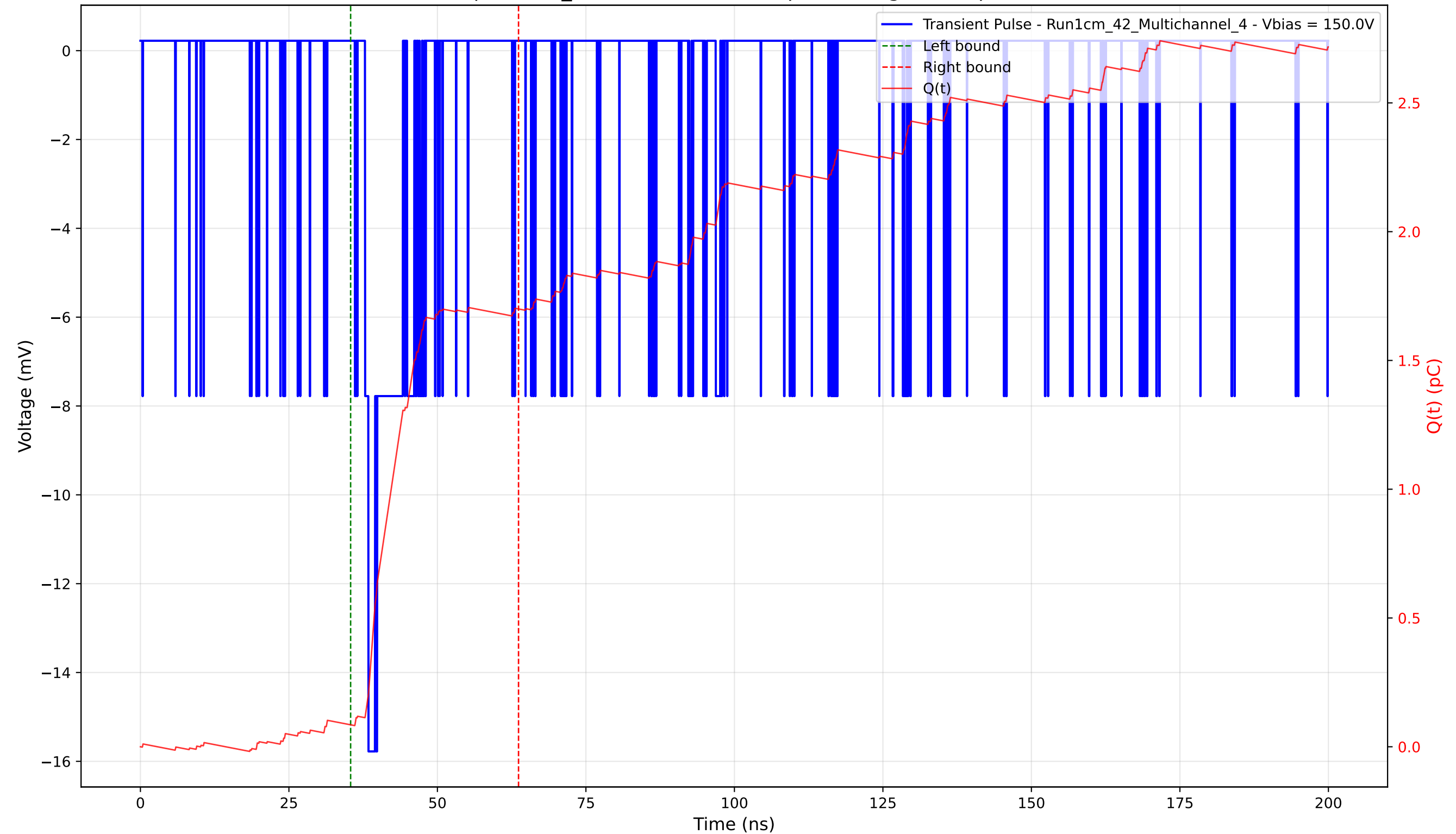
Transient Pulse - Sample: 1cm_42 - Position: 5055.0 \mu\text{m} - Charge: 1.61 pC - Rise Time: 0.59 ns
