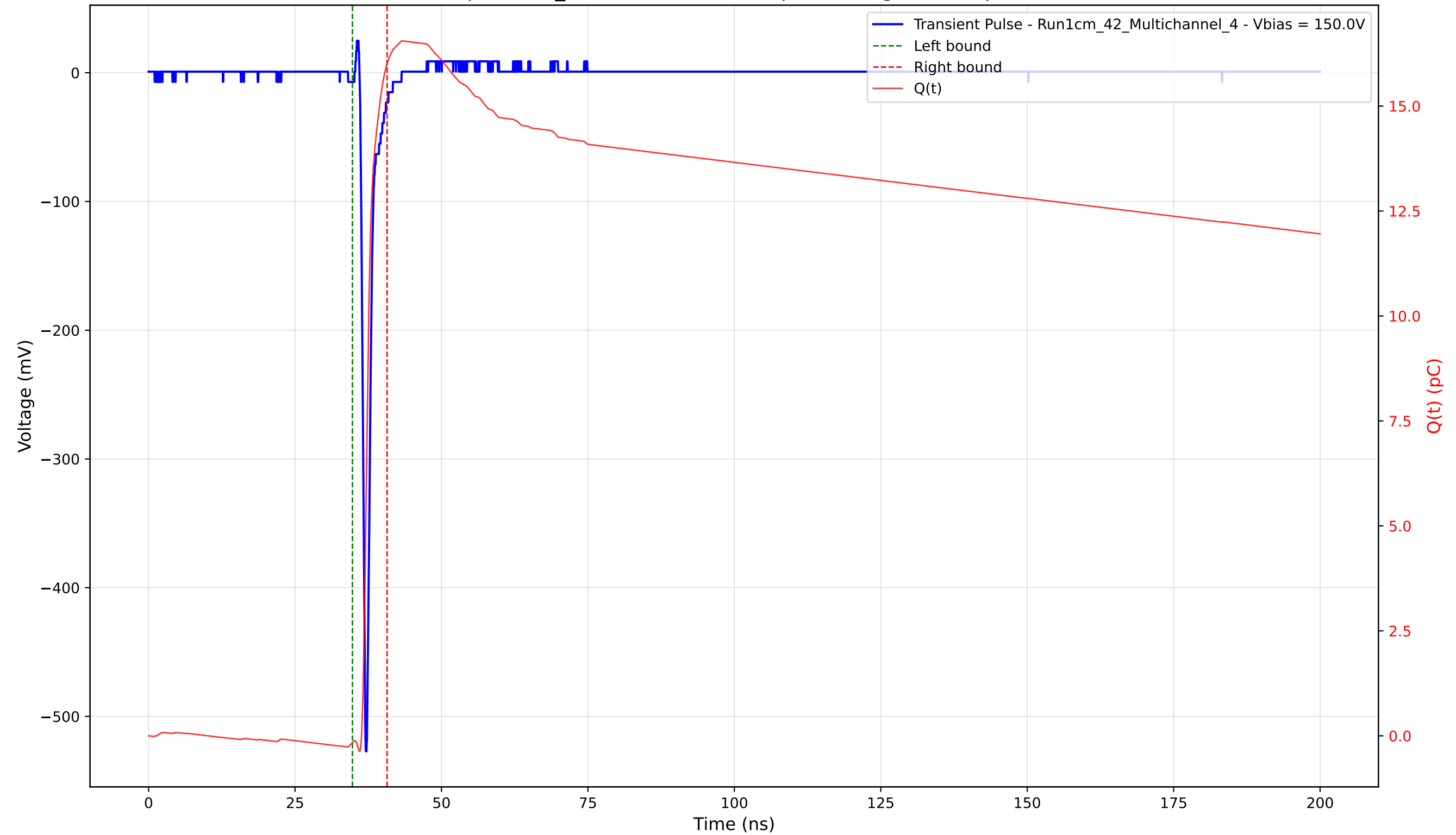
Transient Pulse - Sample: 1cm_42 - Position: 2405.0 \mu\text{m} - Charge: 16.17 pC - Rise Time: 0.71 ns
