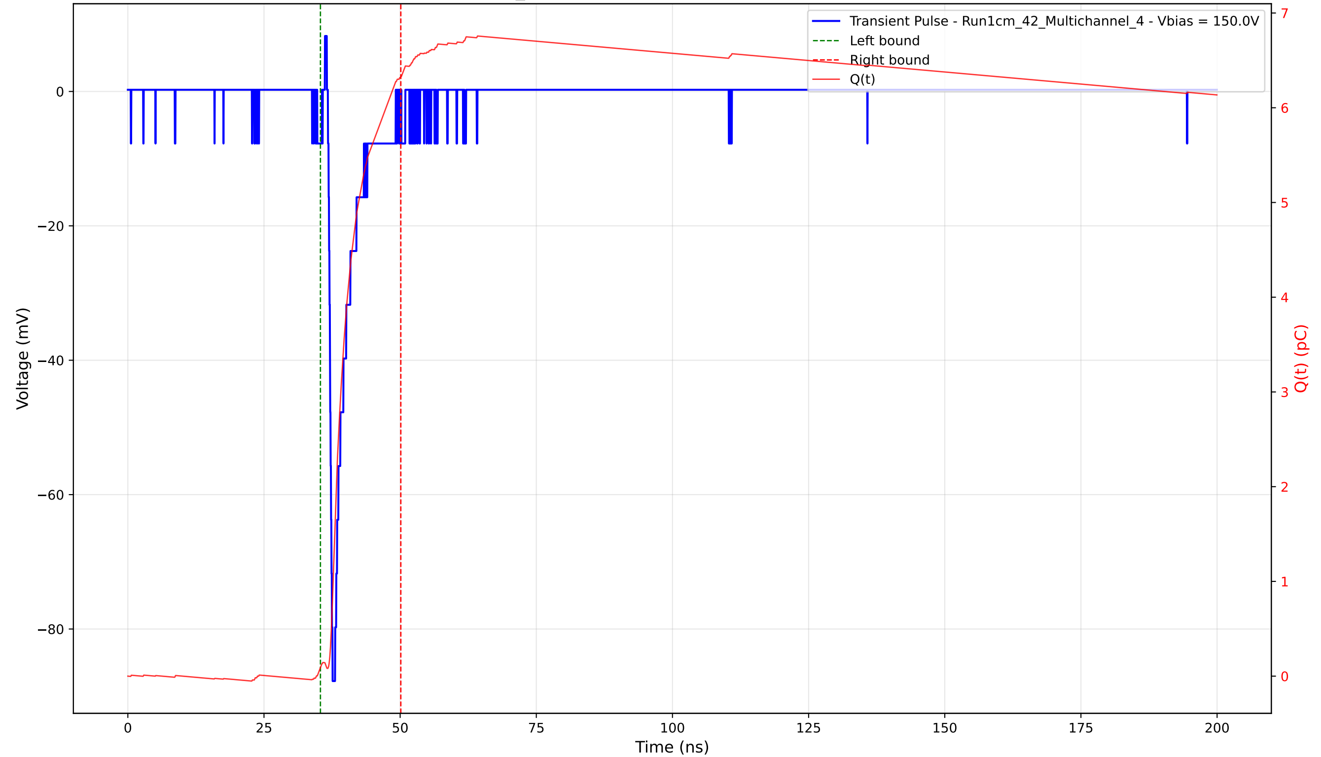
Transient Pulse - Sample: 1cm_42 - Position: 3450.0 \mu\text{m} - Charge: 6.24 pC - Rise Time: 0.63 ns
