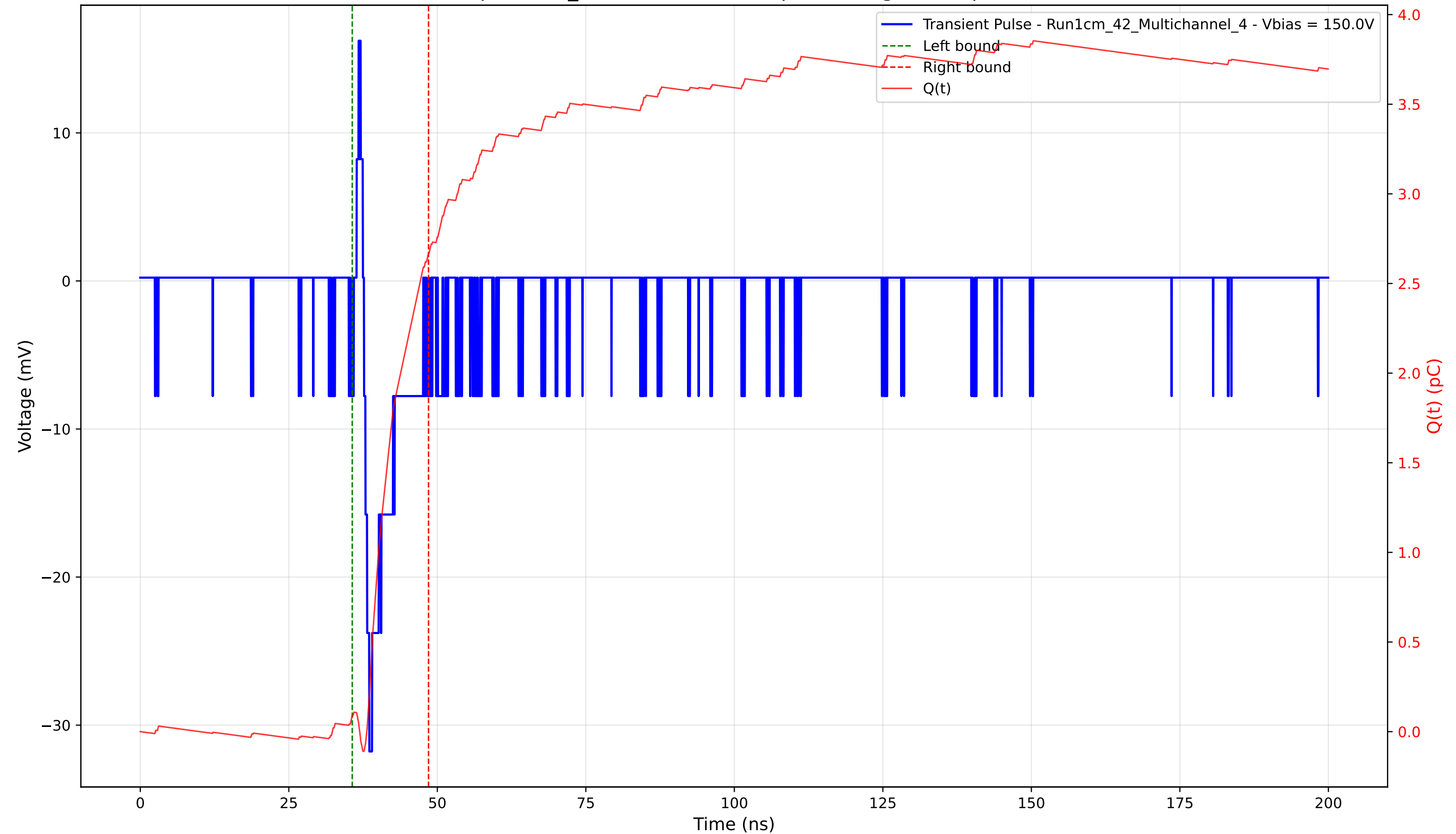
Transient Pulse - Sample: 1cm_42 - Position: 395.0 \mu\text{m} - Charge: 2.58 pC - Rise Time: 0.90 ns
