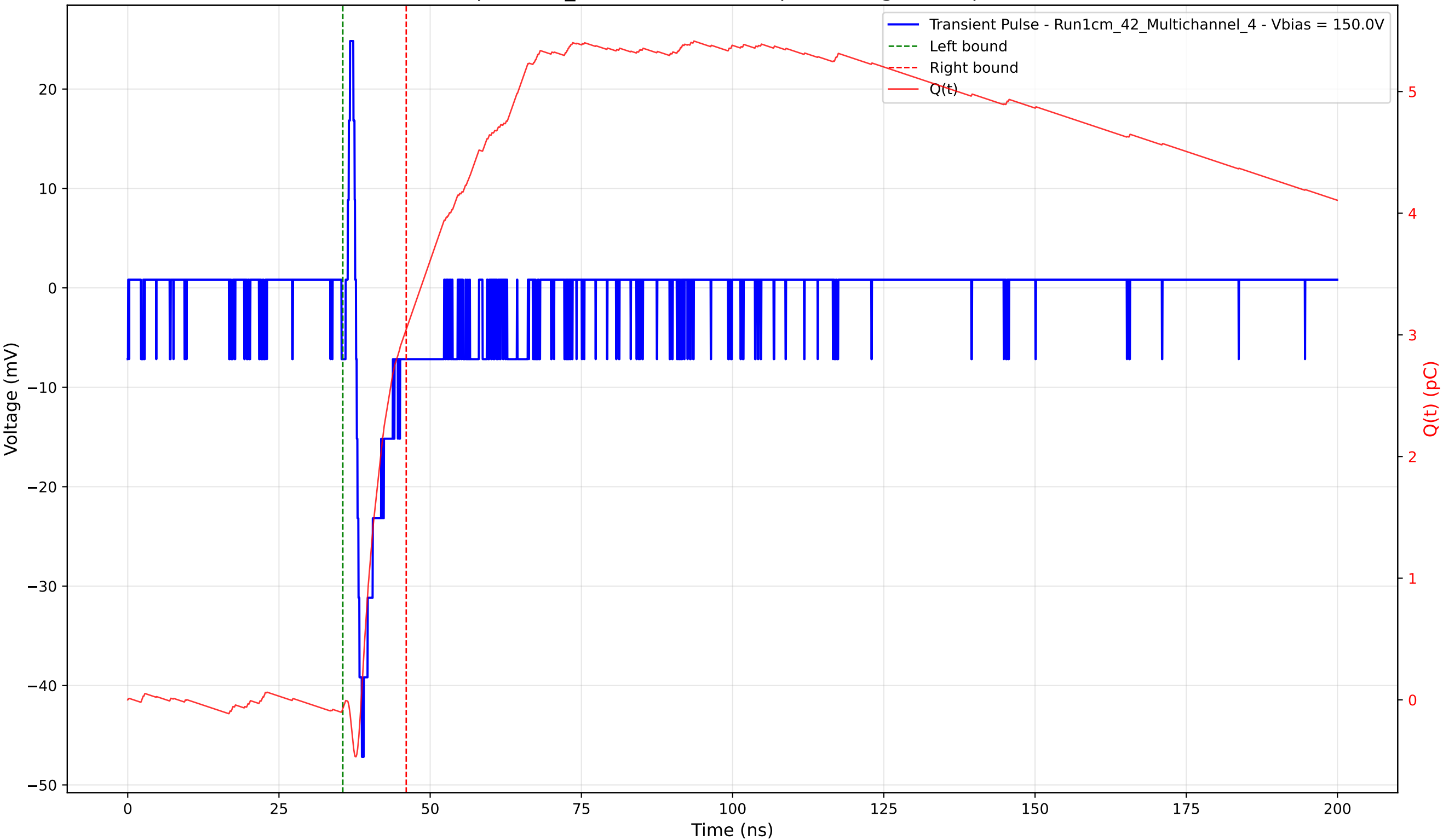
Transient Pulse - Sample: 1cm_42 - Position: 635.0 \mu\text{m} - Charge: 3.12 pC - Rise Time: 0.98 ns
