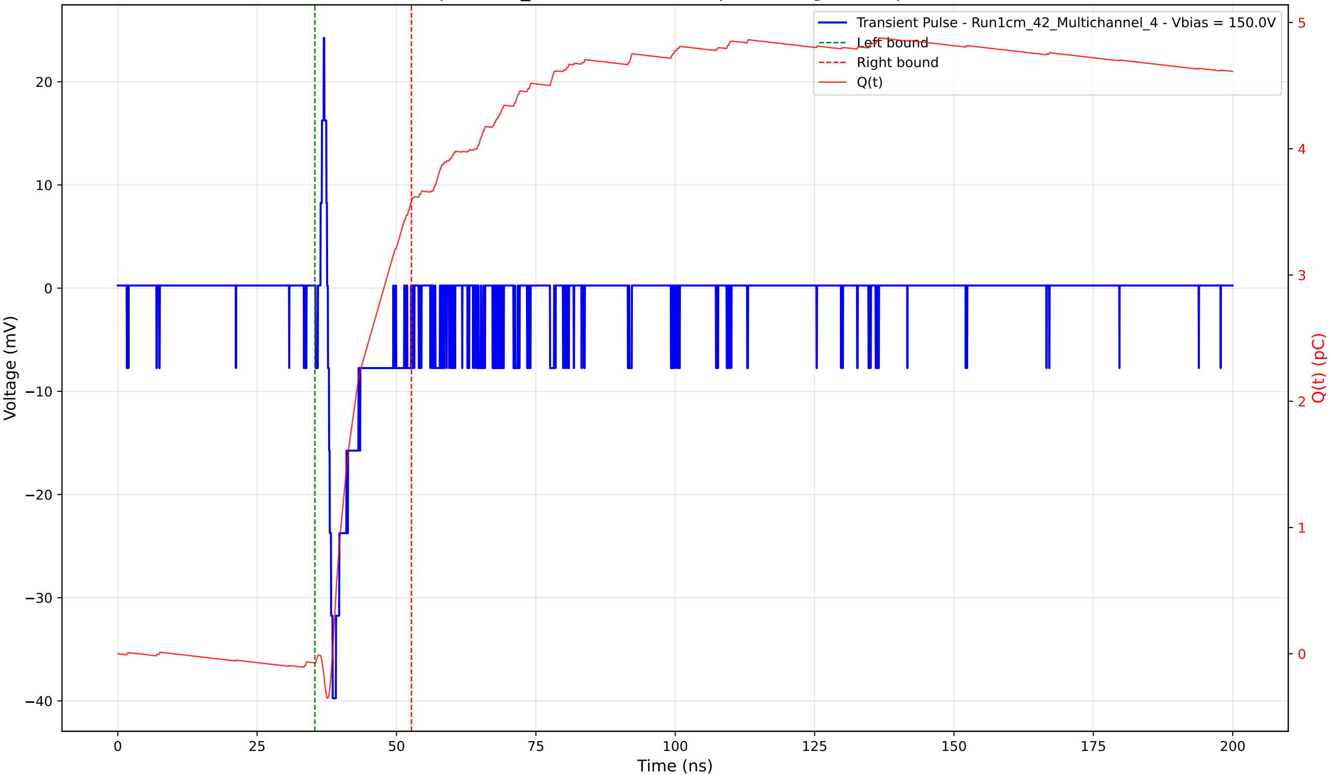
Transient Pulse - Sample: 1cm_42 - Position: 520.0 \mu\text{m} - Charge: 3.65 pC - Rise Time: 0.86 ns
