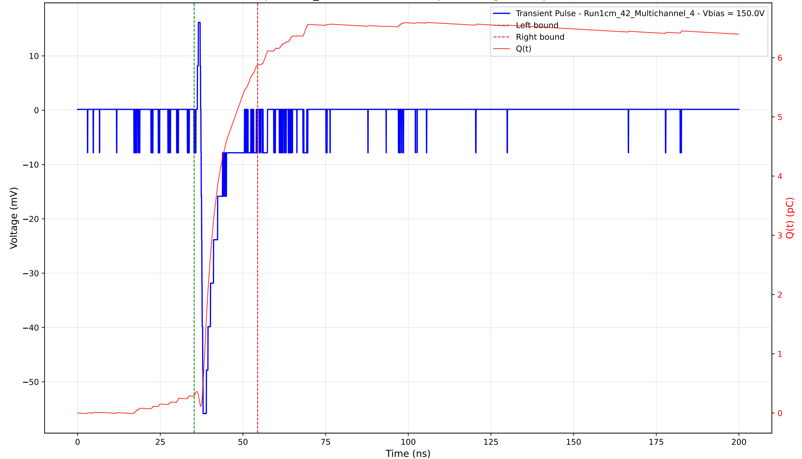
Transient Pulse - Sample: 1cm_42 - Position: 3760.0 \mu\text{m} - Charge: 5.58 pC - Rise Time: 0.65 ns
