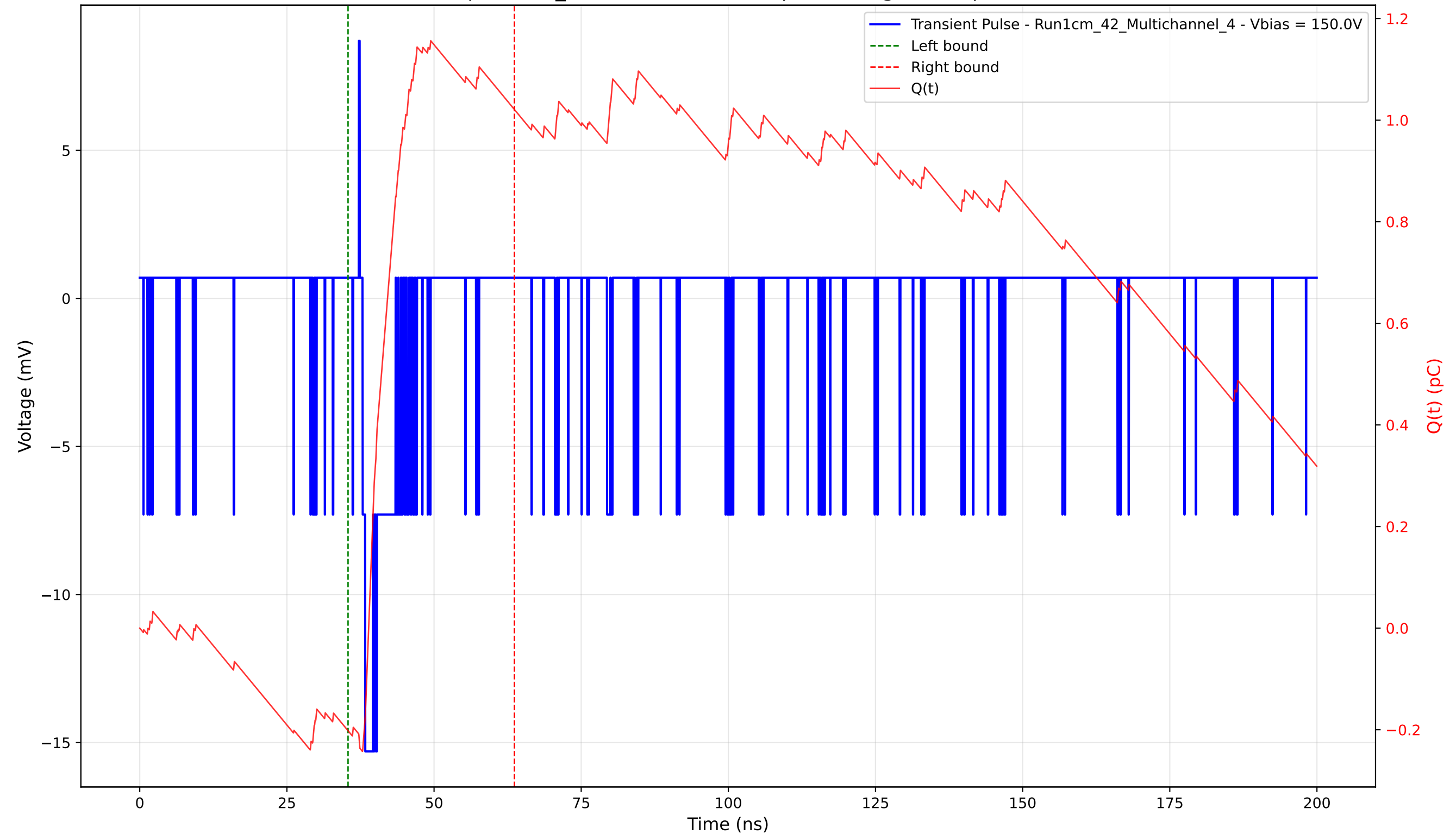
Transient Pulse - Sample: 1cm_42 - Position: 5045.0 \mu\text{m} - Charge: 1.22 pC - Rise Time: 0.47 ns
