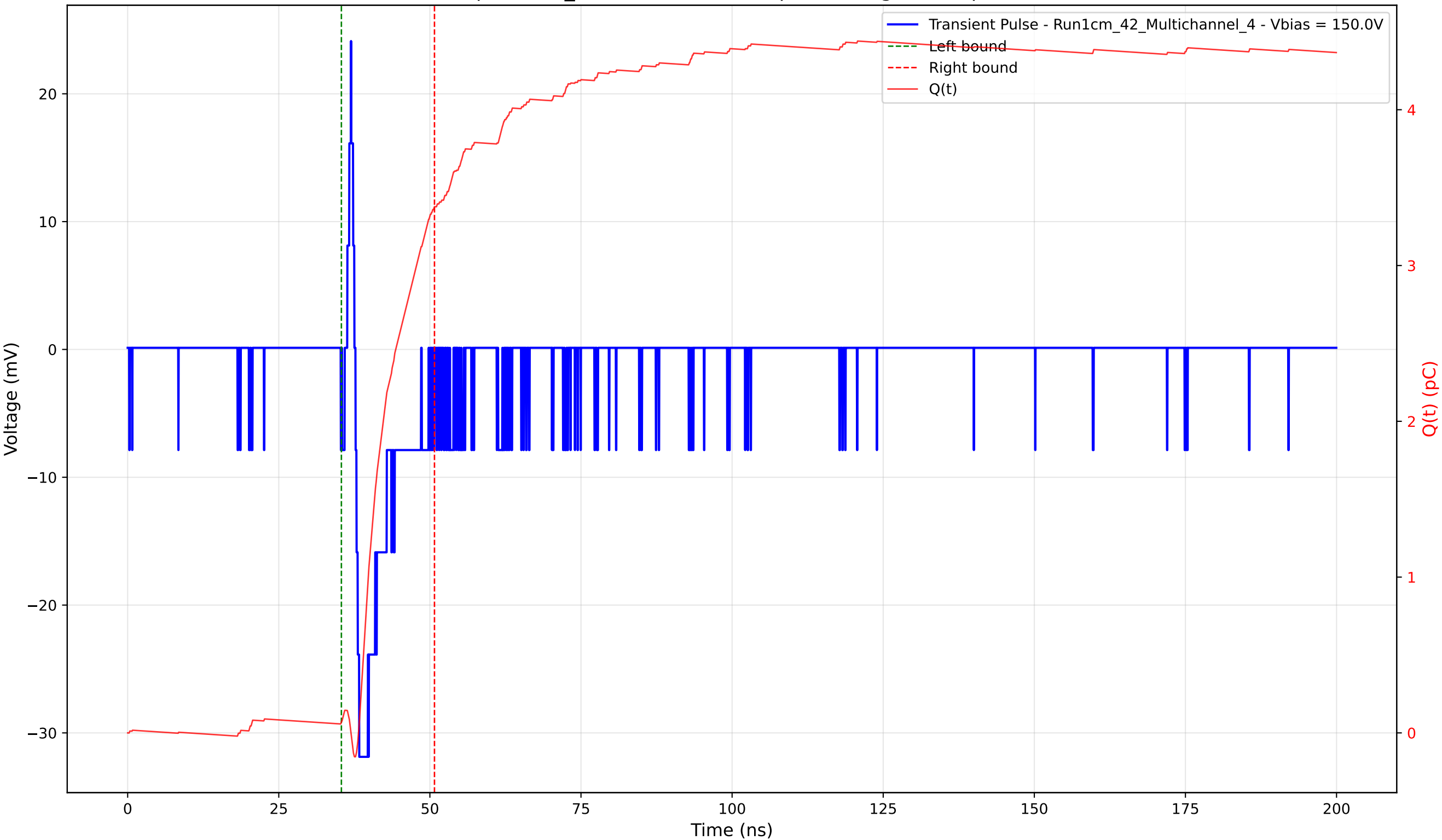
Transient Pulse - Sample: 1cm_42 - Position: 485.0 \mu\text{m} - Charge: 3.30 pC - Rise Time: 0.62 ns
