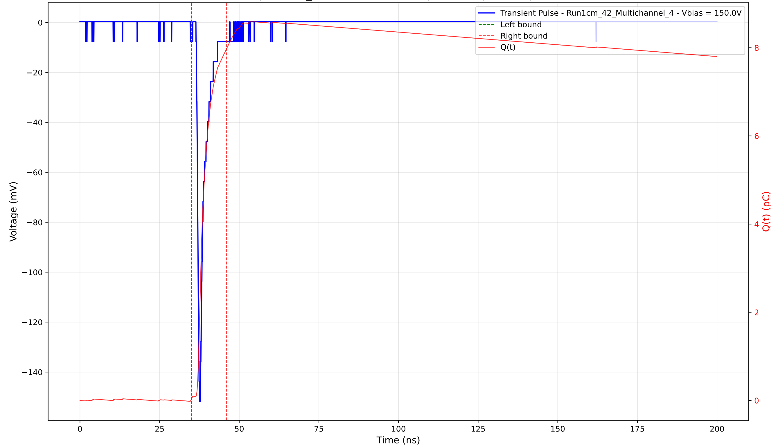
Transient Pulse - Sample: 1cm_42 - Position: 3205.0 \mu\text{m} - Charge: 7.94 pC - Rise Time: 0.84 ns
