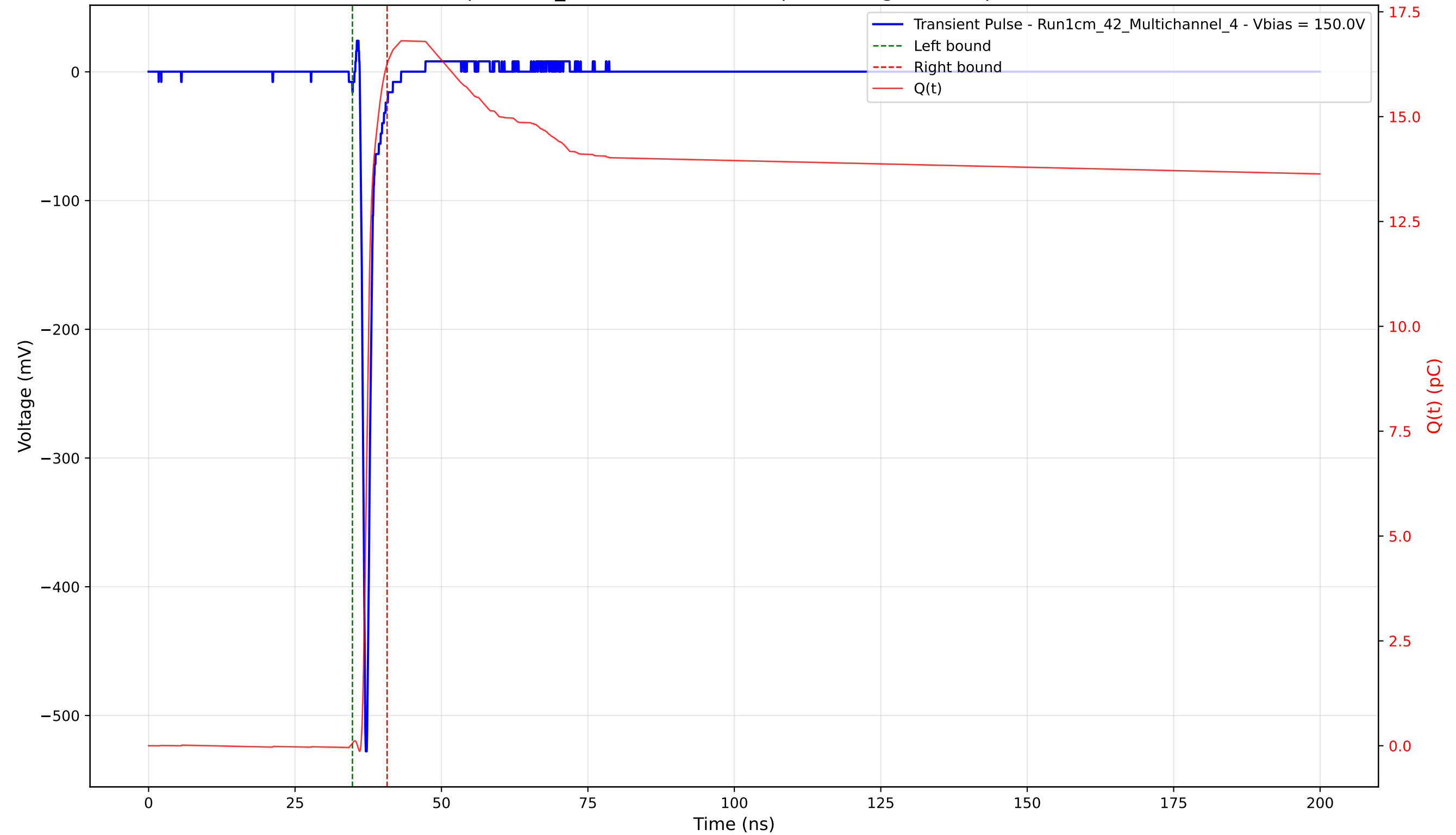
Transient Pulse - Sample: 1cm_42 - Position: 2435.0 \mu\text{m} - Charge: 16.20 pC - Rise Time: 0.72 ns
