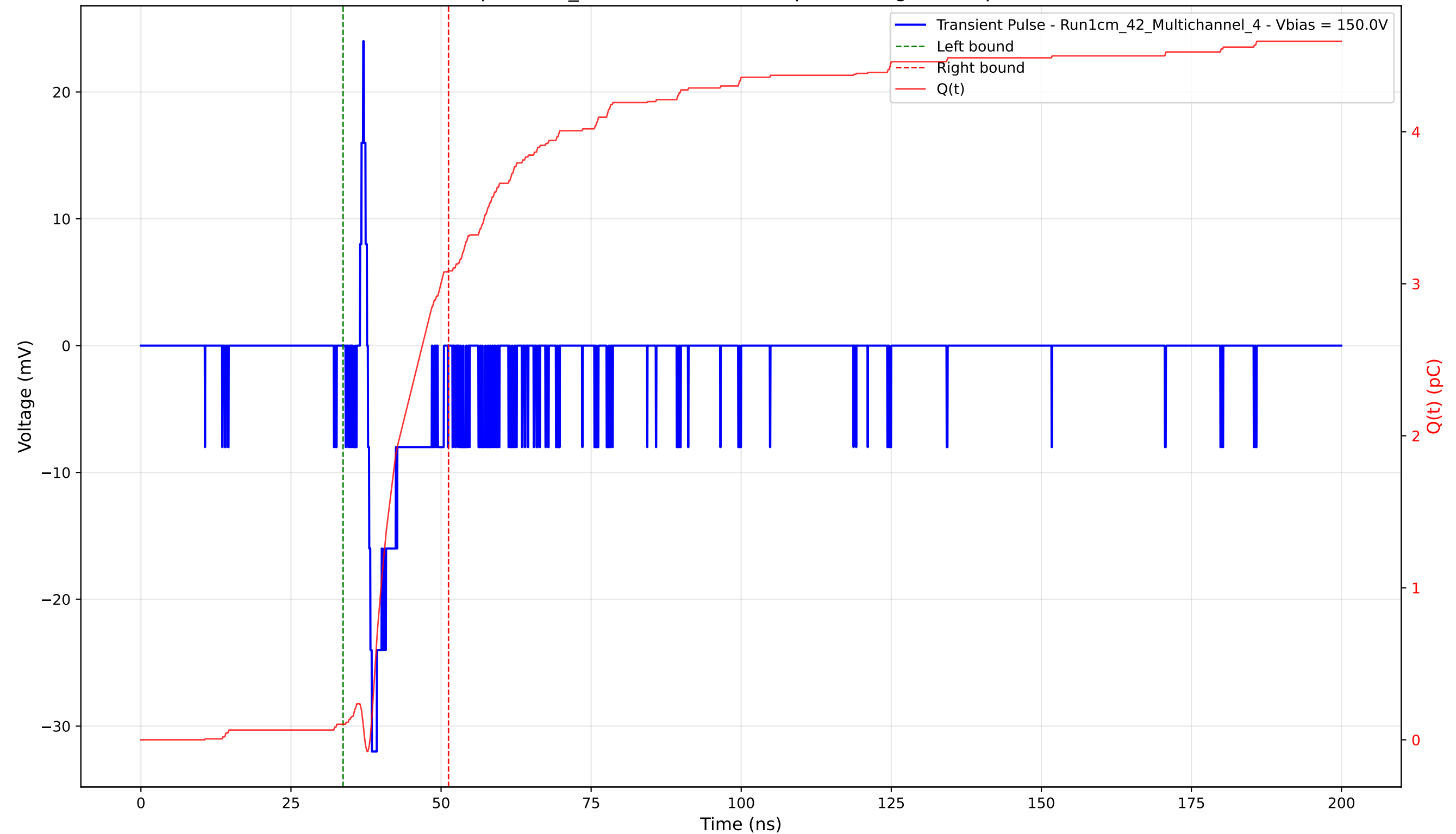
Transient Pulse - Sample: 1cm_42 - Position: 4495.0 \mu\text{m} - Charge: 2.98 pC - Rise Time: 0.66 ns
