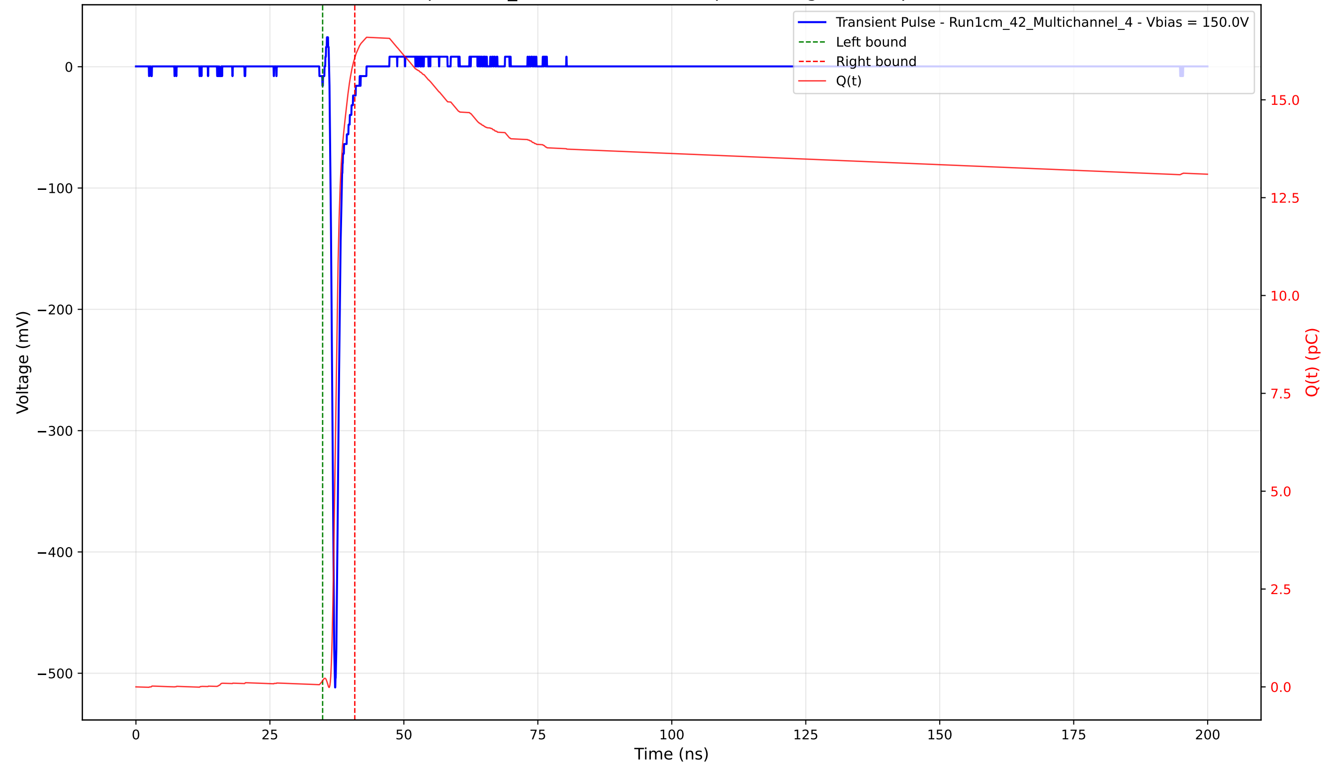
Transient Pulse - Sample: 1cm_42 - Position: 2675.0 \mu\text{m} - Charge: 15.92 pC - Rise Time: 0.72 ns
