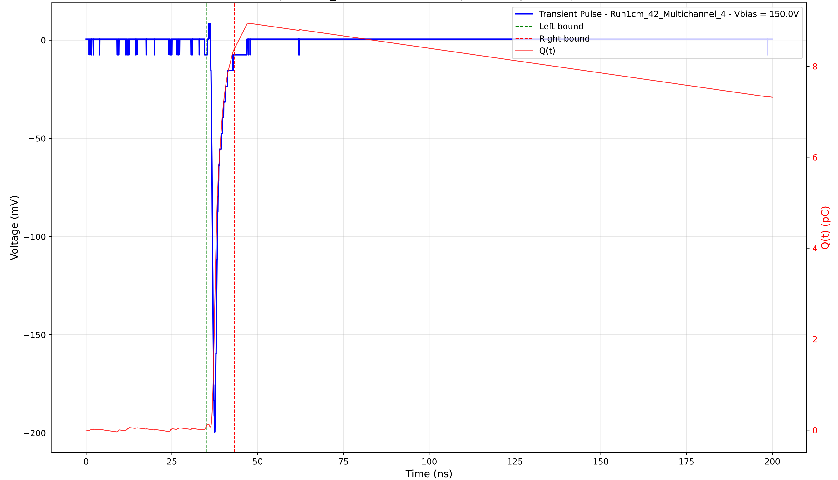
Transient Pulse - Sample: 1cm_42 - Position: 3065.0 \mu\text{m} - Charge: 8.30 pC - Rise Time: 0.82 ns
