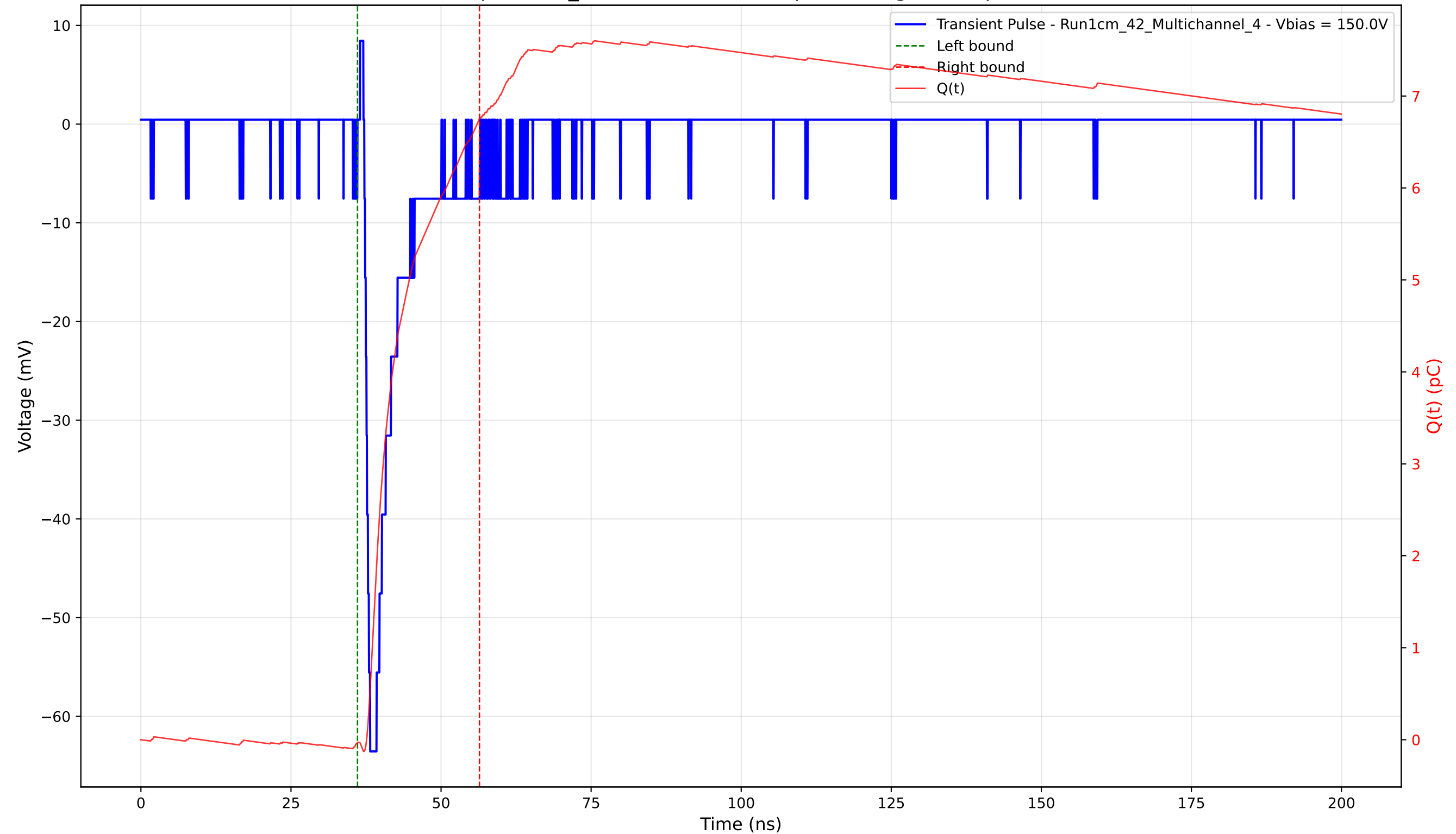
Transient Pulse - Sample: 1cm_42 - Position: 1275.0 \mu\text{m} - Charge: 6.79 pC - Rise Time: 0.97 ns
