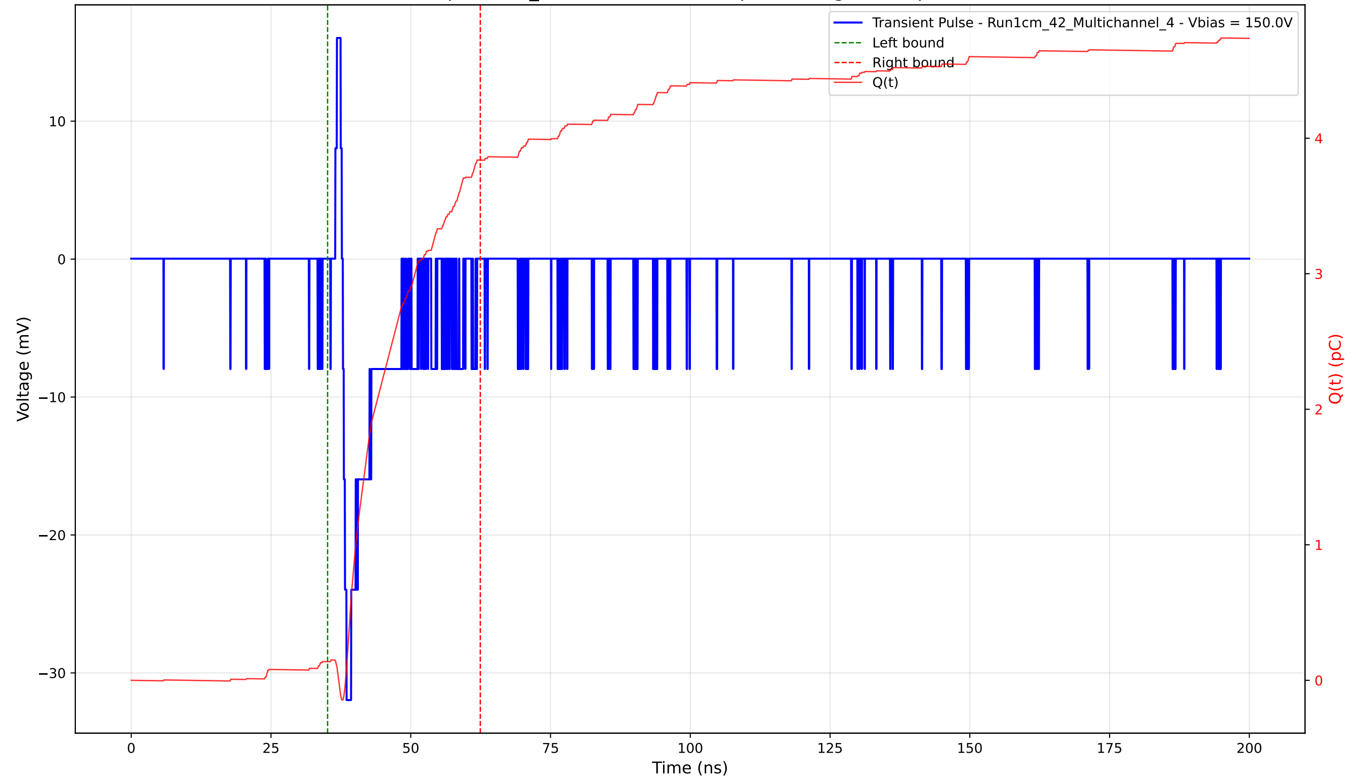
Transient Pulse - Sample: 1cm_42 - Position: 4540.0 \mu\text{m} - Charge: 3.70 pC - Rise Time: 0.66 ns
