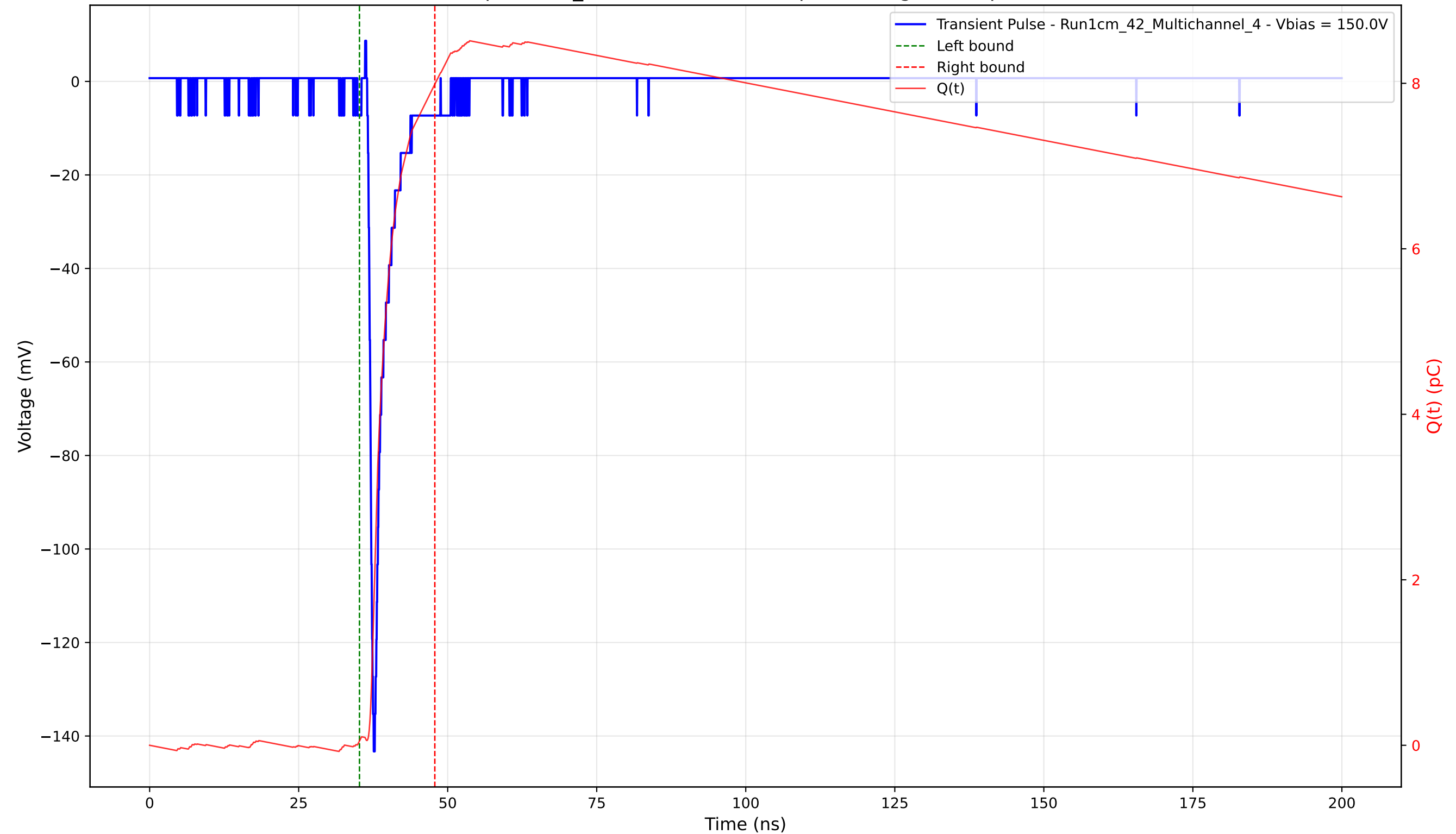
Transient Pulse - Sample: 1cm_42 - Position: 3285.0 \mu\text{m} - Charge: 7.94 pC - Rise Time: 0.84 ns
