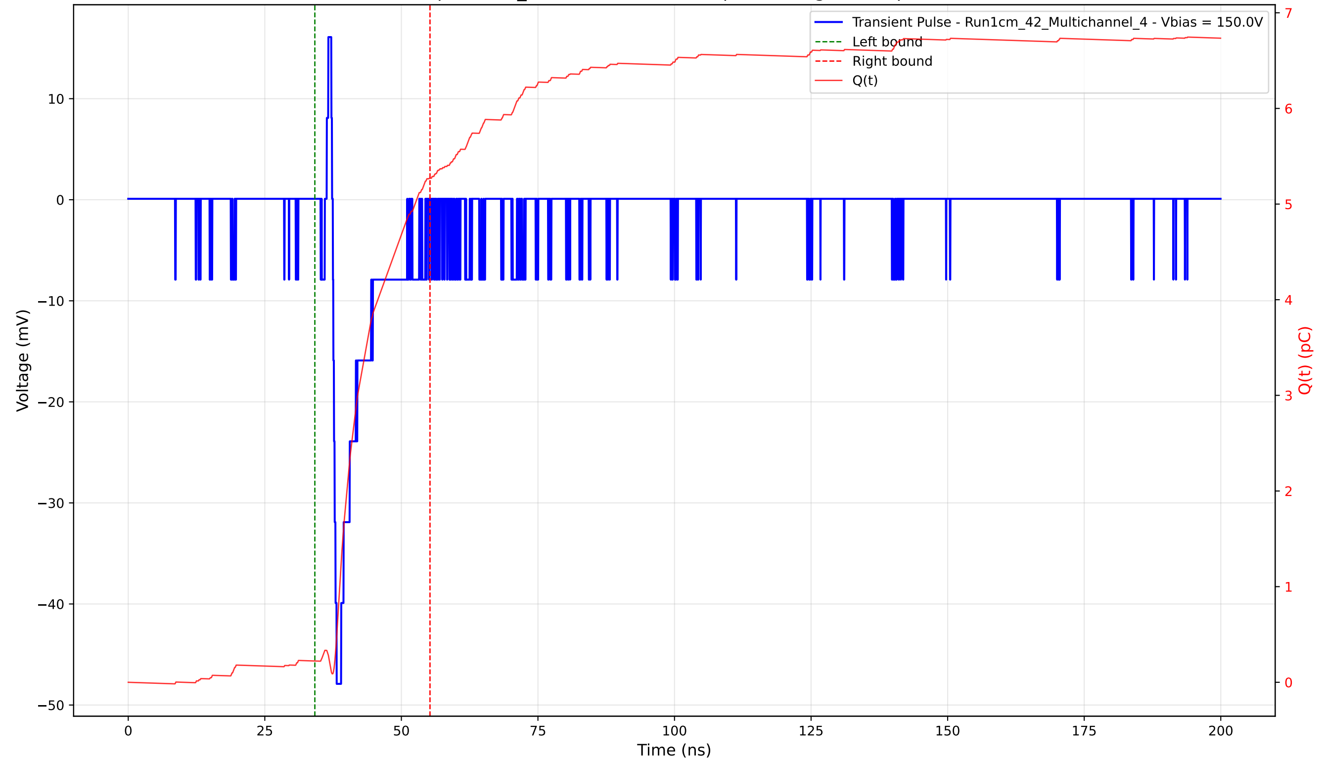
Transient Pulse - Sample: 1cm_42 - Position: 3920.0 \mu\text{m} - Charge: 5.05 pC - Rise Time: 0.70 ns
