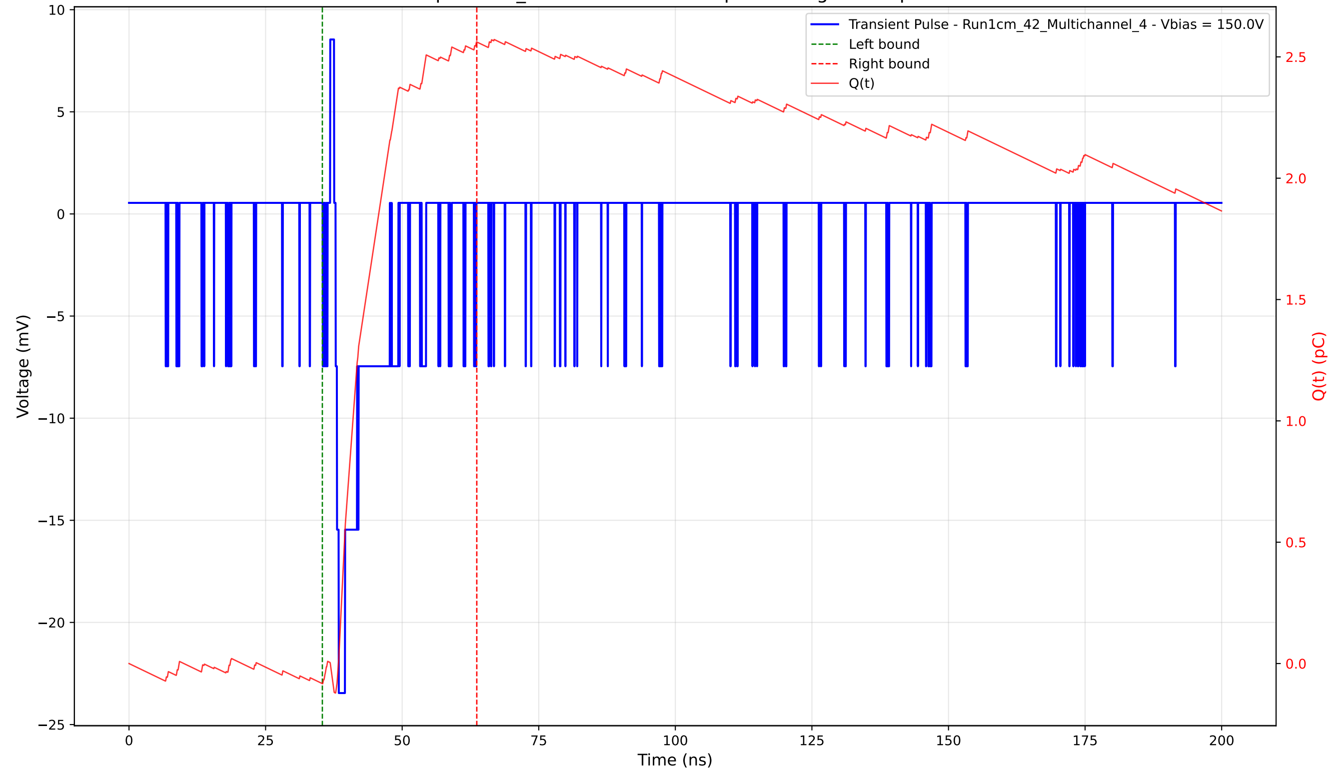
Transient Pulse - Sample: 1cm_42 - Position: 4955.0 \mu\text{m} - Charge: 2.64 pC - Rise Time: 0.59 ns
