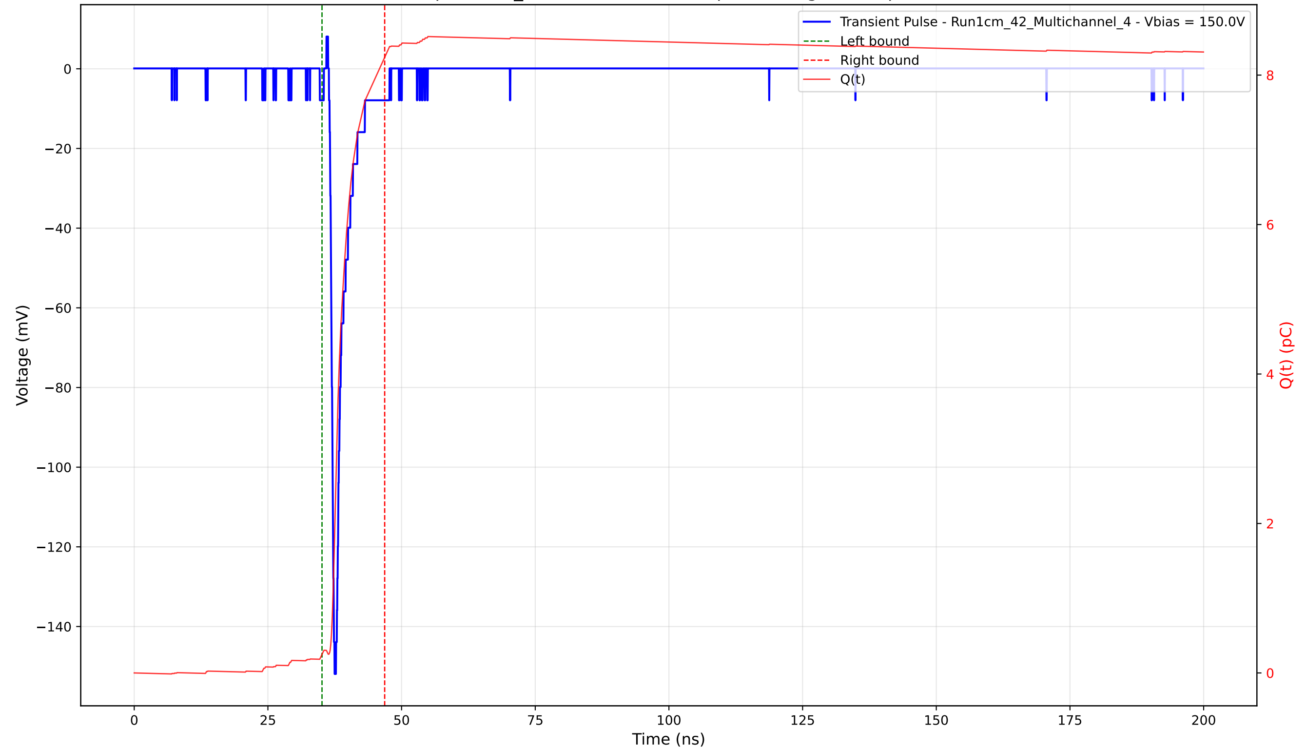
Transient Pulse - Sample: 1cm_42 - Position: 3200.0 \mu\text{m} - Charge: 7.99 pC - Rise Time: 0.80 ns
