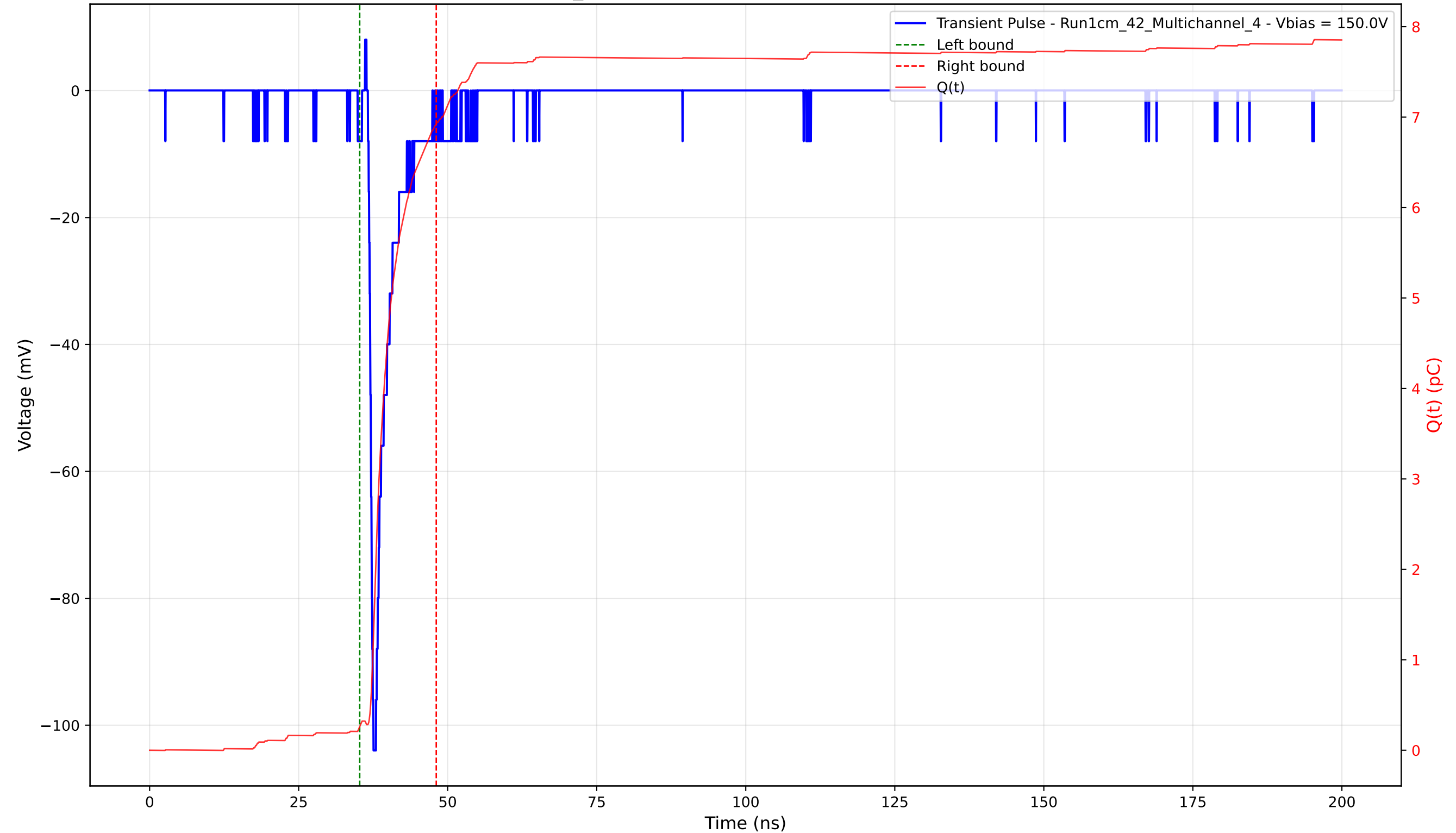
Transient Pulse - Sample: 1cm_42 - Position: 3400.0 \mu\text{m} - Charge: 6.66 pC - Rise Time: 0.71 ns
