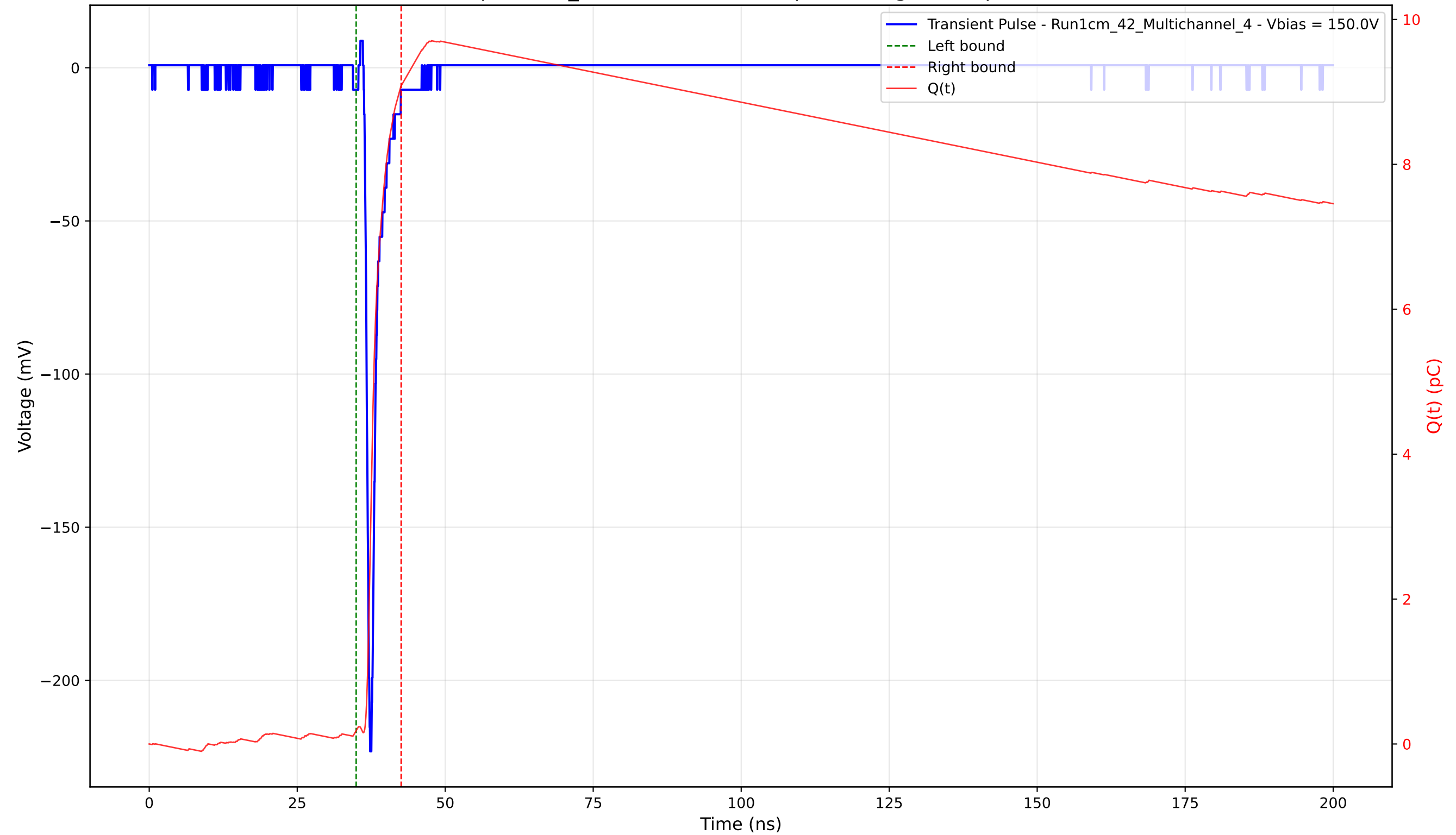
Transient Pulse - Sample: 1cm_42 - Position: 3020.0 \mu\text{m} - Charge: 8.90 pC - Rise Time: 0.77 ns
