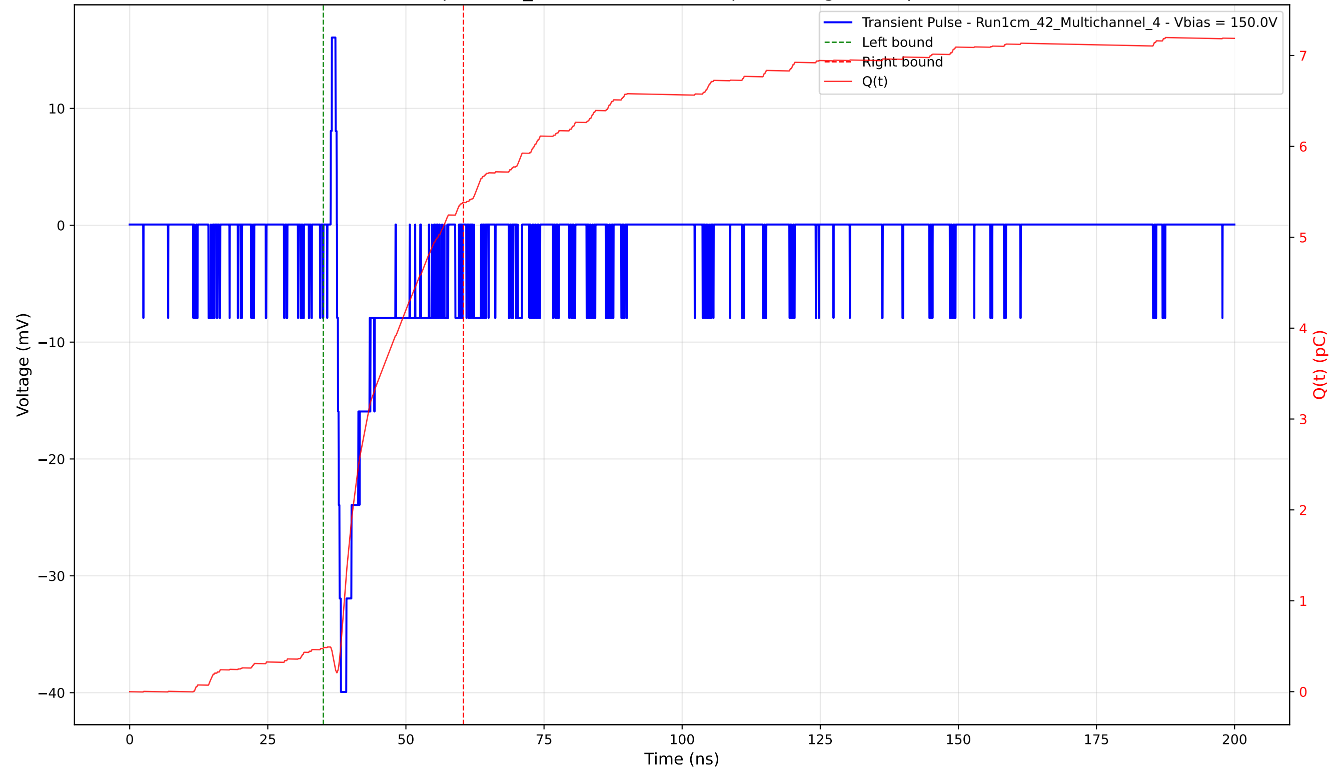
Transient Pulse - Sample: 1cm_42 - Position: 4025.0 \mu\text{m} - Charge: 4.90 pC - Rise Time: 0.70 ns
