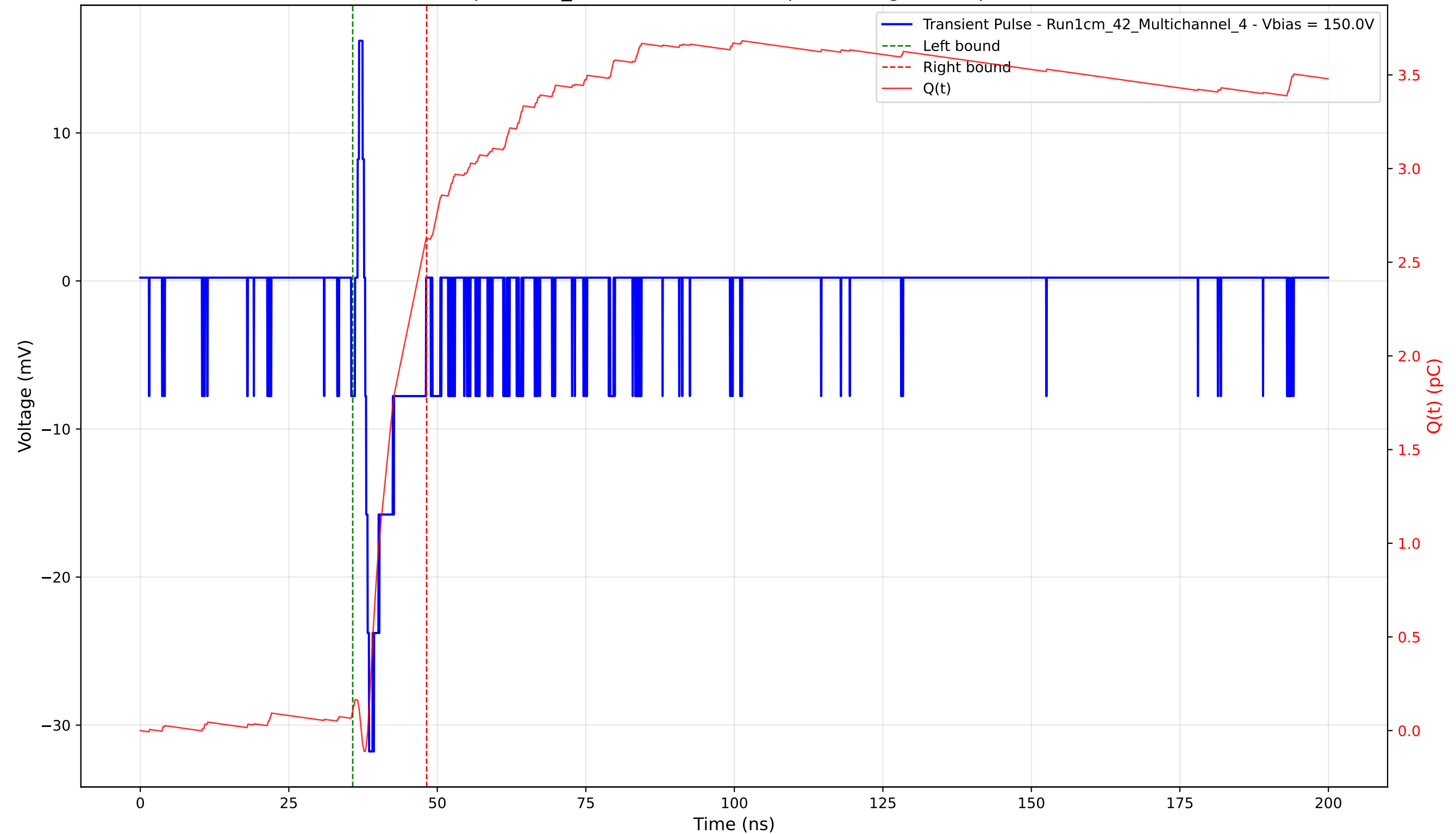
Transient Pulse - Sample: 1cm_42 - Position: 4595.0 \mu\text{m} - Charge: 2.52 pC - Rise Time: 0.66 ns
