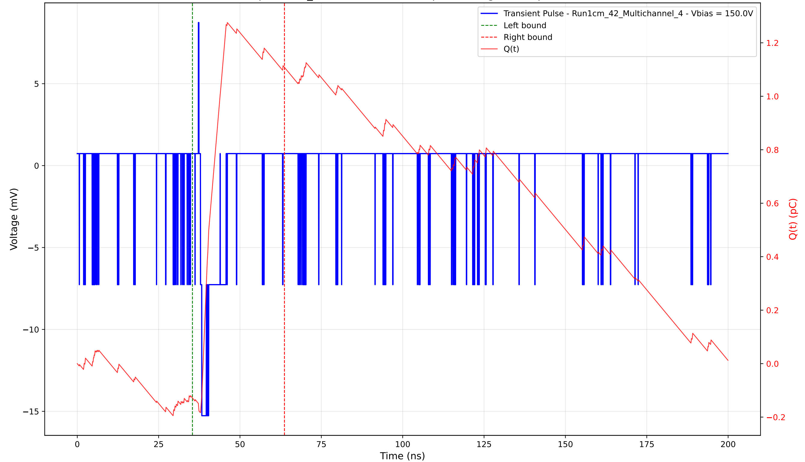
Transient Pulse - Sample: 1cm_42 - Position: 5030.0 \mu\text{m} - Charge: 1.24 pC - Rise Time: 0.44 ns
