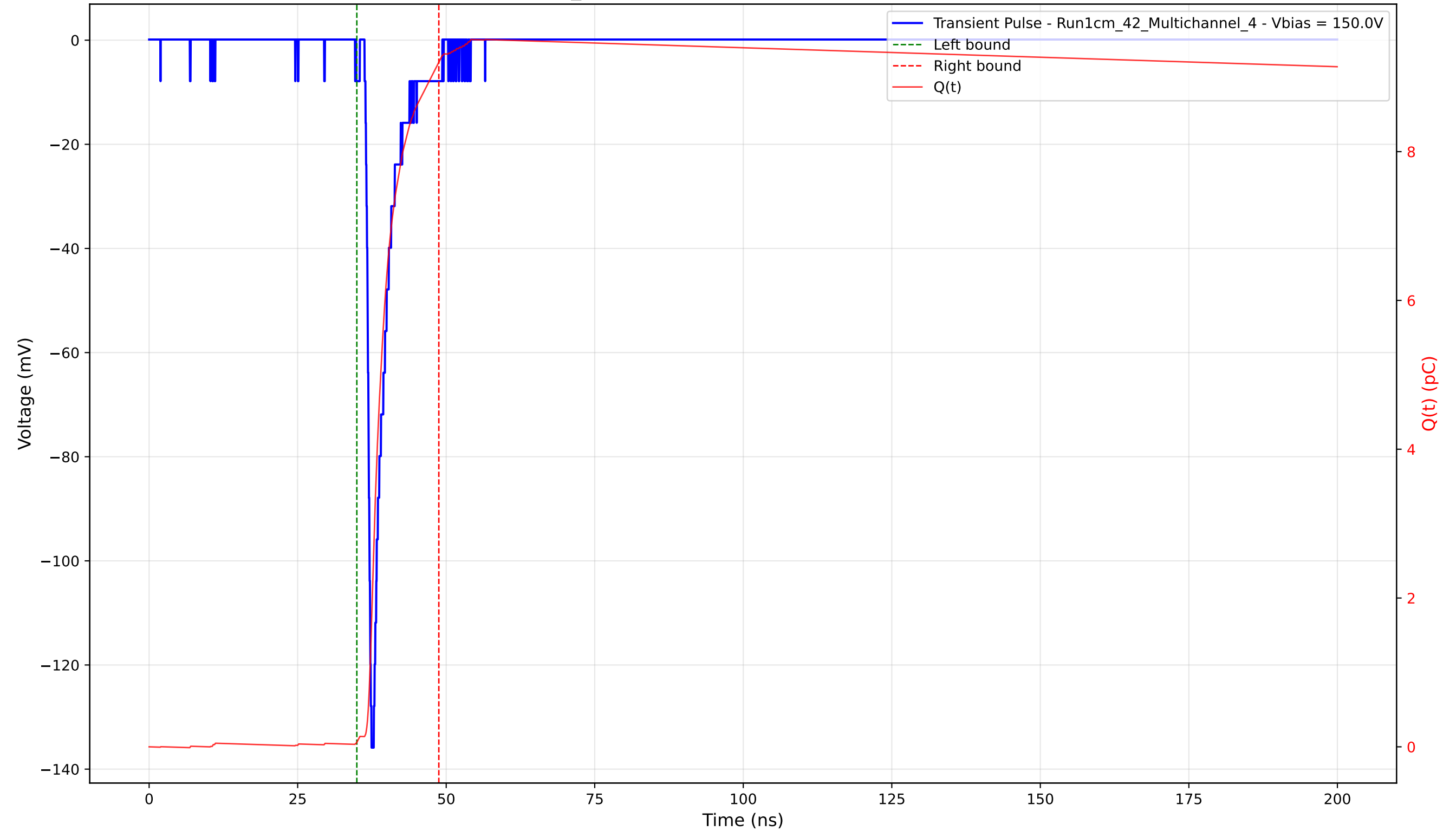
Transient Pulse - Sample: 1cm_42 - Position: 1710.0 \mu\text{m} - Charge: 9.14 pC - Rise Time: 0.89 ns
