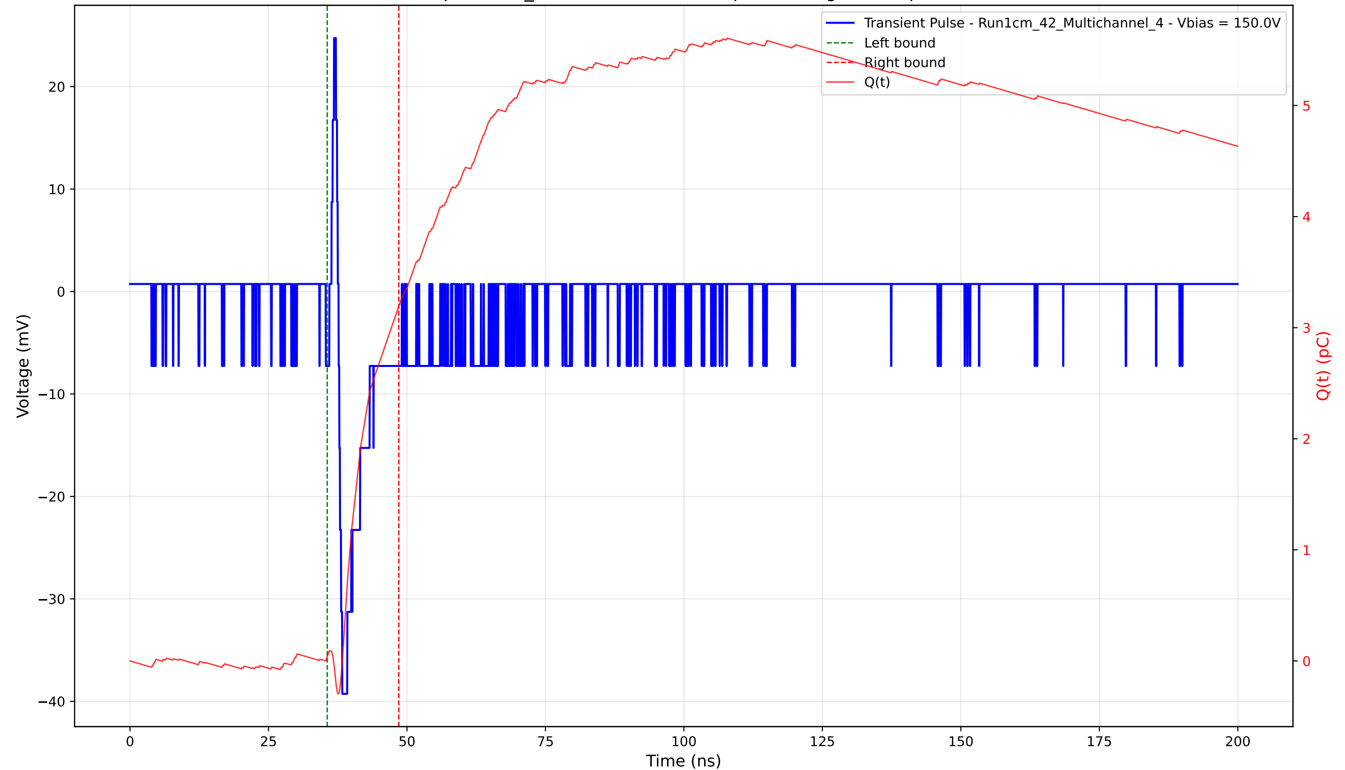
Transient Pulse - Sample: 1cm_42 - Position: 4130.0 \mu\text{m} - Charge: 3.16 pC - Rise Time: 0.66 ns
