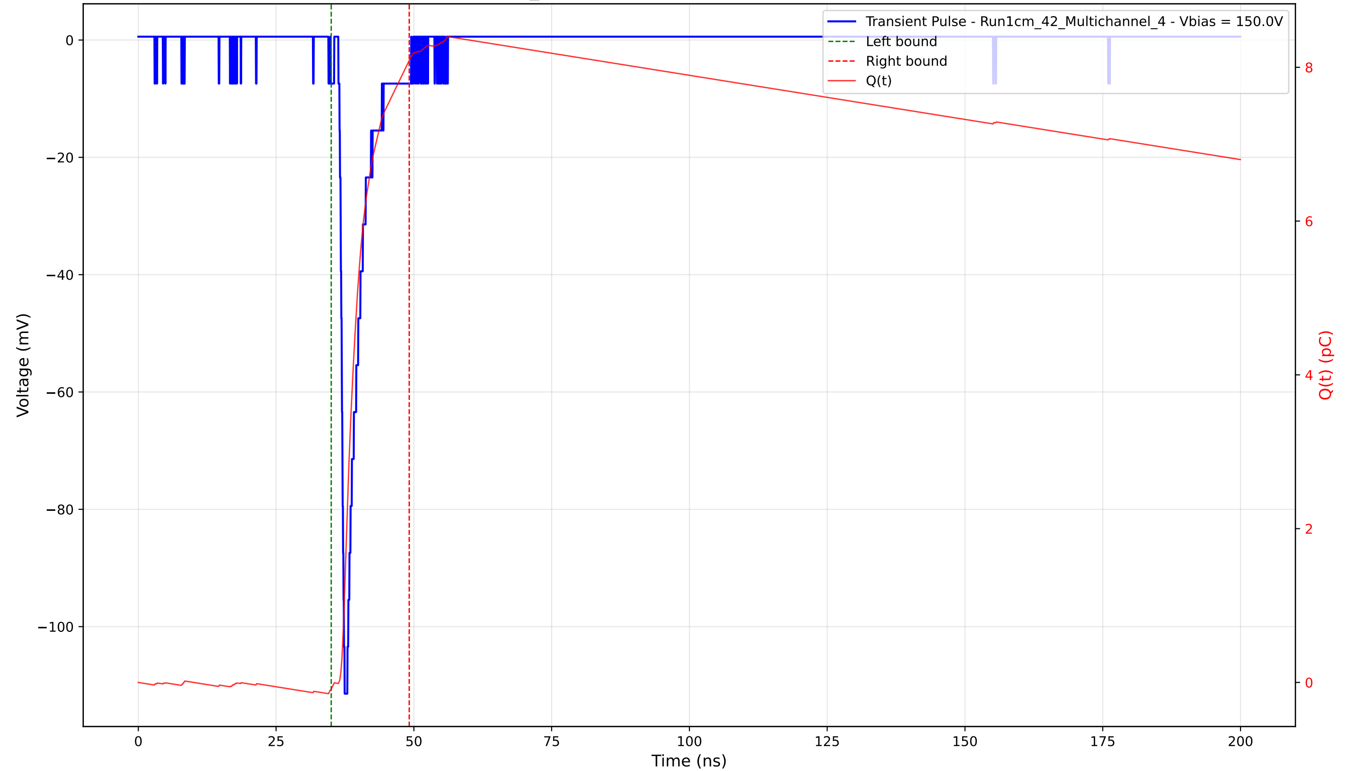
Transient Pulse - Sample: 1cm_42 - Position: 1650.0 \mu\text{m} - Charge: 8.18 pC - Rise Time: 0.82 ns
