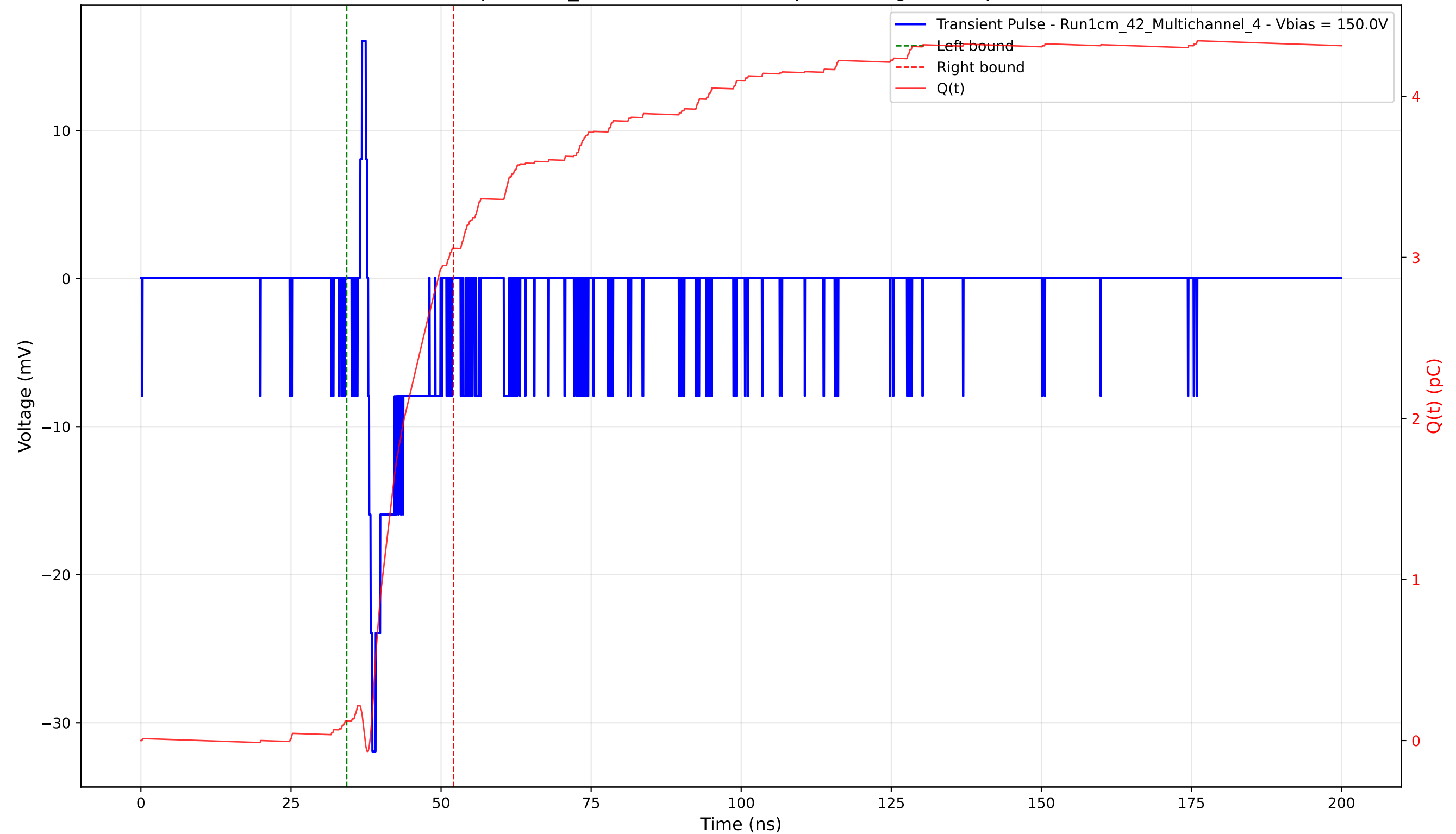
Transient Pulse - Sample: 1cm_42 - Position: 4550.0 \mu\text{m} - Charge: 2.93 pC - Rise Time: 0.70 ns
