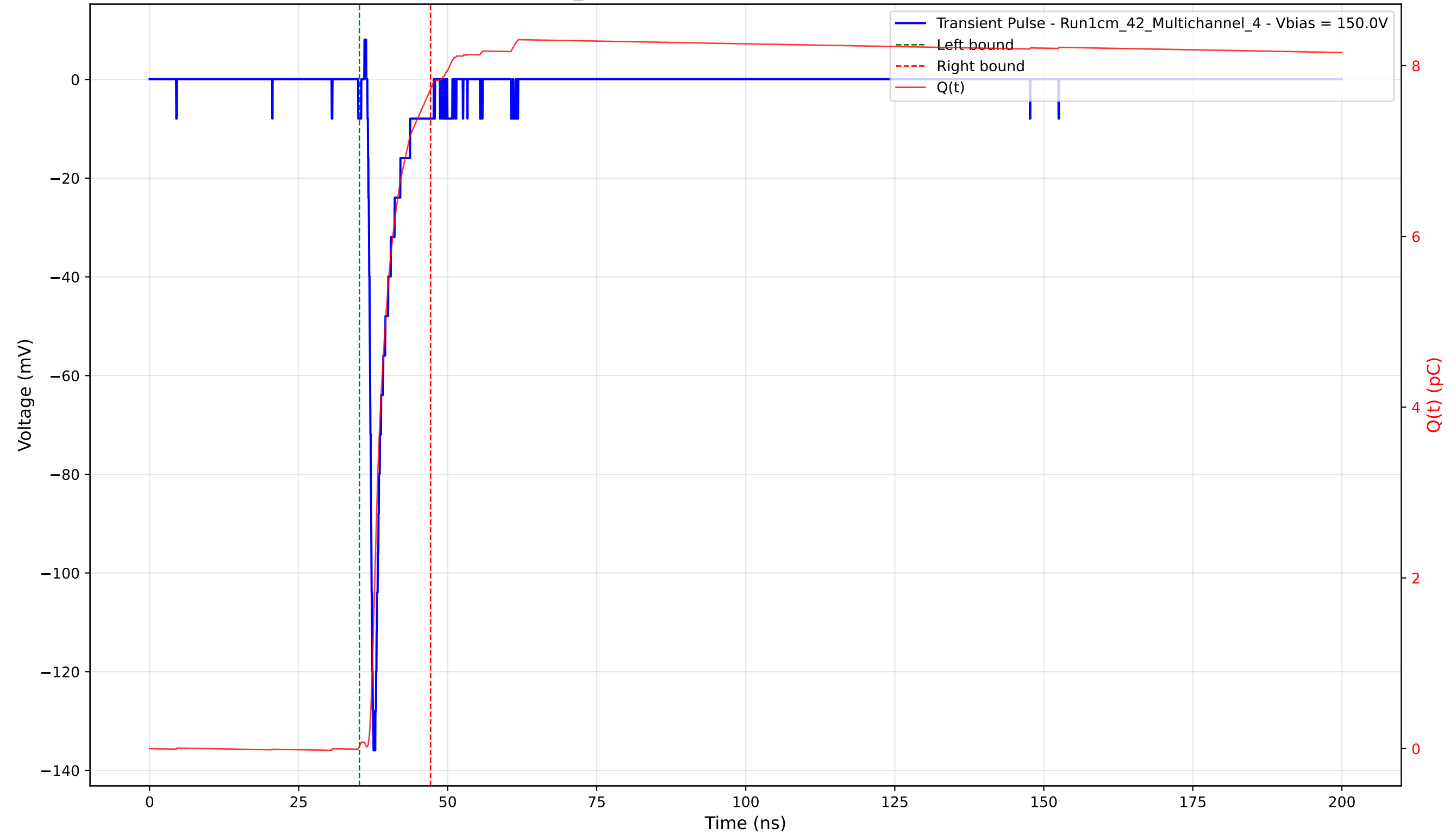
Transient Pulse - Sample: 1cm_42 - Position: 3315.0 \mu\text{m} - Charge: 7.70 pC - Rise Time: 0.81 ns
