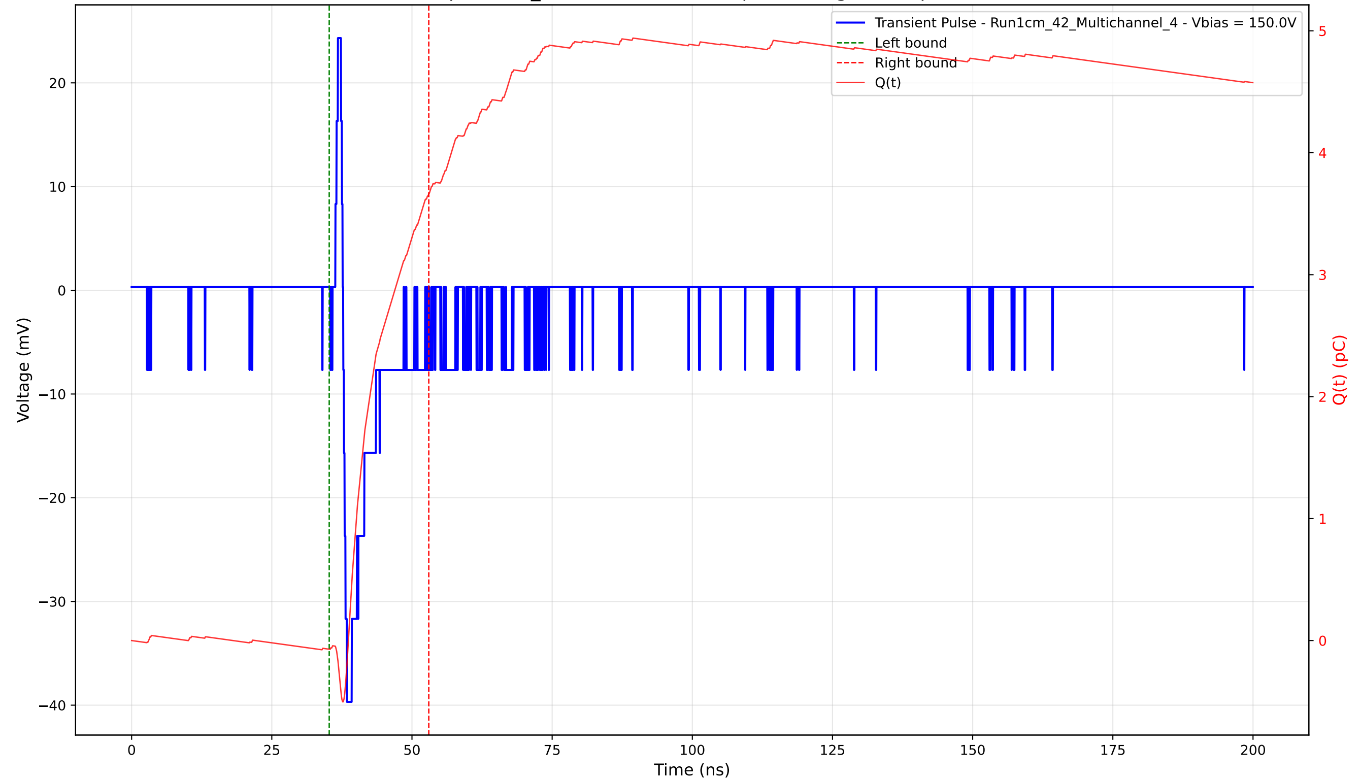
Transient Pulse - Sample: 1cm_42 - Position: 4230.0 \mu\text{m} - Charge: 3.74 pC - Rise Time: 0.66 ns
