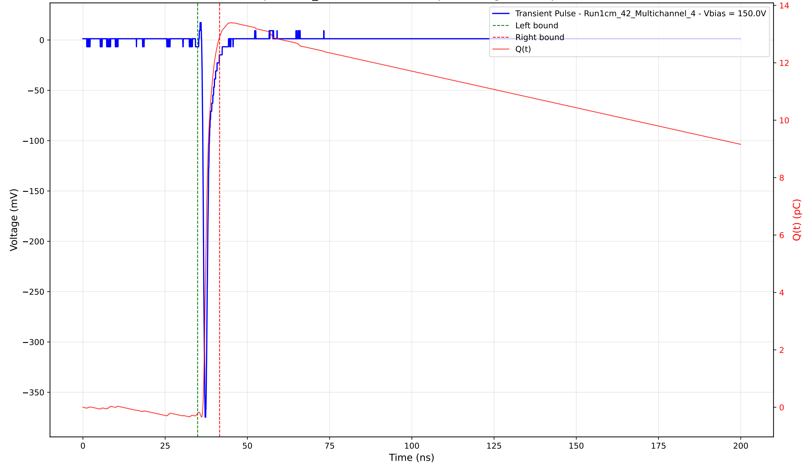
Transient Pulse - Sample: 1cm_42 - Position: 2140.0 \mu\text{m} - Charge: 13.12 pC - Rise Time: 0.72 ns
