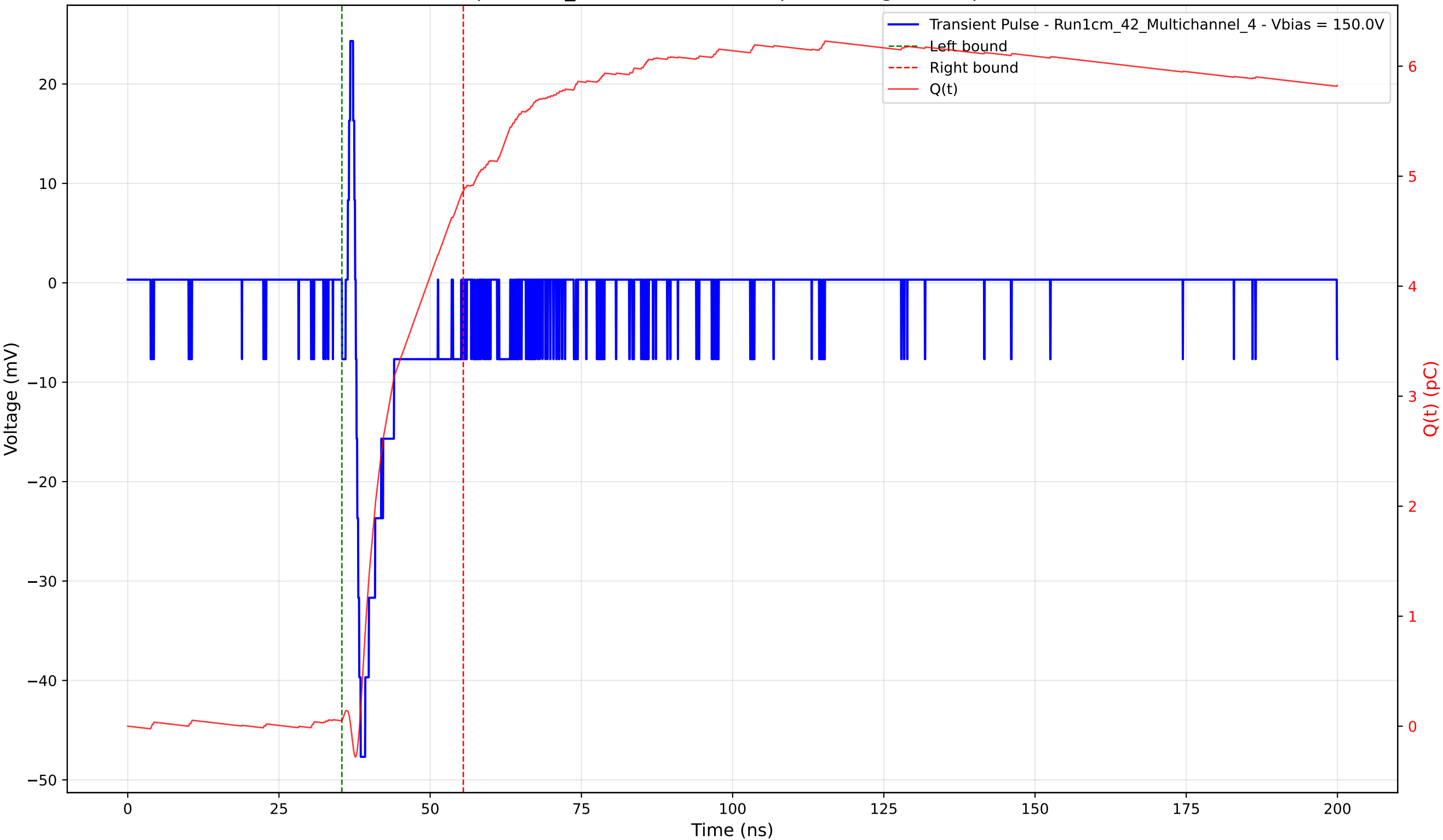
Transient Pulse - Sample: 1cm_42 - Position: 840.0 \mu\text{m} - Charge: 4.81 pC - Rise Time: 0.82 ns
