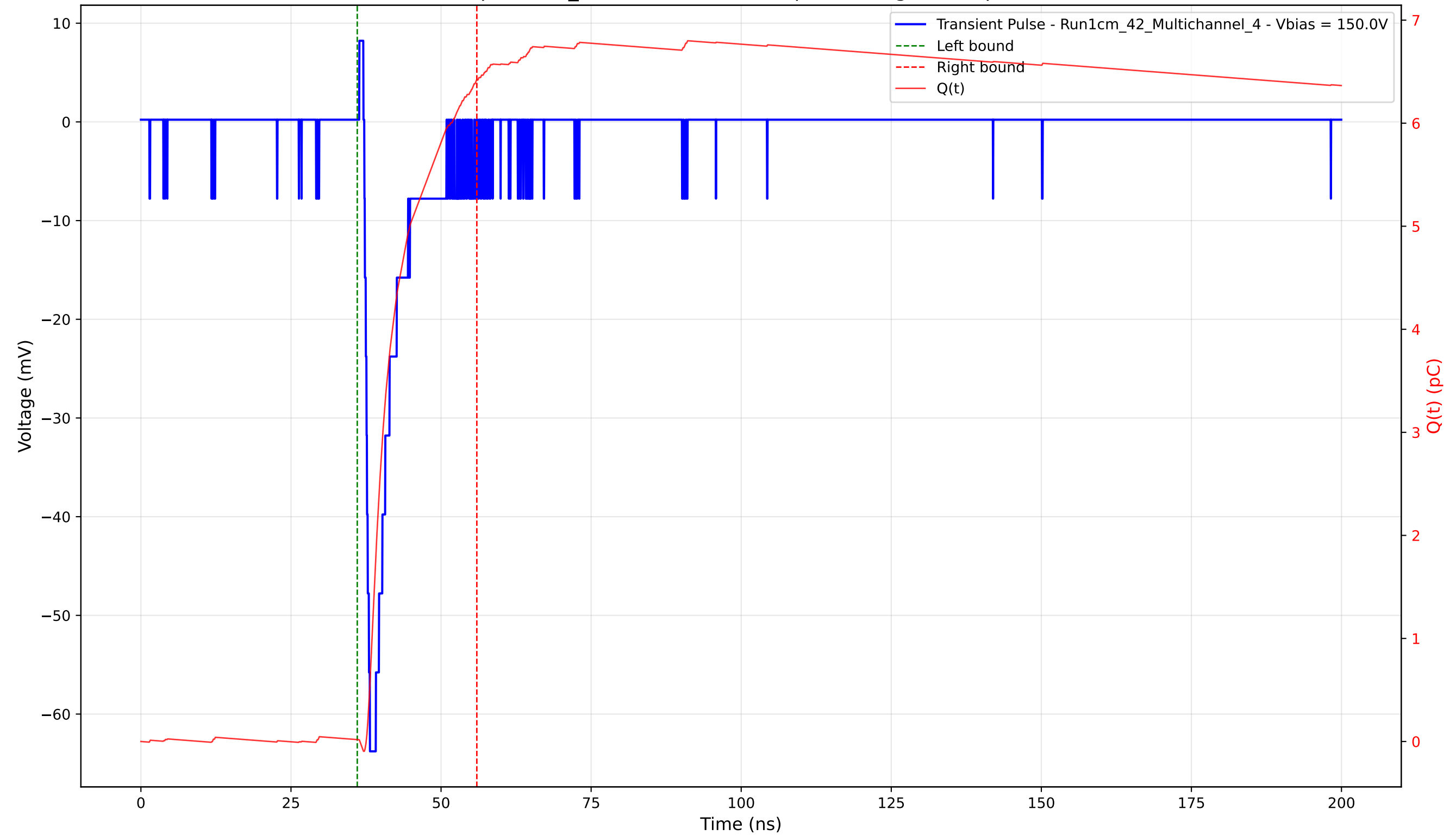
Transient Pulse - Sample: 1cm_42 - Position: 1285.0 \mu\text{m} - Charge: 6.40 pC - Rise Time: 0.93 ns
