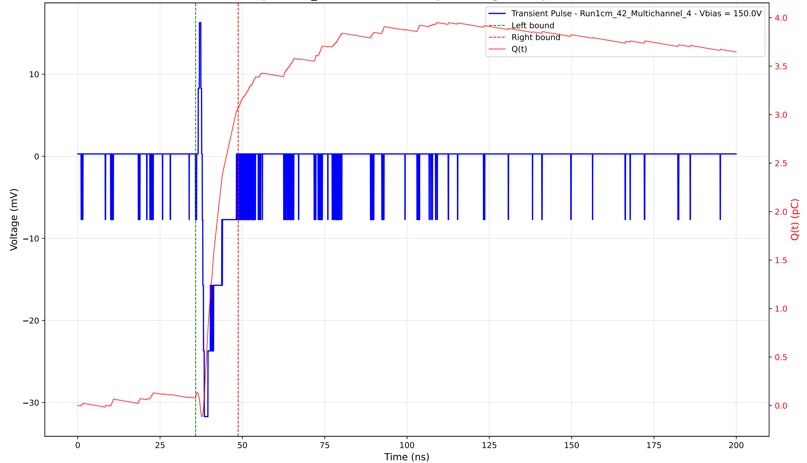
Transient Pulse - Sample: 1cm_42 - Position: 4750.0 \mu\text{m} - Charge: 2.98 pC - Rise Time: 0.62 ns
