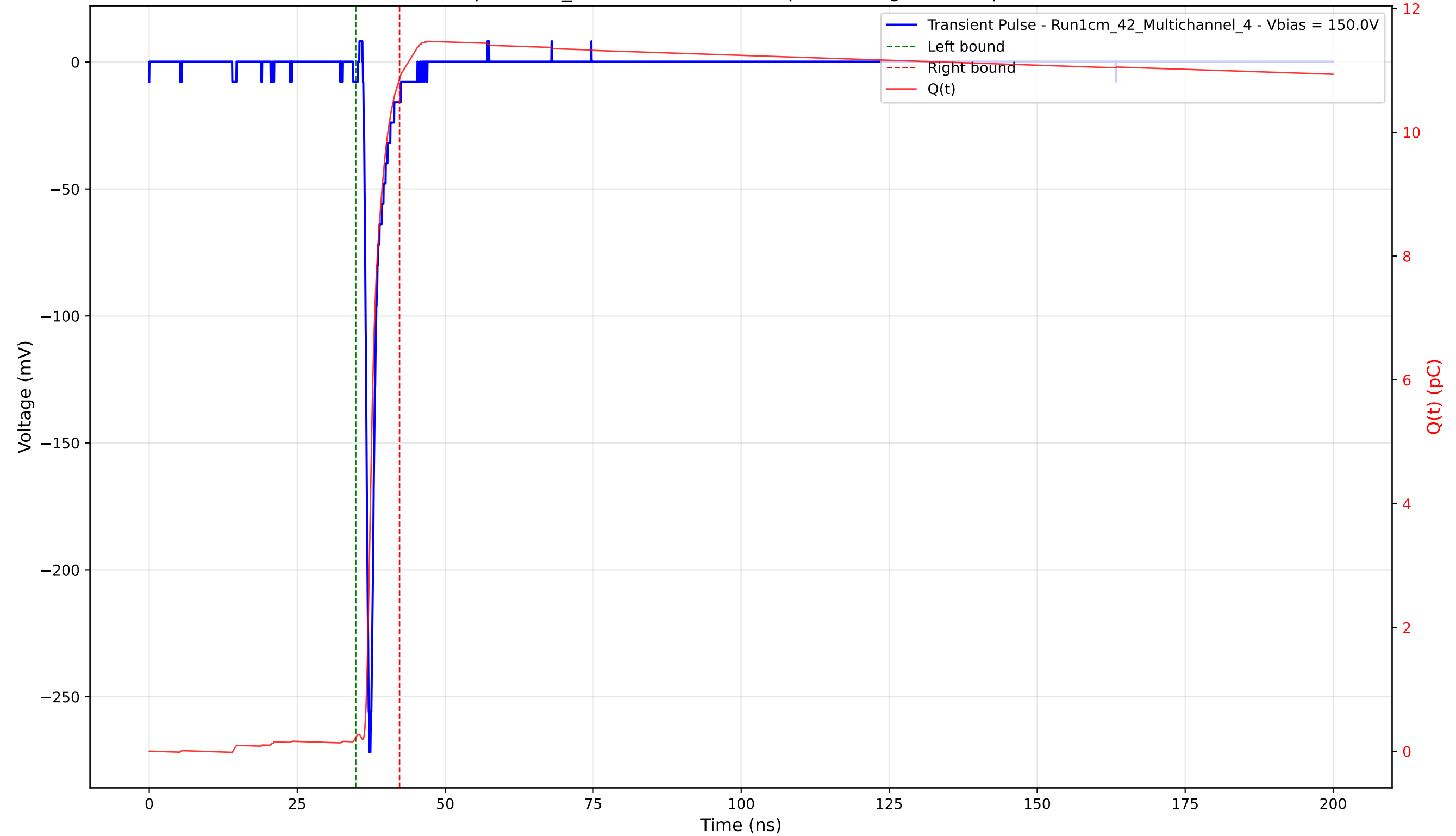
Transient Pulse - Sample: 1cm_42 - Position: 2055.0 \mu\text{m} - Charge: 10.64 pC - Rise Time: 0.73 ns
