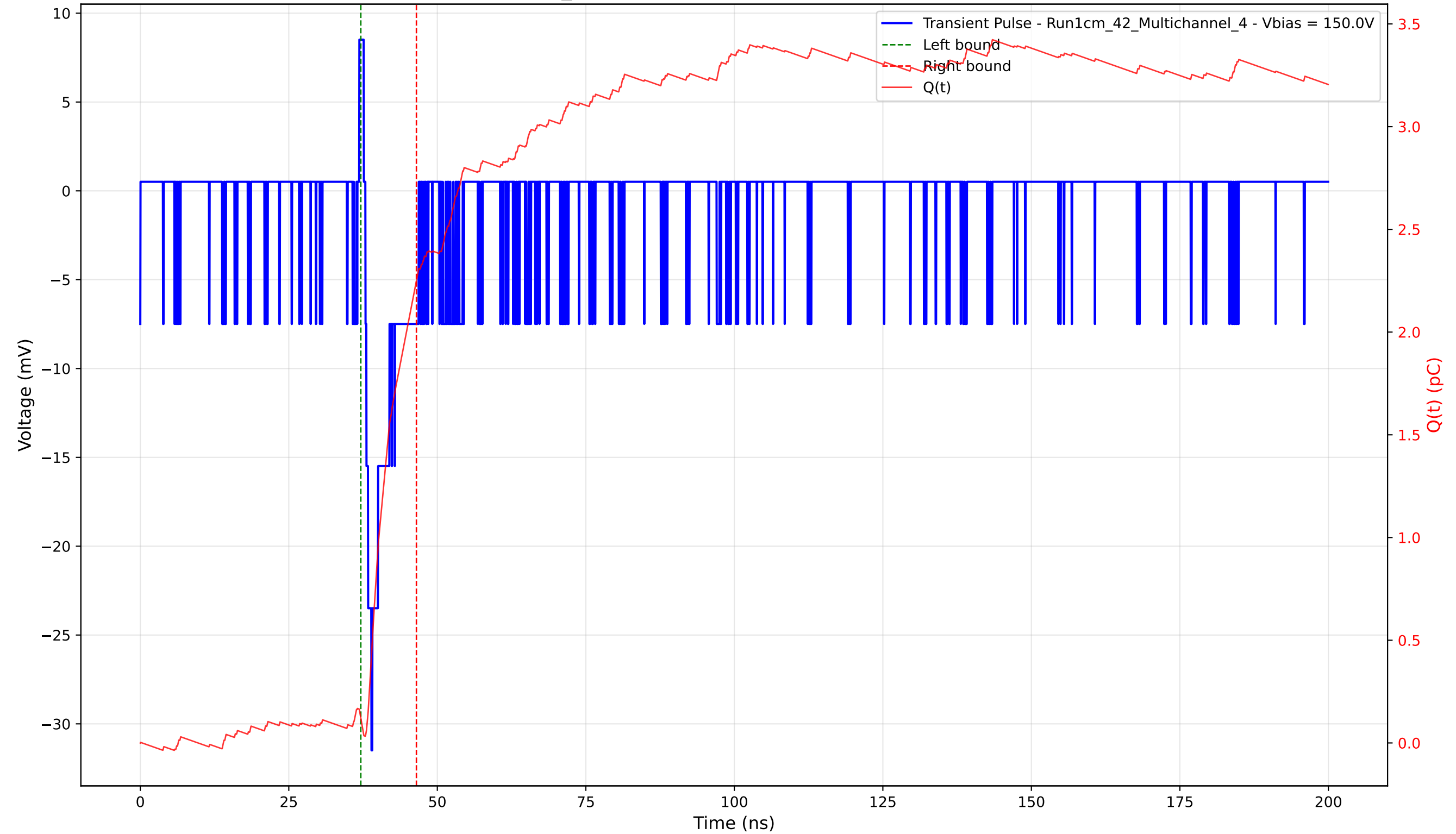
Transient Pulse - Sample: 1cm_42 - Position: 4920.0 \mu\text{m} - Charge: 2.13 pC - Rise Time: 1.02 ns
