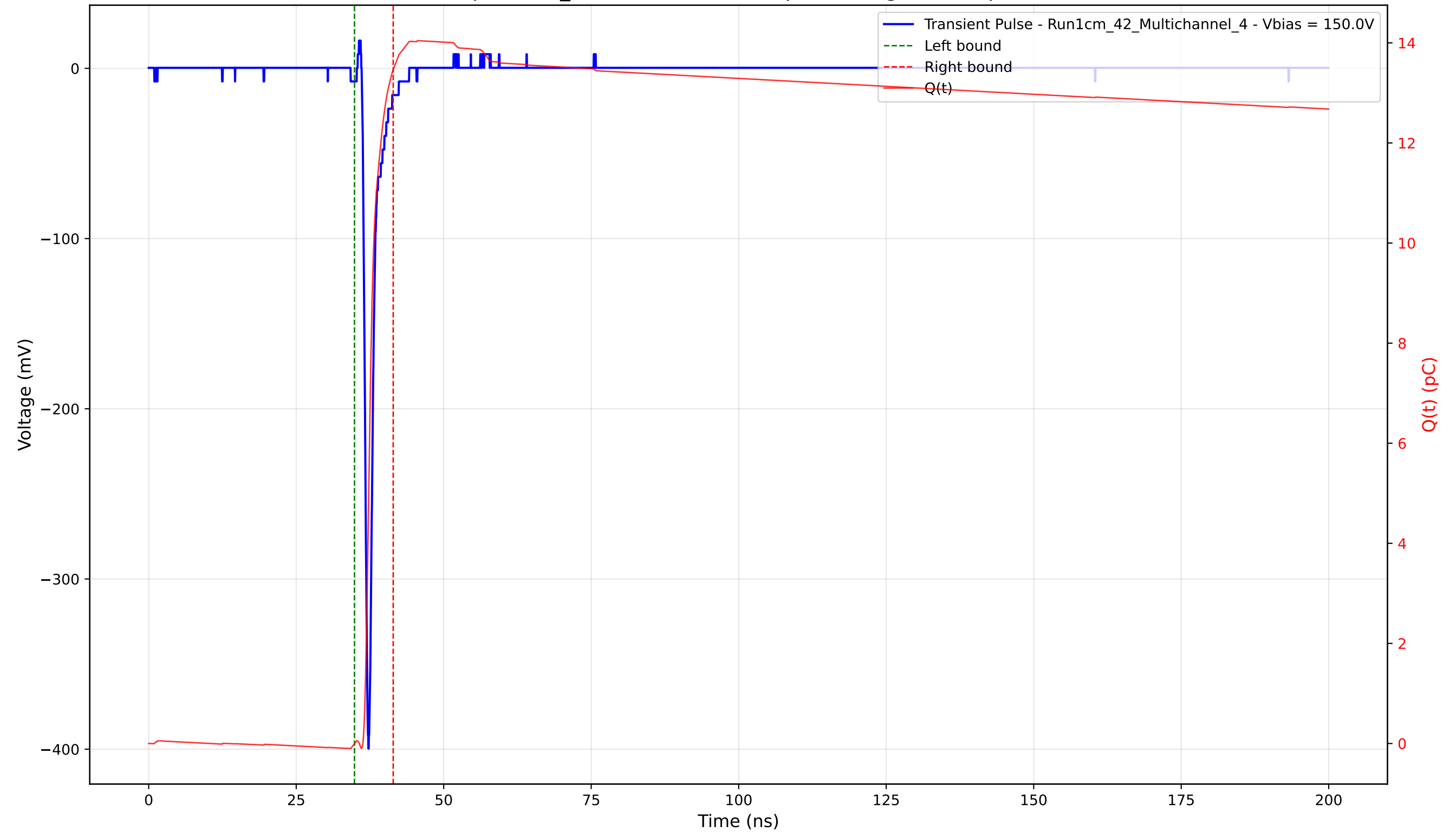
Transient Pulse - Sample: 1cm_42 - Position: 2860.0 \mu\text{m} - Charge: 13.47 pC - Rise Time: 0.72 ns
