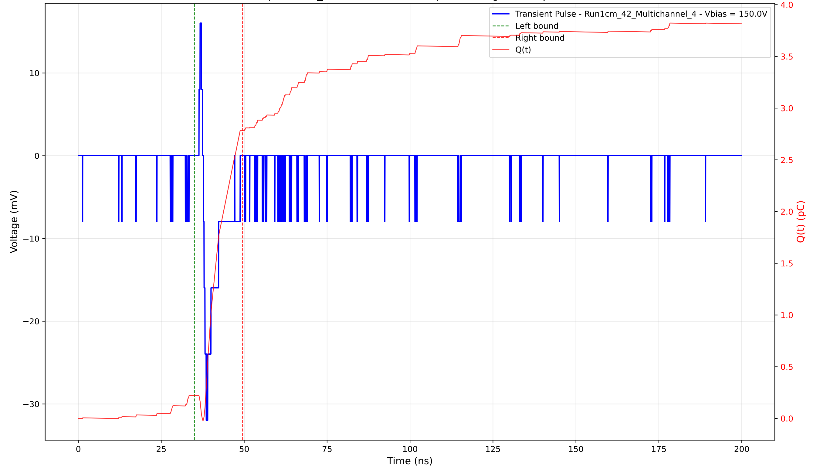
Transient Pulse - Sample: 1cm_42 - Position: 380.0 \mu\text{m} - Charge: 2.56 pC - Rise Time: 0.86 ns
