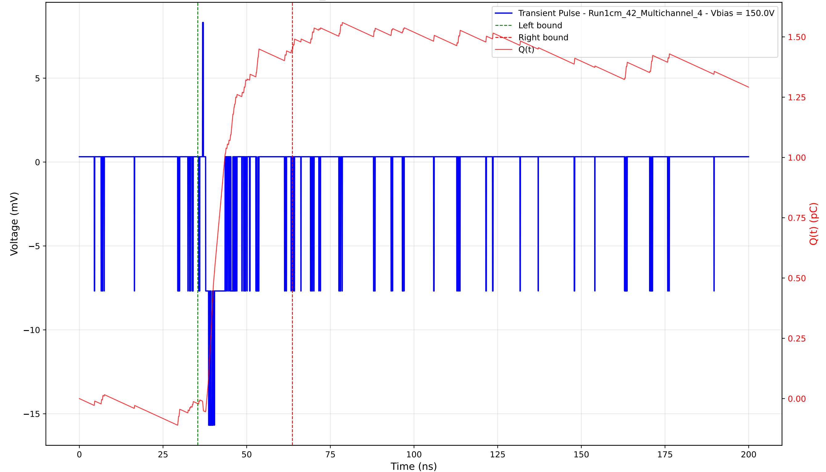
Transient Pulse - Sample: 1cm_42 - Position: 145.0 \mu\text{m} - Charge: 1.46 pC - Rise Time: 0.91 ns
