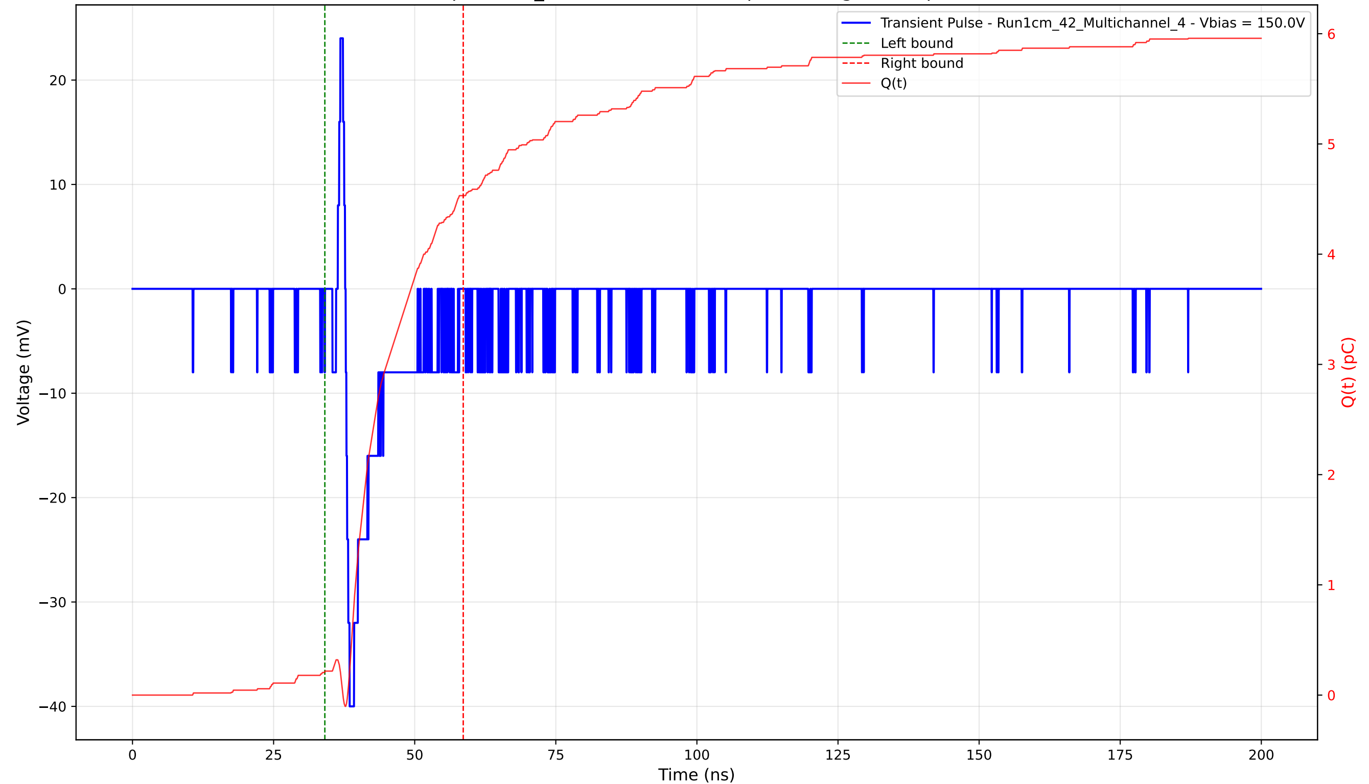
Transient Pulse - Sample: 1cm_42 - Position: 4335.0 \mu\text{m} - Charge: 4.32 pC - Rise Time: 0.70 ns
