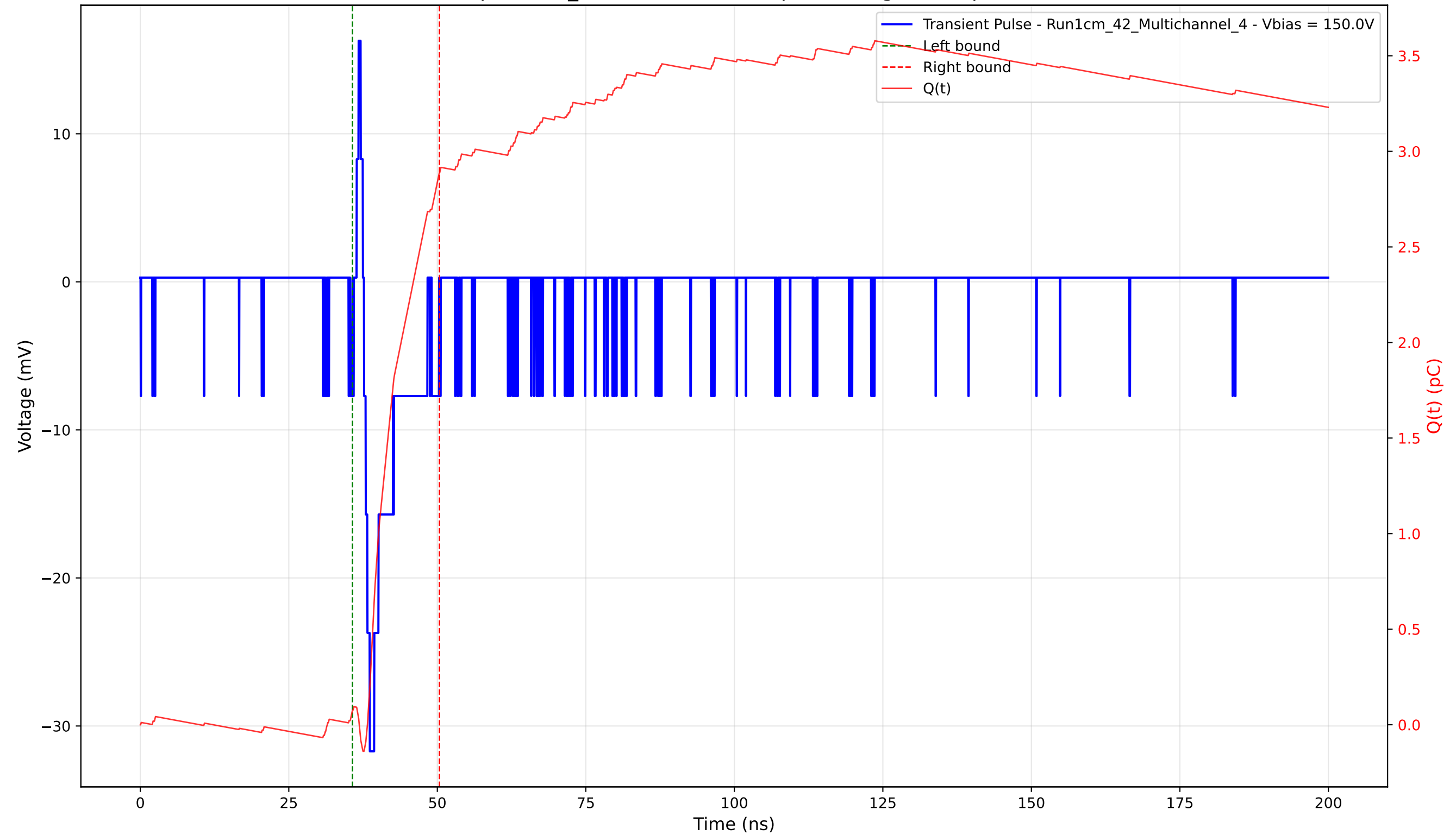
Transient Pulse - Sample: 1cm_42 - Position: 390.0 \mu\text{m} - Charge: 2.81 pC - Rise Time: 0.98 ns
