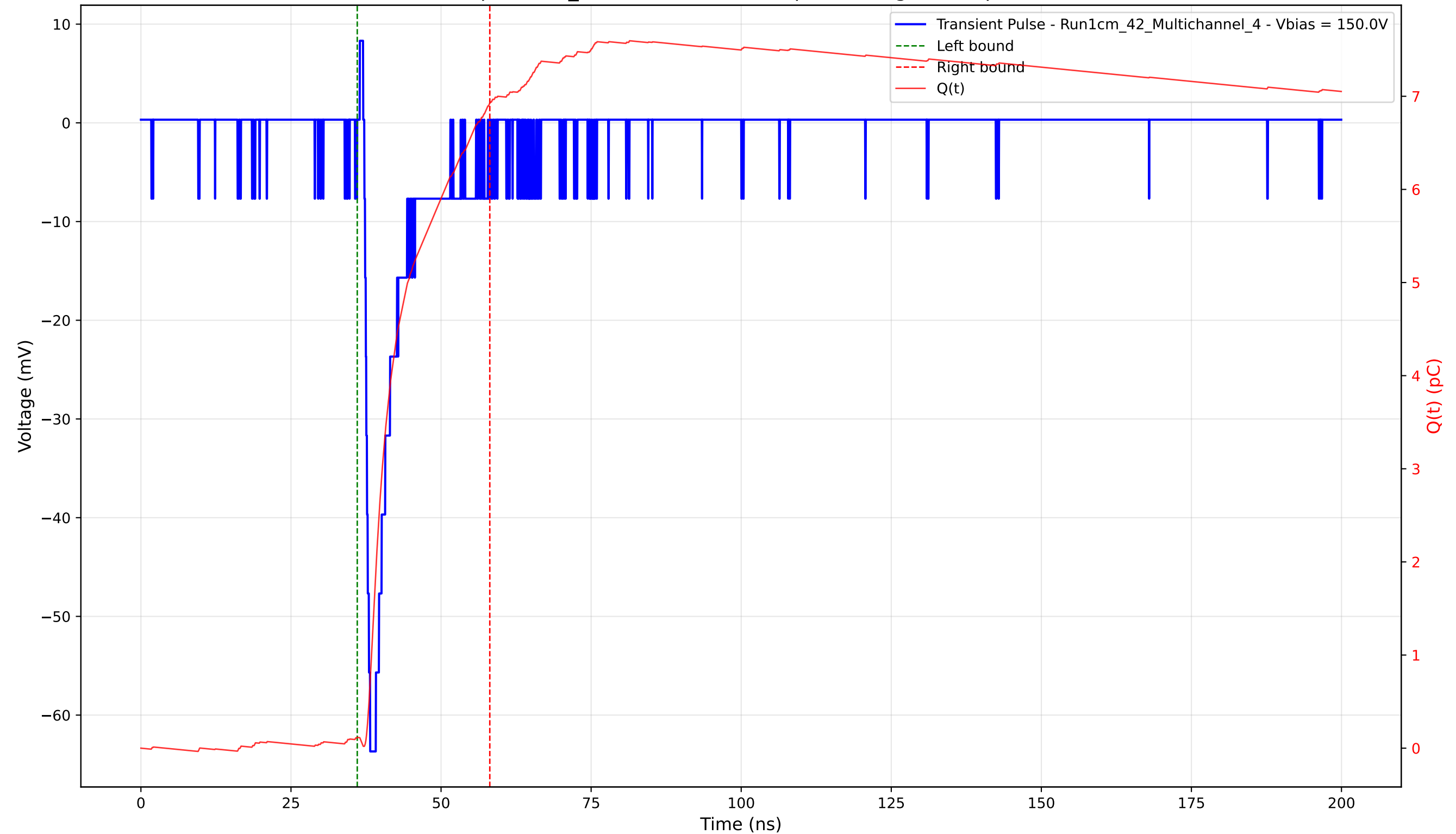
Transient Pulse - Sample: 1cm_42 - Position: 1300.0 \mu\text{m} - Charge: 6.81 pC - Rise Time: 0.97 ns
