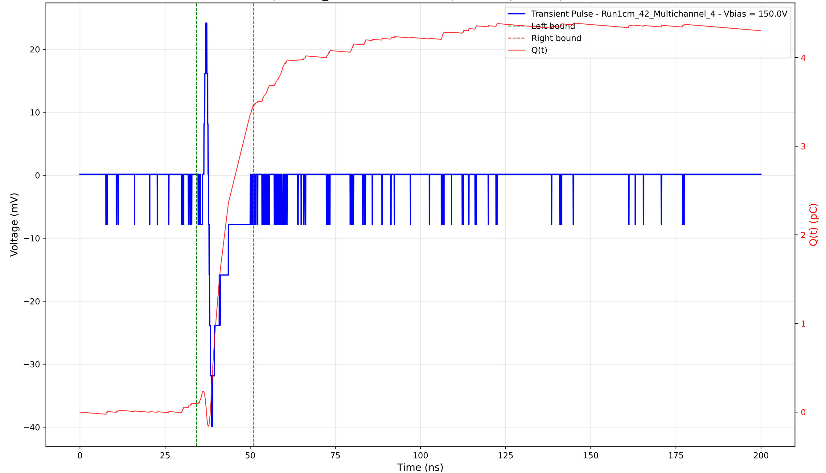
Transient Pulse - Sample: 1cm_42 - Position: 4400.0 \mu\text{m} - Charge: 3.36 pC - Rise Time: 0.90 ns
