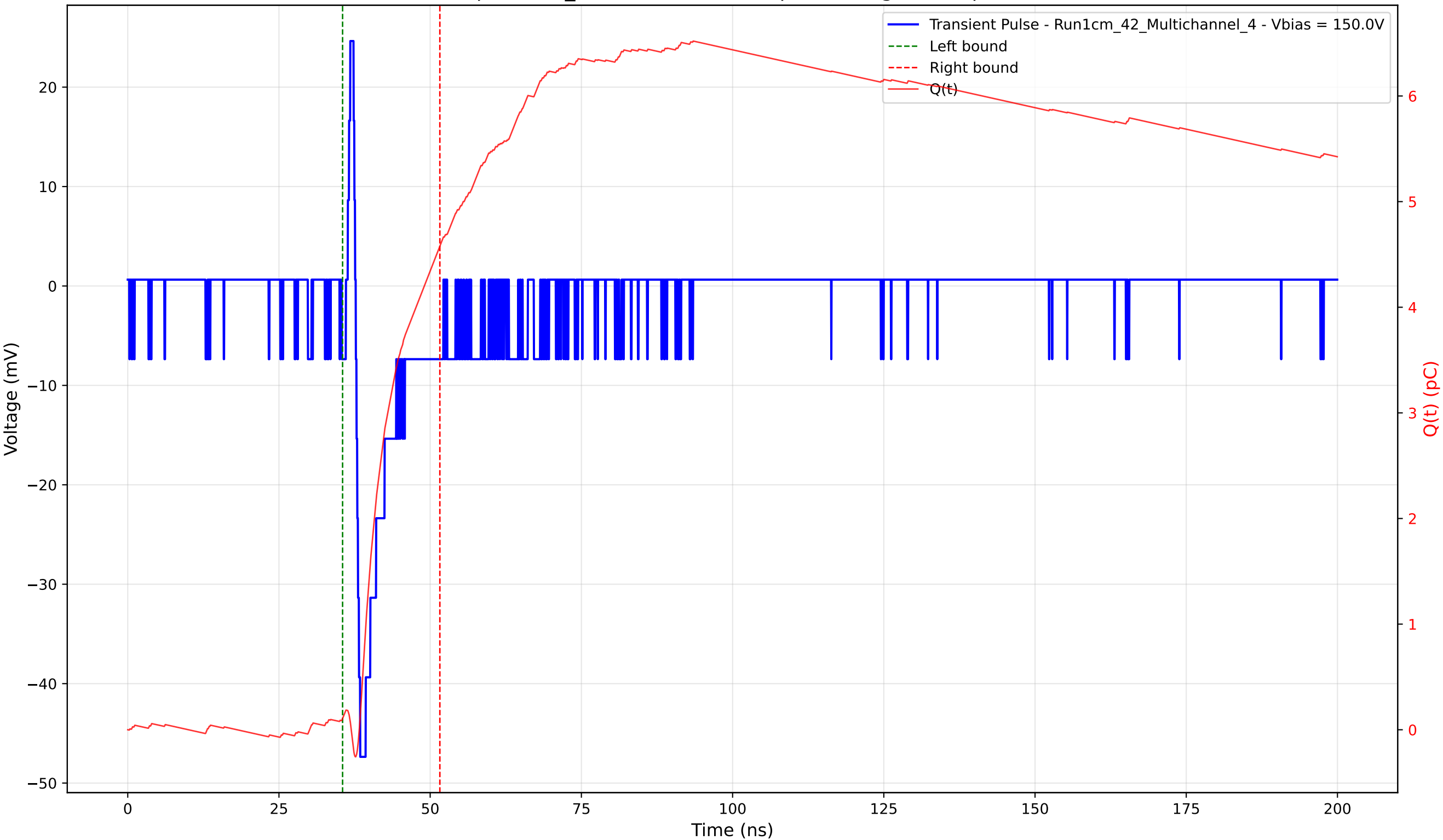
Transient Pulse - Sample: 1cm_42 - Position: 720.0 \mu\text{m} - Charge: 4.47 pC - Rise Time: 0.74 ns
