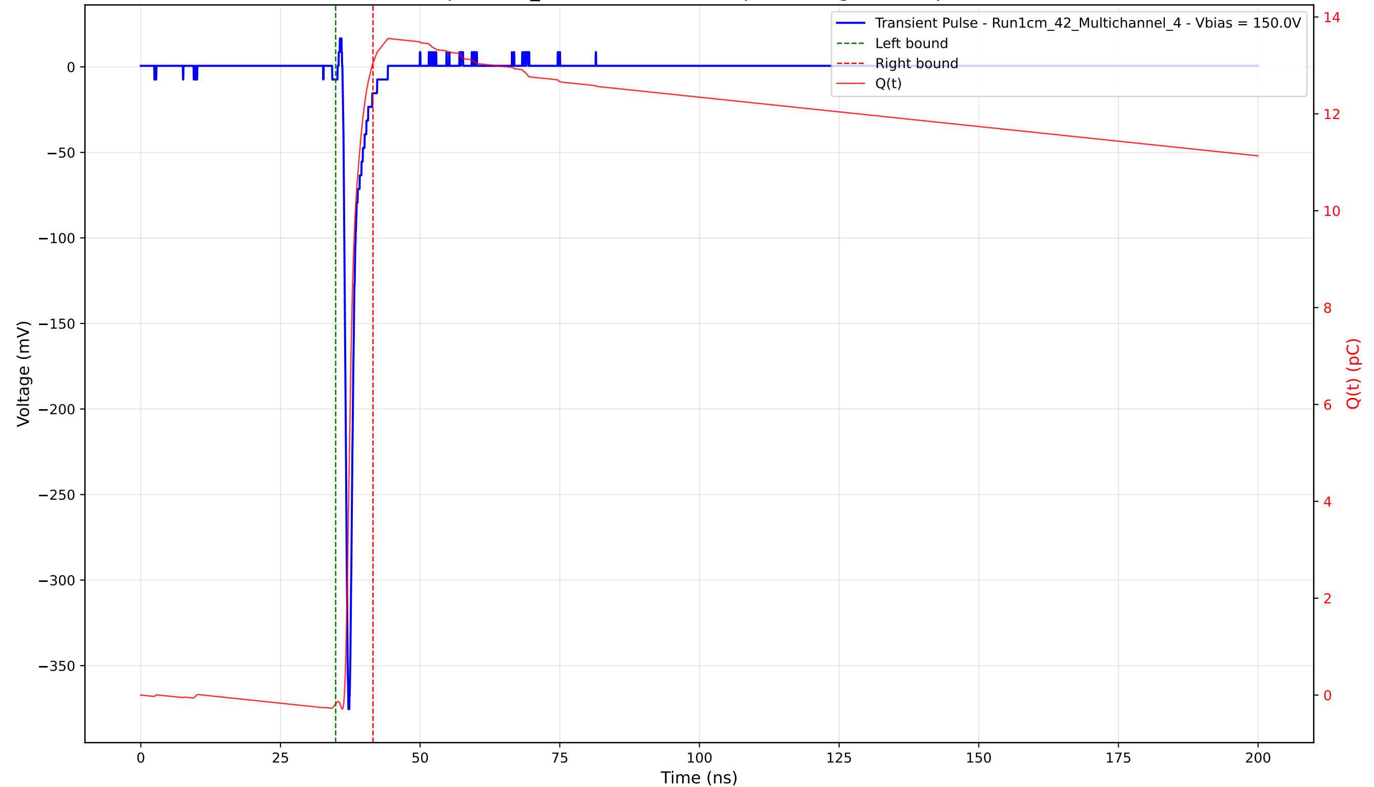
Transient Pulse - Sample: 1cm_42 - Position: 2145.0 \mu\text{m} - Charge: 13.23 pC - Rise Time: 0.70 ns
