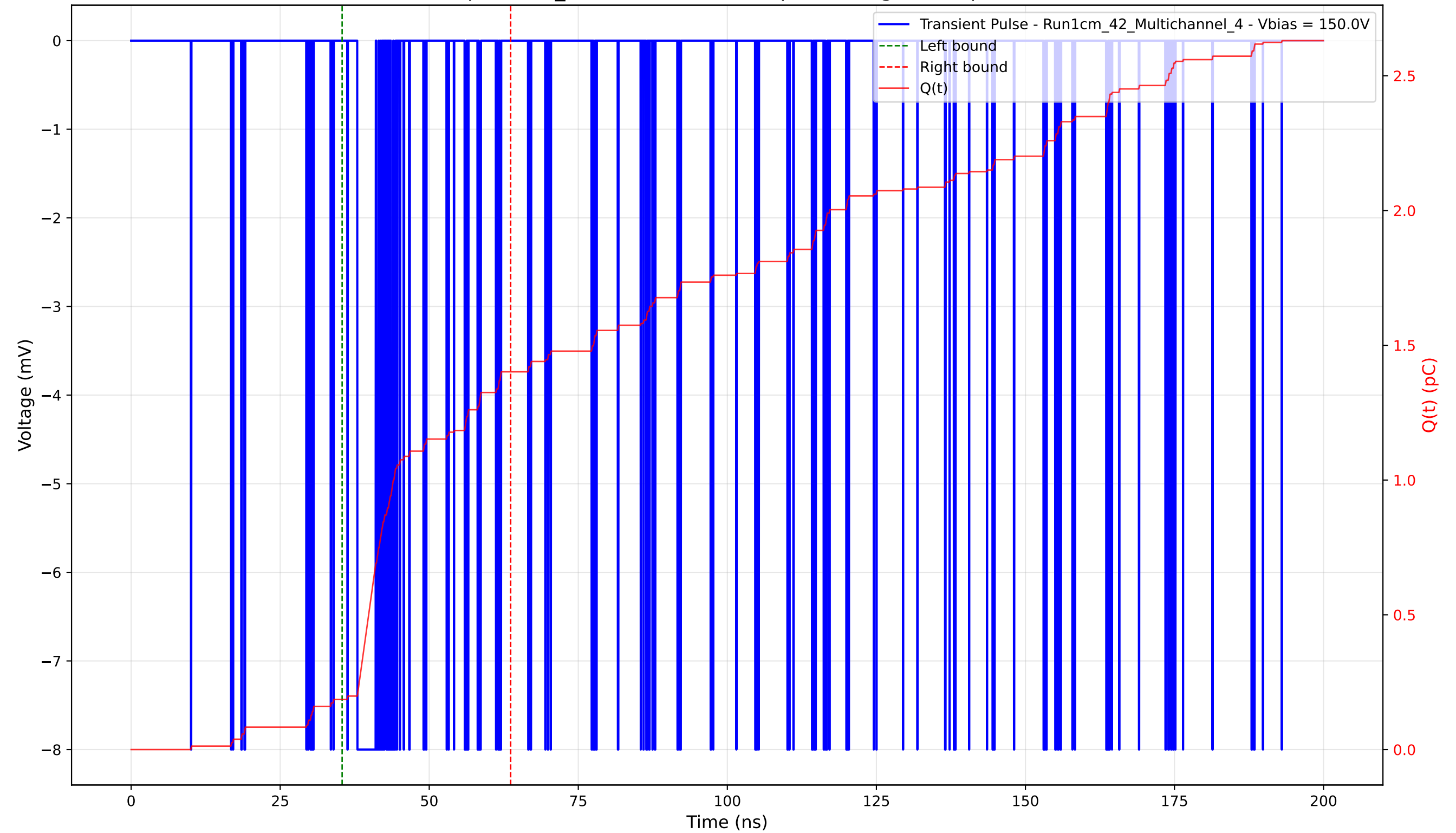
Transient Pulse - Sample: 1cm_42 - Position: 5115.0 \mu\text{m} - Charge: 1.22 pC - Rise Time: 0.04 ns
