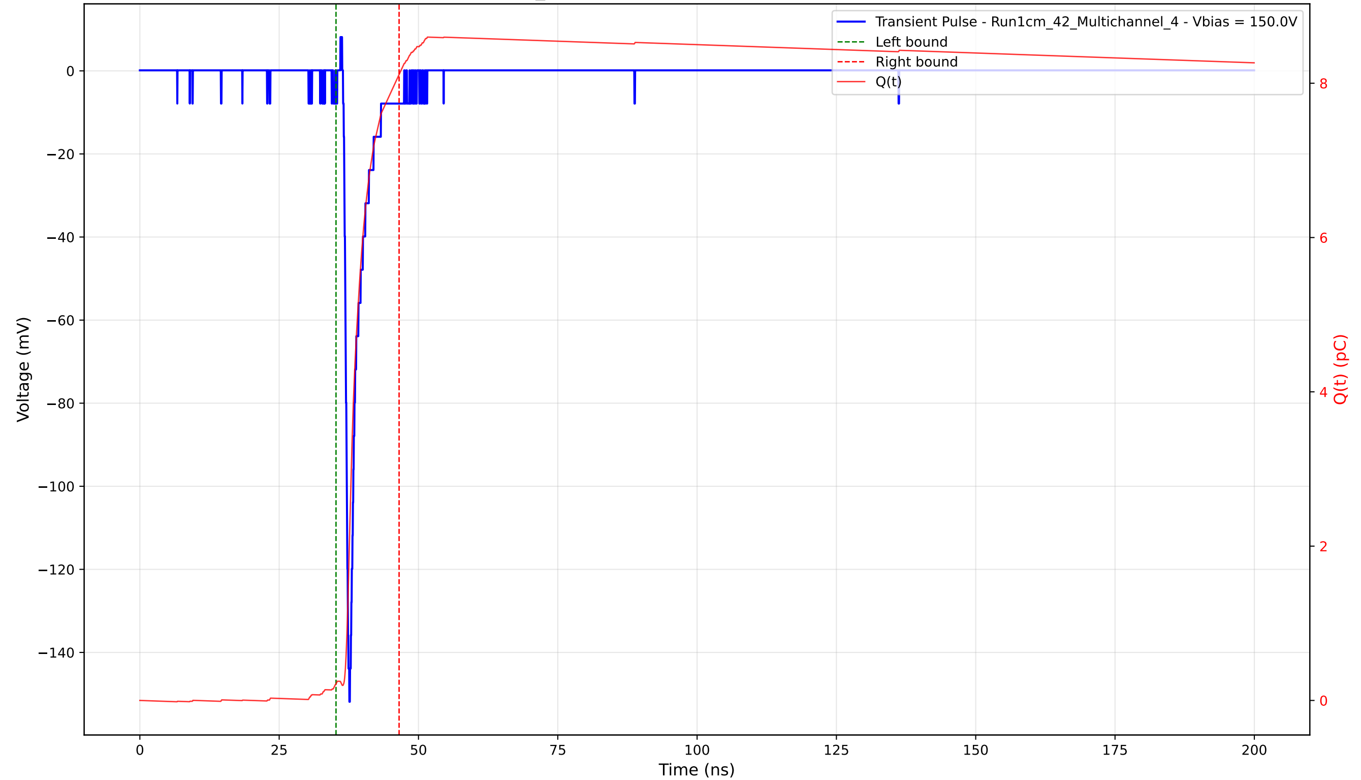
Transient Pulse - Sample: 1cm_42 - Position: 3225.0 \mu\text{m} - Charge: 7.90 pC - Rise Time: 0.84 ns
