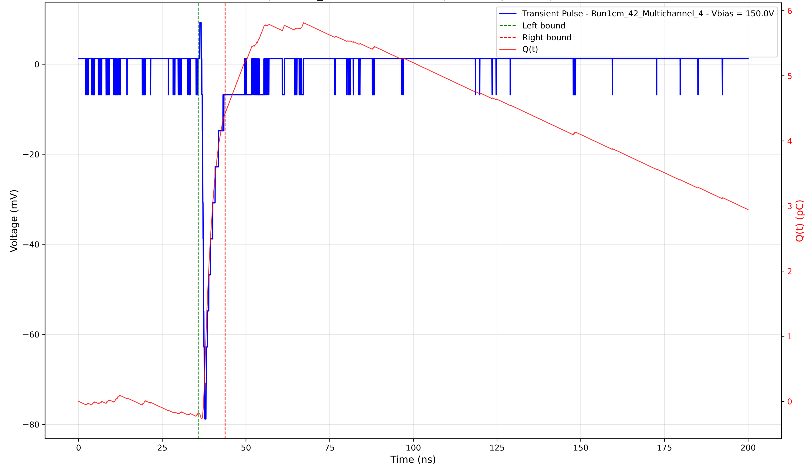
Transient Pulse - Sample: 1cm_42 - Position: 3495.0 \mu\text{m} - Charge: 4.60 pC - Rise Time: 0.79 ns
