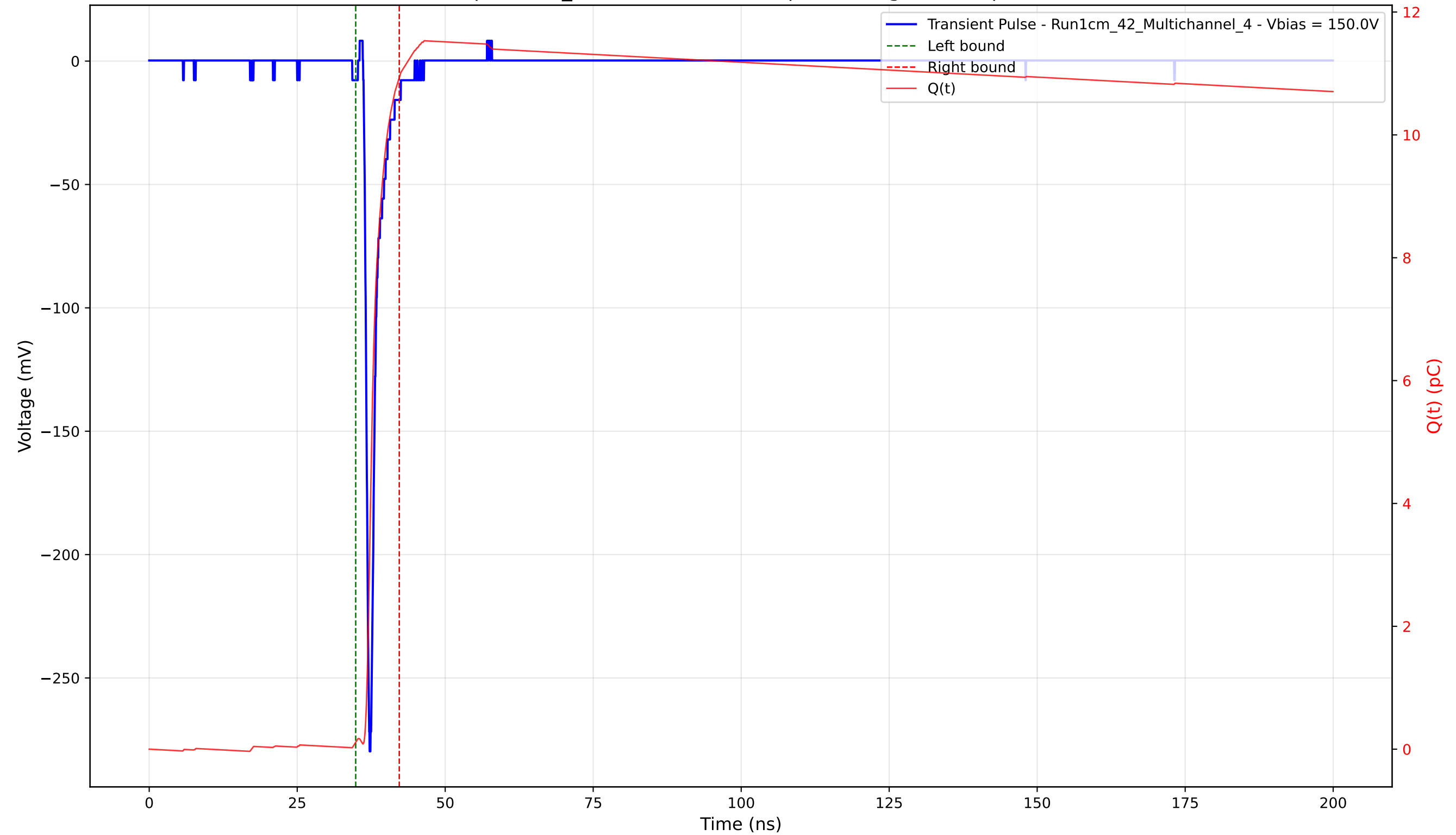
Transient Pulse - Sample: 1cm_42 - Position: 2060.0 \mu\text{m} - Charge: 10.82 pC - Rise Time: 0.76 ns
