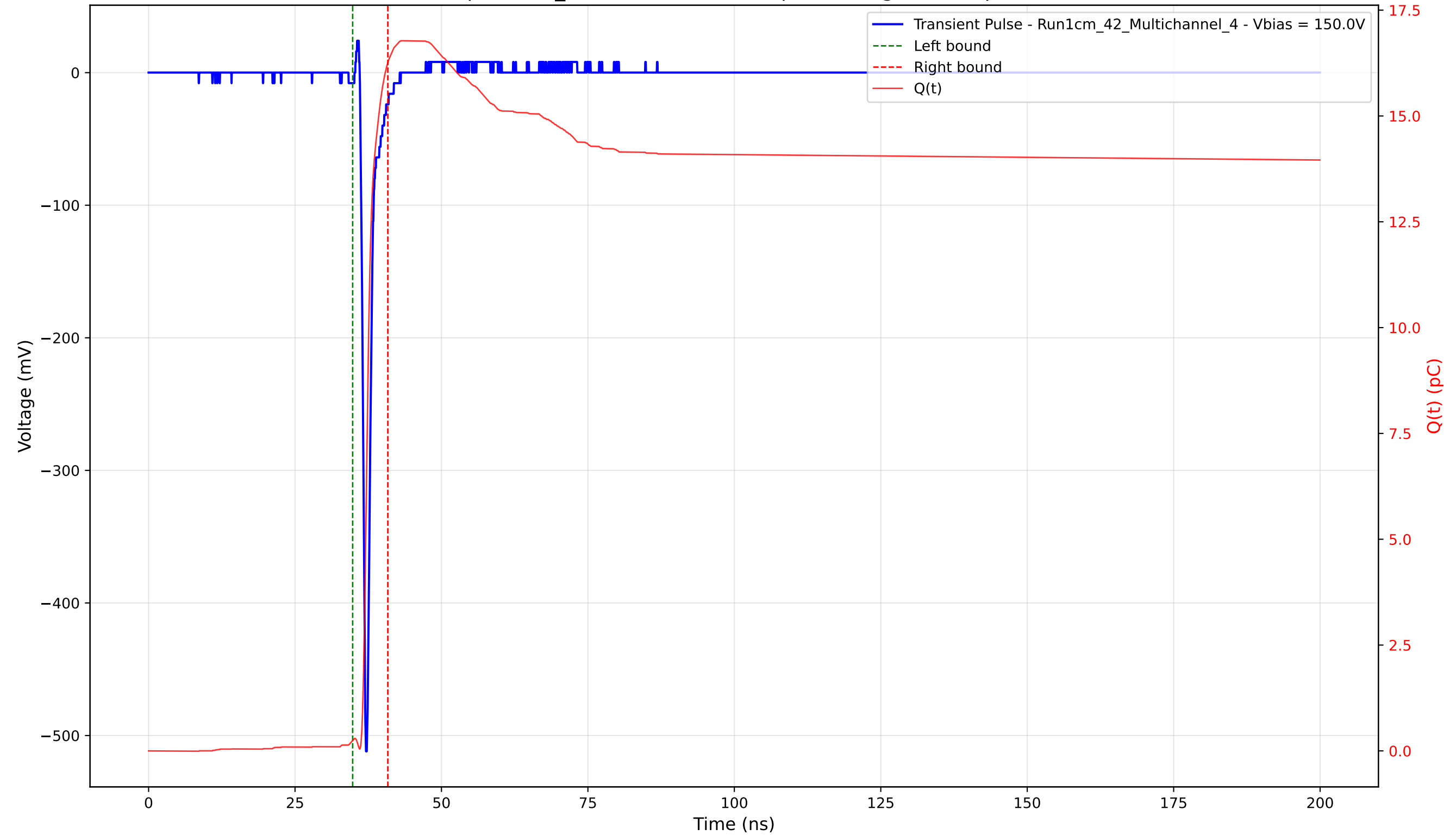
Transient Pulse - Sample: 1cm_42 - Position: 2665.0 \mu\text{m} - Charge: 16.01 pC - Rise Time: 0.72 ns
