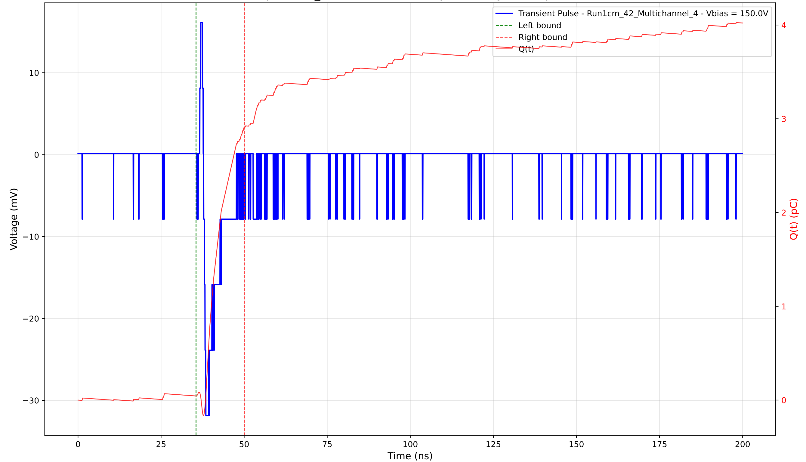
Transient Pulse - Sample: 1cm_42 - Position: 4835.0 \mu\text{m} - Charge: 2.87 pC - Rise Time: 0.66 ns
