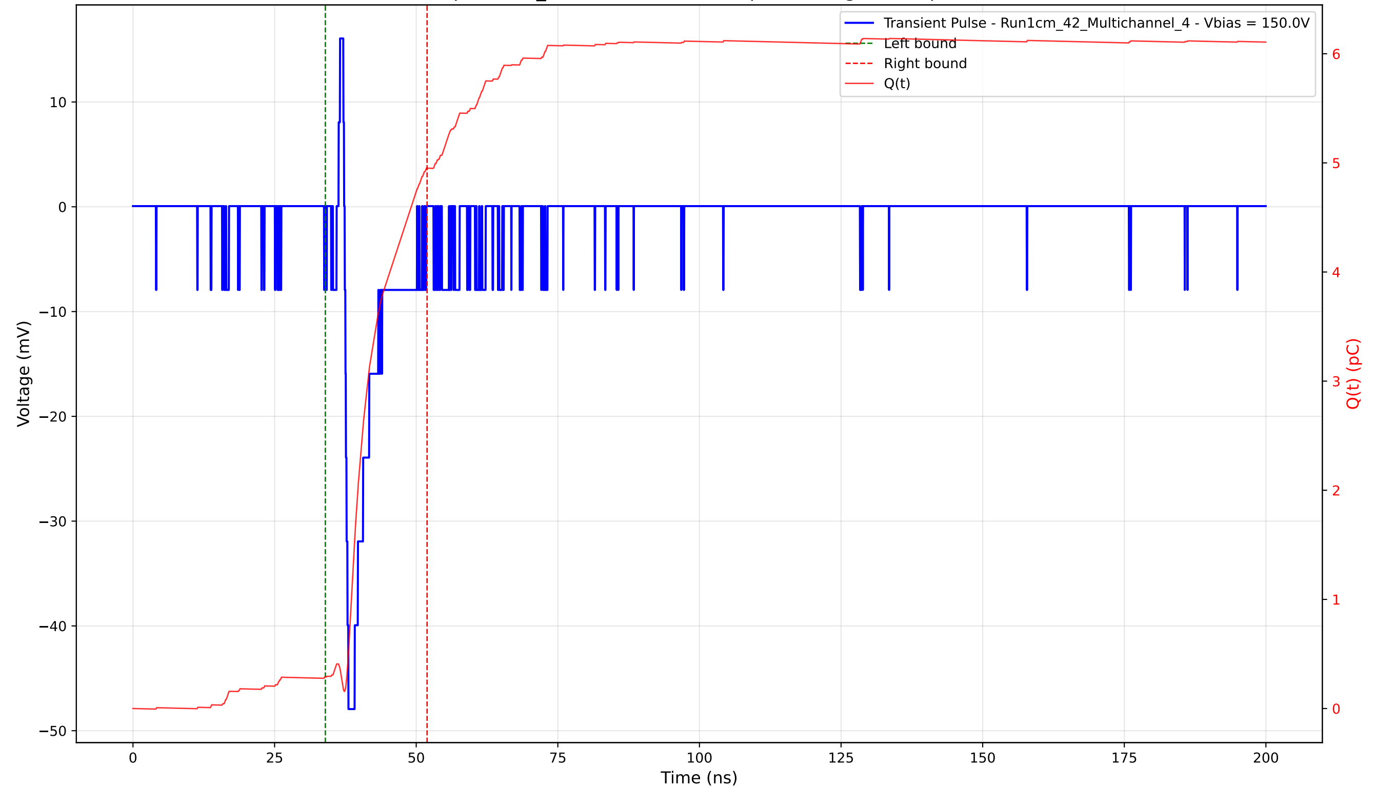
Transient Pulse - Sample: 1cm_42 - Position: 3880.0 \mu\text{m} - Charge: 4.66 pC - Rise Time: 0.66 ns
