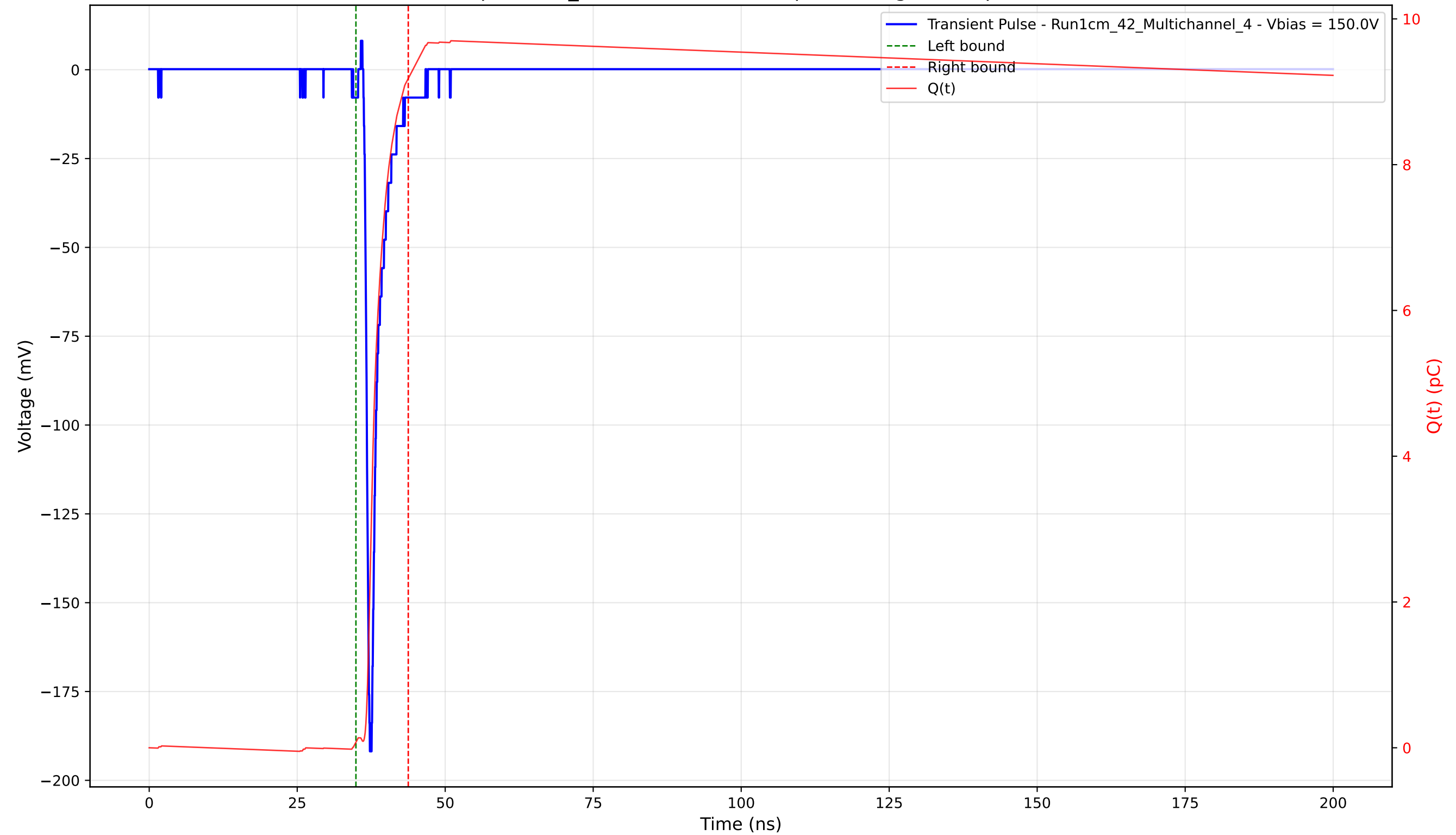
Transient Pulse - Sample: 1cm_42 - Position: 1955.0 \mu\text{m} - Charge: 9.10 pC - Rise Time: 0.78 ns
