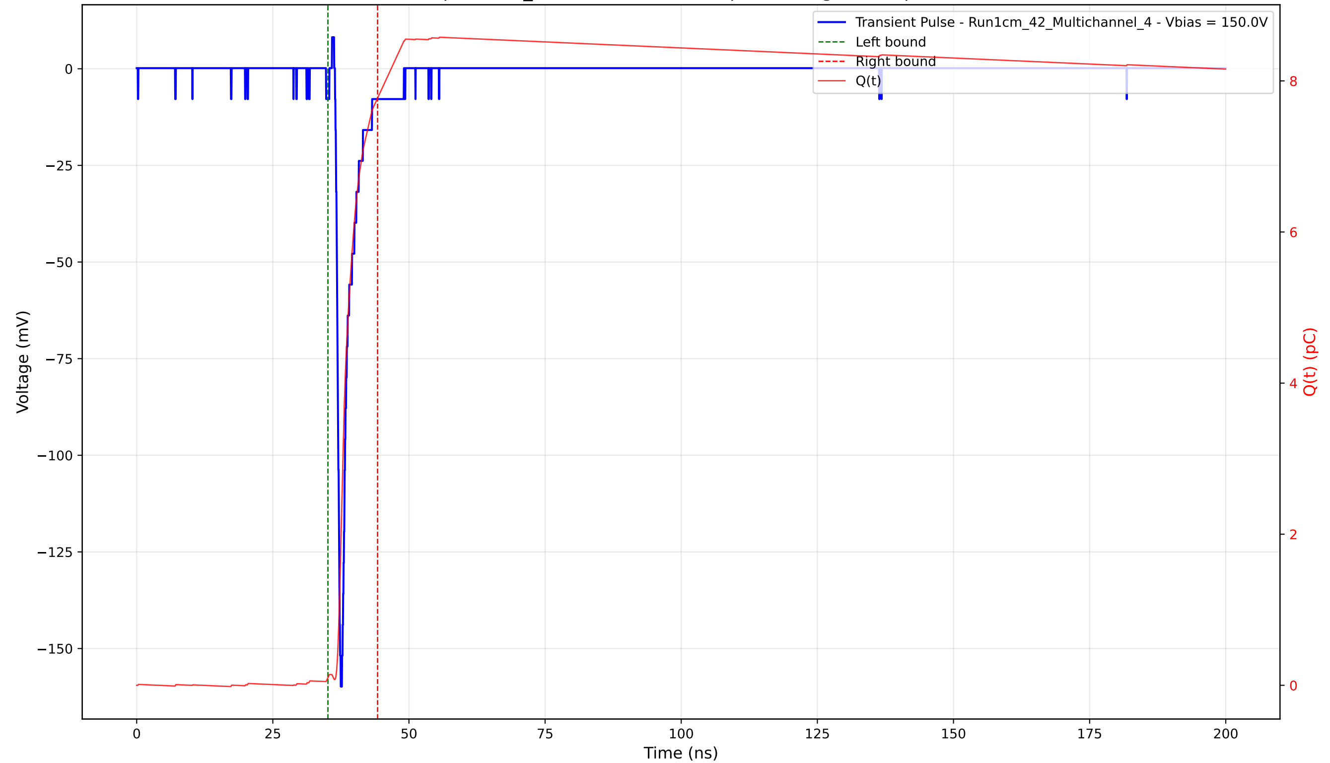
Transient Pulse - Sample: 1cm_42 - Position: 3170.0 \mu\text{m} - Charge: 7.67 pC - Rise Time: 0.80 ns
