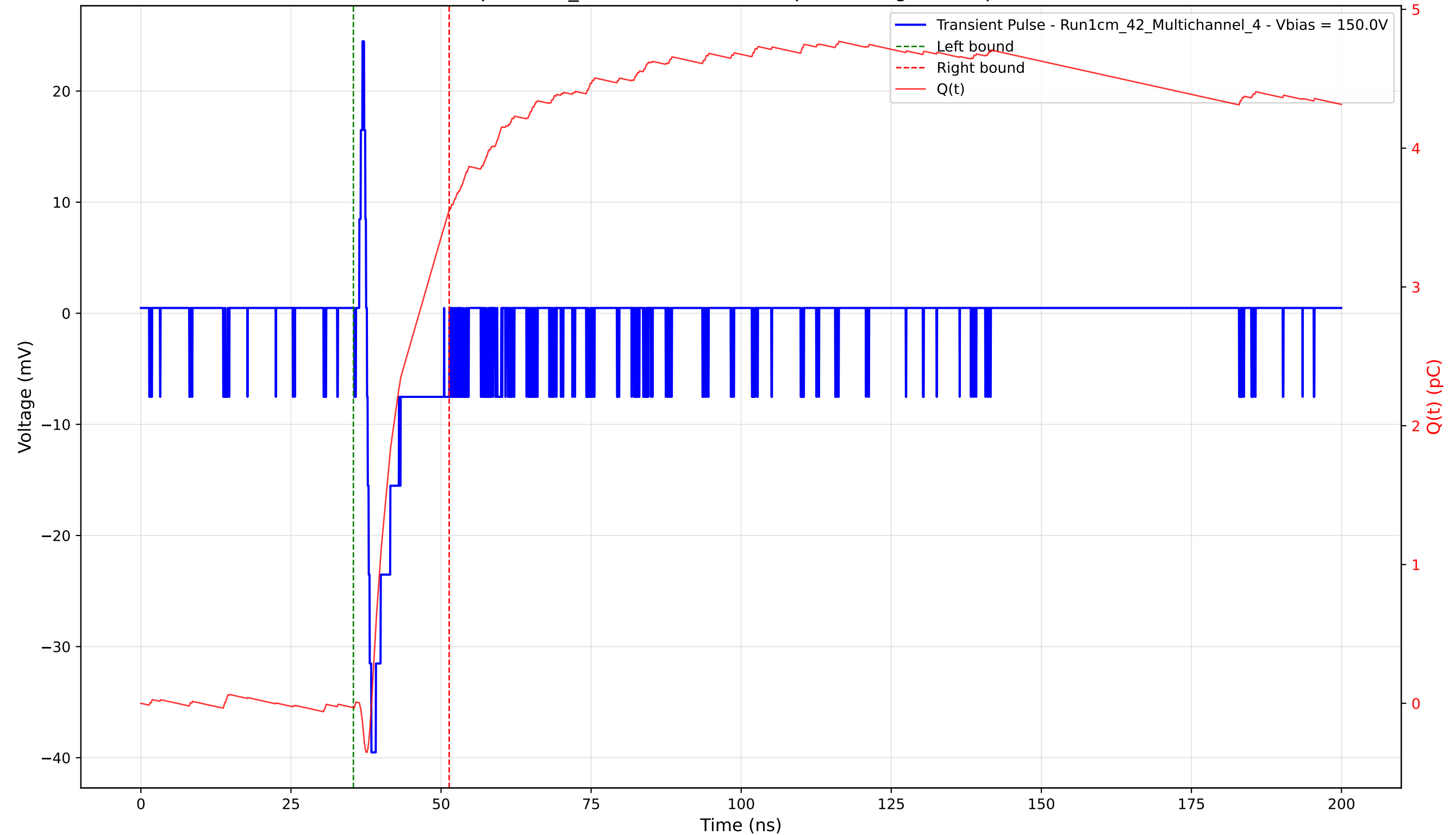
Transient Pulse - Sample: 1cm_42 - Position: 4120.0 \mu\text{m} - Charge: 3.59 pC - Rise Time: 0.74 ns
