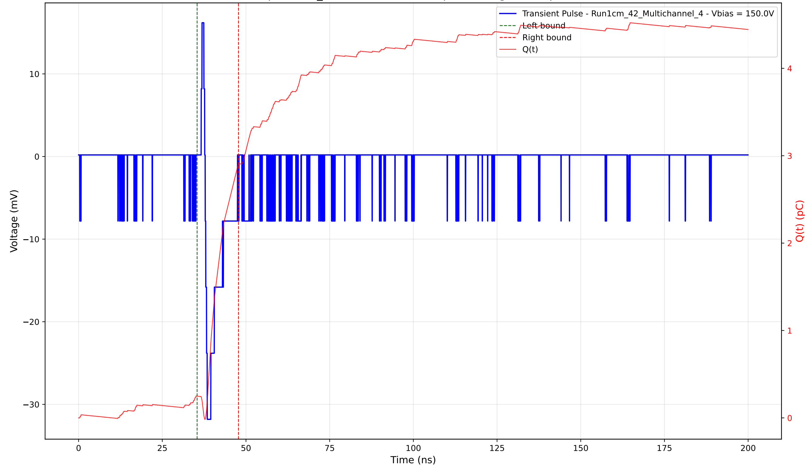
Transient Pulse - Sample: 1cm_42 - Position: 4685.0 \mu\text{m} - Charge: 2.65 pC - Rise Time: 0.62 ns
