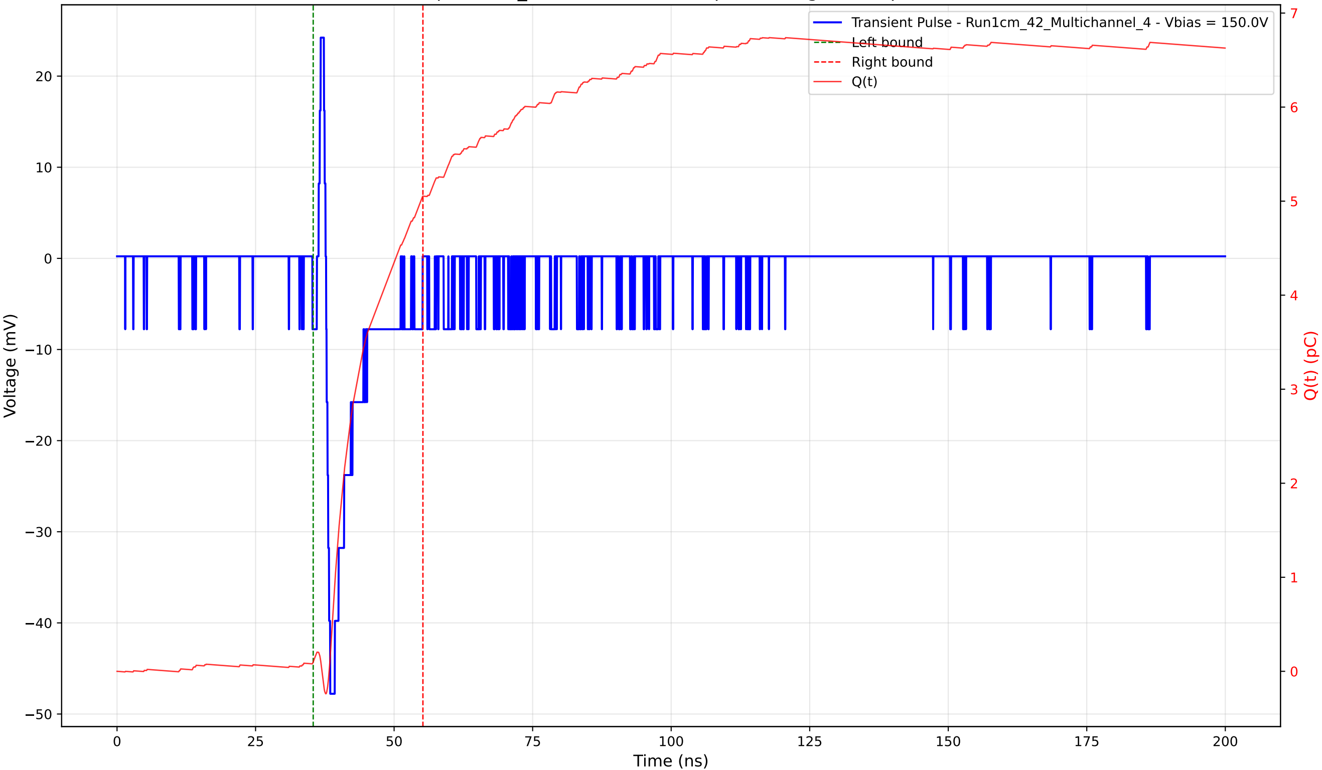
Transient Pulse - Sample: 1cm_42 - Position: 815.0 \mu\text{m} - Charge: 4.95 pC - Rise Time: 0.74 ns
