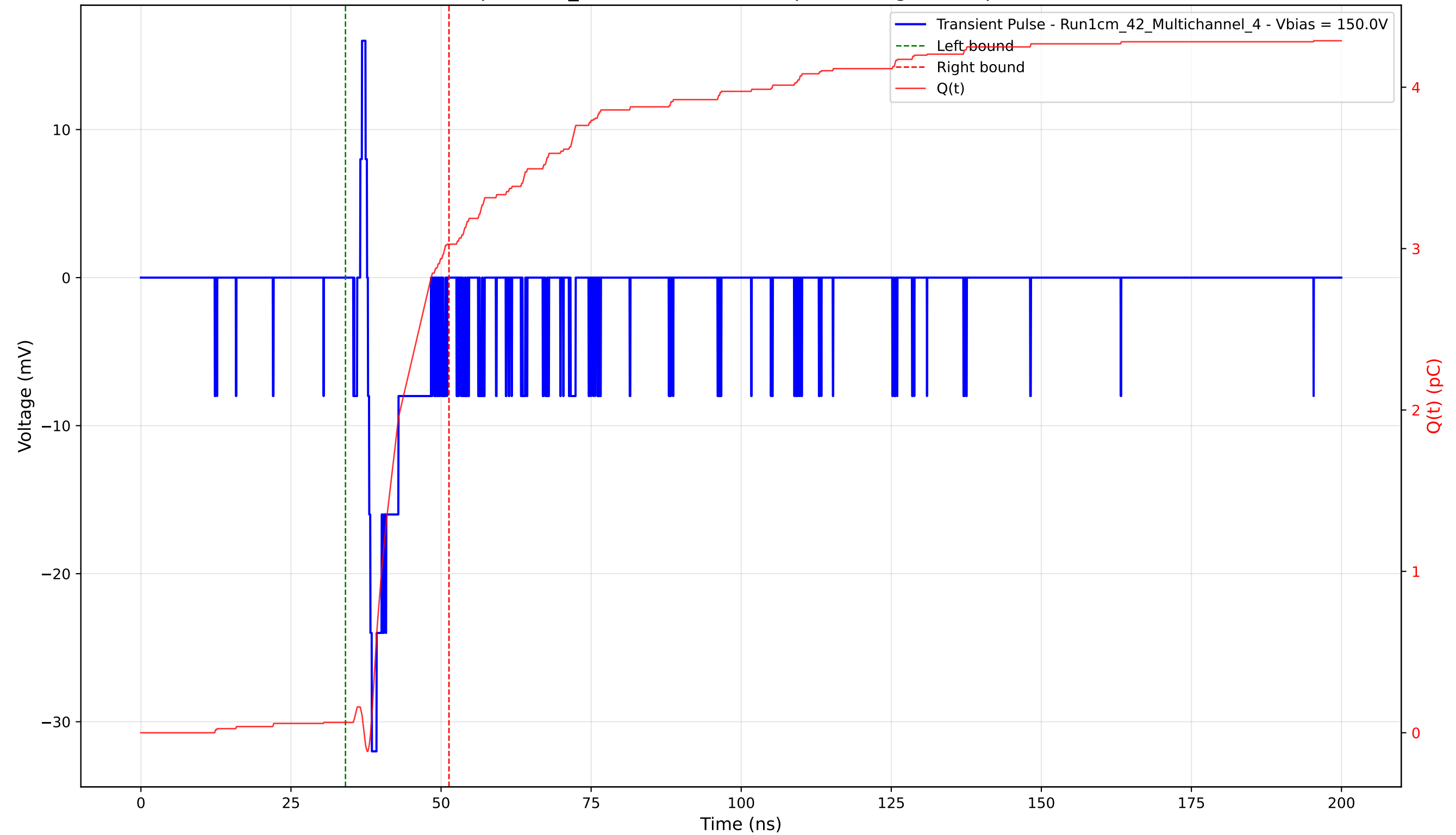
Transient Pulse - Sample: 1cm_42 - Position: 4640.0 \mu\text{m} - Charge: 2.96 pC - Rise Time: 0.66 ns
