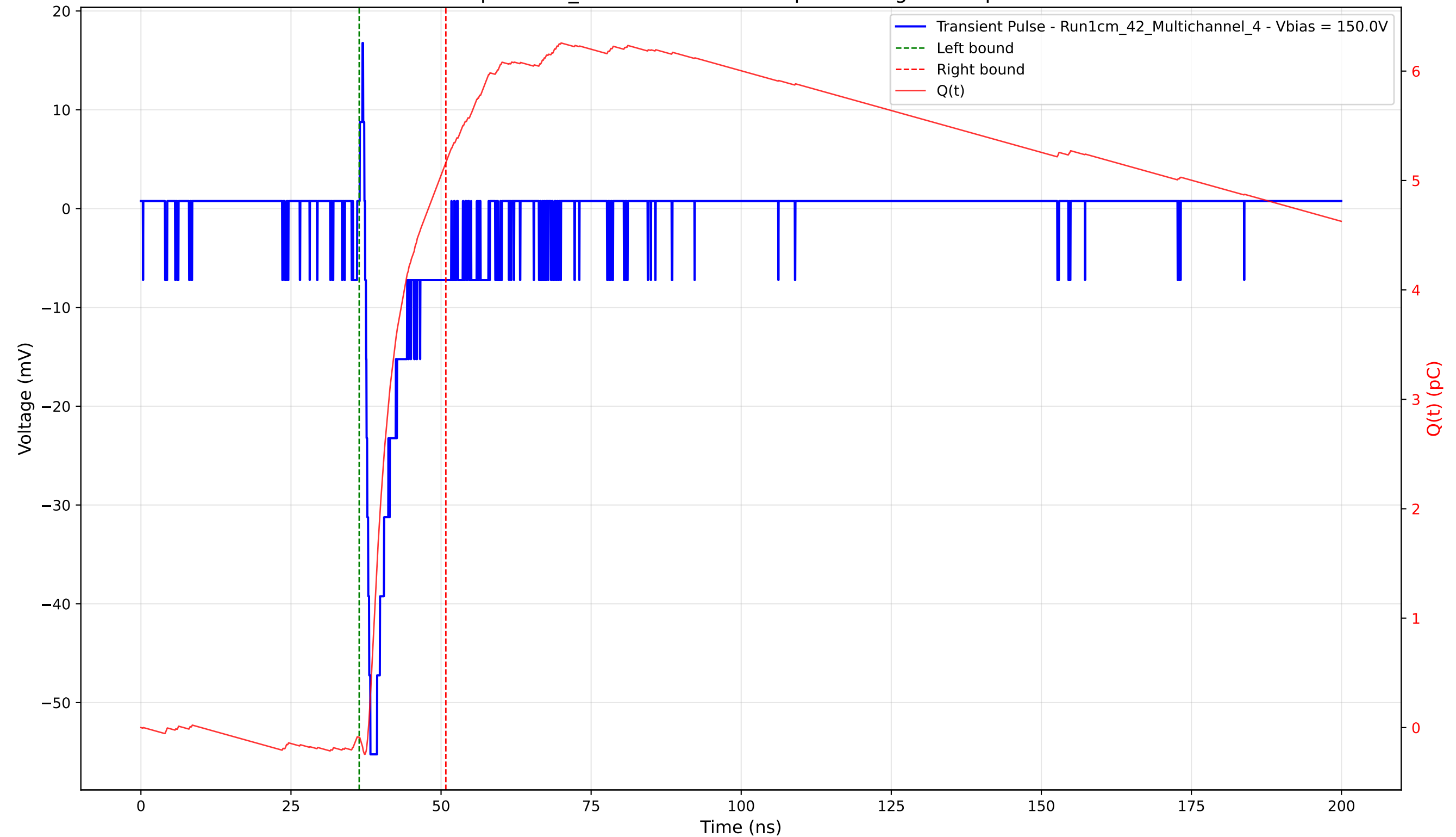
Transient Pulse - Sample: 1cm_42 - Position: 1150.0 \mu\text{m} - Charge: 5.25 pC - Rise Time: 0.89 ns
