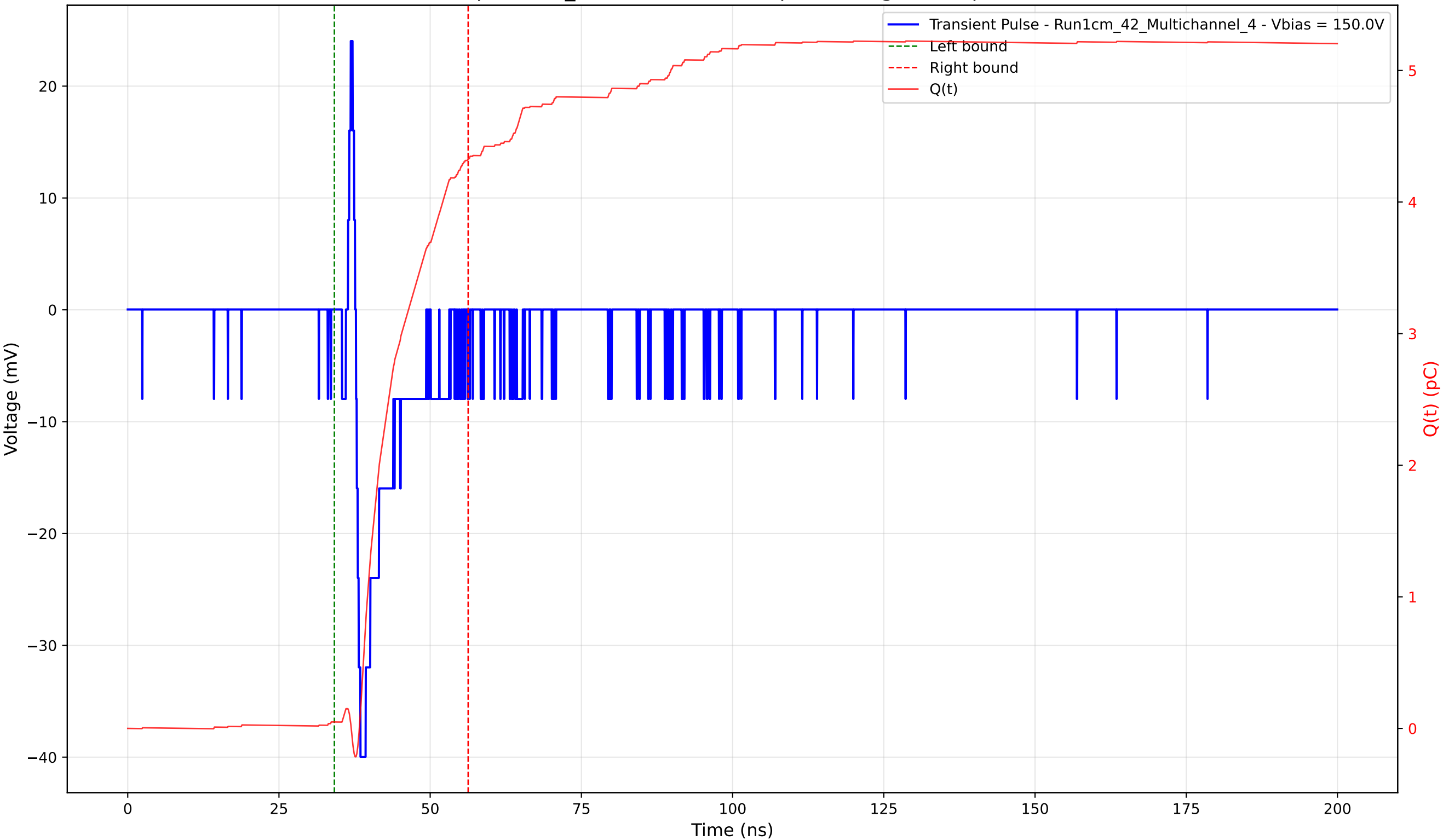
Transient Pulse - Sample: 1cm_42 - Position: 570.0 \mu\text{m} - Charge: 4.28 pC - Rise Time: 0.74 ns
