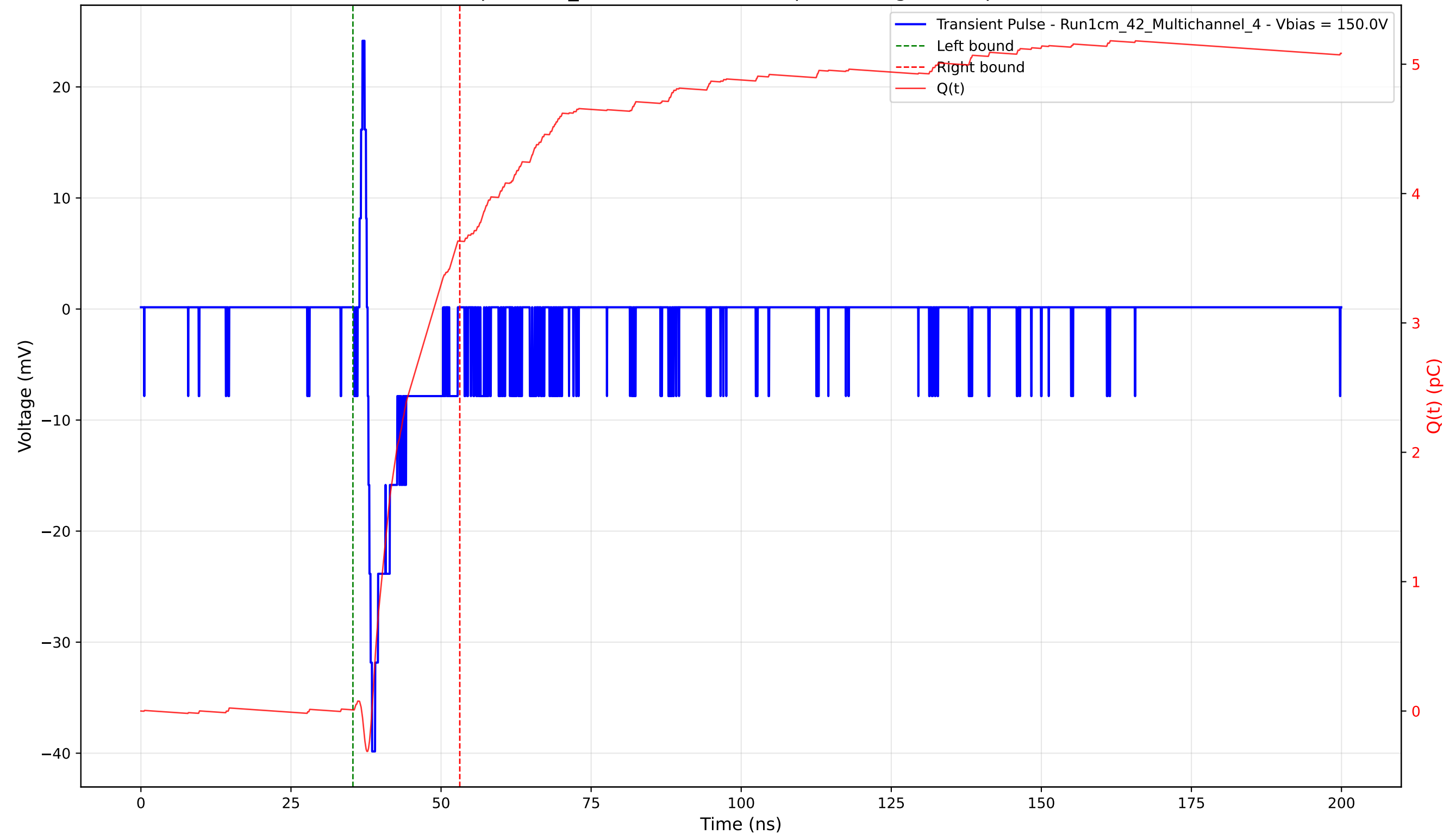
Transient Pulse - Sample: 1cm_42 - Position: 4395.0 \mu\text{m} - Charge: 3.62 pC - Rise Time: 0.74 ns
