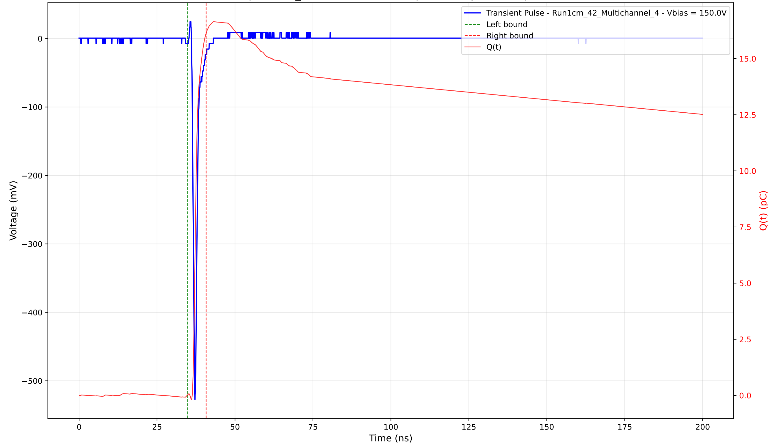
Transient Pulse - Sample: 1cm_42 - Position: 2635.0 \mu\text{m} - Charge: 16.09 pC - Rise Time: 0.68 ns
