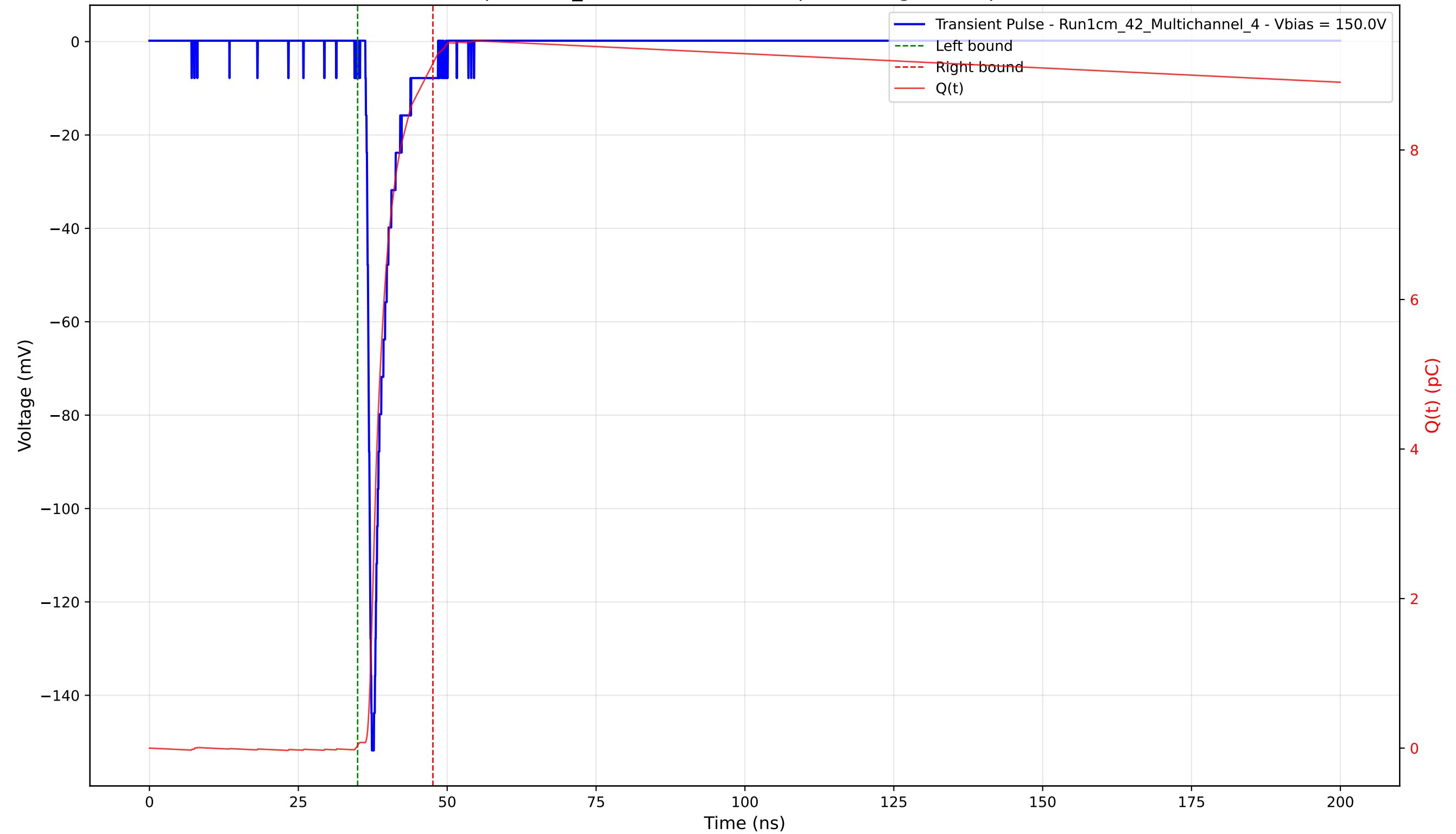
Transient Pulse - Sample: 1cm_42 - Position: 1840.0 \mu\text{m} - Charge: 9.12 pC - Rise Time: 0.92 ns
