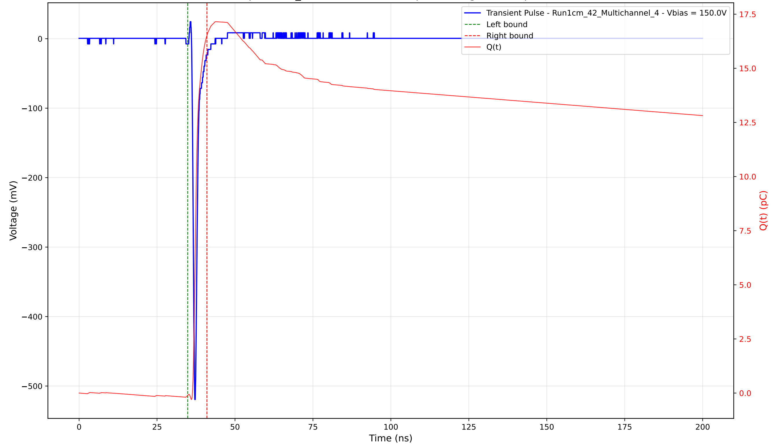
Transient Pulse - Sample: 1cm_42 - Position: 2310.0 \mu\text{m} - Charge: 16.62 pC - Rise Time: 0.69 ns
