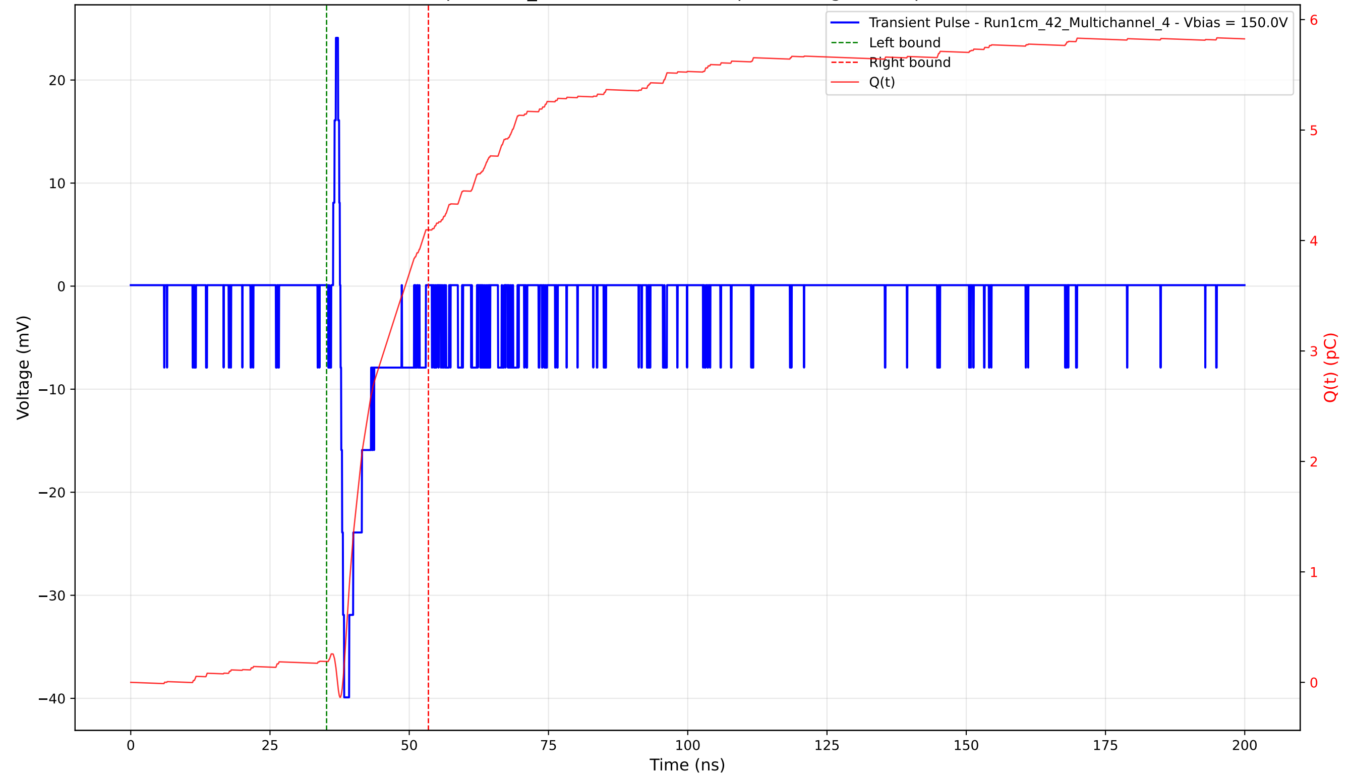
Transient Pulse - Sample: 1cm_42 - Position: 4135.0 \mu\text{m} - Charge: 3.91 pC - Rise Time: 0.66 ns
