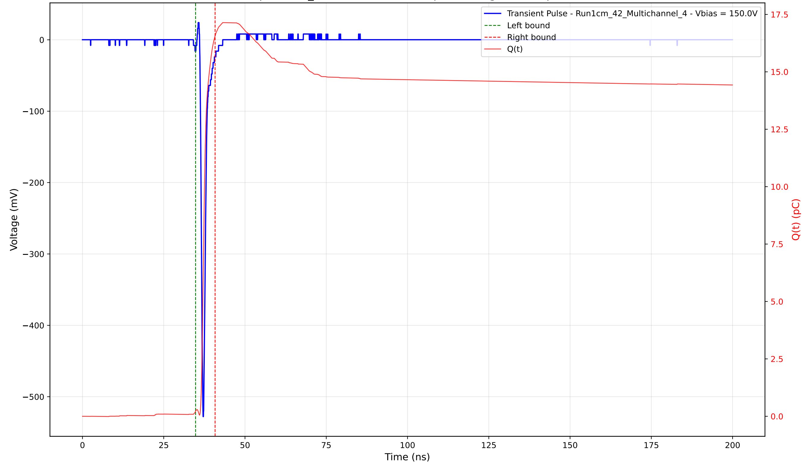
Transient Pulse - Sample: 1cm_42 - Position: 2390.0 \mu\text{m} - Charge: 16.35 pC - Rise Time: 0.74 ns
