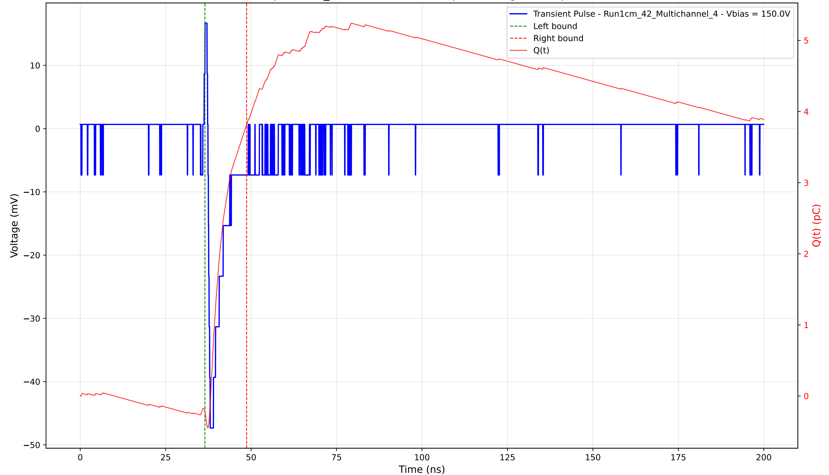
Transient Pulse - Sample: 1cm_42 - Position: 3890.0 \mu\text{m} - Charge: 4.04 pC - Rise Time: 0.66 ns
