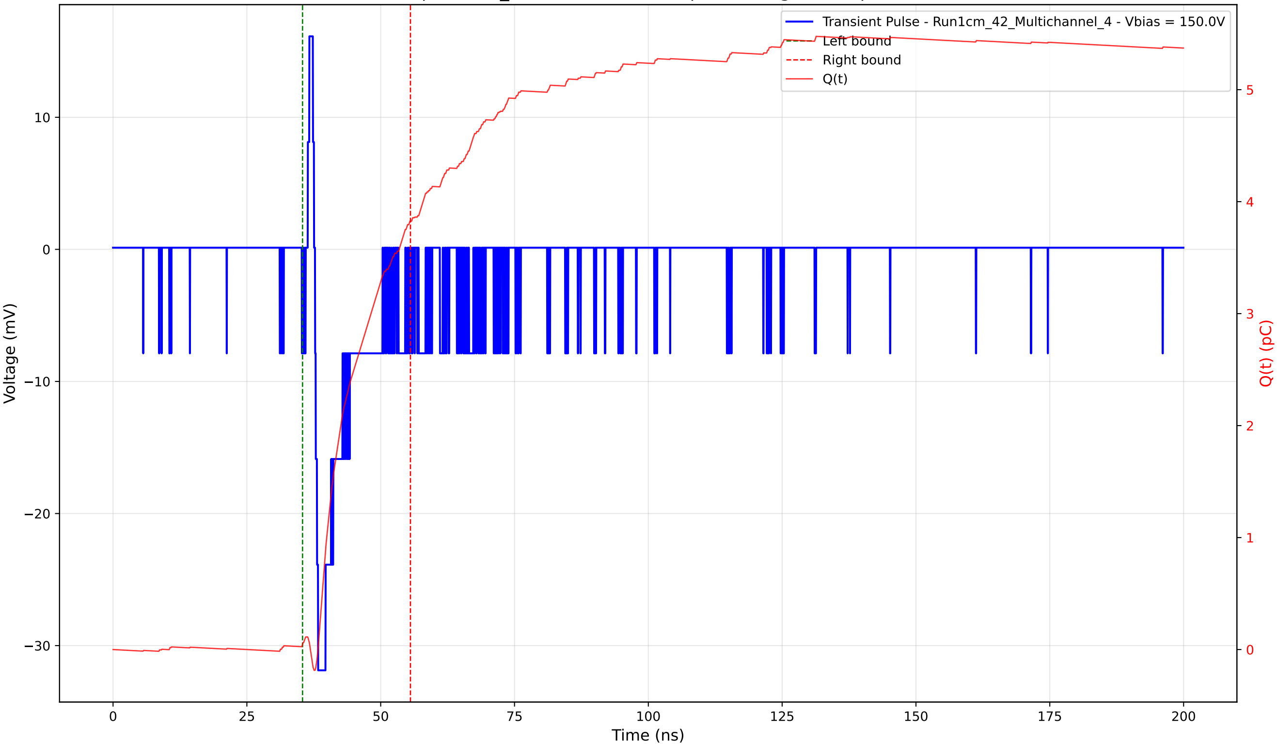
Transient Pulse - Sample: 1cm_42 - Position: 480.0 \mu\text{m} - Charge: 3.78 pC - Rise Time: 0.58 ns
