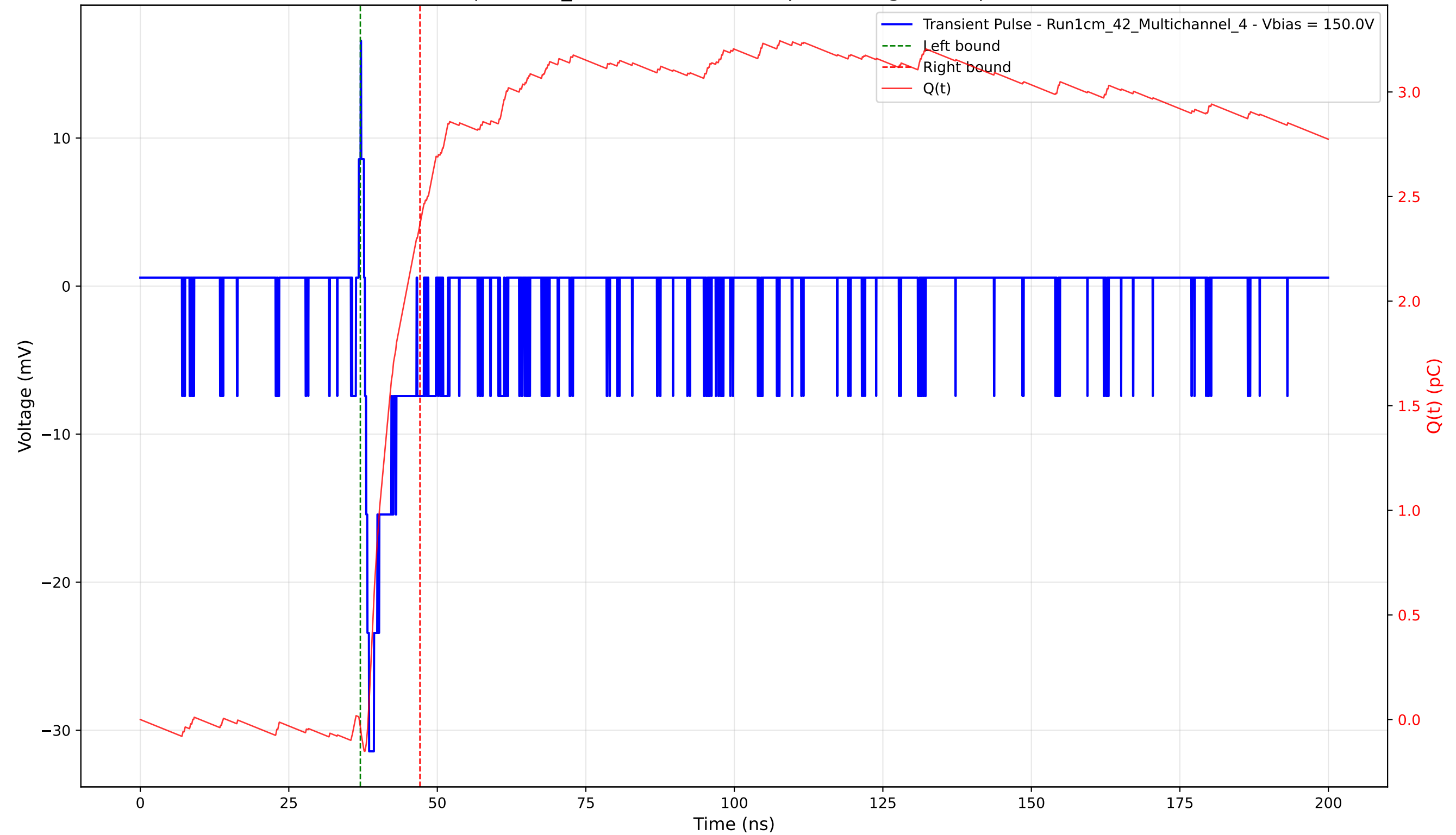
Transient Pulse - Sample: 1cm_42 - Position: 4880.0 \mu\text{m} - Charge: 2.40 pC - Rise Time: 0.71 ns
