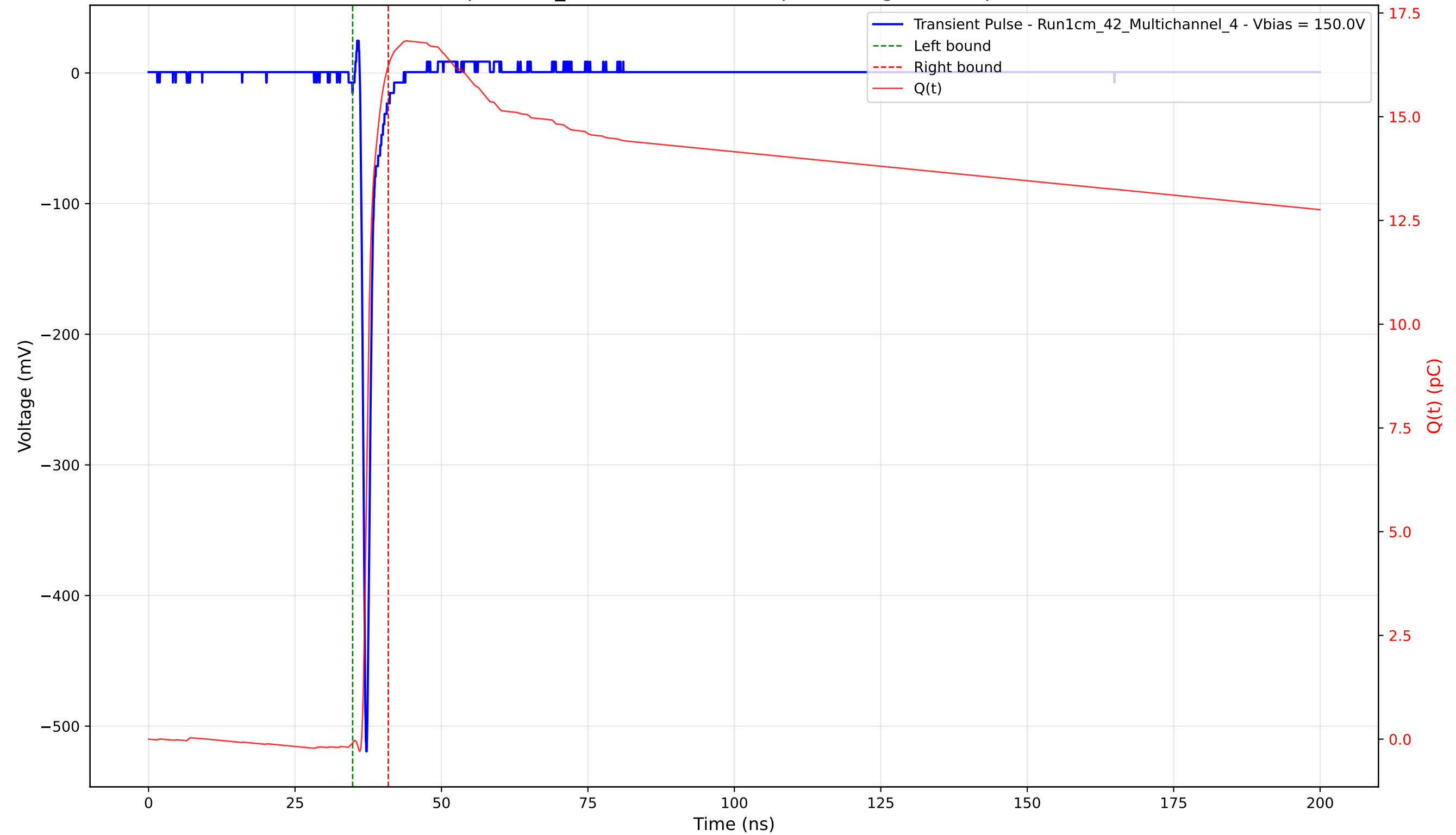
Transient Pulse - Sample: 1cm_42 - Position: 2330.0 \mu\text{m} - Charge: 16.31 pC - Rise Time: 0.72 ns
