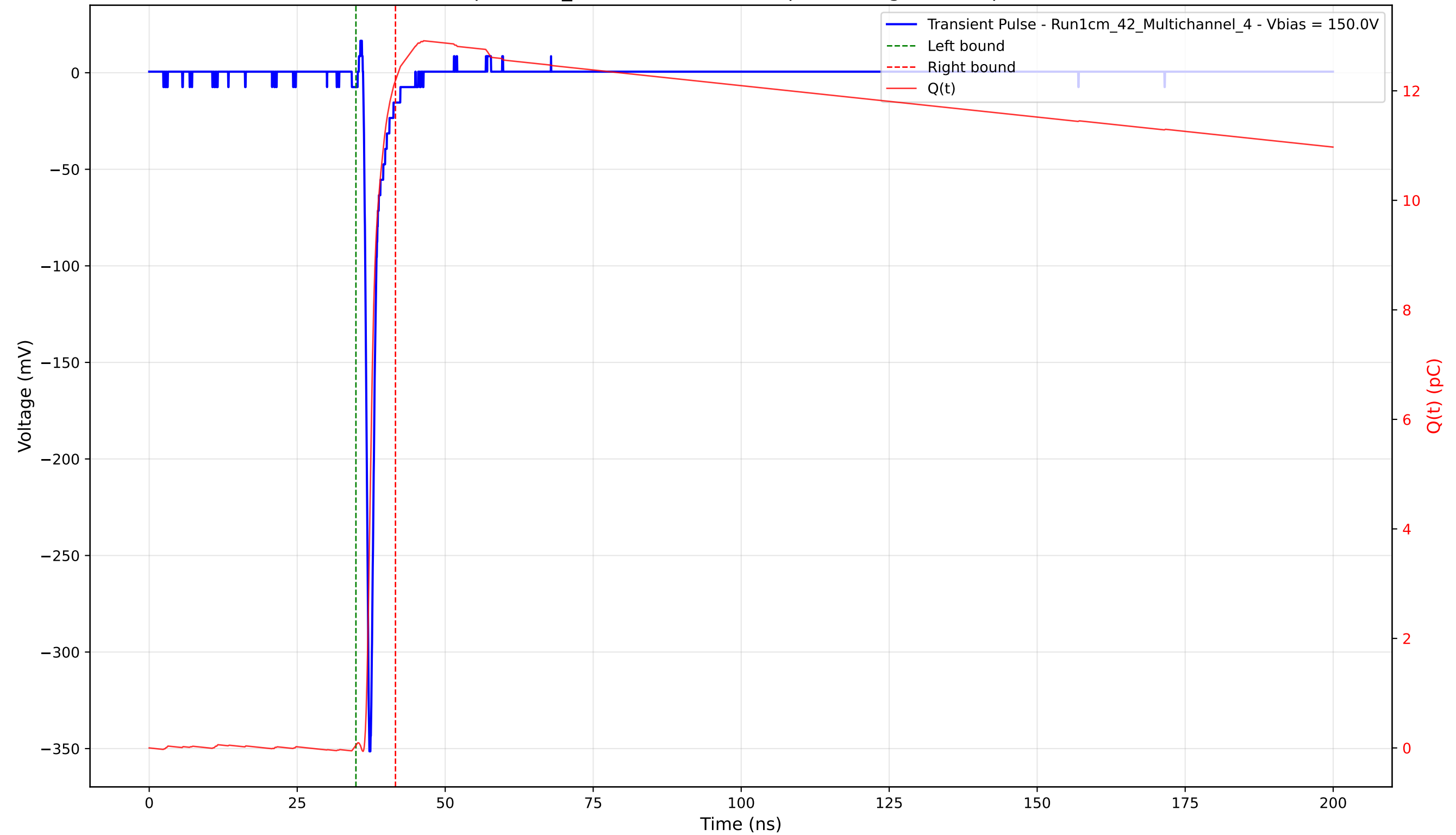
Transient Pulse - Sample: 1cm_42 - Position: 2895.0 \mu\text{m} - Charge: 12.14 pC - Rise Time: 0.73 ns
