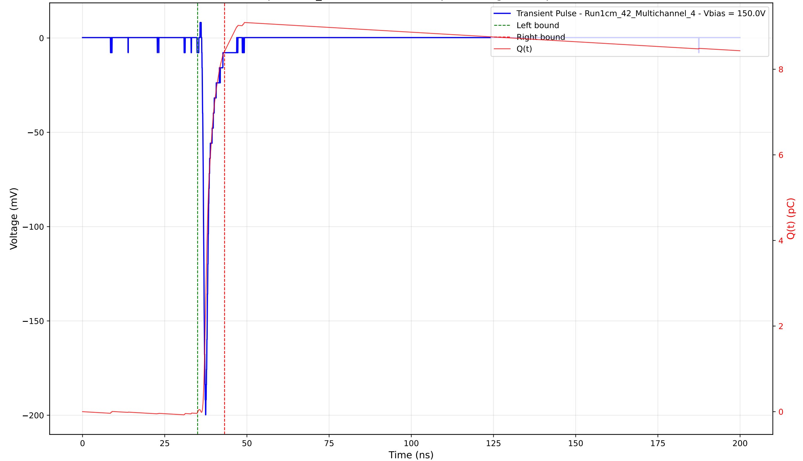
Transient Pulse - Sample: 1cm_42 - Position: 3070.0 \mu\text{m} - Charge: 8.43 pC - Rise Time: 0.82 ns
