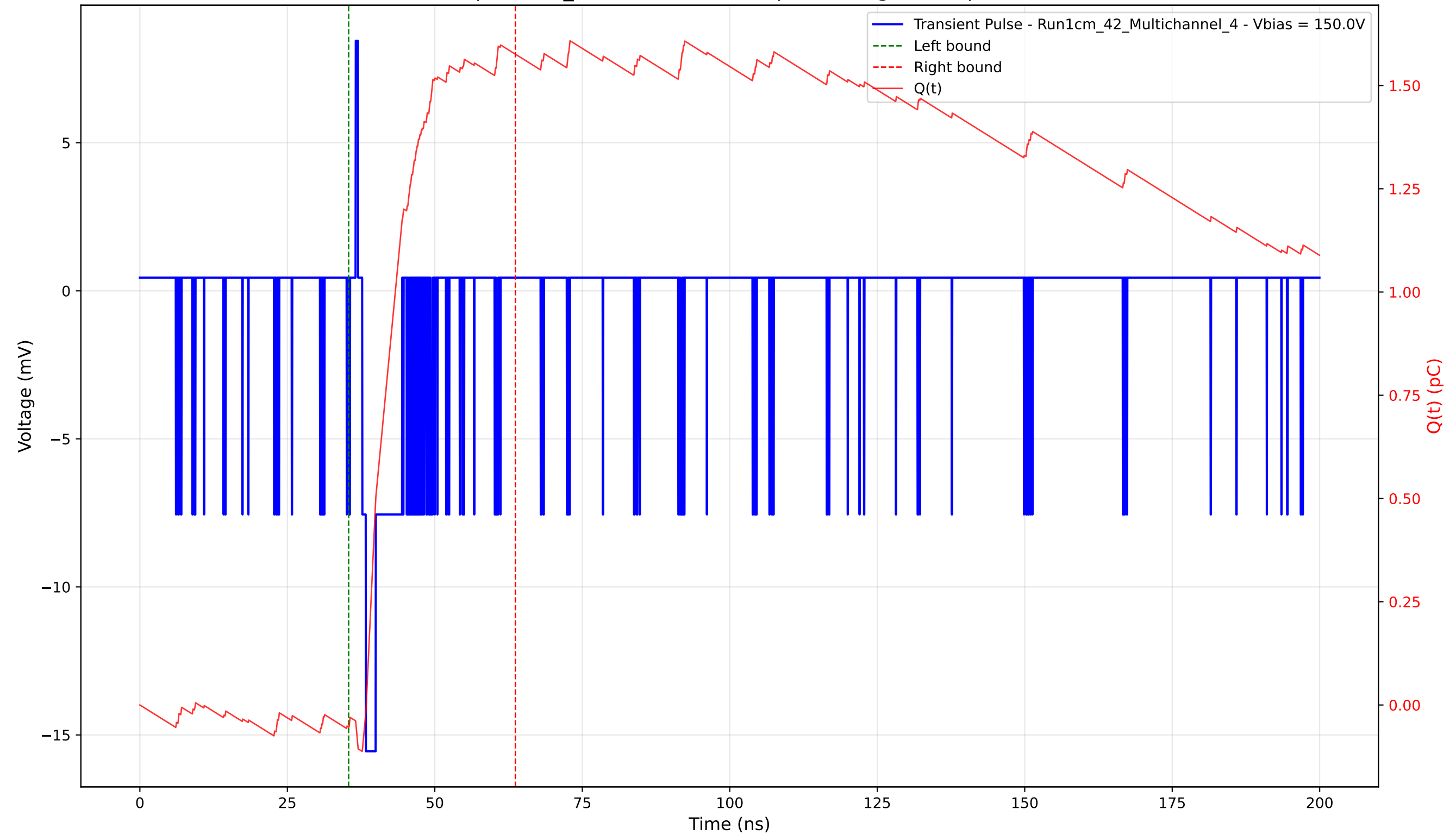
Transient Pulse - Sample: 1cm_42 - Position: 155.0 \mu\text{m} - Charge: 1.63 pC - Rise Time: 0.63 ns
