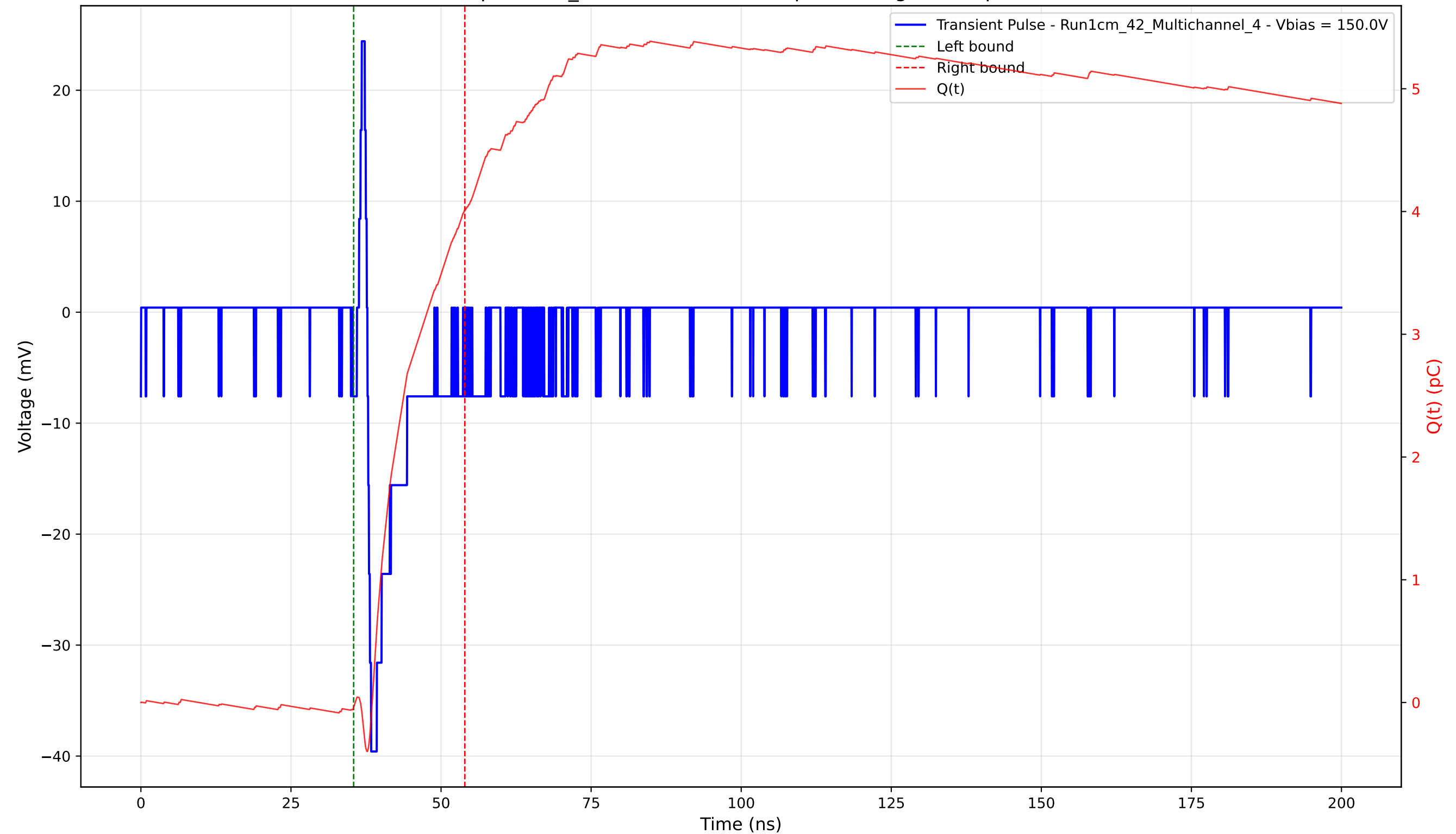
Transient Pulse - Sample: 1cm_42 - Position: 4215.0 \mu\text{m} - Charge: 4.05 pC - Rise Time: 0.62 ns
