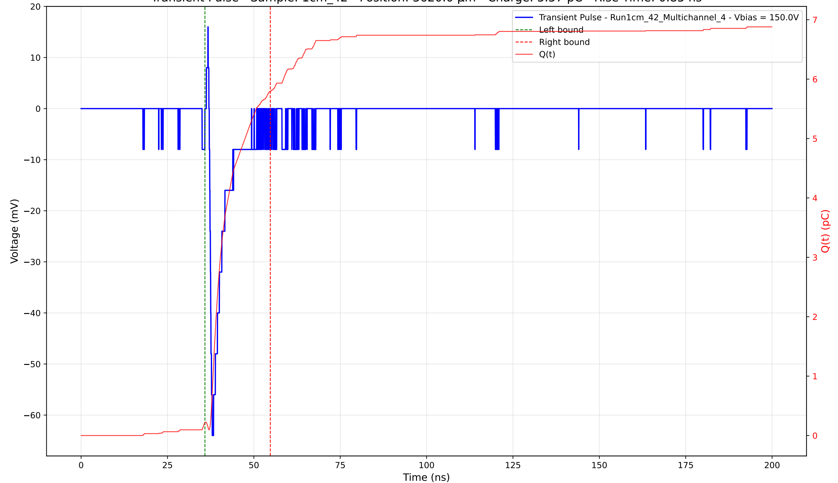
Transient Pulse - Sample: 1cm_42 - Position: 3620.0 \mu\text{m} - Charge: 5.57 pC - Rise Time: 0.85 ns
