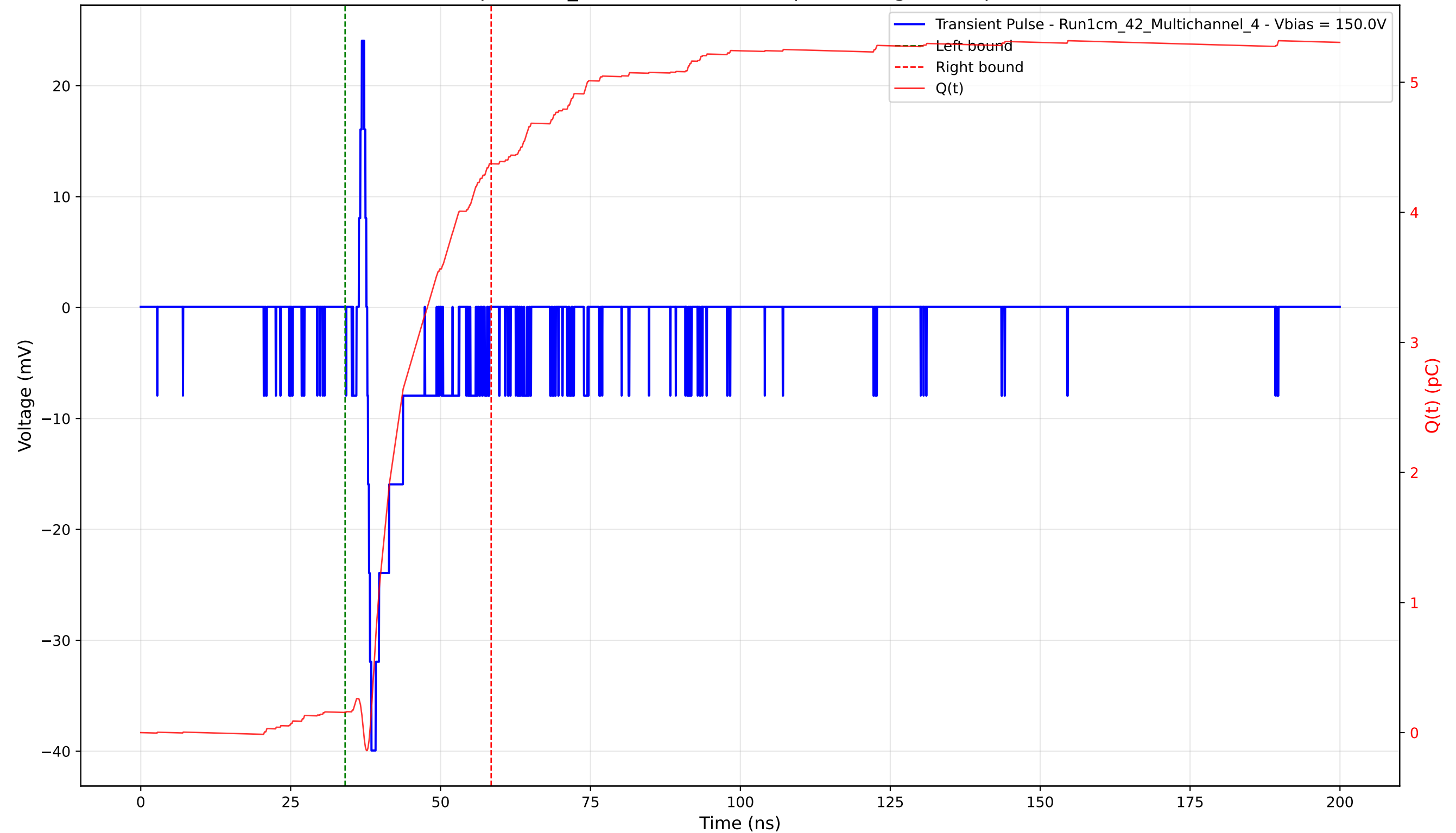
Transient Pulse - Sample: 1cm_42 - Position: 4375.0 \mu\text{m} - Charge: 4.22 pC - Rise Time: 0.70 ns
