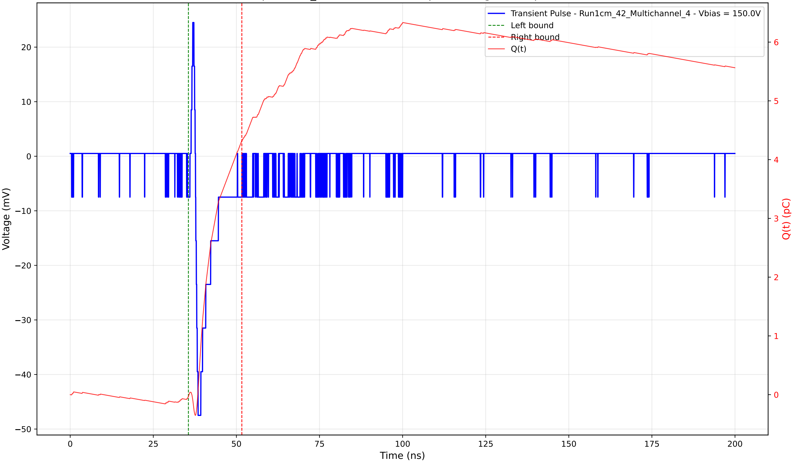
Transient Pulse - Sample: 1cm_42 - Position: 875.0 \mu\text{m} - Charge: 4.35 pC - Rise Time: 0.78 ns
