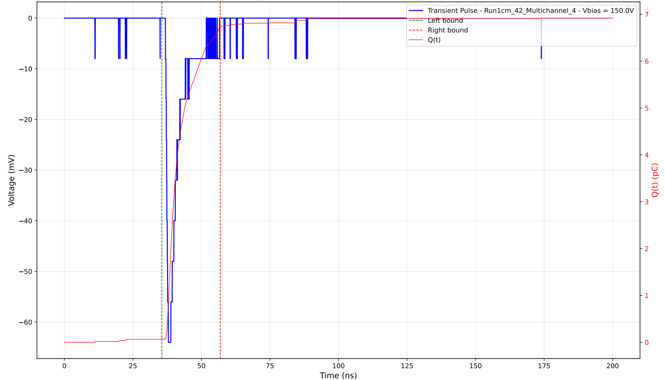
Transient Pulse - Sample: 1cm_42 - Position: 1430.0 \mu\text{m} - Charge: 6.67 pC - Rise Time: 1.05 ns
