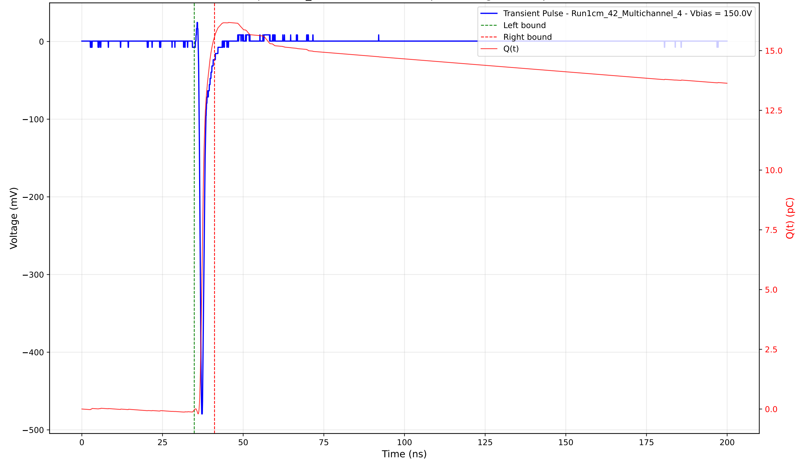
Transient Pulse - Sample: 1cm_42 - Position: 2760.0 \mu\text{m} - Charge: 15.62 pC - Rise Time: 0.74 ns
