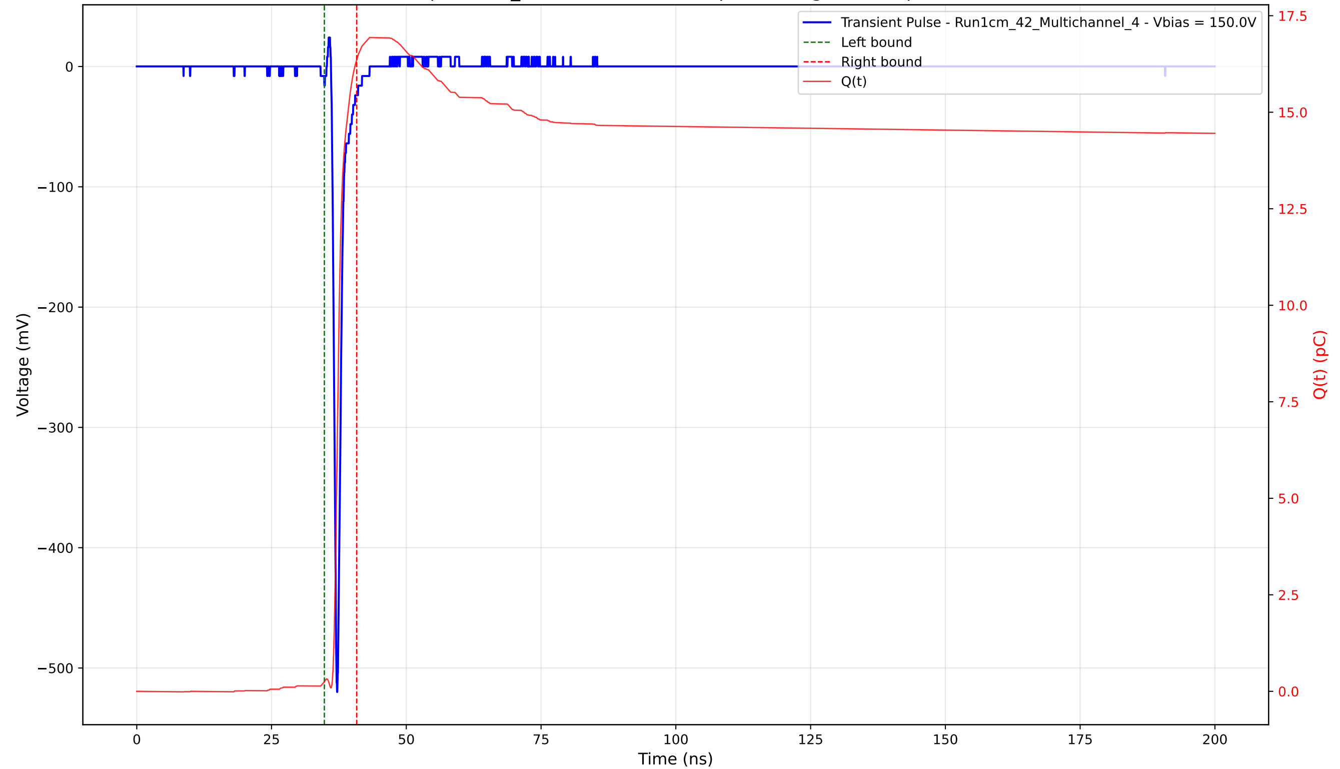
Transient Pulse - Sample: 1cm_42 - Position: 2660.0 \mu\text{m} - Charge: 16.11 pC - Rise Time: 0.69 ns
