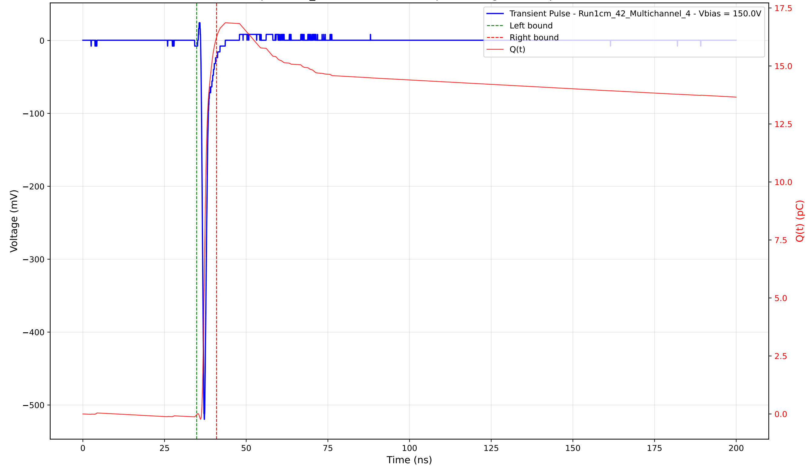
Transient Pulse - Sample: 1cm_42 - Position: 2345.0 \mu\text{m} - Charge: 16.27 pC - Rise Time: 0.74 ns
