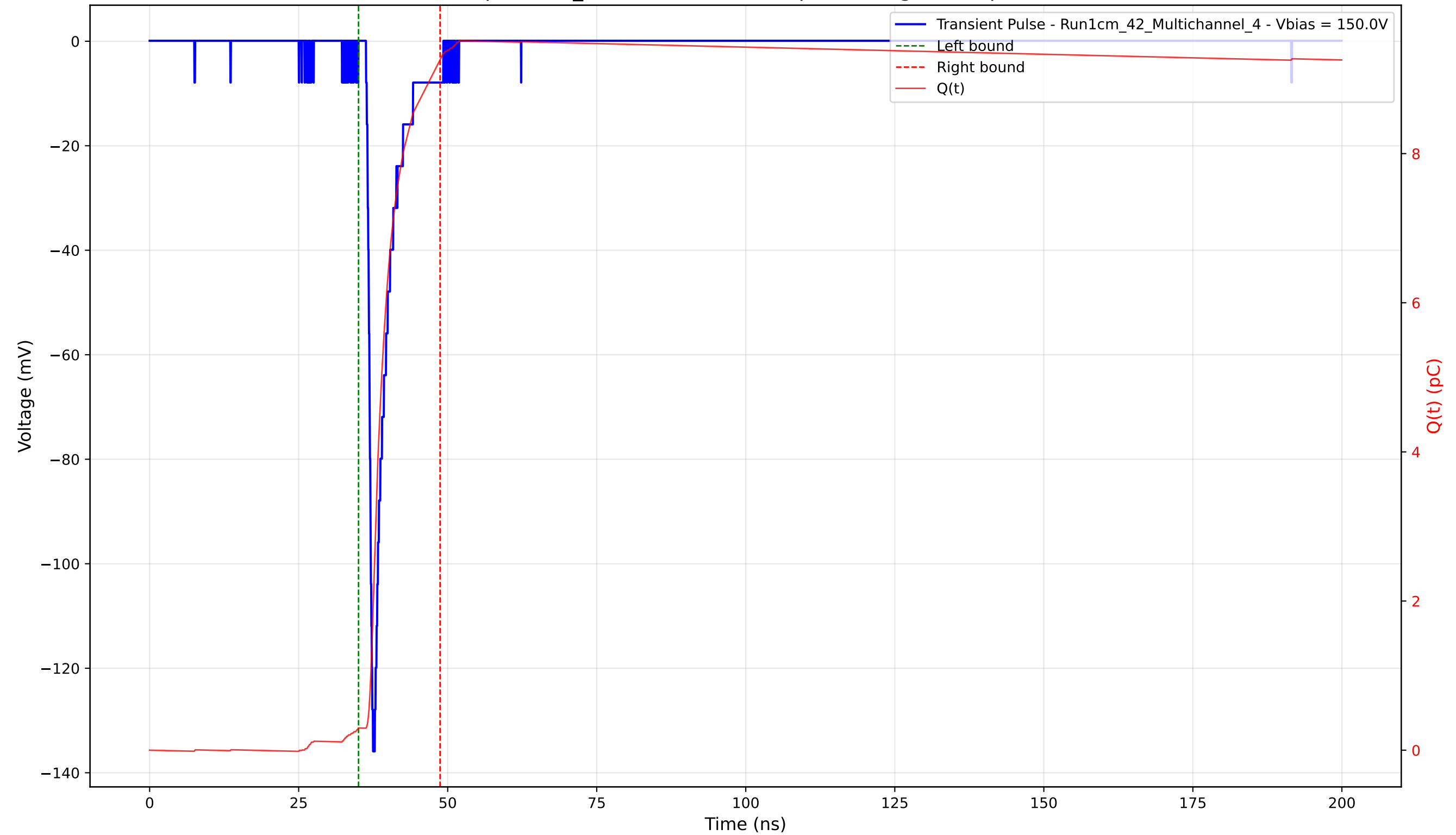
Transient Pulse - Sample: 1cm_42 - Position: 1705.0 \mu\text{m} - Charge: 8.96 pC - Rise Time: 0.93 ns
