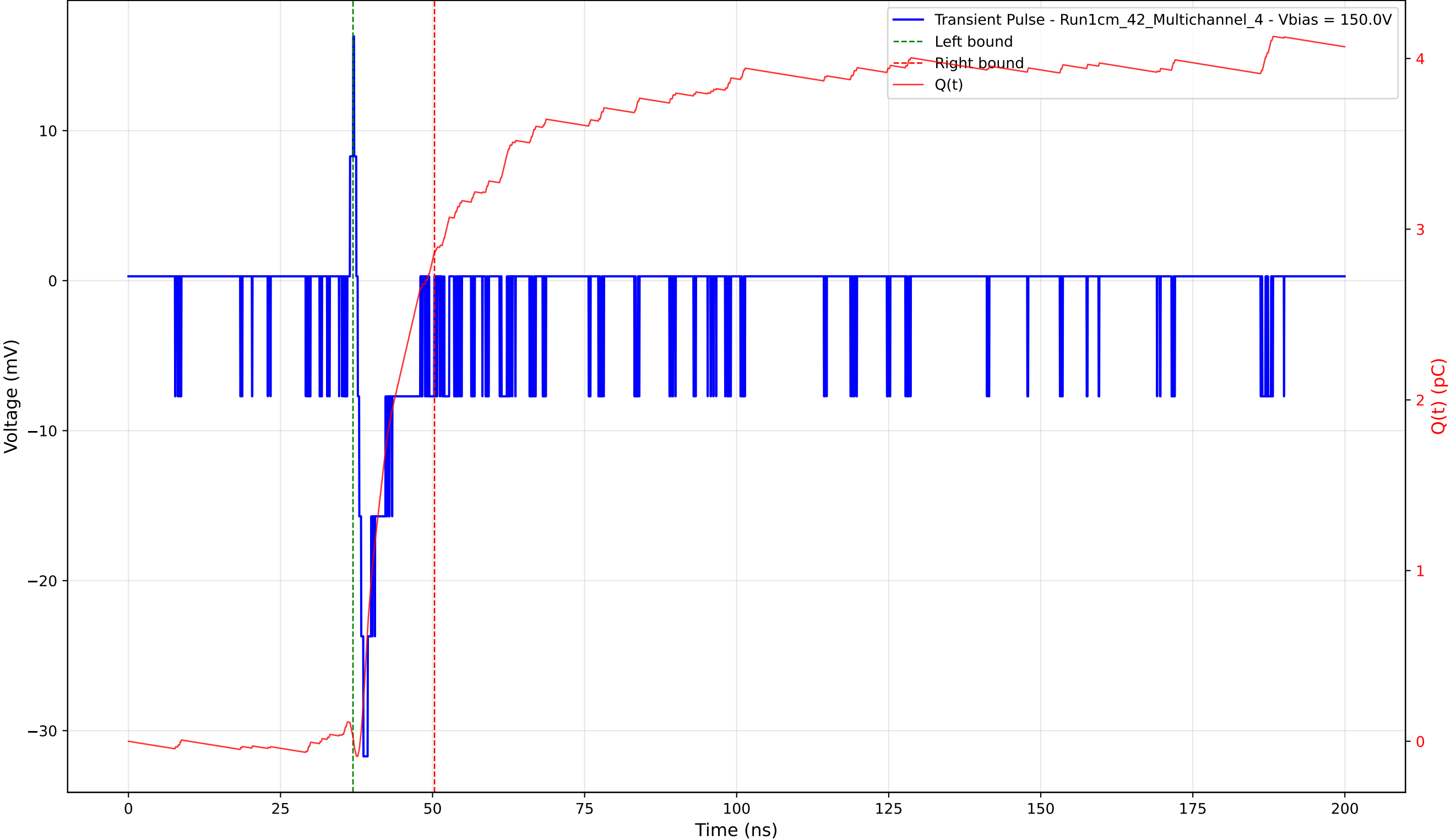
Transient Pulse - Sample: 1cm_42 - Position: 370.0 \mu\text{m} - Charge: 2.84 pC - Rise Time: 0.94 ns
