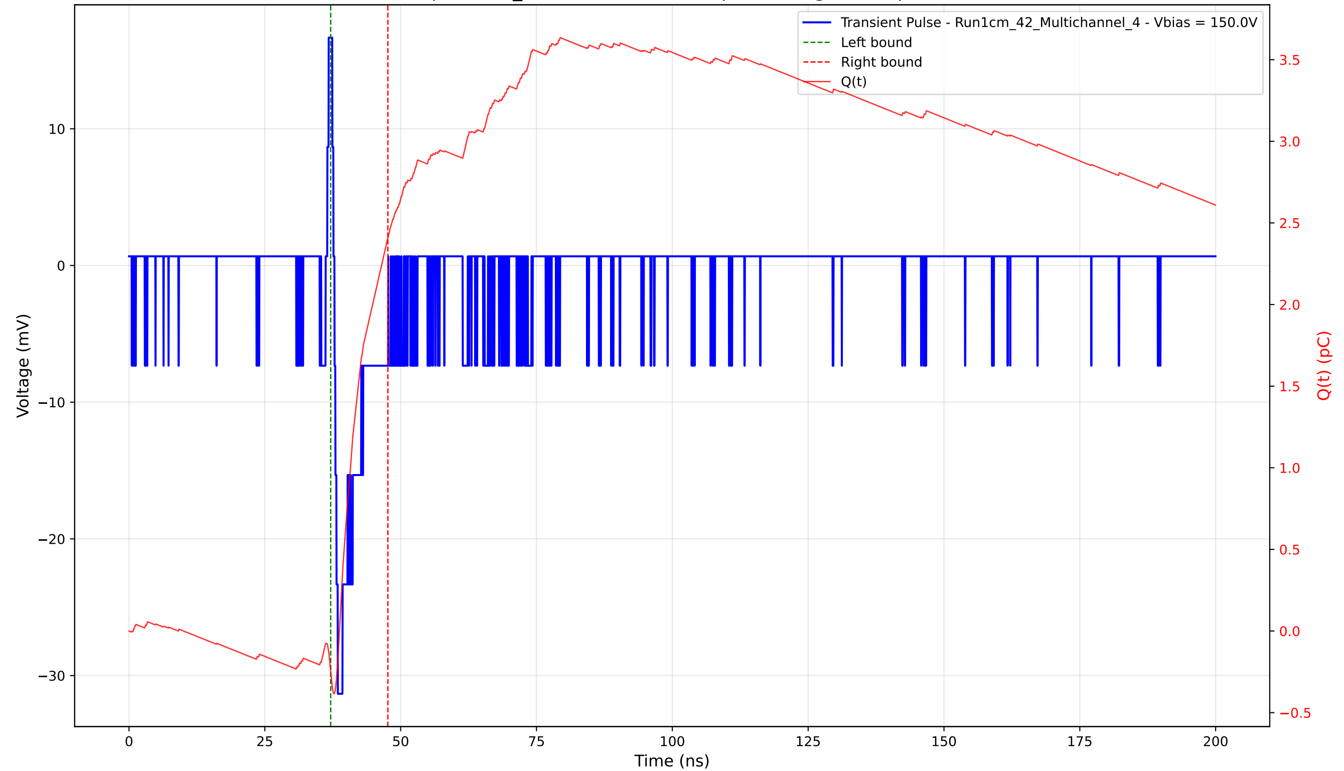
Transient Pulse - Sample: 1cm_42 - Position: 4480.0 \mu\text{m} - Charge: 2.66 pC - Rise Time: 0.63 ns
