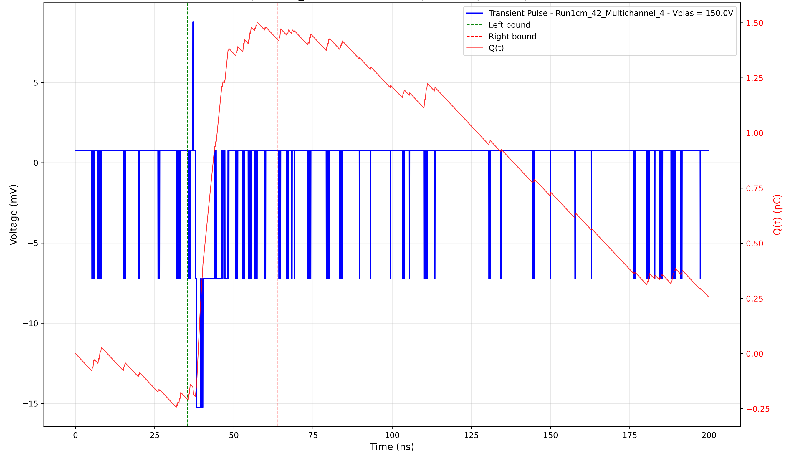
Transient Pulse - Sample: 1cm_42 - Position: 5035.0 \mu\text{m} - Charge: 1.64 pC - Rise Time: 0.44 ns
