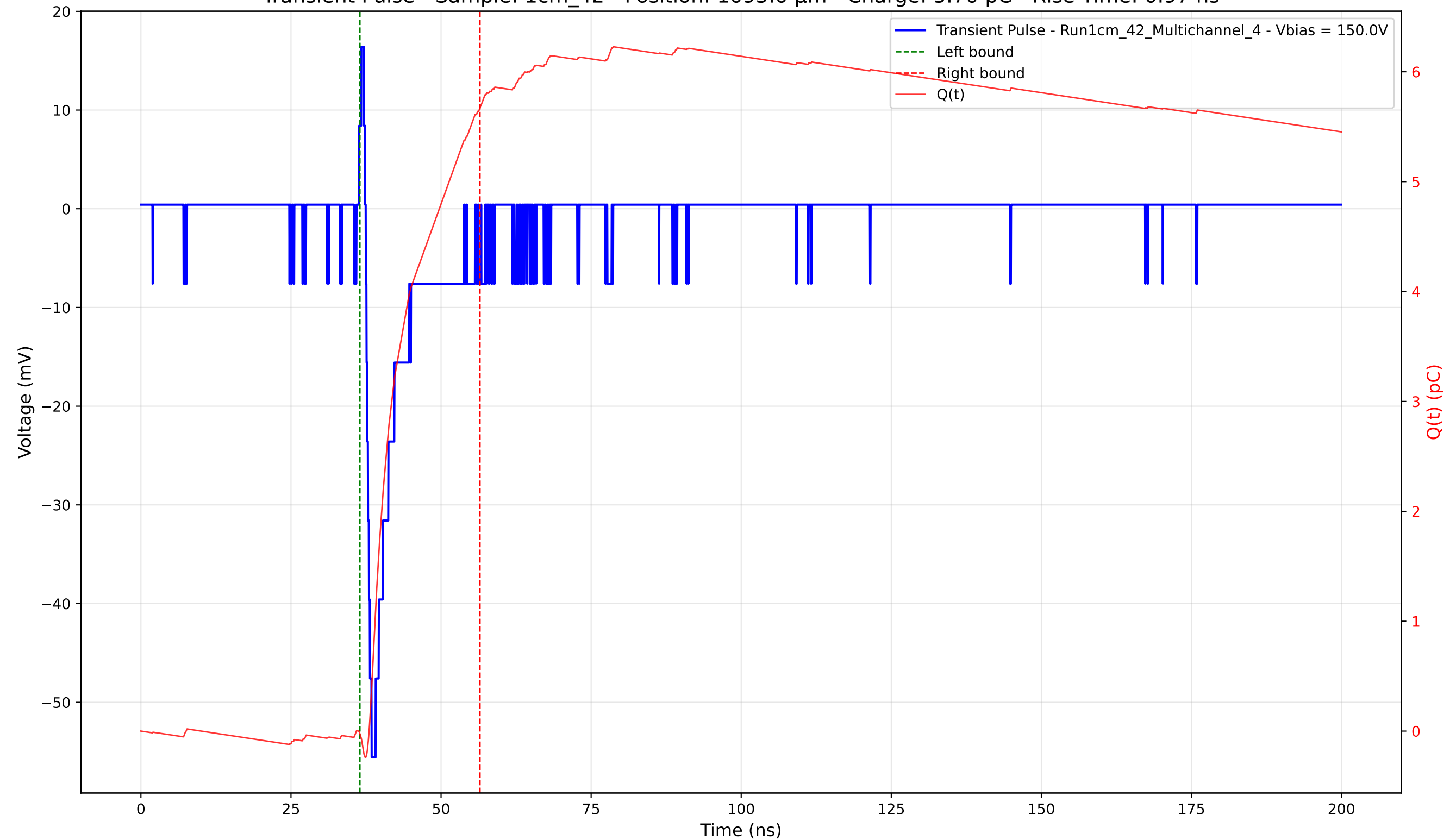
Transient Pulse - Sample: 1cm_42 - Position: 1095.0 \mu\text{m} - Charge: 5.70 pC - Rise Time: 0.97 ns
