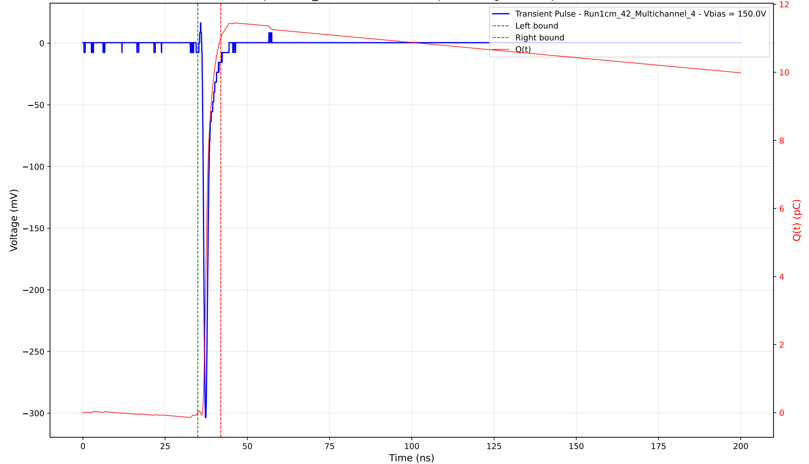
Transient Pulse - Sample: 1cm_42 - Position: 2935.0 \mu\text{m} - Charge: 11.00 pC - Rise Time: 0.73 ns
