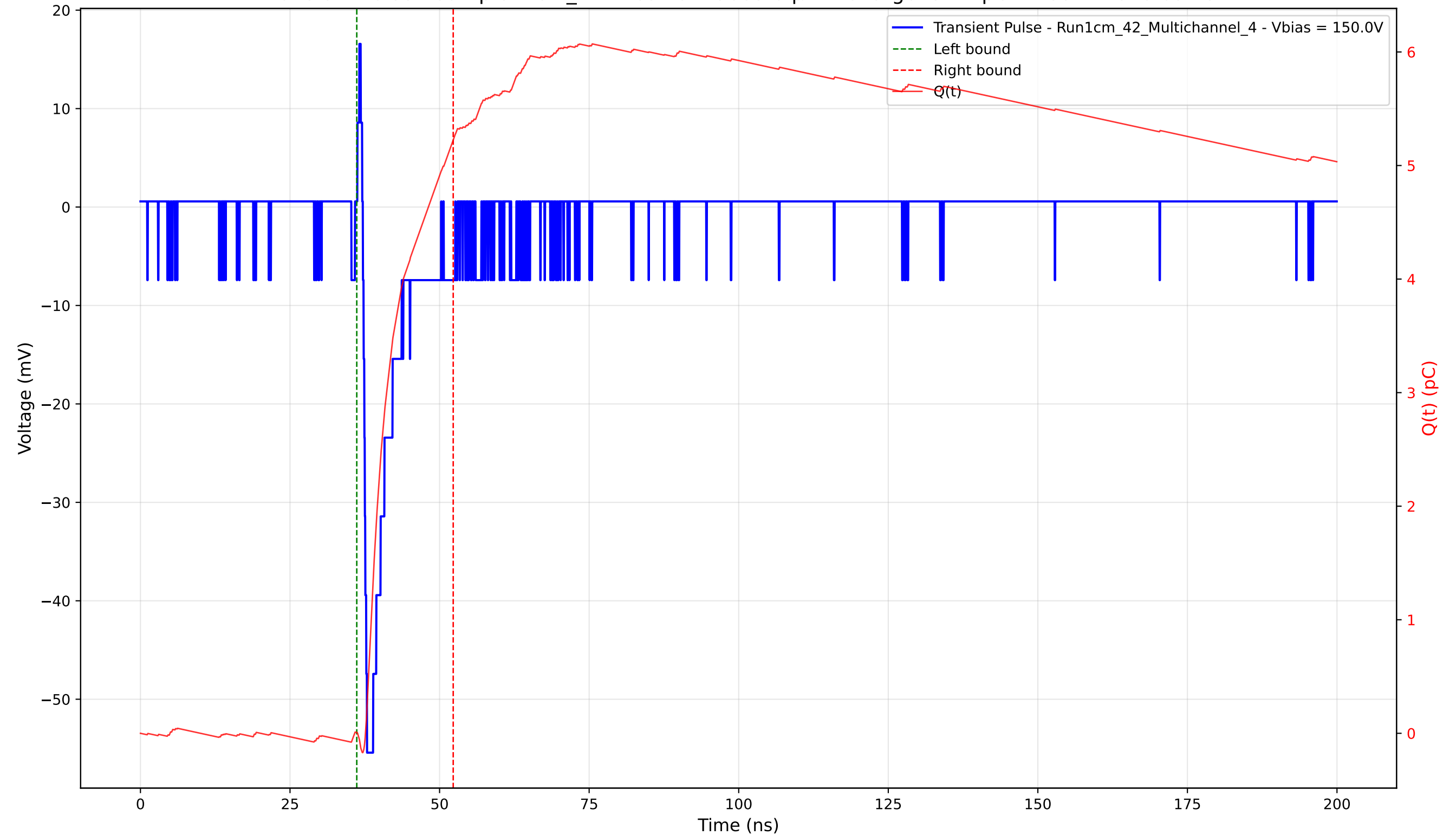
Transient Pulse - Sample: 1cm_42 - Position: 3685.0 \mu\text{m} - Charge: 5.22 pC - Rise Time: 0.69 ns
