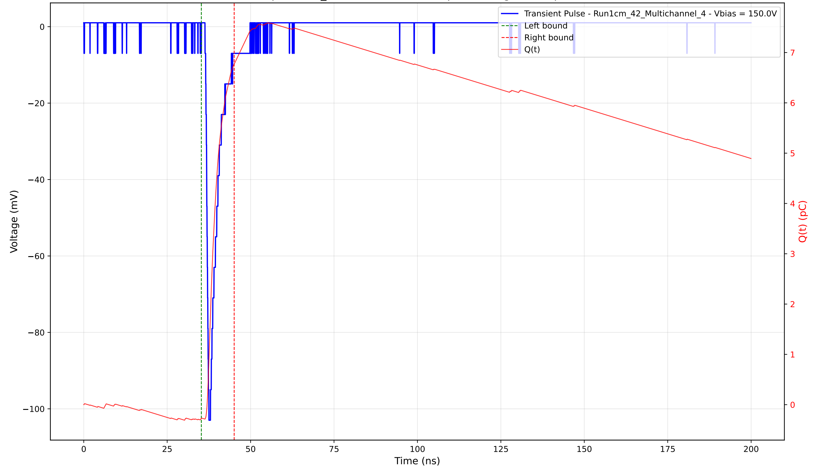
Transient Pulse - Sample: 1cm_42 - Position: 1625.0 \mu\text{m} - Charge: 7.04 pC - Rise Time: 0.82 ns
