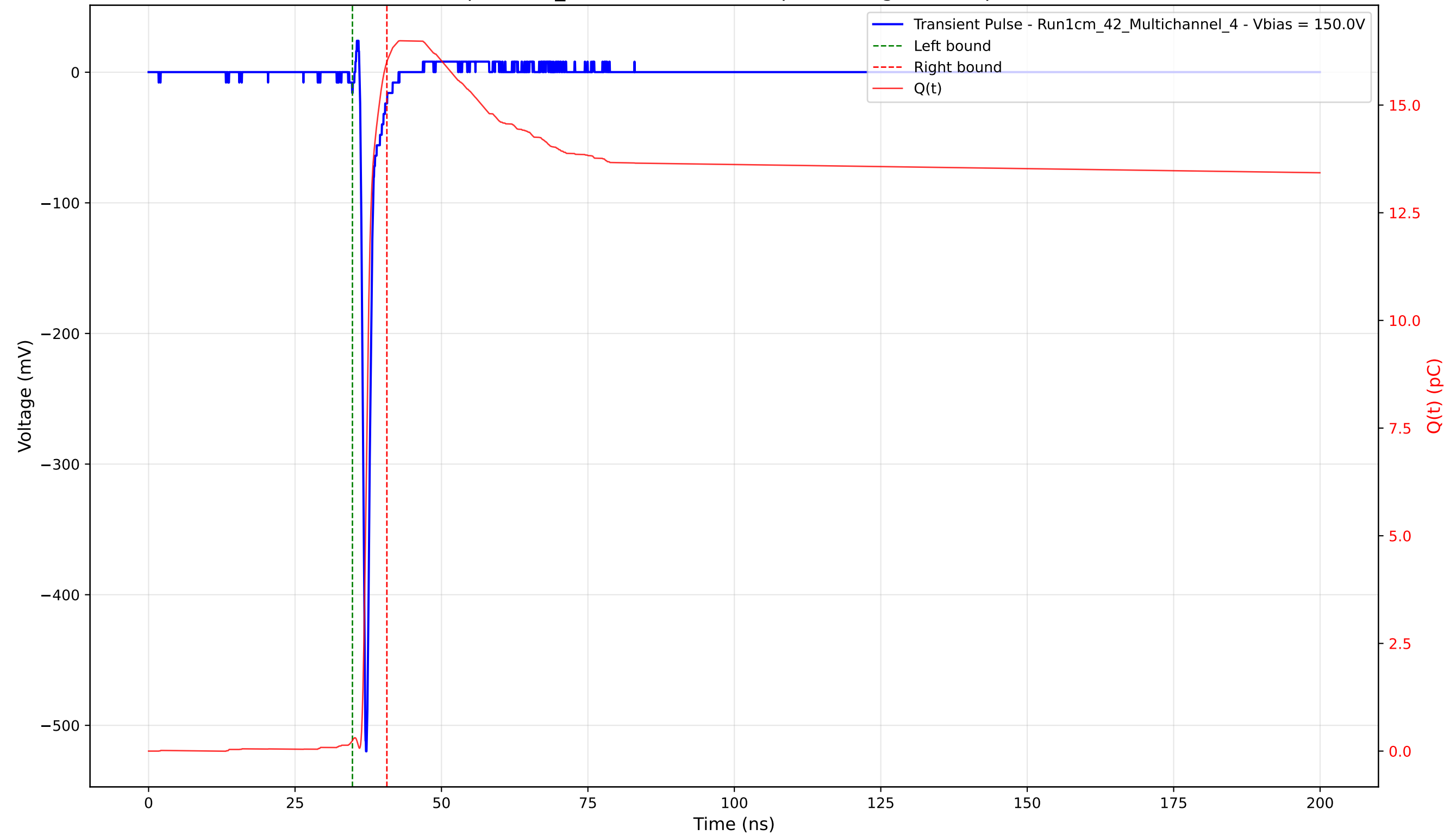
Transient Pulse - Sample: 1cm_42 - Position: 2550.0 \mu\text{m} - Charge: 15.76 pC - Rise Time: 0.72 ns
