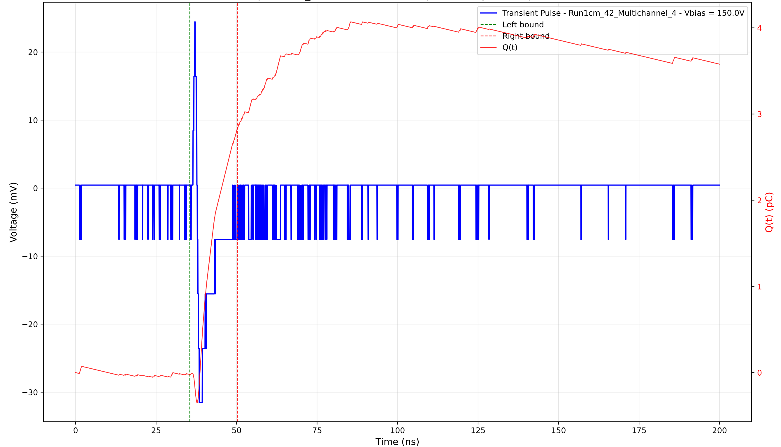
Transient Pulse - Sample: 1cm_42 - Position: 4475.0 \mu\text{m} - Charge: 2.85 pC - Rise Time: 0.62 ns
