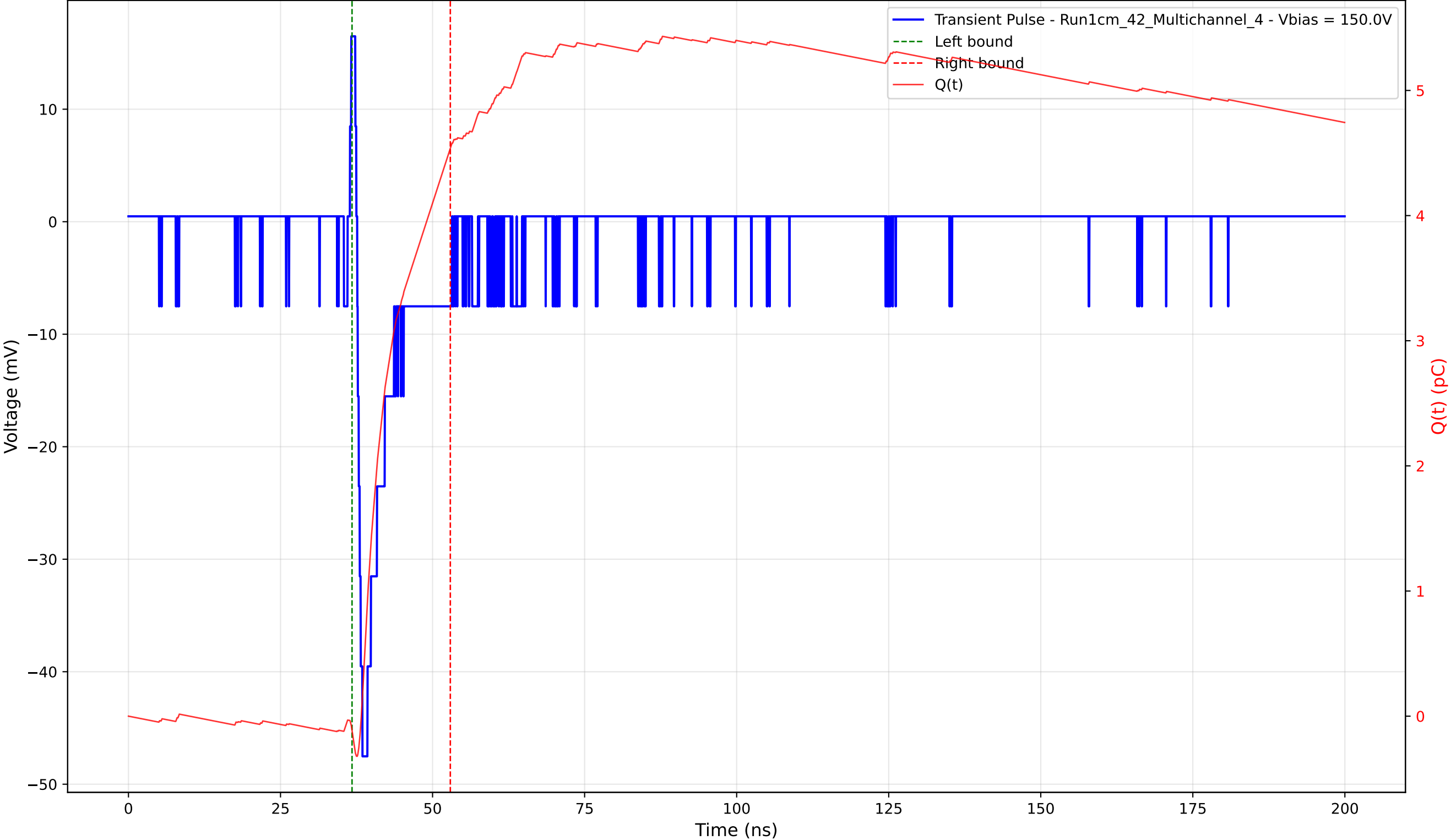
Transient Pulse - Sample: 1cm_42 - Position: 980.0 \mu\text{m} - Charge: 4.66 pC - Rise Time: 0.86 ns
