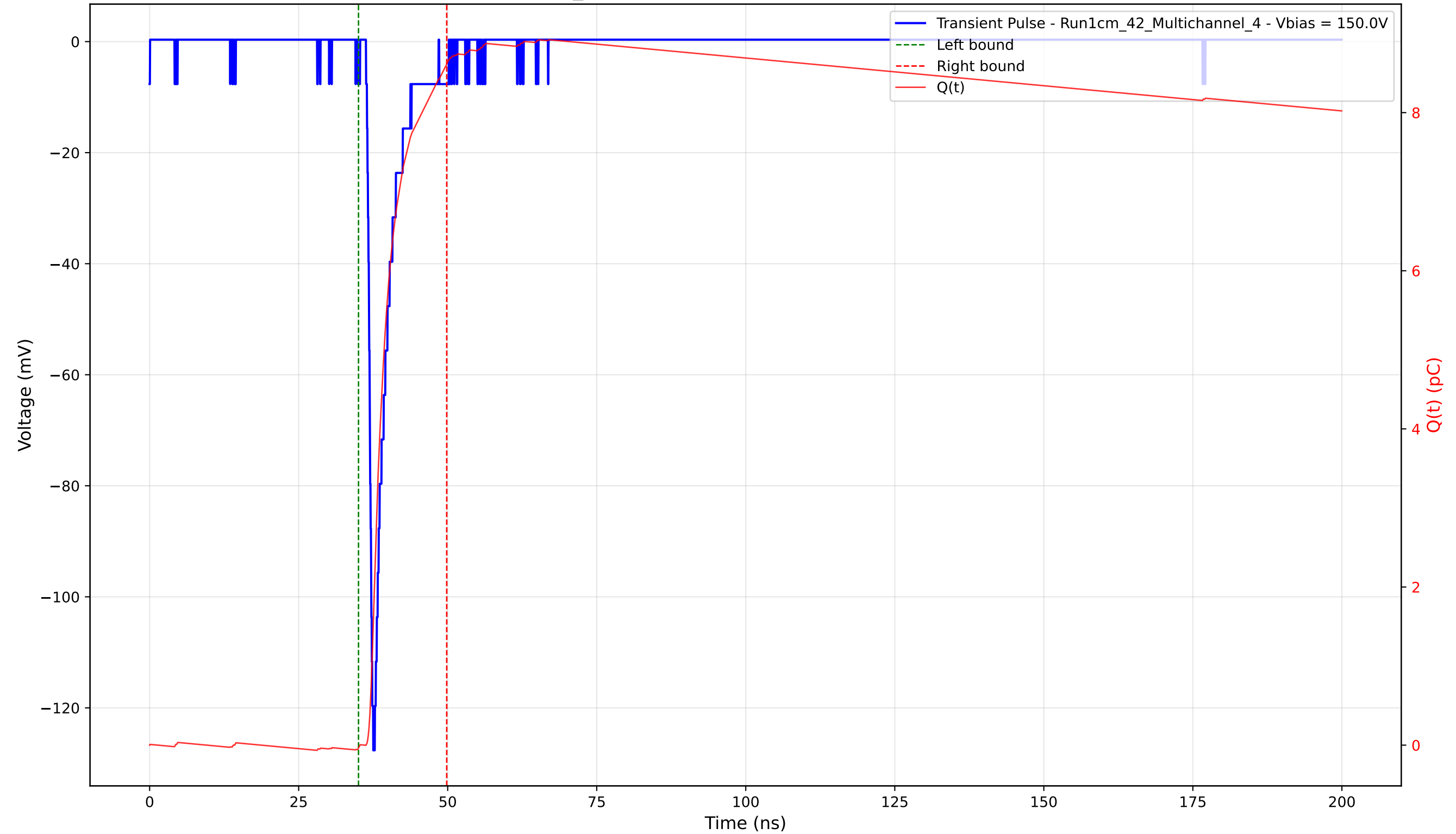
Transient Pulse - Sample: 1cm_42 - Position: 1685.0 \mu\text{m} - Charge: 8.65 pC - Rise Time: 0.89 ns
