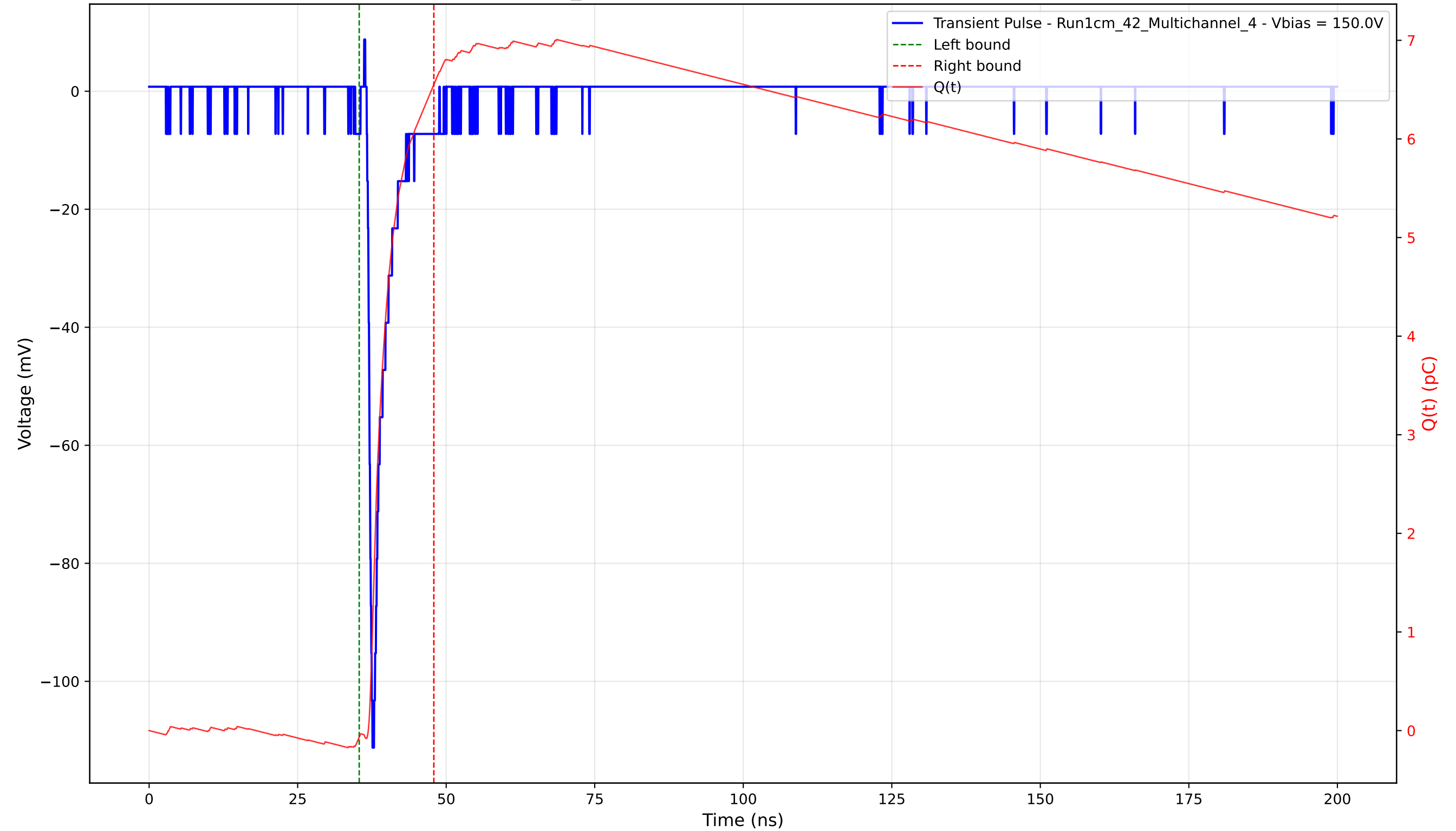
Transient Pulse - Sample: 1cm_42 - Position: 3390.0 \mu\text{m} - Charge: 6.62 pC - Rise Time: 0.78 ns
