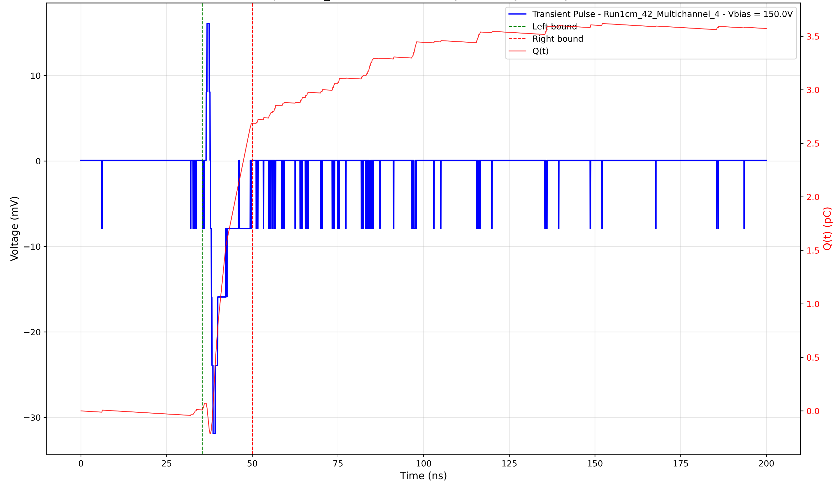
Transient Pulse - Sample: 1cm_42 - Position: 4570.0 \mu\text{m} - Charge: 2.68 pC - Rise Time: 0.74 ns
