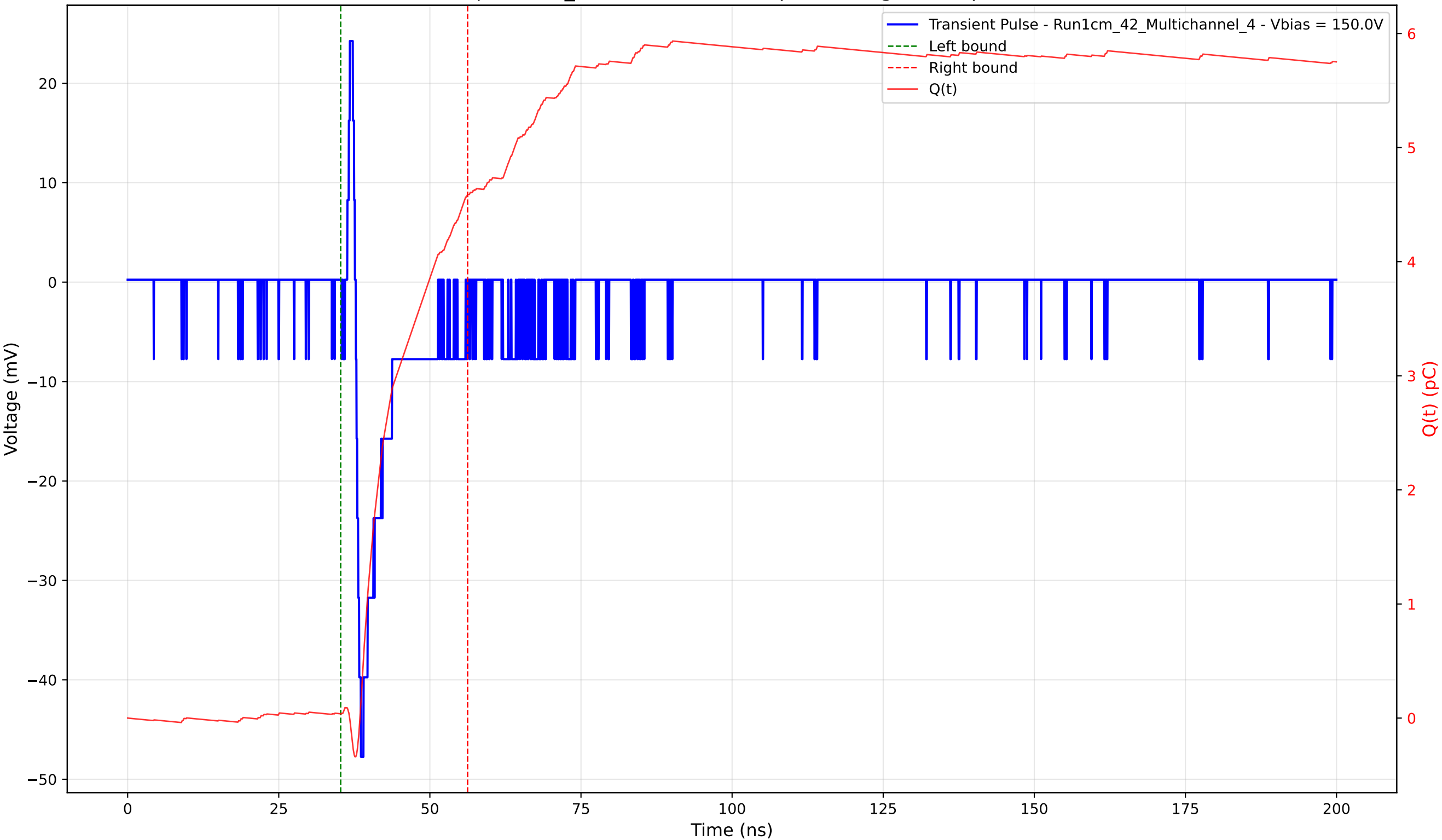
Transient Pulse - Sample: 1cm_42 - Position: 640.0 \mu\text{m} - Charge: 4.55 pC - Rise Time: 0.86 ns
