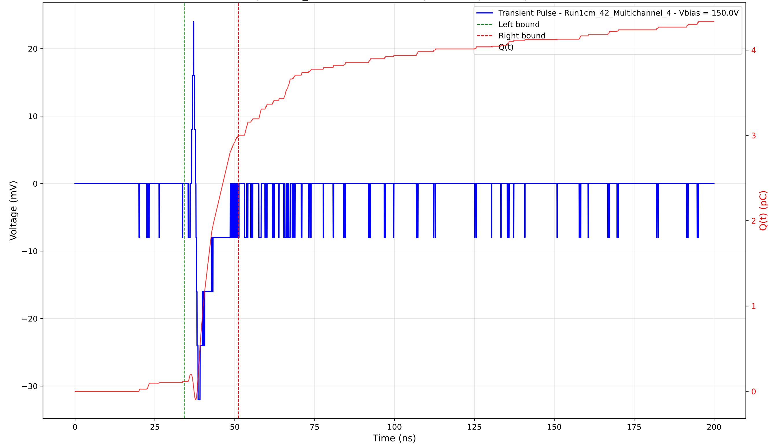
Transient Pulse - Sample: 1cm_42 - Position: 4545.0 \mu\text{m} - Charge: 2.88 pC - Rise Time: 0.66 ns
