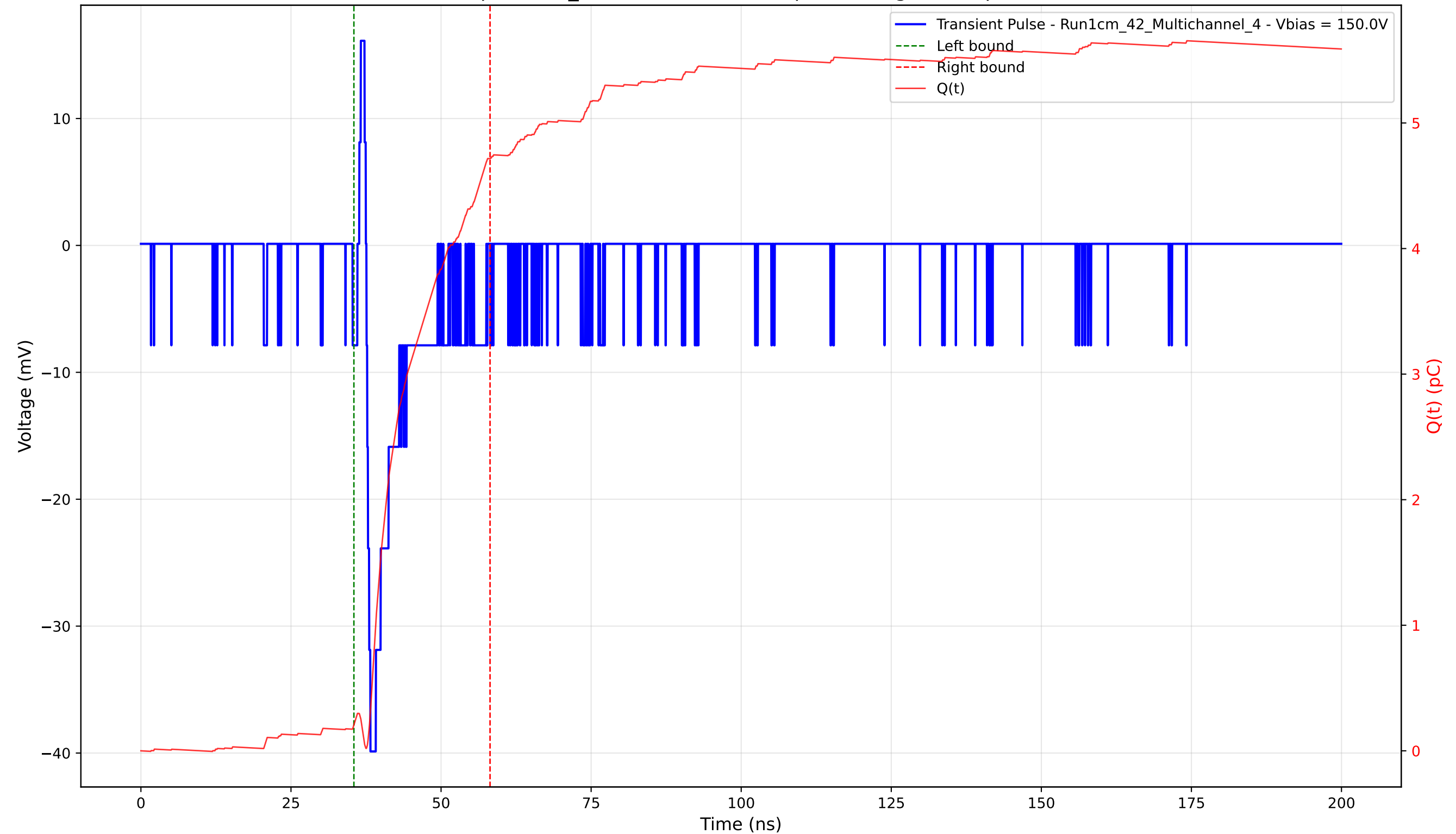
Transient Pulse - Sample: 1cm_42 - Position: 4040.0 \mu\text{m} - Charge: 4.51 pC - Rise Time: 0.66 ns
