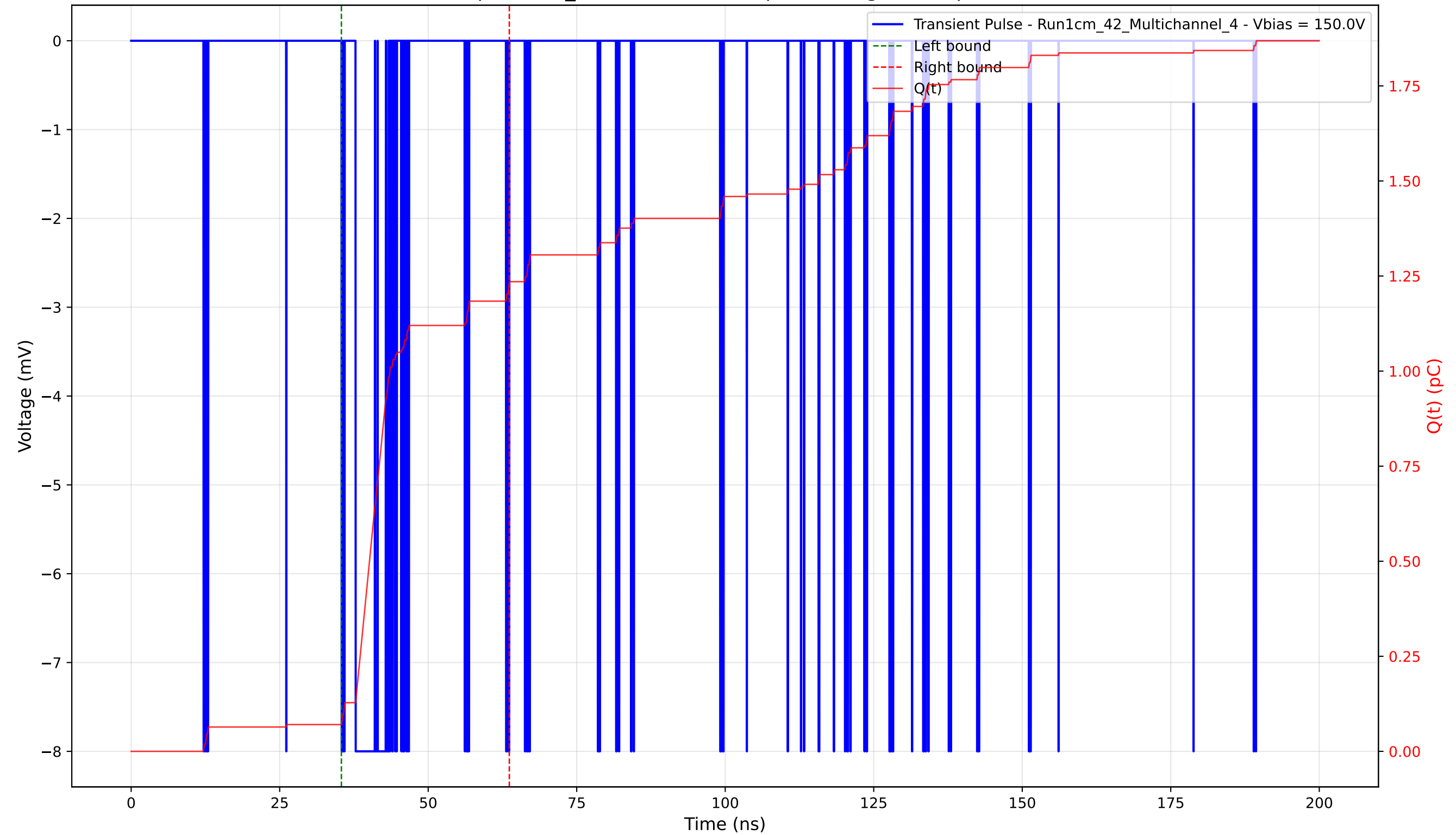
Transient Pulse - Sample: 1cm_42 - Position: 90.0 \mu\text{m} - Charge: 1.16 pC - Rise Time: 0.04 ns
