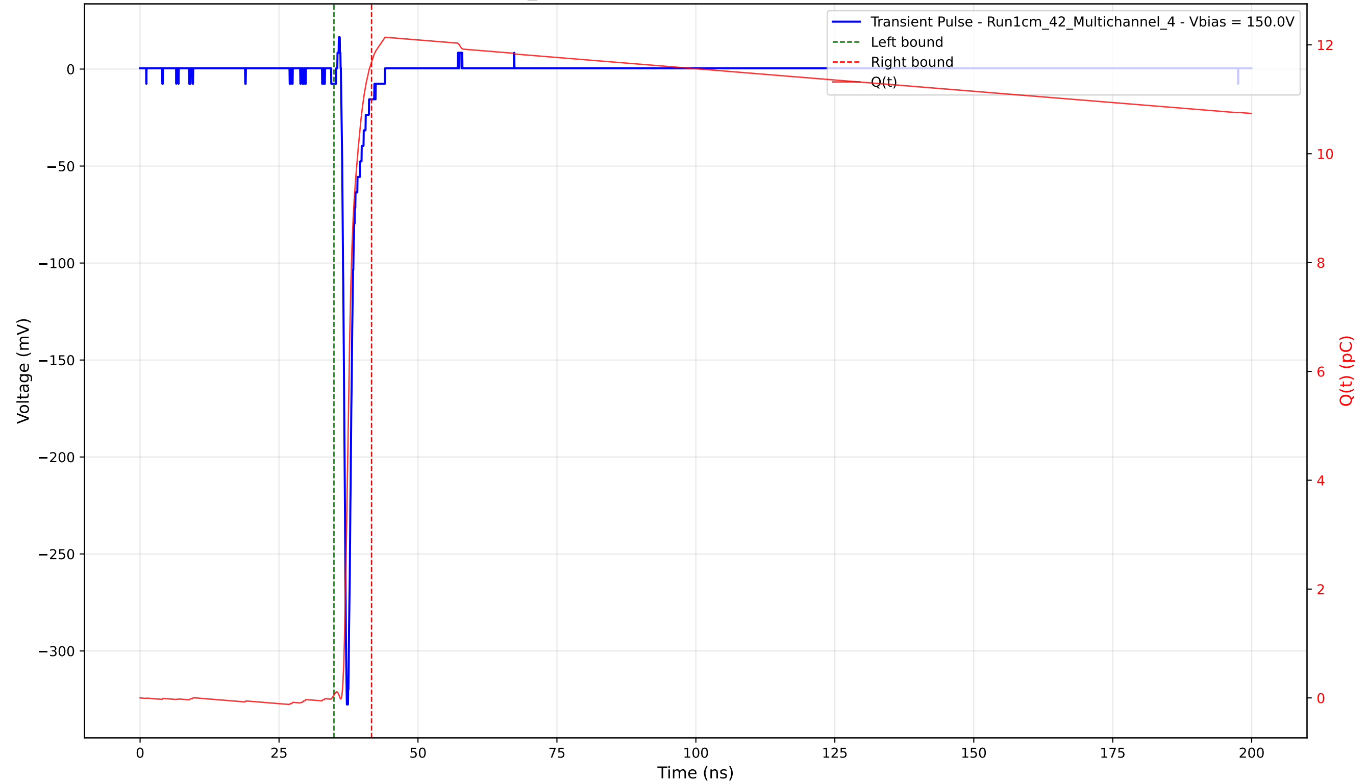
Transient Pulse - Sample: 1cm_42 - Position: 2910.0 \mu\text{m} - Charge: 11.63 pC - Rise Time: 0.75 ns
