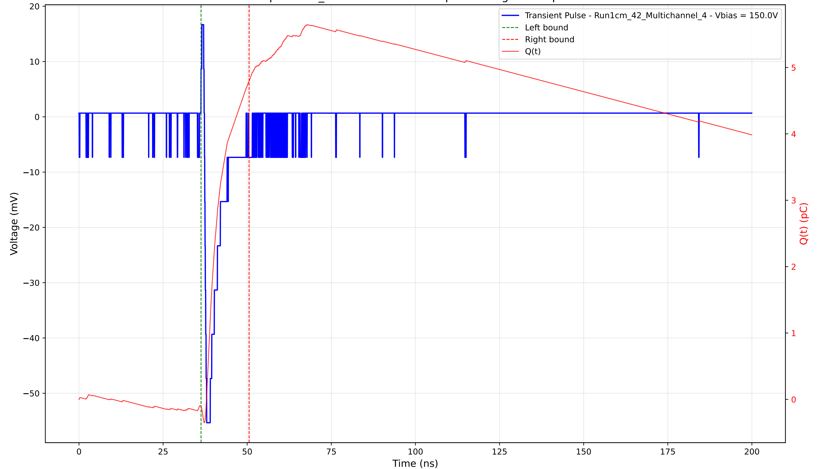
Transient Pulse - Sample: 1cm_42 - Position: 3740.0 \mu\text{m} - Charge: 4.90 pC - Rise Time: 0.65 ns
