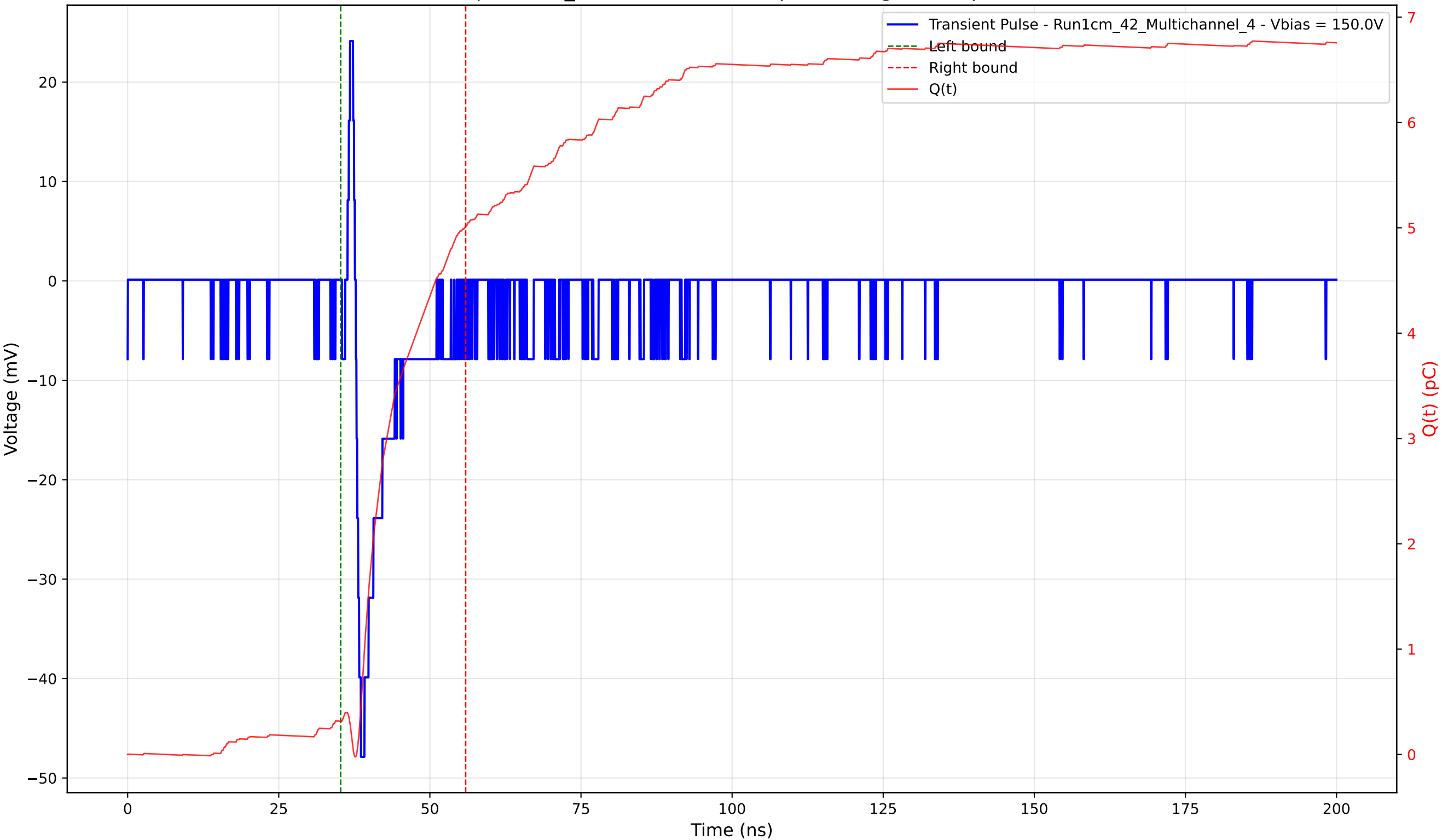
Transient Pulse - Sample: 1cm_42 - Position: 650.0 \mu\text{m} - Charge: 4.70 pC - Rise Time: 0.86 ns
