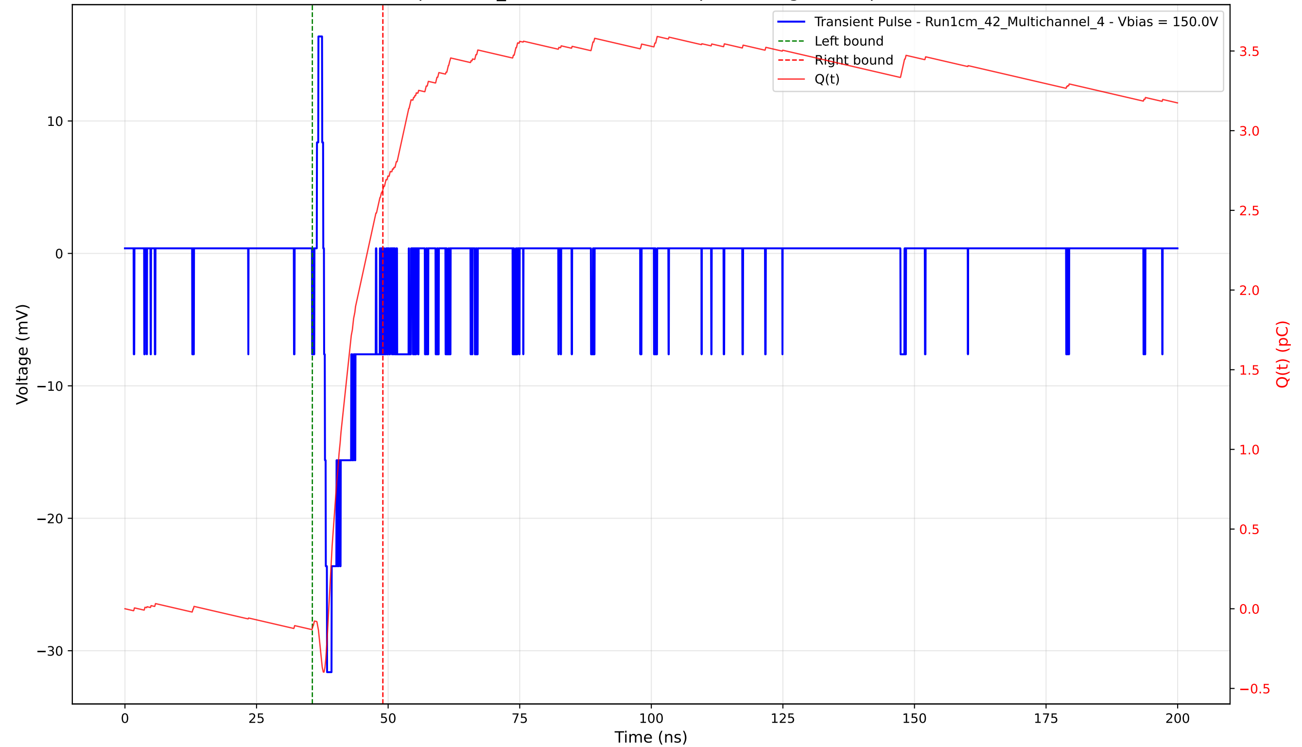
Transient Pulse - Sample: 1cm_42 - Position: 4485.0 \mu\text{m} - Charge: 2.75 pC - Rise Time: 0.58 ns
