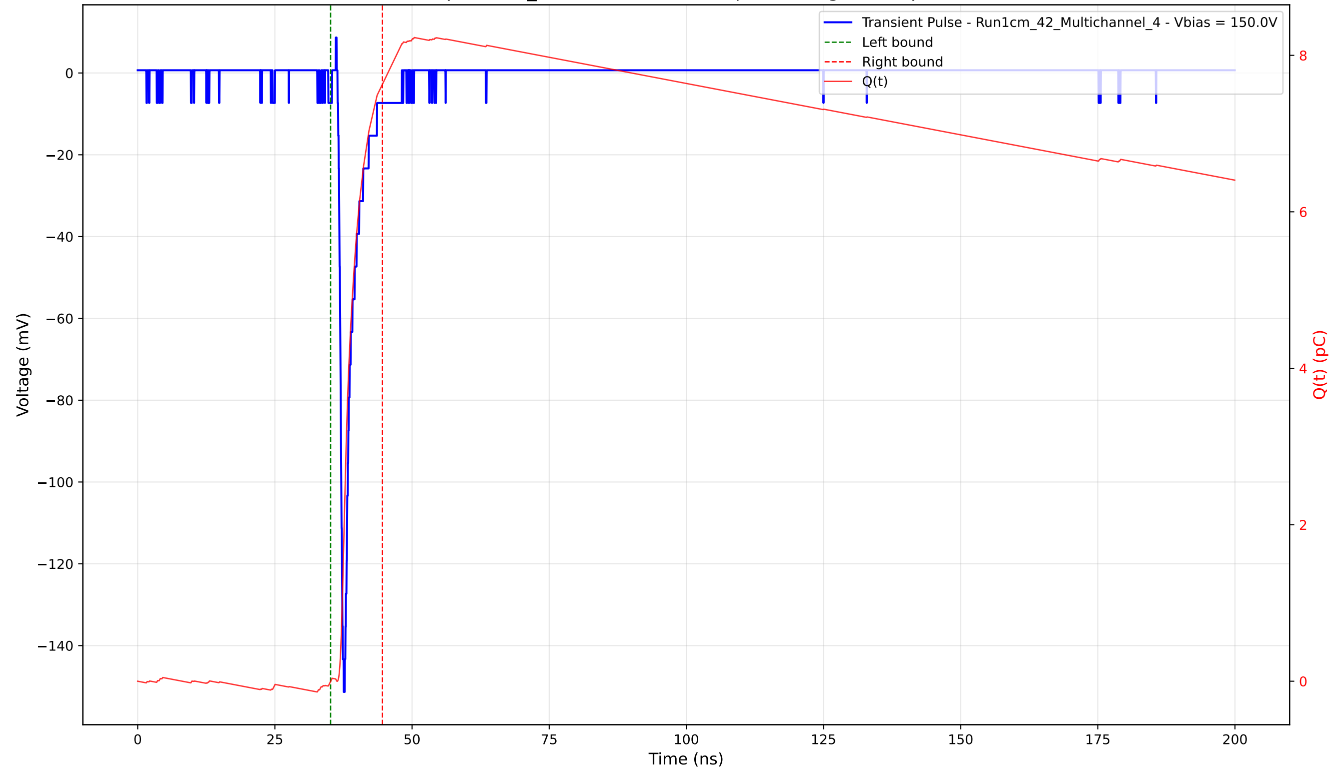
Transient Pulse - Sample: 1cm_42 - Position: 3215.0 \mu\text{m} - Charge: 7.63 pC - Rise Time: 0.84 ns
