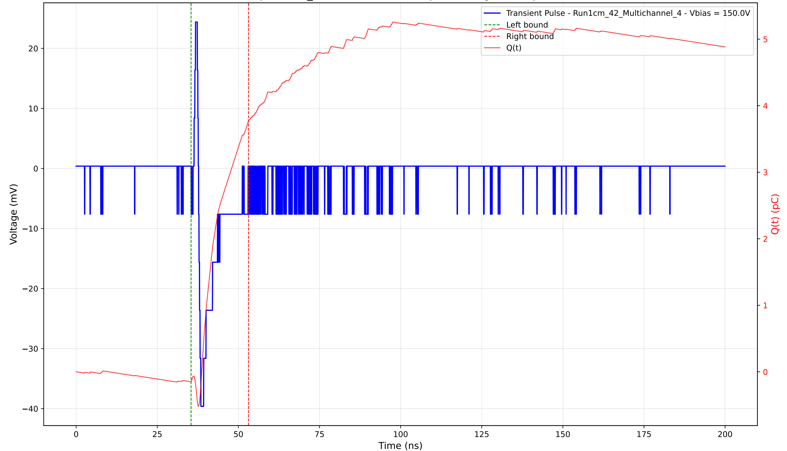
Transient Pulse - Sample: 1cm_42 - Position: 4275.0 \mu\text{m} - Charge: 3.91 pC - Rise Time: 0.70 ns
