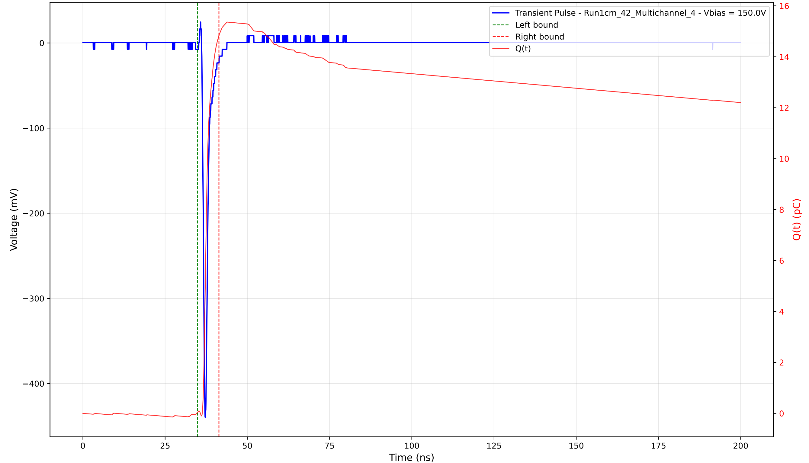
Transient Pulse - Sample: 1cm_42 - Position: 2190.0 \mu\text{m} - Charge: 14.79 pC - Rise Time: 0.74 ns
