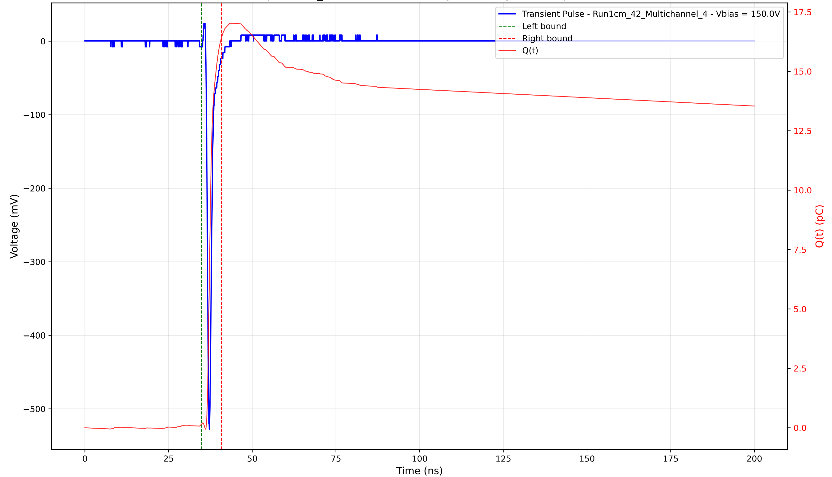
Transient Pulse - Sample: 1cm_42 - Position: 2365.0 \mu\text{m} - Charge: 16.28 pC - Rise Time: 0.68 ns
