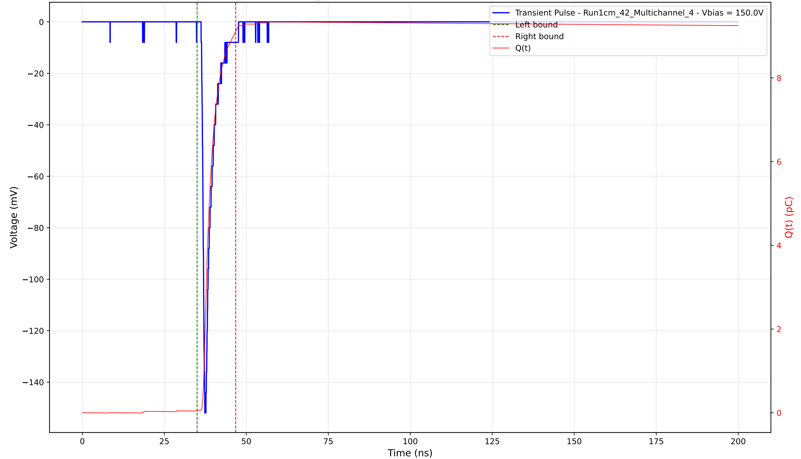
Transient Pulse - Sample: 1cm_42 - Position: 1825.0 \mu\text{m} - Charge: 9.05 pC - Rise Time: 0.88 ns
