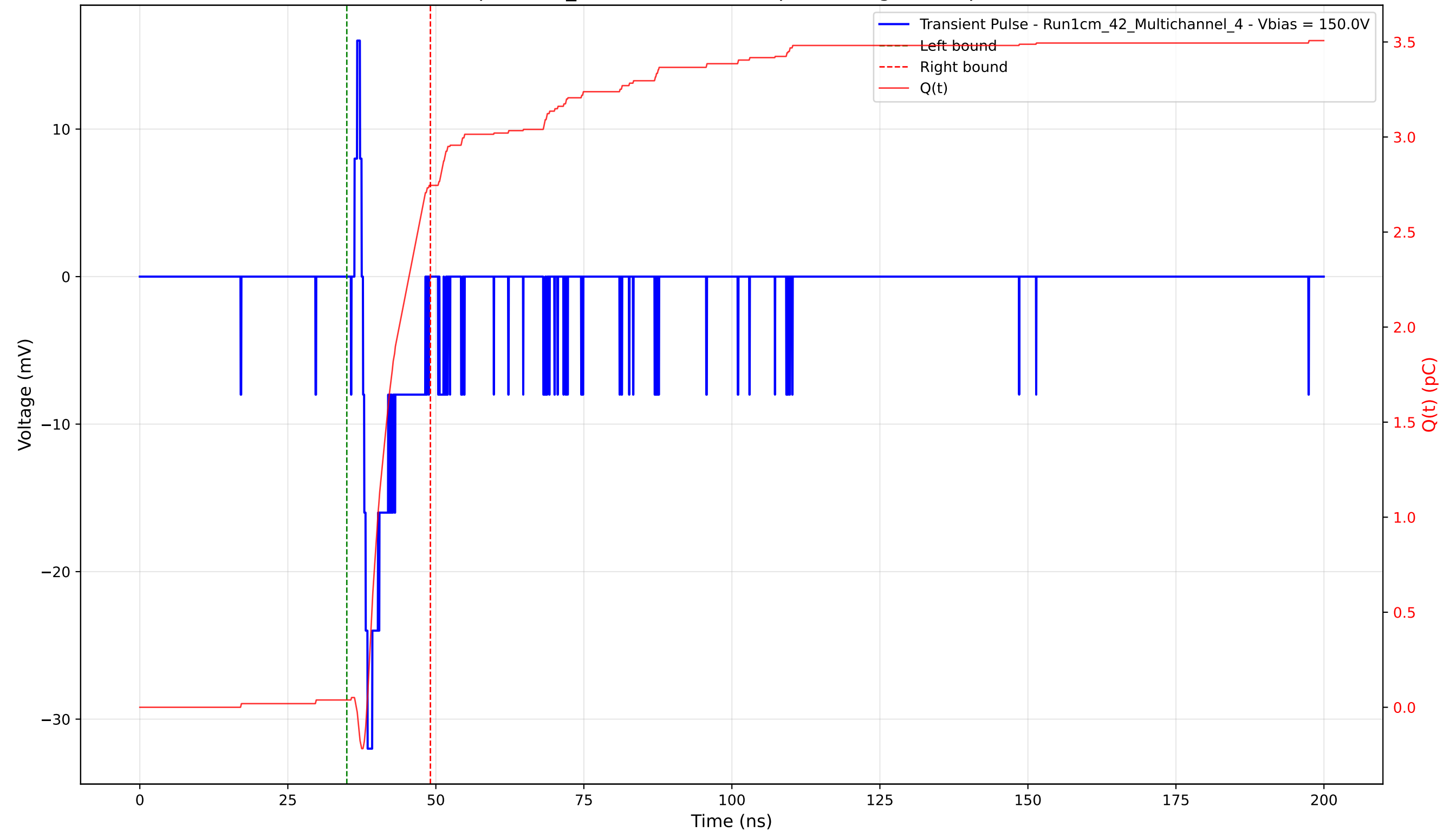
Transient Pulse - Sample: 1cm_42 - Position: 405.0 \mu\text{m} - Charge: 2.71 pC - Rise Time: 0.78 ns
