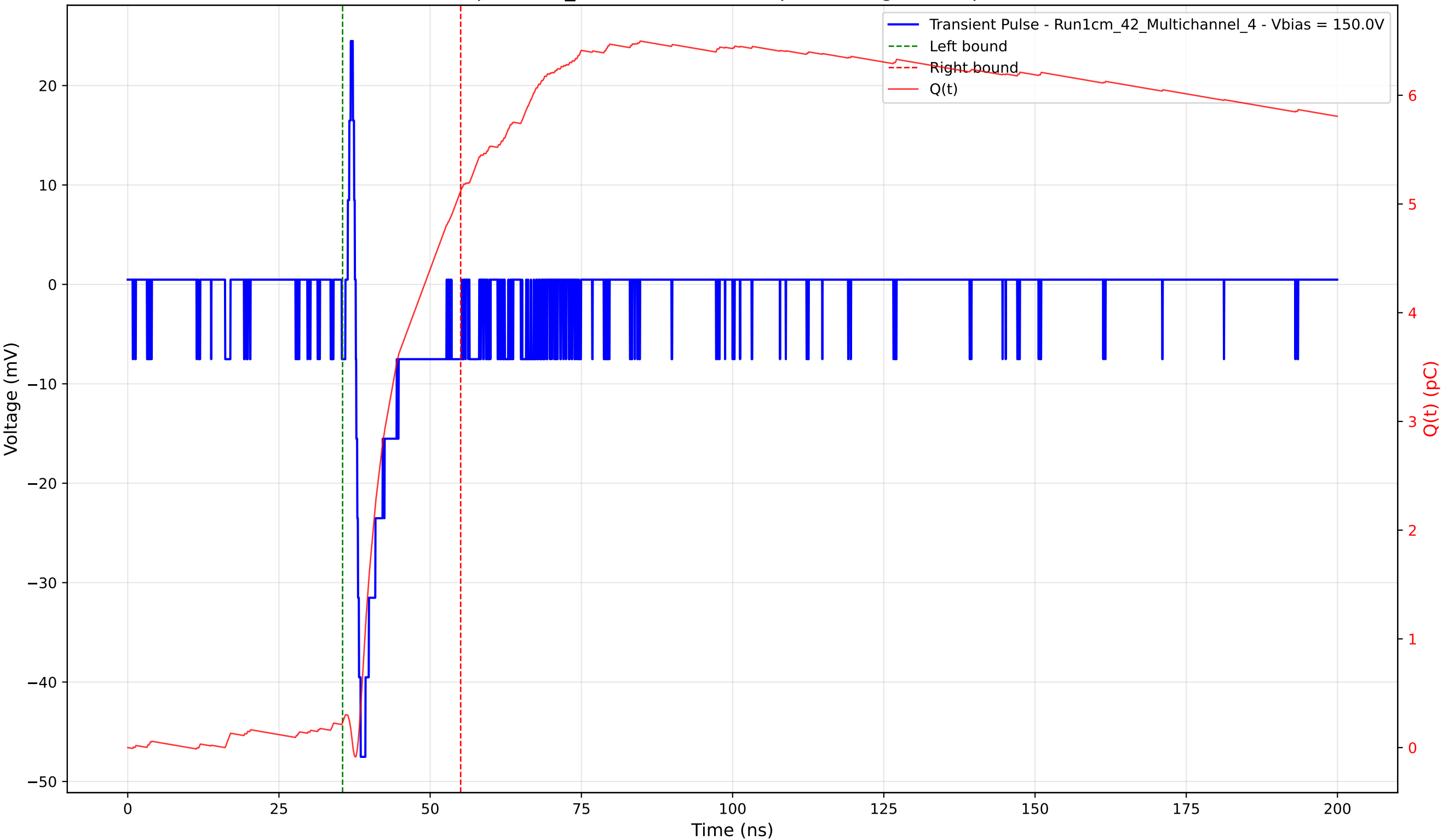
Transient Pulse - Sample: 1cm_42 - Position: 890.0 \mu\text{m} - Charge: 4.89 pC - Rise Time: 0.82 ns
