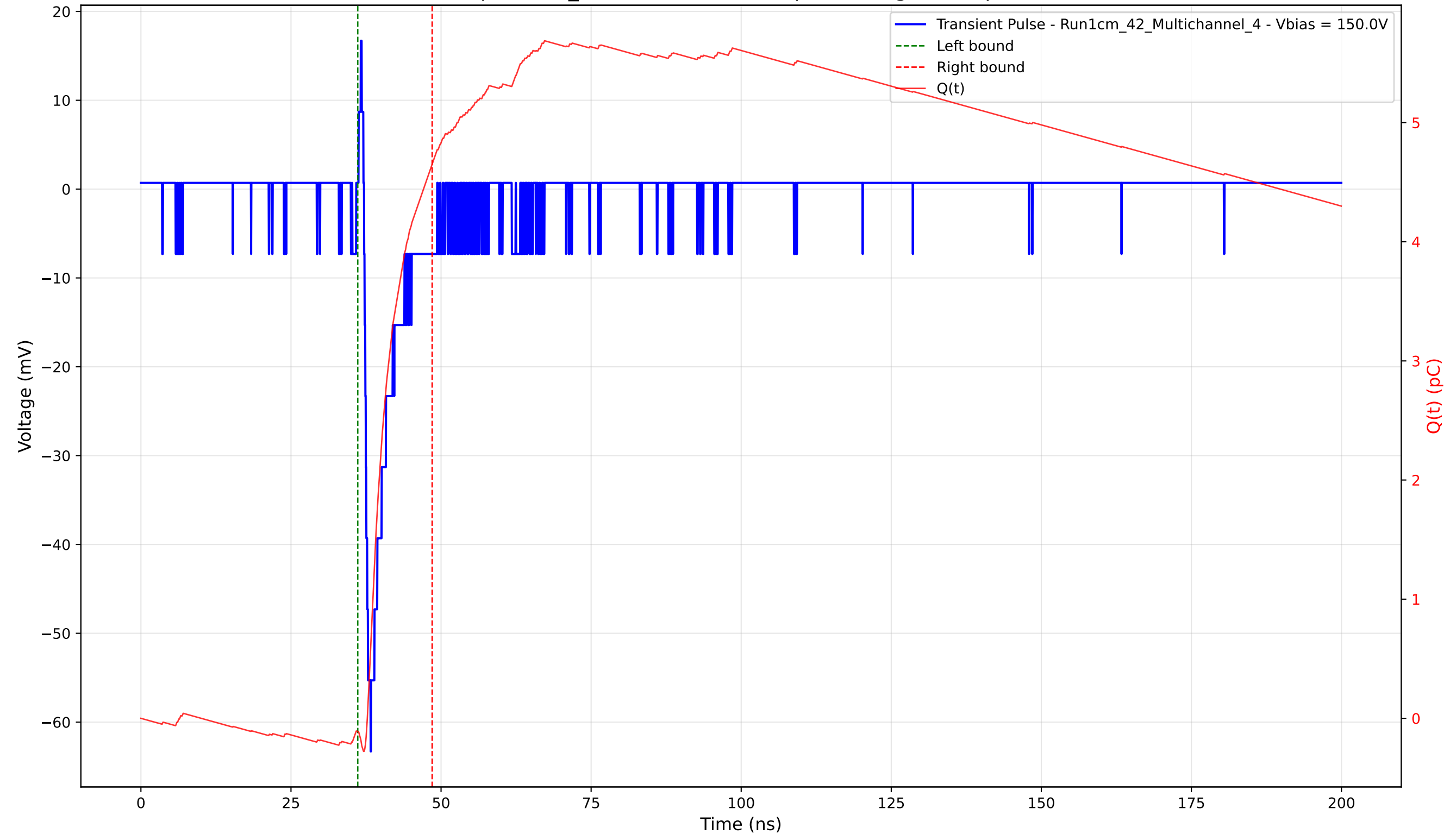
Transient Pulse - Sample: 1cm_42 - Position: 3670.0 \mu\text{m} - Charge: 4.76 pC - Rise Time: 1.09 ns
