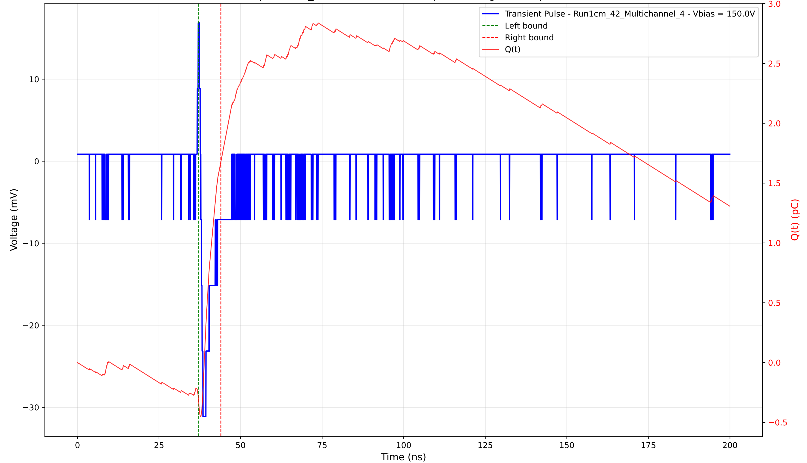
Transient Pulse - Sample: 1cm_42 - Position: 4845.0 \mu\text{m} - Charge: 2.01 pC - Rise Time: 0.67 ns
