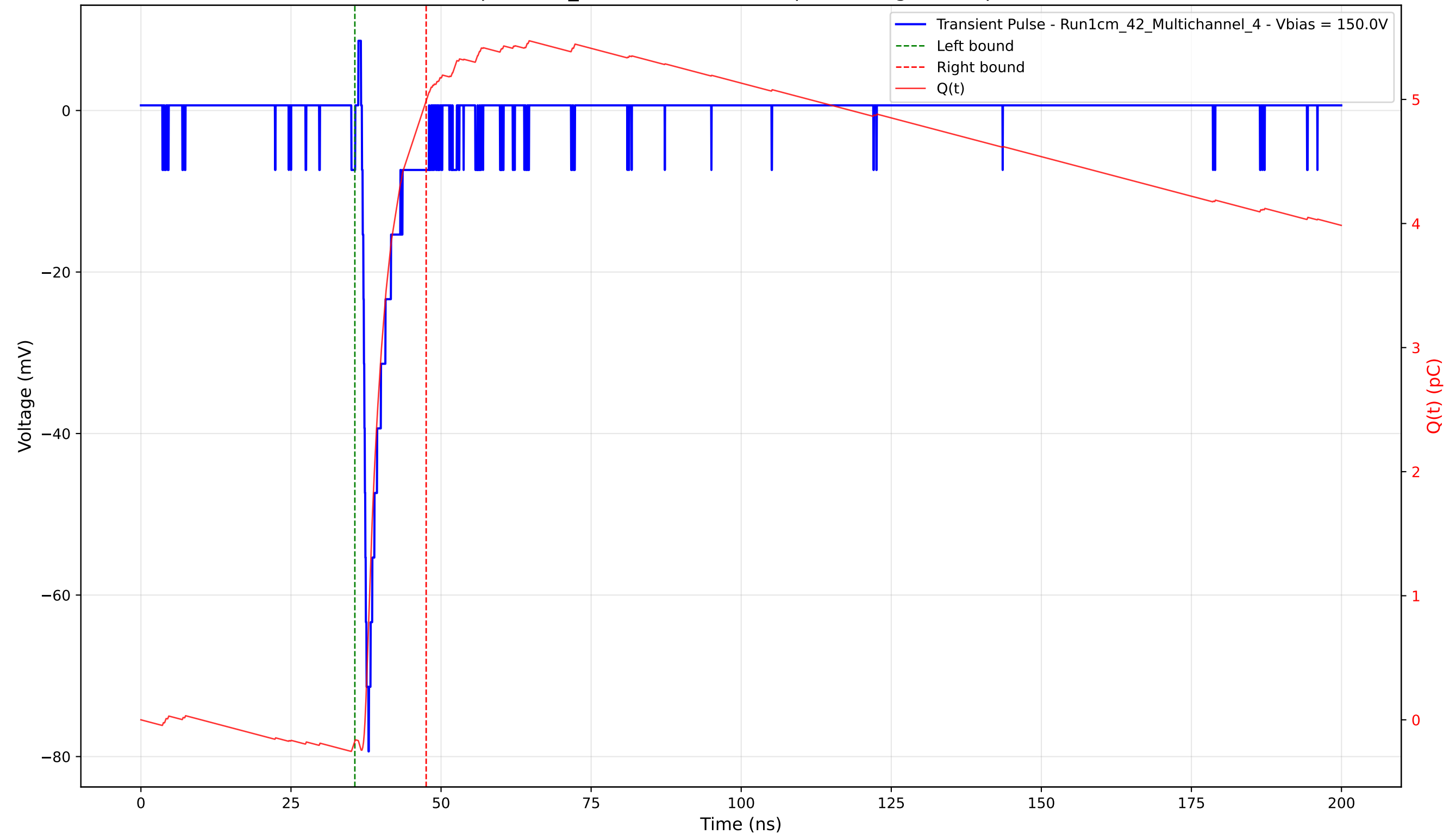
Transient Pulse - Sample: 1cm_42 - Position: 3505.0 \mu\text{m} - Charge: 5.16 pC - Rise Time: 1.00 ns
