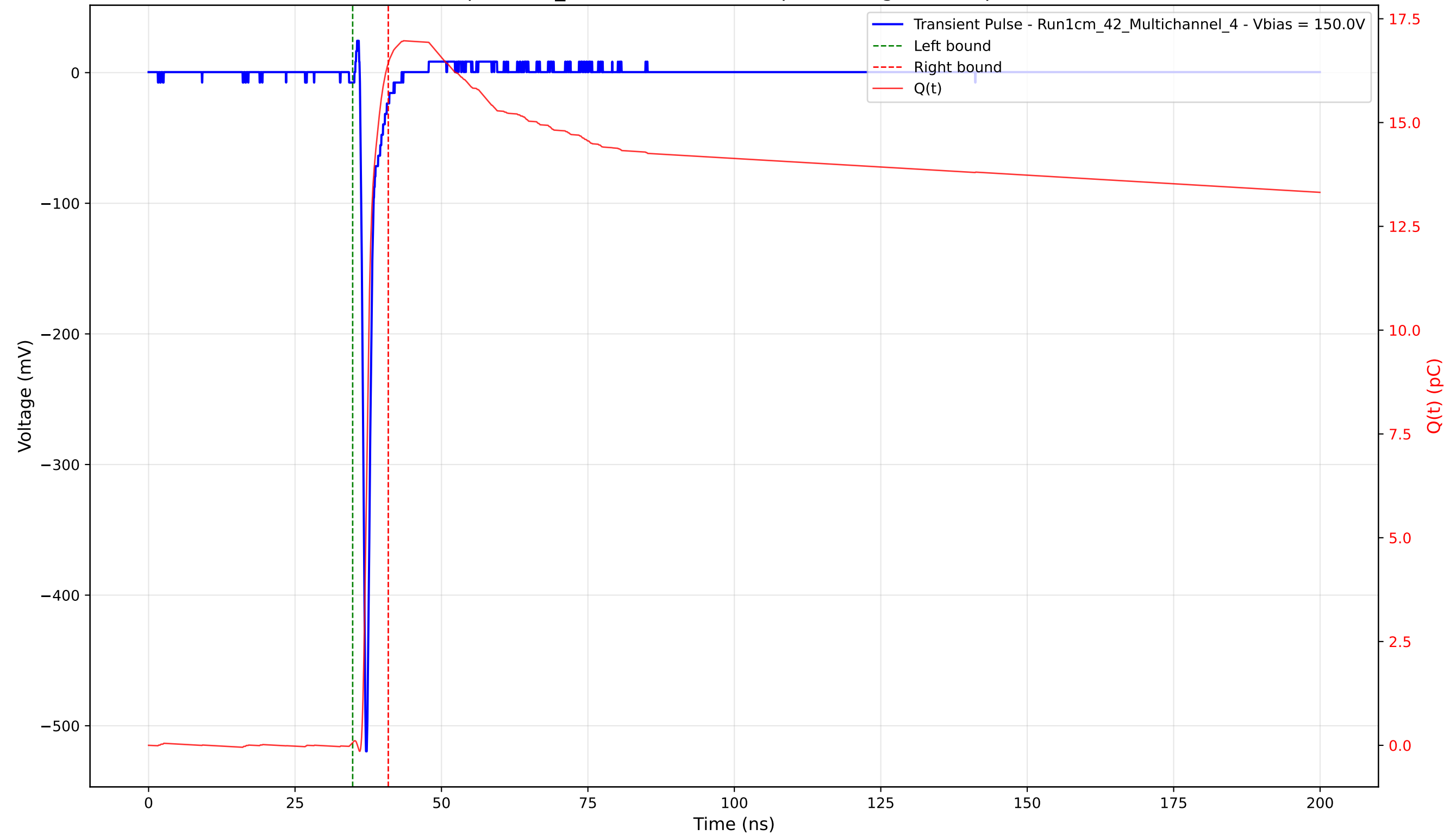
Transient Pulse - Sample: 1cm_42 - Position: 2350.0 \mu\text{m} - Charge: 16.37 pC - Rise Time: 0.69 ns
