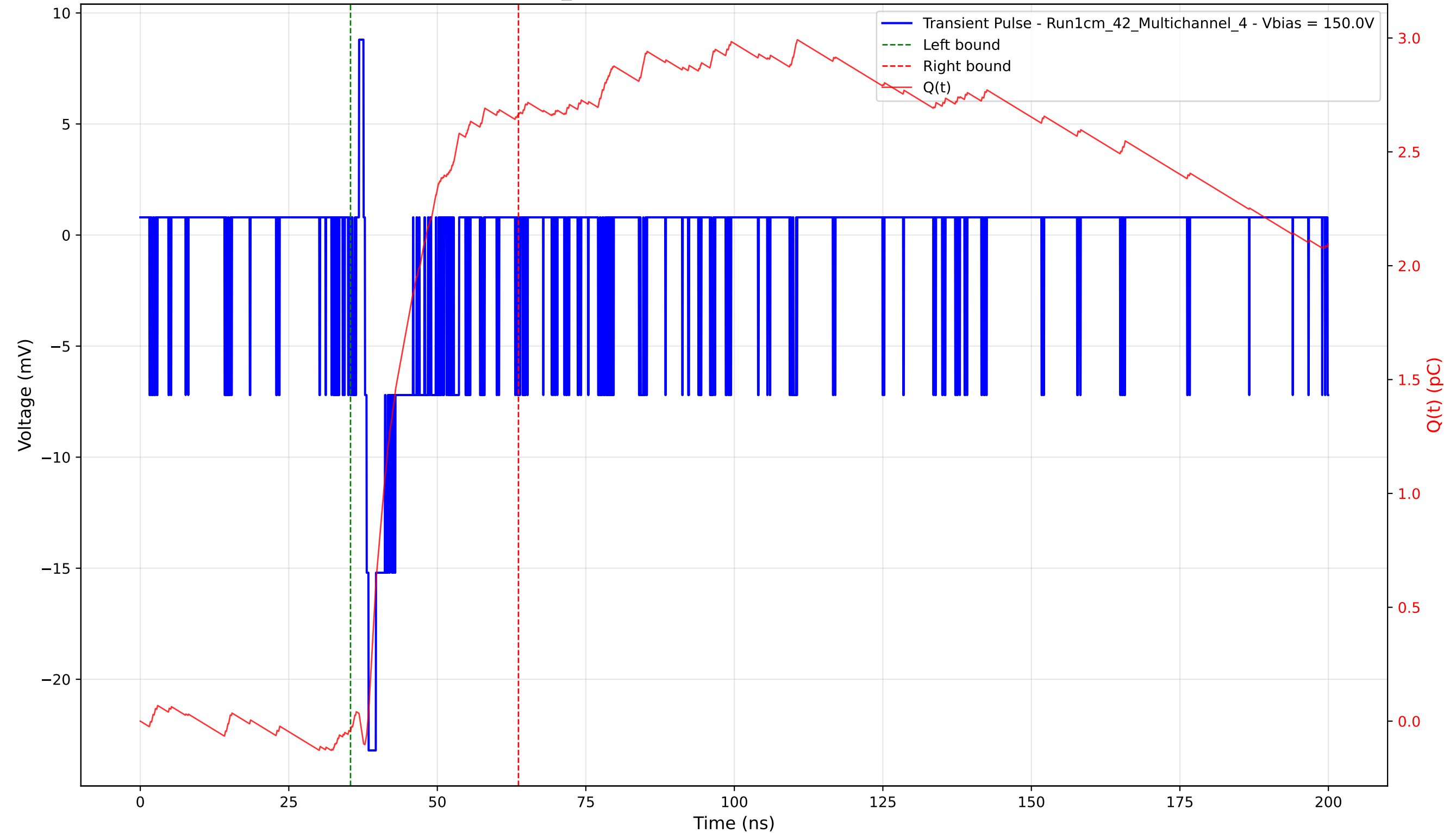
Transient Pulse - Sample: 1cm_42 - Position: 4950.0 \mu\text{m} - Charge: 2.70 pC - Rise Time: 0.63 ns
