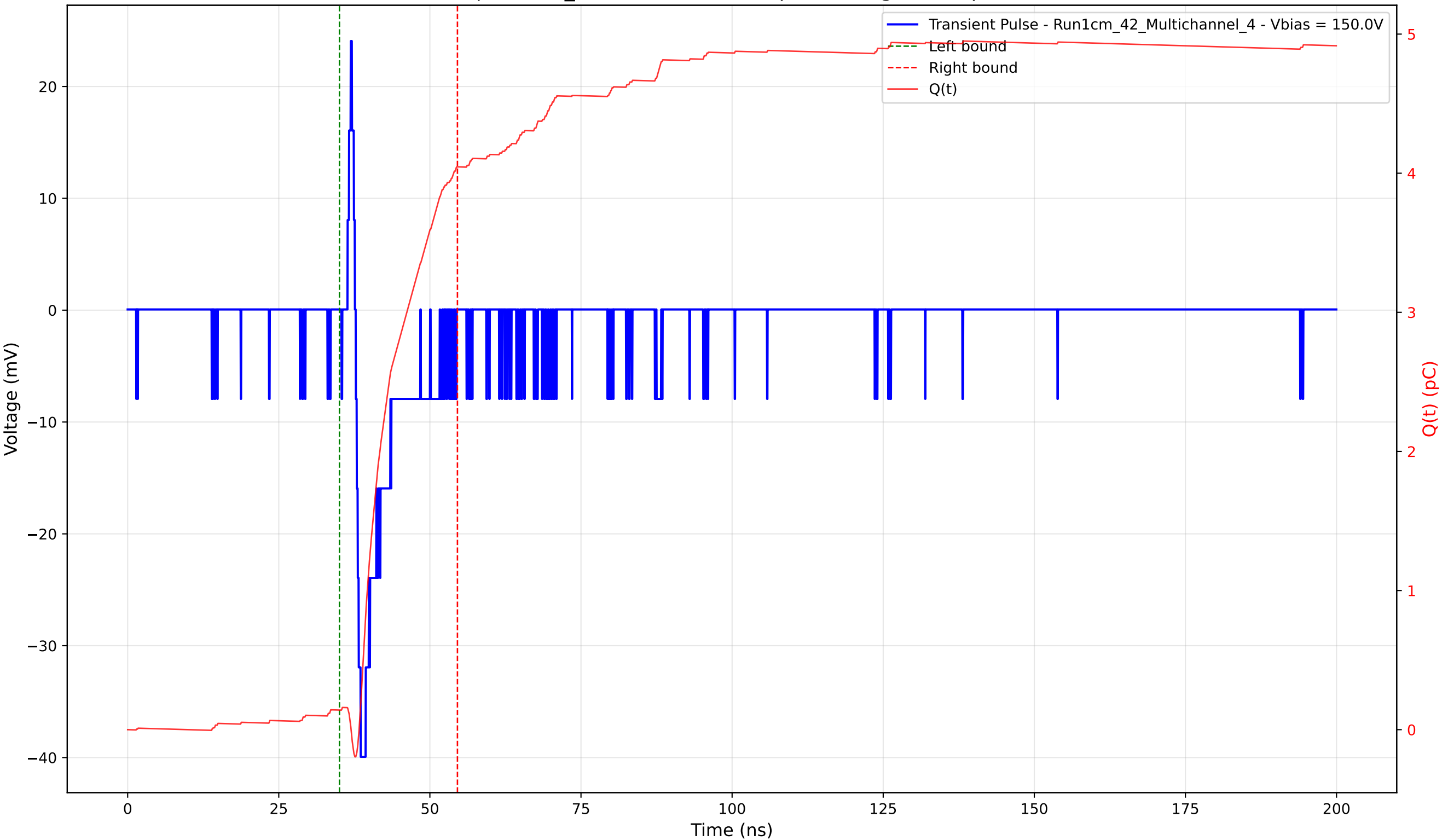
Transient Pulse - Sample: 1cm_42 - Position: 555.0 \mu\text{m} - Charge: 3.90 pC - Rise Time: 0.82 ns
