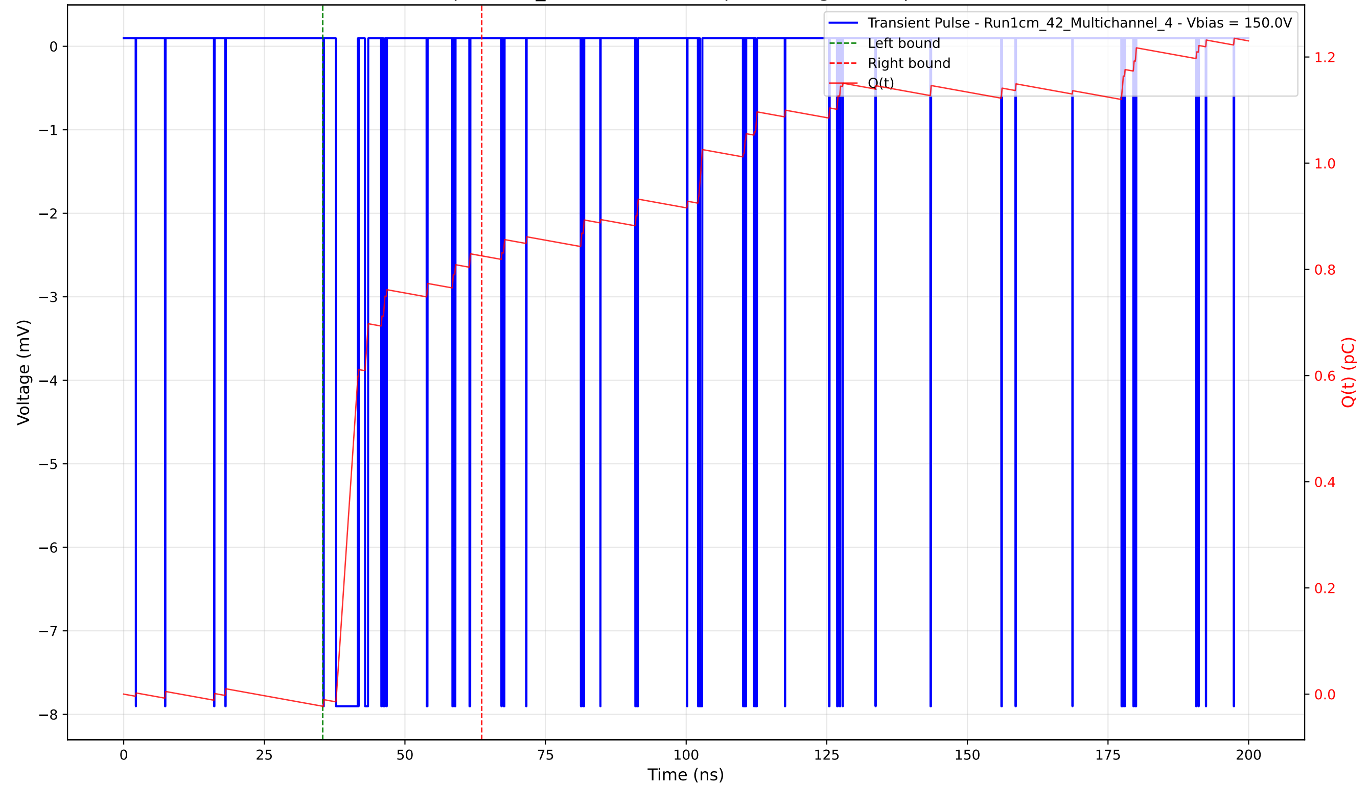
Transient Pulse - Sample: 1cm_42 - Position: 55.0 \mu\text{m} - Charge: 0.85 pC - Rise Time: 0.04 ns
