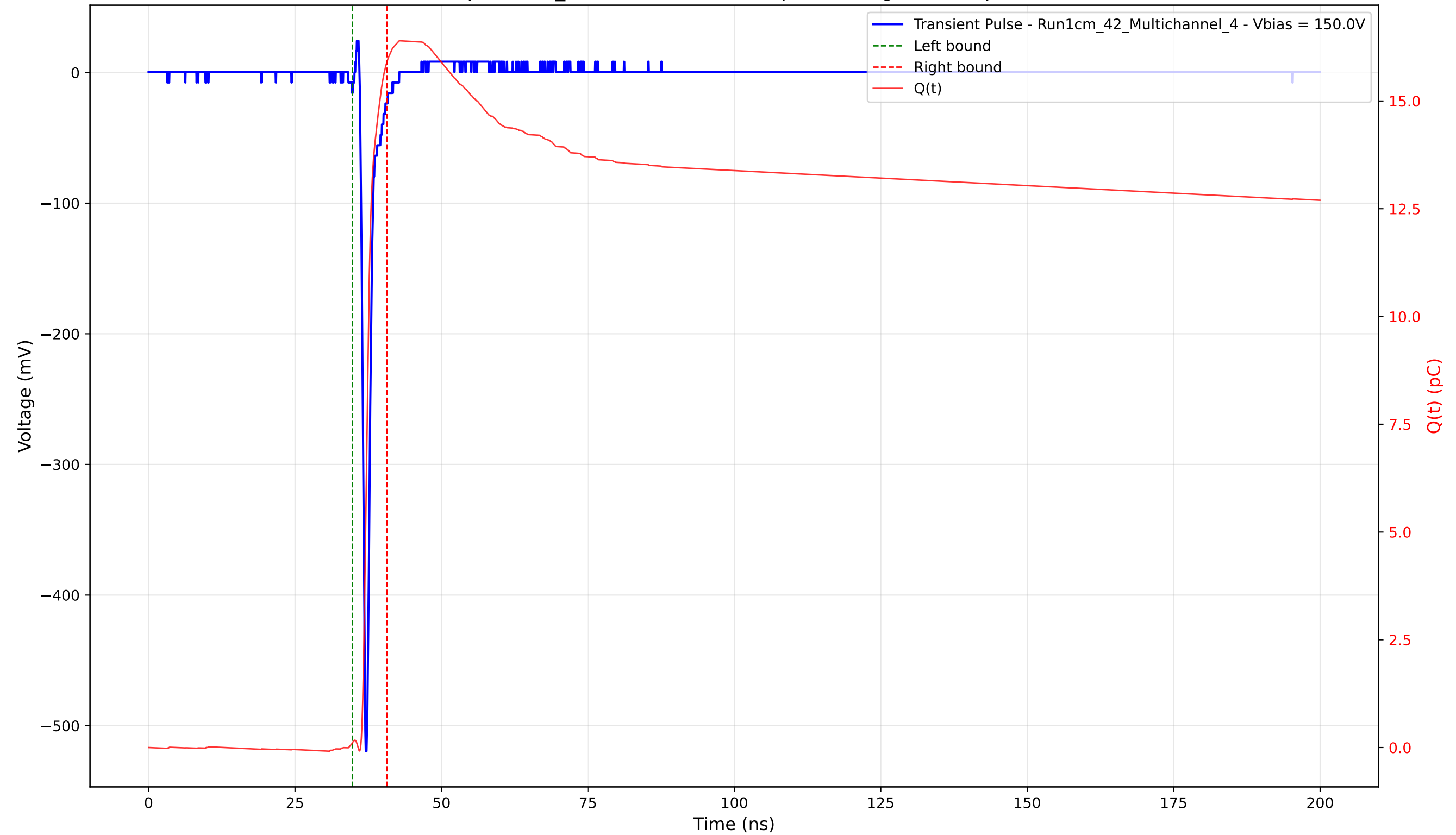
Transient Pulse - Sample: 1cm_42 - Position: 2560.0 \mu\text{m} - Charge: 15.80 pC - Rise Time: 0.72 ns
