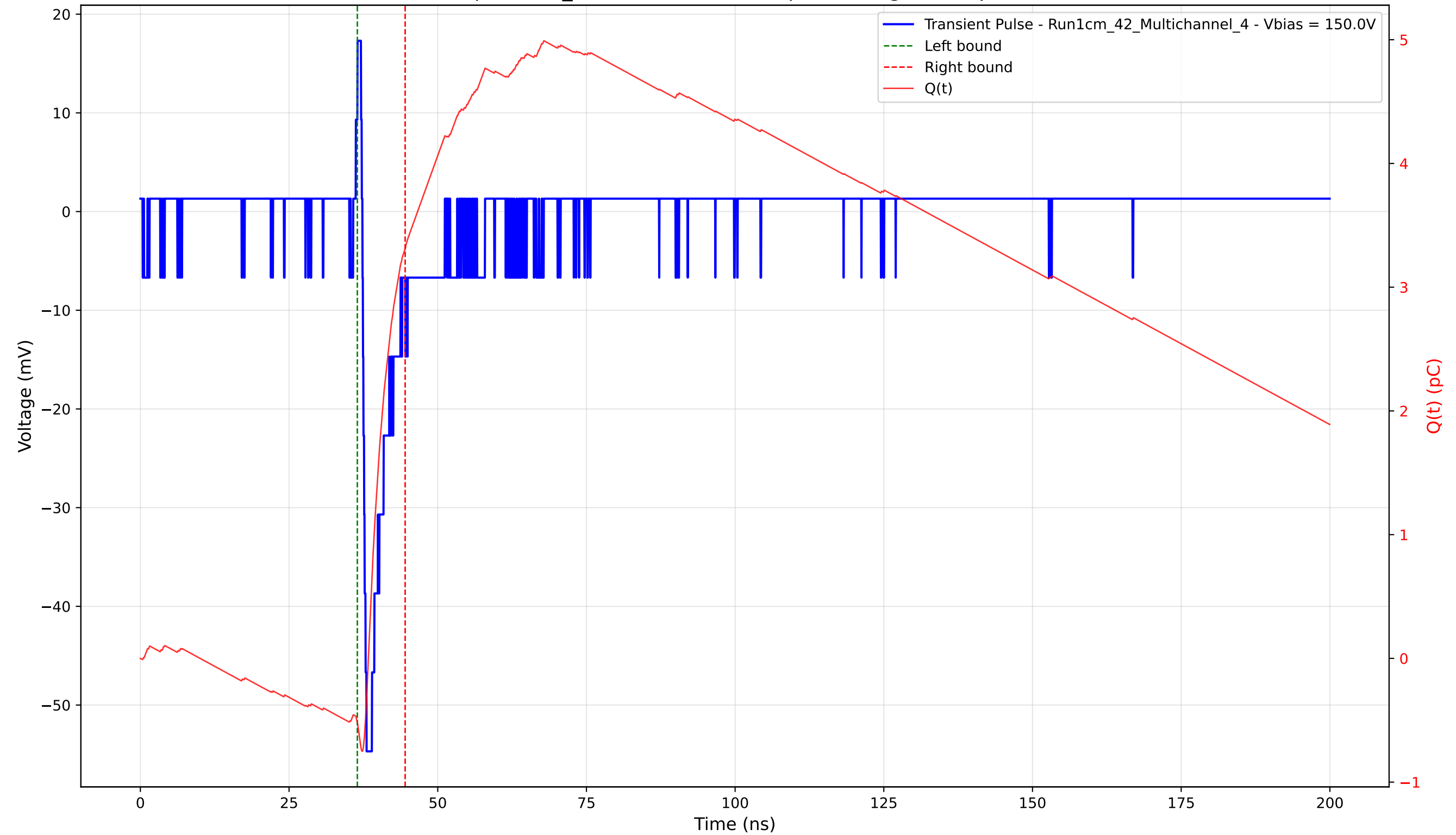
Transient Pulse - Sample: 1cm_42 - Position: 3820.0 \mu\text{m} - Charge: 3.82 pC - Rise Time: 0.69 ns
