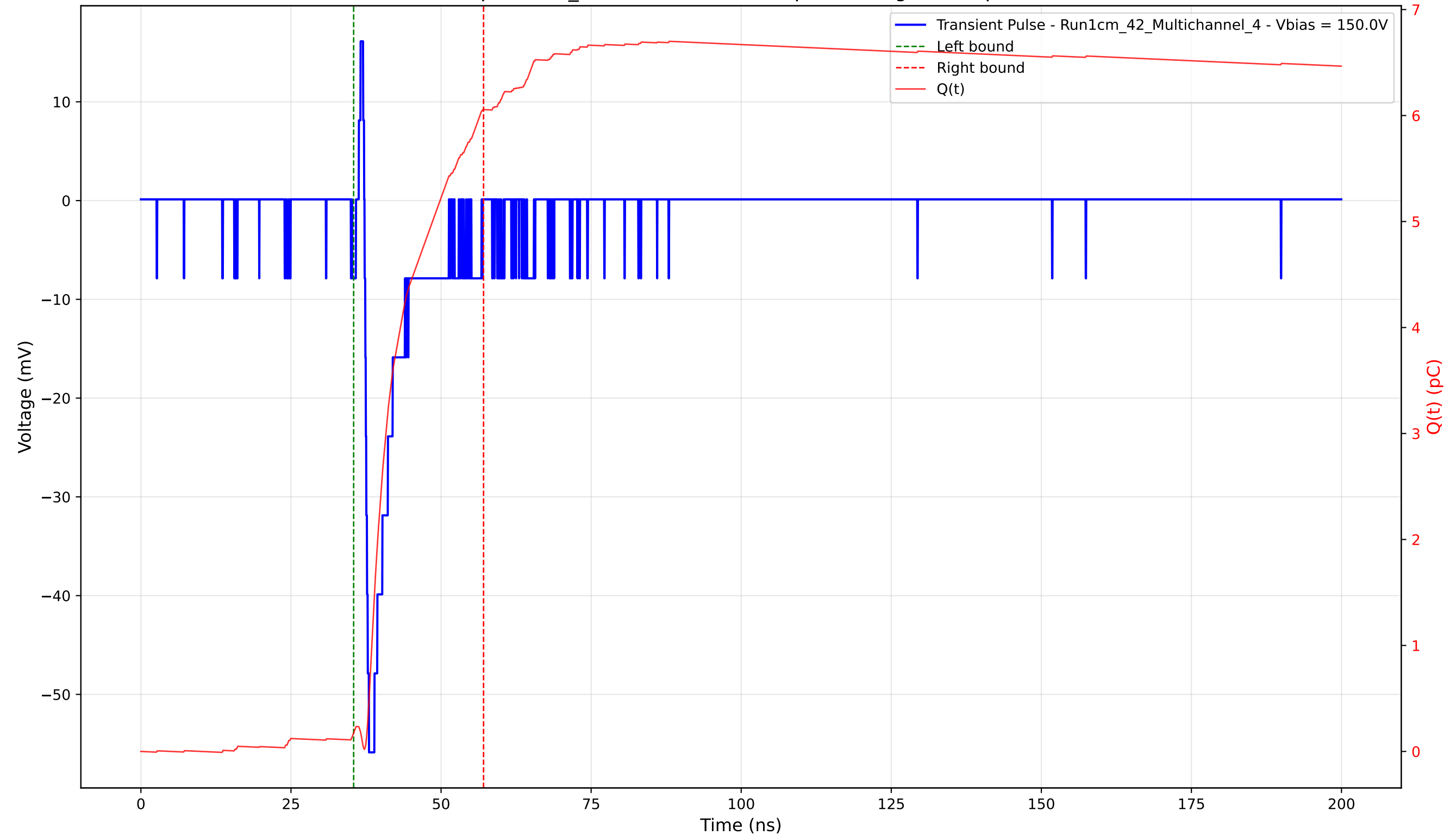
Transient Pulse - Sample: 1cm_42 - Position: 3735.0 \mu\text{m} - Charge: 5.88 pC - Rise Time: 0.73 ns
