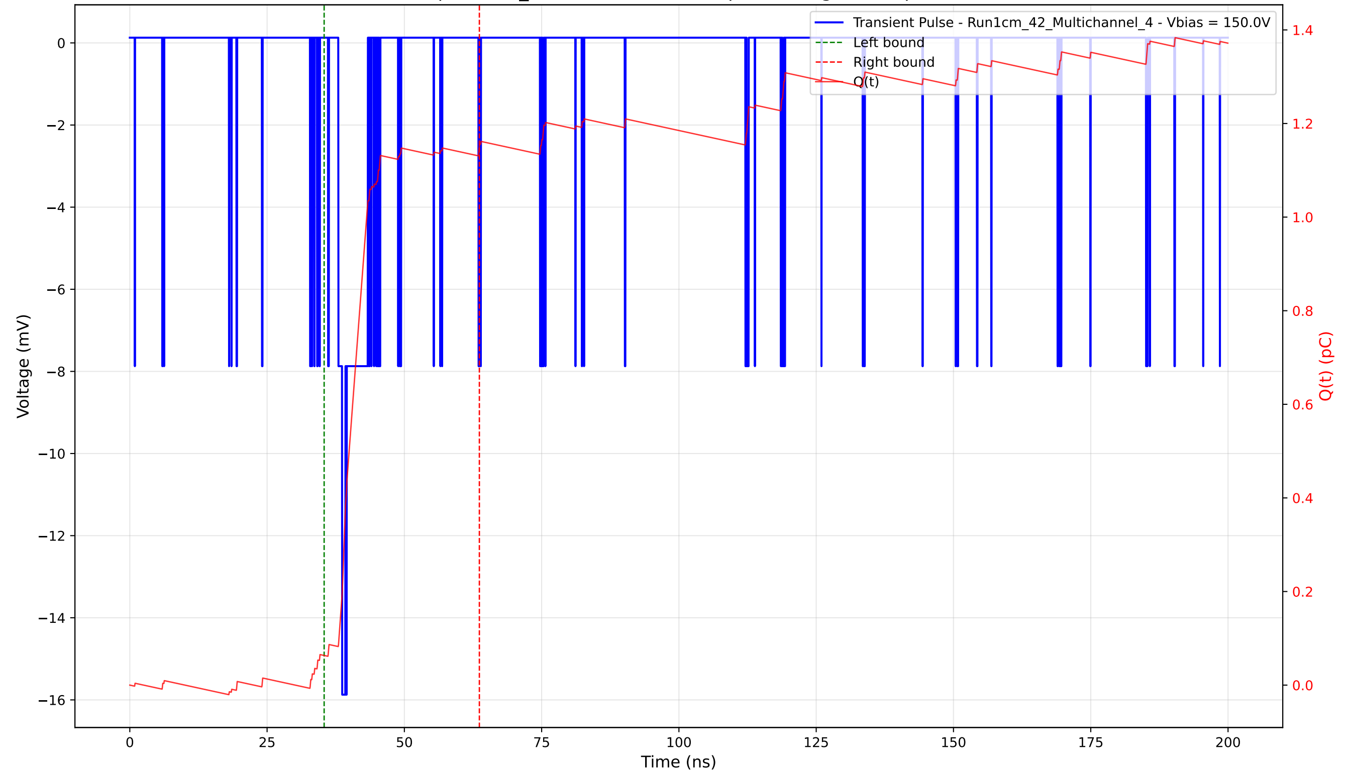
Transient Pulse - Sample: 1cm_42 - Position: 5070.0 \mu\text{m} - Charge: 1.09 pC - Rise Time: 0.71 ns
