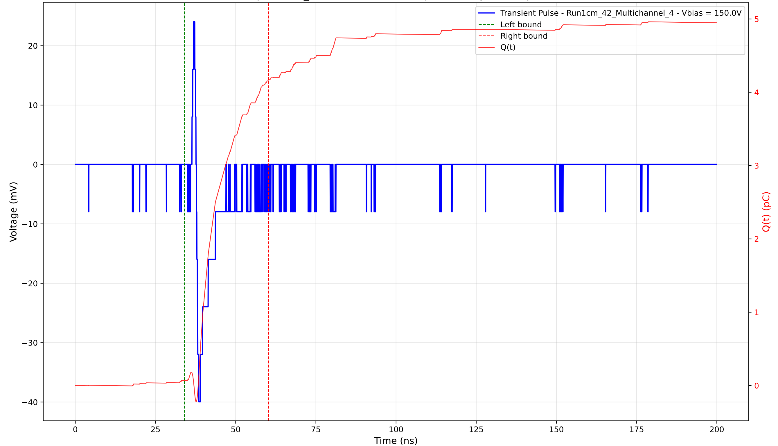
Transient Pulse - Sample: 1cm_42 - Position: 4370.0 \mu\text{m} - Charge: 4.10 pC - Rise Time: 0.78 ns
