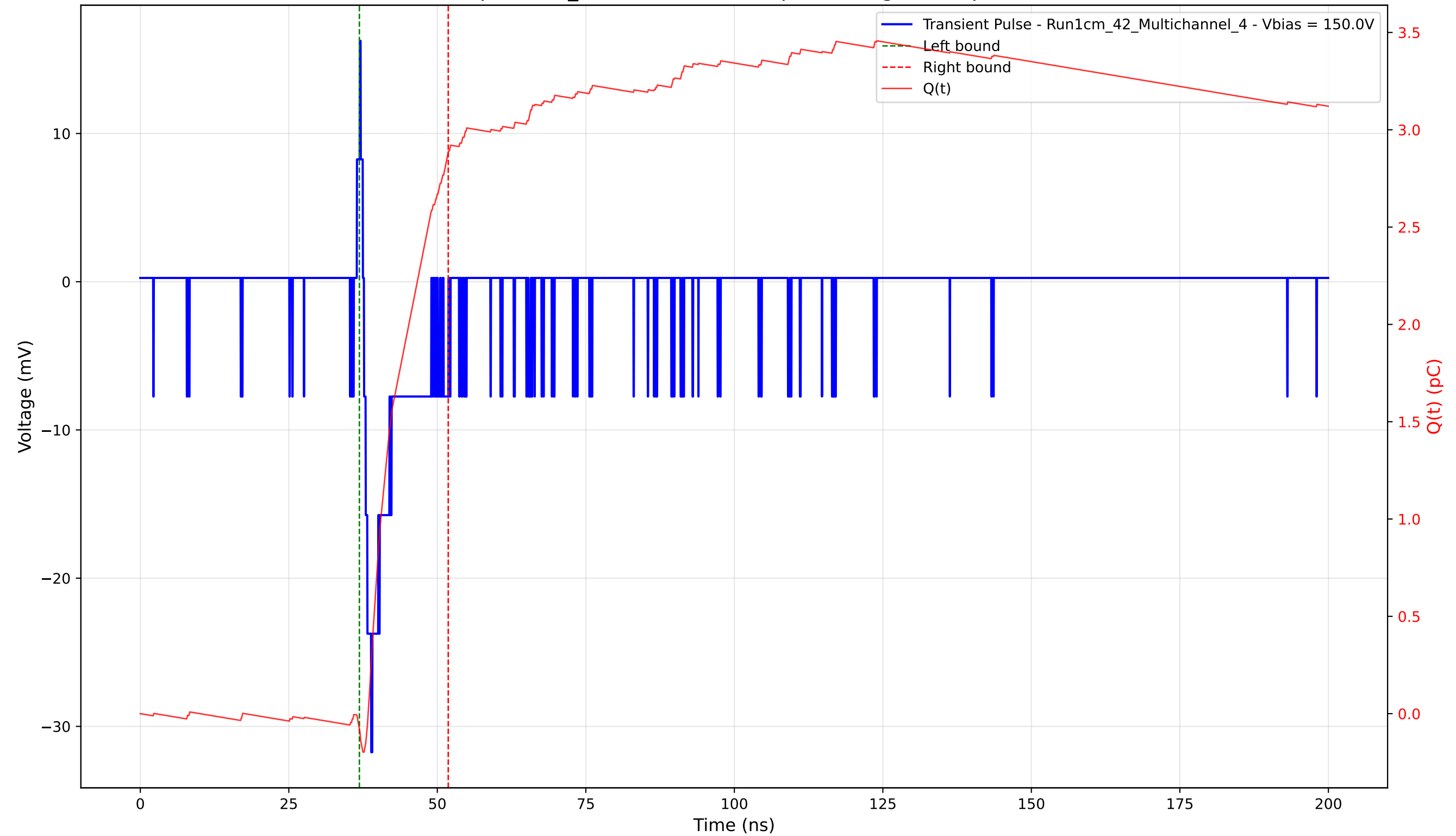
Transient Pulse - Sample: 1cm_42 - Position: 365.0 \mu\text{m} - Charge: 2.96 pC - Rise Time: 1.22 ns
