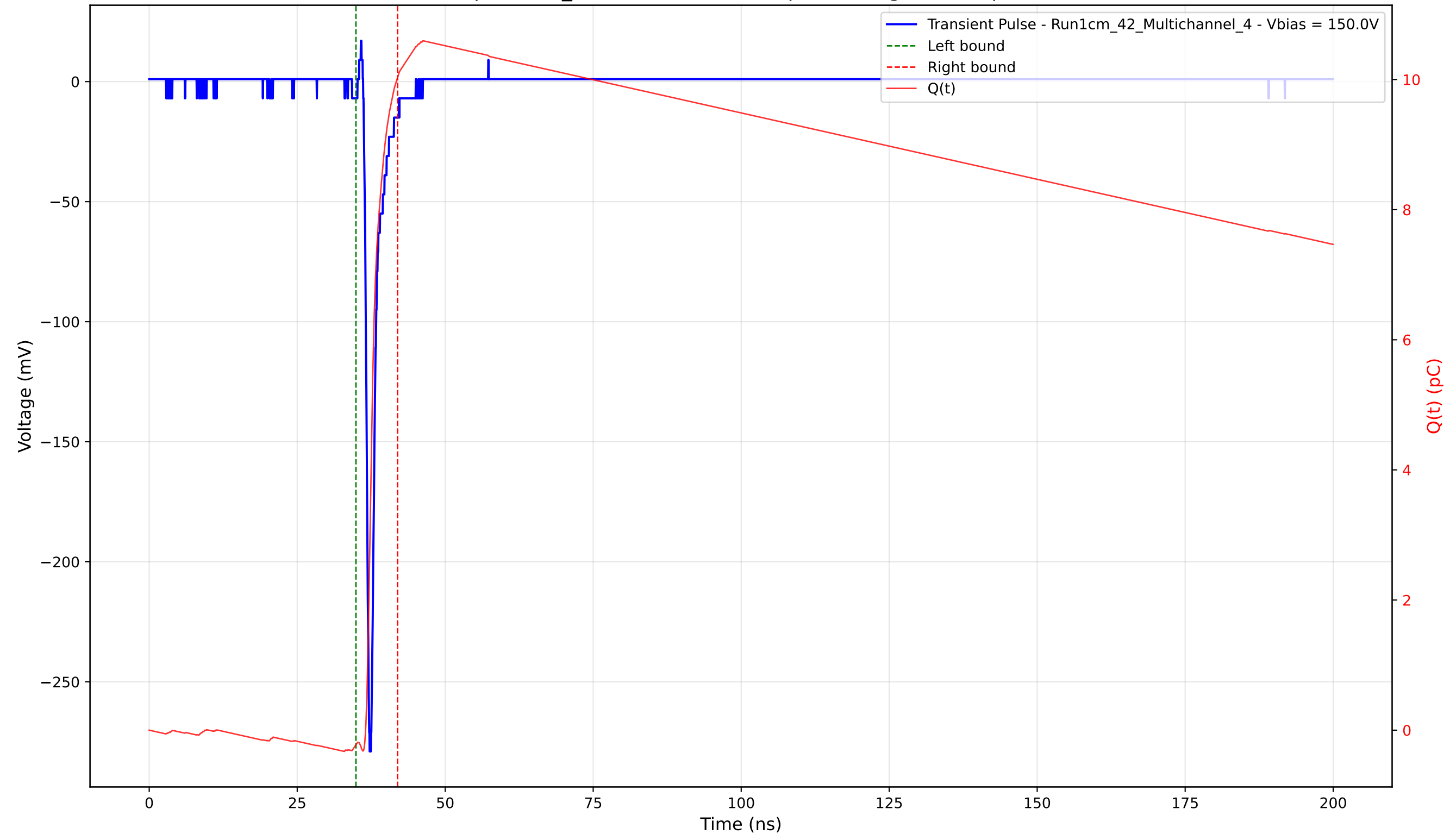
Transient Pulse - Sample: 1cm_42 - Position: 2955.0 \mu\text{m} - Charge: 10.26 pC - Rise Time: 0.76 ns
