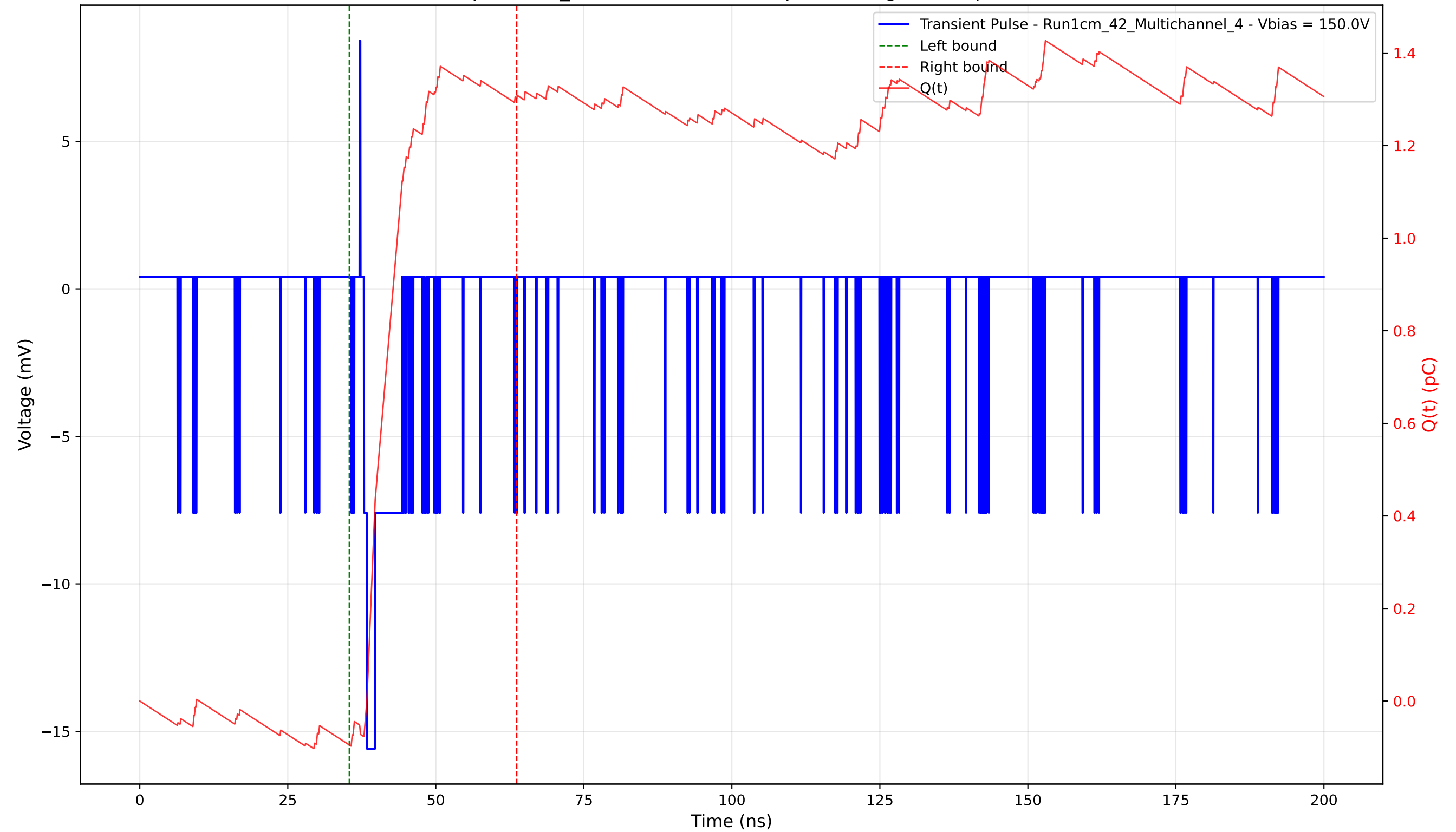
Transient Pulse - Sample: 1cm_42 - Position: 5040.0 \mu\text{m} - Charge: 1.40 pC - Rise Time: 0.51 ns
