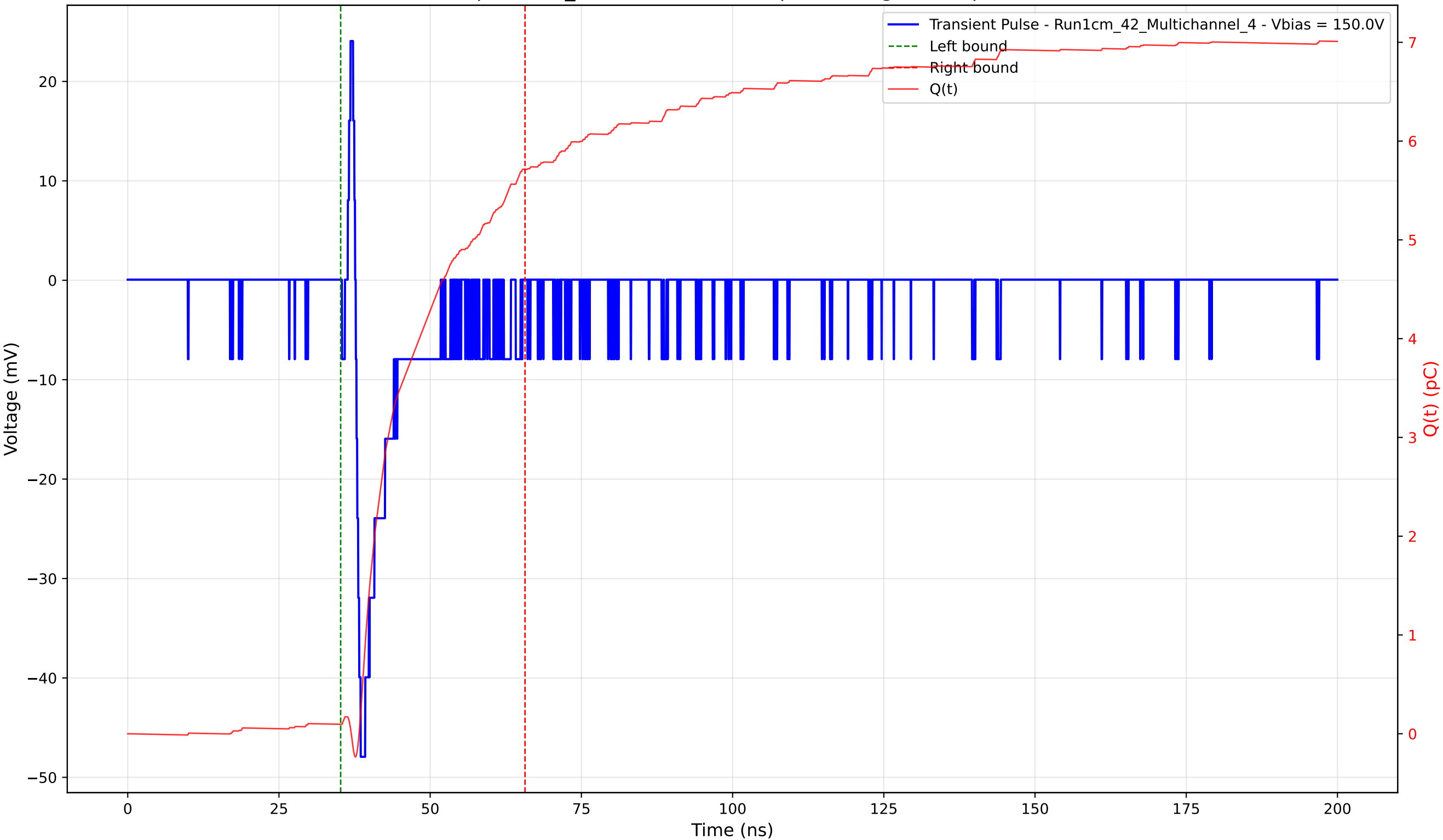
Transient Pulse - Sample: 1cm_42 - Position: 845.0 \mu\text{m} - Charge: 5.62 pC - Rise Time: 0.82 ns
