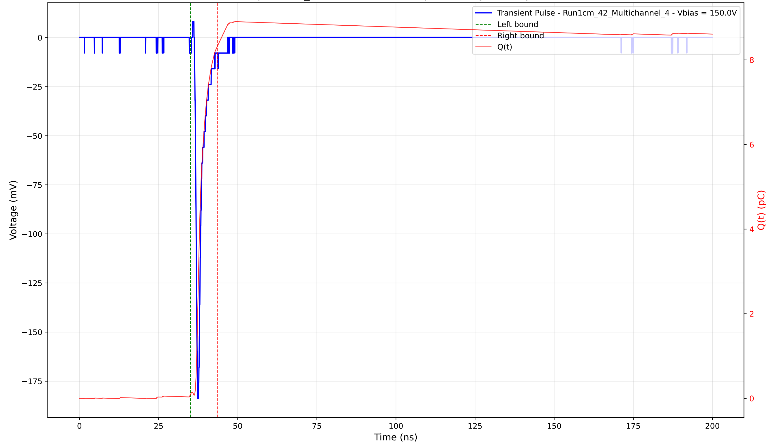
Transient Pulse - Sample: 1cm_42 - Position: 3090.0 \mu\text{m} - Charge: 8.22 pC - Rise Time: 0.78 ns
