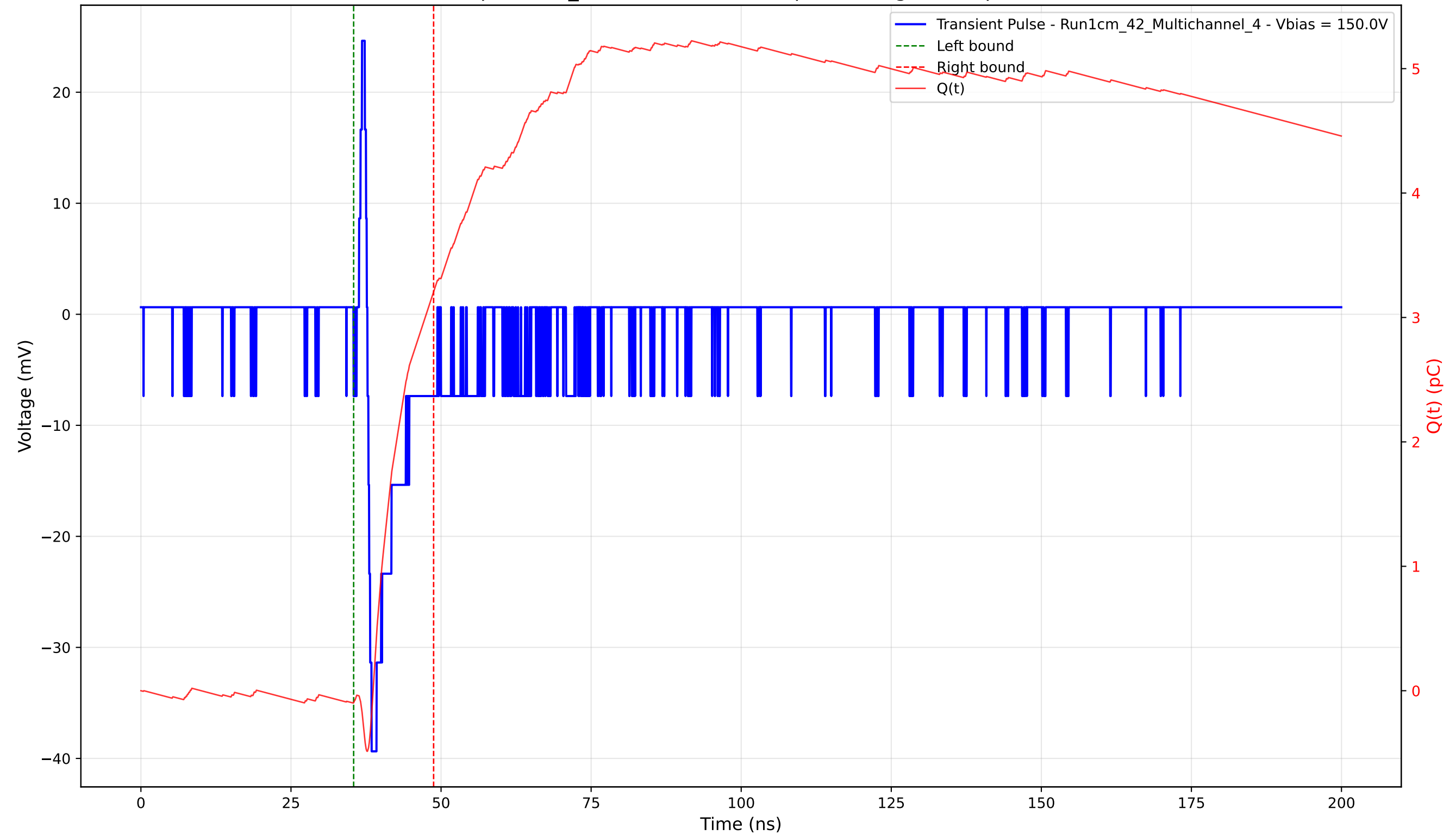
Transient Pulse - Sample: 1cm_42 - Position: 4315.0 \mu\text{m} - Charge: 3.31 pC - Rise Time: 0.70 ns
