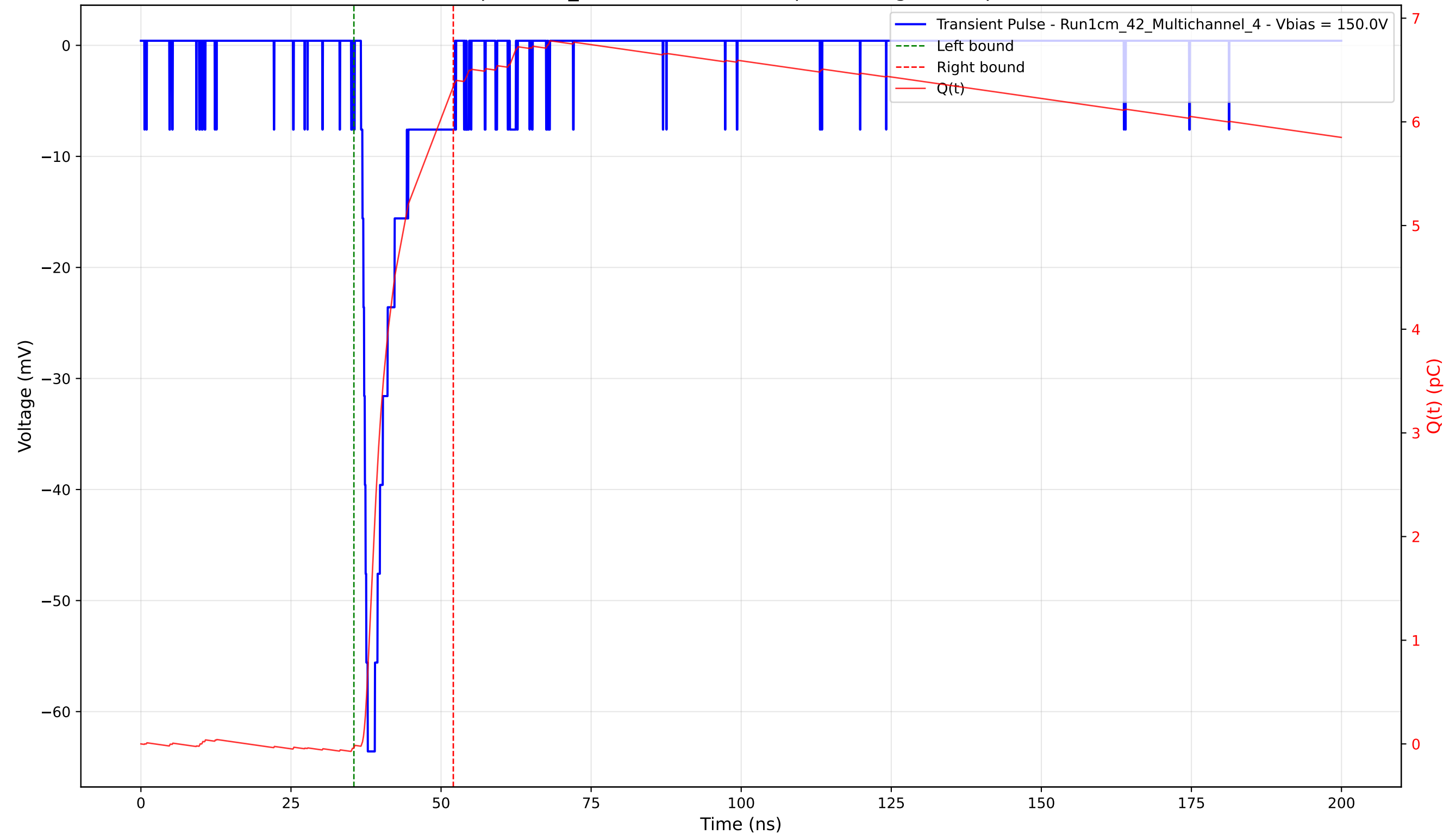
Transient Pulse - Sample: 1cm_42 - Position: 1465.0 \mu\text{m} - Charge: 6.38 pC - Rise Time: 1.13 ns
