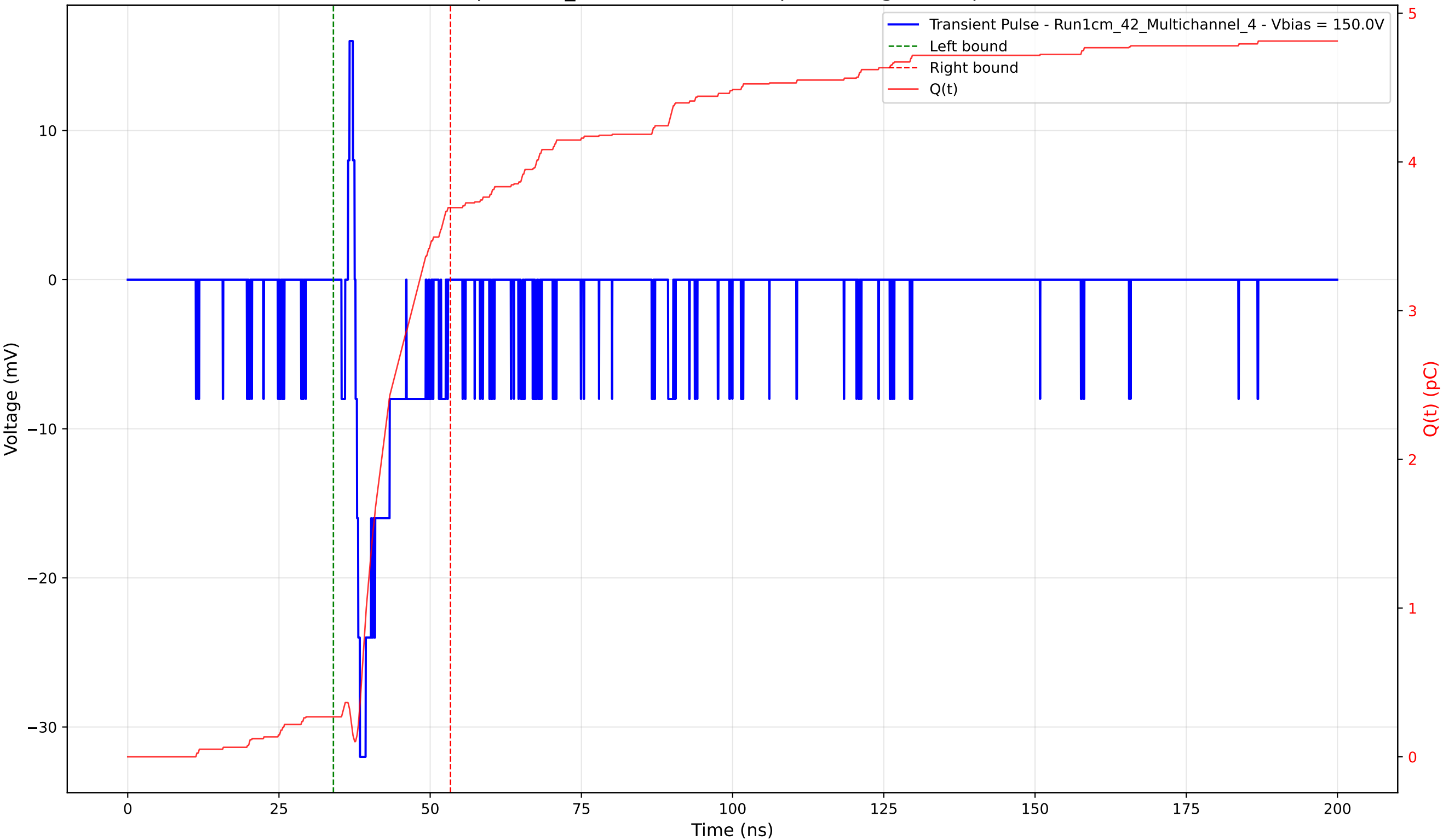
Transient Pulse - Sample: 1cm_42 - Position: 425.0 \mu\text{m} - Charge: 3.42 pC - Rise Time: 0.74 ns
