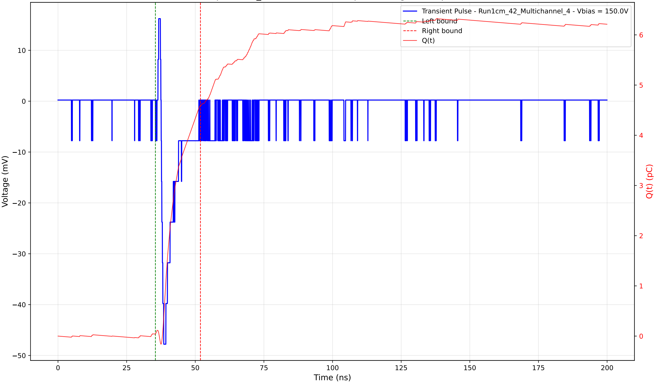
Transient Pulse - Sample: 1cm_42 - Position: 985.0 \mu\text{m} - Charge: 4.54 pC - Rise Time: 0.94 ns
