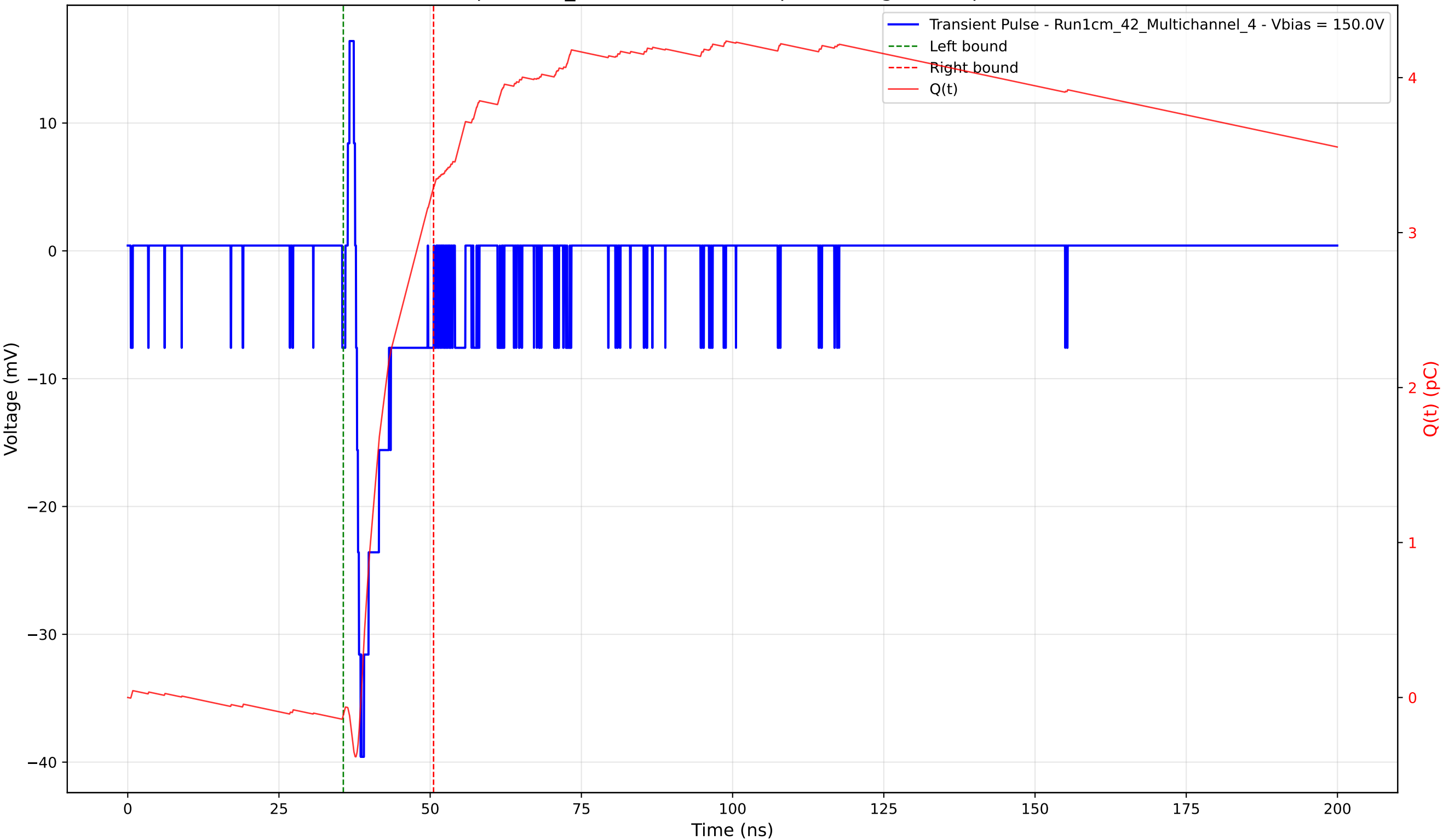
Transient Pulse - Sample: 1cm_42 - Position: 515.0 \mu\text{m} - Charge: 3.41 pC - Rise Time: 0.78 ns
