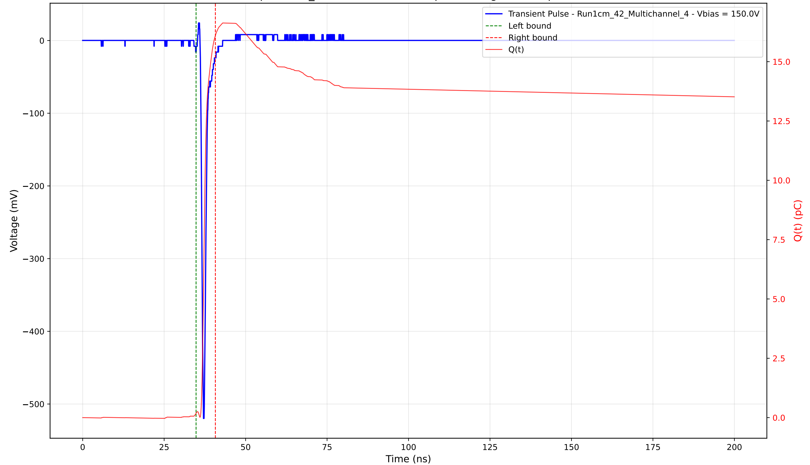
Transient Pulse - Sample: 1cm_42 - Position: 2555.0 \mu\text{m} - Charge: 15.91 pC - Rise Time: 0.72 ns
