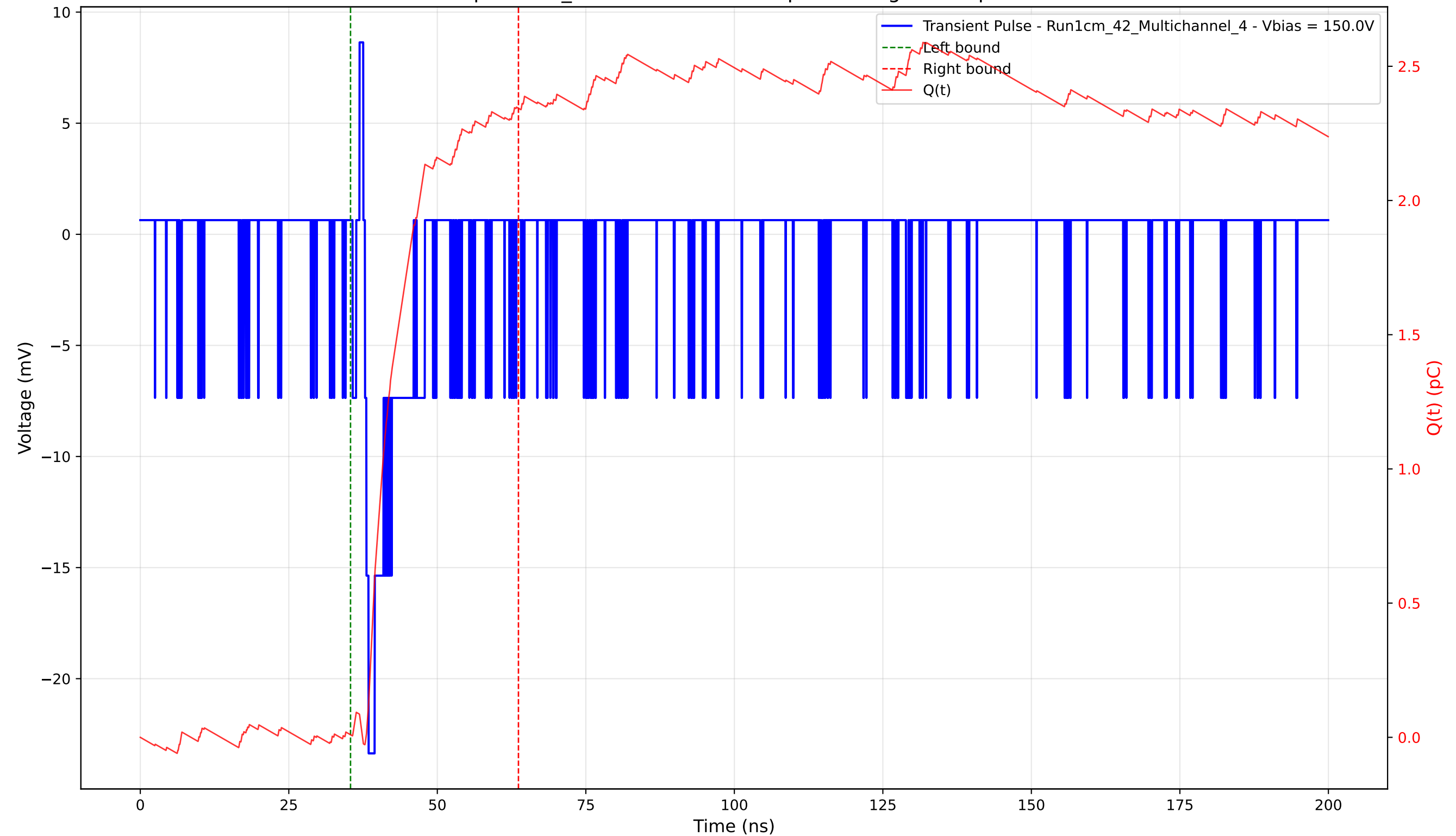
Transient Pulse - Sample: 1cm_42 - Position: 4965.0 \mu\text{m} - Charge: 2.33 pC - Rise Time: 0.63 ns
