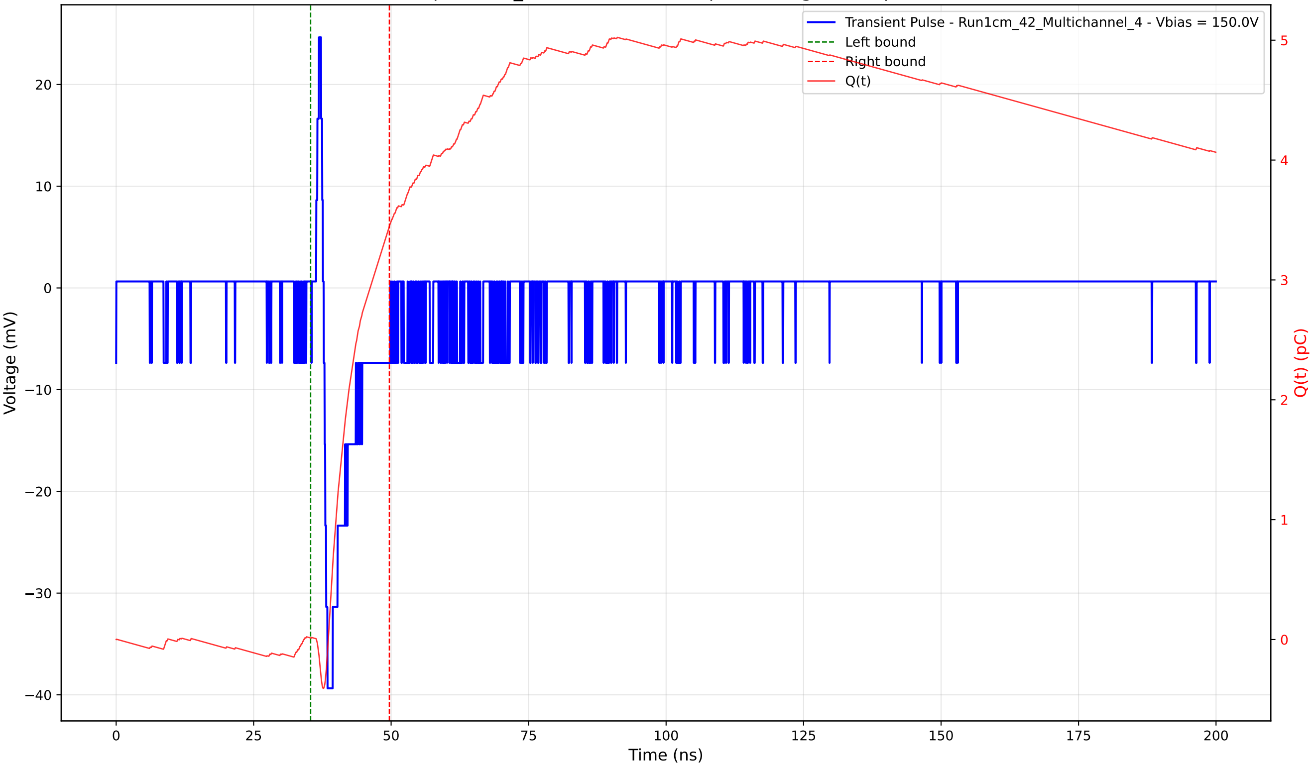
Transient Pulse - Sample: 1cm_42 - Position: 585.0 \mu\text{m} - Charge: 3.44 pC - Rise Time: 0.70 ns
