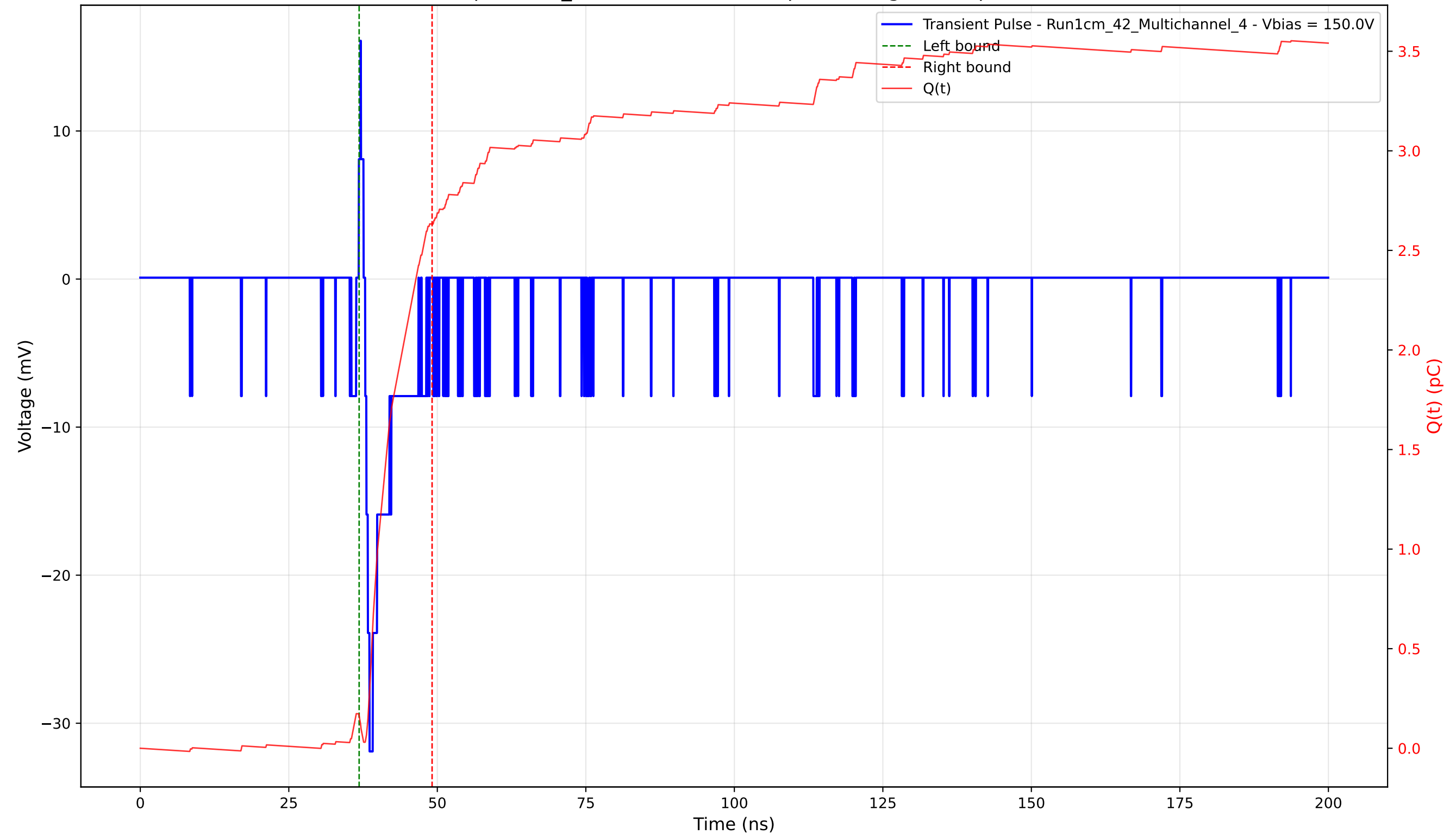
Transient Pulse - Sample: 1cm_42 - Position: 4895.0 \mu\text{m} - Charge: 2.47 pC - Rise Time: 0.74 ns
