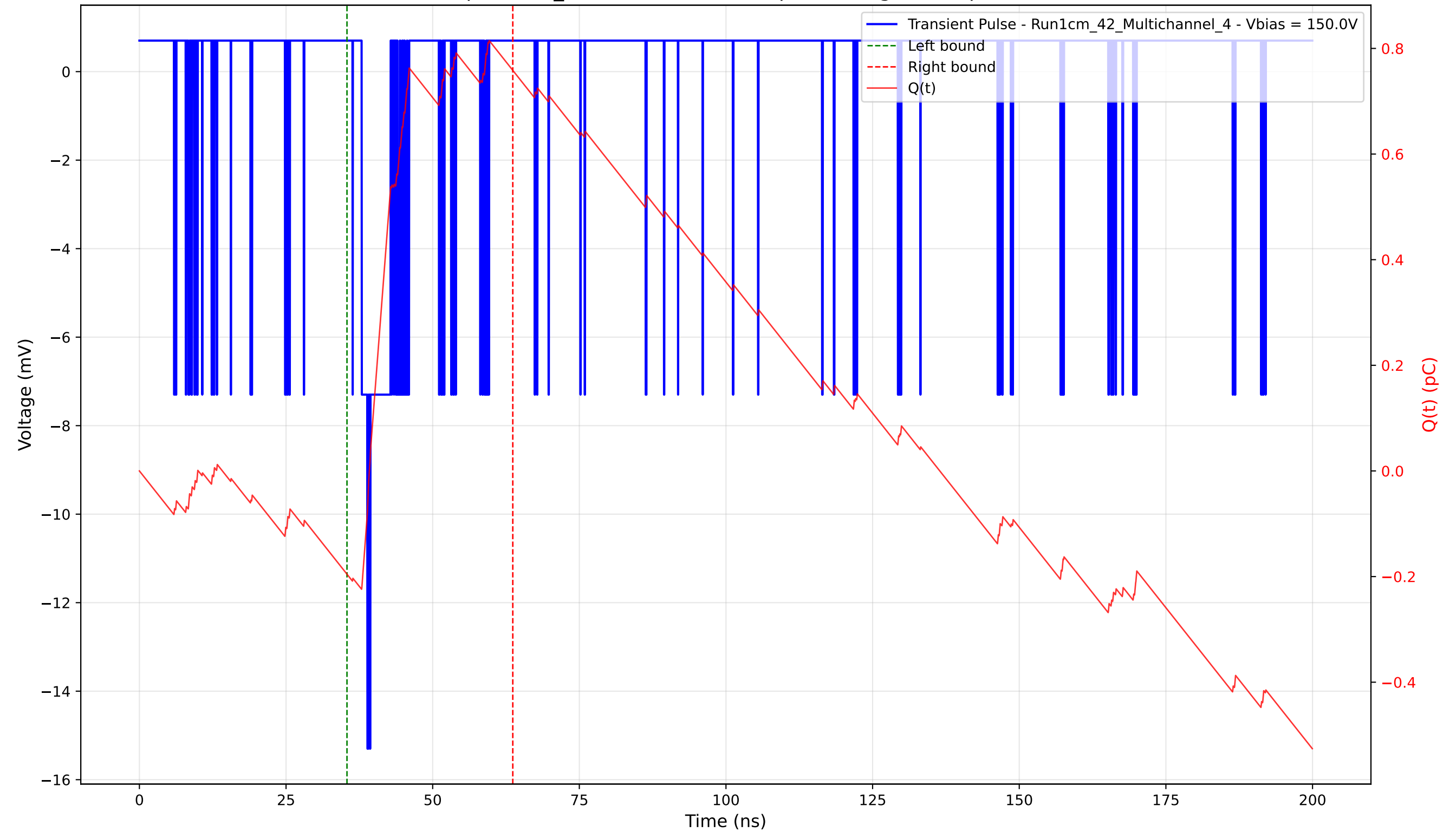
Transient Pulse - Sample: 1cm_42 - Position: 5085.0 \mu\text{m} - Charge: 0.95 pC - Rise Time: 0.99 ns
