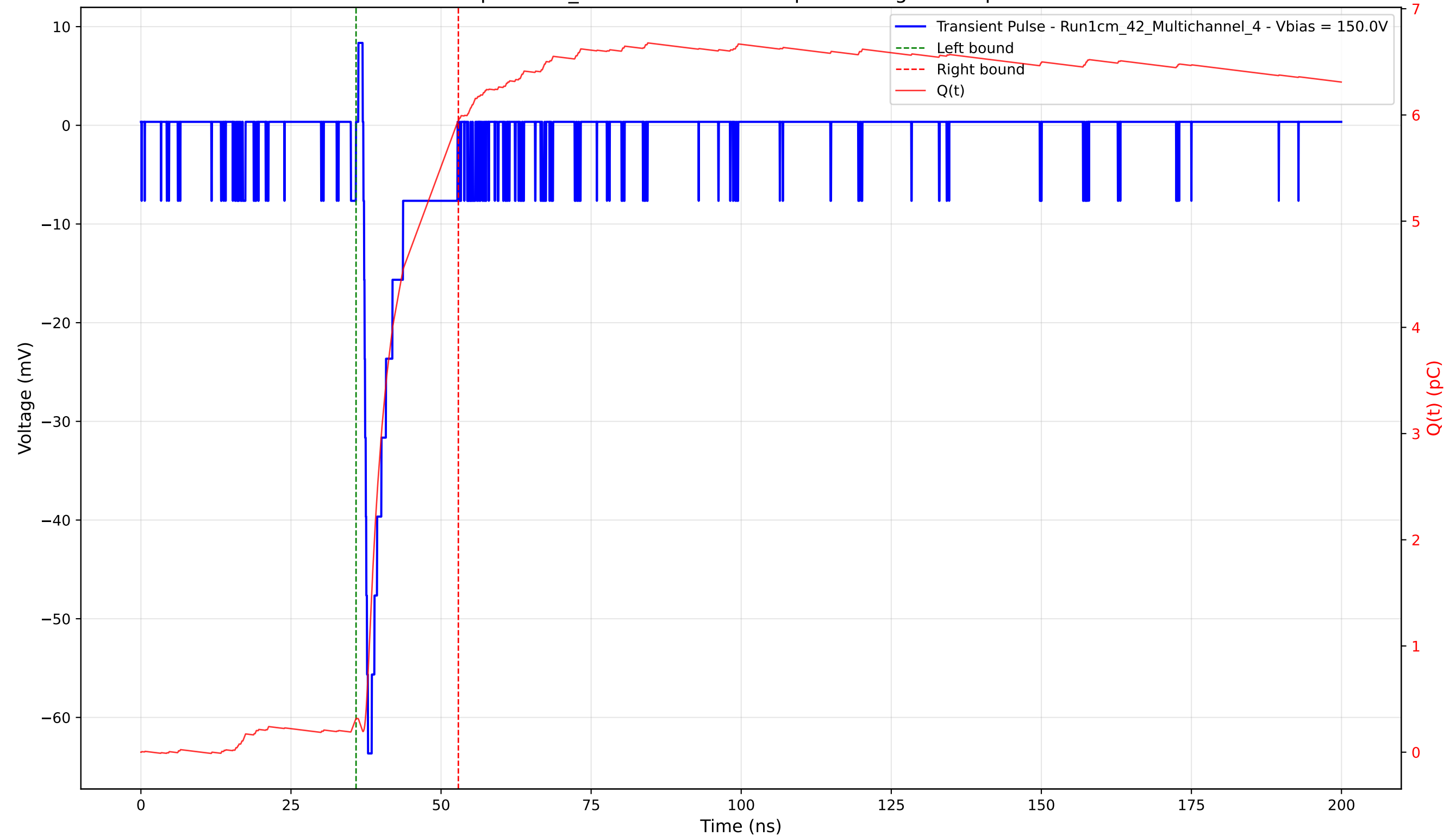
Transient Pulse - Sample: 1cm_42 - Position: 3610.0 \mu\text{m} - Charge: 5.62 pC - Rise Time: 0.77 ns
