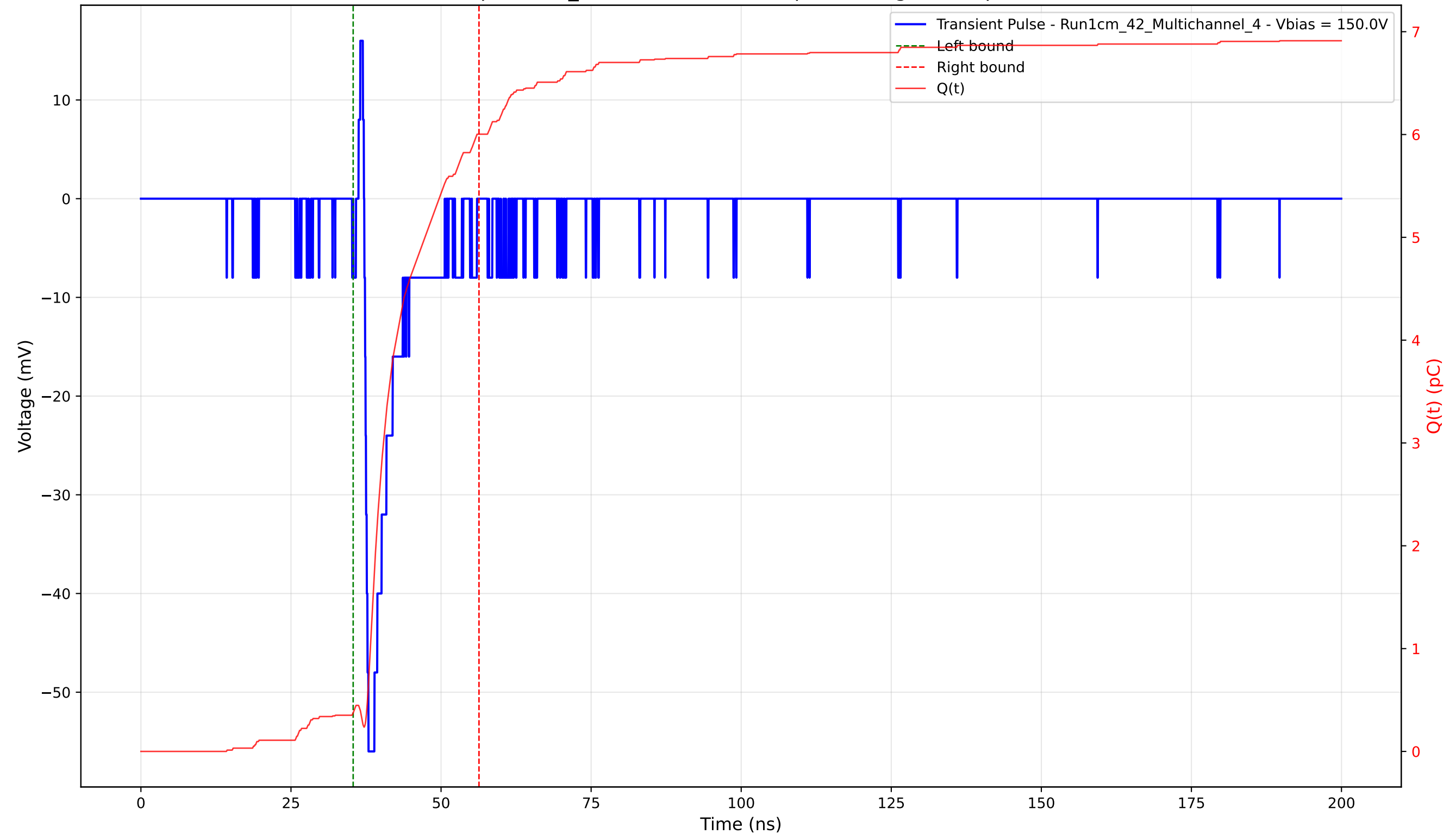
Transient Pulse - Sample: 1cm_42 - Position: 3710.0 \mu\text{m} - Charge: 5.63 pC - Rise Time: 0.69 ns
