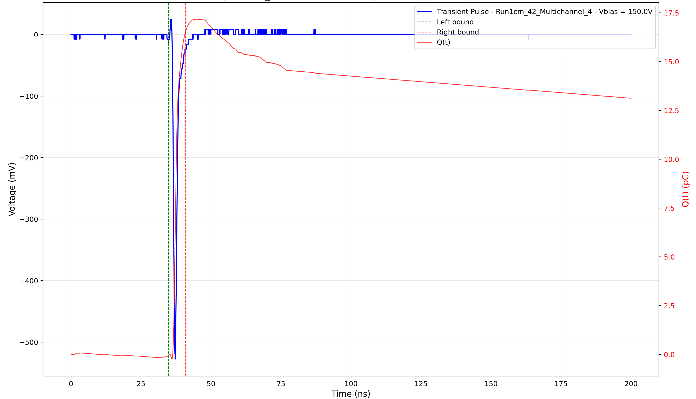
Transient Pulse - Sample: 1cm_42 - Position: 2325.0 \mu\text{m} - Charge: 16.59 pC - Rise Time: 0.73 ns
