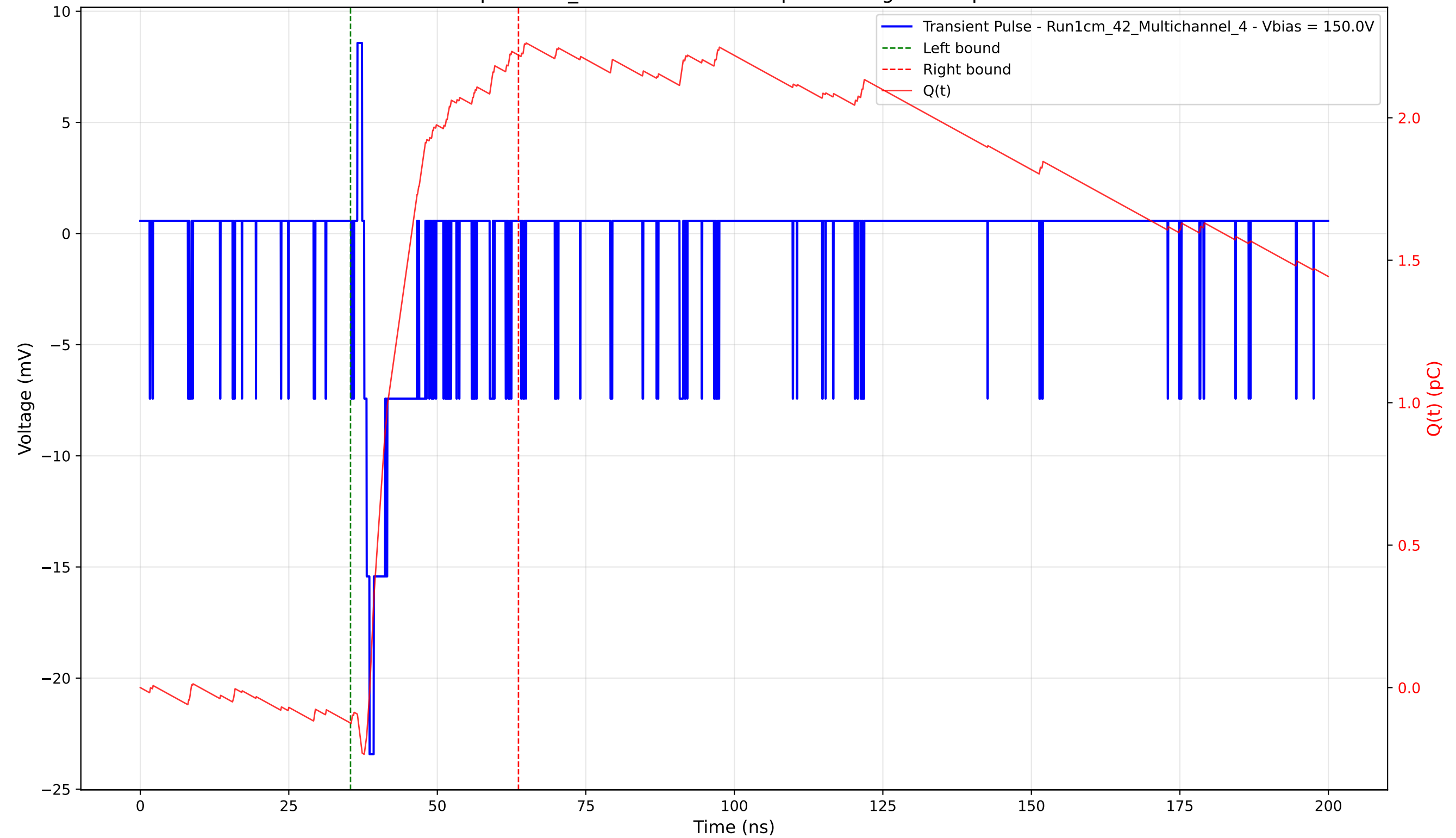
Transient Pulse - Sample: 1cm_42 - Position: 225.0 \mu\text{m} - Charge: 2.34 pC - Rise Time: 0.91 ns
