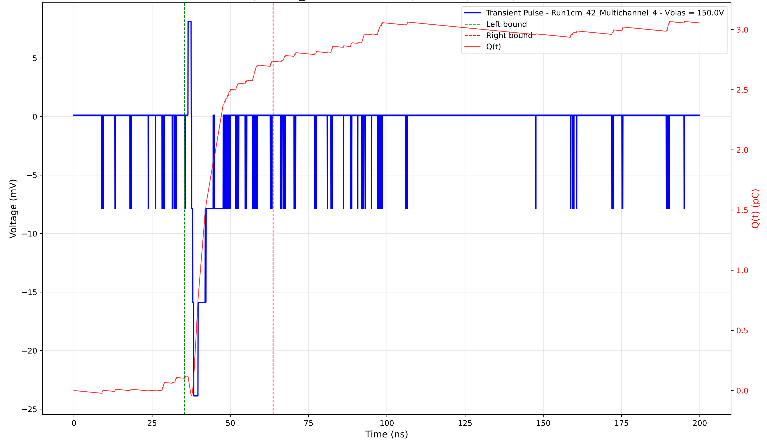
Transient Pulse - Sample: 1cm_42 - Position: 325.0 \mu\text{m} - Charge: 2.64 pC - Rise Time: 0.67 ns
