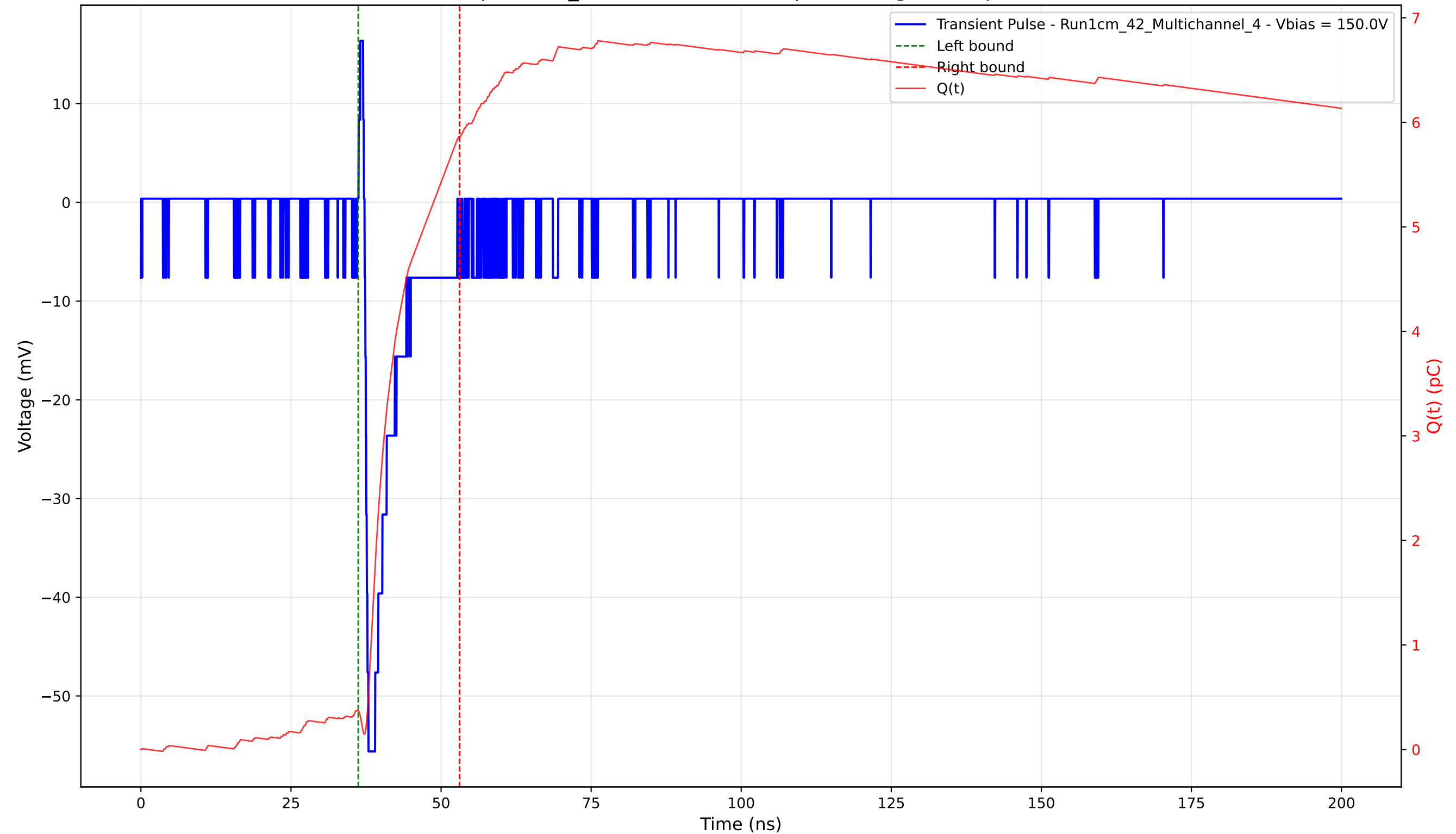
Transient Pulse - Sample: 1cm_42 - Position: 3720.0 \mu\text{m} - Charge: 5.49 pC - Rise Time: 0.65 ns
