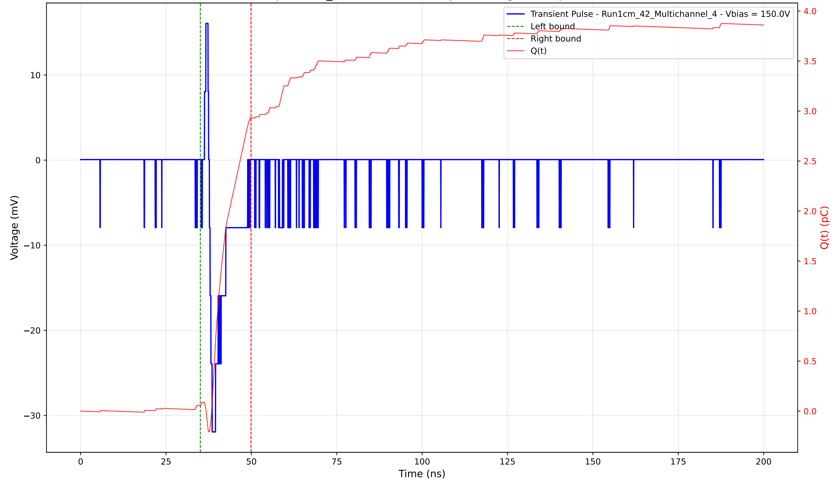
Transient Pulse - Sample: 1cm_42 - Position: 420.0 \mu\text{m} - Charge: 2.87 pC - Rise Time: 0.82 ns
