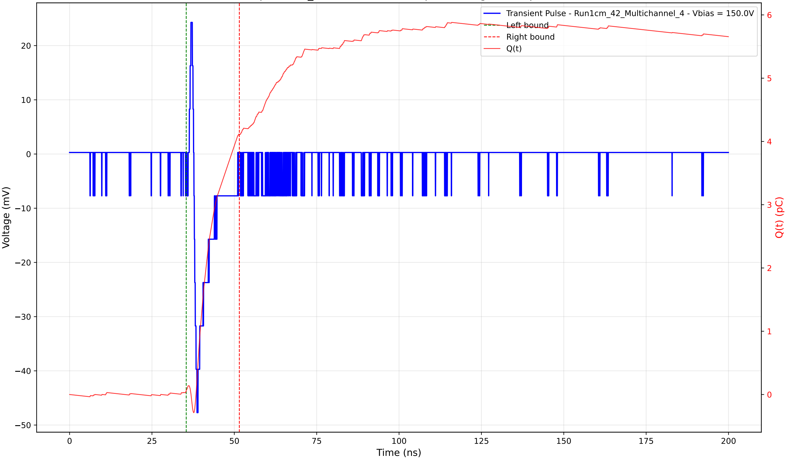
Transient Pulse - Sample: 1cm_42 - Position: 615.0 \mu\text{m} - Charge: 4.05 pC - Rise Time: 0.94 ns
