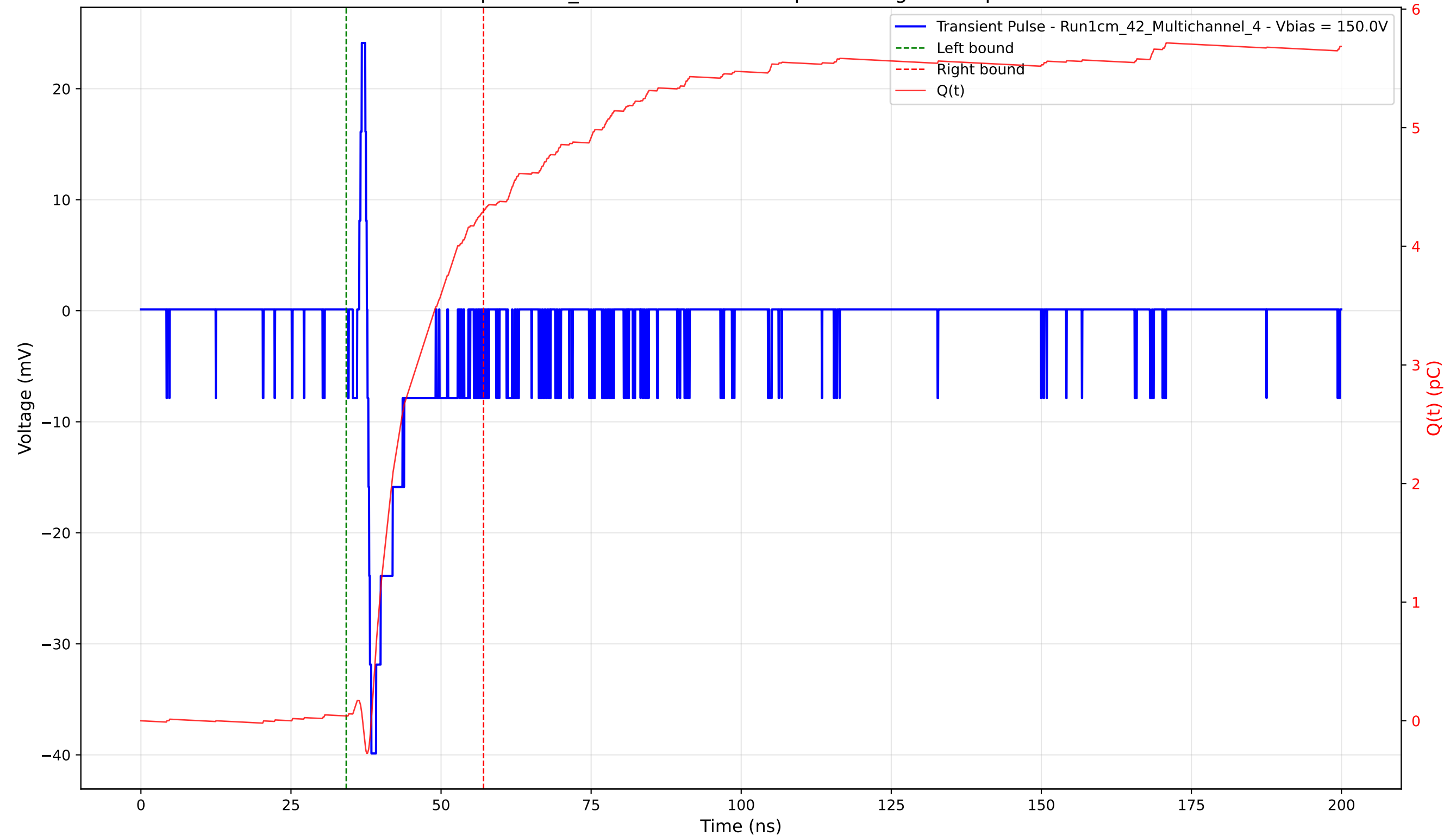
Transient Pulse - Sample: 1cm_42 - Position: 4305.0 \mu\text{m} - Charge: 4.26 pC - Rise Time: 0.66 ns
