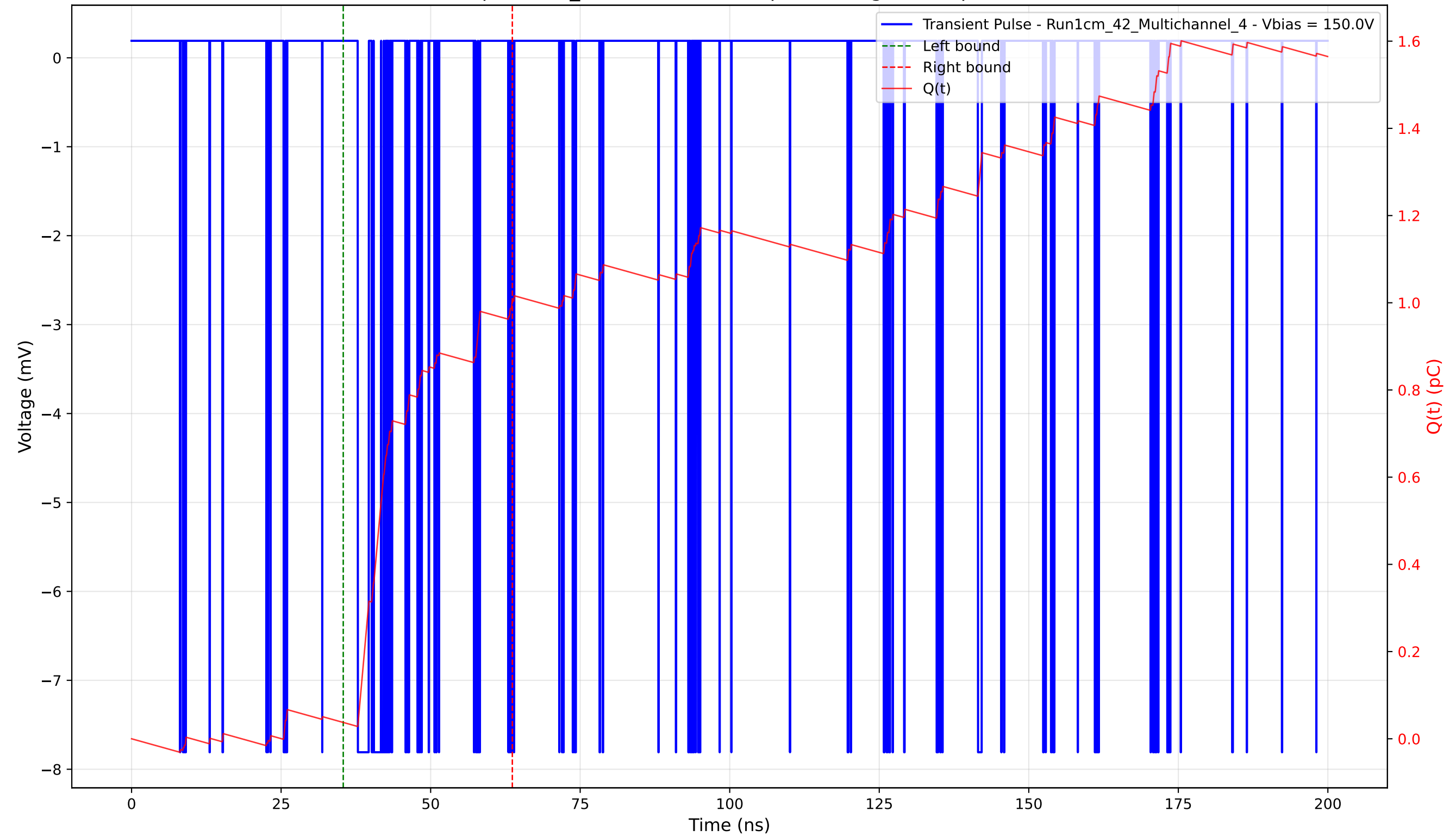
Transient Pulse - Sample: 1cm_42 - Position: 45.0 \mu\text{m} - Charge: 0.97 pC - Rise Time: 0.04 ns
