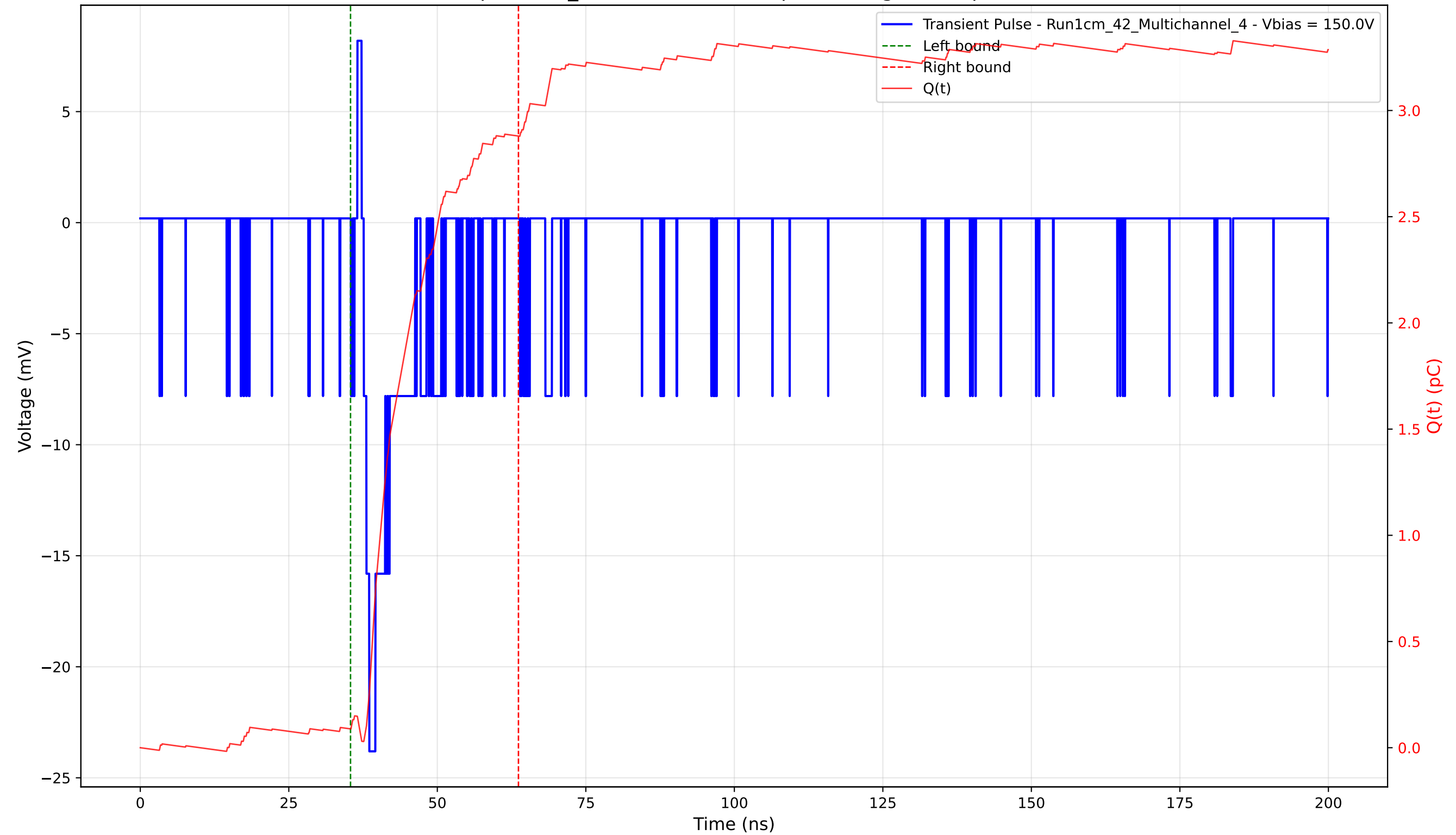
Transient Pulse - Sample: 1cm_42 - Position: 265.0 \mu\text{m} - Charge: 2.79 pC - Rise Time: 0.95 ns
