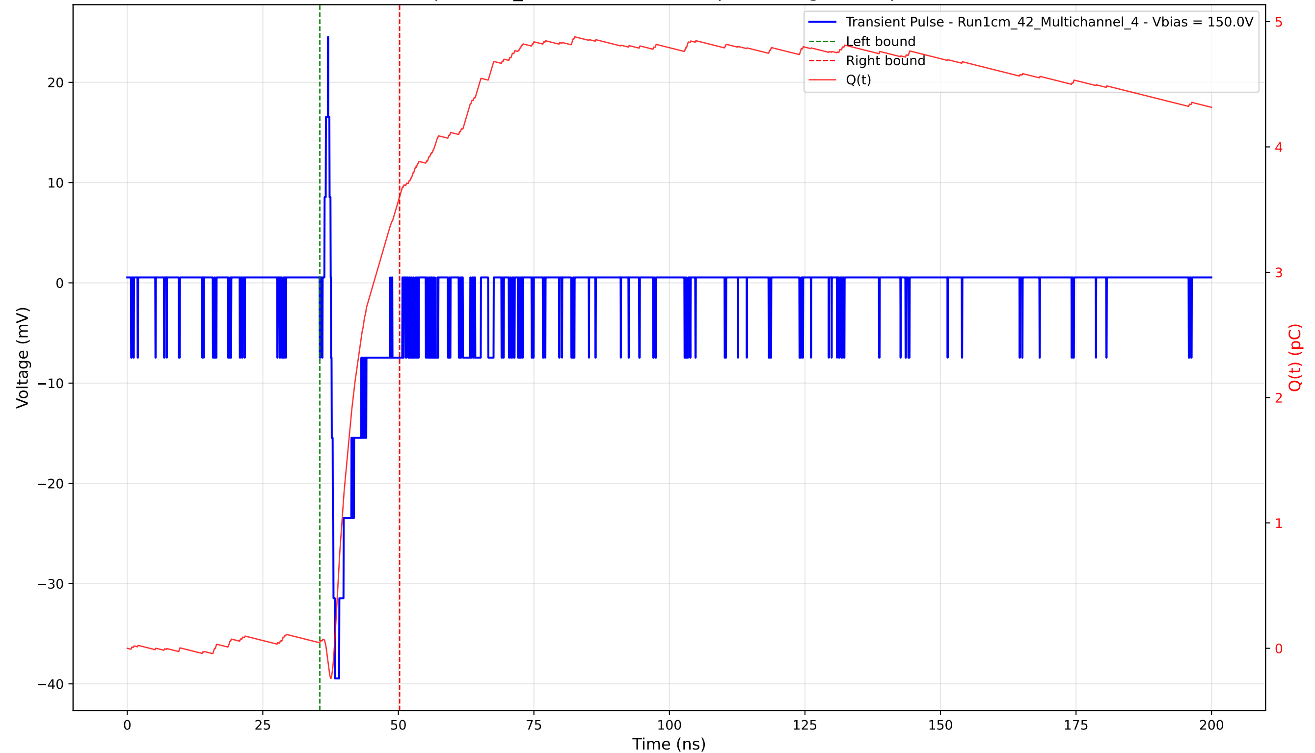
Transient Pulse - Sample: 1cm_42 - Position: 4060.0 \mu\text{m} - Charge: 3.56 pC - Rise Time: 0.74 ns
