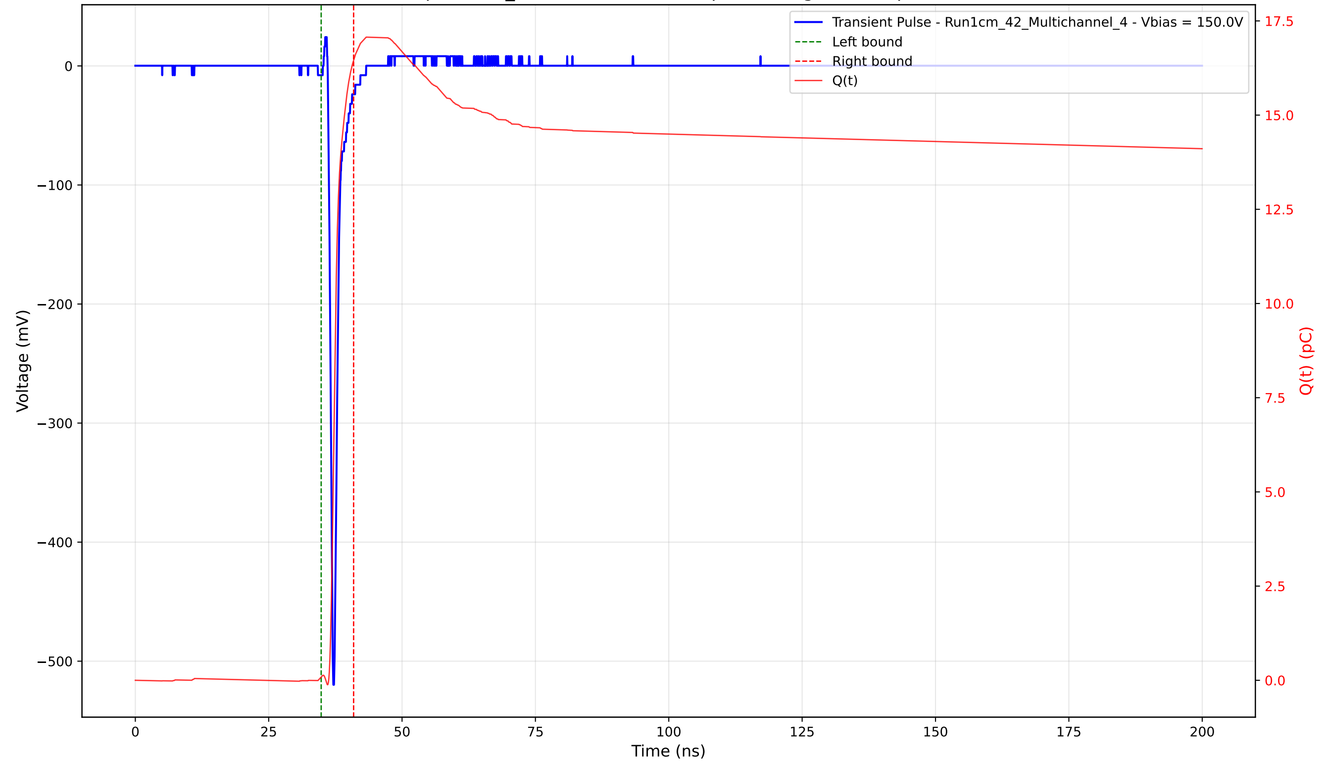
Transient Pulse - Sample: 1cm_42 - Position: 2355.0 \mu\text{m} - Charge: 16.37 pC - Rise Time: 0.72 ns
