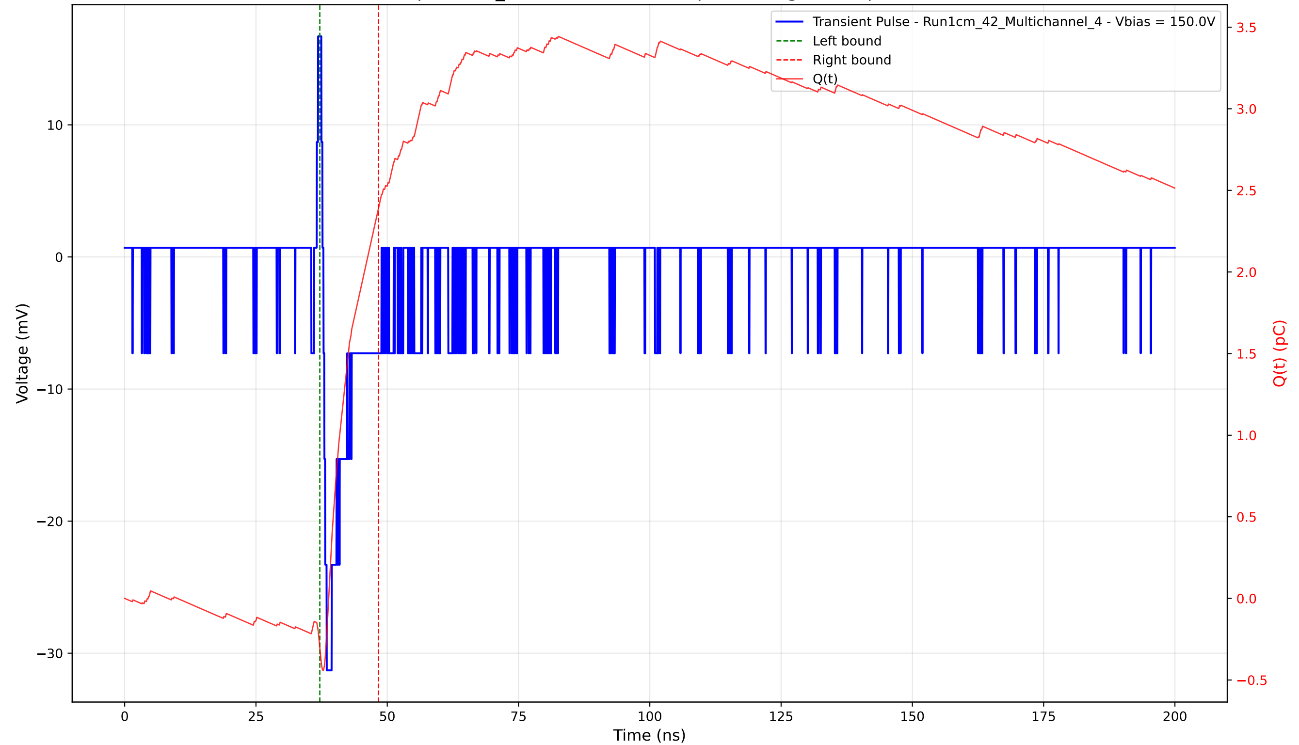
Transient Pulse - Sample: 1cm_42 - Position: 4675.0 \mu\text{m} - Charge: 2.69 pC - Rise Time: 0.63 ns
