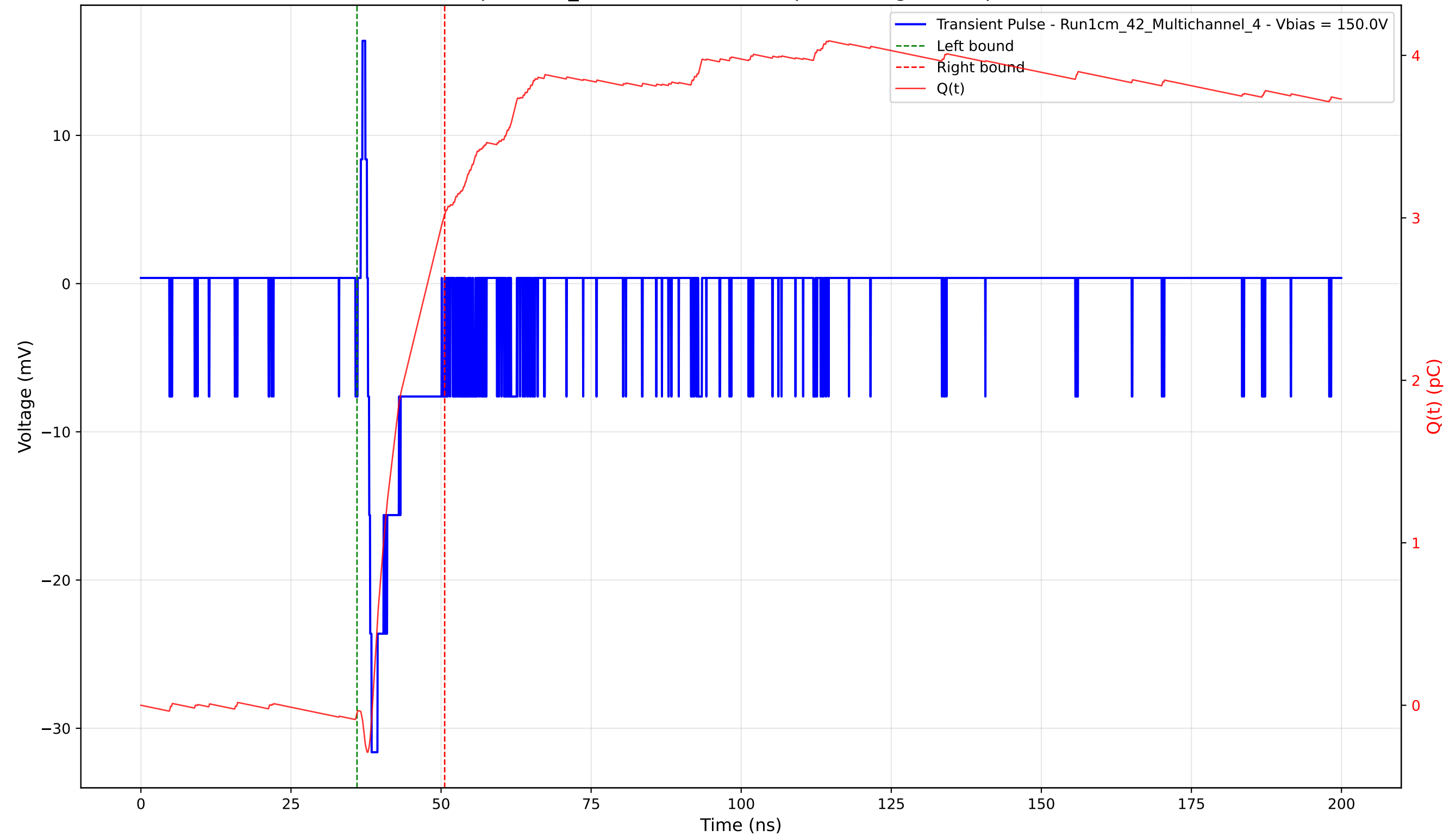
Transient Pulse - Sample: 1cm_42 - Position: 4655.0 \mu\text{m} - Charge: 3.07 pC - Rise Time: 0.62 ns
