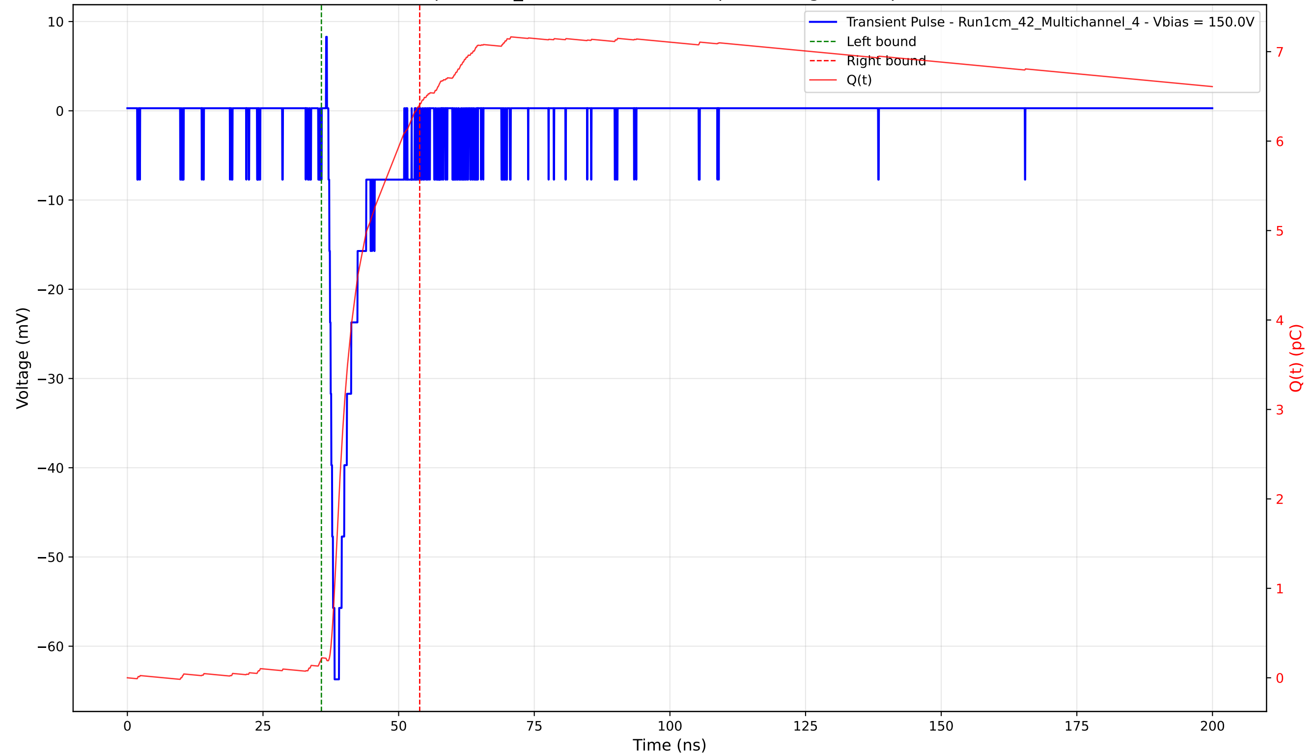
Transient Pulse - Sample: 1cm_42 - Position: 1365.0 \mu\text{m} - Charge: 6.20 pC - Rise Time: 1.13 ns
