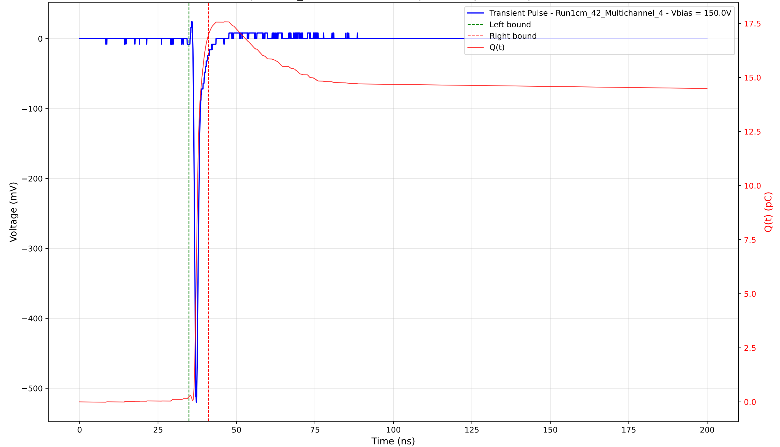
Transient Pulse - Sample: 1cm_42 - Position: 2295.0 \mu\text{m} - Charge: 16.72 pC - Rise Time: 0.72 ns
