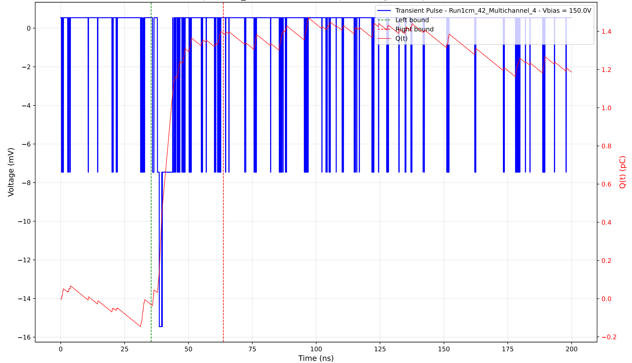
Transient Pulse - Sample: 1cm_42 - Position: 5075.0 \mu\text{m} - Charge: 1.42 pC - Rise Time: 0.75 ns
