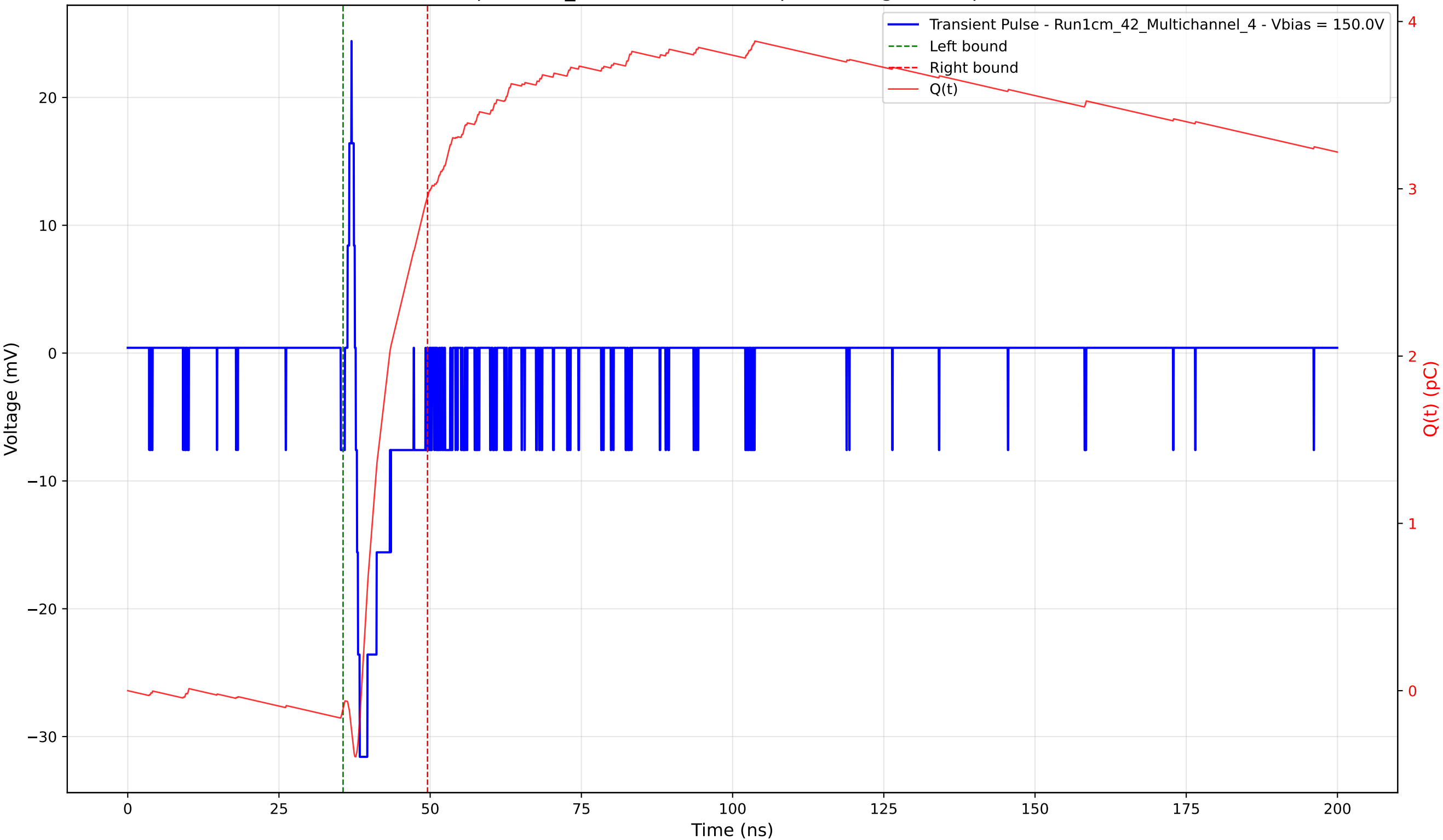
Transient Pulse - Sample: 1cm_42 - Position: 490.0 \mu\text{m} - Charge: 3.06 pC - Rise Time: 0.66 ns
