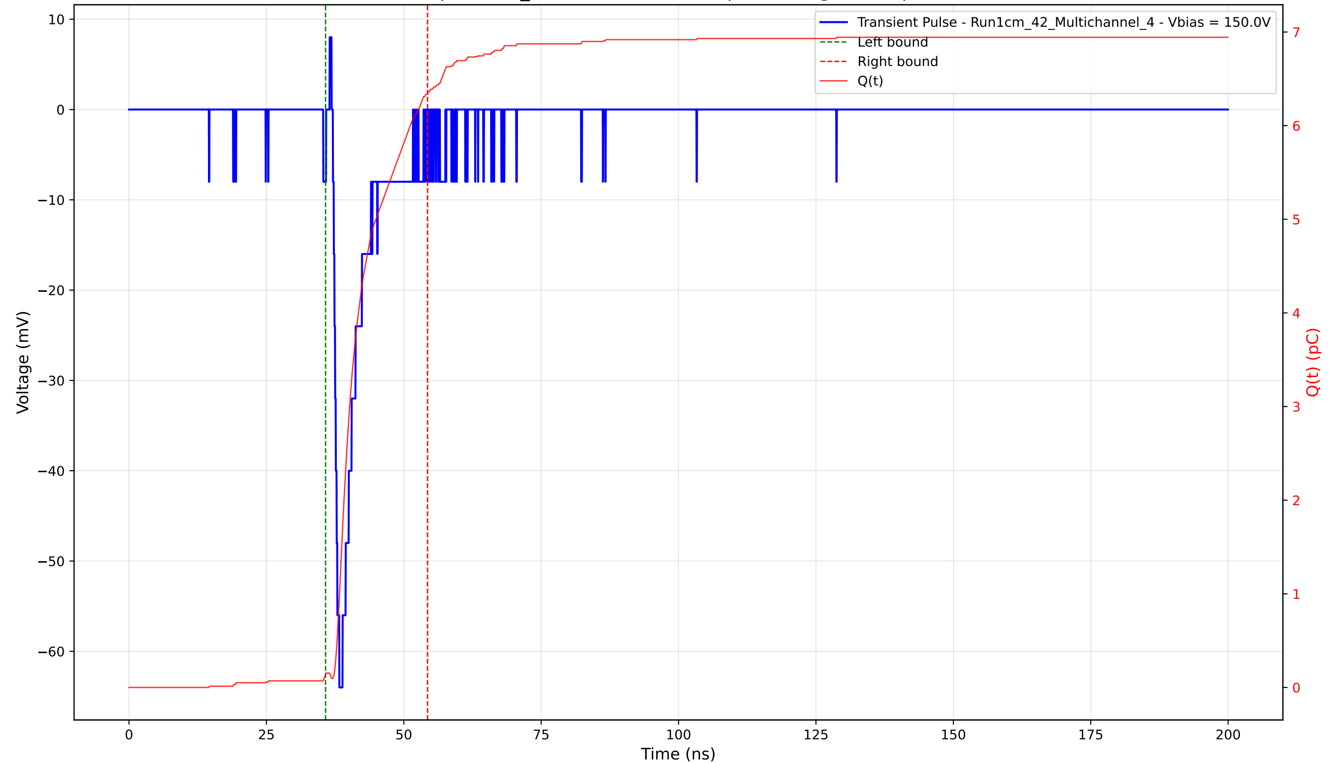
Transient Pulse - Sample: 1cm_42 - Position: 1355.0 \mu\text{m} - Charge: 6.20 pC - Rise Time: 1.17 ns
