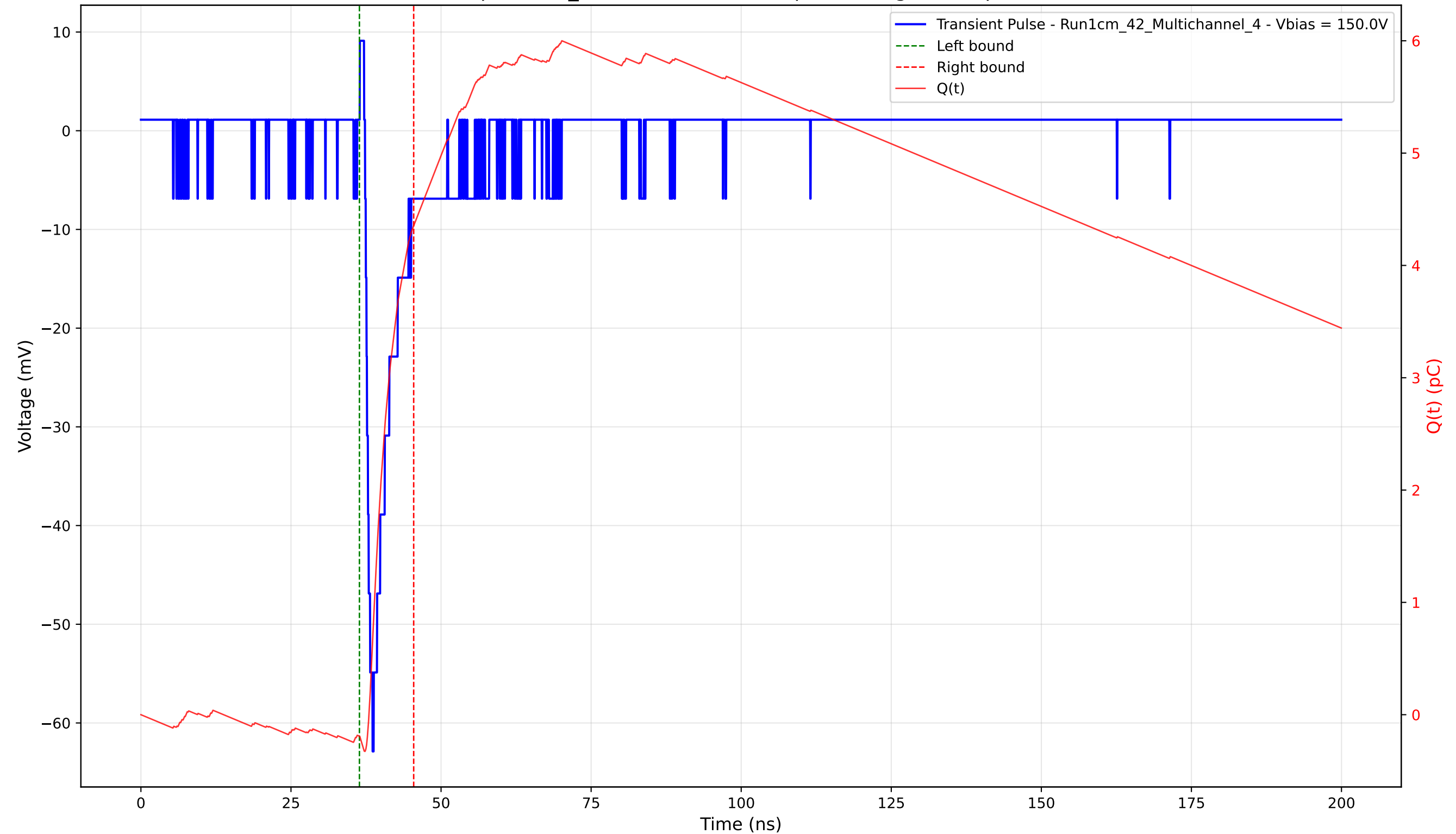
Transient Pulse - Sample: 1cm_42 - Position: 1175.0 \mu\text{m} - Charge: 4.54 pC - Rise Time: 1.24 ns
