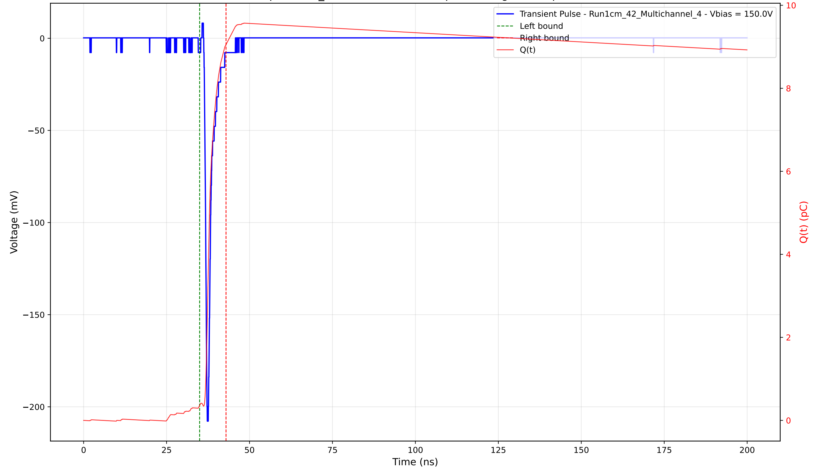
Transient Pulse - Sample: 1cm_42 - Position: 3040.0 \mu\text{m} - Charge: 8.69 pC - Rise Time: 0.75 ns
