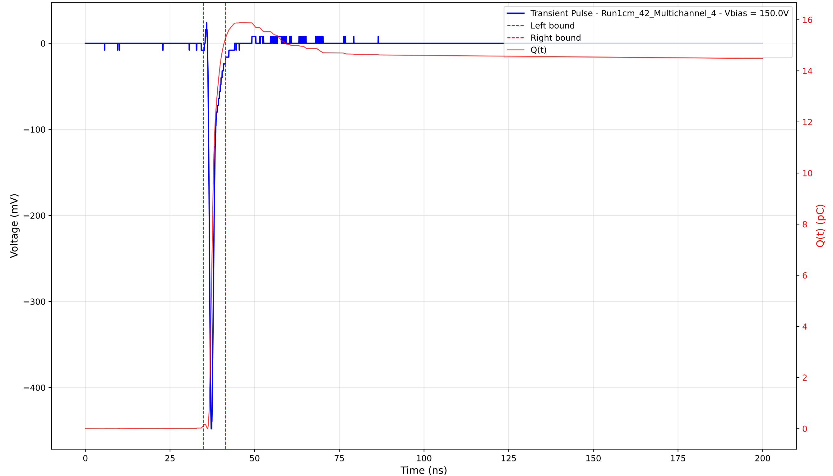
Transient Pulse - Sample: 1cm_42 - Position: 2200.0 \mu\text{m} - Charge: 15.16 pC - Rise Time: 0.70 ns
