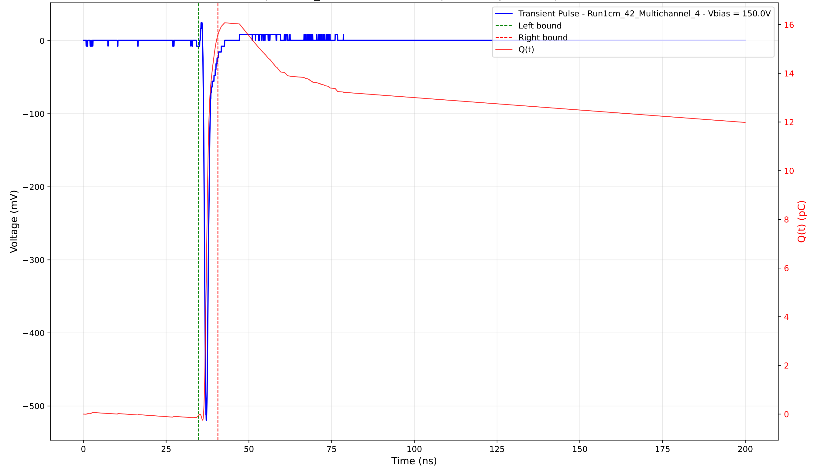
Transient Pulse - Sample: 1cm_42 - Position: 2530.0 \mu\text{m} - Charge: 15.63 pC - Rise Time: 0.72 ns
