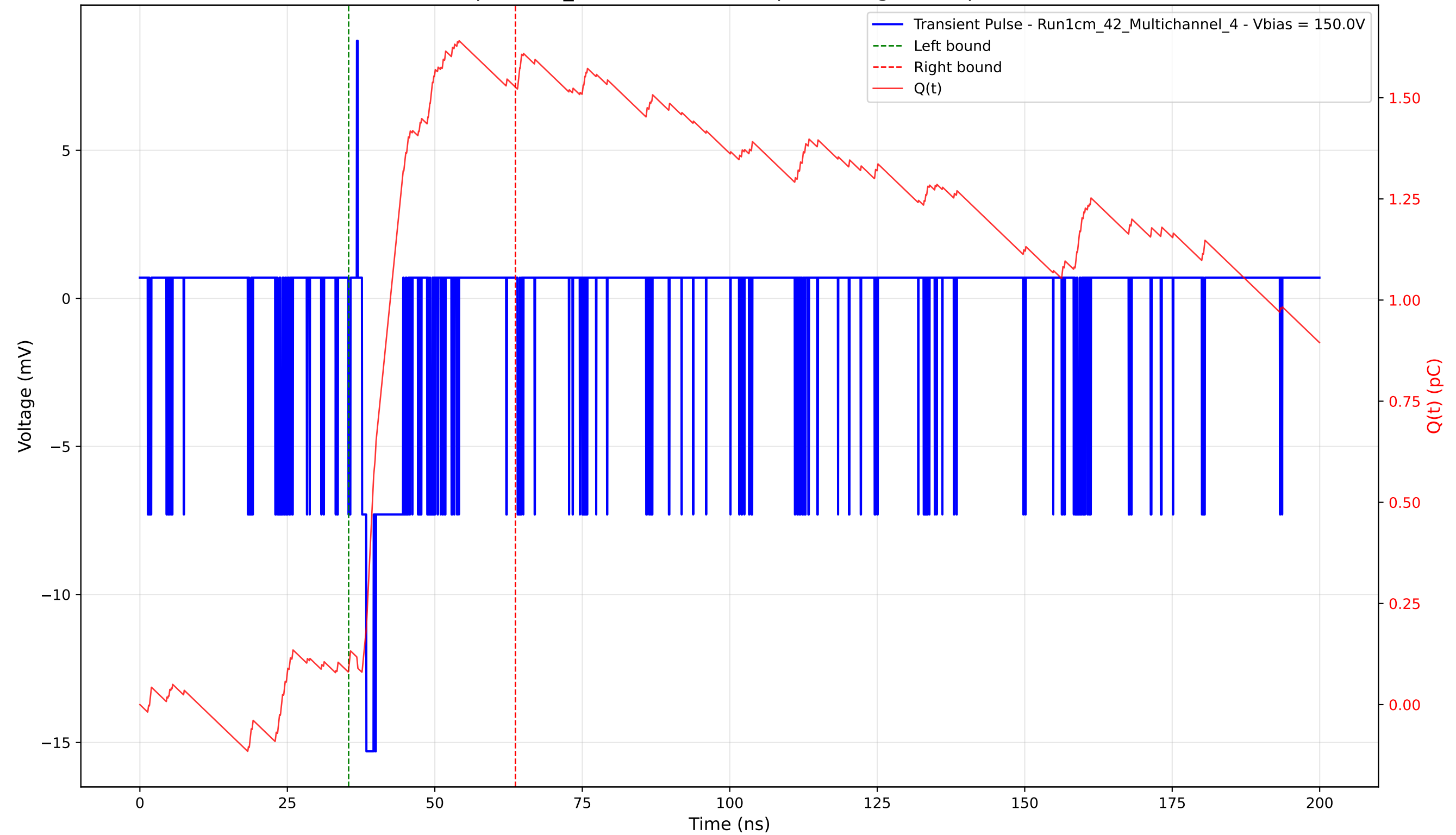
Transient Pulse - Sample: 1cm_42 - Position: 150.0 \mu\text{m} - Charge: 1.44 pC - Rise Time: 0.75 ns
