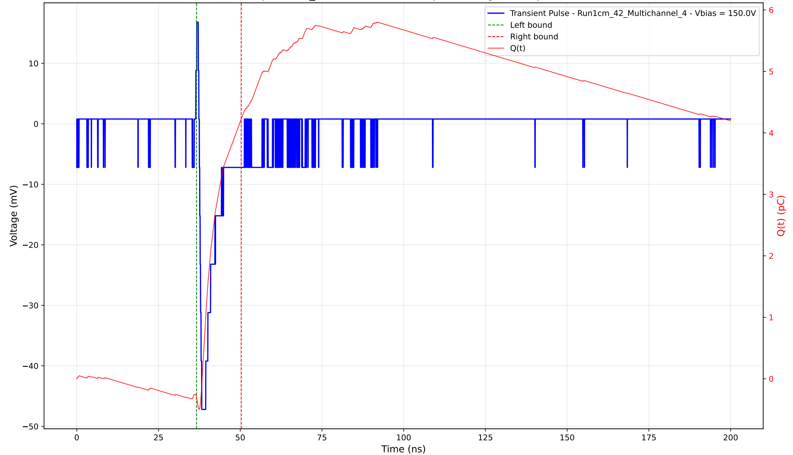
Transient Pulse - Sample: 1cm_42 - Position: 1065.0 \mu\text{m} - Charge: 4.52 pC - Rise Time: 0.74 ns
