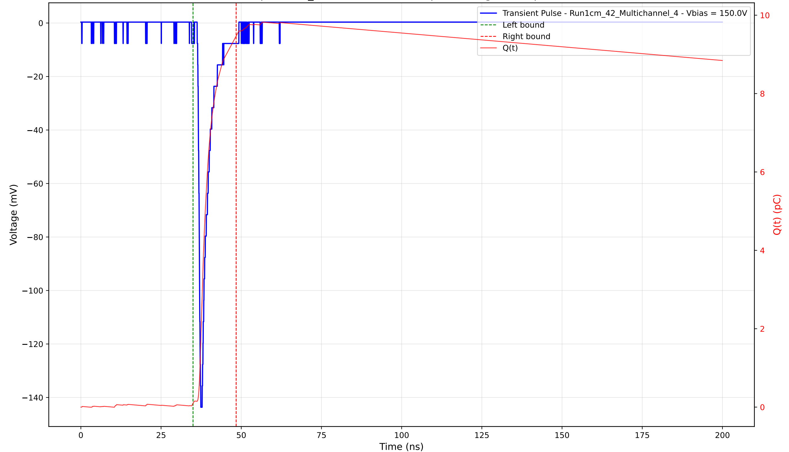
Transient Pulse - Sample: 1cm_42 - Position: 1750.0 \mu\text{m} - Charge: 9.37 pC - Rise Time: 0.85 ns
