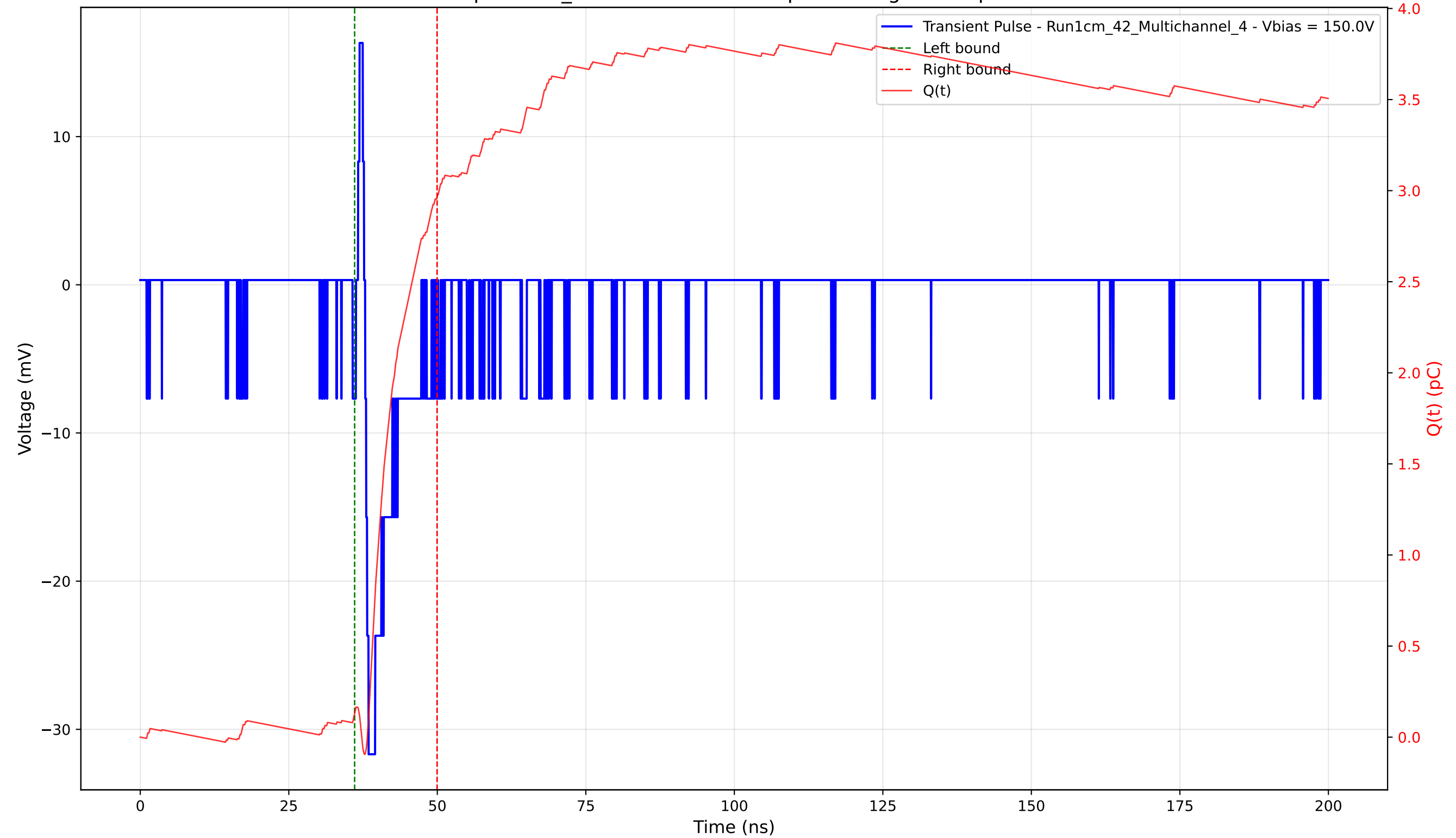
Transient Pulse - Sample: 1cm_42 - Position: 4815.0 \mu\text{m} - Charge: 2.84 pC - Rise Time: 0.58 ns
