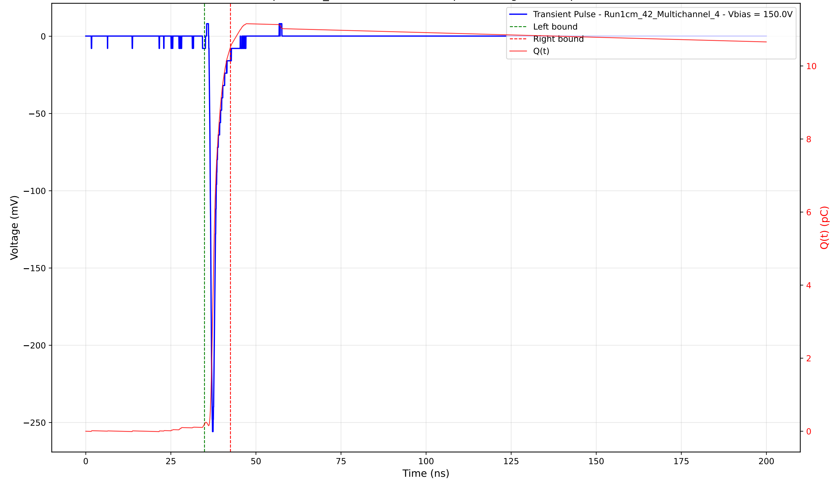
Transient Pulse - Sample: 1cm_42 - Position: 2040.0 \mu\text{m} - Charge: 10.33 pC - Rise Time: 0.78 ns
