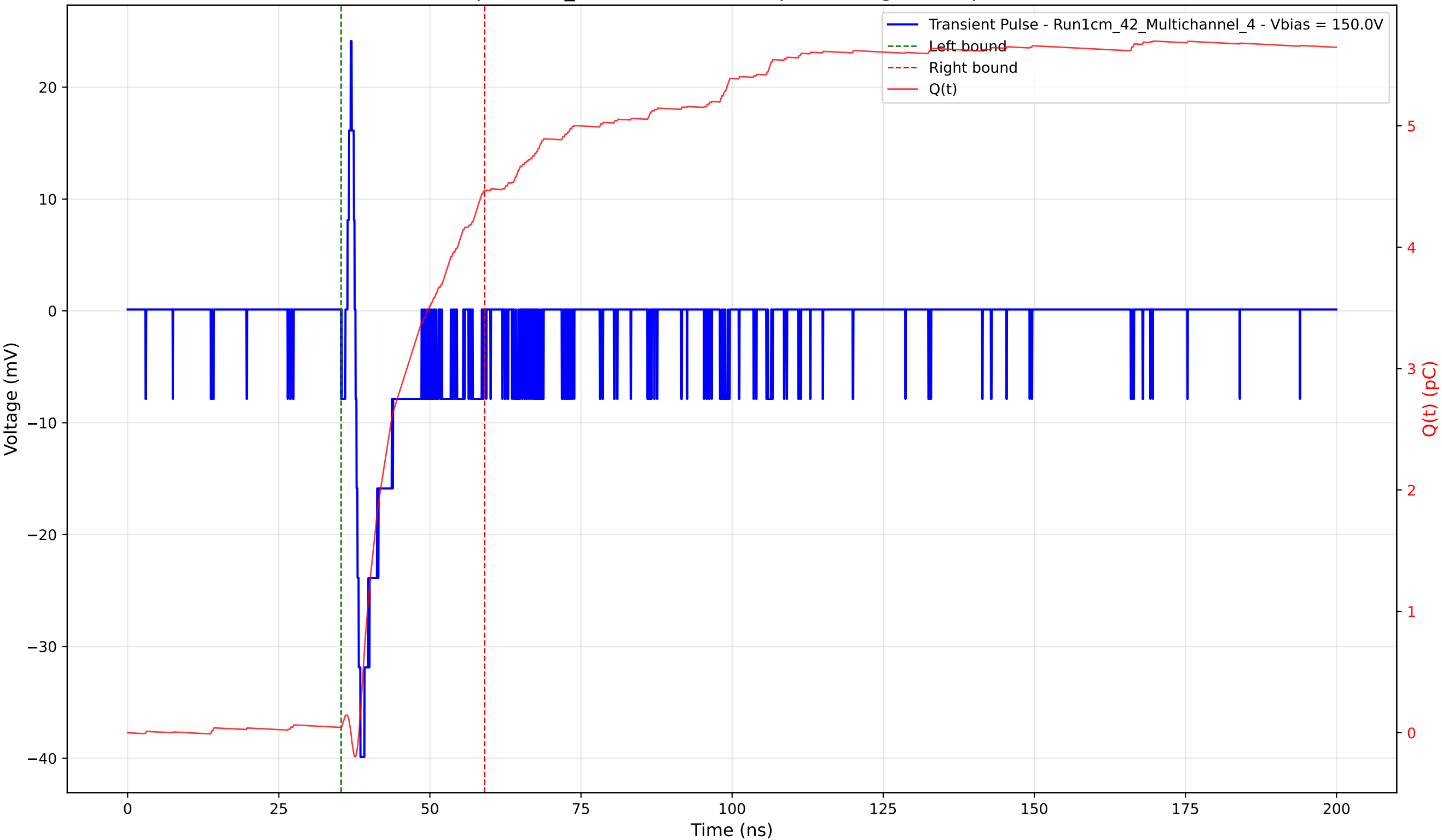
Transient Pulse - Sample: 1cm_42 - Position: 545.0 \mu\text{m} - Charge: 4.42 pC - Rise Time: 0.82 ns
