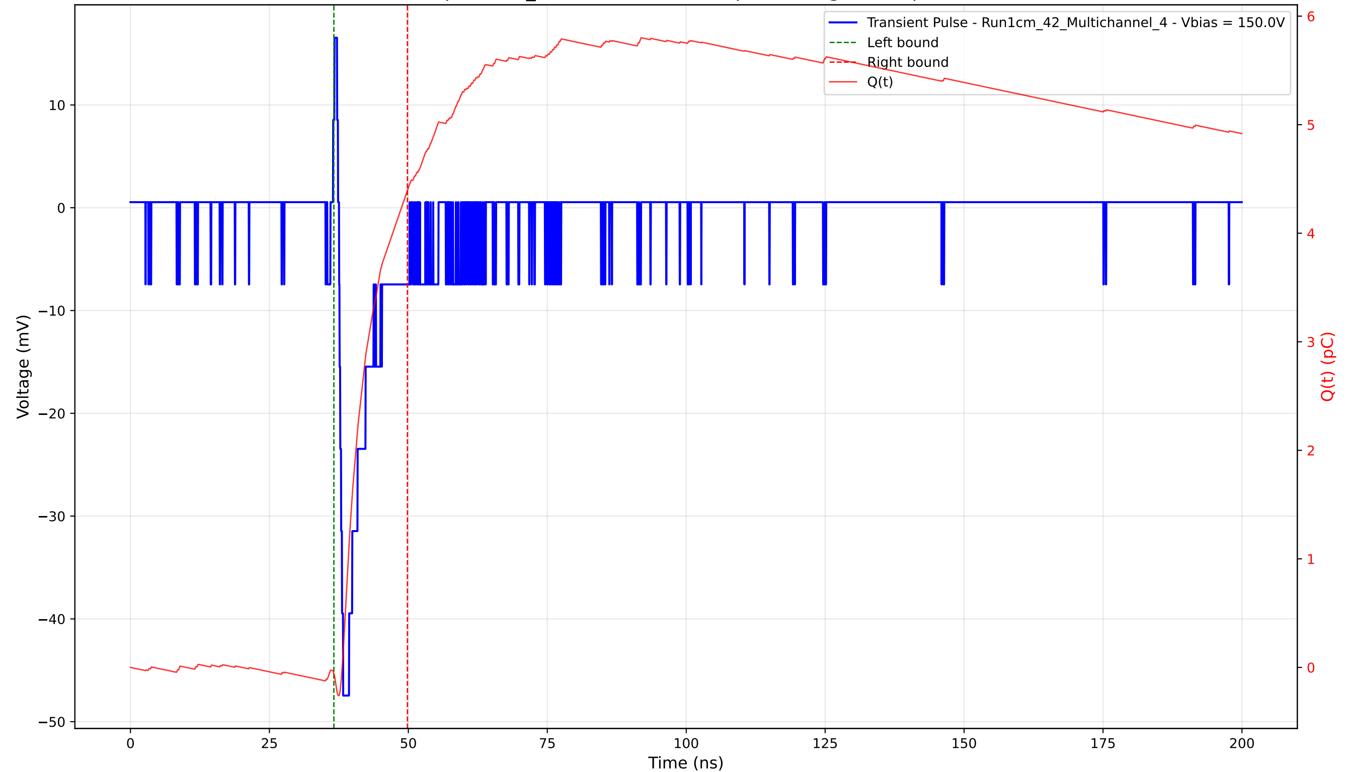
Transient Pulse - Sample: 1cm_42 - Position: 1040.0 \mu\text{m} - Charge: 4.45 pC - Rise Time: 0.74 ns
