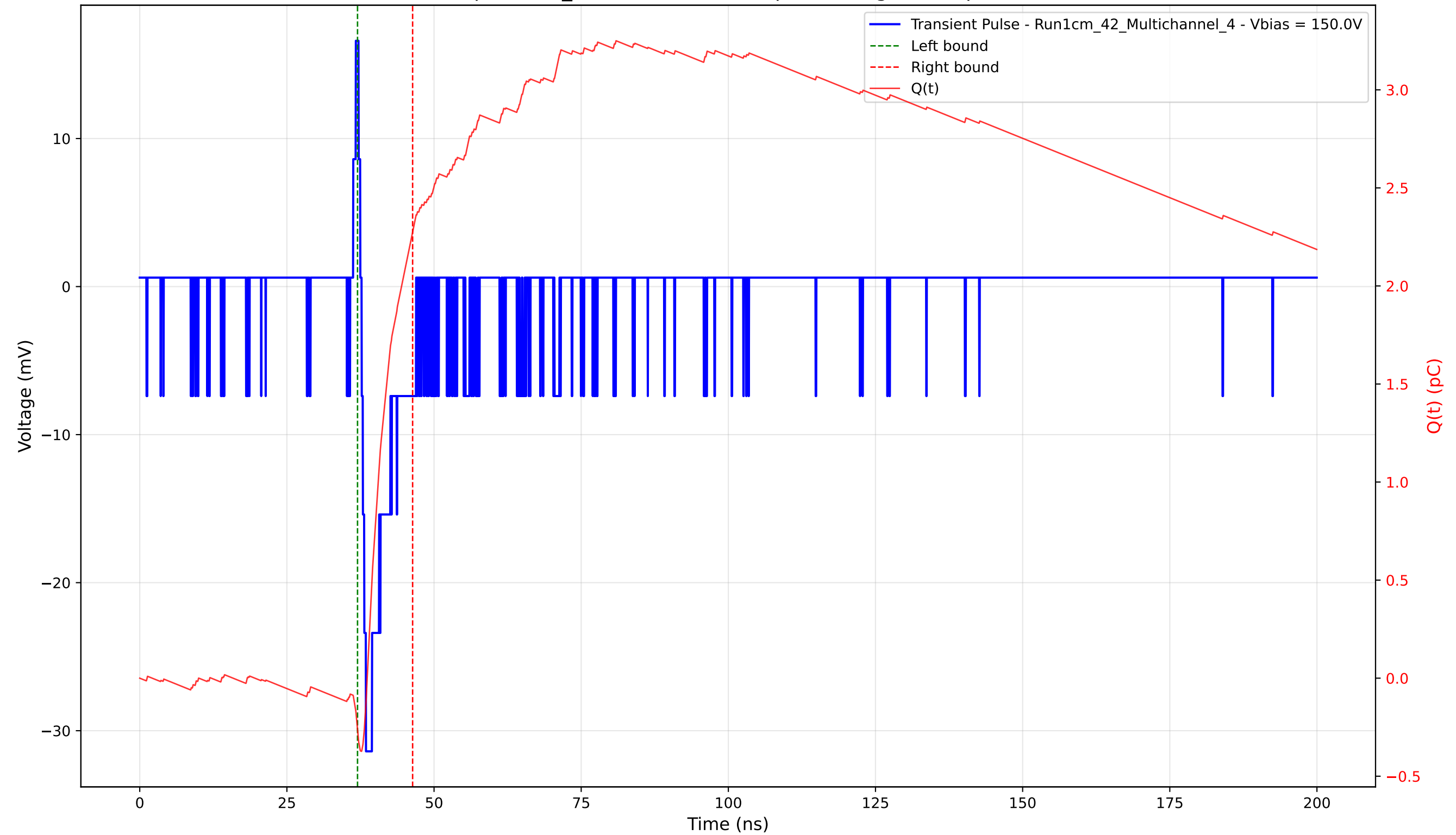
Transient Pulse - Sample: 1cm_42 - Position: 430.0 \mu\text{m} - Charge: 2.54 pC - Rise Time: 0.75 ns
