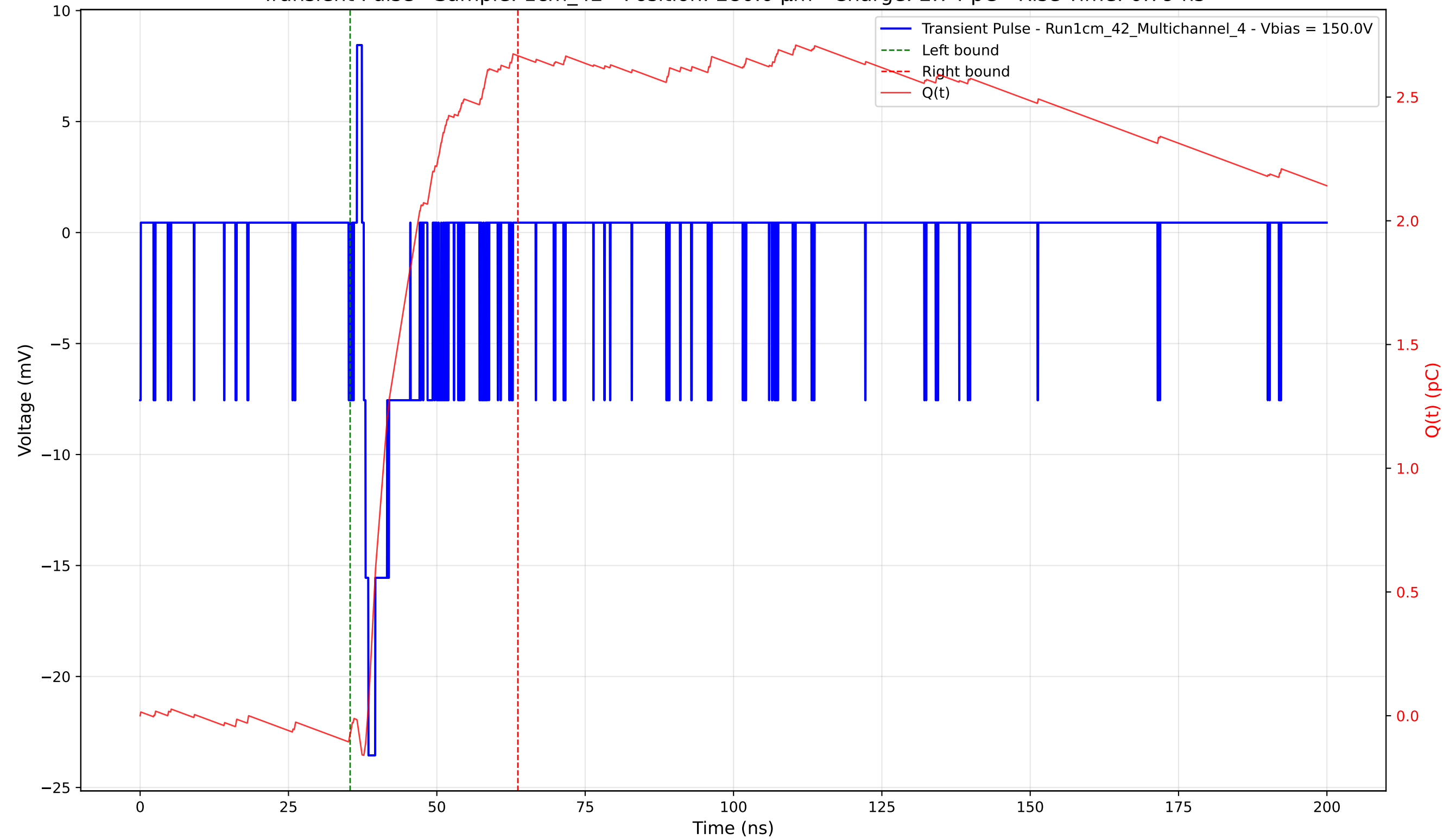
Transient Pulse - Sample: 1cm_42 - Position: 280.0 \mu\text{m} - Charge: 2.74 pC - Rise Time: 0.79 ns
