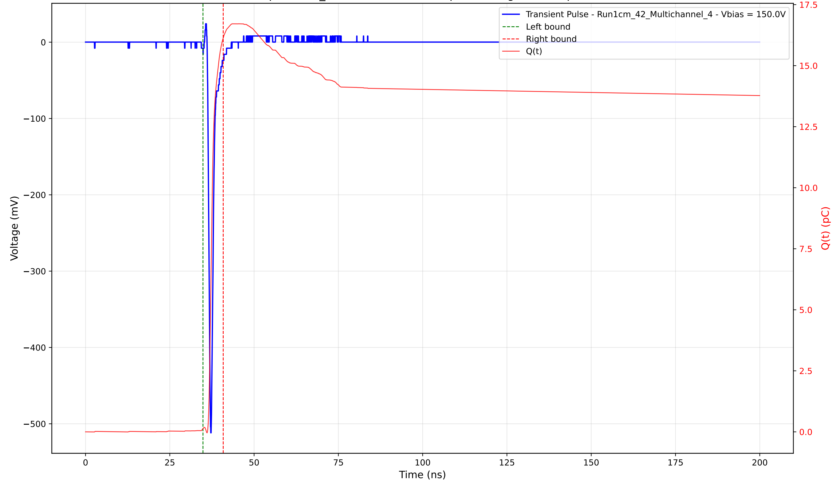
Transient Pulse - Sample: 1cm_42 - Position: 2680.0 \mu\text{m} - Charge: 16.01 pC - Rise Time: 0.74 ns
