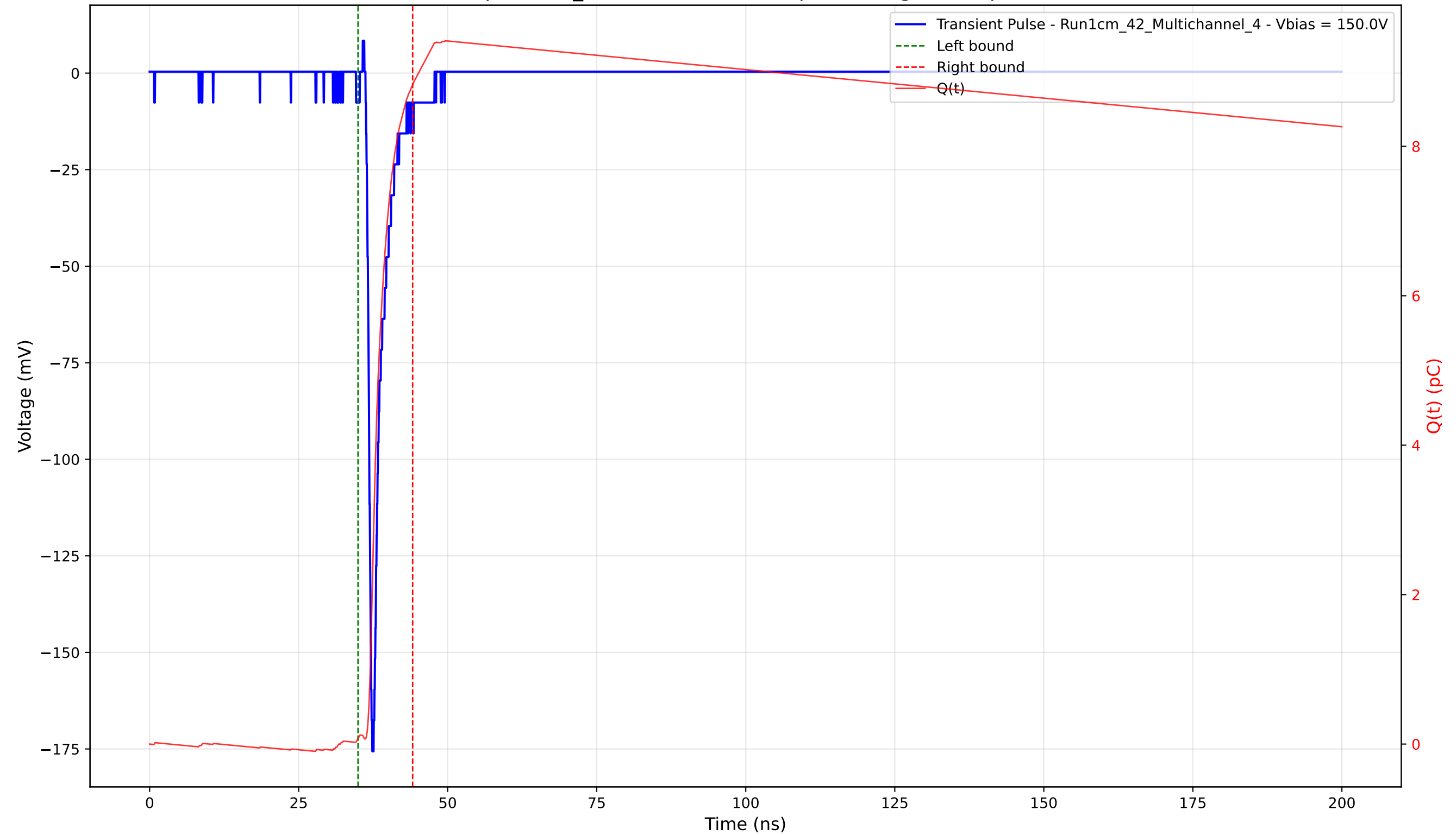
Transient Pulse - Sample: 1cm_42 - Position: 1910.0 \mu\text{m} - Charge: 8.74 pC - Rise Time: 0.79 ns
