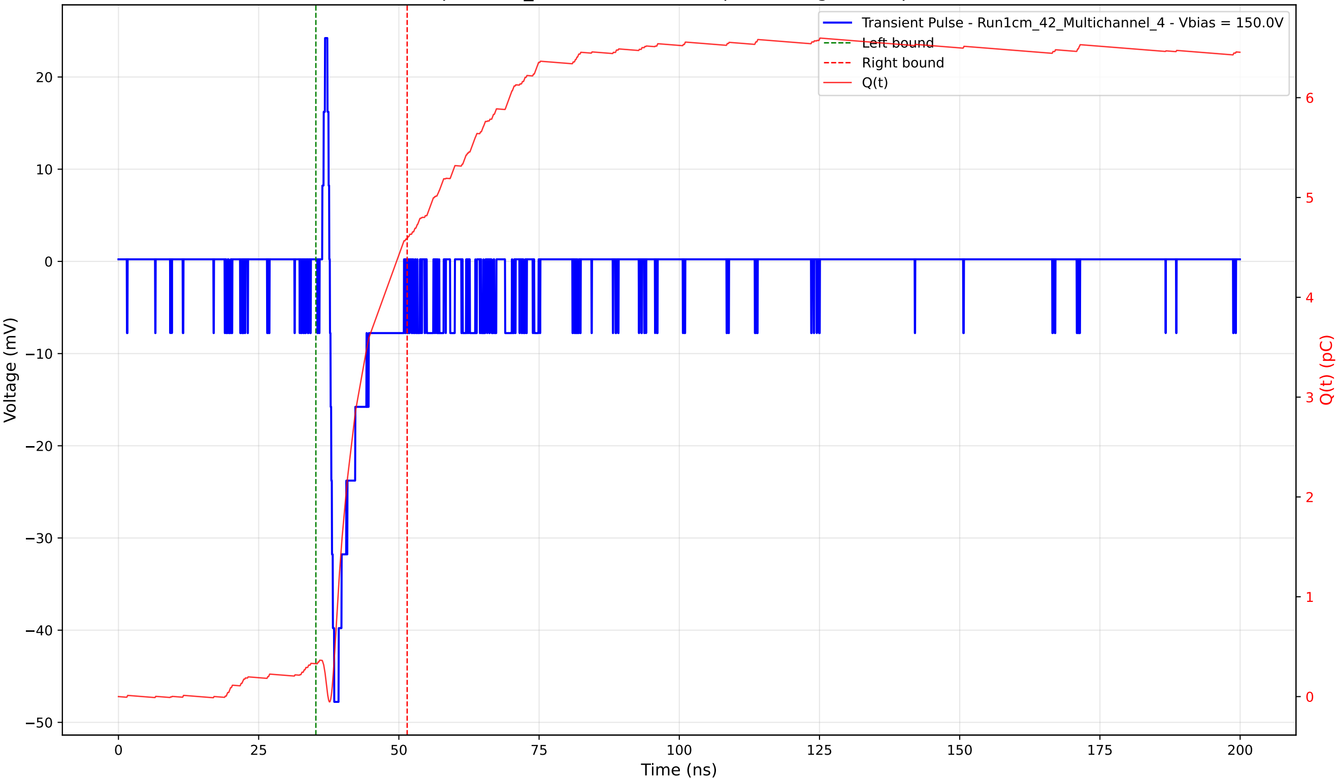
Transient Pulse - Sample: 1cm_42 - Position: 865.0 \mu\text{m} - Charge: 4.26 pC - Rise Time: 0.78 ns
