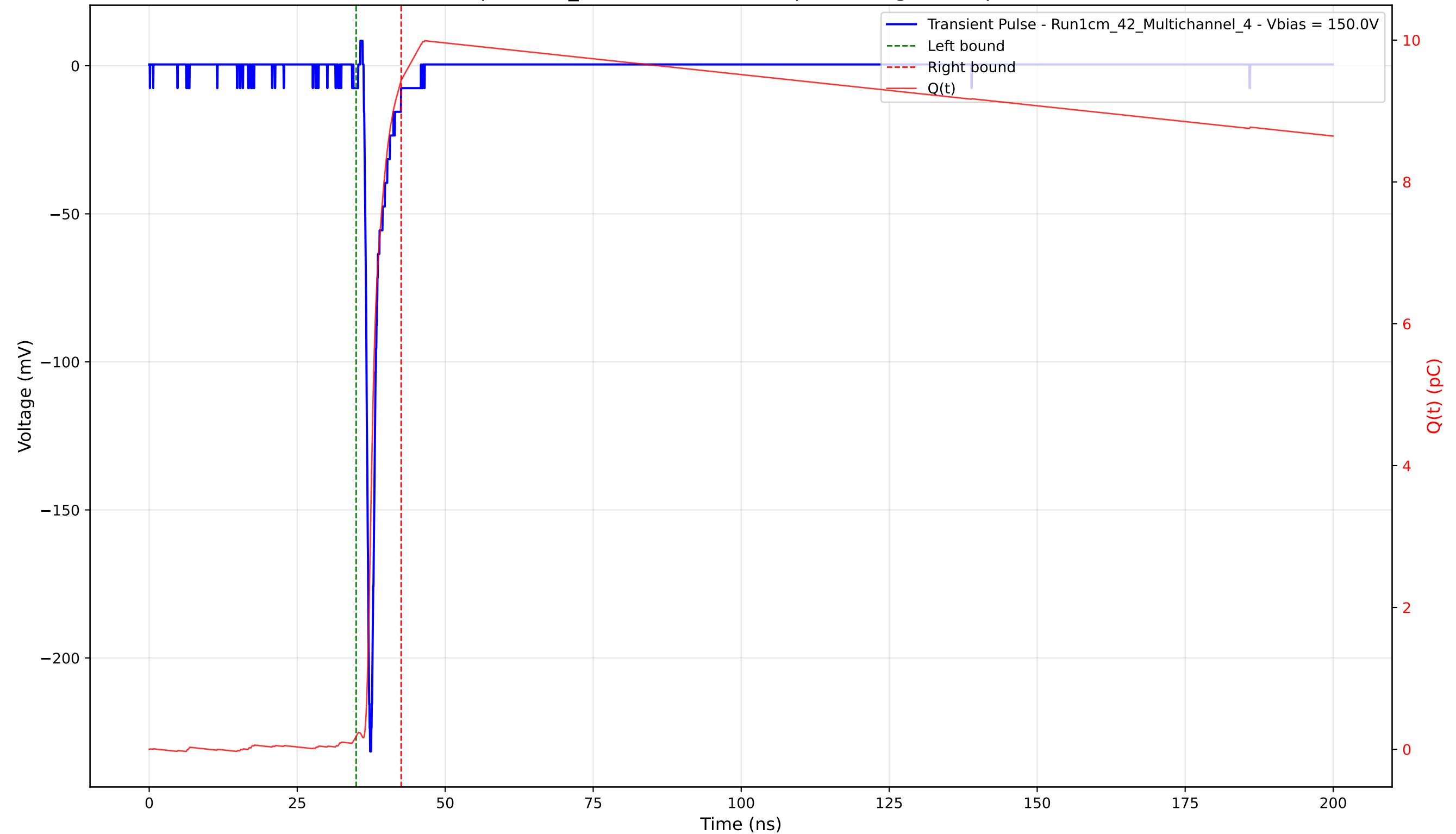
Transient Pulse - Sample: 1cm_42 - Position: 3010.0 \mu\text{m} - Charge: 9.25 pC - Rise Time: 0.80 ns
