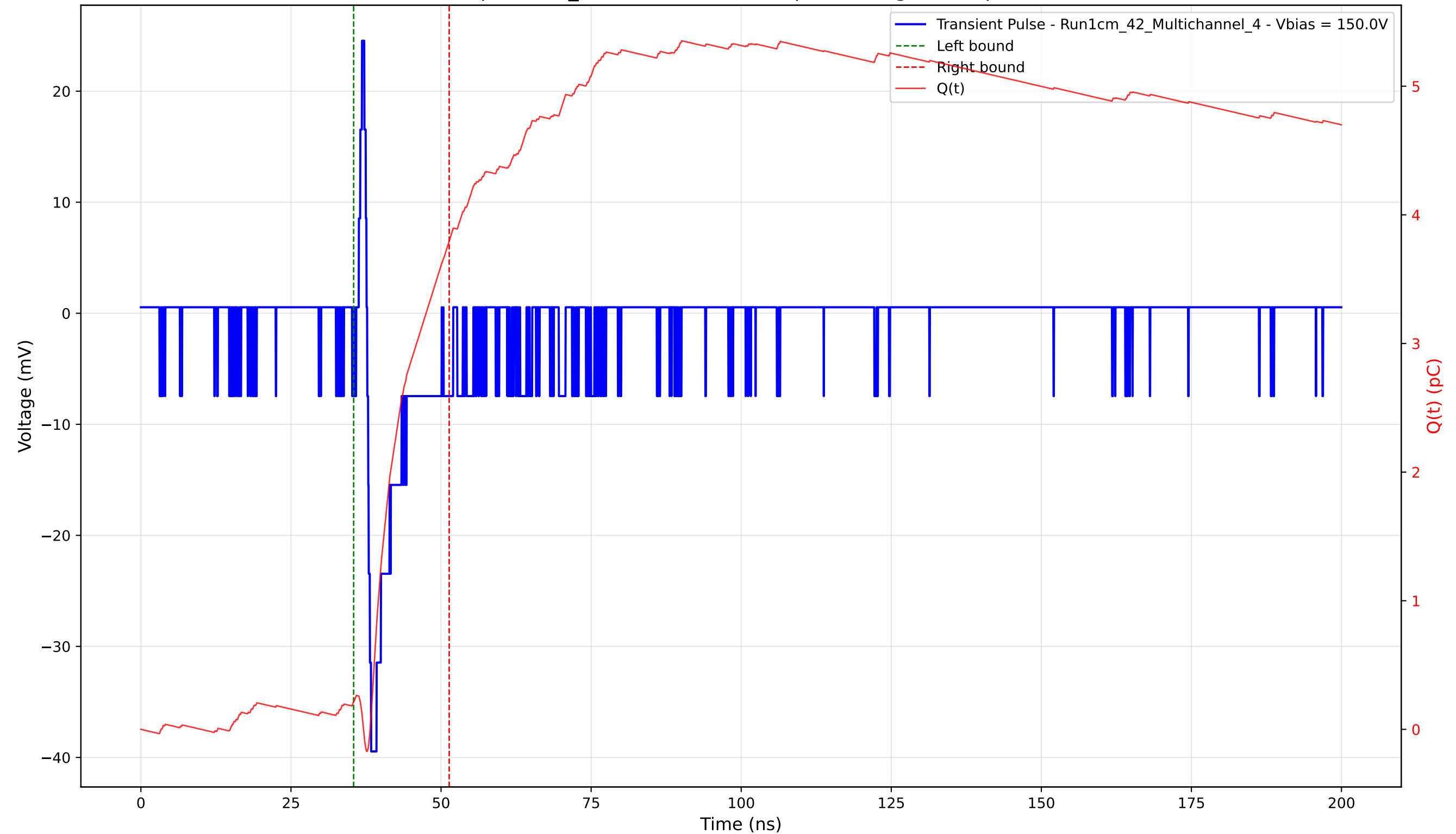
Transient Pulse - Sample: 1cm_42 - Position: 4195.0 \mu\text{m} - Charge: 3.58 pC - Rise Time: 0.66 ns
