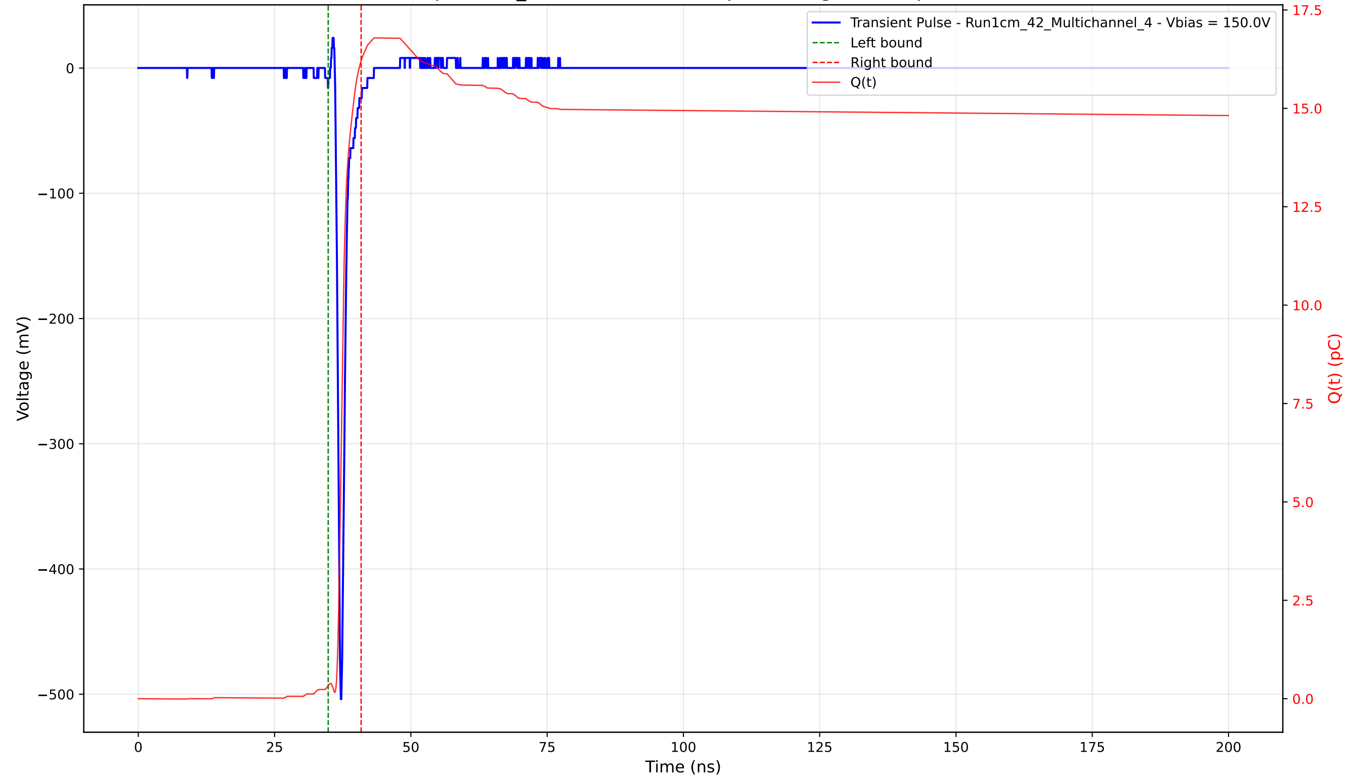
Transient Pulse - Sample: 1cm_42 - Position: 2700.0 \mu\text{m} - Charge: 15.88 pC - Rise Time: 0.73 ns
