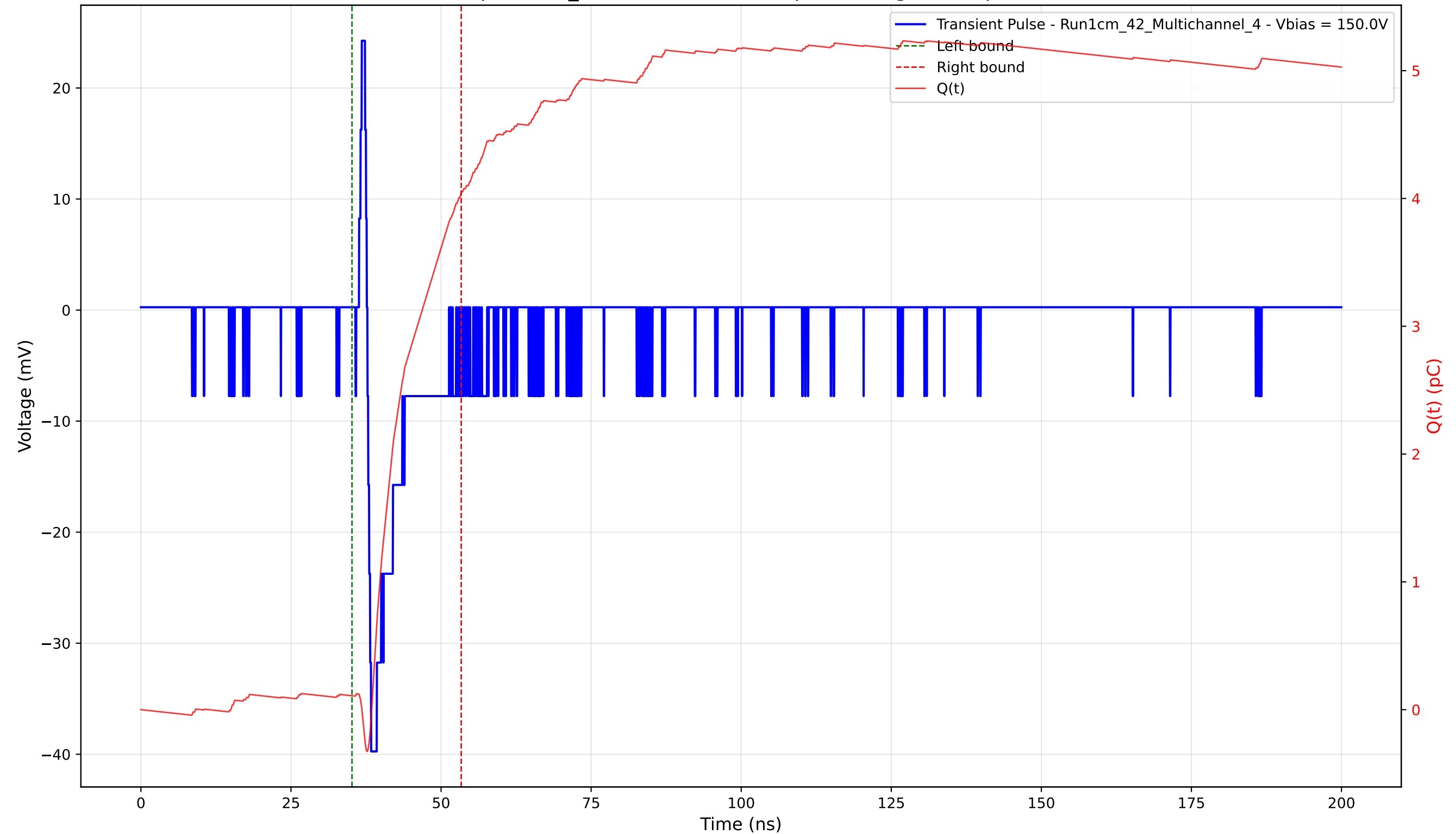
Transient Pulse - Sample: 1cm_42 - Position: 4240.0 \mu\text{m} - Charge: 3.94 pC - Rise Time: 0.62 ns
