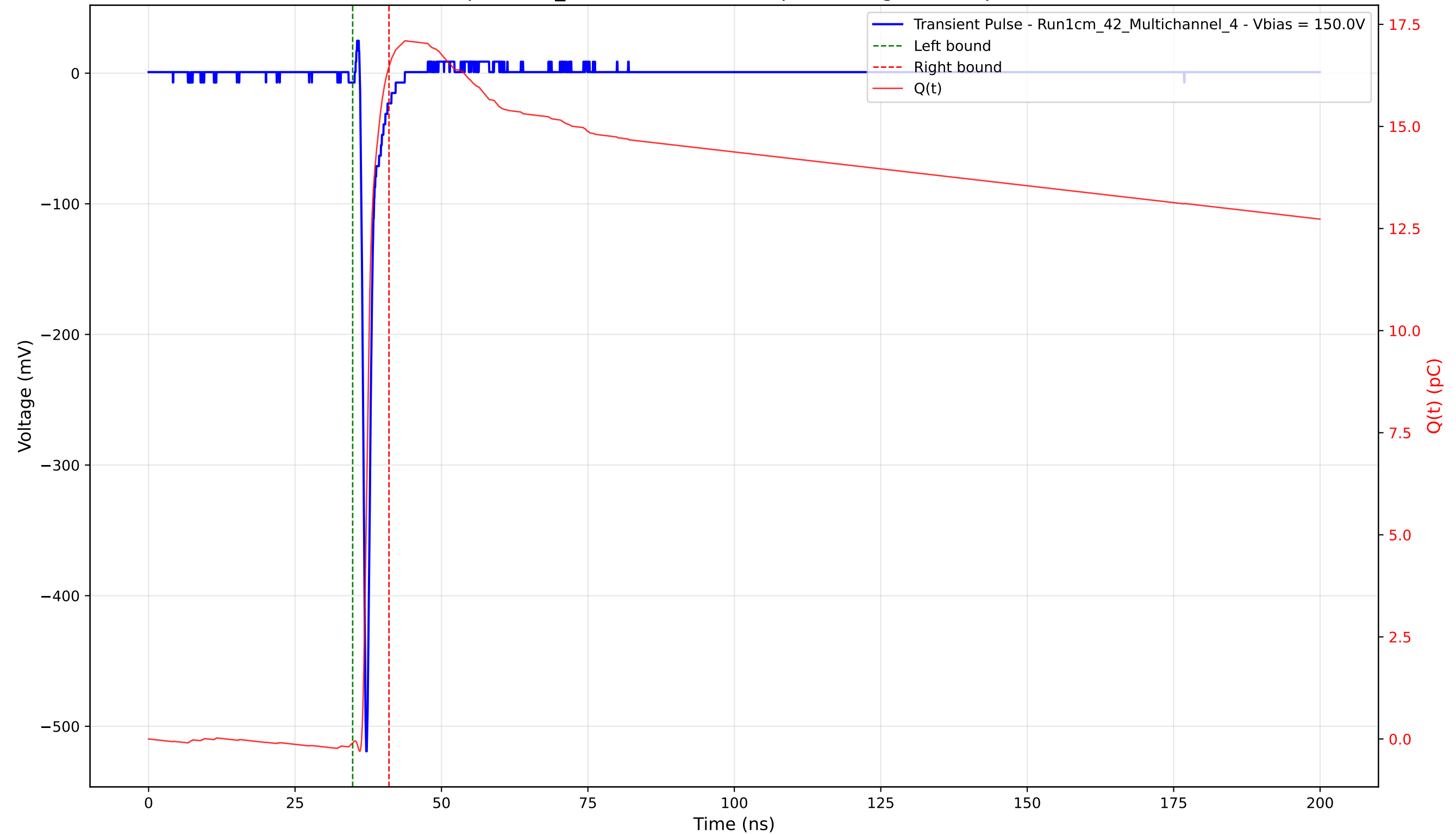
Transient Pulse - Sample: 1cm_42 - Position: 2285.0 \mu\text{m} - Charge: 16.56 pC - Rise Time: 0.72 ns
