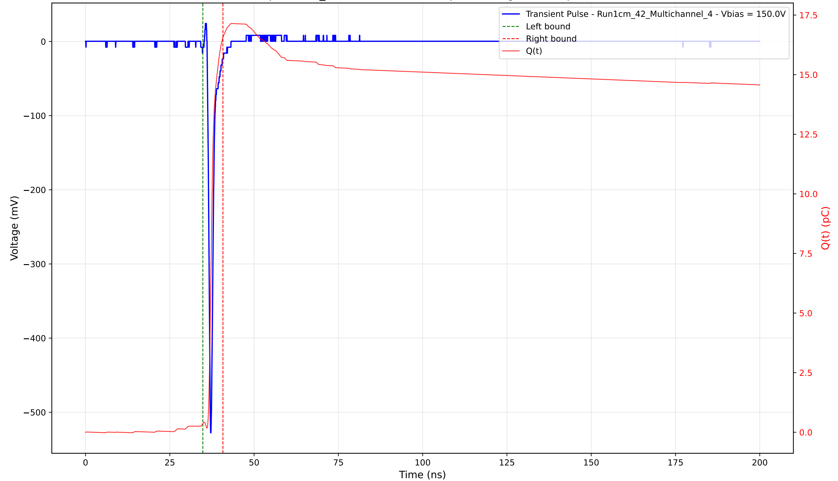
Transient Pulse - Sample: 1cm_42 - Position: 2400.0 \mu\text{m} - Charge: 16.19 pC - Rise Time: 0.74 ns
