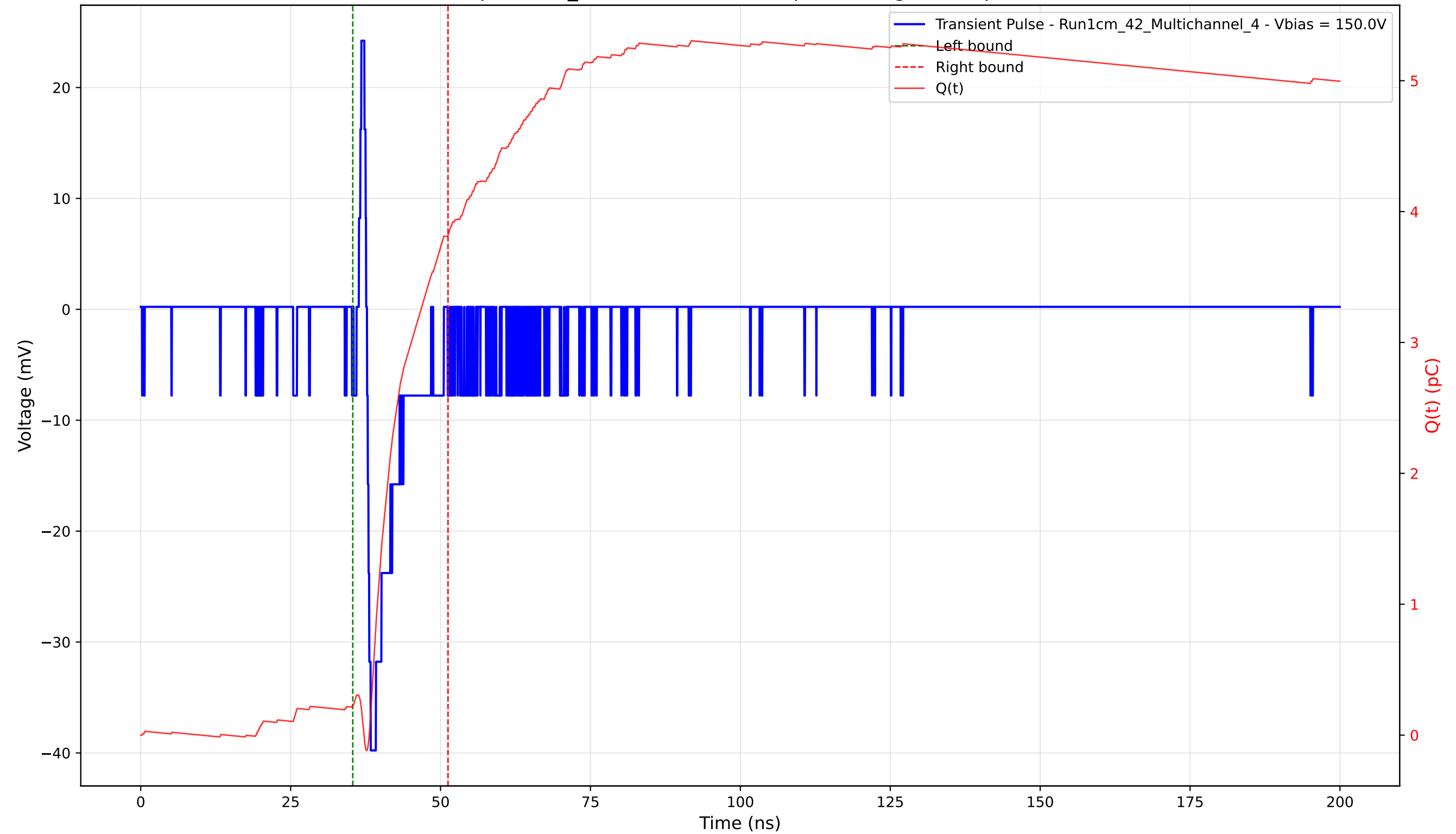
Transient Pulse - Sample: 1cm_42 - Position: 4210.0 \mu\text{m} - Charge: 3.59 pC - Rise Time: 0.62 ns
