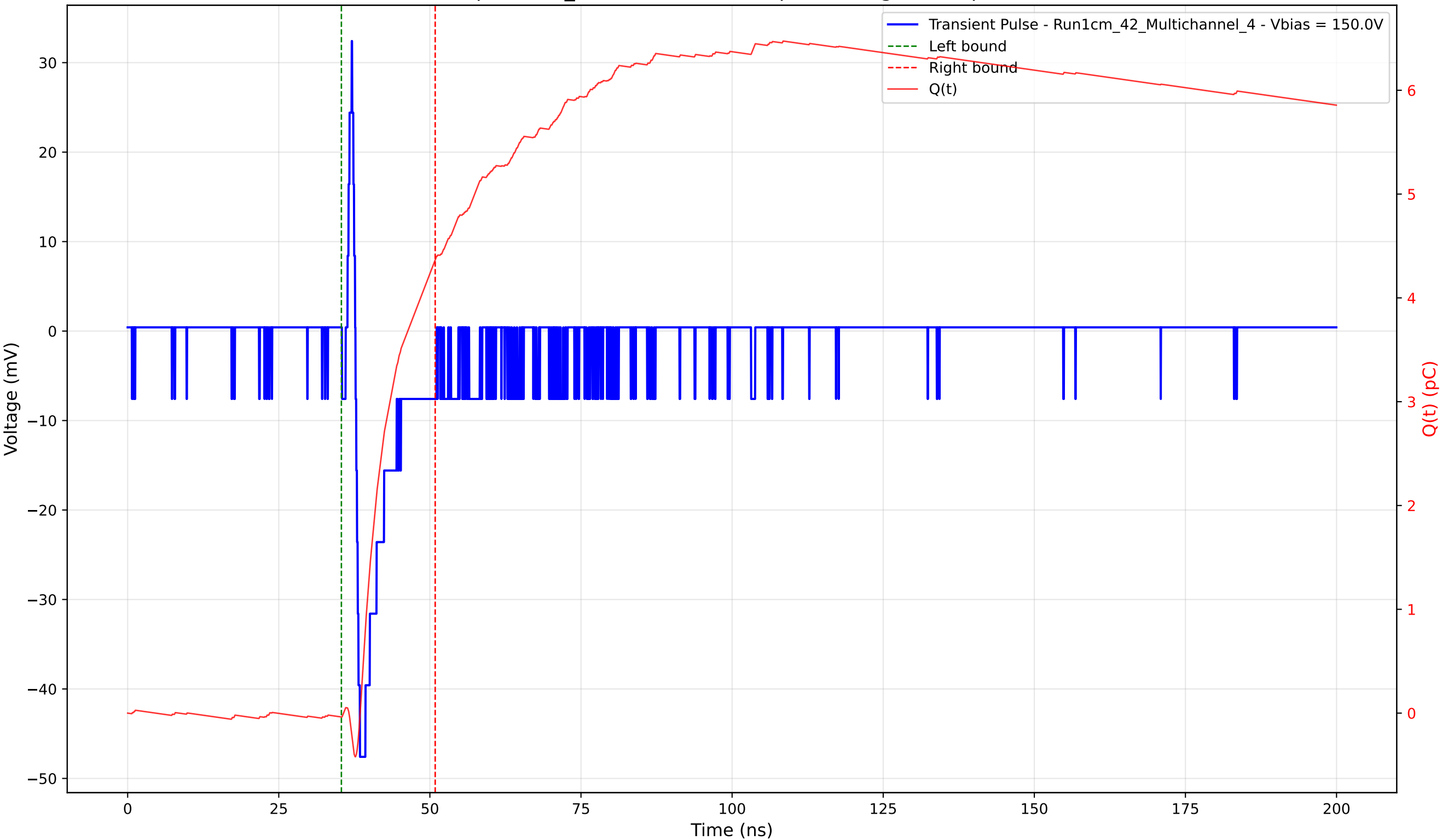
Transient Pulse - Sample: 1cm_42 - Position: 770.0 \mu\text{m} - Charge: 4.41 pC - Rise Time: 0.74 ns
