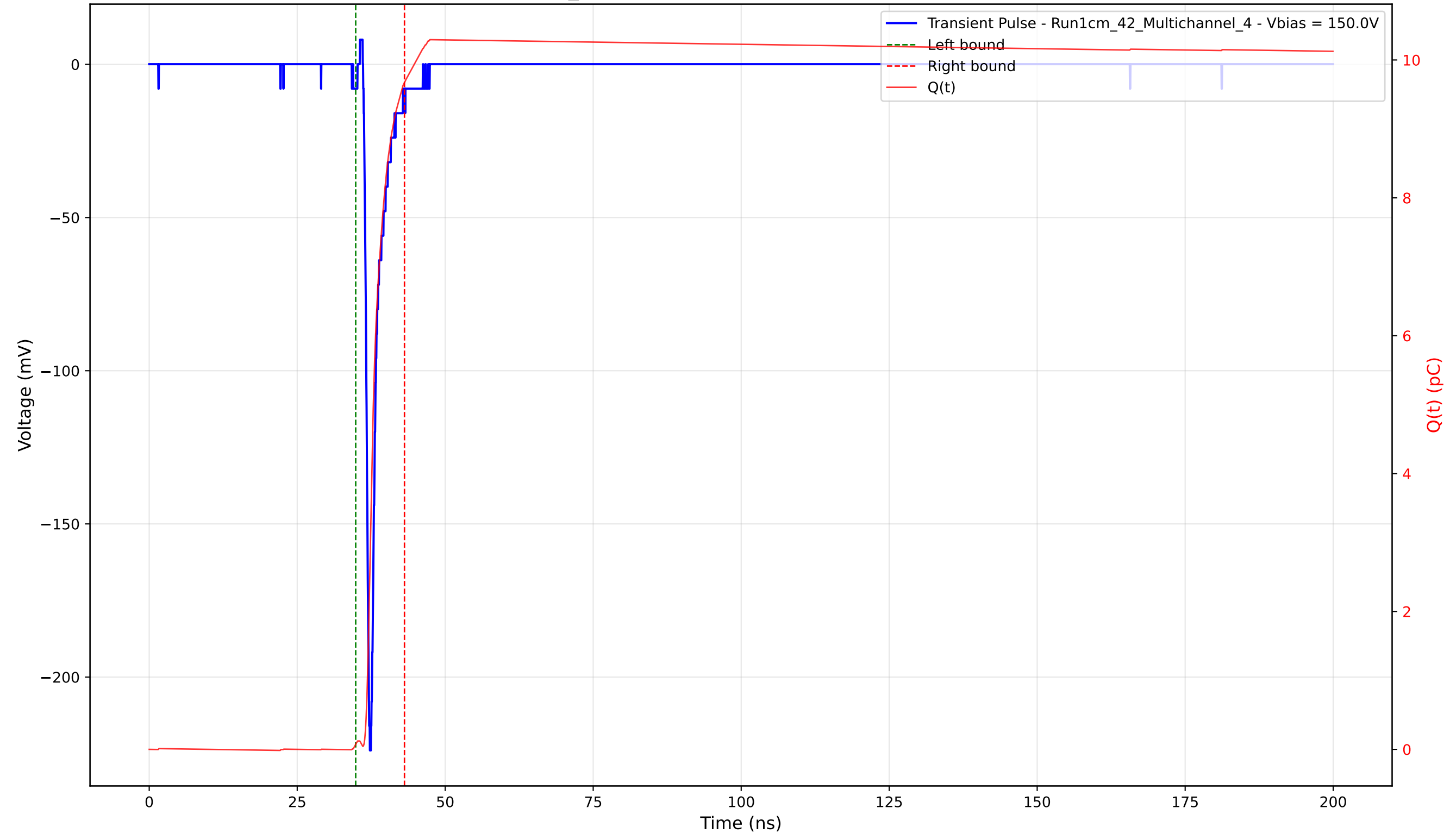
Transient Pulse - Sample: 1cm_42 - Position: 2000.0 \mu\text{m} - Charge: 9.60 pC - Rise Time: 0.78 ns
