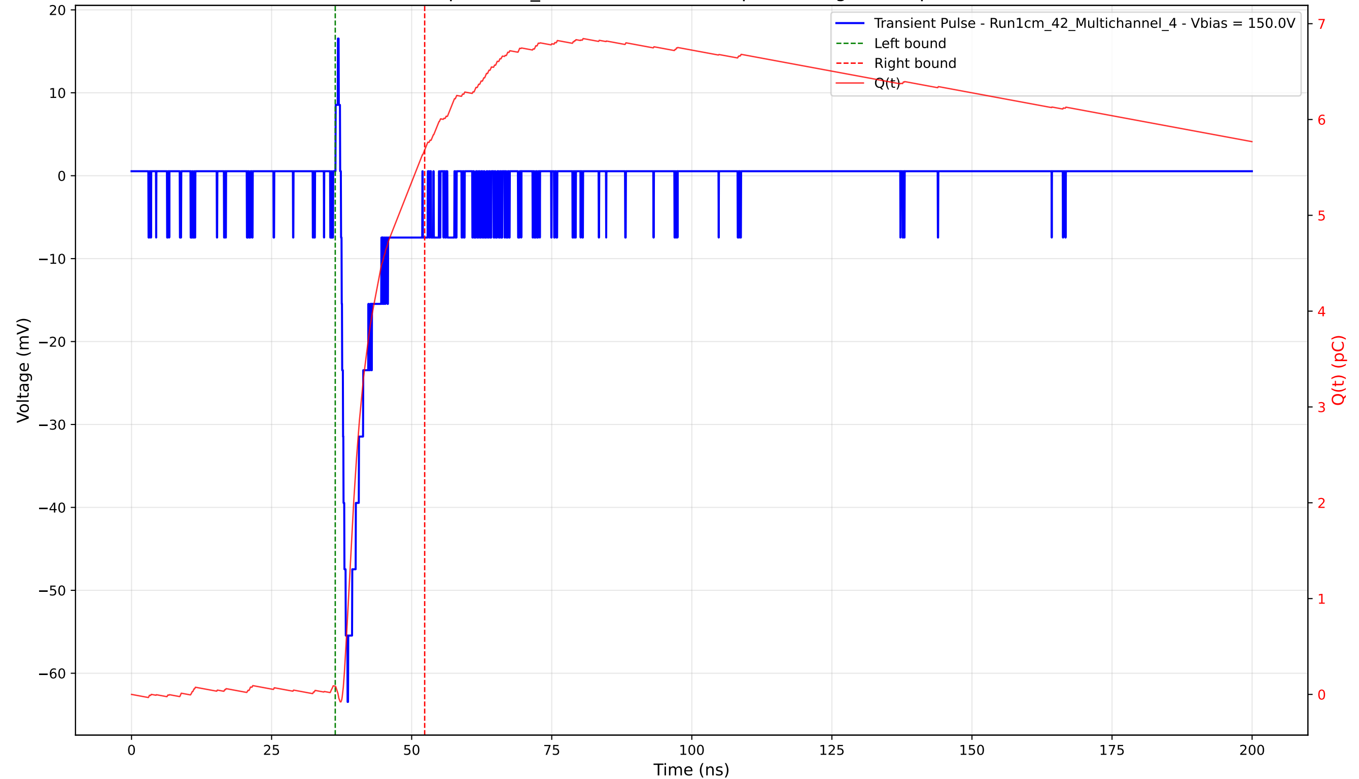
Transient Pulse - Sample: 1cm_42 - Position: 1155.0 \mu\text{m} - Charge: 5.60 pC - Rise Time: 1.17 ns
