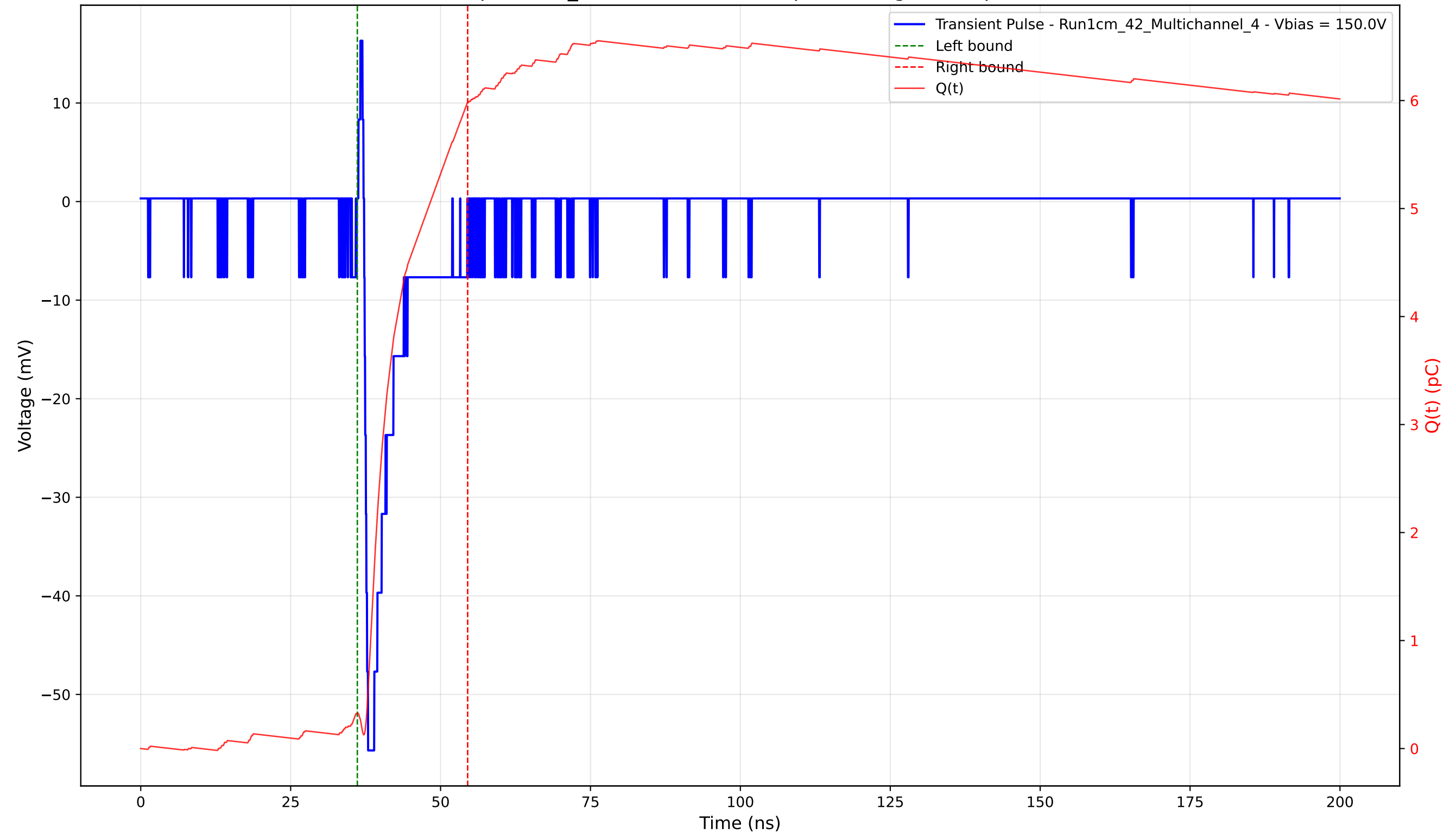
Transient Pulse - Sample: 1cm_42 - Position: 3705.0 \mu\text{m} - Charge: 5.66 pC - Rise Time: 0.65 ns
