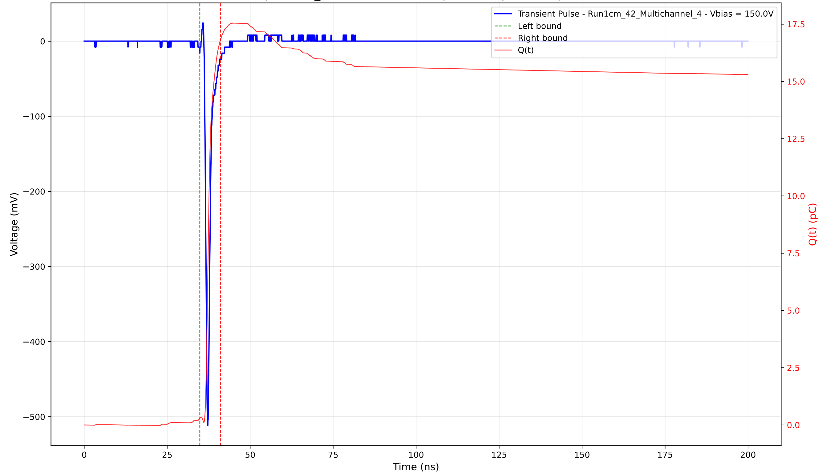
Transient Pulse - Sample: 1cm_42 - Position: 2260.0 \mu\text{m} - Charge: 16.55 pC - Rise Time: 0.72 ns
