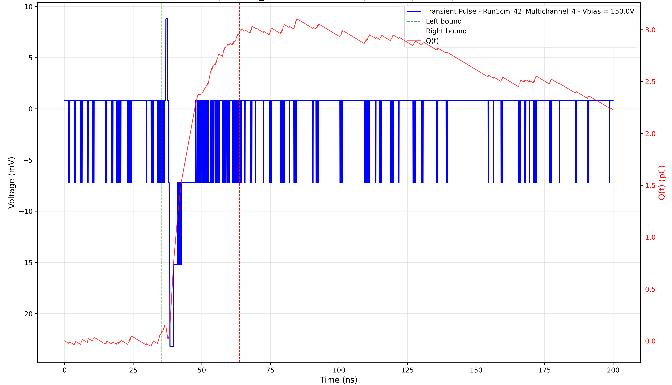
Transient Pulse - Sample: 1cm_42 - Position: 4945.0 \mu\text{m} - Charge: 2.87 pC - Rise Time: 0.59 ns
