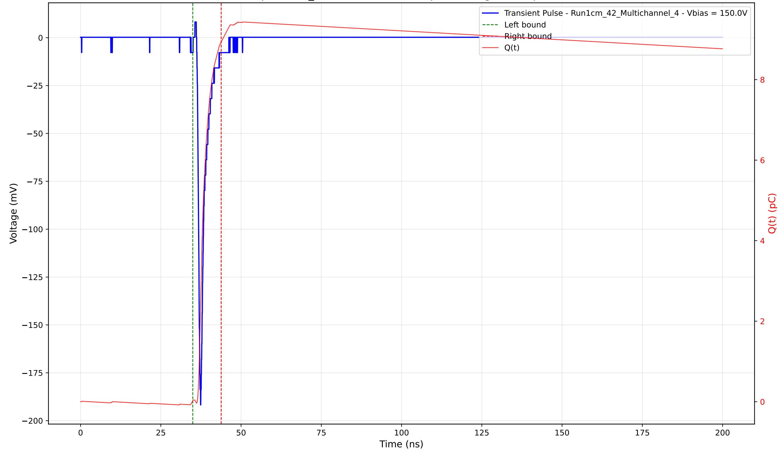
Transient Pulse - Sample: 1cm_42 - Position: 1945.0 \mu\text{m} - Charge: 8.91 pC - Rise Time: 0.82 ns
