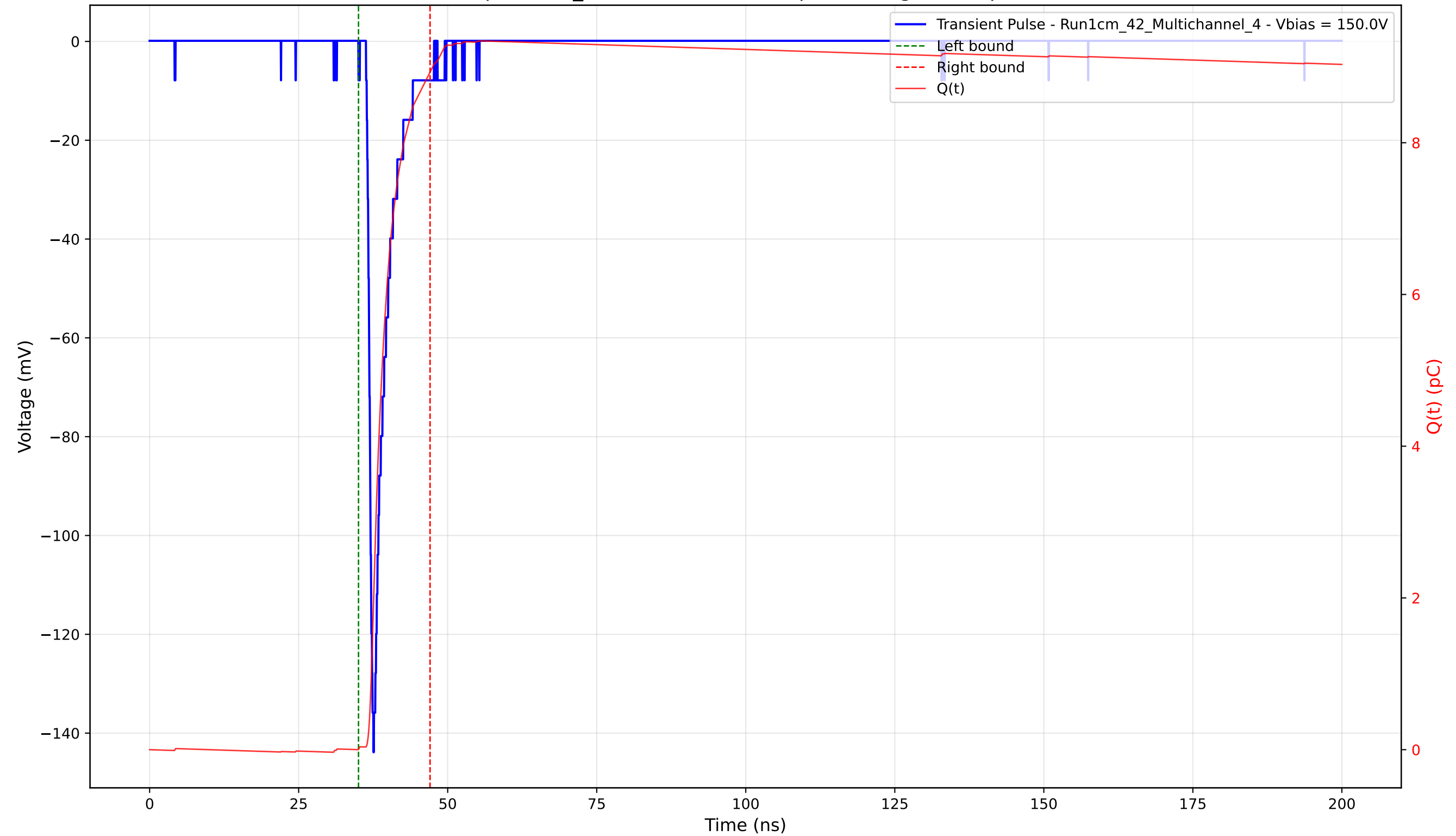
Transient Pulse - Sample: 1cm_42 - Position: 1720.0 \mu\text{m} - Charge: 8.93 pC - Rise Time: 0.97 ns
