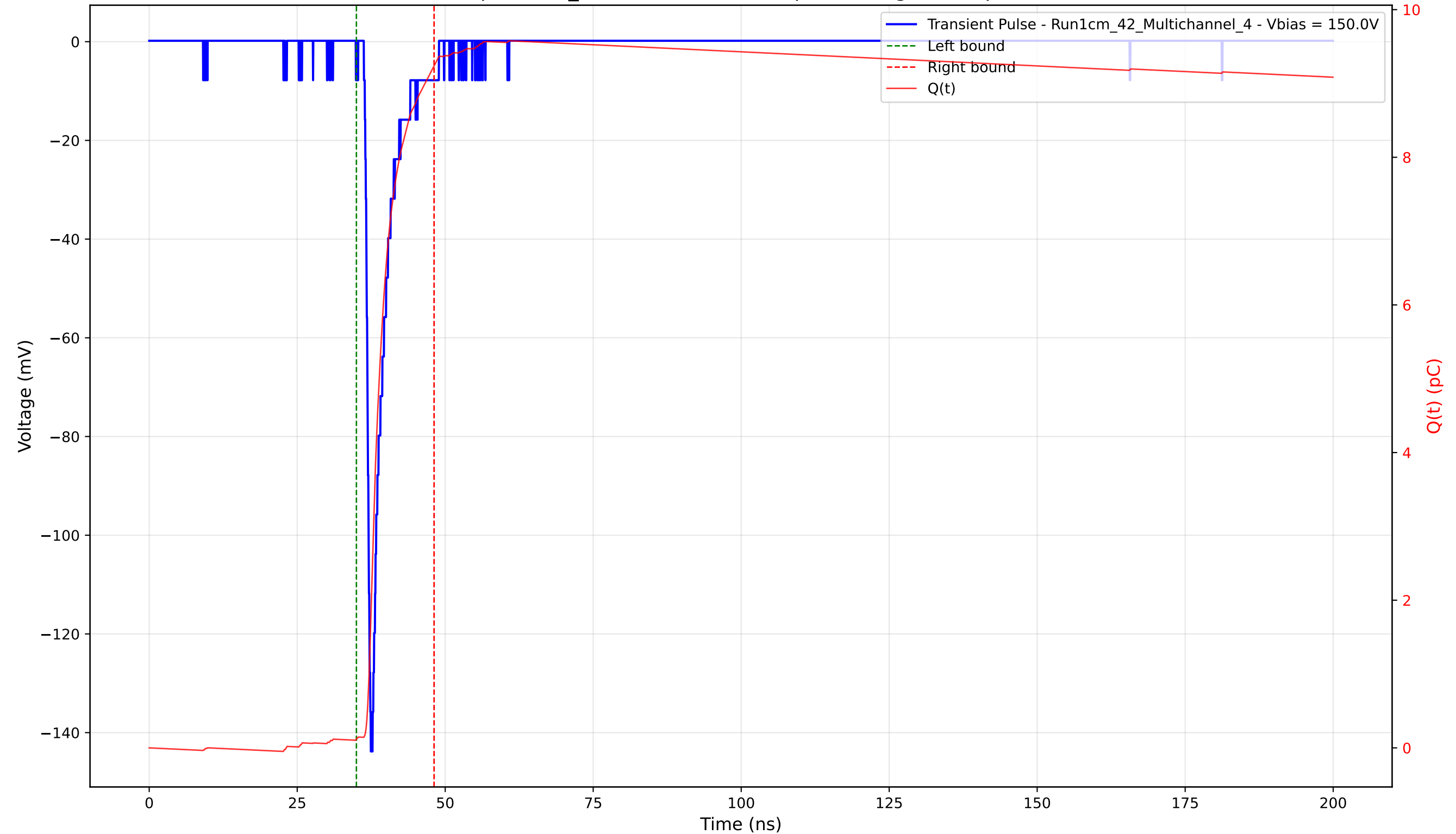
Transient Pulse - Sample: 1cm_42 - Position: 1730.0 \mu\text{m} - Charge: 9.12 pC - Rise Time: 0.93 ns
