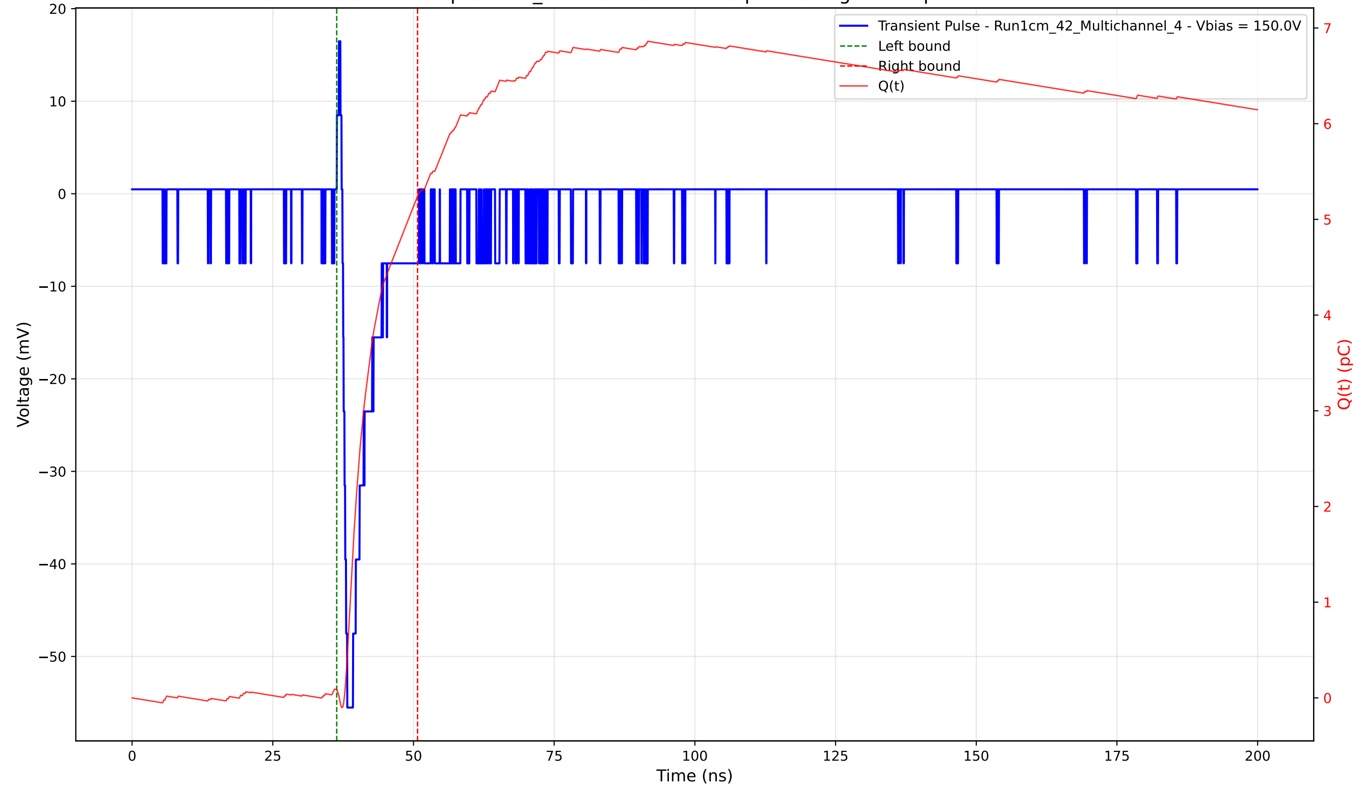
Transient Pulse - Sample: 1cm_42 - Position: 1135.0 \mu\text{m} - Charge: 5.16 pC - Rise Time: 0.85 ns
