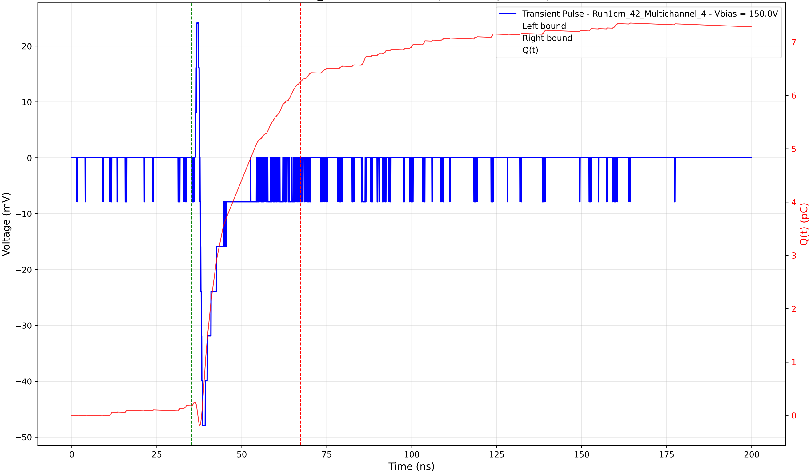
Transient Pulse - Sample: 1cm_42 - Position: 675.0 \mu\text{m} - Charge: 6.08 pC - Rise Time: 0.78 ns
