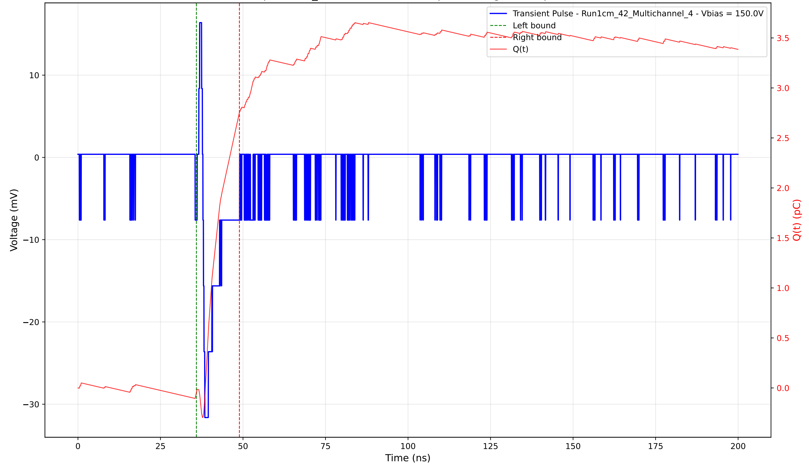
Transient Pulse - Sample: 1cm_42 - Position: 4695.0 \mu\text{m} - Charge: 2.81 pC - Rise Time: 0.58 ns
