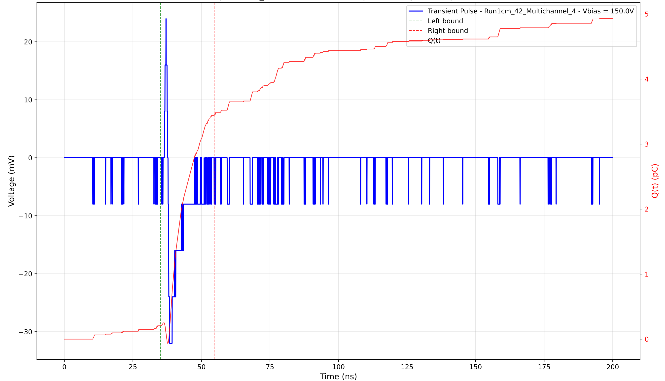
Transient Pulse - Sample: 1cm_42 - Position: 4455.0 \mu\text{m} - Charge: 3.23 pC - Rise Time: 0.58 ns
