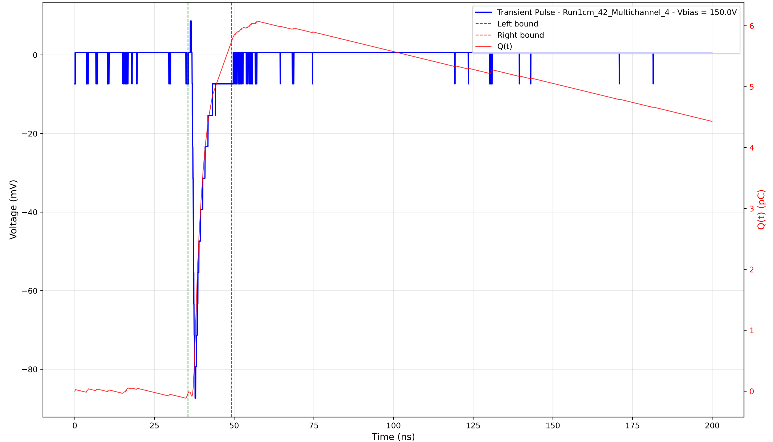
Transient Pulse - Sample: 1cm_42 - Position: 3470.0 \mu\text{m} - Charge: 5.78 pC - Rise Time: 0.71 ns
