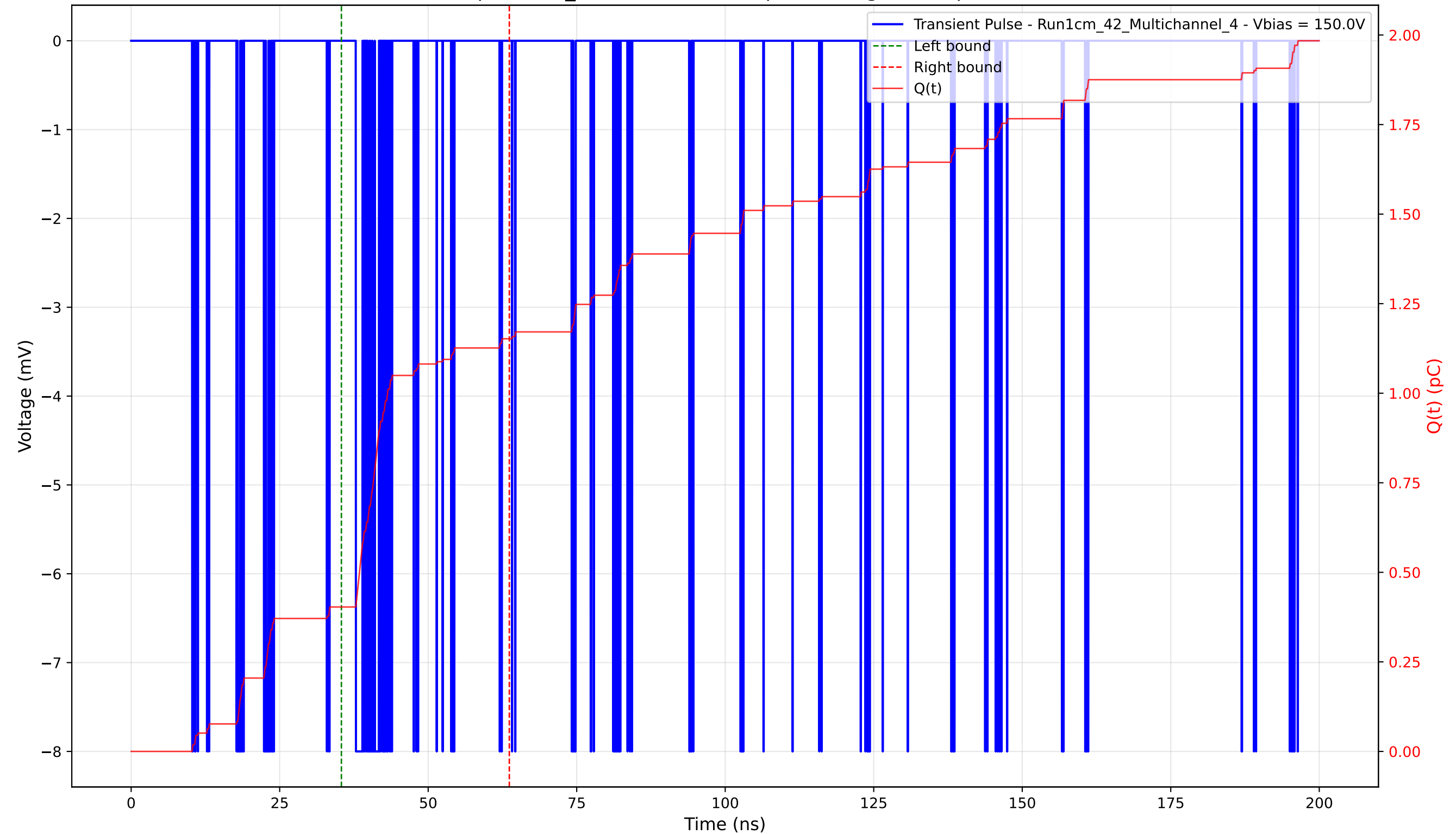
Transient Pulse - Sample: 1cm_42 - Position: 35.0 \mu\text{m} - Charge: 0.75 pC - Rise Time: 0.04 ns
