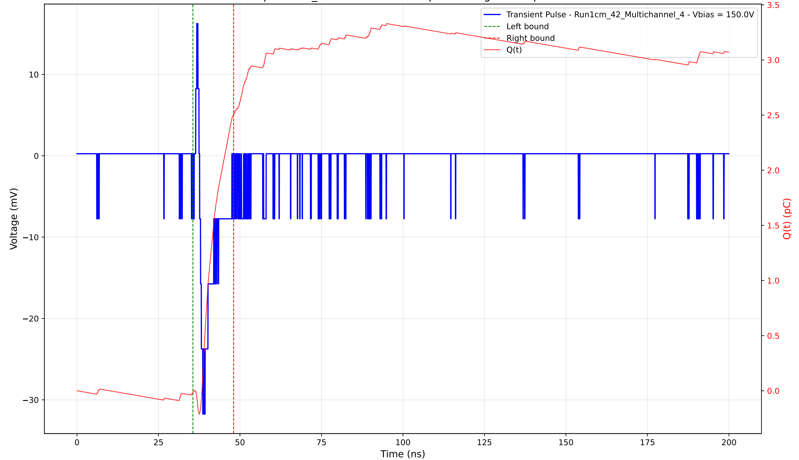
Transient Pulse - Sample: 1cm_42 - Position: 375.0 \mu\text{m} - Charge: 2.53 pC - Rise Time: 0.98 ns
