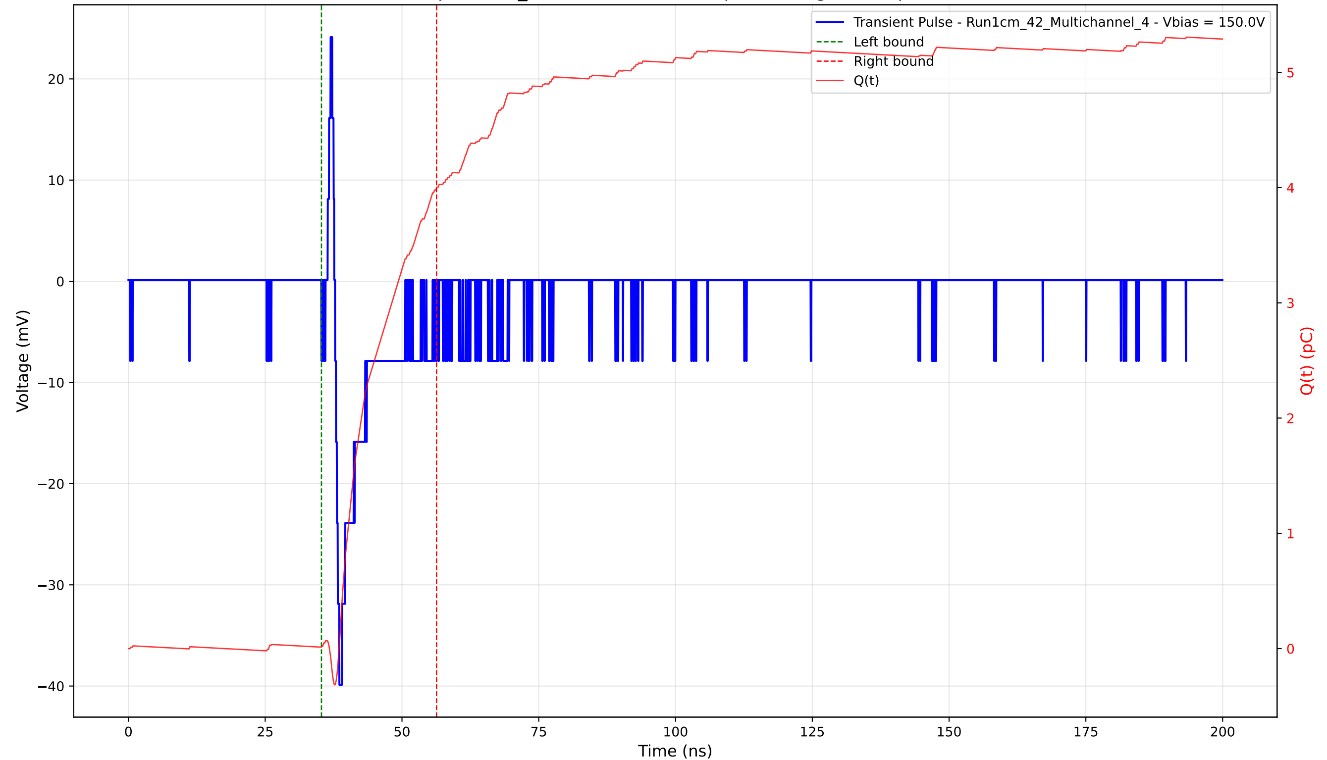
Transient Pulse - Sample: 1cm_42 - Position: 4390.0 \mu\text{m} - Charge: 3.98 pC - Rise Time: 0.78 ns
