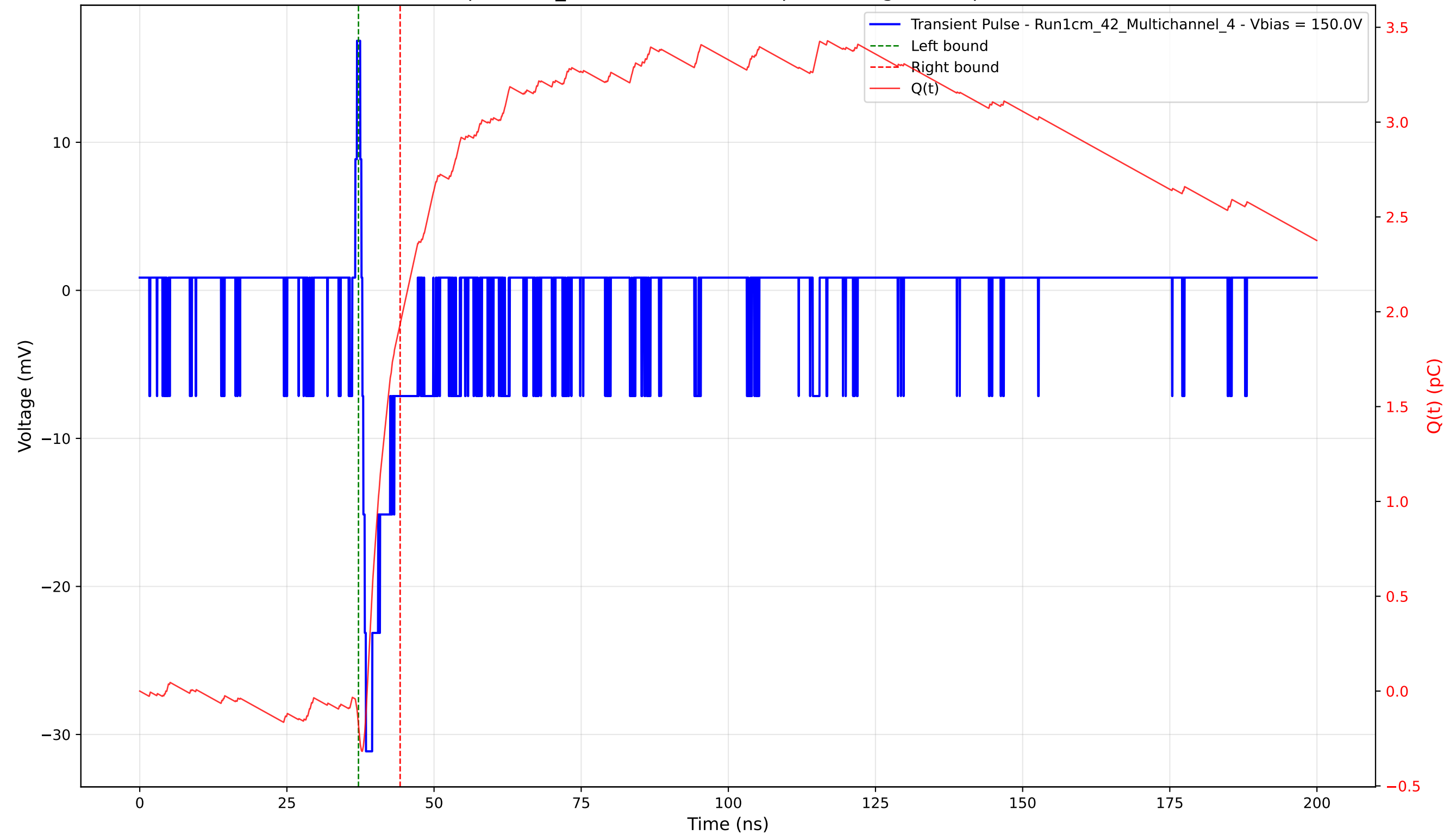
Transient Pulse - Sample: 1cm_42 - Position: 4720.0 \mu\text{m} - Charge: 2.11 pC - Rise Time: 0.63 ns
