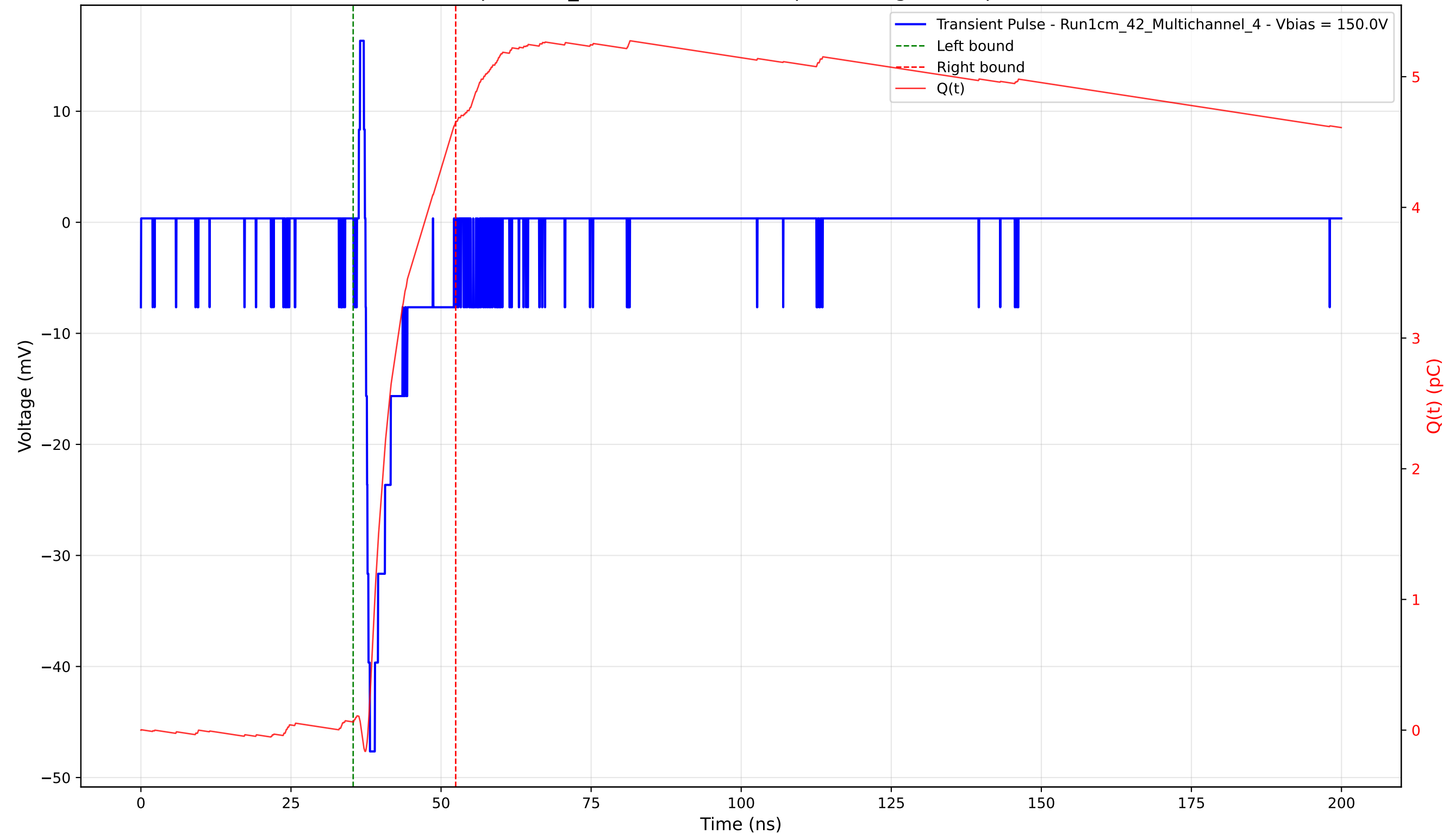
Transient Pulse - Sample: 1cm_42 - Position: 3910.0 \mu\text{m} - Charge: 4.59 pC - Rise Time: 0.74 ns
