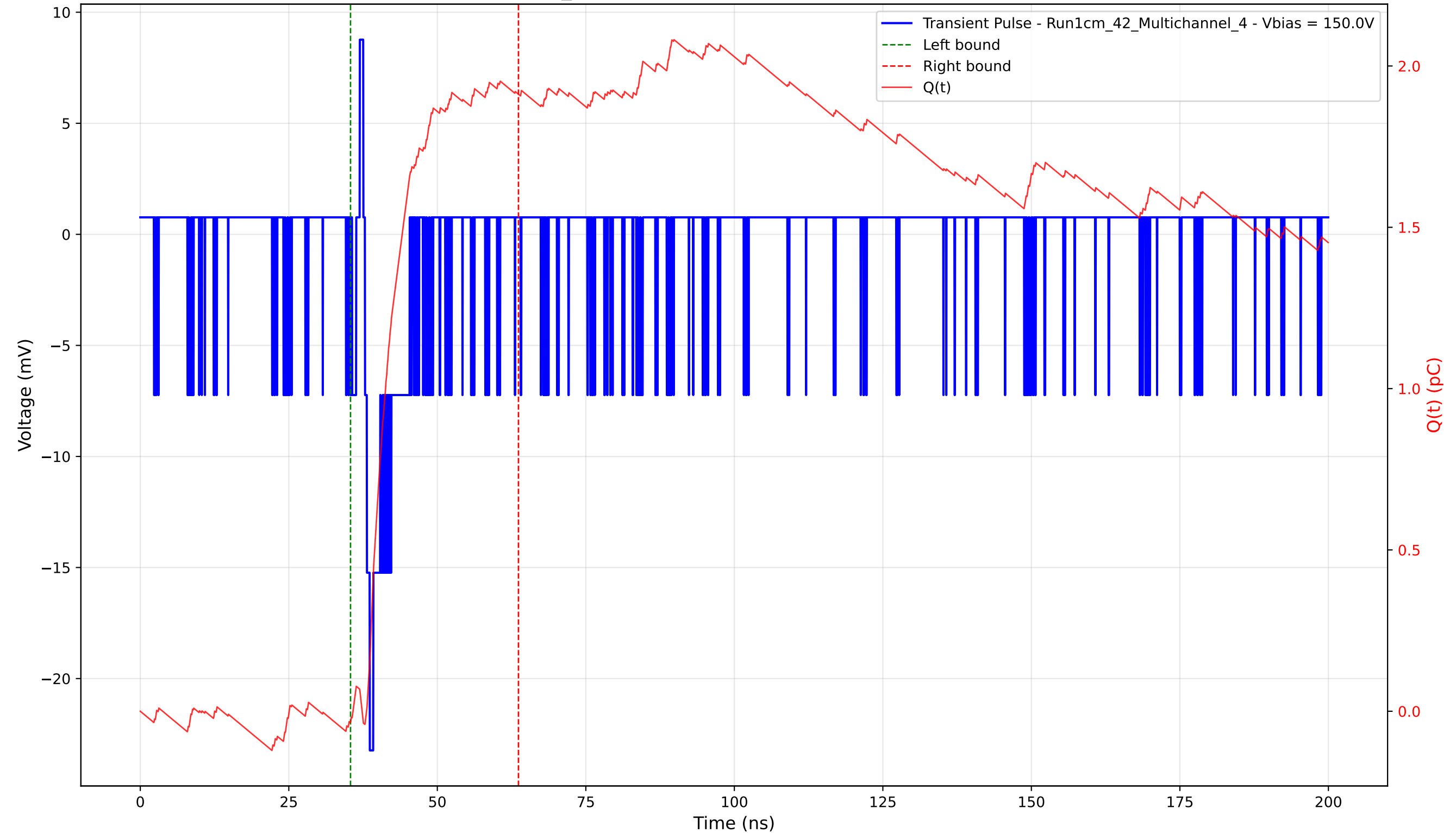
Transient Pulse - Sample: 1cm_42 - Position: 4990.0 \mu\text{m} - Charge: 1.95 pC - Rise Time: 0.83 ns
