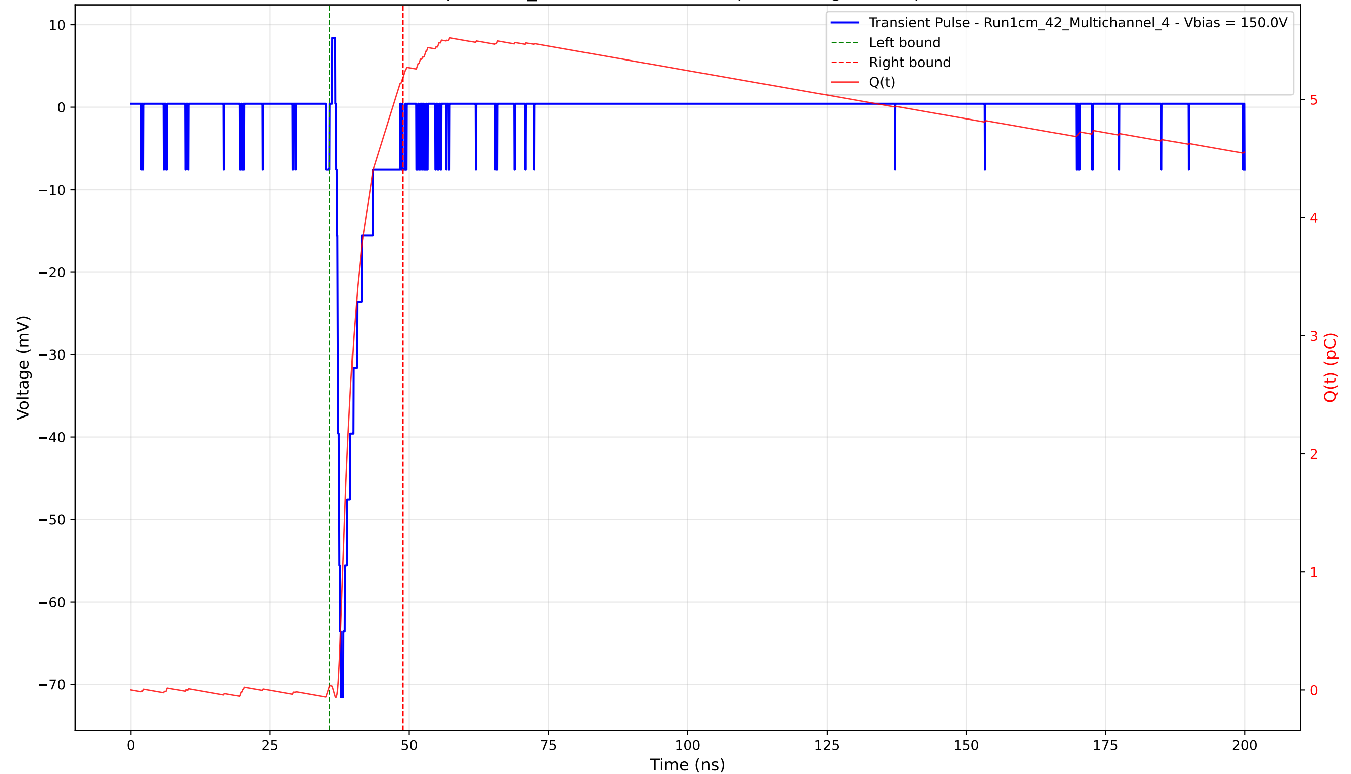
Transient Pulse - Sample: 1cm_42 - Position: 3535.0 \mu\text{m} - Charge: 5.15 pC - Rise Time: 0.84 ns
