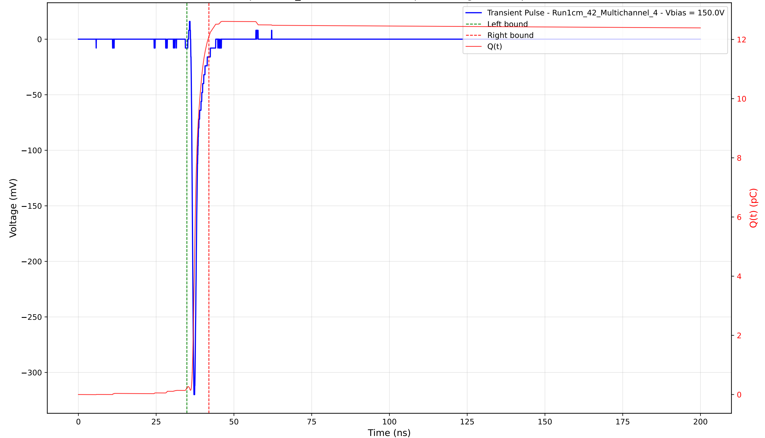
Transient Pulse - Sample: 1cm_42 - Position: 2100.0 \mu\text{m} - Charge: 11.88 pC - Rise Time: 0.72 ns
