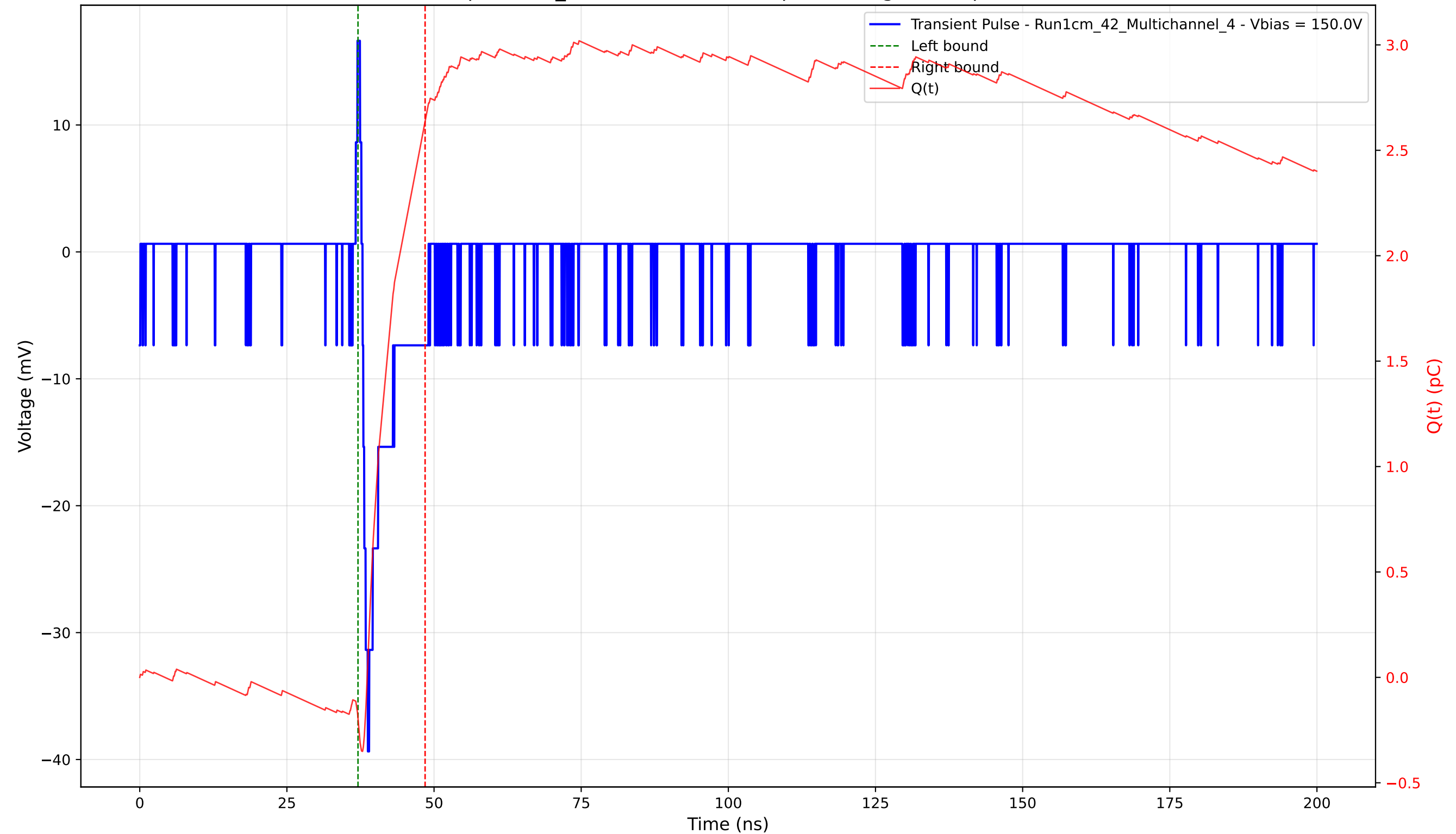
Transient Pulse - Sample: 1cm_42 - Position: 4785.0 \mu\text{m} - Charge: 2.83 pC - Rise Time: 0.90 ns
