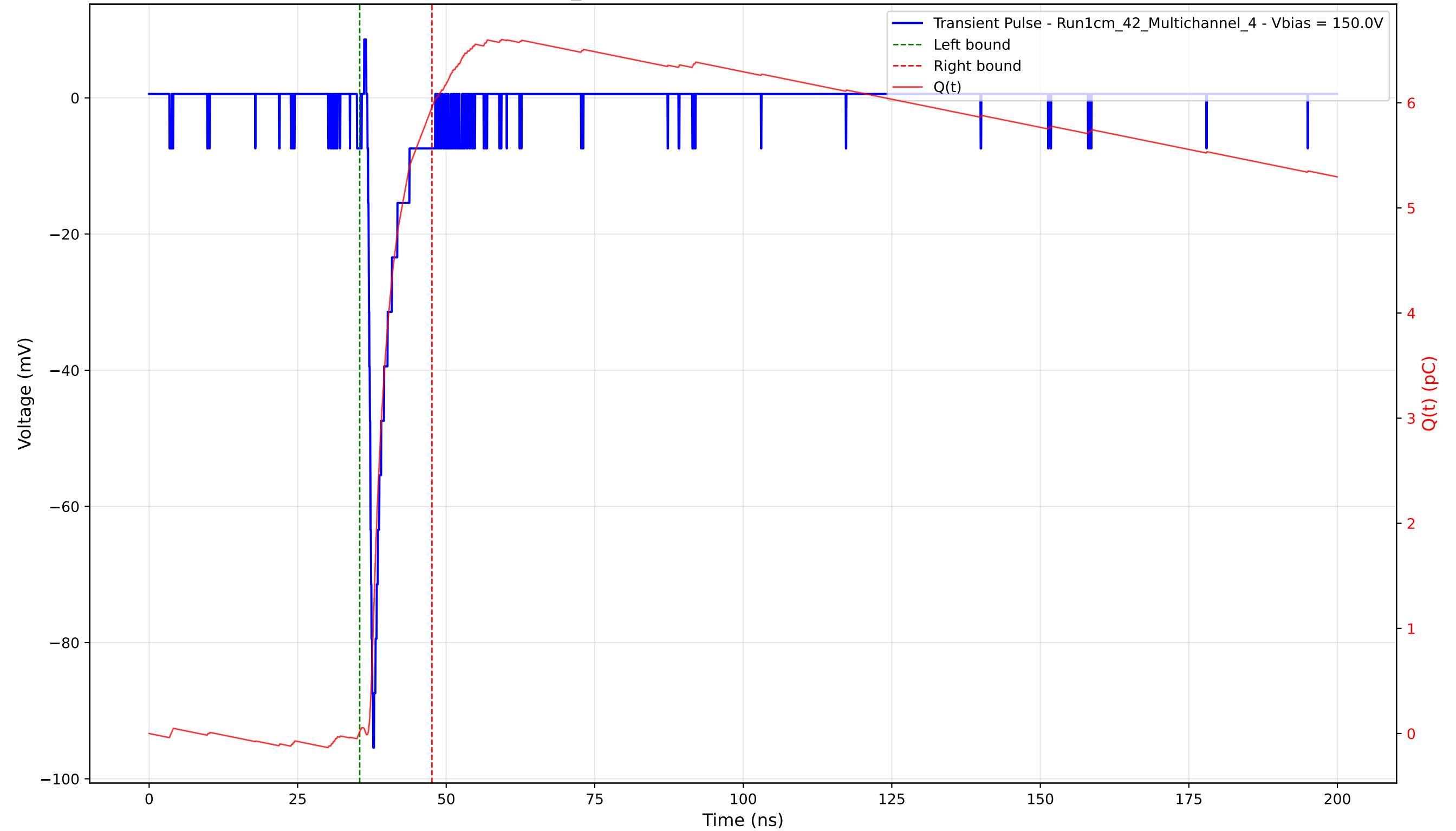
Transient Pulse - Sample: 1cm_42 - Position: 3445.0 \mu\text{m} - Charge: 5.94 pC - Rise Time: 0.71 ns
