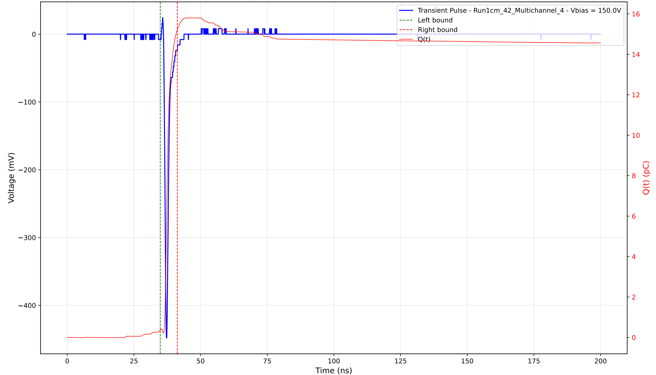
Transient Pulse - Sample: 1cm_42 - Position: 2820.0 \mu\text{m} - Charge: 14.86 pC - Rise Time: 0.76 ns
