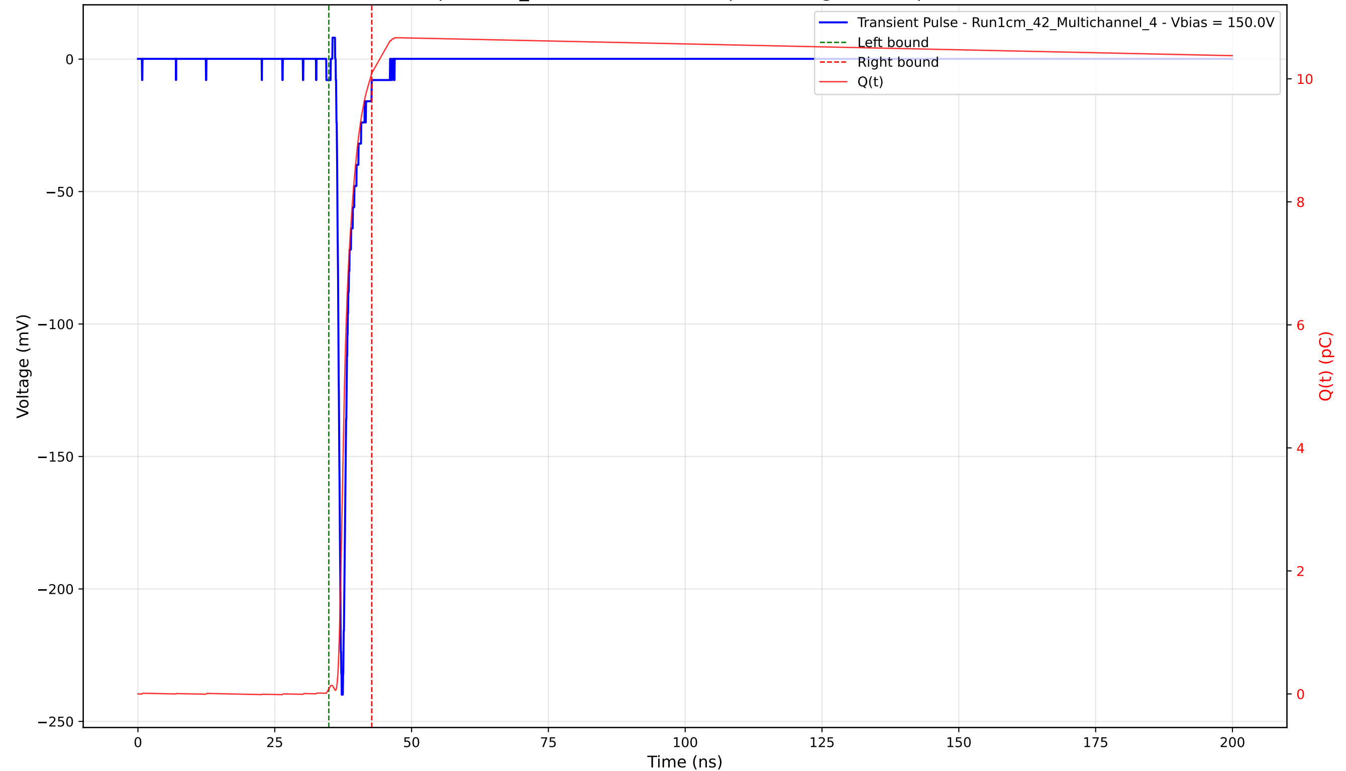
Transient Pulse - Sample: 1cm_42 - Position: 2020.0 \mu\text{m} - Charge: 10.01 pC - Rise Time: 0.76 ns
