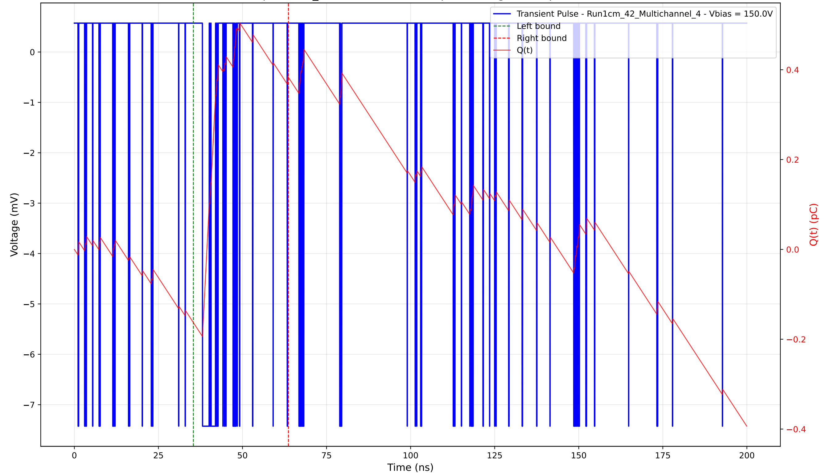
Transient Pulse - Sample: 1cm_42 - Position: 5150.0 \mu\text{m} - Charge: 0.55 pC - Rise Time: 0.04 ns
