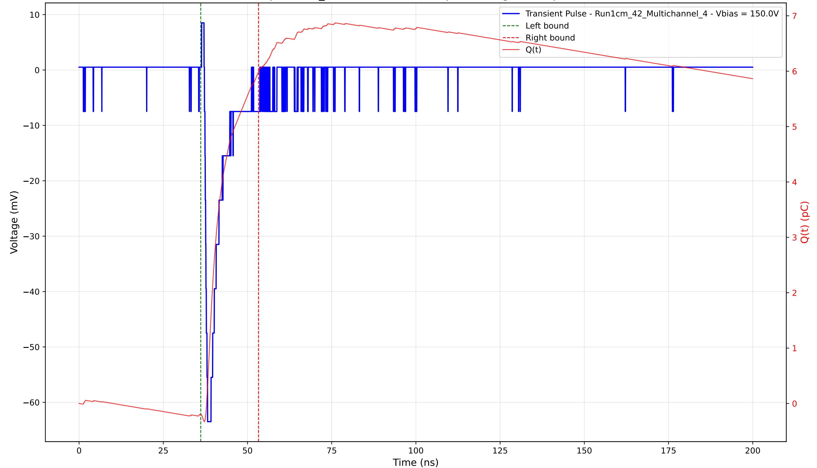
Transient Pulse - Sample: 1cm_42 - Position: 1255.0 \mu\text{m} - Charge: 6.20 pC - Rise Time: 0.93 ns
