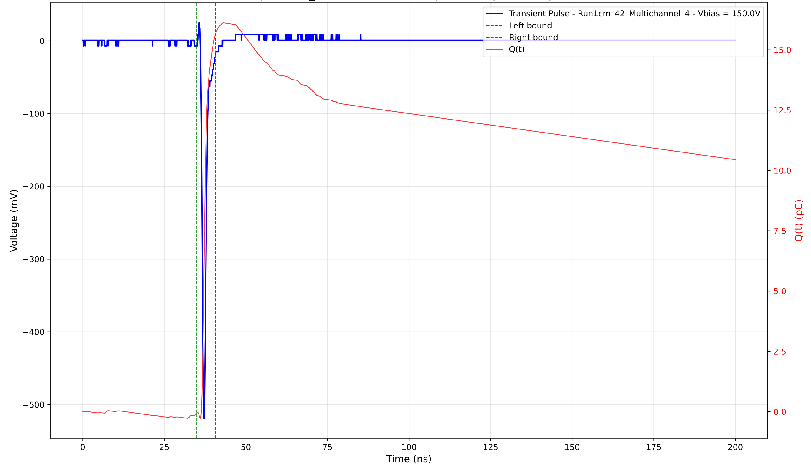
Transient Pulse - Sample: 1cm_42 - Position: 2515.0 \mu\text{m} - Charge: 15.70 pC - Rise Time: 0.72 ns
