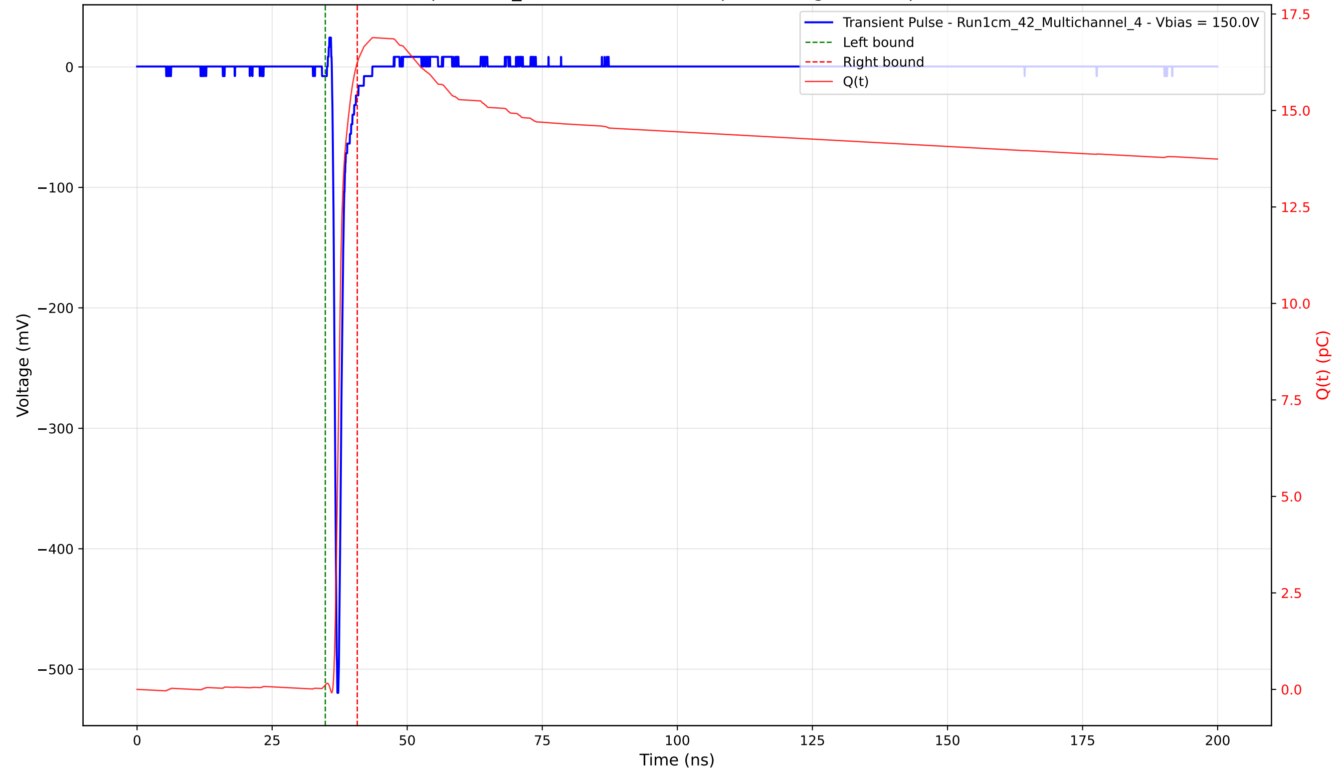
Transient Pulse - Sample: 1cm_42 - Position: 2395.0 \mu\text{m} - Charge: 16.12 pC - Rise Time: 0.70 ns
