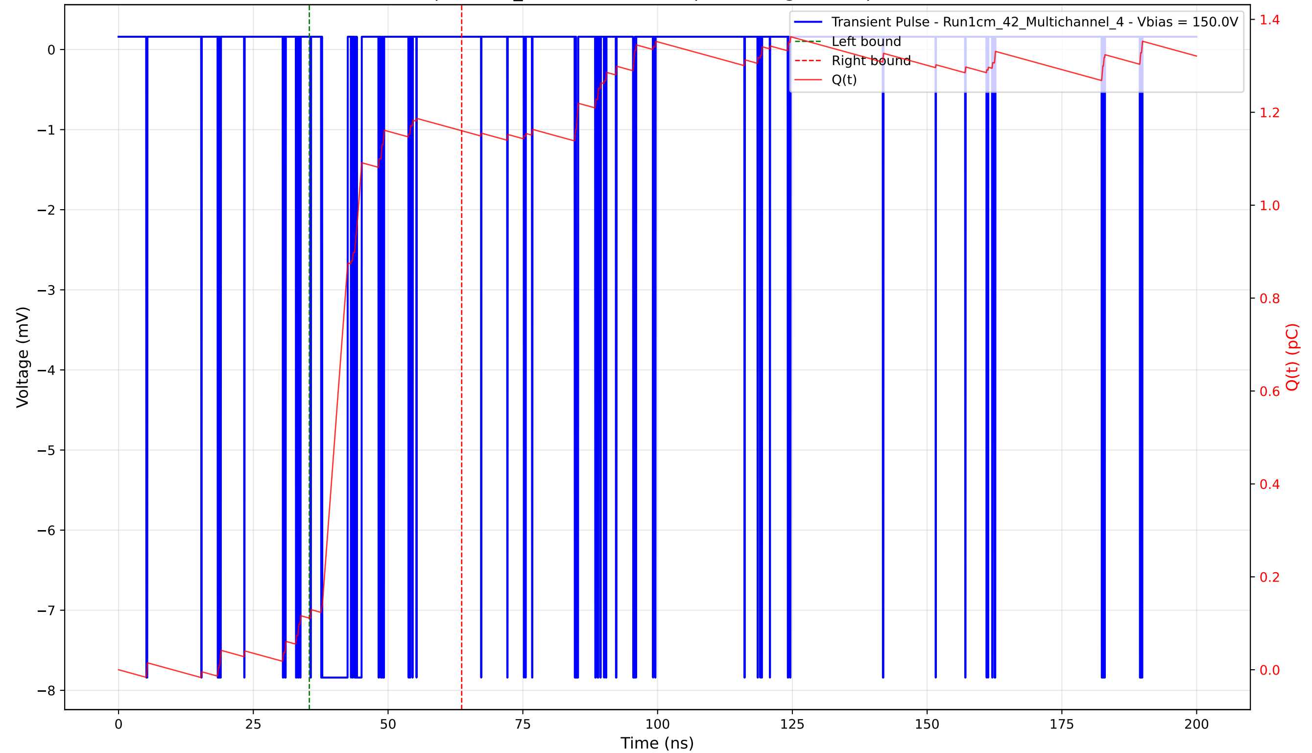
Transient Pulse - Sample: 1cm_42 - Position: 95.0 \mu\text{m} - Charge: 1.05 pC - Rise Time: 0.04 ns
