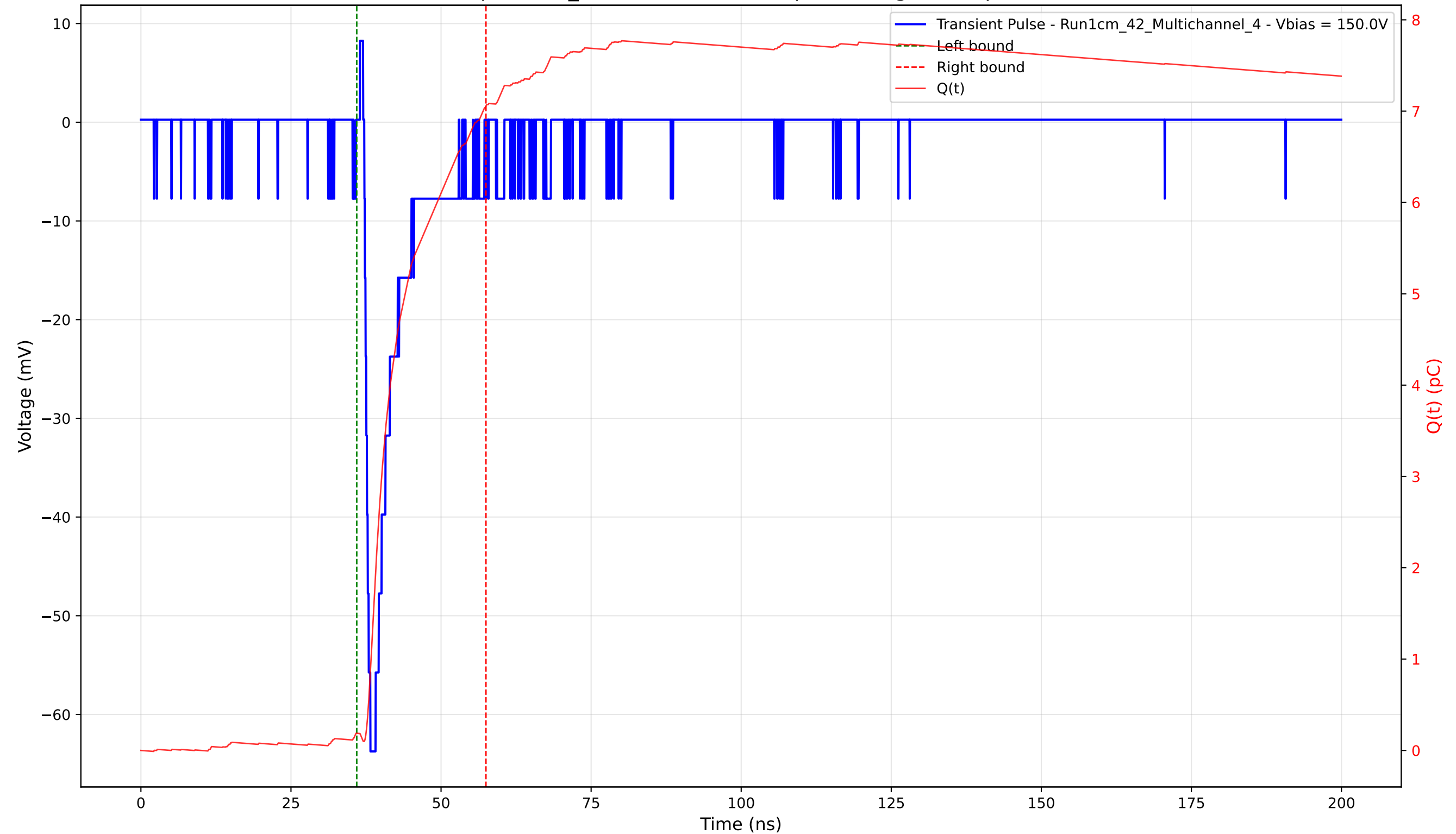
Transient Pulse - Sample: 1cm_42 - Position: 1290.0 \mu\text{m} - Charge: 6.87 pC - Rise Time: 1.01 ns
