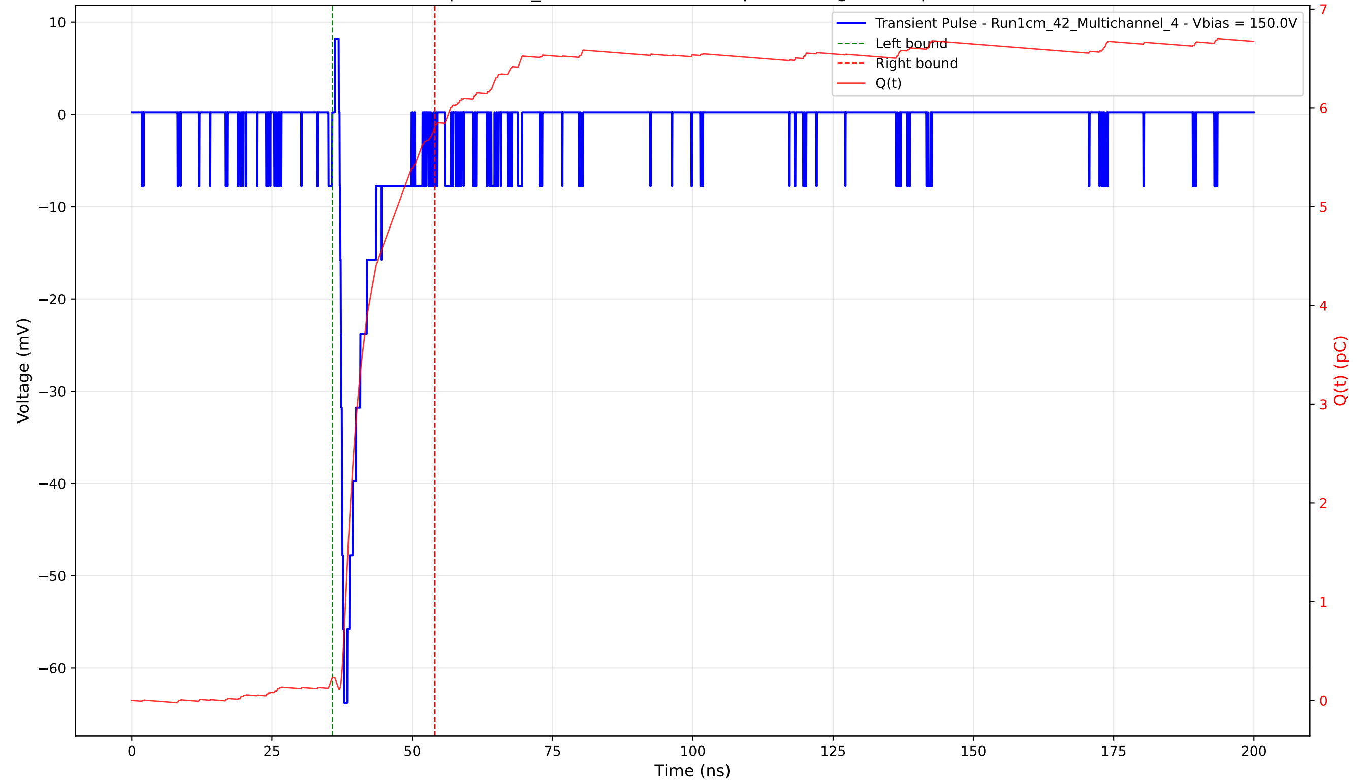
Transient Pulse - Sample: 1cm_42 - Position: 3605.0 \mu\text{m} - Charge: 5.57 pC - Rise Time: 0.81 ns
