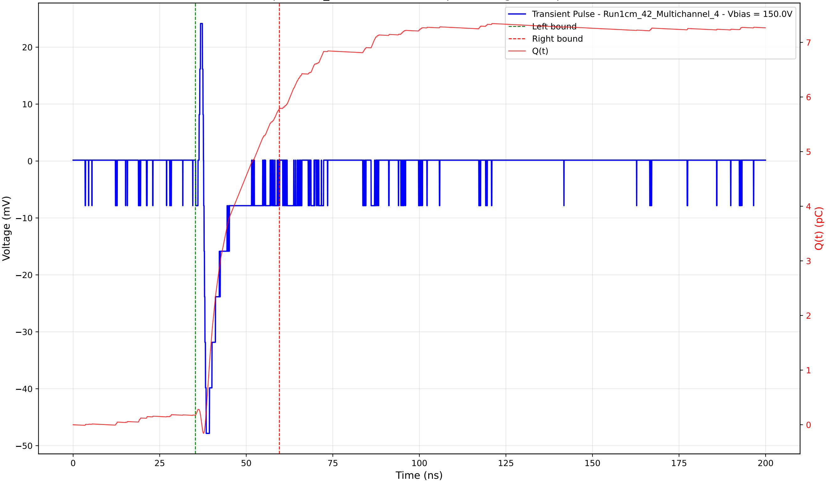
Transient Pulse - Sample: 1cm_42 - Position: 790.0 \mu\text{m} - Charge: 5.61 pC - Rise Time: 0.74 ns
