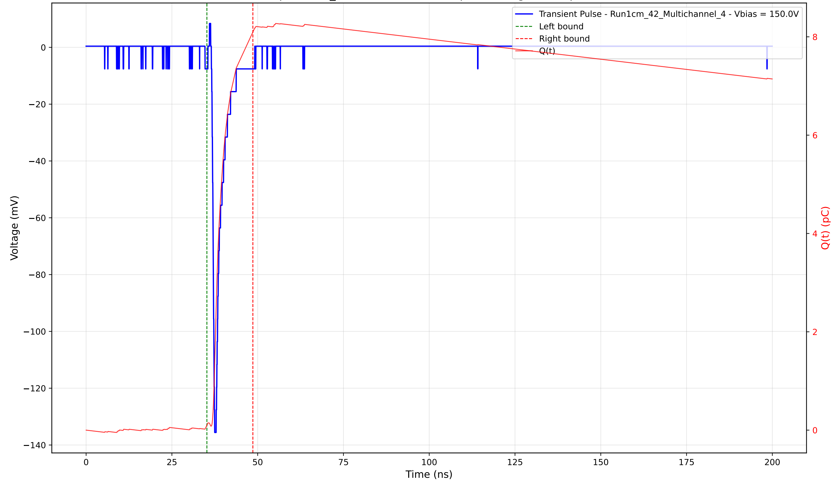
Transient Pulse - Sample: 1cm_42 - Position: 3290.0 \mu\text{m} - Charge: 8.00 pC - Rise Time: 0.77 ns
