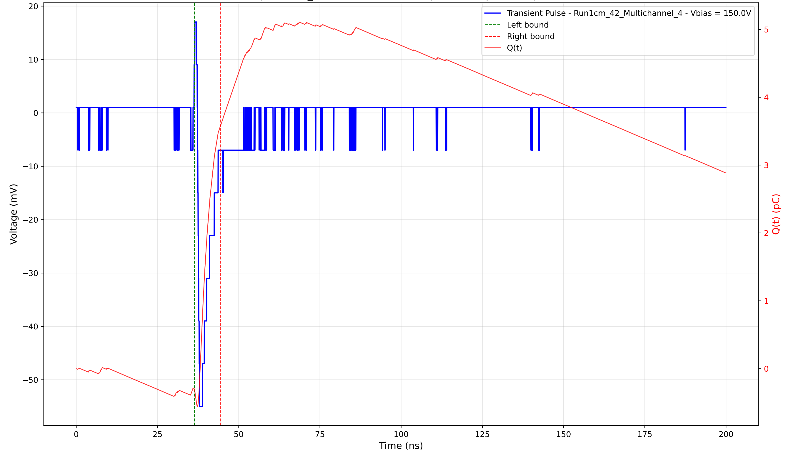
Transient Pulse - Sample: 1cm_42 - Position: 3780.0 \mu\text{m} - Charge: 3.91 pC - Rise Time: 0.69 ns
