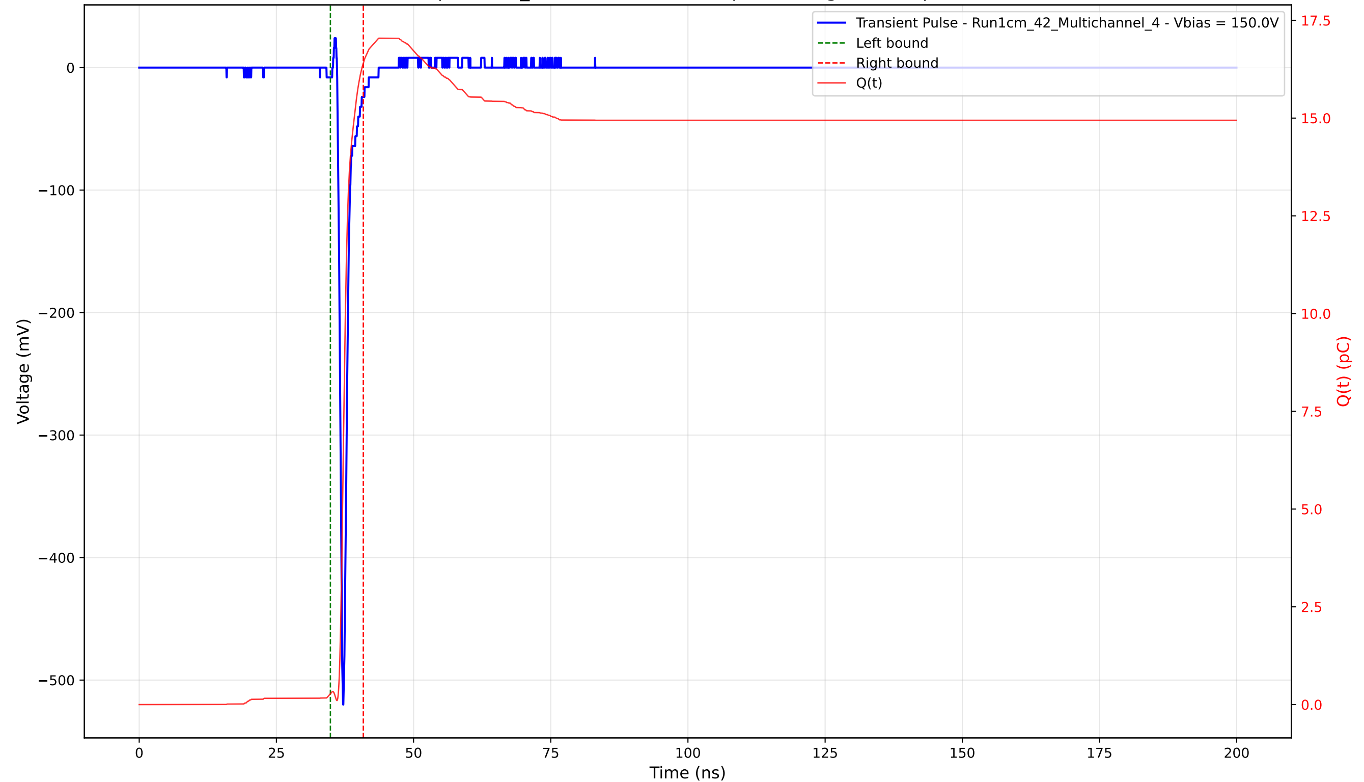
Transient Pulse - Sample: 1cm_42 - Position: 2670.0 \mu\text{m} - Charge: 16.13 pC - Rise Time: 0.74 ns
