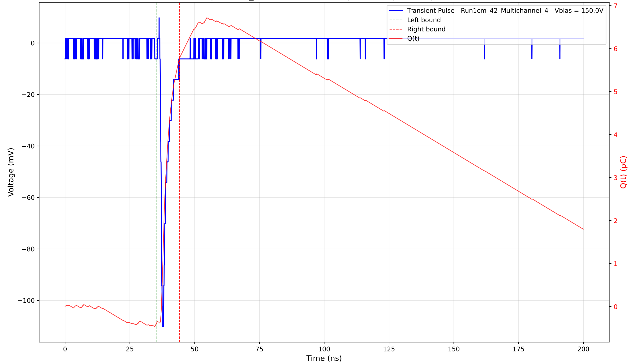
Transient Pulse - Sample: 1cm_42 - Position: 3375.0 \mu\text{m} - Charge: 6.13 pC - Rise Time: 0.74 ns
