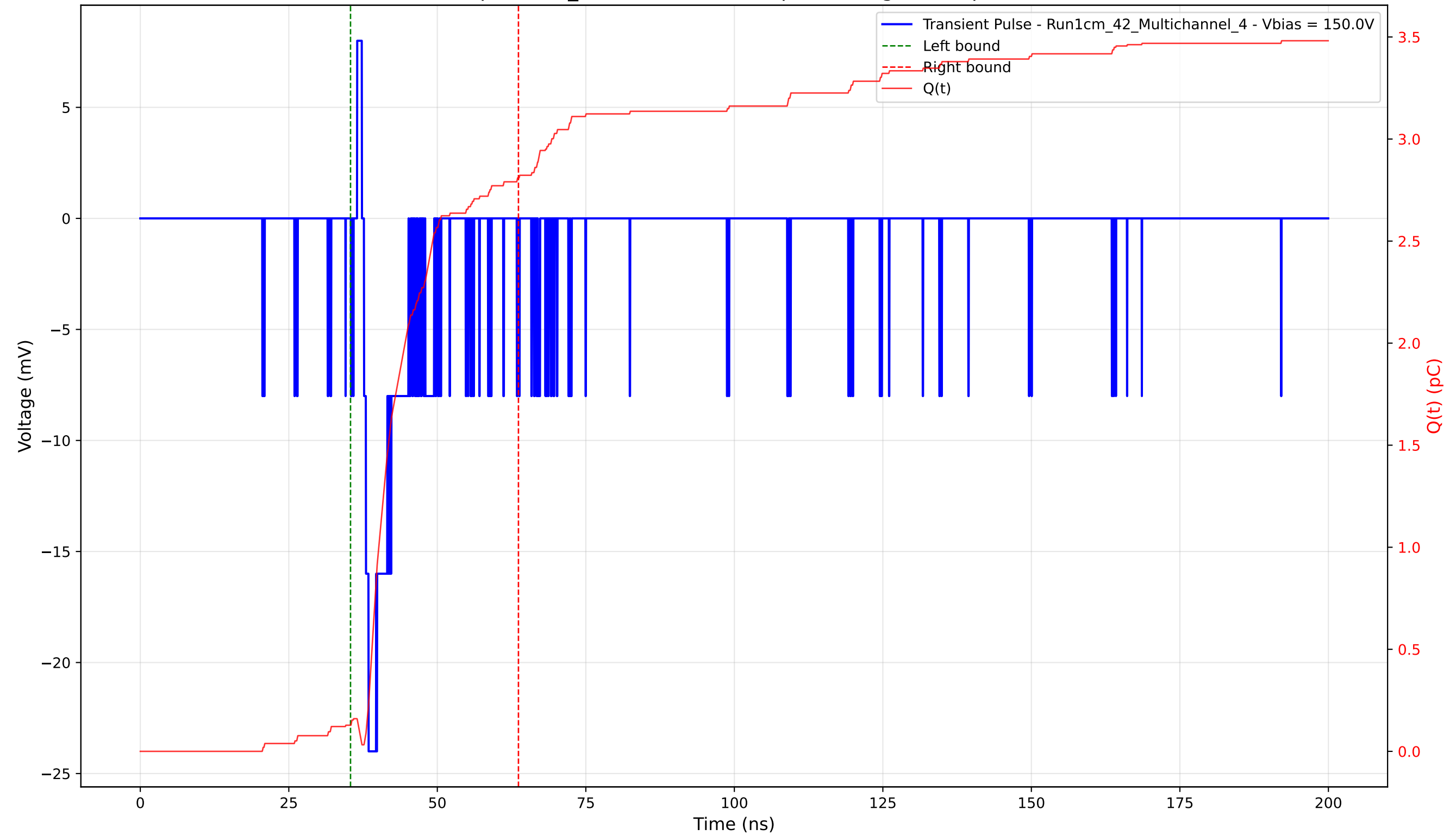
Transient Pulse - Sample: 1cm_42 - Position: 310.0 \mu\text{m} - Charge: 2.68 pC - Rise Time: 0.79 ns
