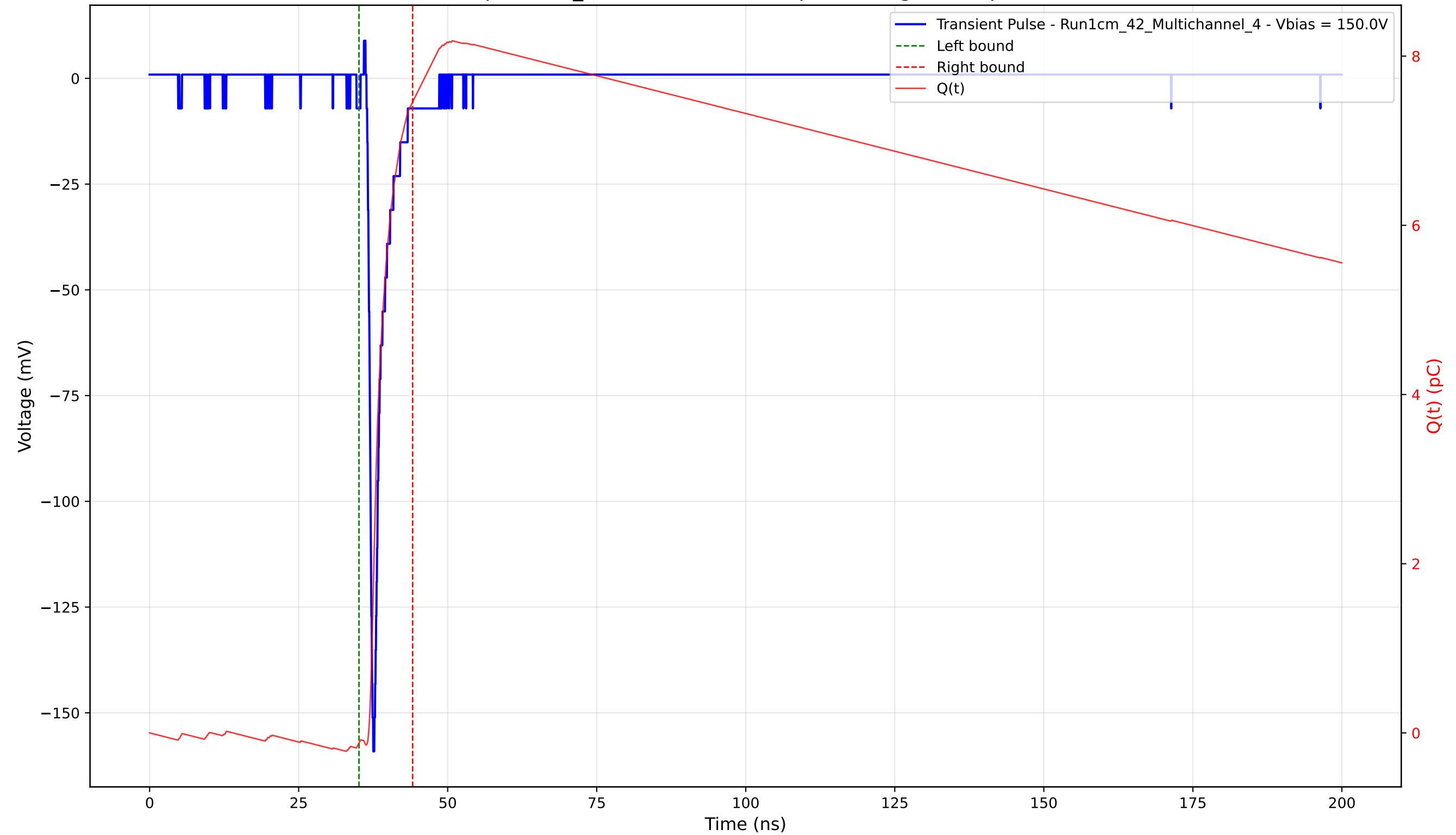
Transient Pulse - Sample: 1cm_42 - Position: 3175.0 \mu\text{m} - Charge: 7.58 pC - Rise Time: 0.84 ns
