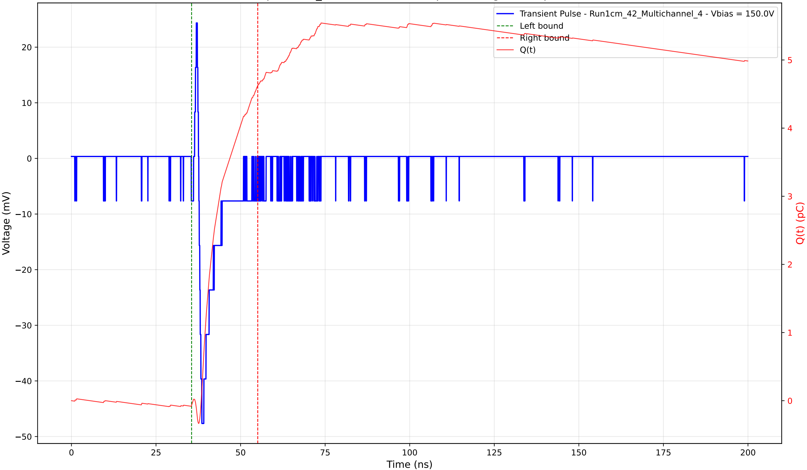
Transient Pulse - Sample: 1cm_42 - Position: 905.0 \mu\text{m} - Charge: 4.69 pC - Rise Time: 0.90 ns
