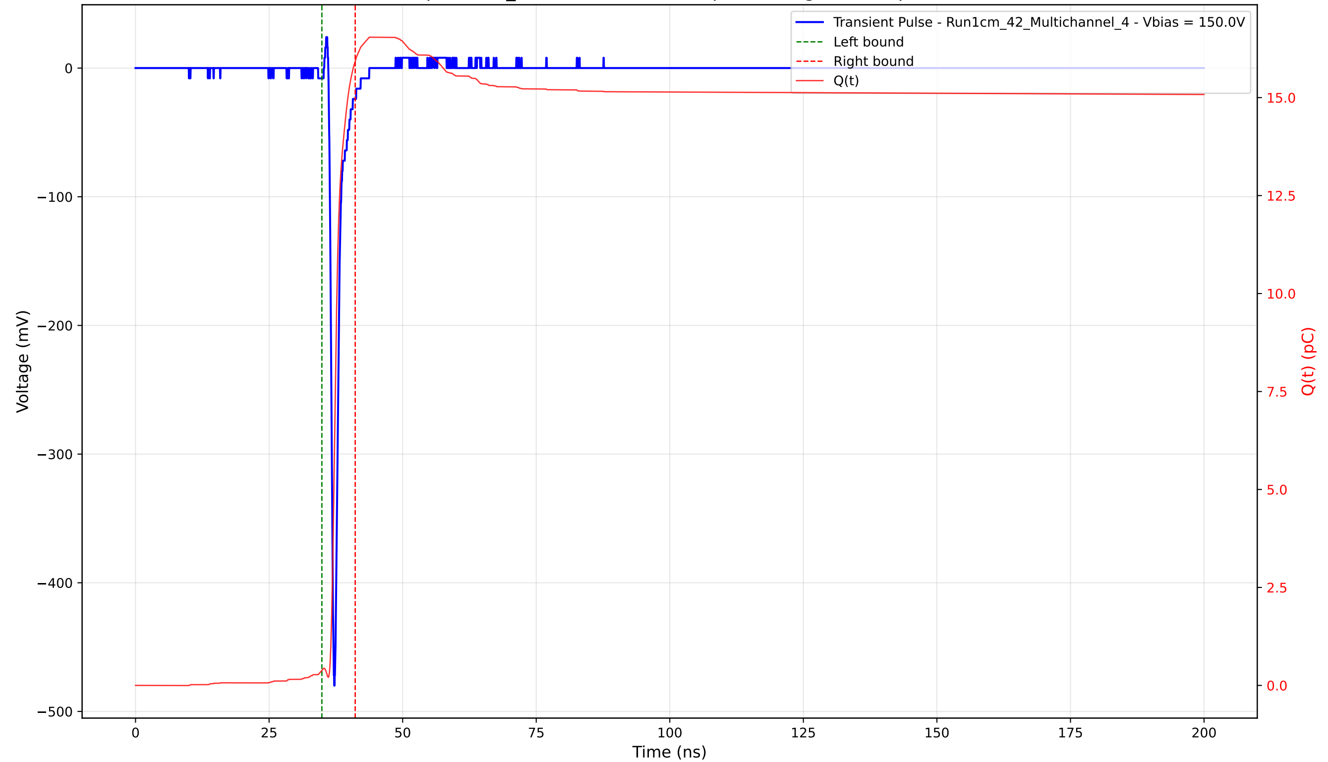
Transient Pulse - Sample: 1cm_42 - Position: 2780.0 \mu\text{m} - Charge: 15.55 pC - Rise Time: 0.72 ns
