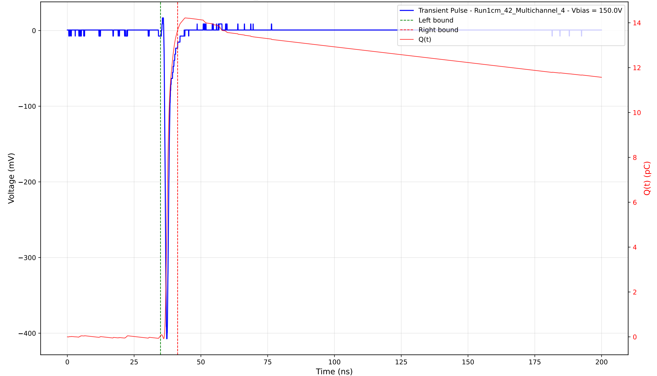
Transient Pulse - Sample: 1cm_42 - Position: 2850.0 \mu\text{m} - Charge: 13.63 pC - Rise Time: 0.73 ns
