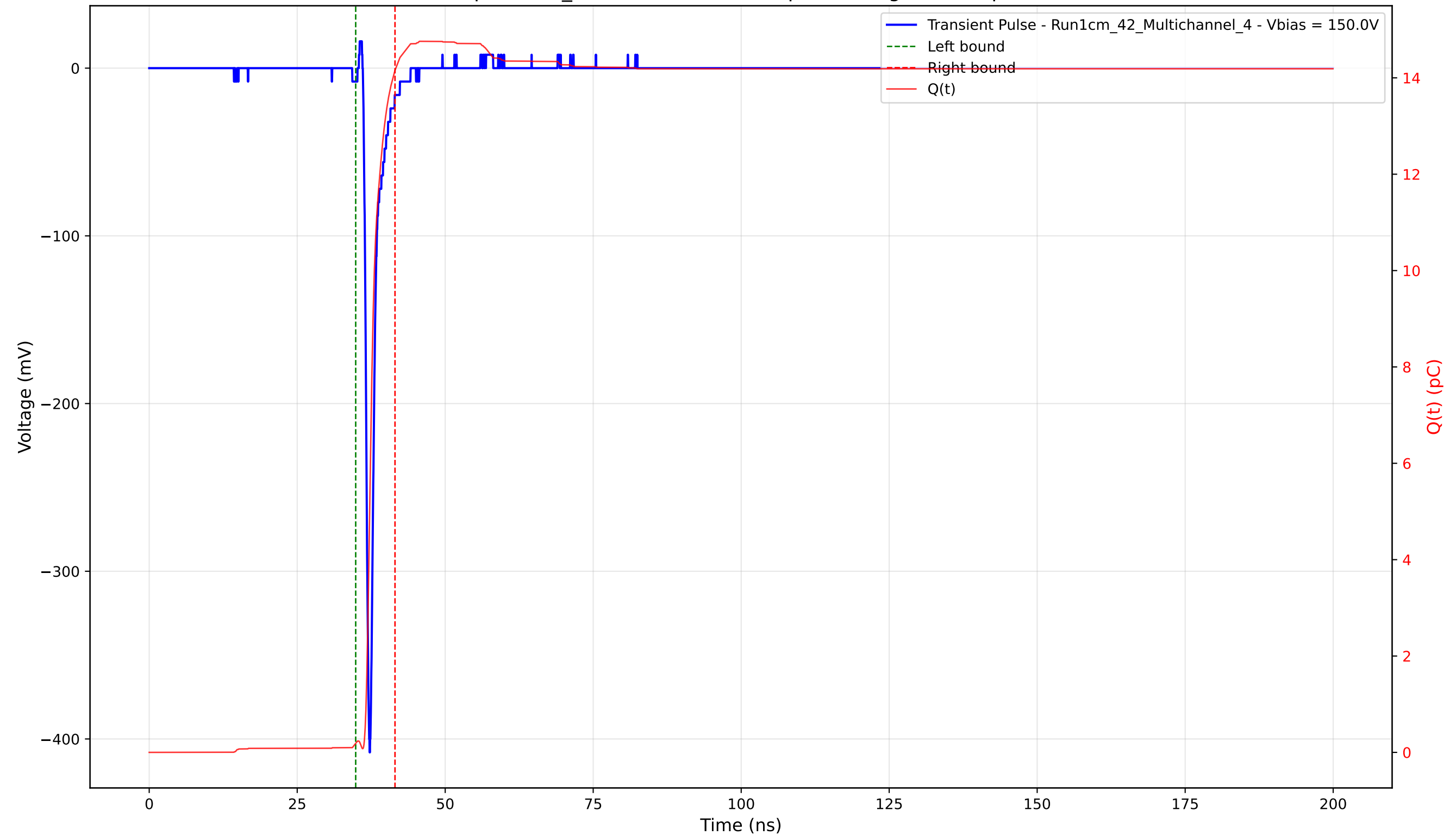
Transient Pulse - Sample: 1cm_42 - Position: 2160.0 \mu\text{m} - Charge: 13.97 pC - Rise Time: 0.75 ns
