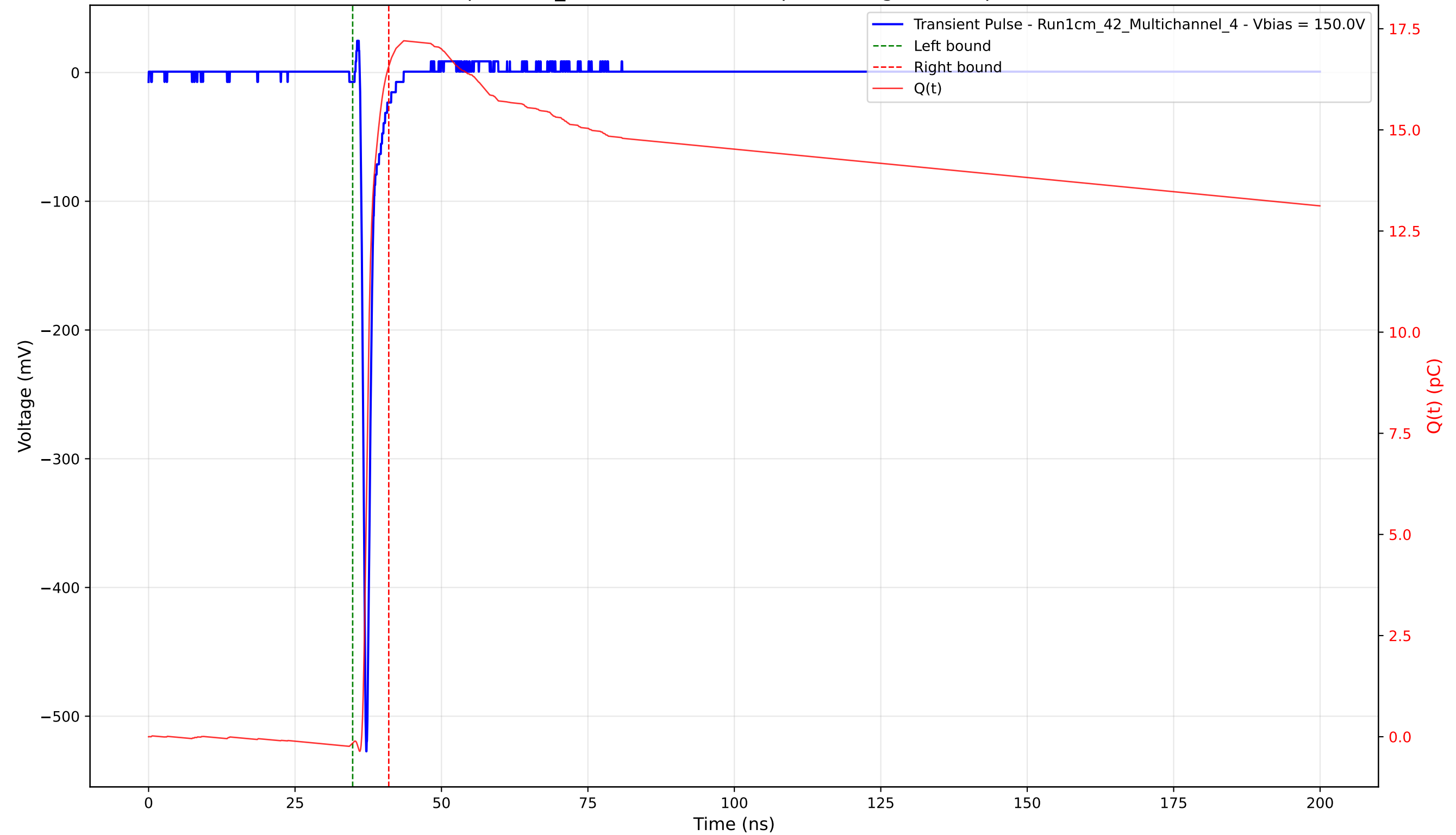
Transient Pulse - Sample: 1cm_42 - Position: 2290.0 \mu\text{m} - Charge: 16.73 pC - Rise Time: 0.70 ns
