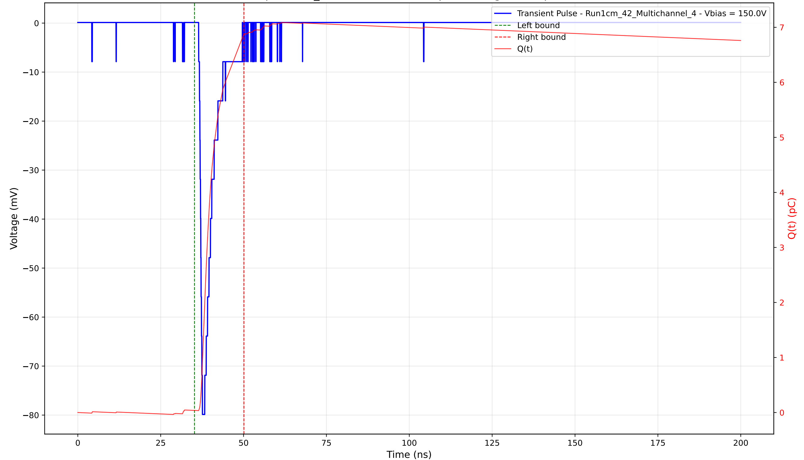
Transient Pulse - Sample: 1cm_42 - Position: 1550.0 \mu\text{m} - Charge: 6.82 pC - Rise Time: 0.92 ns
