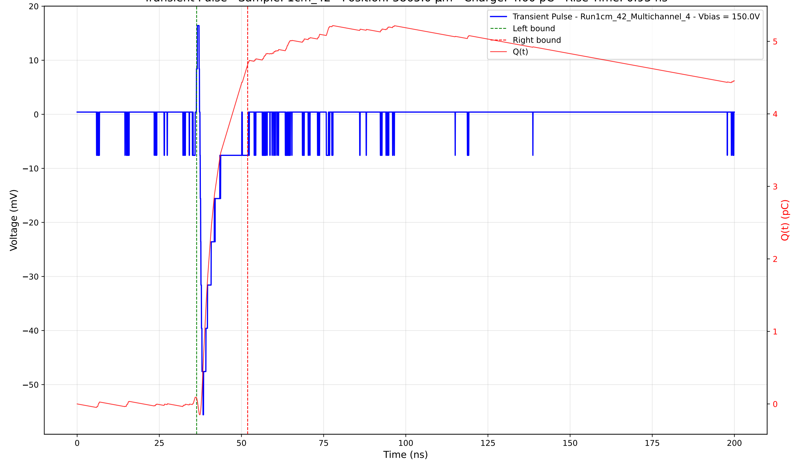
Transient Pulse - Sample: 1cm_42 - Position: 3865.0 \mu\text{m} - Charge: 4.60 pC - Rise Time: 0.93 ns
