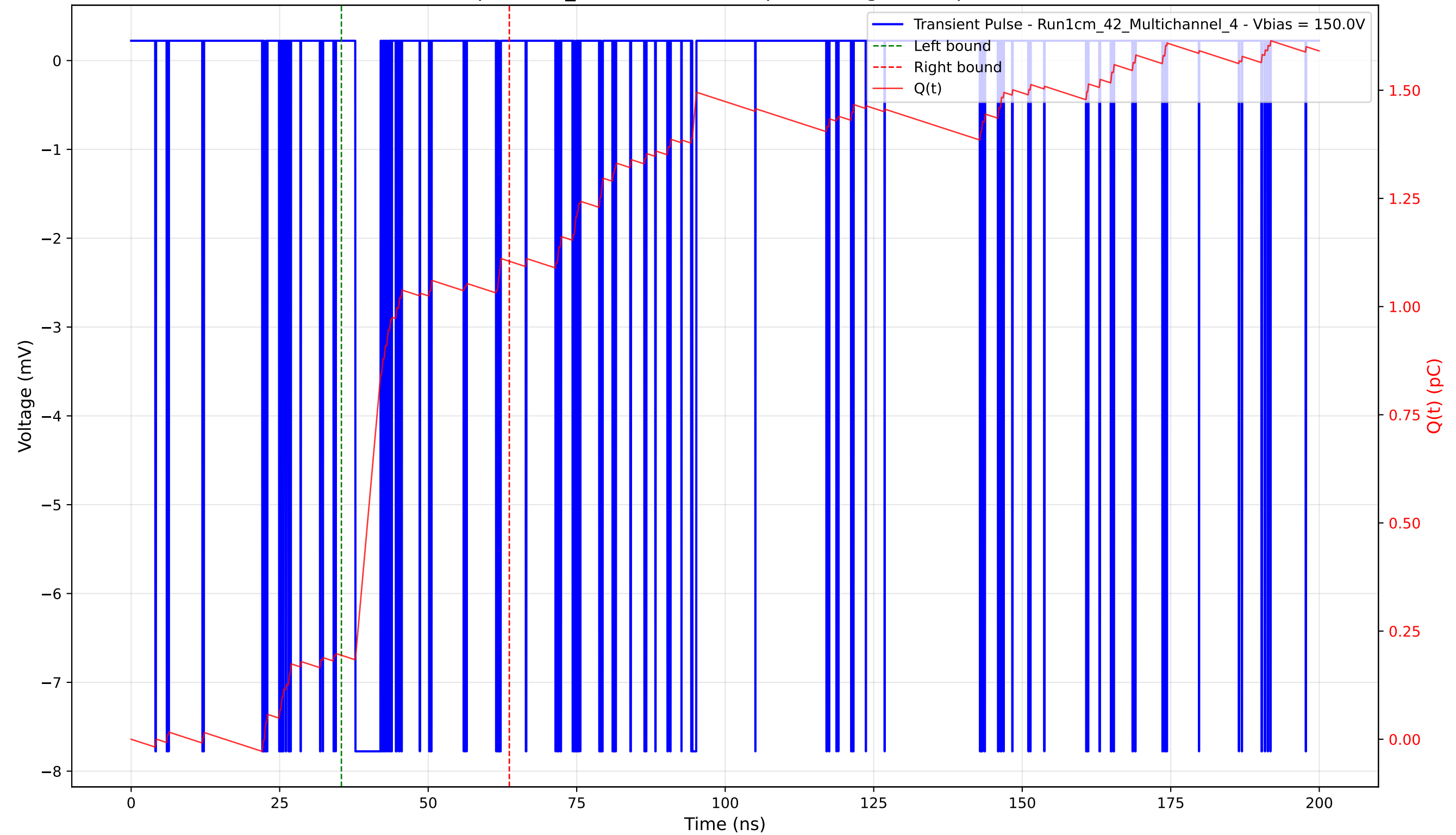
Transient Pulse - Sample: 1cm_42 - Position: 70.0 \mu\text{m} - Charge: 0.91 pC - Rise Time: 0.04 ns
