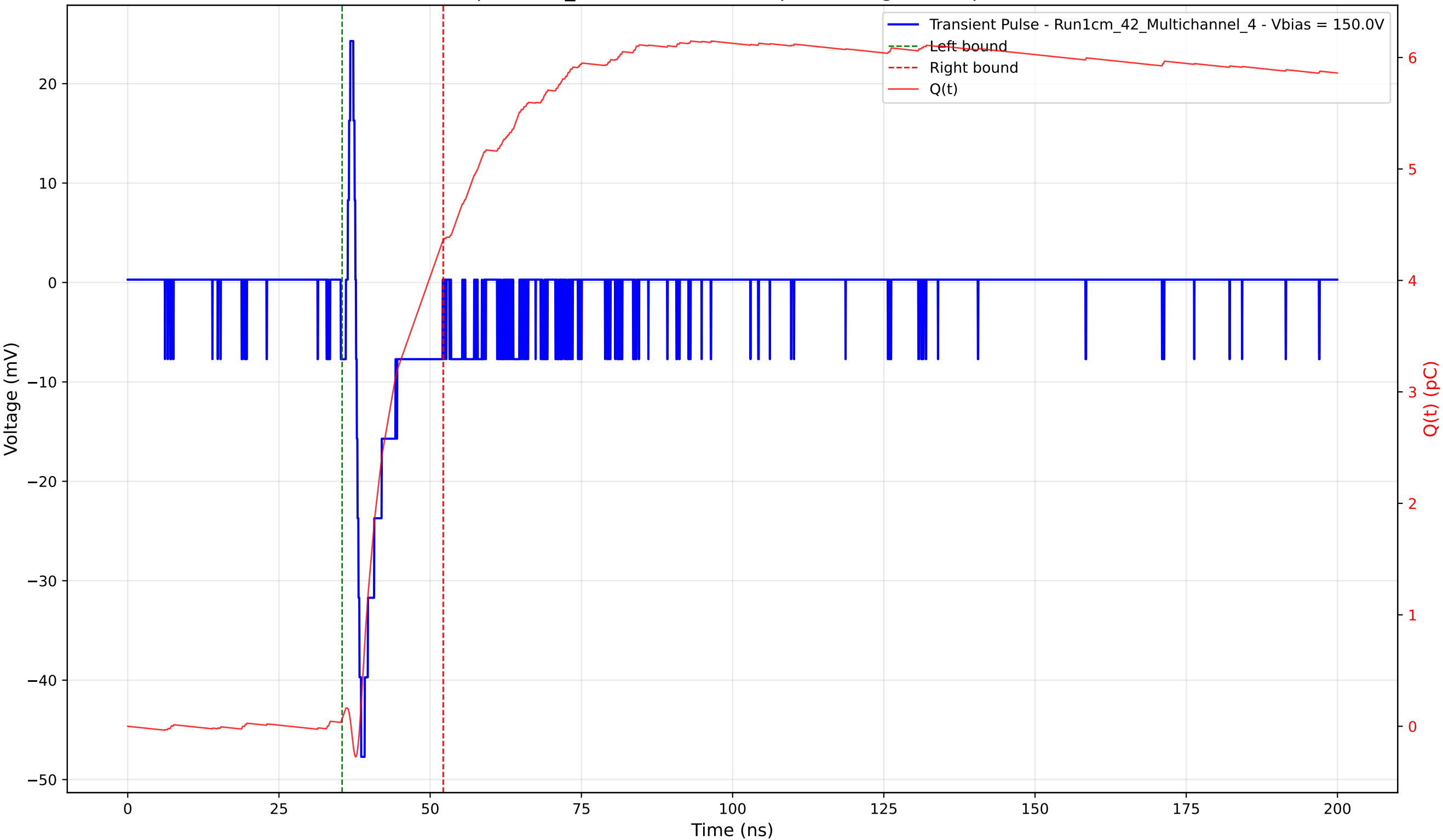
Transient Pulse - Sample: 1cm_42 - Position: 645.0 \mu\text{m} - Charge: 4.28 pC - Rise Time: 0.86 ns
