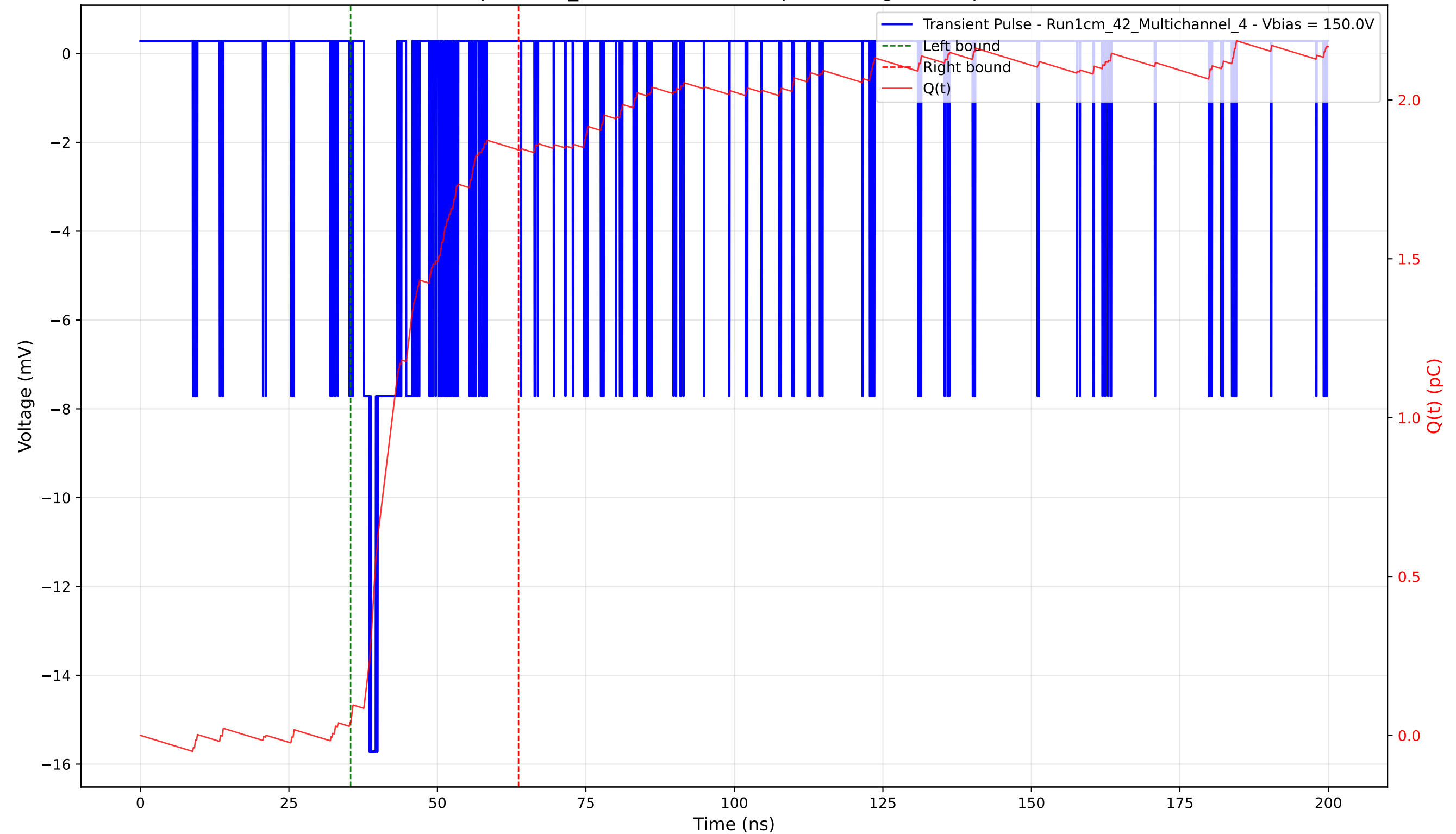
Transient Pulse - Sample: 1cm_42 - Position: 135.0 \mu\text{m} - Charge: 1.80 pC - Rise Time: 0.95 ns
