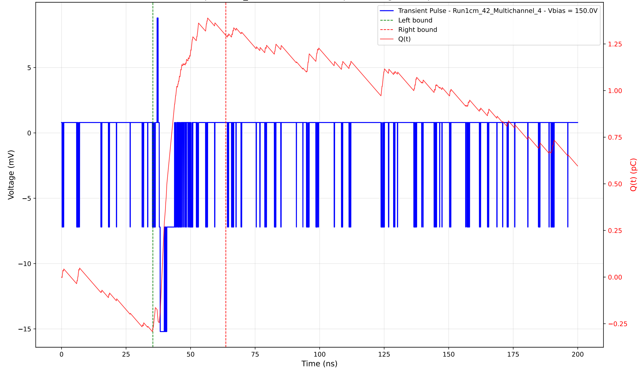
Transient Pulse - Sample: 1cm_42 - Position: 5025.0 \mu\text{m} - Charge: 1.57 pC - Rise Time: 0.40 ns
