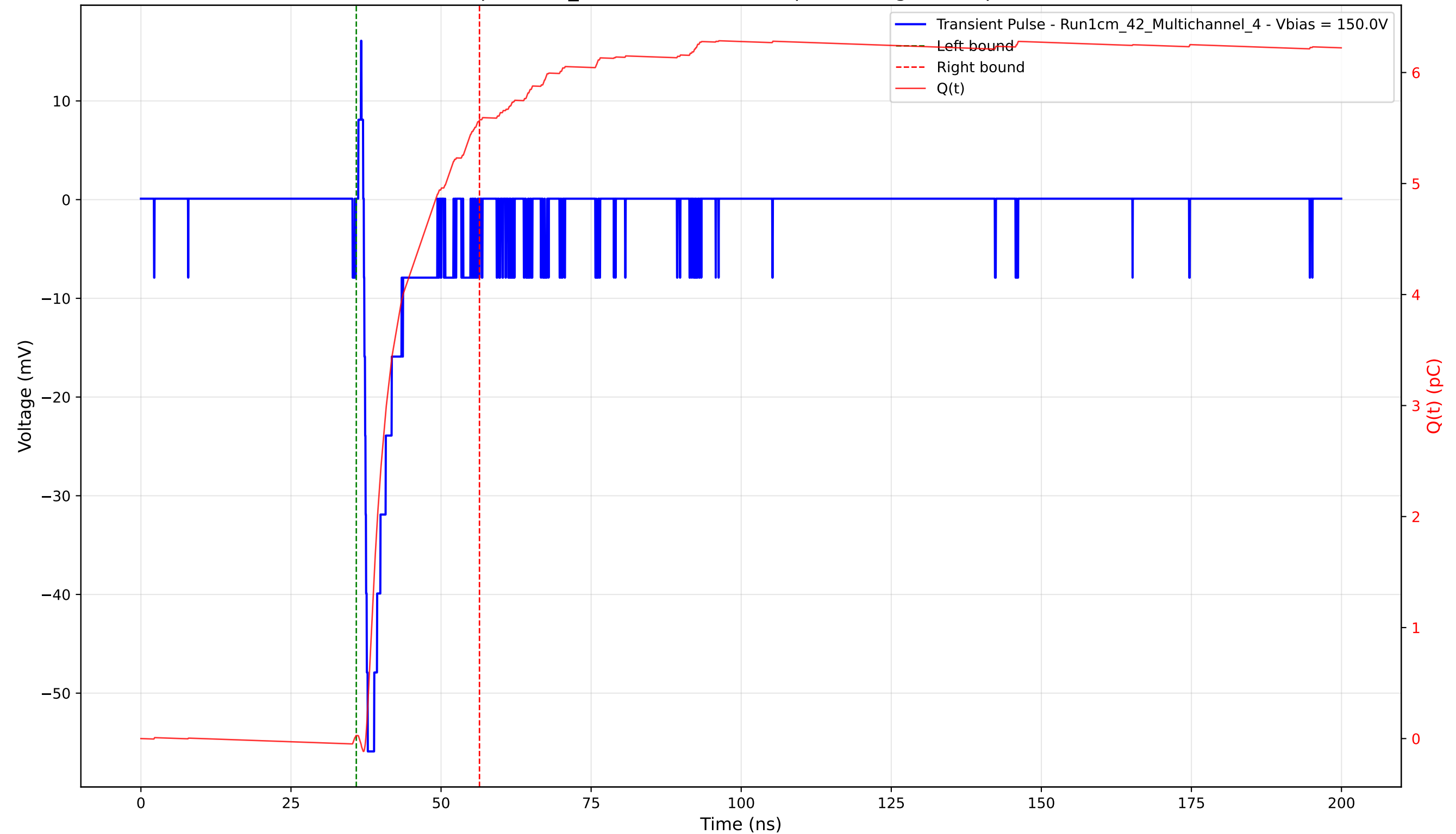
Transient Pulse - Sample: 1cm_42 - Position: 3645.0 \mu\text{m} - Charge: 5.54 pC - Rise Time: 0.65 ns
