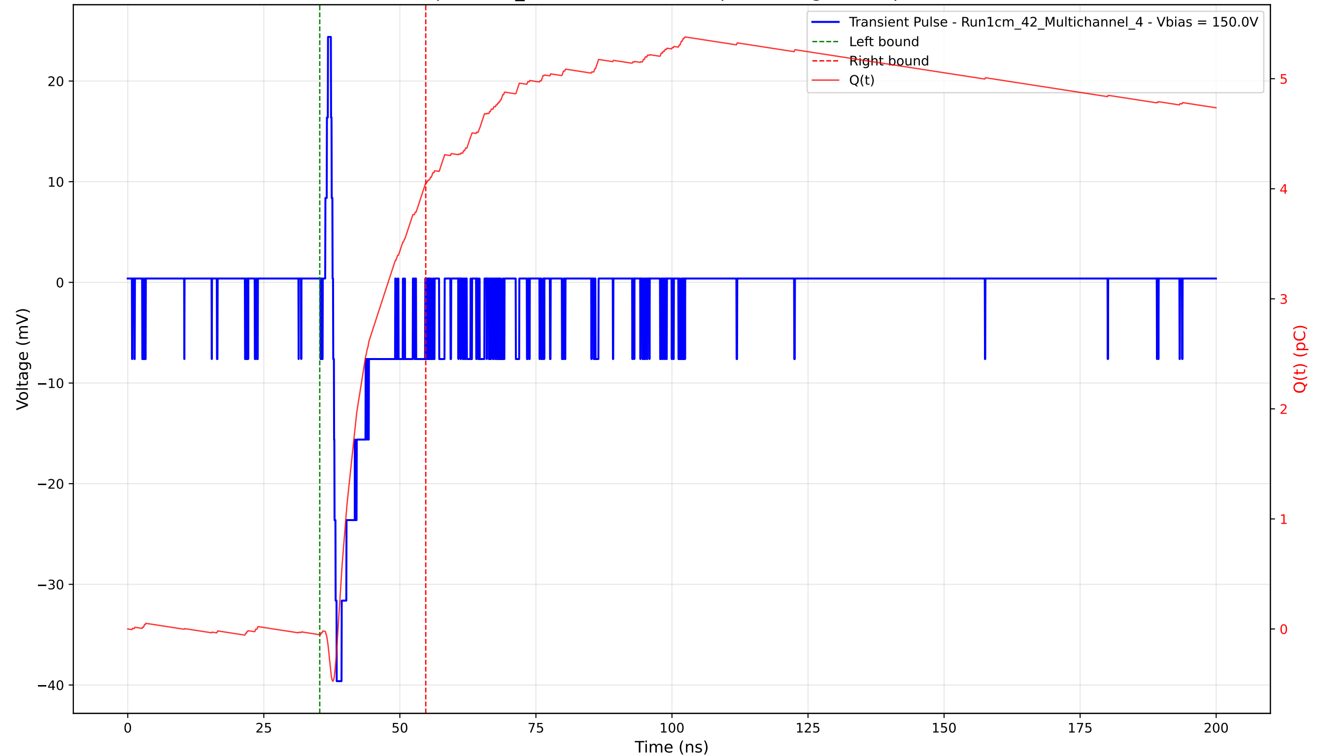
Transient Pulse - Sample: 1cm_42 - Position: 4235.0 \mu\text{m} - Charge: 4.09 pC - Rise Time: 0.66 ns
