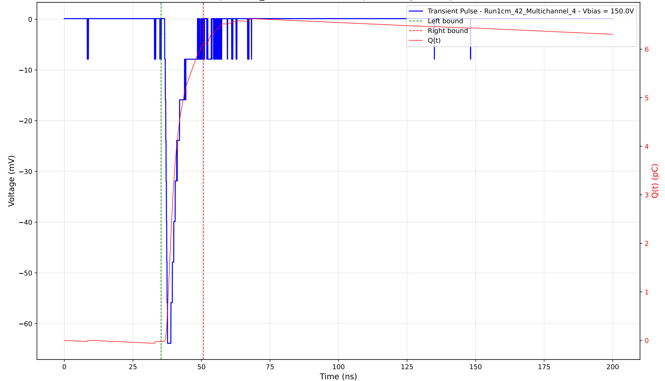
Transient Pulse - Sample: 1cm_42 - Position: 1495.0 \mu\text{m} - Charge: 6.12 pC - Rise Time: 1.05 ns
