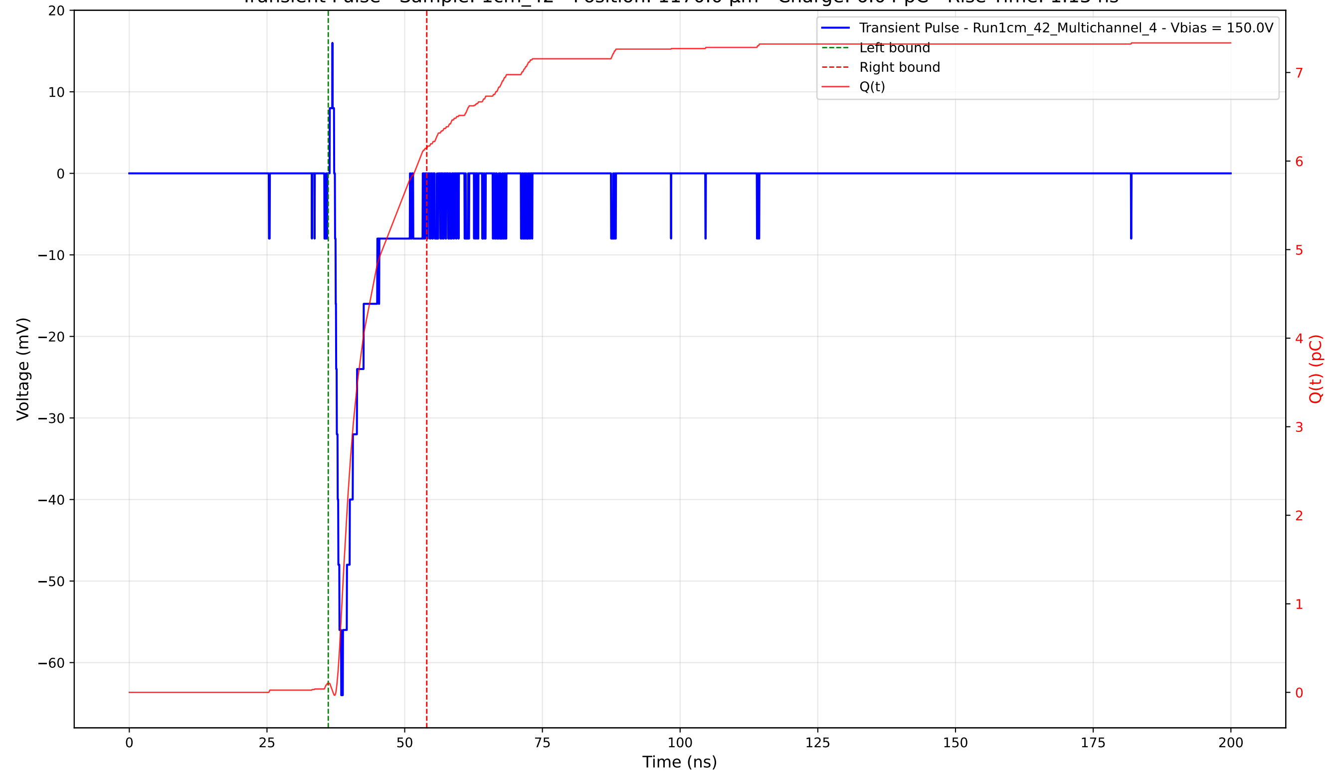
Transient Pulse - Sample: 1cm_42 - Position: 1170.0 \mu\text{m} - Charge: 6.04 pC - Rise Time: 1.13 ns
