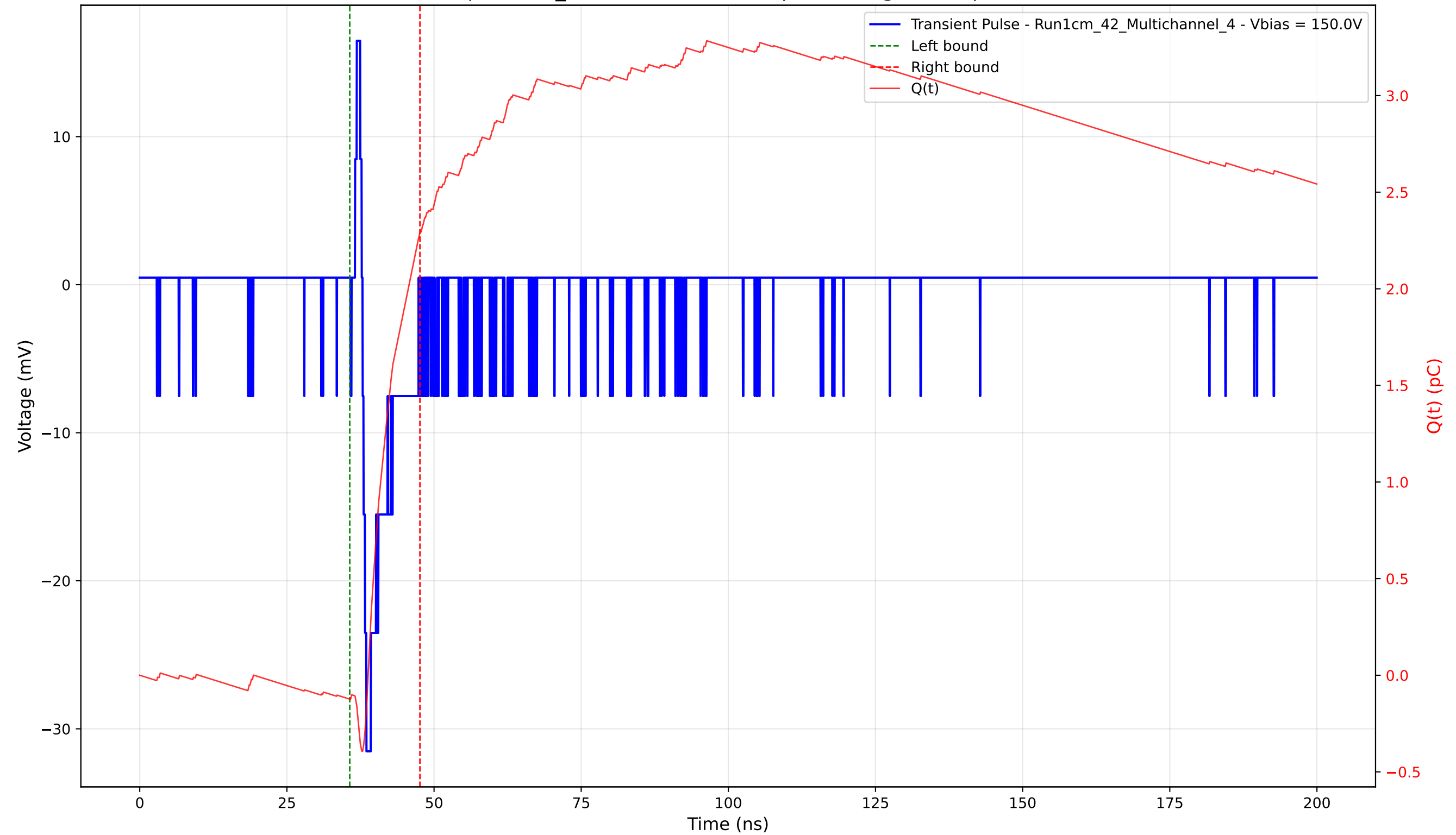
Transient Pulse - Sample: 1cm_42 - Position: 4605.0 \mu\text{m} - Charge: 2.42 pC - Rise Time: 0.66 ns
