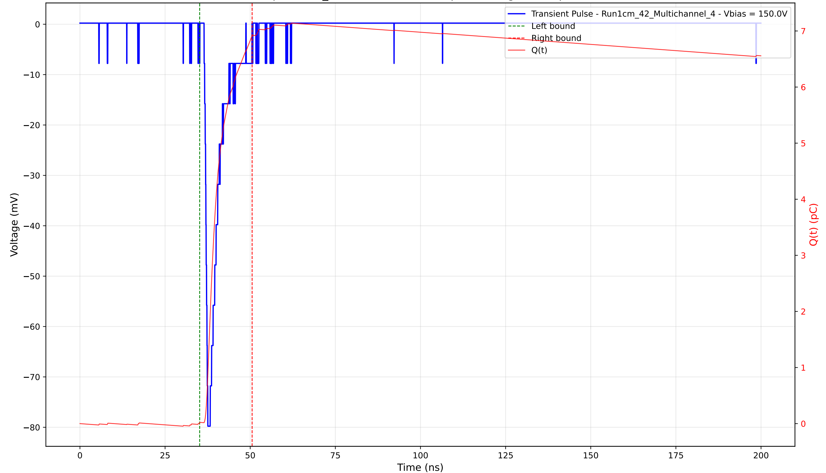
Transient Pulse - Sample: 1cm_42 - Position: 1555.0 \mu\text{m} - Charge: 6.90 pC - Rise Time: 0.96 ns
