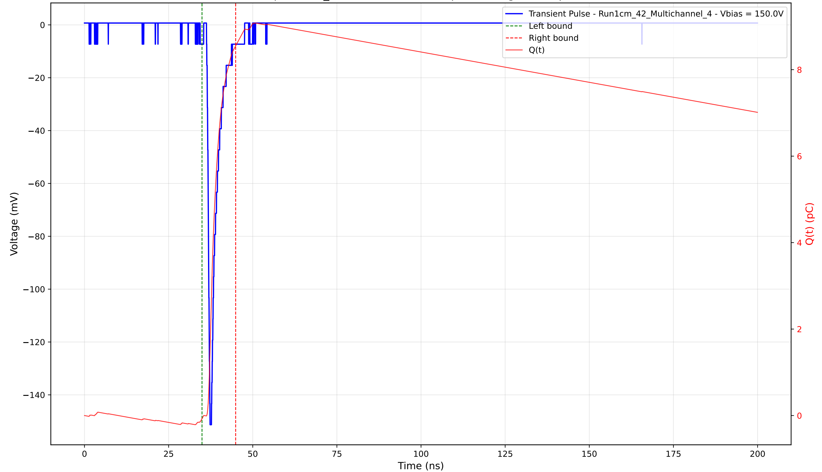
Transient Pulse - Sample: 1cm_42 - Position: 1845.0 \mu\text{m} - Charge: 8.62 pC - Rise Time: 0.88 ns
