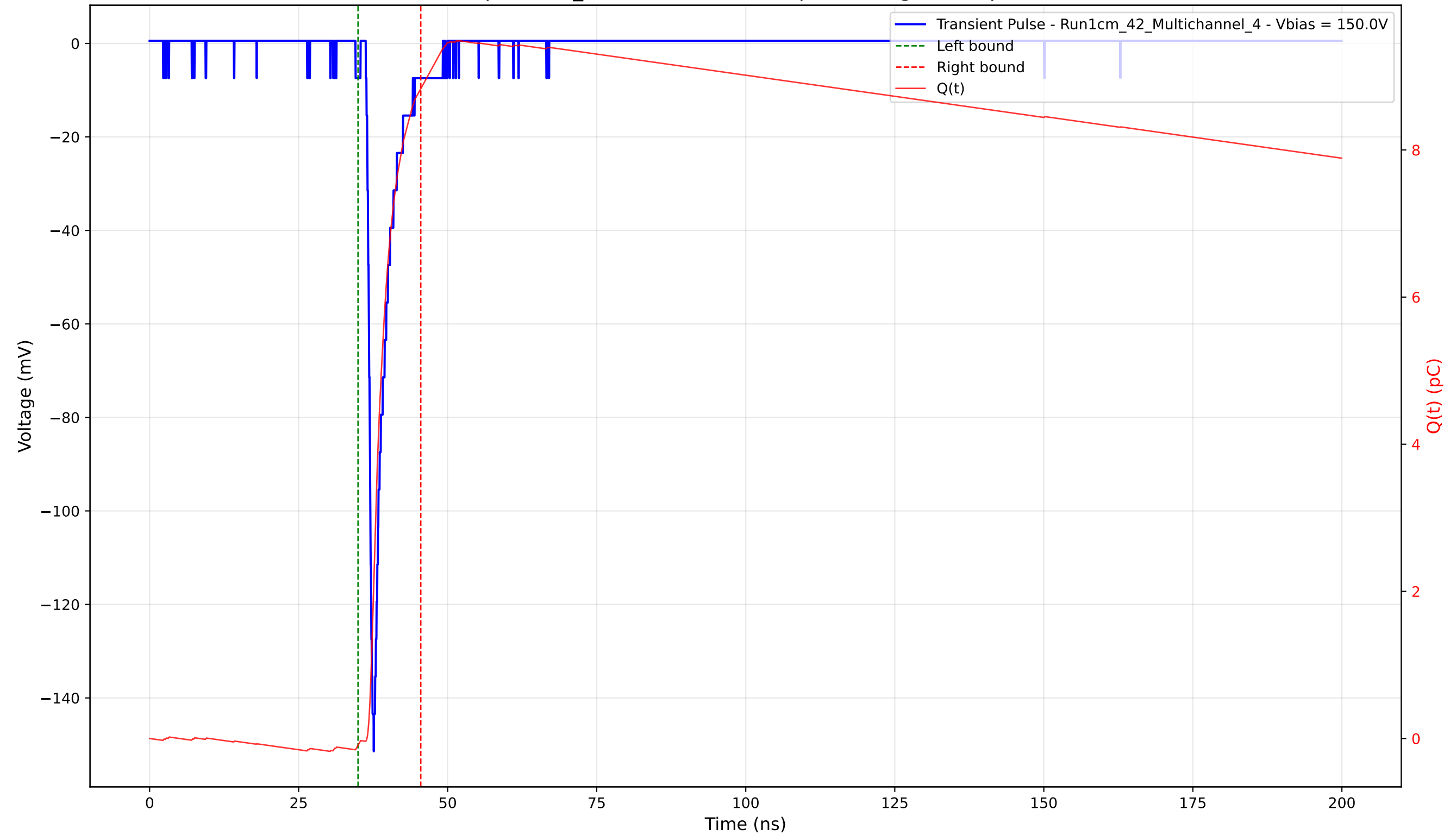
Transient Pulse - Sample: 1cm_42 - Position: 1760.0 \mu\text{m} - Charge: 8.92 pC - Rise Time: 1.00 ns
