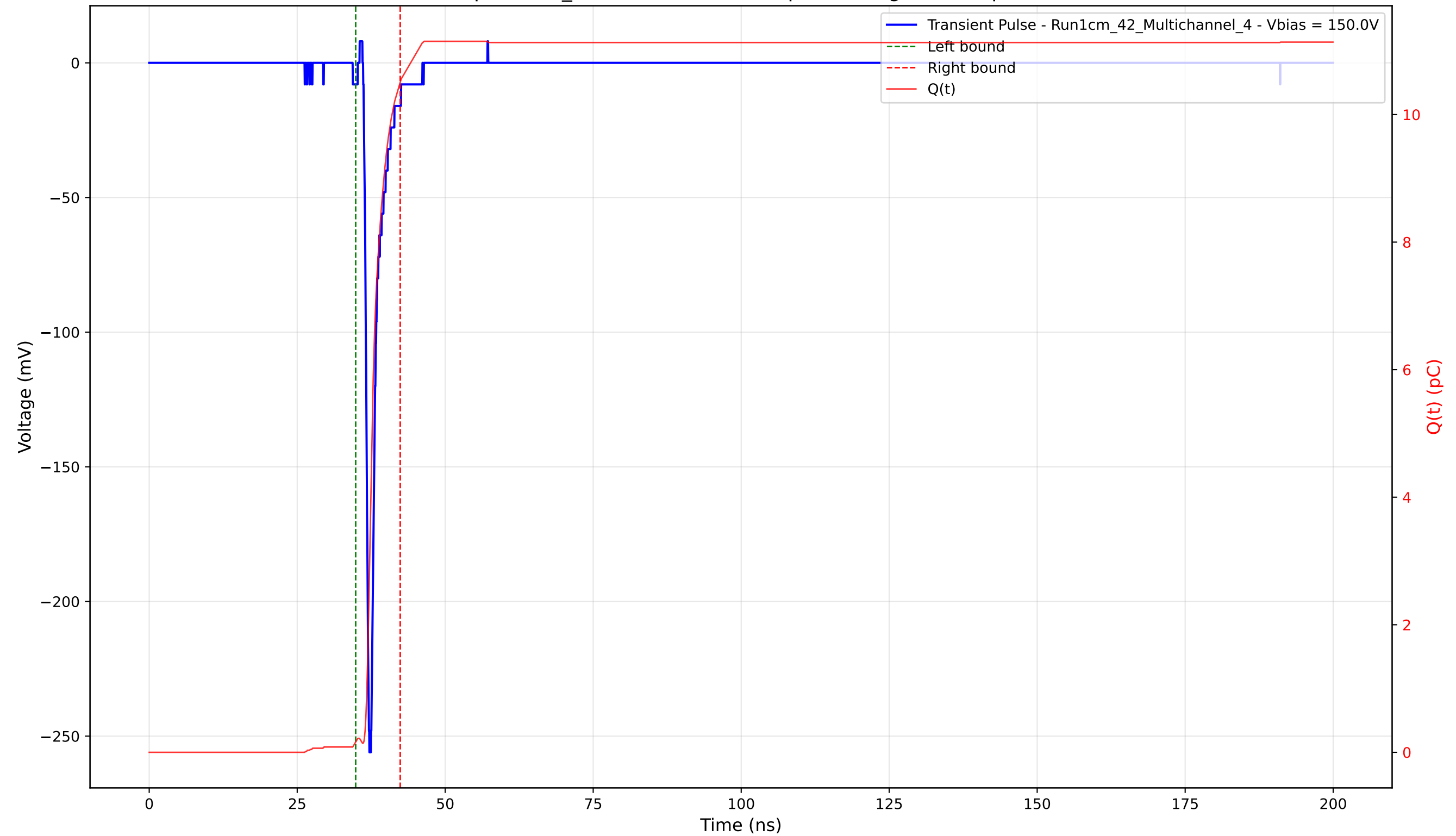
Transient Pulse - Sample: 1cm_42 - Position: 2045.0 \mu\text{m} - Charge: 10.35 pC - Rise Time: 0.74 ns
