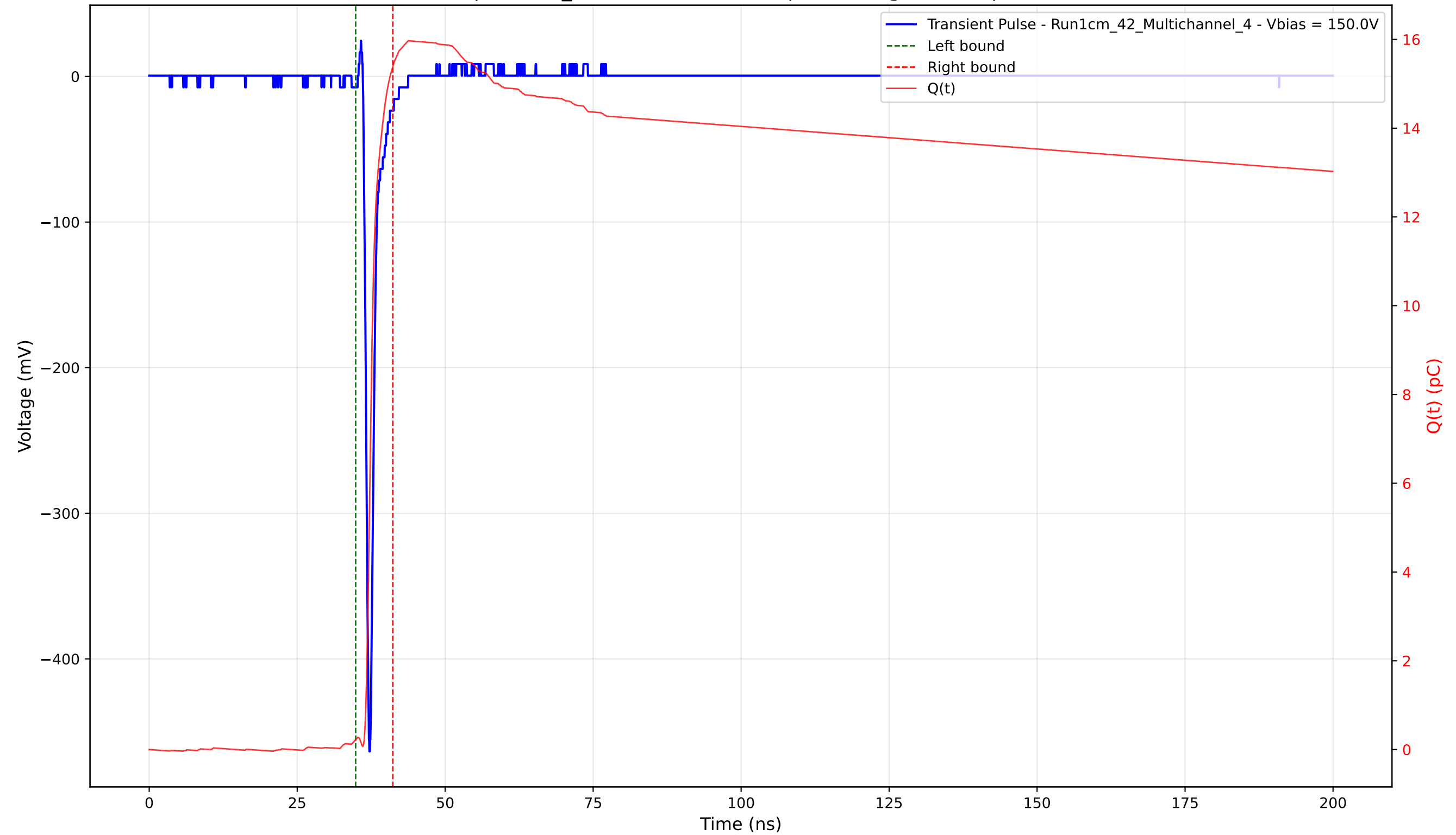
Transient Pulse - Sample: 1cm_42 - Position: 2800.0 \mu\text{m} - Charge: 15.17 pC - Rise Time: 0.71 ns
