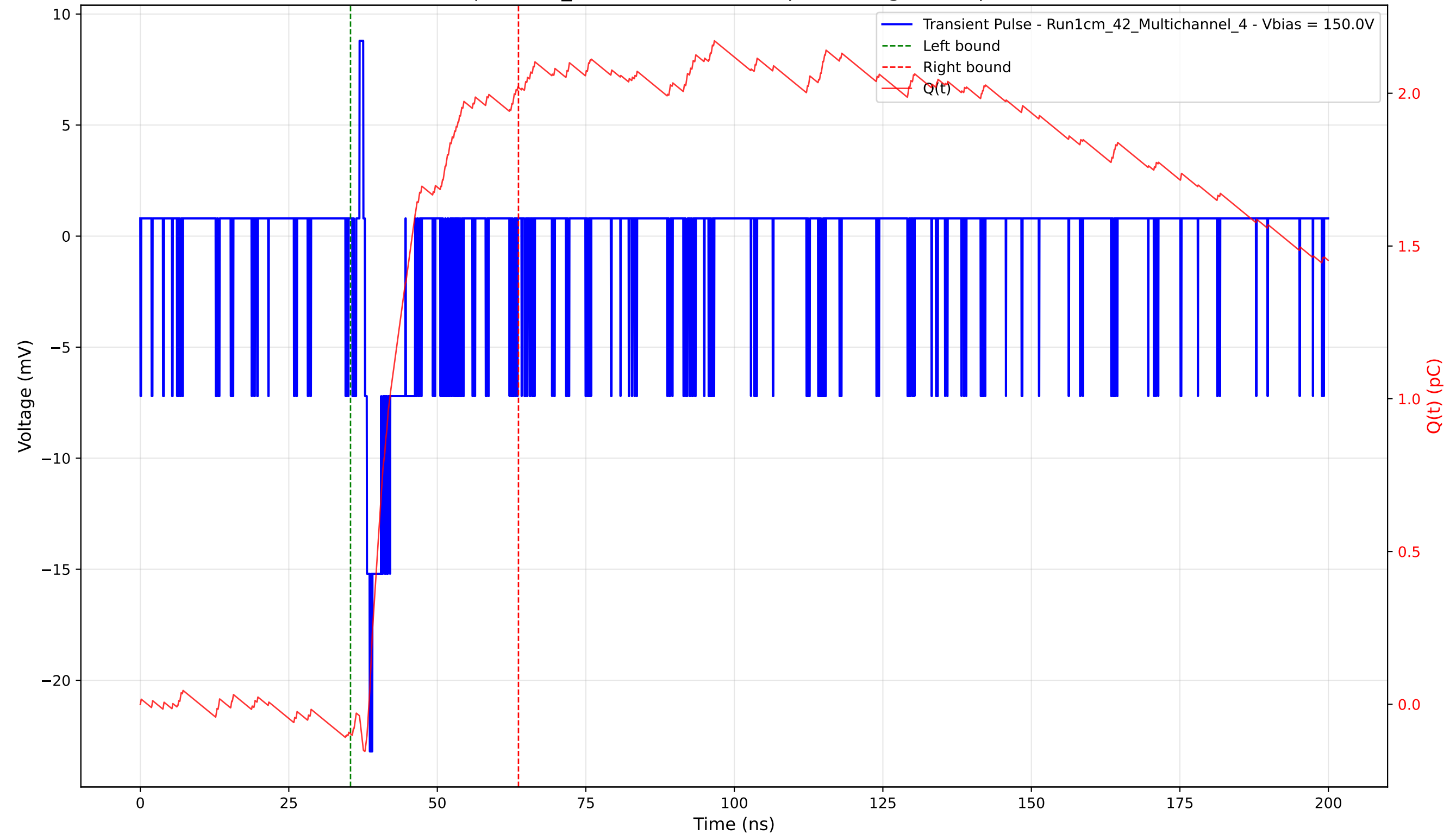
Transient Pulse - Sample: 1cm_42 - Position: 5000.0 \mu\text{m} - Charge: 2.12 pC - Rise Time: 0.83 ns
