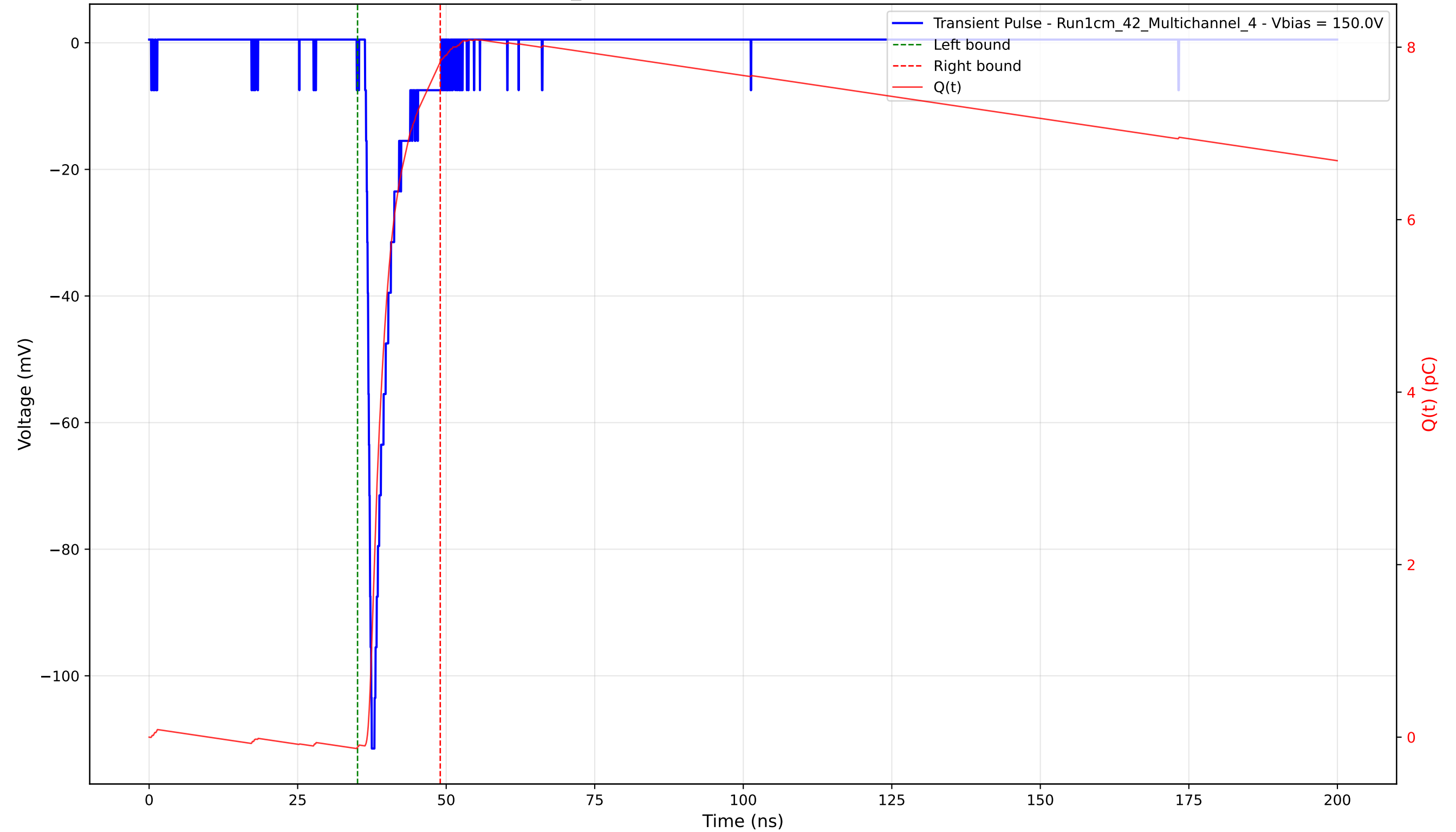
Transient Pulse - Sample: 1cm_42 - Position: 1645.0 \mu\text{m} - Charge: 7.94 pC - Rise Time: 0.90 ns
