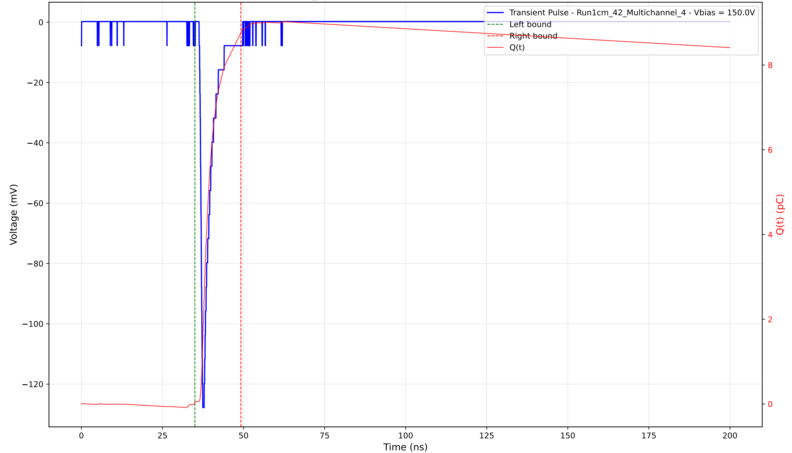
Transient Pulse - Sample: 1cm_42 - Position: 1690.0 \mu\text{m} - Charge: 8.73 pC - Rise Time: 0.85 ns
