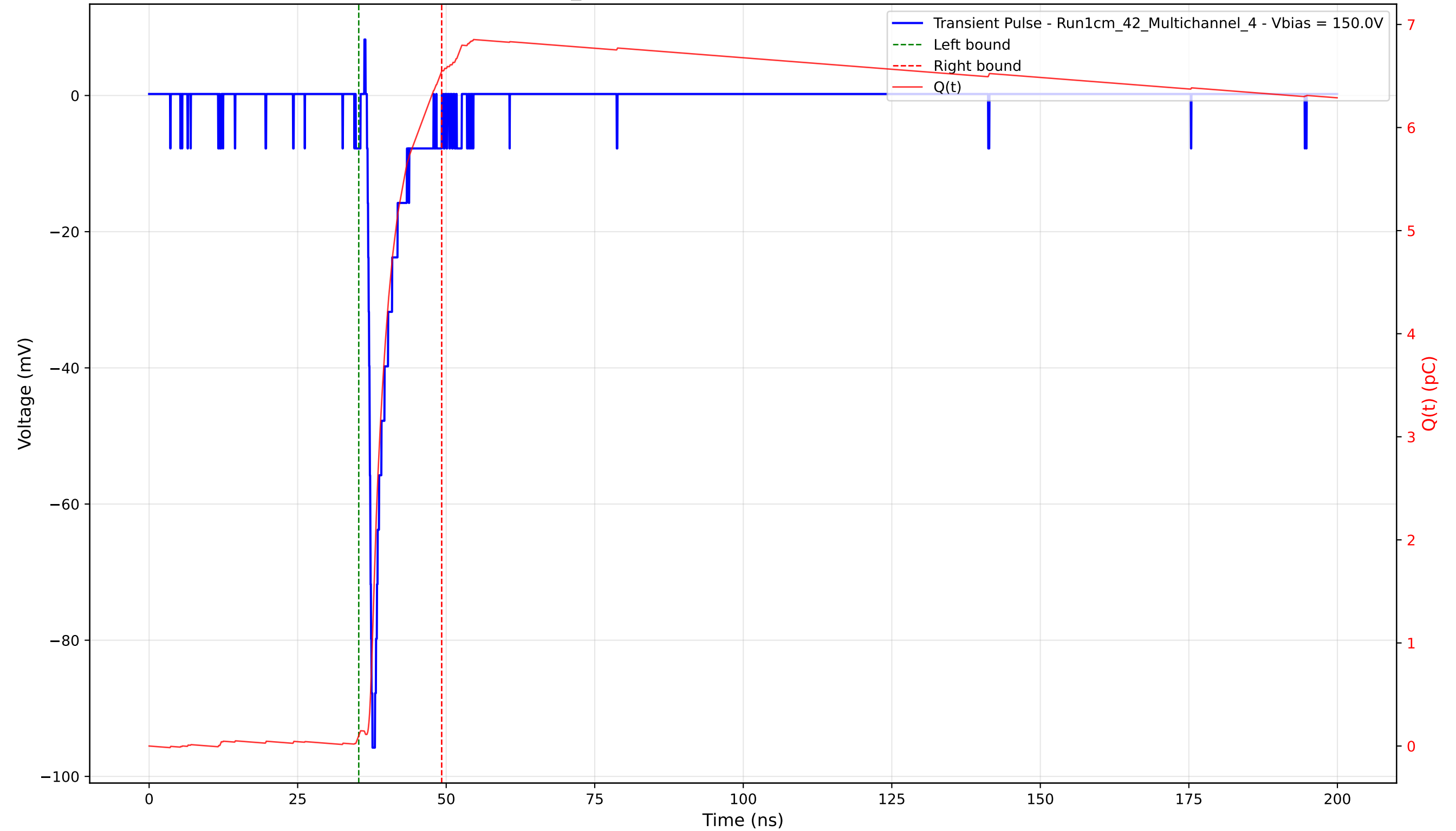
Transient Pulse - Sample: 1cm_42 - Position: 3425.0 \mu\text{m} - Charge: 6.45 pC - Rise Time: 0.67 ns
