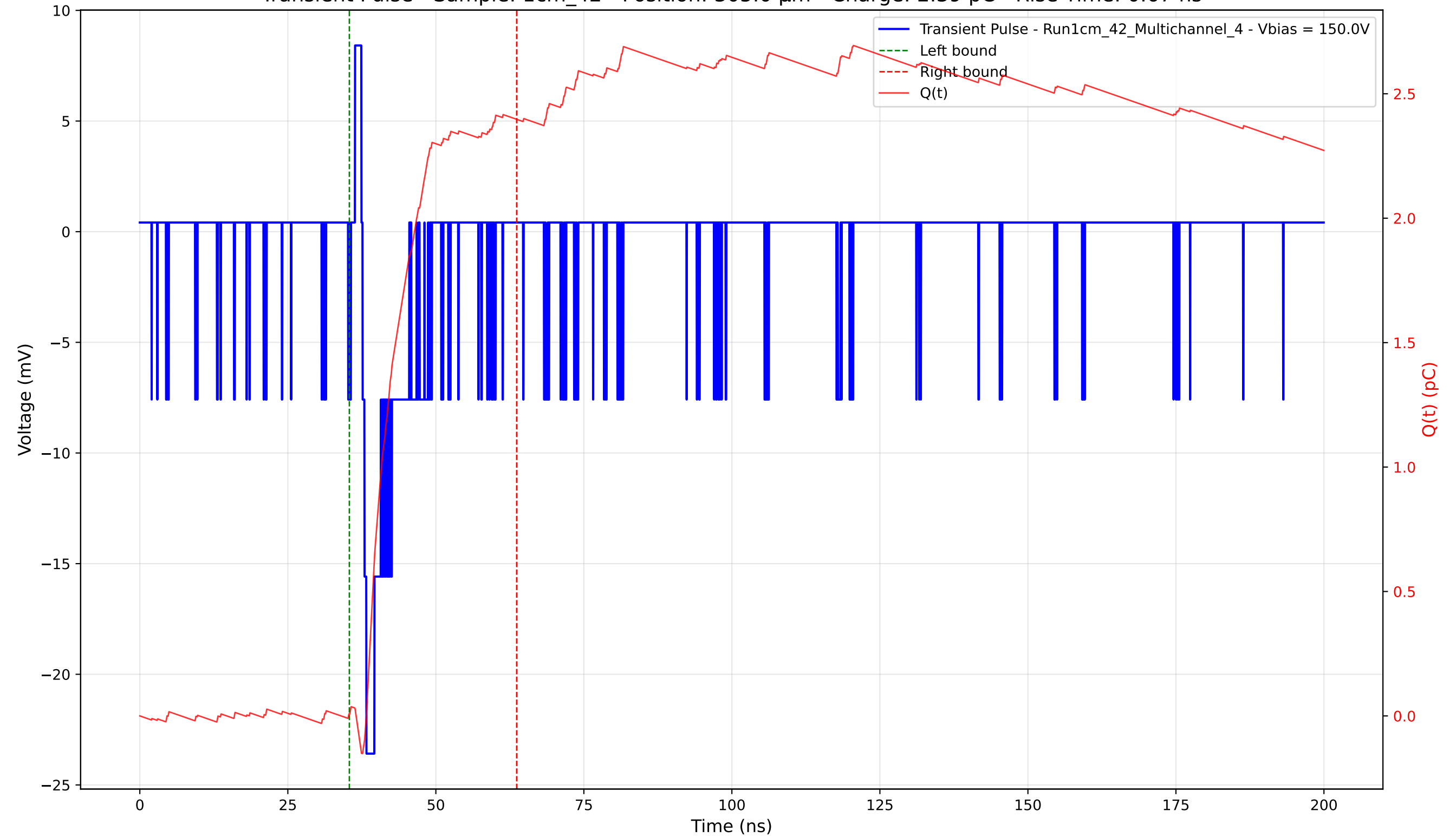
Transient Pulse - Sample: 1cm_42 - Position: 305.0 \mu\text{m} - Charge: 2.39 pC - Rise Time: 0.67 ns
