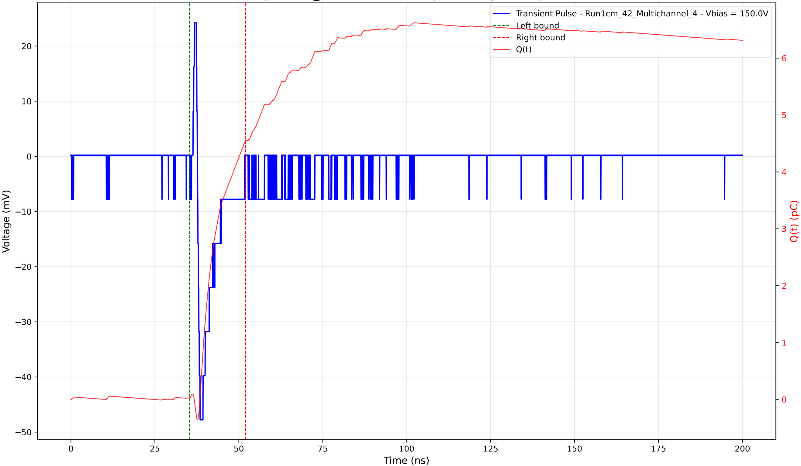
Transient Pulse - Sample: 1cm_42 - Position: 715.0 \mu\text{m} - Charge: 4.53 pC - Rise Time: 0.74 ns
