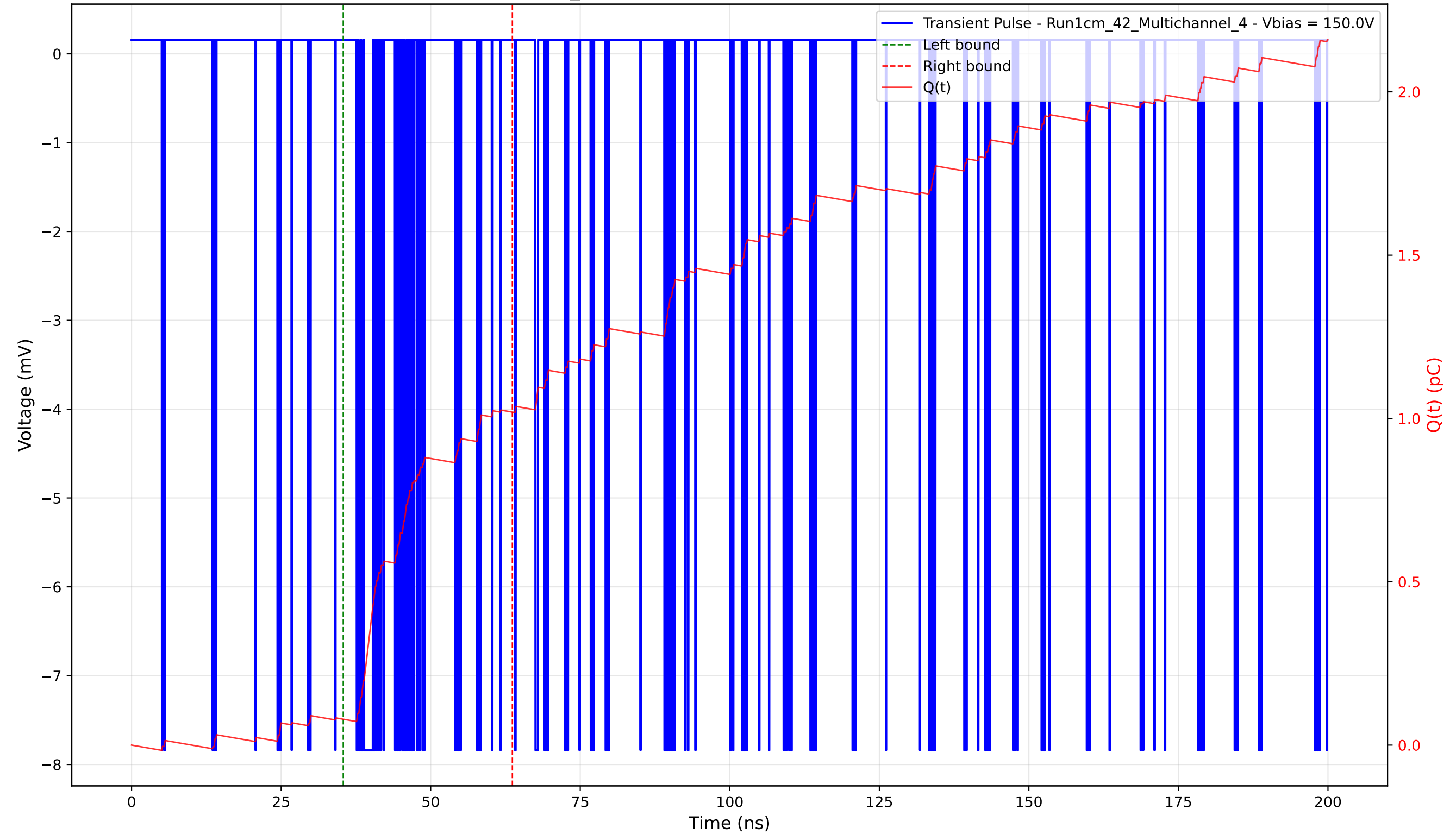
Transient Pulse - Sample: 1cm_42 - Position: 30.0 \mu\text{m} - Charge: 0.94 pC - Rise Time: 0.04 ns
