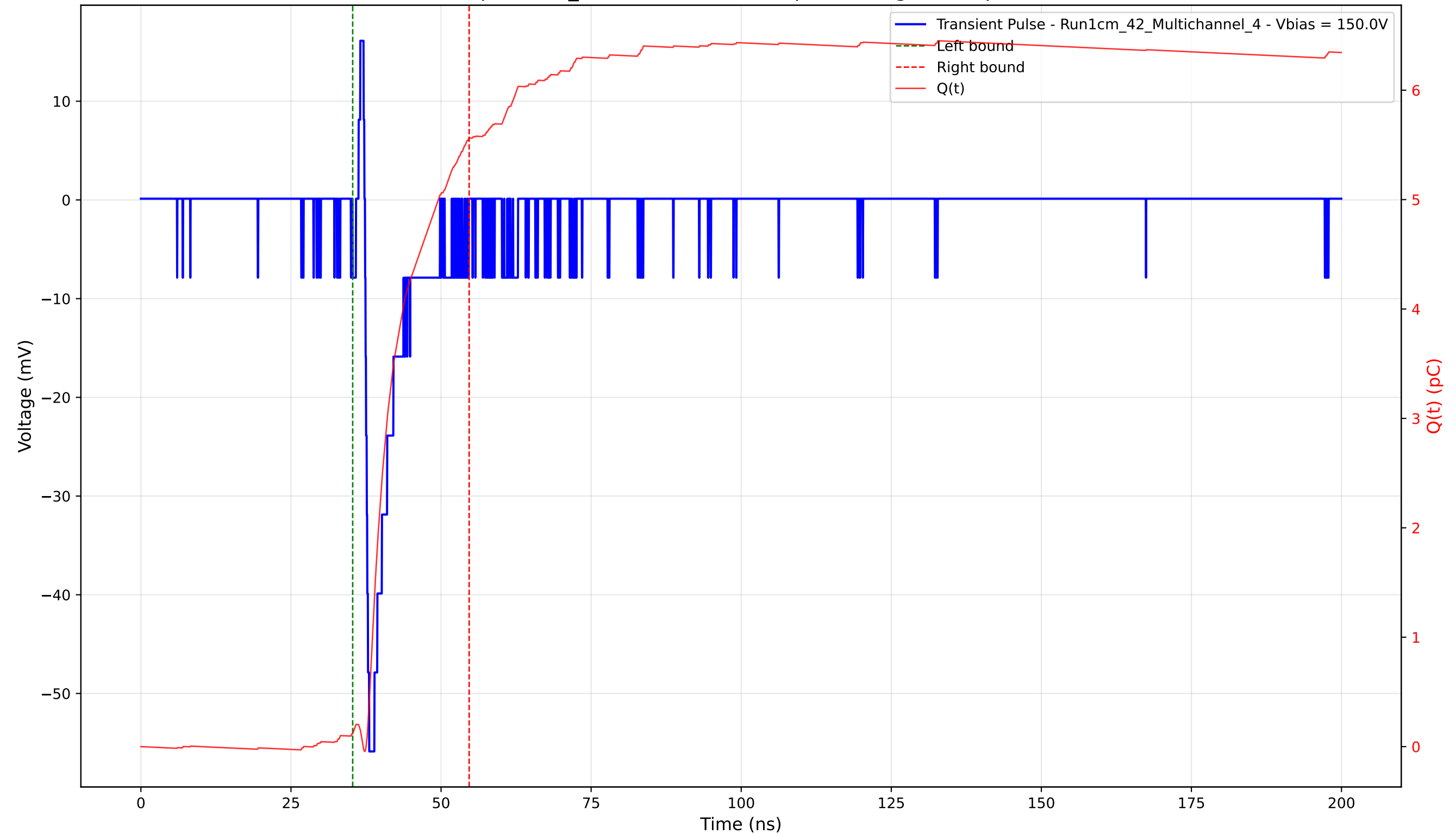
Transient Pulse - Sample: 1cm_42 - Position: 3795.0 \mu\text{m} - Charge: 5.44 pC - Rise Time: 0.69 ns
