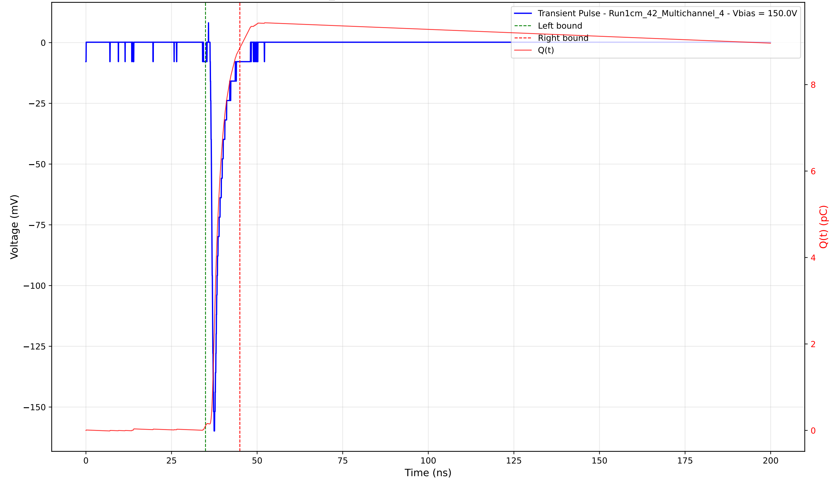
Transient Pulse - Sample: 1cm_42 - Position: 1860.0 \mu\text{m} - Charge: 8.74 pC - Rise Time: 0.88 ns
