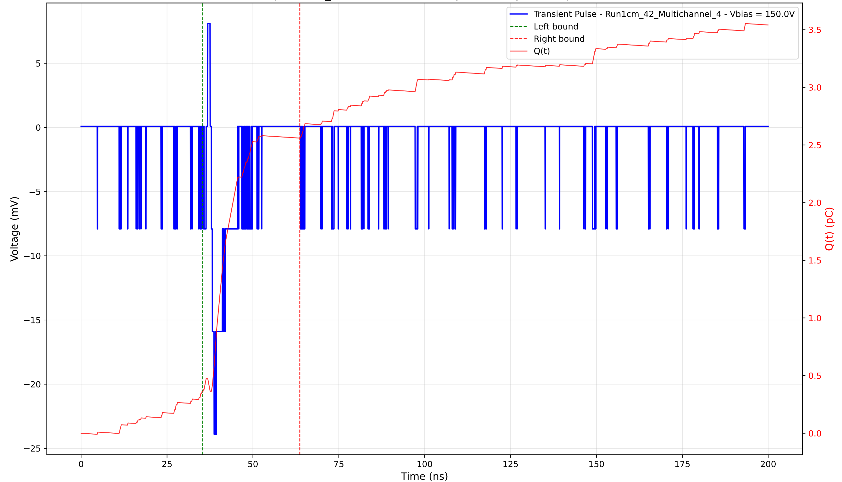
Transient Pulse - Sample: 1cm_42 - Position: 4980.0 \mu\text{m} - Charge: 2.20 pC - Rise Time: 0.83 ns
