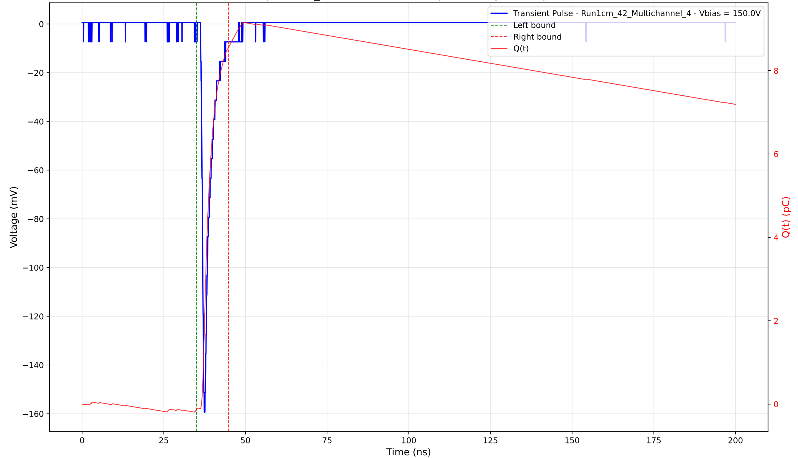
Transient Pulse - Sample: 1cm_42 - Position: 1855.0 \mu\text{m} - Charge: 8.70 pC - Rise Time: 0.88 ns
