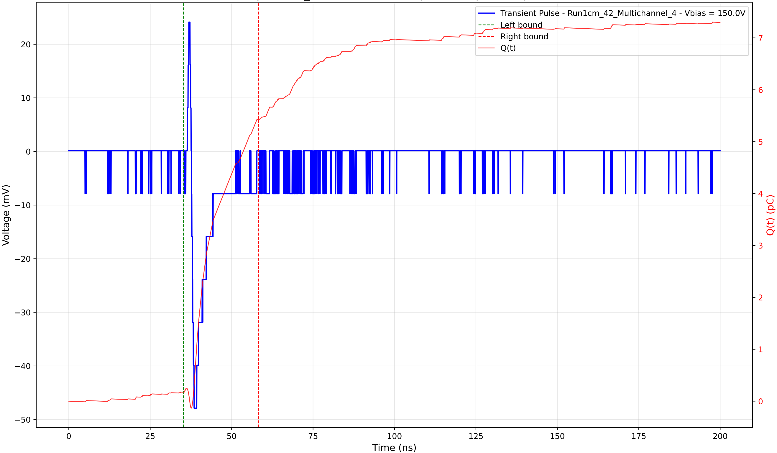
Transient Pulse - Sample: 1cm_42 - Position: 880.0 \mu\text{m} - Charge: 5.25 pC - Rise Time: 0.82 ns
