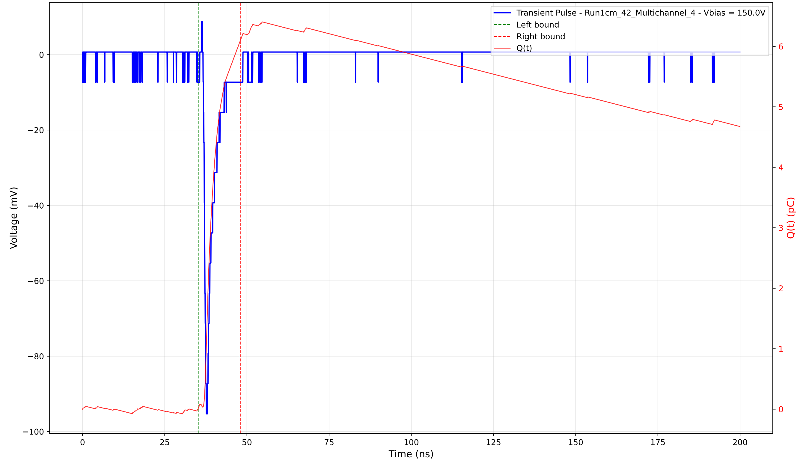
Transient Pulse - Sample: 1cm_42 - Position: 3430.0 \mu\text{m} - Charge: 6.05 pC - Rise Time: 0.71 ns
