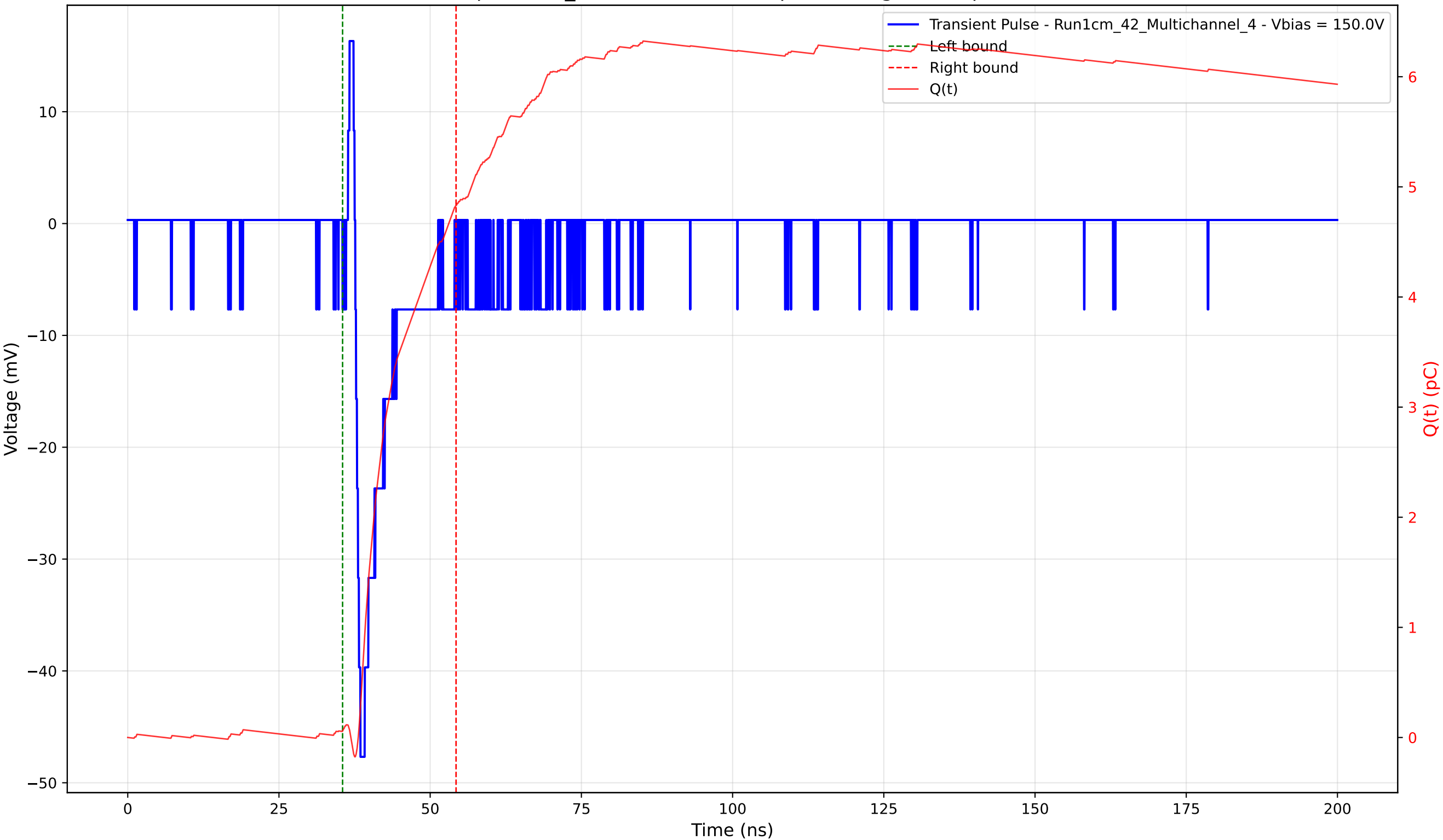
Transient Pulse - Sample: 1cm_42 - Position: 930.0 \mu\text{m} - Charge: 4.77 pC - Rise Time: 0.86 ns
