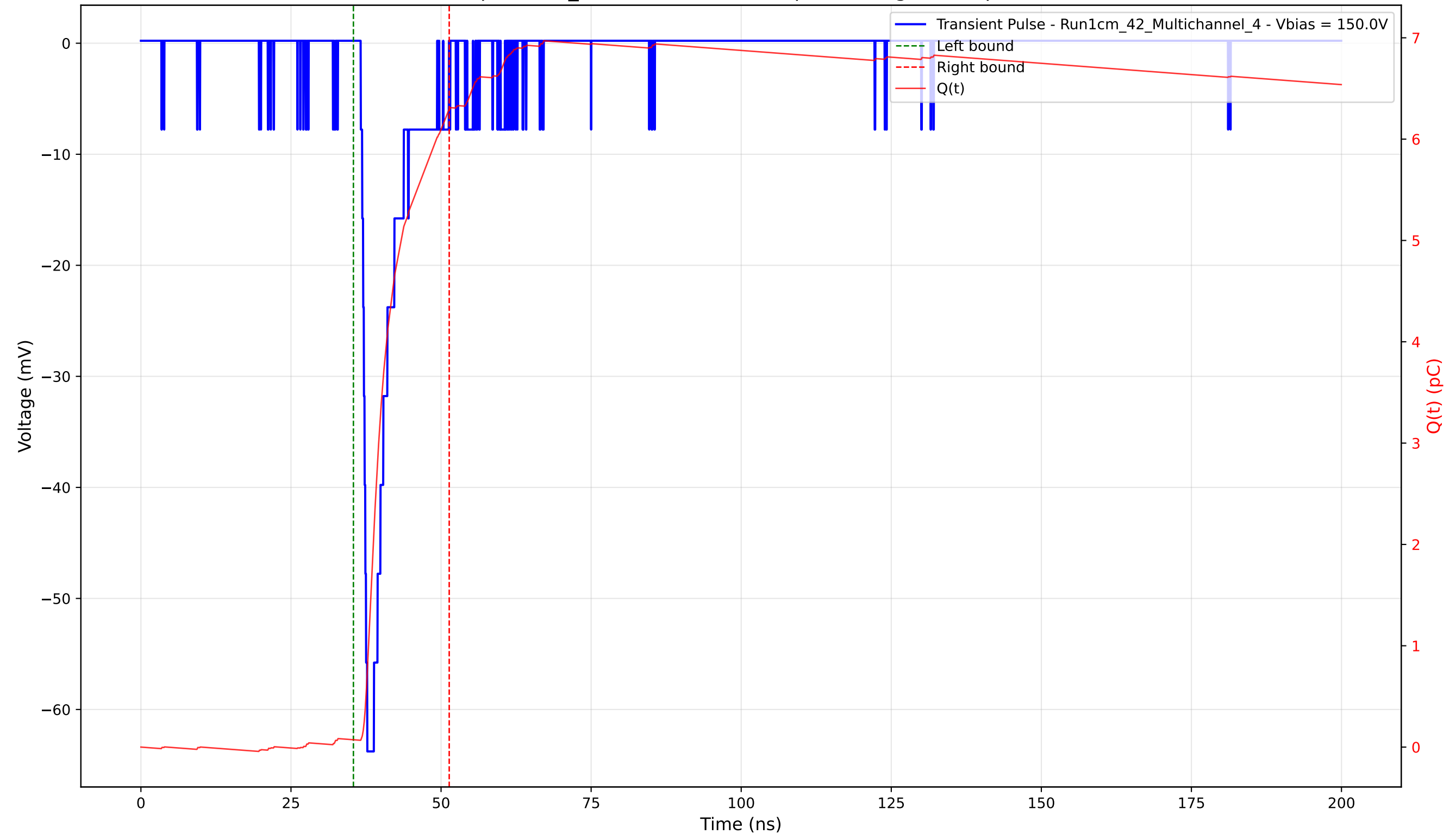
Transient Pulse - Sample: 1cm_42 - Position: 1475.0 \mu\text{m} - Charge: 6.22 pC - Rise Time: 1.09 ns
