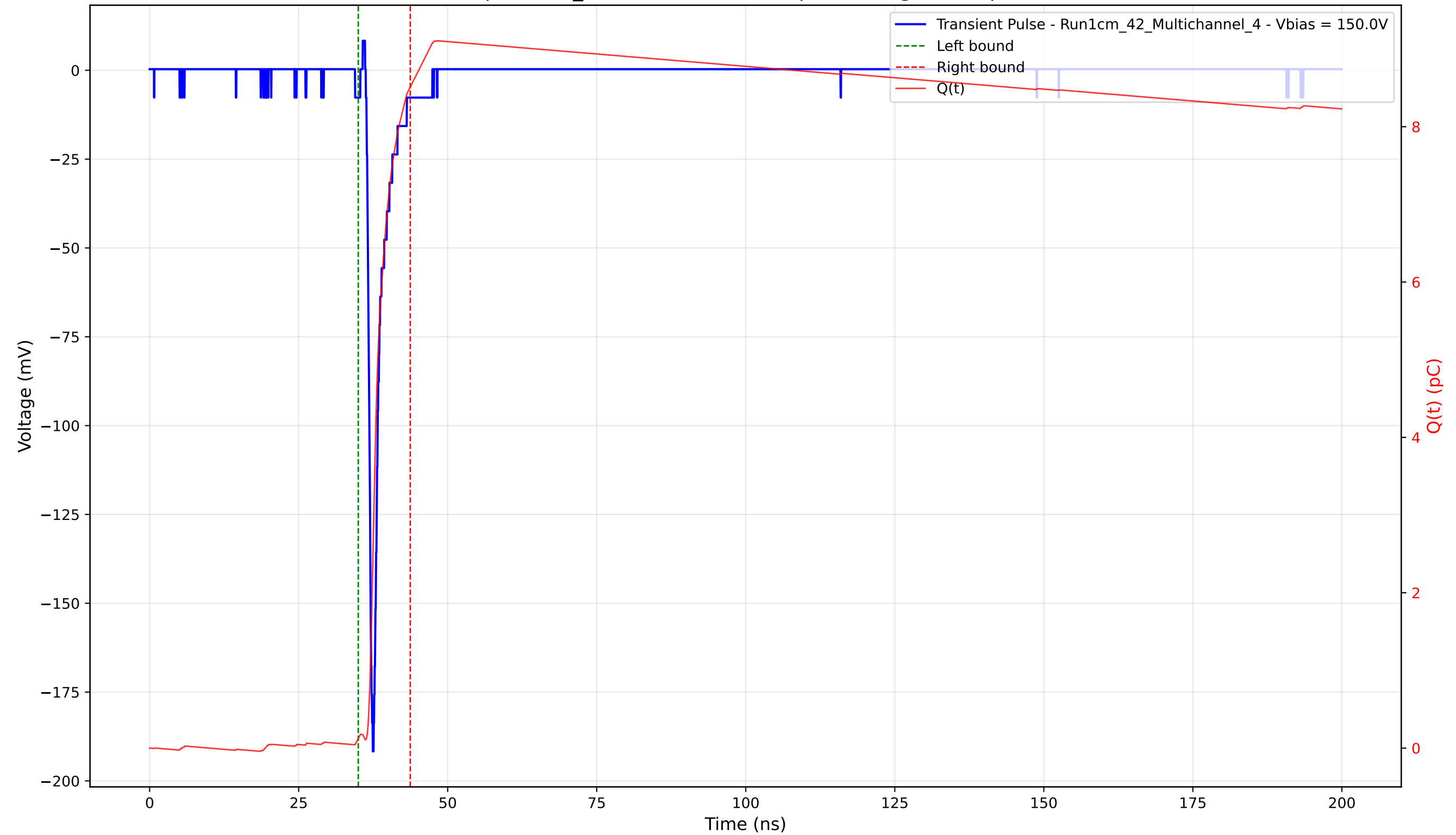
Transient Pulse - Sample: 1cm_42 - Position: 3085.0 \mu\text{m} - Charge: 8.39 pC - Rise Time: 0.82 ns
