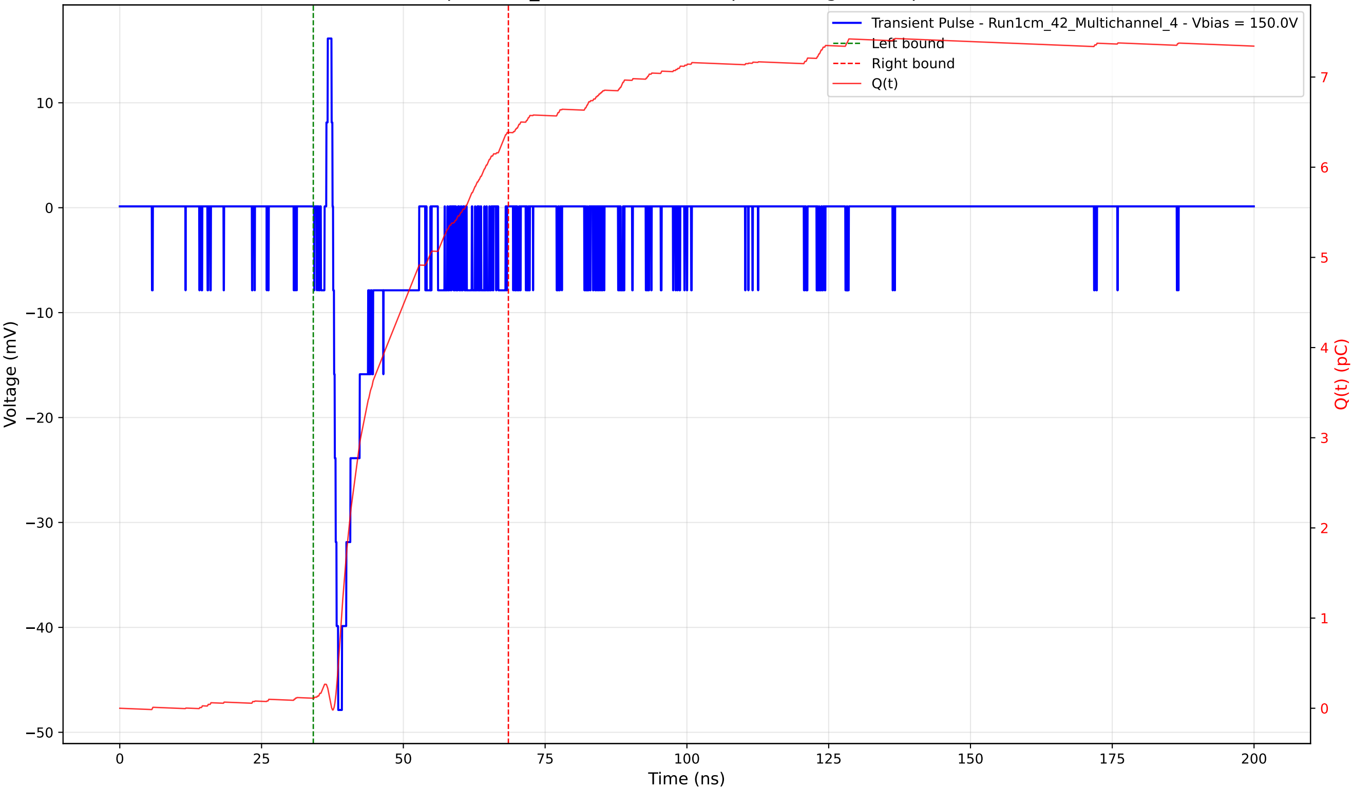
Transient Pulse - Sample: 1cm_42 - Position: 935.0 \mu\text{m} - Charge: 6.27 pC - Rise Time: 0.90 ns
