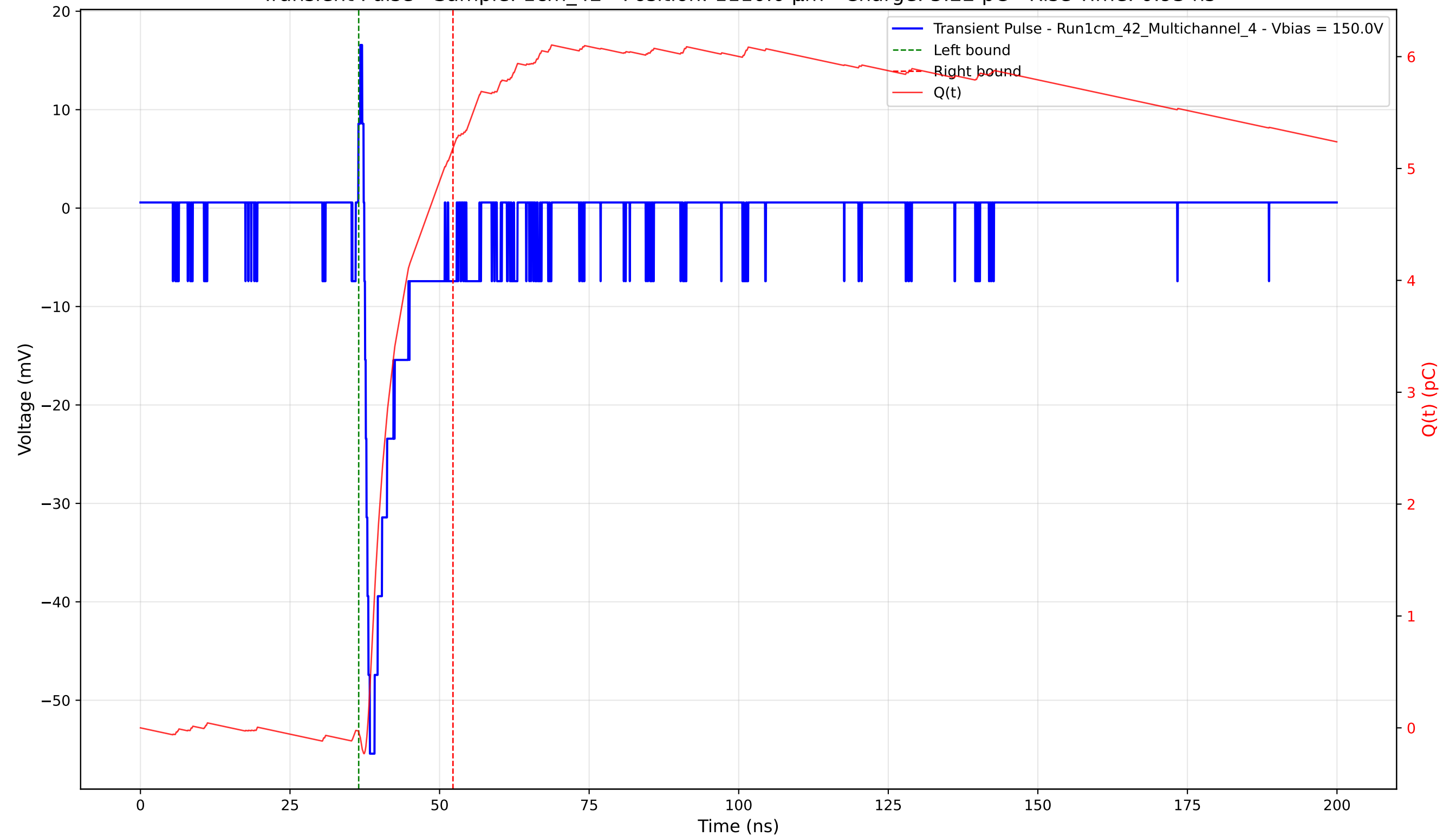
Transient Pulse - Sample: 1cm_42 - Position: 1110.0 \mu\text{m} - Charge: 5.22 pC - Rise Time: 0.93 ns
