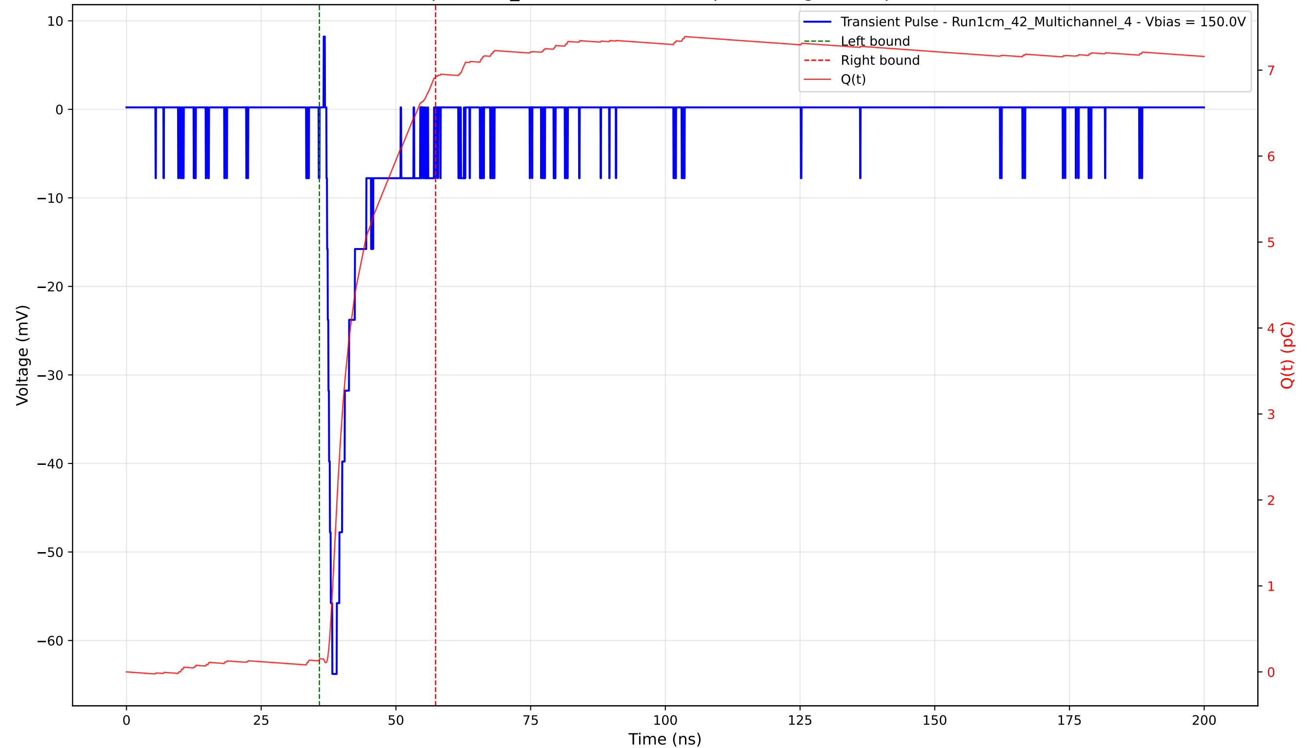
Transient Pulse - Sample: 1cm_42 - Position: 1360.0 \mu\text{m} - Charge: 6.77 pC - Rise Time: 1.09 ns
