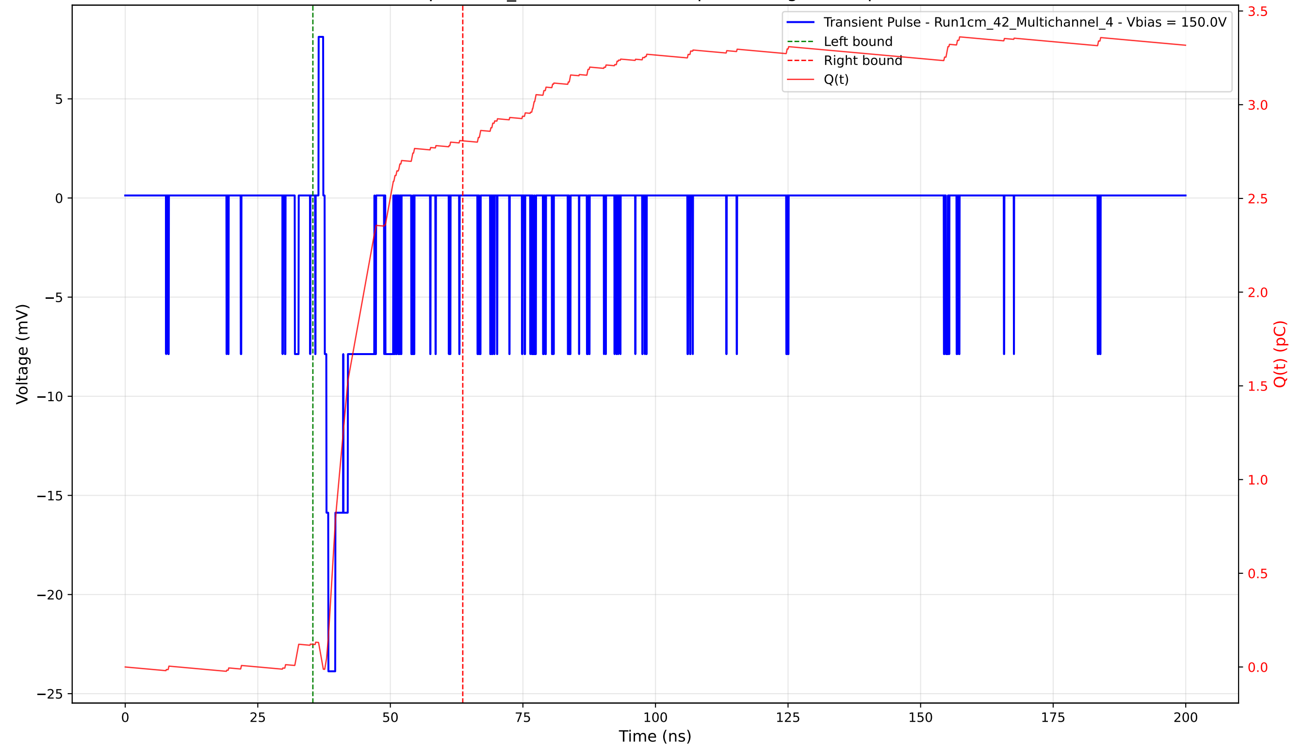
Transient Pulse - Sample: 1cm_42 - Position: 300.0 \mu\text{m} - Charge: 2.69 pC - Rise Time: 0.71 ns
