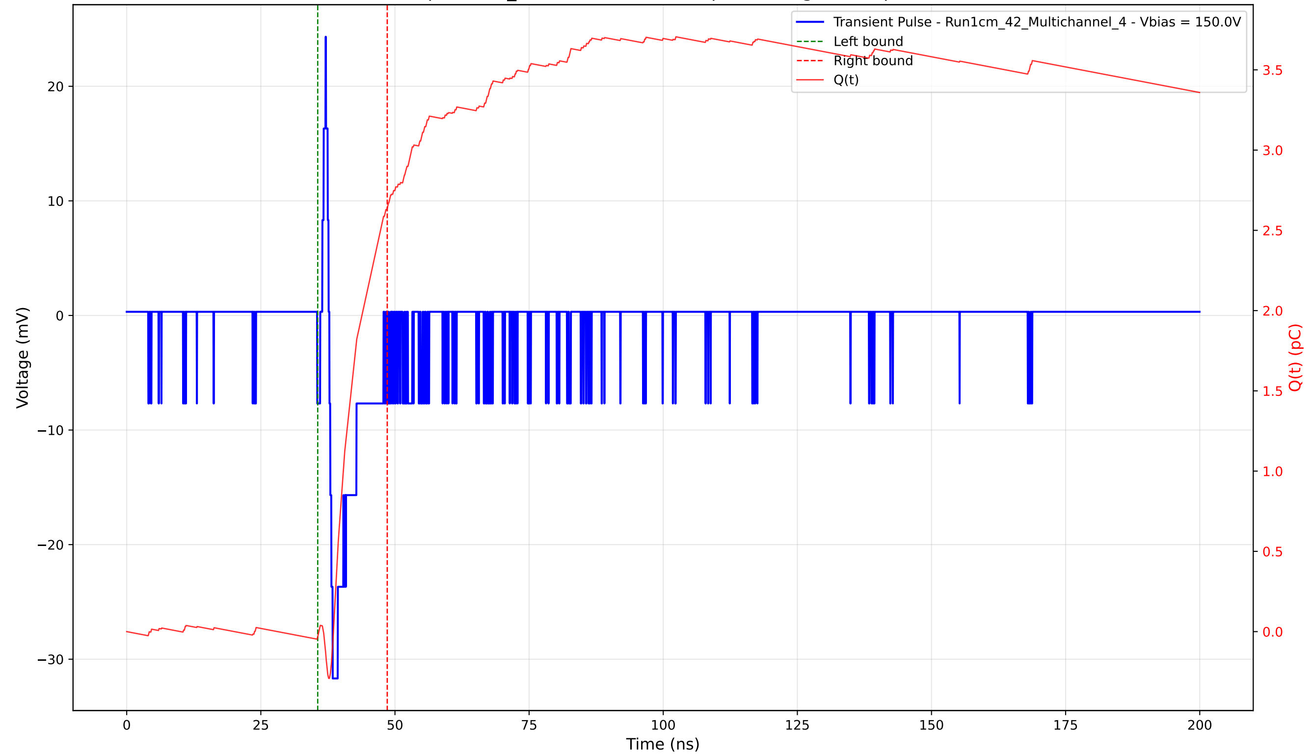
Transient Pulse - Sample: 1cm_42 - Position: 4460.0 \mu\text{m} - Charge: 2.67 pC - Rise Time: 0.62 ns
