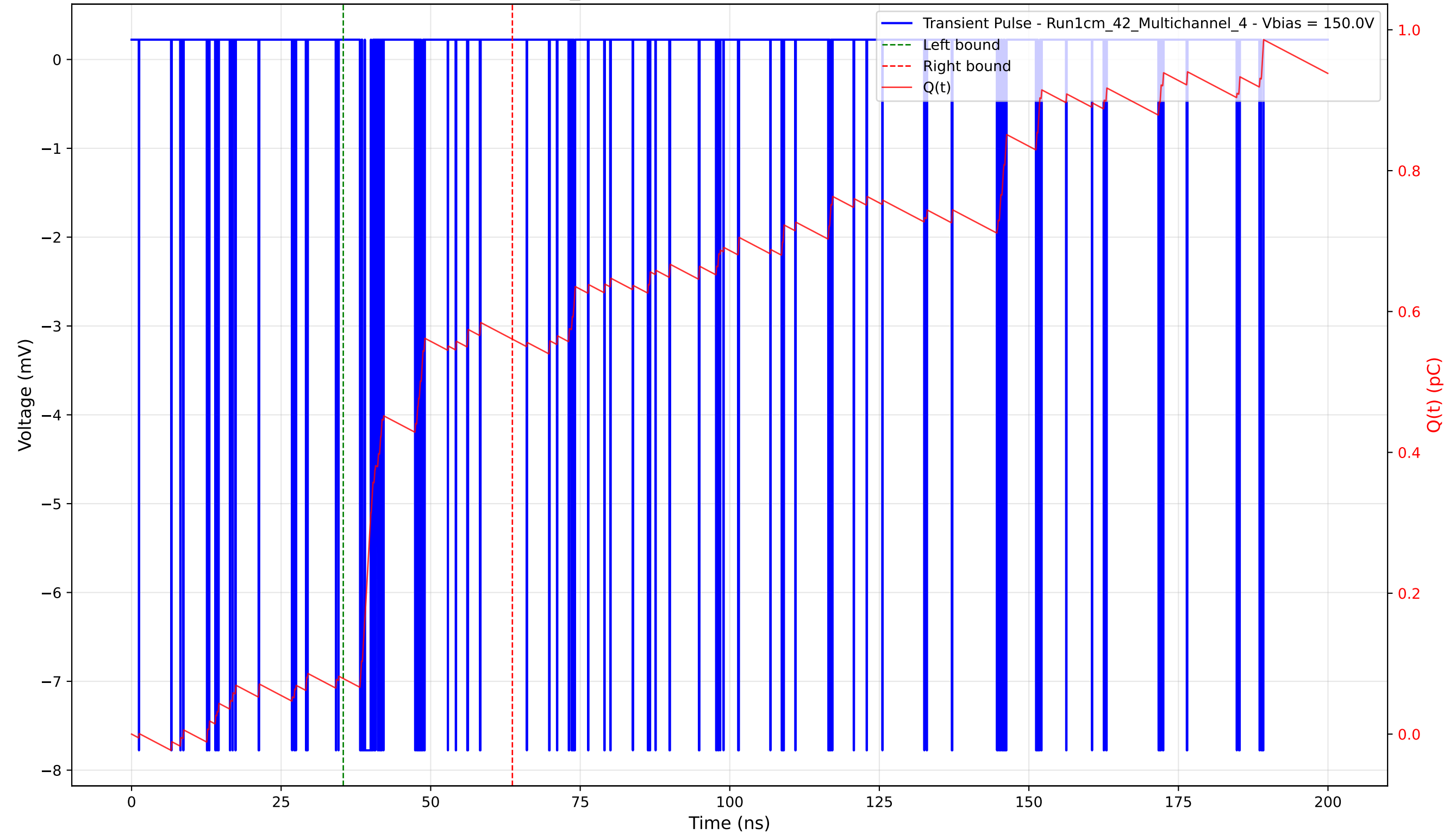
Transient Pulse - Sample: 1cm_42 - Position: 20.0 \mu\text{m} - Charge: 0.48 pC - Rise Time: 0.04 ns
