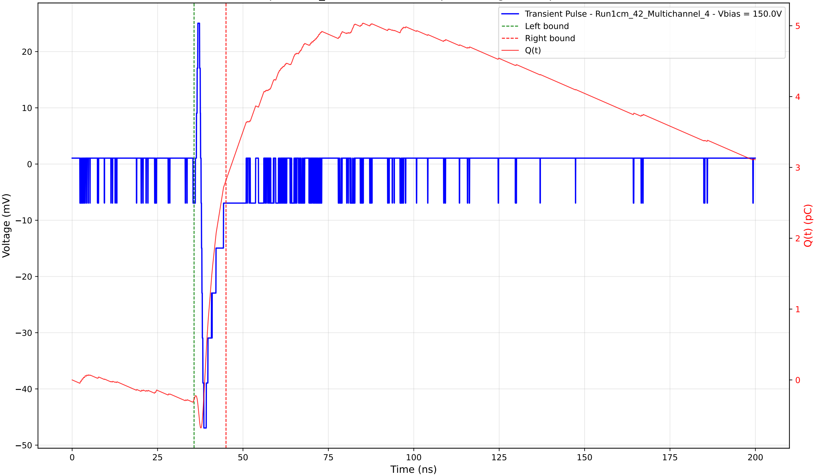
Transient Pulse - Sample: 1cm_42 - Position: 685.0 \mu\text{m} - Charge: 3.09 pC - Rise Time: 0.82 ns
