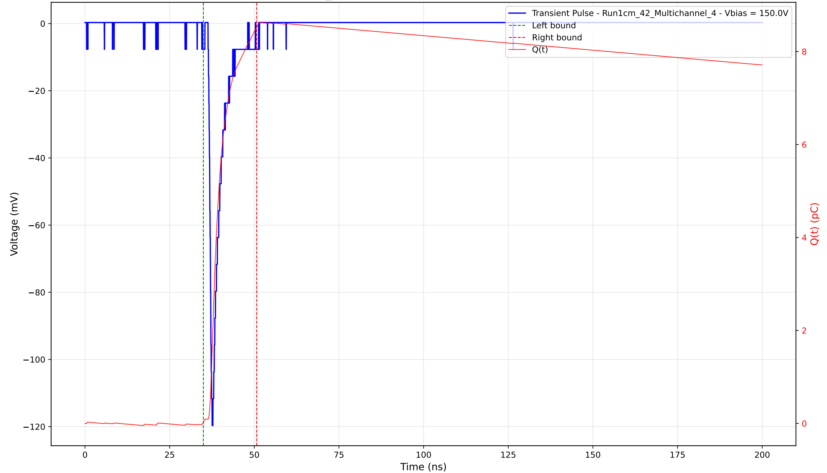
Transient Pulse - Sample: 1cm_42 - Position: 1660.0 \mu\text{m} - Charge: 8.50 pC - Rise Time: 0.94 ns
