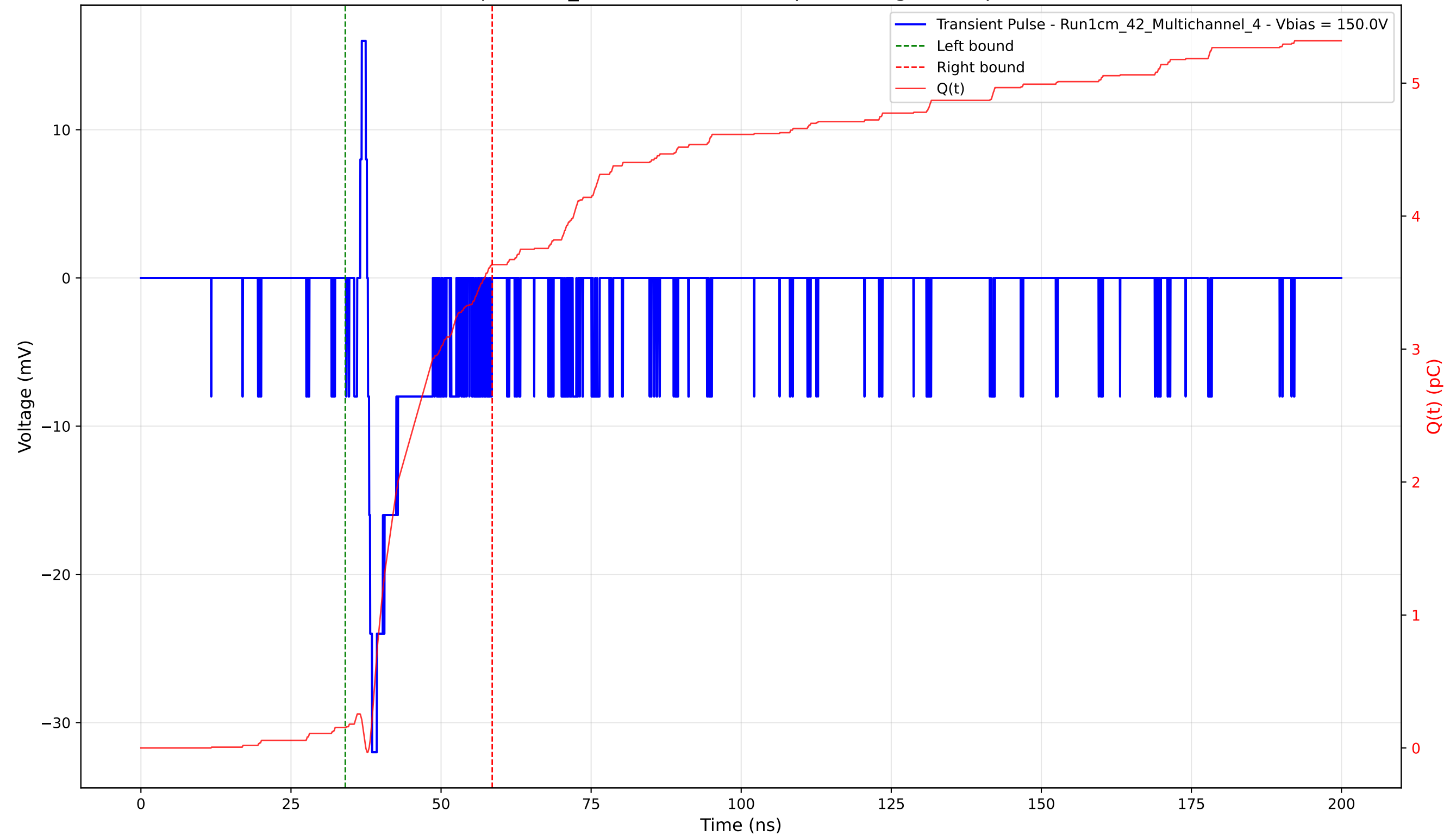
Transient Pulse - Sample: 1cm_42 - Position: 4525.0 \mu\text{m} - Charge: 3.48 pC - Rise Time: 0.70 ns
