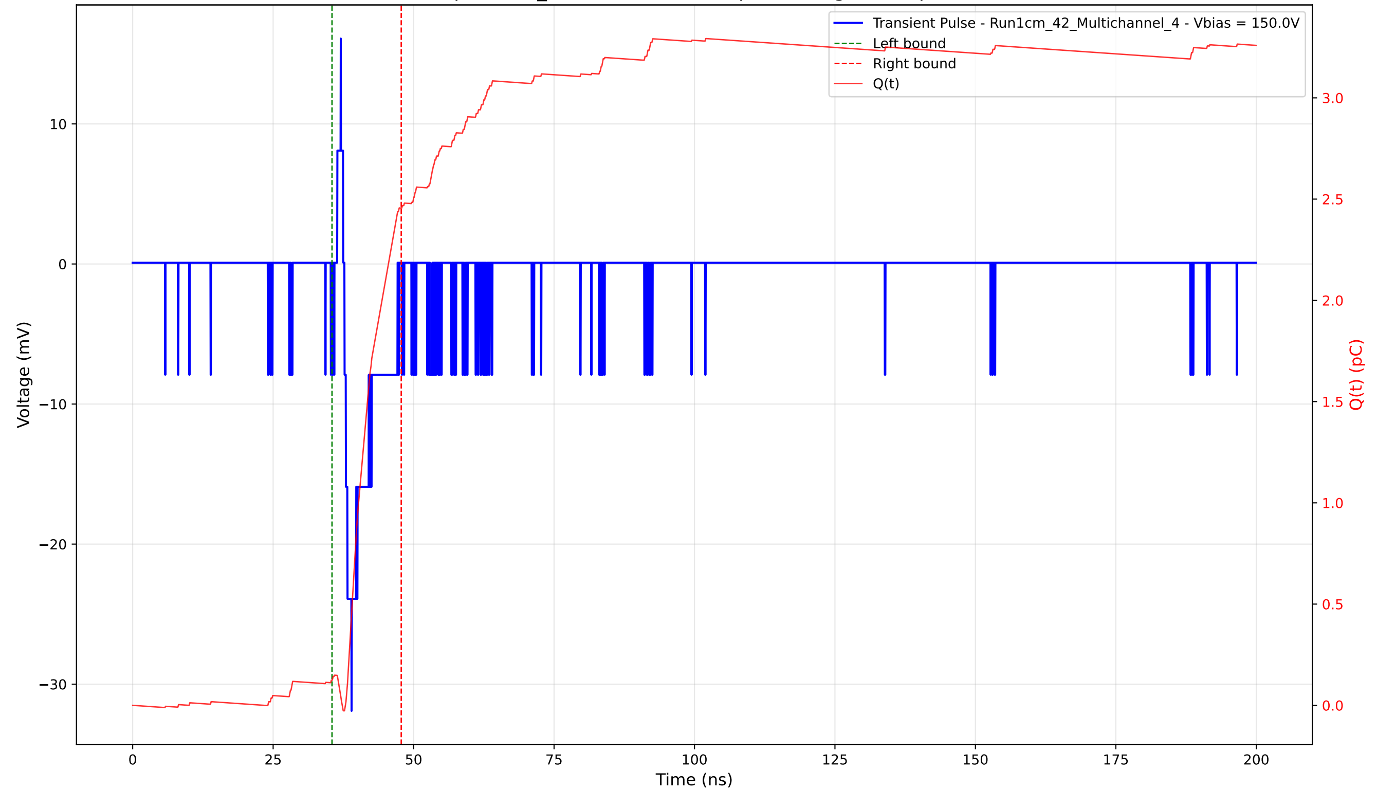
Transient Pulse - Sample: 1cm_42 - Position: 345.0 \mu\text{m} - Charge: 2.33 pC - Rise Time: 1.26 ns
