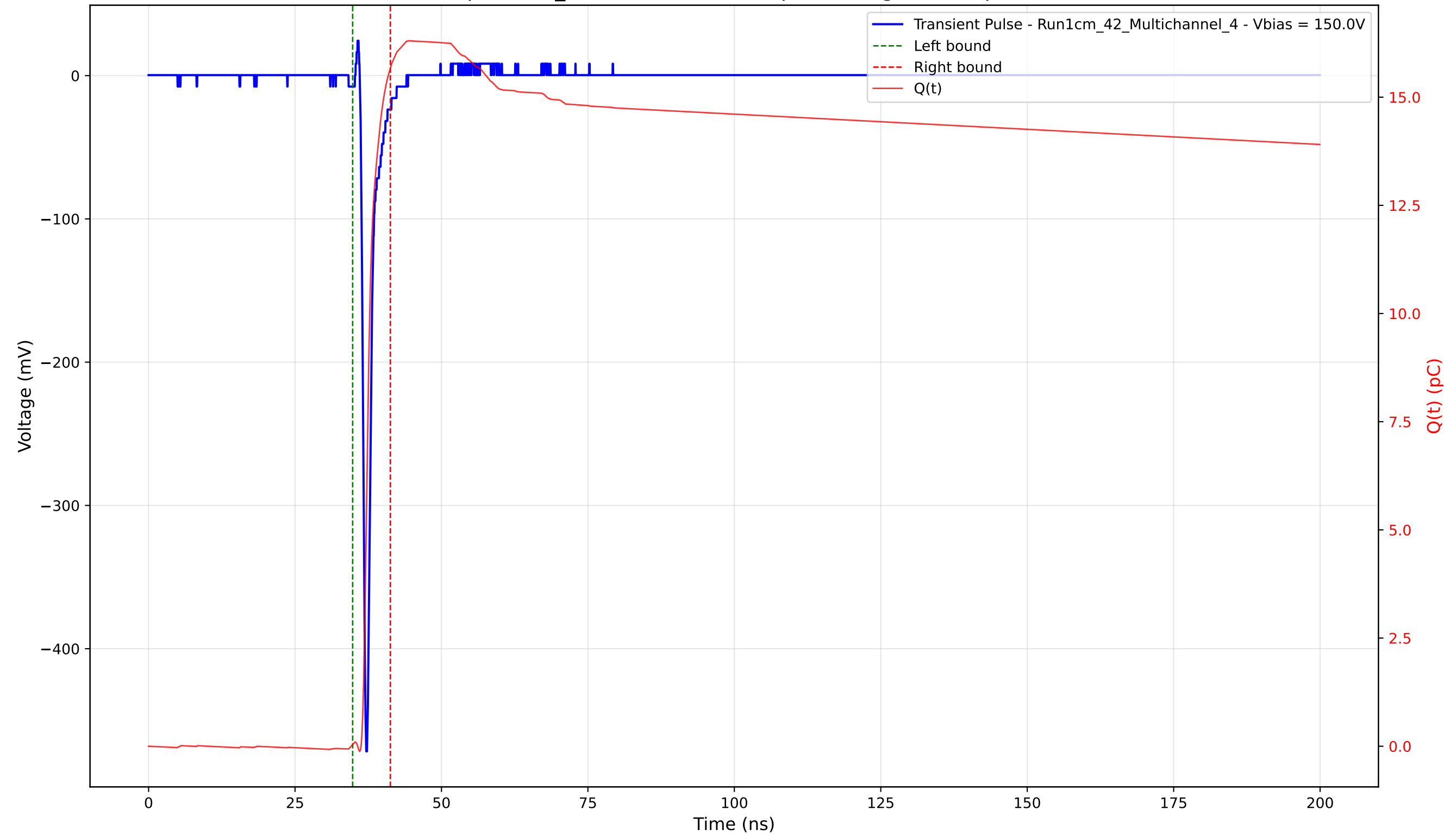
Transient Pulse - Sample: 1cm_42 - Position: 2210.0 \mu\text{m} - Charge: 15.63 pC - Rise Time: 0.69 ns
