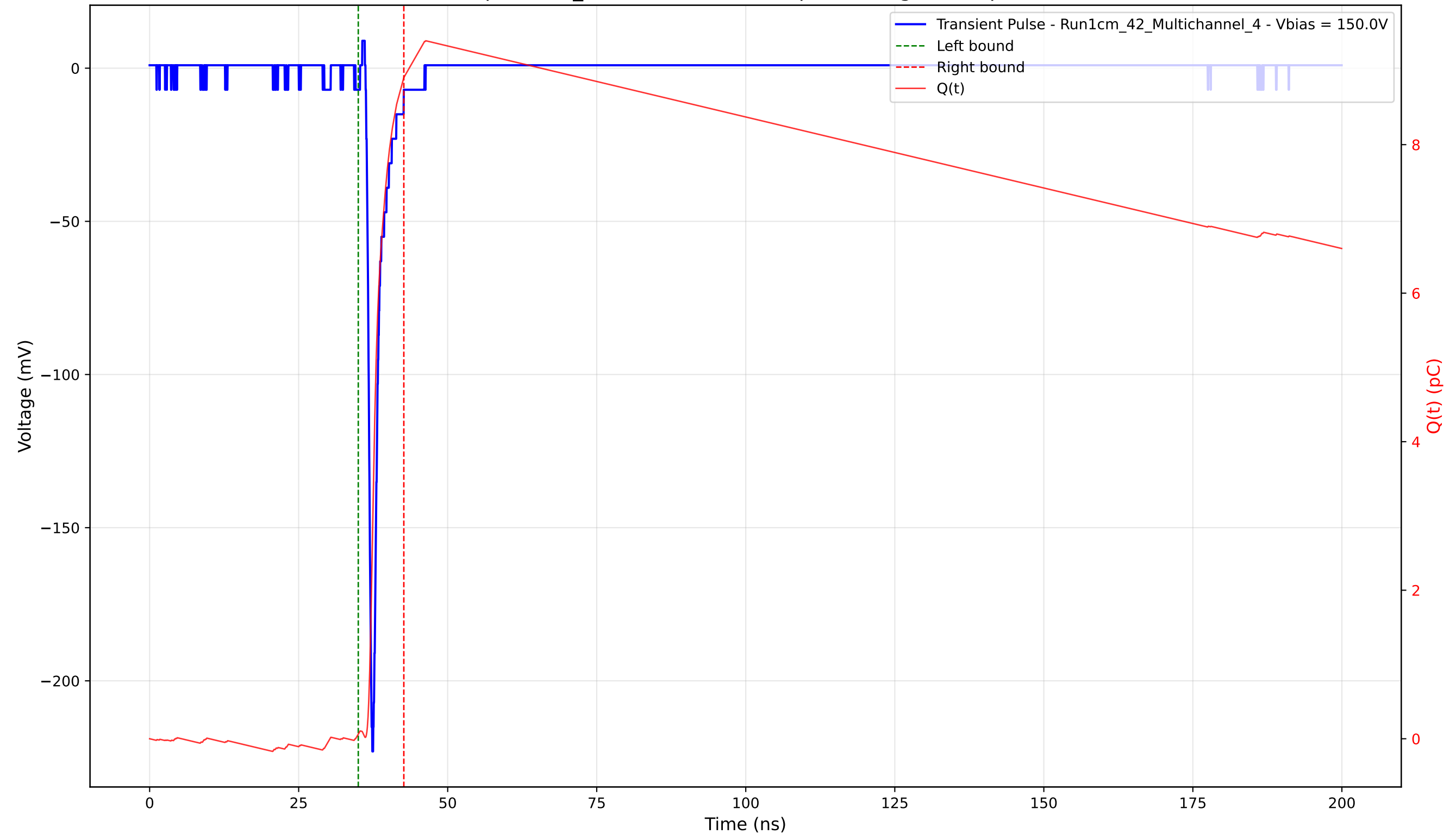
Transient Pulse - Sample: 1cm_42 - Position: 3025.0 \mu\text{m} - Charge: 8.84 pC - Rise Time: 0.81 ns
