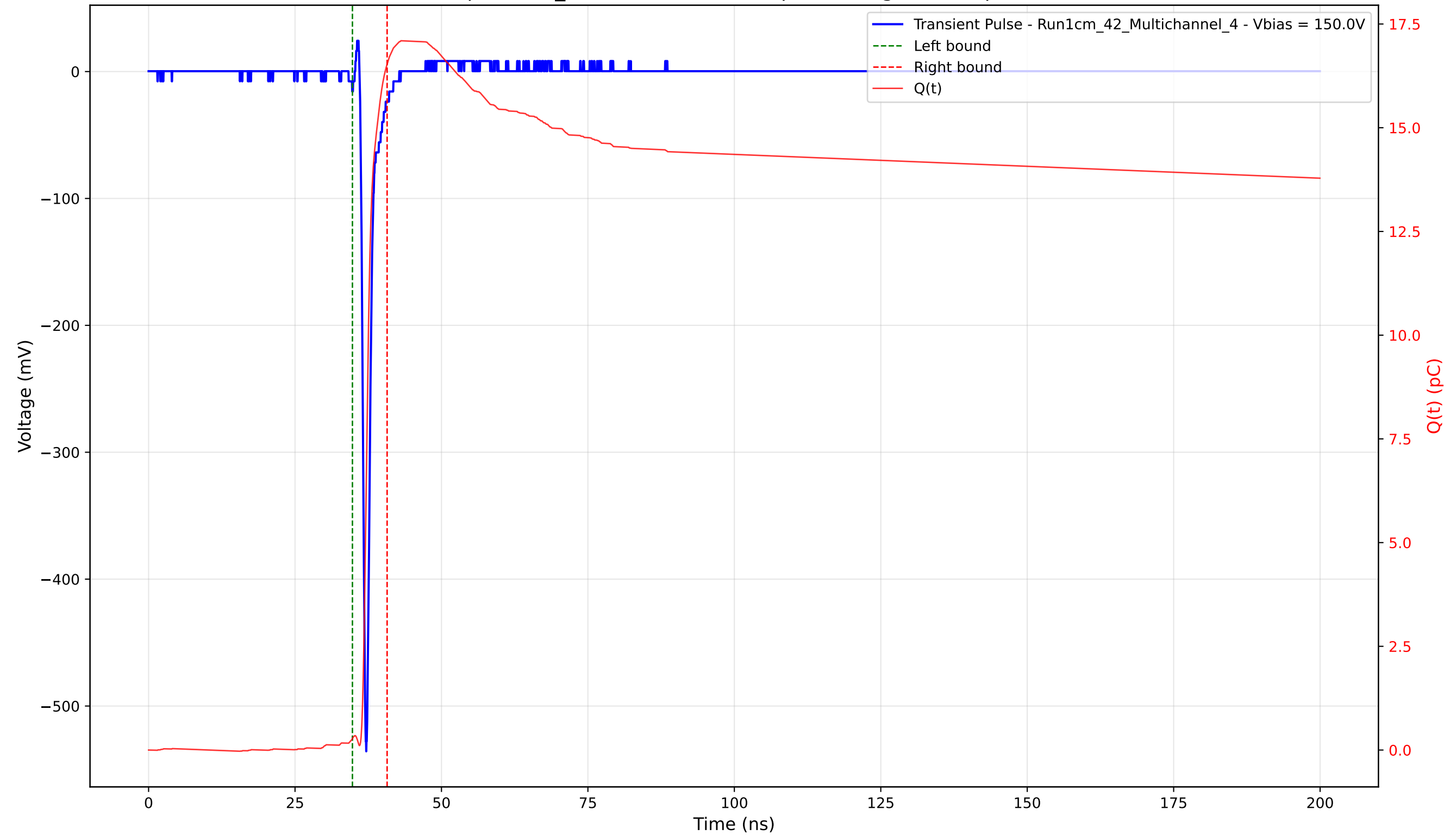
Transient Pulse - Sample: 1cm_42 - Position: 2420.0 \mu\text{m} - Charge: 16.26 pC - Rise Time: 0.73 ns
