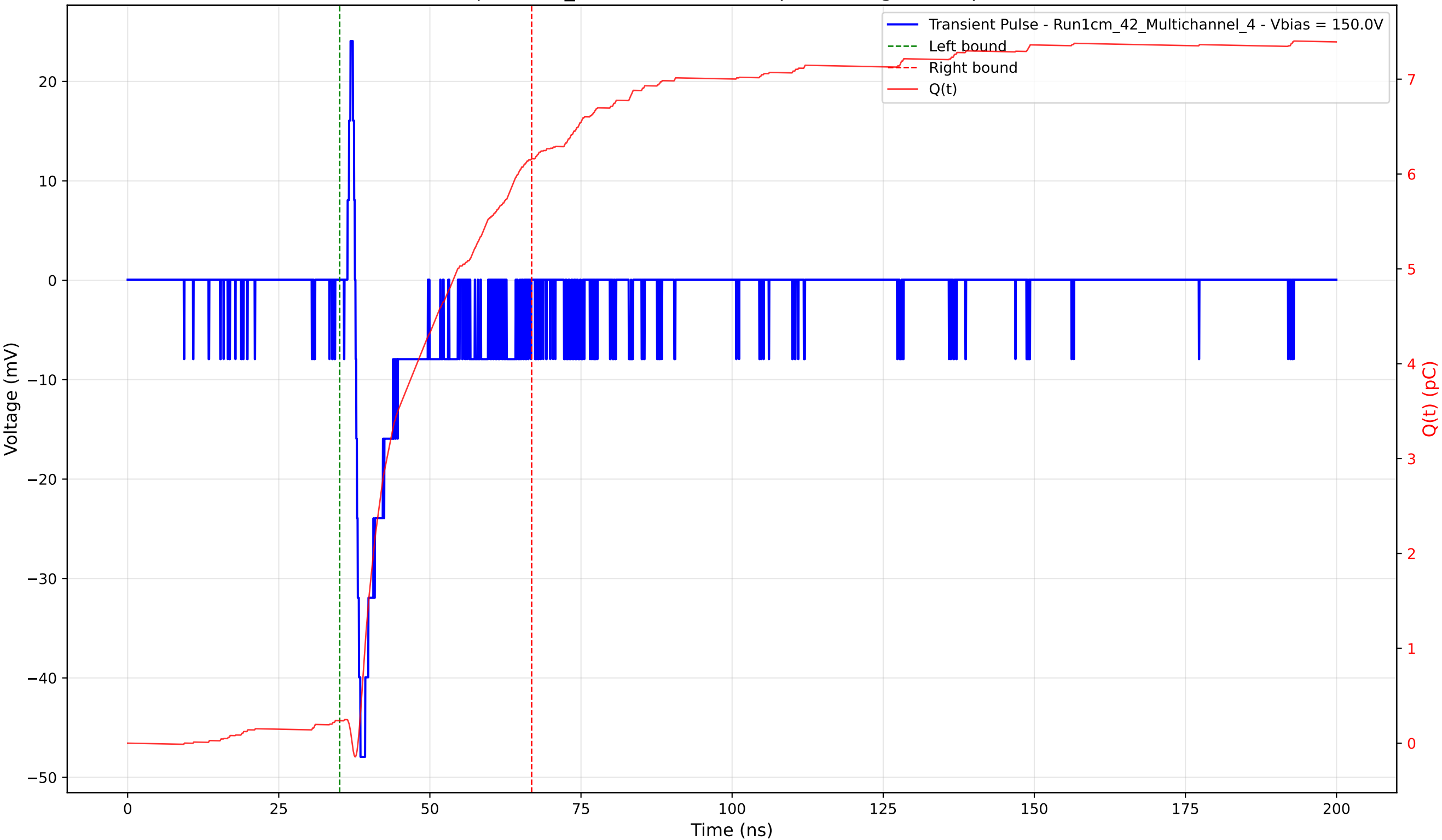
Transient Pulse - Sample: 1cm_42 - Position: 870.0 \mu\text{m} - Charge: 5.92 pC - Rise Time: 0.82 ns
