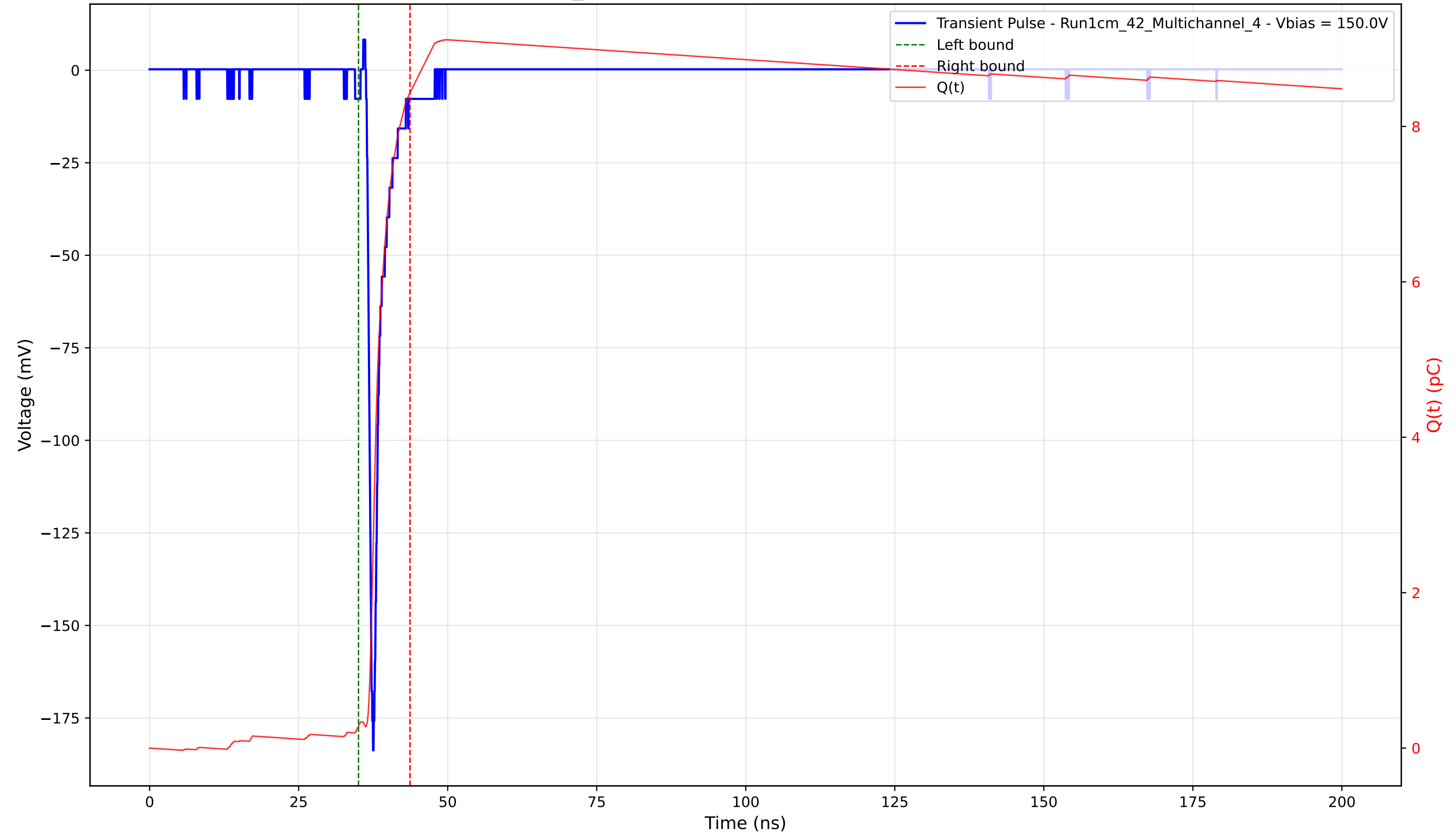
Transient Pulse - Sample: 1cm_42 - Position: 3105.0 \mu\text{m} - Charge: 8.15 pC - Rise Time: 0.79 ns
