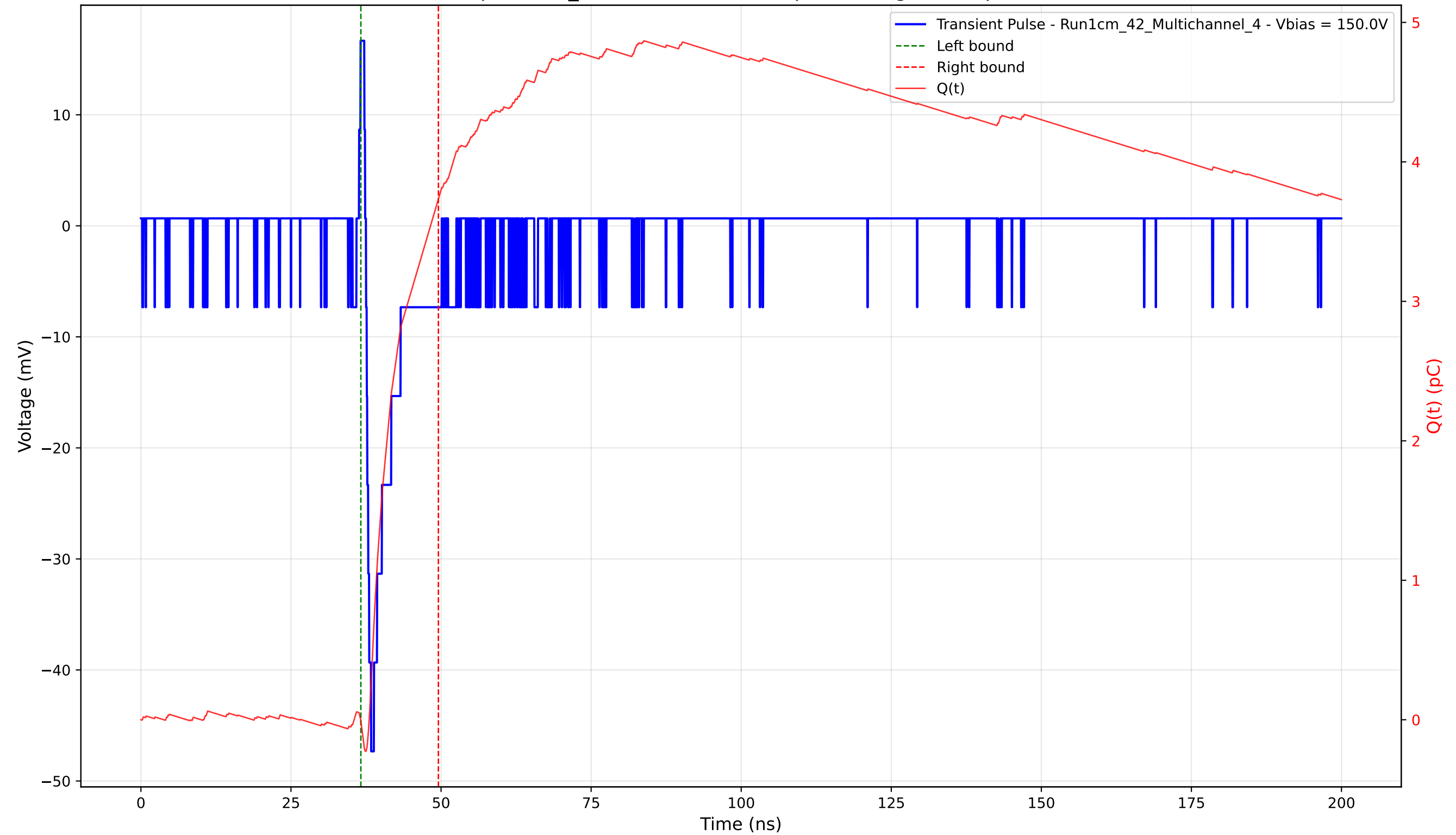
Transient Pulse - Sample: 1cm_42 - Position: 3955.0 \mu\text{m} - Charge: 3.75 pC - Rise Time: 0.86 ns
