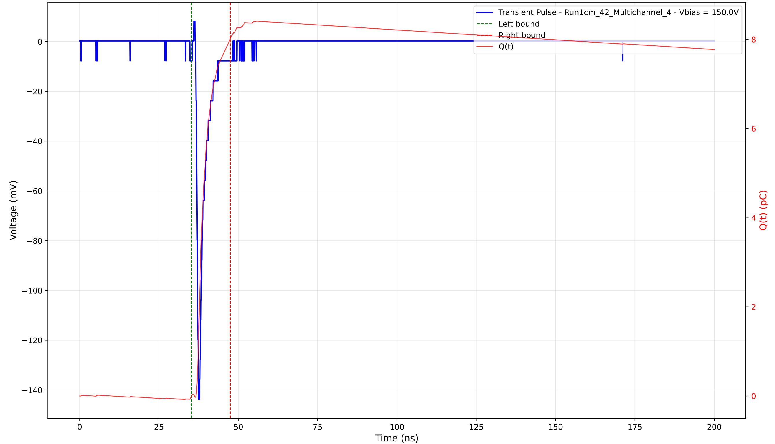
Transient Pulse - Sample: 1cm_42 - Position: 3265.0 \mu\text{m} - Charge: 8.02 pC - Rise Time: 0.77 ns
