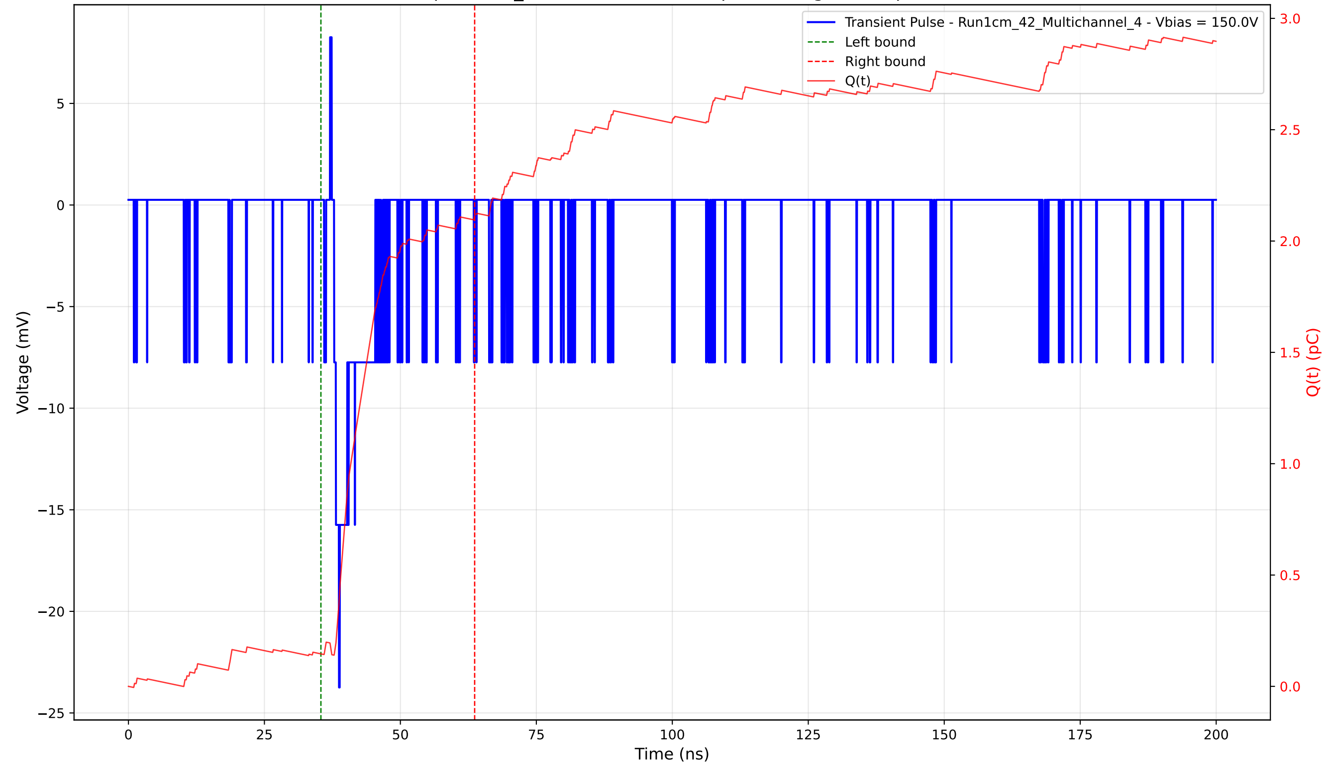
Transient Pulse - Sample: 1cm_42 - Position: 4995.0 \mu\text{m} - Charge: 1.97 pC - Rise Time: 0.91 ns
