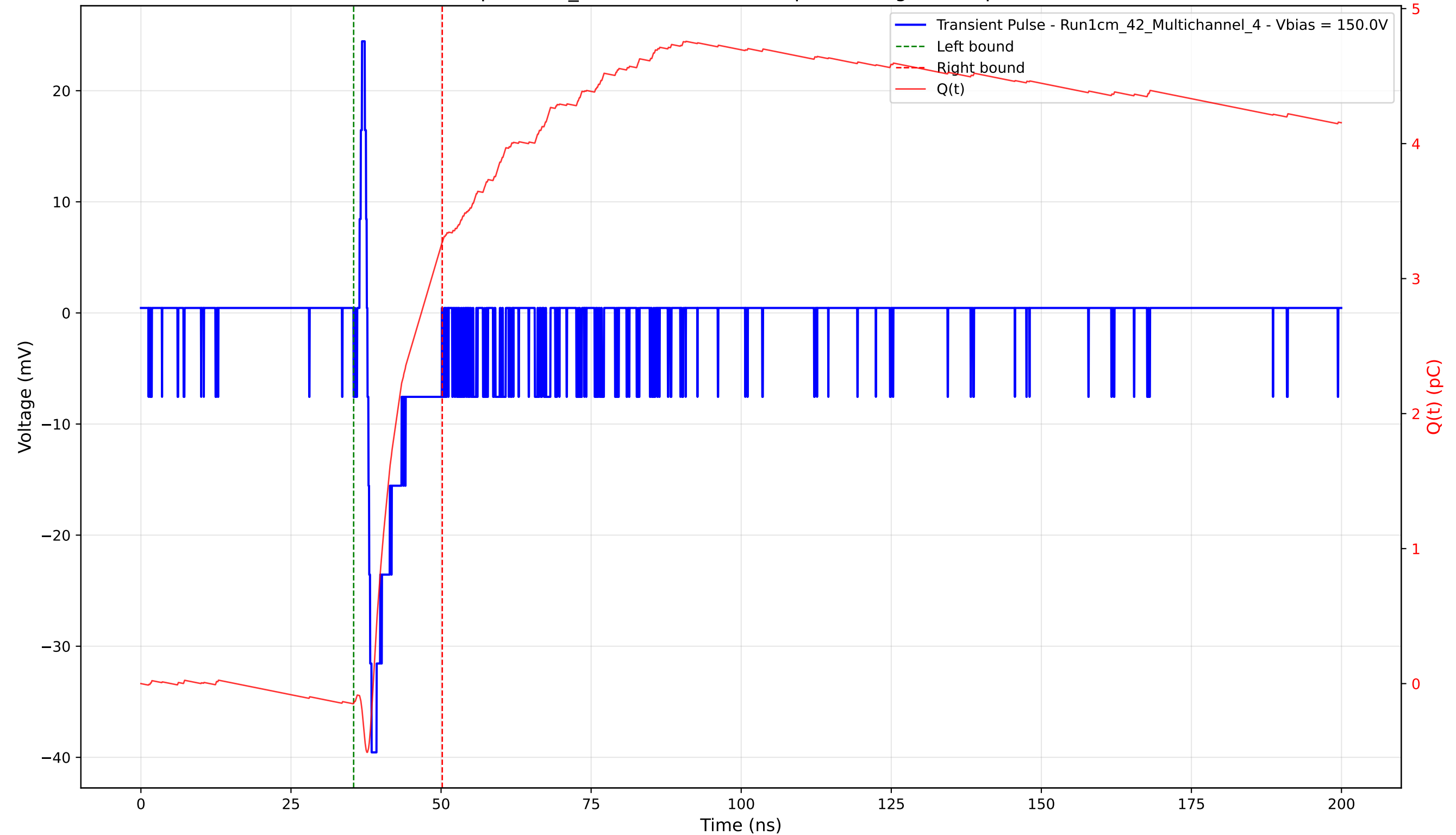
Transient Pulse - Sample: 1cm_42 - Position: 4325.0 \mu\text{m} - Charge: 3.41 pC - Rise Time: 0.70 ns
