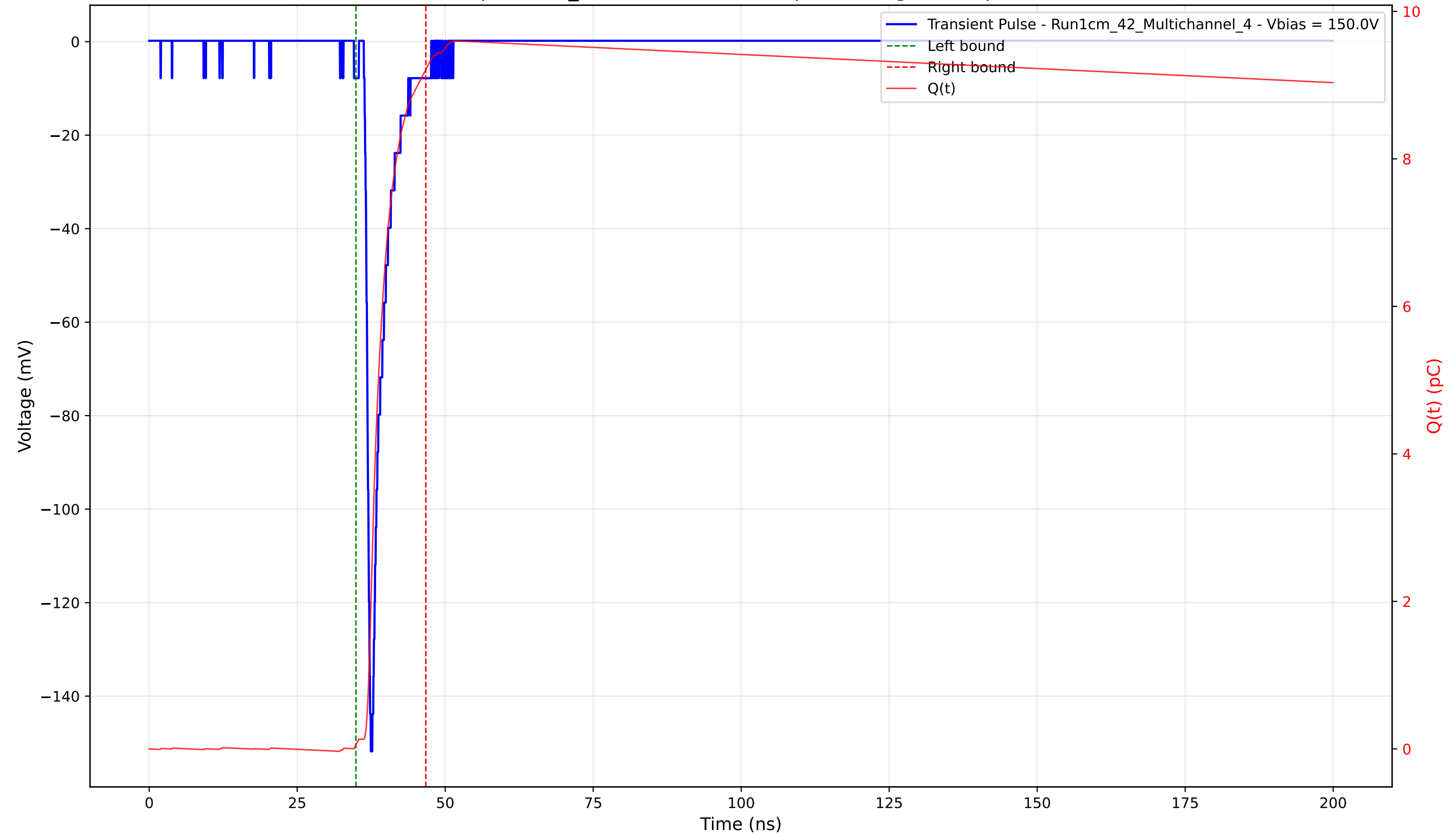
Transient Pulse - Sample: 1cm_42 - Position: 1785.0 \mu\text{m} - Charge: 9.16 pC - Rise Time: 0.92 ns
