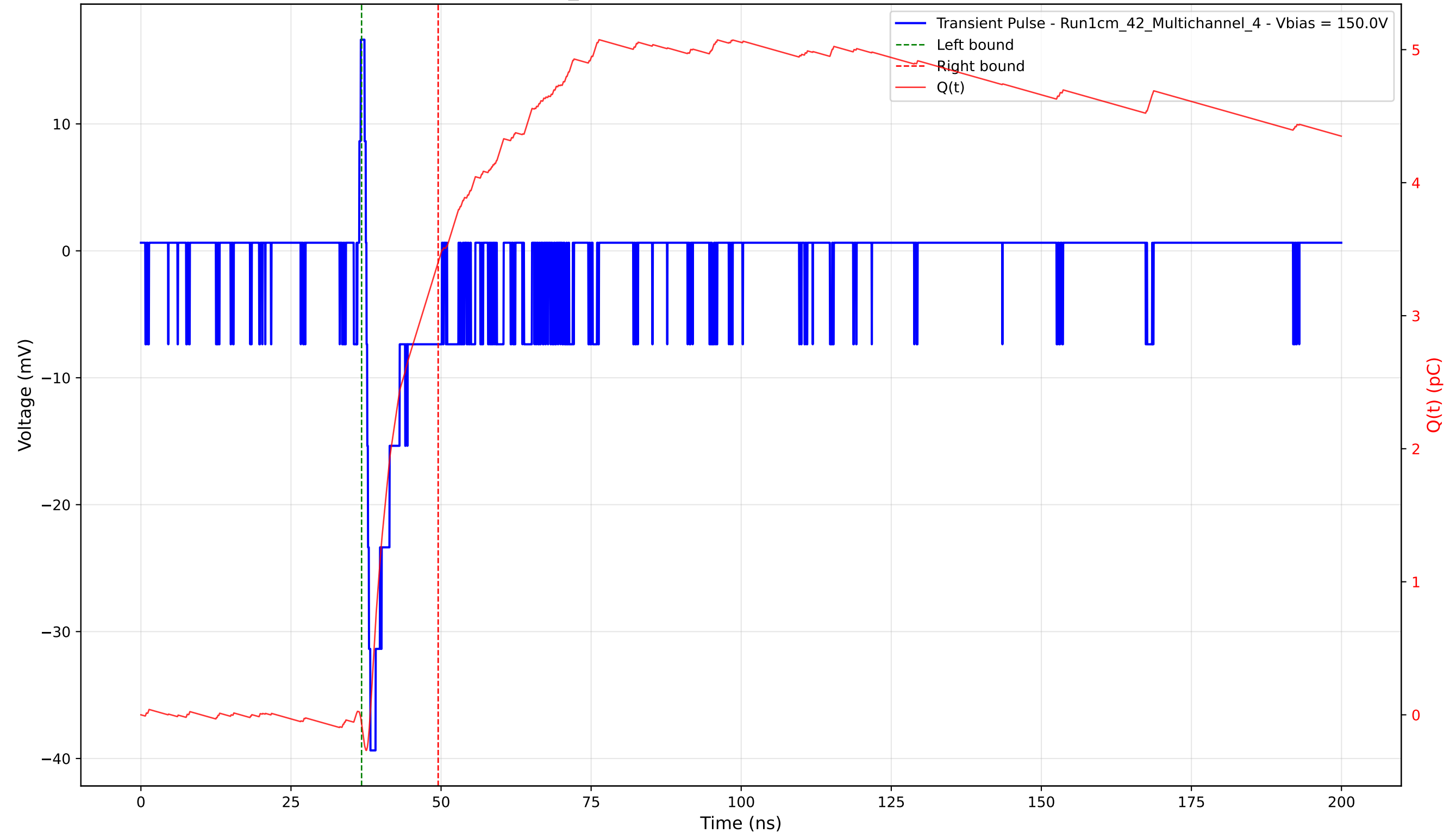
Transient Pulse - Sample: 1cm_42 - Position: 4030.0 \mu\text{m} - Charge: 3.47 pC - Rise Time: 0.66 ns
