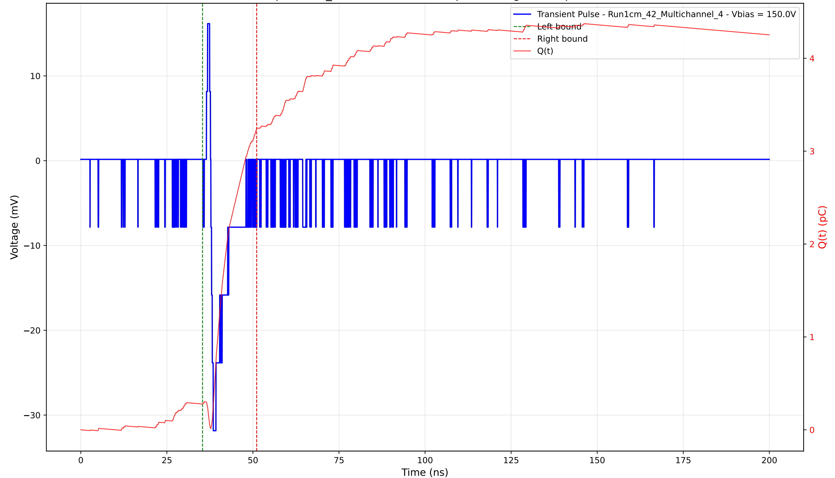
Transient Pulse - Sample: 1cm_42 - Position: 4625.0 \mu\text{m} - Charge: 2.96 pC - Rise Time: 0.70 ns
