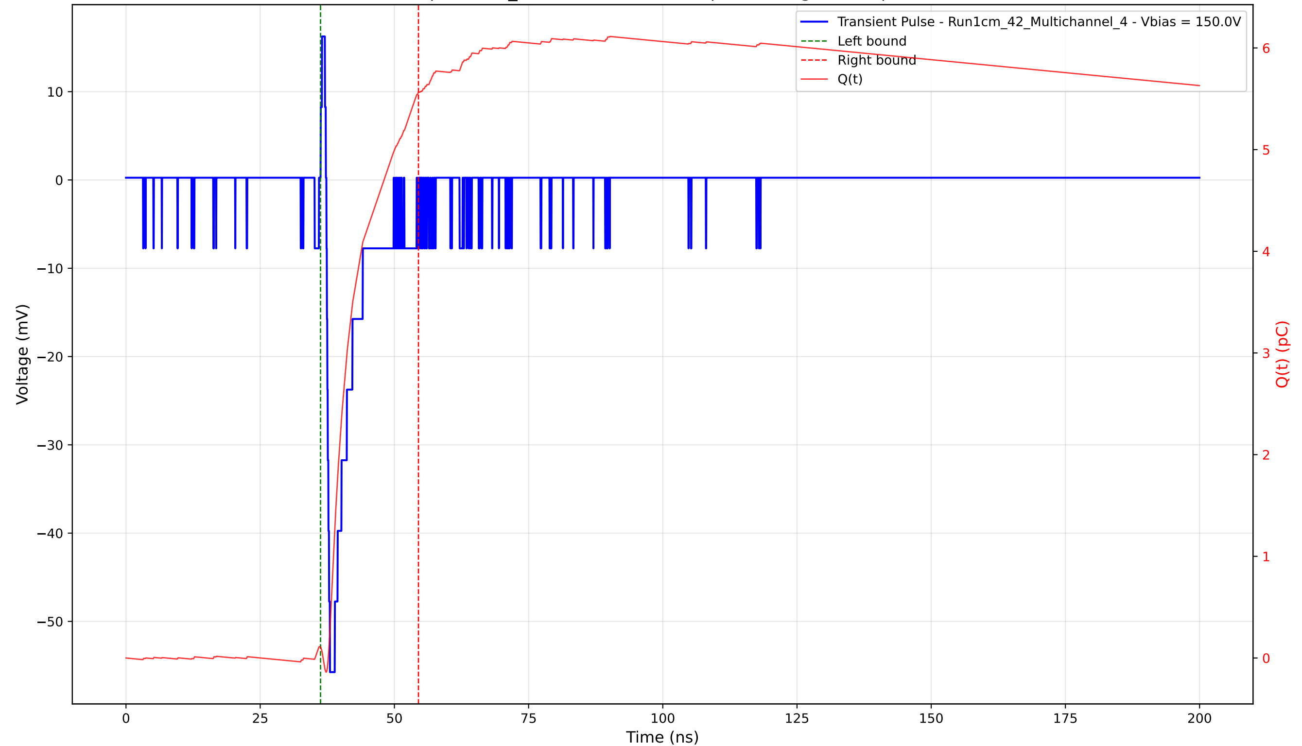
Transient Pulse - Sample: 1cm_42 - Position: 3785.0 \mu\text{m} - Charge: 5.46 pC - Rise Time: 0.65 ns
