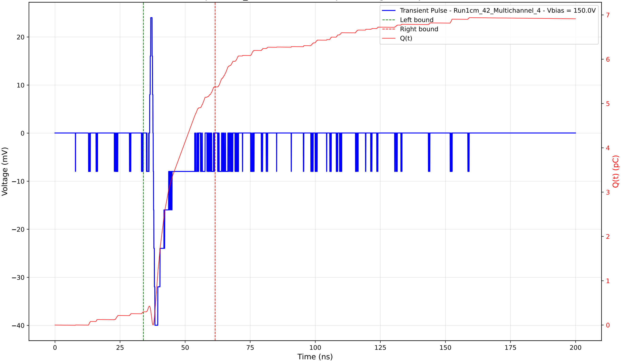
Transient Pulse - Sample: 1cm_42 - Position: 610.0 \mu\text{m} - Charge: 5.08 pC - Rise Time: 0.66 ns
