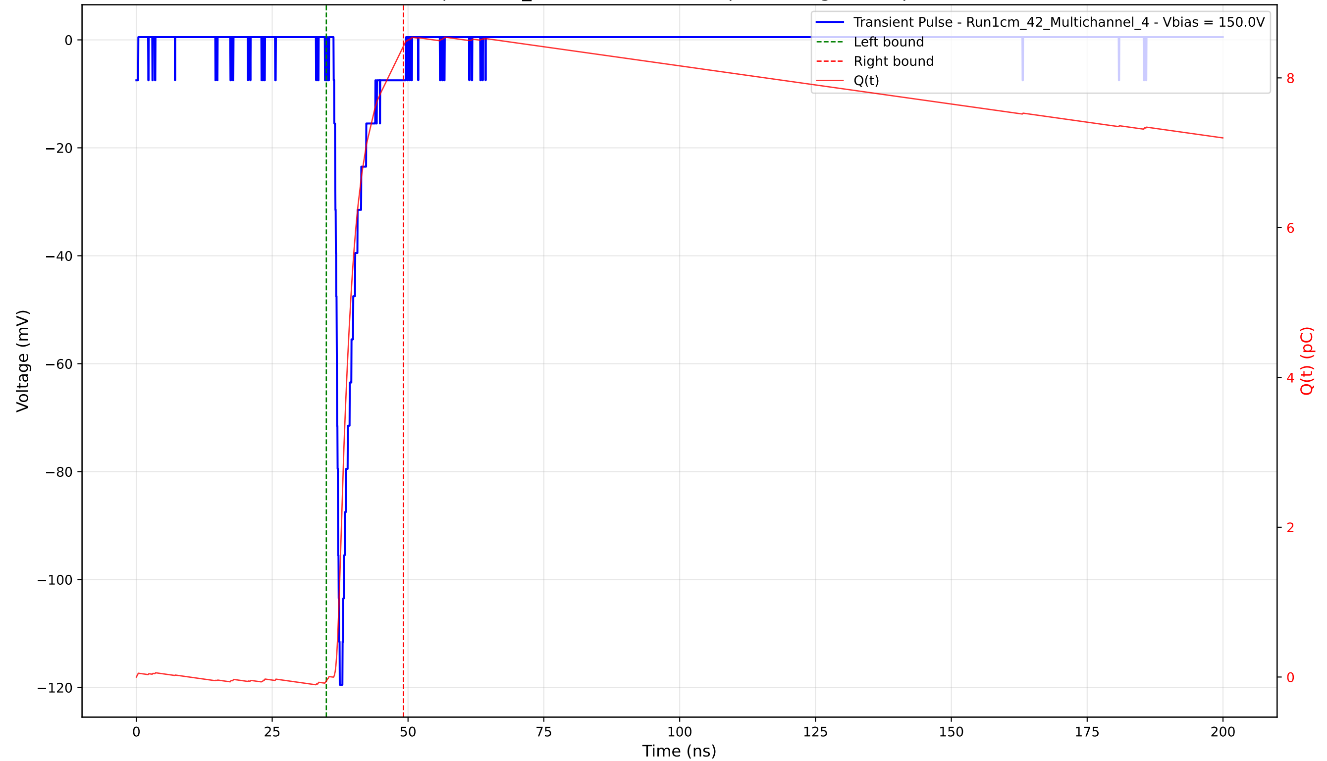
Transient Pulse - Sample: 1cm_42 - Position: 1675.0 \mu\text{m} - Charge: 8.48 pC - Rise Time: 0.90 ns
