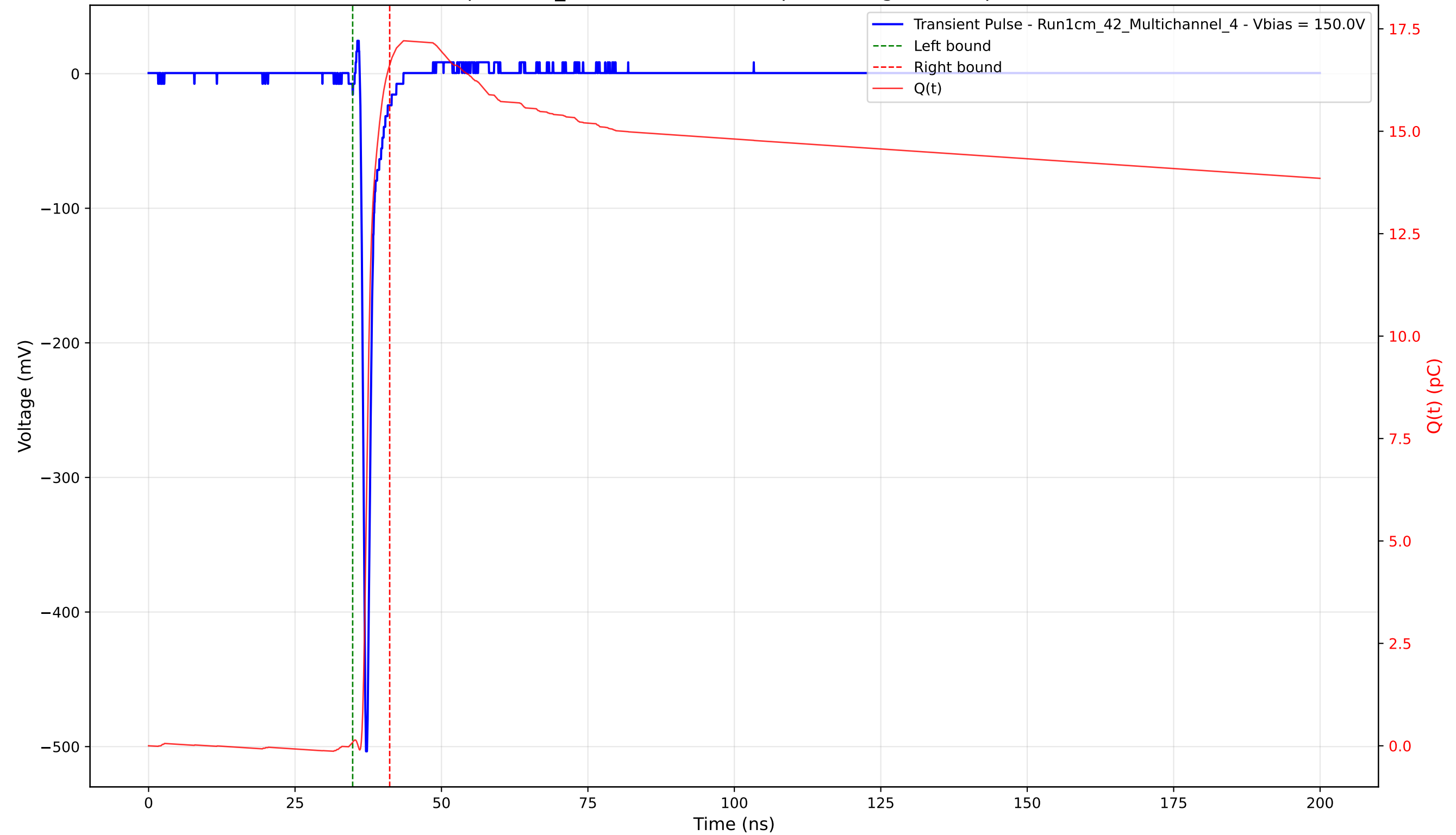
Transient Pulse - Sample: 1cm_42 - Position: 2250.0 \mu\text{m} - Charge: 16.54 pC - Rise Time: 0.73 ns
