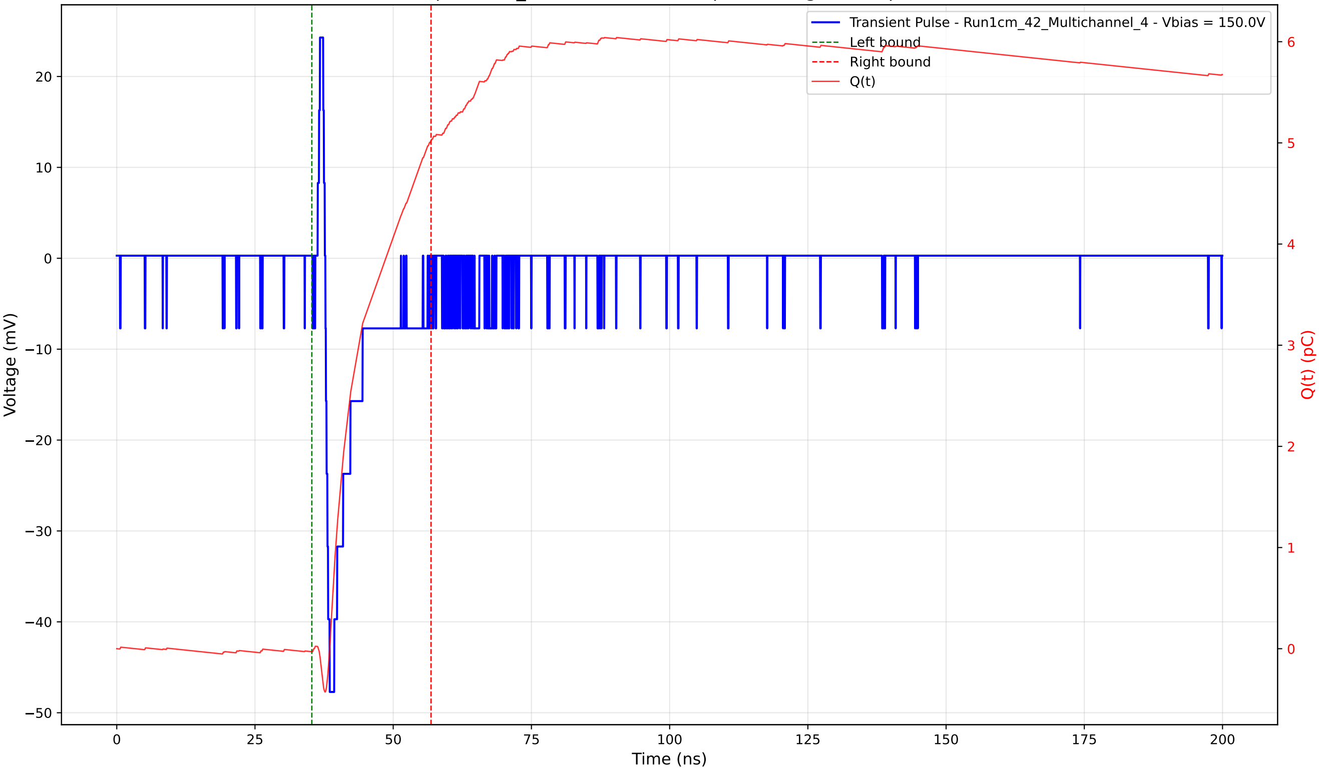
Transient Pulse - Sample: 1cm_42 - Position: 700.0 \mu\text{m} - Charge: 5.05 pC - Rise Time: 0.78 ns
