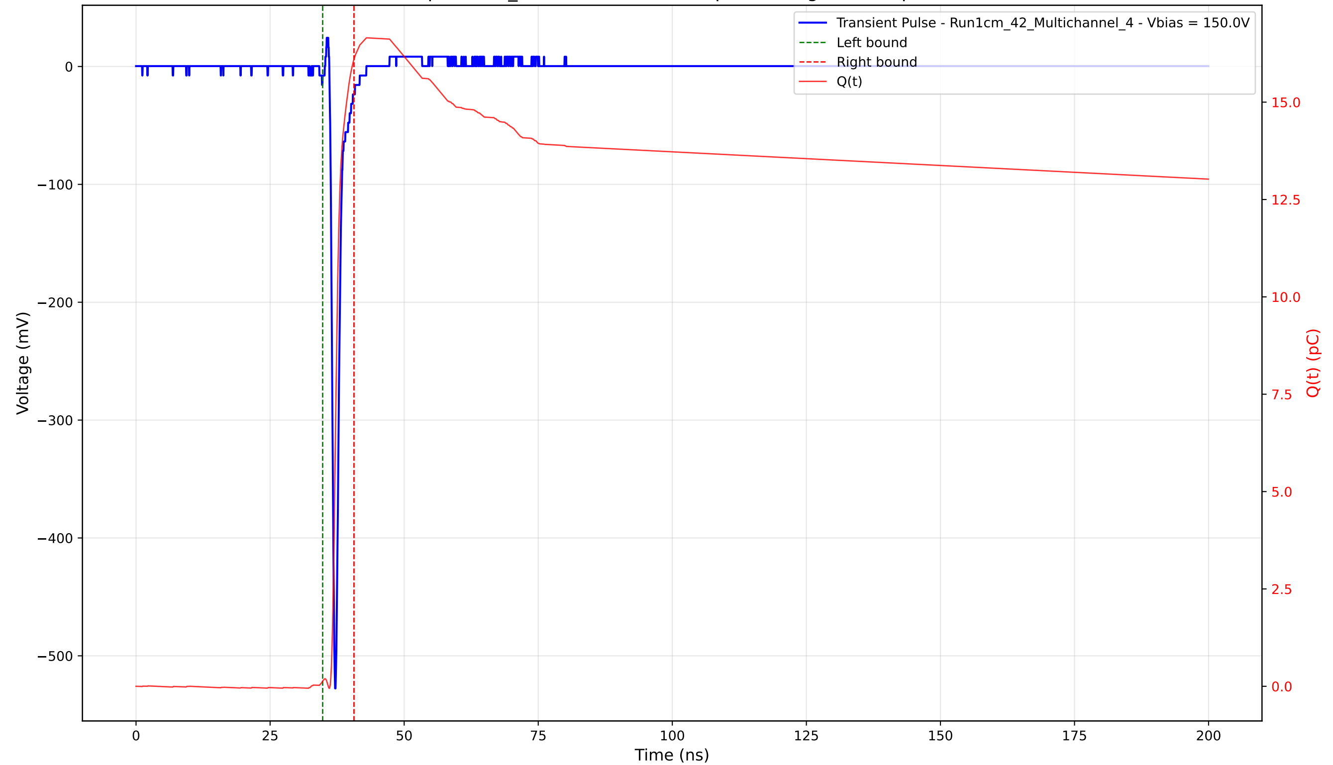
Transient Pulse - Sample: 1cm_42 - Position: 2600.0 \mu\text{m} - Charge: 15.97 pC - Rise Time: 0.72 ns
