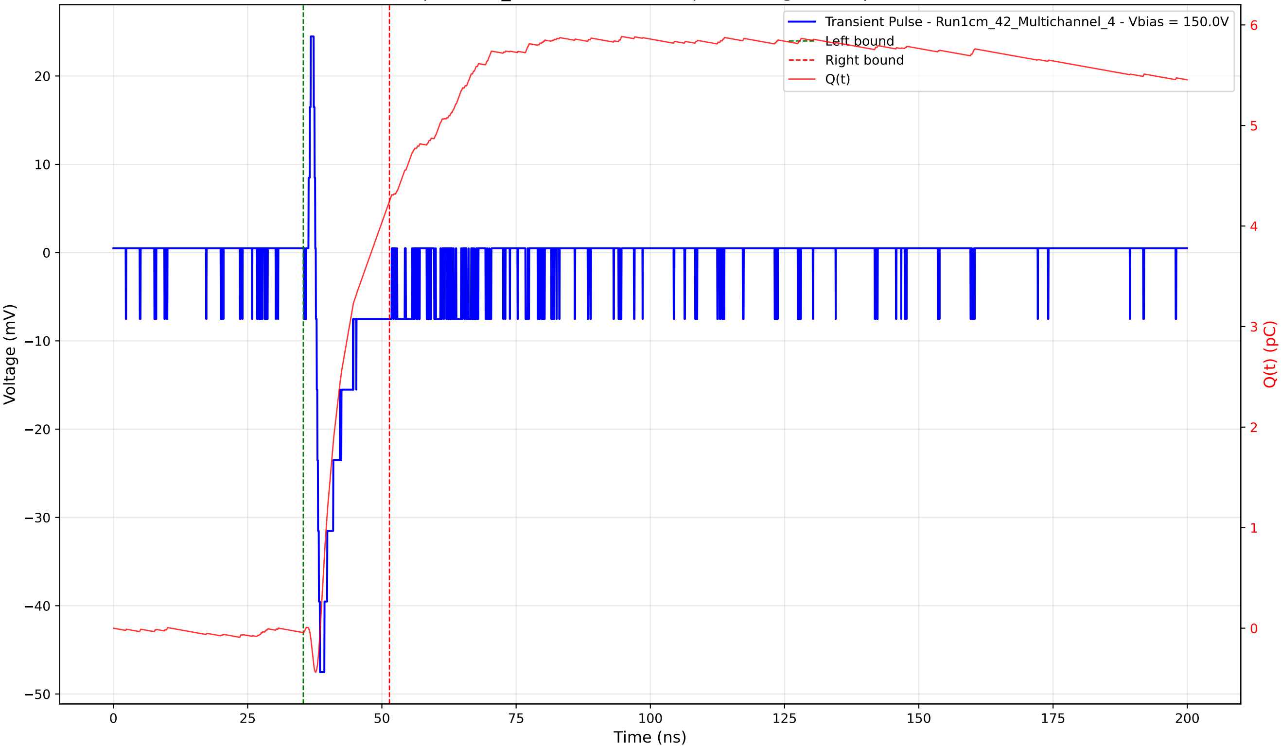
Transient Pulse - Sample: 1cm_42 - Position: 680.0 \mu\text{m} - Charge: 4.29 pC - Rise Time: 0.78 ns
