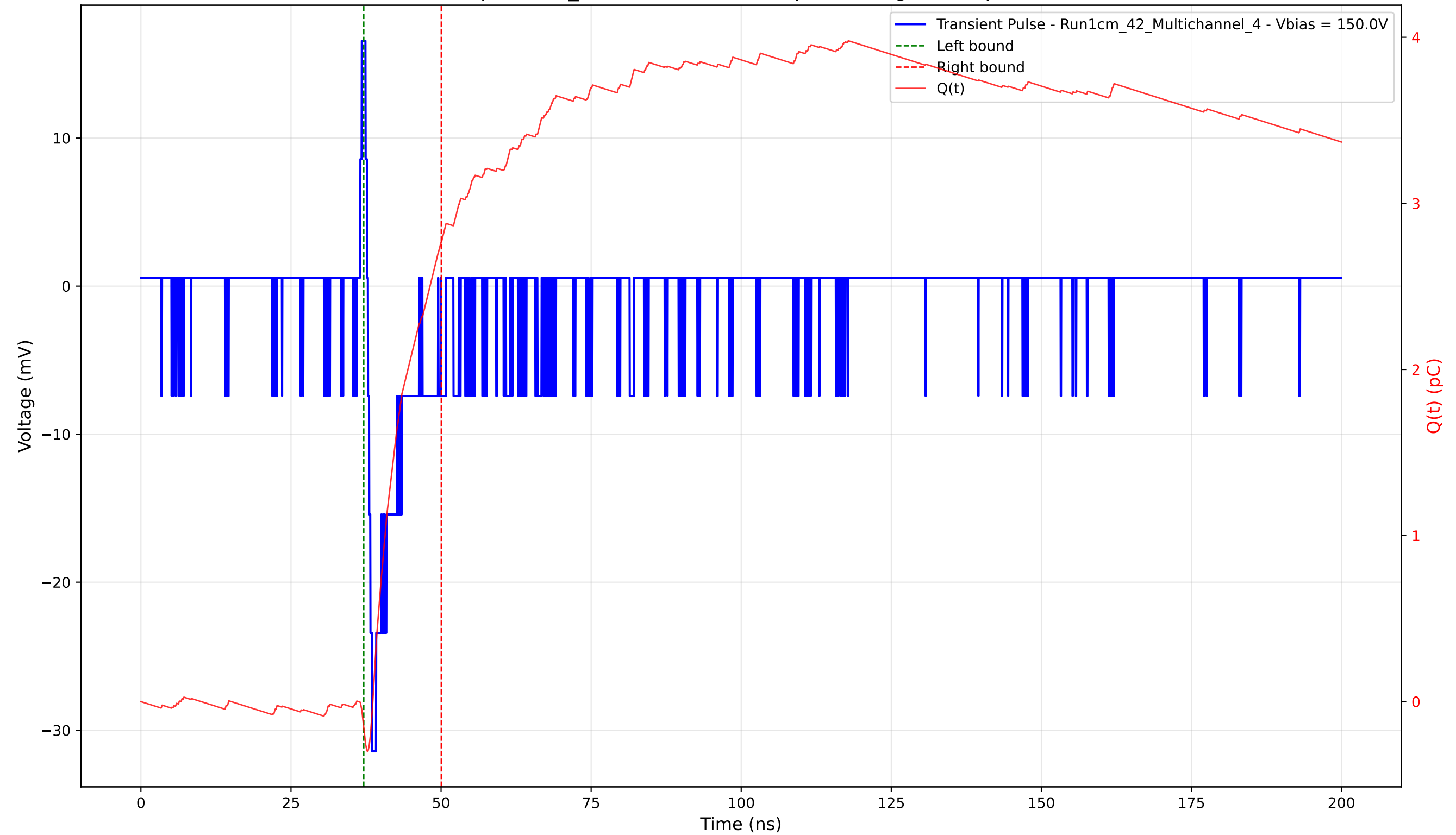
Transient Pulse - Sample: 1cm_42 - Position: 4560.0 \mu\text{m} - Charge: 2.92 pC - Rise Time: 0.71 ns
