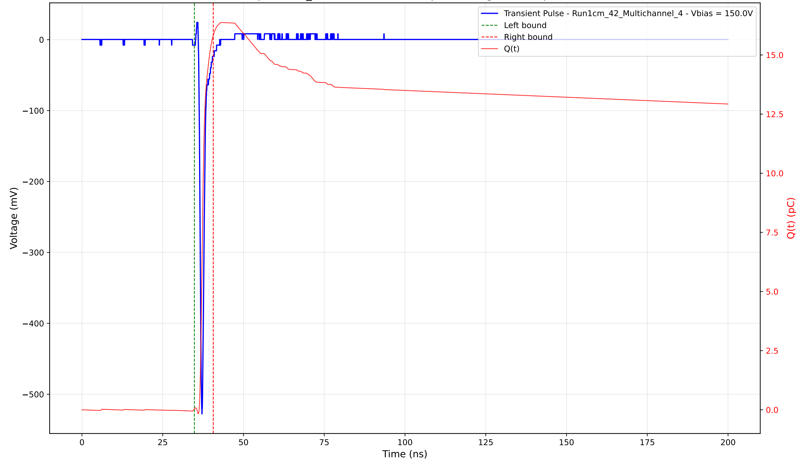
Transient Pulse - Sample: 1cm_42 - Position: 2495.0 \mu\text{m} - Charge: 15.79 pC - Rise Time: 0.70 ns
