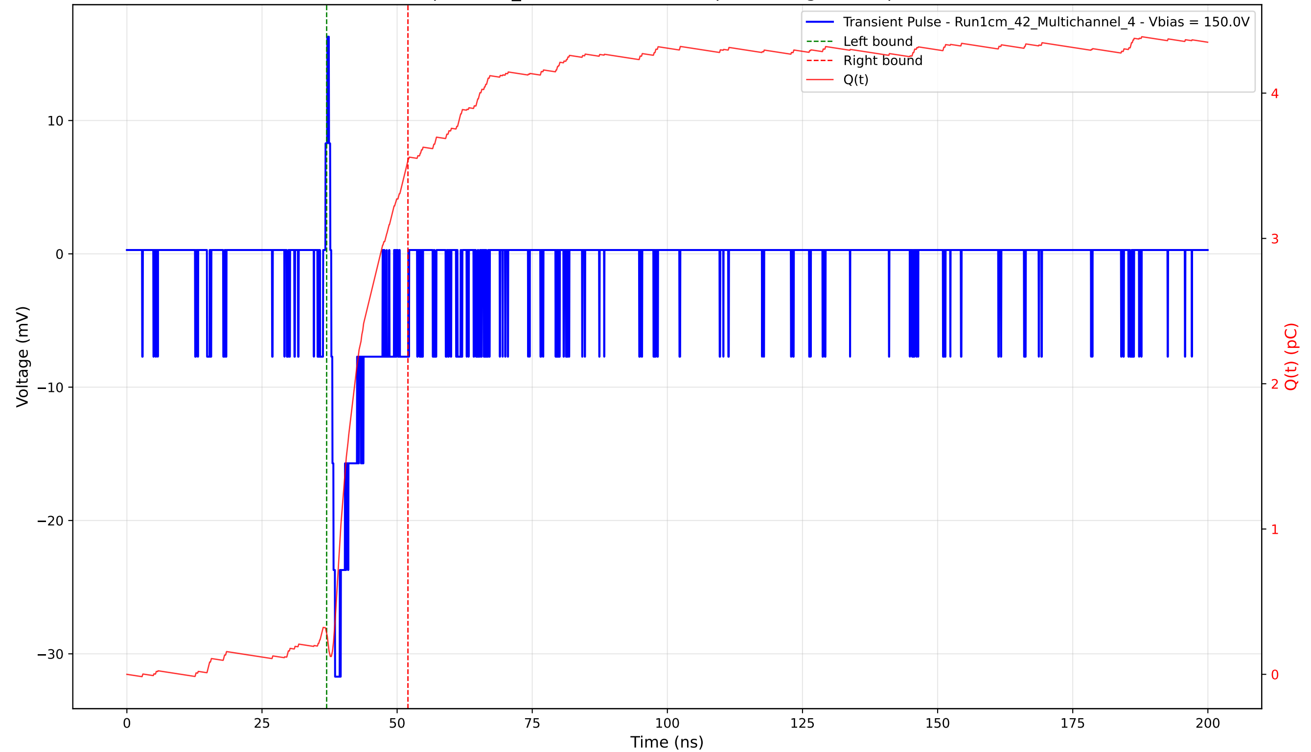
Transient Pulse - Sample: 1cm_42 - Position: 4850.0 \mu\text{m} - Charge: 3.25 pC - Rise Time: 0.70 ns
