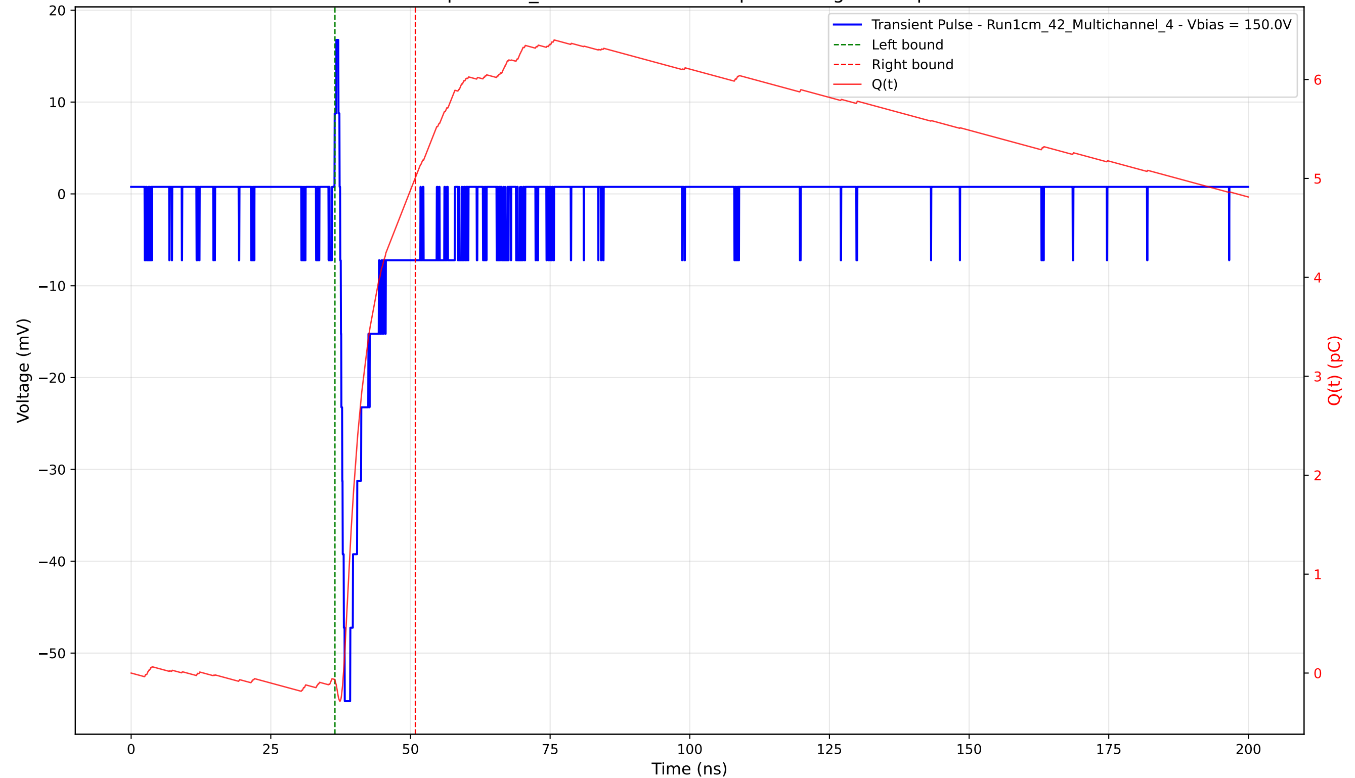
Transient Pulse - Sample: 1cm_42 - Position: 1125.0 \mu\text{m} - Charge: 5.09 pC - Rise Time: 0.81 ns
