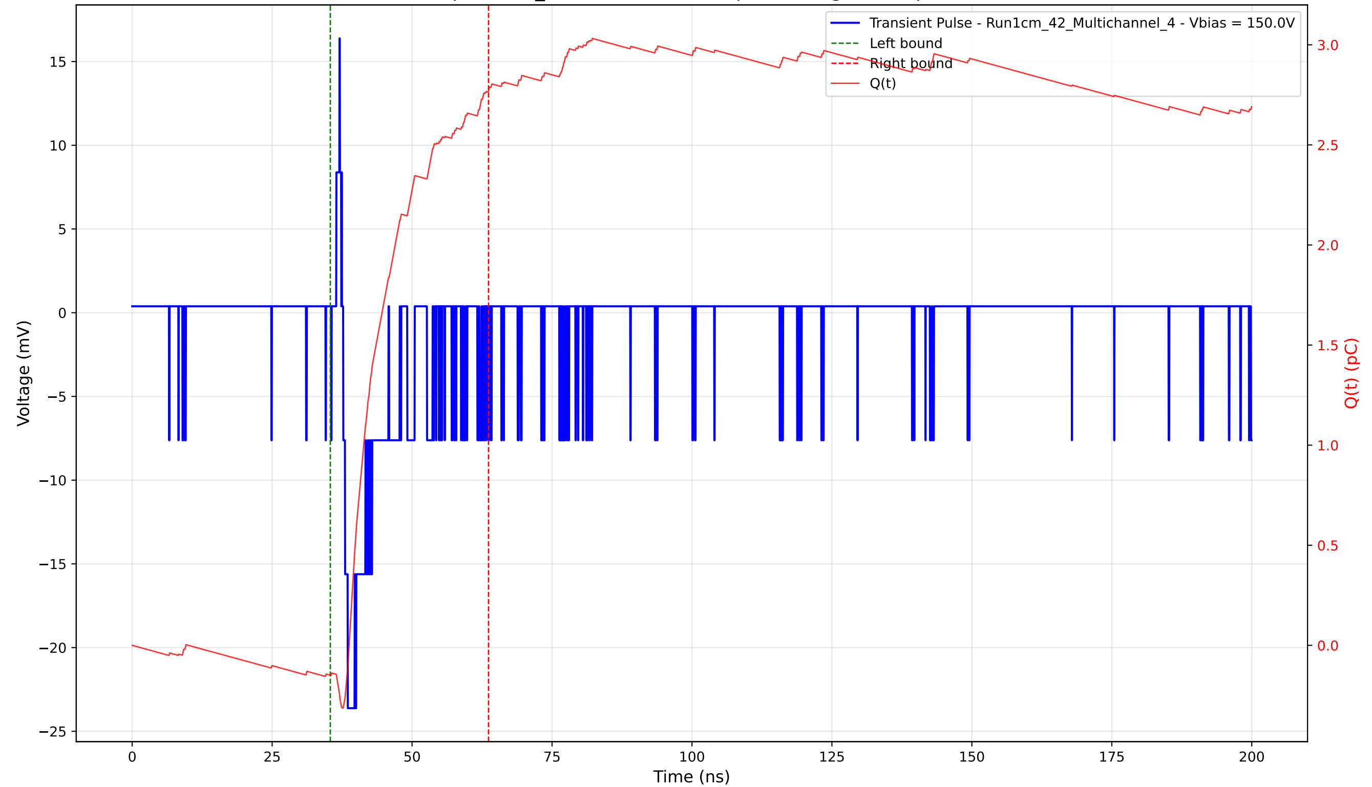
Transient Pulse - Sample: 1cm_42 - Position: 330.0 \mu\text{m} - Charge: 2.92 pC - Rise Time: 0.83 ns
