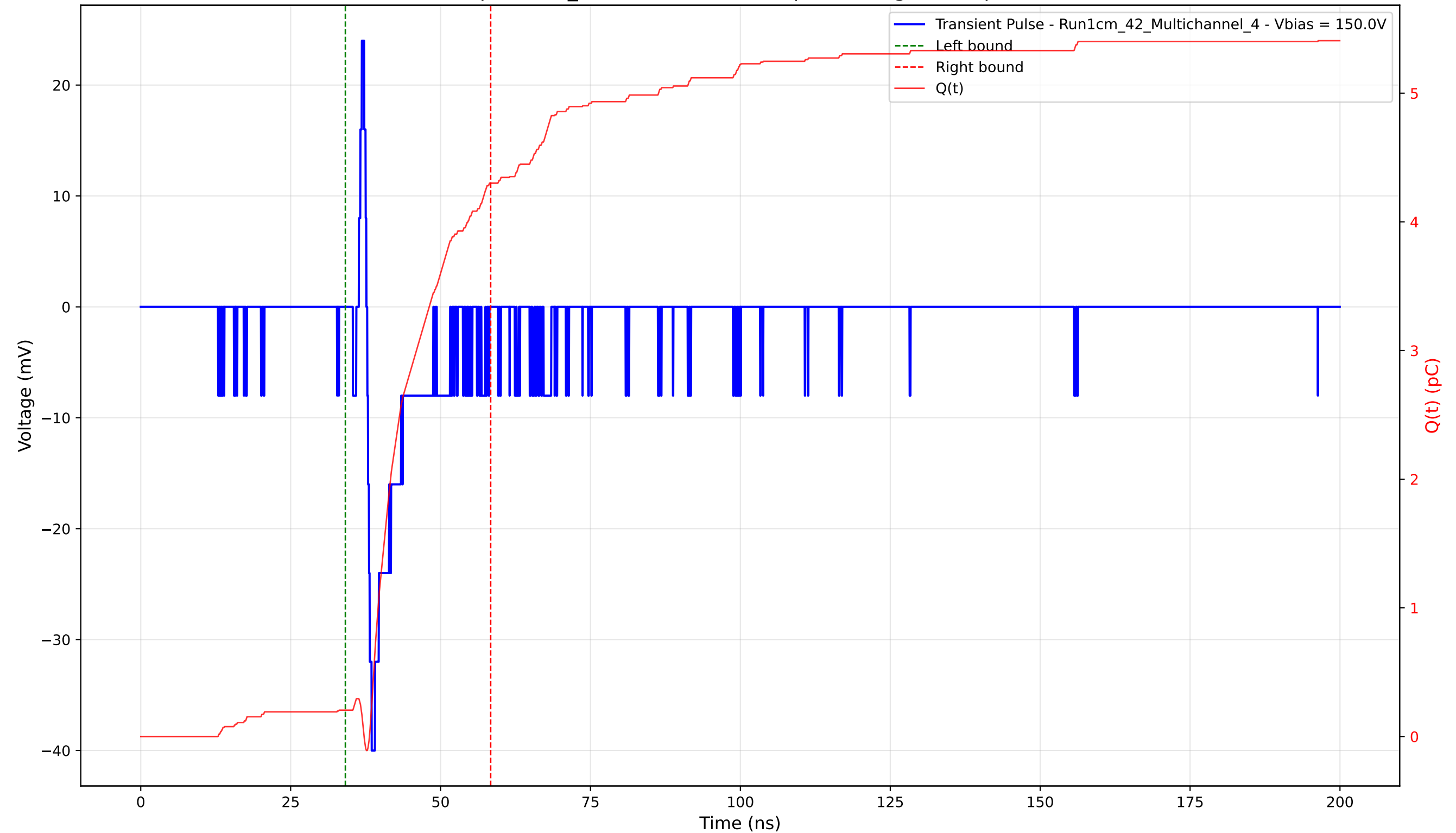
Transient Pulse - Sample: 1cm_42 - Position: 4360.0 \mu\text{m} - Charge: 4.10 pC - Rise Time: 0.74 ns
