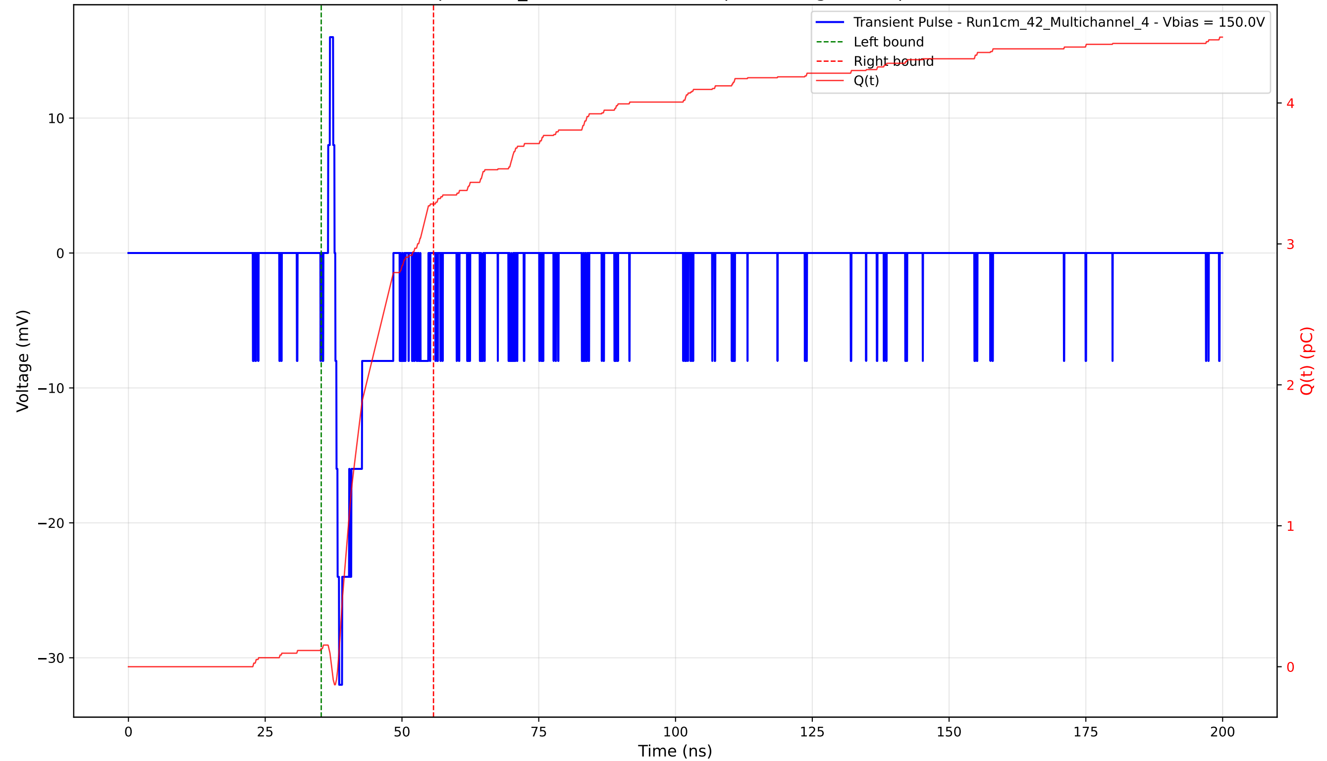
Transient Pulse - Sample: 1cm_42 - Position: 4565.0 \mu\text{m} - Charge: 3.16 pC - Rise Time: 0.70 ns
