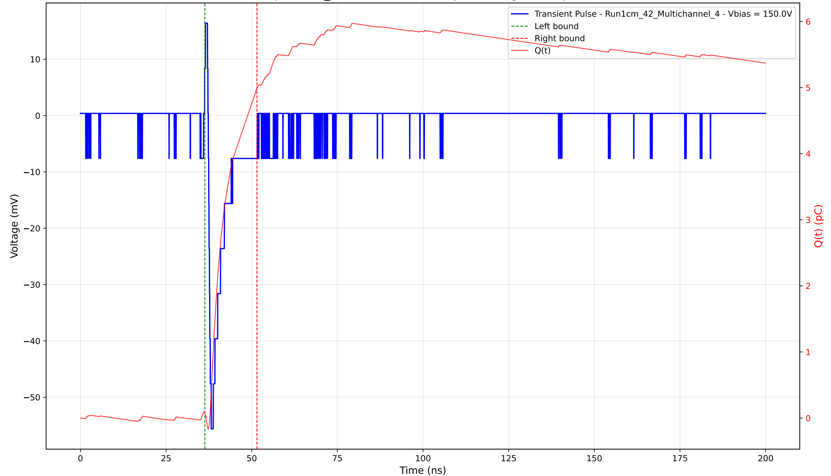
Transient Pulse - Sample: 1cm_42 - Position: 3840.0 \mu\text{m} - Charge: 4.91 pC - Rise Time: 0.85 ns
