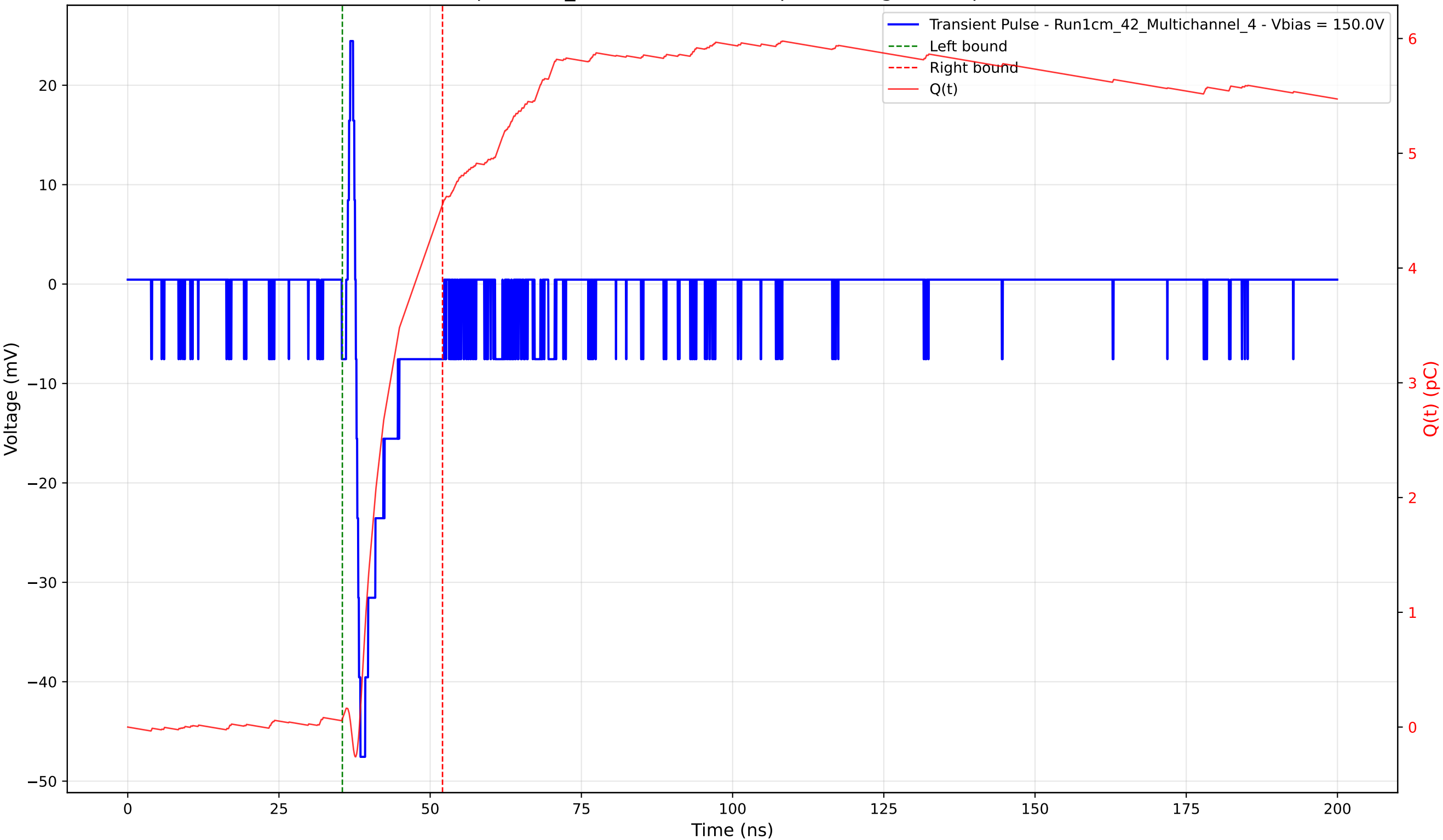
Transient Pulse - Sample: 1cm_42 - Position: 830.0 \mu\text{m} - Charge: 4.49 pC - Rise Time: 0.78 ns
