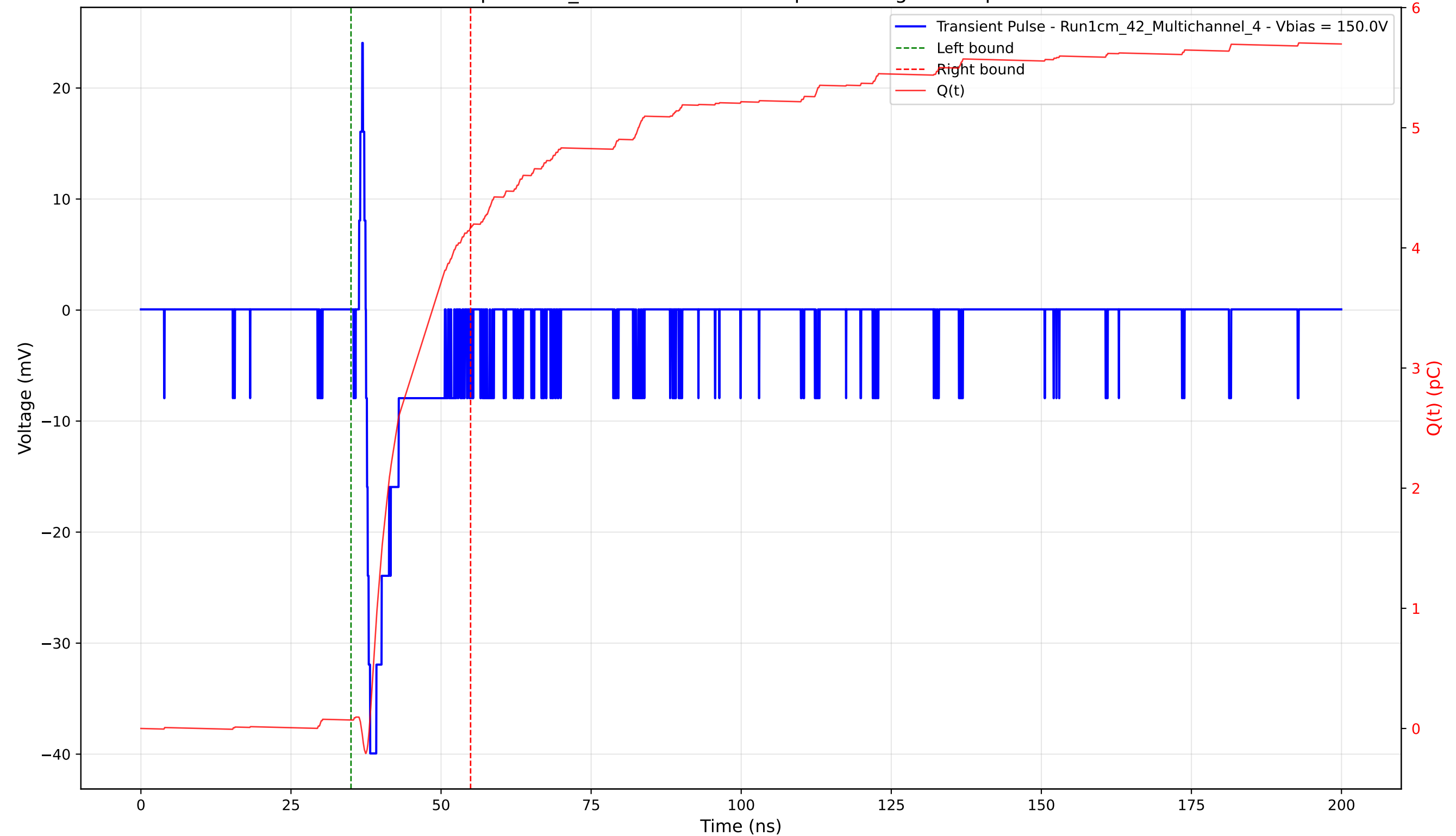
Transient Pulse - Sample: 1cm_42 - Position: 4000.0 \mu\text{m} - Charge: 4.10 pC - Rise Time: 0.70 ns
