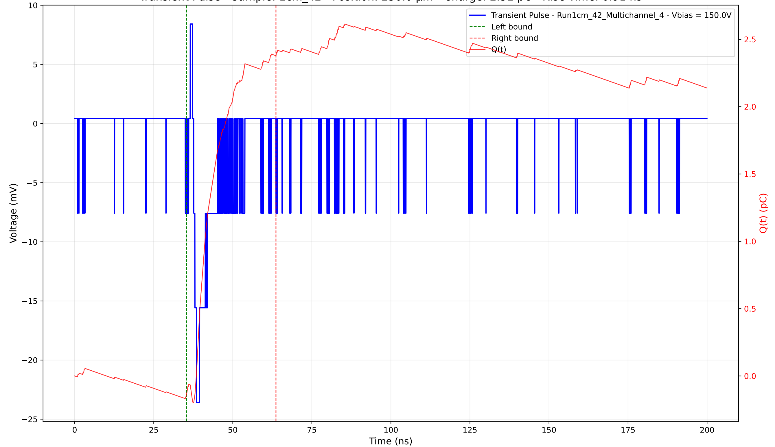
Transient Pulse - Sample: 1cm_42 - Position: 250.0 \mu\text{m} - Charge: 2.51 pC - Rise Time: 0.91 ns
