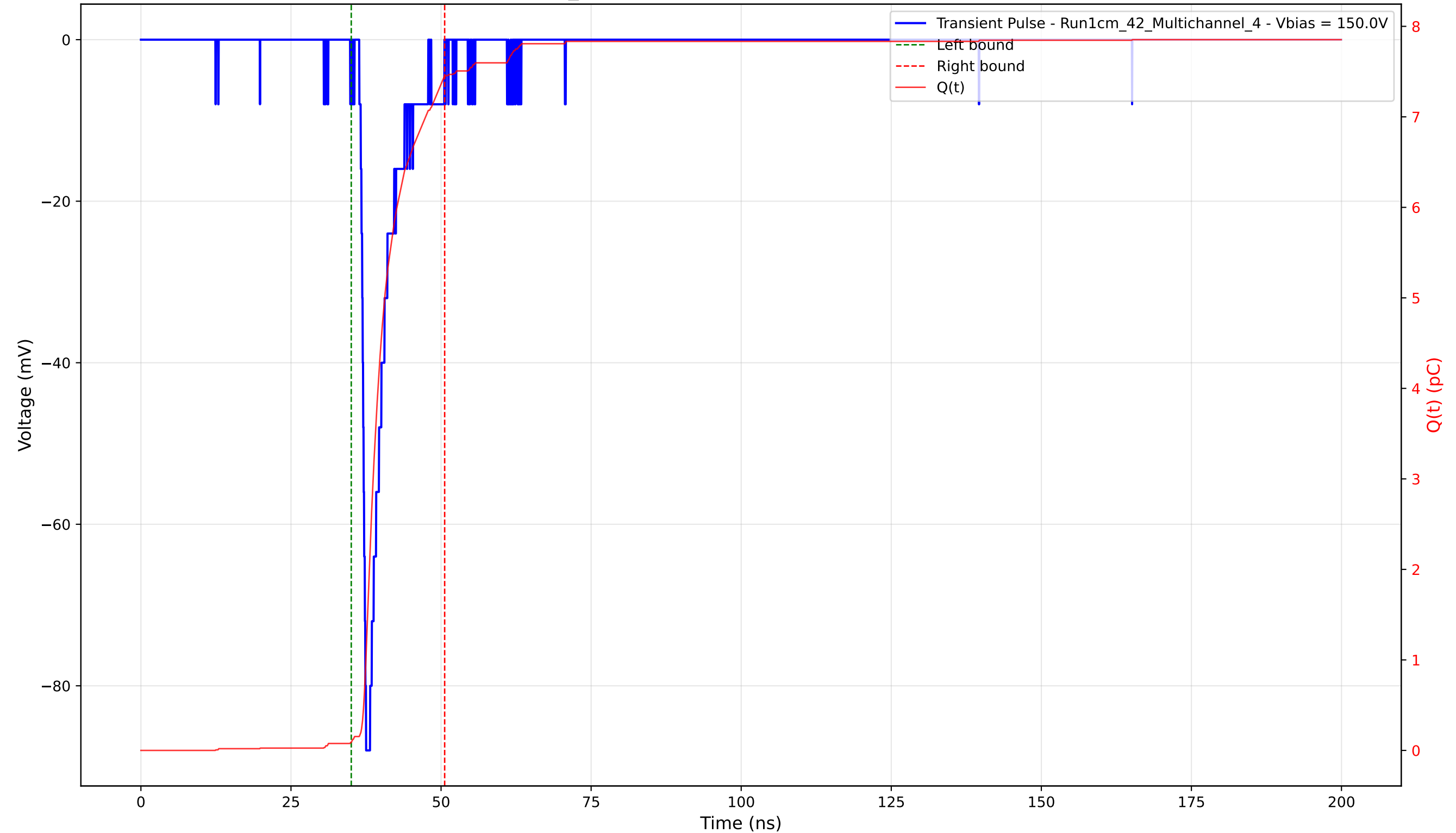
Transient Pulse - Sample: 1cm_42 - Position: 1580.0 \mu\text{m} - Charge: 7.36 pC - Rise Time: 0.80 ns
