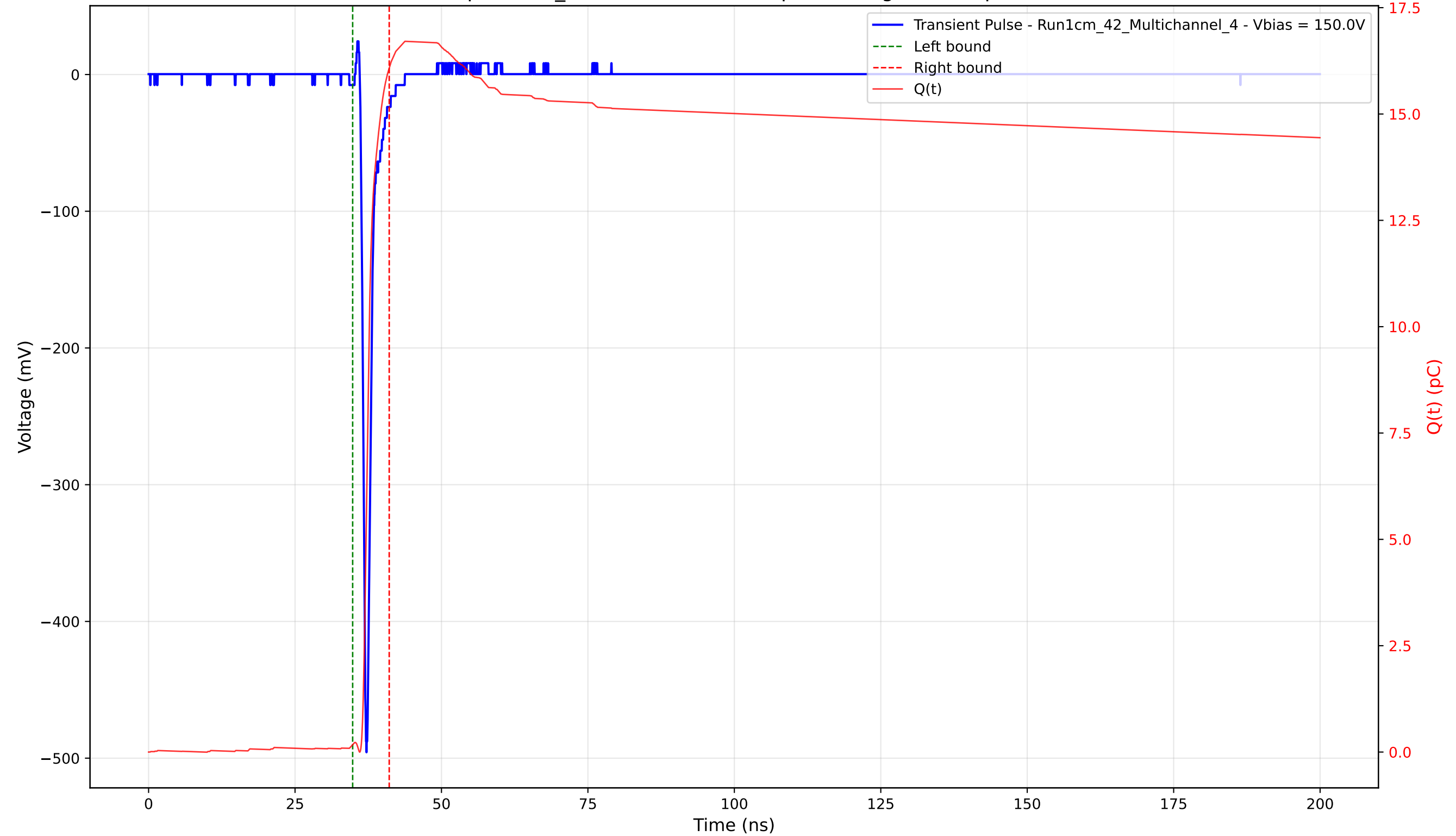
Transient Pulse - Sample: 1cm_42 - Position: 2745.0 \mu\text{m} - Charge: 15.91 pC - Rise Time: 0.71 ns
