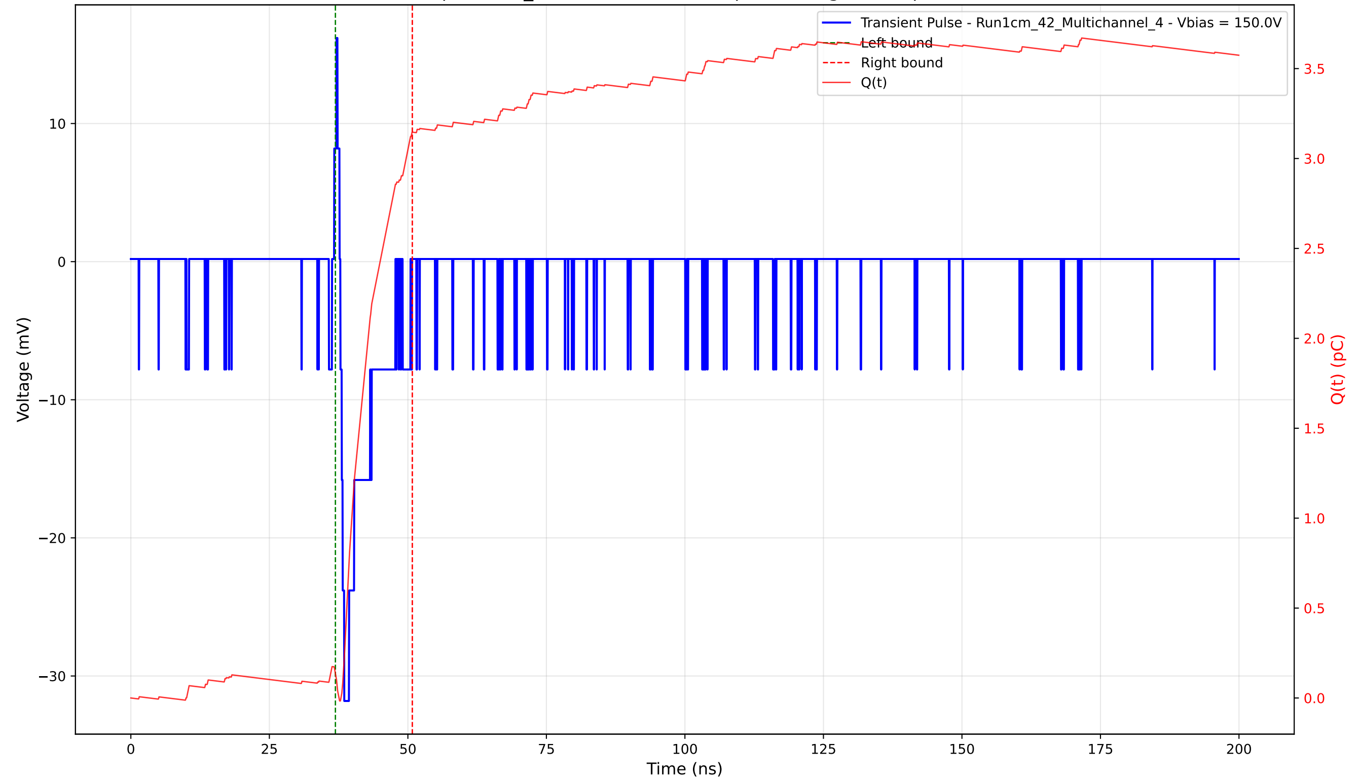
Transient Pulse - Sample: 1cm_42 - Position: 4865.0 \mu\text{m} - Charge: 3.01 pC - Rise Time: 0.70 ns
