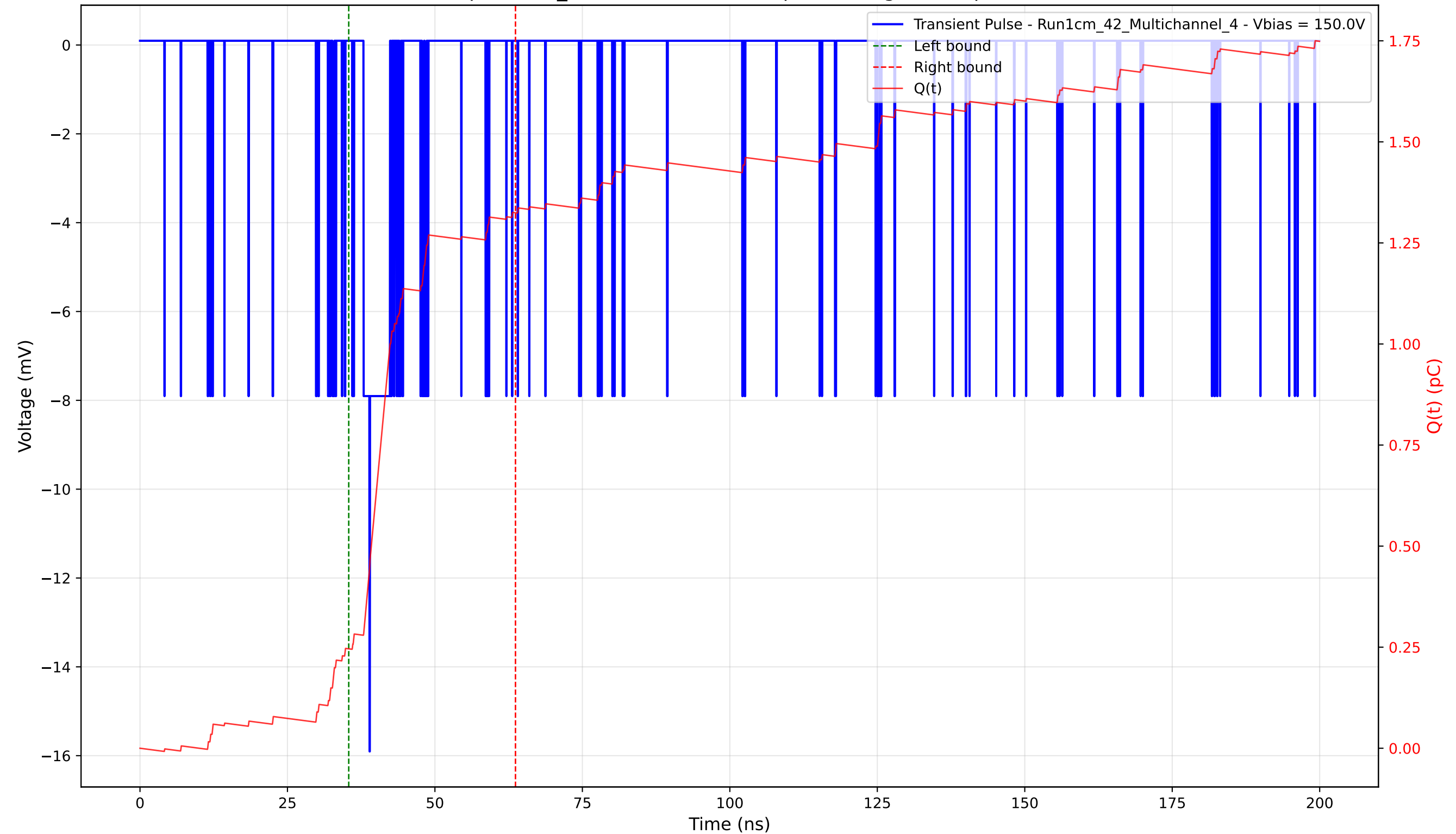
Transient Pulse - Sample: 1cm_42 - Position: 5105.0 \mu\text{m} - Charge: 1.08 pC - Rise Time: 1.03 ns
