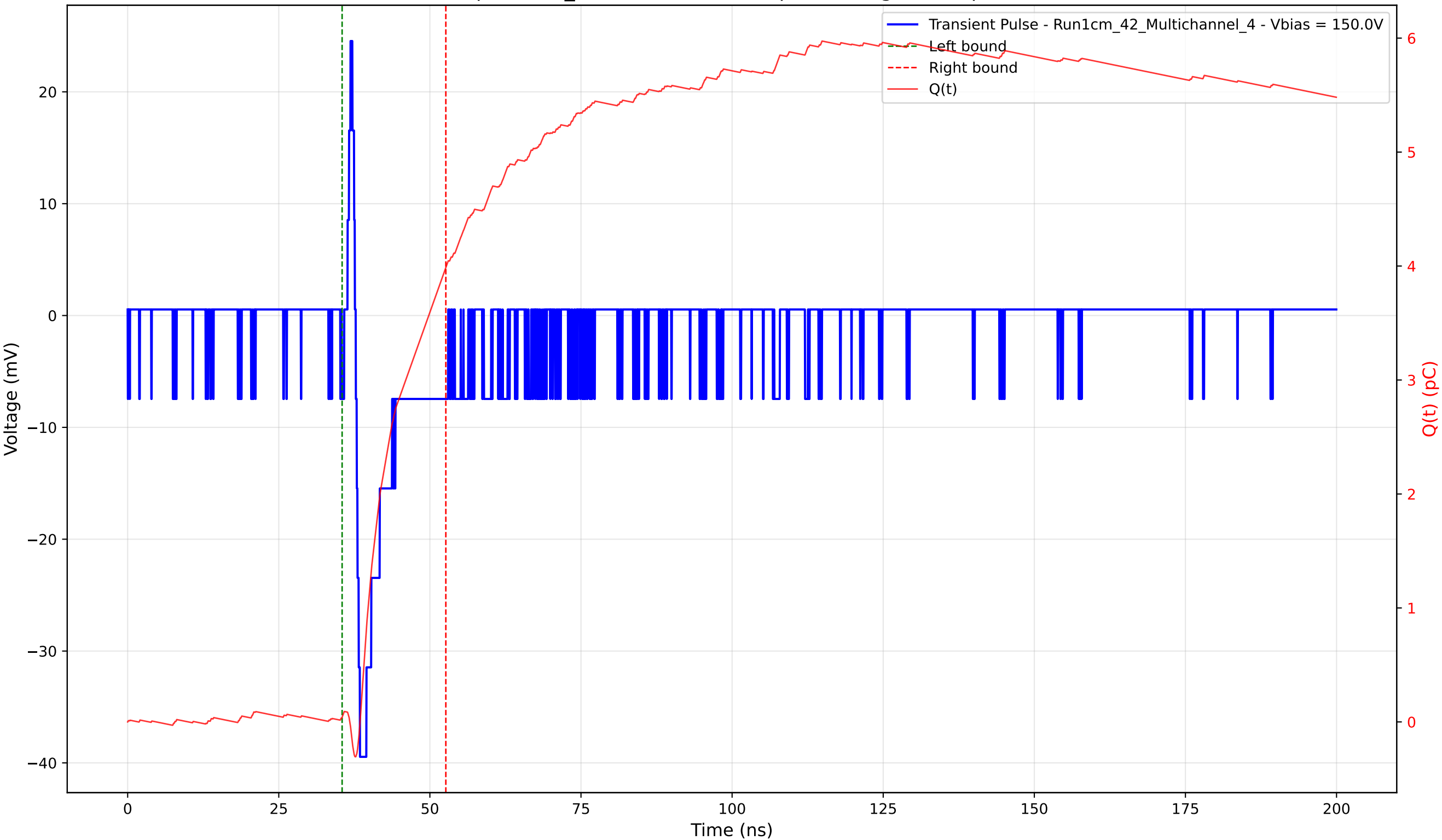
Transient Pulse - Sample: 1cm_42 - Position: 590.0 \mu\text{m} - Charge: 3.95 pC - Rise Time: 0.70 ns
