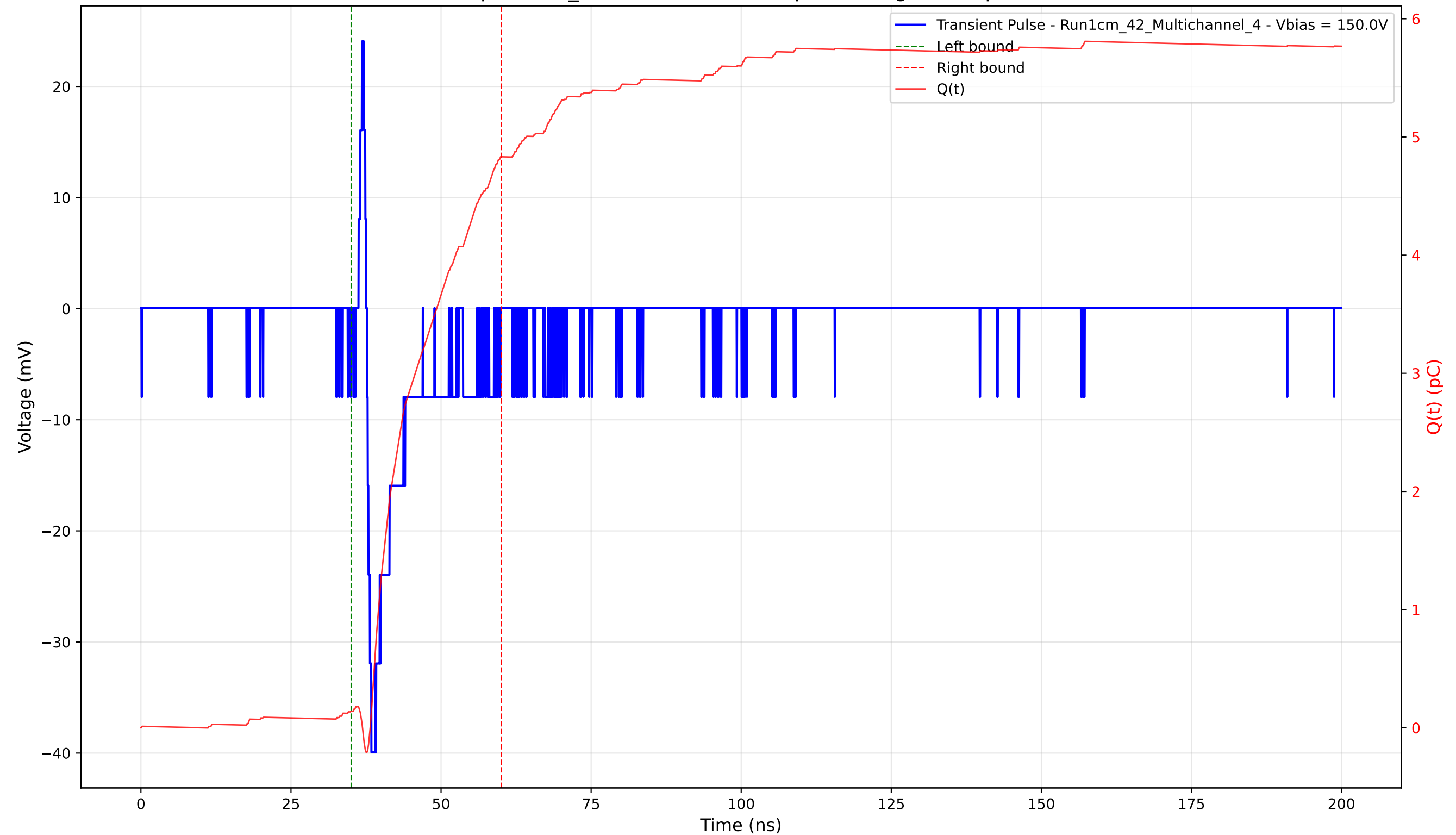
Transient Pulse - Sample: 1cm_42 - Position: 4105.0 \mu\text{m} - Charge: 4.69 pC - Rise Time: 0.74 ns
