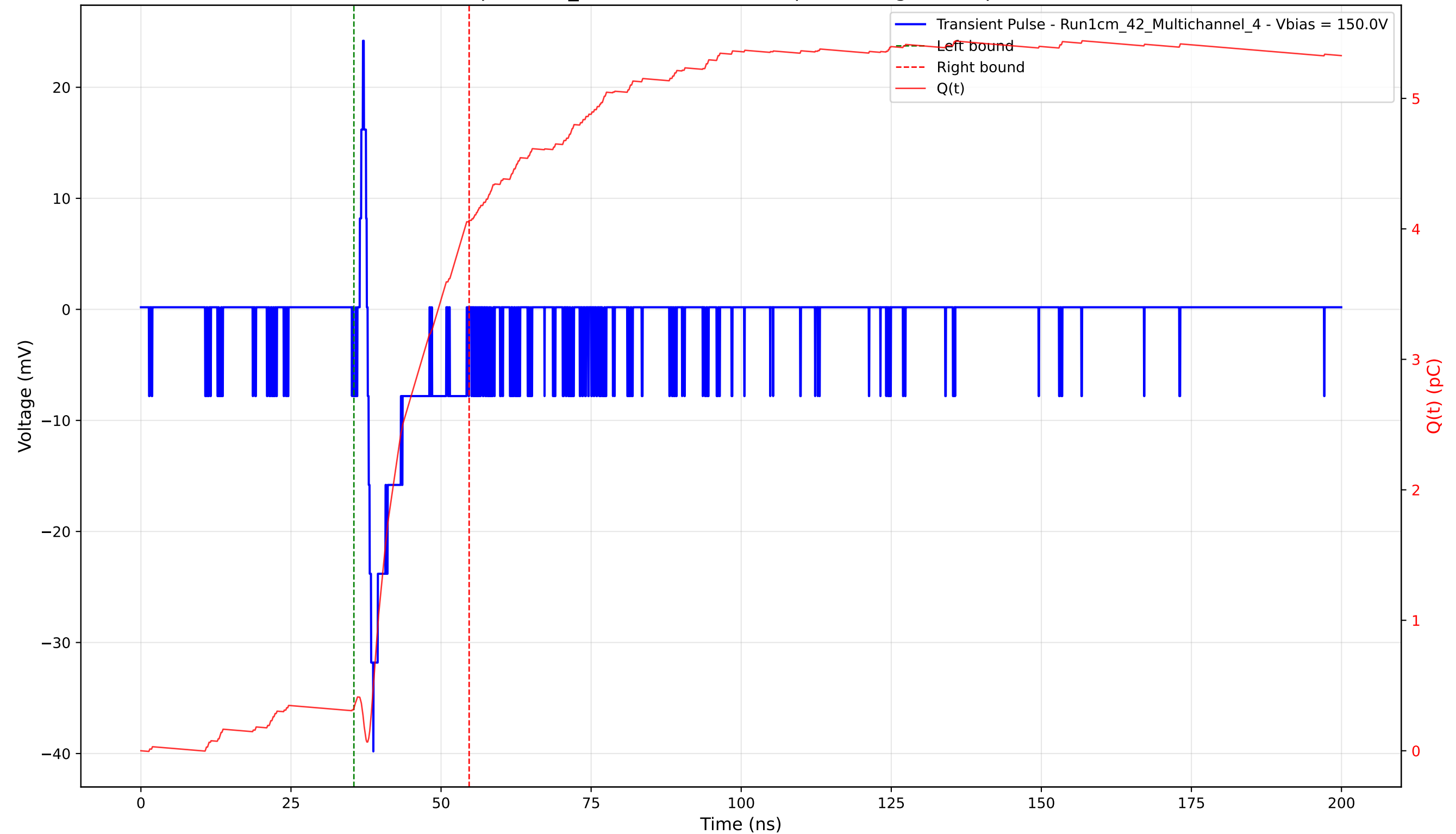
Transient Pulse - Sample: 1cm_42 - Position: 4430.0 \mu\text{m} - Charge: 3.74 pC - Rise Time: 0.94 ns
