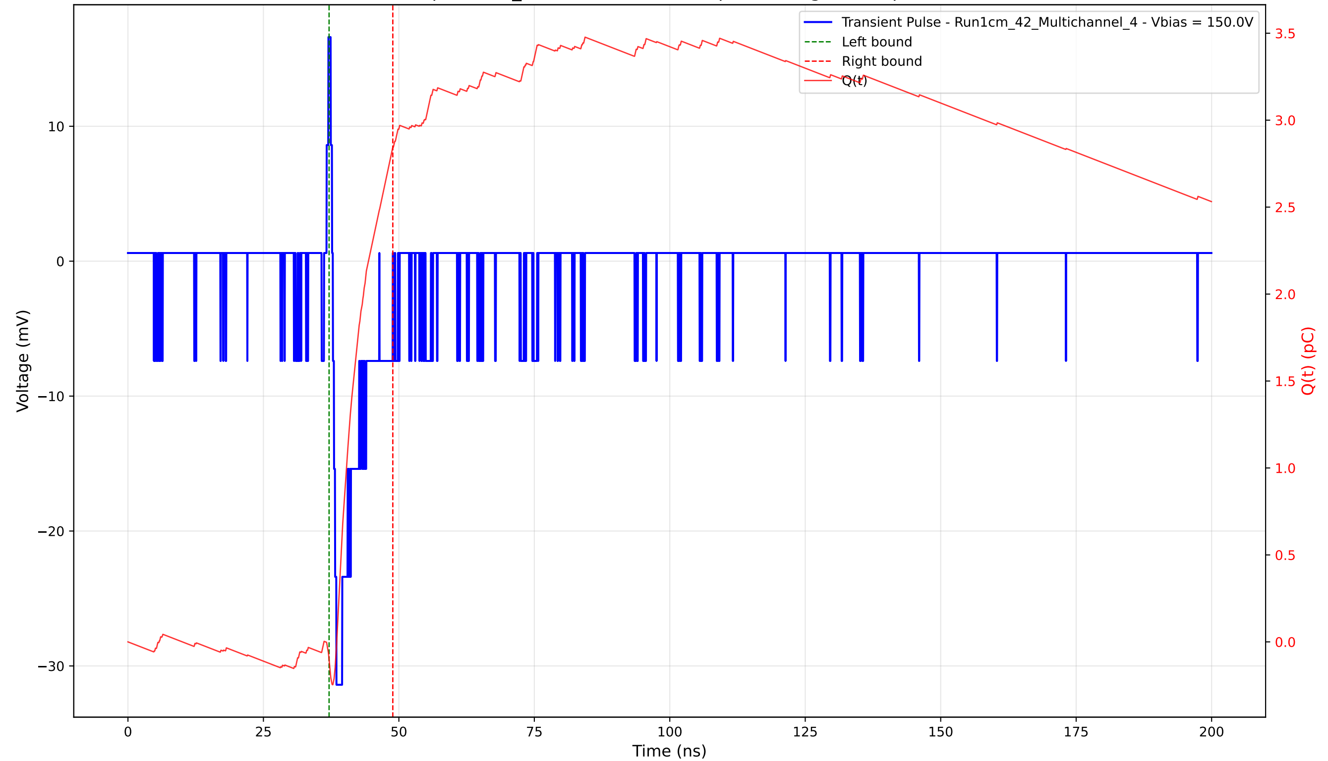
Transient Pulse - Sample: 1cm_42 - Position: 4755.0 \mu\text{m} - Charge: 2.95 pC - Rise Time: 0.67 ns
