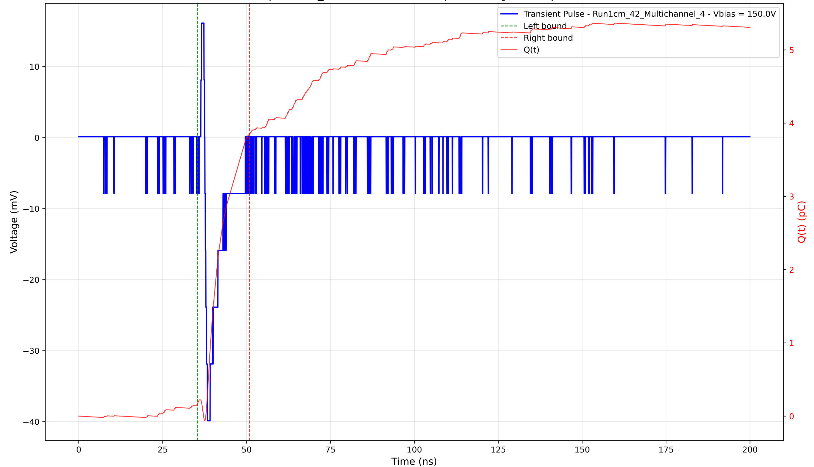
Transient Pulse - Sample: 1cm_42 - Position: 4055.0 \mu\text{m} - Charge: 3.69 pC - Rise Time: 0.74 ns
