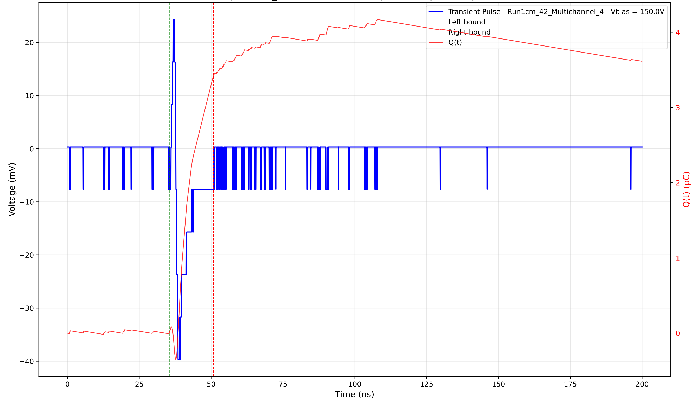
Transient Pulse - Sample: 1cm_42 - Position: 4355.0 \mu\text{m} - Charge: 3.42 pC - Rise Time: 0.74 ns
