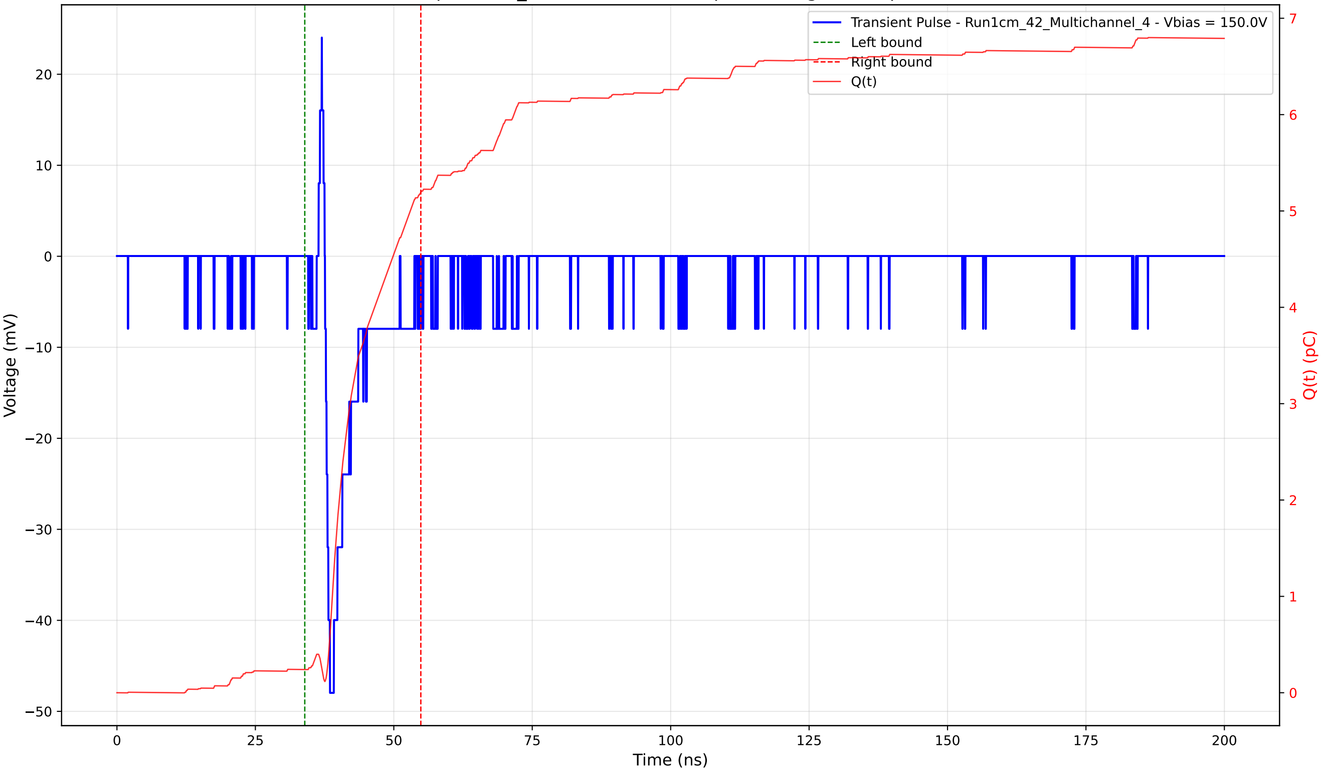
Transient Pulse - Sample: 1cm_42 - Position: 970.0 \mu\text{m} - Charge: 4.96 pC - Rise Time: 0.90 ns
