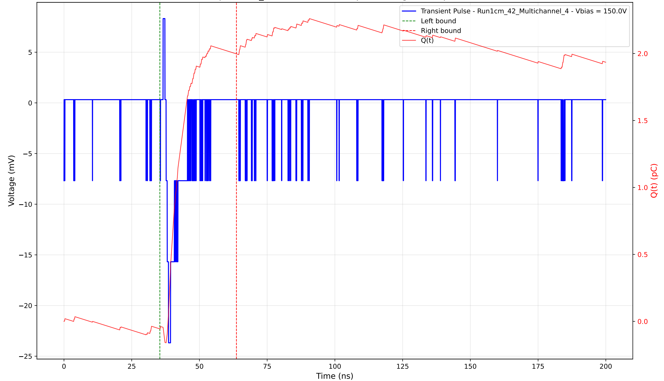
Transient Pulse - Sample: 1cm_42 - Position: 235.0 \mu\text{m} - Charge: 2.05 pC - Rise Time: 0.91 ns
