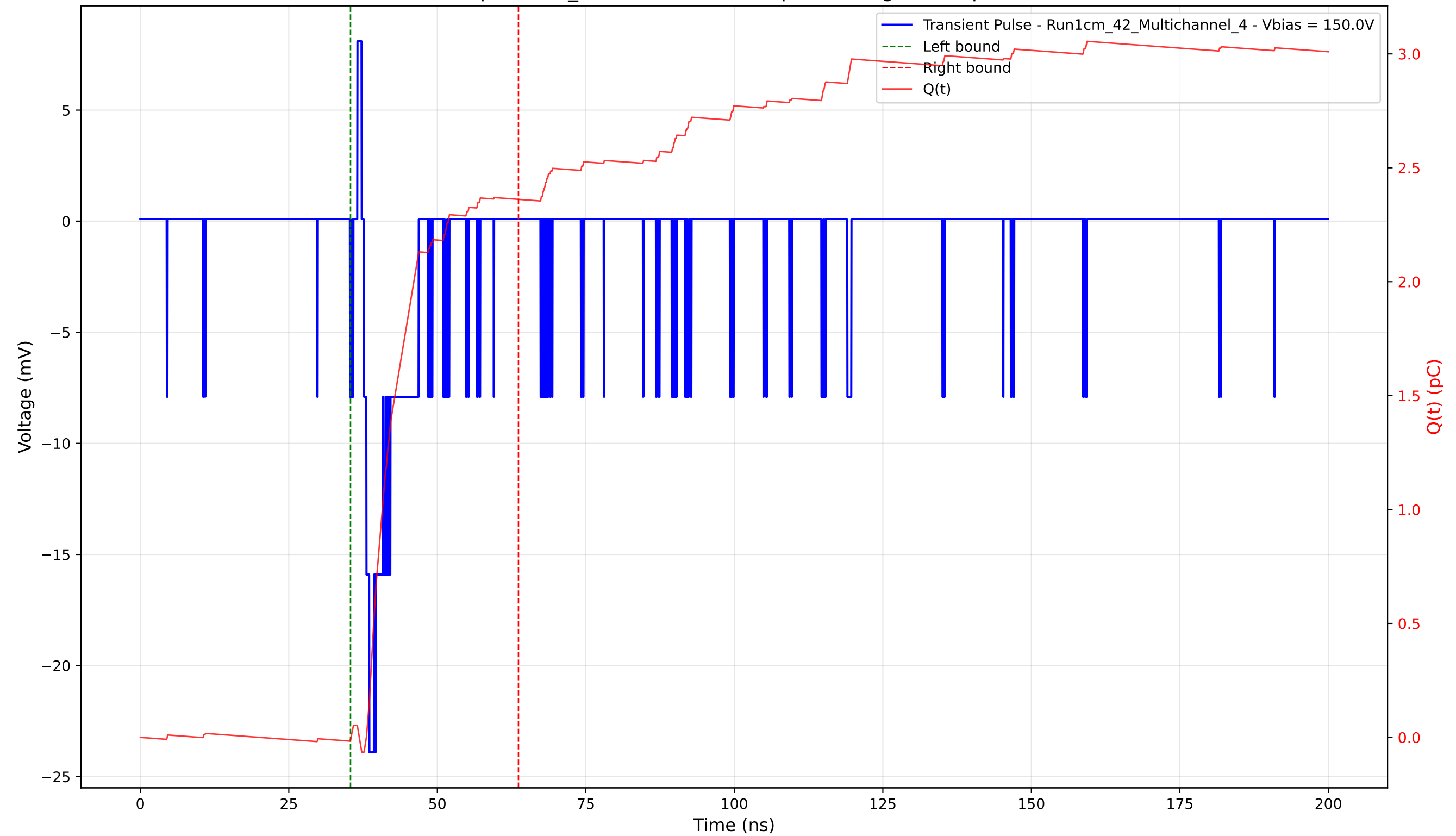
Transient Pulse - Sample: 1cm_42 - Position: 275.0 \mu\text{m} - Charge: 2.37 pC - Rise Time: 0.91 ns
