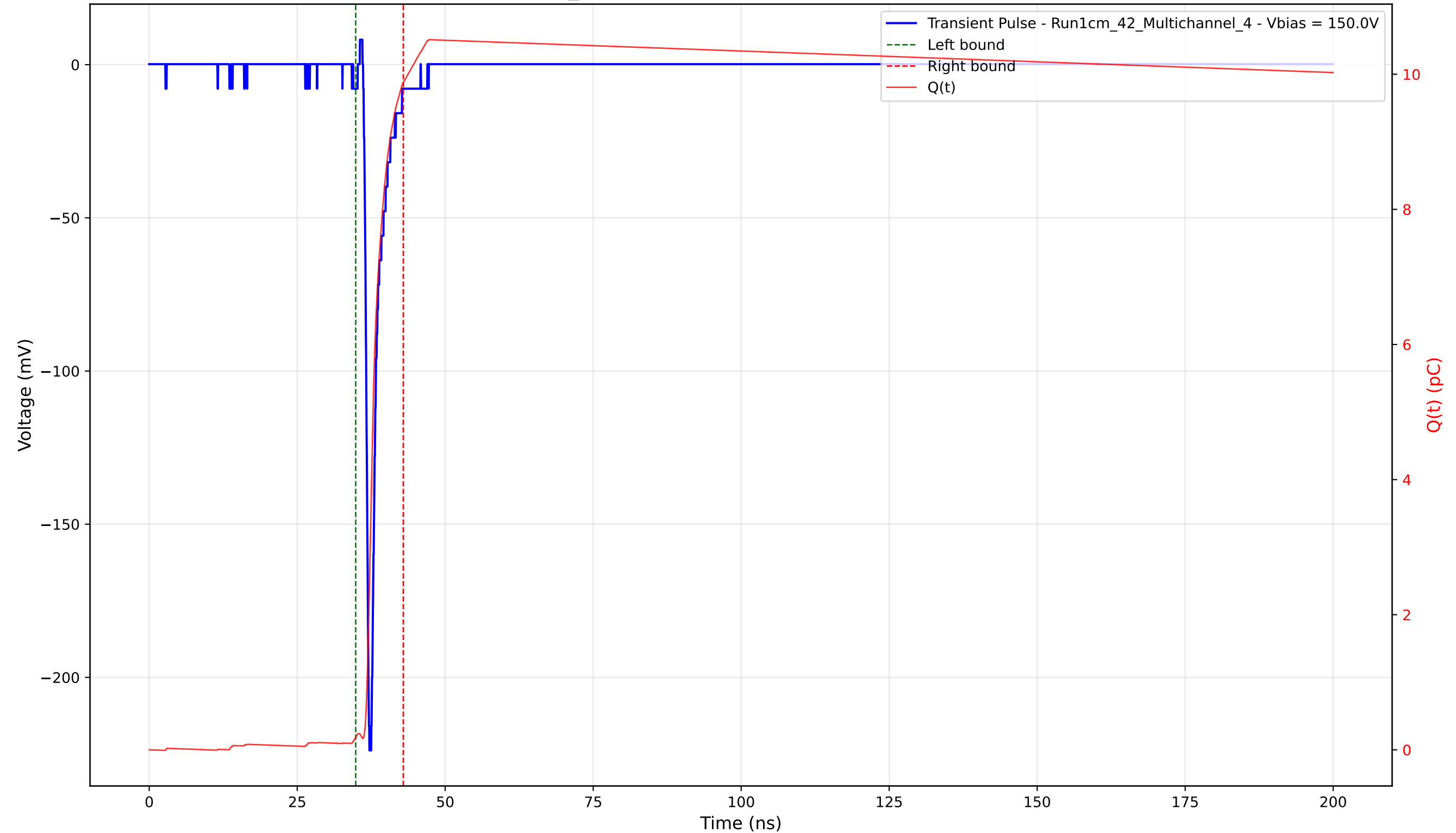
Transient Pulse - Sample: 1cm_42 - Position: 2005.0 \mu\text{m} - Charge: 9.69 pC - Rise Time: 0.78 ns
