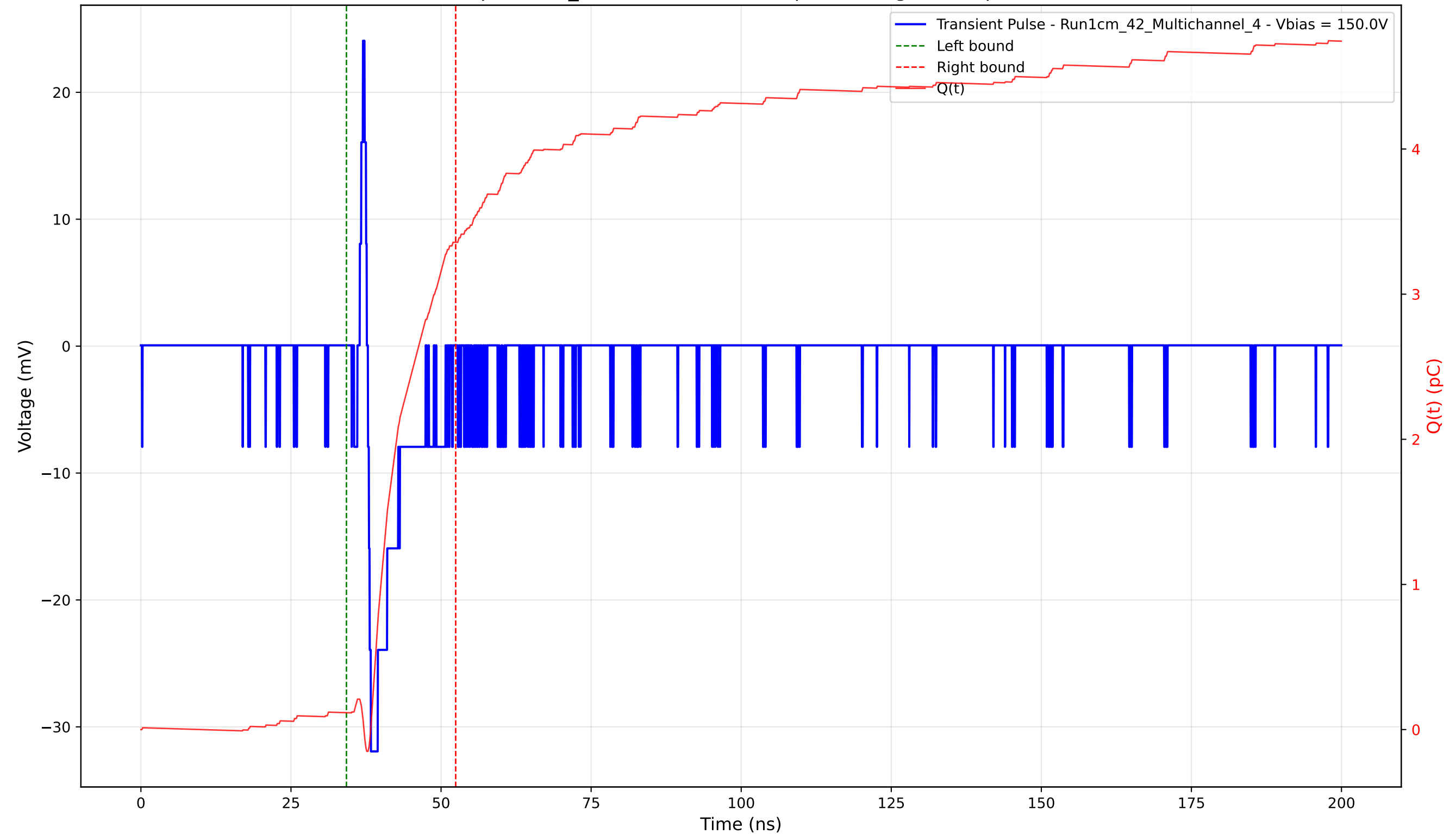
Transient Pulse - Sample: 1cm_42 - Position: 4415.0 \mu\text{m} - Charge: 3.24 pC - Rise Time: 0.50 ns
