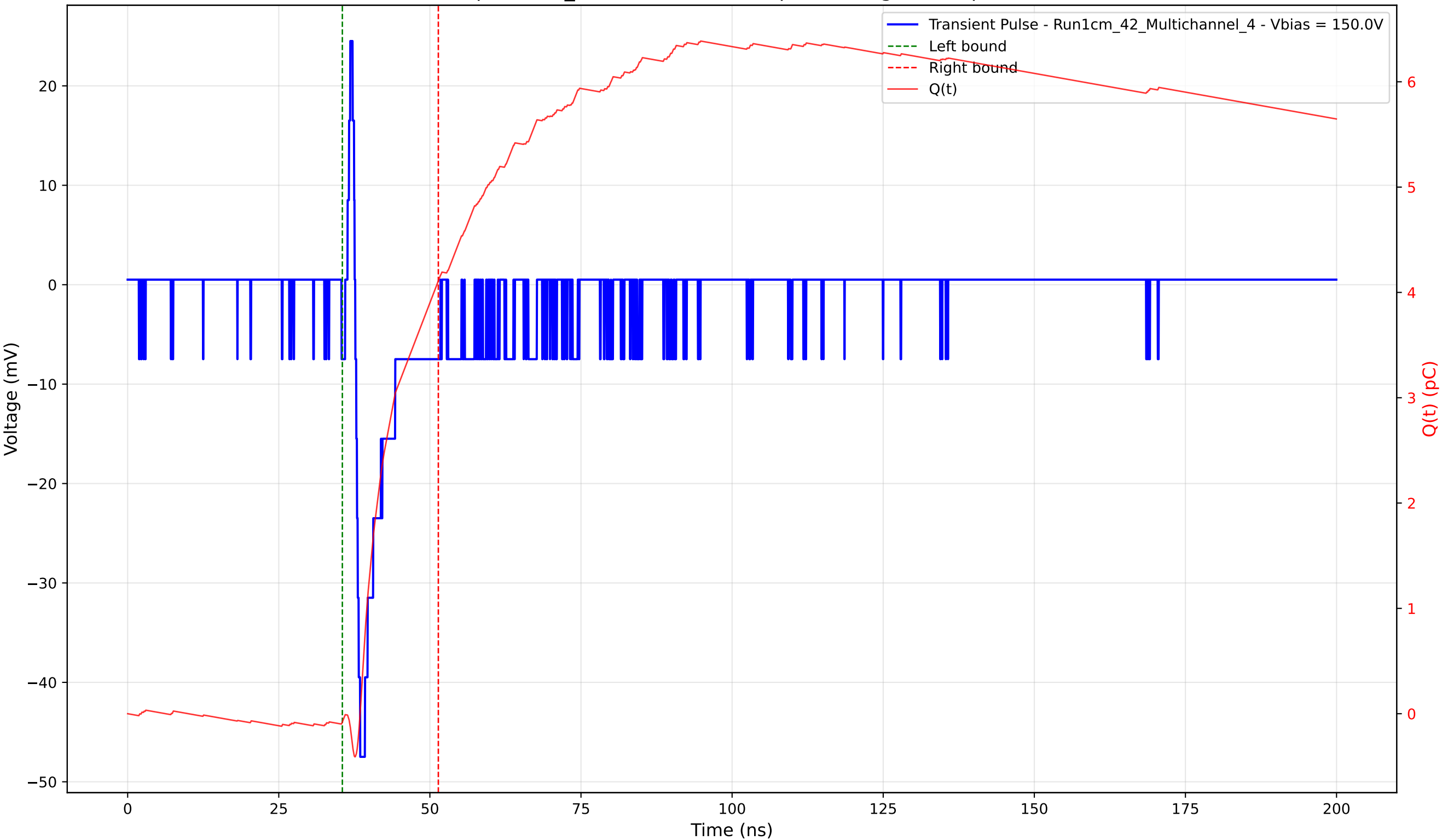
Transient Pulse - Sample: 1cm_42 - Position: 885.0 \mu\text{m} - Charge: 4.19 pC - Rise Time: 0.82 ns
