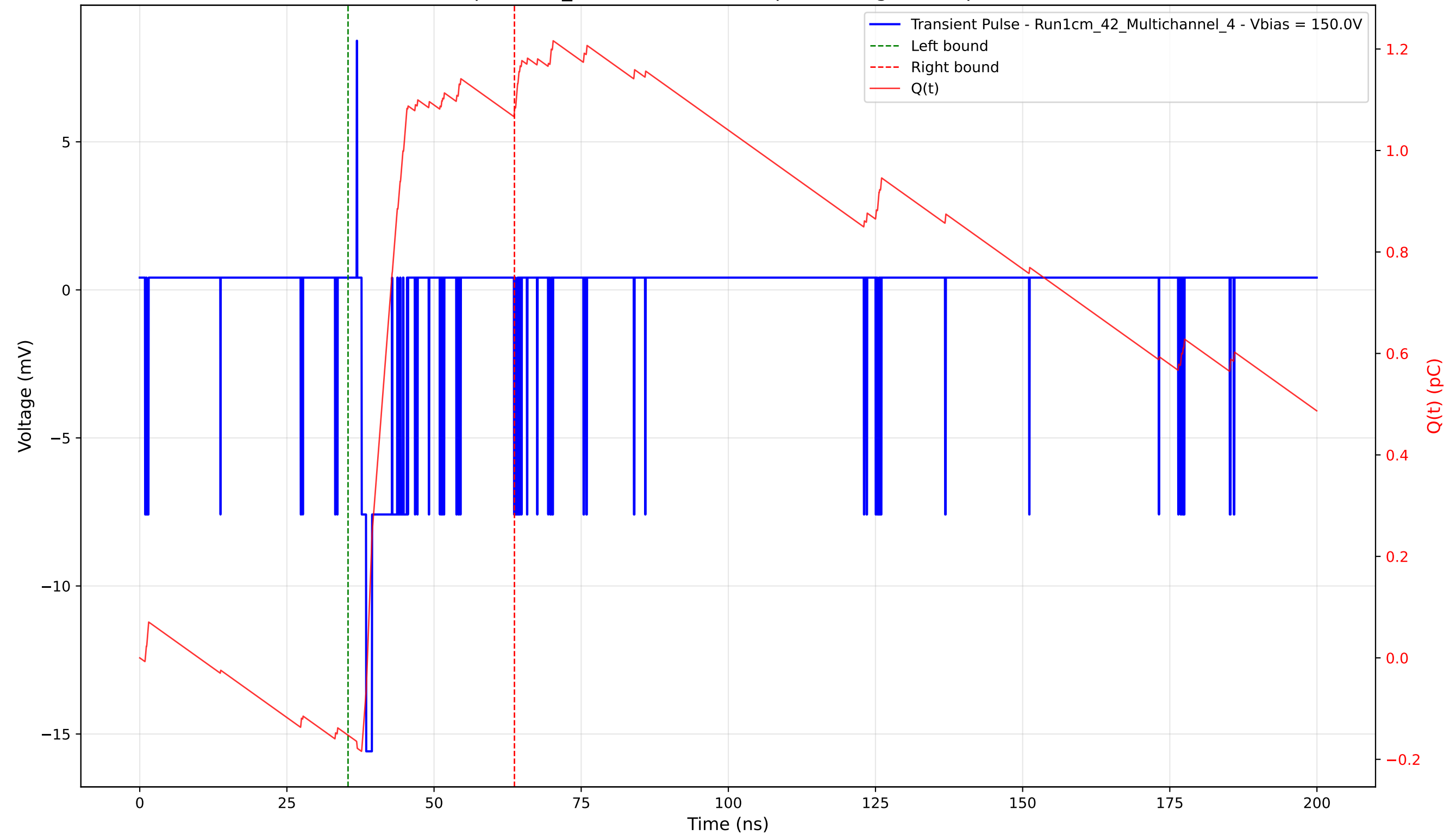
Transient Pulse - Sample: 1cm_42 - Position: 140.0 \mu\text{m} - Charge: 1.23 pC - Rise Time: 0.79 ns
