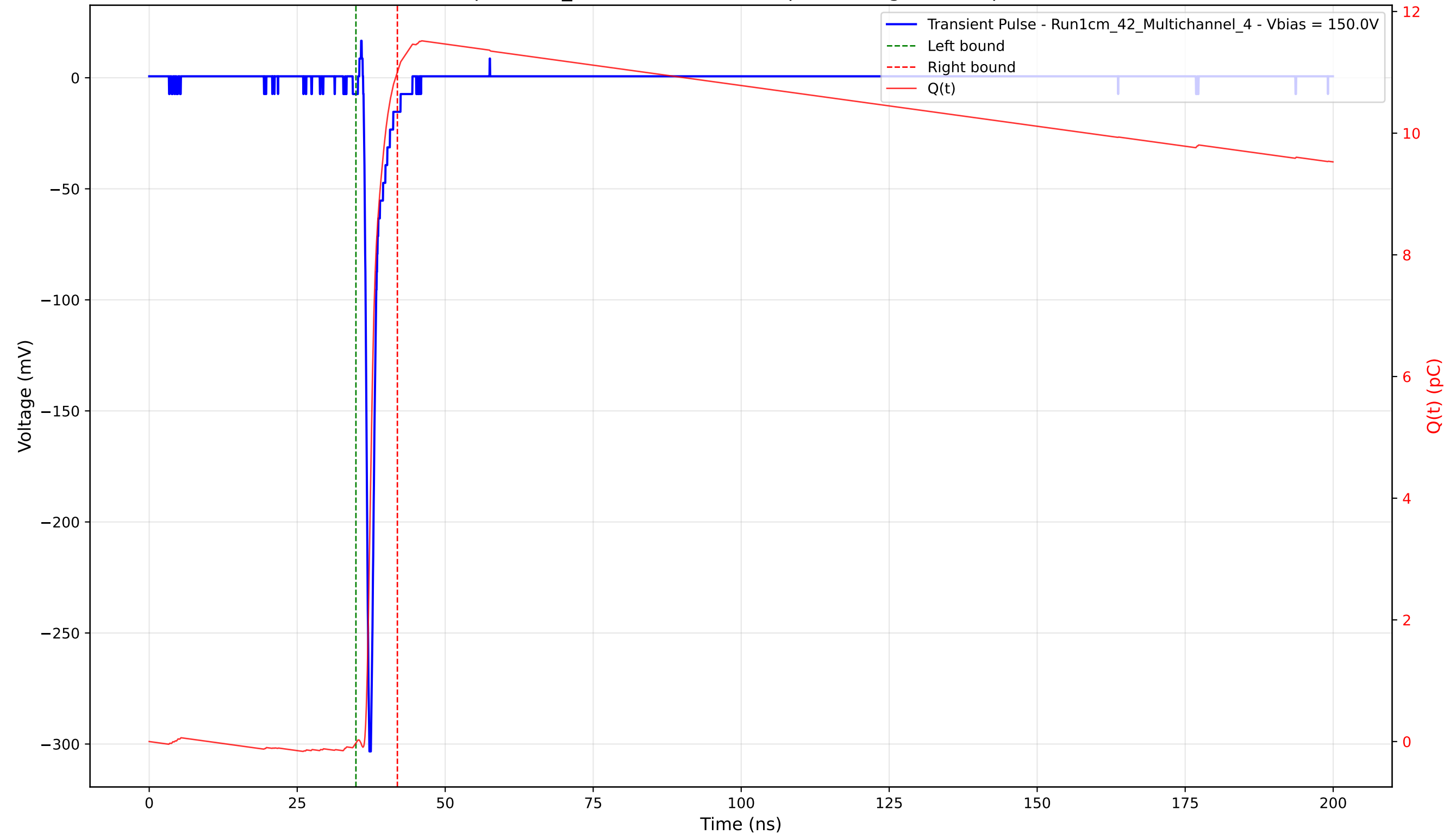
Transient Pulse - Sample: 1cm_42 - Position: 2930.0 \mu\text{m} - Charge: 11.03 pC - Rise Time: 0.73 ns
