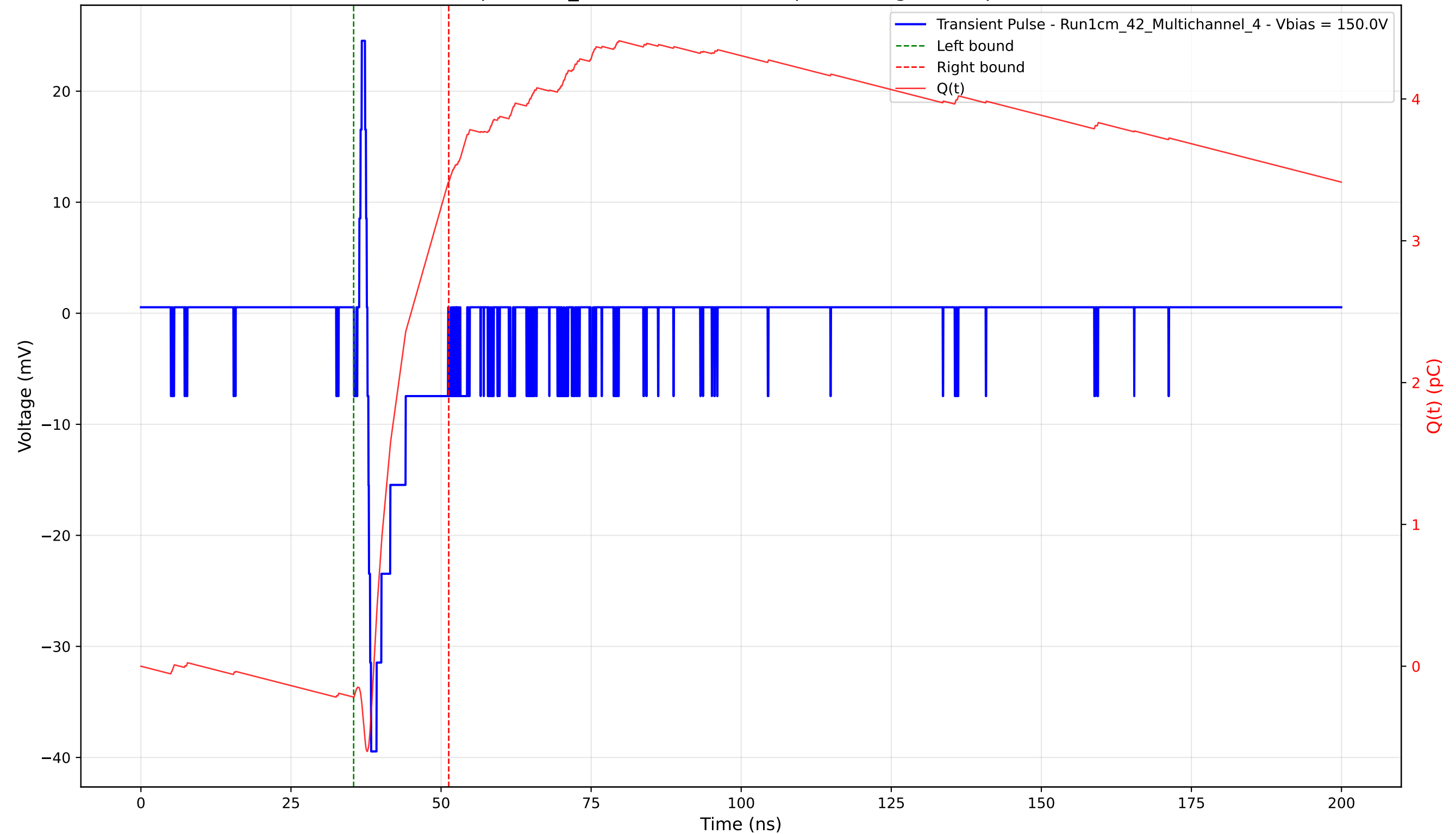
Transient Pulse - Sample: 1cm_42 - Position: 4270.0 \mu\text{m} - Charge: 3.63 pC - Rise Time: 0.62 ns
