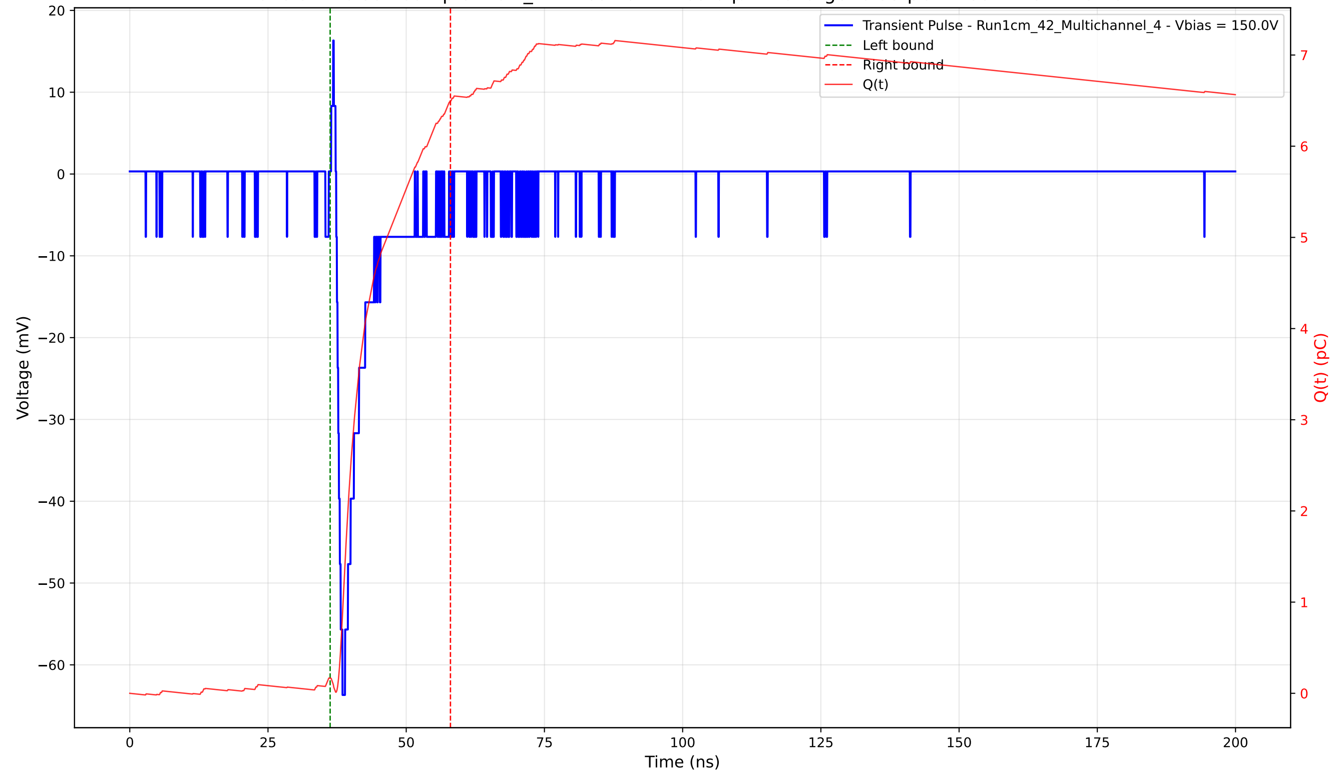
Transient Pulse - Sample: 1cm_42 - Position: 1165.0 \mu\text{m} - Charge: 6.33 pC - Rise Time: 1.13 ns
