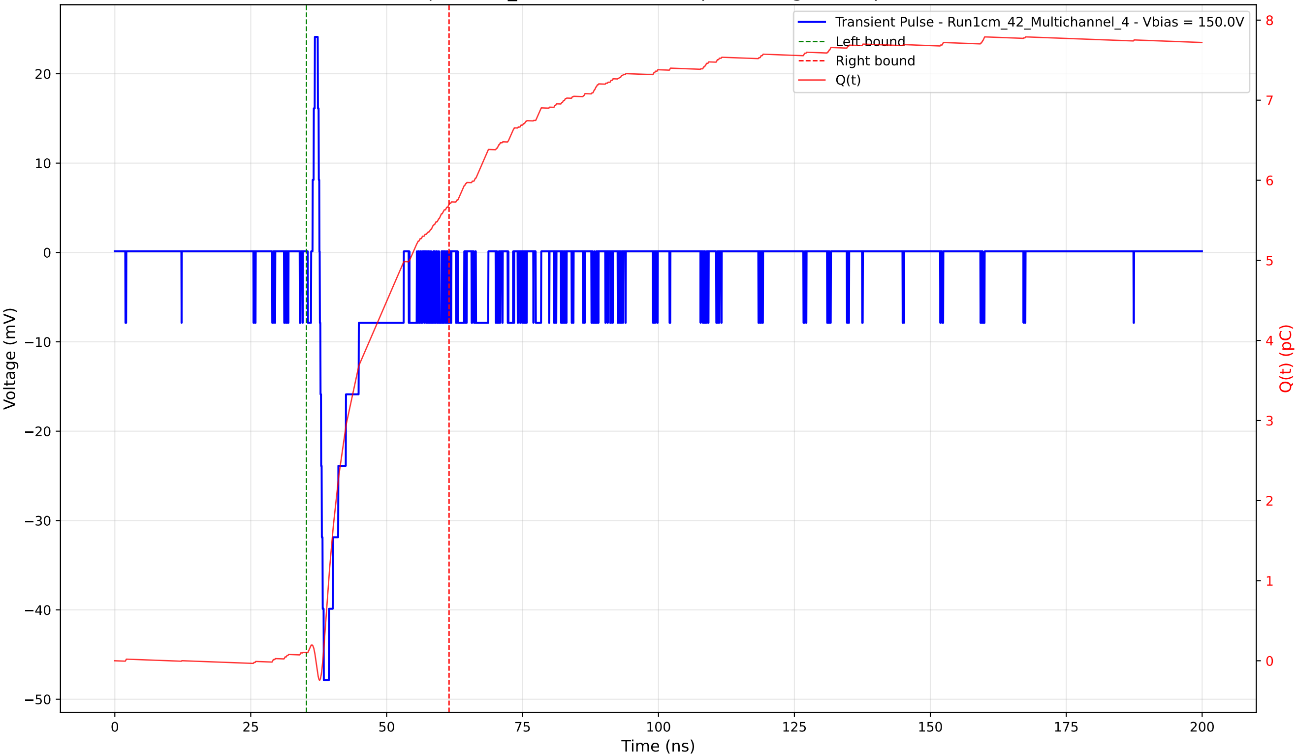
Transient Pulse - Sample: 1cm_42 - Position: 780.0 \mu\text{m} - Charge: 5.60 pC - Rise Time: 0.74 ns
