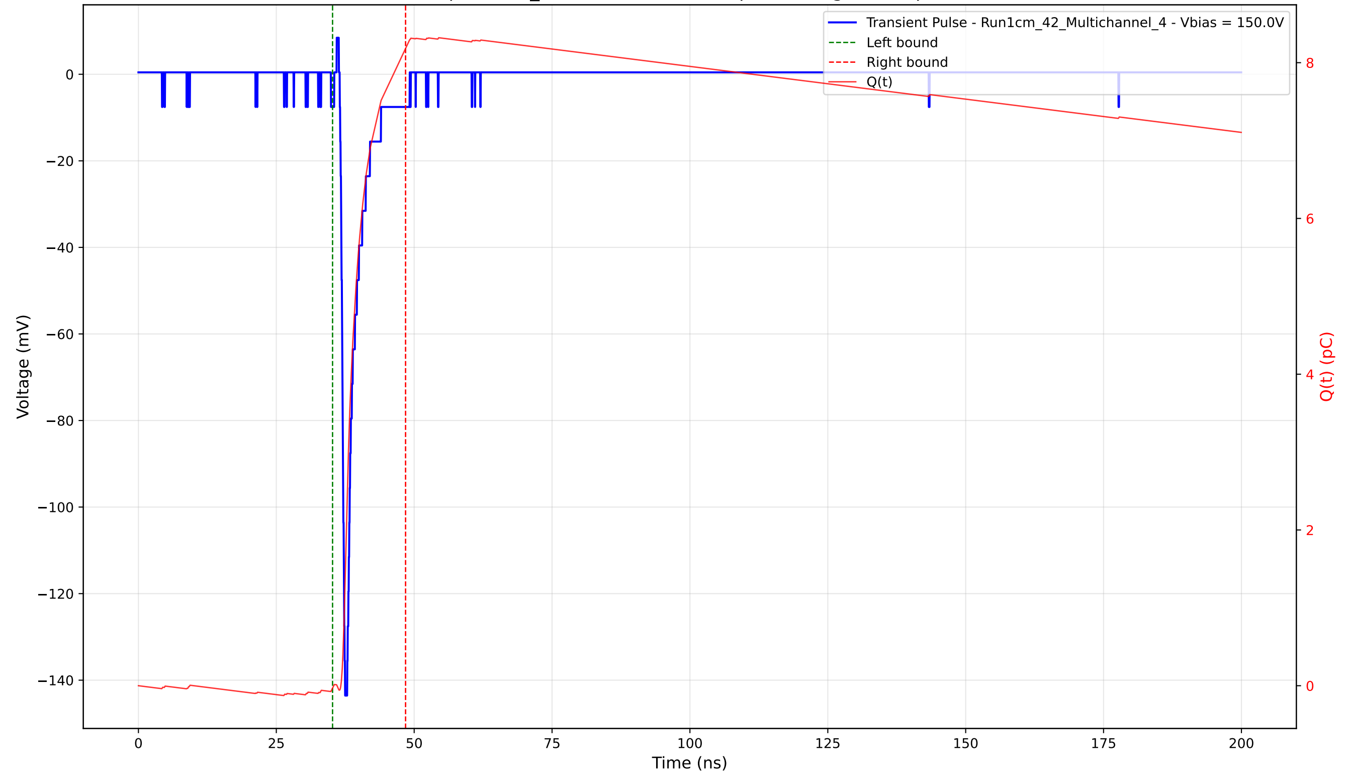
Transient Pulse - Sample: 1cm_42 - Position: 3260.0 \mu\text{m} - Charge: 8.21 pC - Rise Time: 0.81 ns
