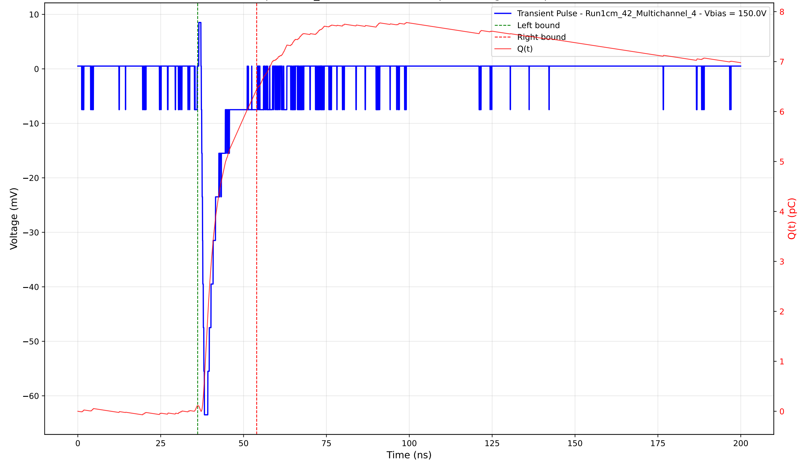
Transient Pulse - Sample: 1cm_42 - Position: 1225.0 \mu\text{m} - Charge: 6.34 pC - Rise Time: 0.93 ns
