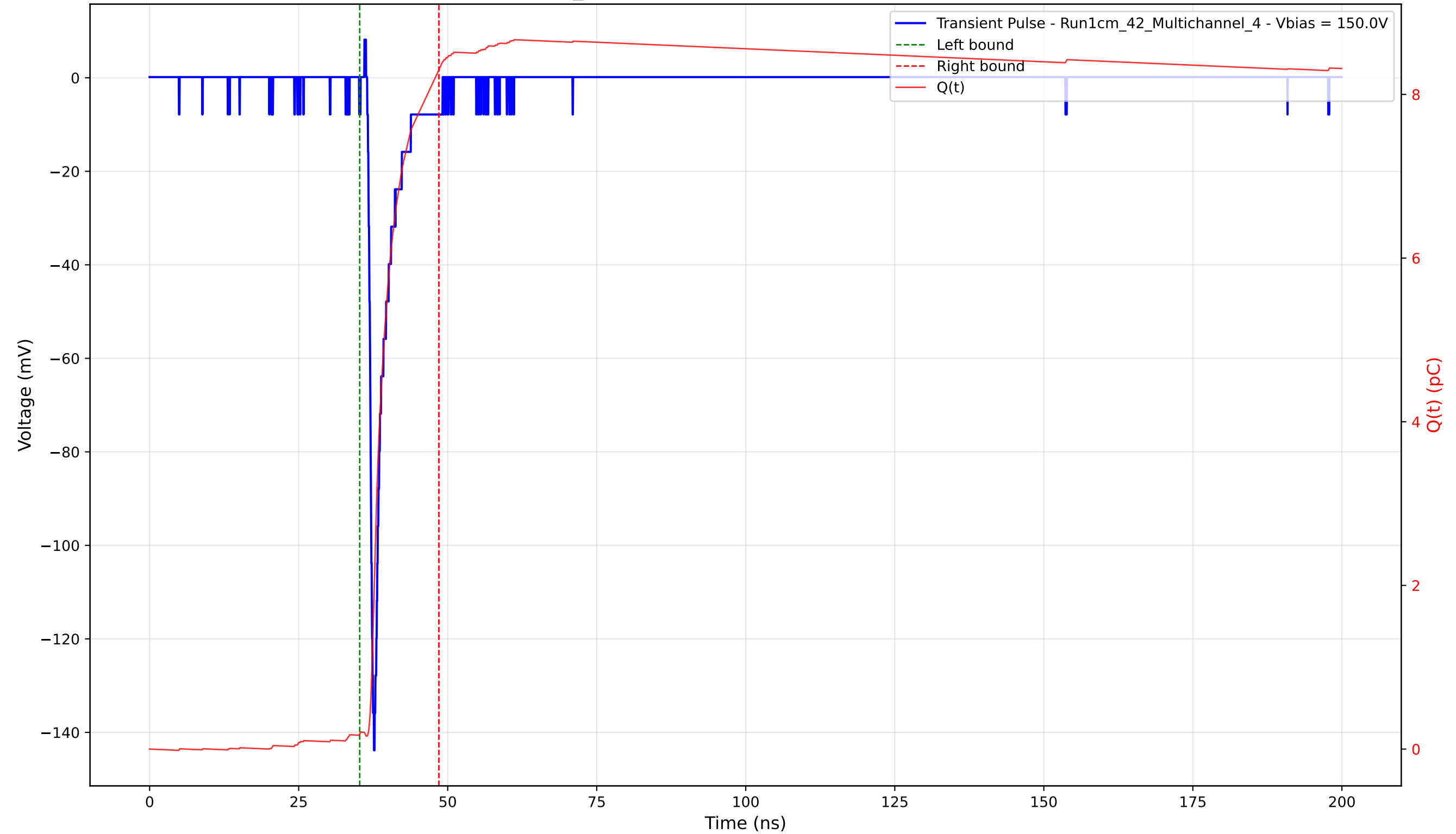
Transient Pulse - Sample: 1cm_42 - Position: 3295.0 \mu\text{m} - Charge: 8.12 pC - Rise Time: 0.85 ns
