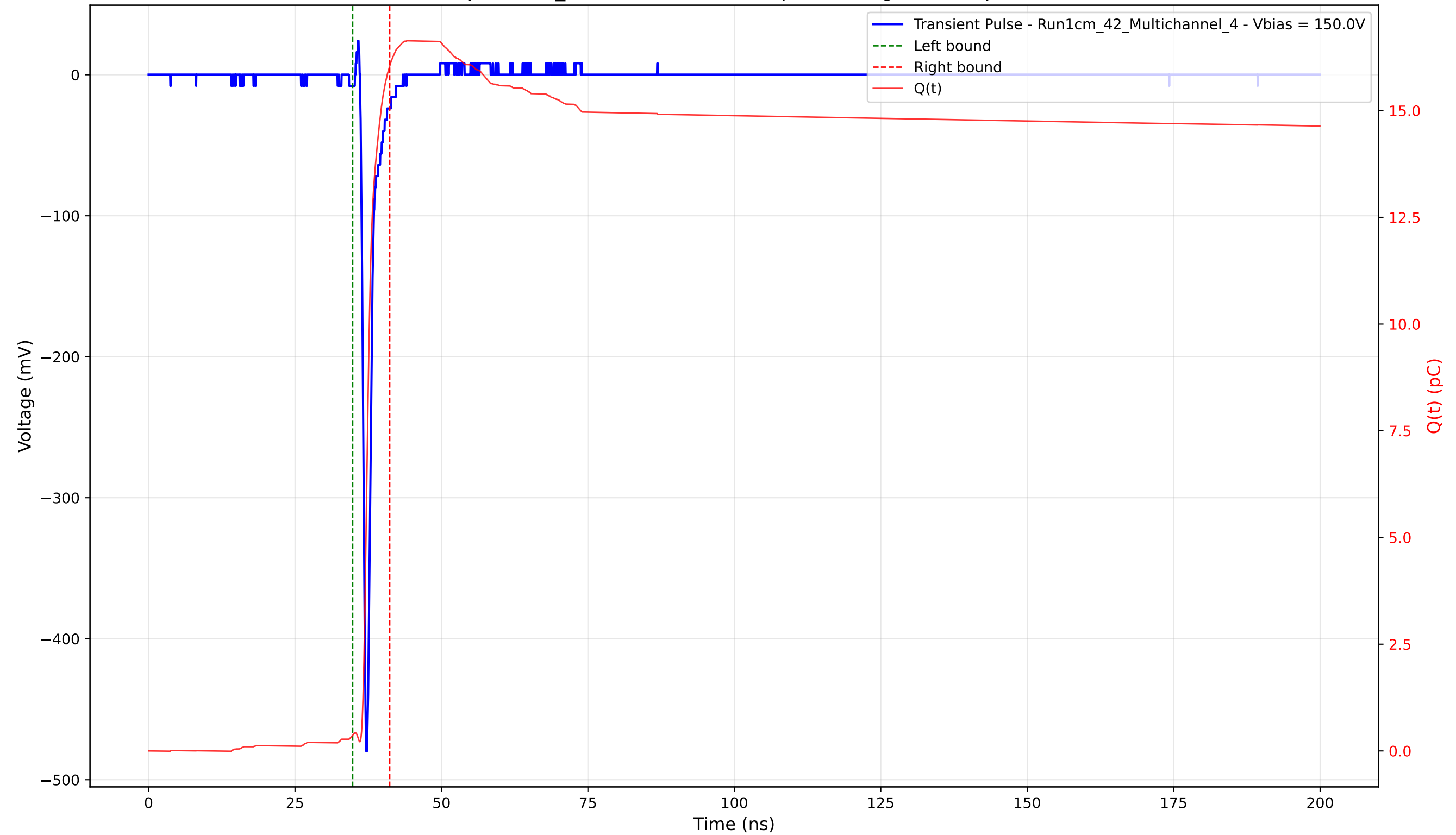
Transient Pulse - Sample: 1cm_42 - Position: 2770.0 \mu\text{m} - Charge: 15.68 pC - Rise Time: 0.74 ns
