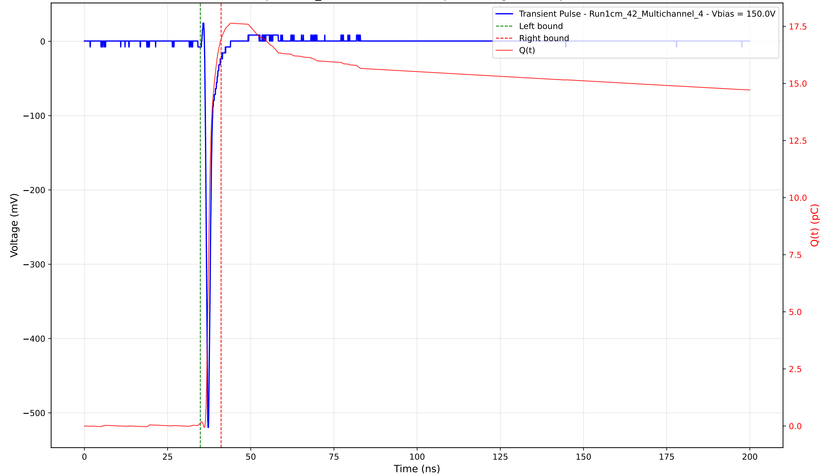
Transient Pulse - Sample: 1cm_42 - Position: 2275.0 \mu\text{m} - Charge: 16.81 pC - Rise Time: 0.72 ns
