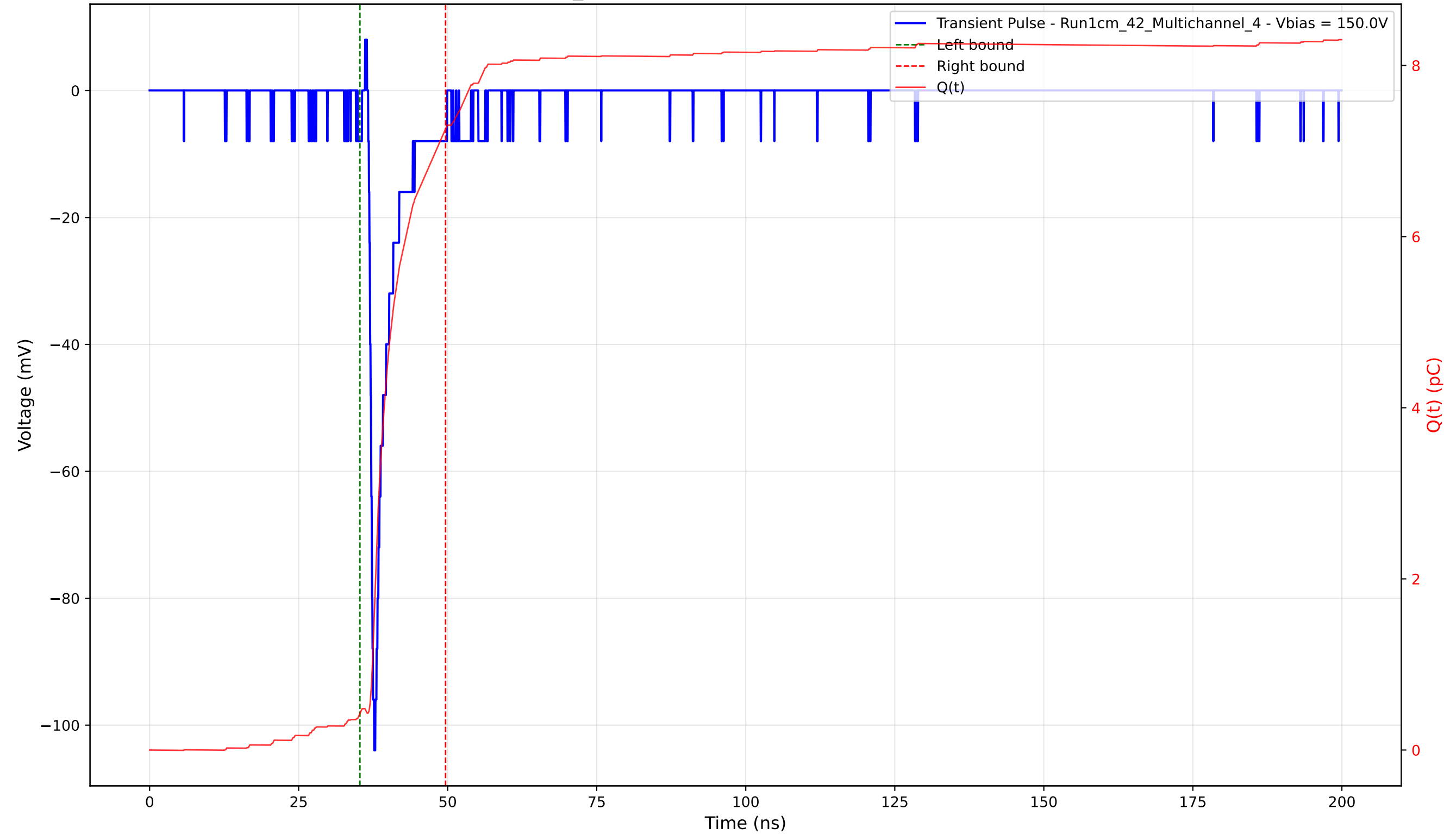
Transient Pulse - Sample: 1cm_42 - Position: 3415.0 \mu\text{m} - Charge: 6.83 pC - Rise Time: 0.71 ns
