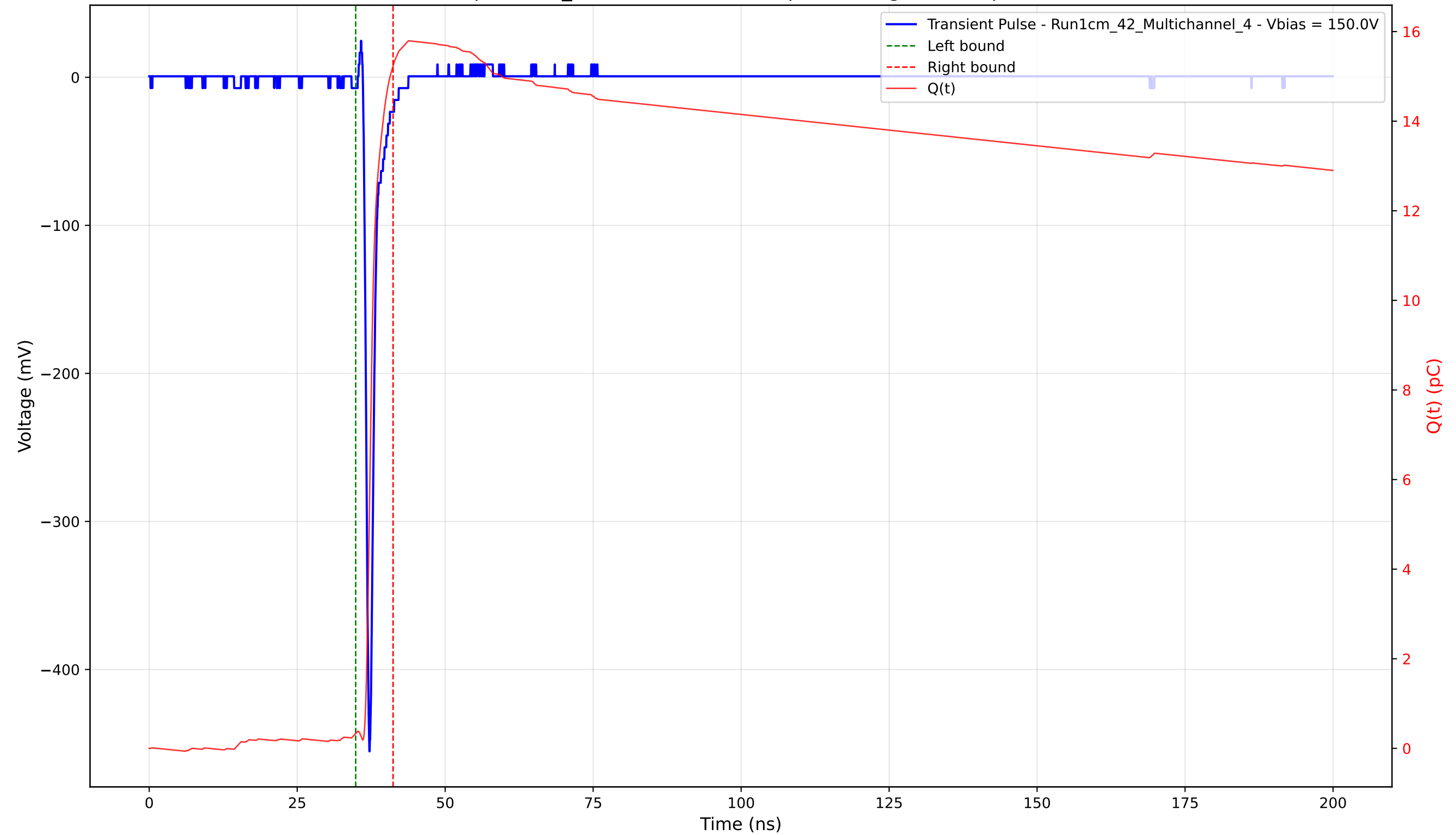
Transient Pulse - Sample: 1cm_42 - Position: 2815.0 \mu\text{m} - Charge: 14.91 pC - Rise Time: 0.72 ns
