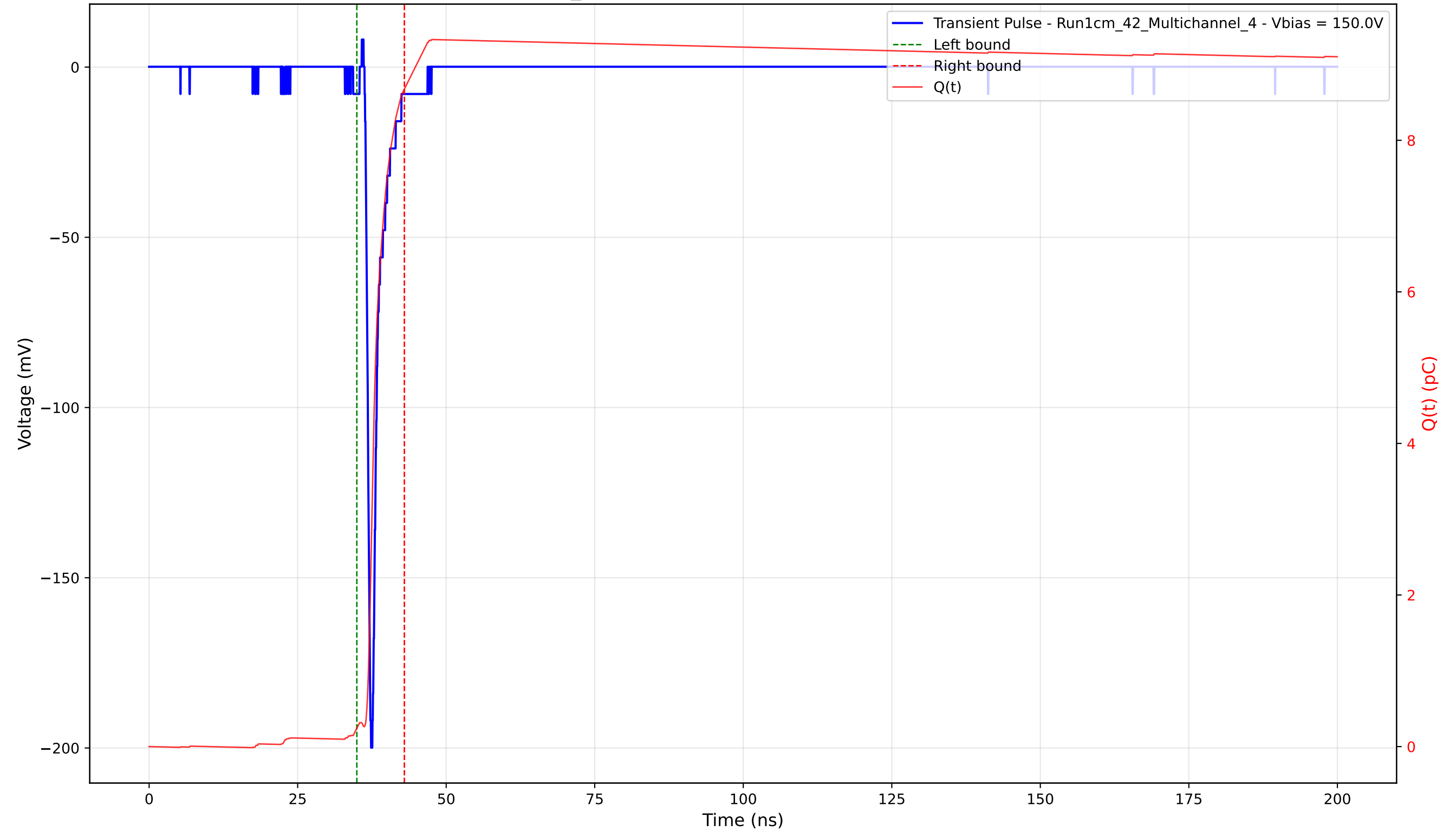
Transient Pulse - Sample: 1cm_42 - Position: 3055.0 \mu\text{m} - Charge: 8.43 pC - Rise Time: 0.76 ns
