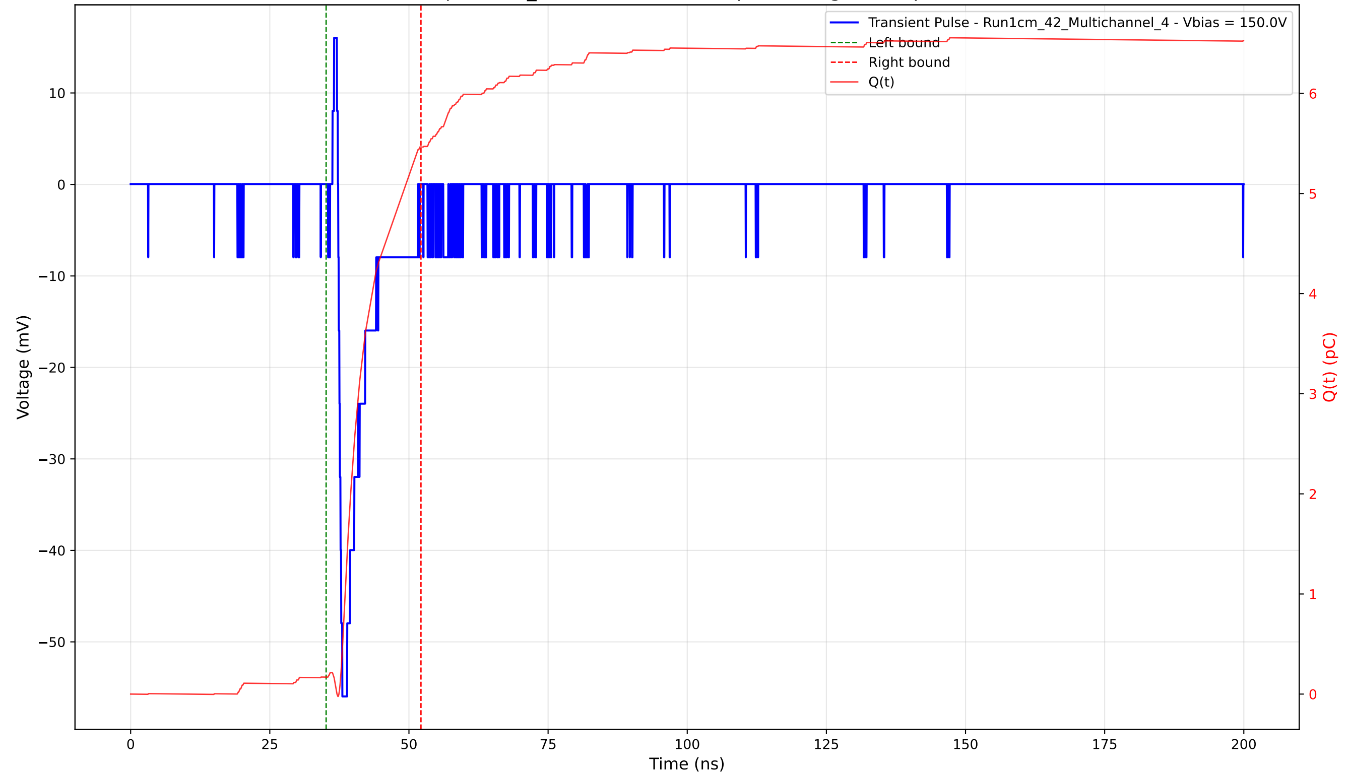
Transient Pulse - Sample: 1cm_42 - Position: 3775.0 \mu\text{m} - Charge: 5.29 pC - Rise Time: 0.73 ns
