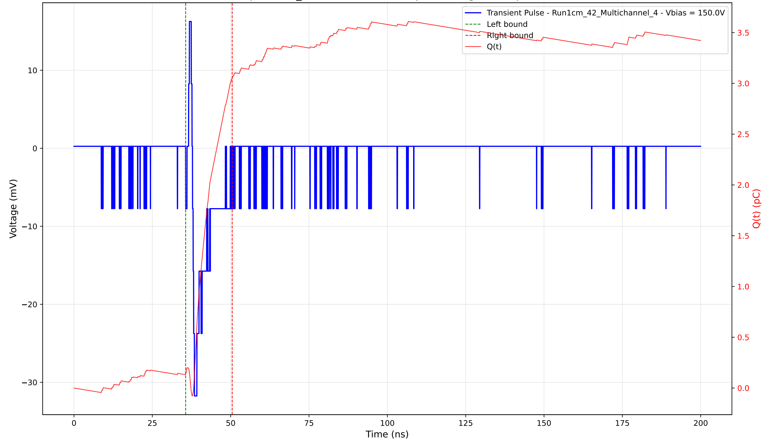
Transient Pulse - Sample: 1cm_42 - Position: 4580.0 \mu\text{m} - Charge: 2.92 pC - Rise Time: 0.62 ns
