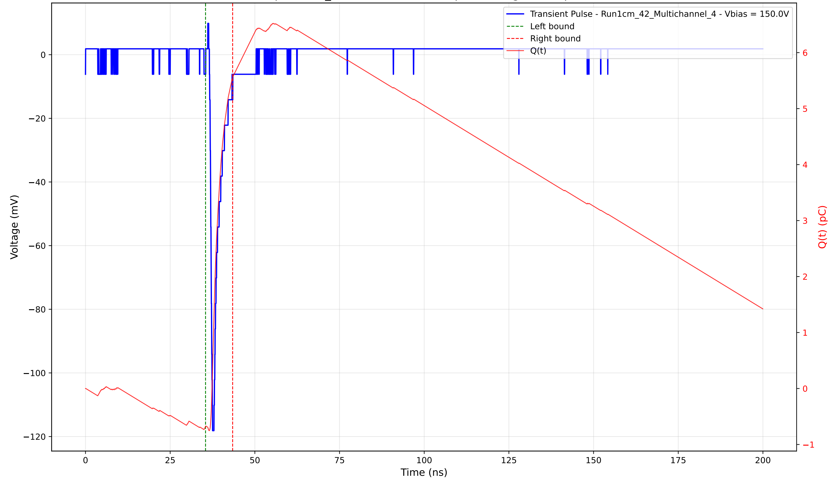
Transient Pulse - Sample: 1cm_42 - Position: 3350.0 \mu\text{m} - Charge: 6.23 pC - Rise Time: 0.77 ns
