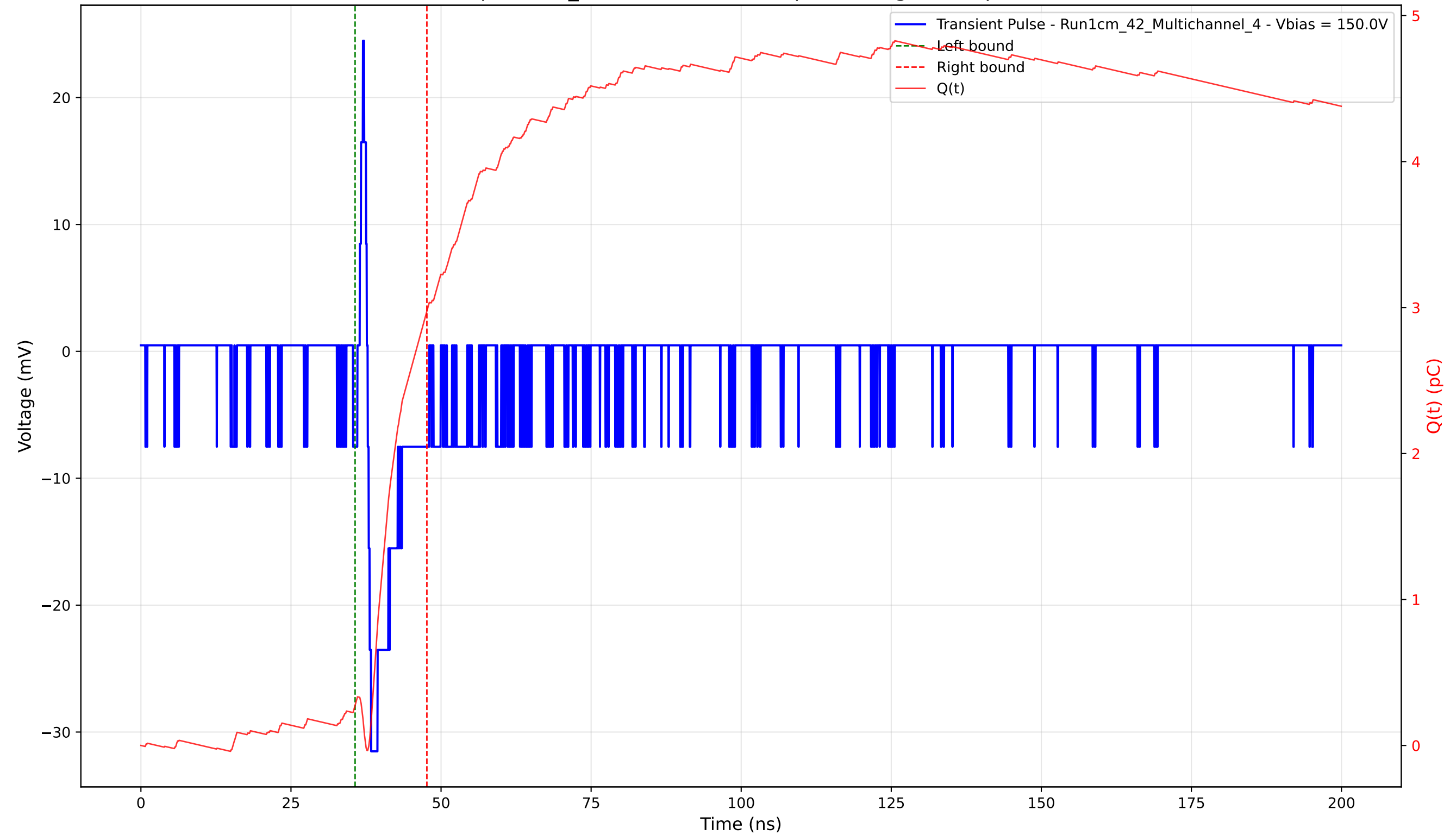
Transient Pulse - Sample: 1cm_42 - Position: 4435.0 \mu\text{m} - Charge: 2.70 pC - Rise Time: 0.58 ns
