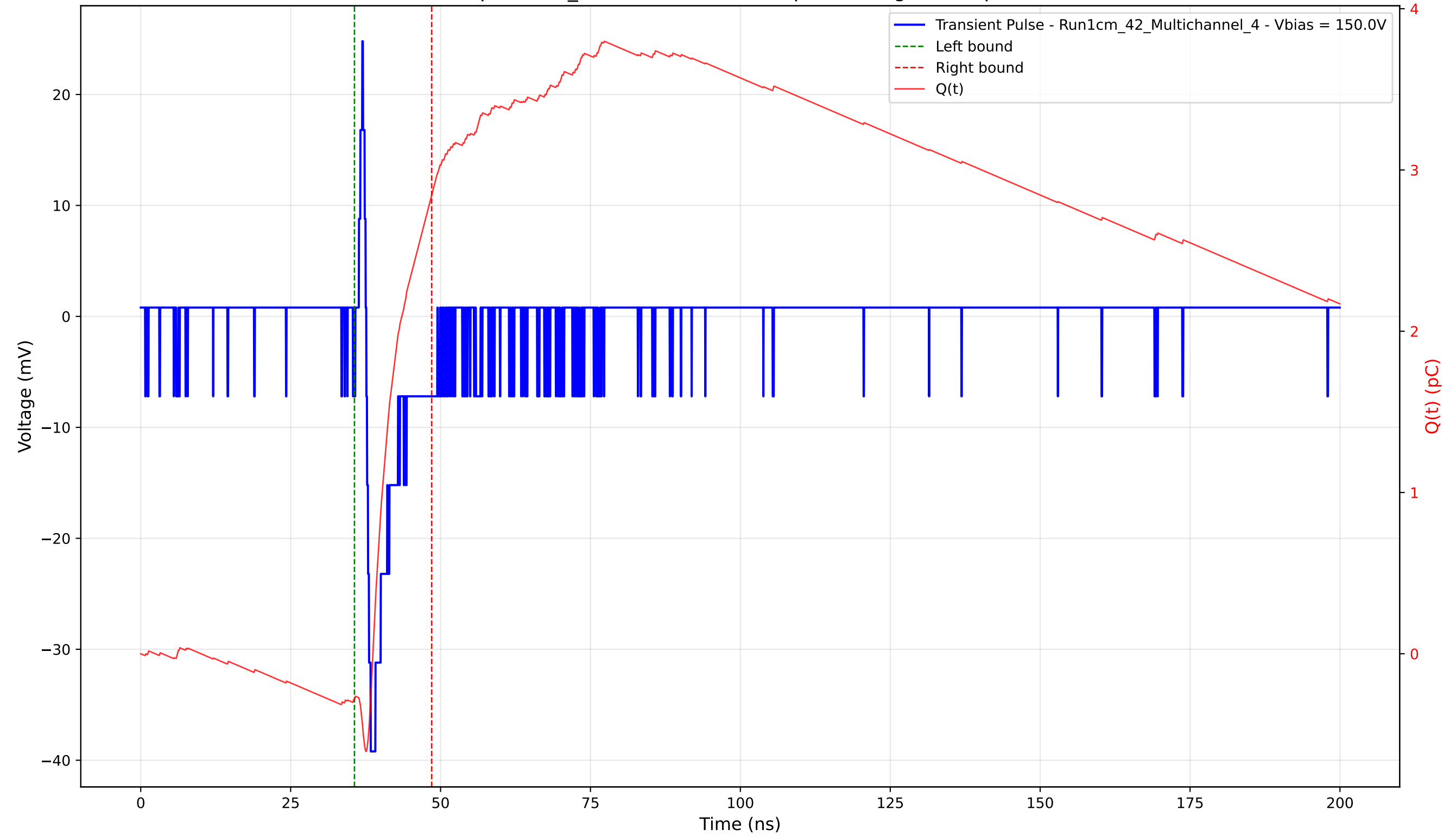
Transient Pulse - Sample: 1cm_42 - Position: 4090.0 \mu\text{m} - Charge: 3.13 pC - Rise Time: 0.74 ns
