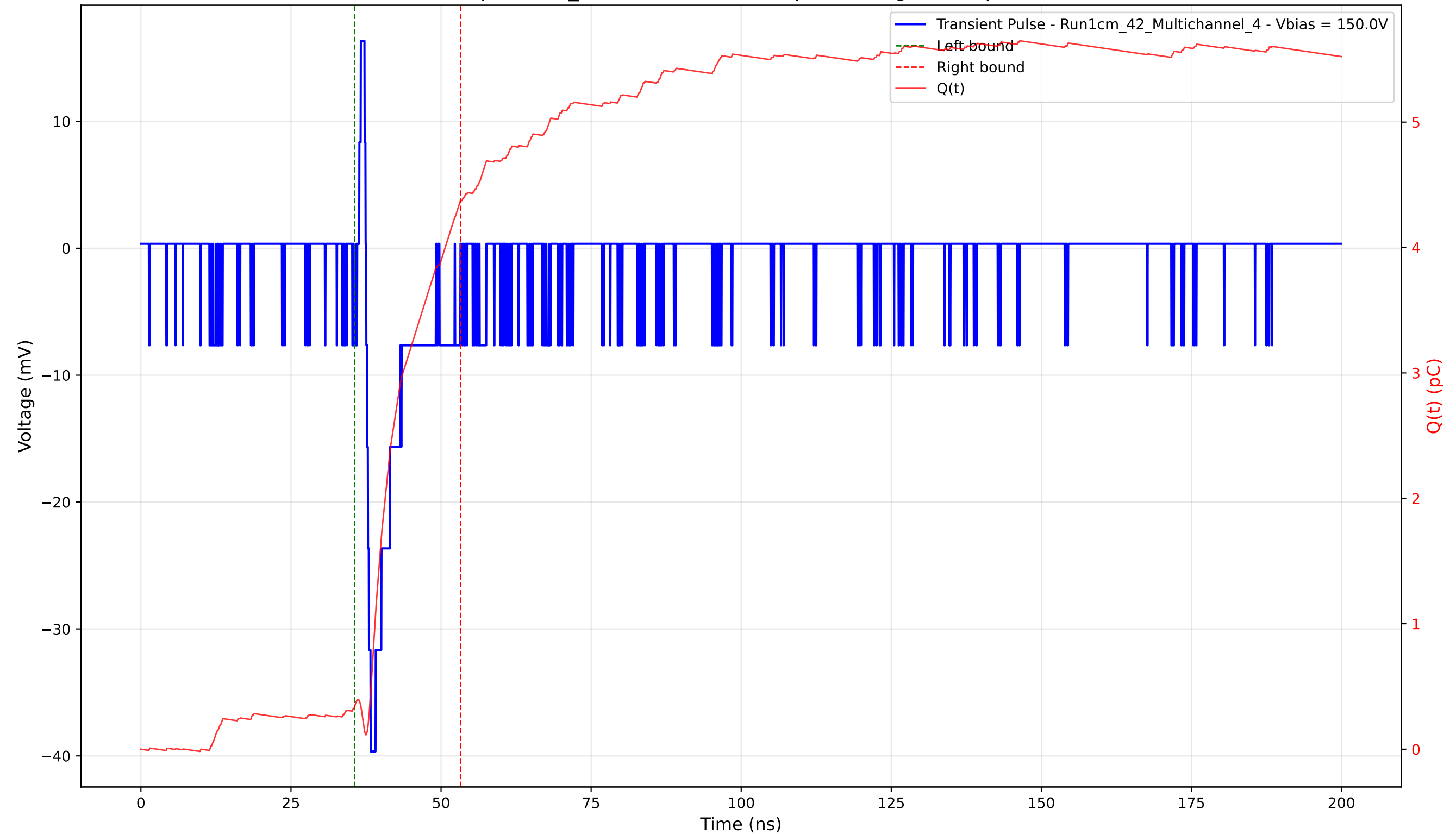
Transient Pulse - Sample: 1cm_42 - Position: 4035.0 \mu\text{m} - Charge: 4.03 pC - Rise Time: 0.74 ns
