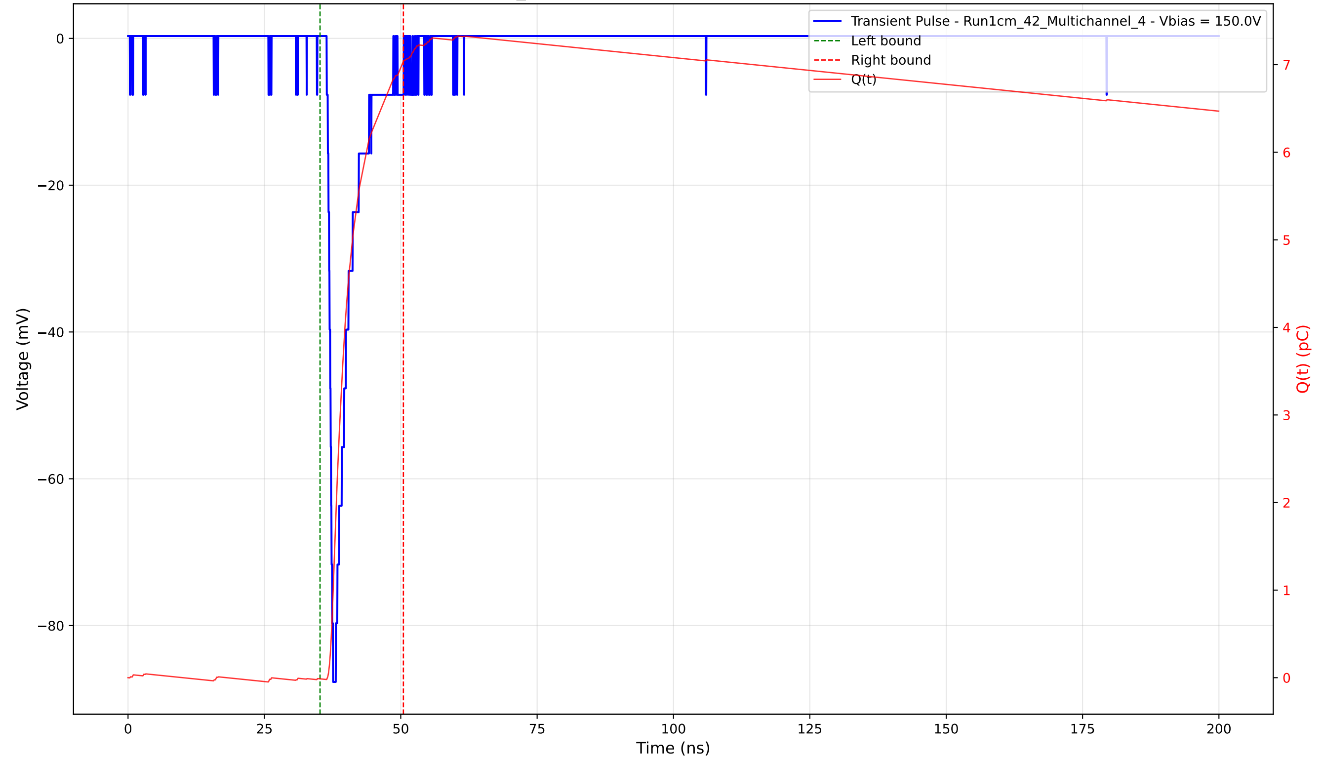
Transient Pulse - Sample: 1cm_42 - Position: 1575.0 \mu\text{m} - Charge: 7.05 pC - Rise Time: 0.83 ns
