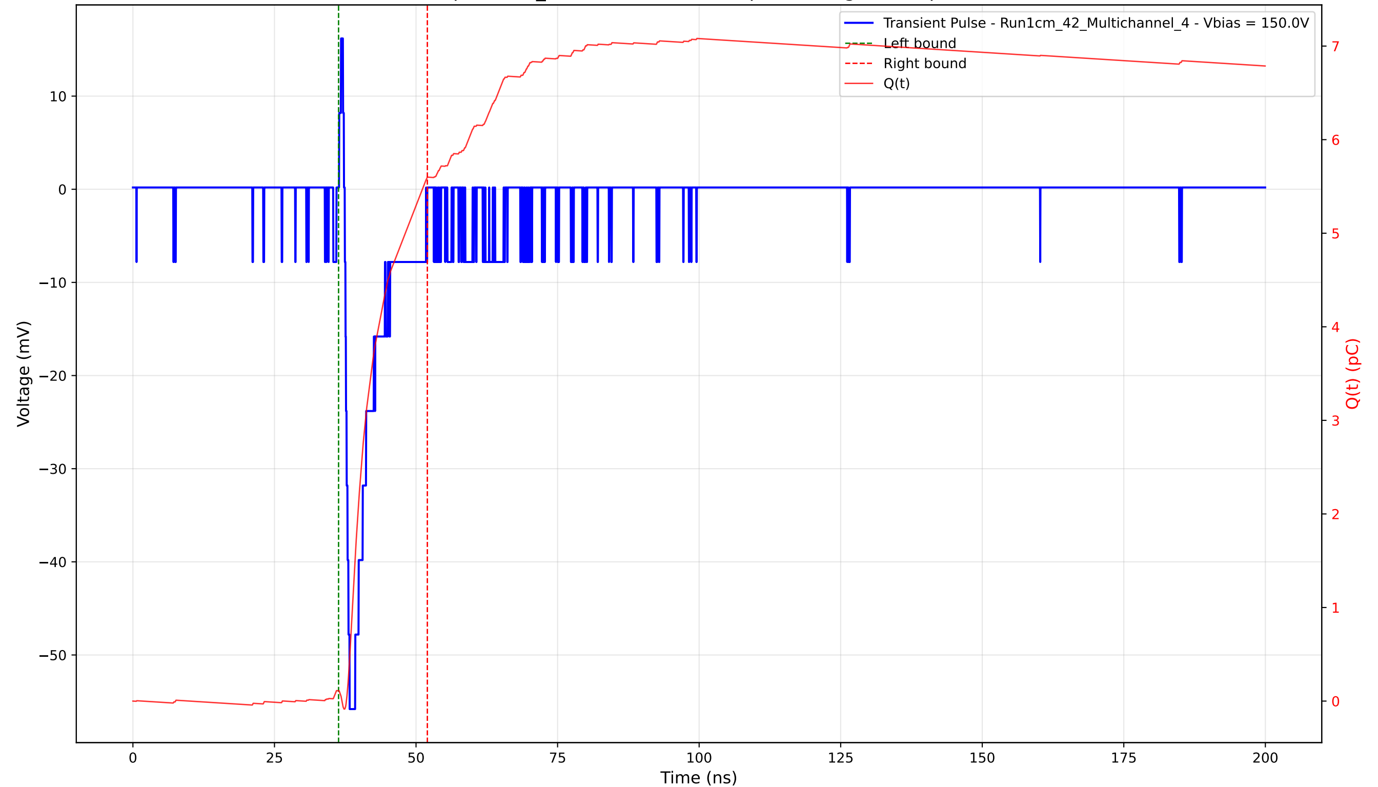
Transient Pulse - Sample: 1cm_42 - Position: 1130.0 \mu\text{m} - Charge: 5.49 pC - Rise Time: 0.85 ns
