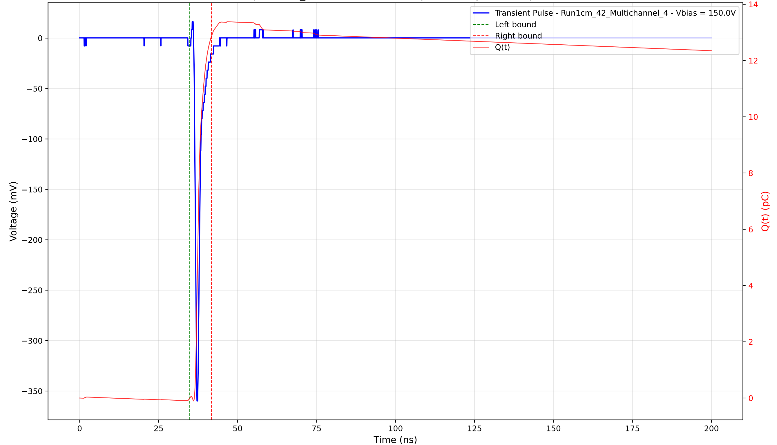
Transient Pulse - Sample: 1cm_42 - Position: 2130.0 \mu\text{m} - Charge: 12.84 pC - Rise Time: 0.72 ns
