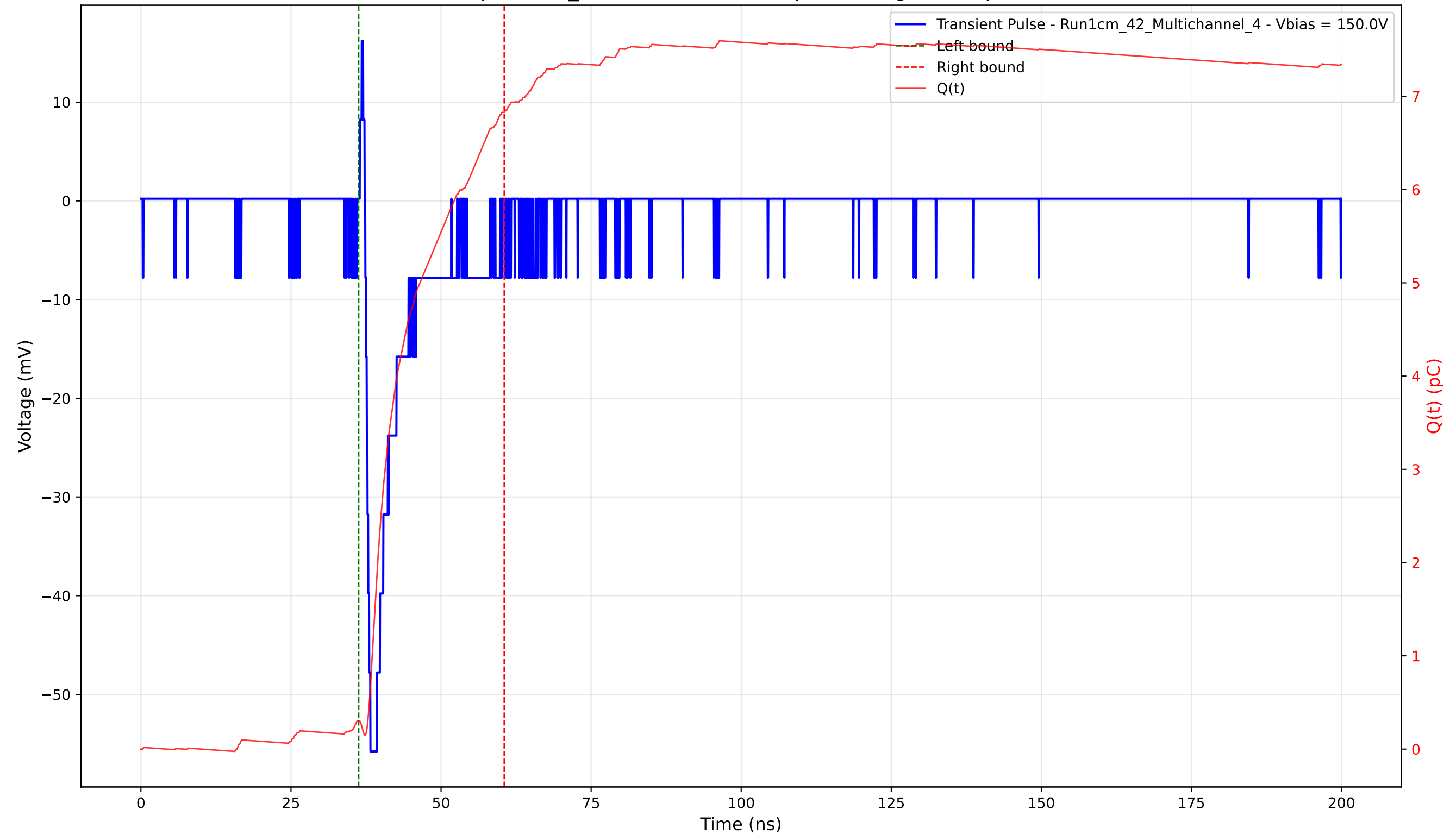
Transient Pulse - Sample: 1cm_42 - Position: 1140.0 \mu\text{m} - Charge: 6.52 pC - Rise Time: 0.85 ns
