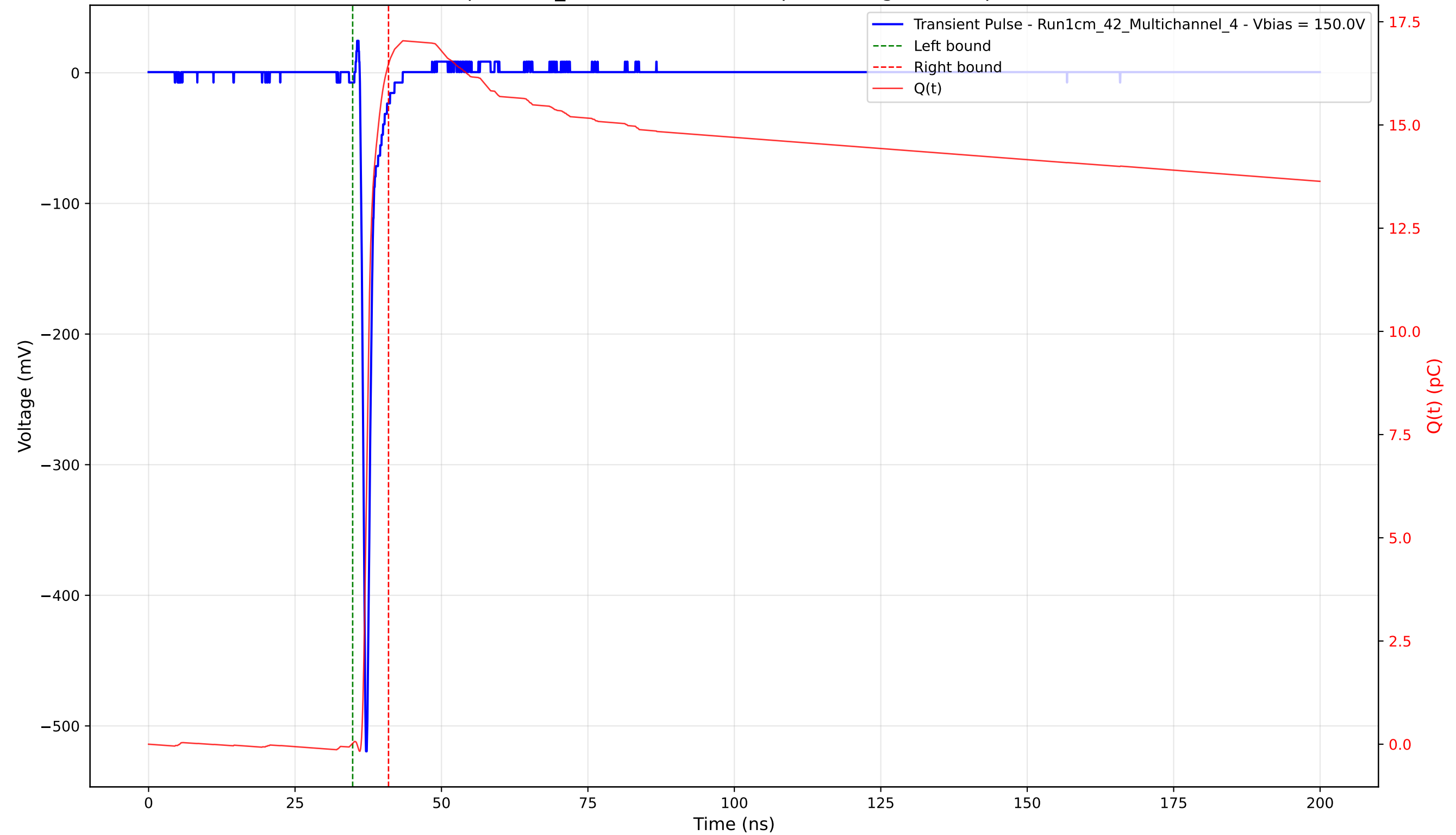
Transient Pulse - Sample: 1cm_42 - Position: 2335.0 \mu\text{m} - Charge: 16.45 pC - Rise Time: 0.69 ns
