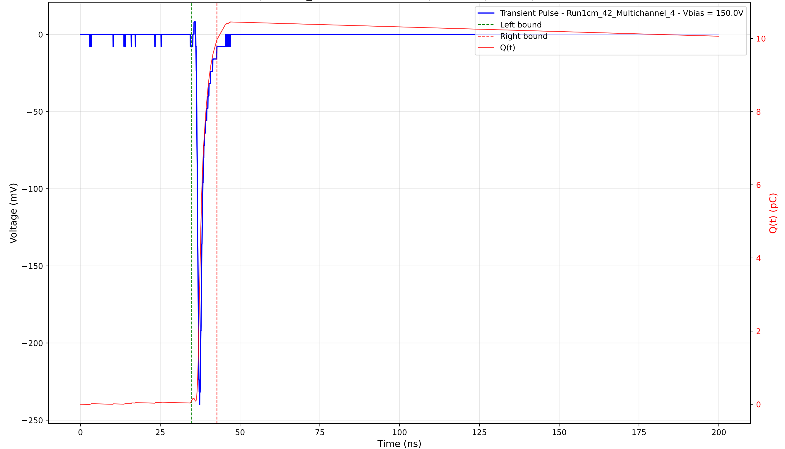
Transient Pulse - Sample: 1cm_42 - Position: 2015.0 \mu\text{m} - Charge: 9.86 pC - Rise Time: 0.80 ns
