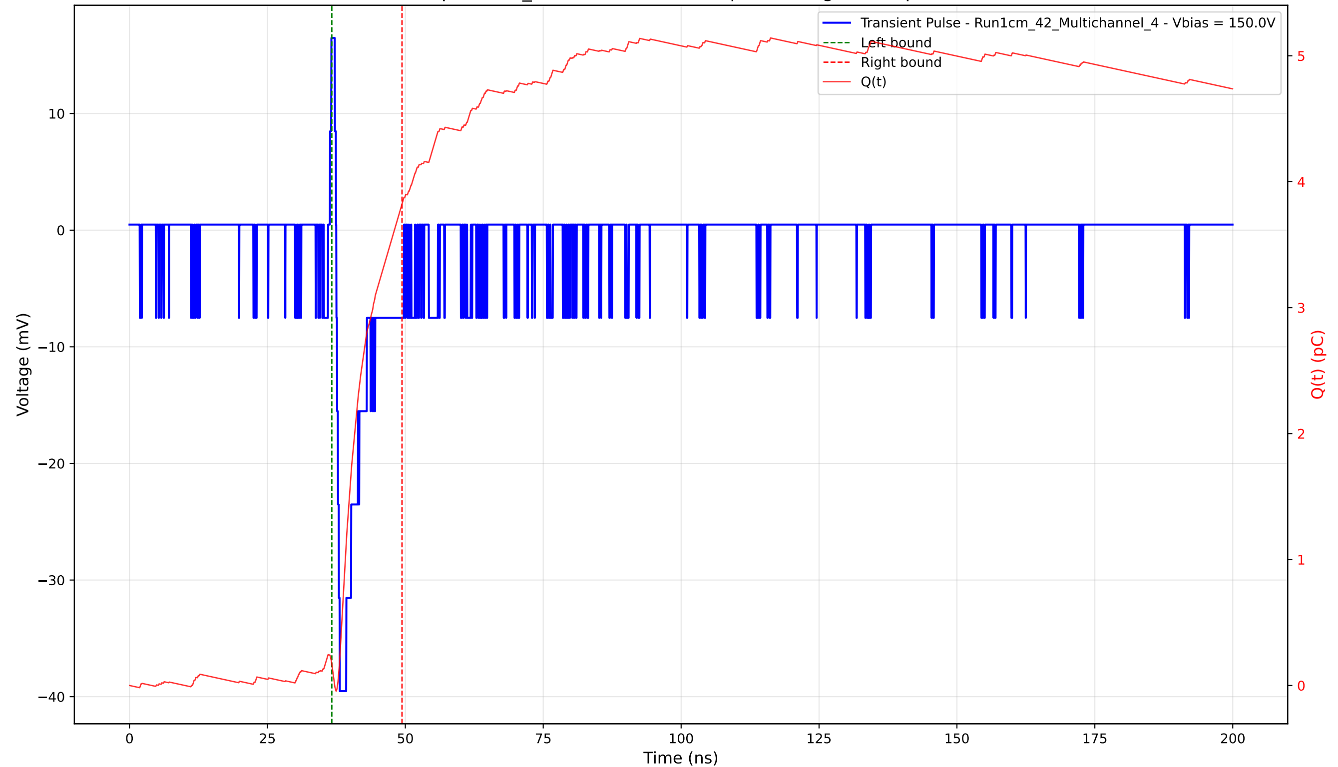
Transient Pulse - Sample: 1cm_42 - Position: 4005.0 \mu\text{m} - Charge: 3.66 pC - Rise Time: 0.62 ns
