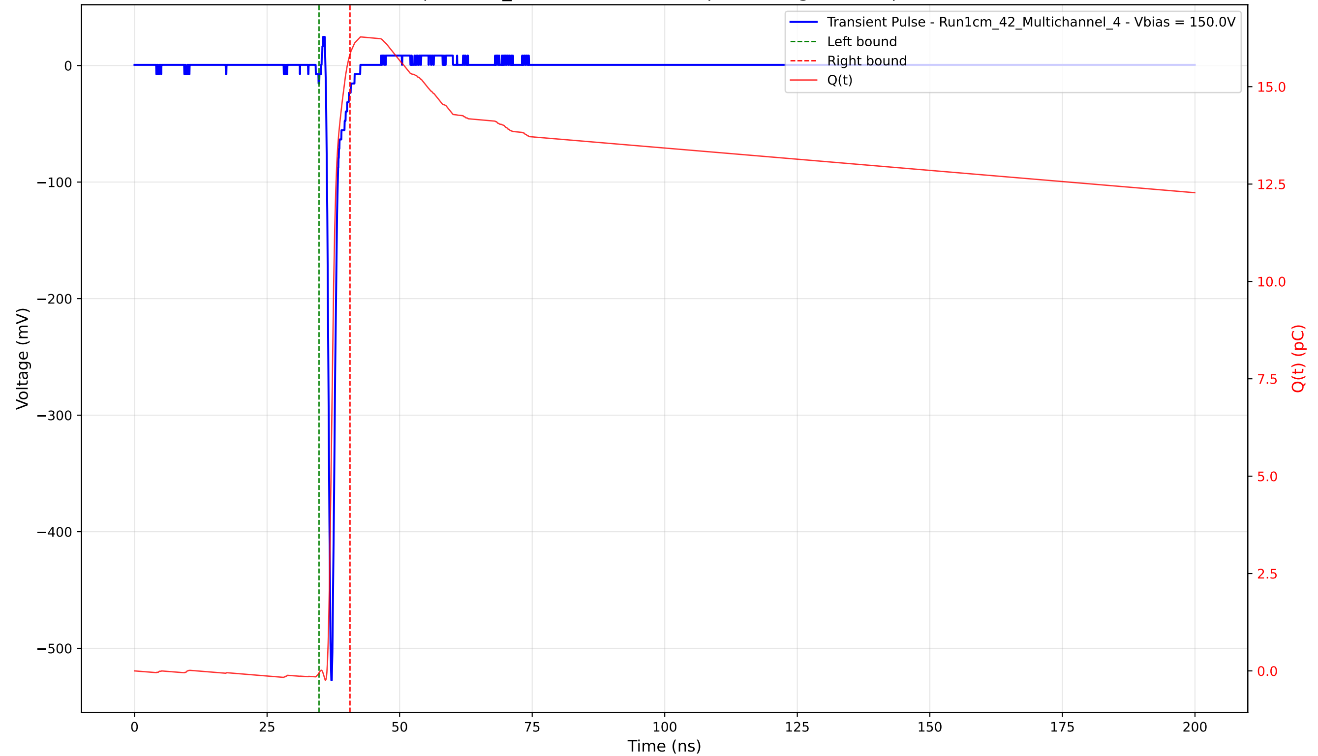
Transient Pulse - Sample: 1cm_42 - Position: 2470.0 \mu\text{m} - Charge: 15.88 pC - Rise Time: 0.71 ns
