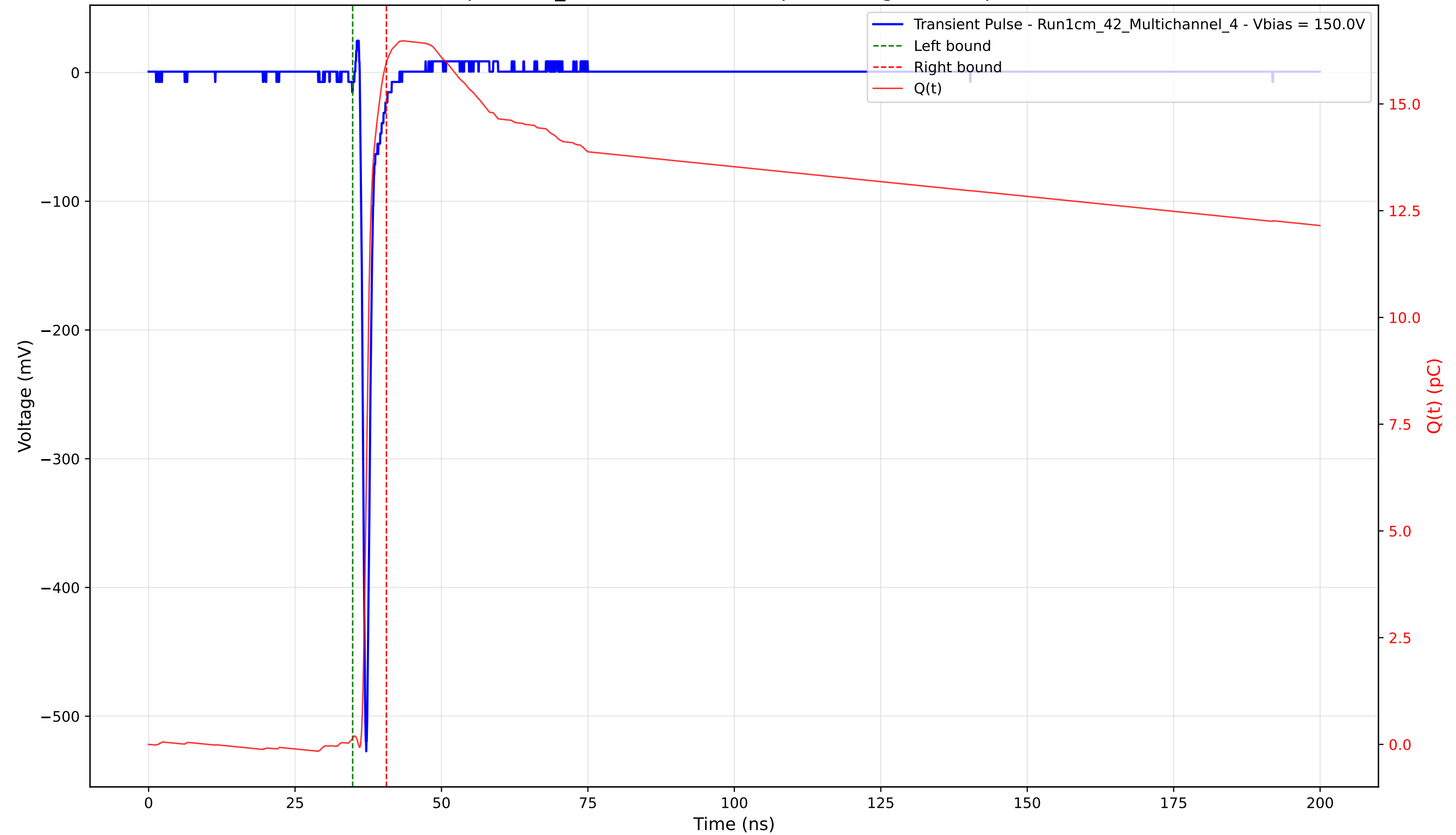
Transient Pulse - Sample: 1cm_42 - Position: 2595.0 \mu\text{m} - Charge: 15.82 pC - Rise Time: 0.73 ns
