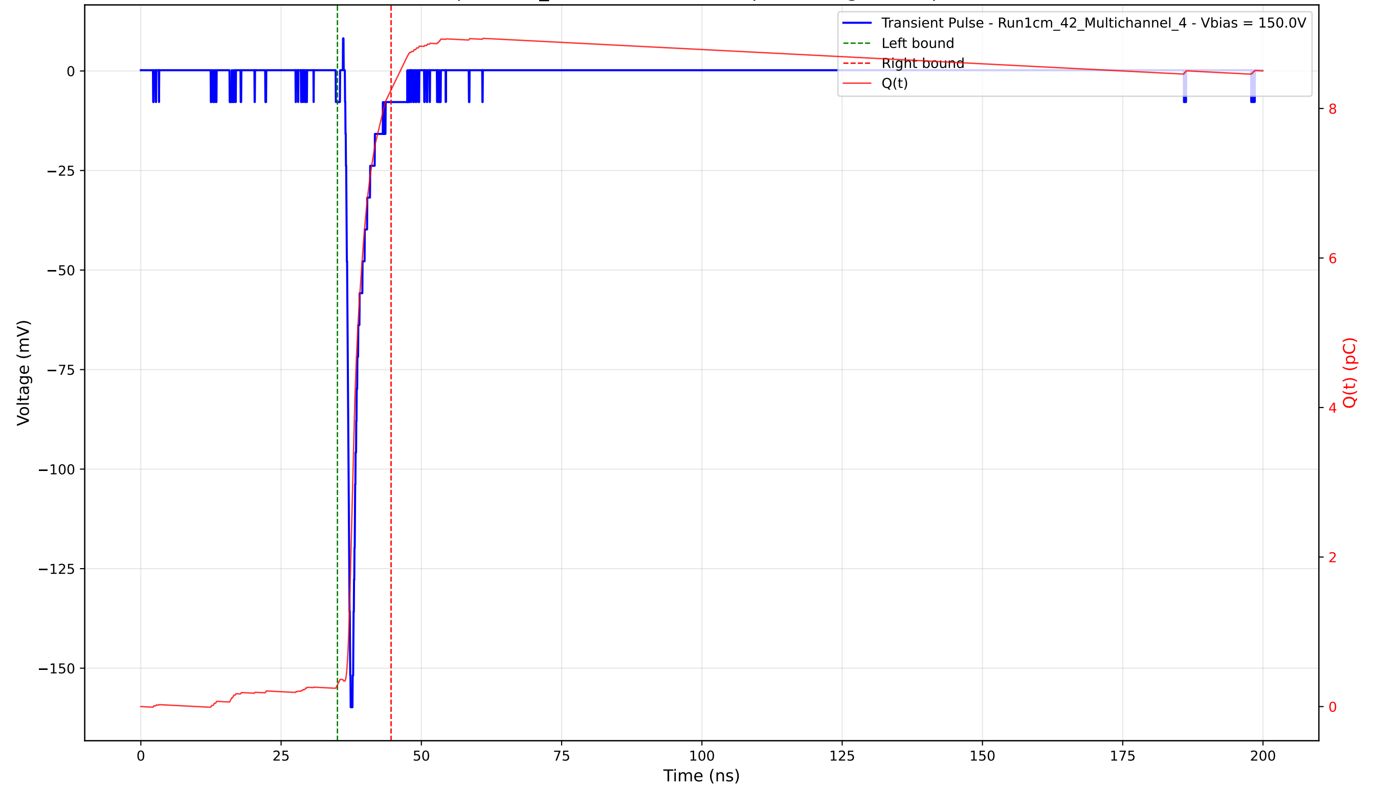
Transient Pulse - Sample: 1cm_42 - Position: 3165.0 \mu\text{m} - Charge: 7.96 pC - Rise Time: 0.80 ns
