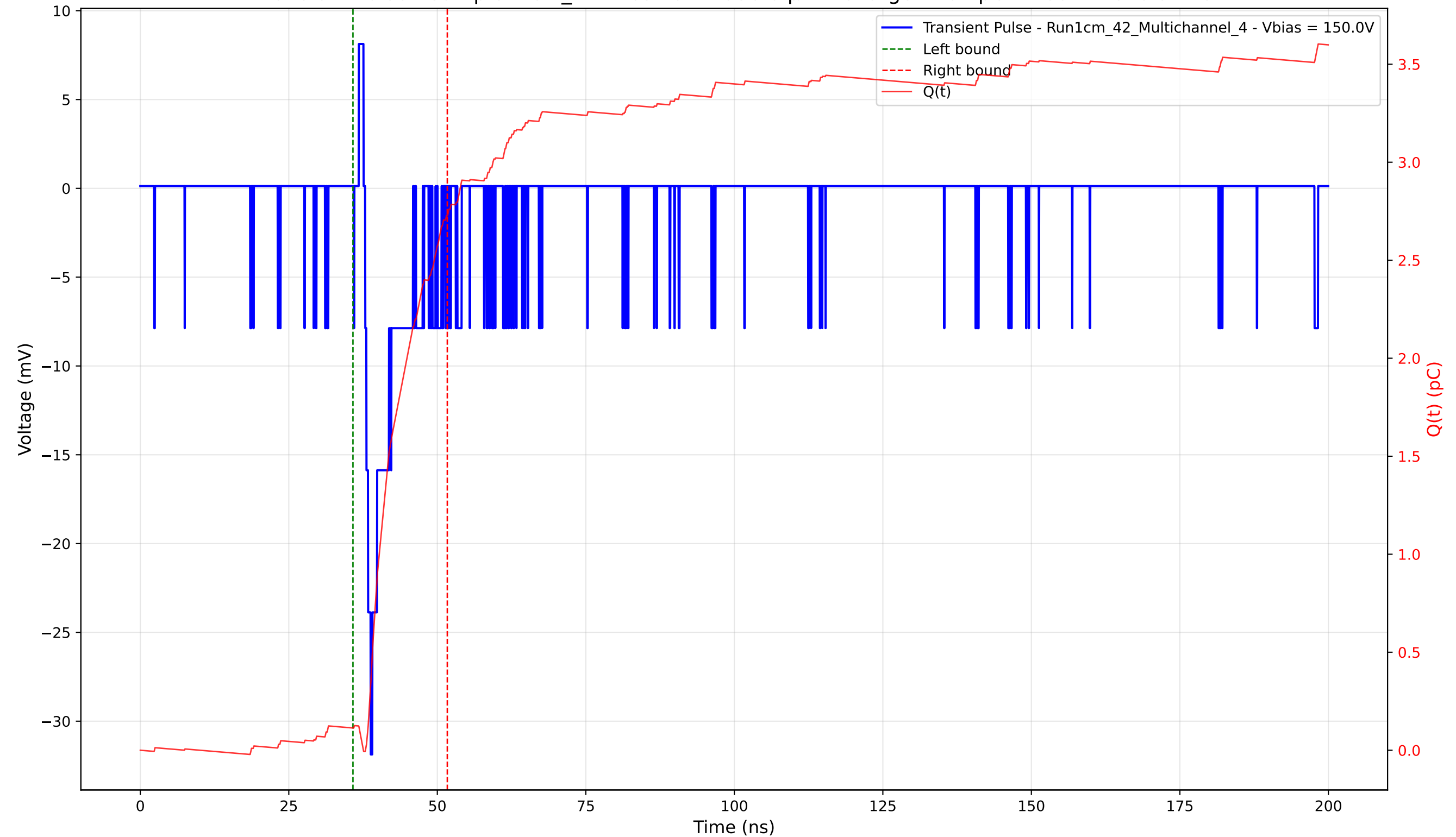
Transient Pulse - Sample: 1cm_42 - Position: 4930.0 \mu\text{m} - Charge: 2.62 pC - Rise Time: 0.94 ns
