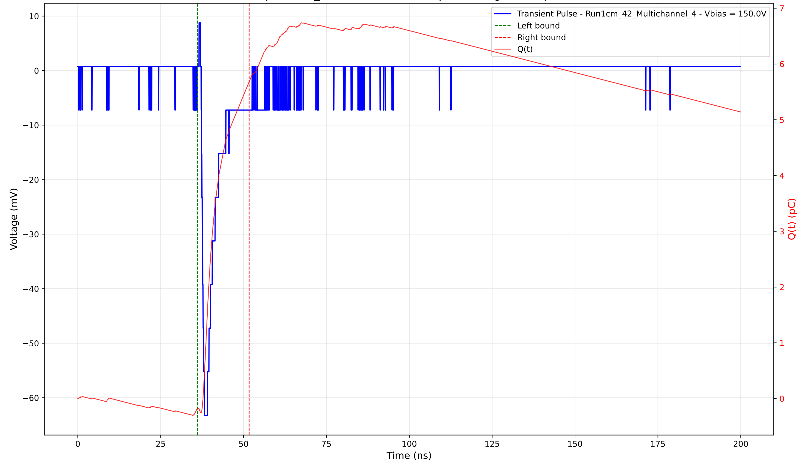
Transient Pulse - Sample: 1cm_42 - Position: 1305.0 \mu\text{m} - Charge: 5.86 pC - Rise Time: 1.05 ns
