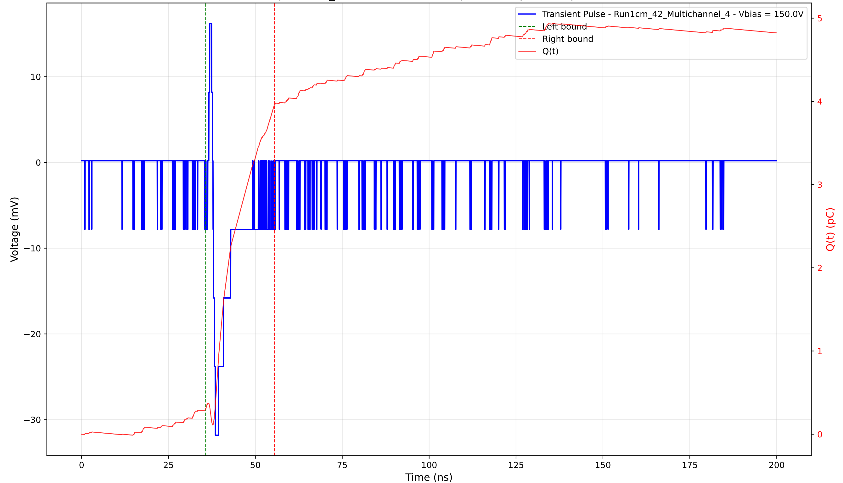
Transient Pulse - Sample: 1cm_42 - Position: 4705.0 \mu\text{m} - Charge: 3.66 pC - Rise Time: 0.66 ns
