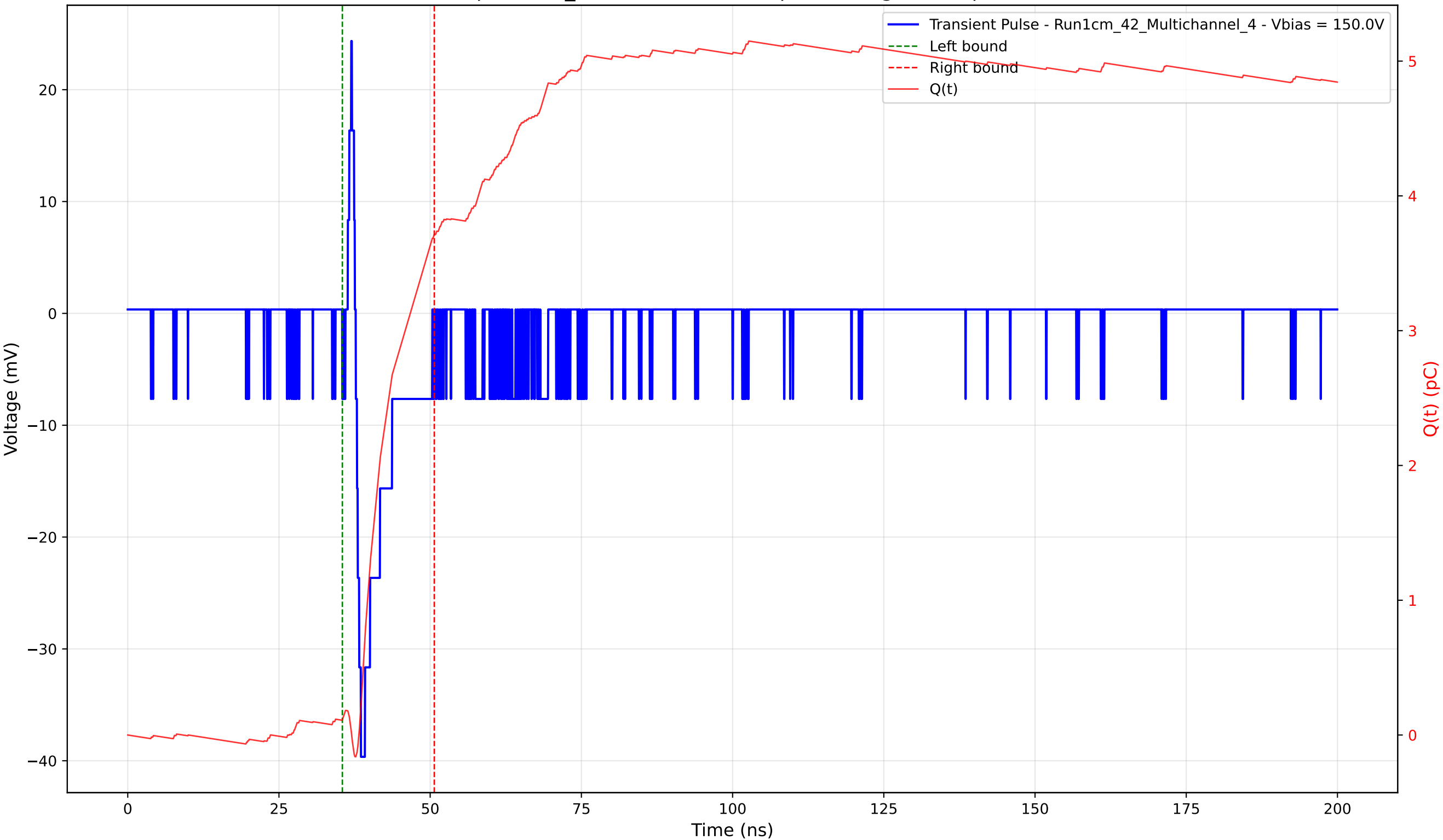
Transient Pulse - Sample: 1cm_42 - Position: 530.0 \mu\text{m} - Charge: 3.60 pC - Rise Time: 0.86 ns
