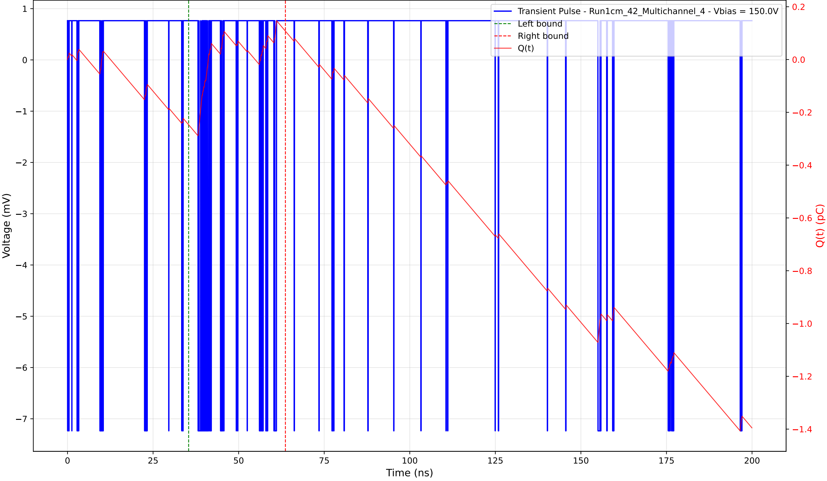
Transient Pulse - Sample: 1cm_42 - Position: 25.0 \mu\text{m} - Charge: 0.36 pC - Rise Time: 0.00 ns (N/A)
