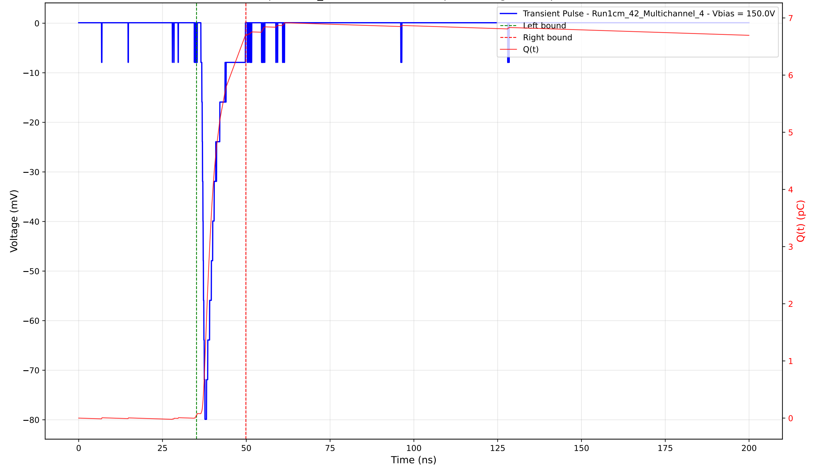
Transient Pulse - Sample: 1cm_42 - Position: 1540.0 \mu\text{m} - Charge: 6.66 pC - Rise Time: 0.96 ns
