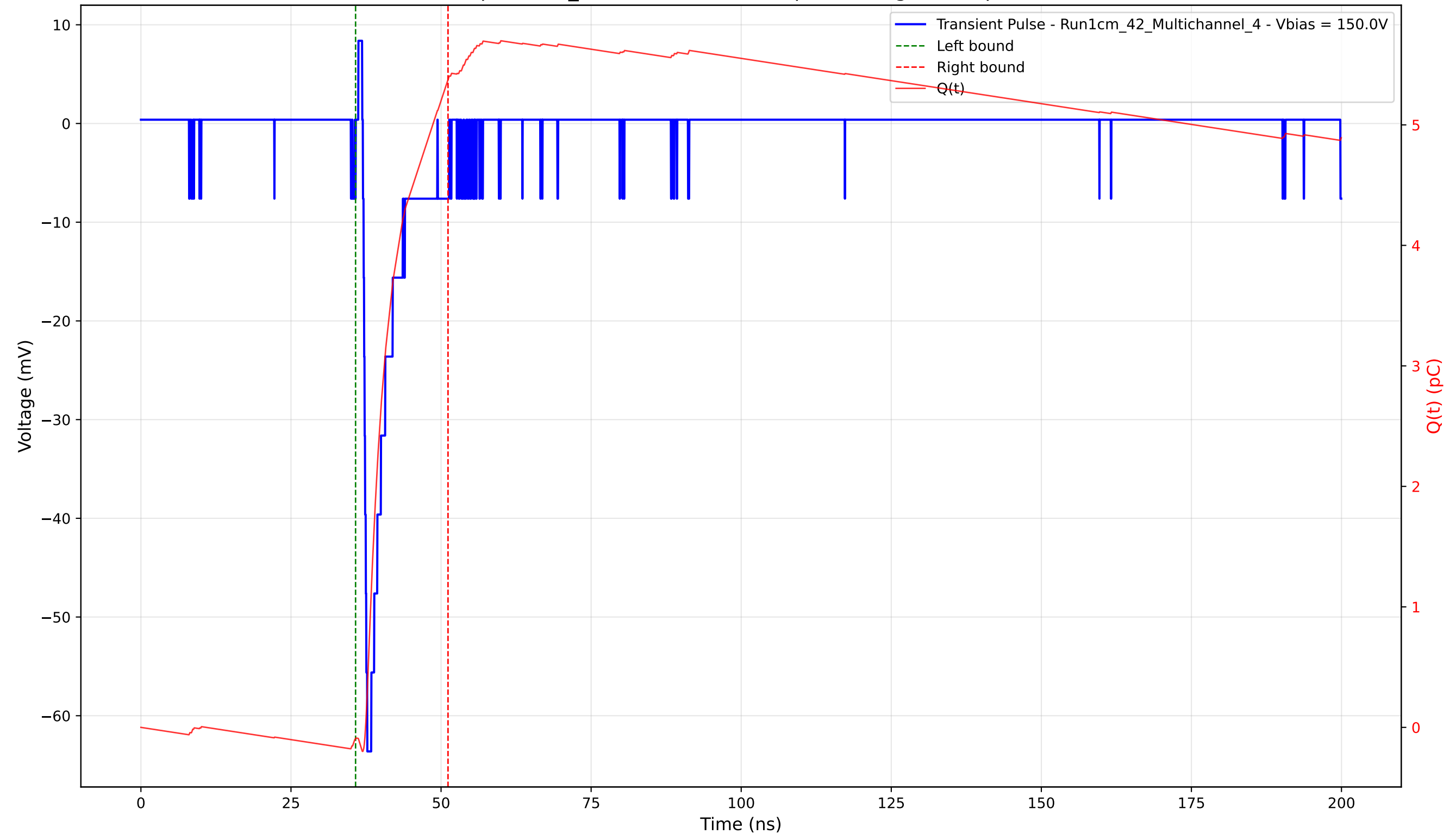
Transient Pulse - Sample: 1cm_42 - Position: 3560.0 \mu\text{m} - Charge: 5.47 pC - Rise Time: 0.73 ns
