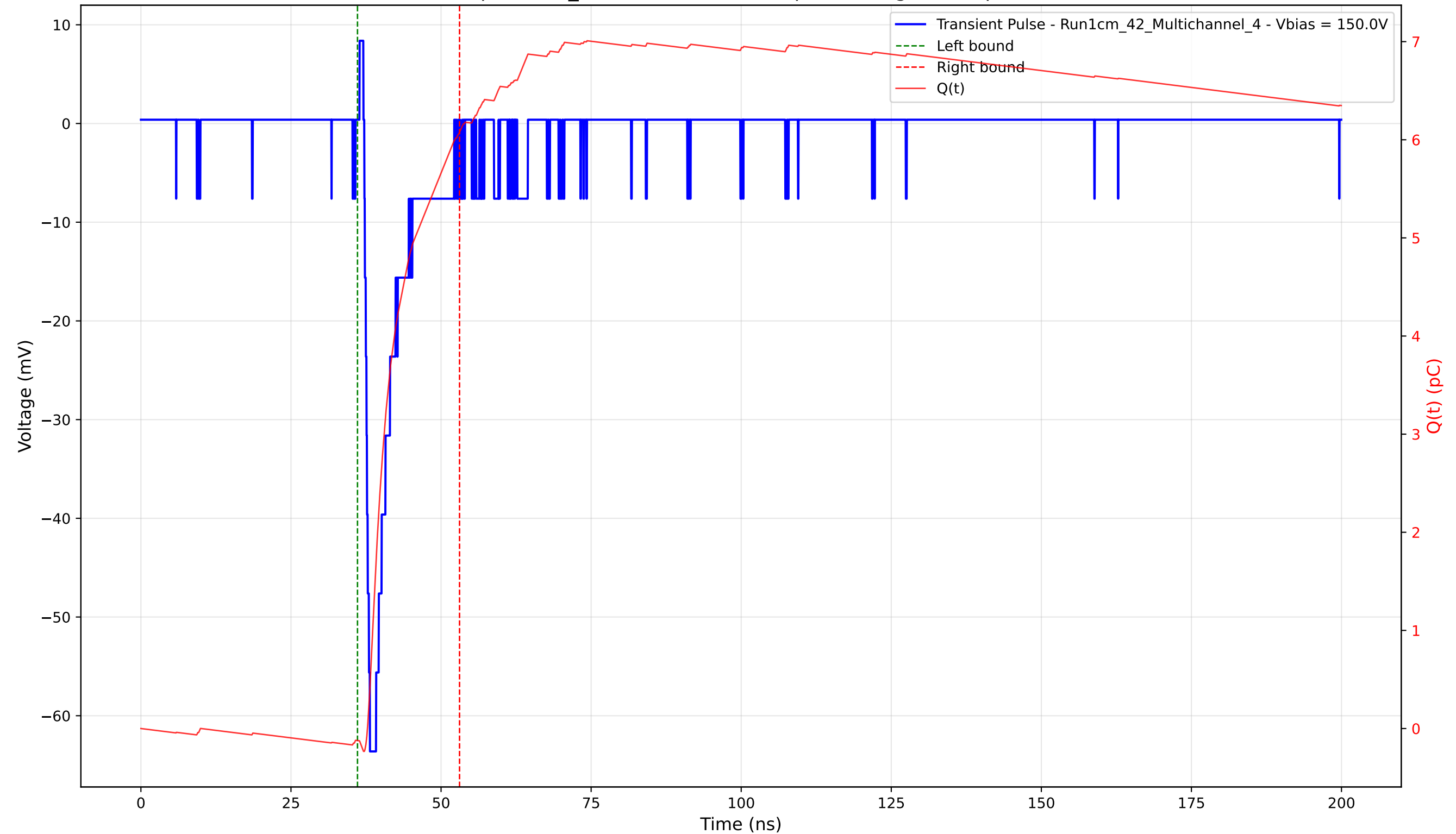
Transient Pulse - Sample: 1cm_42 - Position: 1280.0 \mu\text{m} - Charge: 6.20 pC - Rise Time: 0.93 ns
