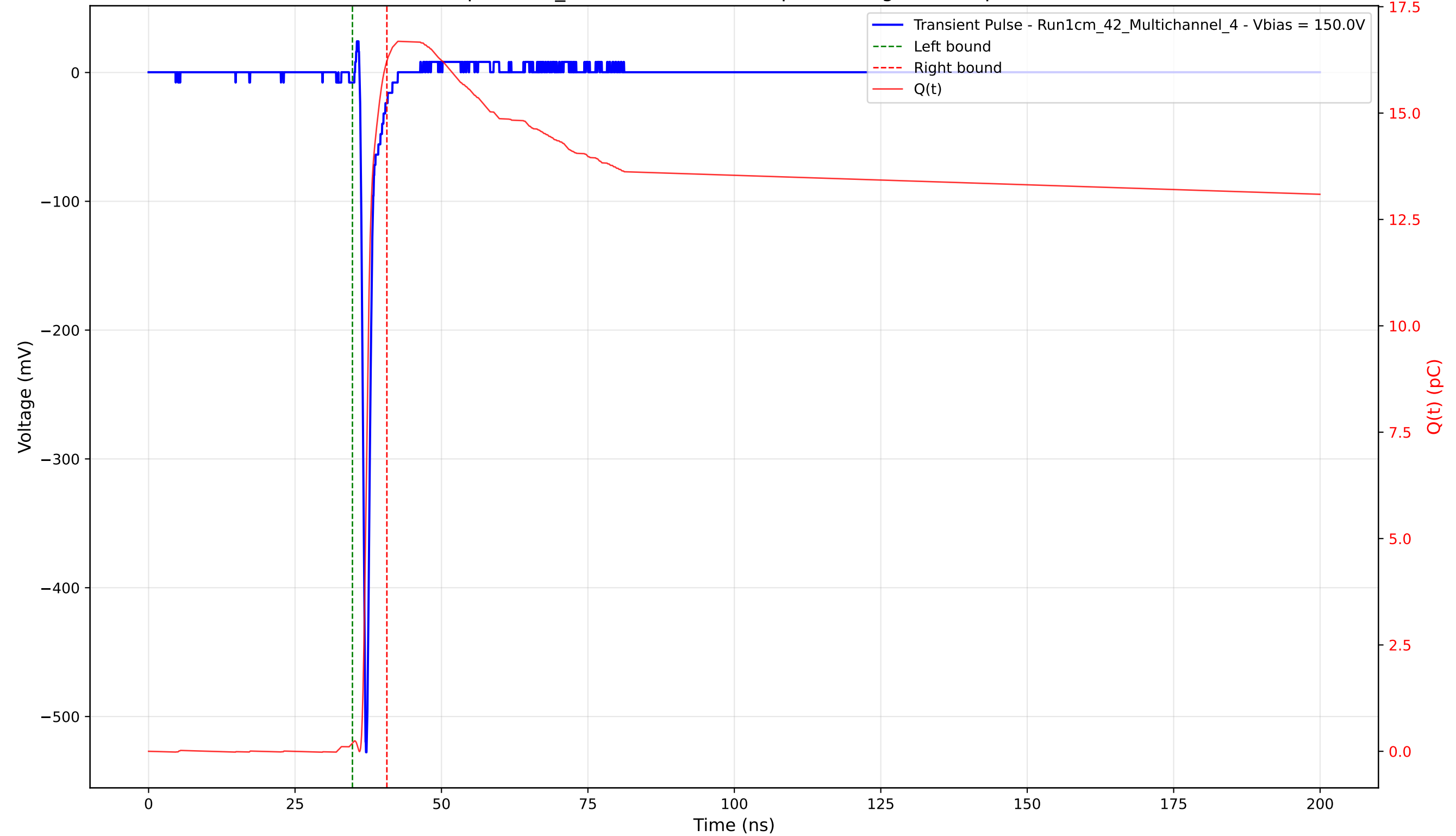
Transient Pulse - Sample: 1cm_42 - Position: 2455.0 \mu\text{m} - Charge: 16.03 pC - Rise Time: 0.72 ns
