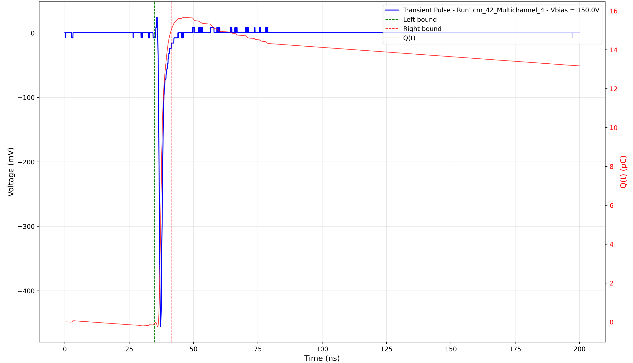
Transient Pulse - Sample: 1cm_42 - Position: 2195.0 \mu\text{m} - Charge: 15.06 pC - Rise Time: 0.72 ns
