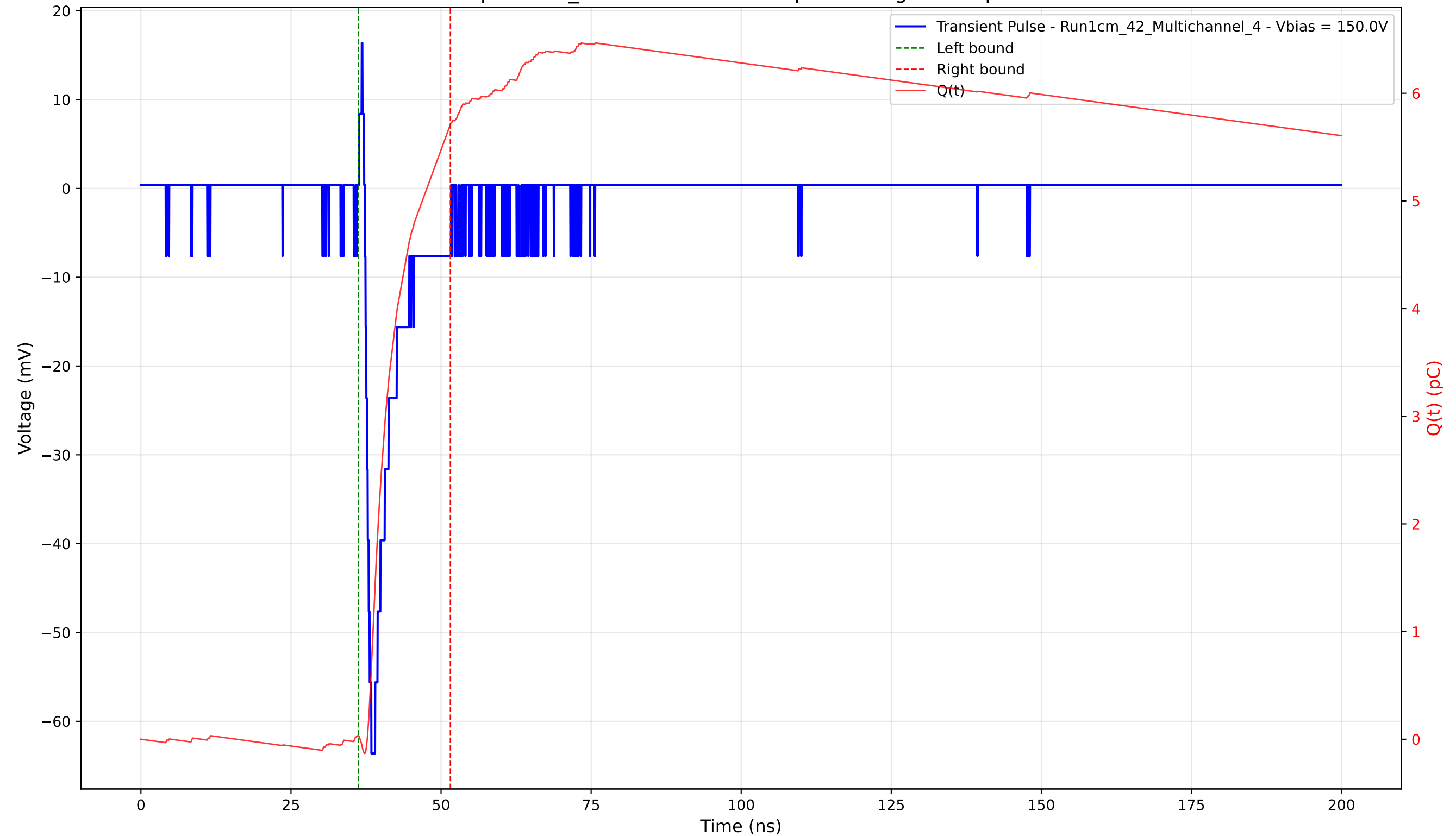
Transient Pulse - Sample: 1cm_42 - Position: 1185.0 \mu\text{m} - Charge: 5.68 pC - Rise Time: 1.05 ns
