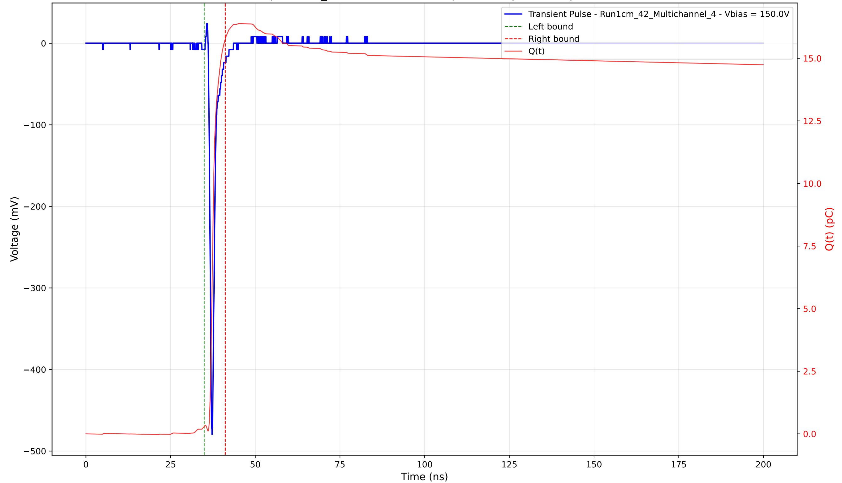
Transient Pulse - Sample: 1cm_42 - Position: 2775.0 \mu\text{m} - Charge: 15.47 pC - Rise Time: 0.72 ns
