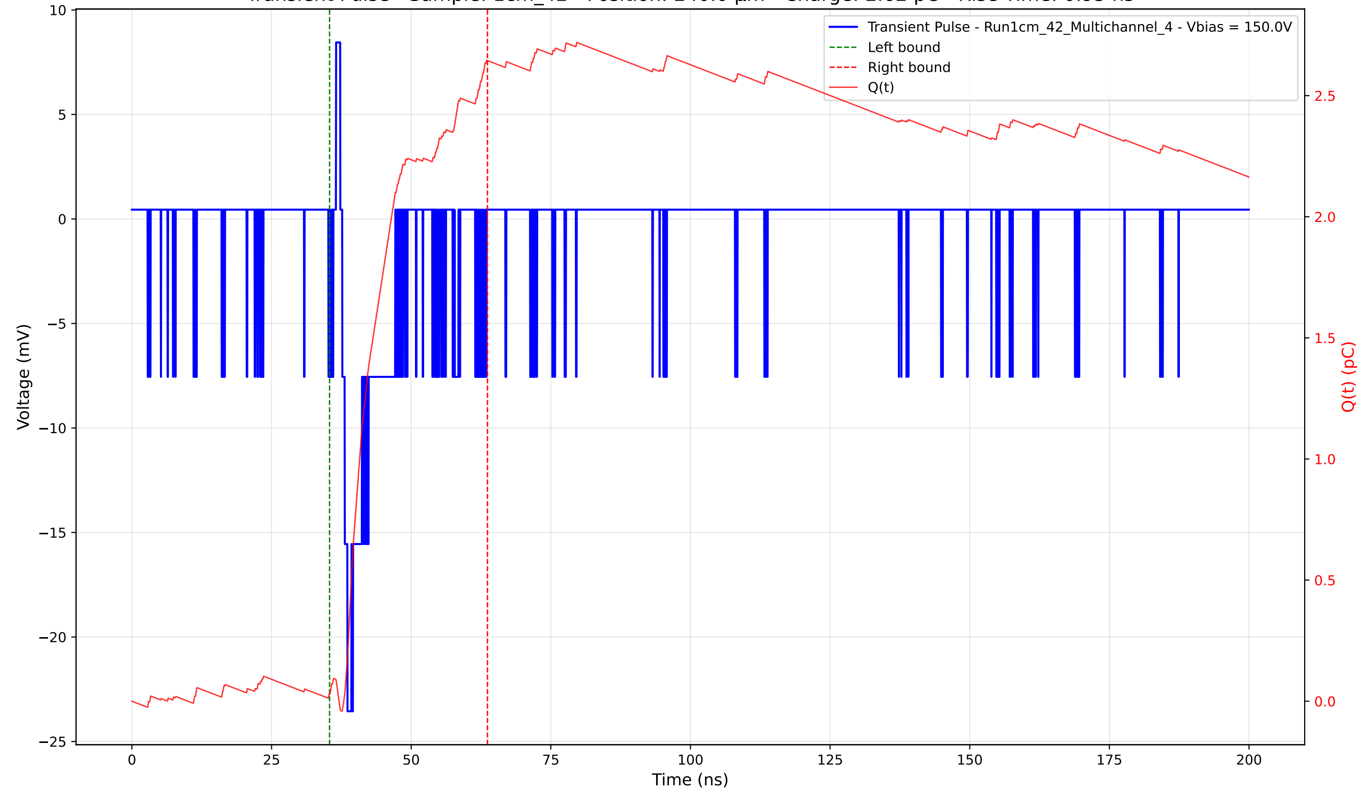
Transient Pulse - Sample: 1cm_42 - Position: 240.0 \mu\text{m} - Charge: 2.62 pC - Rise Time: 0.95 ns
