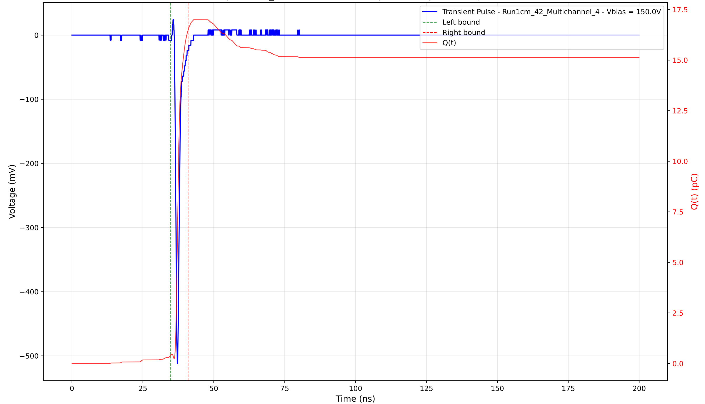
Transient Pulse - Sample: 1cm_42 - Position: 2685.0 \mu\text{m} - Charge: 16.06 pC - Rise Time: 0.74 ns
