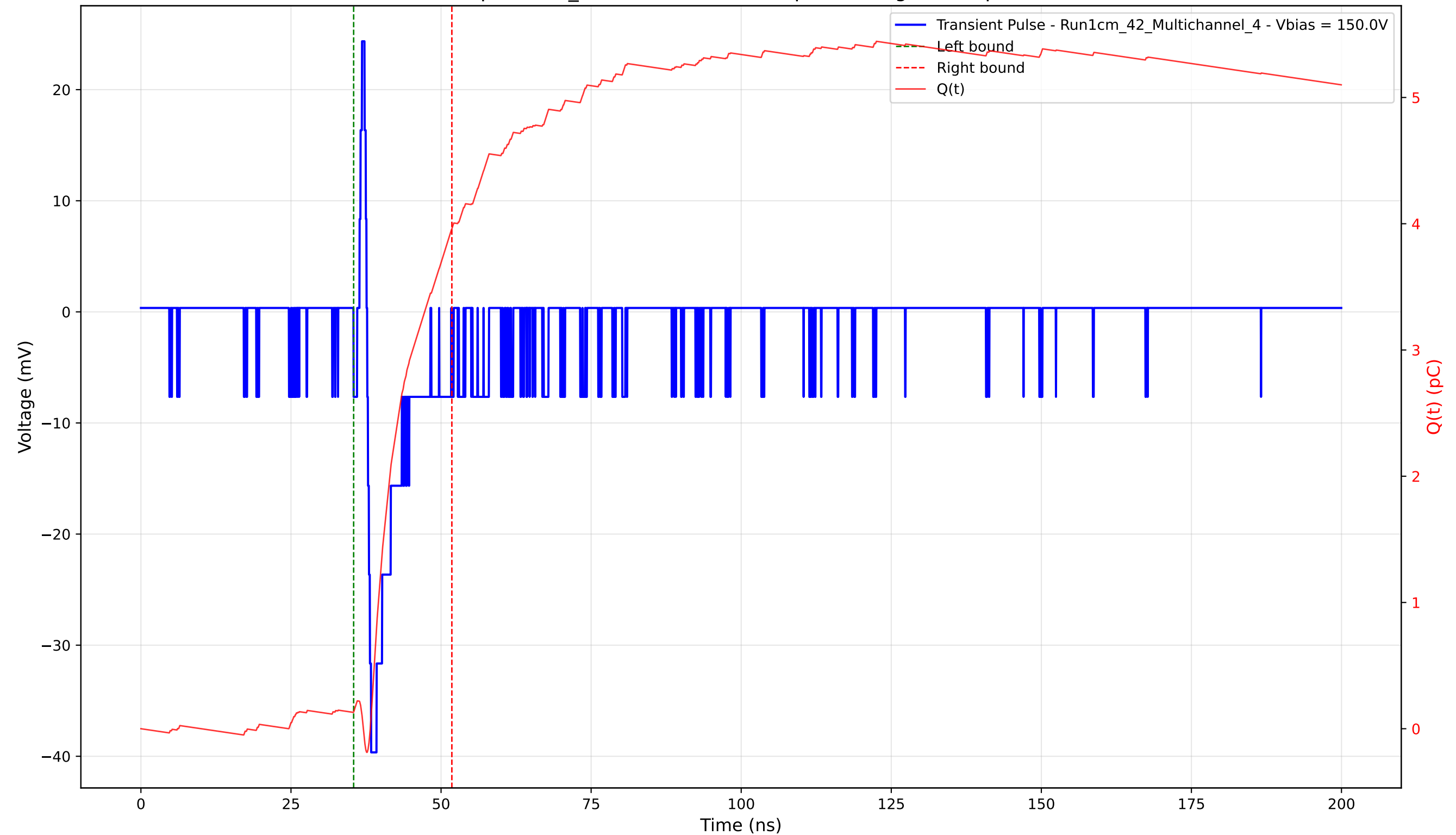
Transient Pulse - Sample: 1cm_42 - Position: 4180.0 \mu\text{m} - Charge: 3.83 pC - Rise Time: 0.66 ns
