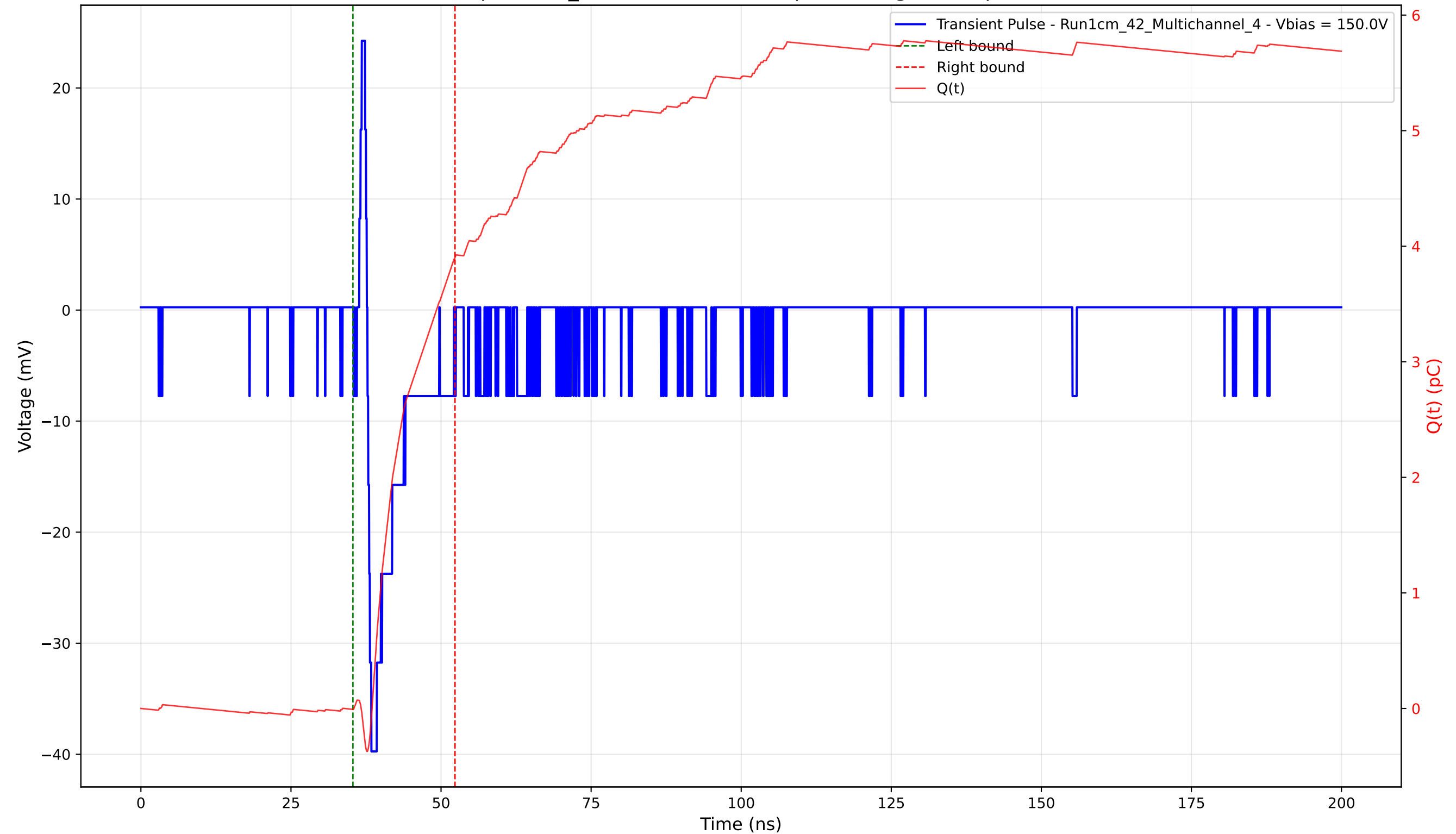
Transient Pulse - Sample: 1cm_42 - Position: 4255.0 \mu\text{m} - Charge: 3.91 pC - Rise Time: 0.66 ns
