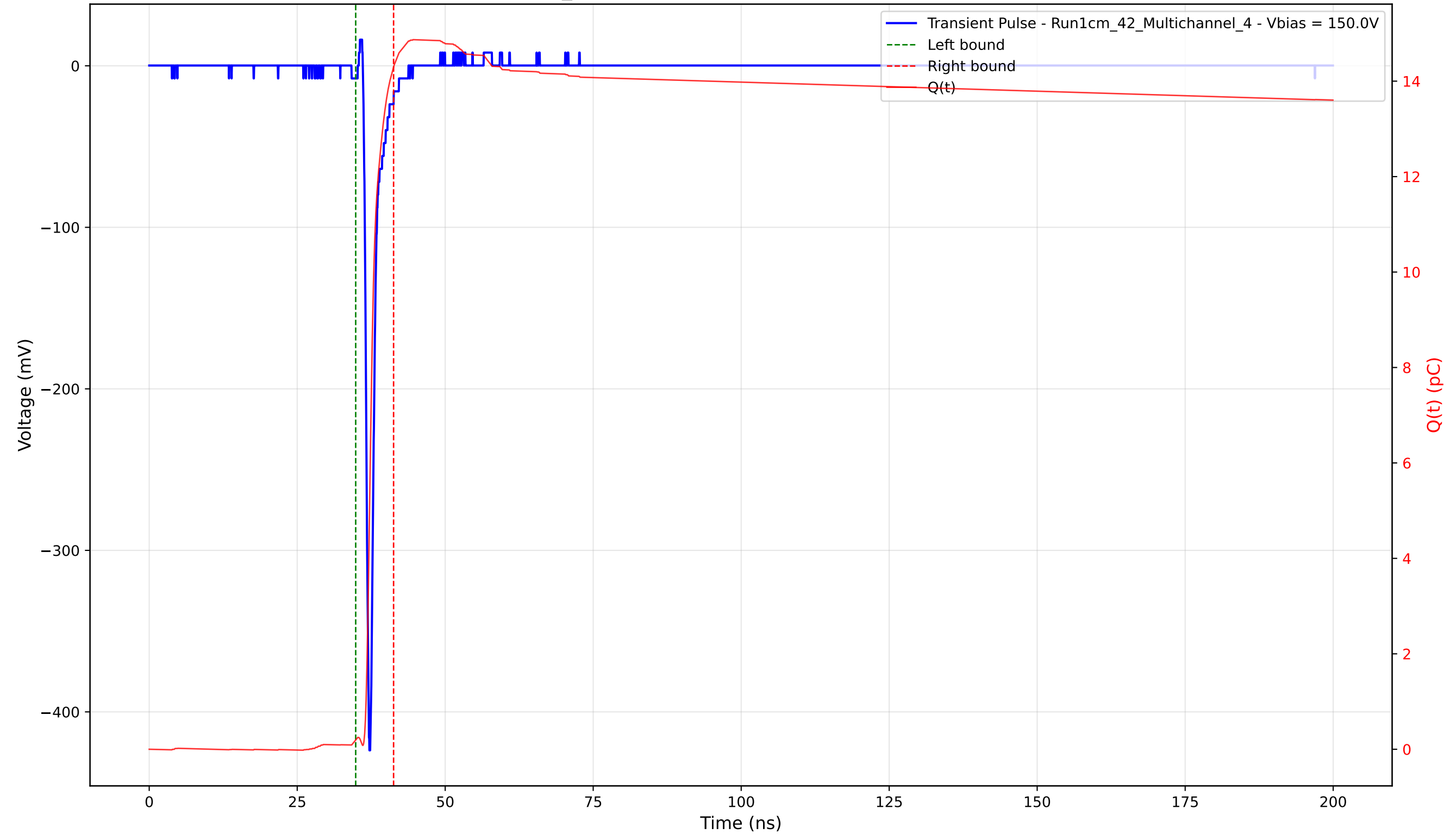
Transient Pulse - Sample: 1cm_42 - Position: 2835.0 \mu\text{m} - Charge: 14.11 pC - Rise Time: 0.74 ns
