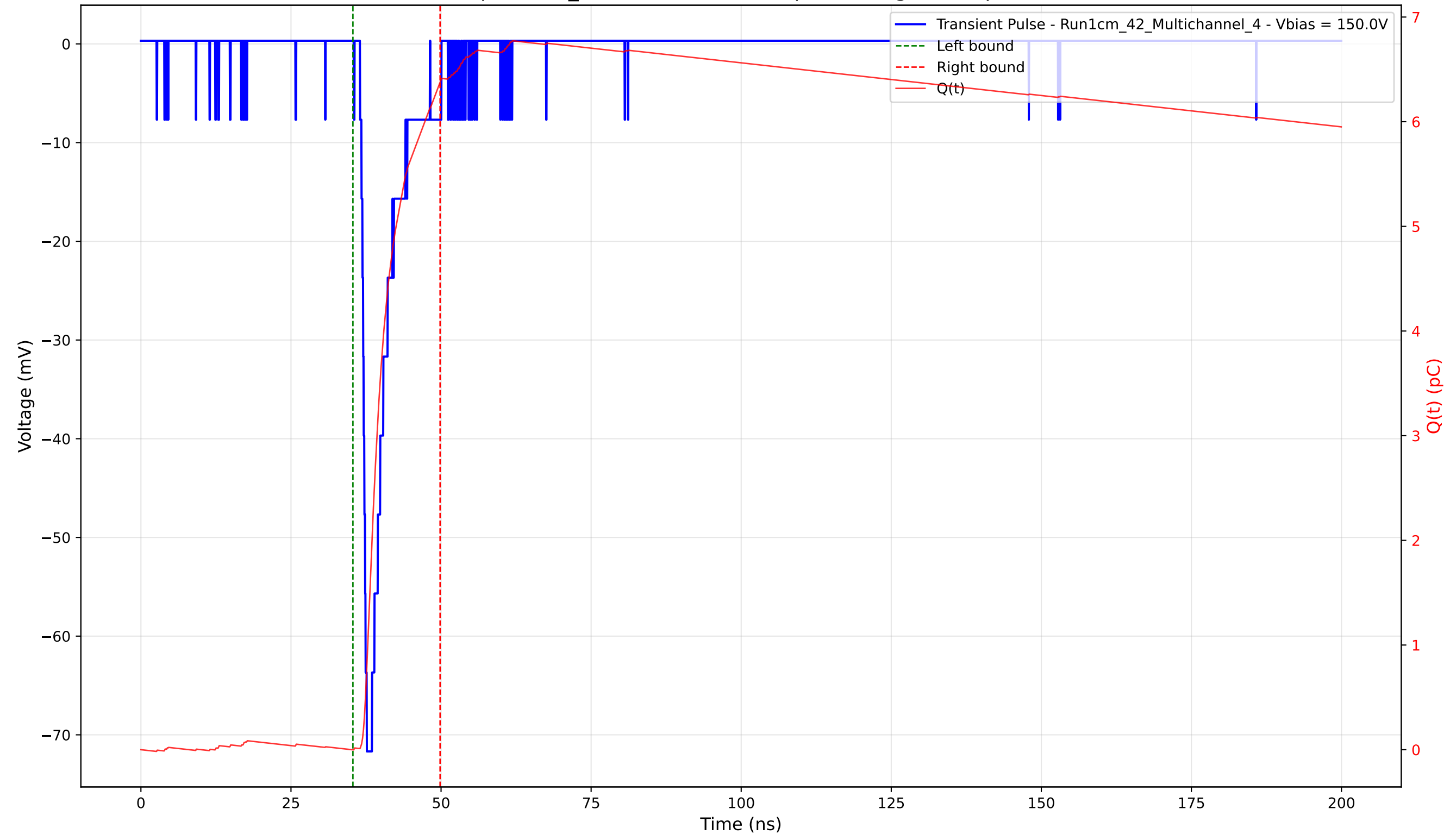
Transient Pulse - Sample: 1cm_42 - Position: 1525.0 \mu\text{m} - Charge: 6.38 pC - Rise Time: 1.12 ns
