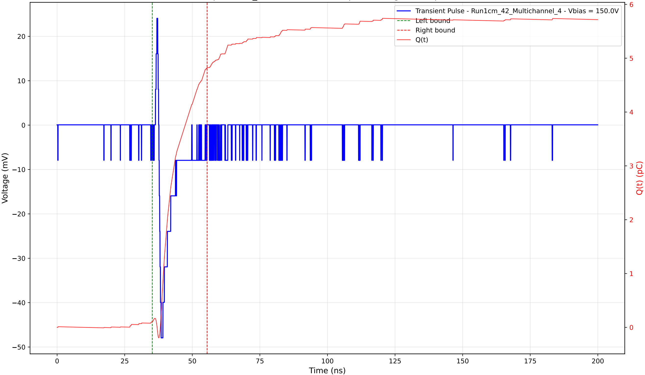
Transient Pulse - Sample: 1cm_42 - Position: 915.0 \mu\text{m} - Charge: 4.71 pC - Rise Time: 0.82 ns
