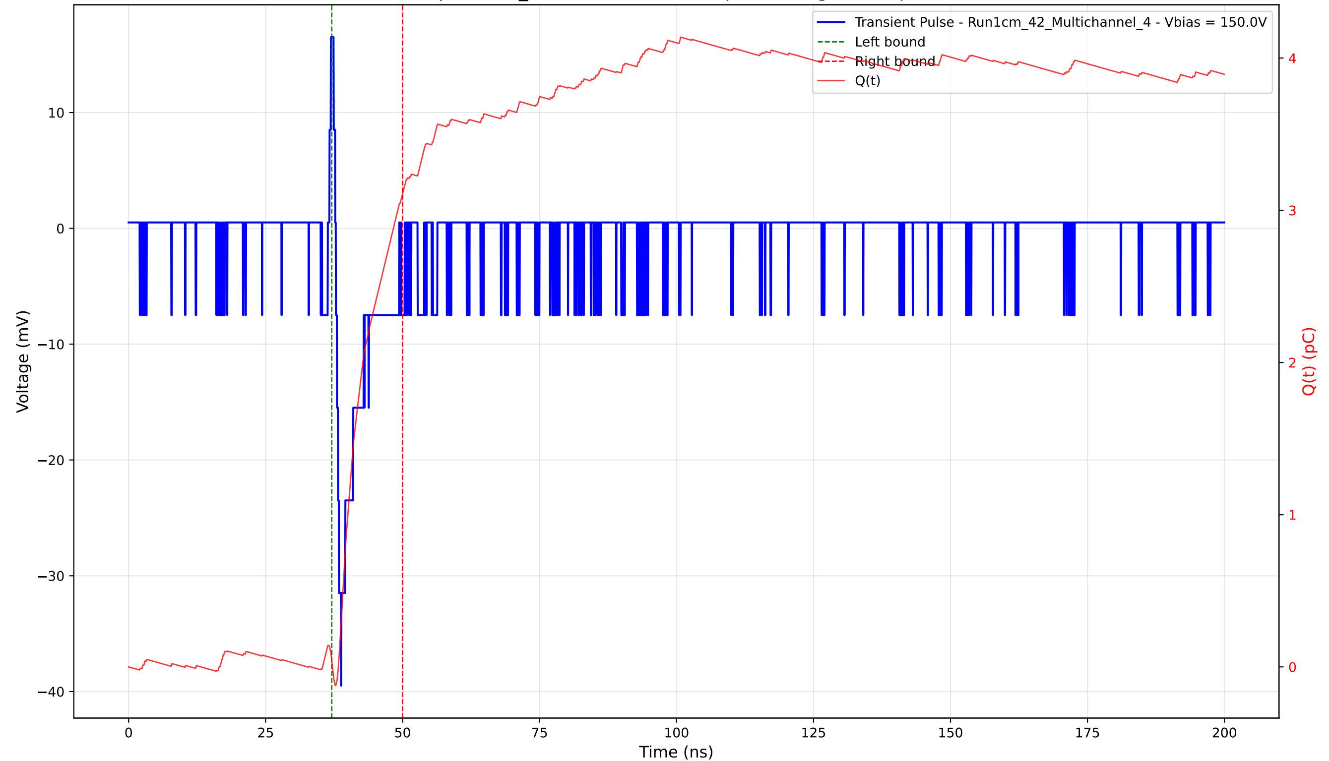
Transient Pulse - Sample: 1cm_42 - Position: 4740.0 \mu\text{m} - Charge: 3.07 pC - Rise Time: 0.98 ns
