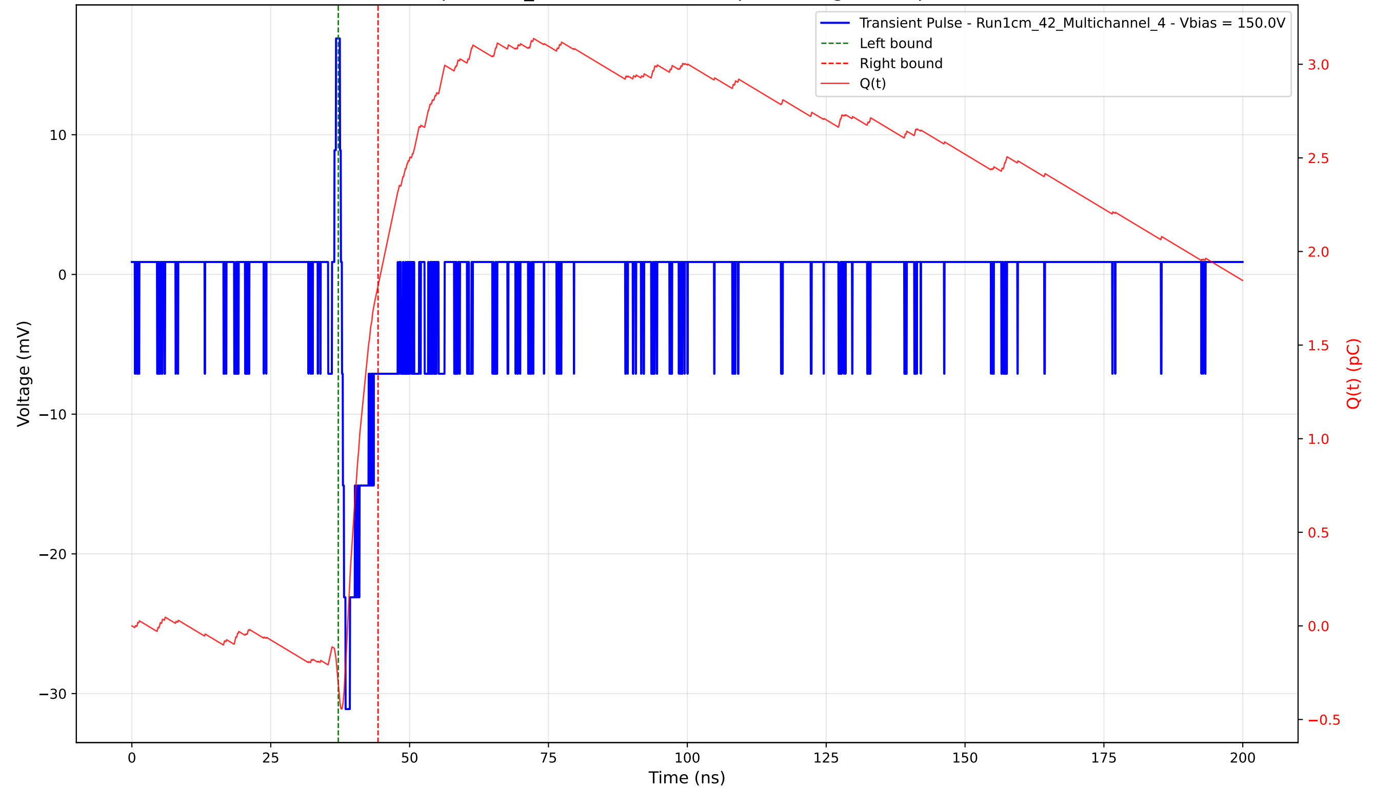
Transient Pulse - Sample: 1cm_42 - Position: 4490.0 \mu\text{m} - Charge: 2.13 pC - Rise Time: 0.67 ns
