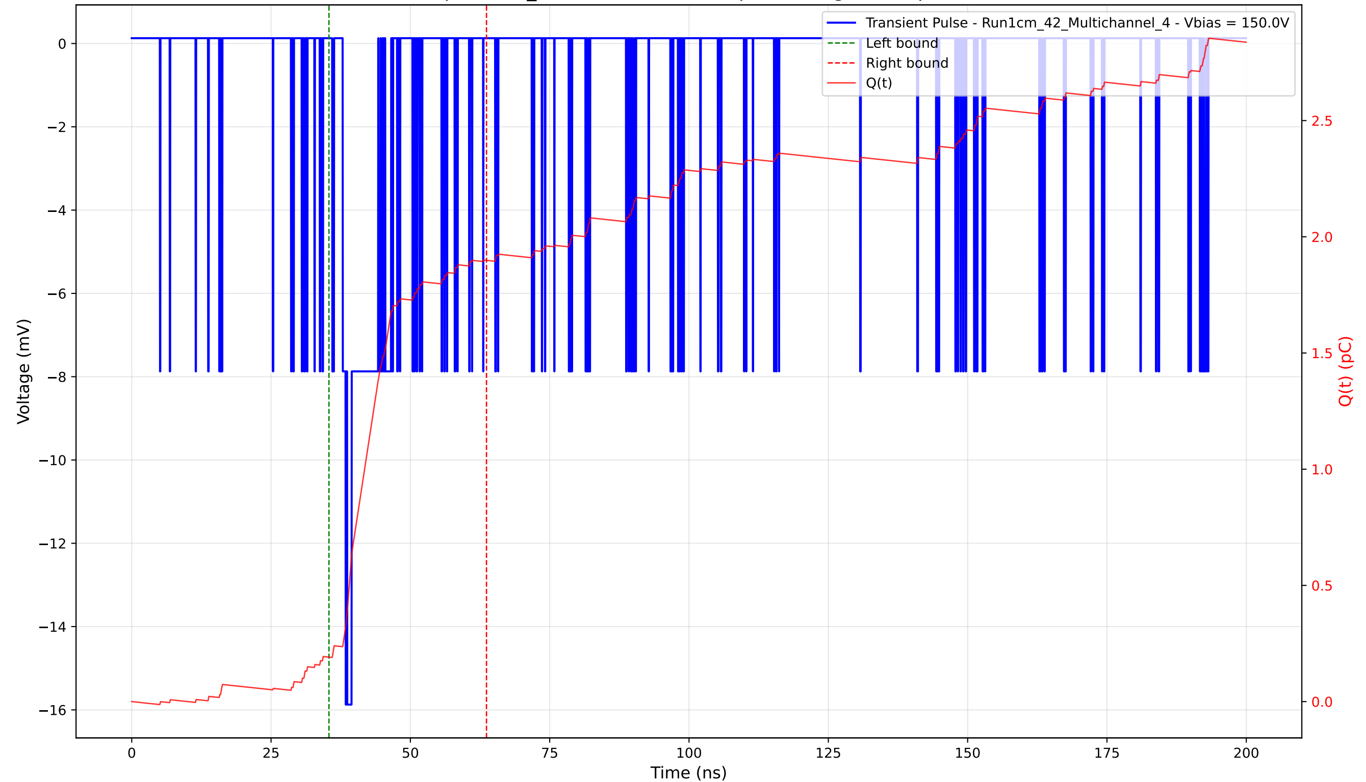
Transient Pulse - Sample: 1cm_42 - Position: 5060.0 \mu\text{m} - Charge: 1.71 pC - Rise Time: 0.55 ns
