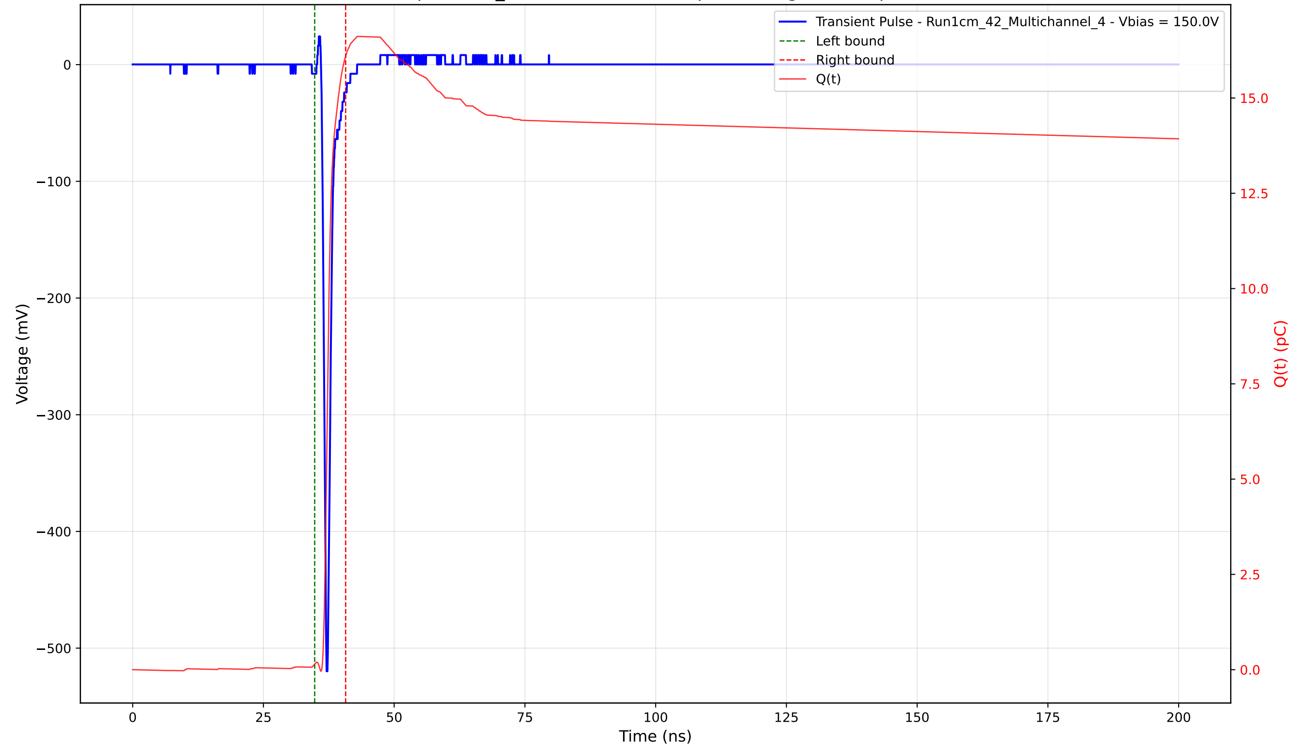
Transient Pulse - Sample: 1cm_42 - Position: 2610.0 \mu\text{m} - Charge: 15.95 pC - Rise Time: 0.72 ns
