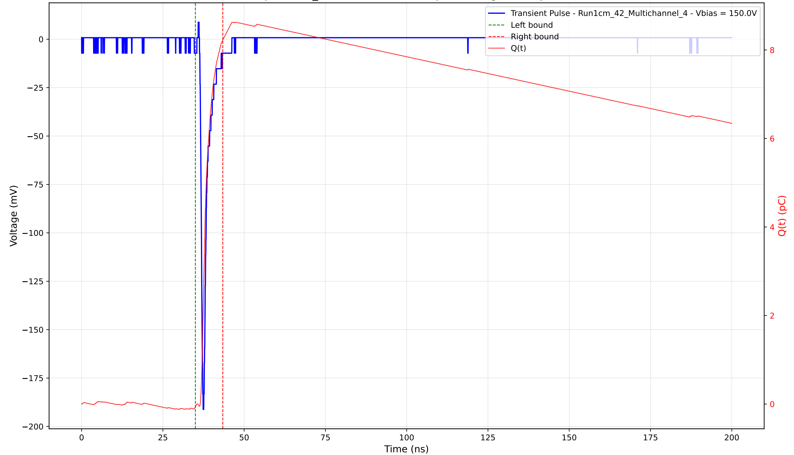
Transient Pulse - Sample: 1cm_42 - Position: 3080.0 \mu\text{m} - Charge: 8.29 pC - Rise Time: 0.80 ns
