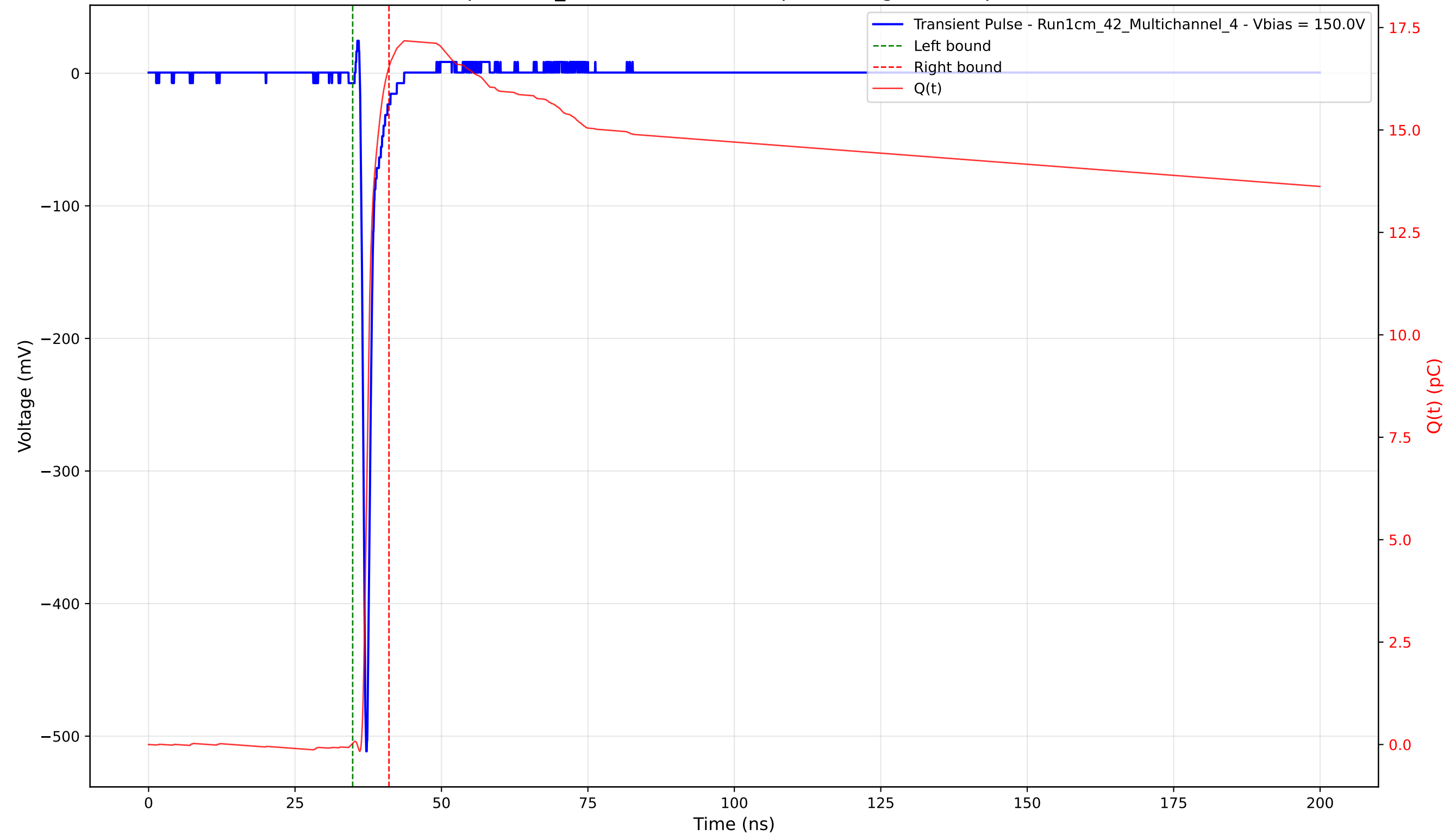
Transient Pulse - Sample: 1cm_42 - Position: 2265.0 \mu\text{m} - Charge: 16.51 pC - Rise Time: 0.72 ns
