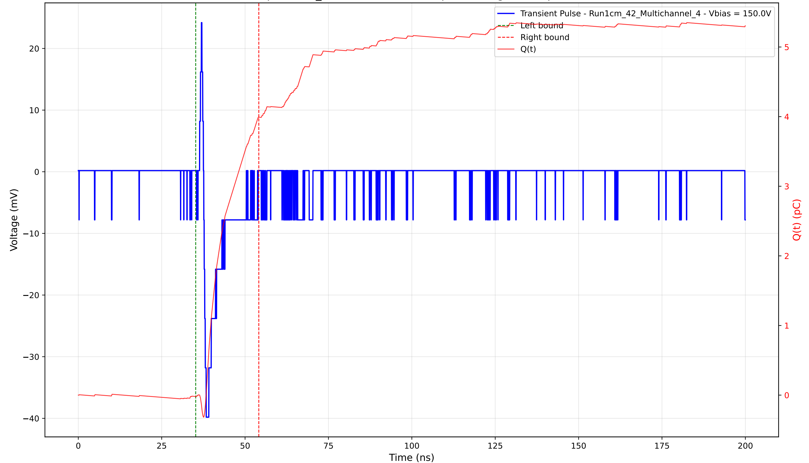
Transient Pulse - Sample: 1cm_42 - Position: 4085.0 \mu\text{m} - Charge: 4.01 pC - Rise Time: 0.74 ns
