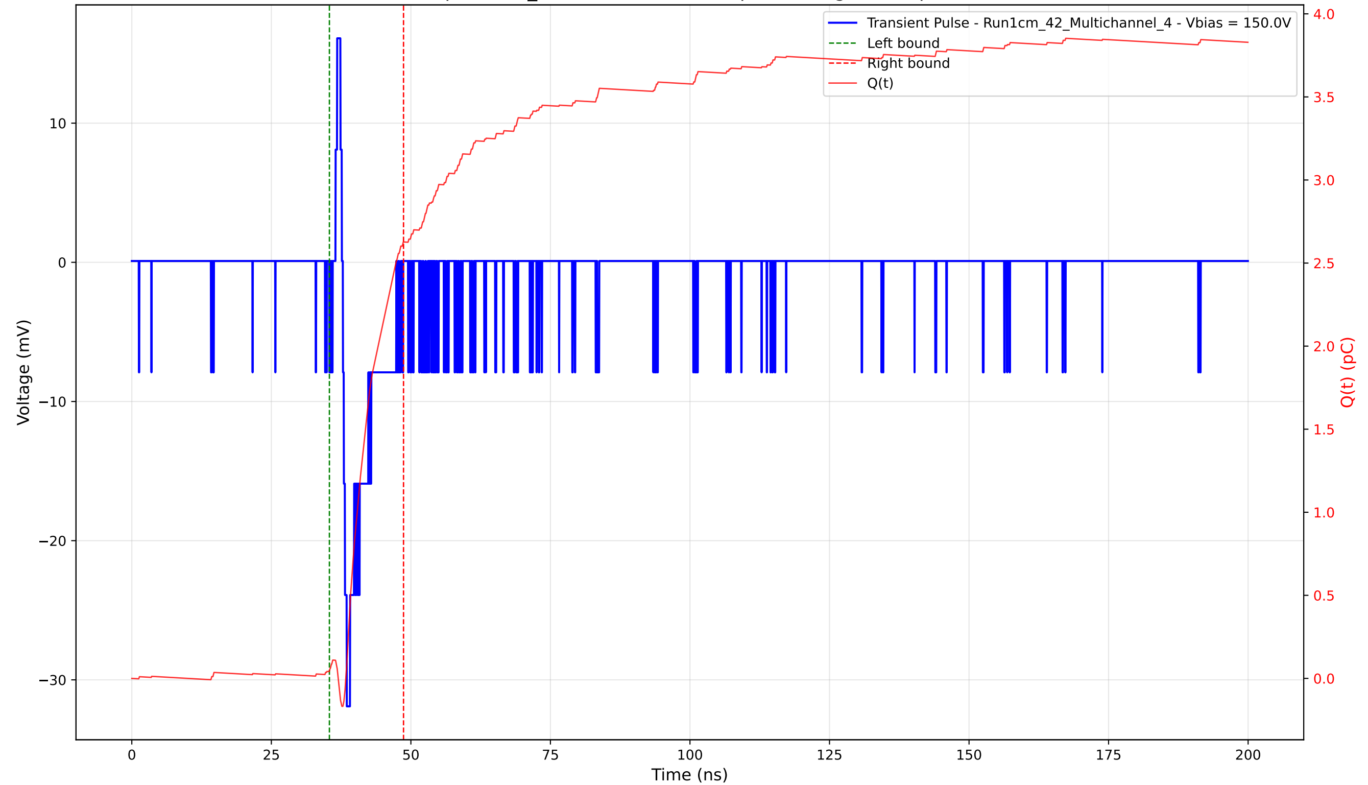
Transient Pulse - Sample: 1cm_42 - Position: 4555.0 \mu\text{m} - Charge: 2.58 pC - Rise Time: 0.70 ns
