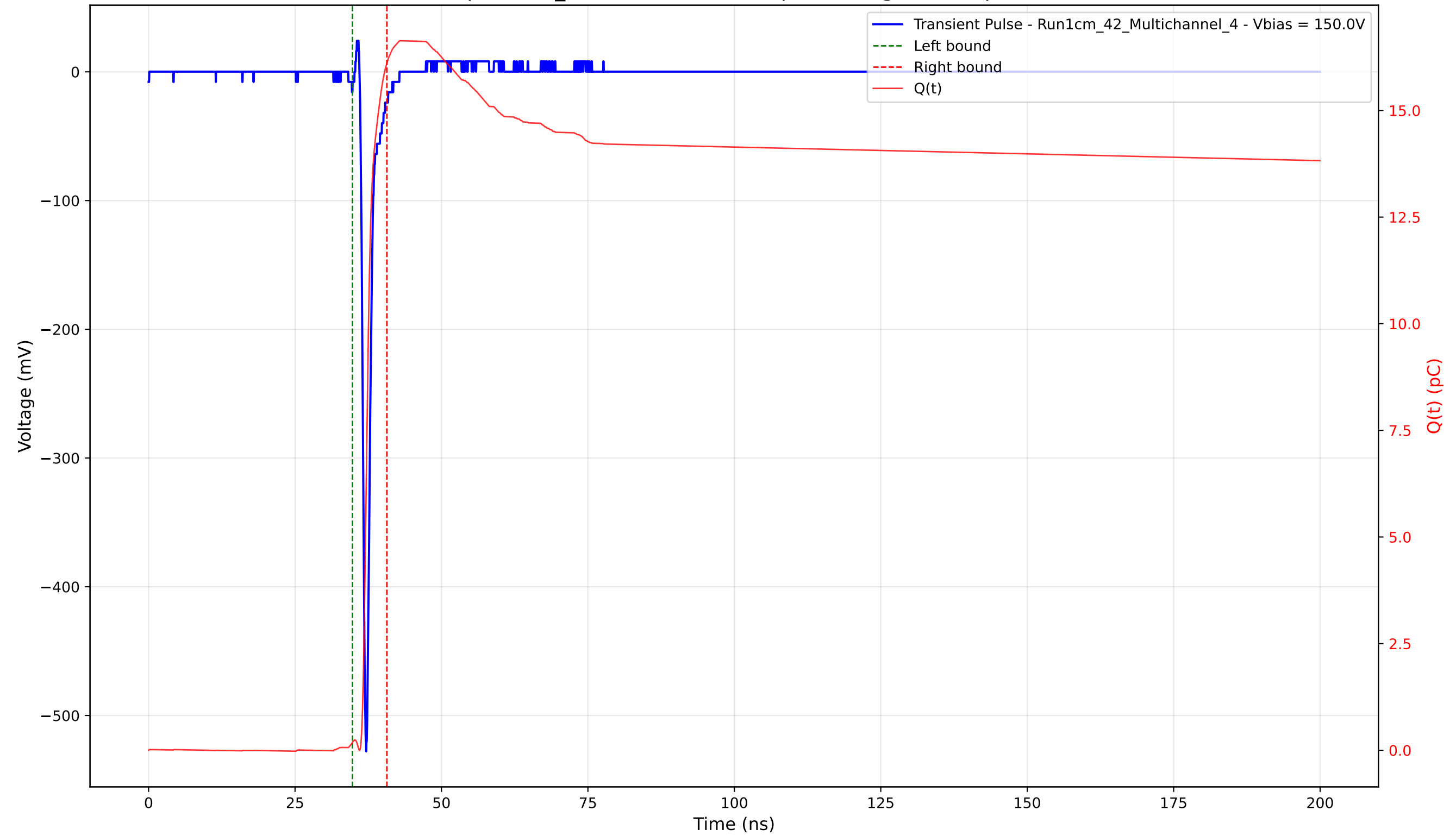
Transient Pulse - Sample: 1cm_42 - Position: 2575.0 \mu\text{m} - Charge: 15.92 pC - Rise Time: 0.70 ns
