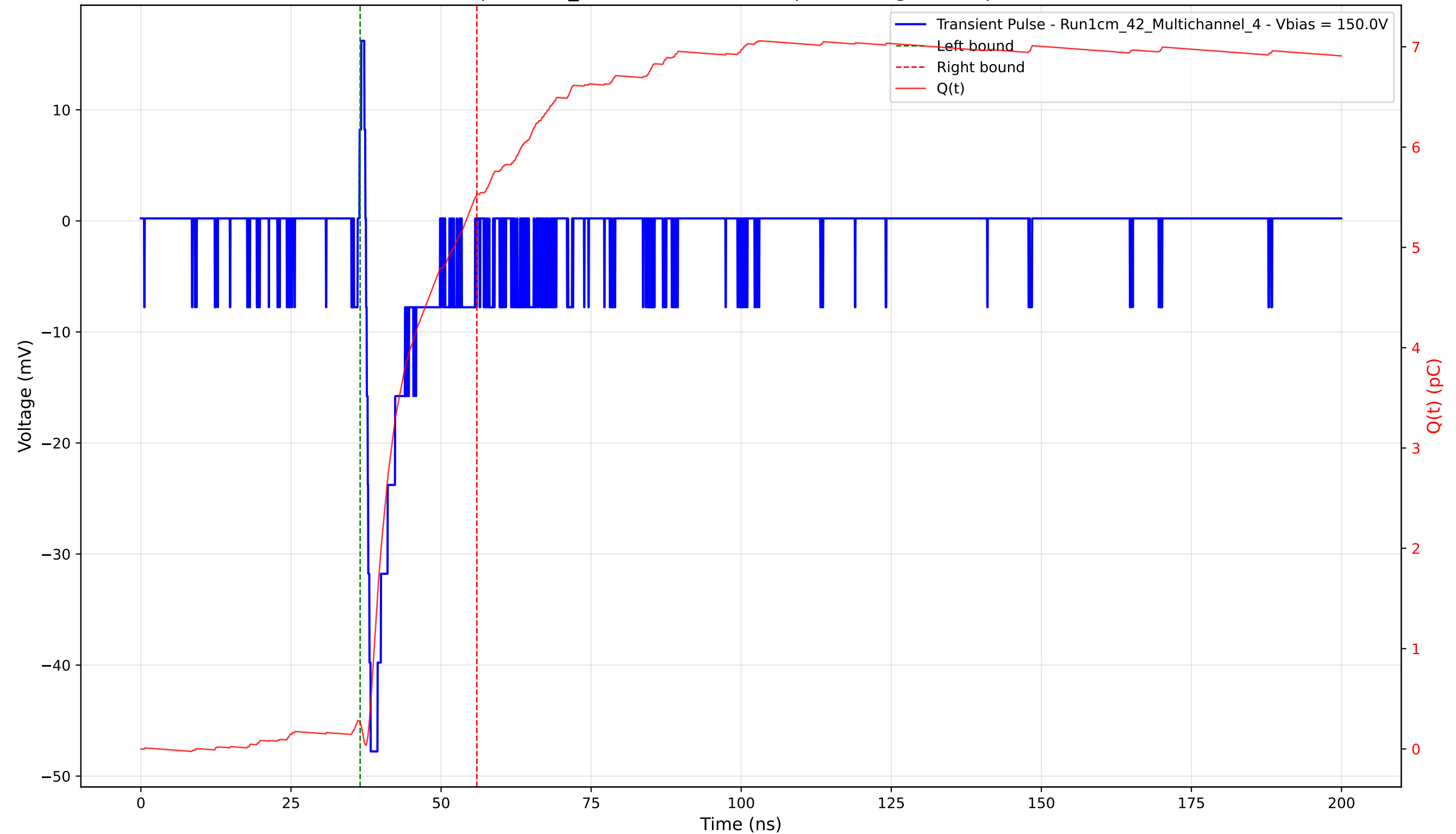
Transient Pulse - Sample: 1cm_42 - Position: 1050.0 \mu\text{m} - Charge: 5.26 pC - Rise Time: 0.78 ns
