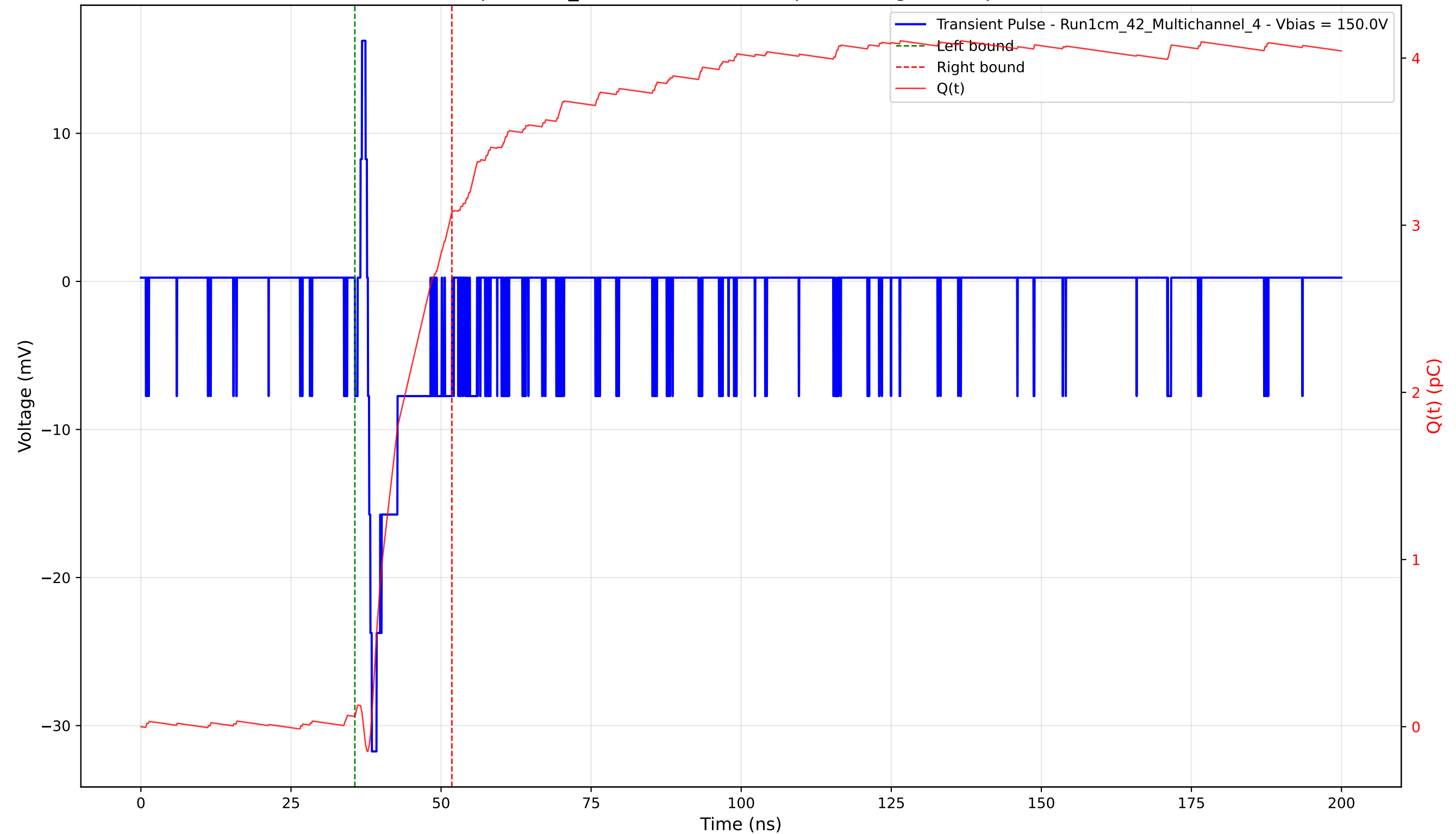
Transient Pulse - Sample: 1cm_42 - Position: 4590.0 \mu\text{m} - Charge: 3.02 pC - Rise Time: 0.66 ns
