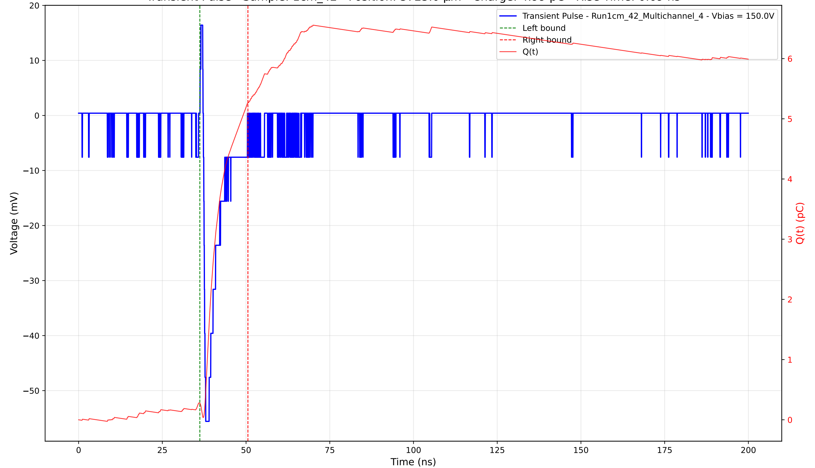
Transient Pulse - Sample: 1cm_42 - Position: 3725.0 \mu\text{m} - Charge: 4.99 pC - Rise Time: 0.69 ns
