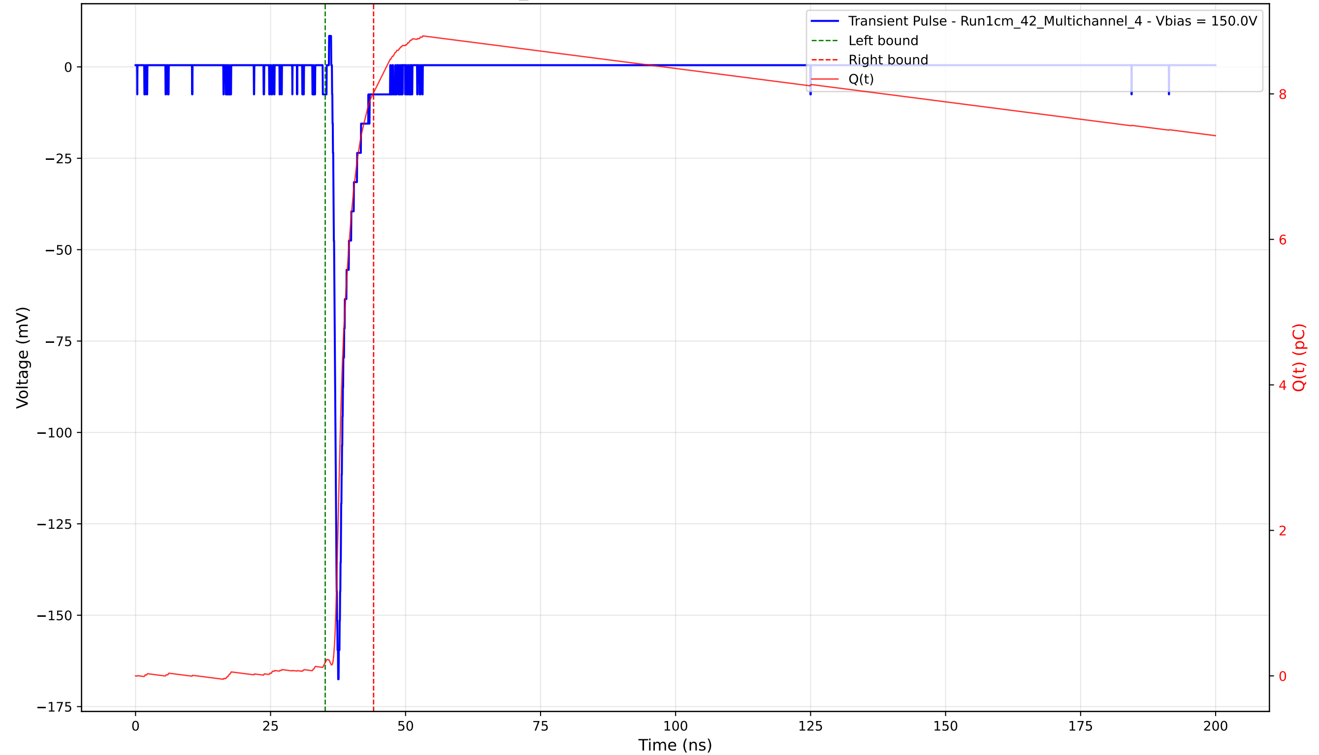
Transient Pulse - Sample: 1cm_42 - Position: 3155.0 \mu\text{m} - Charge: 7.83 pC - Rise Time: 0.79 ns
