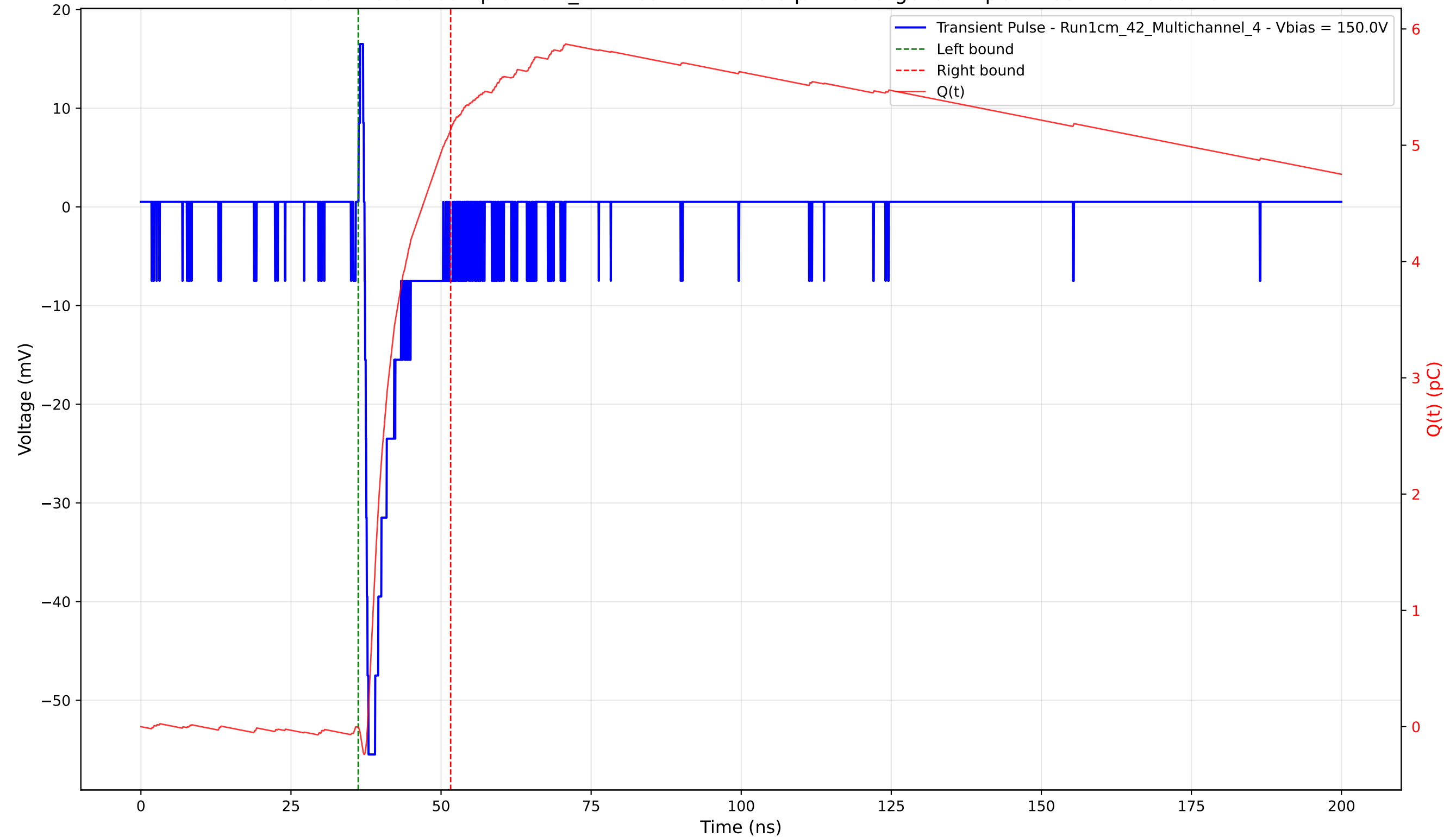
Transient Pulse - Sample: 1cm_42 - Position: 3730.0 \mu\text{m} - Charge: 5.14 pC - Rise Time: 0.65 ns
