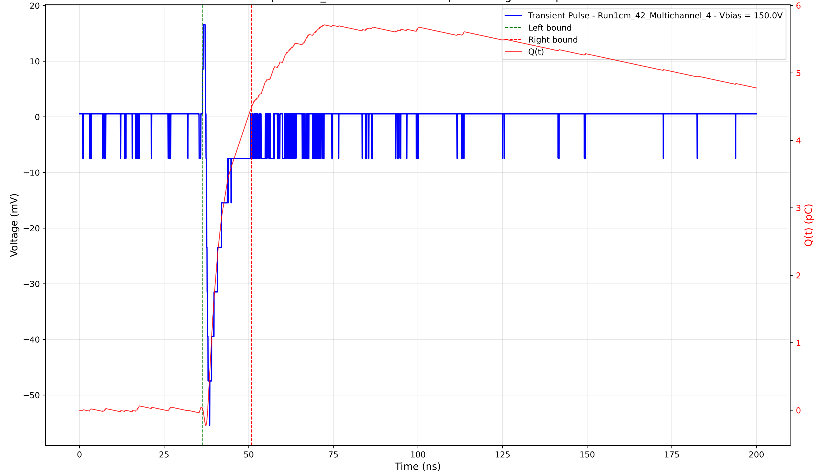
Transient Pulse - Sample: 1cm_42 - Position: 3885.0 \mu\text{m} - Charge: 4.48 pC - Rise Time: 1.05 ns
