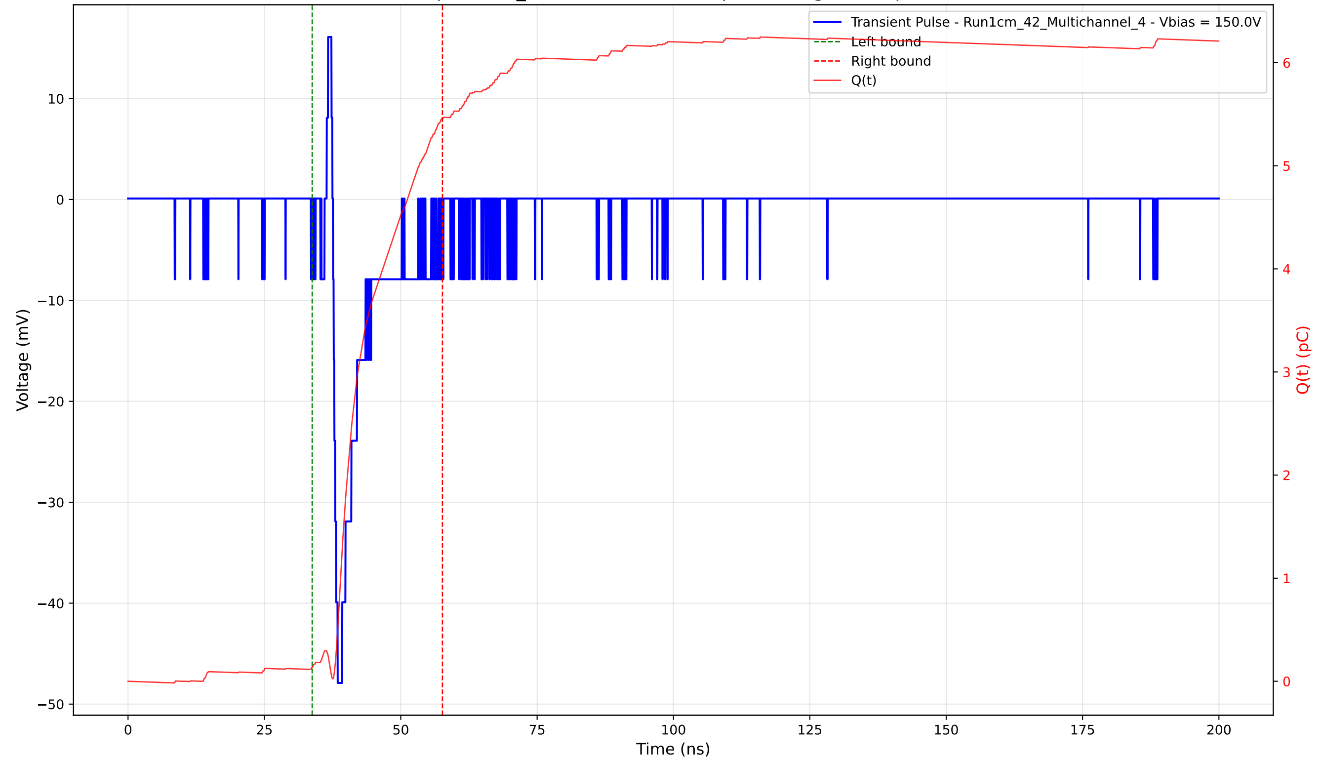
Transient Pulse - Sample: 1cm_42 - Position: 1000.0 \mu\text{m} - Charge: 5.32 pC - Rise Time: 0.86 ns
