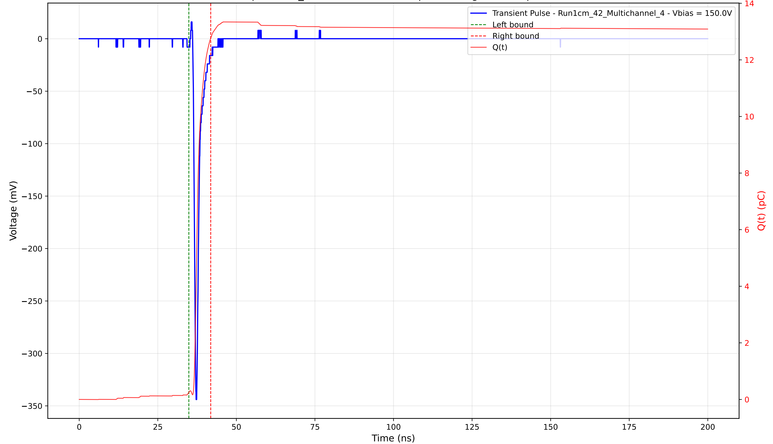
Transient Pulse - Sample: 1cm_42 - Position: 2115.0 \mu\text{m} - Charge: 12.52 pC - Rise Time: 0.74 ns
