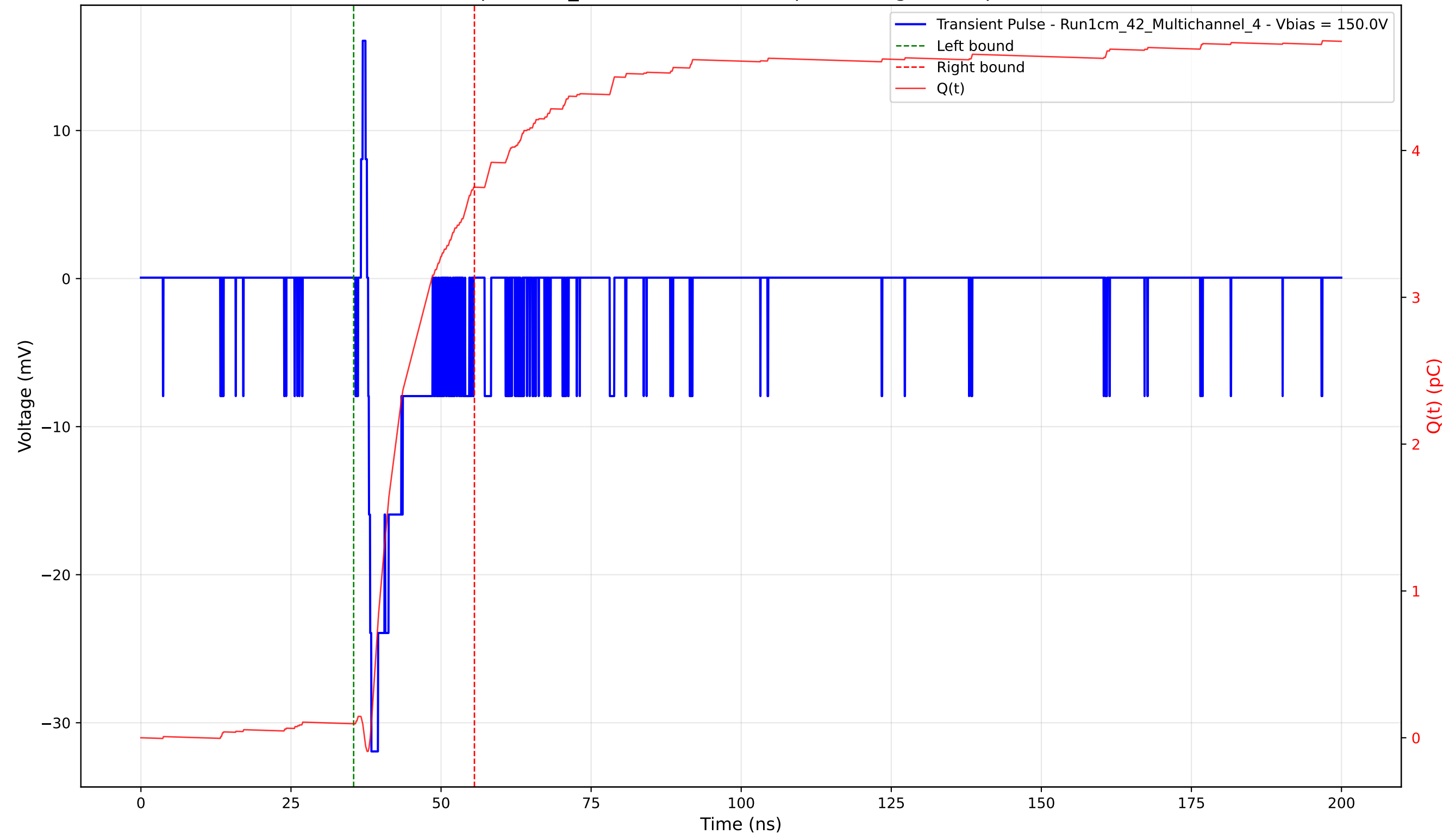
Transient Pulse - Sample: 1cm_42 - Position: 4775.0 \mu\text{m} - Charge: 3.65 pC - Rise Time: 0.54 ns
