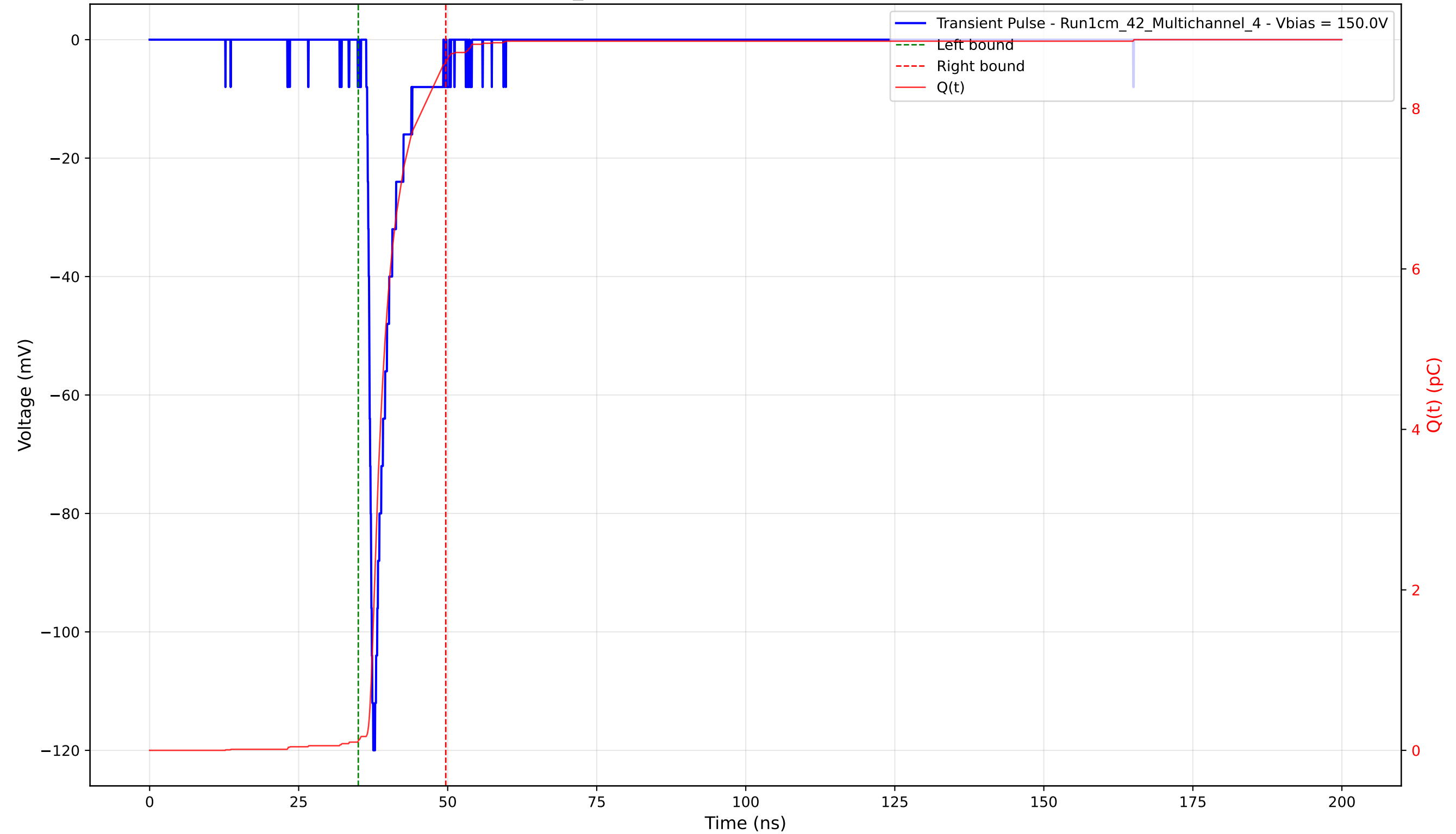
Transient Pulse - Sample: 1cm_42 - Position: 1665.0 \mu\text{m} - Charge: 8.47 pC - Rise Time: 0.86 ns
