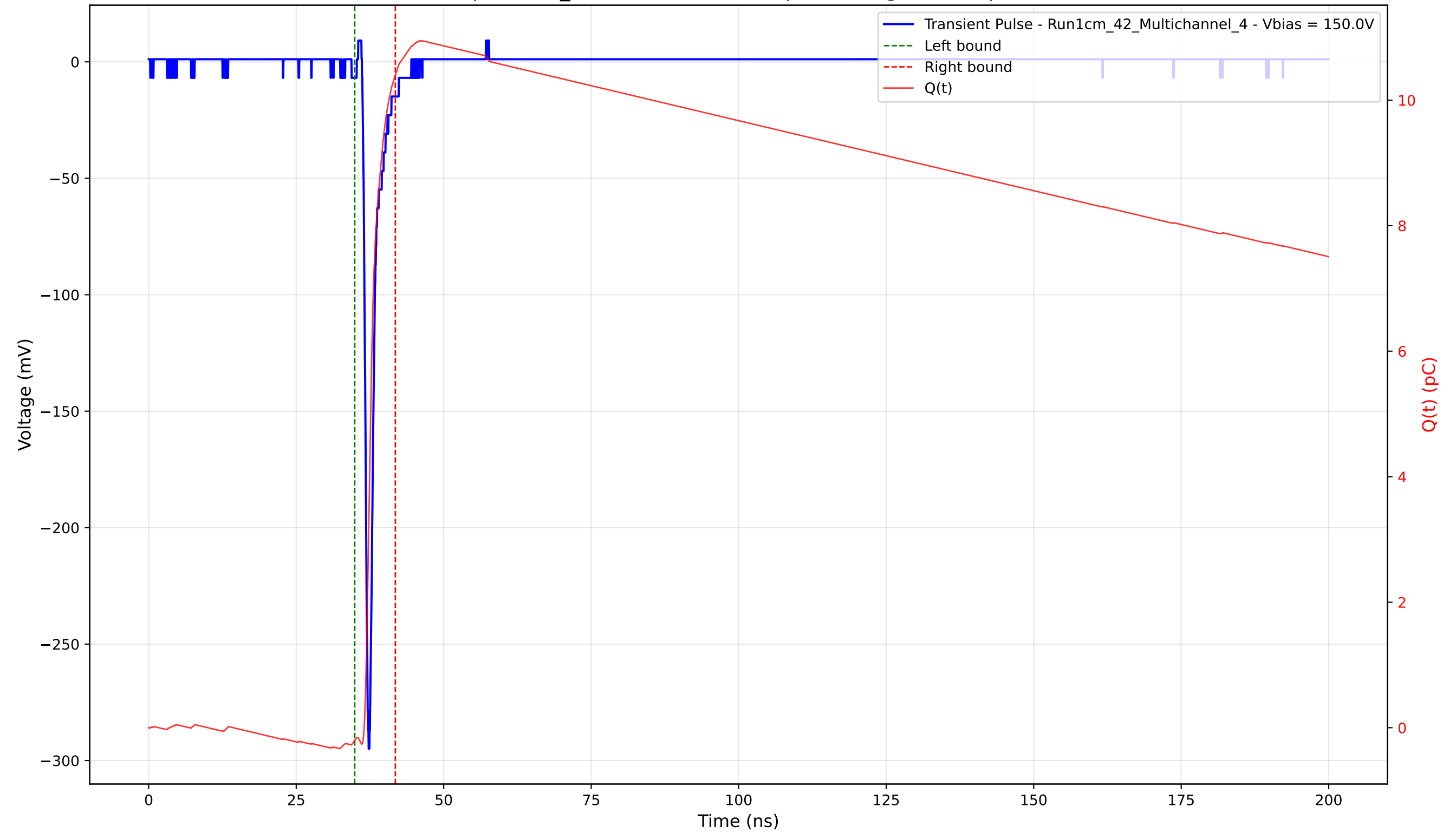
Transient Pulse - Sample: 1cm_42 - Position: 2940.0 \mu\text{m} - Charge: 10.60 pC - Rise Time: 0.74 ns
