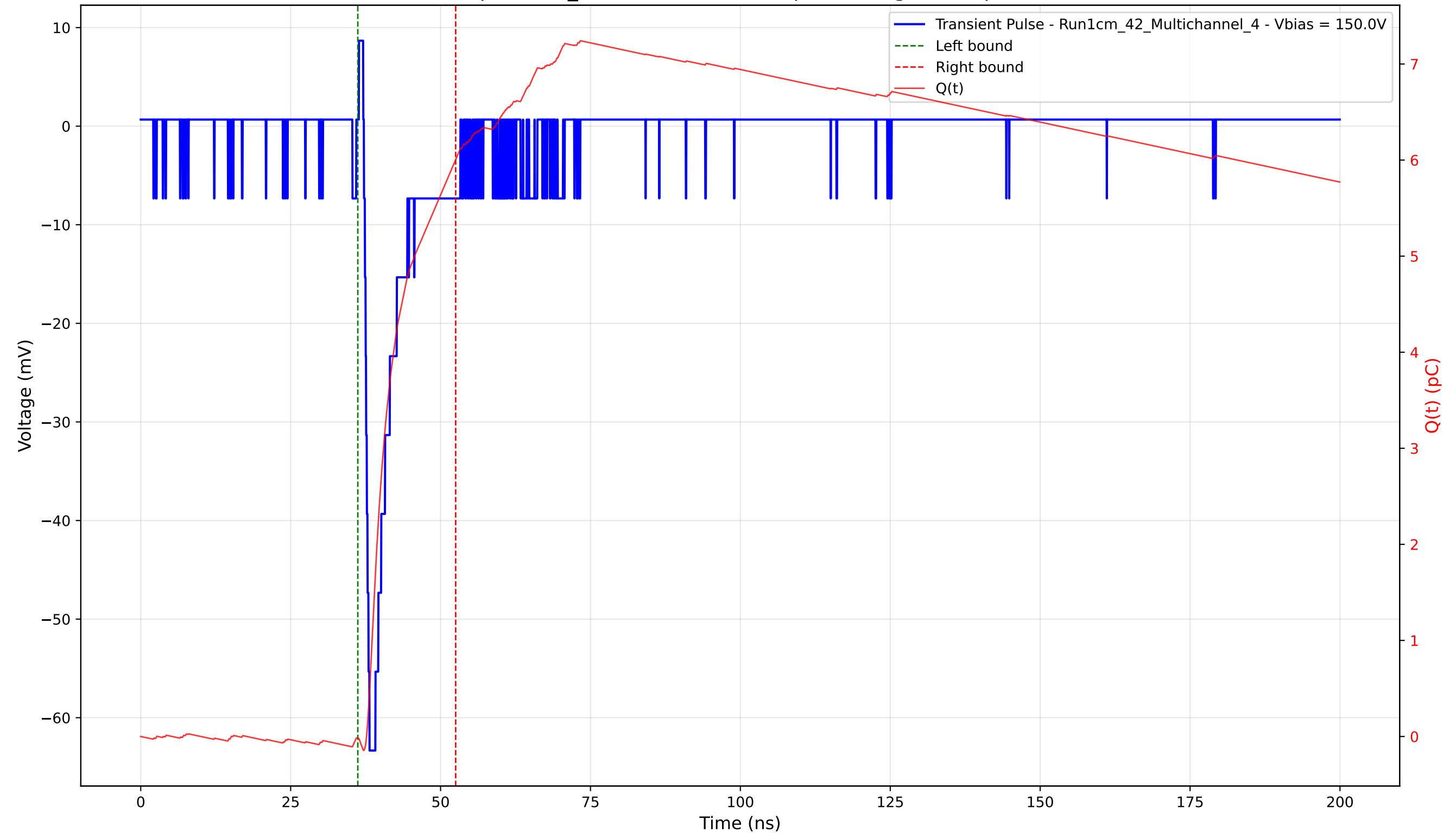
Transient Pulse - Sample: 1cm_42 - Position: 1250.0 \mu\text{m} - Charge: 6.02 pC - Rise Time: 0.93 ns
