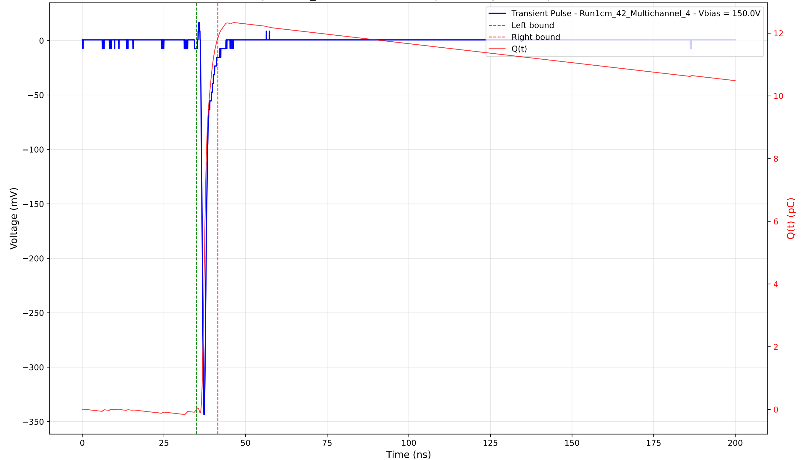
Transient Pulse - Sample: 1cm_42 - Position: 2900.0 \mu\text{m} - Charge: 11.85 pC - Rise Time: 0.73 ns
