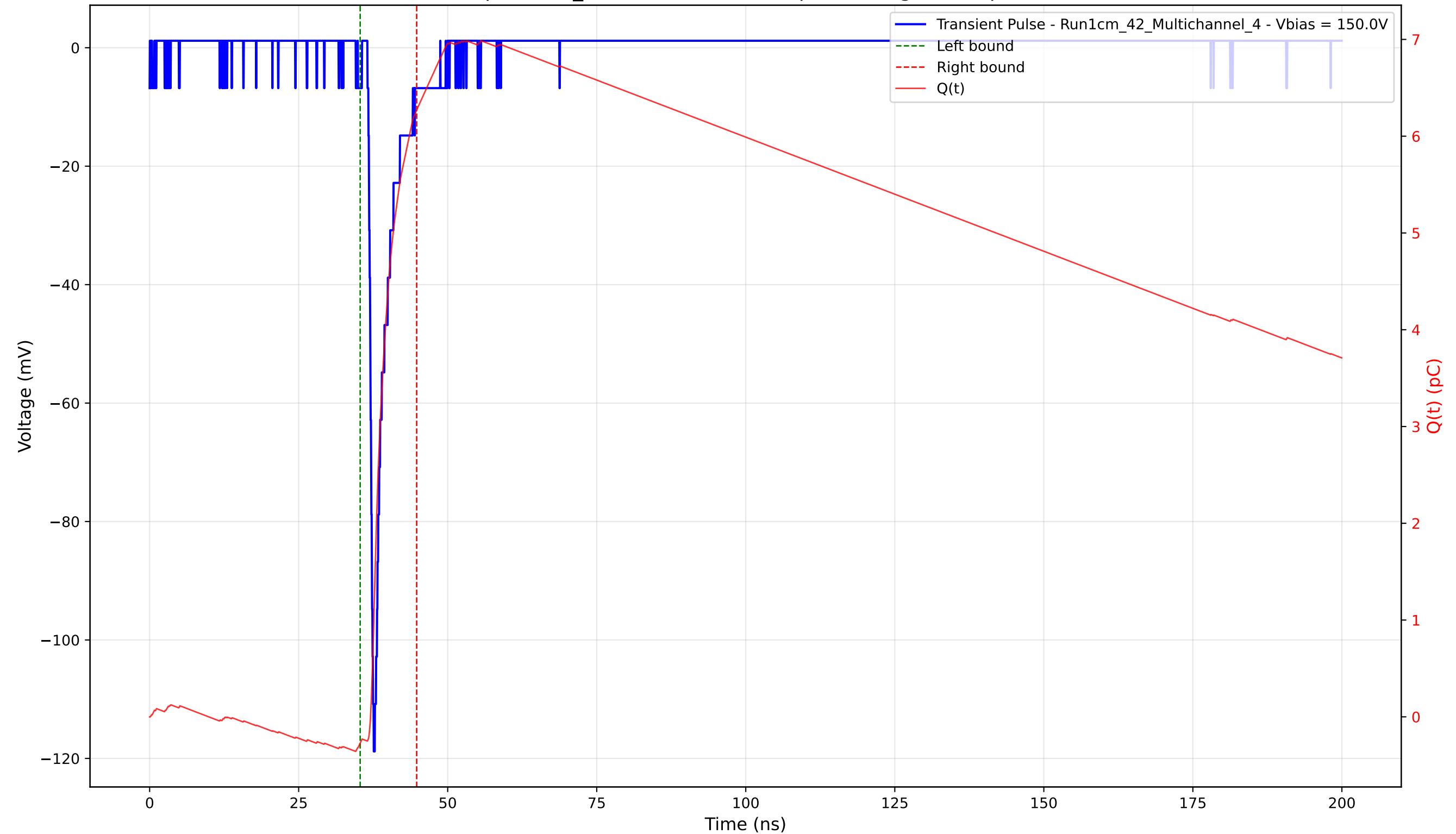
Transient Pulse - Sample: 1cm_42 - Position: 3370.0 \mu\text{m} - Charge: 6.54 pC - Rise Time: 0.77 ns
