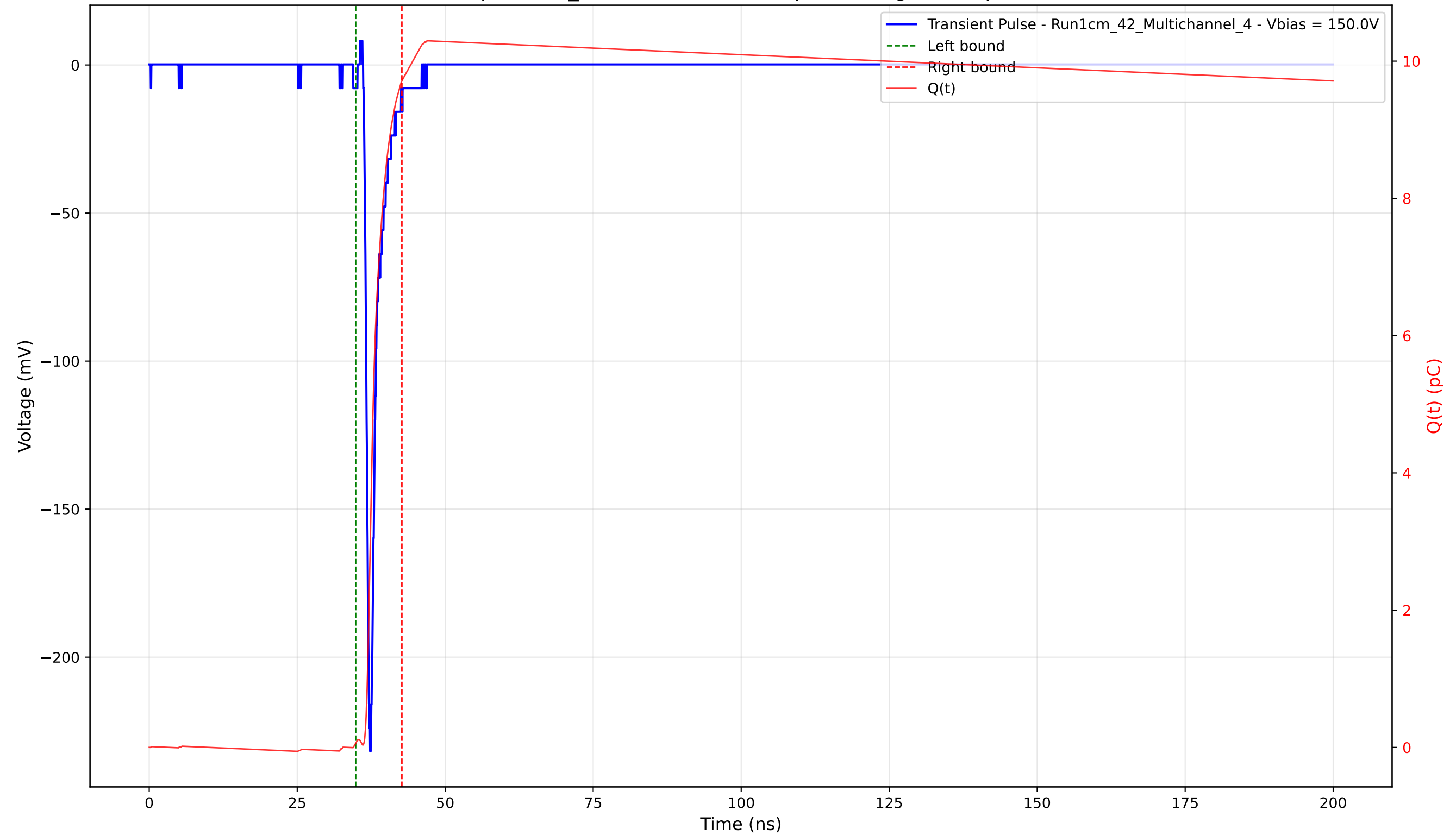
Transient Pulse - Sample: 1cm_42 - Position: 2010.0 \mu\text{m} - Charge: 9.65 pC - Rise Time: 0.80 ns
