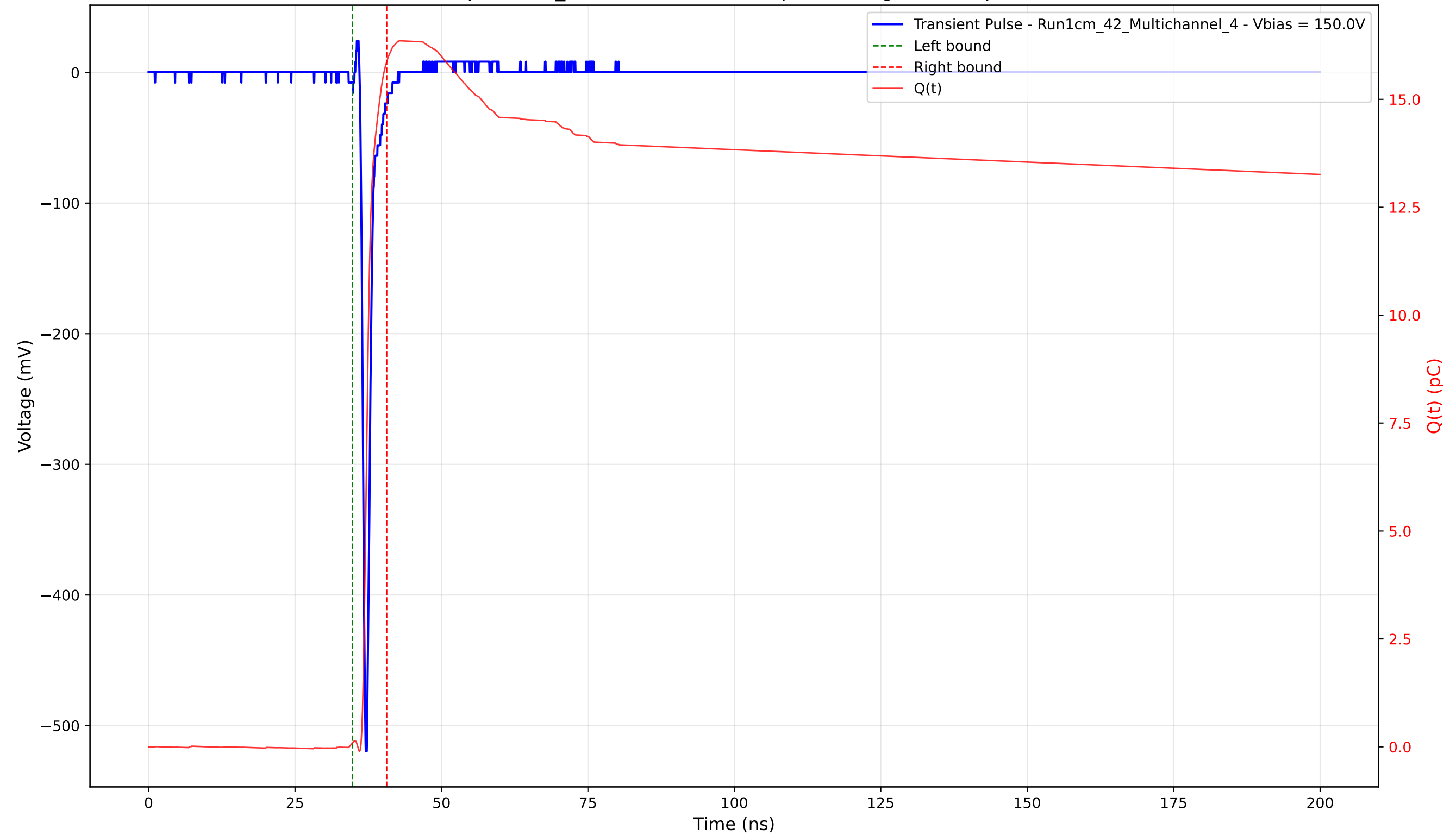
Transient Pulse - Sample: 1cm_42 - Position: 2540.0 \mu\text{m} - Charge: 15.78 pC - Rise Time: 0.72 ns
