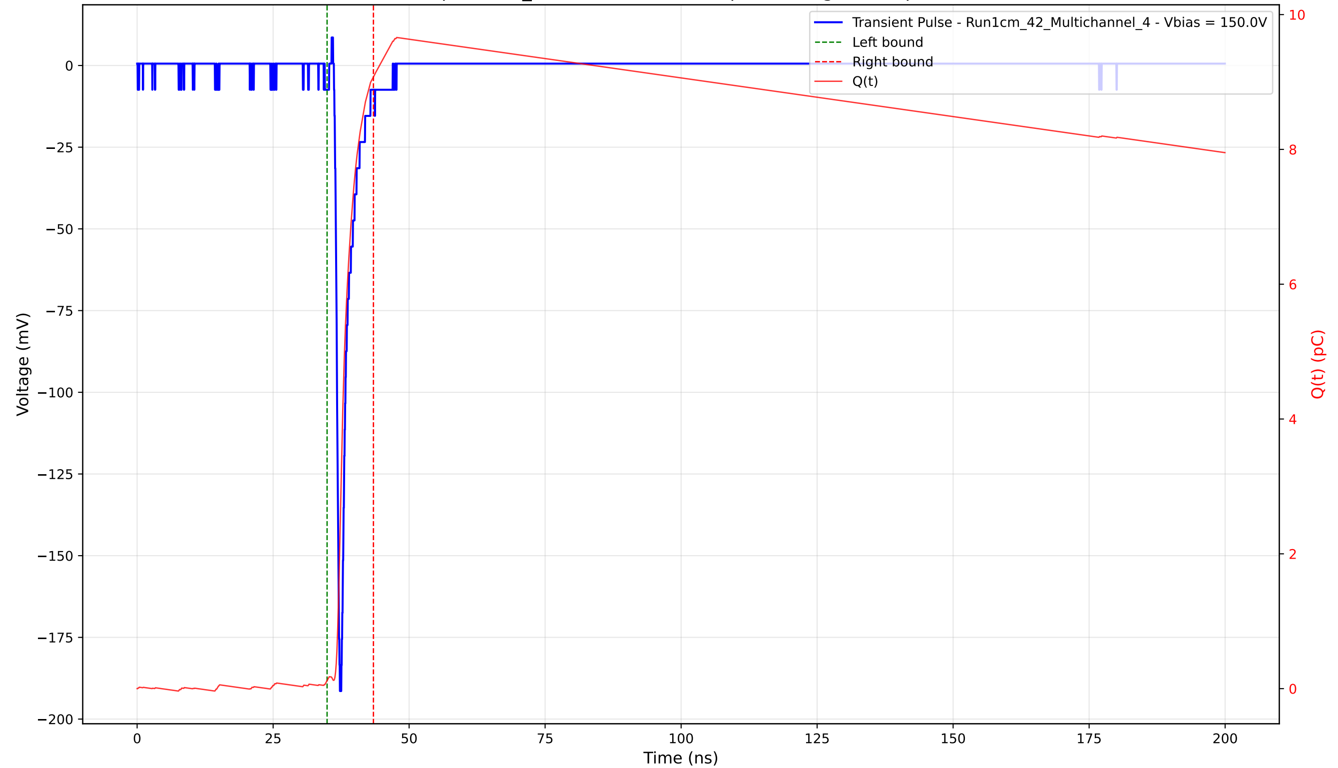
Transient Pulse - Sample: 1cm_42 - Position: 1950.0 \mu\text{m} - Charge: 8.95 pC - Rise Time: 0.78 ns
