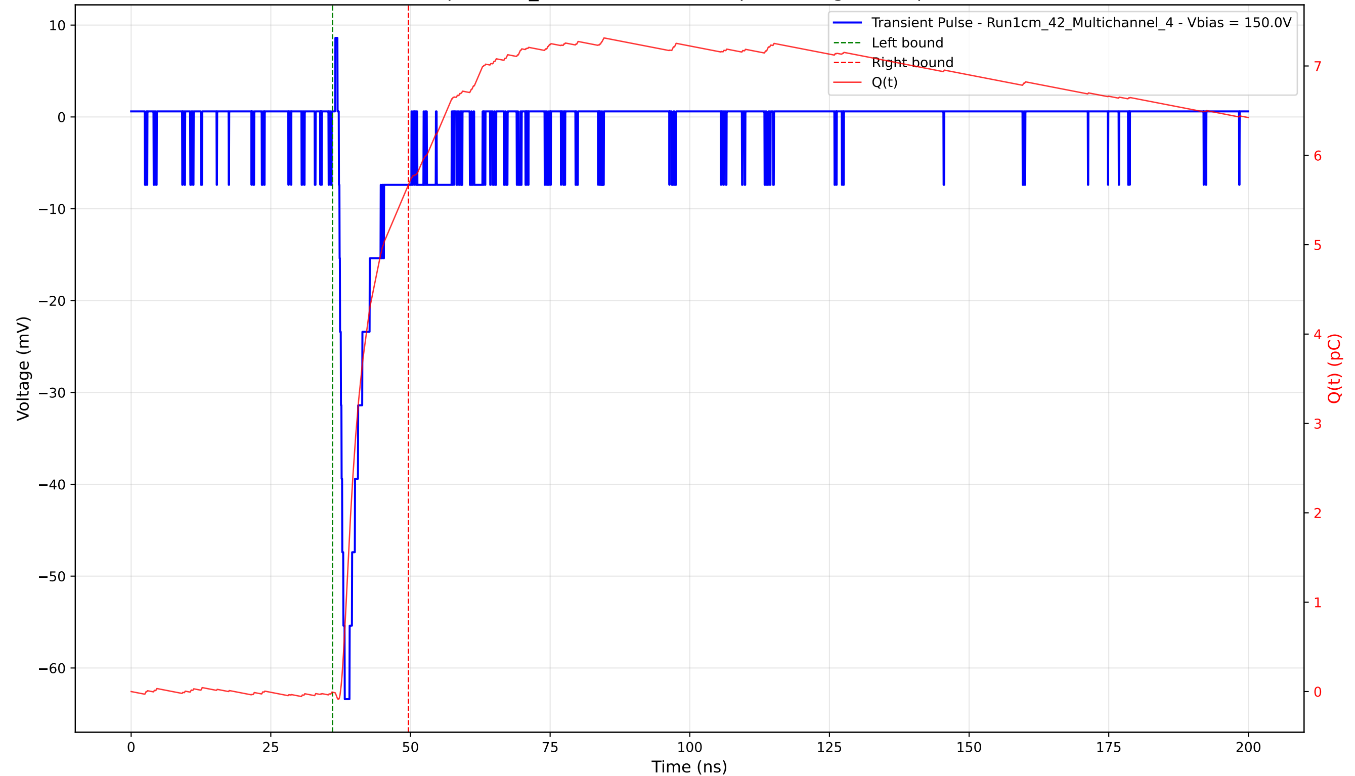
Transient Pulse - Sample: 1cm_42 - Position: 1320.0 \mu\text{m} - Charge: 5.68 pC - Rise Time: 1.05 ns
