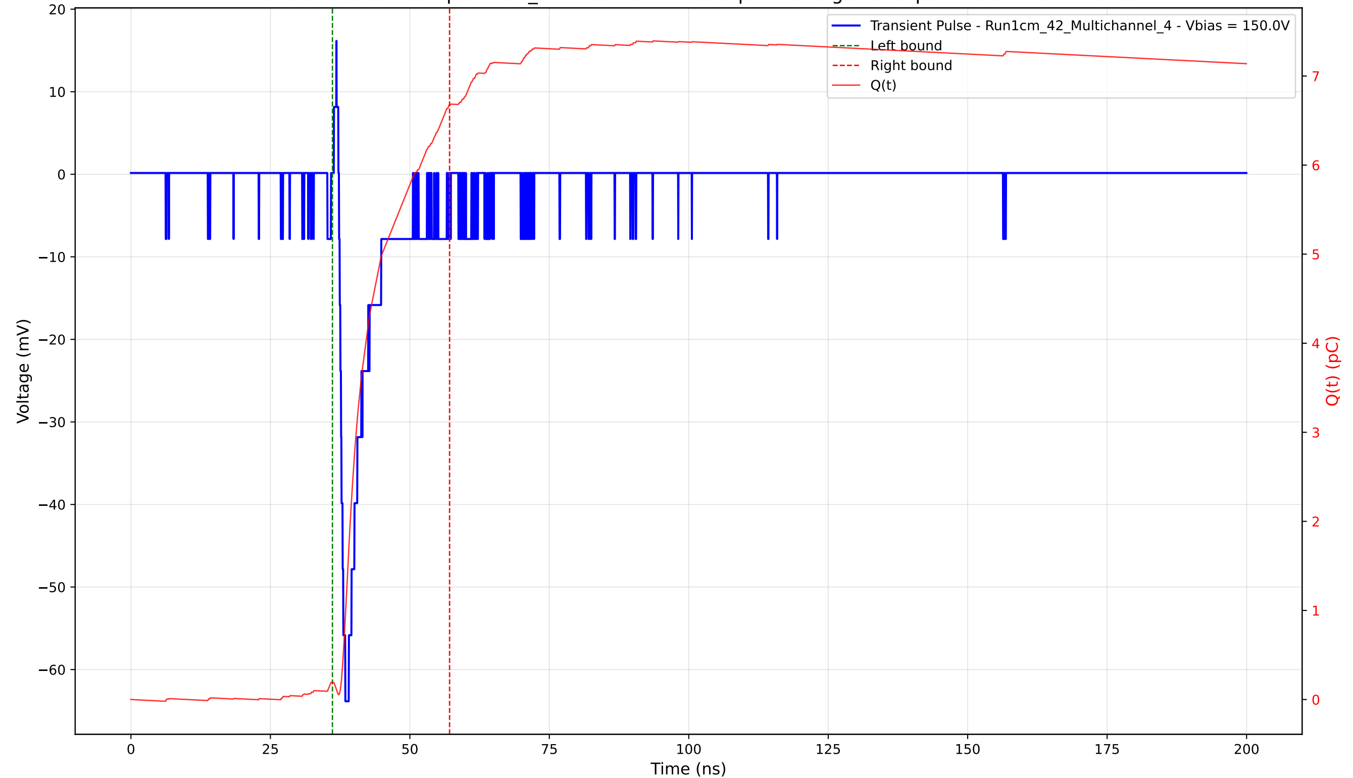
Transient Pulse - Sample: 1cm_42 - Position: 1200.0 \mu\text{m} - Charge: 6.49 pC - Rise Time: 1.13 ns
