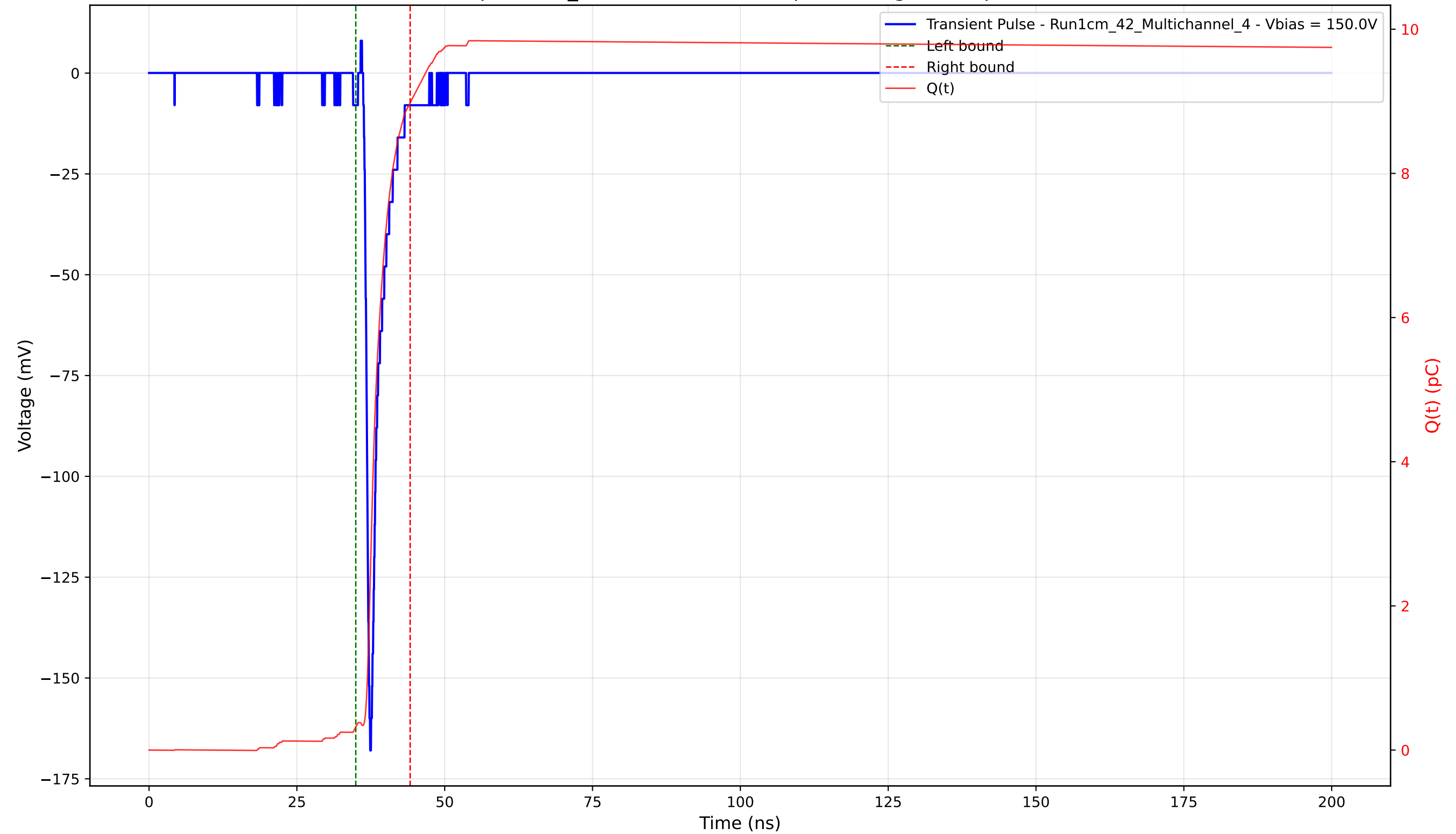
Transient Pulse - Sample: 1cm_42 - Position: 1885.0 \mu\text{m} - Charge: 8.66 pC - Rise Time: 0.80 ns
