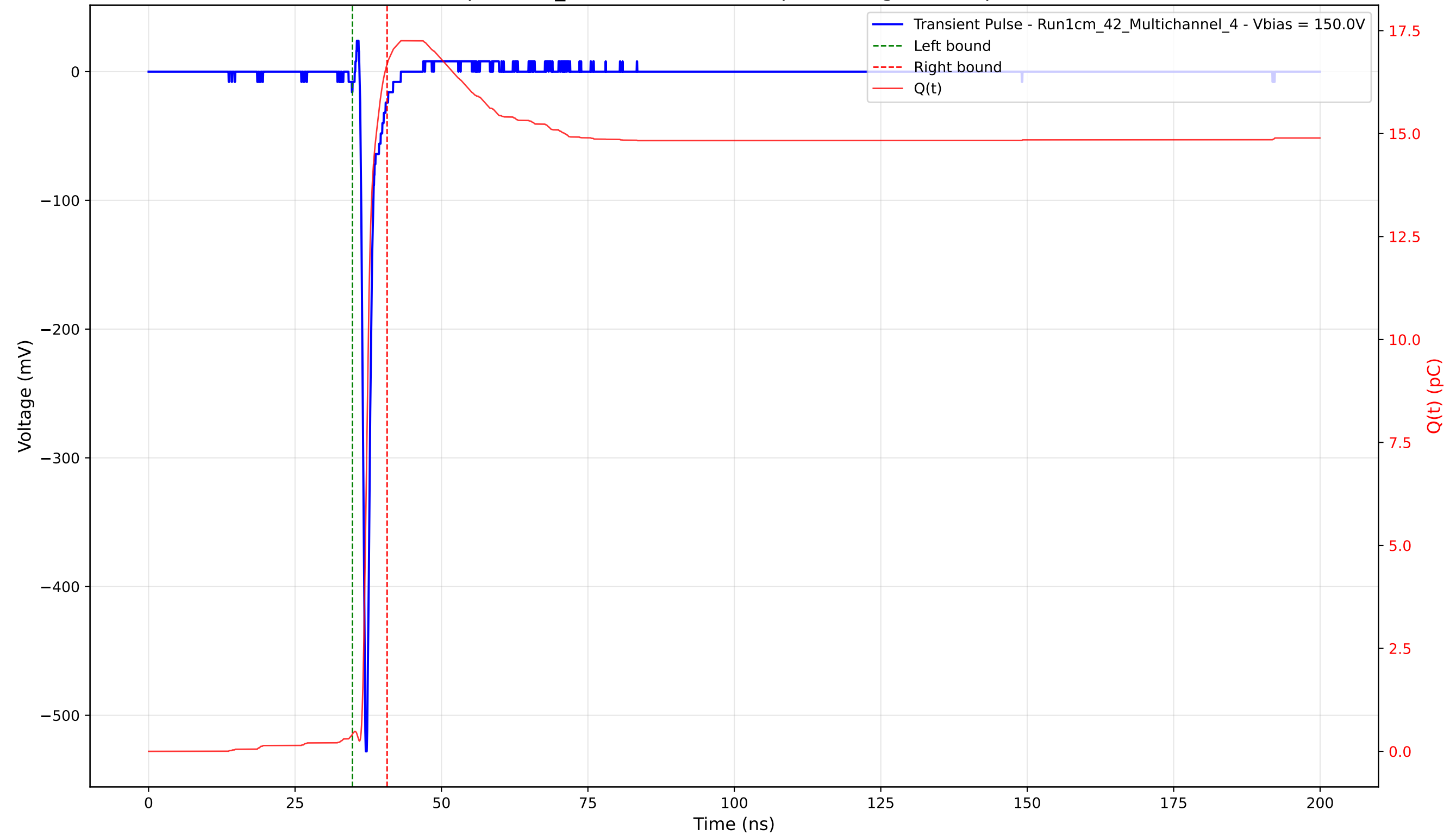
Transient Pulse - Sample: 1cm_42 - Position: 2415.0 \mu\text{m} - Charge: 16.27 pC - Rise Time: 0.72 ns
