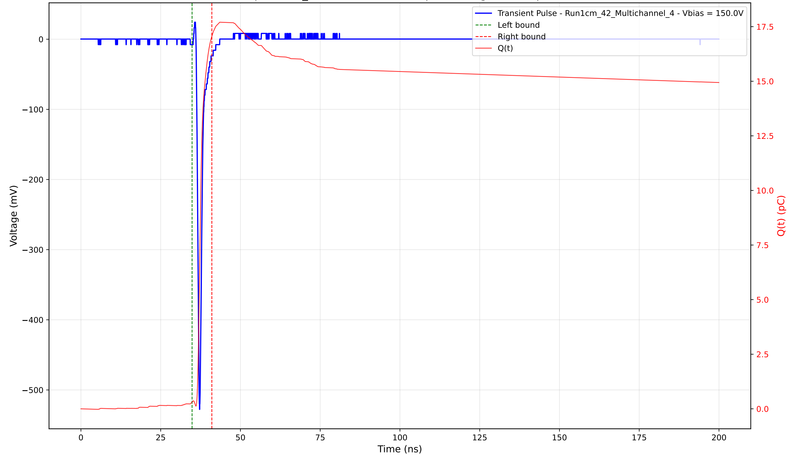
Transient Pulse - Sample: 1cm_42 - Position: 2300.0 \mu\text{m} - Charge: 16.75 pC - Rise Time: 0.70 ns
