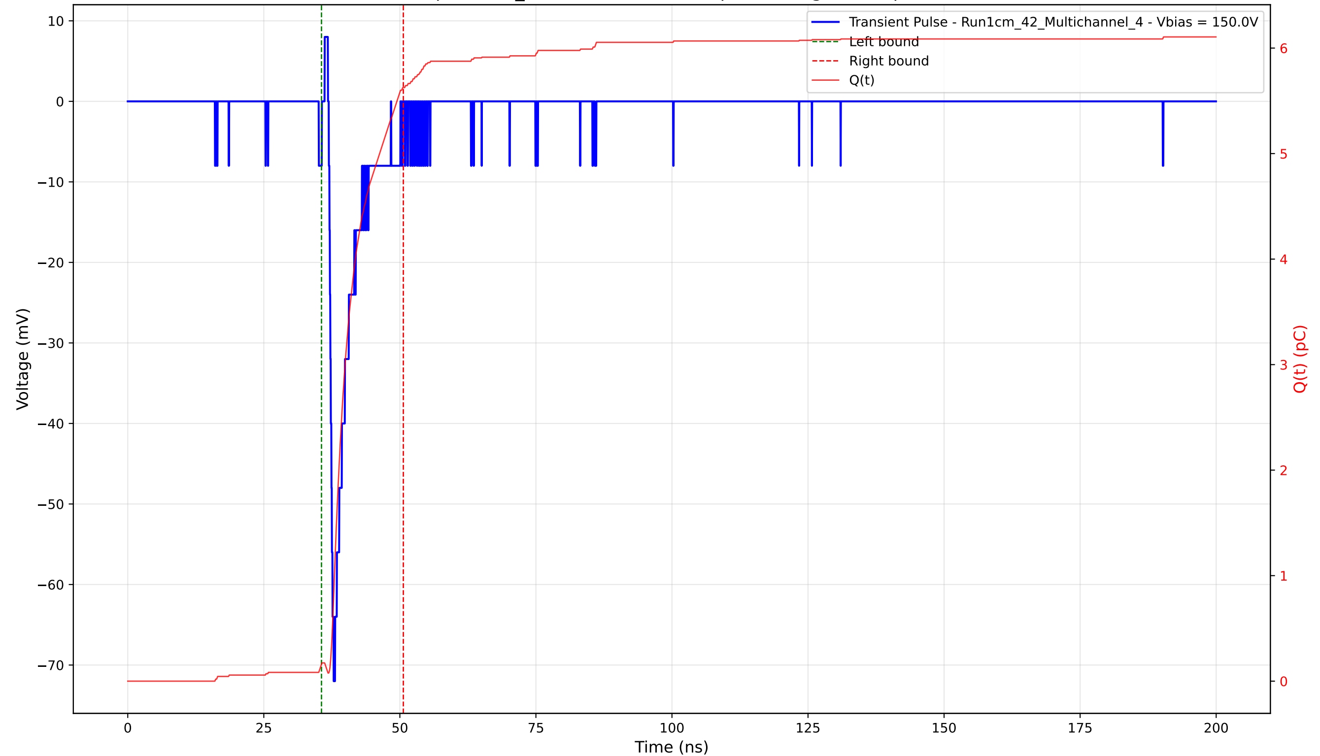
Transient Pulse - Sample: 1cm_42 - Position: 3545.0 \mu\text{m} - Charge: 5.46 pC - Rise Time: 0.88 ns
