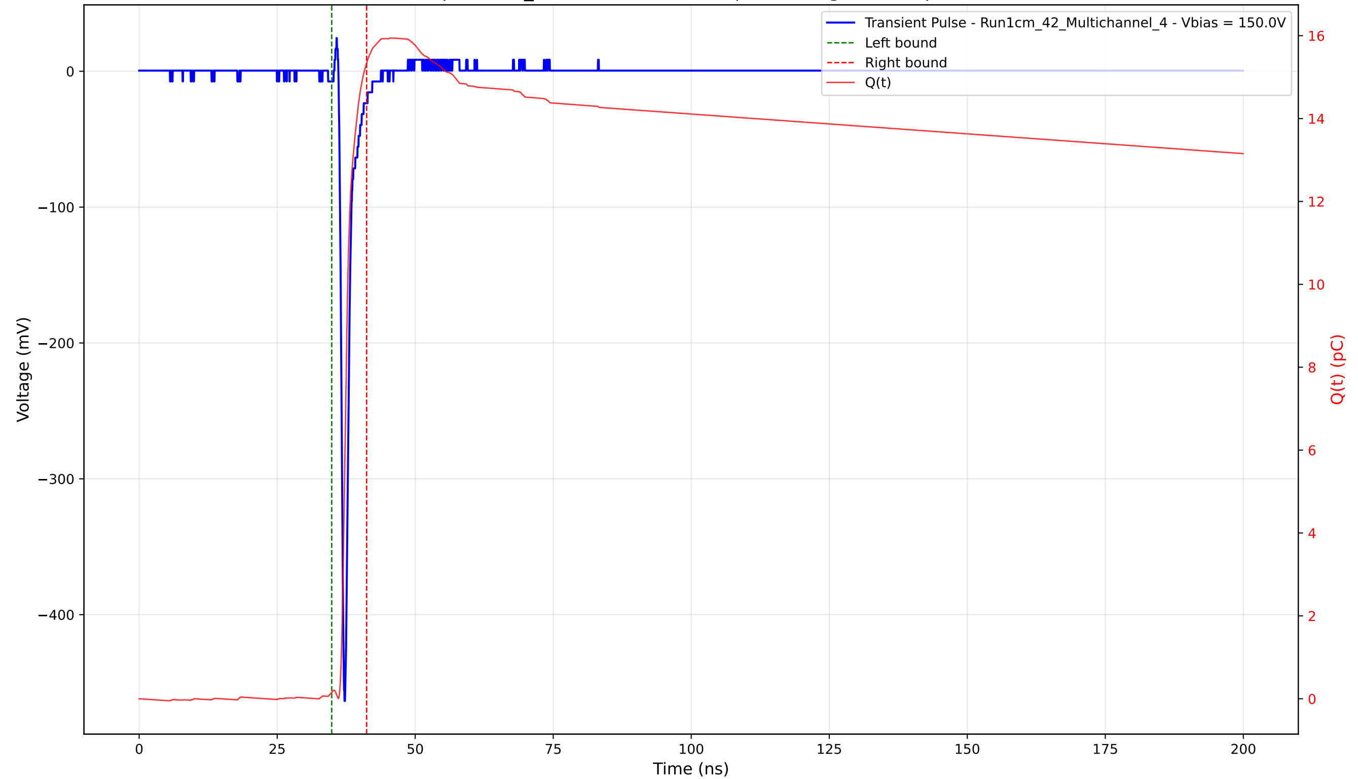
Transient Pulse - Sample: 1cm_42 - Position: 2795.0 \mu\text{m} - Charge: 15.18 pC - Rise Time: 0.71 ns
