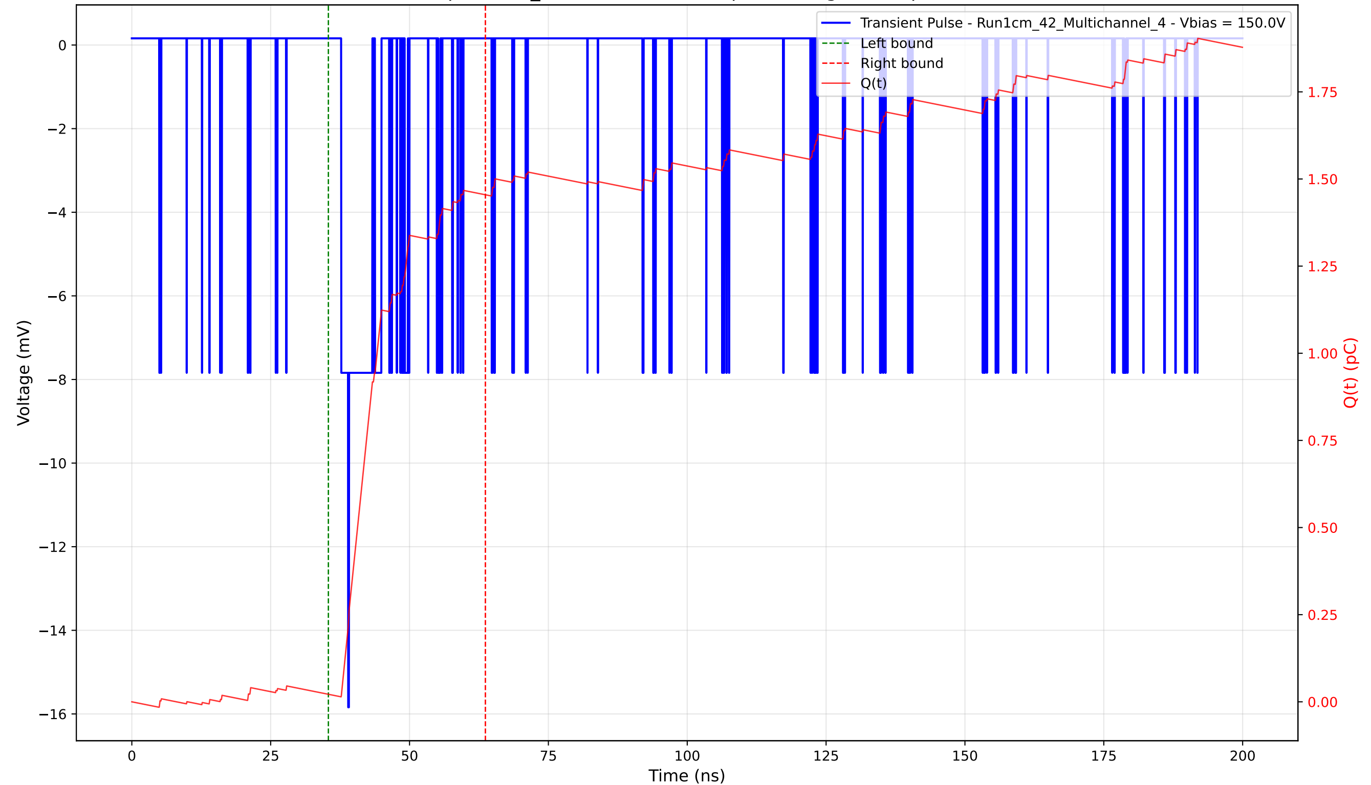
Transient Pulse - Sample: 1cm_42 - Position: 120.0 \mu\text{m} - Charge: 1.43 pC - Rise Time: 1.27 ns
