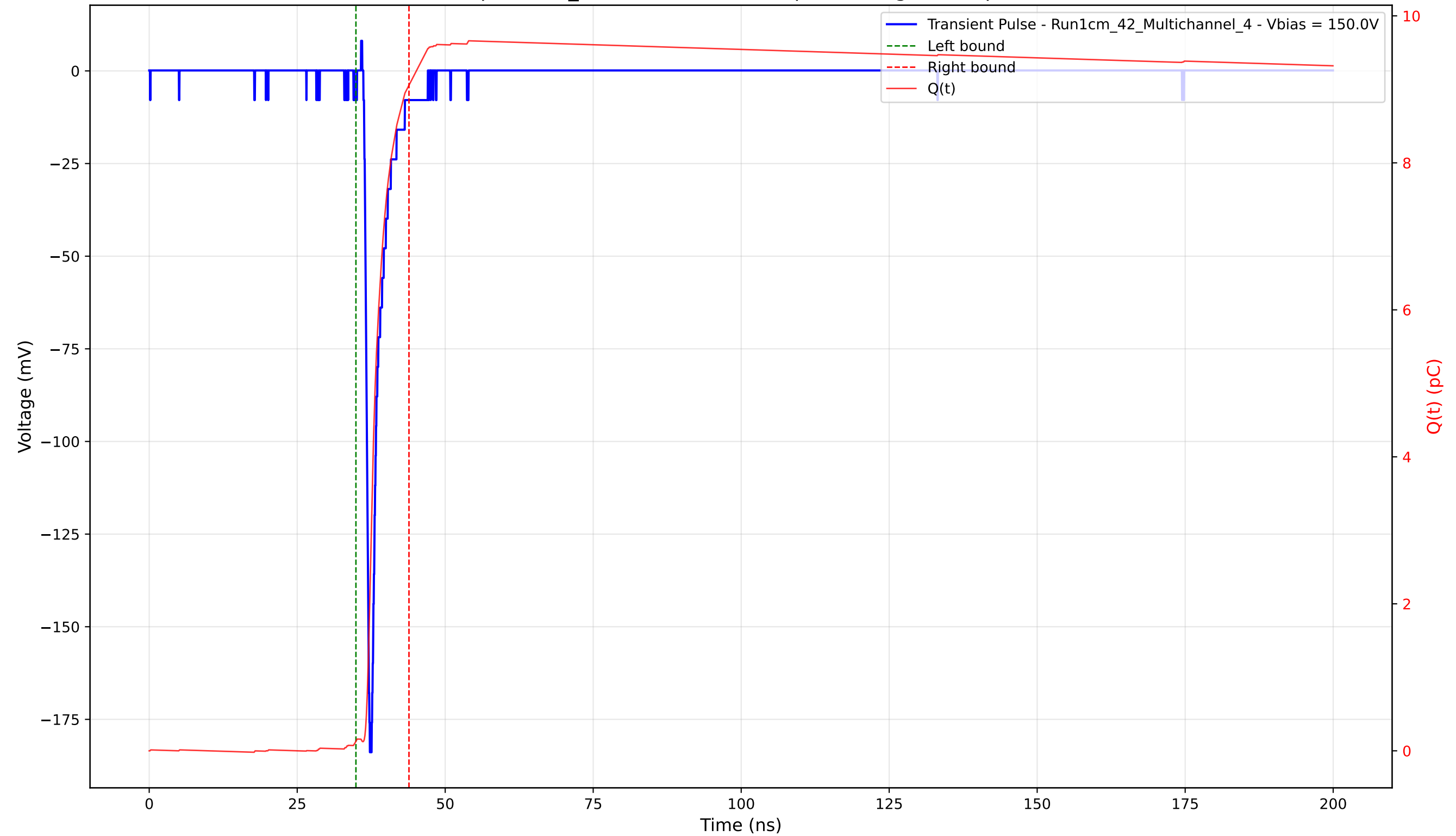
Transient Pulse - Sample: 1cm_42 - Position: 1940.0 \mu\text{m} - Charge: 8.92 pC - Rise Time: 0.79 ns
