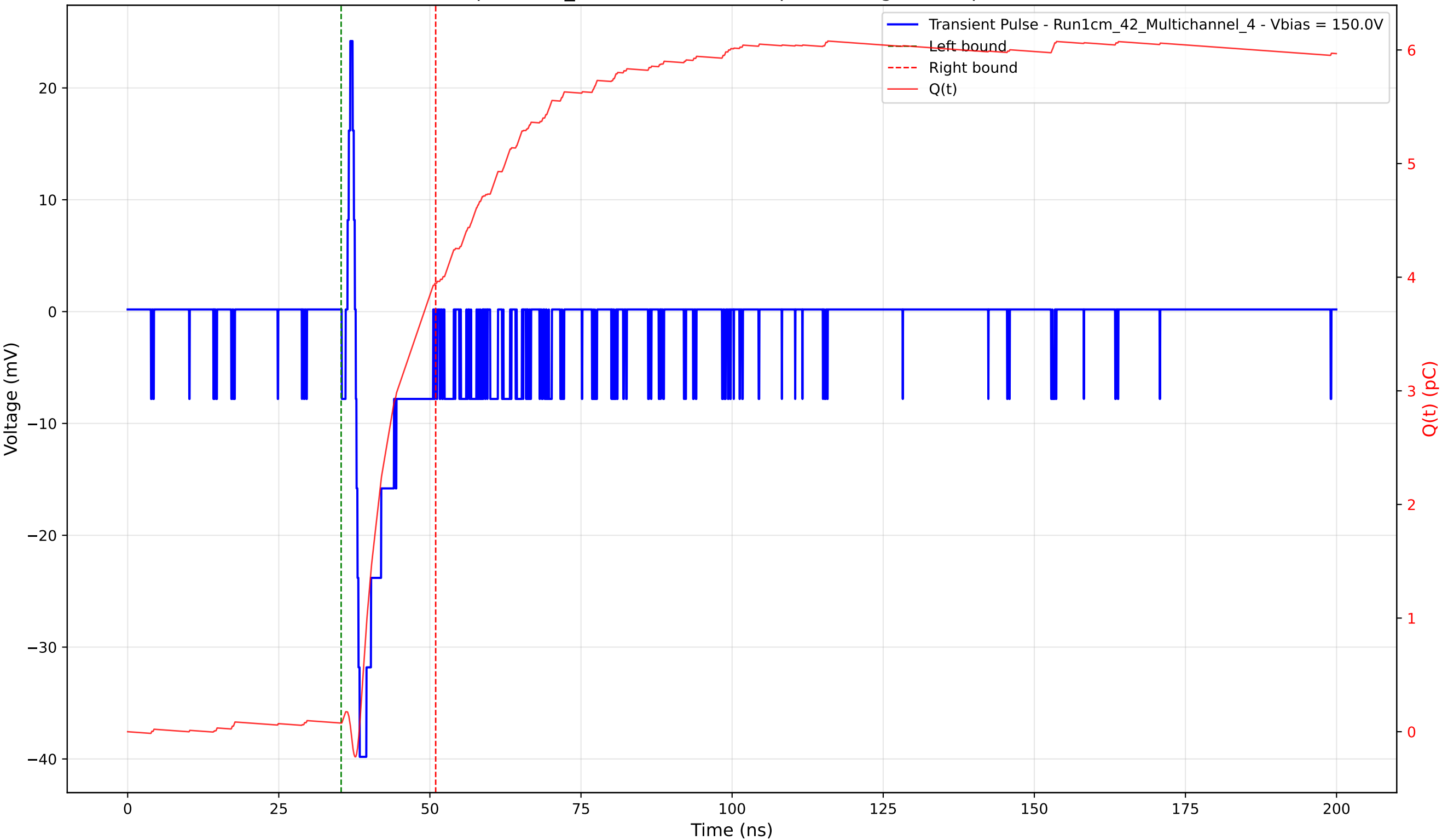
Transient Pulse - Sample: 1cm_42 - Position: 600.0 \mu\text{m} - Charge: 3.87 pC - Rise Time: 0.66 ns
