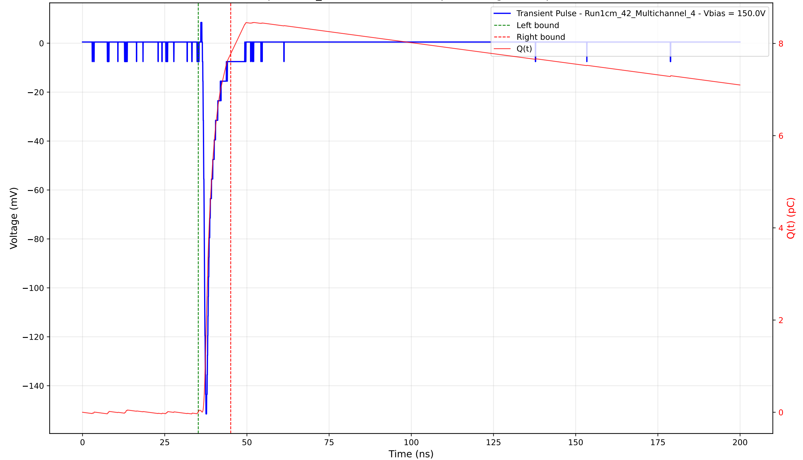
Transient Pulse - Sample: 1cm_42 - Position: 3230.0 \mu\text{m} - Charge: 7.77 pC - Rise Time: 0.84 ns
