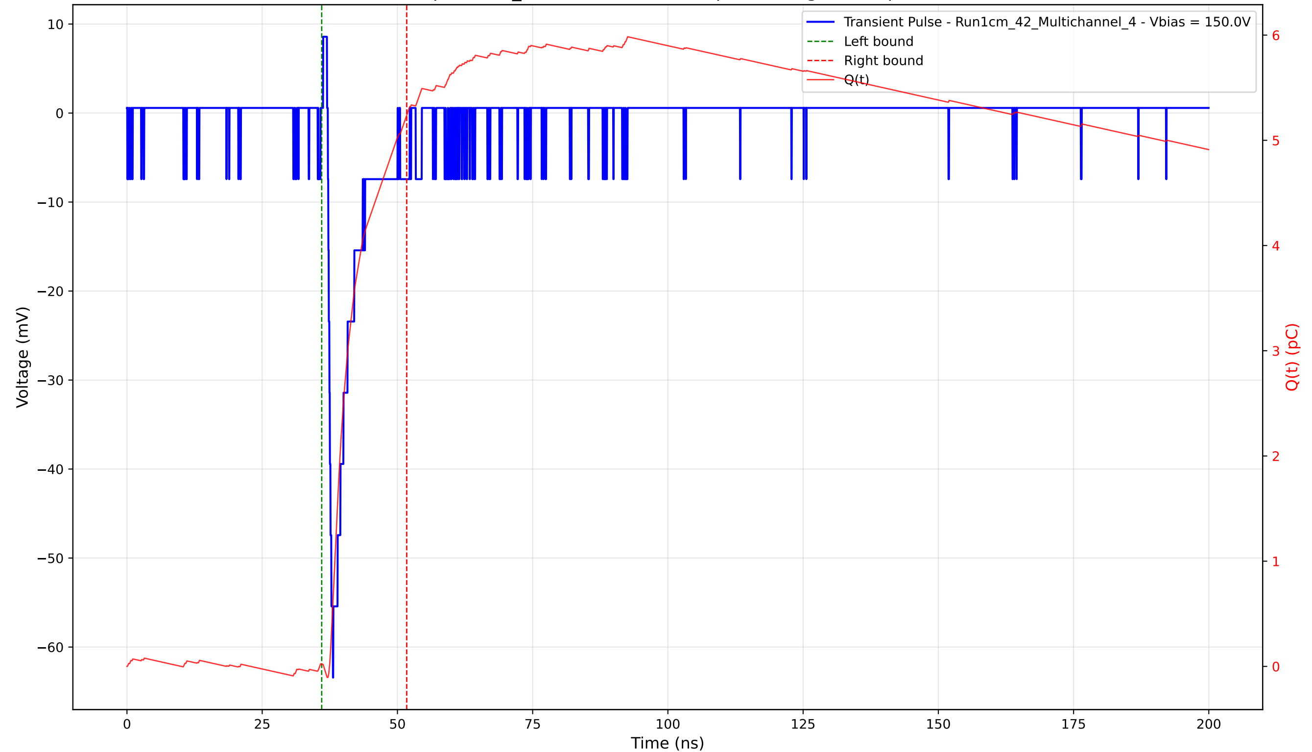
Transient Pulse - Sample: 1cm_42 - Position: 3635.0 \mu\text{m} - Charge: 5.22 pC - Rise Time: 0.93 ns
