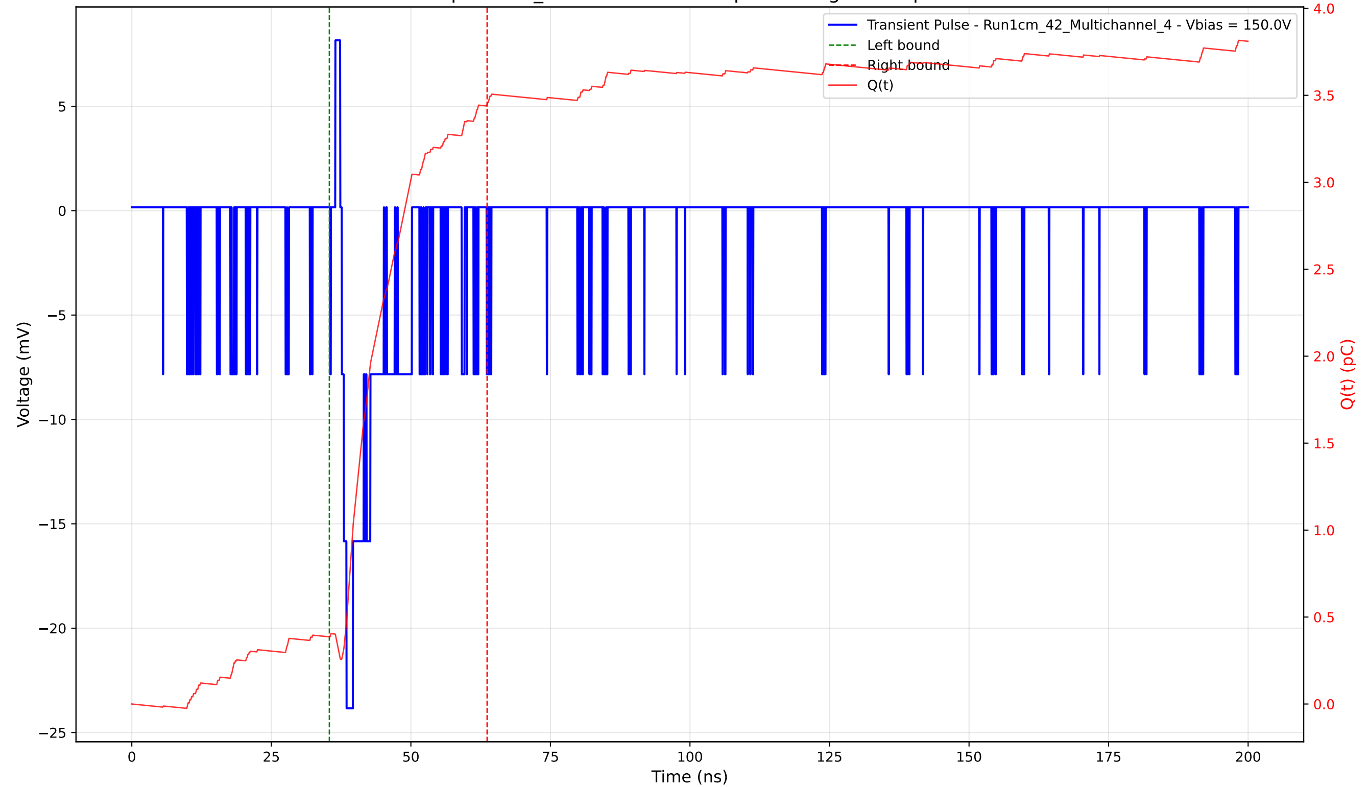
Transient Pulse - Sample: 1cm_42 - Position: 285.0 \mu\text{m} - Charge: 3.06 pC - Rise Time: 0.87 ns
