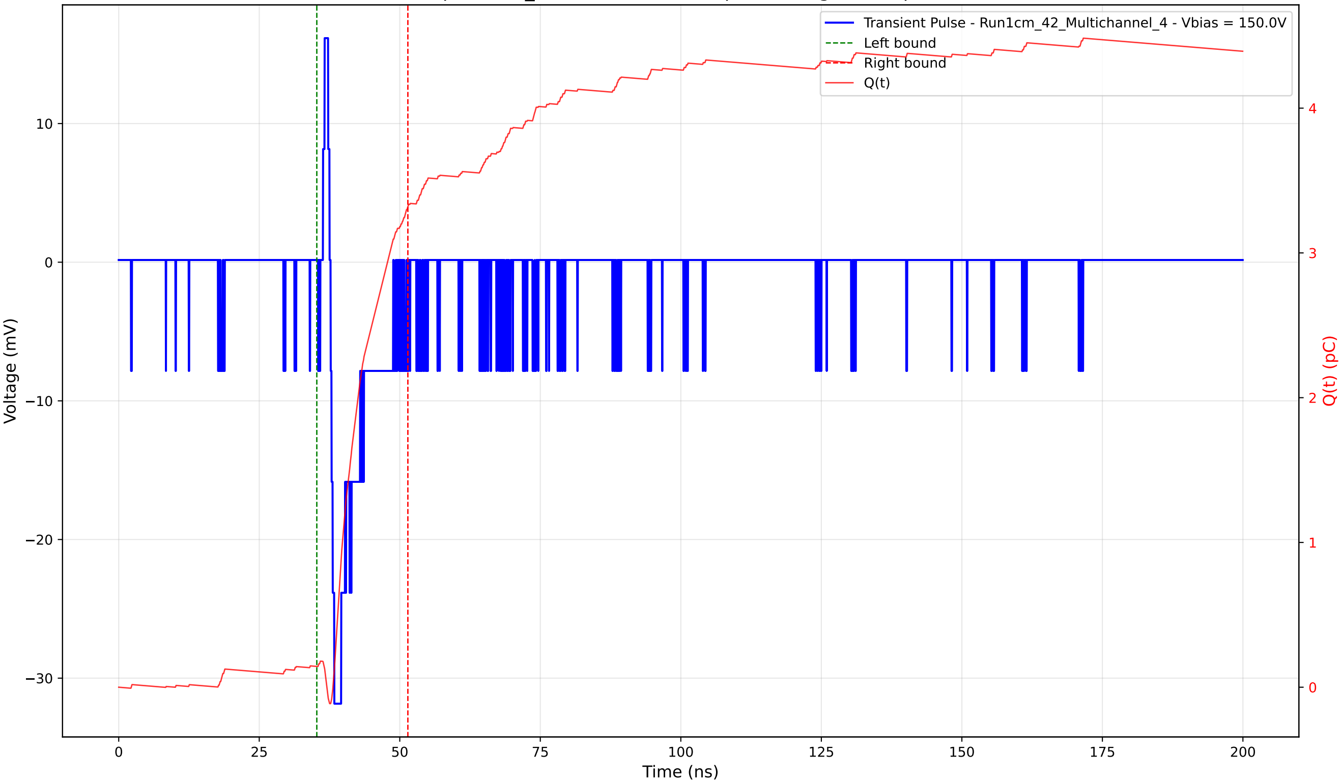
Transient Pulse - Sample: 1cm_42 - Position: 455.0 \mu\text{m} - Charge: 3.18 pC - Rise Time: 0.66 ns
