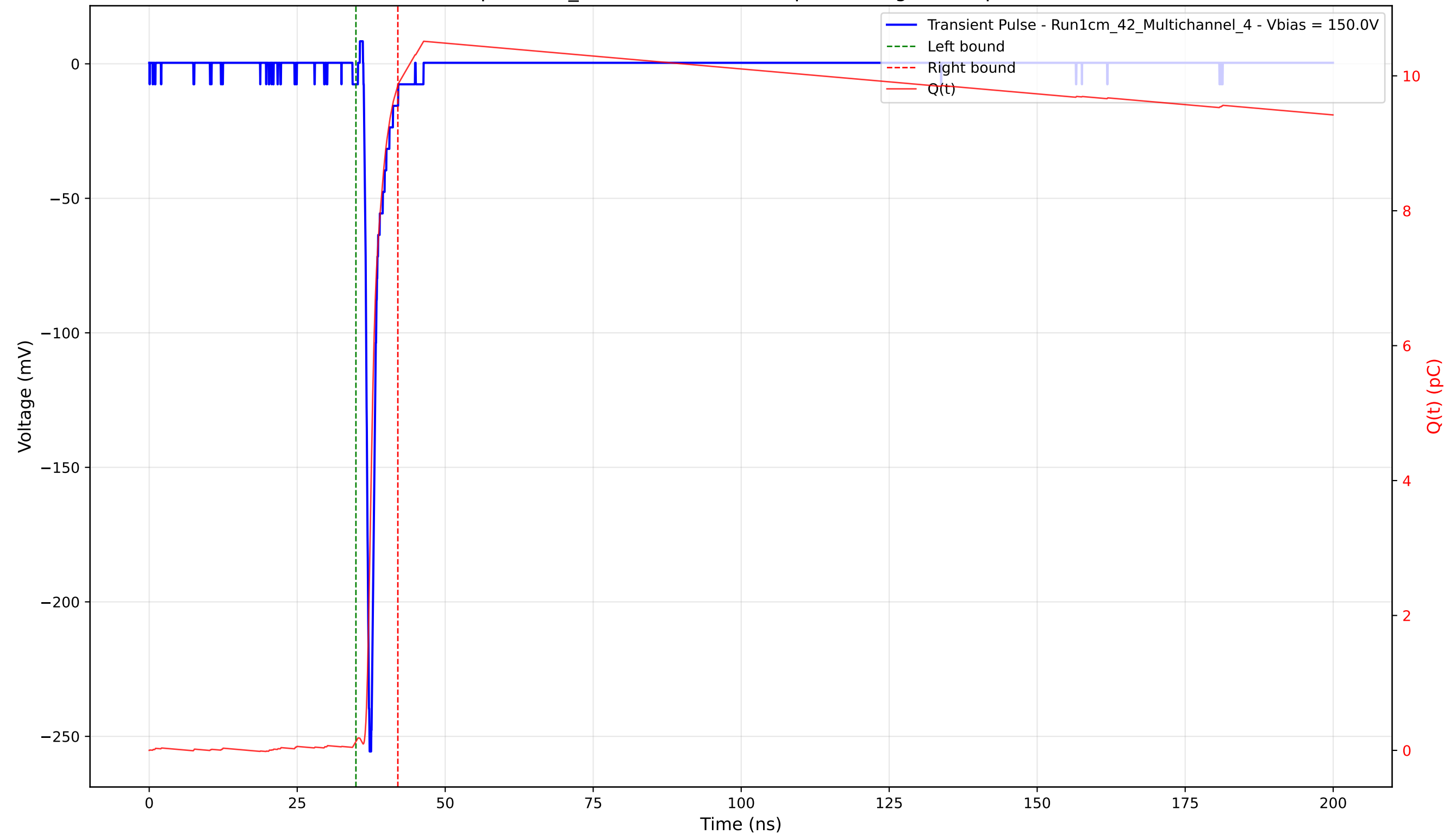
Transient Pulse - Sample: 1cm_42 - Position: 2980.0 \mu\text{m} - Charge: 9.73 pC - Rise Time: 0.74 ns
