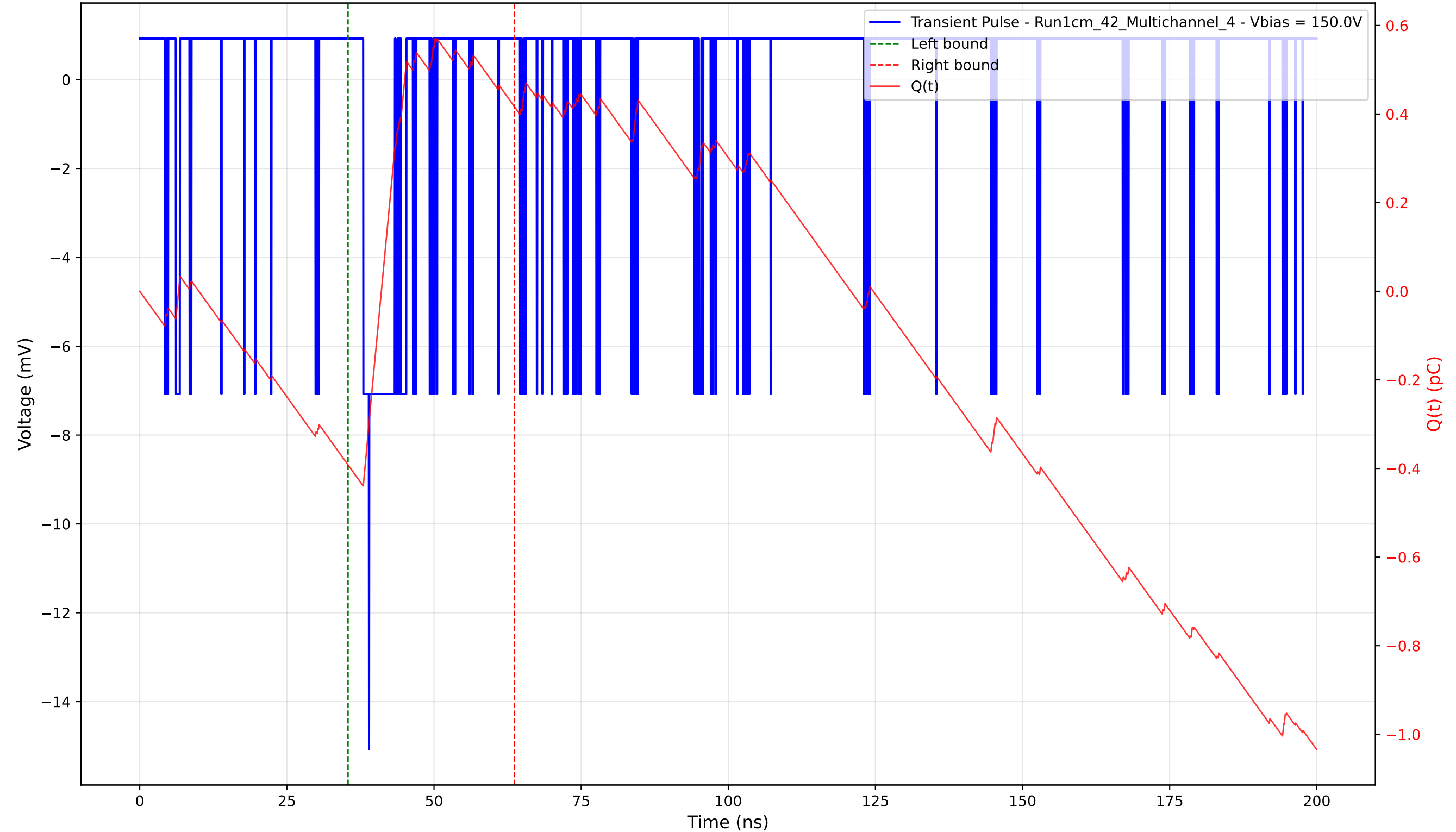
Transient Pulse - Sample: 1cm_42 - Position: 5090.0 \mu\text{m} - Charge: 0.81 pC - Rise Time: 1.00 ns
