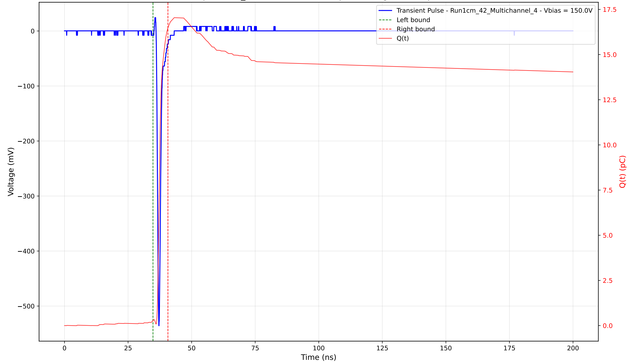
Transient Pulse - Sample: 1cm_42 - Position: 2440.0 \mu\text{m} - Charge: 16.20 pC - Rise Time: 0.73 ns
