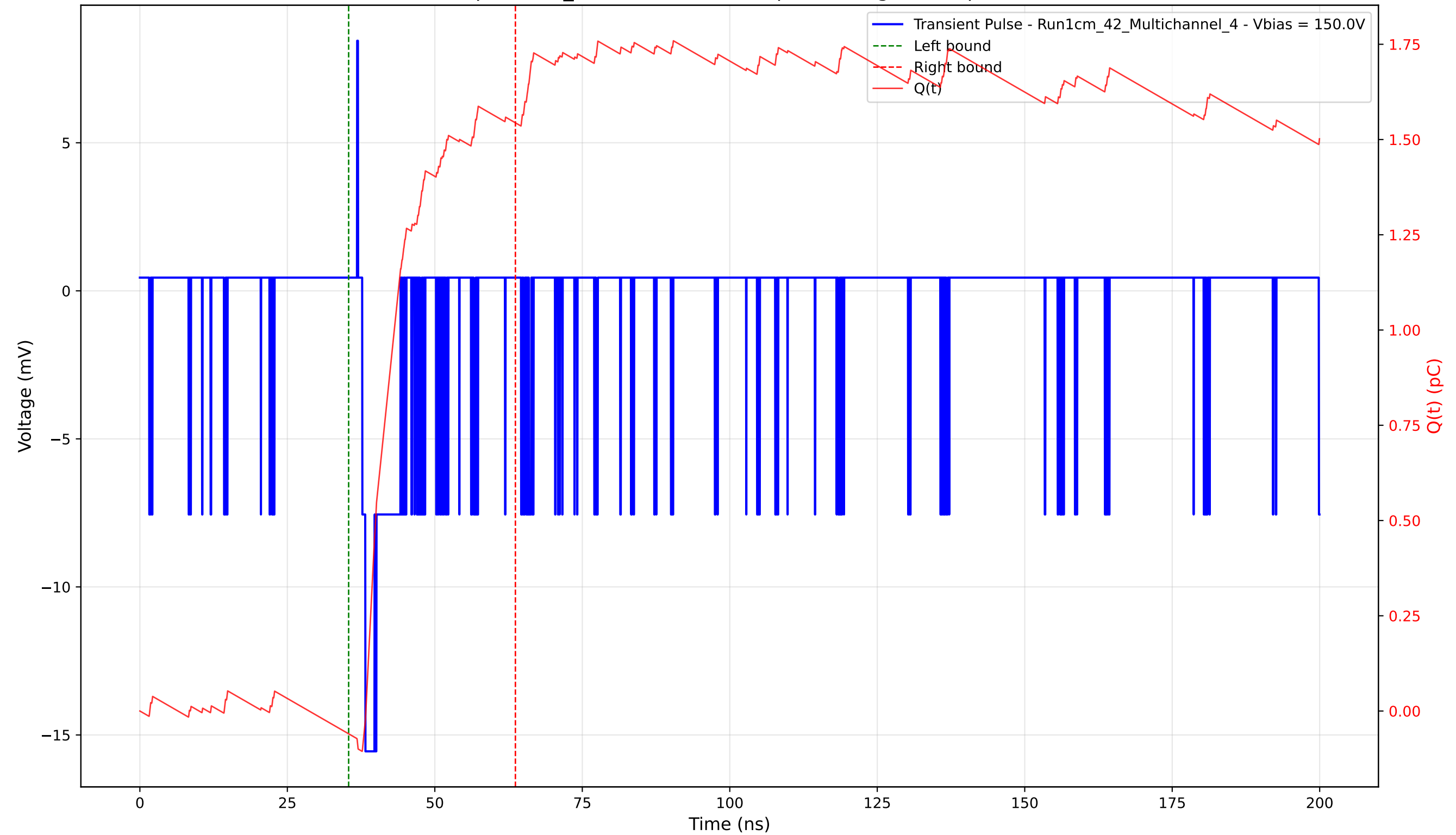
Transient Pulse - Sample: 1cm_42 - Position: 160.0 \mu\text{m} - Charge: 1.60 pC - Rise Time: 0.55 ns
