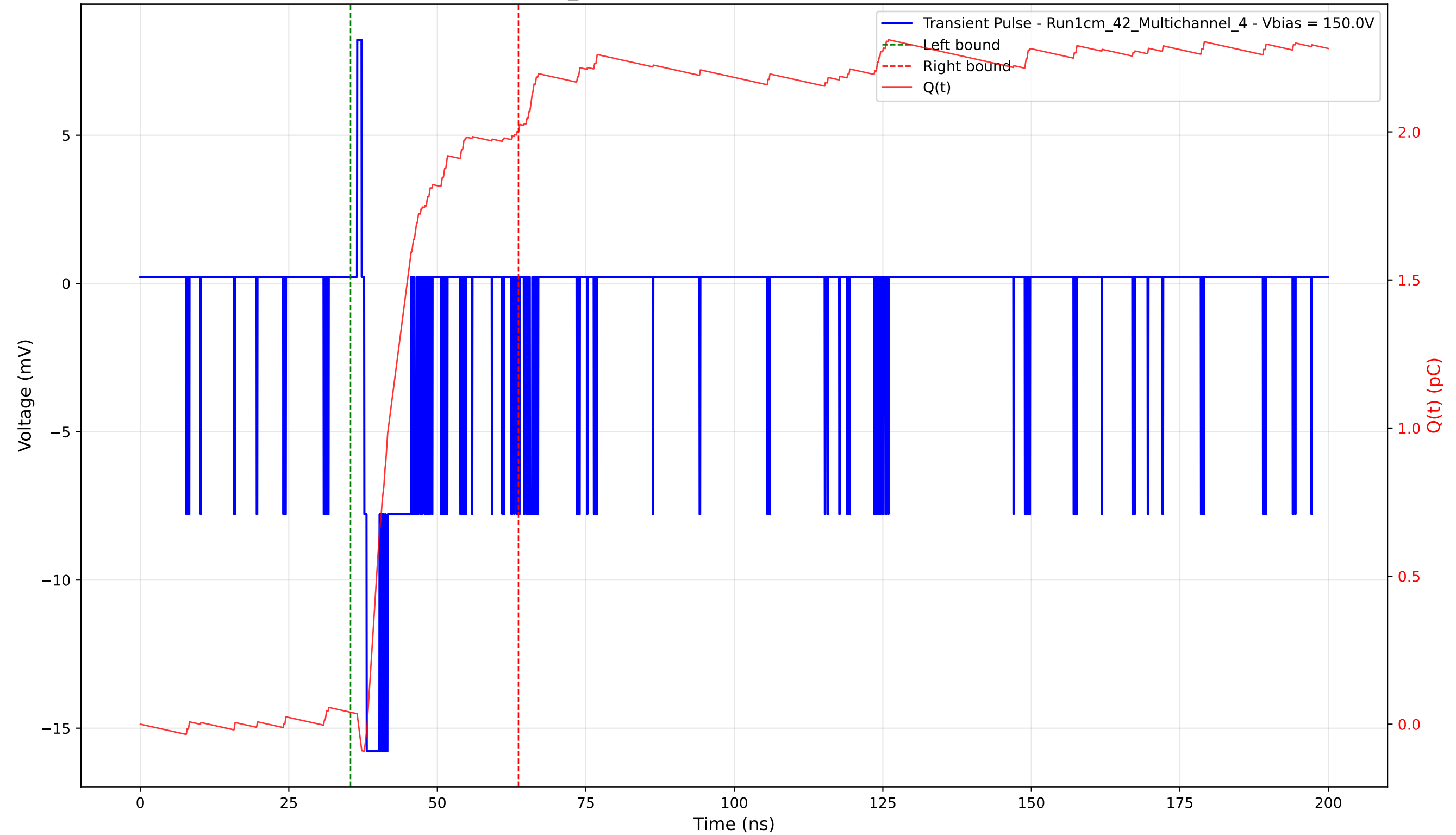
Transient Pulse - Sample: 1cm_42 - Position: 205.0 \mu\text{m} - Charge: 1.96 pC - Rise Time: 0.43 ns
