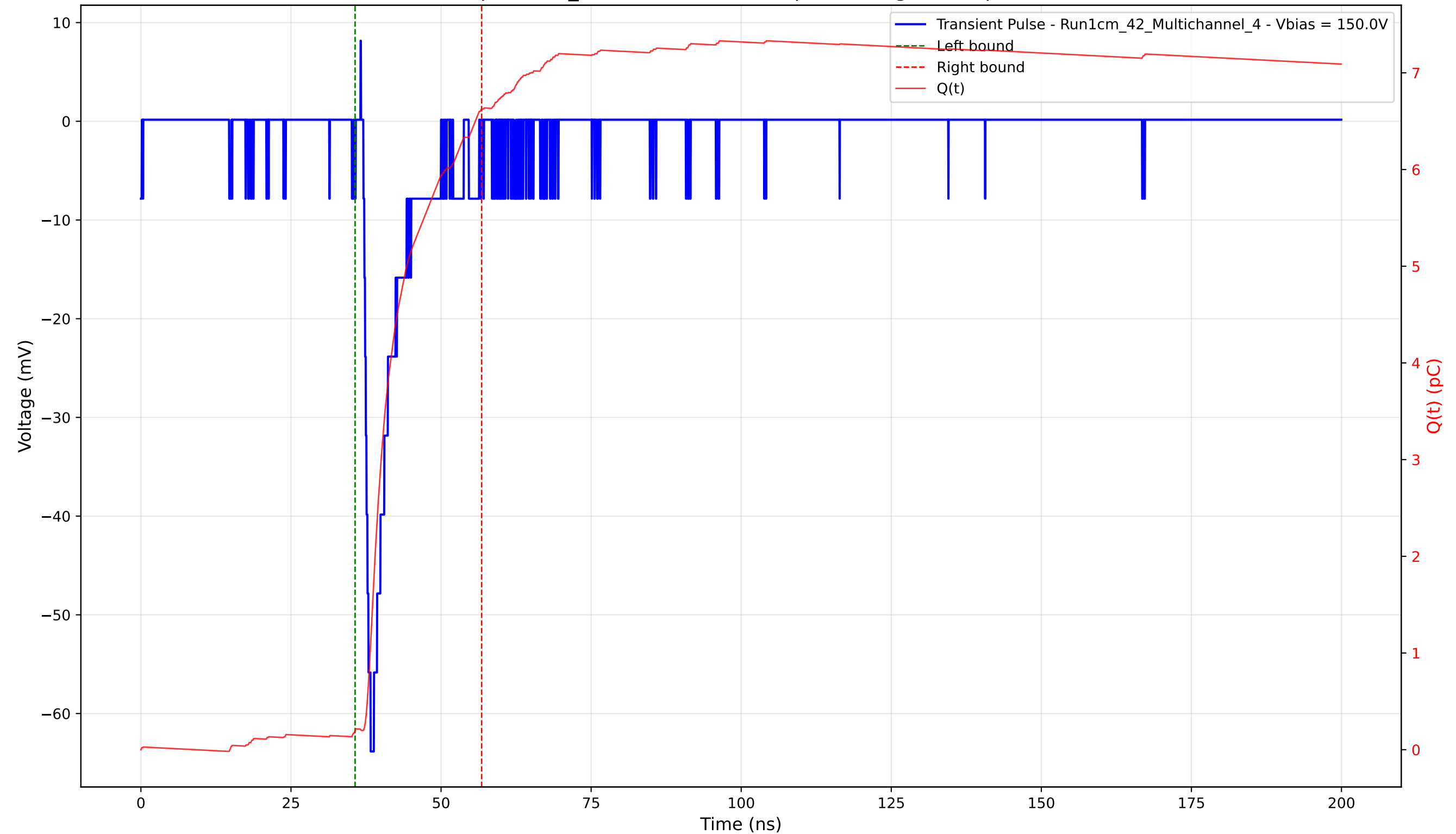
Transient Pulse - Sample: 1cm_42 - Position: 1370.0 \mu\text{m} - Charge: 6.43 pC - Rise Time: 1.21 ns
