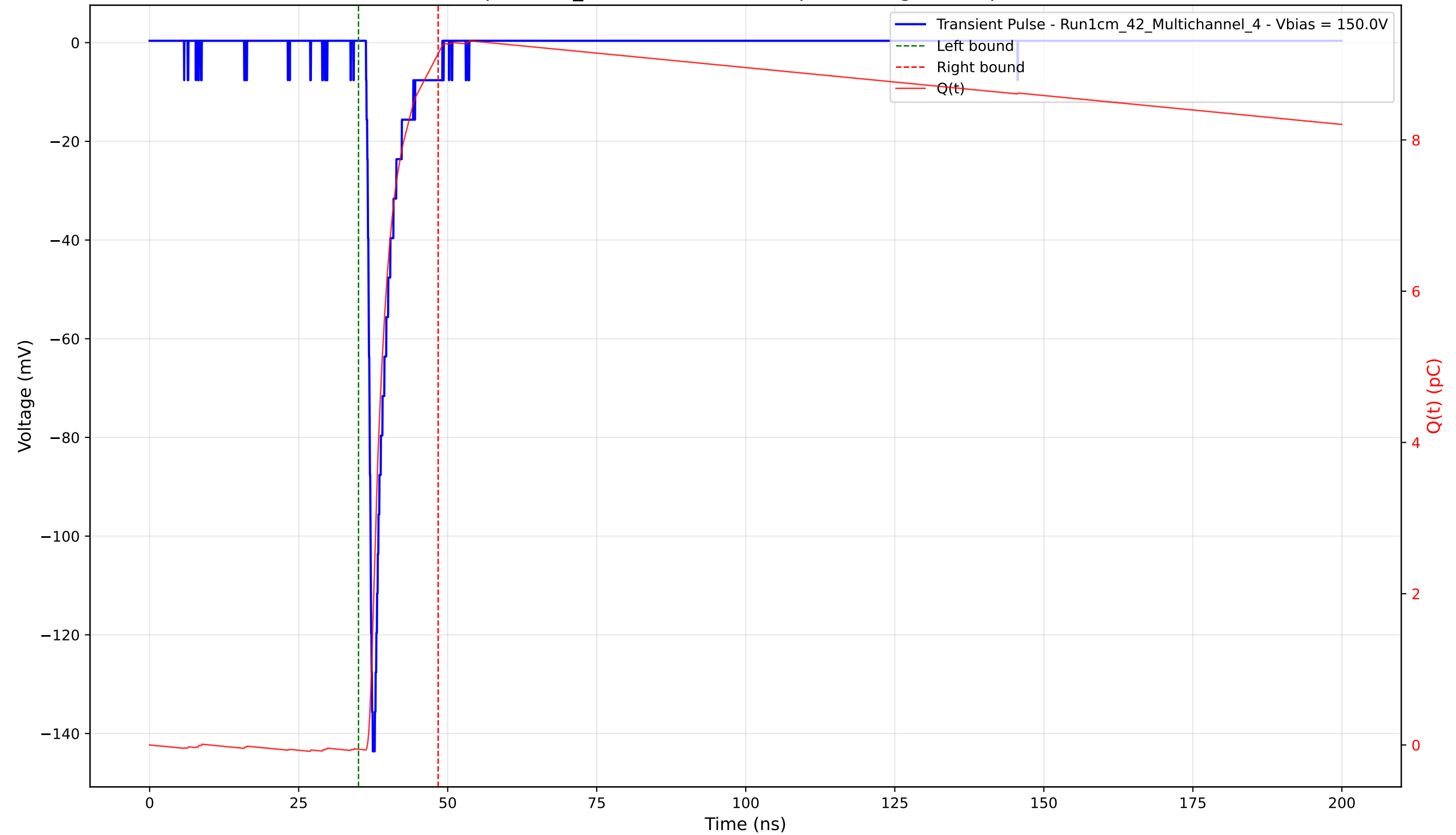
Transient Pulse - Sample: 1cm_42 - Position: 1735.0 \mu\text{m} - Charge: 9.20 pC - Rise Time: 0.93 ns
