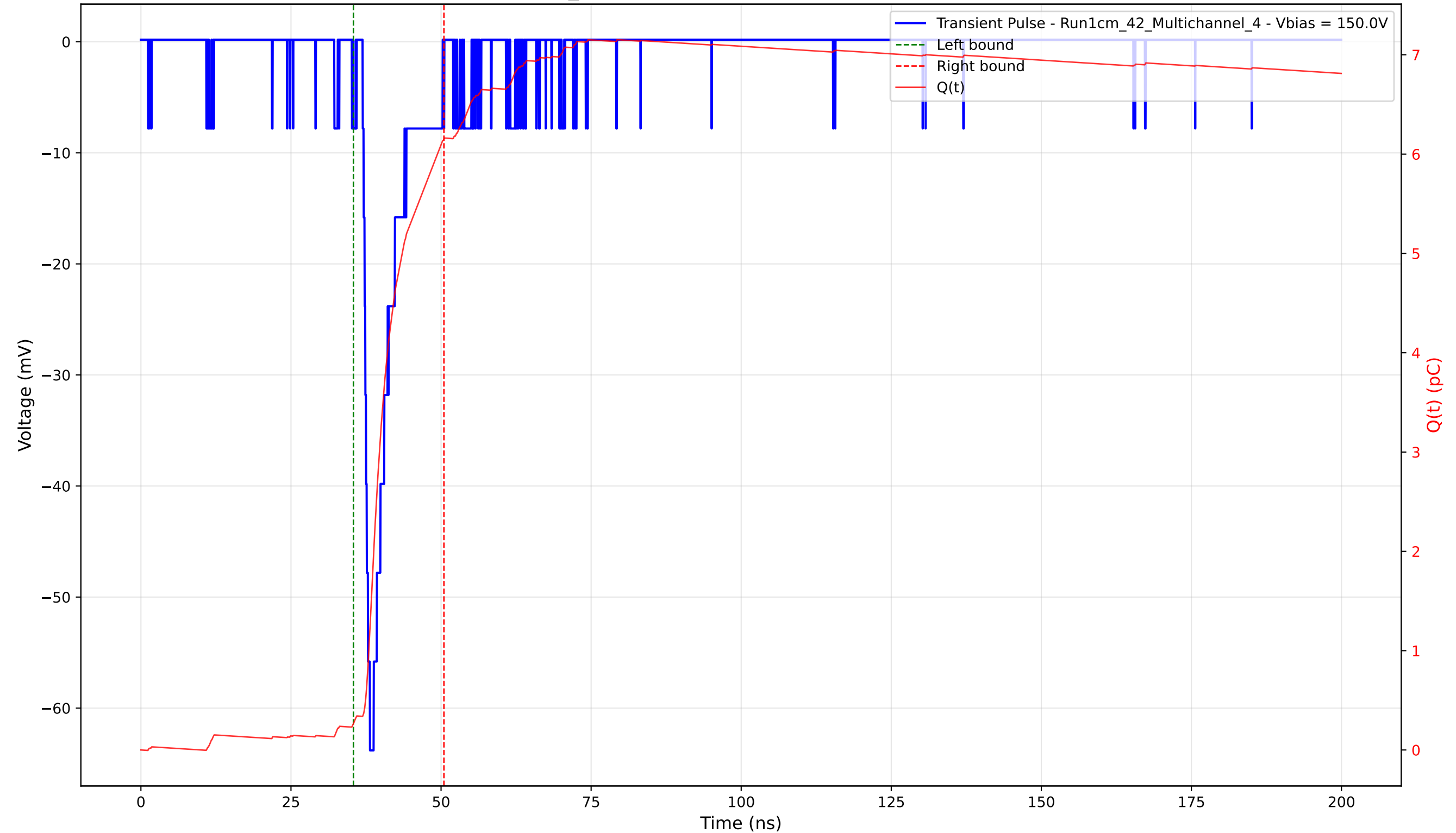
Transient Pulse - Sample: 1cm_42 - Position: 1405.0 \mu\text{m} - Charge: 5.89 pC - Rise Time: 1.21 ns
