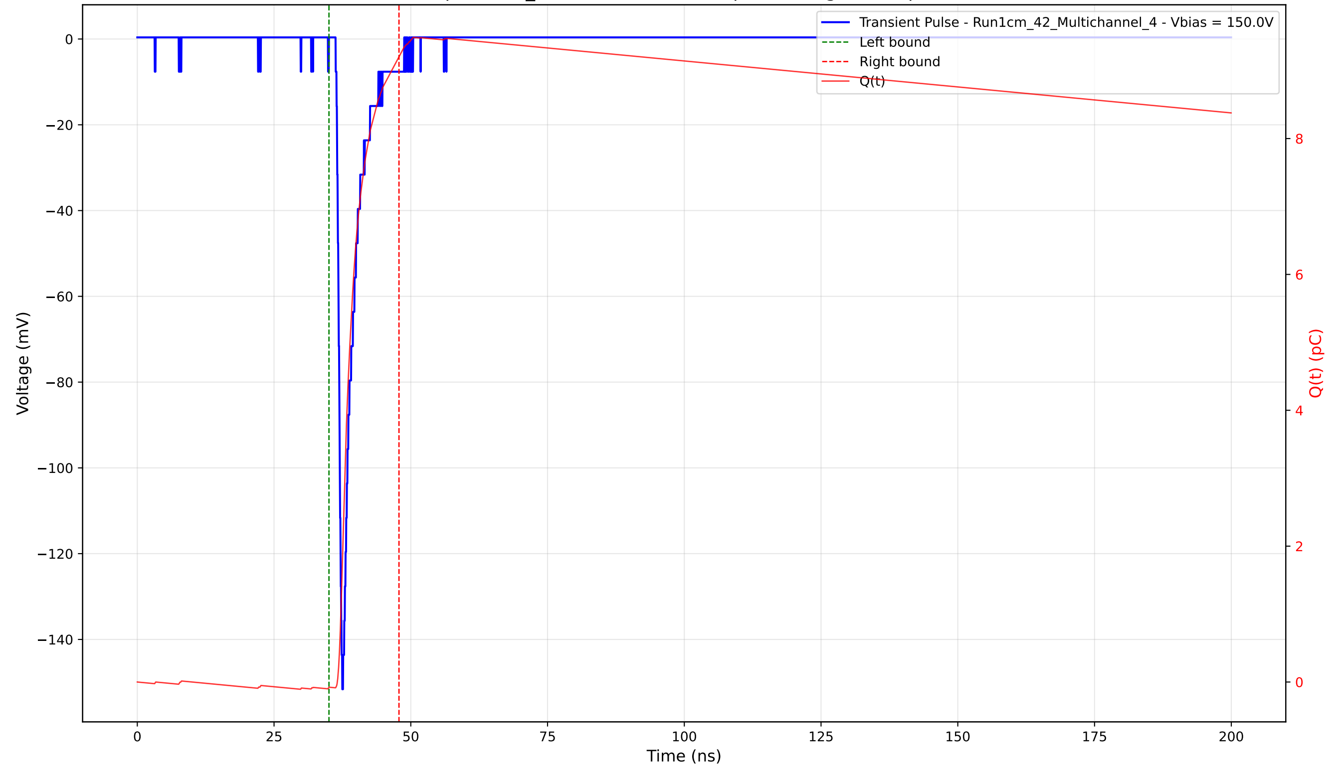
Transient Pulse - Sample: 1cm_42 - Position: 1775.0 \mu\text{m} - Charge: 9.28 pC - Rise Time: 0.92 ns
