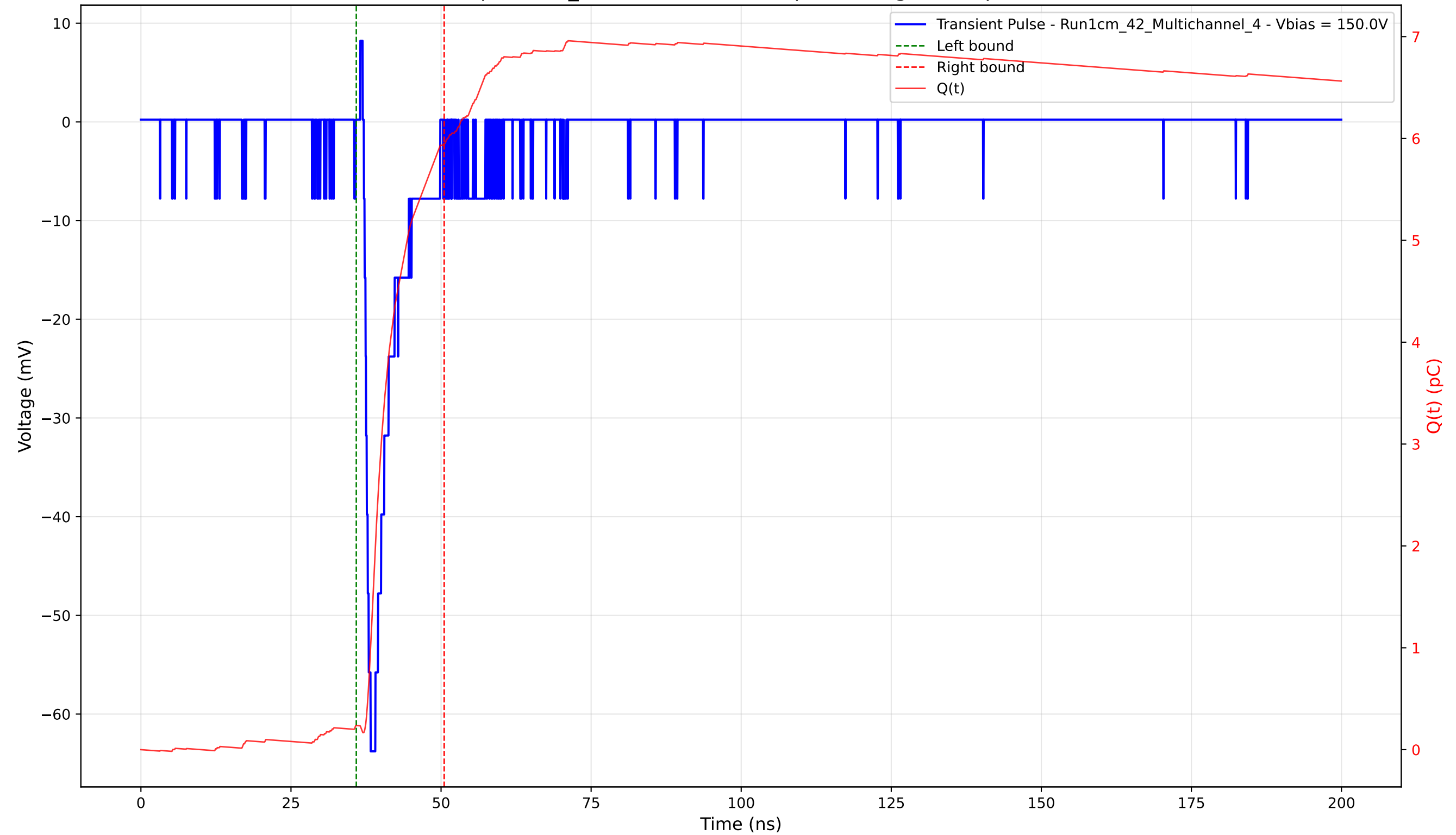
Transient Pulse - Sample: 1cm_42 - Position: 1330.0 \mu\text{m} - Charge: 5.71 pC - Rise Time: 1.13 ns
