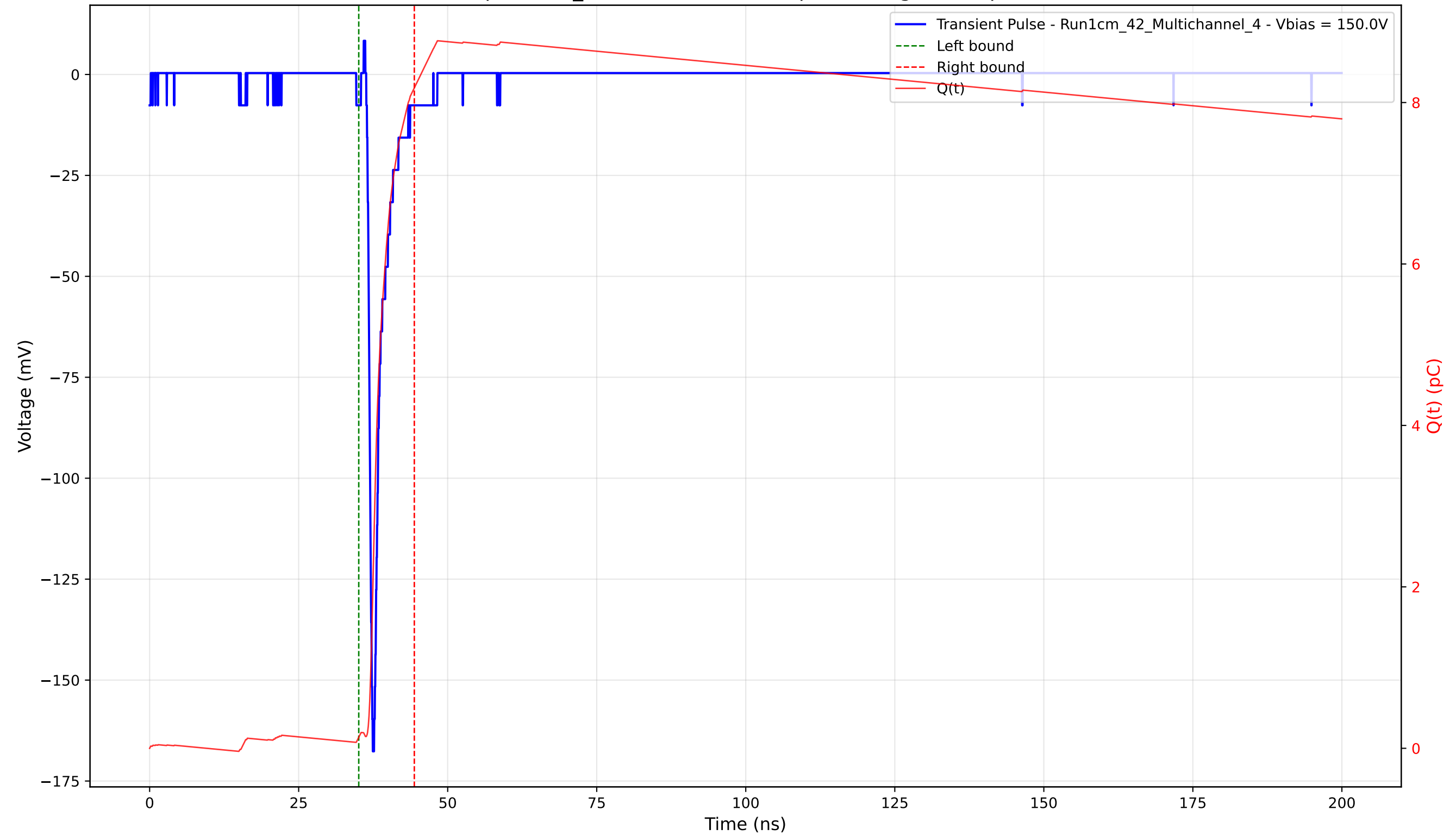
Transient Pulse - Sample: 1cm_42 - Position: 3145.0 \mu\text{m} - Charge: 8.04 pC - Rise Time: 0.75 ns
