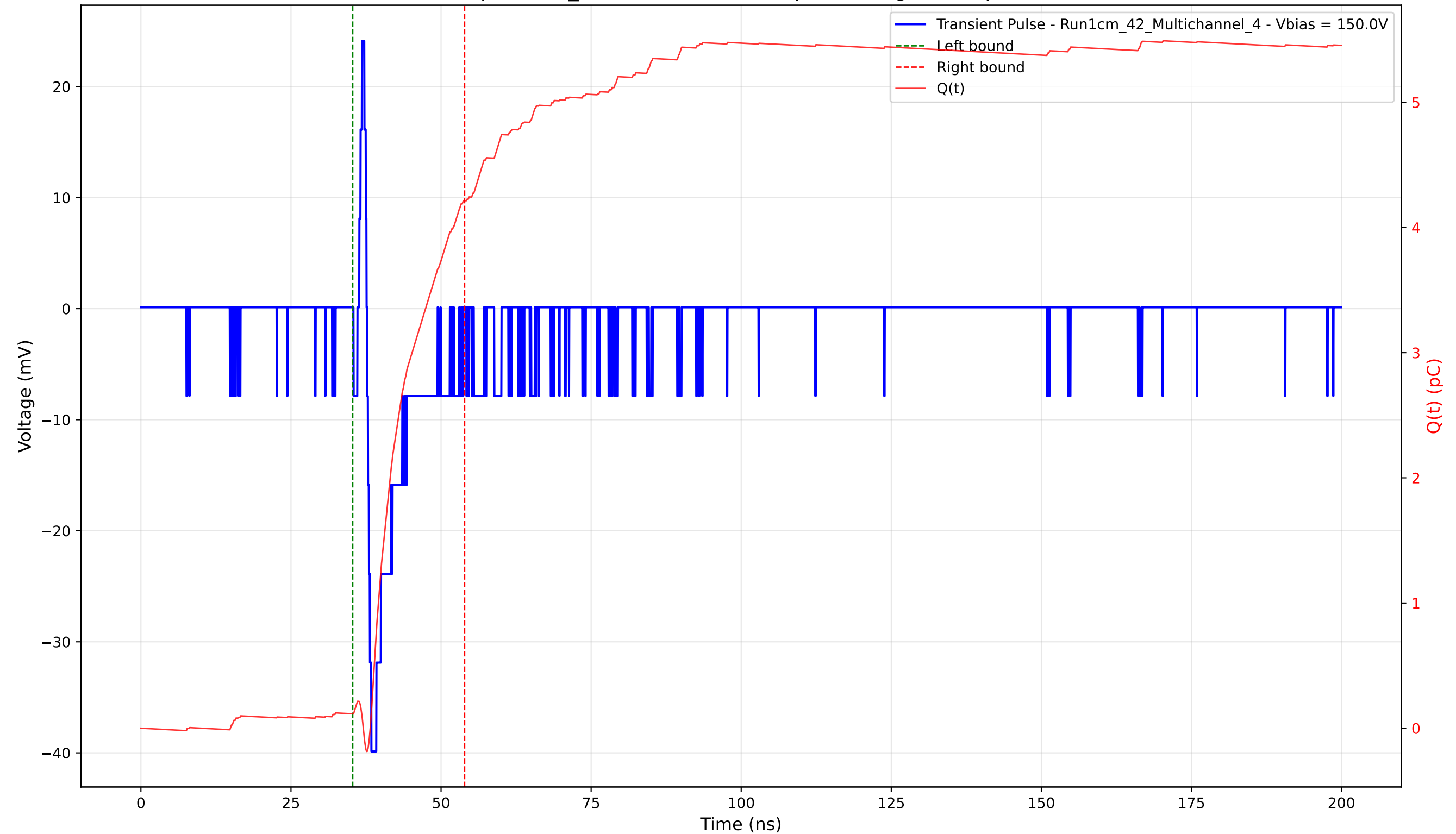
Transient Pulse - Sample: 1cm_42 - Position: 4175.0 \mu\text{m} - Charge: 4.10 pC - Rise Time: 0.70 ns
