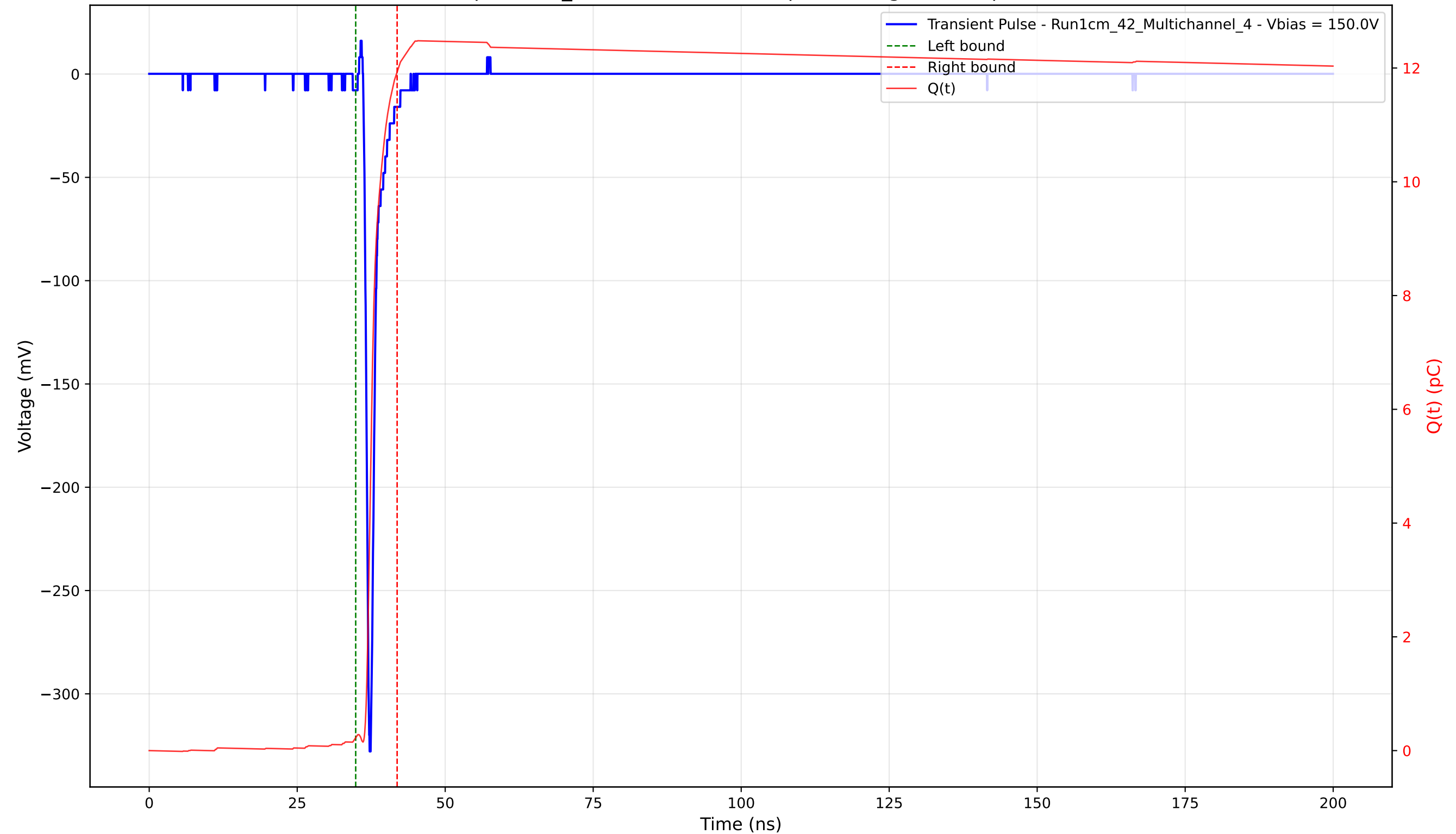
Transient Pulse - Sample: 1cm_42 - Position: 2915.0 \mu\text{m} - Charge: 11.70 pC - Rise Time: 0.75 ns
