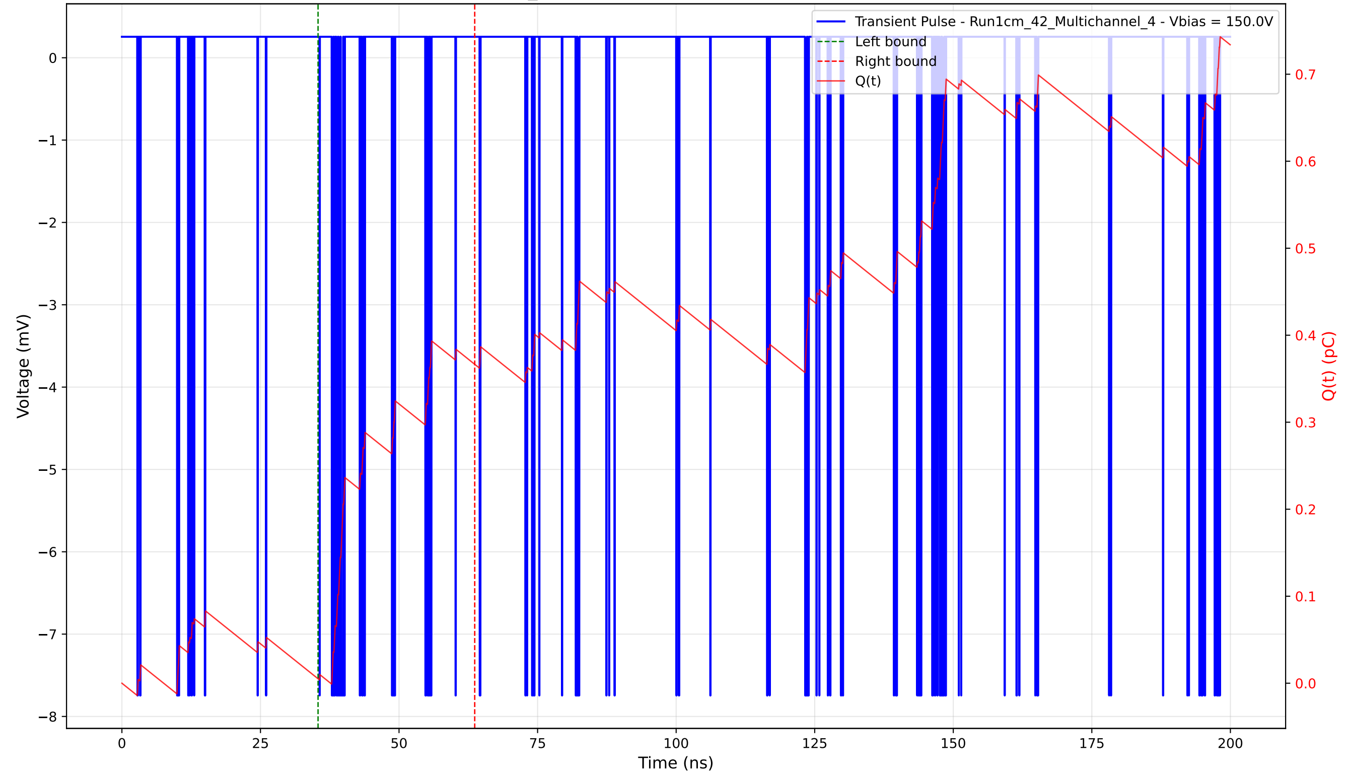
Transient Pulse - Sample: 1cm_42 - Position: 15.0 \mu\text{m} - Charge: 0.36 pC - Rise Time: 0.04 ns
