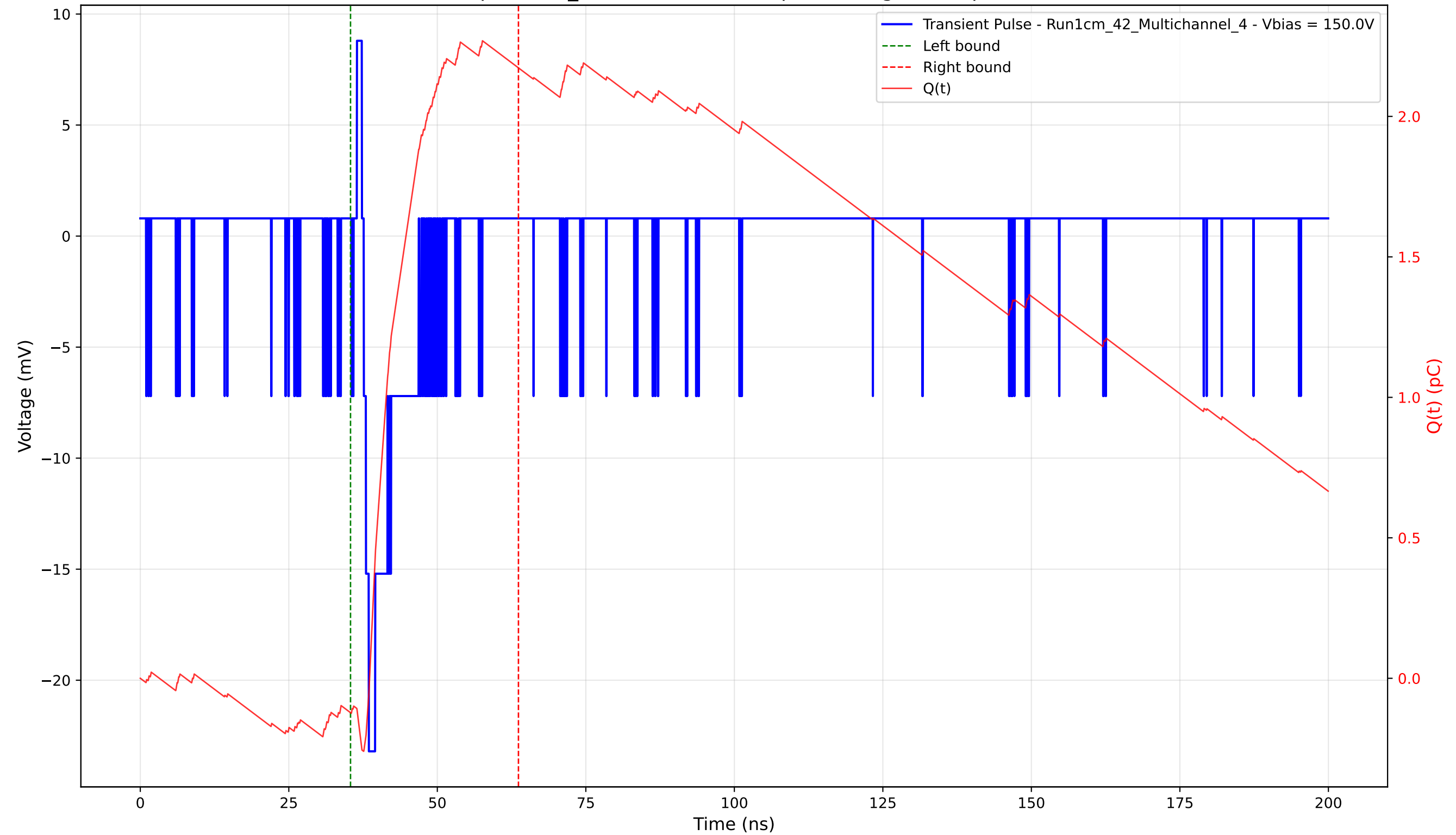
Transient Pulse - Sample: 1cm_42 - Position: 290.0 \mu\text{m} - Charge: 2.30 pC - Rise Time: 0.87 ns
