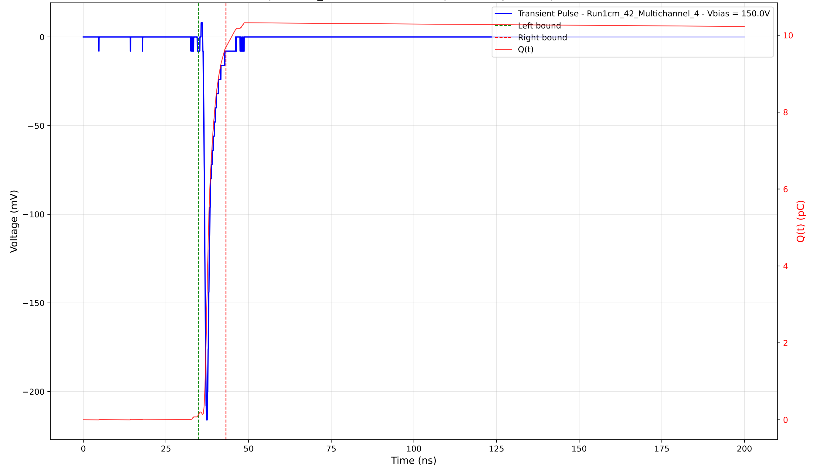
Transient Pulse - Sample: 1cm_42 - Position: 1990.0 \mu\text{m} - Charge: 9.55 pC - Rise Time: 0.78 ns
