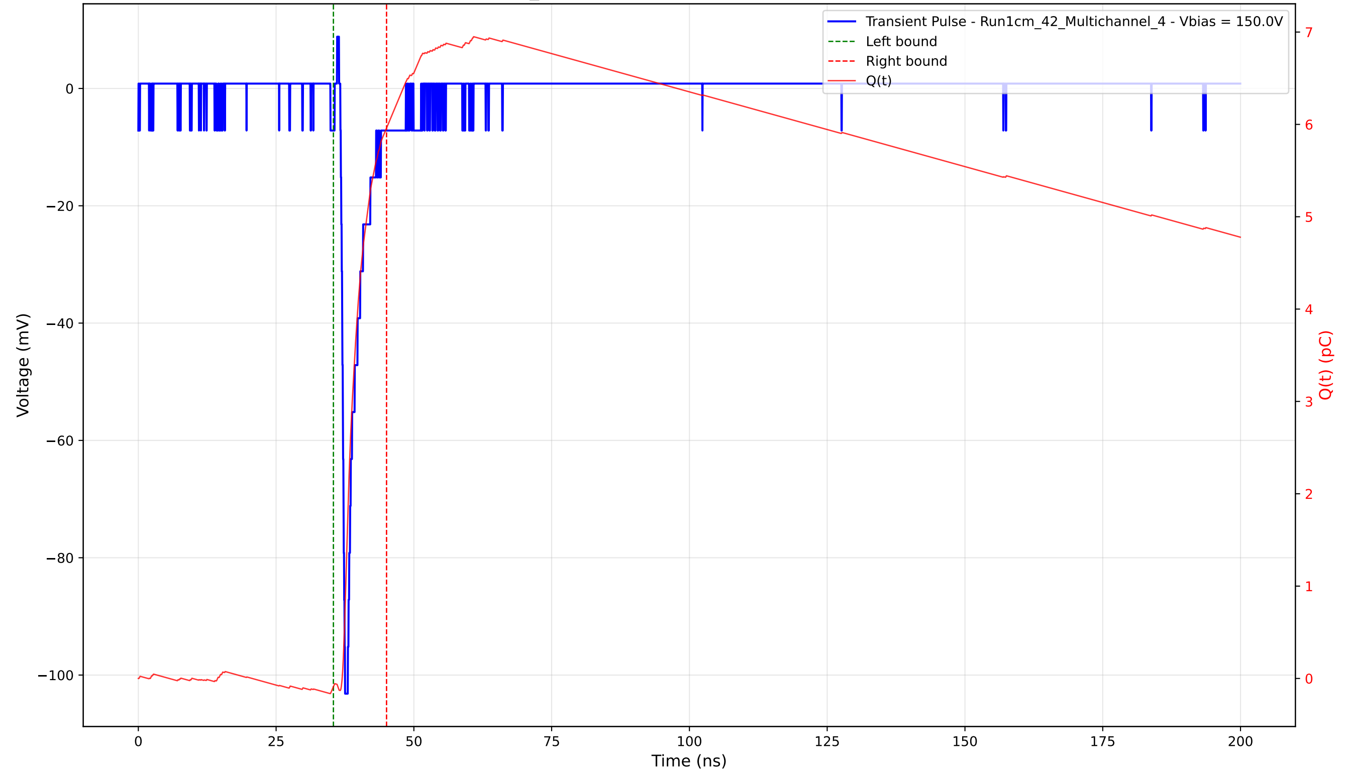
Transient Pulse - Sample: 1cm_42 - Position: 3395.0 \mu\text{m} - Charge: 6.05 pC - Rise Time: 0.70 ns
