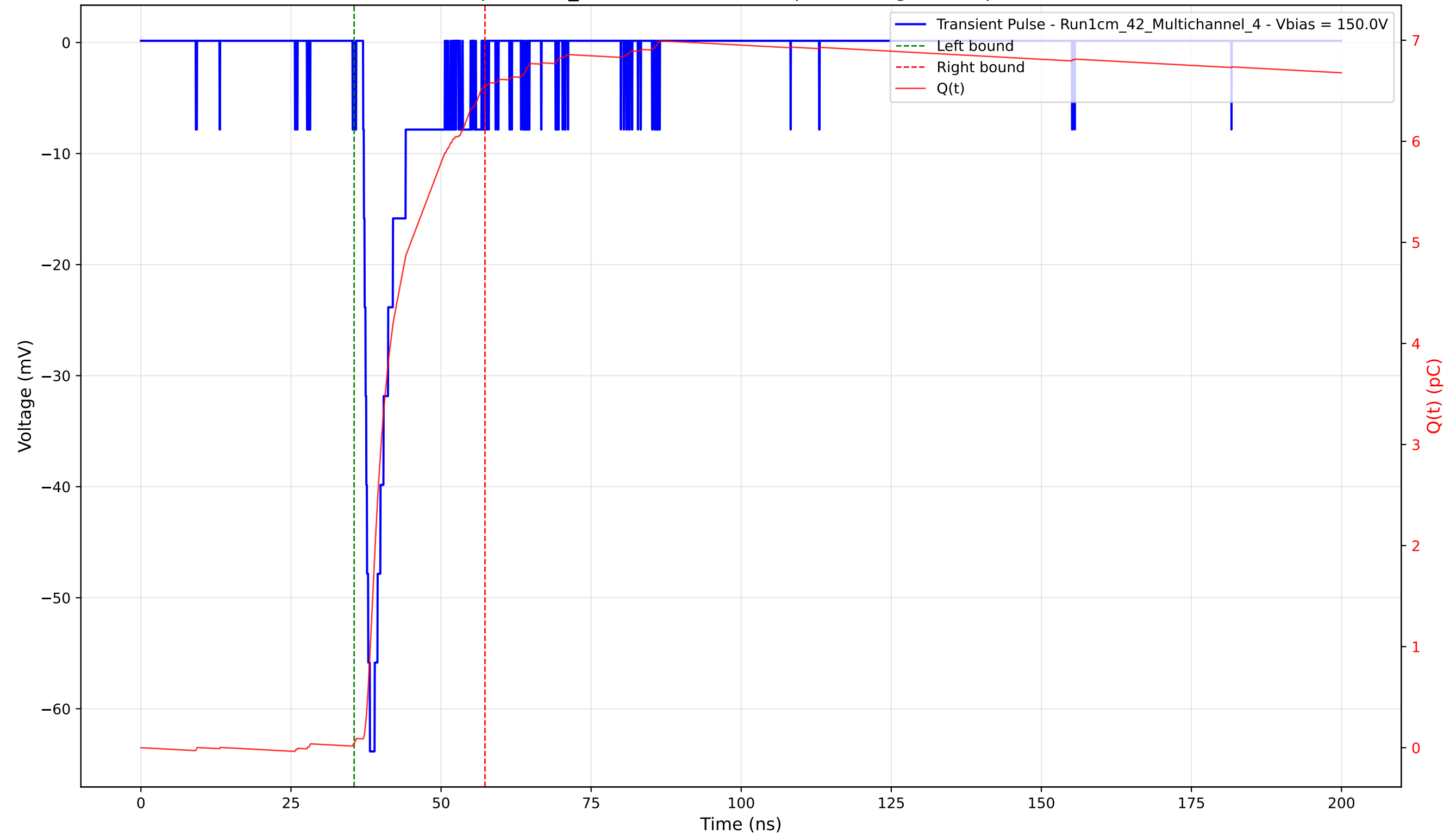
Transient Pulse - Sample: 1cm_42 - Position: 1395.0 \mu\text{m} - Charge: 6.50 pC - Rise Time: 1.13 ns
