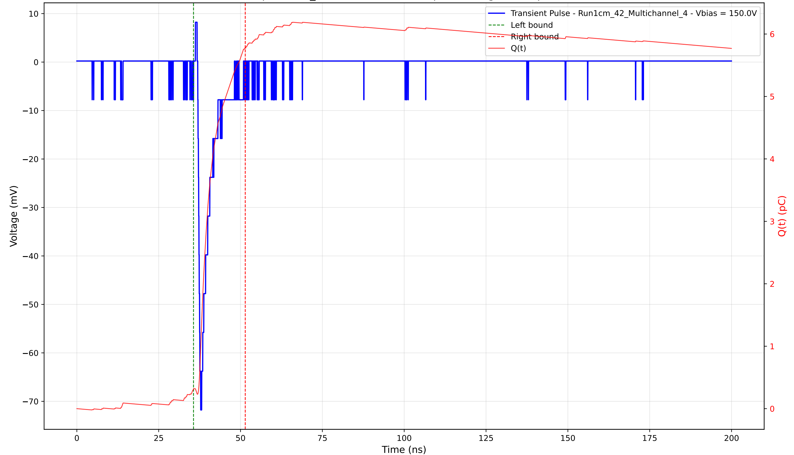
Transient Pulse - Sample: 1cm_42 - Position: 3540.0 \mu\text{m} - Charge: 5.46 pC - Rise Time: 0.88 ns
