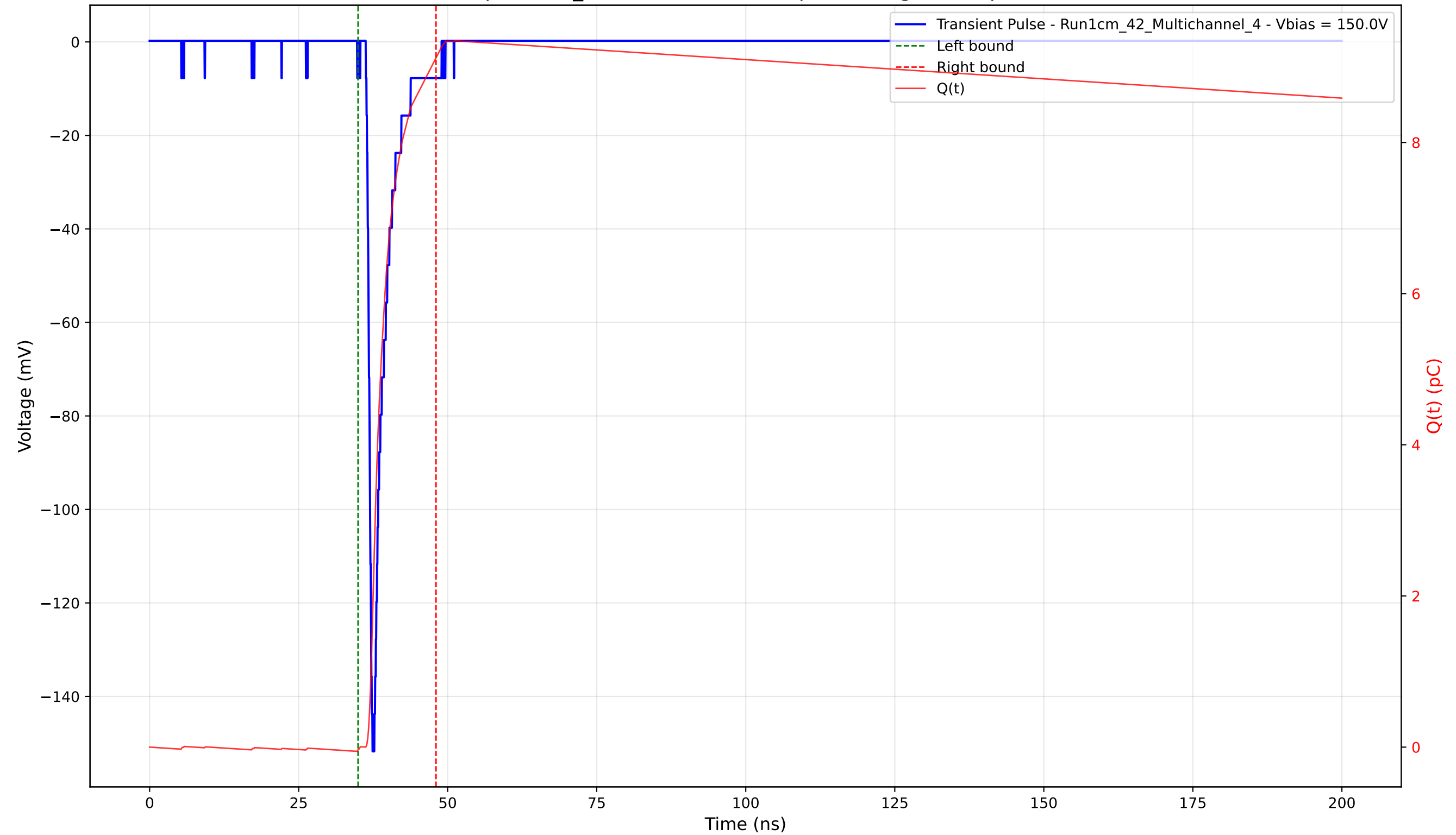
Transient Pulse - Sample: 1cm_42 - Position: 1835.0 \mu\text{m} - Charge: 9.16 pC - Rise Time: 0.88 ns
