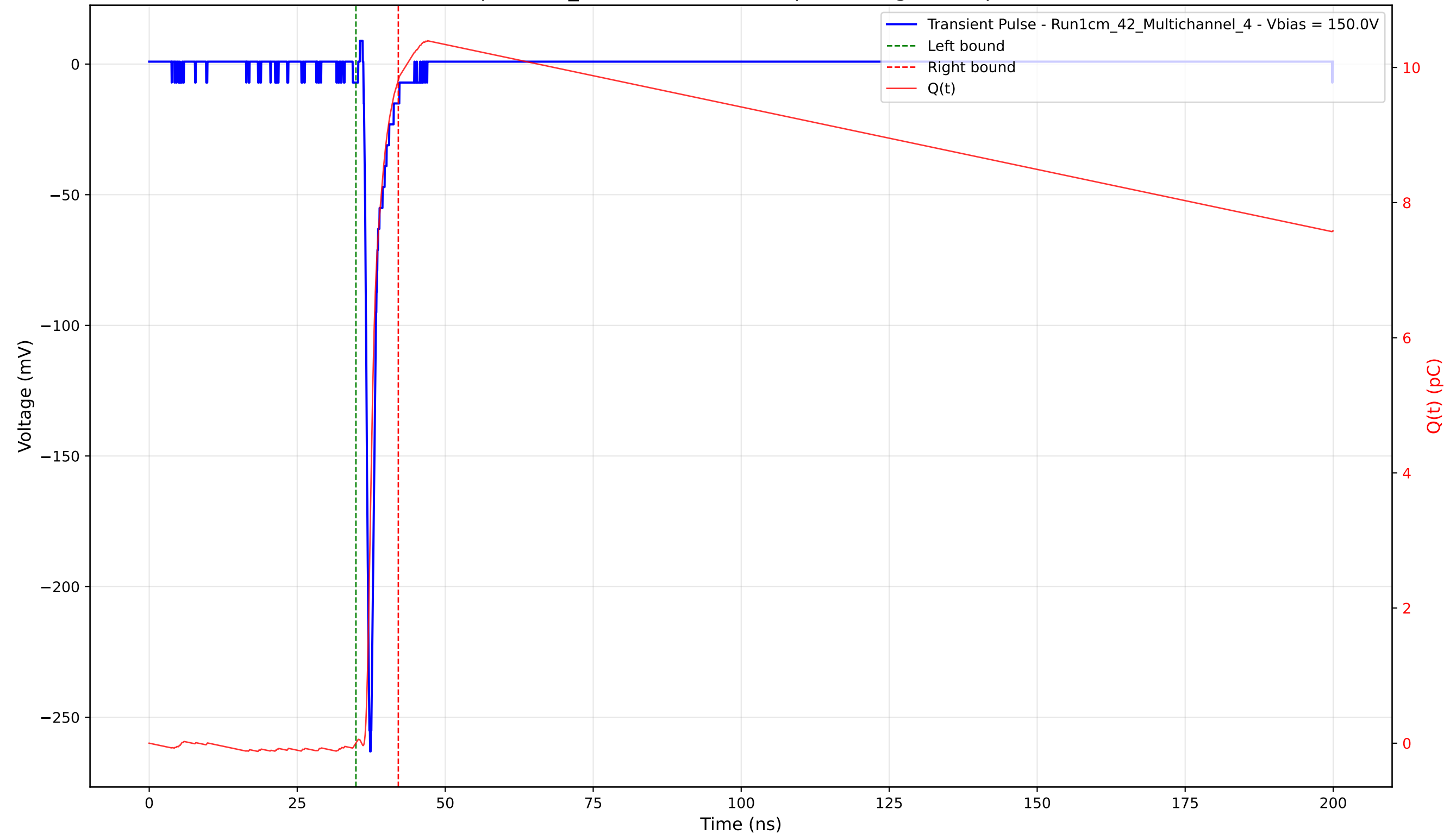
Transient Pulse - Sample: 1cm_42 - Position: 2975.0 \mu\text{m} - Charge: 9.81 pC - Rise Time: 0.77 ns
