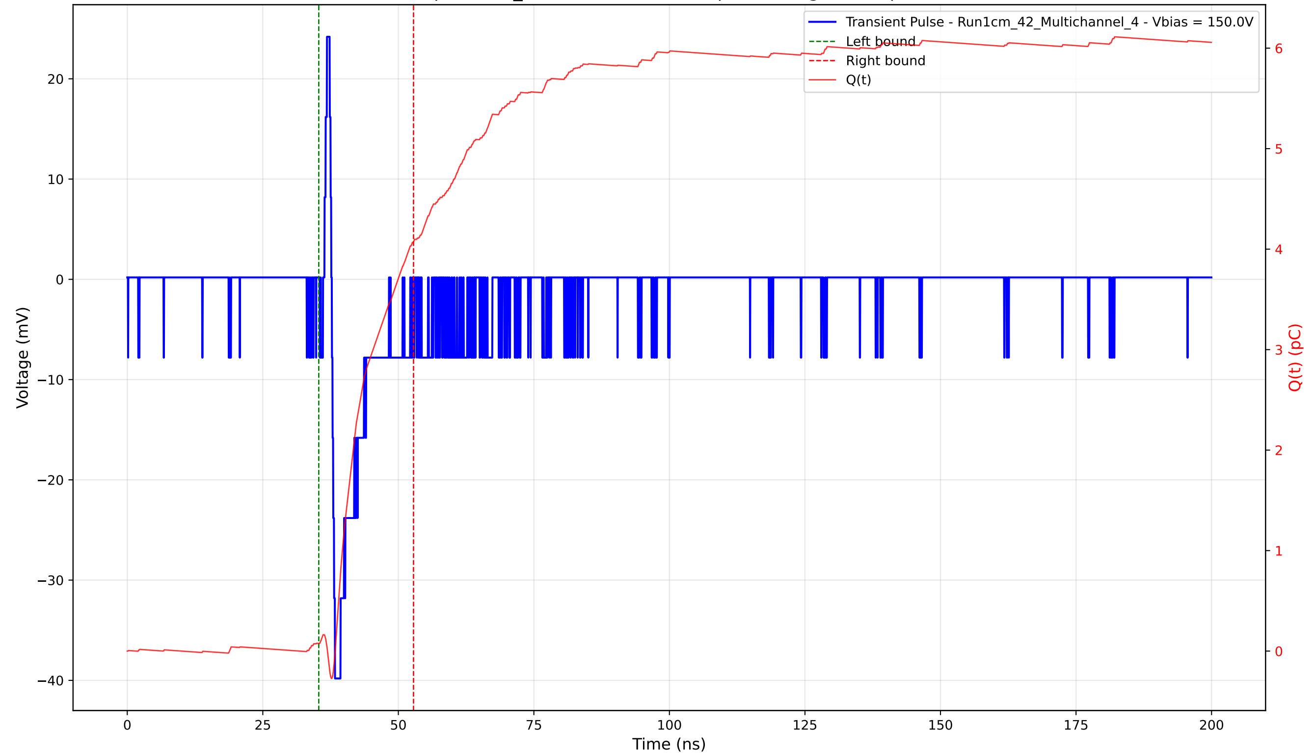
Transient Pulse - Sample: 1cm_42 - Position: 4310.0 \mu\text{m} - Charge: 3.99 pC - Rise Time: 0.58 ns
