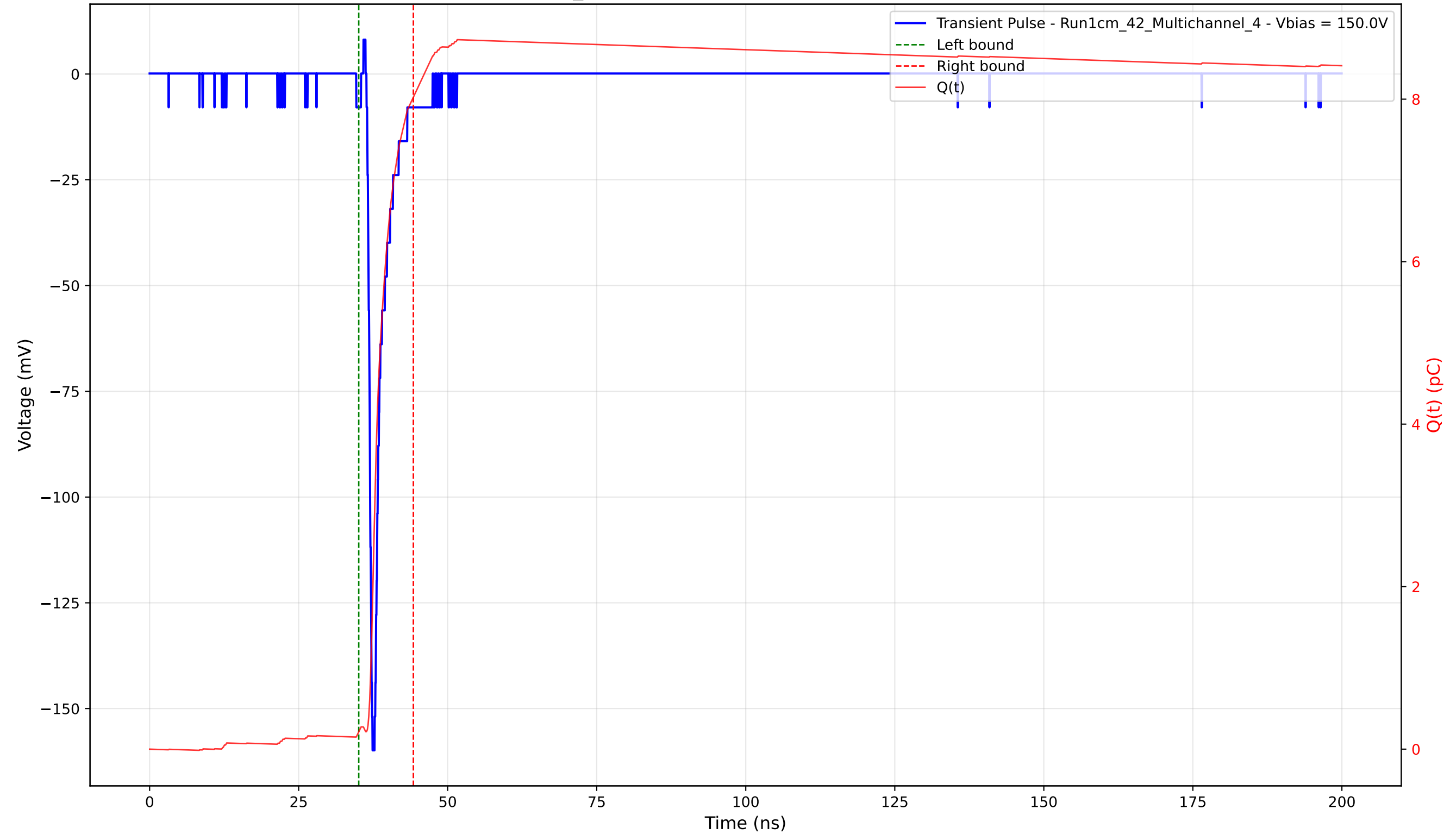
Transient Pulse - Sample: 1cm_42 - Position: 3150.0 \mu\text{m} - Charge: 7.81 pC - Rise Time: 0.80 ns
