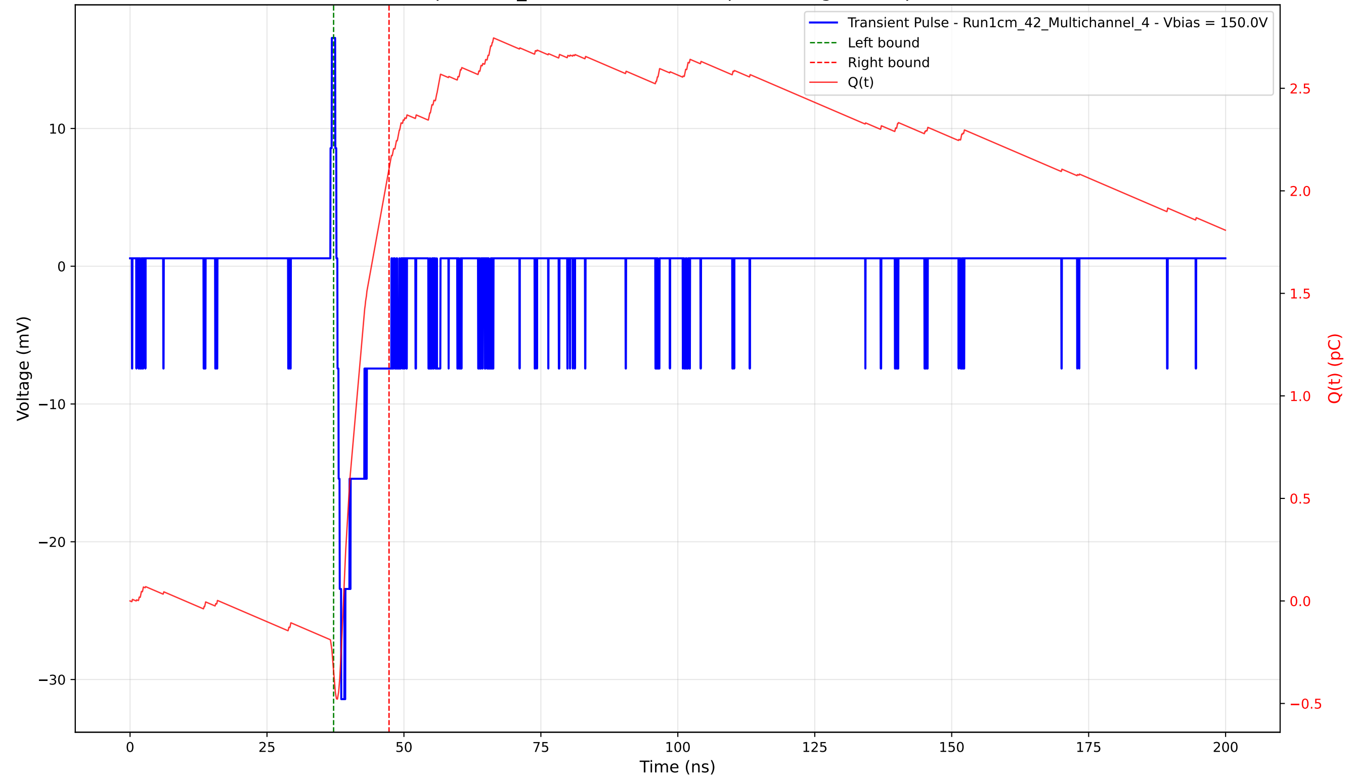
Transient Pulse - Sample: 1cm_42 - Position: 4575.0 \mu\text{m} - Charge: 2.45 pC - Rise Time: 0.71 ns
