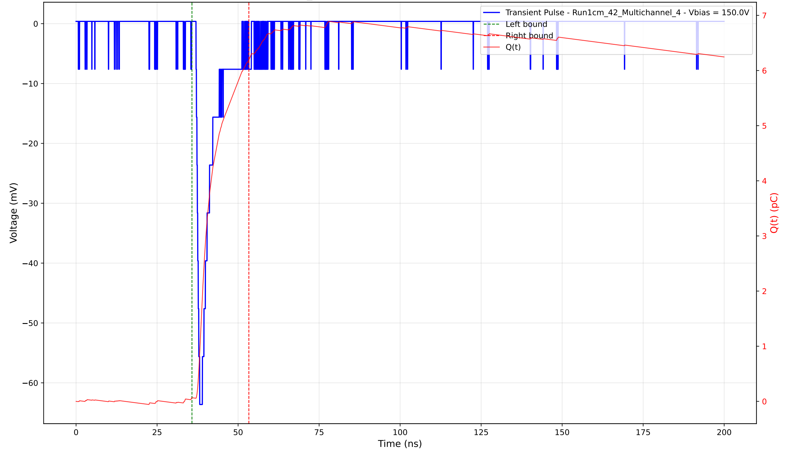
Transient Pulse - Sample: 1cm_42 - Position: 1385.0 \mu\text{m} - Charge: 6.12 pC - Rise Time: 1.13 ns
