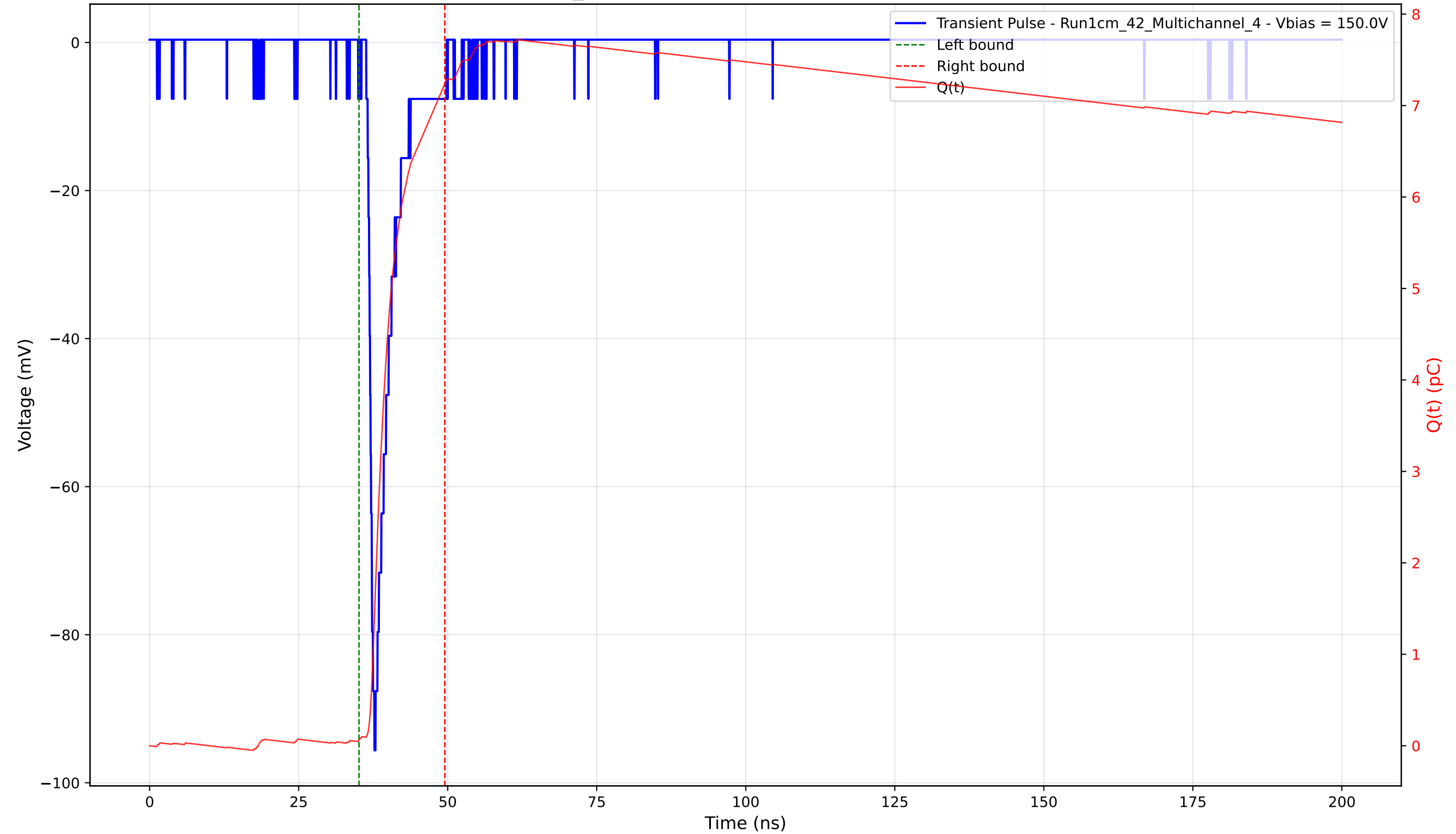
Transient Pulse - Sample: 1cm_42 - Position: 1590.0 \mu\text{m} - Charge: 7.17 pC - Rise Time: 0.91 ns
