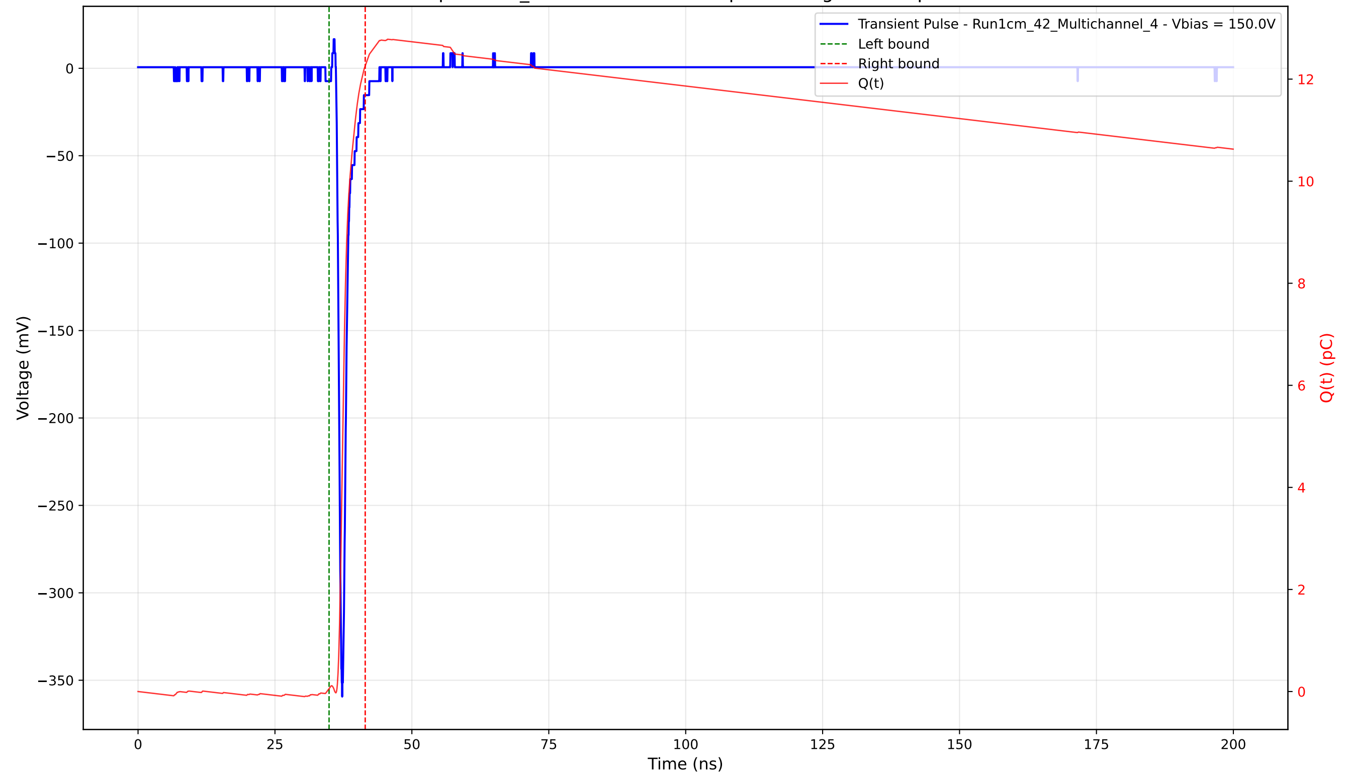
Transient Pulse - Sample: 1cm_42 - Position: 2890.0 \mu\text{m} - Charge: 12.20 pC - Rise Time: 0.78 ns
