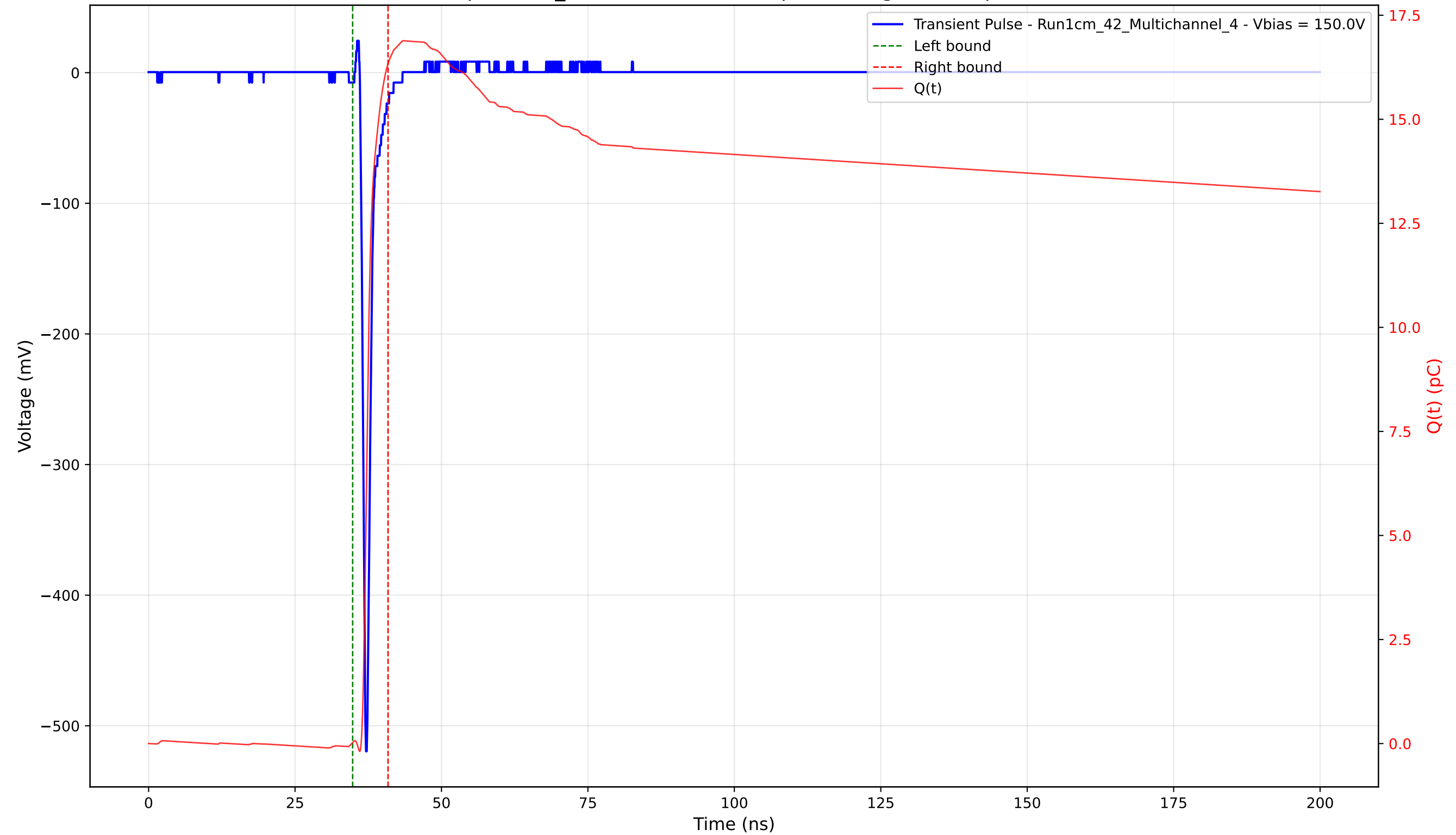
Transient Pulse - Sample: 1cm_42 - Position: 2360.0 \mu\text{m} - Charge: 16.31 pC - Rise Time: 0.72 ns
