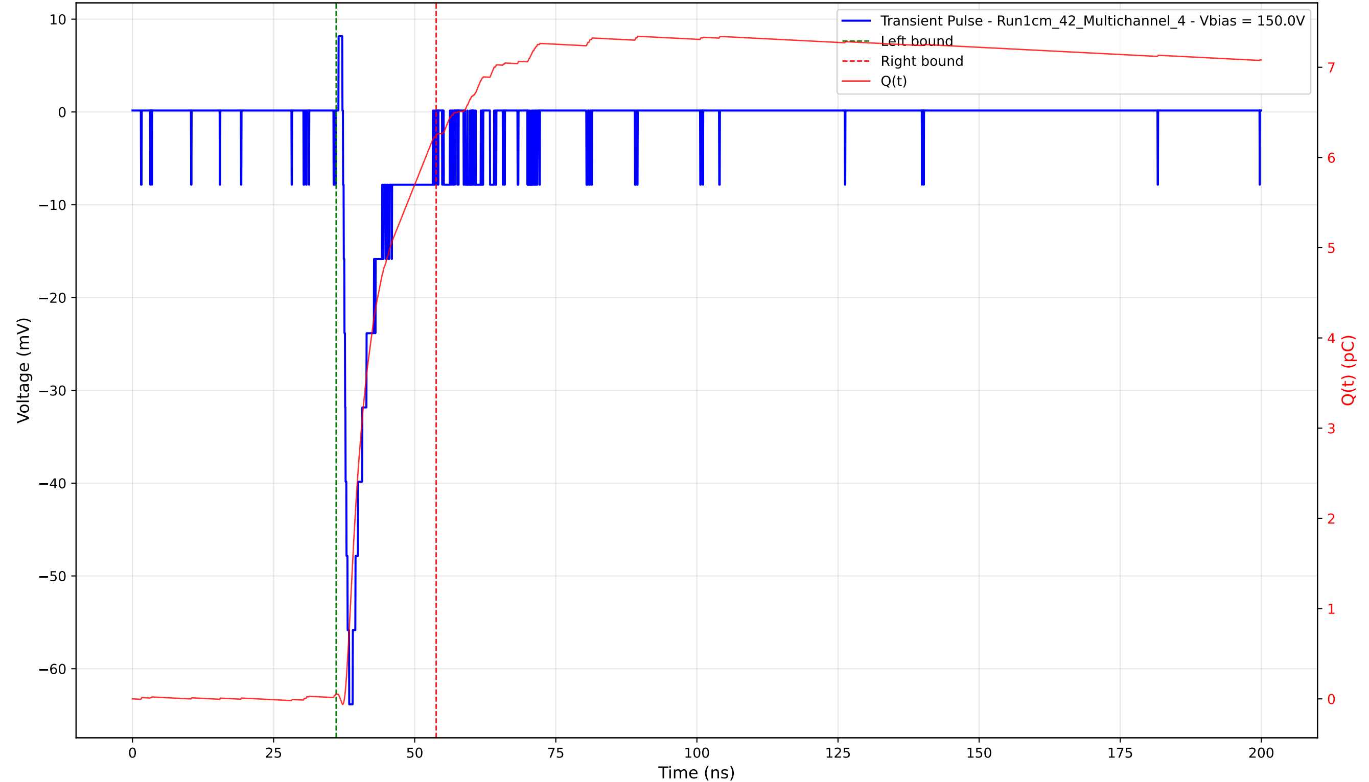
Transient Pulse - Sample: 1cm_42 - Position: 1195.0 \mu\text{m} - Charge: 6.19 pC - Rise Time: 1.09 ns
