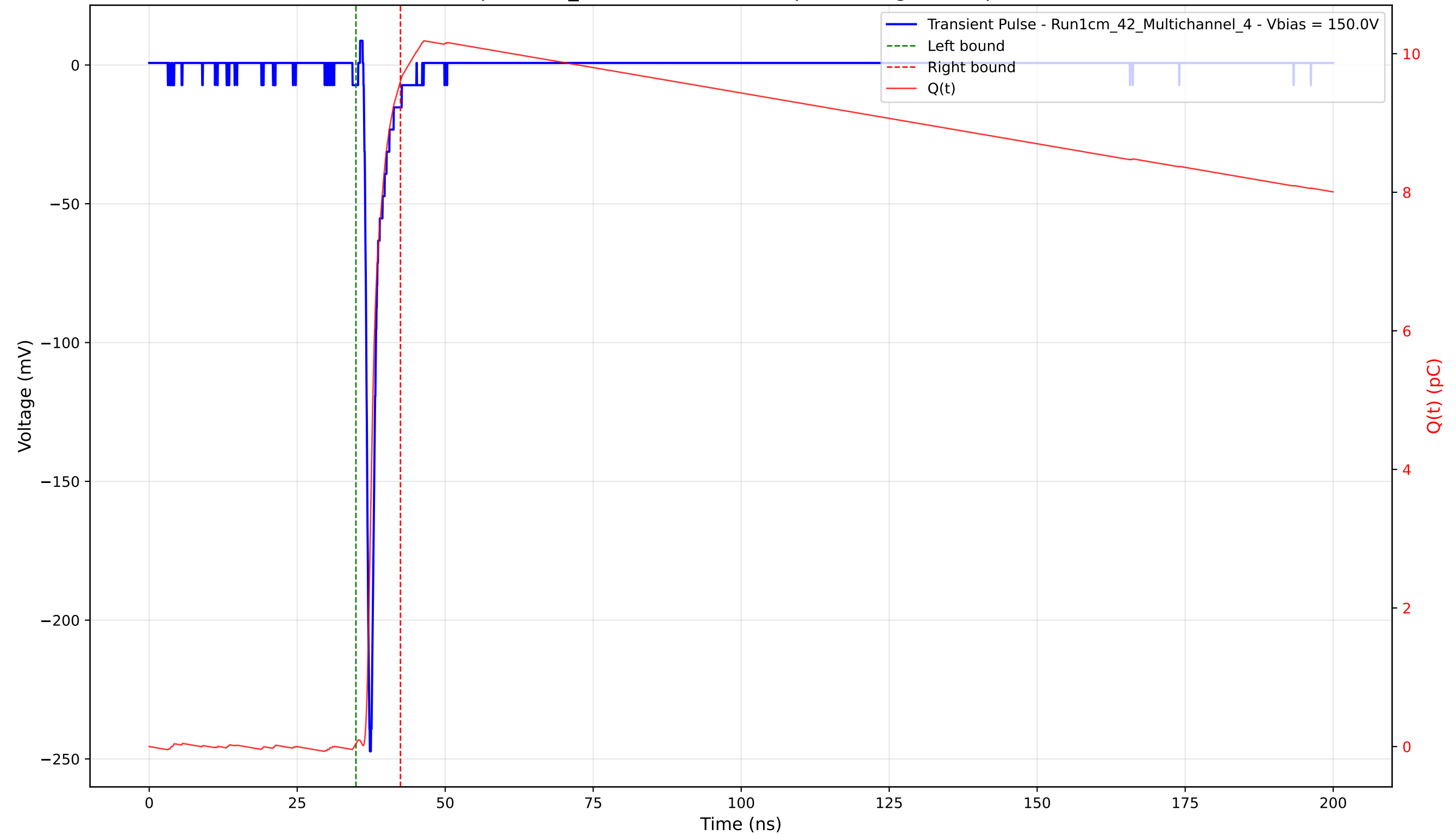
Transient Pulse - Sample: 1cm_42 - Position: 2990.0 \mu\text{m} - Charge: 9.56 pC - Rise Time: 0.79 ns
