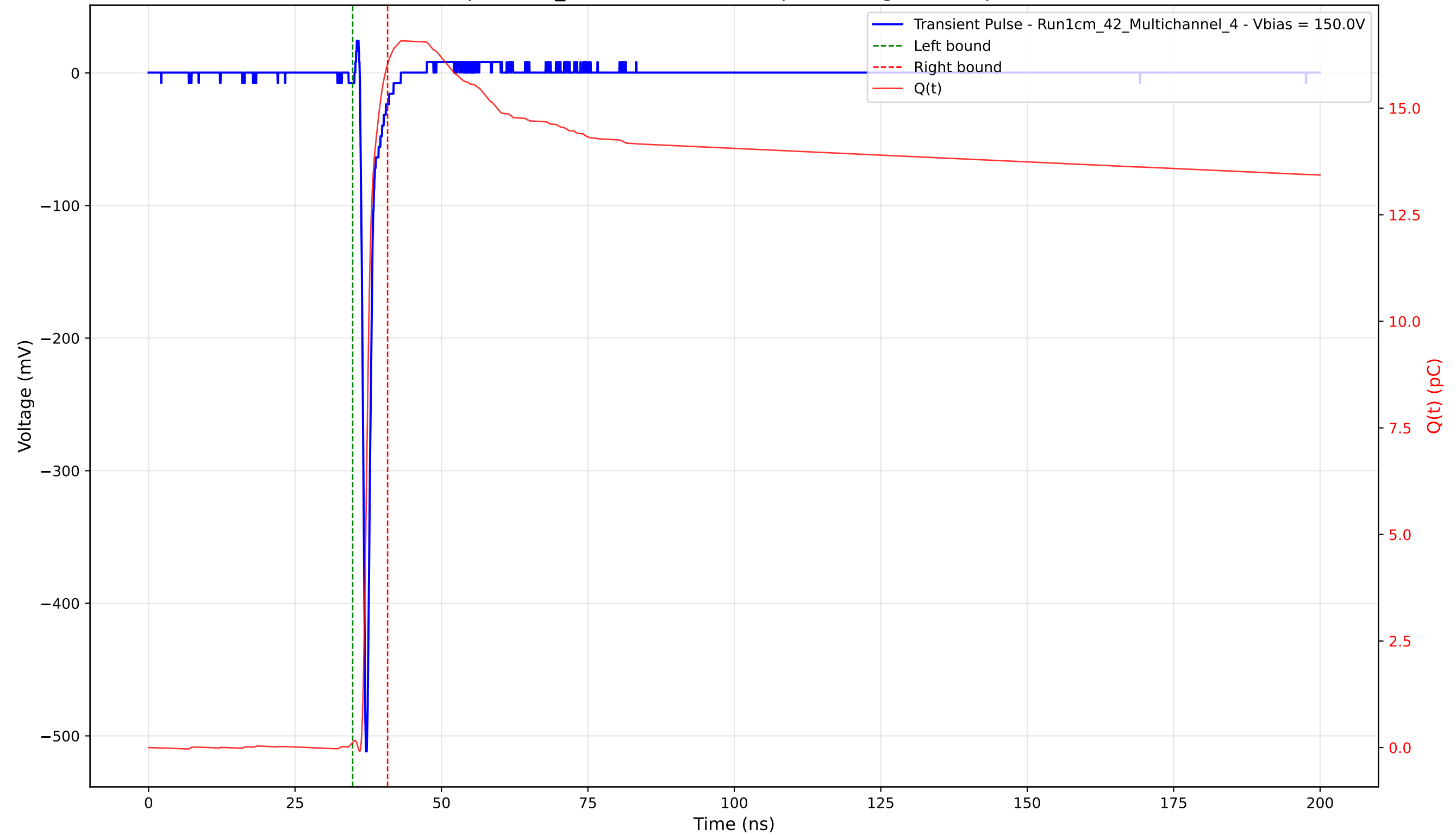
Transient Pulse - Sample: 1cm_42 - Position: 2655.0 \mu\text{m} - Charge: 15.91 pC - Rise Time: 0.72 ns
