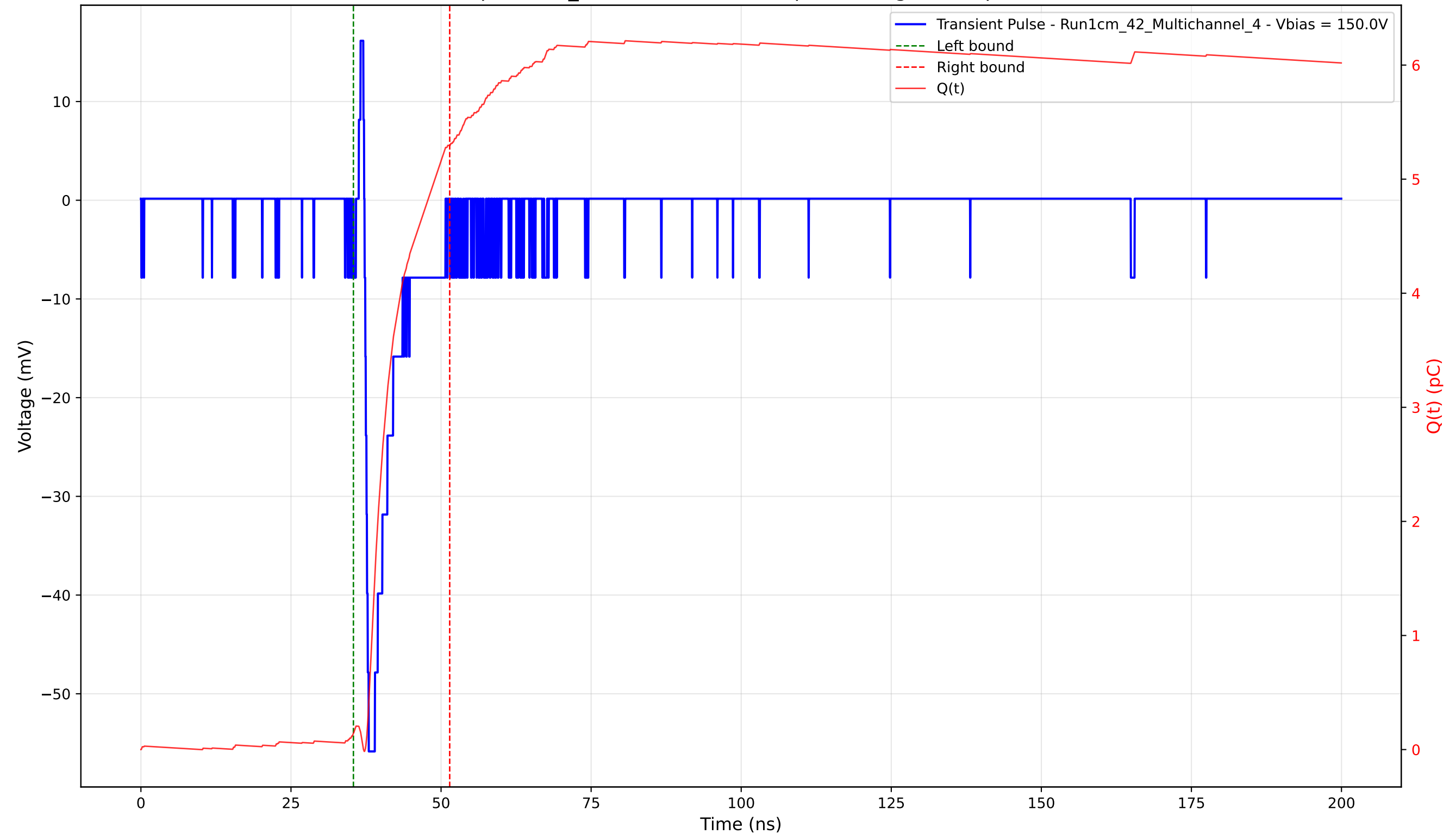
Transient Pulse - Sample: 1cm_42 - Position: 3750.0 \mu\text{m} - Charge: 5.15 pC - Rise Time: 0.69 ns
