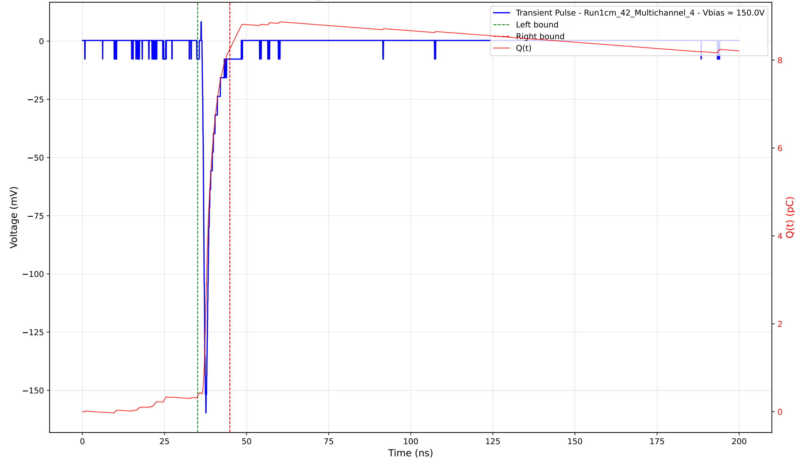
Transient Pulse - Sample: 1cm_42 - Position: 3190.0 \mu\text{m} - Charge: 7.90 pC - Rise Time: 0.88 ns
