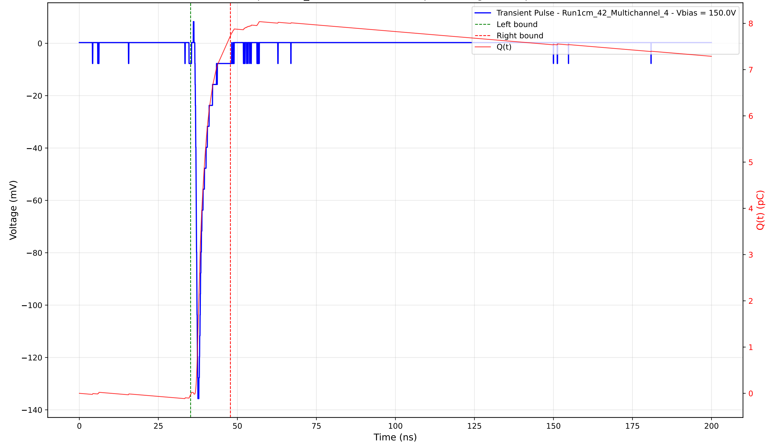
Transient Pulse - Sample: 1cm_42 - Position: 3310.0 \mu\text{m} - Charge: 7.76 pC - Rise Time: 0.81 ns
