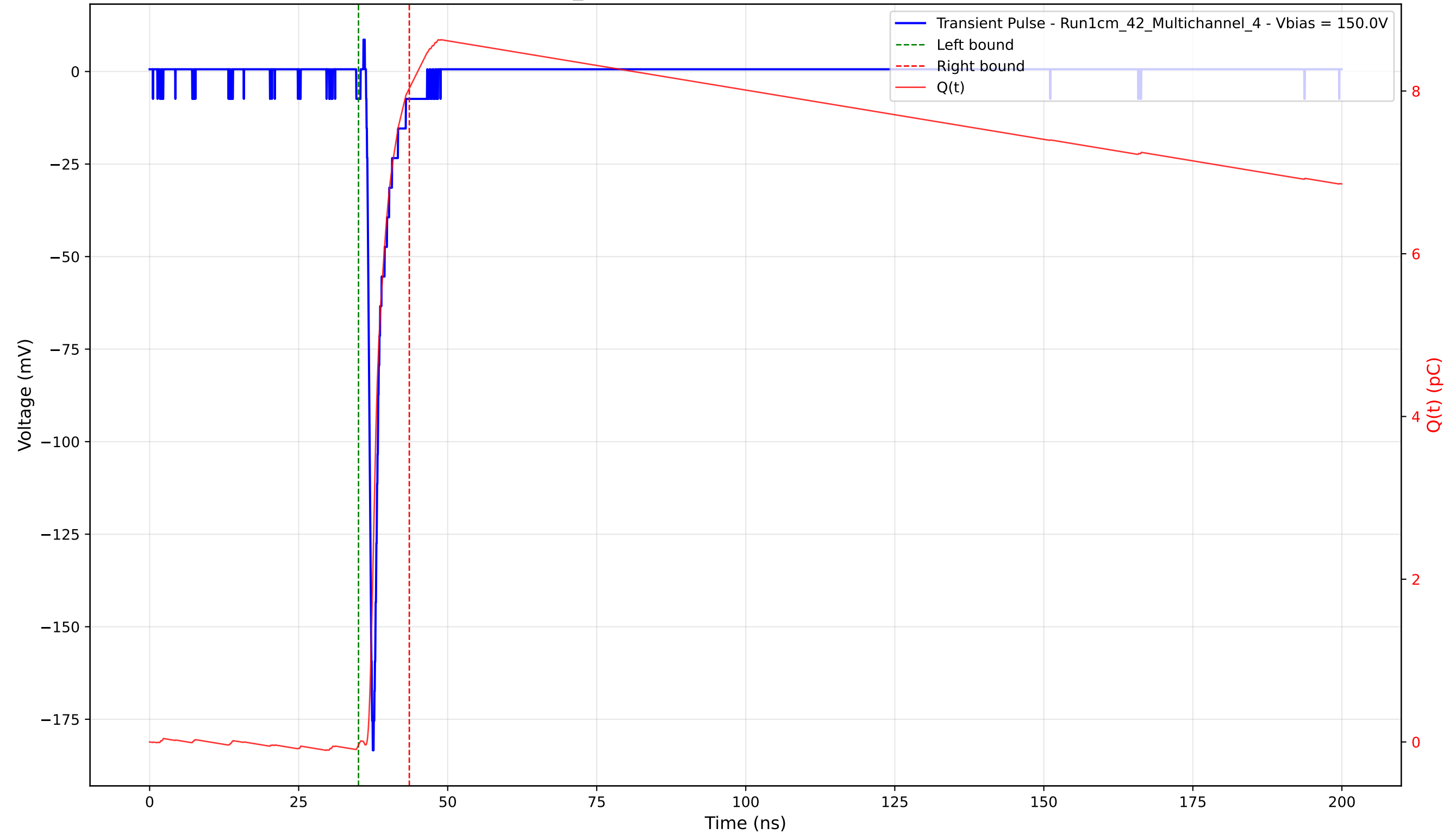
Transient Pulse - Sample: 1cm_42 - Position: 3100.0 \mu\text{m} - Charge: 8.07 pC - Rise Time: 0.81 ns
