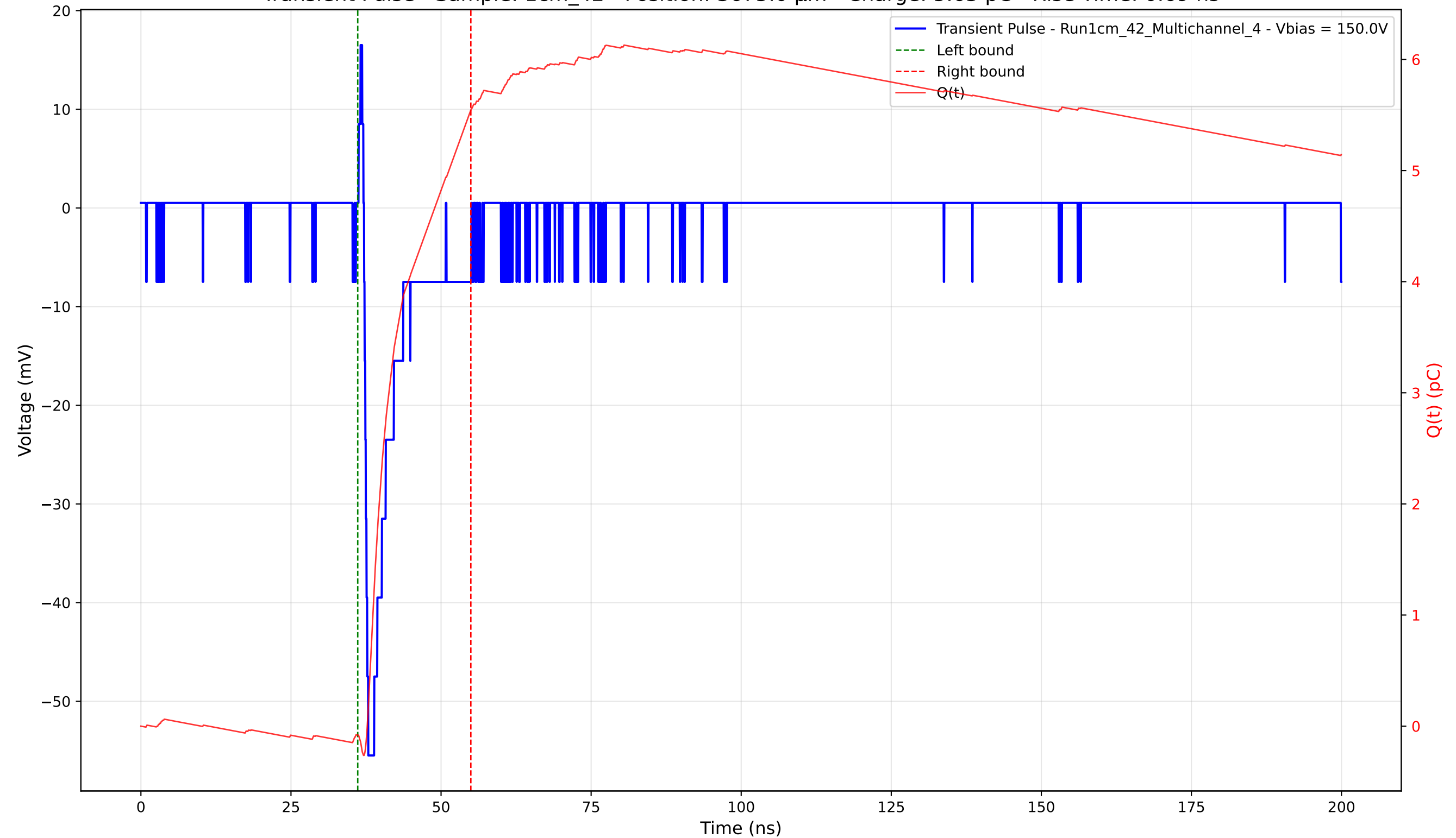
Transient Pulse - Sample: 1cm_42 - Position: 3675.0 \mu\text{m} - Charge: 5.63 pC - Rise Time: 0.69 ns
