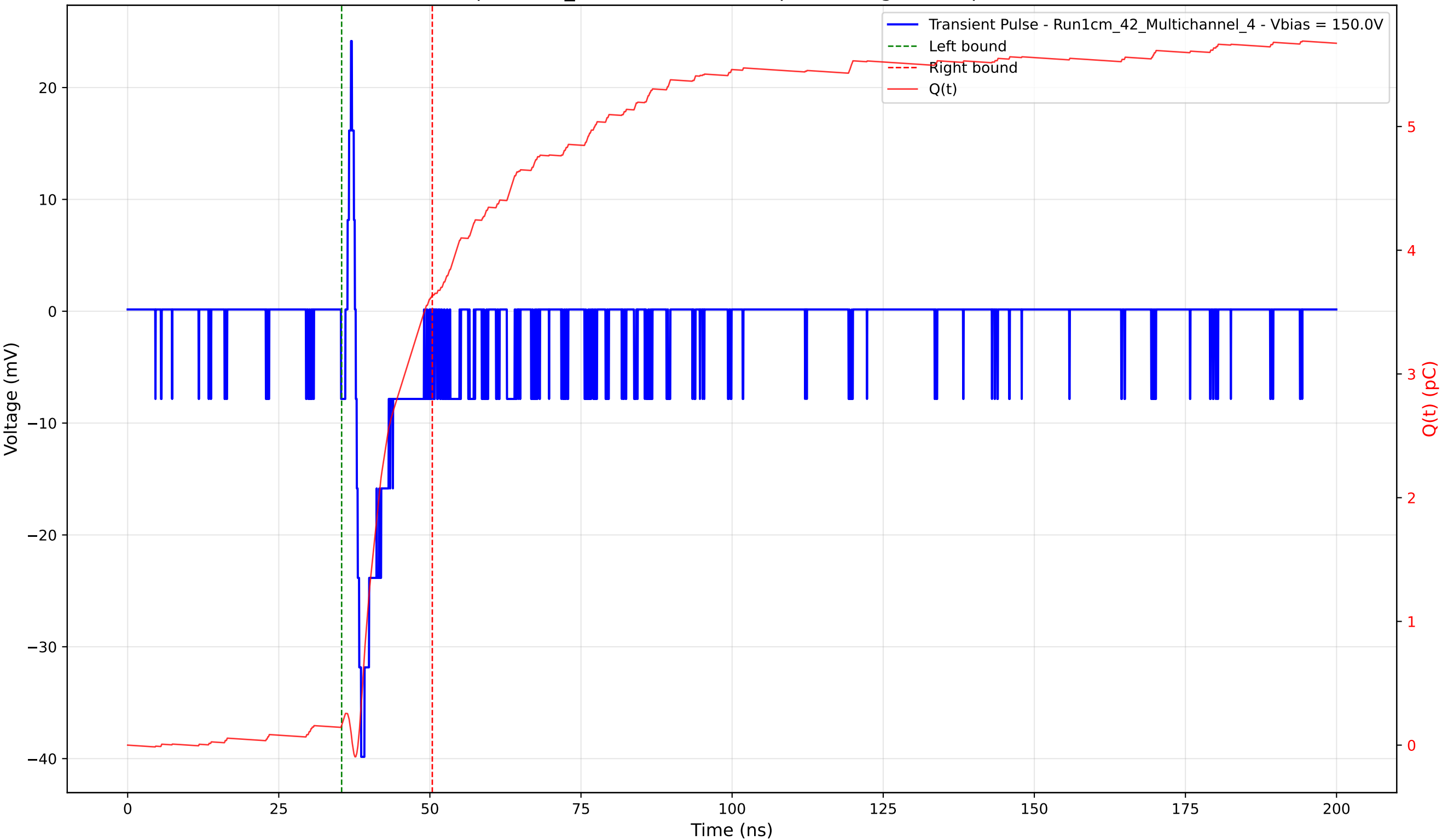
Transient Pulse - Sample: 1cm_42 - Position: 535.0 \mu\text{m} - Charge: 3.48 pC - Rise Time: 0.90 ns
