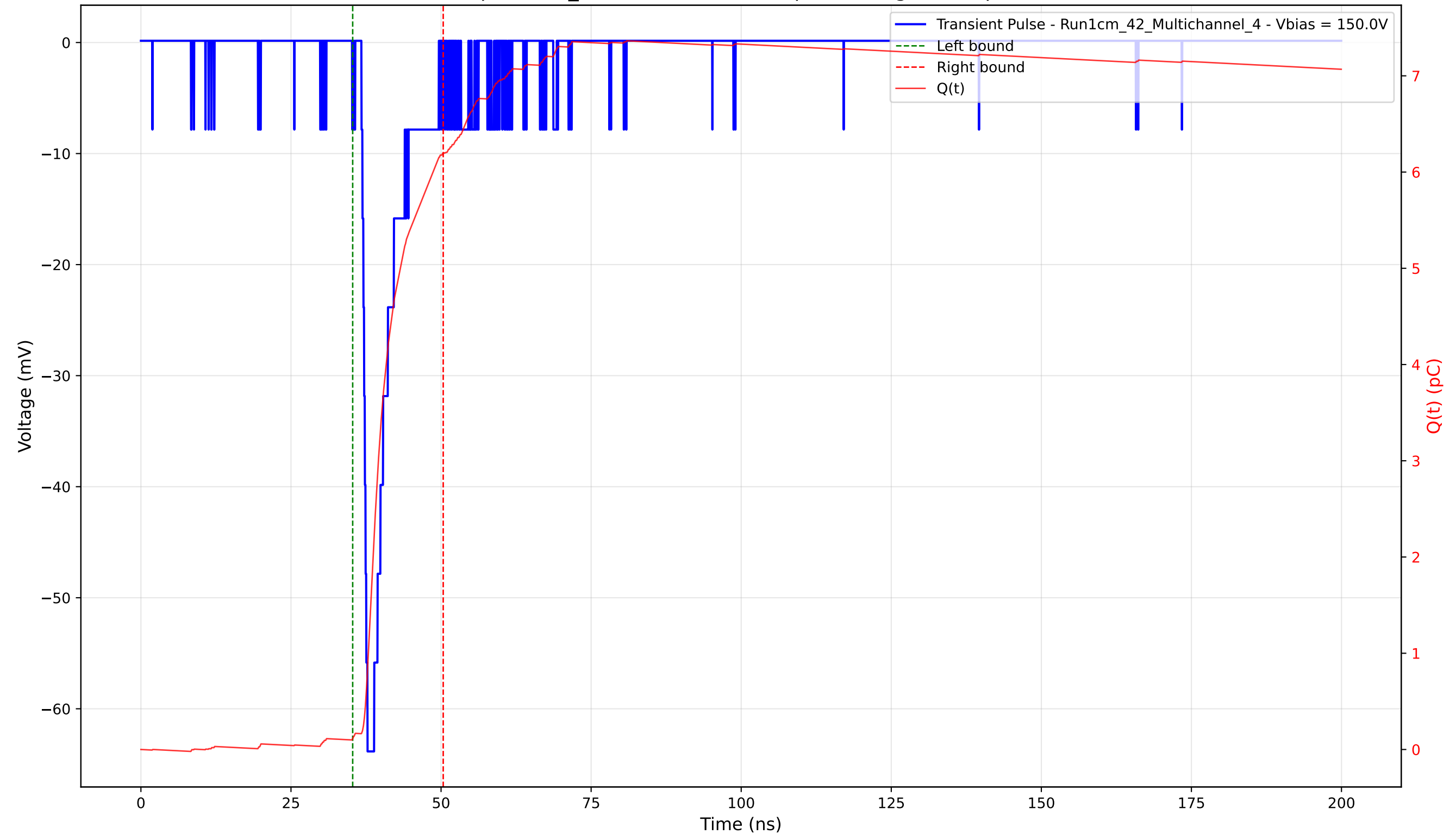
Transient Pulse - Sample: 1cm_42 - Position: 1470.0 \mu\text{m} - Charge: 6.08 pC - Rise Time: 1.01 ns
