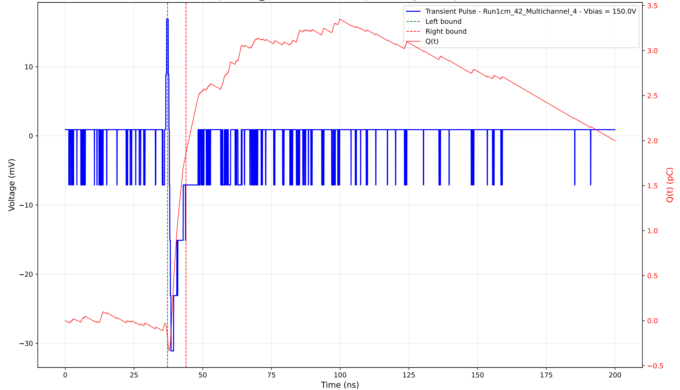
Transient Pulse - Sample: 1cm_42 - Position: 4690.0 \mu\text{m} - Charge: 2.07 pC - Rise Time: 0.63 ns
