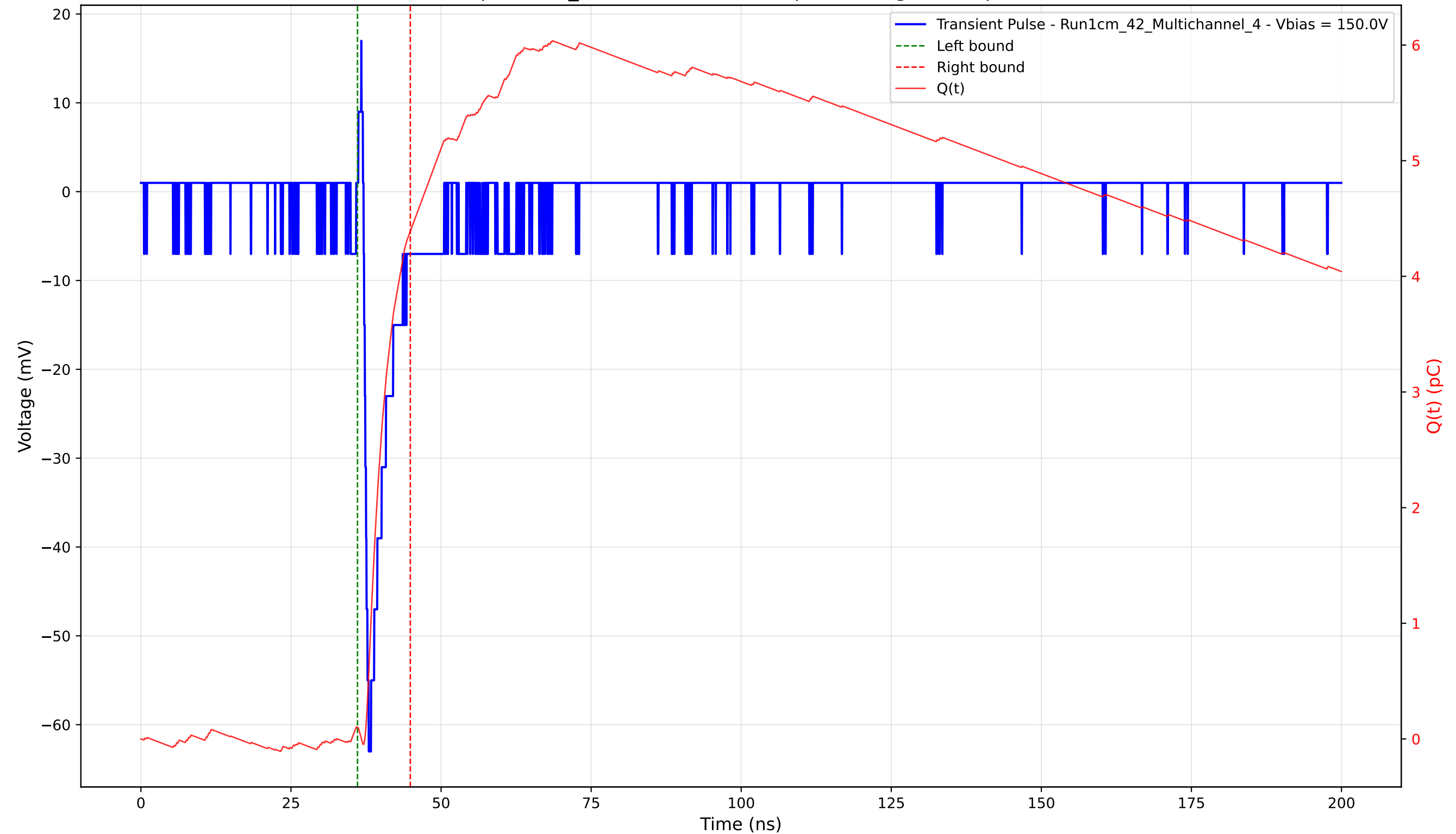
Transient Pulse - Sample: 1cm_42 - Position: 3630.0 \mu\text{m} - Charge: 4.29 pC - Rise Time: 0.84 ns
