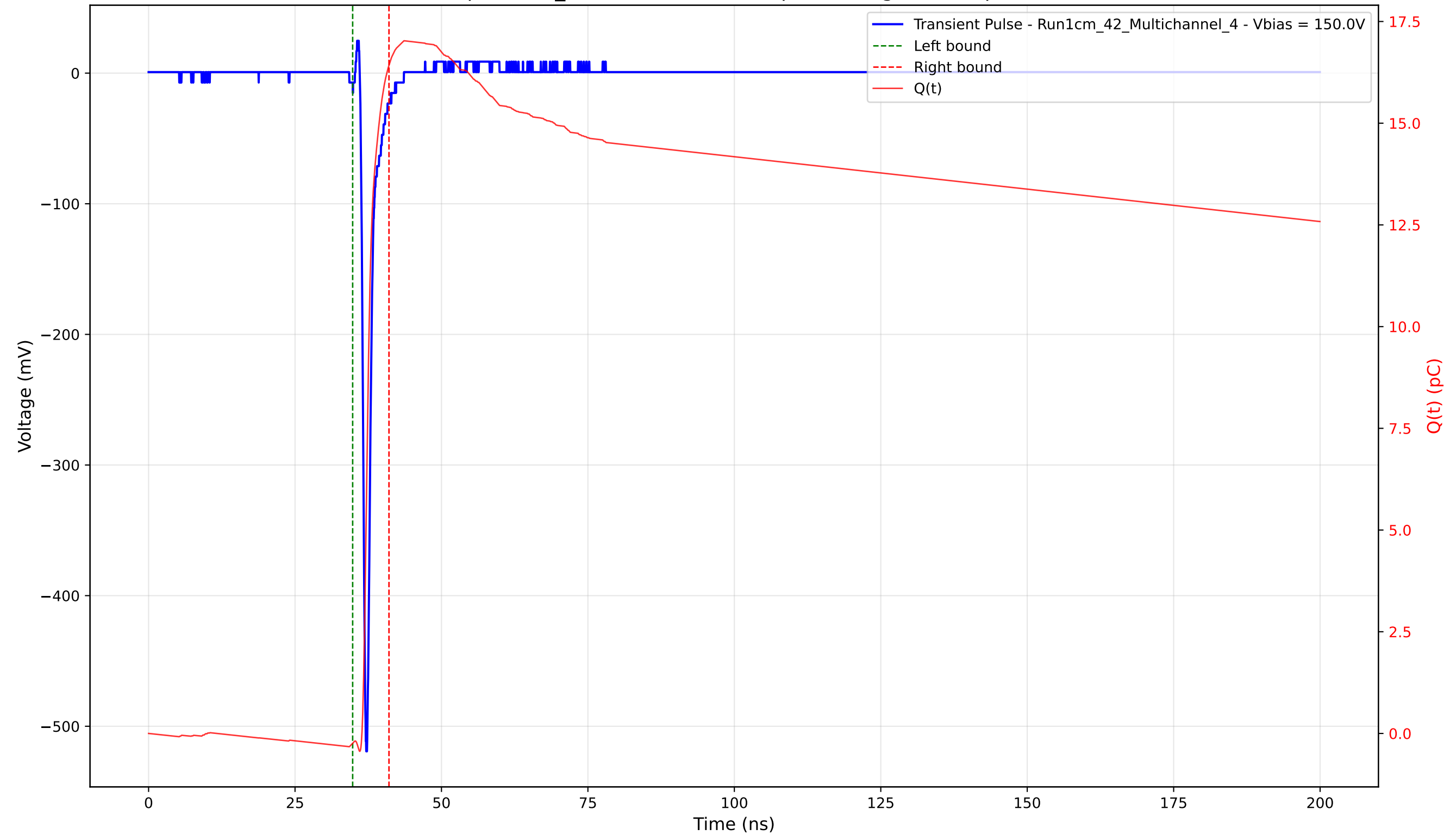
Transient Pulse - Sample: 1cm_42 - Position: 2280.0 \mu\text{m} - Charge: 16.67 pC - Rise Time: 0.72 ns
