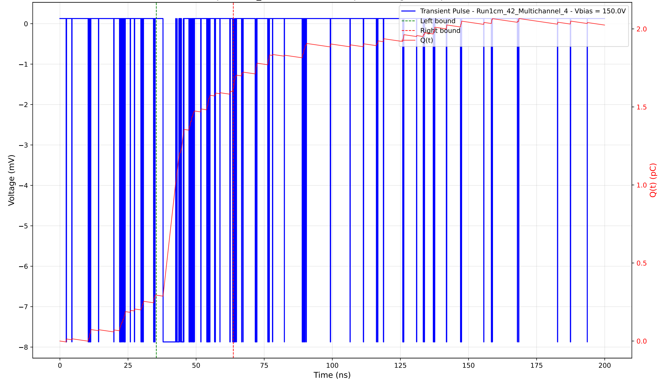
Transient Pulse - Sample: 1cm_42 - Position: 100.0 \mu\text{m} - Charge: 1.33 pC - Rise Time: 0.04 ns
