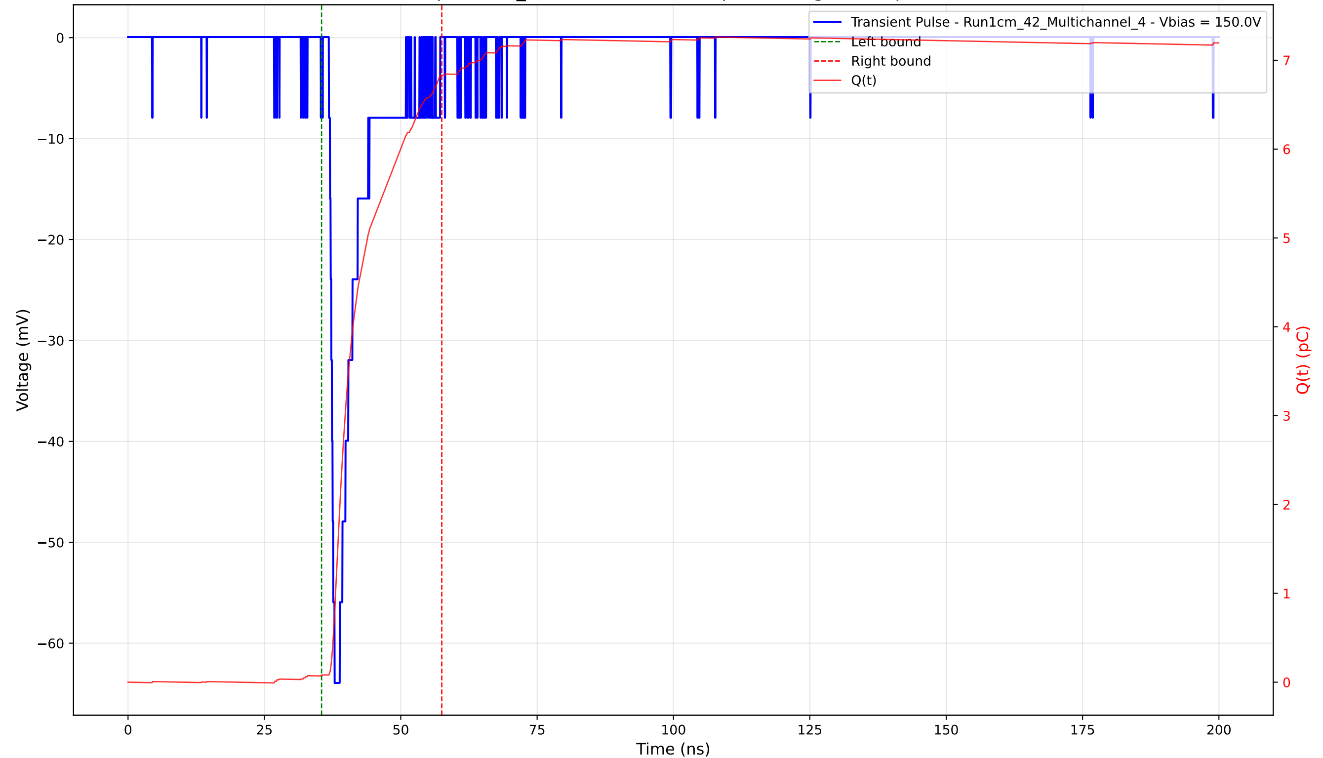
Transient Pulse - Sample: 1cm_42 - Position: 1445.0 \mu\text{m} - Charge: 6.76 pC - Rise Time: 1.05 ns
