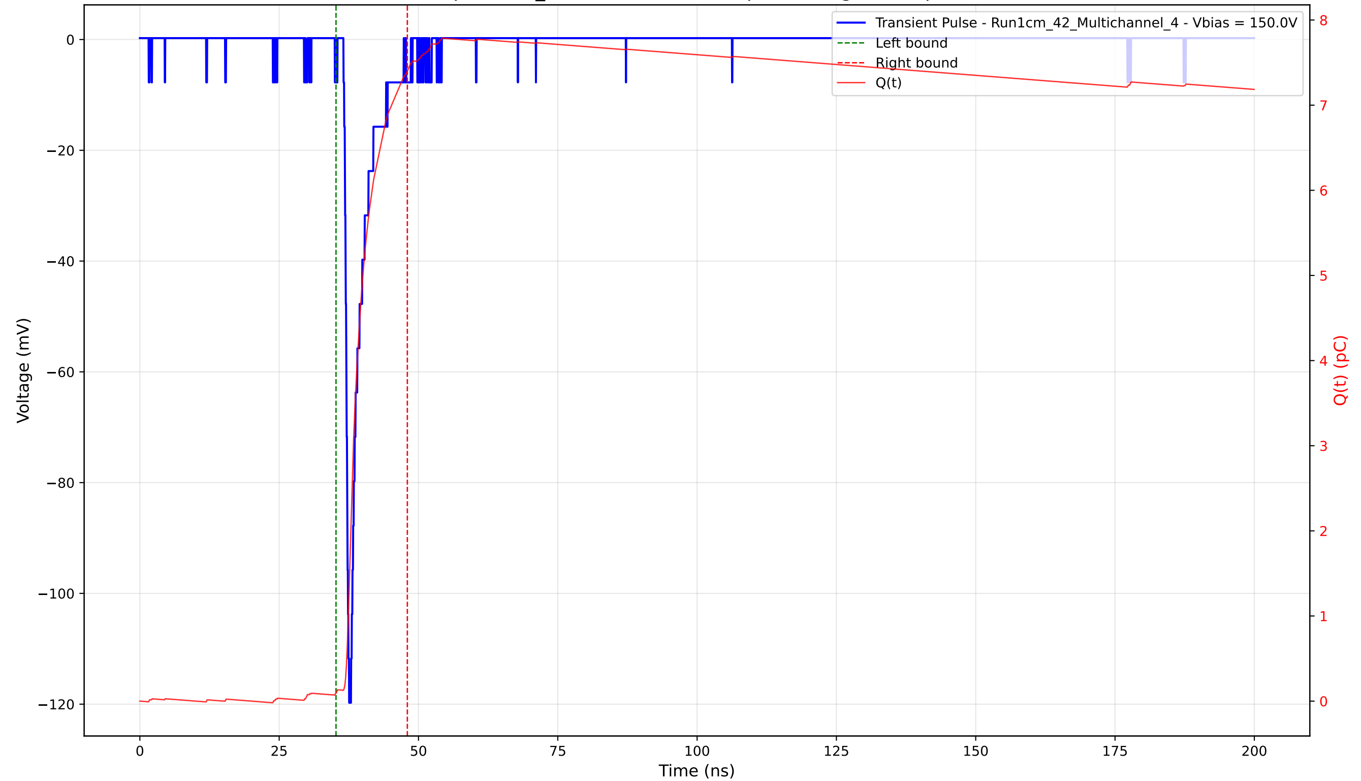
Transient Pulse - Sample: 1cm_42 - Position: 3360.0 \mu\text{m} - Charge: 7.31 pC - Rise Time: 0.78 ns
