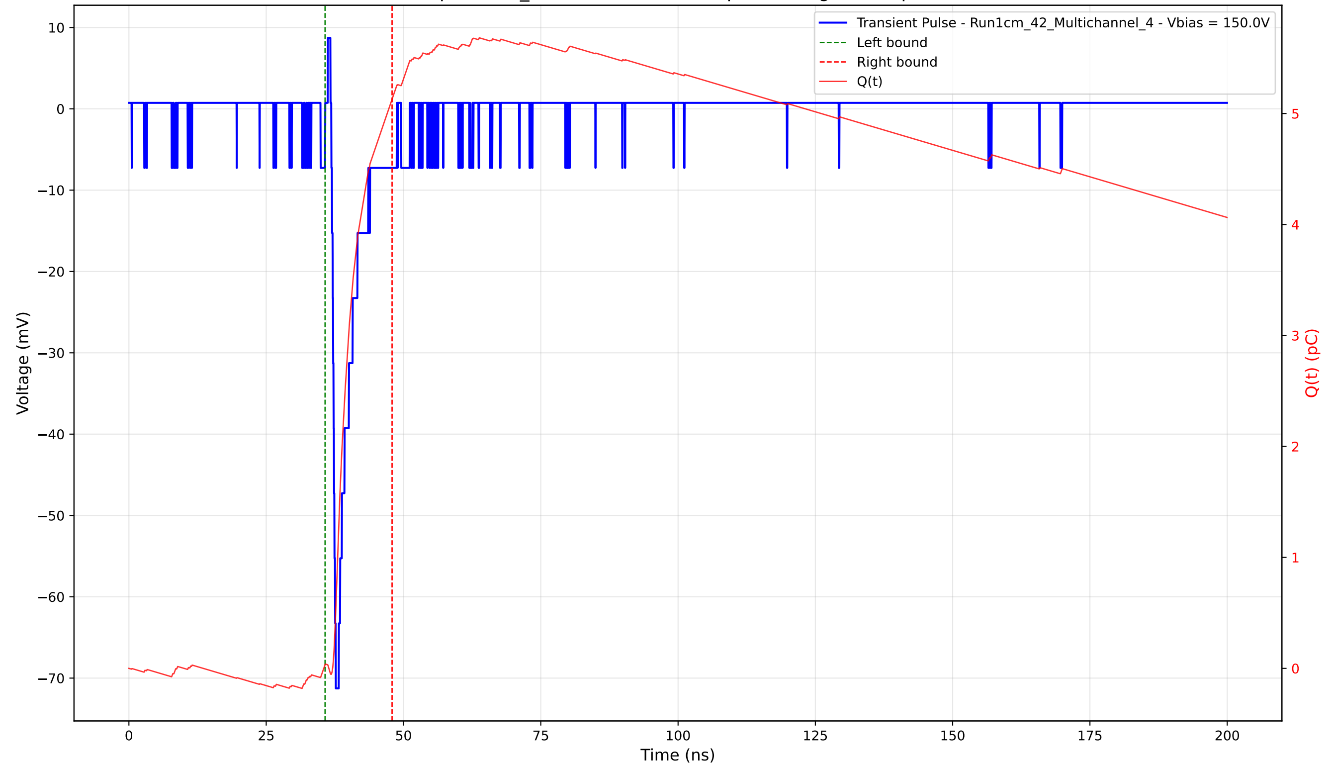
Transient Pulse - Sample: 1cm_42 - Position: 3525.0 \mu\text{m} - Charge: 5.09 pC - Rise Time: 0.80 ns
