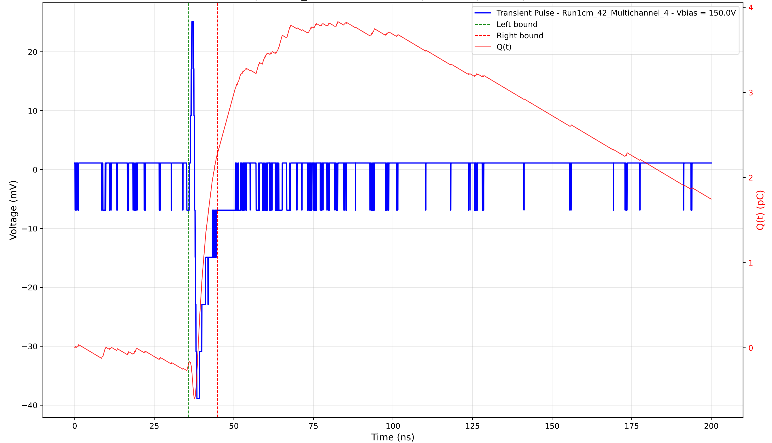
Transient Pulse - Sample: 1cm_42 - Position: 4155.0 \mu\text{m} - Charge: 2.48 pC - Rise Time: 0.70 ns
