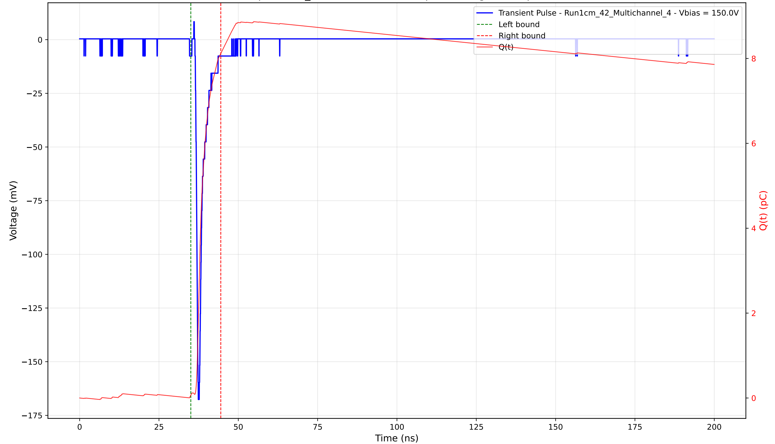
Transient Pulse - Sample: 1cm_42 - Position: 3130.0 \mu\text{m} - Charge: 8.05 pC - Rise Time: 0.75 ns
