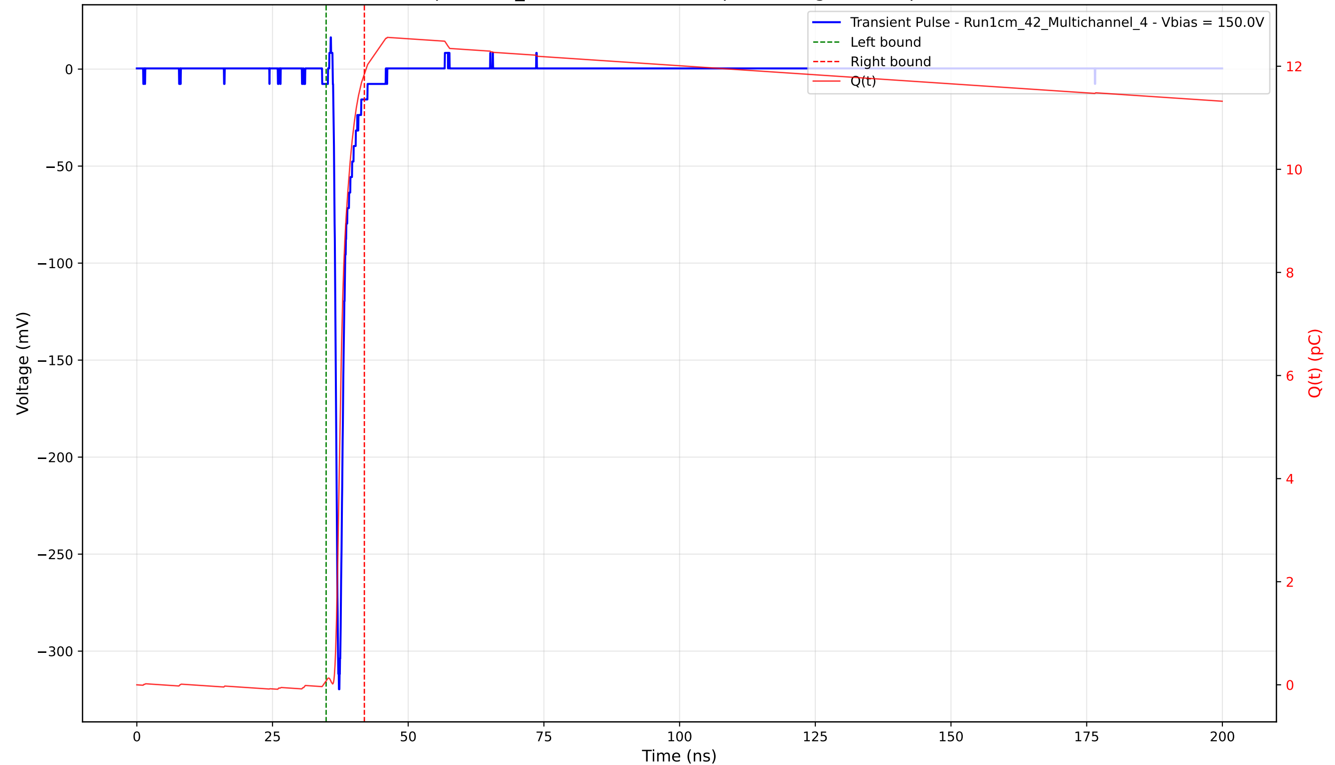
Transient Pulse - Sample: 1cm_42 - Position: 2095.0 \mu\text{m} - Charge: 11.77 pC - Rise Time: 0.72 ns
