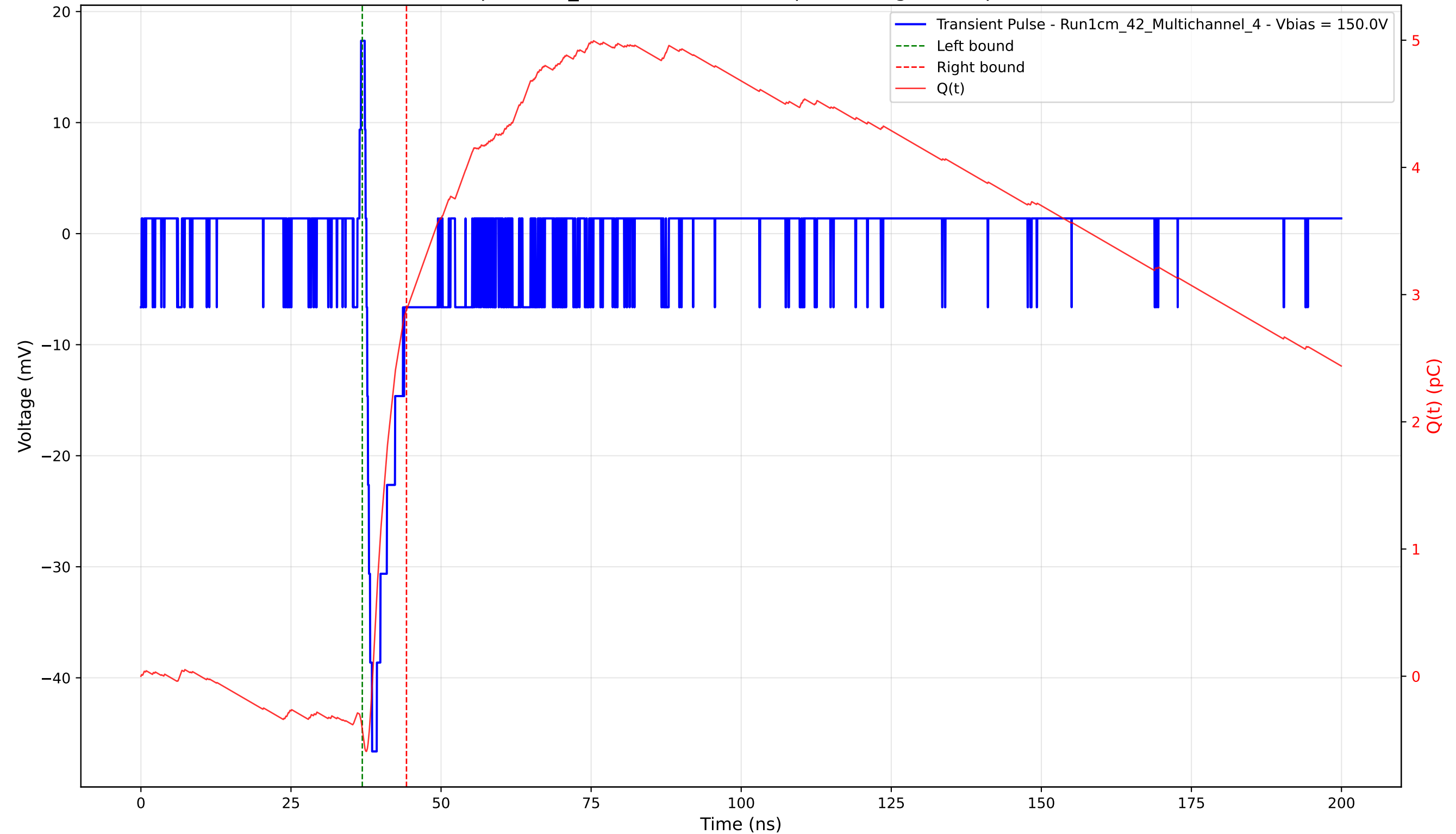
Transient Pulse - Sample: 1cm_42 - Position: 1005.0 \mu\text{m} - Charge: 3.30 pC - Rise Time: 0.93 ns
