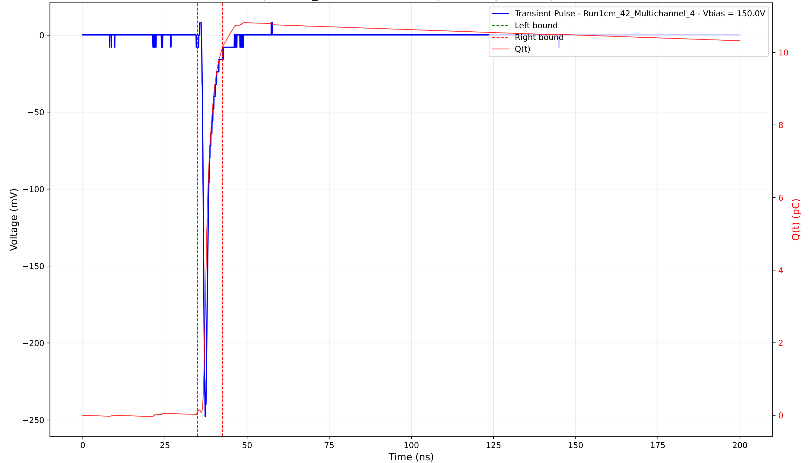
Transient Pulse - Sample: 1cm_42 - Position: 2025.0 \mu\text{m} - Charge: 10.05 pC - Rise Time: 0.79 ns
