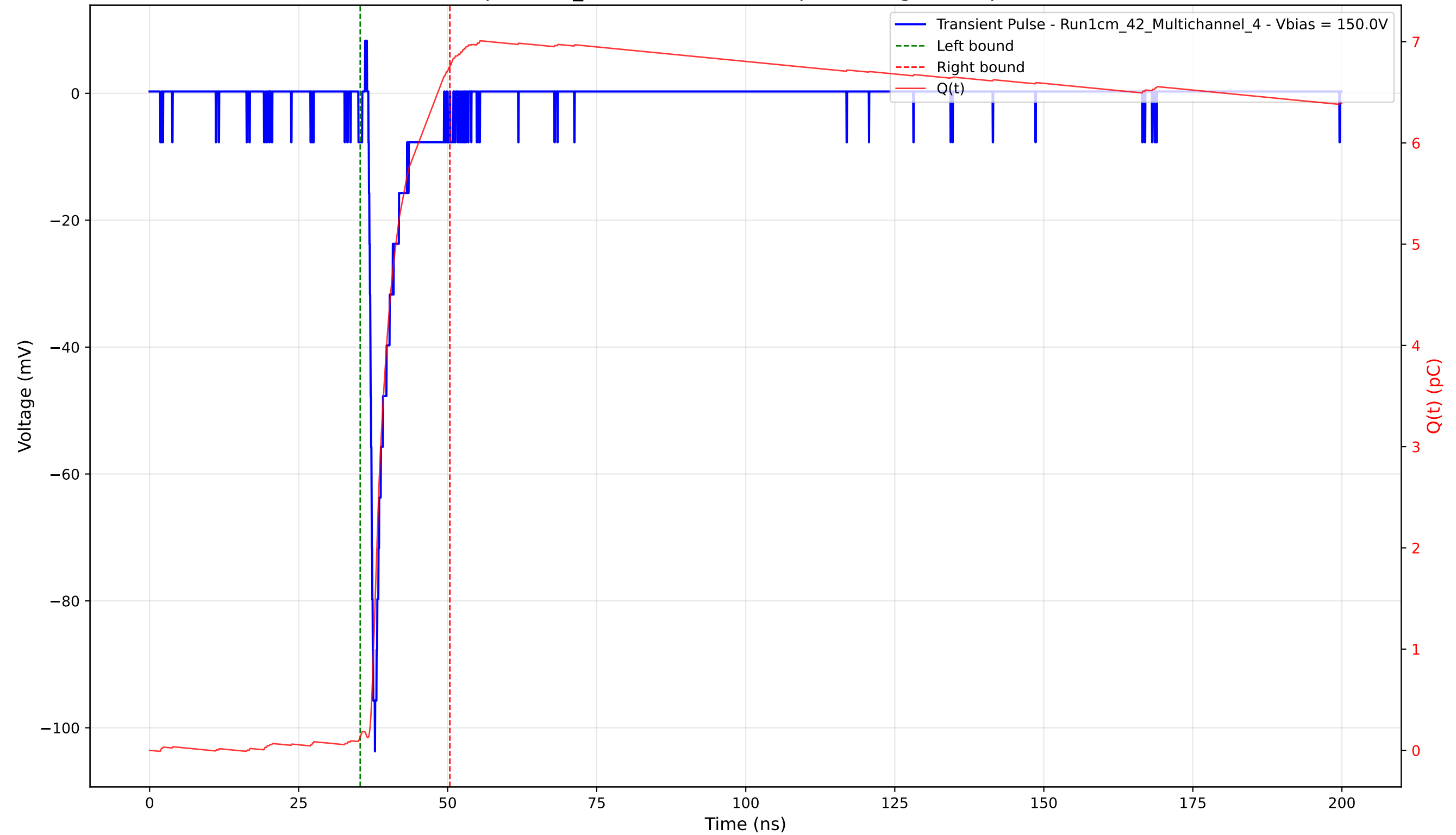
Transient Pulse - Sample: 1cm_42 - Position: 3420.0 \mu\text{m} - Charge: 6.62 pC - Rise Time: 0.75 ns
