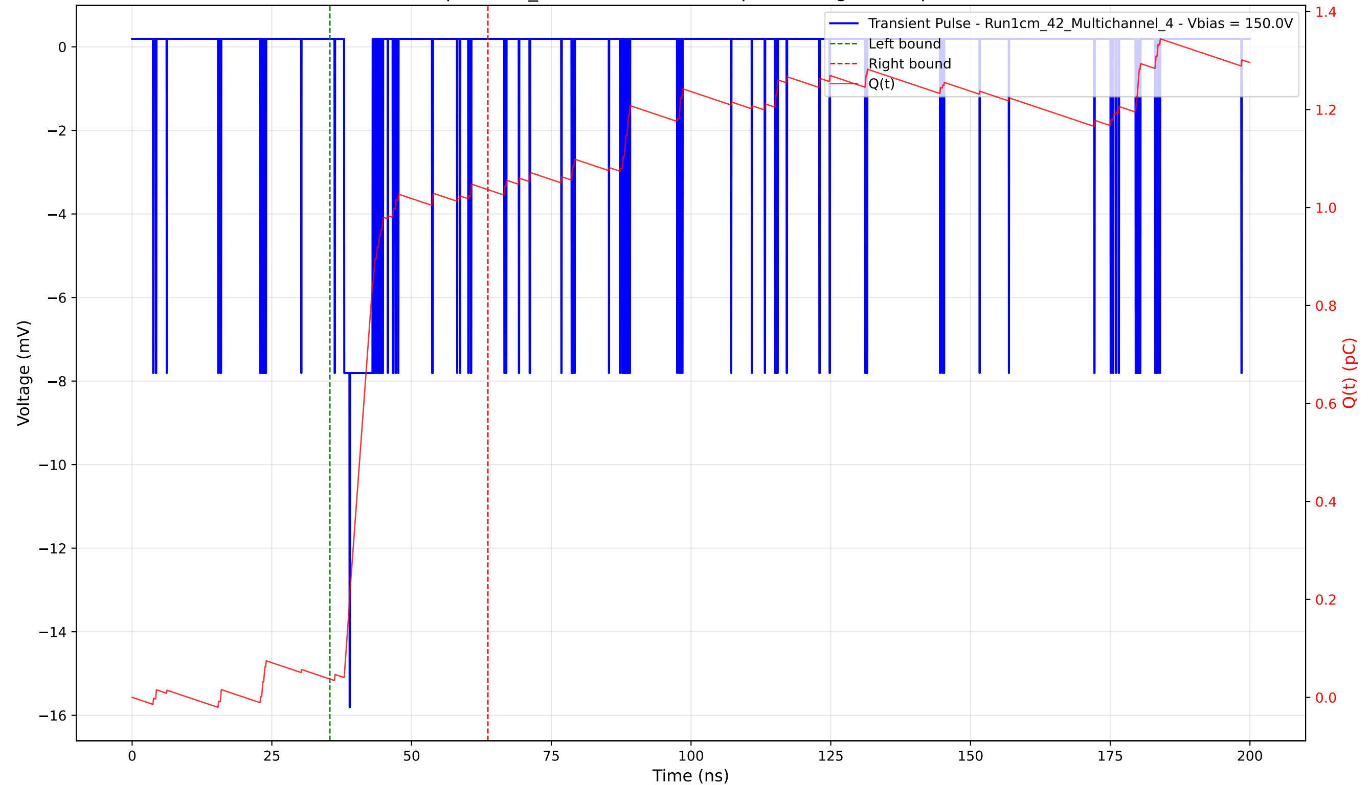
Transient Pulse - Sample: 1cm_42 - Position: 5100.0 \mu\text{m} - Charge: 1.00 pC - Rise Time: 0.99 ns
