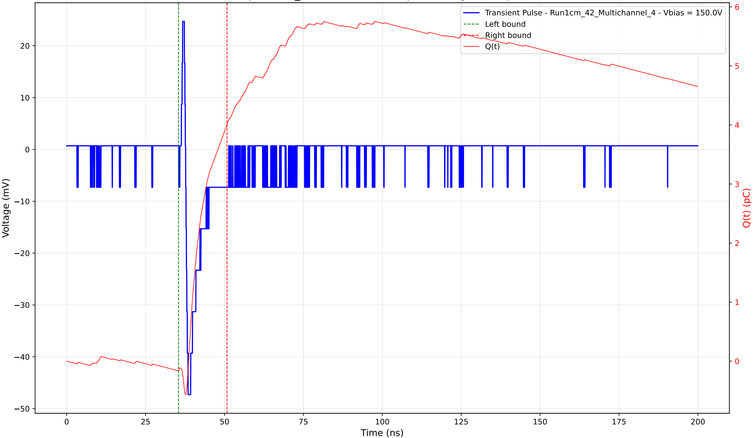
Transient Pulse - Sample: 1cm_42 - Position: 825.0 \mu\text{m} - Charge: 4.17 pC - Rise Time: 0.78 ns
