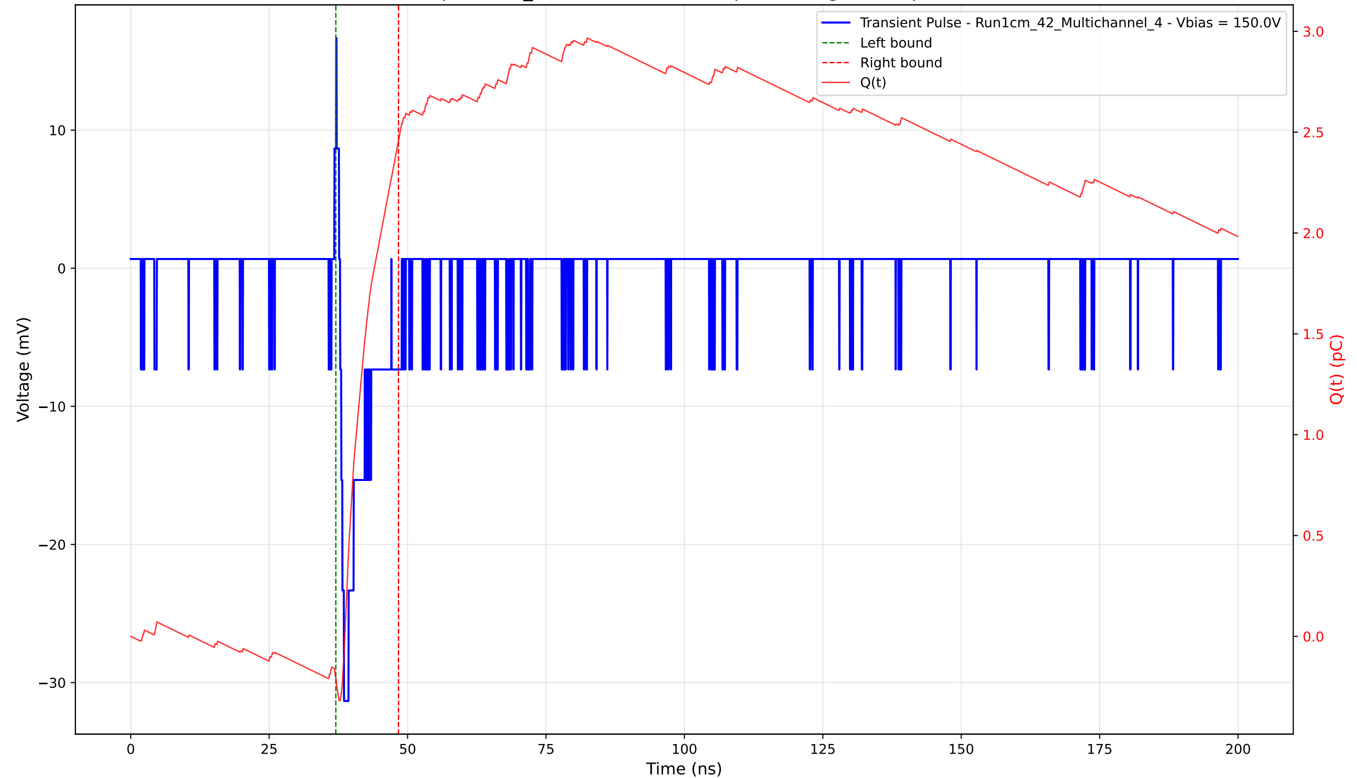
Transient Pulse - Sample: 1cm_42 - Position: 4870.0 \mu\text{m} - Charge: 2.66 pC - Rise Time: 0.71 ns
