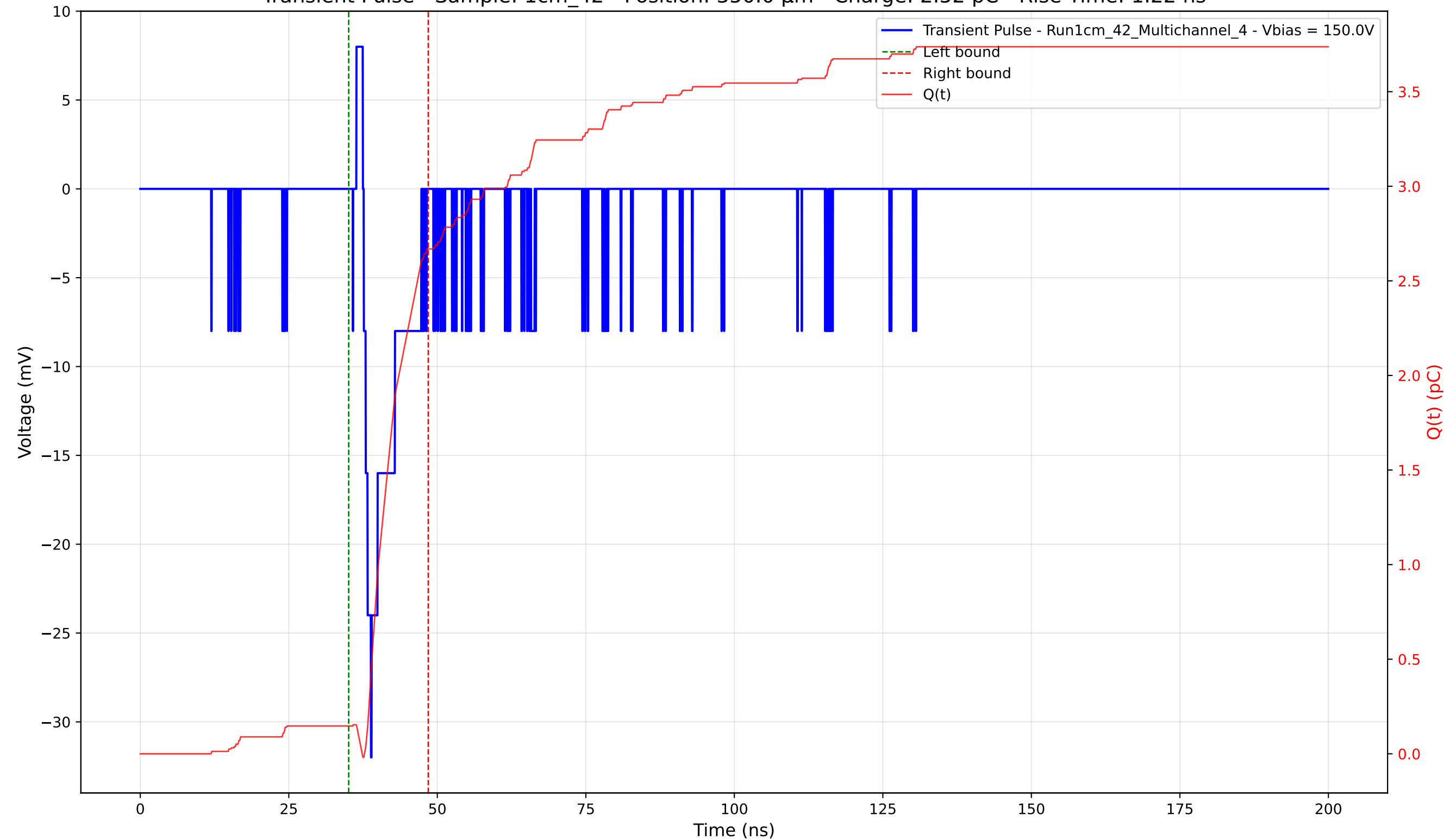
Transient Pulse - Sample: 1cm_42 - Position: 350.0 \mu\text{m} - Charge: 2.52 pC - Rise Time: 1.22 ns
