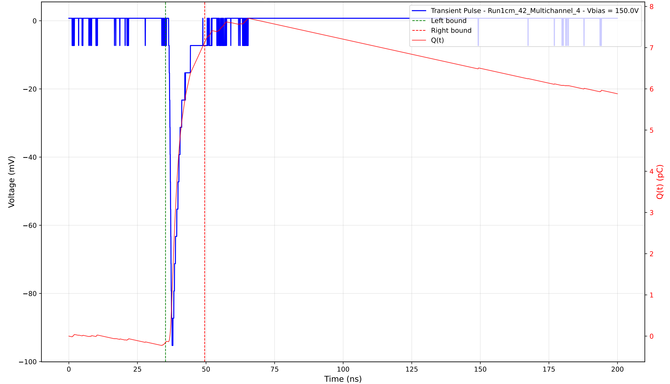
Transient Pulse - Sample: 1cm_42 - Position: 1595.0 \mu\text{m} - Charge: 7.28 pC - Rise Time: 0.87 ns
