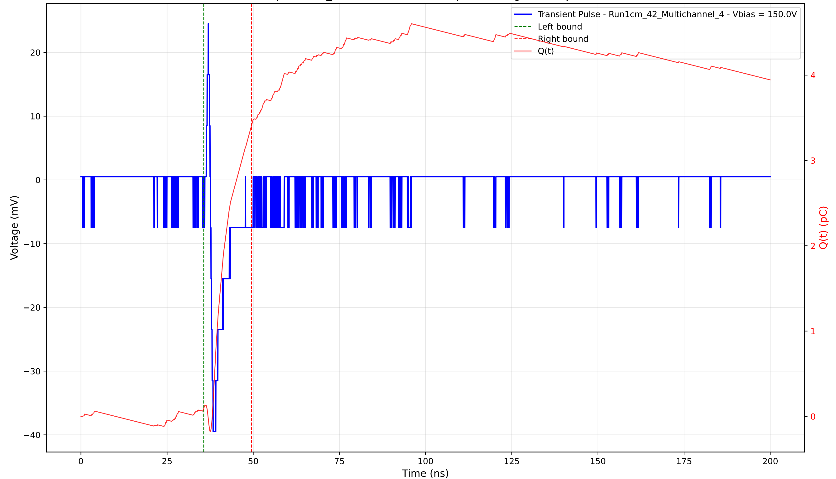
Transient Pulse - Sample: 1cm_42 - Position: 4065.0 \mu\text{m} - Charge: 3.31 pC - Rise Time: 0.78 ns
