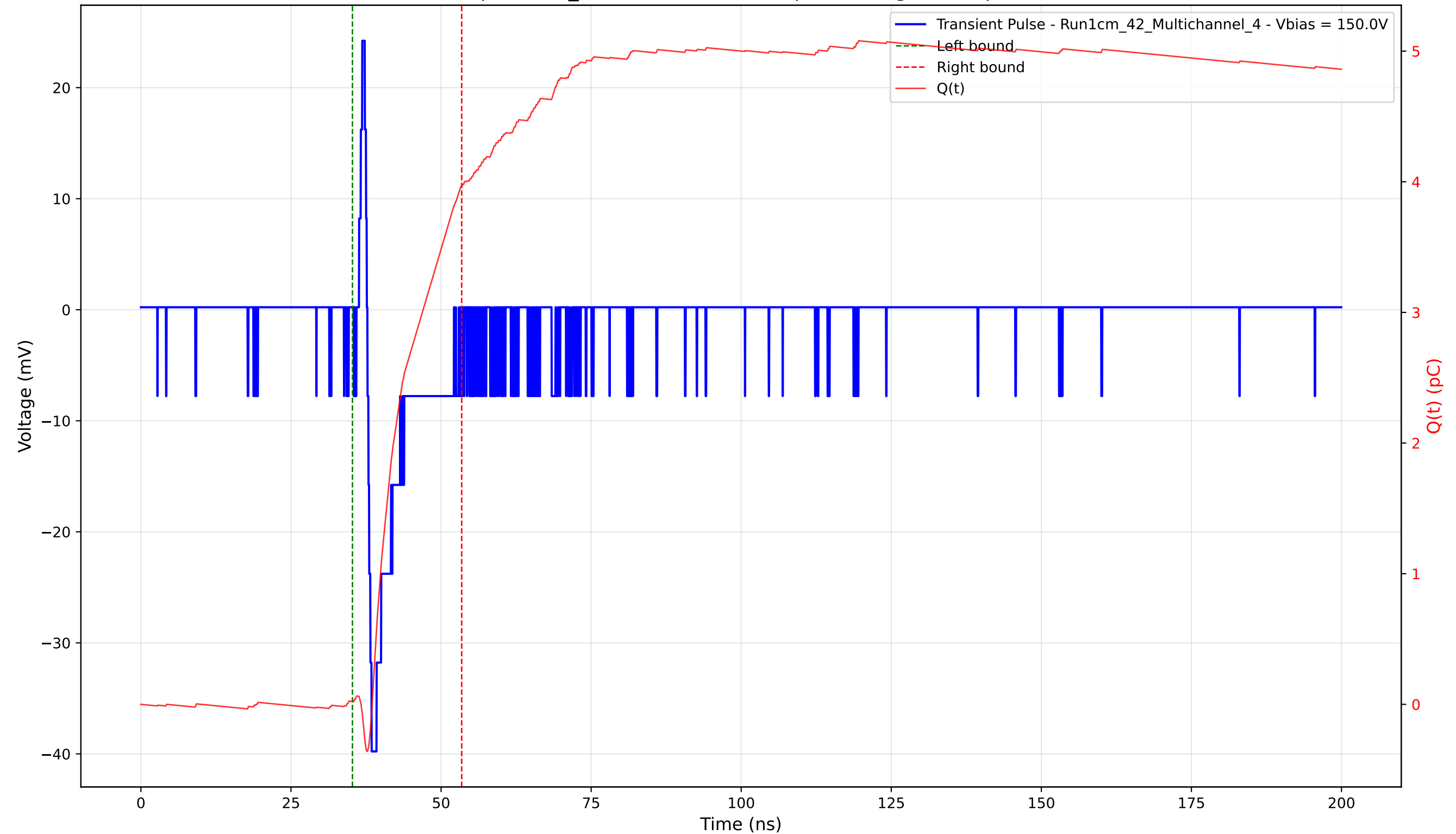
Transient Pulse - Sample: 1cm_42 - Position: 4340.0 \mu\text{m} - Charge: 3.94 pC - Rise Time: 0.70 ns
