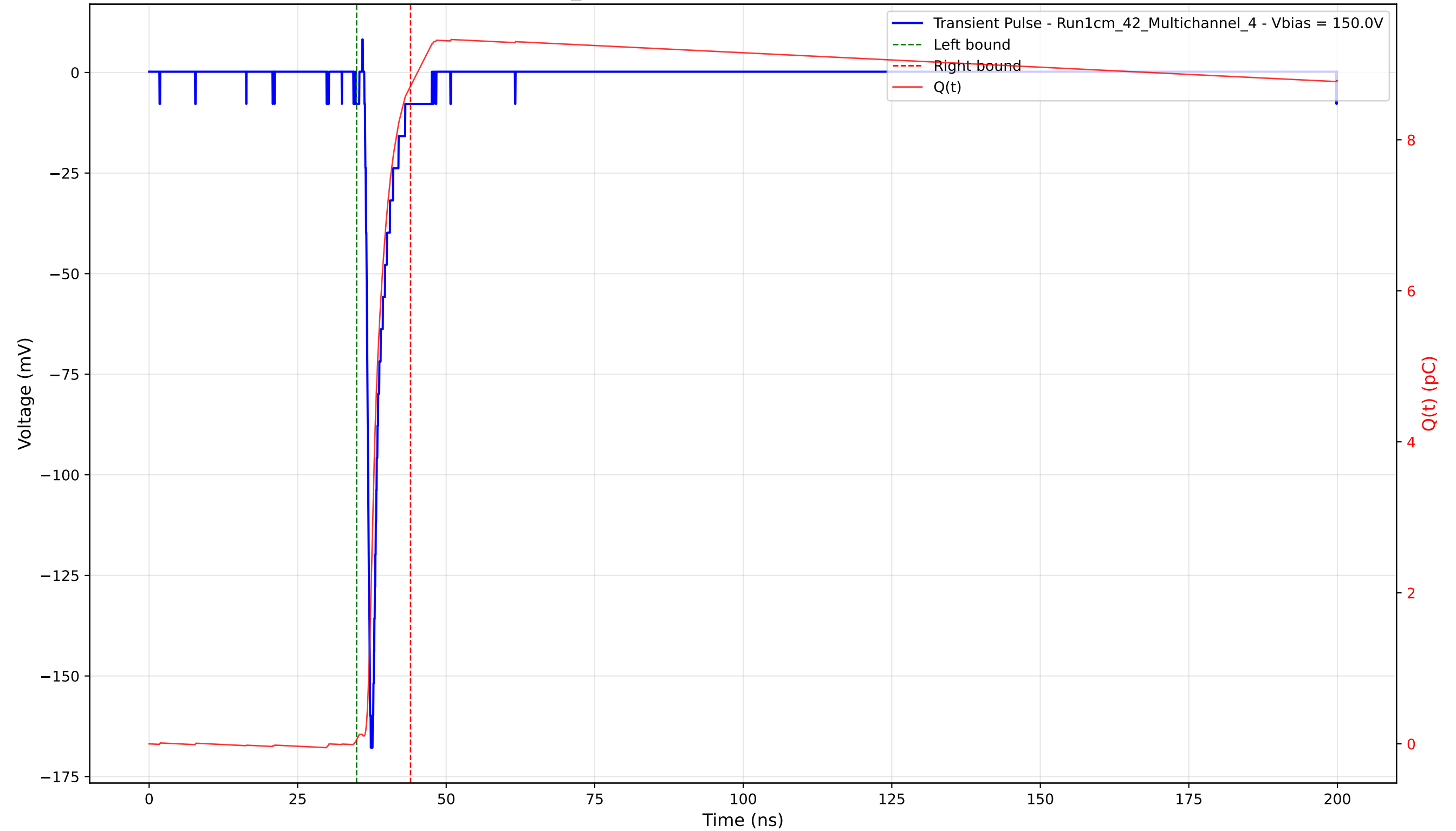
Transient Pulse - Sample: 1cm_42 - Position: 1900.0 \mu\text{m} - Charge: 8.66 pC - Rise Time: 0.79 ns
