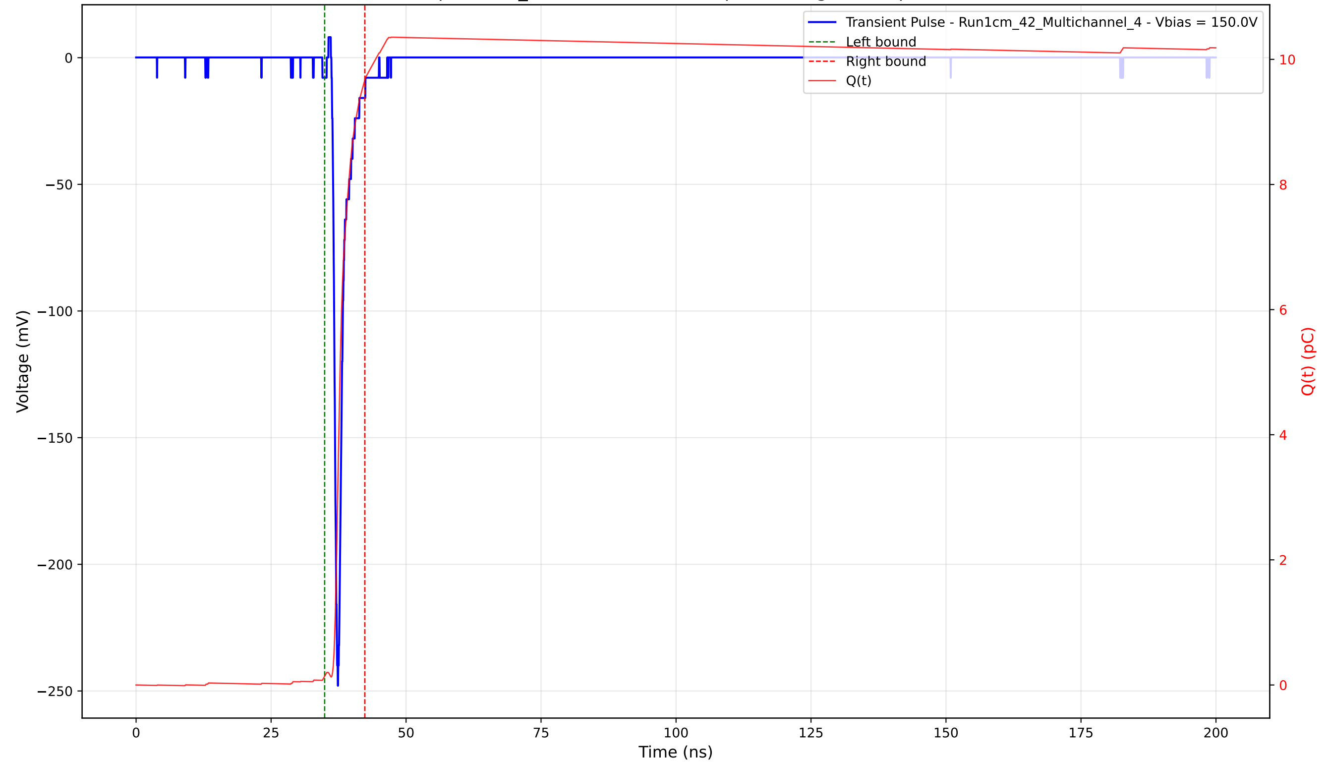
Transient Pulse - Sample: 1cm_42 - Position: 2995.0 \mu\text{m} - Charge: 9.53 pC - Rise Time: 0.79 ns
