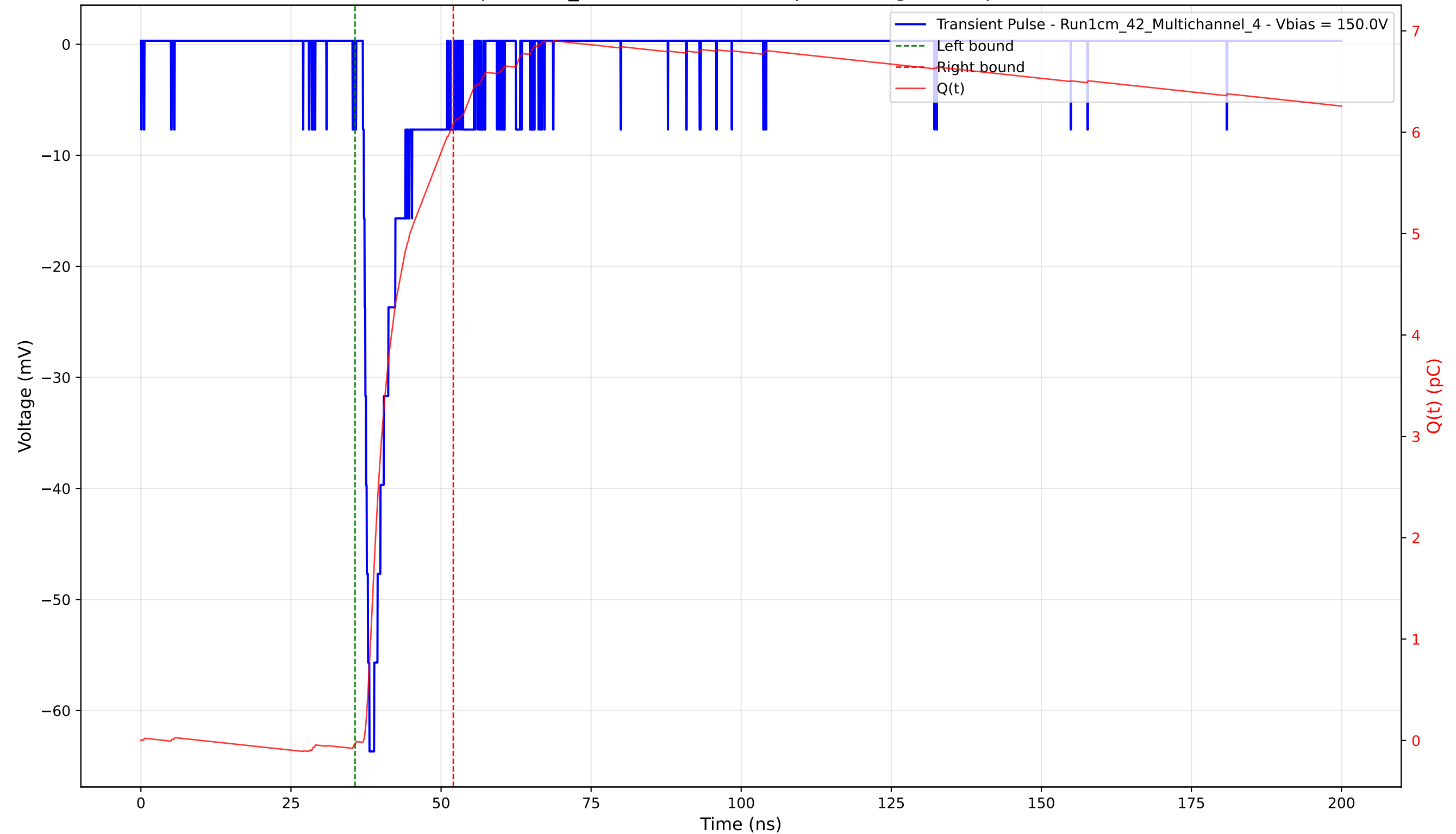
Transient Pulse - Sample: 1cm_42 - Position: 1400.0 \mu\text{m} - Charge: 6.12 pC - Rise Time: 1.09 ns
