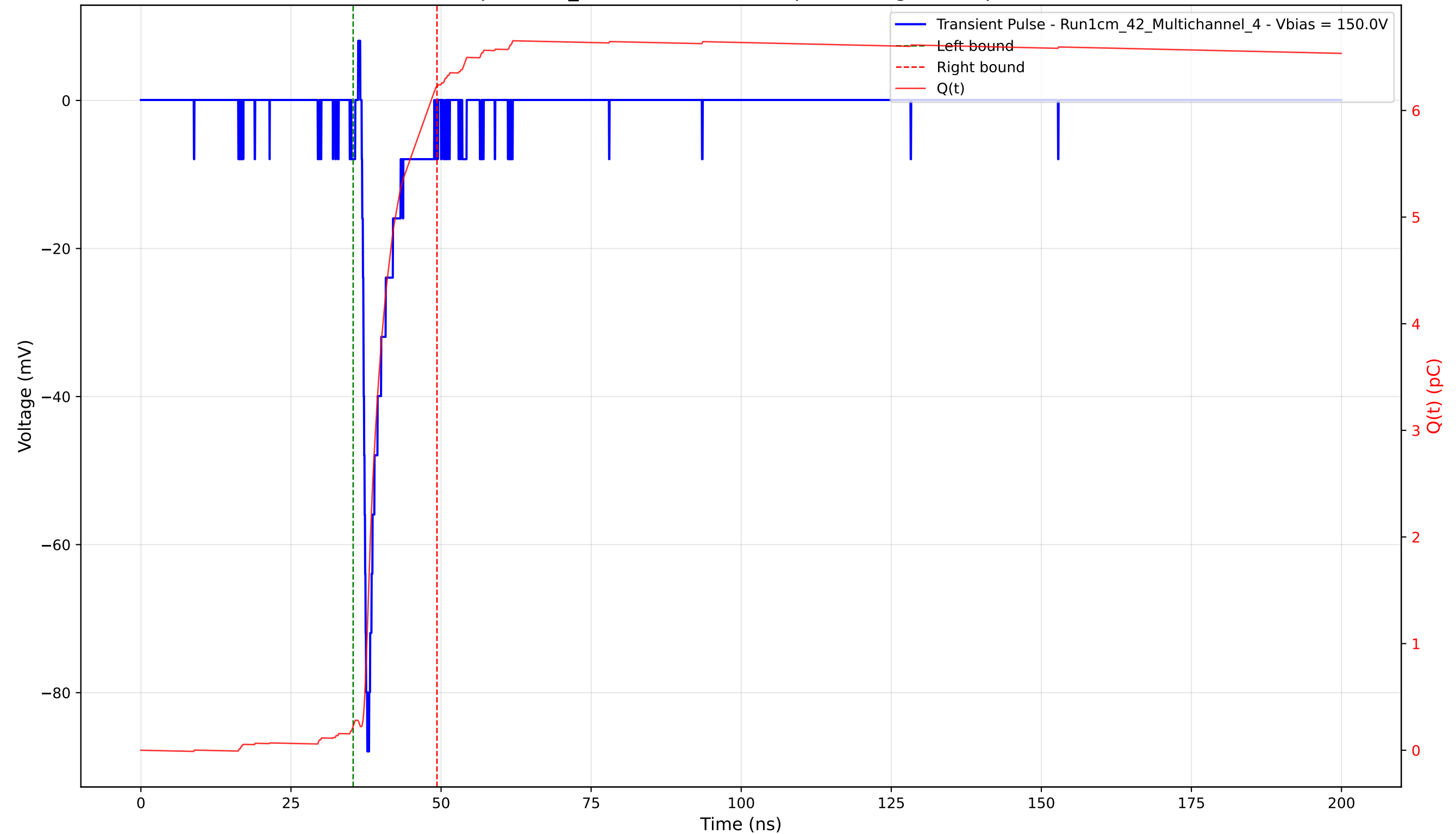
Transient Pulse - Sample: 1cm_42 - Position: 3465.0 \mu\text{m} - Charge: 6.00 pC - Rise Time: 0.68 ns
