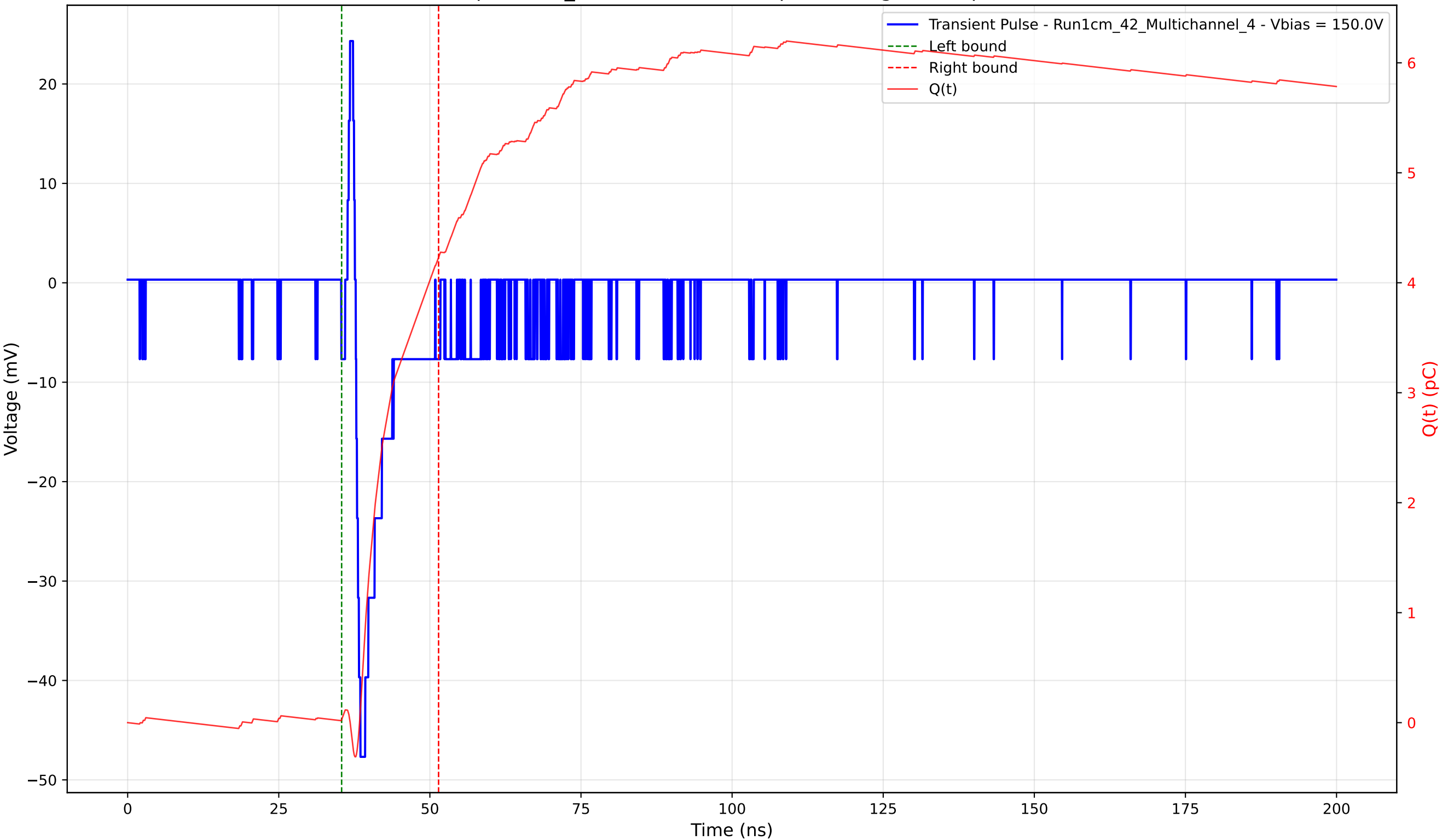
Transient Pulse - Sample: 1cm_42 - Position: 850.0 \mu\text{m} - Charge: 4.20 pC - Rise Time: 0.78 ns
