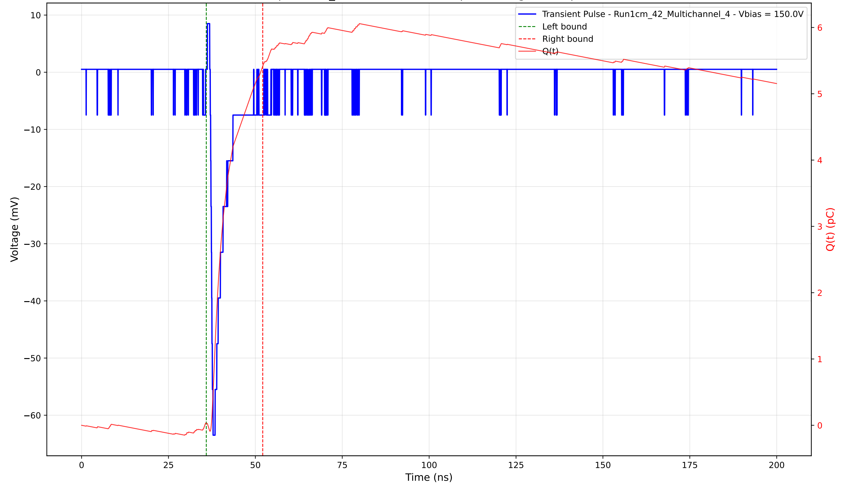
Transient Pulse - Sample: 1cm_42 - Position: 3595.0 \mu\text{m} - Charge: 5.39 pC - Rise Time: 0.81 ns
