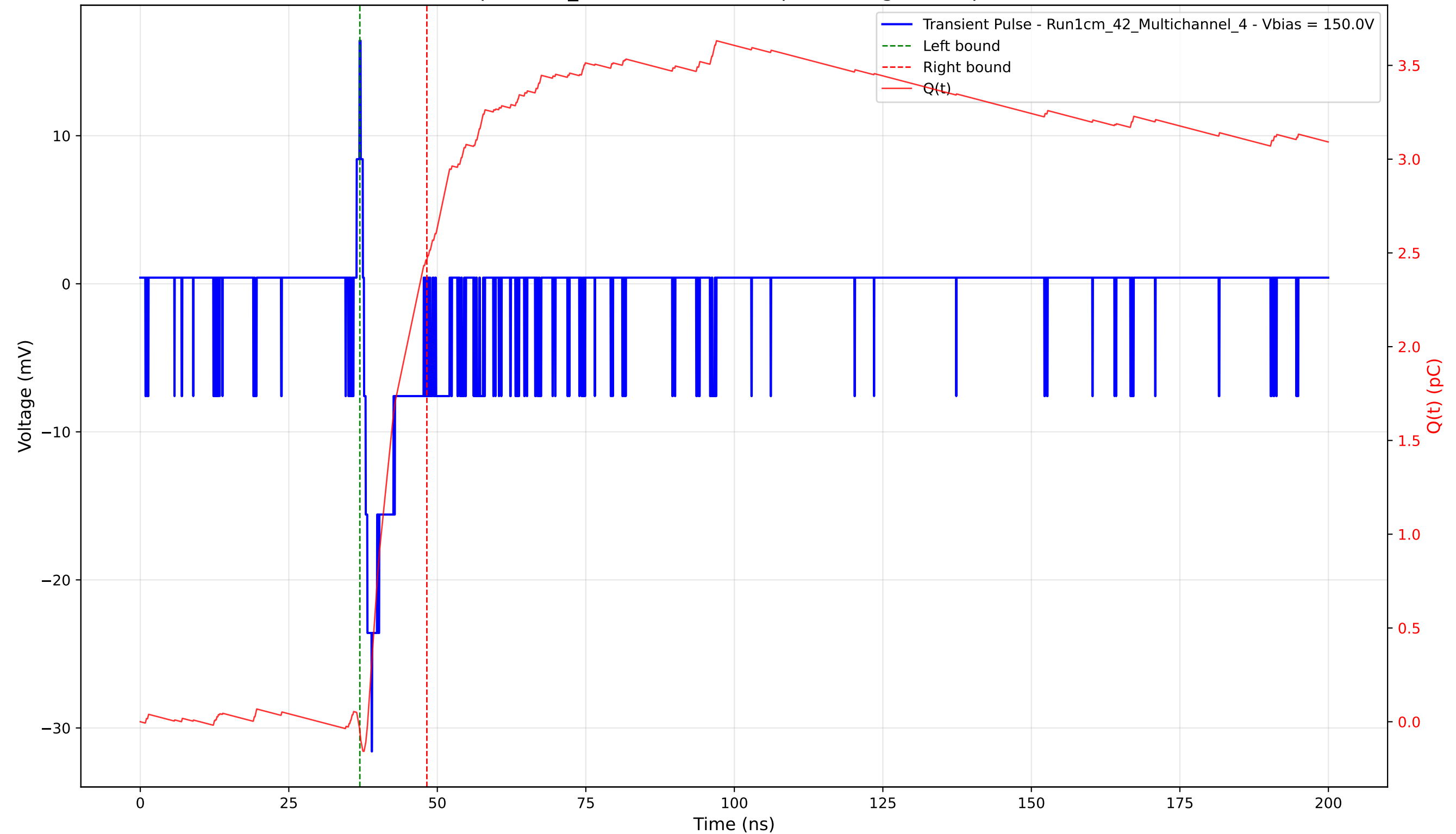
Transient Pulse - Sample: 1cm_42 - Position: 360.0 \mu\text{m} - Charge: 2.51 pC - Rise Time: 1.30 ns
