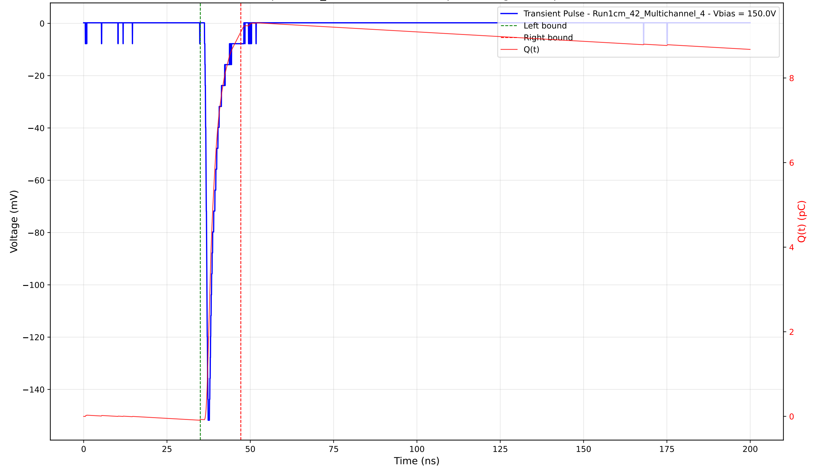
Transient Pulse - Sample: 1cm_42 - Position: 1815.0 \mu\text{m} - Charge: 9.16 pC - Rise Time: 0.88 ns
