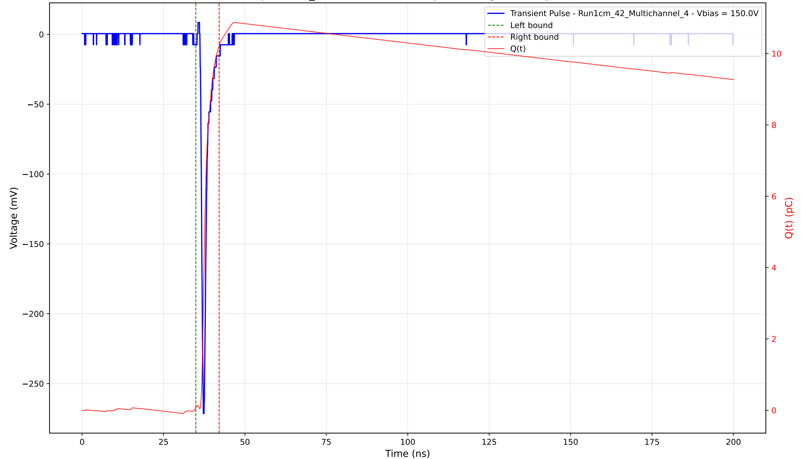
Transient Pulse - Sample: 1cm_42 - Position: 2965.0 \mu\text{m} - Charge: 10.15 pC - Rise Time: 0.77 ns
