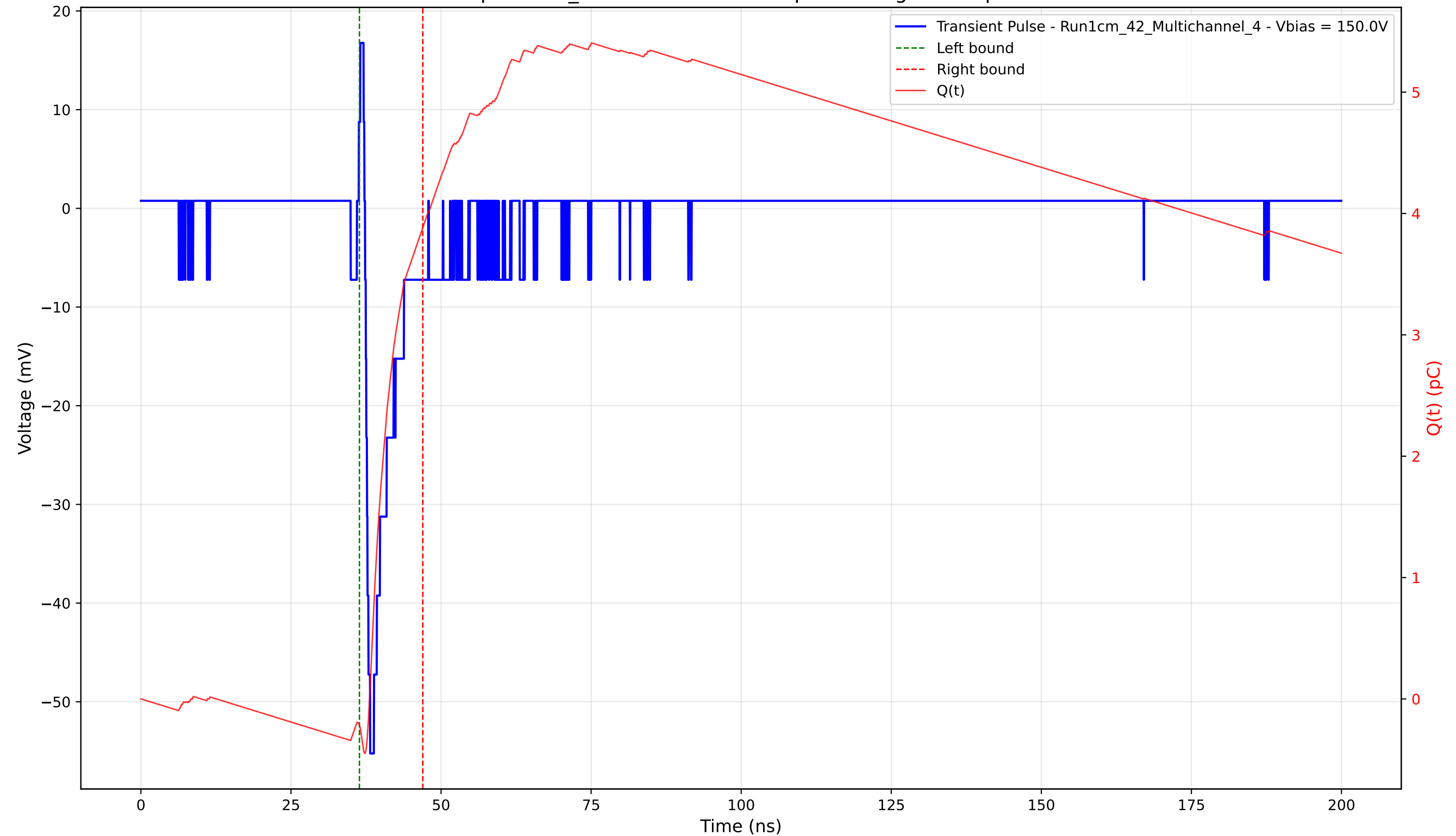
Transient Pulse - Sample: 1cm_42 - Position: 3845.0 \mu\text{m} - Charge: 4.10 pC - Rise Time: 0.85 ns
