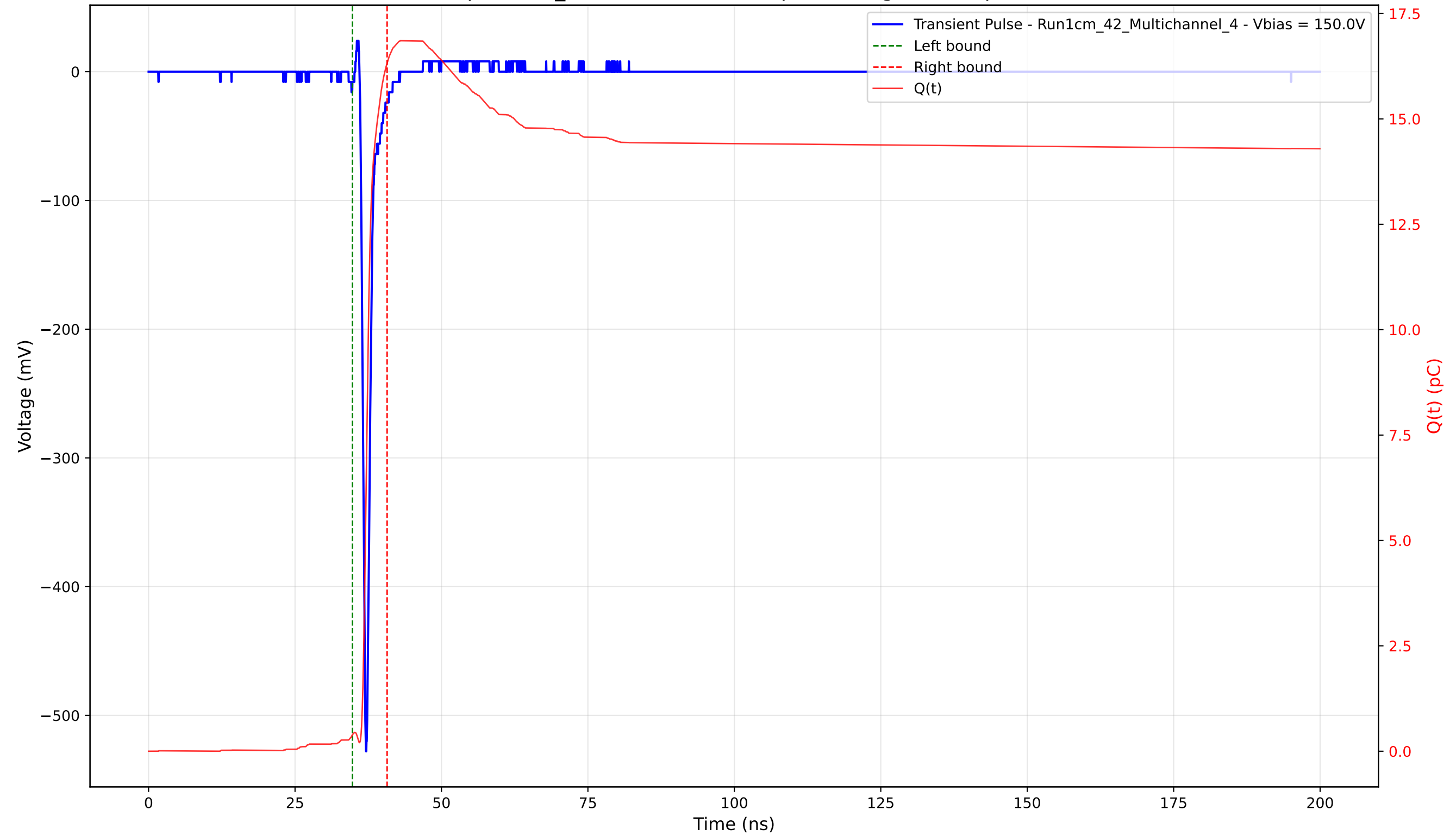
Transient Pulse - Sample: 1cm_42 - Position: 2460.0 \mu\text{m} - Charge: 15.93 pC - Rise Time: 0.72 ns
