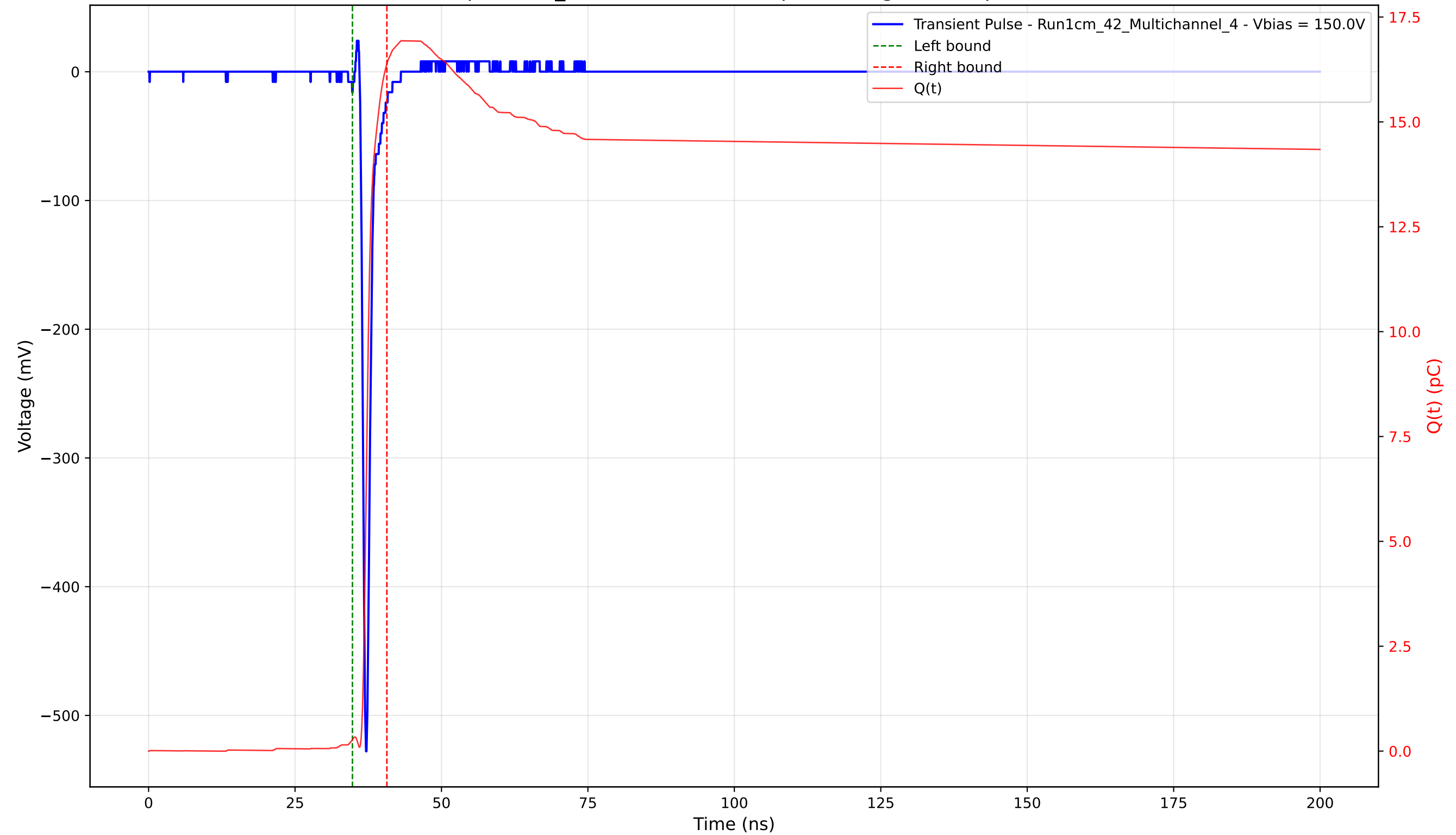
Transient Pulse - Sample: 1cm_42 - Position: 2425.0 \mu\text{m} - Charge: 16.11 pC - Rise Time: 0.72 ns
