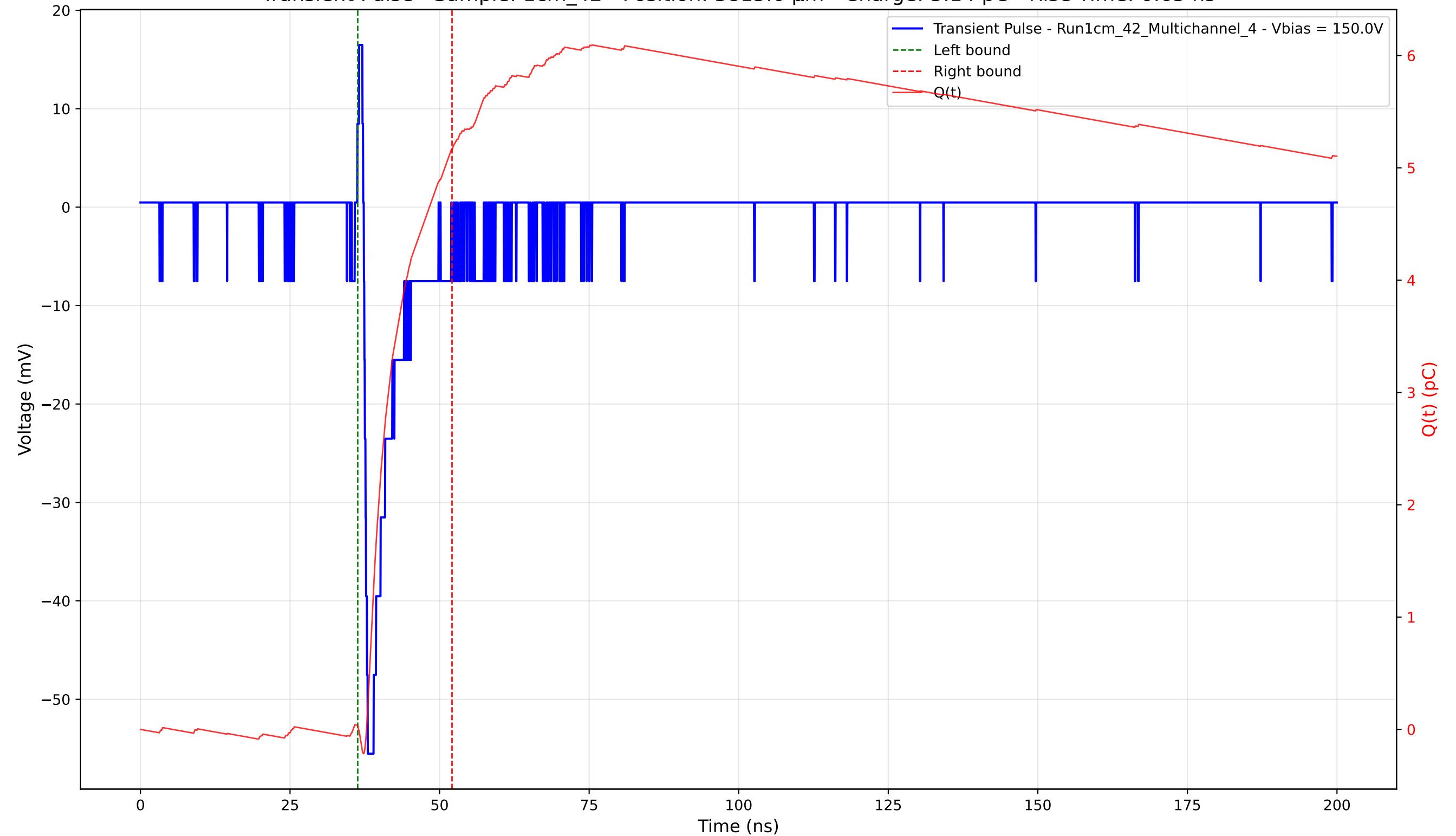
Transient Pulse - Sample: 1cm_42 - Position: 3815.0 \mu\text{m} - Charge: 5.14 pC - Rise Time: 0.65 ns
