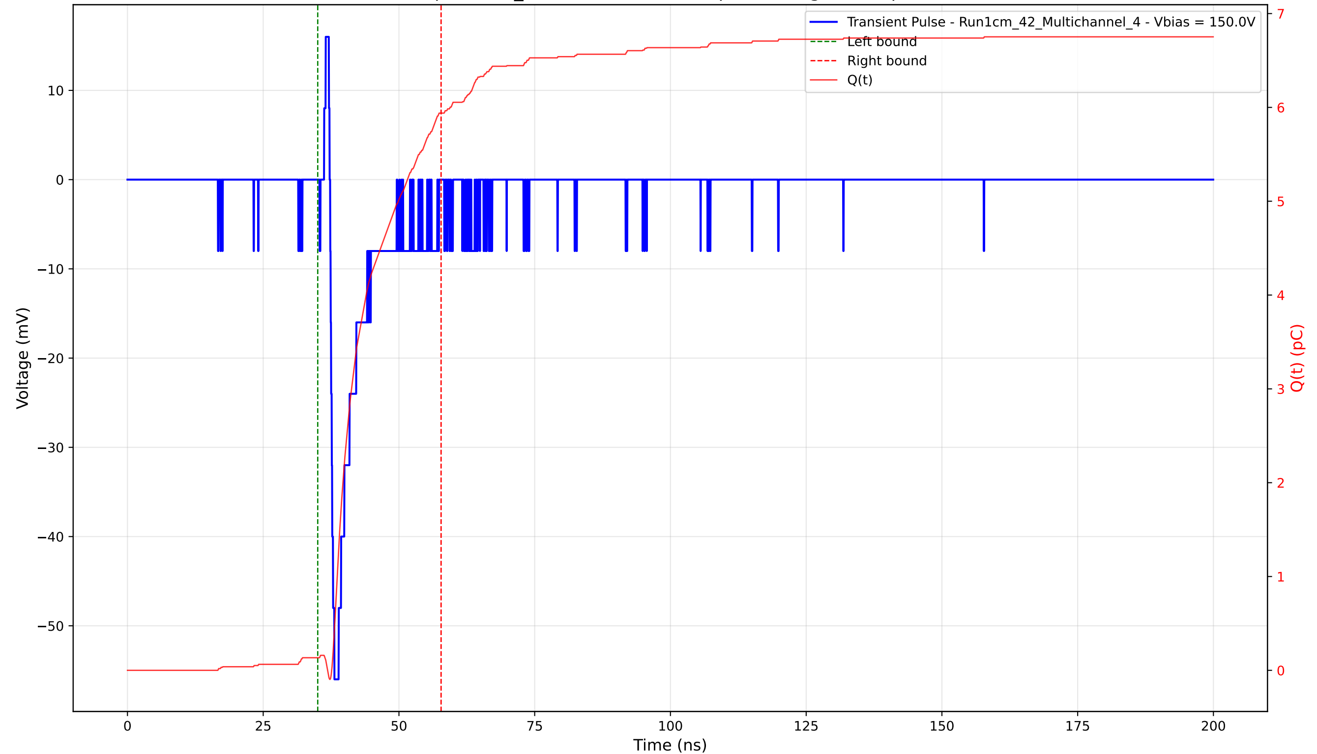
Transient Pulse - Sample: 1cm_42 - Position: 3825.0 \mu\text{m} - Charge: 5.80 pC - Rise Time: 0.77 ns
