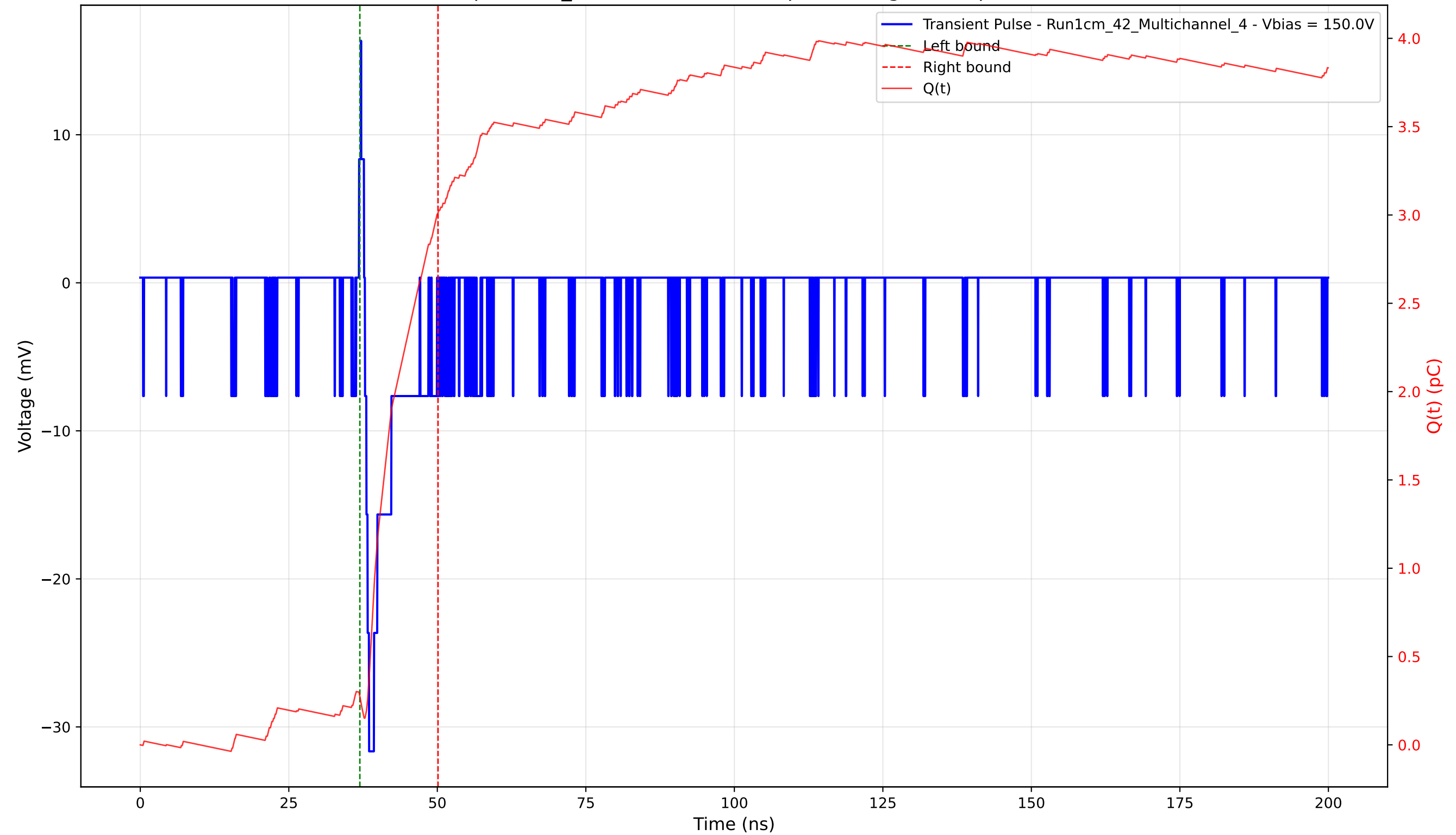
Transient Pulse - Sample: 1cm_42 - Position: 4885.0 \mu\text{m} - Charge: 2.74 pC - Rise Time: 0.70 ns
