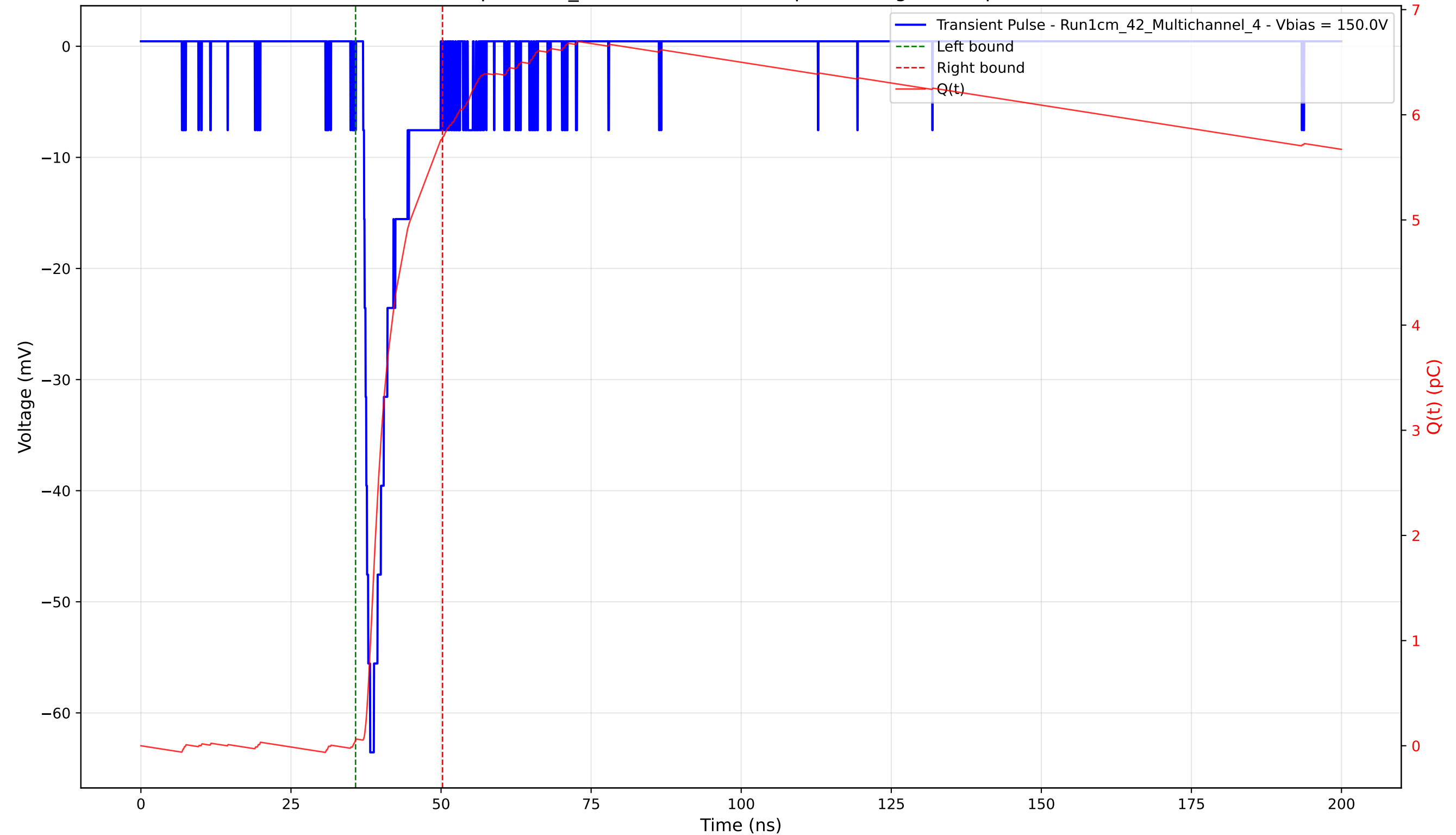
Transient Pulse - Sample: 1cm_42 - Position: 1390.0 \mu\text{m} - Charge: 5.73 pC - Rise Time: 1.17 ns
