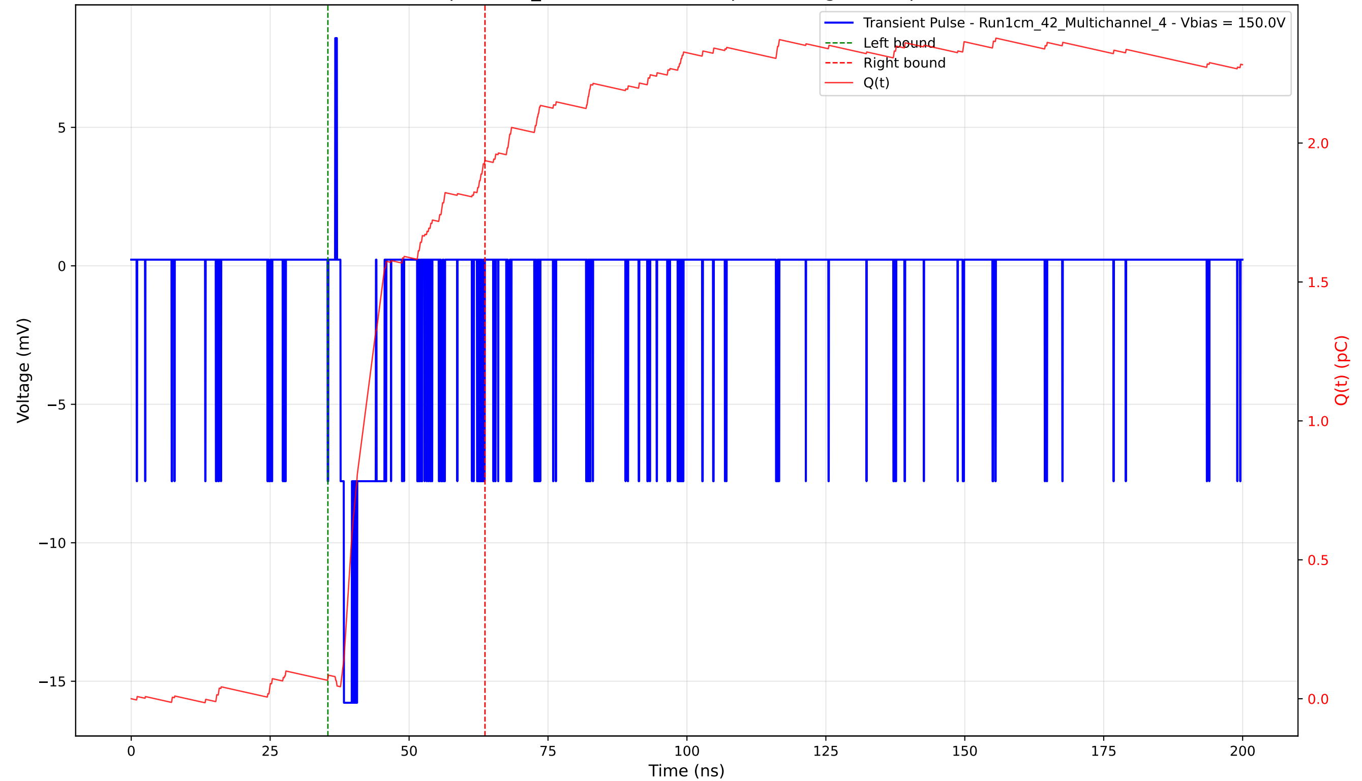
Transient Pulse - Sample: 1cm_42 - Position: 165.0 \mu\text{m} - Charge: 1.86 pC - Rise Time: 0.63 ns
