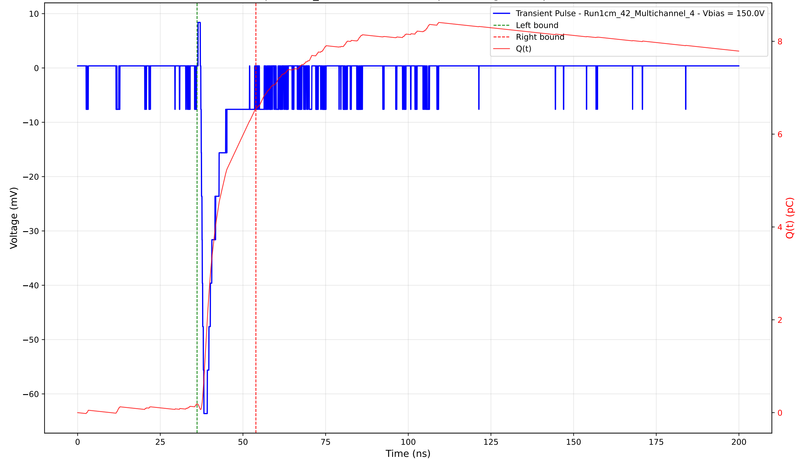
Transient Pulse - Sample: 1cm_42 - Position: 1230.0 \mu\text{m} - Charge: 6.36 pC - Rise Time: 0.93 ns
