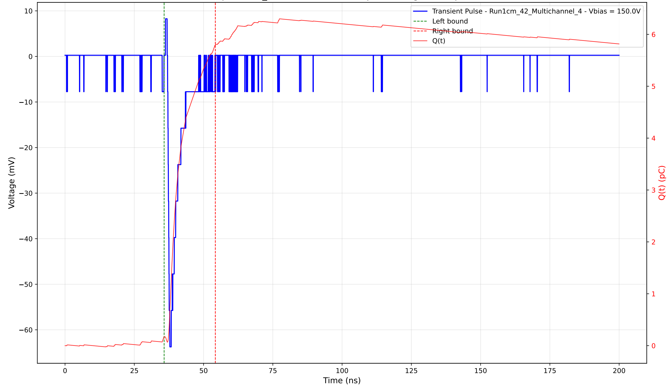
Transient Pulse - Sample: 1cm_42 - Position: 3585.0 \mu\text{m} - Charge: 5.62 pC - Rise Time: 0.81 ns
