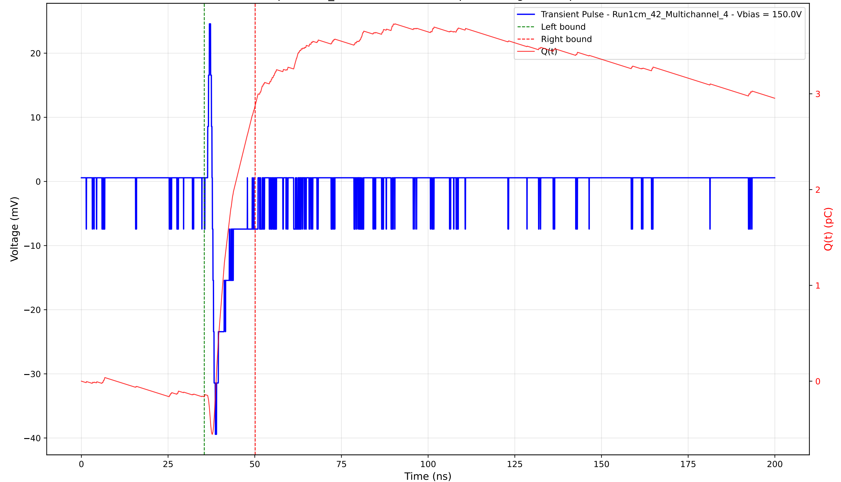
Transient Pulse - Sample: 1cm_42 - Position: 4410.0 \mu\text{m} - Charge: 3.04 pC - Rise Time: 0.86 ns
