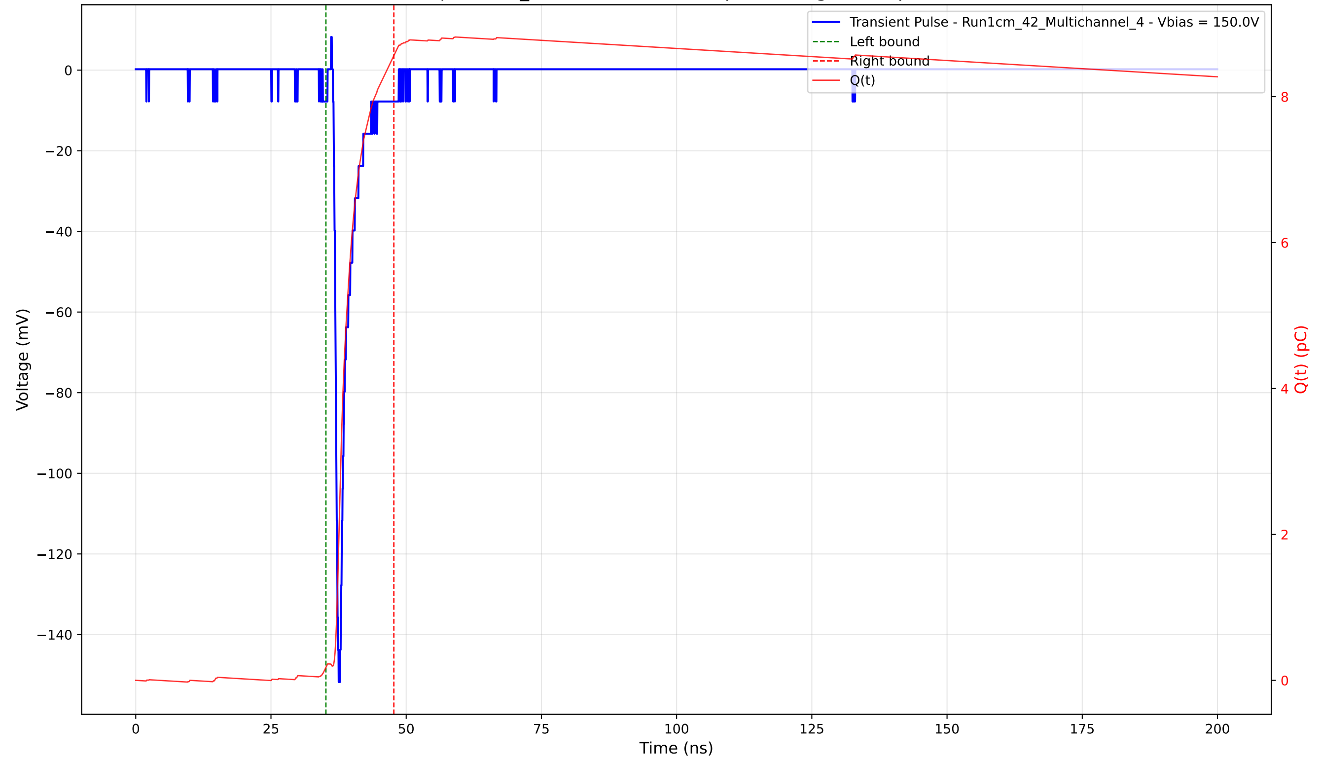
Transient Pulse - Sample: 1cm_42 - Position: 3220.0 \mu\text{m} - Charge: 8.39 pC - Rise Time: 0.80 ns
