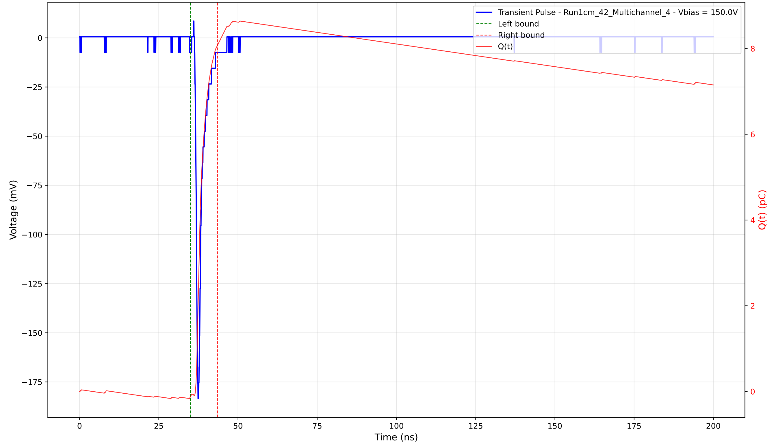
Transient Pulse - Sample: 1cm_42 - Position: 3095.0 \mu\text{m} - Charge: 8.19 pC - Rise Time: 0.79 ns
