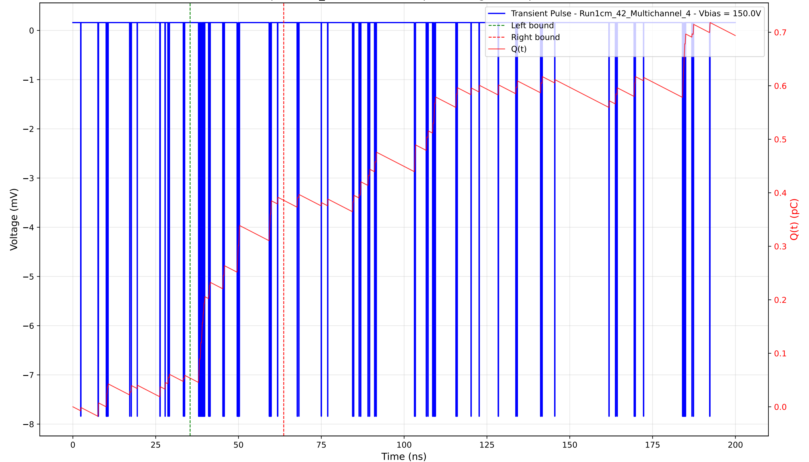
Transient Pulse - Sample: 1cm_42 - Position: 0.0 \mu\text{m} - Charge: 0.33 pC - Rise Time: 0.04 ns
