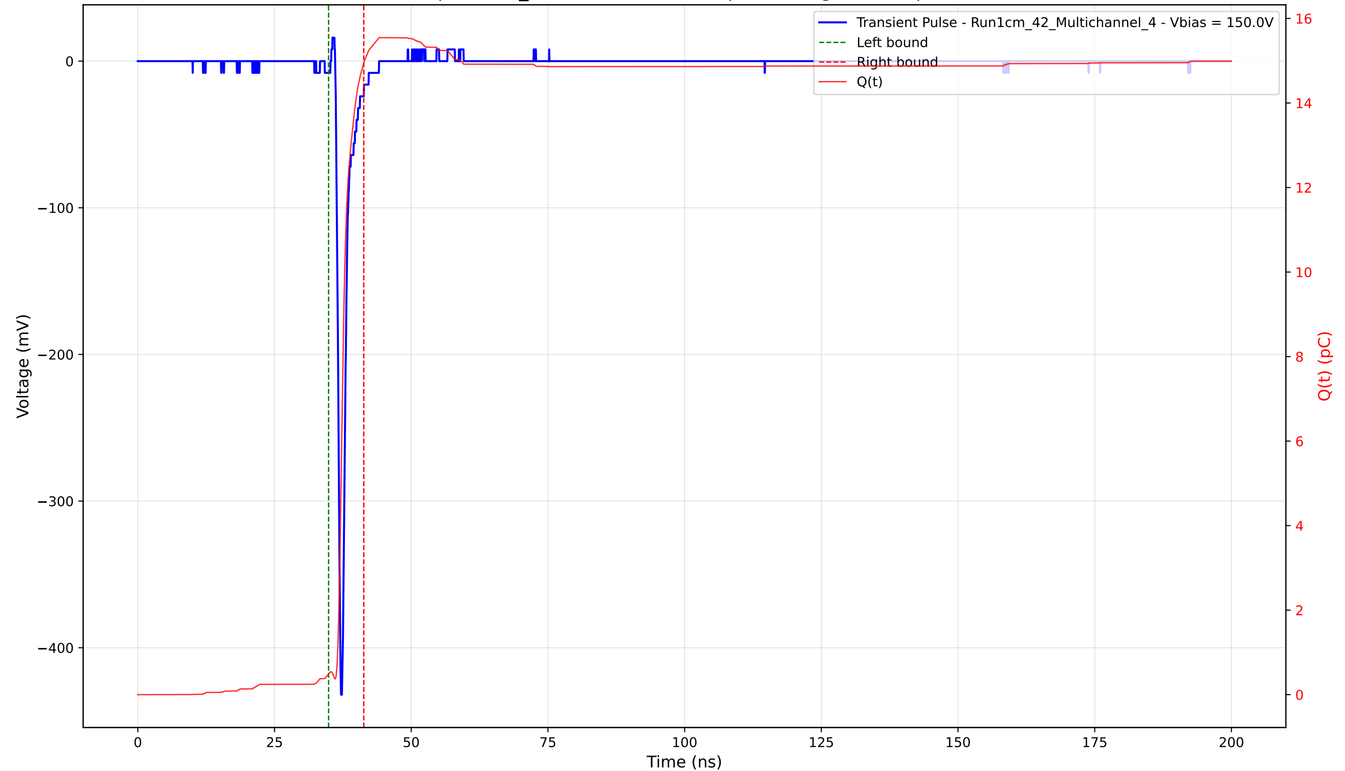
Transient Pulse - Sample: 1cm_42 - Position: 2830.0 \mu\text{m} - Charge: 14.46 pC - Rise Time: 0.73 ns
