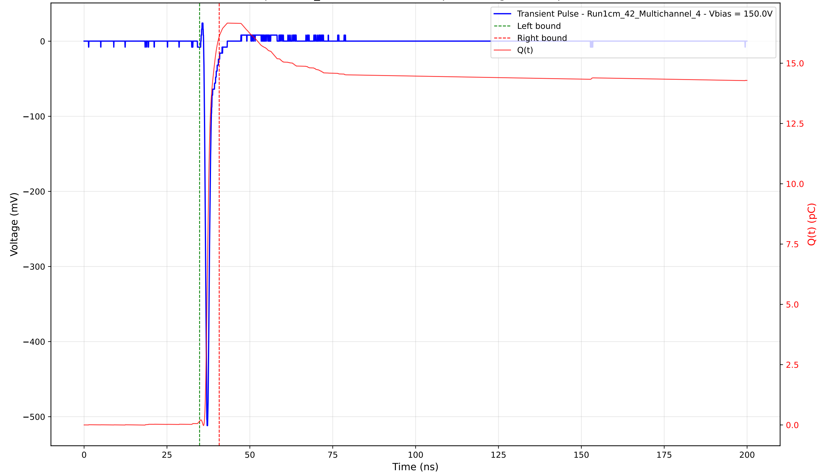
Transient Pulse - Sample: 1cm_42 - Position: 2645.0 \mu\text{m} - Charge: 15.95 pC - Rise Time: 0.66 ns
