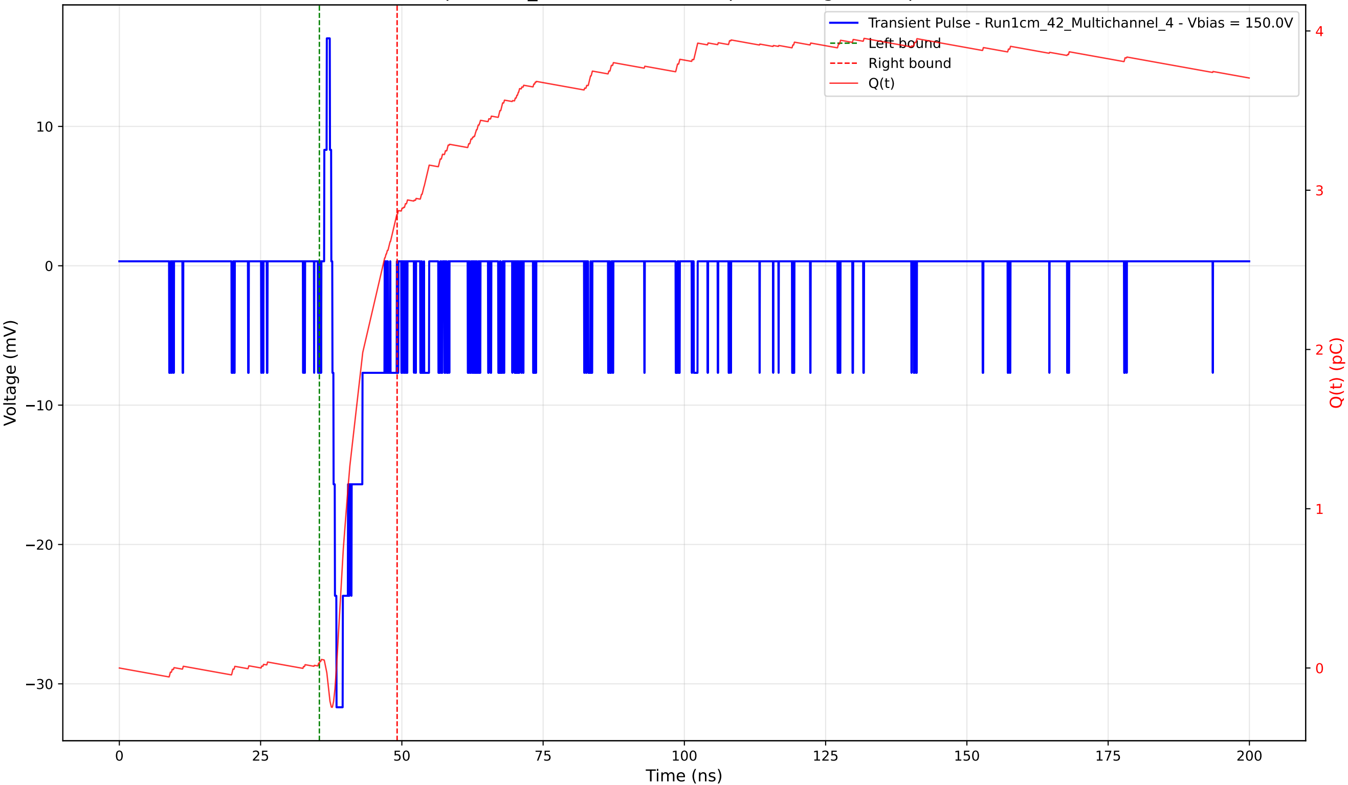
Transient Pulse - Sample: 1cm_42 - Position: 445.0 \mu\text{m} - Charge: 2.82 pC - Rise Time: 0.74 ns
