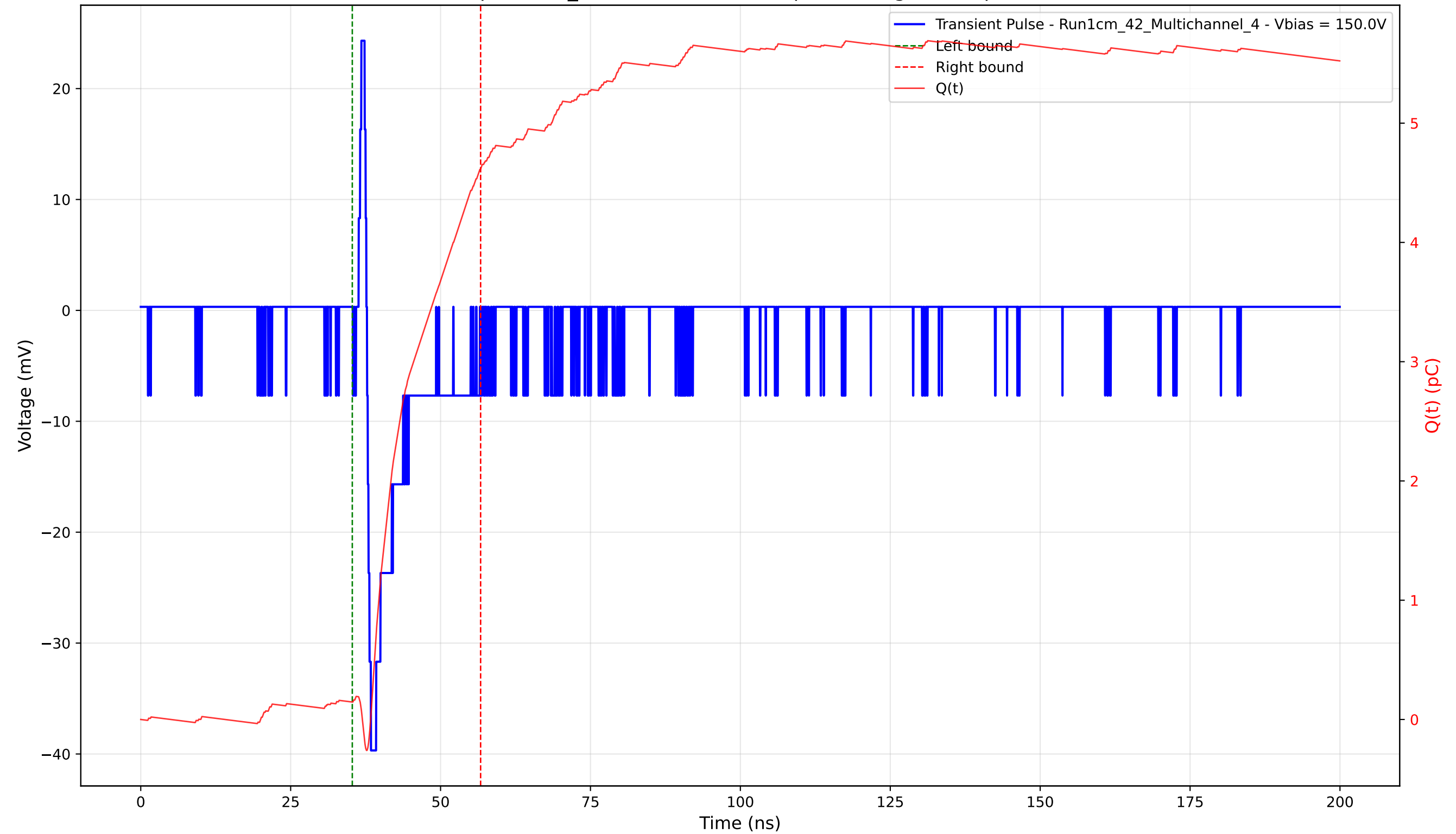
Transient Pulse - Sample: 1cm_42 - Position: 4245.0 \mu\text{m} - Charge: 4.47 pC - Rise Time: 0.66 ns
