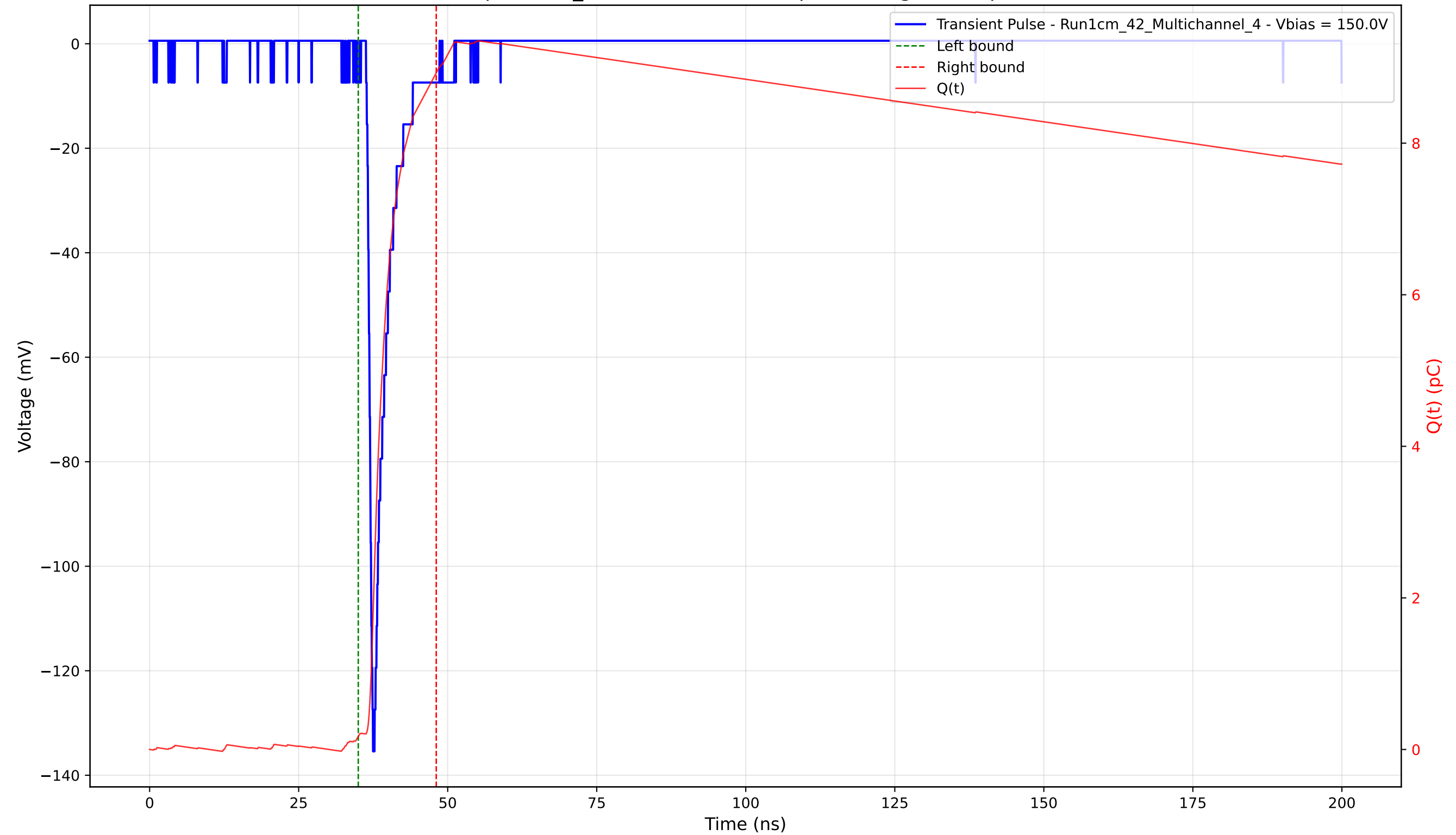
Transient Pulse - Sample: 1cm_42 - Position: 1700.0 \mu\text{m} - Charge: 8.76 pC - Rise Time: 0.97 ns
