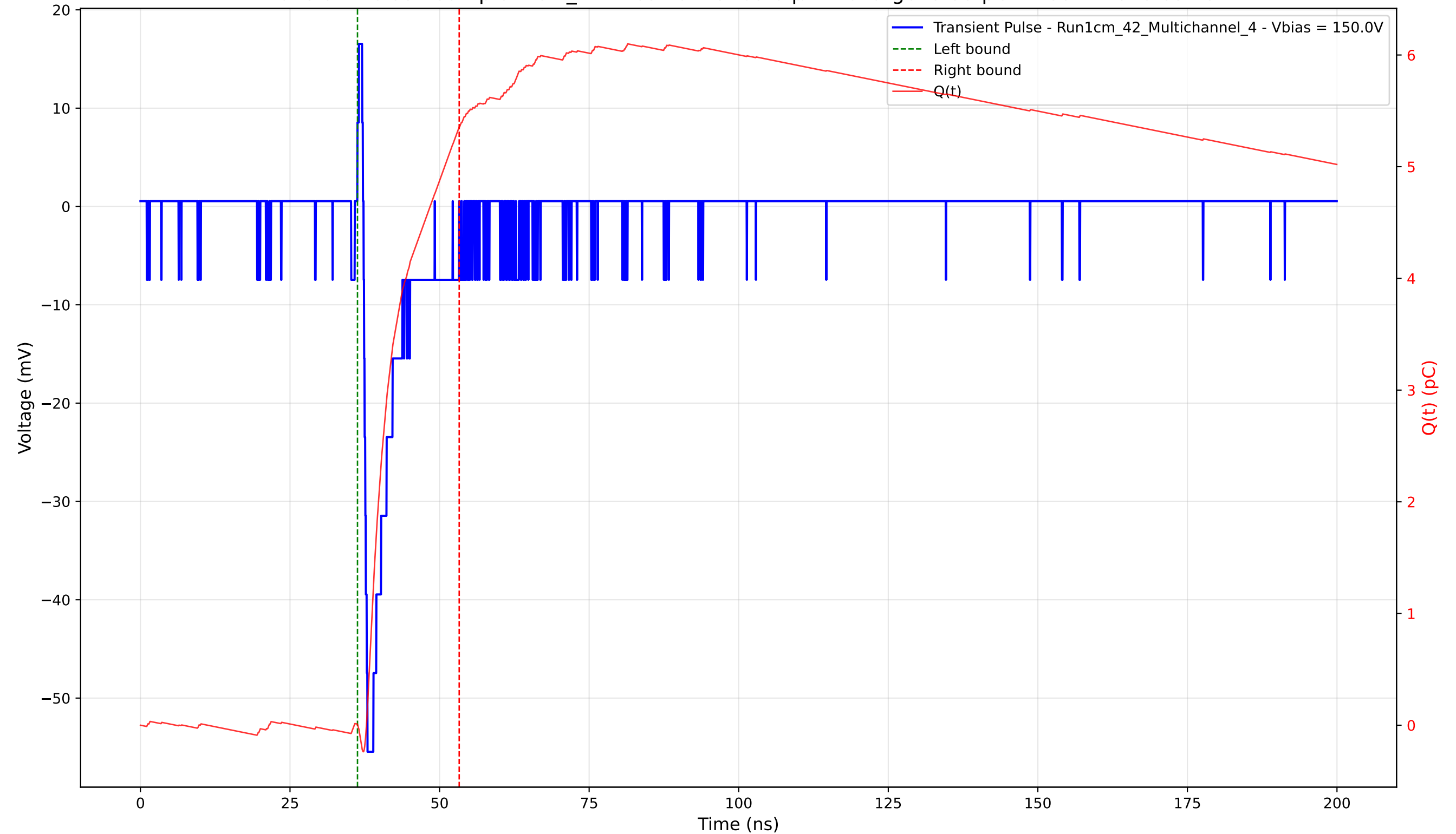
Transient Pulse - Sample: 1cm_42 - Position: 3765.0 \mu\text{m} - Charge: 5.35 pC - Rise Time: 0.65 ns
