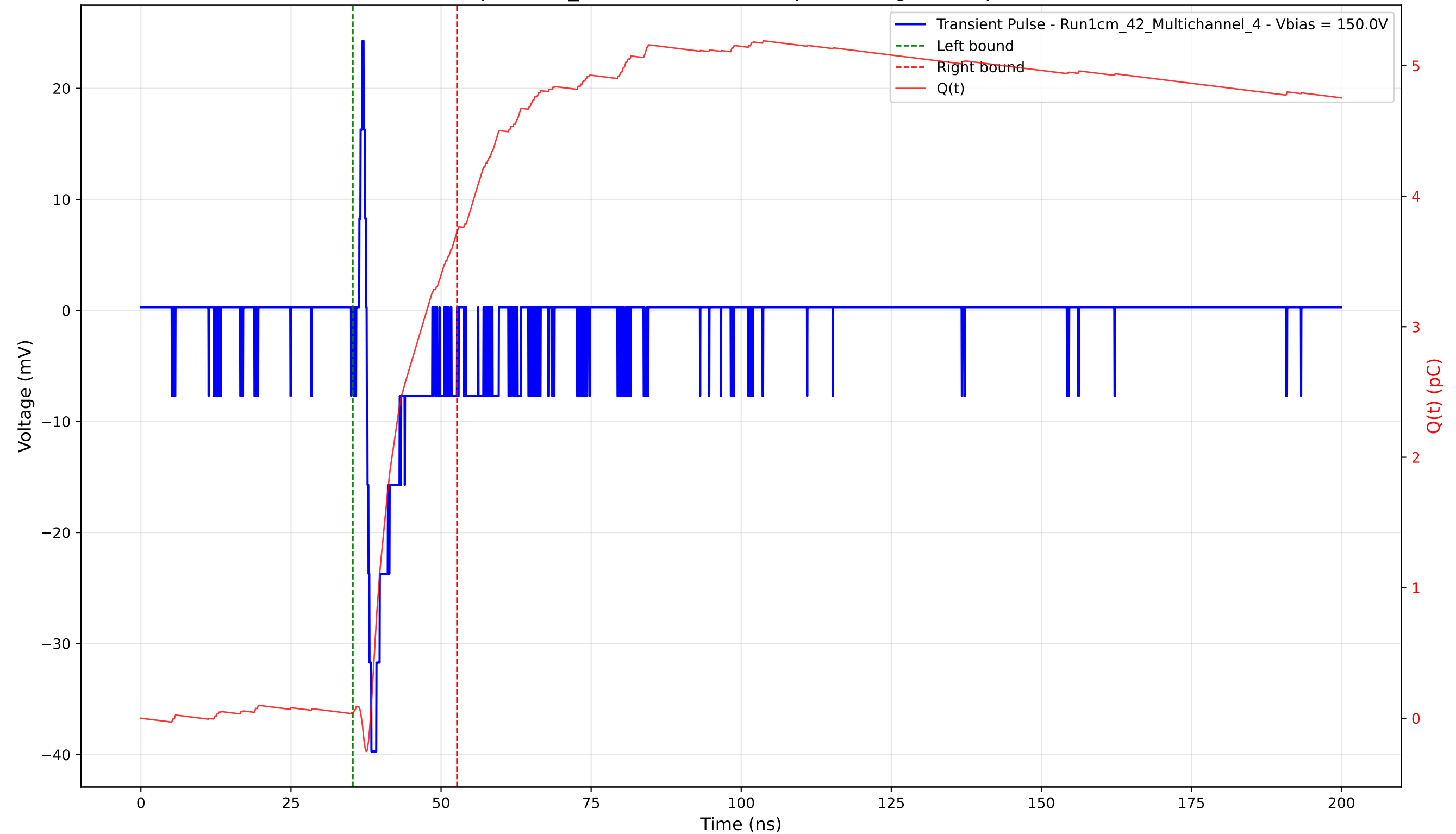
Transient Pulse - Sample: 1cm_42 - Position: 4080.0 \mu\text{m} - Charge: 3.69 pC - Rise Time: 0.78 ns
