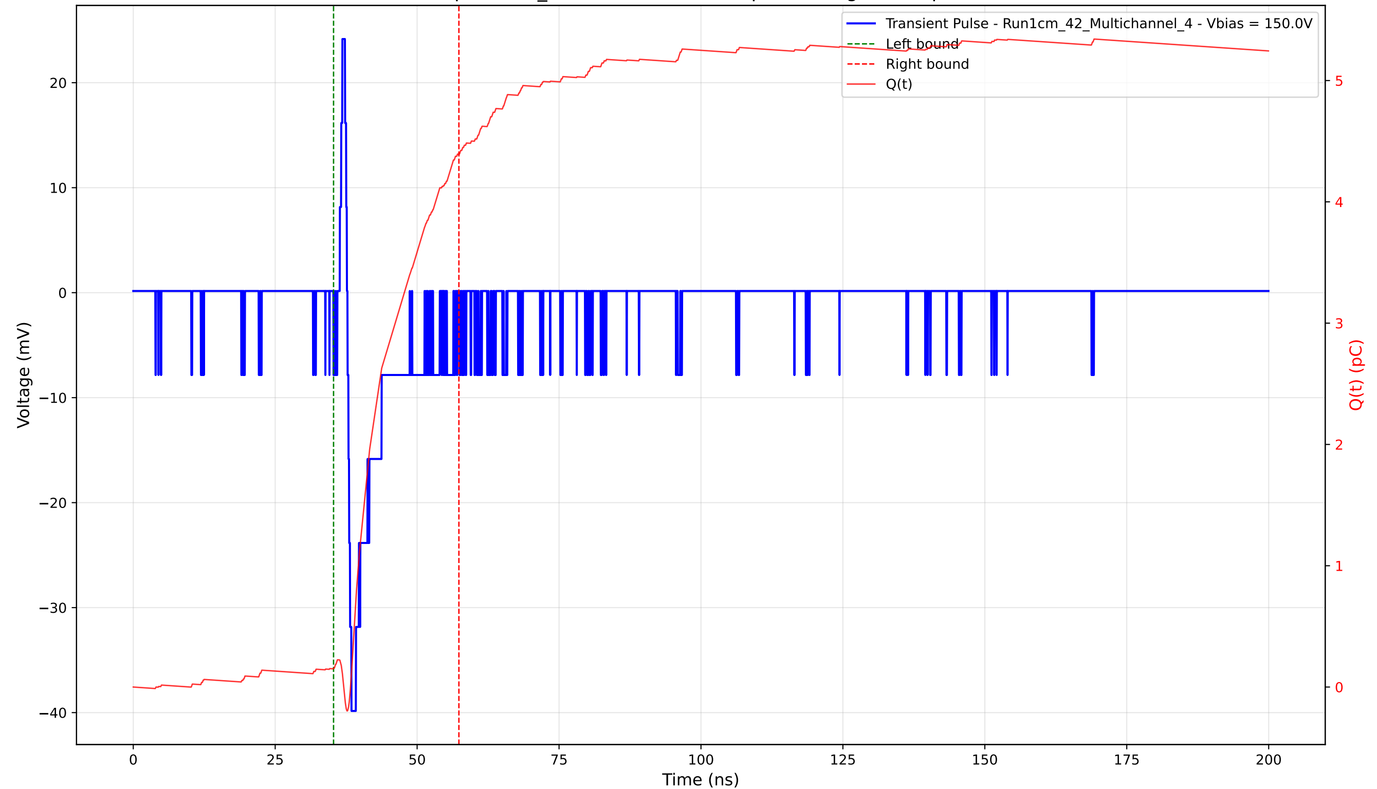
Transient Pulse - Sample: 1cm_42 - Position: 4345.0 \mu\text{m} - Charge: 4.24 pC - Rise Time: 0.70 ns
