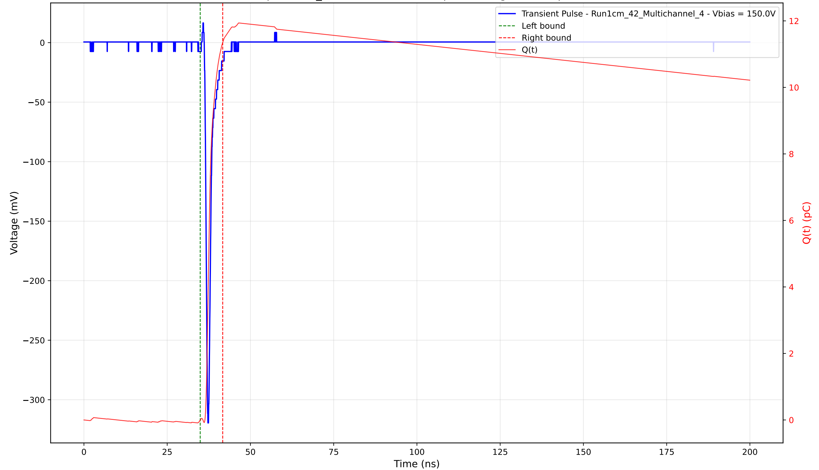
Transient Pulse - Sample: 1cm_42 - Position: 2920.0 \mu\text{m} - Charge: 11.35 pC - Rise Time: 0.72 ns
