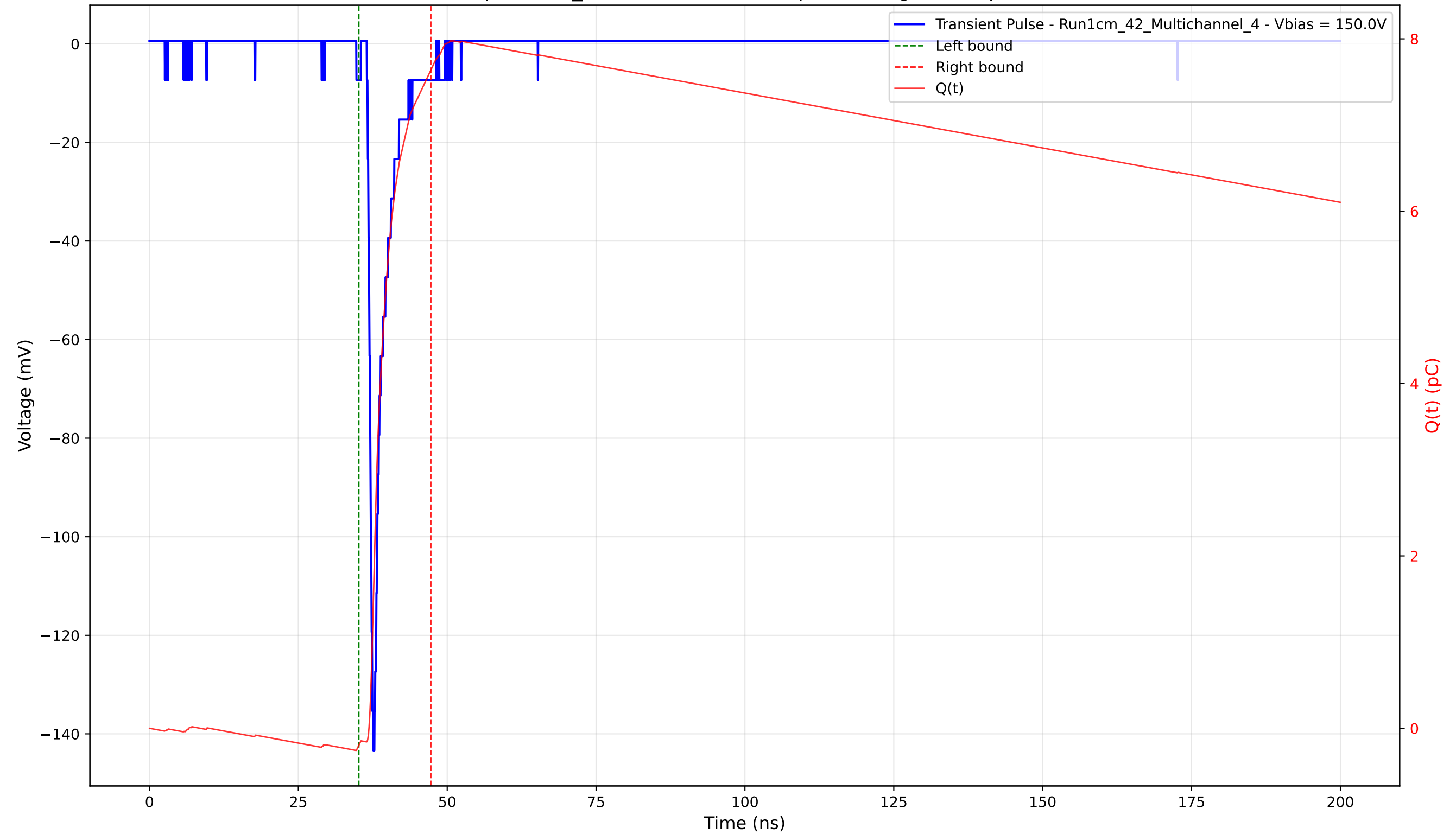
Transient Pulse - Sample: 1cm_42 - Position: 3280.0 \mu\text{m} - Charge: 7.83 pC - Rise Time: 0.81 ns
