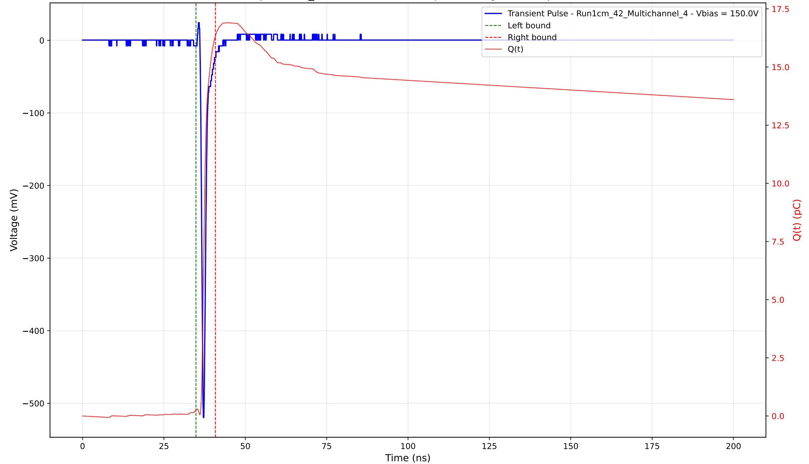
Transient Pulse - Sample: 1cm_42 - Position: 2640.0 \mu\text{m} - Charge: 16.09 pC - Rise Time: 0.72 ns
