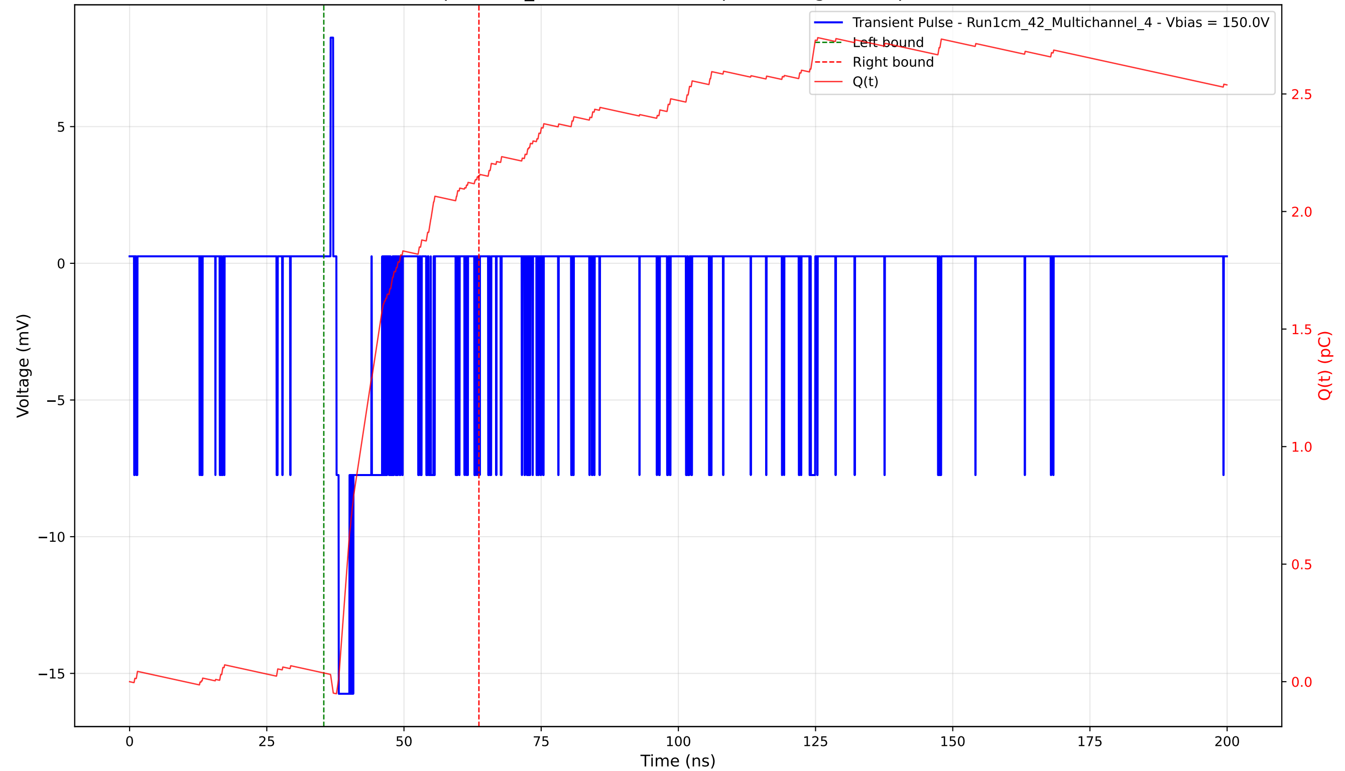
Transient Pulse - Sample: 1cm_42 - Position: 190.0 \mu\text{m} - Charge: 2.12 pC - Rise Time: 0.43 ns
