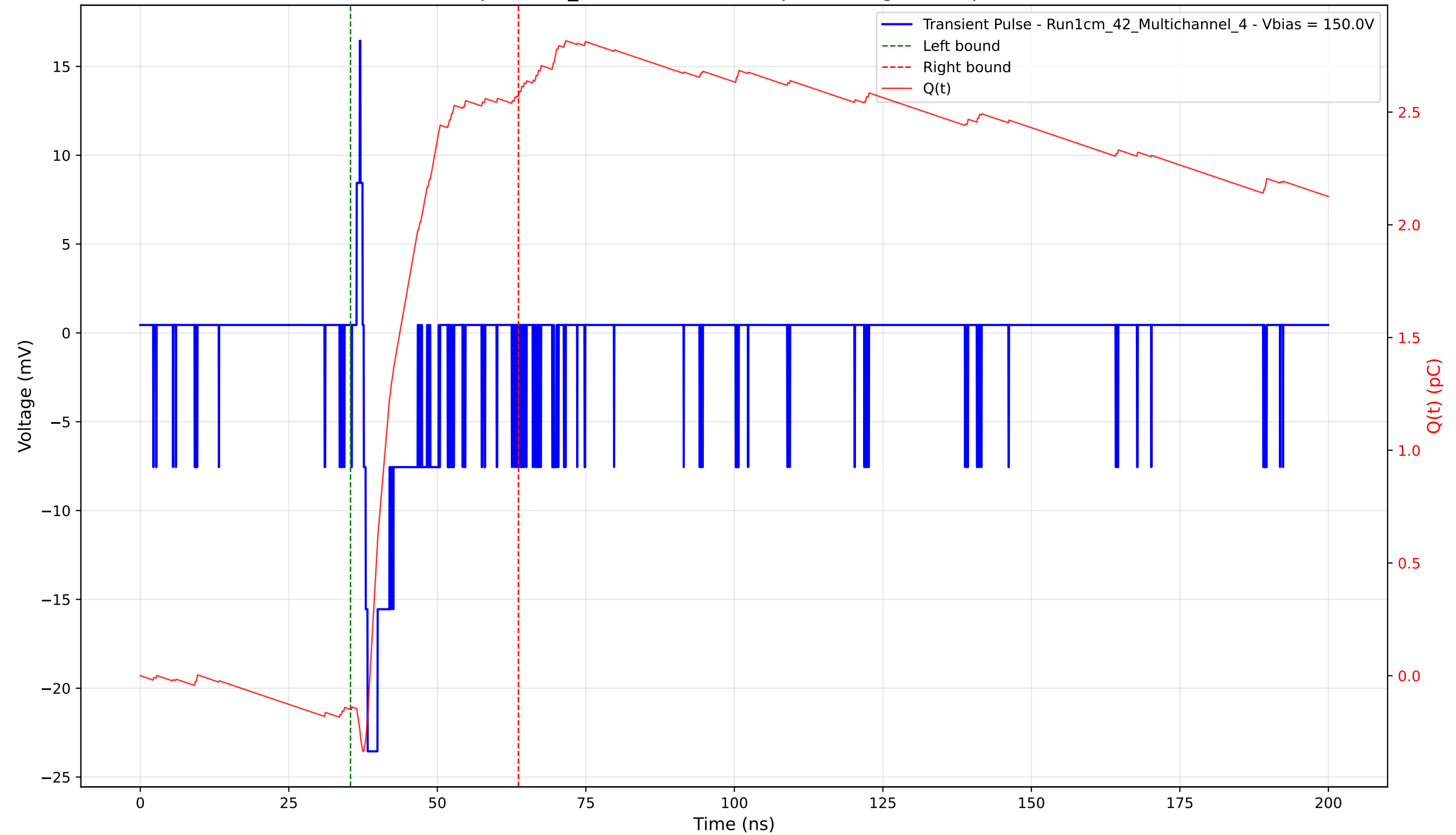
Transient Pulse - Sample: 1cm_42 - Position: 340.0 \mu\text{m} - Charge: 2.72 pC - Rise Time: 0.67 ns
