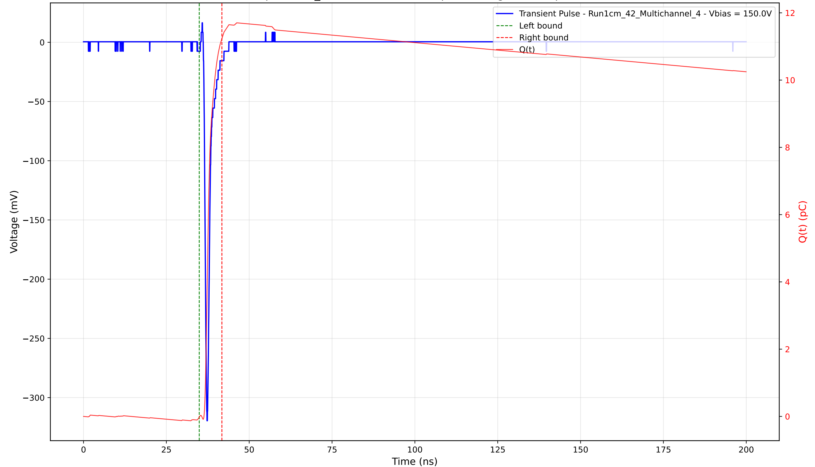
Transient Pulse - Sample: 1cm_42 - Position: 2925.0 \mu\text{m} - Charge: 11.25 pC - Rise Time: 0.76 ns
