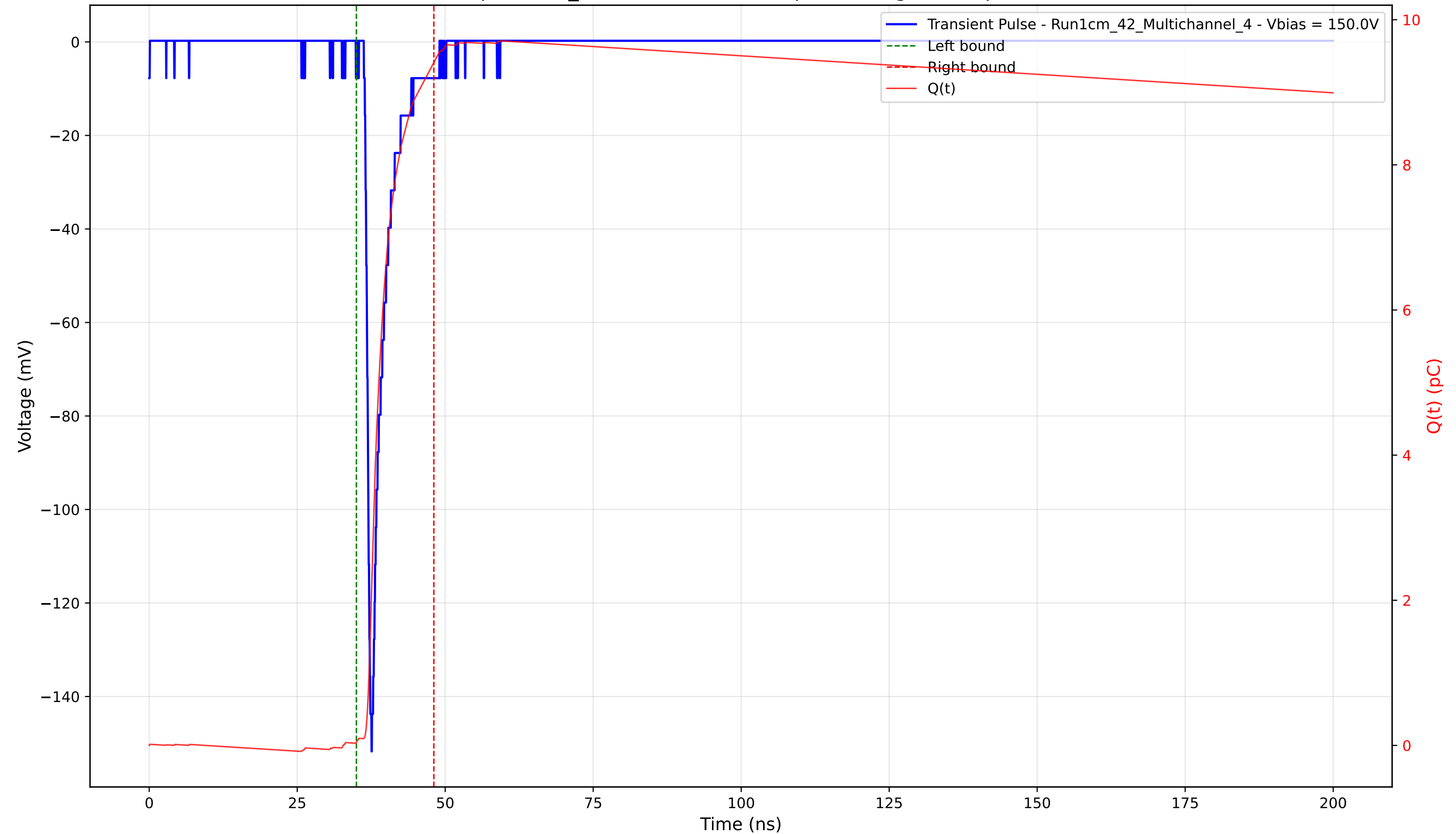
Transient Pulse - Sample: 1cm_42 - Position: 1755.0 \mu\text{m} - Charge: 9.37 pC - Rise Time: 0.92 ns
