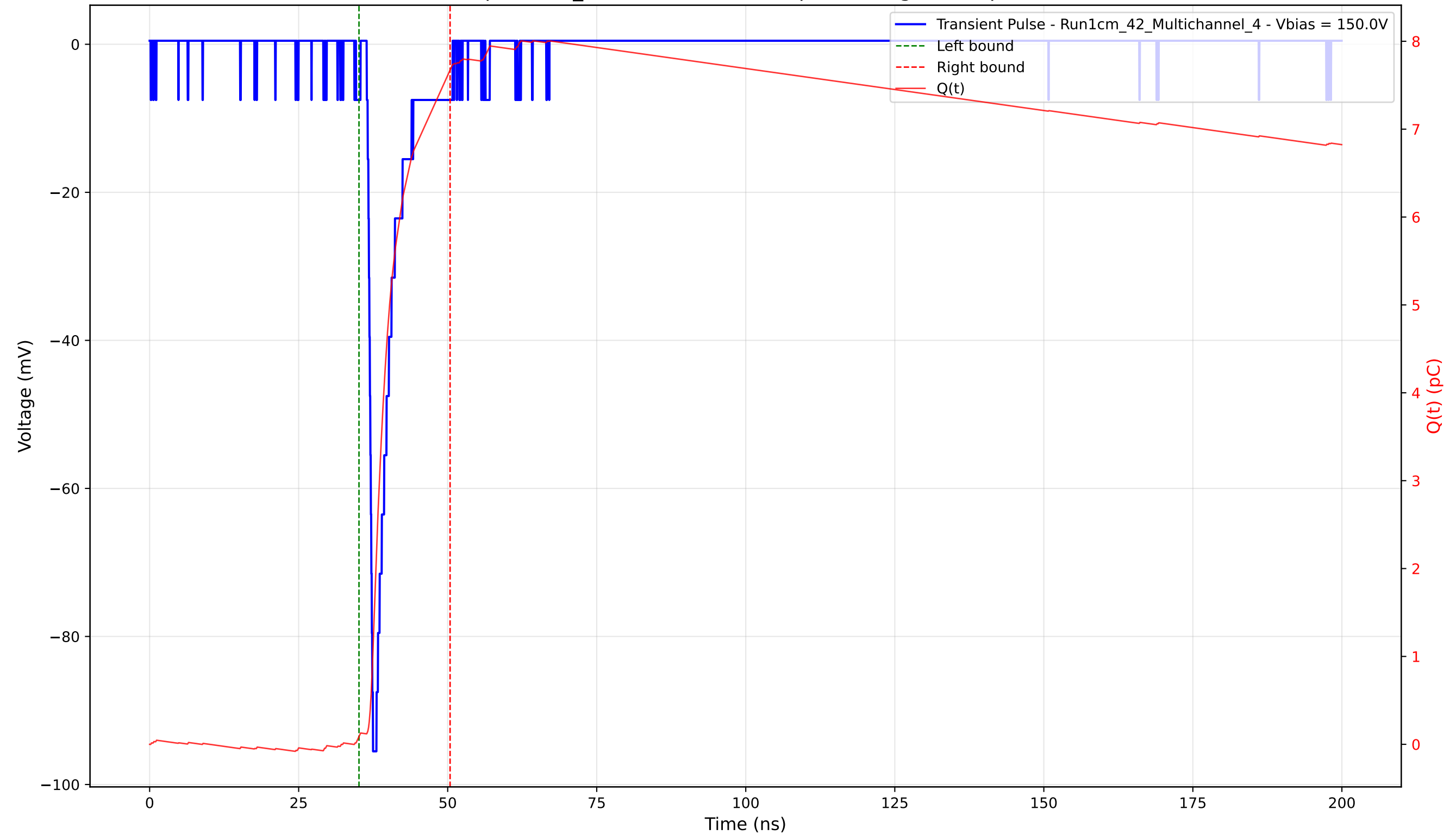
Transient Pulse - Sample: 1cm_42 - Position: 1605.0 \mu\text{m} - Charge: 7.59 pC - Rise Time: 0.79 ns
