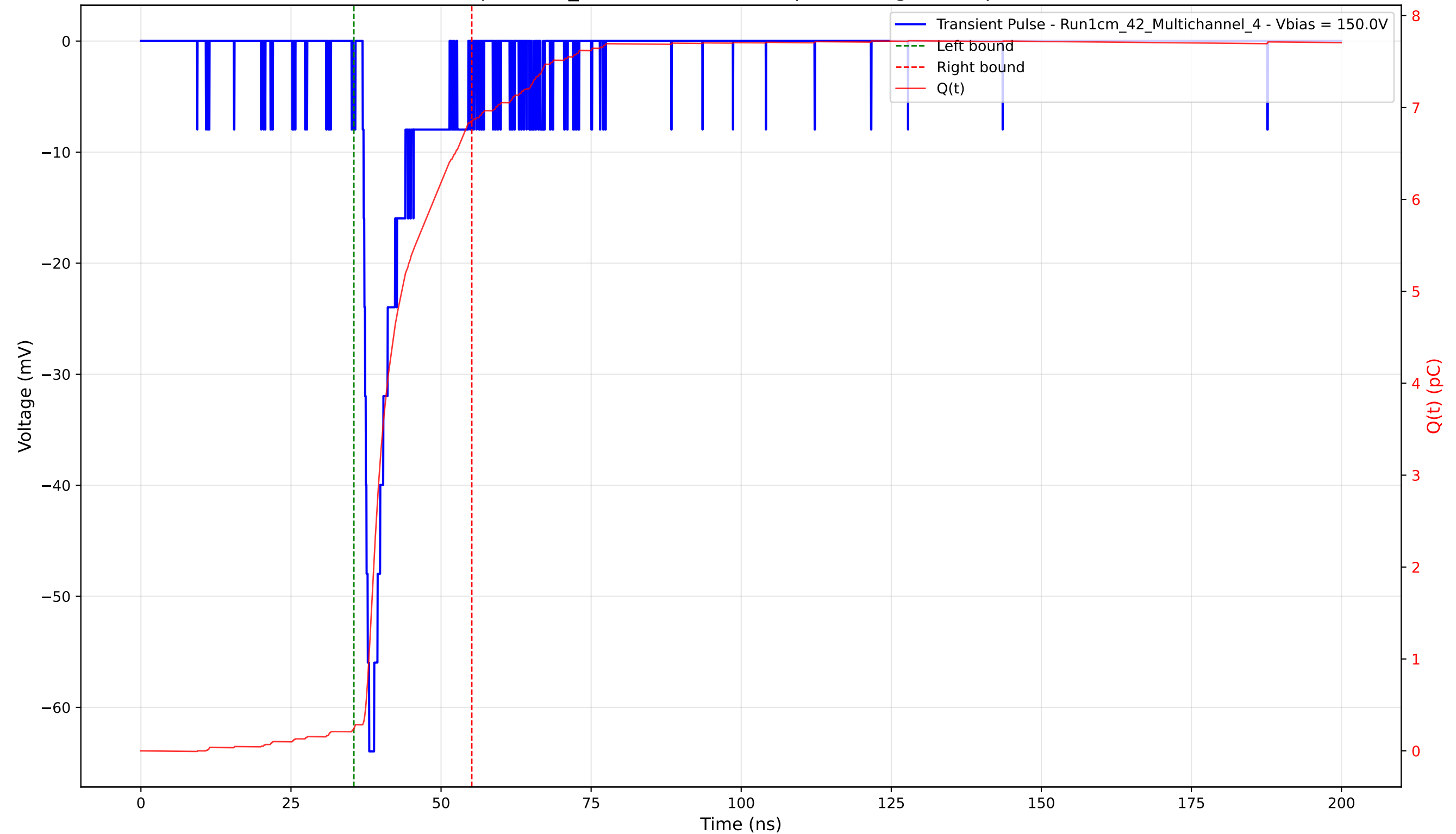
Transient Pulse - Sample: 1cm_42 - Position: 1410.0 \mu\text{m} - Charge: 6.61 pC - Rise Time: 1.09 ns
