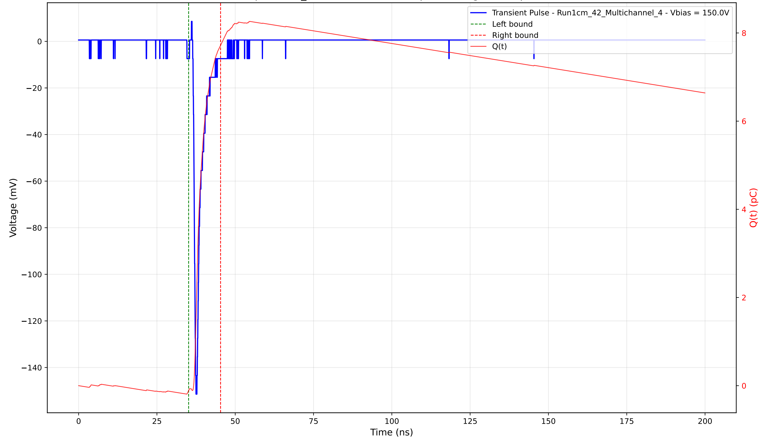
Transient Pulse - Sample: 1cm_42 - Position: 3195.0 \mu\text{m} - Charge: 7.83 pC - Rise Time: 0.80 ns
