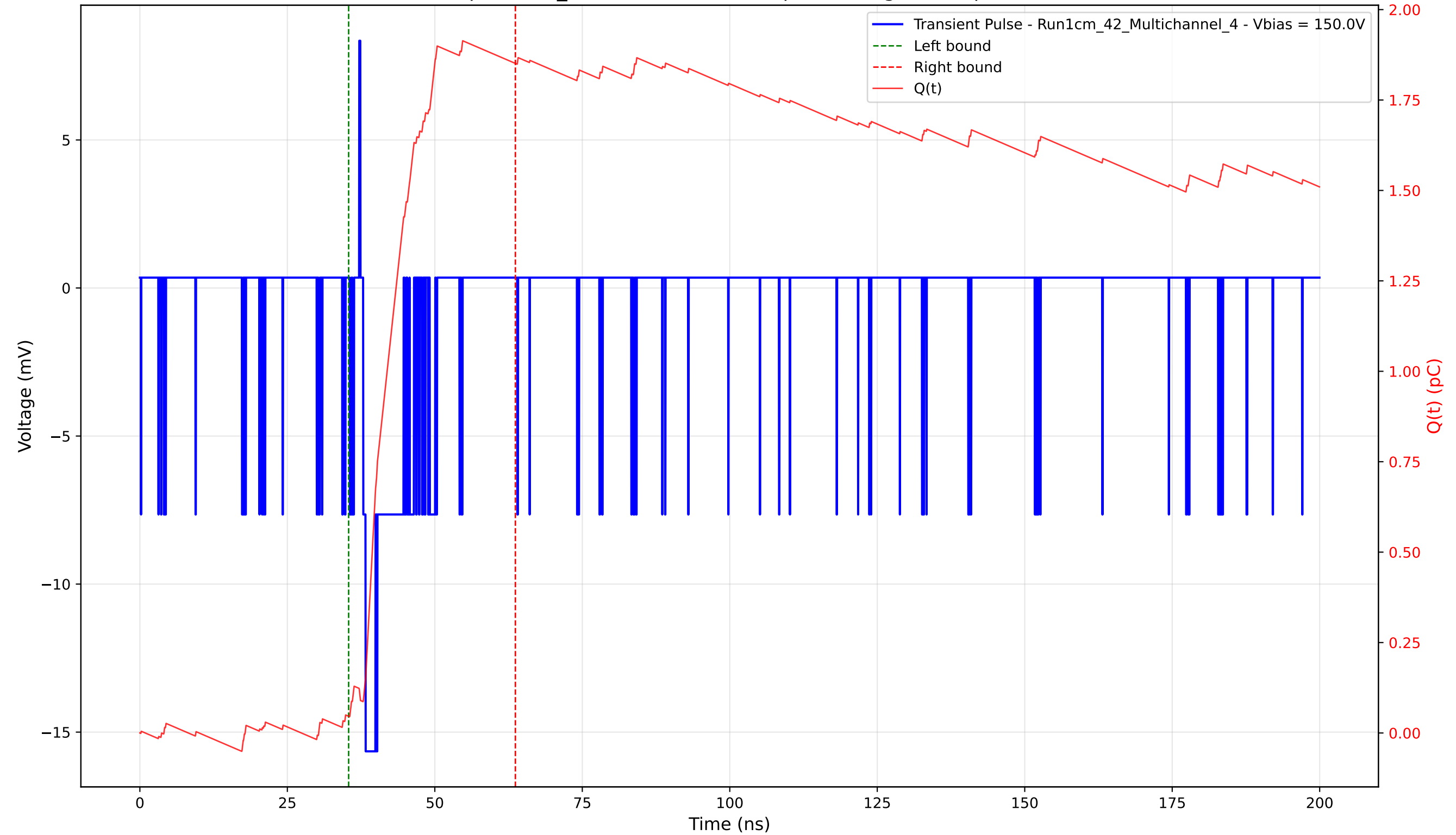
Transient Pulse - Sample: 1cm_42 - Position: 5015.0 \mu\text{m} - Charge: 1.81 pC - Rise Time: 0.43 ns
