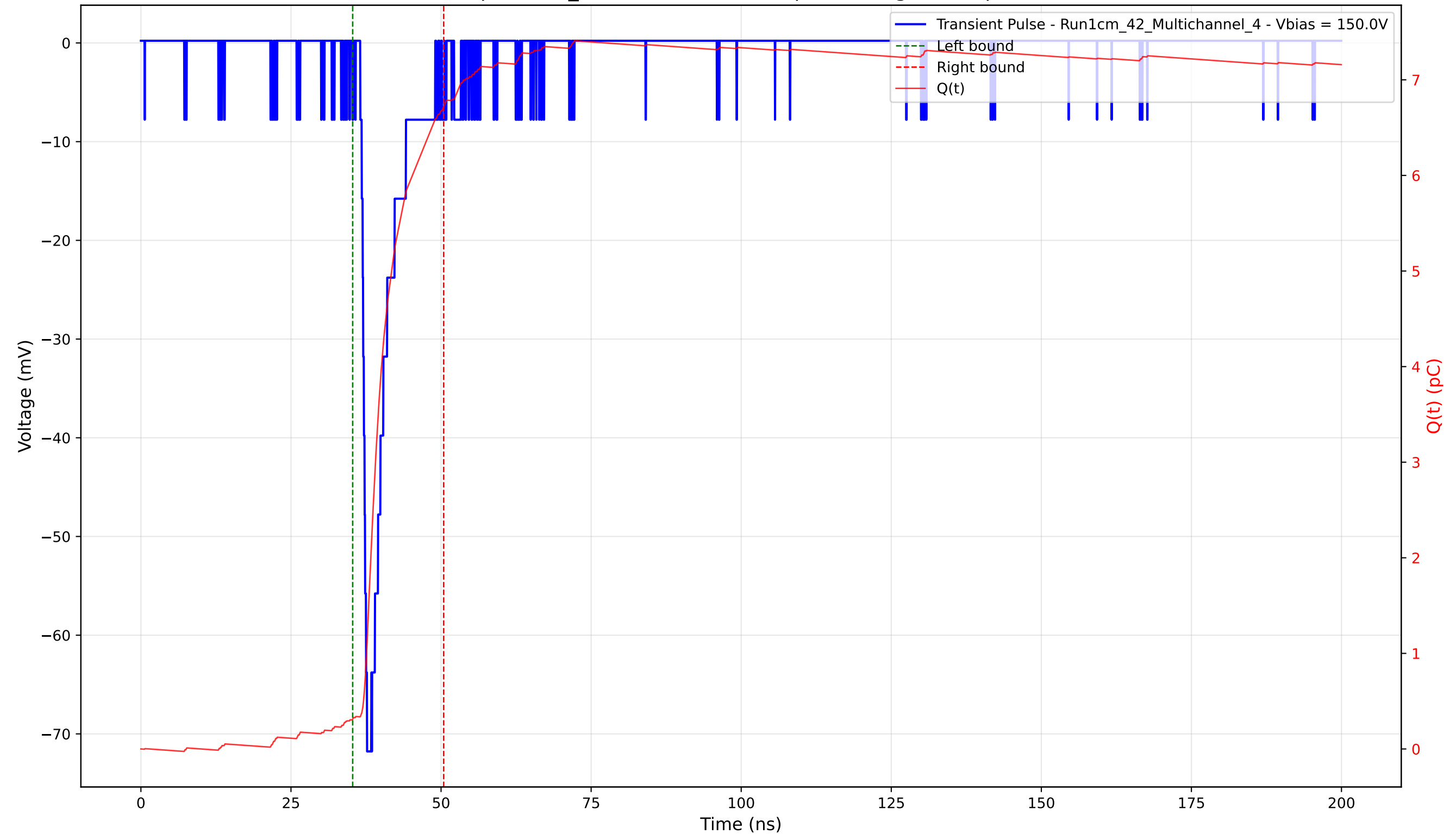
Transient Pulse - Sample: 1cm_42 - Position: 1510.0 \mu\text{m} - Charge: 6.41 pC - Rise Time: 1.12 ns
