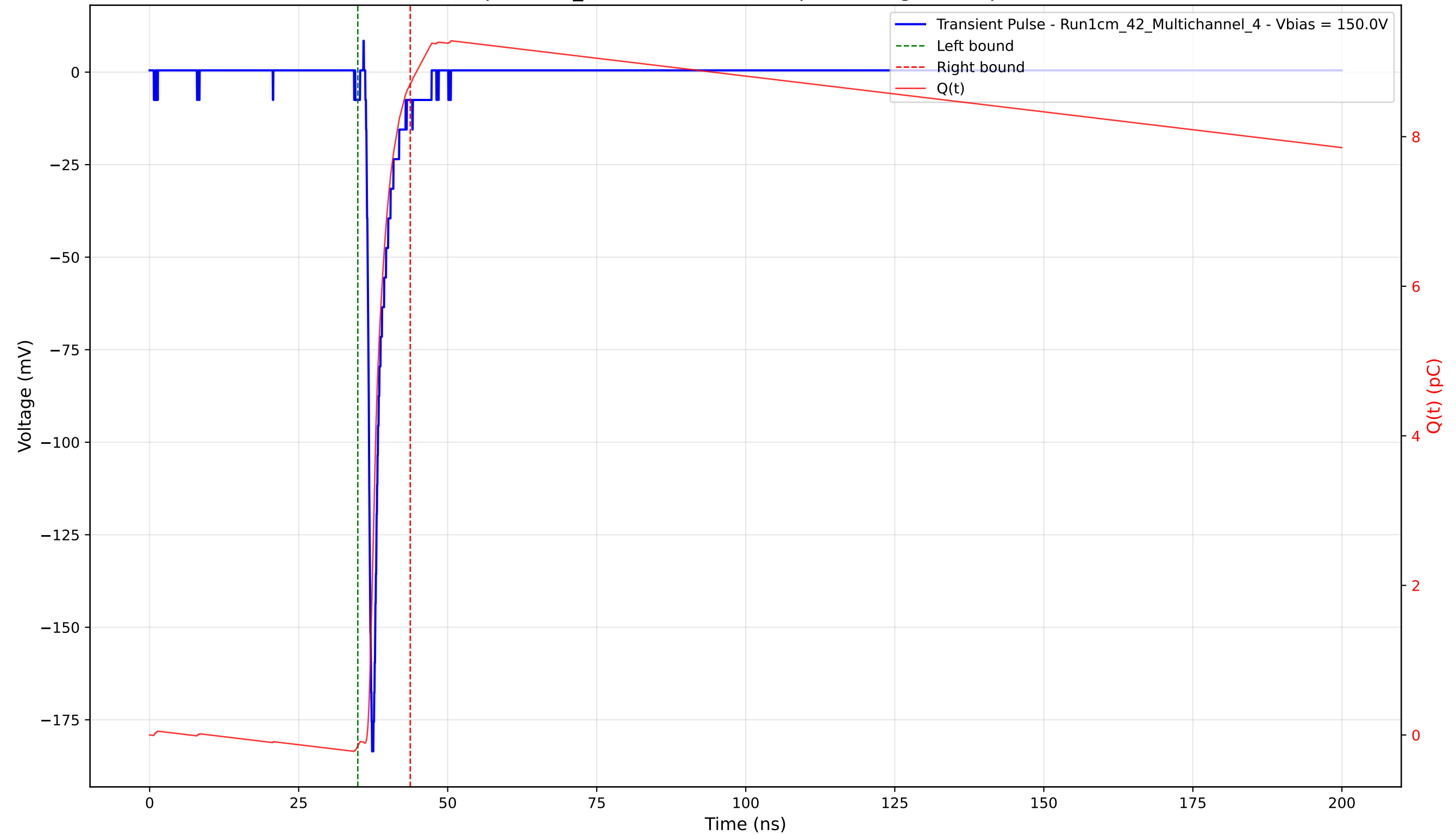
Transient Pulse - Sample: 1cm_42 - Position: 1930.0 \mu\text{m} - Charge: 8.84 pC - Rise Time: 0.79 ns
