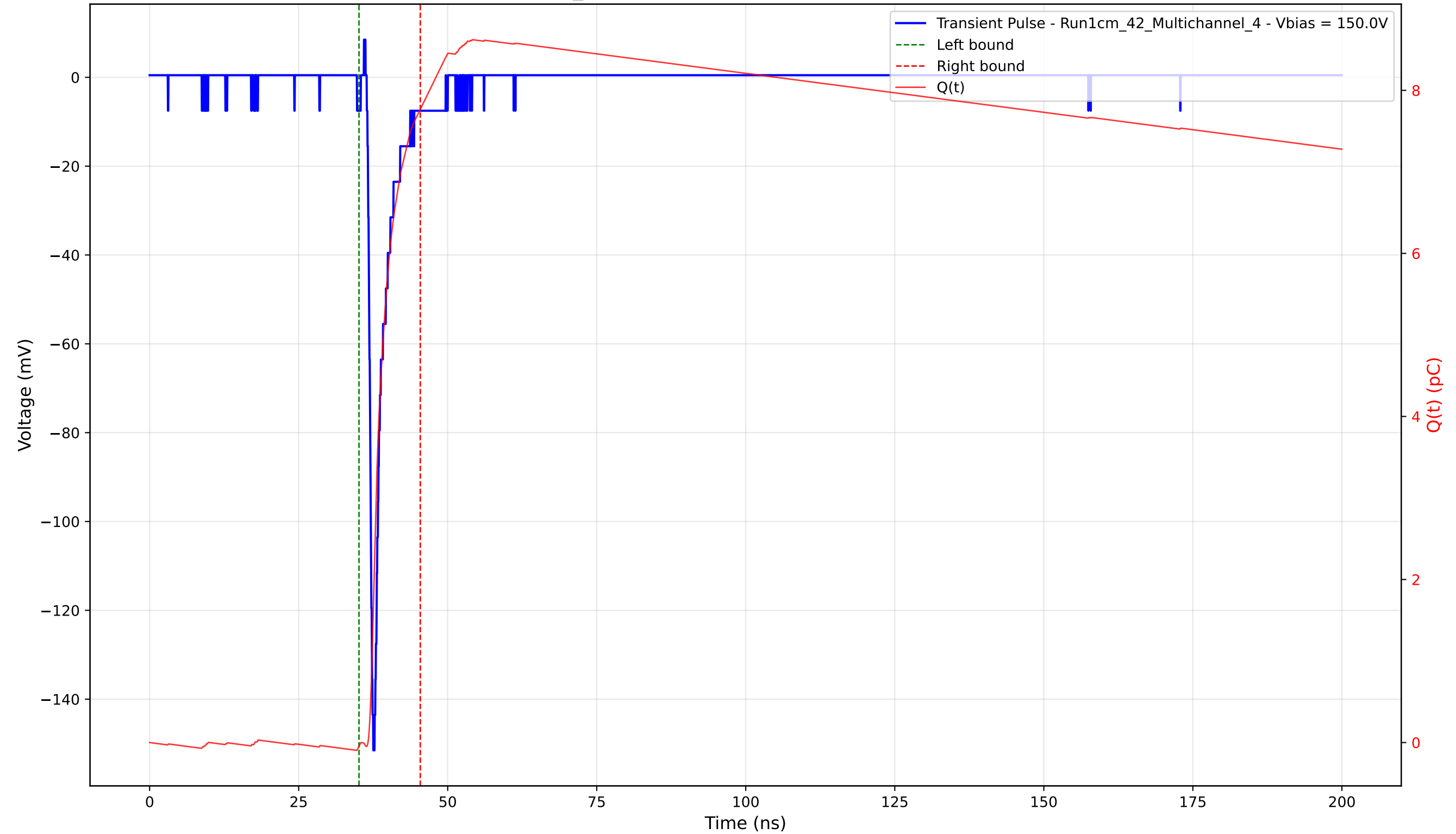
Transient Pulse - Sample: 1cm_42 - Position: 3210.0 \mu\text{m} - Charge: 7.81 pC - Rise Time: 0.84 ns
