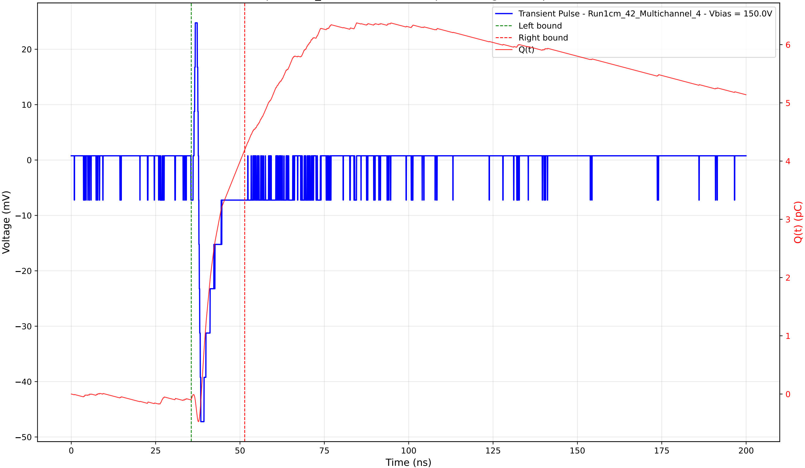
Transient Pulse - Sample: 1cm_42 - Position: 755.0 \mu\text{m} - Charge: 4.28 pC - Rise Time: 0.66 ns
