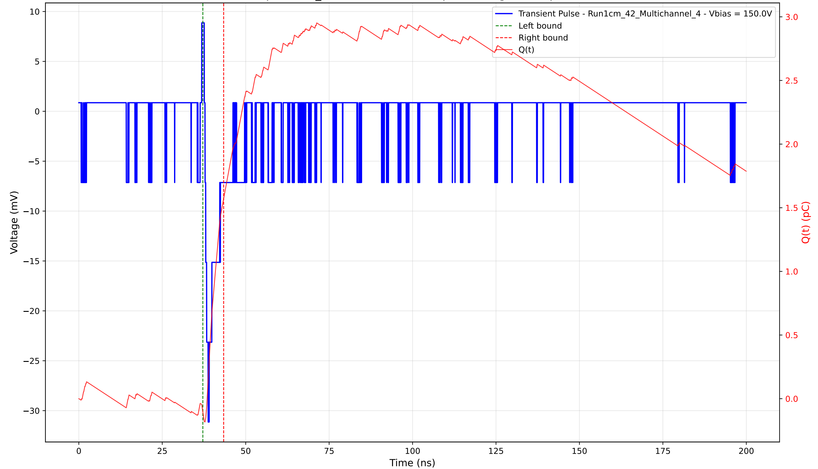
Transient Pulse - Sample: 1cm_42 - Position: 4910.0 \mu\text{m} - Charge: 1.68 pC - Rise Time: 0.95 ns
