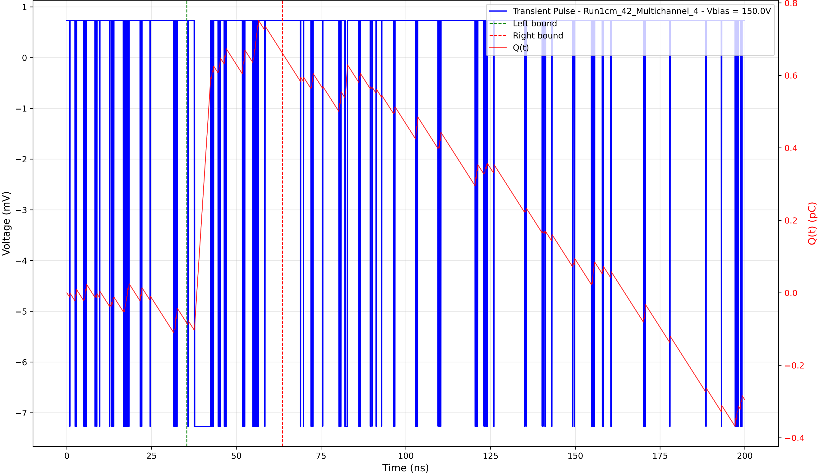
Transient Pulse - Sample: 1cm_42 - Position: 80.0 \mu\text{m} - Charge: 0.74 pC - Rise Time: 0.00 ns (N/A)
