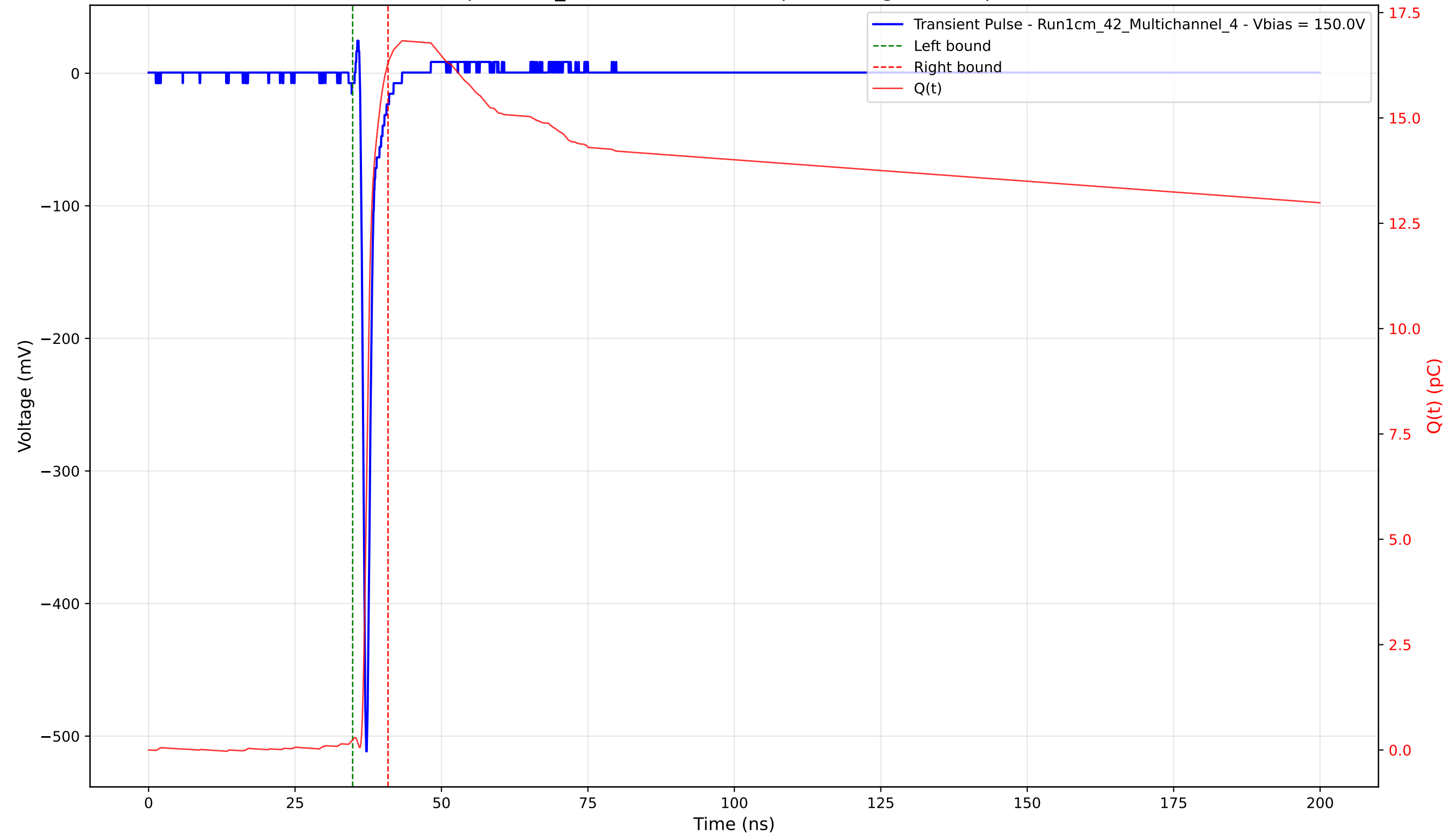
Transient Pulse - Sample: 1cm_42 - Position: 2695.0 \mu\text{m} - Charge: 16.05 pC - Rise Time: 0.73 ns
