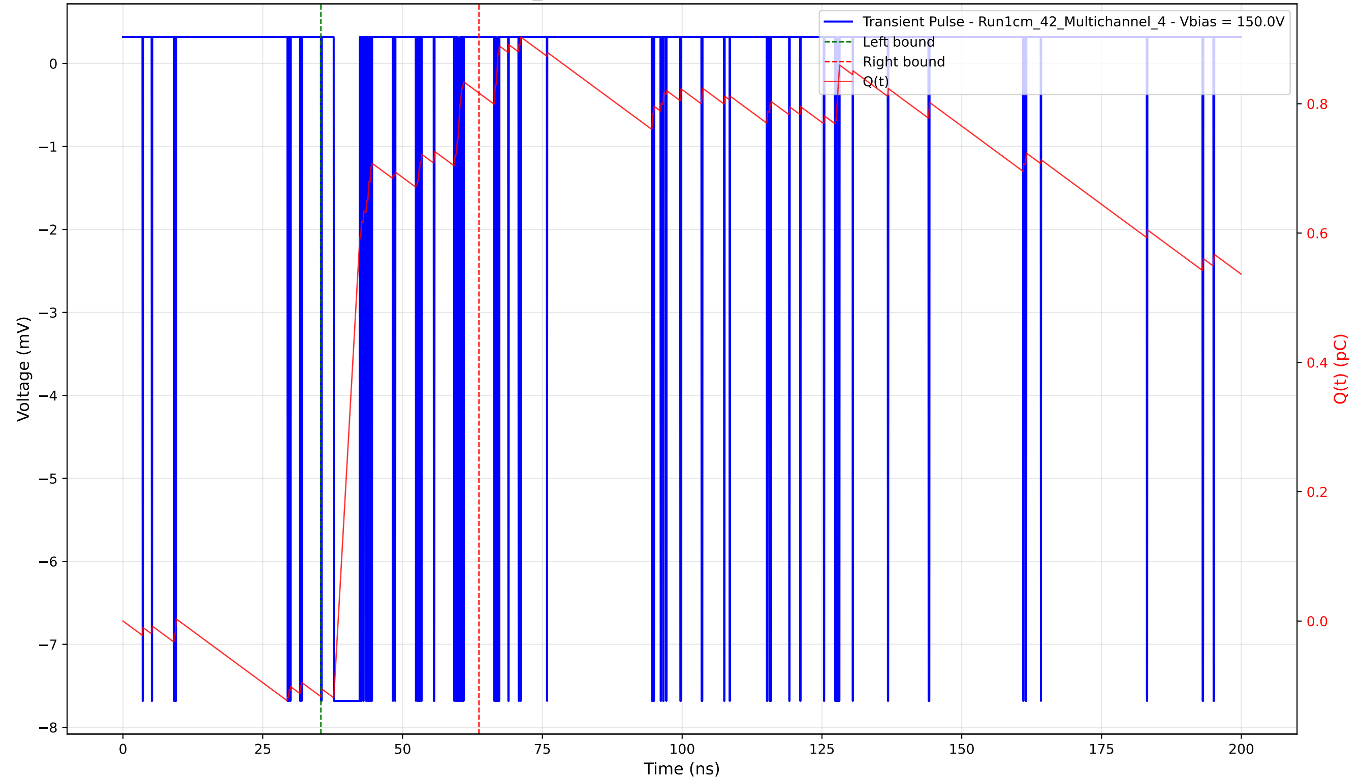
Transient Pulse - Sample: 1cm_42 - Position: 65.0 \mu\text{m} - Charge: 0.93 pC - Rise Time: 0.04 ns
