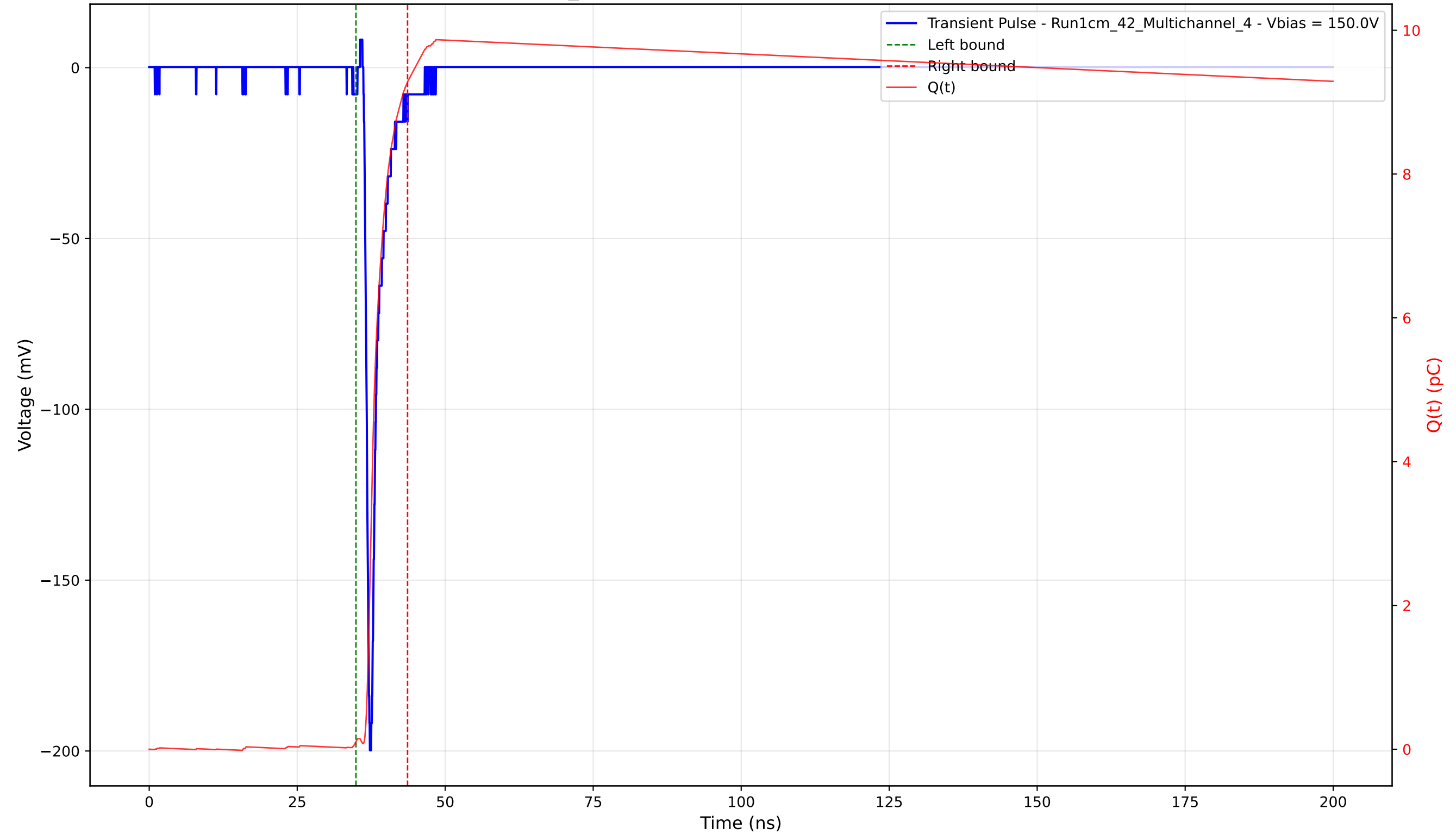
Transient Pulse - Sample: 1cm_42 - Position: 1965.0 \mu\text{m} - Charge: 9.17 pC - Rise Time: 0.78 ns
