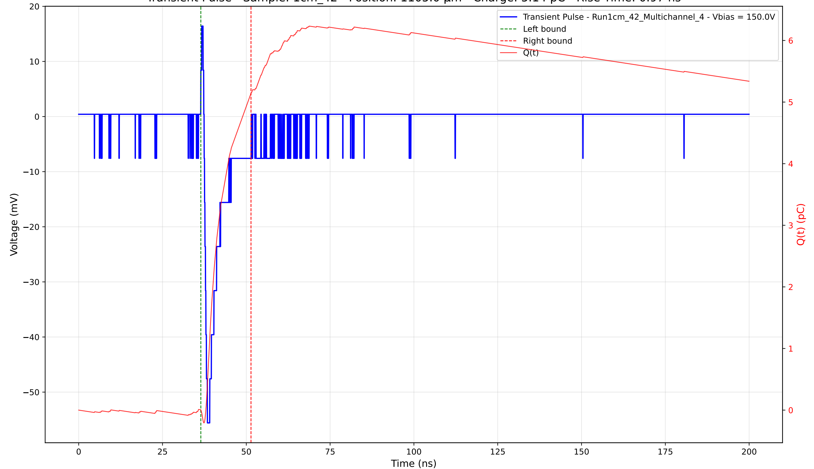
Transient Pulse - Sample: 1cm_42 - Position: 1105.0 \mu\text{m} - Charge: 5.14 pC - Rise Time: 0.97 ns
