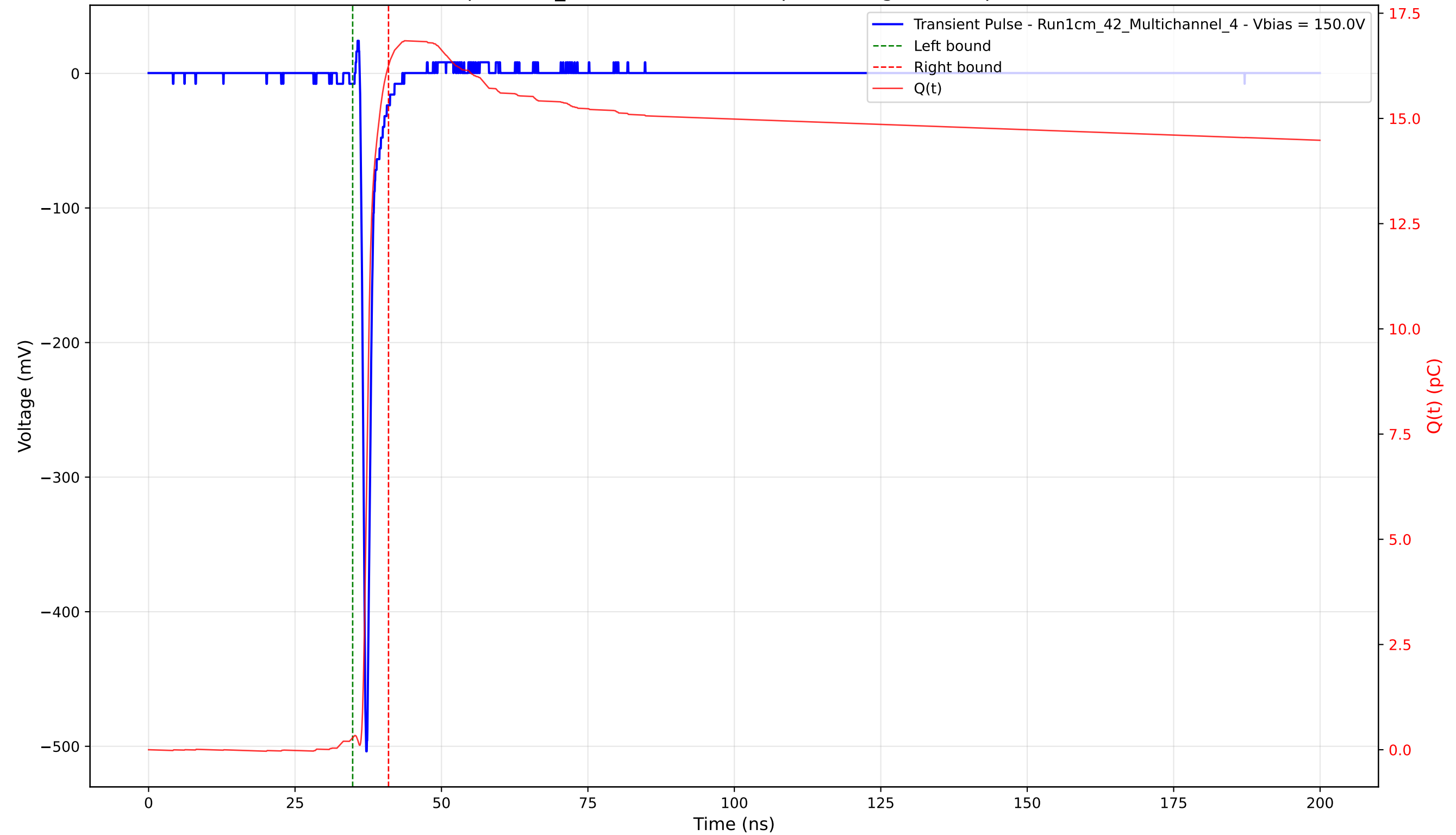
Transient Pulse - Sample: 1cm_42 - Position: 2705.0 \mu\text{m} - Charge: 15.97 pC - Rise Time: 0.73 ns
