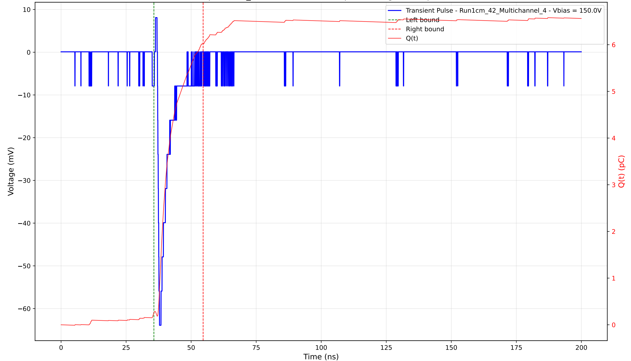
Transient Pulse - Sample: 1cm_42 - Position: 3600.0 \mu\text{m} - Charge: 5.77 pC - Rise Time: 0.77 ns
