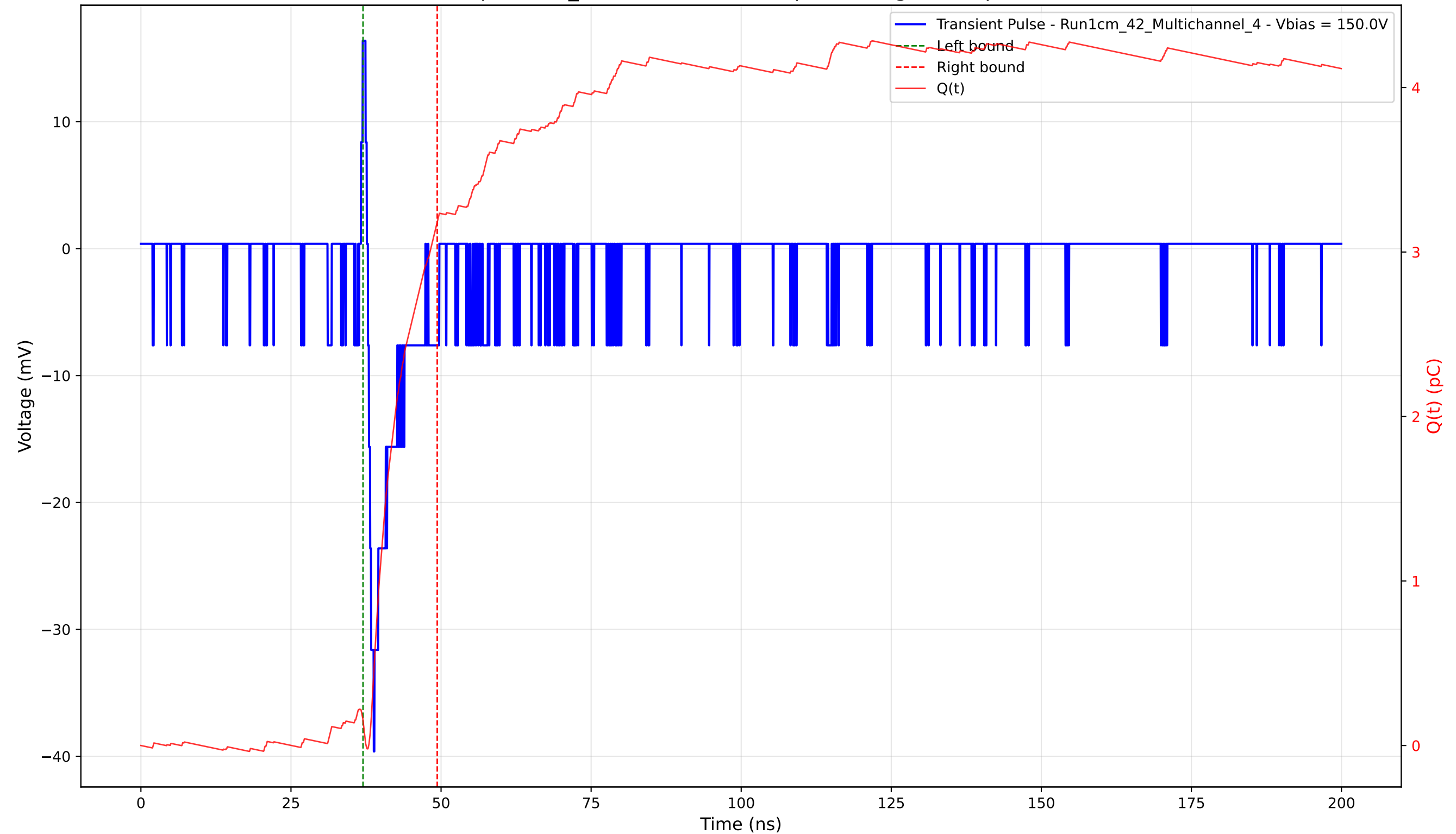
Transient Pulse - Sample: 1cm_42 - Position: 4800.0 \mu\text{m} - Charge: 3.03 pC - Rise Time: 0.98 ns
