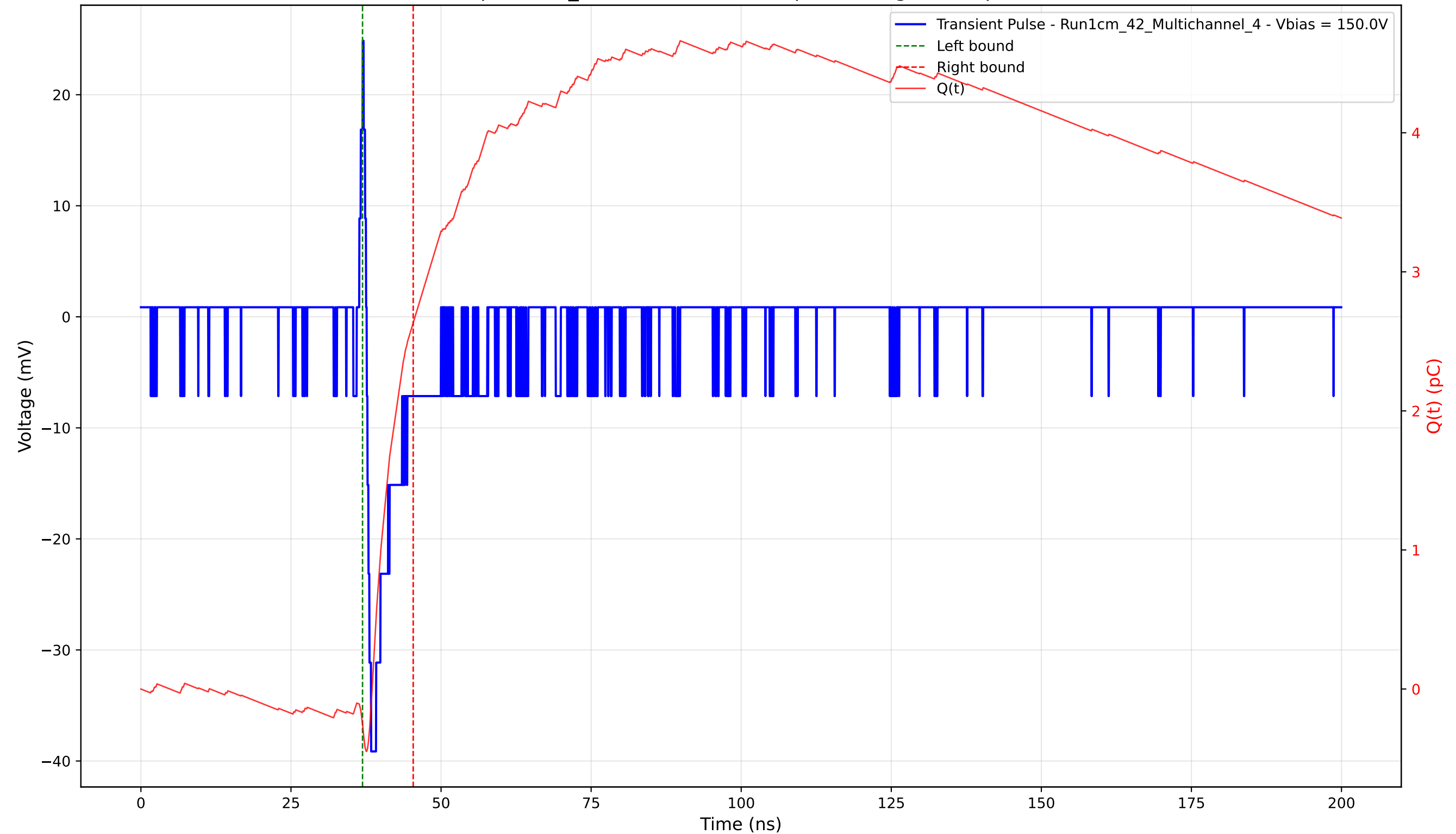
Transient Pulse - Sample: 1cm_42 - Position: 4115.0 \mu\text{m} - Charge: 2.89 pC - Rise Time: 0.74 ns
