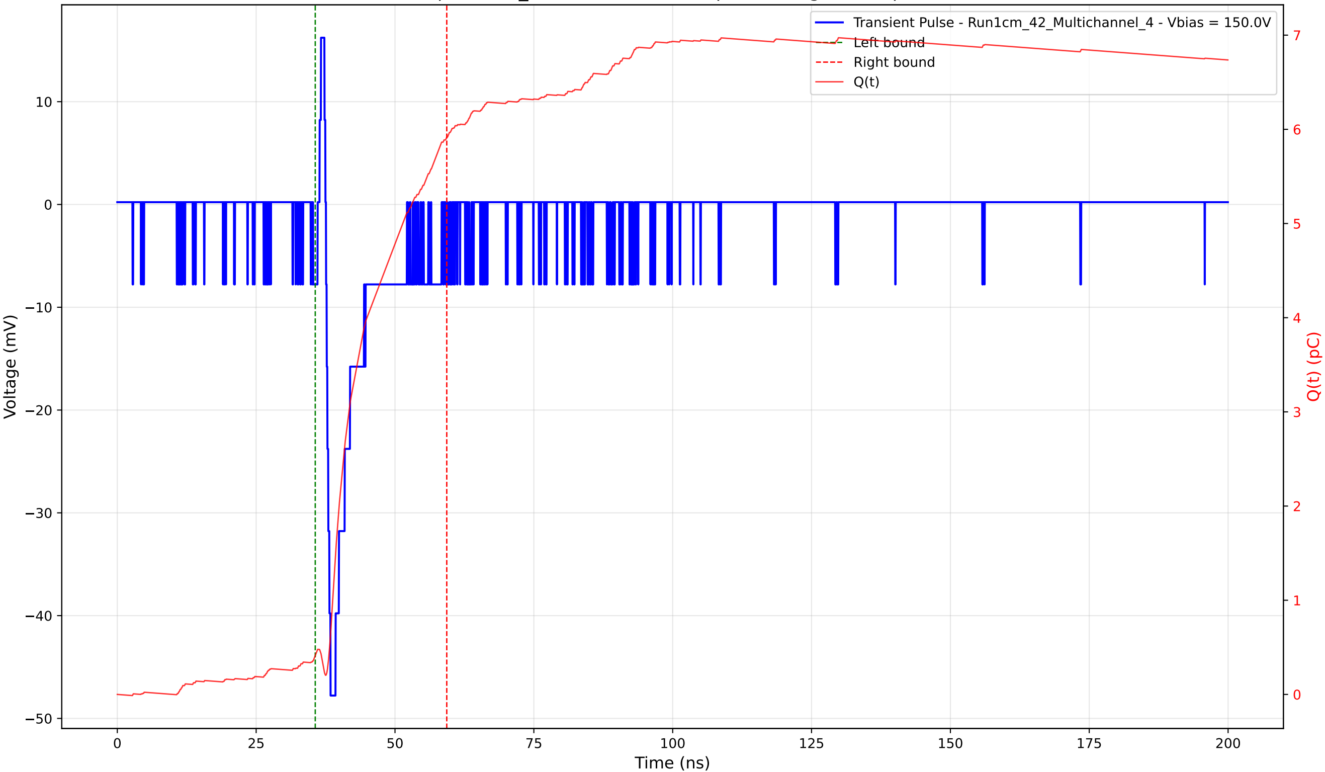
Transient Pulse - Sample: 1cm_42 - Position: 990.0 \mu\text{m} - Charge: 5.50 pC - Rise Time: 0.82 ns
