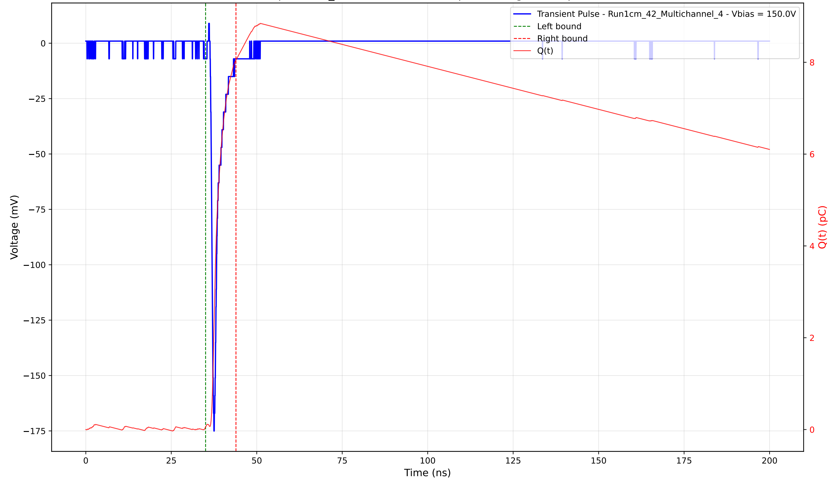
Transient Pulse - Sample: 1cm_42 - Position: 3125.0 \mu\text{m} - Charge: 7.99 pC - Rise Time: 0.79 ns
