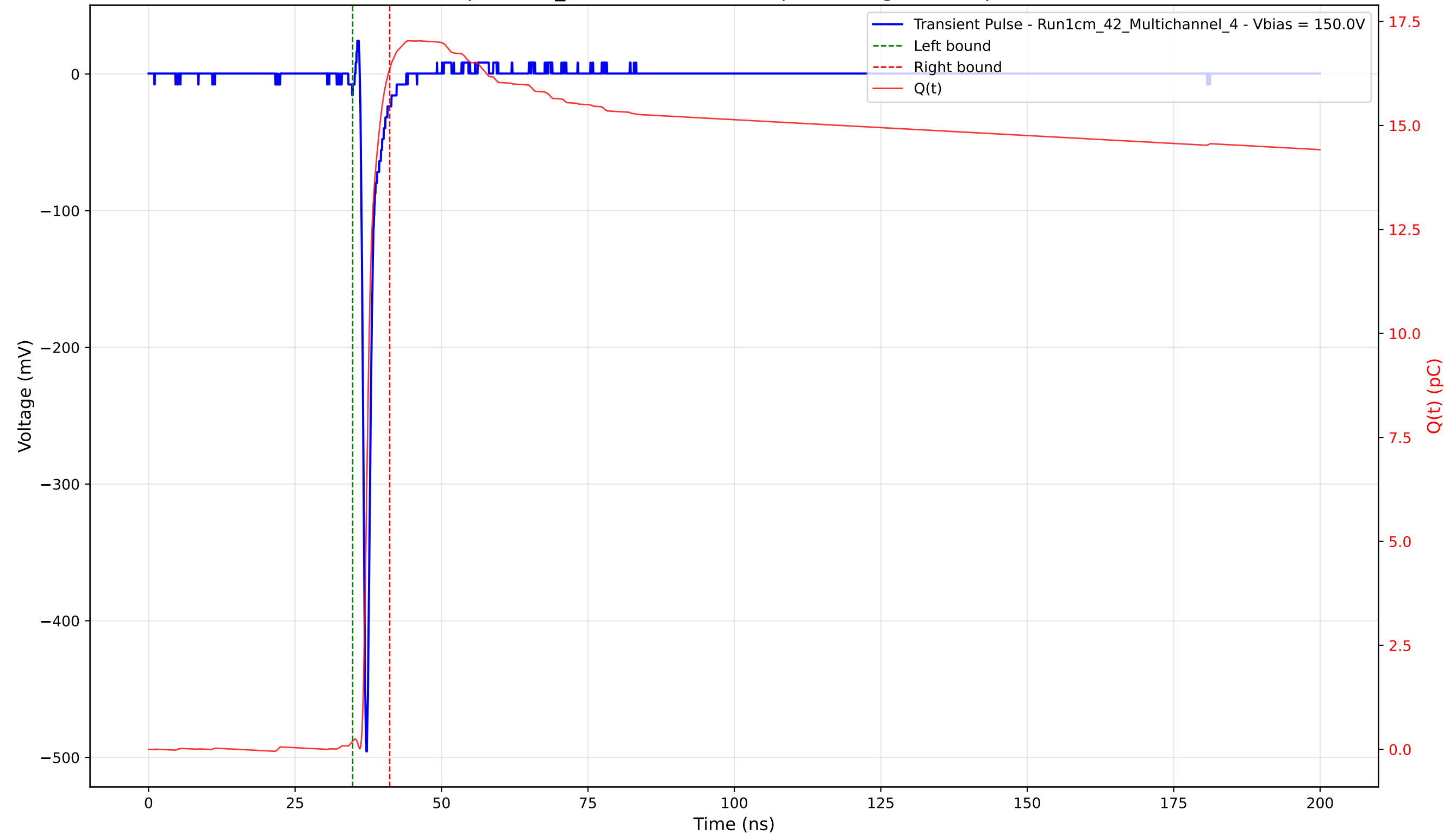
Transient Pulse - Sample: 1cm_42 - Position: 2230.0 \mu\text{m} - Charge: 16.16 pC - Rise Time: 0.73 ns
