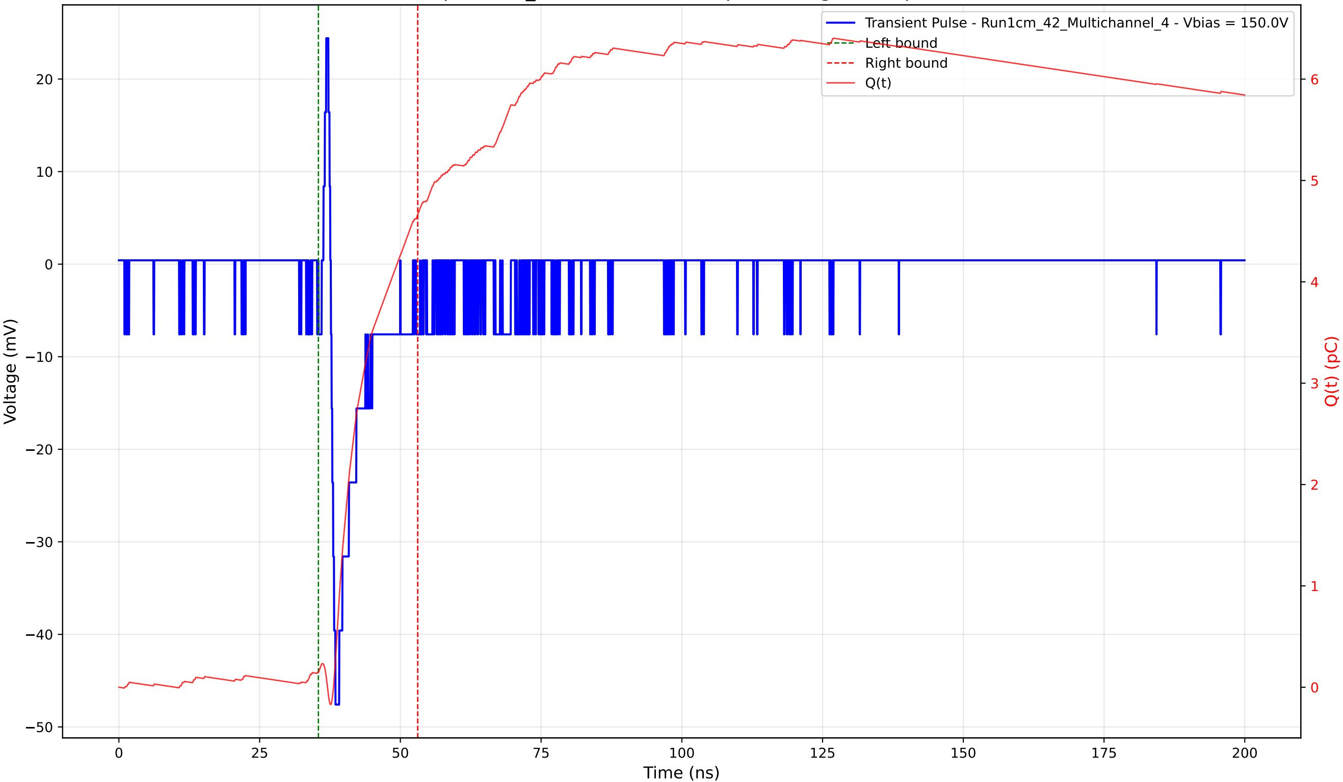
Transient Pulse - Sample: 1cm_42 - Position: 895.0 \mu\text{m} - Charge: 4.52 pC - Rise Time: 0.82 ns
