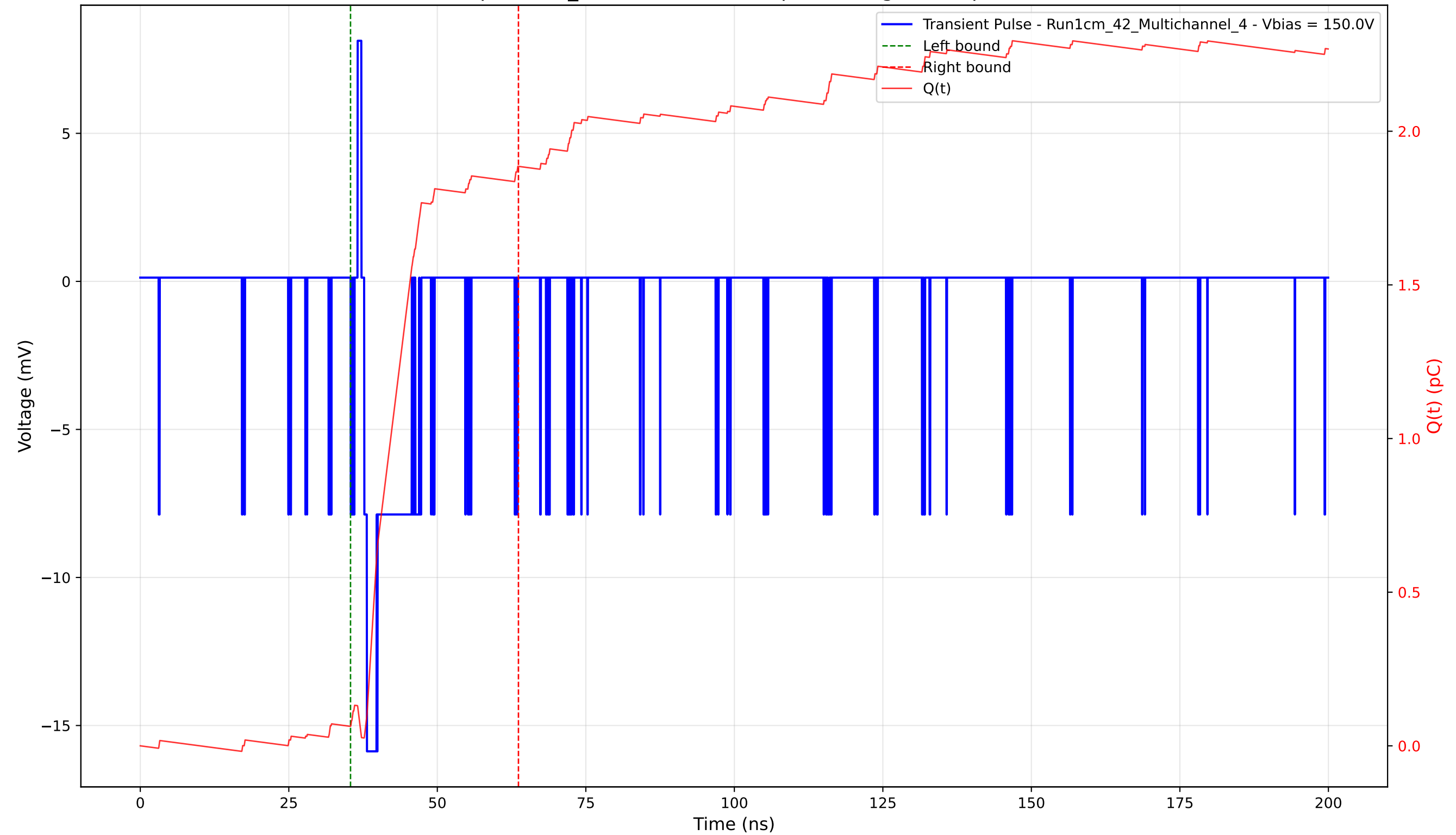
Transient Pulse - Sample: 1cm_42 - Position: 180.0 \mu\text{m} - Charge: 1.82 pC - Rise Time: 0.47 ns
