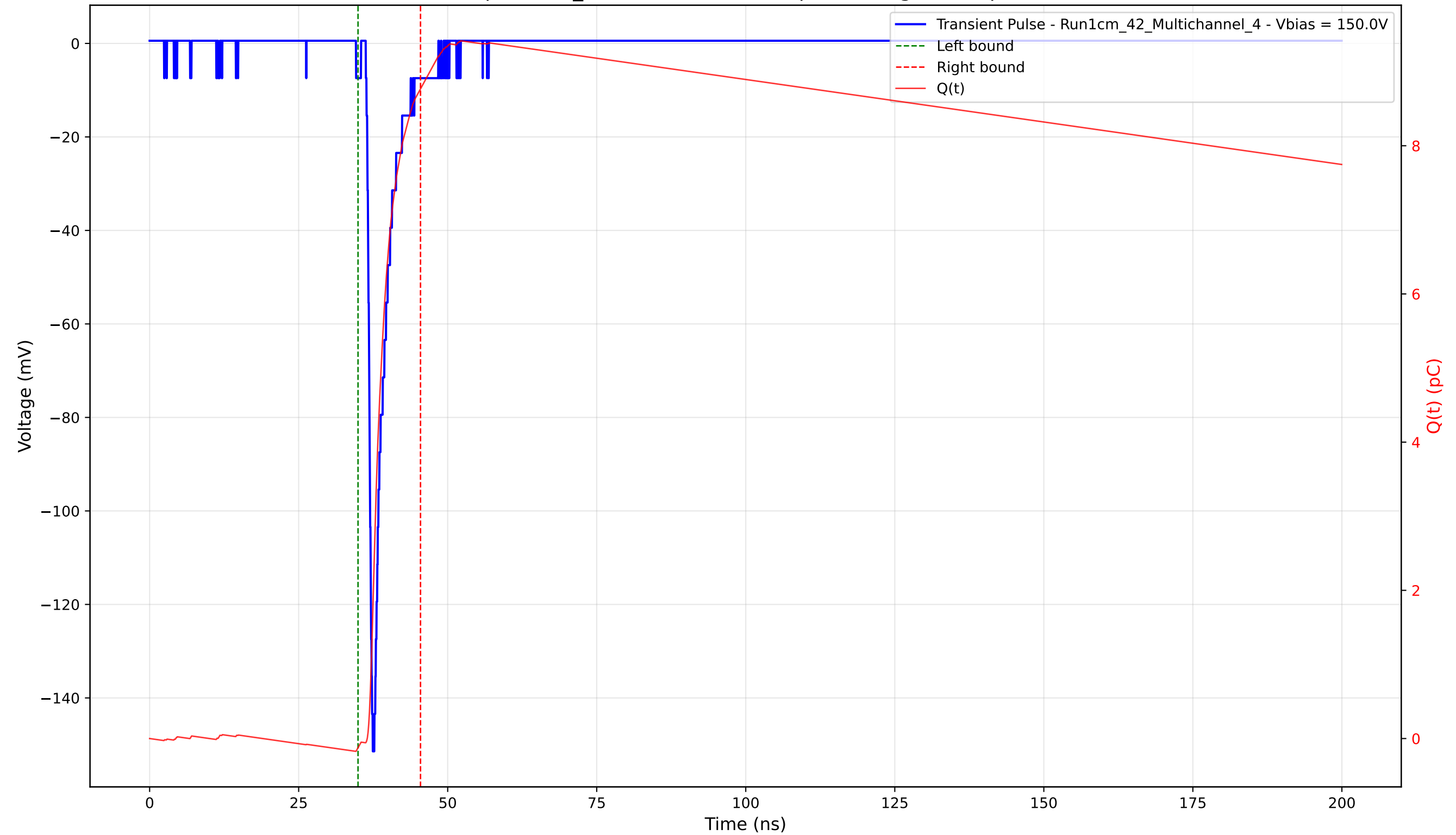
Transient Pulse - Sample: 1cm_42 - Position: 1800.0 \mu\text{m} - Charge: 8.89 pC - Rise Time: 0.92 ns
