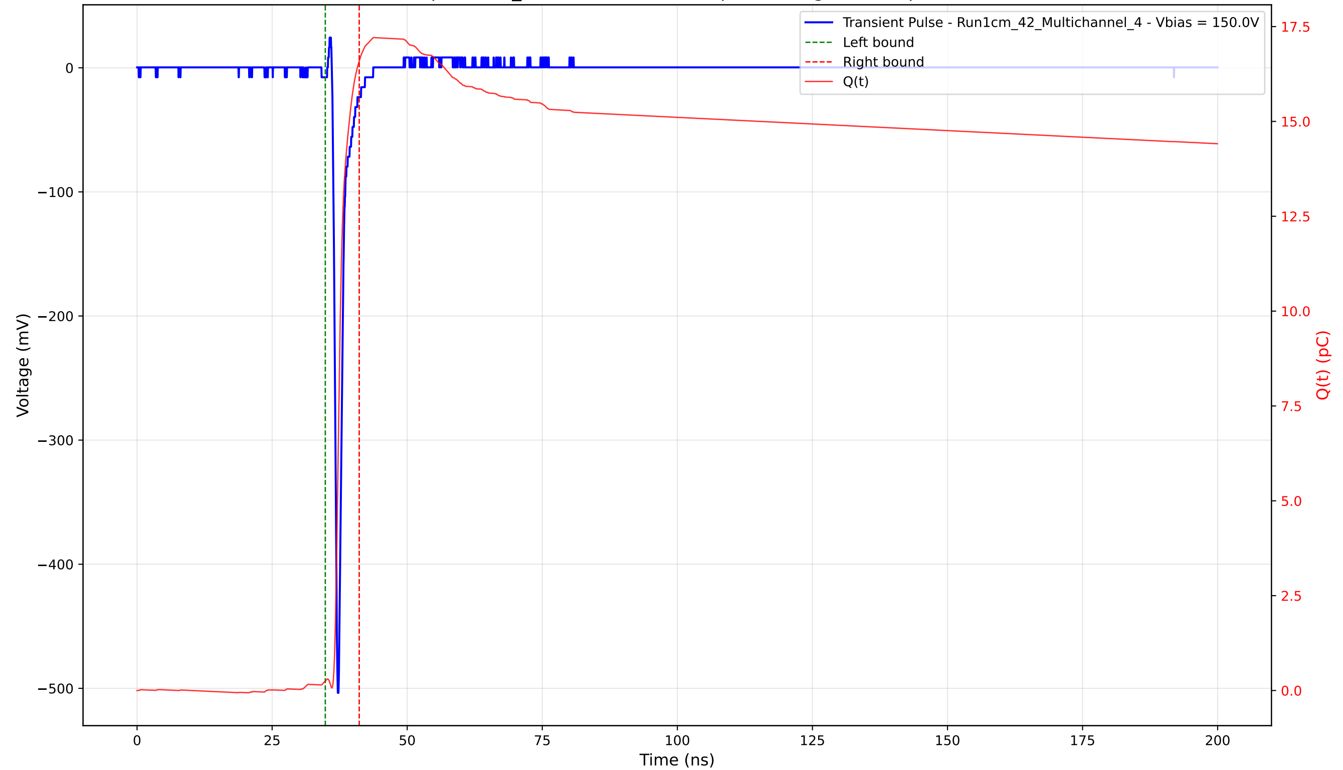
Transient Pulse - Sample: 1cm_42 - Position: 2240.0 \mu\text{m} - Charge: 16.34 pC - Rise Time: 0.70 ns
