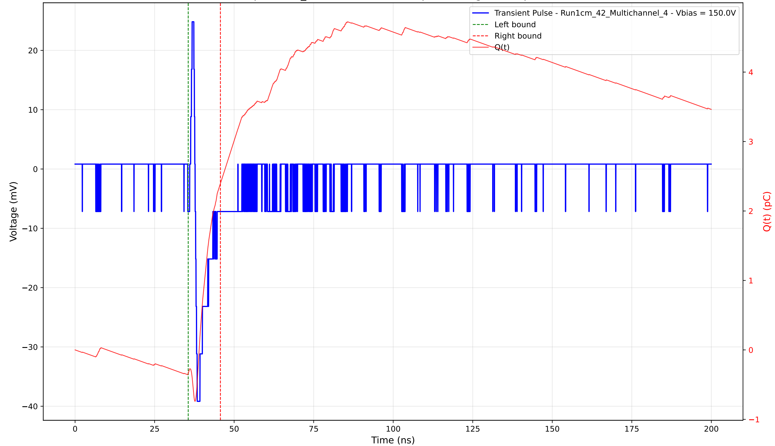
Transient Pulse - Sample: 1cm_42 - Position: 4285.0 \mu\text{m} - Charge: 2.73 pC - Rise Time: 0.66 ns
