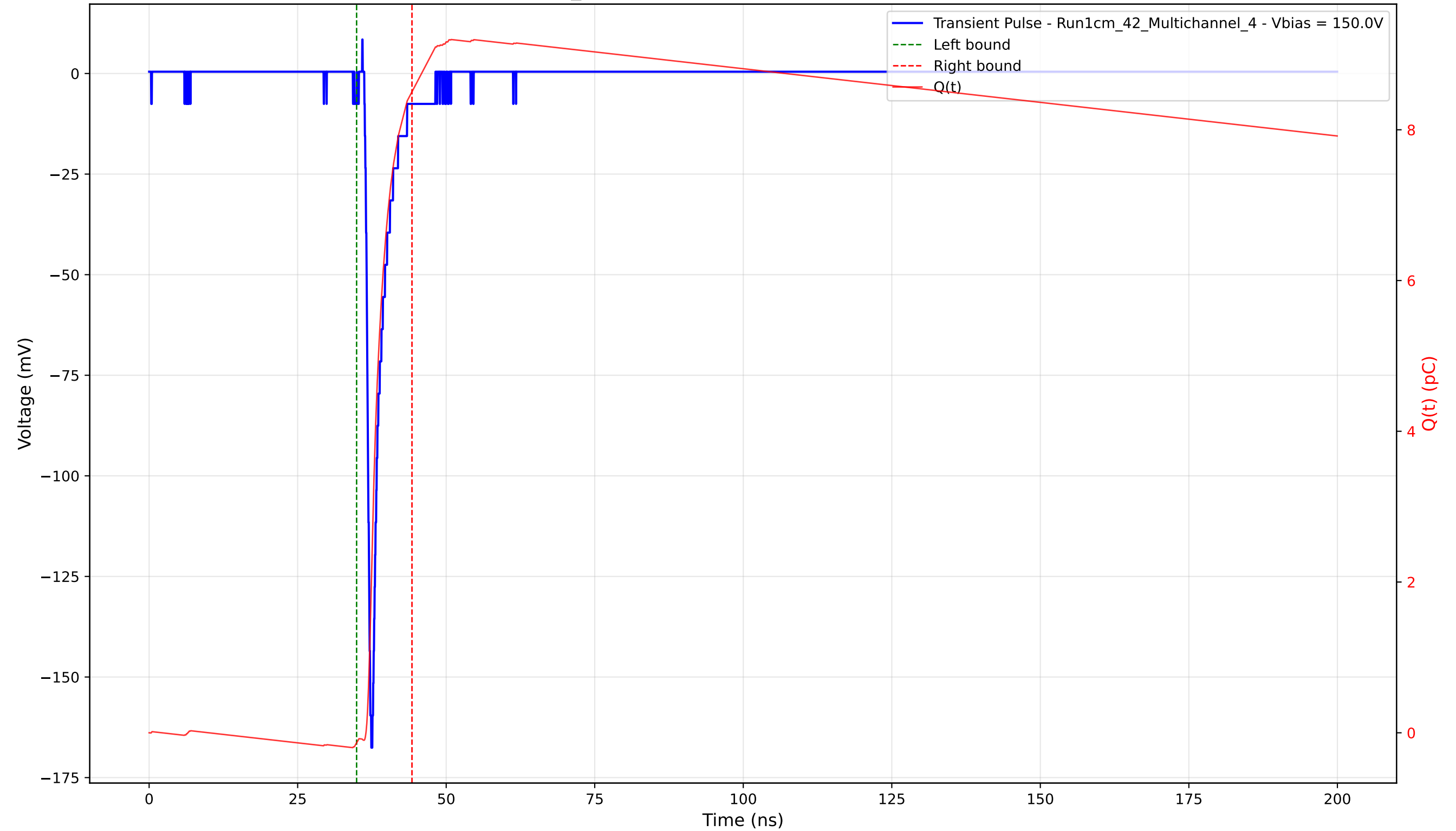
Transient Pulse - Sample: 1cm_42 - Position: 1890.0 \mu\text{m} - Charge: 8.63 pC - Rise Time: 0.83 ns
