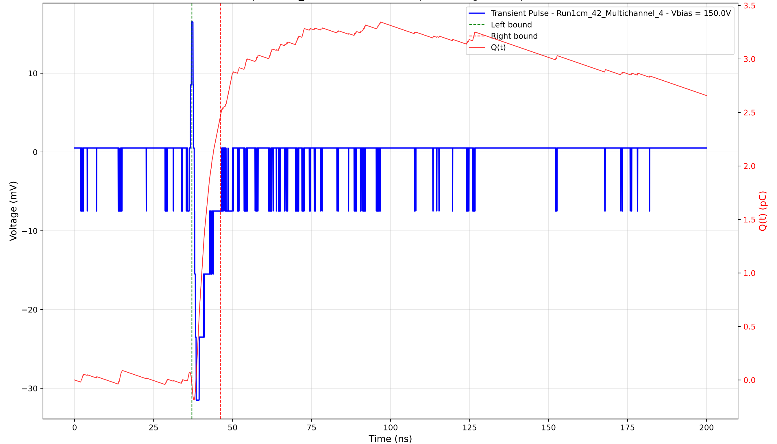
Transient Pulse - Sample: 1cm_42 - Position: 4770.0 \mu\text{m} - Charge: 2.50 pC - Rise Time: 0.62 ns
