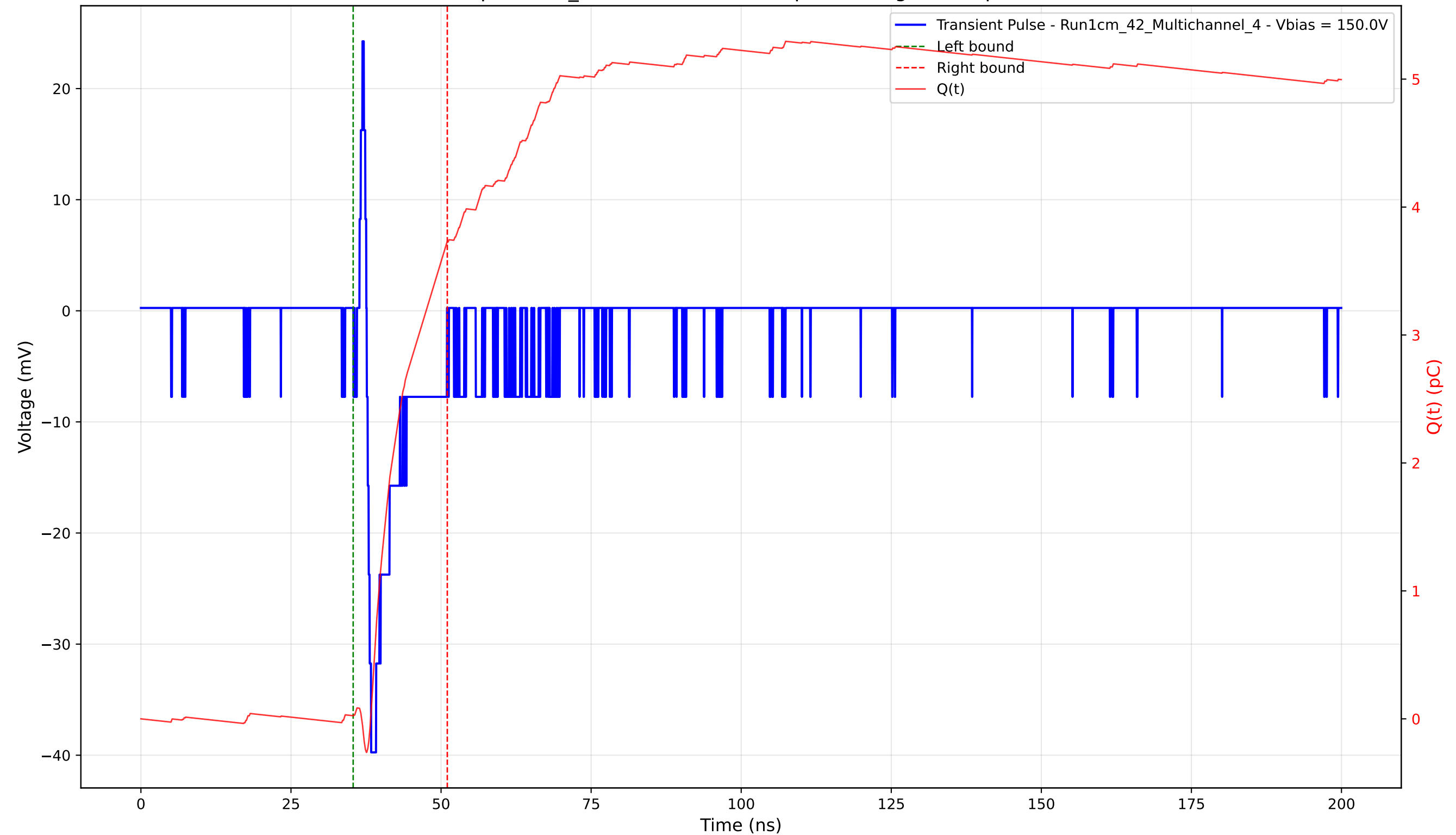
Transient Pulse - Sample: 1cm_42 - Position: 4100.0 \mu\text{m} - Charge: 3.70 pC - Rise Time: 0.74 ns
