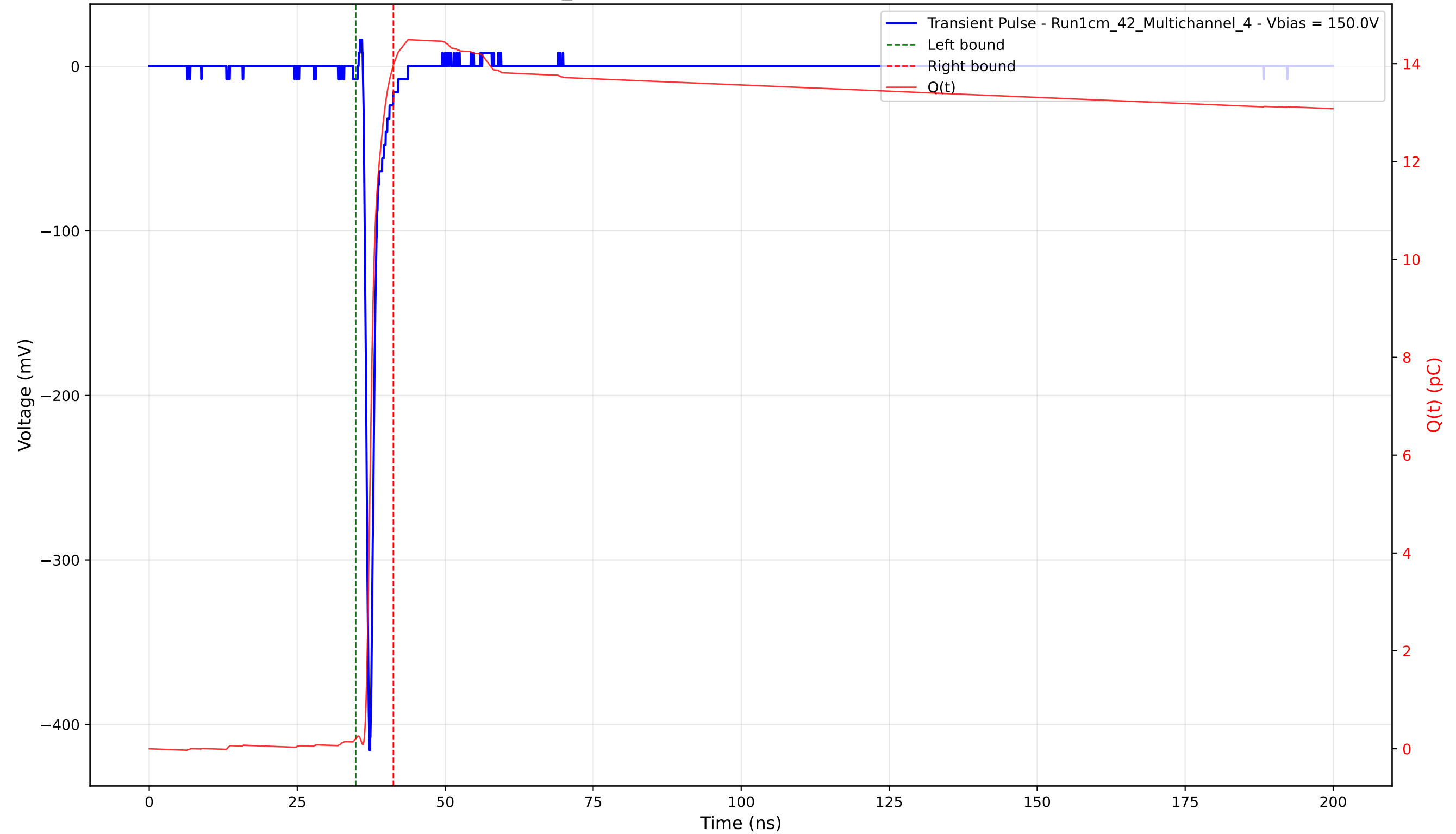
Transient Pulse - Sample: 1cm_42 - Position: 2845.0 \mu\text{m} - Charge: 13.77 pC - Rise Time: 0.73 ns
