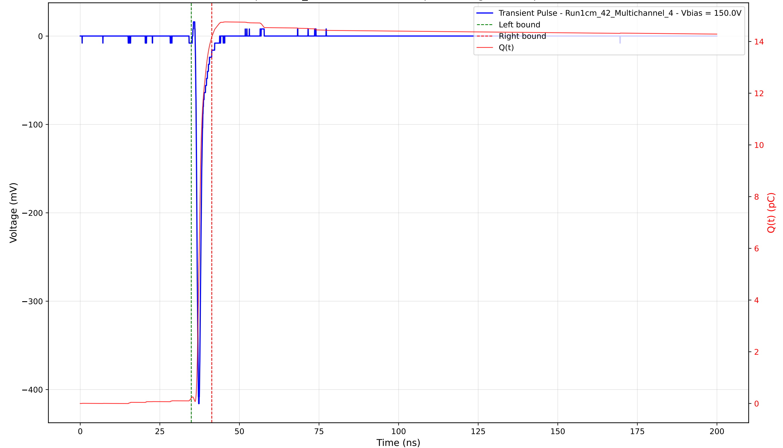
Transient Pulse - Sample: 1cm_42 - Position: 2840.0 \mu\text{m} - Charge: 13.97 pC - Rise Time: 0.75 ns
