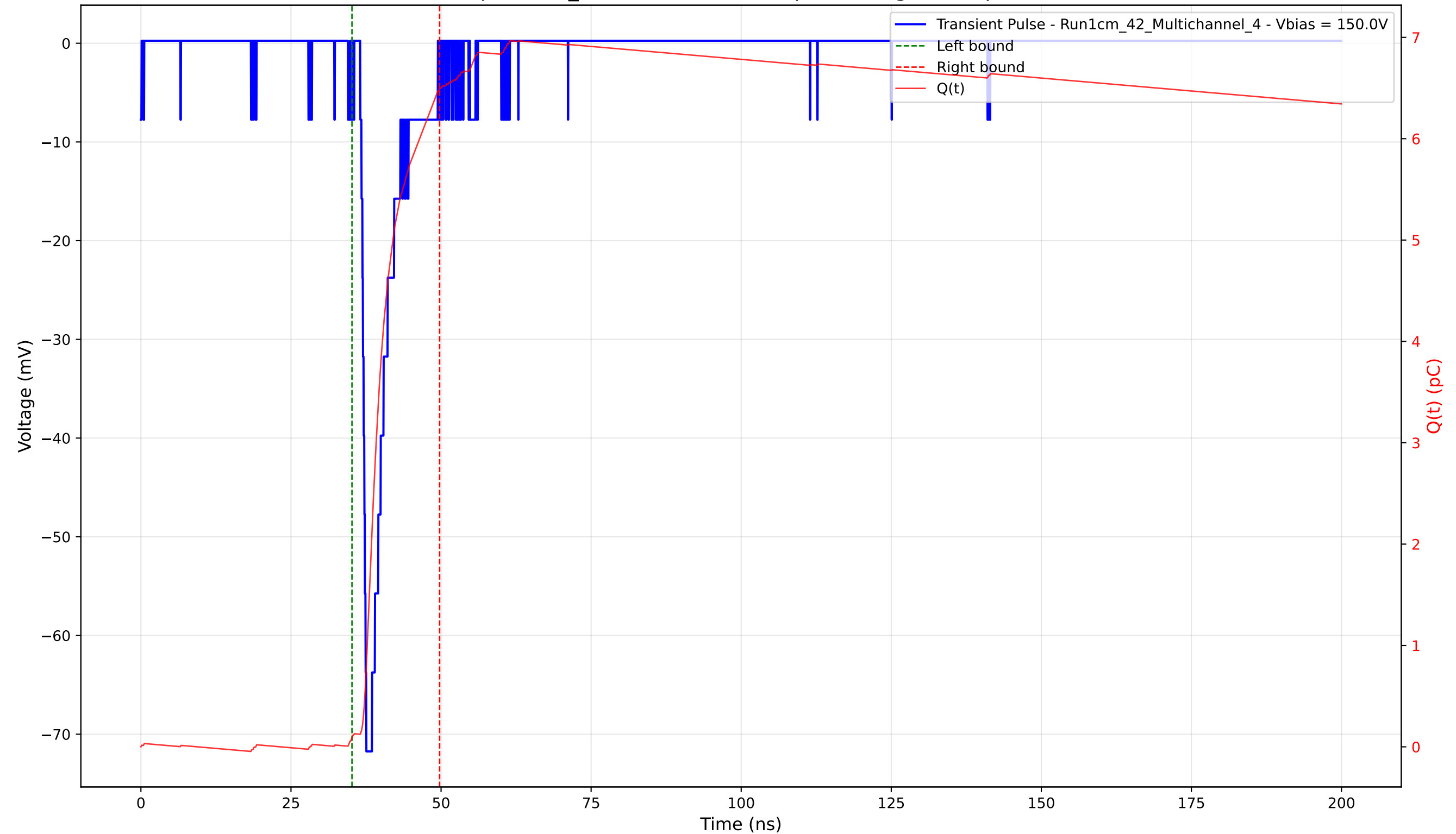
Transient Pulse - Sample: 1cm_42 - Position: 1520.0 \mu\text{m} - Charge: 6.41 pC - Rise Time: 1.00 ns
