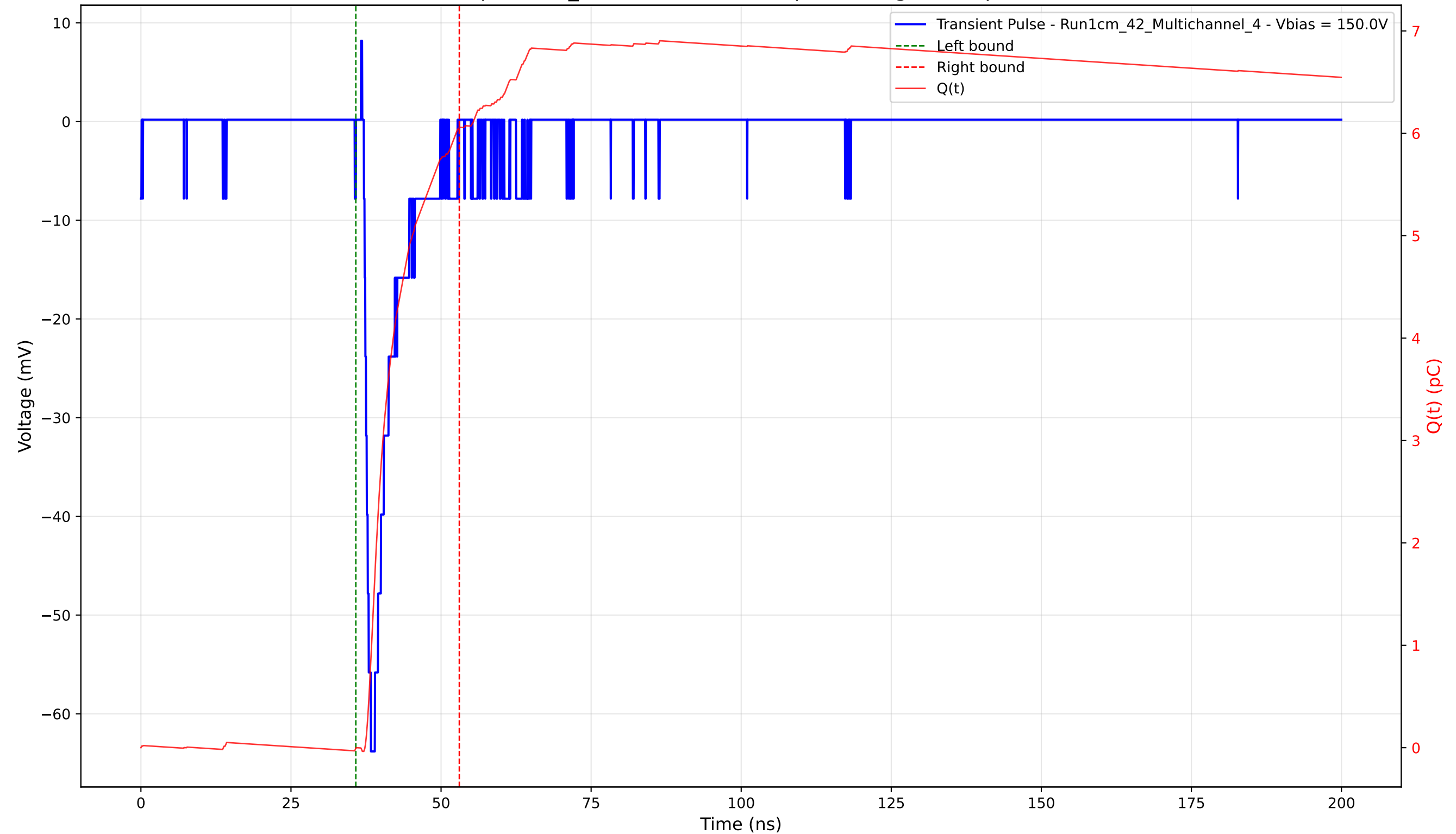
Transient Pulse - Sample: 1cm_42 - Position: 1350.0 \mu\text{m} - Charge: 6.06 pC - Rise Time: 1.17 ns
