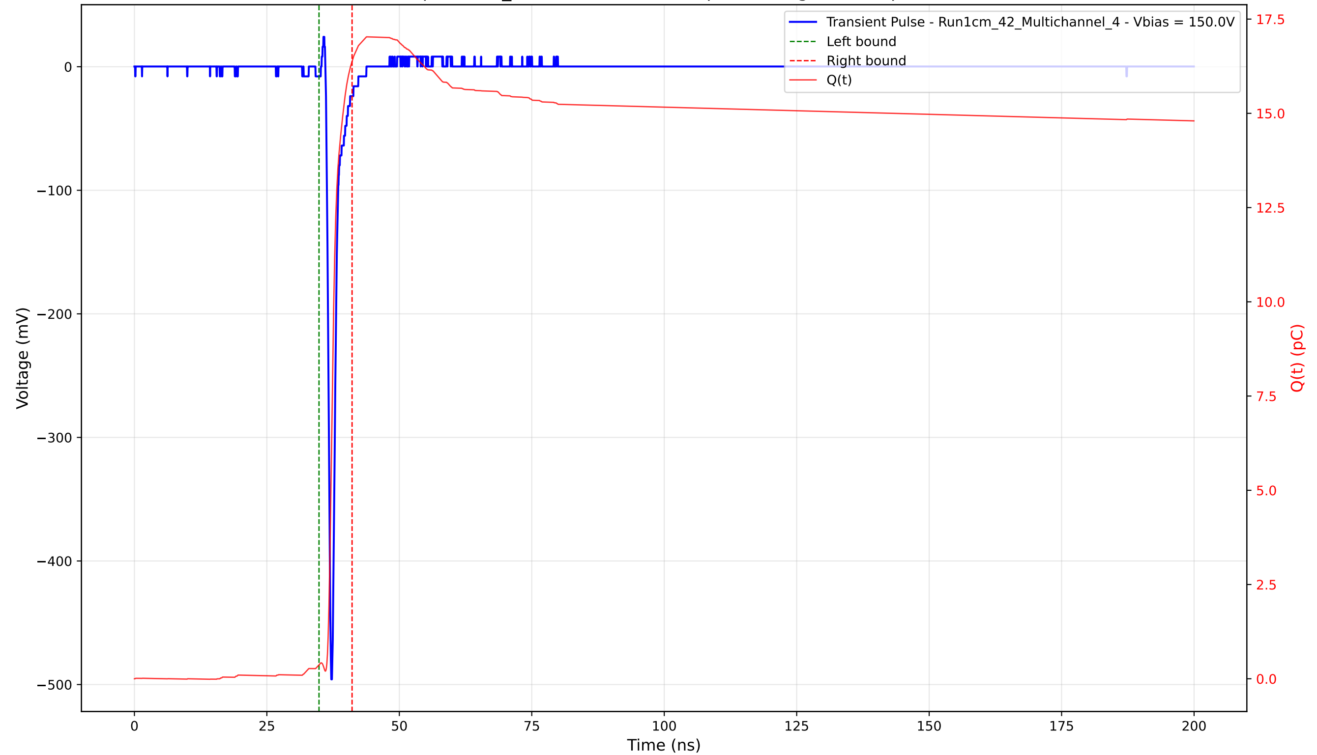
Transient Pulse - Sample: 1cm_42 - Position: 2735.0 \mu\text{m} - Charge: 16.01 pC - Rise Time: 0.73 ns
