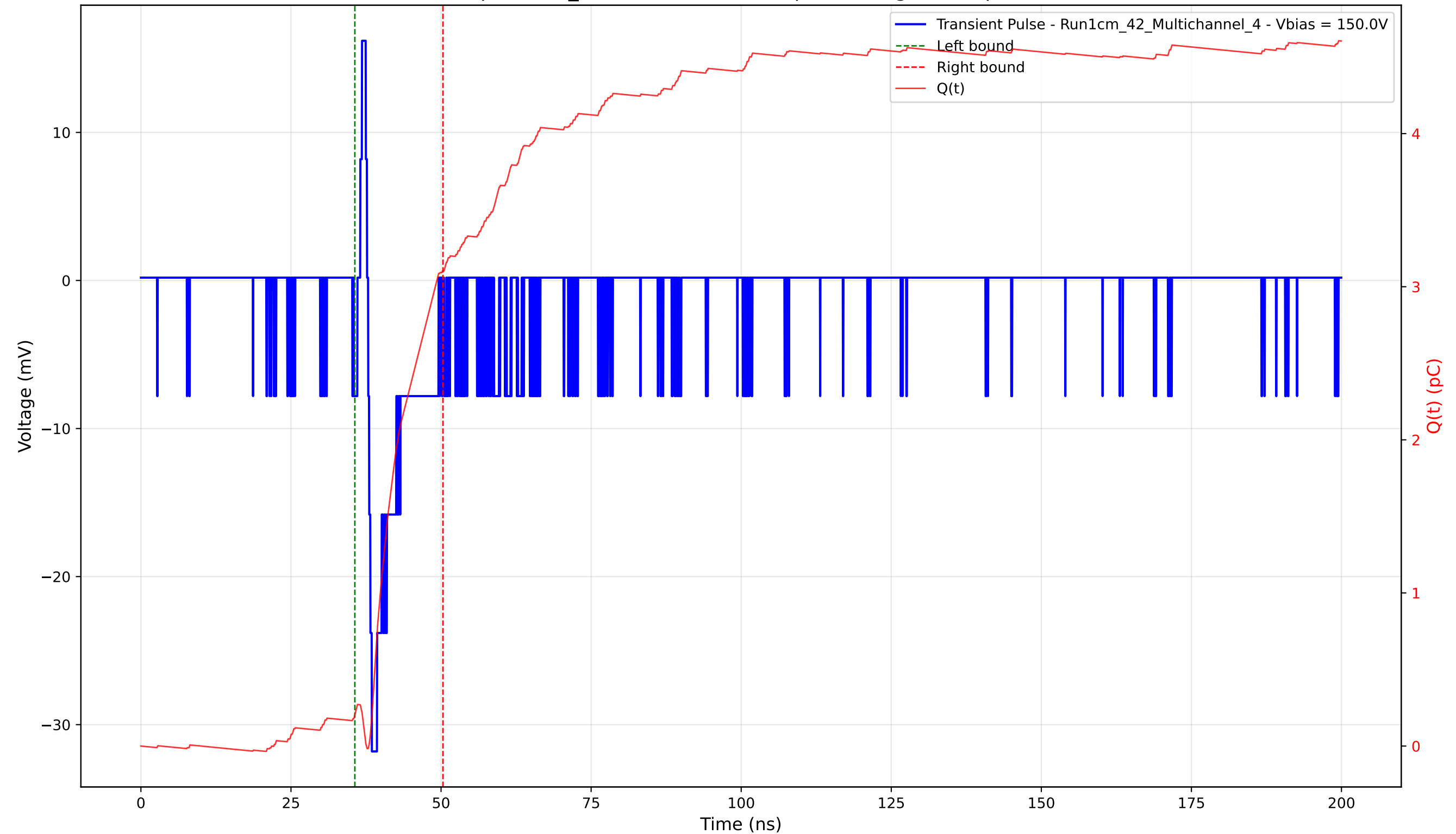
Transient Pulse - Sample: 1cm_42 - Position: 4635.0 \mu\text{m} - Charge: 2.90 pC - Rise Time: 0.62 ns
