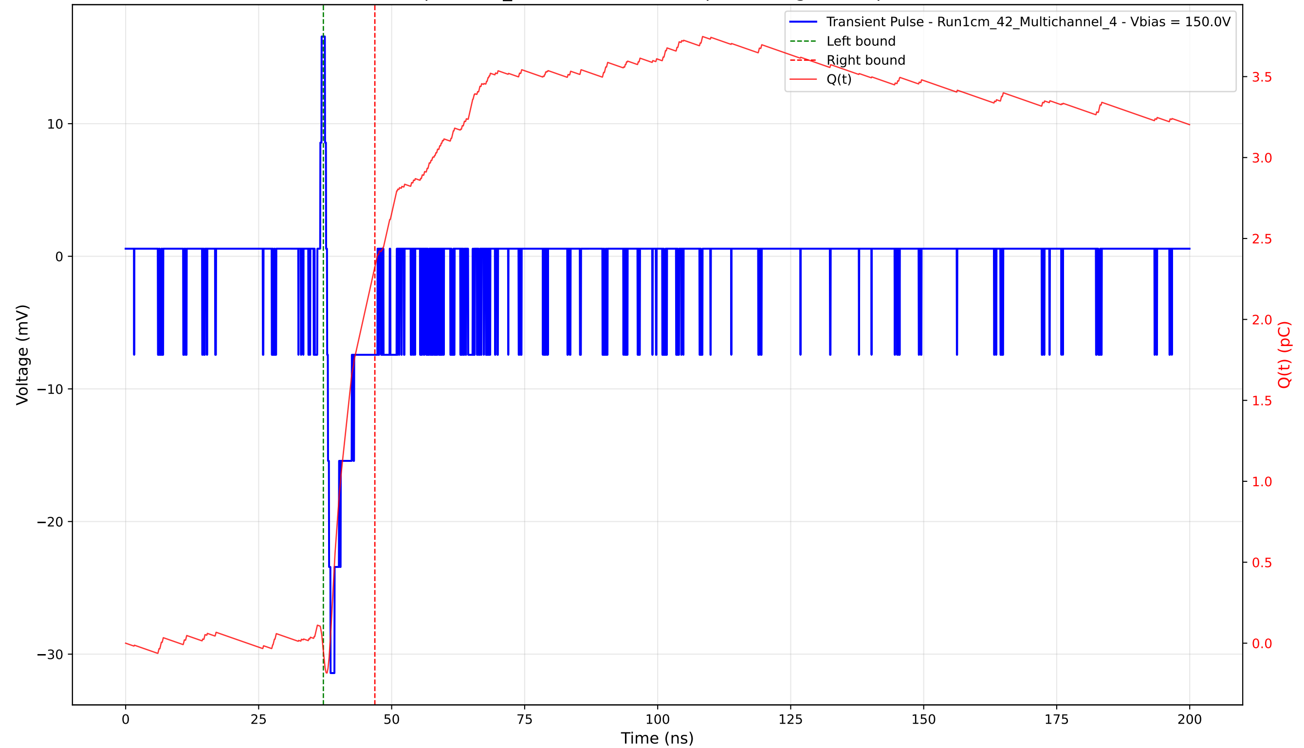
Transient Pulse - Sample: 1cm_42 - Position: 4530.0 \mu\text{m} - Charge: 2.38 pC - Rise Time: 0.67 ns
