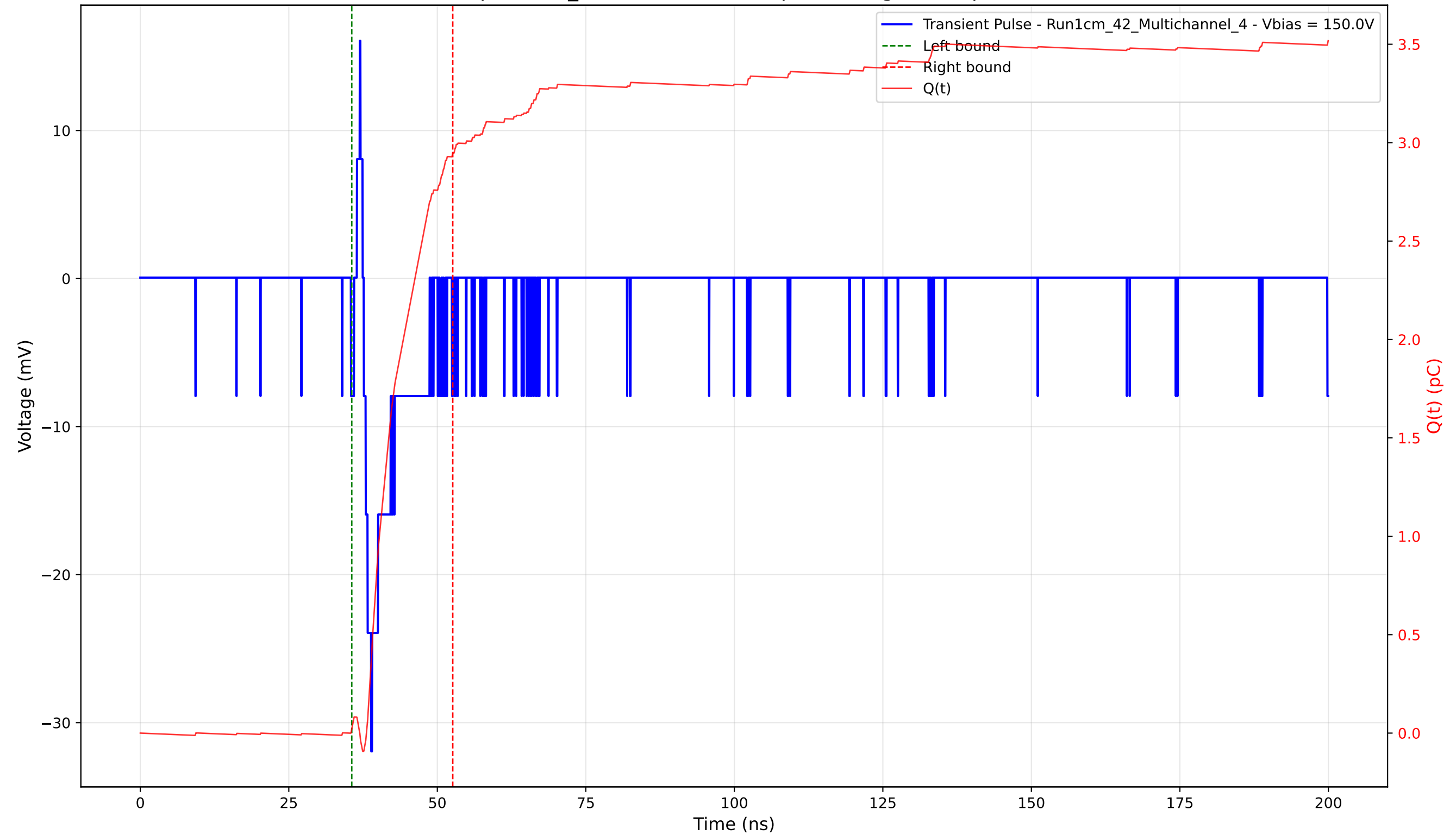
Transient Pulse - Sample: 1cm_42 - Position: 355.0 \mu\text{m} - Charge: 2.93 pC - Rise Time: 1.26 ns
