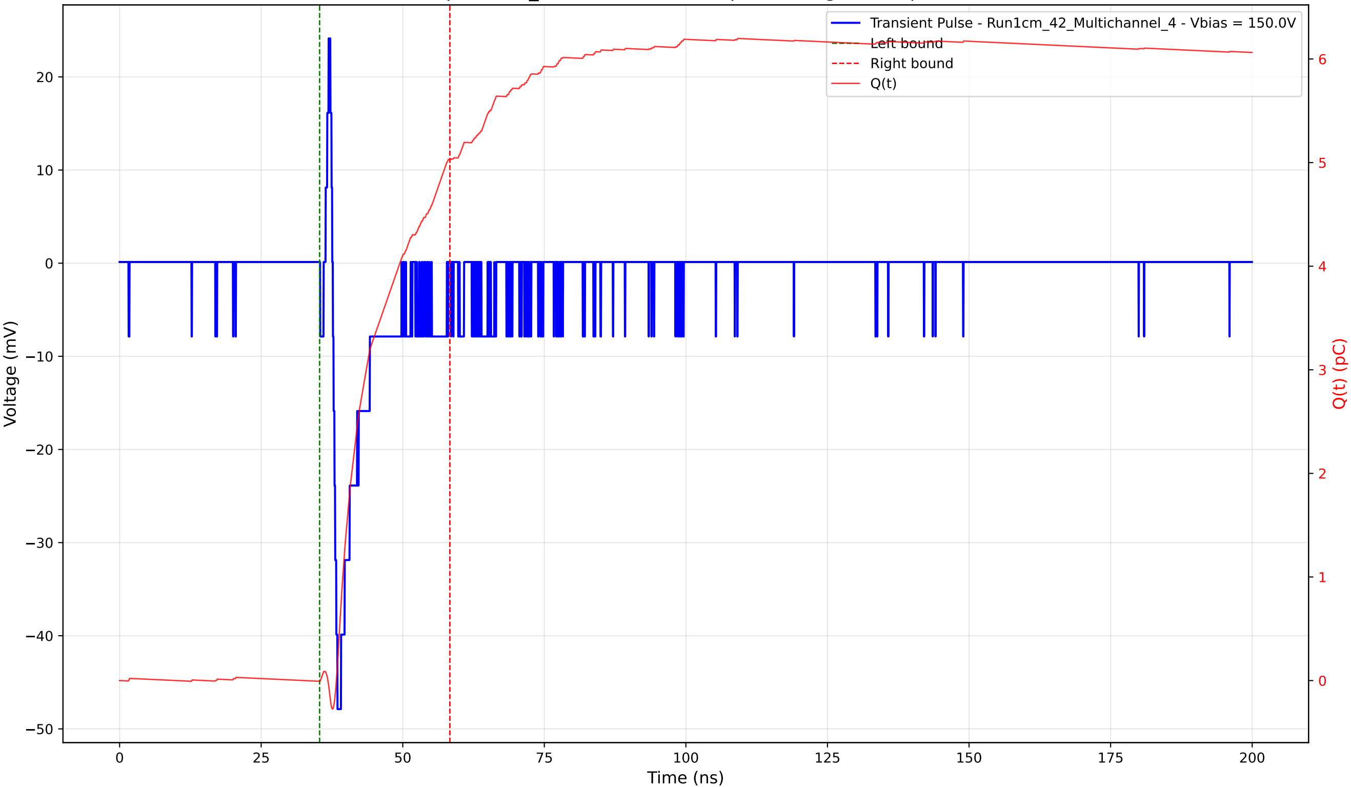
Transient Pulse - Sample: 1cm_42 - Position: 900.0 \mu\text{m} - Charge: 5.04 pC - Rise Time: 0.82 ns
