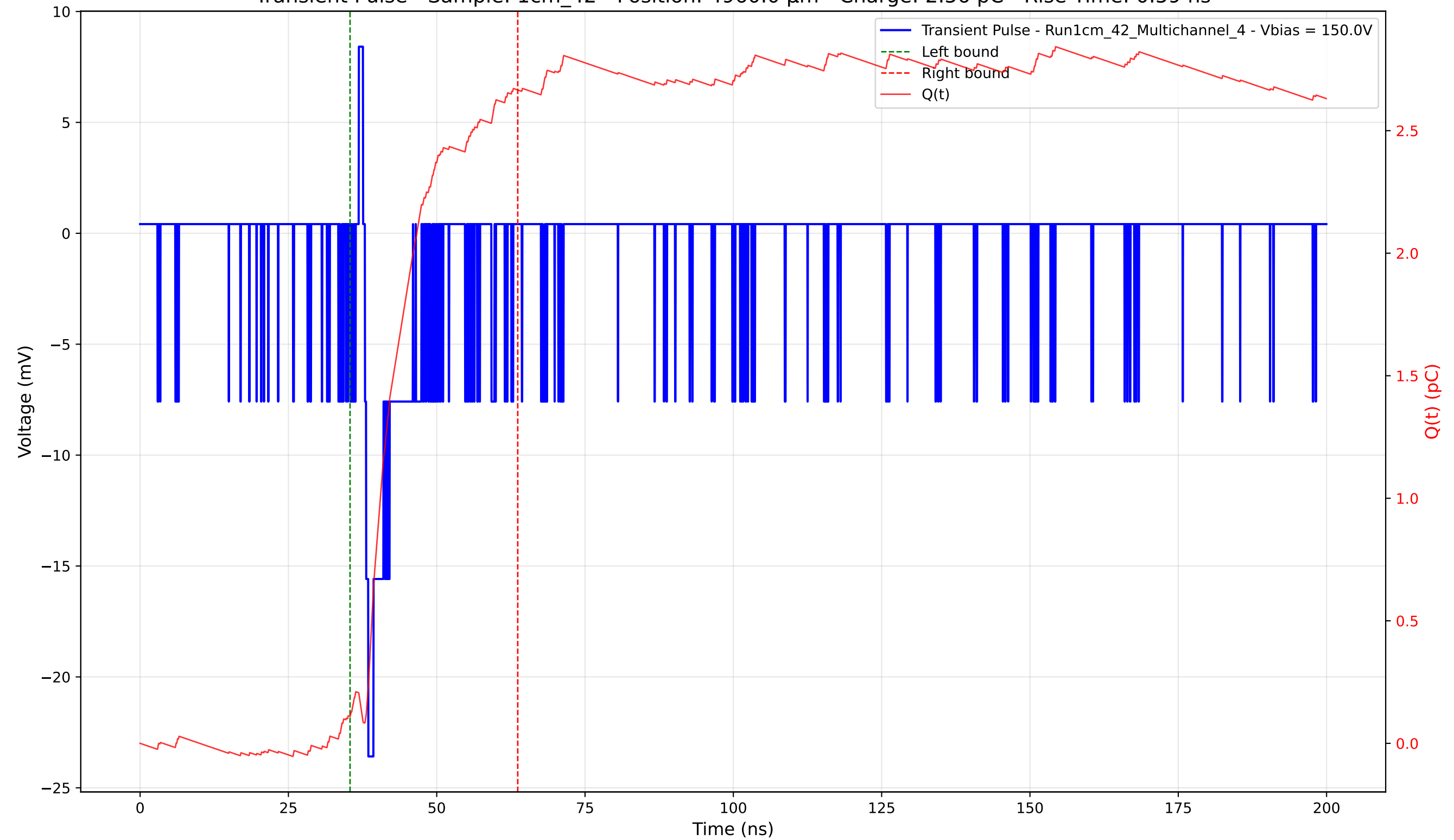
Transient Pulse - Sample: 1cm_42 - Position: 4960.0 \mu\text{m} - Charge: 2.56 pC - Rise Time: 0.59 ns
