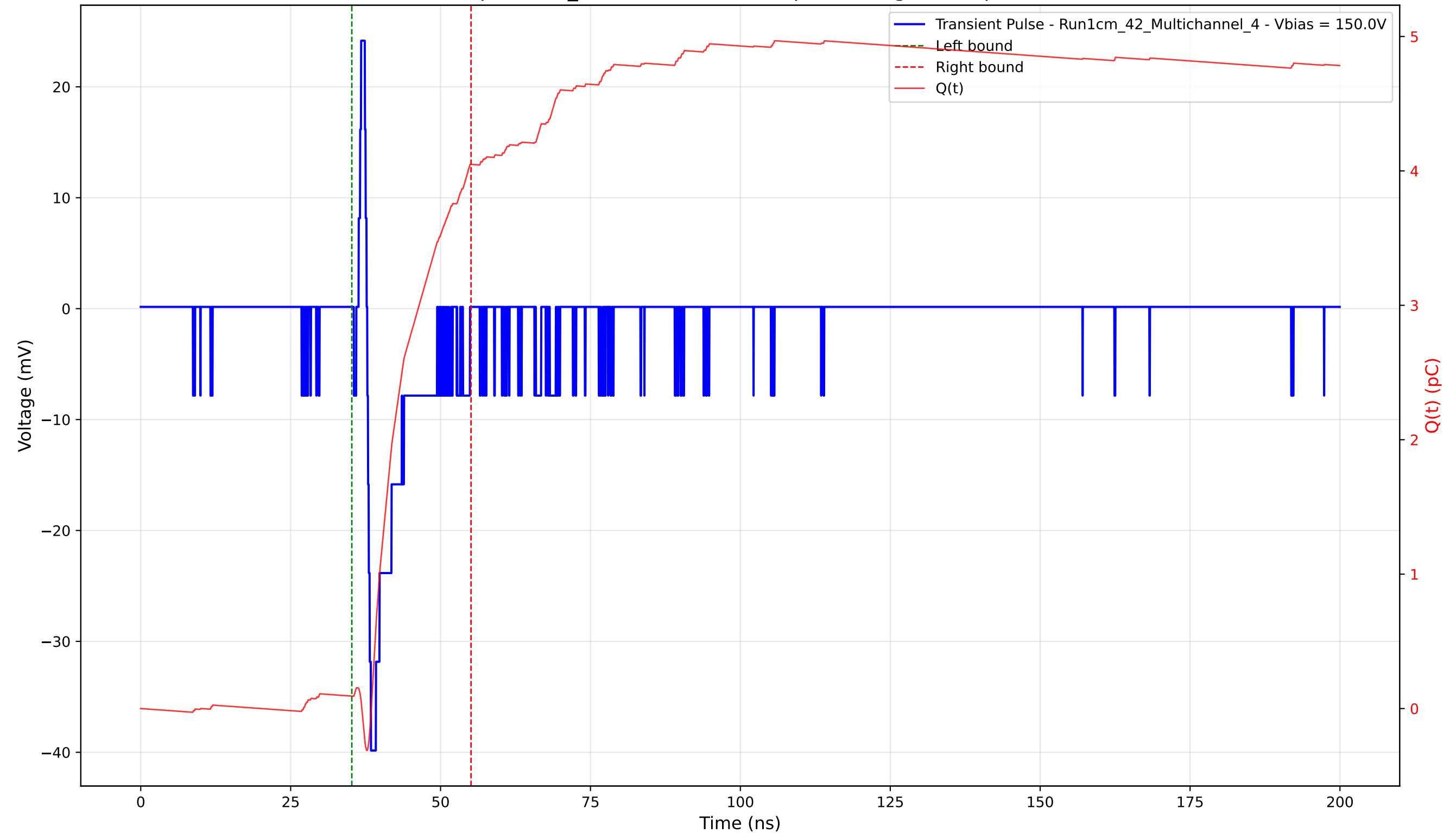
Transient Pulse - Sample: 1cm_42 - Position: 4320.0 \mu\text{m} - Charge: 3.96 pC - Rise Time: 0.62 ns
