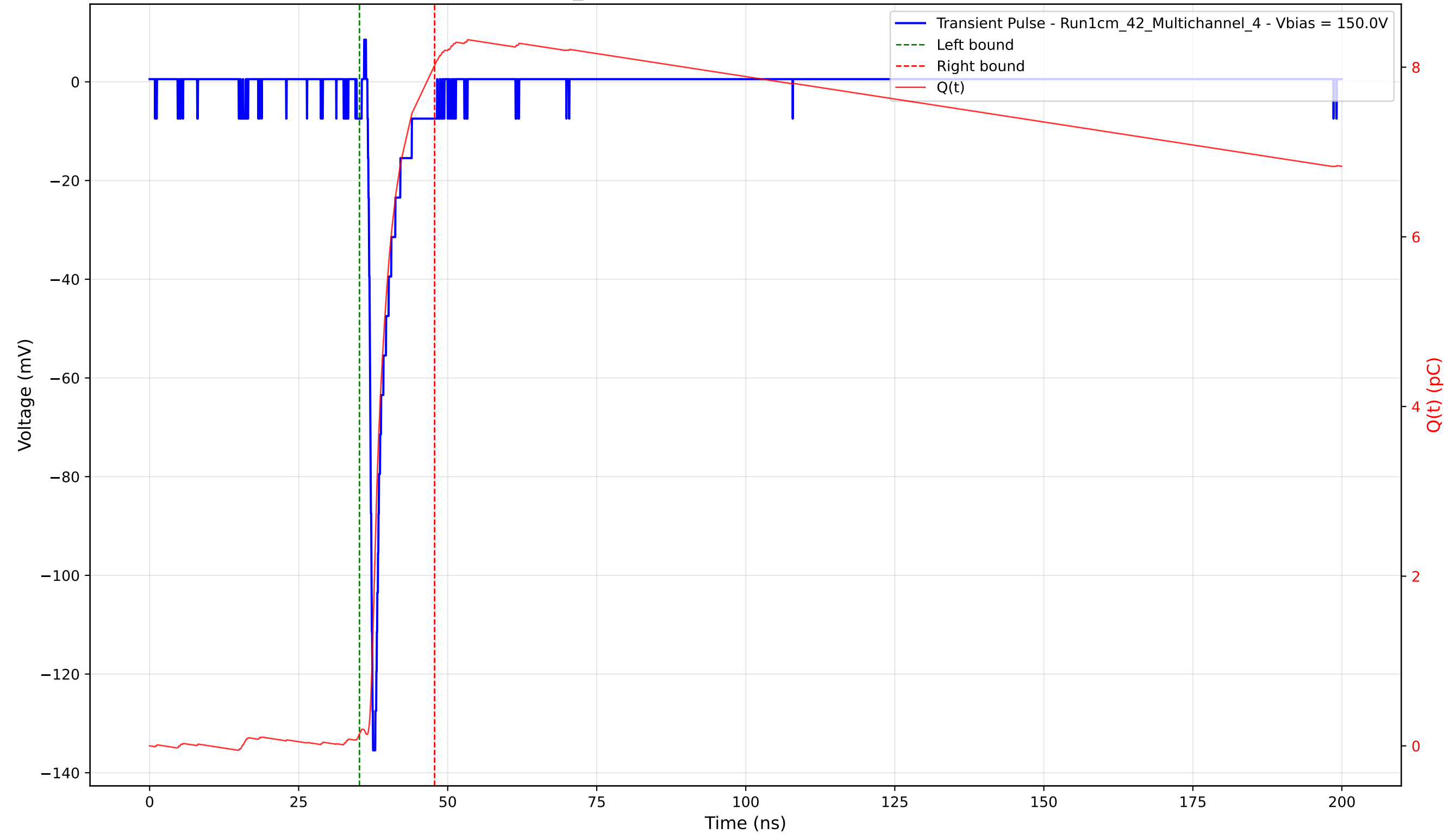
Transient Pulse - Sample: 1cm_42 - Position: 3300.0 \mu\text{m} - Charge: 7.88 pC - Rise Time: 0.77 ns
