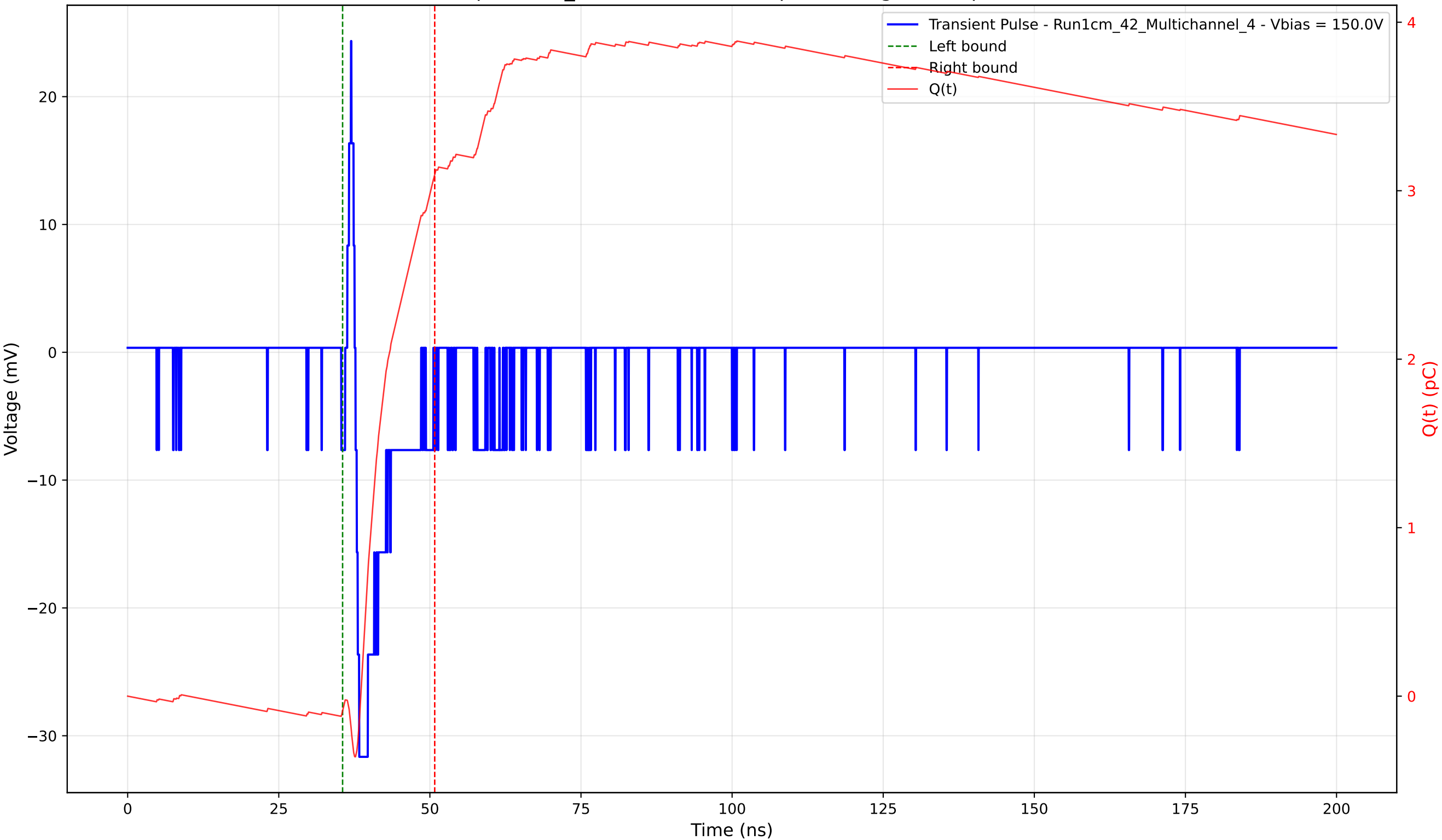
Transient Pulse - Sample: 1cm_42 - Position: 500.0 \mu\text{m} - Charge: 3.18 pC - Rise Time: 0.62 ns
