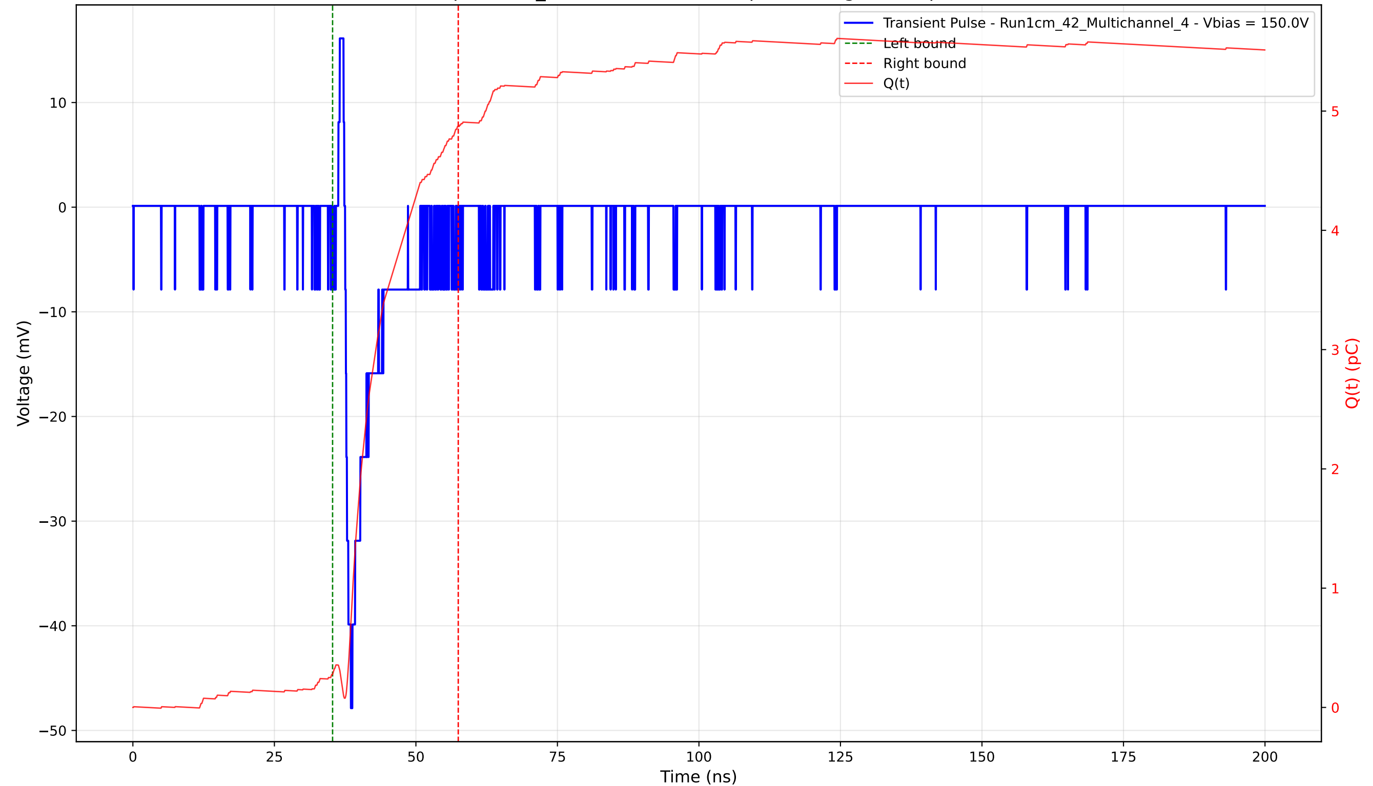
Transient Pulse - Sample: 1cm_42 - Position: 3965.0 \mu\text{m} - Charge: 4.59 pC - Rise Time: 1.02 ns
