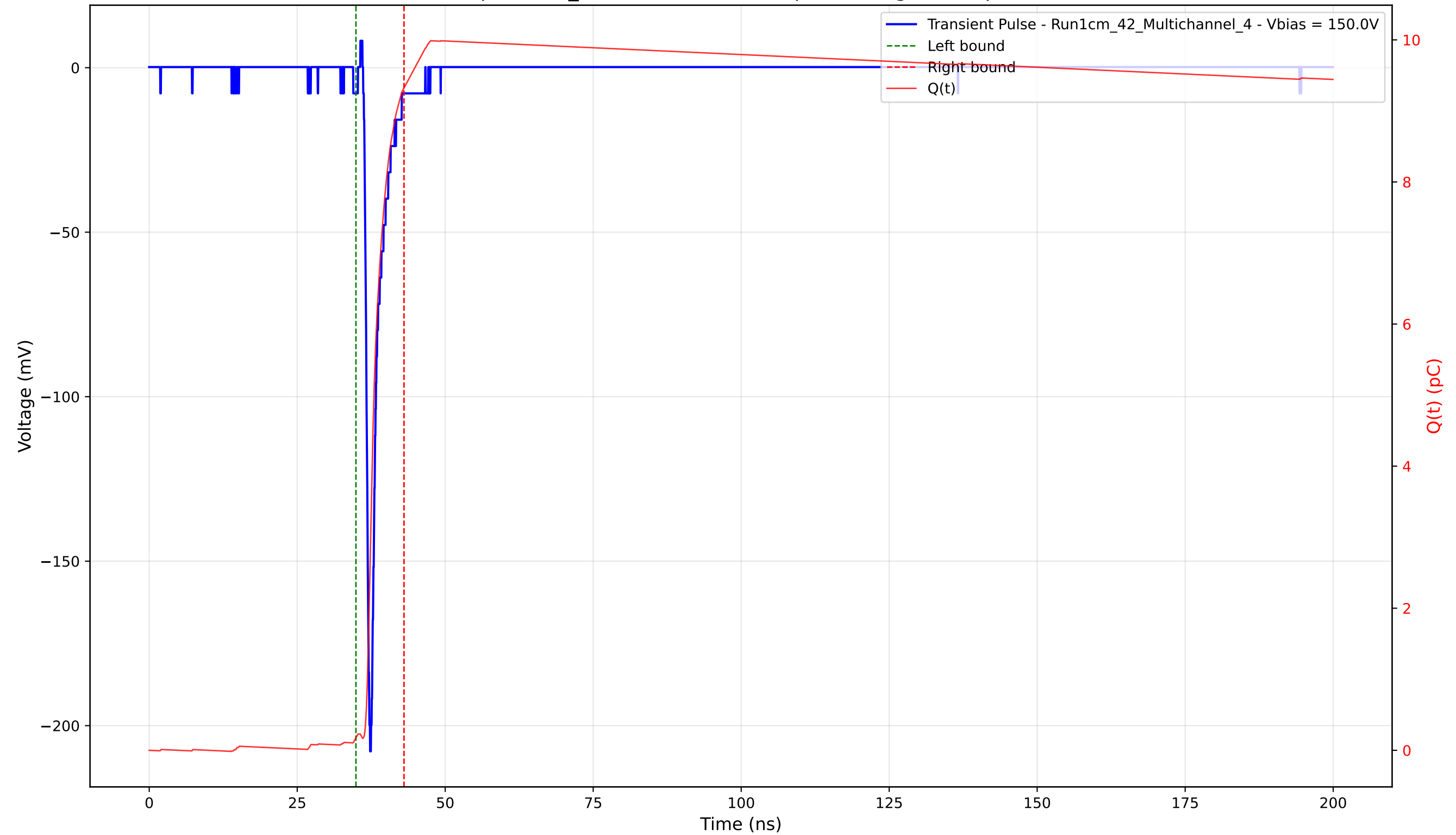
Transient Pulse - Sample: 1cm_42 - Position: 1975.0 \mu\text{m} - Charge: 9.15 pC - Rise Time: 0.79 ns
