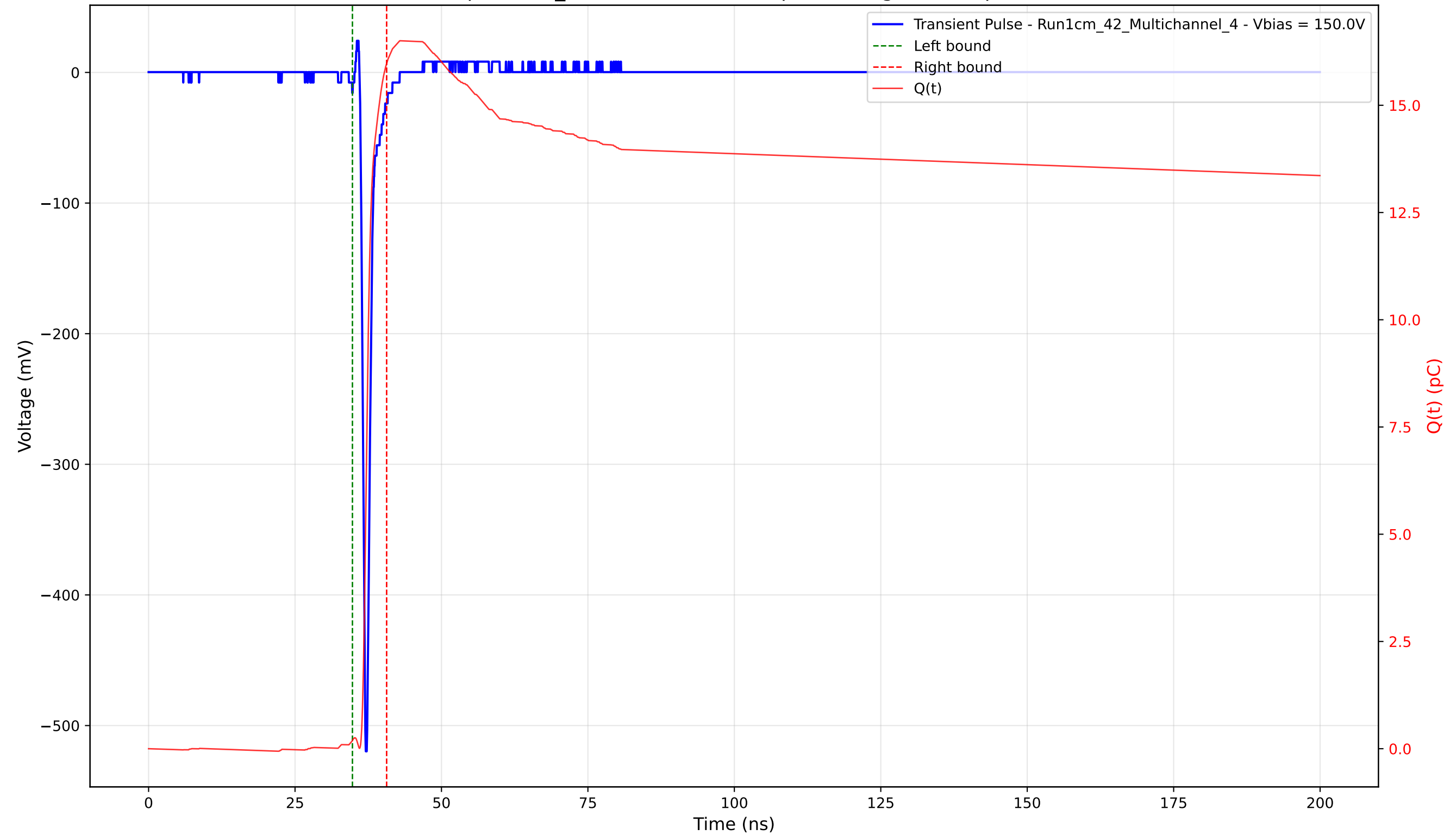
Transient Pulse - Sample: 1cm_42 - Position: 2485.0 \mu\text{m} - Charge: 15.78 pC - Rise Time: 0.67 ns
