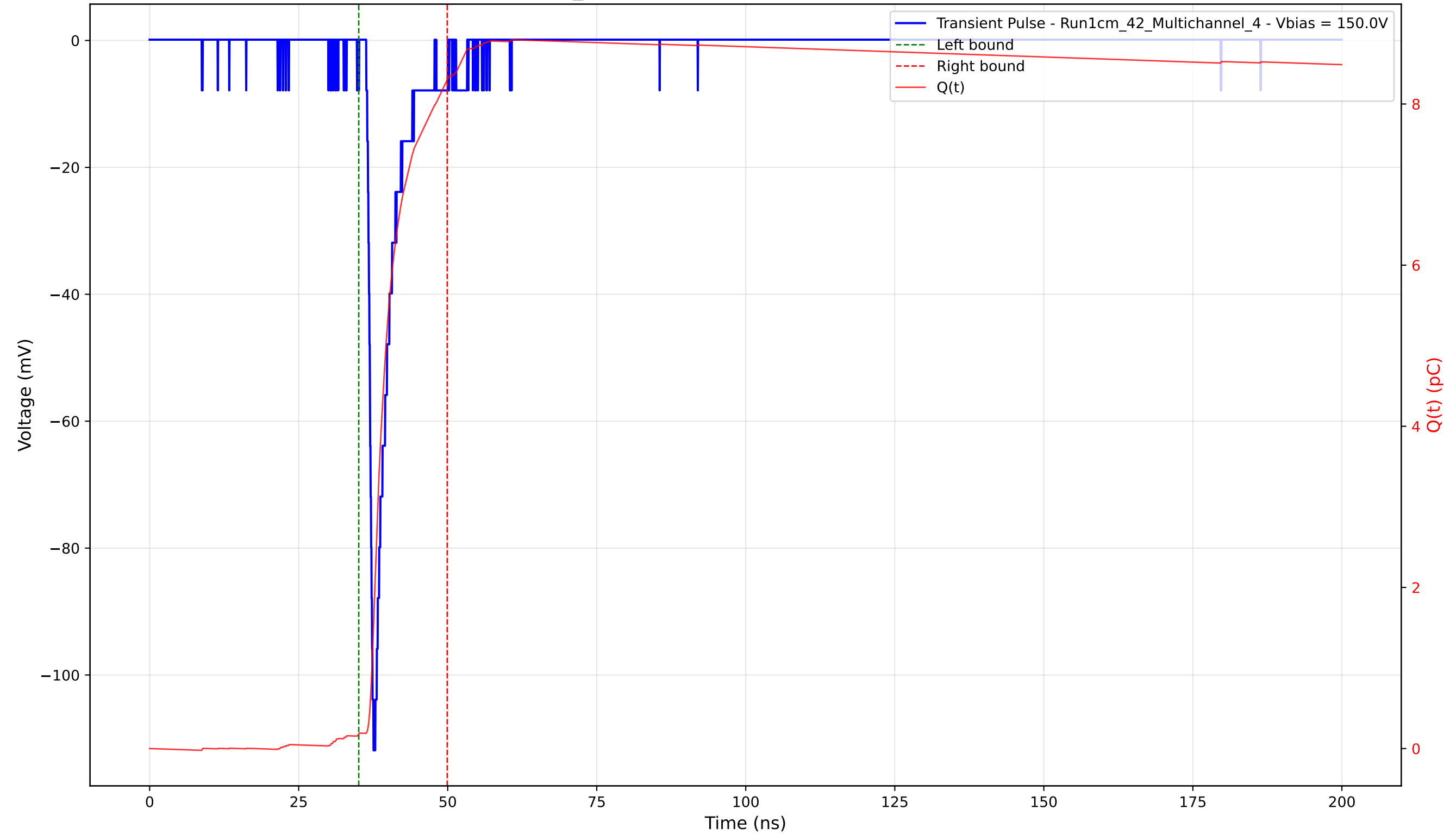
Transient Pulse - Sample: 1cm_42 - Position: 1640.0 \mu\text{m} - Charge: 8.12 pC - Rise Time: 0.90 ns
