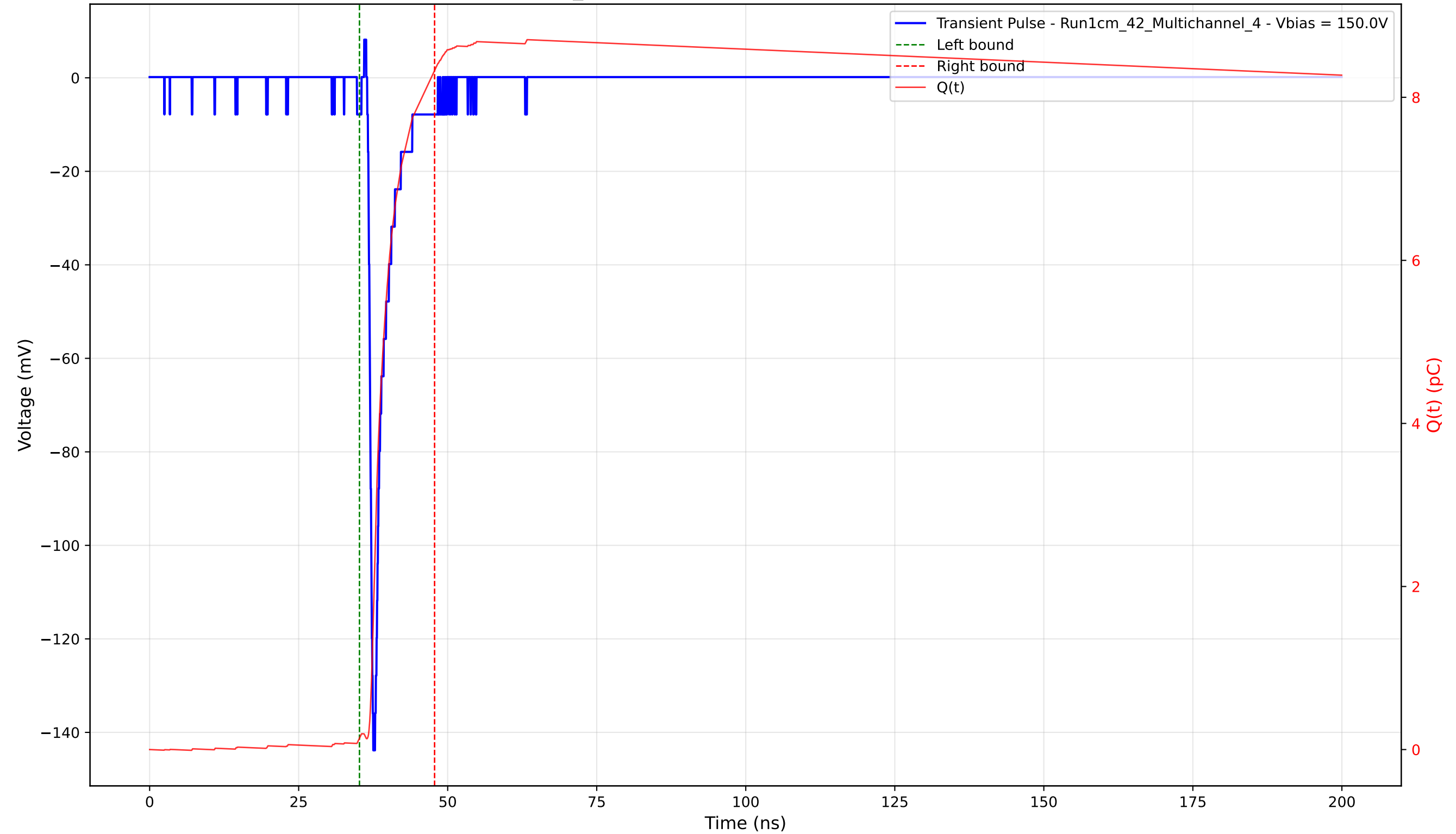
Transient Pulse - Sample: 1cm_42 - Position: 3255.0 \mu\text{m} - Charge: 8.19 pC - Rise Time: 0.81 ns
