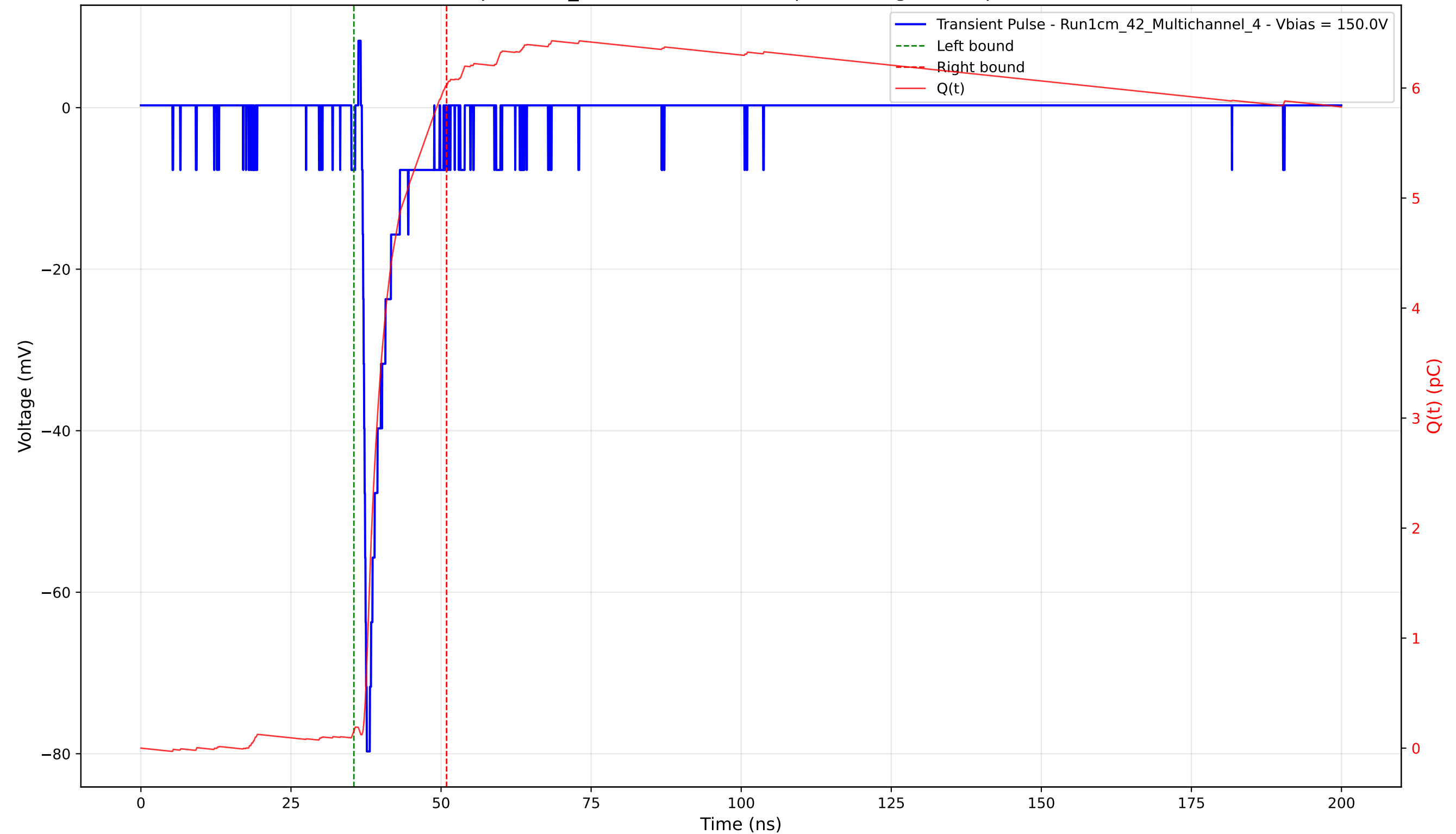
Transient Pulse - Sample: 1cm_42 - Position: 3485.0 \mu\text{m} - Charge: 5.86 pC - Rise Time: 0.72 ns
