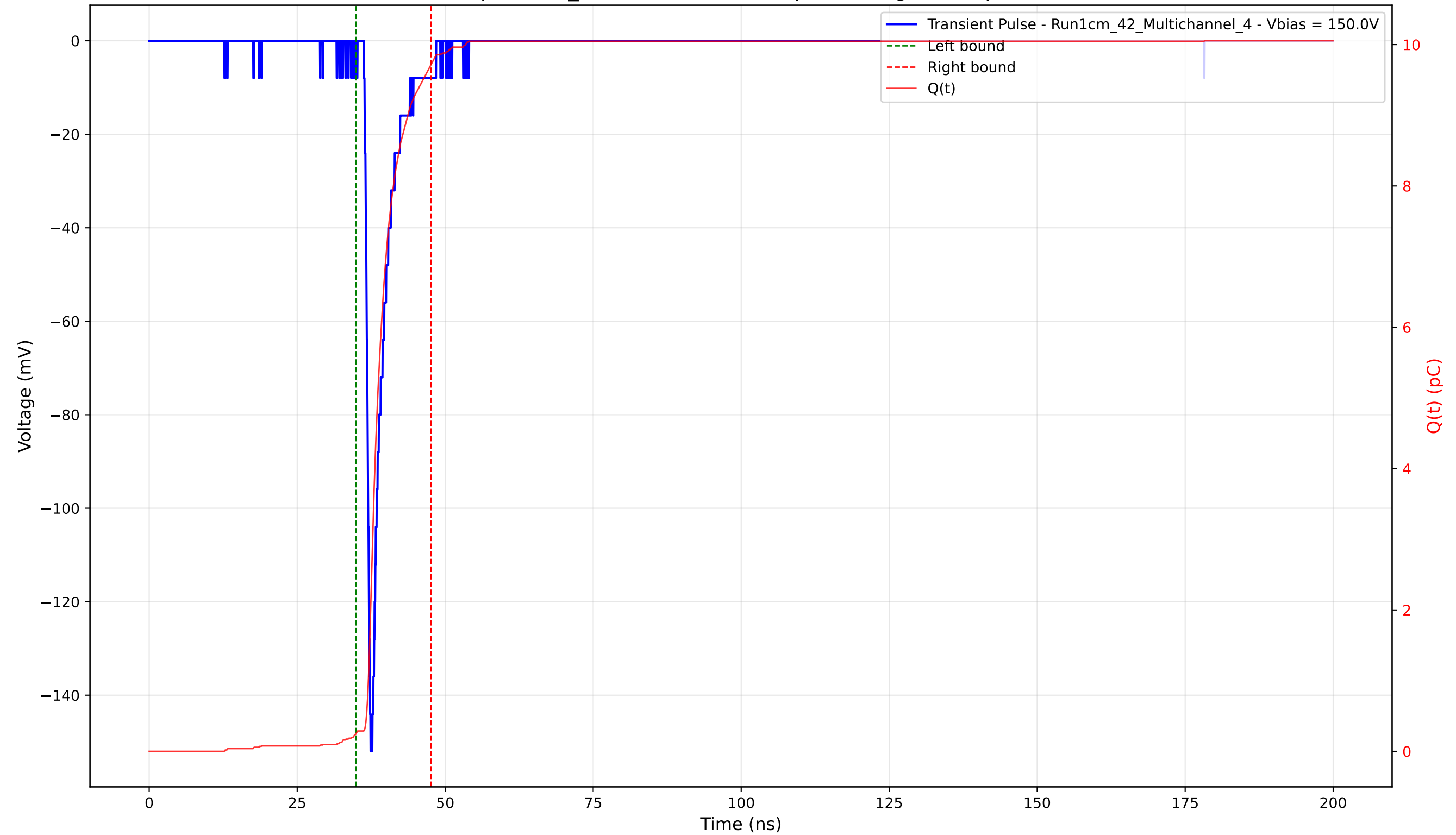
Transient Pulse - Sample: 1cm_42 - Position: 1790.0 \mu\text{m} - Charge: 9.47 pC - Rise Time: 0.92 ns
