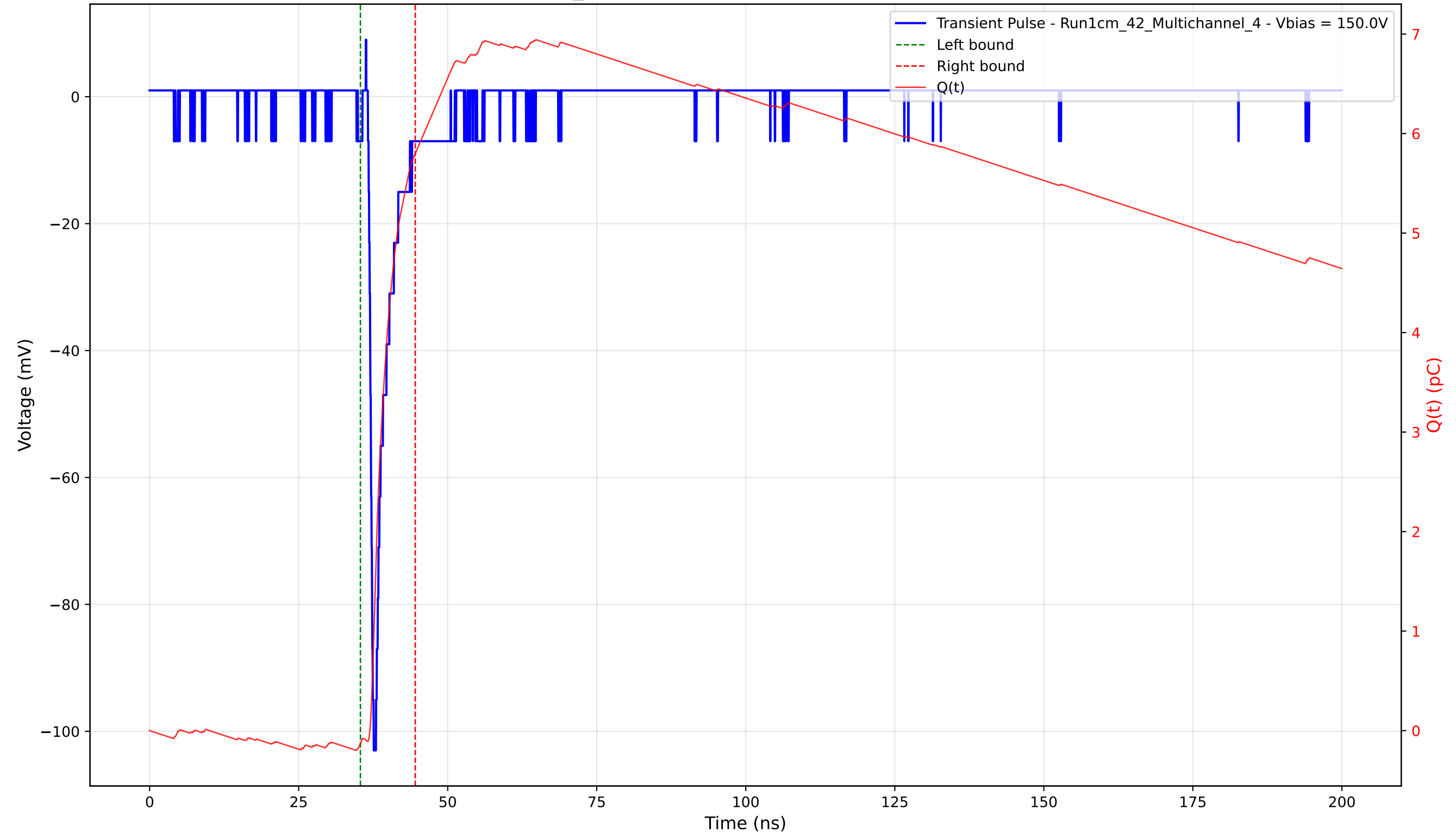
Transient Pulse - Sample: 1cm_42 - Position: 3405.0 \mu\text{m} - Charge: 5.92 pC - Rise Time: 0.70 ns
