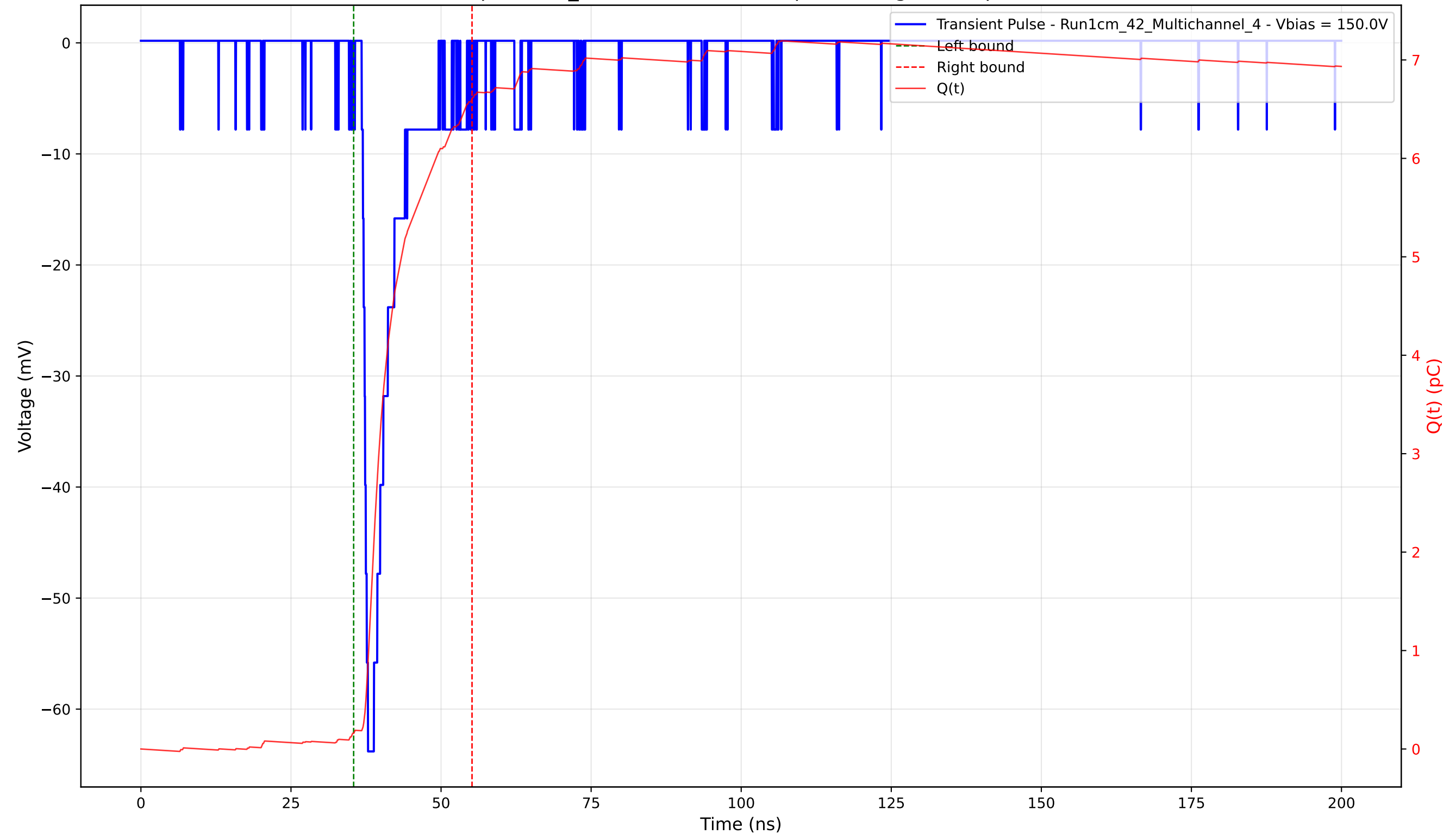
Transient Pulse - Sample: 1cm_42 - Position: 1450.0 \mu\text{m} - Charge: 6.45 pC - Rise Time: 1.05 ns
