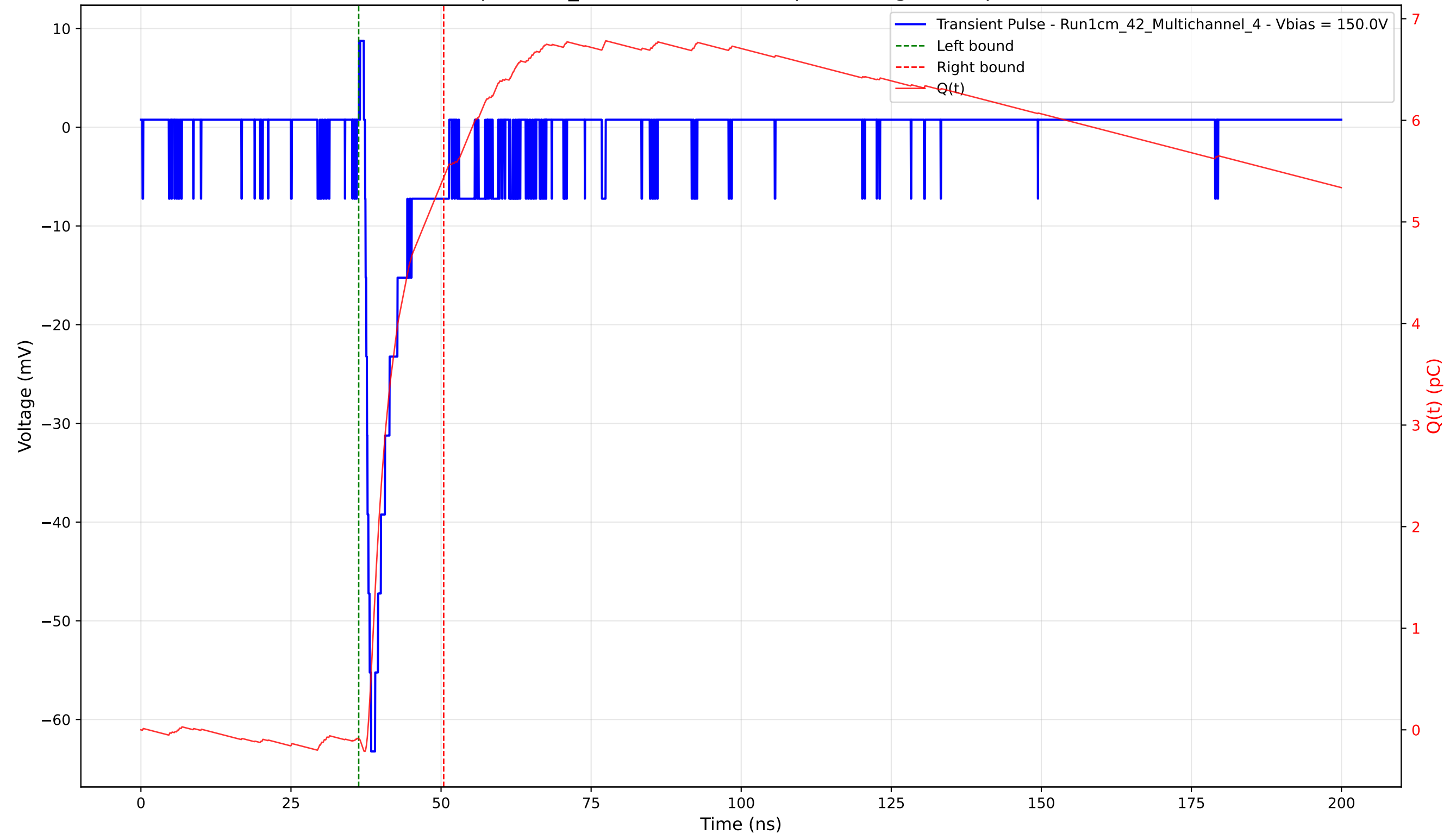
Transient Pulse - Sample: 1cm_42 - Position: 1190.0 \mu\text{m} - Charge: 5.53 pC - Rise Time: 1.01 ns
