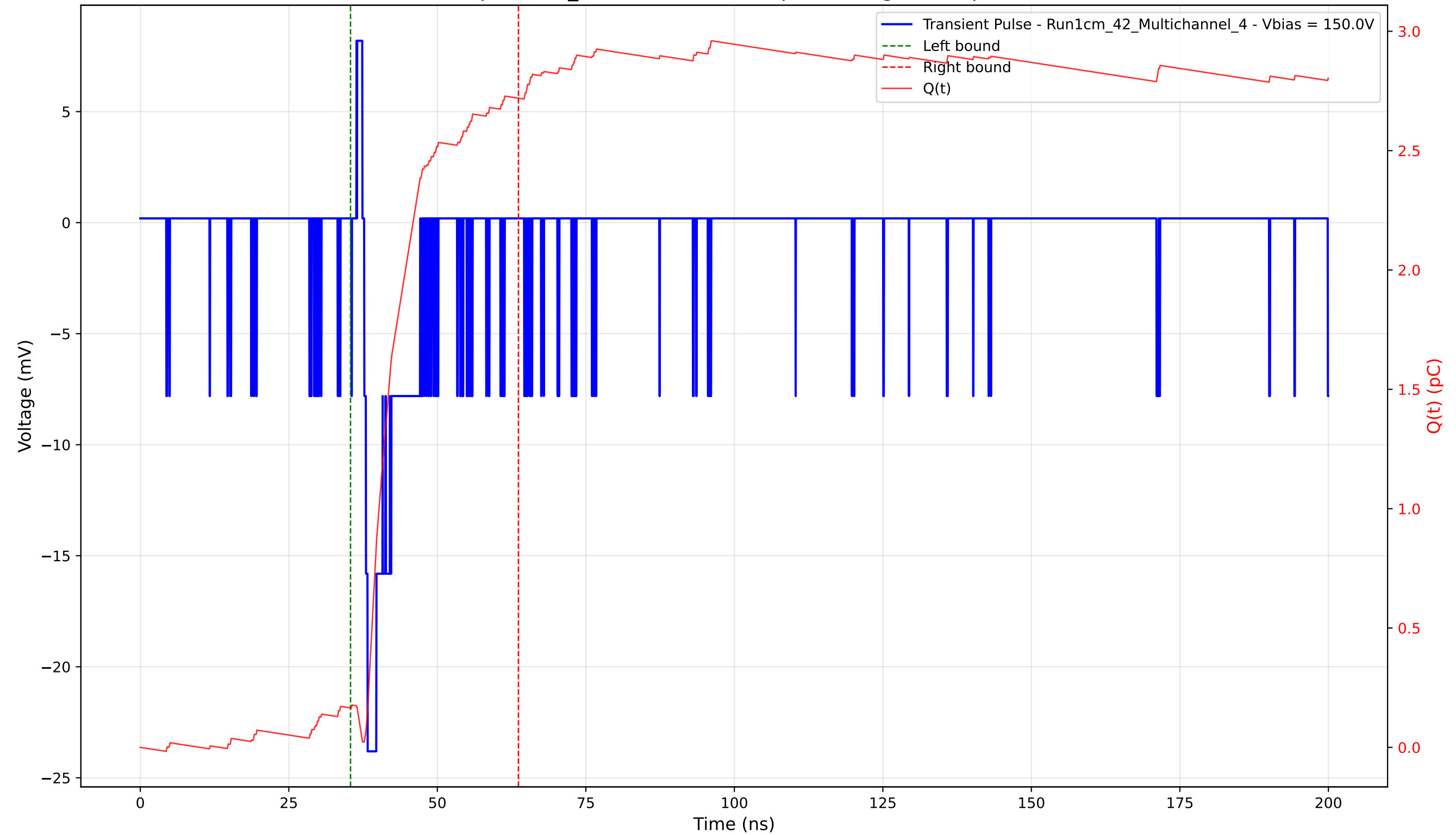
Transient Pulse - Sample: 1cm_42 - Position: 315.0 \mu\text{m} - Charge: 2.55 pC - Rise Time: 0.59 ns
