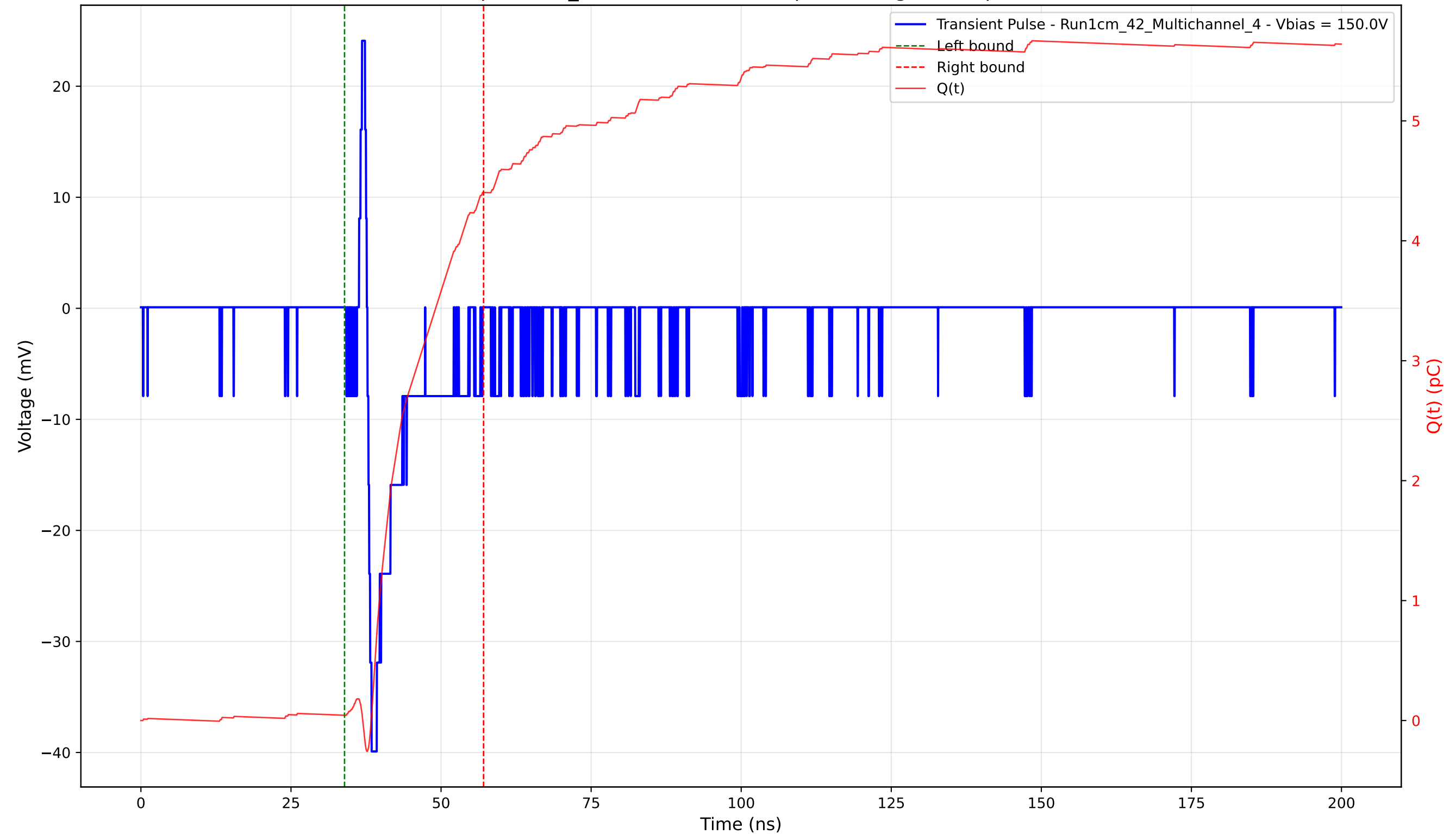
Transient Pulse - Sample: 1cm_42 - Position: 4295.0 \mu\text{m} - Charge: 4.36 pC - Rise Time: 0.70 ns
