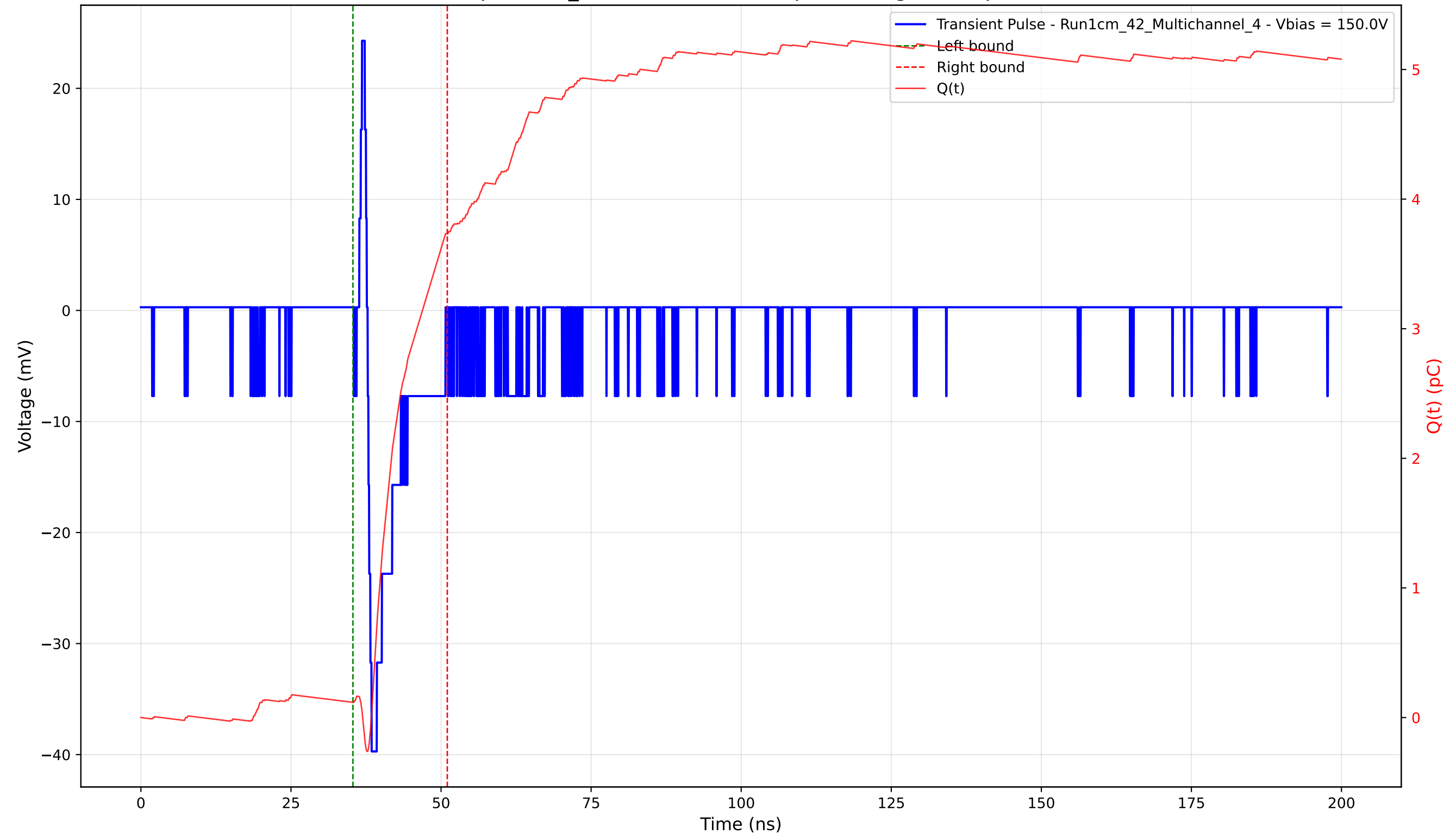
Transient Pulse - Sample: 1cm_42 - Position: 4290.0 \mu\text{m} - Charge: 3.62 pC - Rise Time: 0.66 ns
