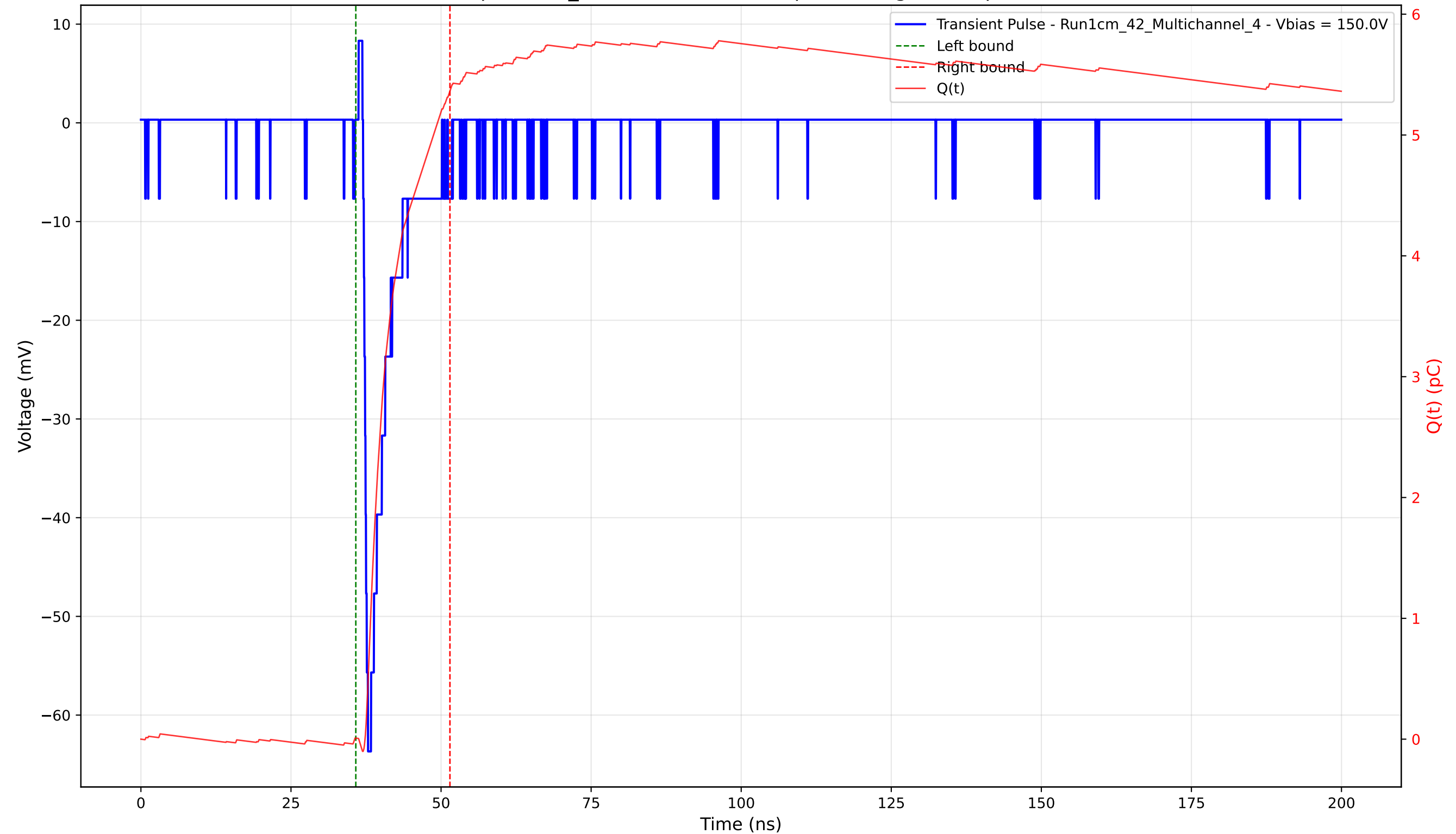
Transient Pulse - Sample: 1cm_42 - Position: 3590.0 \mu\text{m} - Charge: 5.36 pC - Rise Time: 0.81 ns
