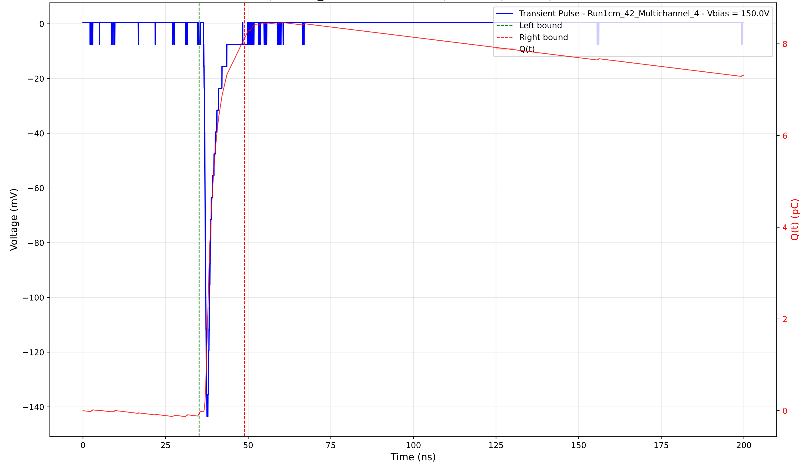
Transient Pulse - Sample: 1cm_42 - Position: 3270.0 \mu\text{m} - Charge: 8.19 pC - Rise Time: 0.85 ns
