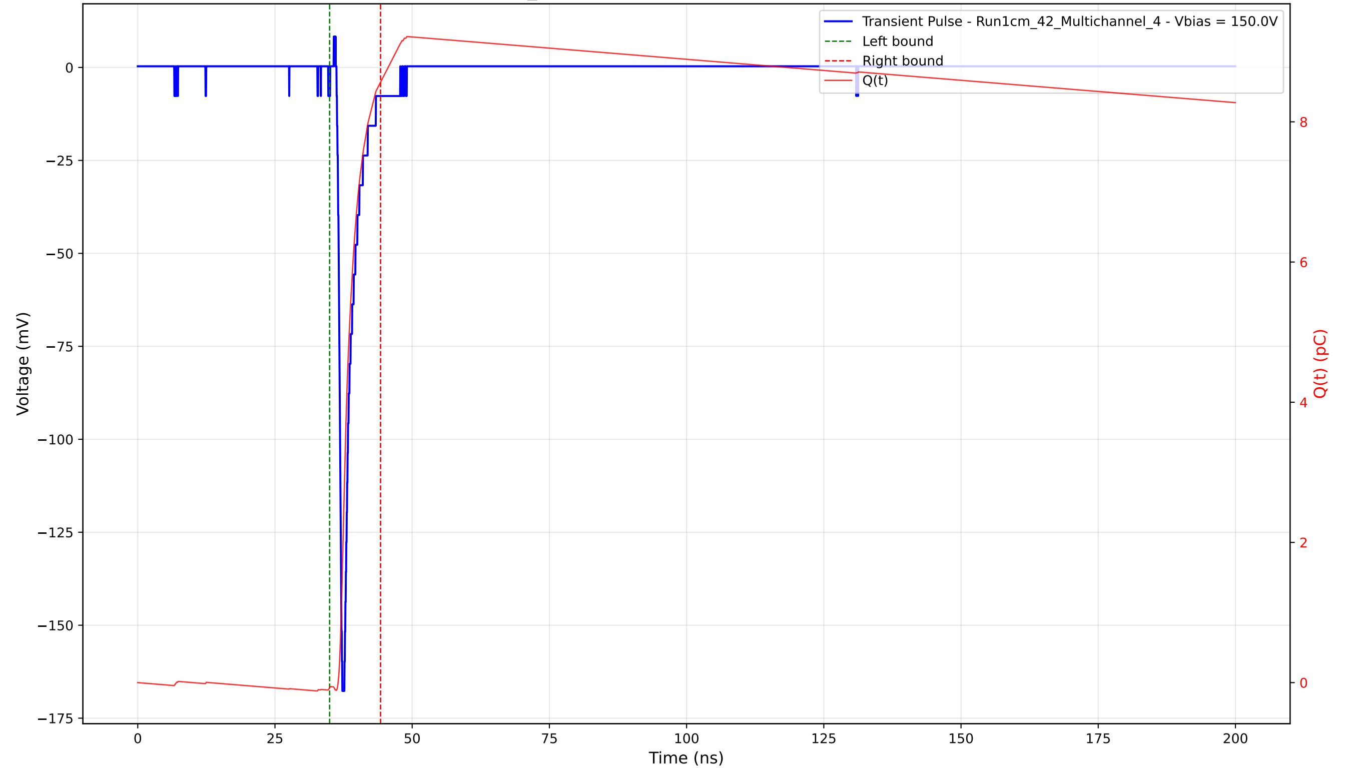
Transient Pulse - Sample: 1cm_42 - Position: 1905.0 \mu\text{m} - Charge: 8.64 pC - Rise Time: 0.75 ns
