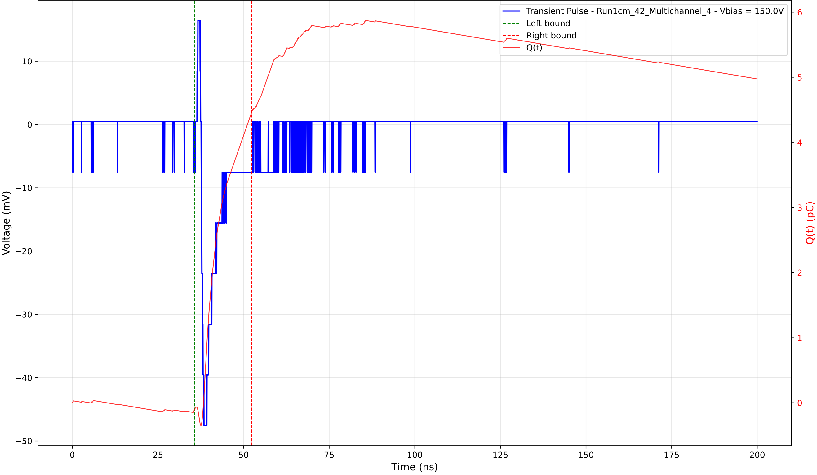
Transient Pulse - Sample: 1cm_42 - Position: 995.0 \mu\text{m} - Charge: 4.56 pC - Rise Time: 0.82 ns
