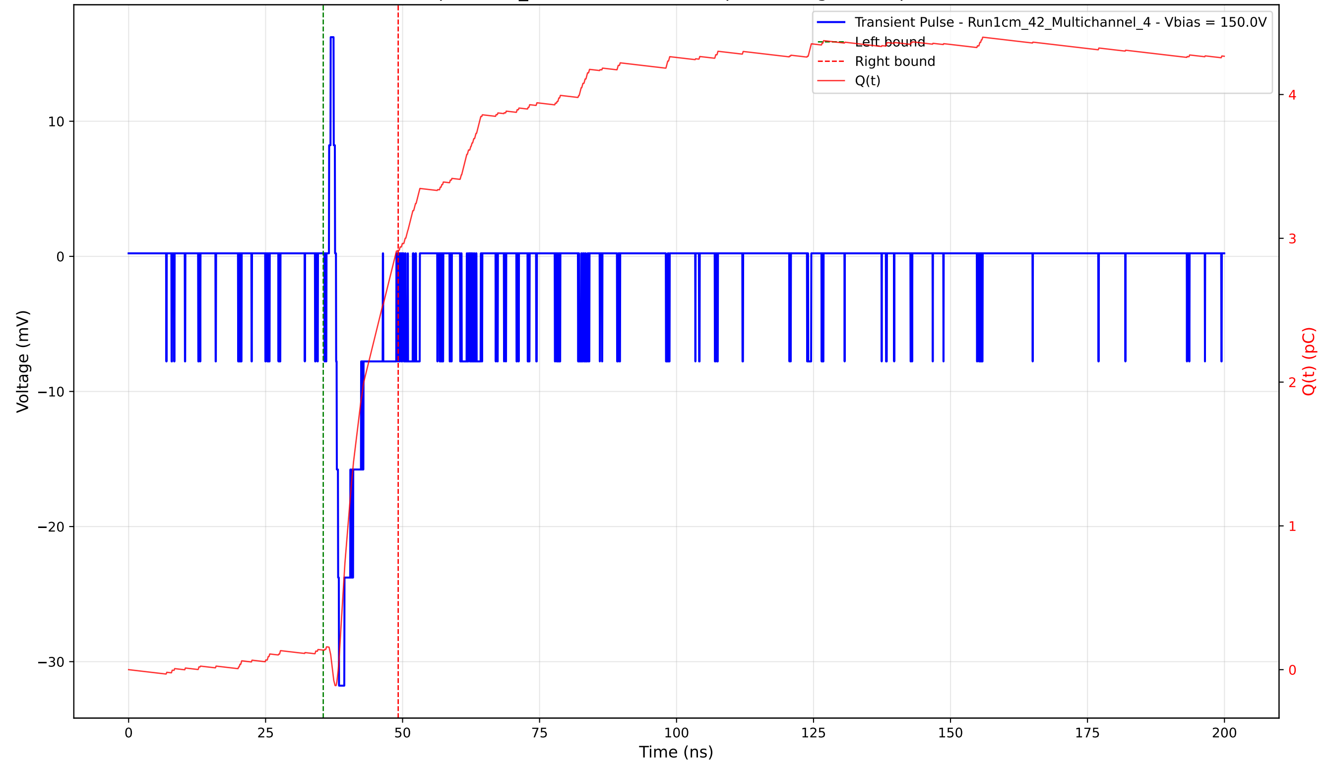
Transient Pulse - Sample: 1cm_42 - Position: 4660.0 \mu\text{m} - Charge: 2.78 pC - Rise Time: 0.54 ns
