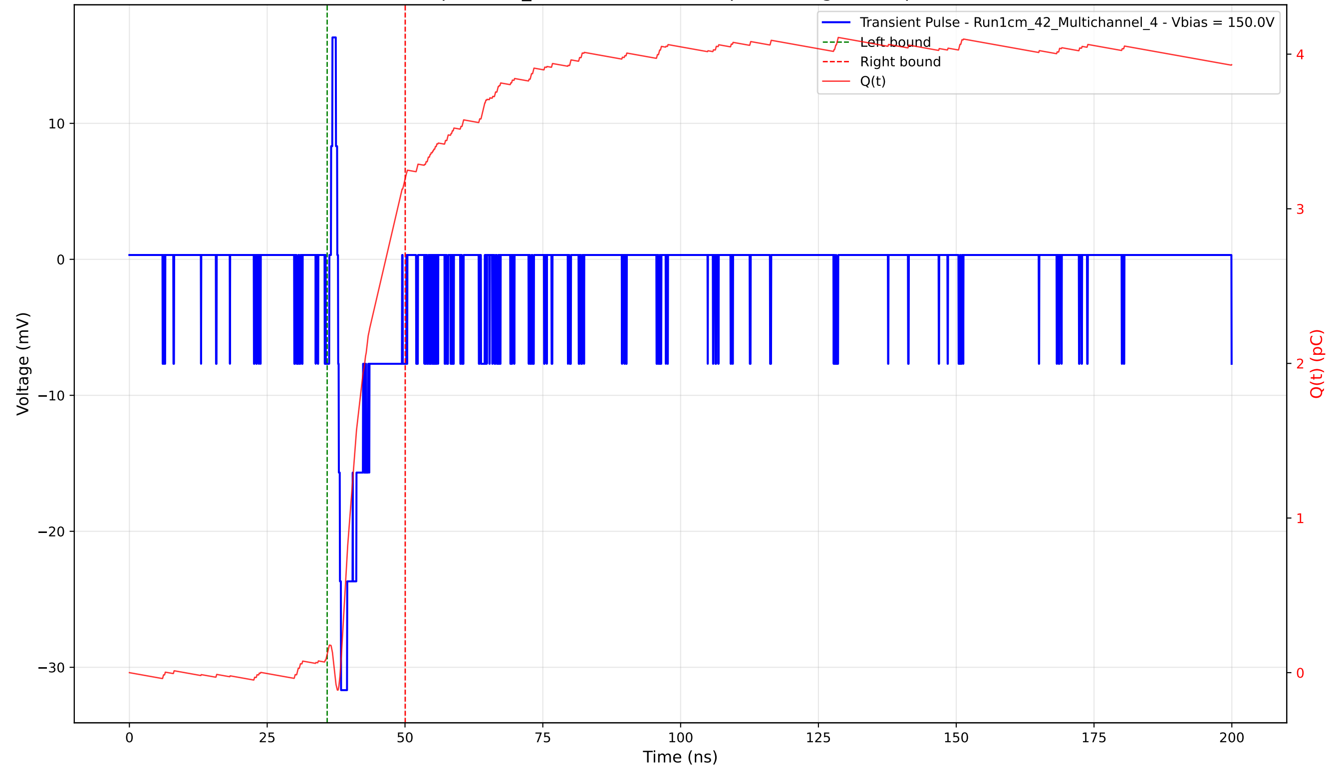
Transient Pulse - Sample: 1cm_42 - Position: 4730.0 \mu\text{m} - Charge: 3.08 pC - Rise Time: 0.54 ns
