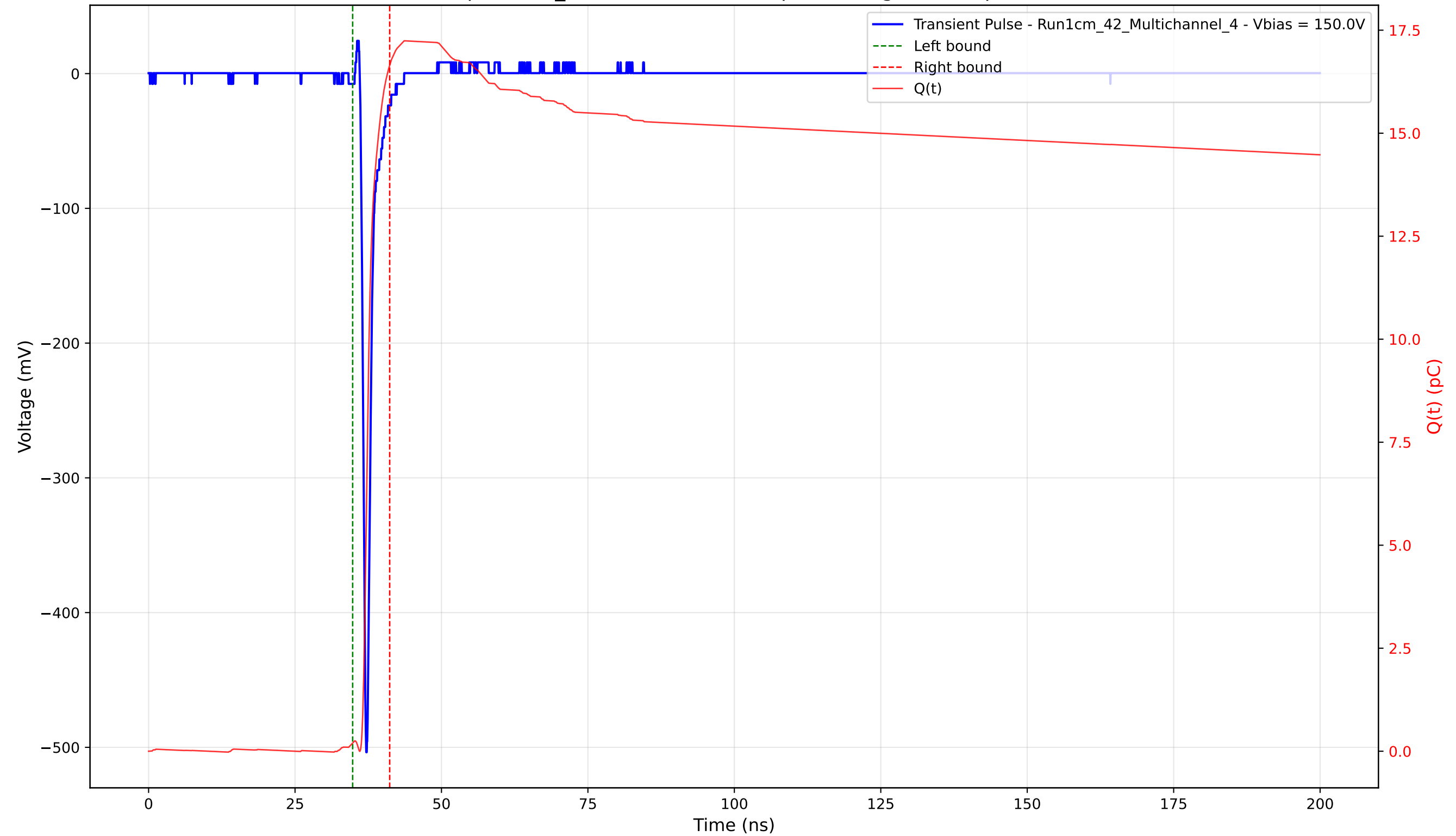
Transient Pulse - Sample: 1cm_42 - Position: 2245.0 \mu\text{m} - Charge: 16.45 pC - Rise Time: 0.70 ns
