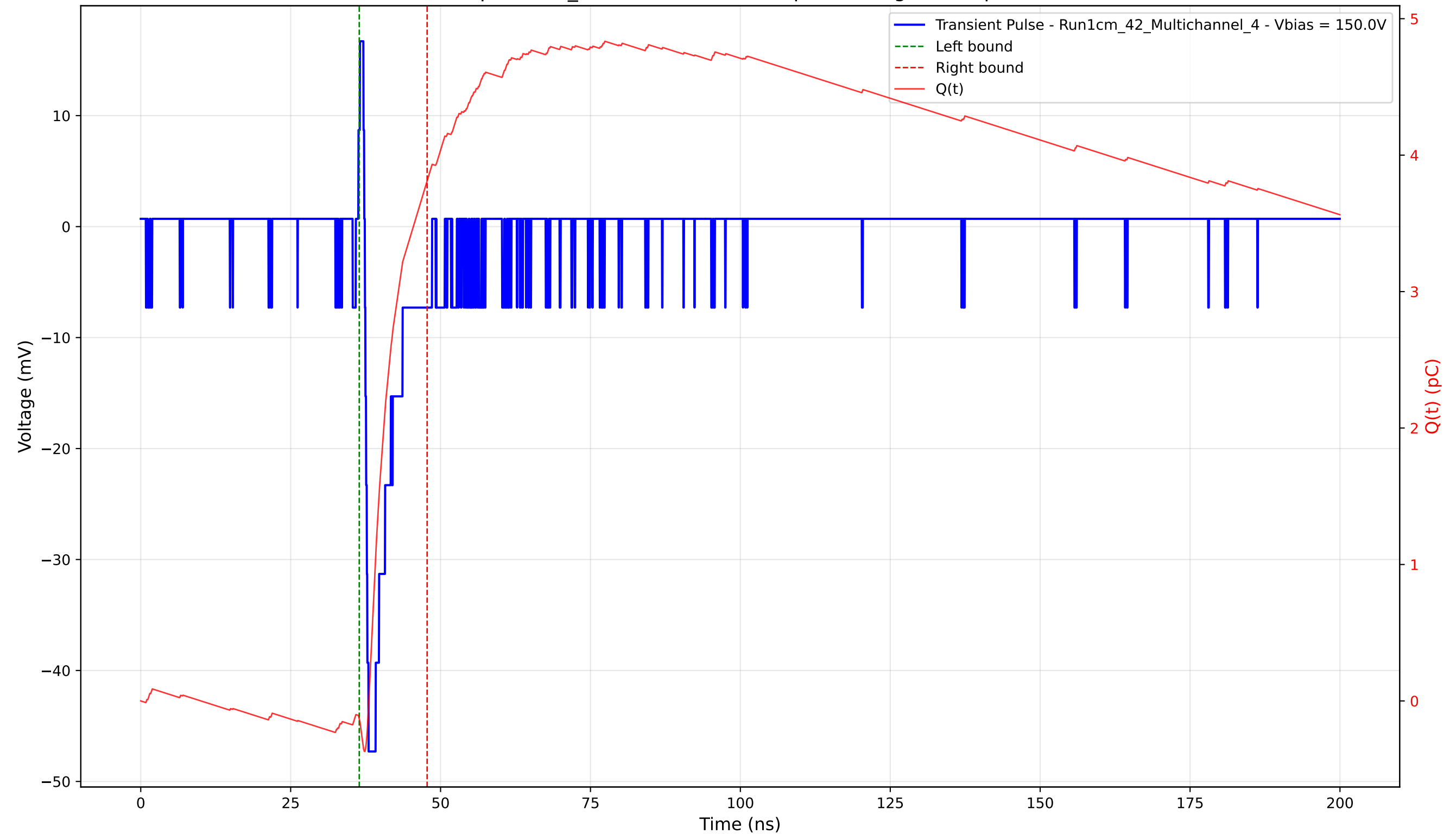
Transient Pulse - Sample: 1cm_42 - Position: 3870.0 \mu\text{m} - Charge: 3.94 pC - Rise Time: 0.62 ns
