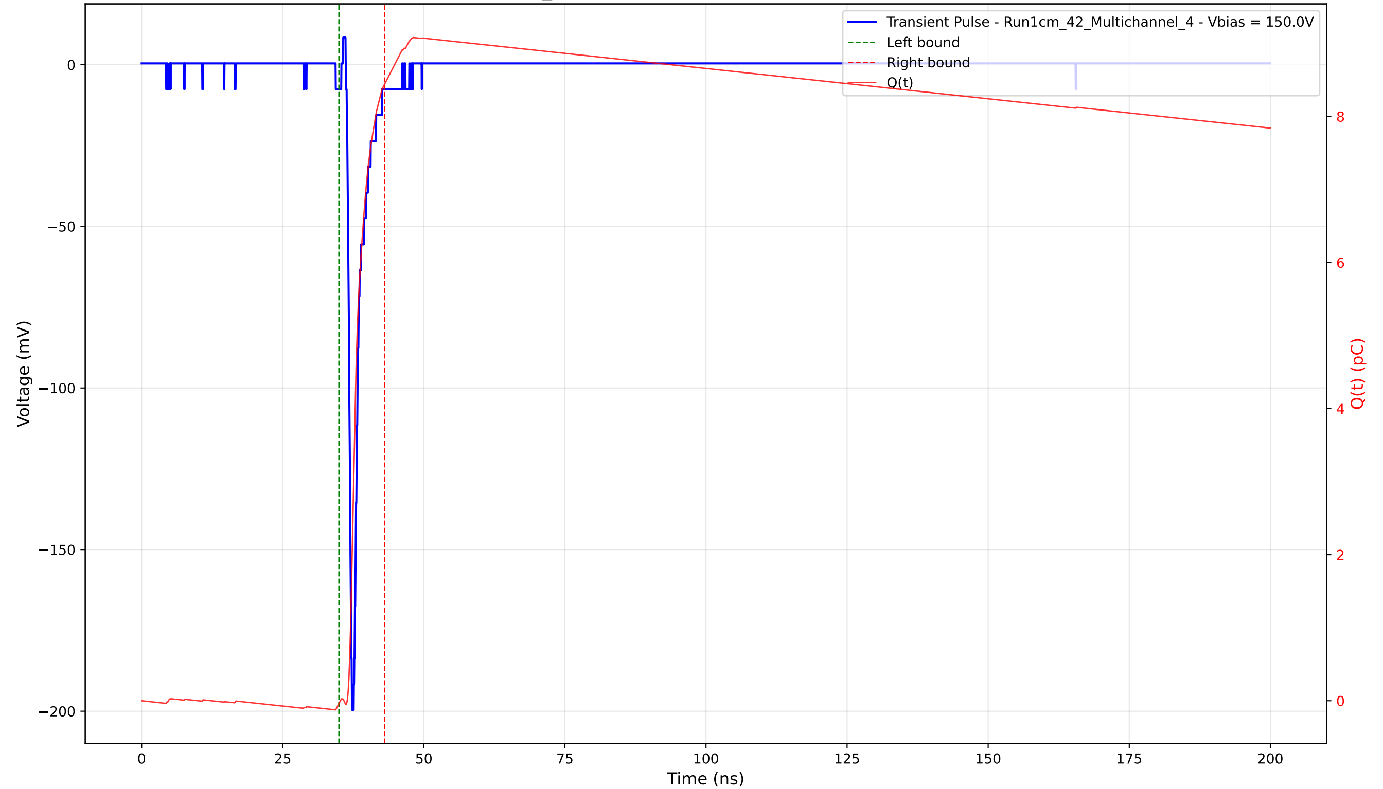
Transient Pulse - Sample: 1cm_42 - Position: 3050.0 \mu\text{m} - Charge: 8.48 pC - Rise Time: 0.78 ns
