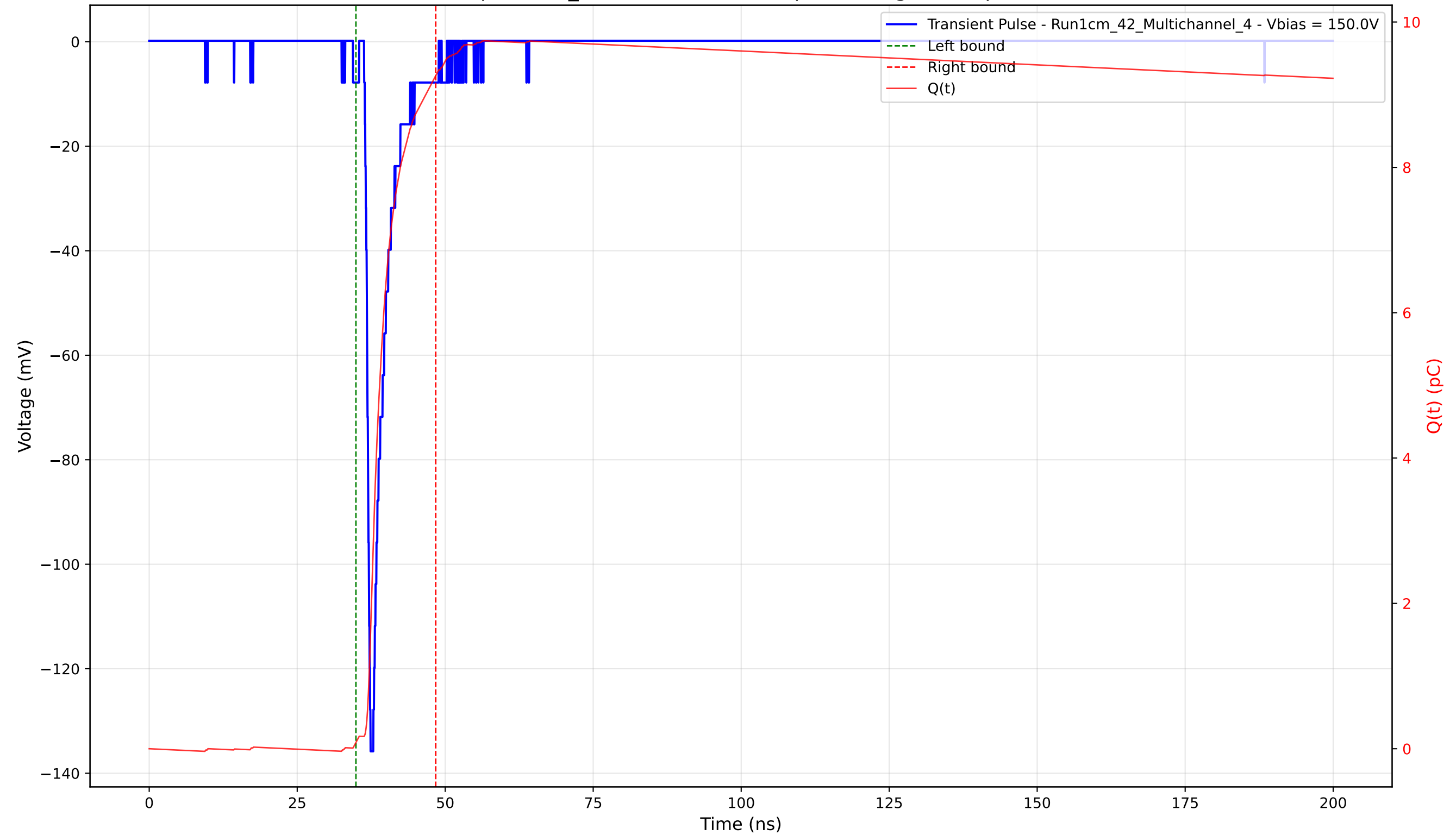
Transient Pulse - Sample: 1cm_42 - Position: 1715.0 \mu\text{m} - Charge: 9.18 pC - Rise Time: 0.89 ns
