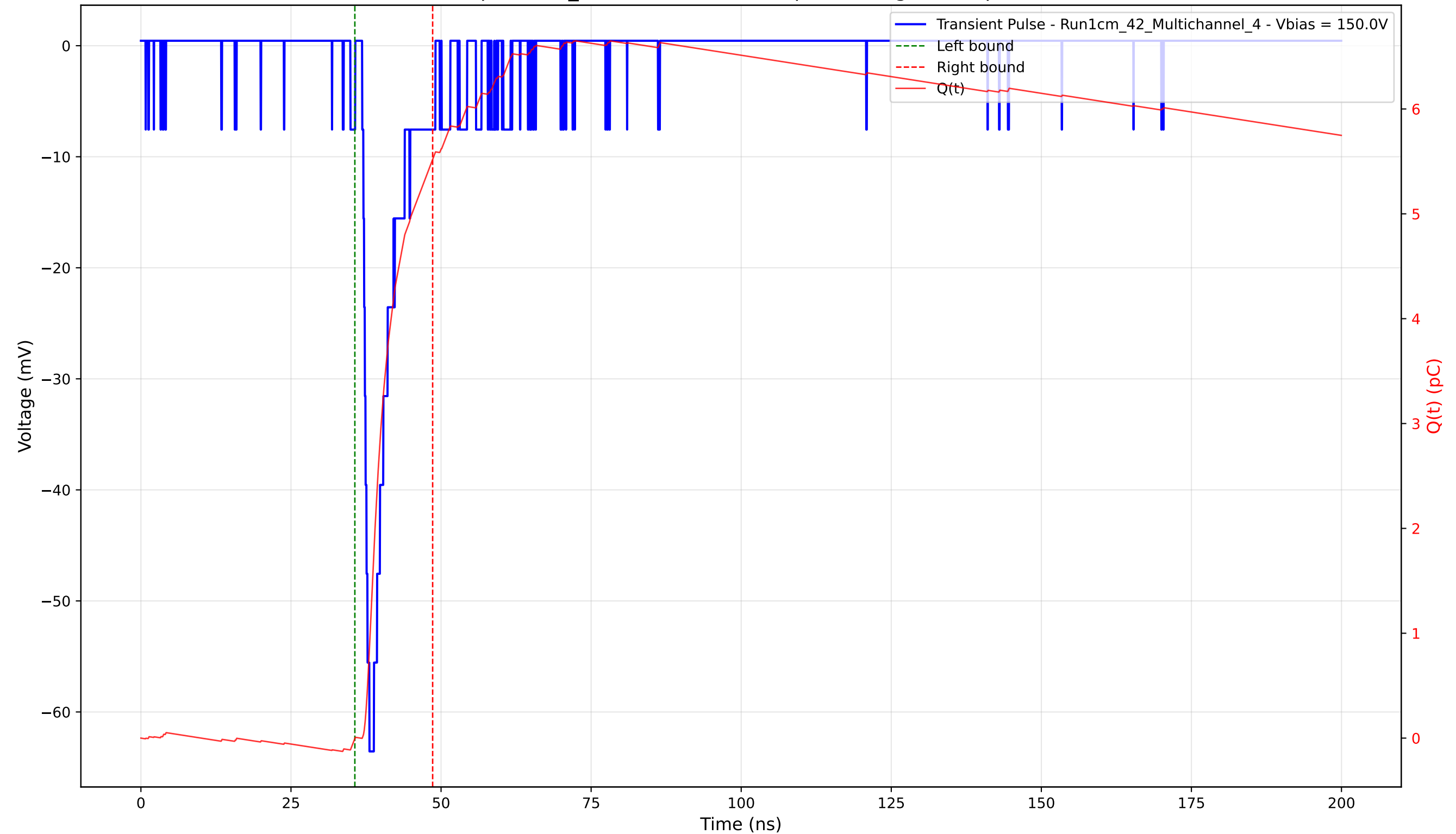
Transient Pulse - Sample: 1cm_42 - Position: 1425.0 \mu\text{m} - Charge: 5.52 pC - Rise Time: 1.21 ns
