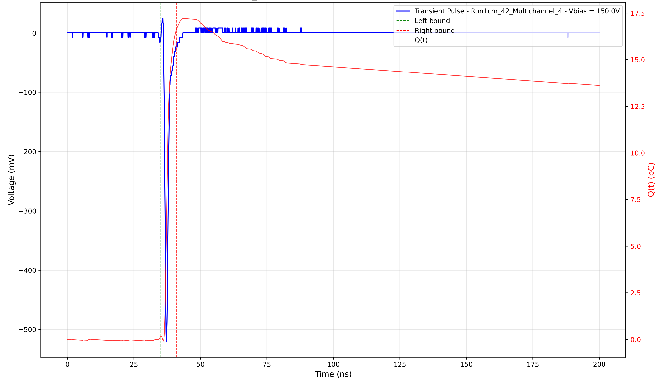
Transient Pulse - Sample: 1cm_42 - Position: 2320.0 \mu\text{m} - Charge: 16.46 pC - Rise Time: 0.72 ns
