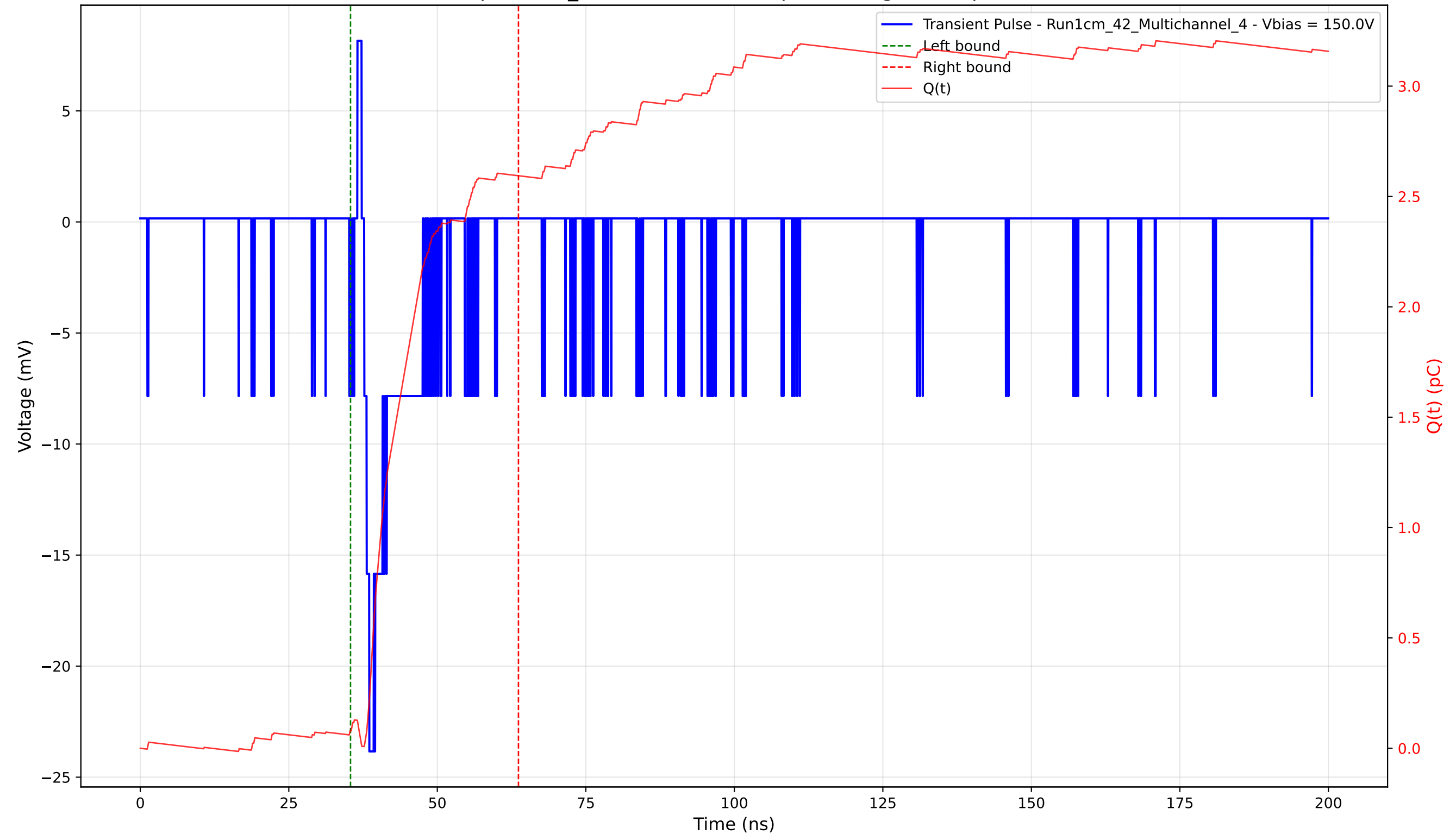
Transient Pulse - Sample: 1cm_42 - Position: 245.0 \mu\text{m} - Charge: 2.51 pC - Rise Time: 0.87 ns
