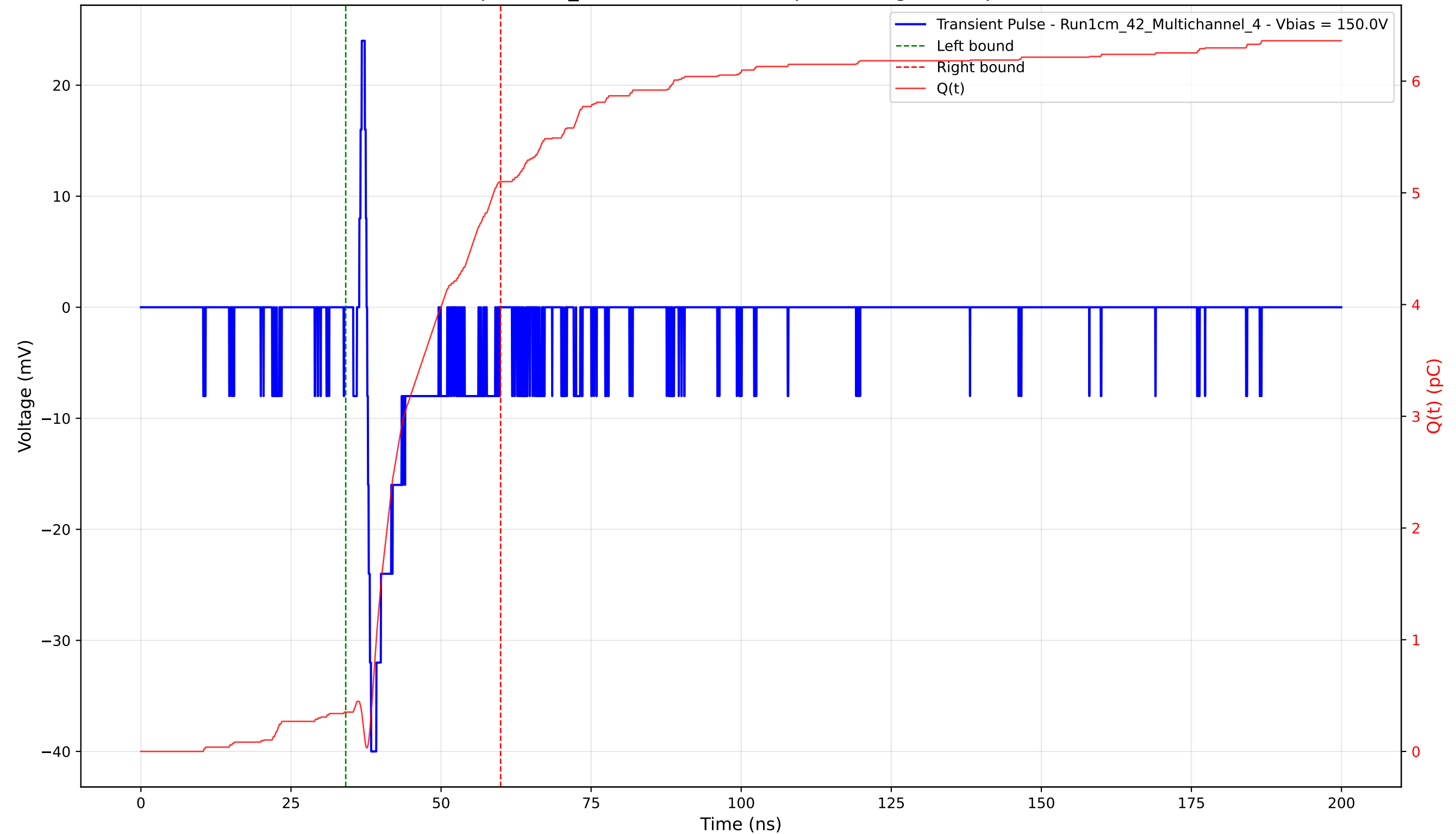
Transient Pulse - Sample: 1cm_42 - Position: 4190.0 \mu\text{m} - Charge: 4.75 pC - Rise Time: 0.66 ns
