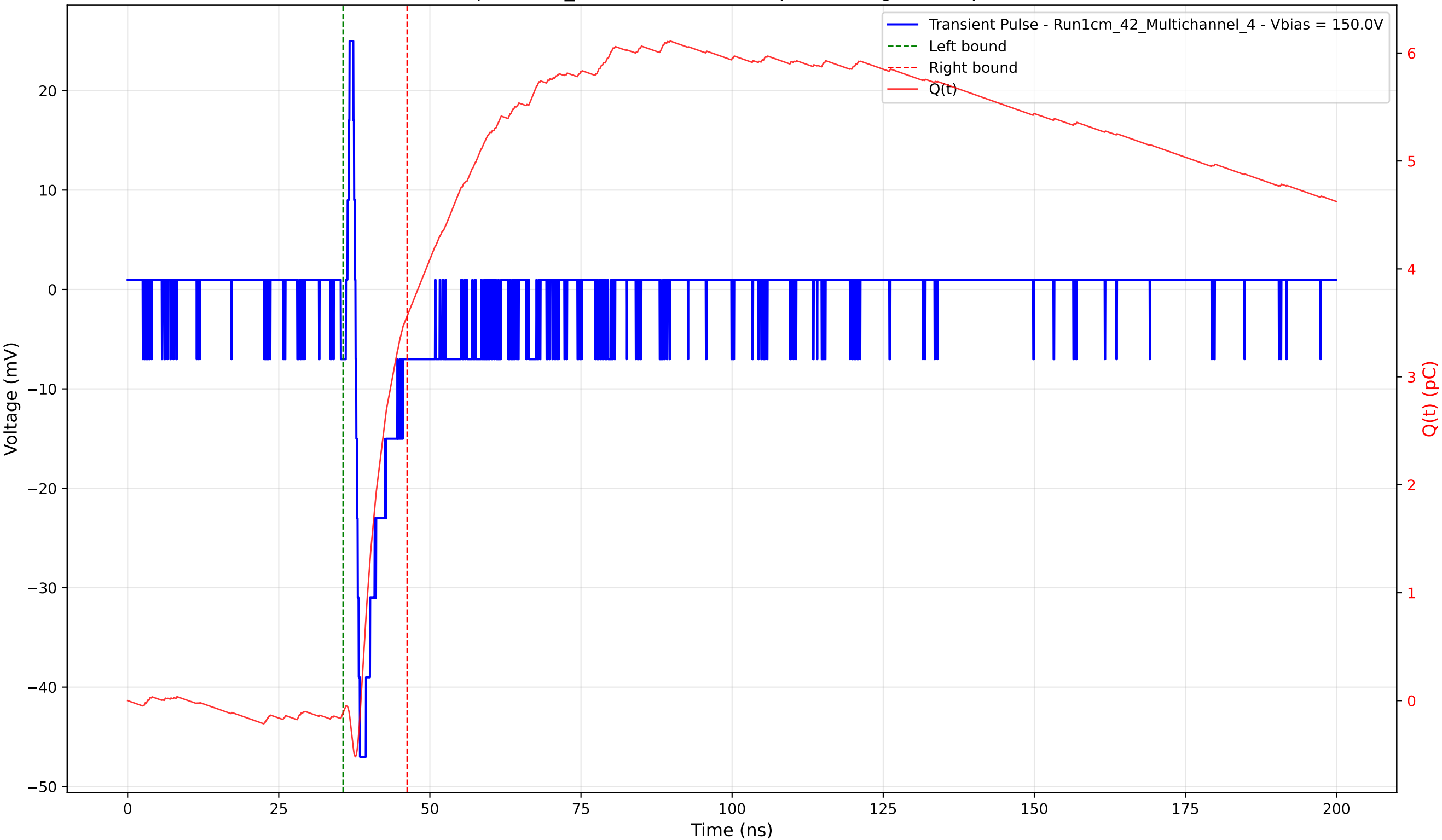
Transient Pulse - Sample: 1cm_42 - Position: 760.0 \mu\text{m} - Charge: 3.68 pC - Rise Time: 0.74 ns
