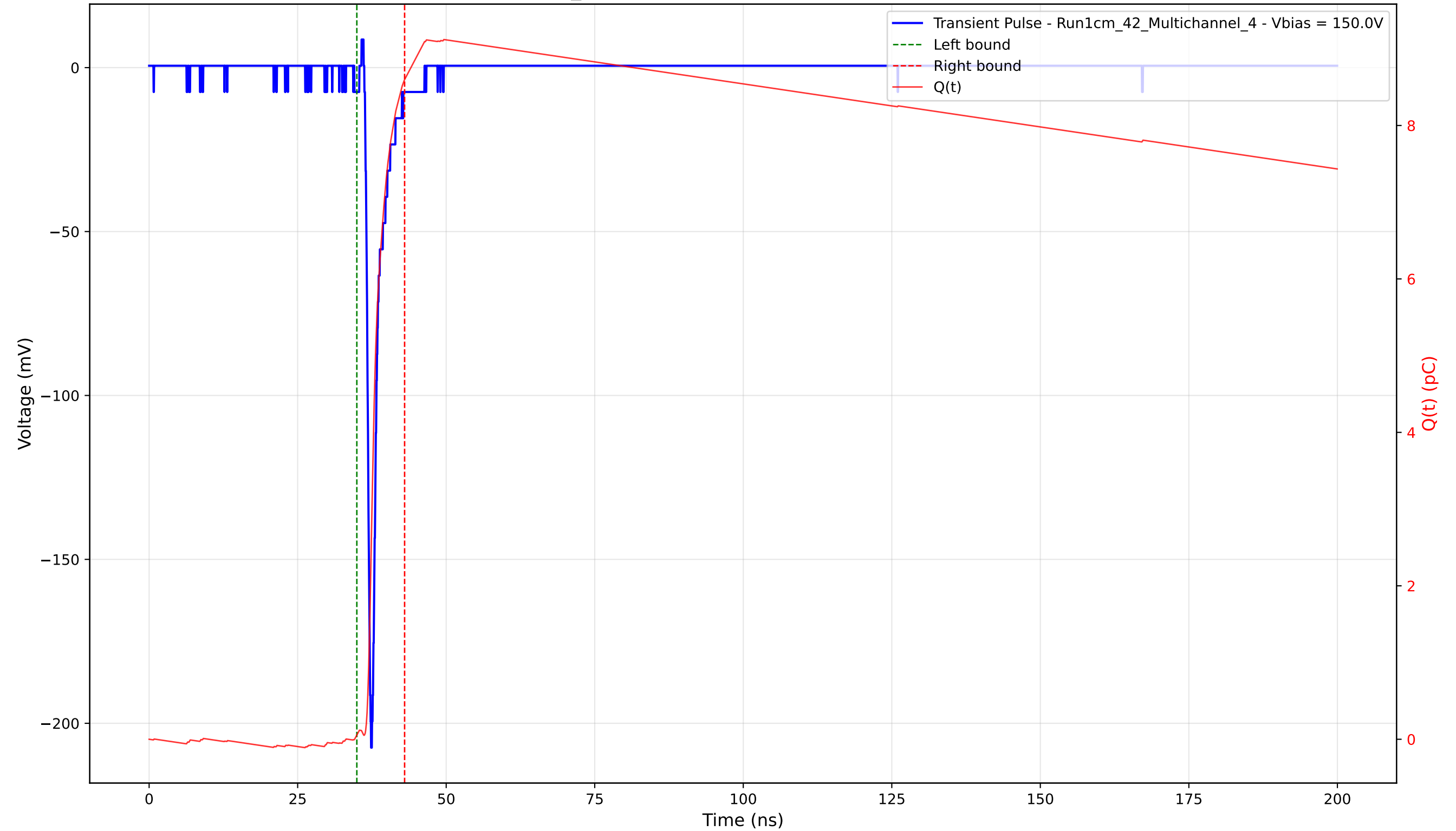
Transient Pulse - Sample: 1cm_42 - Position: 3045.0 \mu\text{m} - Charge: 8.54 pC - Rise Time: 0.81 ns
