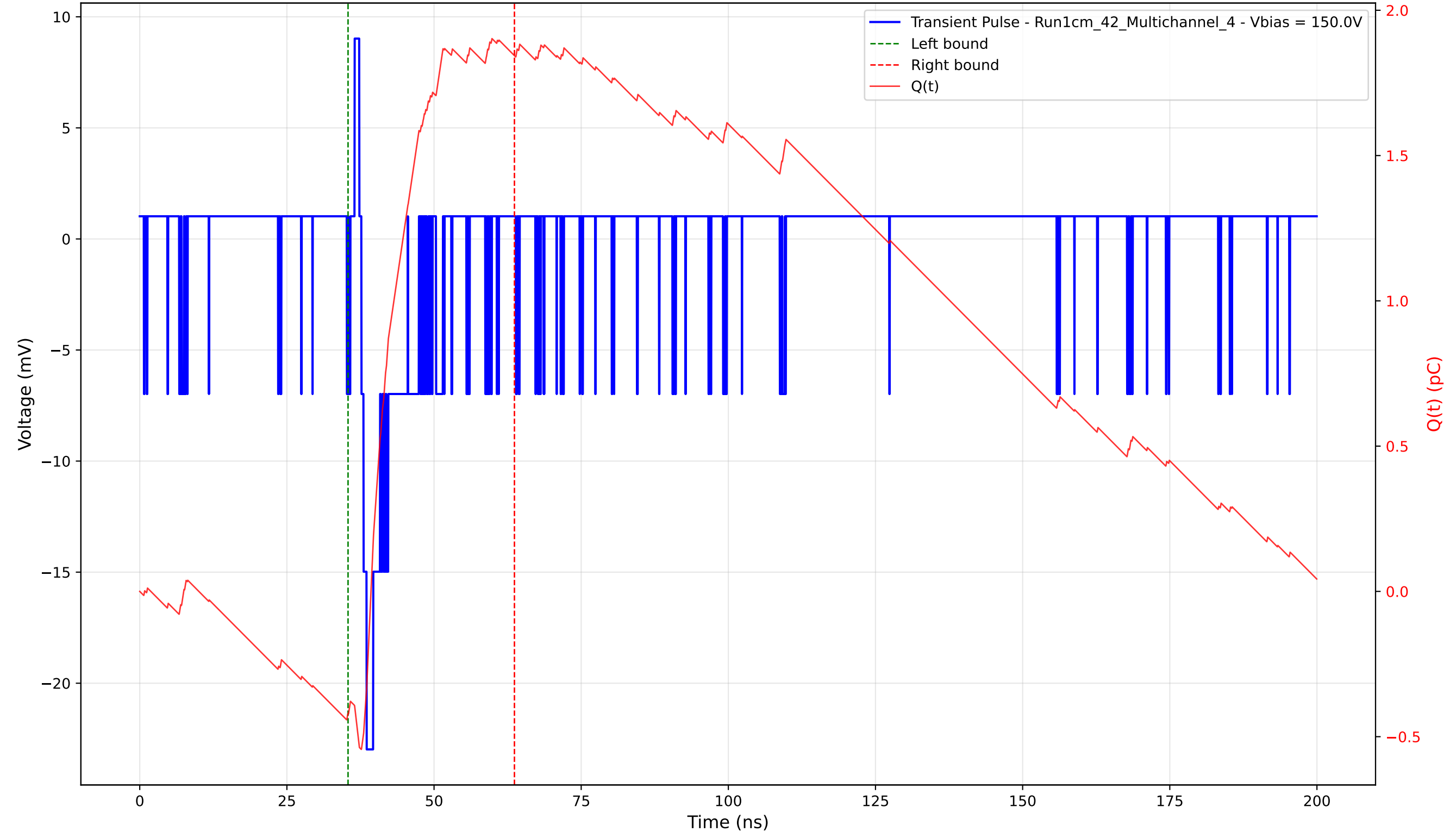
Transient Pulse - Sample: 1cm_42 - Position: 260.0 \mu\text{m} - Charge: 2.27 pC - Rise Time: 0.91 ns
