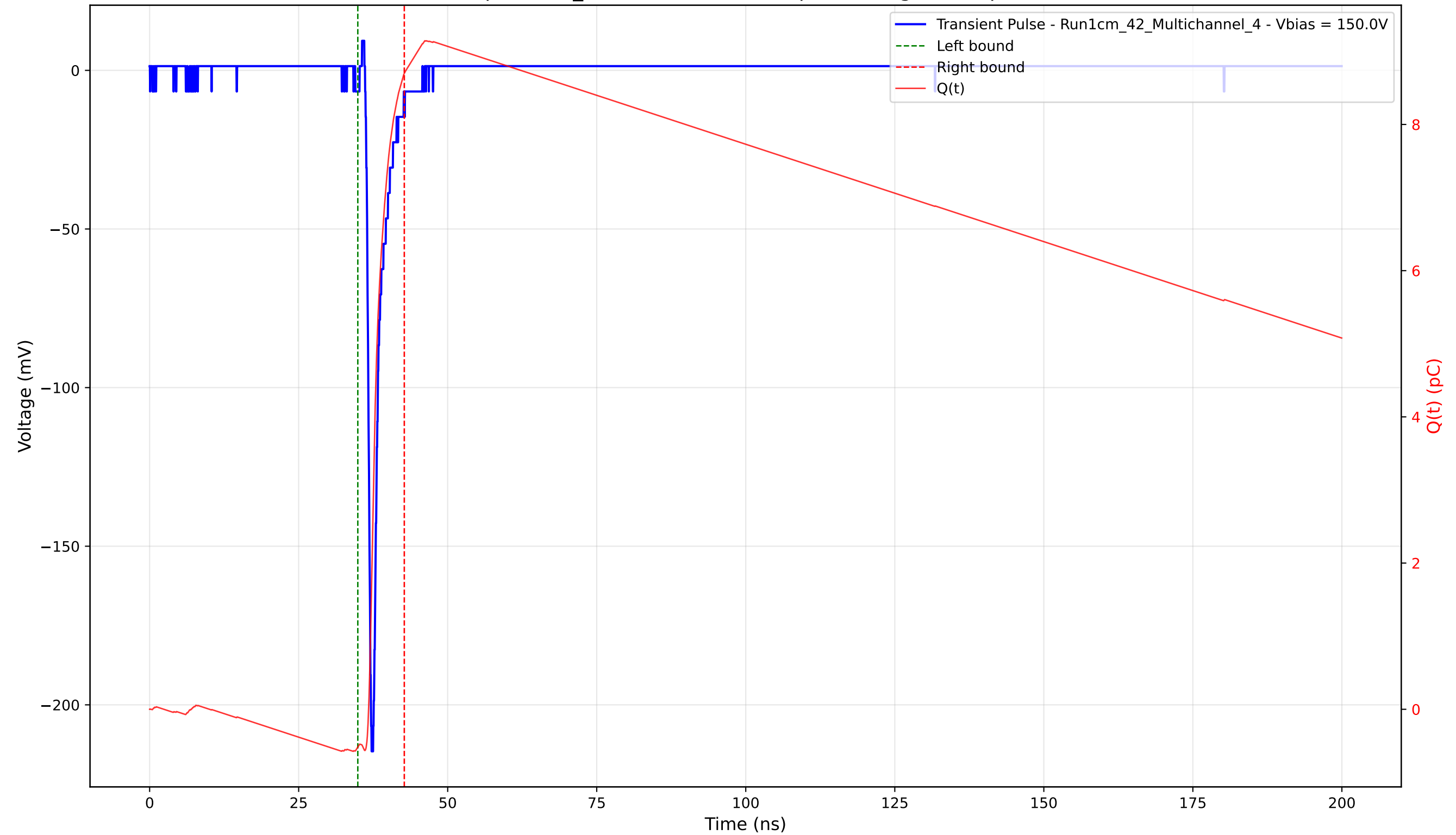
Transient Pulse - Sample: 1cm_42 - Position: 1995.0 \mu\text{m} - Charge: 9.21 pC - Rise Time: 0.78 ns
