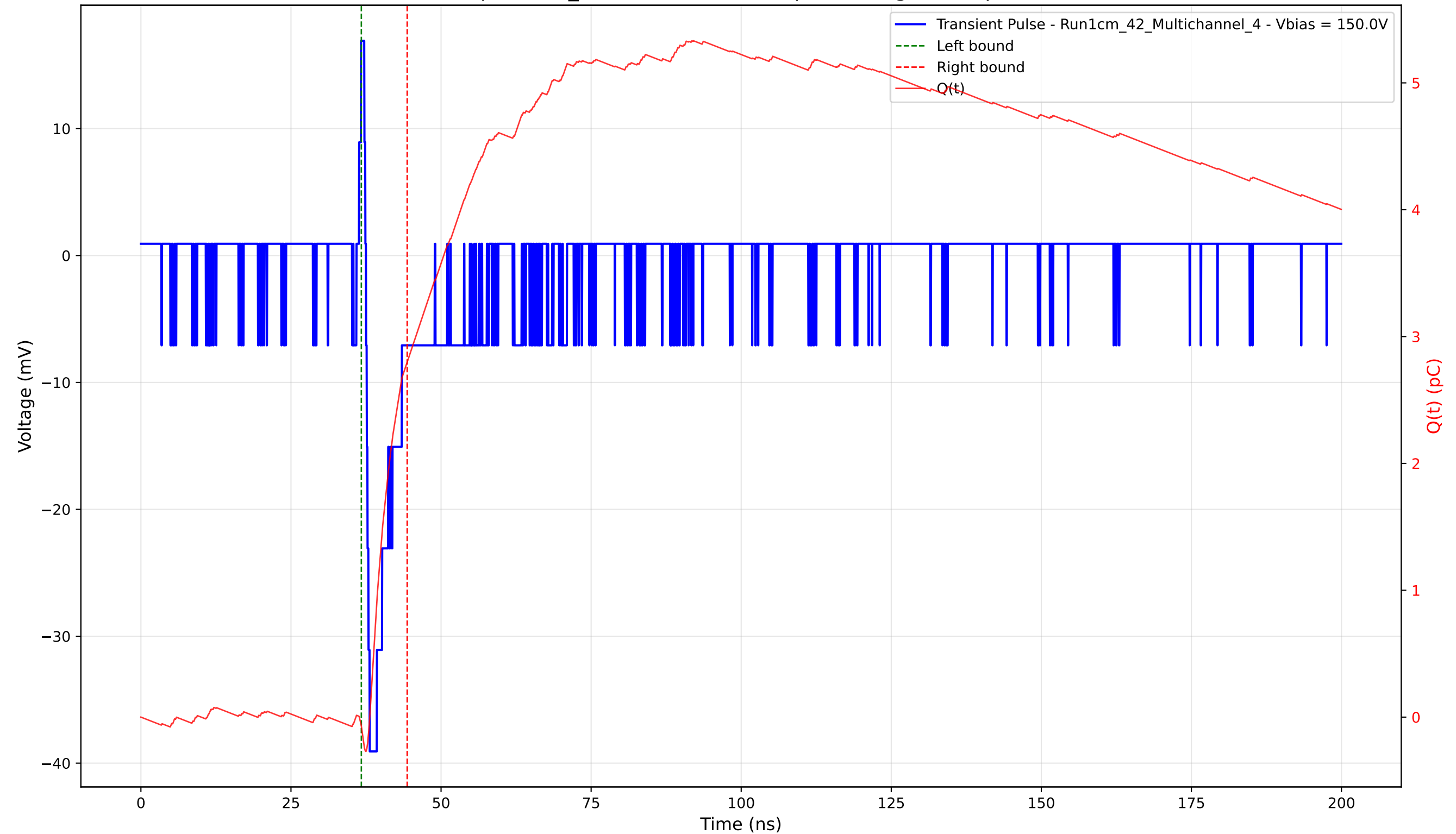
Transient Pulse - Sample: 1cm_42 - Position: 3990.0 \mu\text{m} - Charge: 2.87 pC - Rise Time: 0.62 ns
