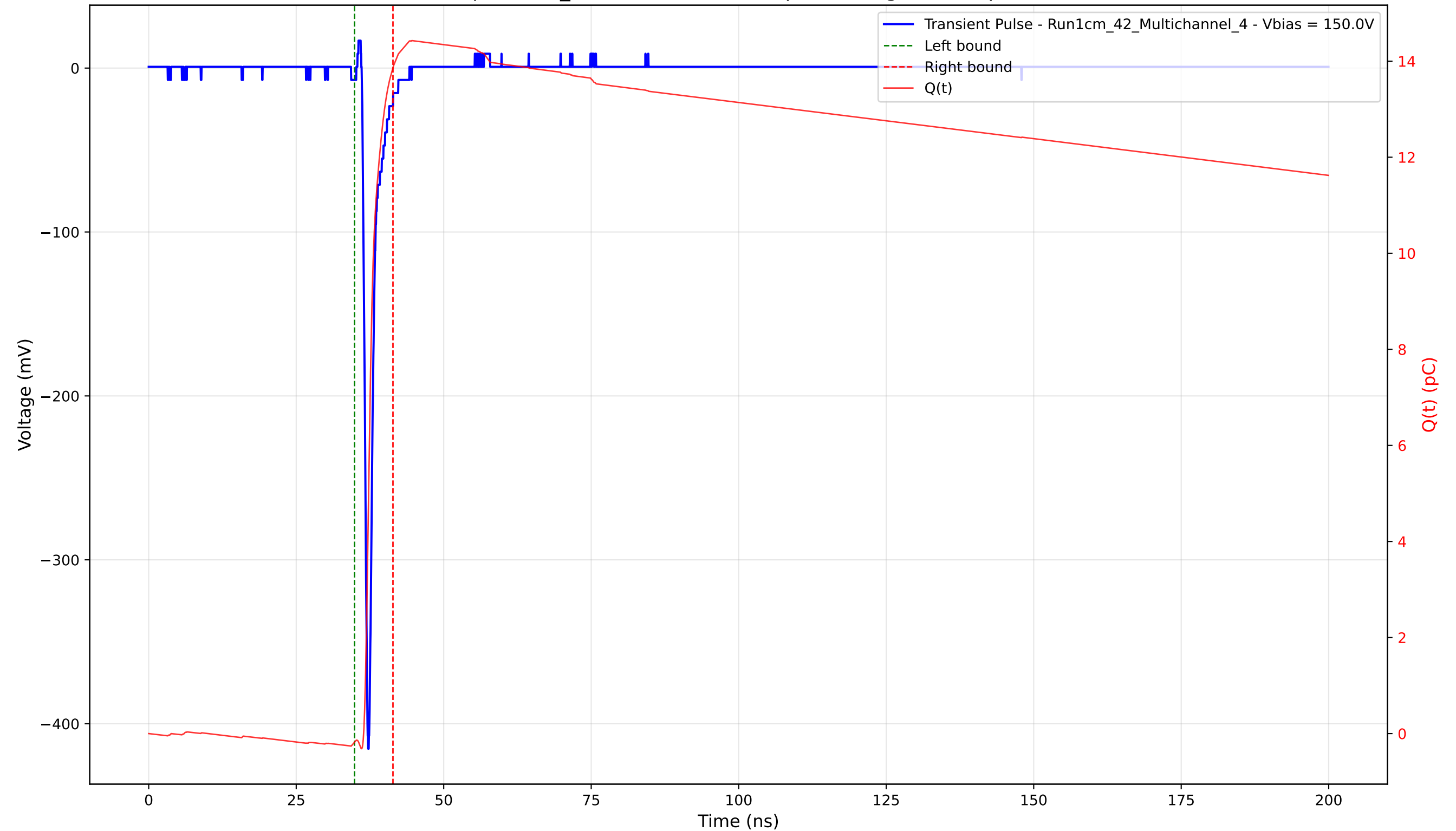
Transient Pulse - Sample: 1cm_42 - Position: 2170.0 \mu\text{m} - Charge: 14.05 pC - Rise Time: 0.74 ns
