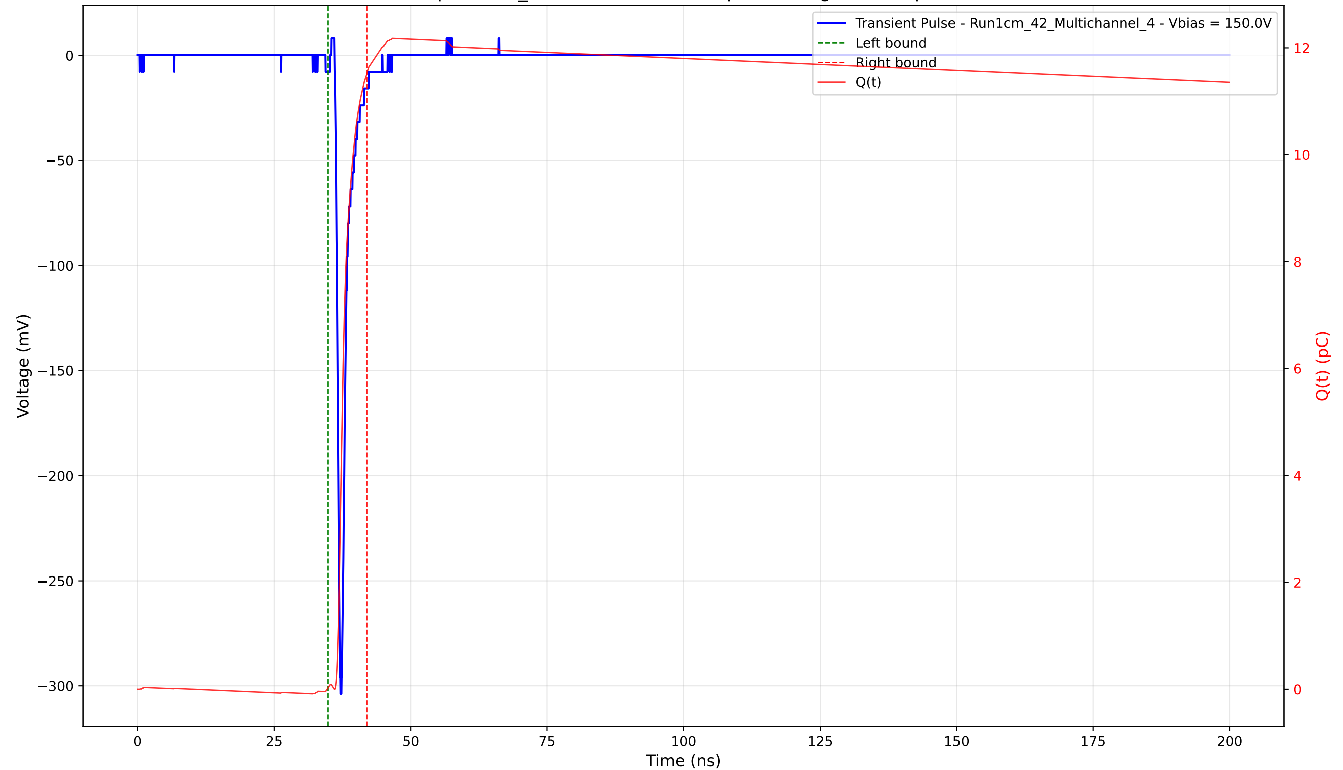
Transient Pulse - Sample: 1cm_42 - Position: 2085.0 \mu\text{m} - Charge: 11.50 pC - Rise Time: 0.74 ns
