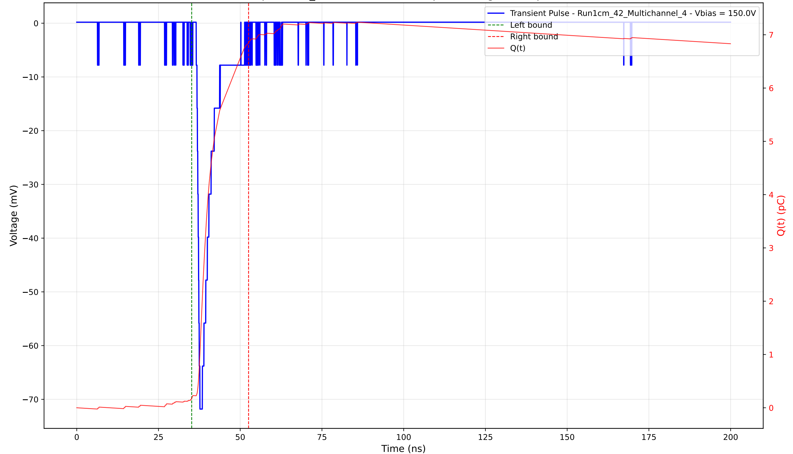
Transient Pulse - Sample: 1cm_42 - Position: 1515.0 \mu\text{m} - Charge: 6.67 pC - Rise Time: 1.12 ns
