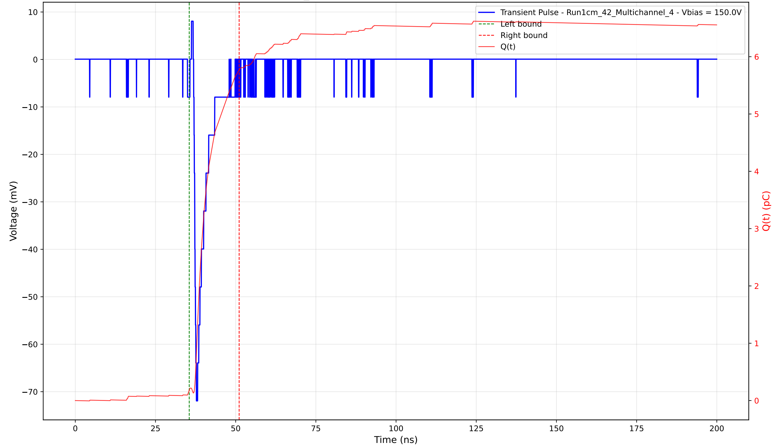
Transient Pulse - Sample: 1cm_42 - Position: 3530.0 \mu\text{m} - Charge: 5.59 pC - Rise Time: 0.84 ns
