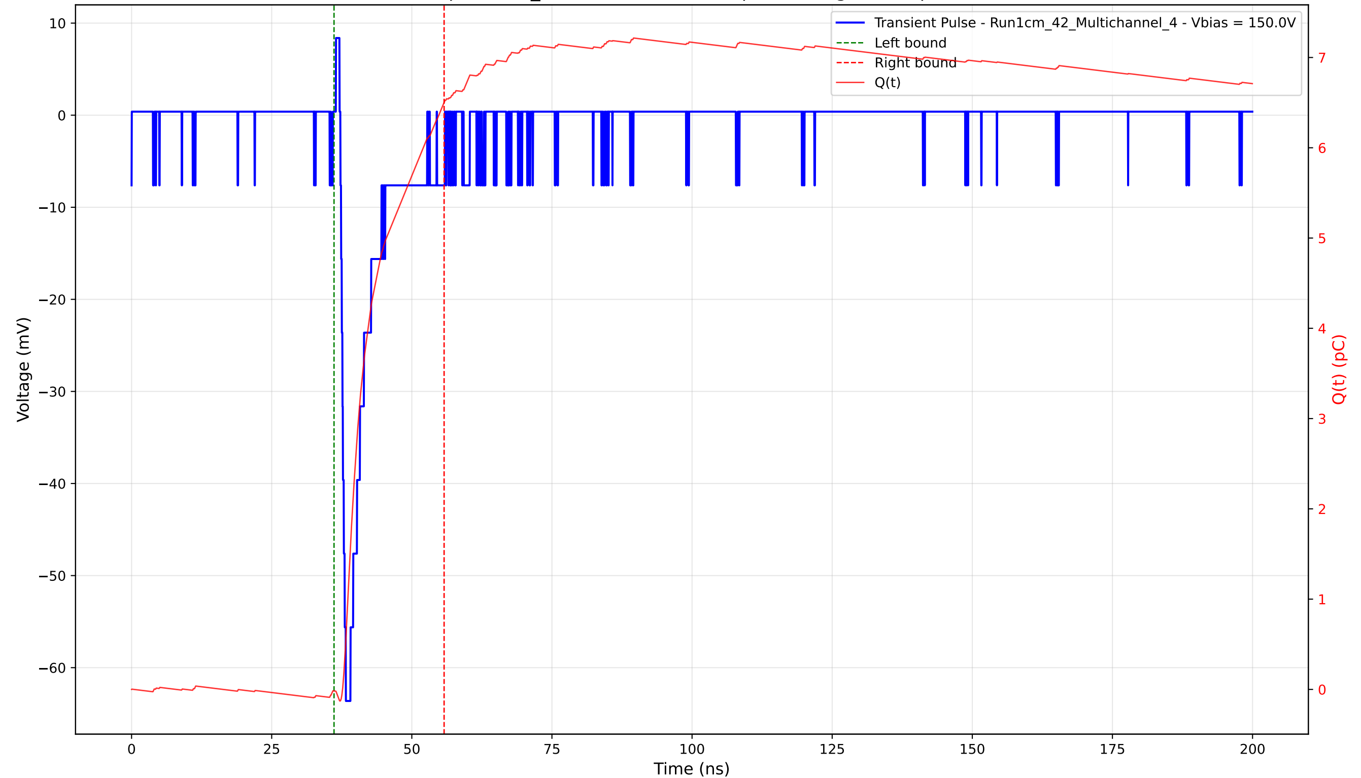
Transient Pulse - Sample: 1cm_42 - Position: 1220.0 \mu\text{m} - Charge: 6.52 pC - Rise Time: 0.97 ns
