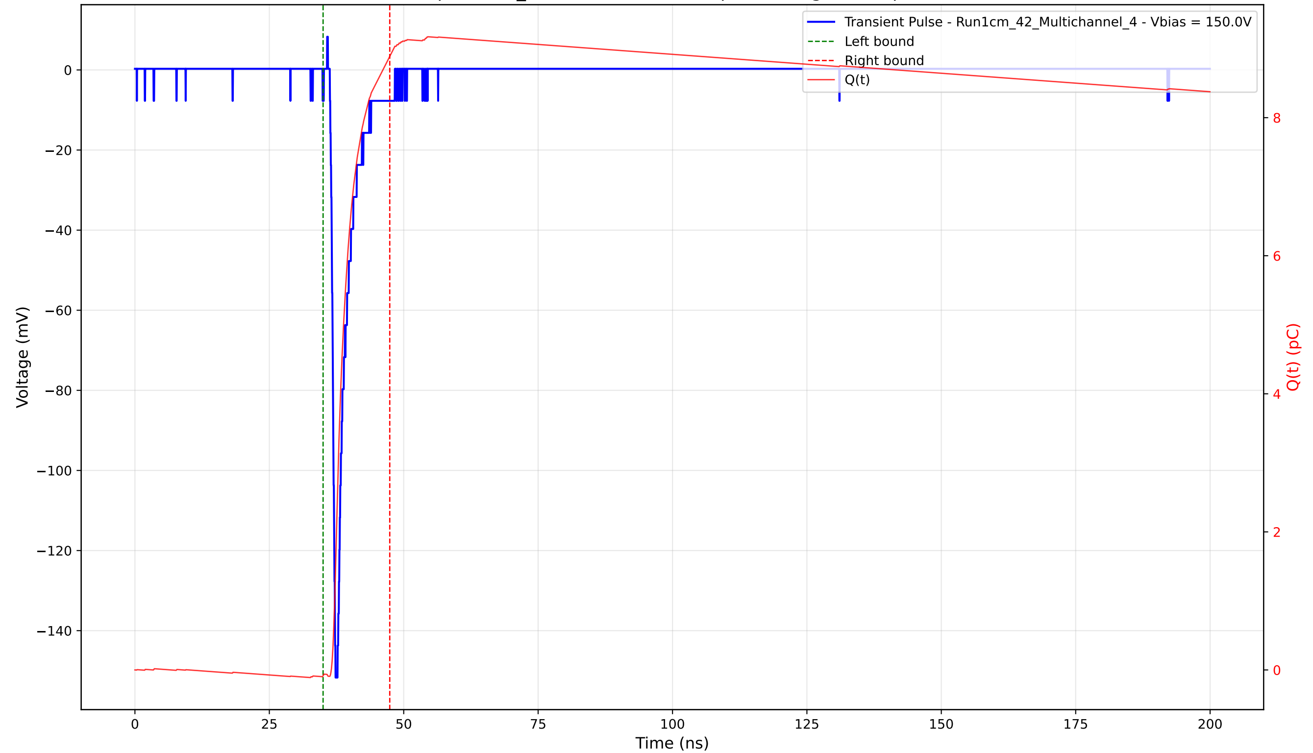
Transient Pulse - Sample: 1cm_42 - Position: 1850.0 \mu\text{m} - Charge: 8.97 pC - Rise Time: 0.88 ns
