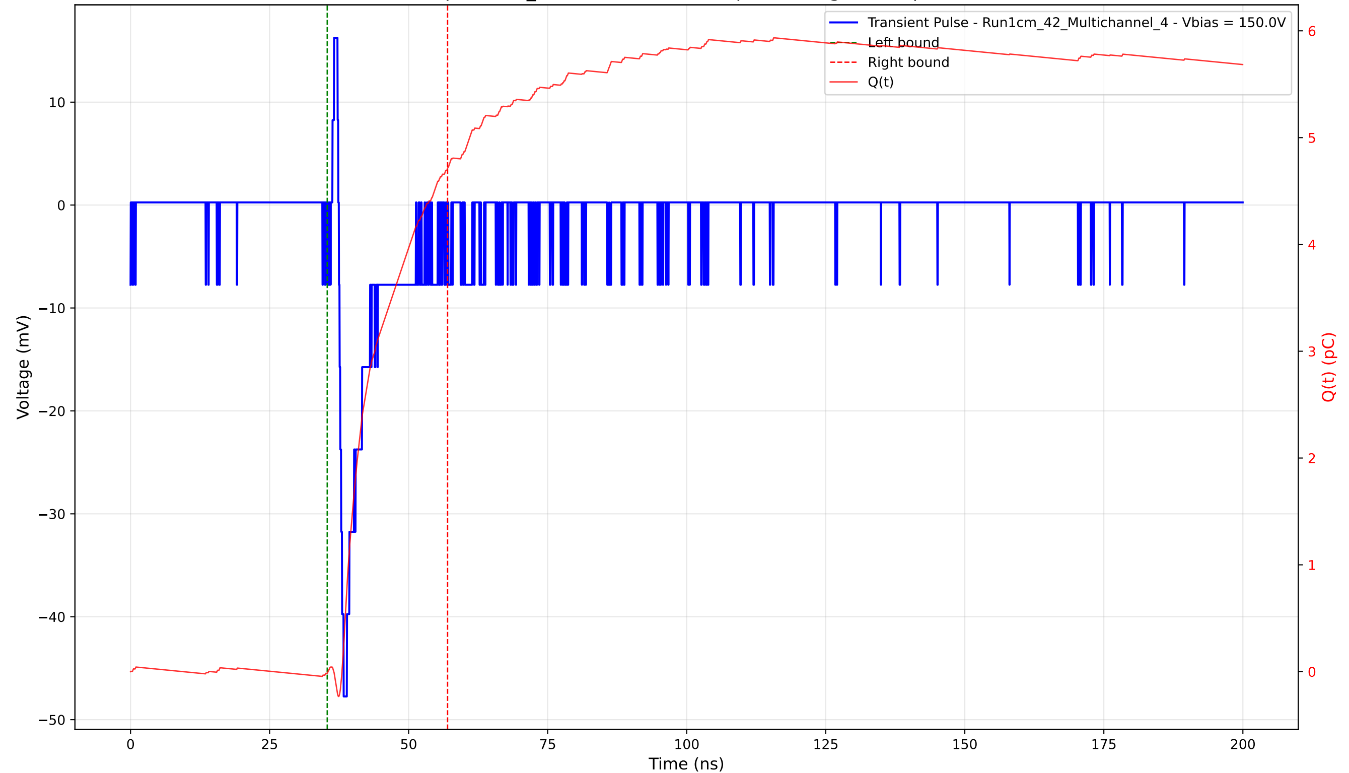
Transient Pulse - Sample: 1cm_42 - Position: 3945.0 \mu\text{m} - Charge: 4.73 pC - Rise Time: 0.86 ns
