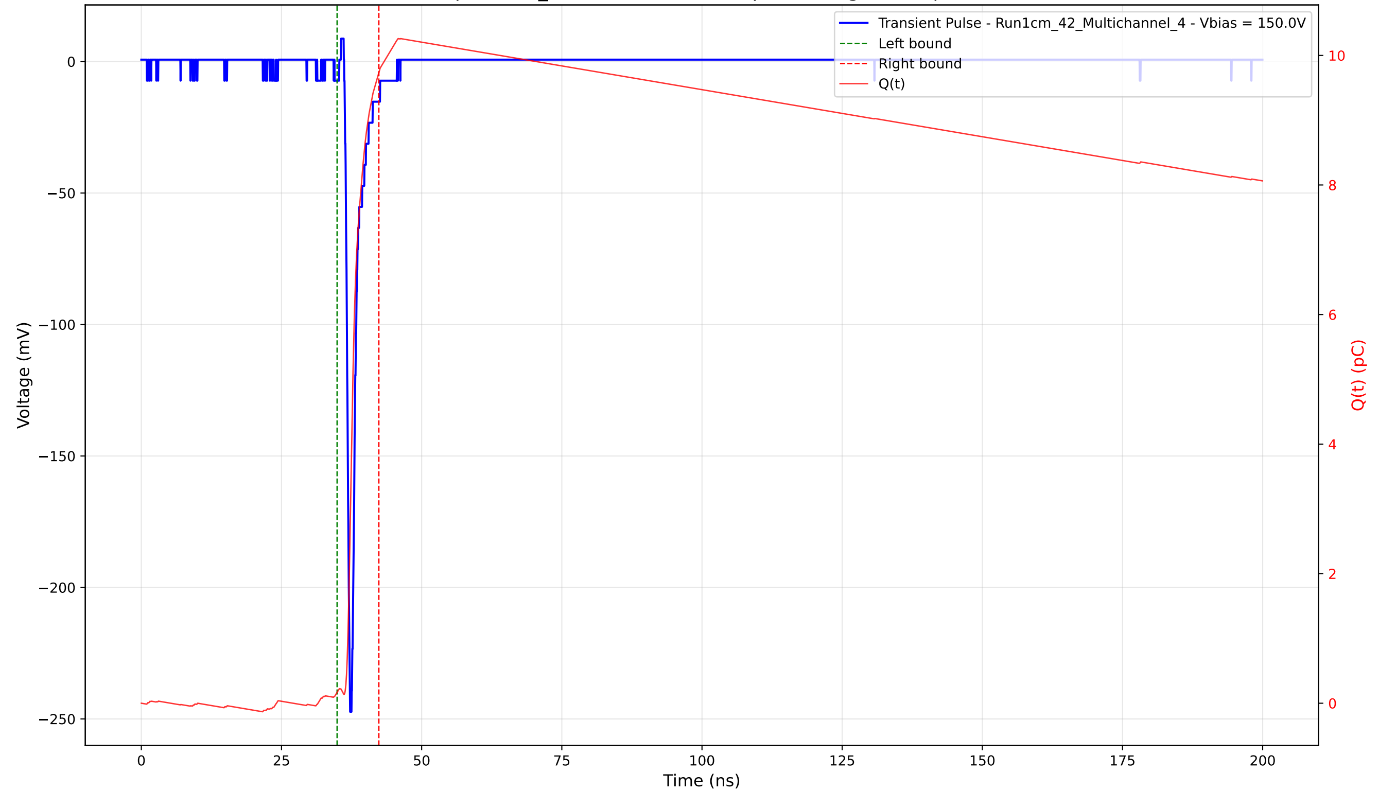
Transient Pulse - Sample: 1cm_42 - Position: 2985.0 \mu\text{m} - Charge: 9.56 pC - Rise Time: 0.79 ns
