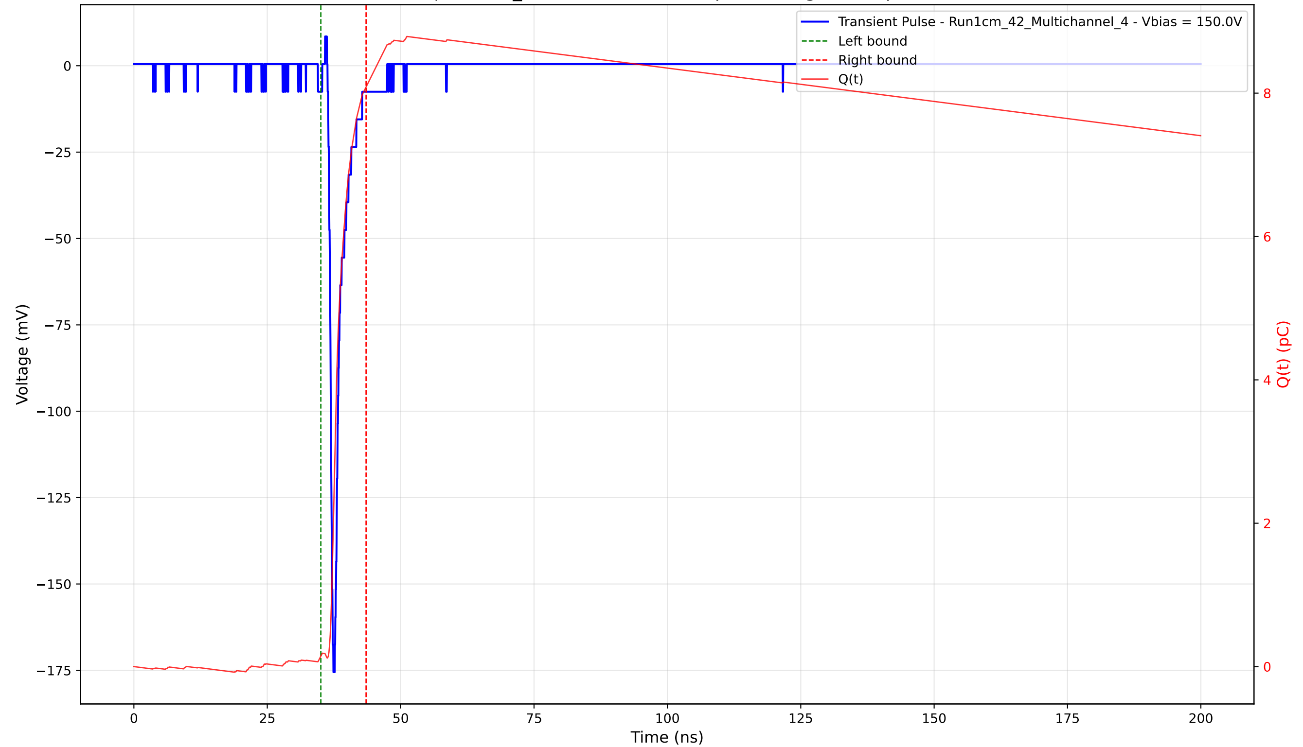
Transient Pulse - Sample: 1cm_42 - Position: 3110.0 \mu\text{m} - Charge: 7.94 pC - Rise Time: 0.78 ns
