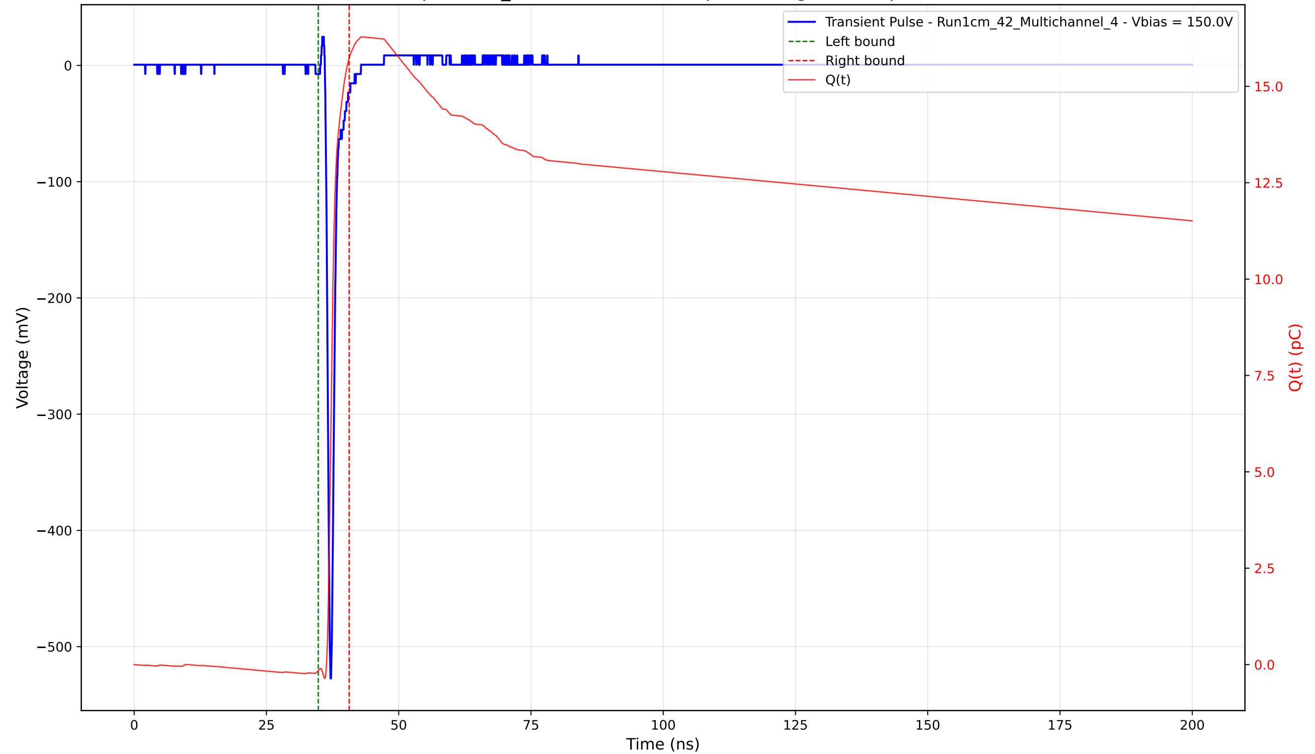
Transient Pulse - Sample: 1cm_42 - Position: 2445.0 \mu\text{m} - Charge: 15.89 pC - Rise Time: 0.71 ns
