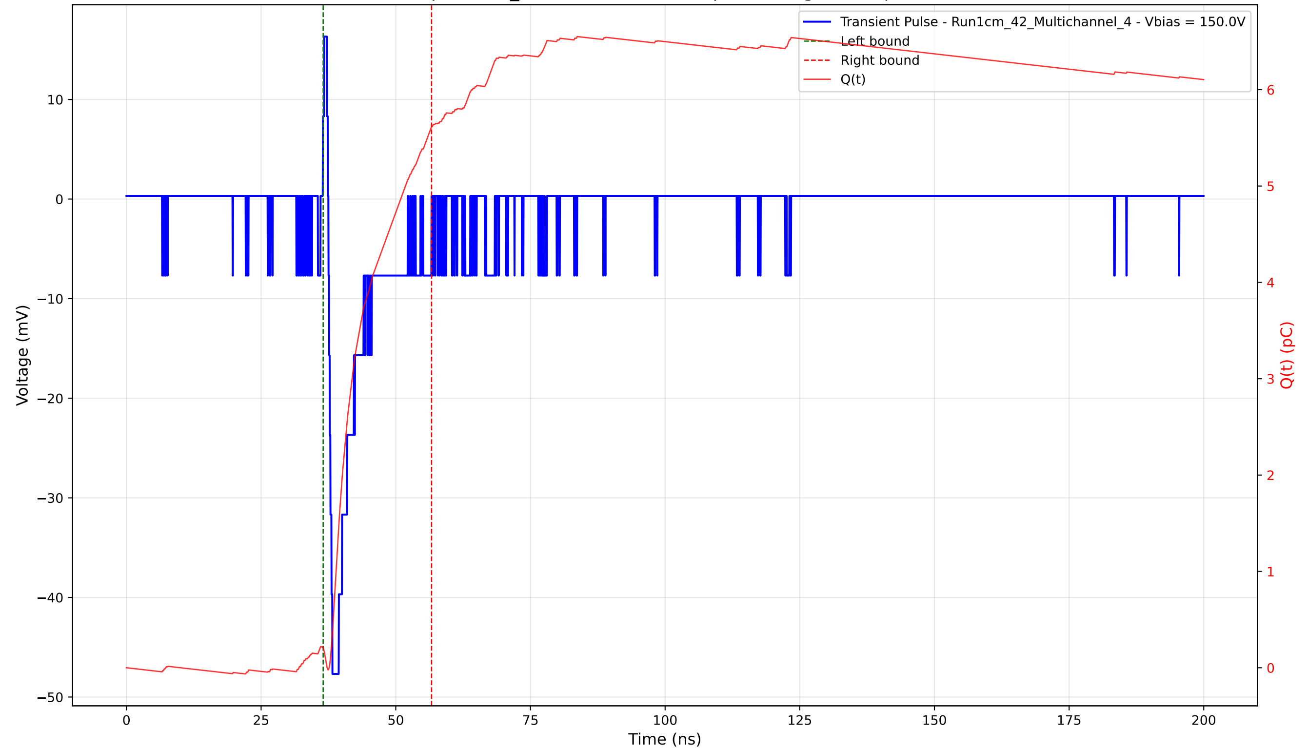
Transient Pulse - Sample: 1cm_42 - Position: 1055.0 \mu\text{m} - Charge: 5.41 pC - Rise Time: 0.74 ns
