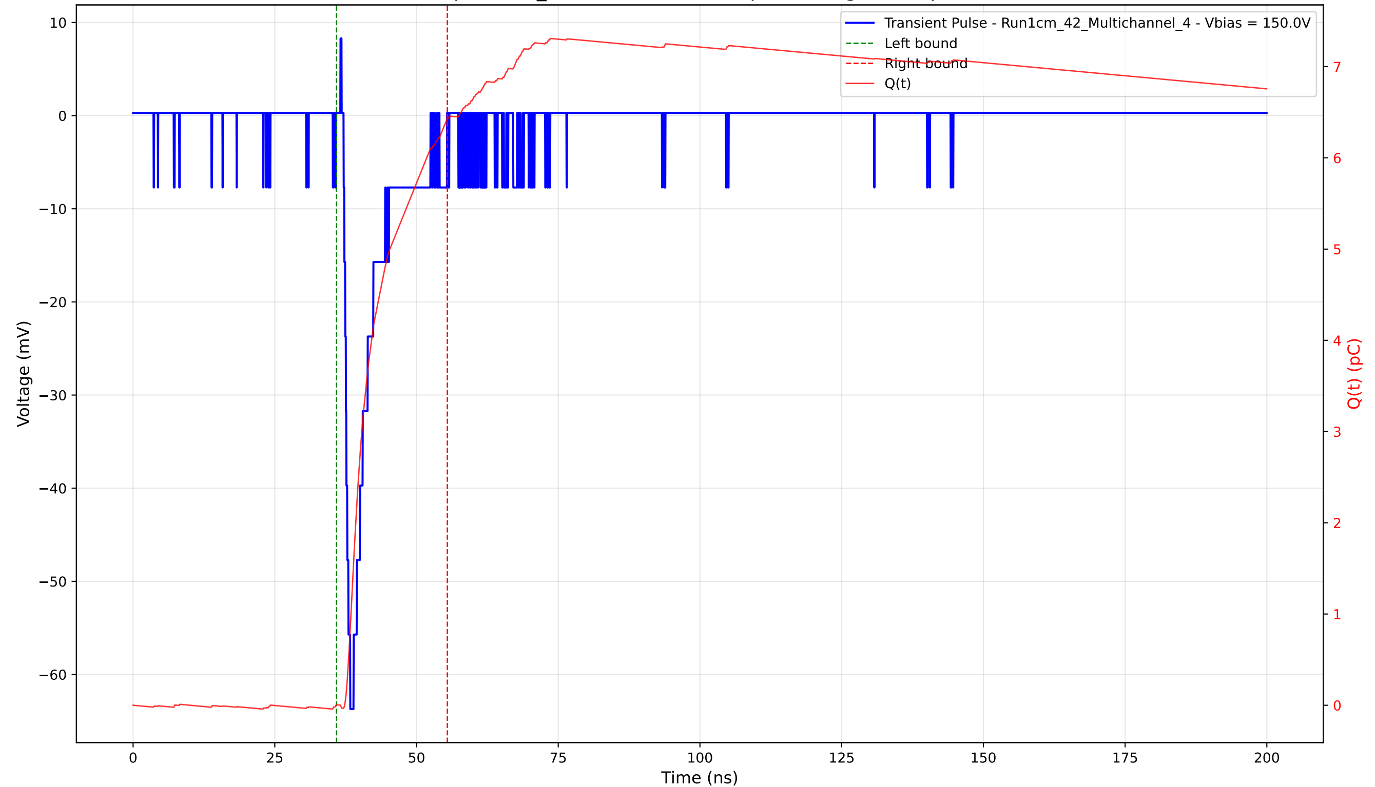
Transient Pulse - Sample: 1cm_42 - Position: 1340.0 \mu\text{m} - Charge: 6.42 pC - Rise Time: 1.17 ns
