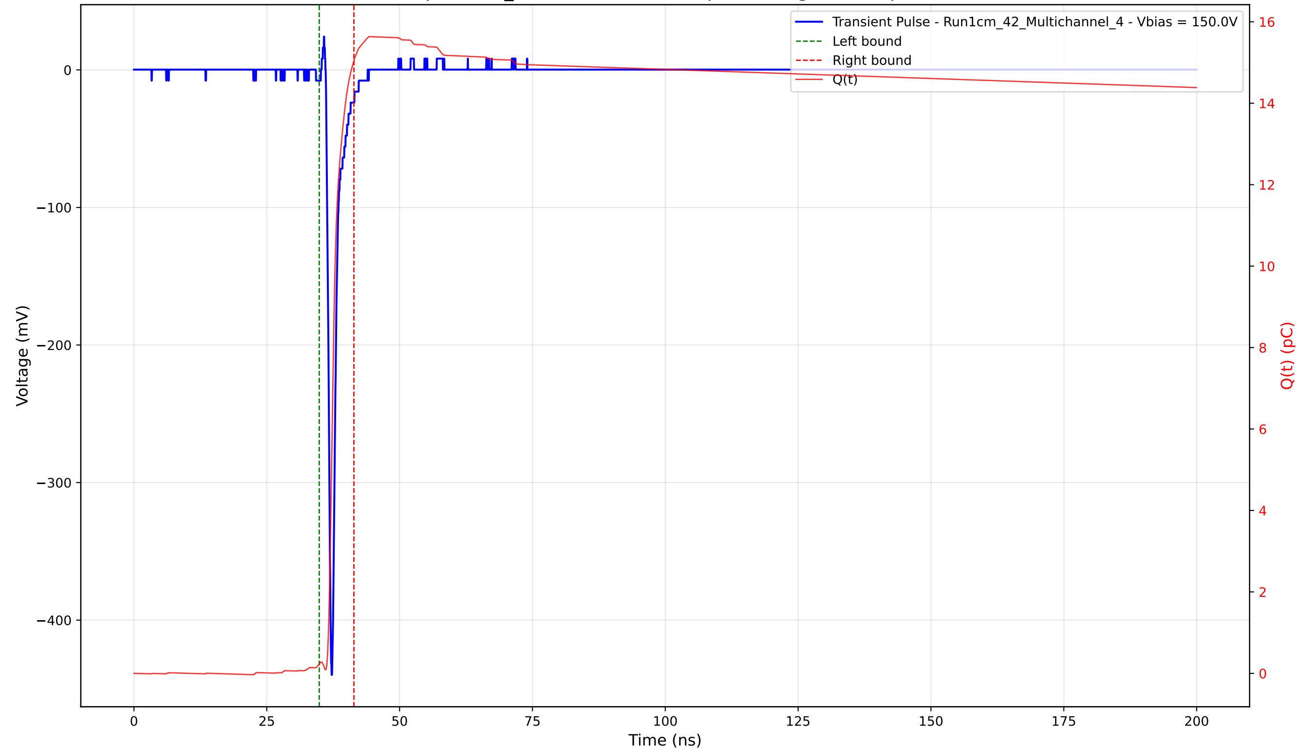
Transient Pulse - Sample: 1cm_42 - Position: 2185.0 \mu\text{m} - Charge: 14.82 pC - Rise Time: 0.74 ns
