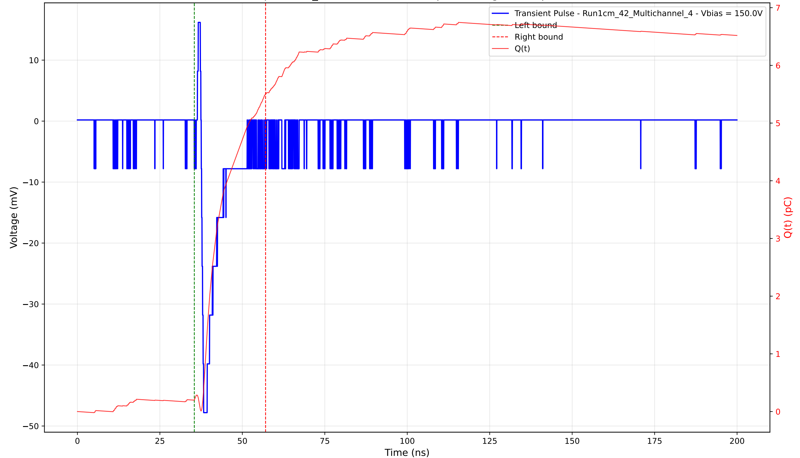
Transient Pulse - Sample: 1cm_42 - Position: 1030.0 \mu\text{m} - Charge: 5.31 pC - Rise Time: 0.74 ns
