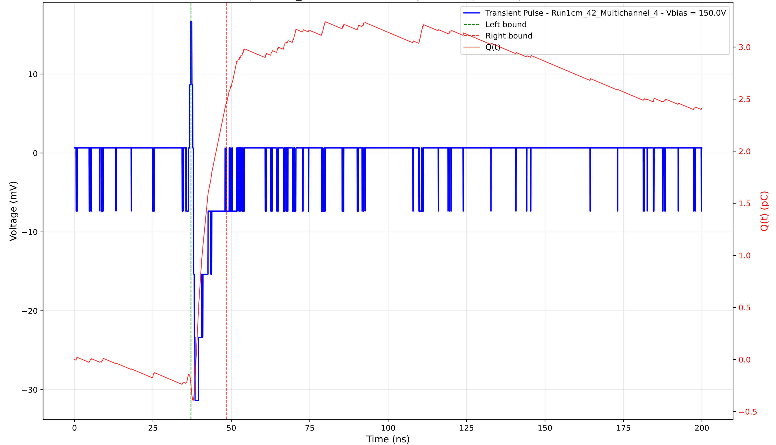
Transient Pulse - Sample: 1cm_42 - Position: 4820.0 \mu\text{m} - Charge: 2.70 pC - Rise Time: 0.59 ns
