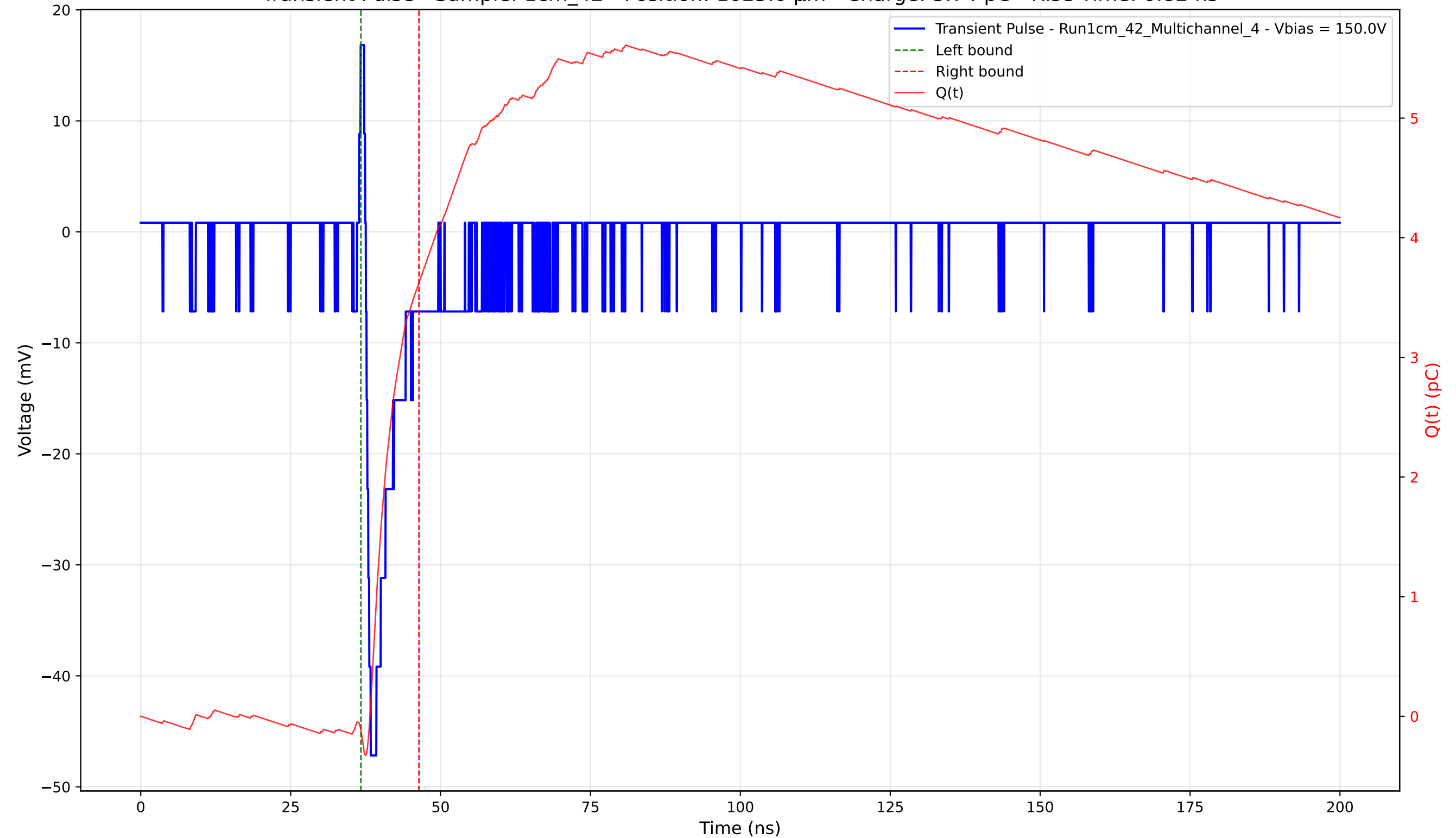
Transient Pulse - Sample: 1cm_42 - Position: 1025.0 \mu\text{m} - Charge: 3.74 pC - Rise Time: 0.82 ns
