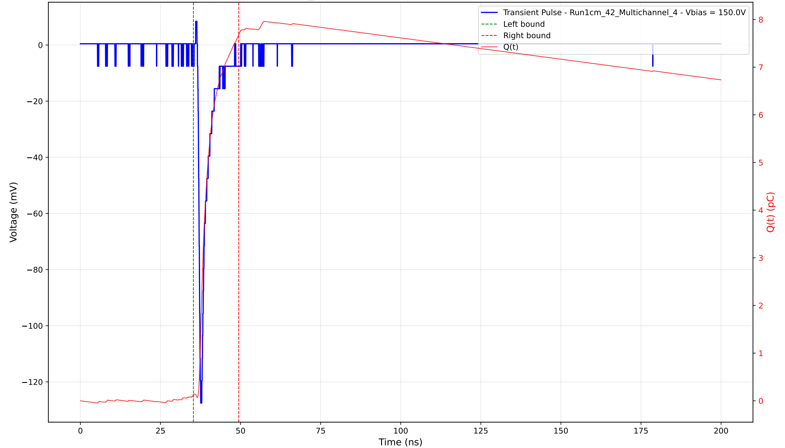
Transient Pulse - Sample: 1cm_42 - Position: 3340.0 \mu\text{m} - Charge: 7.55 pC - Rise Time: 0.77 ns
