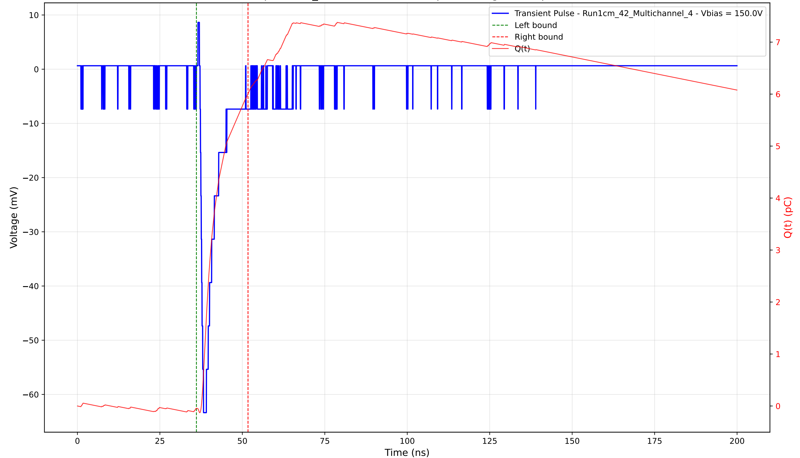
Transient Pulse - Sample: 1cm_42 - Position: 1315.0 \mu\text{m} - Charge: 6.05 pC - Rise Time: 1.05 ns
