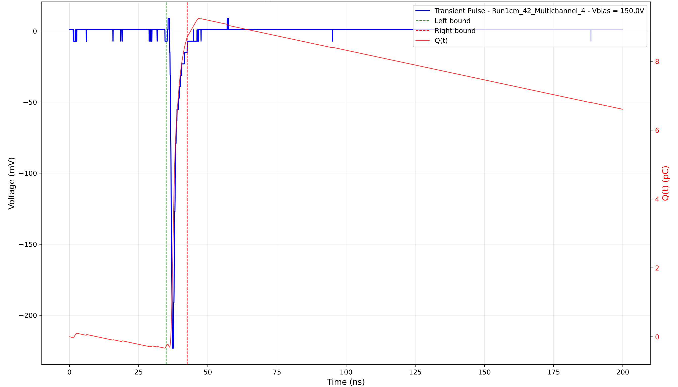
Transient Pulse - Sample: 1cm_42 - Position: 3015.0 \mu\text{m} - Charge: 8.98 pC - Rise Time: 0.77 ns
