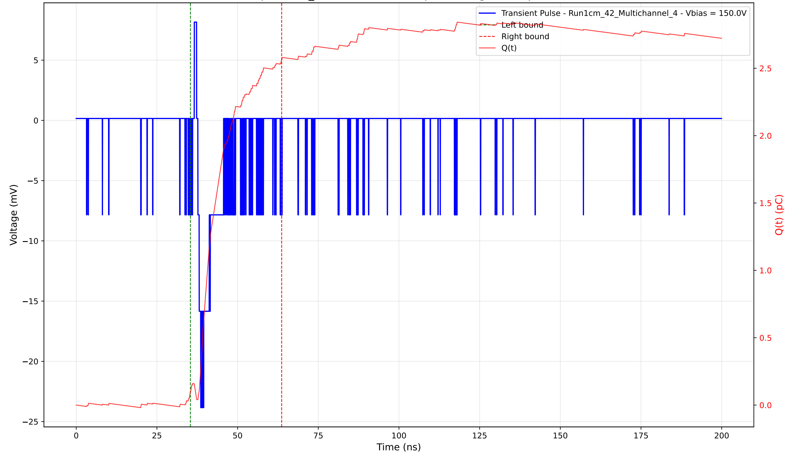
Transient Pulse - Sample: 1cm_42 - Position: 220.0 \mu\text{m} - Charge: 2.46 pC - Rise Time: 0.91 ns
