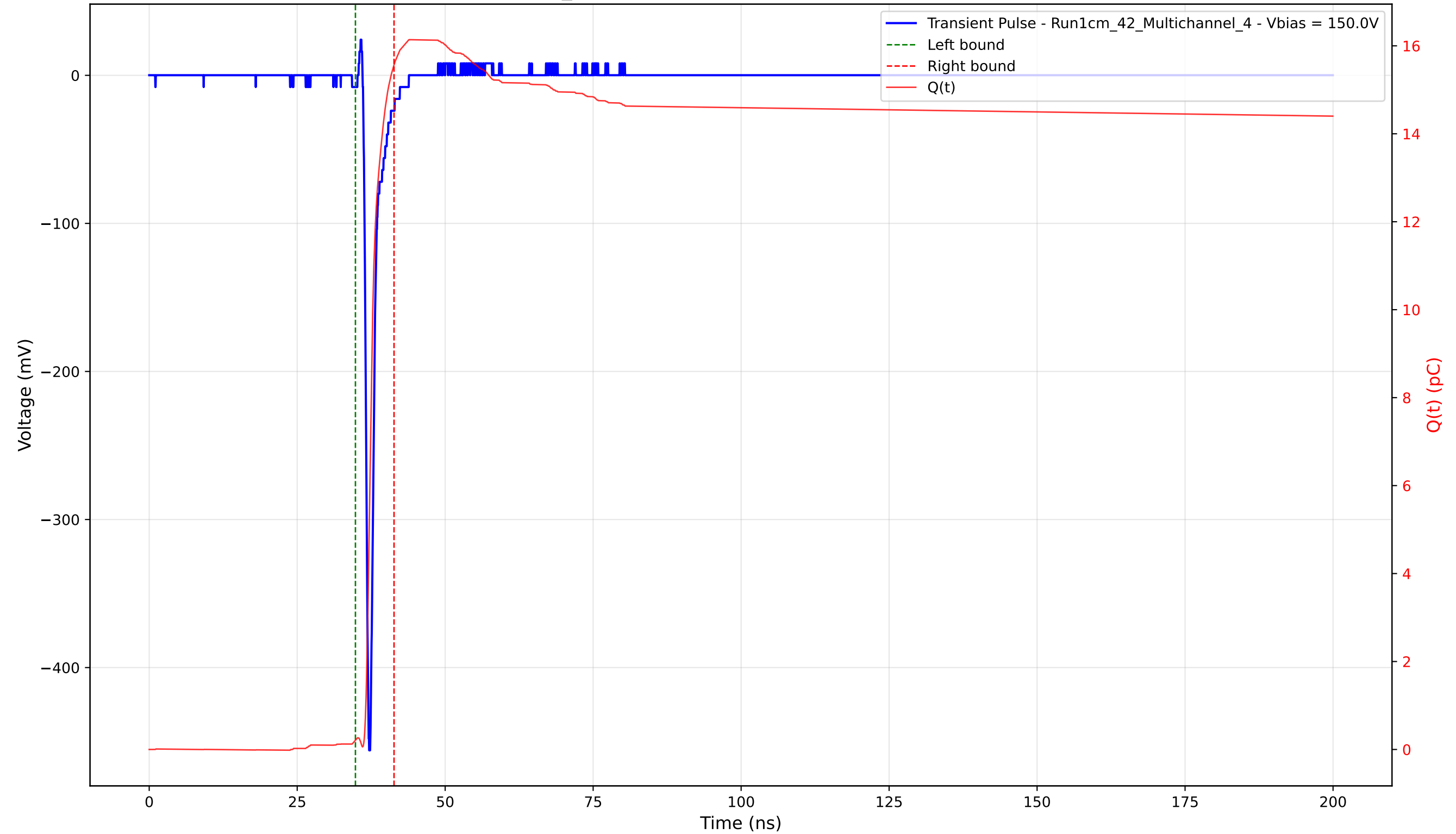
Transient Pulse - Sample: 1cm_42 - Position: 2205.0 \mu\text{m} - Charge: 15.36 pC - Rise Time: 0.70 ns
