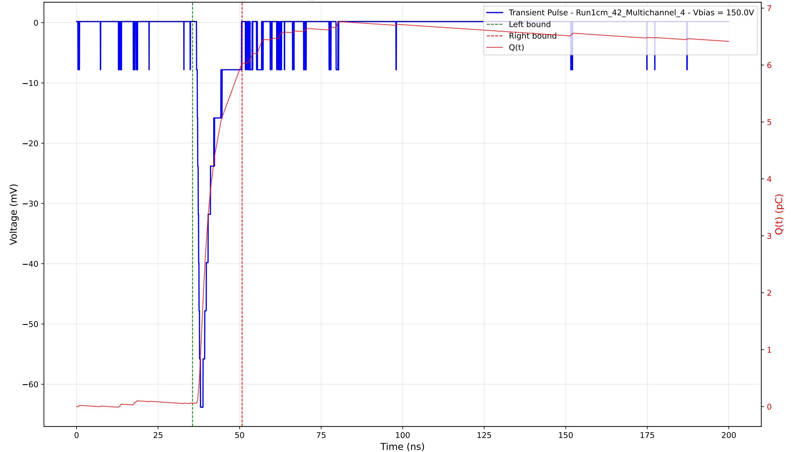
Transient Pulse - Sample: 1cm_42 - Position: 1435.0 \mu\text{m} - Charge: 5.97 pC - Rise Time: 1.21 ns
