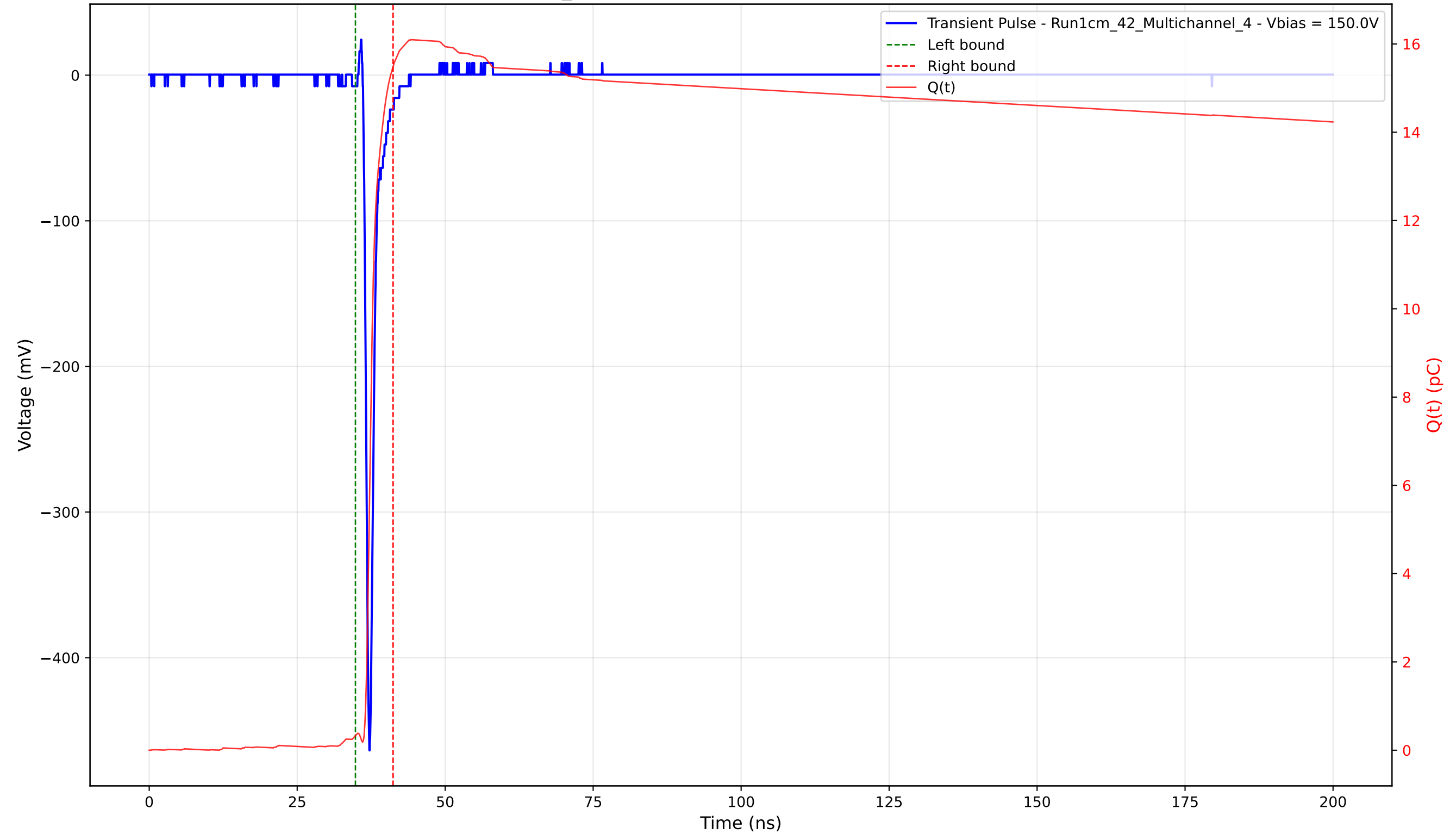
Transient Pulse - Sample: 1cm_42 - Position: 2805.0 \mu\text{m} - Charge: 15.16 pC - Rise Time: 0.73 ns
