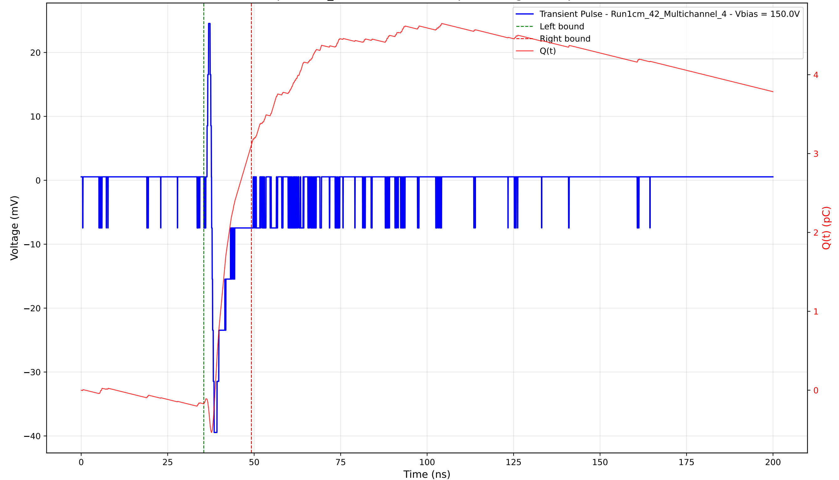
Transient Pulse - Sample: 1cm_42 - Position: 4185.0 \mu\text{m} - Charge: 3.28 pC - Rise Time: 0.74 ns
