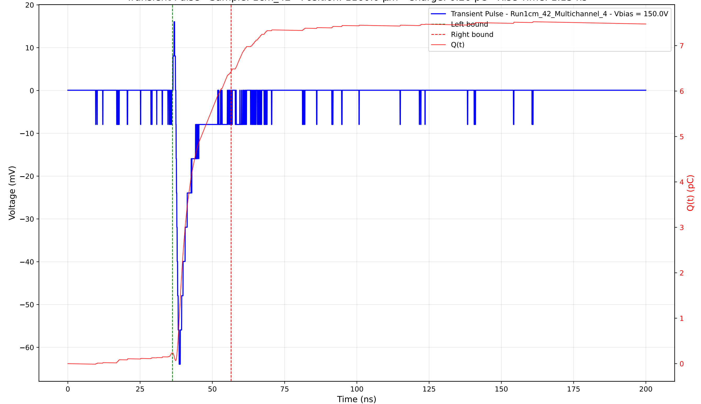
Transient Pulse - Sample: 1cm_42 - Position: 1160.0 \mu\text{m} - Charge: 6.20 pC - Rise Time: 1.13 ns
