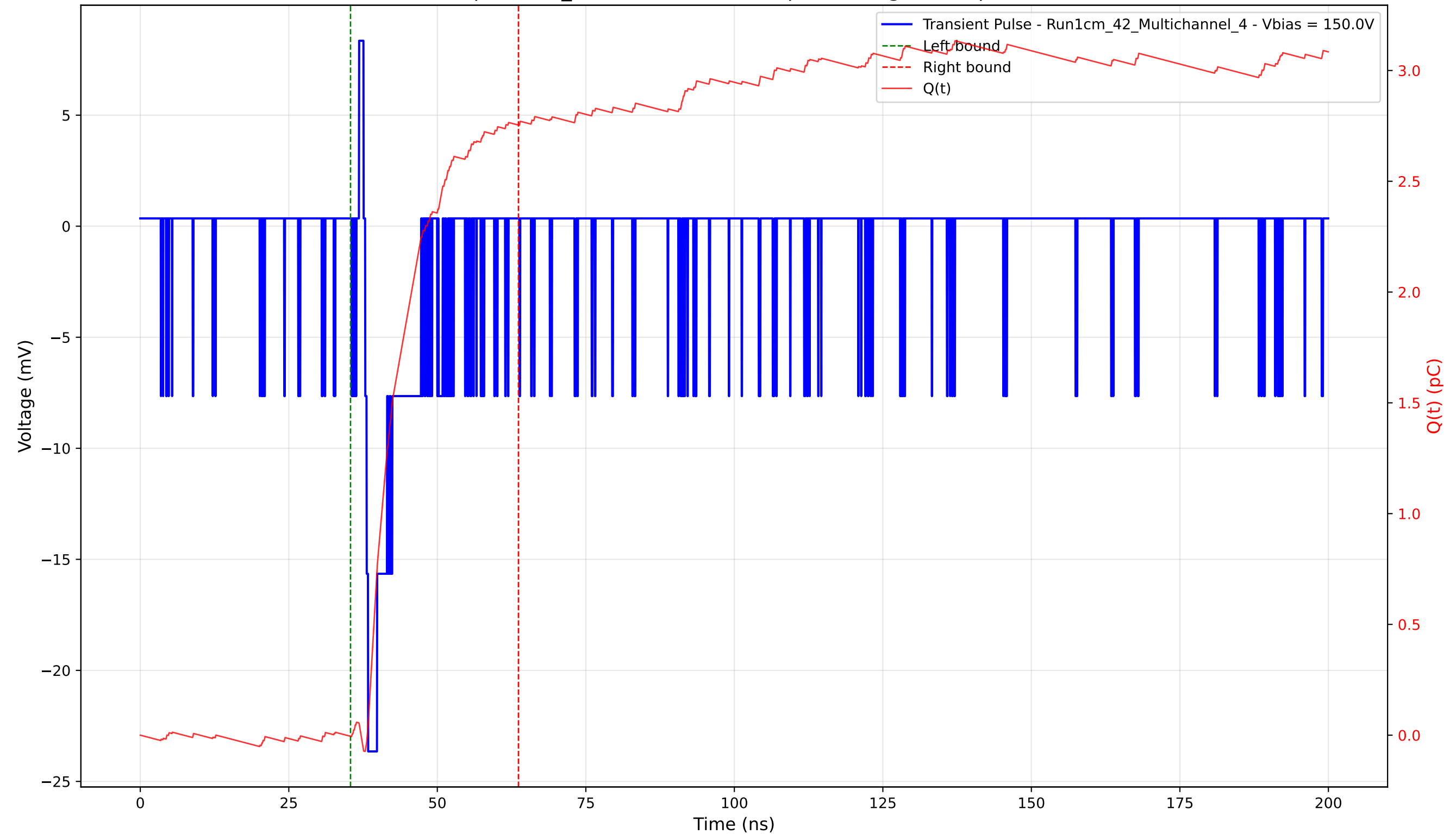
Transient Pulse - Sample: 1cm_42 - Position: 4925.0 \mu\text{m} - Charge: 2.76 pC - Rise Time: 0.51 ns
