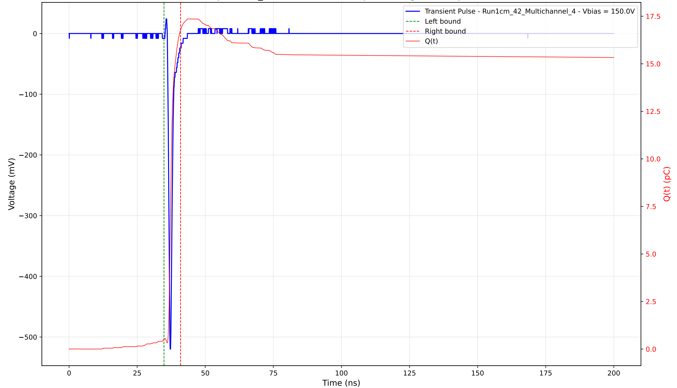
Transient Pulse - Sample: 1cm_42 - Position: 2370.0 \mu\text{m} - Charge: 16.27 pC - Rise Time: 0.72 ns
