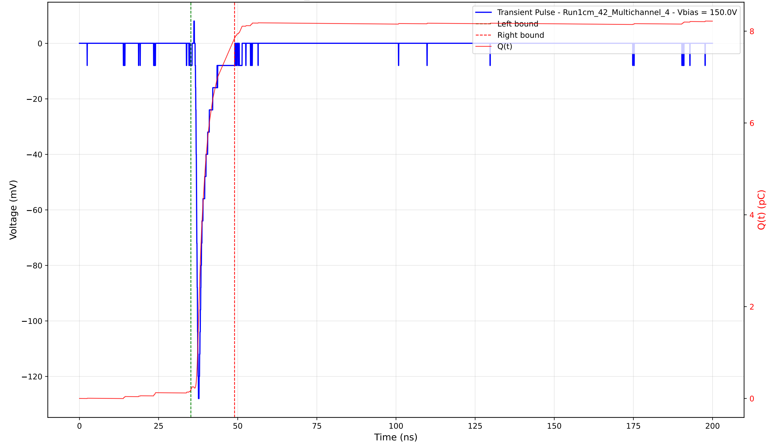
Transient Pulse - Sample: 1cm_42 - Position: 3345.0 \mu\text{m} - Charge: 7.66 pC - Rise Time: 0.82 ns
