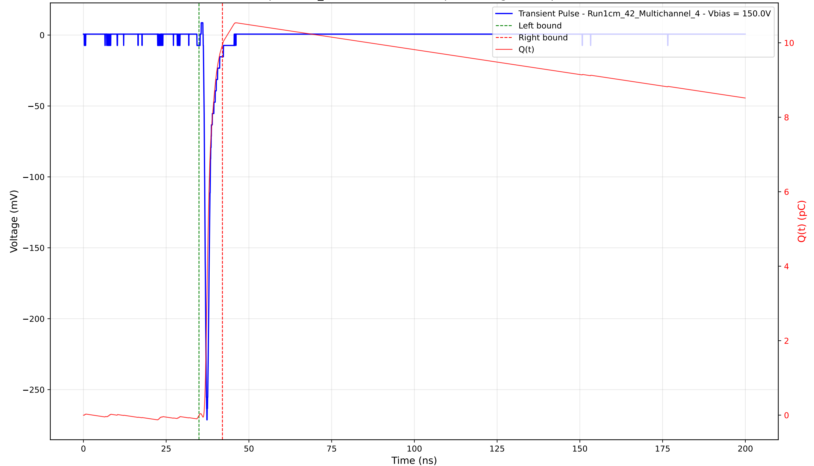
Transient Pulse - Sample: 1cm_42 - Position: 2970.0 \mu\text{m} - Charge: 9.96 pC - Rise Time: 0.77 ns
