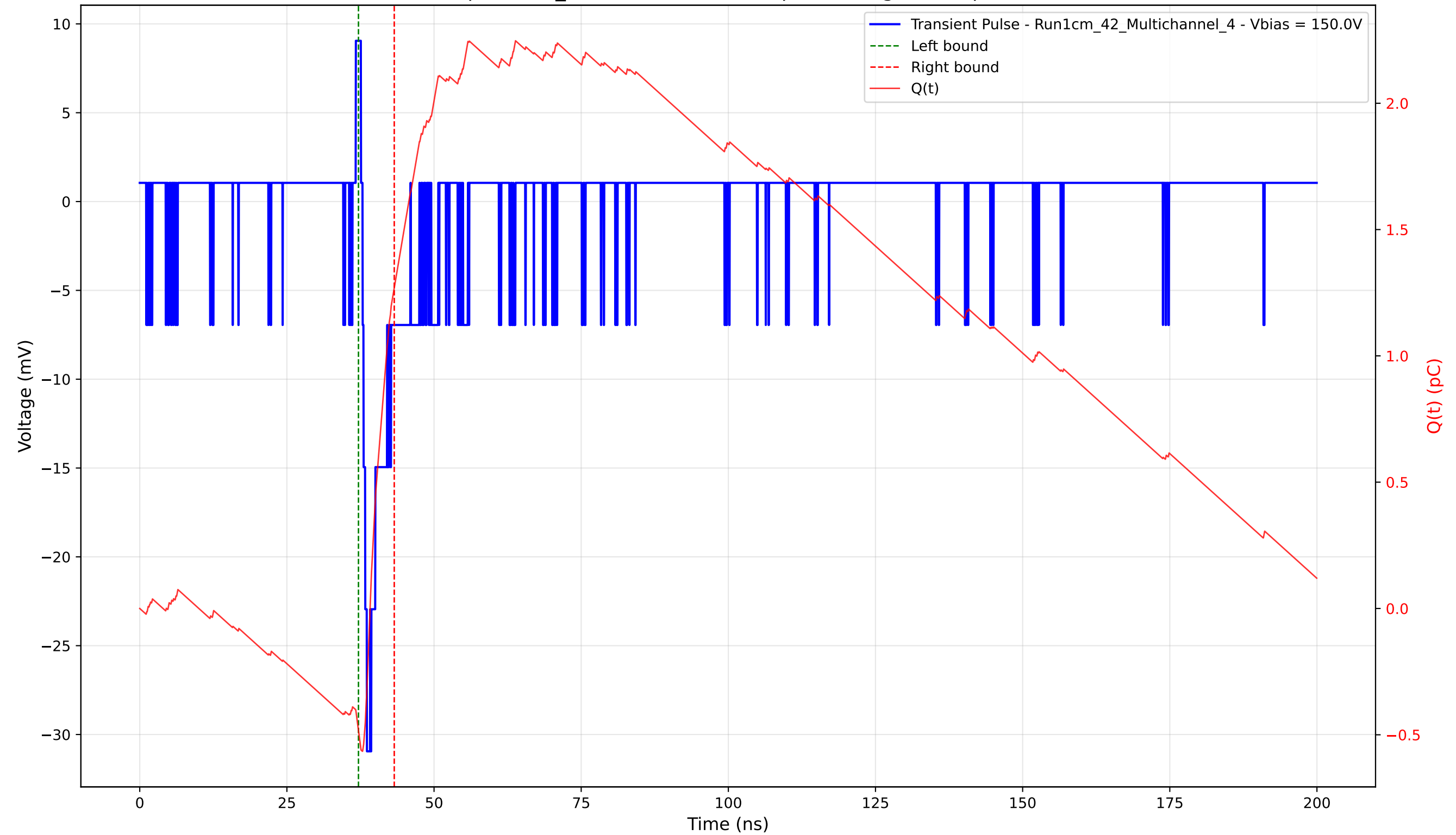
Transient Pulse - Sample: 1cm_42 - Position: 4890.0 \mu\text{m} - Charge: 1.75 pC - Rise Time: 0.75 ns
