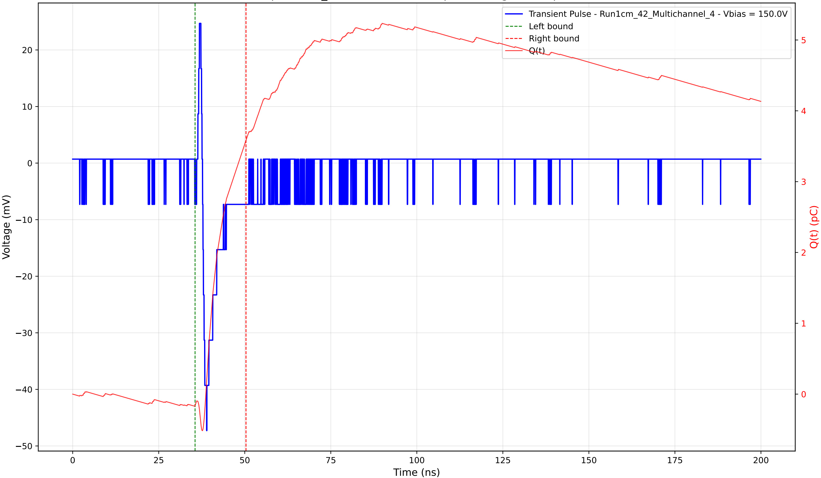
Transient Pulse - Sample: 1cm_42 - Position: 625.0 \mu\text{m} - Charge: 3.74 pC - Rise Time: 1.22 ns
