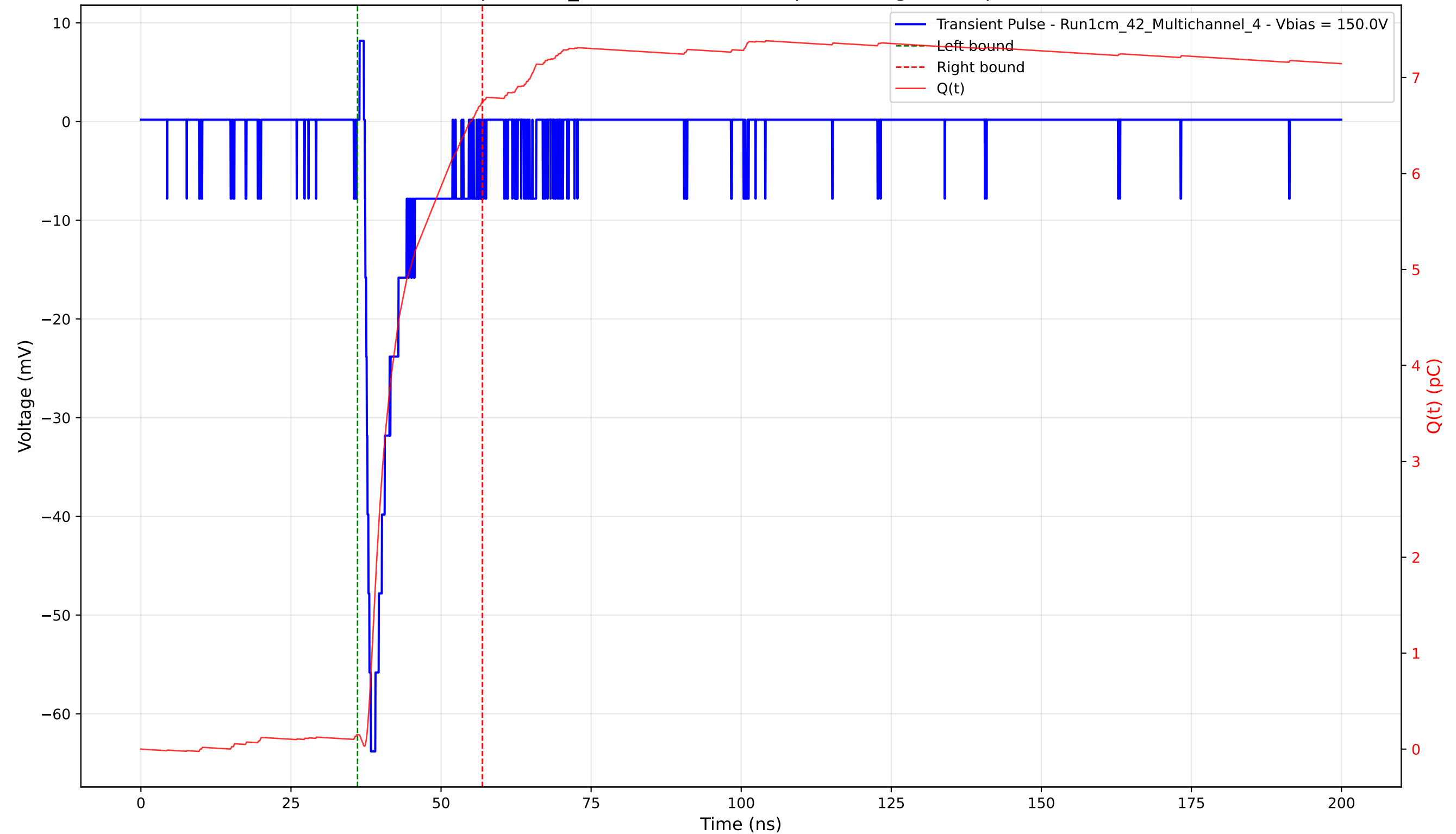
Transient Pulse - Sample: 1cm_42 - Position: 1205.0 \mu\text{m} - Charge: 6.60 pC - Rise Time: 1.01 ns
