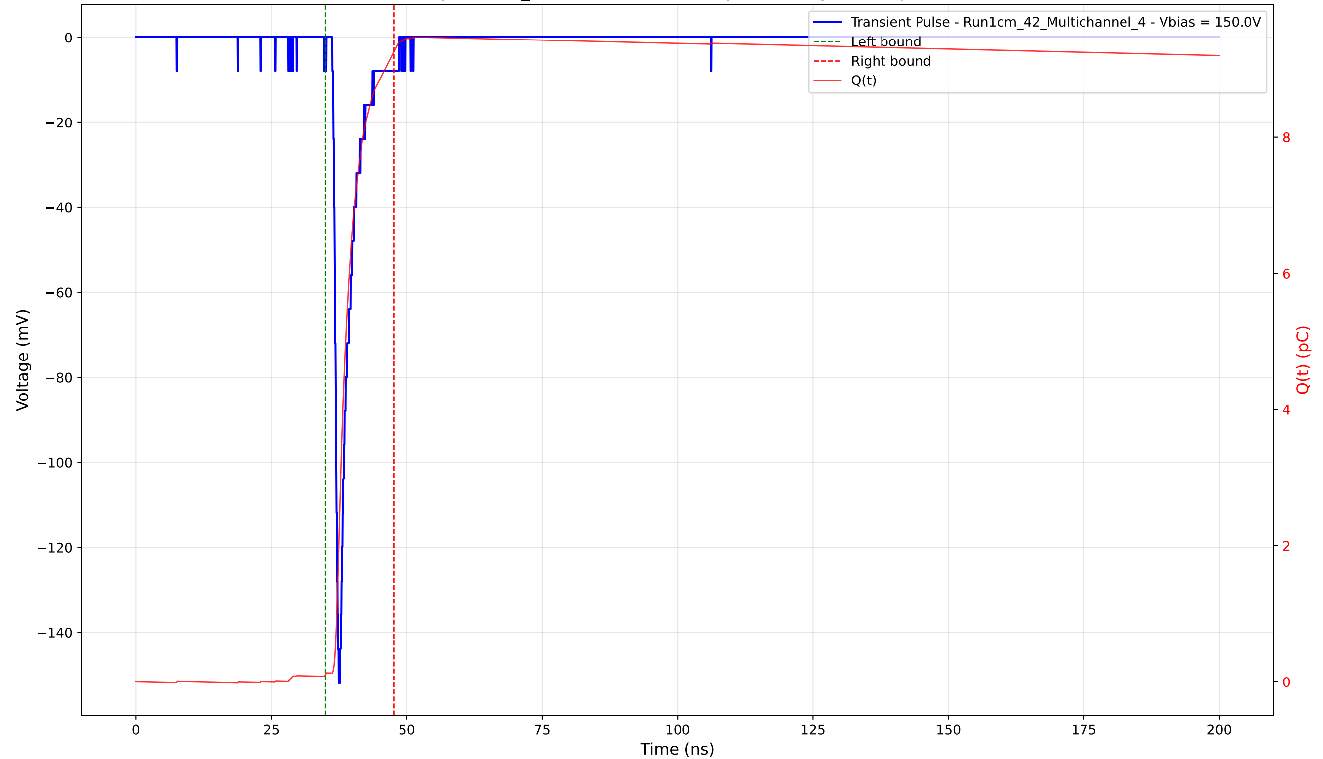
Transient Pulse - Sample: 1cm_42 - Position: 1820.0 \mu\text{m} - Charge: 9.15 pC - Rise Time: 0.92 ns
