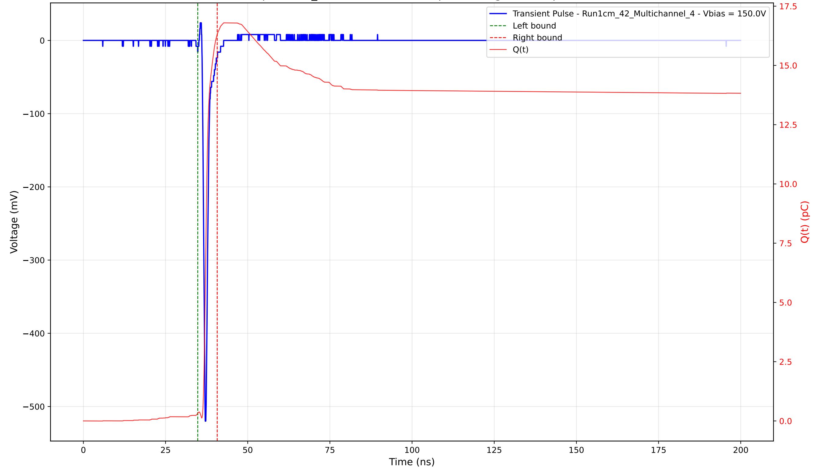
Transient Pulse - Sample: 1cm_42 - Position: 2615.0 \mu\text{m} - Charge: 15.99 pC - Rise Time: 0.70 ns
