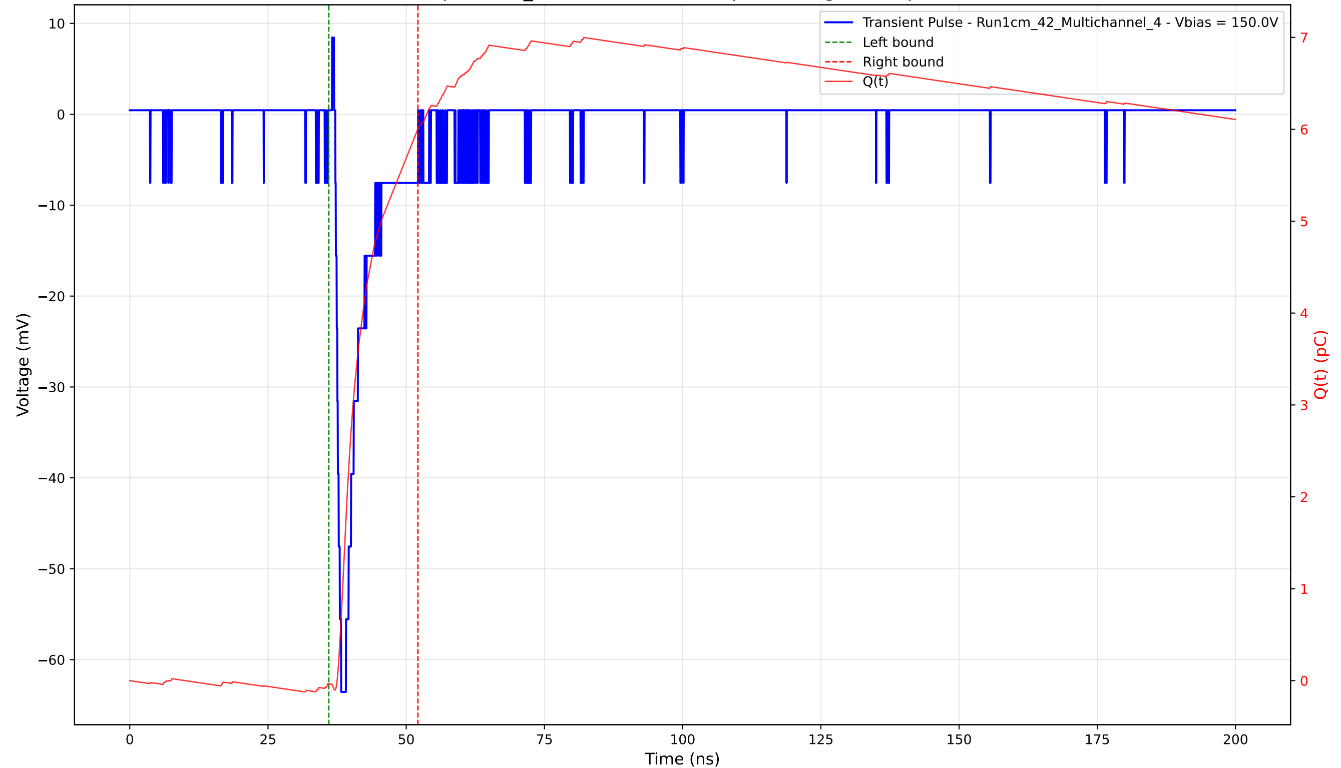
Transient Pulse - Sample: 1cm_42 - Position: 1335.0 \mu\text{m} - Charge: 6.04 pC - Rise Time: 1.05 ns
