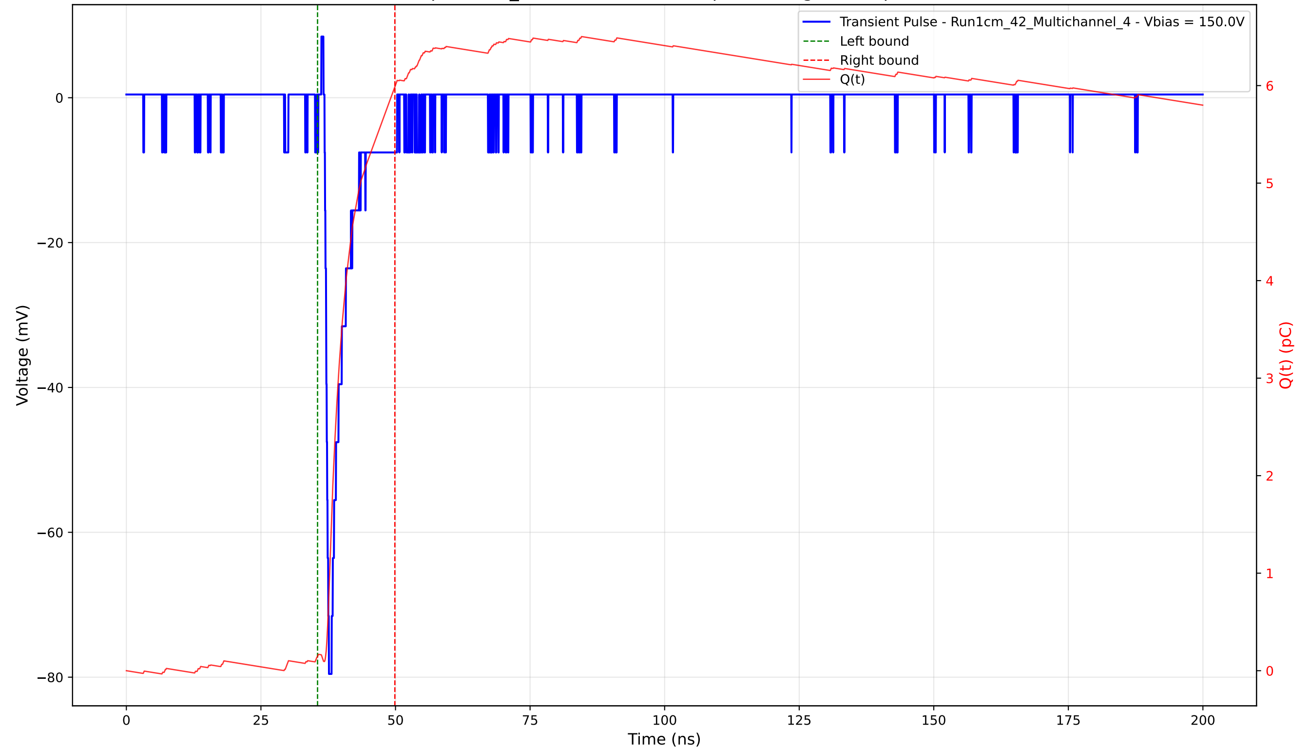
Transient Pulse - Sample: 1cm_42 - Position: 3480.0 \mu\text{m} - Charge: 5.84 pC - Rise Time: 0.76 ns
