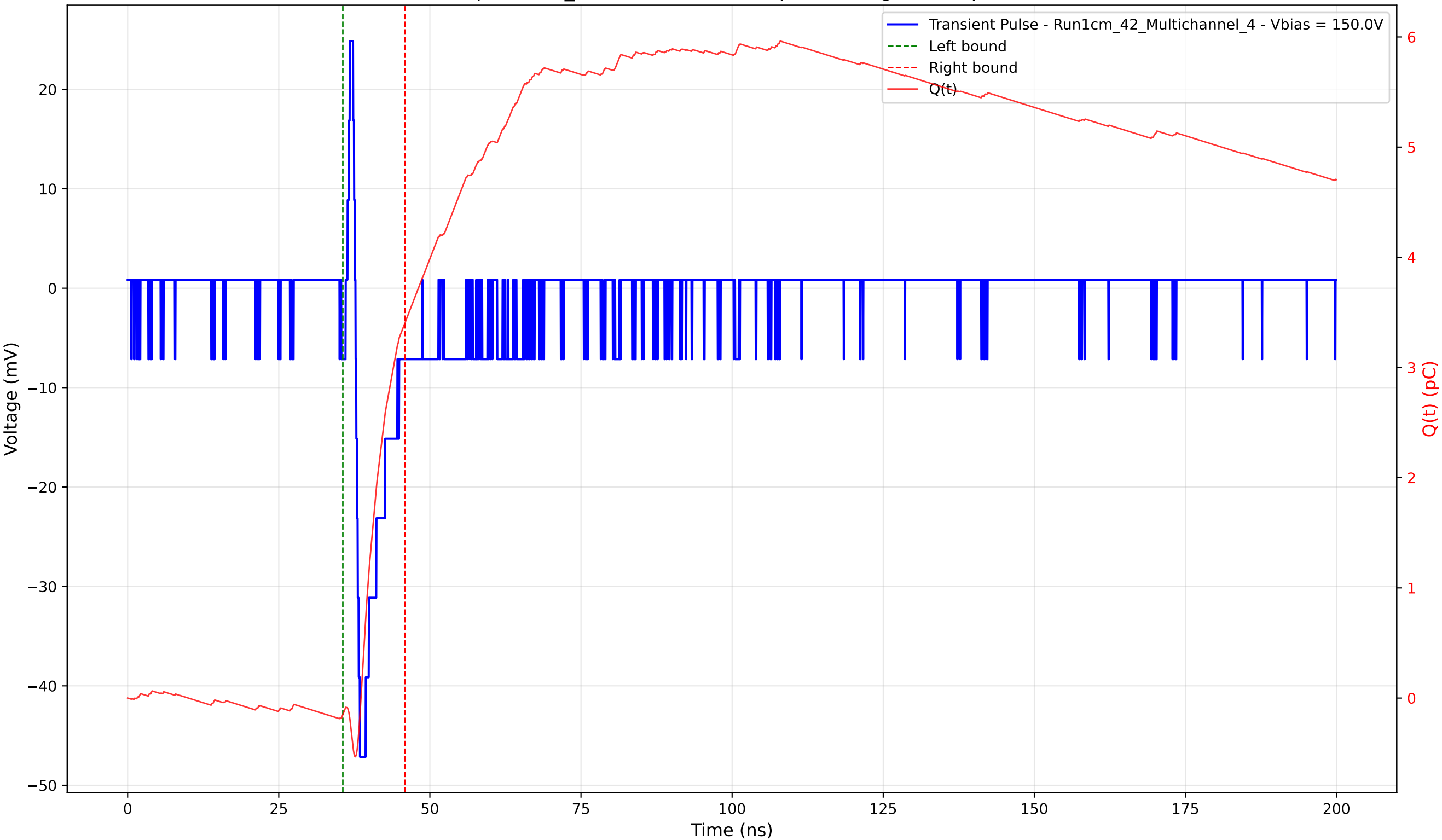
Transient Pulse - Sample: 1cm_42 - Position: 800.0 \mu\text{m} - Charge: 3.55 pC - Rise Time: 0.74 ns
