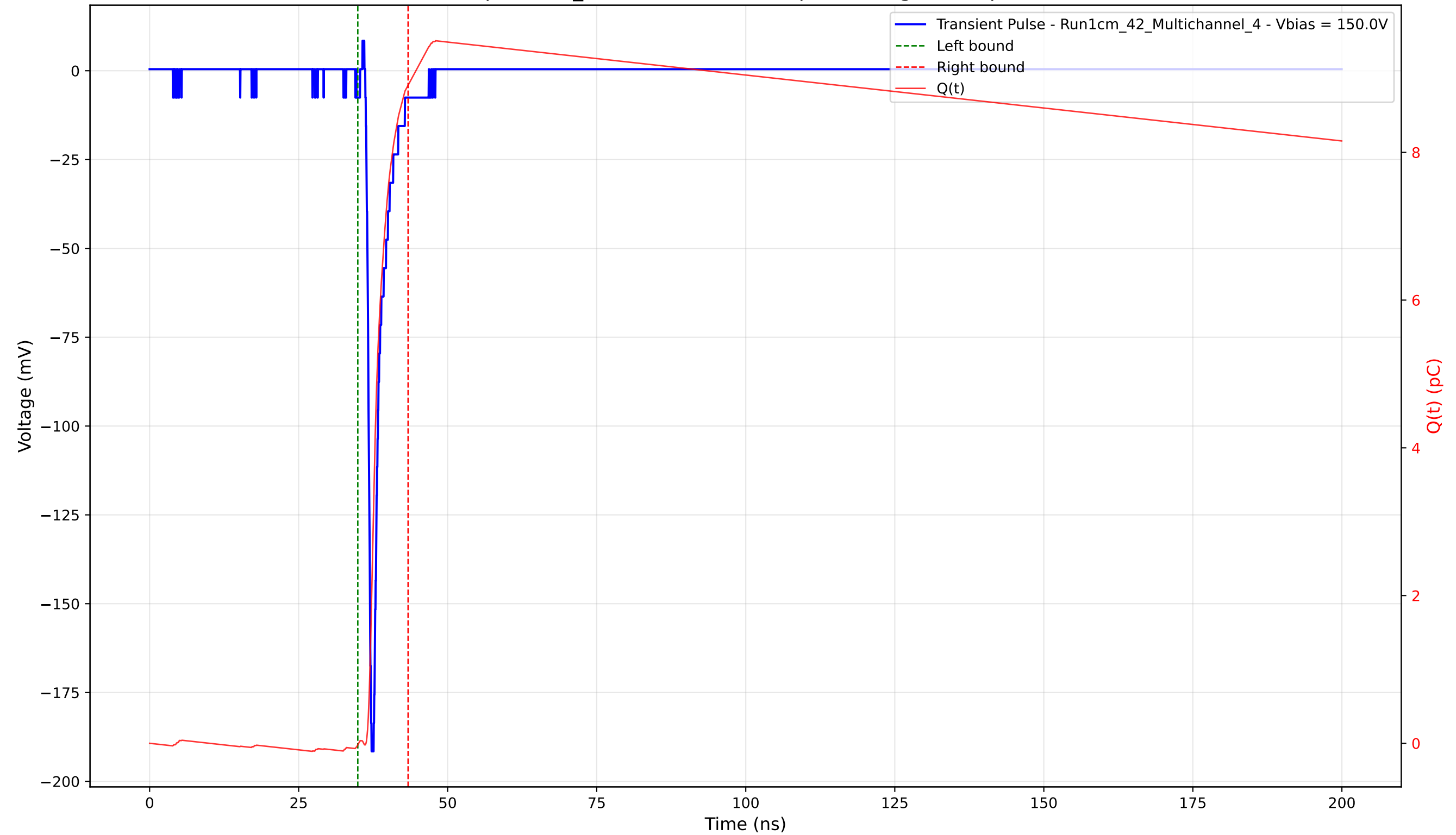
Transient Pulse - Sample: 1cm_42 - Position: 1960.0 \mu\text{m} - Charge: 8.93 pC - Rise Time: 0.77 ns
