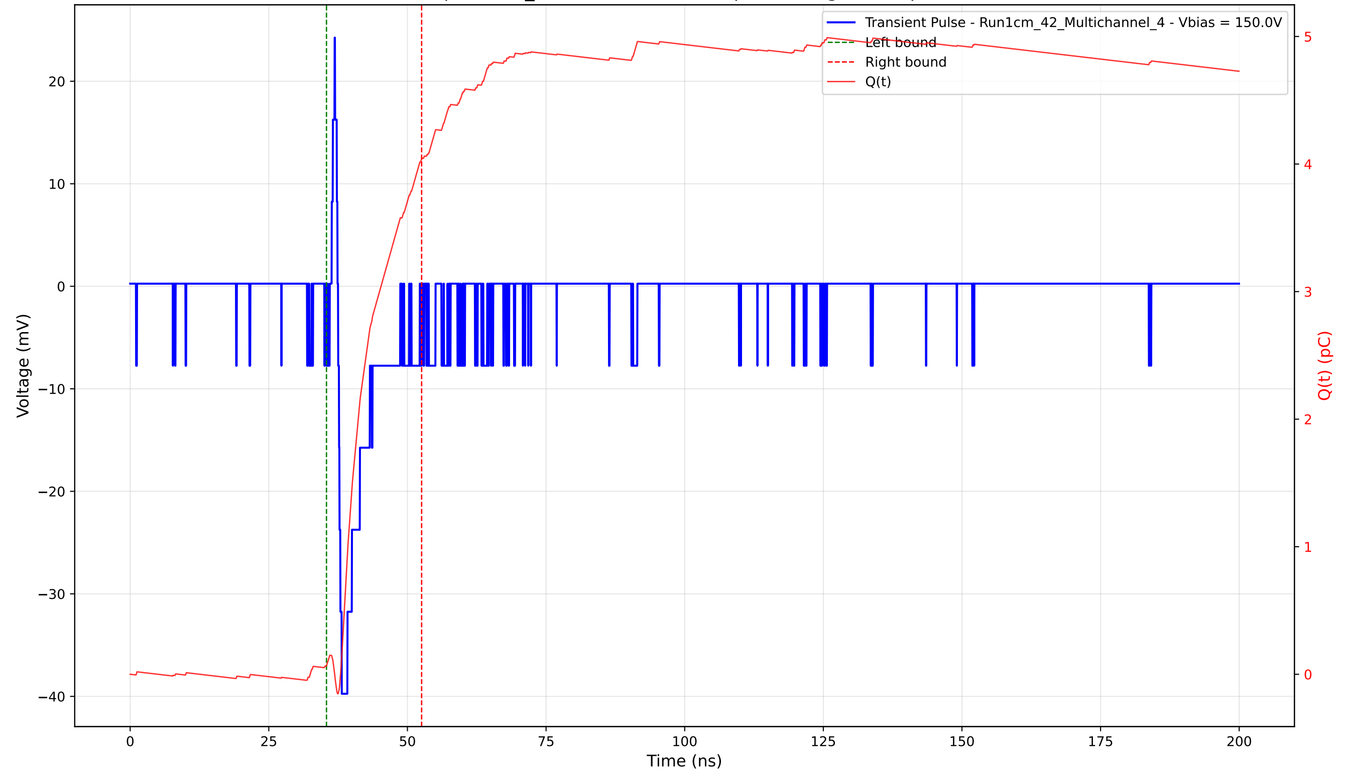
Transient Pulse - Sample: 1cm_42 - Position: 3985.0 \mu\text{m} - Charge: 3.98 pC - Rise Time: 0.66 ns
