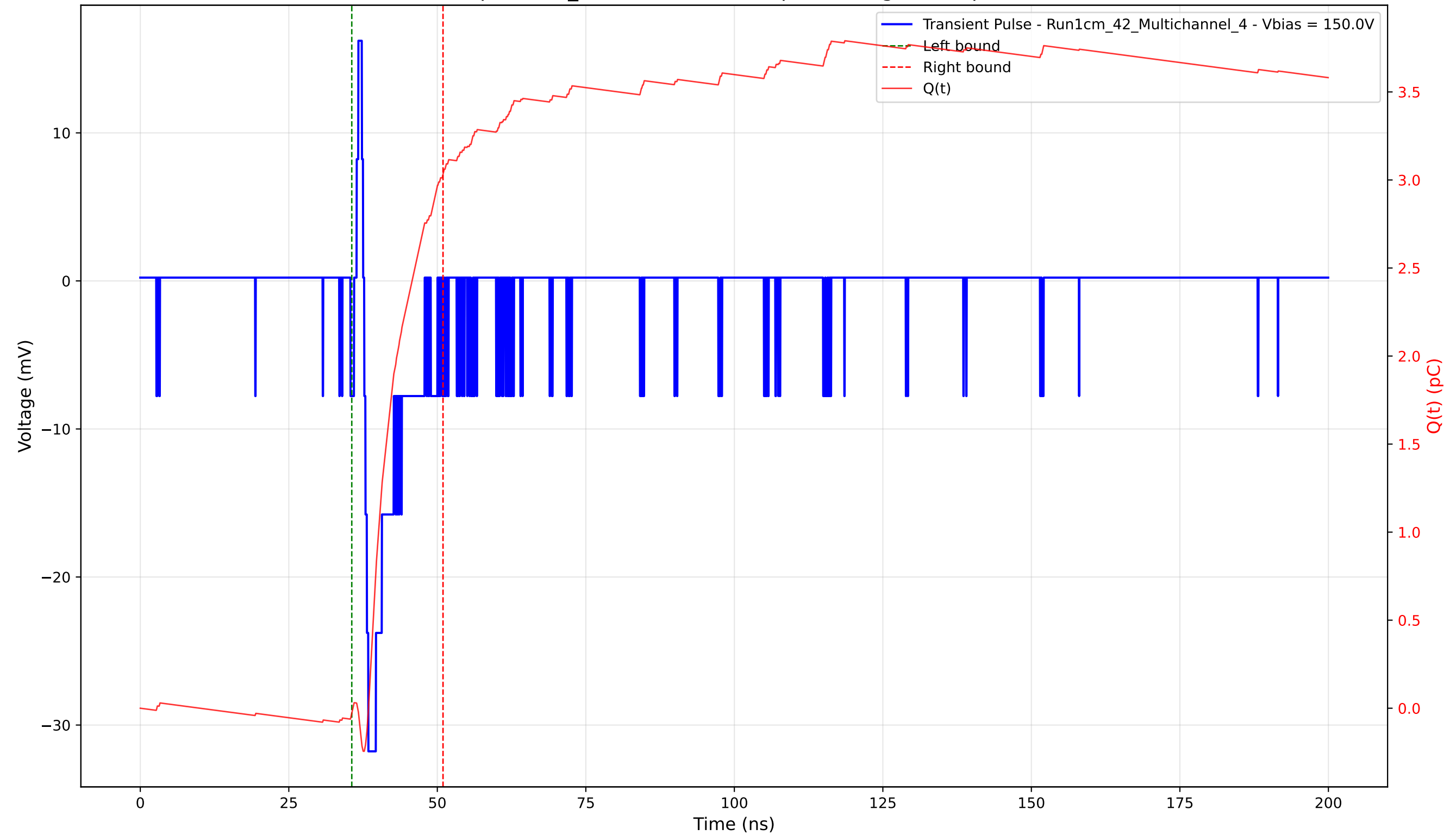
Transient Pulse - Sample: 1cm_42 - Position: 440.0 \mu\text{m} - Charge: 3.06 pC - Rise Time: 0.70 ns
