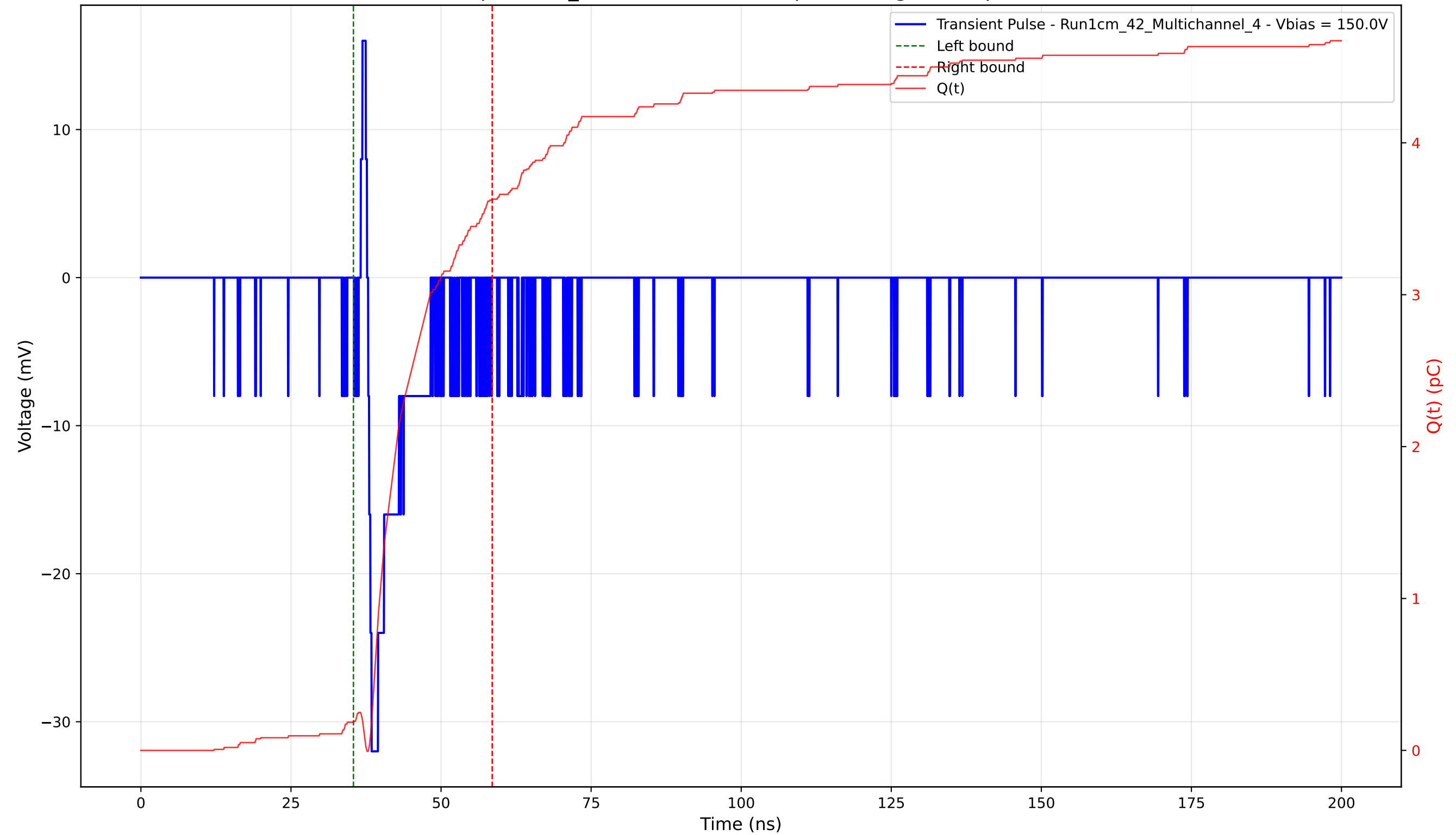
Transient Pulse - Sample: 1cm_42 - Position: 4715.0 \mu\text{m} - Charge: 3.44 pC - Rise Time: 0.58 ns
