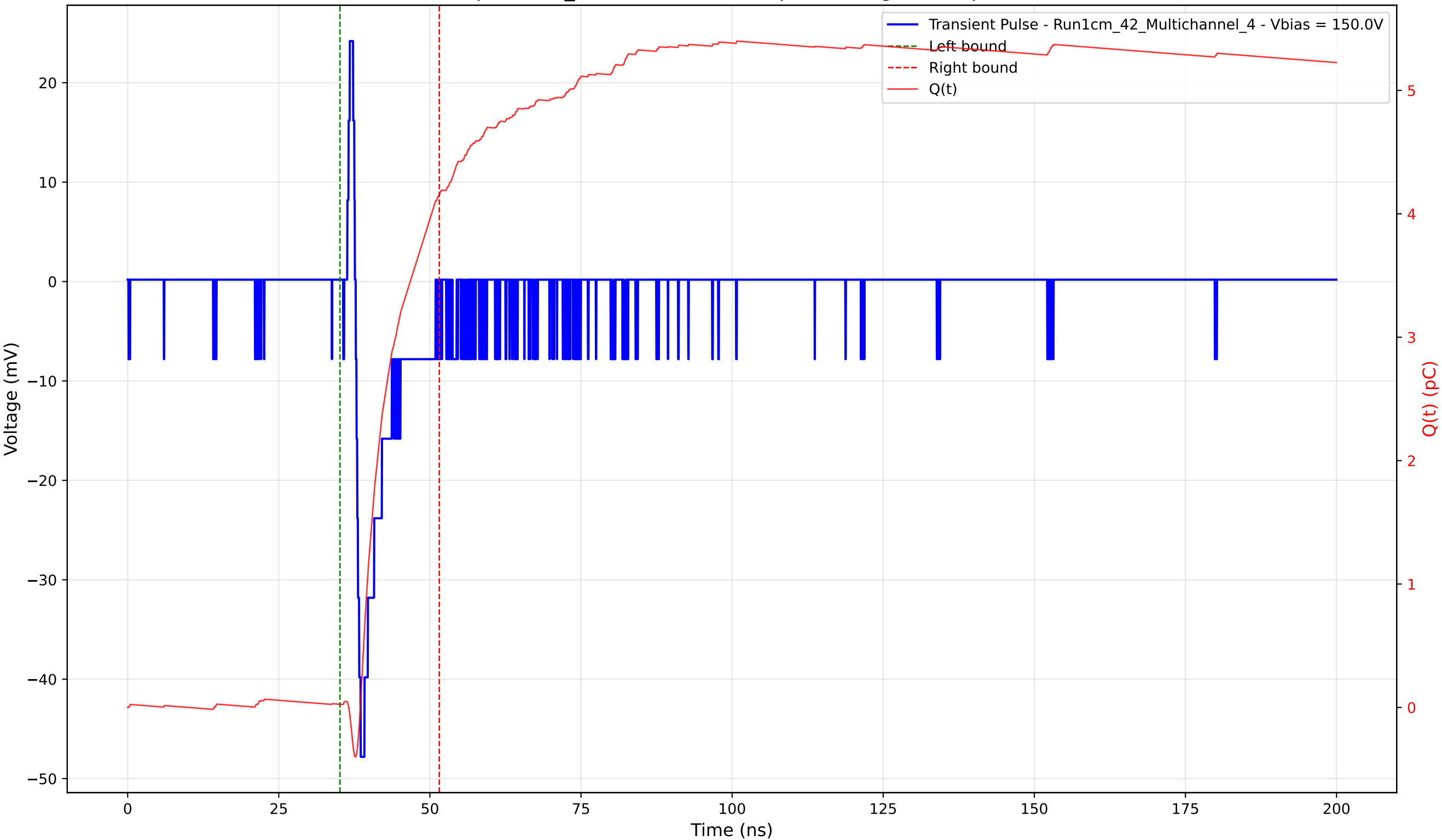
Transient Pulse - Sample: 1cm_42 - Position: 660.0 \mu\text{m} - Charge: 4.13 pC - Rise Time: 0.82 ns
