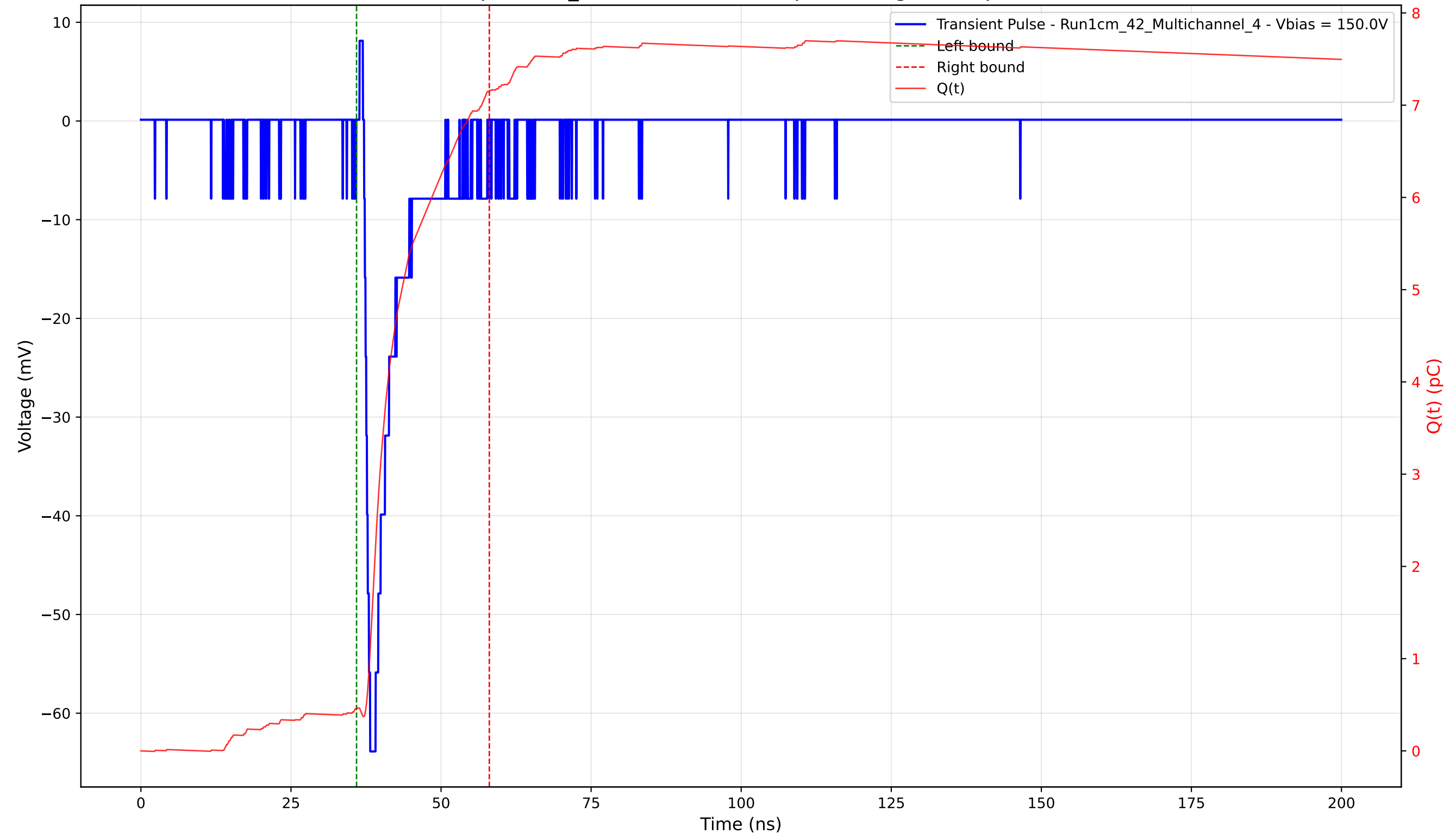
Transient Pulse - Sample: 1cm_42 - Position: 1325.0 \mu\text{m} - Charge: 6.69 pC - Rise Time: 1.01 ns
