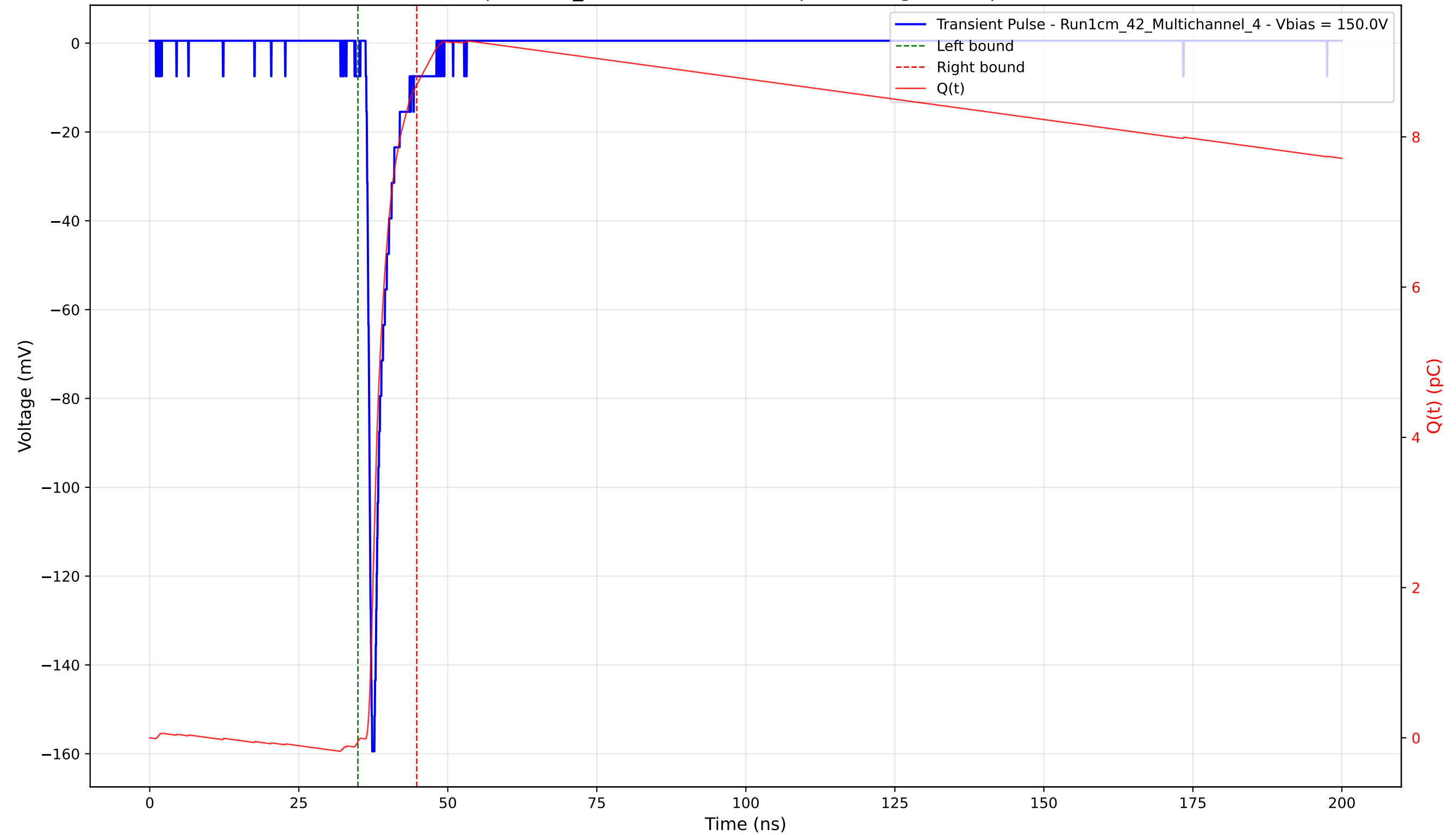
Transient Pulse - Sample: 1cm_42 - Position: 1875.0 \mu\text{m} - Charge: 8.74 pC - Rise Time: 0.84 ns
