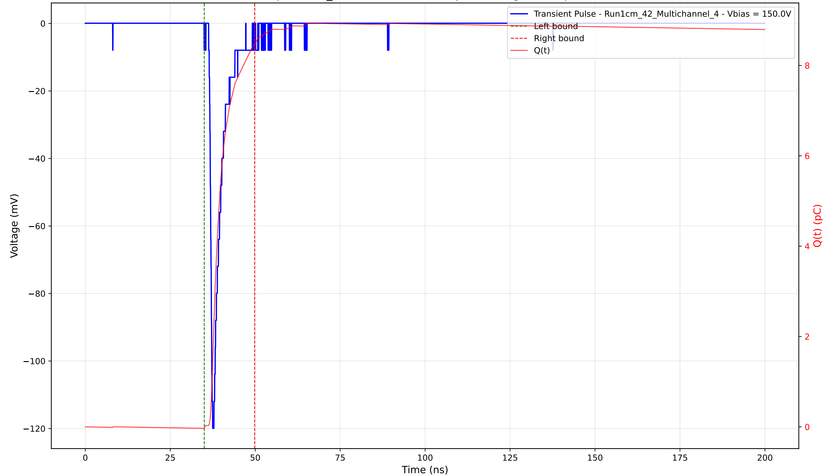
Transient Pulse - Sample: 1cm_42 - Position: 1670.0 \mu\text{m} - Charge: 8.49 pC - Rise Time: 0.86 ns
