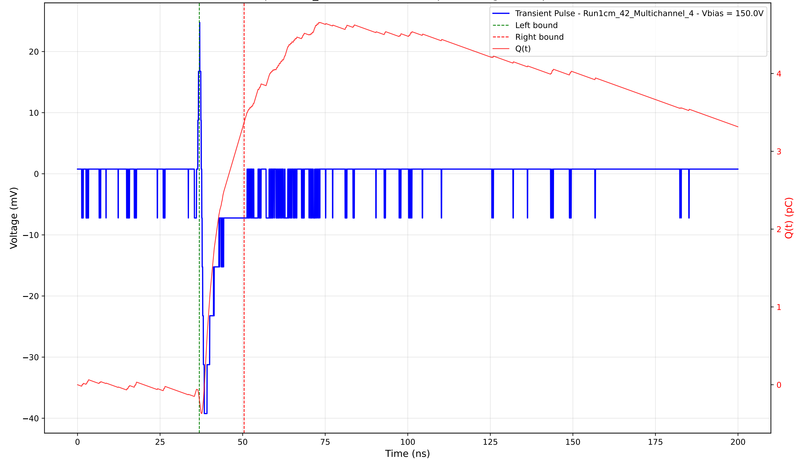
Transient Pulse - Sample: 1cm_42 - Position: 4070.0 \mu\text{m} - Charge: 3.56 pC - Rise Time: 0.78 ns
