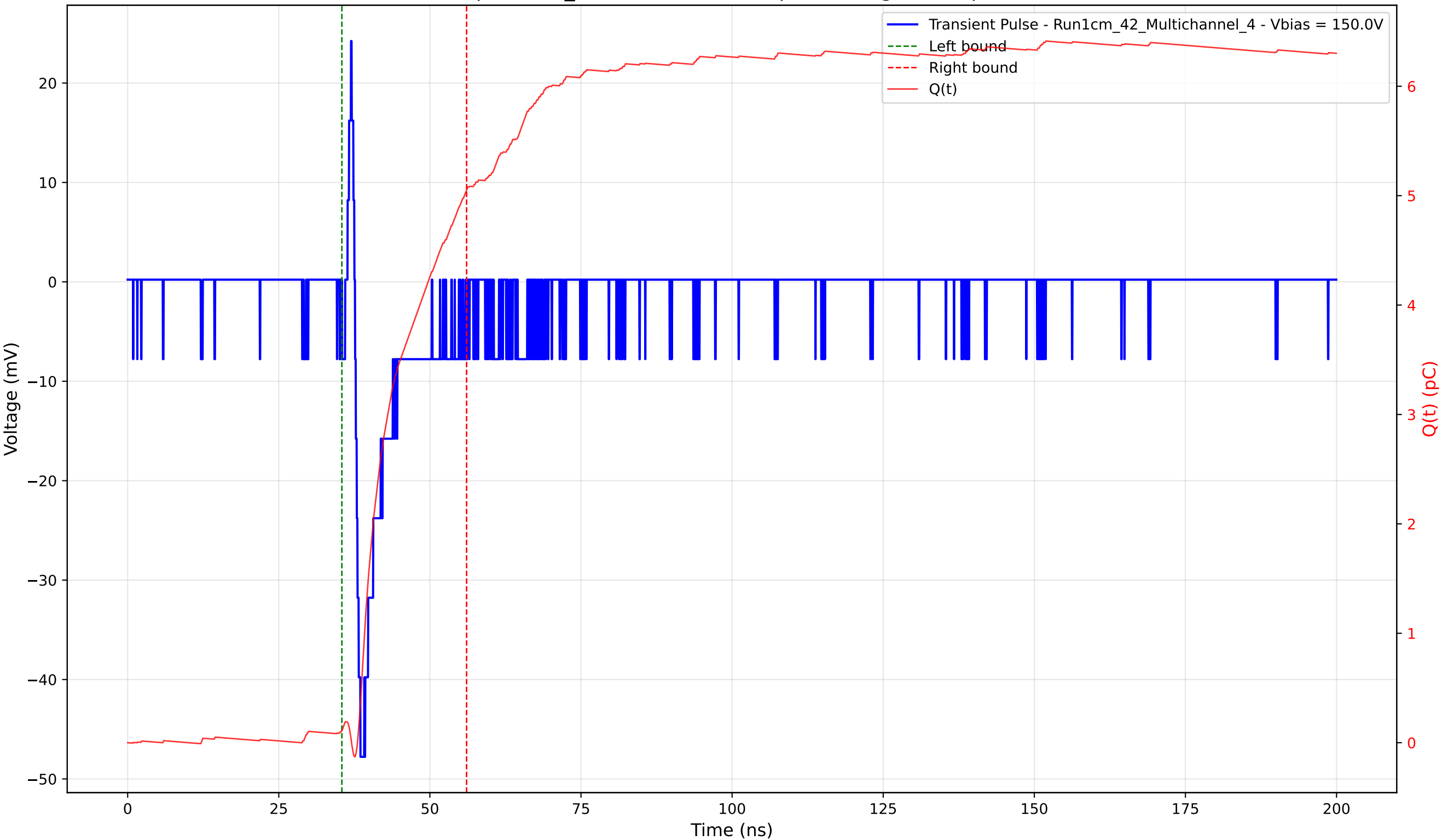
Transient Pulse - Sample: 1cm_42 - Position: 950.0 \mu\text{m} - Charge: 4.94 pC - Rise Time: 0.90 ns
