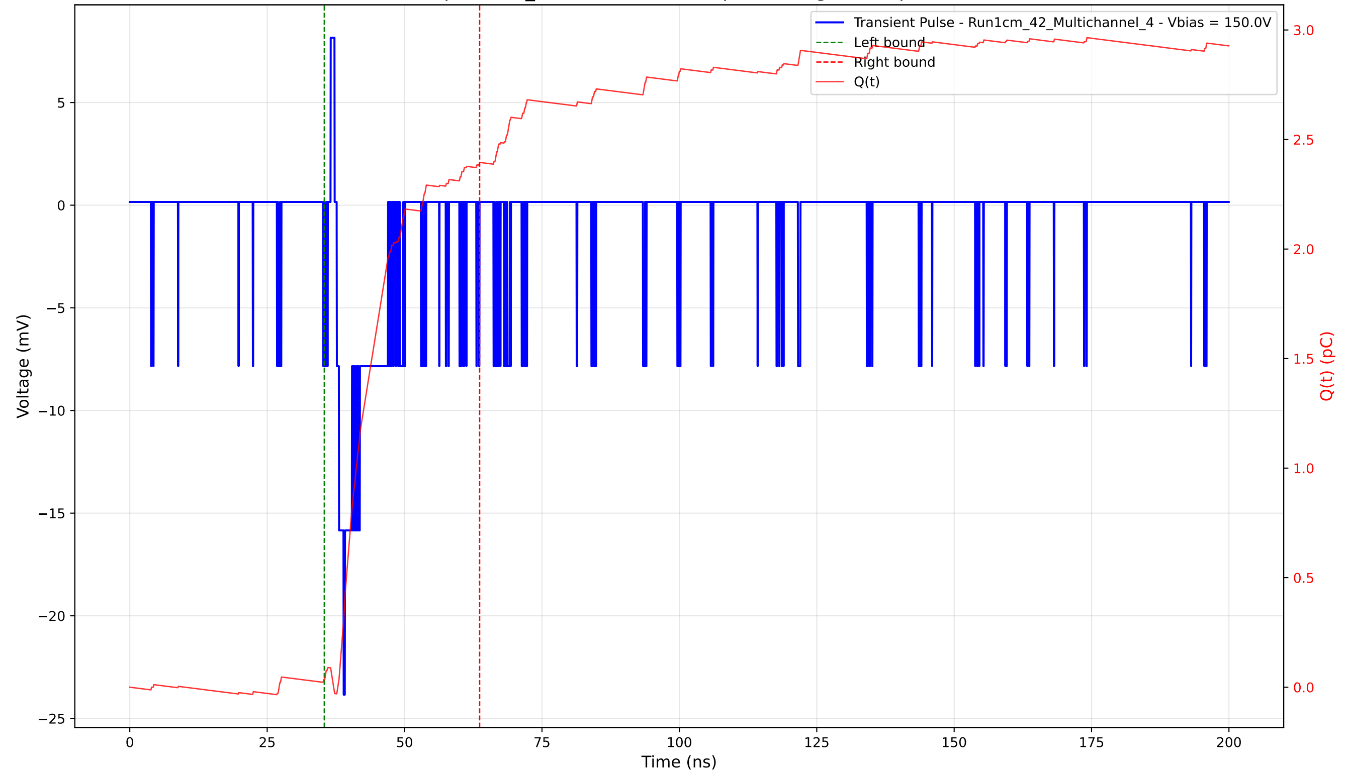
Transient Pulse - Sample: 1cm_42 - Position: 210.0 \mu\text{m} - Charge: 2.36 pC - Rise Time: 1.27 ns
