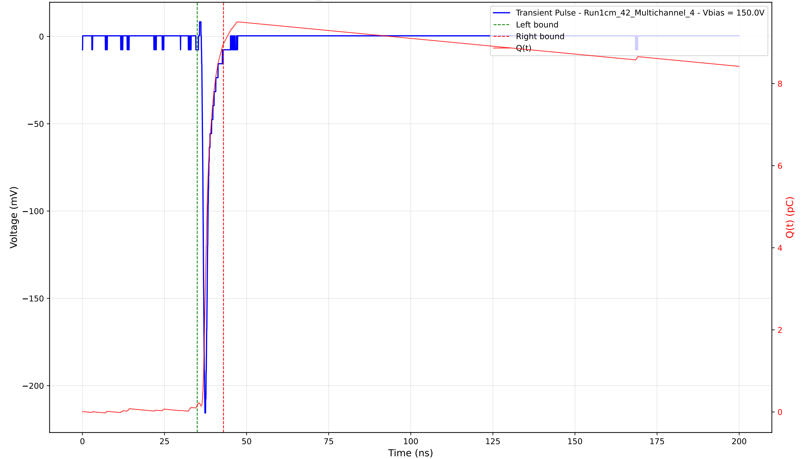
Transient Pulse - Sample: 1cm_42 - Position: 3035.0 \mu\text{m} - Charge: 8.81 pC - Rise Time: 0.78 ns
