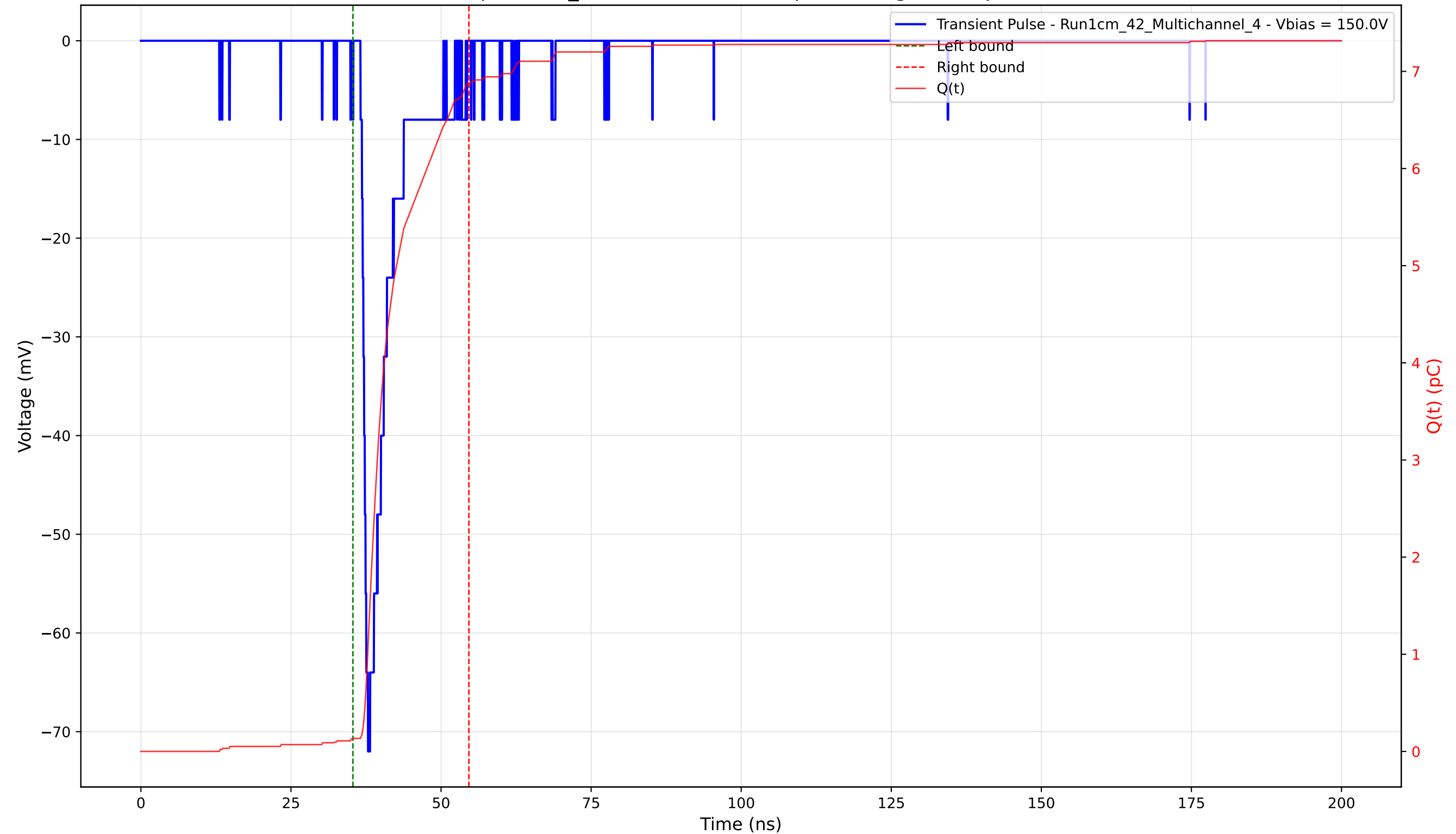
Transient Pulse - Sample: 1cm_42 - Position: 1500.0 \mu\text{m} - Charge: 6.75 pC - Rise Time: 1.24 ns
