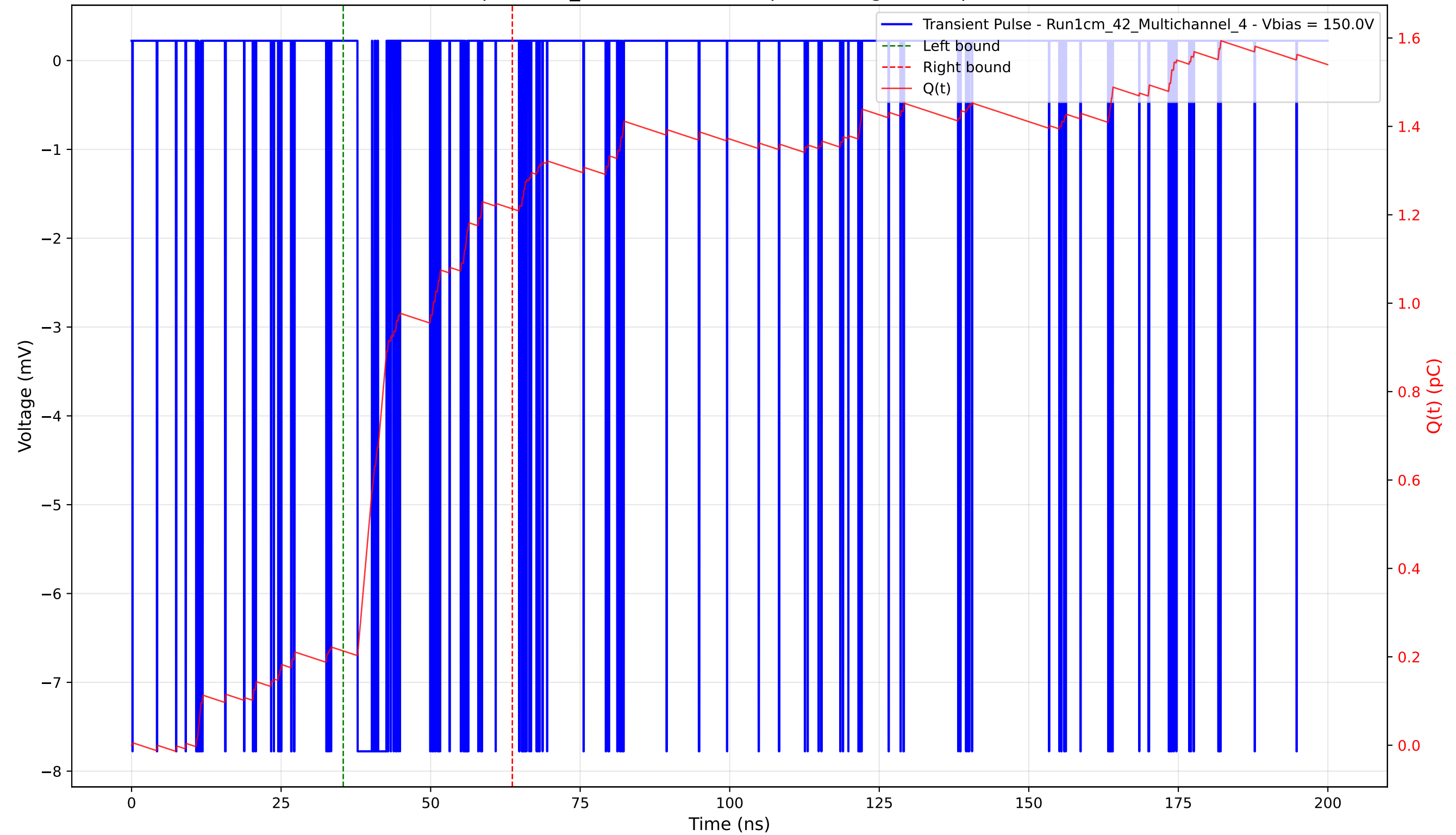
Transient Pulse - Sample: 1cm_42 - Position: 75.0 \mu\text{m} - Charge: 1.00 pC - Rise Time: 0.04 ns
