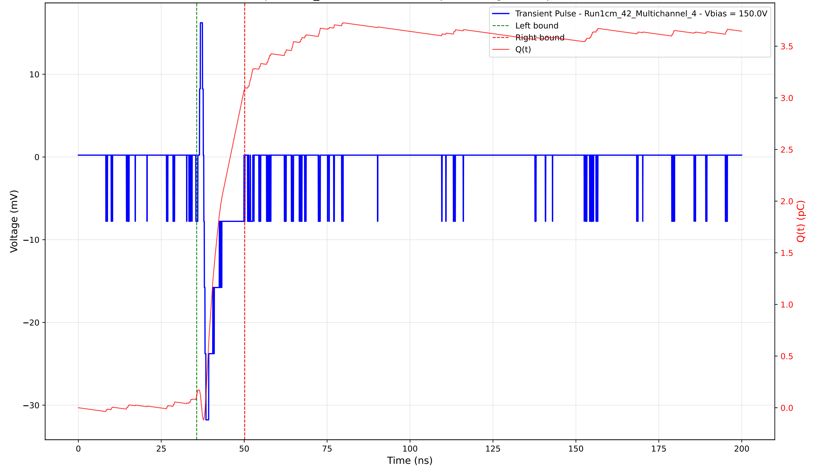
Transient Pulse - Sample: 1cm_42 - Position: 4600.0 \mu\text{m} - Charge: 2.97 pC - Rise Time: 0.66 ns
