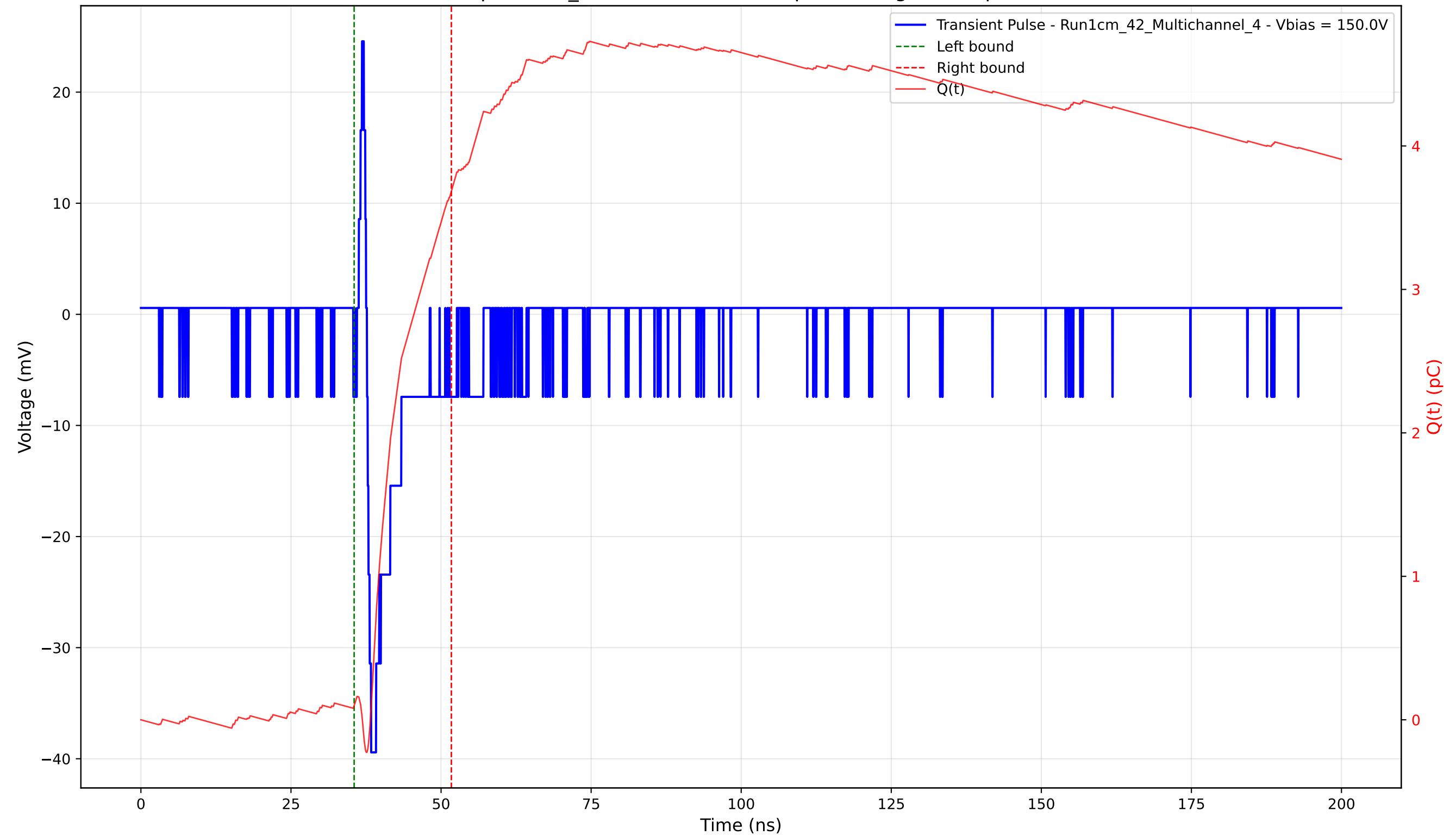
Transient Pulse - Sample: 1cm_42 - Position: 4125.0 \mu\text{m} - Charge: 3.58 pC - Rise Time: 0.70 ns
