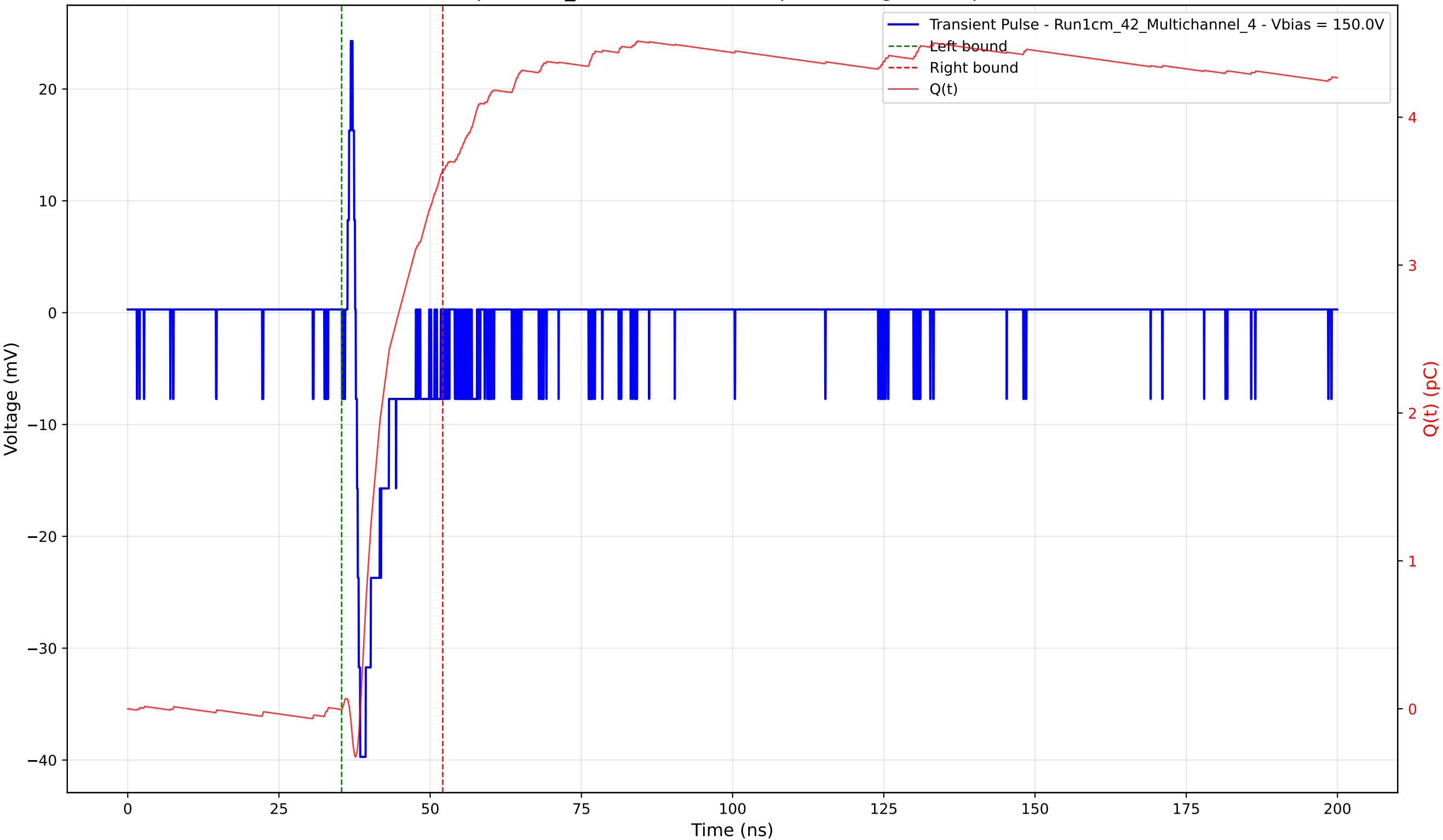
Transient Pulse - Sample: 1cm_42 - Position: 575.0 \mu\text{m} - Charge: 3.64 pC - Rise Time: 0.74 ns
