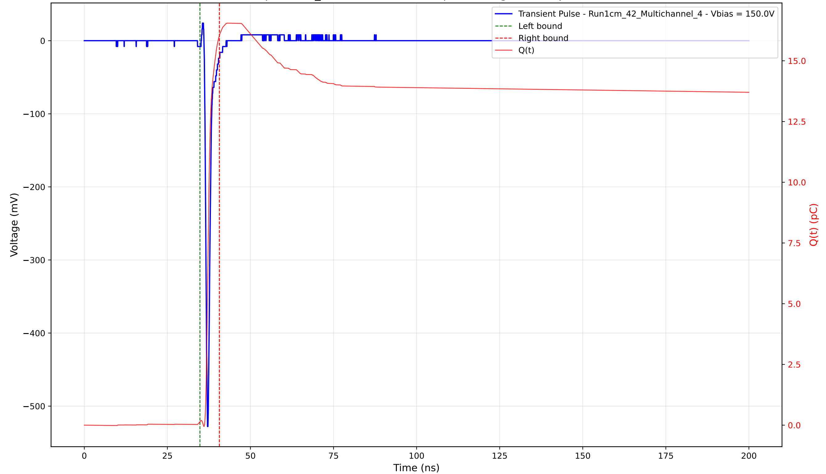
Transient Pulse - Sample: 1cm_42 - Position: 2480.0 \mu\text{m} - Charge: 15.90 pC - Rise Time: 0.72 ns
