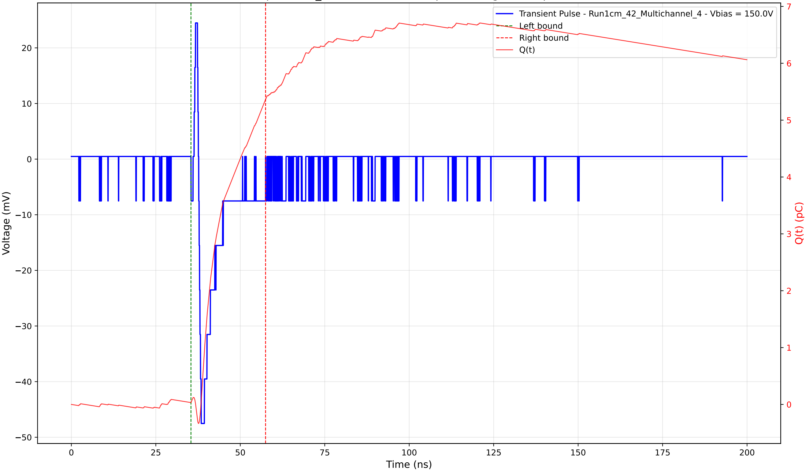
Transient Pulse - Sample: 1cm_42 - Position: 745.0 \mu\text{m} - Charge: 5.33 pC - Rise Time: 0.74 ns
