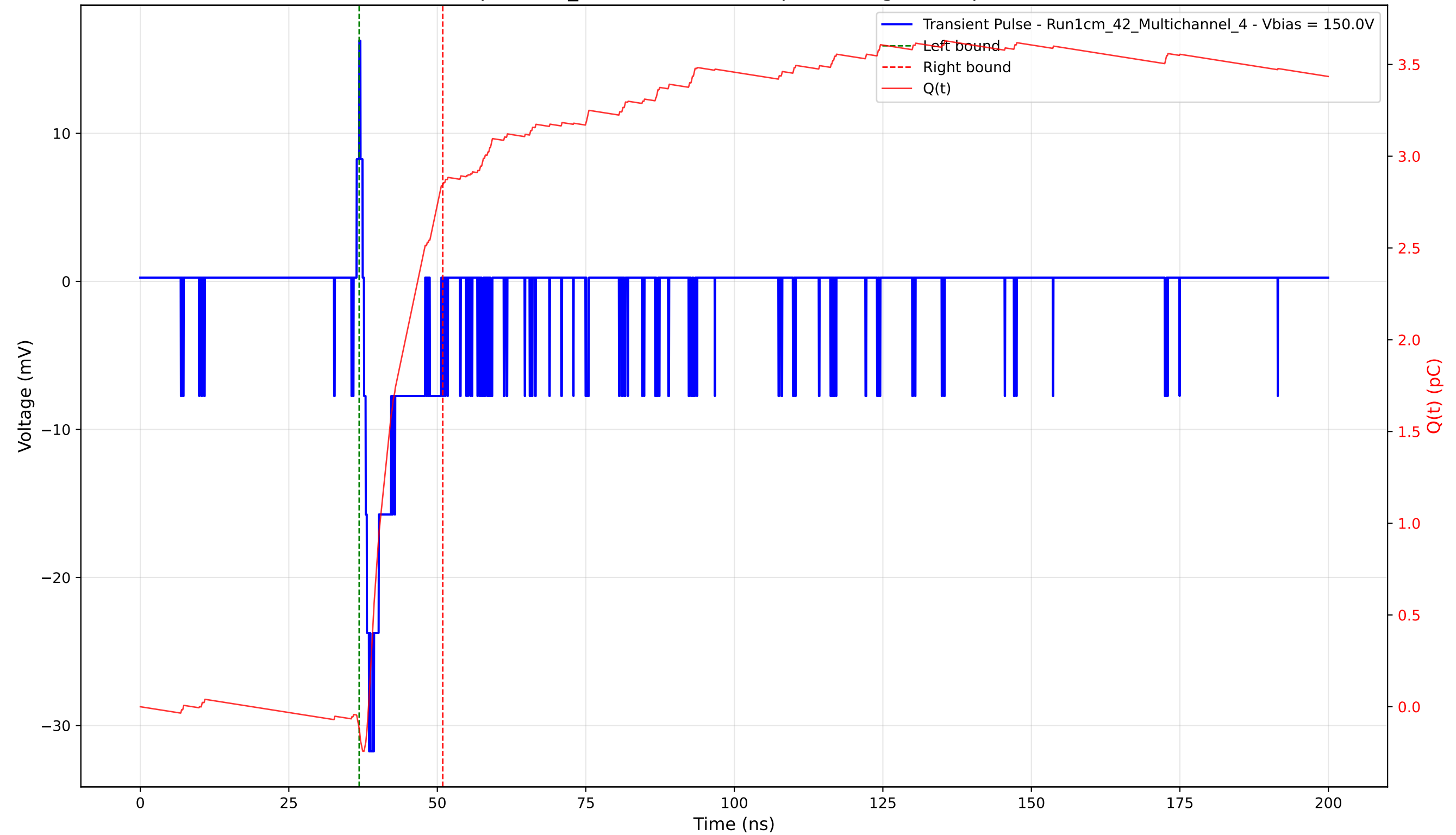
Transient Pulse - Sample: 1cm_42 - Position: 385.0 \mu\text{m} - Charge: 2.96 pC - Rise Time: 0.86 ns
