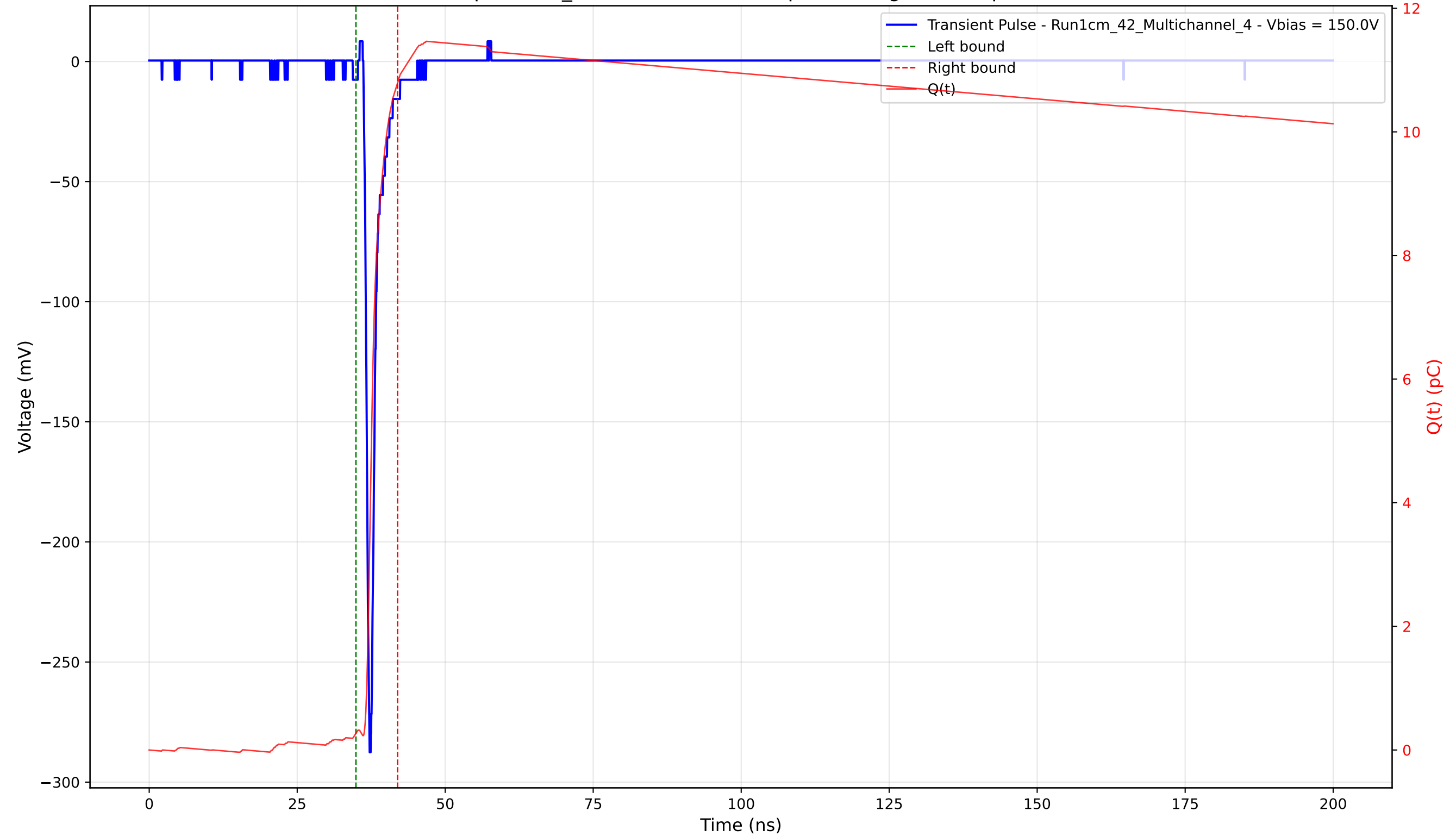
Transient Pulse - Sample: 1cm_42 - Position: 2950.0 \mu\text{m} - Charge: 10.52 pC - Rise Time: 0.79 ns
