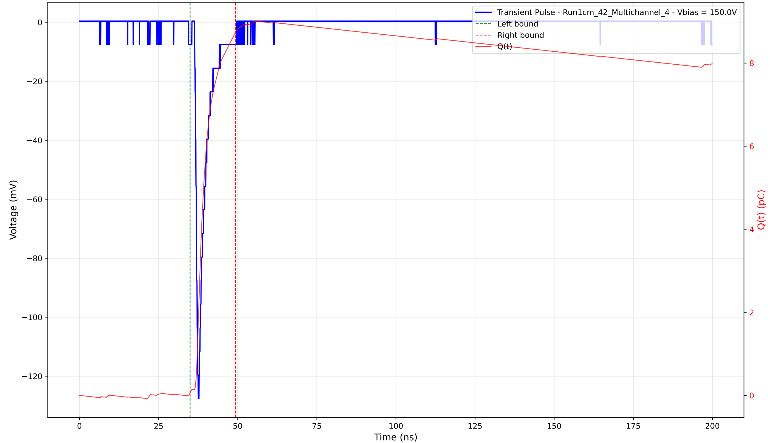
Transient Pulse - Sample: 1cm_42 - Position: 1680.0 \mu\text{m} - Charge: 8.68 pC - Rise Time: 0.93 ns
