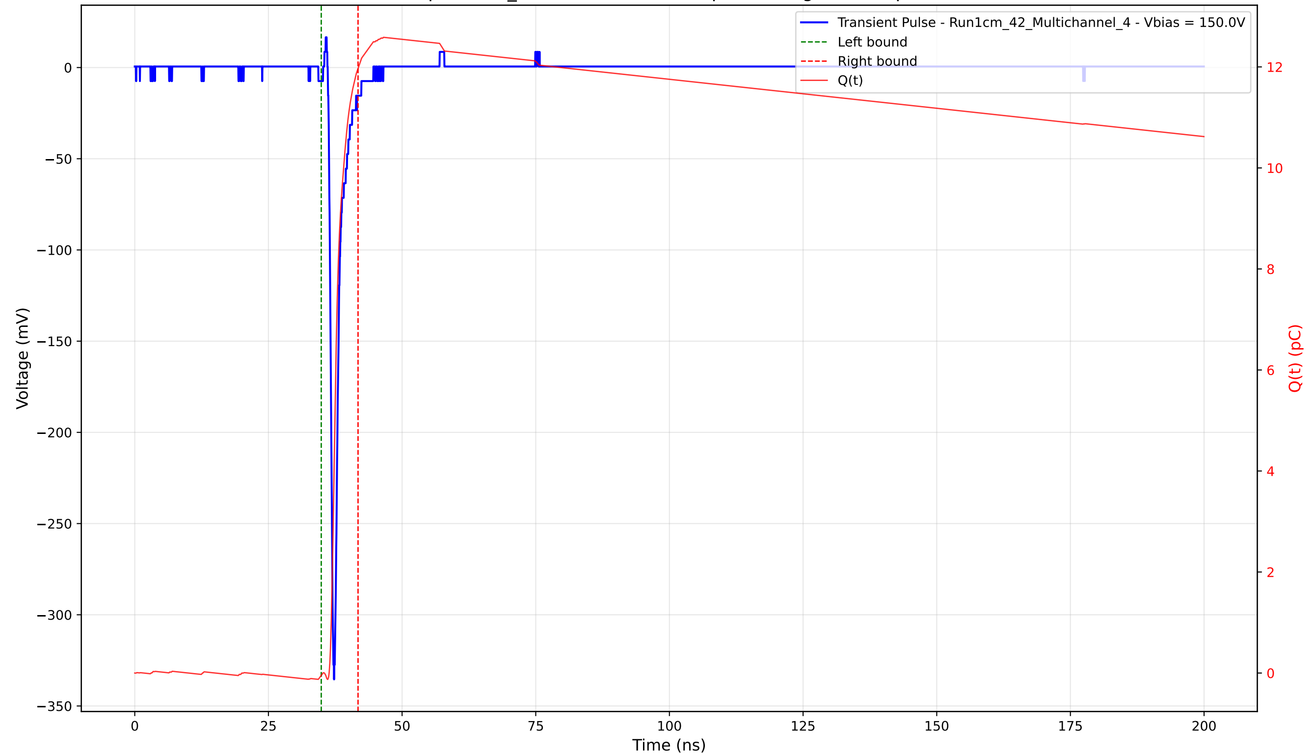
Transient Pulse - Sample: 1cm_42 - Position: 2105.0 \mu\text{m} - Charge: 12.02 pC - Rise Time: 0.75 ns
