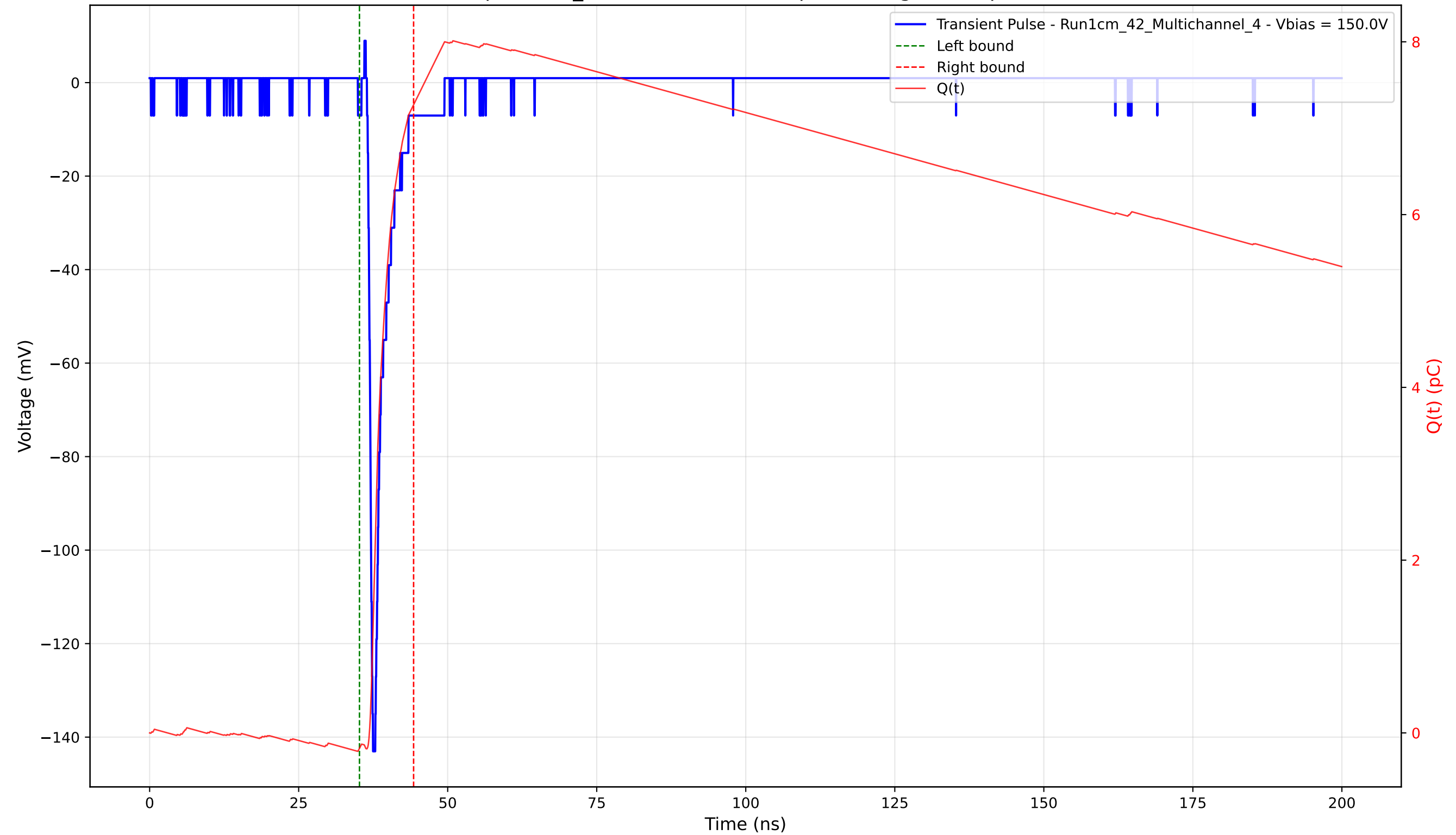
Transient Pulse - Sample: 1cm_42 - Position: 3240.0 \mu\text{m} - Charge: 7.45 pC - Rise Time: 0.80 ns
