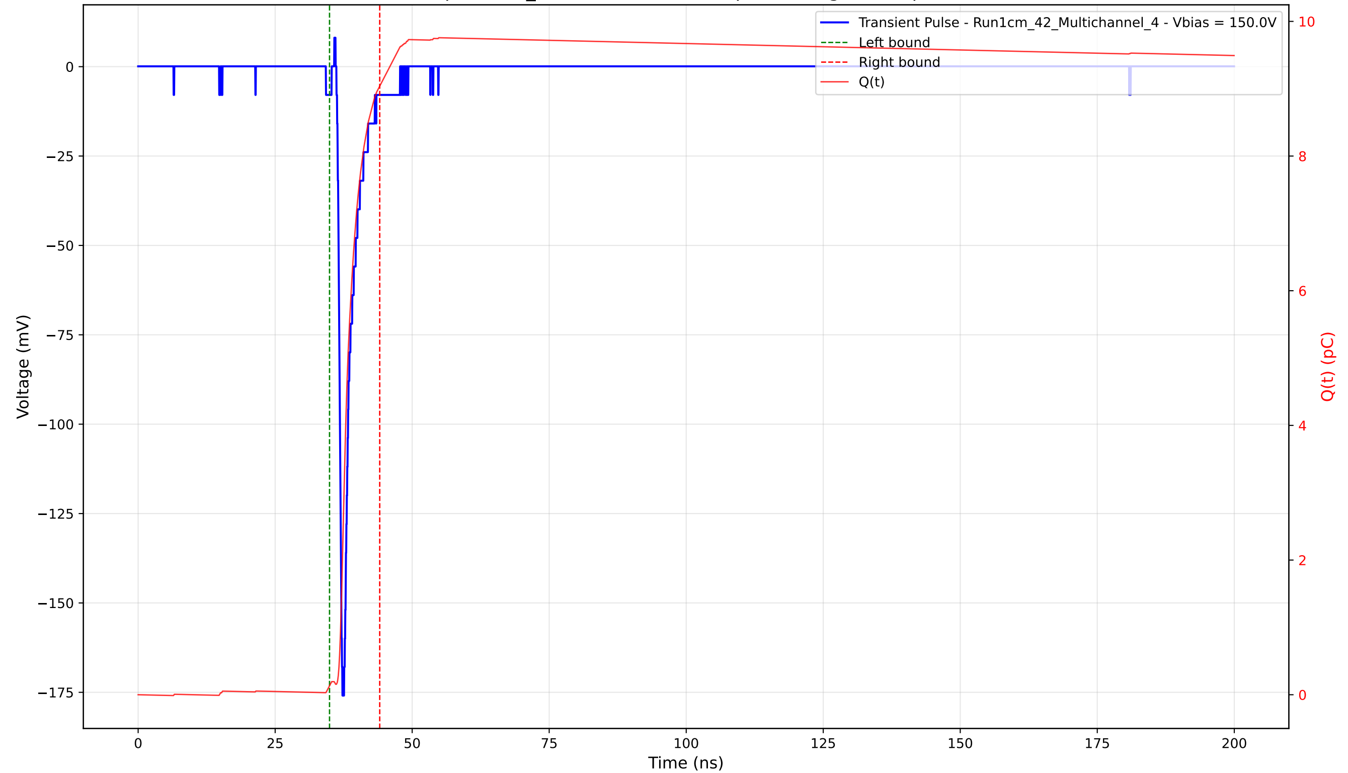
Transient Pulse - Sample: 1cm_42 - Position: 1920.0 \mu\text{m} - Charge: 8.90 pC - Rise Time: 0.75 ns
