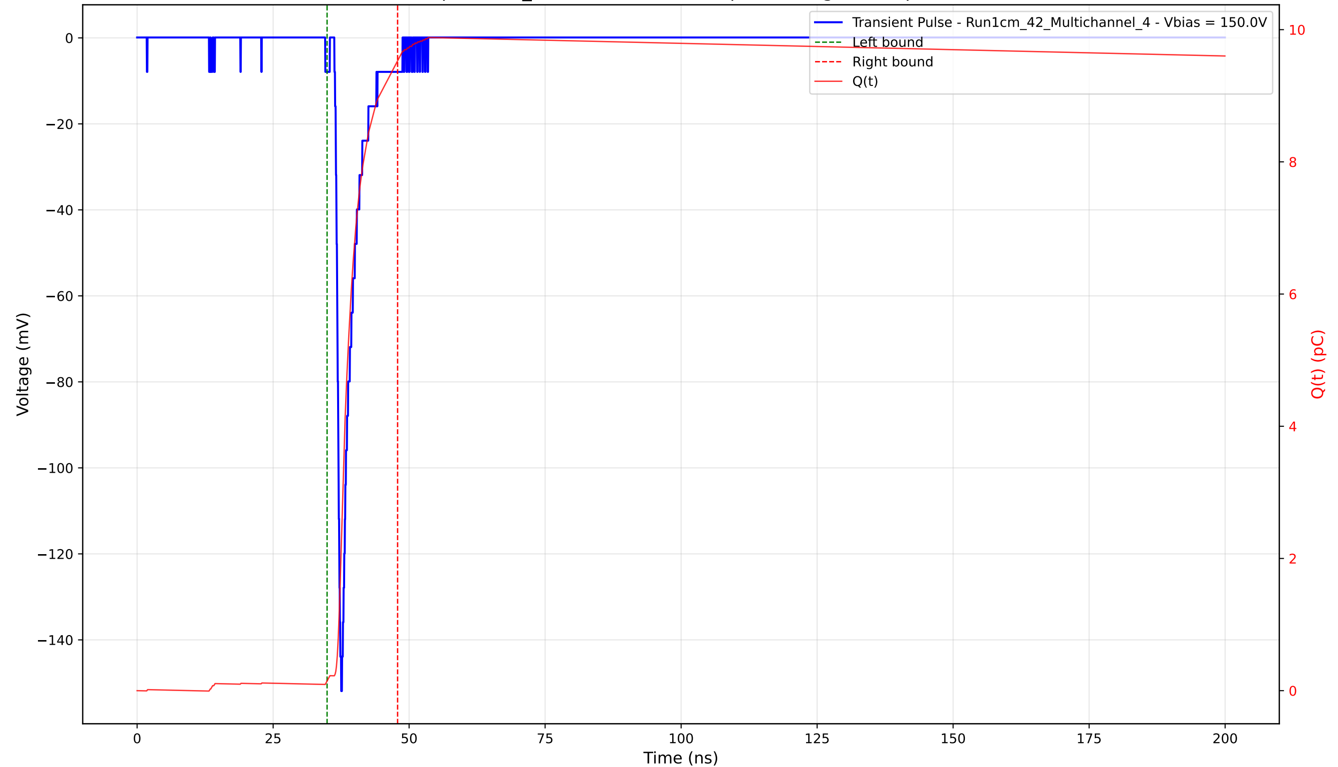
Transient Pulse - Sample: 1cm_42 - Position: 1765.0 \mu\text{m} - Charge: 9.38 pC - Rise Time: 0.96 ns
