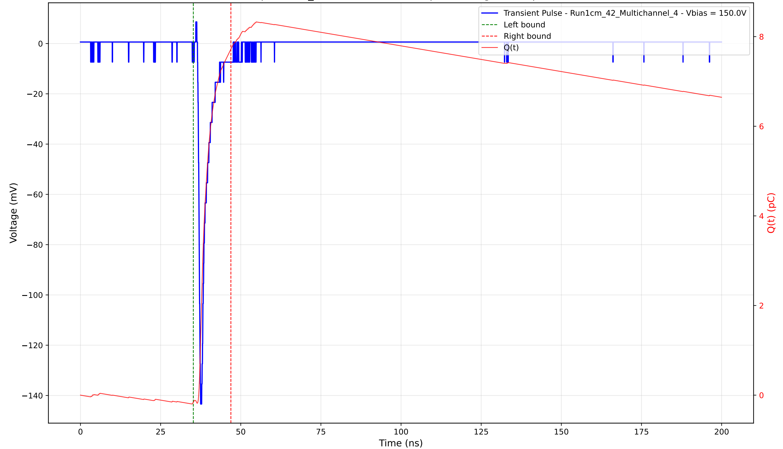
Transient Pulse - Sample: 1cm_42 - Position: 3245.0 \mu\text{m} - Charge: 7.88 pC - Rise Time: 0.81 ns
