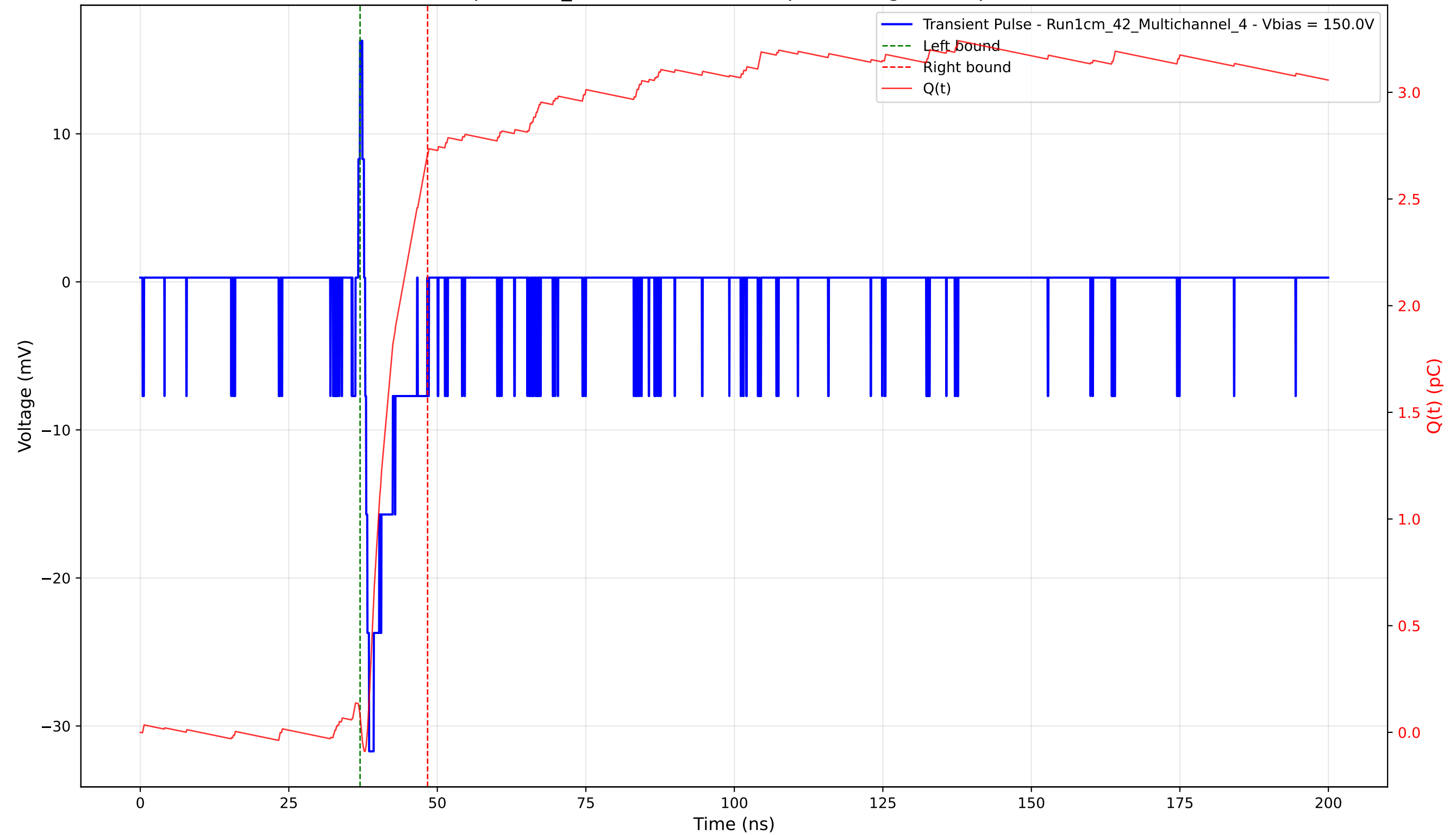
Transient Pulse - Sample: 1cm_42 - Position: 4855.0 \mu\text{m} - Charge: 2.62 pC - Rise Time: 0.66 ns
