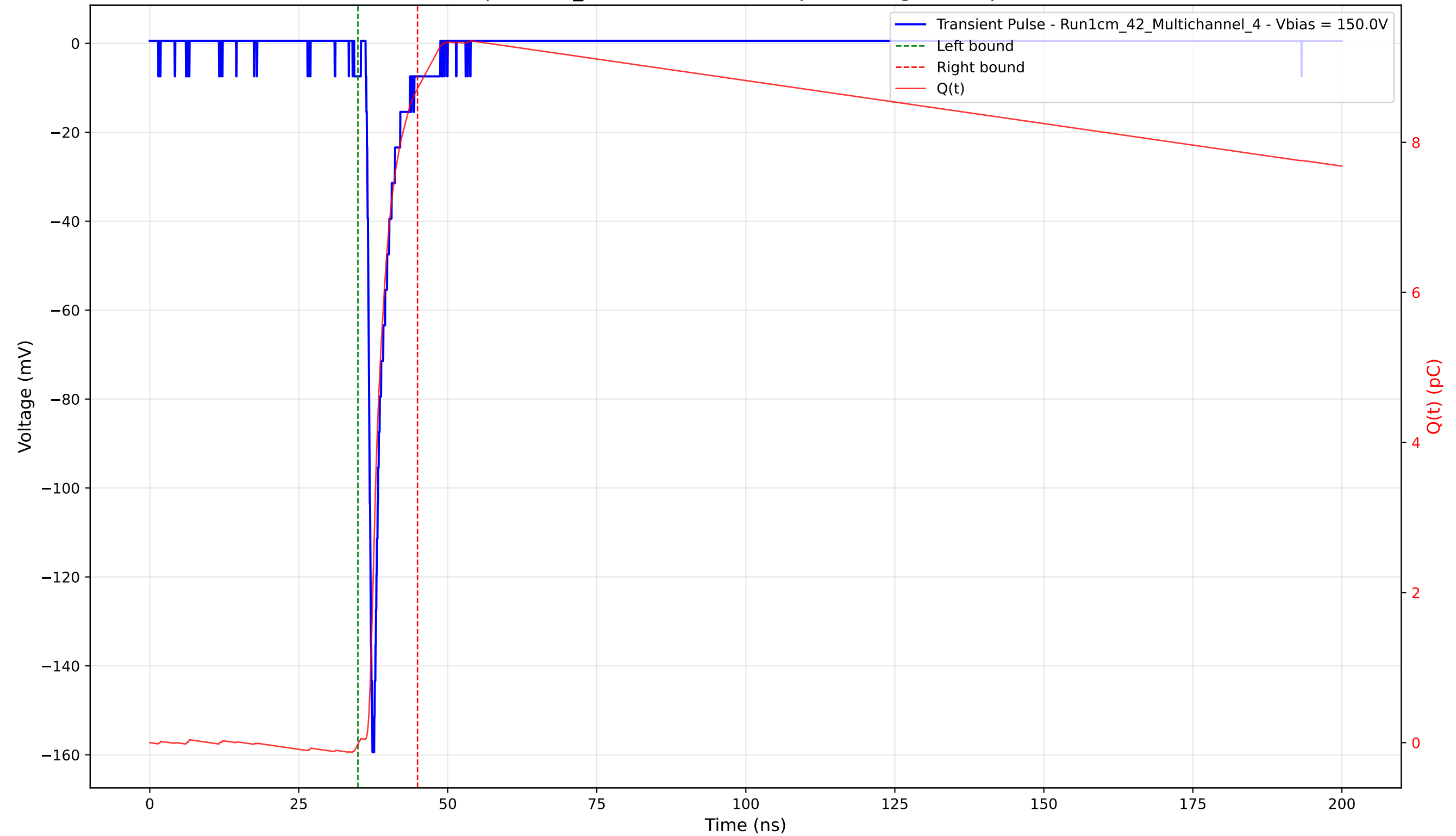
Transient Pulse - Sample: 1cm_42 - Position: 1870.0 \mu\text{m} - Charge: 8.74 pC - Rise Time: 0.88 ns
