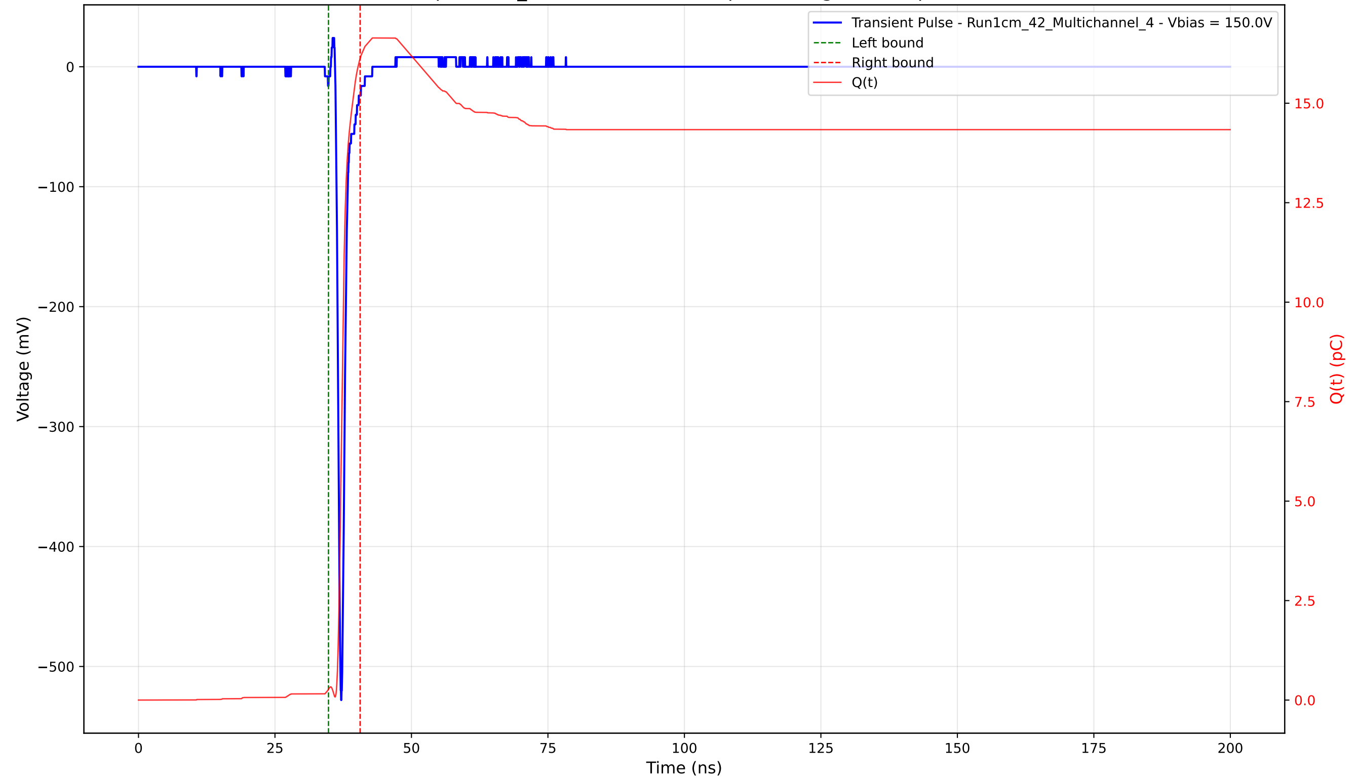
Transient Pulse - Sample: 1cm_42 - Position: 2505.0 \mu\text{m} - Charge: 15.85 pC - Rise Time: 0.72 ns
