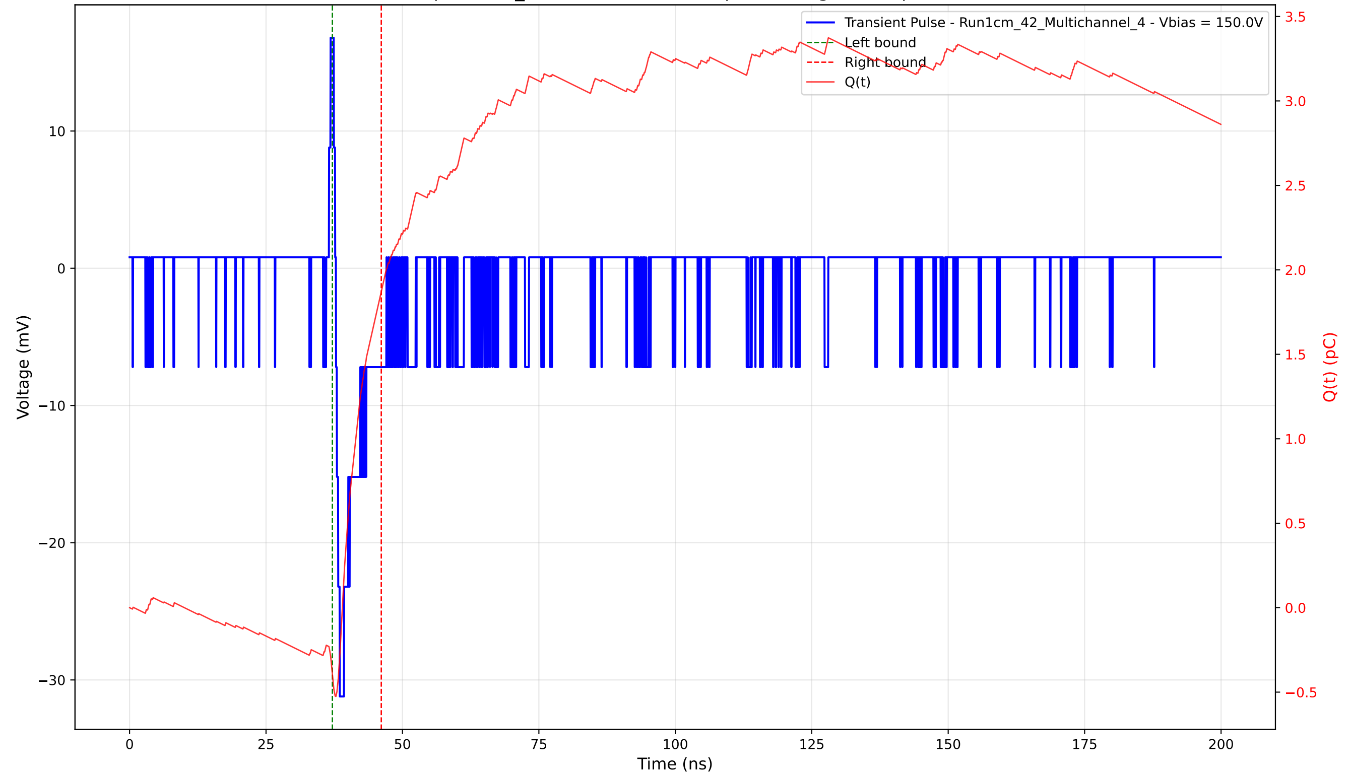
Transient Pulse - Sample: 1cm_42 - Position: 4585.0 \mu\text{m} - Charge: 2.27 pC - Rise Time: 0.71 ns
