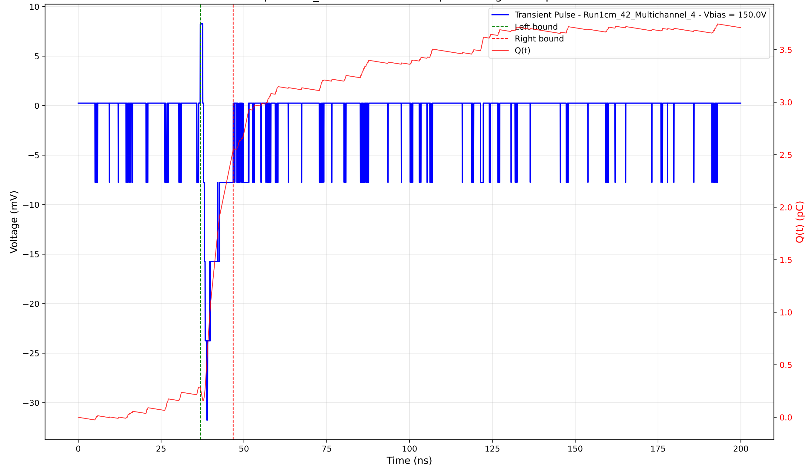
Transient Pulse - Sample: 1cm_42 - Position: 4915.0 \mu\text{m} - Charge: 2.28 pC - Rise Time: 0.98 ns
