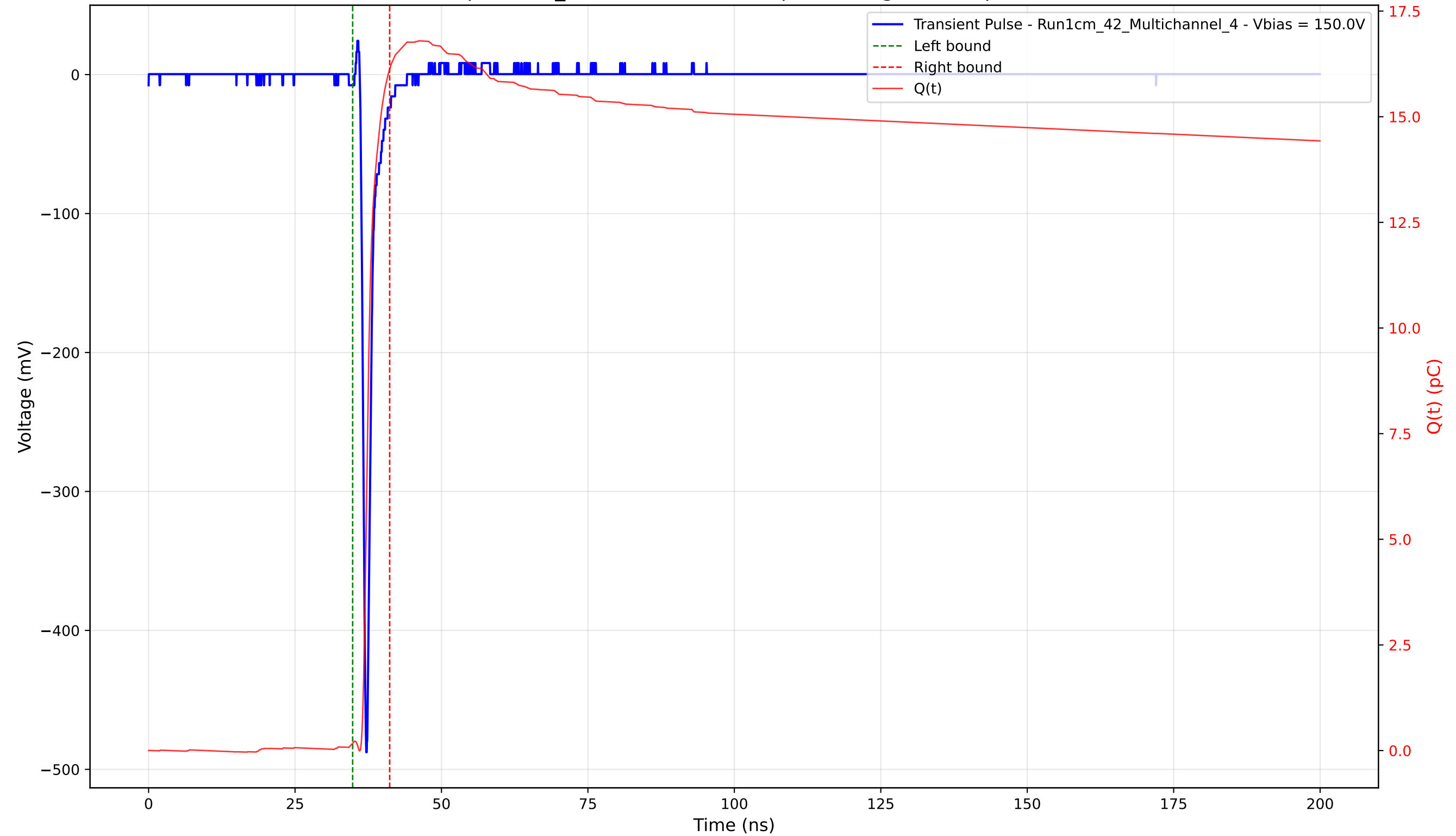
Transient Pulse - Sample: 1cm_42 - Position: 2225.0 \mu\text{m} - Charge: 15.95 pC - Rise Time: 0.76 ns
