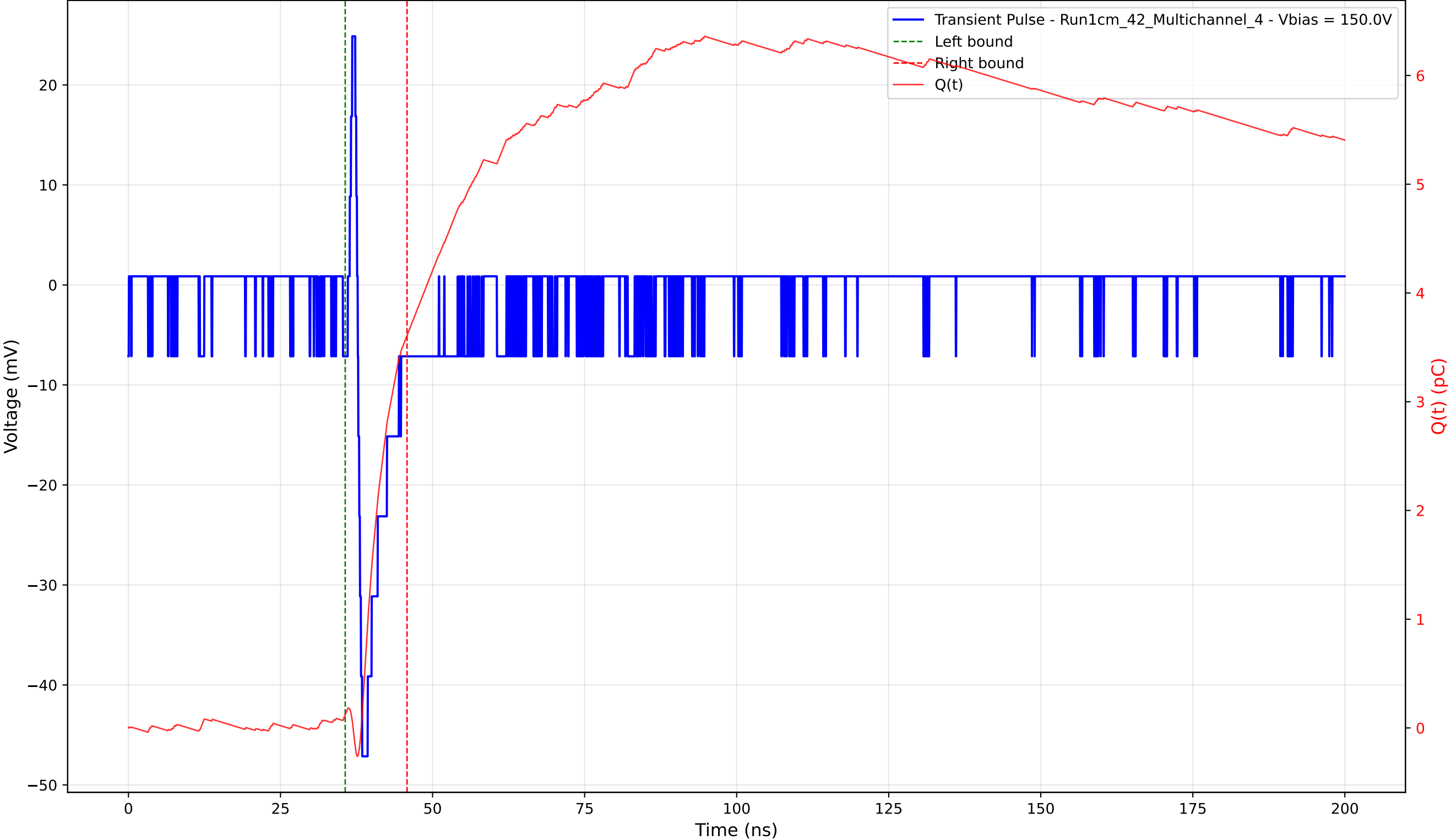
Transient Pulse - Sample: 1cm_42 - Position: 795.0 \mu\text{m} - Charge: 3.49 pC - Rise Time: 0.74 ns
