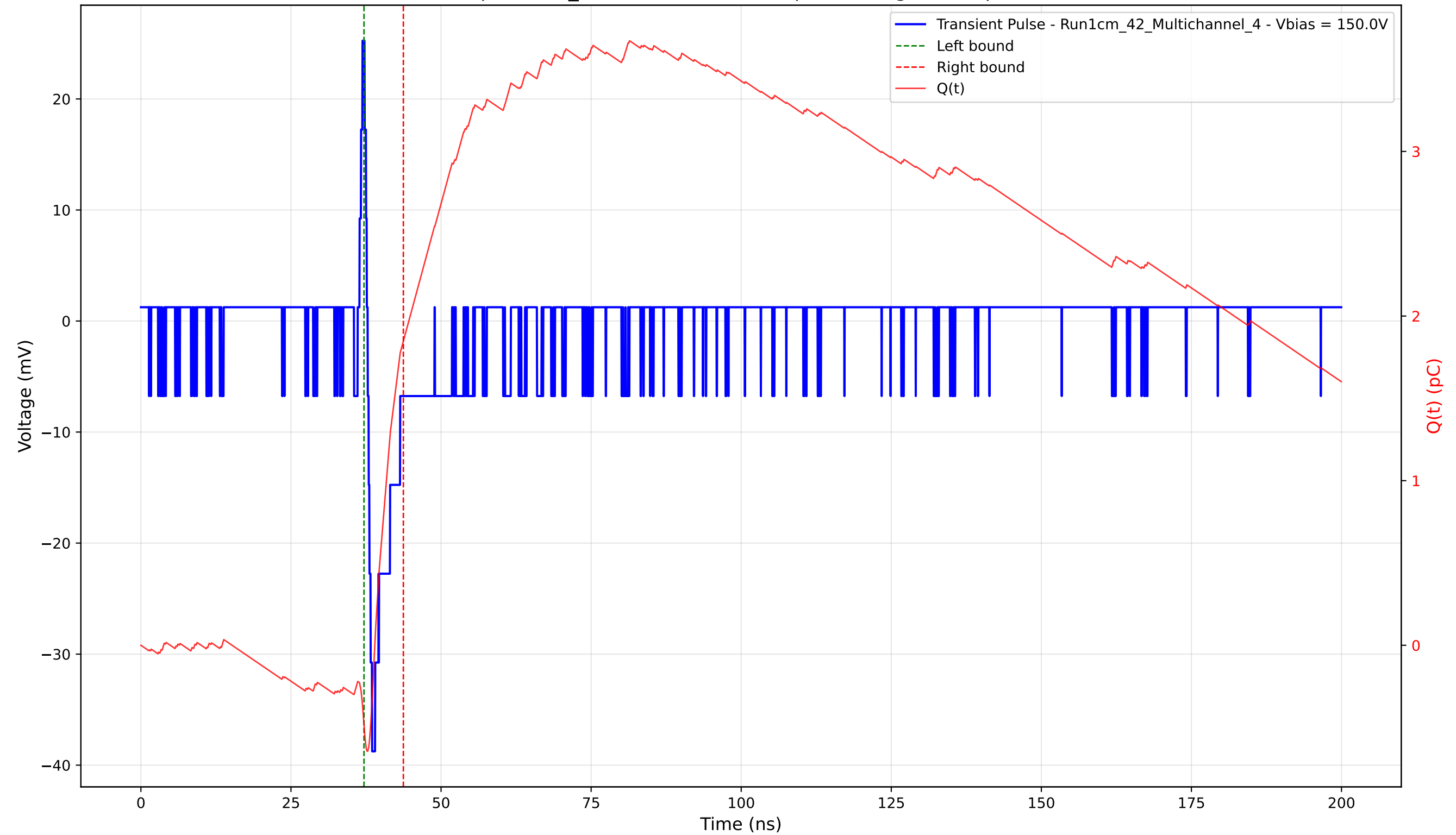
Transient Pulse - Sample: 1cm_42 - Position: 4385.0 \mu\text{m} - Charge: 2.33 pC - Rise Time: 0.74 ns
