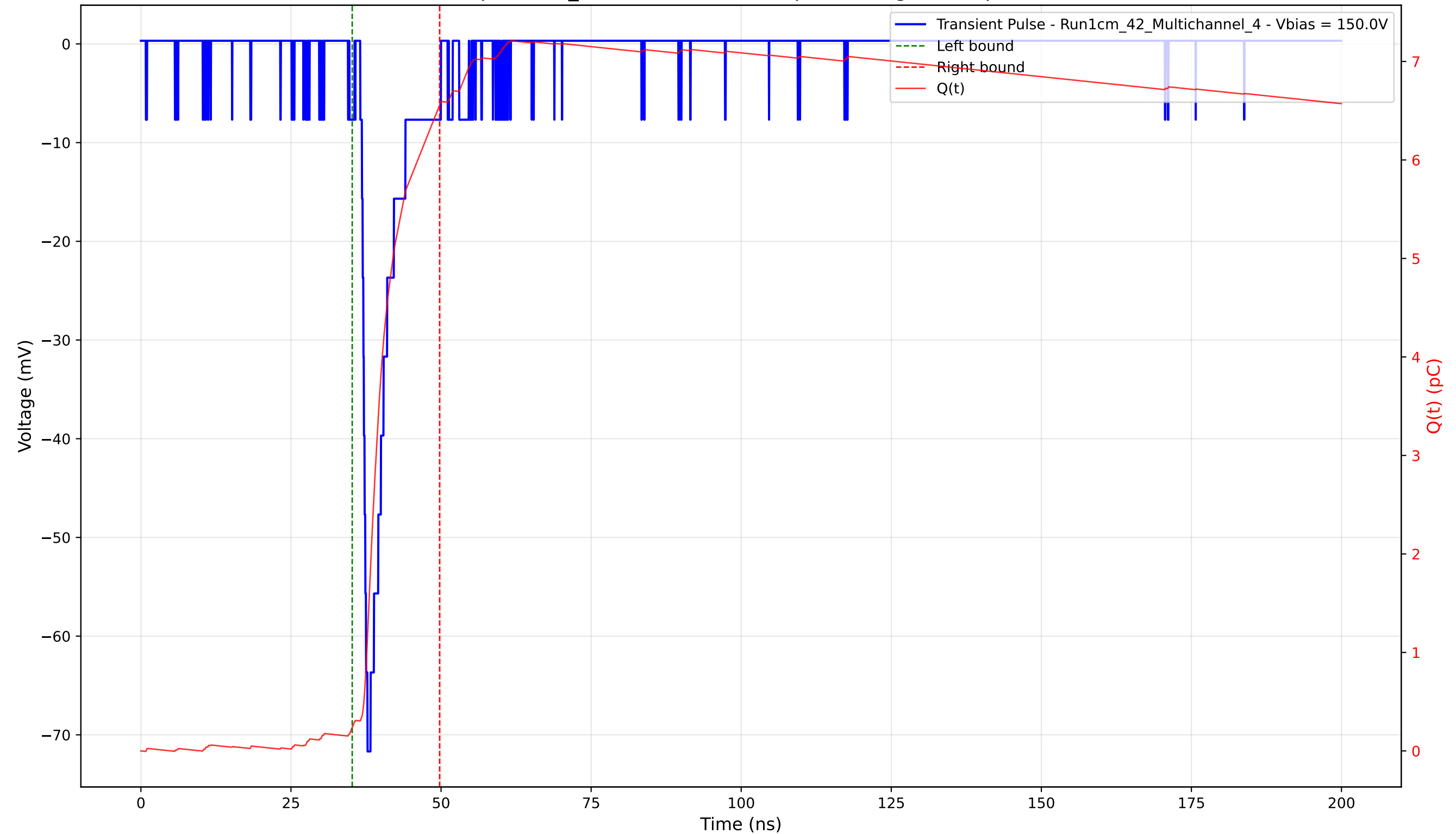
Transient Pulse - Sample: 1cm_42 - Position: 1505.0 \mu\text{m} - Charge: 6.32 pC - Rise Time: 1.20 ns
