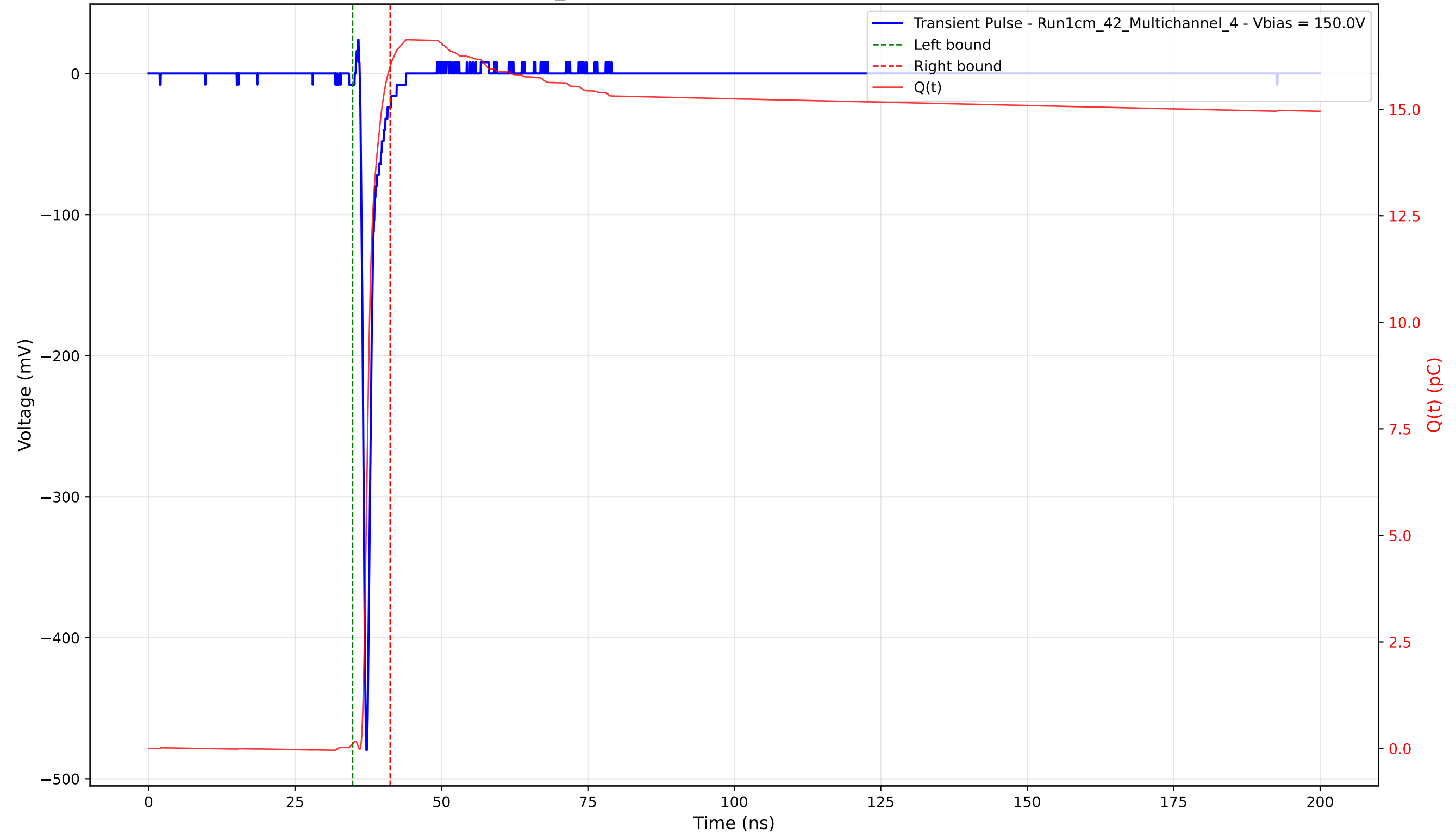
Transient Pulse - Sample: 1cm_42 - Position: 2215.0 \mu\text{m} - Charge: 15.89 pC - Rise Time: 0.74 ns
