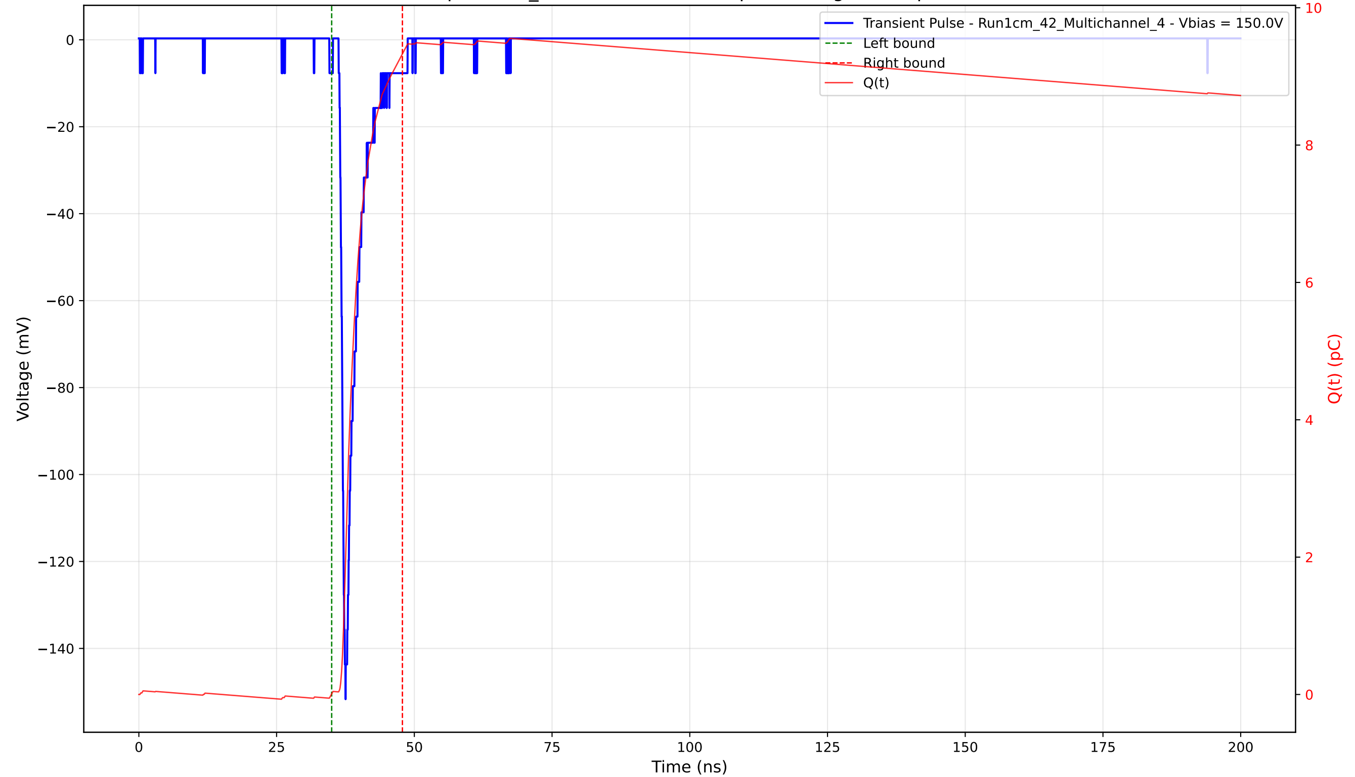
Transient Pulse - Sample: 1cm_42 - Position: 1745.0 \mu\text{m} - Charge: 9.32 pC - Rise Time: 0.96 ns
