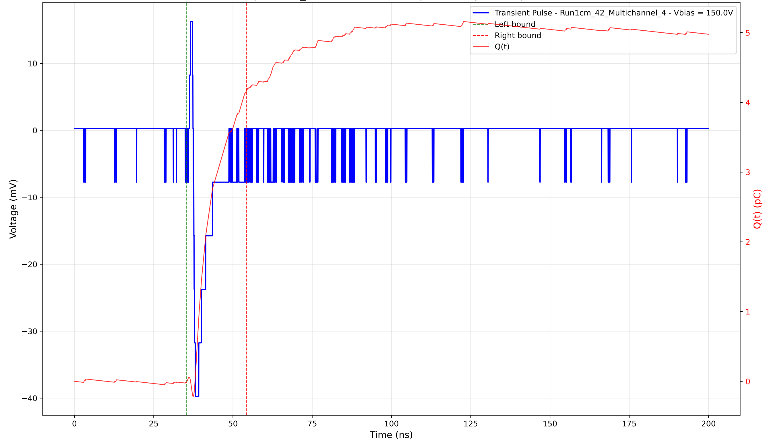
Transient Pulse - Sample: 1cm_42 - Position: 3995.0 \mu\text{m} - Charge: 4.16 pC - Rise Time: 0.66 ns
