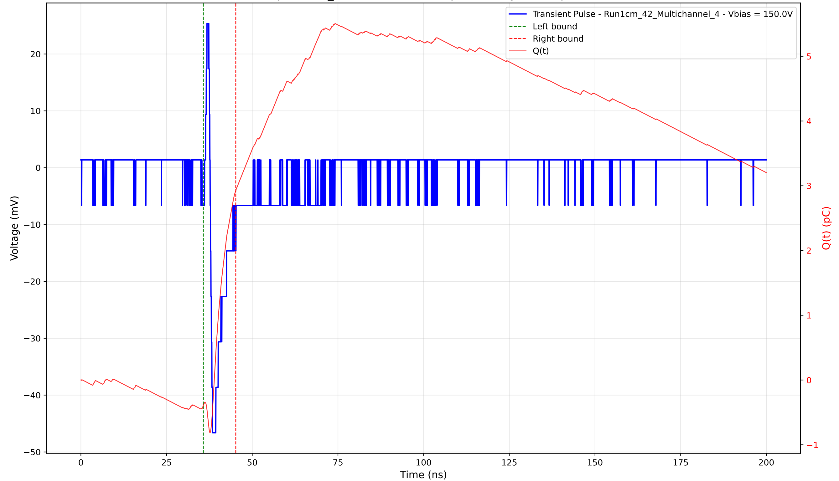
Transient Pulse - Sample: 1cm_42 - Position: 805.0 \mu\text{m} - Charge: 3.31 pC - Rise Time: 0.73 ns
