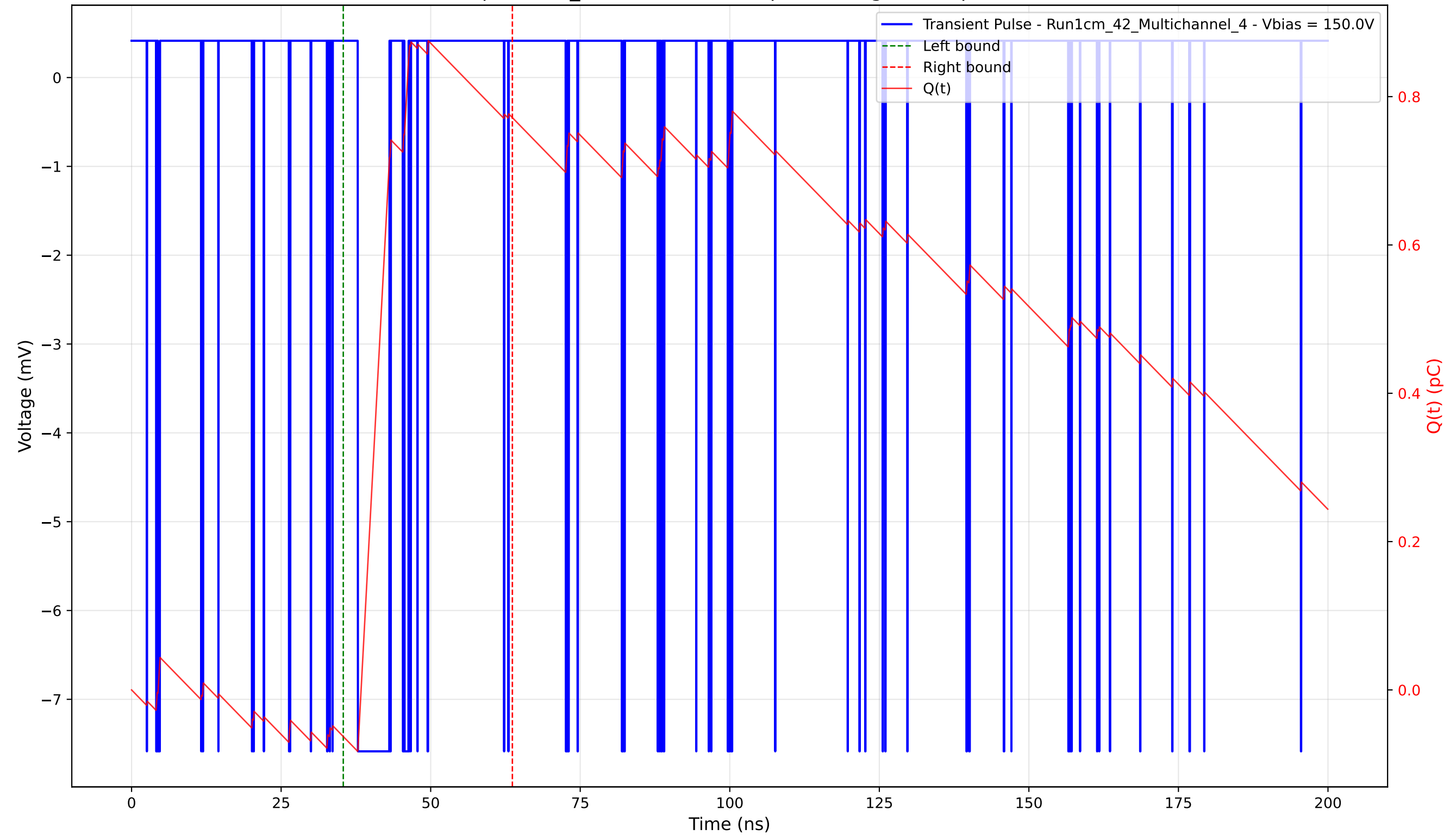
Transient Pulse - Sample: 1cm_42 - Position: 85.0 \mu\text{m} - Charge: 0.83 pC - Rise Time: 0.04 ns
