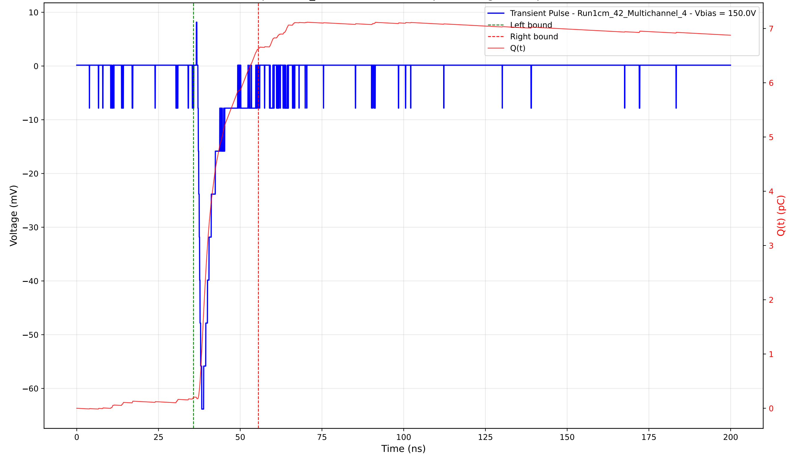
Transient Pulse - Sample: 1cm_42 - Position: 1375.0 \mu\text{m} - Charge: 6.43 pC - Rise Time: 1.17 ns
