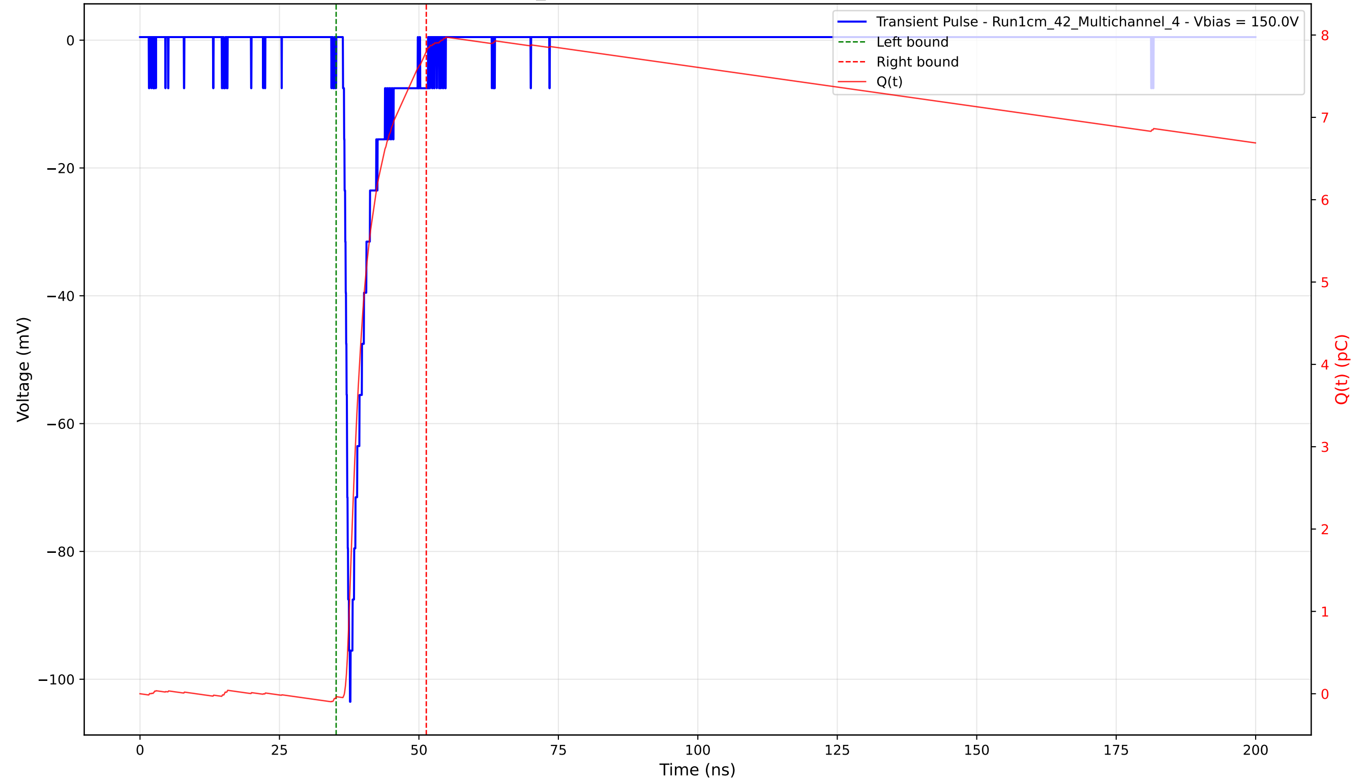
Transient Pulse - Sample: 1cm_42 - Position: 1610.0 \mu\text{m} - Charge: 7.84 pC - Rise Time: 0.91 ns
