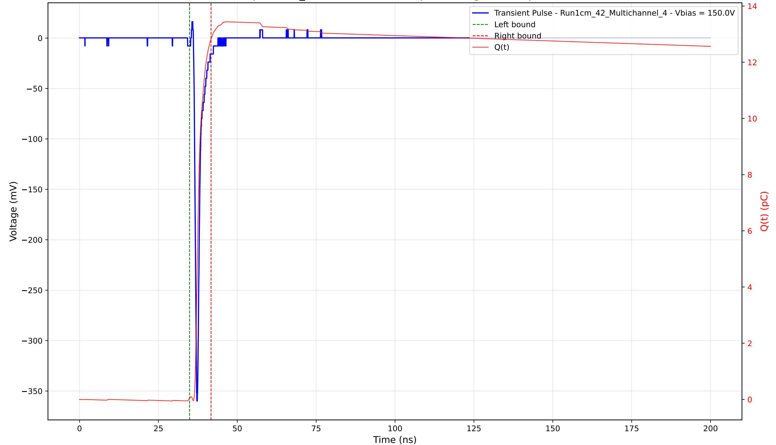
Transient Pulse - Sample: 1cm_42 - Position: 2125.0 \mu\text{m} - Charge: 12.78 pC - Rise Time: 0.76 ns
