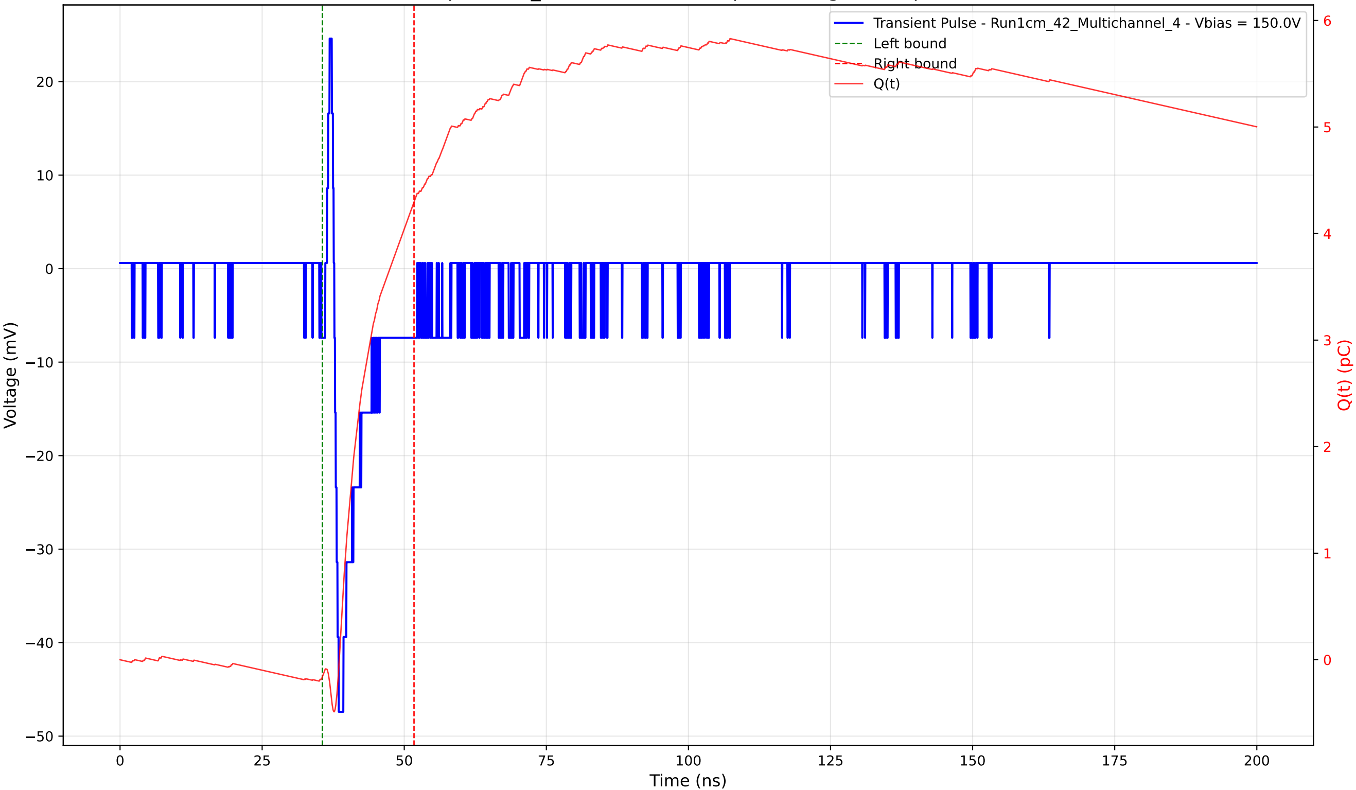
Transient Pulse - Sample: 1cm_42 - Position: 855.0 \mu\text{m} - Charge: 4.46 pC - Rise Time: 0.78 ns
