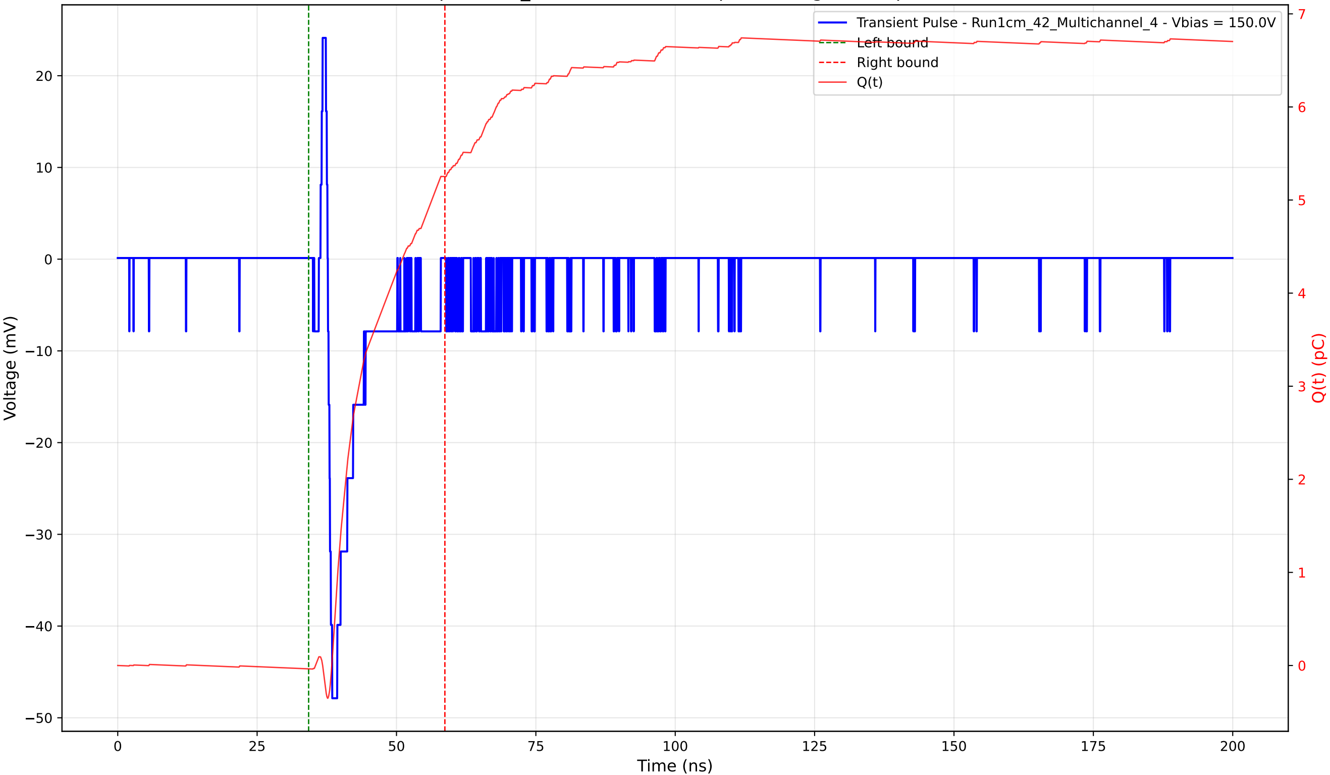
Transient Pulse - Sample: 1cm_42 - Position: 710.0 \mu\text{m} - Charge: 5.29 pC - Rise Time: 0.78 ns
