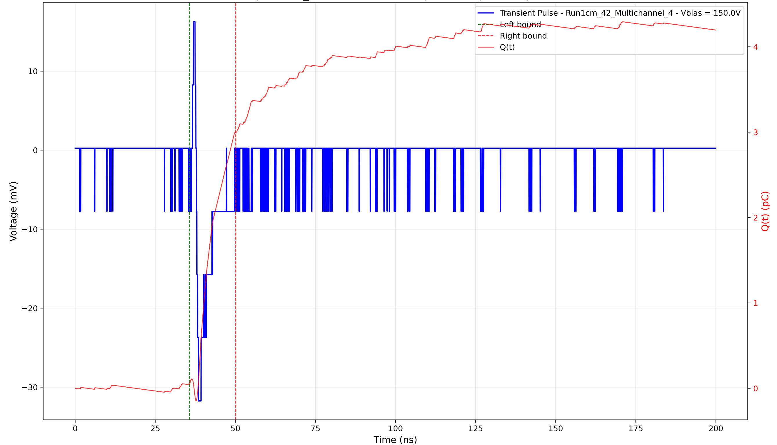
Transient Pulse - Sample: 1cm_42 - Position: 4665.0 \mu\text{m} - Charge: 2.95 pC - Rise Time: 0.66 ns
