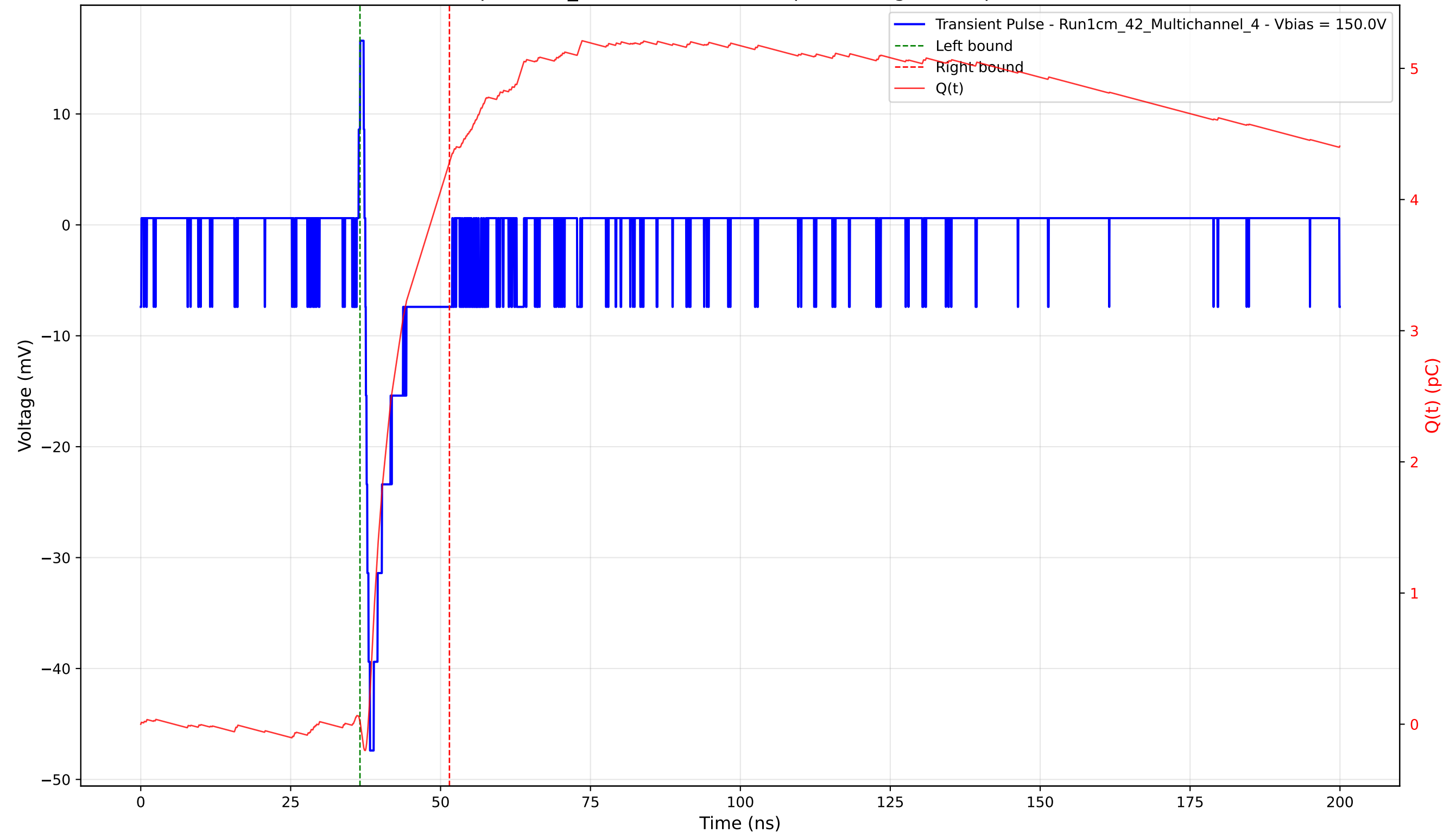
Transient Pulse - Sample: 1cm_42 - Position: 3930.0 \mu\text{m} - Charge: 4.26 pC - Rise Time: 0.78 ns
