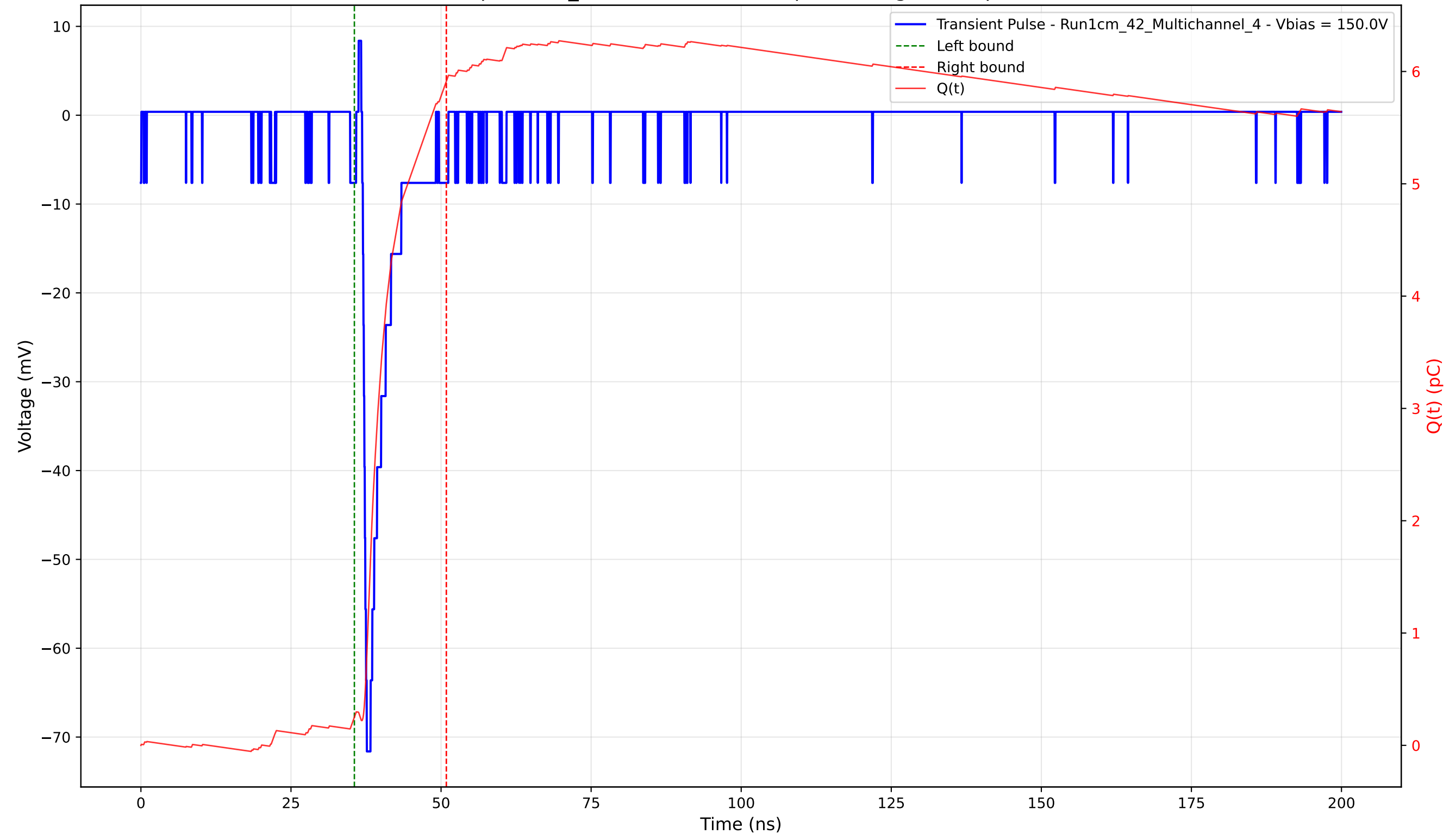
Transient Pulse - Sample: 1cm_42 - Position: 3515.0 \mu\text{m} - Charge: 5.66 pC - Rise Time: 0.76 ns
