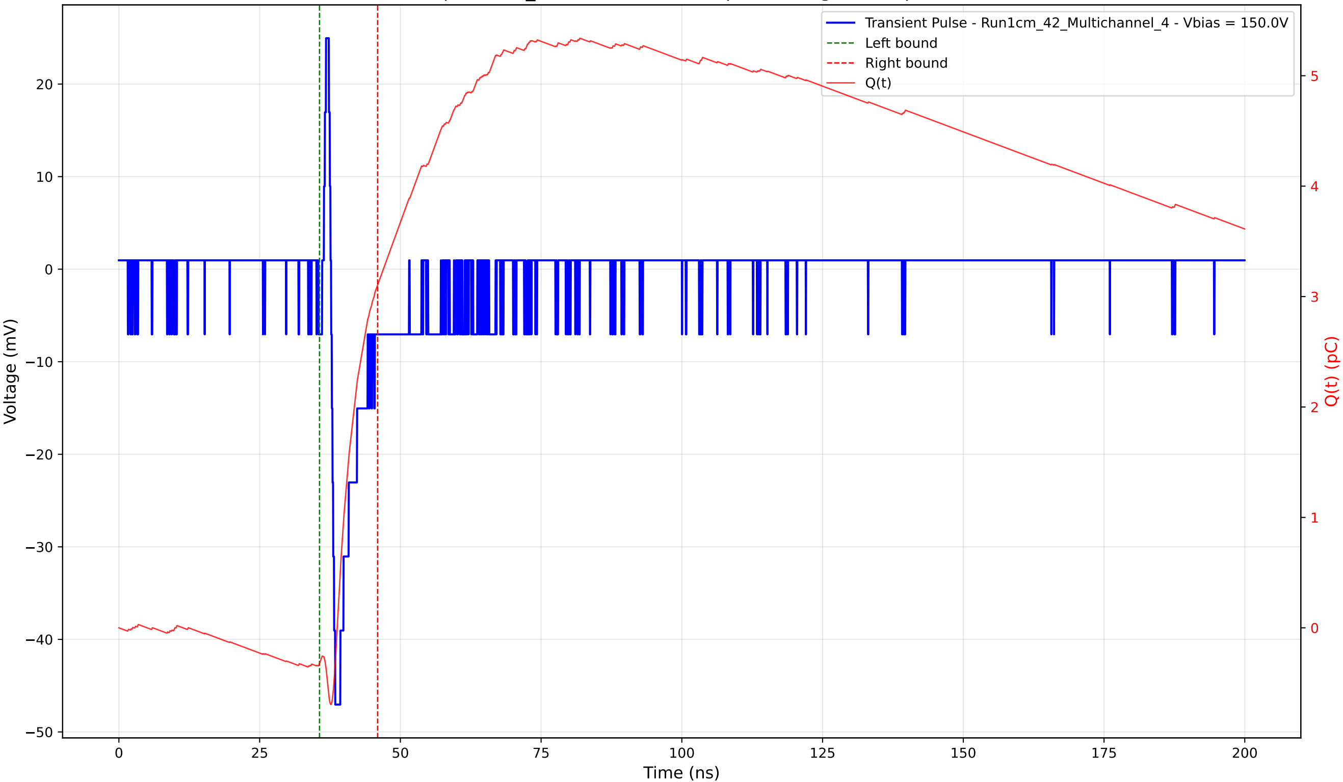
Transient Pulse - Sample: 1cm_42 - Position: 810.0 \mu\text{m} - Charge: 3.43 pC - Rise Time: 0.74 ns
