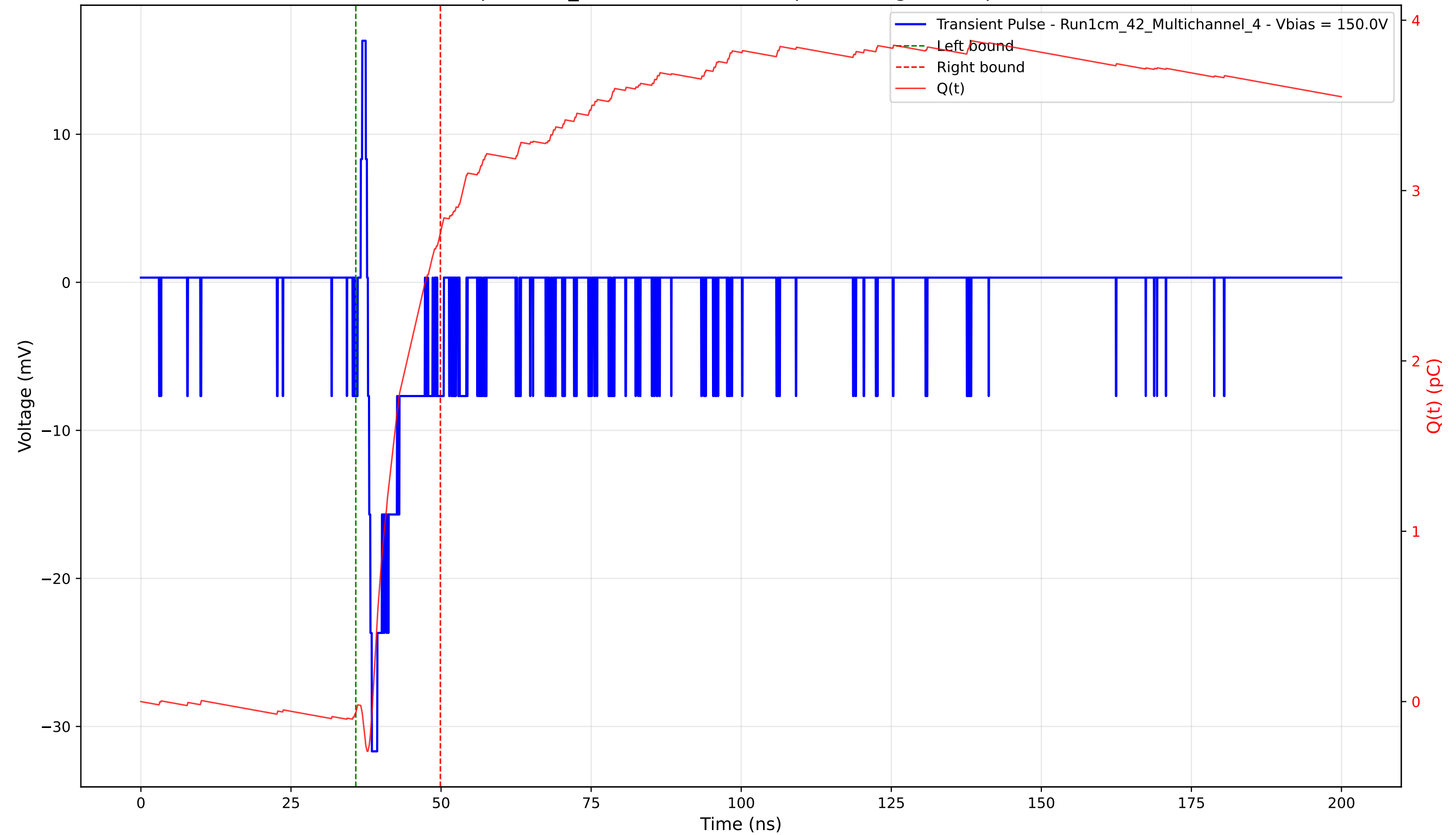
Transient Pulse - Sample: 1cm_42 - Position: 4680.0 \mu\text{m} - Charge: 2.82 pC - Rise Time: 0.66 ns
