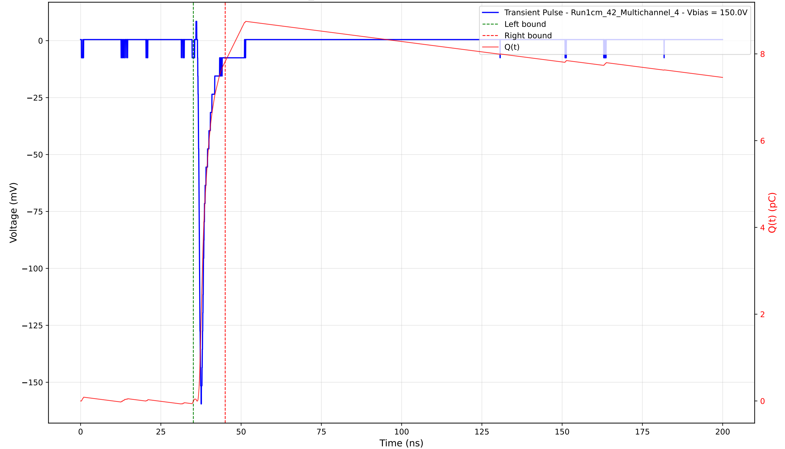
Transient Pulse - Sample: 1cm_42 - Position: 3185.0 \mu\text{m} - Charge: 7.83 pC - Rise Time: 0.84 ns
