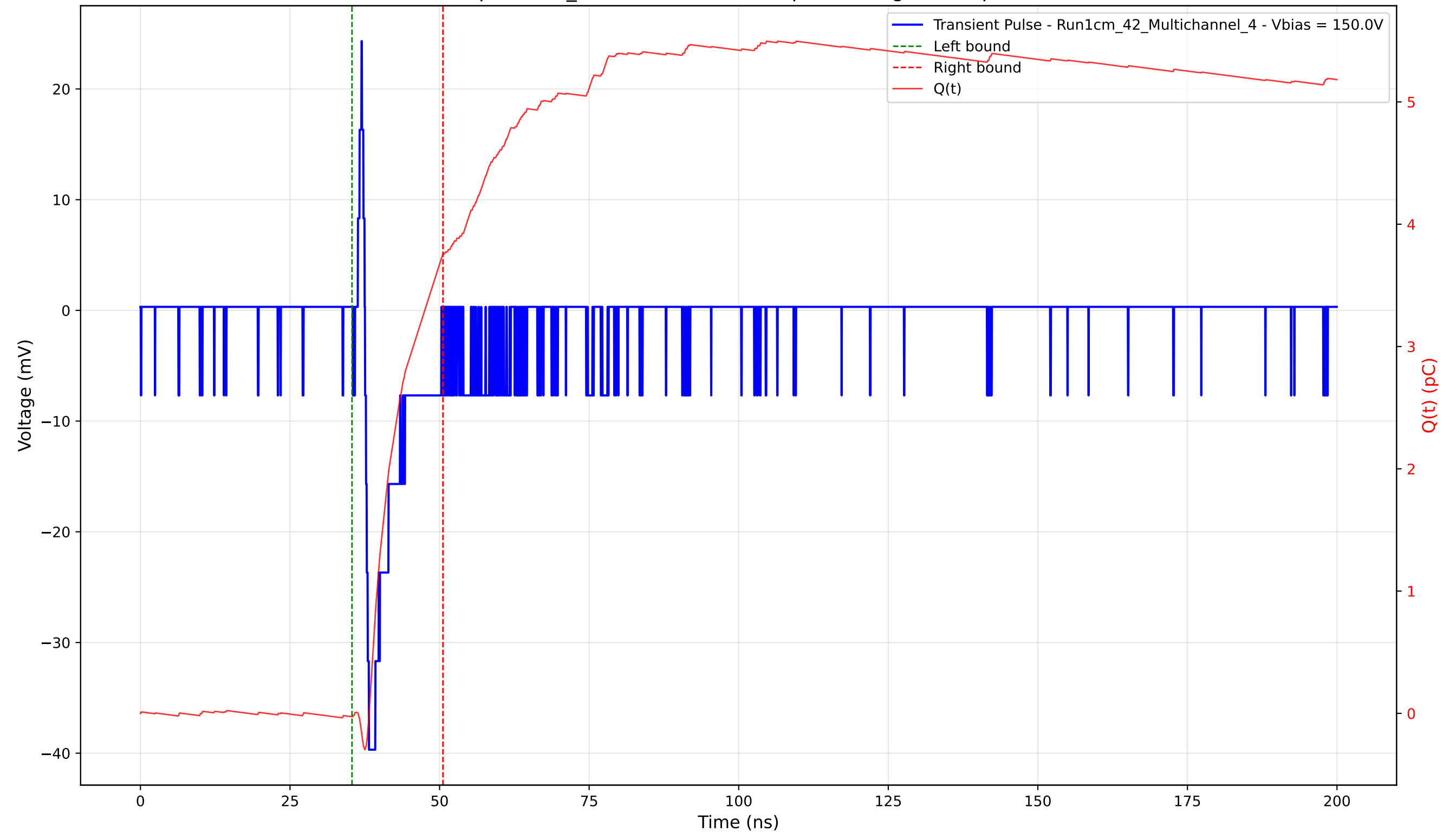
Transient Pulse - Sample: 1cm_42 - Position: 4015.0 \mu\text{m} - Charge: 3.78 pC - Rise Time: 0.66 ns
