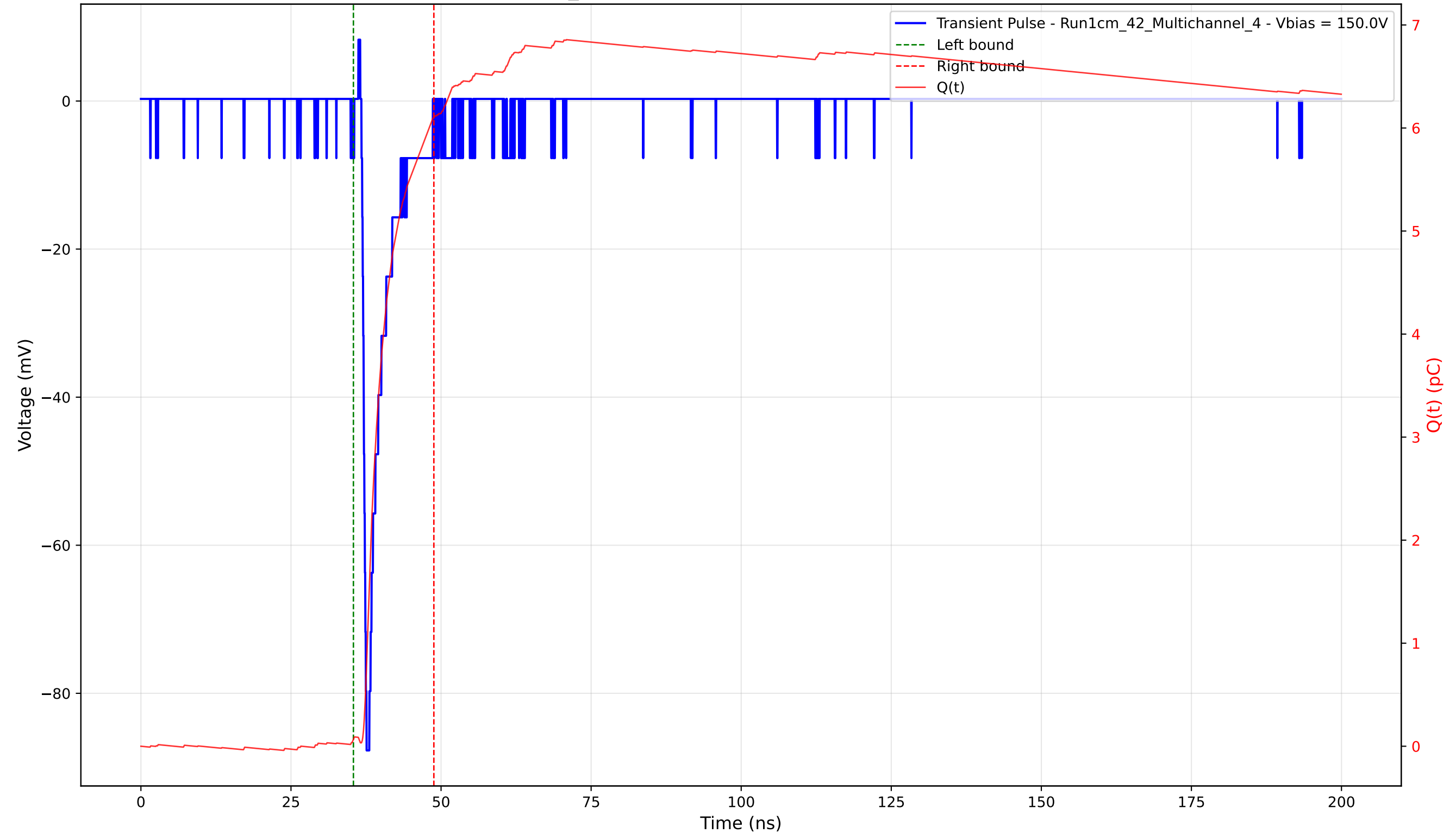
Transient Pulse - Sample: 1cm_42 - Position: 3455.0 \mu\text{m} - Charge: 6.03 pC - Rise Time: 0.63 ns
