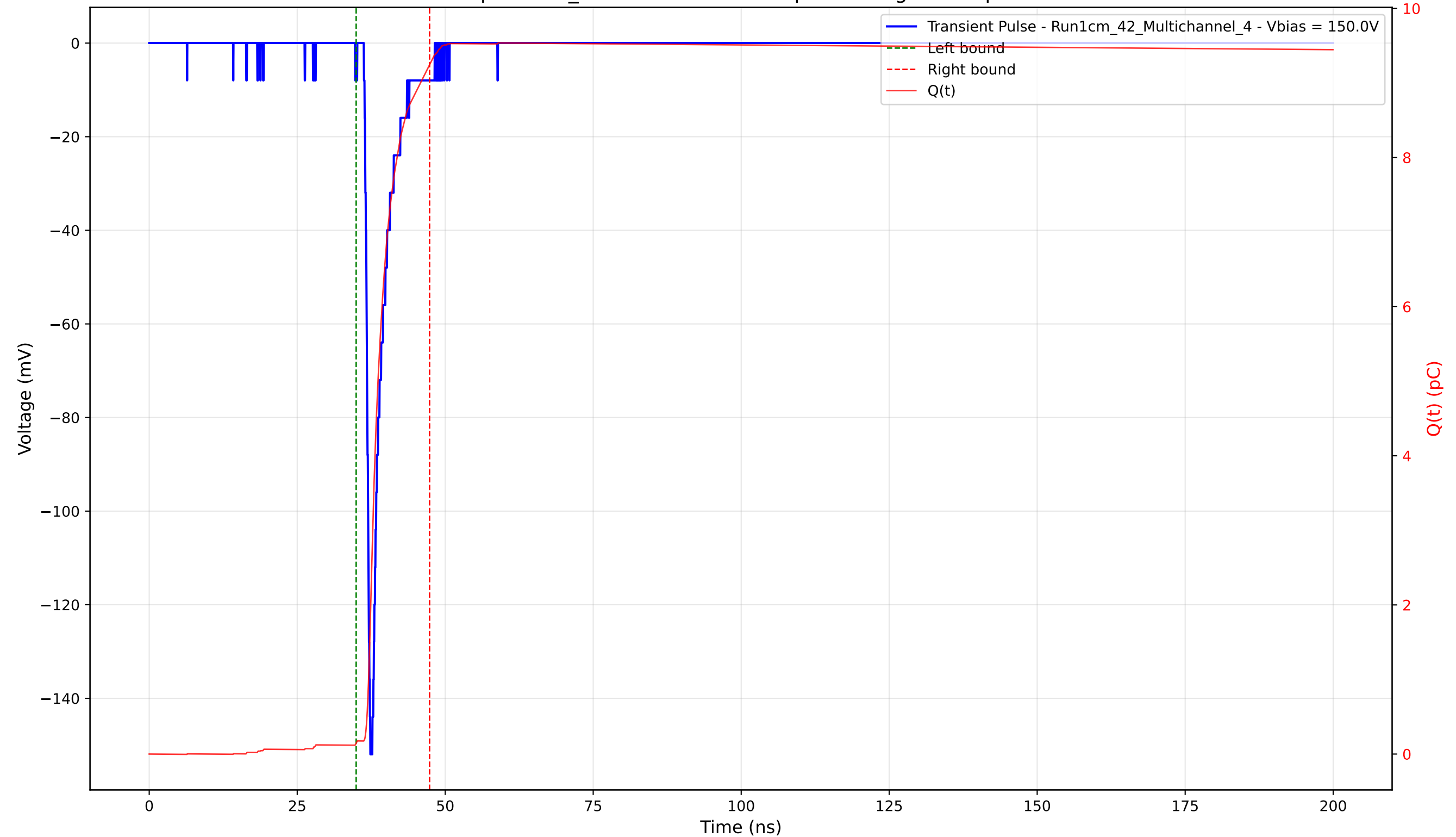
Transient Pulse - Sample: 1cm_42 - Position: 1830.0 \mu\text{m} - Charge: 9.10 pC - Rise Time: 0.88 ns
