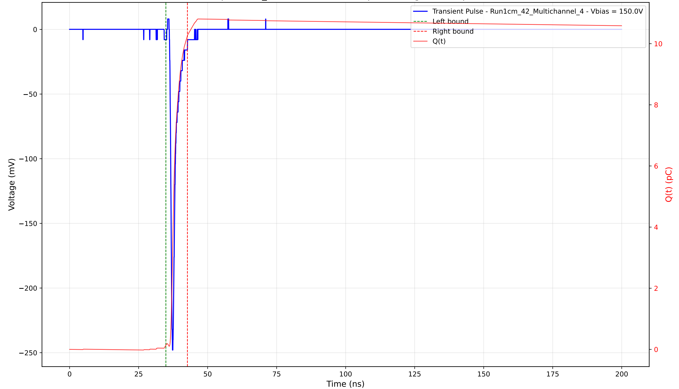
Transient Pulse - Sample: 1cm_42 - Position: 2030.0 \mu\text{m} - Charge: 10.13 pC - Rise Time: 0.75 ns
