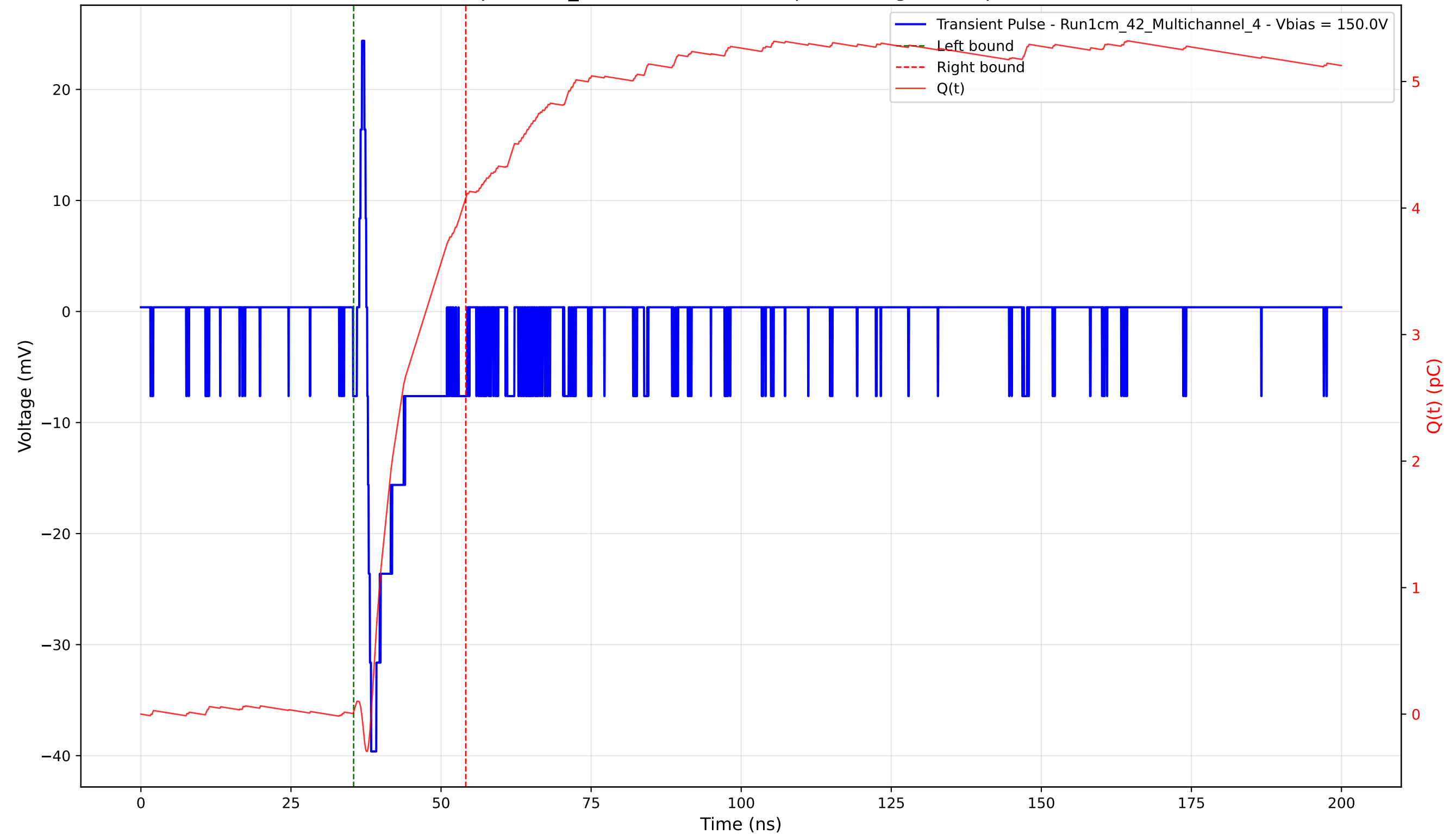
Transient Pulse - Sample: 1cm_42 - Position: 4160.0 \mu\text{m} - Charge: 4.06 pC - Rise Time: 0.66 ns
