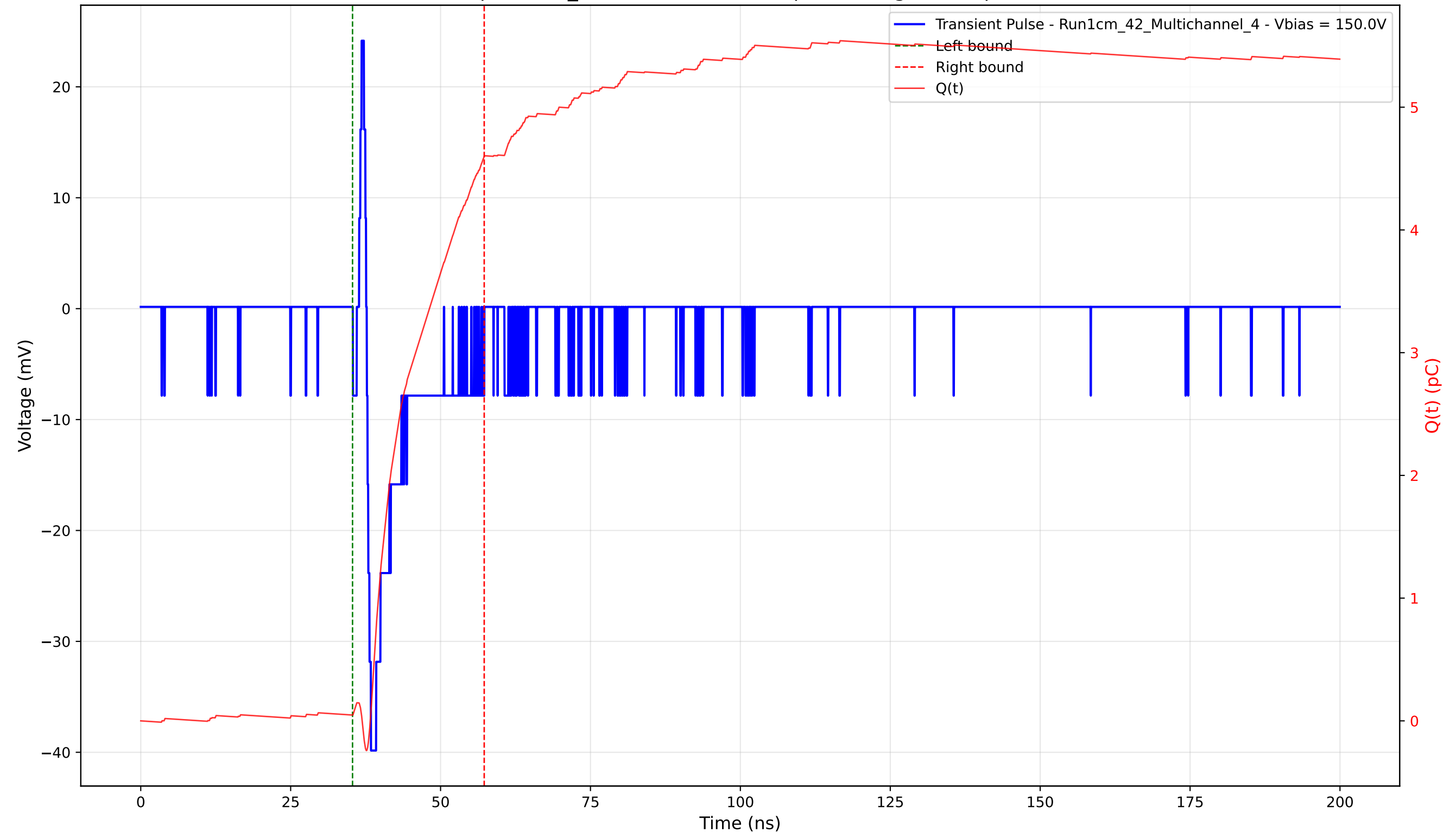
Transient Pulse - Sample: 1cm_42 - Position: 4170.0 \mu\text{m} - Charge: 4.55 pC - Rise Time: 0.70 ns
