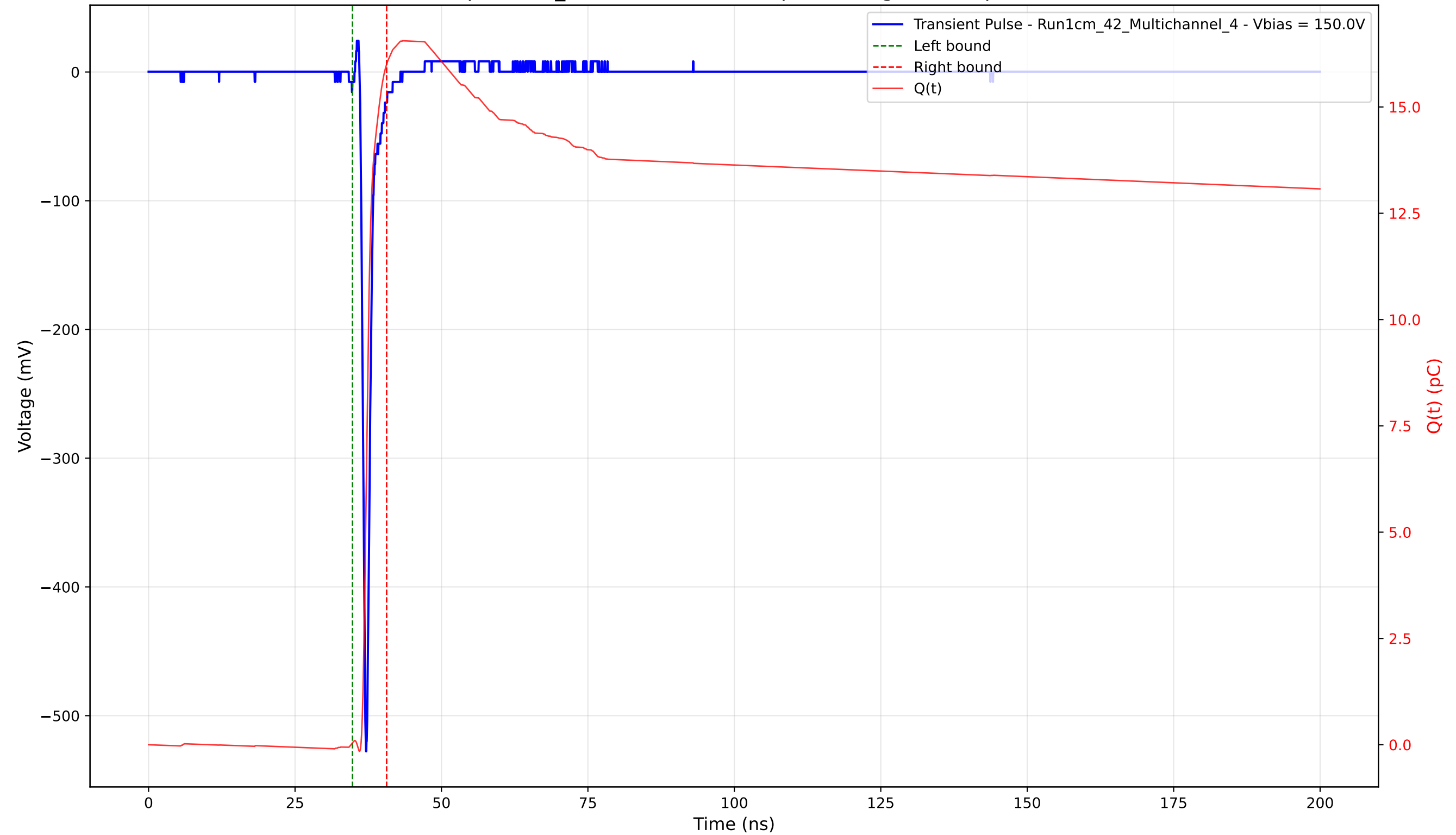
Transient Pulse - Sample: 1cm_42 - Position: 2570.0 \mu\text{m} - Charge: 15.96 pC - Rise Time: 0.72 ns
