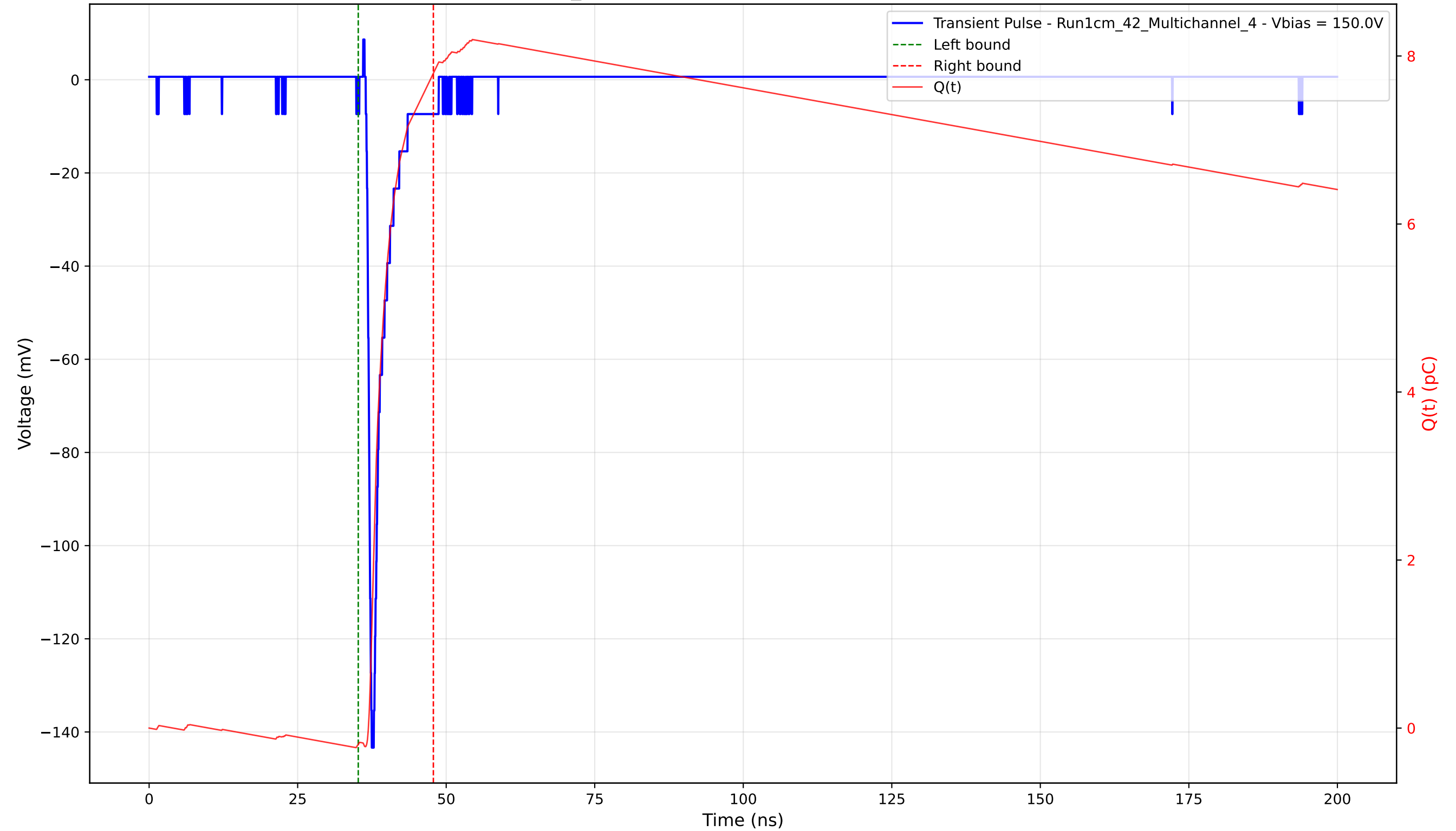
Transient Pulse - Sample: 1cm_42 - Position: 3250.0 \mu\text{m} - Charge: 7.99 pC - Rise Time: 0.81 ns
