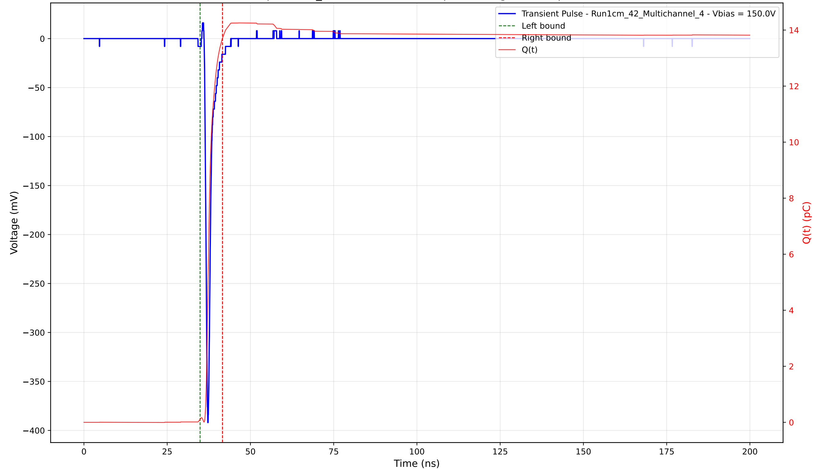
Transient Pulse - Sample: 1cm_42 - Position: 2150.0 \mu\text{m} - Charge: 13.60 pC - Rise Time: 0.76 ns
