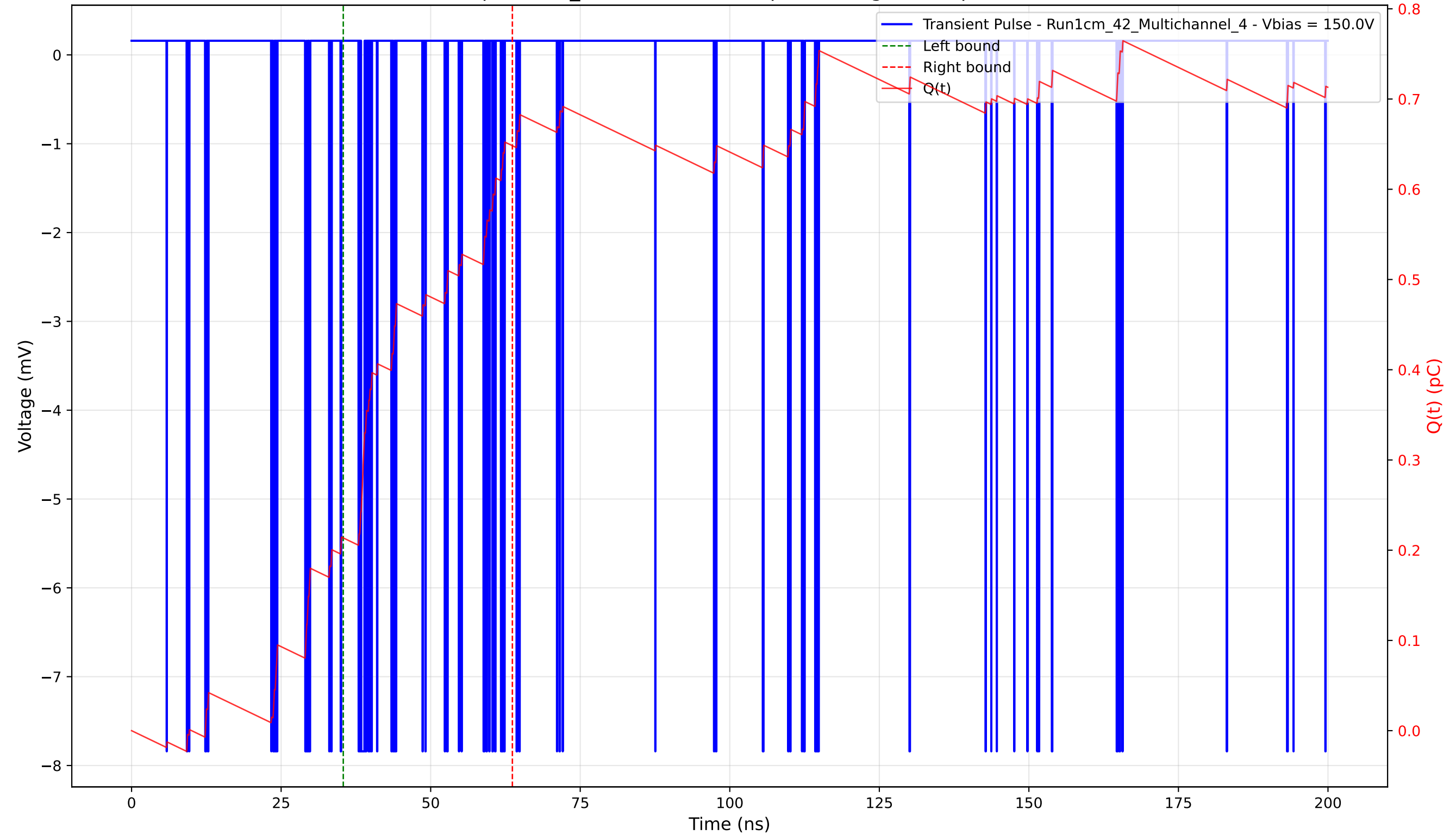
Transient Pulse - Sample: 1cm_42 - Position: 10.0 \mu\text{m} - Charge: 0.43 pC - Rise Time: 0.04 ns
