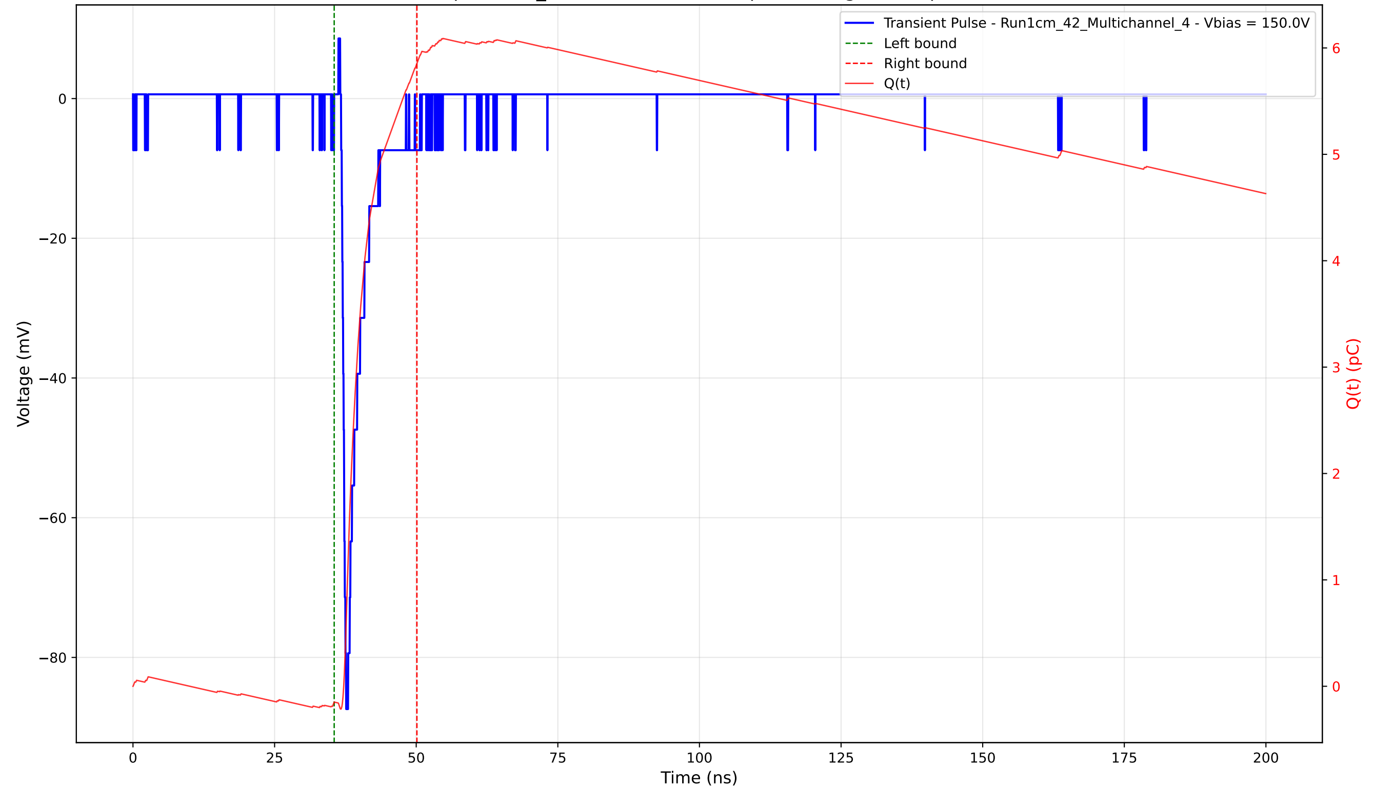
Transient Pulse - Sample: 1cm_42 - Position: 3460.0 \mu\text{m} - Charge: 6.00 pC - Rise Time: 0.67 ns
