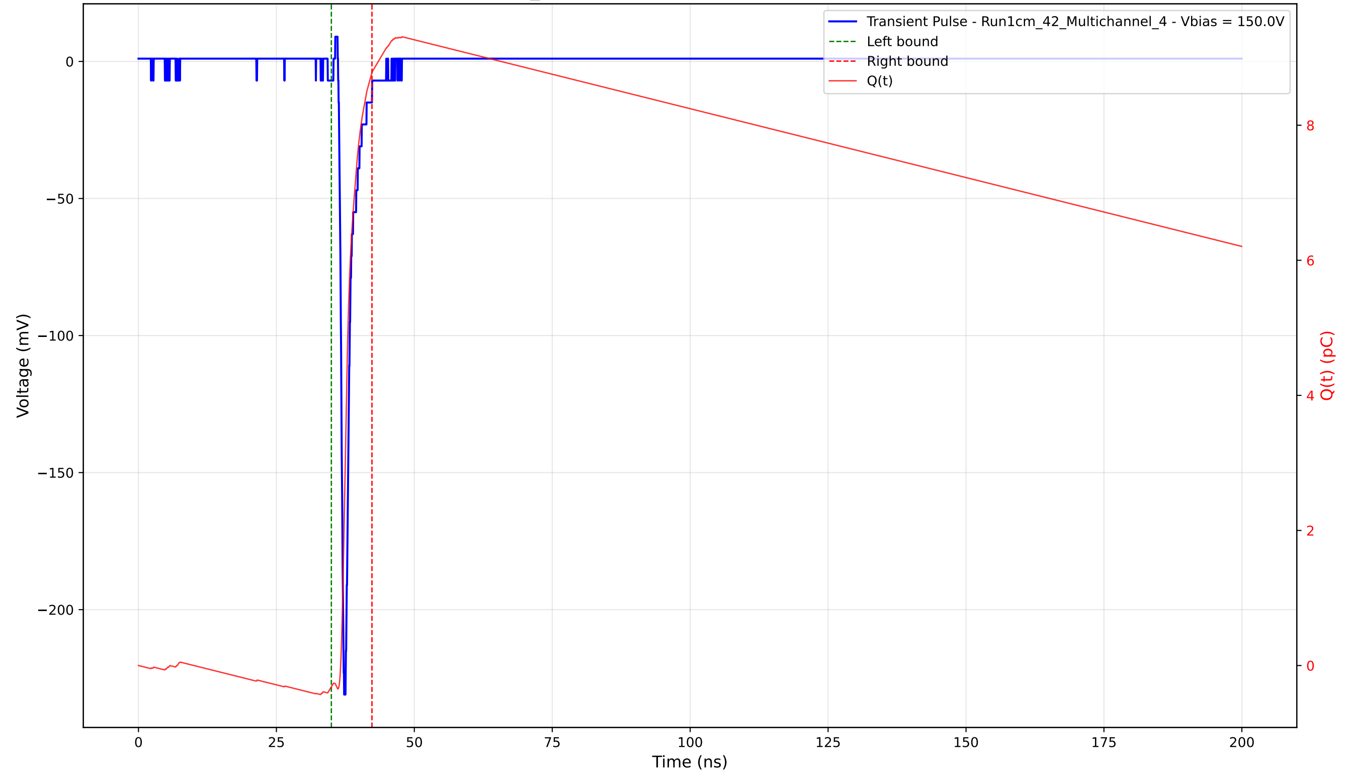
Transient Pulse - Sample: 1cm_42 - Position: 3005.0 \mu\text{m} - Charge: 9.09 pC - Rise Time: 0.76 ns
