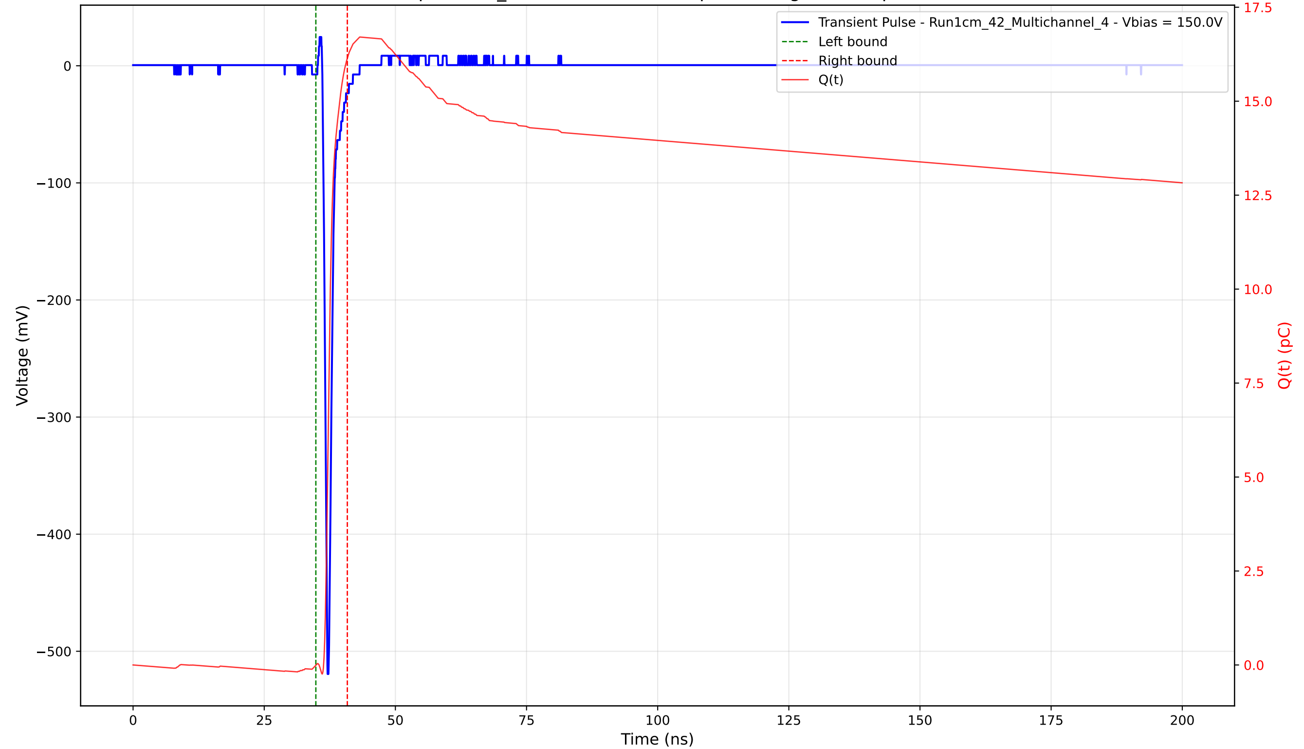
Transient Pulse - Sample: 1cm_42 - Position: 2375.0 \mu\text{m} - Charge: 16.15 pC - Rise Time: 0.72 ns
