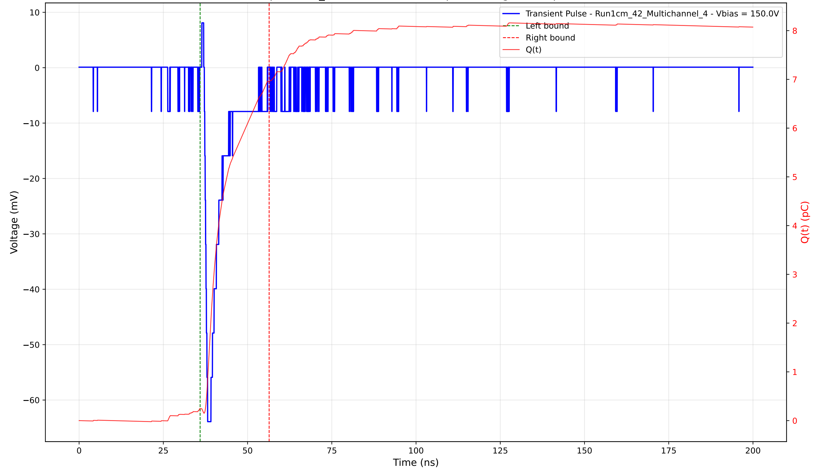
Transient Pulse - Sample: 1cm_42 - Position: 1310.0 \mu\text{m} - Charge: 6.72 pC - Rise Time: 0.97 ns
