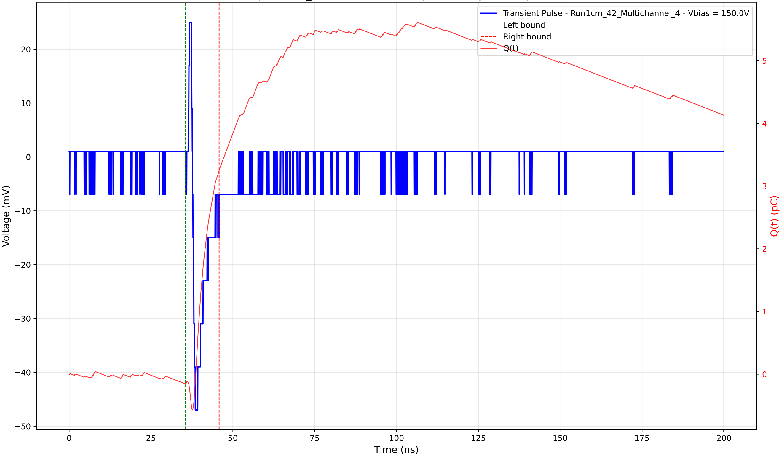
Transient Pulse - Sample: 1cm_42 - Position: 820.0 \mu\text{m} - Charge: 3.41 pC - Rise Time: 0.82 ns
