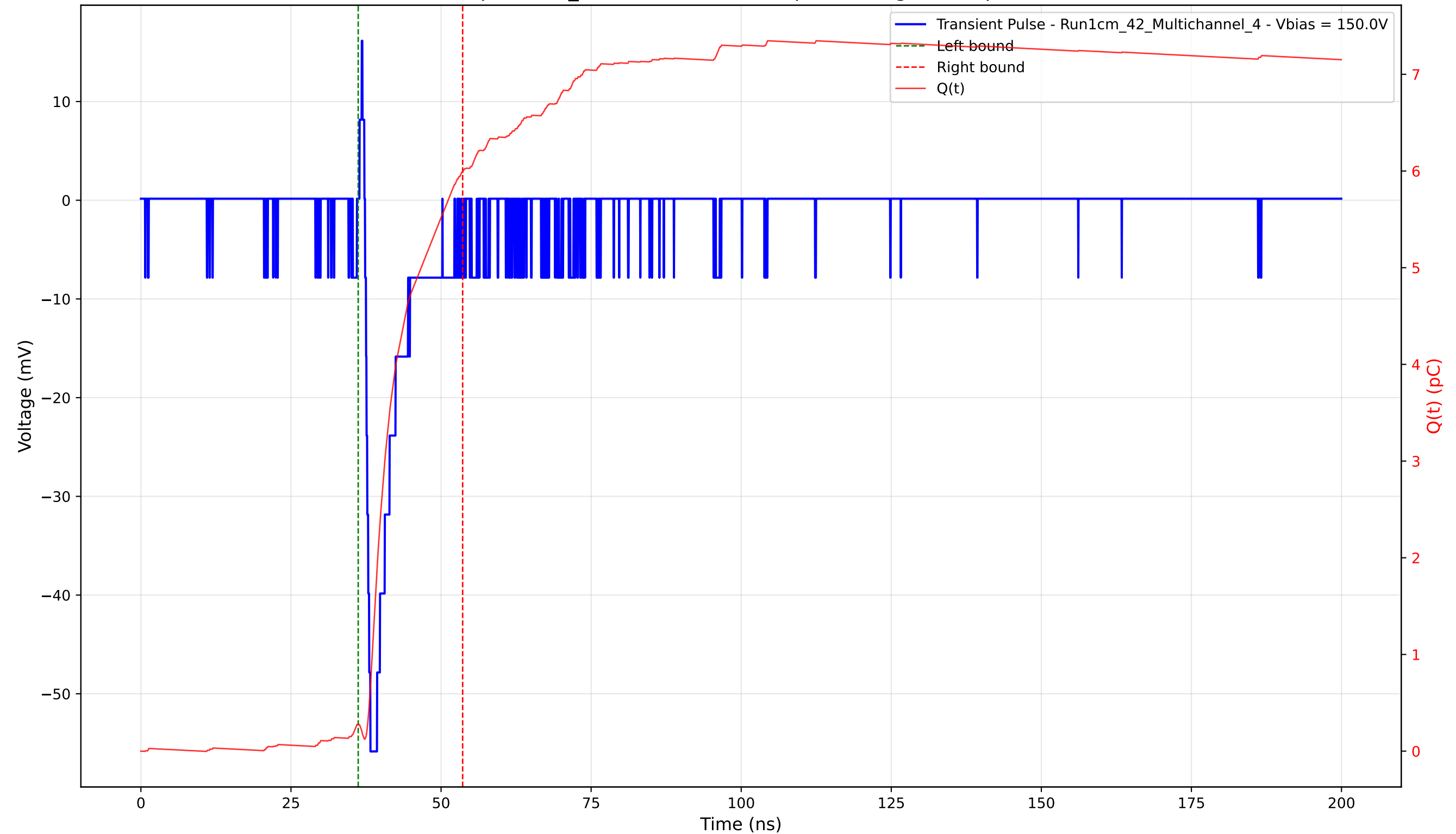
Transient Pulse - Sample: 1cm_42 - Position: 1145.0 \mu\text{m} - Charge: 5.71 pC - Rise Time: 0.89 ns
