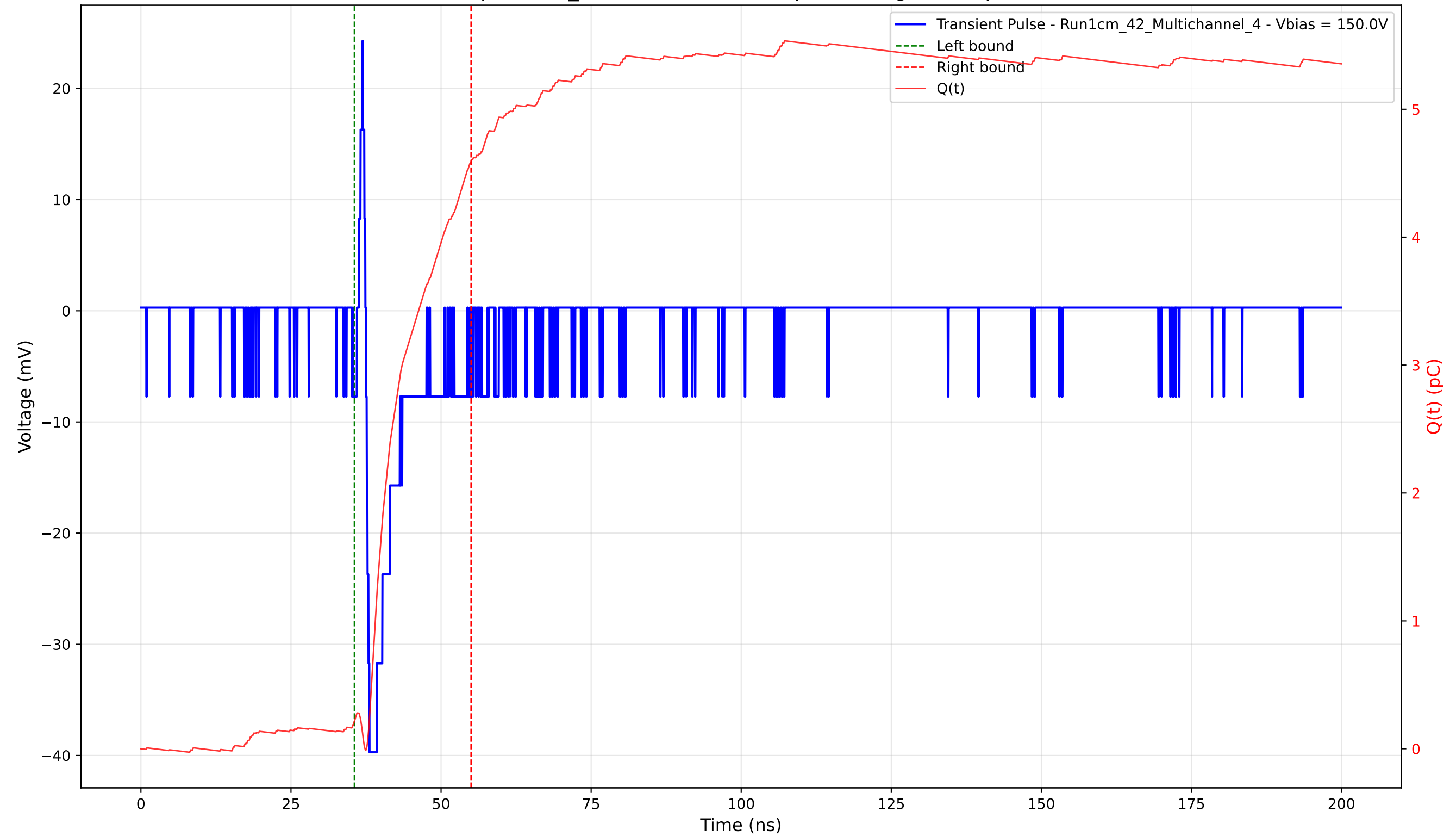
Transient Pulse - Sample: 1cm_42 - Position: 3975.0 \mu\text{m} - Charge: 4.37 pC - Rise Time: 0.58 ns
