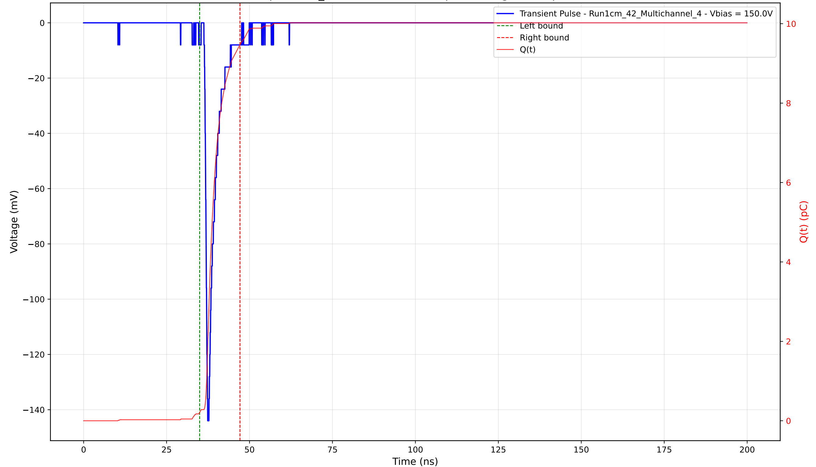
Transient Pulse - Sample: 1cm_42 - Position: 1740.0 \mu\text{m} - Charge: 9.27 pC - Rise Time: 0.89 ns
