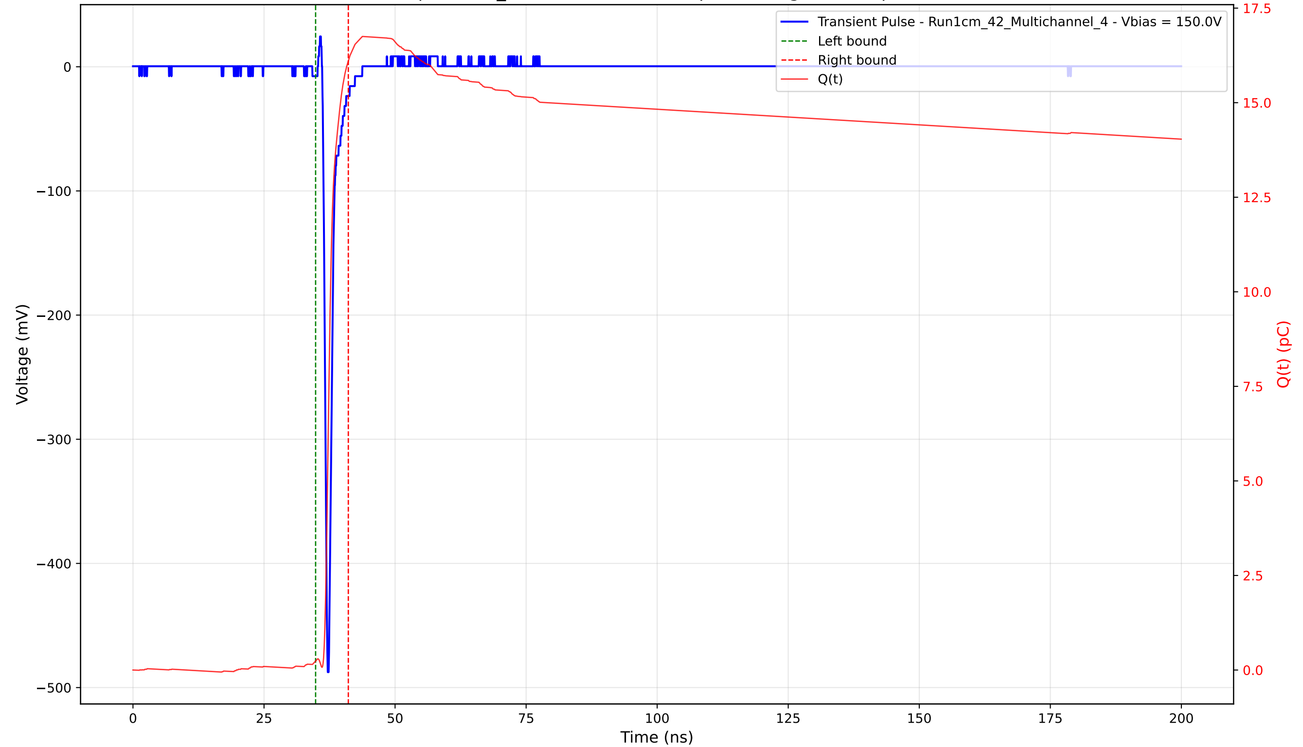
Transient Pulse - Sample: 1cm_42 - Position: 2755.0 \mu\text{m} - Charge: 15.87 pC - Rise Time: 0.74 ns
