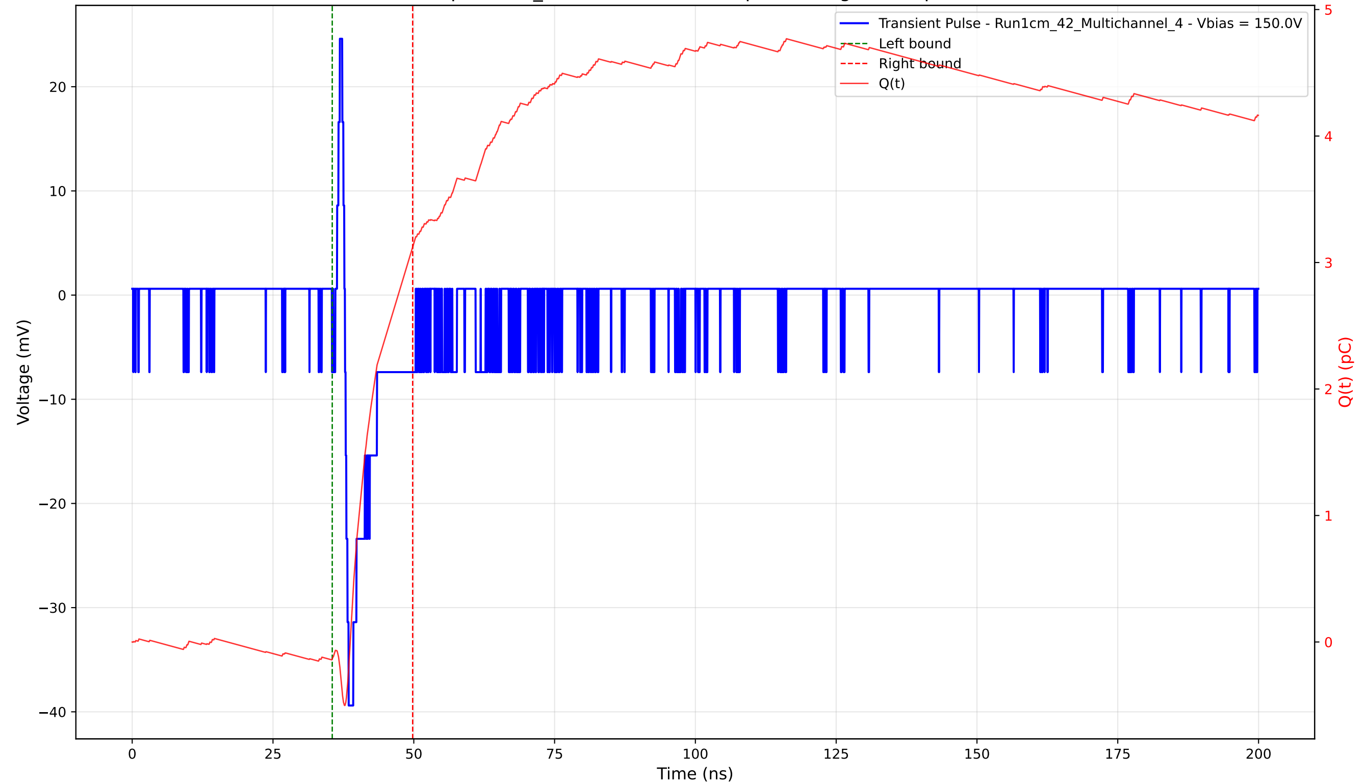
Transient Pulse - Sample: 1cm_42 - Position: 4350.0 \mu\text{m} - Charge: 3.26 pC - Rise Time: 0.66 ns
