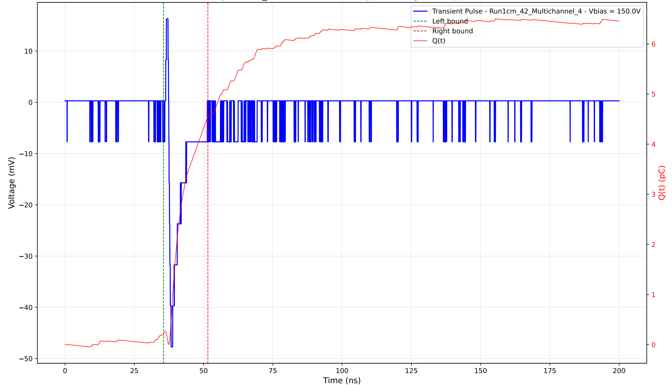
Transient Pulse - Sample: 1cm_42 - Position: 3935.0 \mu\text{m} - Charge: 4.32 pC - Rise Time: 0.82 ns
