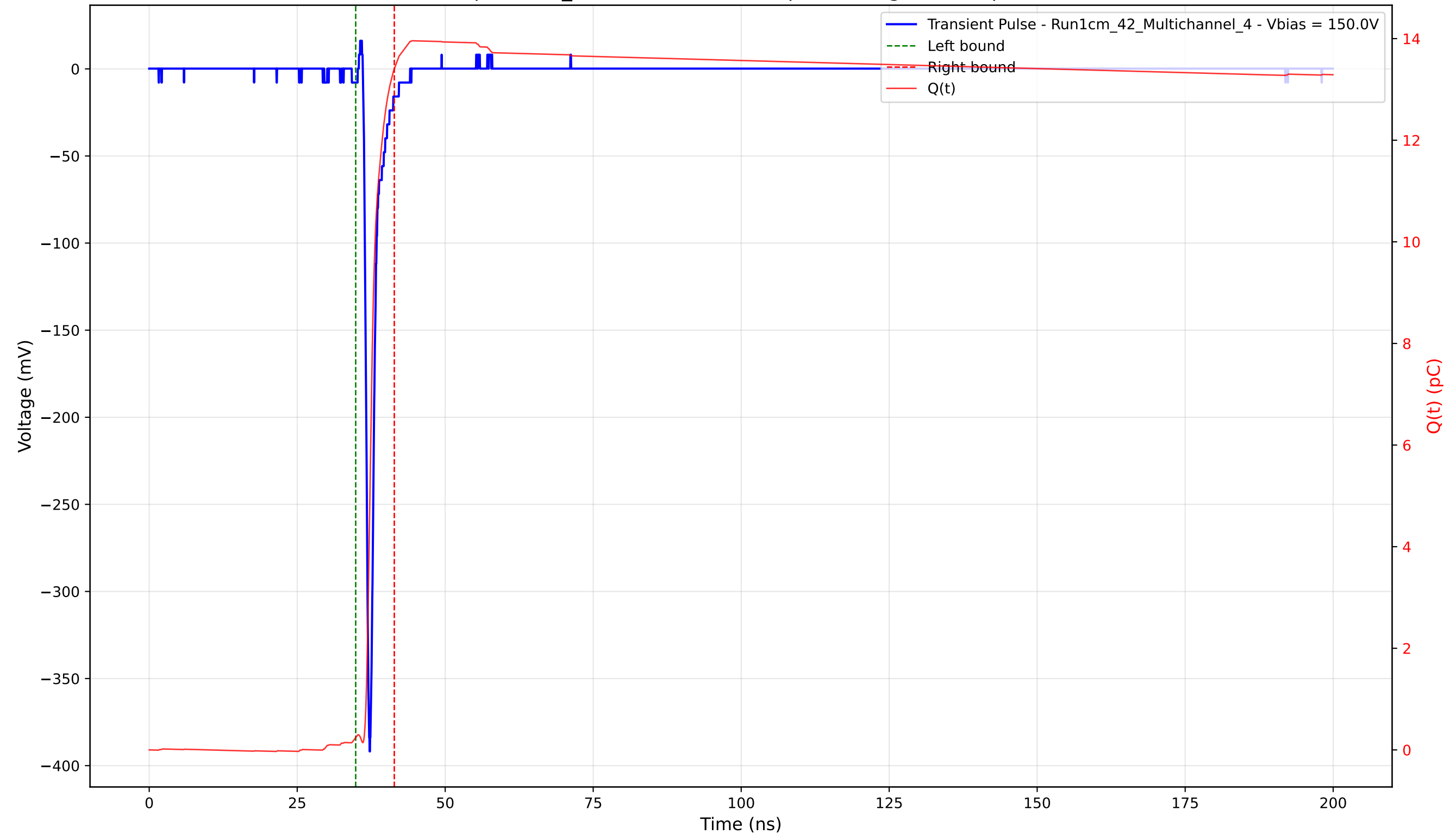
Transient Pulse - Sample: 1cm_42 - Position: 2865.0 \mu\text{m} - Charge: 13.16 pC - Rise Time: 0.73 ns
