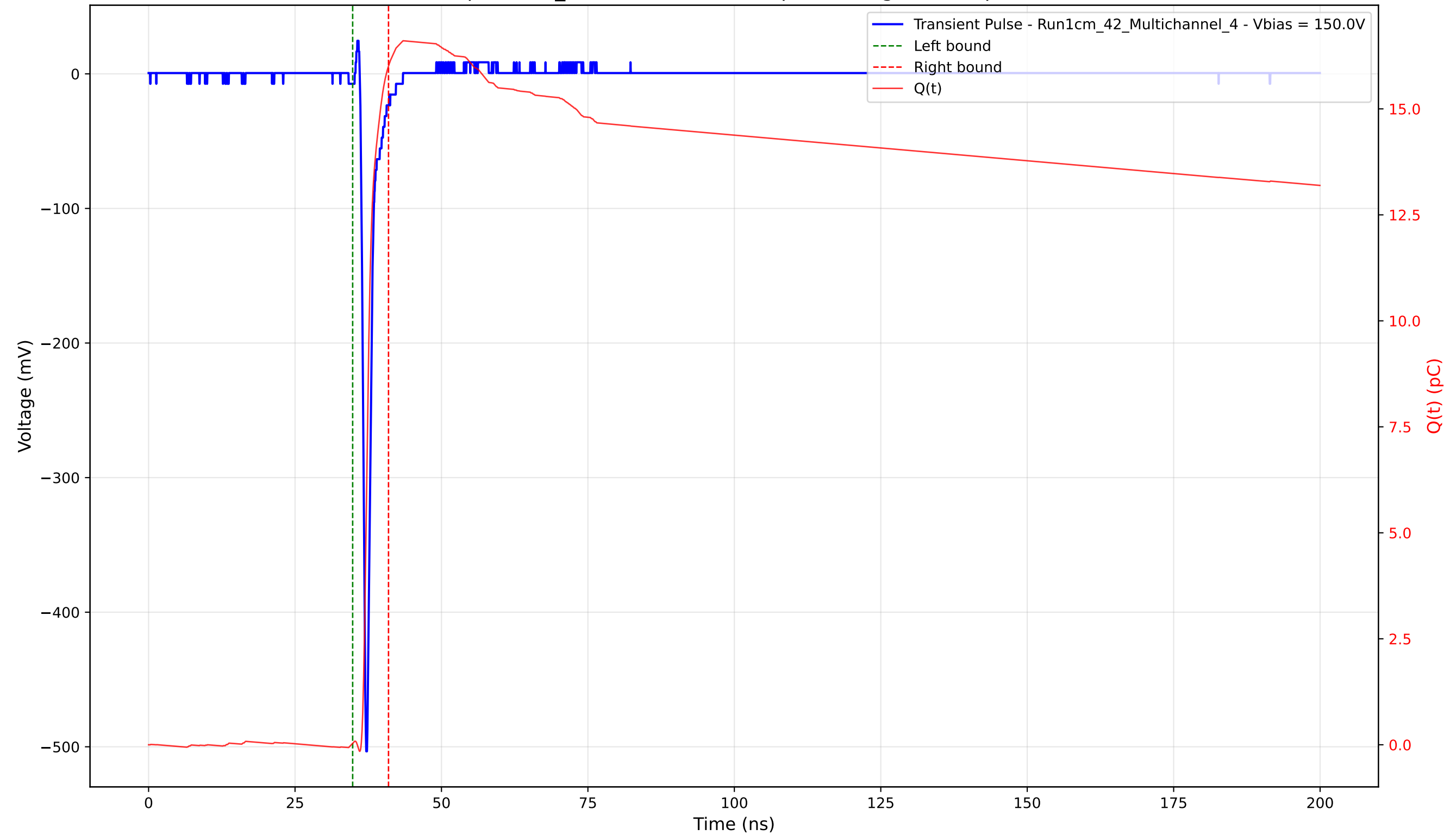
Transient Pulse - Sample: 1cm_42 - Position: 2710.0 \mu\text{m} - Charge: 15.98 pC - Rise Time: 0.75 ns
