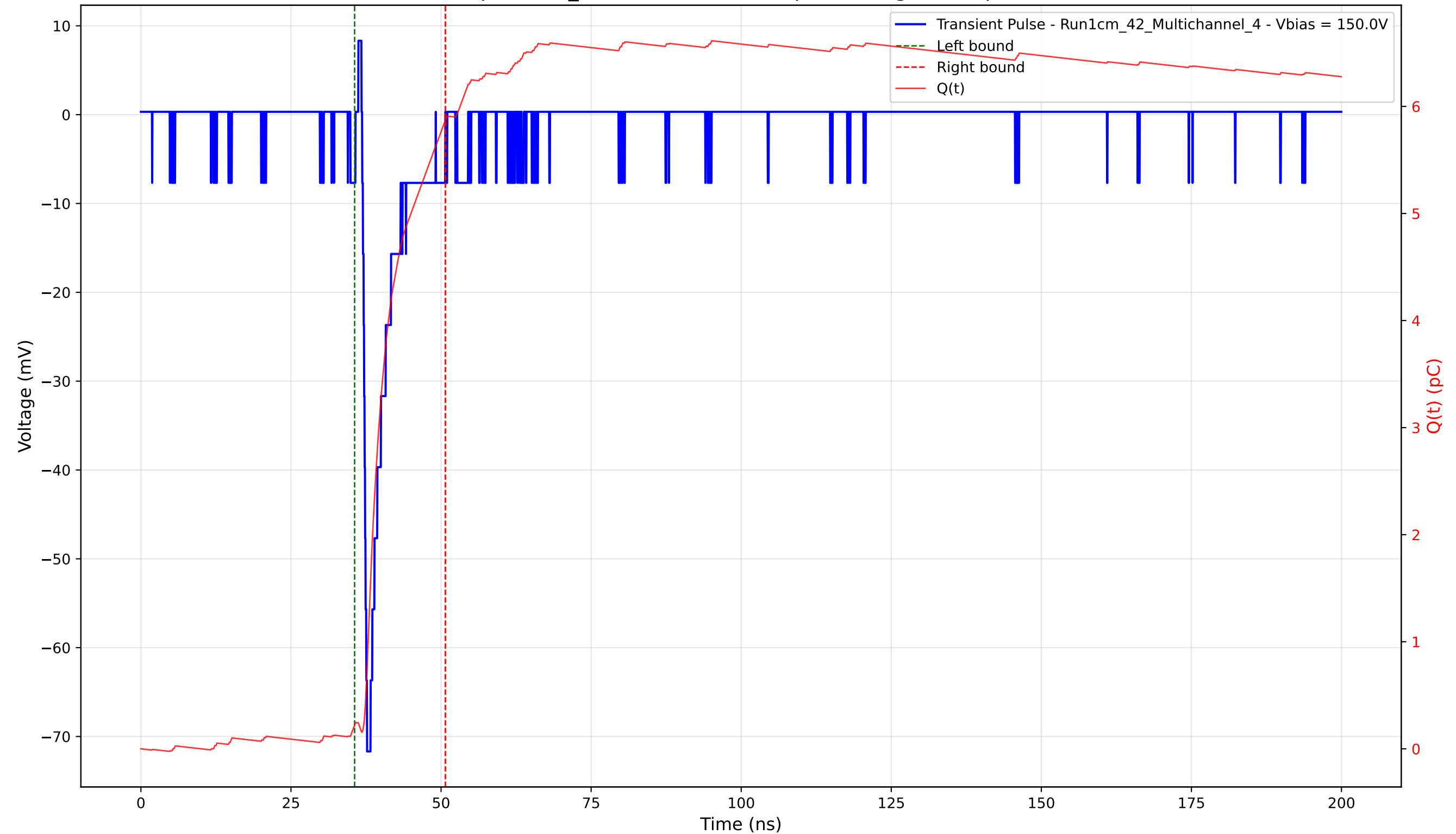
Transient Pulse - Sample: 1cm_42 - Position: 3520.0 \mu\text{m} - Charge: 5.65 pC - Rise Time: 0.80 ns
