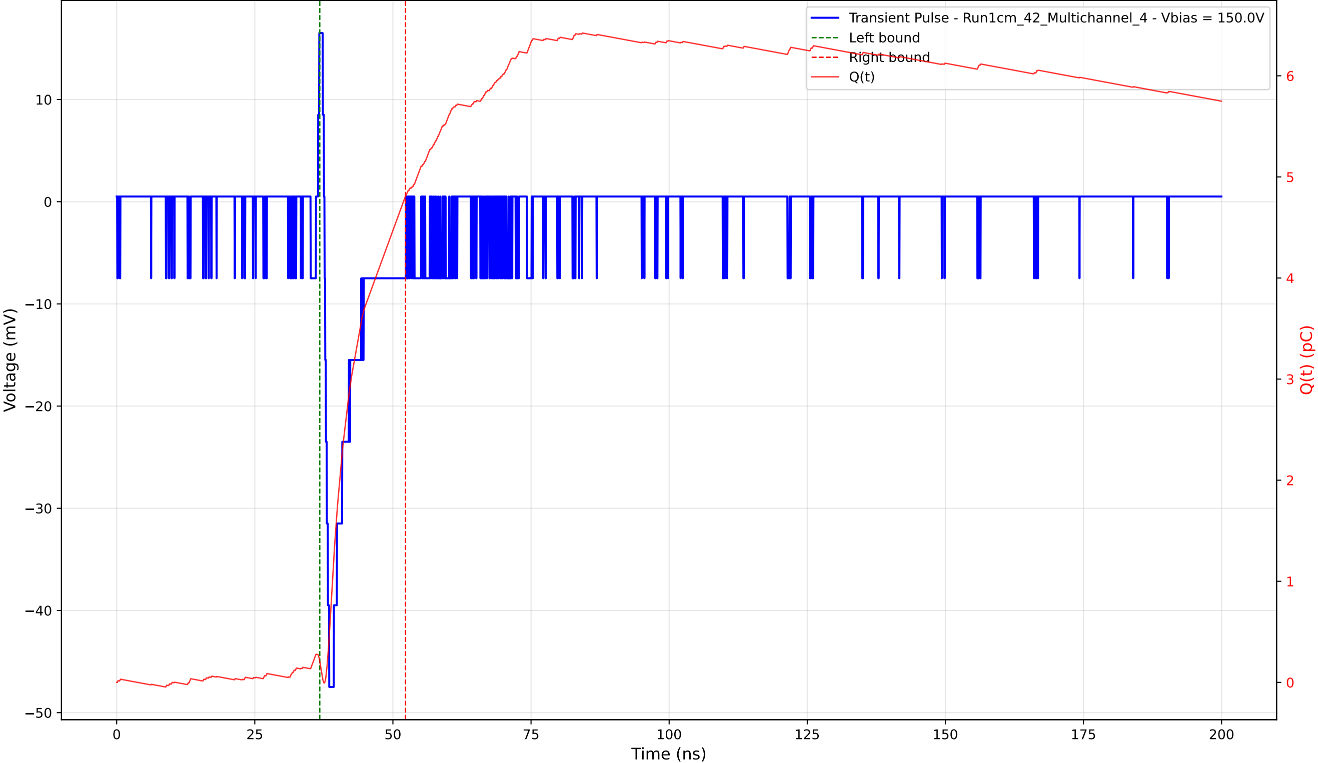
Transient Pulse - Sample: 1cm_42 - Position: 955.0 \mu\text{m} - Charge: 4.61 pC - Rise Time: 0.86 ns
