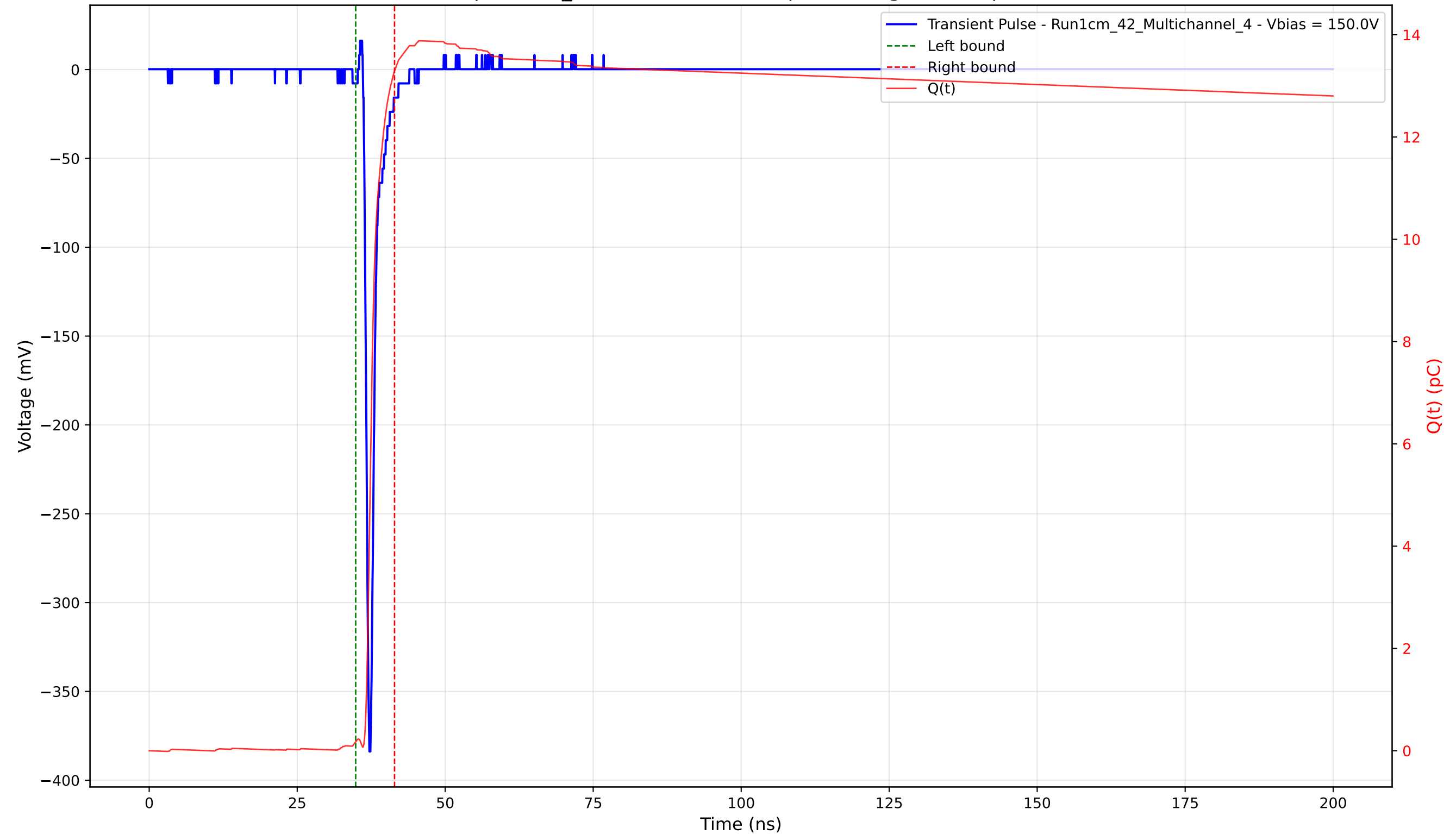
Transient Pulse - Sample: 1cm_42 - Position: 2870.0 \mu\text{m} - Charge: 13.12 pC - Rise Time: 0.74 ns
