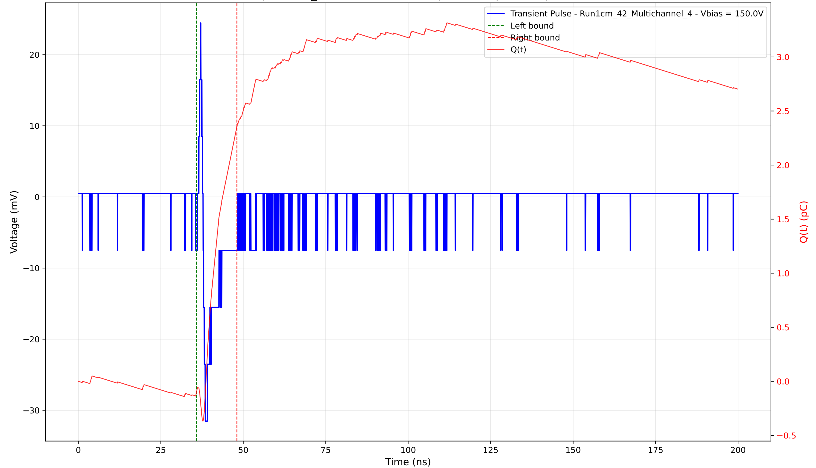
Transient Pulse - Sample: 1cm_42 - Position: 4510.0 \mu\text{m} - Charge: 2.46 pC - Rise Time: 0.66 ns
