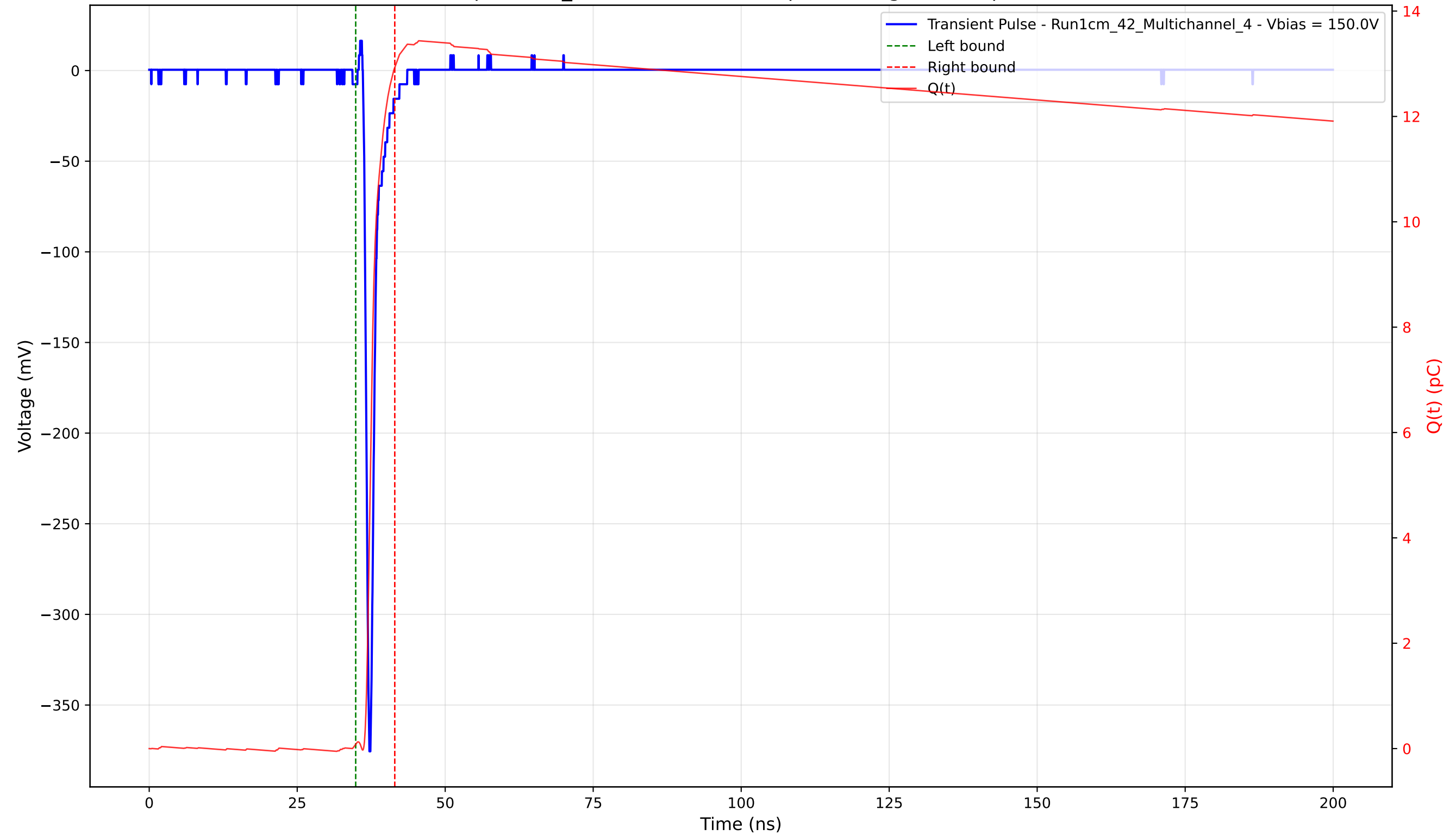
Transient Pulse - Sample: 1cm_42 - Position: 2875.0 \mu\text{m} - Charge: 12.85 pC - Rise Time: 0.74 ns
