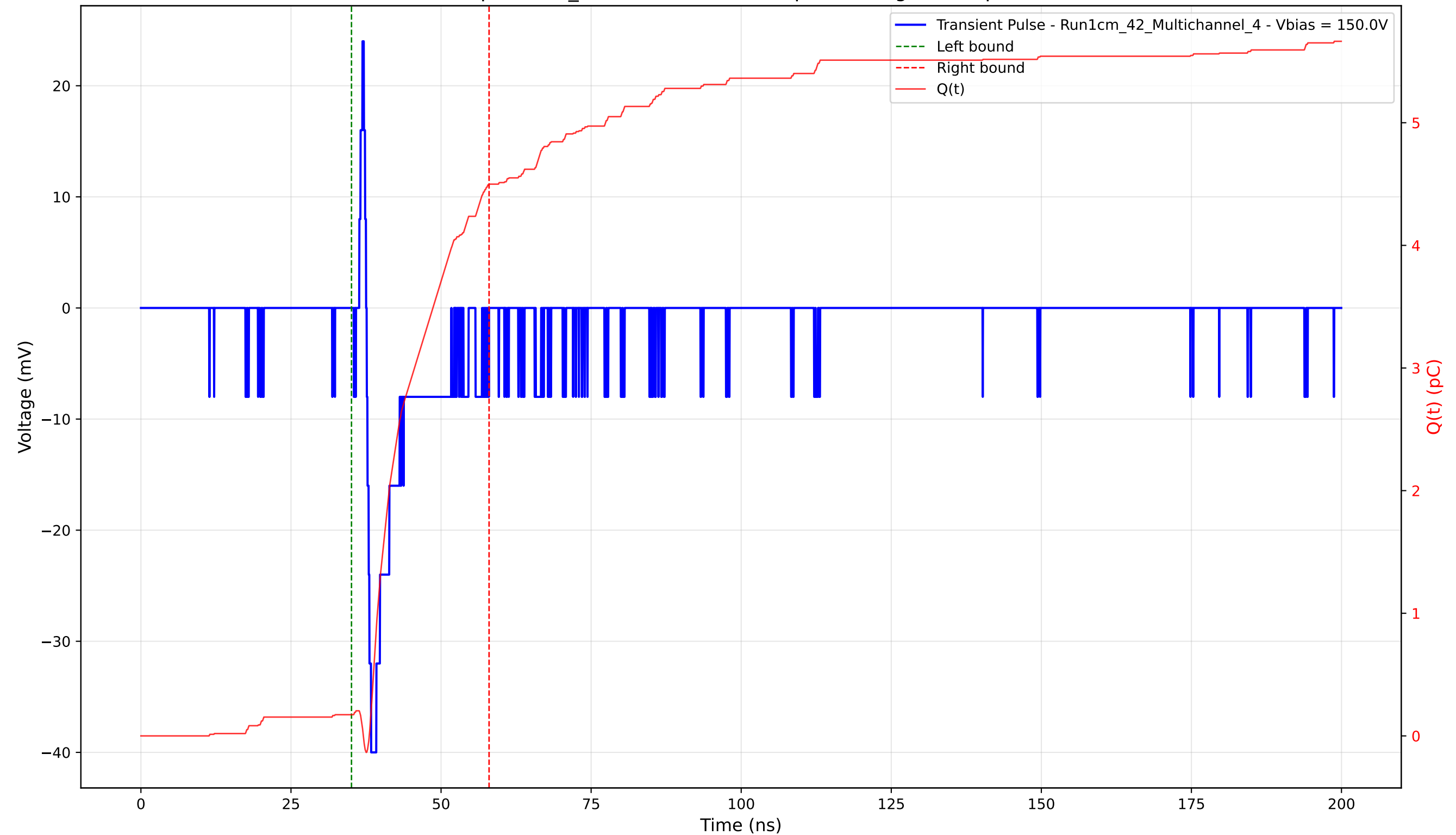
Transient Pulse - Sample: 1cm_42 - Position: 4095.0 \mu\text{m} - Charge: 4.33 pC - Rise Time: 0.74 ns
