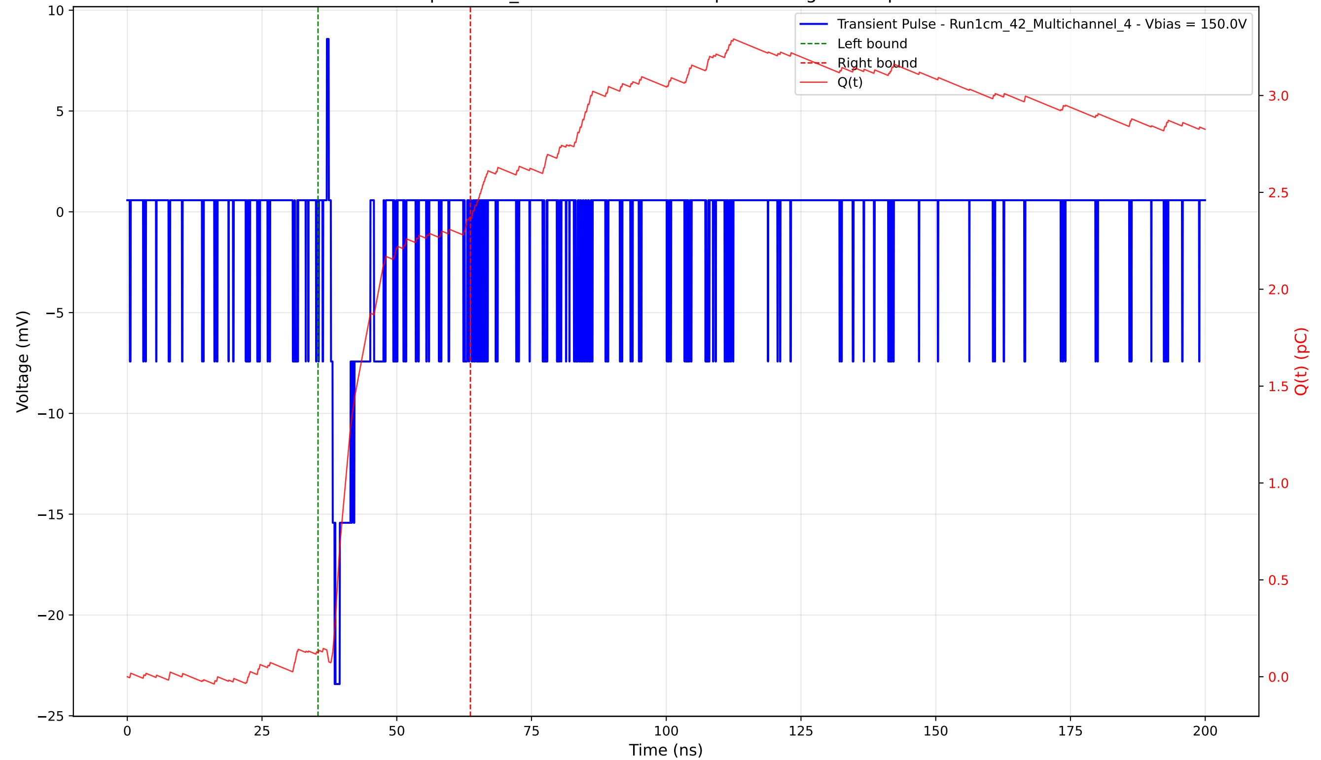
Transient Pulse - Sample: 1cm_42 - Position: 4970.0 \mu\text{m} - Charge: 2.24 pC - Rise Time: 0.71 ns
