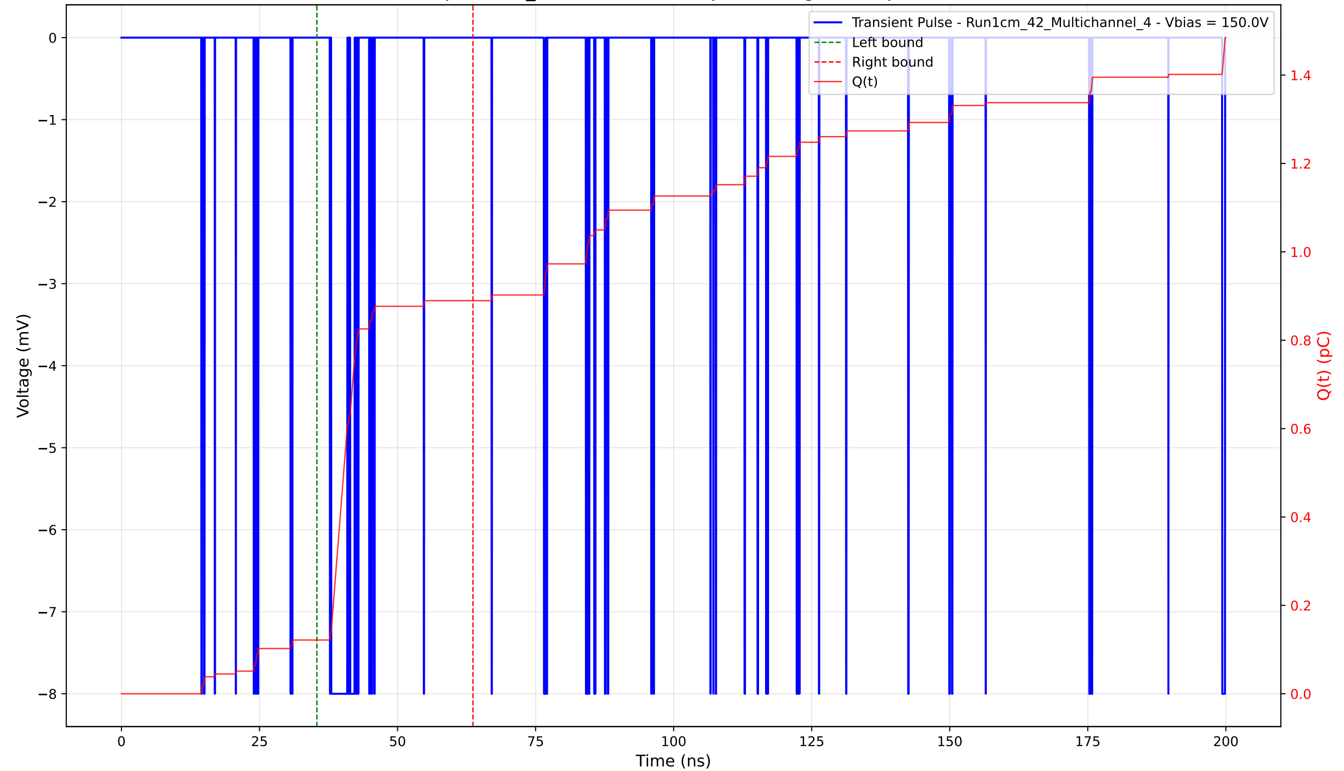
Transient Pulse - Sample: 1cm_42 - Position: 60.0 \mu\text{m} - Charge: 0.77 pC - Rise Time: 0.04 ns
