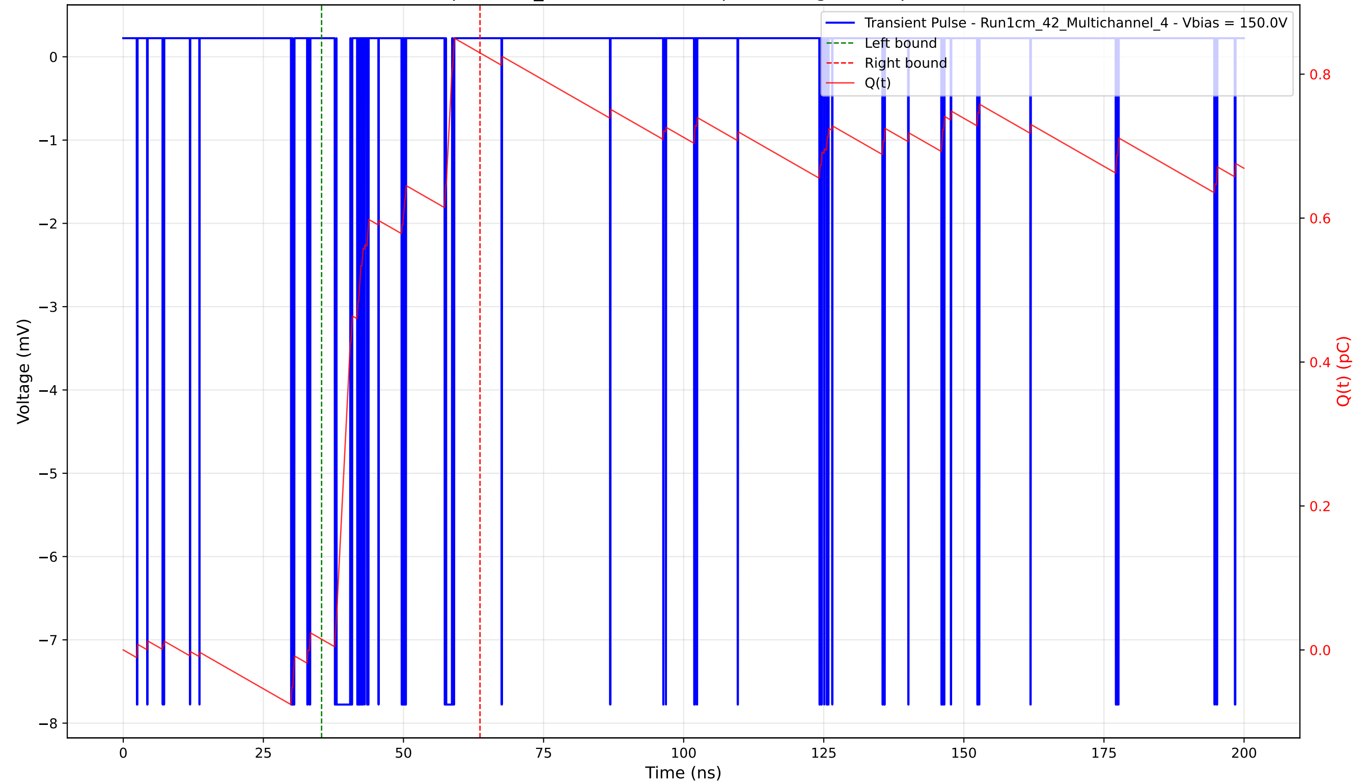
Transient Pulse - Sample: 1cm_42 - Position: 50.0 \mu\text{m} - Charge: 0.81 pC - Rise Time: 0.04 ns
