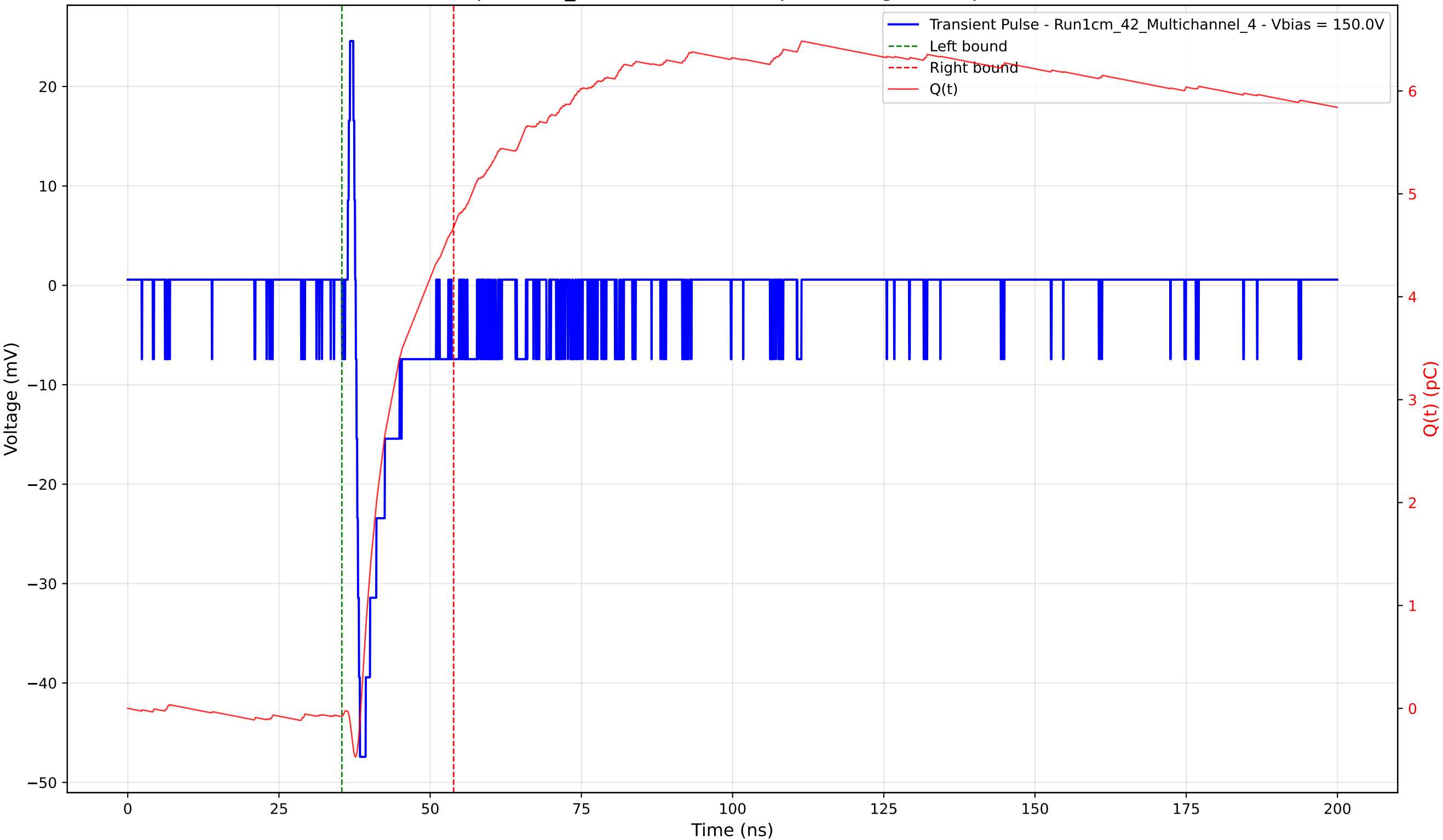
Transient Pulse - Sample: 1cm_42 - Position: 775.0 \mu\text{m} - Charge: 4.76 pC - Rise Time: 0.70 ns
