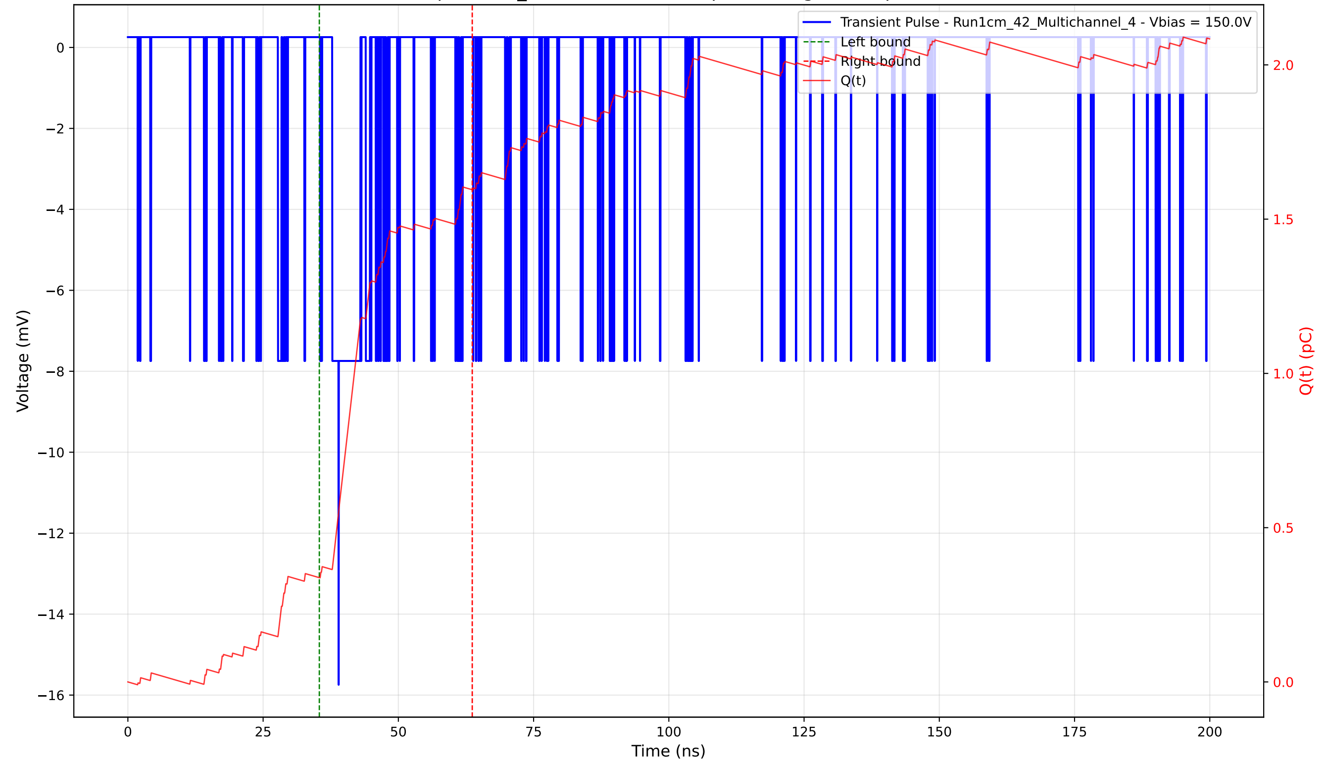
Transient Pulse - Sample: 1cm_42 - Position: 105.0 \mu\text{m} - Charge: 1.26 pC - Rise Time: 1.19 ns
