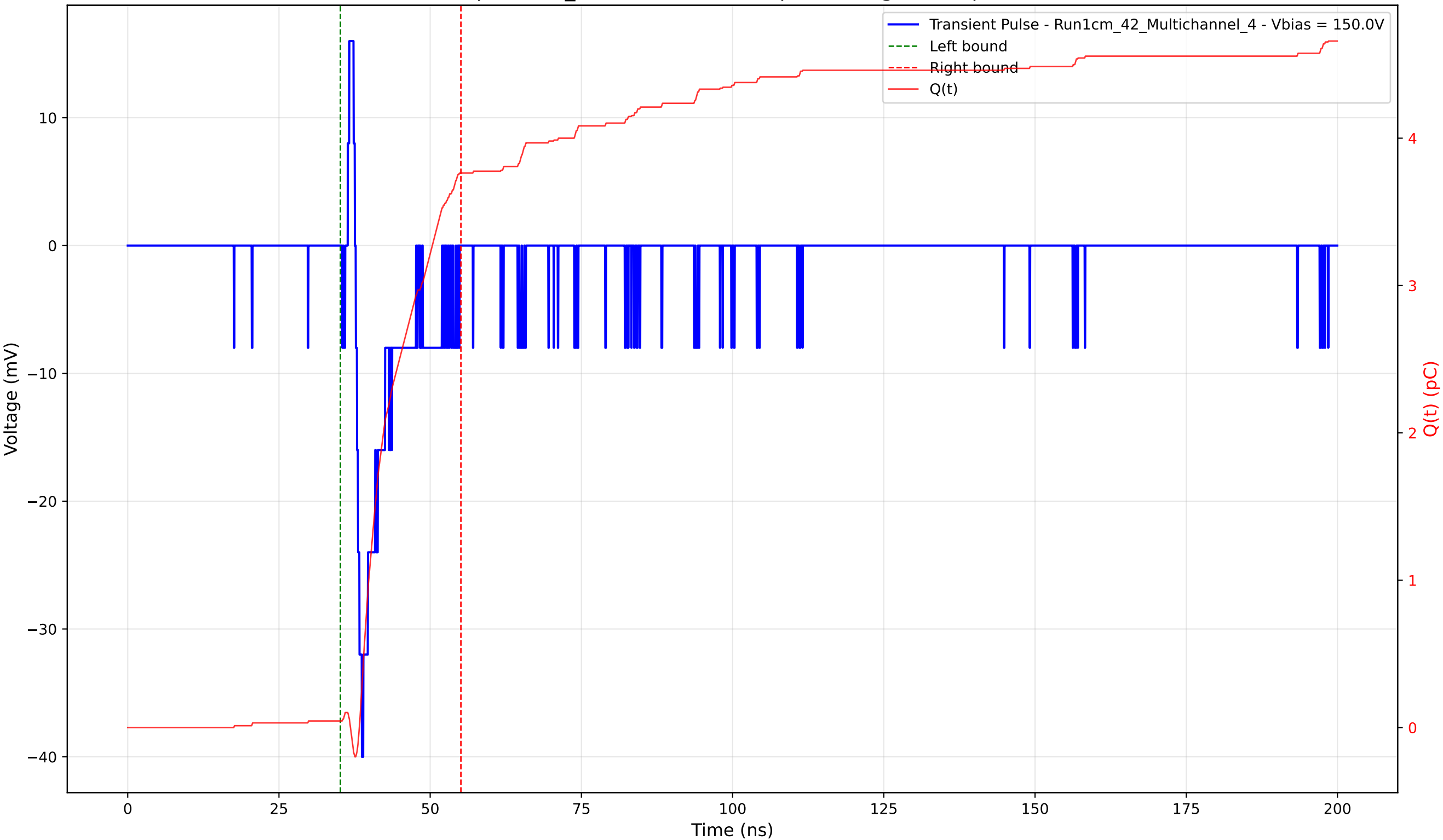
Transient Pulse - Sample: 1cm_42 - Position: 495.0 \mu\text{m} - Charge: 3.72 pC - Rise Time: 1.02 ns
