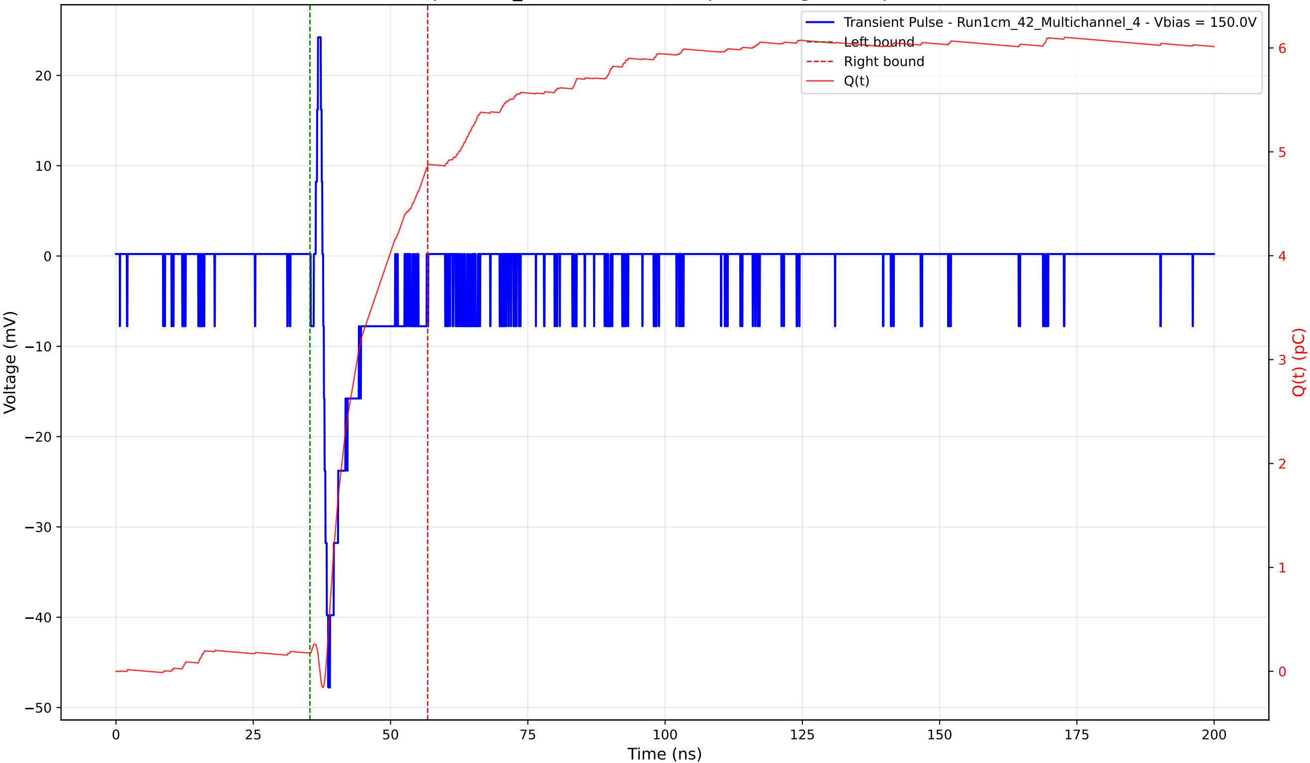
Transient Pulse - Sample: 1cm_42 - Position: 630.0 \mu\text{m} - Charge: 4.69 pC - Rise Time: 0.94 ns
