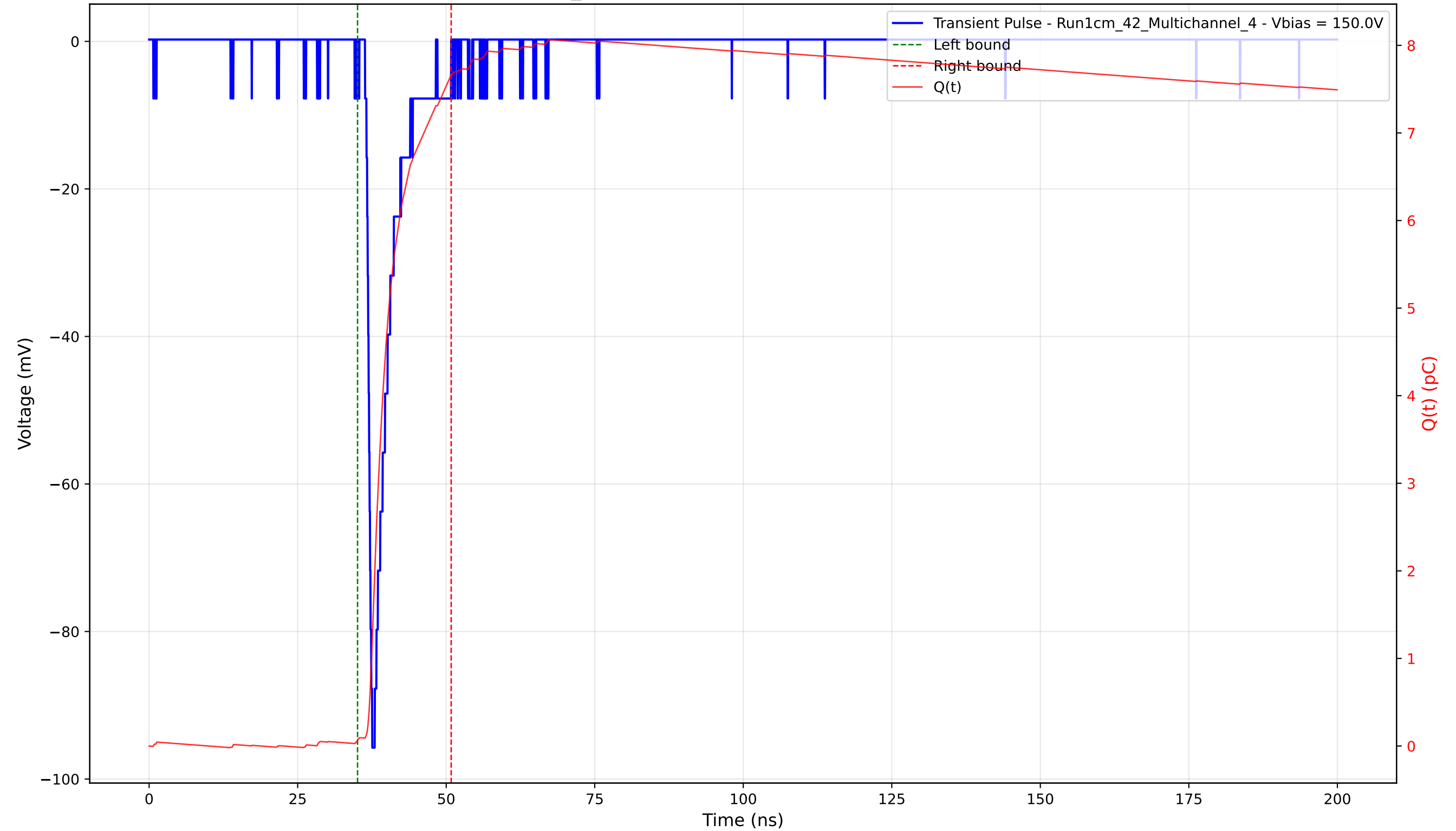
Transient Pulse - Sample: 1cm_42 - Position: 1600.0 \mu\text{m} - Charge: 7.60 pC - Rise Time: 0.83 ns
