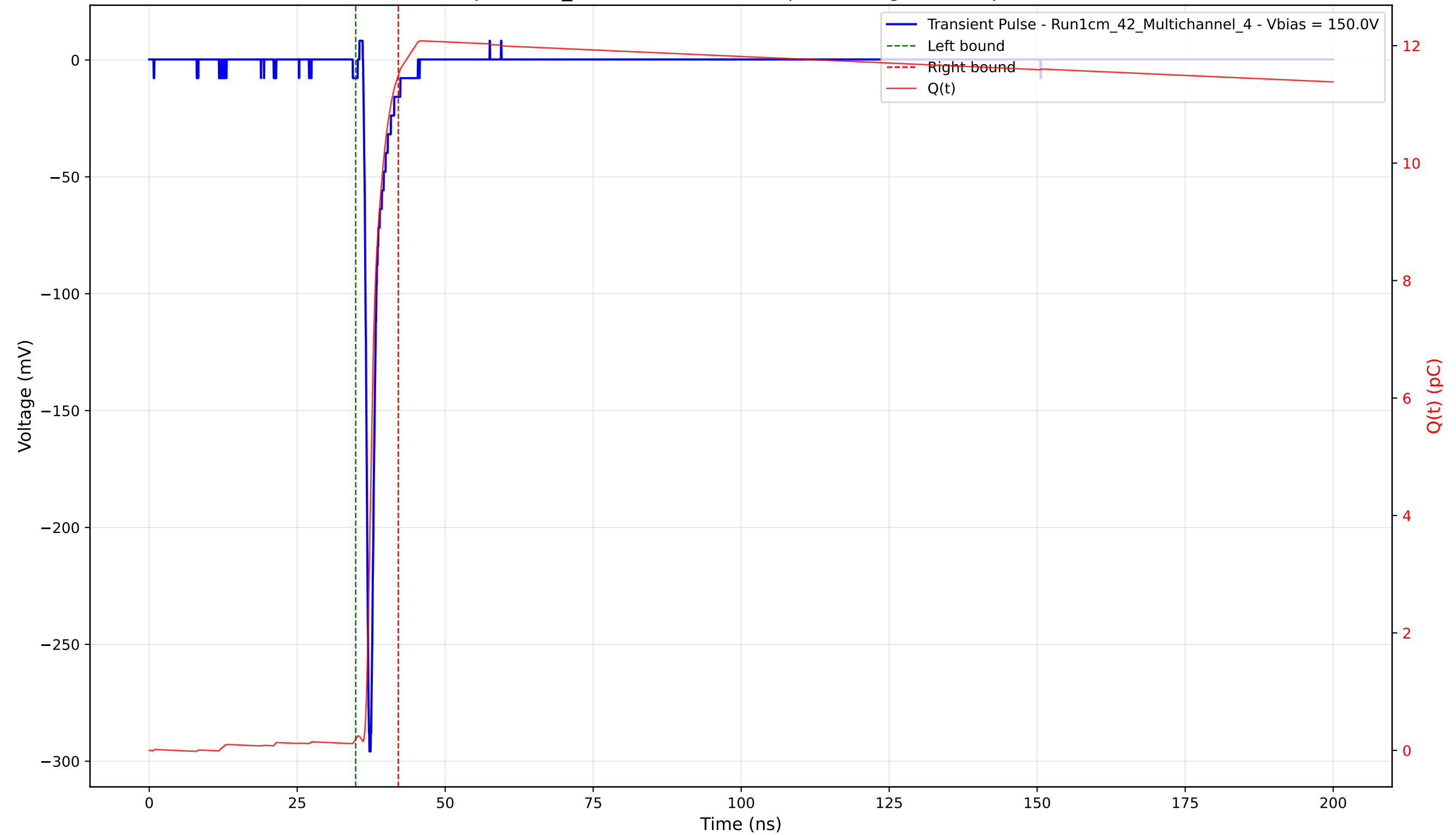
Transient Pulse - Sample: 1cm_42 - Position: 2080.0 \mu\text{m} - Charge: 11.31 pC - Rise Time: 0.74 ns
