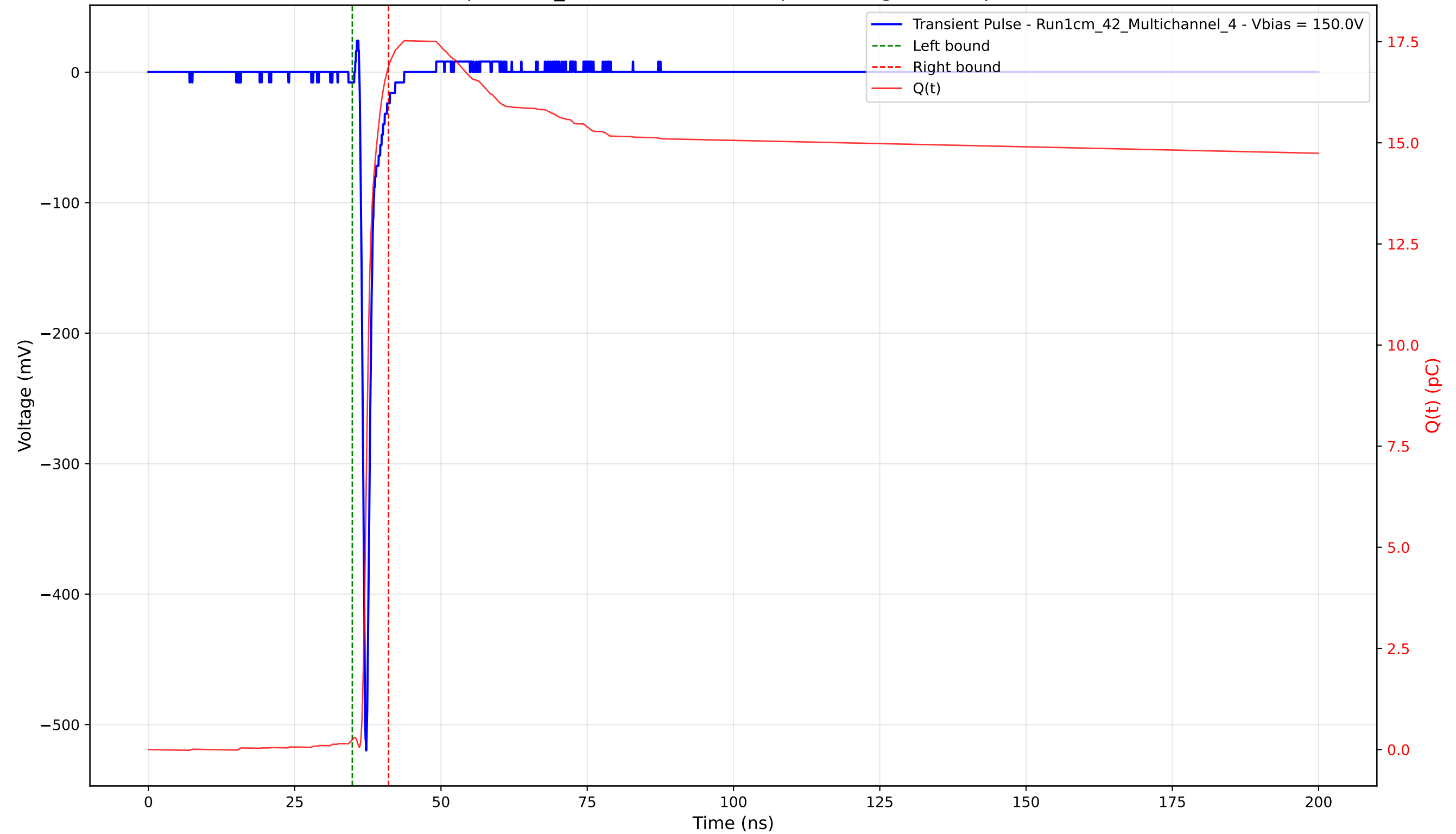
Transient Pulse - Sample: 1cm_42 - Position: 2270.0 \mu\text{m} - Charge: 16.65 pC - Rise Time: 0.74 ns
