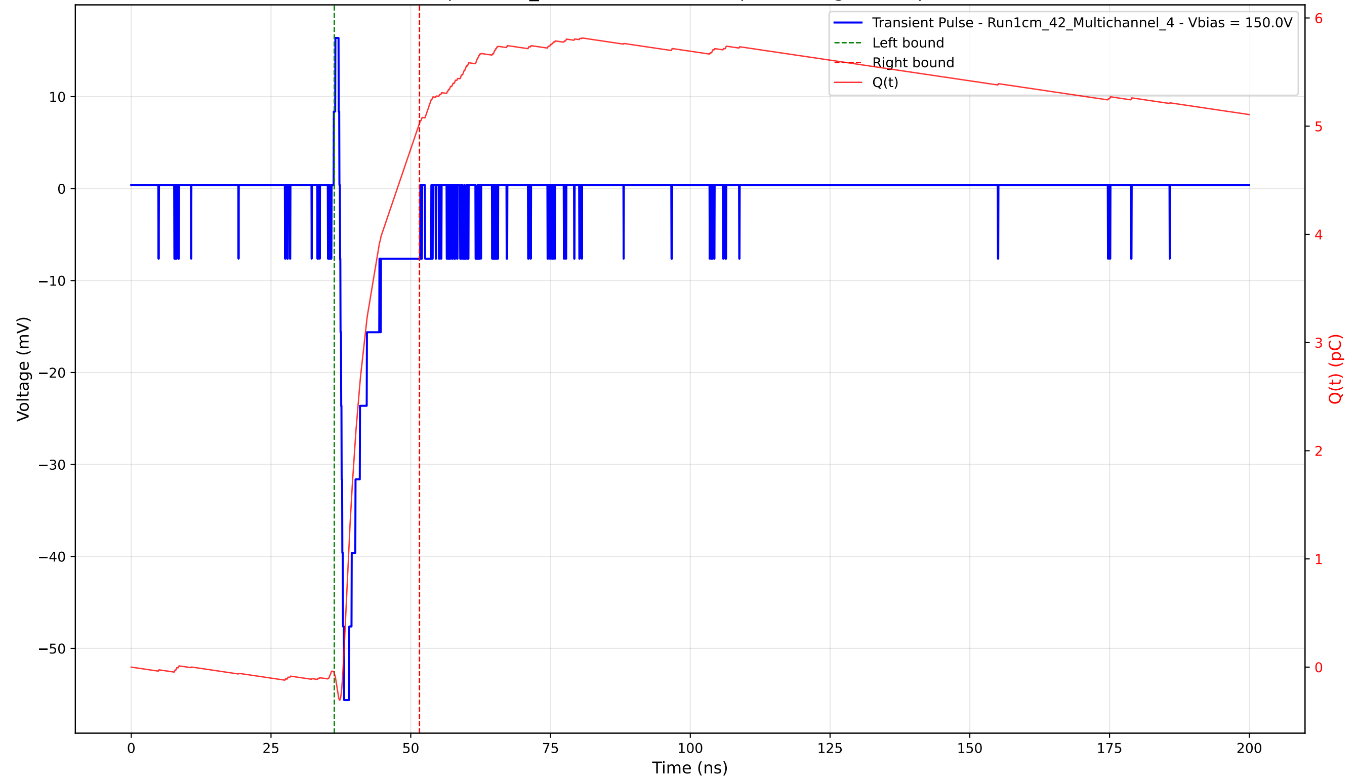
Transient Pulse - Sample: 1cm_42 - Position: 3810.0 \mu\text{m} - Charge: 5.09 pC - Rise Time: 0.73 ns
