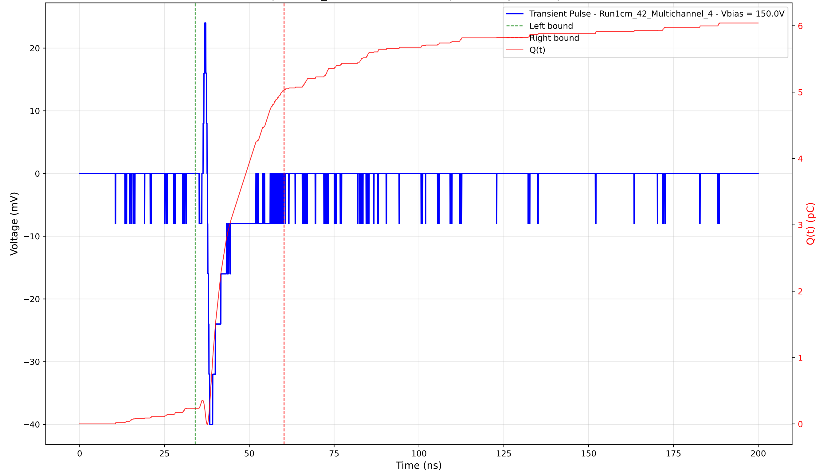
Transient Pulse - Sample: 1cm_42 - Position: 4140.0 \mu\text{m} - Charge: 4.80 pC - Rise Time: 0.70 ns
