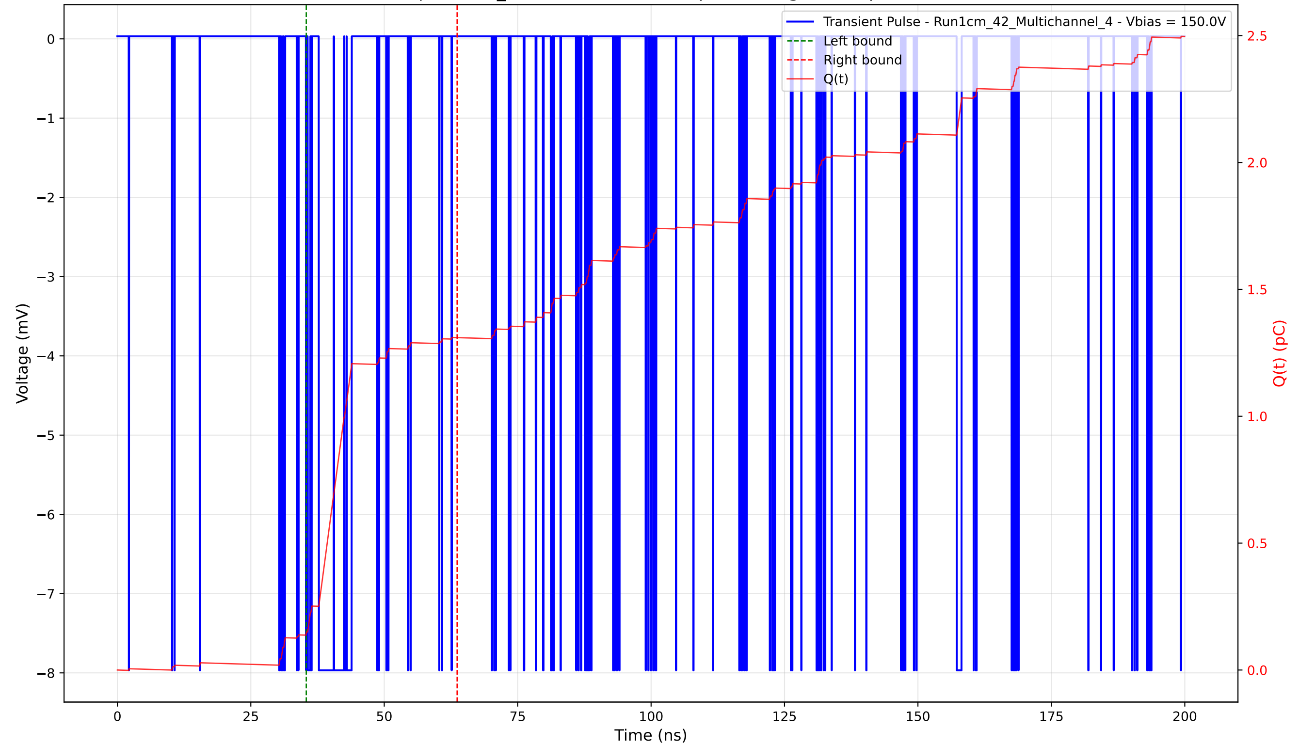
Transient Pulse - Sample: 1cm_42 - Position: 5140.0 \mu\text{m} - Charge: 1.16 pC - Rise Time: 0.04 ns
