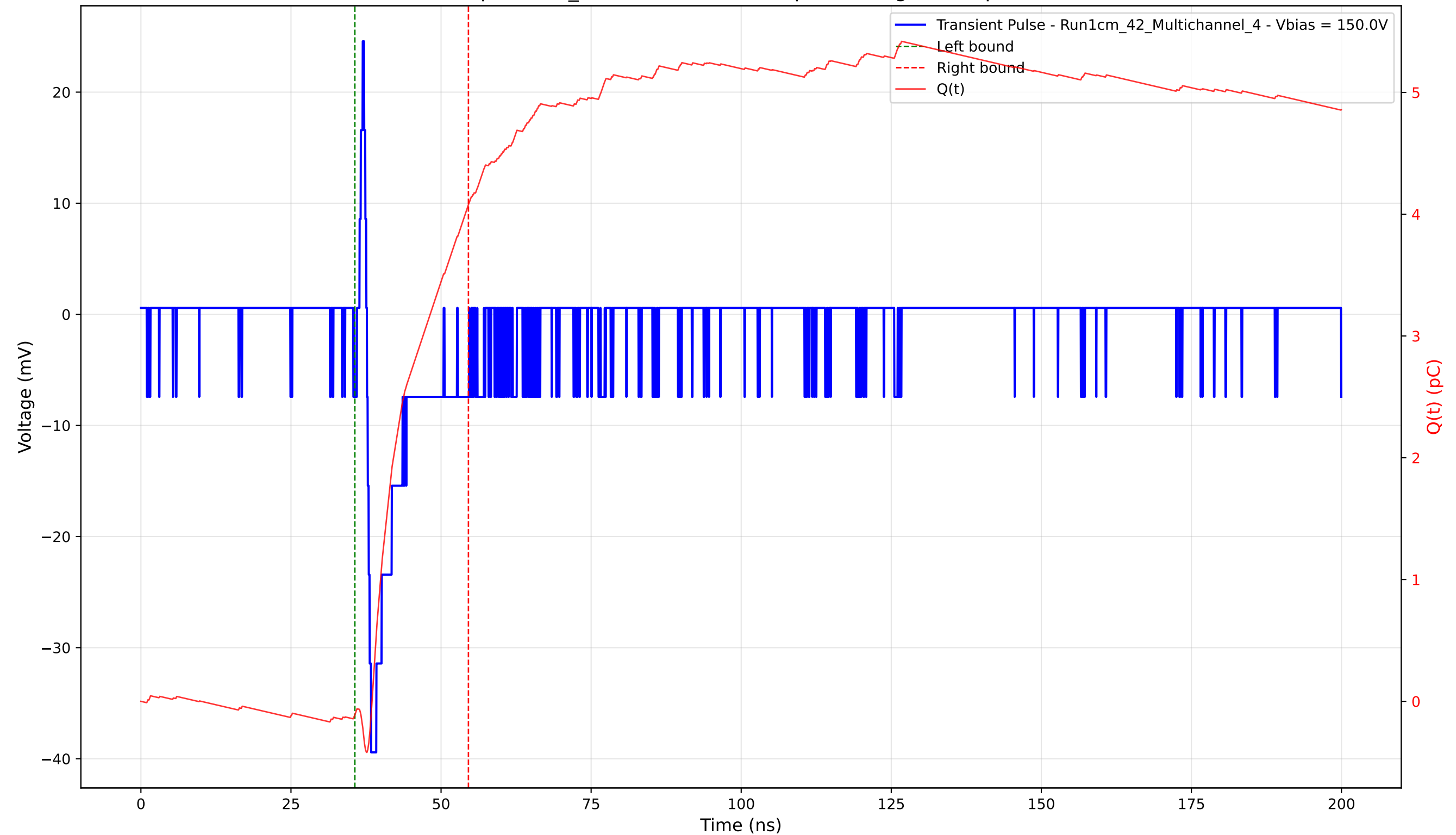
Transient Pulse - Sample: 1cm_42 - Position: 4145.0 \mu\text{m} - Charge: 4.19 pC - Rise Time: 0.70 ns
