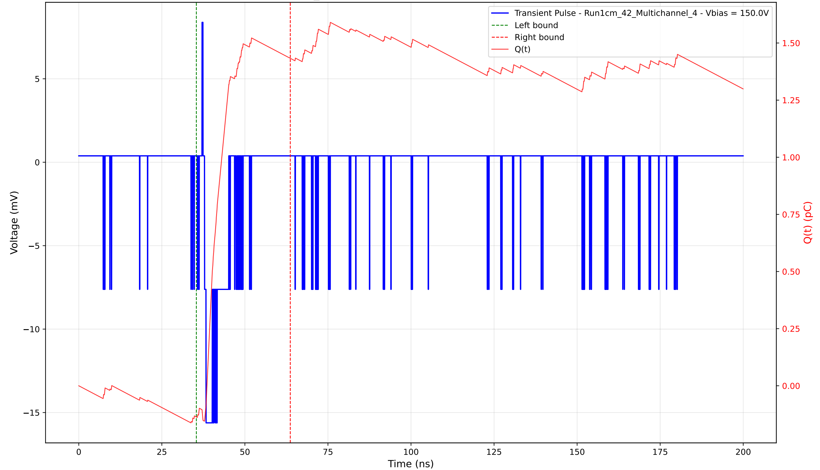
Transient Pulse - Sample: 1cm_42 - Position: 5010.0 \mu\text{m} - Charge: 1.57 pC - Rise Time: 0.47 ns
