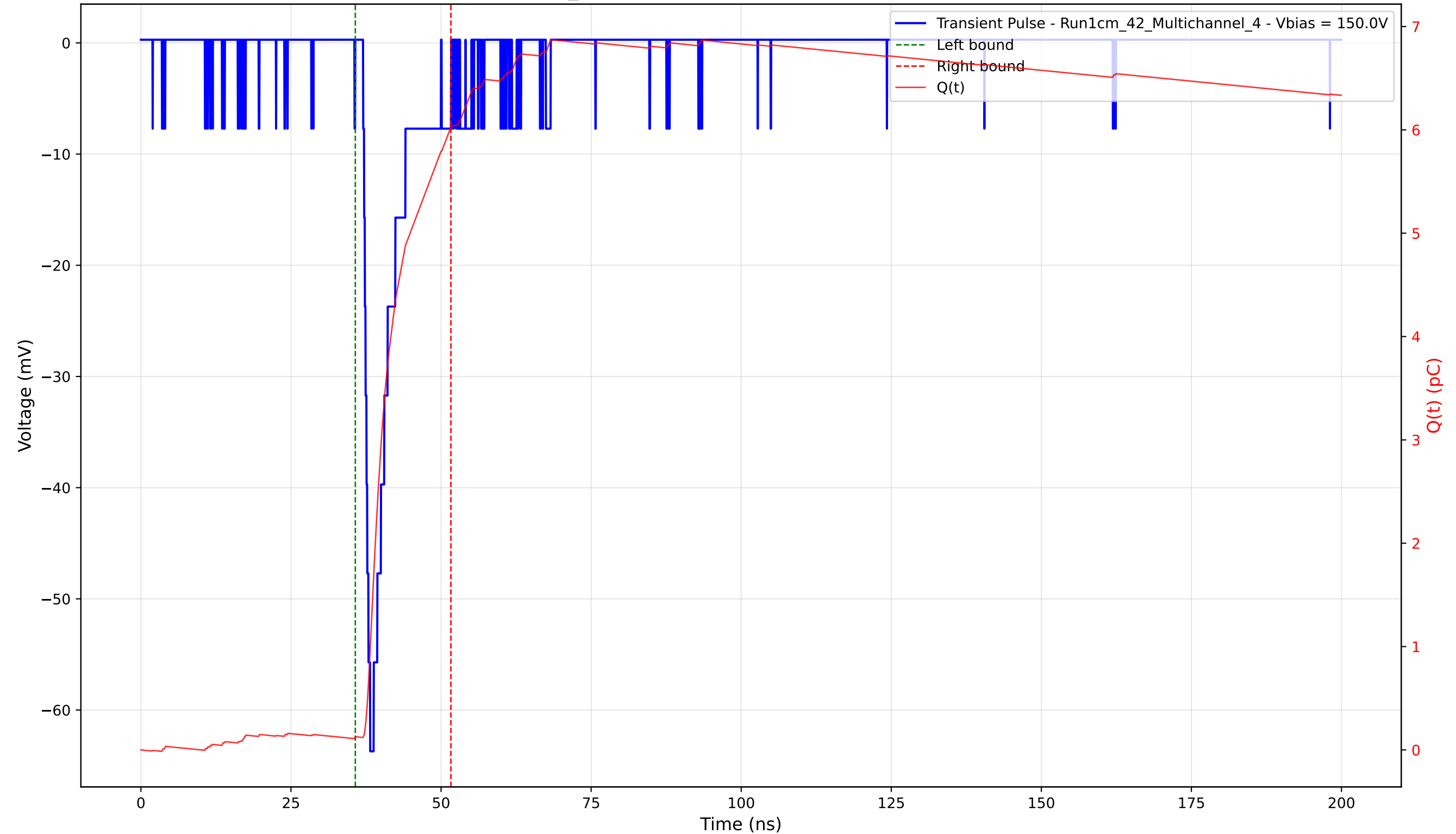
Transient Pulse - Sample: 1cm_42 - Position: 1380.0 \mu\text{m} - Charge: 5.90 pC - Rise Time: 1.17 ns
