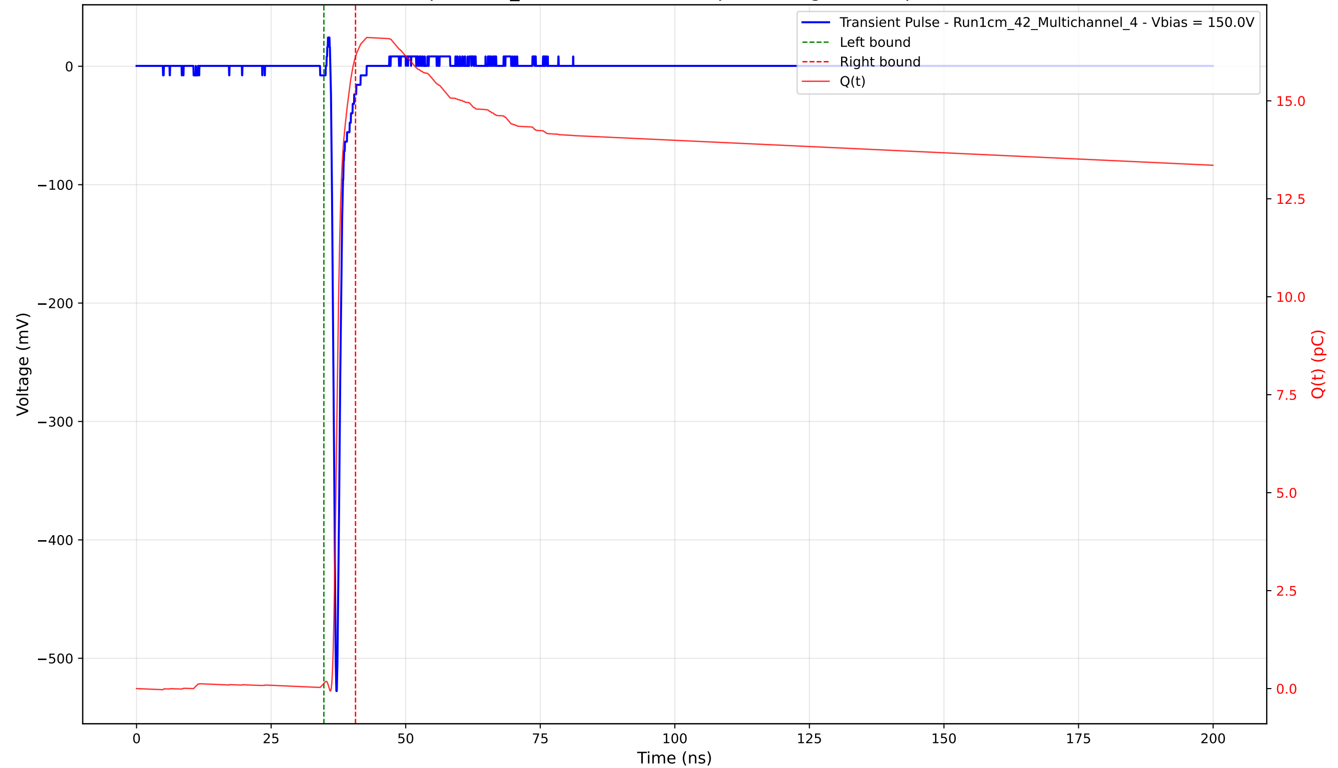
Transient Pulse - Sample: 1cm_42 - Position: 2585.0 \mu\text{m} - Charge: 15.99 pC - Rise Time: 0.72 ns
