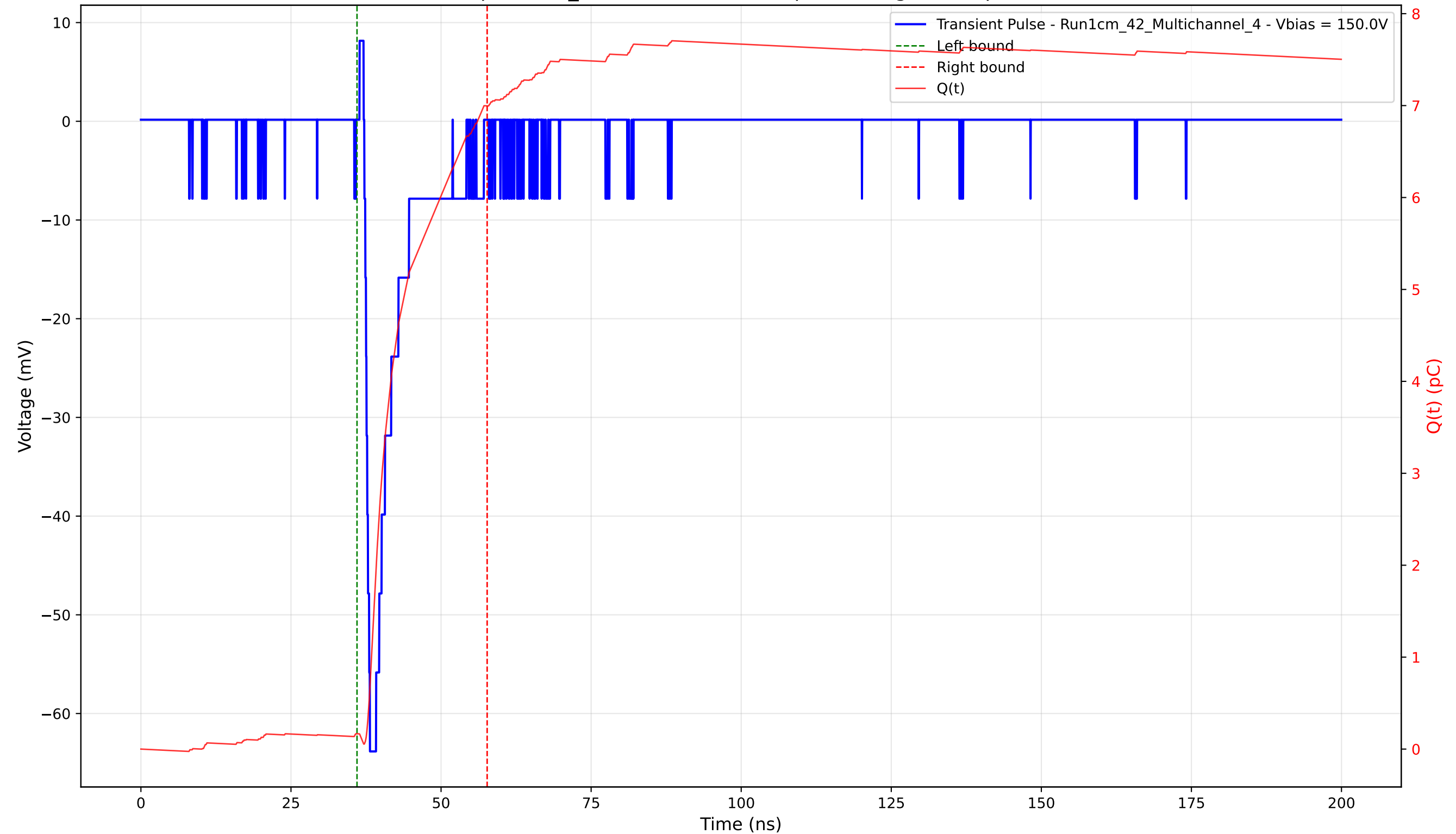
Transient Pulse - Sample: 1cm_42 - Position: 1240.0 \mu\text{m} - Charge: 6.83 pC - Rise Time: 0.93 ns
