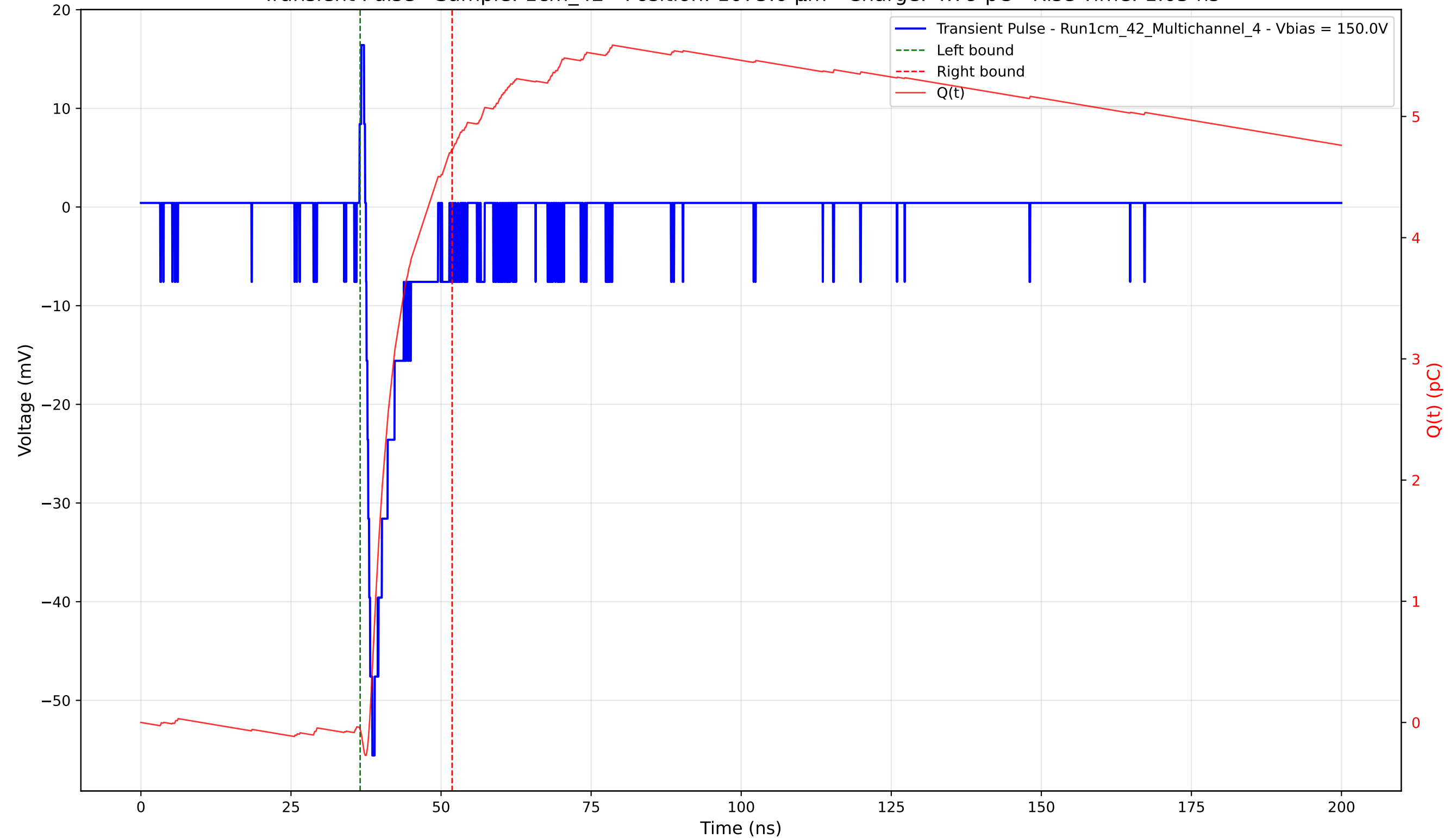
Transient Pulse - Sample: 1cm_42 - Position: 1075.0 \mu\text{m} - Charge: 4.79 pC - Rise Time: 1.05 ns
