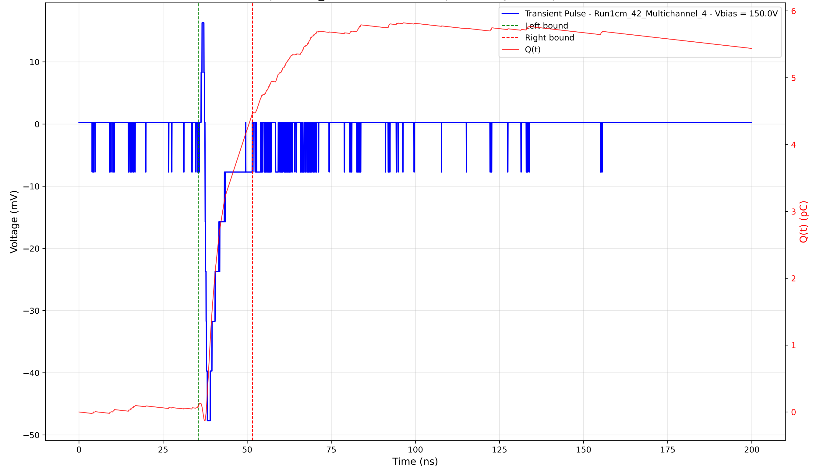
Transient Pulse - Sample: 1cm_42 - Position: 3915.0 \mu\text{m} - Charge: 4.38 pC - Rise Time: 0.70 ns
