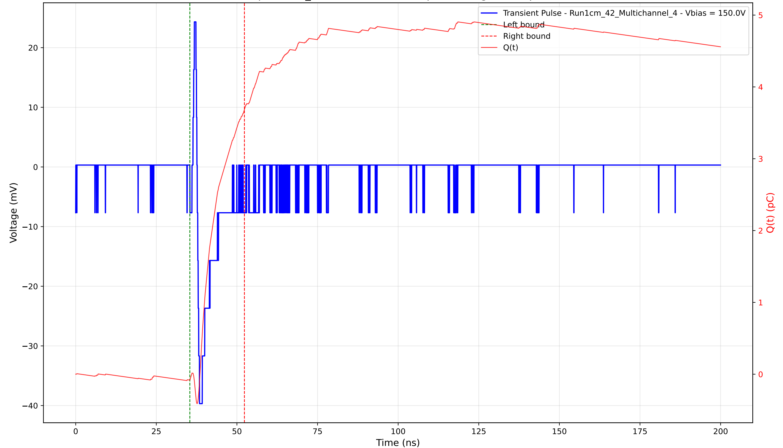
Transient Pulse - Sample: 1cm_42 - Position: 4205.0 \mu\text{m} - Charge: 3.77 pC - Rise Time: 0.70 ns
