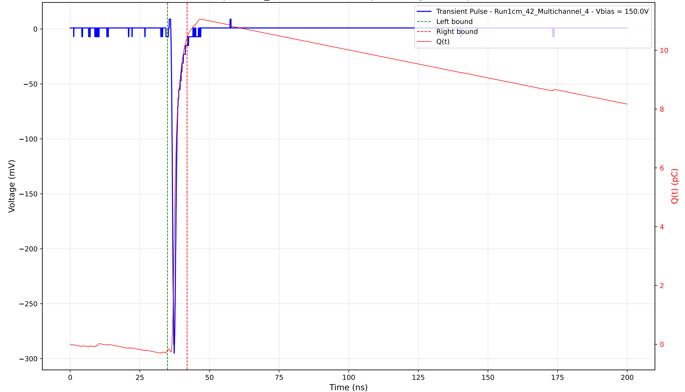
Transient Pulse - Sample: 1cm_42 - Position: 2945.0 \mu\text{m} - Charge: 10.64 pC - Rise Time: 0.78 ns
