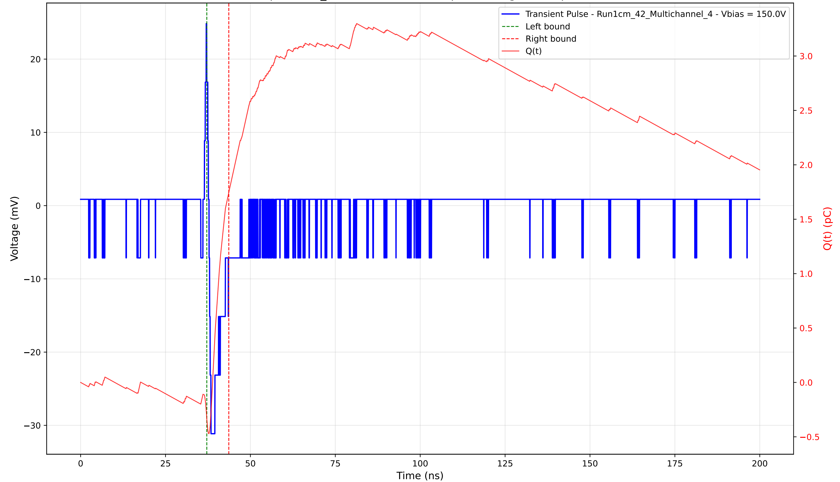
Transient Pulse - Sample: 1cm_42 - Position: 4450.0 \mu\text{m} - Charge: 2.09 pC - Rise Time: 0.59 ns
