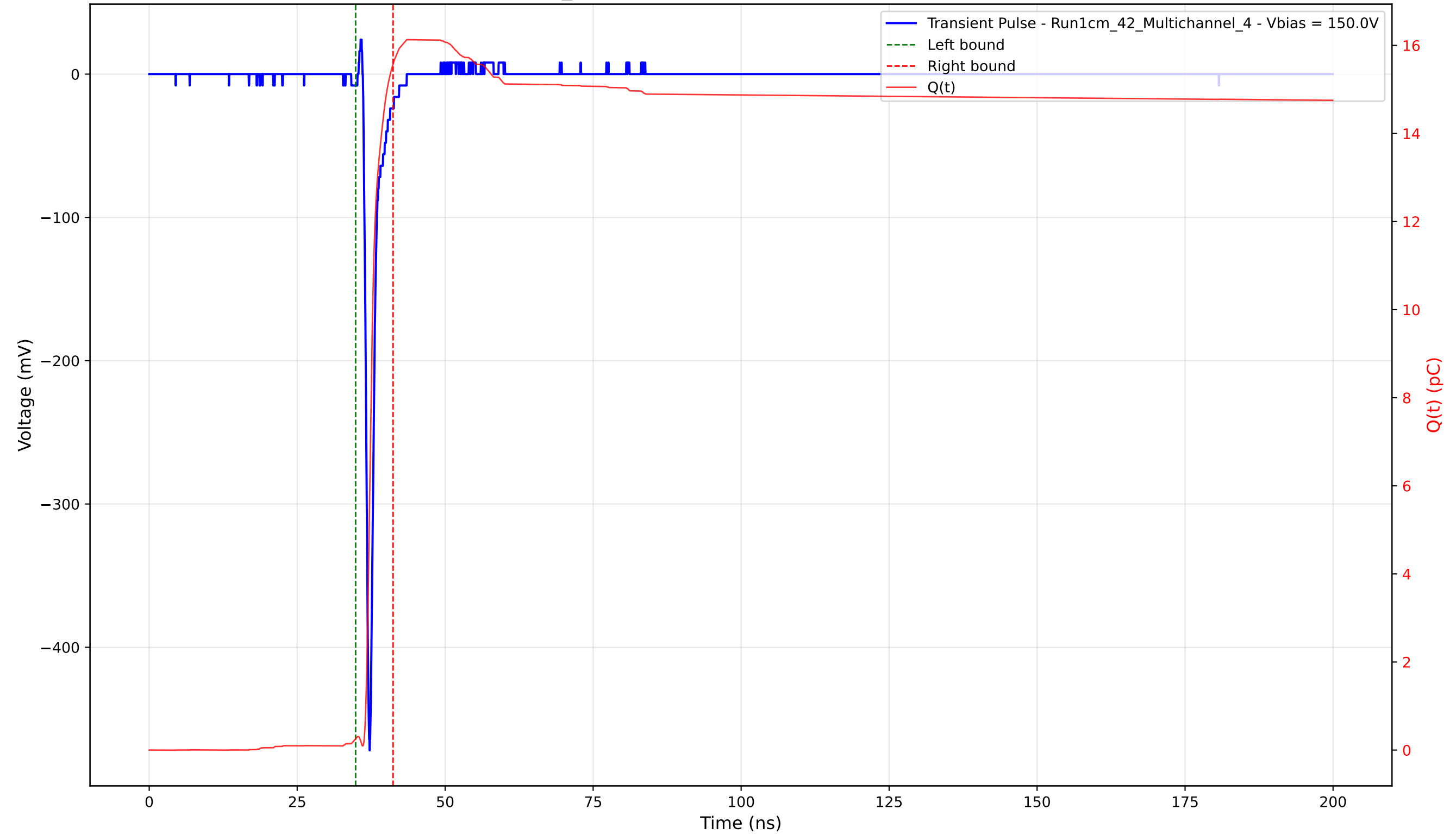
Transient Pulse - Sample: 1cm_42 - Position: 2790.0 \mu\text{m} - Charge: 15.32 pC - Rise Time: 0.71 ns
