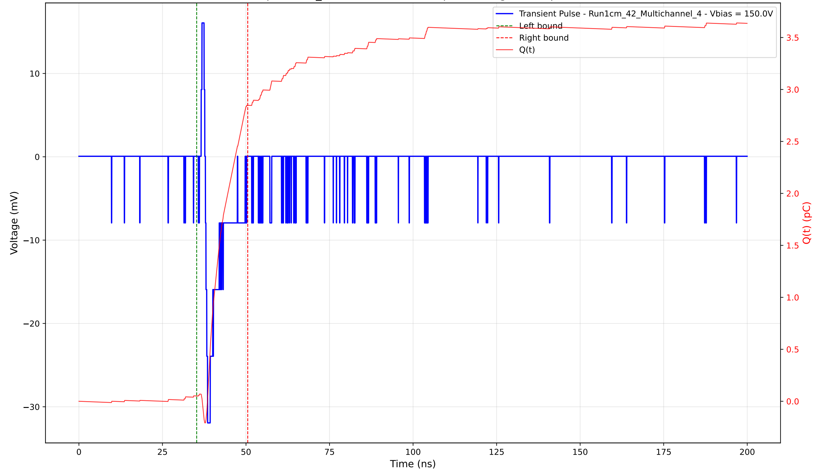
Transient Pulse - Sample: 1cm_42 - Position: 4610.0 \mu\text{m} - Charge: 2.80 pC - Rise Time: 0.66 ns
