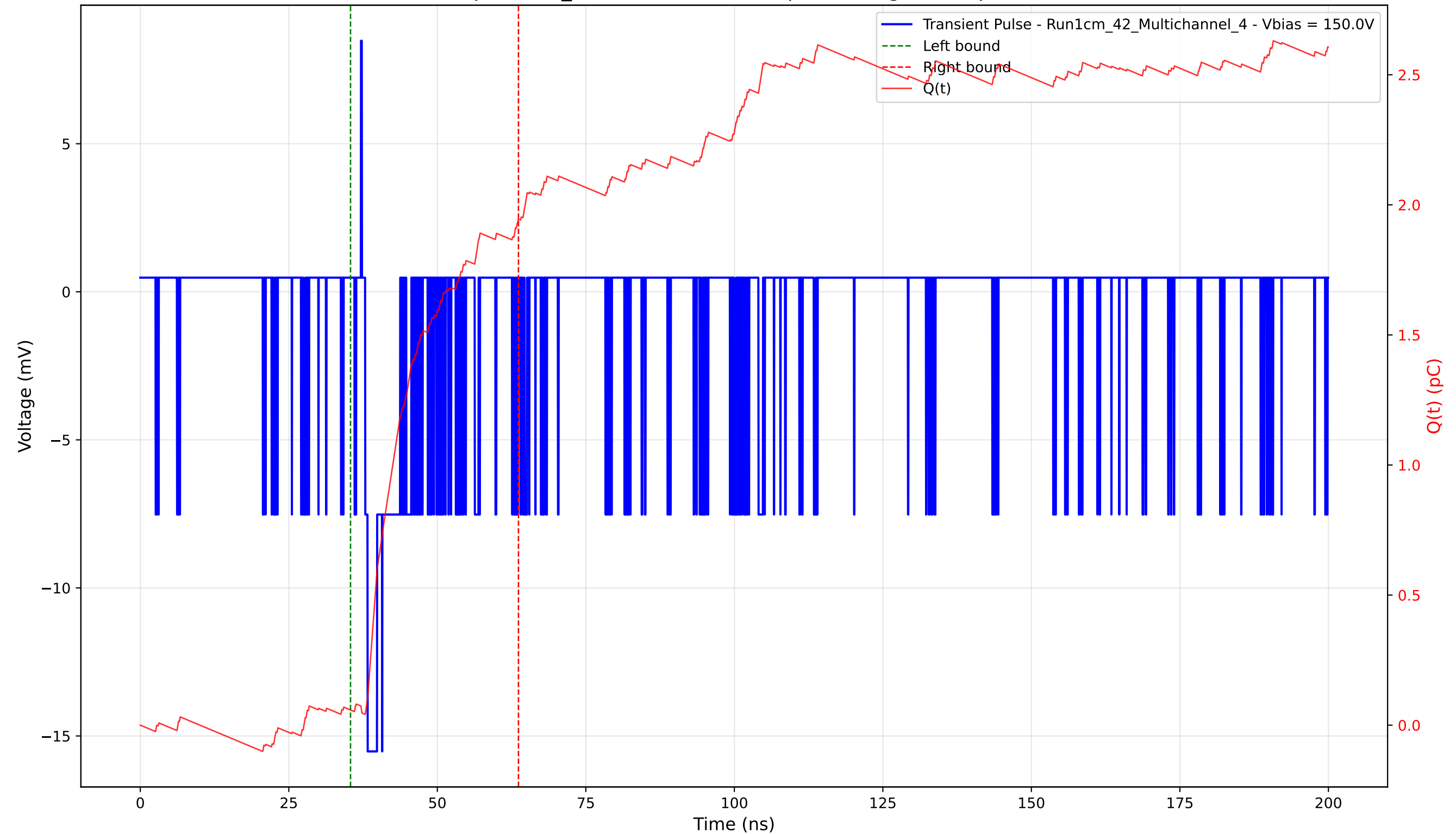
Transient Pulse - Sample: 1cm_42 - Position: 5020.0 \mu\text{m} - Charge: 1.89 pC - Rise Time: 0.43 ns
