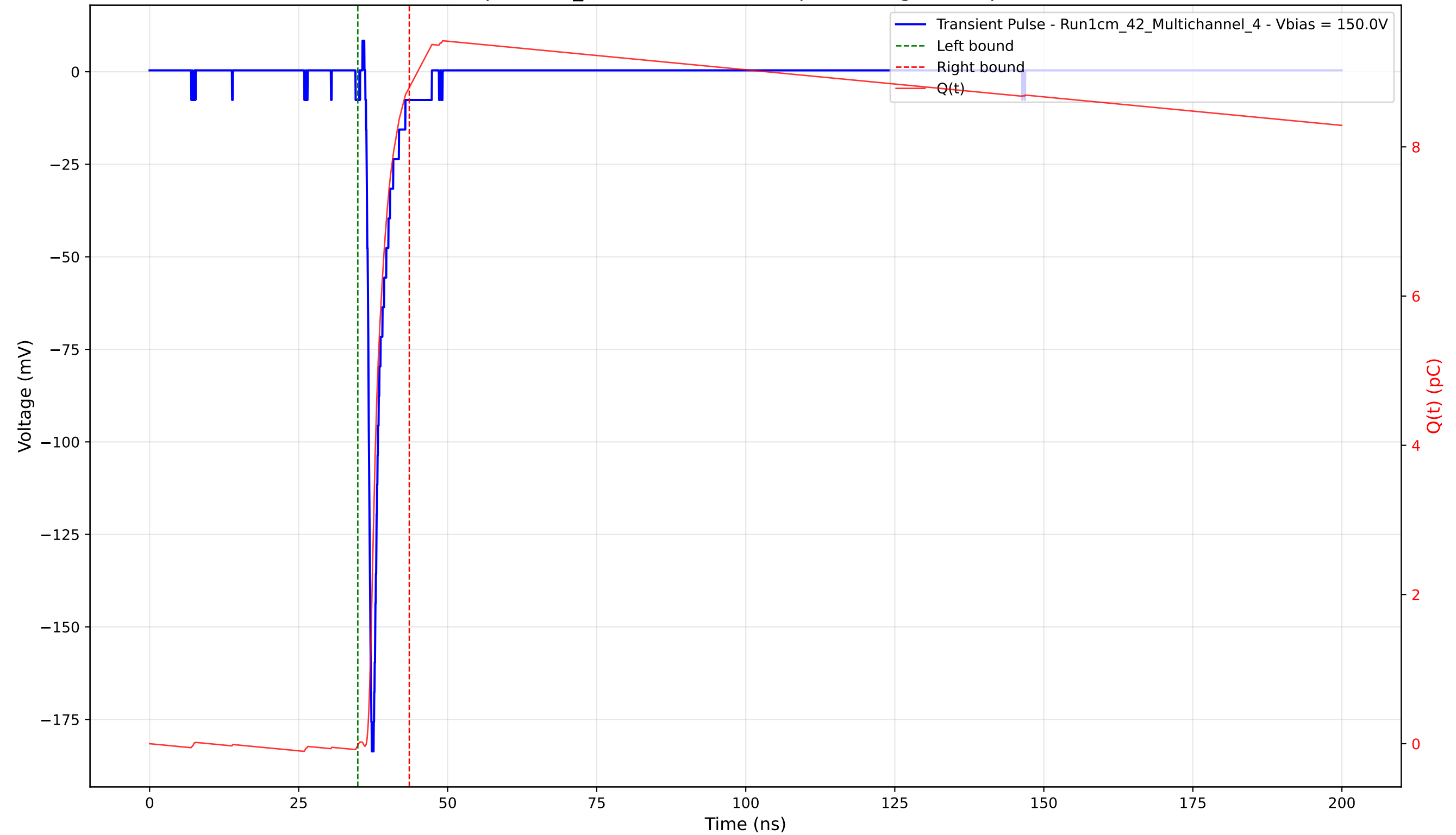
Transient Pulse - Sample: 1cm_42 - Position: 1935.0 \mu\text{m} - Charge: 8.82 pC - Rise Time: 0.75 ns
