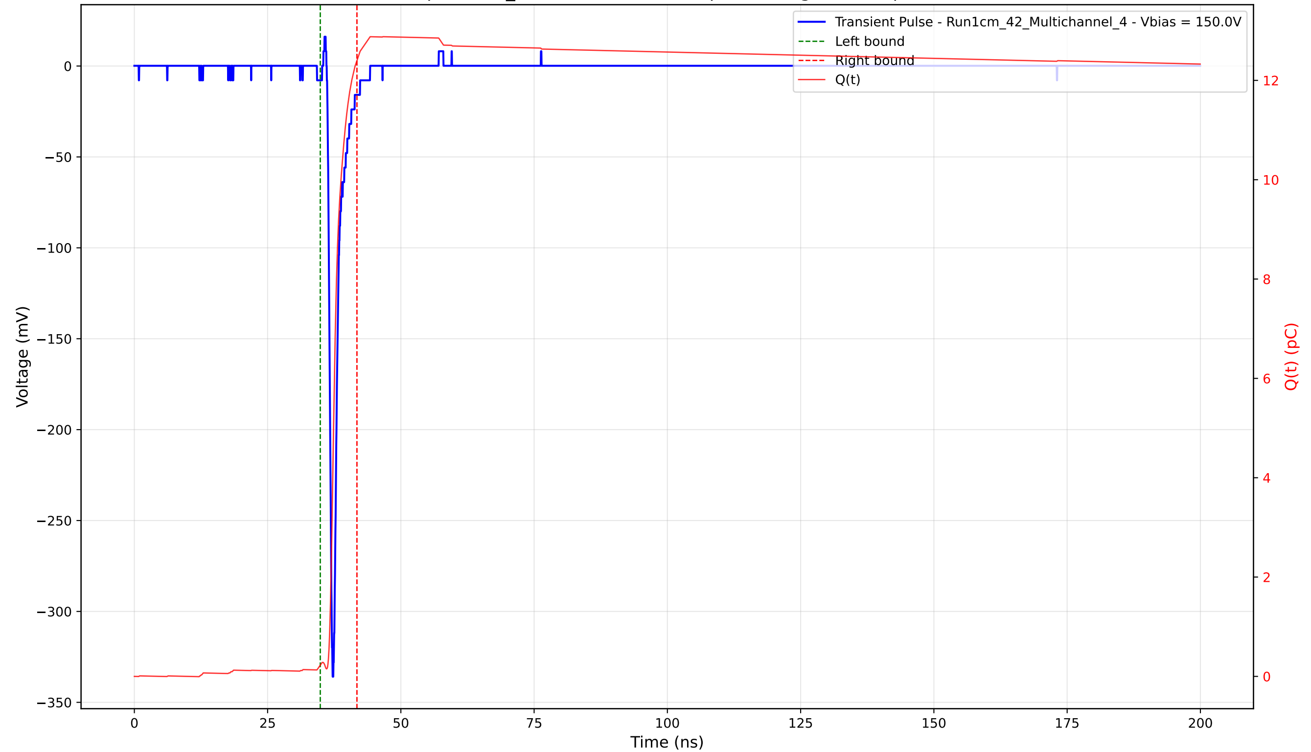
Transient Pulse - Sample: 1cm_42 - Position: 2110.0 \mu\text{m} - Charge: 12.17 pC - Rise Time: 0.73 ns
