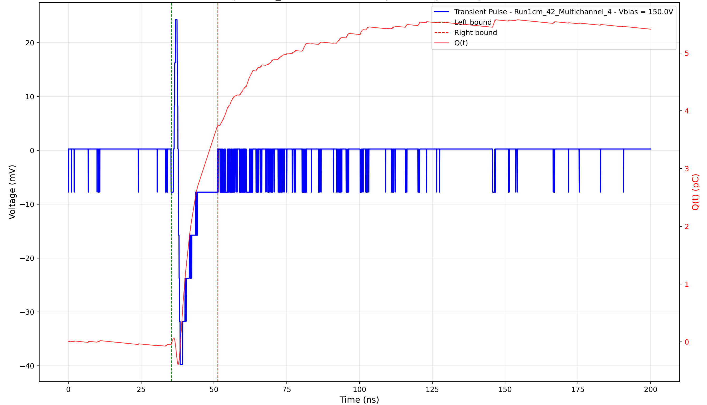
Transient Pulse - Sample: 1cm_42 - Position: 4260.0 \mu\text{m} - Charge: 3.77 pC - Rise Time: 0.66 ns
