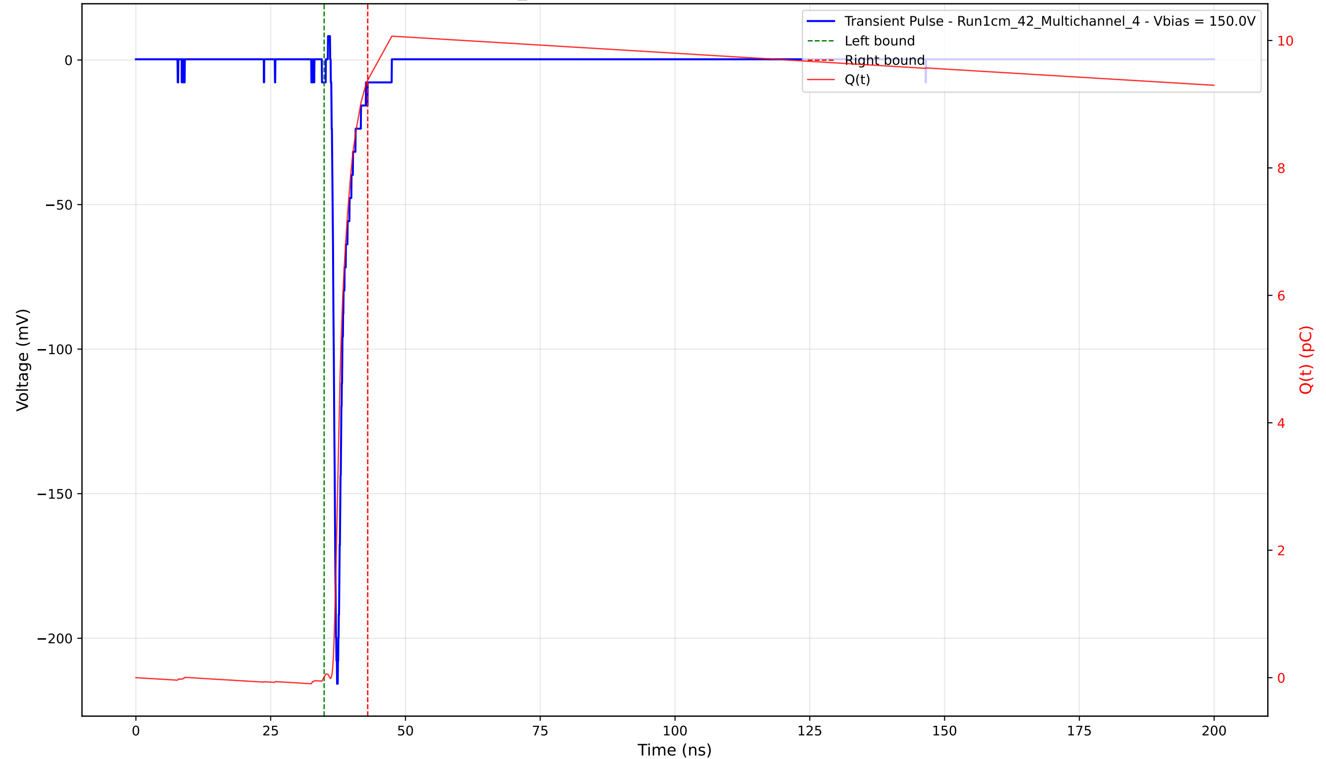
Transient Pulse - Sample: 1cm_42 - Position: 1985.0 \mu\text{m} - Charge: 9.37 pC - Rise Time: 0.81 ns
