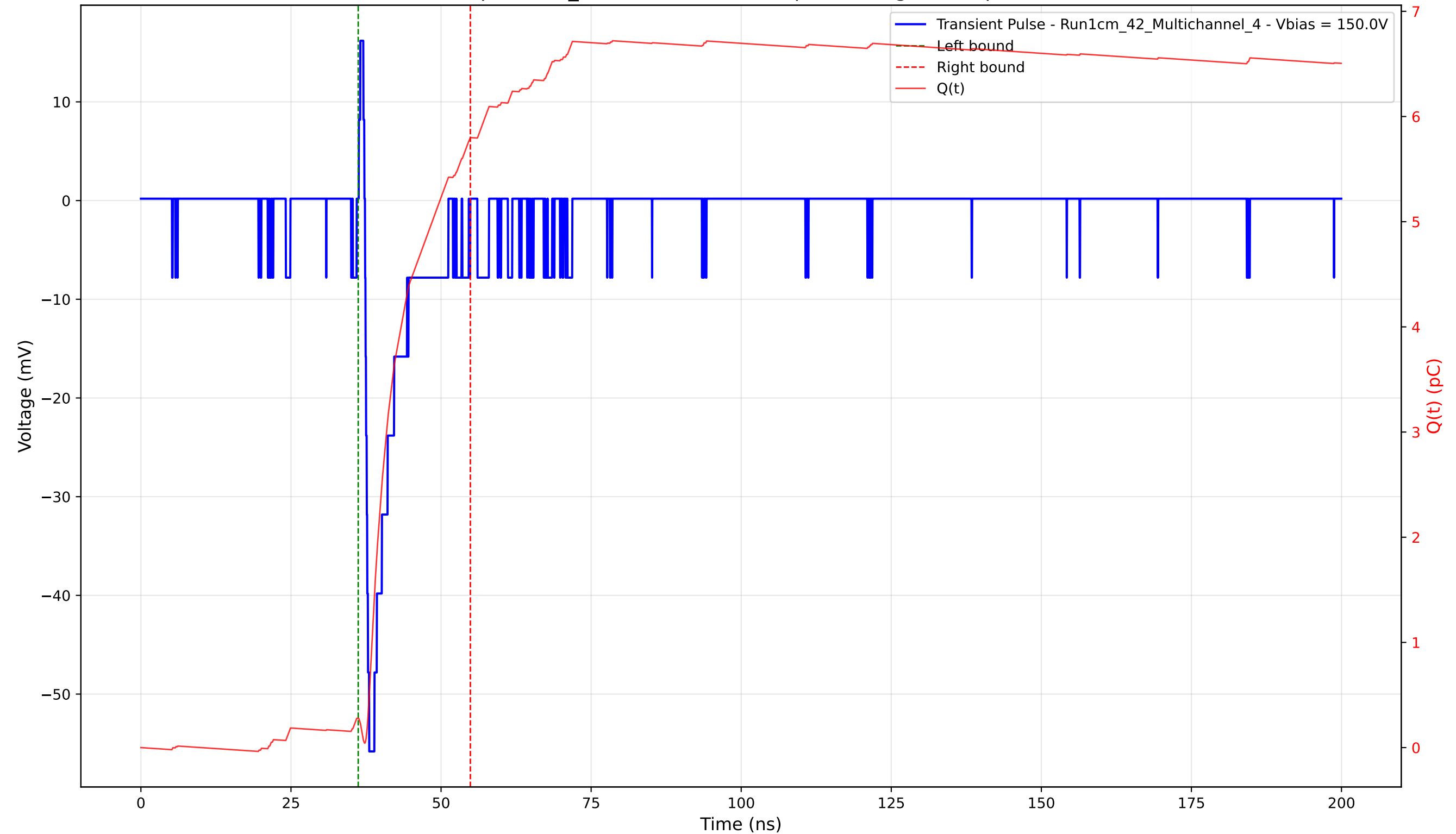
Transient Pulse - Sample: 1cm_42 - Position: 3790.0 \mu\text{m} - Charge: 5.52 pC - Rise Time: 0.69 ns
