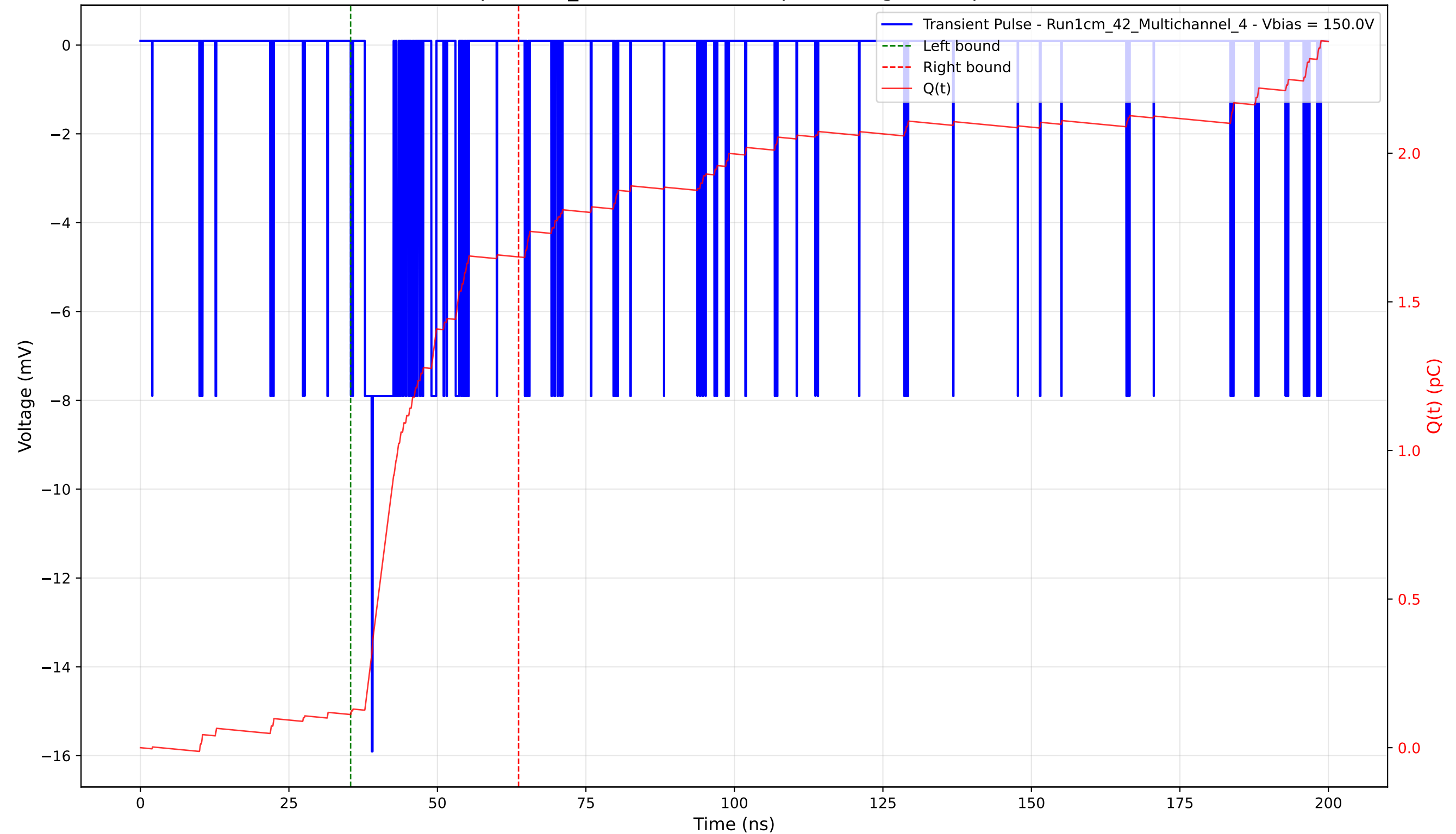
Transient Pulse - Sample: 1cm_42 - Position: 110.0 \mu\text{m} - Charge: 1.54 pC - Rise Time: 1.19 ns
