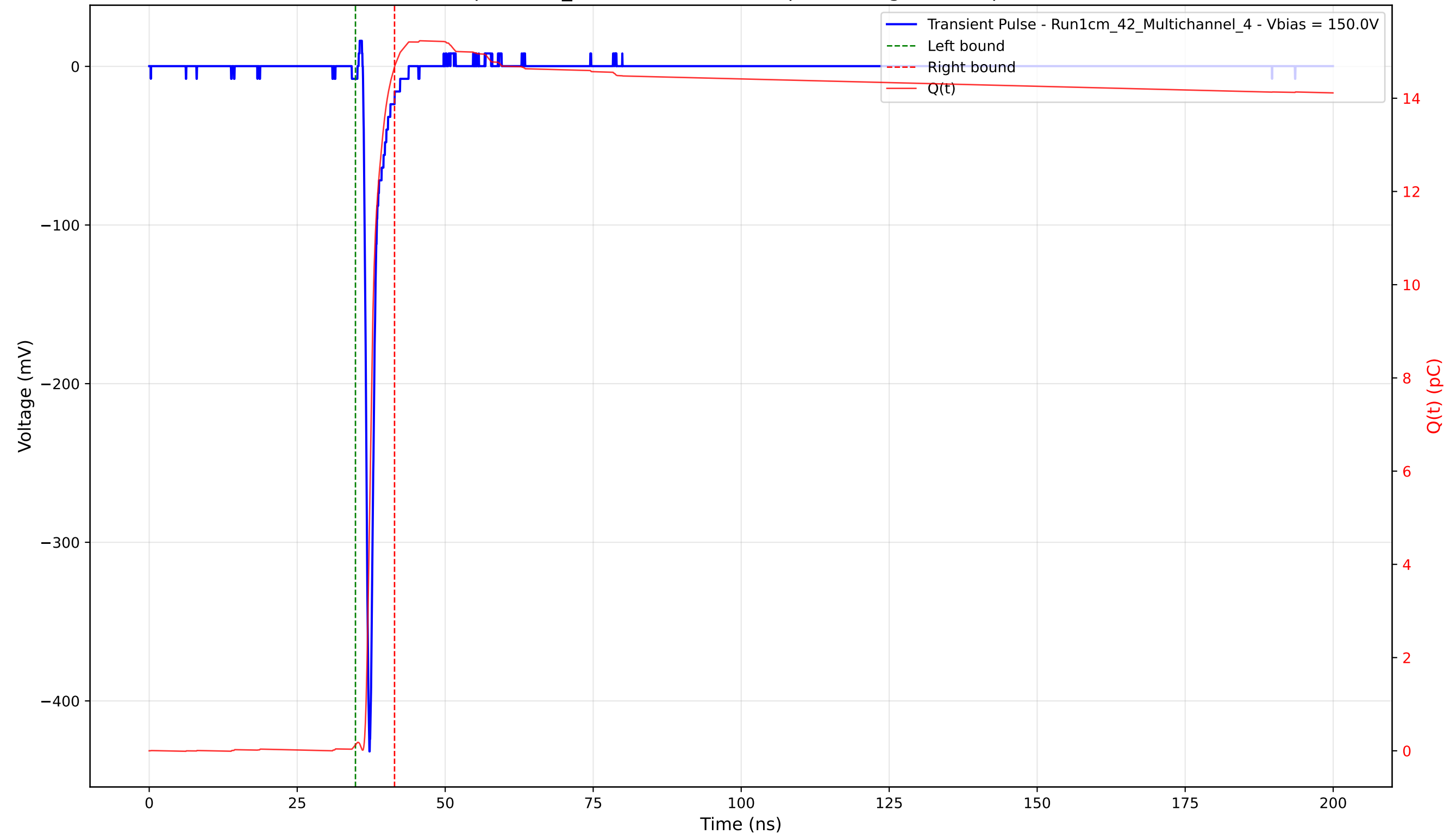
Transient Pulse - Sample: 1cm_42 - Position: 2180.0 \mu\text{m} - Charge: 14.55 pC - Rise Time: 0.74 ns
