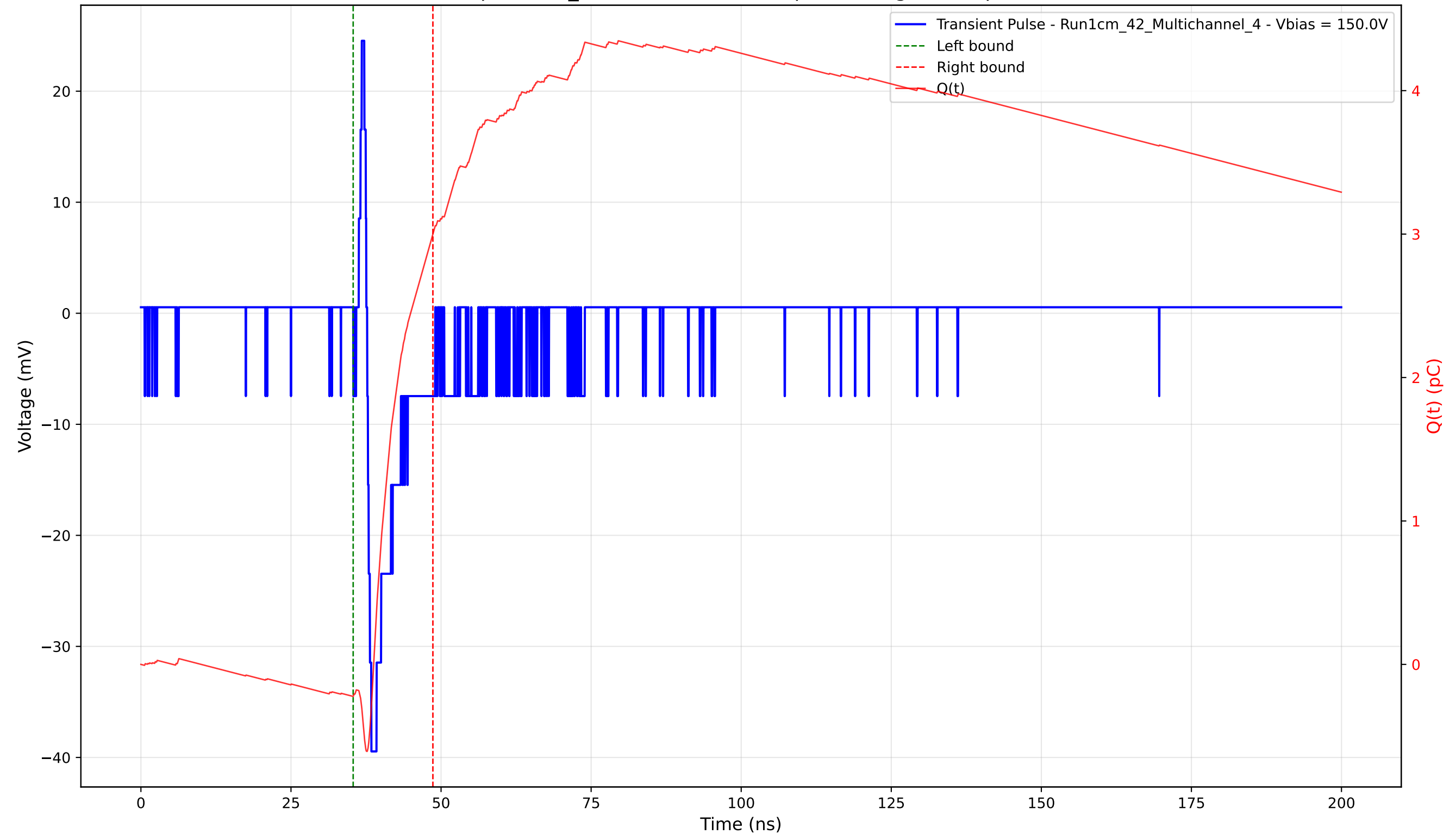
Transient Pulse - Sample: 1cm_42 - Position: 4150.0 \mu\text{m} - Charge: 3.23 pC - Rise Time: 0.70 ns
