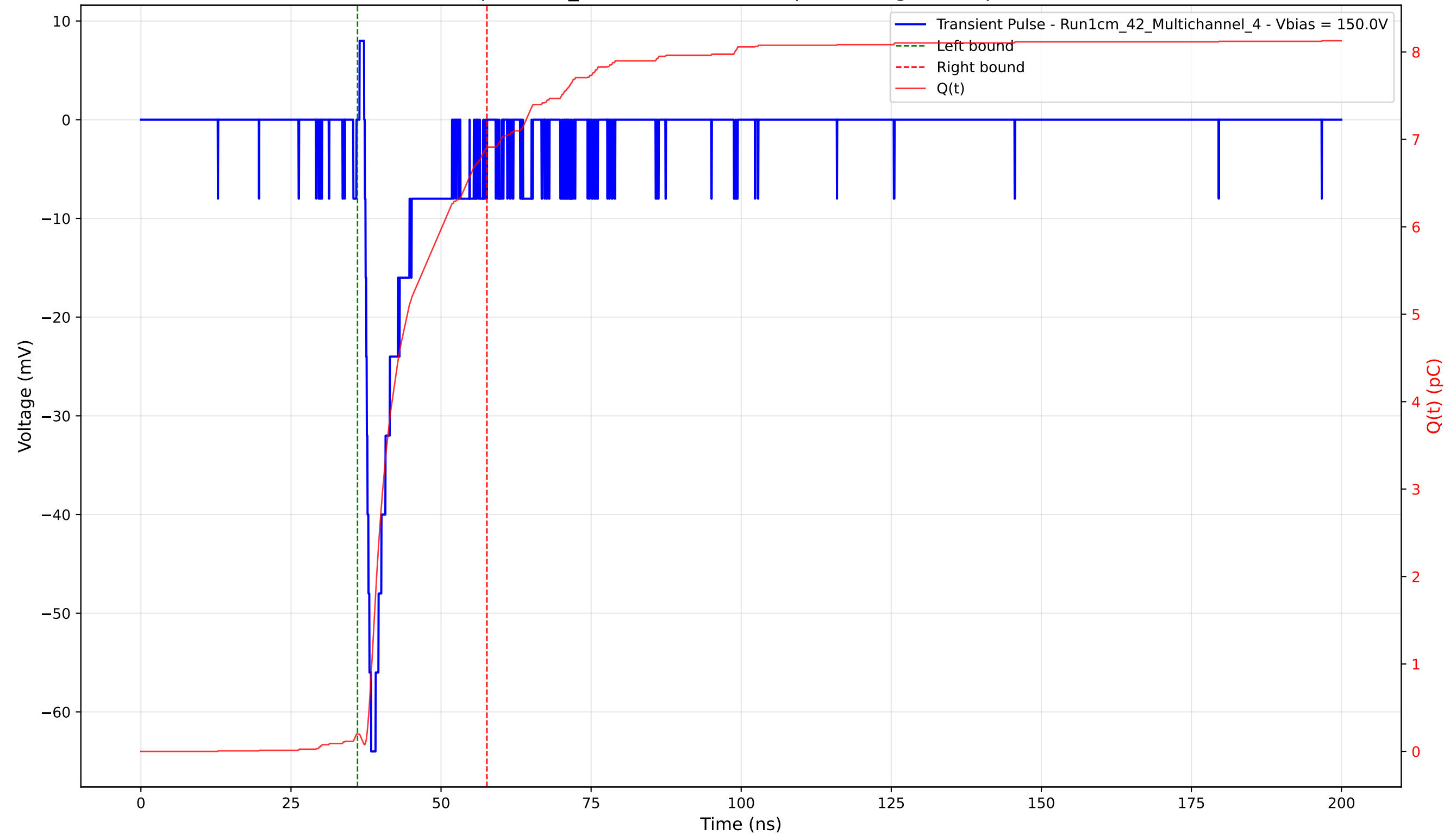
Transient Pulse - Sample: 1cm_42 - Position: 1210.0 \mu\text{m} - Charge: 6.71 pC - Rise Time: 1.05 ns
