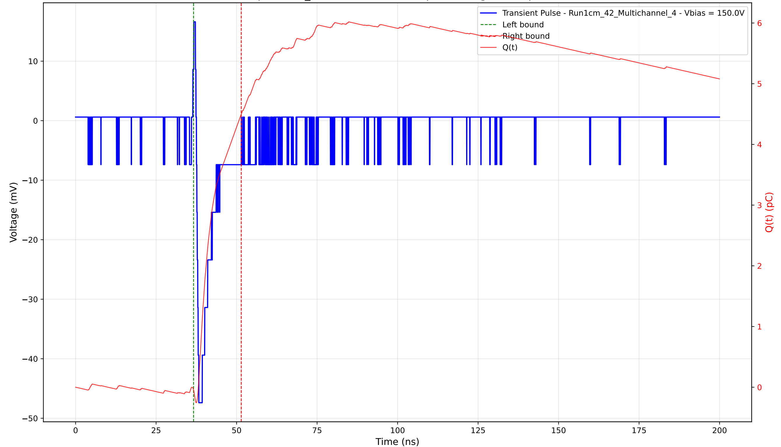
Transient Pulse - Sample: 1cm_42 - Position: 1035.0 \mu\text{m} - Charge: 4.54 pC - Rise Time: 0.74 ns
