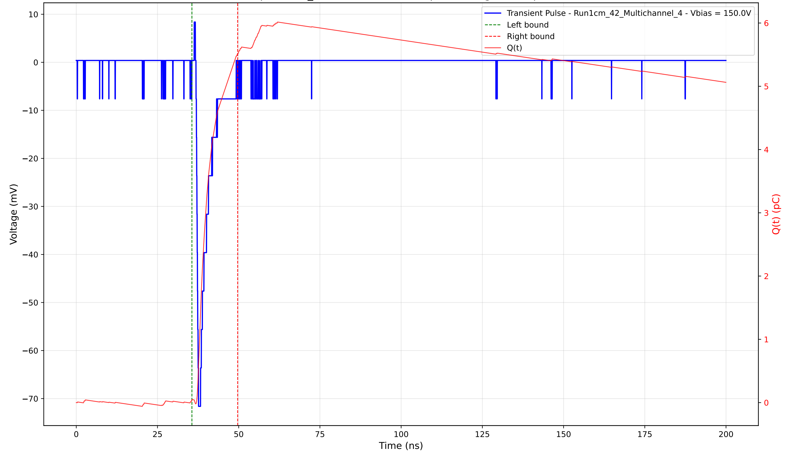
Transient Pulse - Sample: 1cm_42 - Position: 3510.0 \mu\text{m} - Charge: 5.47 pC - Rise Time: 0.76 ns
