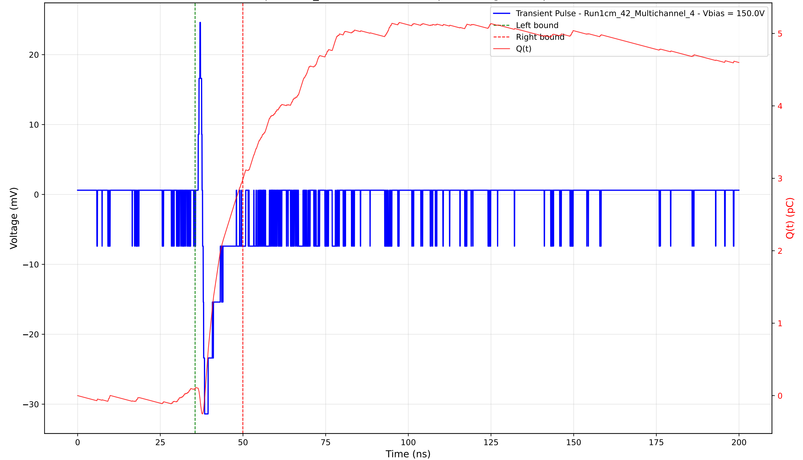
Transient Pulse - Sample: 1cm_42 - Position: 4440.0 \mu\text{m} - Charge: 2.90 pC - Rise Time: 0.63 ns
