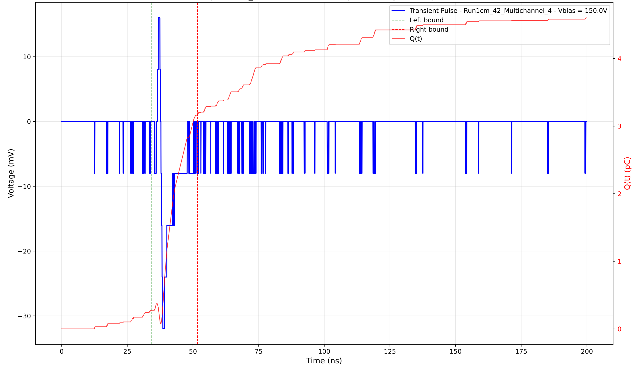
Transient Pulse - Sample: 1cm_42 - Position: 4535.0 \mu\text{m} - Charge: 2.91 pC - Rise Time: 0.74 ns
