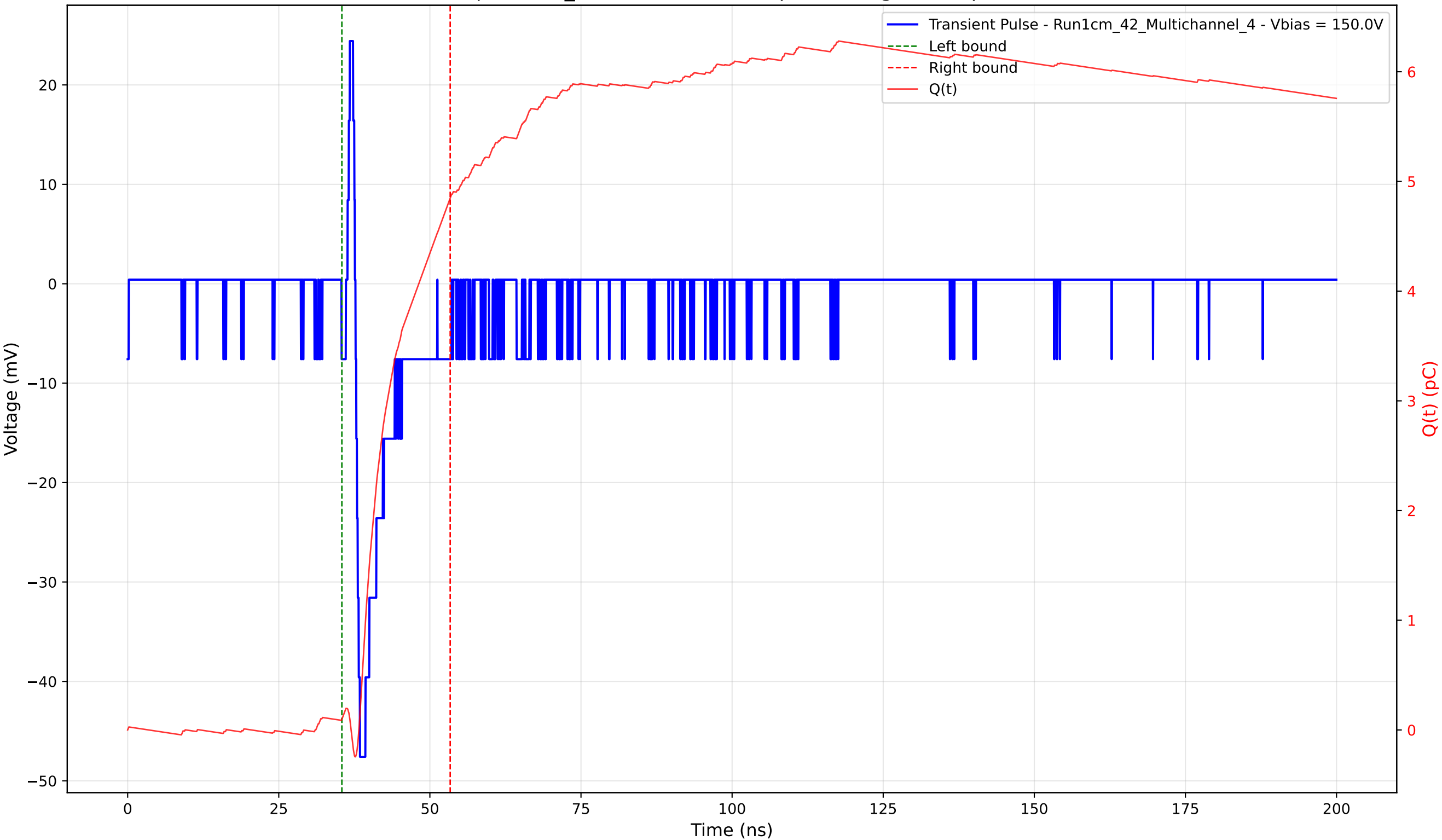
Transient Pulse - Sample: 1cm_42 - Position: 765.0 \mu\text{m} - Charge: 4.75 pC - Rise Time: 0.74 ns
