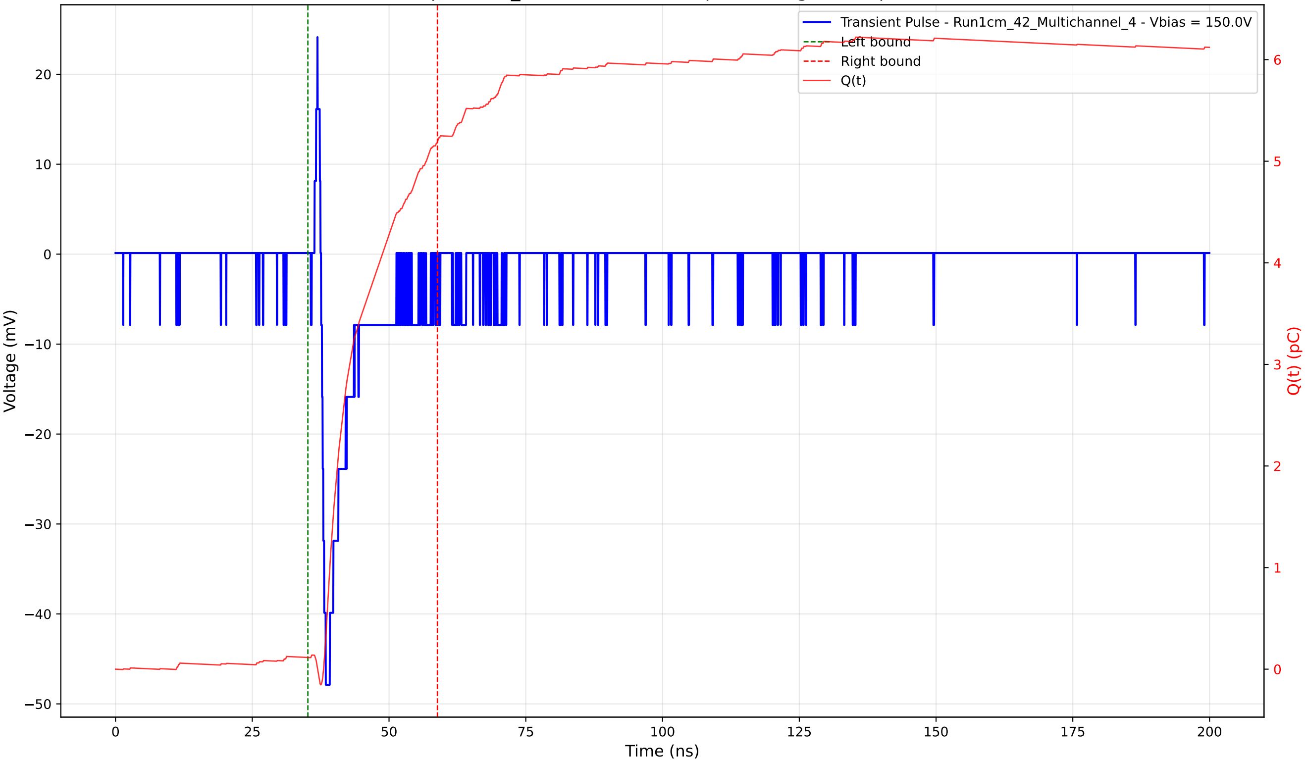
Transient Pulse - Sample: 1cm_42 - Position: 975.0 \mu\text{m} - Charge: 5.08 pC - Rise Time: 0.86 ns
