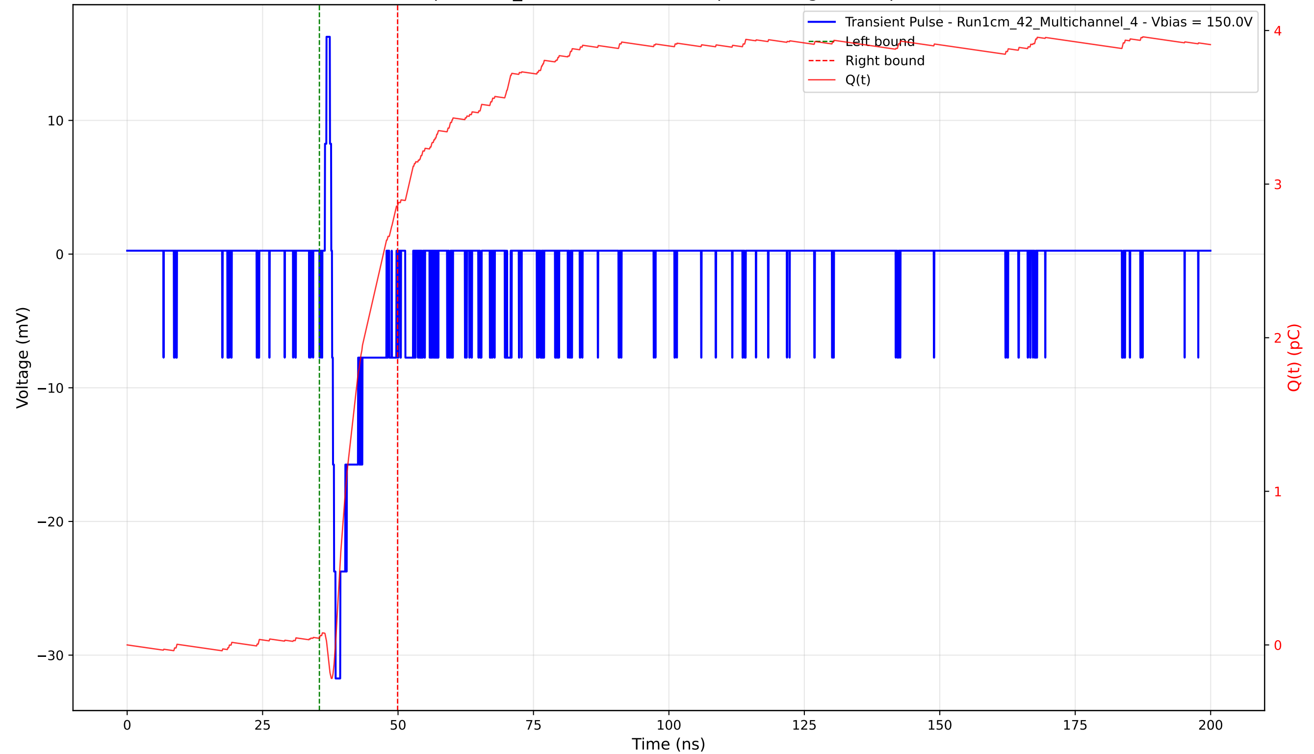
Transient Pulse - Sample: 1cm_42 - Position: 4505.0 \mu\text{m} - Charge: 2.82 pC - Rise Time: 0.66 ns
