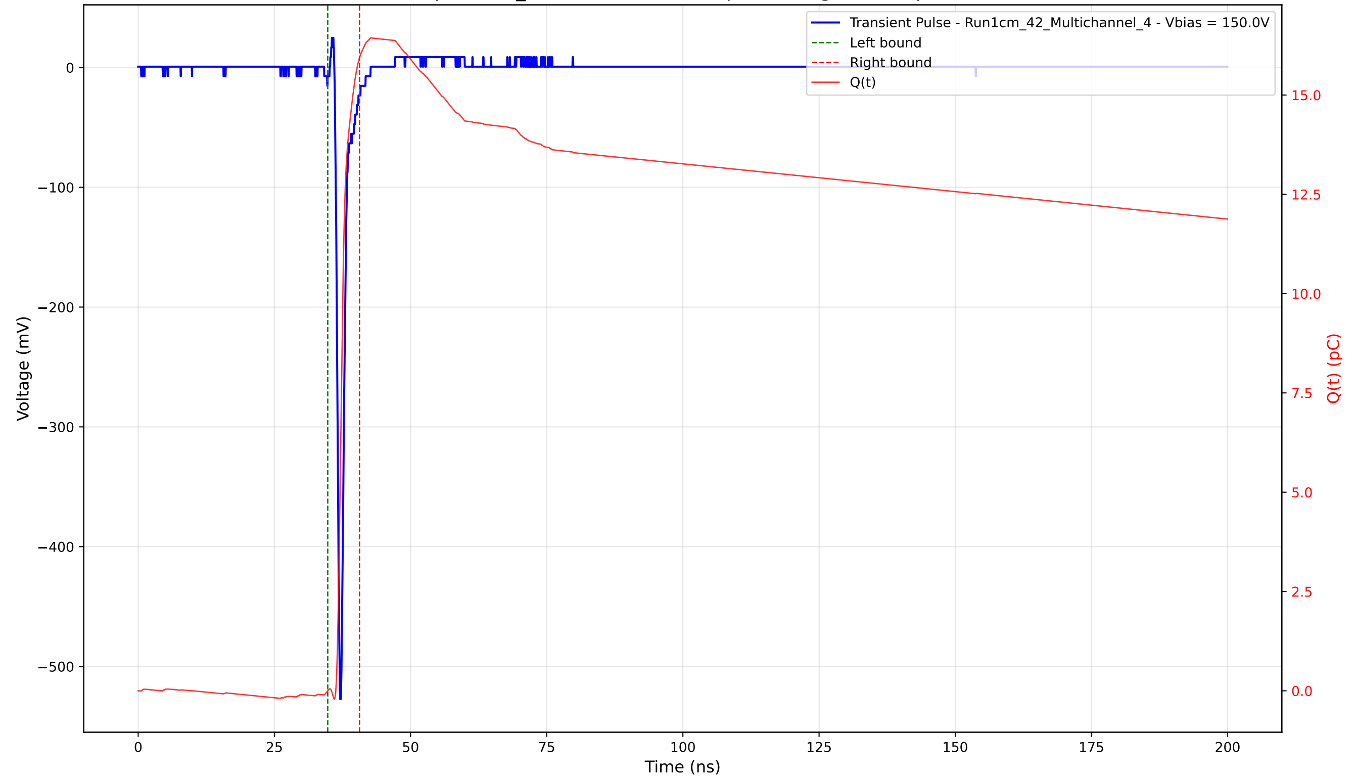
Transient Pulse - Sample: 1cm_42 - Position: 2465.0 \mu\text{m} - Charge: 15.94 pC - Rise Time: 0.71 ns
