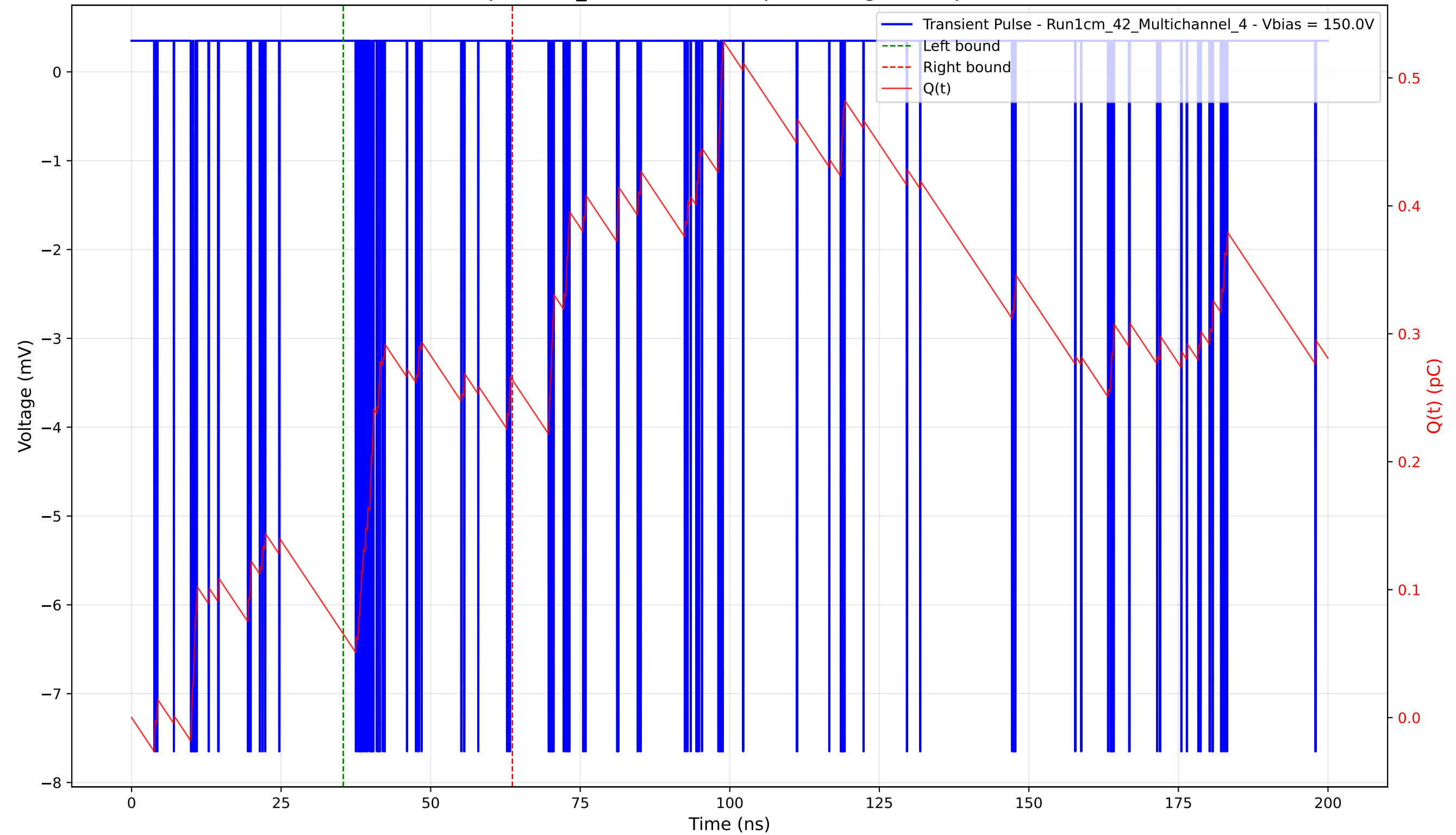
Transient Pulse - Sample: 1cm_42 - Position: 5.0 \mu\text{m} - Charge: 0.20 pC - Rise Time: 0.04 ns
