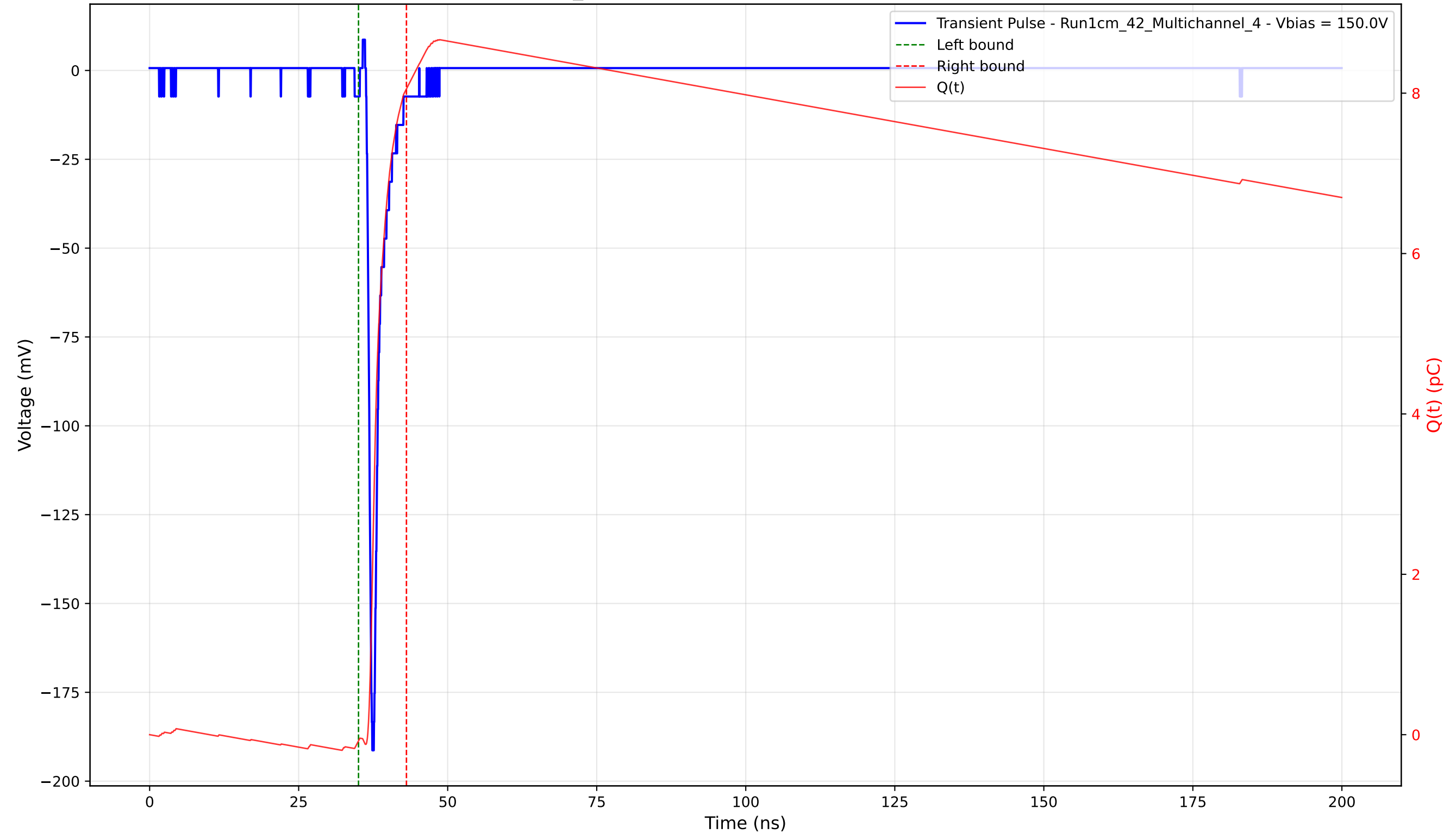
Transient Pulse - Sample: 1cm_42 - Position: 3075.0 \mu\text{m} - Charge: 8.13 pC - Rise Time: 0.78 ns
