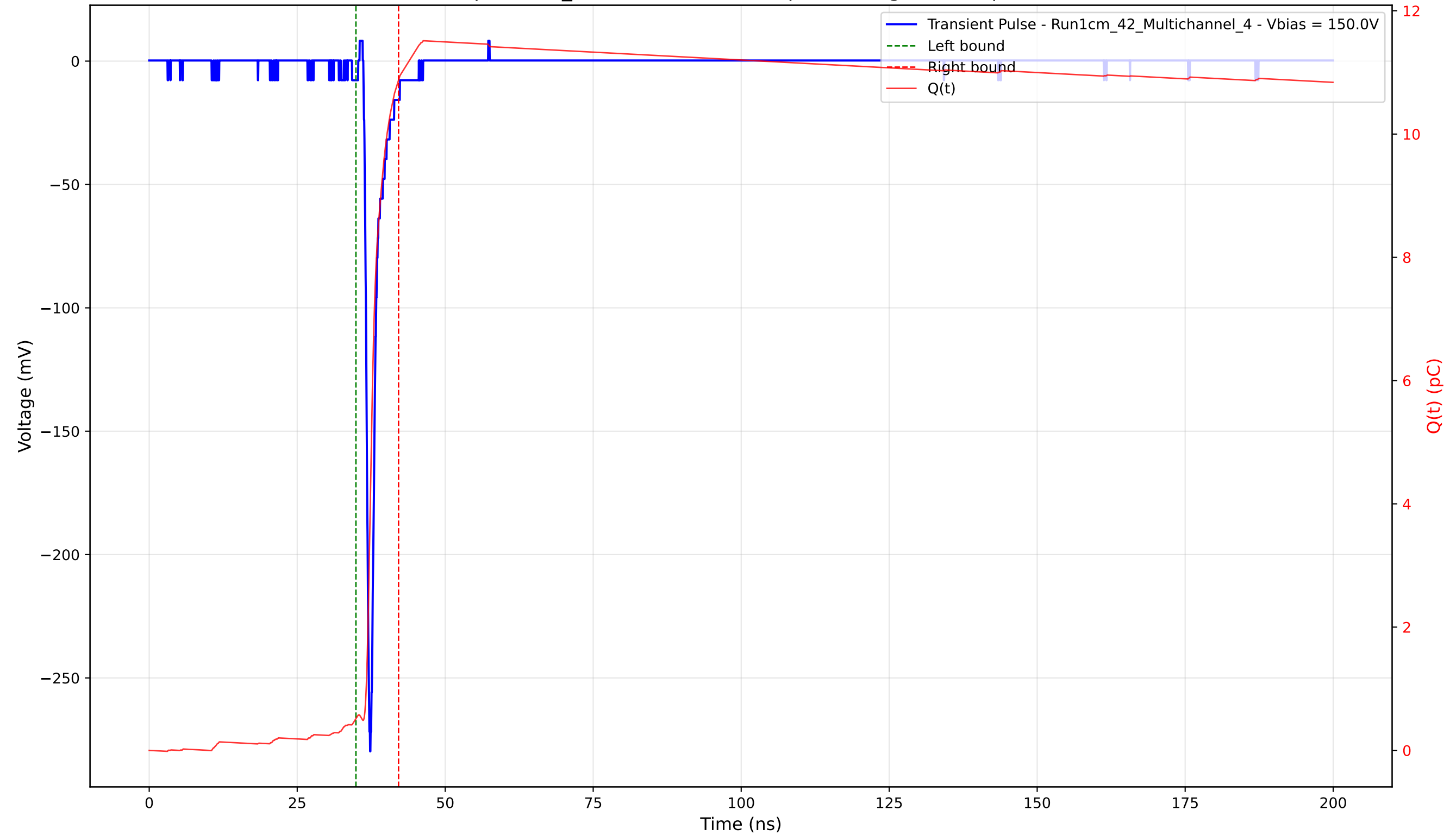
Transient Pulse - Sample: 1cm_42 - Position: 2960.0 \mu\text{m} - Charge: 10.36 pC - Rise Time: 0.76 ns
