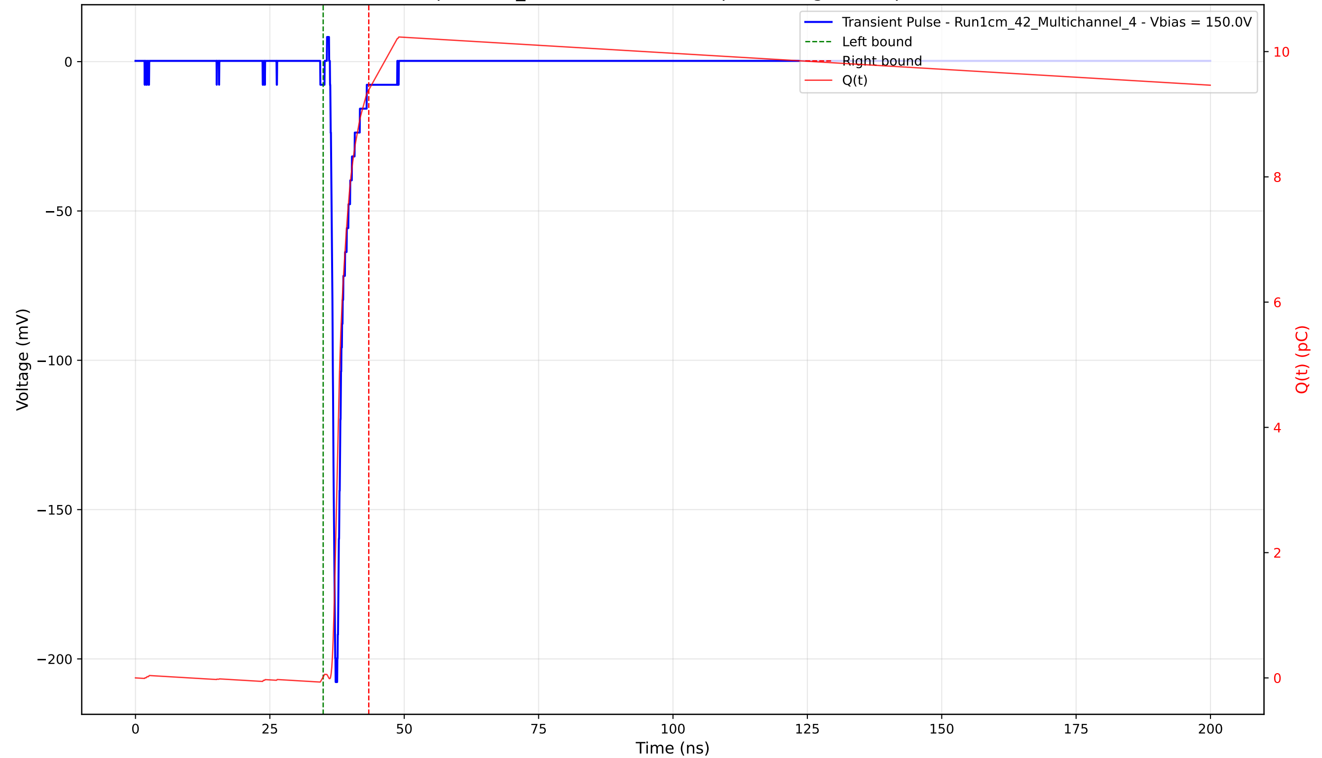
Transient Pulse - Sample: 1cm_42 - Position: 1980.0 \mu\text{m} - Charge: 9.37 pC - Rise Time: 0.79 ns
