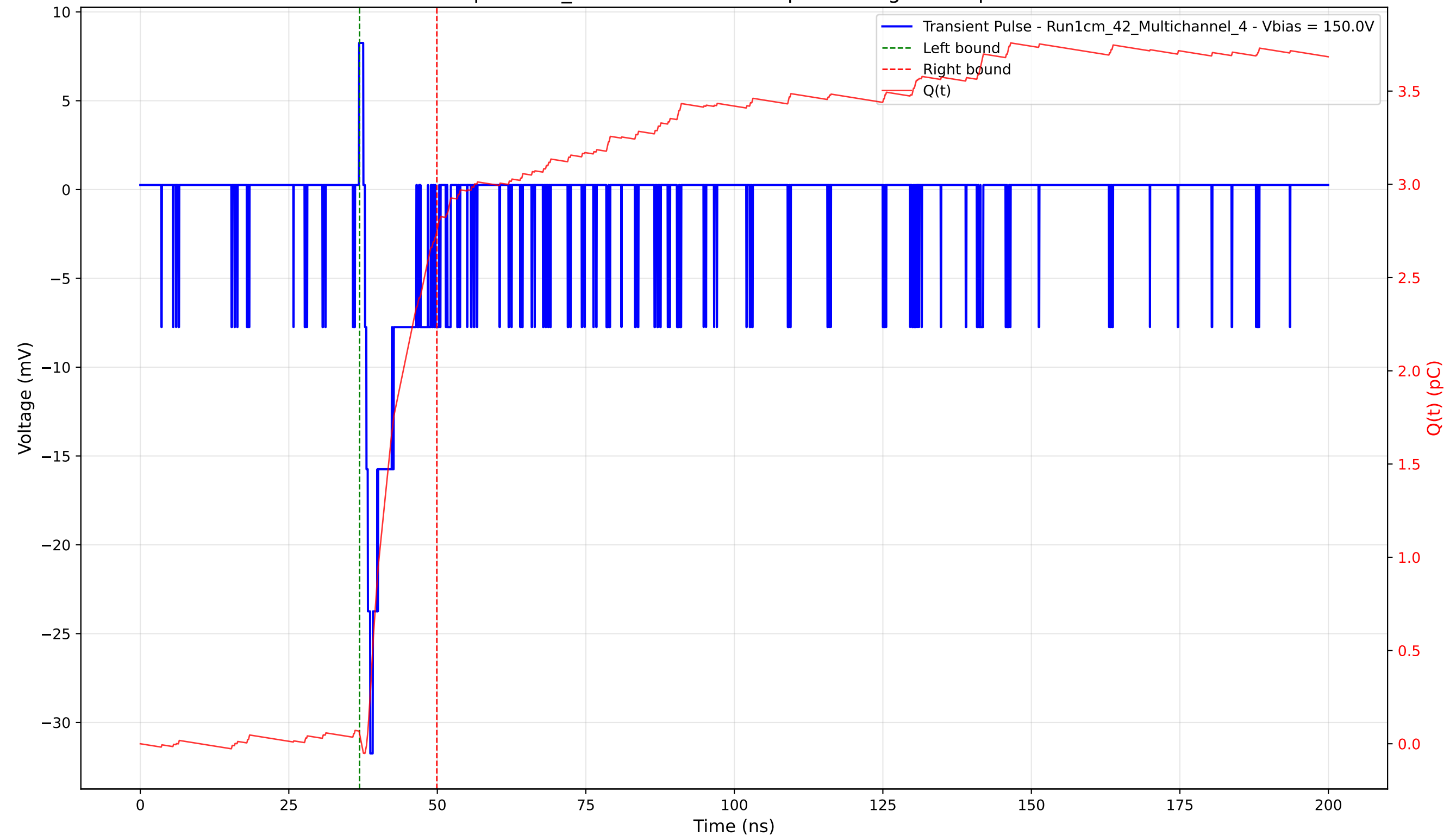
Transient Pulse - Sample: 1cm_42 - Position: 4905.0 \mu\text{m} - Charge: 2.70 pC - Rise Time: 0.90 ns
