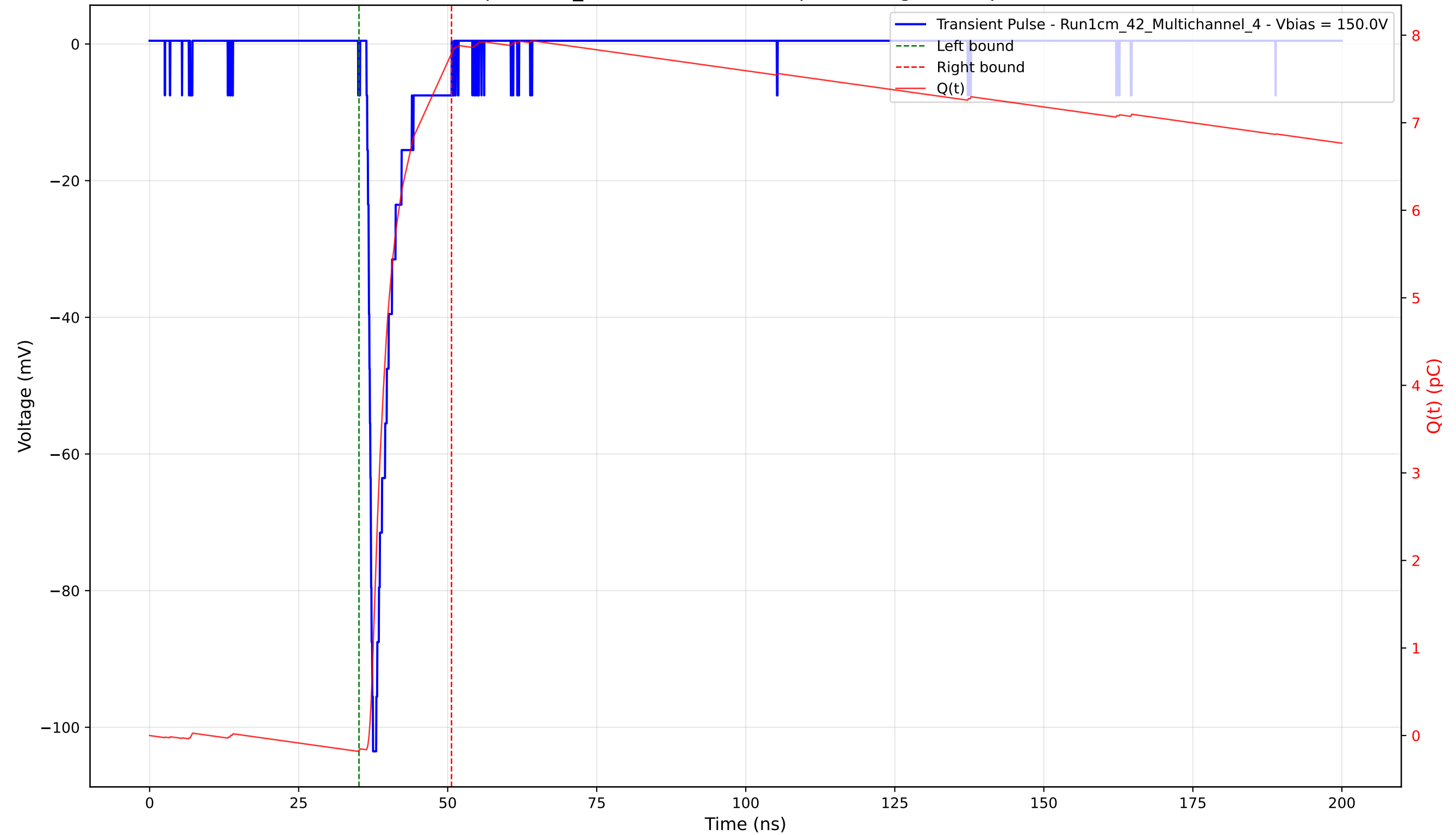
Transient Pulse - Sample: 1cm_42 - Position: 1630.0 \mu\text{m} - Charge: 7.96 pC - Rise Time: 0.87 ns
