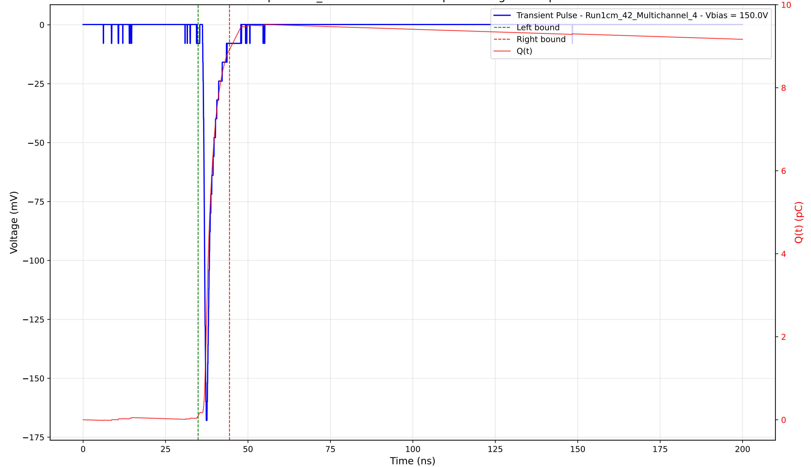
Transient Pulse - Sample: 1cm_42 - Position: 1895.0 \mu\text{m} - Charge: 8.83 pC - Rise Time: 0.80 ns
