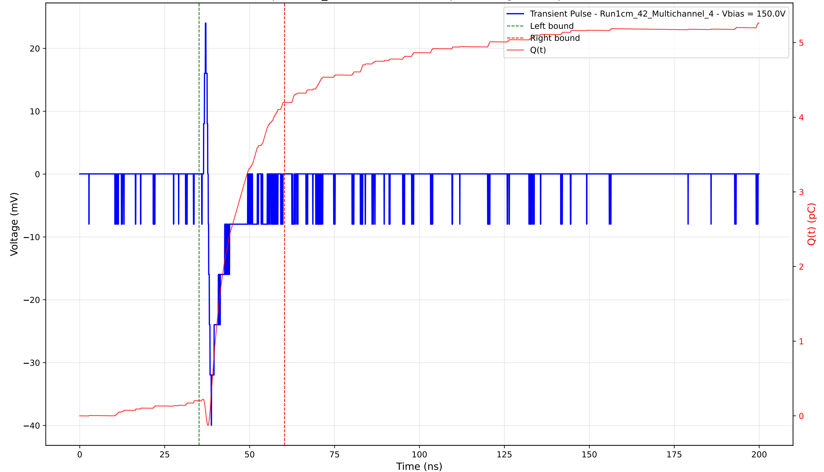
Transient Pulse - Sample: 1cm_42 - Position: 4420.0 \mu\text{m} - Charge: 4.00 pC - Rise Time: 0.90 ns
