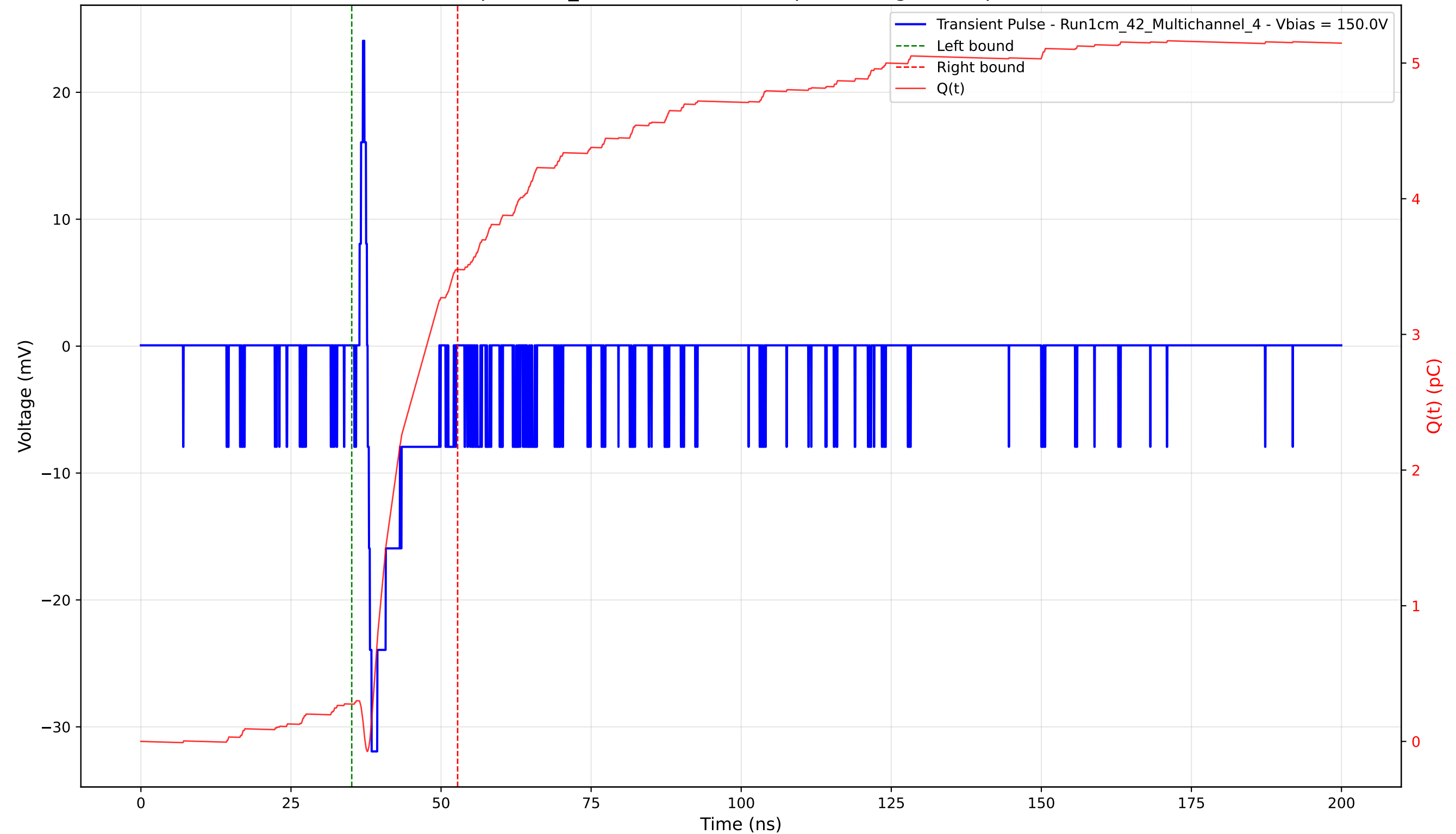
Transient Pulse - Sample: 1cm_42 - Position: 4445.0 \mu\text{m} - Charge: 3.20 pC - Rise Time: 0.66 ns
