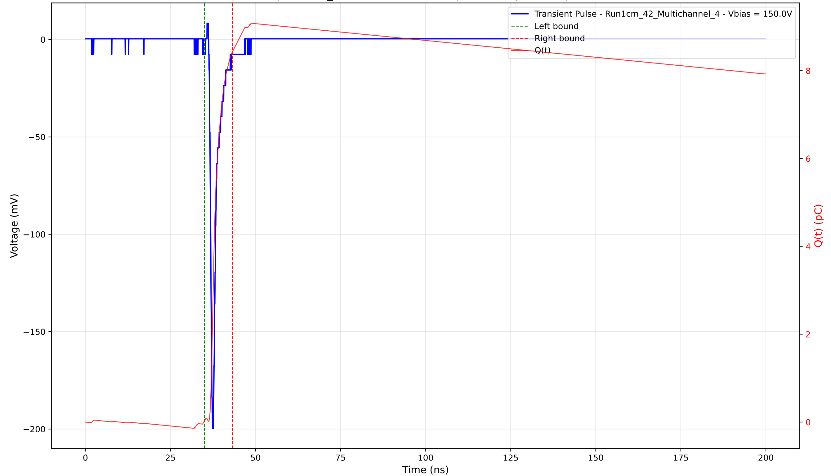
Transient Pulse - Sample: 1cm_42 - Position: 3060.0 \mu\text{m} - Charge: 8.39 pC - Rise Time: 0.78 ns
