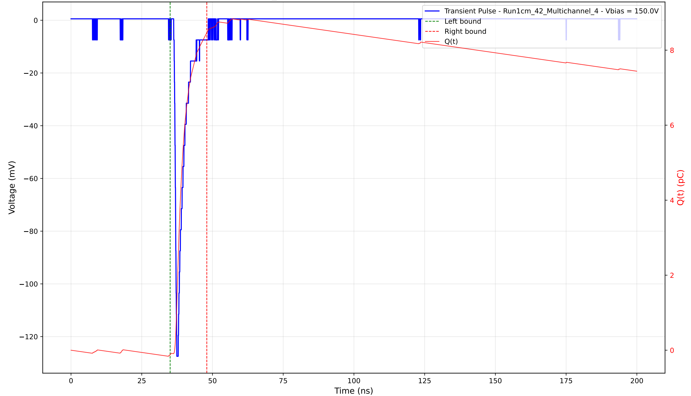
Transient Pulse - Sample: 1cm_42 - Position: 1695.0 \mu\text{m} - Charge: 8.58 pC - Rise Time: 0.85 ns
