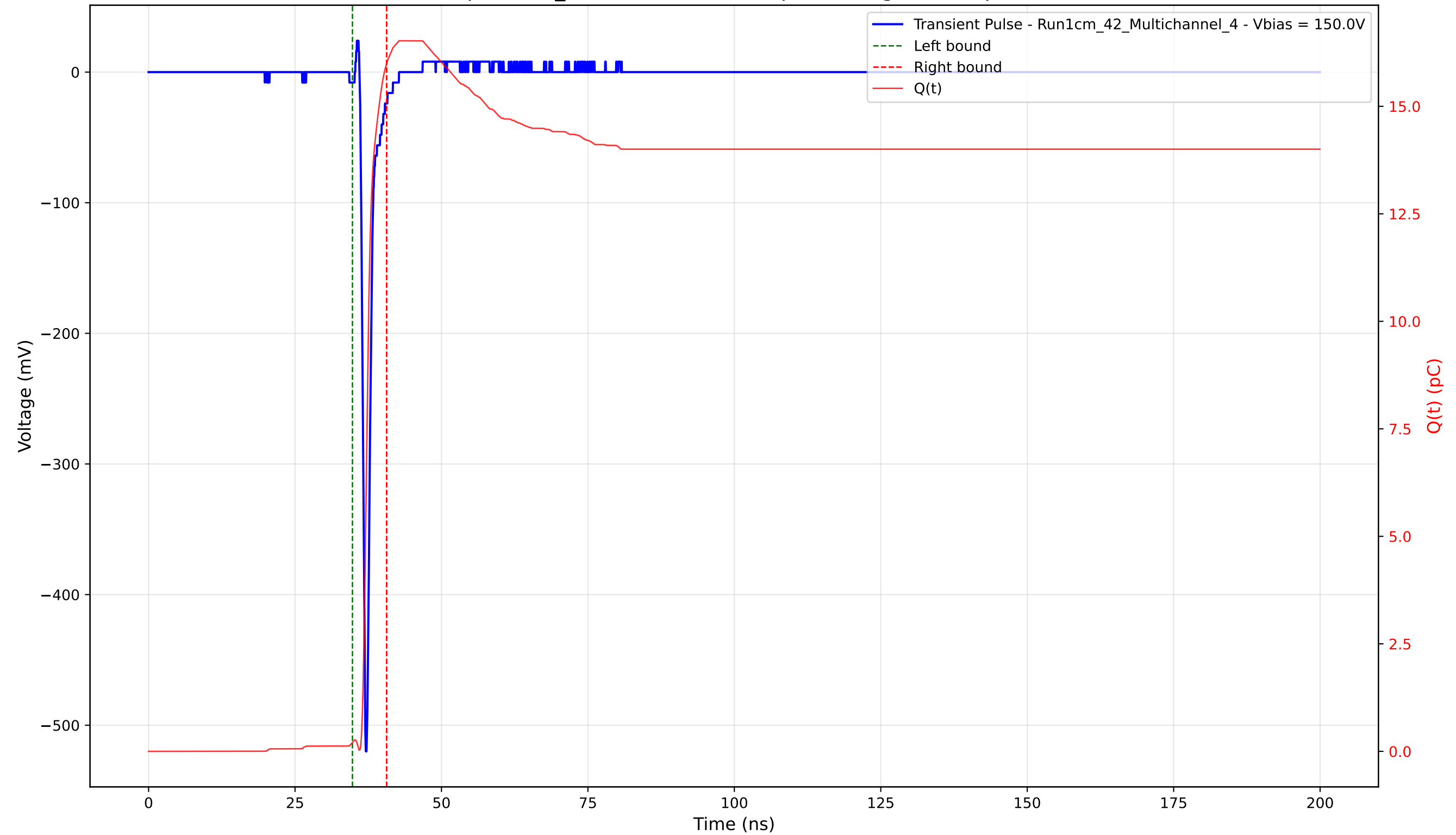
Transient Pulse - Sample: 1cm_42 - Position: 2545.0 \mu\text{m} - Charge: 15.79 pC - Rise Time: 0.72 ns
