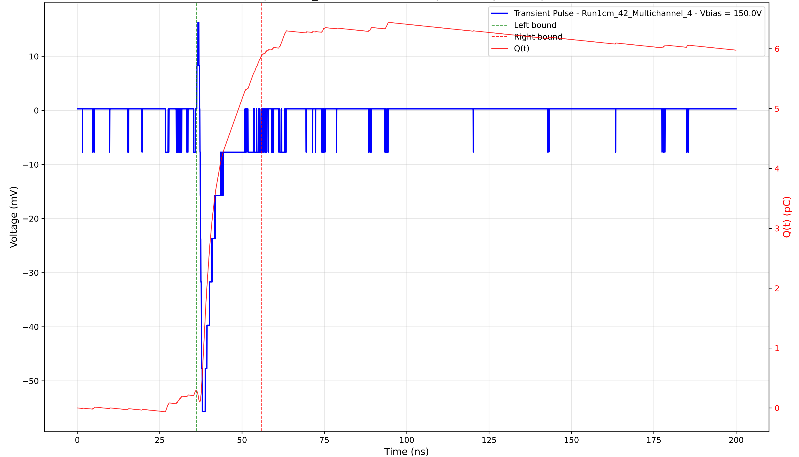
Transient Pulse - Sample: 1cm_42 - Position: 3680.0 \mu\text{m} - Charge: 5.59 pC - Rise Time: 0.69 ns
