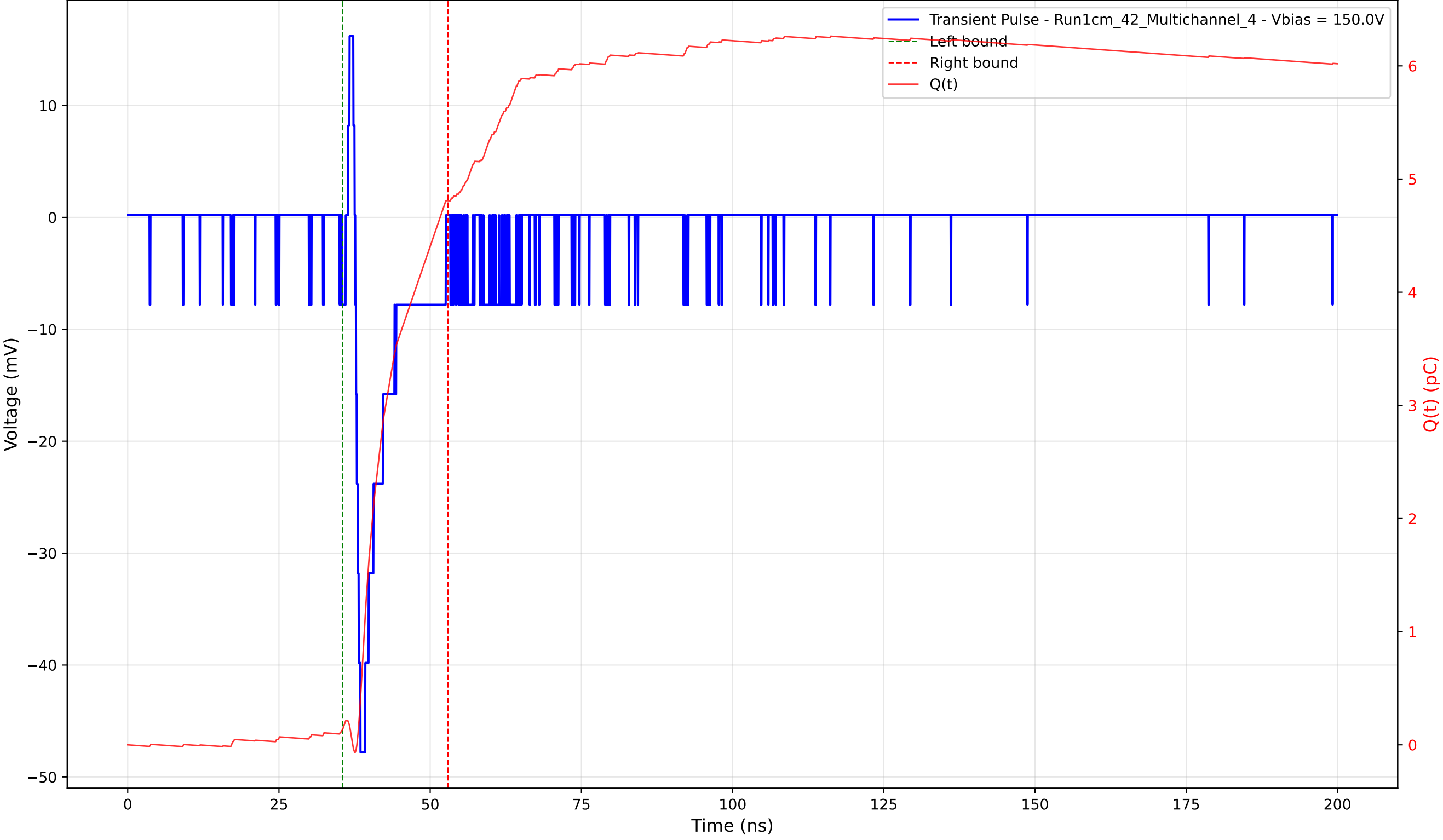
Transient Pulse - Sample: 1cm_42 - Position: 965.0 \mu\text{m} - Charge: 4.67 pC - Rise Time: 0.86 ns
