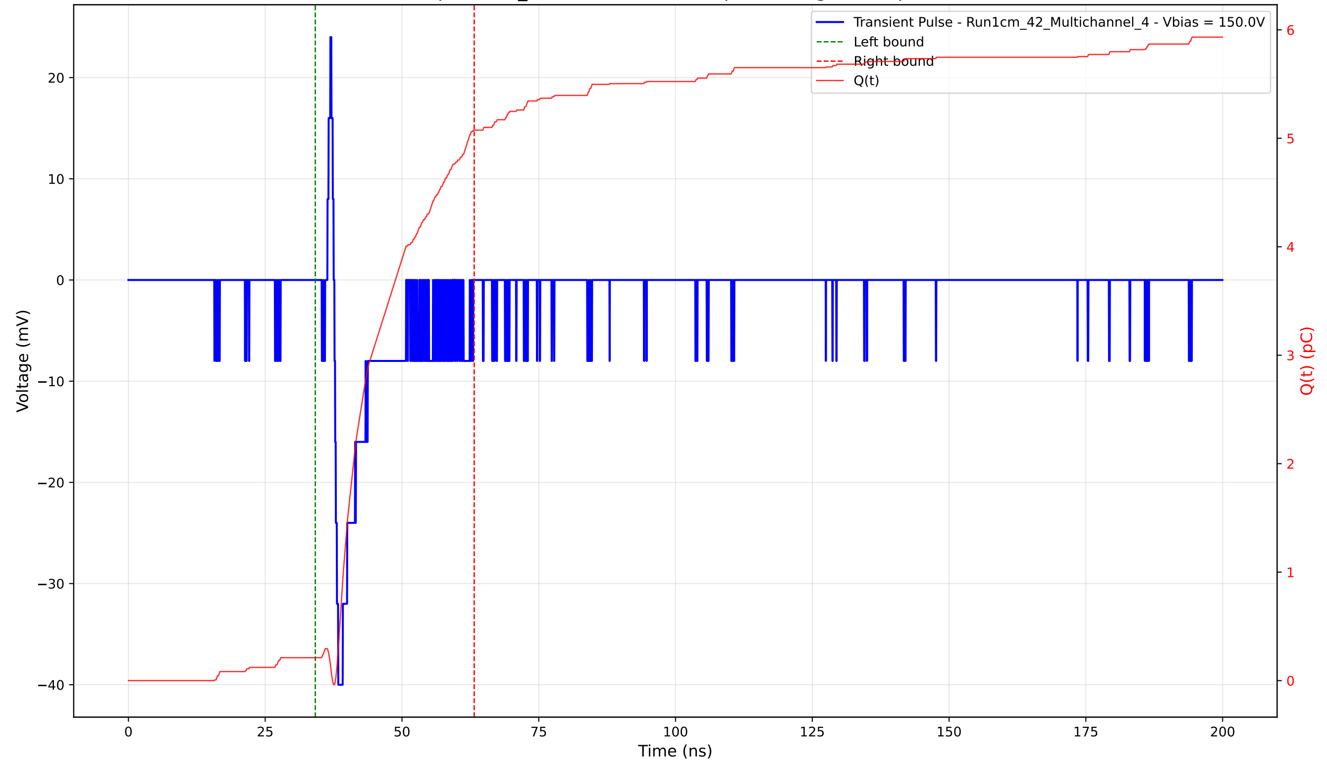
Transient Pulse - Sample: 1cm_42 - Position: 4110.0 \mu\text{m} - Charge: 4.86 pC - Rise Time: 0.70 ns
