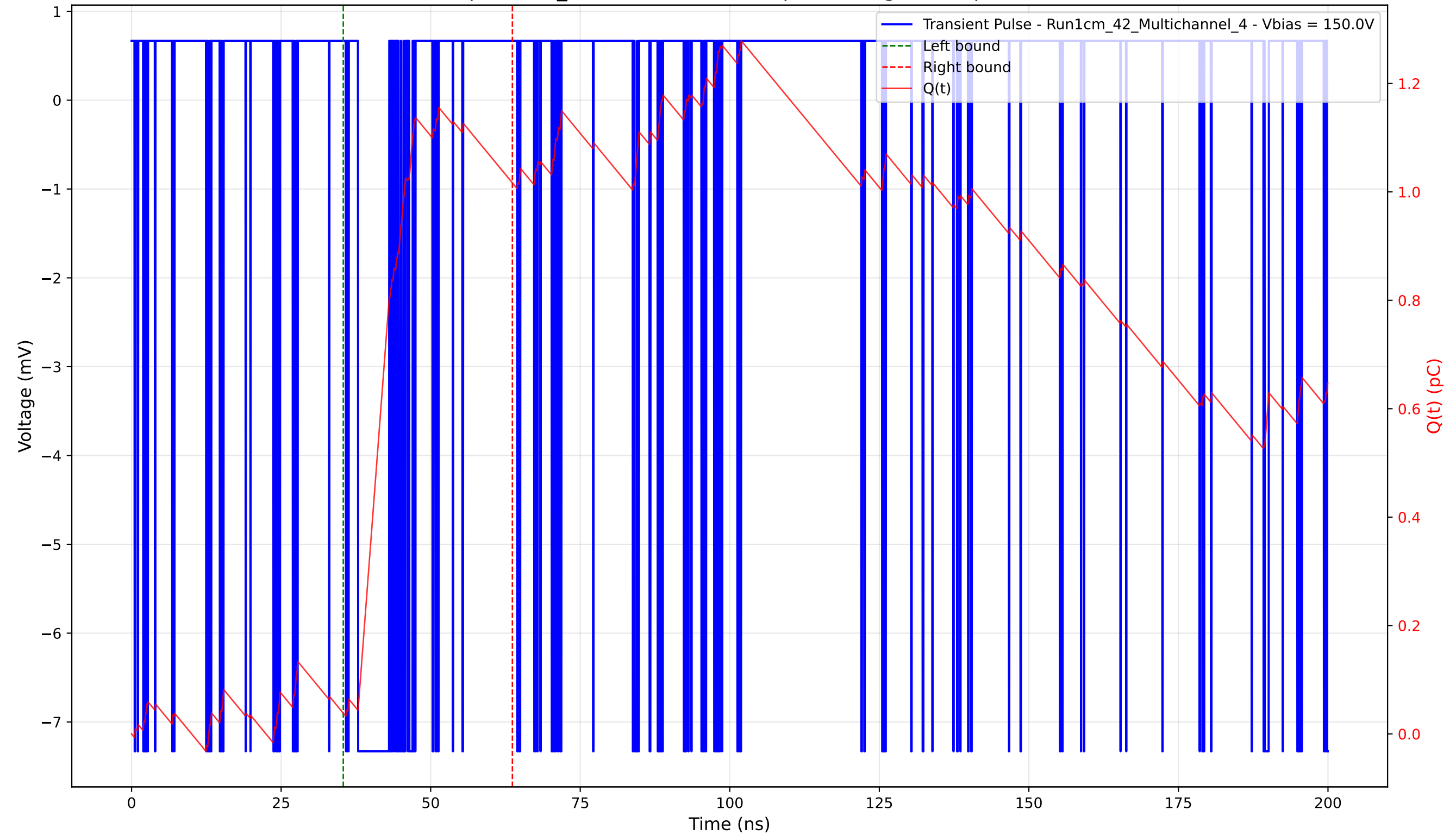
Transient Pulse - Sample: 1cm_42 - Position: 5130.0 \mu\text{m} - Charge: 0.98 pC - Rise Time: 0.04 ns
