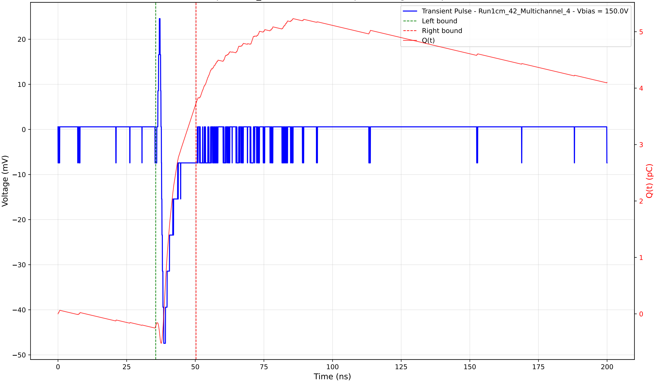
Transient Pulse - Sample: 1cm_42 - Position: 925.0 \mu\text{m} - Charge: 3.95 pC - Rise Time: 0.86 ns
