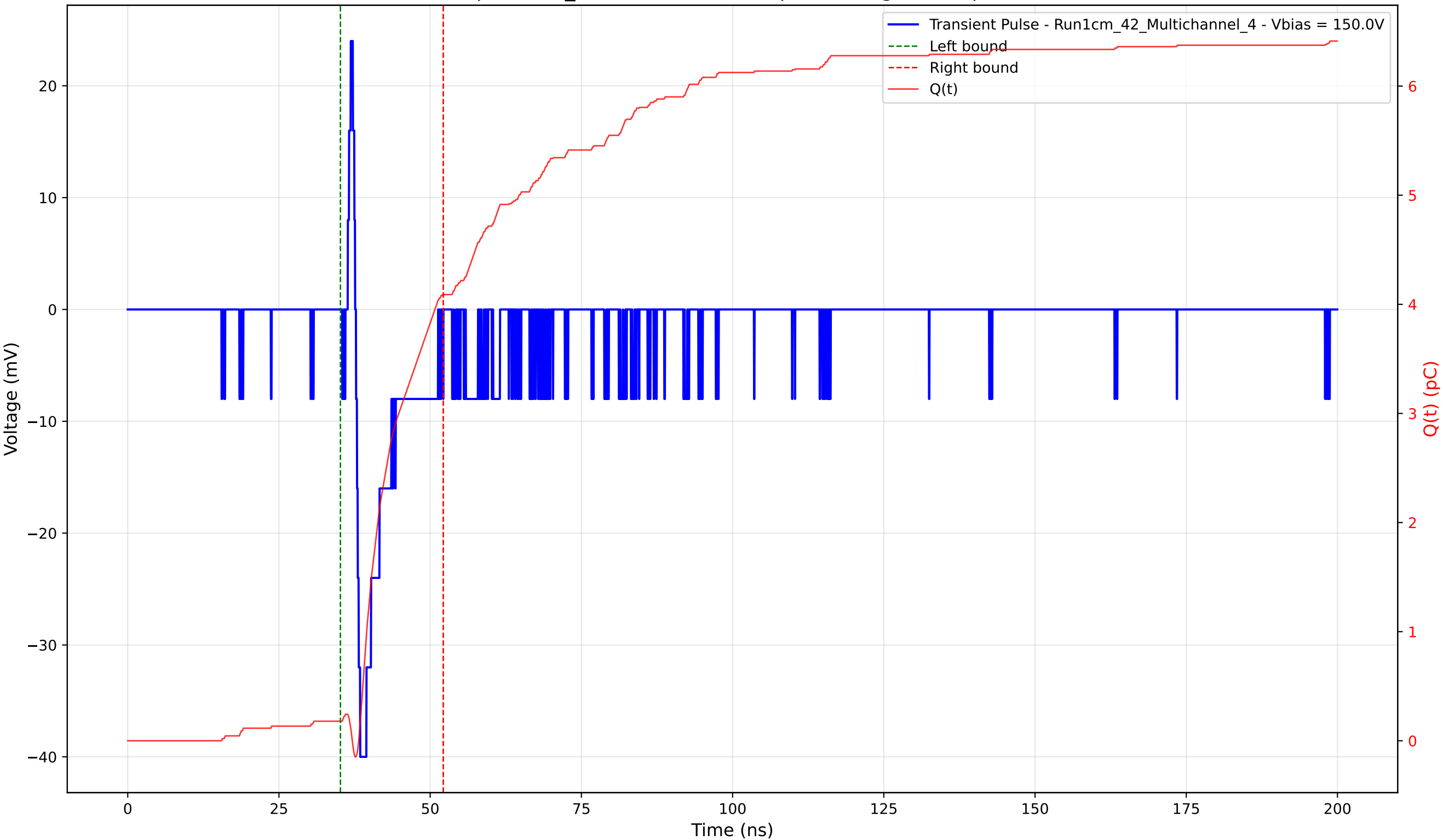
Transient Pulse - Sample: 1cm_42 - Position: 580.0 \mu\text{m} - Charge: 3.91 pC - Rise Time: 0.70 ns
