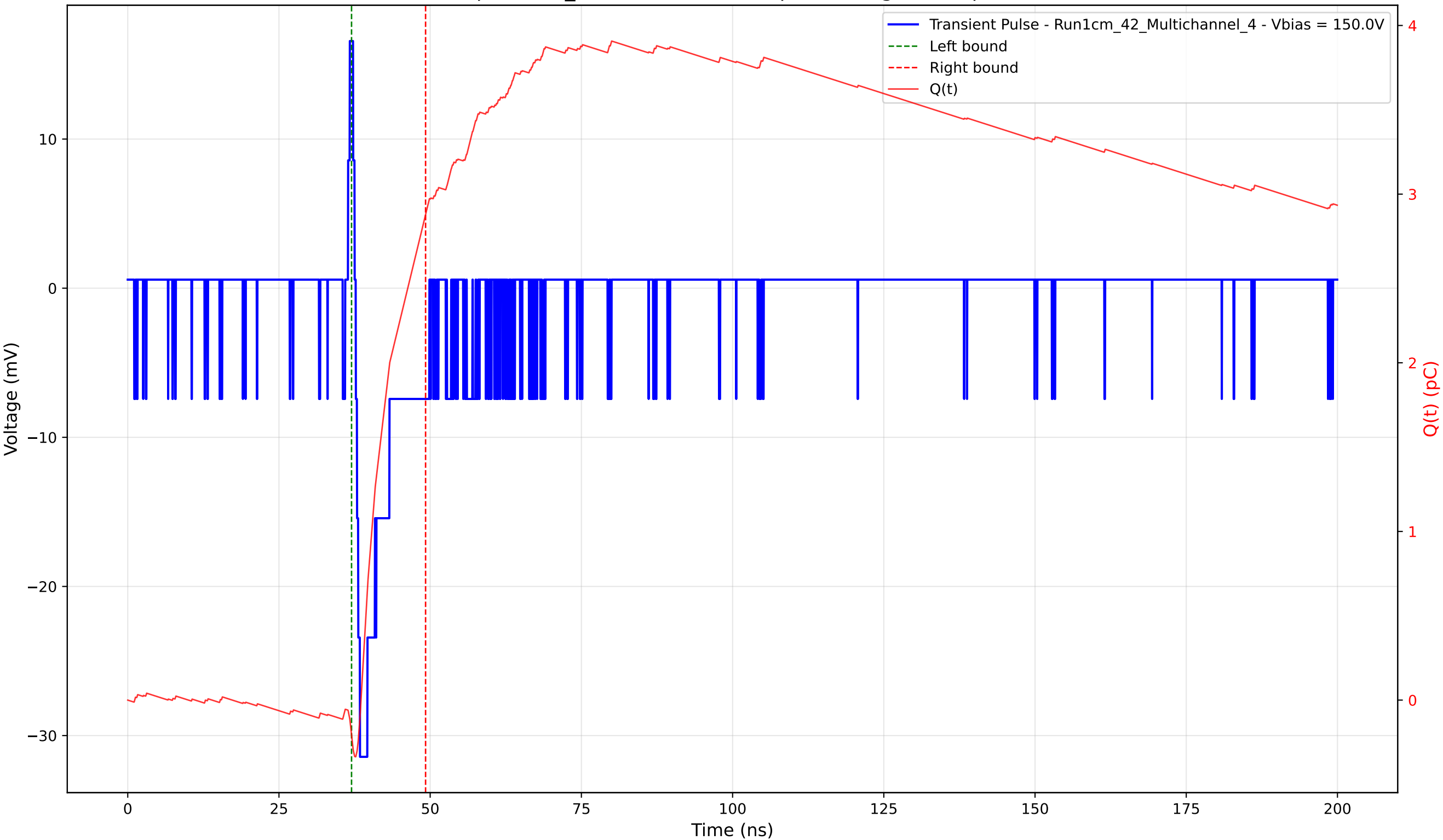
Transient Pulse - Sample: 1cm_42 - Position: 460.0 \mu\text{m} - Charge: 3.09 pC - Rise Time: 0.71 ns
