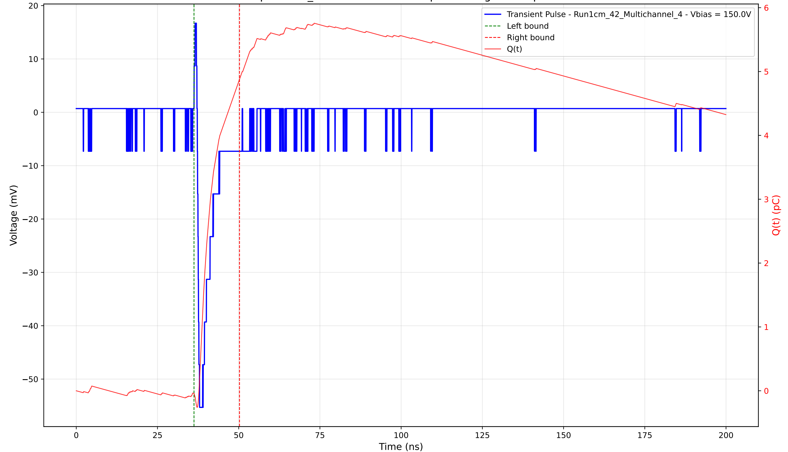
Transient Pulse - Sample: 1cm_42 - Position: 3715.0 \mu\text{m} - Charge: 4.92 pC - Rise Time: 0.69 ns
