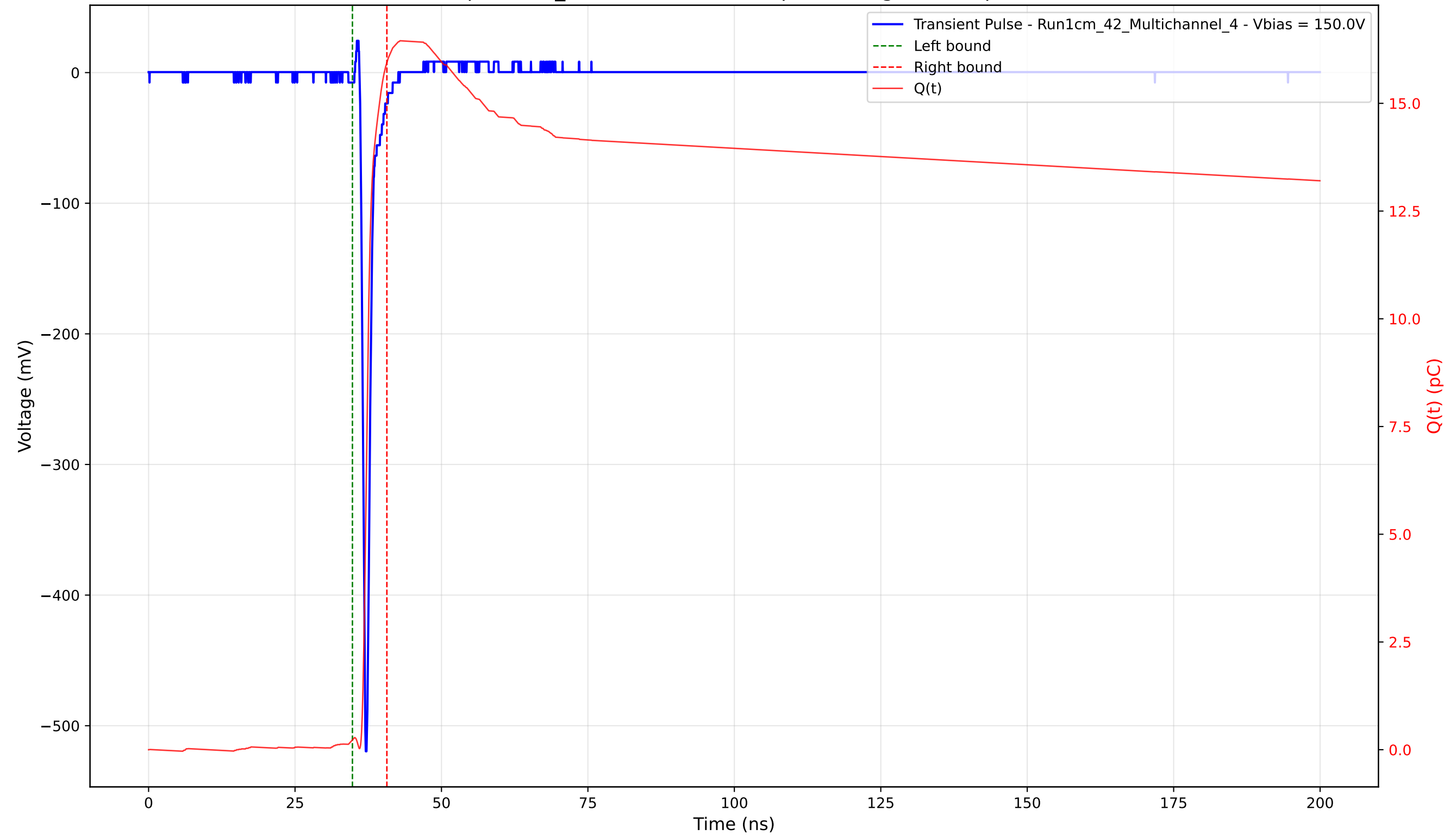
Transient Pulse - Sample: 1cm_42 - Position: 2535.0 \mu\text{m} - Charge: 15.72 pC - Rise Time: 0.72 ns
