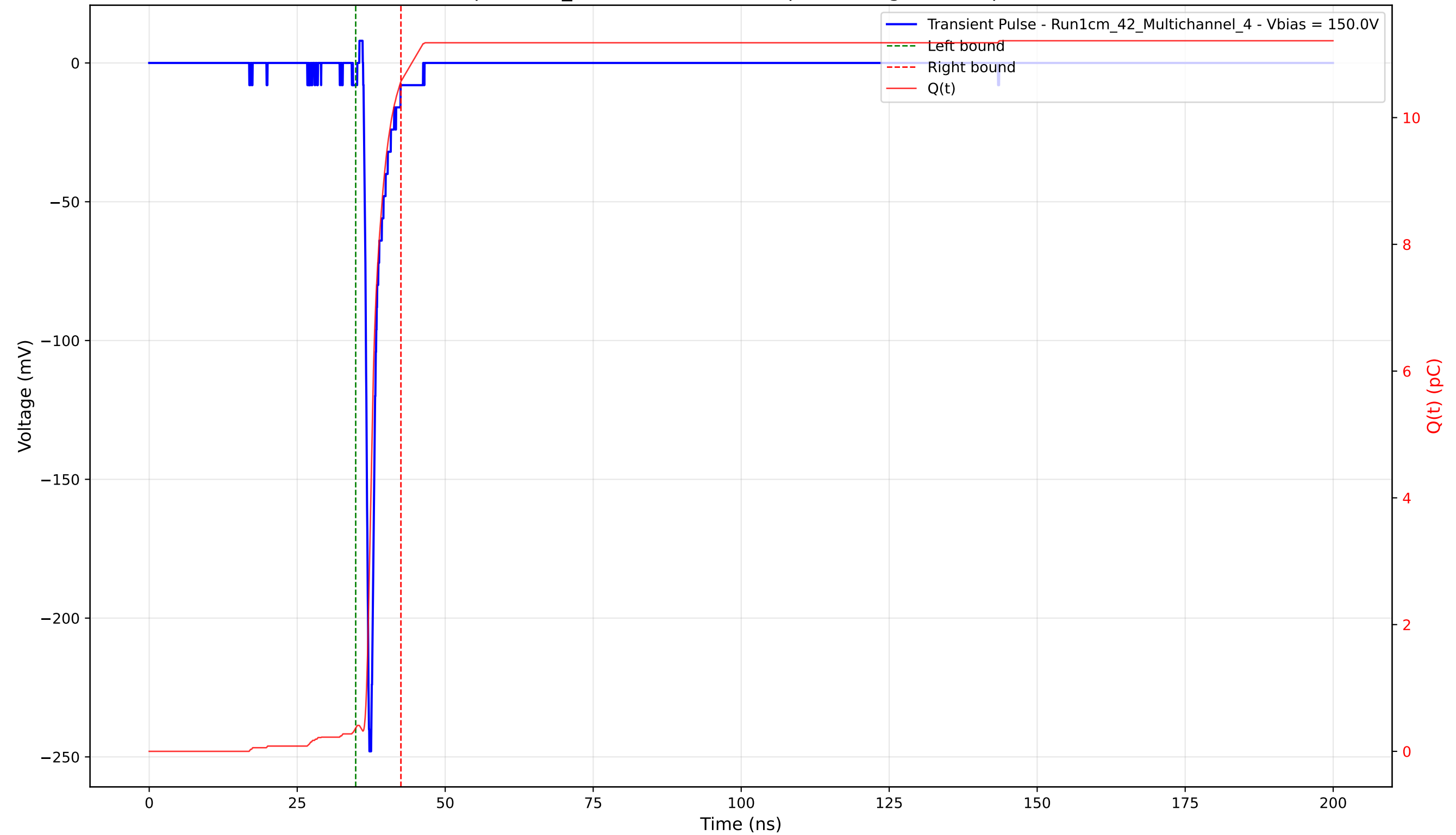
Transient Pulse - Sample: 1cm_42 - Position: 2035.0 \mu\text{m} - Charge: 10.20 pC - Rise Time: 0.75 ns
