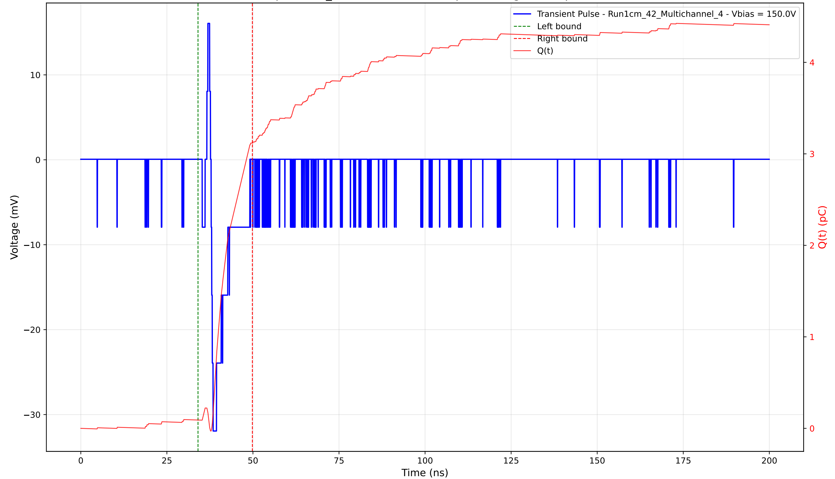
Transient Pulse - Sample: 1cm_42 - Position: 4735.0 \mu\text{m} - Charge: 3.03 pC - Rise Time: 0.58 ns
