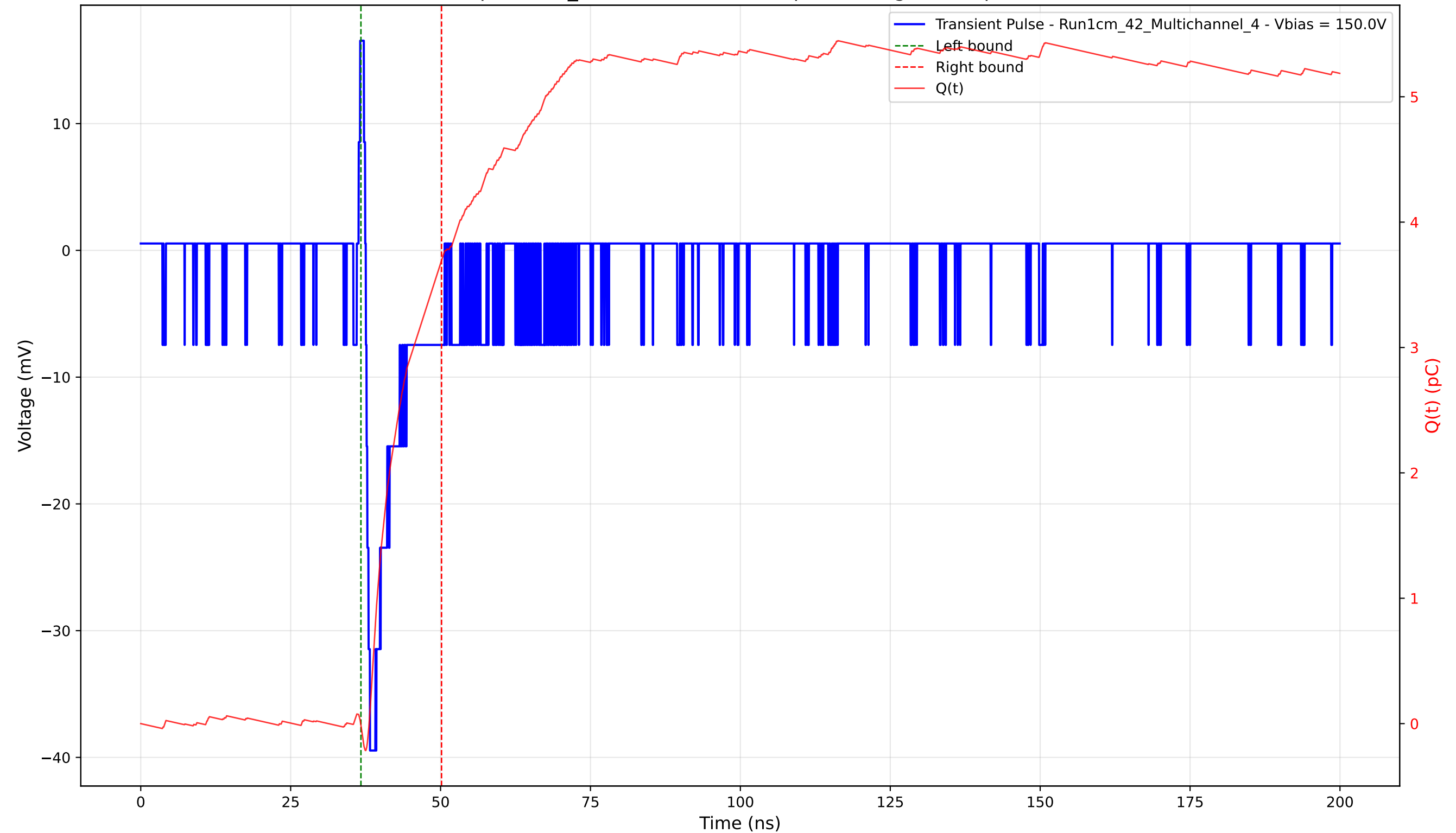
Transient Pulse - Sample: 1cm_42 - Position: 4010.0 \mu\text{m} - Charge: 3.71 pC - Rise Time: 0.70 ns
