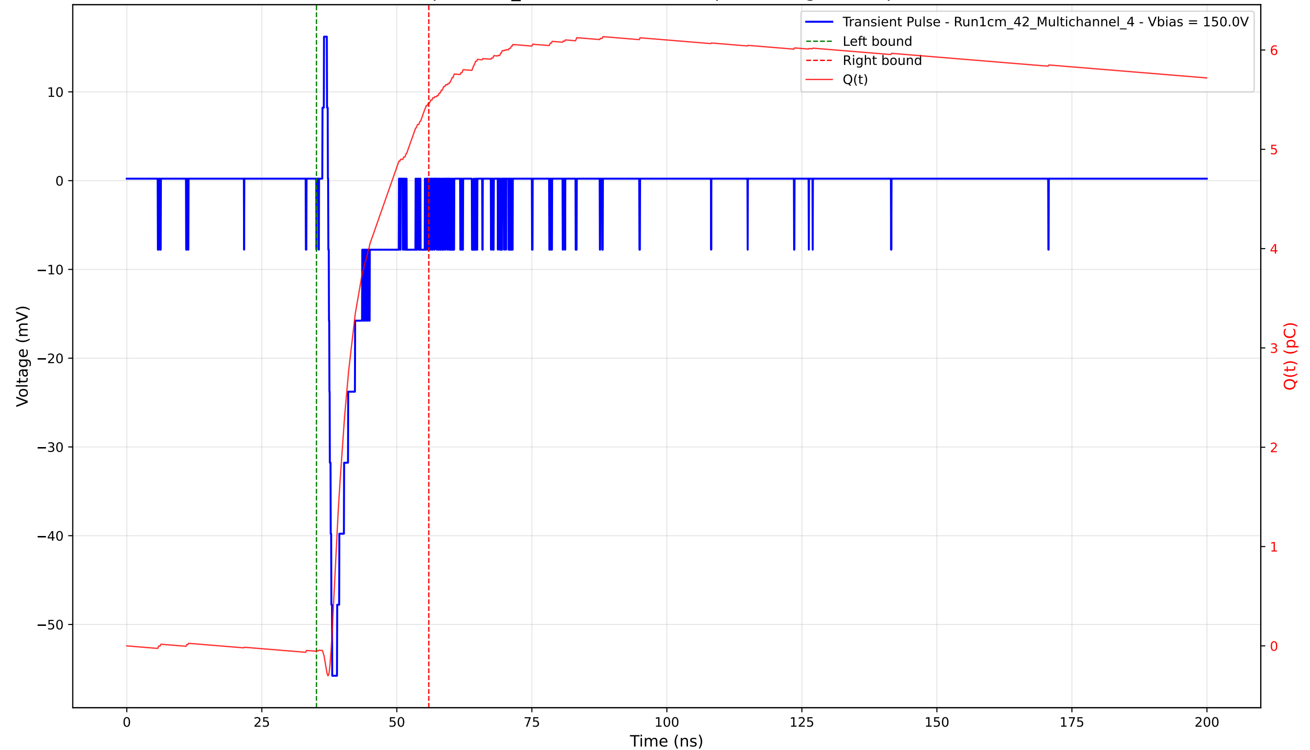
Transient Pulse - Sample: 1cm_42 - Position: 3800.0 \mu\text{m} - Charge: 5.52 pC - Rise Time: 0.73 ns
