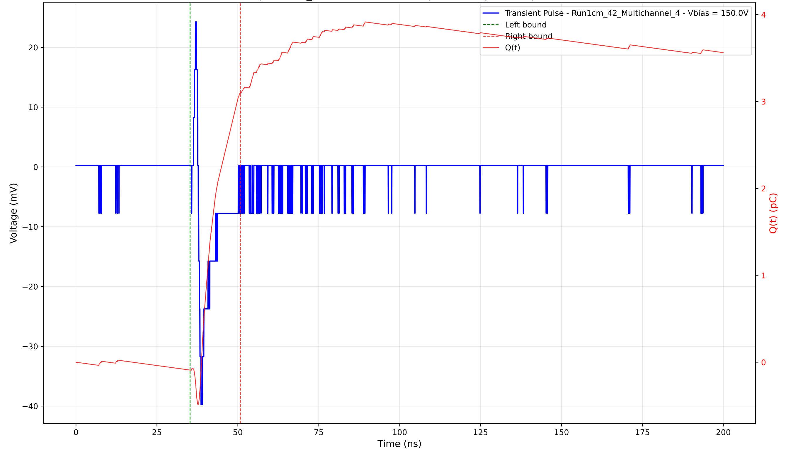
Transient Pulse - Sample: 1cm_42 - Position: 4405.0 \mu\text{m} - Charge: 3.18 pC - Rise Time: 0.86 ns
