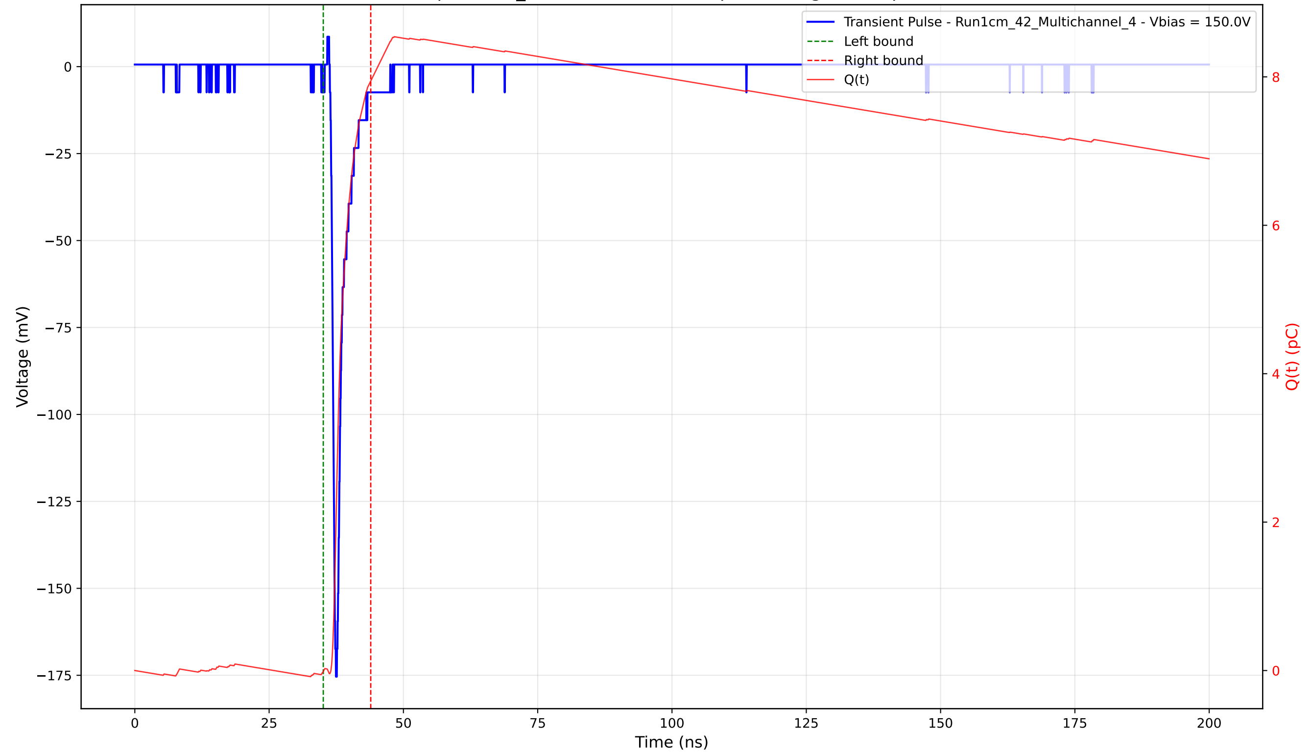
Transient Pulse - Sample: 1cm_42 - Position: 3120.0 \mu\text{m} - Charge: 7.96 pC - Rise Time: 0.75 ns
