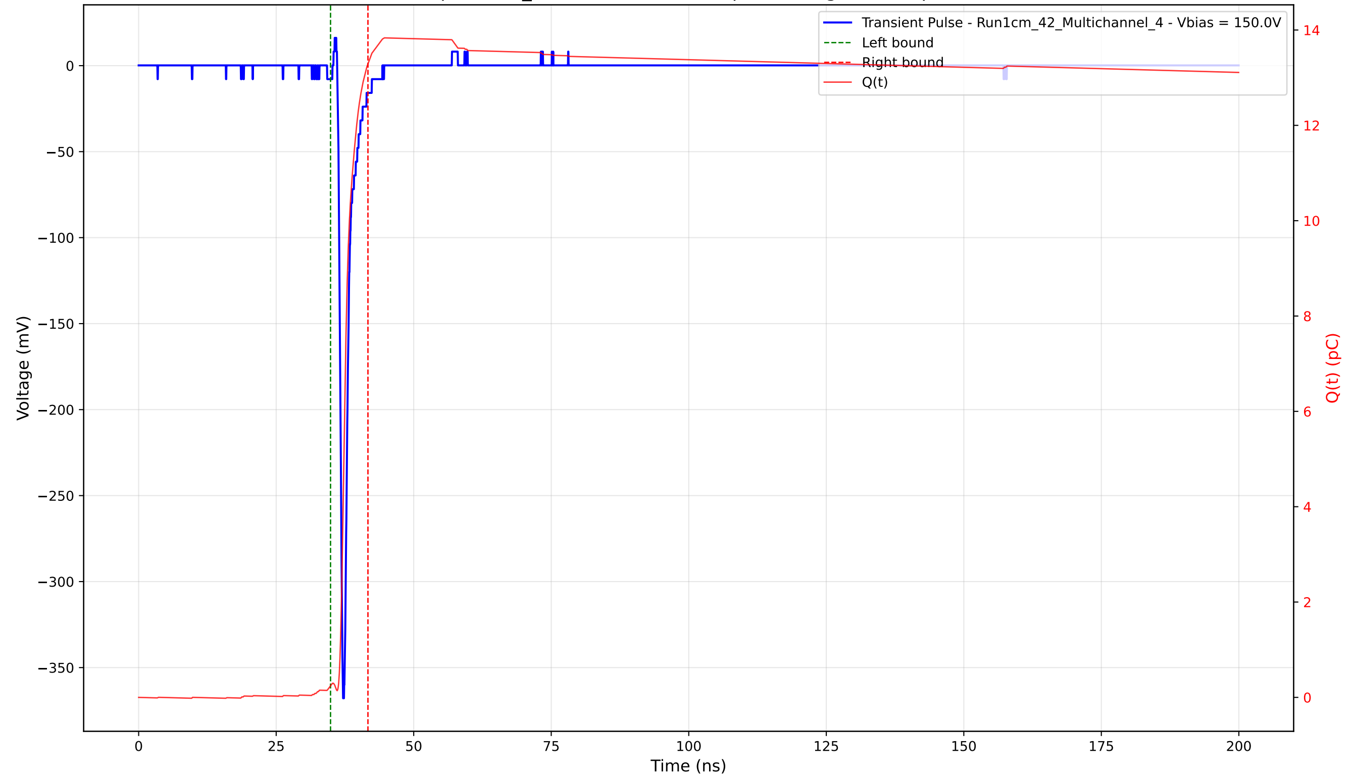
Transient Pulse - Sample: 1cm_42 - Position: 2135.0 \mu\text{m} - Charge: 13.04 pC - Rise Time: 0.71 ns
