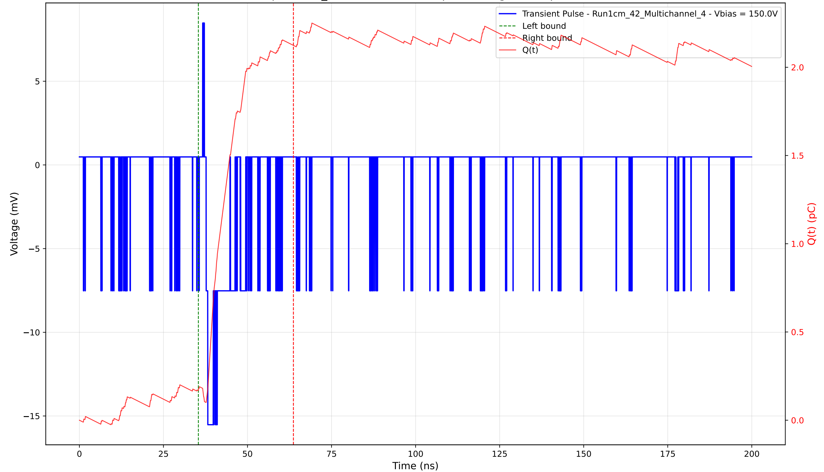
Transient Pulse - Sample: 1cm_42 - Position: 185.0 \mu\text{m} - Charge: 1.95 pC - Rise Time: 0.51 ns
