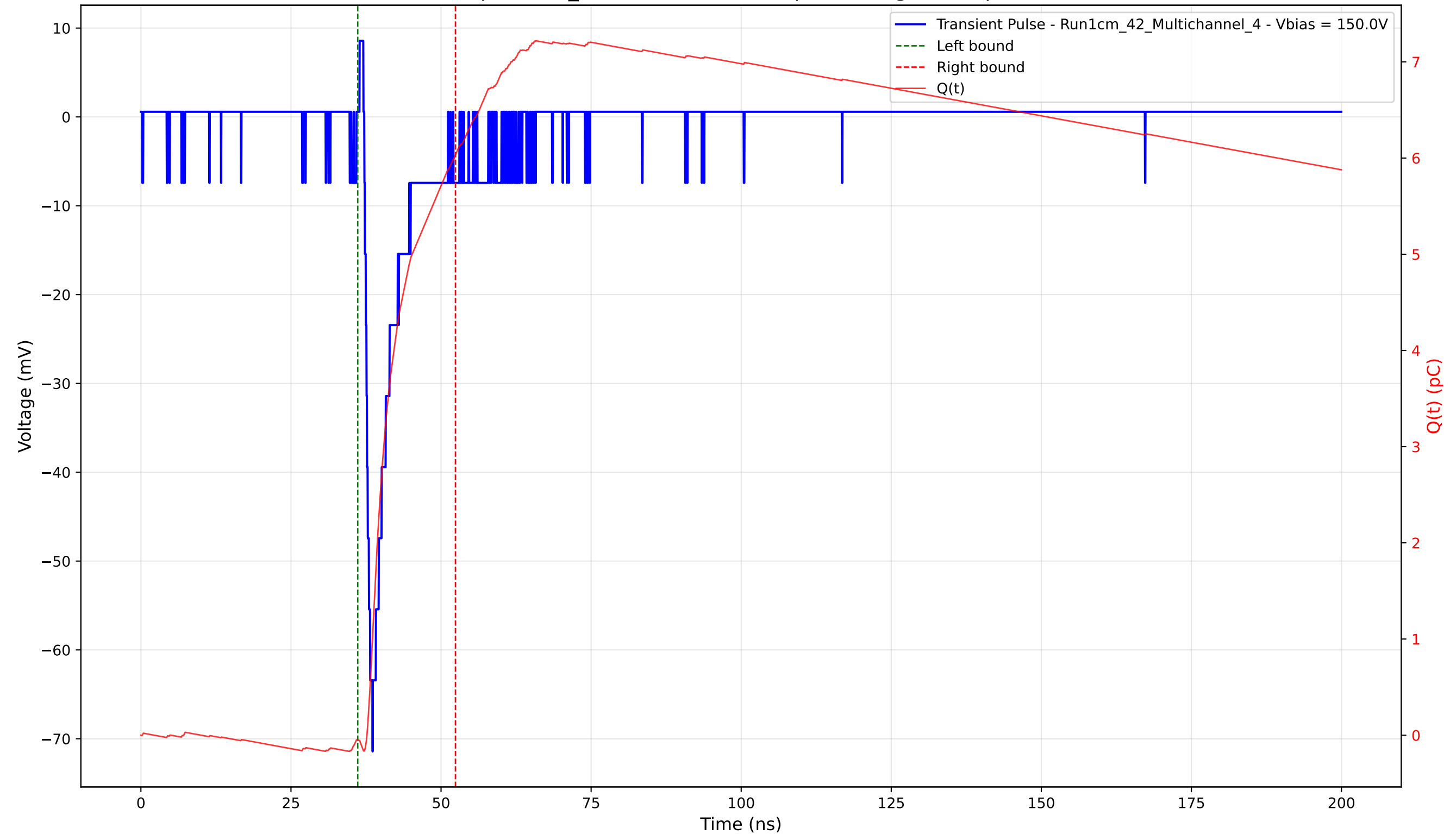
Transient Pulse - Sample: 1cm_42 - Position: 1260.0 \mu\text{m} - Charge: 6.08 pC - Rise Time: 1.36 ns
