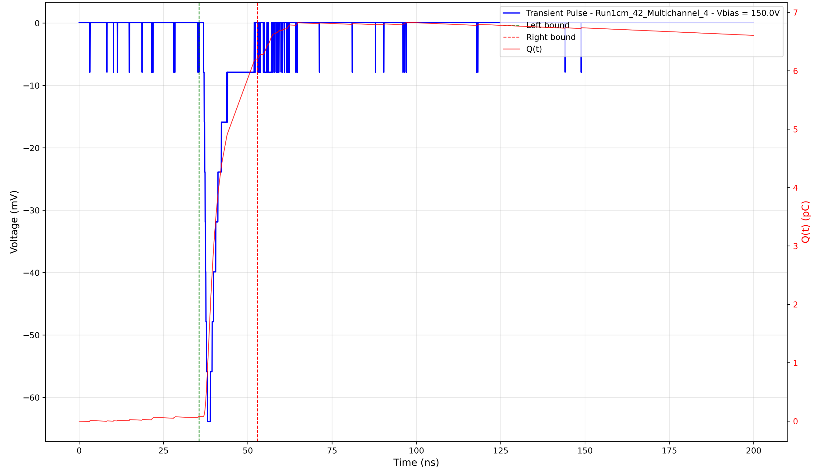
Transient Pulse - Sample: 1cm_42 - Position: 1420.0 \mu\text{m} - Charge: 6.12 pC - Rise Time: 1.17 ns
