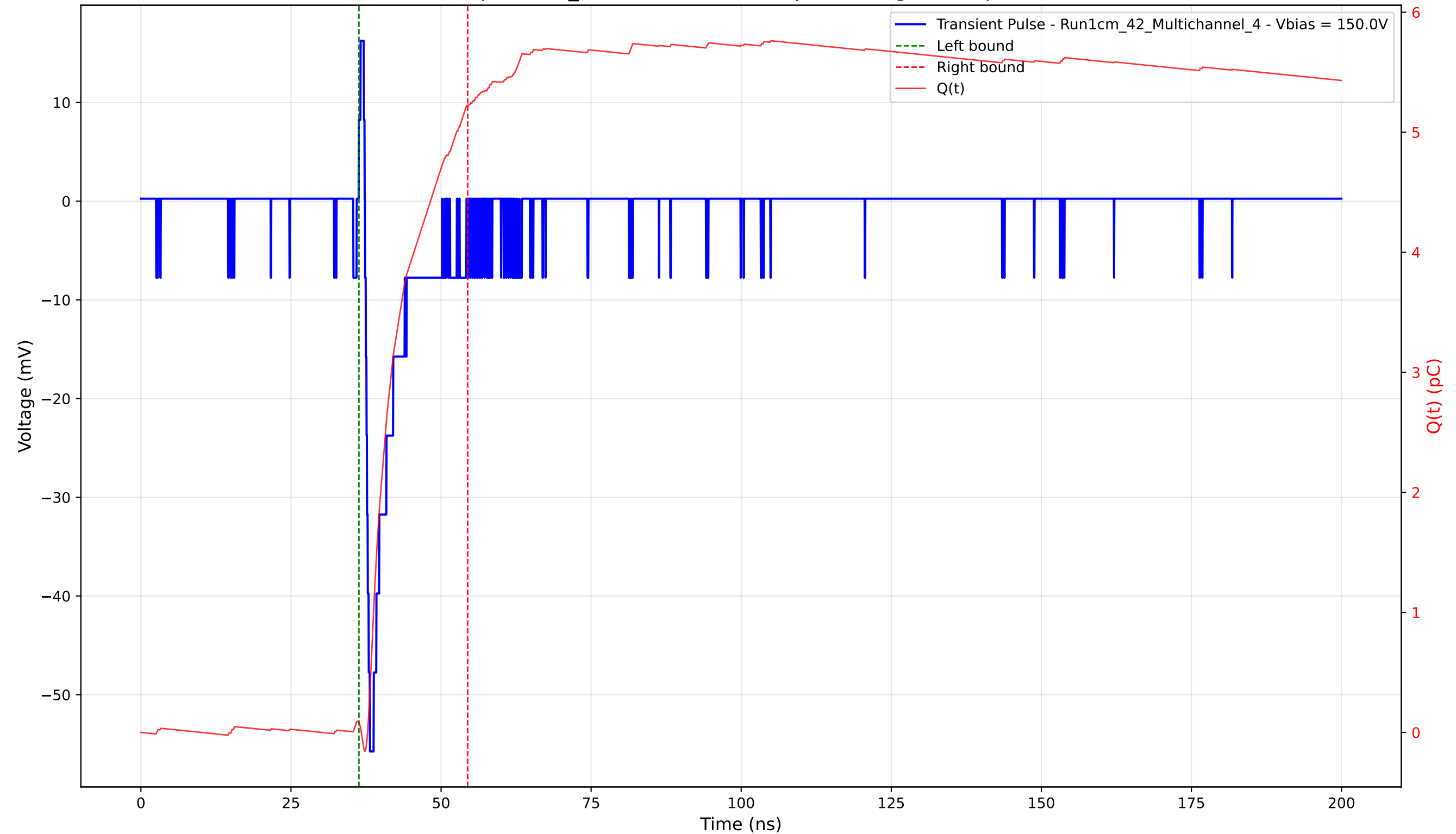
Transient Pulse - Sample: 1cm_42 - Position: 3855.0 \mu\text{m} - Charge: 5.13 pC - Rise Time: 0.81 ns
