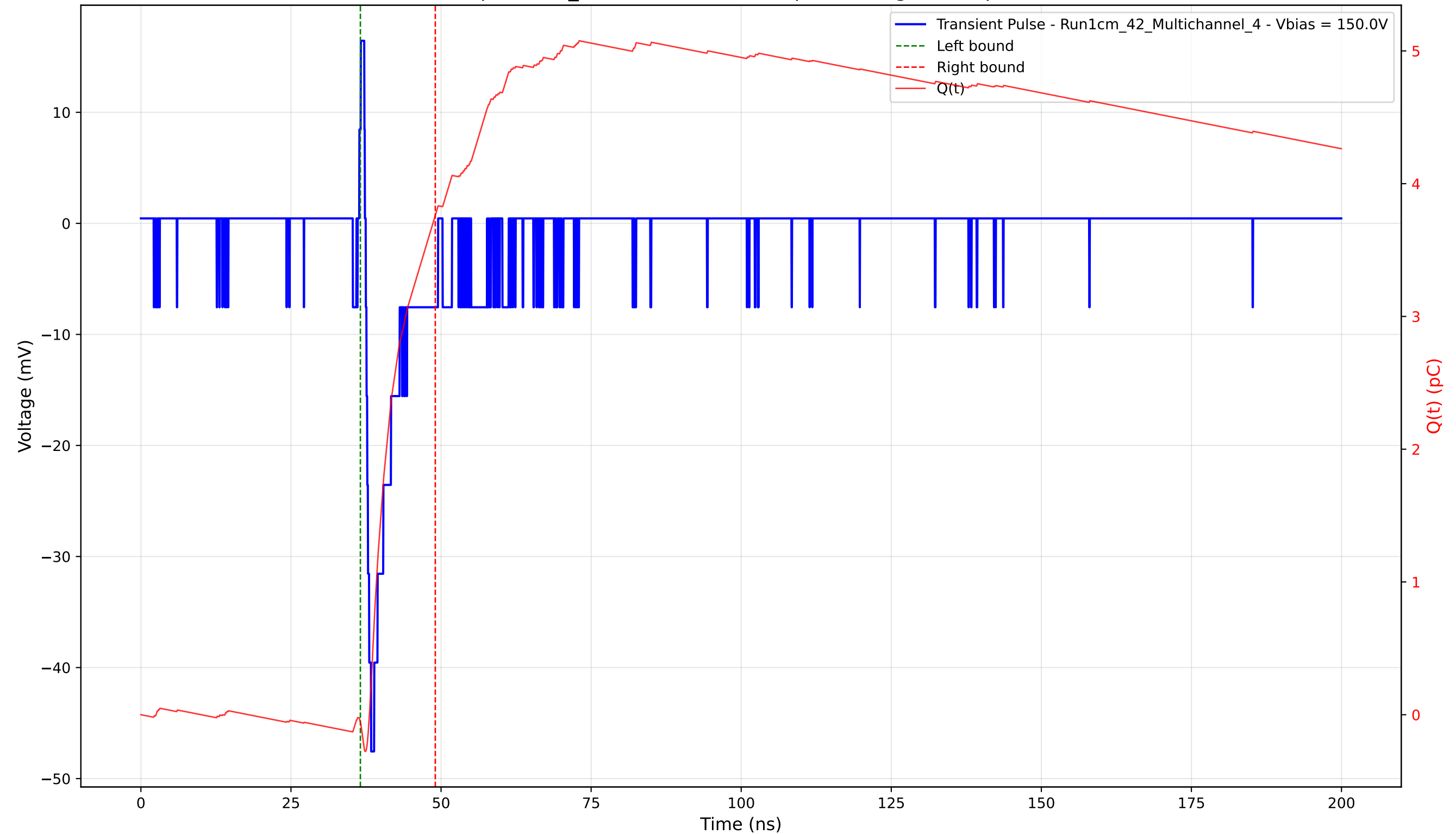
Transient Pulse - Sample: 1cm_42 - Position: 3940.0 \mu\text{m} - Charge: 3.82 pC - Rise Time: 0.90 ns
