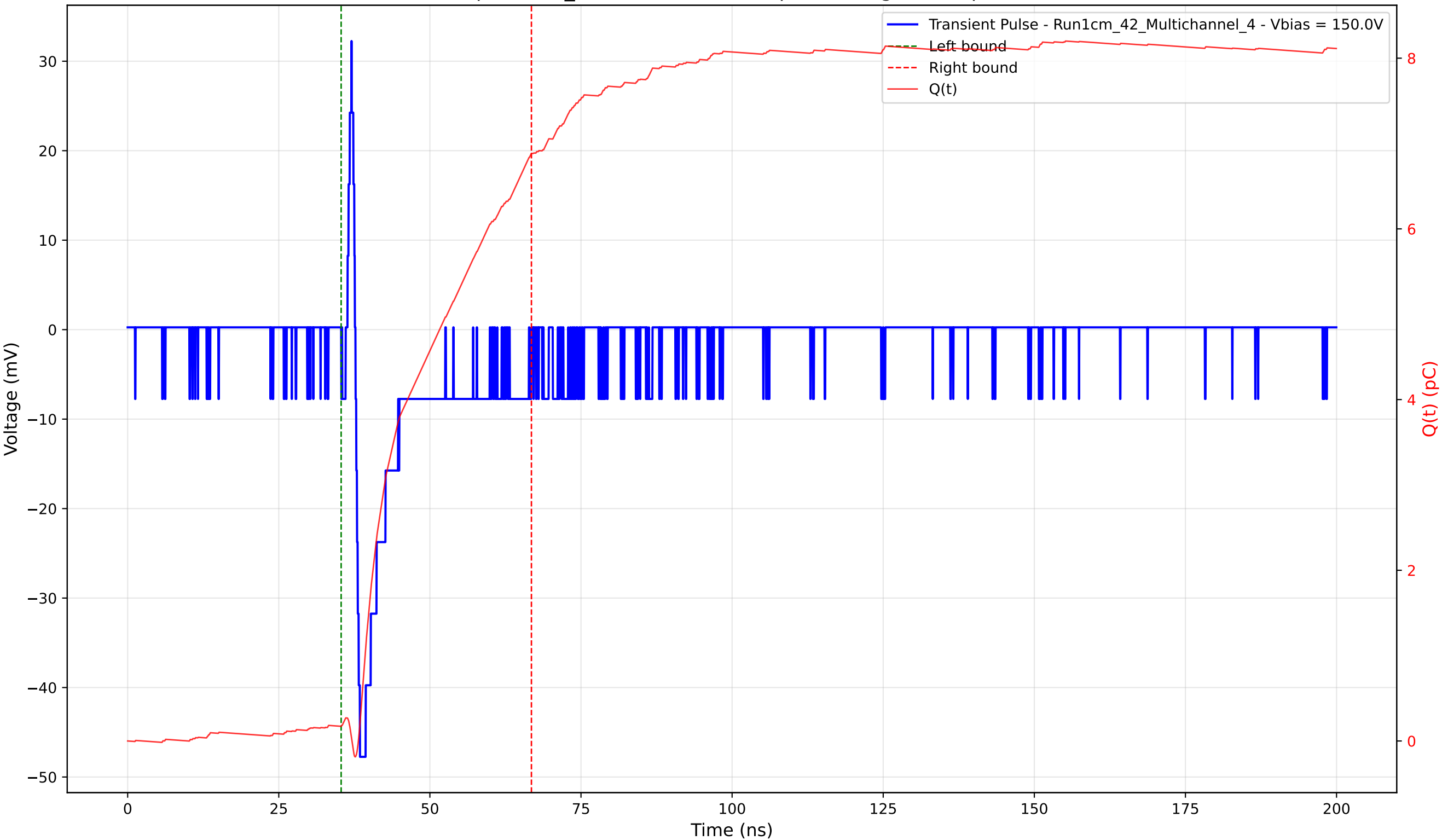
Transient Pulse - Sample: 1cm_42 - Position: 735.0 \mu\text{m} - Charge: 6.71 pC - Rise Time: 0.74 ns
