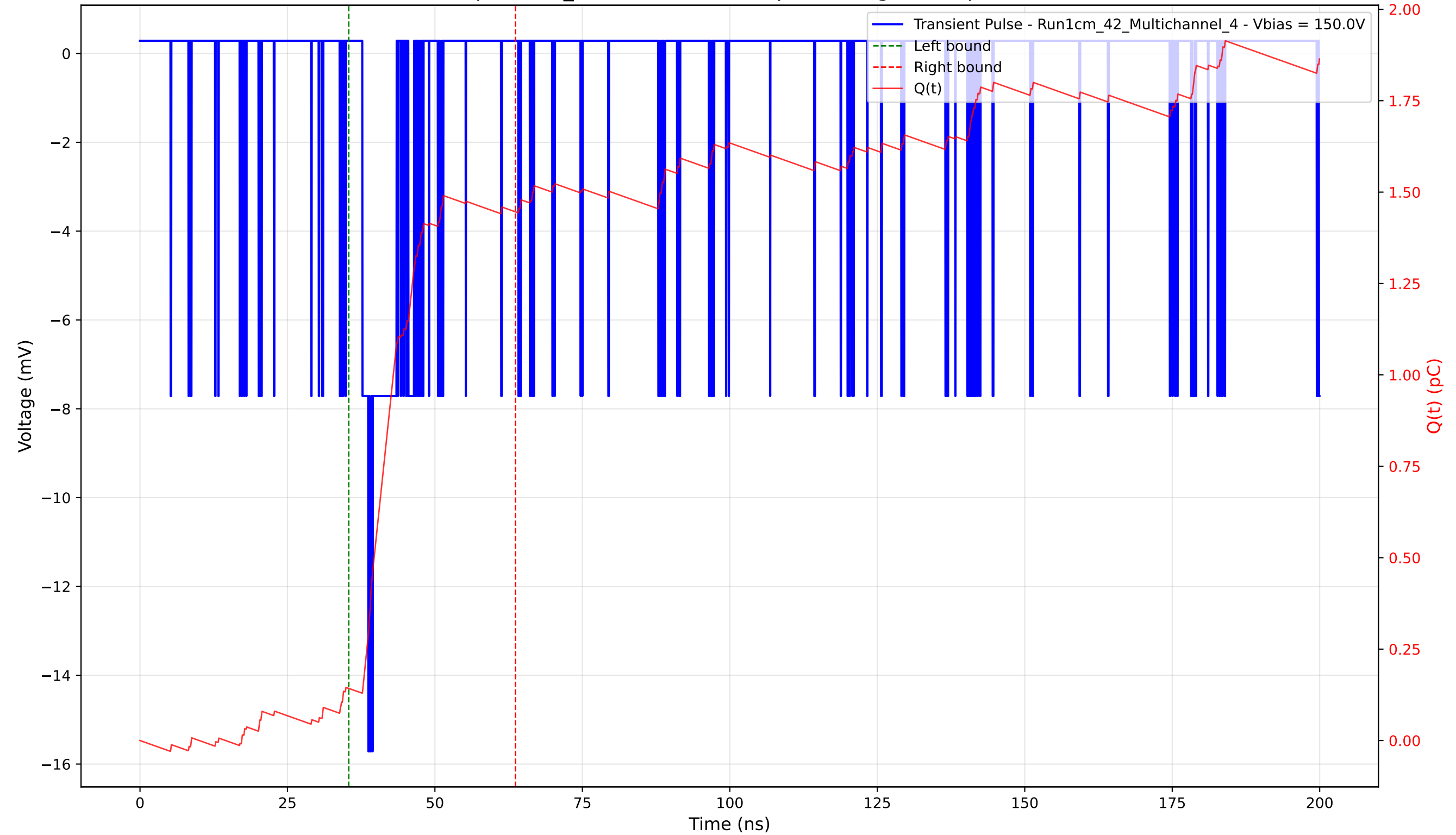
Transient Pulse - Sample: 1cm_42 - Position: 125.0 \mu\text{m} - Charge: 1.30 pC - Rise Time: 1.03 ns
