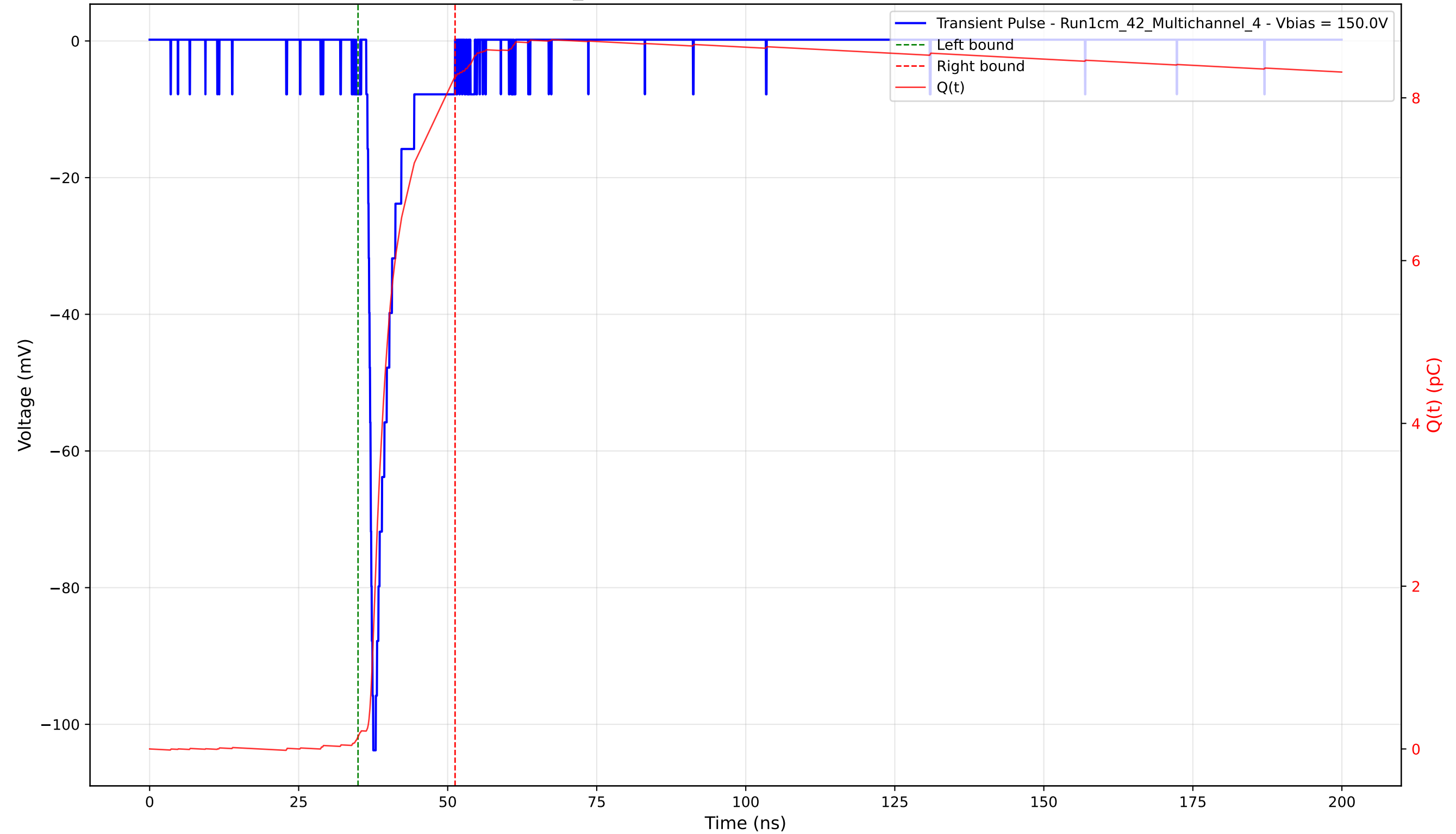
Transient Pulse - Sample: 1cm_42 - Position: 1620.0 \mu\text{m} - Charge: 8.11 pC - Rise Time: 0.87 ns
