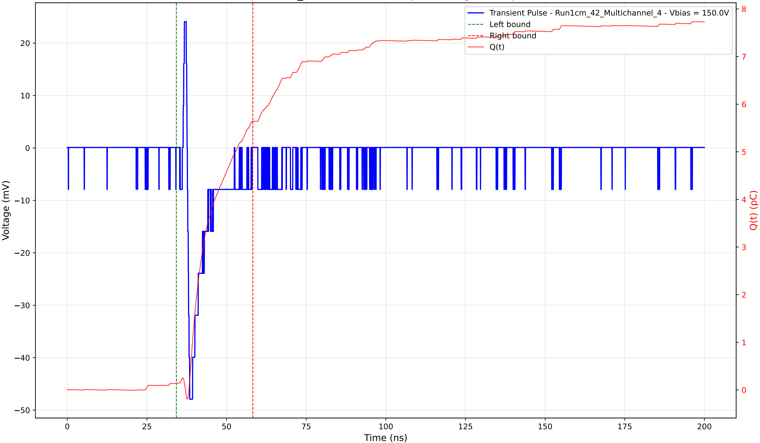
Transient Pulse - Sample: 1cm_42 - Position: 740.0 \mu\text{m} - Charge: 5.50 pC - Rise Time: 0.74 ns
