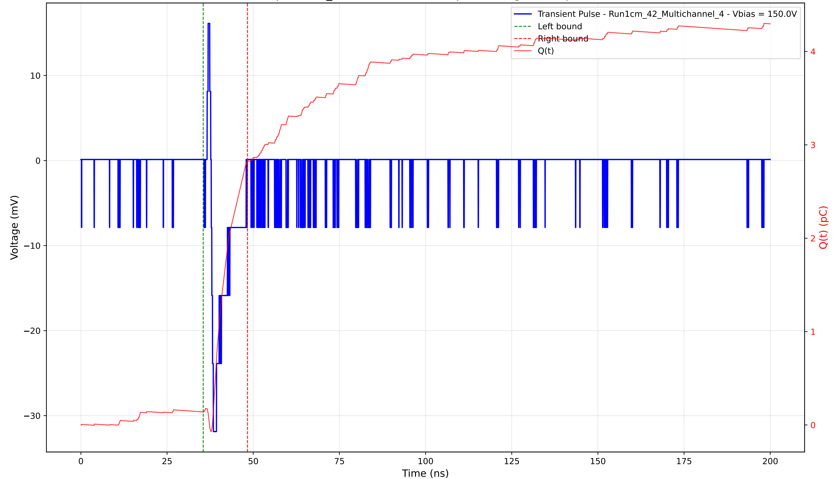
Transient Pulse - Sample: 1cm_42 - Position: 4670.0 \mu\text{m} - Charge: 2.69 pC - Rise Time: 0.62 ns
