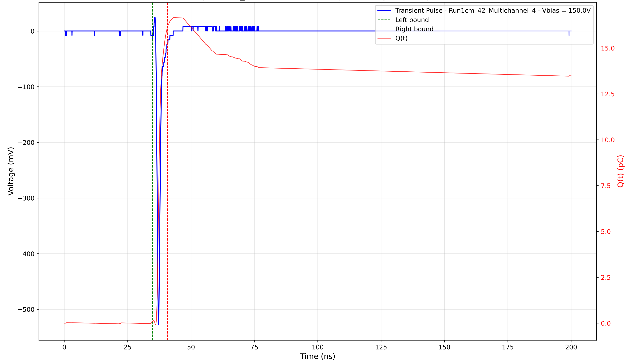
Transient Pulse - Sample: 1cm_42 - Position: 2620.0 \mu\text{m} - Charge: 16.05 pC - Rise Time: 0.68 ns
