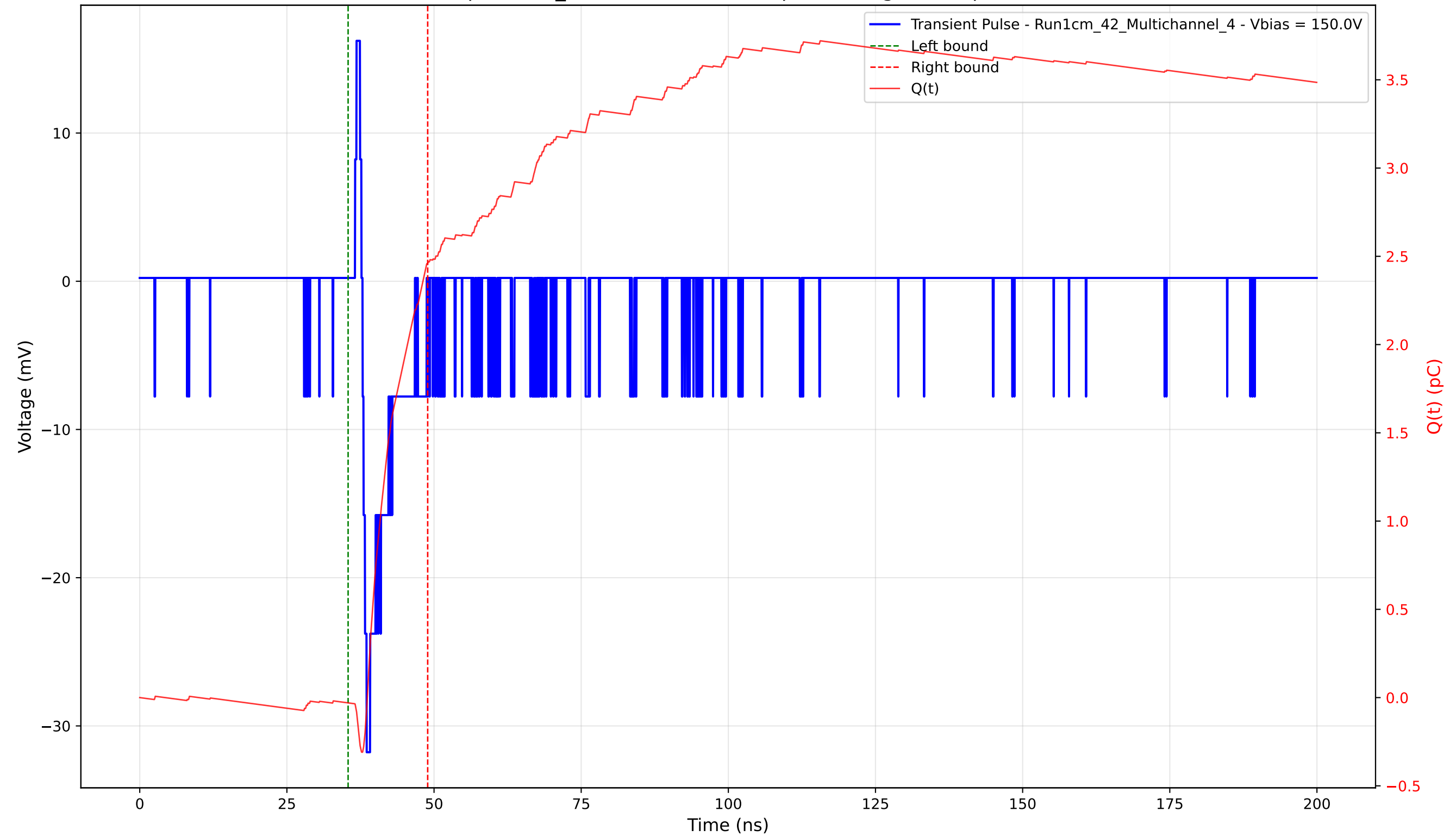
Transient Pulse - Sample: 1cm_42 - Position: 4615.0 \mu\text{m} - Charge: 2.49 pC - Rise Time: 0.70 ns
