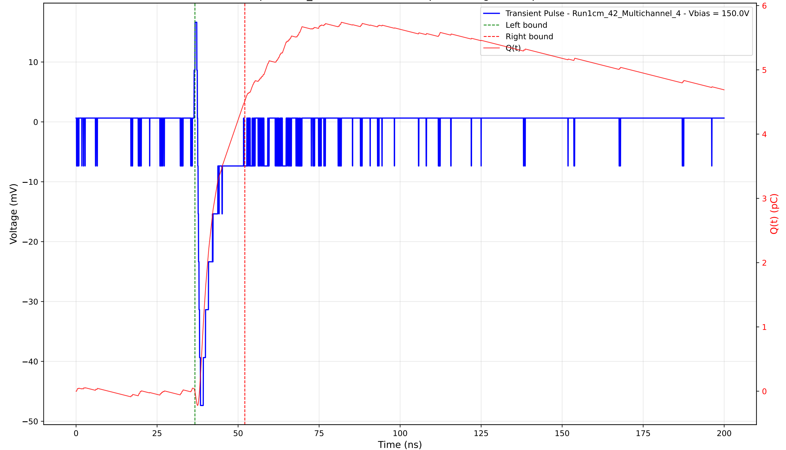
Transient Pulse - Sample: 1cm_42 - Position: 1020.0 \mu\text{m} - Charge: 4.52 pC - Rise Time: 0.86 ns
