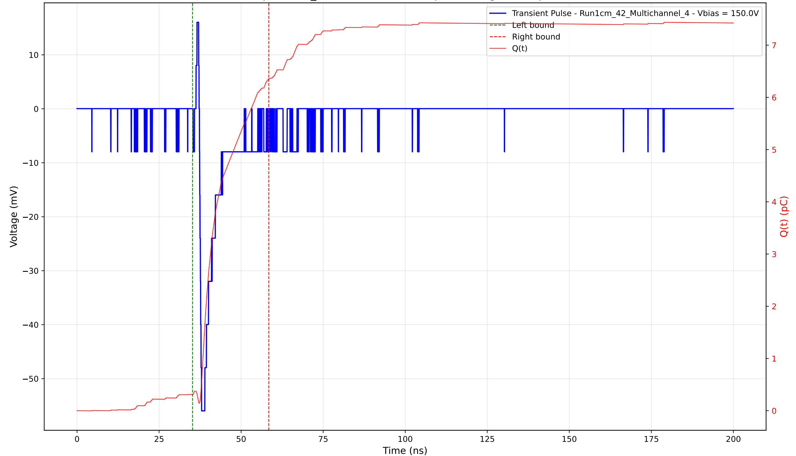
Transient Pulse - Sample: 1cm_42 - Position: 3770.0 \mu\text{m} - Charge: 6.05 pC - Rise Time: 0.65 ns
