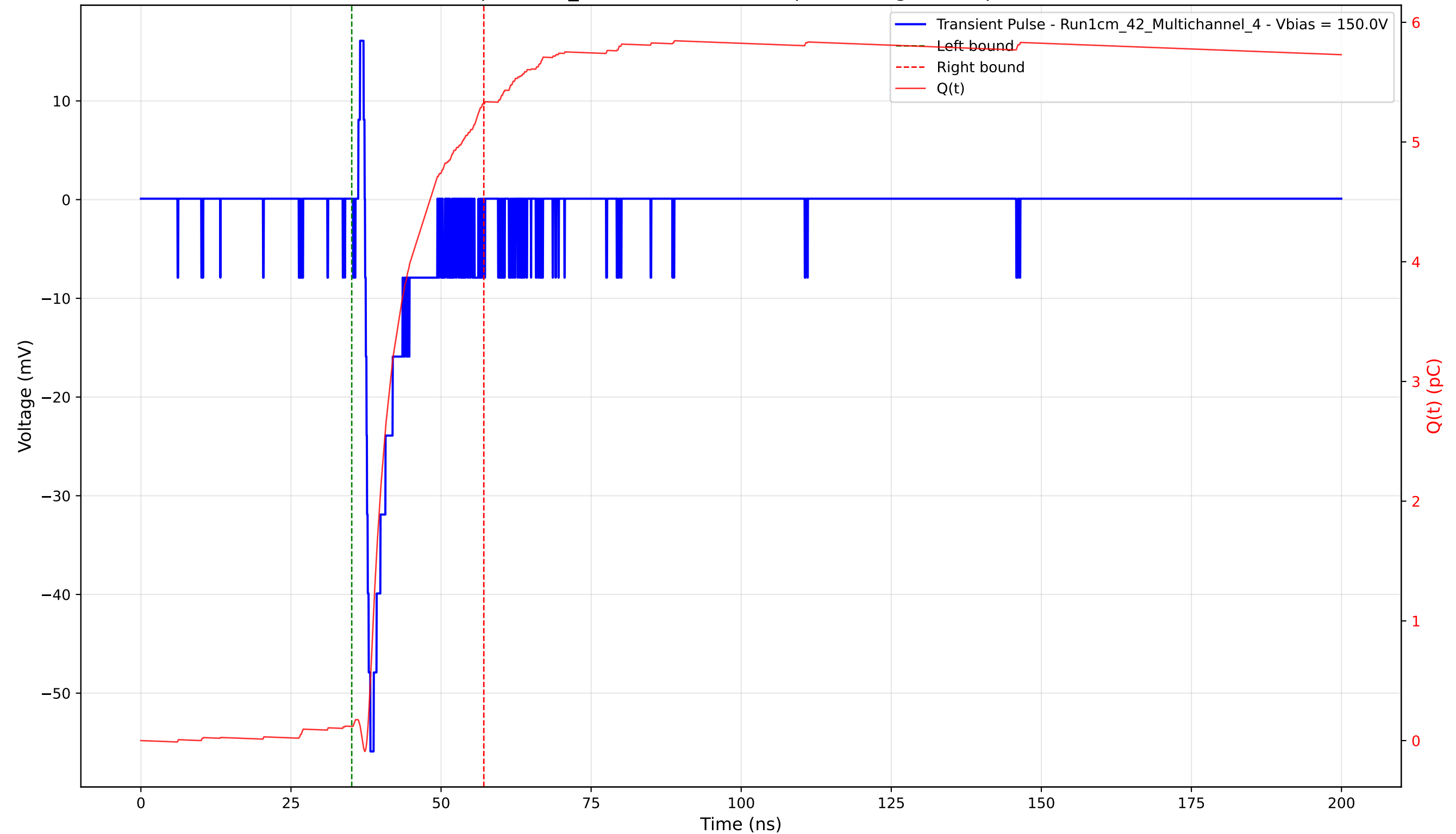
Transient Pulse - Sample: 1cm_42 - Position: 3850.0 \mu\text{m} - Charge: 5.20 pC - Rise Time: 0.89 ns
