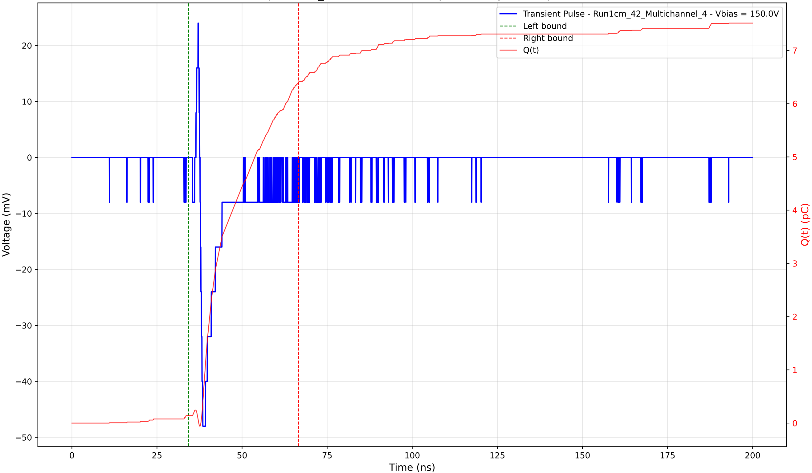
Transient Pulse - Sample: 1cm_42 - Position: 910.0 \mu\text{m} - Charge: 6.26 pC - Rise Time: 0.82 ns
