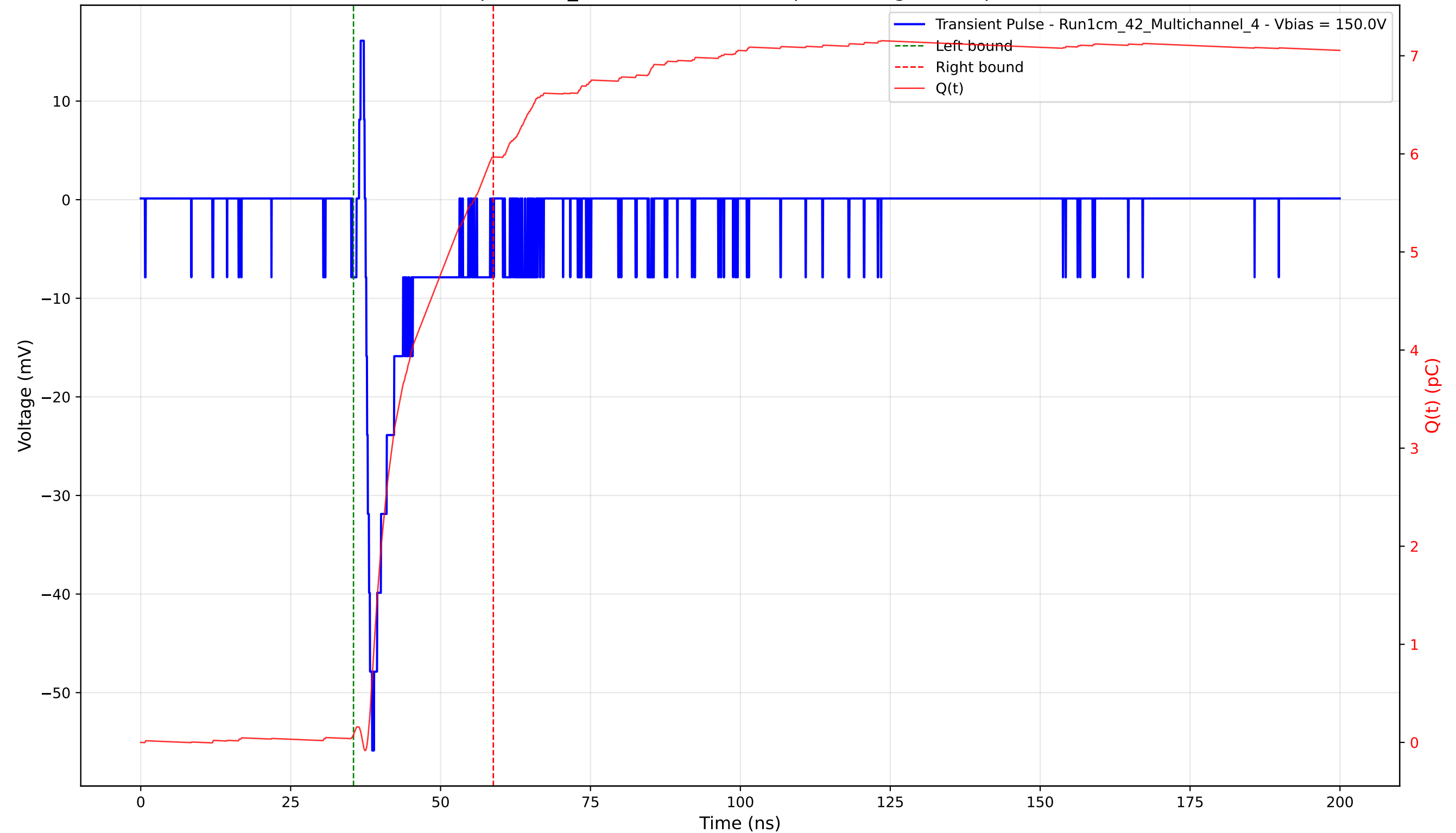
Transient Pulse - Sample: 1cm_42 - Position: 1060.0 \mu\text{m} - Charge: 5.88 pC - Rise Time: 1.09 ns
