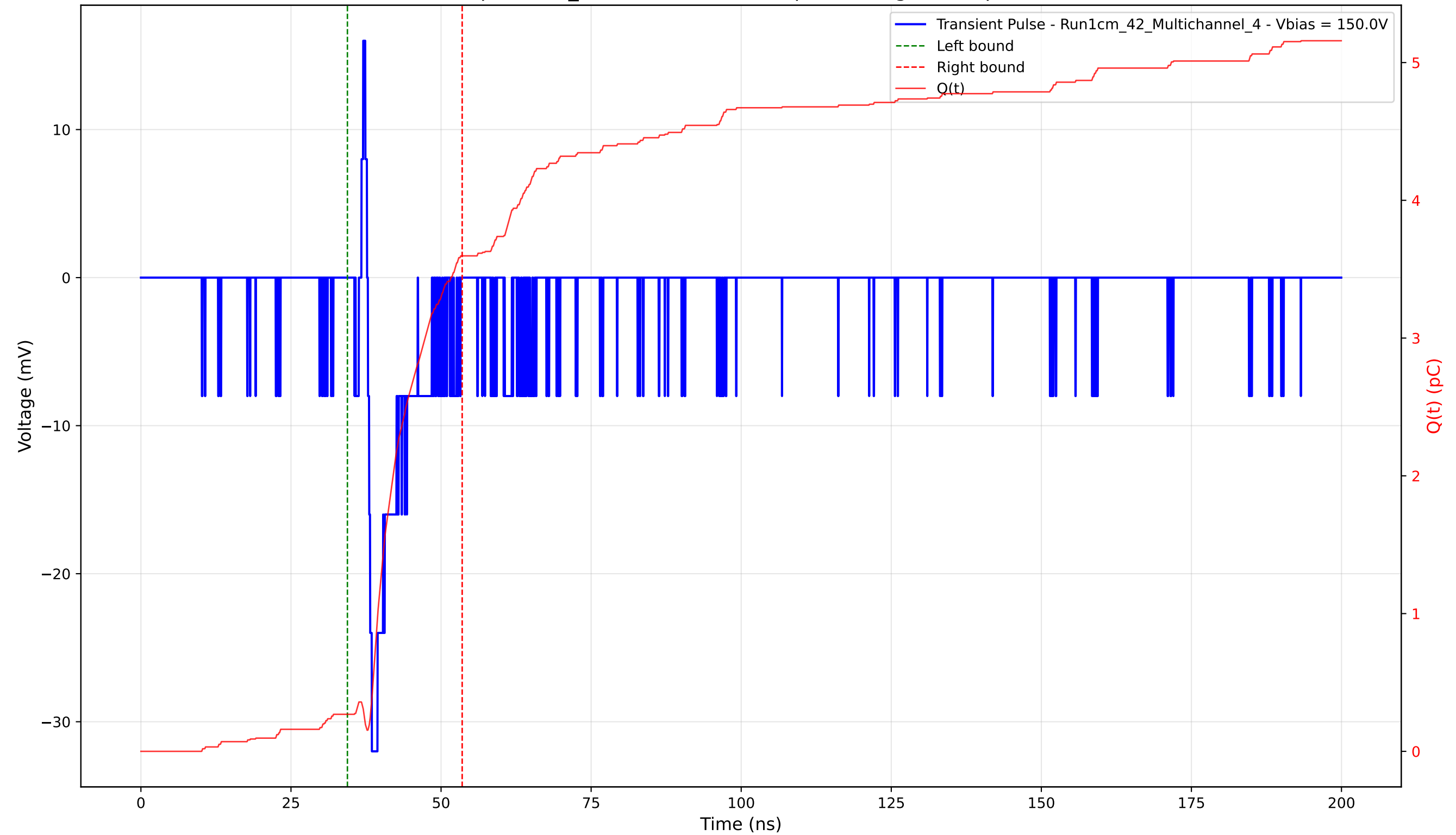
Transient Pulse - Sample: 1cm_42 - Position: 4840.0 \mu\text{m} - Charge: 3.33 pC - Rise Time: 0.66 ns
