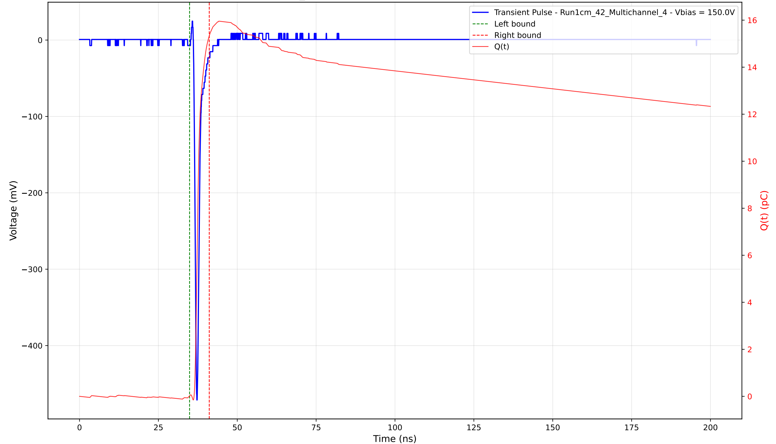
Transient Pulse - Sample: 1cm_42 - Position: 2785.0 \mu\text{m} - Charge: 15.31 pC - Rise Time: 0.74 ns
