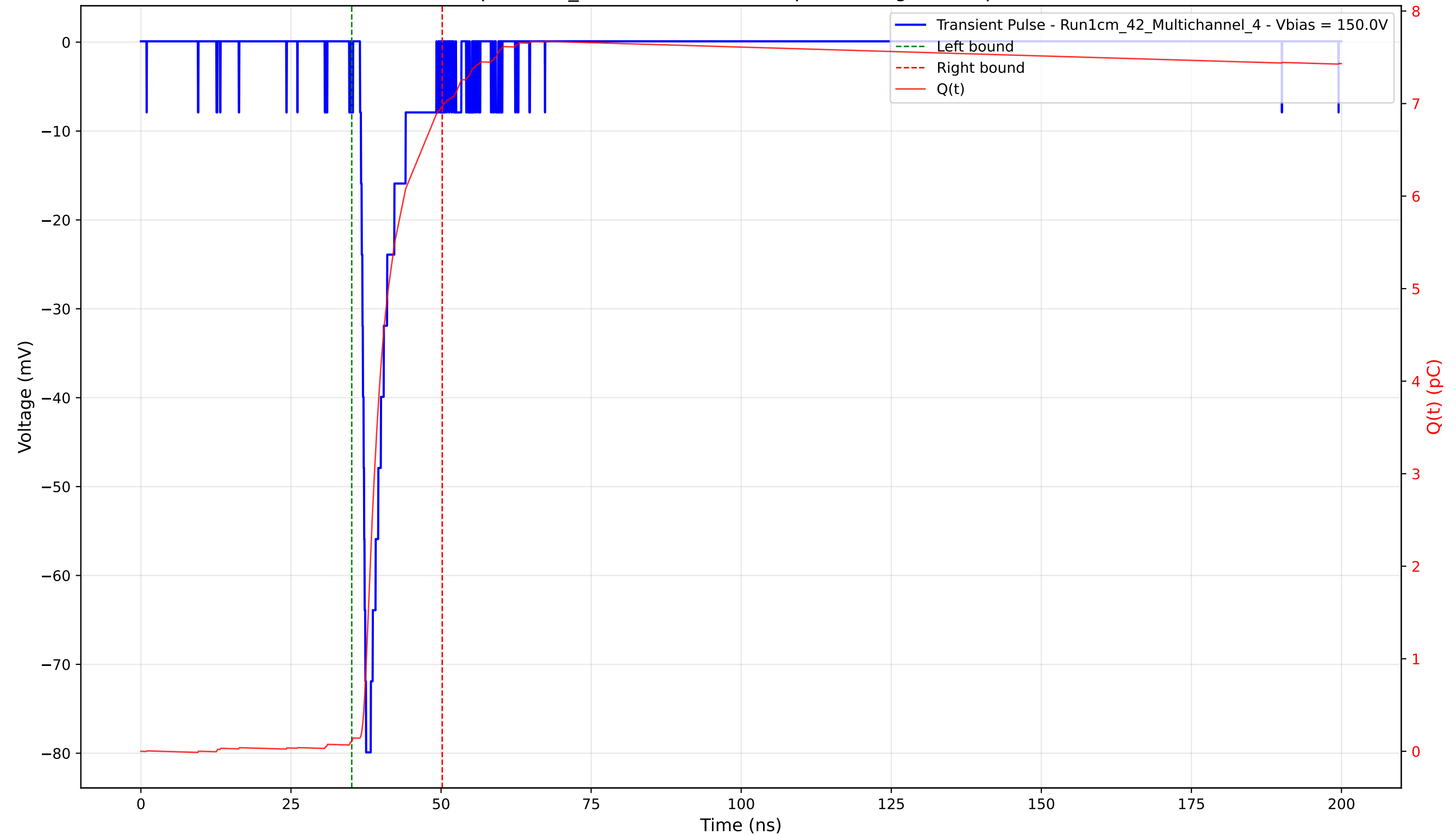
Transient Pulse - Sample: 1cm_42 - Position: 1560.0 \mu\text{m} - Charge: 6.86 pC - Rise Time: 0.88 ns
