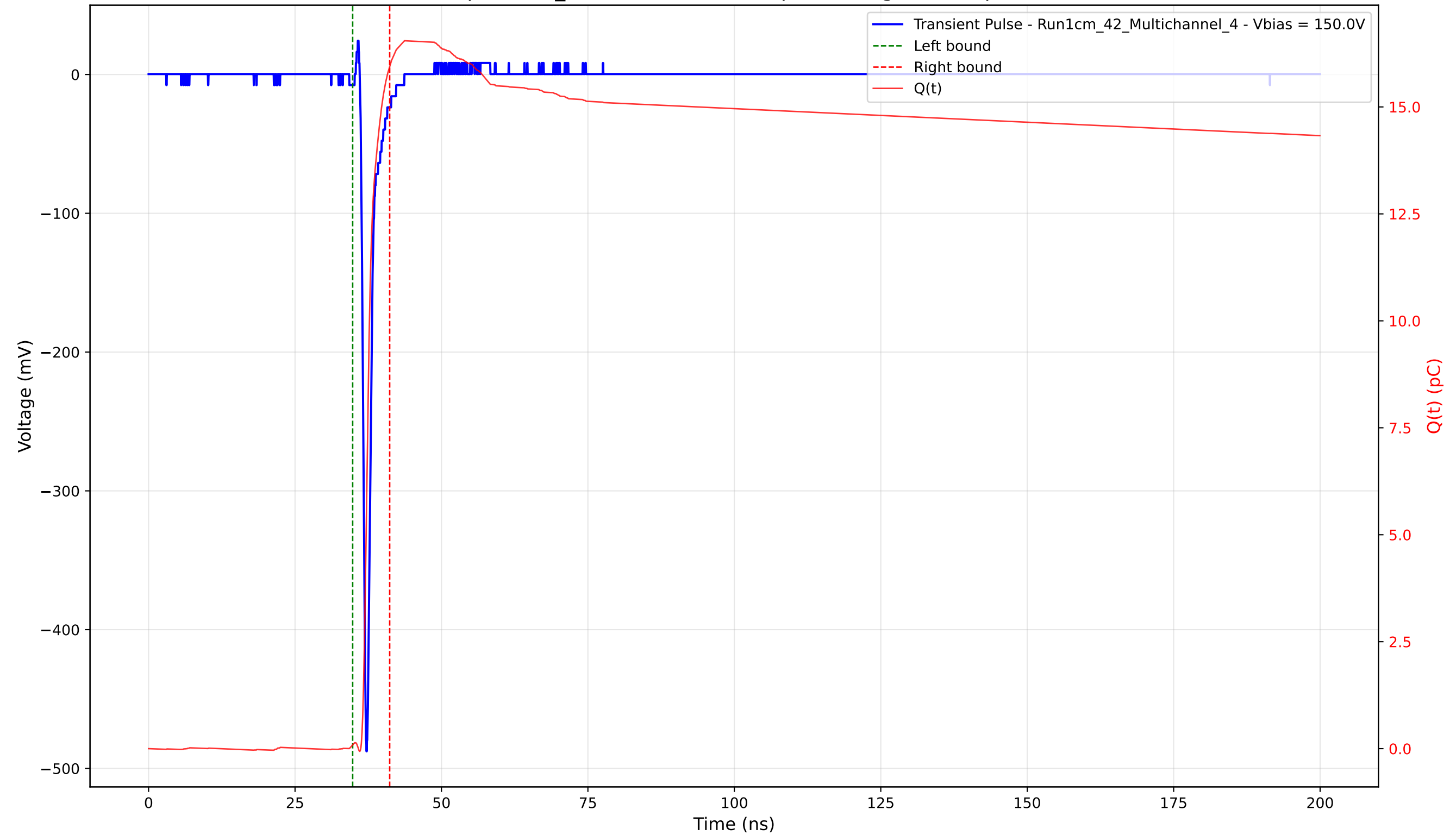
Transient Pulse - Sample: 1cm_42 - Position: 2765.0 \mu\text{m} - Charge: 15.86 pC - Rise Time: 0.76 ns
