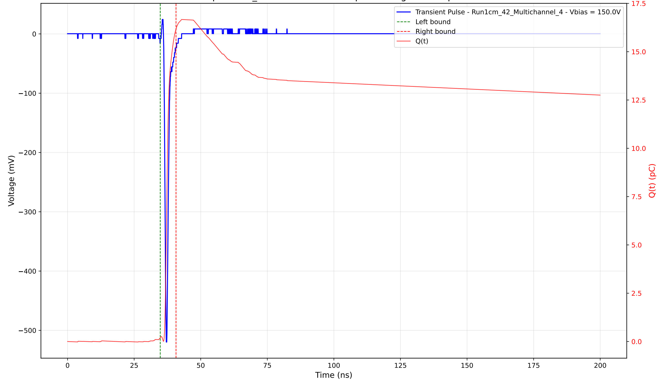
Transient Pulse - Sample: 1cm_42 - Position: 2590.0 \mu\text{m} - Charge: 15.97 pC - Rise Time: 0.72 ns
