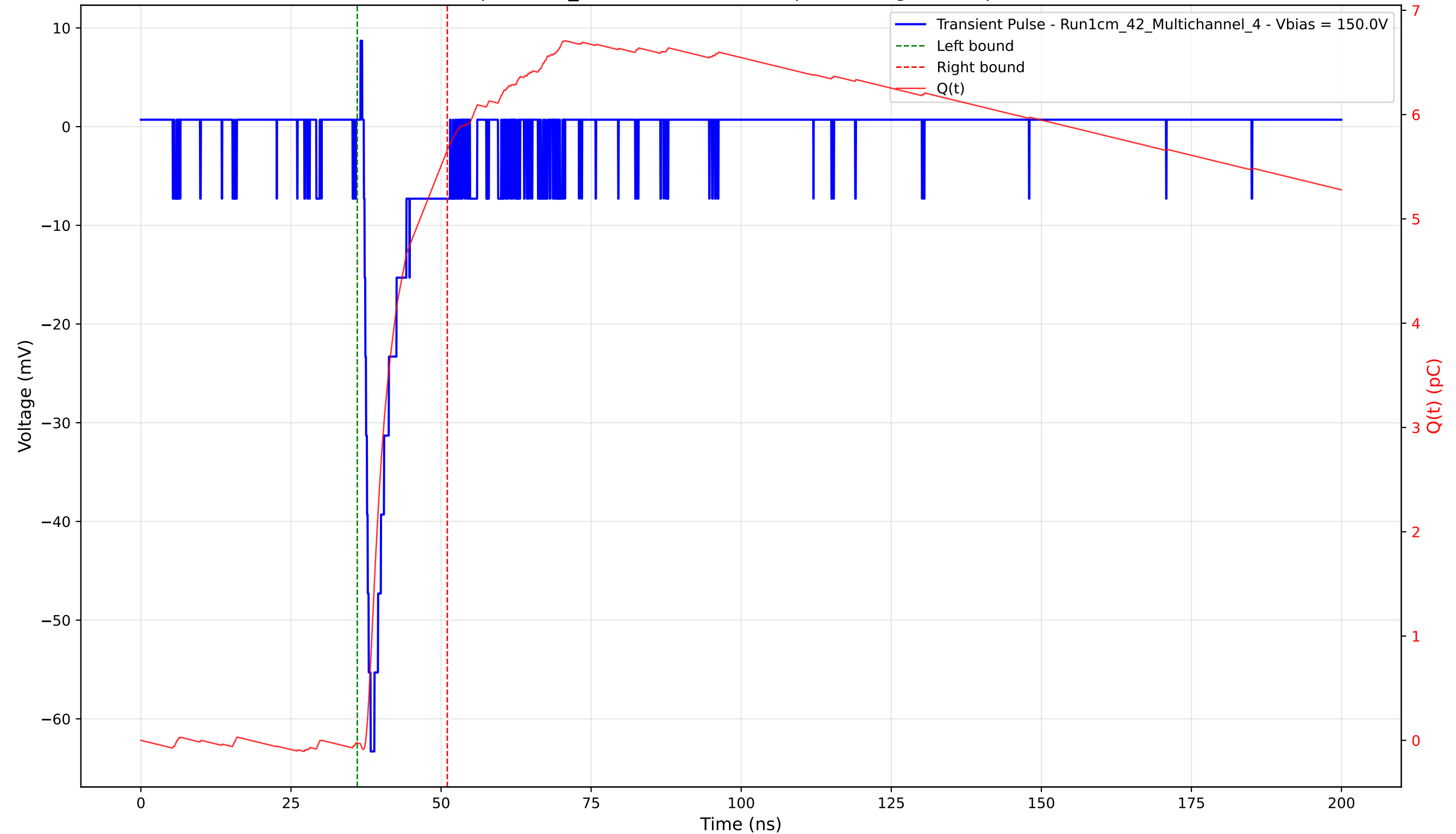
Transient Pulse - Sample: 1cm_42 - Position: 1345.0 \mu\text{m} - Charge: 5.69 pC - Rise Time: 1.13 ns
