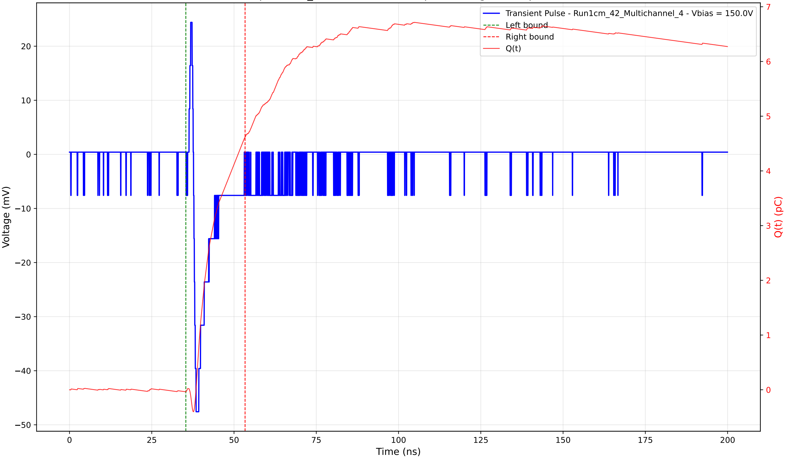
Transient Pulse - Sample: 1cm_42 - Position: 860.0 \mu\text{m} - Charge: 4.66 pC - Rise Time: 0.78 ns
