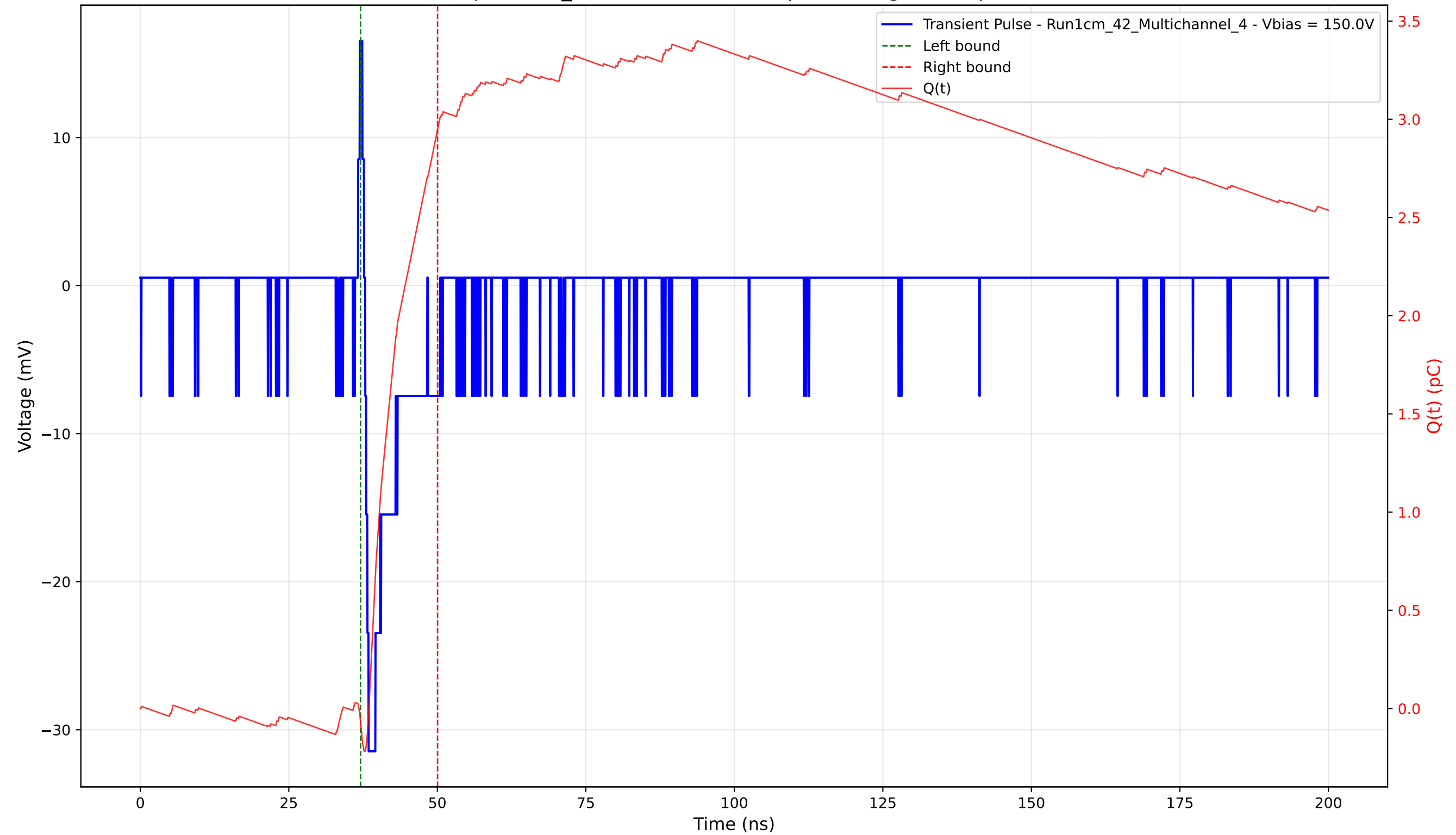
Transient Pulse - Sample: 1cm_42 - Position: 4780.0 \mu\text{m} - Charge: 3.02 pC - Rise Time: 0.58 ns
