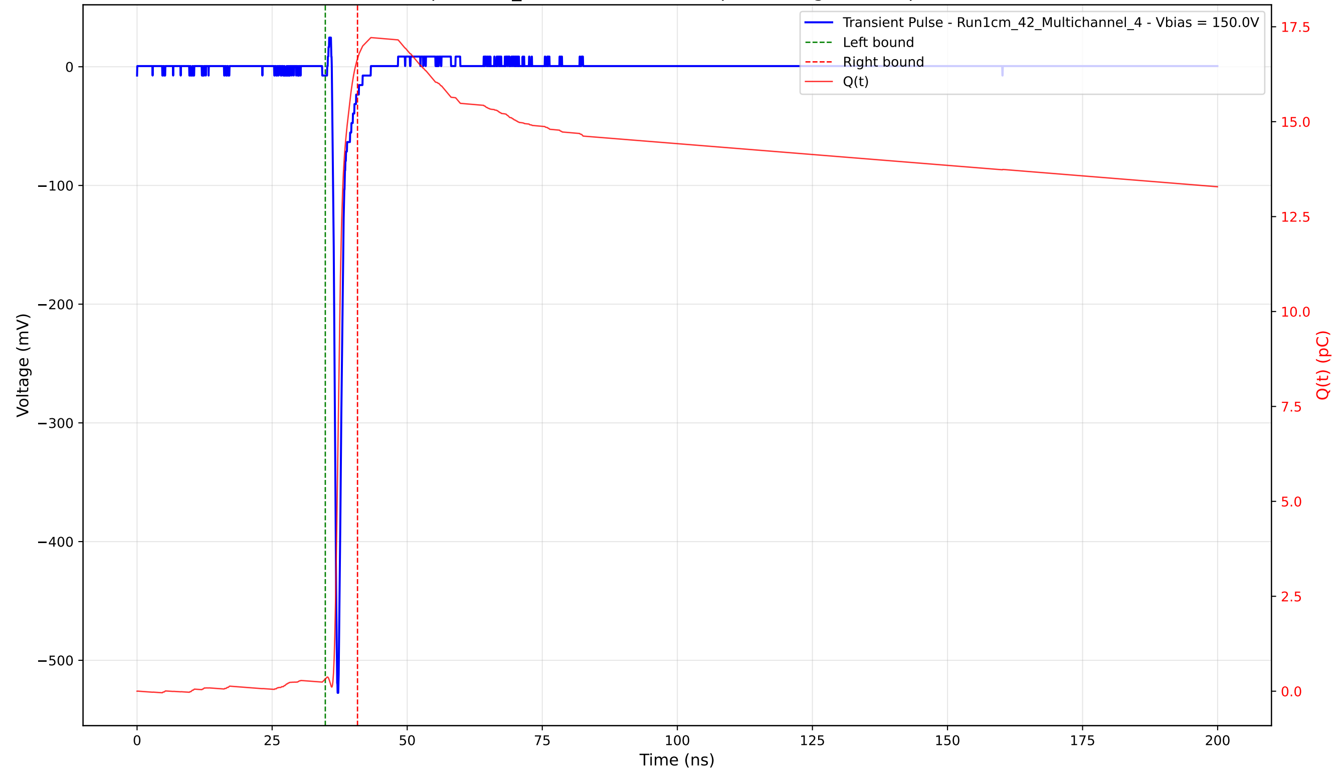
Transient Pulse - Sample: 1cm_42 - Position: 2385.0 \mu\text{m} - Charge: 16.33 pC - Rise Time: 0.71 ns
