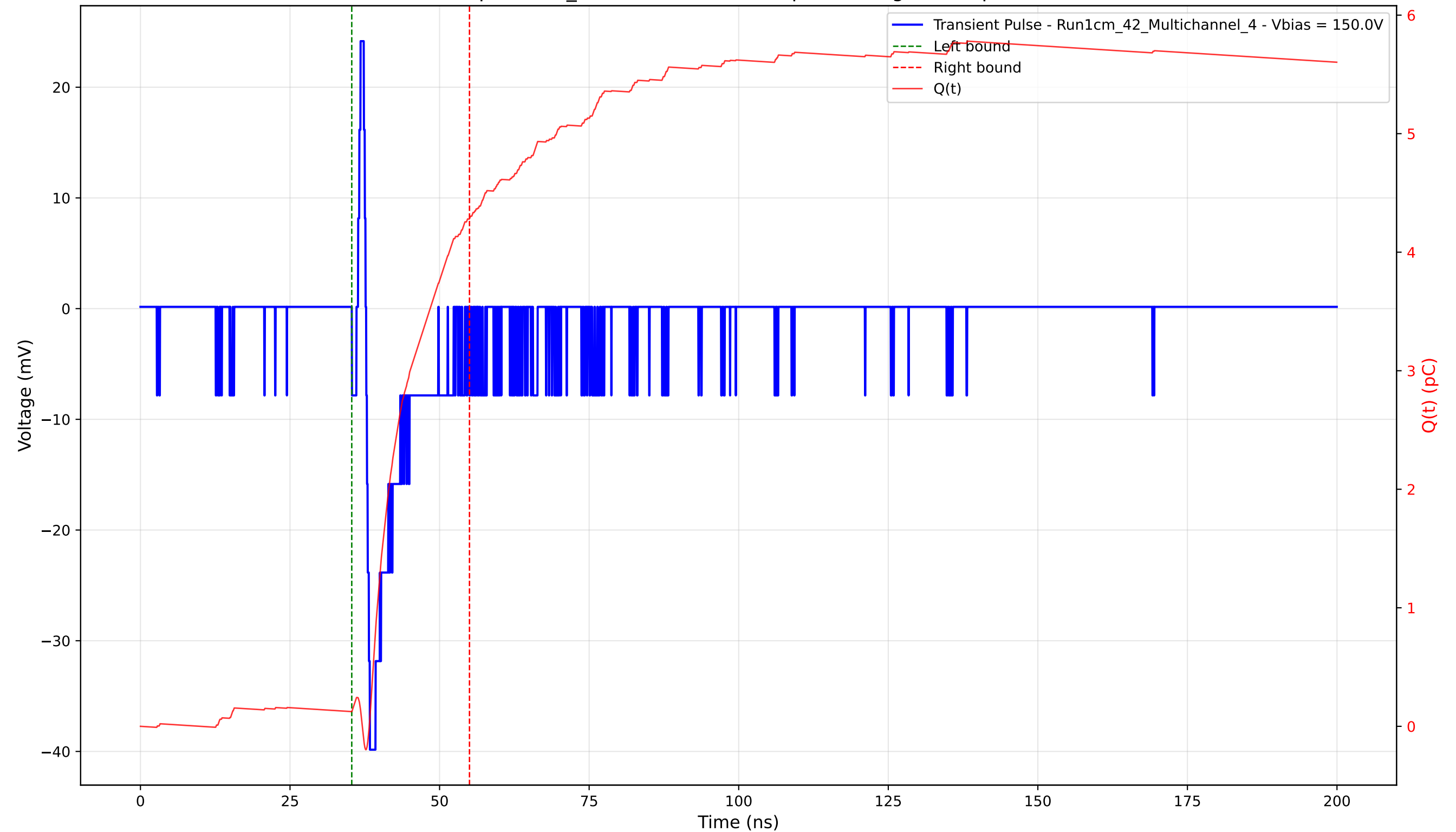
Transient Pulse - Sample: 1cm_42 - Position: 4265.0 \mu\text{m} - Charge: 4.16 pC - Rise Time: 0.62 ns
