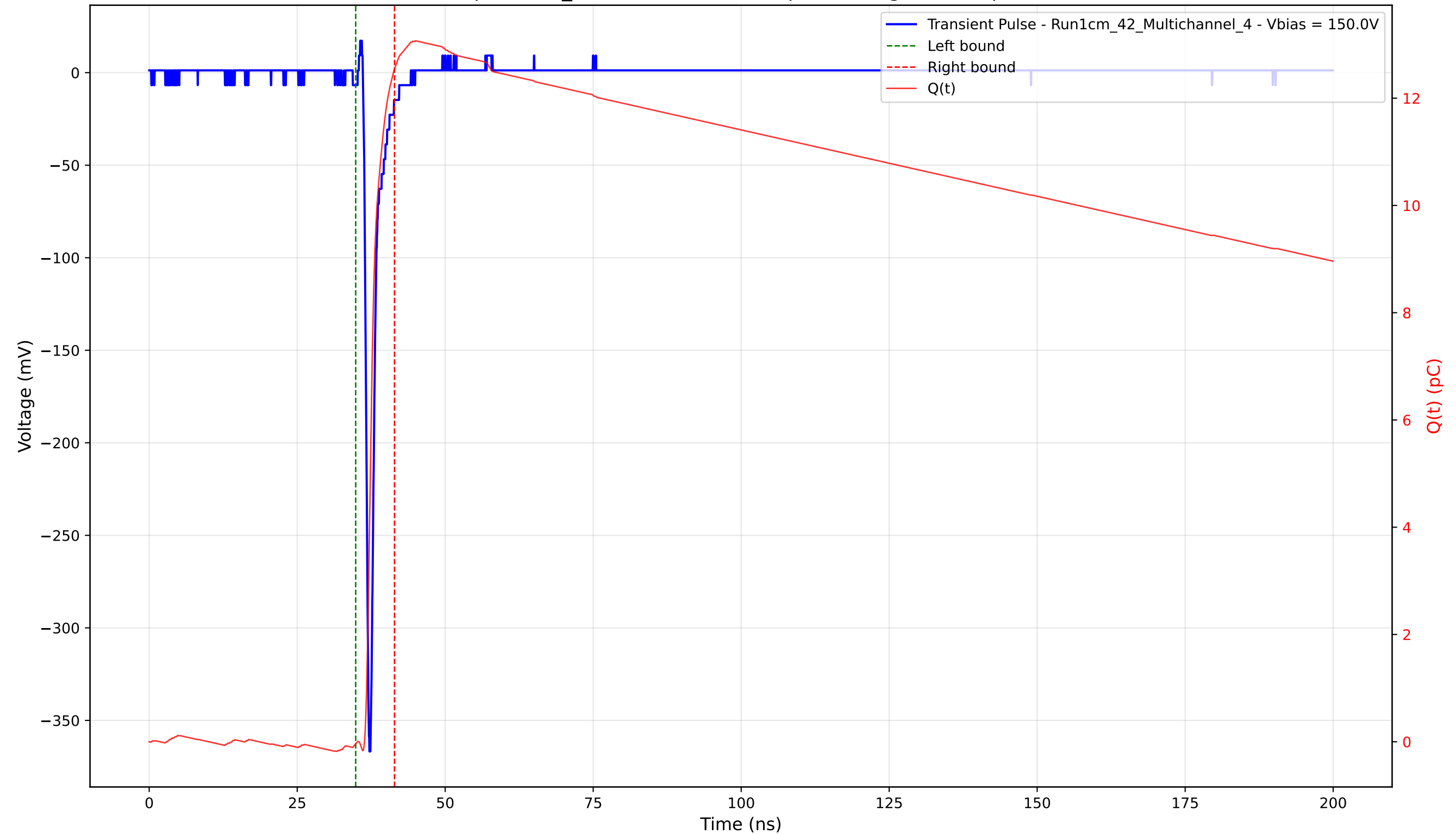
Transient Pulse - Sample: 1cm_42 - Position: 2880.0 \mu\text{m} - Charge: 12.59 pC - Rise Time: 0.71 ns
