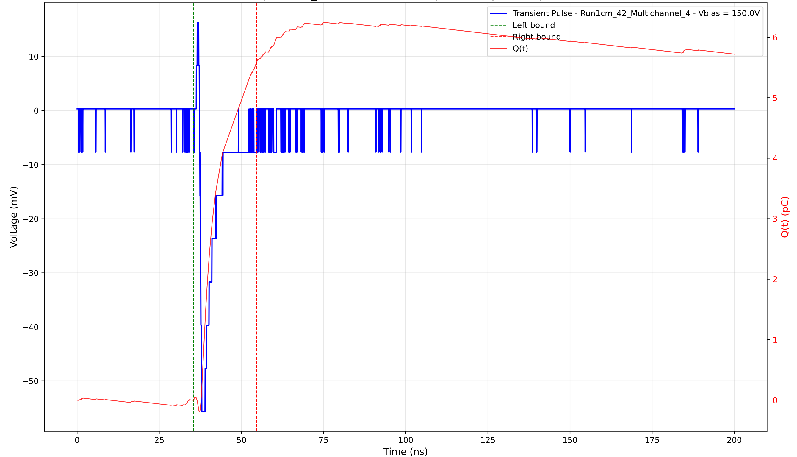
Transient Pulse - Sample: 1cm_42 - Position: 3745.0 \mu\text{m} - Charge: 5.60 pC - Rise Time: 0.69 ns
