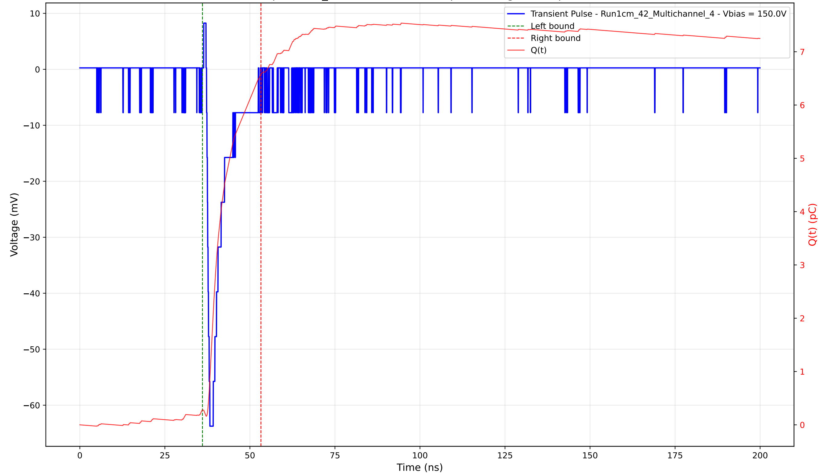
Transient Pulse - Sample: 1cm_42 - Position: 1245.0 \mu\text{m} - Charge: 6.30 pC - Rise Time: 0.97 ns
