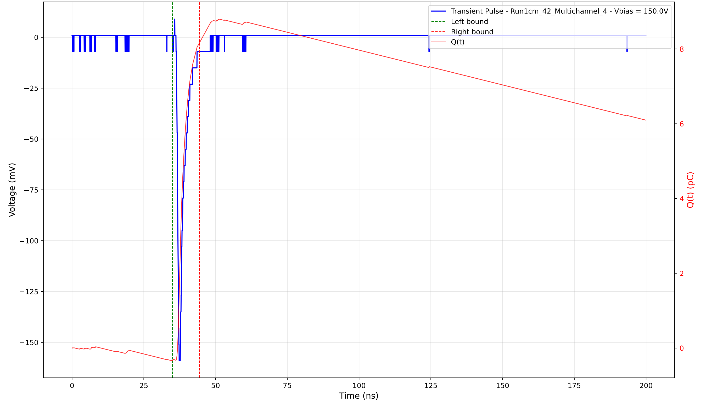
Transient Pulse - Sample: 1cm_42 - Position: 1880.0 \mu\text{m} - Charge: 8.49 pC - Rise Time: 0.84 ns
