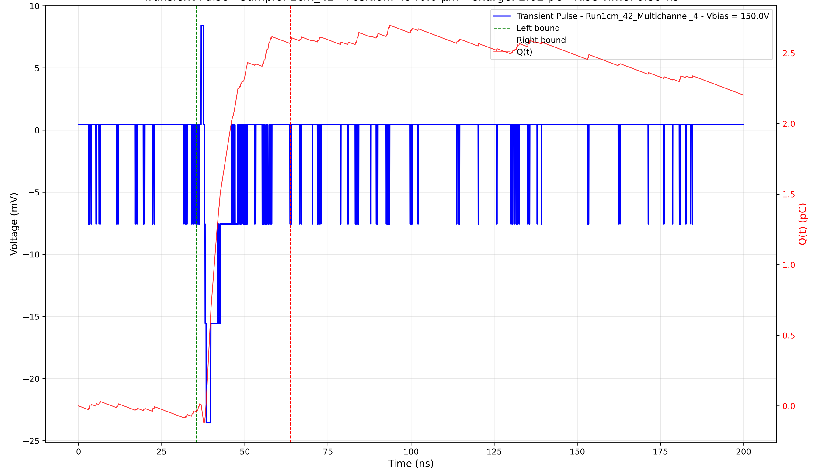
Transient Pulse - Sample: 1cm_42 - Position: 4940.0 \mu\text{m} - Charge: 2.62 pC - Rise Time: 0.59 ns
