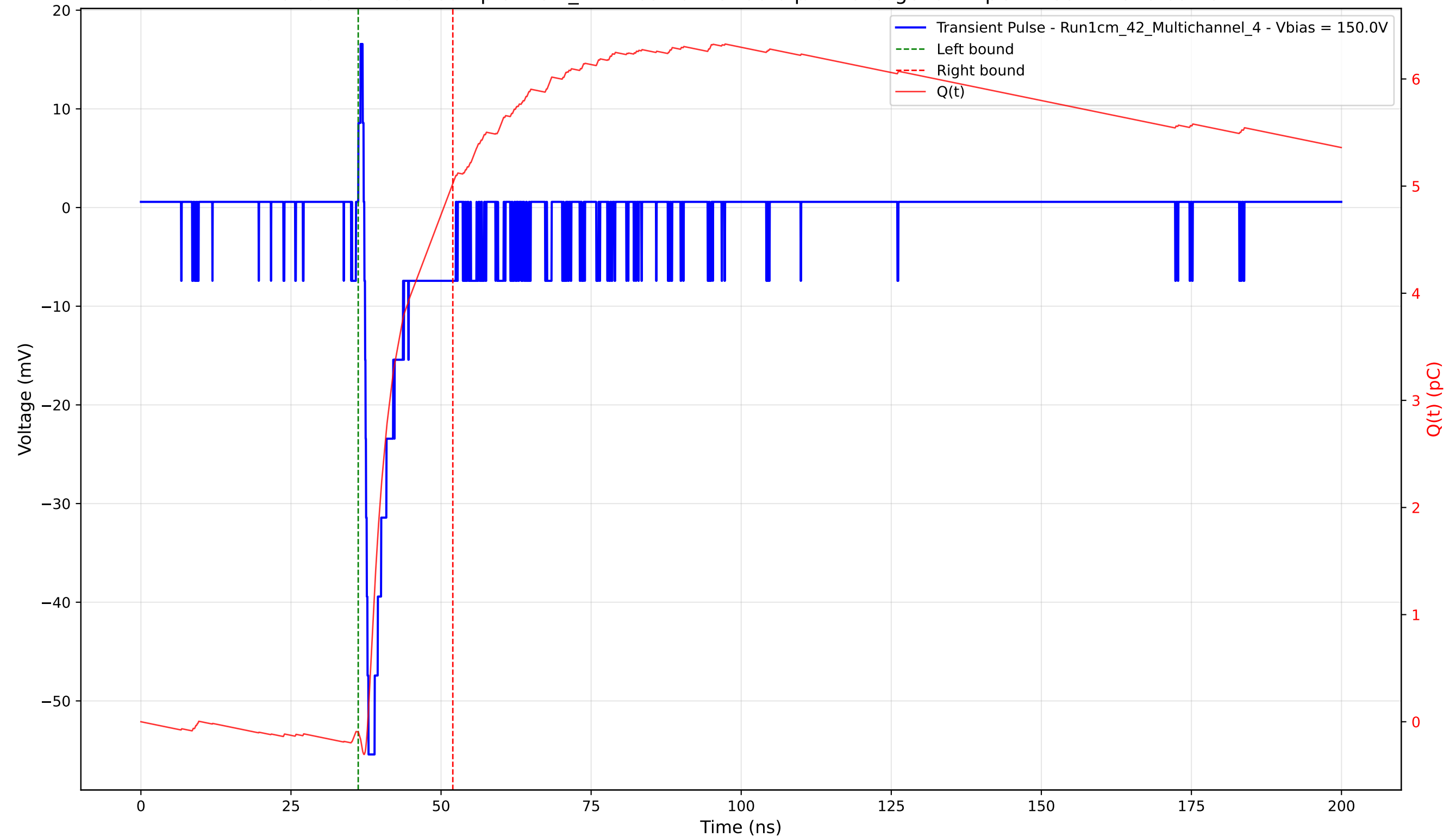
Transient Pulse - Sample: 1cm_42 - Position: 3700.0 \mu\text{m} - Charge: 5.12 pC - Rise Time: 0.69 ns
