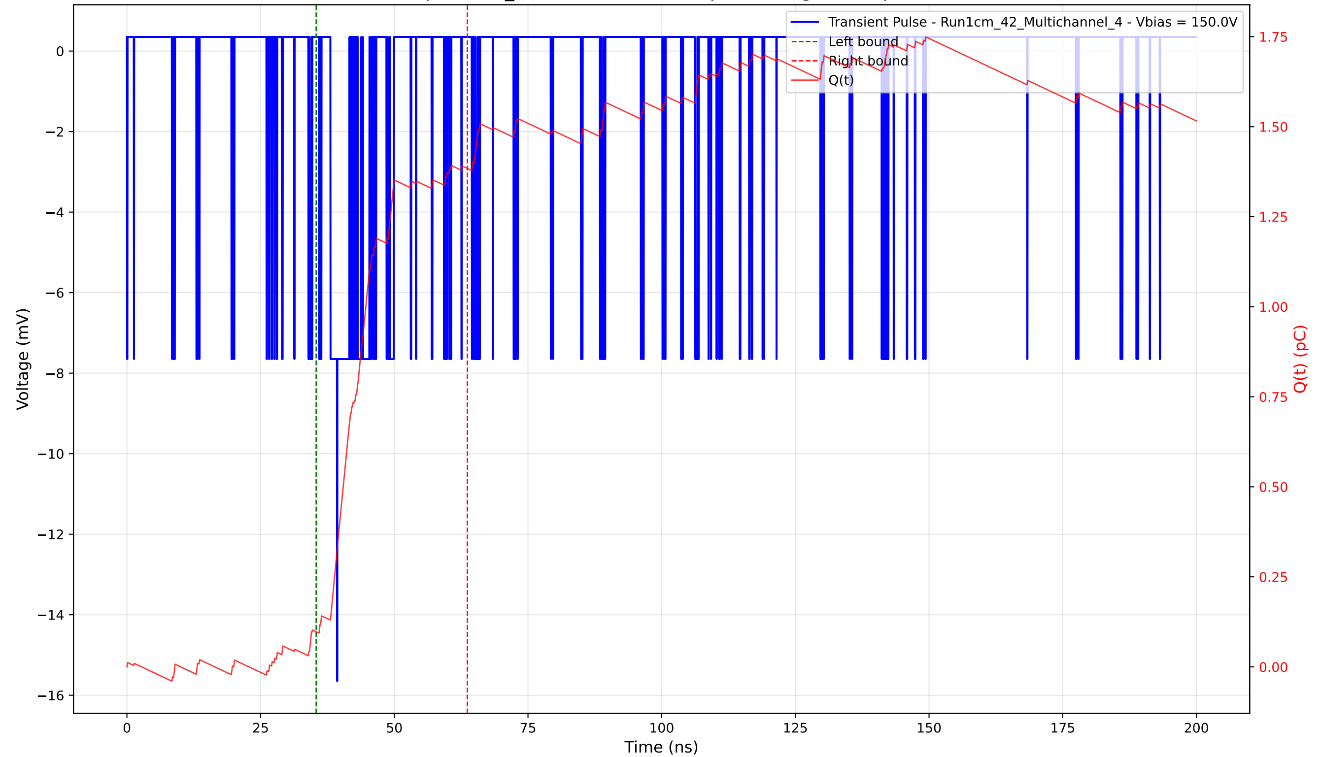
Transient Pulse - Sample: 1cm_42 - Position: 5110.0 \mu\text{m} - Charge: 1.29 pC - Rise Time: 1.27 ns
