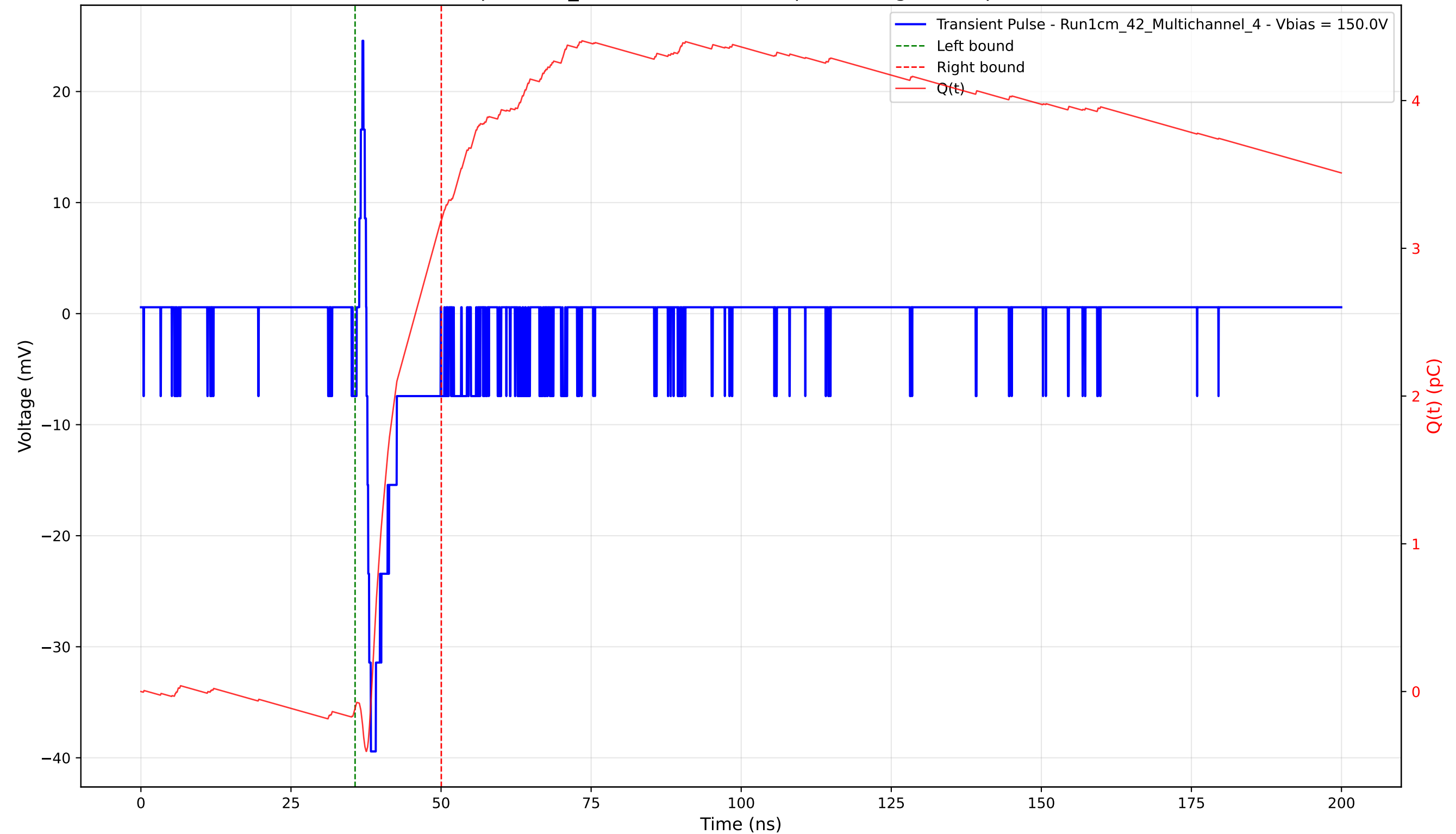
Transient Pulse - Sample: 1cm_42 - Position: 4075.0 \mu\text{m} - Charge: 3.30 pC - Rise Time: 0.74 ns
