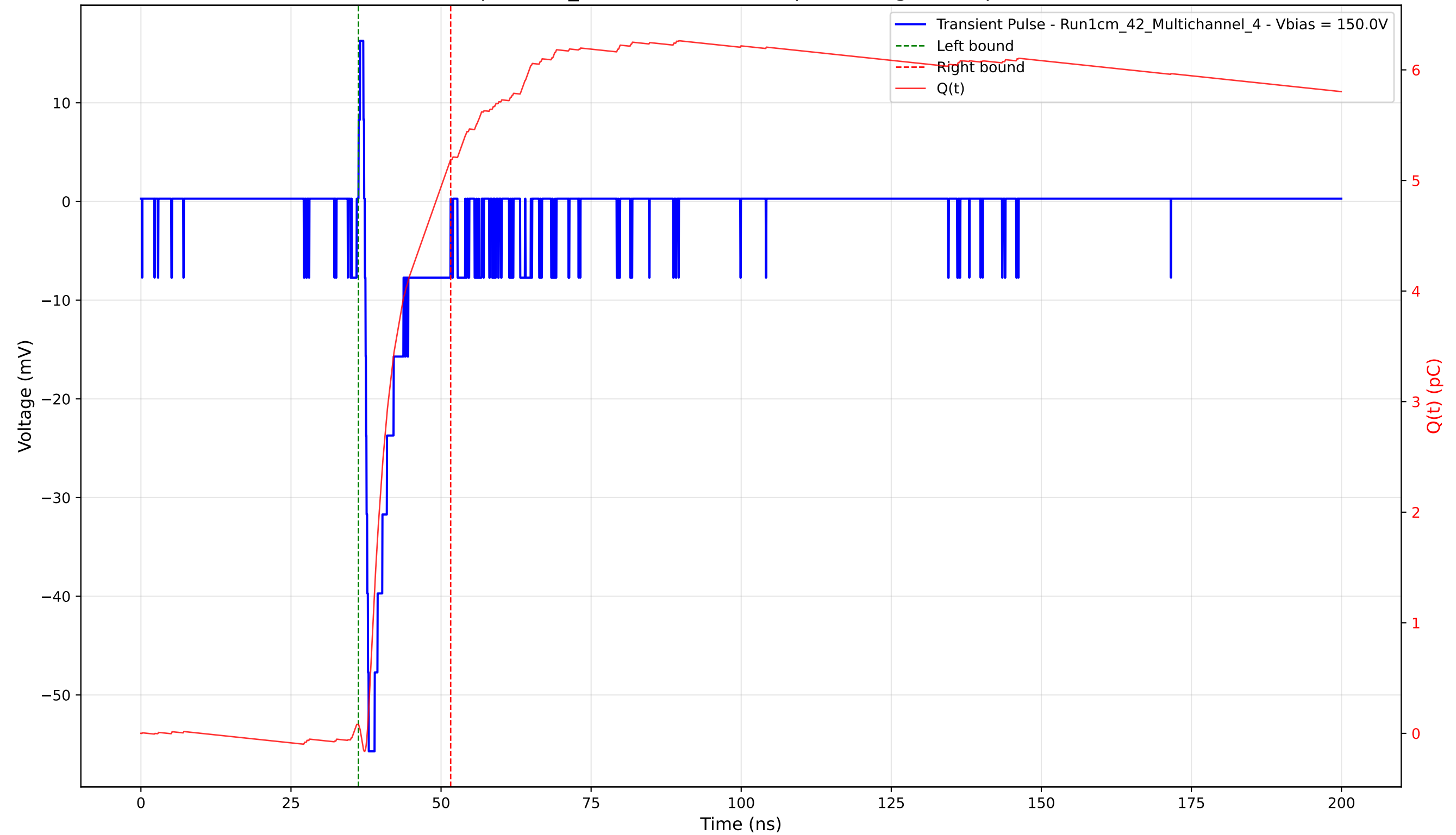
Transient Pulse - Sample: 1cm_42 - Position: 3755.0 \mu\text{m} - Charge: 5.11 pC - Rise Time: 0.65 ns
