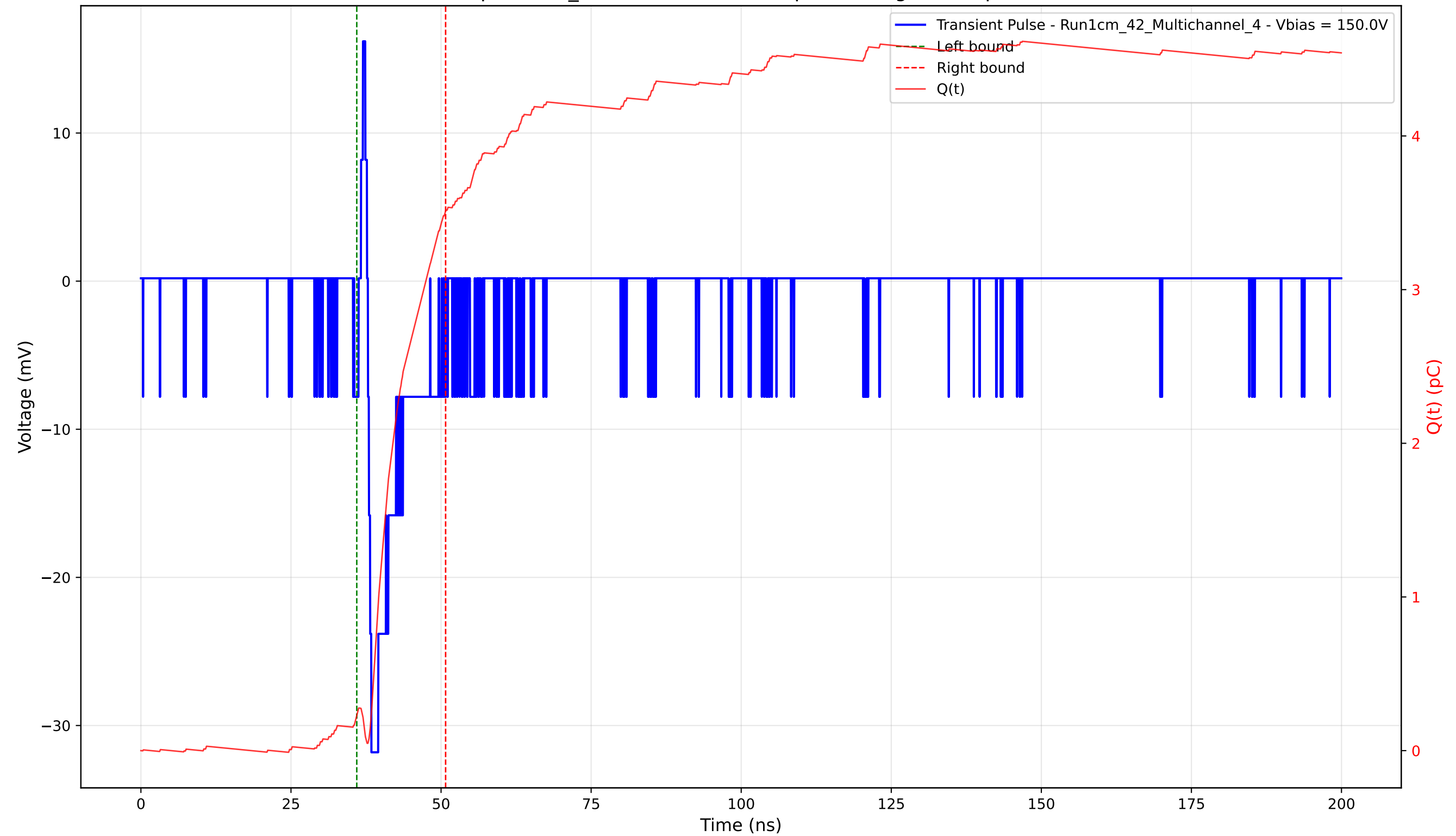
Transient Pulse - Sample: 1cm_42 - Position: 4765.0 \mu\text{m} - Charge: 3.28 pC - Rise Time: 0.58 ns
