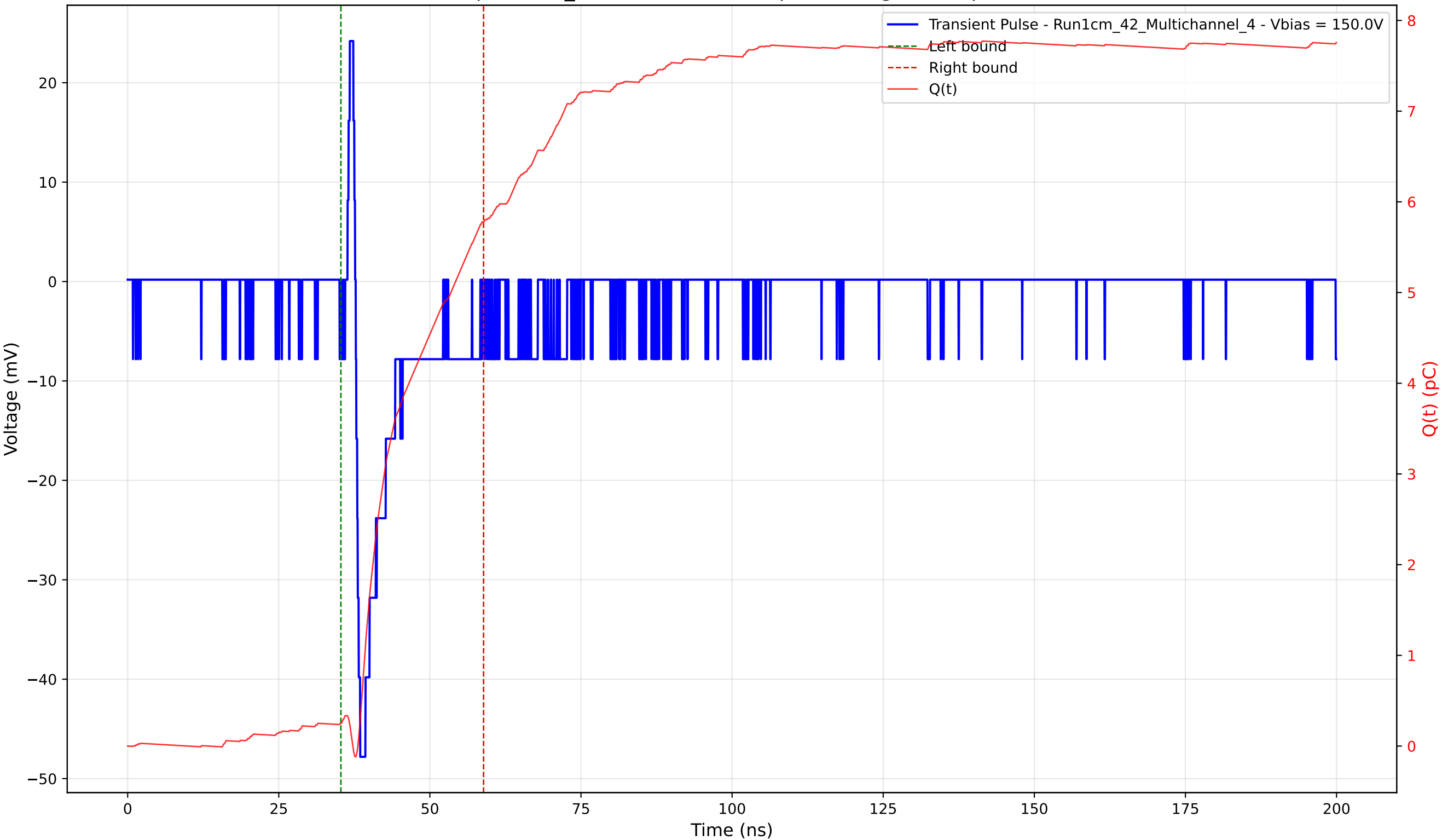
Transient Pulse - Sample: 1cm_42 - Position: 750.0 \mu\text{m} - Charge: 5.53 pC - Rise Time: 0.74 ns
