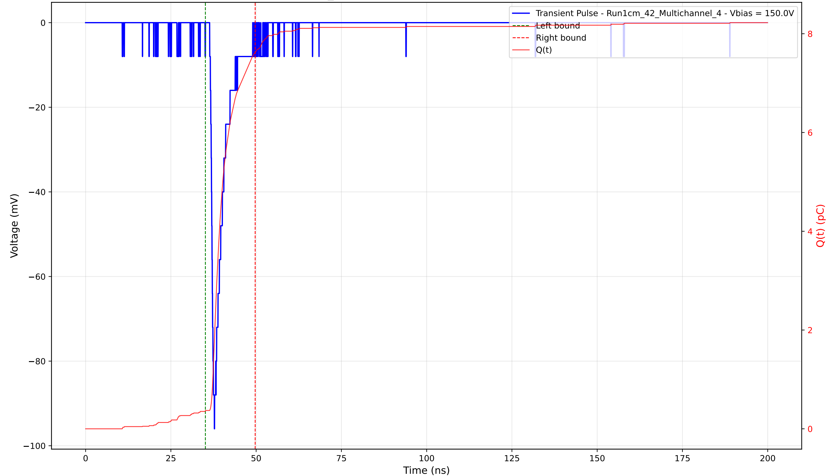
Transient Pulse - Sample: 1cm_42 - Position: 1585.0 \mu\text{m} - Charge: 7.26 pC - Rise Time: 0.91 ns
