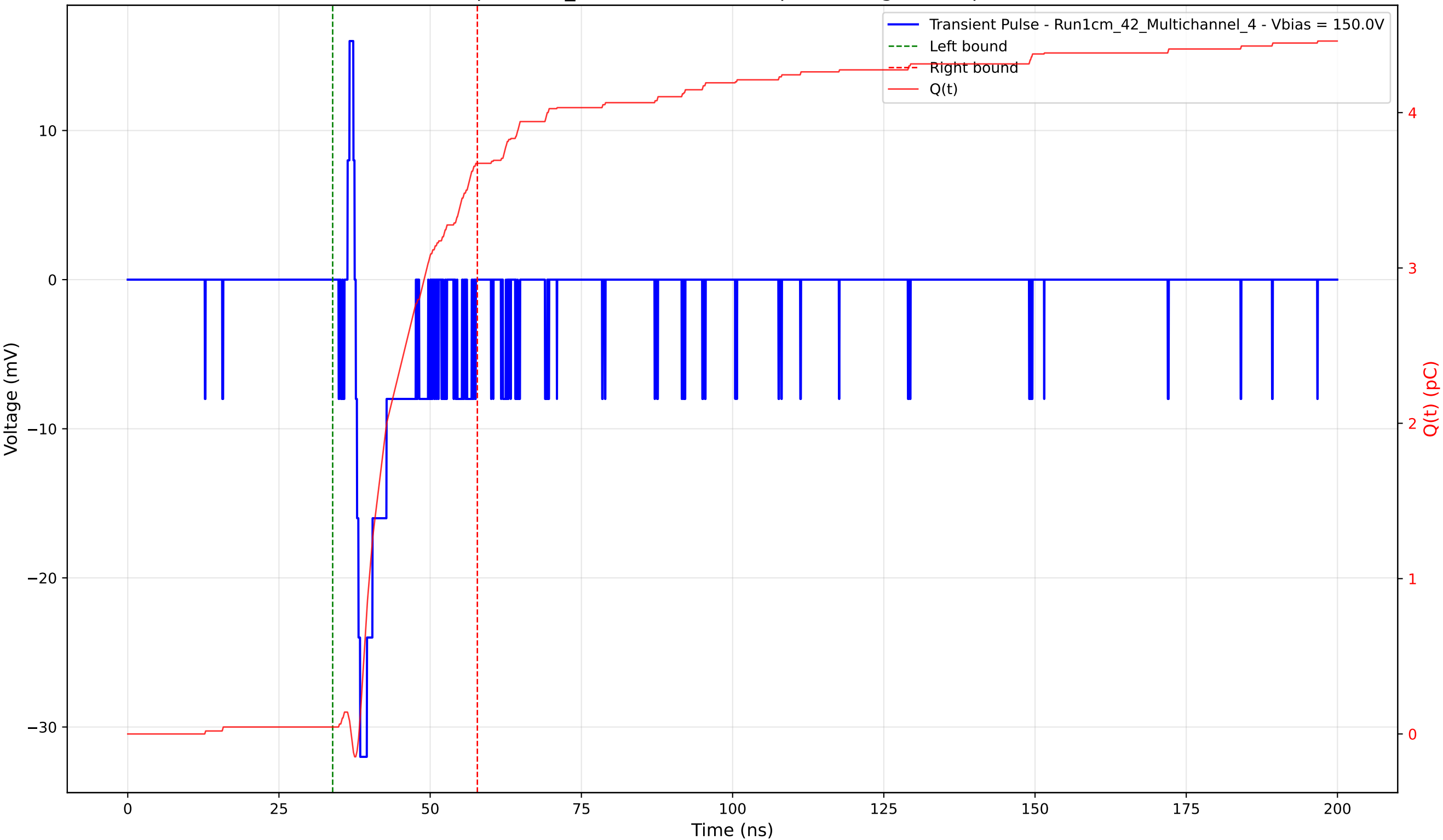
Transient Pulse - Sample: 1cm_42 - Position: 435.0 \mu\text{m} - Charge: 3.63 pC - Rise Time: 0.74 ns
