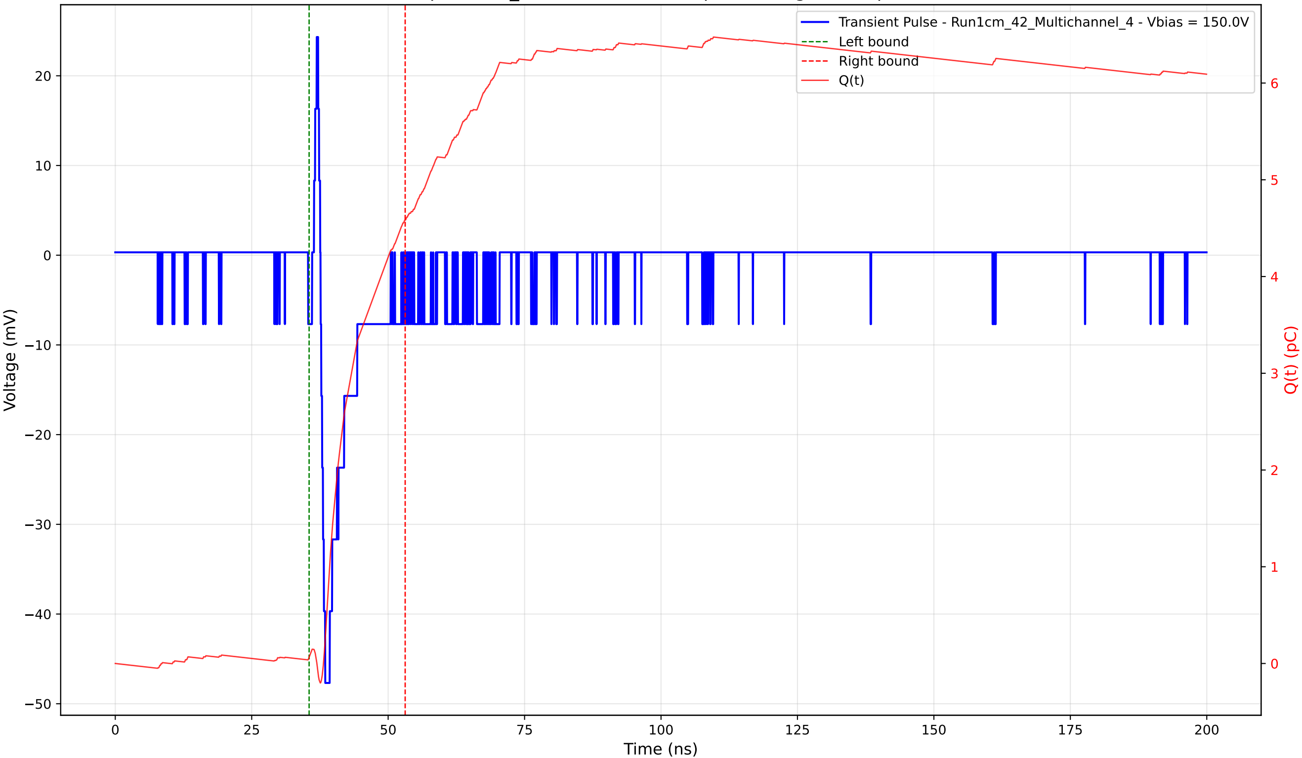
Transient Pulse - Sample: 1cm_42 - Position: 945.0 \mu\text{m} - Charge: 4.52 pC - Rise Time: 0.86 ns
