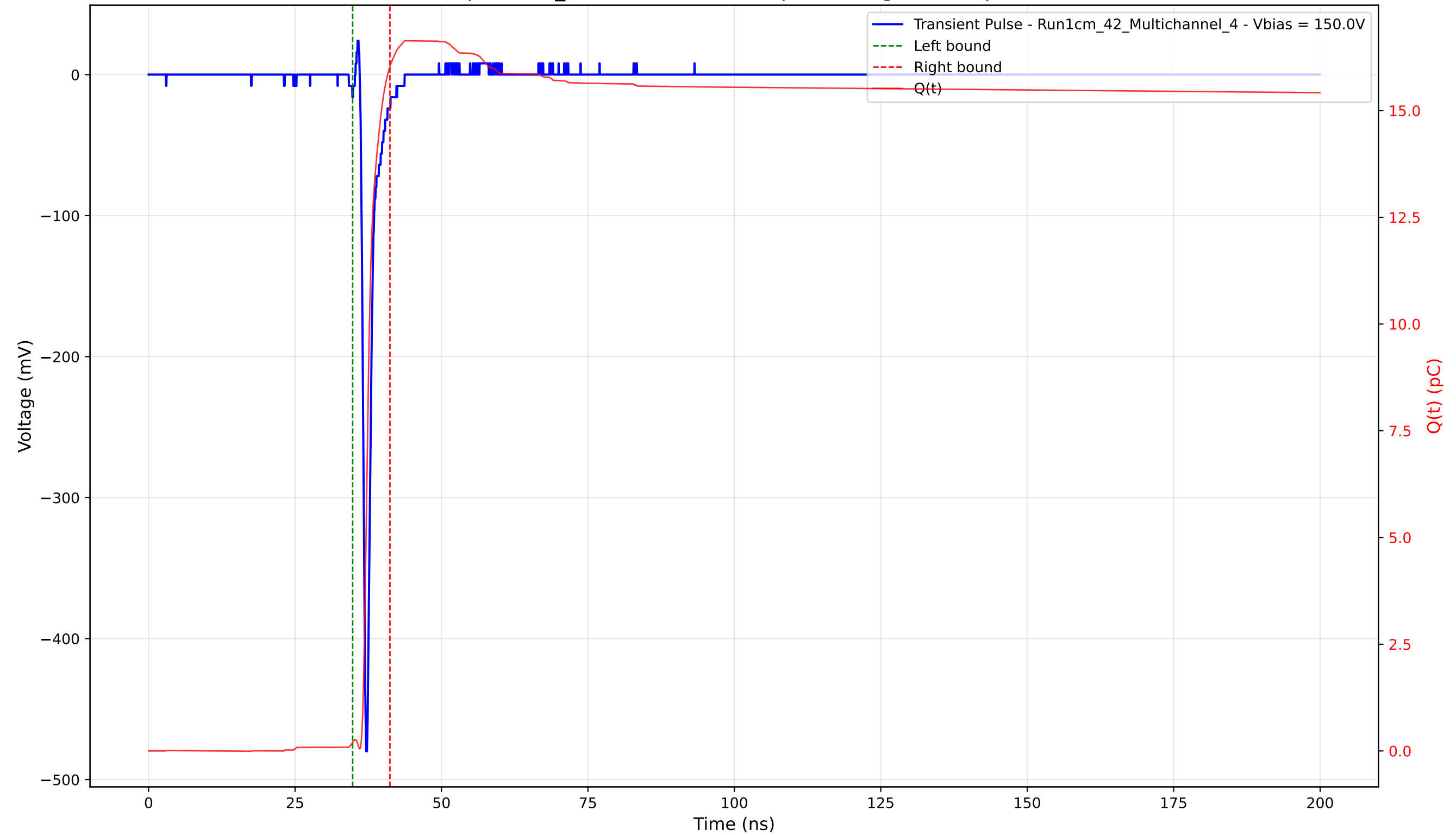
Transient Pulse - Sample: 1cm_42 - Position: 2220.0 \mu\text{m} - Charge: 15.84 pC - Rise Time: 0.74 ns
