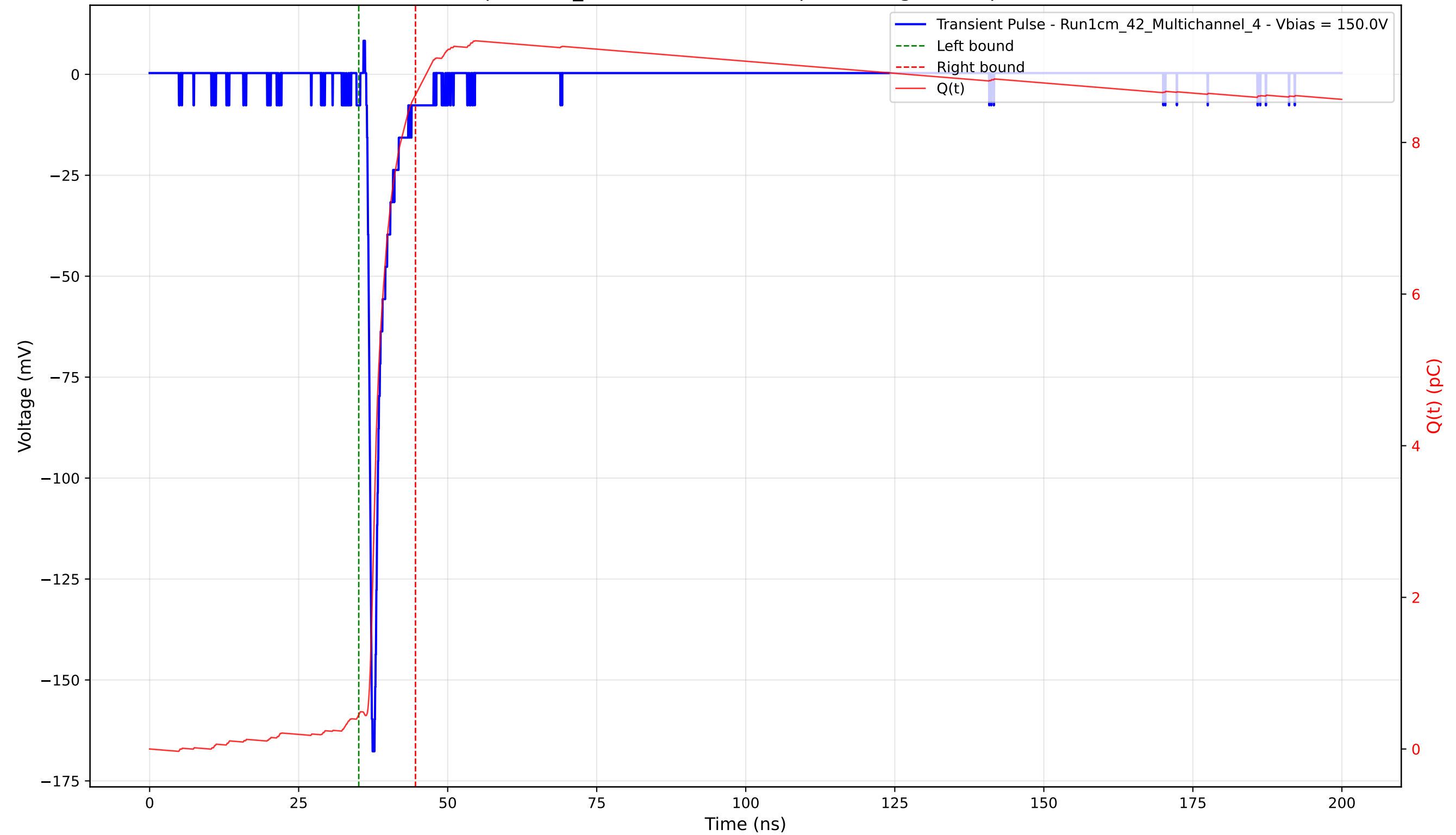
Transient Pulse - Sample: 1cm_42 - Position: 3140.0 \mu\text{m} - Charge: 8.18 pC - Rise Time: 0.71 ns
