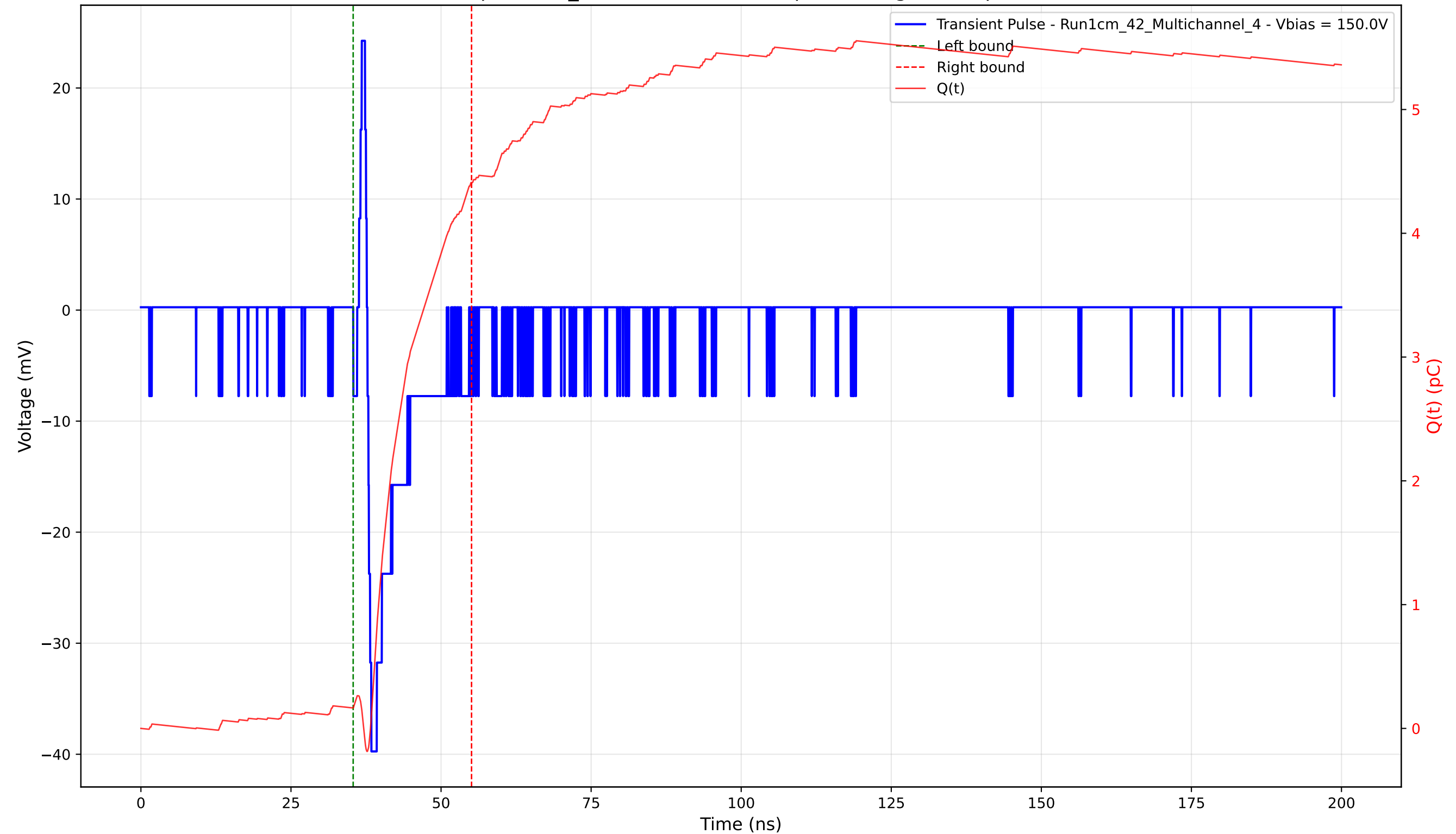
Transient Pulse - Sample: 1cm_42 - Position: 4300.0 \mu\text{m} - Charge: 4.25 pC - Rise Time: 0.66 ns
