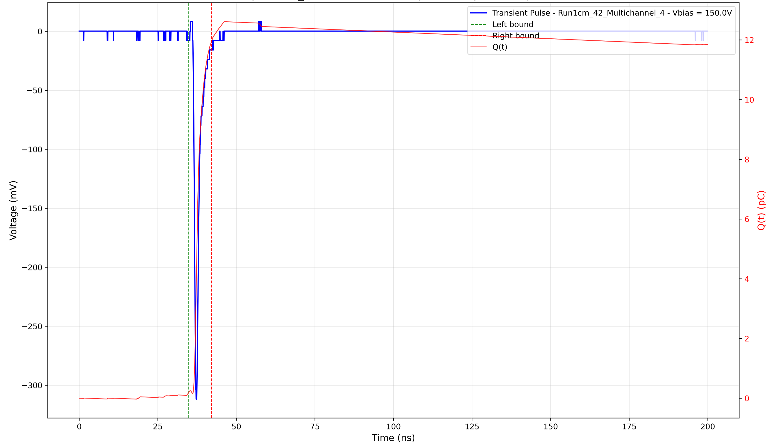
Transient Pulse - Sample: 1cm_42 - Position: 2090.0 \mu\text{m} - Charge: 11.73 pC - Rise Time: 0.73 ns
