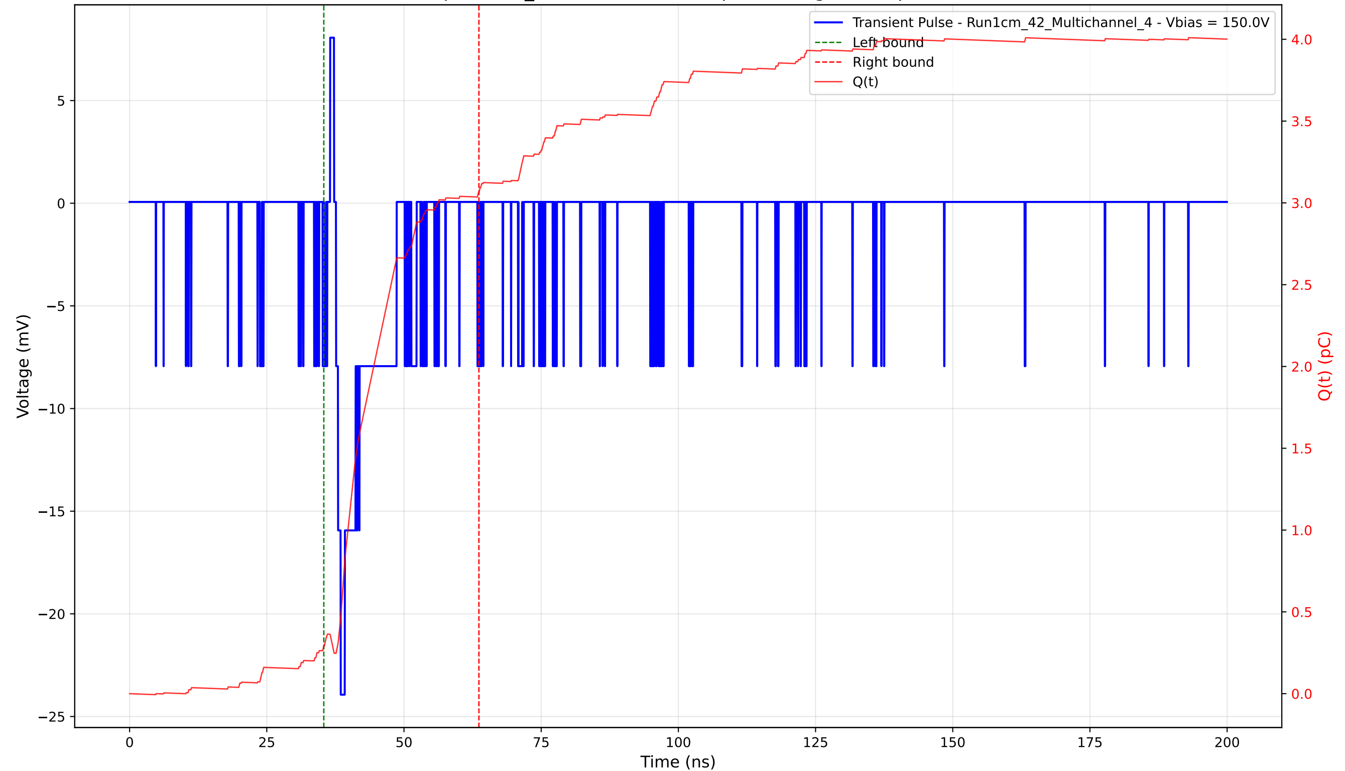
Transient Pulse - Sample: 1cm_42 - Position: 255.0 \mu\text{m} - Charge: 2.77 pC - Rise Time: 0.87 ns
