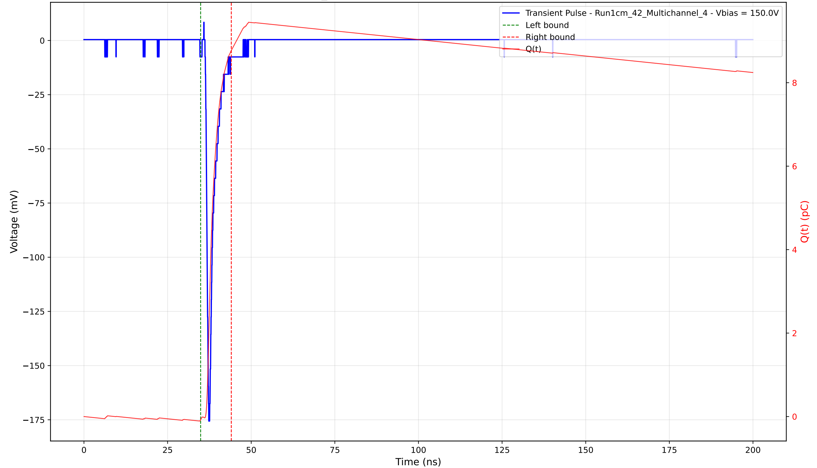
Transient Pulse - Sample: 1cm_42 - Position: 1915.0 \mu\text{m} - Charge: 8.85 pC - Rise Time: 0.79 ns
