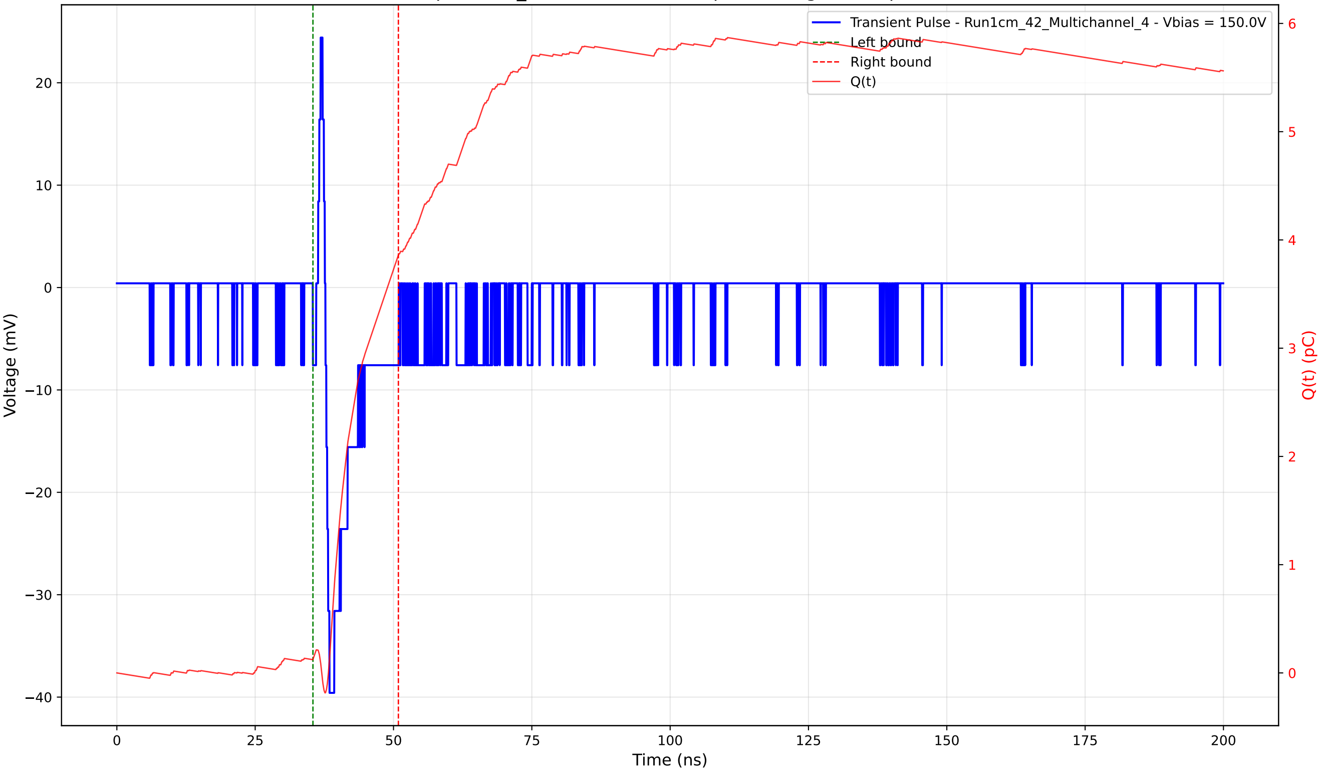
Transient Pulse - Sample: 1cm_42 - Position: 595.0 \mu\text{m} - Charge: 3.74 pC - Rise Time: 0.74 ns
