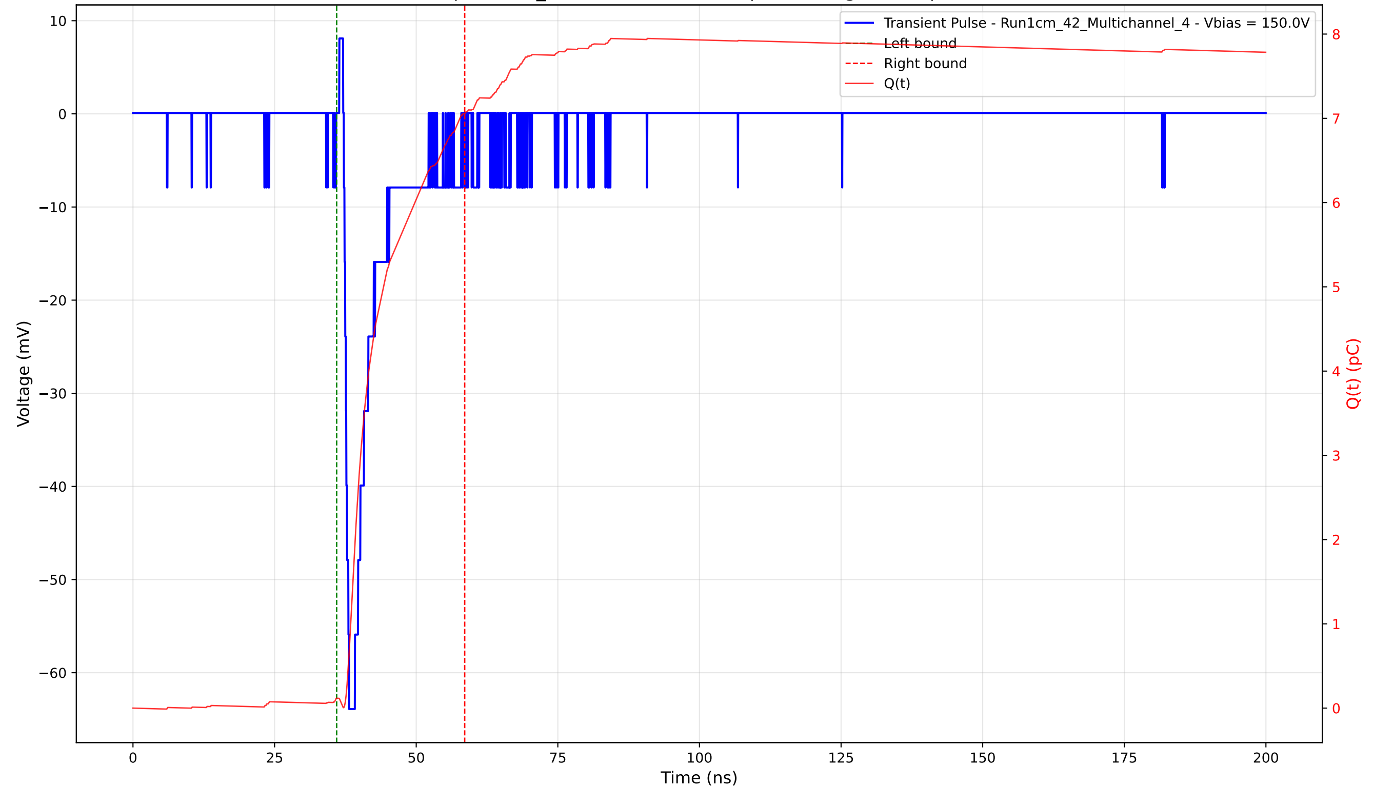
Transient Pulse - Sample: 1cm_42 - Position: 1270.0 \mu\text{m} - Charge: 6.94 pC - Rise Time: 0.93 ns
