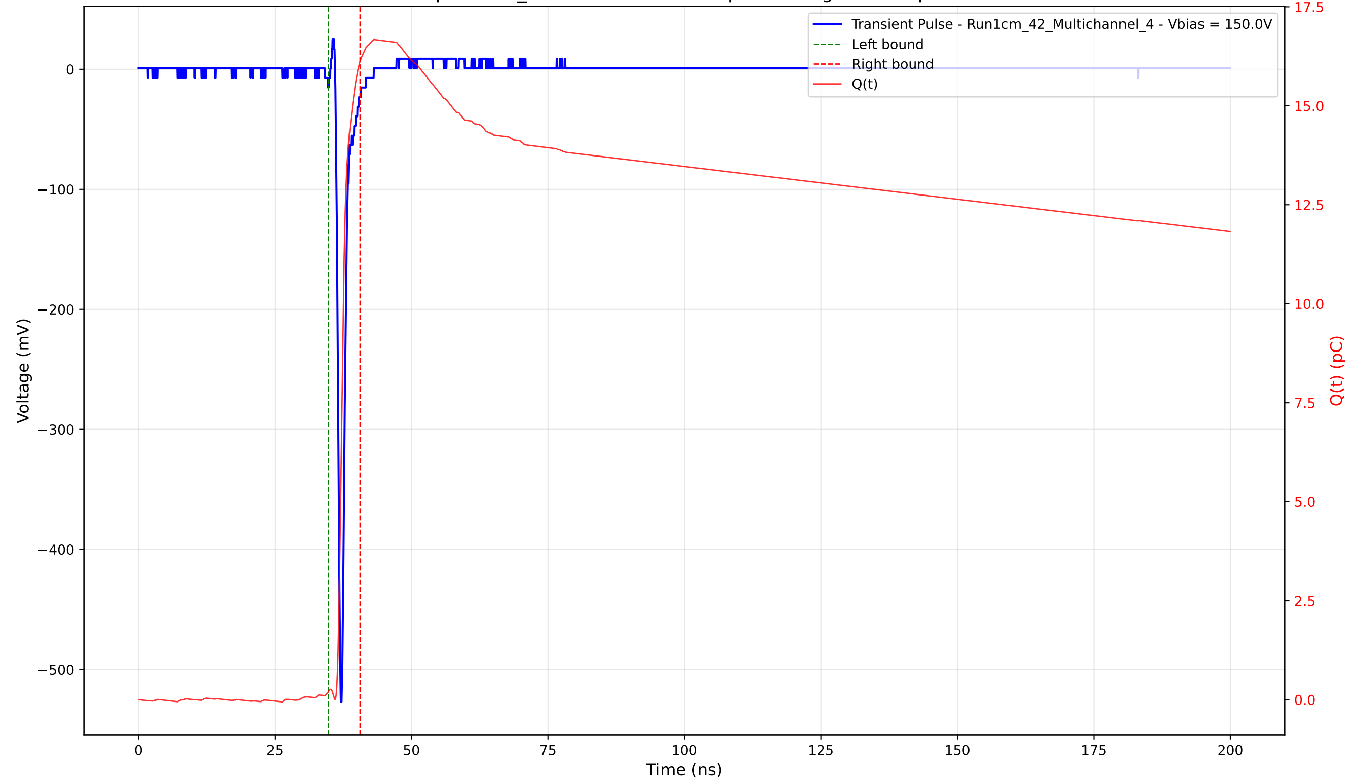
Transient Pulse - Sample: 1cm_42 - Position: 2580.0 \mu\text{m} - Charge: 15.92 pC - Rise Time: 0.71 ns
