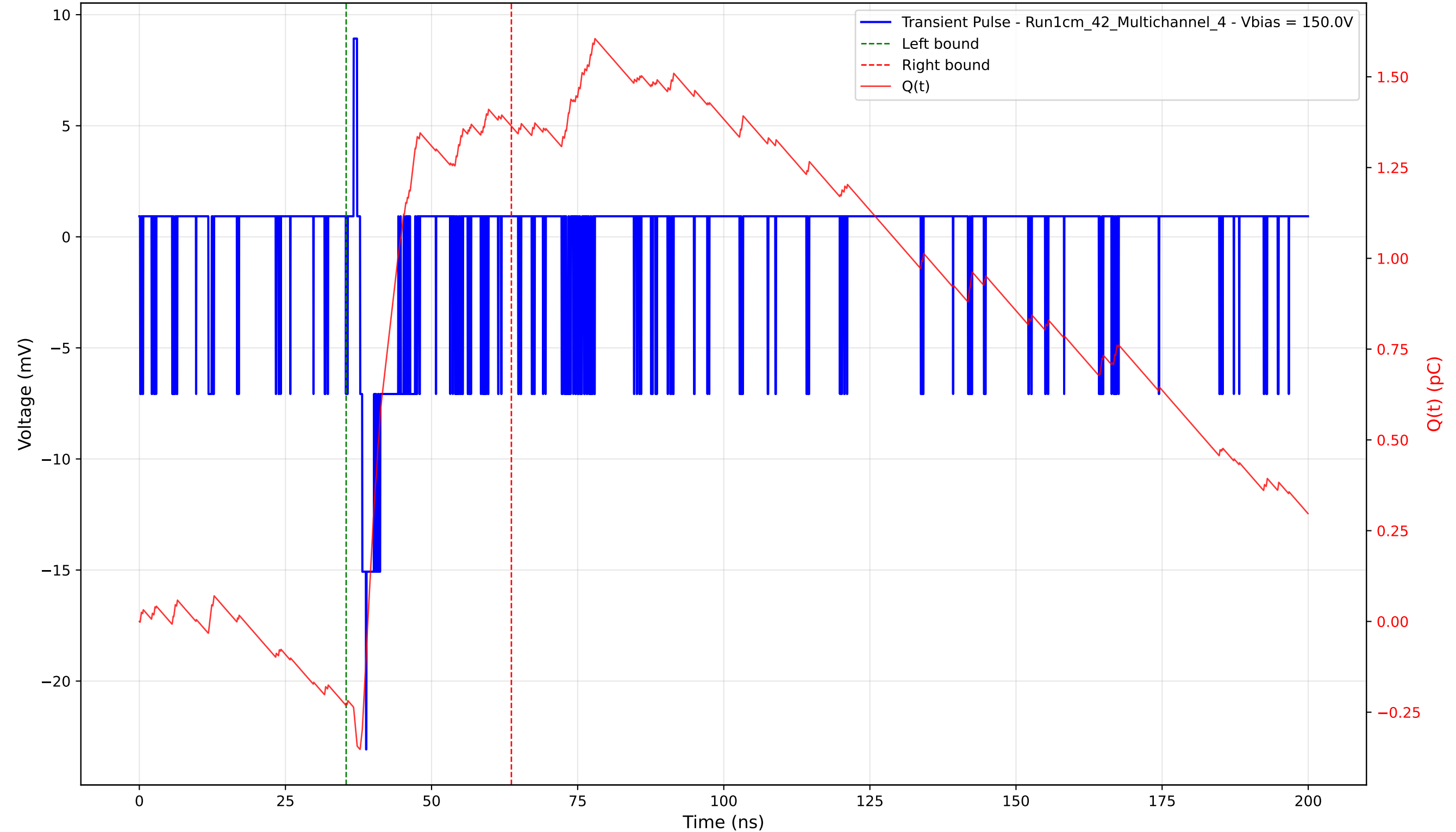
Transient Pulse - Sample: 1cm_42 - Position: 195.0 \mu\text{m} - Charge: 1.59 pC - Rise Time: 1.03 ns
