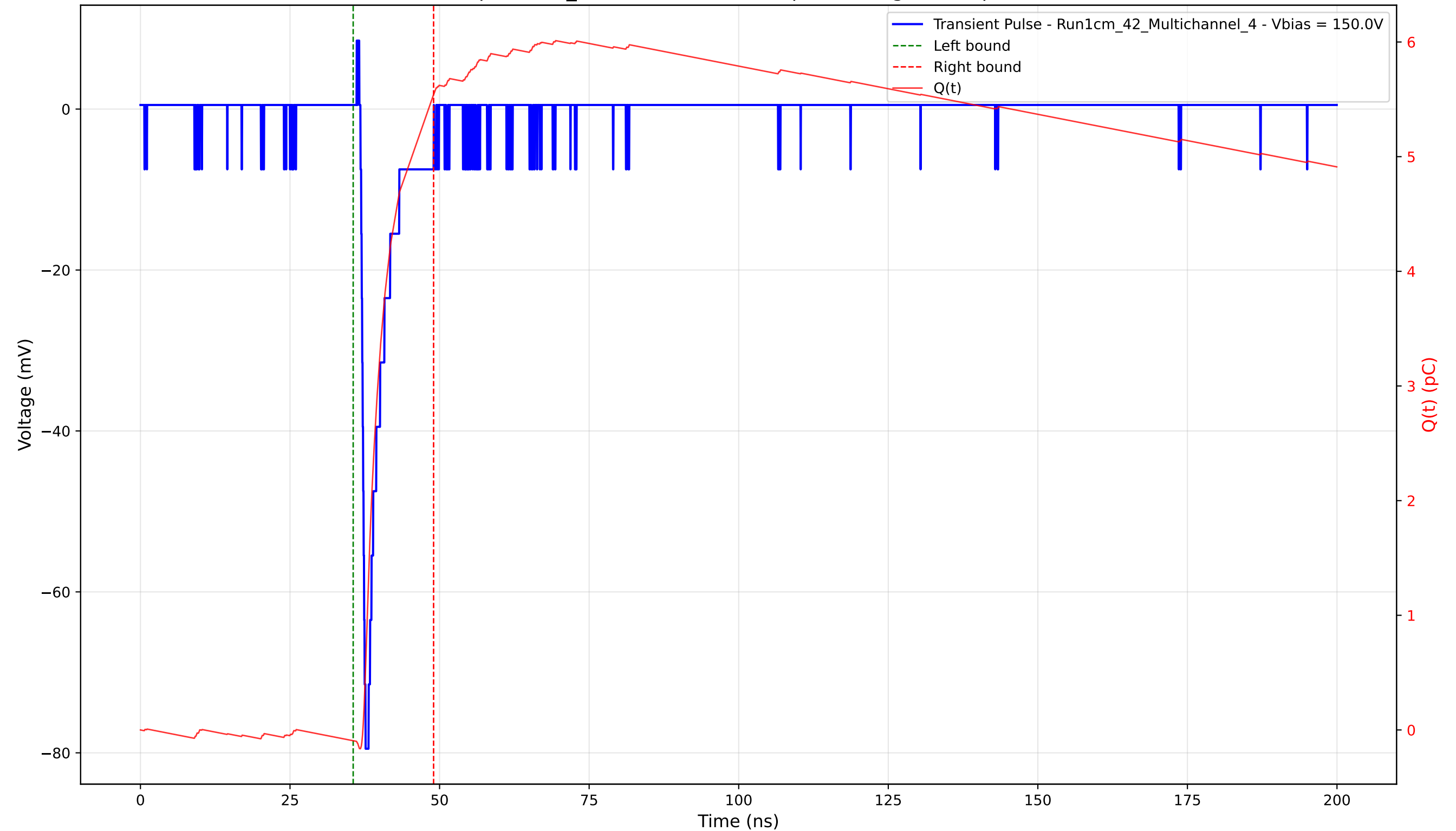
Transient Pulse - Sample: 1cm_42 - Position: 3475.0 \mu\text{m} - Charge: 5.64 pC - Rise Time: 0.76 ns
