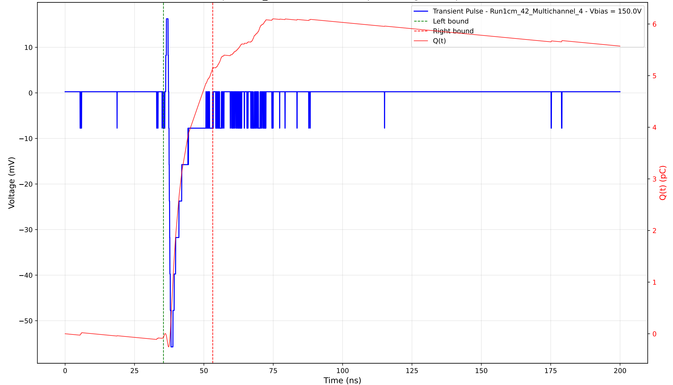
Transient Pulse - Sample: 1cm_42 - Position: 3835.0 \mu\text{m} - Charge: 5.21 pC - Rise Time: 0.81 ns
