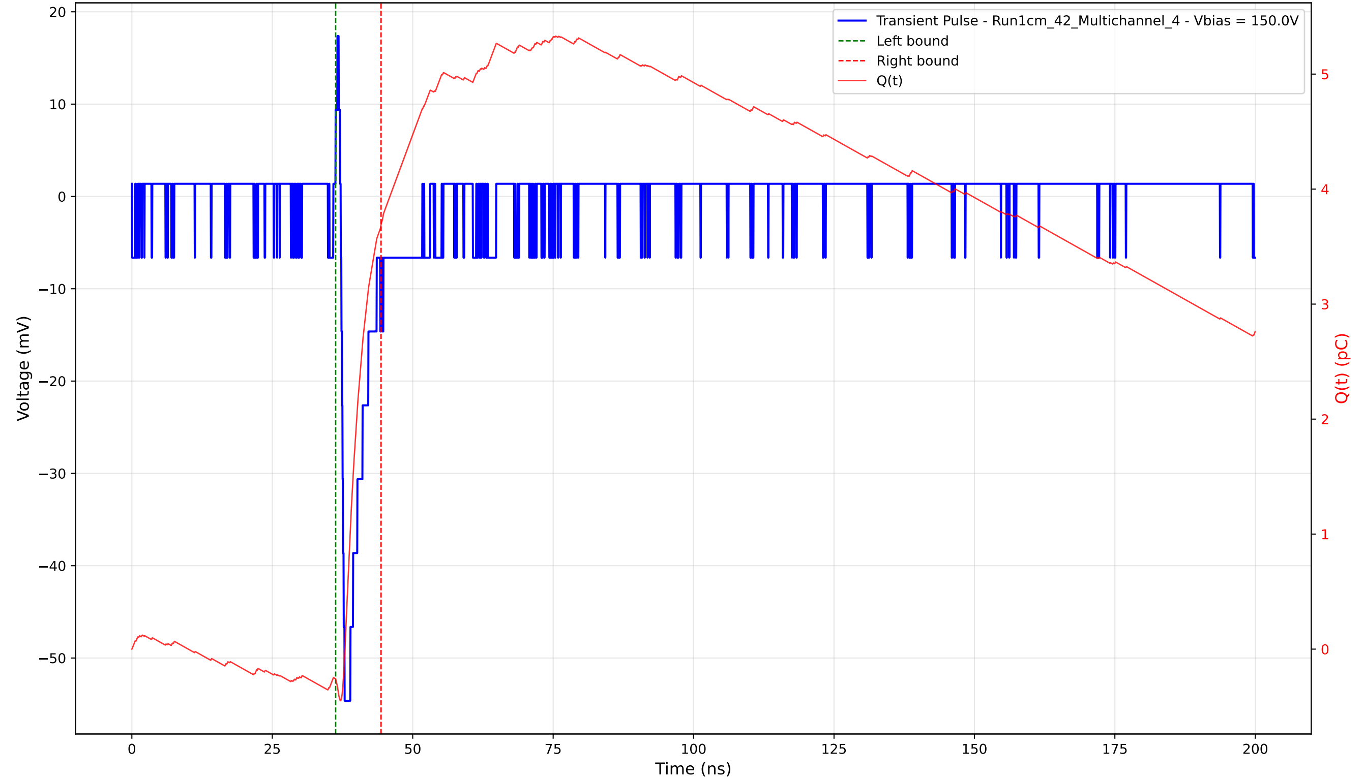
Transient Pulse - Sample: 1cm_42 - Position: 3690.0 \mu\text{m} - Charge: 3.95 pC - Rise Time: 0.69 ns
