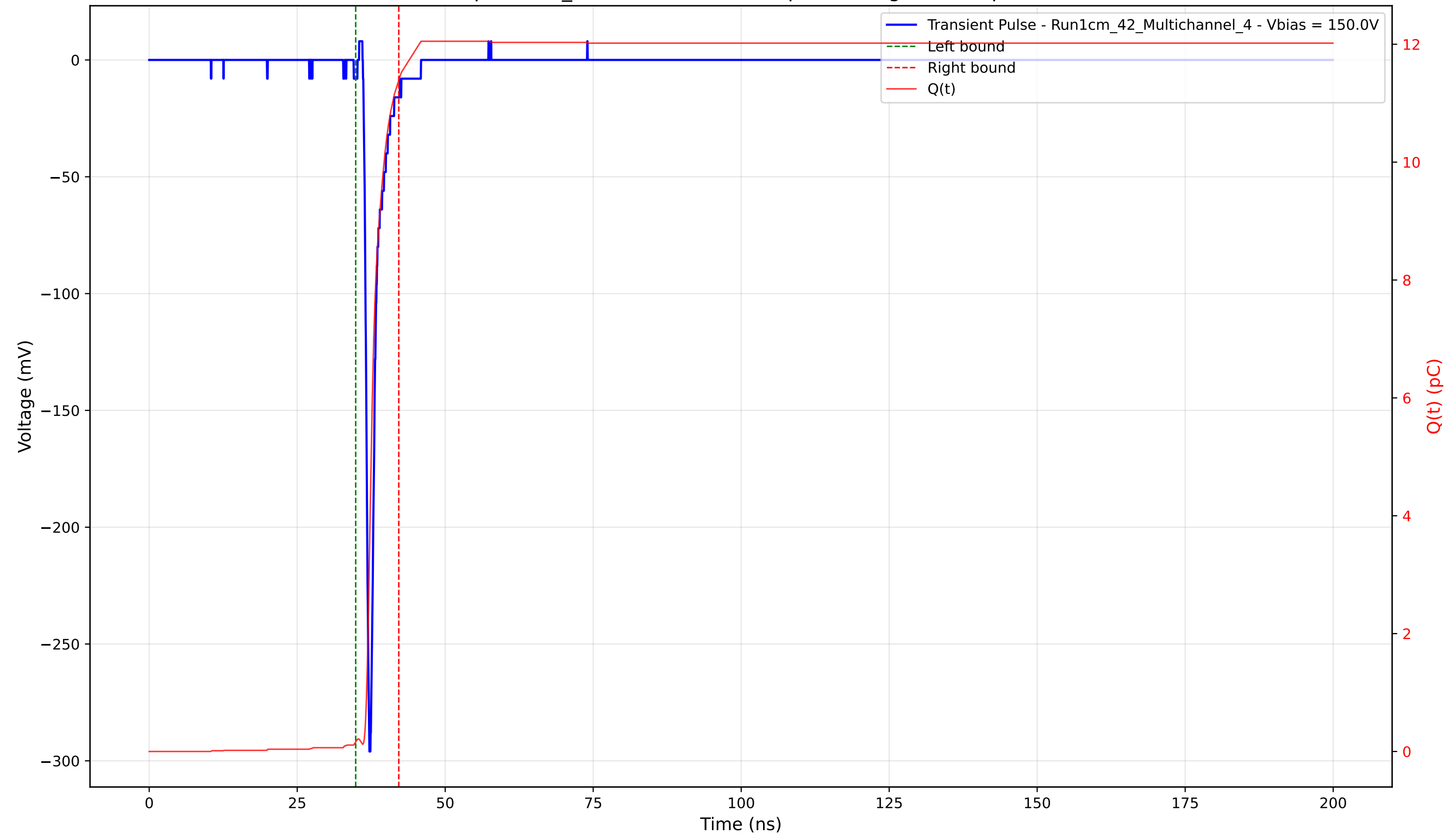
Transient Pulse - Sample: 1cm_42 - Position: 2075.0 \mu\text{m} - Charge: 11.23 pC - Rise Time: 0.78 ns
