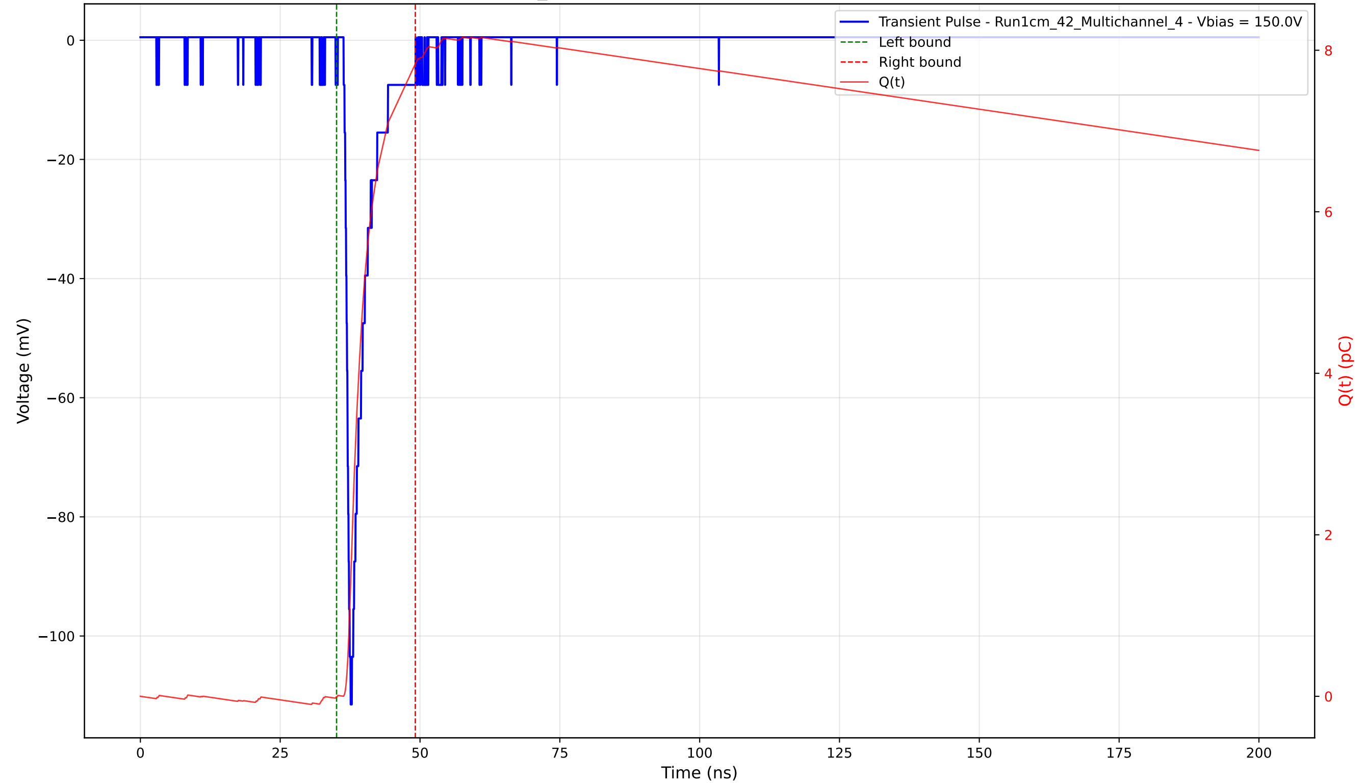
Transient Pulse - Sample: 1cm_42 - Position: 1635.0 \mu\text{m} - Charge: 7.84 pC - Rise Time: 0.94 ns
