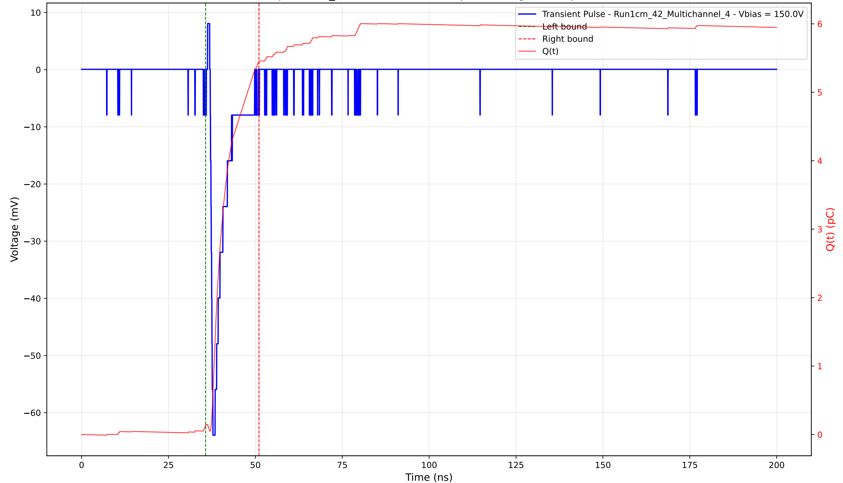
Transient Pulse - Sample: 1cm_42 - Position: 3575.0 \mu\text{m} - Charge: 5.31 pC - Rise Time: 0.77 ns
