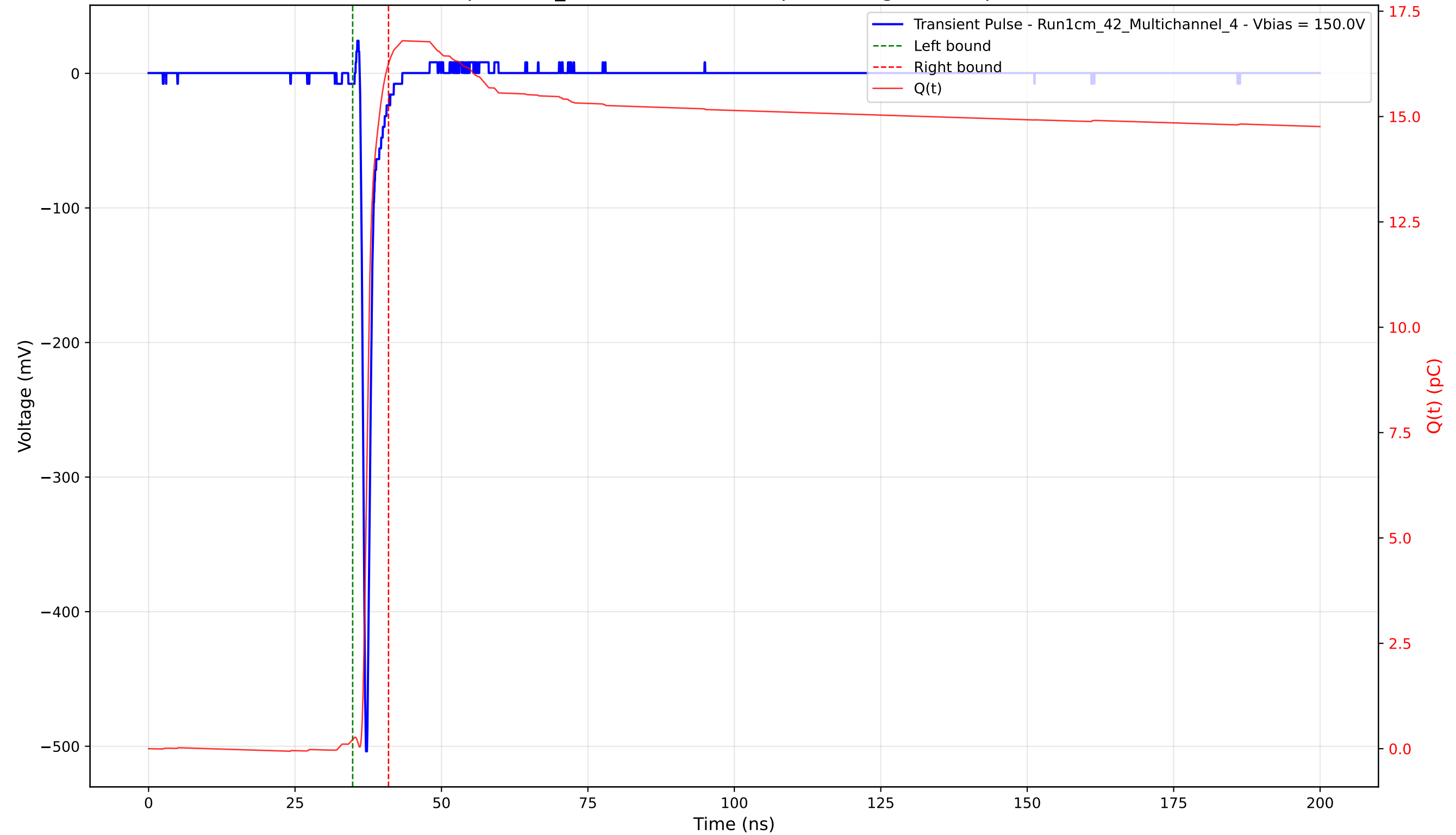
Transient Pulse - Sample: 1cm_42 - Position: 2690.0 \mu\text{m} - Charge: 16.04 pC - Rise Time: 0.70 ns
