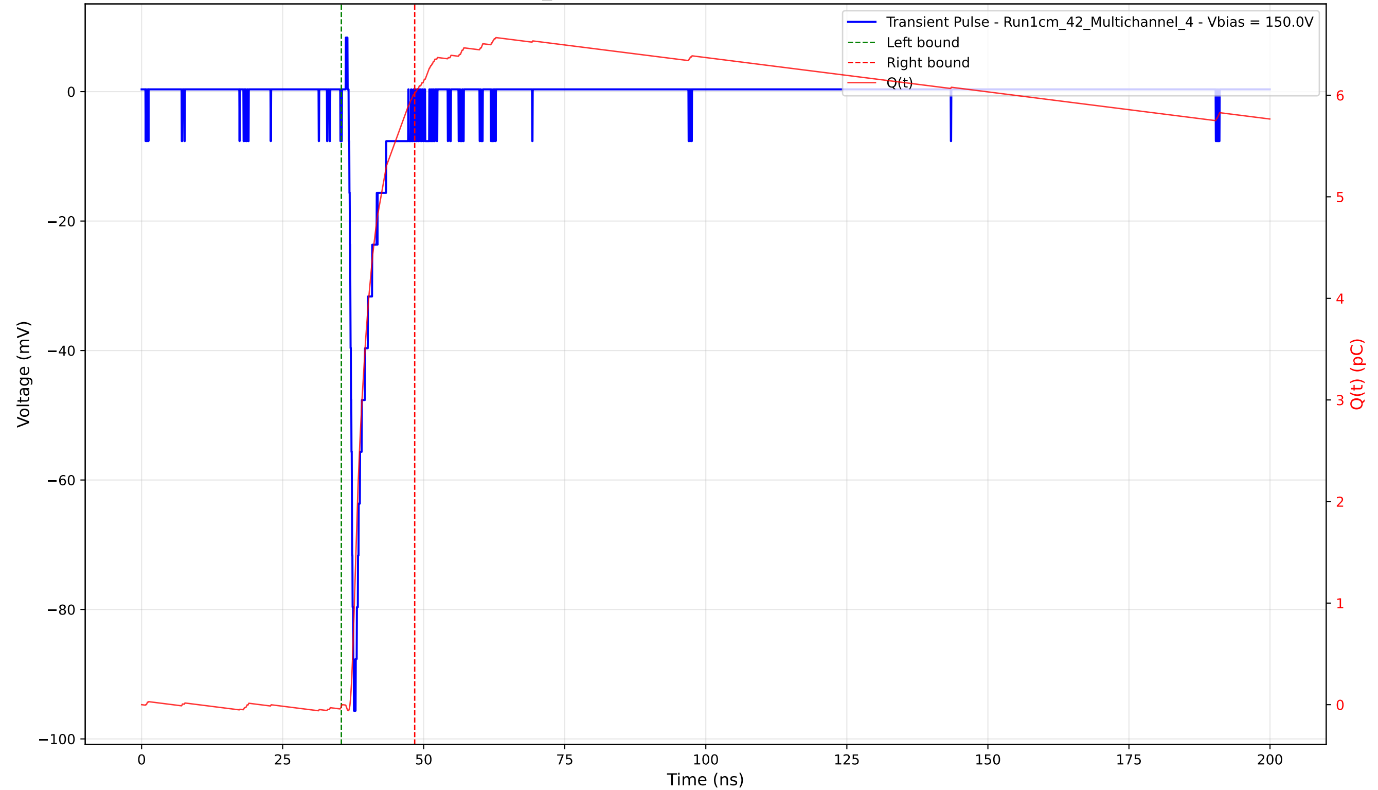
Transient Pulse - Sample: 1cm_42 - Position: 3435.0 \mu\text{m} - Charge: 6.03 pC - Rise Time: 0.71 ns
