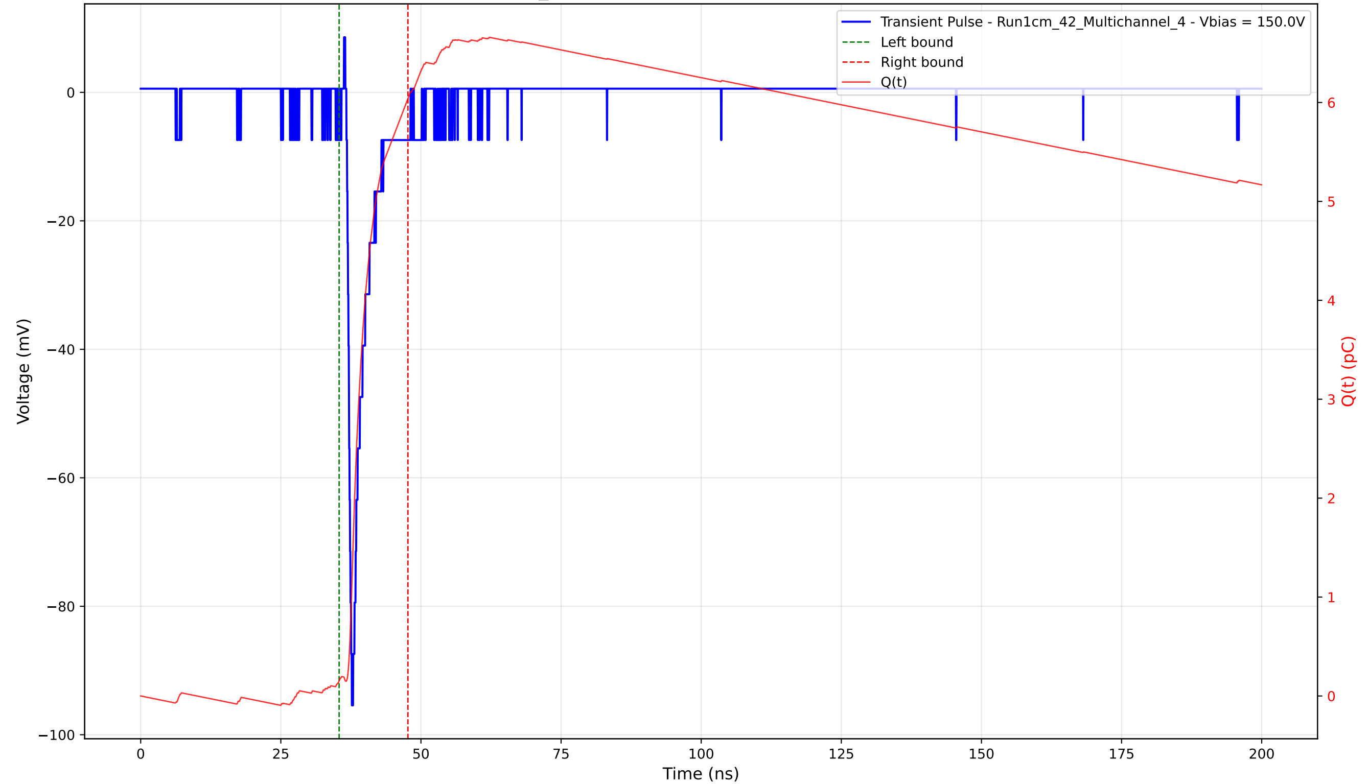
Transient Pulse - Sample: 1cm_42 - Position: 3440.0 \mu\text{m} - Charge: 5.89 pC - Rise Time: 0.75 ns
