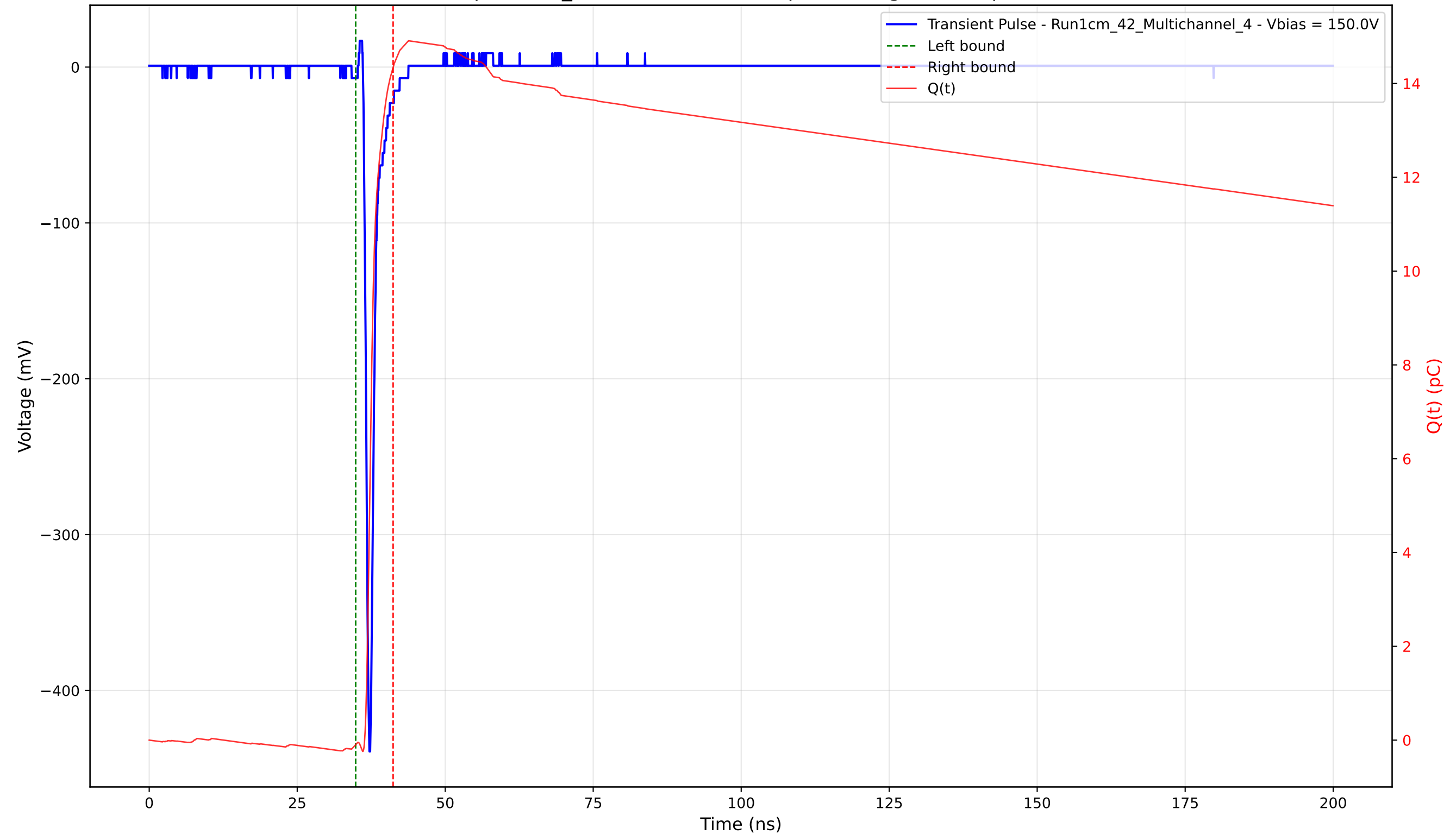
Transient Pulse - Sample: 1cm_42 - Position: 2825.0 \mu\text{m} - Charge: 14.44 pC - Rise Time: 0.72 ns
