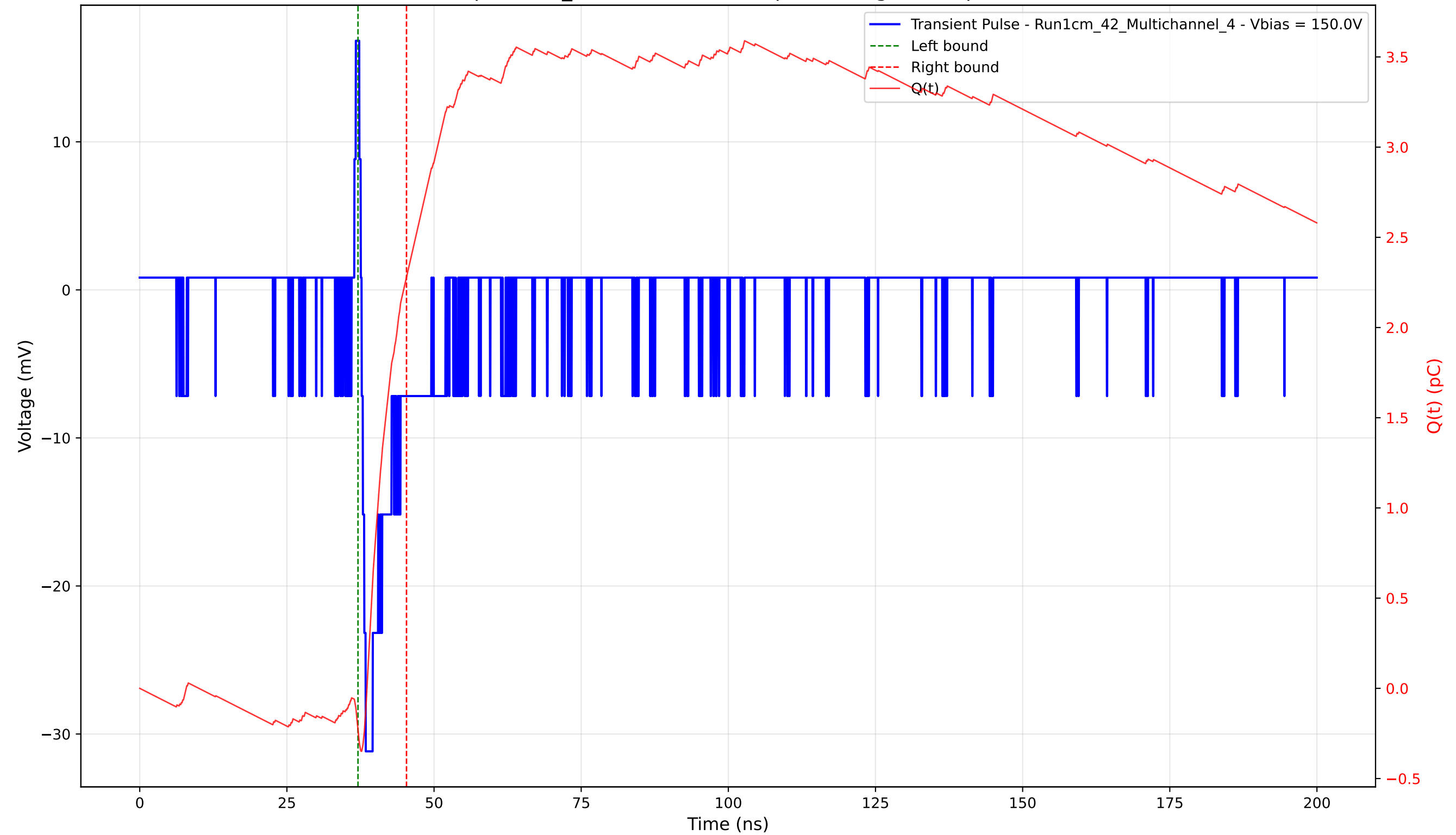
Transient Pulse - Sample: 1cm_42 - Position: 465.0 \mu\text{m} - Charge: 2.51 pC - Rise Time: 0.71 ns
