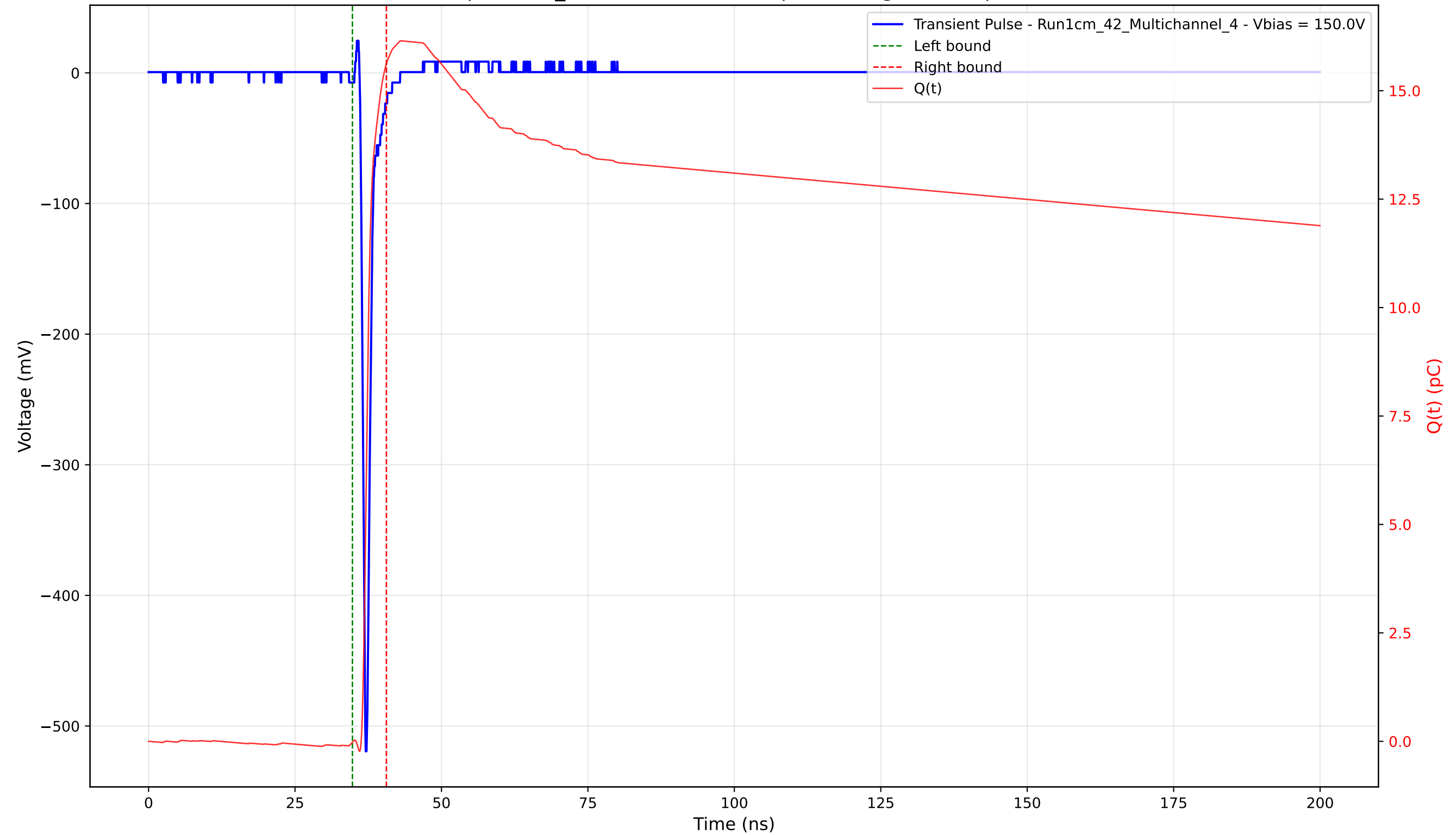
Transient Pulse - Sample: 1cm_42 - Position: 2525.0 \mu\text{m} - Charge: 15.65 pC - Rise Time: 0.72 ns
