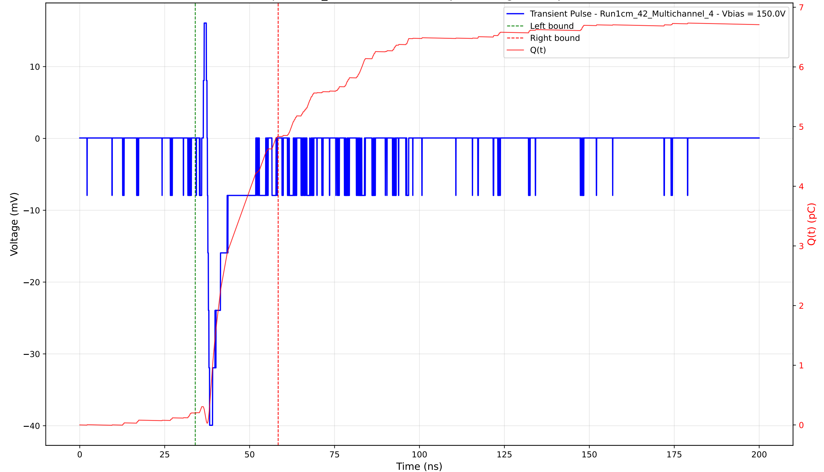
Transient Pulse - Sample: 1cm_42 - Position: 4050.0 \mu\text{m} - Charge: 4.63 pC - Rise Time: 0.66 ns
