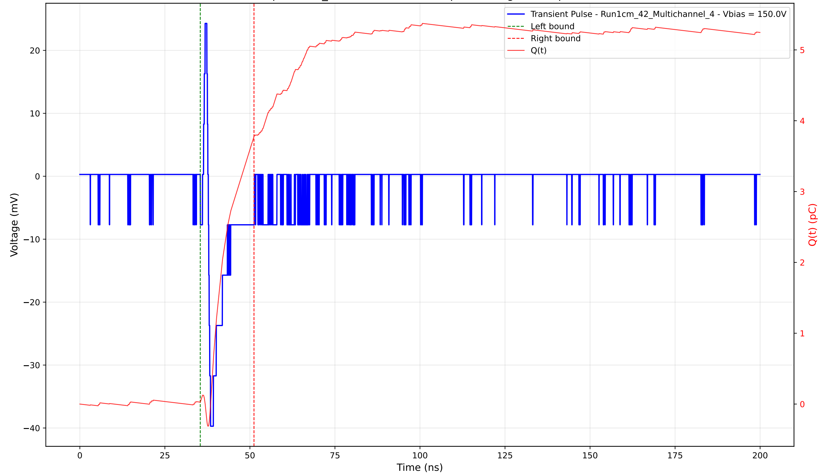
Transient Pulse - Sample: 1cm_42 - Position: 4330.0 \mu\text{m} - Charge: 3.75 pC - Rise Time: 0.66 ns
