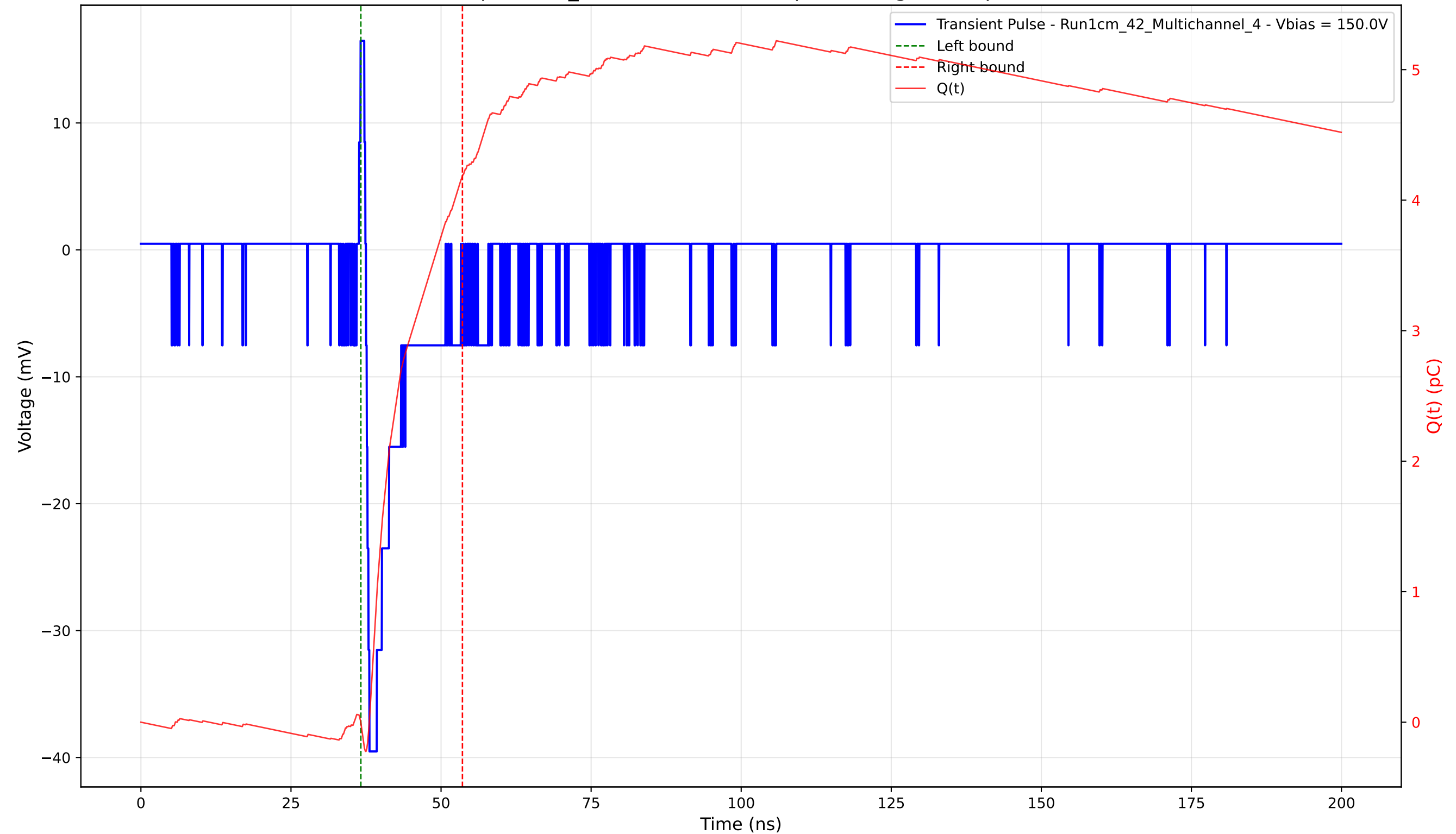
Transient Pulse - Sample: 1cm_42 - Position: 3980.0 \mu\text{m} - Charge: 4.19 pC - Rise Time: 0.58 ns
