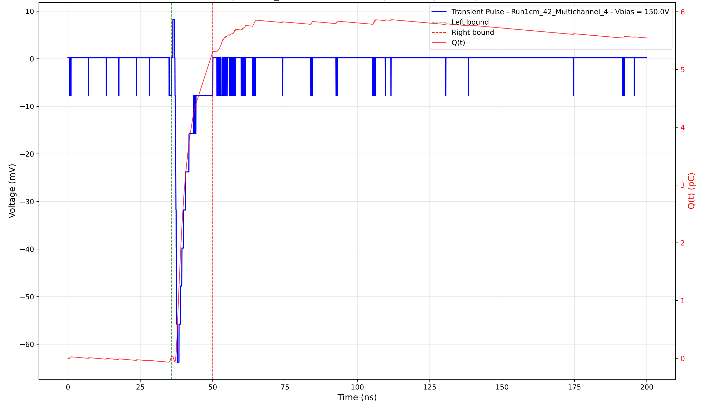
Transient Pulse - Sample: 1cm_42 - Position: 3570.0 \mu\text{m} - Charge: 5.29 pC - Rise Time: 0.77 ns
