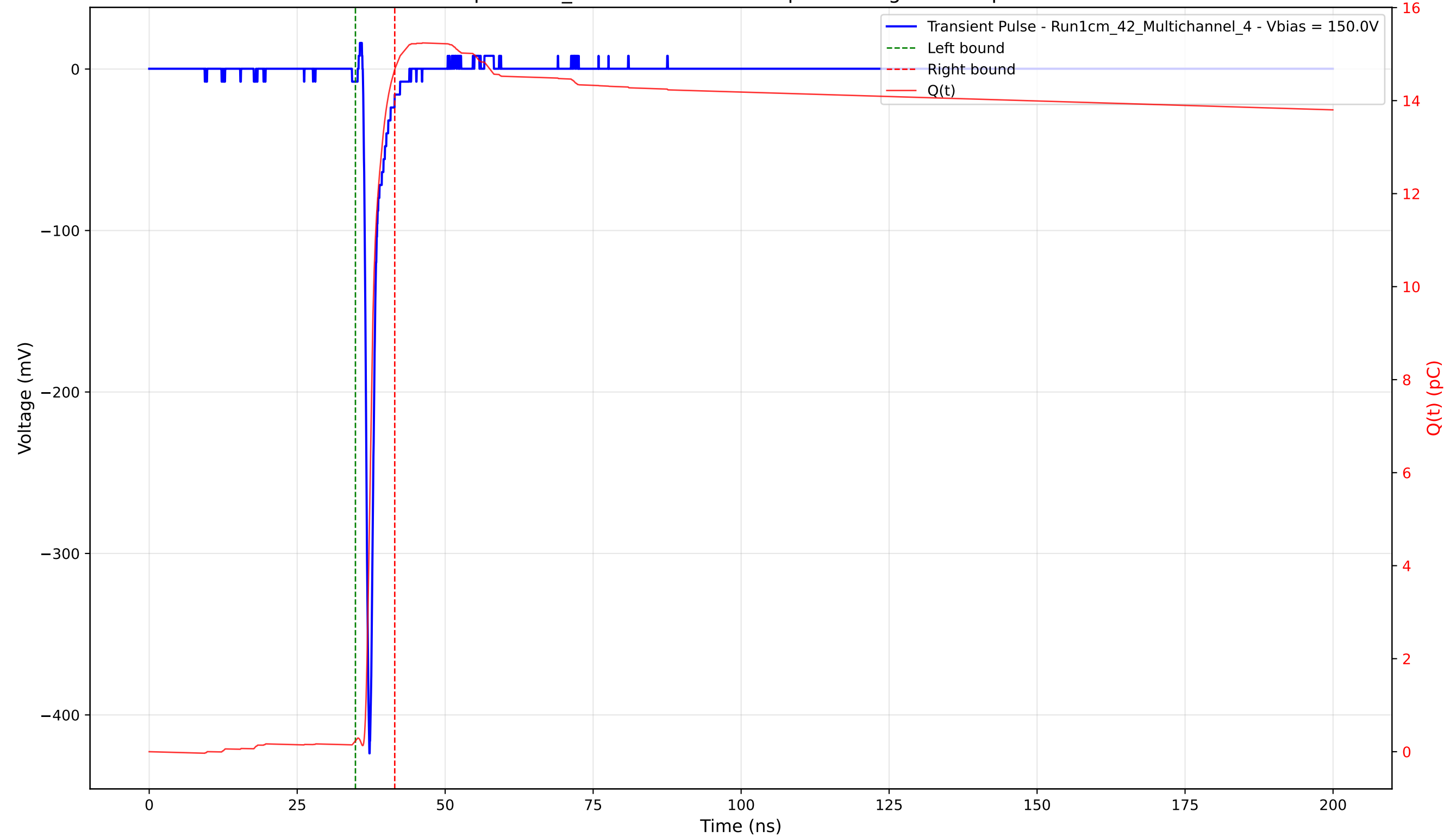
Transient Pulse - Sample: 1cm_42 - Position: 2175.0 \mu\text{m} - Charge: 14.44 pC - Rise Time: 0.74 ns
