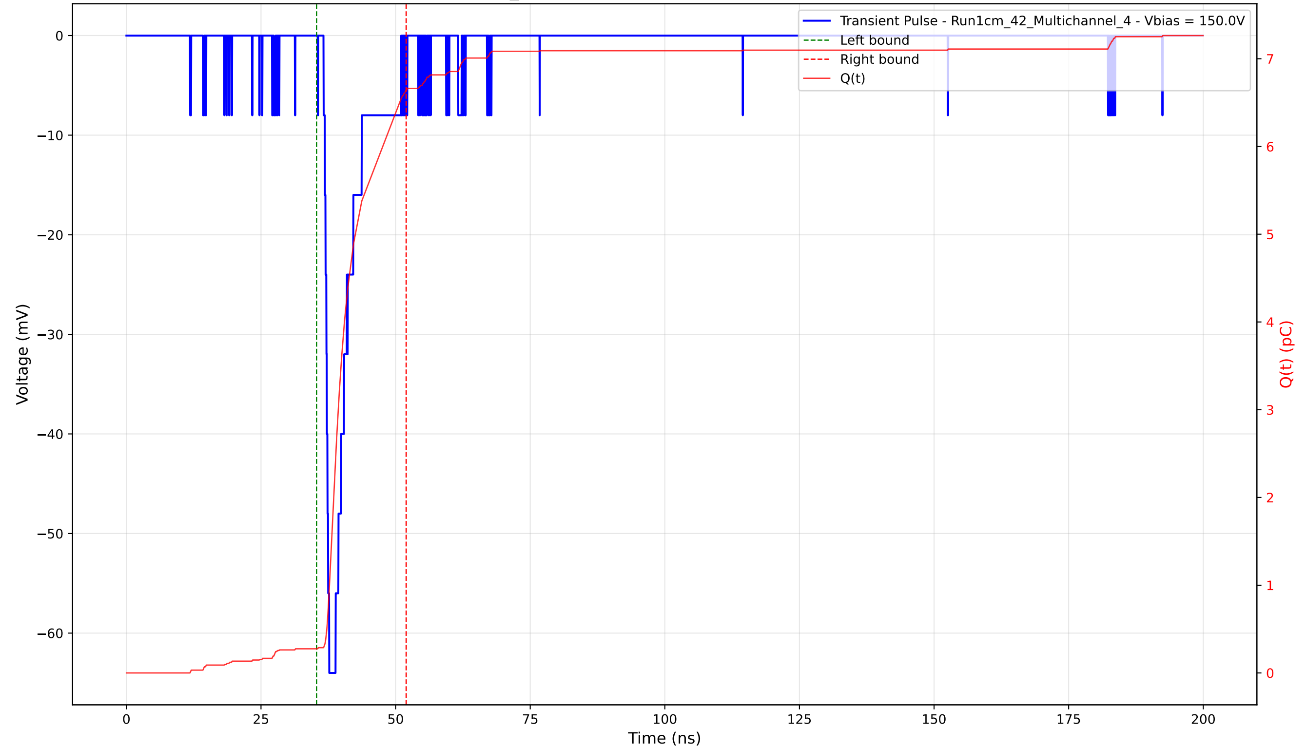
Transient Pulse - Sample: 1cm_42 - Position: 1485.0 \mu\text{m} - Charge: 6.36 pC - Rise Time: 1.05 ns
