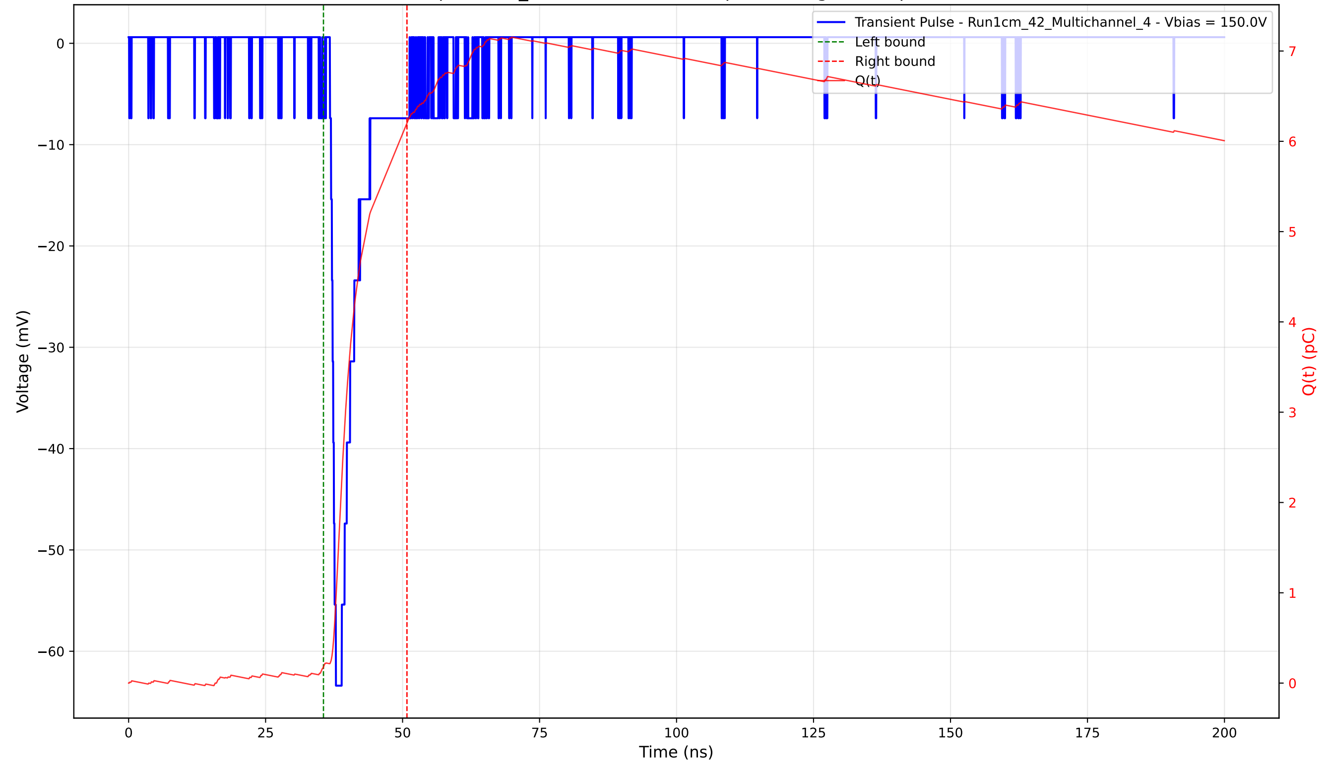
Transient Pulse - Sample: 1cm_42 - Position: 1460.0 \mu\text{m} - Charge: 6.02 pC - Rise Time: 1.09 ns
