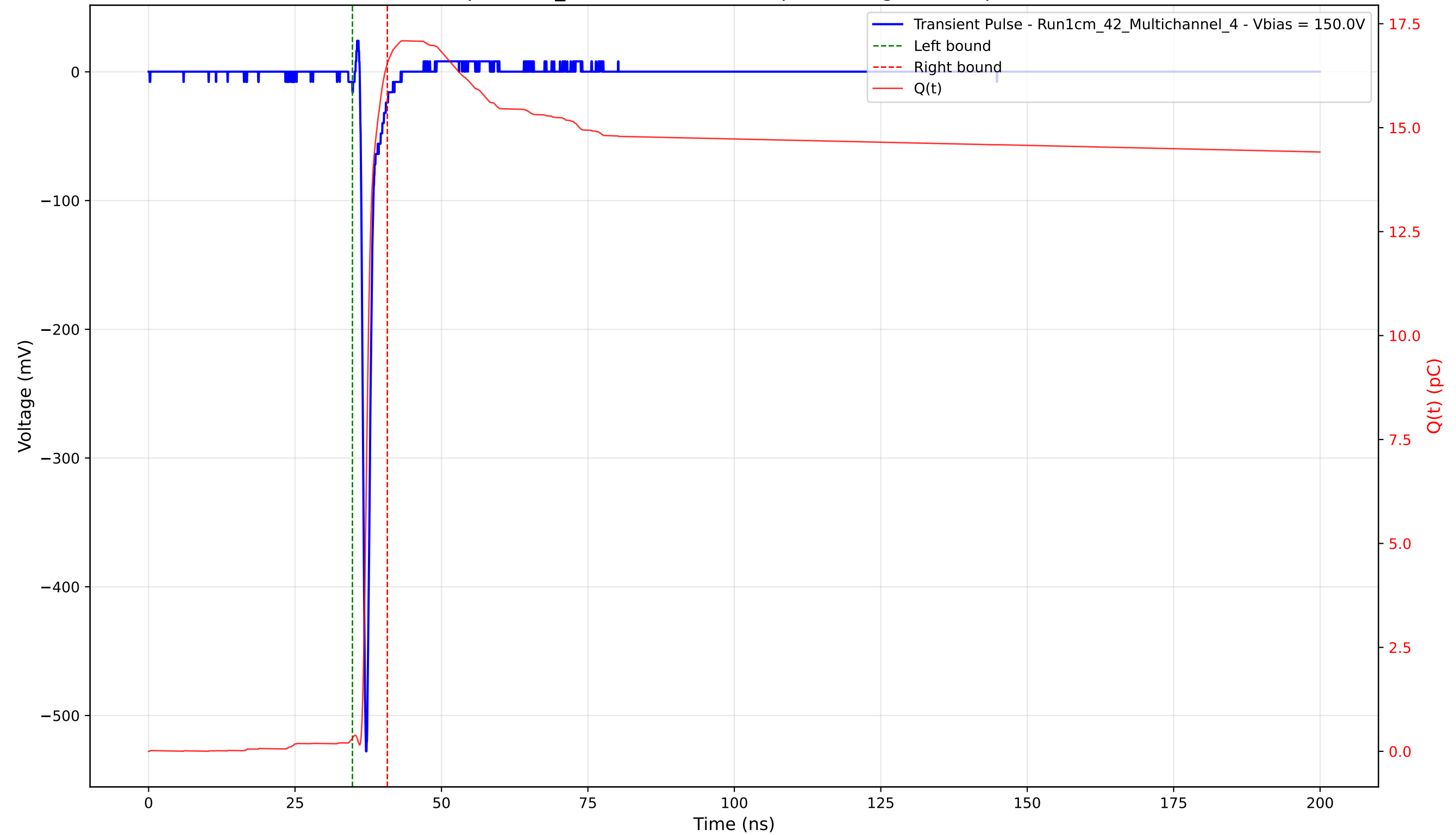
Transient Pulse - Sample: 1cm_42 - Position: 2605.0 \mu\text{m} - Charge: 16.23 pC - Rise Time: 0.72 ns
