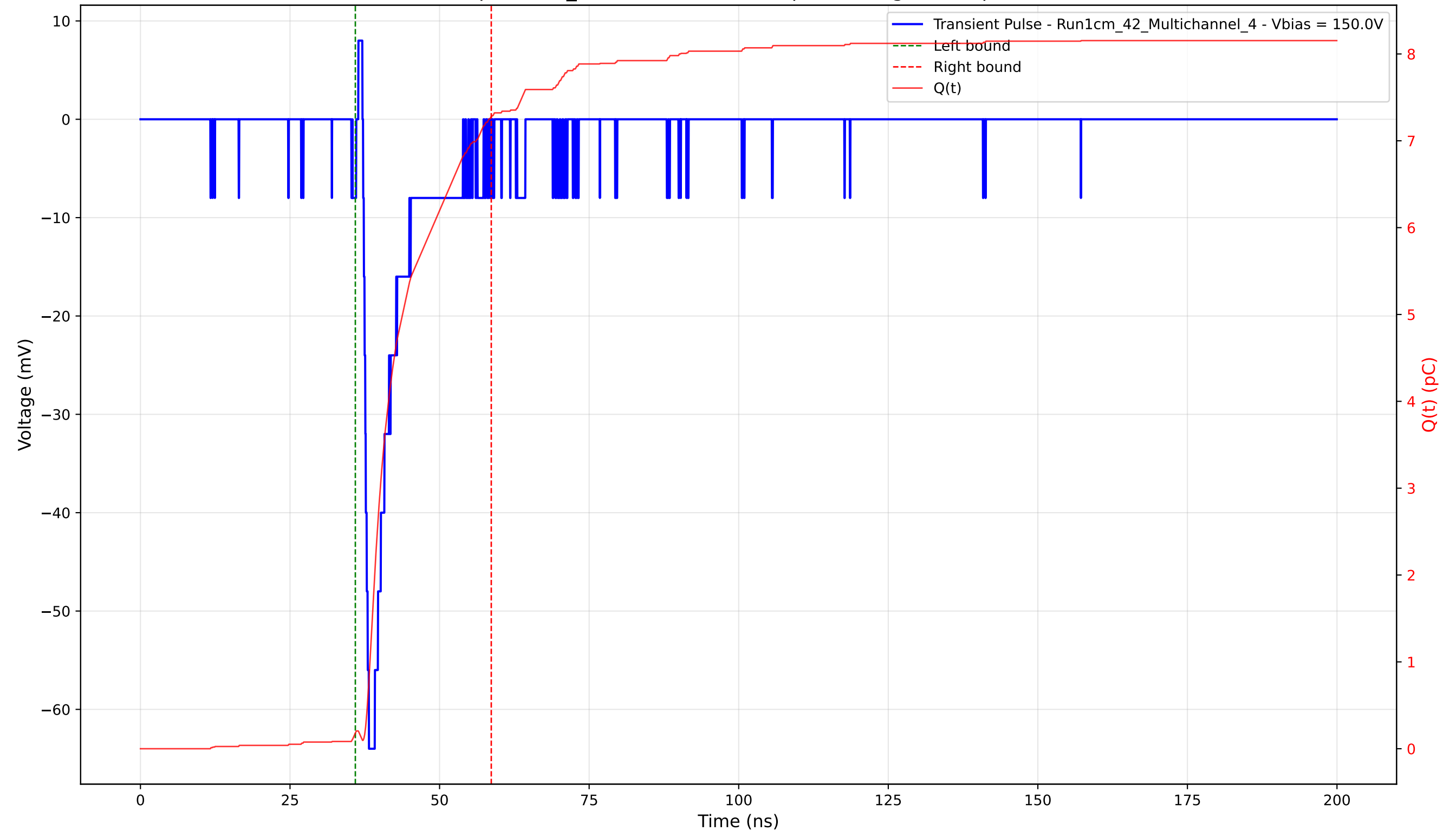
Transient Pulse - Sample: 1cm_42 - Position: 1265.0 \mu\text{m} - Charge: 7.09 pC - Rise Time: 0.97 ns
