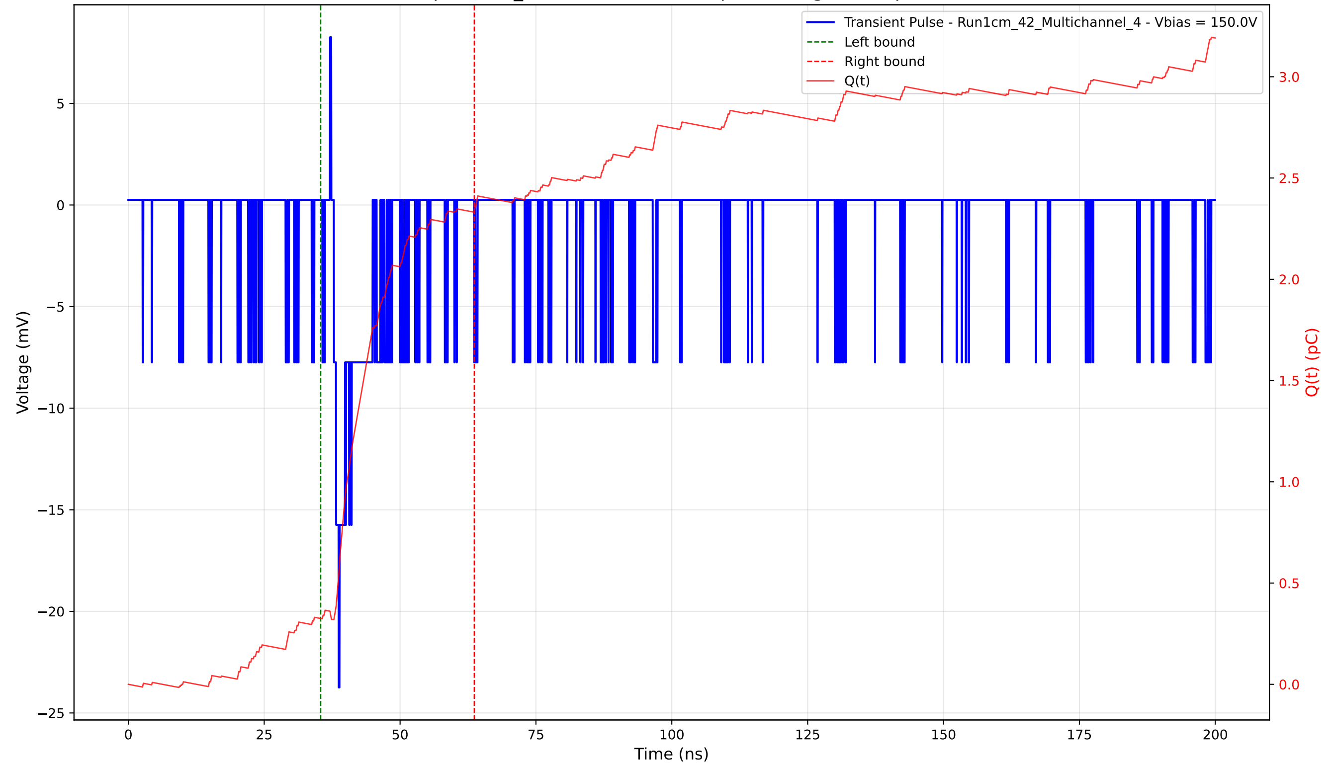
Transient Pulse - Sample: 1cm_42 - Position: 5005.0 \mu\text{m} - Charge: 2.01 pC - Rise Time: 0.91 ns
