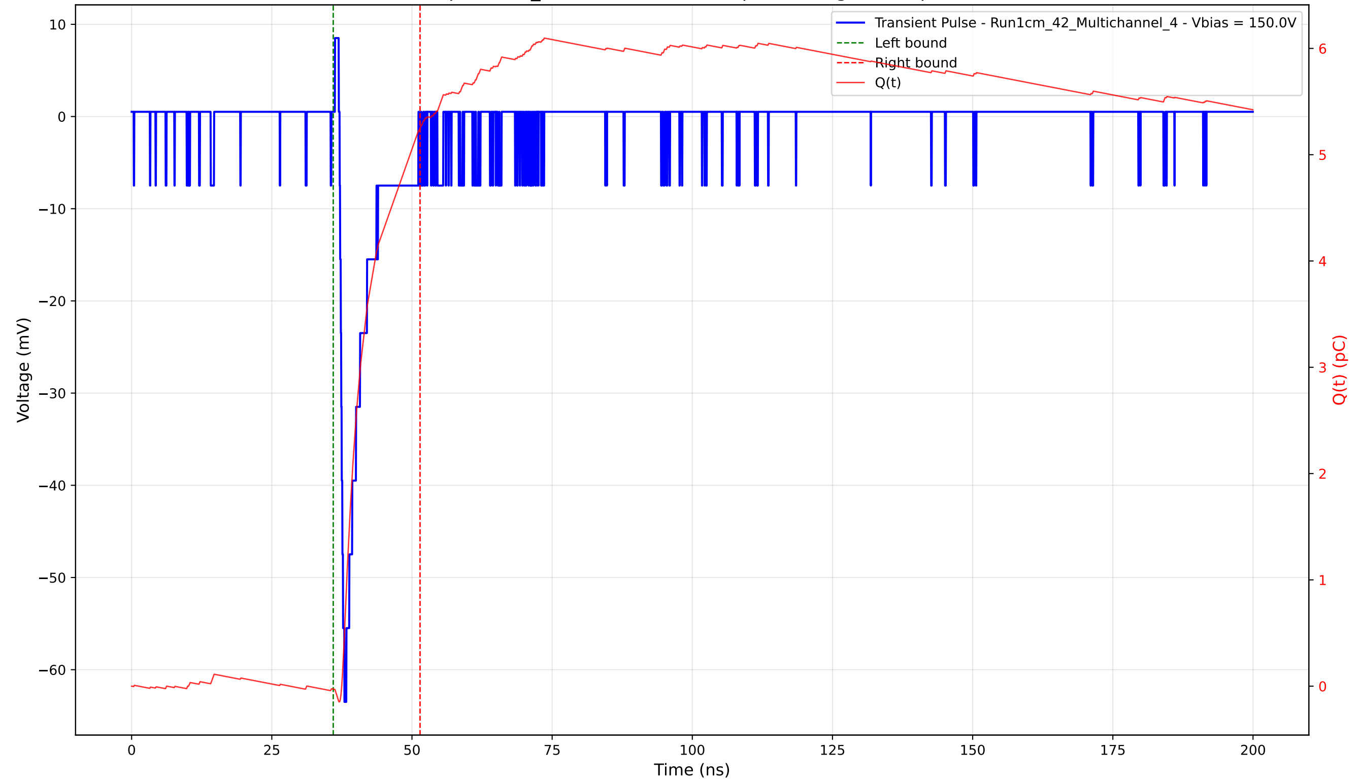
Transient Pulse - Sample: 1cm_42 - Position: 3615.0 \mu\text{m} - Charge: 5.28 pC - Rise Time: 0.85 ns
