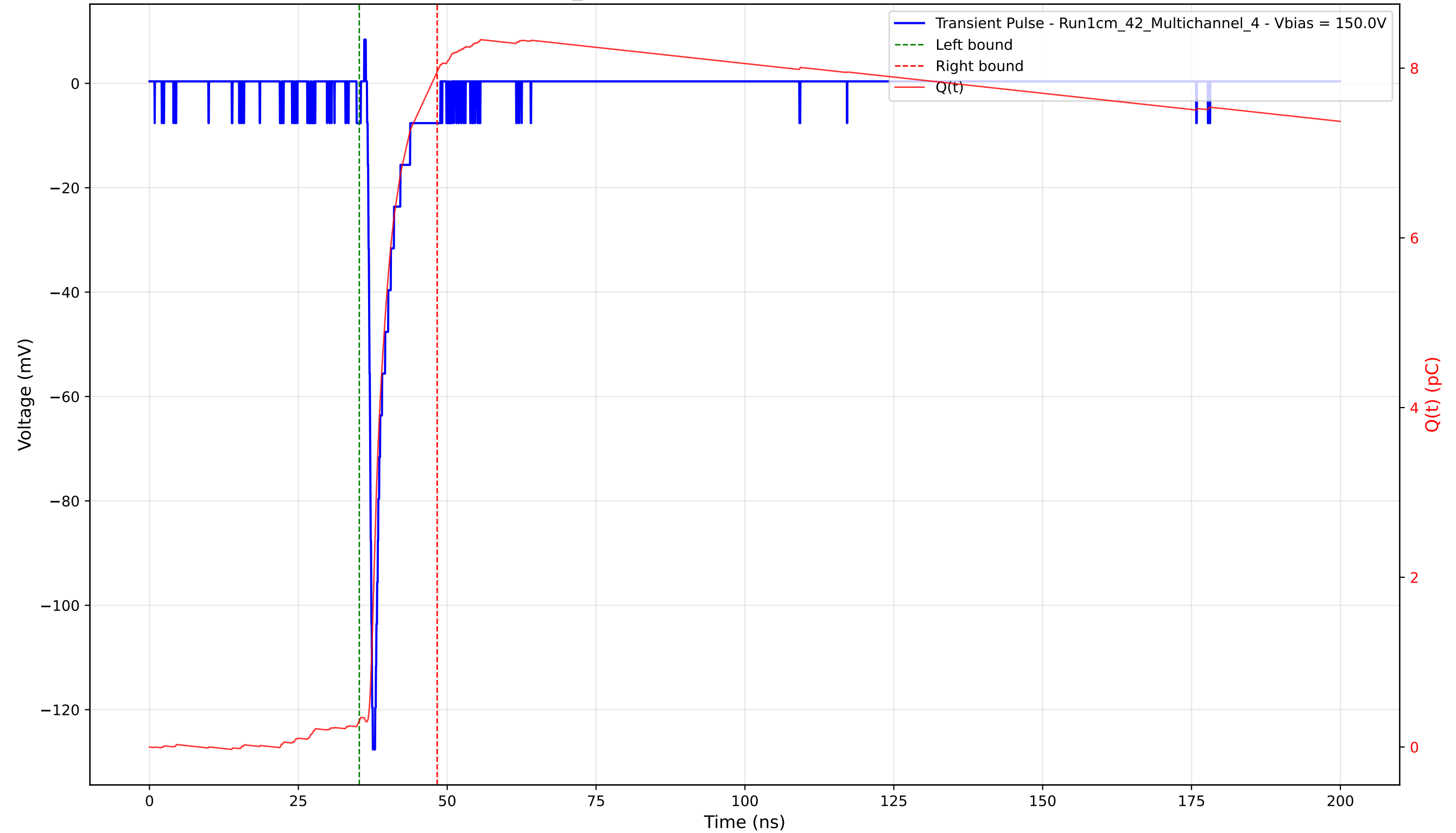
Transient Pulse - Sample: 1cm_42 - Position: 3330.0 \mu\text{m} - Charge: 7.65 pC - Rise Time: 0.73 ns
