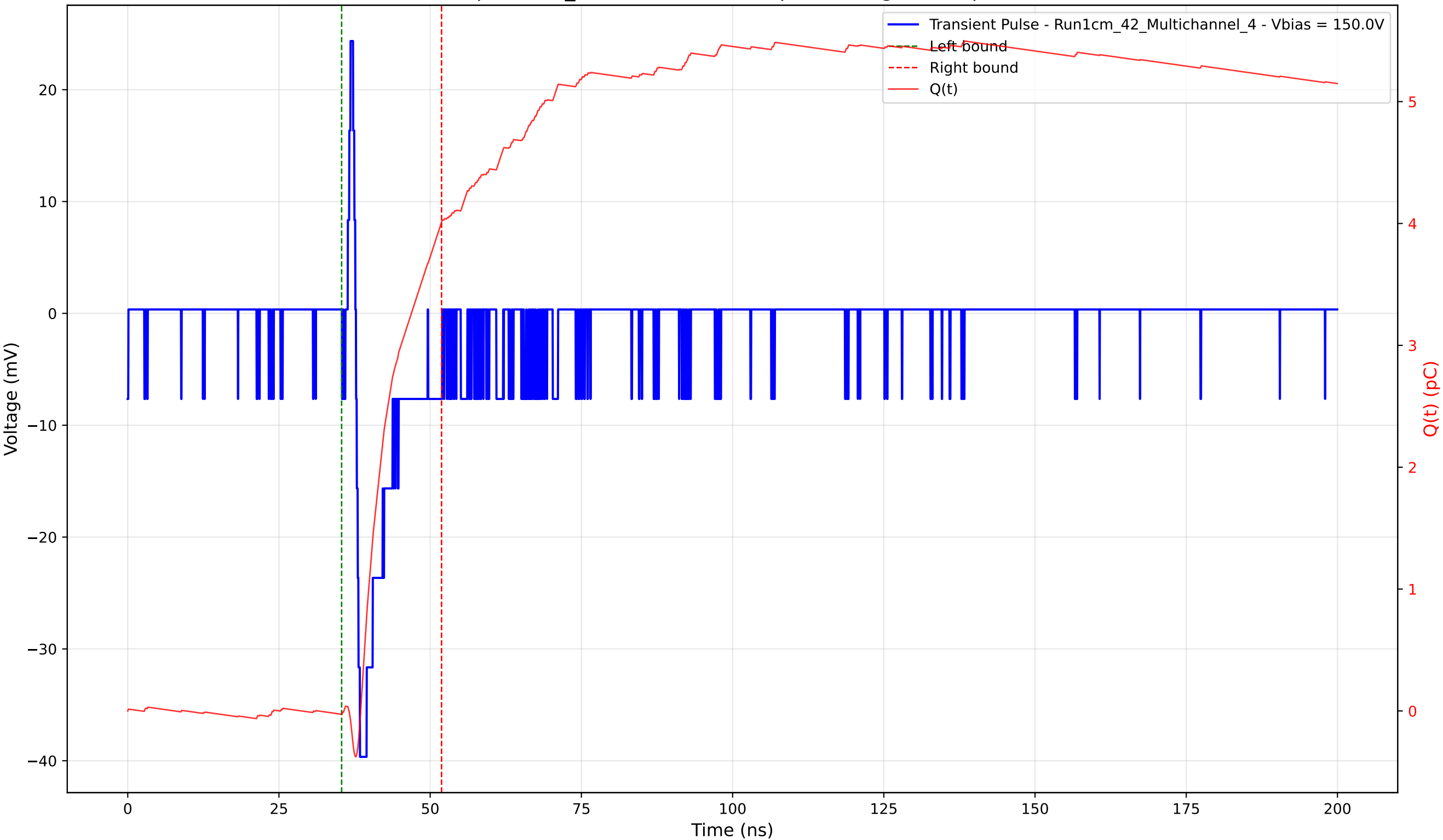
Transient Pulse - Sample: 1cm_42 - Position: 620.0 \mu\text{m} - Charge: 4.04 pC - Rise Time: 0.66 ns
