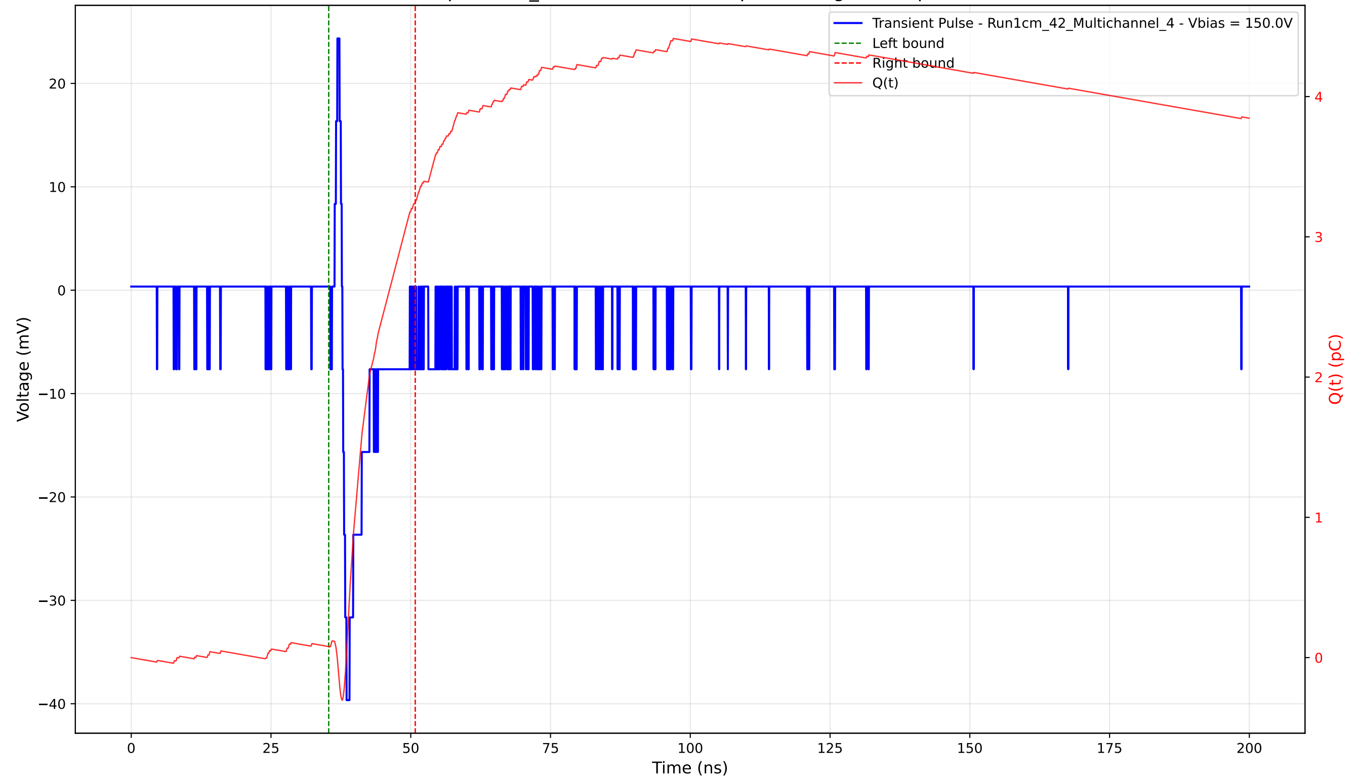
Transient Pulse - Sample: 1cm_42 - Position: 4380.0 \mu\text{m} - Charge: 3.17 pC - Rise Time: 0.74 ns
