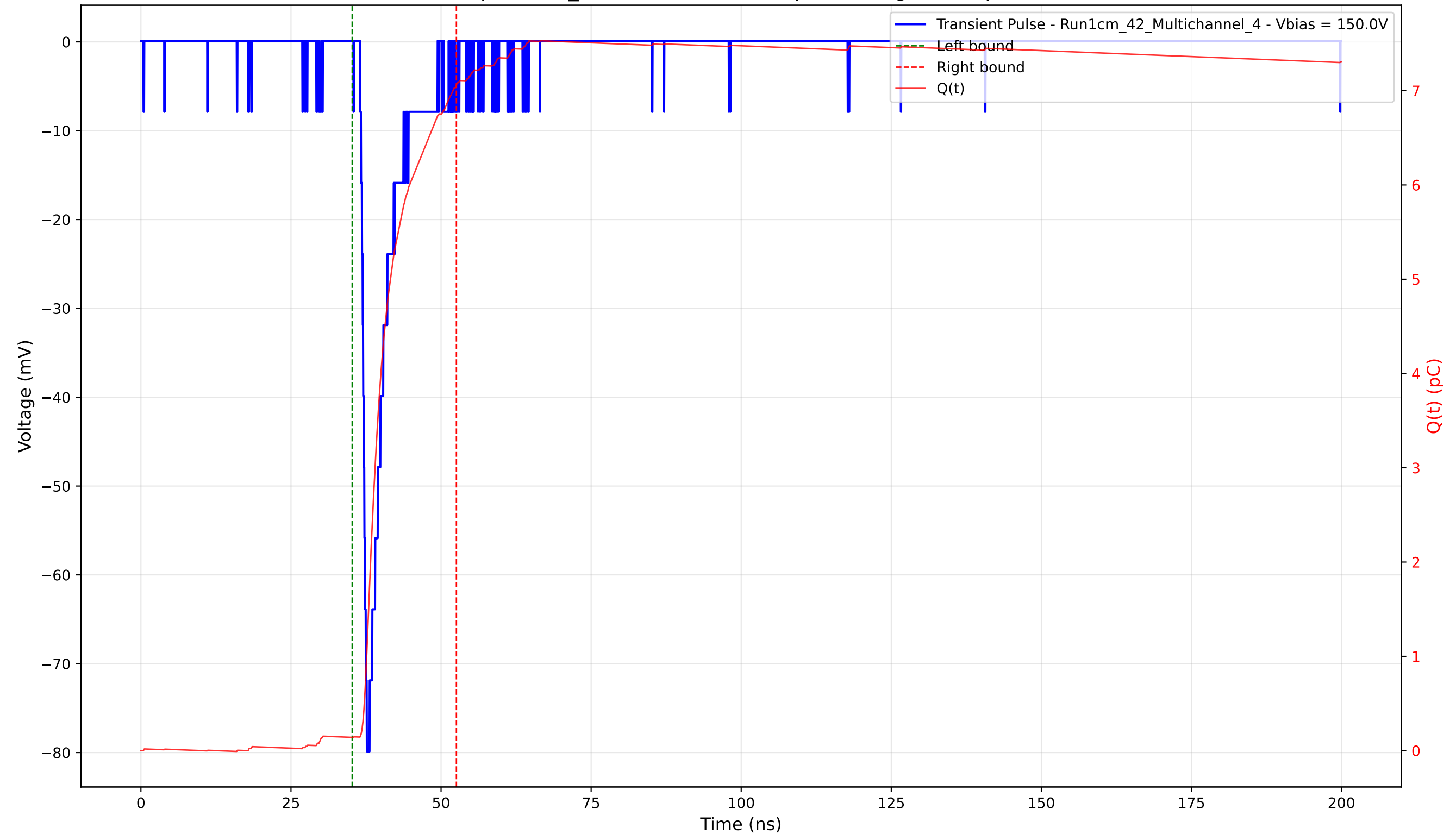
Transient Pulse - Sample: 1cm_42 - Position: 1545.0 \mu\text{m} - Charge: 6.92 pC - Rise Time: 1.00 ns
