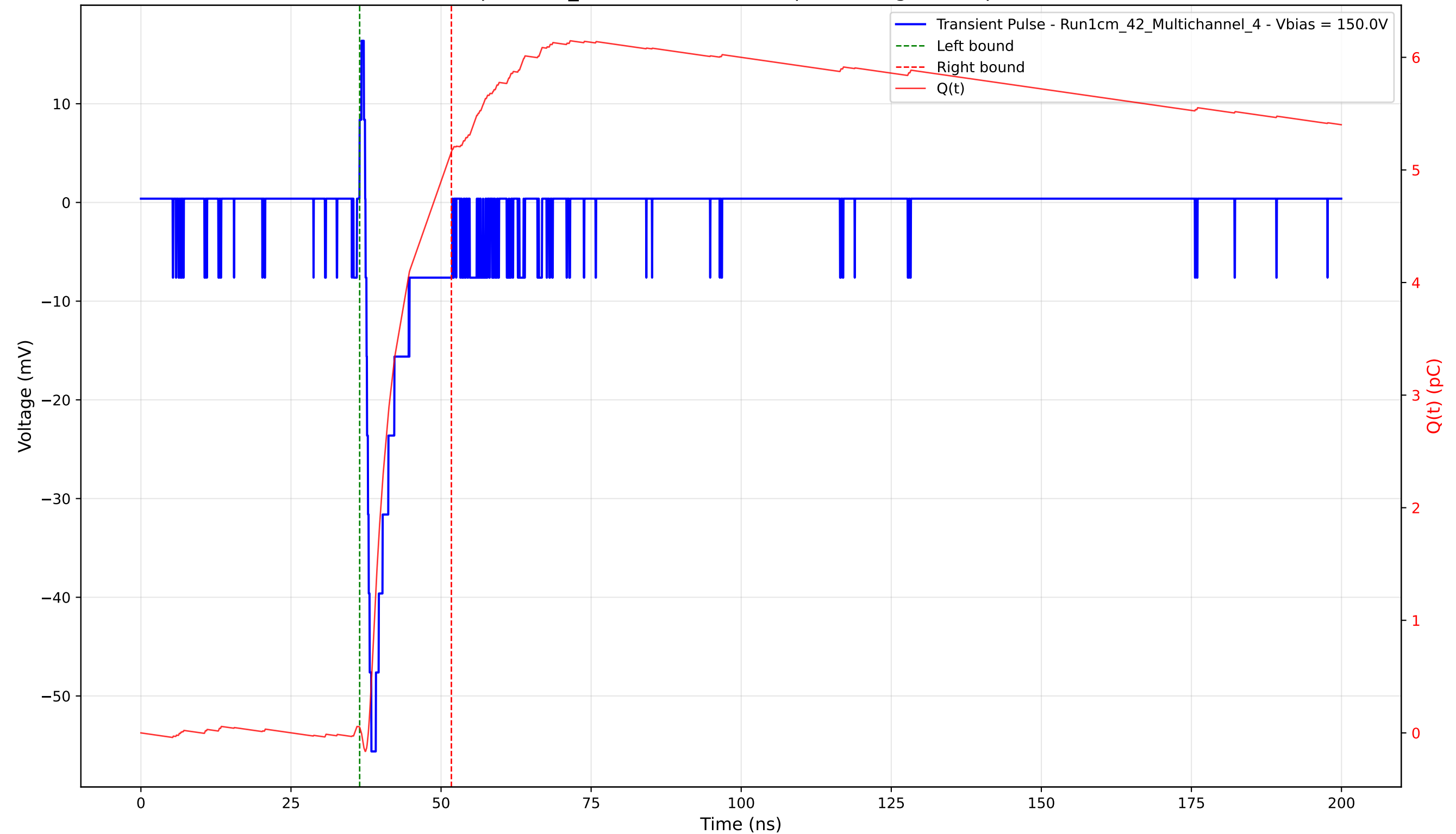
Transient Pulse - Sample: 1cm_42 - Position: 1100.0 \mu\text{m} - Charge: 5.11 pC - Rise Time: 0.97 ns
