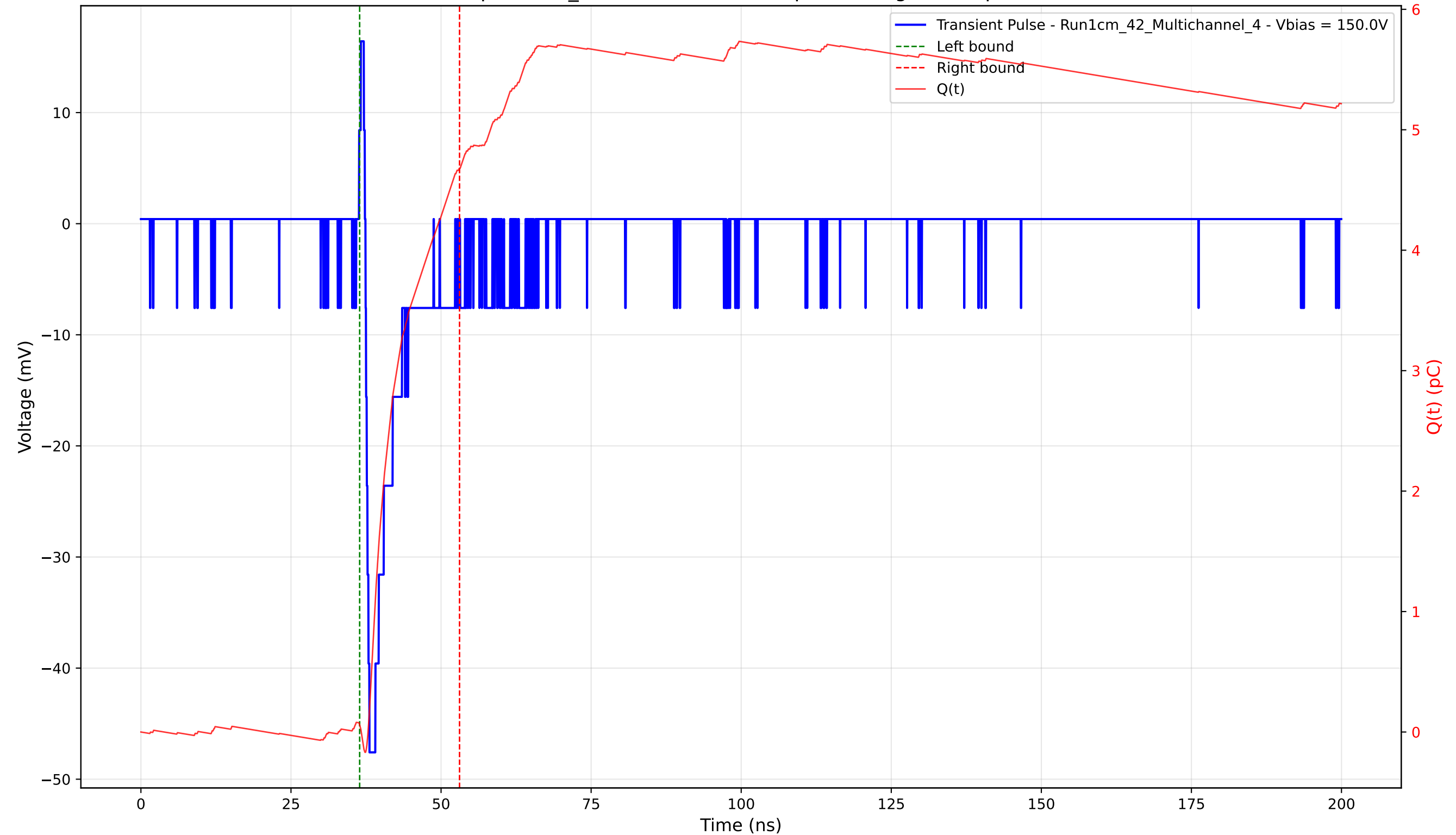
Transient Pulse - Sample: 1cm_42 - Position: 3895.0 \mu\text{m} - Charge: 4.62 pC - Rise Time: 0.66 ns
