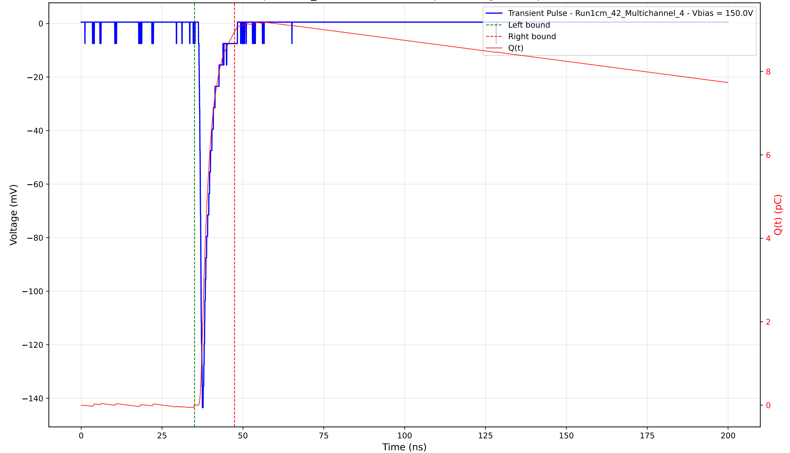
Transient Pulse - Sample: 1cm_42 - Position: 1725.0 \mu\text{m} - Charge: 8.97 pC - Rise Time: 0.97 ns
