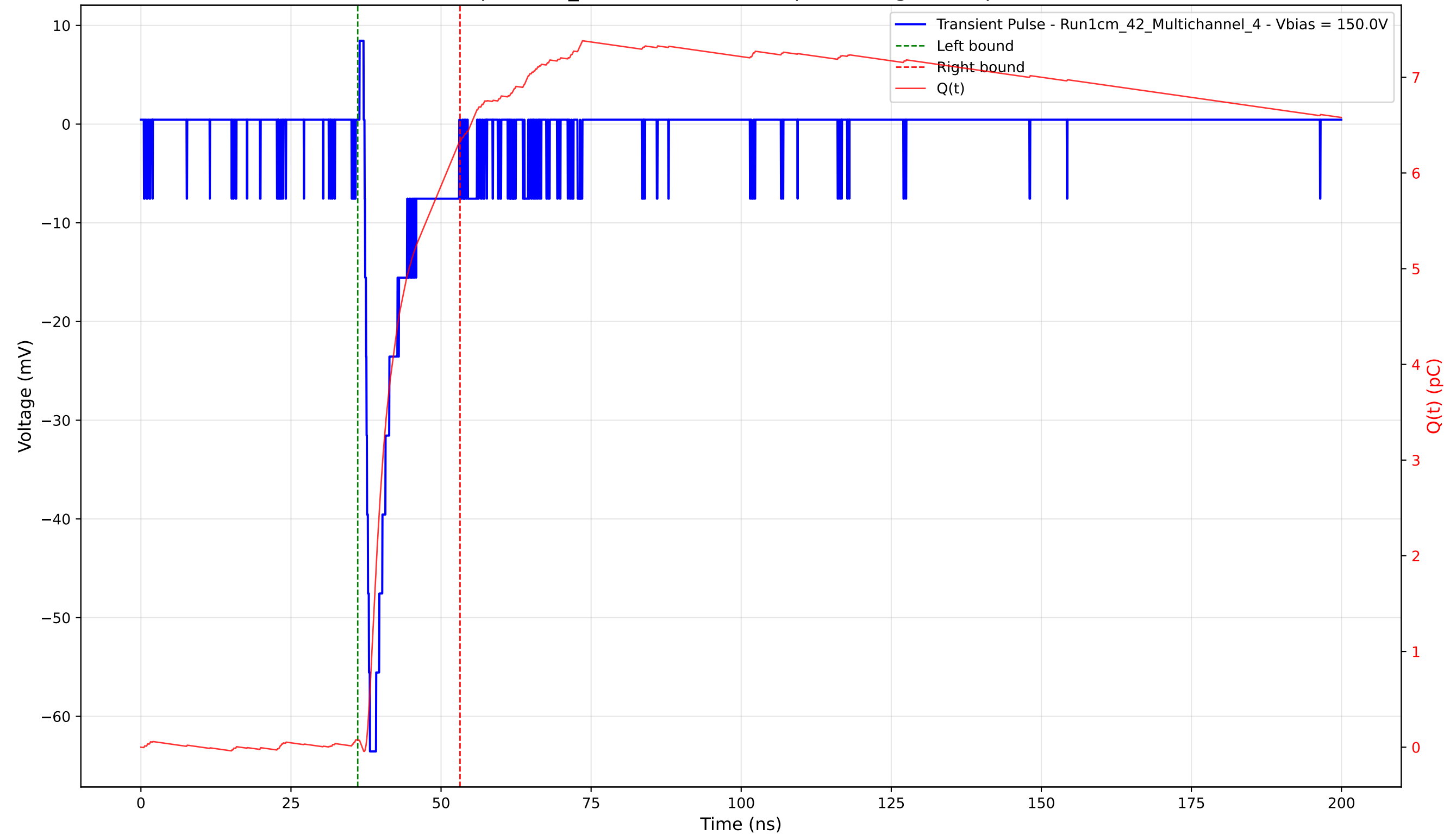
Transient Pulse - Sample: 1cm_42 - Position: 1235.0 \mu\text{m} - Charge: 6.25 pC - Rise Time: 0.89 ns
