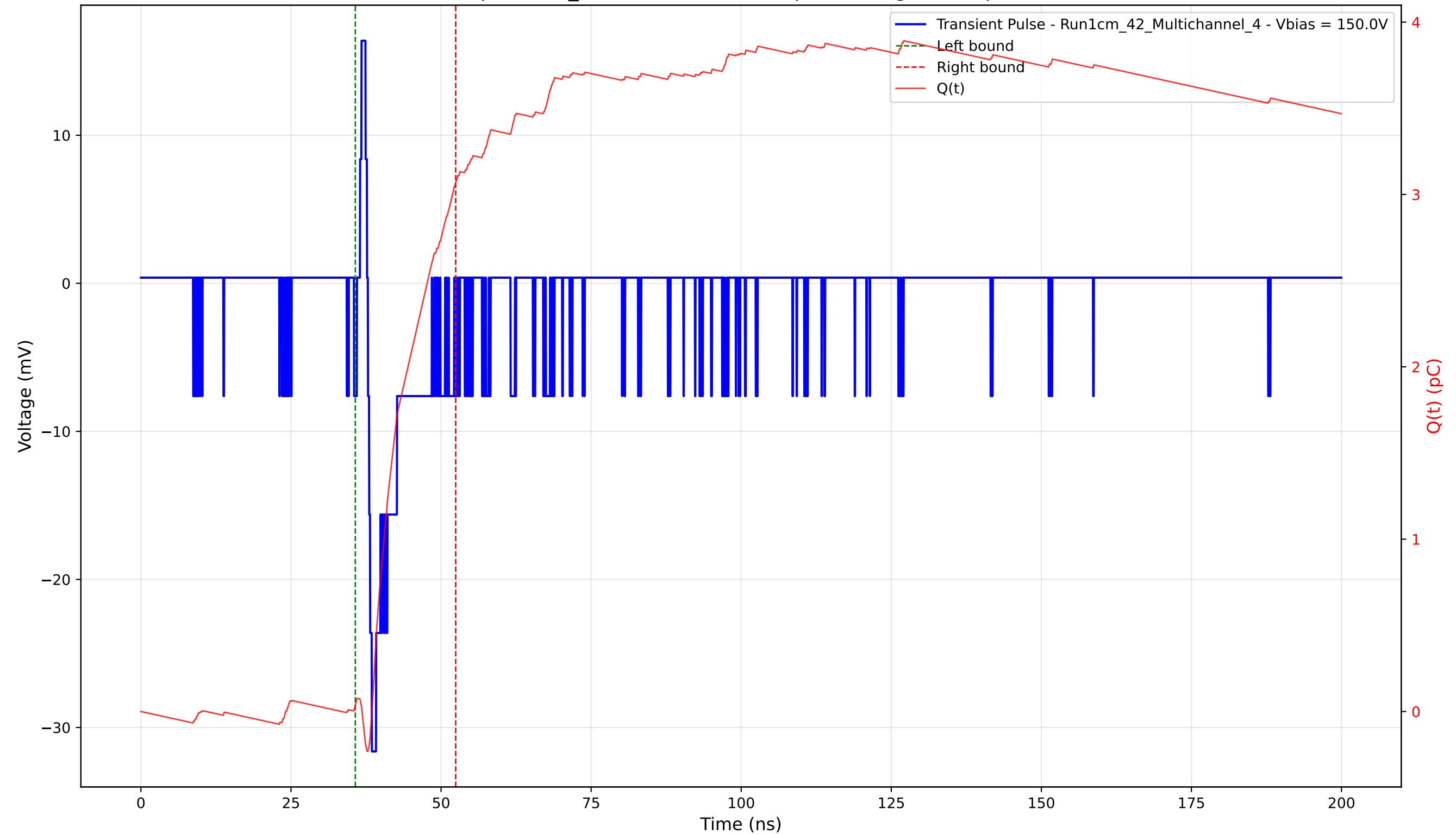
Transient Pulse - Sample: 1cm_42 - Position: 4520.0 \mu\text{m} - Charge: 3.03 pC - Rise Time: 0.66 ns
