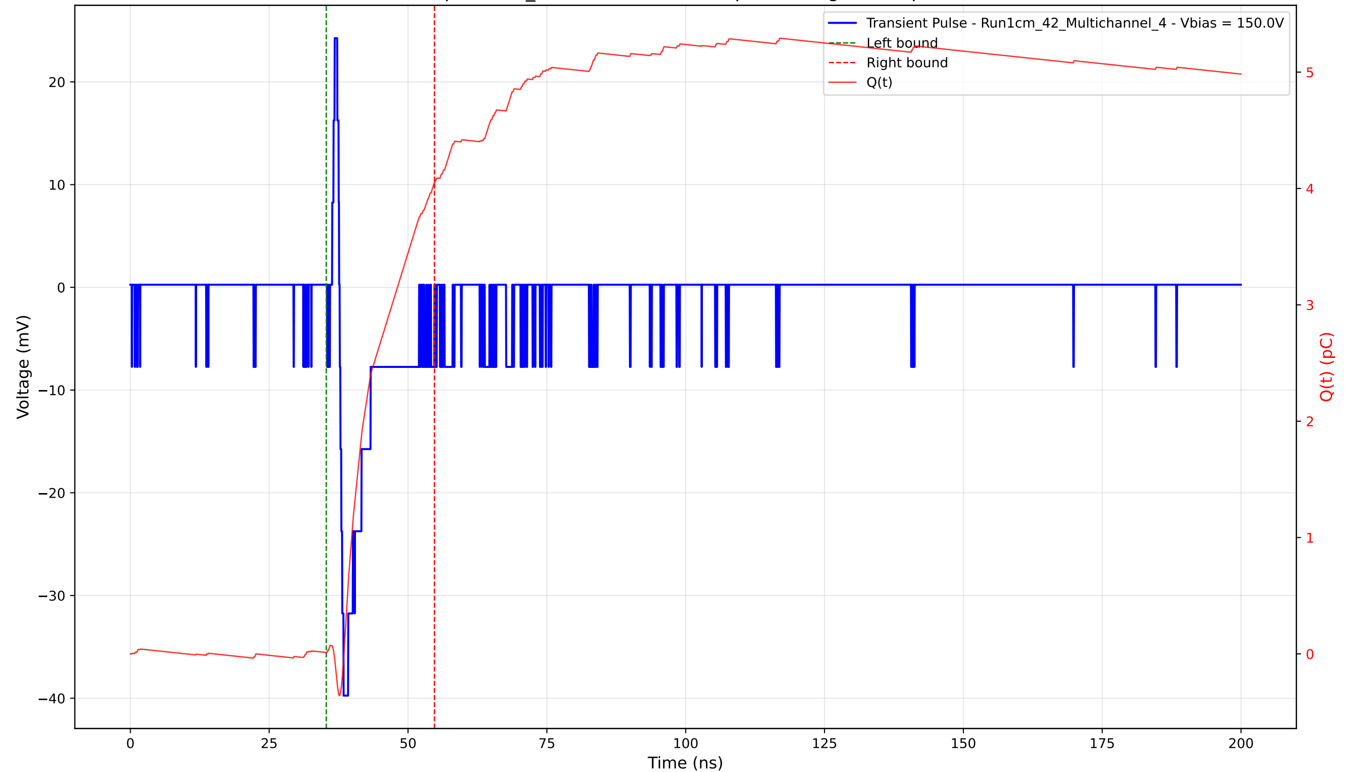
Transient Pulse - Sample: 1cm_42 - Position: 4200.0 \mu\text{m} - Charge: 4.04 pC - Rise Time: 0.70 ns
