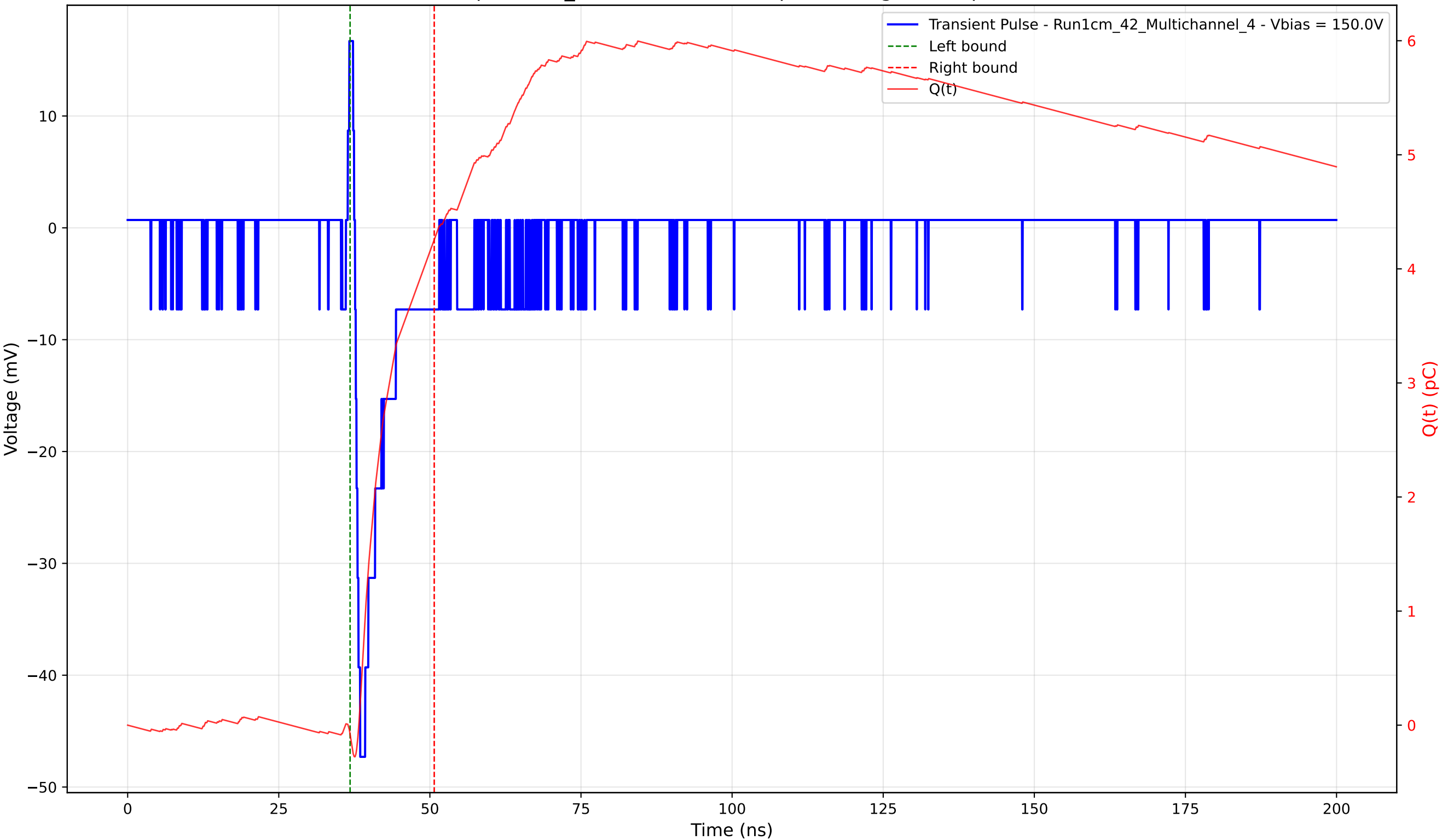
Transient Pulse - Sample: 1cm_42 - Position: 960.0 \mu\text{m} - Charge: 4.34 pC - Rise Time: 0.86 ns
