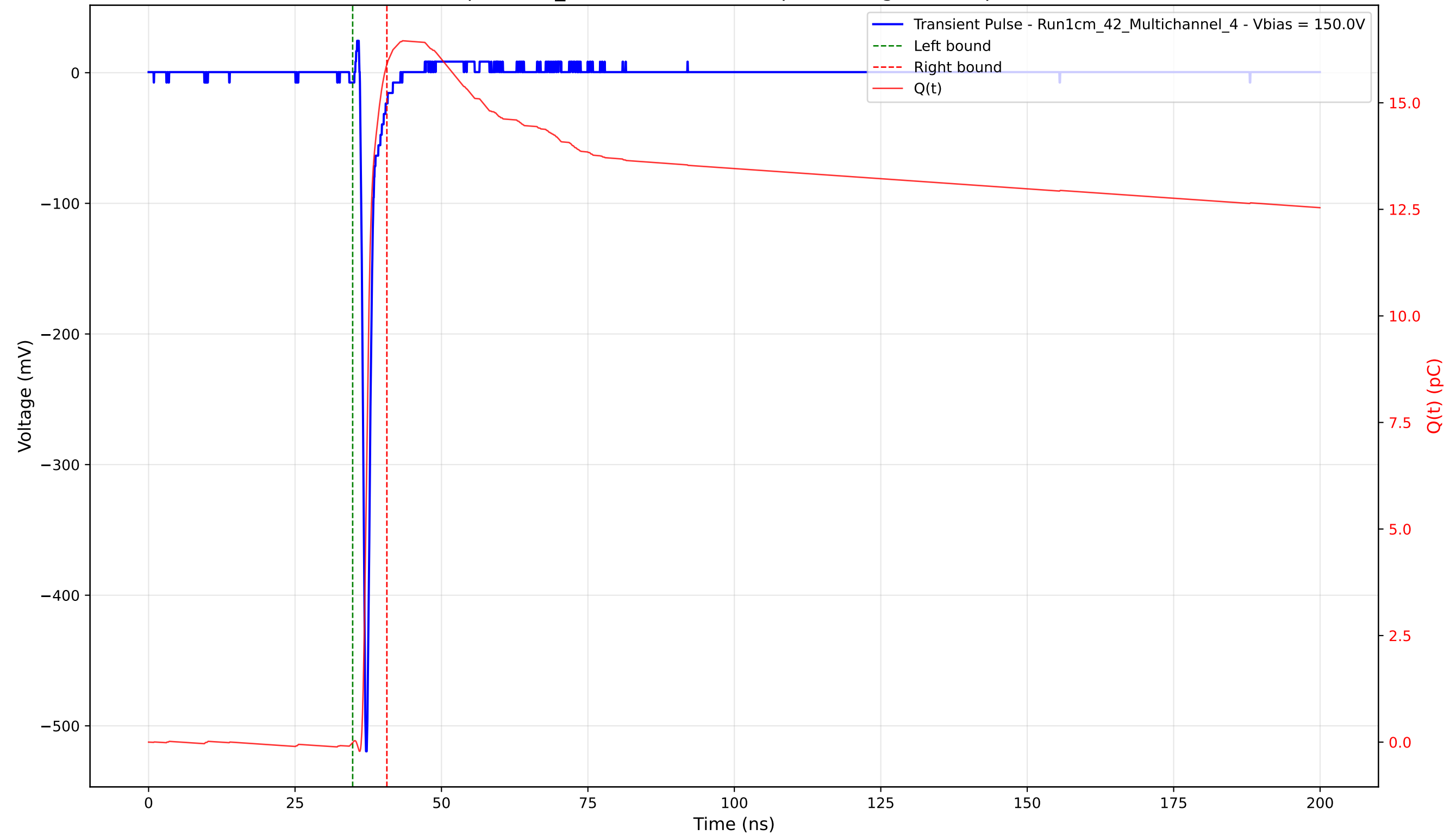
Transient Pulse - Sample: 1cm_42 - Position: 2625.0 \mu\text{m} - Charge: 15.91 pC - Rise Time: 0.72 ns
