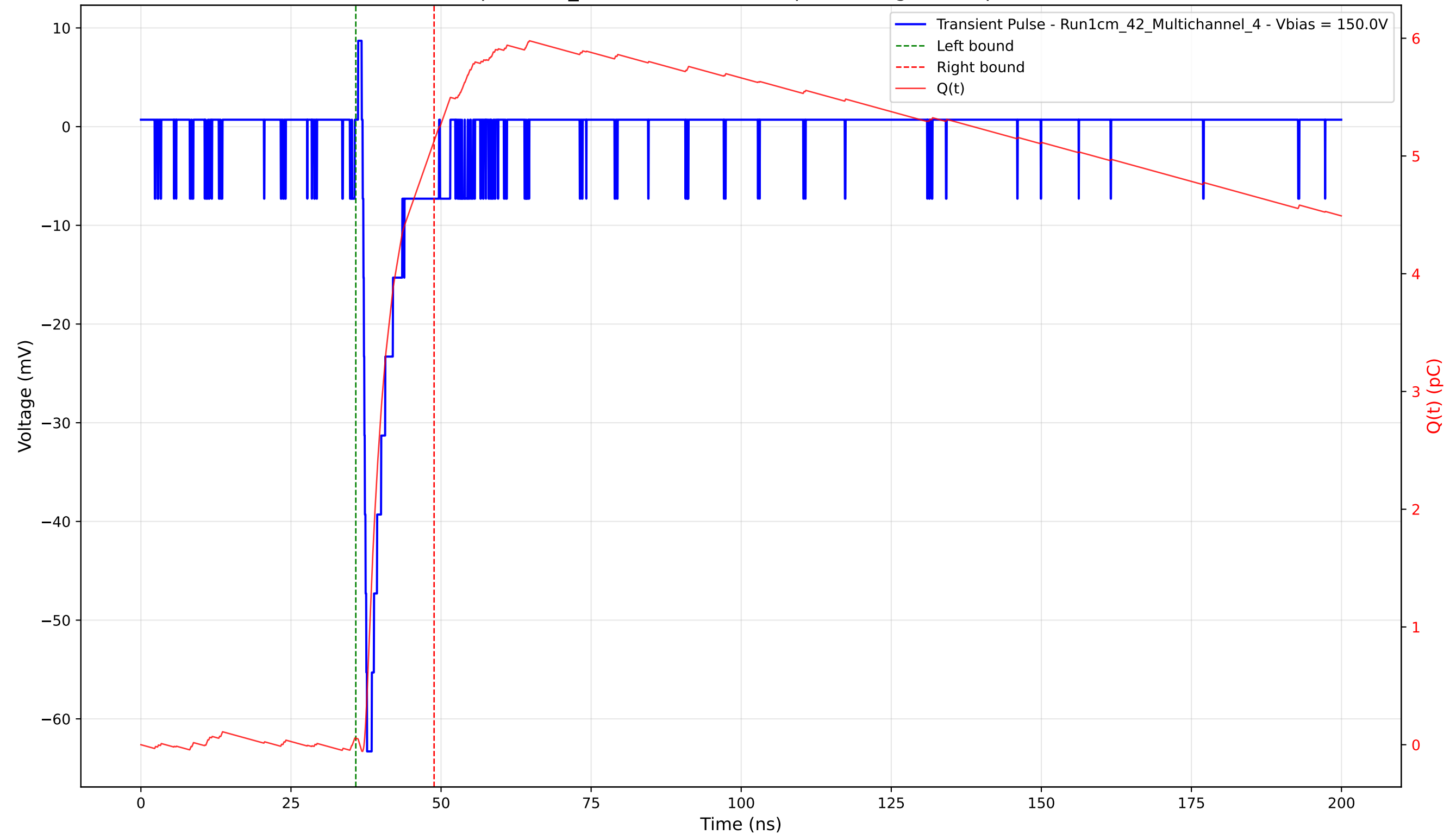
Transient Pulse - Sample: 1cm_42 - Position: 3555.0 \mu\text{m} - Charge: 5.07 pC - Rise Time: 0.73 ns
