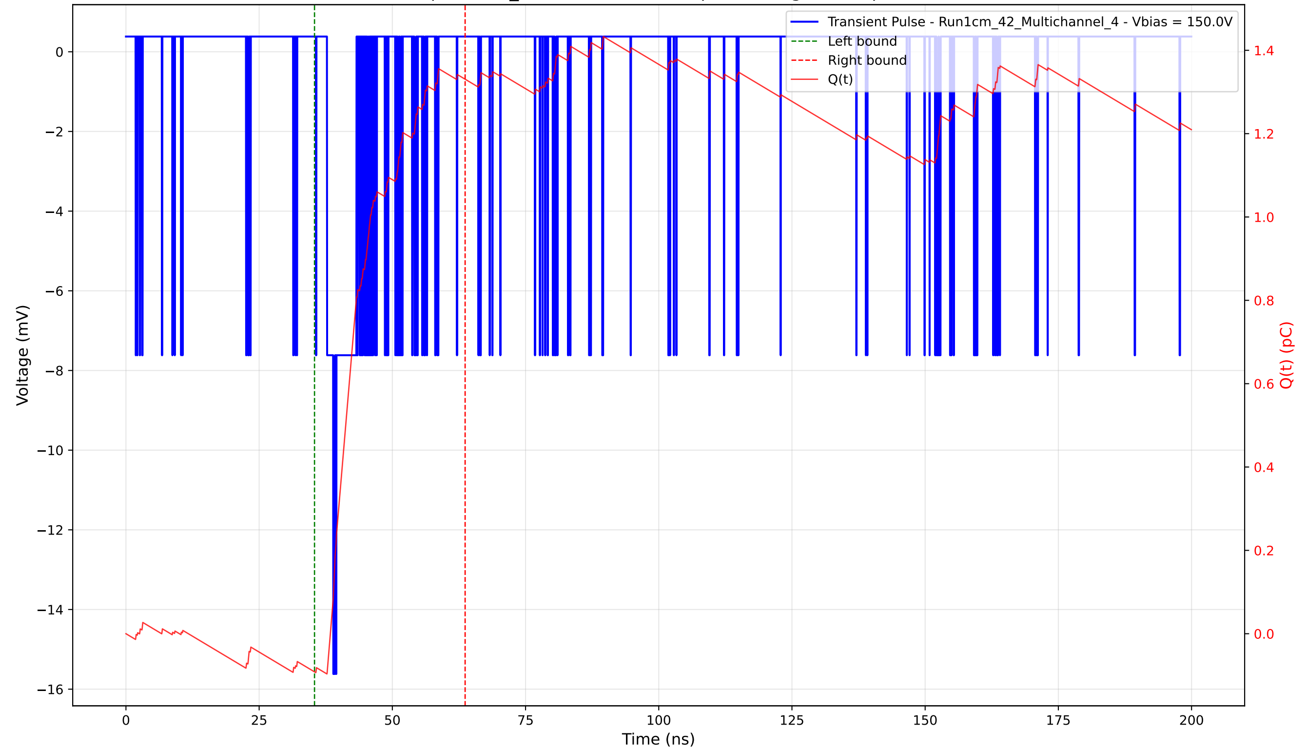
Transient Pulse - Sample: 1cm_42 - Position: 115.0 \mu\text{m} - Charge: 1.42 pC - Rise Time: 1.19 ns
