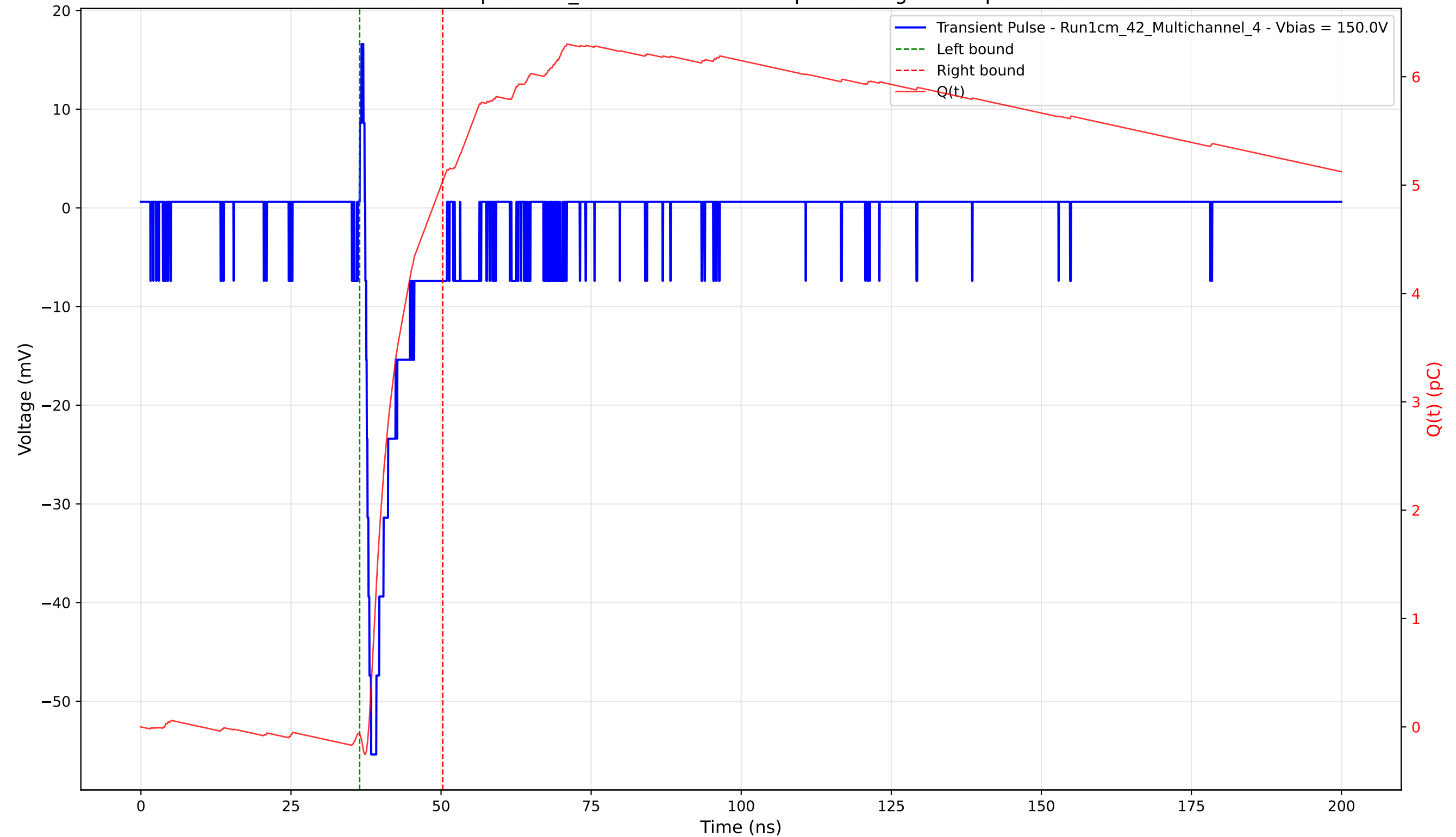
Transient Pulse - Sample: 1cm_42 - Position: 1120.0 \mu\text{m} - Charge: 5.10 pC - Rise Time: 0.97 ns
