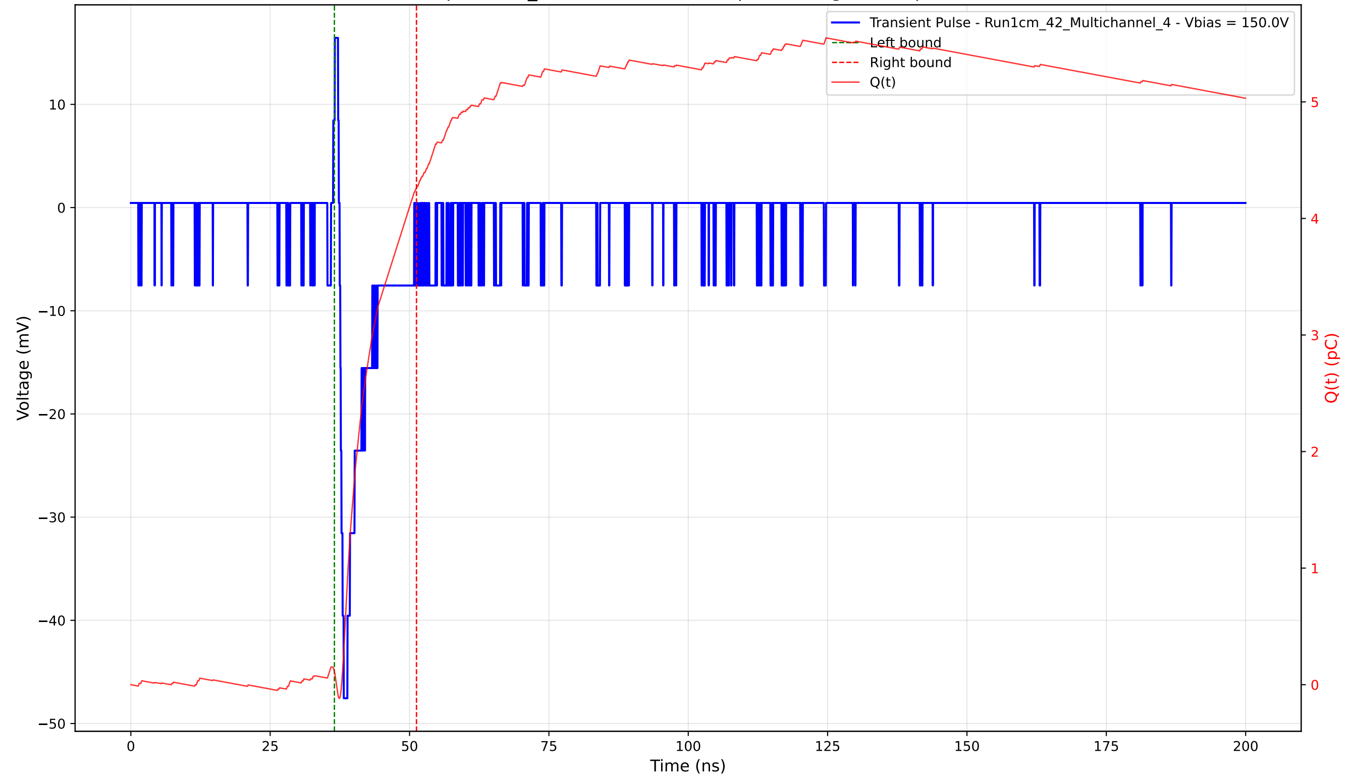
Transient Pulse - Sample: 1cm_42 - Position: 3950.0 \mu\text{m} - Charge: 4.14 pC - Rise Time: 0.74 ns
