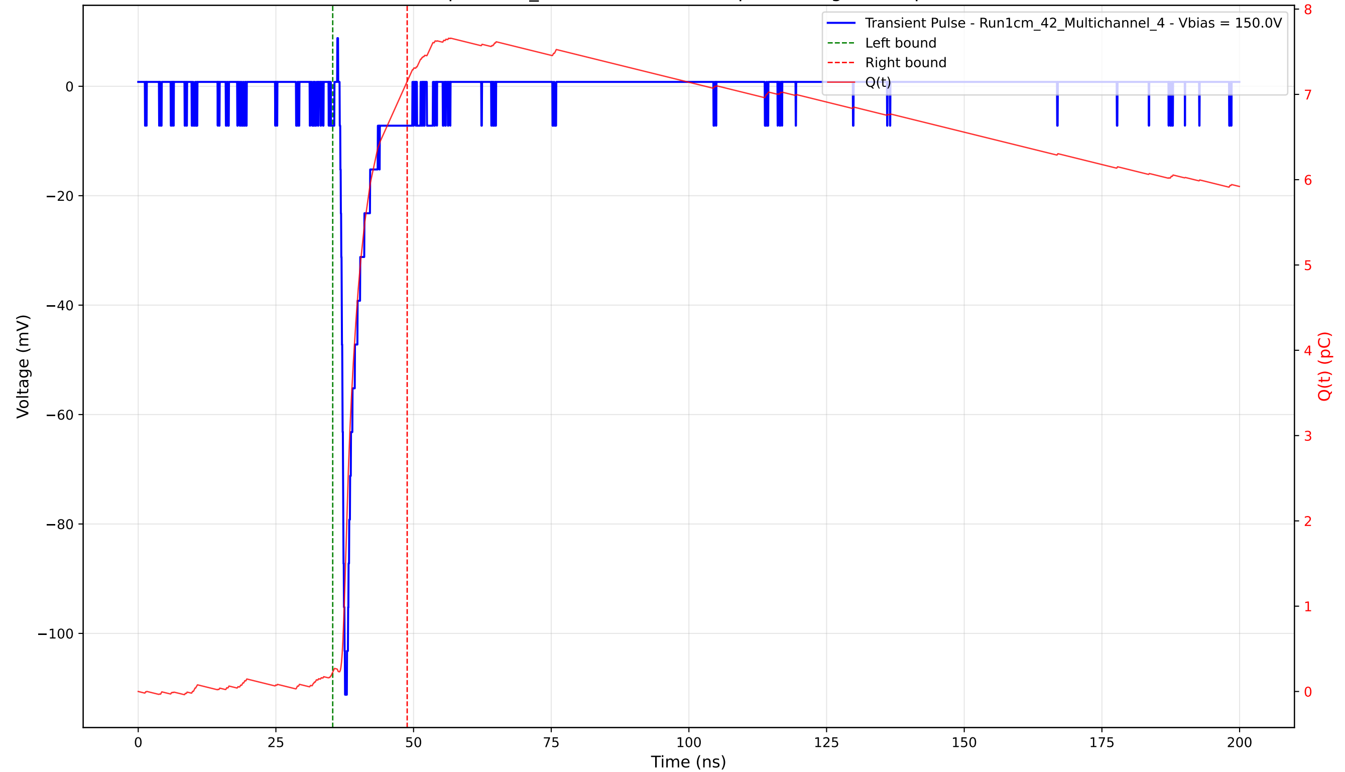
Transient Pulse - Sample: 1cm_42 - Position: 3380.0 \mu\text{m} - Charge: 6.93 pC - Rise Time: 0.78 ns
