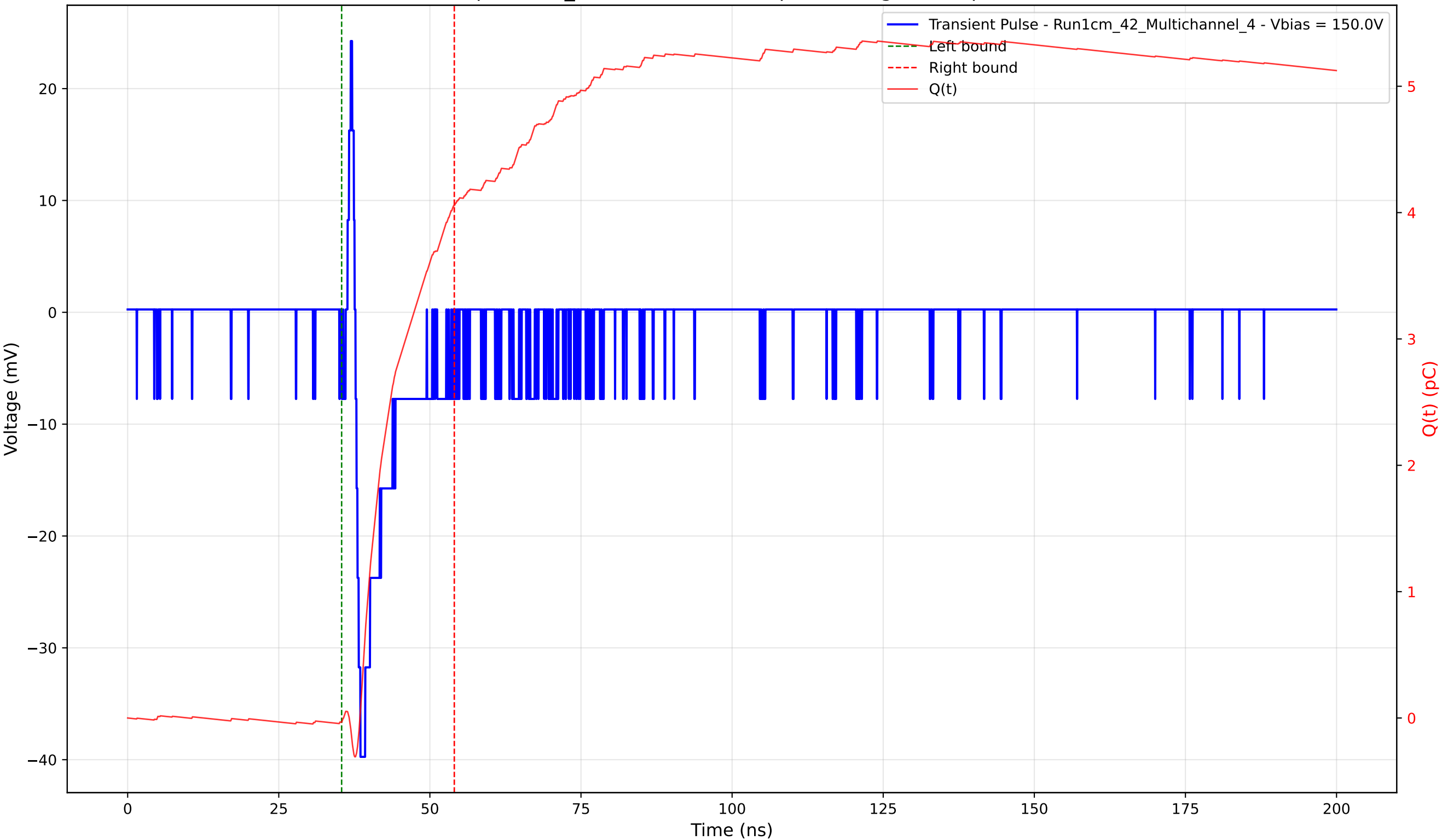
Transient Pulse - Sample: 1cm_42 - Position: 560.0 \mu\text{m} - Charge: 4.09 pC - Rise Time: 0.82 ns
