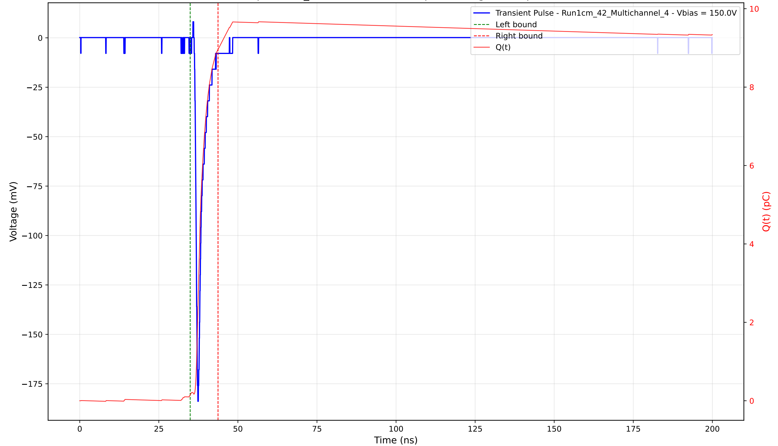
Transient Pulse - Sample: 1cm_42 - Position: 1925.0 \mu\text{m} - Charge: 8.81 pC - Rise Time: 0.79 ns
