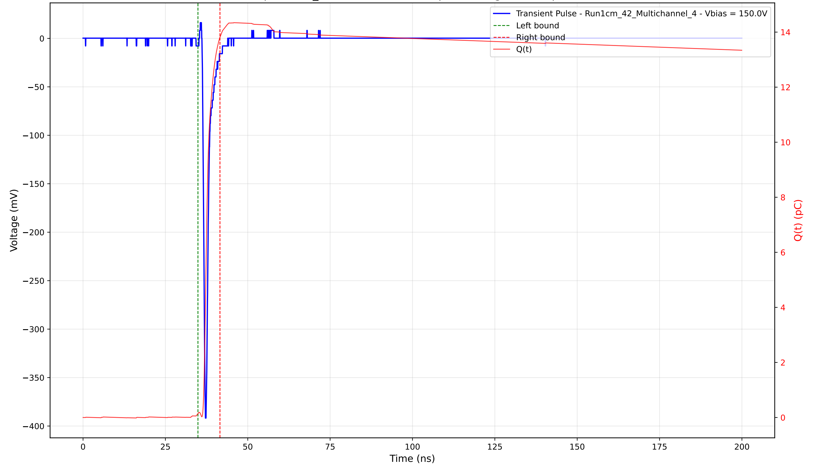
Transient Pulse - Sample: 1cm_42 - Position: 2155.0 \mu\text{m} - Charge: 13.67 pC - Rise Time: 0.71 ns
