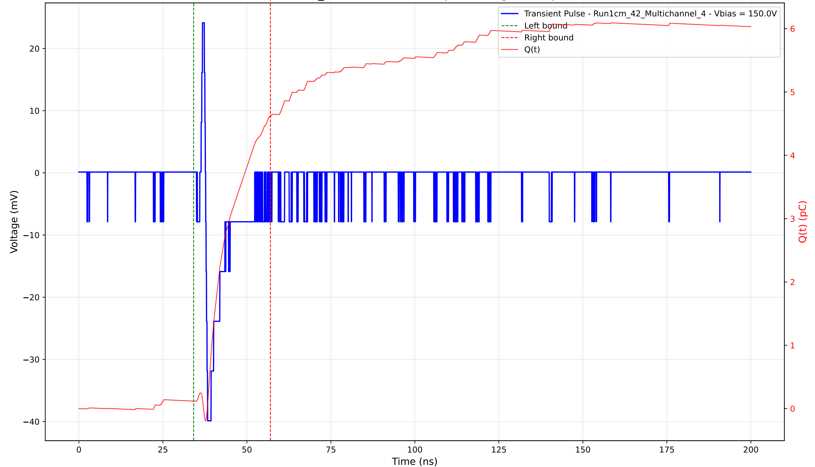
Transient Pulse - Sample: 1cm_42 - Position: 4280.0 \mu\text{m} - Charge: 4.50 pC - Rise Time: 0.58 ns
