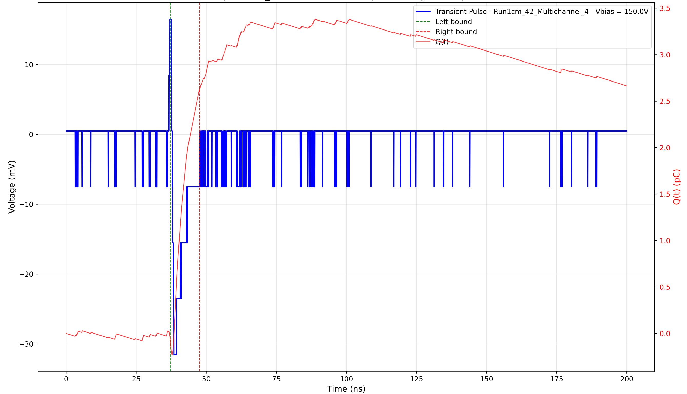
Transient Pulse - Sample: 1cm_42 - Position: 4710.0 \mu\text{m} - Charge: 2.71 pC - Rise Time: 0.62 ns
