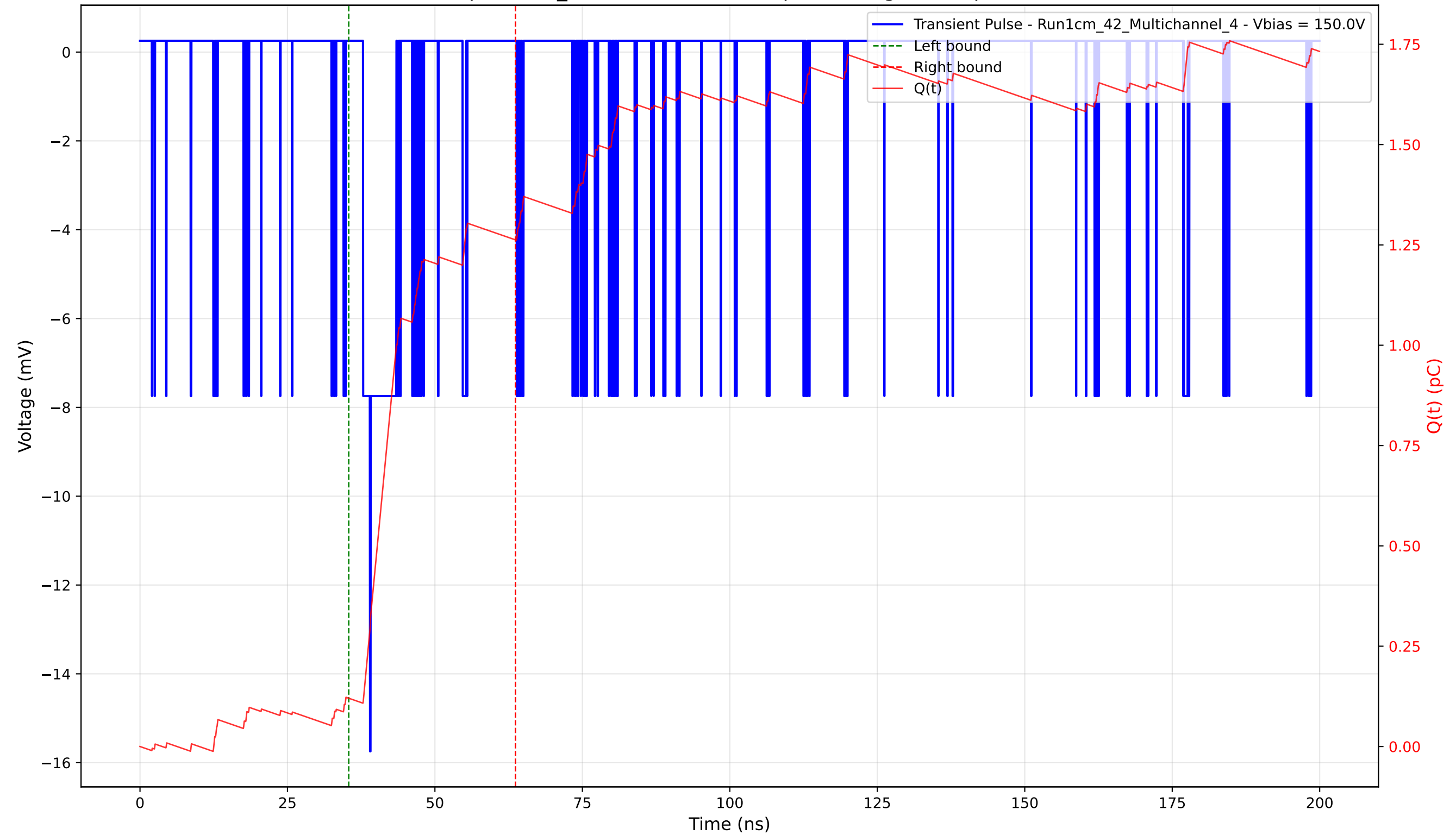
Transient Pulse - Sample: 1cm_42 - Position: 5095.0 \mu\text{m} - Charge: 1.14 pC - Rise Time: 1.19 ns
