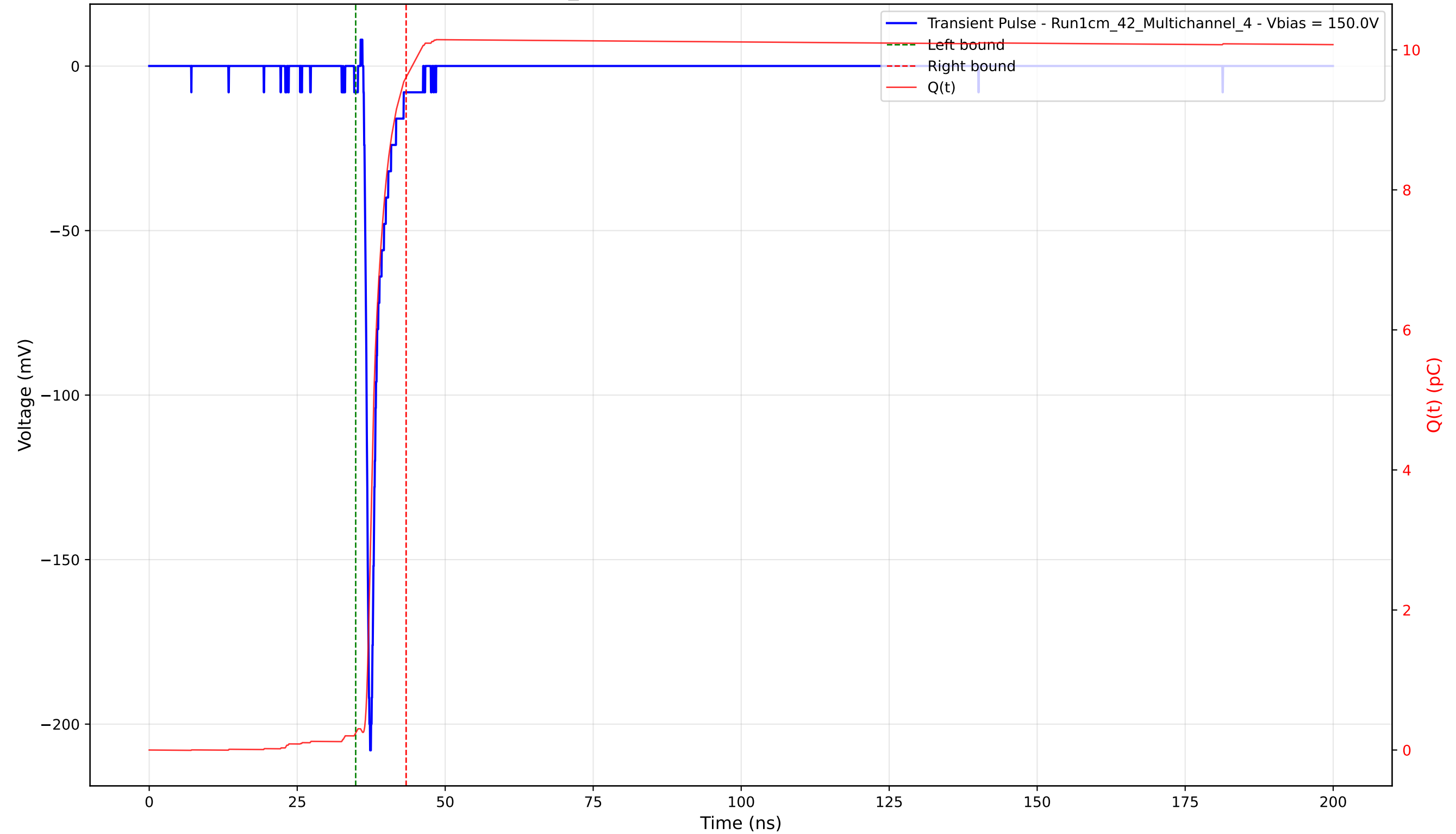
Transient Pulse - Sample: 1cm_42 - Position: 1970.0 \mu\text{m} - Charge: 9.36 pC - Rise Time: 0.82 ns
