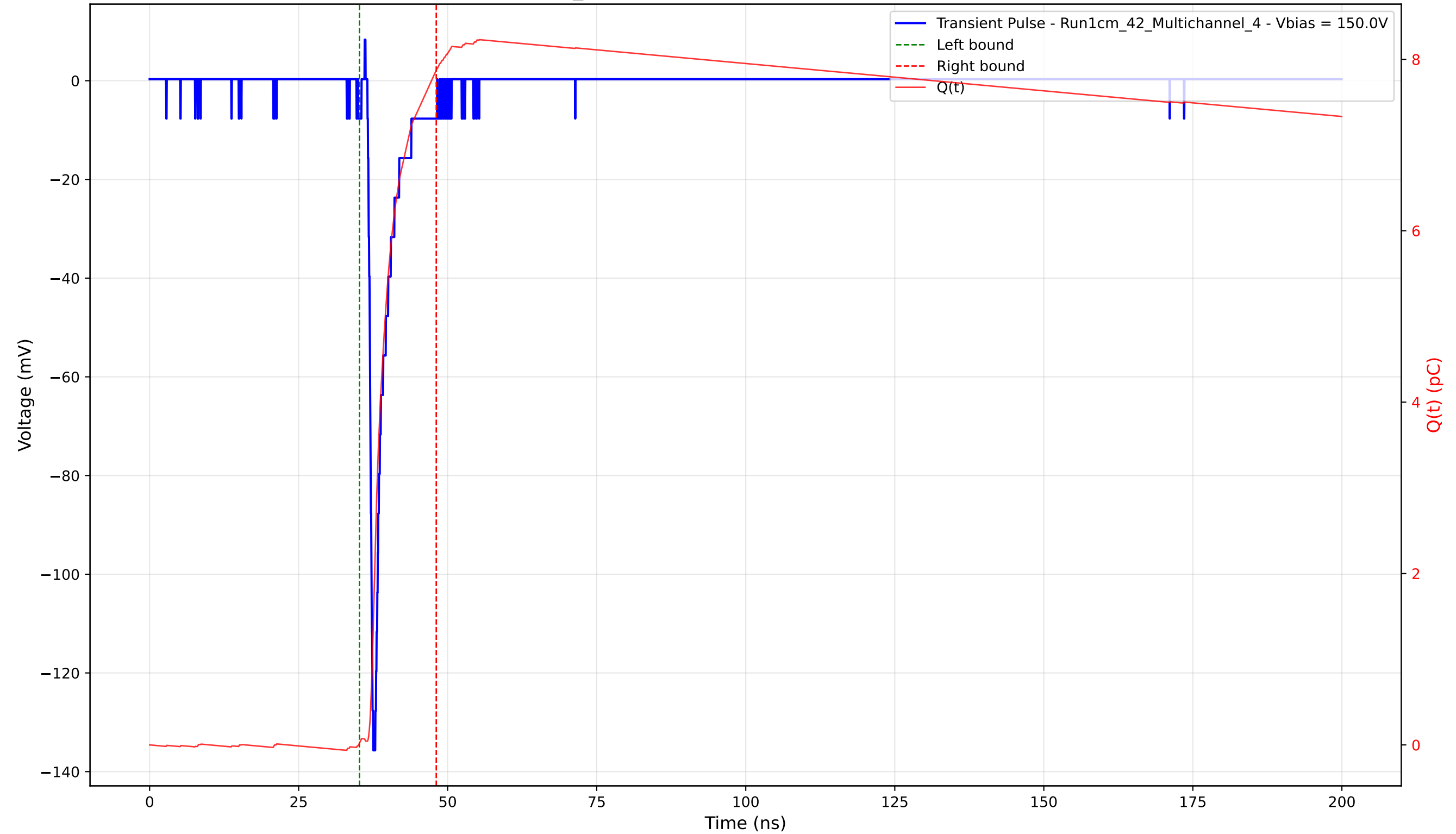
Transient Pulse - Sample: 1cm_42 - Position: 3305.0 \mu\text{m} - Charge: 7.85 pC - Rise Time: 0.77 ns
