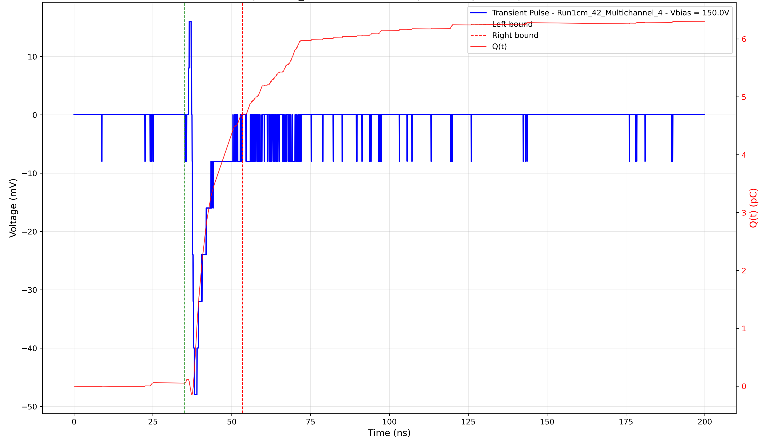
Transient Pulse - Sample: 1cm_42 - Position: 3905.0 \mu\text{m} - Charge: 4.65 pC - Rise Time: 0.74 ns
