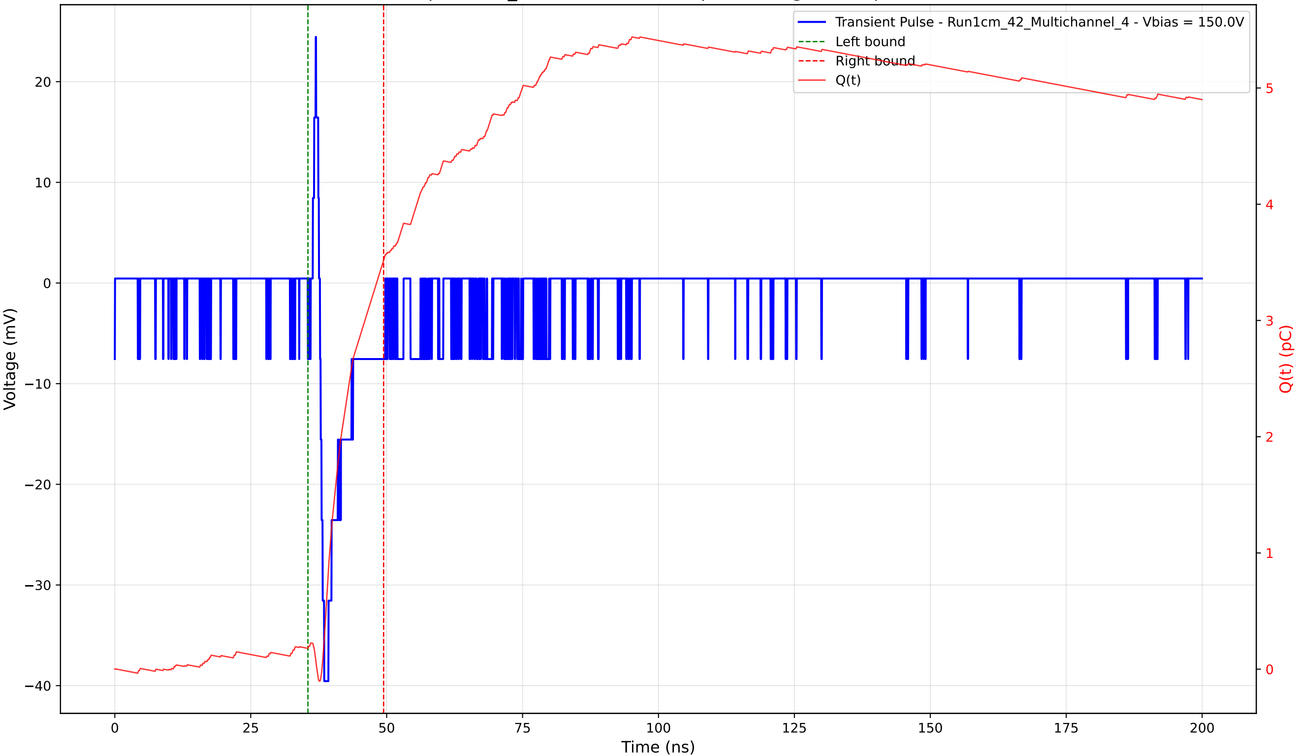
Transient Pulse - Sample: 1cm_42 - Position: 540.0 \mu\text{m} - Charge: 3.34 pC - Rise Time: 0.78 ns
