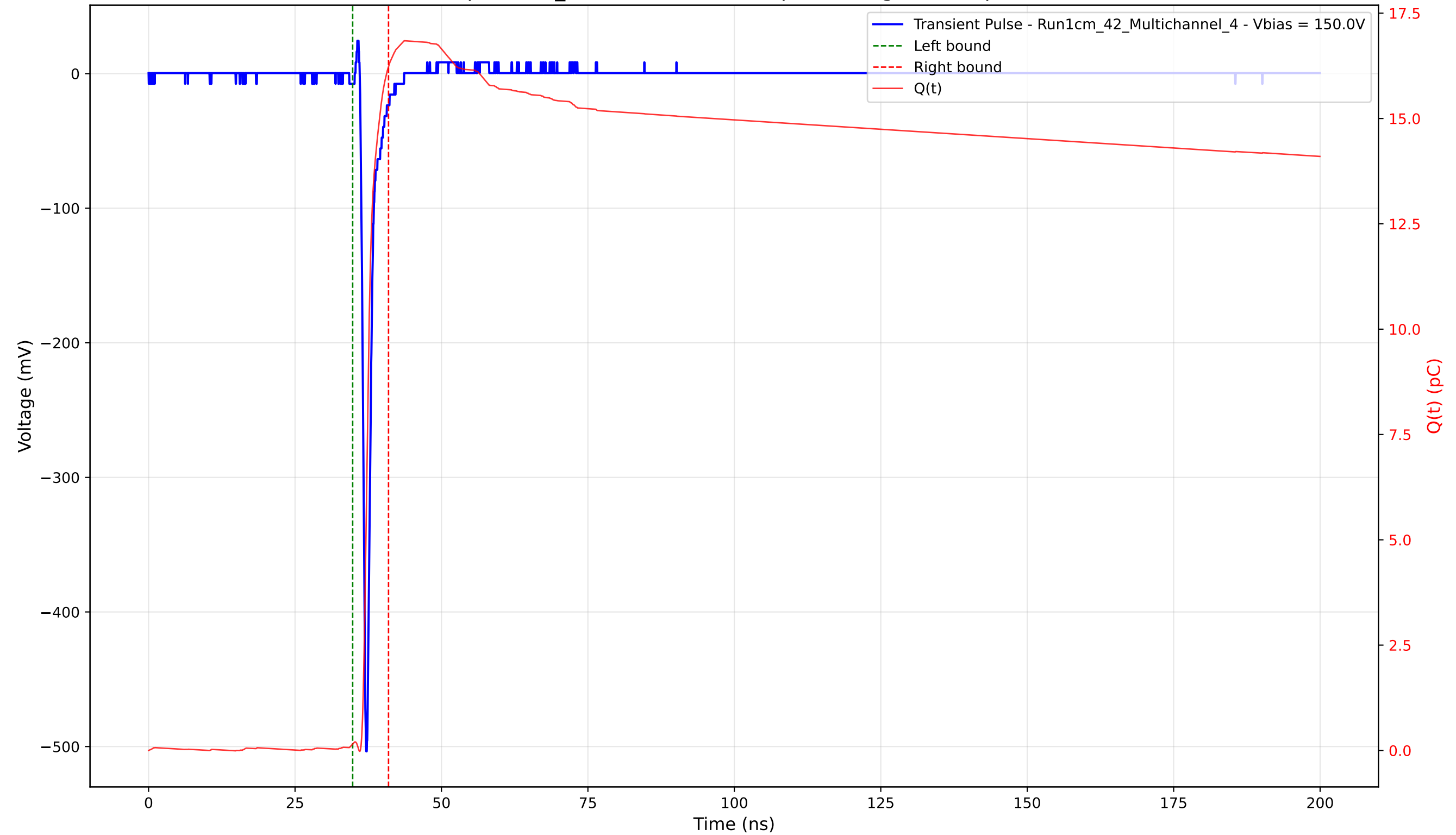
Transient Pulse - Sample: 1cm_42 - Position: 2725.0 \mu\text{m} - Charge: 16.08 pC - Rise Time: 0.73 ns
