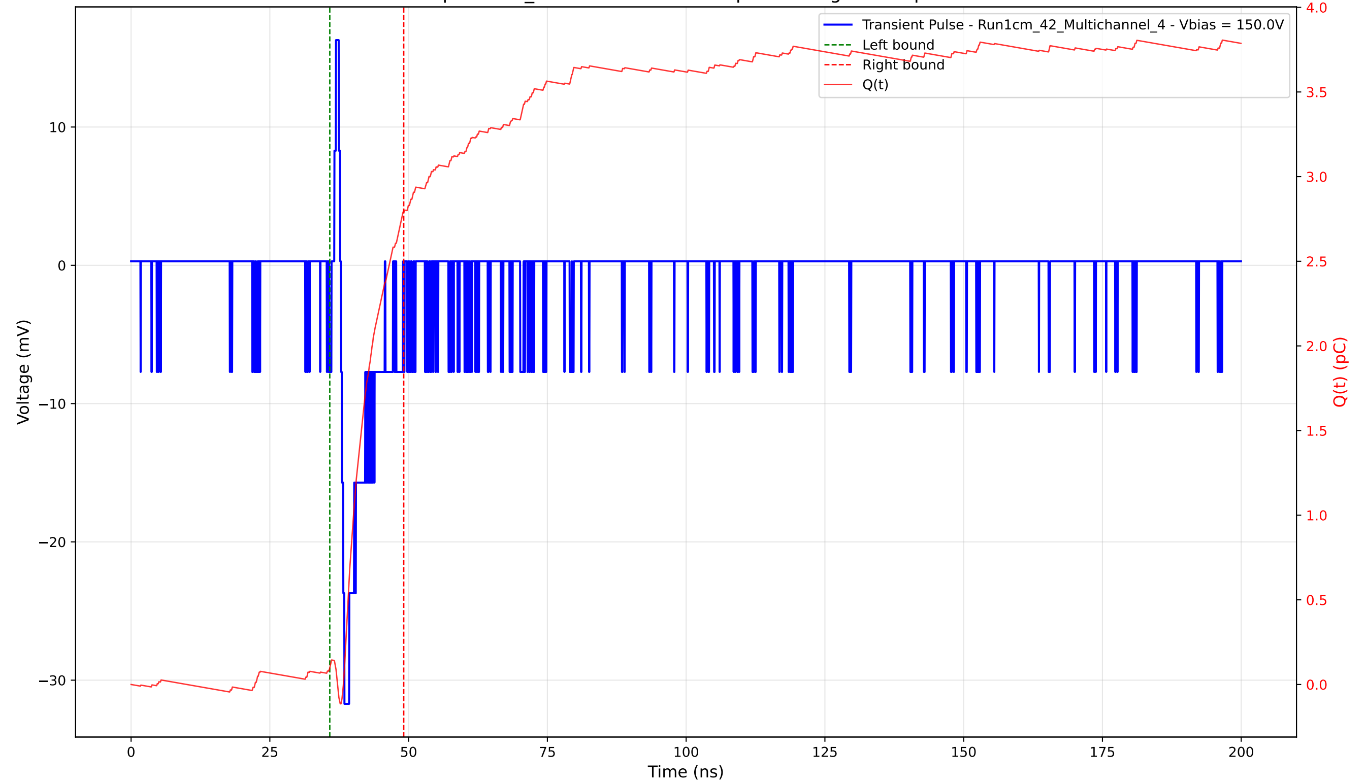
Transient Pulse - Sample: 1cm_42 - Position: 4650.0 \mu\text{m} - Charge: 2.69 pC - Rise Time: 0.62 ns
