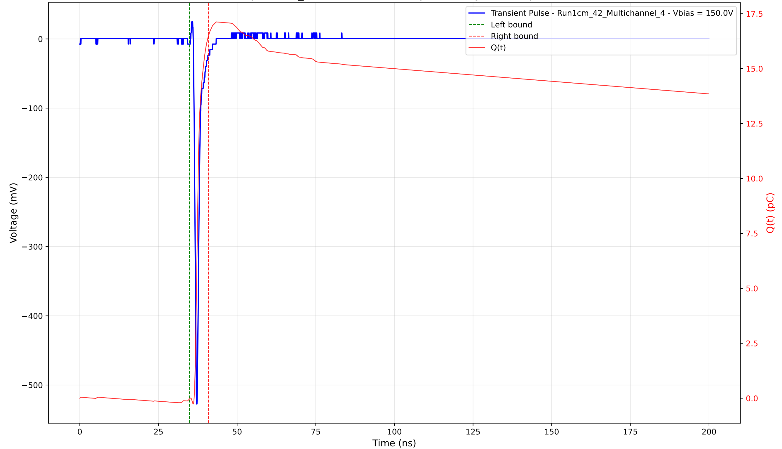
Transient Pulse - Sample: 1cm_42 - Position: 2340.0 \mu\text{m} - Charge: 16.55 pC - Rise Time: 0.73 ns
