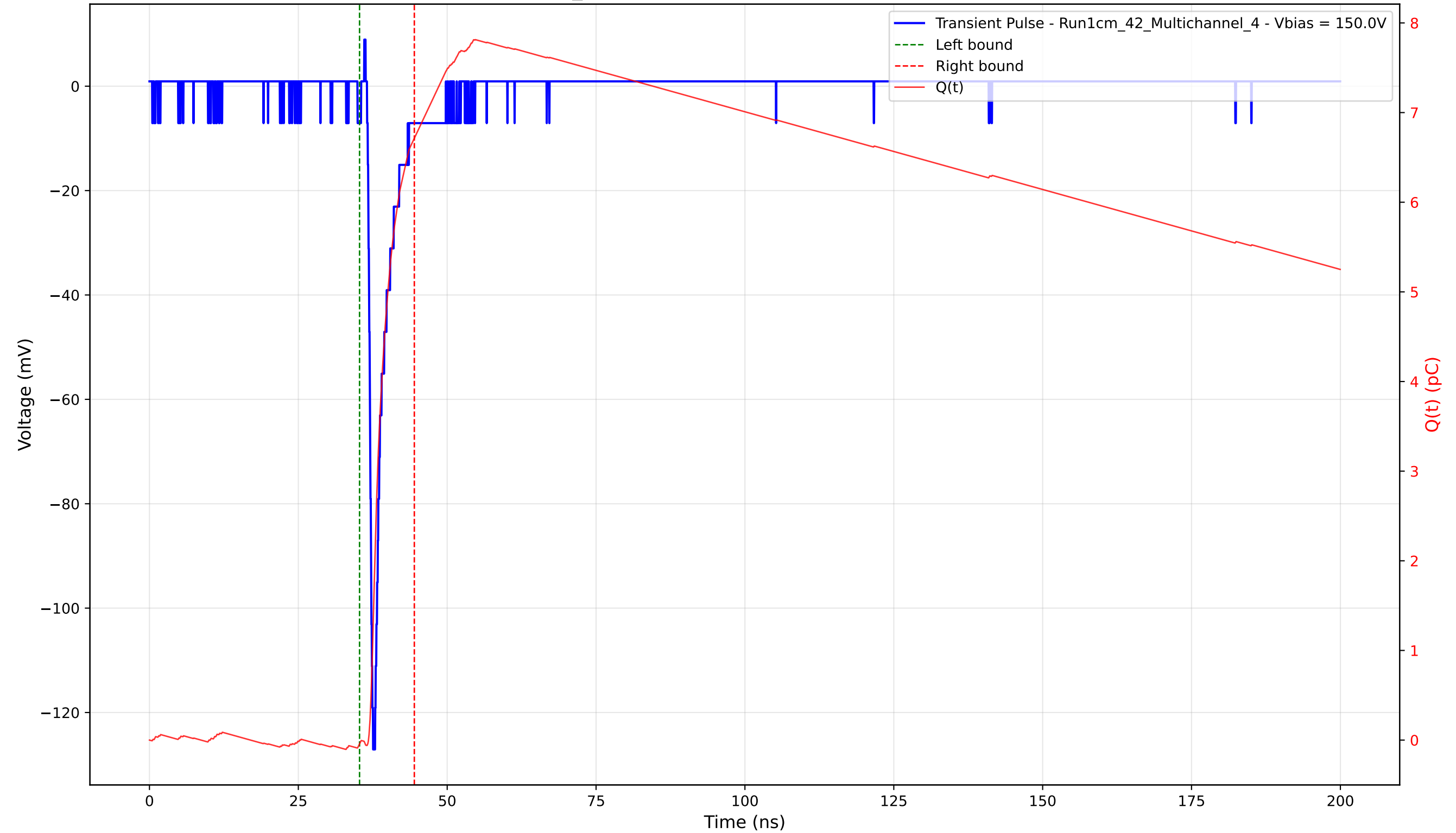
Transient Pulse - Sample: 1cm_42 - Position: 3335.0 \mu\text{m} - Charge: 6.75 pC - Rise Time: 0.77 ns
