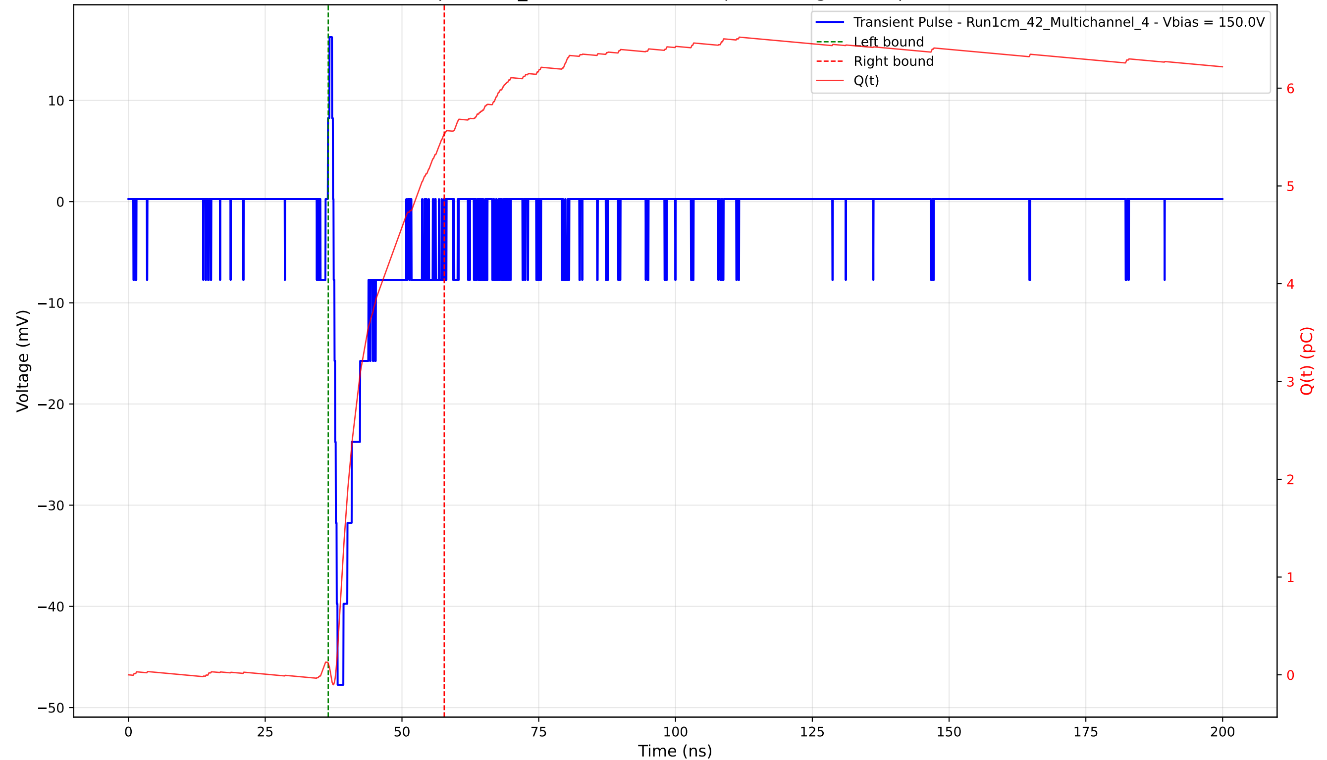
Transient Pulse - Sample: 1cm_42 - Position: 1045.0 \mu\text{m} - Charge: 5.41 pC - Rise Time: 0.74 ns
