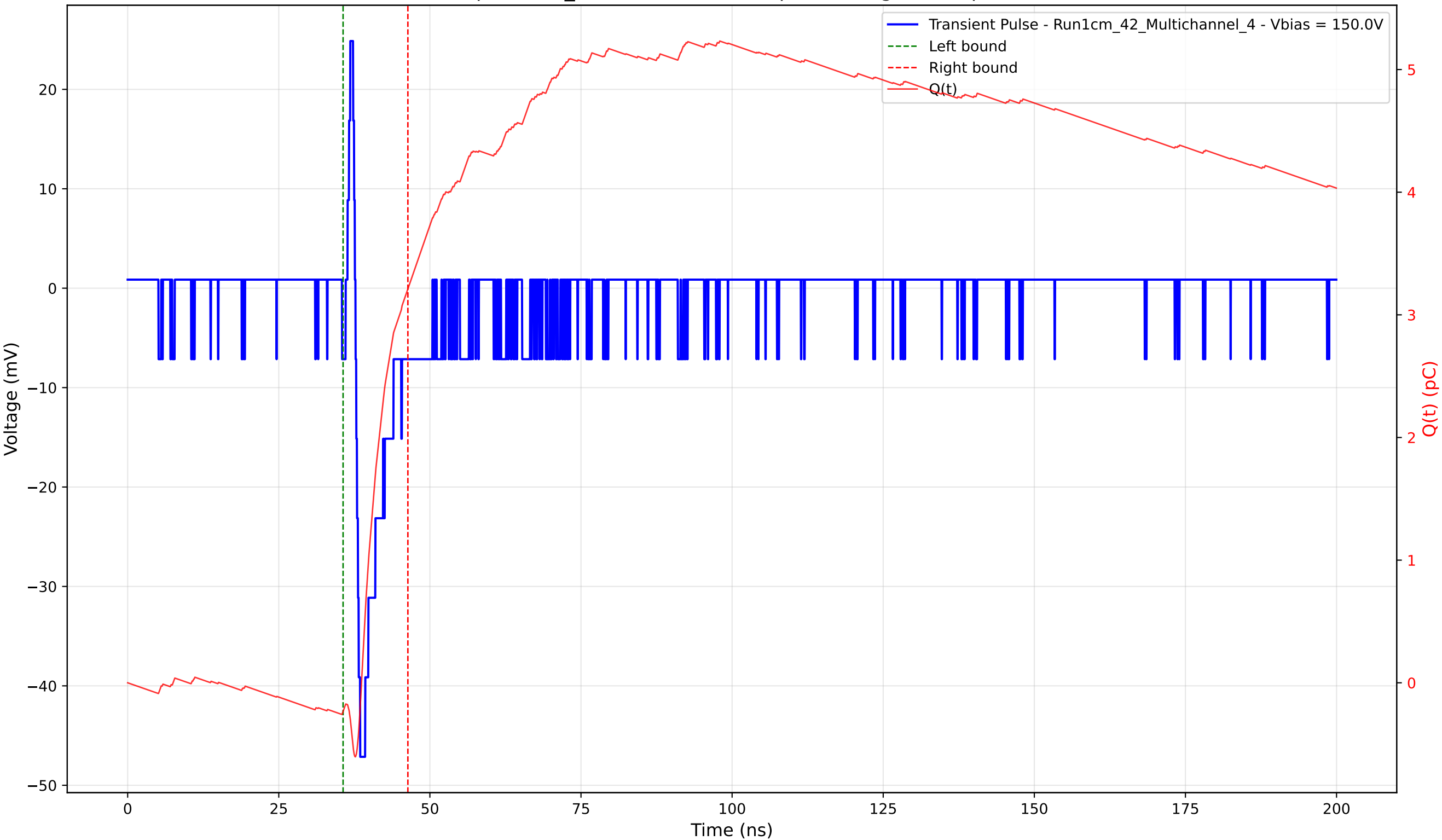
Transient Pulse - Sample: 1cm_42 - Position: 835.0 \mu\text{m} - Charge: 3.44 pC - Rise Time: 0.78 ns
