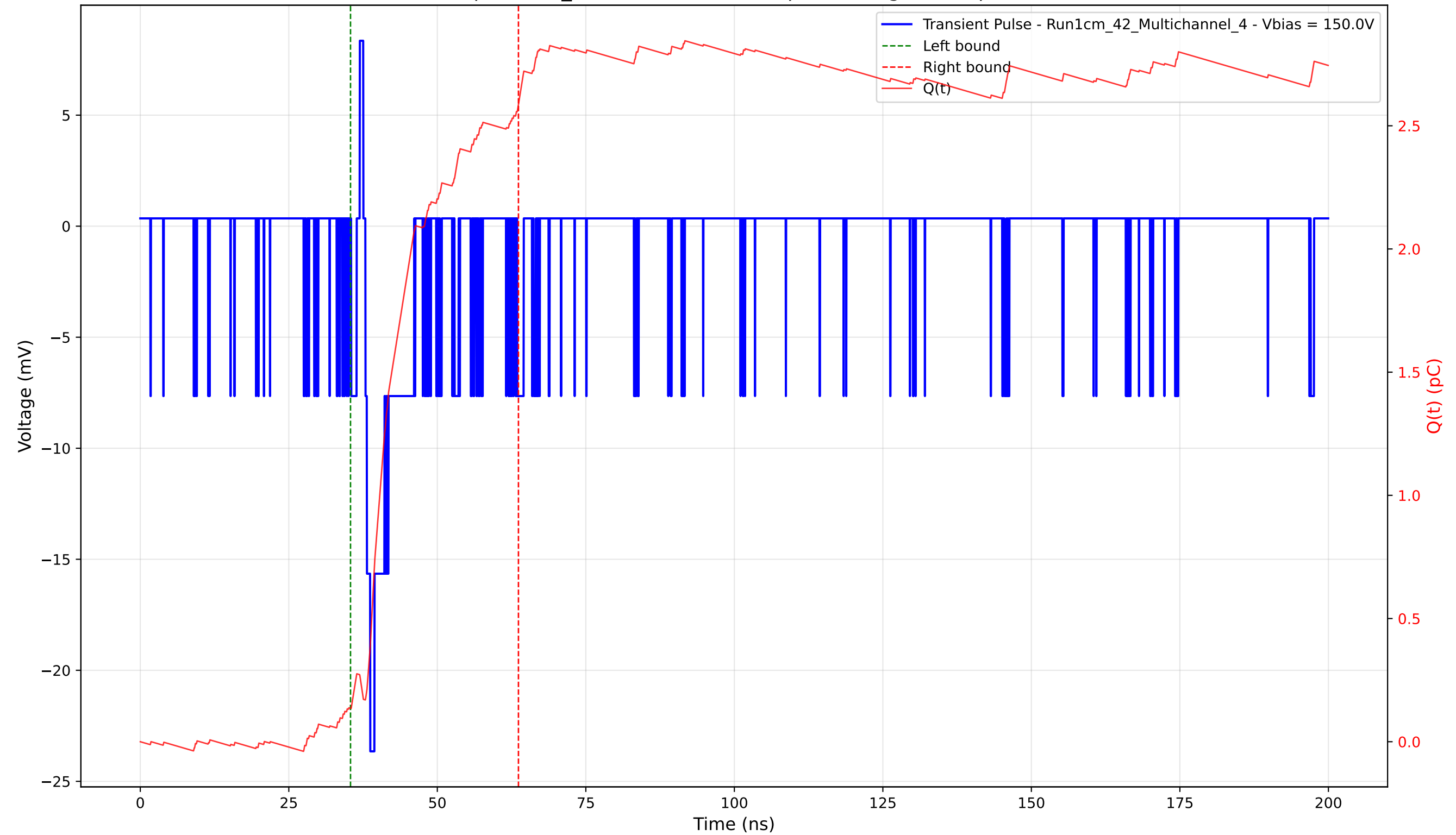
Transient Pulse - Sample: 1cm_42 - Position: 4975.0 \mu\text{m} - Charge: 2.45 pC - Rise Time: 0.83 ns
