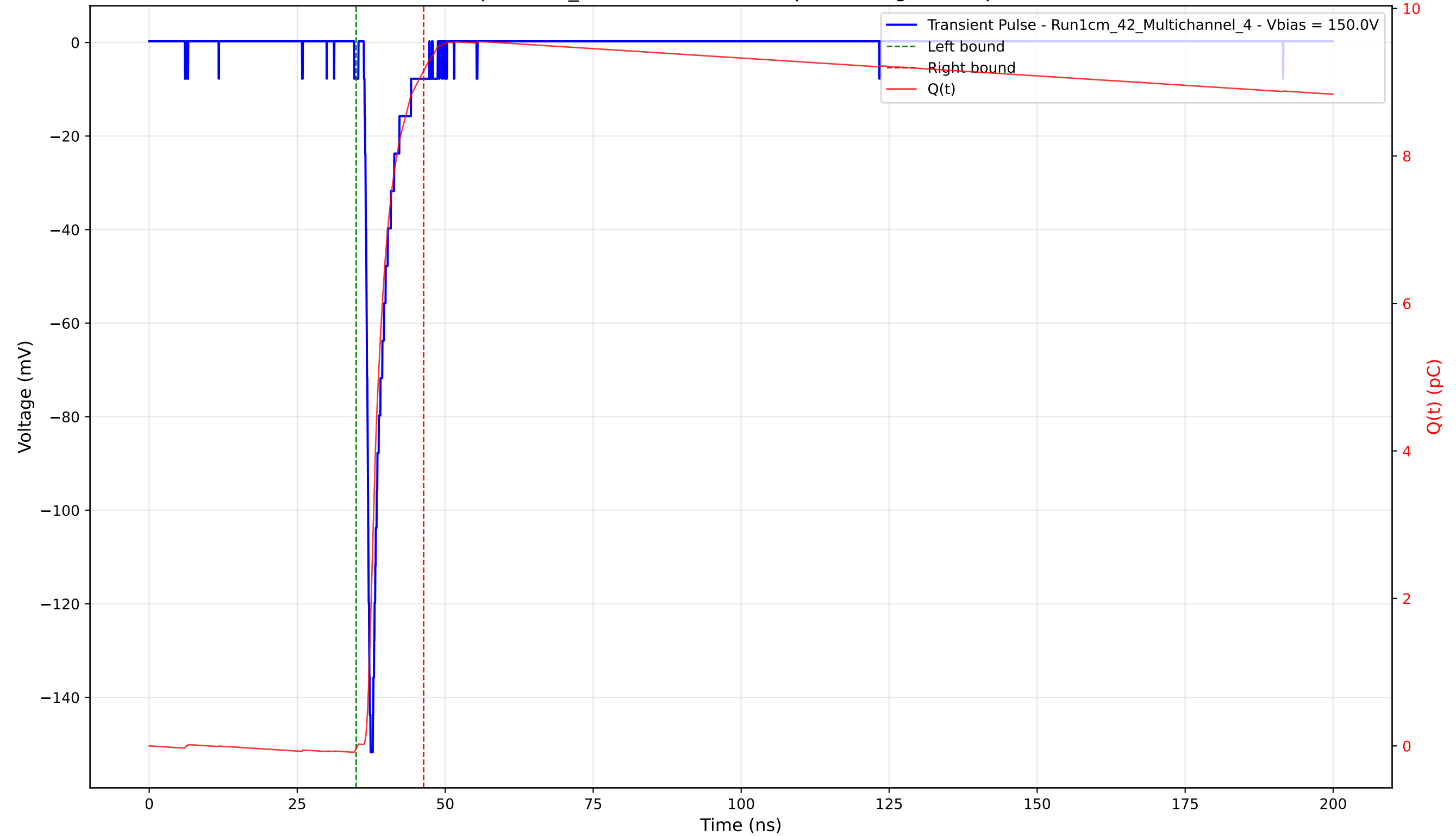
Transient Pulse - Sample: 1cm_42 - Position: 1805.0 \mu\text{m} - Charge: 9.19 pC - Rise Time: 0.88 ns
