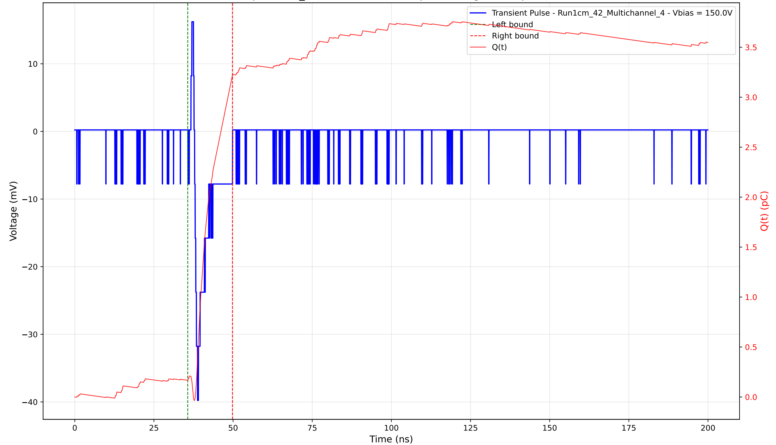
Transient Pulse - Sample: 1cm_42 - Position: 4805.0 \mu\text{m} - Charge: 3.06 pC - Rise Time: 0.94 ns
