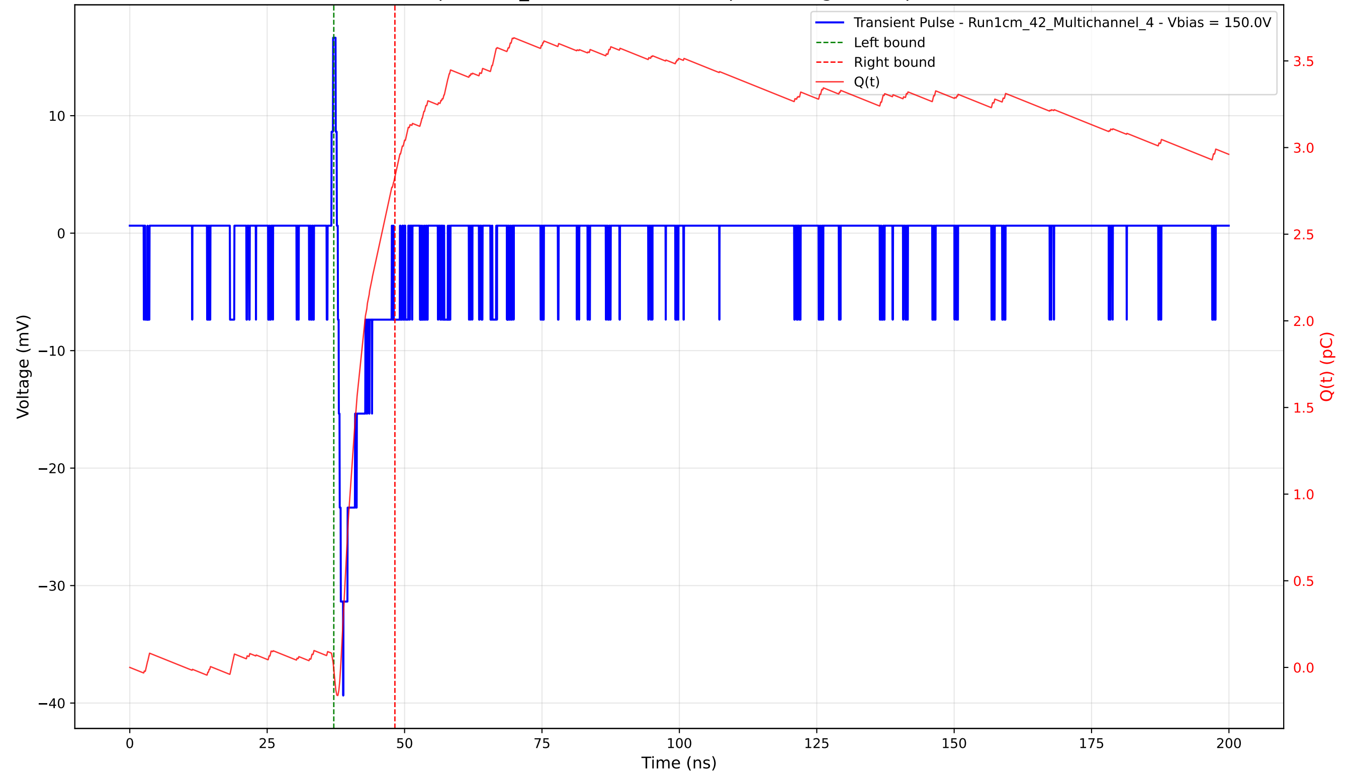
Transient Pulse - Sample: 1cm_42 - Position: 4825.0 \mu\text{m} - Charge: 2.84 pC - Rise Time: 0.98 ns
