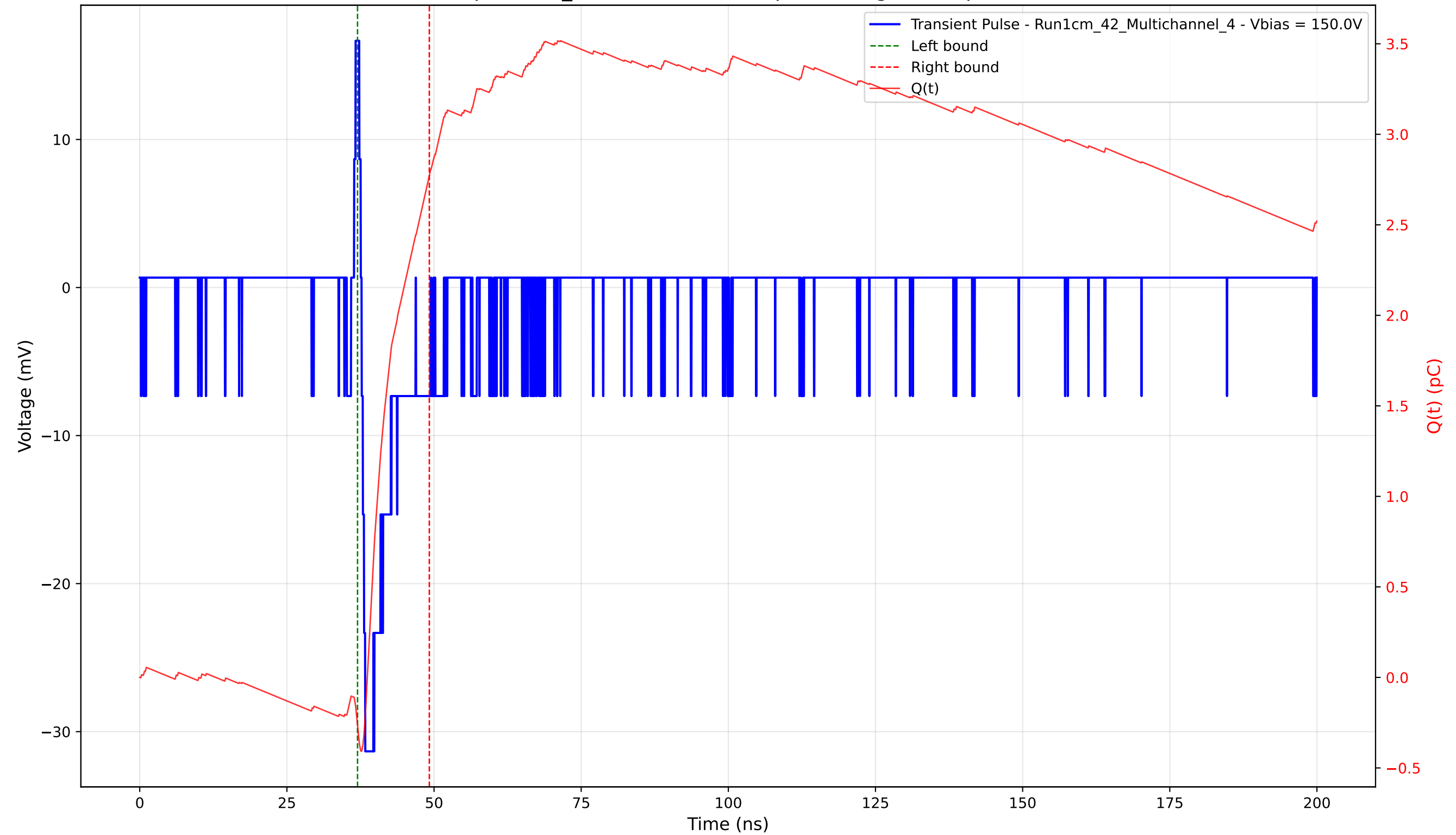
Transient Pulse - Sample: 1cm_42 - Position: 470.0 \mu\text{m} - Charge: 3.04 pC - Rise Time: 0.63 ns
