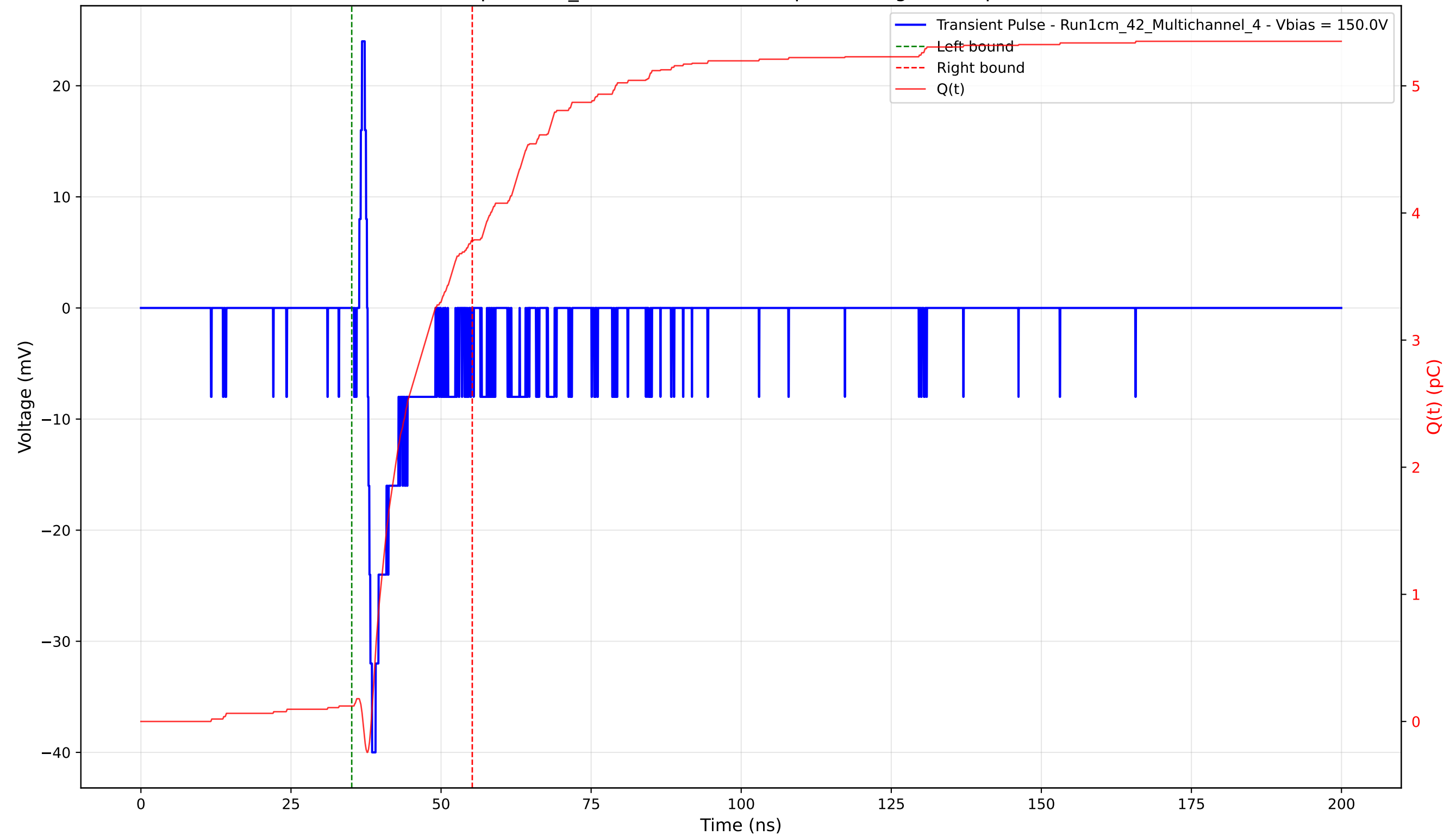
Transient Pulse - Sample: 1cm_42 - Position: 4365.0 \mu\text{m} - Charge: 3.66 pC - Rise Time: 0.74 ns
