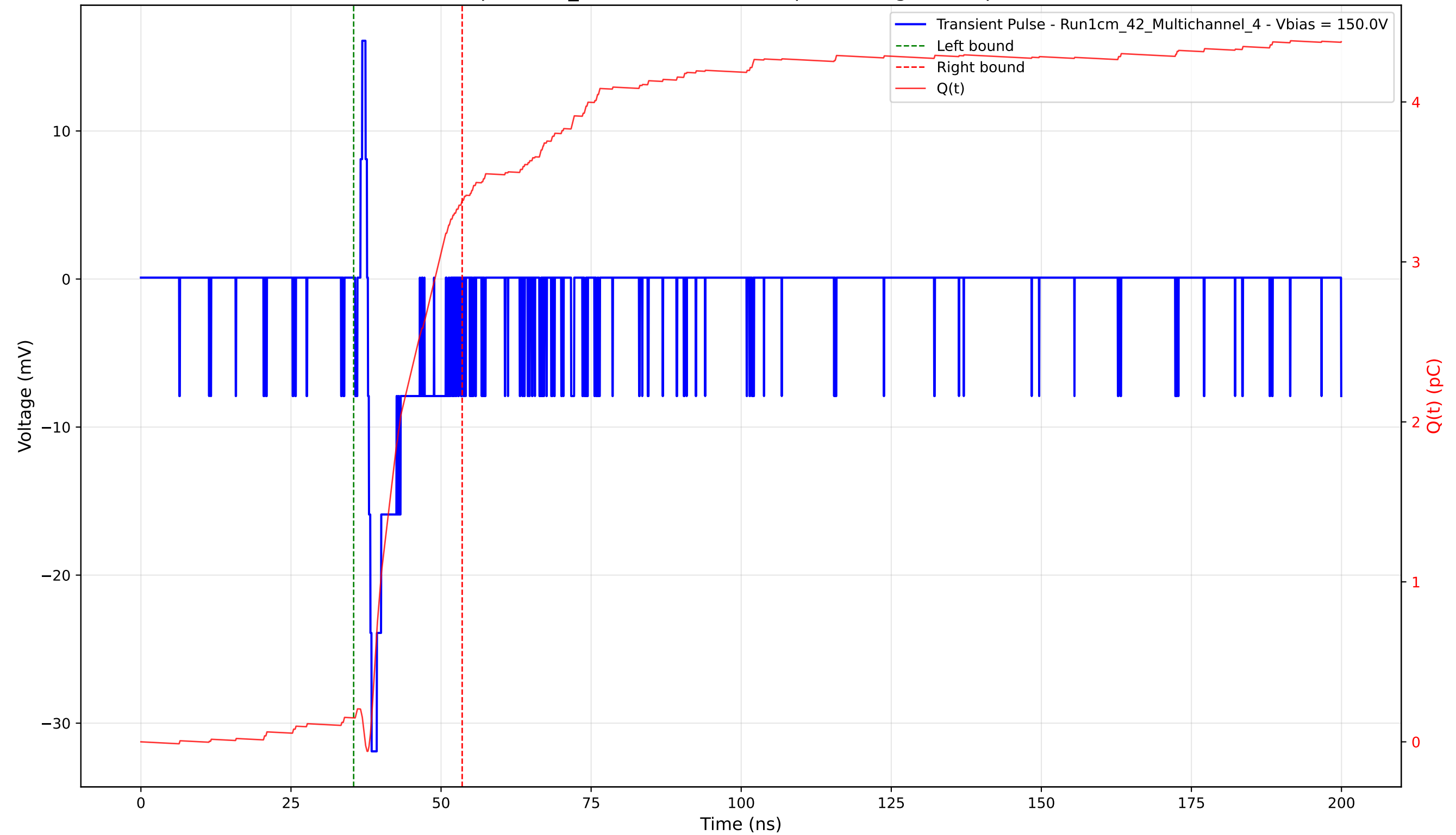
Transient Pulse - Sample: 1cm_42 - Position: 4645.0 \mu\text{m} - Charge: 3.24 pC - Rise Time: 0.62 ns
