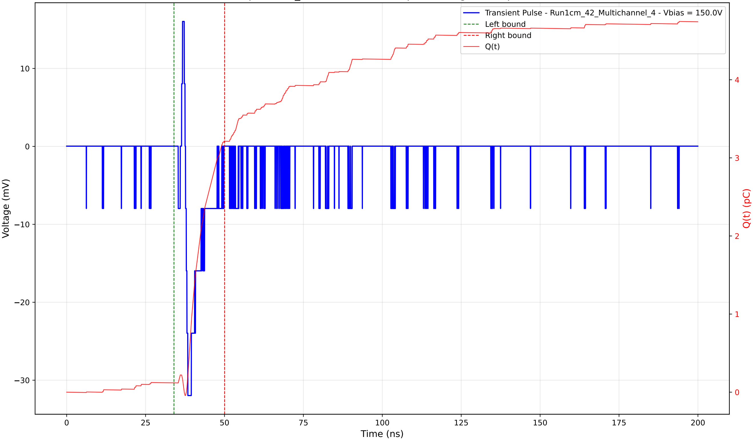
Transient Pulse - Sample: 1cm_42 - Position: 450.0 \mu\text{m} - Charge: 3.09 pC - Rise Time: 0.74 ns
