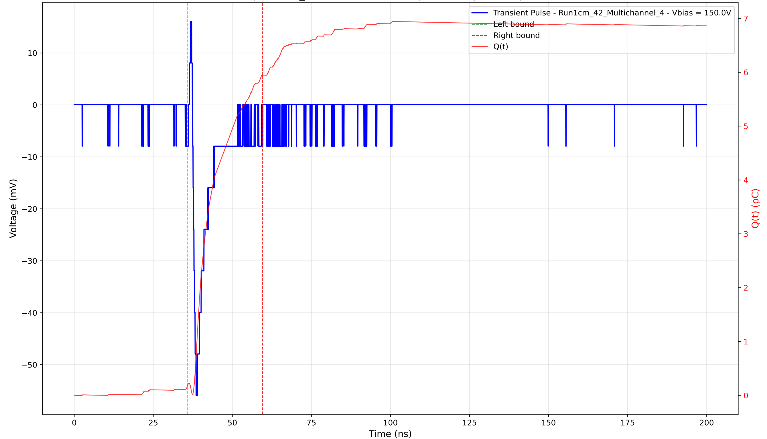
Transient Pulse - Sample: 1cm_42 - Position: 1080.0 \mu\text{m} - Charge: 5.79 pC - Rise Time: 1.09 ns
