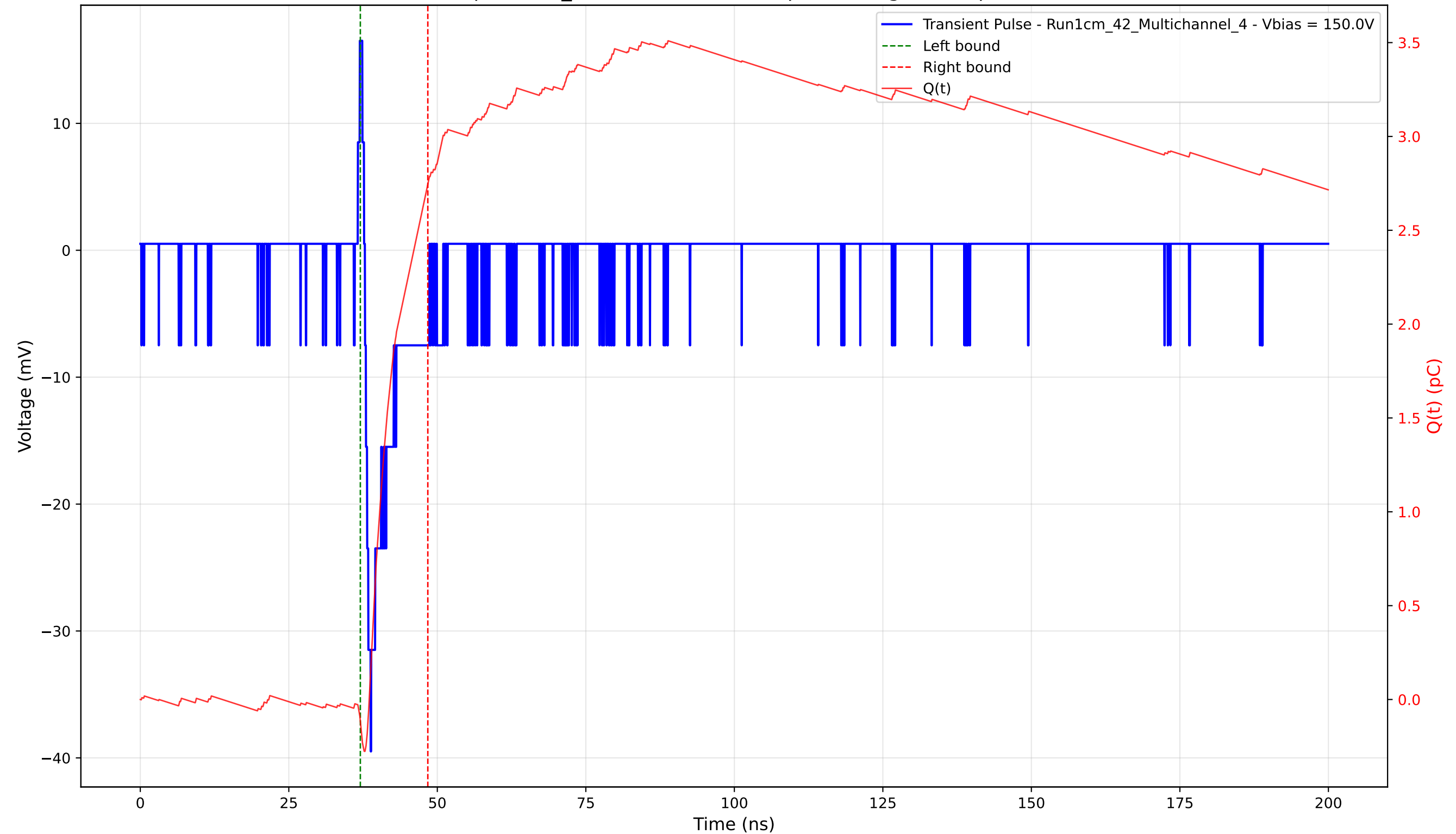
Transient Pulse - Sample: 1cm_42 - Position: 4760.0 \mu\text{m} - Charge: 2.86 pC - Rise Time: 0.98 ns
