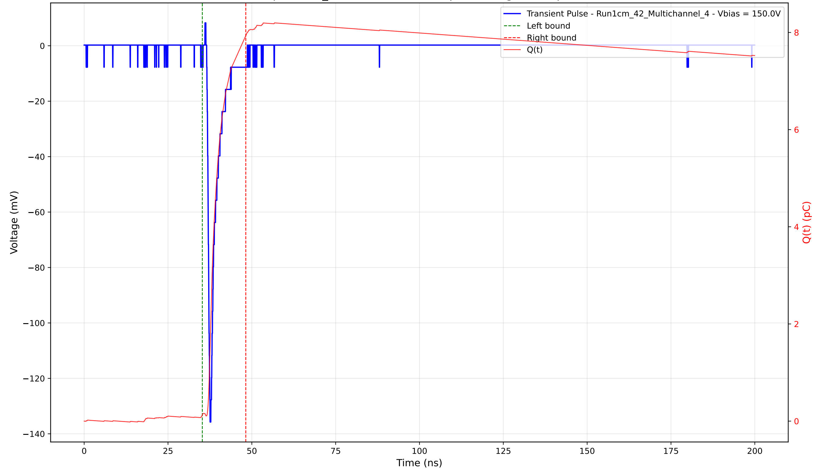
Transient Pulse - Sample: 1cm_42 - Position: 3320.0 \mu\text{m} - Charge: 7.81 pC - Rise Time: 0.85 ns
