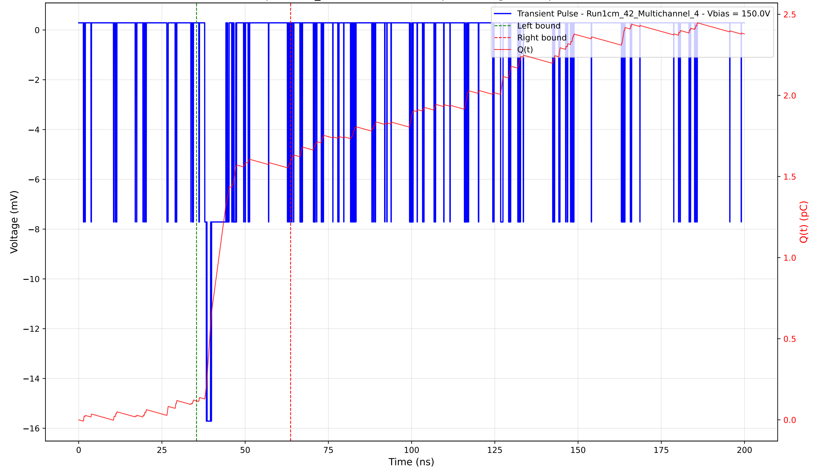
Transient Pulse - Sample: 1cm_42 - Position: 5050.0 \mu\text{m} - Charge: 1.48 pC - Rise Time: 0.51 ns
