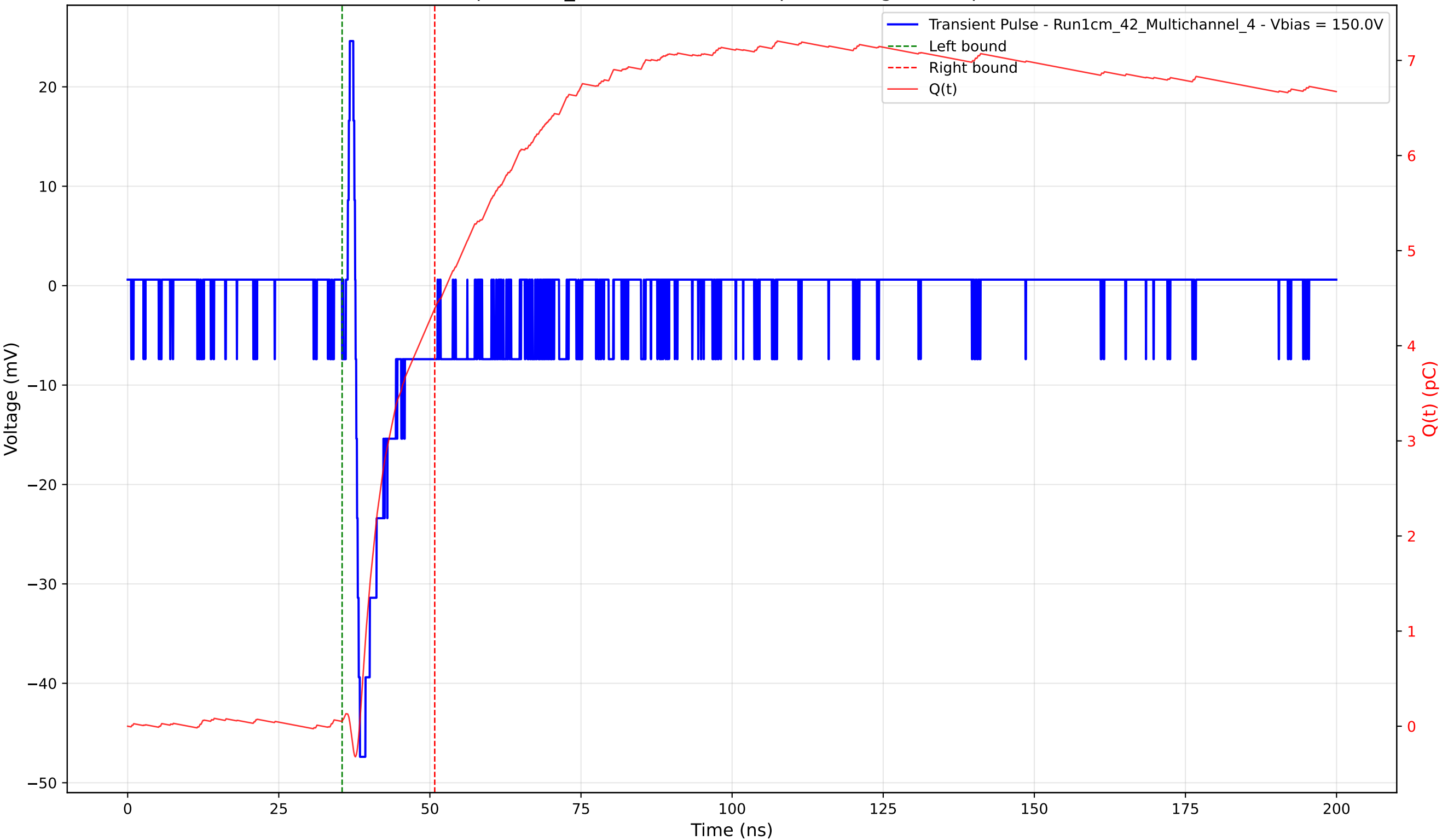
Transient Pulse - Sample: 1cm_42 - Position: 785.0 \mu\text{m} - Charge: 4.34 pC - Rise Time: 0.74 ns
