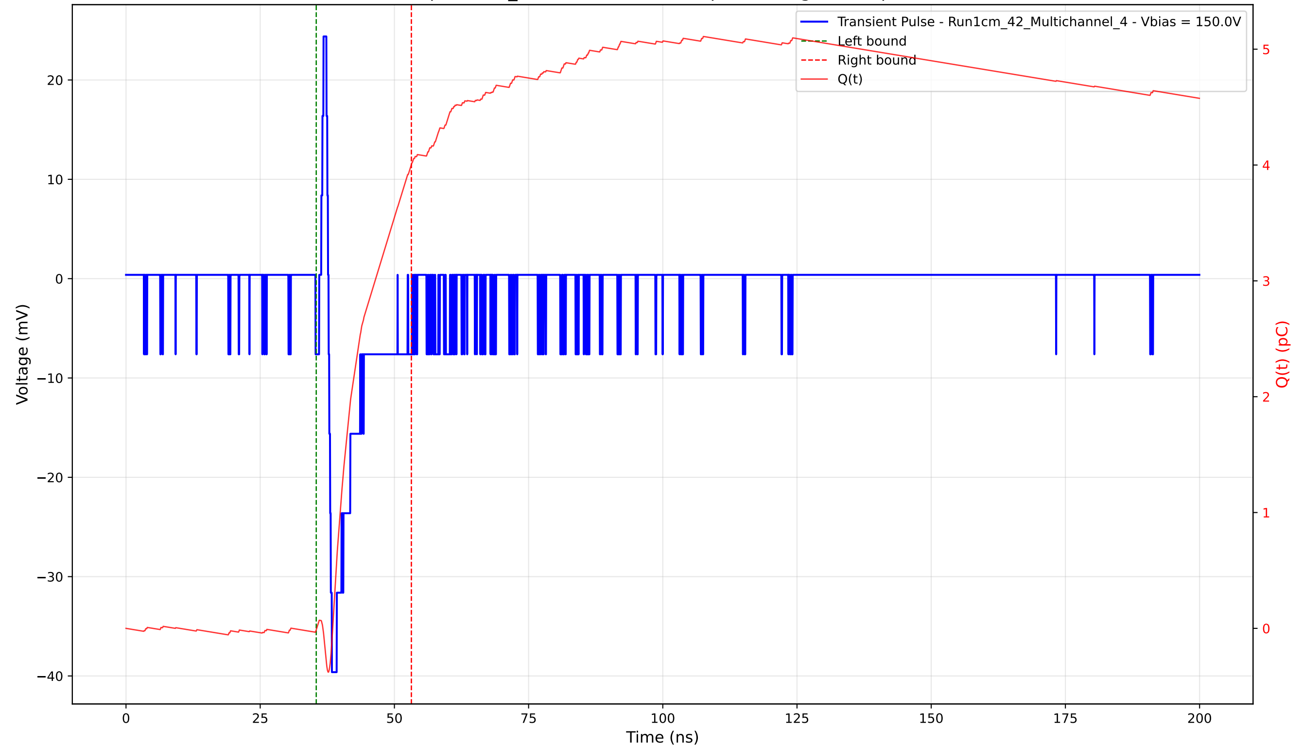
Transient Pulse - Sample: 1cm_42 - Position: 4250.0 \mu\text{m} - Charge: 4.02 pC - Rise Time: 0.62 ns
