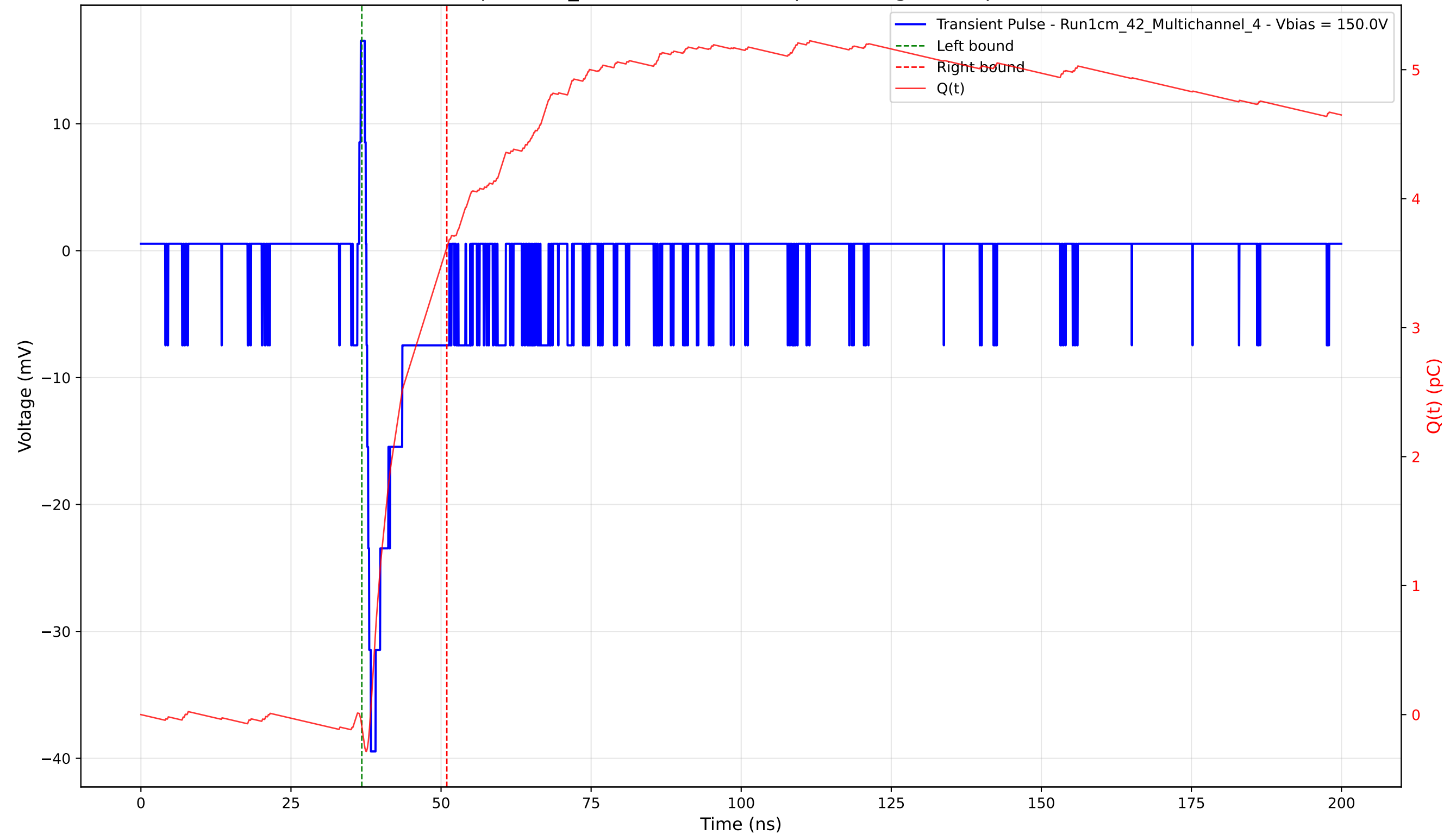
Transient Pulse - Sample: 1cm_42 - Position: 4045.0 \mu\text{m} - Charge: 3.72 pC - Rise Time: 0.74 ns
