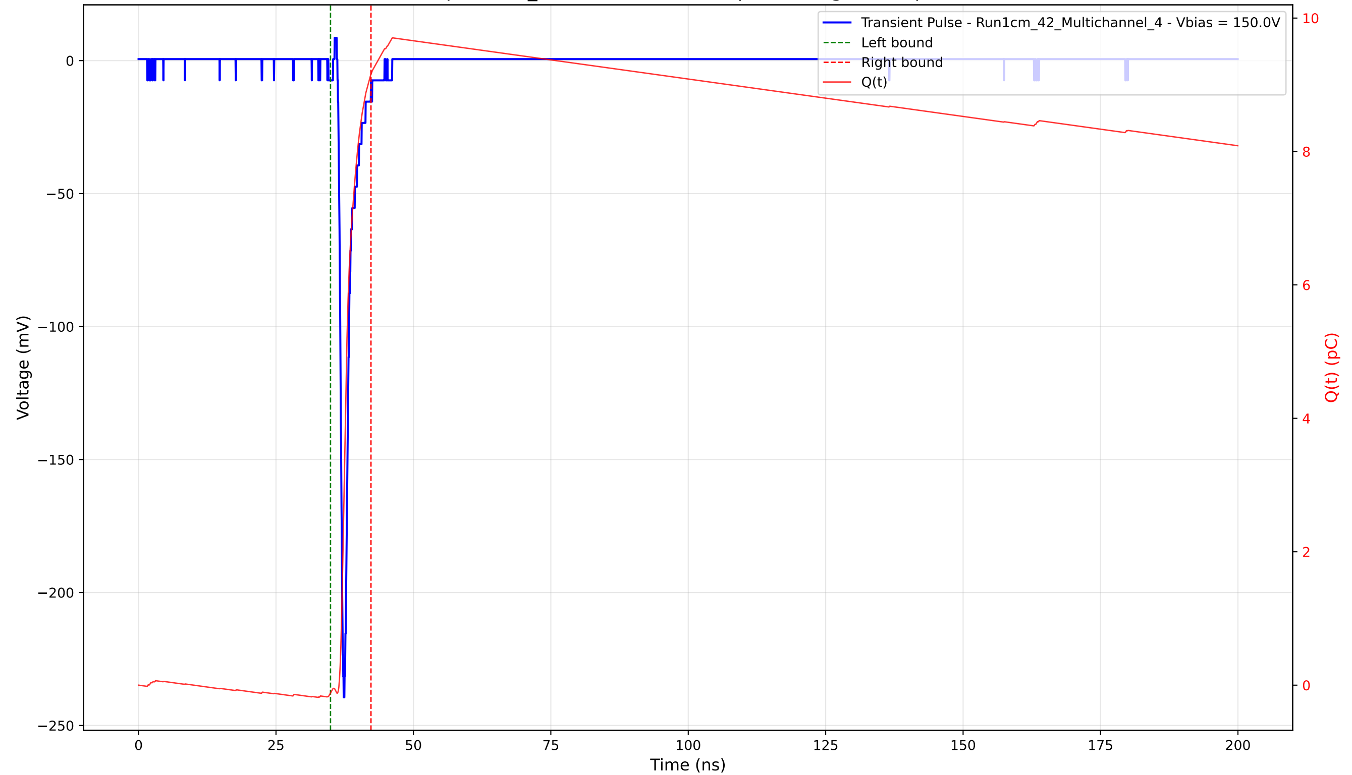
Transient Pulse - Sample: 1cm_42 - Position: 3000.0 \mu\text{m} - Charge: 9.28 pC - Rise Time: 0.80 ns
