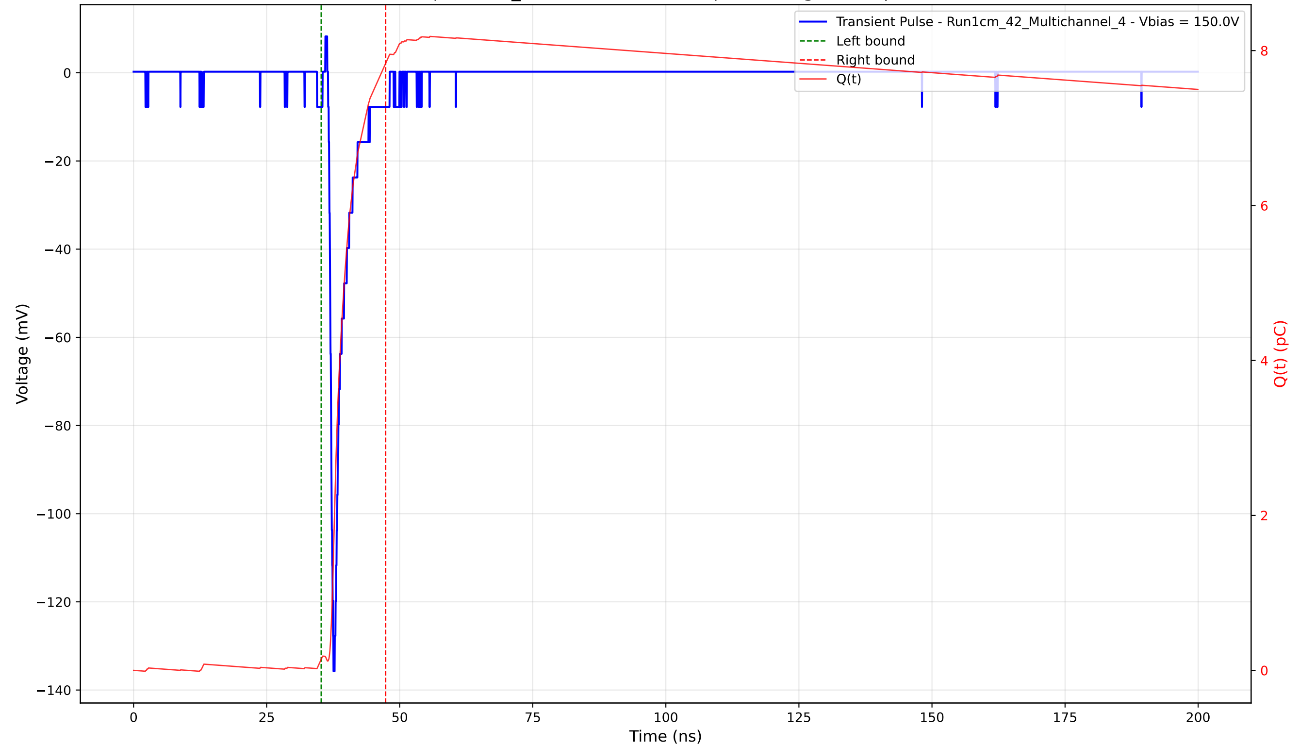
Transient Pulse - Sample: 1cm_42 - Position: 3325.0 \mu\text{m} - Charge: 7.69 pC - Rise Time: 0.81 ns
