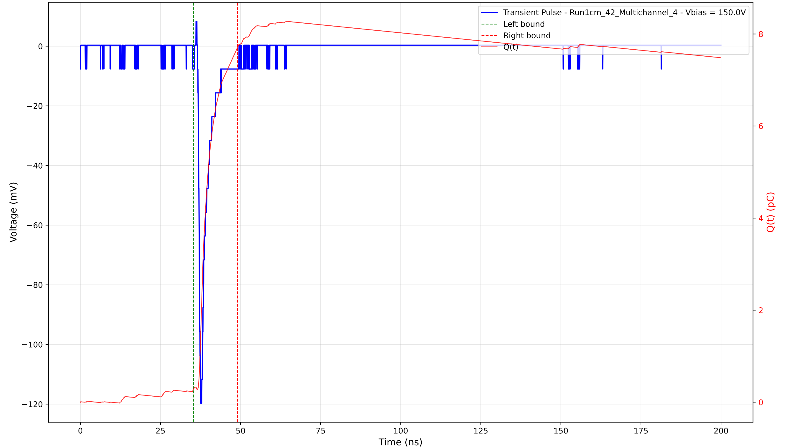
Transient Pulse - Sample: 1cm_42 - Position: 3355.0 \mu\text{m} - Charge: 7.43 pC - Rise Time: 0.74 ns
