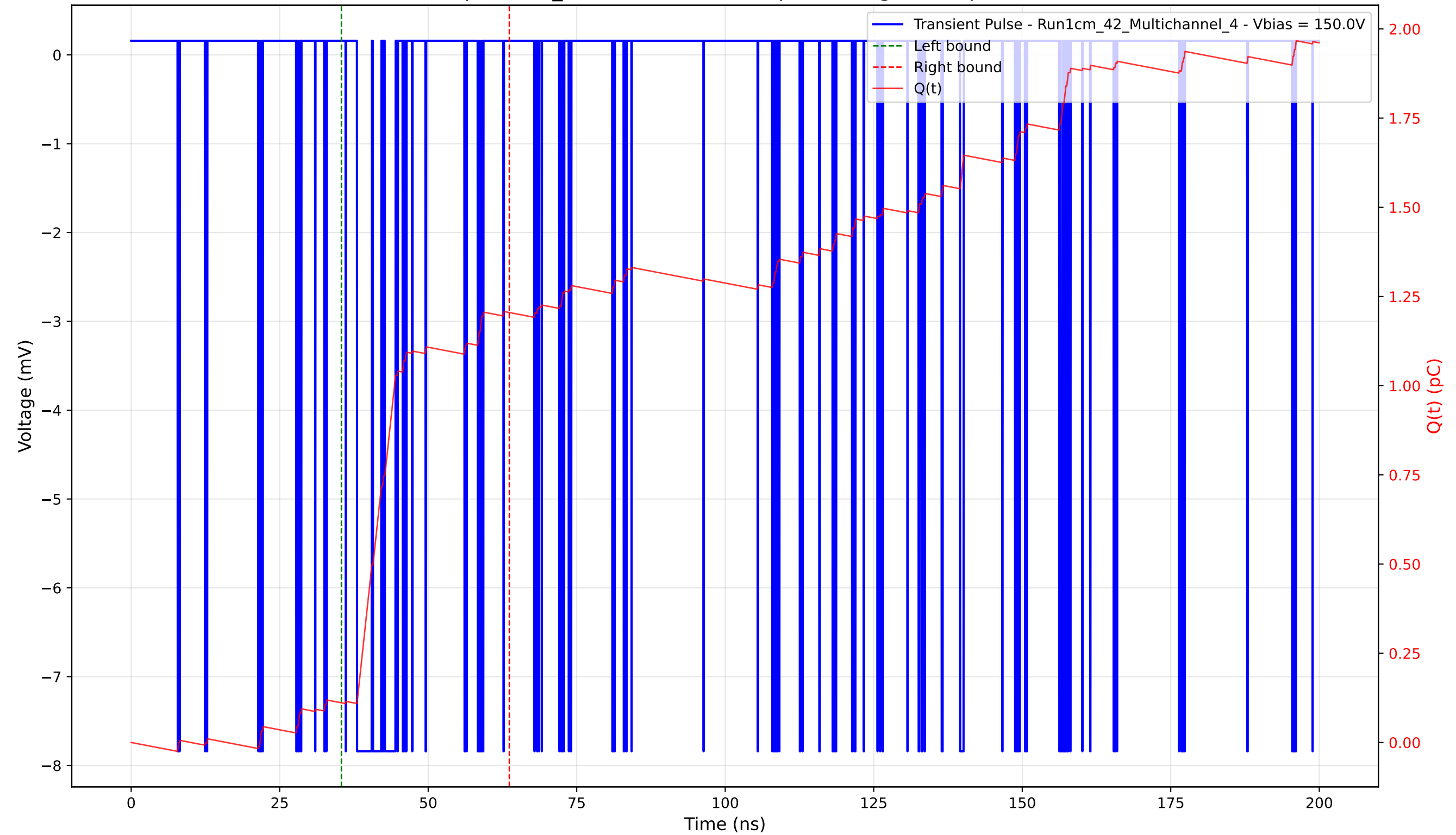
Transient Pulse - Sample: 1cm_42 - Position: 5135.0 \mu\text{m} - Charge: 1.09 pC - Rise Time: 0.04 ns
