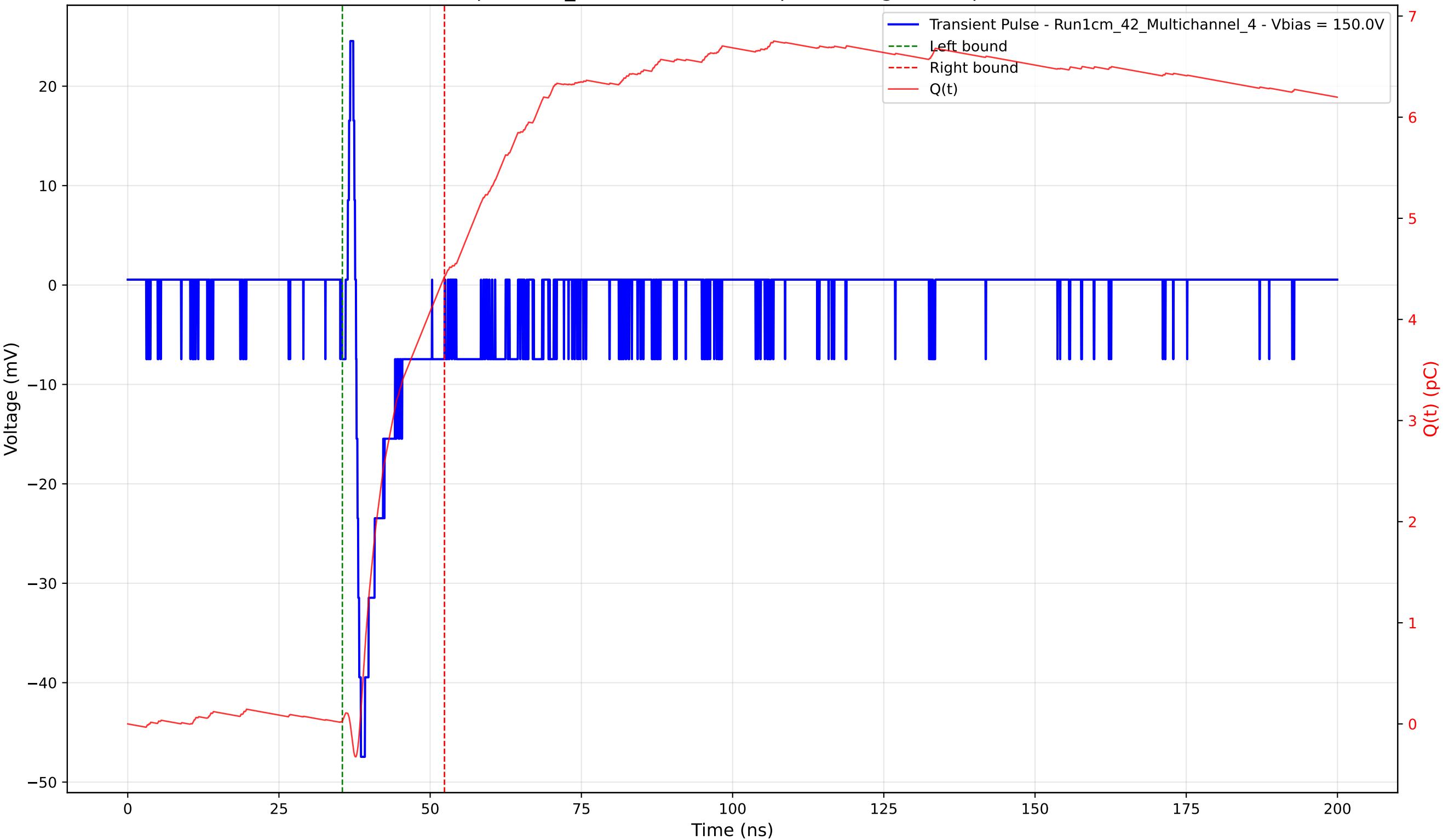
Transient Pulse - Sample: 1cm_42 - Position: 670.0 \mu\text{m} - Charge: 4.40 pC - Rise Time: 0.82 ns
