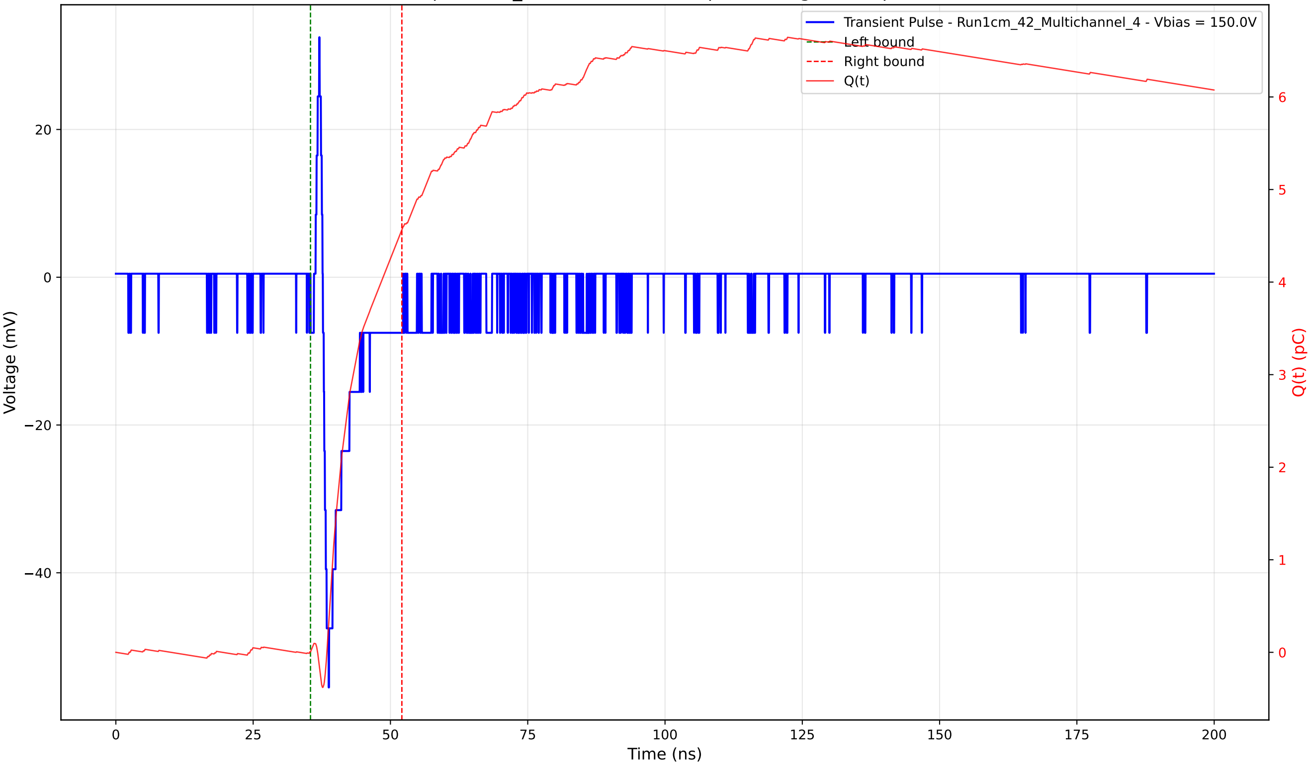
Transient Pulse - Sample: 1cm_42 - Position: 725.0 \mu\text{m} - Charge: 4.56 pC - Rise Time: 1.05 ns
