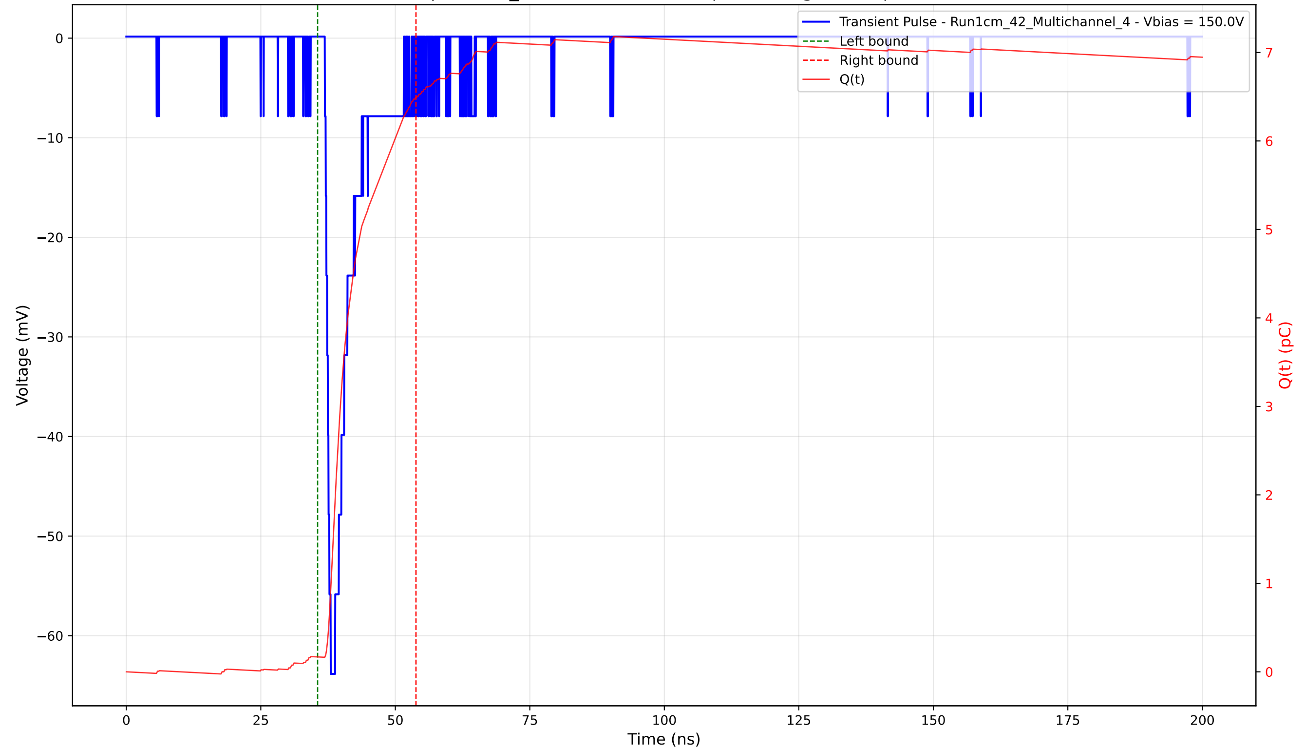
Transient Pulse - Sample: 1cm_42 - Position: 1415.0 \mu\text{m} - Charge: 6.32 pC - Rise Time: 1.09 ns
