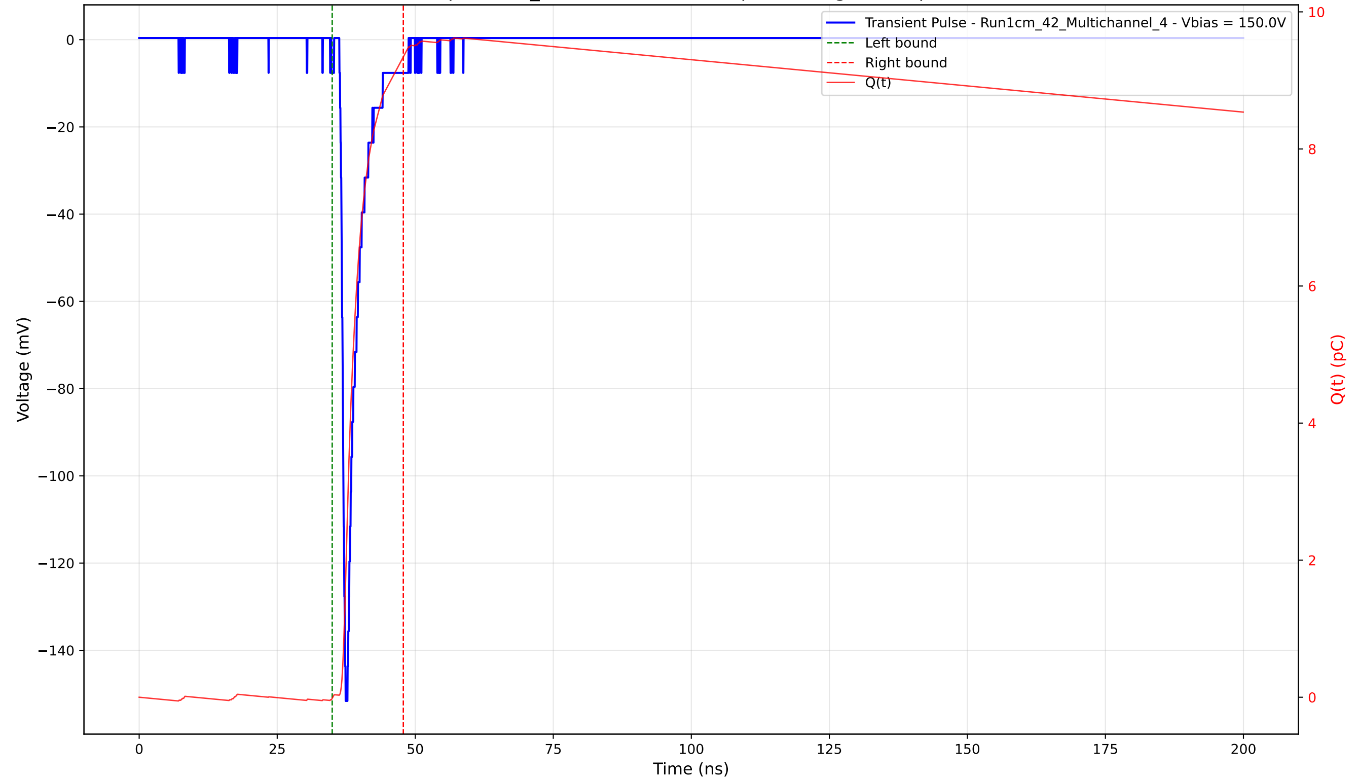
Transient Pulse - Sample: 1cm_42 - Position: 1795.0 \mu\text{m} - Charge: 9.36 pC - Rise Time: 0.92 ns
