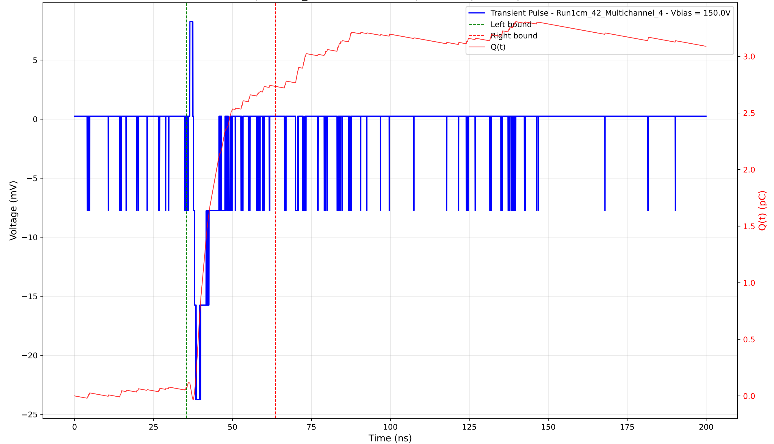
Transient Pulse - Sample: 1cm_42 - Position: 295.0 \mu\text{m} - Charge: 2.66 pC - Rise Time: 0.67 ns
