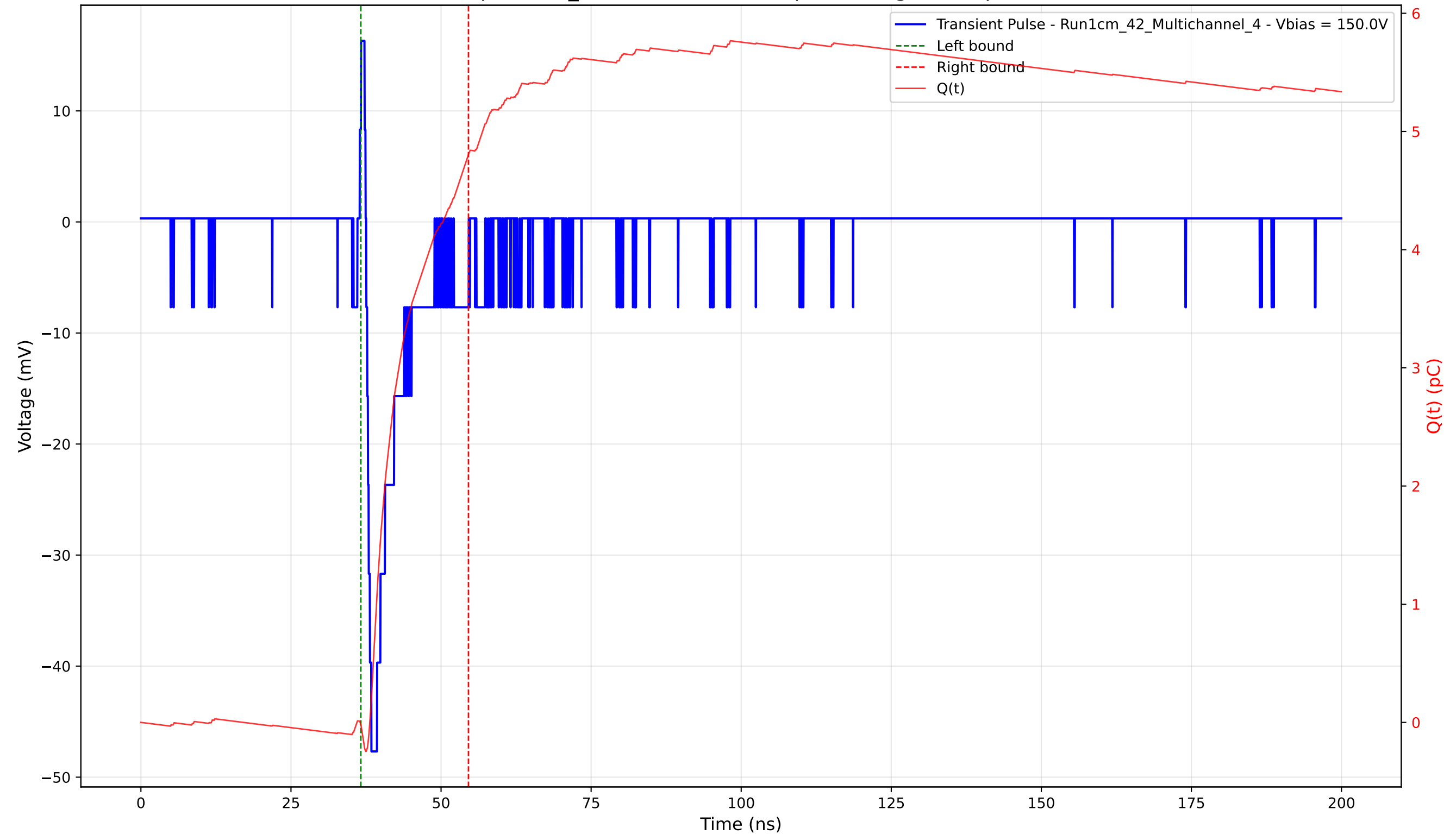
Transient Pulse - Sample: 1cm_42 - Position: 1010.0 \mu\text{m} - Charge: 4.83 pC - Rise Time: 0.86 ns
