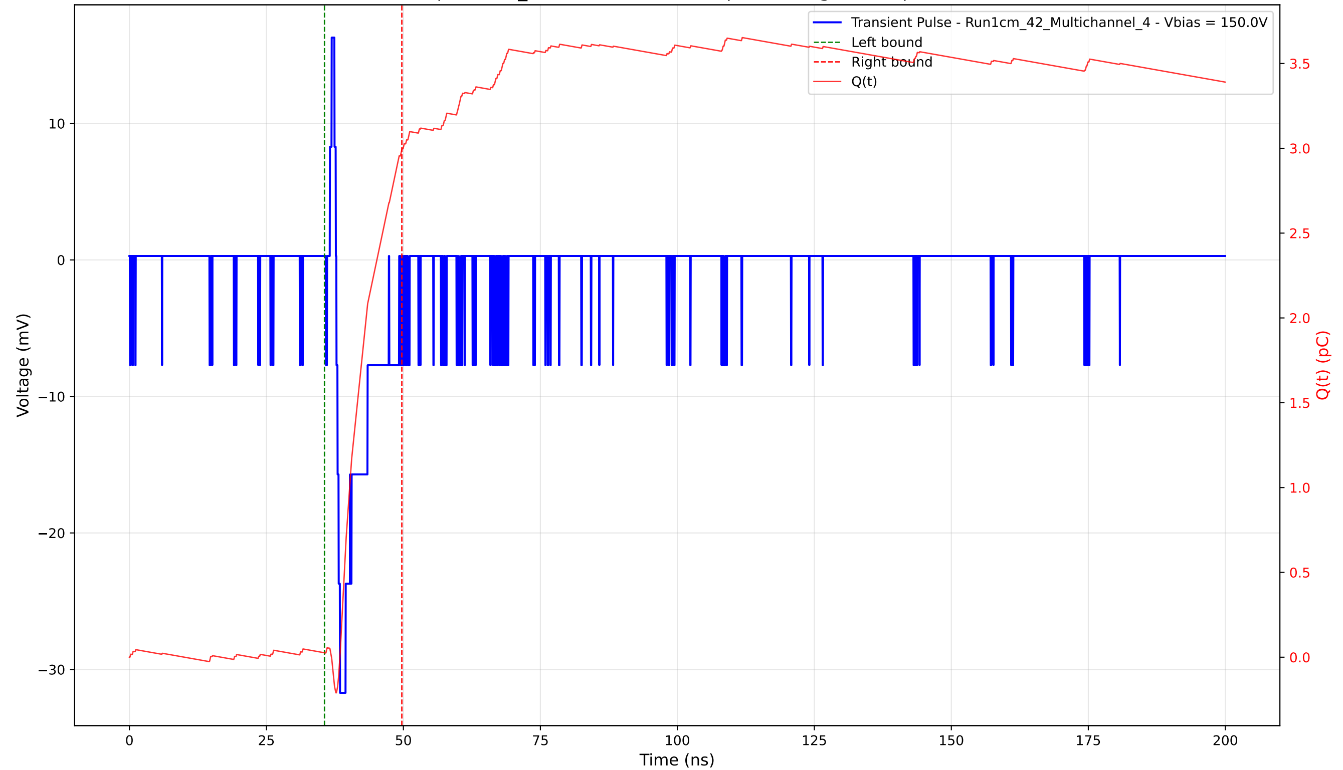
Transient Pulse - Sample: 1cm_42 - Position: 4700.0 \mu\text{m} - Charge: 2.97 pC - Rise Time: 0.66 ns
