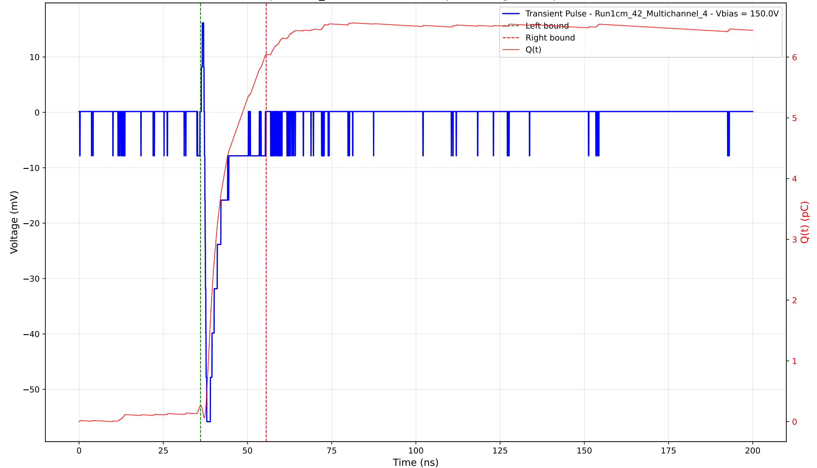
Transient Pulse - Sample: 1cm_42 - Position: 3695.0 \mu\text{m} - Charge: 5.79 pC - Rise Time: 0.69 ns
