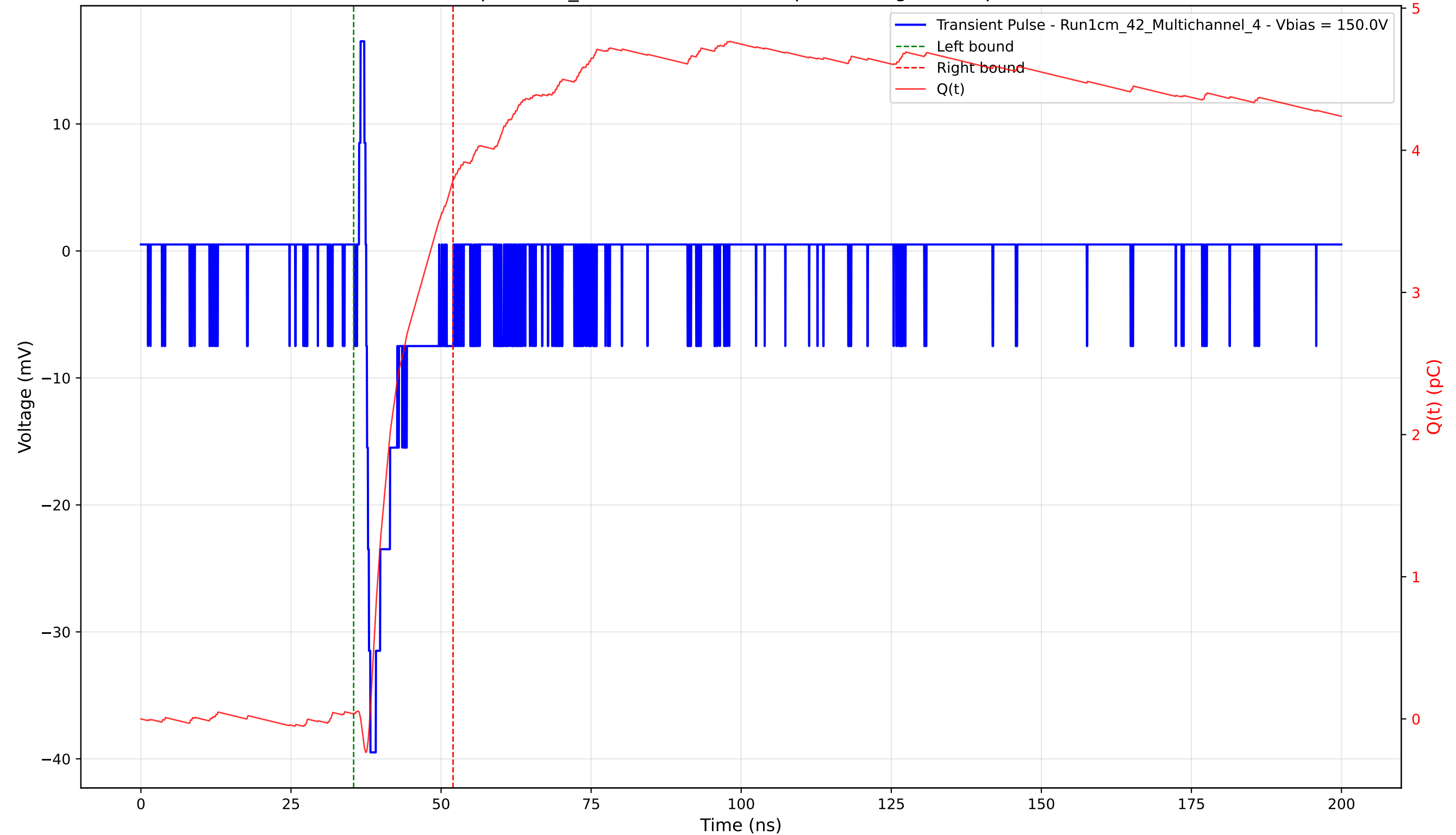
Transient Pulse - Sample: 1cm_42 - Position: 4020.0 \mu\text{m} - Charge: 3.76 pC - Rise Time: 0.70 ns
