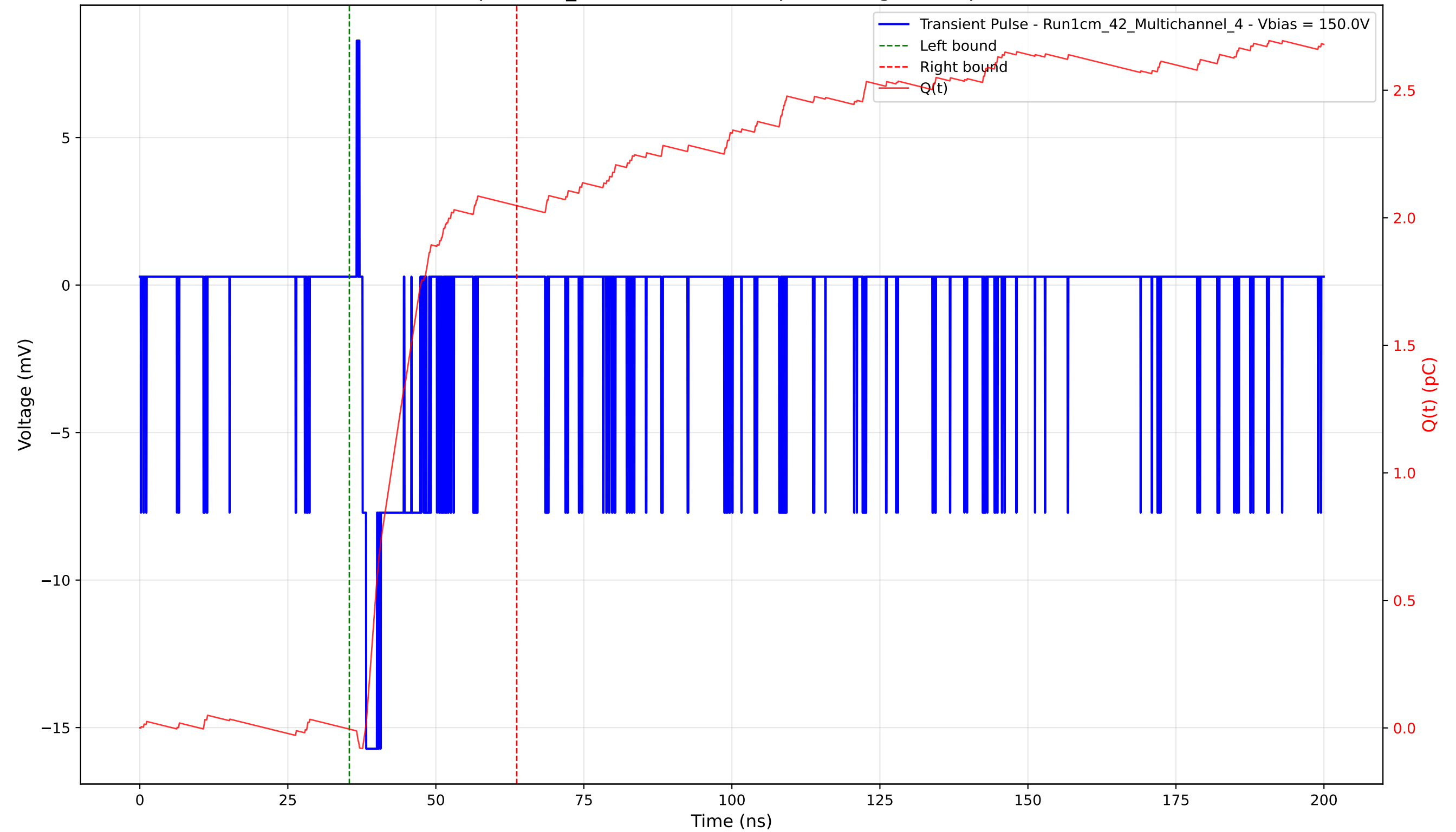
Transient Pulse - Sample: 1cm_42 - Position: 170.0 \mu\text{m} - Charge: 2.05 pC - Rise Time: 0.63 ns
