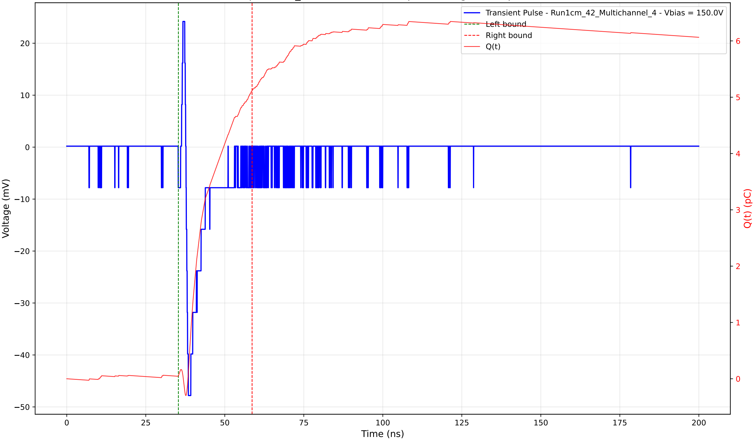
Transient Pulse - Sample: 1cm_42 - Position: 695.0 \mu\text{m} - Charge: 5.06 pC - Rise Time: 0.74 ns
