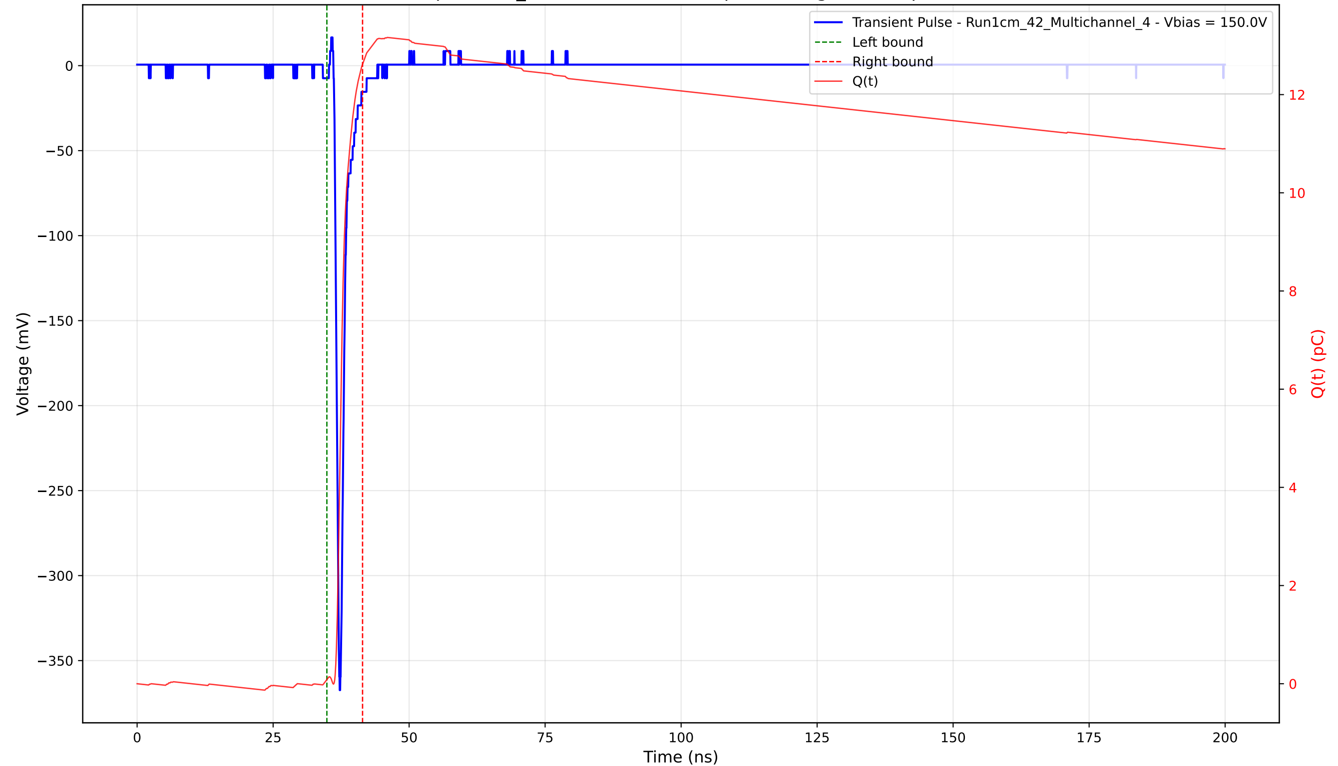
Transient Pulse - Sample: 1cm_42 - Position: 2885.0 \mu\text{m} - Charge: 12.53 pC - Rise Time: 0.72 ns
