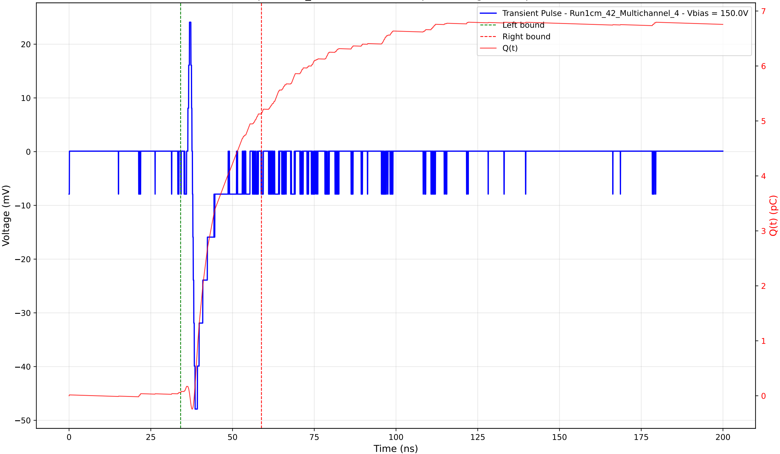
Transient Pulse - Sample: 1cm_42 - Position: 665.0 \mu\text{m} - Charge: 5.08 pC - Rise Time: 0.82 ns
