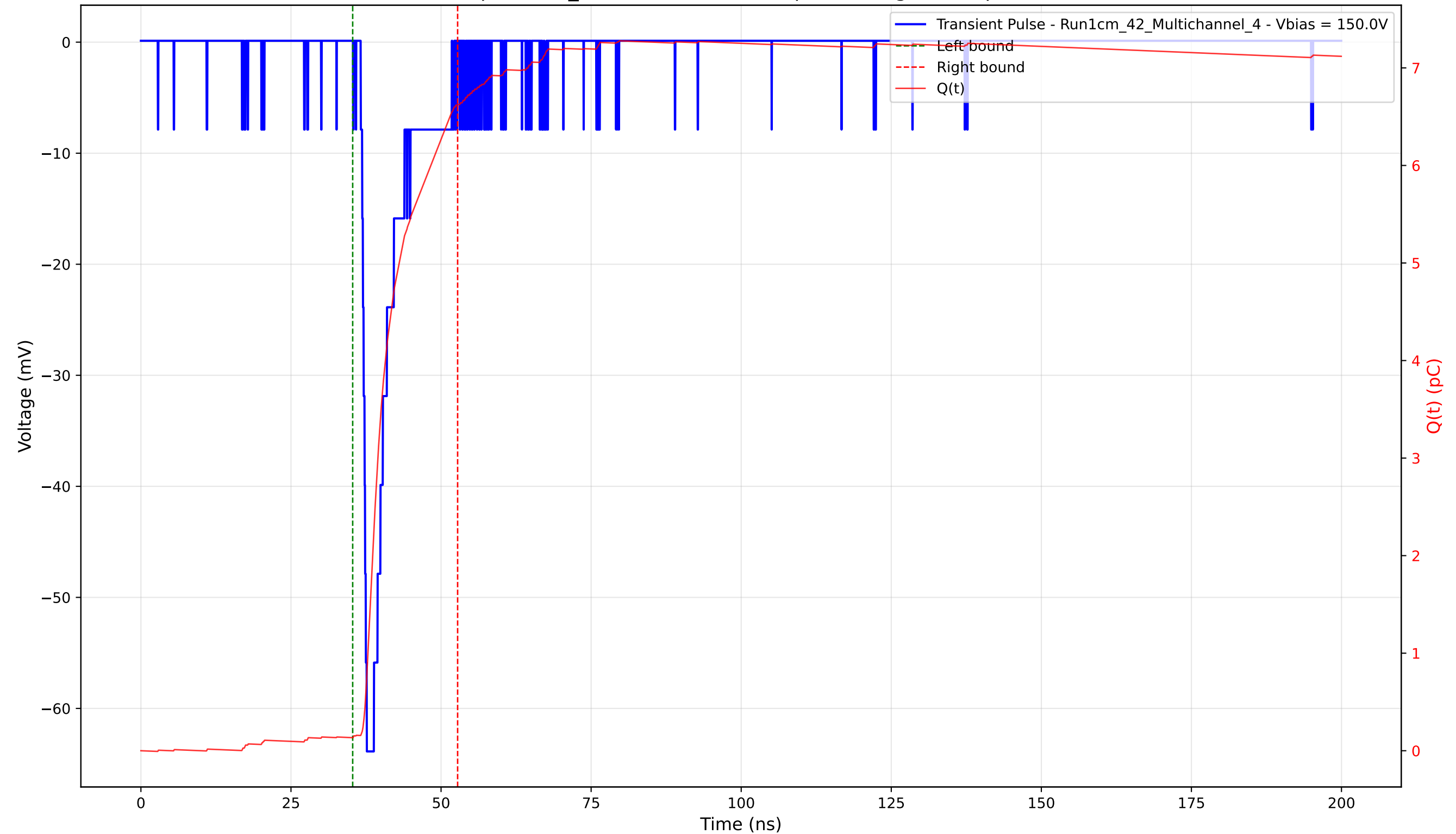
Transient Pulse - Sample: 1cm_42 - Position: 1490.0 \mu\text{m} - Charge: 6.49 pC - Rise Time: 1.01 ns
