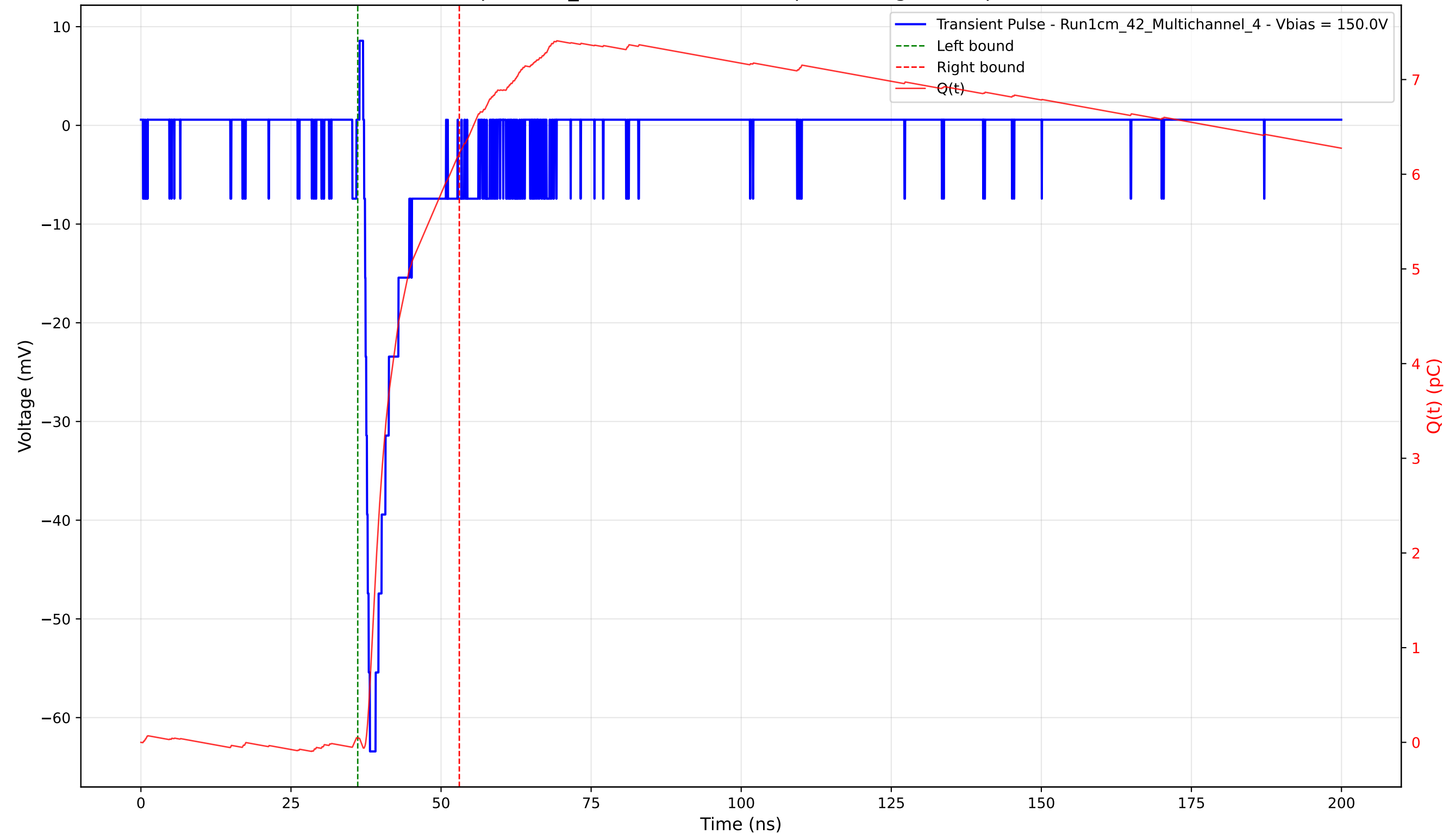
Transient Pulse - Sample: 1cm_42 - Position: 1295.0 \mu\text{m} - Charge: 6.17 pC - Rise Time: 0.97 ns
