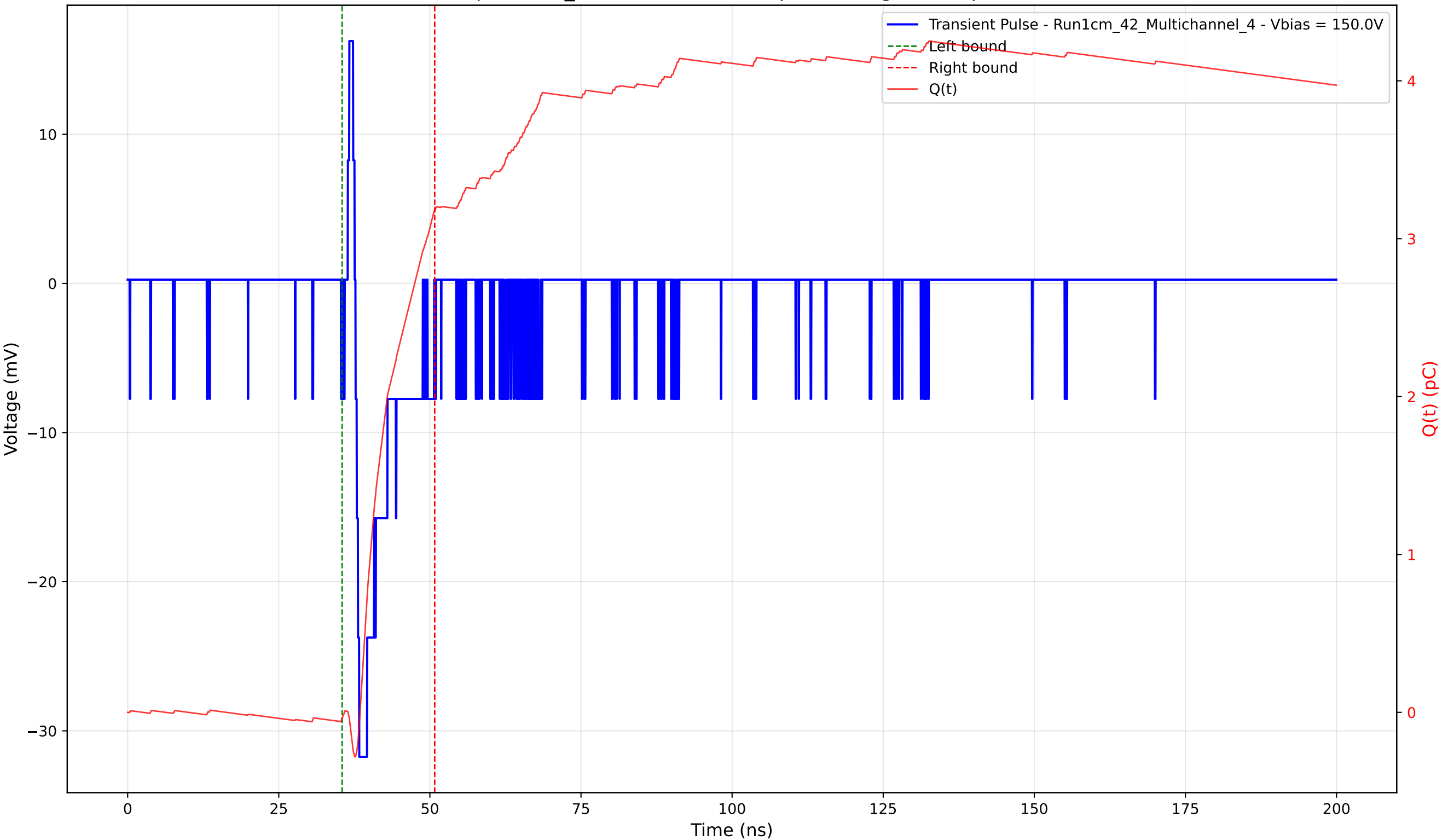
Transient Pulse - Sample: 1cm_42 - Position: 475.0 \mu\text{m} - Charge: 3.21 pC - Rise Time: 0.62 ns
