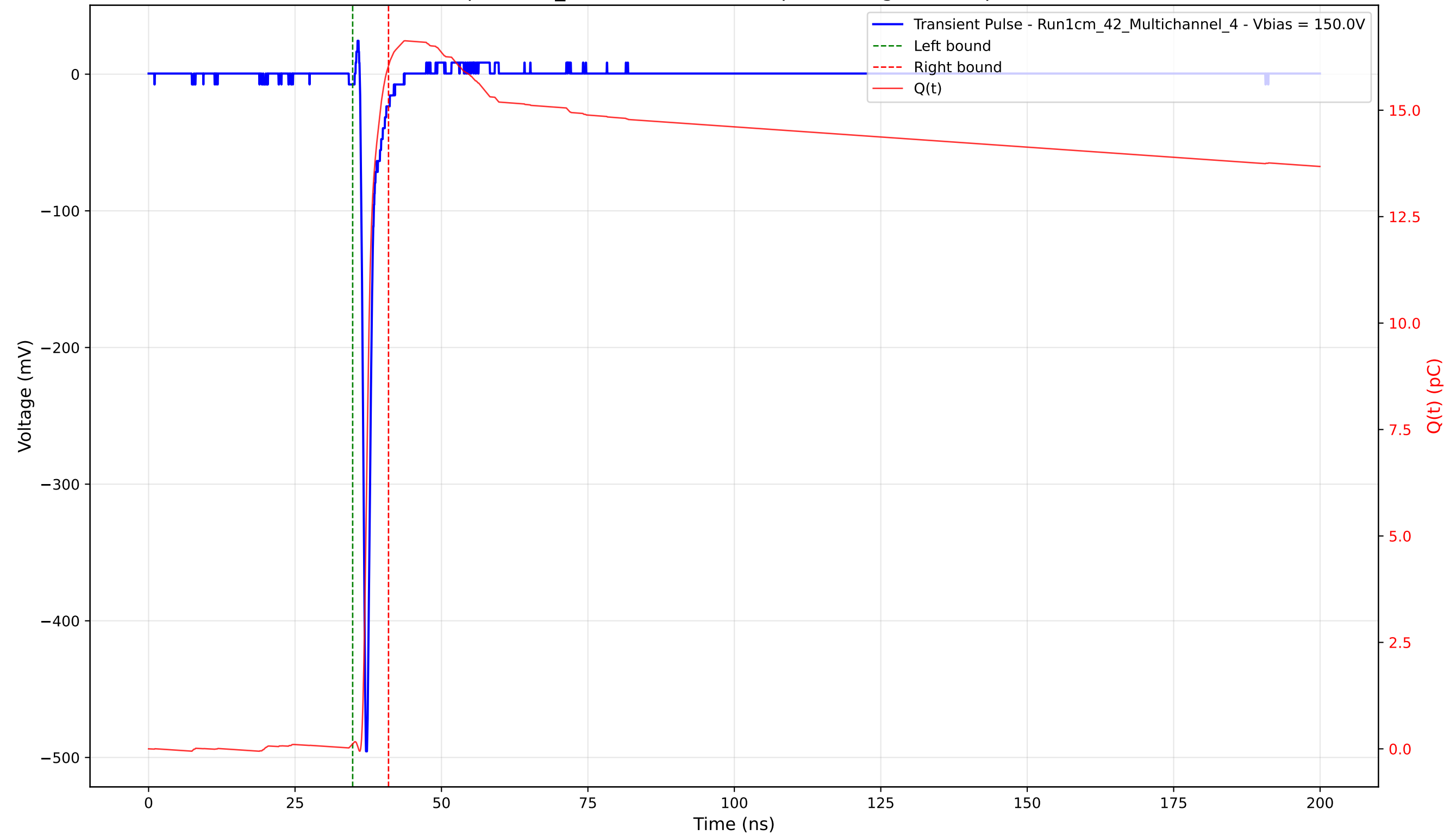
Transient Pulse - Sample: 1cm_42 - Position: 2715.0 \mu\text{m} - Charge: 15.93 pC - Rise Time: 0.73 ns
