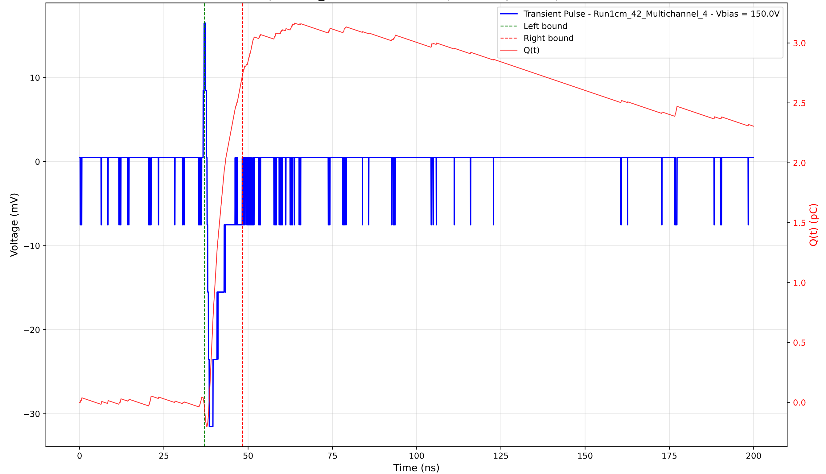
Transient Pulse - Sample: 1cm_42 - Position: 4830.0 \mu\text{m} - Charge: 2.78 pC - Rise Time: 0.66 ns
