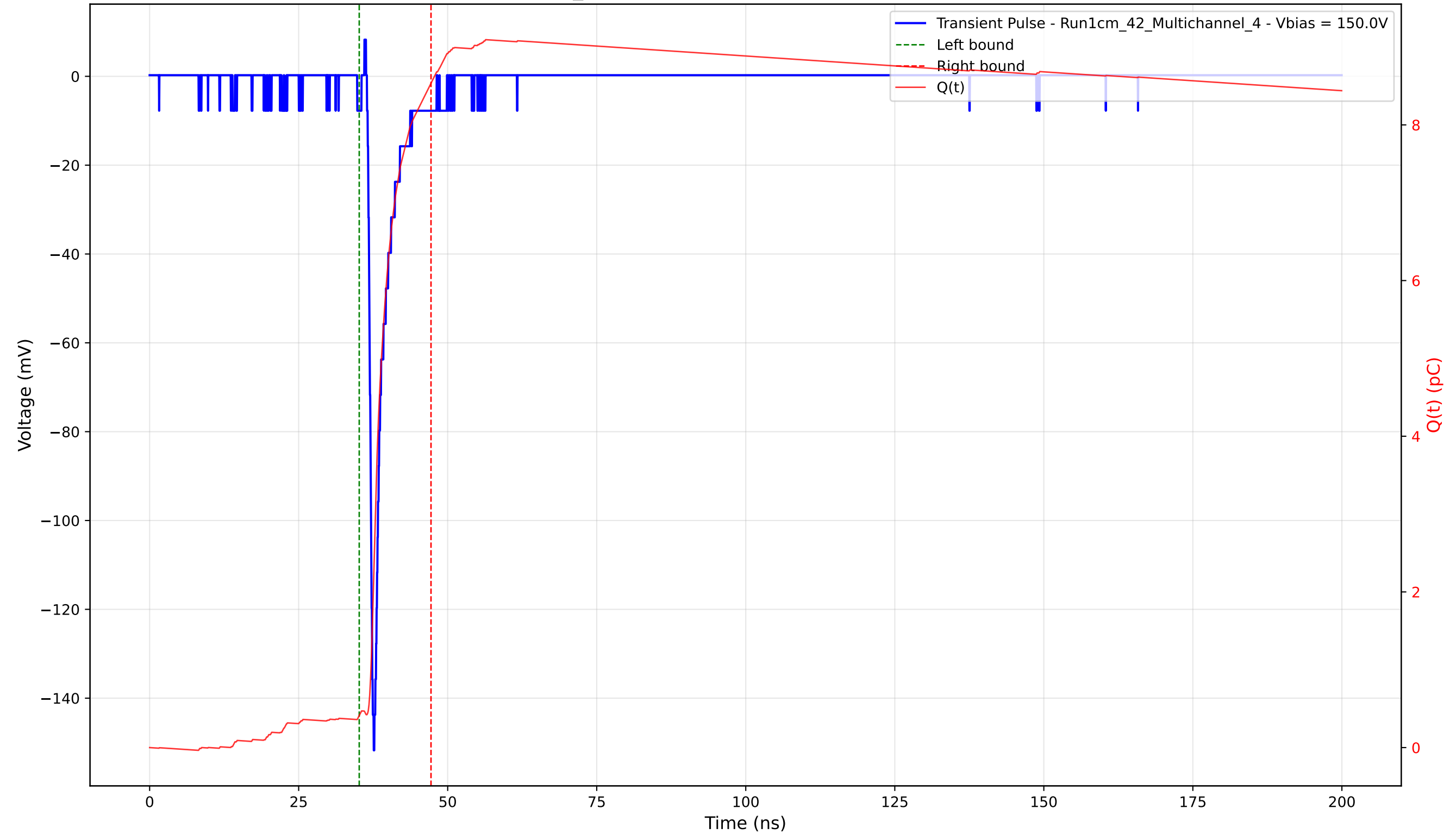
Transient Pulse - Sample: 1cm_42 - Position: 3235.0 \mu\text{m} - Charge: 8.12 pC - Rise Time: 0.84 ns
