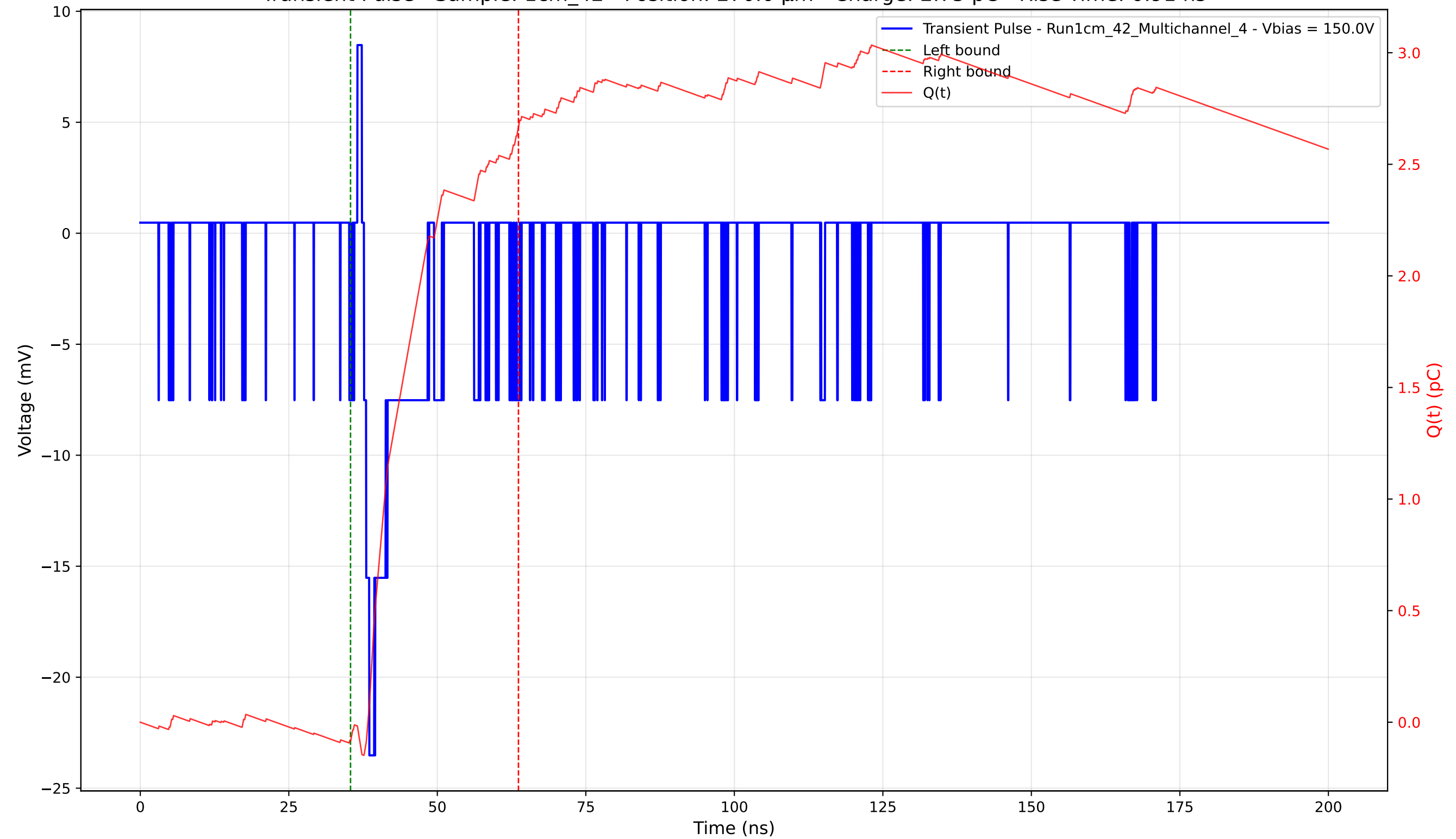
Transient Pulse - Sample: 1cm_42 - Position: 270.0 \mu\text{m} - Charge: 2.75 pC - Rise Time: 0.91 ns
