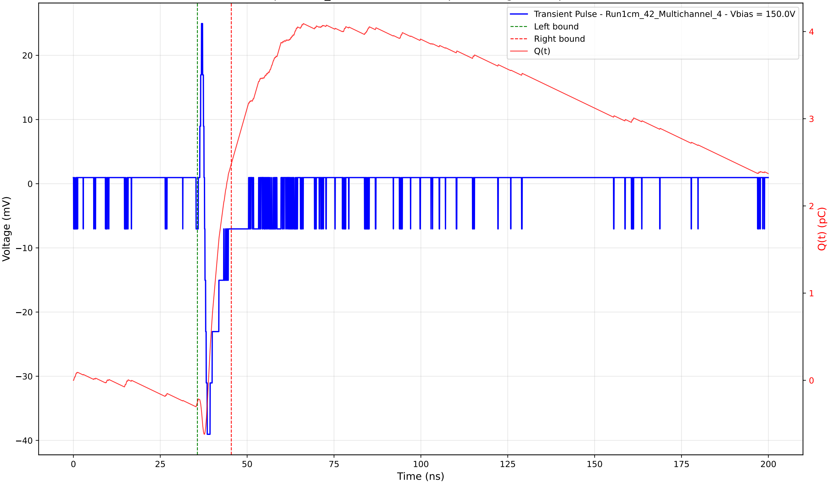
Transient Pulse - Sample: 1cm_42 - Position: 550.0 \mu\text{m} - Charge: 2.73 pC - Rise Time: 0.78 ns
