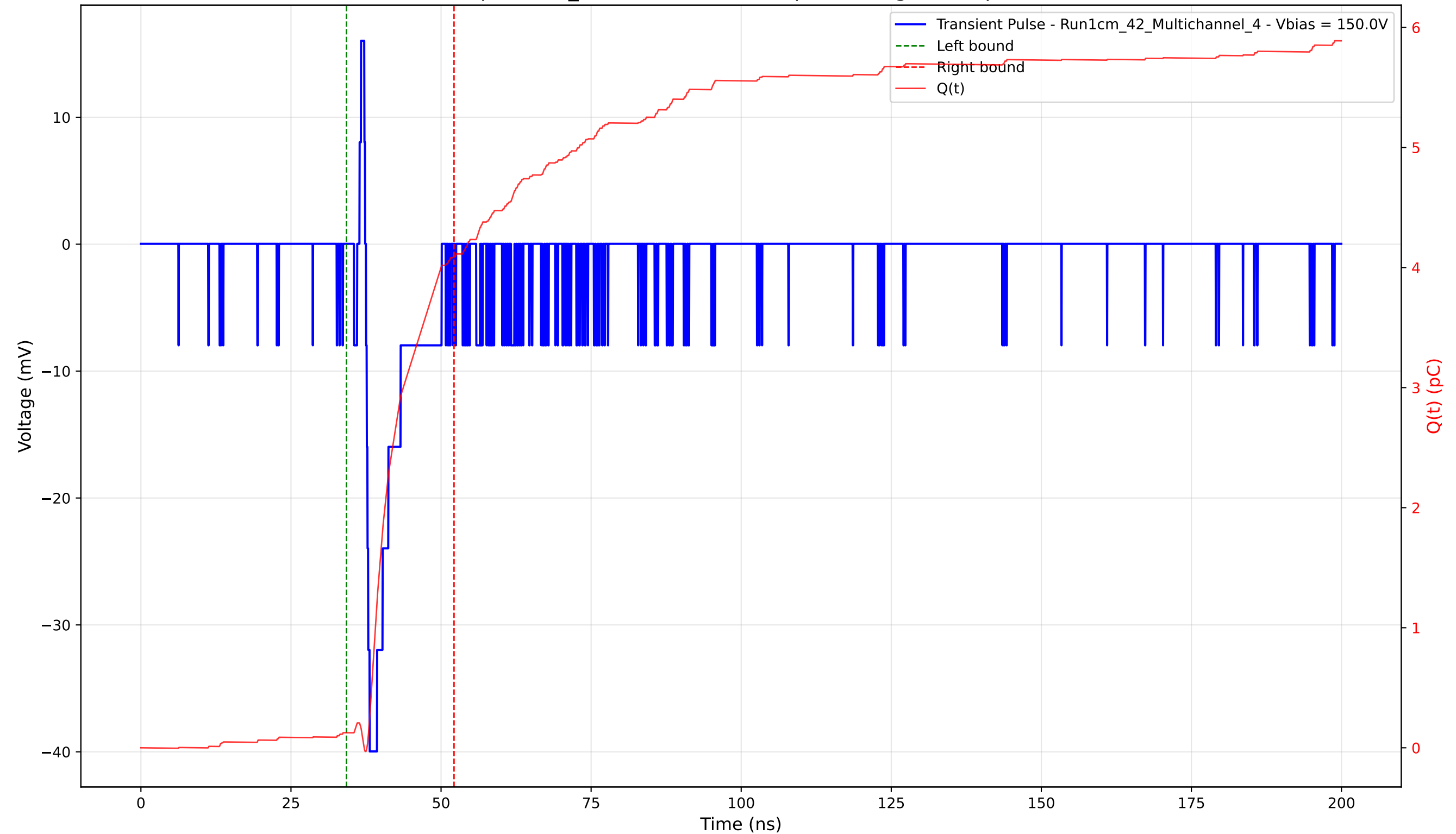
Transient Pulse - Sample: 1cm_42 - Position: 3970.0 \mu\text{m} - Charge: 3.96 pC - Rise Time: 0.62 ns
