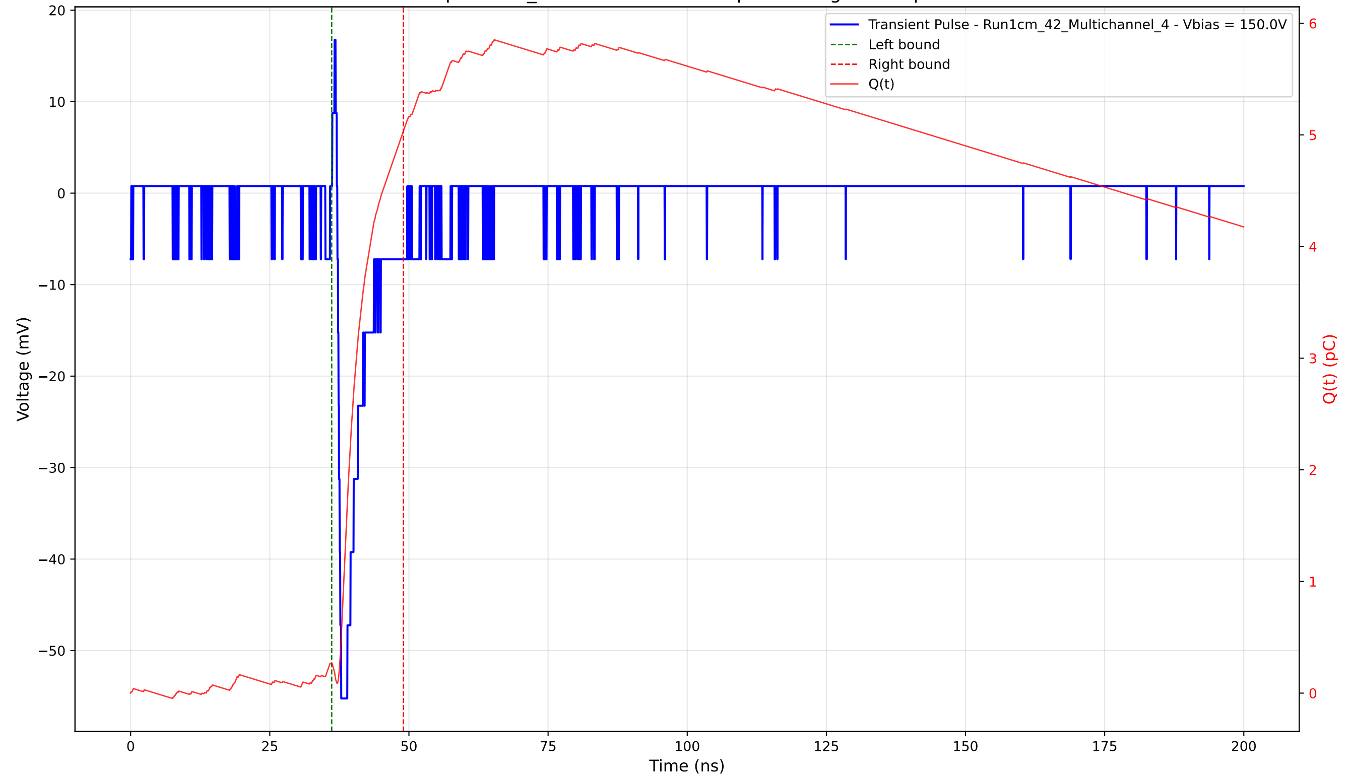
Transient Pulse - Sample: 1cm_42 - Position: 3655.0 \mu\text{m} - Charge: 4.77 pC - Rise Time: 0.69 ns
