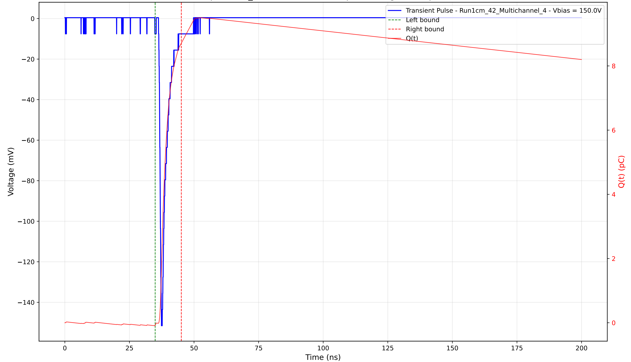
Transient Pulse - Sample: 1cm_42 - Position: 1810.0 \mu\text{m} - Charge: 8.78 pC - Rise Time: 0.92 ns
