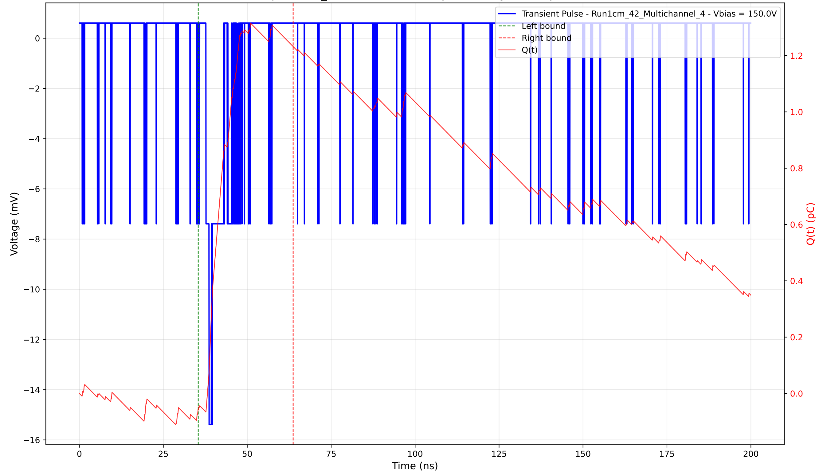
Transient Pulse - Sample: 1cm_42 - Position: 130.0 \mu\text{m} - Charge: 1.29 pC - Rise Time: 0.95 ns
