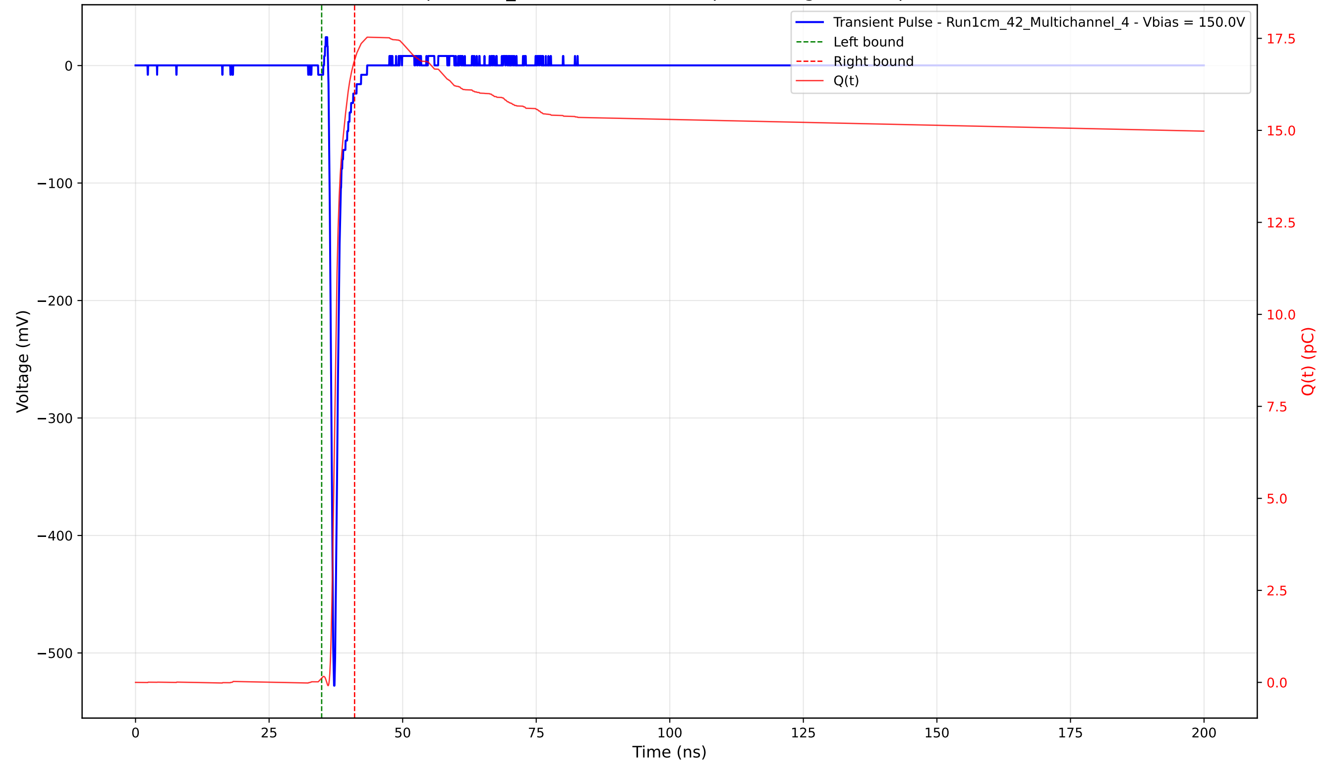
Transient Pulse - Sample: 1cm_42 - Position: 2315.0 \mu\text{m} - Charge: 16.79 pC - Rise Time: 0.74 ns
