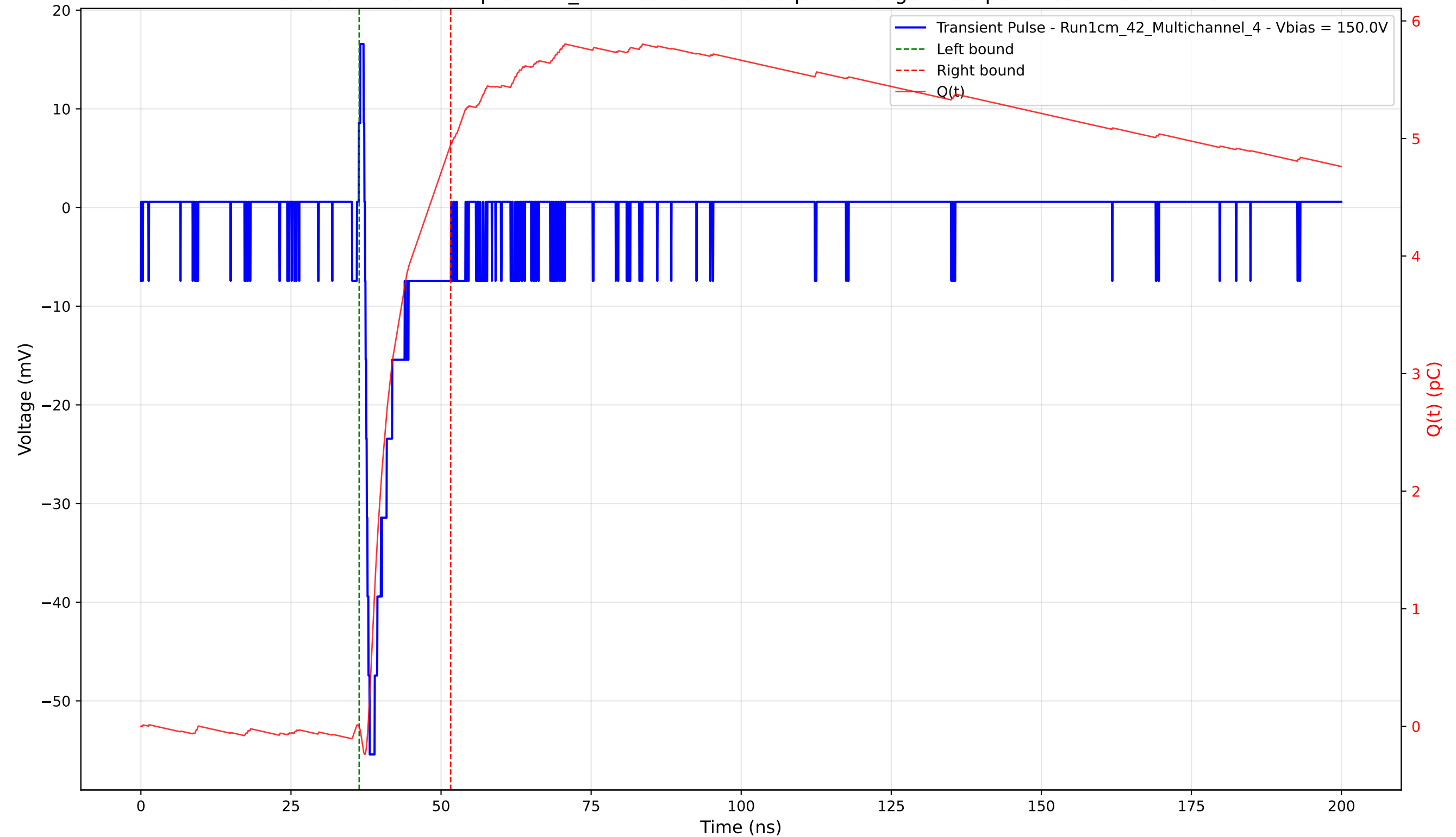
Transient Pulse - Sample: 1cm_42 - Position: 3830.0 \mu\text{m} - Charge: 4.95 pC - Rise Time: 0.77 ns
