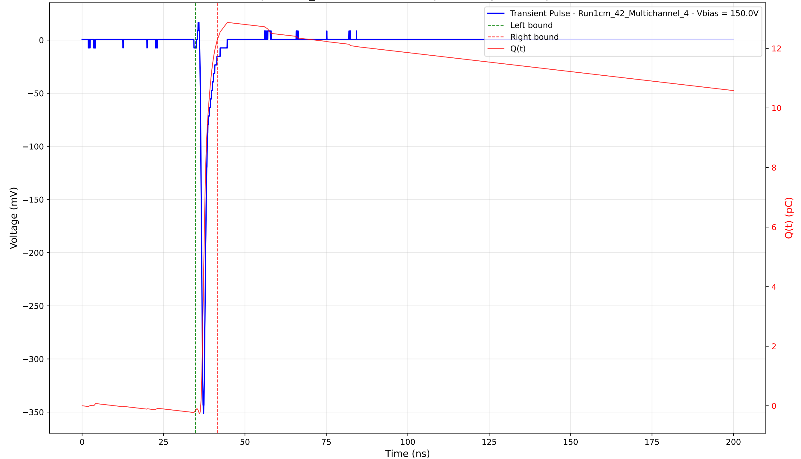
Transient Pulse - Sample: 1cm_42 - Position: 2120.0 \mu\text{m} - Charge: 12.48 pC - Rise Time: 0.77 ns
