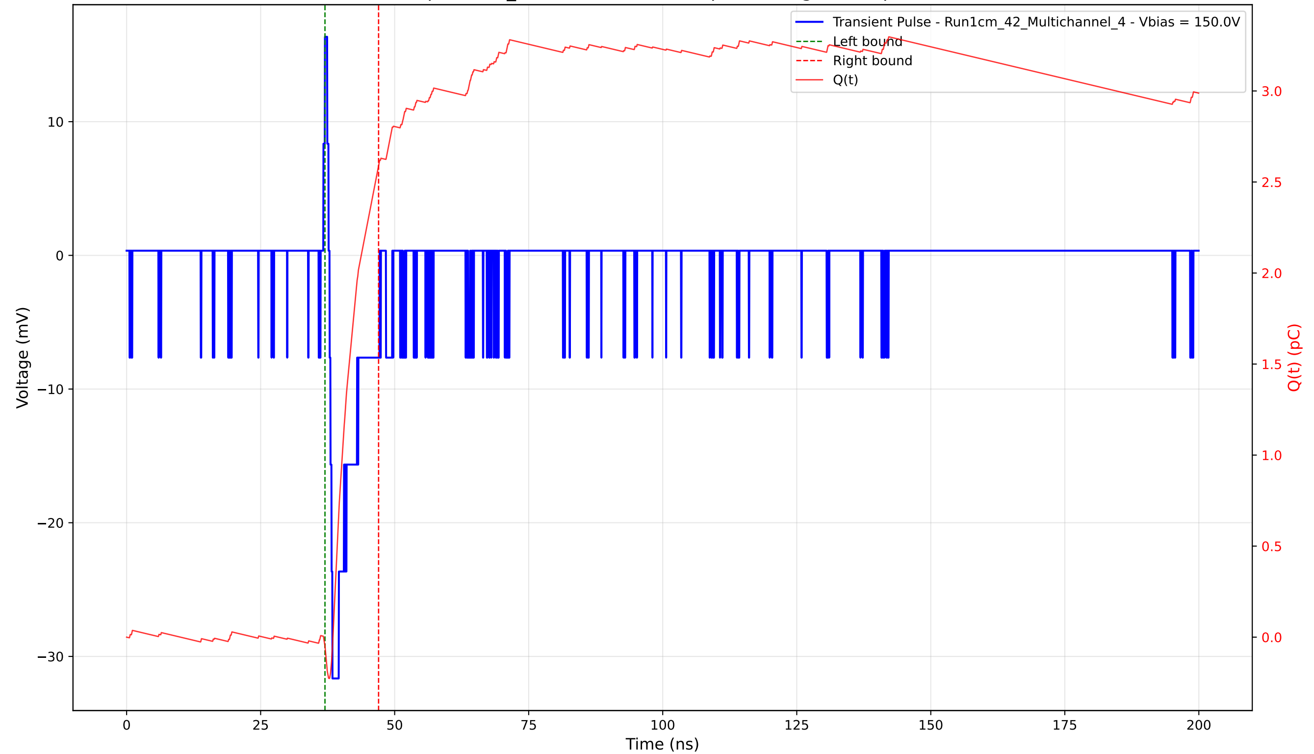
Transient Pulse - Sample: 1cm_42 - Position: 4810.0 \mu\text{m} - Charge: 2.64 pC - Rise Time: 0.54 ns
