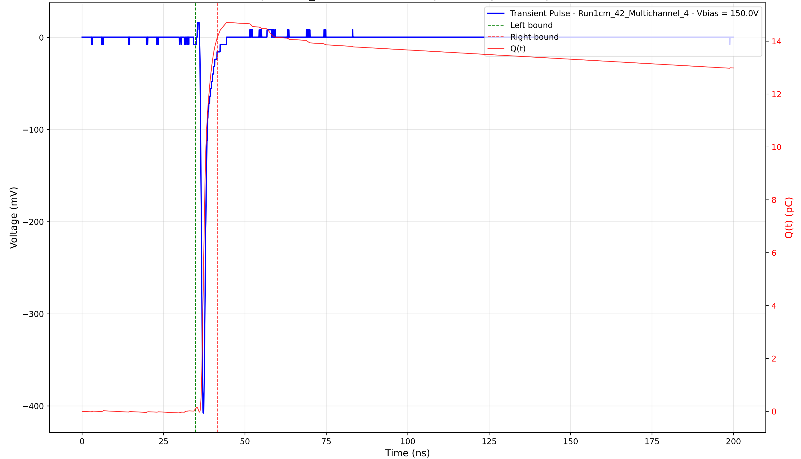
Transient Pulse - Sample: 1cm_42 - Position: 2165.0 \mu\text{m} - Charge: 14.02 pC - Rise Time: 0.71 ns
