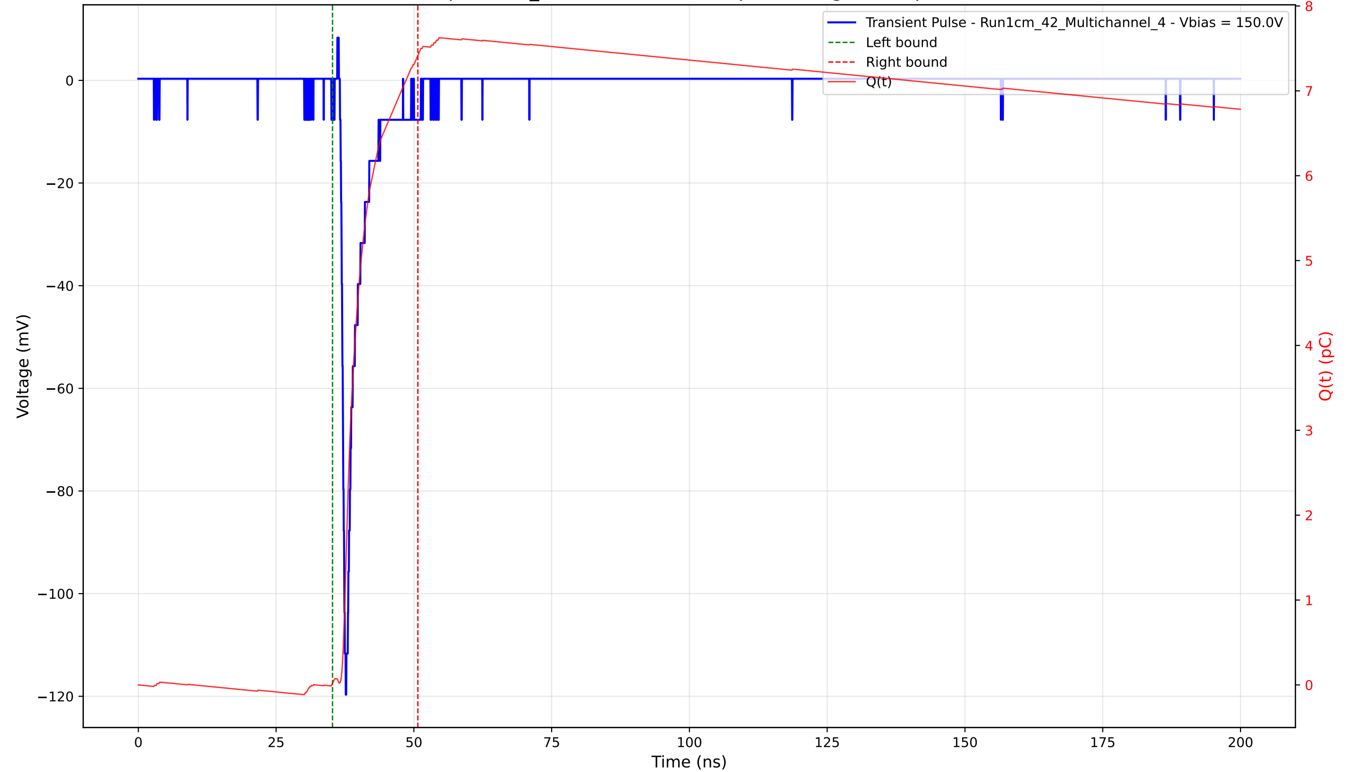
Transient Pulse - Sample: 1cm_42 - Position: 3365.0 \mu\text{m} - Charge: 7.40 pC - Rise Time: 0.78 ns
