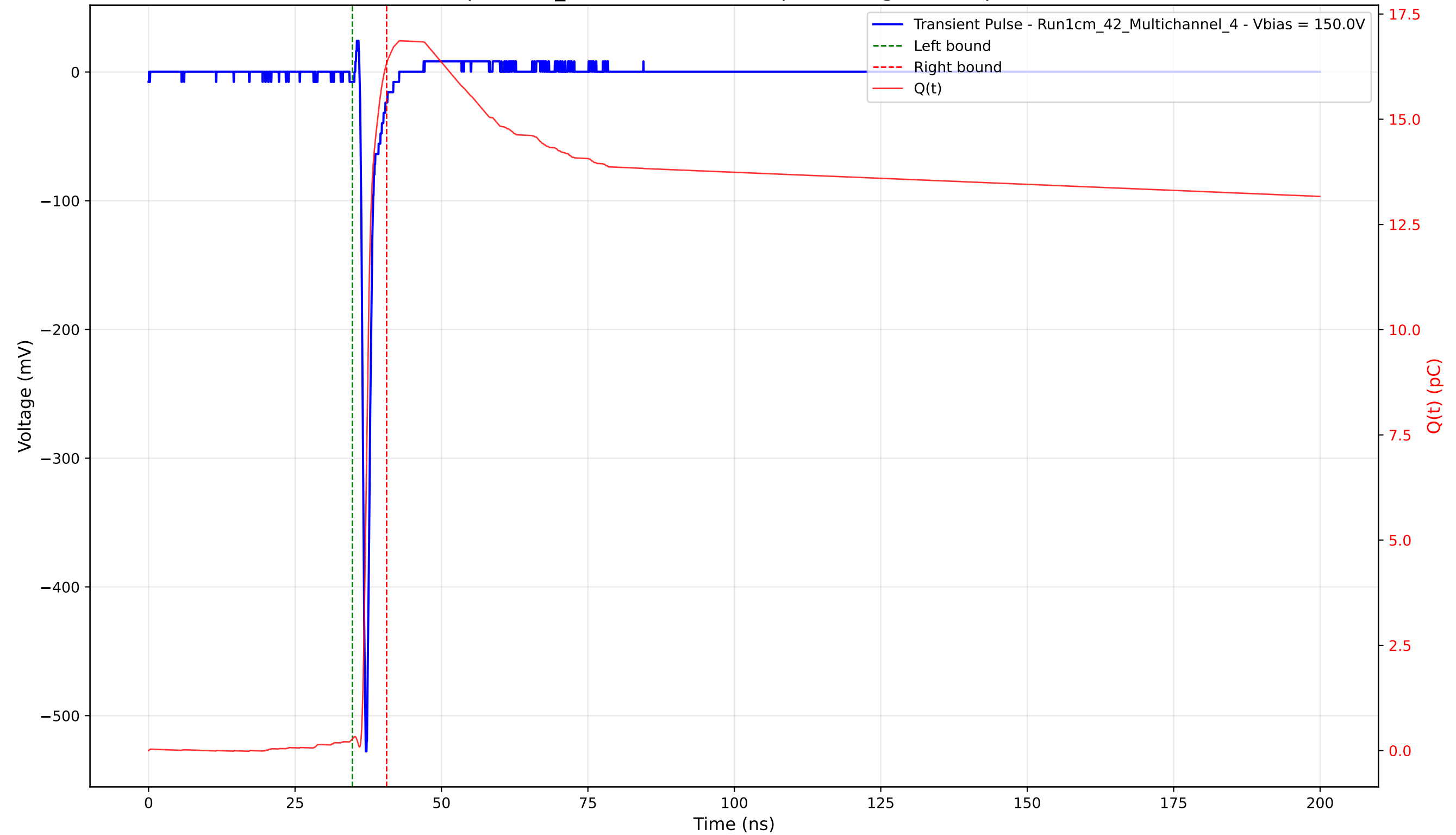
Transient Pulse - Sample: 1cm_42 - Position: 2450.0 \mu\text{m} - Charge: 16.05 pC - Rise Time: 0.72 ns
