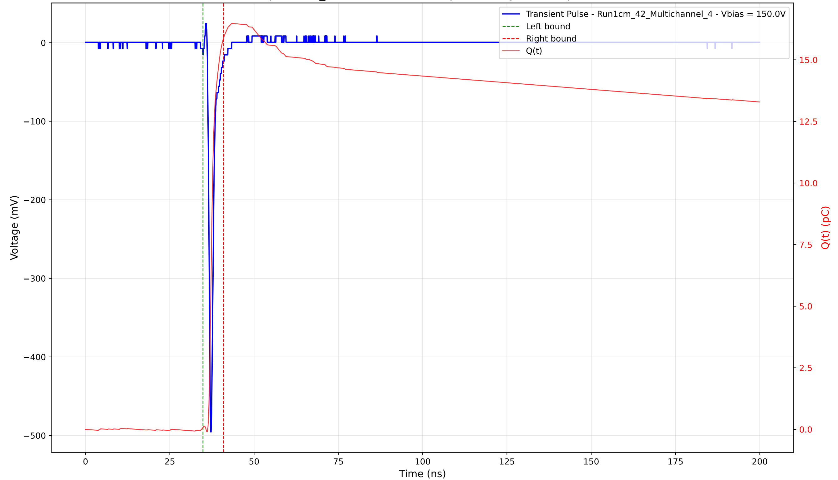
Transient Pulse - Sample: 1cm_42 - Position: 2720.0 \mu\text{m} - Charge: 15.82 pC - Rise Time: 0.73 ns
