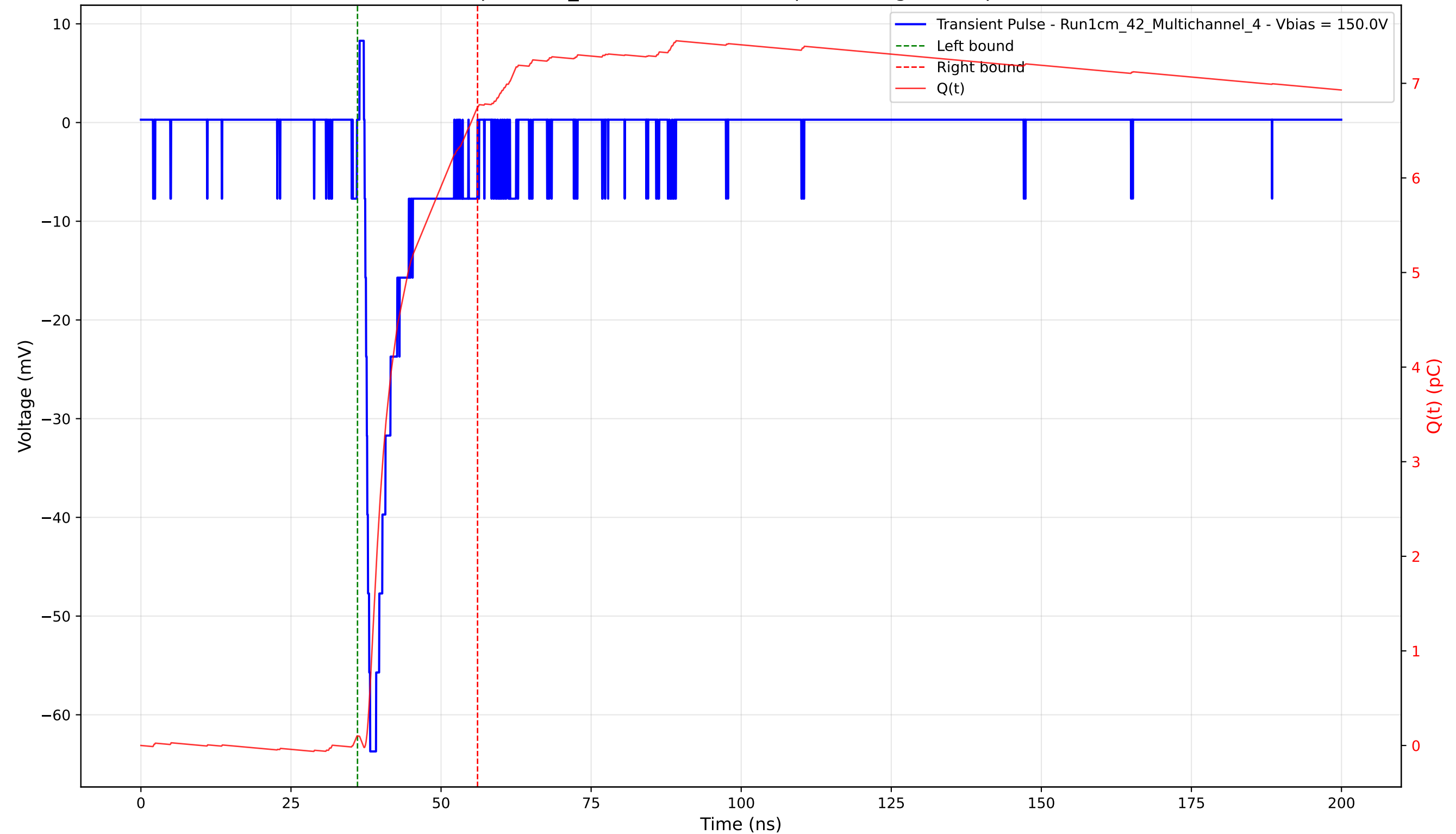
Transient Pulse - Sample: 1cm_42 - Position: 1215.0 \mu\text{m} - Charge: 6.65 pC - Rise Time: 0.93 ns
