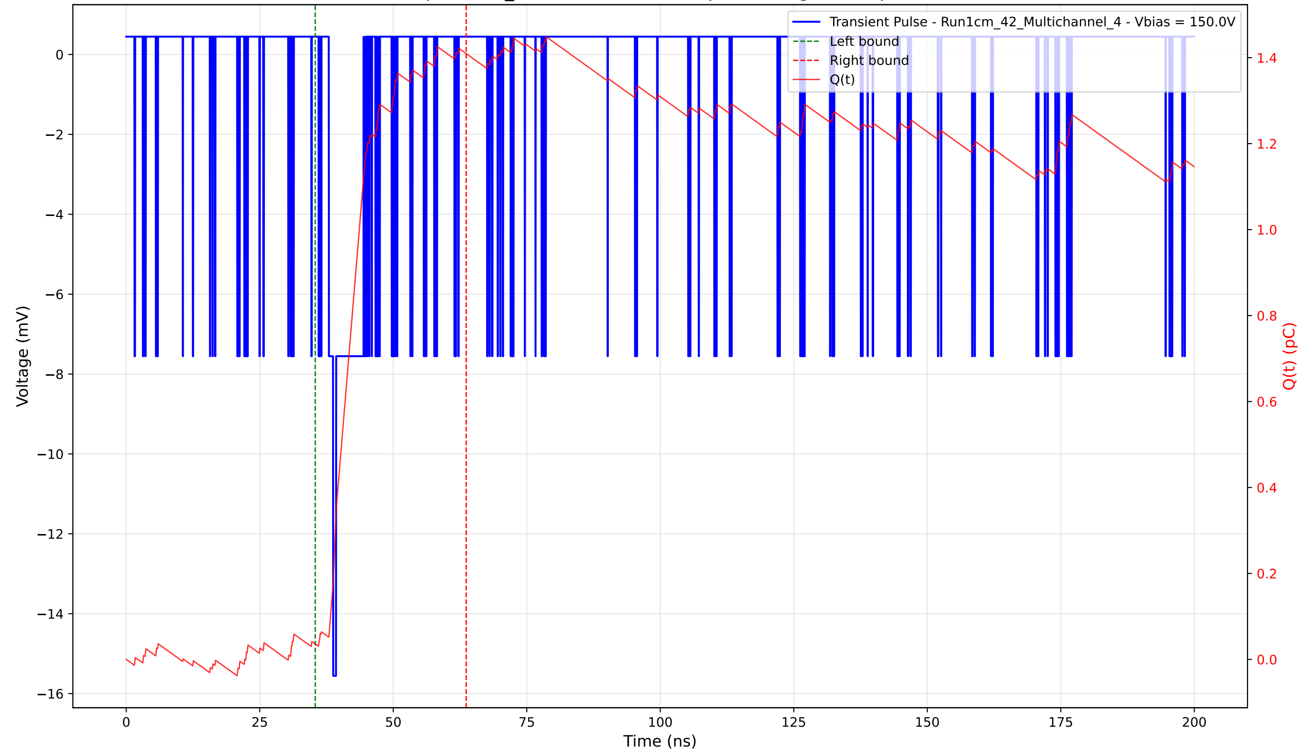
Transient Pulse - Sample: 1cm_42 - Position: 5080.0 \mu\text{m} - Charge: 1.37 pC - Rise Time: 0.83 ns
