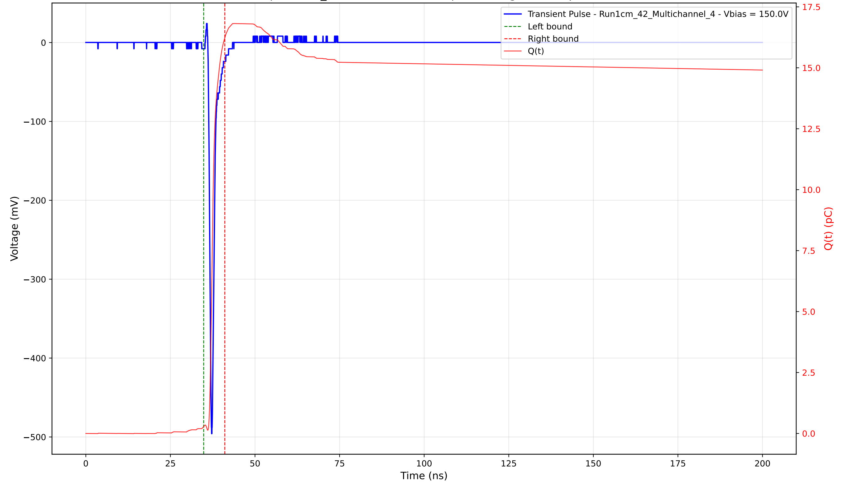
Transient Pulse - Sample: 1cm_42 - Position: 2740.0 \mu\text{m} - Charge: 15.95 pC - Rise Time: 0.71 ns
