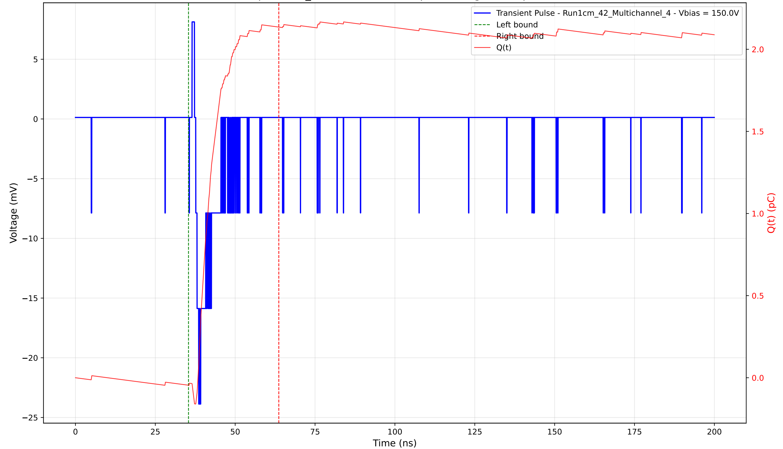
Transient Pulse - Sample: 1cm_42 - Position: 230.0 \mu\text{m} - Charge: 2.18 pC - Rise Time: 0.95 ns
