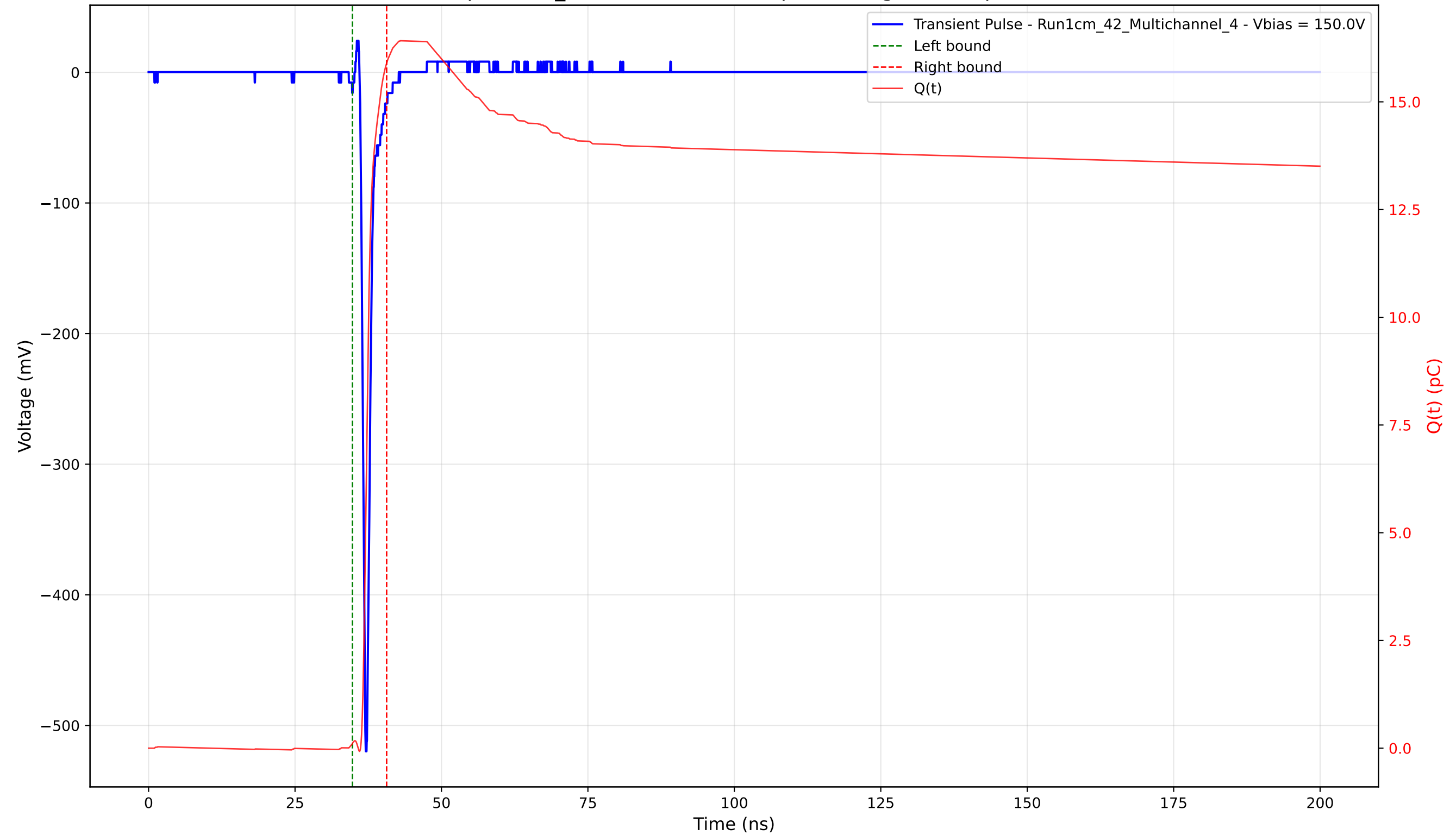
Transient Pulse - Sample: 1cm_42 - Position: 2500.0 \mu\text{m} - Charge: 15.79 pC - Rise Time: 0.72 ns
