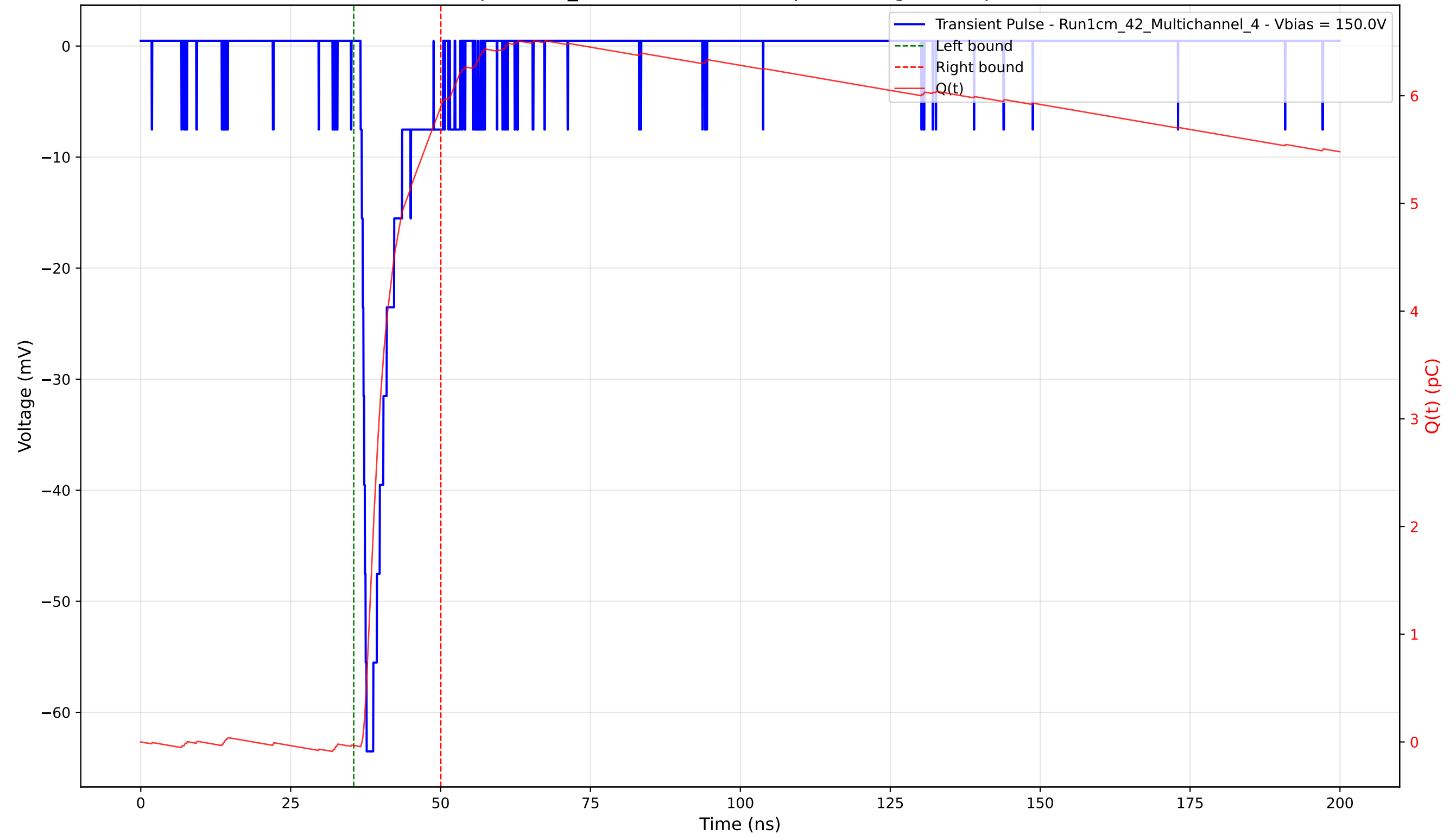
Transient Pulse - Sample: 1cm_42 - Position: 1480.0 \mu\text{m} - Charge: 5.93 pC - Rise Time: 1.01 ns
