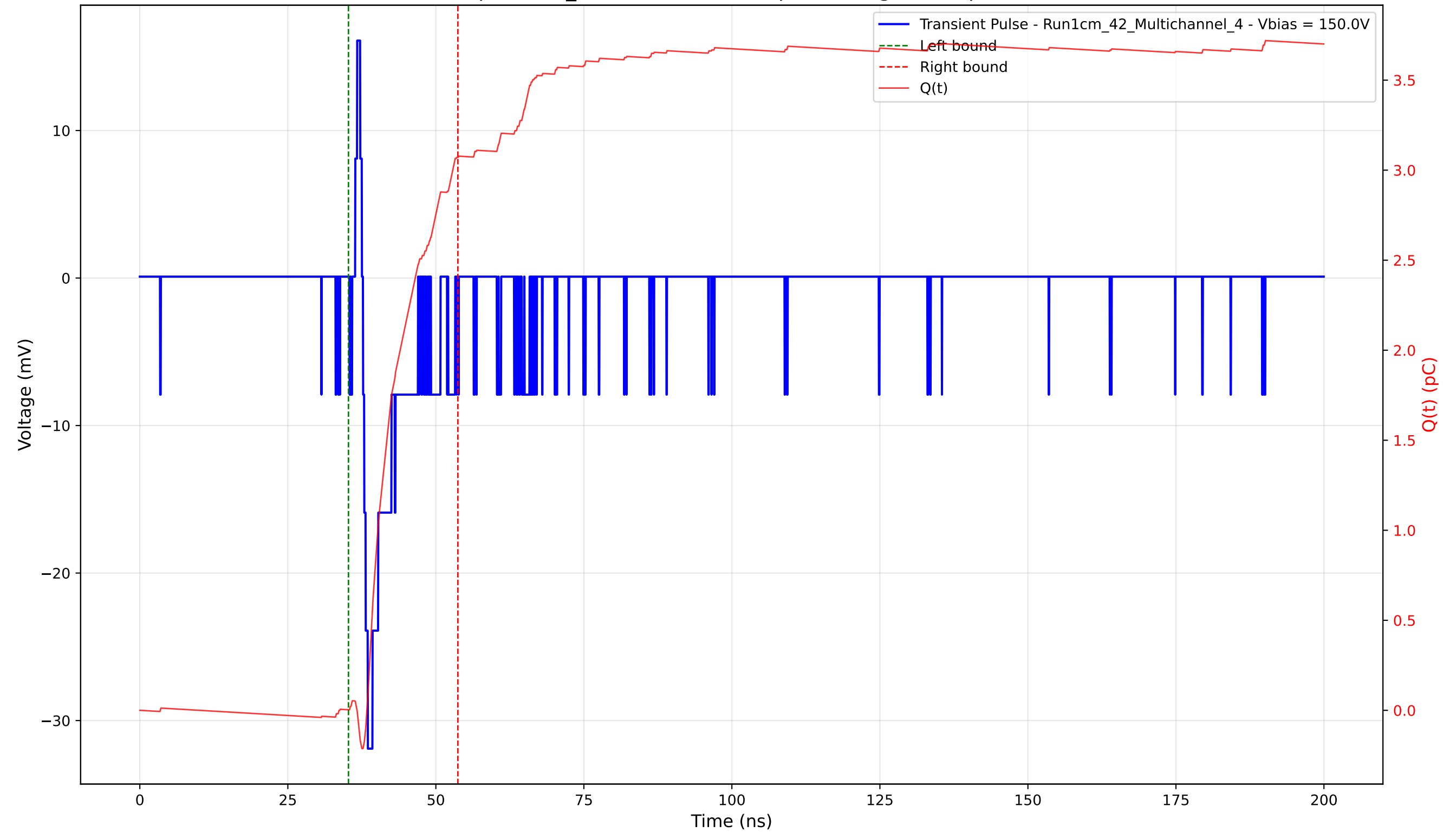
Transient Pulse - Sample: 1cm_42 - Position: 410.0 \mu\text{m} - Charge: 3.07 pC - Rise Time: 0.82 ns
