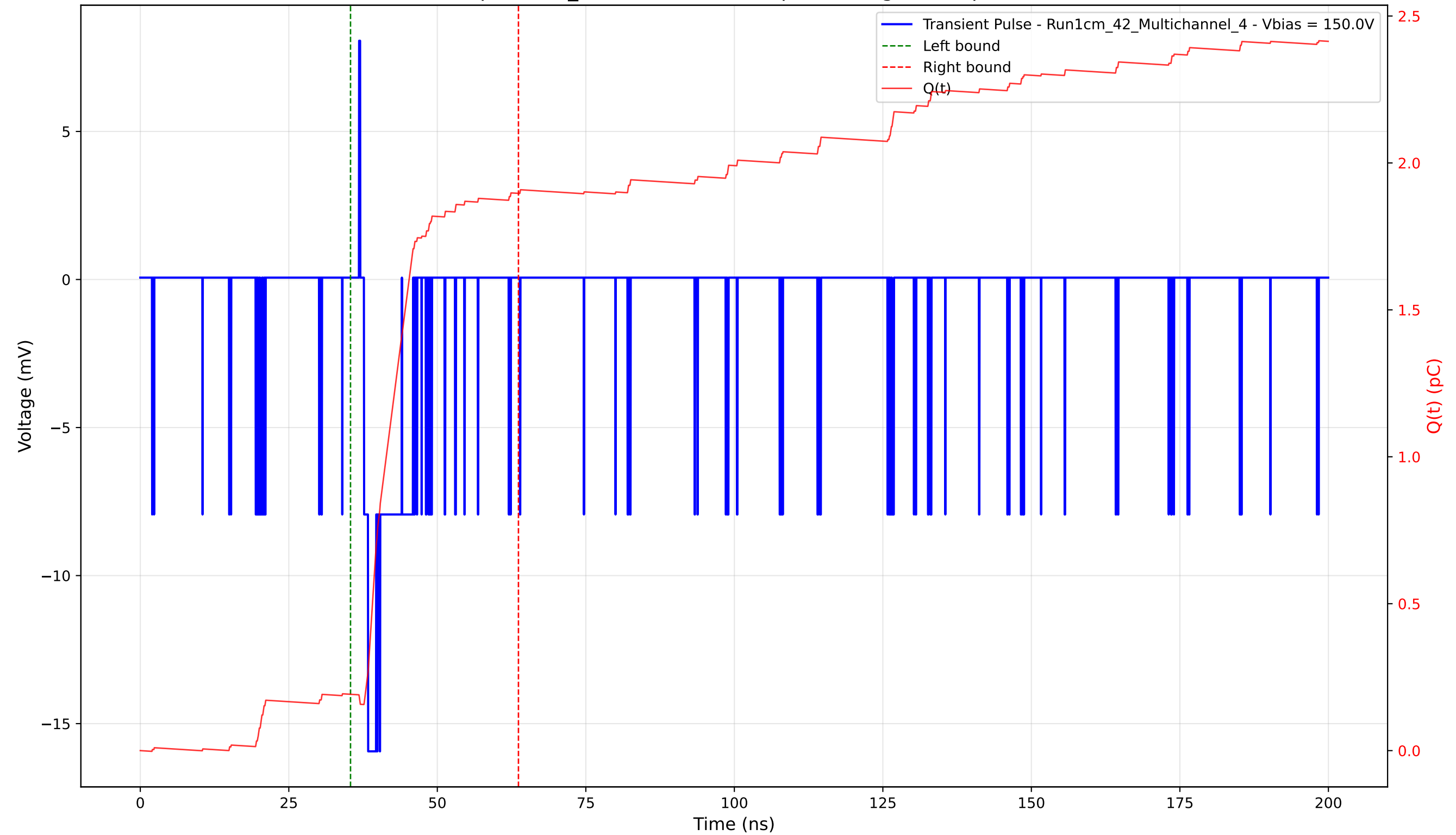
Transient Pulse - Sample: 1cm_42 - Position: 175.0 \mu\text{m} - Charge: 1.70 pC - Rise Time: 0.71 ns
