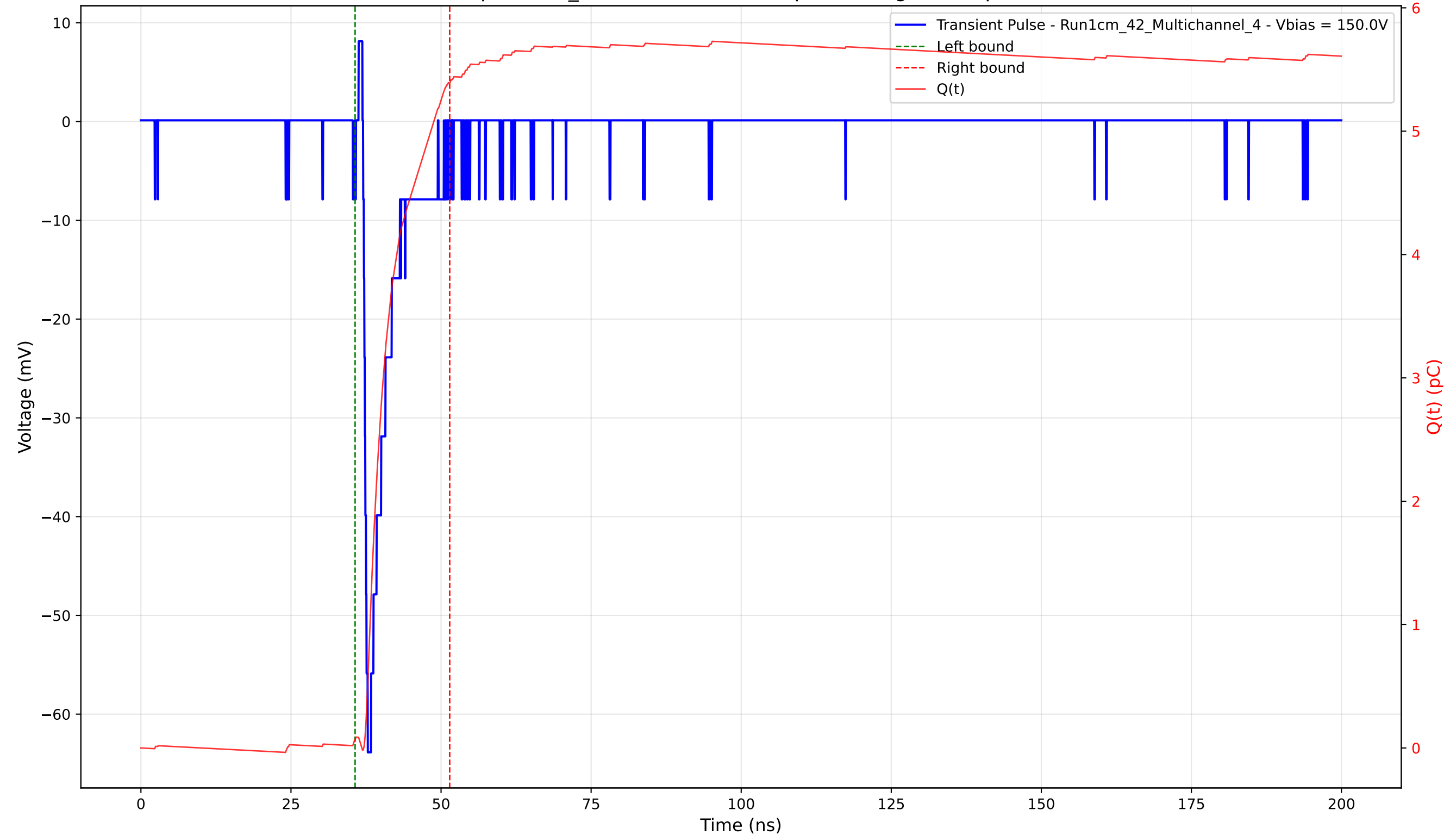
Transient Pulse - Sample: 1cm_42 - Position: 3580.0 \mu\text{m} - Charge: 5.32 pC - Rise Time: 0.77 ns
