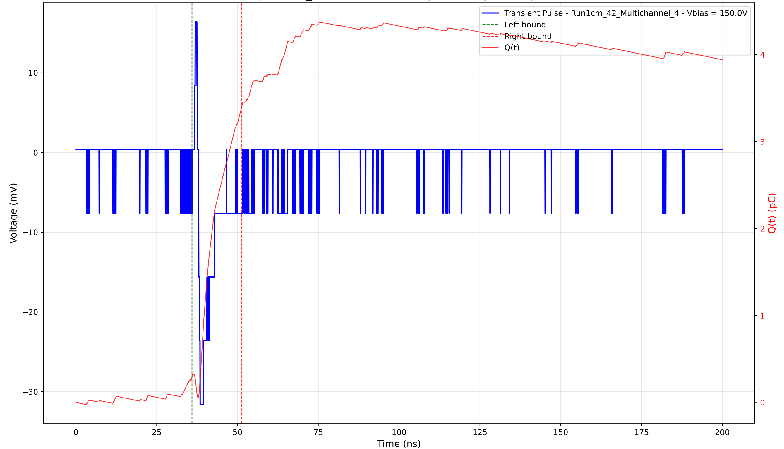
Transient Pulse - Sample: 1cm_42 - Position: 4725.0 \mu\text{m} - Charge: 3.12 pC - Rise Time: 0.58 ns
