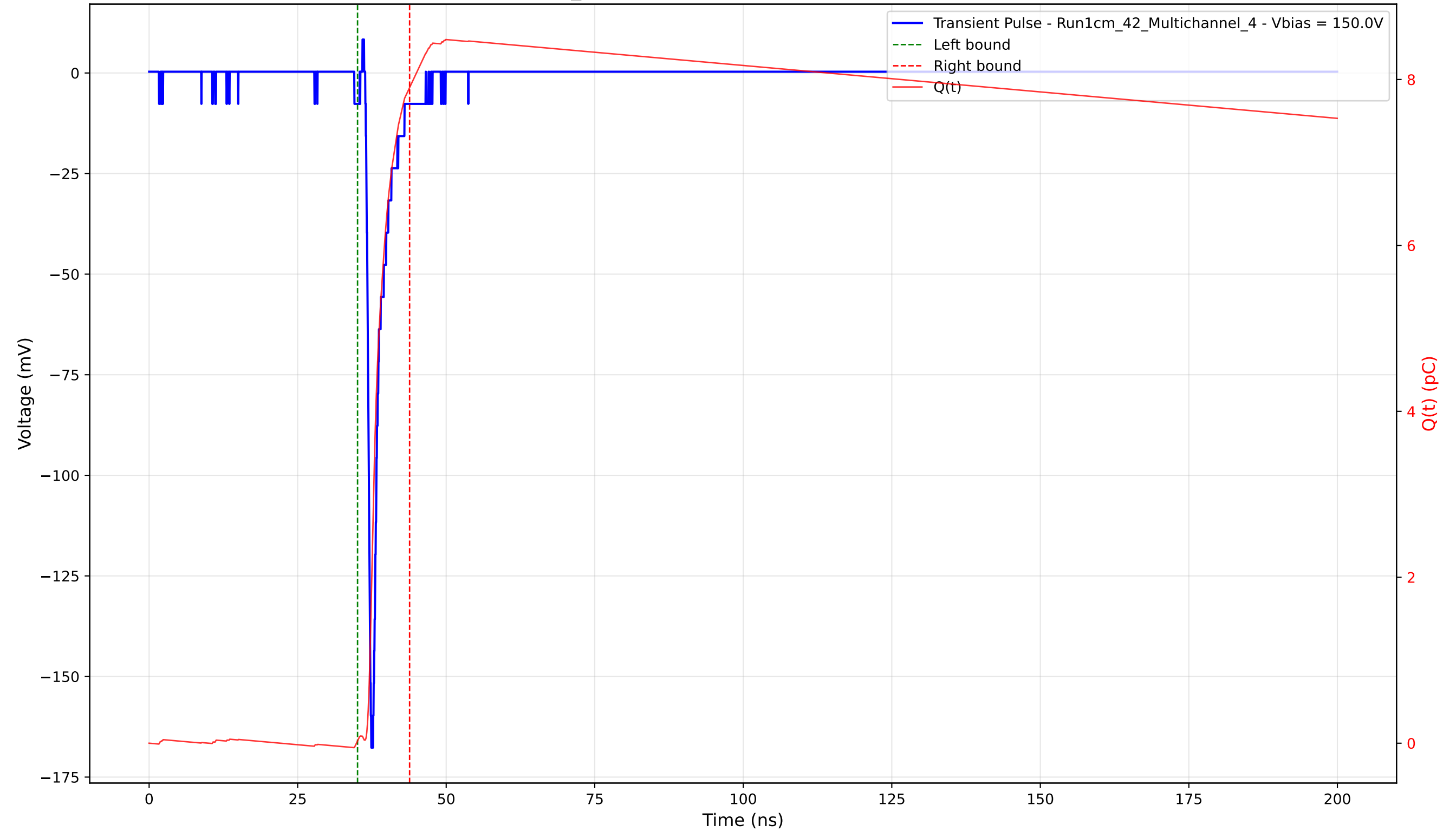
Transient Pulse - Sample: 1cm_42 - Position: 3135.0 \mu\text{m} - Charge: 7.87 pC - Rise Time: 0.71 ns
