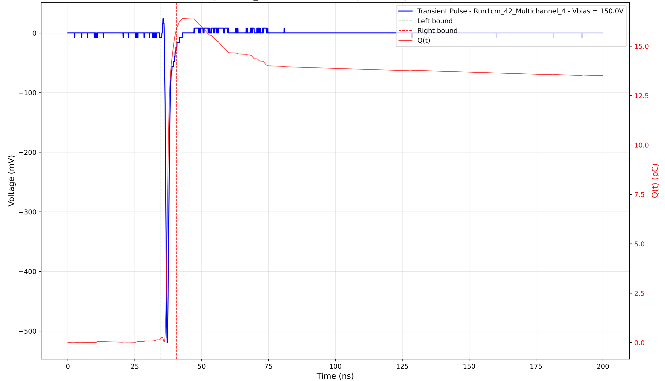
Transient Pulse - Sample: 1cm_42 - Position: 2510.0 \mu\text{m} - Charge: 15.69 pC - Rise Time: 0.72 ns
