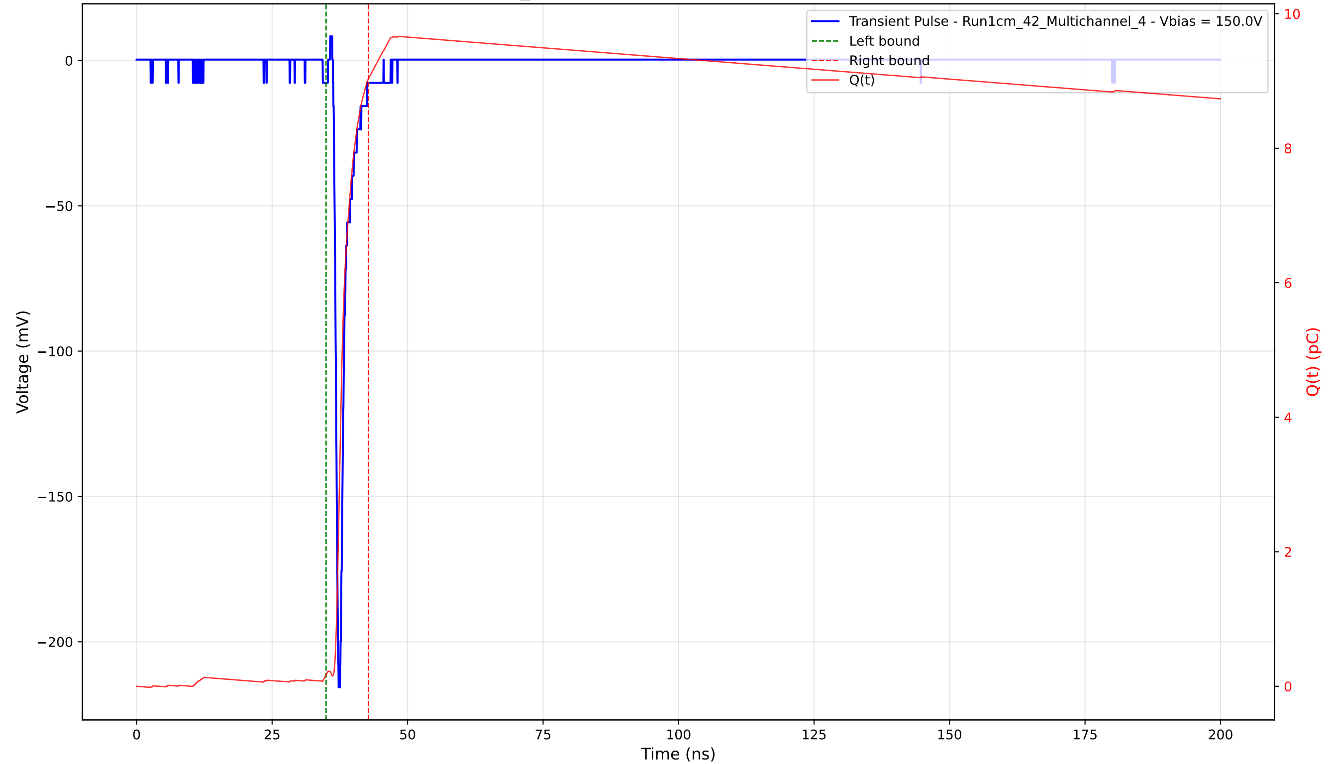
Transient Pulse - Sample: 1cm_42 - Position: 3030.0 \mu\text{m} - Charge: 8.86 pC - Rise Time: 0.74 ns
