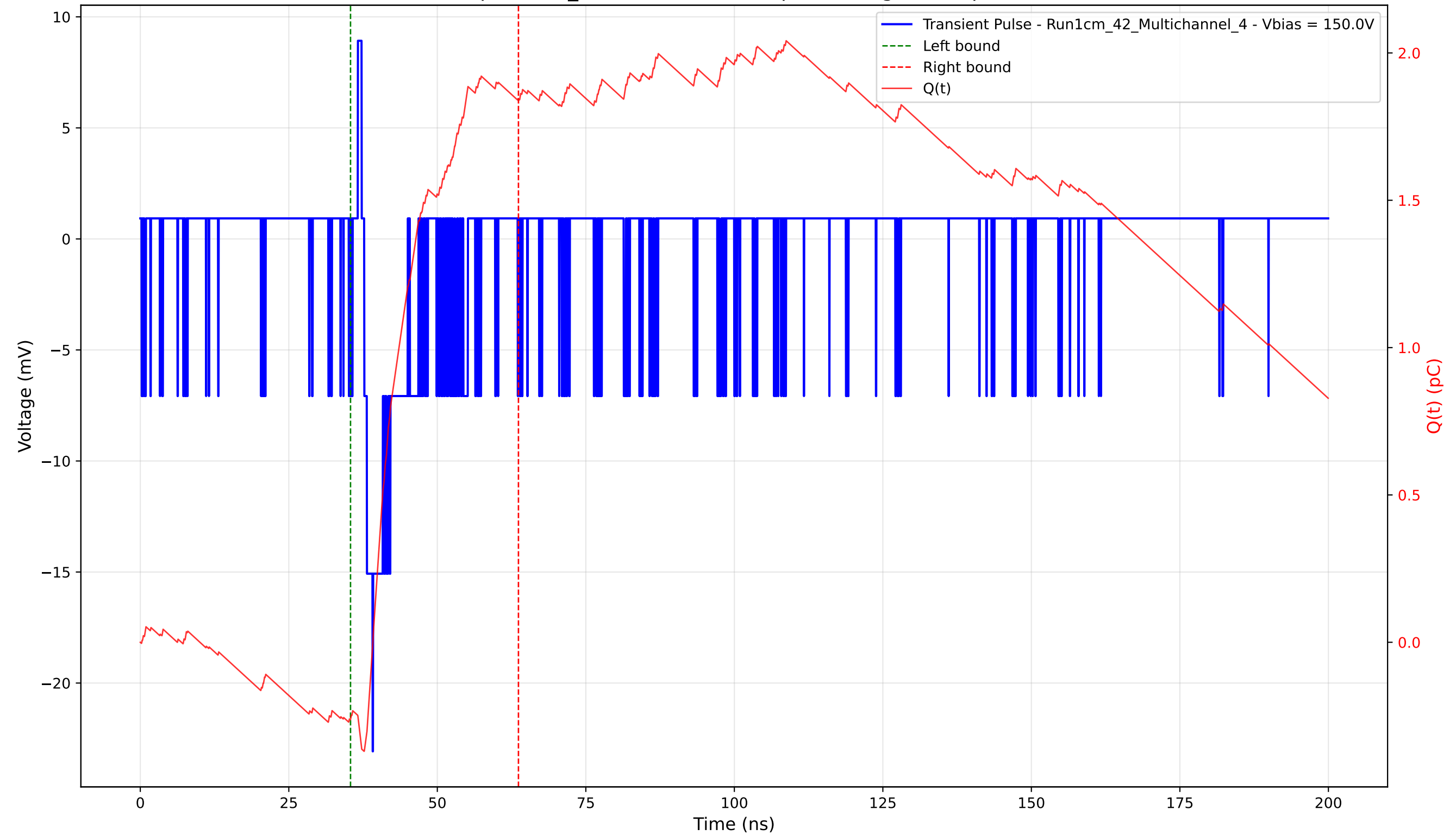
Transient Pulse - Sample: 1cm_42 - Position: 200.0 \mu\text{m} - Charge: 2.11 pC - Rise Time: 1.43 ns
