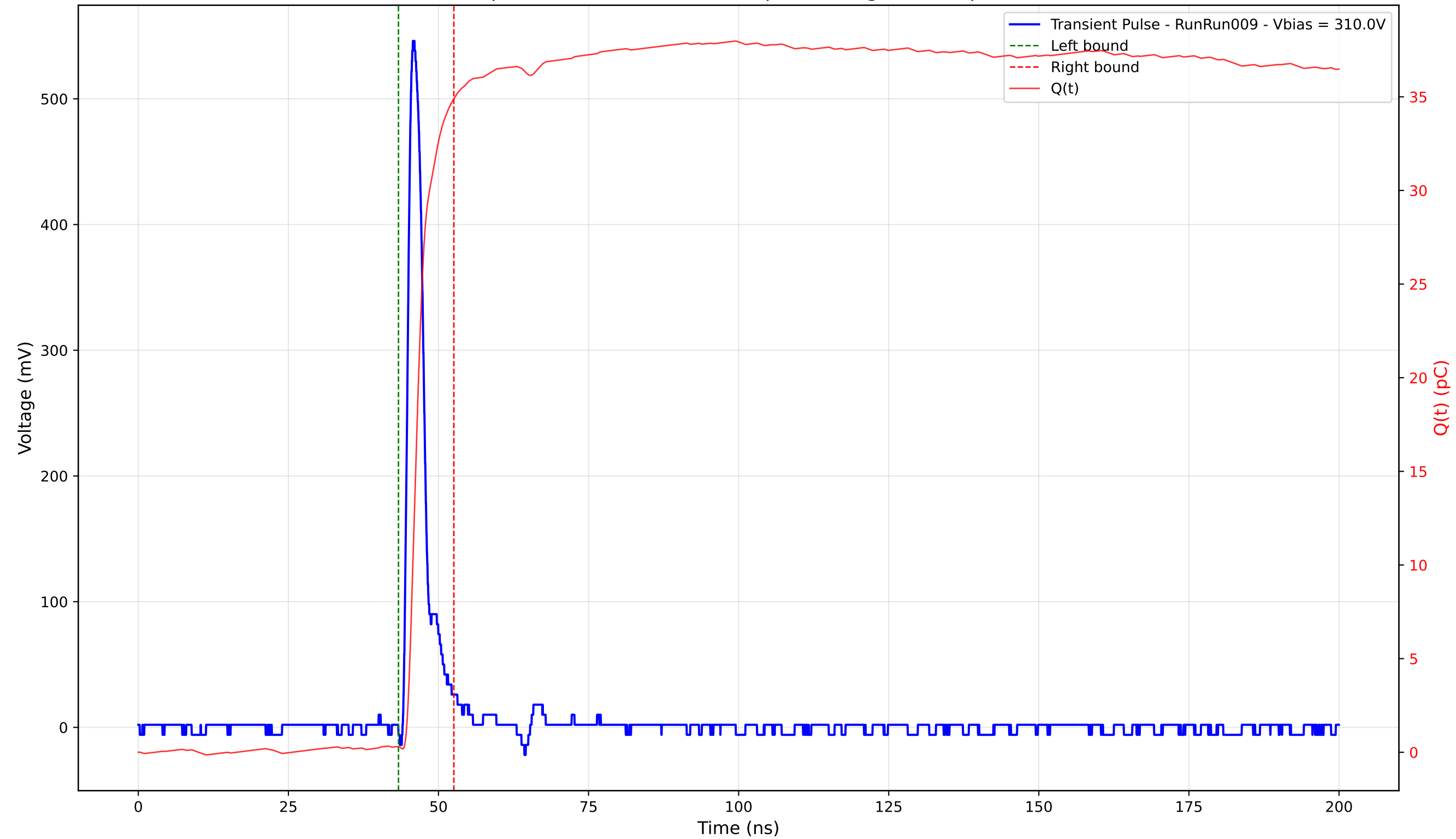
Transient Pulse - Sample: 4003 - Position: 265.0 \mu\text{m} - Charge: 34.58 pC - Rise Time: 1.09 ns
