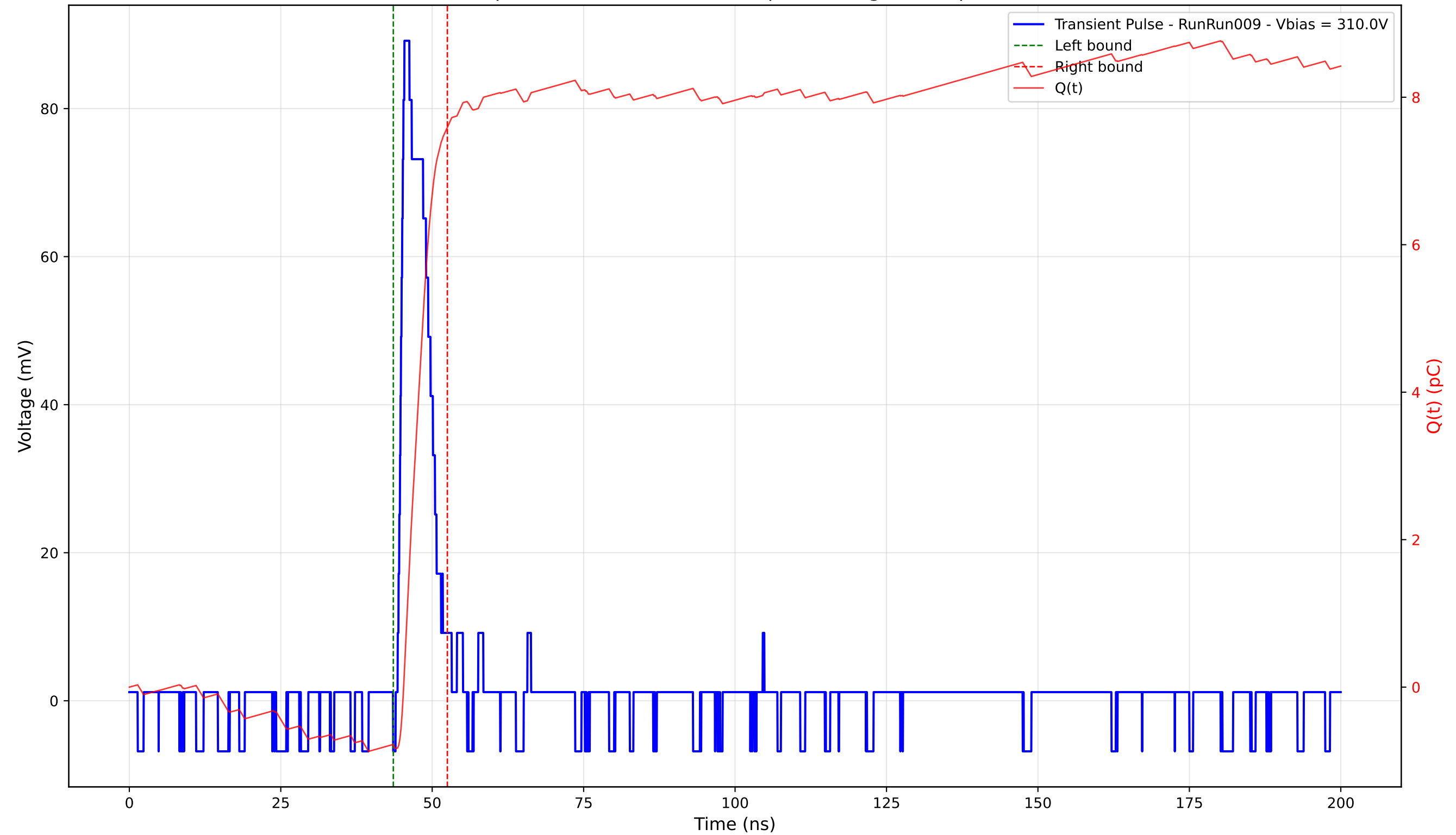
Transient Pulse - Sample: 4003 - Position: 405.0 \mu\text{m} - Charge: 8.38 pC - Rise Time: 0.94 ns
