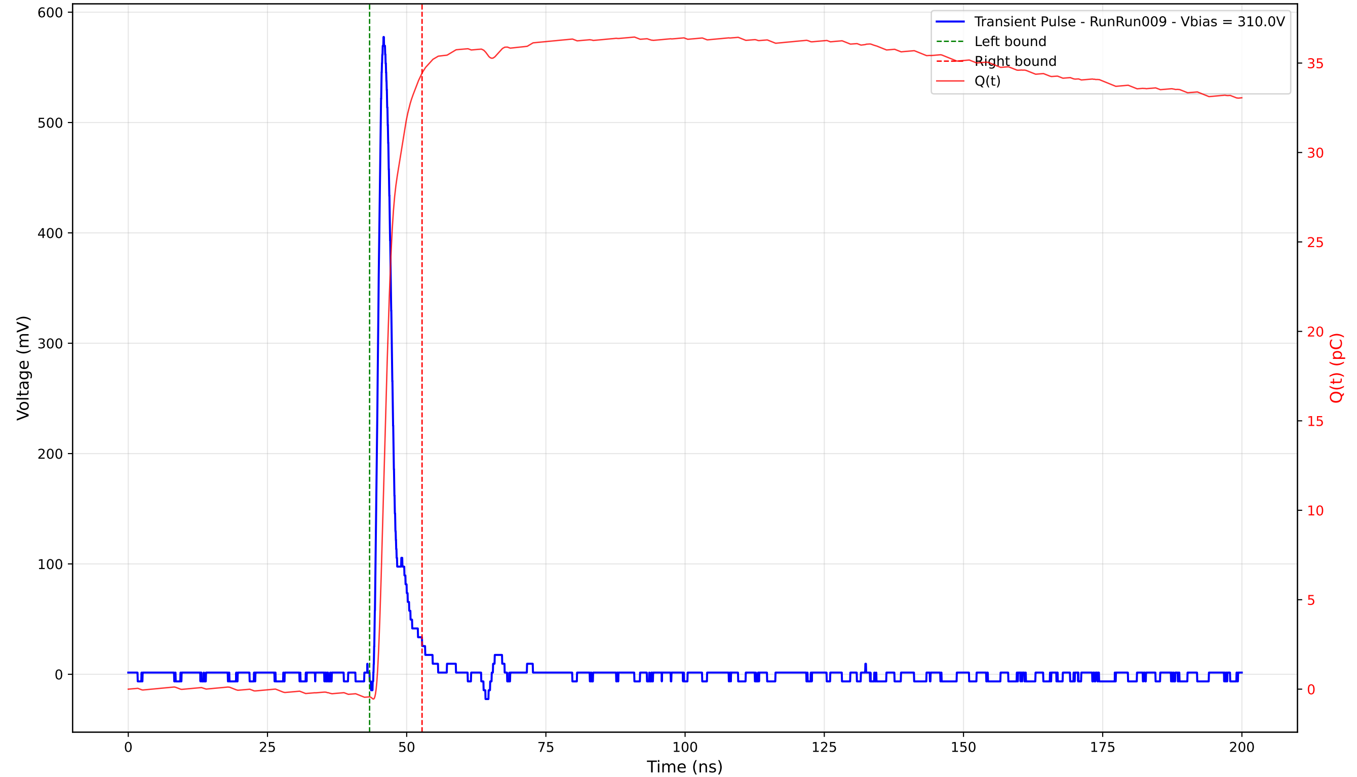
Transient Pulse - Sample: 4003 - Position: 250.0 \mu\text{m} - Charge: 34.87 pC - Rise Time: 1.10 ns
