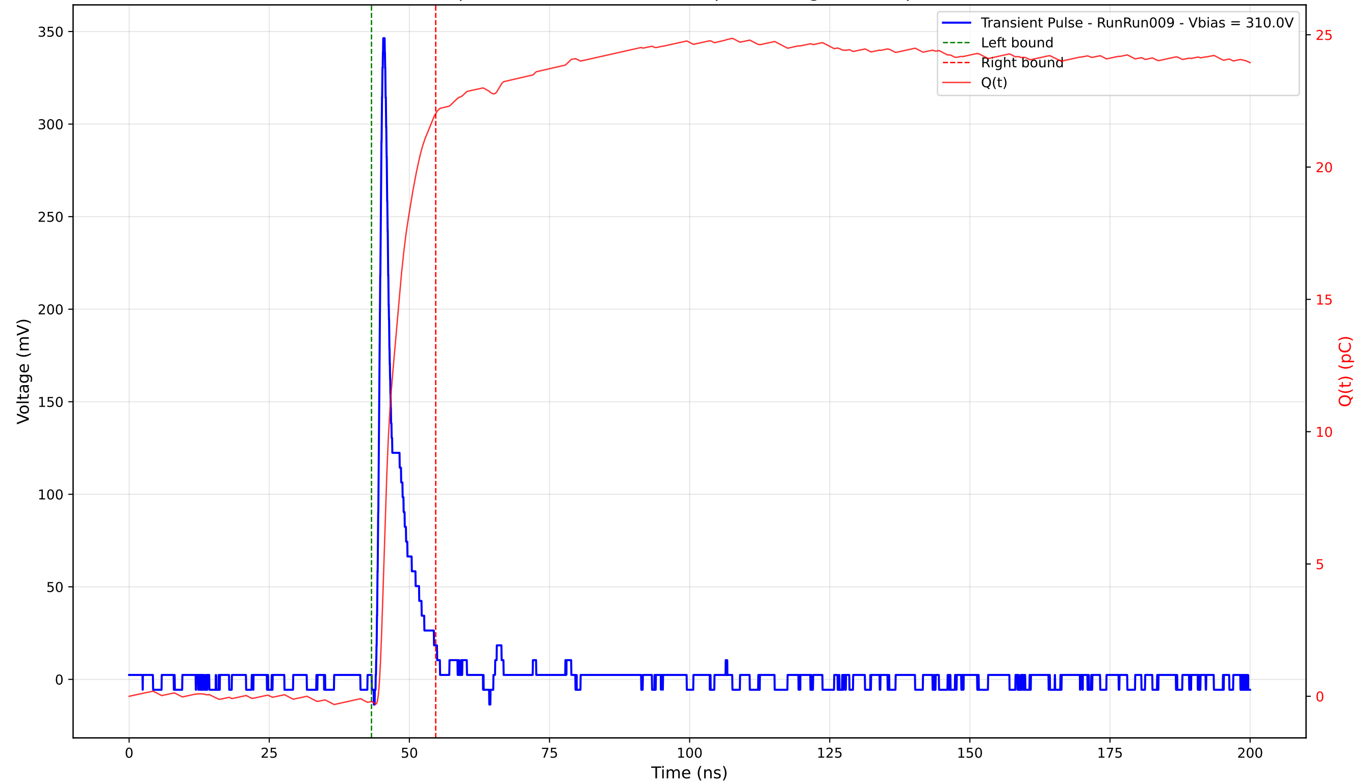
Transient Pulse - Sample: 4003 - Position: 100.0 \mu\text{m} - Charge: 22.22 pC - Rise Time: 0.88 ns
