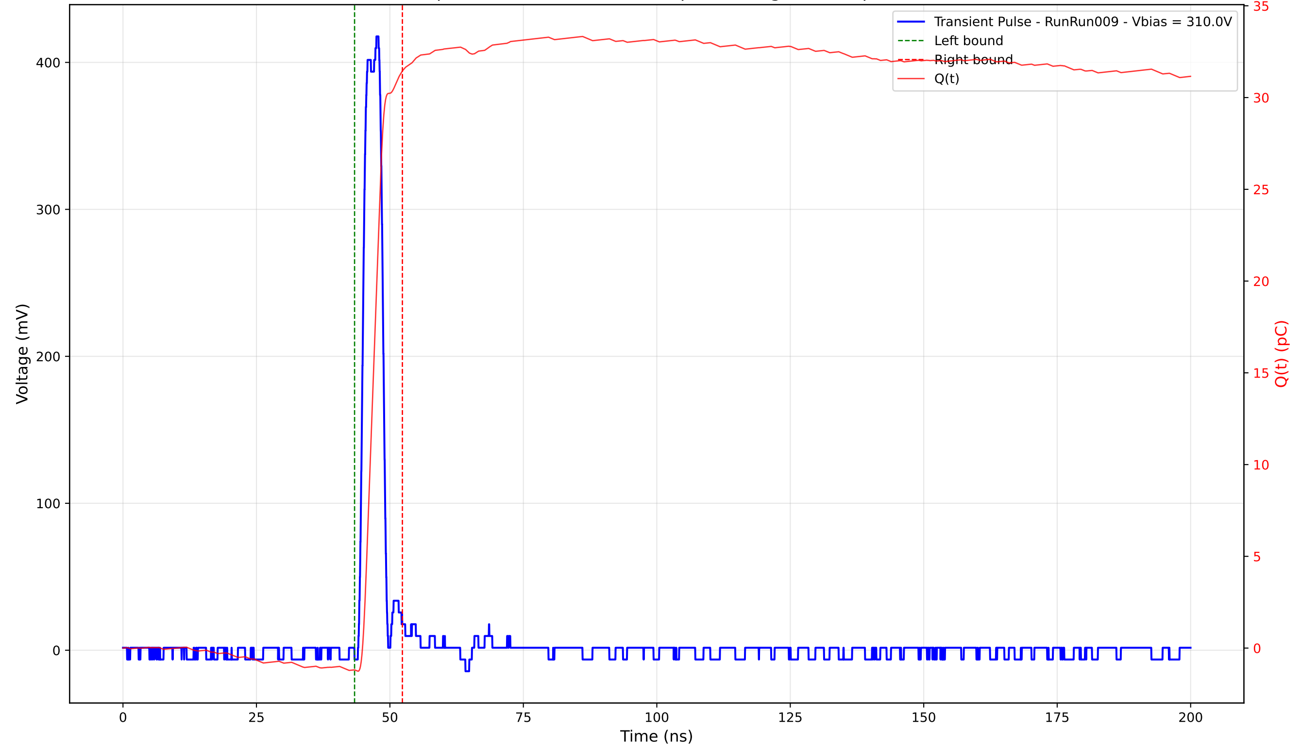
Transient Pulse - Sample: 4003 - Position: 335.0 \mu\text{m} - Charge: 32.64 pC - Rise Time: 1.20 ns
