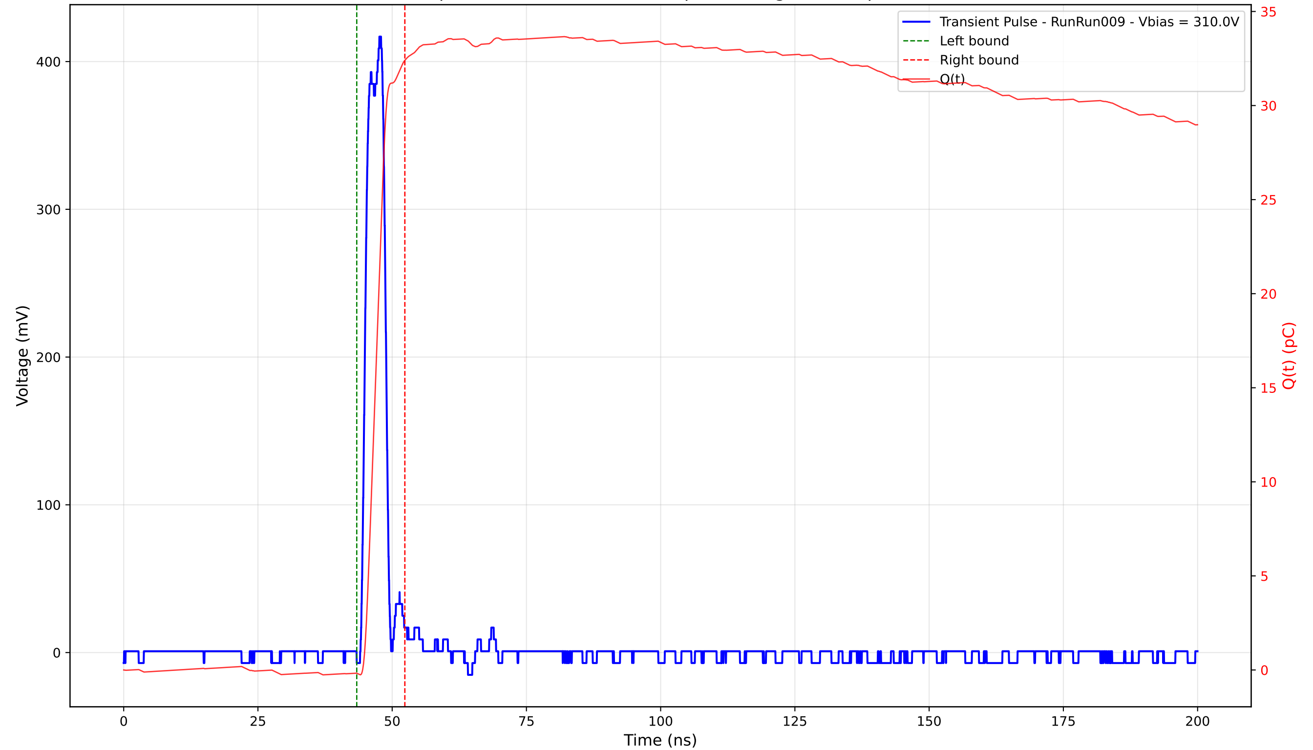
Transient Pulse - Sample: 4003 - Position: 340.0 \mu\text{m} - Charge: 32.57 pC - Rise Time: 1.30 ns
