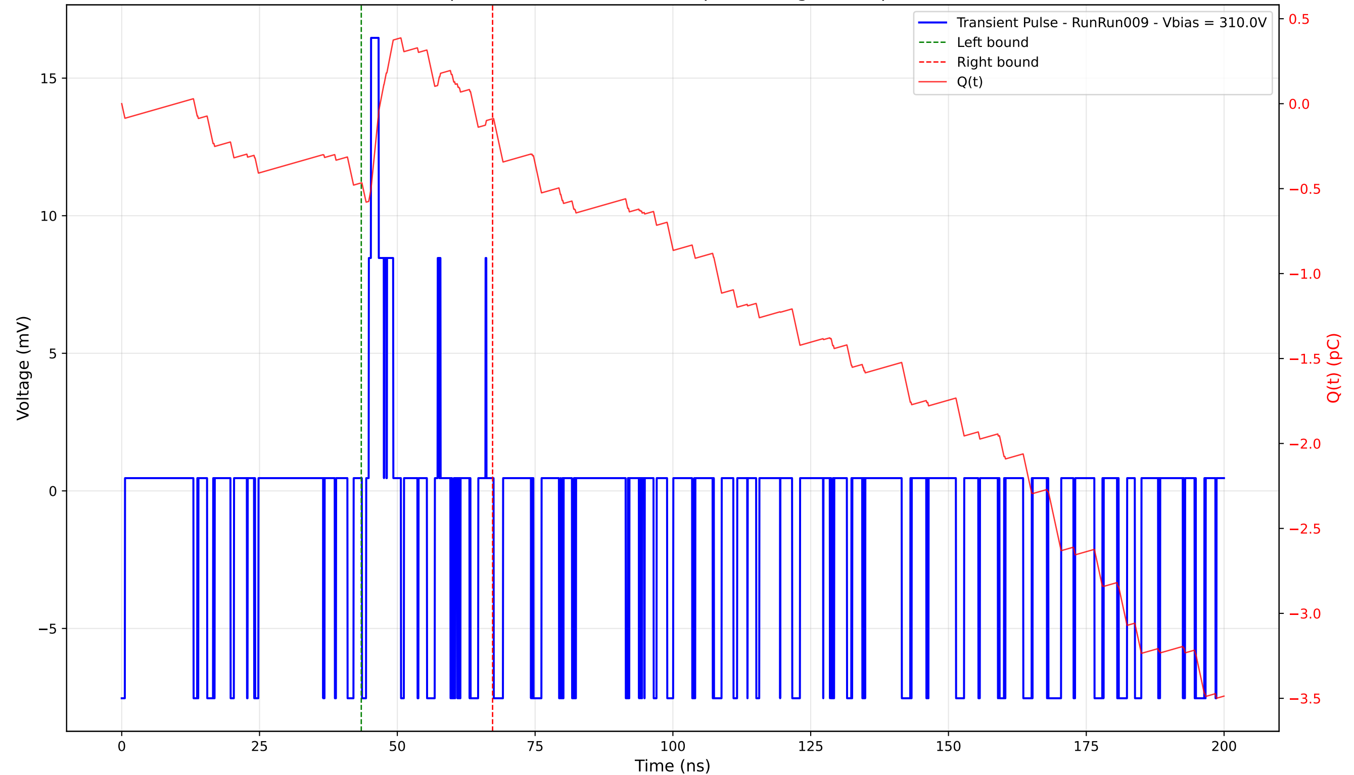
Transient Pulse - Sample: 4003 - Position: 425.0 \mu\text{m} - Charge: 0.38 pC - Rise Time: 0.42 ns
