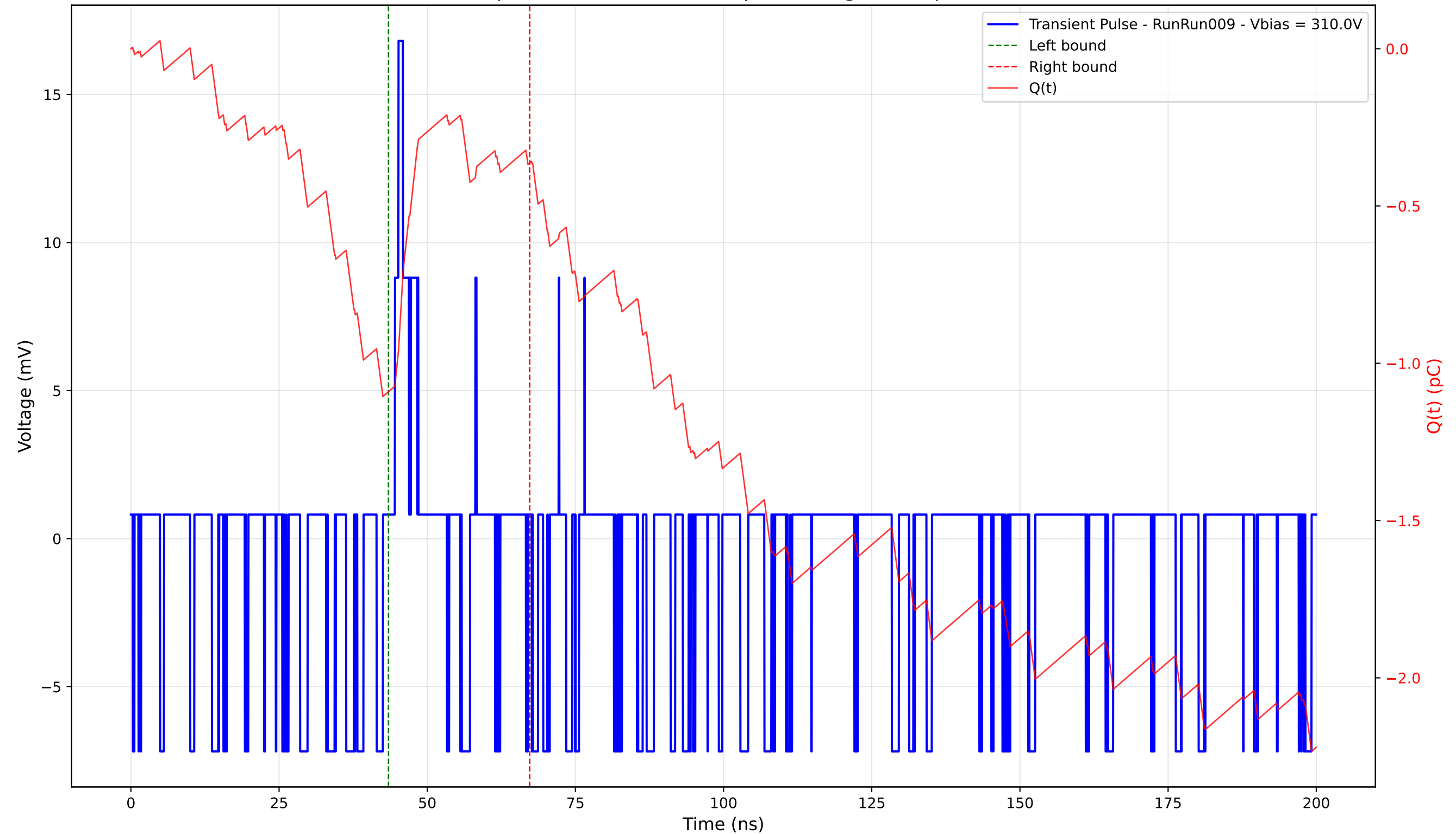
Transient Pulse - Sample: 4003 - Position: 5.0 \mu\text{m} - Charge: 0.73 pC - Rise Time: 0.62 ns
