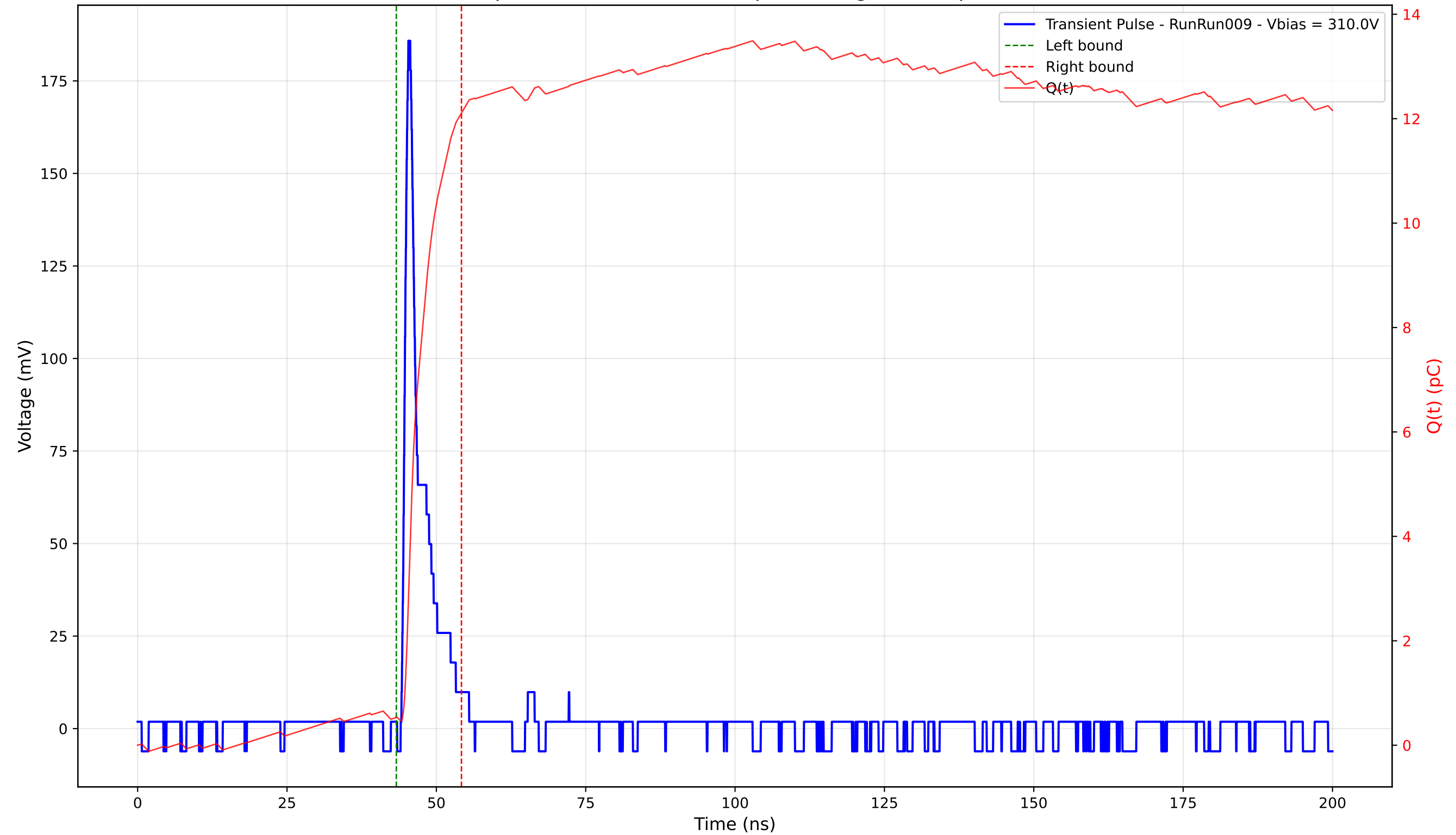
Transient Pulse - Sample: 4003 - Position: 90.0 \mu\text{m} - Charge: 11.58 pC - Rise Time: 0.86 ns
