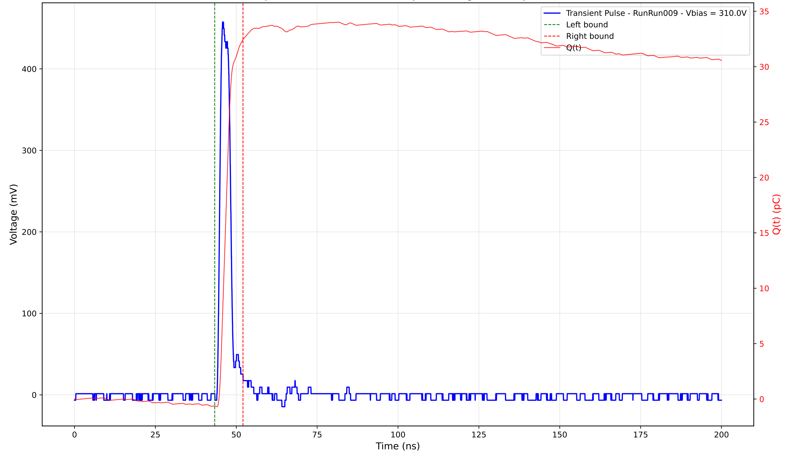
Transient Pulse - Sample: 4003 - Position: 310.0 \mu\text{m} - Charge: 33.07 pC - Rise Time: 1.11 ns
