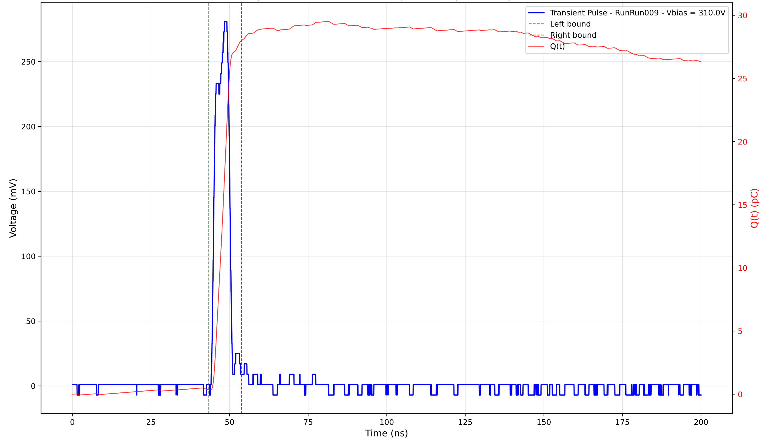
Transient Pulse - Sample: 4003 - Position: 385.0 \mu\text{m} - Charge: 27.60 pC - Rise Time: 3.29 ns
