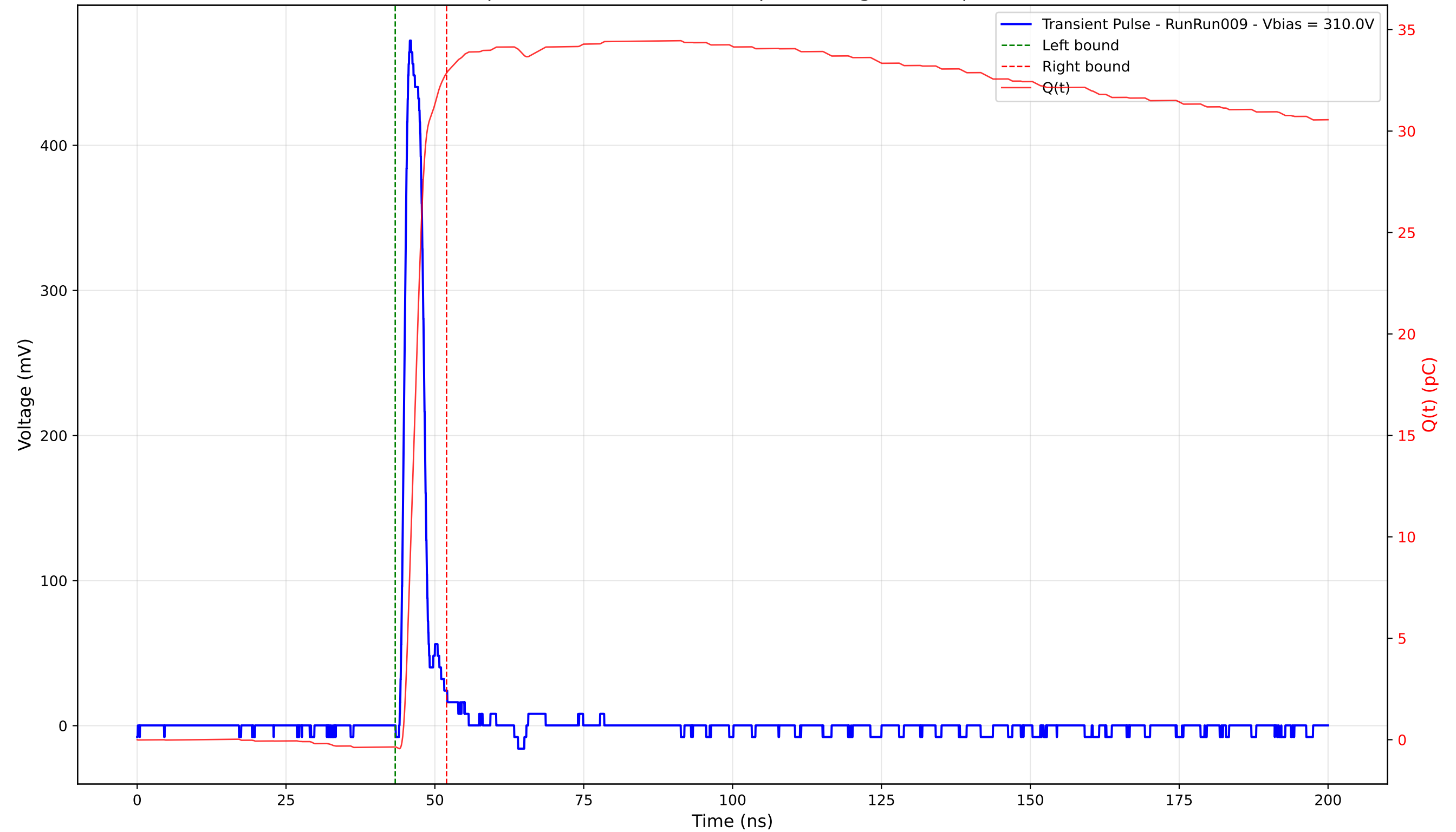
Transient Pulse - Sample: 4003 - Position: 305.0 \mu\text{m} - Charge: 33.22 pC - Rise Time: 1.12 ns
