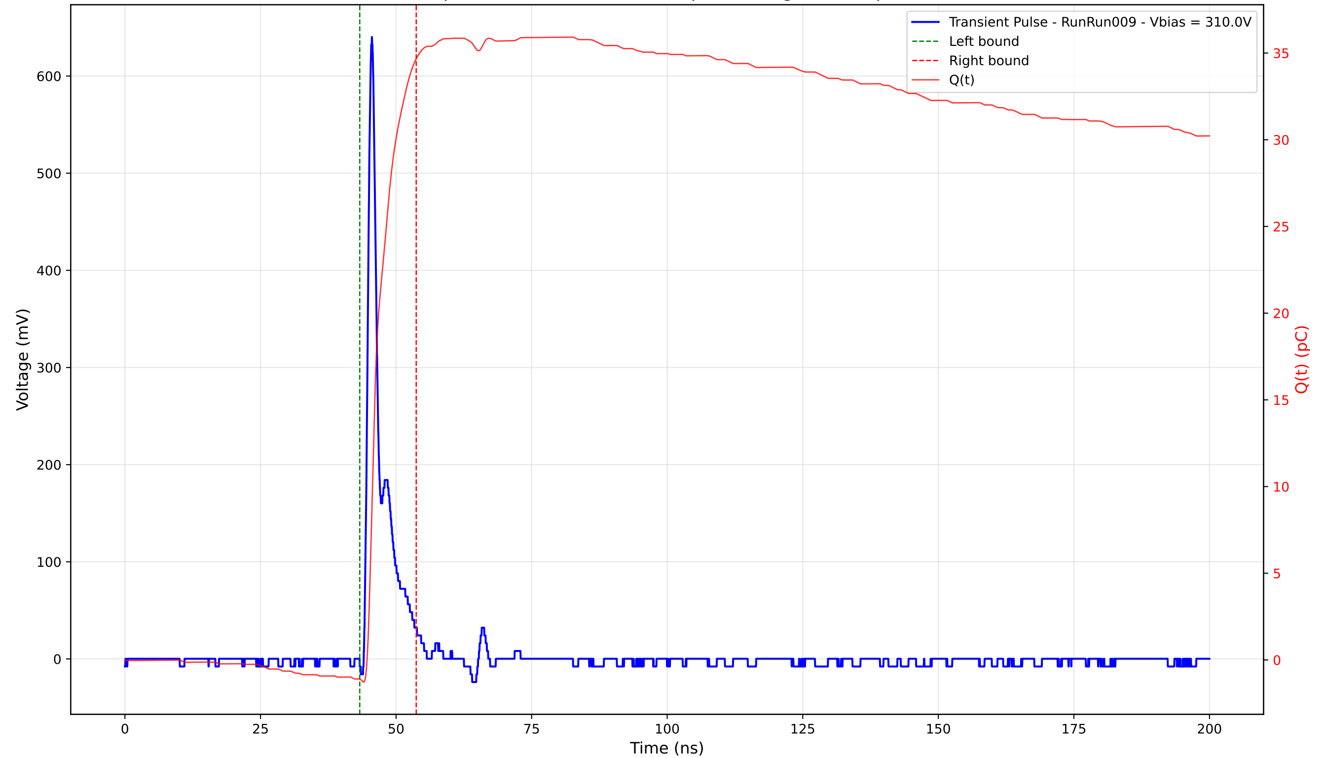
Transient Pulse - Sample: 4003 - Position: 155.0 \mu\text{m} - Charge: 35.77 pC - Rise Time: 0.94 ns
