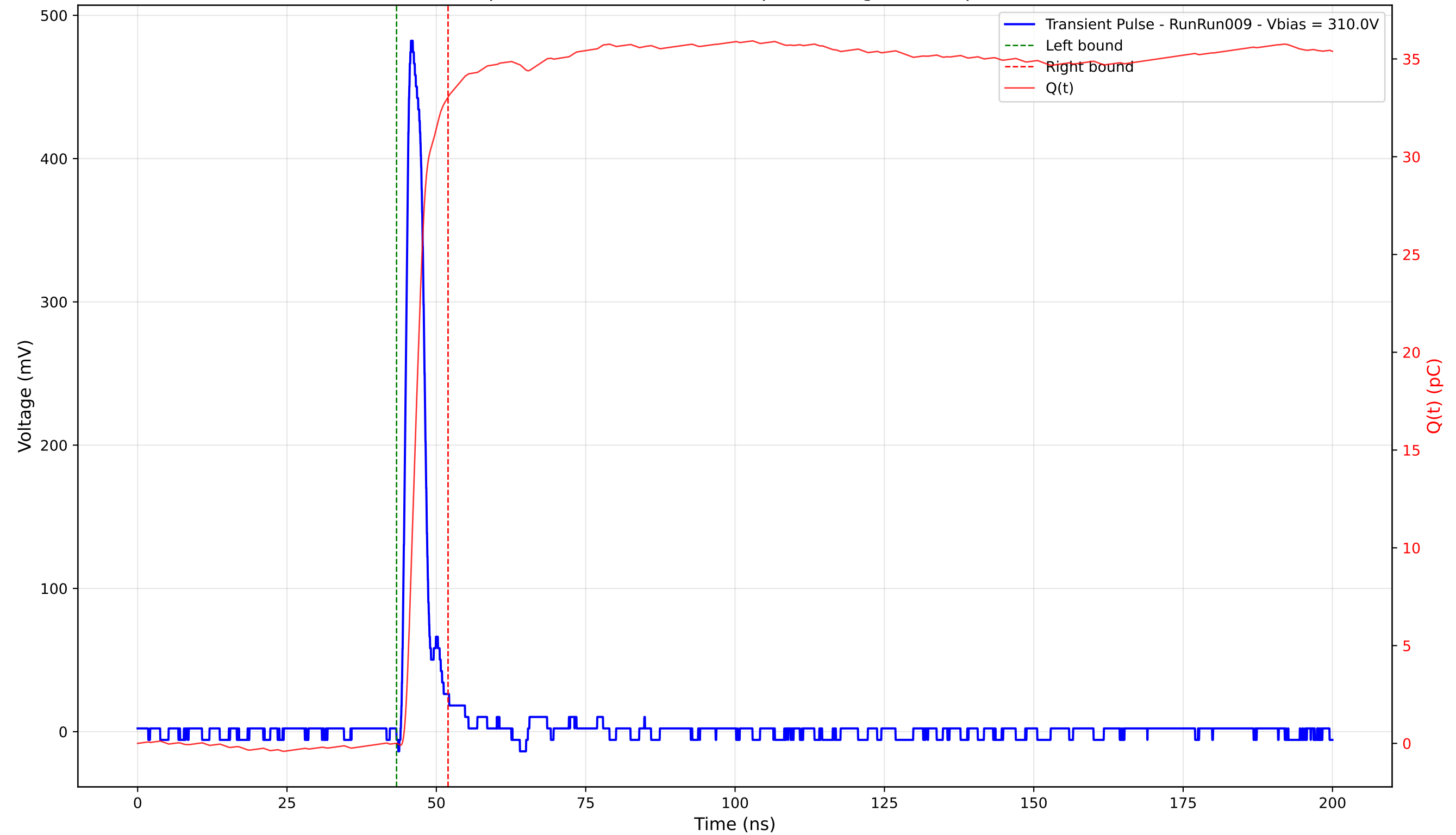
Transient Pulse - Sample: 4003 - Position: 295.0 \mu\text{m} - Charge: 33.05 pC - Rise Time: 1.10 ns
