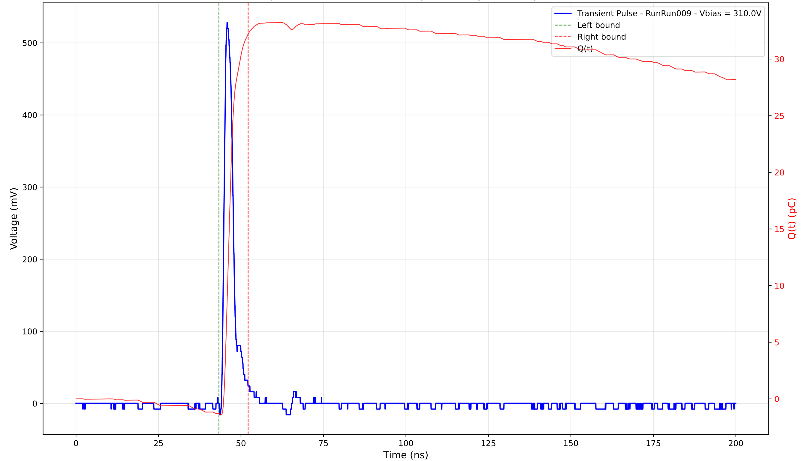
Transient Pulse - Sample: 4003 - Position: 270.0 \mu\text{m} - Charge: 33.48 pC - Rise Time: 1.09 ns
