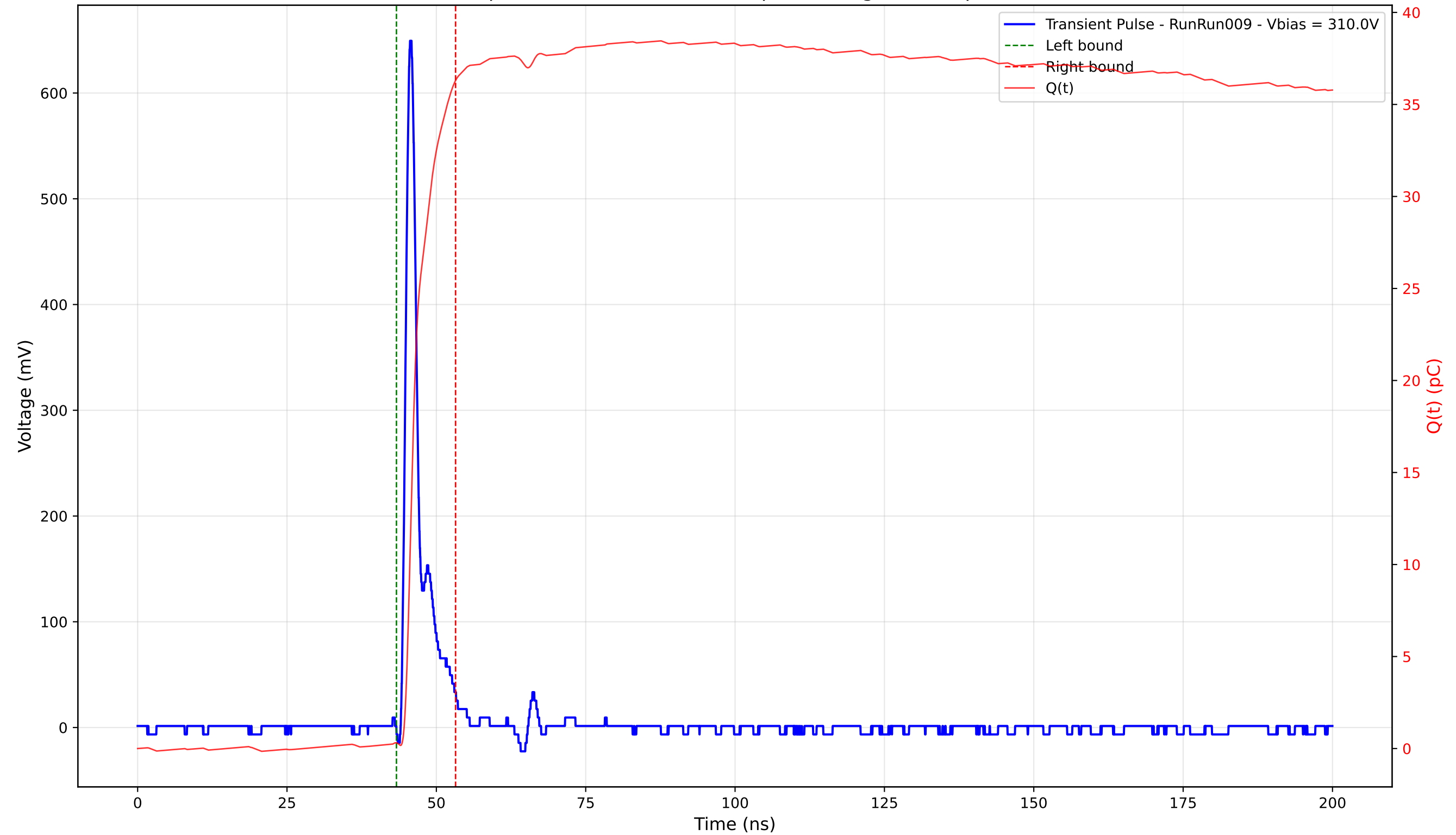
Transient Pulse - Sample: 4003 - Position: 200.0 \mu\text{m} - Charge: 35.99 pC - Rise Time: 1.02 ns
