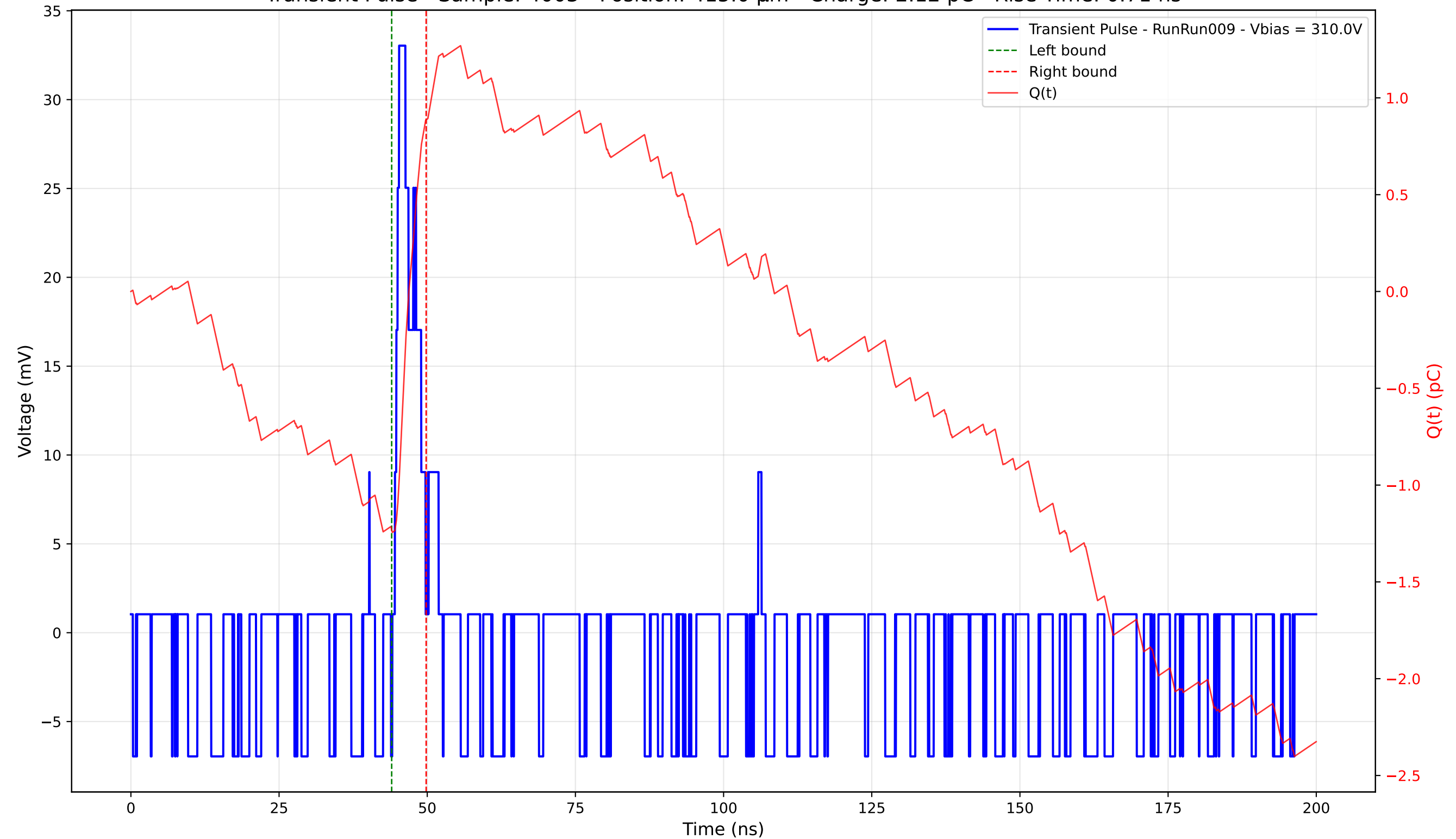
Transient Pulse - Sample: 4003 - Position: 415.0 \mu\text{m} - Charge: 2.12 pC - Rise Time: 0.71 ns
