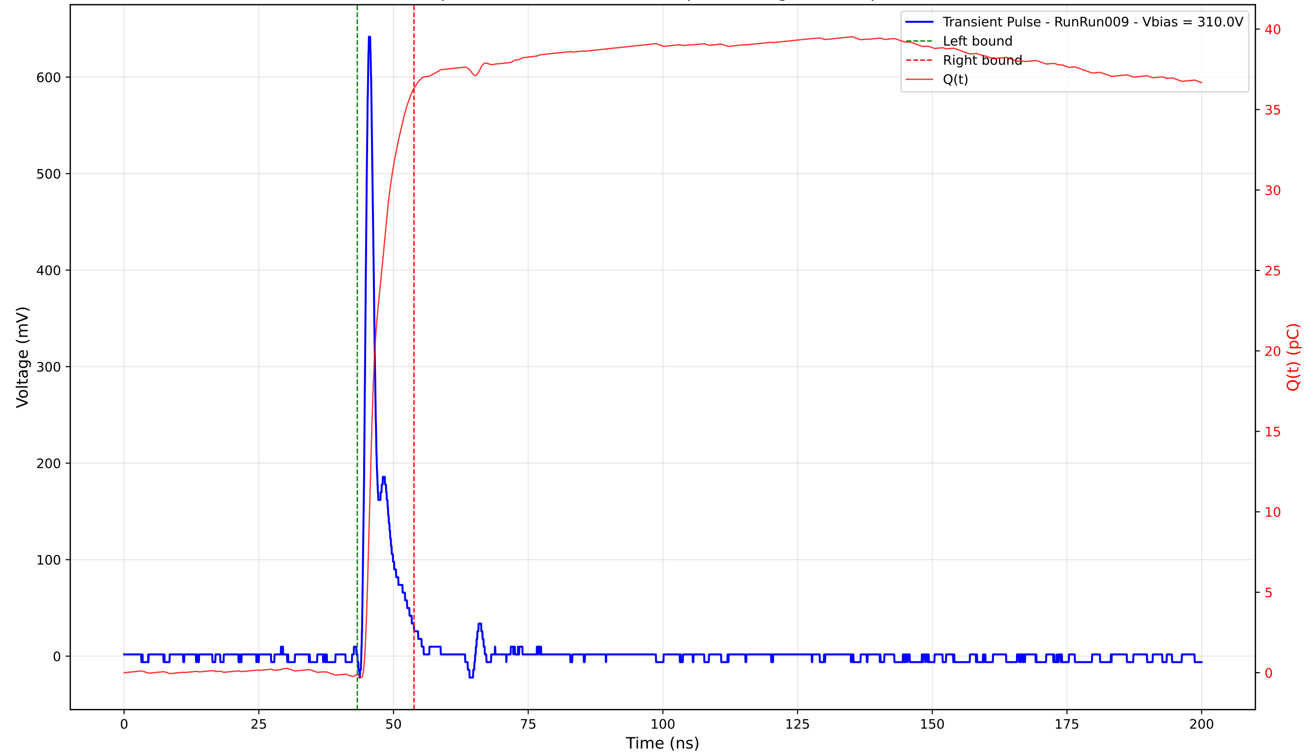
Transient Pulse - Sample: 4003 - Position: 160.0 \mu\text{m} - Charge: 36.45 pC - Rise Time: 0.92 ns
