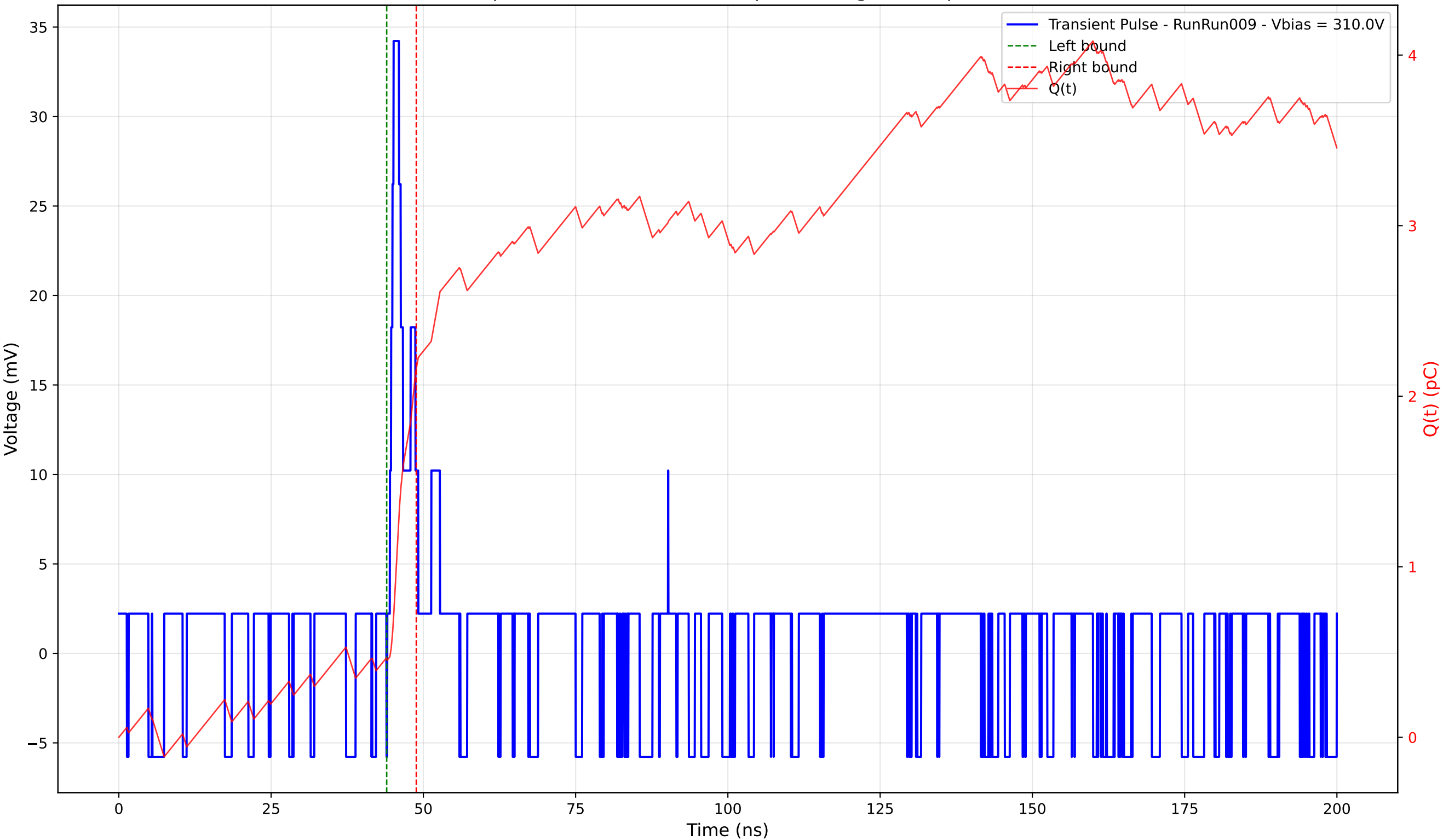
Transient Pulse - Sample: 4003 - Position: 75.0 \mu\text{m} - Charge: 1.70 pC - Rise Time: 0.62 ns
