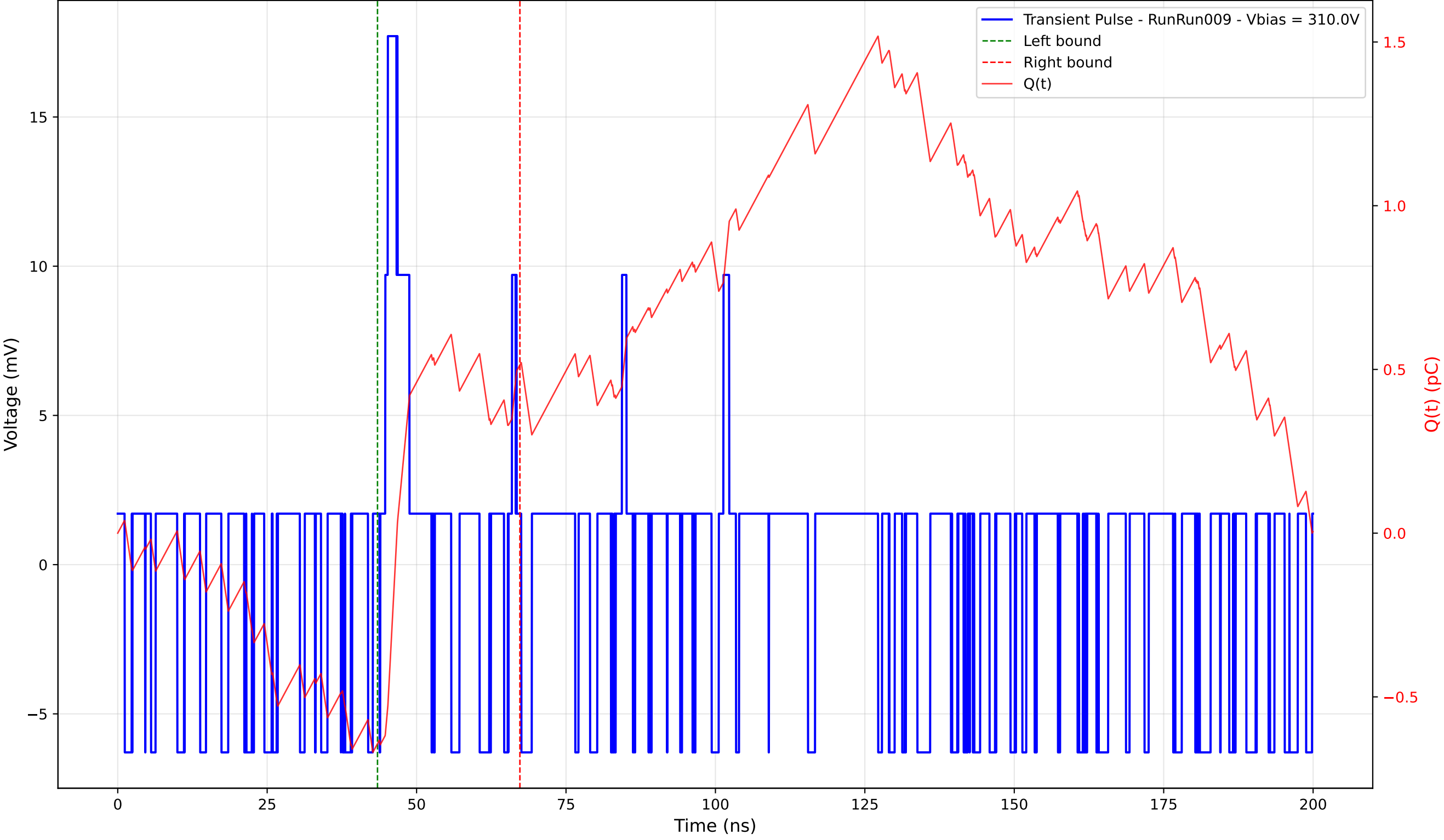
Transient Pulse - Sample: 4003 - Position: 65.0 \mu\text{m} - Charge: 1.16 pC - Rise Time: 0.44 ns
