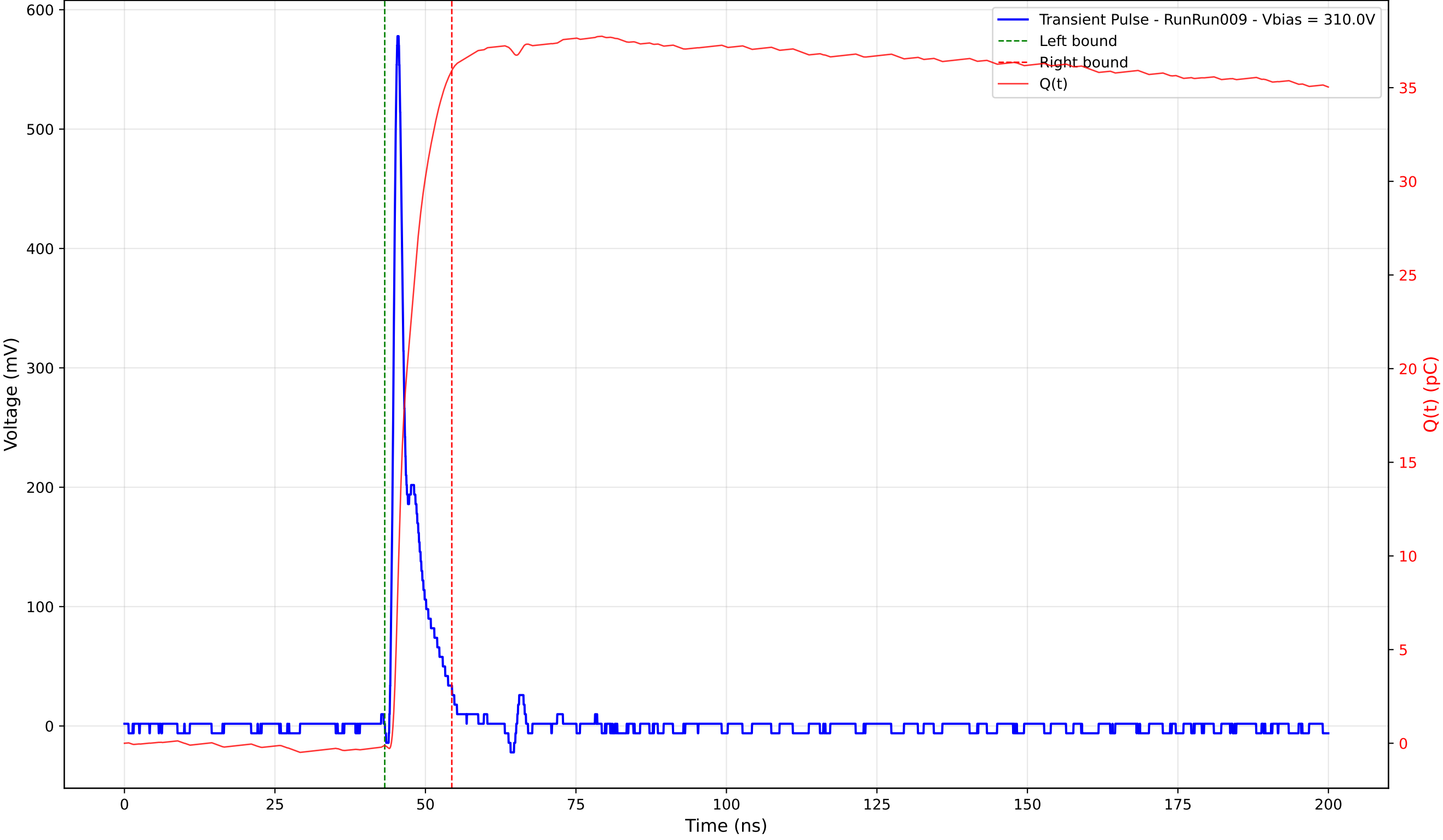
Transient Pulse - Sample: 4003 - Position: 120.0 \mu\text{m} - Charge: 36.05 pC - Rise Time: 0.90 ns
