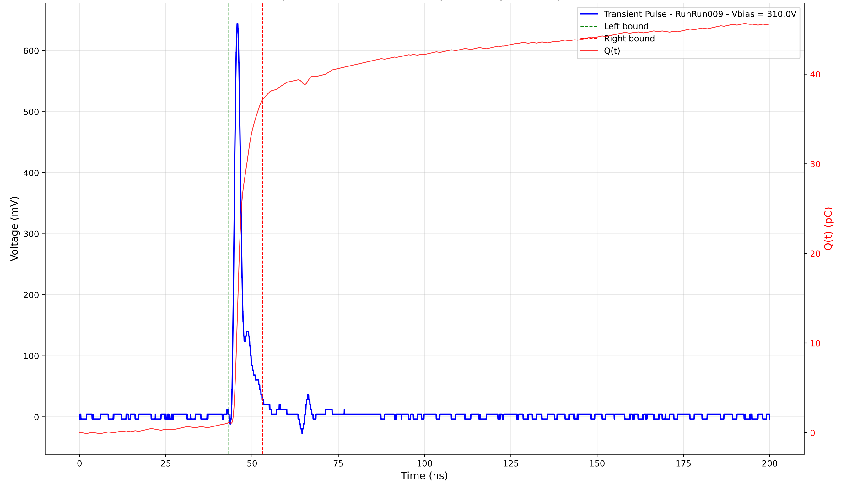
Transient Pulse - Sample: 4003 - Position: 210.0 \mu\text{m} - Charge: 36.02 pC - Rise Time: 1.07 ns
