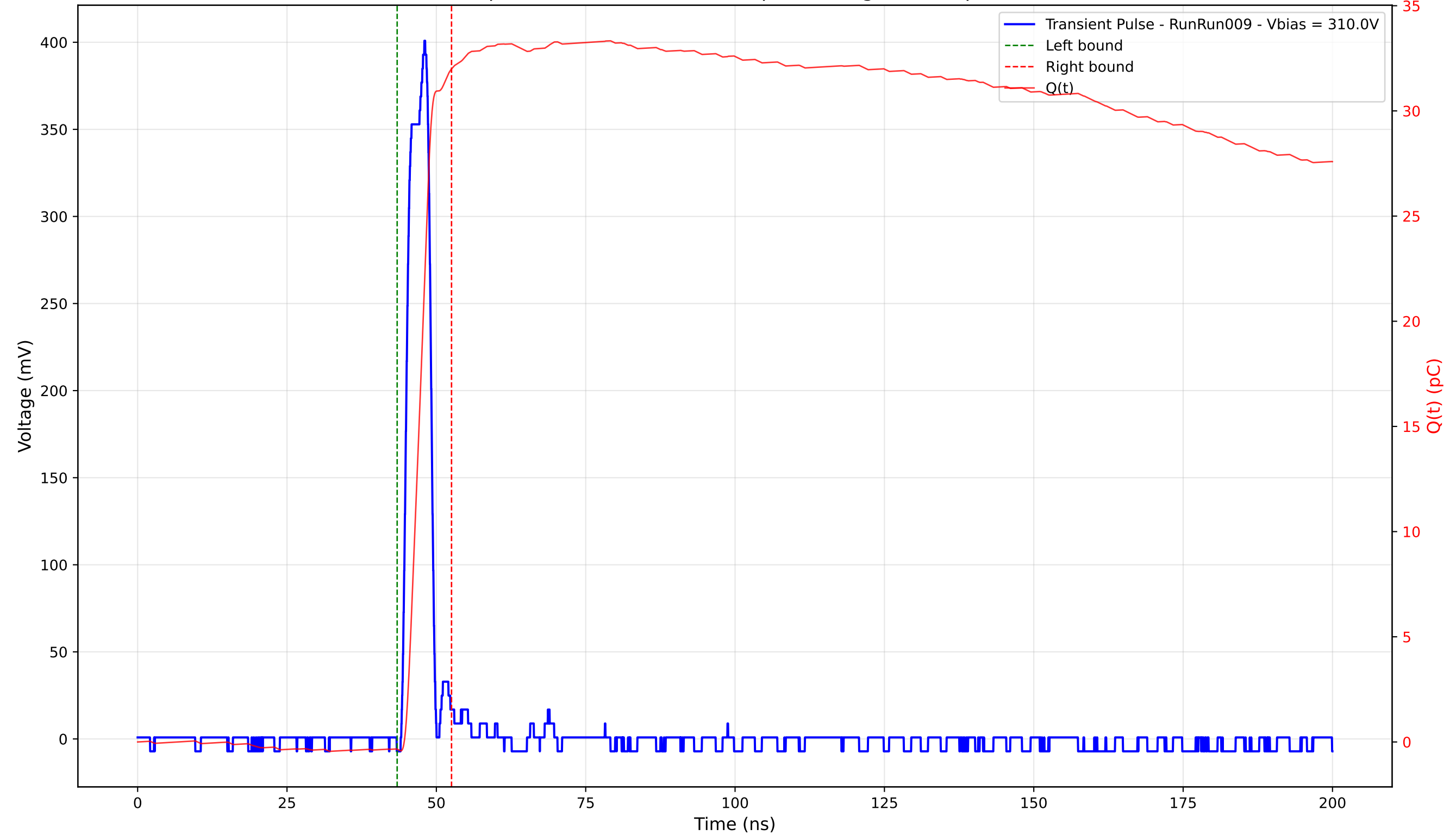
Transient Pulse - Sample: 4003 - Position: 355.0 \mu\text{m} - Charge: 32.34 pC - Rise Time: 2.80 ns
