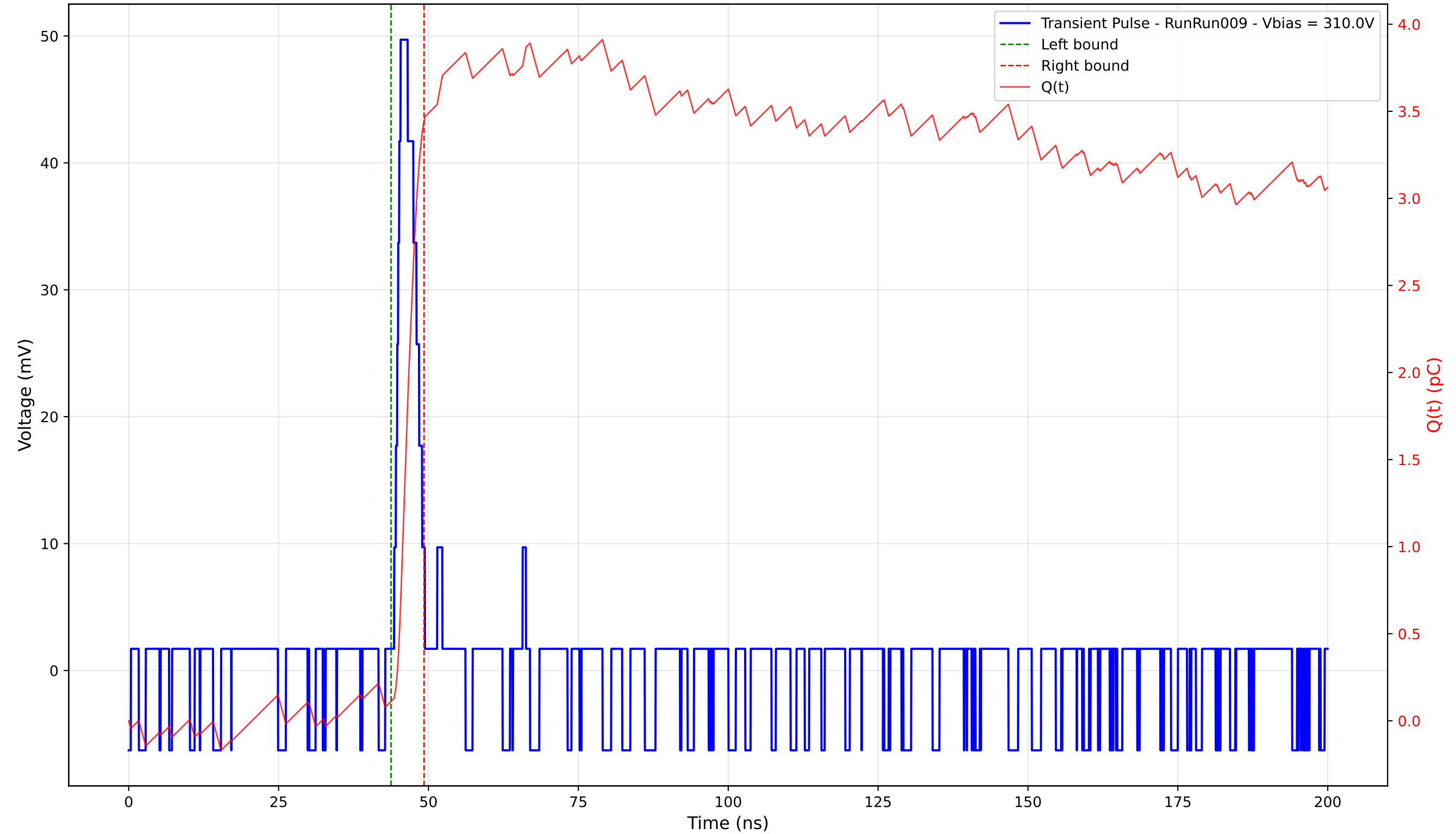
Transient Pulse - Sample: 4003 - Position: 55.0 \mu\text{m} - Charge: 3.33 pC - Rise Time: 1.07 ns
