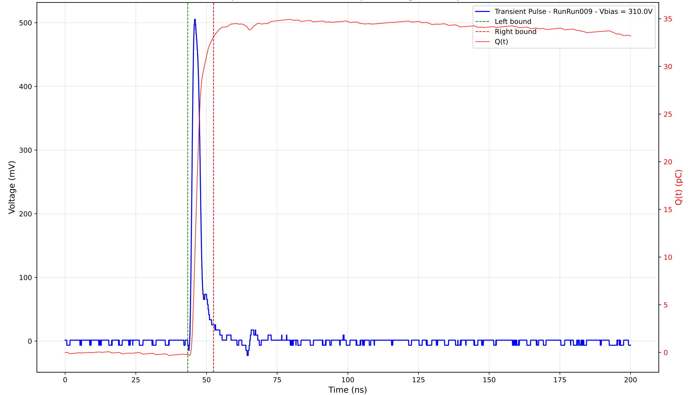
Transient Pulse - Sample: 4003 - Position: 280.0 \mu\text{m} - Charge: 33.28 pC - Rise Time: 1.08 ns
