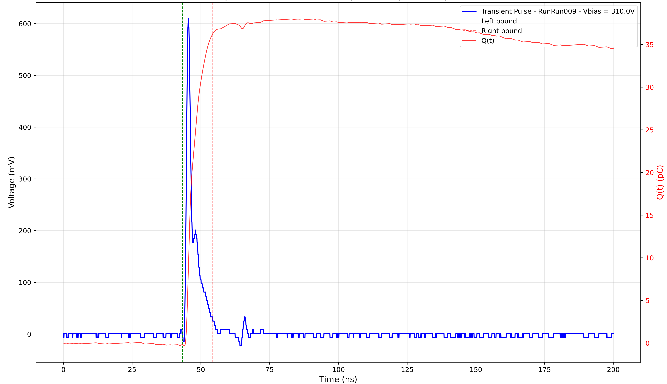
Transient Pulse - Sample: 4003 - Position: 135.0 \mu\text{m} - Charge: 36.29 pC - Rise Time: 0.90 ns
