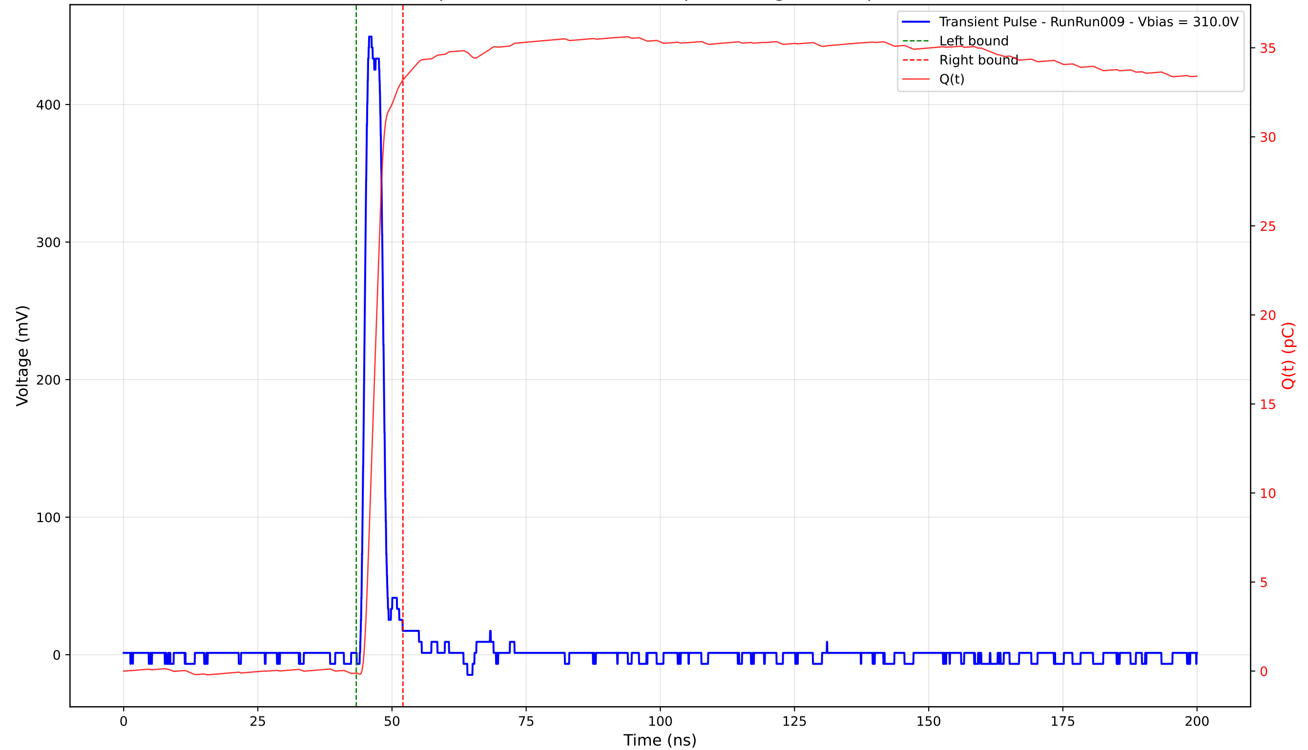
Transient Pulse - Sample: 4003 - Position: 315.0 \mu\text{m} - Charge: 33.31 pC - Rise Time: 1.11 ns
