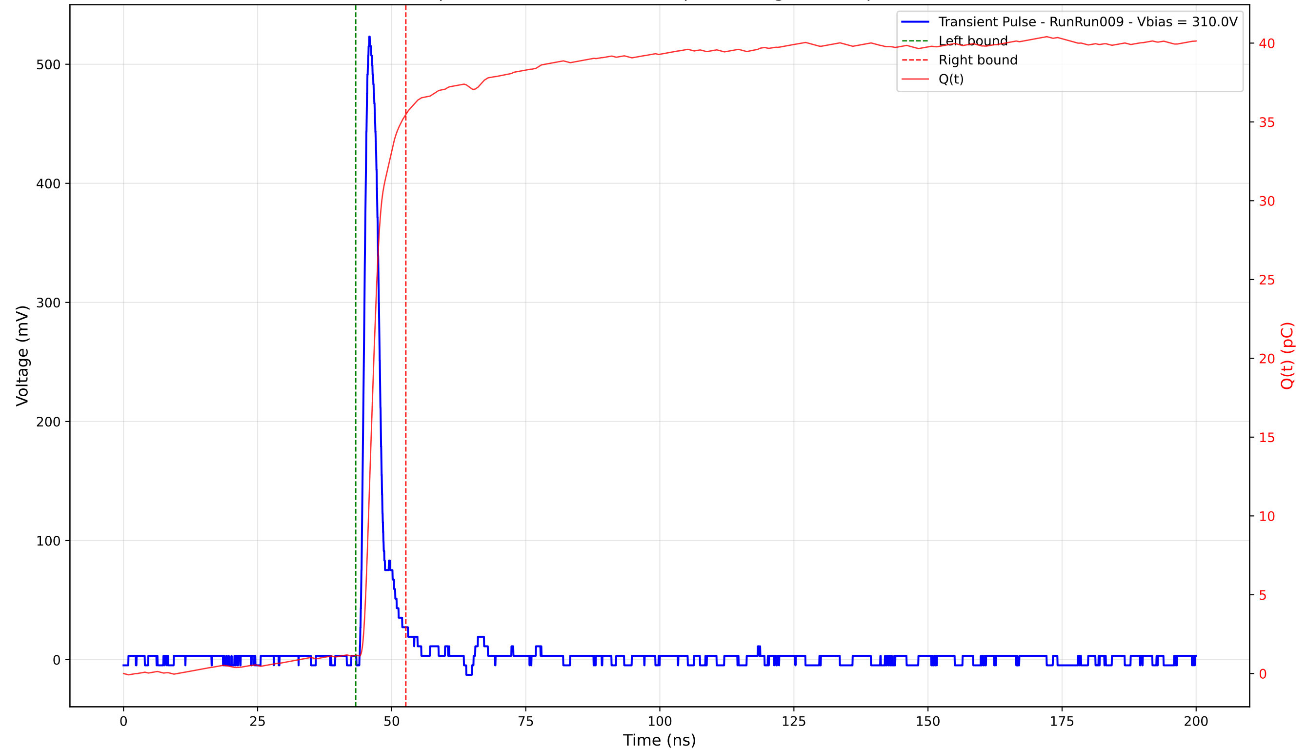
Transient Pulse - Sample: 4003 - Position: 275.0 \mu\text{m} - Charge: 34.32 pC - Rise Time: 1.12 ns
