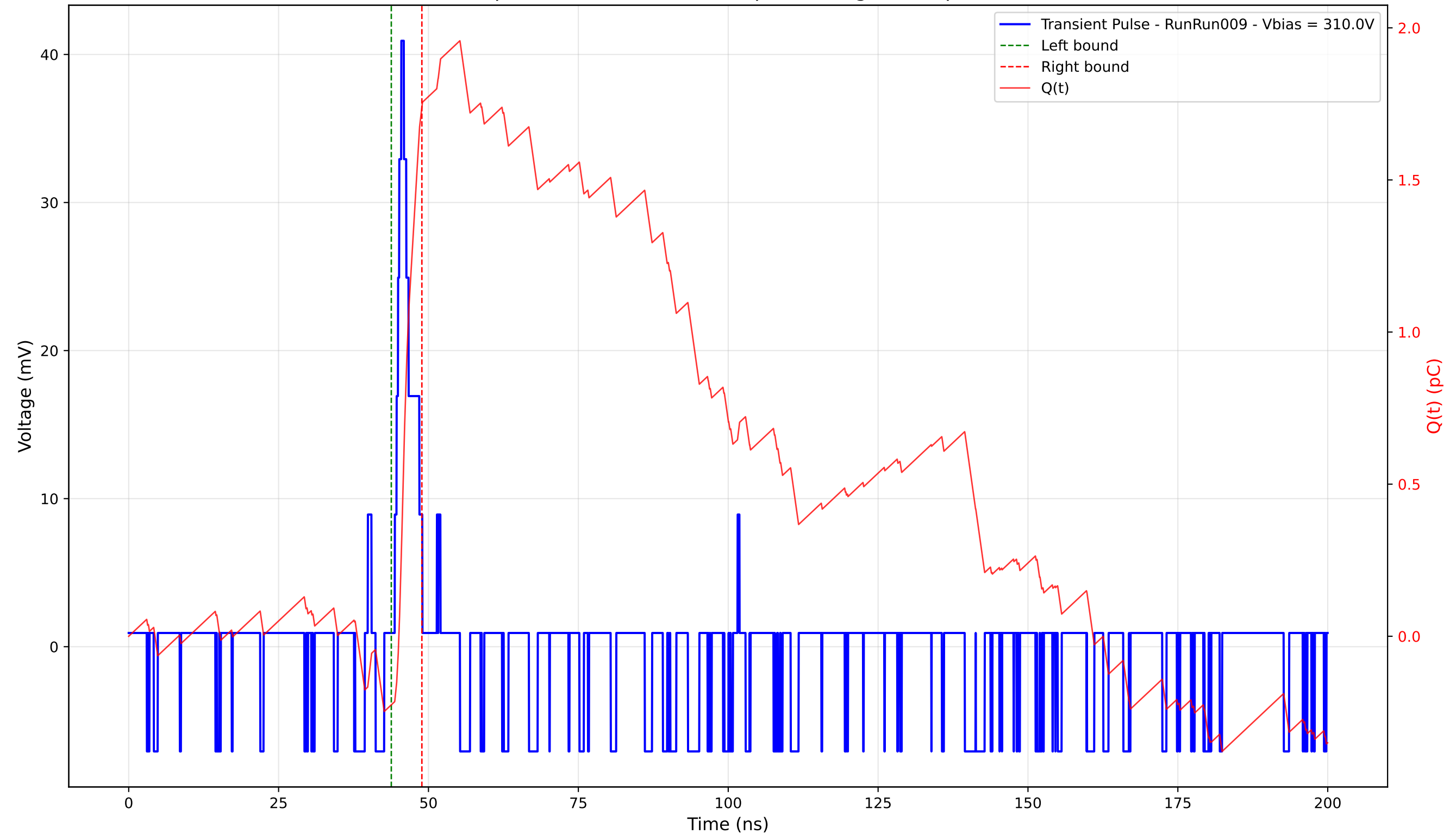
Transient Pulse - Sample: 4003 - Position: 25.0 \mu\text{m} - Charge: 1.97 pC - Rise Time: 1.09 ns
