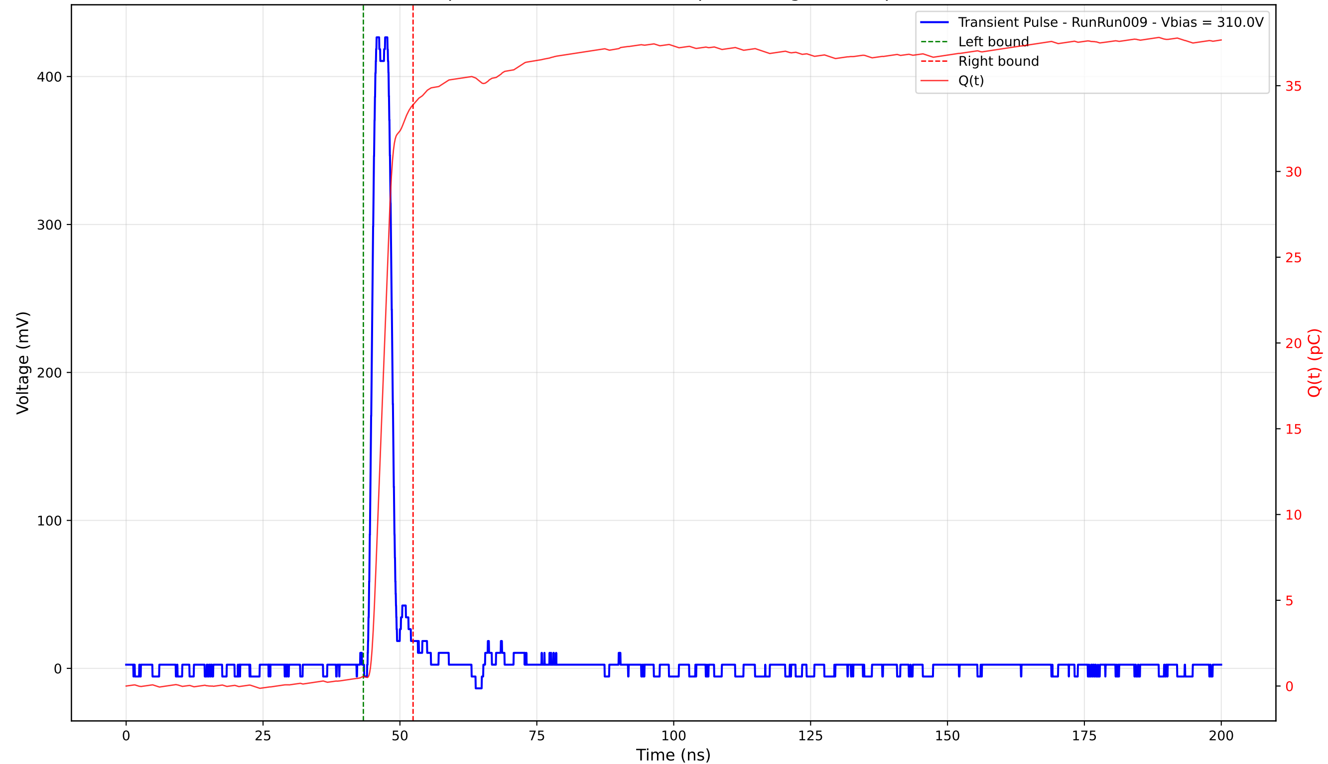
Transient Pulse - Sample: 4003 - Position: 325.0 \mu\text{m} - Charge: 33.34 pC - Rise Time: 1.08 ns
