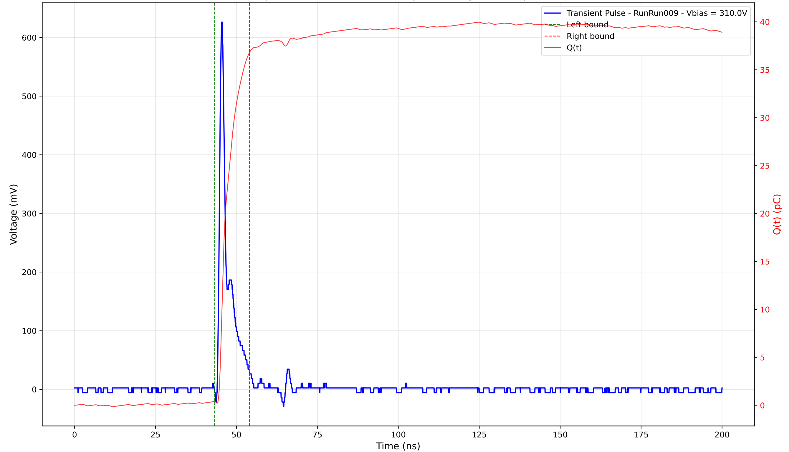
Transient Pulse - Sample: 4003 - Position: 145.0 \mu\text{m} - Charge: 36.39 pC - Rise Time: 0.91 ns
