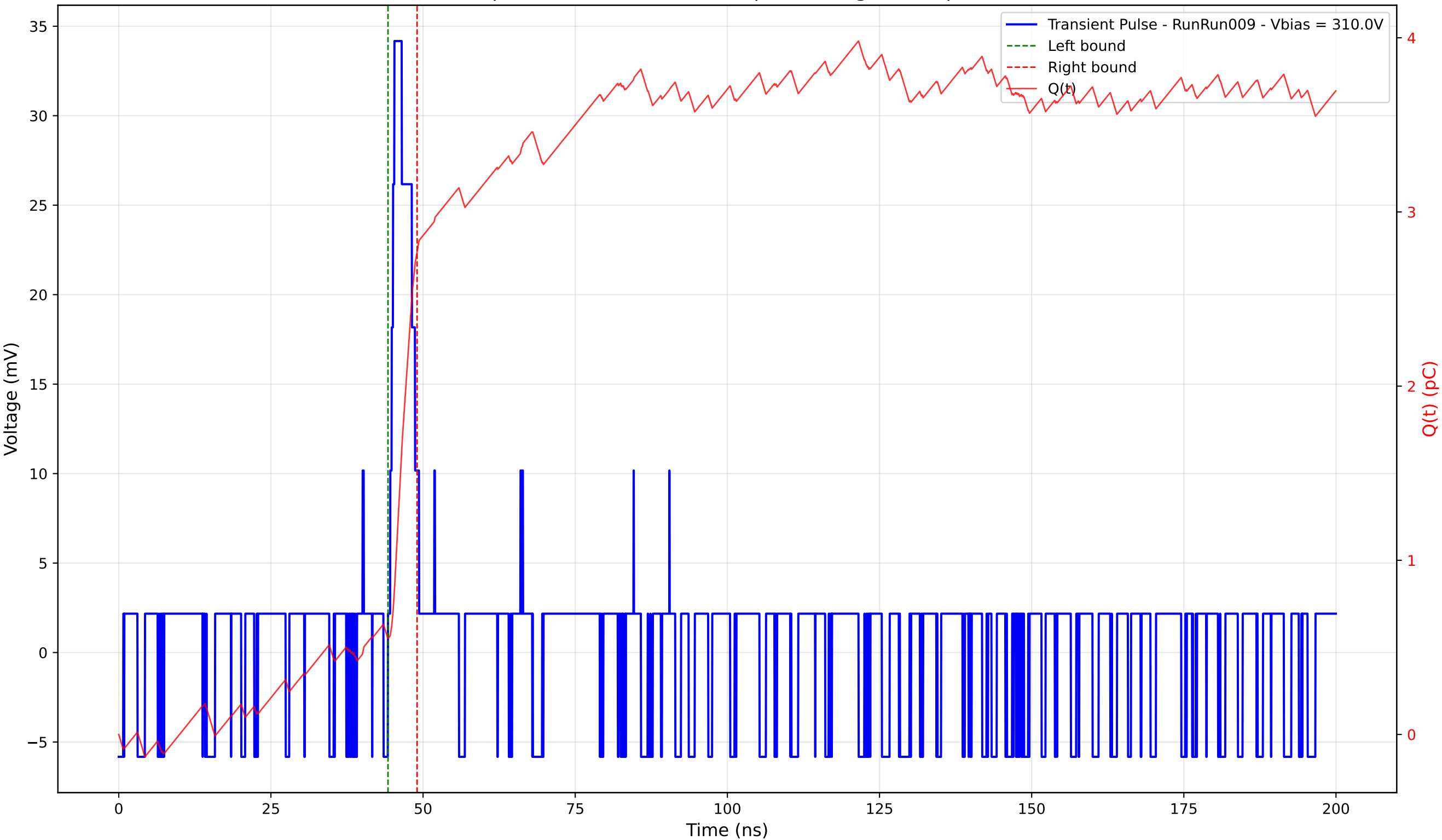
Transient Pulse - Sample: 4003 - Position: 60.0 \mu\text{m} - Charge: 2.22 pC - Rise Time: 0.70 ns
