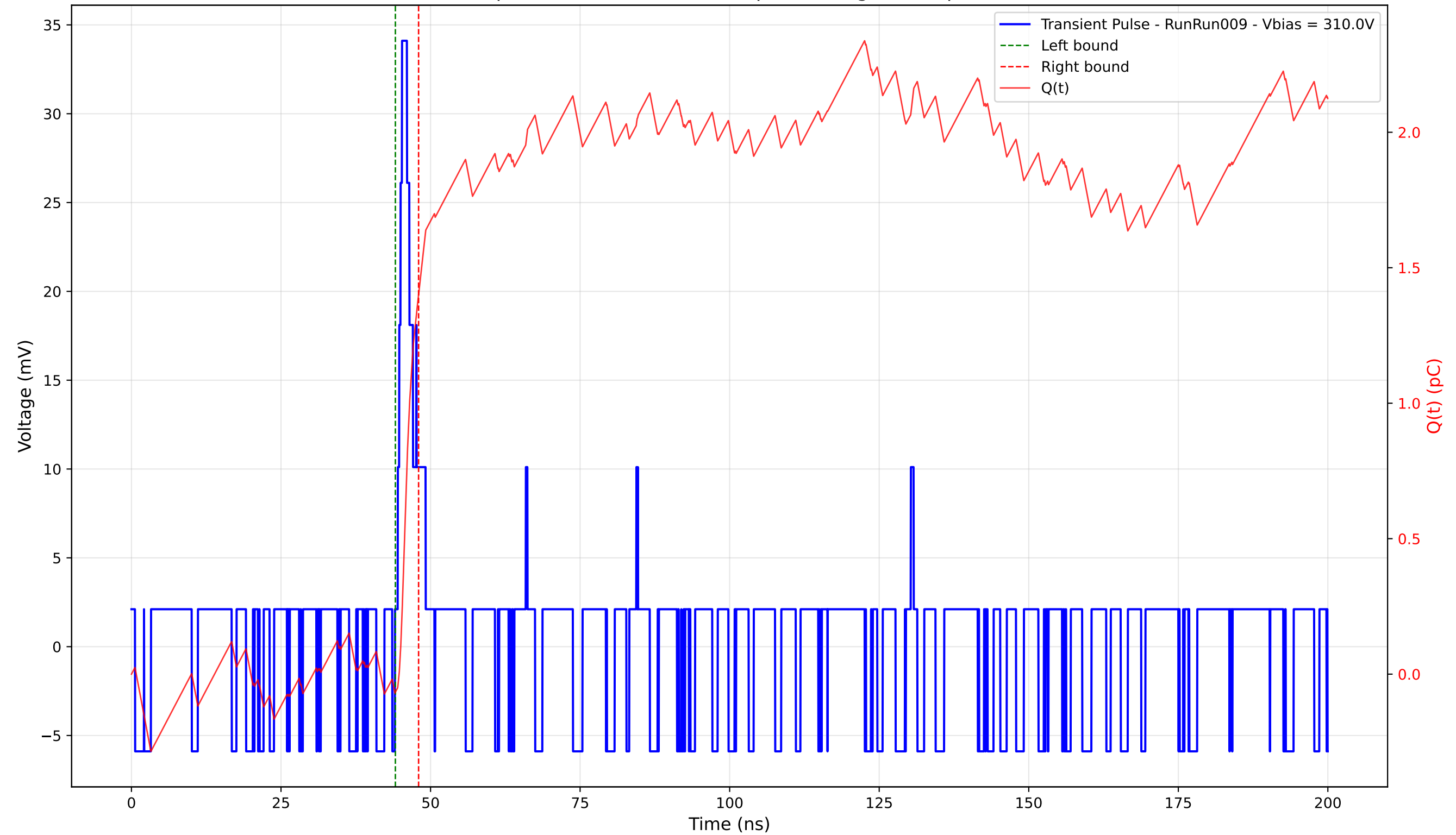
Transient Pulse - Sample: 4003 - Position: 35.0 \mu\text{m} - Charge: 1.47 pC - Rise Time: 0.72 ns
