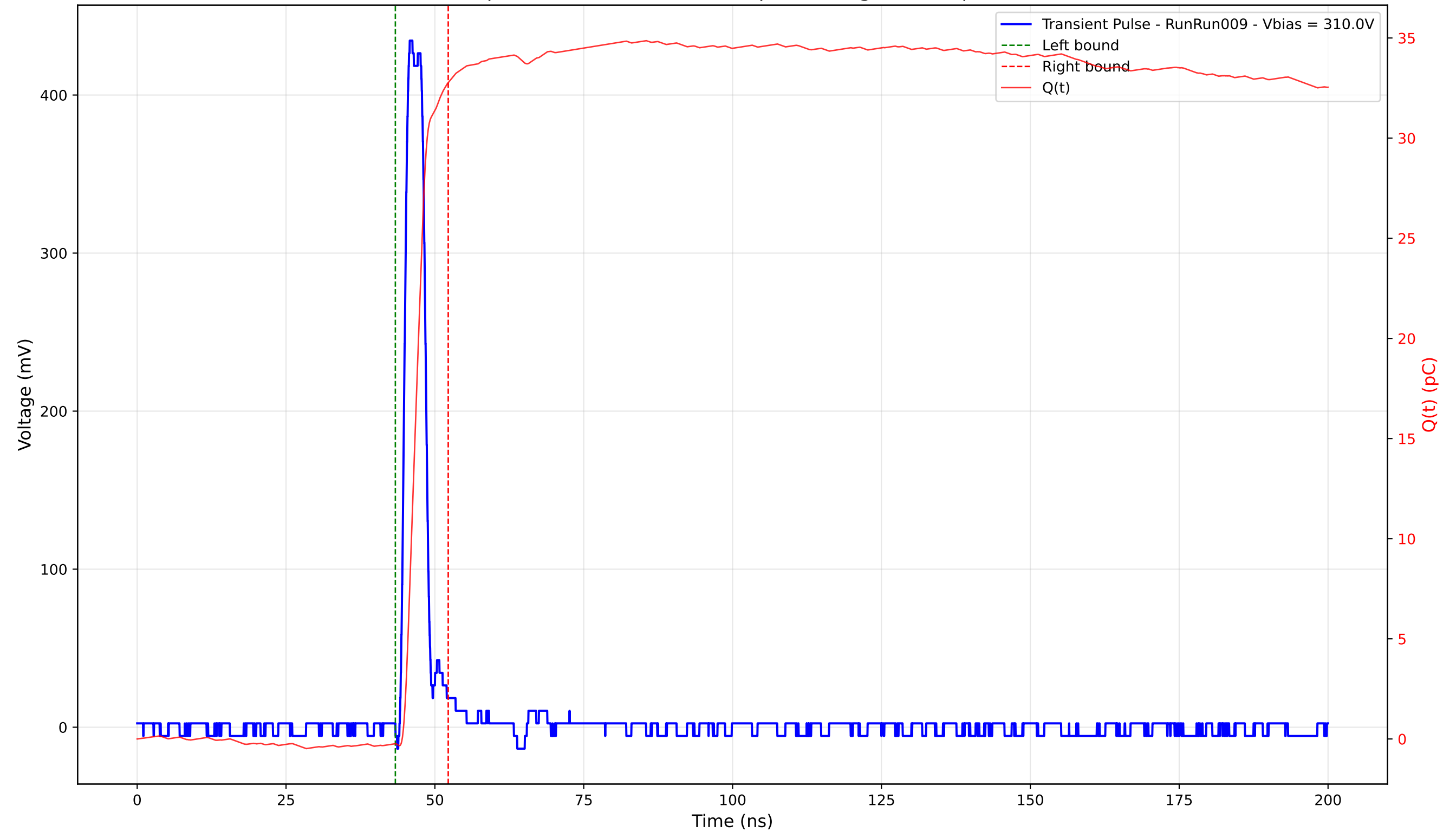
Transient Pulse - Sample: 4003 - Position: 320.0 \mu\text{m} - Charge: 33.00 pC - Rise Time: 1.10 ns
