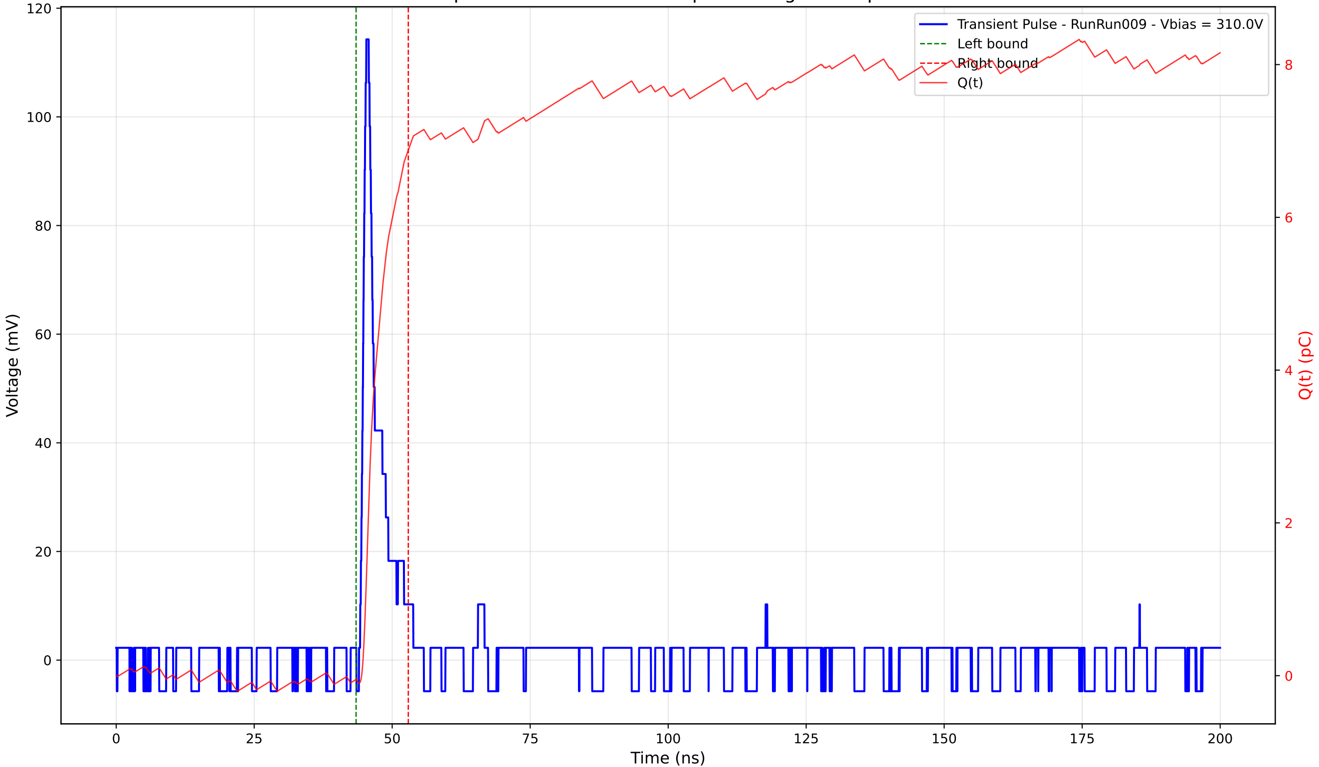
Transient Pulse - Sample: 4003 - Position: 85.0 \mu\text{m} - Charge: 6.93 pC - Rise Time: 0.88 ns
