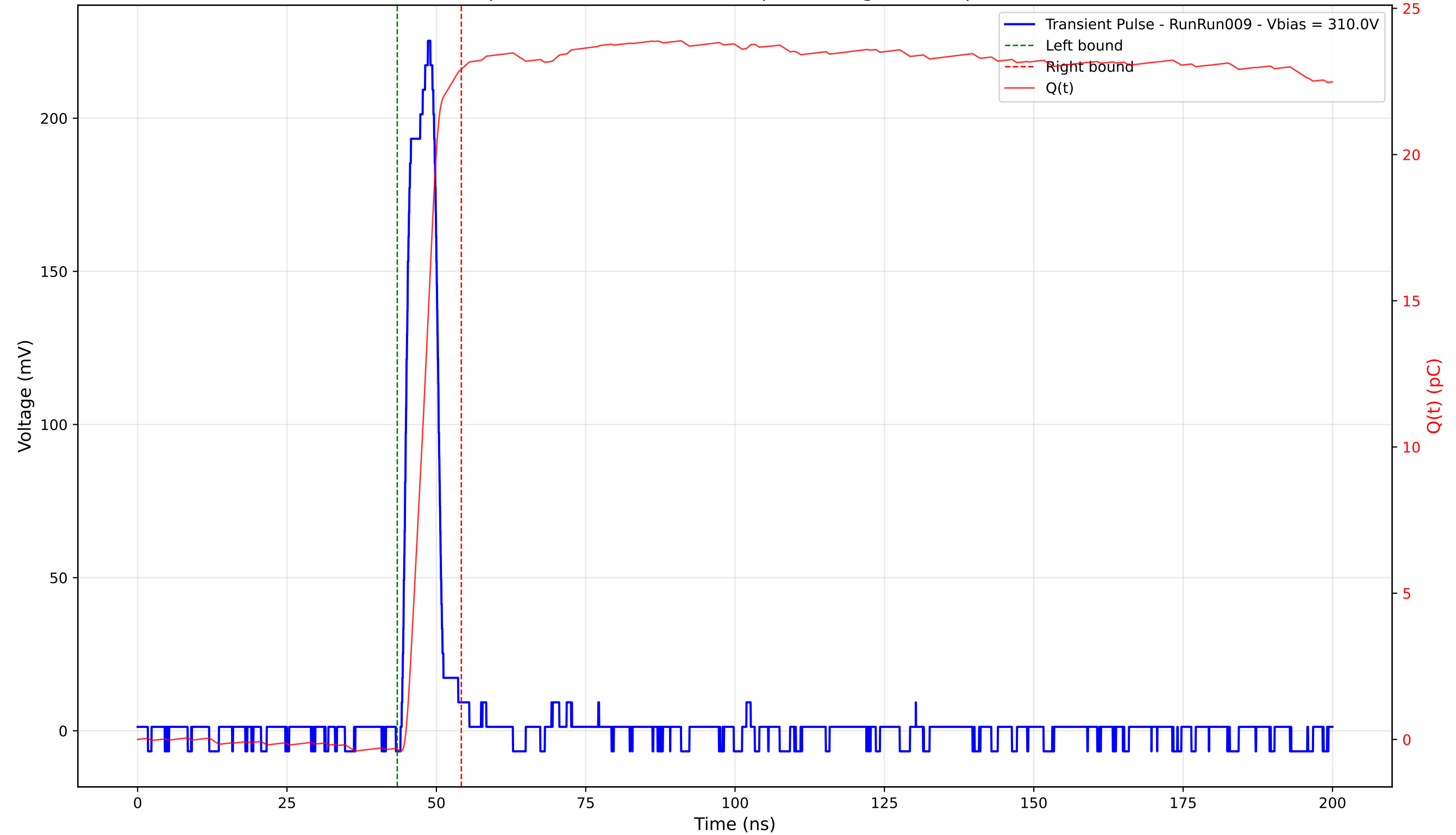
Transient Pulse - Sample: 4003 - Position: 390.0 \mu\text{m} - Charge: 23.26 pC - Rise Time: 3.35 ns
