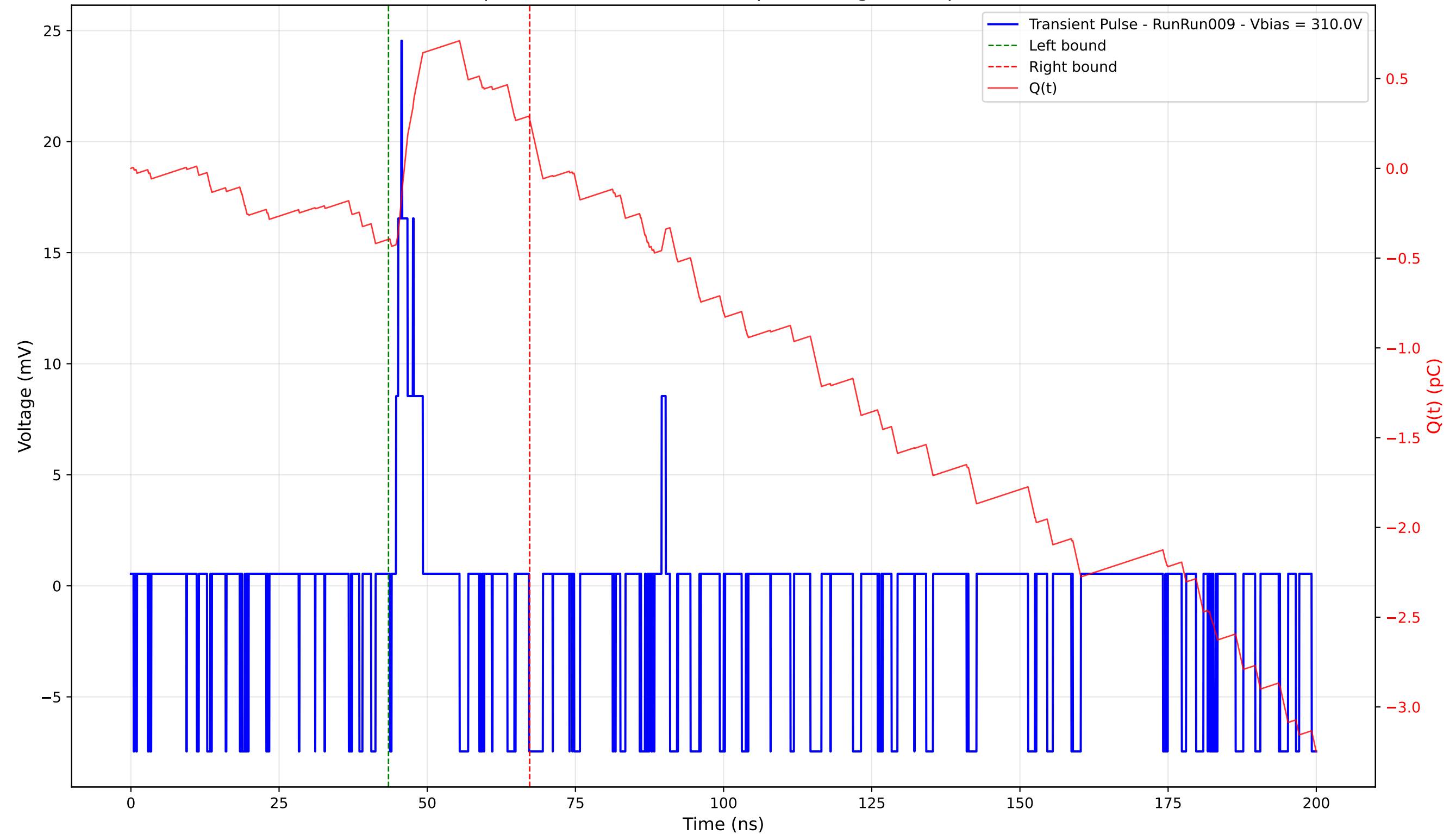
Transient Pulse - Sample: 4003 - Position: 420.0 \mu\text{m} - Charge: 0.67 pC - Rise Time: 0.90 ns
