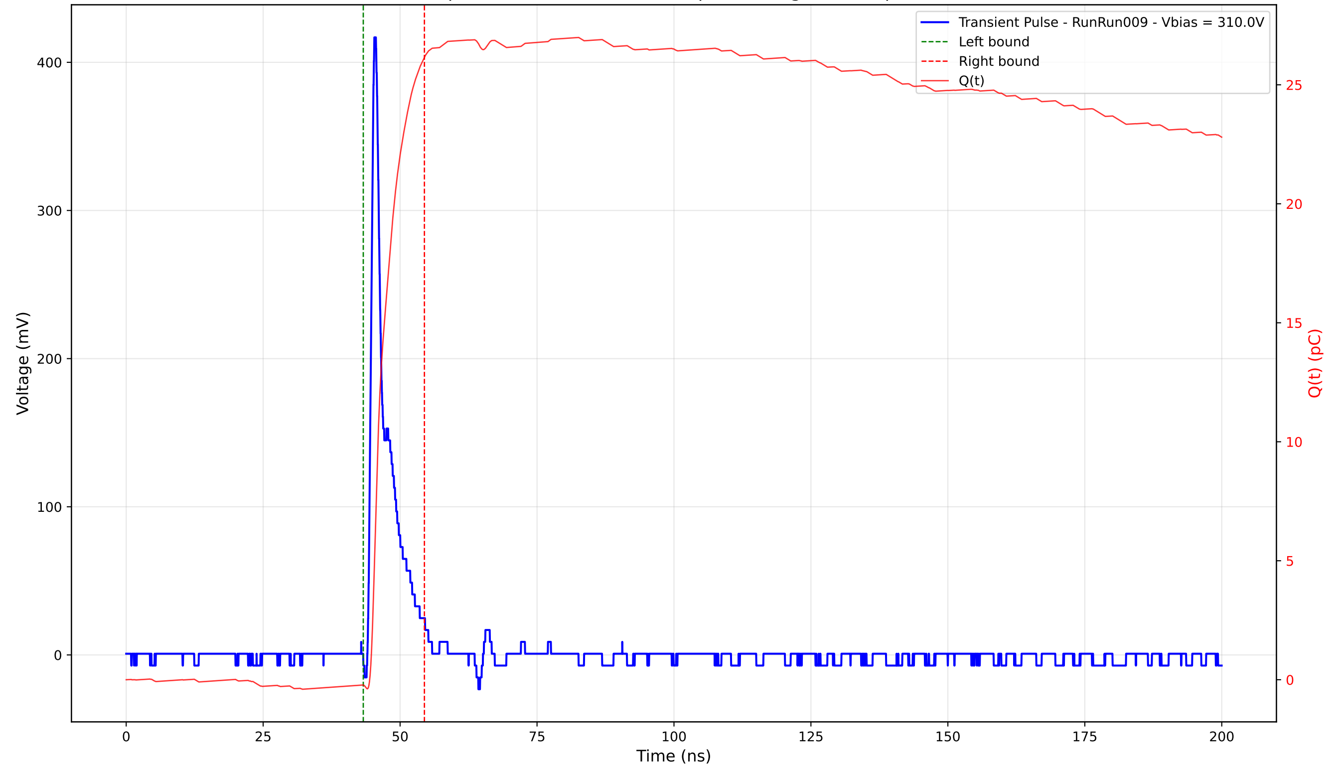
Transient Pulse - Sample: 4003 - Position: 105.0 \mu\text{m} - Charge: 26.38 pC - Rise Time: 0.87 ns
