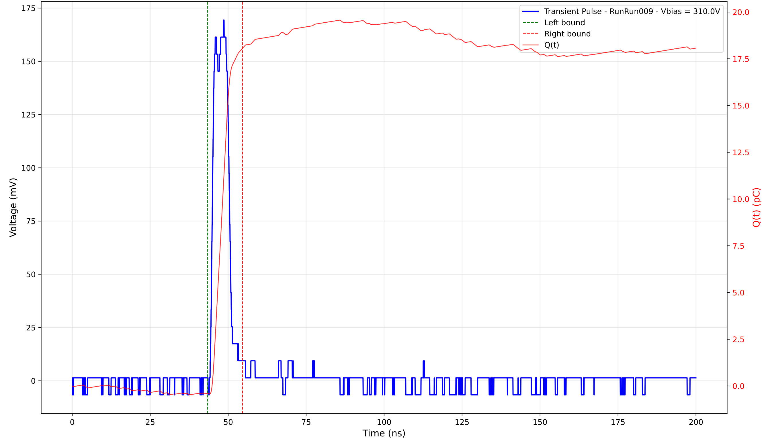
Transient Pulse - Sample: 4003 - Position: 395.0 \mu\text{m} - Charge: 18.46 pC - Rise Time: 1.26 ns
