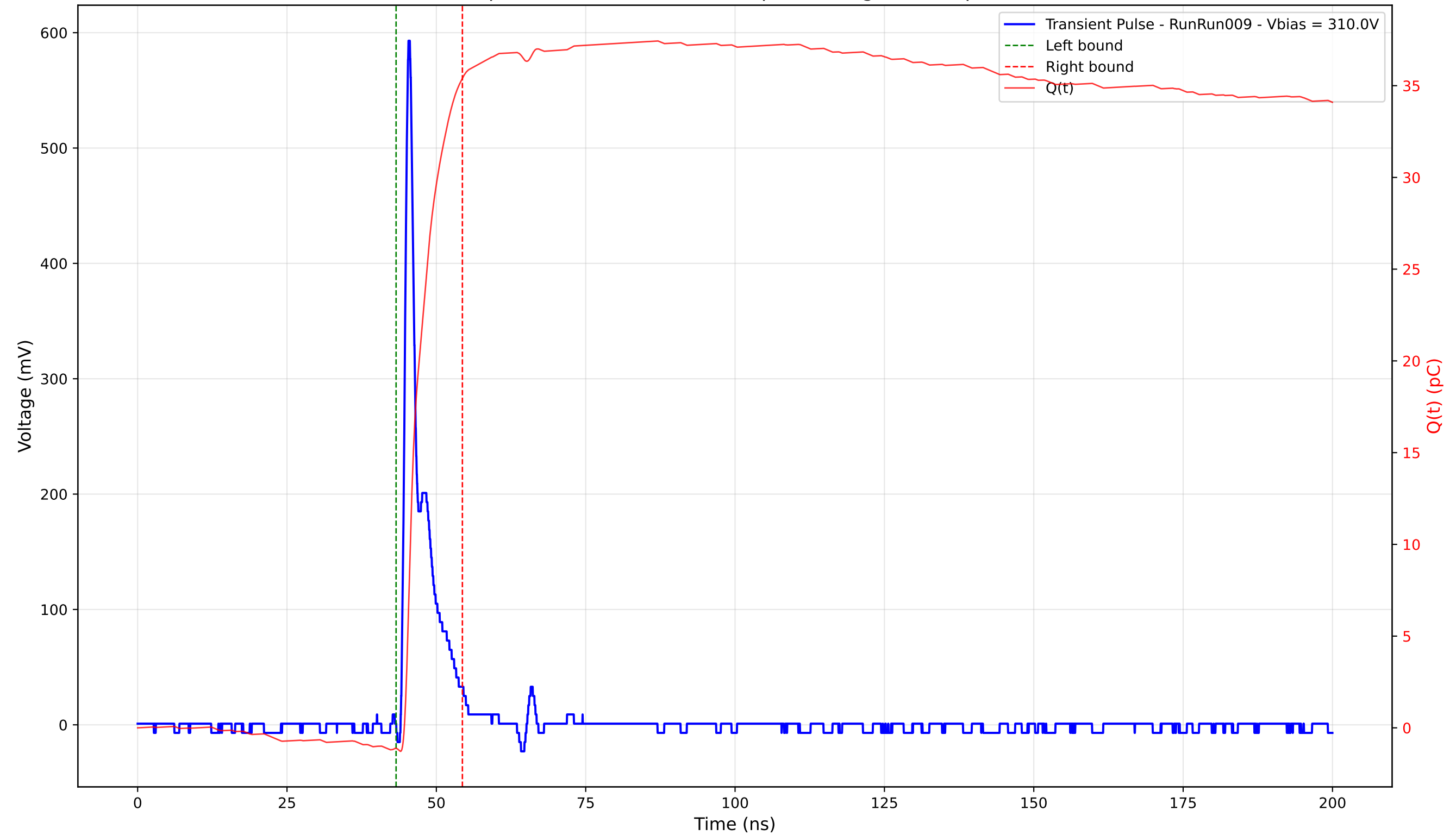
Transient Pulse - Sample: 4003 - Position: 125.0 \mu\text{m} - Charge: 36.52 pC - Rise Time: 0.89 ns
