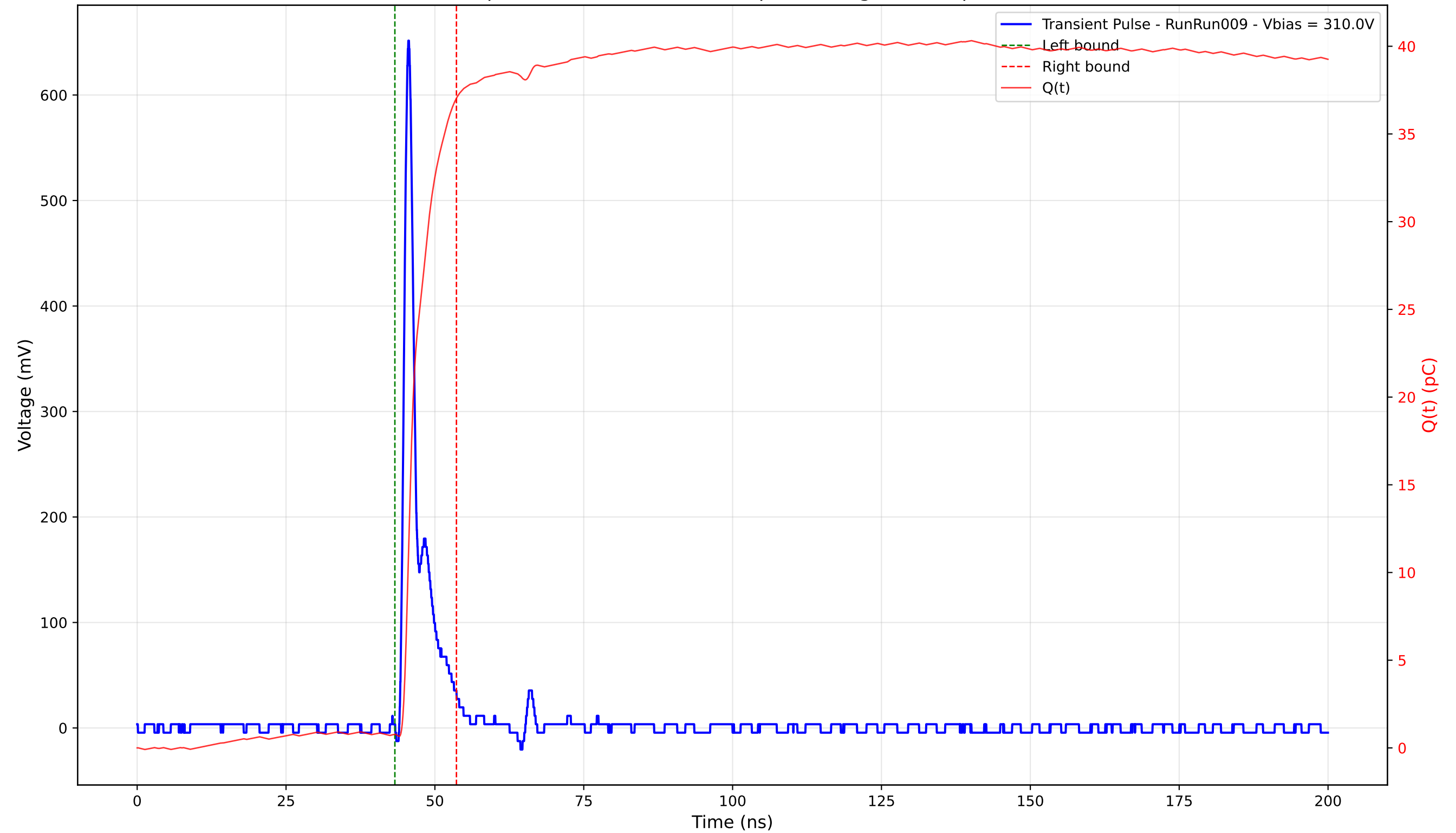
Transient Pulse - Sample: 4003 - Position: 170.0 \mu\text{m} - Charge: 36.27 pC - Rise Time: 0.97 ns
