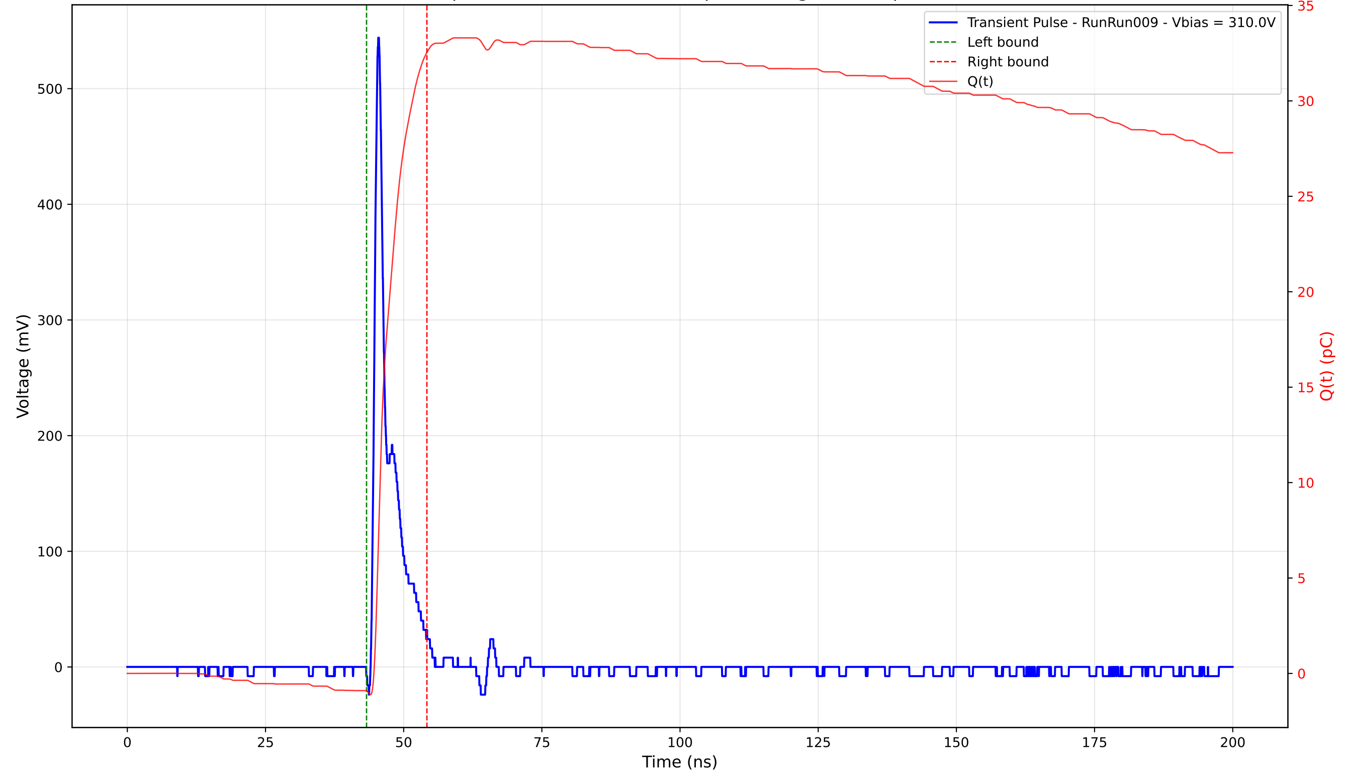
Transient Pulse - Sample: 4003 - Position: 115.0 \mu\text{m} - Charge: 33.45 pC - Rise Time: 0.89 ns
