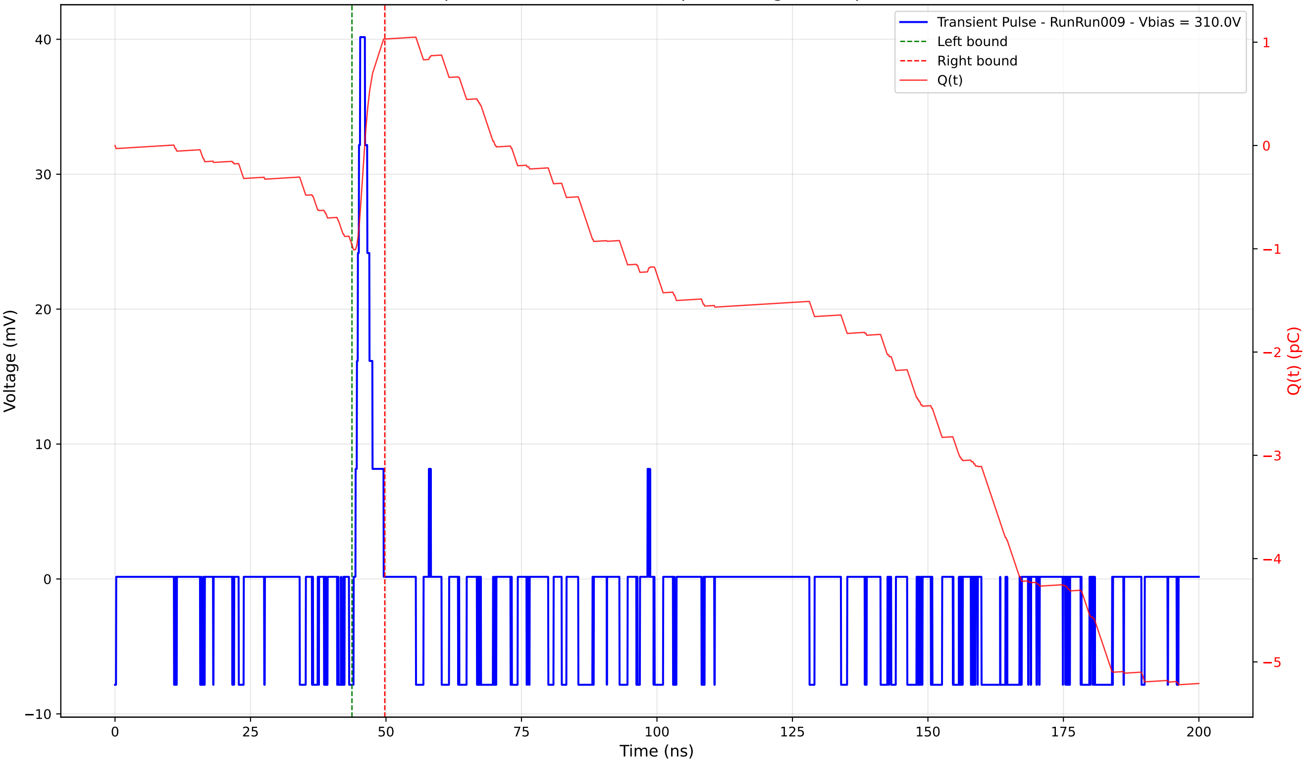
Transient Pulse - Sample: 4003 - Position: 40.0 \mu\text{m} - Charge: 2.00 pC - Rise Time: 0.85 ns
