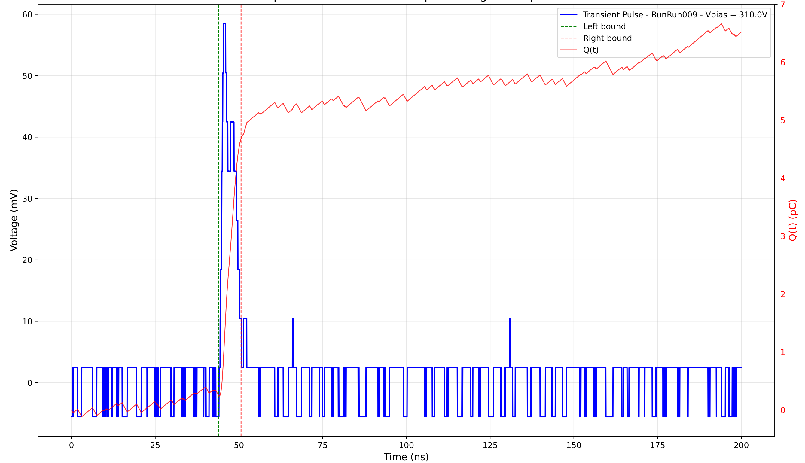
Transient Pulse - Sample: 4003 - Position: 410.0 \mu\text{m} - Charge: 4.43 pC - Rise Time: 0.99 ns
