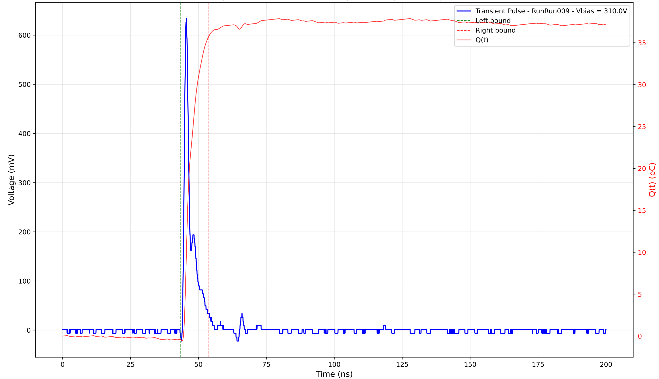
Transient Pulse - Sample: 4003 - Position: 150.0 \mu\text{m} - Charge: 36.20 pC - Rise Time: 0.95 ns
