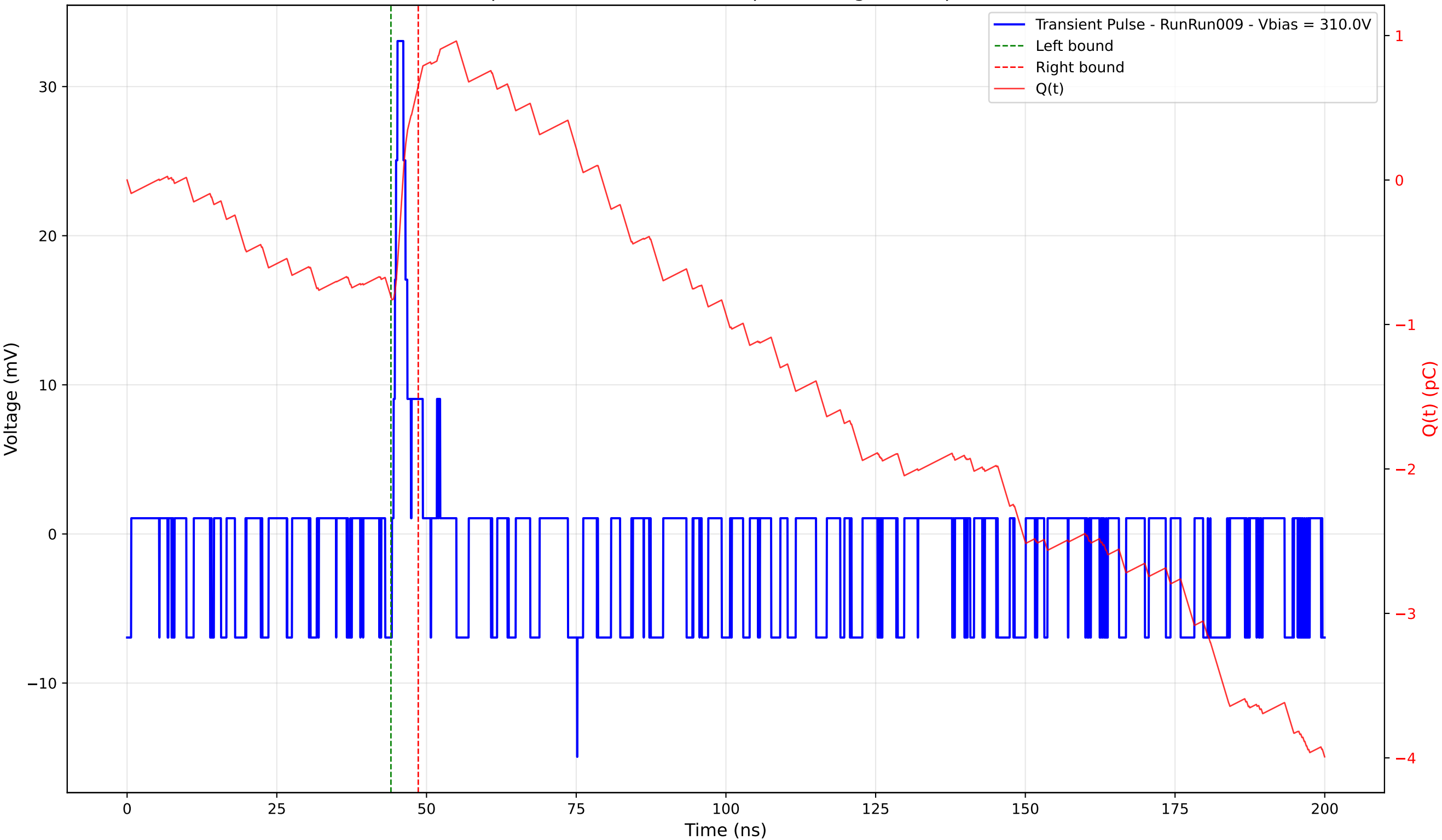
Transient Pulse - Sample: 4003 - Position: 20.0 \mu\text{m} - Charge: 1.46 pC - Rise Time: 0.65 ns
