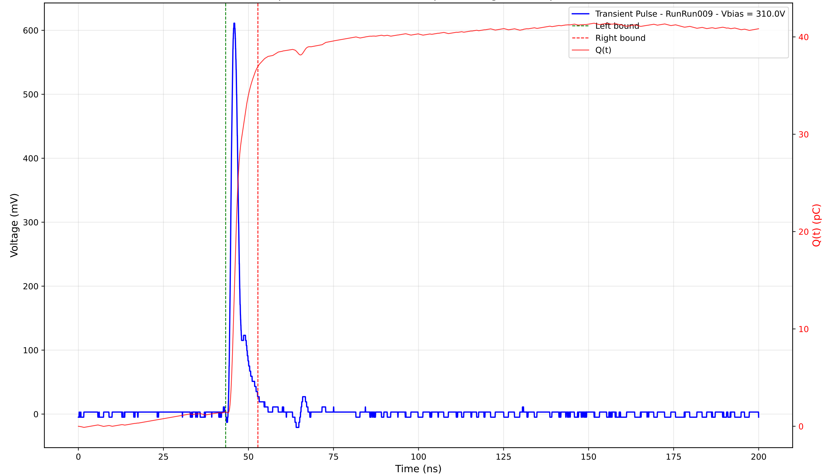
Transient Pulse - Sample: 4003 - Position: 230.0 \mu\text{m} - Charge: 35.49 pC - Rise Time: 1.10 ns
