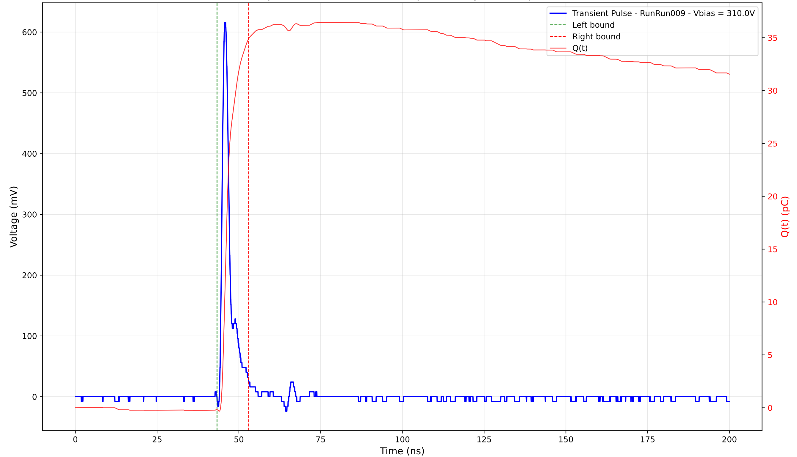
Transient Pulse - Sample: 4003 - Position: 225.0 \mu\text{m} - Charge: 35.01 pC - Rise Time: 1.07 ns
