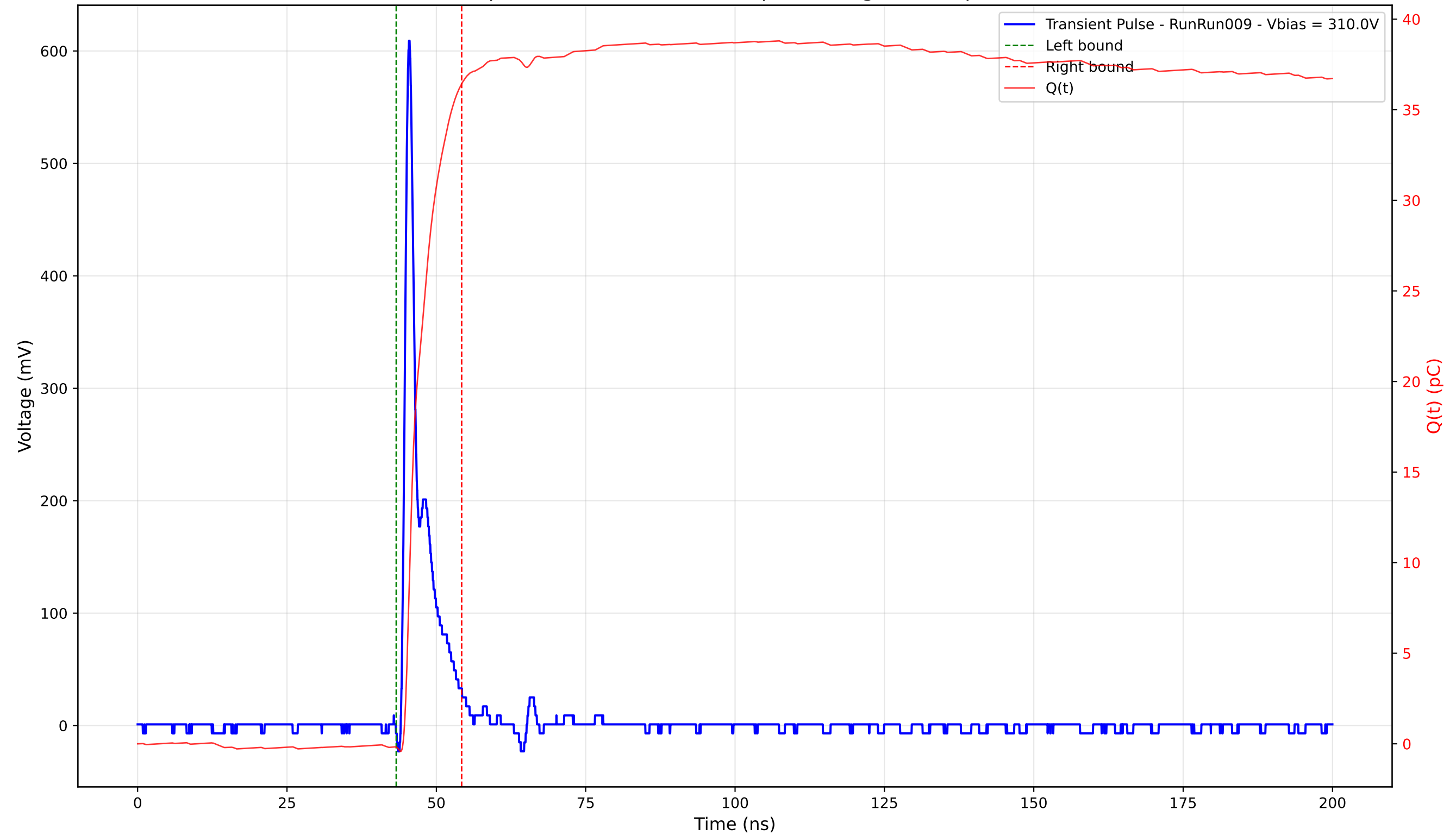
Transient Pulse - Sample: 4003 - Position: 130.0 \mu\text{m} - Charge: 36.61 pC - Rise Time: 0.90 ns
