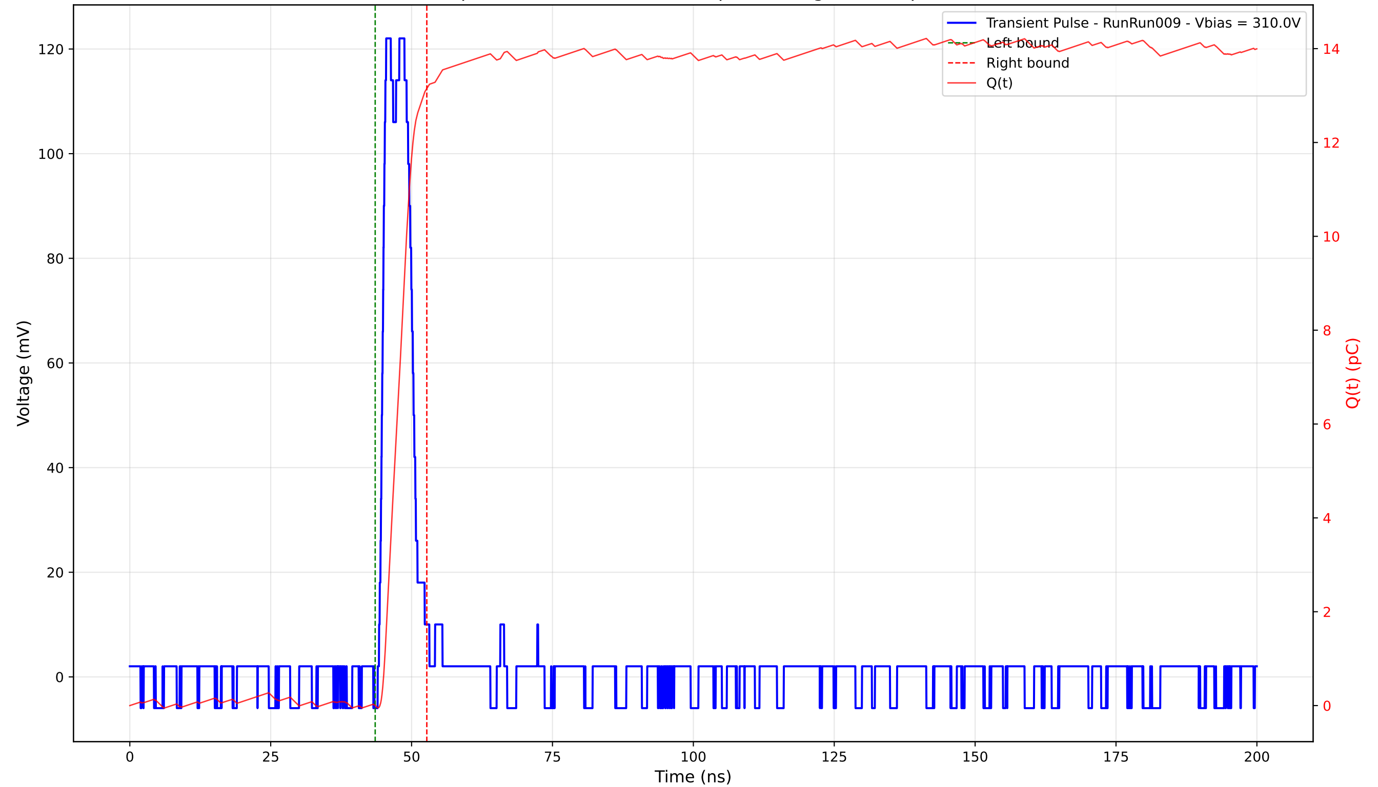
Transient Pulse - Sample: 4003 - Position: 400.0 \mu\text{m} - Charge: 13.15 pC - Rise Time: 1.01 ns
