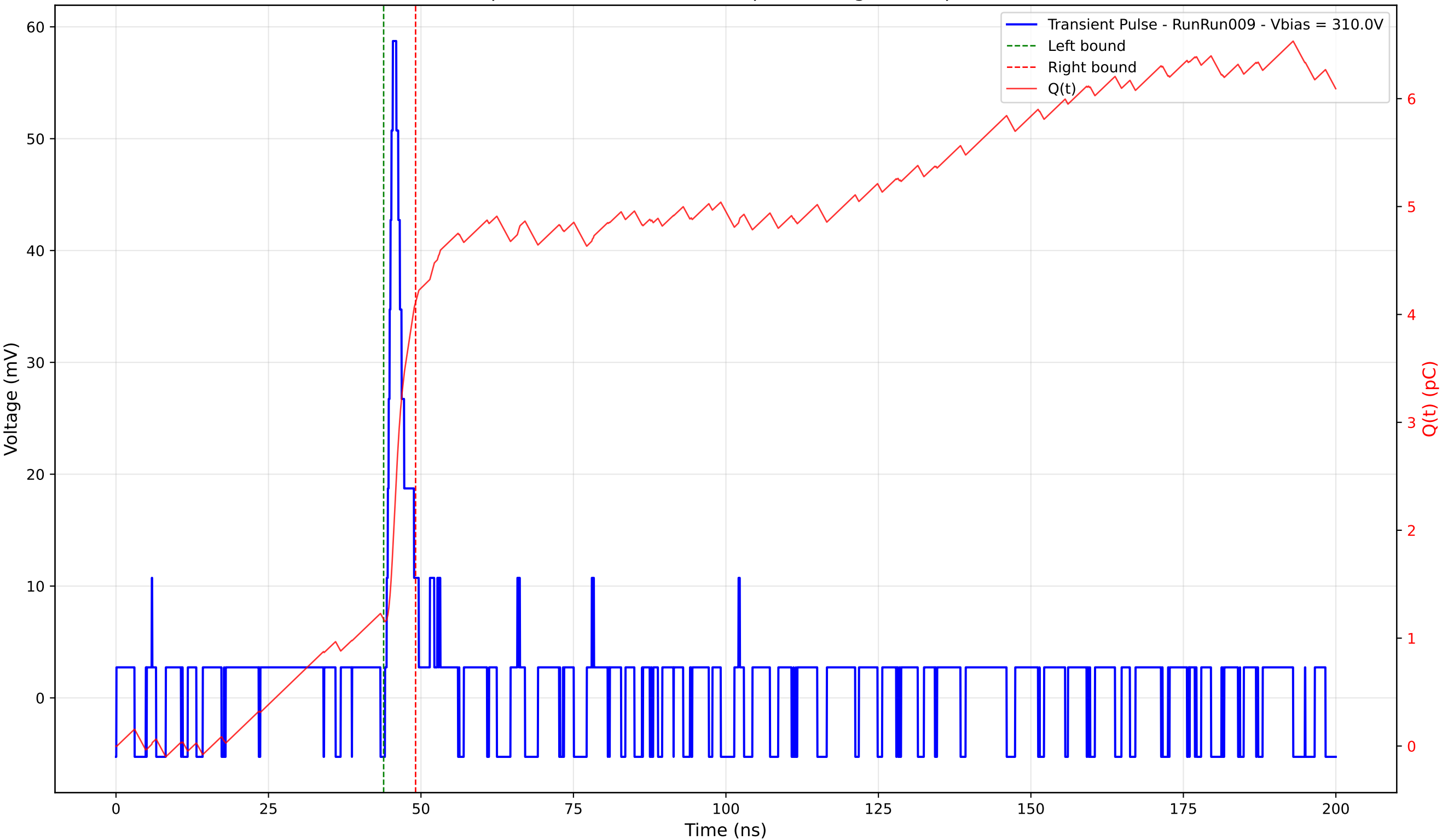
Transient Pulse - Sample: 4003 - Position: 45.0 \mu\text{m} - Charge: 2.94 pC - Rise Time: 1.01 ns
