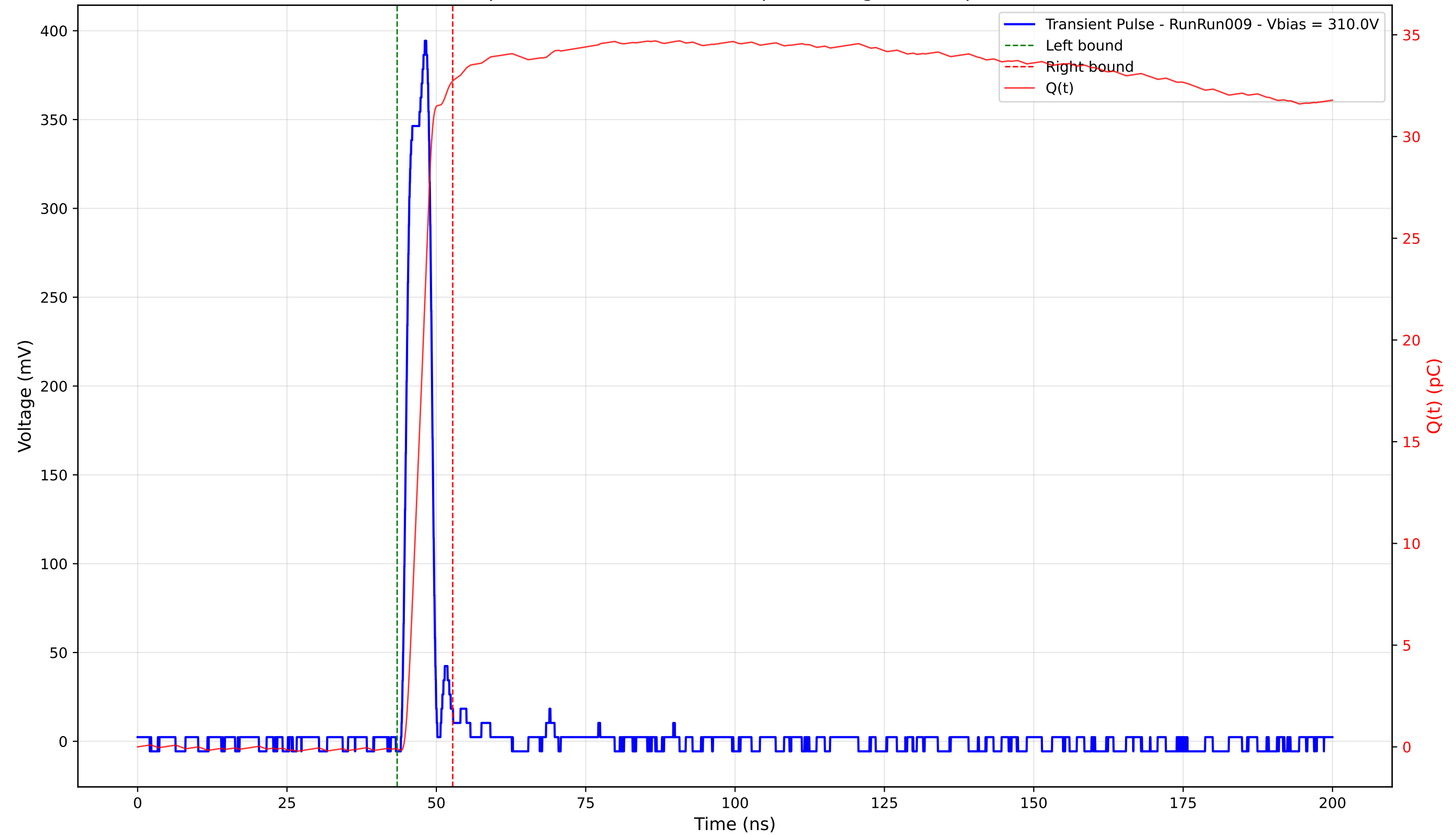
Transient Pulse - Sample: 4003 - Position: 360.0 \mu\text{m} - Charge: 32.84 pC - Rise Time: 2.95 ns
