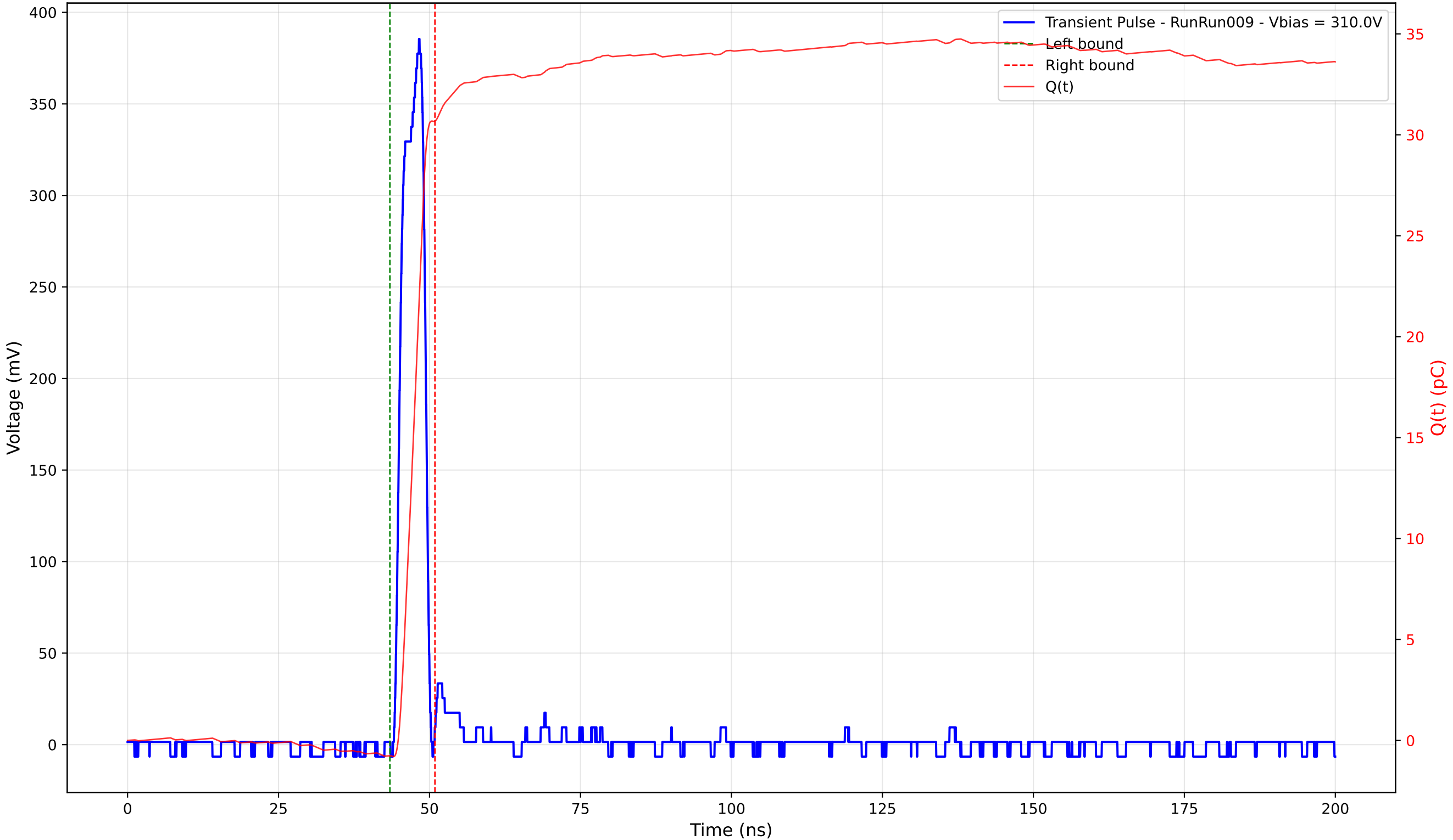
Transient Pulse - Sample: 4003 - Position: 365.0 \mu\text{m} - Charge: 31.43 pC - Rise Time: 3.03 ns
