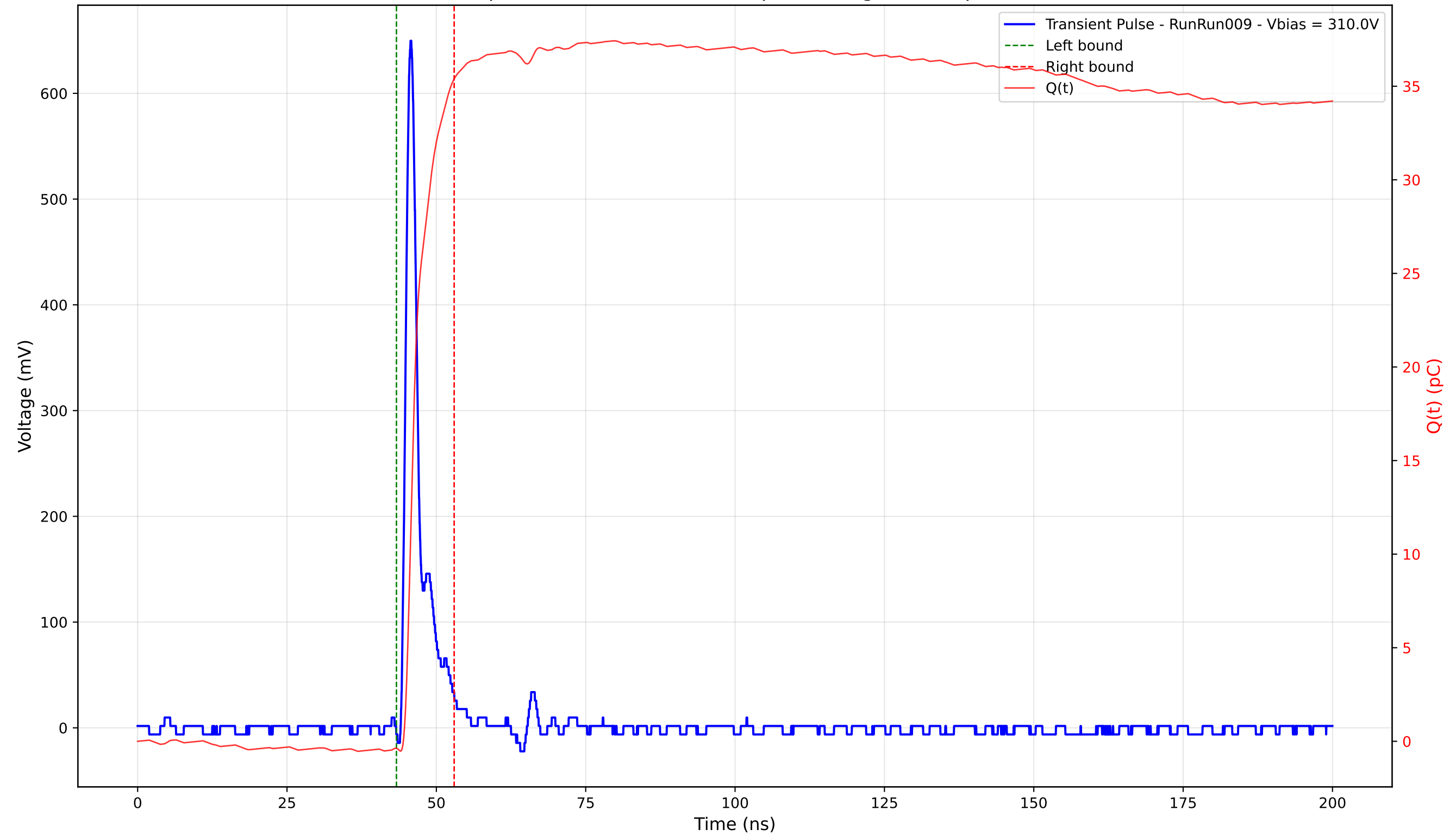
Transient Pulse - Sample: 4003 - Position: 205.0 \mu\text{m} - Charge: 35.77 pC - Rise Time: 1.04 ns
