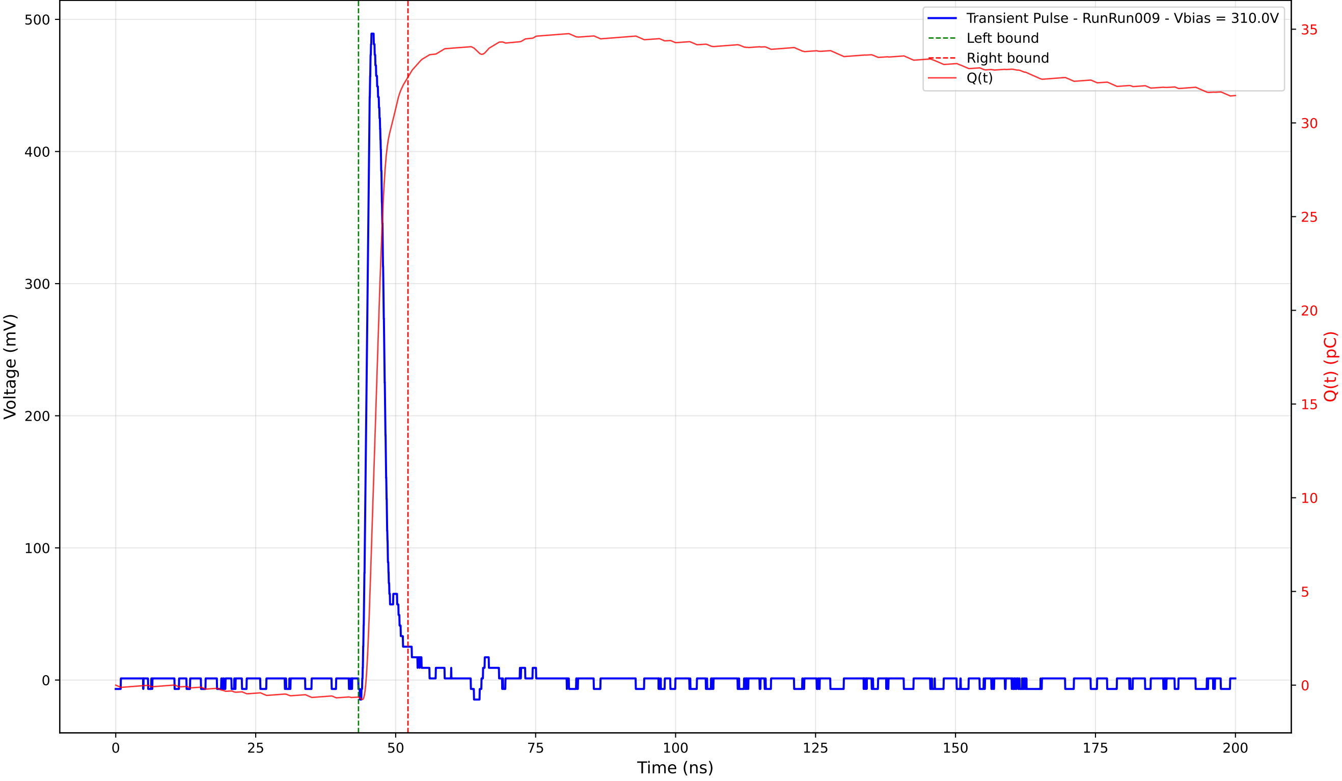
Transient Pulse - Sample: 4003 - Position: 290.0 \mu\text{m} - Charge: 33.09 pC - Rise Time: 1.04 ns
