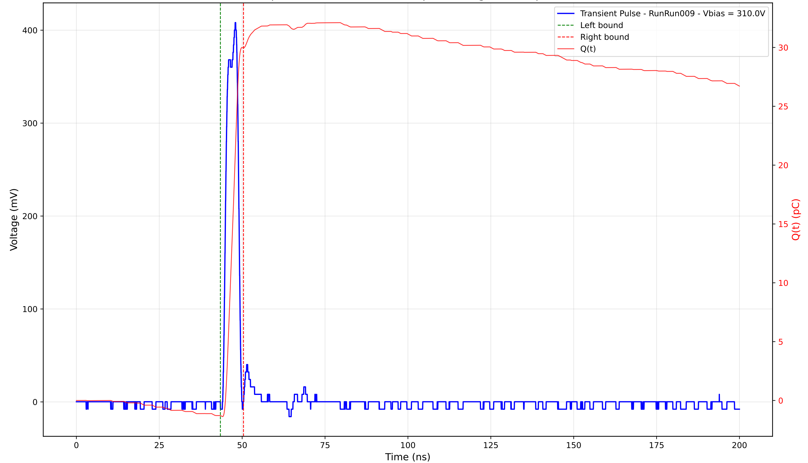
Transient Pulse - Sample: 4003 - Position: 350.0 \mu\text{m} - Charge: 31.24 pC - Rise Time: 1.50 ns
