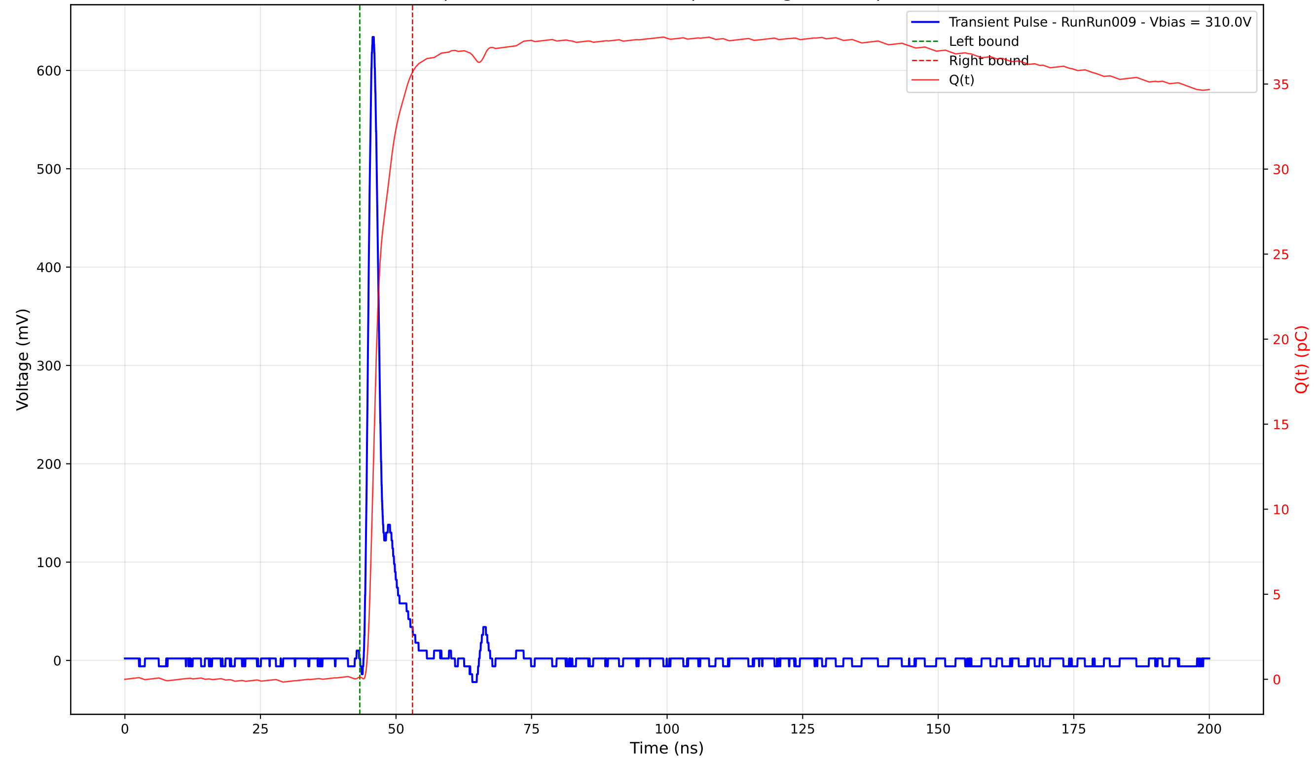
Transient Pulse - Sample: 4003 - Position: 215.0 \mu\text{m} - Charge: 35.58 pC - Rise Time: 1.07 ns
