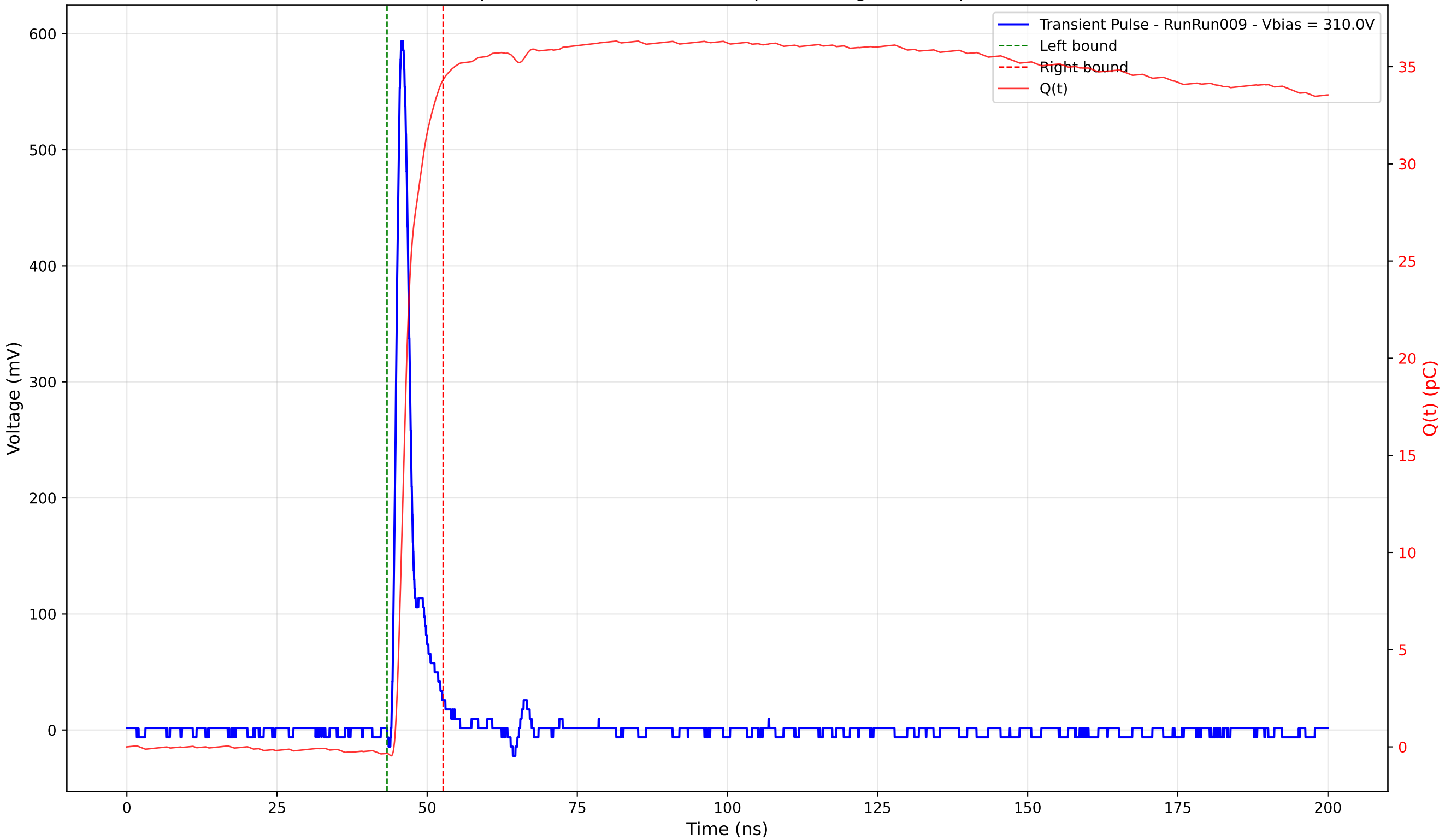
Transient Pulse - Sample: 4003 - Position: 235.0 \mu\text{m} - Charge: 34.65 pC - Rise Time: 1.07 ns
