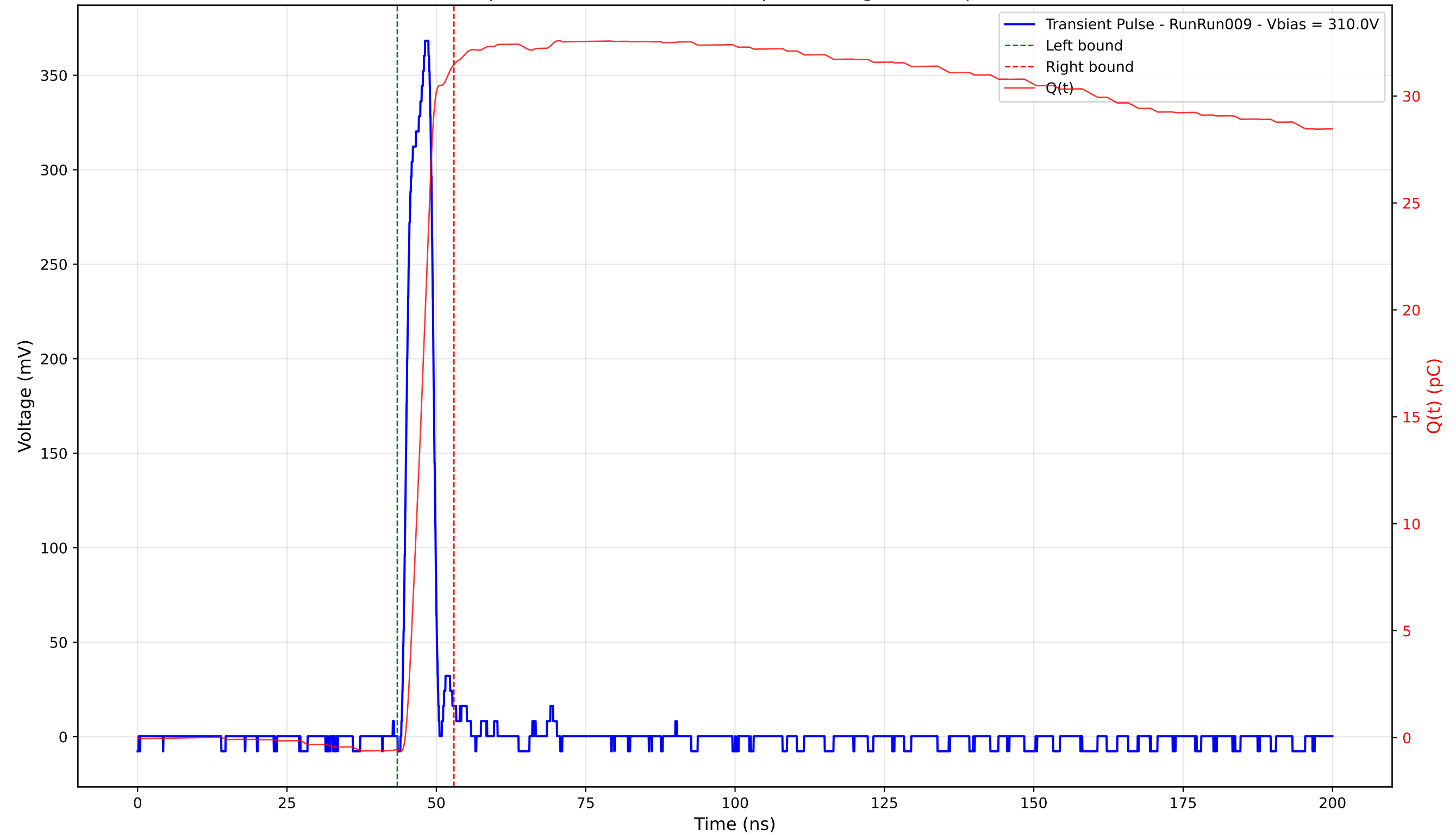
Transient Pulse - Sample: 4003 - Position: 370.0 \mu\text{m} - Charge: 32.04 pC - Rise Time: 2.91 ns
