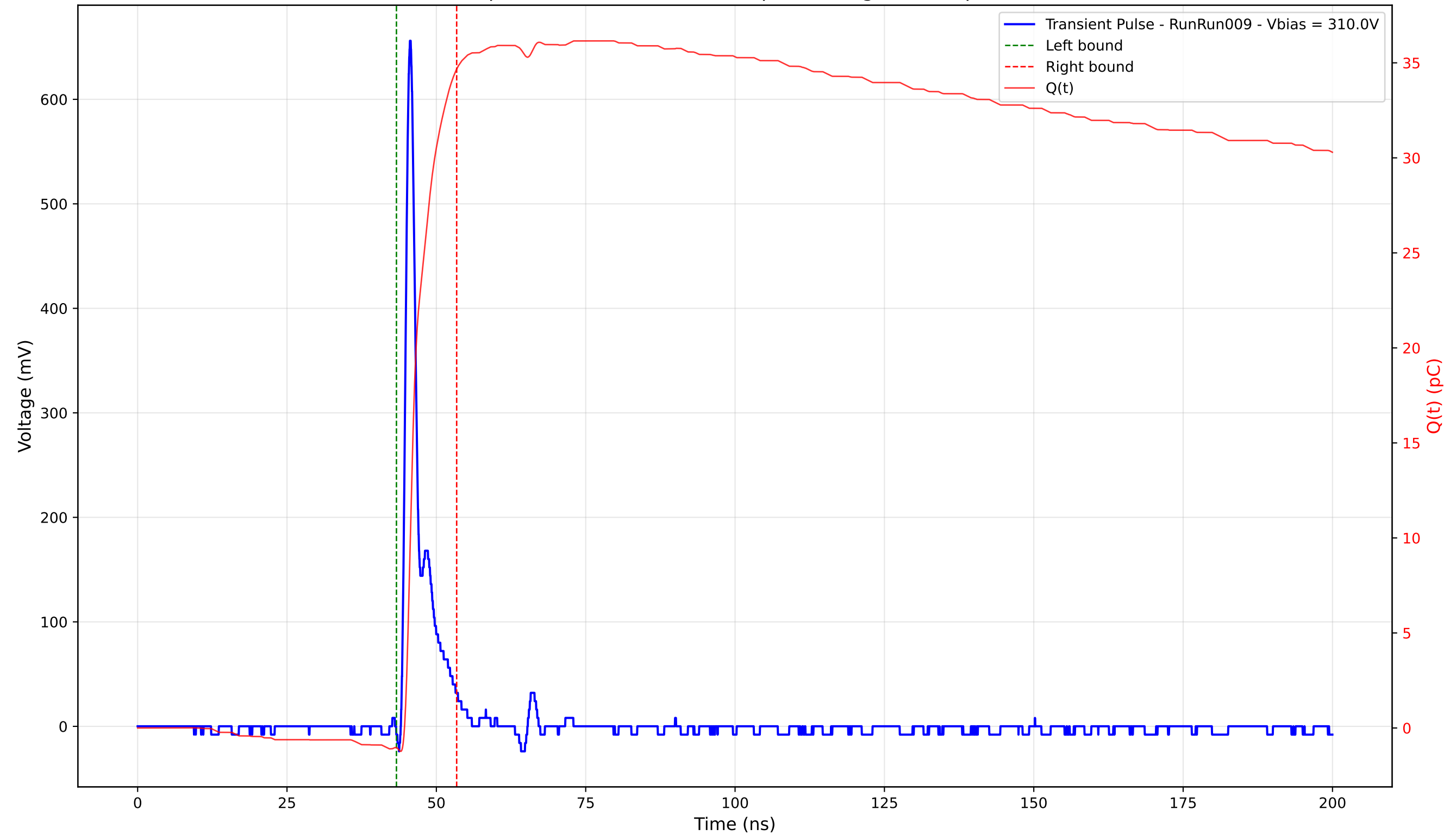
Transient Pulse - Sample: 4003 - Position: 180.0 \mu\text{m} - Charge: 35.70 pC - Rise Time: 0.97 ns
