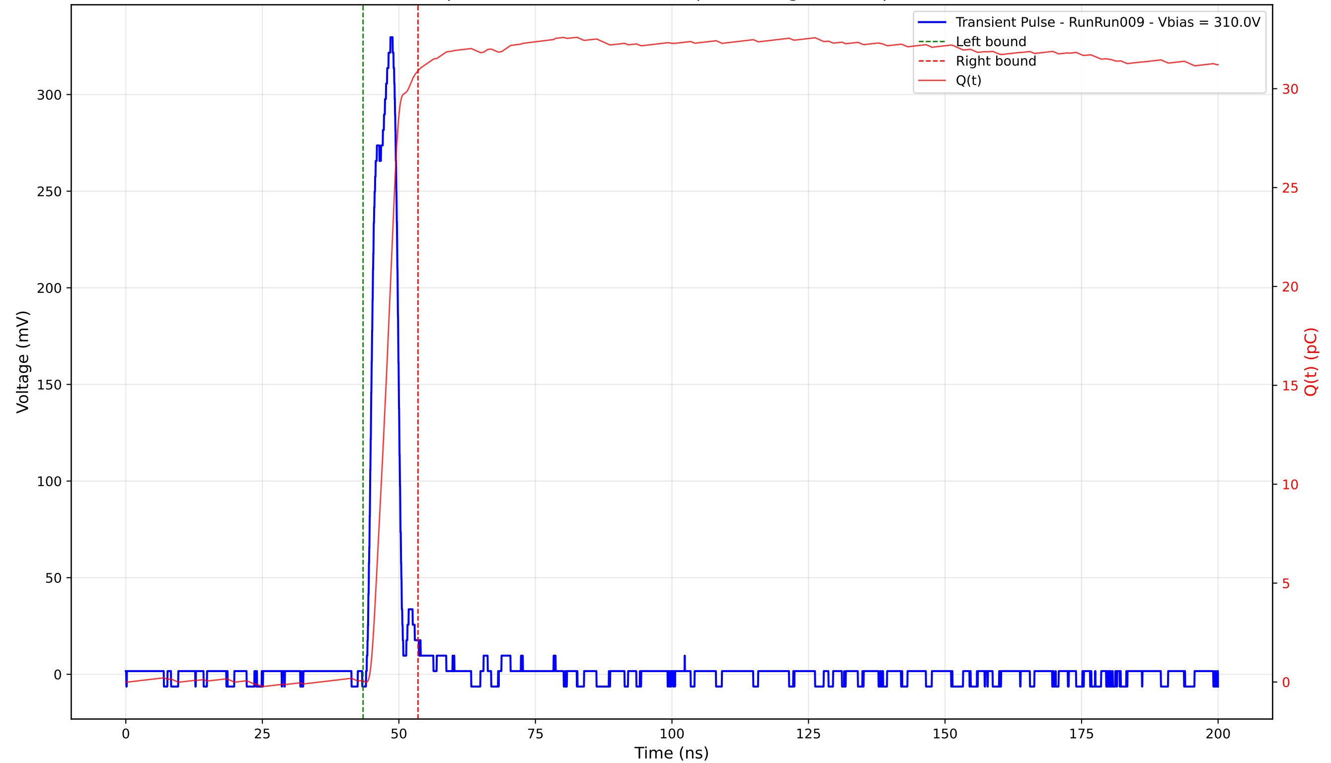
Transient Pulse - Sample: 4003 - Position: 380.0 \mu\text{m} - Charge: 30.86 pC - Rise Time: 3.06 ns
