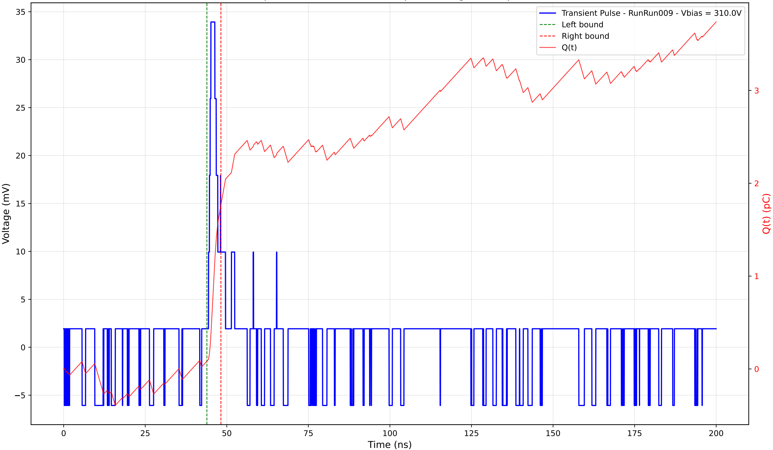
Transient Pulse - Sample: 4003 - Position: 30.0 \mu\text{m} - Charge: 1.68 pC - Rise Time: 0.74 ns
