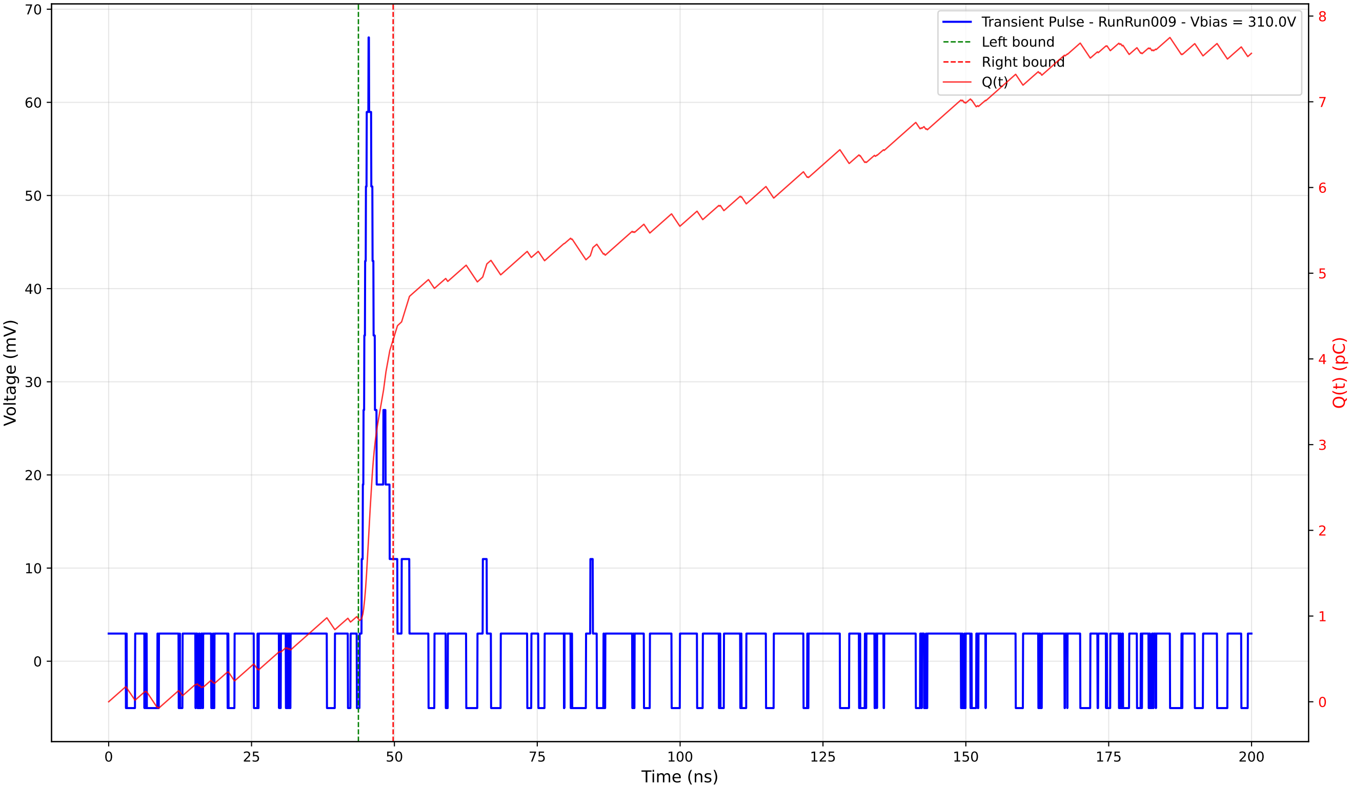
Transient Pulse - Sample: 4003 - Position: 80.0 \mu\text{m} - Charge: 3.26 pC - Rise Time: 1.21 ns
