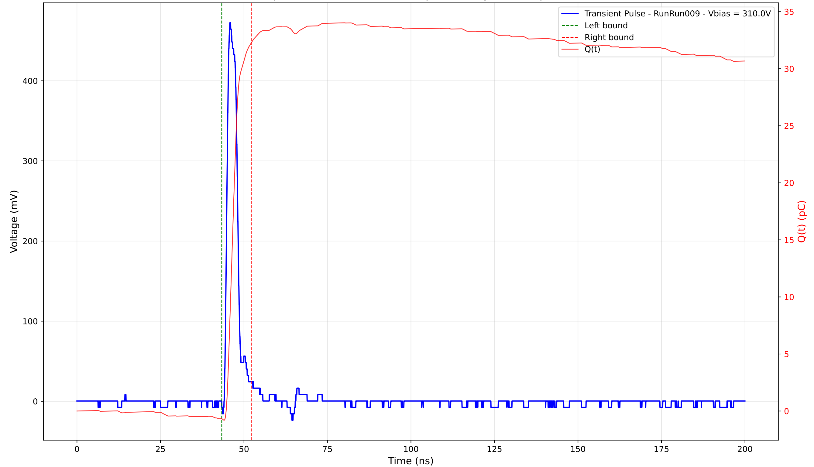
Transient Pulse - Sample: 4003 - Position: 300.0 \mu\text{m} - Charge: 32.93 pC - Rise Time: 1.10 ns
