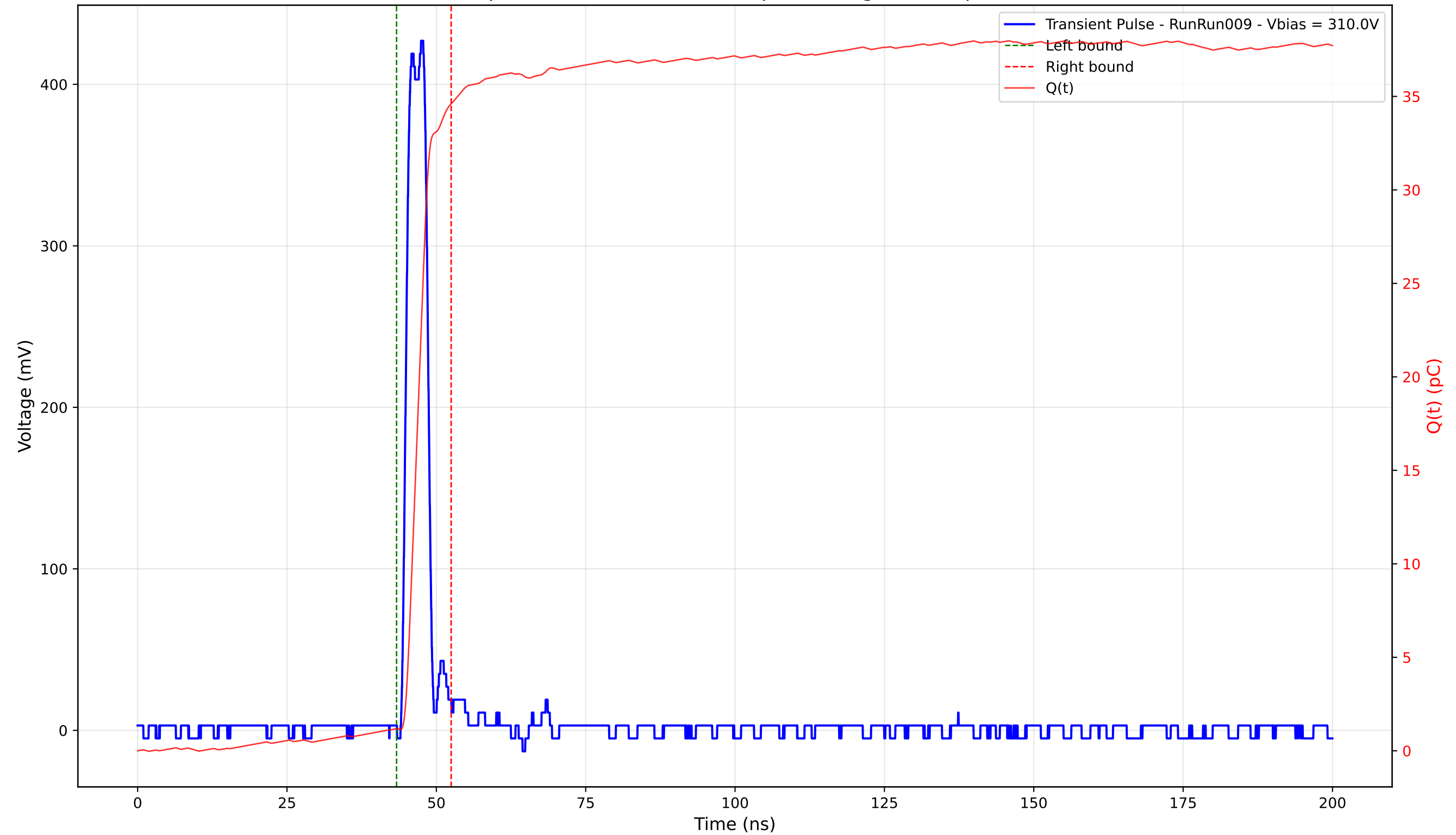
Transient Pulse - Sample: 4003 - Position: 330.0 \mu\text{m} - Charge: 33.42 pC - Rise Time: 1.18 ns
