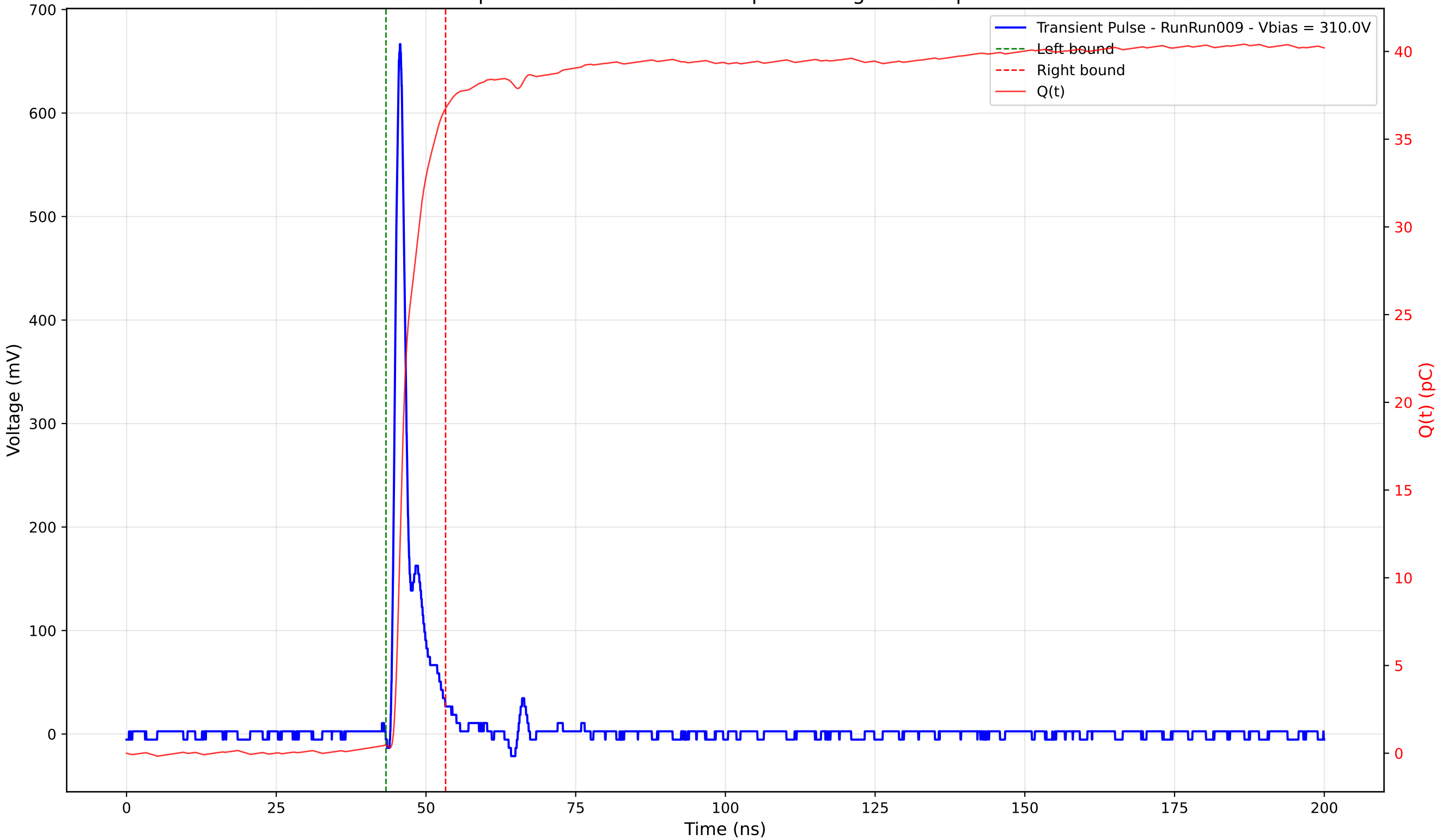
Transient Pulse - Sample: 4003 - Position: 190.0 \mu\text{m} - Charge: 36.30 pC - Rise Time: 1.01 ns
