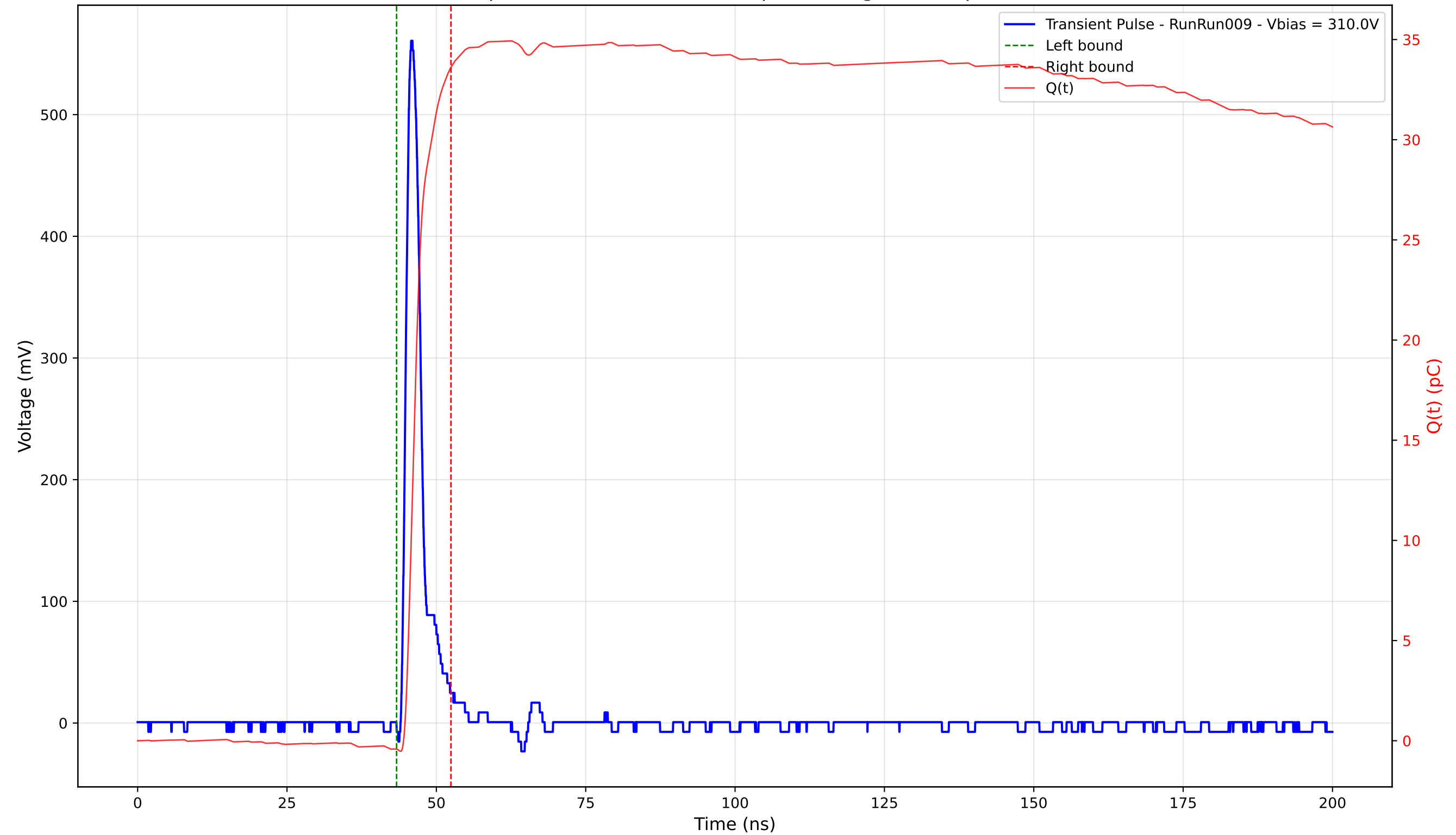
Transient Pulse - Sample: 4003 - Position: 255.0 \mu\text{m} - Charge: 34.02 pC - Rise Time: 1.10 ns
