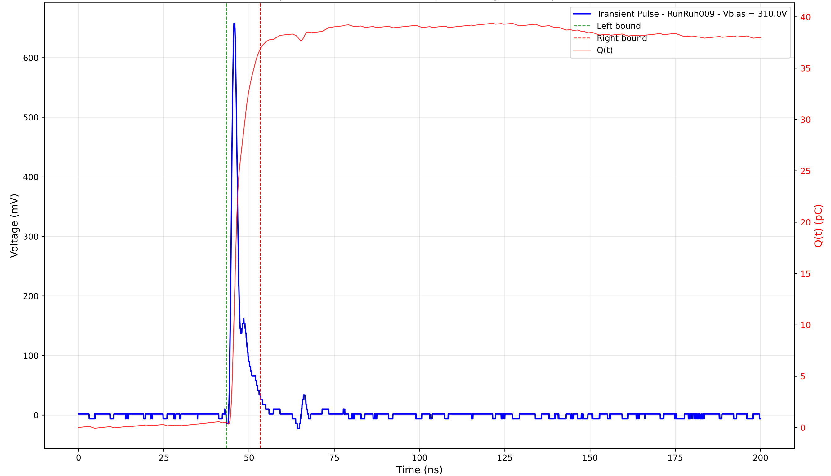
Transient Pulse - Sample: 4003 - Position: 195.0 \mu\text{m} - Charge: 36.37 pC - Rise Time: 1.02 ns
