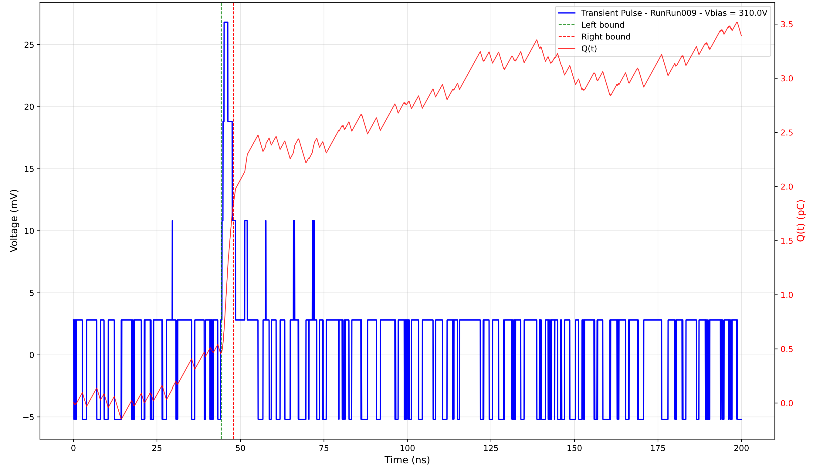
Transient Pulse - Sample: 4003 - Position: 15.0 \mu\text{m} - Charge: 1.39 pC - Rise Time: 0.00 ns (N/A)
