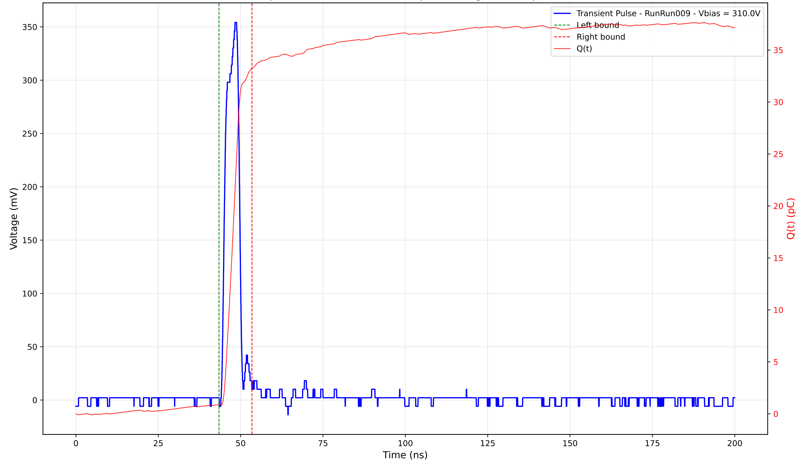
Transient Pulse - Sample: 4003 - Position: 375.0 \mu\text{m} - Charge: 32.37 pC - Rise Time: 3.02 ns
