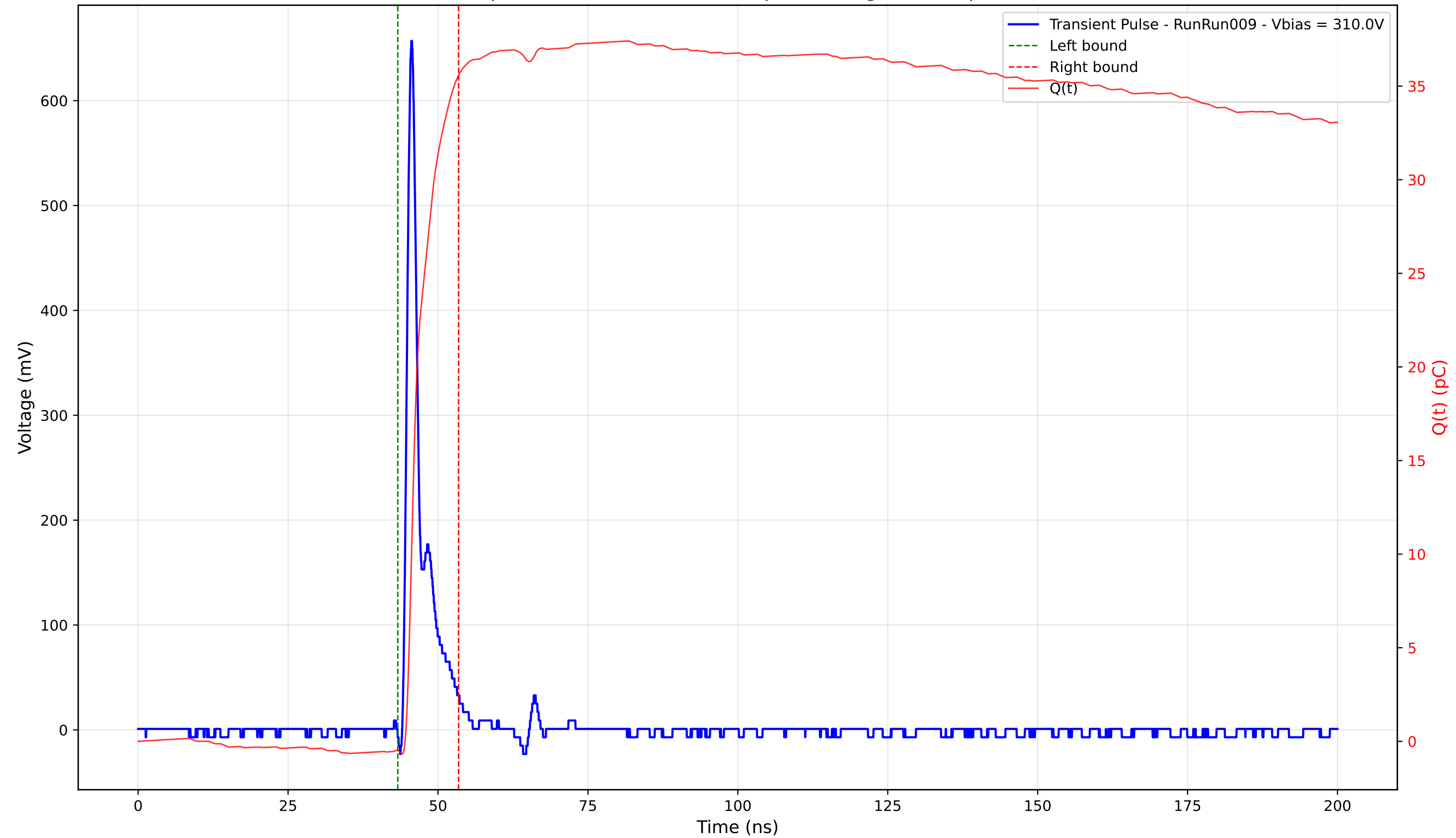
Transient Pulse - Sample: 4003 - Position: 175.0 \mu\text{m} - Charge: 36.07 pC - Rise Time: 0.97 ns
