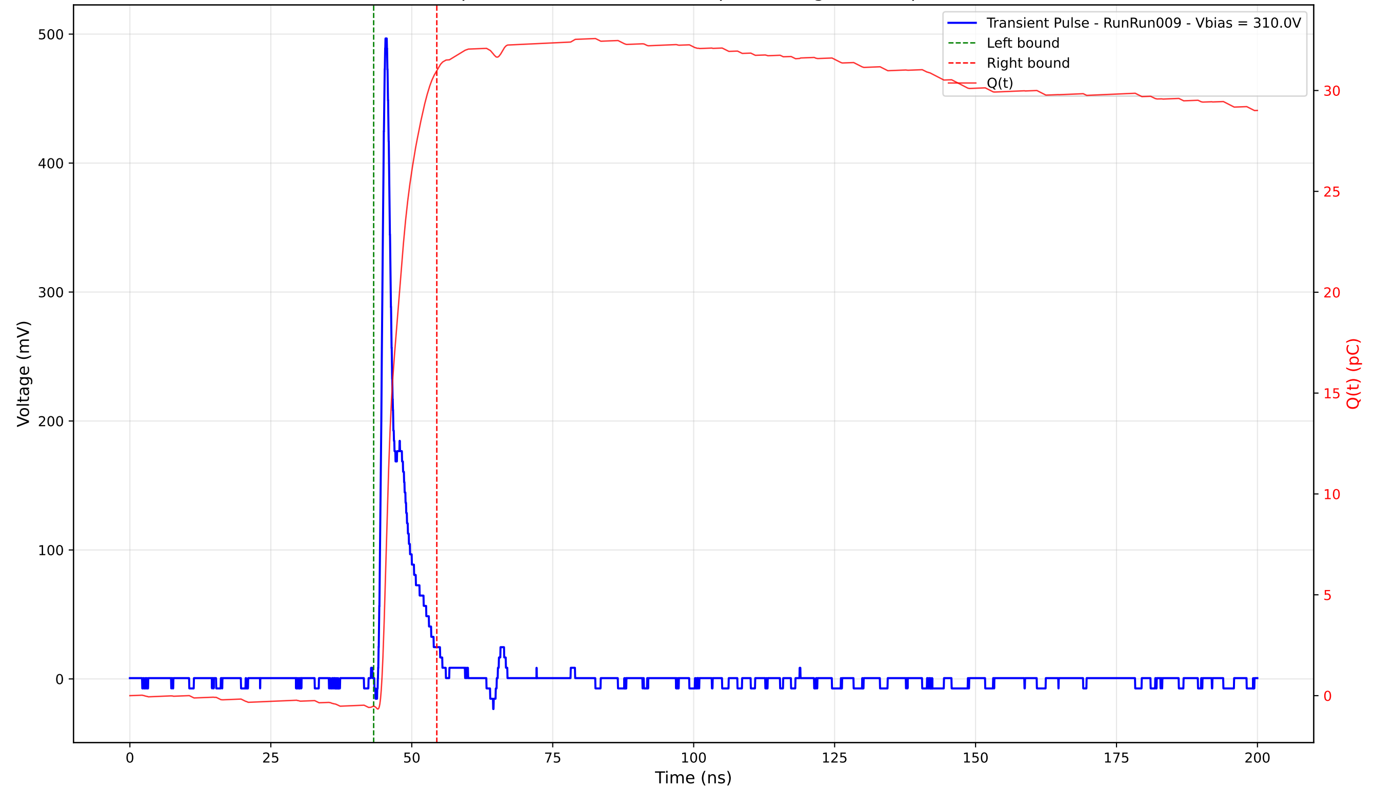
Transient Pulse - Sample: 4003 - Position: 110.0 \mu\text{m} - Charge: 31.52 pC - Rise Time: 0.89 ns
