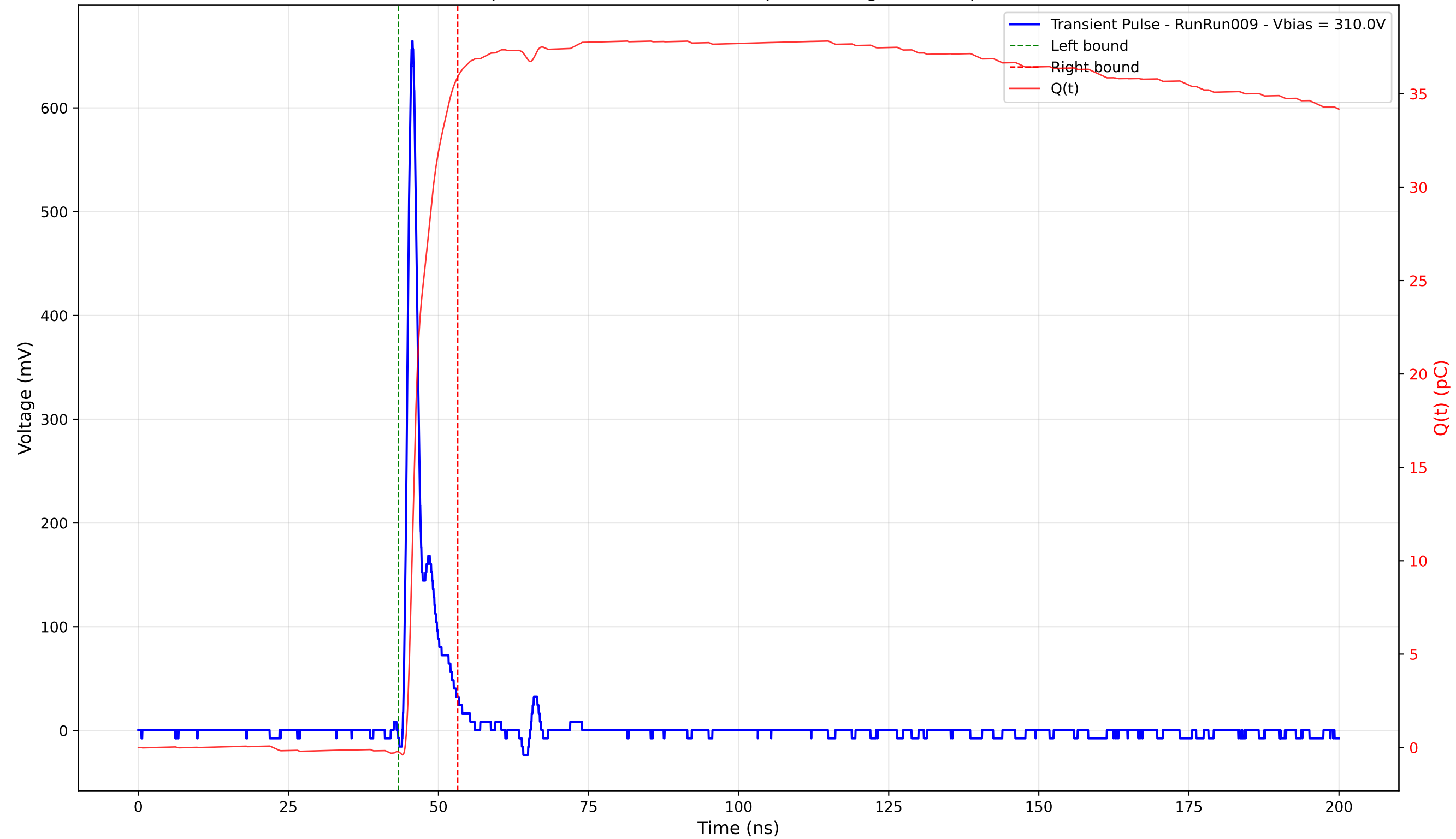
Transient Pulse - Sample: 4003 - Position: 185.0 \mu\text{m} - Charge: 36.13 pC - Rise Time: 1.01 ns
