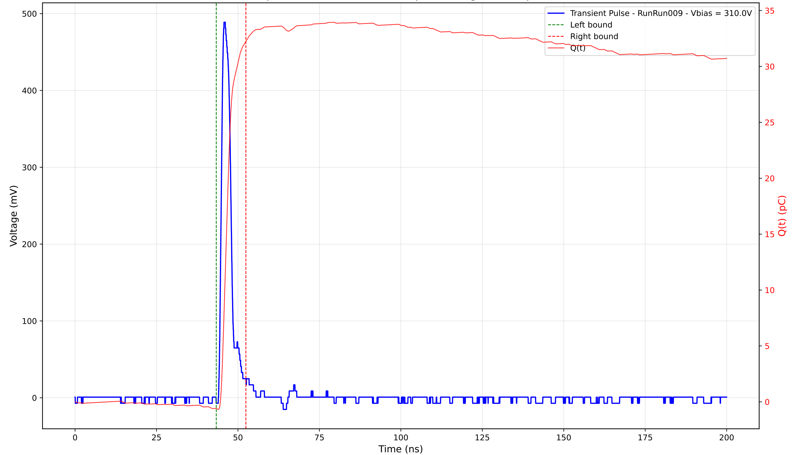
Transient Pulse - Sample: 4003 - Position: 285.0 \mu\text{m} - Charge: 32.84 pC - Rise Time: 1.08 ns
