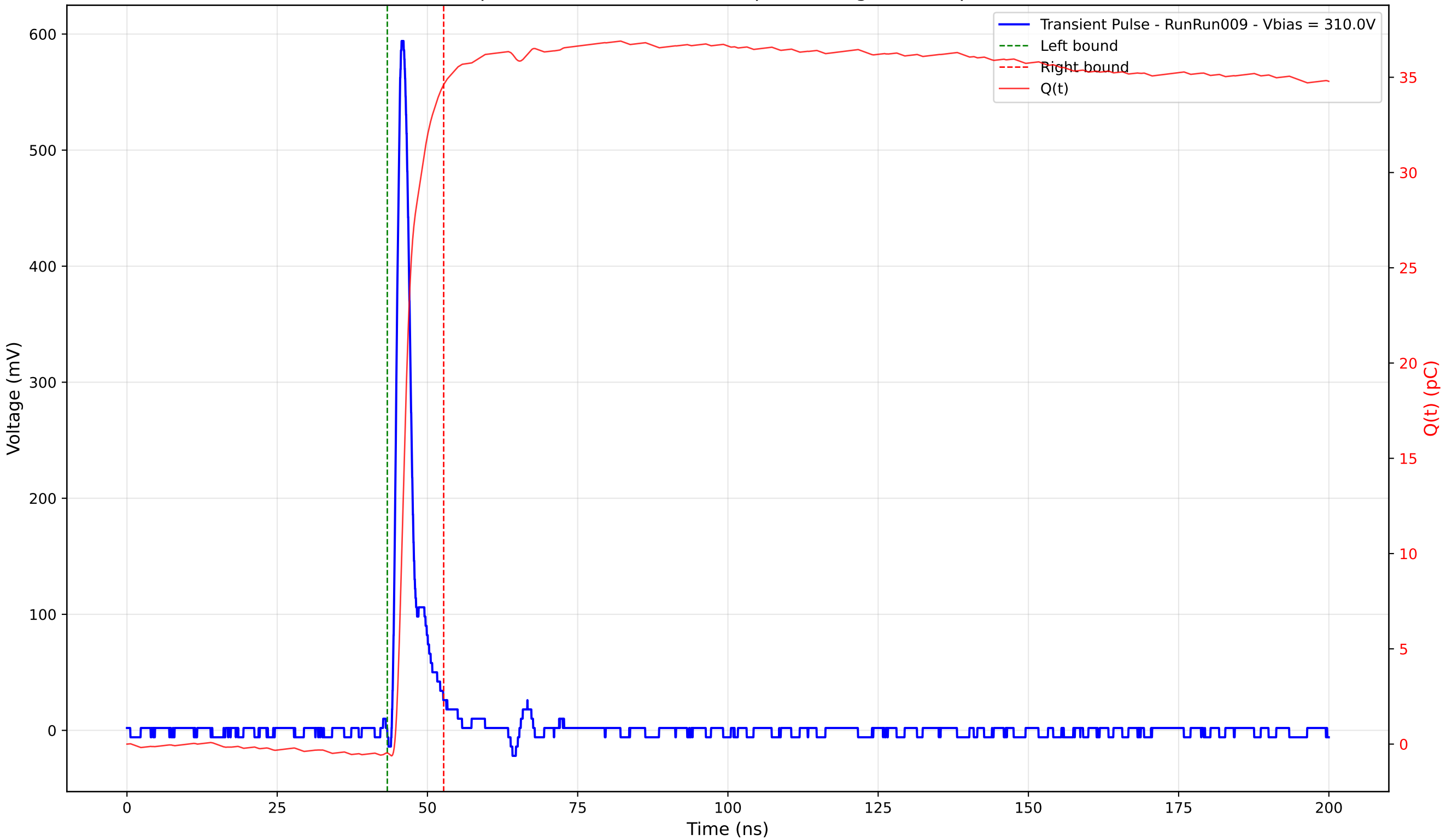
Transient Pulse - Sample: 4003 - Position: 240.0 \mu\text{m} - Charge: 35.08 pC - Rise Time: 1.07 ns
