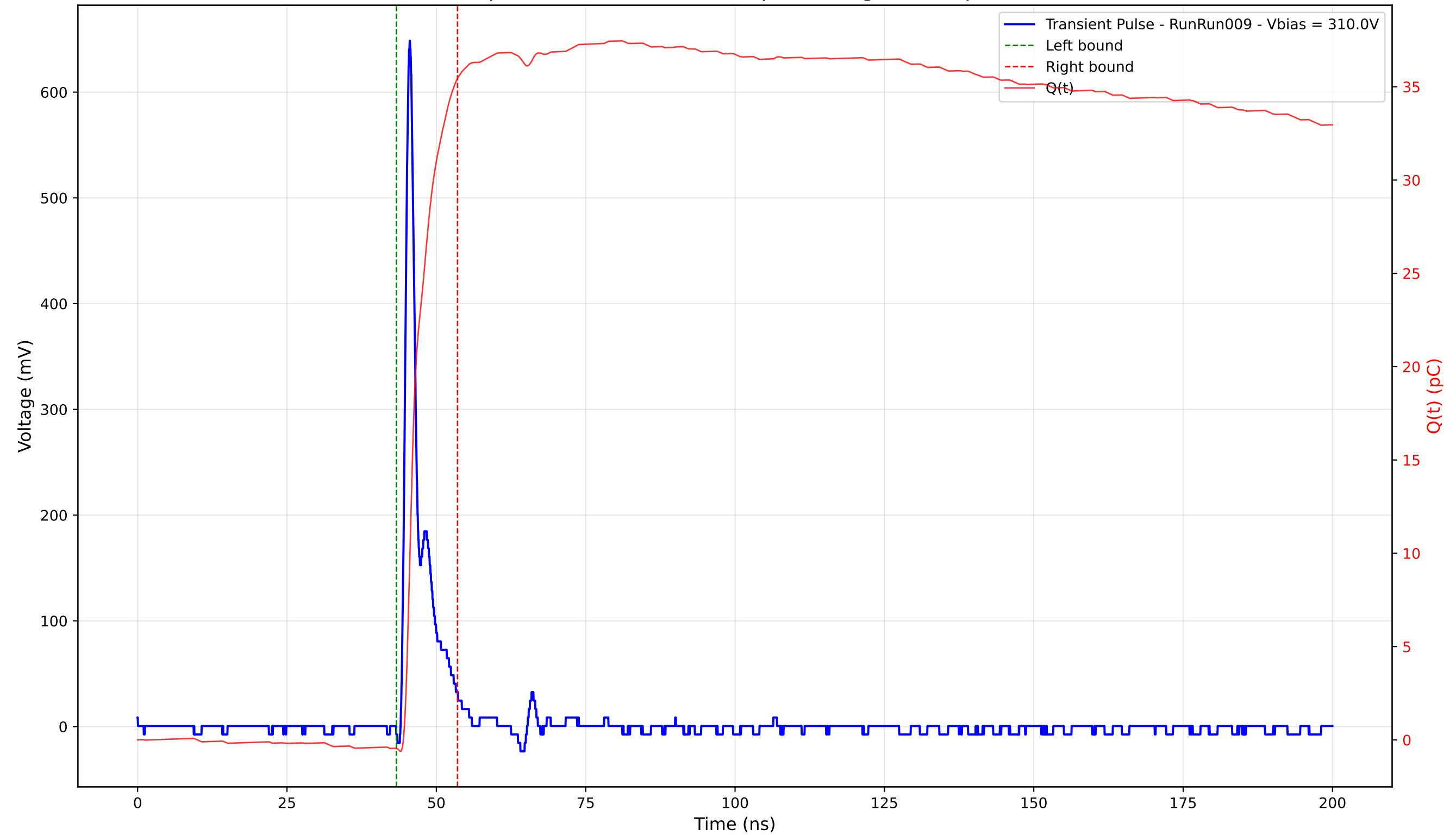
Transient Pulse - Sample: 4003 - Position: 165.0 \mu\text{m} - Charge: 35.89 pC - Rise Time: 0.98 ns
