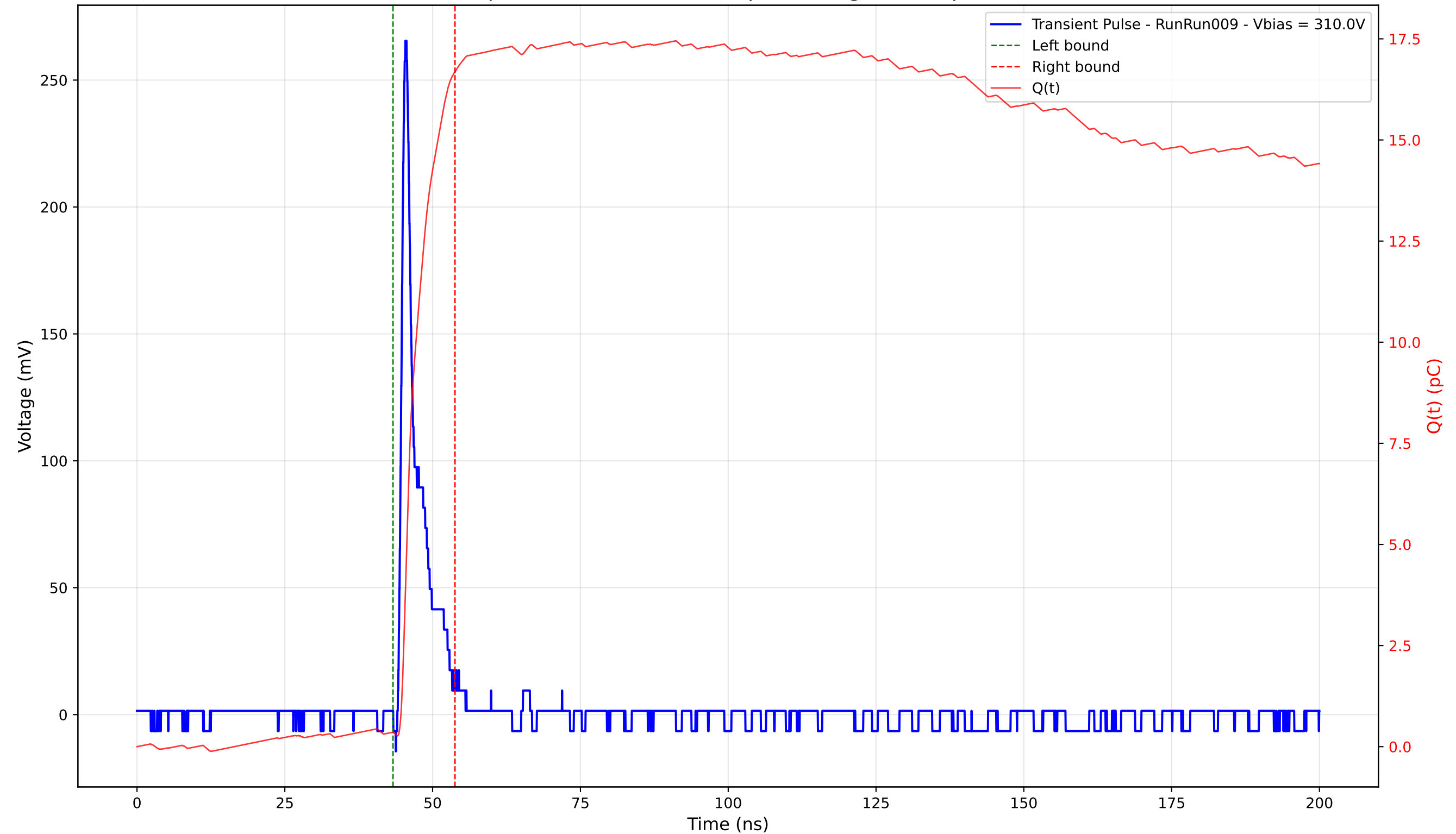
Transient Pulse - Sample: 4003 - Position: 95.0 \mu\text{m} - Charge: 16.32 pC - Rise Time: 0.88 ns
