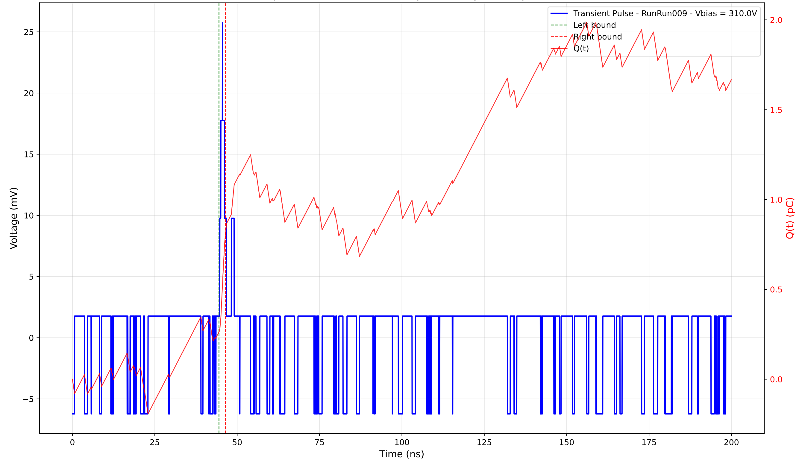
Transient Pulse - Sample: 4003 - Position: 70.0 \mu\text{m} - Charge: 0.55 pC - Rise Time: 0.82 ns
