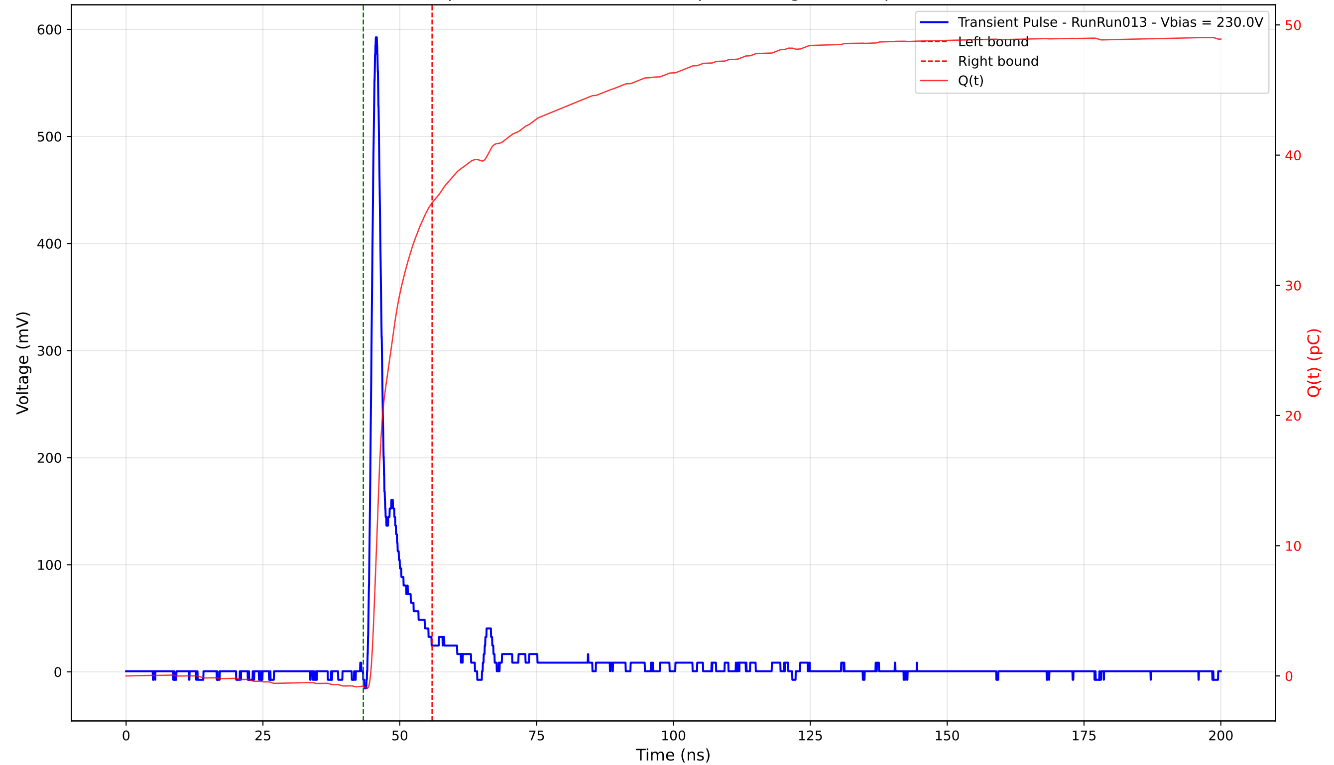
Transient Pulse - Sample: 4003 - Position: 185.0 \mu\text{m} - Charge: 37.14 pC - Rise Time: 1.01 ns
