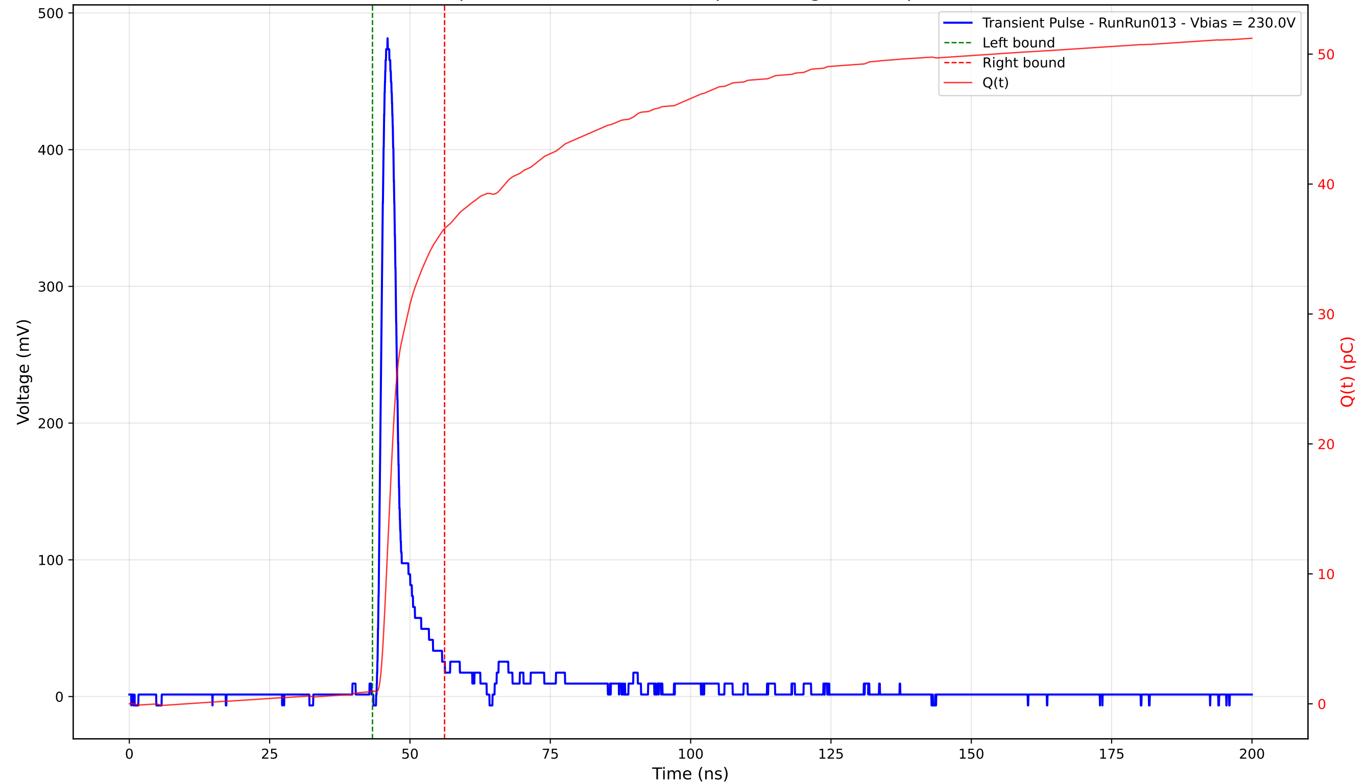
Transient Pulse - Sample: 4003 - Position: 250.0 \mu\text{m} - Charge: 35.60 pC - Rise Time: 1.14 ns
