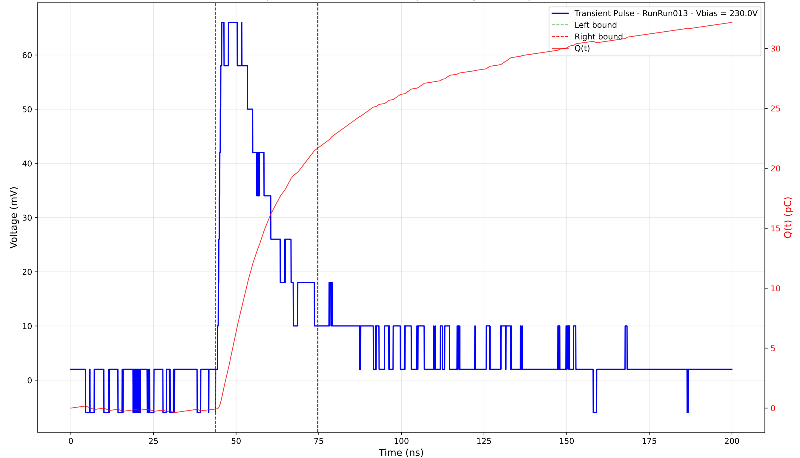
Transient Pulse - Sample: 4003 - Position: 365.0 \mu\text{m} - Charge: 21.74 pC - Rise Time: 1.31 ns
