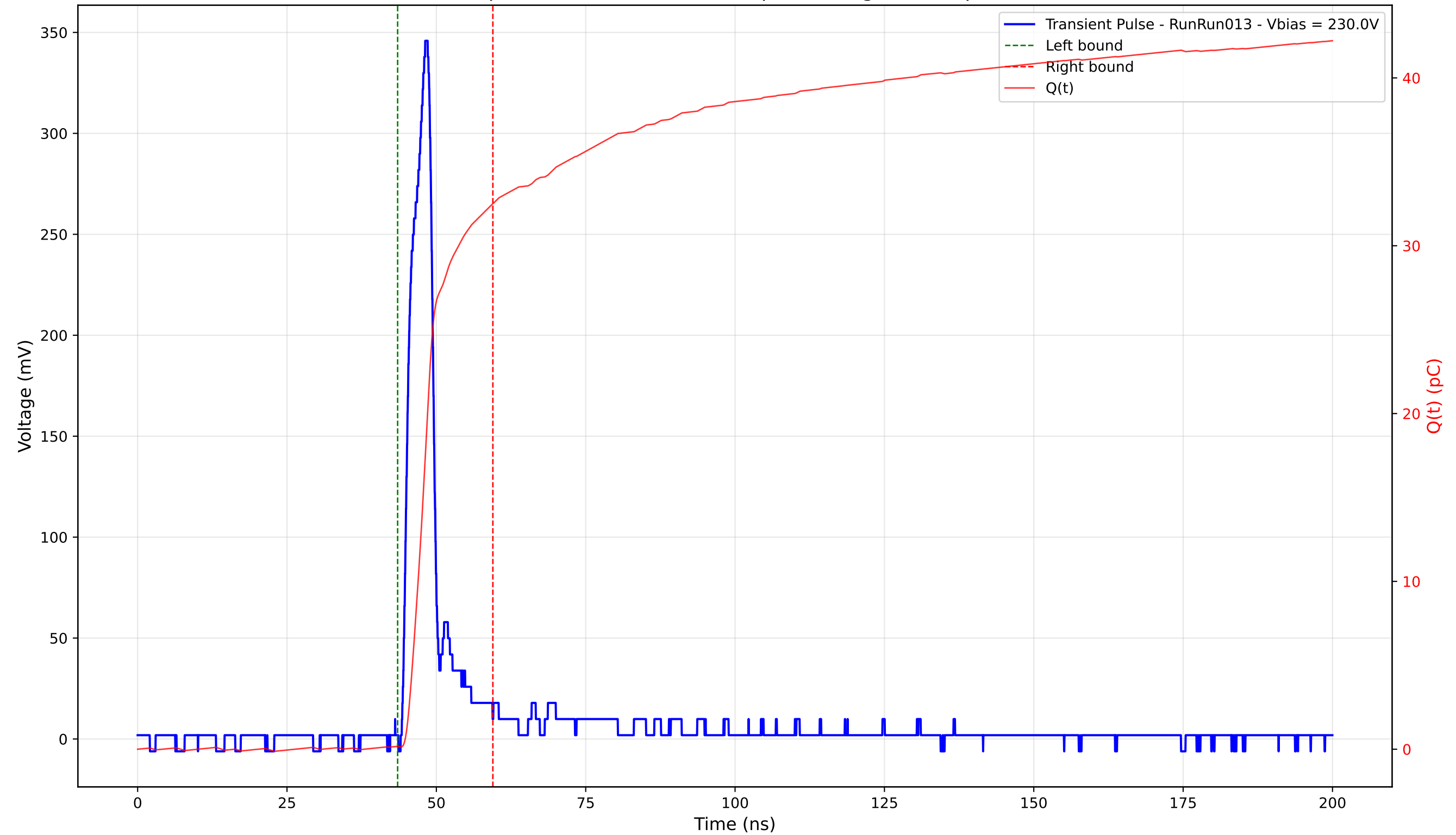
Transient Pulse - Sample: 4003 - Position: 330.0 \mu\text{m} - Charge: 32.33 pC - Rise Time: 3.06 ns
