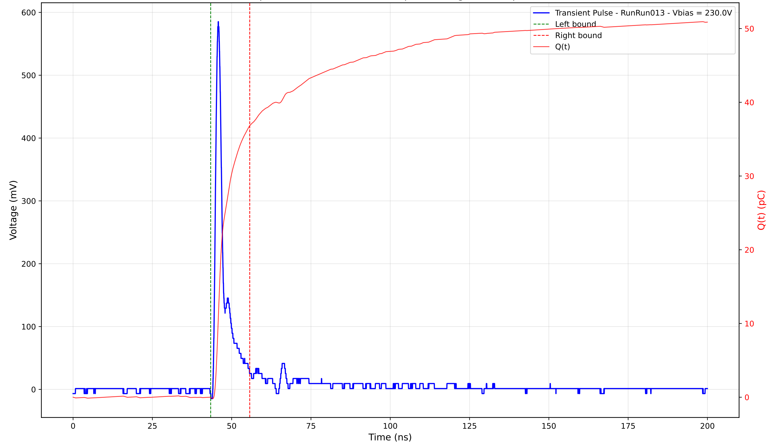
Transient Pulse - Sample: 4003 - Position: 205.0 \mu\text{m} - Charge: 36.84 pC - Rise Time: 1.08 ns
