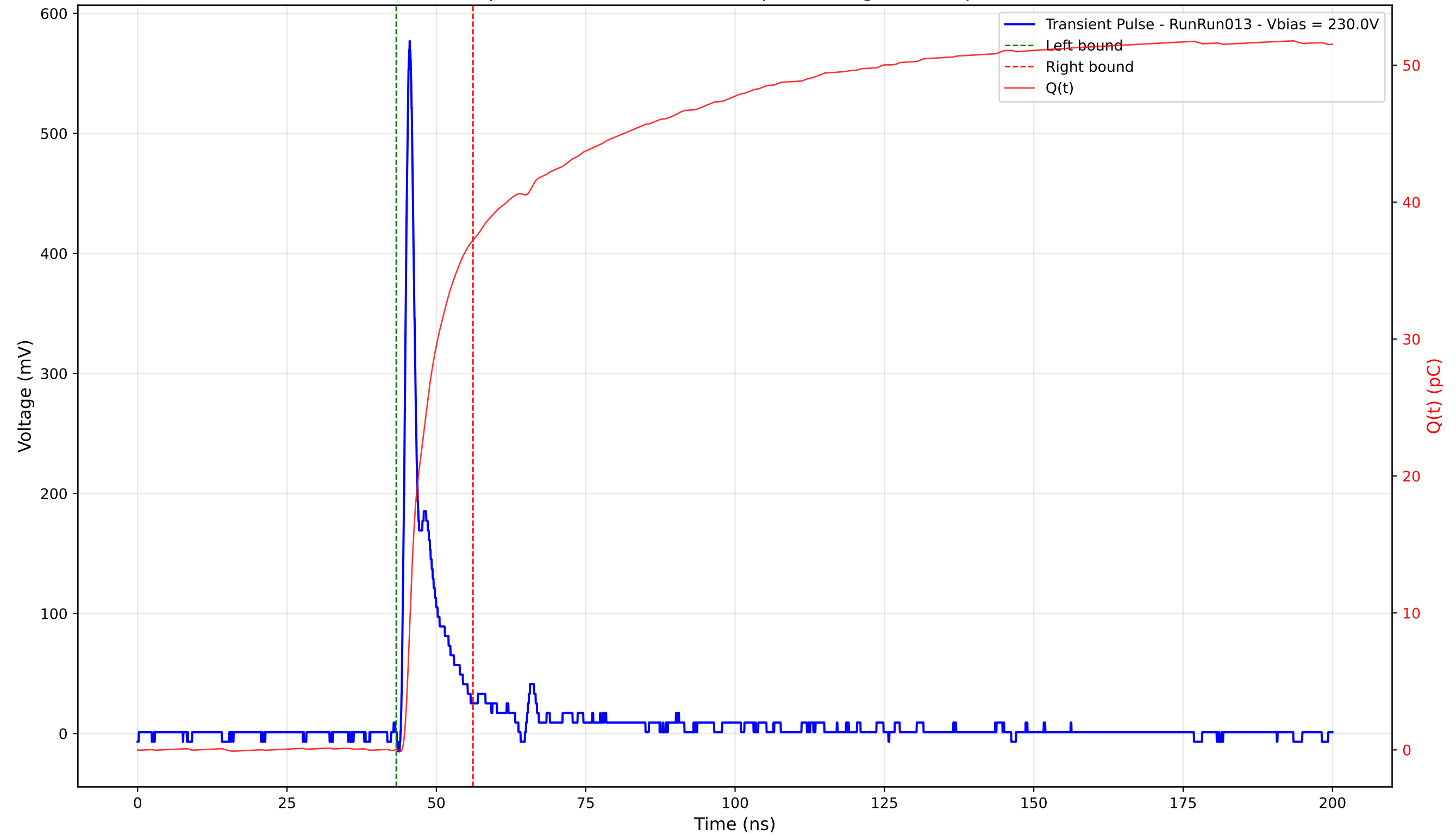
Transient Pulse - Sample: 4003 - Position: 150.0 \mu\text{m} - Charge: 37.21 pC - Rise Time: 0.94 ns
