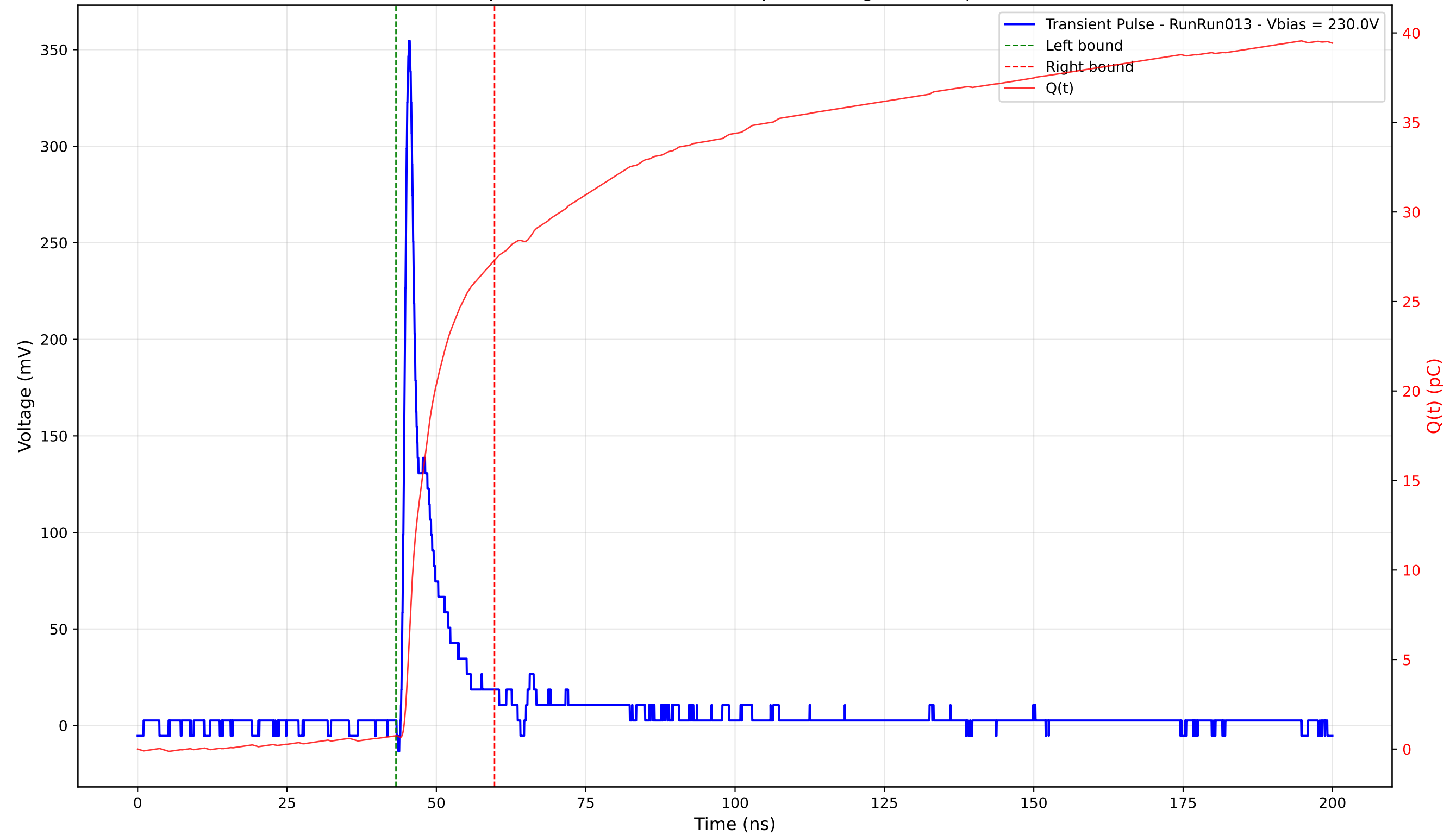
Transient Pulse - Sample: 4003 - Position: 105.0 \mu\text{m} - Charge: 26.56 pC - Rise Time: 0.90 ns
