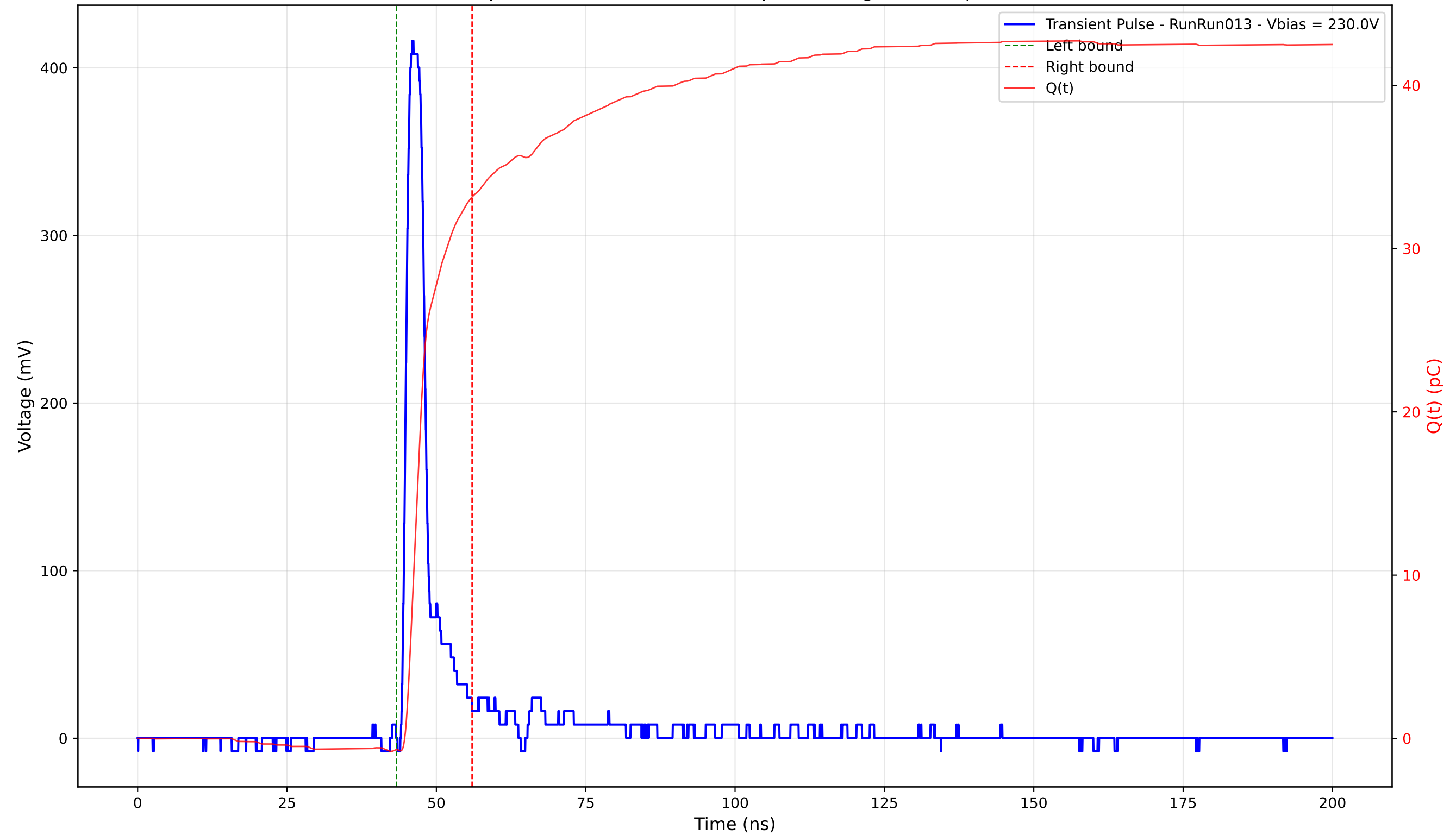
Transient Pulse - Sample: 4003 - Position: 275.0 \mu\text{m} - Charge: 33.86 pC - Rise Time: 1.14 ns
