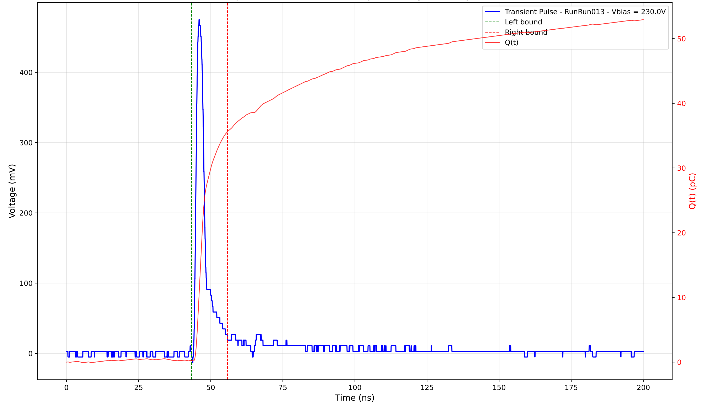
Transient Pulse - Sample: 4003 - Position: 255.0 \mu\text{m} - Charge: 35.34 pC - Rise Time: 1.19 ns
