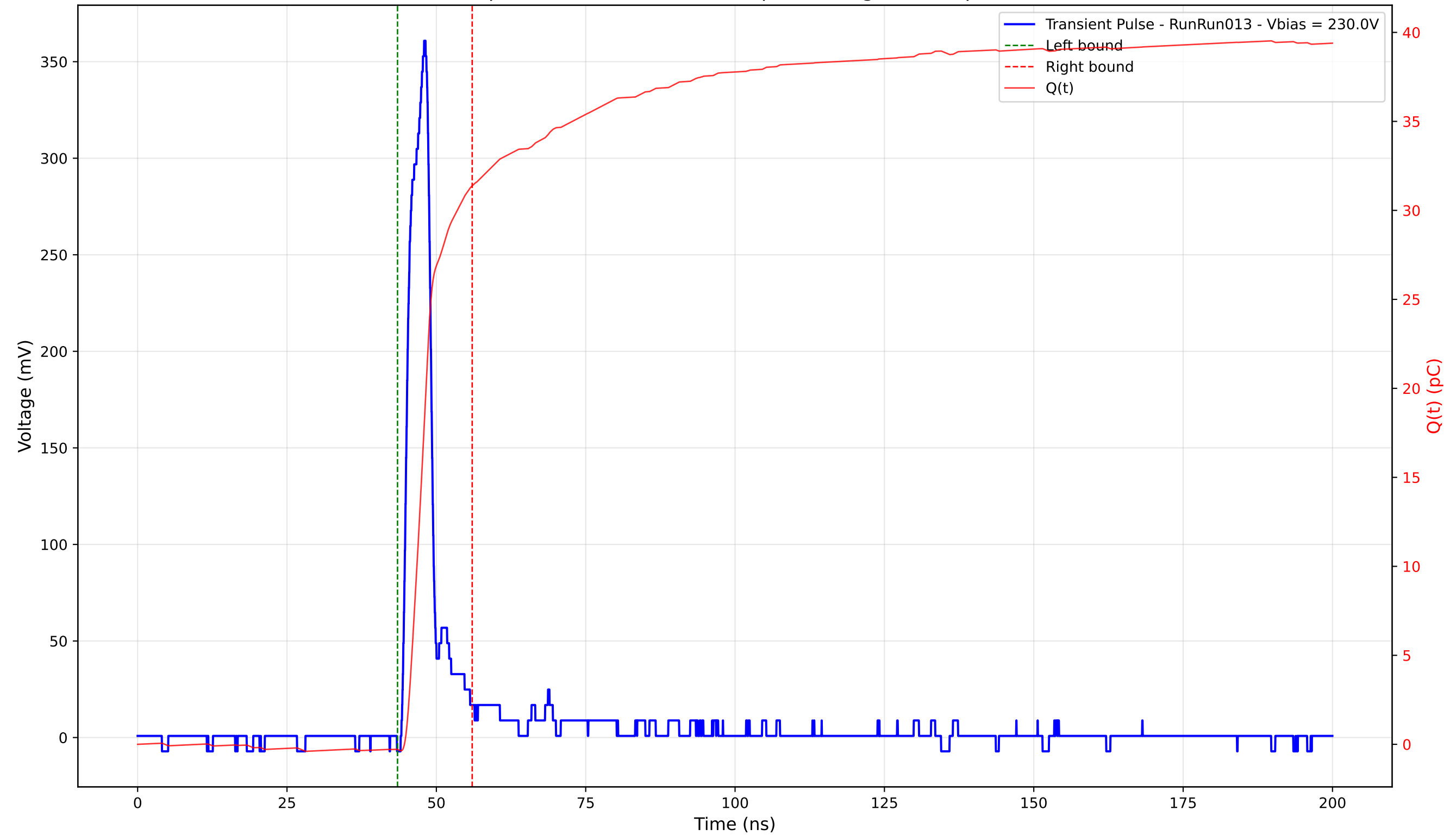
Transient Pulse - Sample: 4003 - Position: 320.0 \mu\text{m} - Charge: 31.67 pC - Rise Time: 2.87 ns
