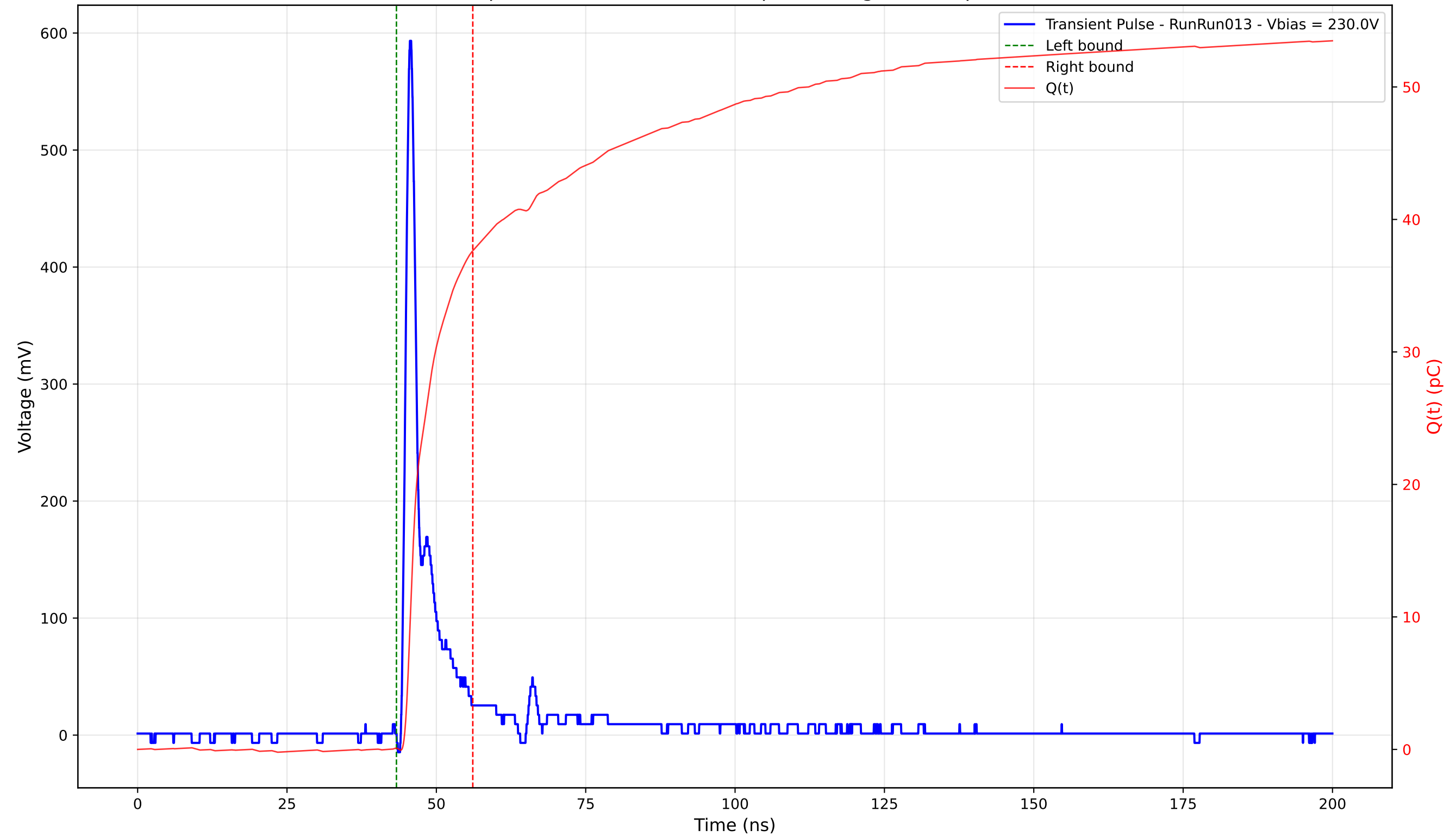
Transient Pulse - Sample: 4003 - Position: 180.0 \mu\text{m} - Charge: 37.54 pC - Rise Time: 1.00 ns
