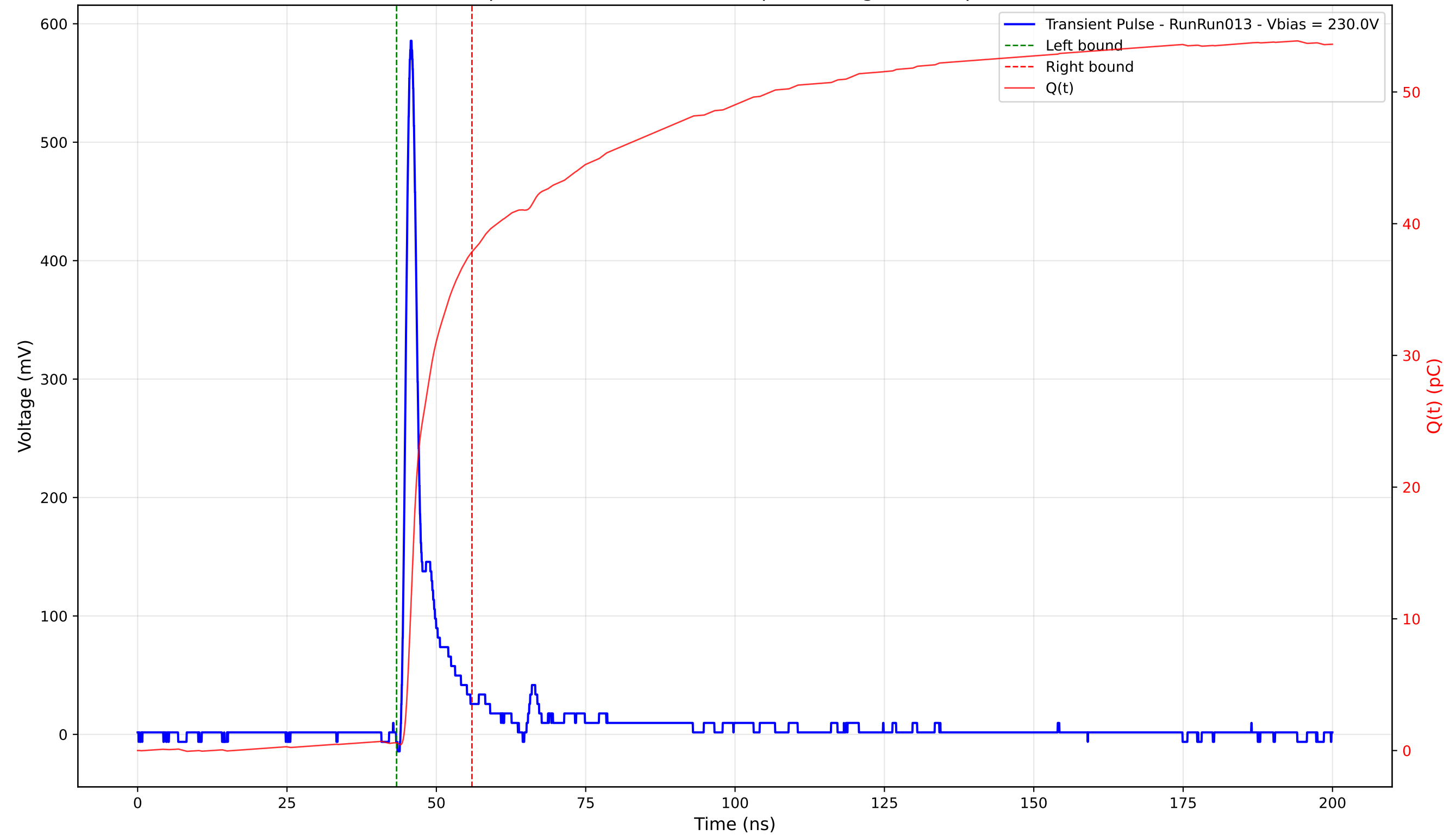
Transient Pulse - Sample: 4003 - Position: 200.0 \mu\text{m} - Charge: 37.27 pC - Rise Time: 1.09 ns
