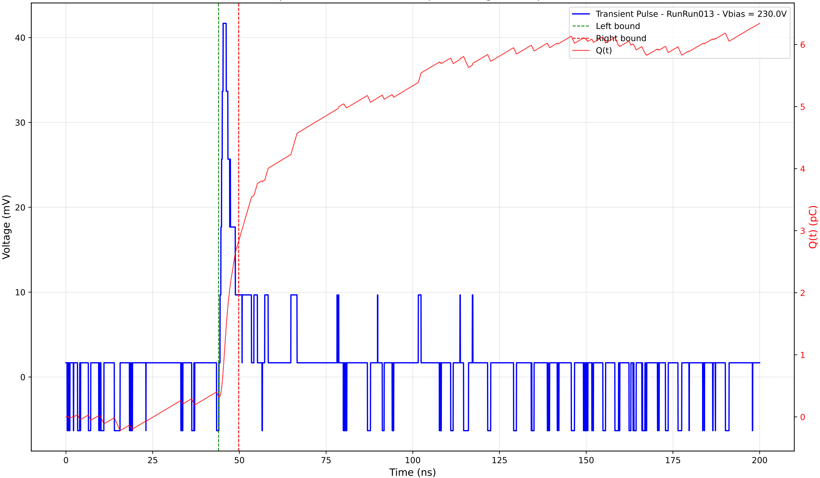
Transient Pulse - Sample: 4003 - Position: 45.0 \mu\text{m} - Charge: 2.50 pC - Rise Time: 0.89 ns
