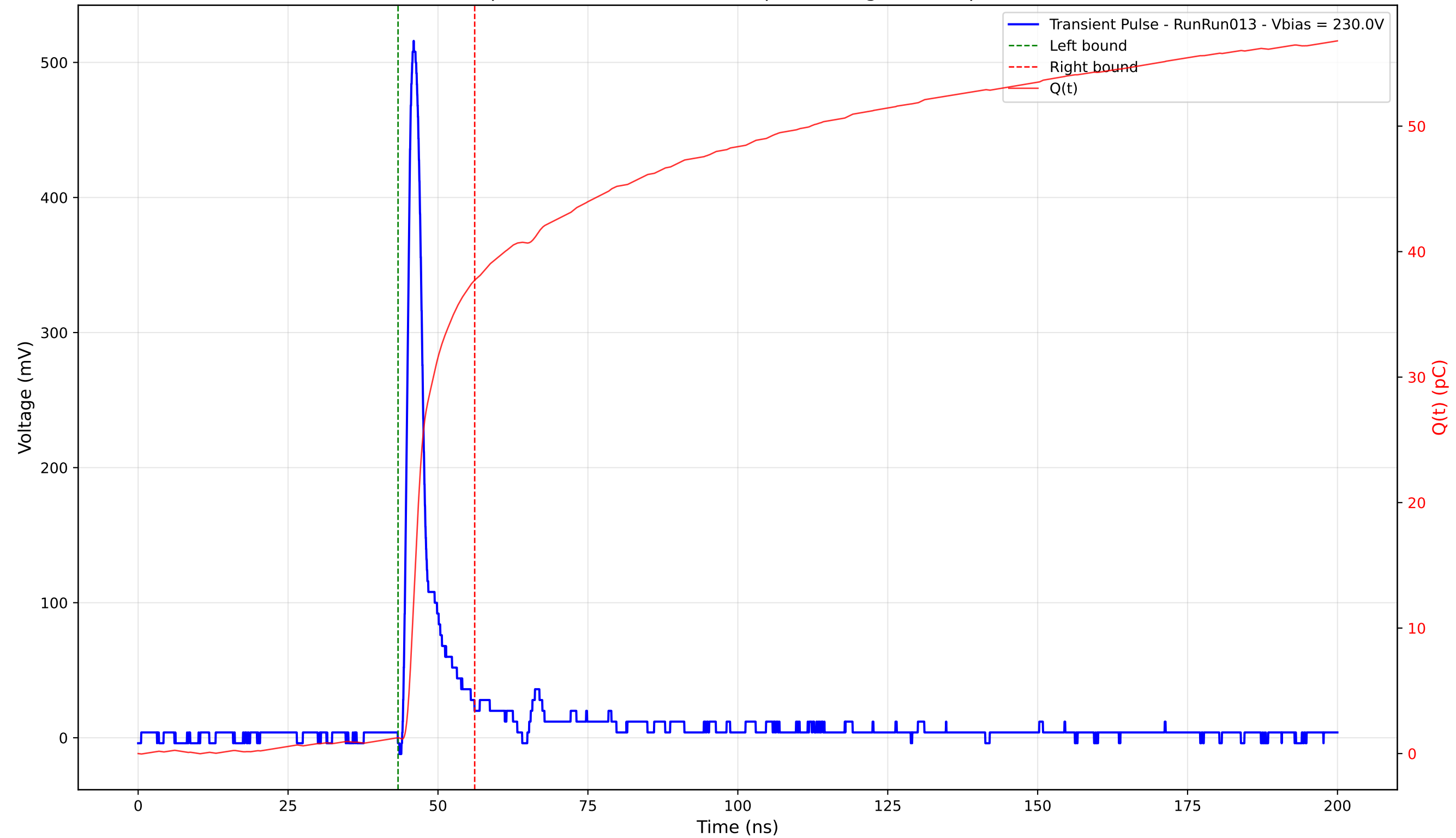
Transient Pulse - Sample: 4003 - Position: 240.0 \mu\text{m} - Charge: 36.47 pC - Rise Time: 1.16 ns
