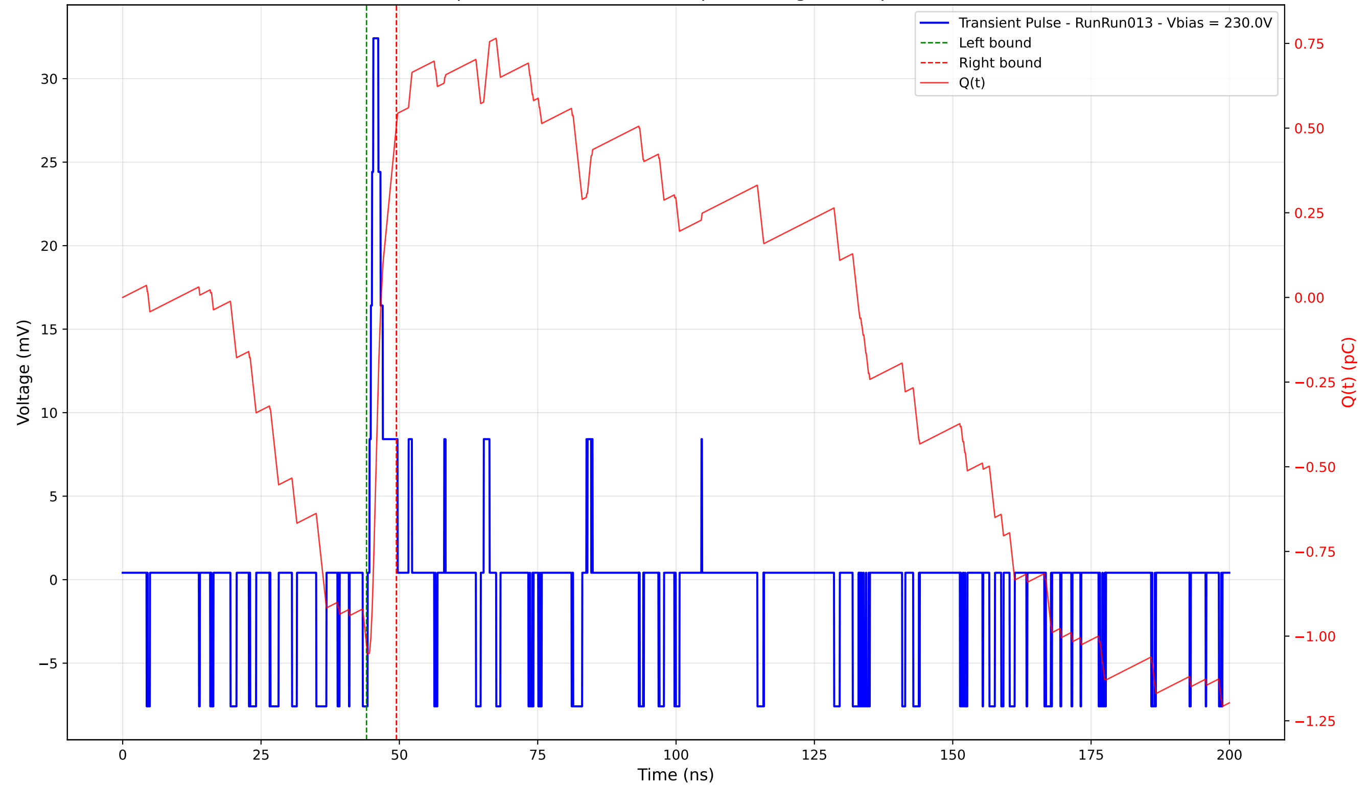
Transient Pulse - Sample: 4003 - Position: 25.0 \mu\text{m} - Charge: 1.53 pC - Rise Time: 0.69 ns
