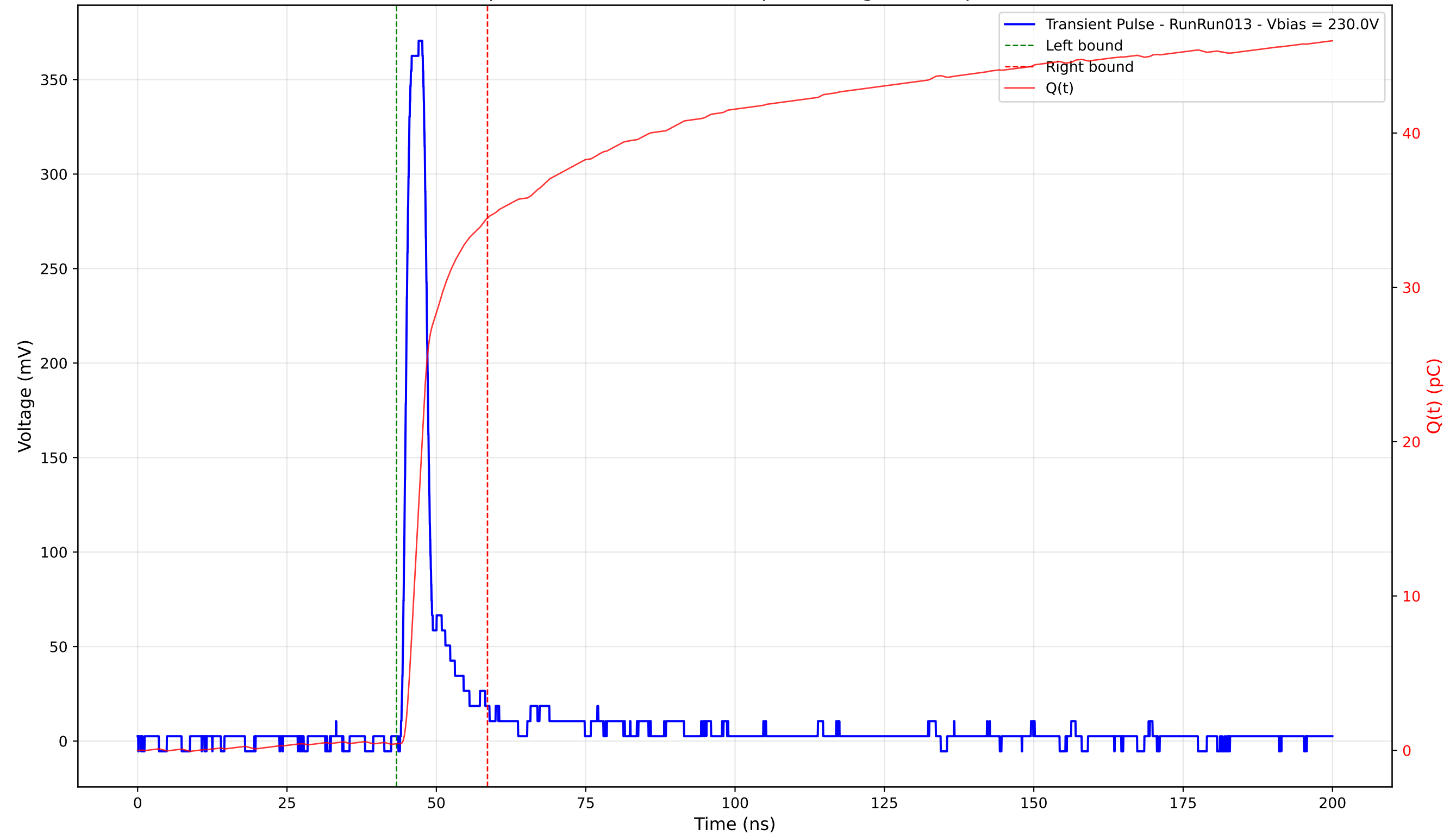
Transient Pulse - Sample: 4003 - Position: 295.0 \mu\text{m} - Charge: 34.06 pC - Rise Time: 1.21 ns
