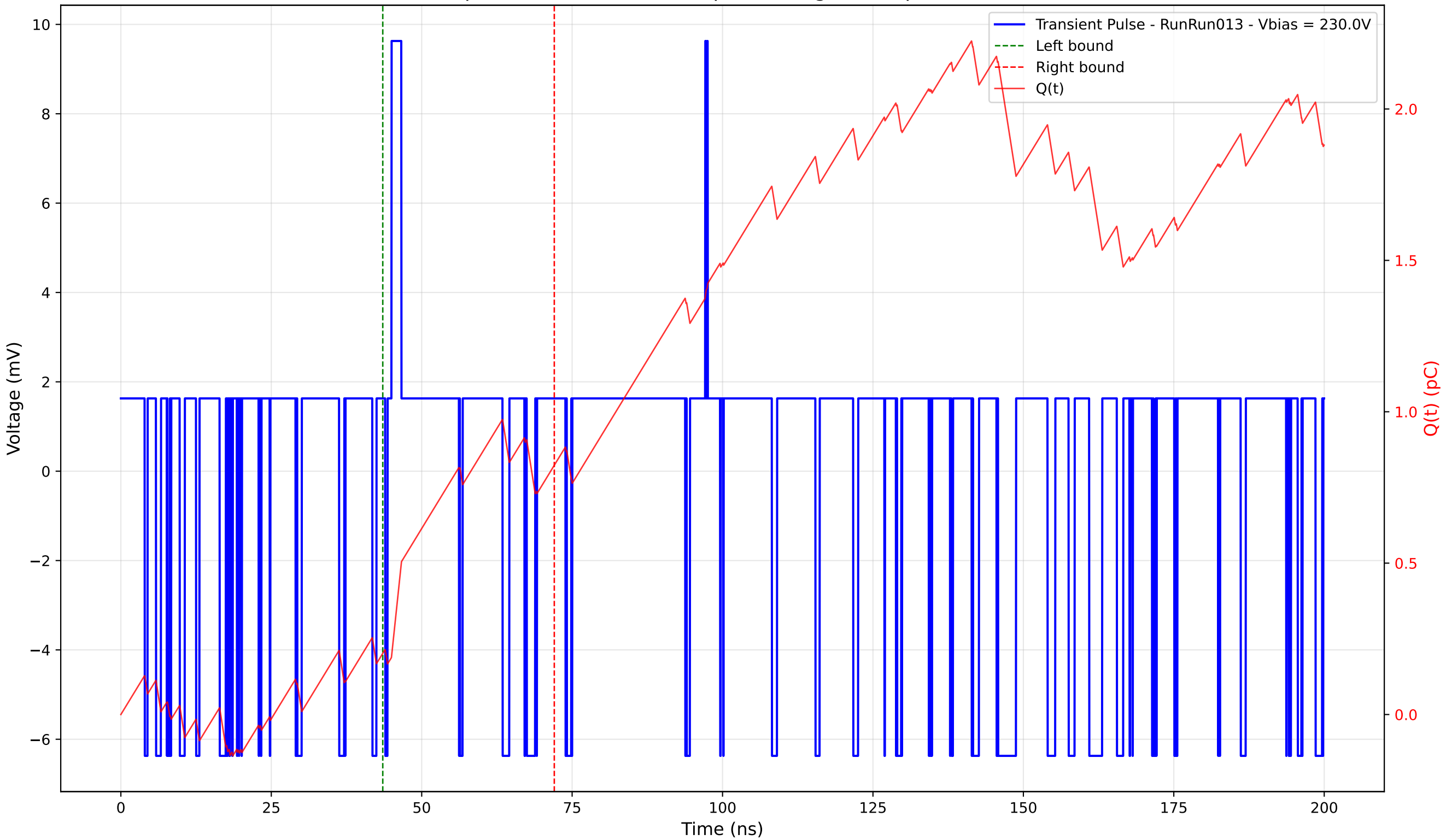
Transient Pulse - Sample: 4003 - Position: 0.0 \mu\text{m} - Charge: 0.62 pC - Rise Time: 0.00 ns (N/A)
