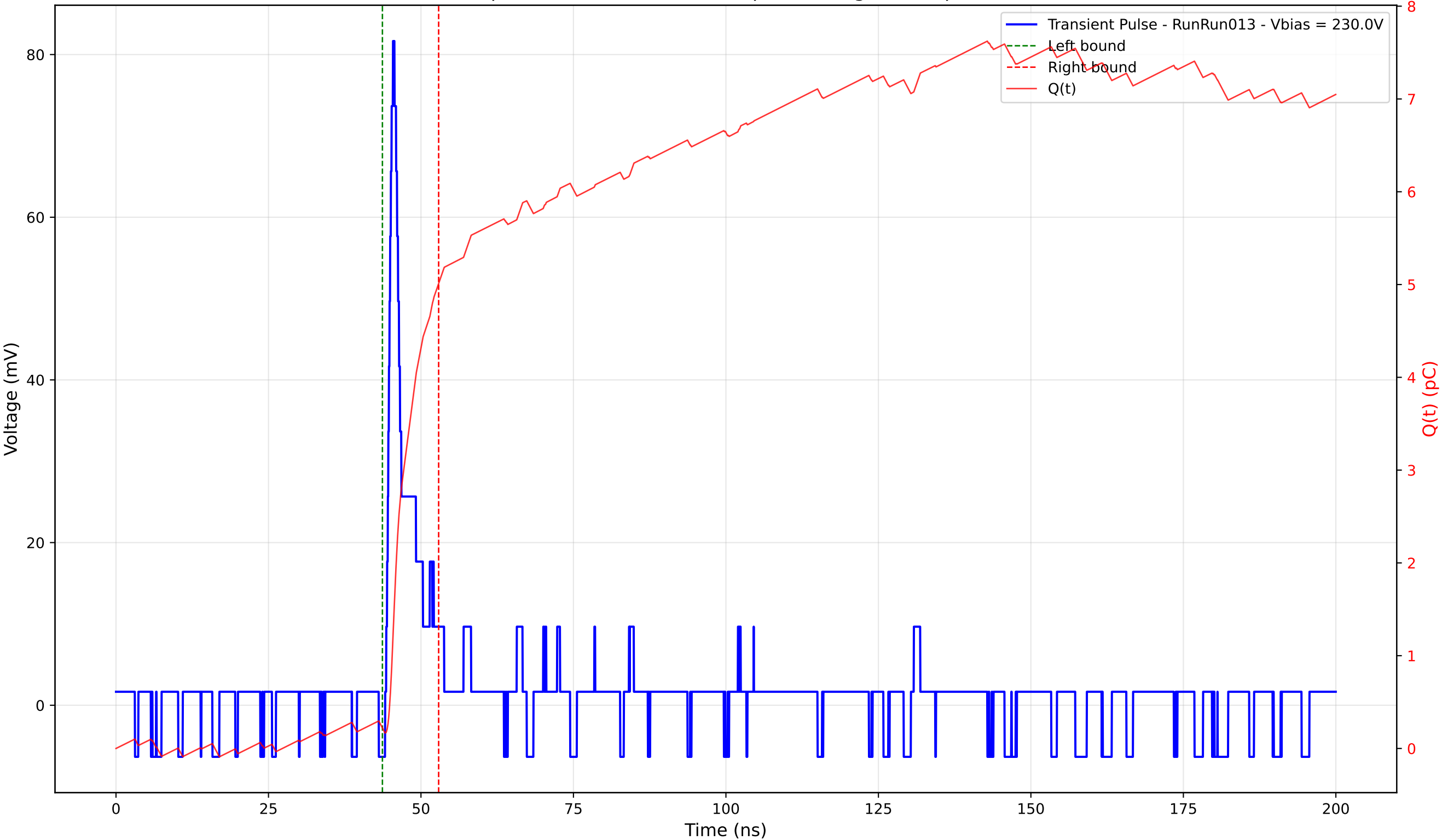
Transient Pulse - Sample: 4003 - Position: 85.0 \mu\text{m} - Charge: 4.79 pC - Rise Time: 0.88 ns
