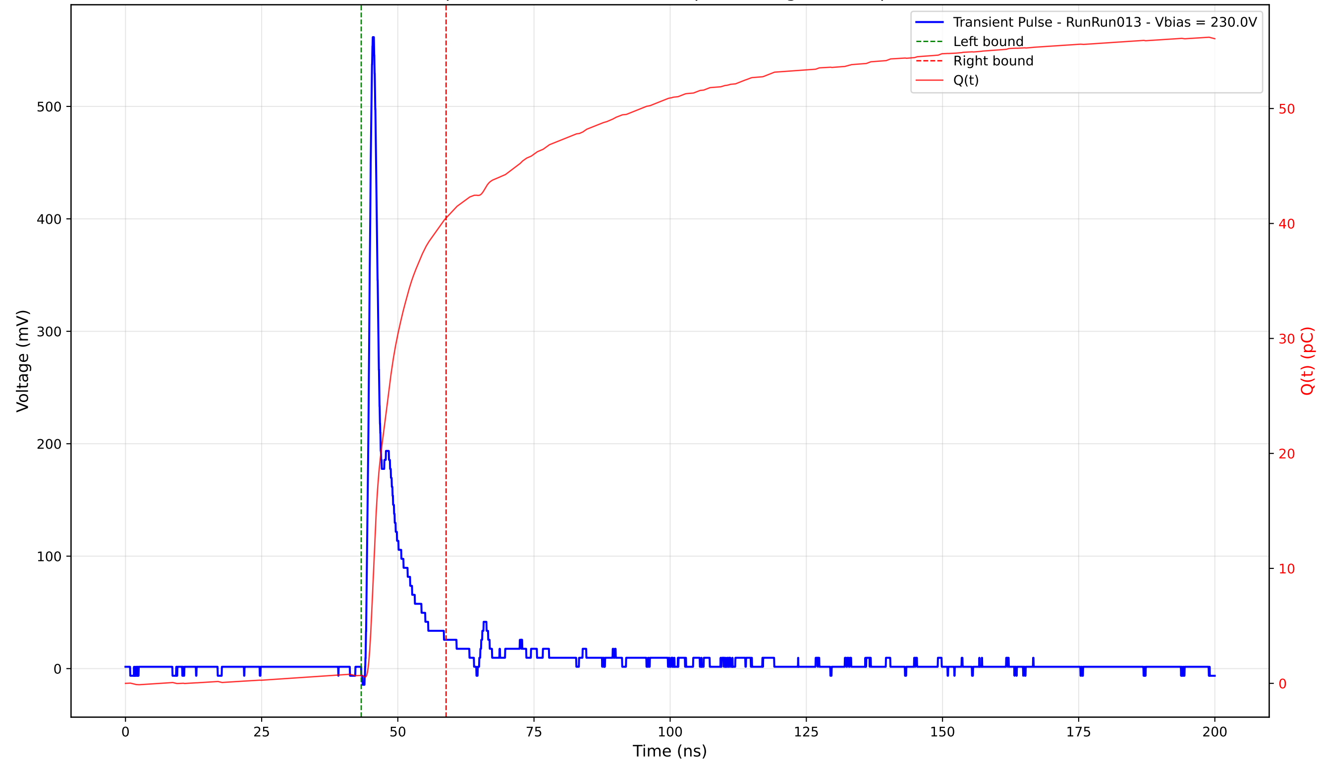
Transient Pulse - Sample: 4003 - Position: 135.0 \mu\text{m} - Charge: 39.78 pC - Rise Time: 0.90 ns
