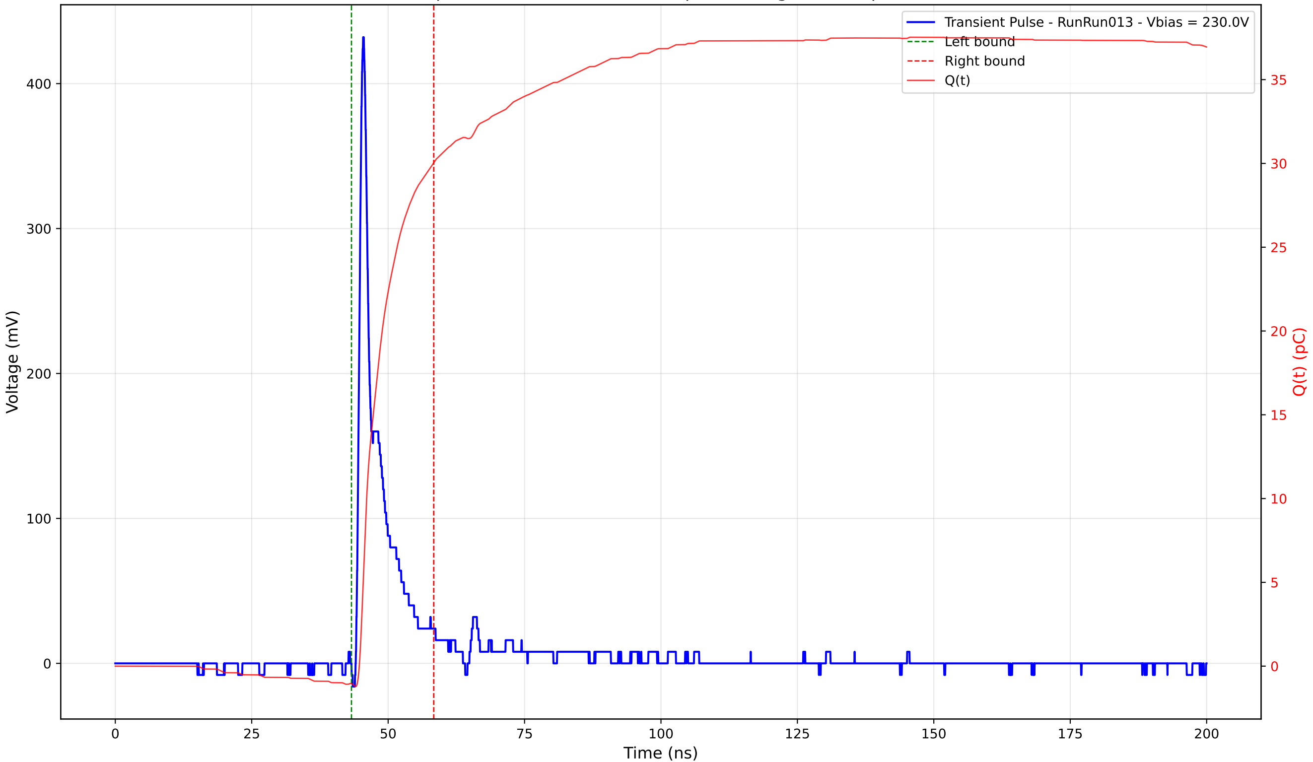
Transient Pulse - Sample: 4003 - Position: 110.0 \mu\text{m} - Charge: 31.09 pC - Rise Time: 0.88 ns
