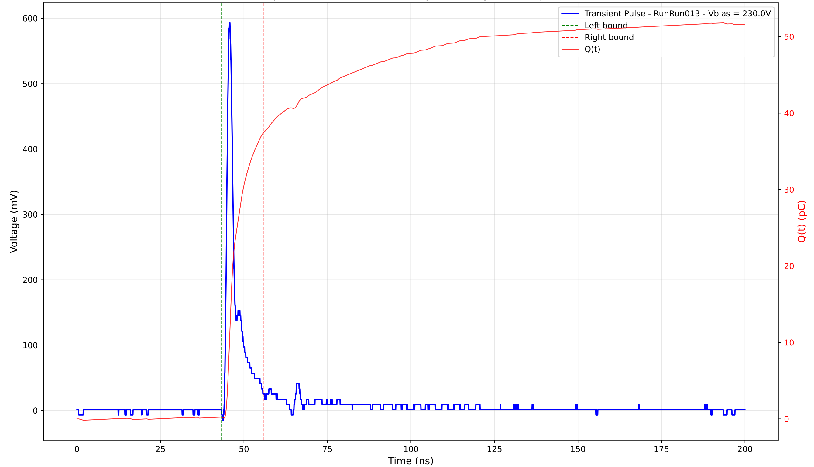
Transient Pulse - Sample: 4003 - Position: 190.0 \mu\text{m} - Charge: 37.13 pC - Rise Time: 1.05 ns
