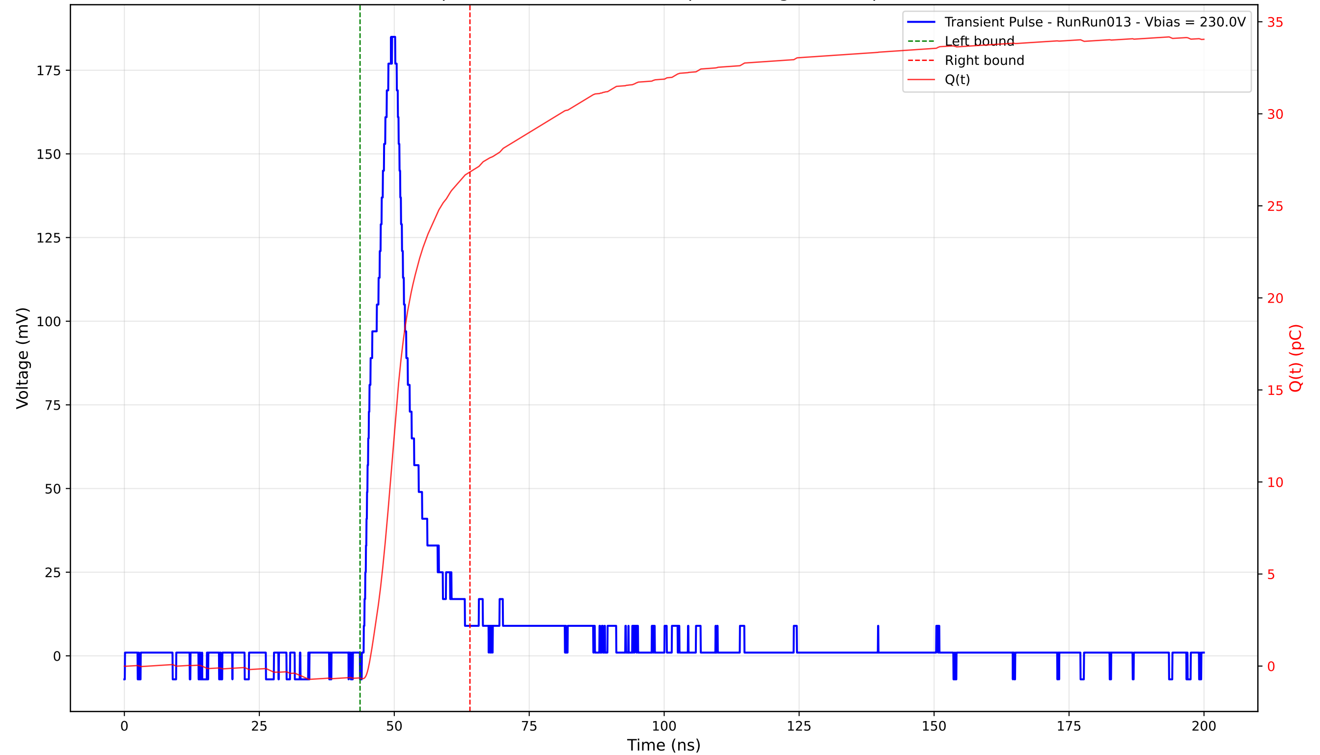
Transient Pulse - Sample: 4003 - Position: 355.0 \mu\text{m} - Charge: 27.48 pC - Rise Time: 4.00 ns
