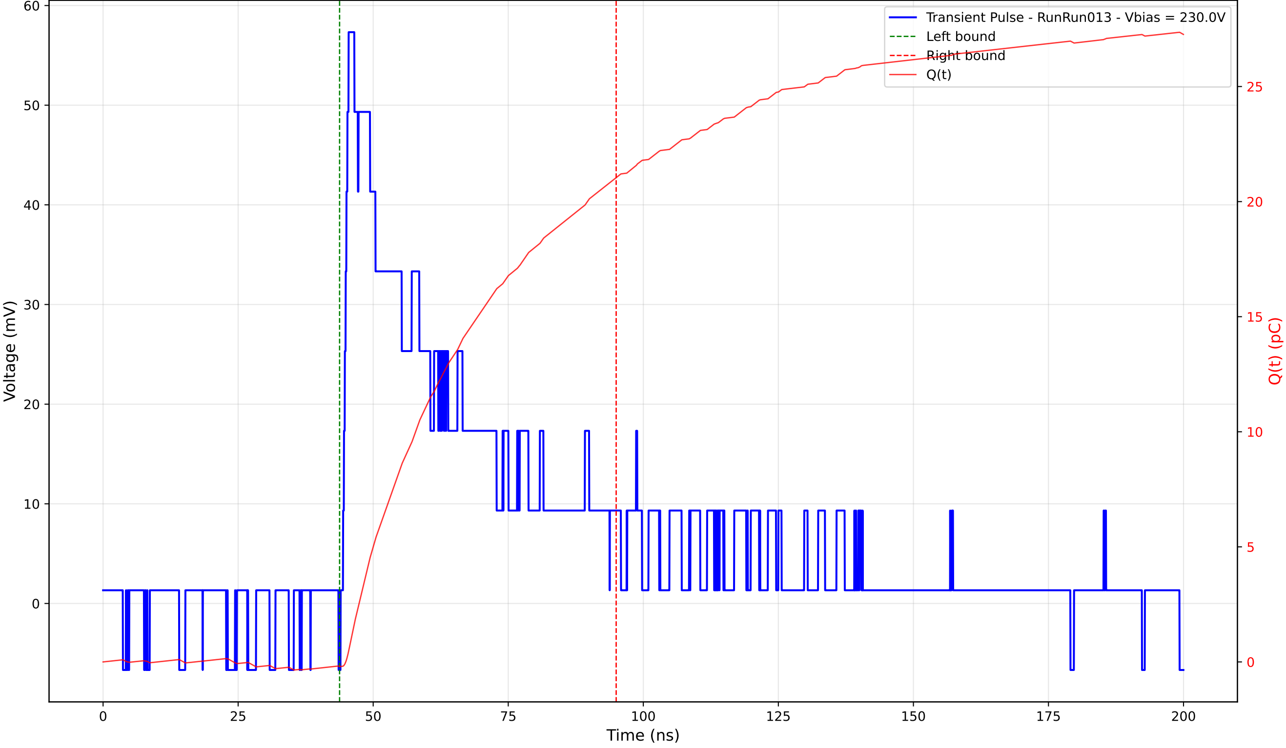
Transient Pulse - Sample: 4003 - Position: 370.0 \mu\text{m} - Charge: 21.22 pC - Rise Time: 1.03 ns
