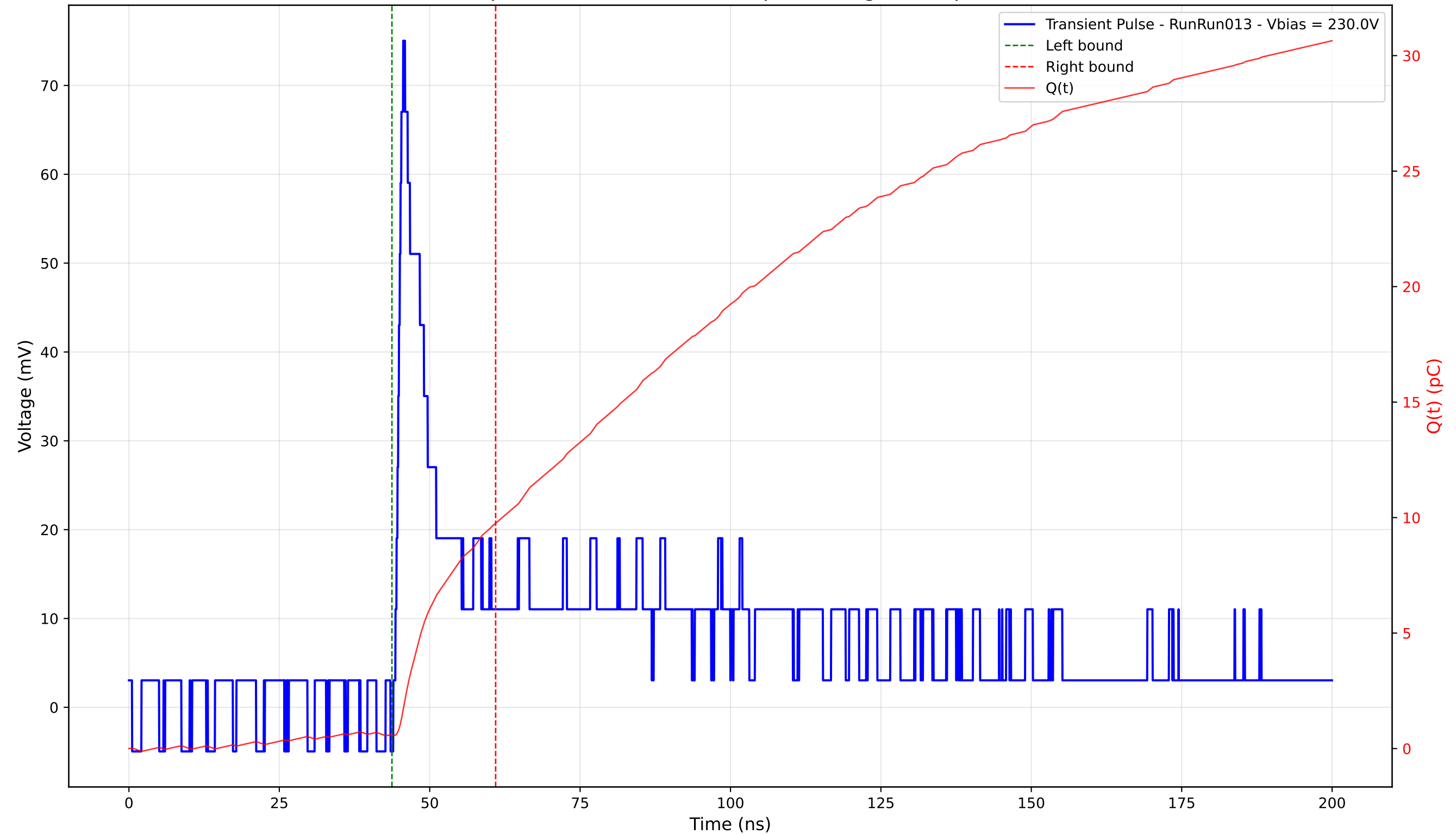
Transient Pulse - Sample: 4003 - Position: 380.0 \mu\text{m} - Charge: 9.18 pC - Rise Time: 1.29 ns
