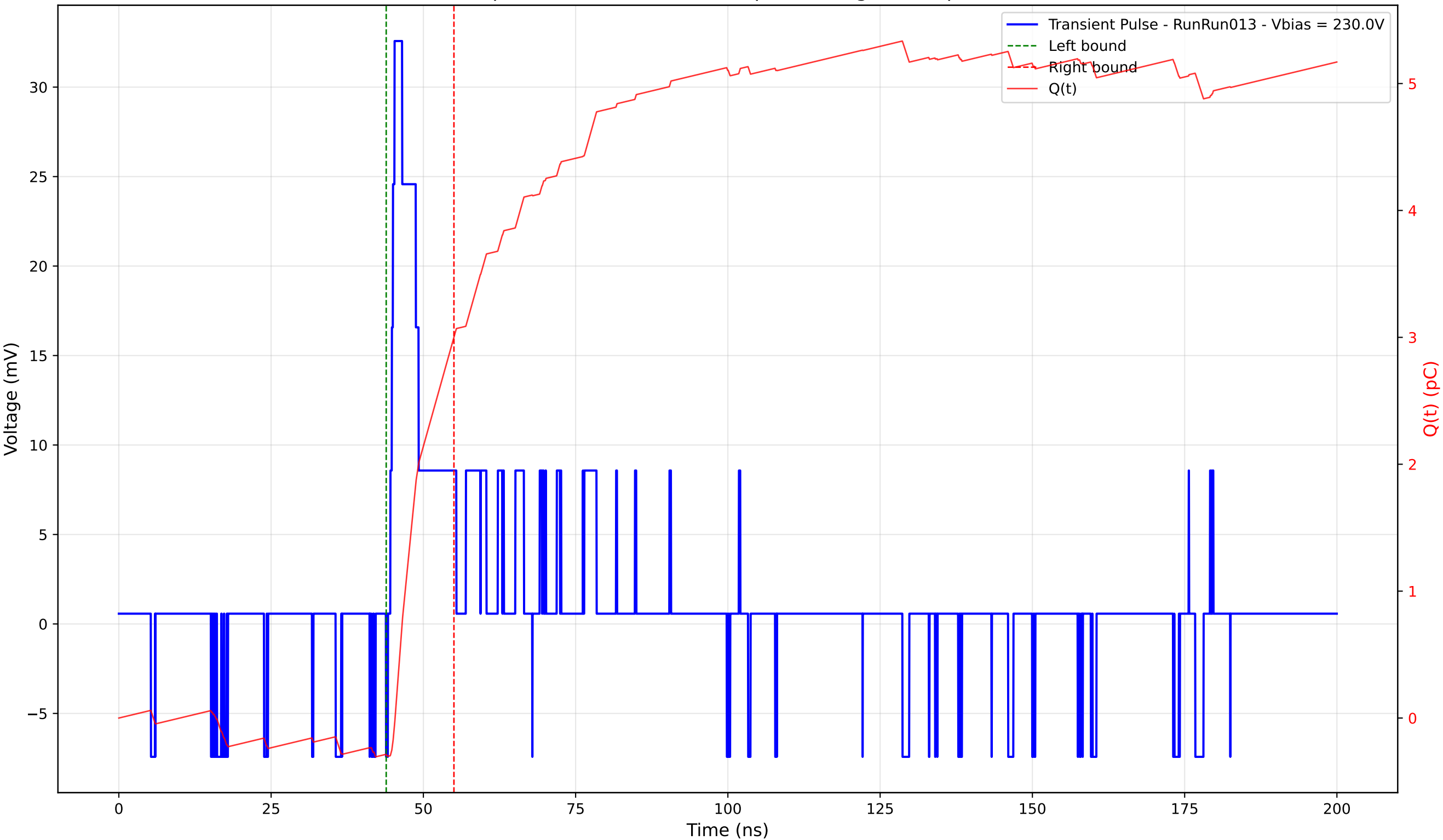
Transient Pulse - Sample: 4003 - Position: 60.0 \mu\text{m} - Charge: 3.30 pC - Rise Time: 0.69 ns
