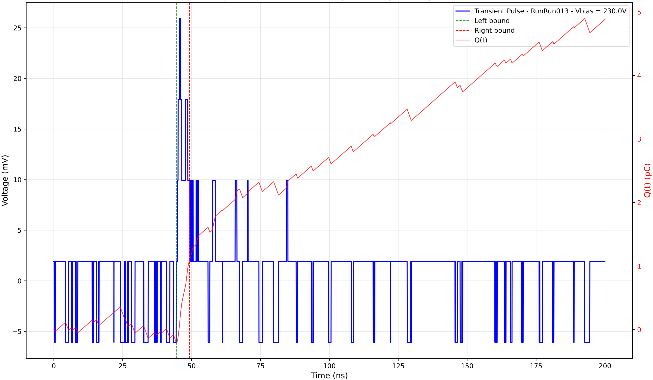
Transient Pulse - Sample: 4003 - Position: 65.0 \mu\text{m} - Charge: 1.30 pC - Rise Time: 0.76 ns
