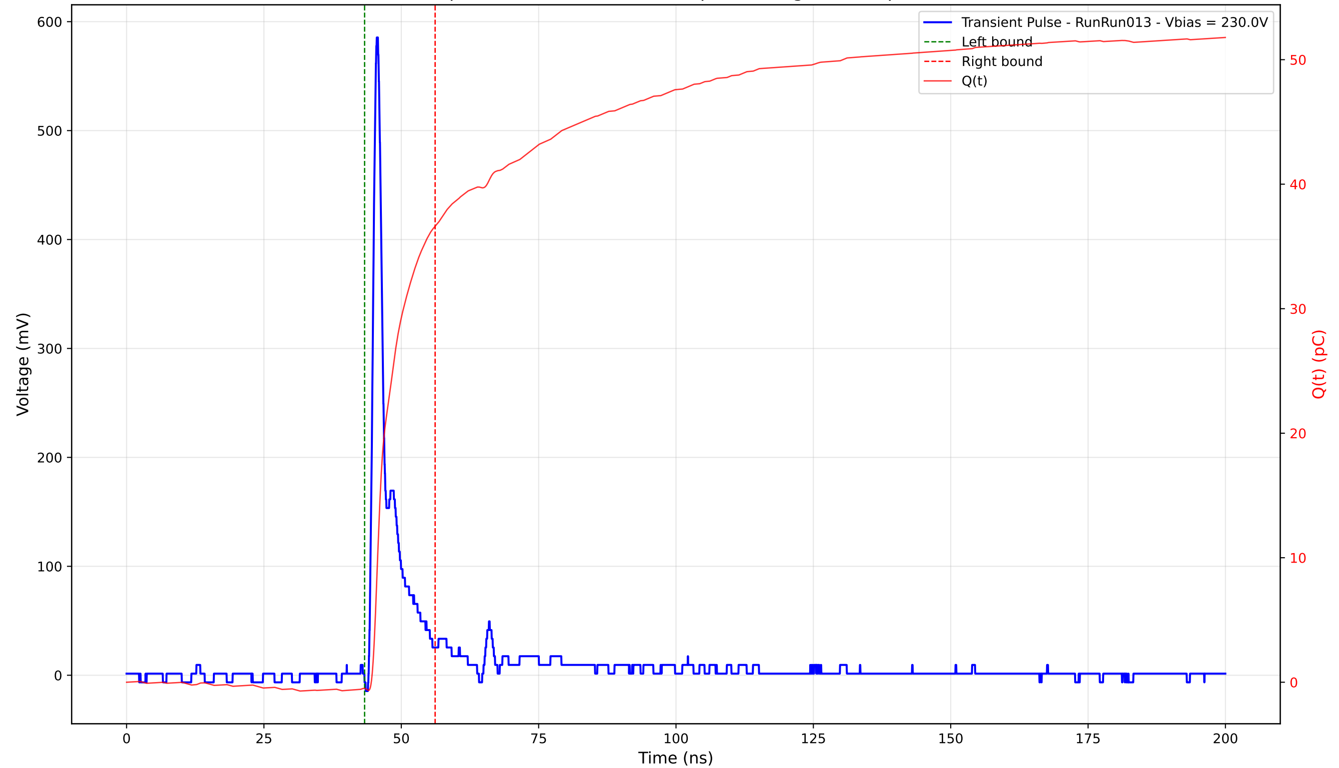
Transient Pulse - Sample: 4003 - Position: 170.0 \mu\text{m} - Charge: 37.11 pC - Rise Time: 0.97 ns
