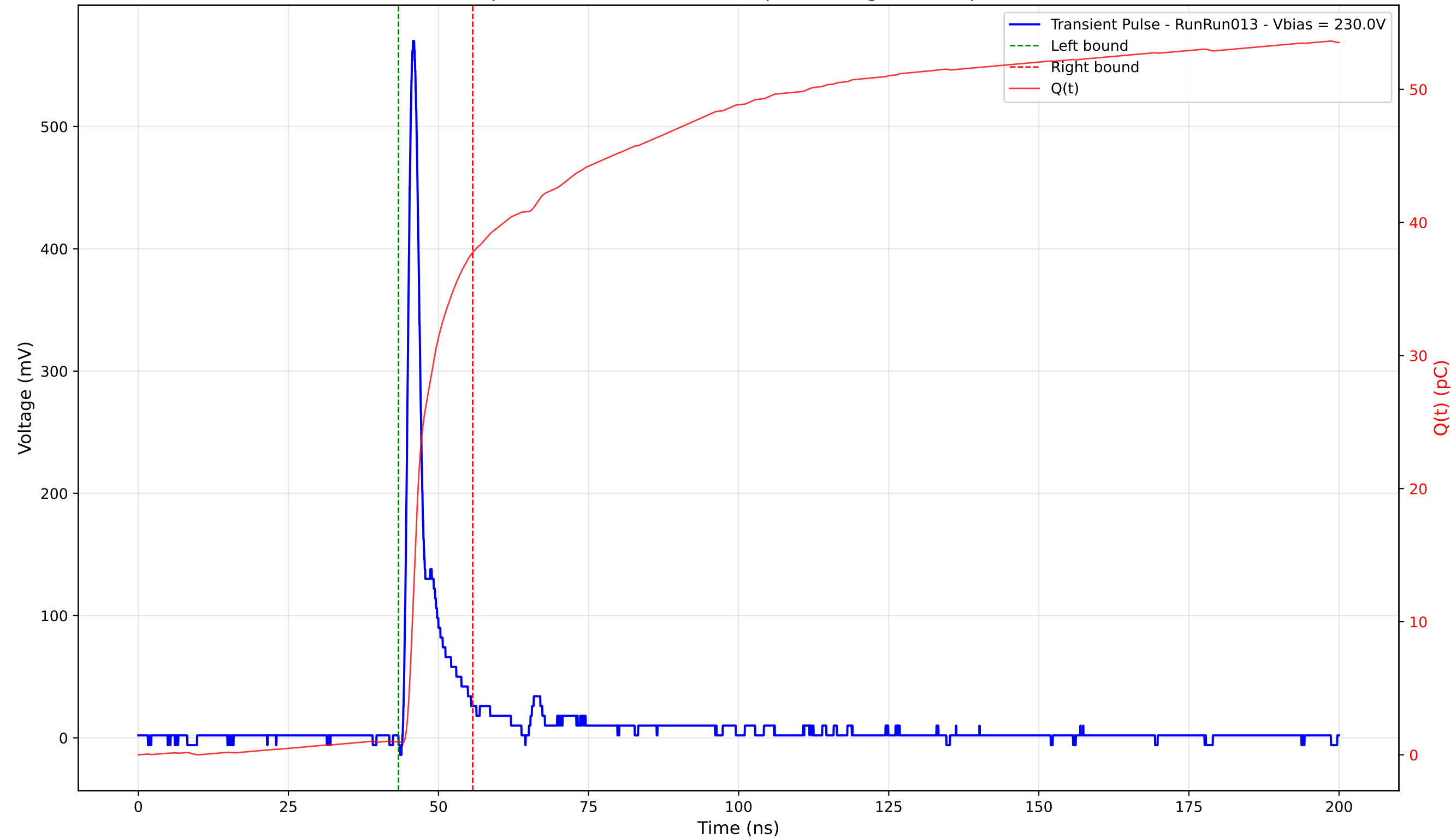
Transient Pulse - Sample: 4003 - Position: 210.0 \mu\text{m} - Charge: 36.75 pC - Rise Time: 1.10 ns
