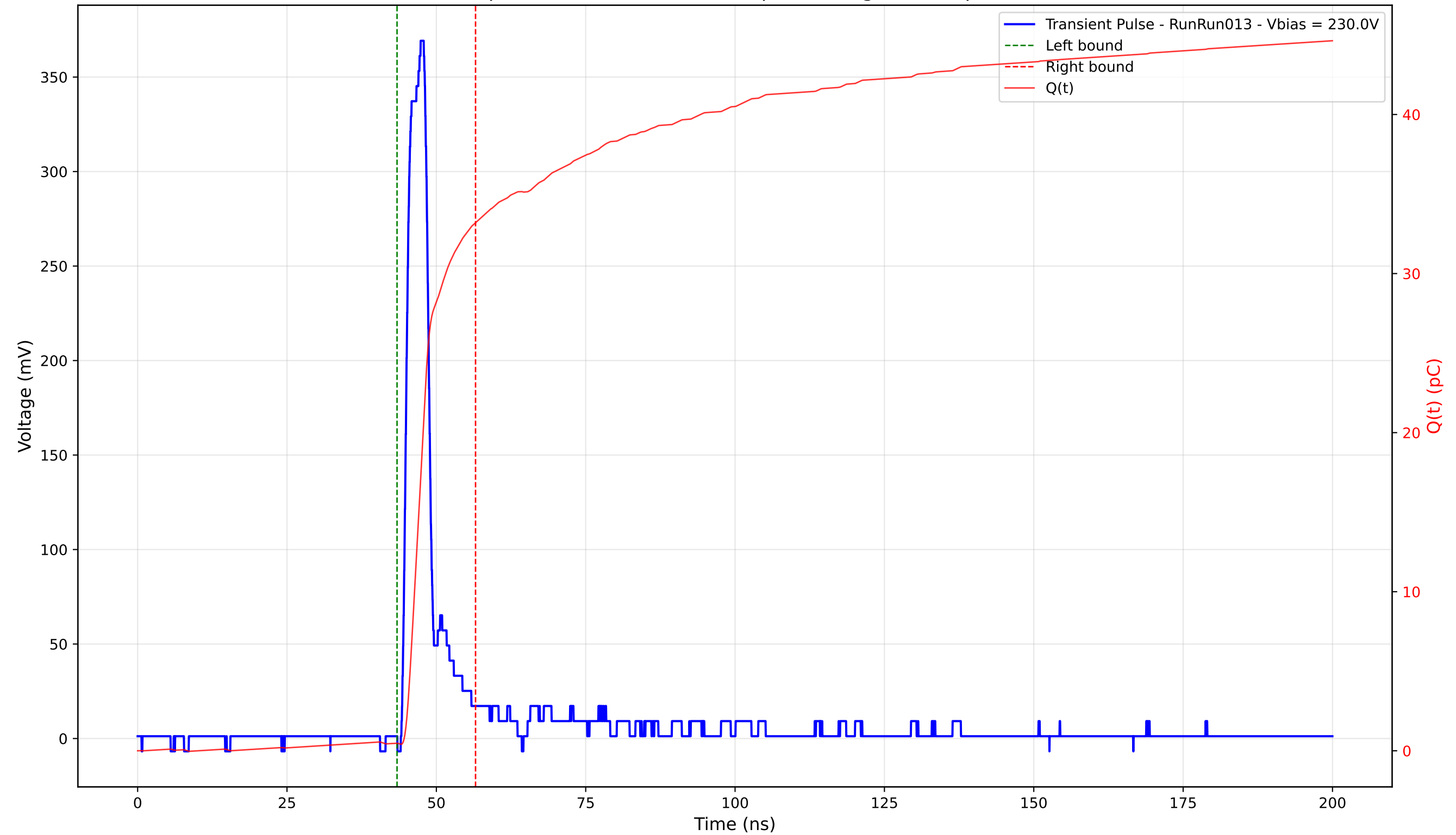
Transient Pulse - Sample: 4003 - Position: 305.0 \mu\text{m} - Charge: 32.72 pC - Rise Time: 1.45 ns
