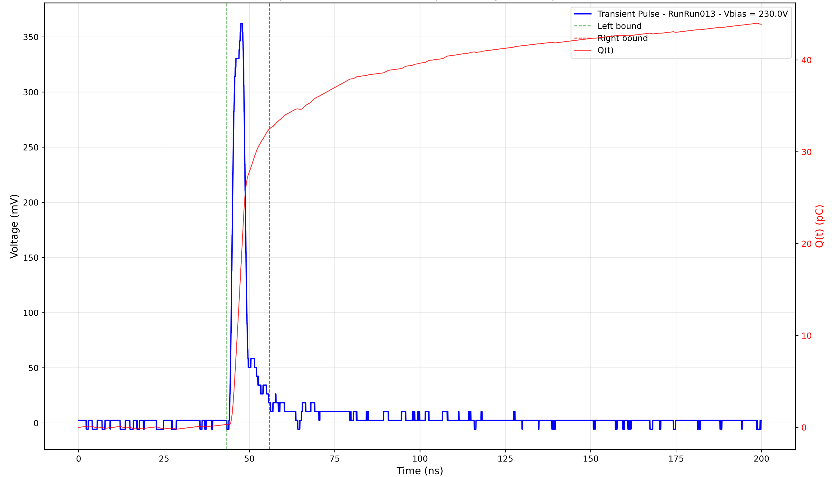
Transient Pulse - Sample: 4003 - Position: 310.0 \mu\text{m} - Charge: 32.20 pC - Rise Time: 1.66 ns
