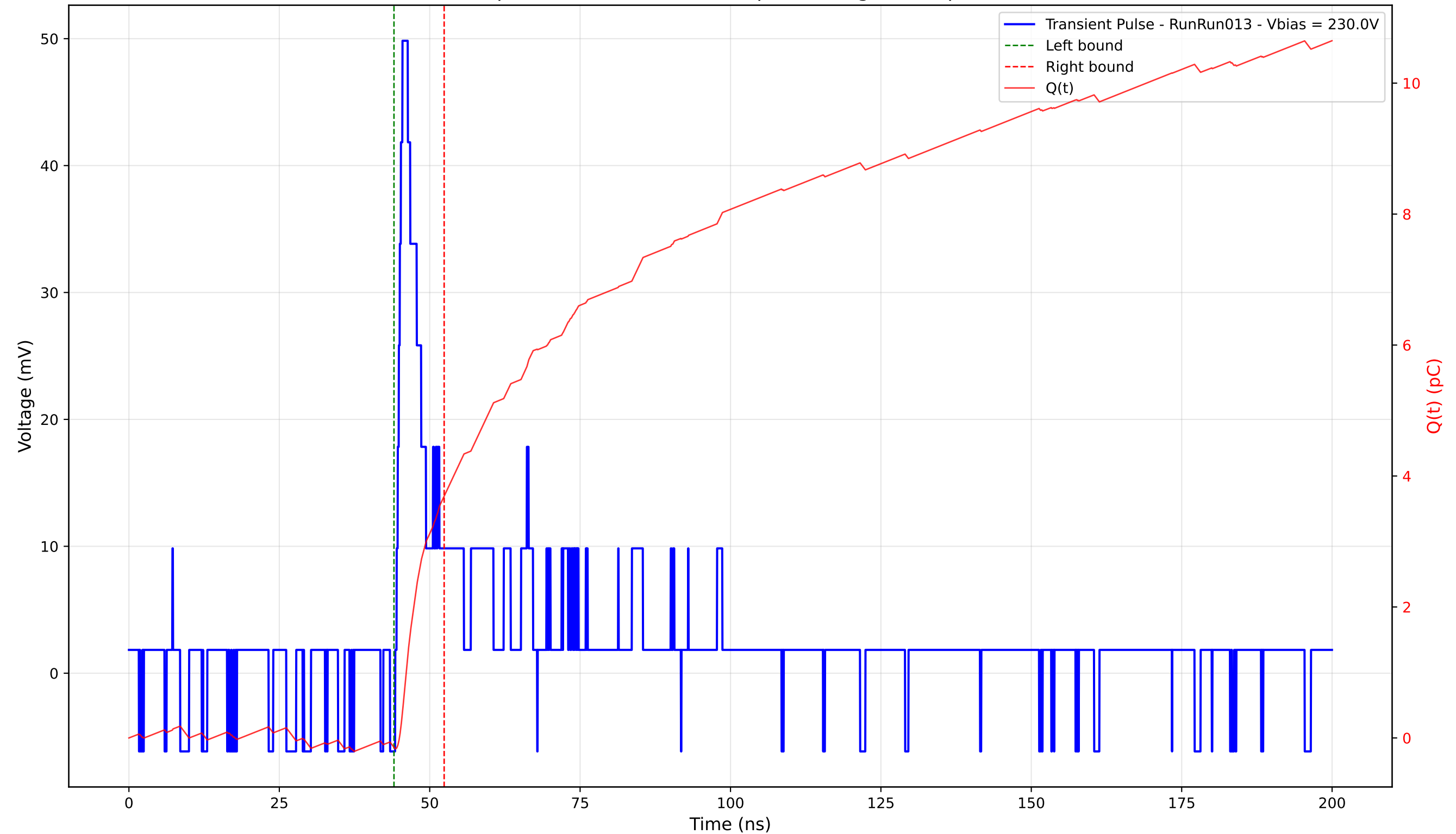
Transient Pulse - Sample: 4003 - Position: 55.0 \mu\text{m} - Charge: 3.84 pC - Rise Time: 0.97 ns
