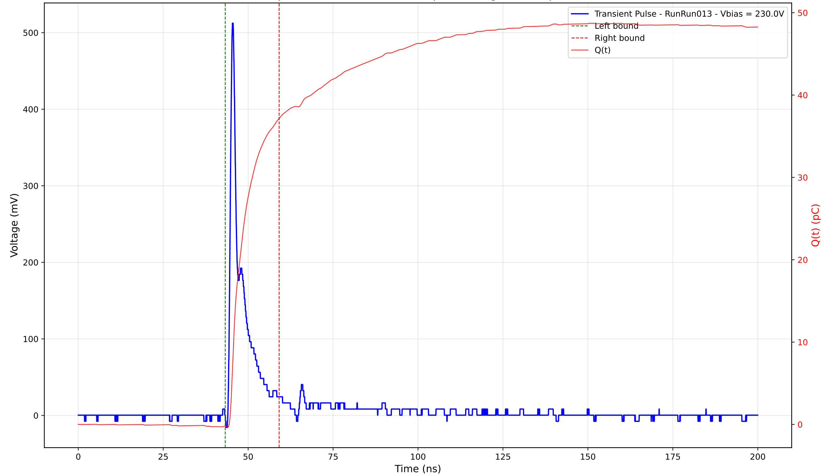
Transient Pulse - Sample: 4003 - Position: 120.0 \mu\text{m} - Charge: 37.36 pC - Rise Time: 0.88 ns
