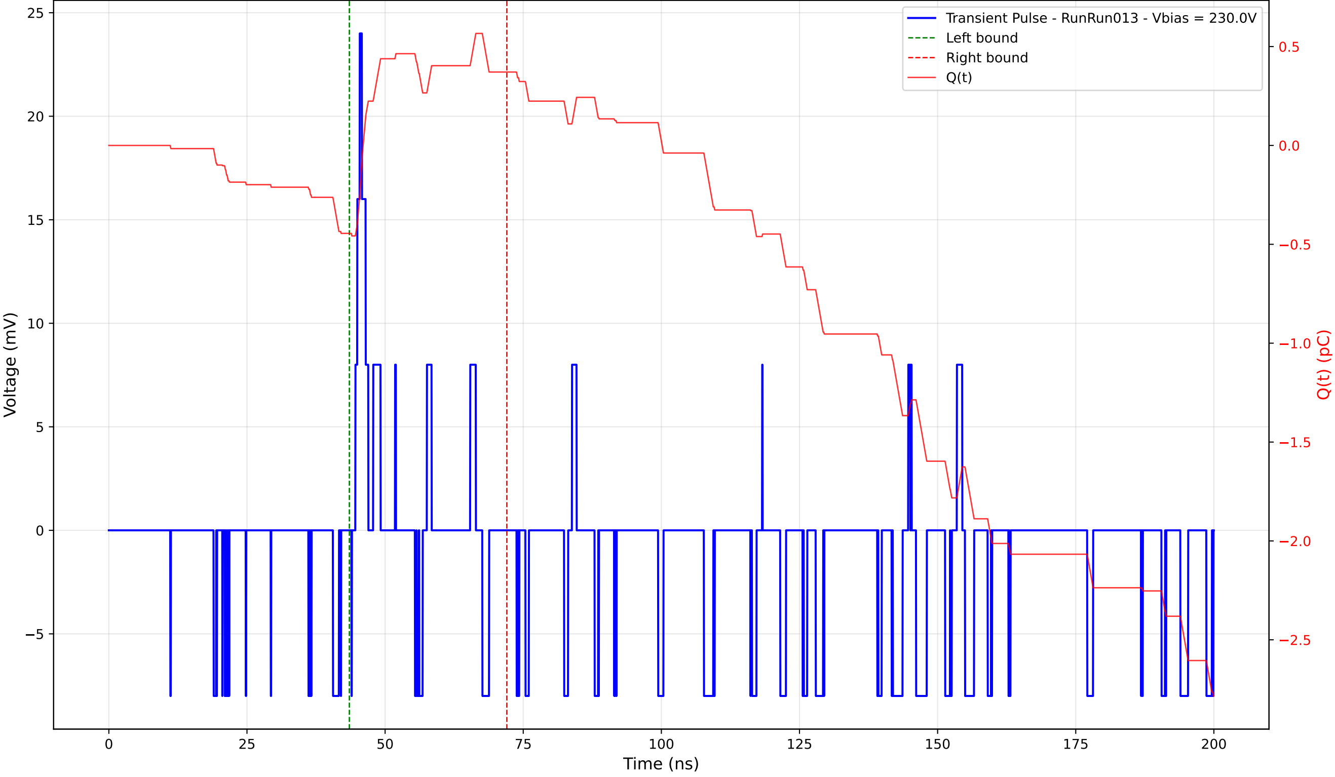
Transient Pulse - Sample: 4003 - Position: 75.0 \mu\text{m} - Charge: 0.82 pC - Rise Time: 0.79 ns
