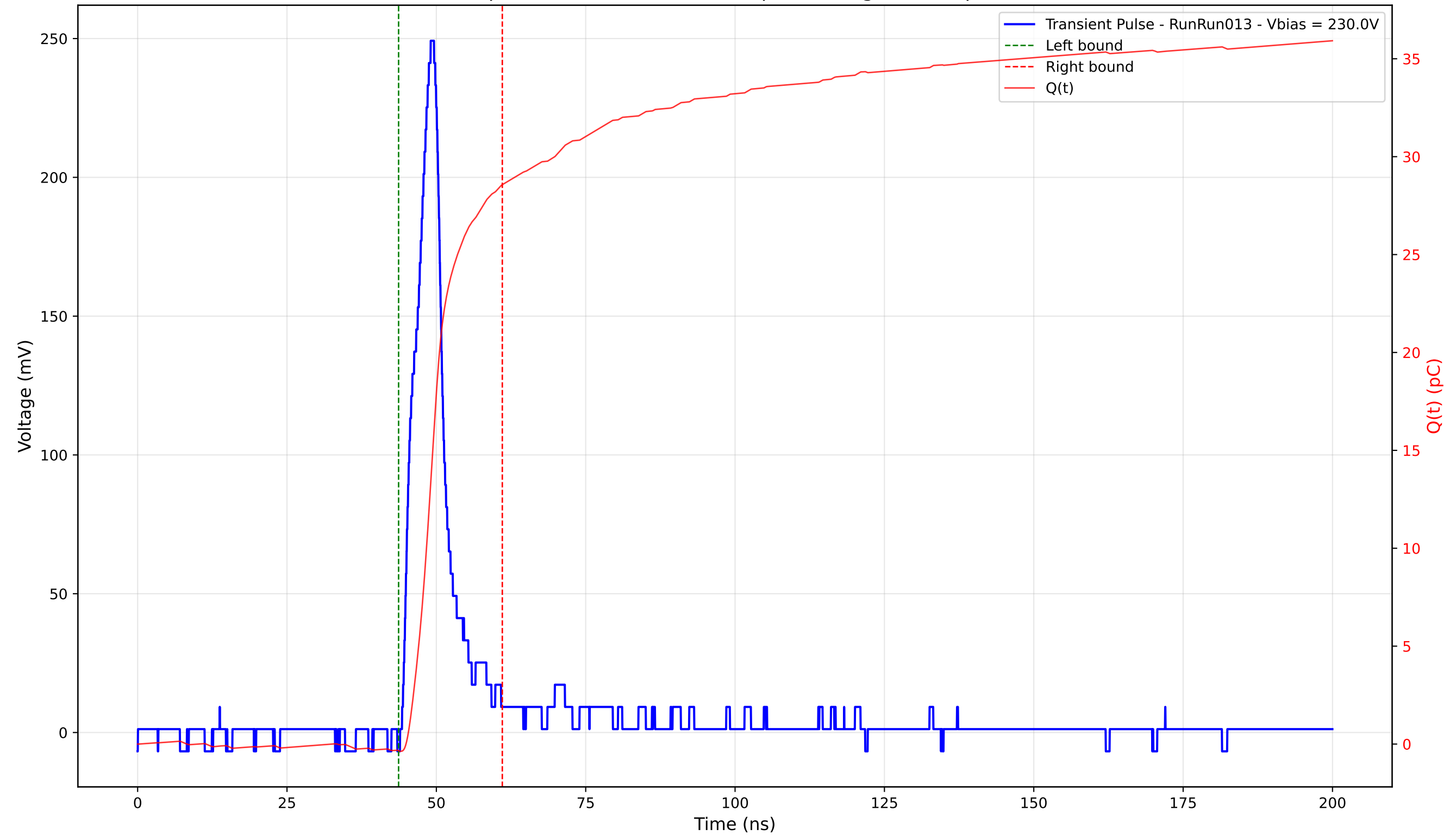
Transient Pulse - Sample: 4003 - Position: 350.0 \mu\text{m} - Charge: 28.91 pC - Rise Time: 3.80 ns
