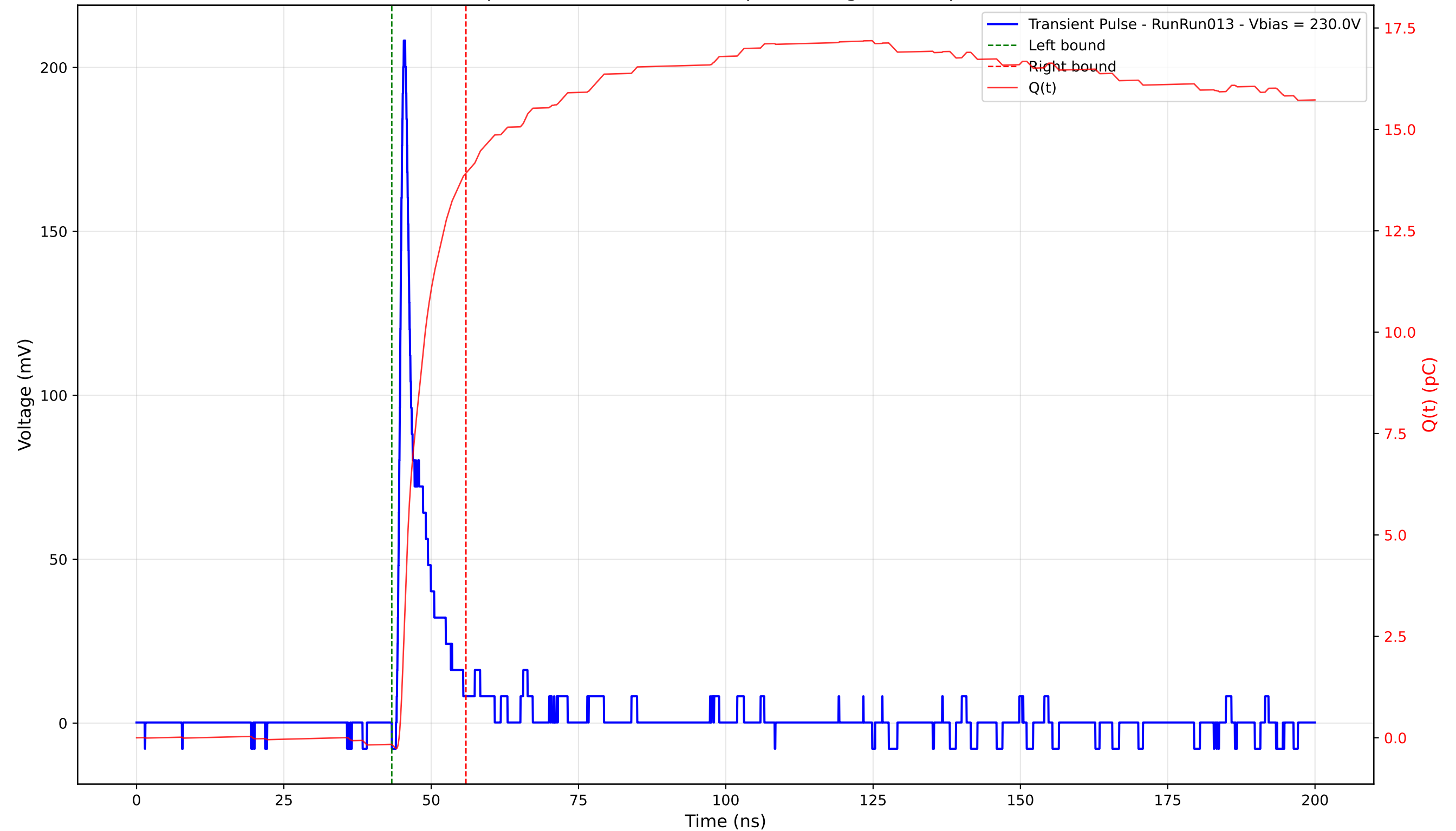
Transient Pulse - Sample: 4003 - Position: 95.0 \mu\text{m} - Charge: 14.08 pC - Rise Time: 0.89 ns
