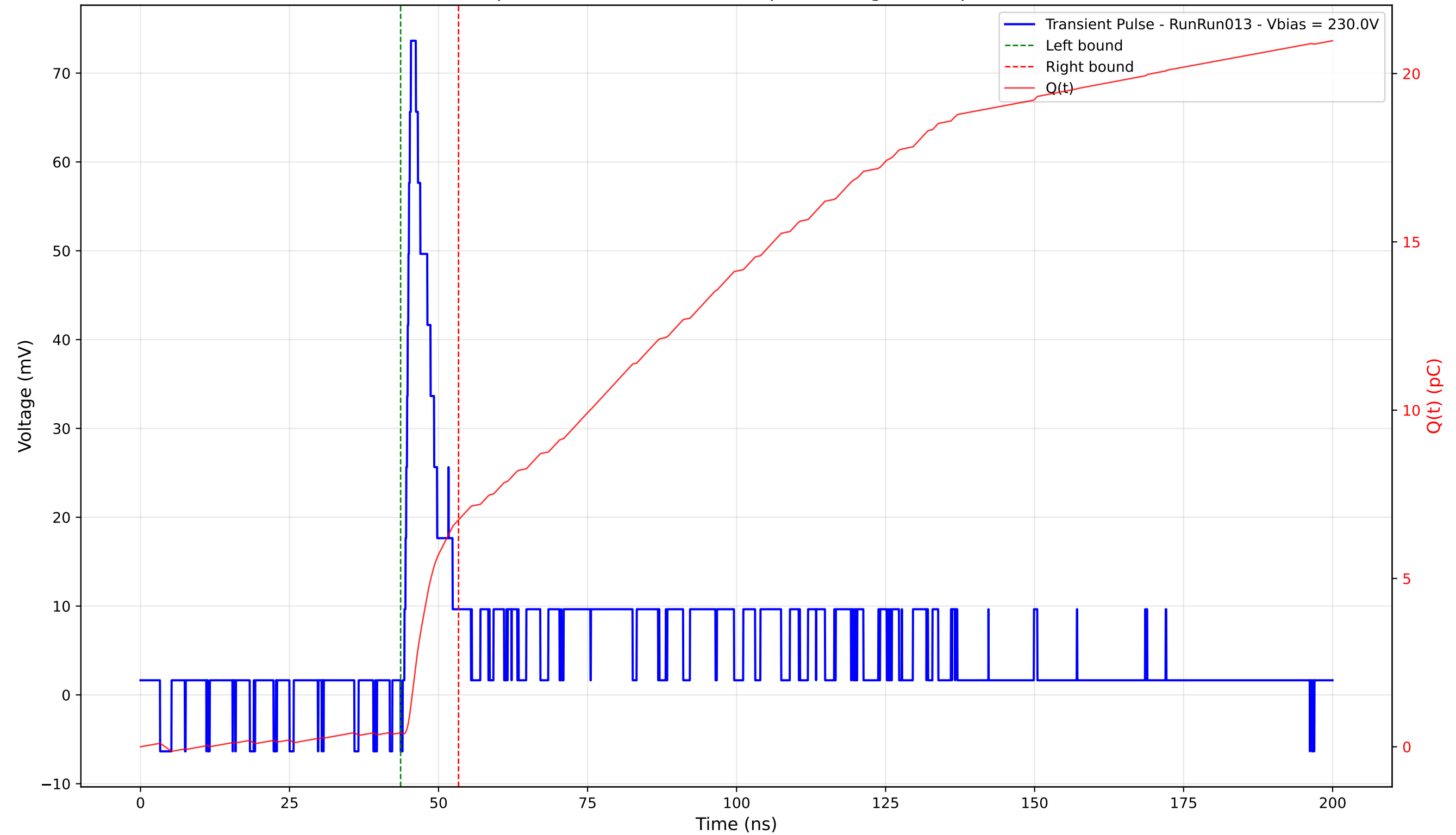
Transient Pulse - Sample: 4003 - Position: 390.0 \mu\text{m} - Charge: 6.33 pC - Rise Time: 1.09 ns
