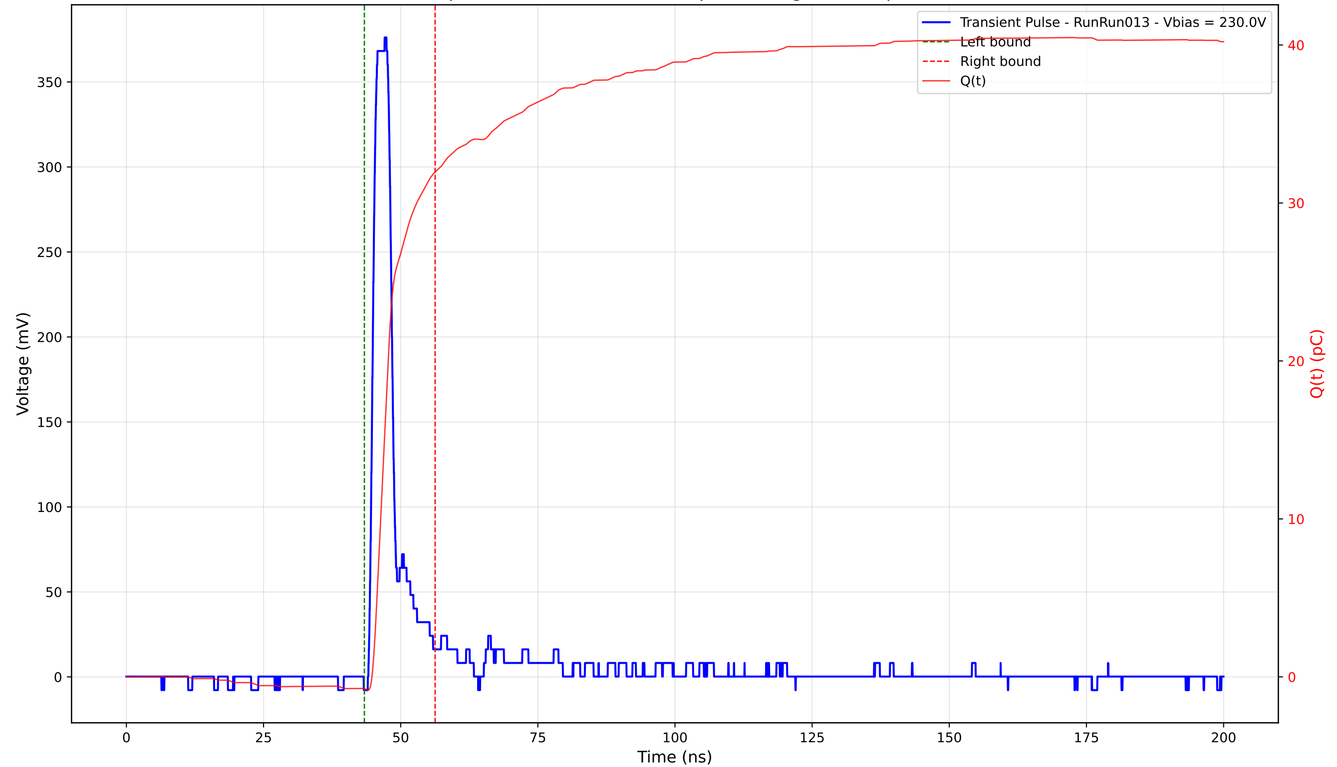
Transient Pulse - Sample: 4003 - Position: 290.0 \mu\text{m} - Charge: 32.70 pC - Rise Time: 1.19 ns
