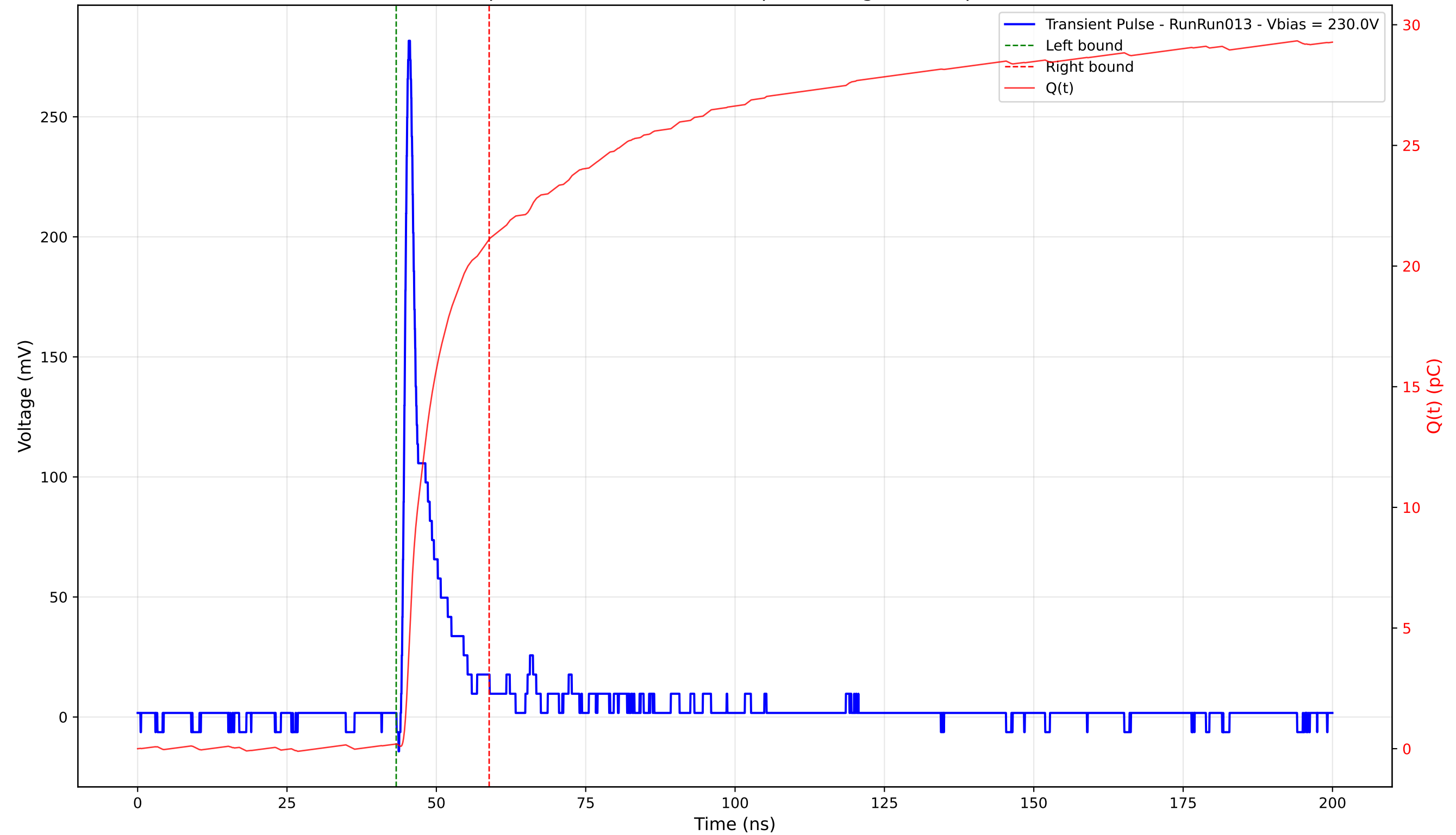
Transient Pulse - Sample: 4003 - Position: 100.0 \mu\text{m} - Charge: 20.92 pC - Rise Time: 0.89 ns
