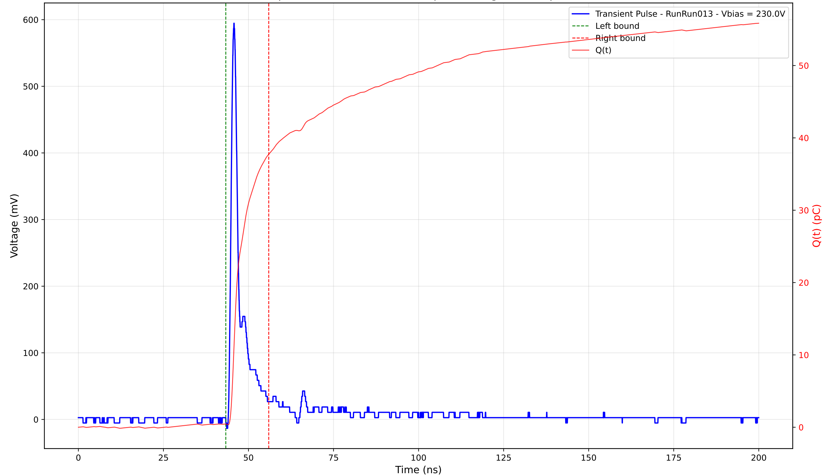
Transient Pulse - Sample: 4003 - Position: 195.0 \mu\text{m} - Charge: 37.27 pC - Rise Time: 1.05 ns
