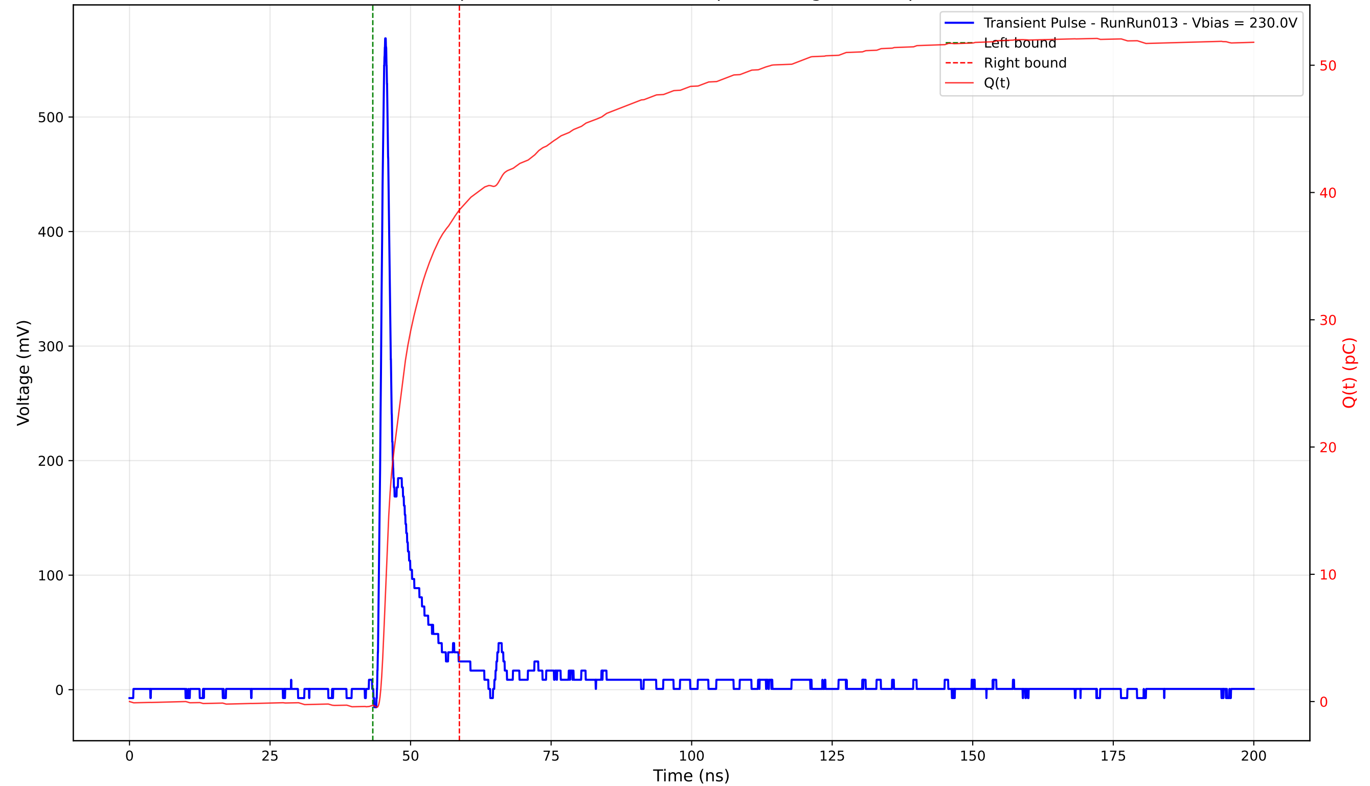
Transient Pulse - Sample: 4003 - Position: 145.0 \mu\text{m} - Charge: 38.93 pC - Rise Time: 0.92 ns
