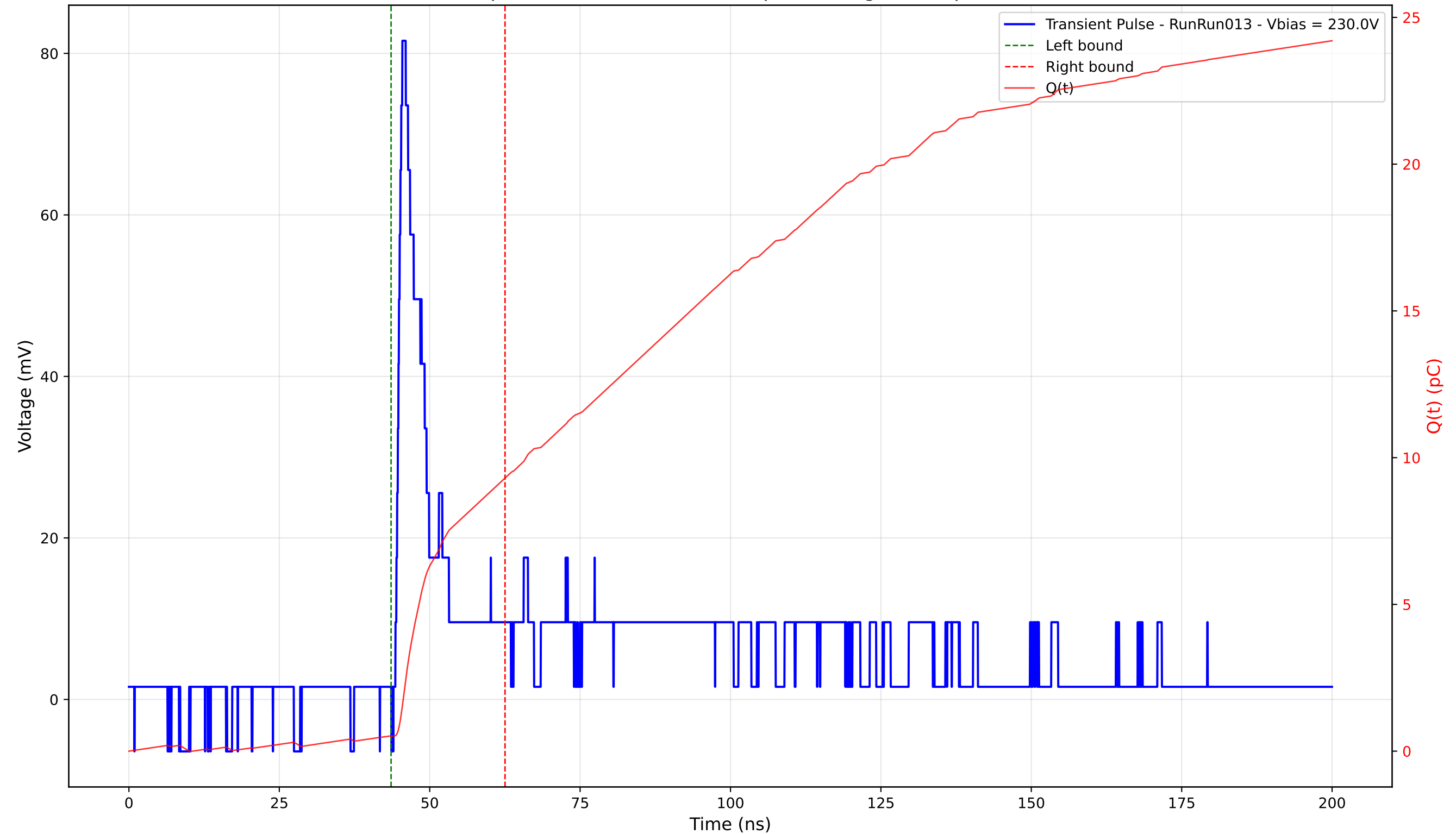
Transient Pulse - Sample: 4003 - Position: 385.0 \mu\text{m} - Charge: 8.79 pC - Rise Time: 0.96 ns
