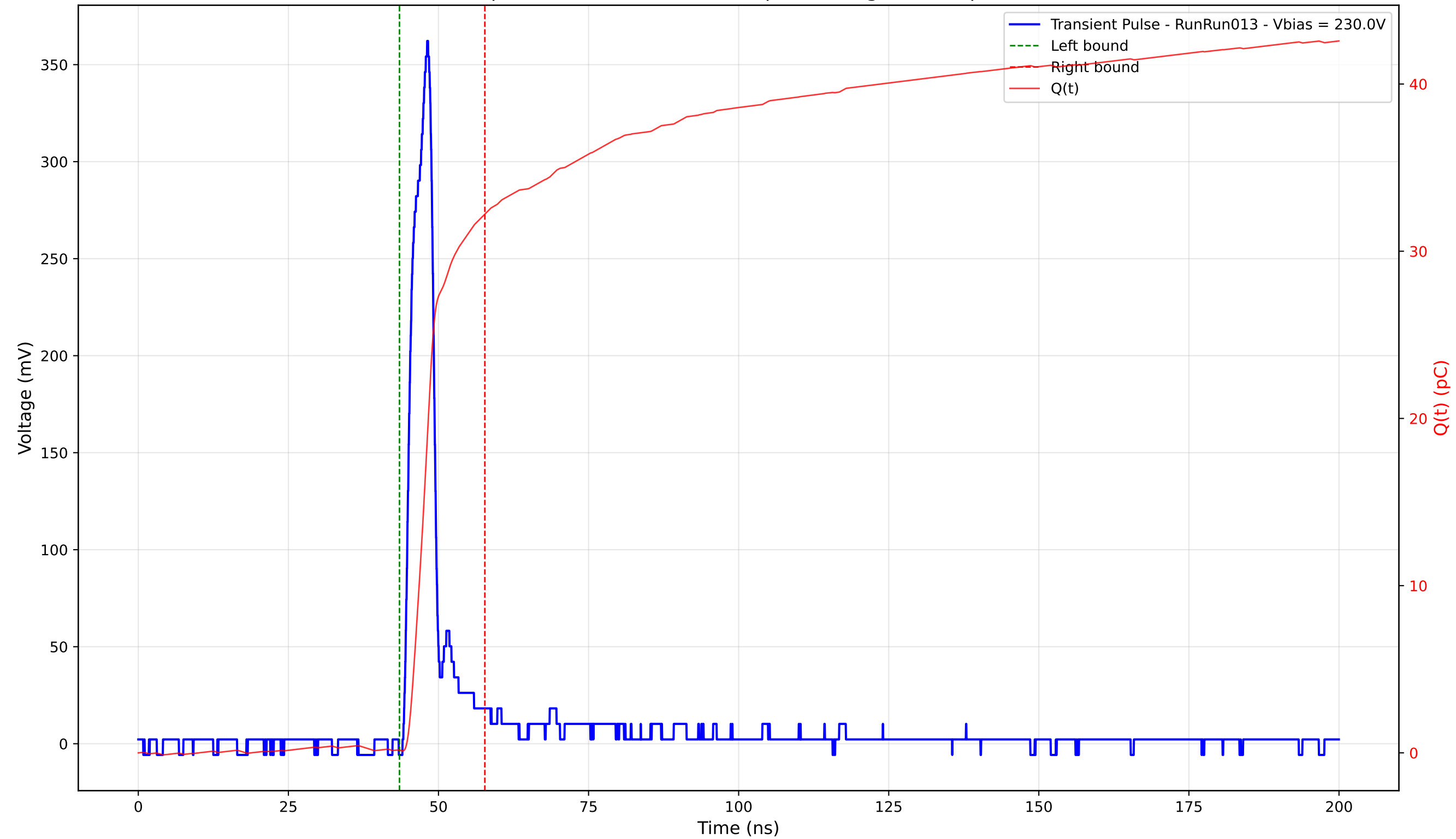
Transient Pulse - Sample: 4003 - Position: 325.0 \mu\text{m} - Charge: 32.05 pC - Rise Time: 3.03 ns
