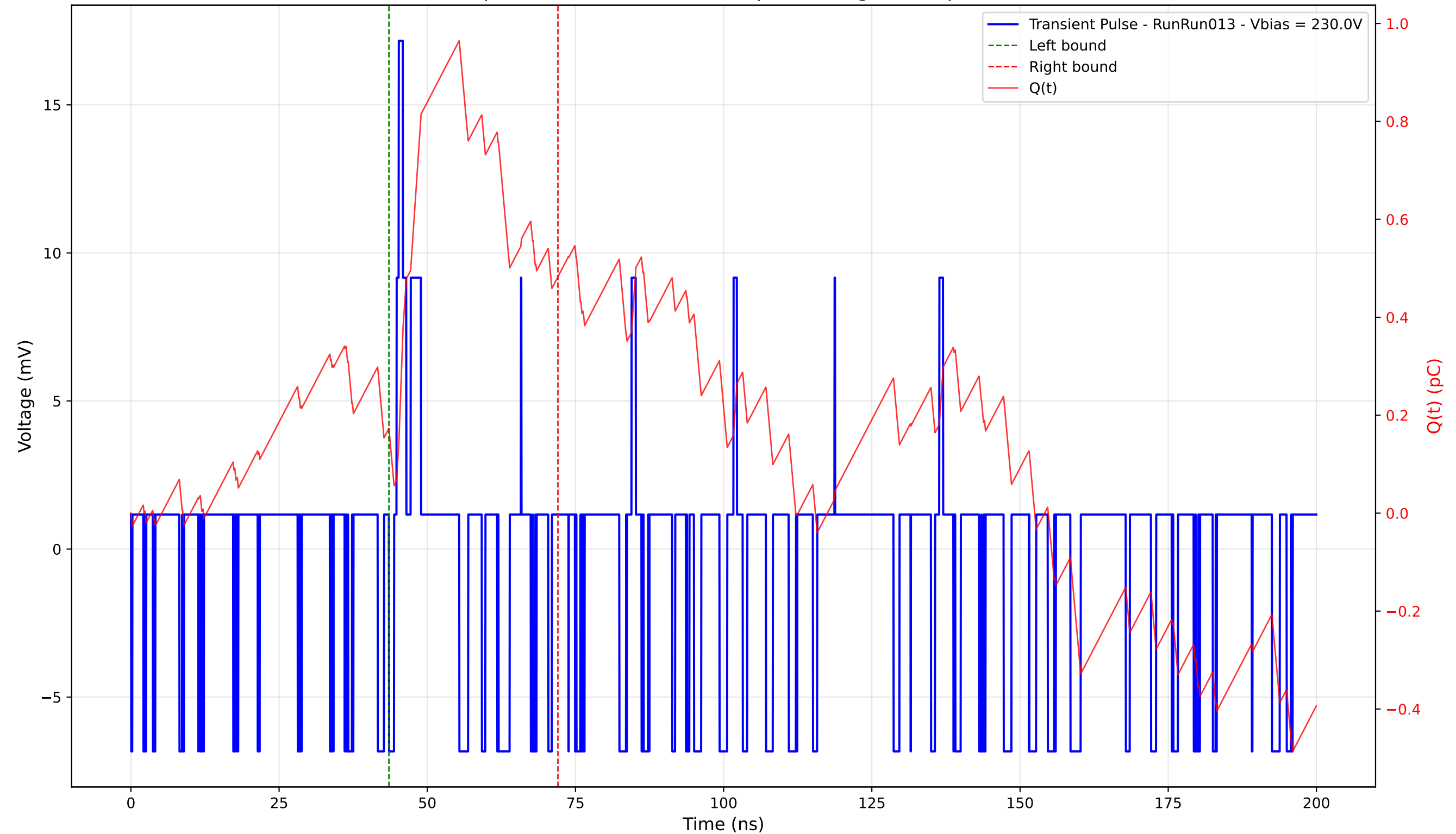
Transient Pulse - Sample: 4003 - Position: 425.0 \mu\text{m} - Charge: 0.31 pC - Rise Time: 0.38 ns
