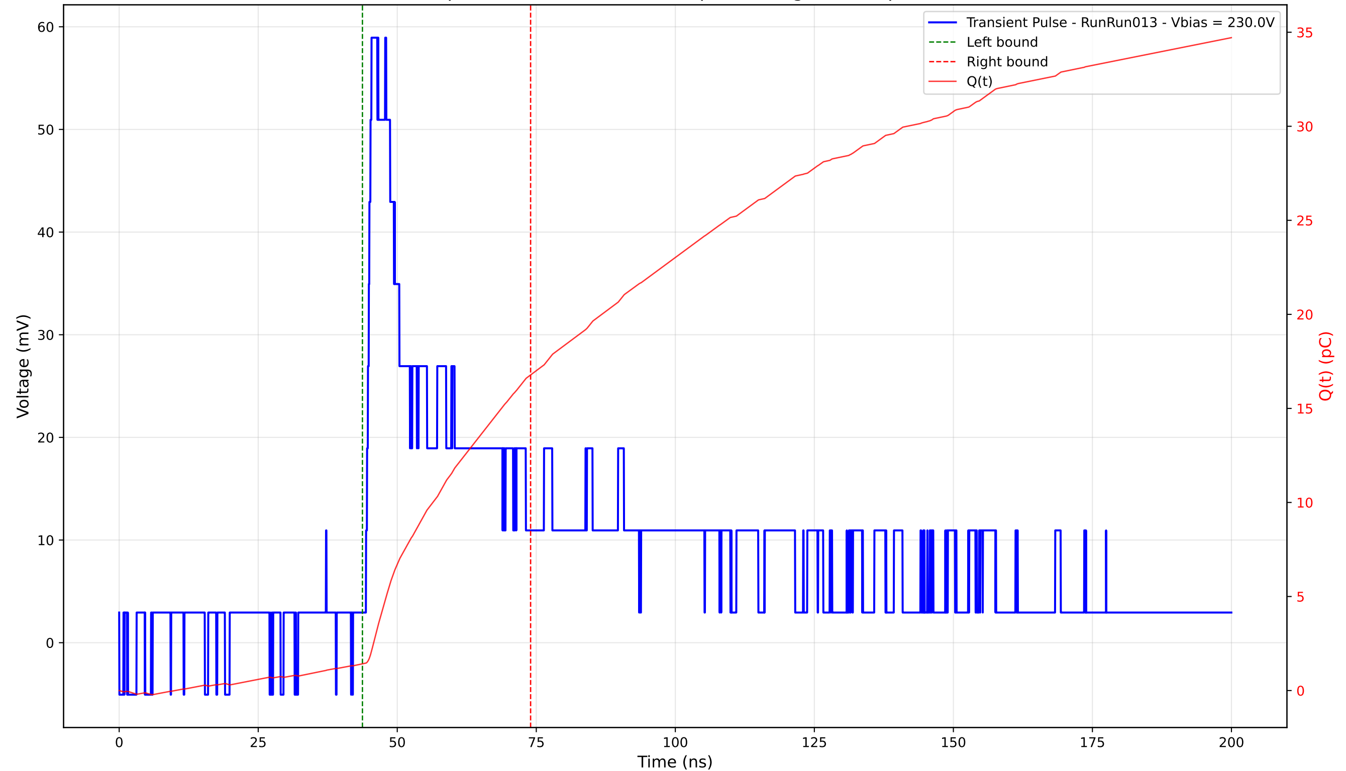
Transient Pulse - Sample: 4003 - Position: 375.0 \mu\text{m} - Charge: 15.36 pC - Rise Time: 0.99 ns
