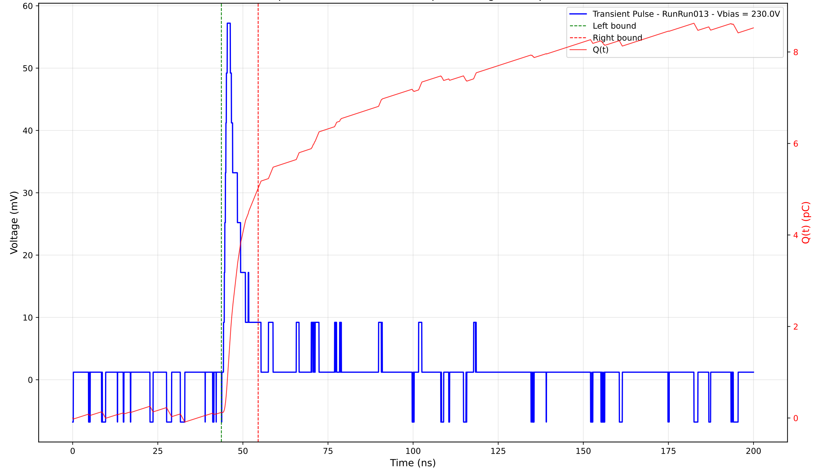
Transient Pulse - Sample: 4003 - Position: 405.0 \mu\text{m} - Charge: 4.90 pC - Rise Time: 1.11 ns
