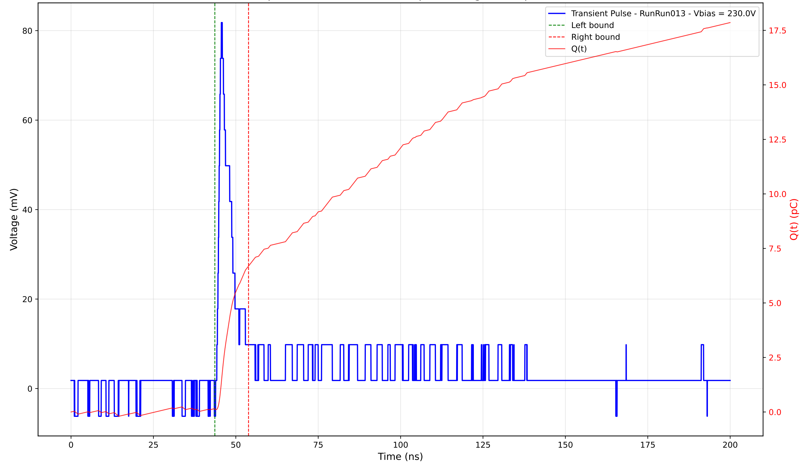
Transient Pulse - Sample: 4003 - Position: 395.0 \mu\text{m} - Charge: 6.56 pC - Rise Time: 1.08 ns
