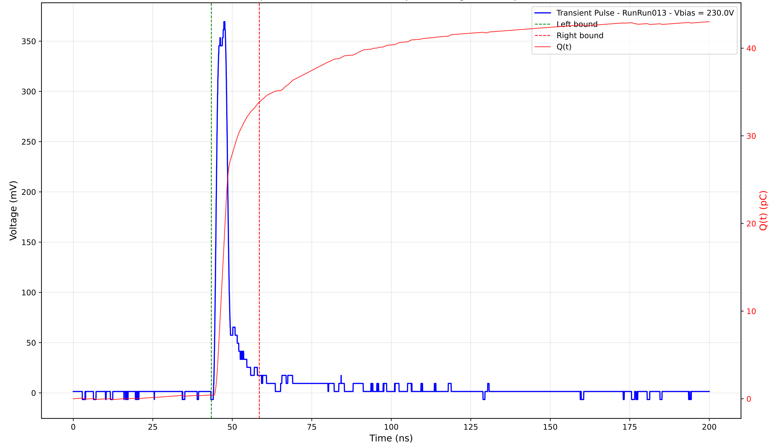
Transient Pulse - Sample: 4003 - Position: 300.0 \mu\text{m} - Charge: 33.41 pC - Rise Time: 1.31 ns
