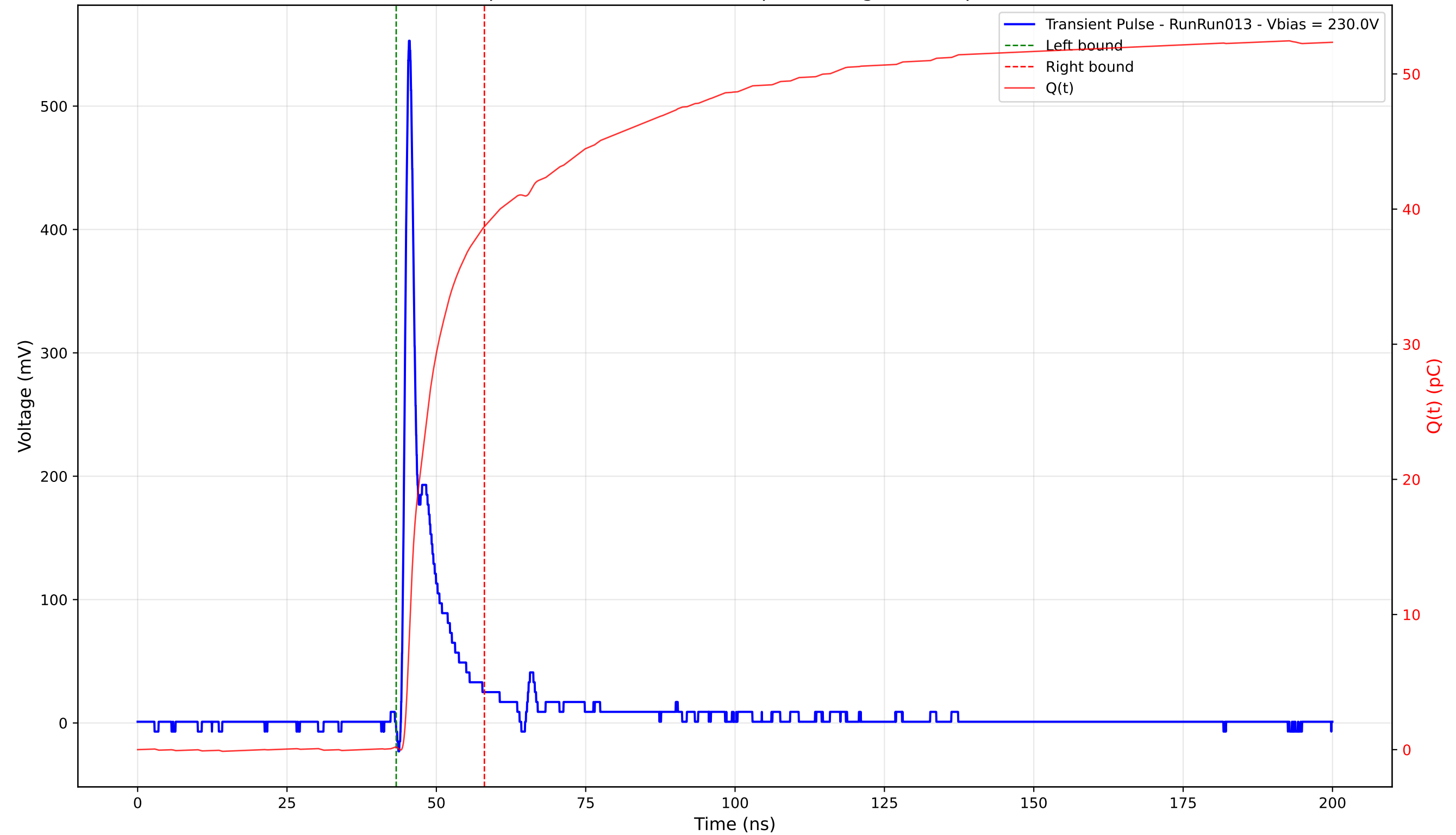
Transient Pulse - Sample: 4003 - Position: 130.0 \mu\text{m} - Charge: 38.52 pC - Rise Time: 0.91 ns
