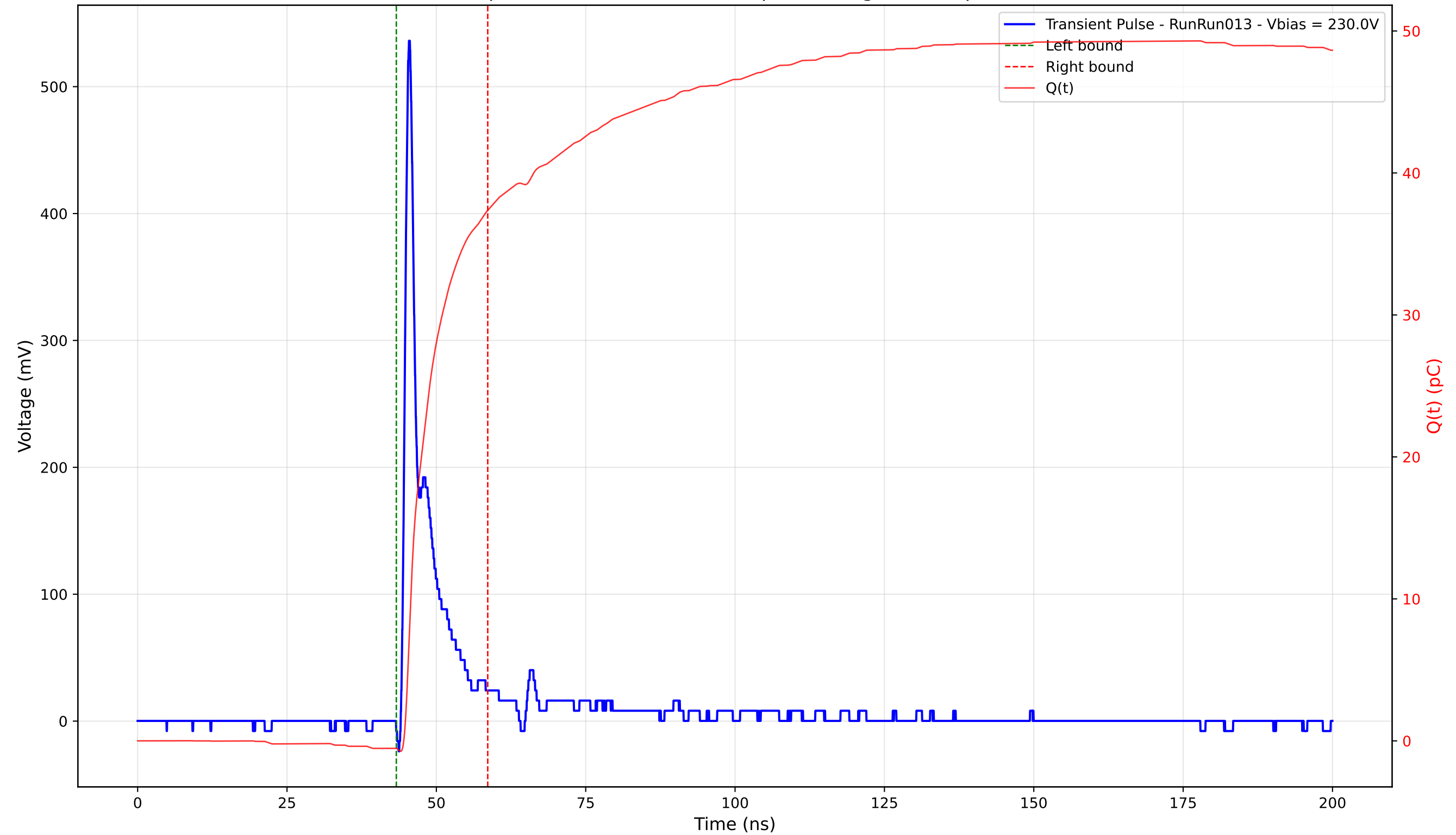
Transient Pulse - Sample: 4003 - Position: 125.0 \mu\text{m} - Charge: 37.89 pC - Rise Time: 0.89 ns
