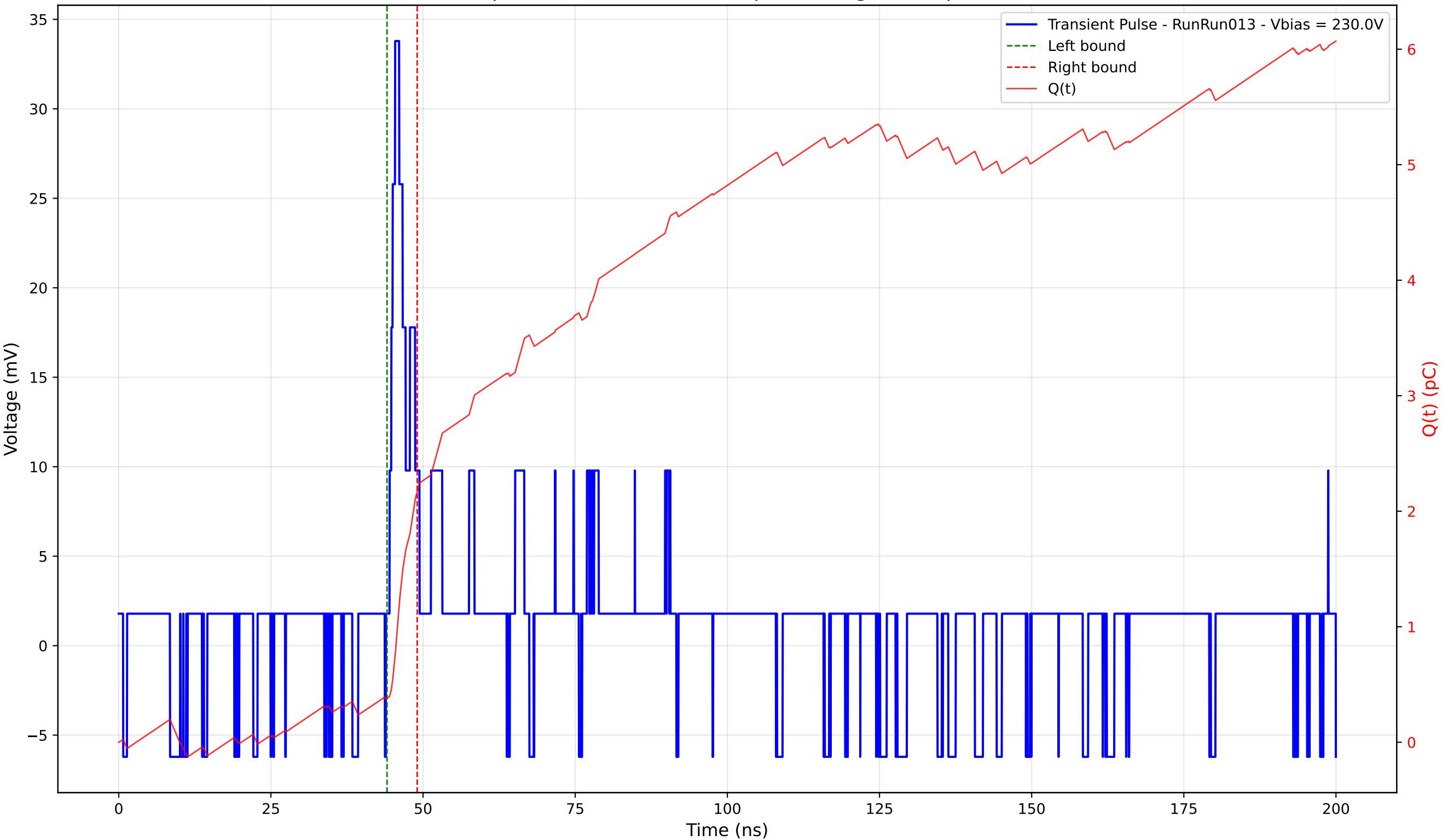
Transient Pulse - Sample: 4003 - Position: 40.0 \mu\text{m} - Charge: 1.79 pC - Rise Time: 0.92 ns
