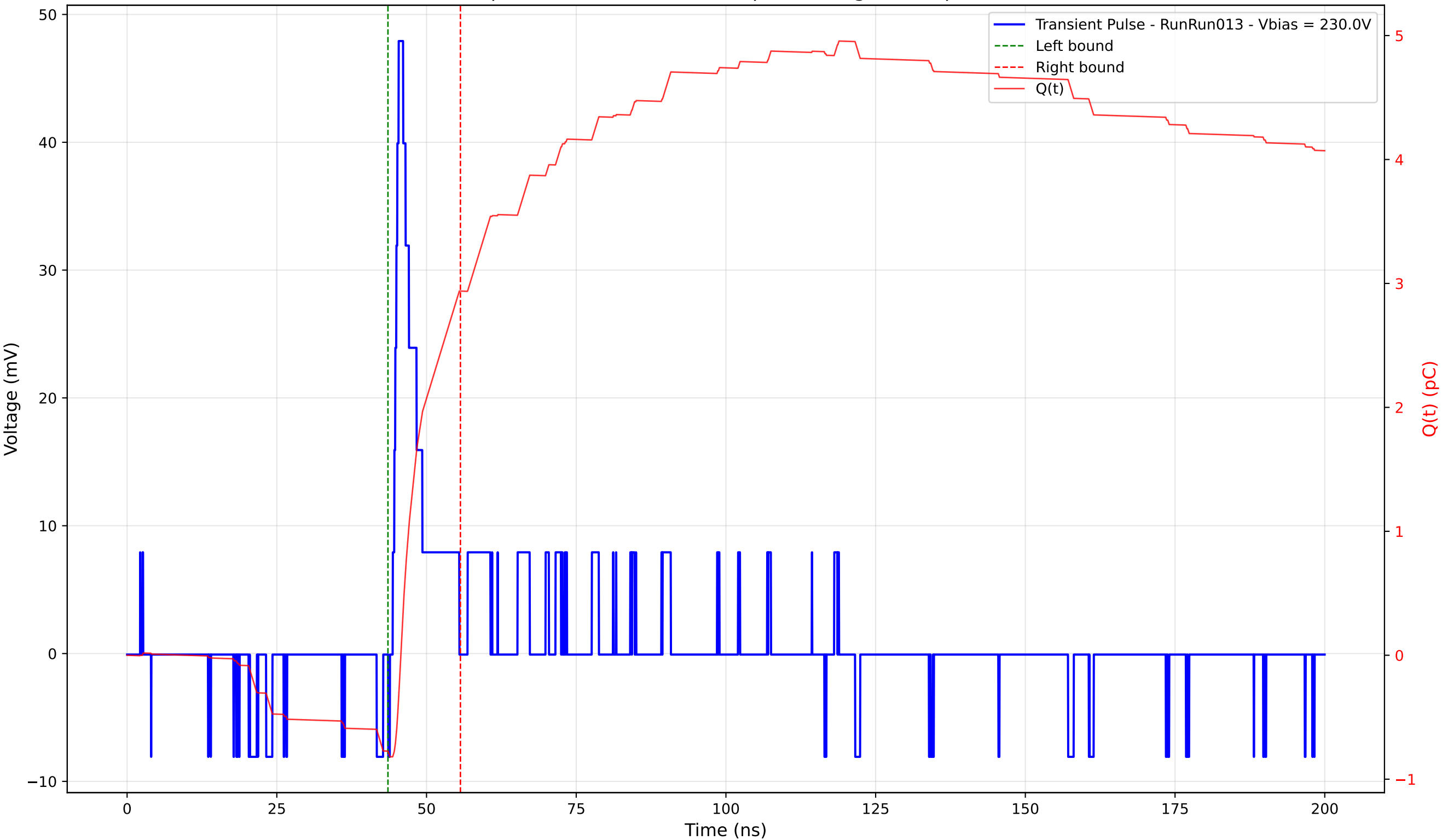
Transient Pulse - Sample: 4003 - Position: 50.0 \mu\text{m} - Charge: 3.71 pC - Rise Time: 0.99 ns
