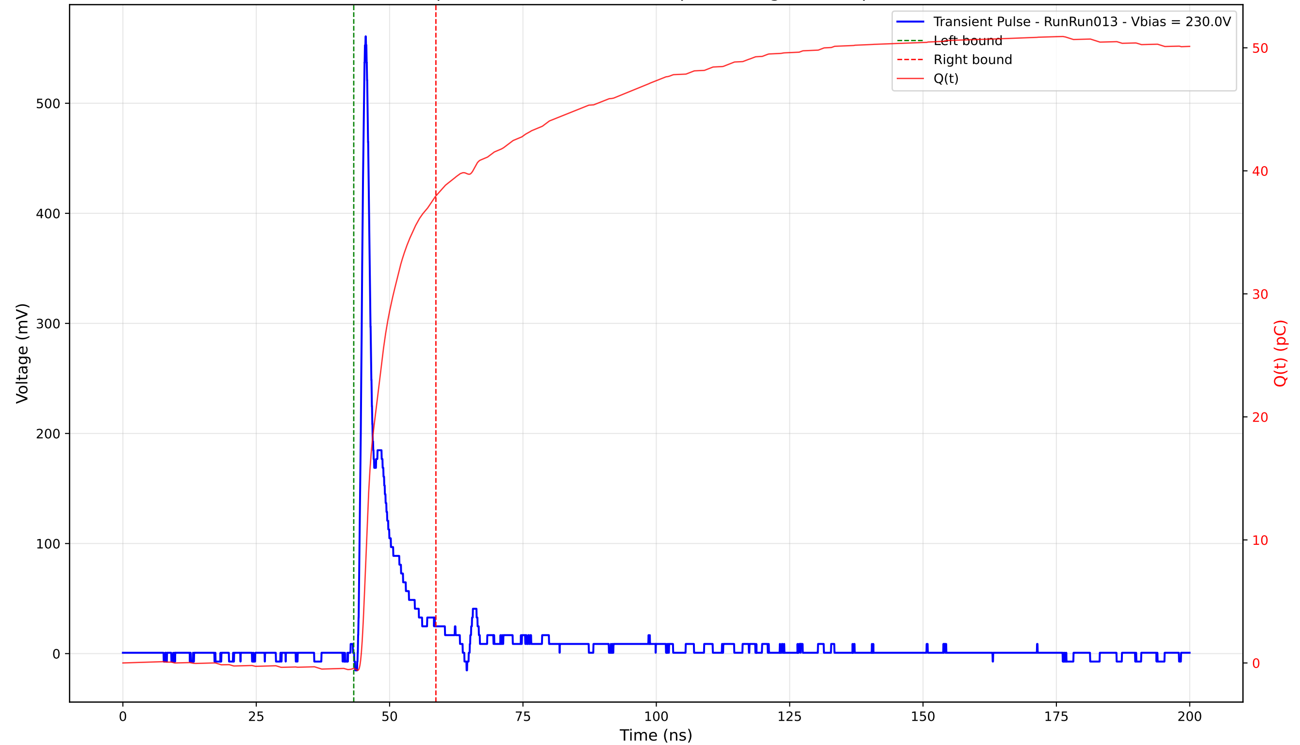
Transient Pulse - Sample: 4003 - Position: 140.0 \mu\text{m} - Charge: 38.41 pC - Rise Time: 0.94 ns
