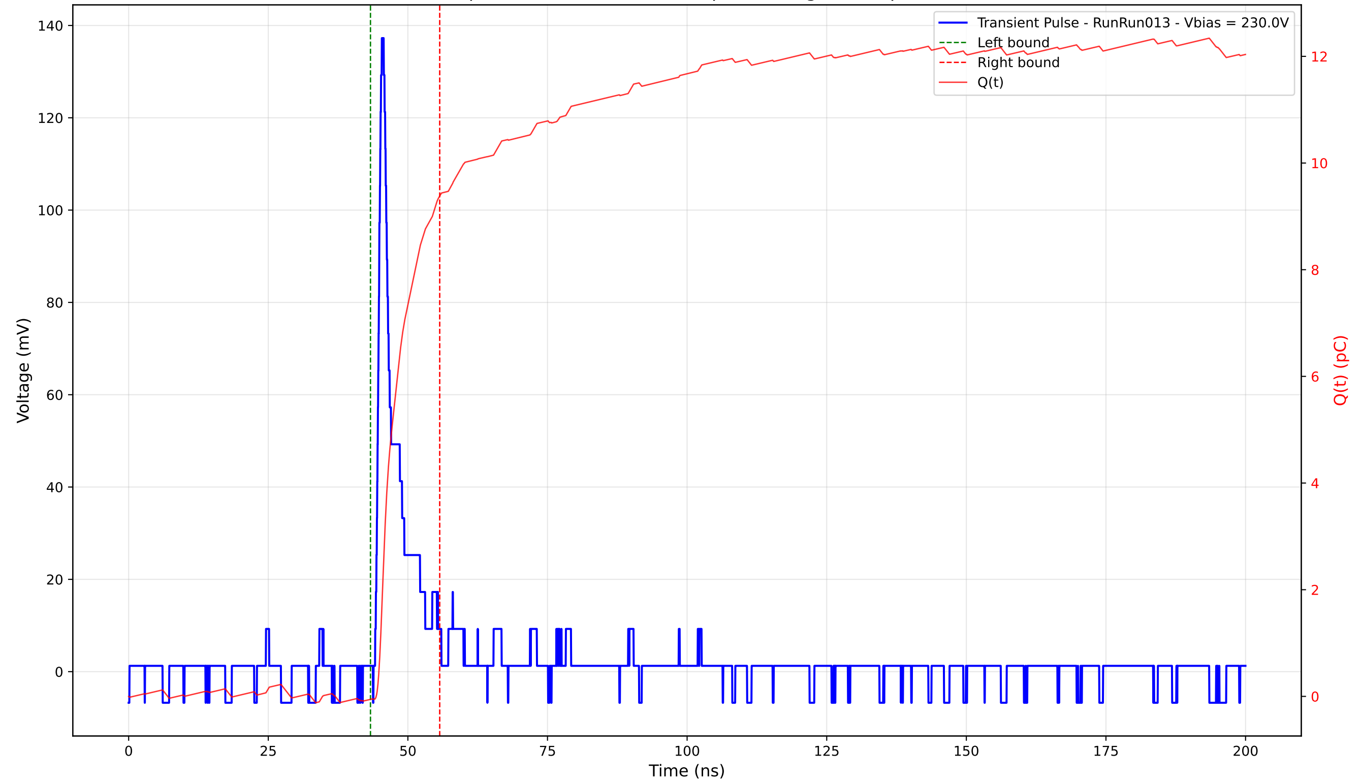
Transient Pulse - Sample: 4003 - Position: 90.0 \mu\text{m} - Charge: 9.44 pC - Rise Time: 0.93 ns
