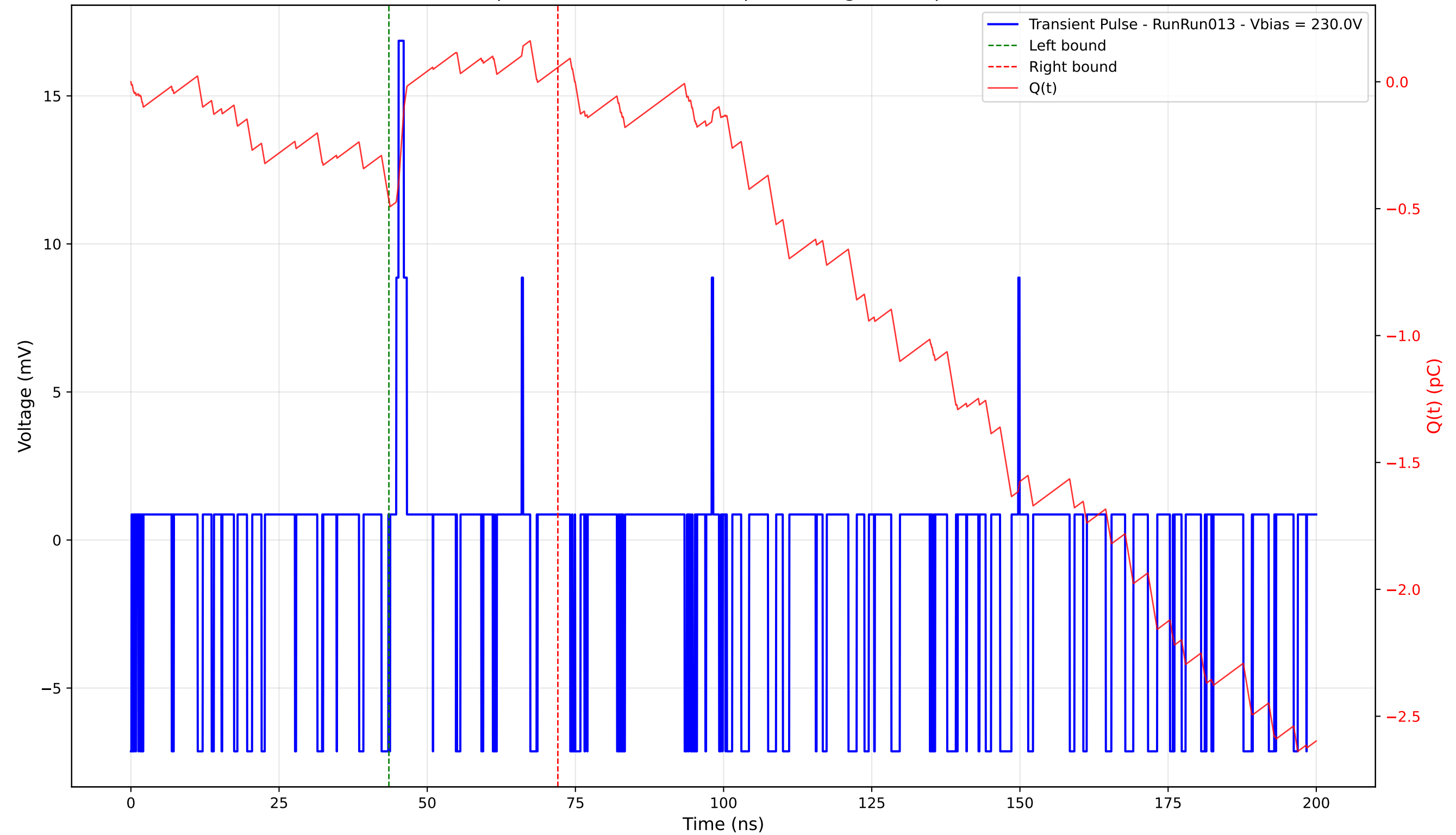
Transient Pulse - Sample: 4003 - Position: 5.0 \mu\text{m} - Charge: 0.52 pC - Rise Time: 0.40 ns
