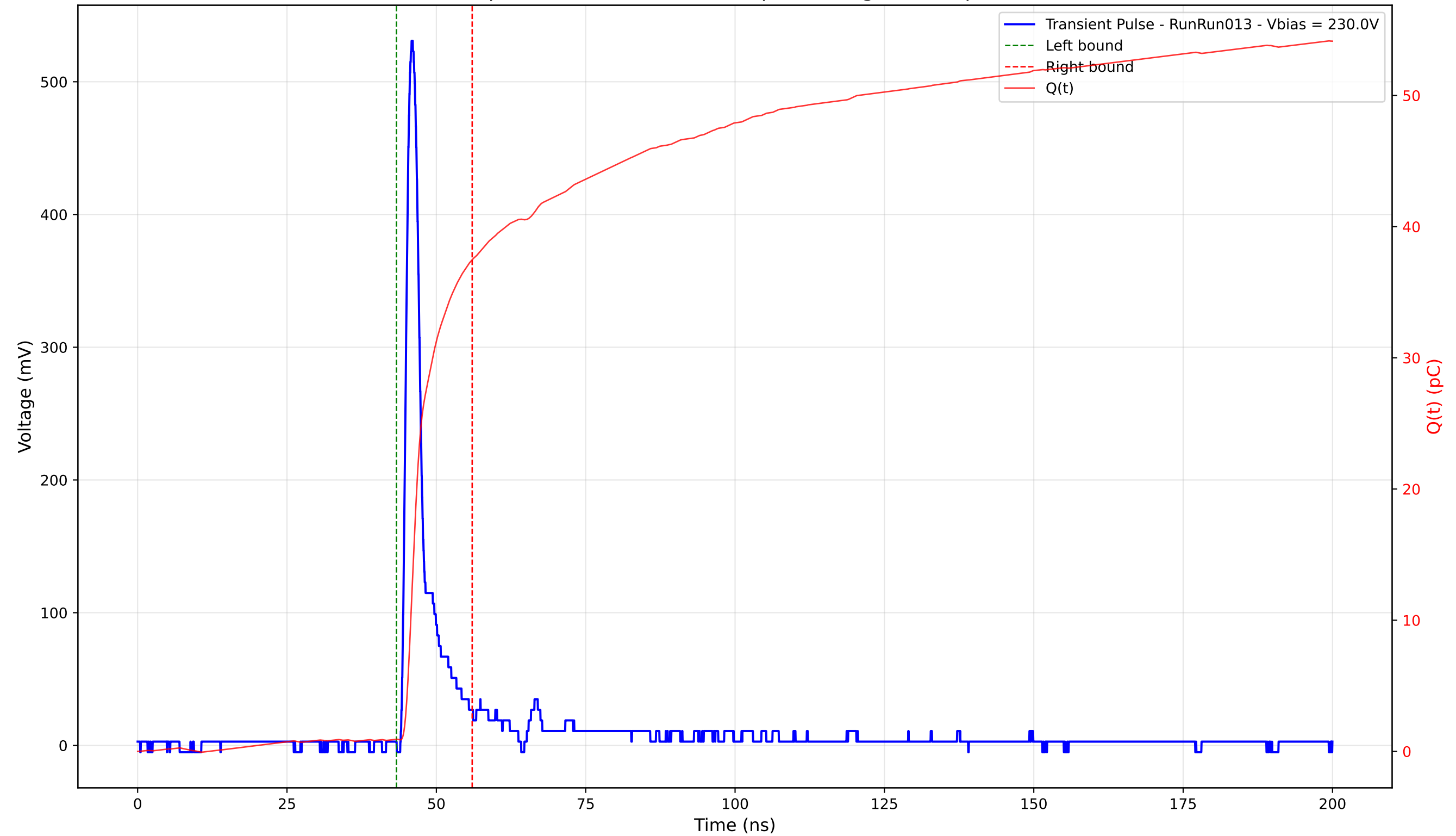
Transient Pulse - Sample: 4003 - Position: 230.0 \mu\text{m} - Charge: 36.55 pC - Rise Time: 1.15 ns
