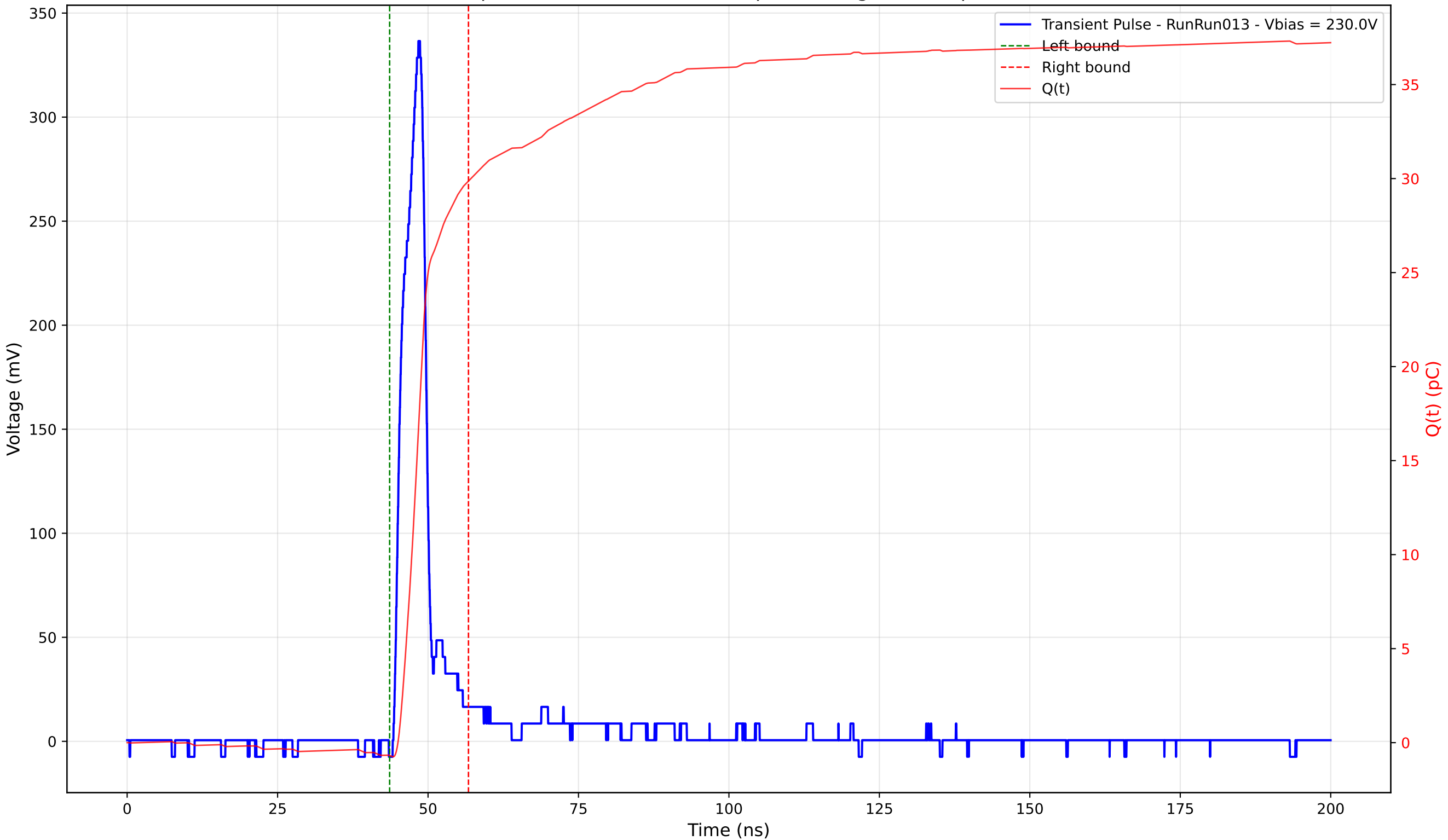
Transient Pulse - Sample: 4003 - Position: 335.0 \mu\text{m} - Charge: 30.55 pC - Rise Time: 3.18 ns
