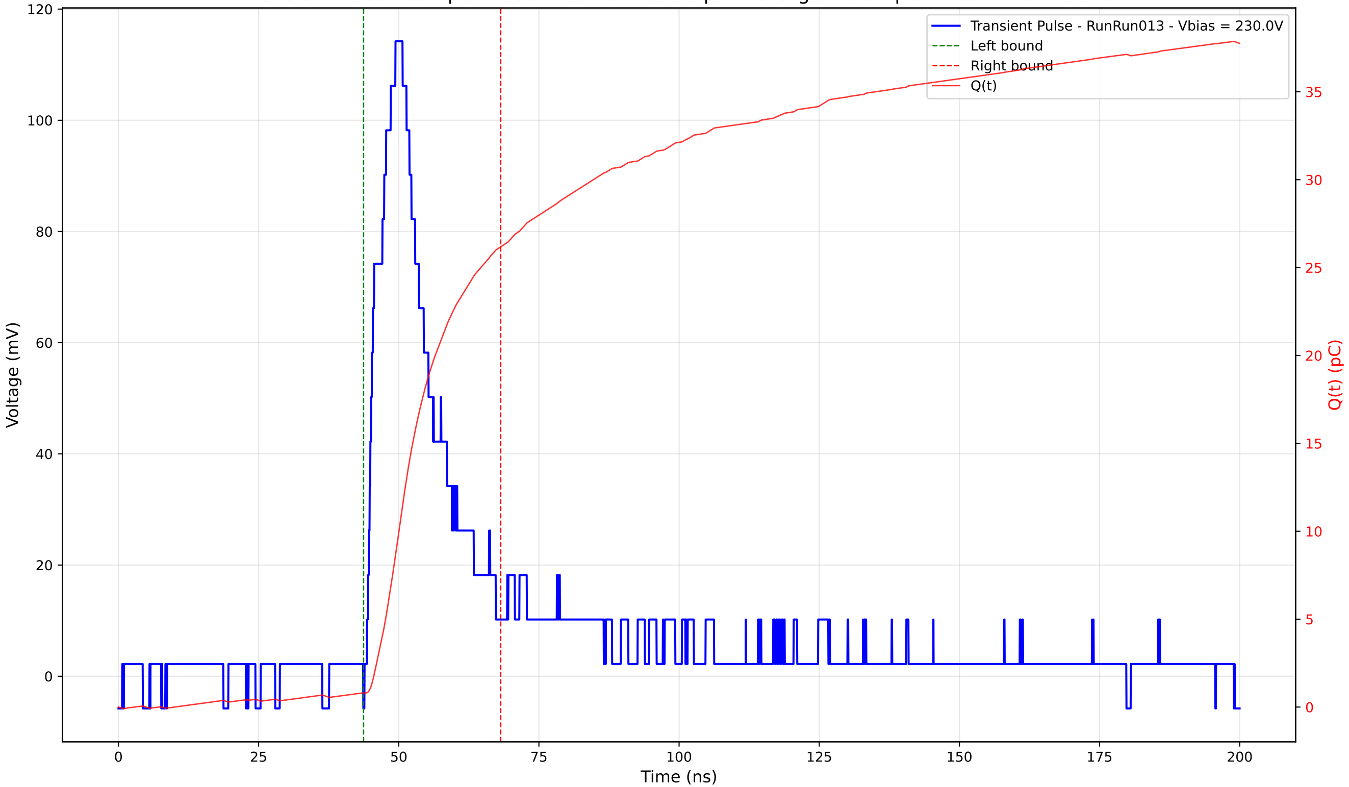
Transient Pulse - Sample: 4003 - Position: 360.0 \mu\text{m} - Charge: 25.37 pC - Rise Time: 4.06 ns
