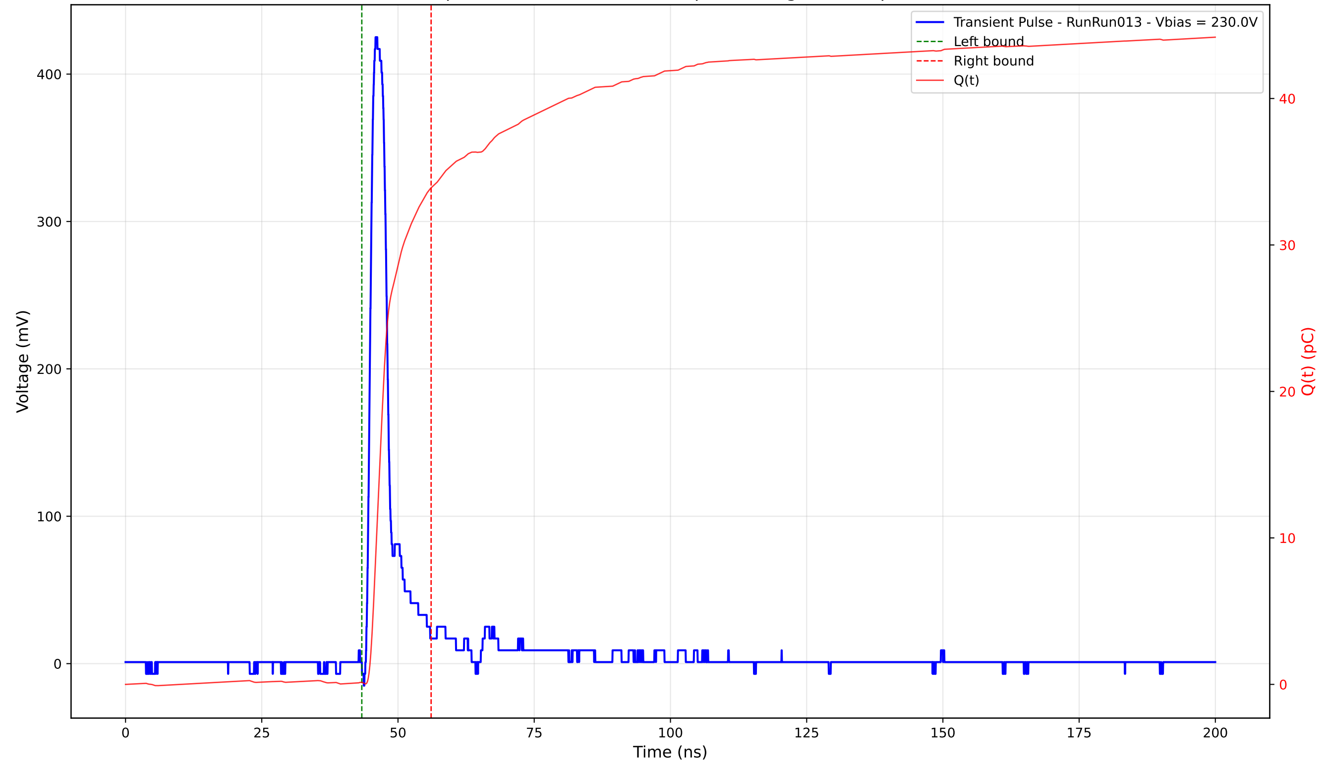
Transient Pulse - Sample: 4003 - Position: 270.0 \mu\text{m} - Charge: 33.76 pC - Rise Time: 1.12 ns
