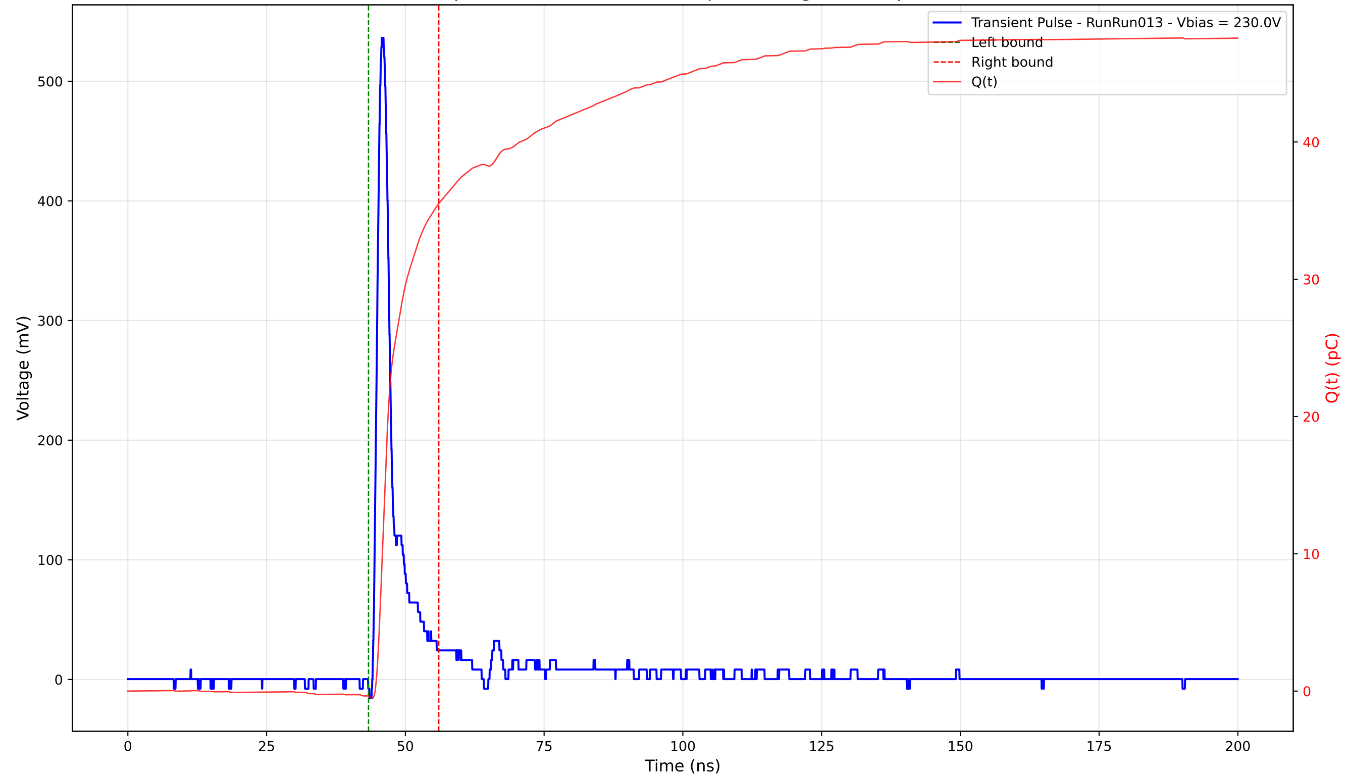
Transient Pulse - Sample: 4003 - Position: 225.0 \mu\text{m} - Charge: 35.87 pC - Rise Time: 1.11 ns
