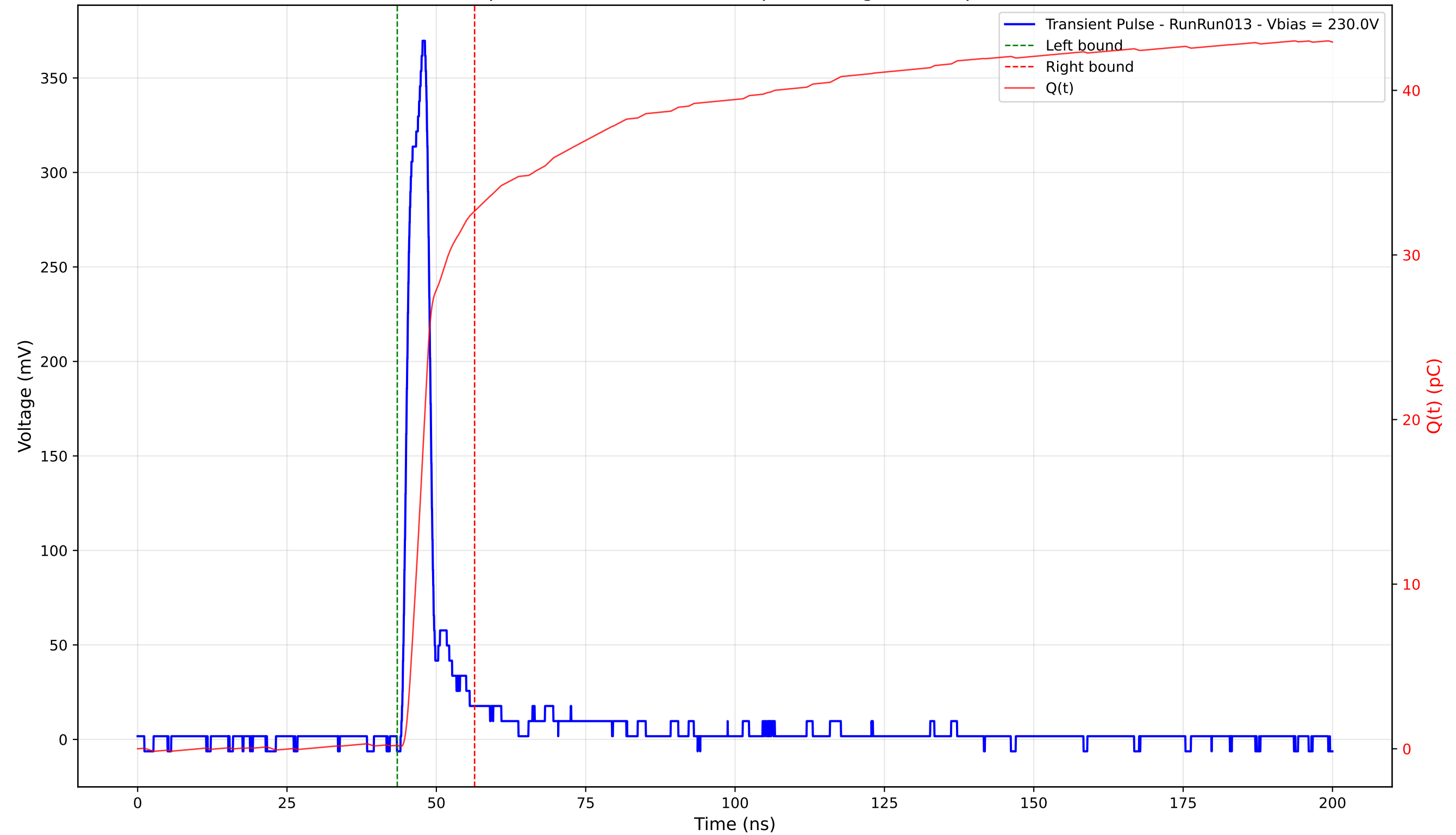
Transient Pulse - Sample: 4003 - Position: 315.0 \mu\text{m} - Charge: 32.46 pC - Rise Time: 2.69 ns
