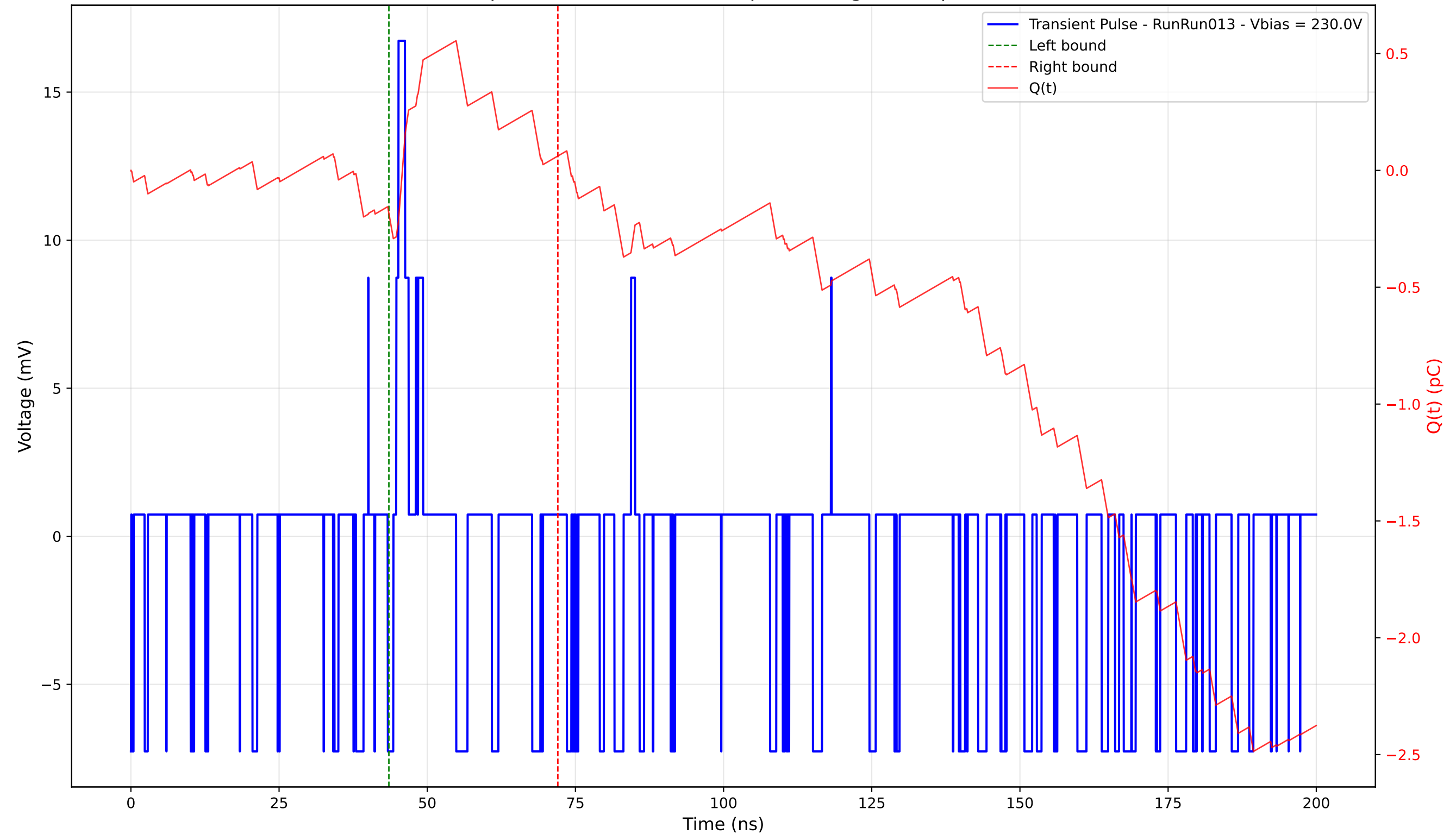
Transient Pulse - Sample: 4003 - Position: 70.0 \mu\text{m} - Charge: 0.25 pC - Rise Time: 0.38 ns
