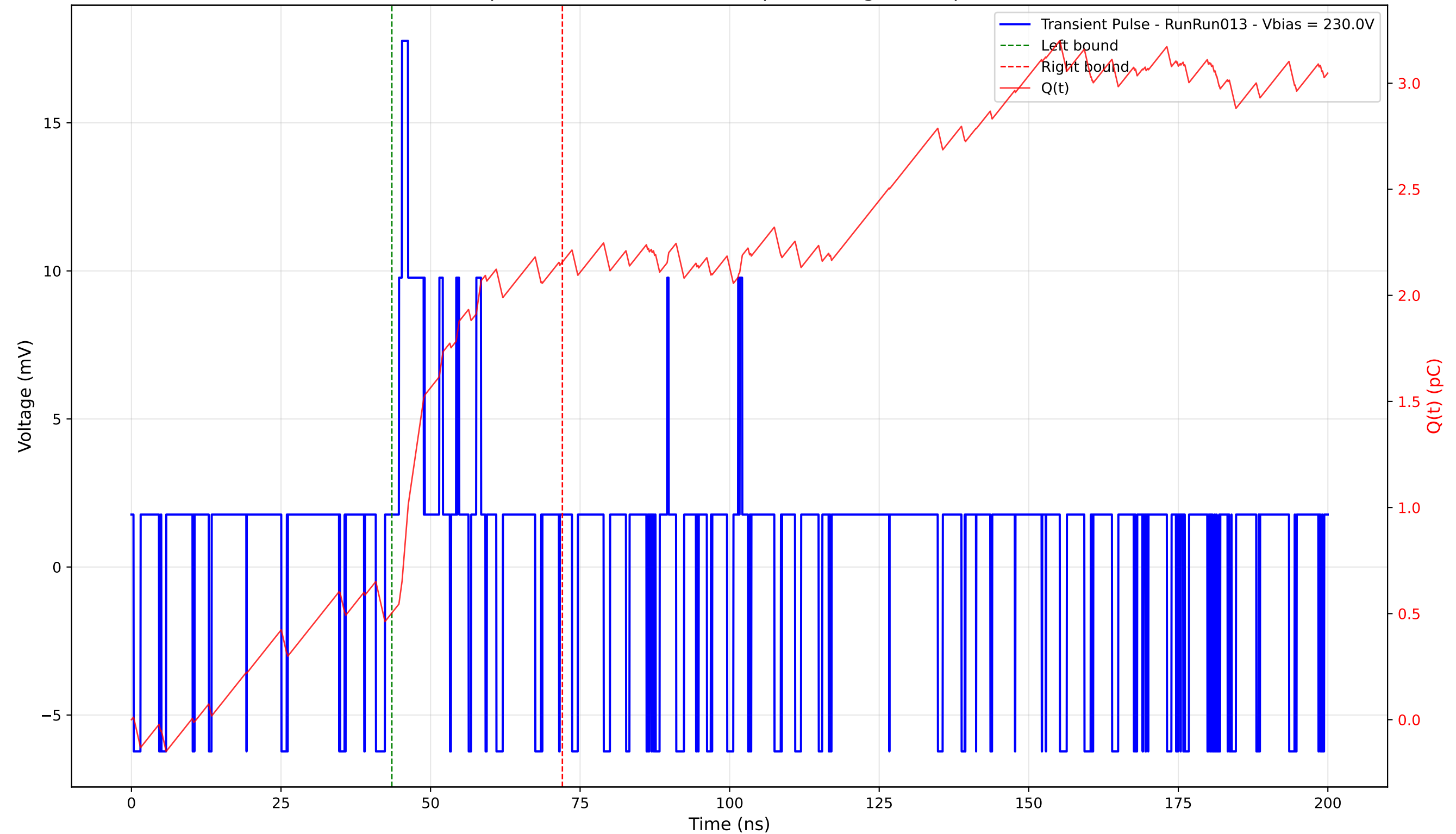
Transient Pulse - Sample: 4003 - Position: 420.0 \mu\text{m} - Charge: 1.65 pC - Rise Time: 0.52 ns
