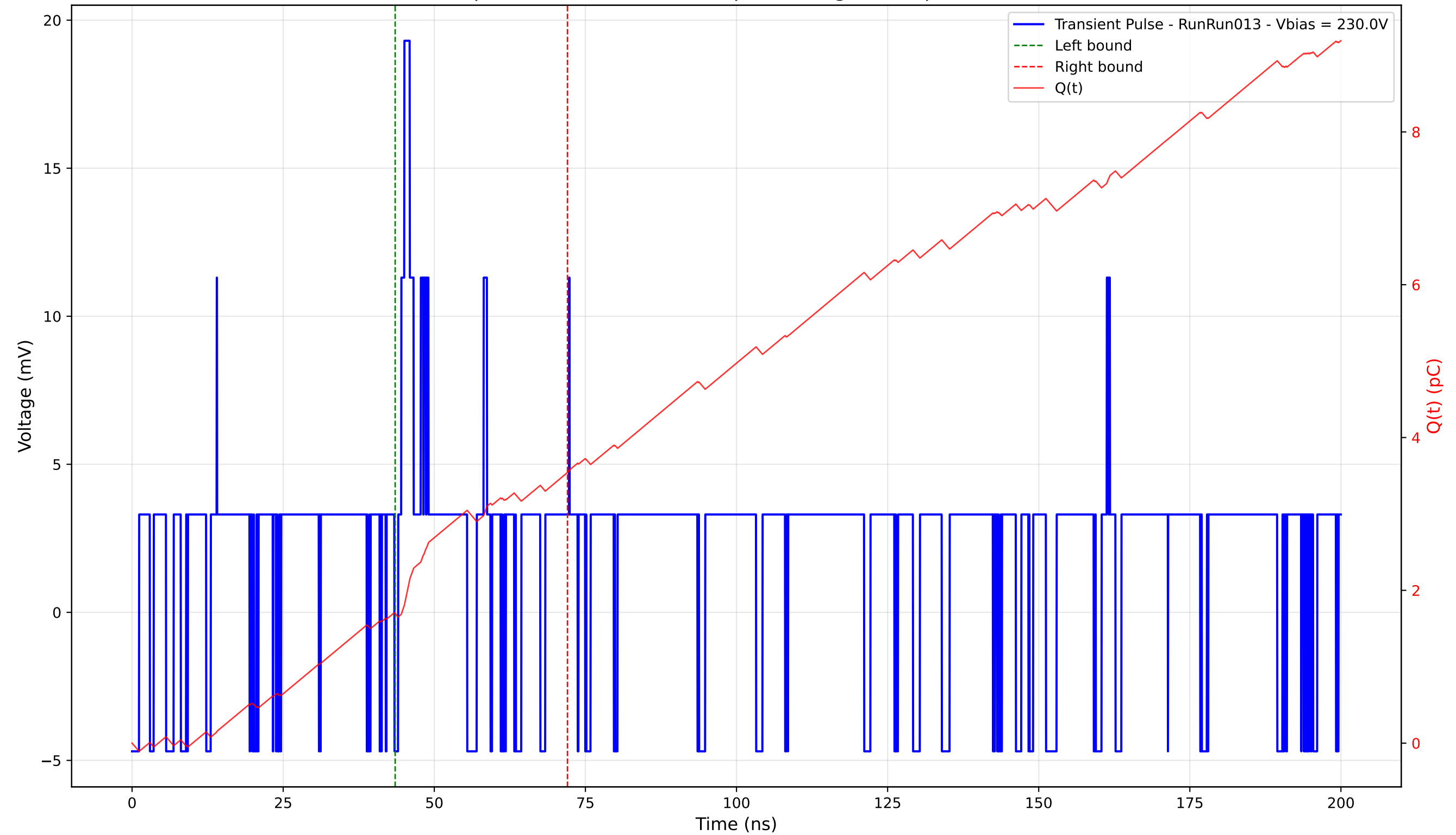
Transient Pulse - Sample: 4003 - Position: 10.0 \mu\text{m} - Charge: 1.85 pC - Rise Time: 0.00 ns (N/A)
