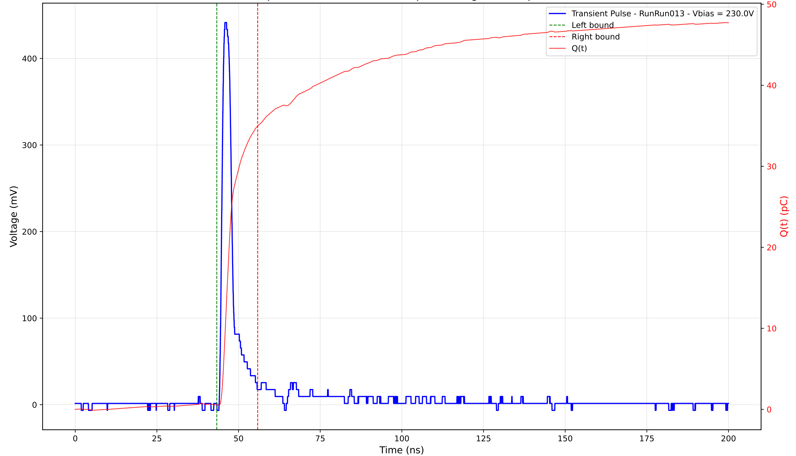
Transient Pulse - Sample: 4003 - Position: 265.0 \mu\text{m} - Charge: 34.40 pC - Rise Time: 1.11 ns
