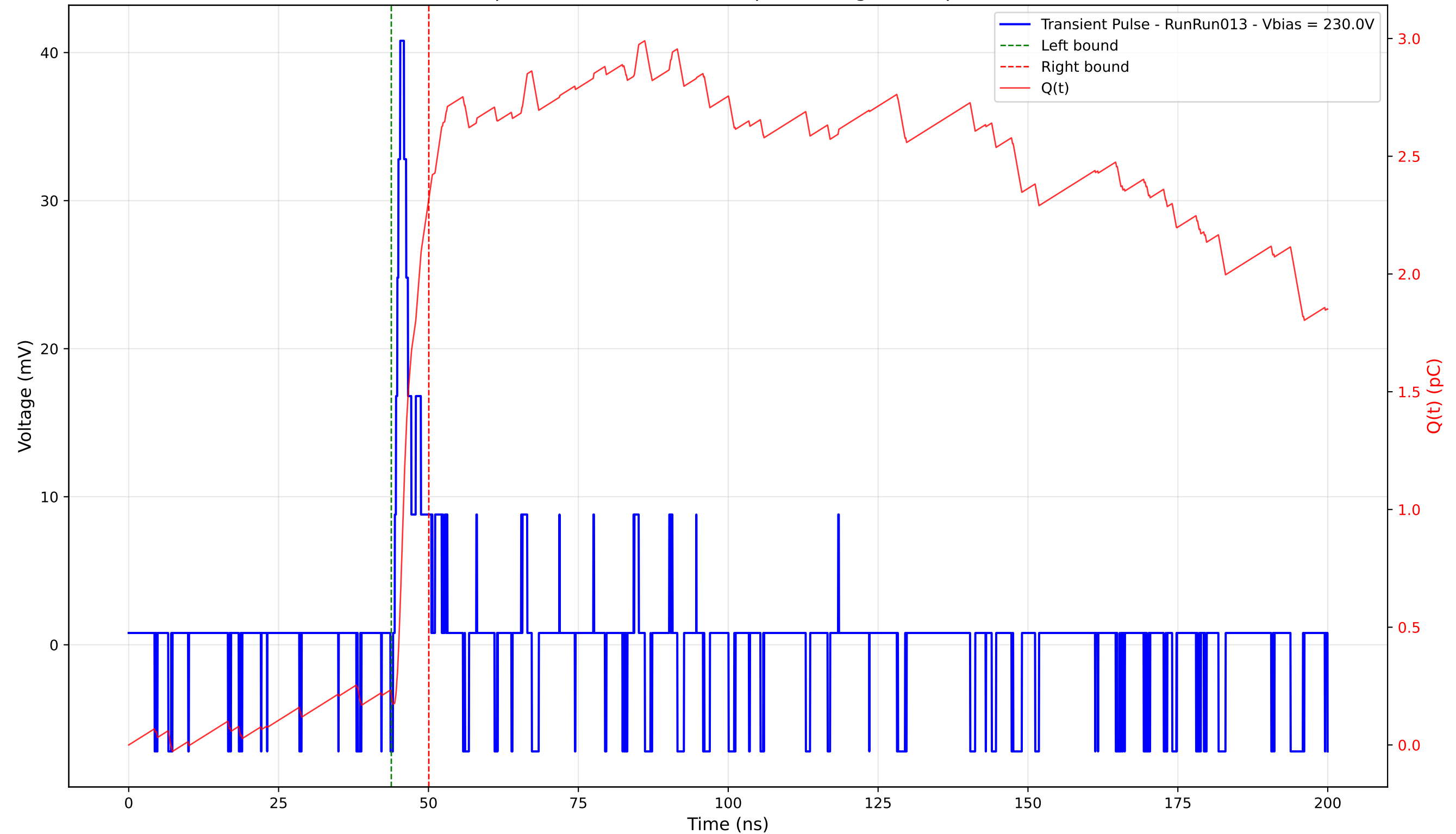
Transient Pulse - Sample: 4003 - Position: 80.0 \mu\text{m} - Charge: 2.11 pC - Rise Time: 0.91 ns
