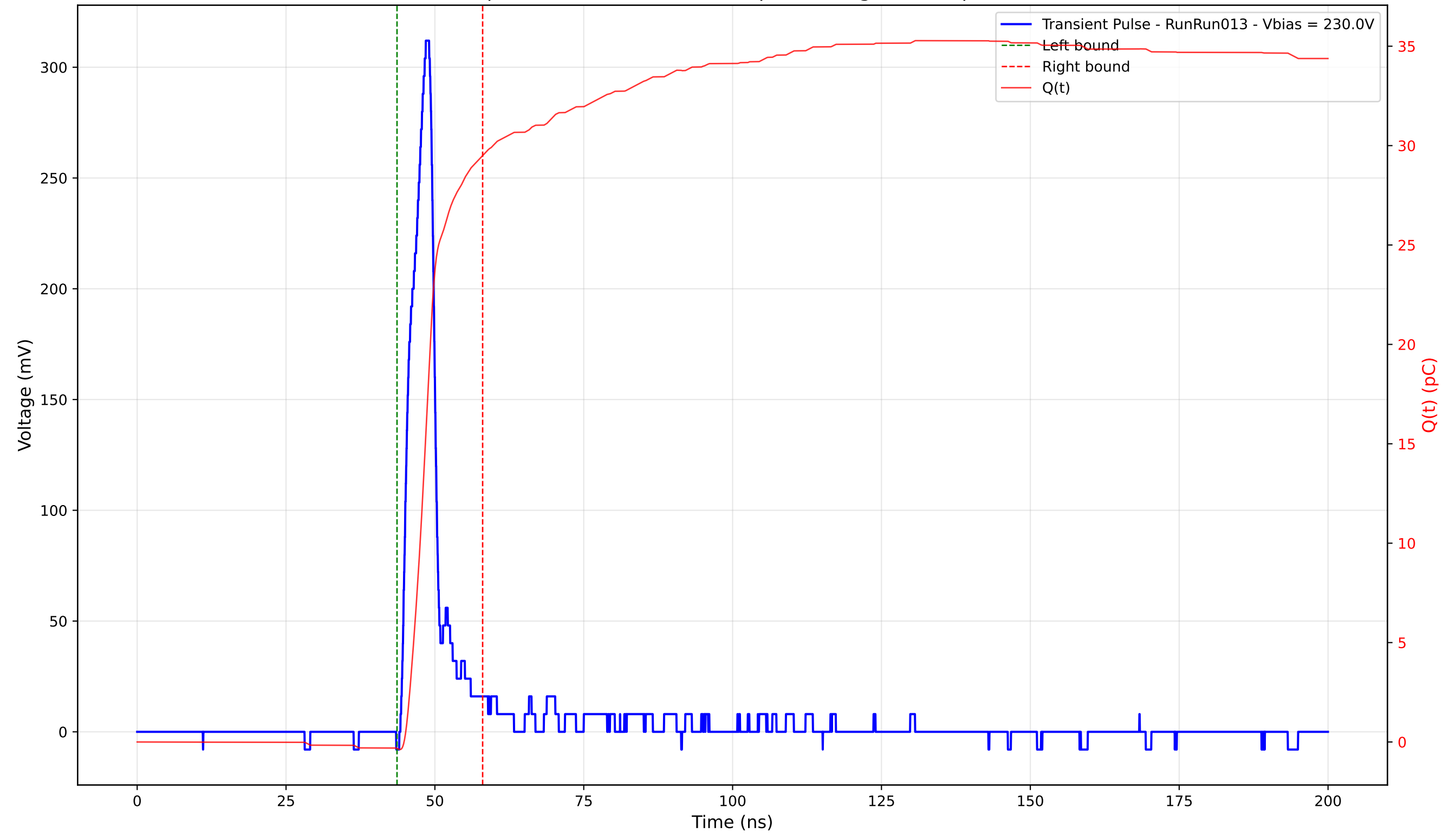
Transient Pulse - Sample: 4003 - Position: 340.0 \mu\text{m} - Charge: 29.83 pC - Rise Time: 3.42 ns
