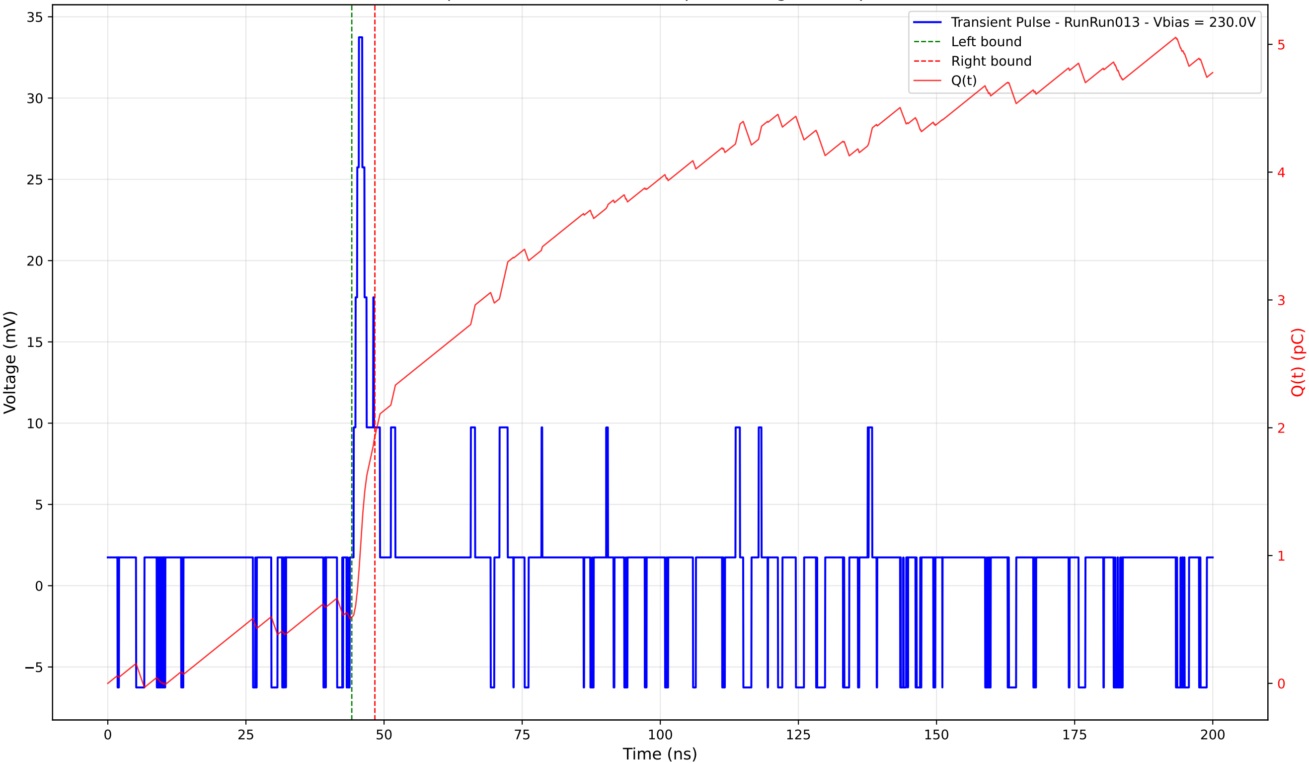
Transient Pulse - Sample: 4003 - Position: 35.0 \mu\text{m} - Charge: 1.41 pC - Rise Time: 0.96 ns
