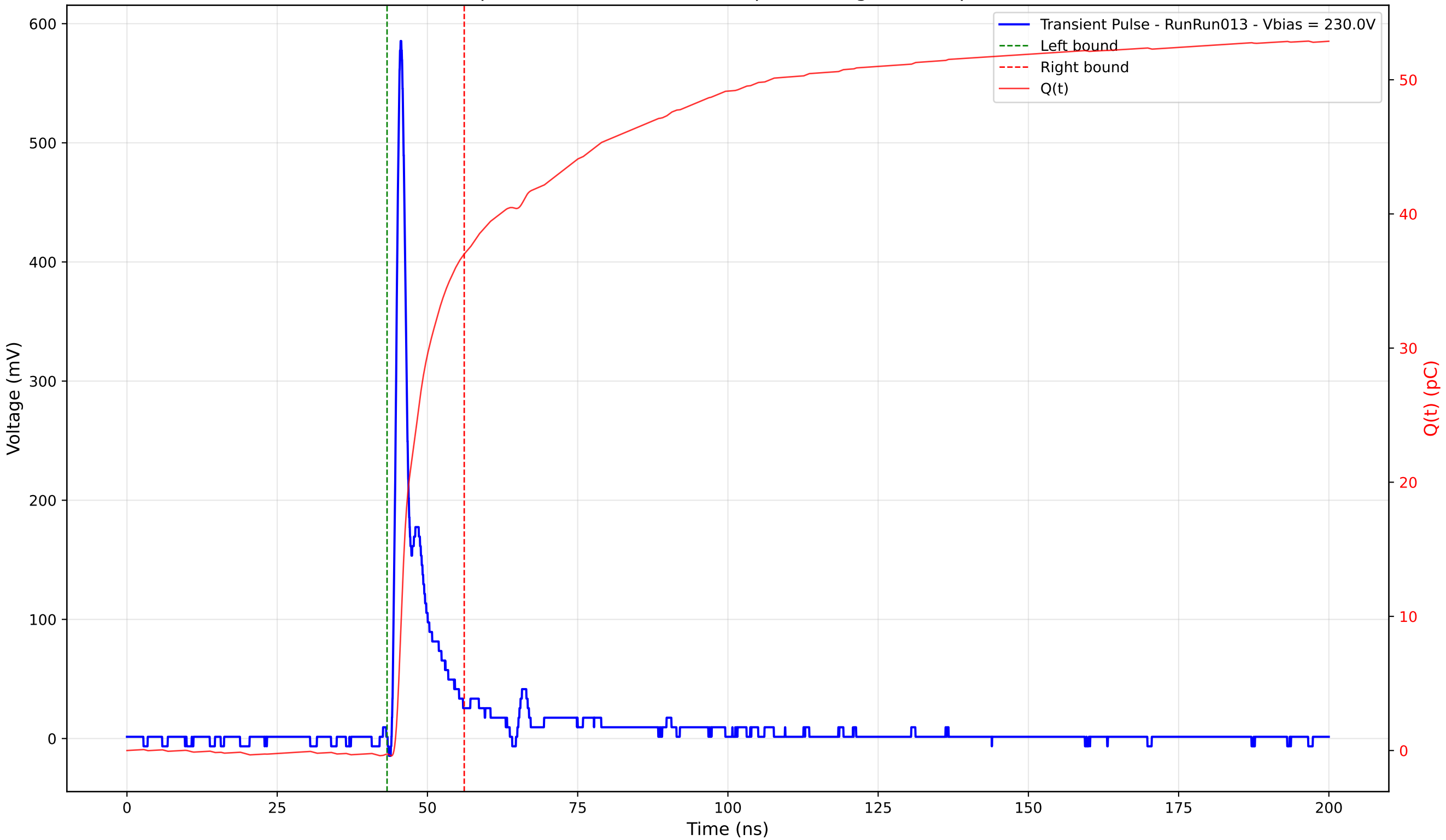
Transient Pulse - Sample: 4003 - Position: 160.0 \mu\text{m} - Charge: 37.27 pC - Rise Time: 0.97 ns
