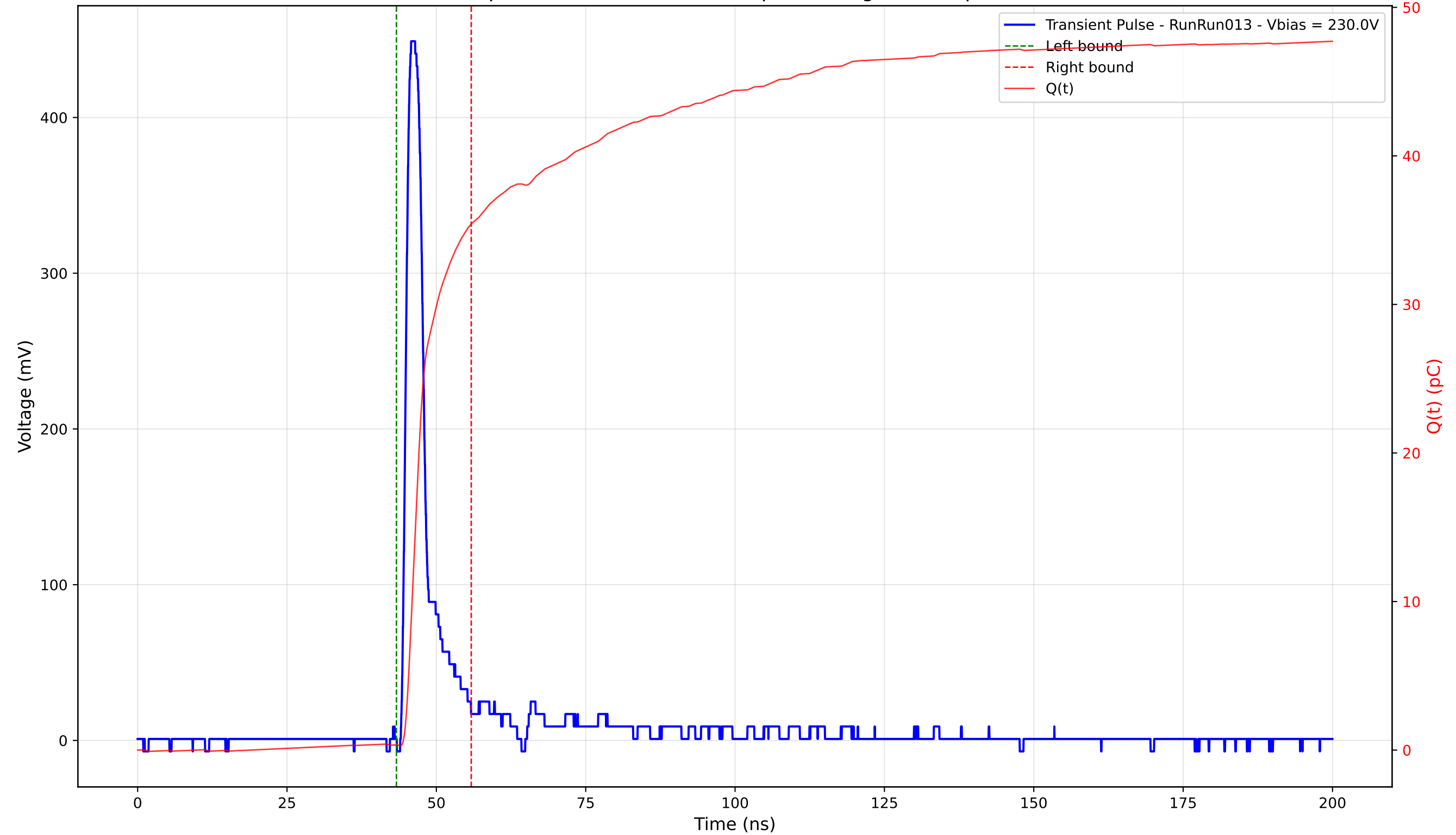
Transient Pulse - Sample: 4003 - Position: 260.0 \mu\text{m} - Charge: 35.06 pC - Rise Time: 1.13 ns
