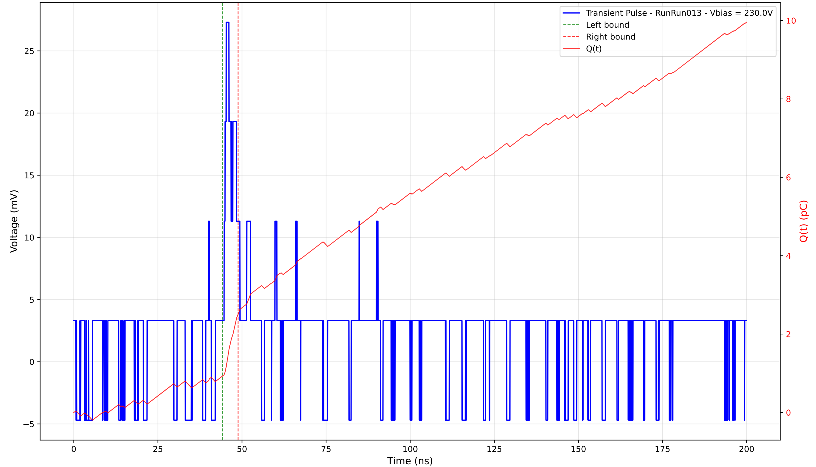
Transient Pulse - Sample: 4003 - Position: 415.0 \mu\text{m} - Charge: 1.57 pC - Rise Time: 0.00 ns (N/A)
