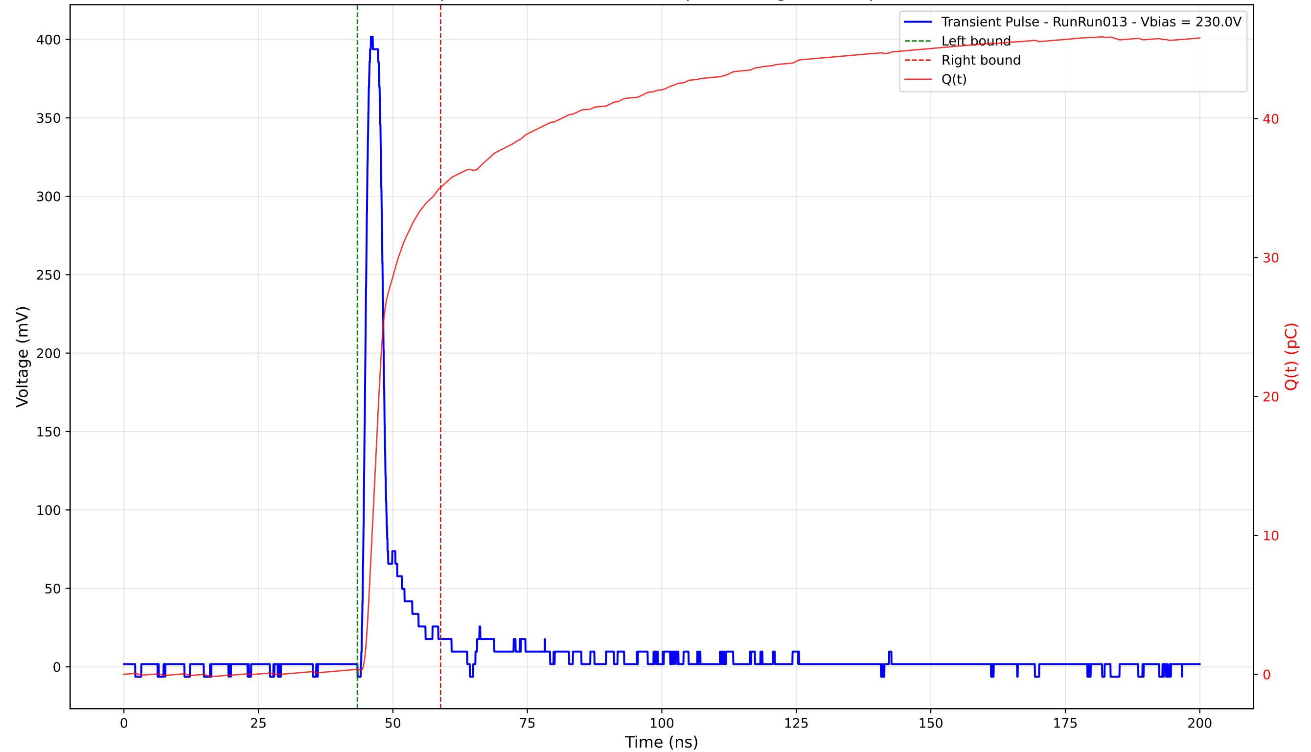
Transient Pulse - Sample: 4003 - Position: 280.0 \mu\text{m} - Charge: 34.68 pC - Rise Time: 1.14 ns
