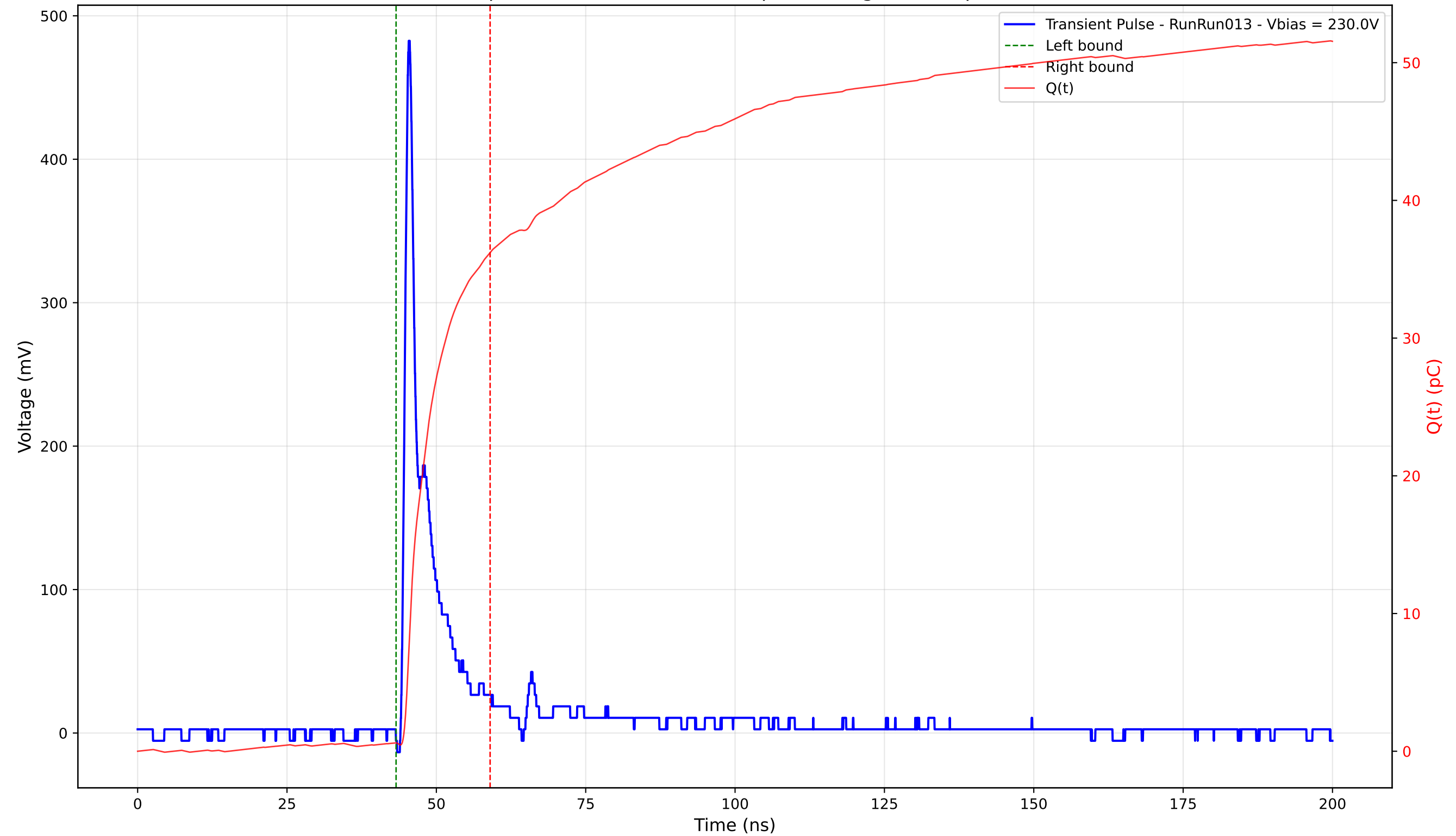
Transient Pulse - Sample: 4003 - Position: 115.0 \mu\text{m} - Charge: 35.60 pC - Rise Time: 0.89 ns
