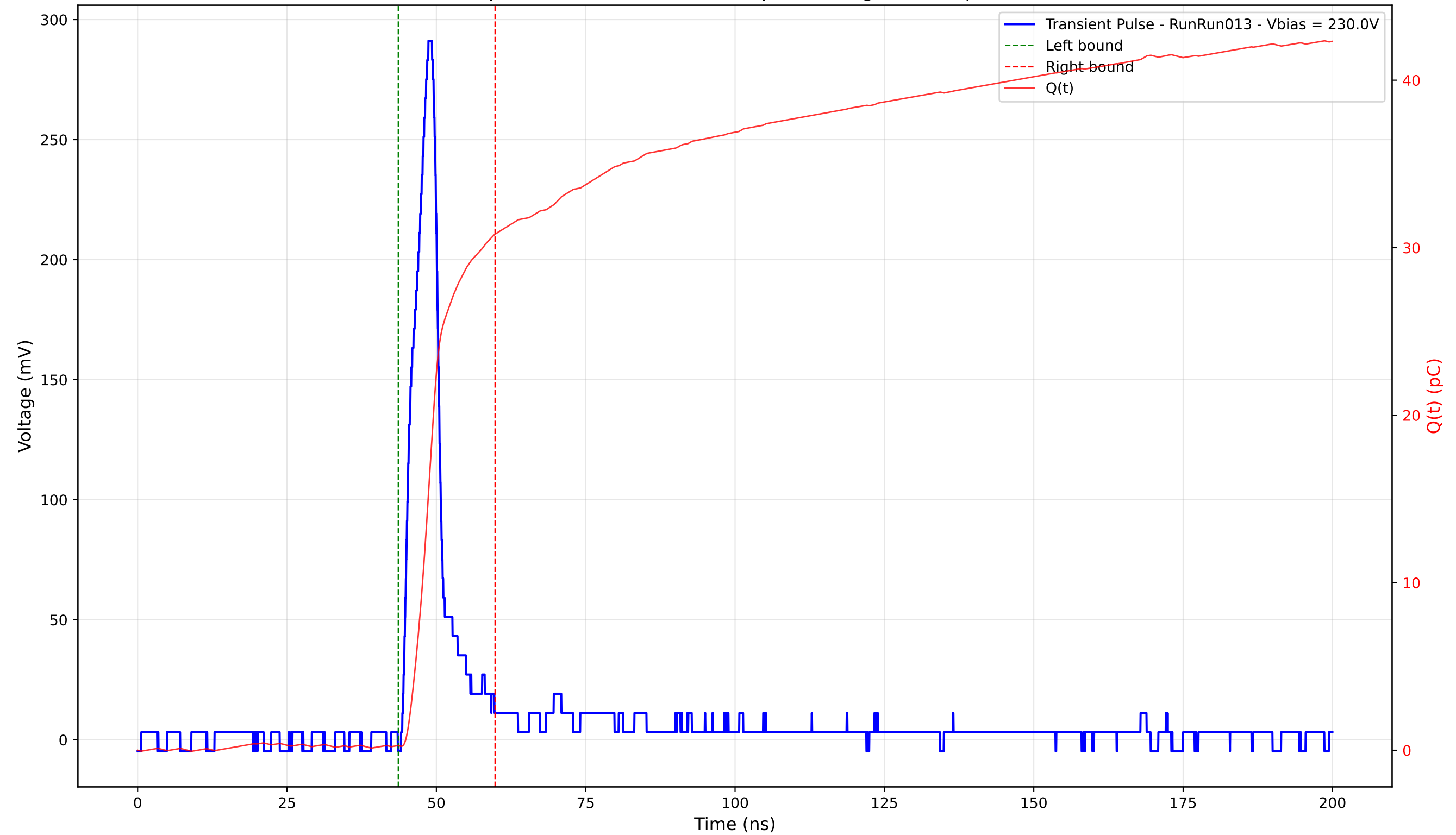
Transient Pulse - Sample: 4003 - Position: 345.0 \mu\text{m} - Charge: 30.54 pC - Rise Time: 3.54 ns
