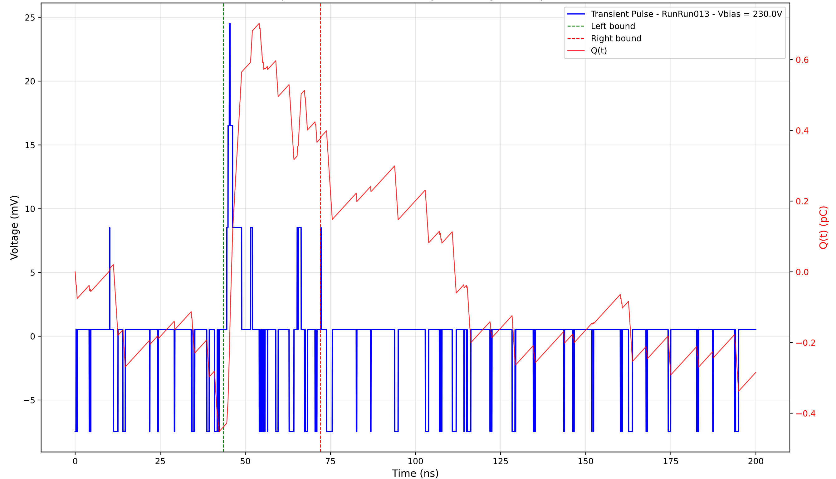
Transient Pulse - Sample: 4003 - Position: 15.0 \mu\text{m} - Charge: 0.82 pC - Rise Time: 0.76 ns
