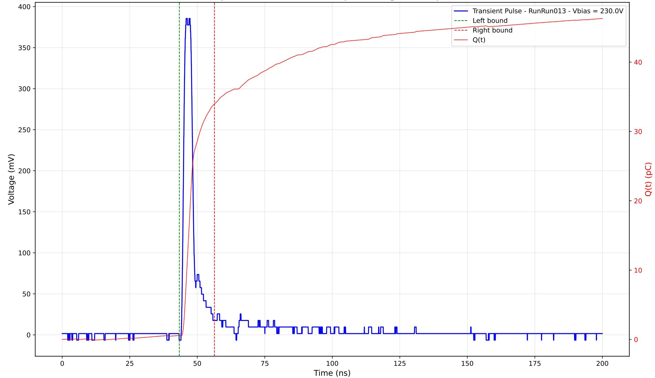
Transient Pulse - Sample: 4003 - Position: 285.0 \mu\text{m} - Charge: 33.40 pC - Rise Time: 1.17 ns
