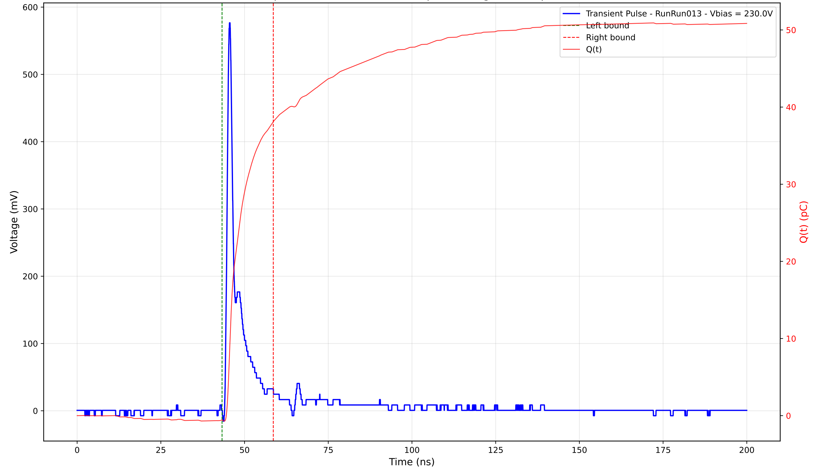
Transient Pulse - Sample: 4003 - Position: 155.0 \mu\text{m} - Charge: 38.69 pC - Rise Time: 0.94 ns
