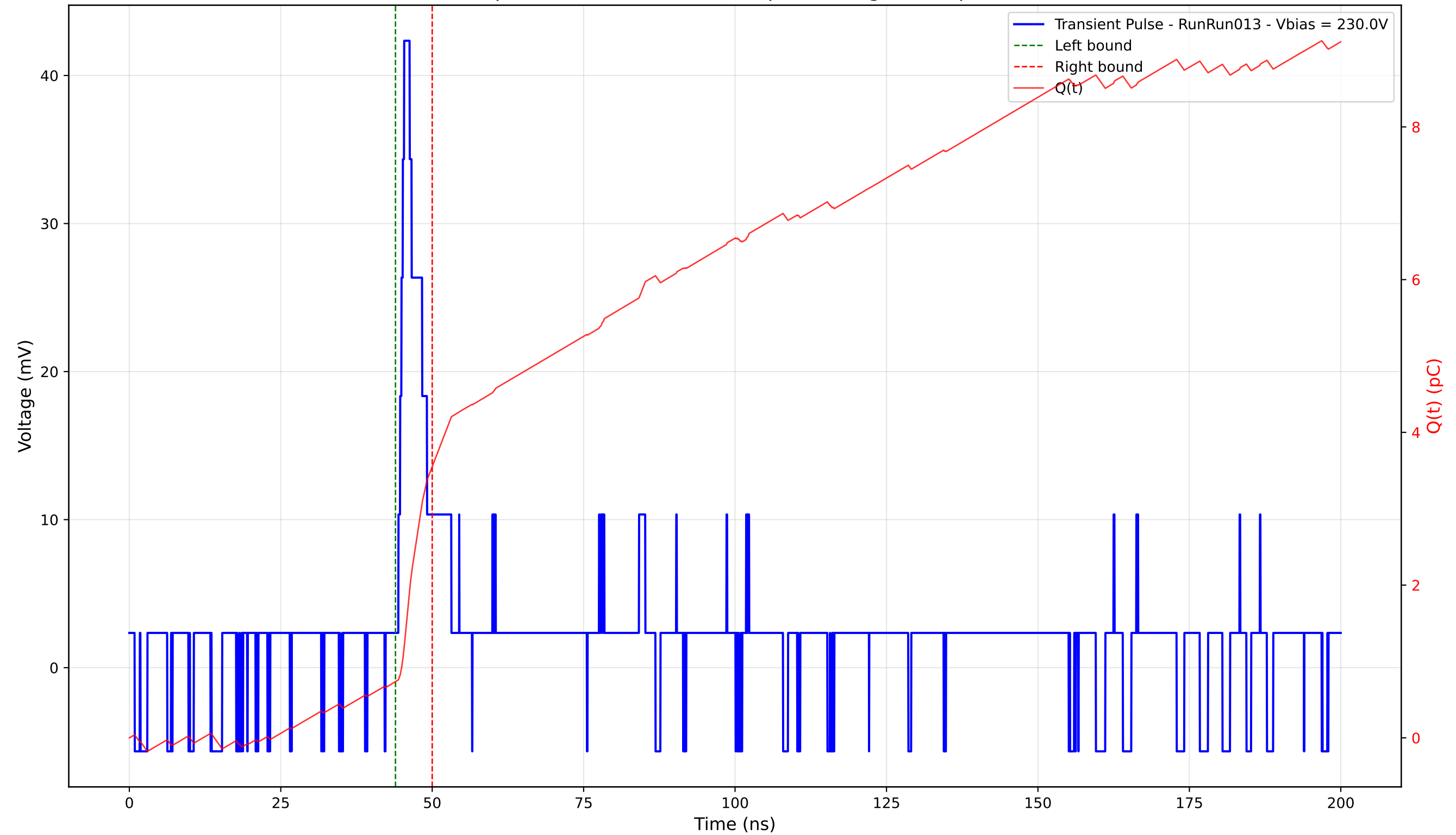
Transient Pulse - Sample: 4003 - Position: 410.0 \mu\text{m} - Charge: 2.82 pC - Rise Time: 0.96 ns
