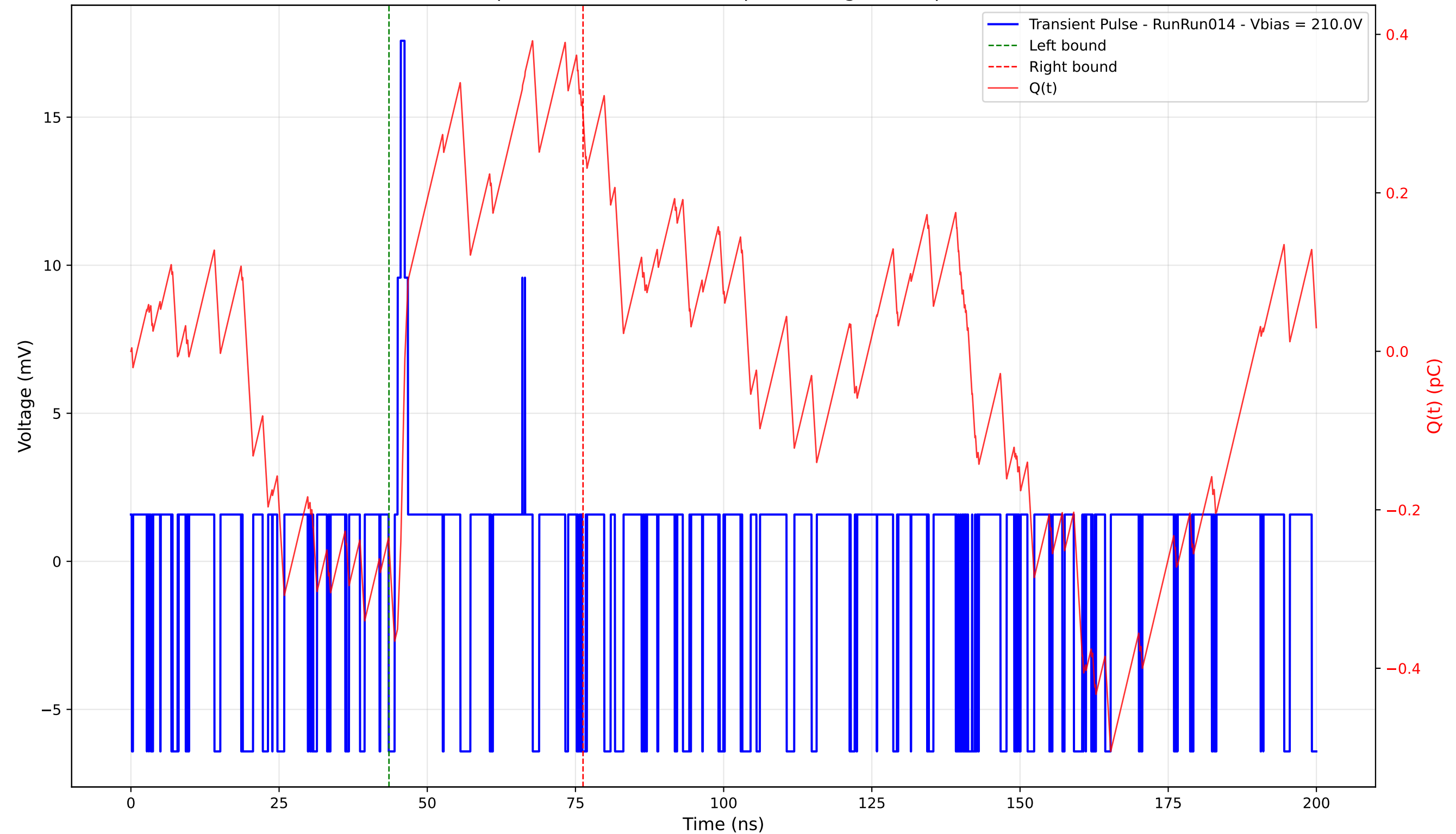
Transient Pulse - Sample: 4003 - Position: 5.0 \mu\text{m} - Charge: 0.54 pC - Rise Time: 0.54 ns
