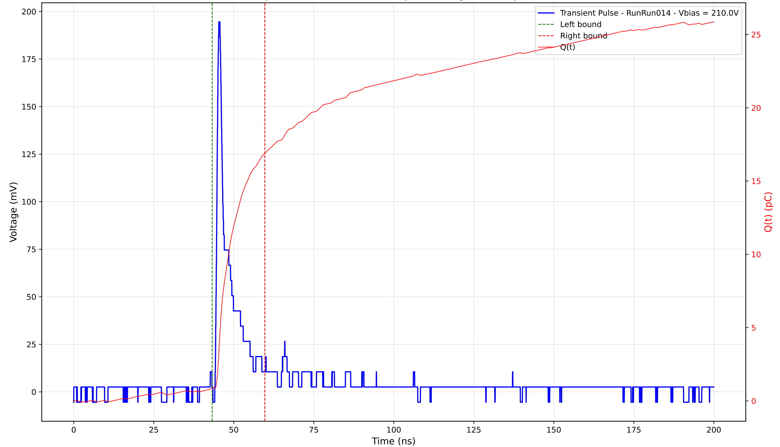
Transient Pulse - Sample: 4003 - Position: 95.0 \mu\text{m} - Charge: 15.97 pC - Rise Time: 0.84 ns
