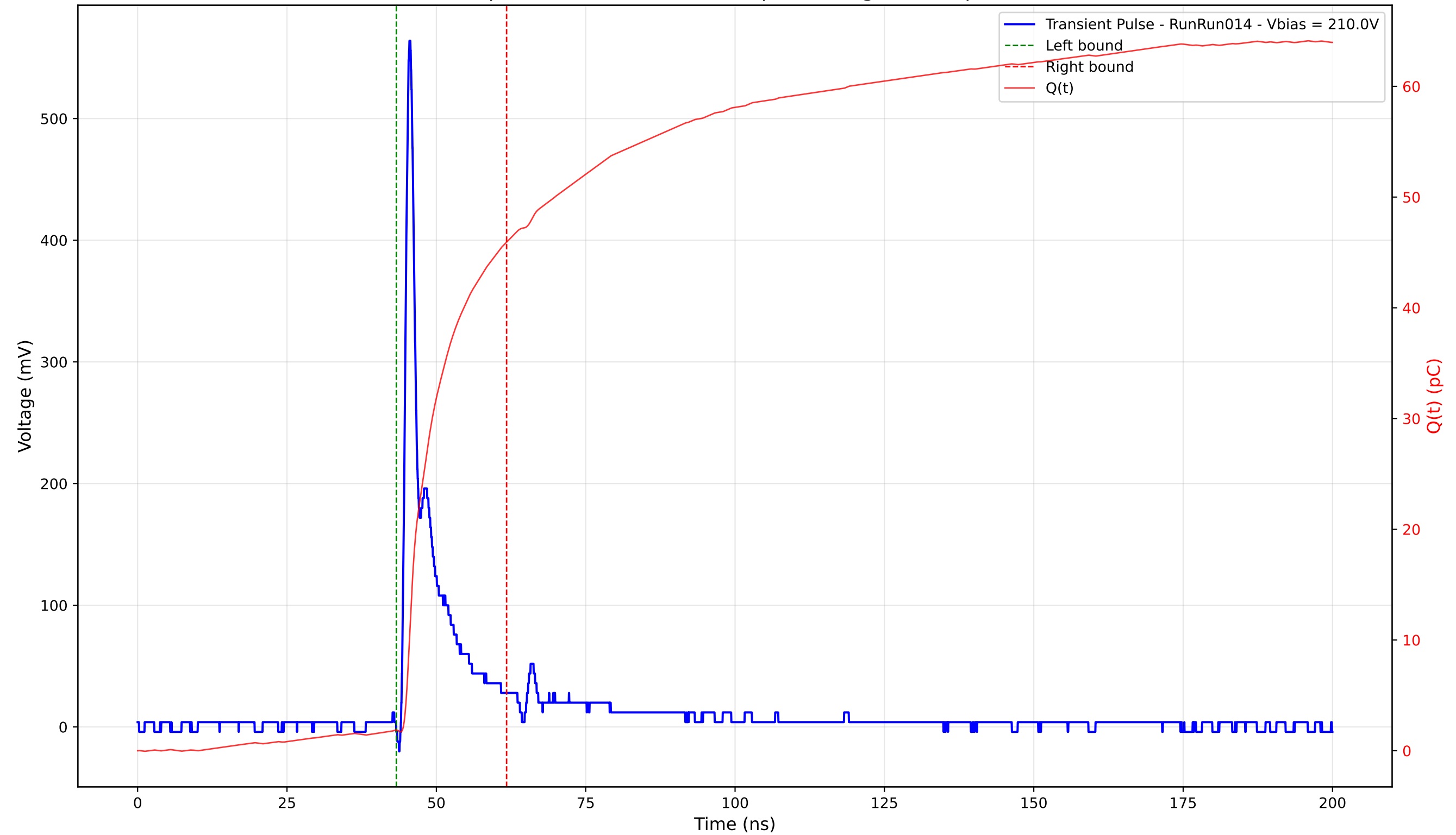
Transient Pulse - Sample: 4003 - Position: 150.0 \mu\text{m} - Charge: 44.07 pC - Rise Time: 0.93 ns
