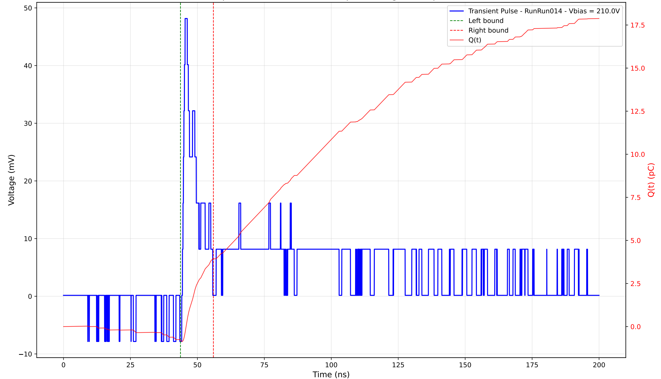
Transient Pulse - Sample: 4003 - Position: 370.0 \mu\text{m} - Charge: 4.72 pC - Rise Time: 0.99 ns
