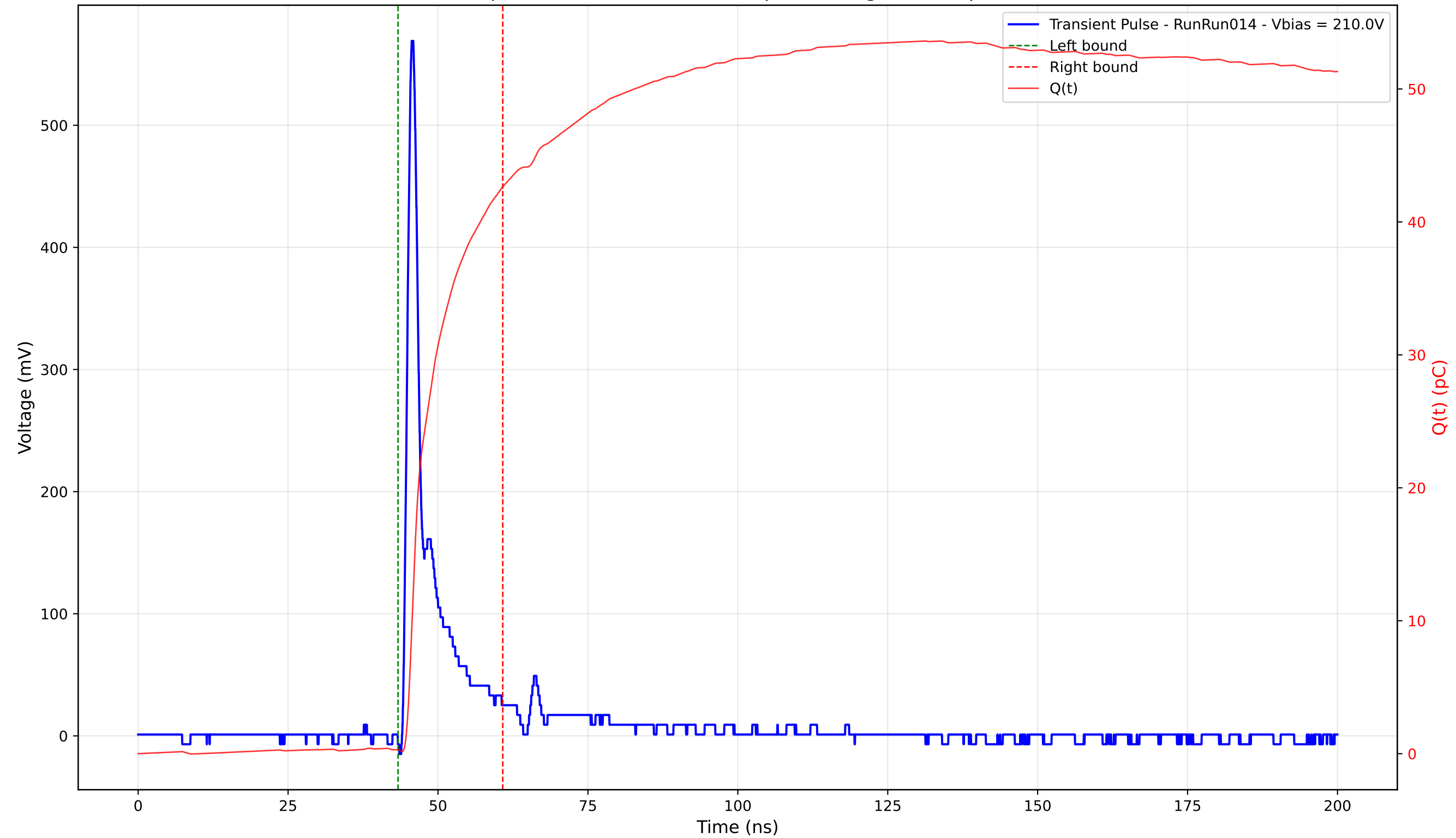
Transient Pulse - Sample: 4003 - Position: 190.0 \mu\text{m} - Charge: 42.34 pC - Rise Time: 1.06 ns
