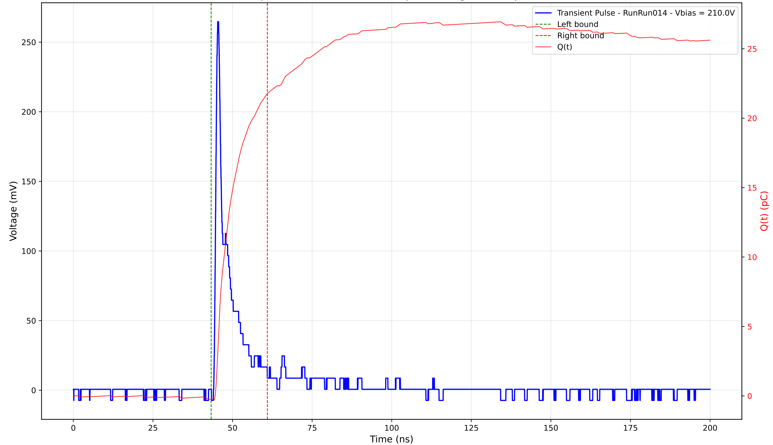
Transient Pulse - Sample: 4003 - Position: 100.0 \mu\text{m} - Charge: 22.02 pC - Rise Time: 0.84 ns
