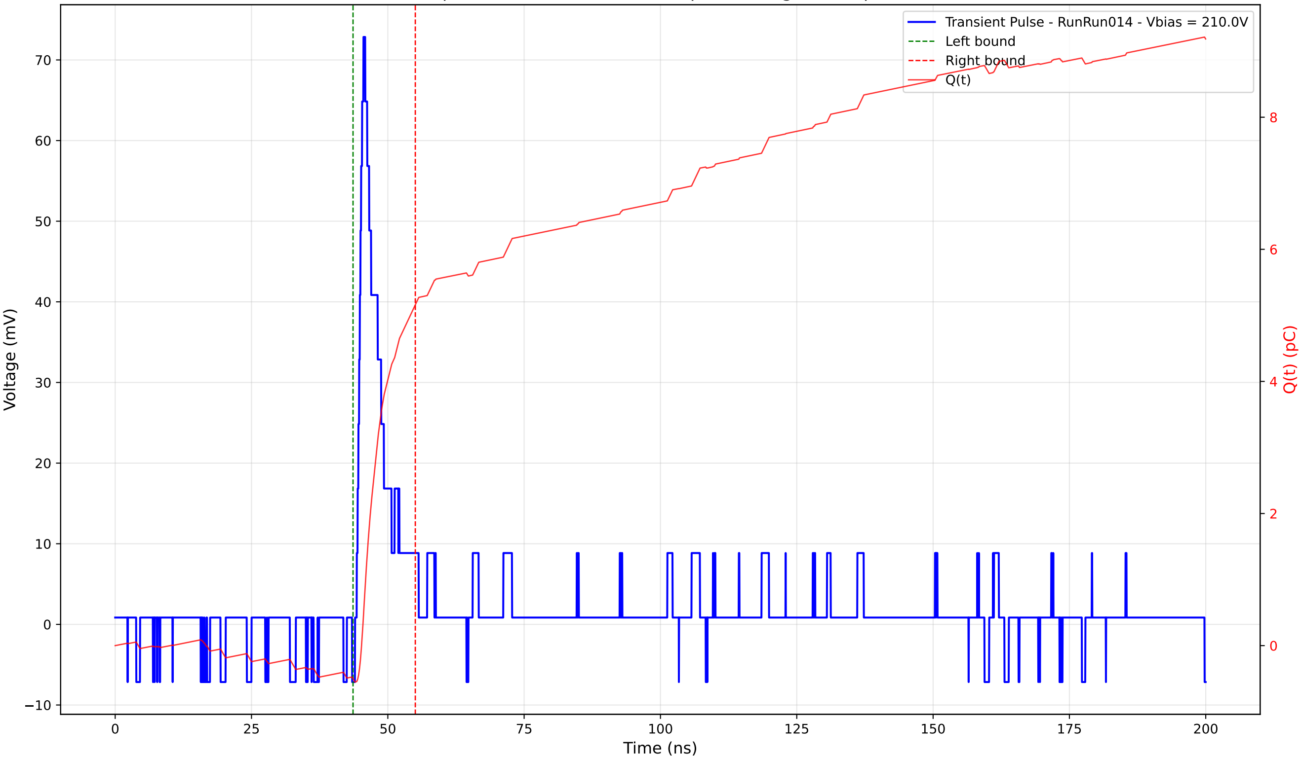
Transient Pulse - Sample: 4003 - Position: 395.0 \mu\text{m} - Charge: 5.67 pC - Rise Time: 1.22 ns
