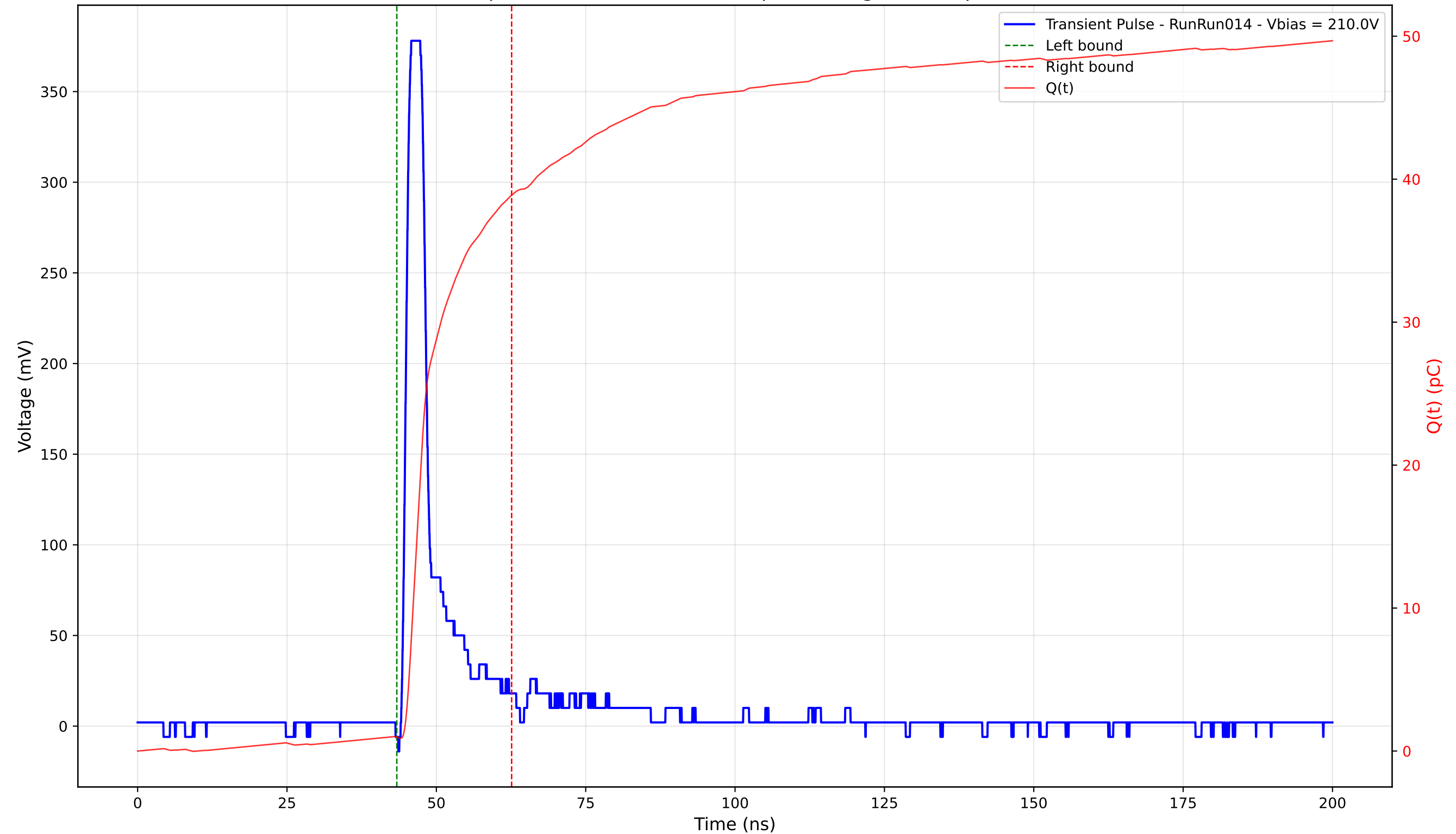
Transient Pulse - Sample: 4003 - Position: 275.0 \mu\text{m} - Charge: 37.88 pC - Rise Time: 1.15 ns
