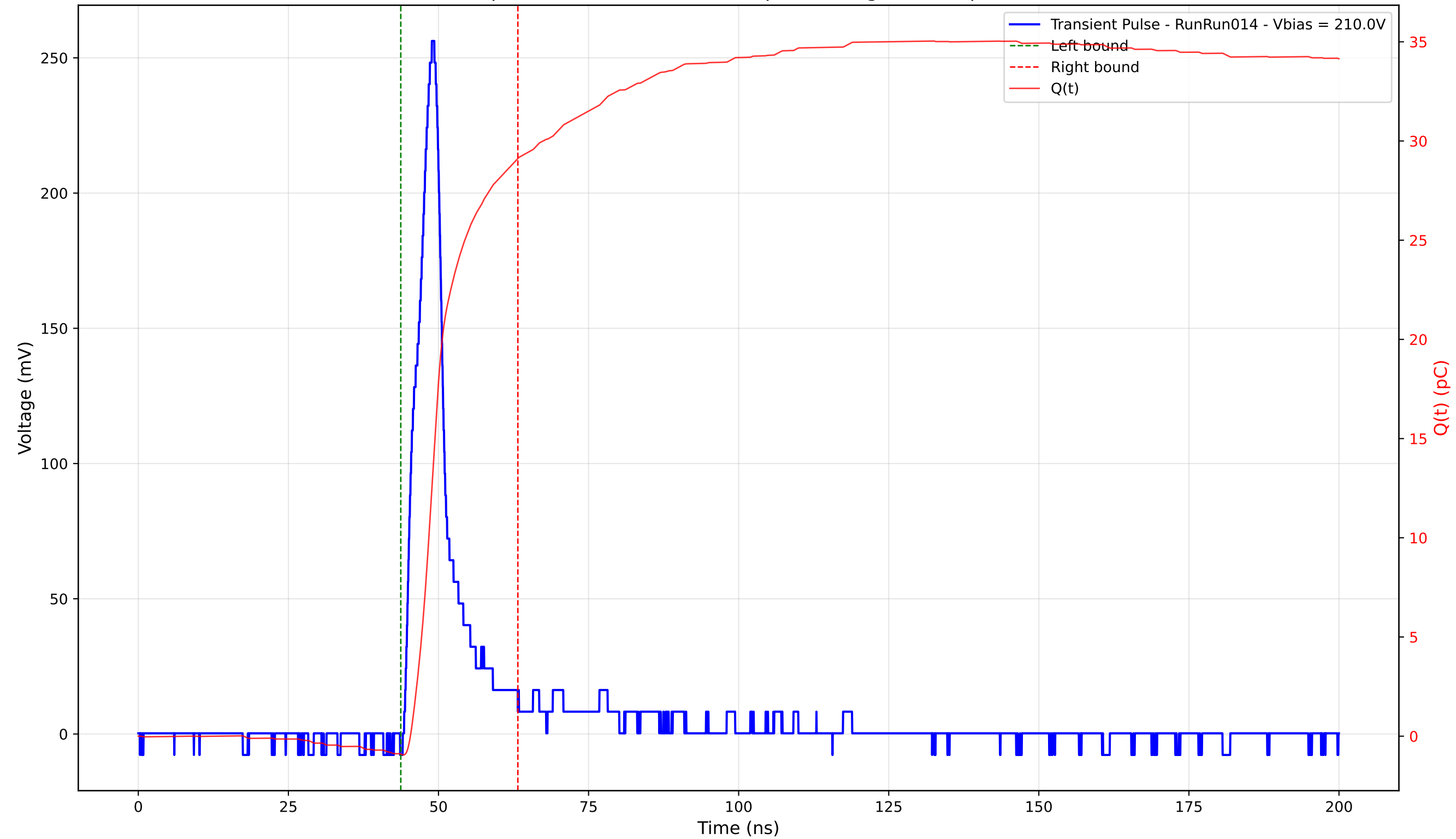
Transient Pulse - Sample: 4003 - Position: 335.0 \mu\text{m} - Charge: 30.02 pC - Rise Time: 3.56 ns
