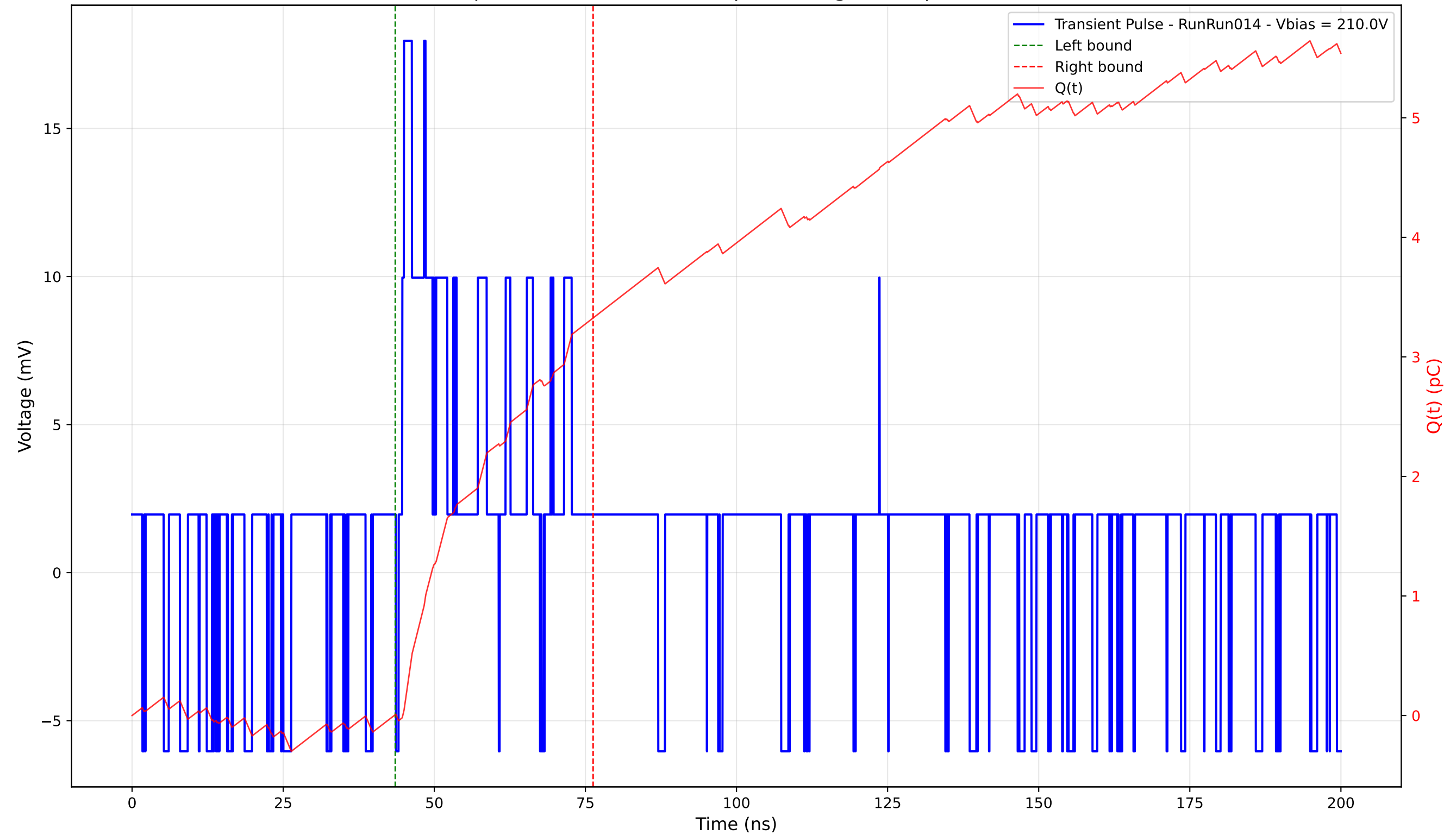
Transient Pulse - Sample: 4003 - Position: 65.0 \mu\text{m} - Charge: 3.32 pC - Rise Time: 0.00 ns (N/A)
