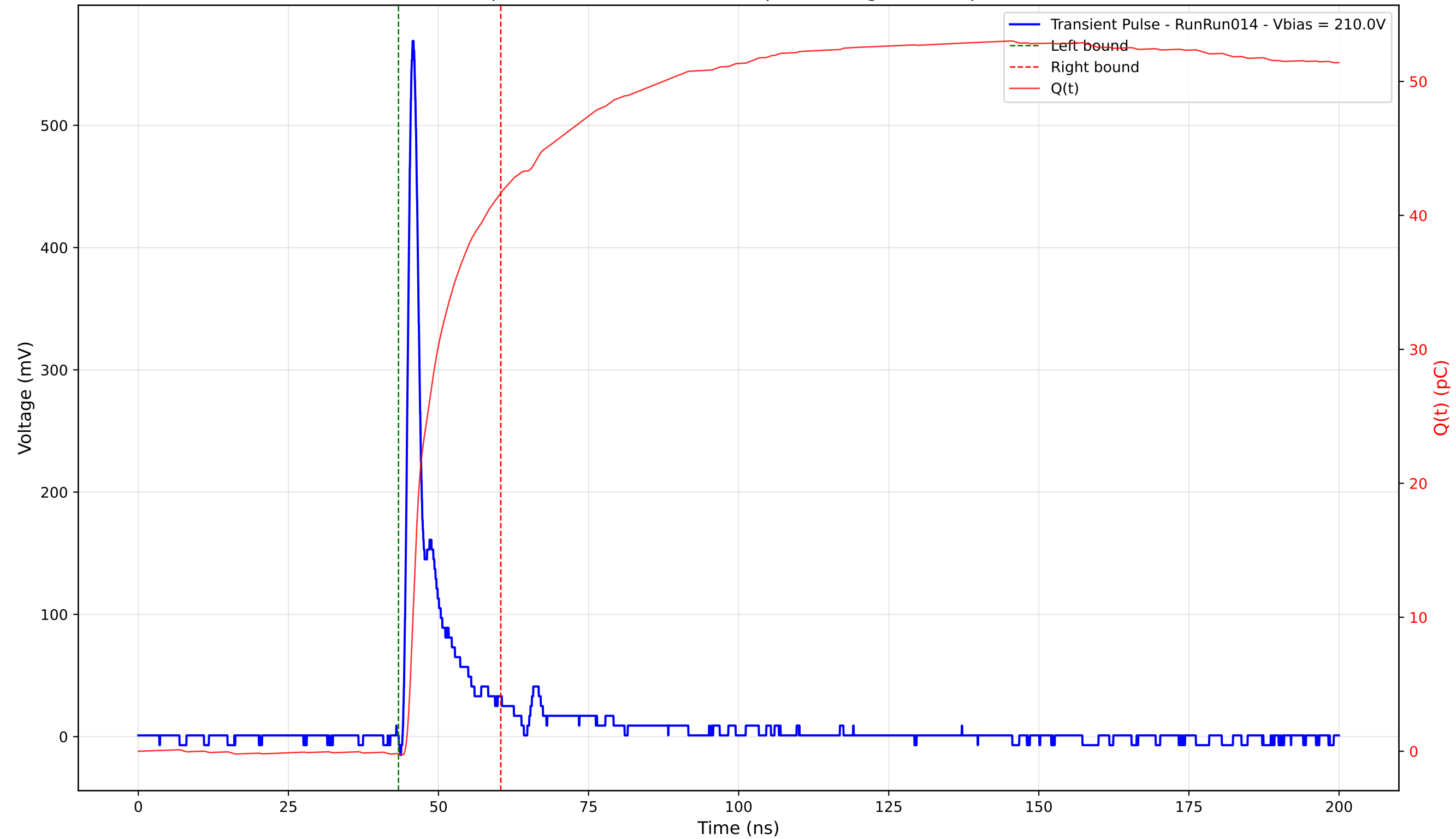
Transient Pulse - Sample: 4003 - Position: 195.0 \mu\text{m} - Charge: 41.85 pC - Rise Time: 1.08 ns
