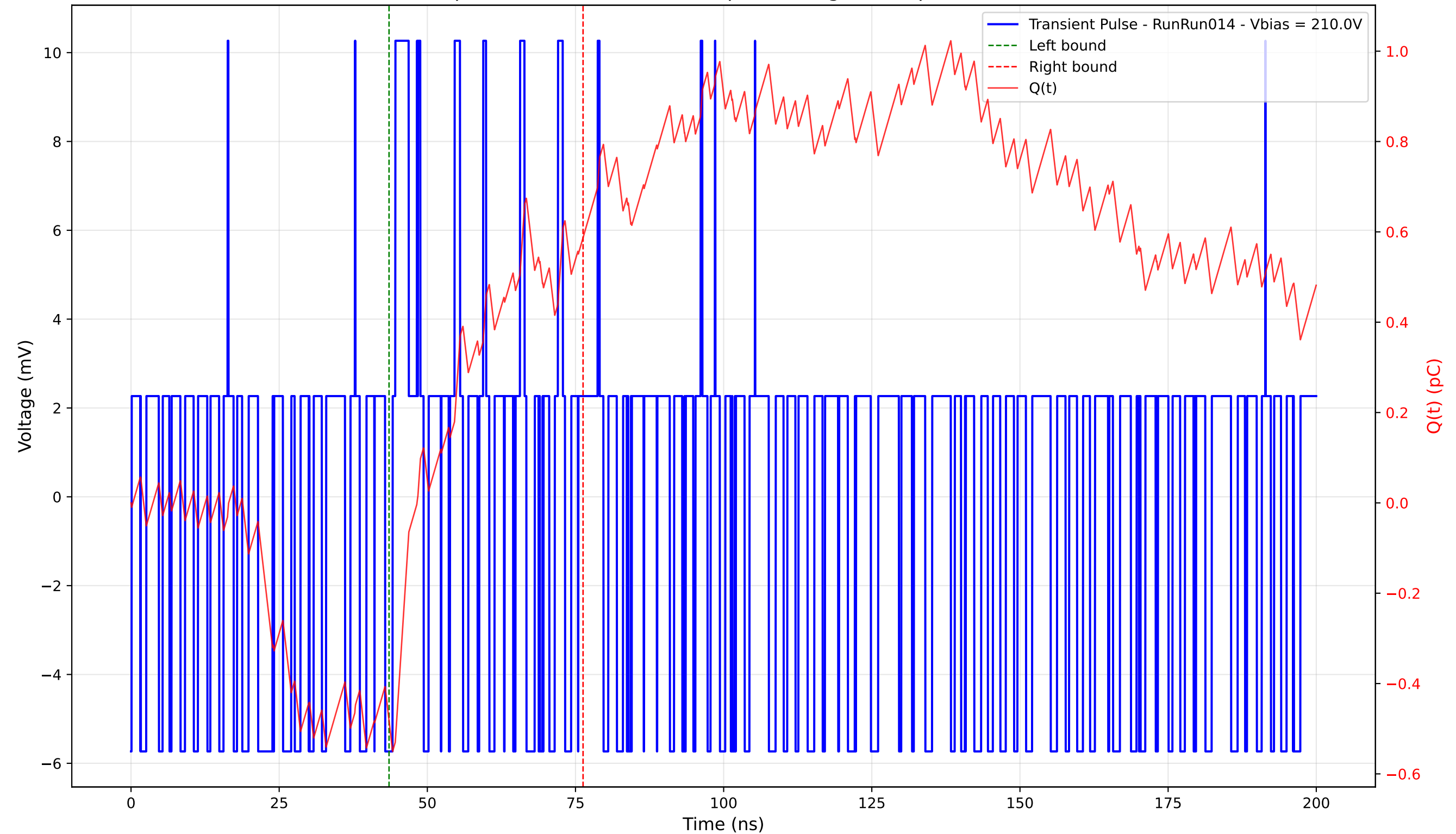
Transient Pulse - Sample: 4003 - Position: 425.0 \mu\text{m} - Charge: 1.07 pC - Rise Time: 0.00 ns (N/A)
