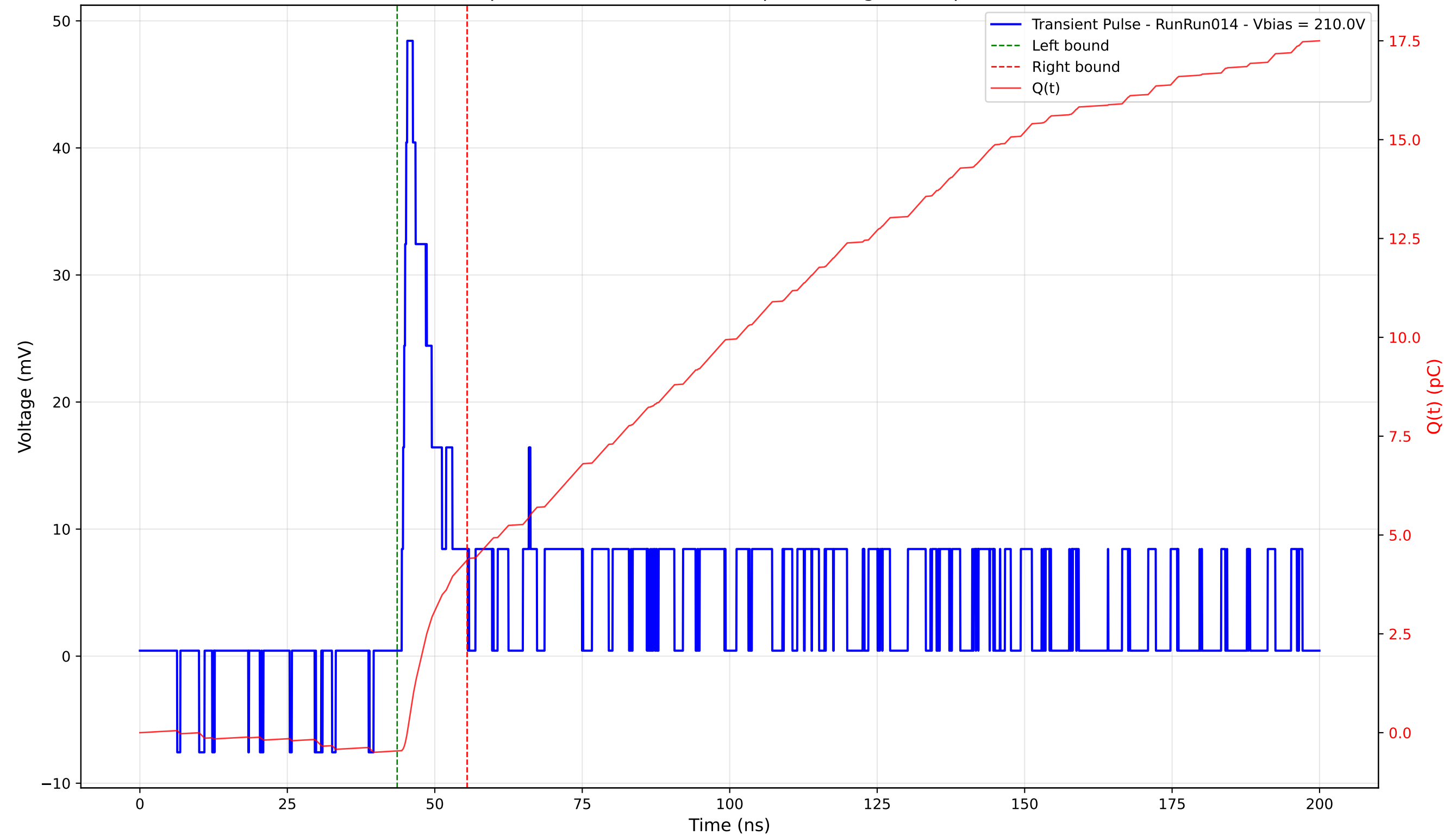
Transient Pulse - Sample: 4003 - Position: 375.0 \mu\text{m} - Charge: 4.83 pC - Rise Time: 0.93 ns
