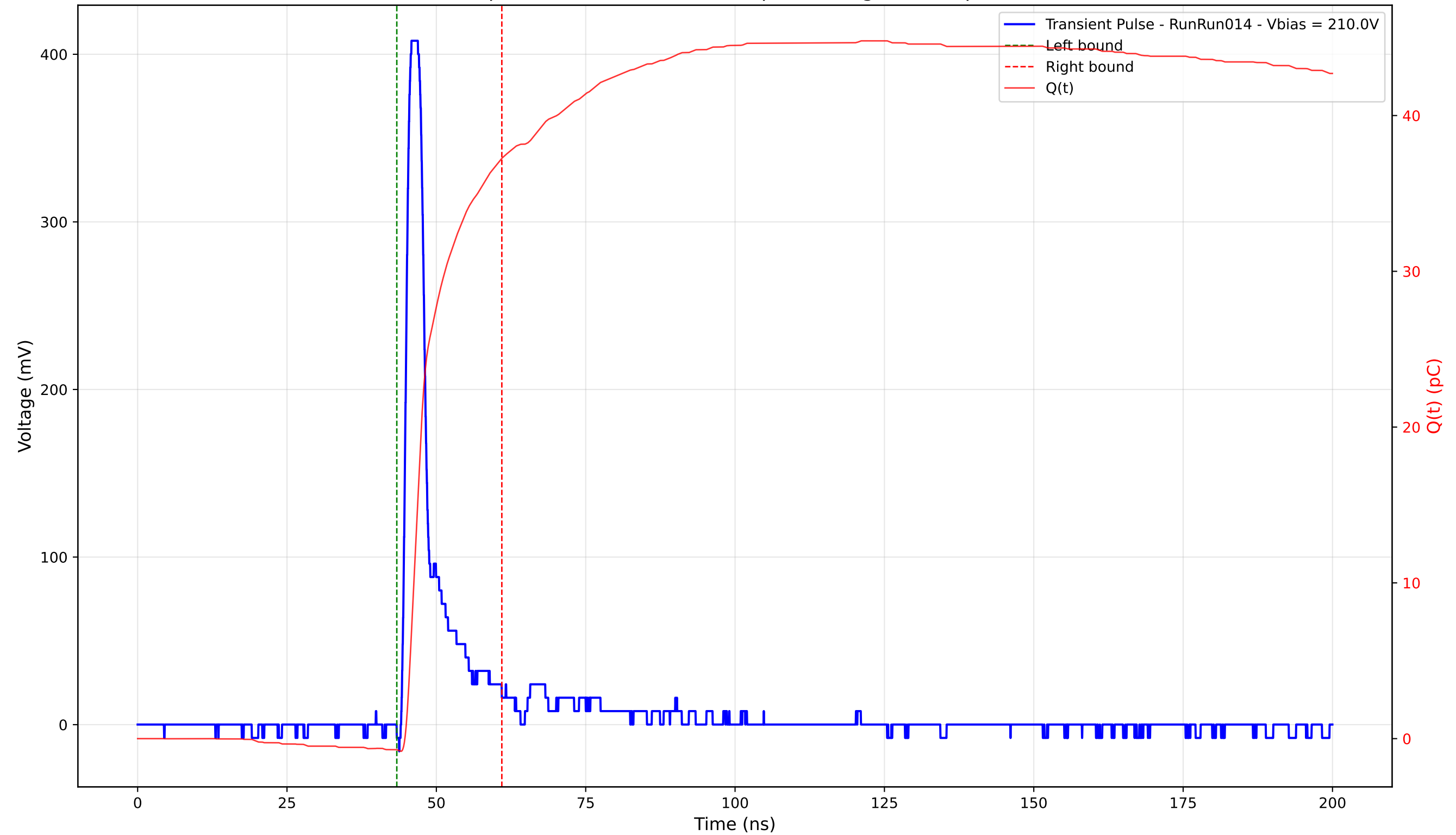
Transient Pulse - Sample: 4003 - Position: 265.0 \mu\text{m} - Charge: 37.97 pC - Rise Time: 1.12 ns
