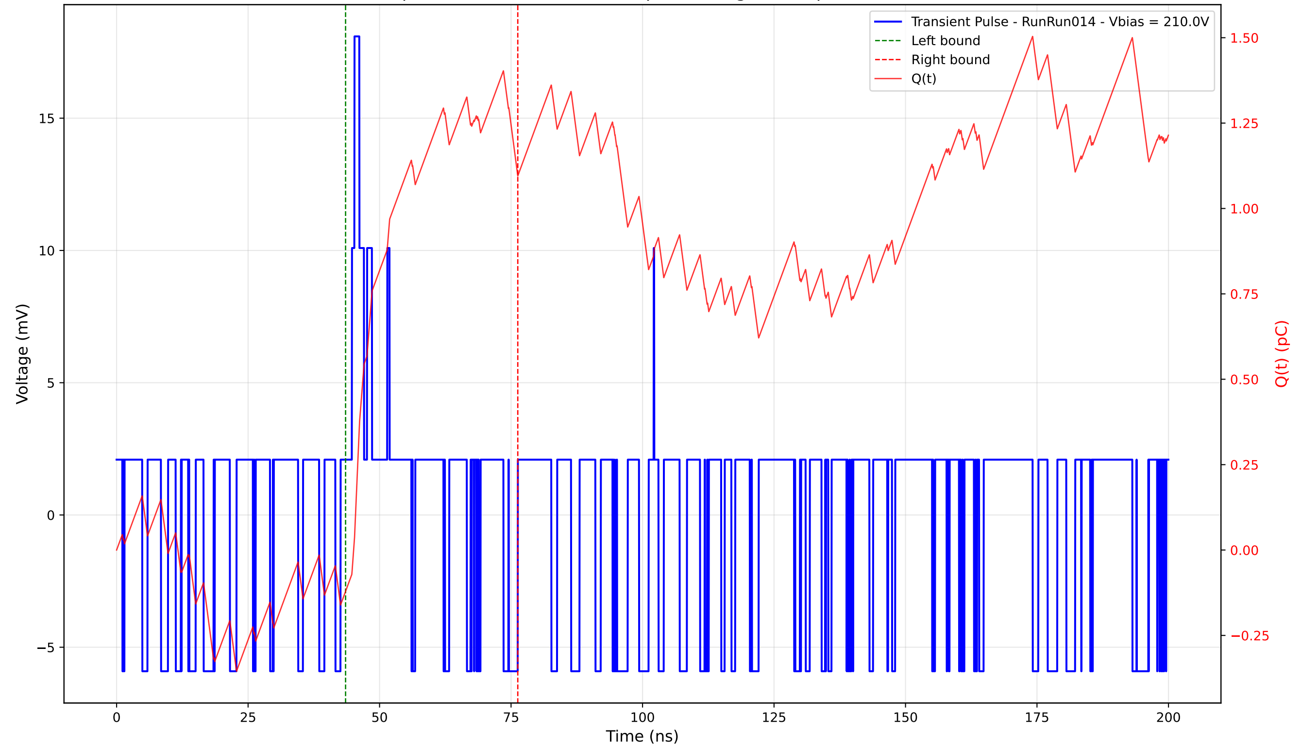
Transient Pulse - Sample: 4003 - Position: 420.0 \mu\text{m} - Charge: 1.22 pC - Rise Time: 0.00 ns (N/A)
