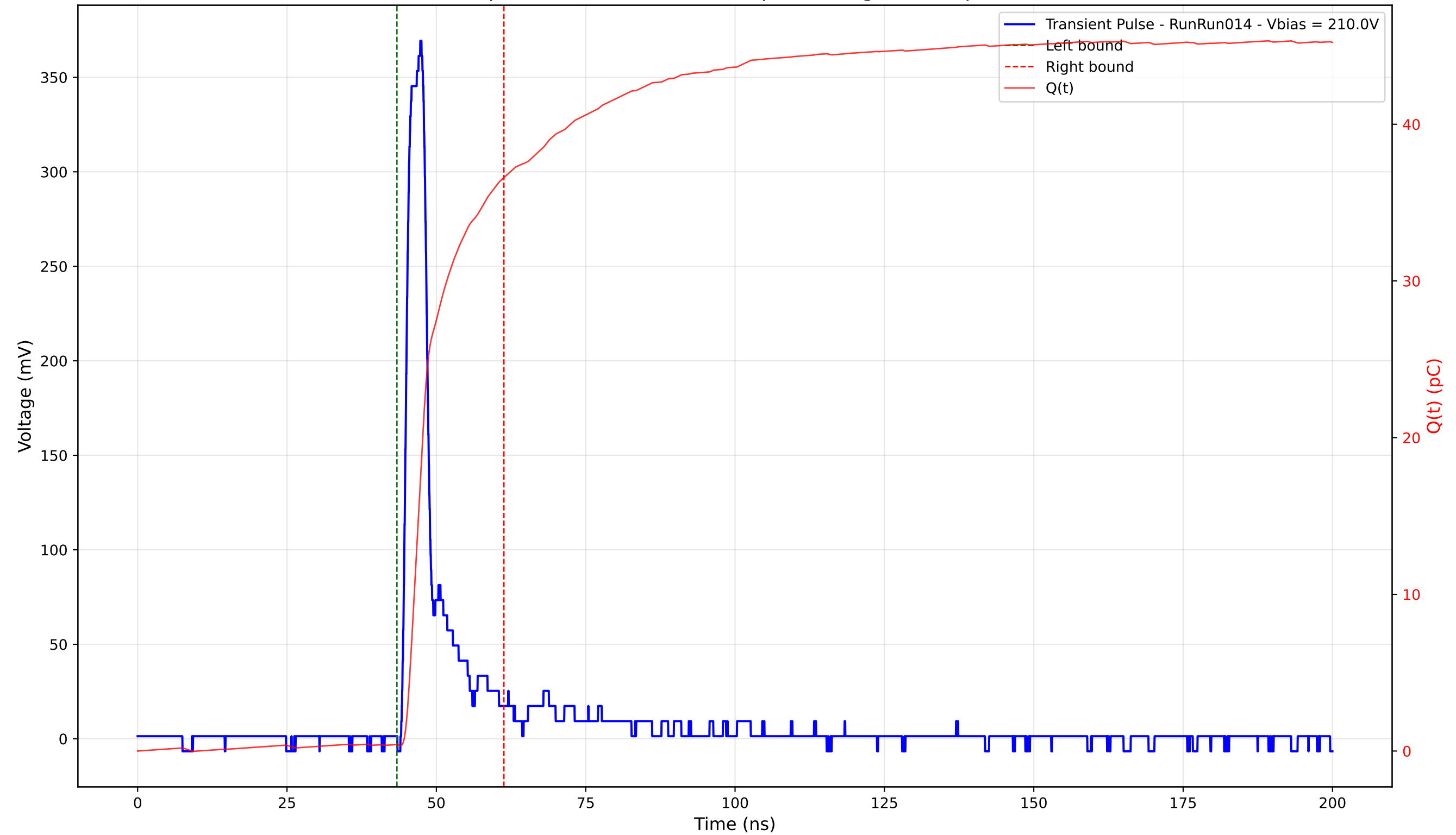
Transient Pulse - Sample: 4003 - Position: 285.0 \mu\text{m} - Charge: 36.18 pC - Rise Time: 1.37 ns
