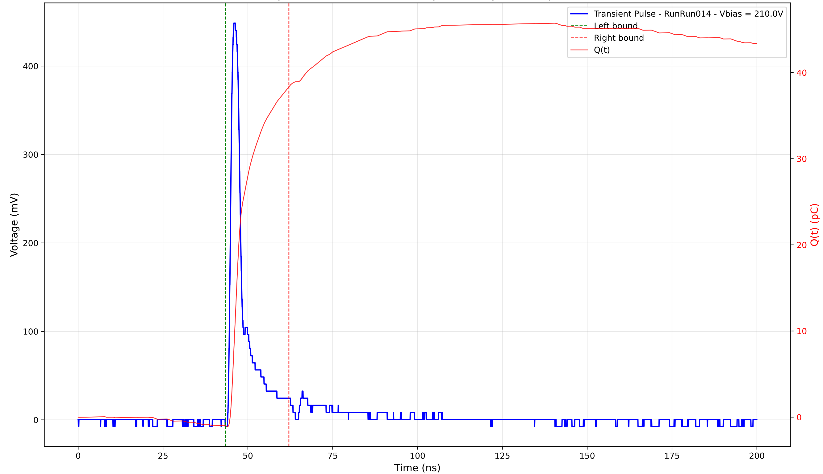
Transient Pulse - Sample: 4003 - Position: 250.0 \mu\text{m} - Charge: 39.35 pC - Rise Time: 1.15 ns
