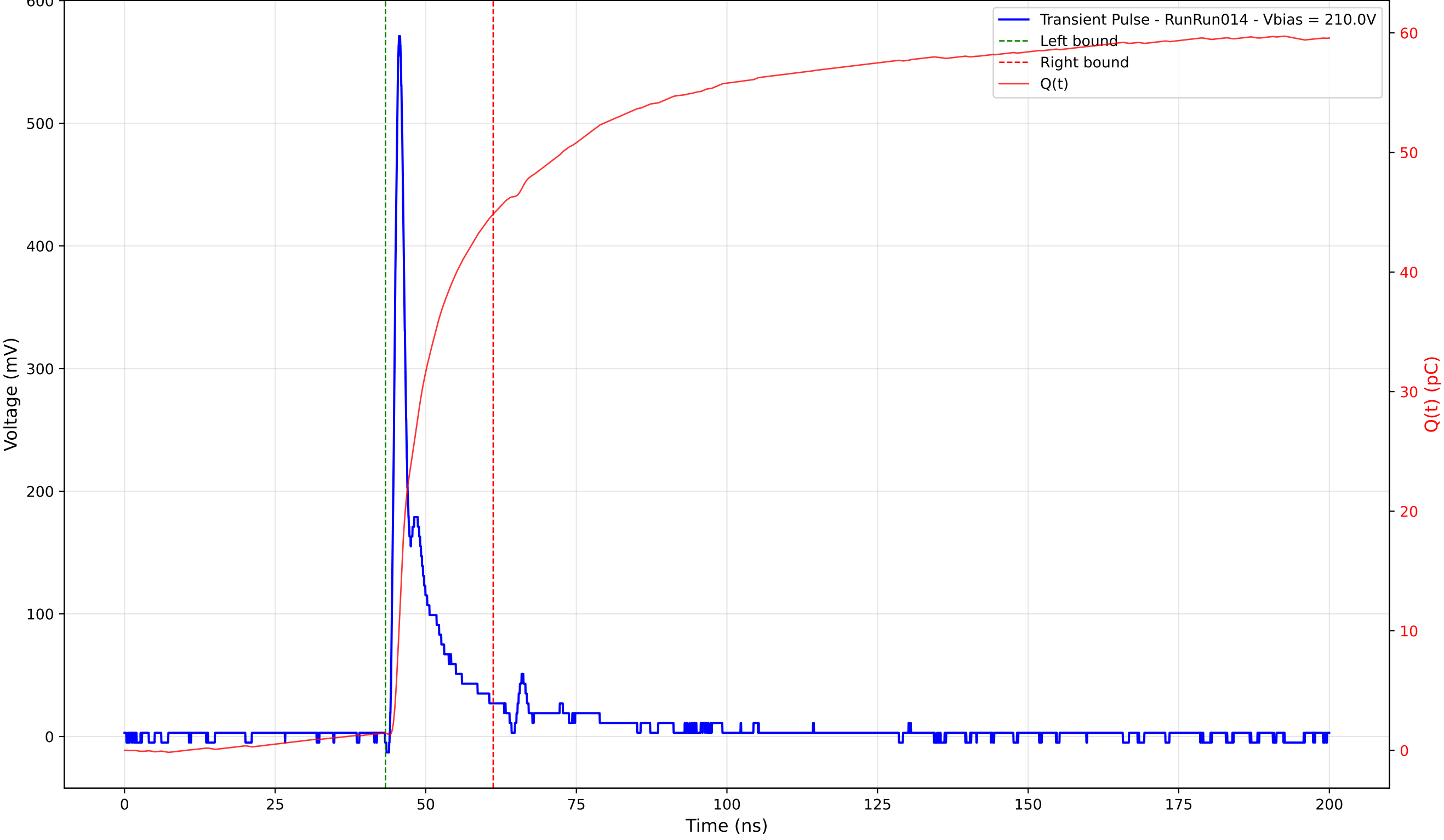
Transient Pulse - Sample: 4003 - Position: 170.0 \mu\text{m} - Charge: 43.40 pC - Rise Time: 1.00 ns
