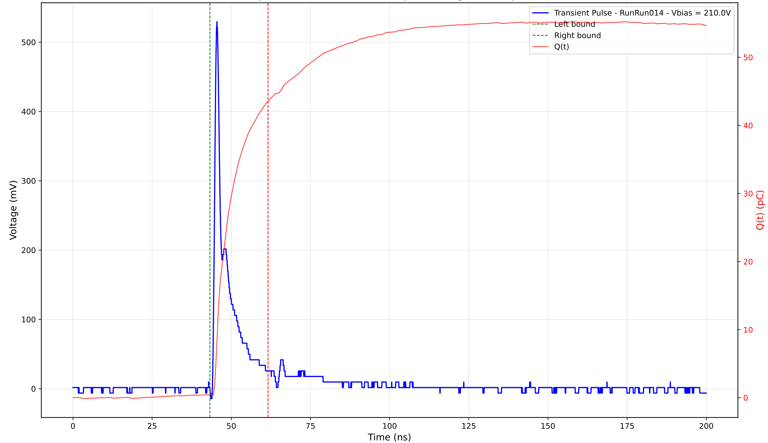
Transient Pulse - Sample: 4003 - Position: 125.0 \mu\text{m} - Charge: 43.08 pC - Rise Time: 0.92 ns
