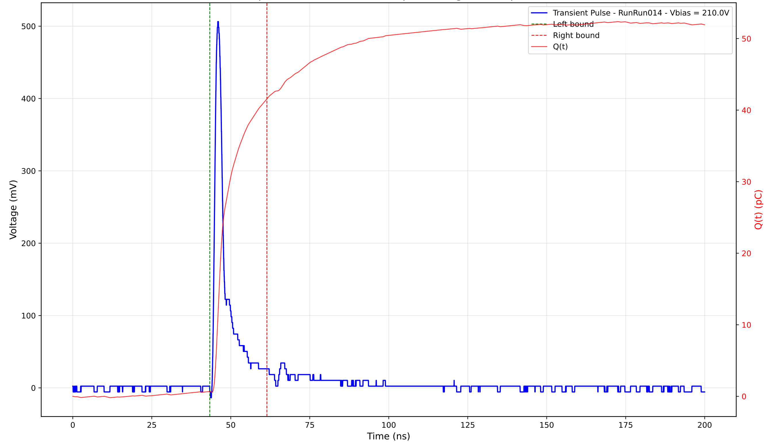
Transient Pulse - Sample: 4003 - Position: 230.0 \mu\text{m} - Charge: 40.90 pC - Rise Time: 1.12 ns
