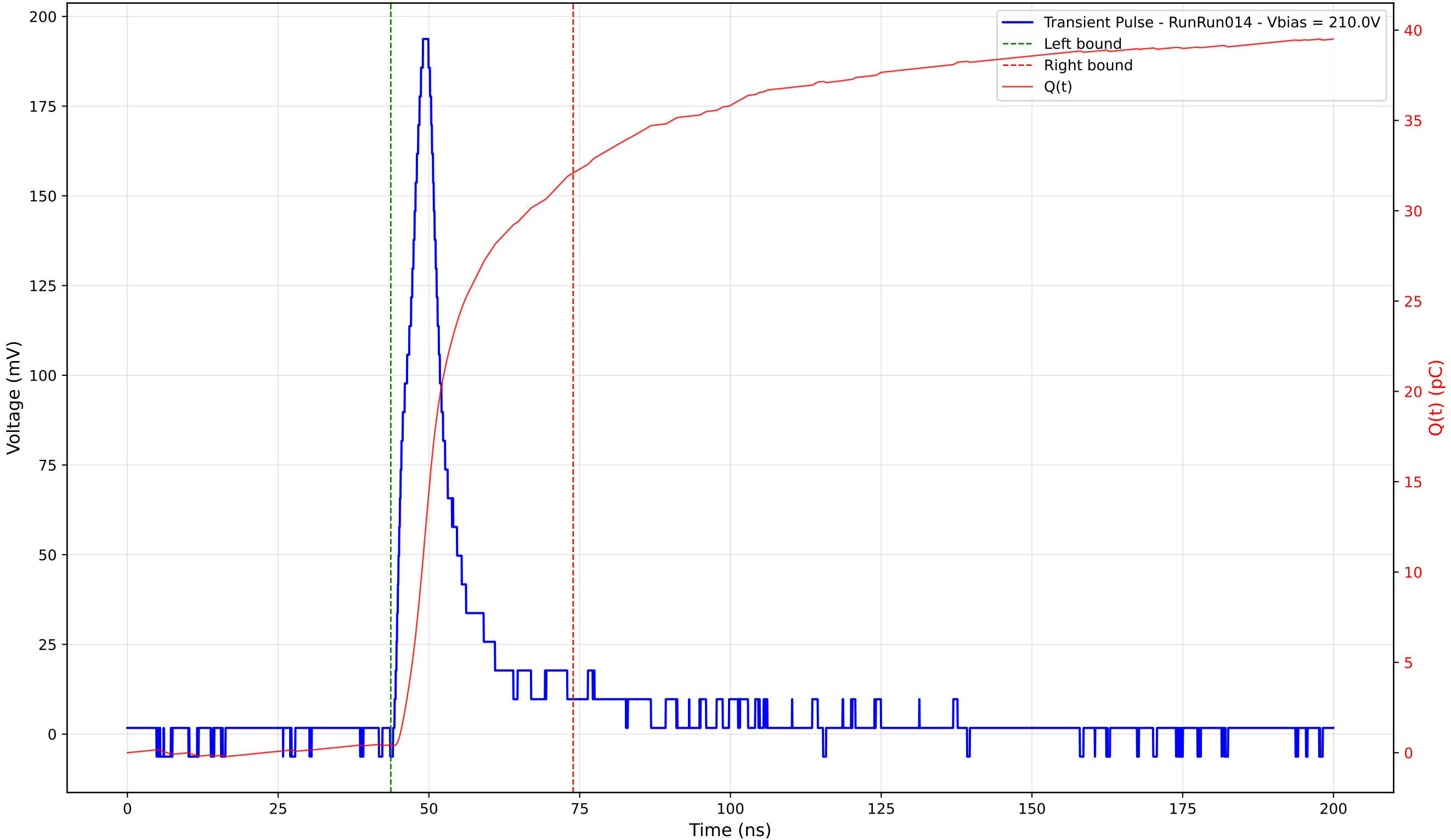
Transient Pulse - Sample: 4003 - Position: 340.0 \mu\text{m} - Charge: 31.67 pC - Rise Time: 3.84 ns
