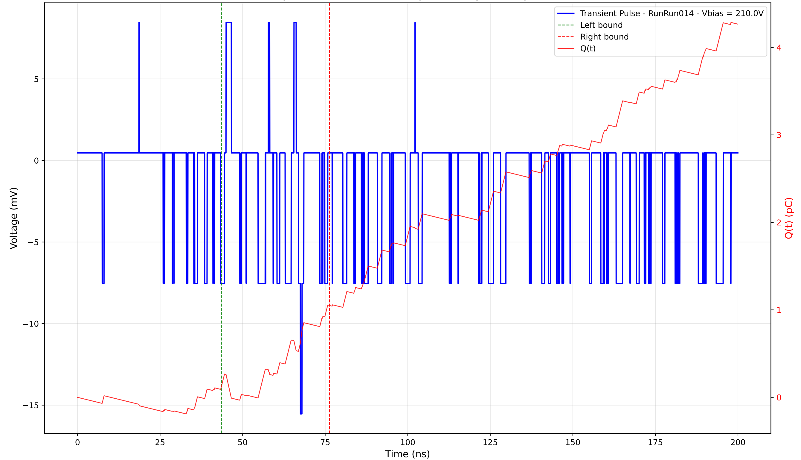
Transient Pulse - Sample: 4003 - Position: 0.0 \mu\text{m} - Charge: 0.93 pC - Rise Time: 0.60 ns
