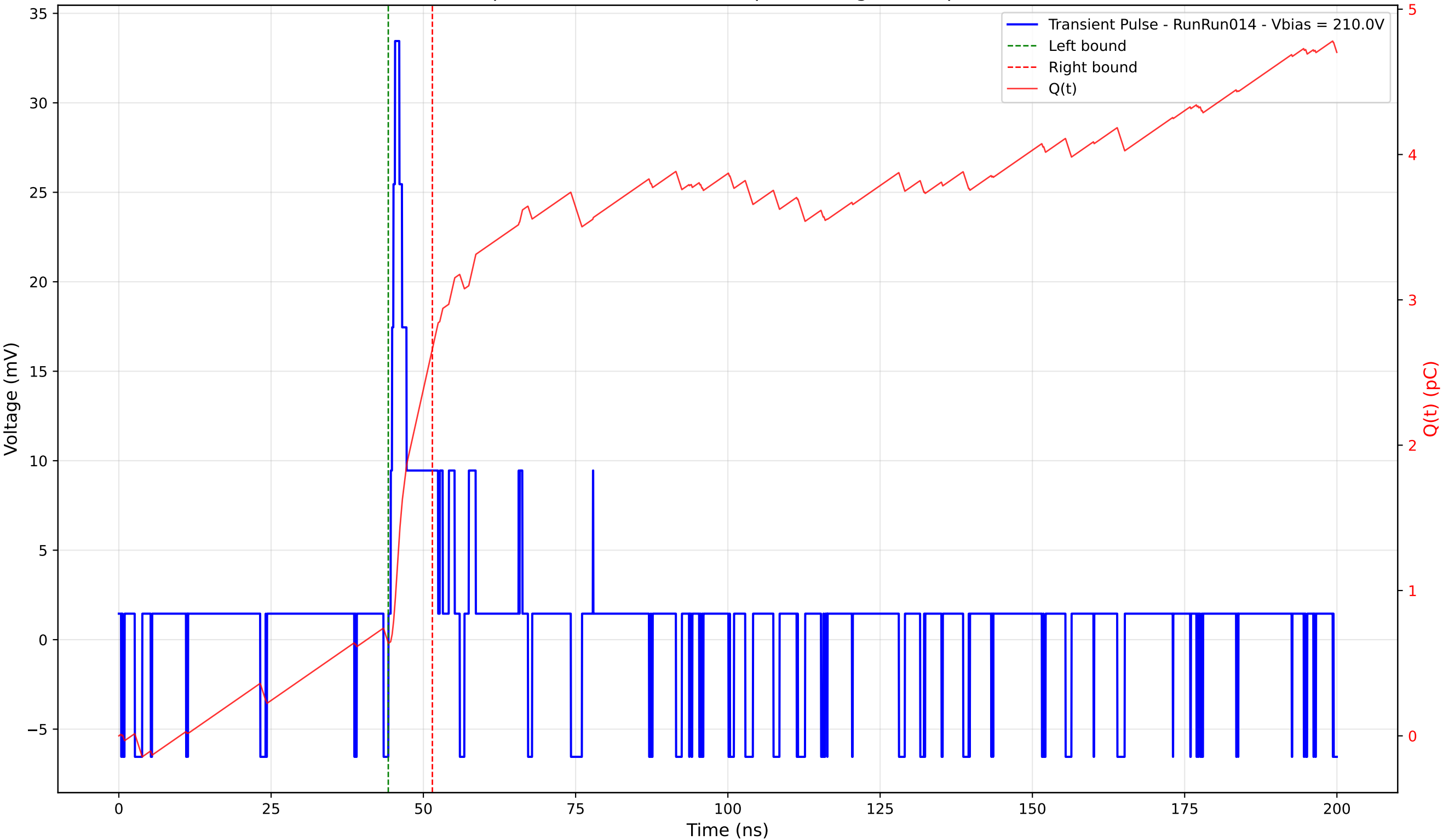
Transient Pulse - Sample: 4003 - Position: 35.0 \mu\text{m} - Charge: 2.03 pC - Rise Time: 0.72 ns
