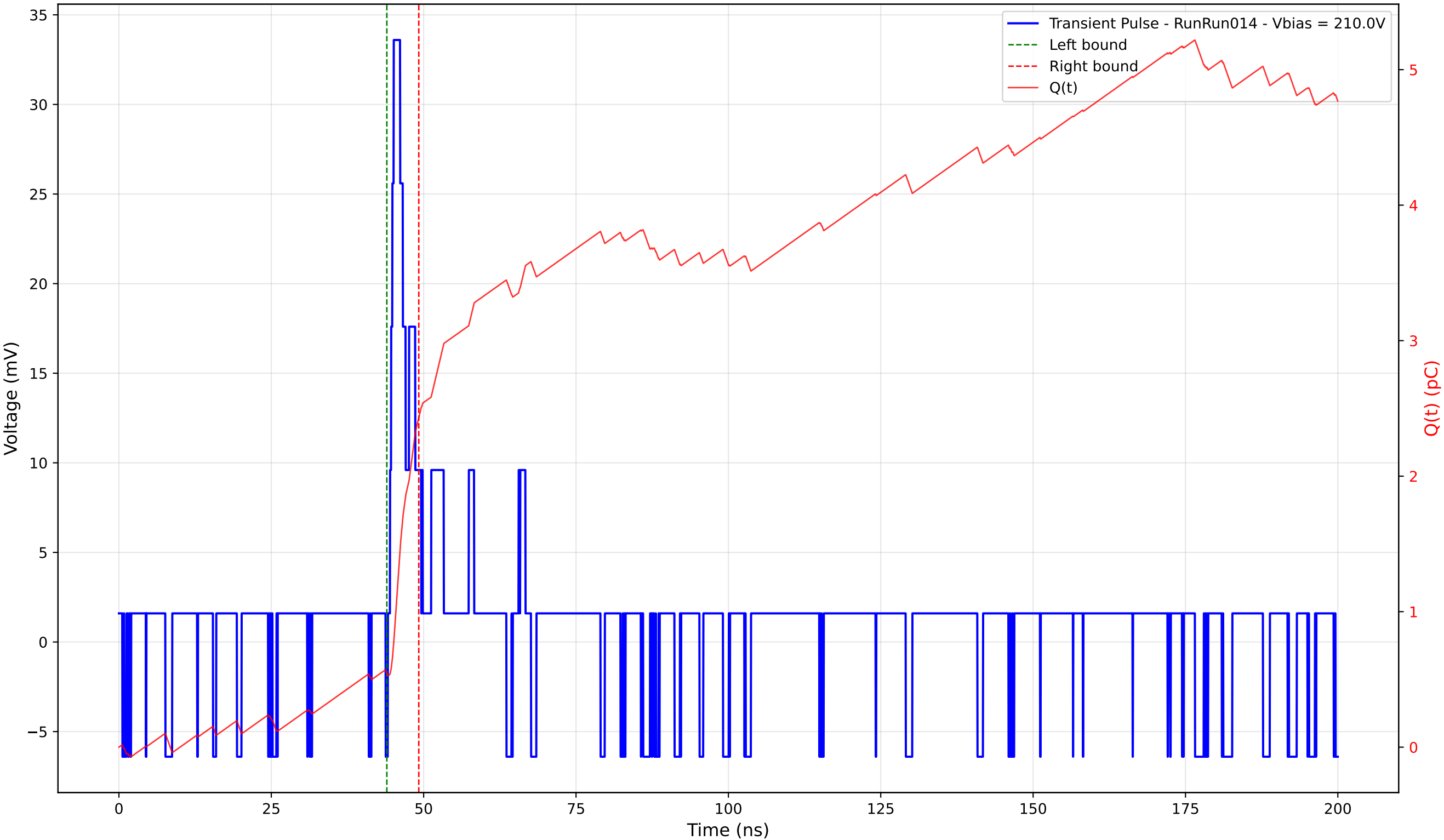
Transient Pulse - Sample: 4003 - Position: 80.0 \mu\text{m} - Charge: 1.89 pC - Rise Time: 0.62 ns
