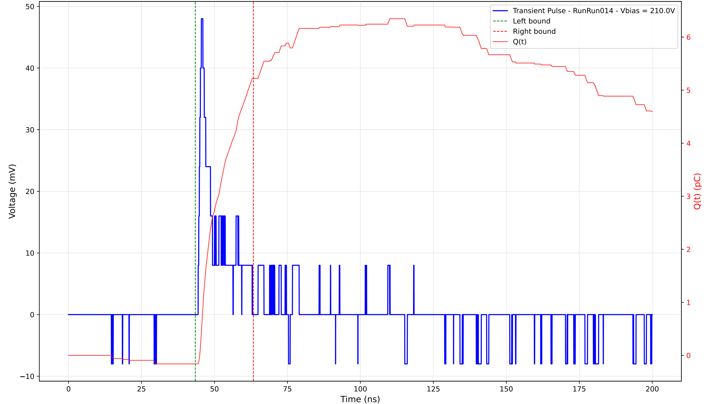
Transient Pulse - Sample: 4003 - Position: 50.0 \mu\text{m} - Charge: 5.38 pC - Rise Time: 1.09 ns
