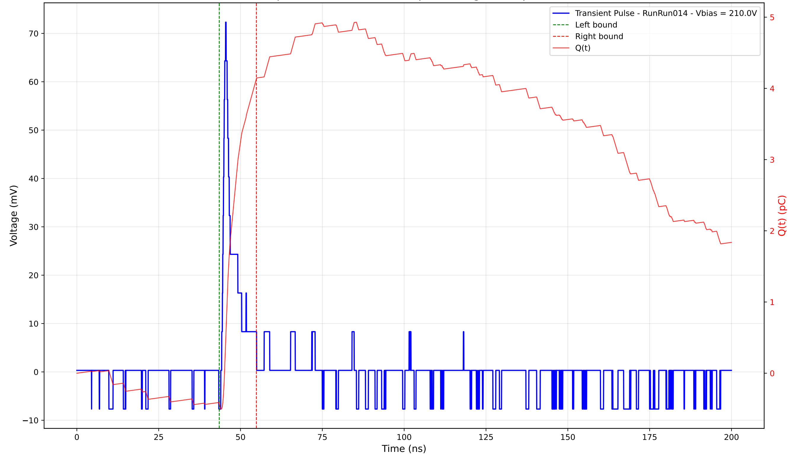
Transient Pulse - Sample: 4003 - Position: 85.0 \mu\text{m} - Charge: 4.57 pC - Rise Time: 1.18 ns
