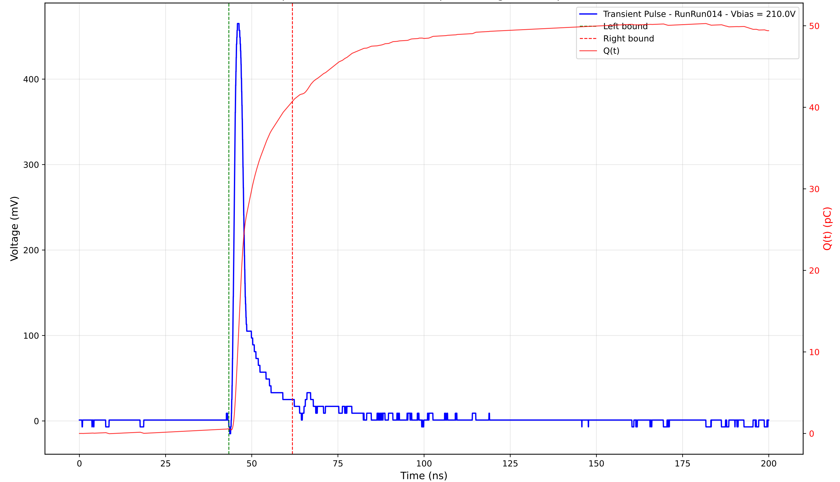
Transient Pulse - Sample: 4003 - Position: 245.0 \mu\text{m} - Charge: 40.16 pC - Rise Time: 1.17 ns
