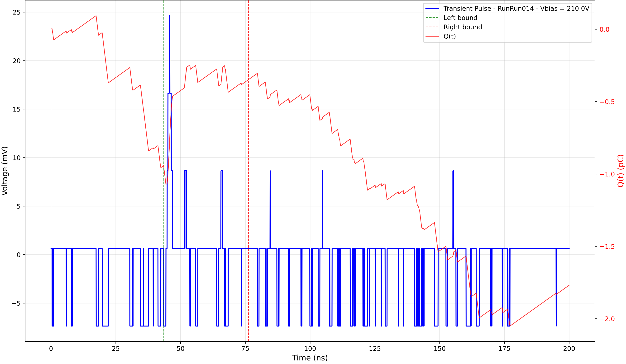
Transient Pulse - Sample: 4003 - Position: 75.0 \mu\text{m} - Charge: 0.61 pC - Rise Time: 0.82 ns
