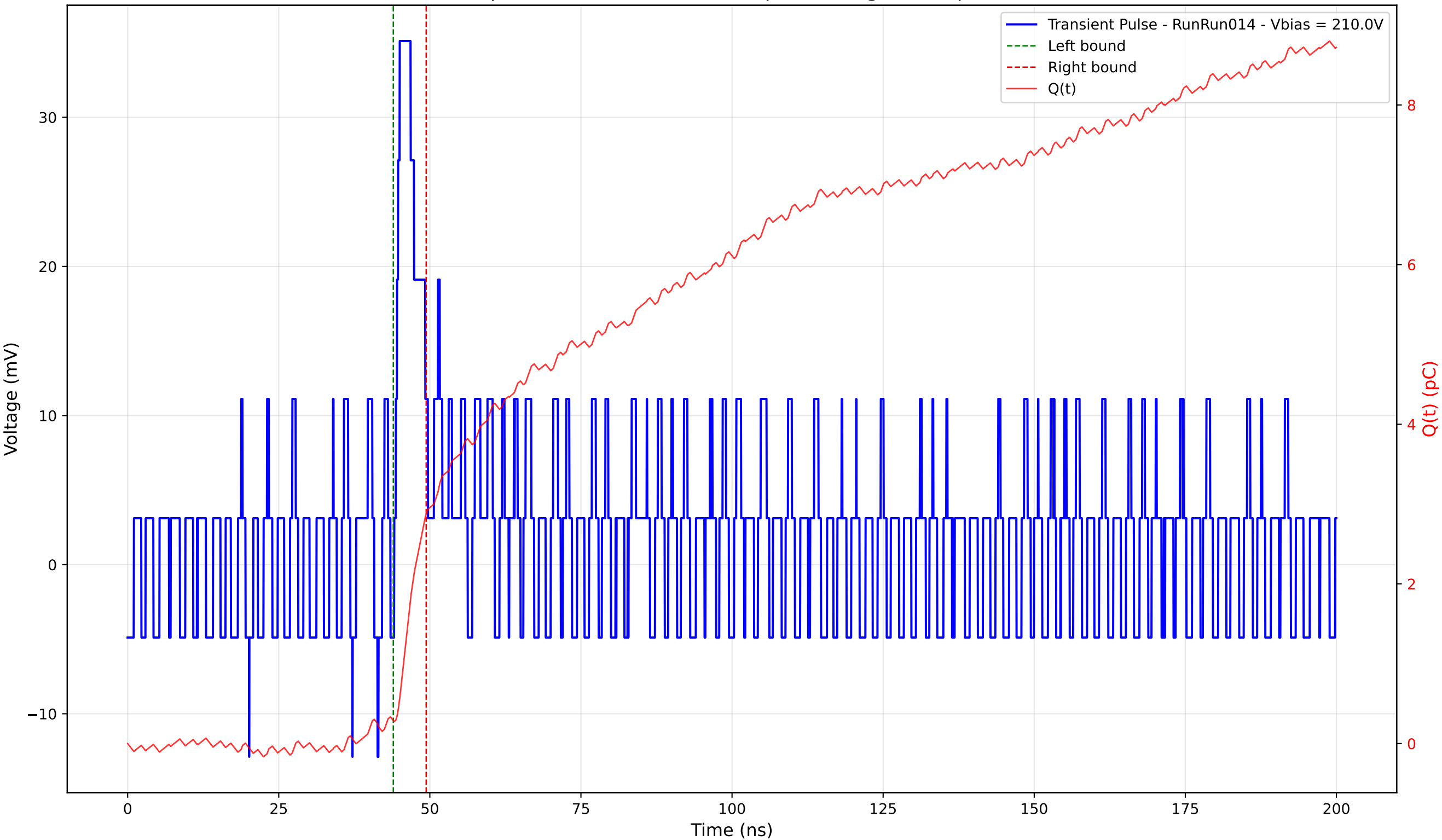
Transient Pulse - Sample: 4003 - Position: 410.0 \mu\text{m} - Charge: 2.59 pC - Rise Time: 0.66 ns
