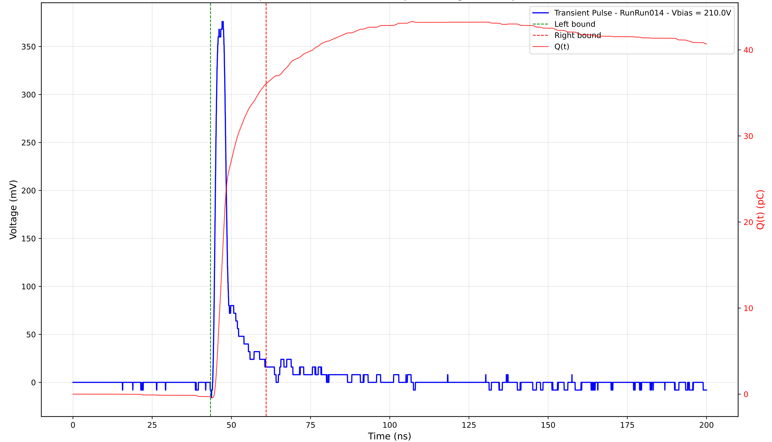
Transient Pulse - Sample: 4003 - Position: 280.0 \mu\text{m} - Charge: 36.39 pC - Rise Time: 1.25 ns
