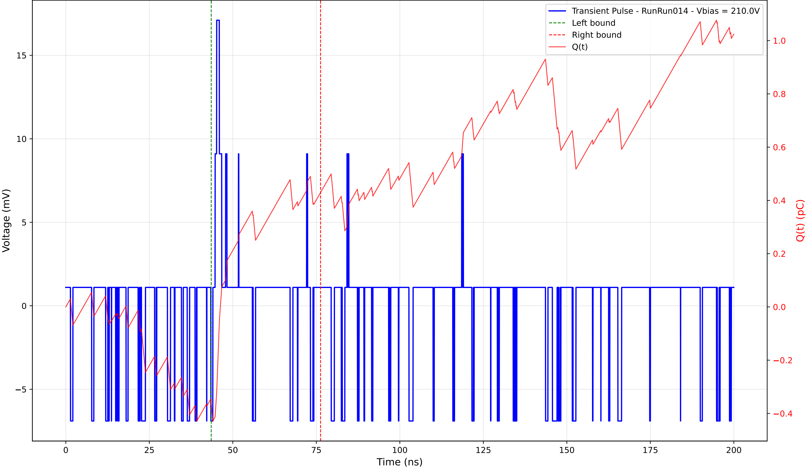
Transient Pulse - Sample: 4003 - Position: 10.0 \mu\text{m} - Charge: 0.79 pC - Rise Time: 0.48 ns
