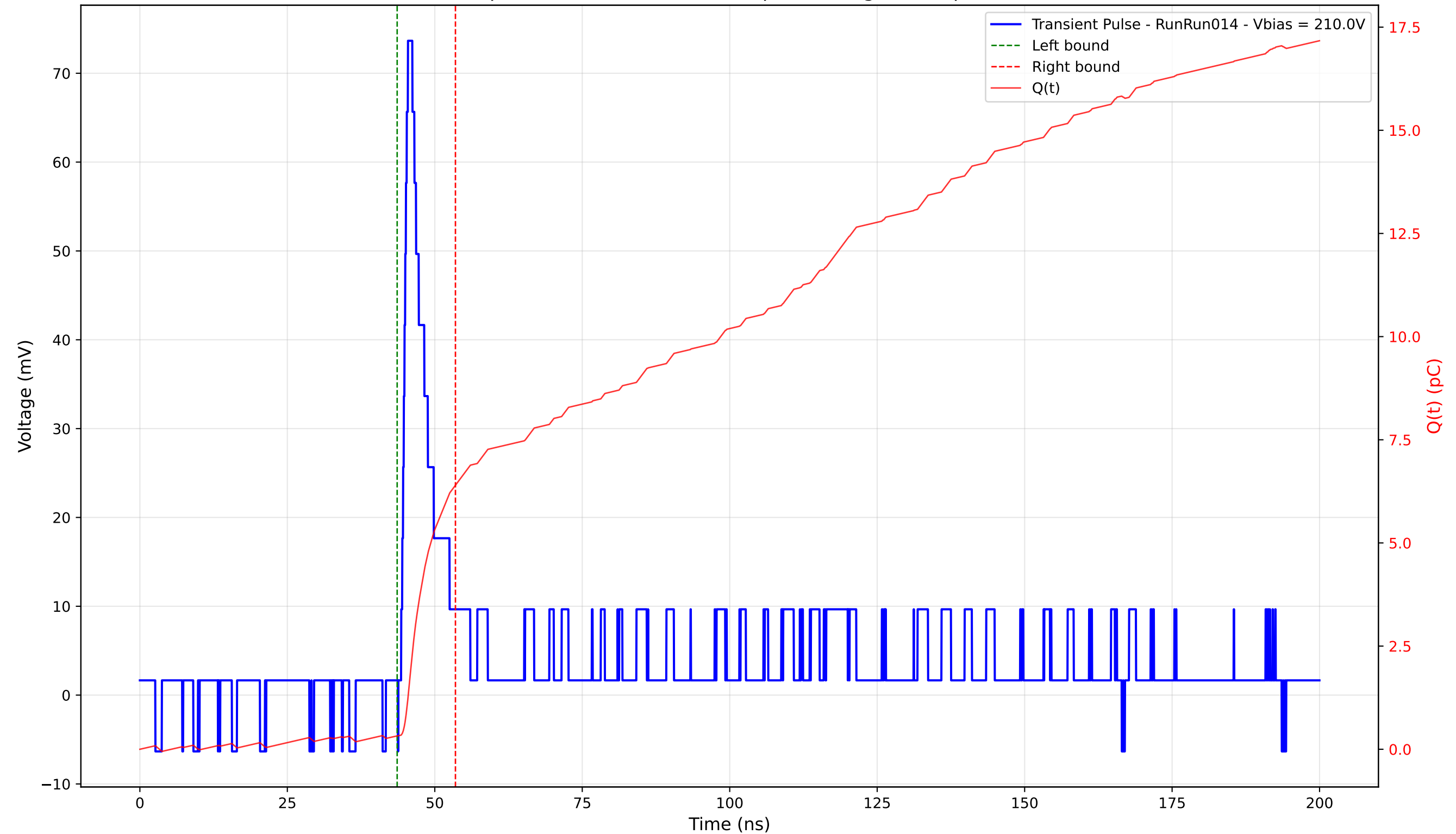
Transient Pulse - Sample: 4003 - Position: 385.0 \mu\text{m} - Charge: 6.07 pC - Rise Time: 1.15 ns
