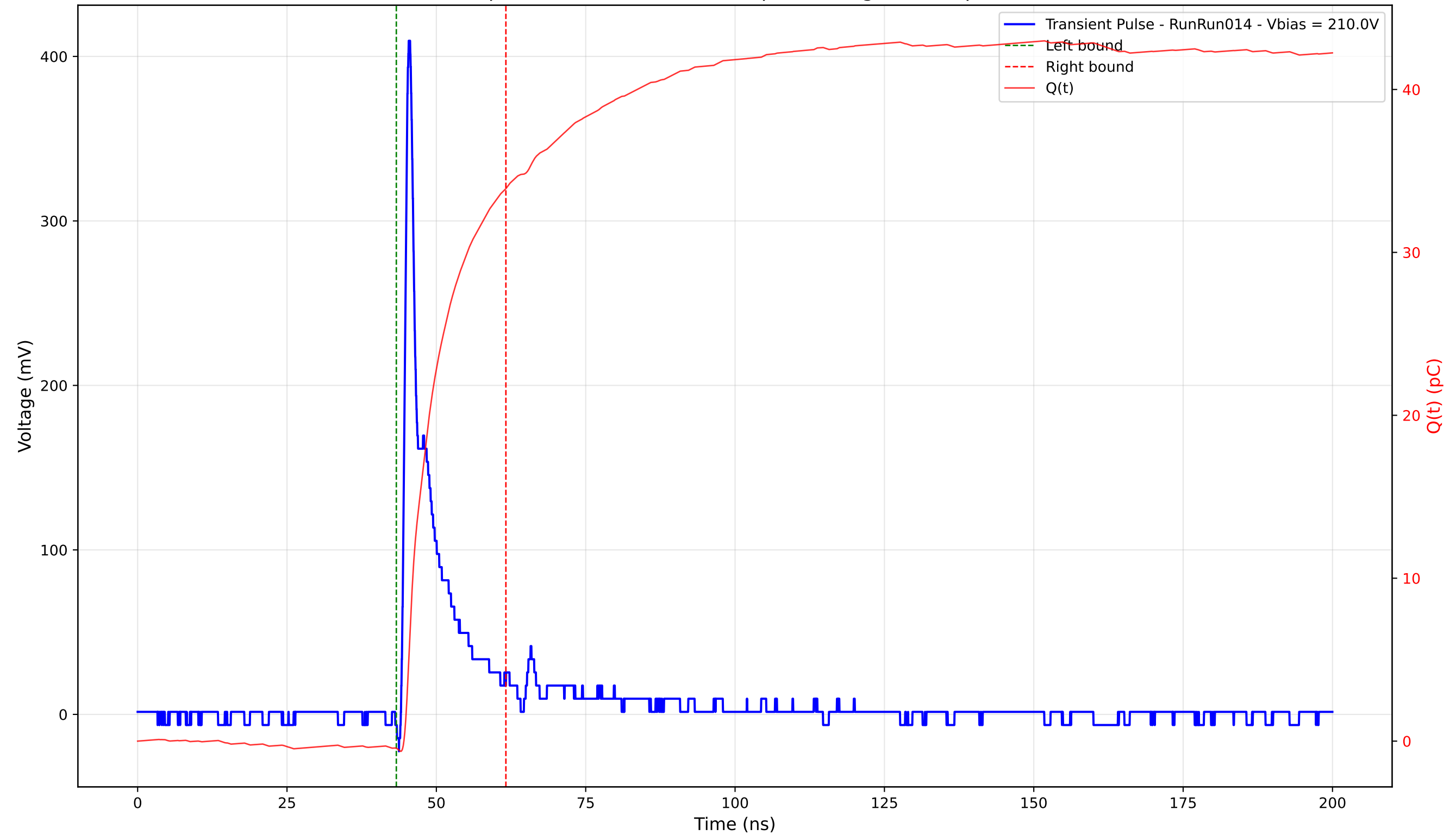
Transient Pulse - Sample: 4003 - Position: 110.0 \mu\text{m} - Charge: 34.35 pC - Rise Time: 0.88 ns
