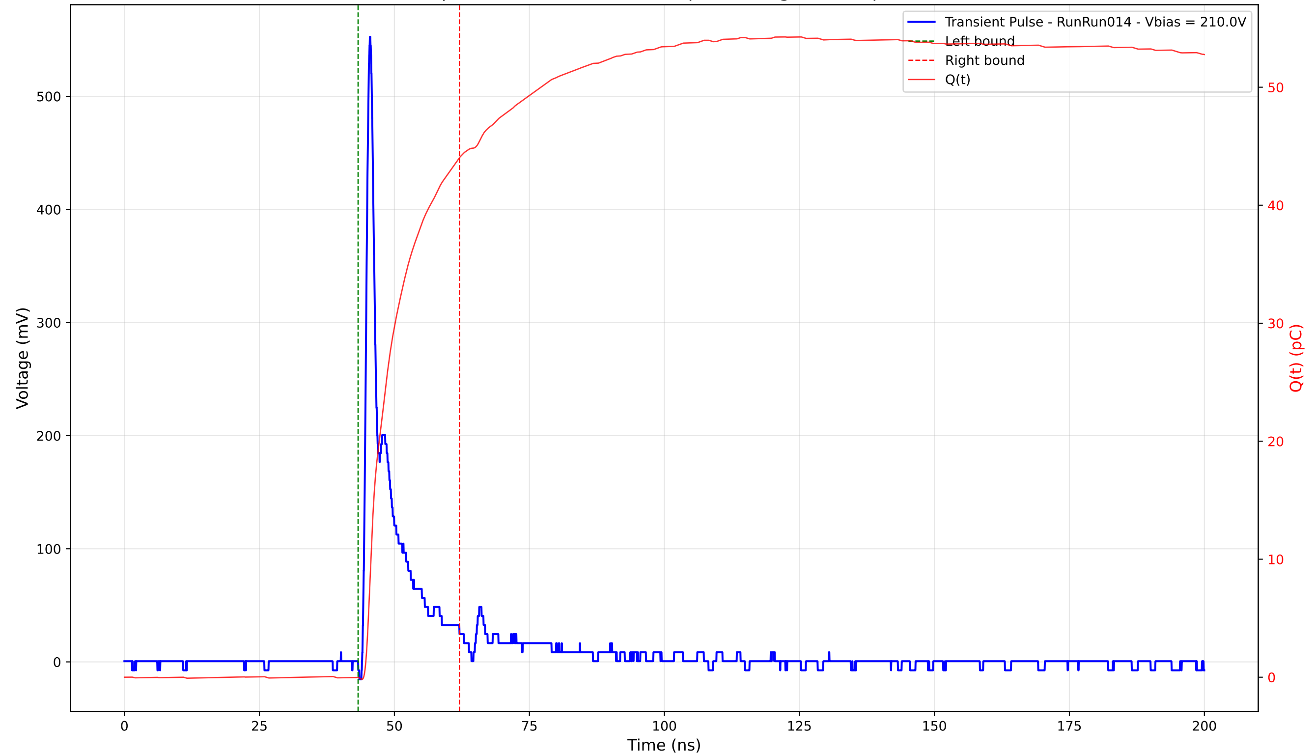
Transient Pulse - Sample: 4003 - Position: 135.0 \mu\text{m} - Charge: 44.07 pC - Rise Time: 0.93 ns
