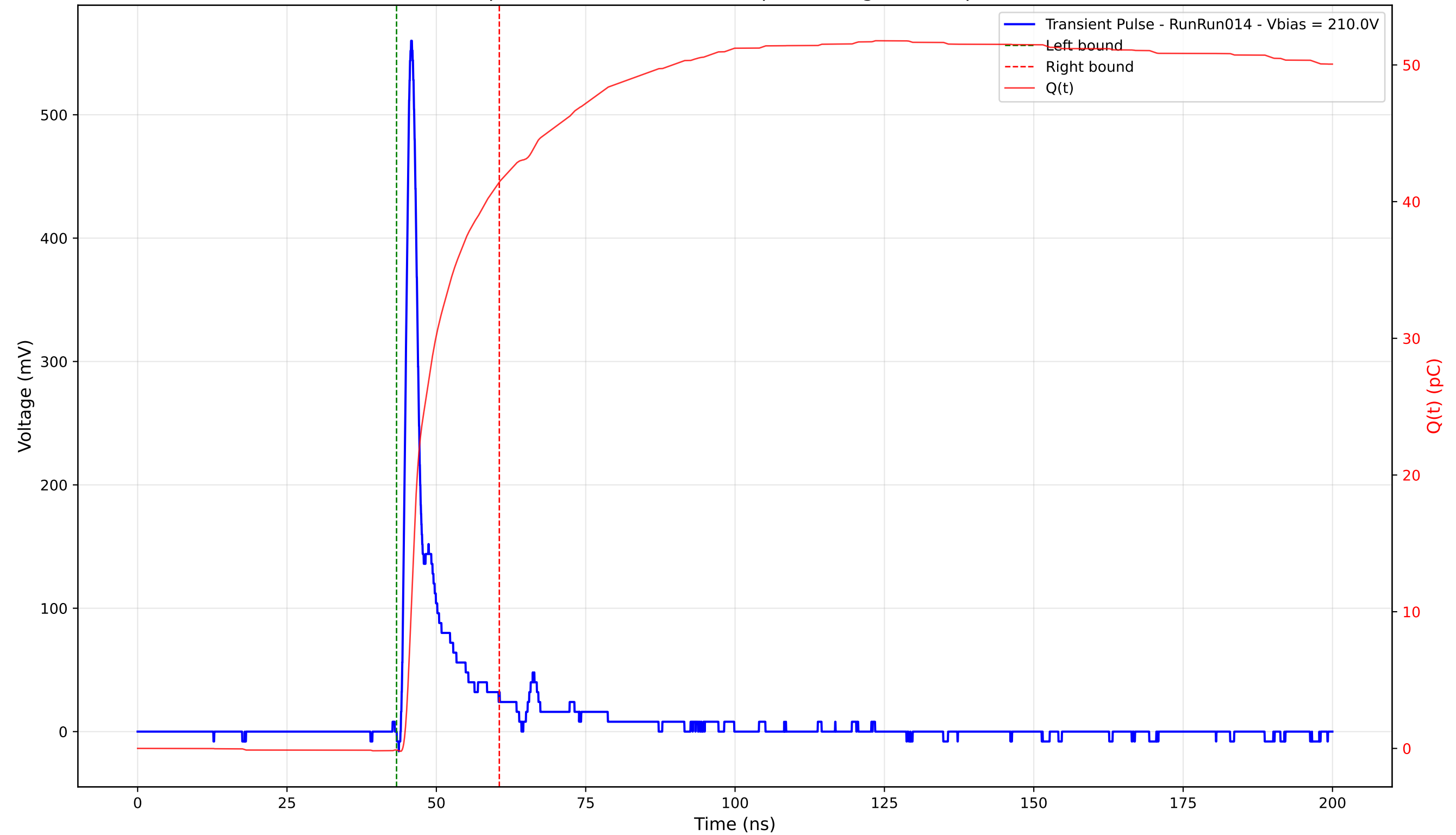
Transient Pulse - Sample: 4003 - Position: 205.0 \mu\text{m} - Charge: 41.55 pC - Rise Time: 1.08 ns
