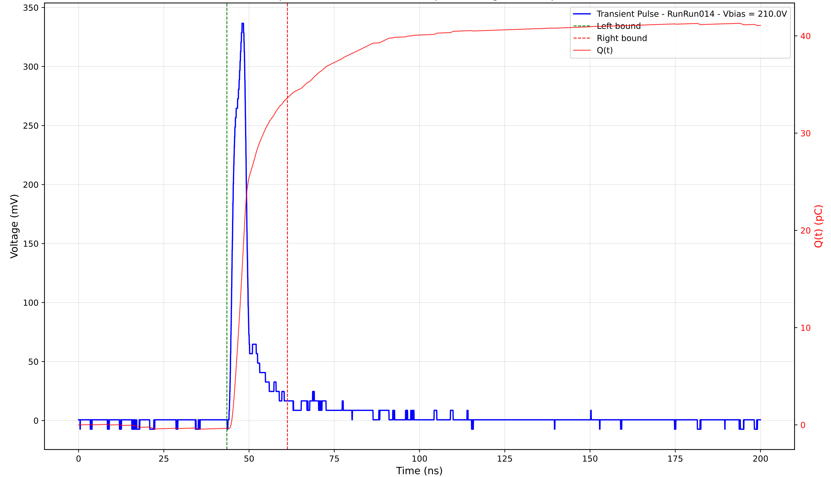
Transient Pulse - Sample: 4003 - Position: 315.0 \mu\text{m} - Charge: 33.97 pC - Rise Time: 2.90 ns
