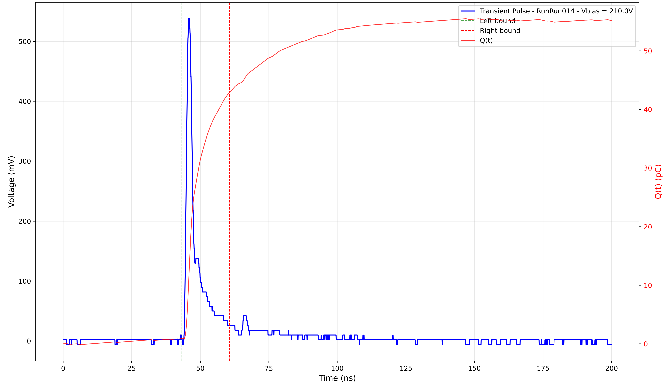
Transient Pulse - Sample: 4003 - Position: 215.0 \mu\text{m} - Charge: 41.98 pC - Rise Time: 1.14 ns
