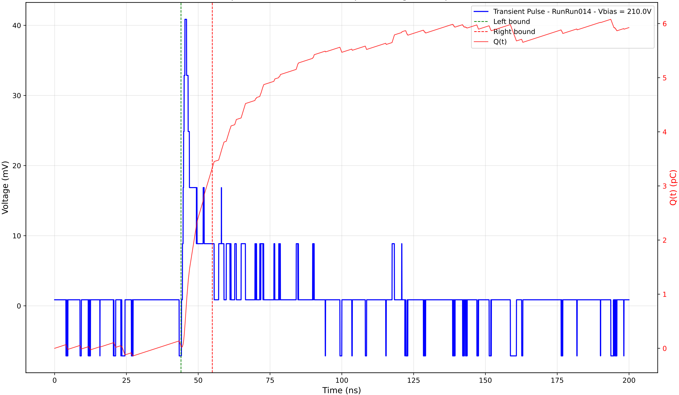
Transient Pulse - Sample: 4003 - Position: 45.0 \mu\text{m} - Charge: 3.30 pC - Rise Time: 0.87 ns
