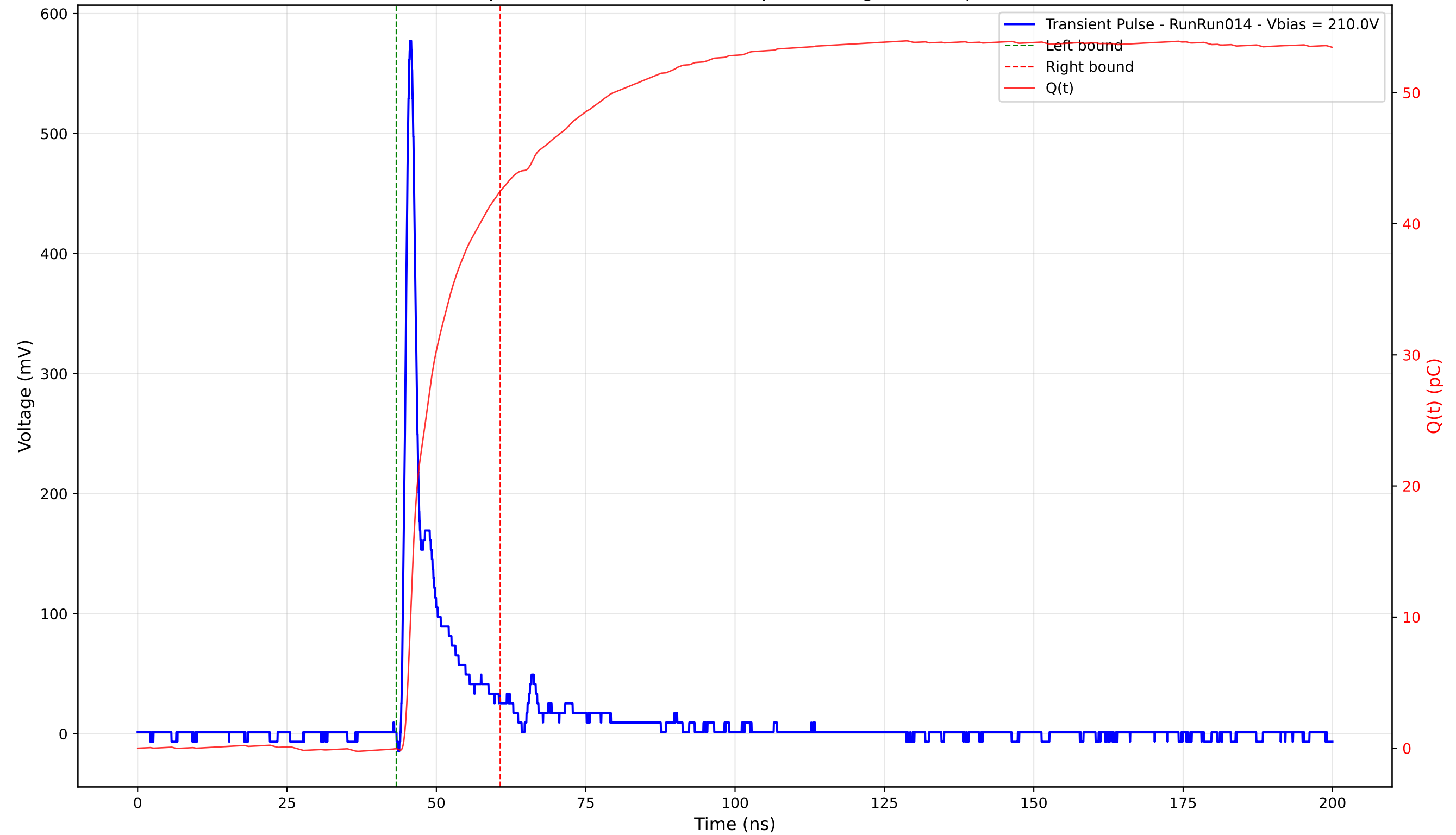
Transient Pulse - Sample: 4003 - Position: 180.0 \mu\text{m} - Charge: 42.53 pC - Rise Time: 1.01 ns
