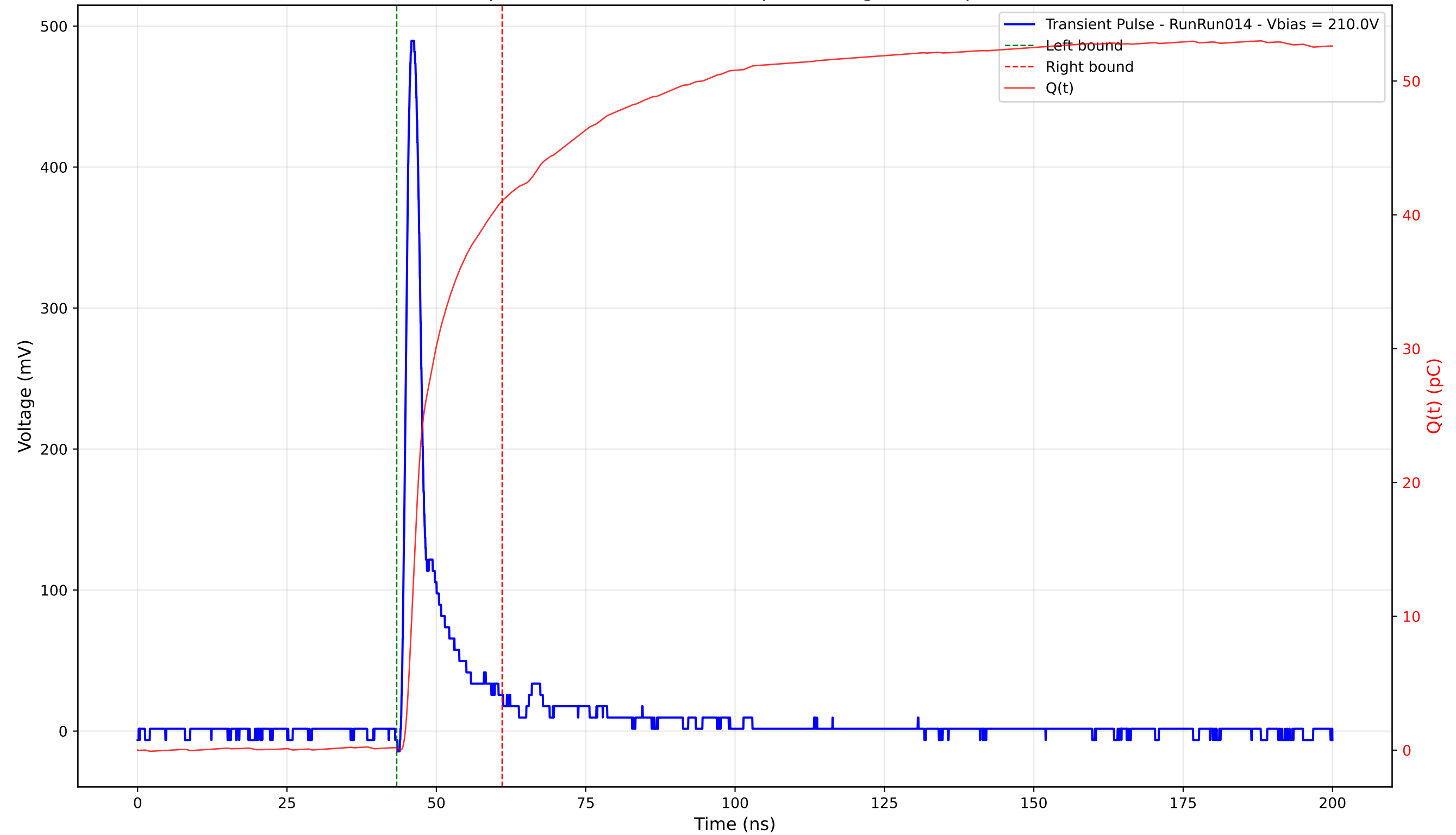
Transient Pulse - Sample: 4003 - Position: 235.0 \mu\text{m} - Charge: 40.89 pC - Rise Time: 1.16 ns
