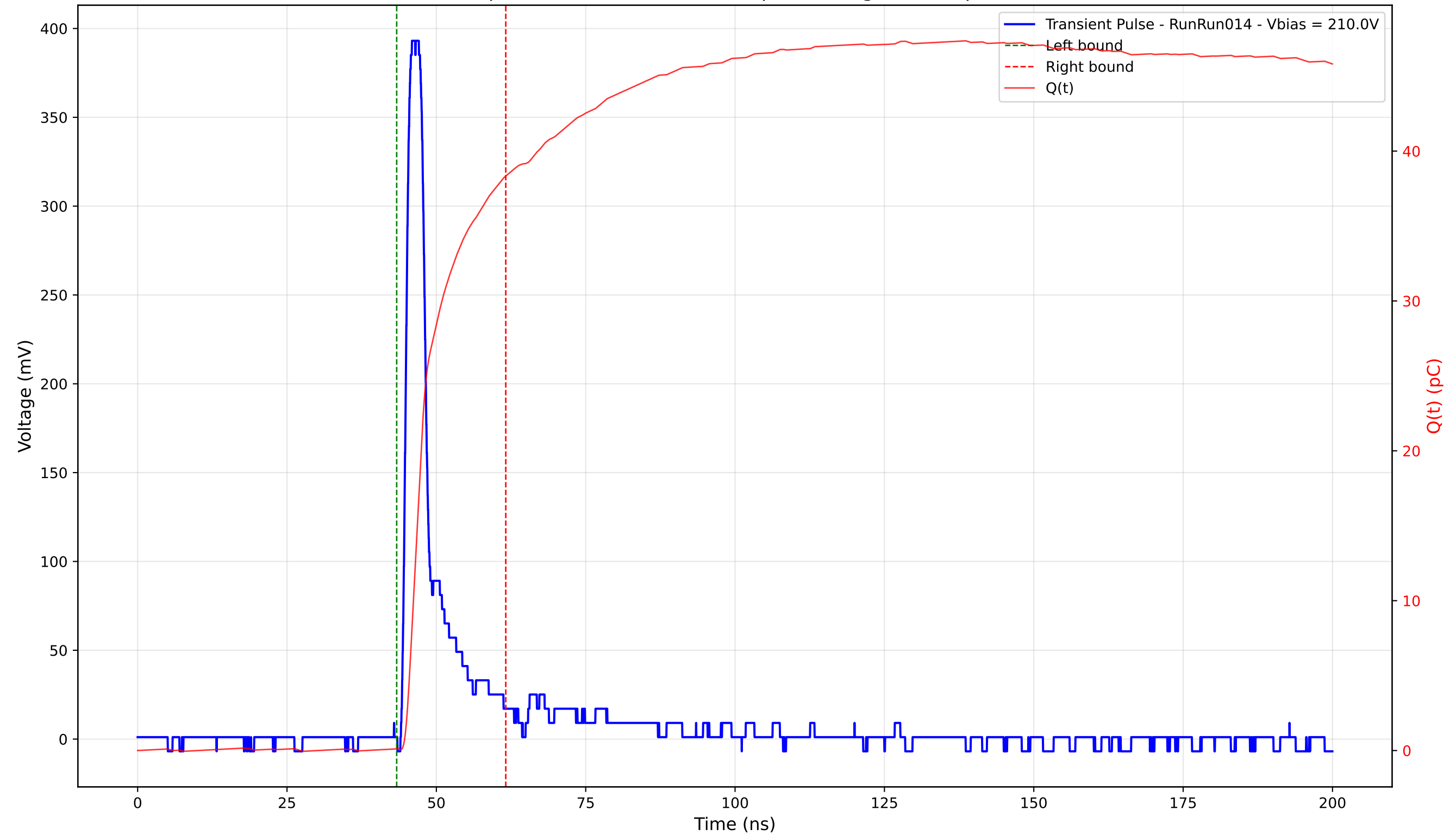
Transient Pulse - Sample: 4003 - Position: 270.0 \mu\text{m} - Charge: 38.21 pC - Rise Time: 1.18 ns
