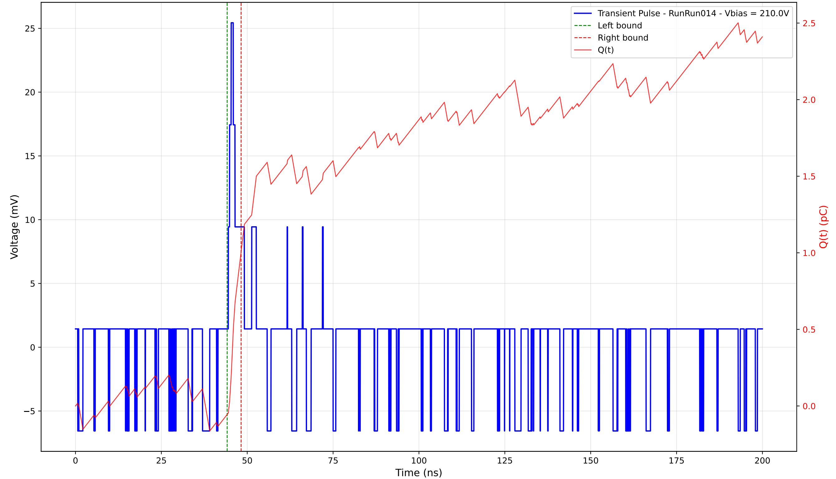
Transient Pulse - Sample: 4003 - Position: 20.0 \mu\text{m} - Charge: 1.07 pC - Rise Time: 0.84 ns
