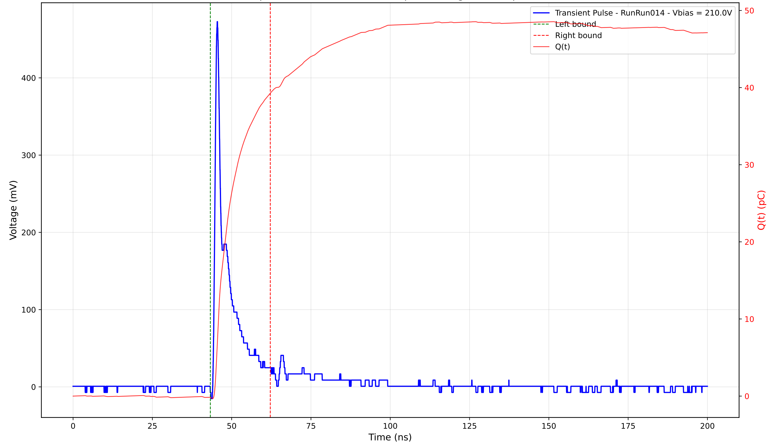
Transient Pulse - Sample: 4003 - Position: 115.0 \mu\text{m} - Charge: 39.43 pC - Rise Time: 0.93 ns
