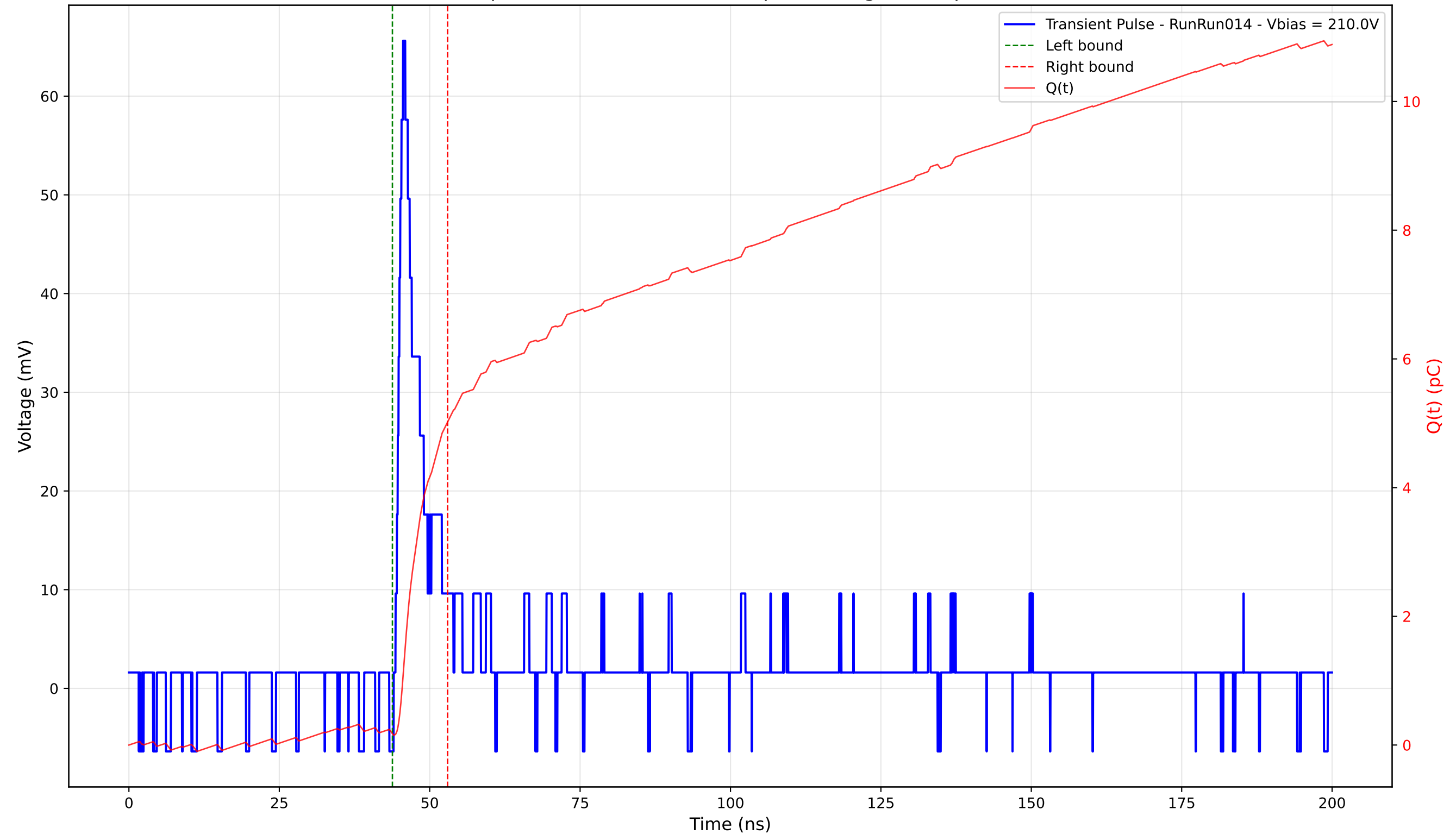
Transient Pulse - Sample: 4003 - Position: 400.0 \mu\text{m} - Charge: 4.85 pC - Rise Time: 1.25 ns
