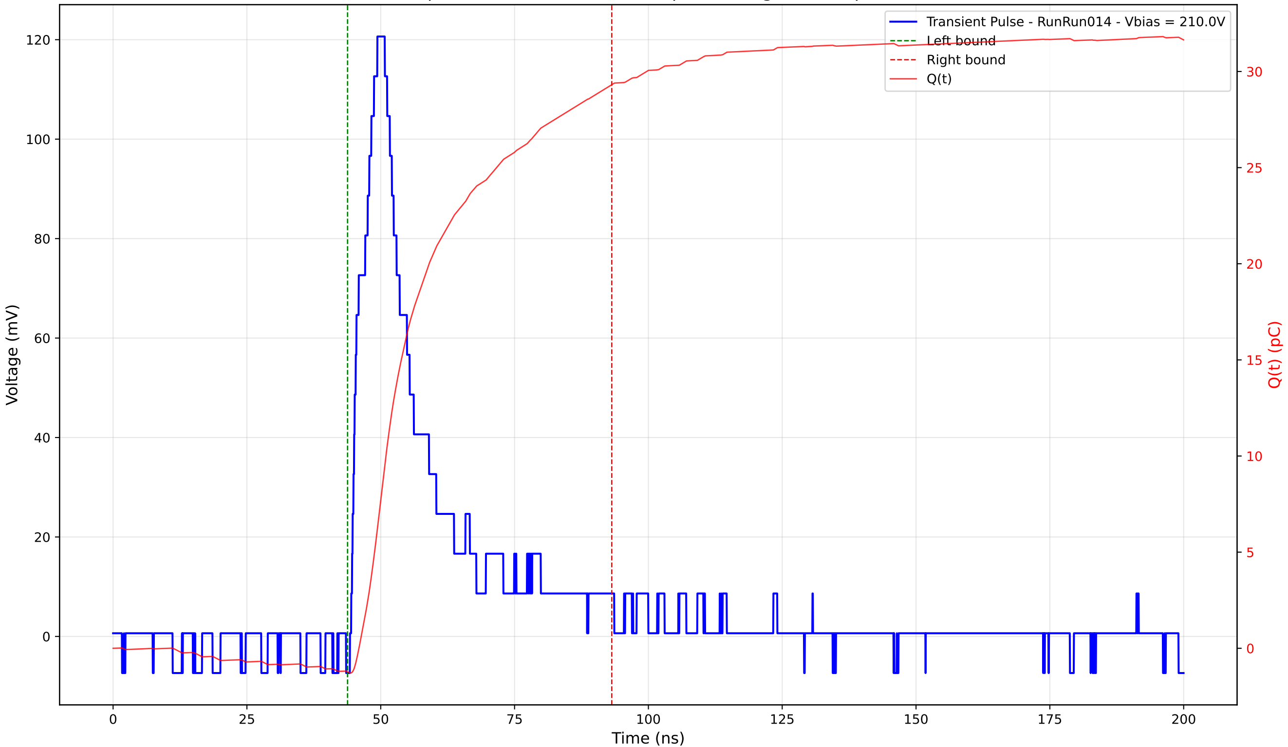
Transient Pulse - Sample: 4003 - Position: 345.0 \mu\text{m} - Charge: 30.54 pC - Rise Time: 4.11 ns
