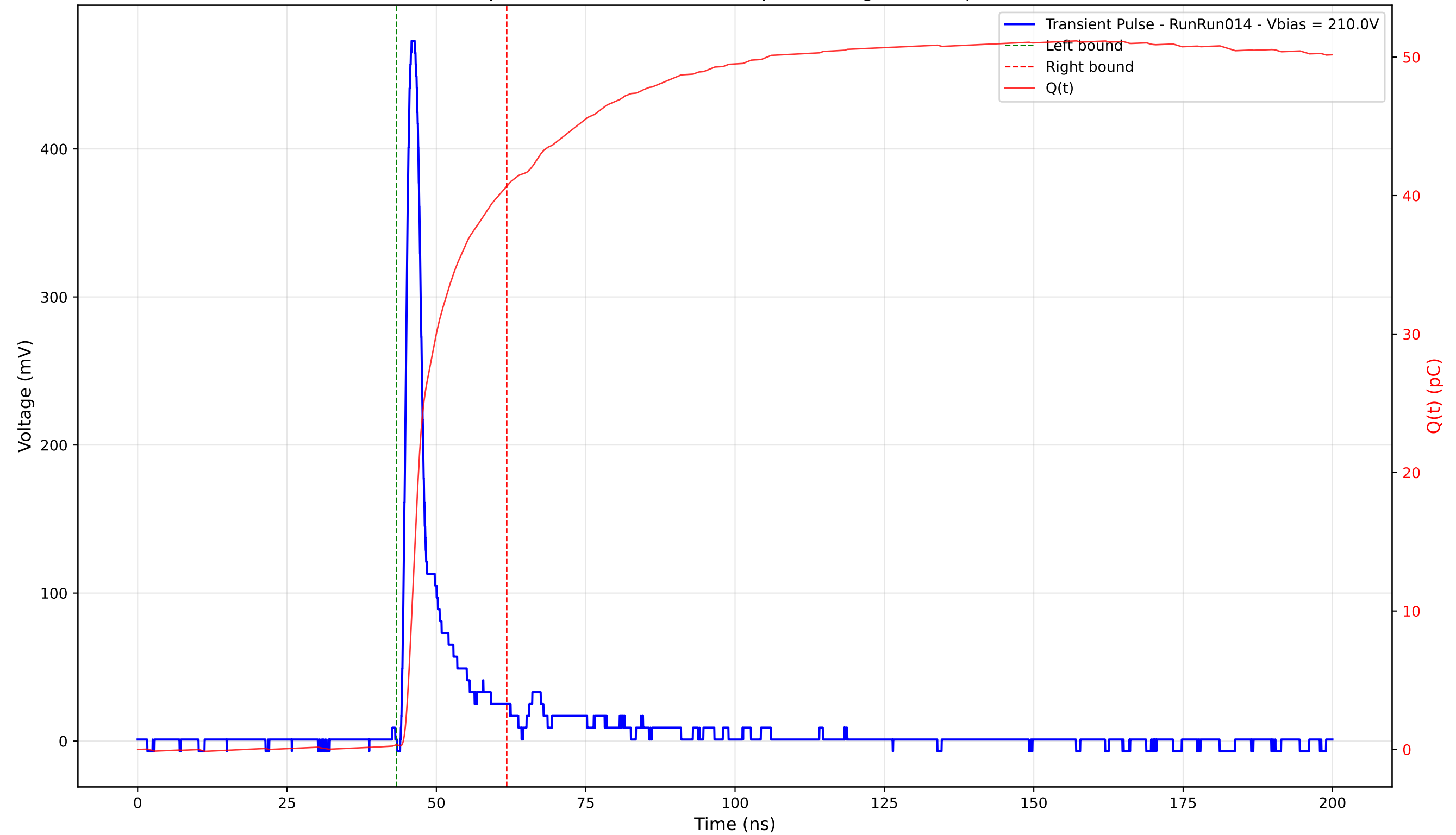
Transient Pulse - Sample: 4003 - Position: 240.0 \mu\text{m} - Charge: 40.36 pC - Rise Time: 1.18 ns
