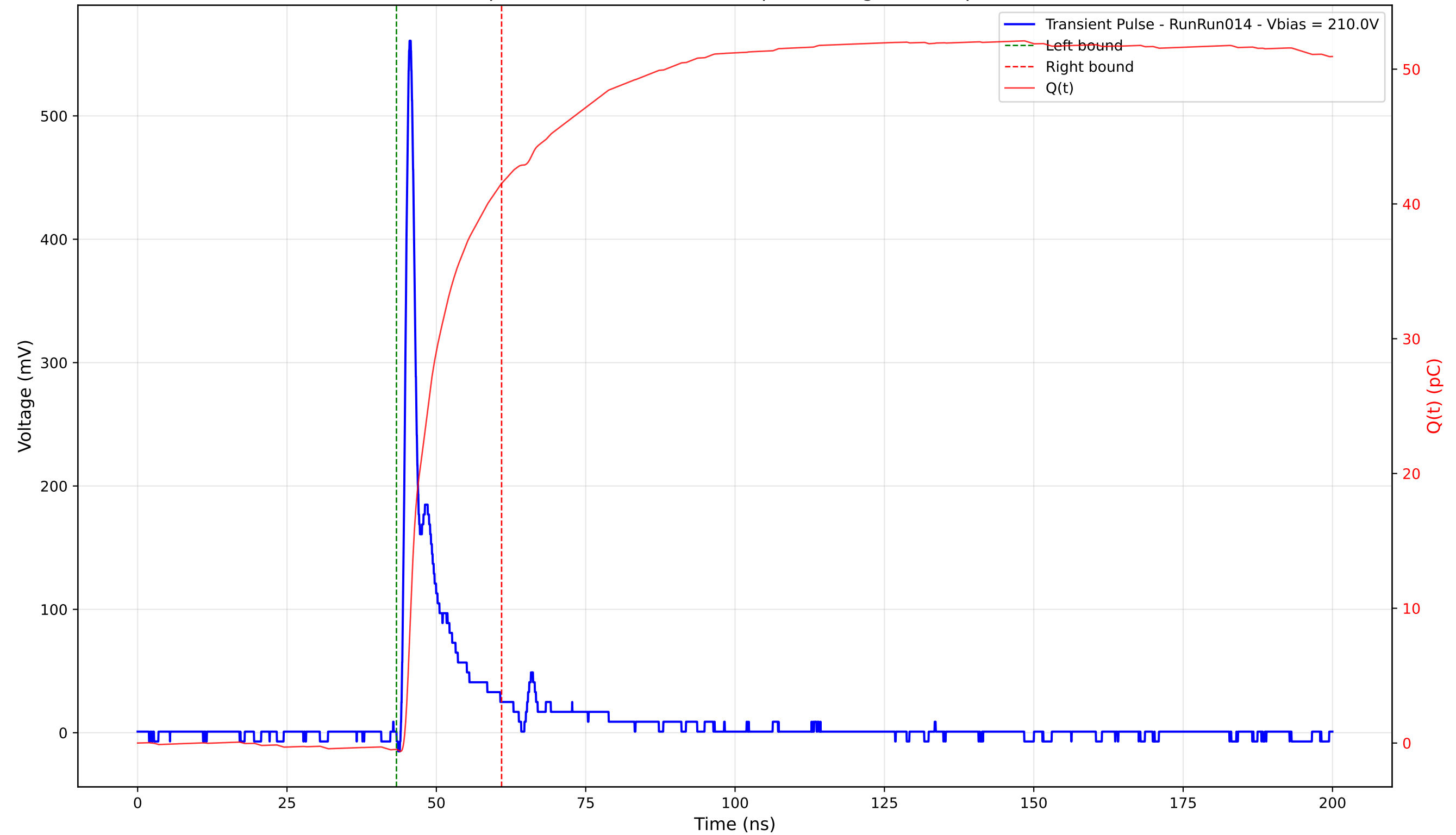
Transient Pulse - Sample: 4003 - Position: 160.0 \mu\text{m} - Charge: 41.99 pC - Rise Time: 0.96 ns
