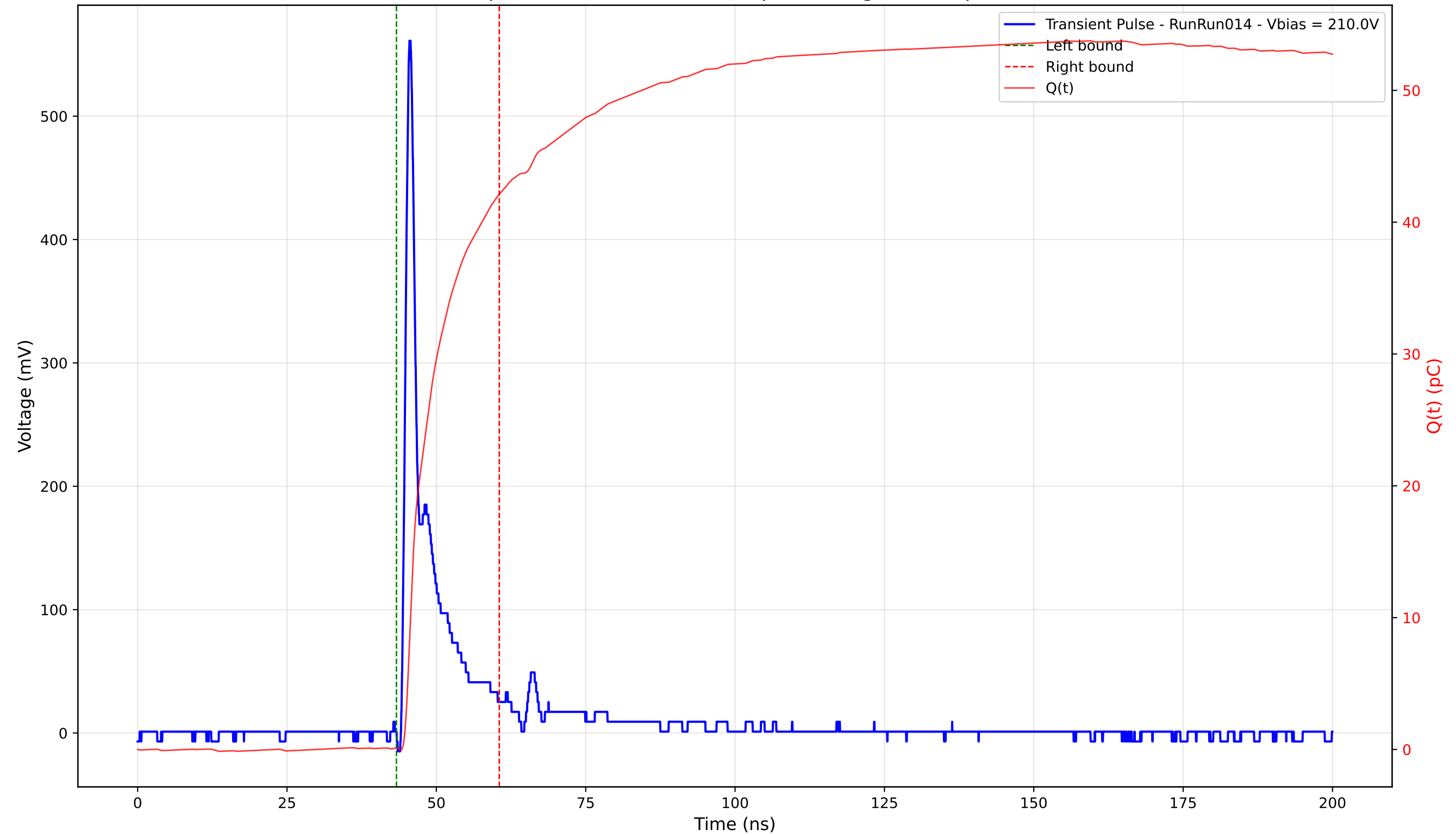
Transient Pulse - Sample: 4003 - Position: 155.0 \mu\text{m} - Charge: 42.01 pC - Rise Time: 0.94 ns
