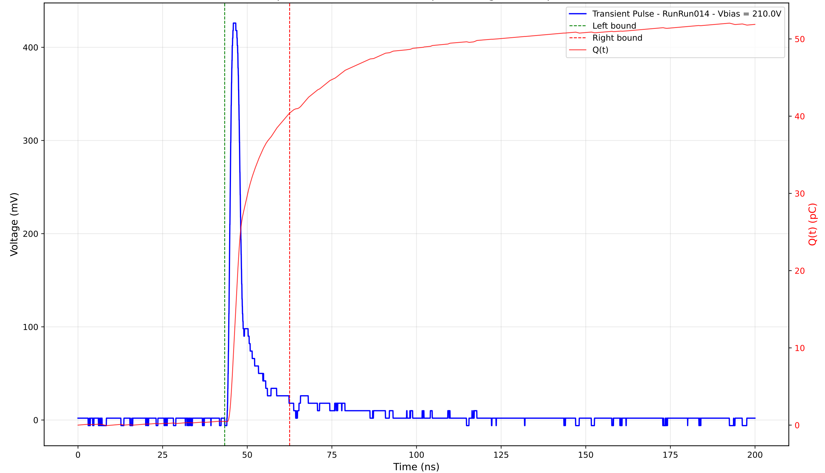
Transient Pulse - Sample: 4003 - Position: 260.0 \mu\text{m} - Charge: 39.91 pC - Rise Time: 1.16 ns
