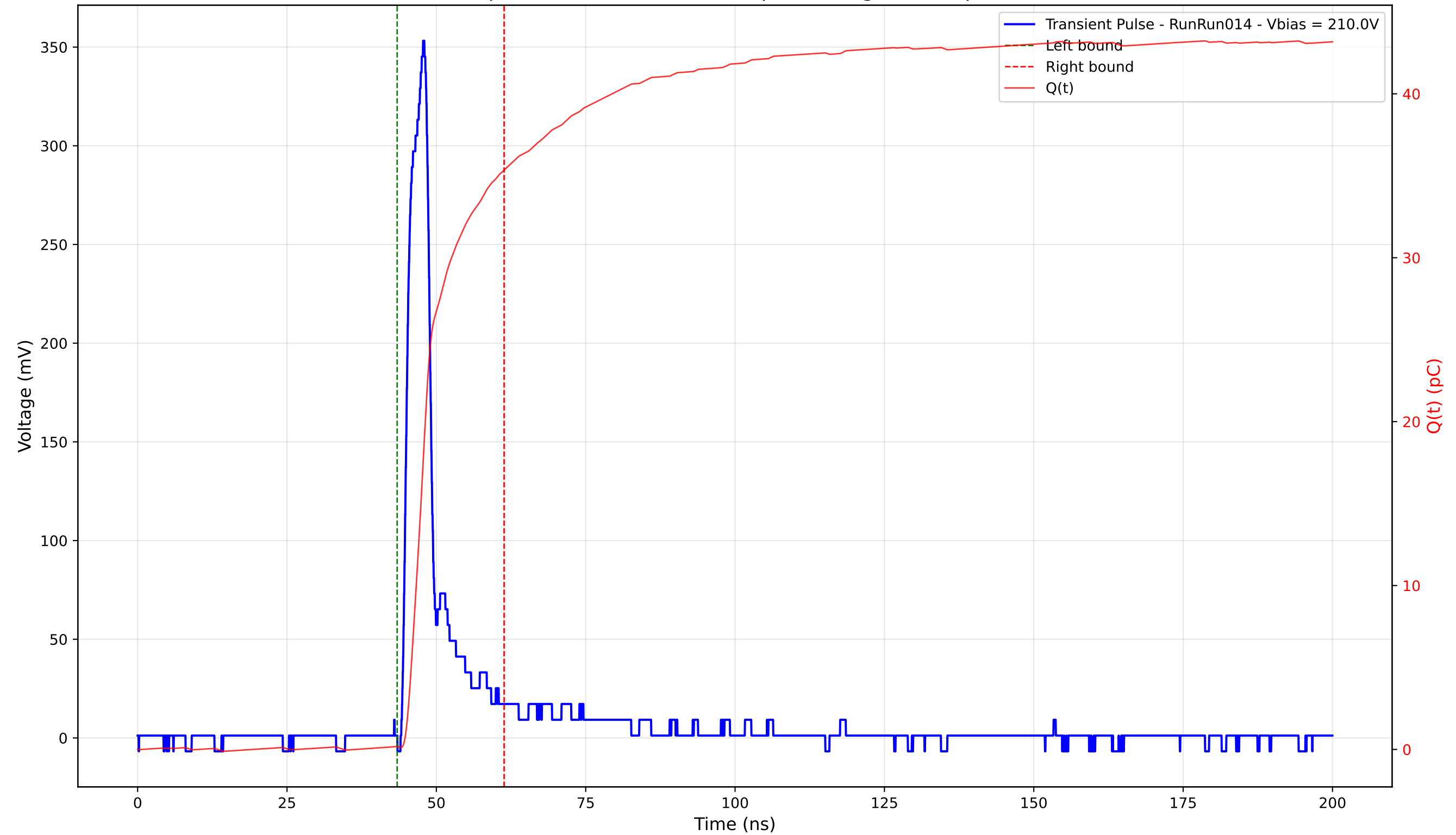
Transient Pulse - Sample: 4003 - Position: 305.0 \mu\text{m} - Charge: 35.17 pC - Rise Time: 2.65 ns
