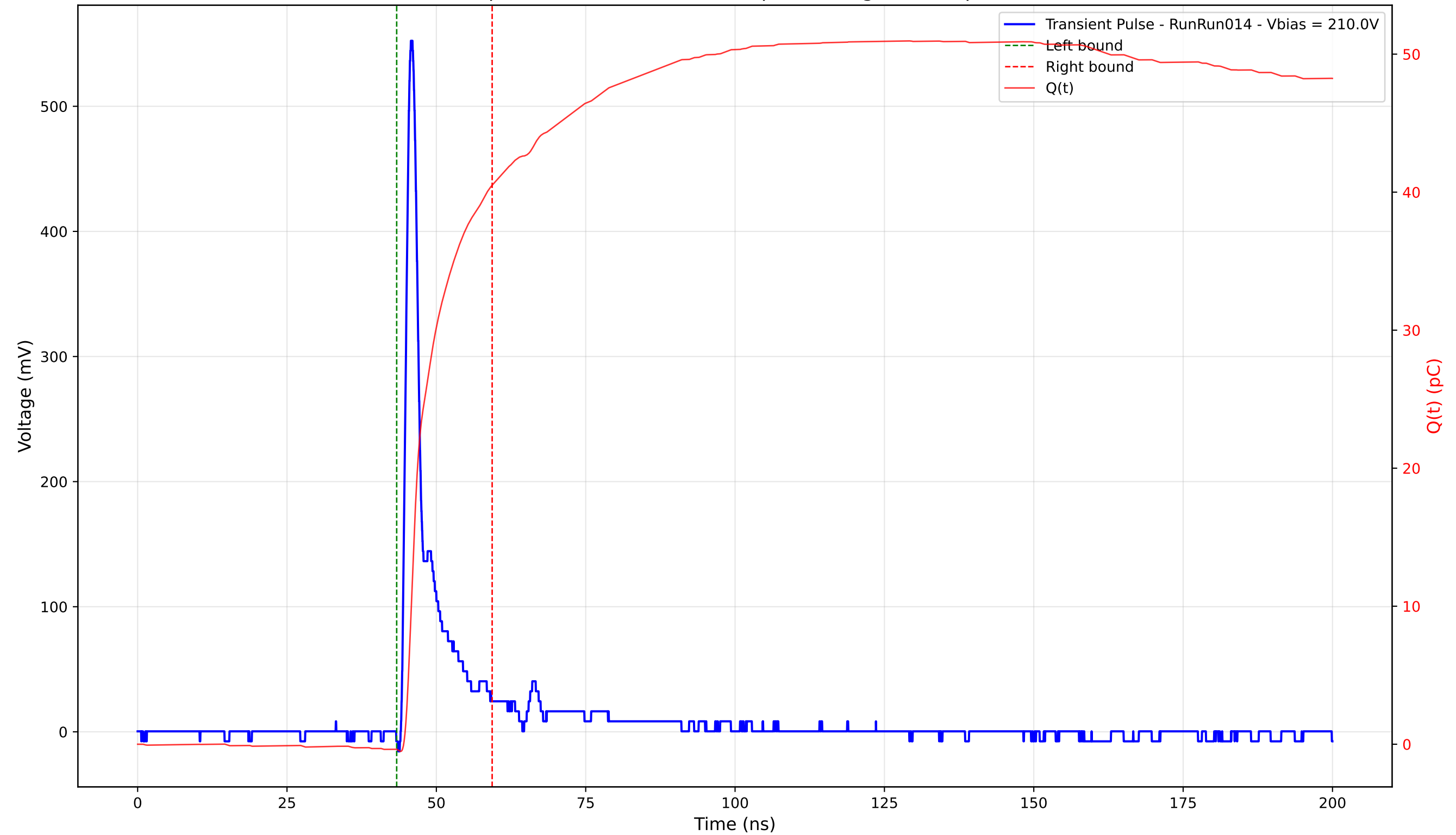
Transient Pulse - Sample: 4003 - Position: 210.0 \mu\text{m} - Charge: 40.87 pC - Rise Time: 1.10 ns
