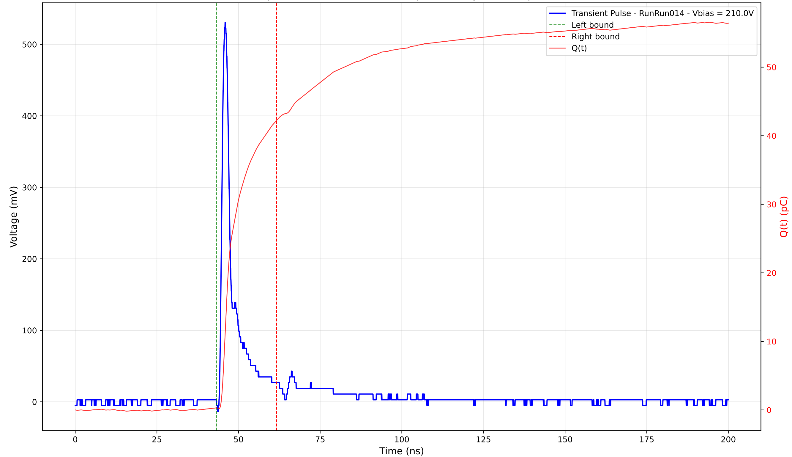
Transient Pulse - Sample: 4003 - Position: 220.0 \mu\text{m} - Charge: 41.91 pC - Rise Time: 1.15 ns
