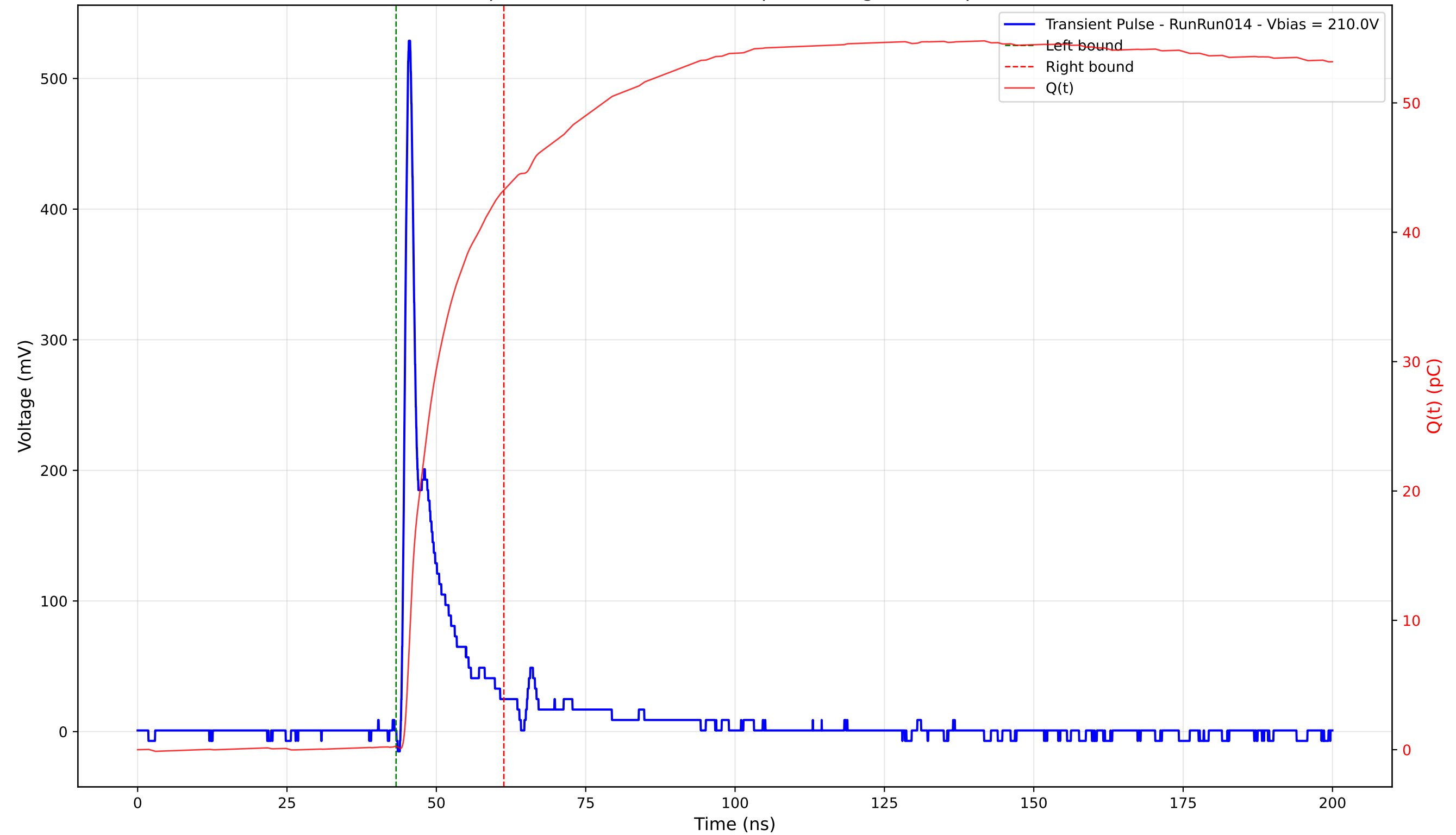
Transient Pulse - Sample: 4003 - Position: 130.0 \mu\text{m} - Charge: 43.00 pC - Rise Time: 0.90 ns
