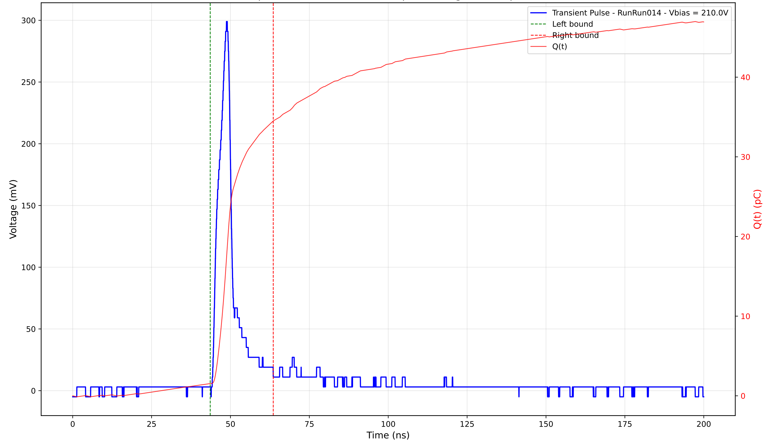
Transient Pulse - Sample: 4003 - Position: 330.0 \mu\text{m} - Charge: 32.97 pC - Rise Time: 3.59 ns
