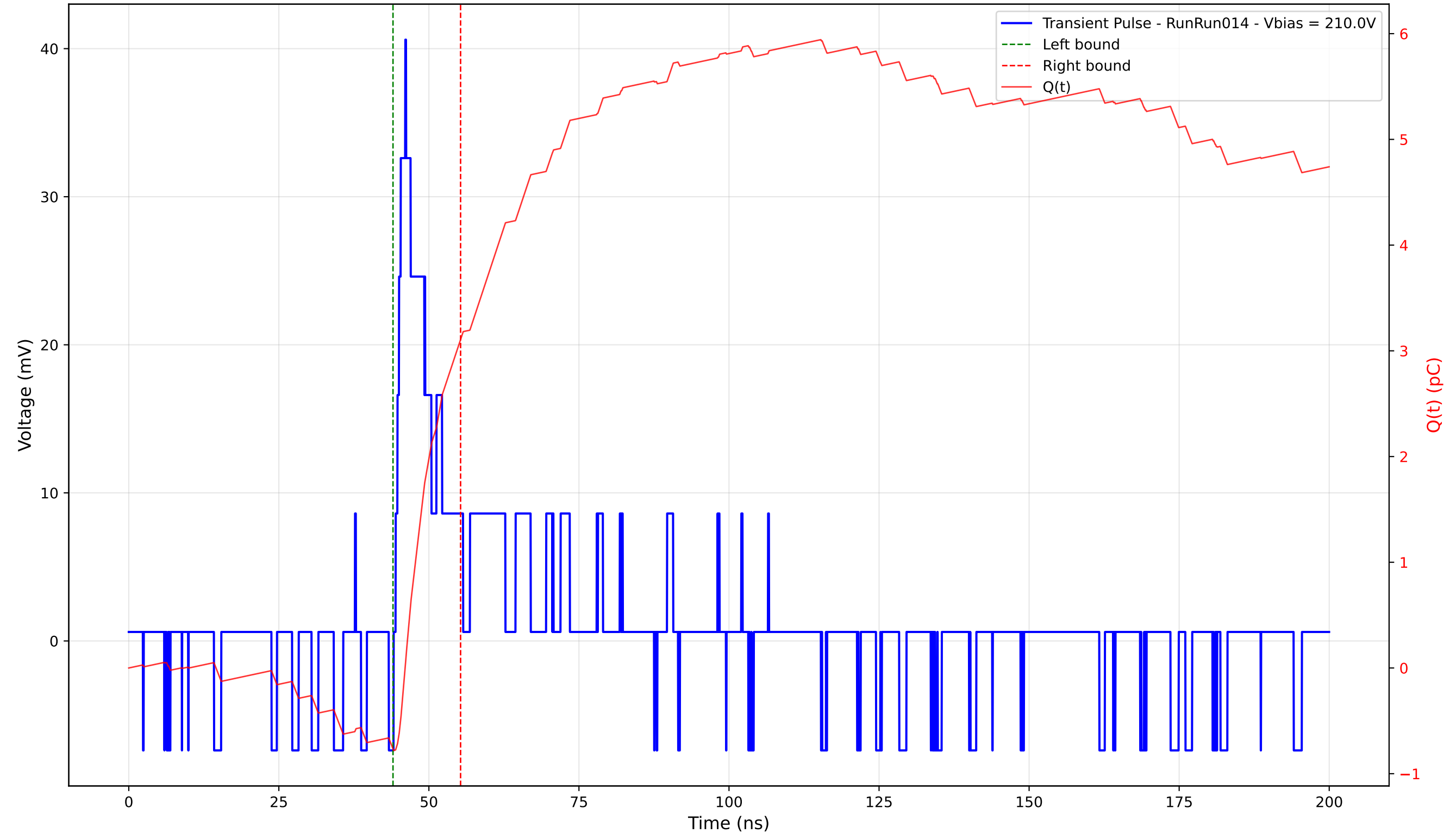
Transient Pulse - Sample: 4003 - Position: 60.0 \mu\text{m} - Charge: 3.88 pC - Rise Time: 1.61 ns
