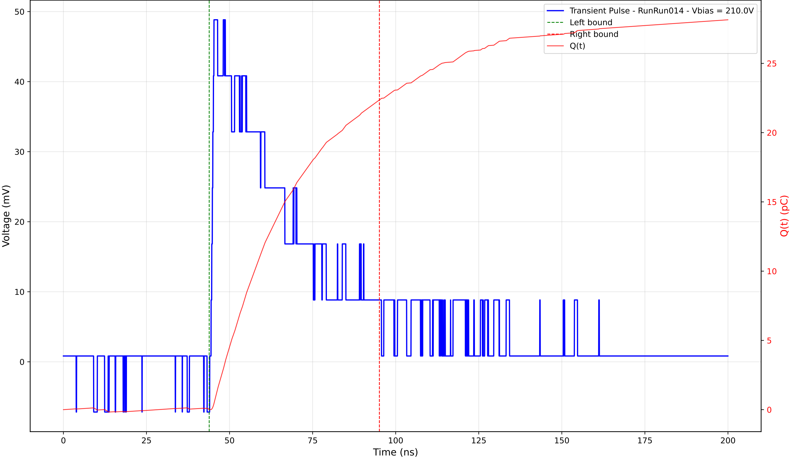
Transient Pulse - Sample: 4003 - Position: 355.0 \mu\text{m} - Charge: 22.36 pC - Rise Time: 0.87 ns
