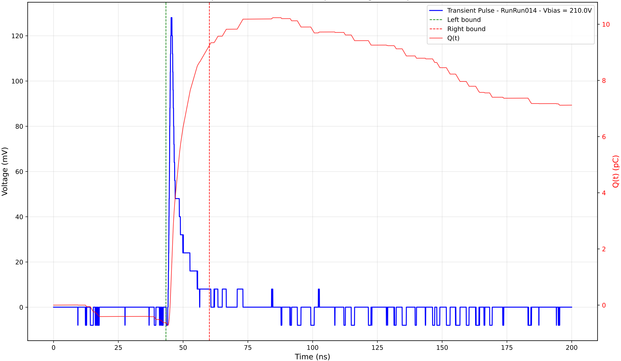
Transient Pulse - Sample: 4003 - Position: 90.0 \mu\text{m} - Charge: 9.87 pC - Rise Time: 0.91 ns
