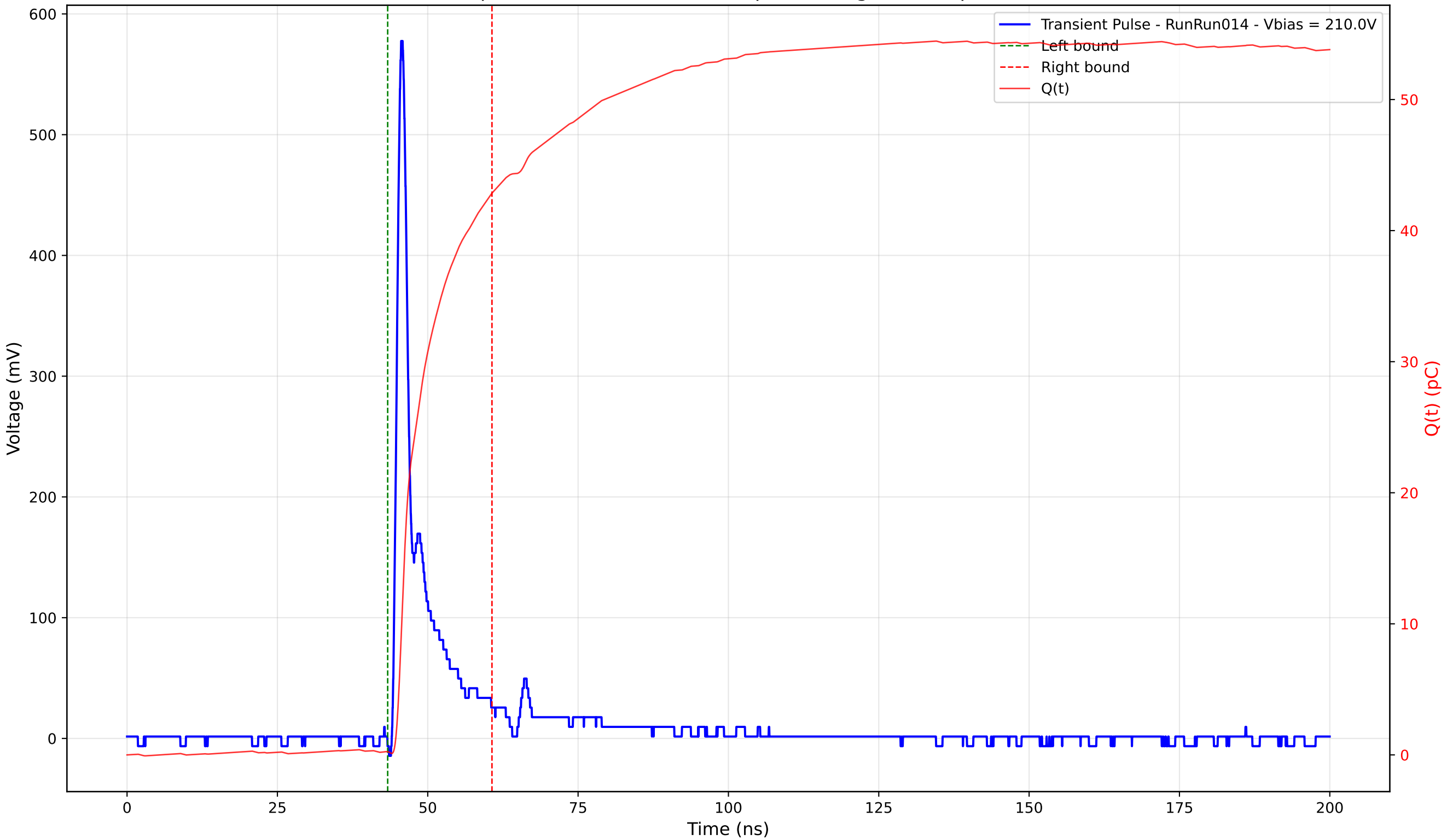
Transient Pulse - Sample: 4003 - Position: 185.0 \mu\text{m} - Charge: 42.61 pC - Rise Time: 1.02 ns
