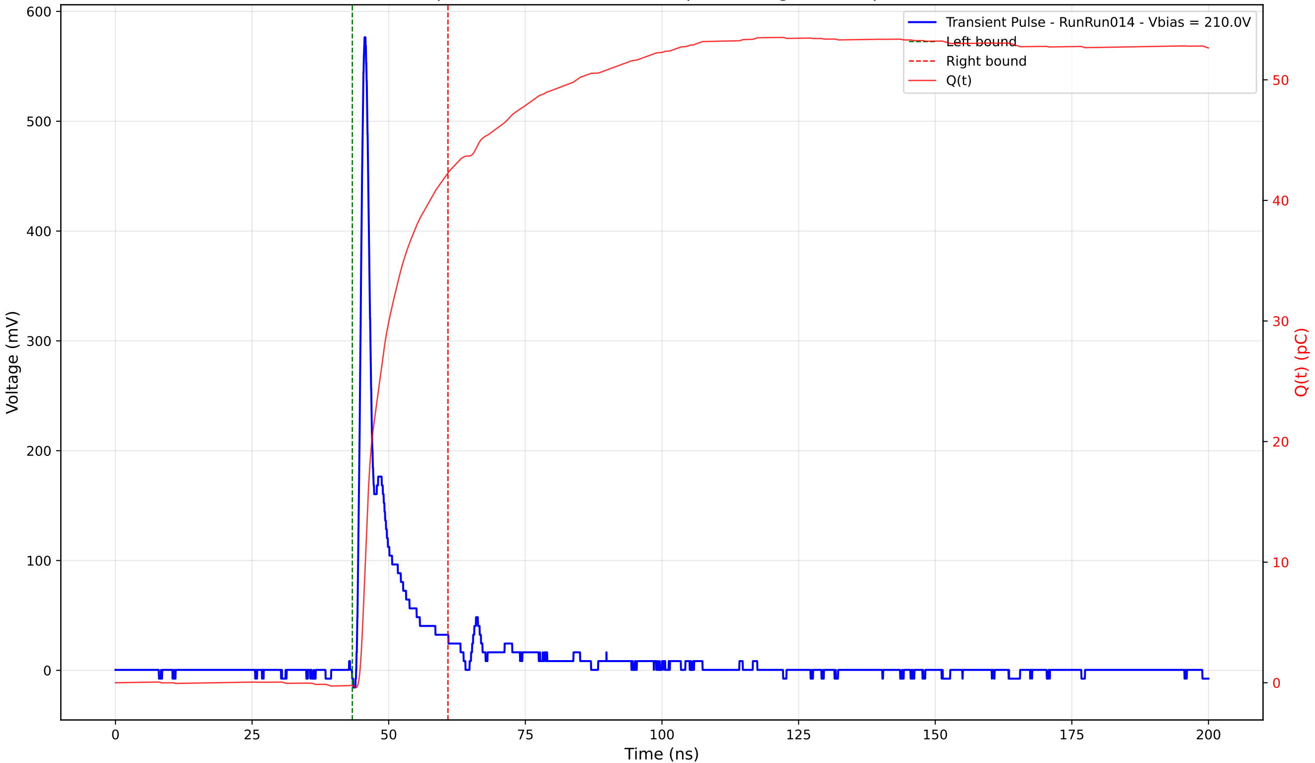
Transient Pulse - Sample: 4003 - Position: 175.0 \mu\text{m} - Charge: 42.52 pC - Rise Time: 0.99 ns
