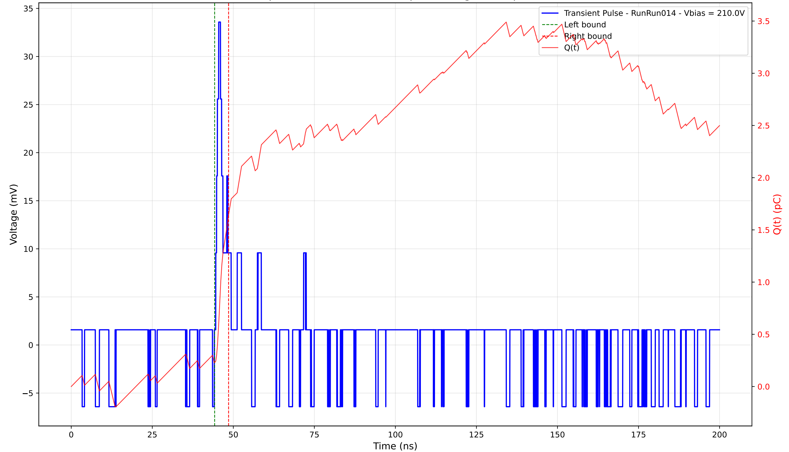
Transient Pulse - Sample: 4003 - Position: 30.0 \mu\text{m} - Charge: 1.41 pC - Rise Time: 0.92 ns
