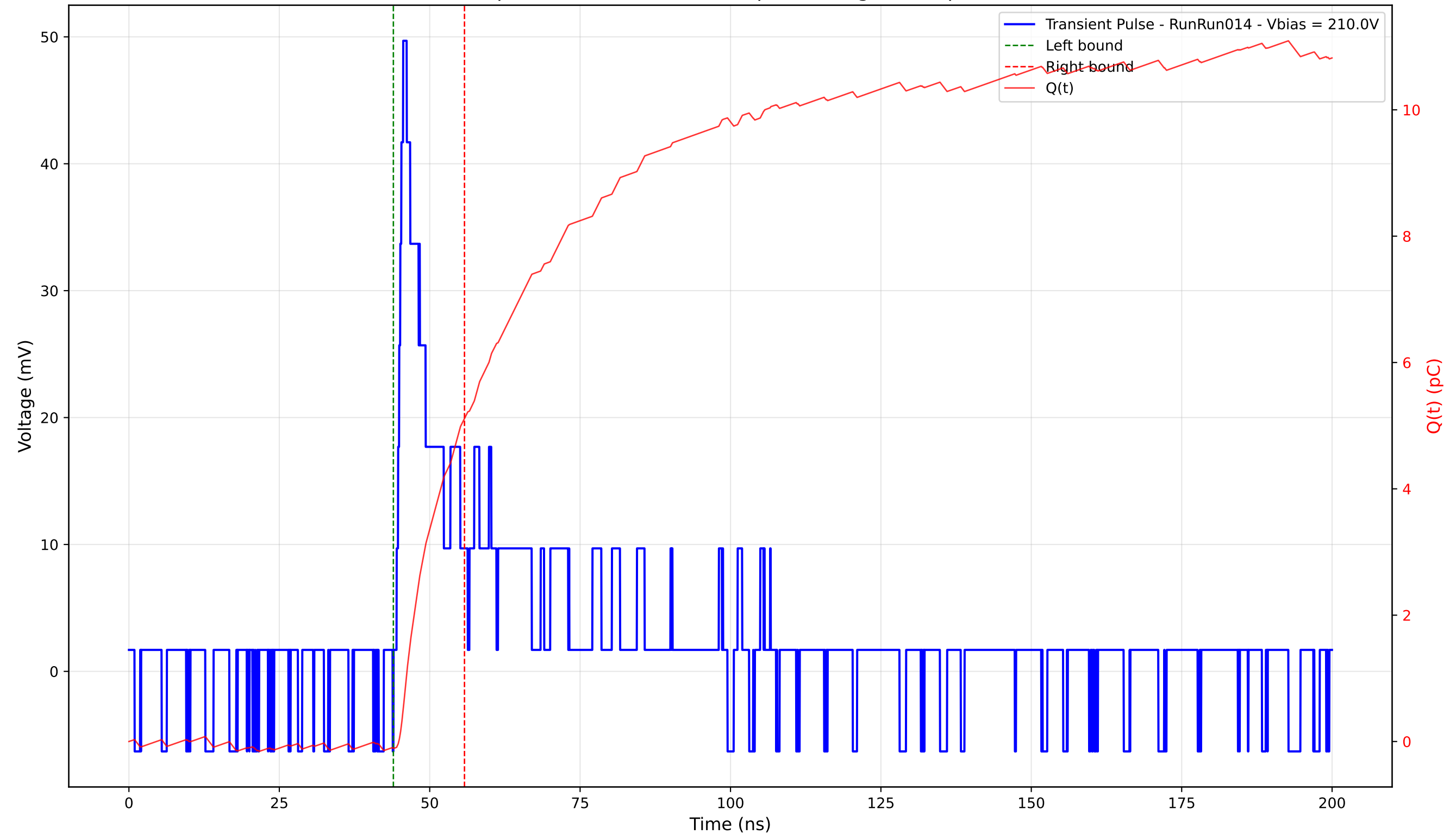
Transient Pulse - Sample: 4003 - Position: 55.0 \mu\text{m} - Charge: 5.23 pC - Rise Time: 1.09 ns
