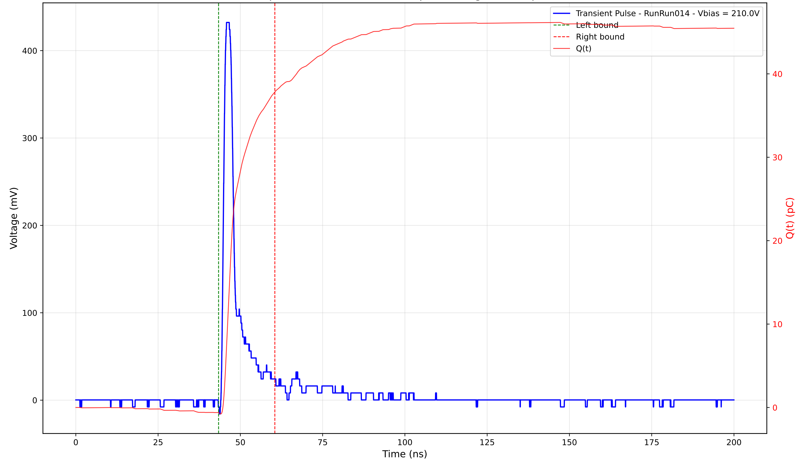
Transient Pulse - Sample: 4003 - Position: 255.0 \mu\text{m} - Charge: 38.45 pC - Rise Time: 1.11 ns
