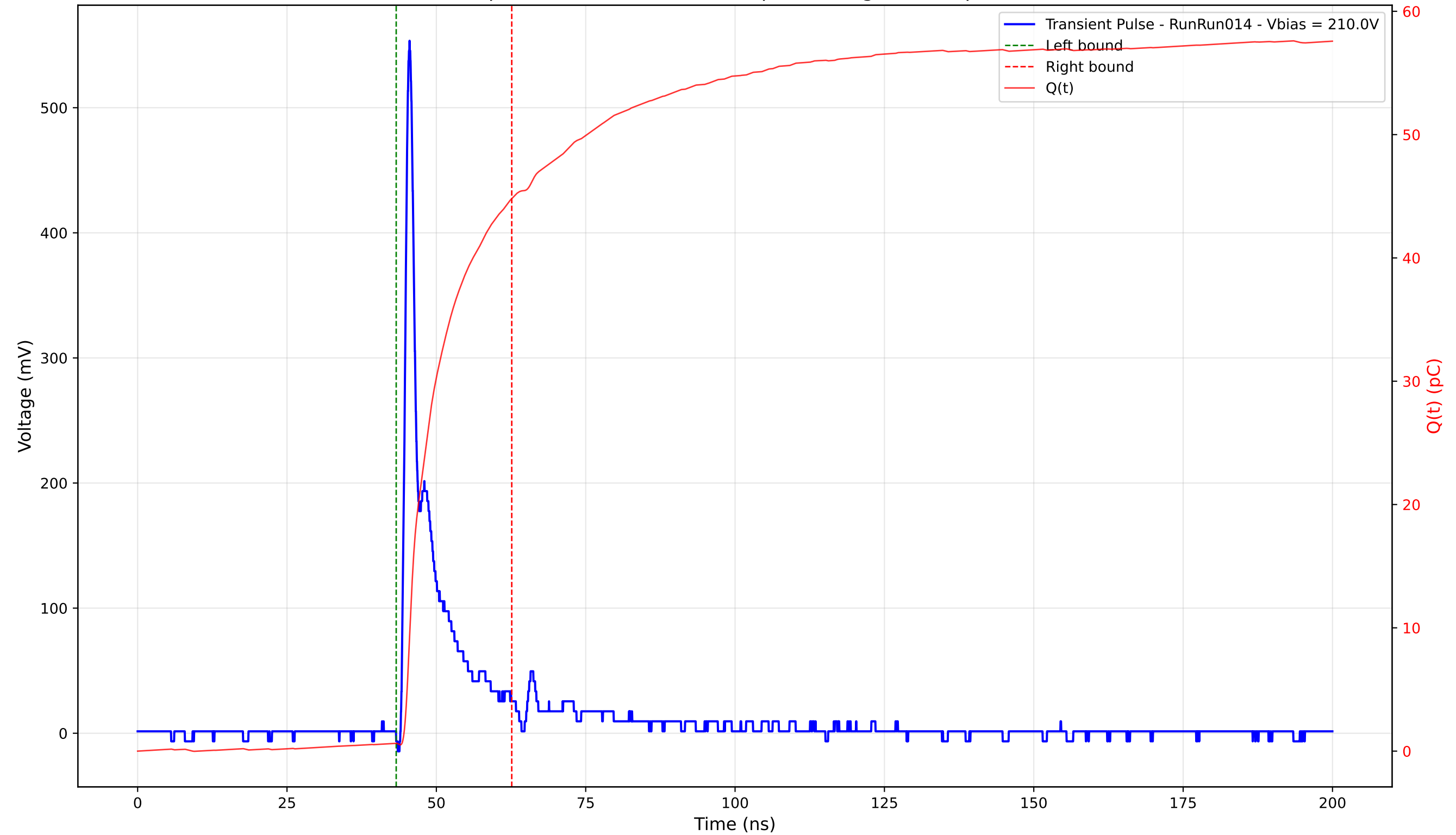
Transient Pulse - Sample: 4003 - Position: 140.0 \mu\text{m} - Charge: 44.17 pC - Rise Time: 0.95 ns
