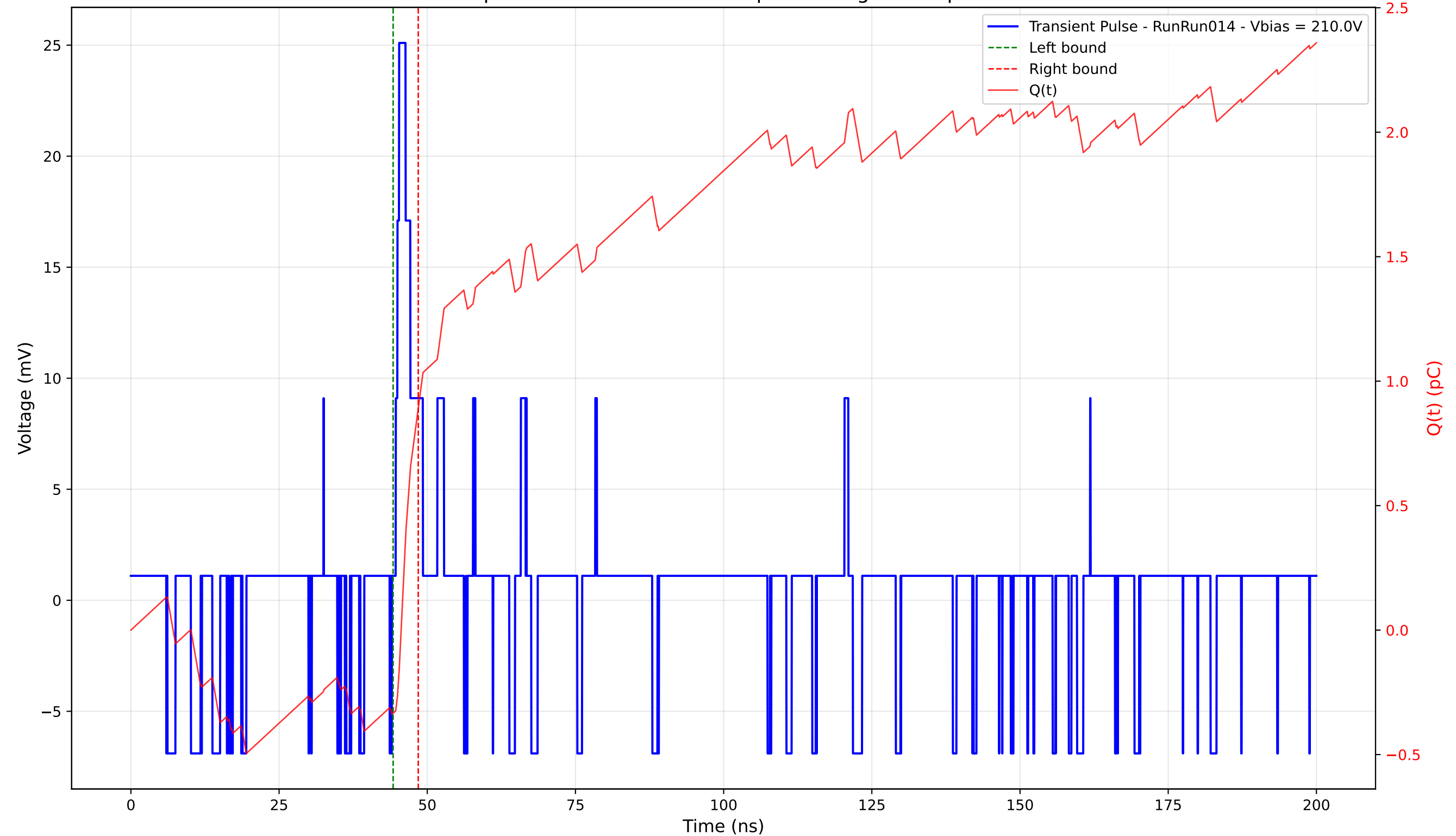
Transient Pulse - Sample: 4003 - Position: 415.0 \mu\text{m} - Charge: 1.23 pC - Rise Time: 0.58 ns
