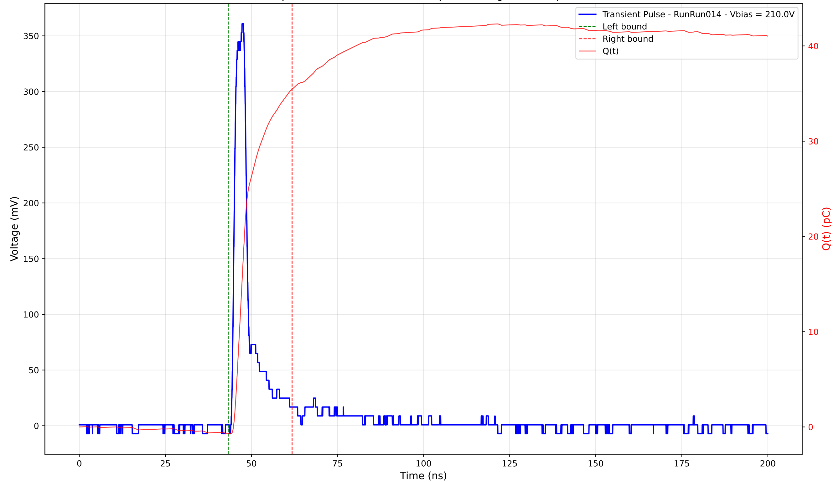
Transient Pulse - Sample: 4003 - Position: 290.0 \mu\text{m} - Charge: 36.11 pC - Rise Time: 1.33 ns
