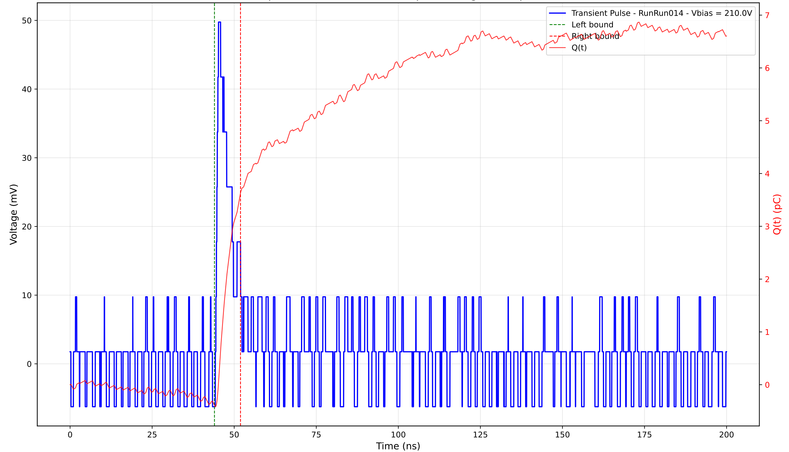
Transient Pulse - Sample: 4003 - Position: 405.0 \mu\text{m} - Charge: 4.02 pC - Rise Time: 0.79 ns
