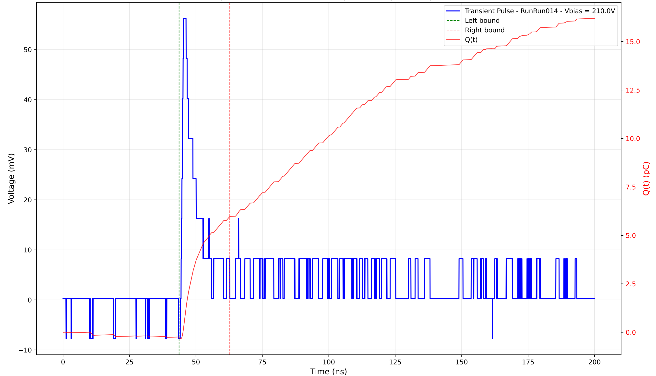
Transient Pulse - Sample: 4003 - Position: 380.0 \mu\text{m} - Charge: 6.25 pC - Rise Time: 0.93 ns
