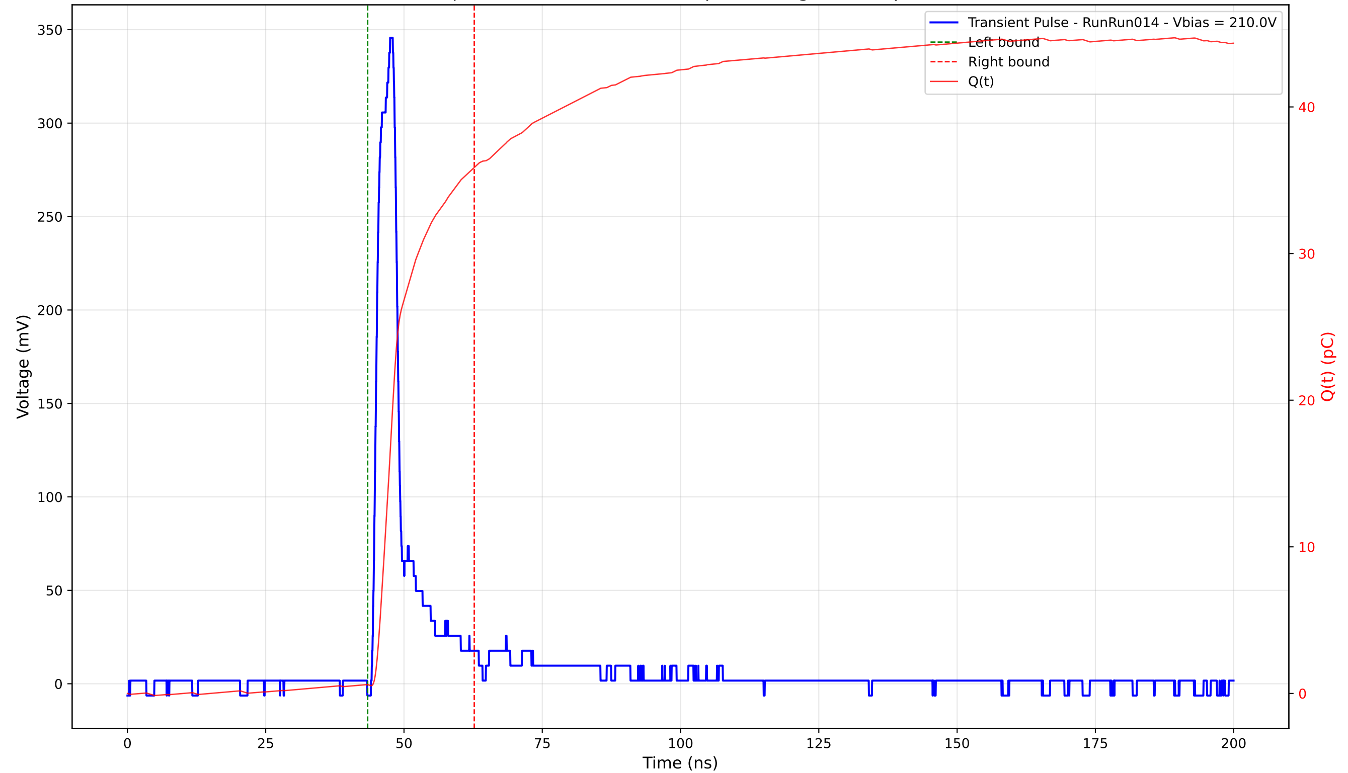
Transient Pulse - Sample: 4003 - Position: 300.0 \mu\text{m} - Charge: 35.28 pC - Rise Time: 2.30 ns
