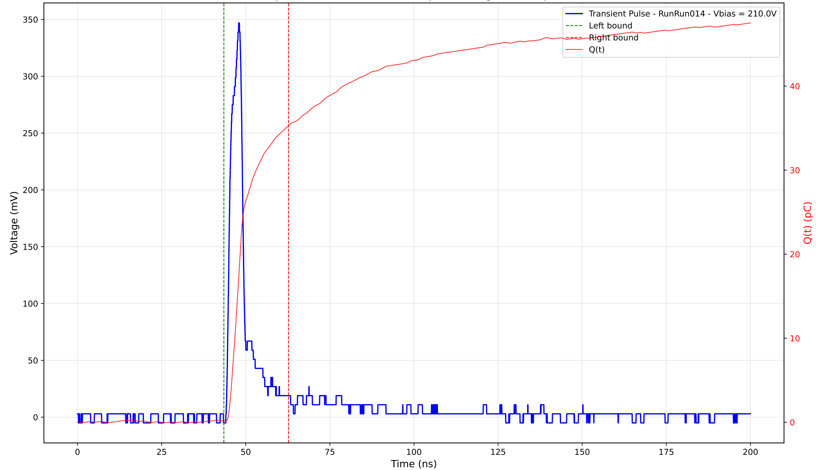
Transient Pulse - Sample: 4003 - Position: 310.0 \mu\text{m} - Charge: 35.13 pC - Rise Time: 2.82 ns
