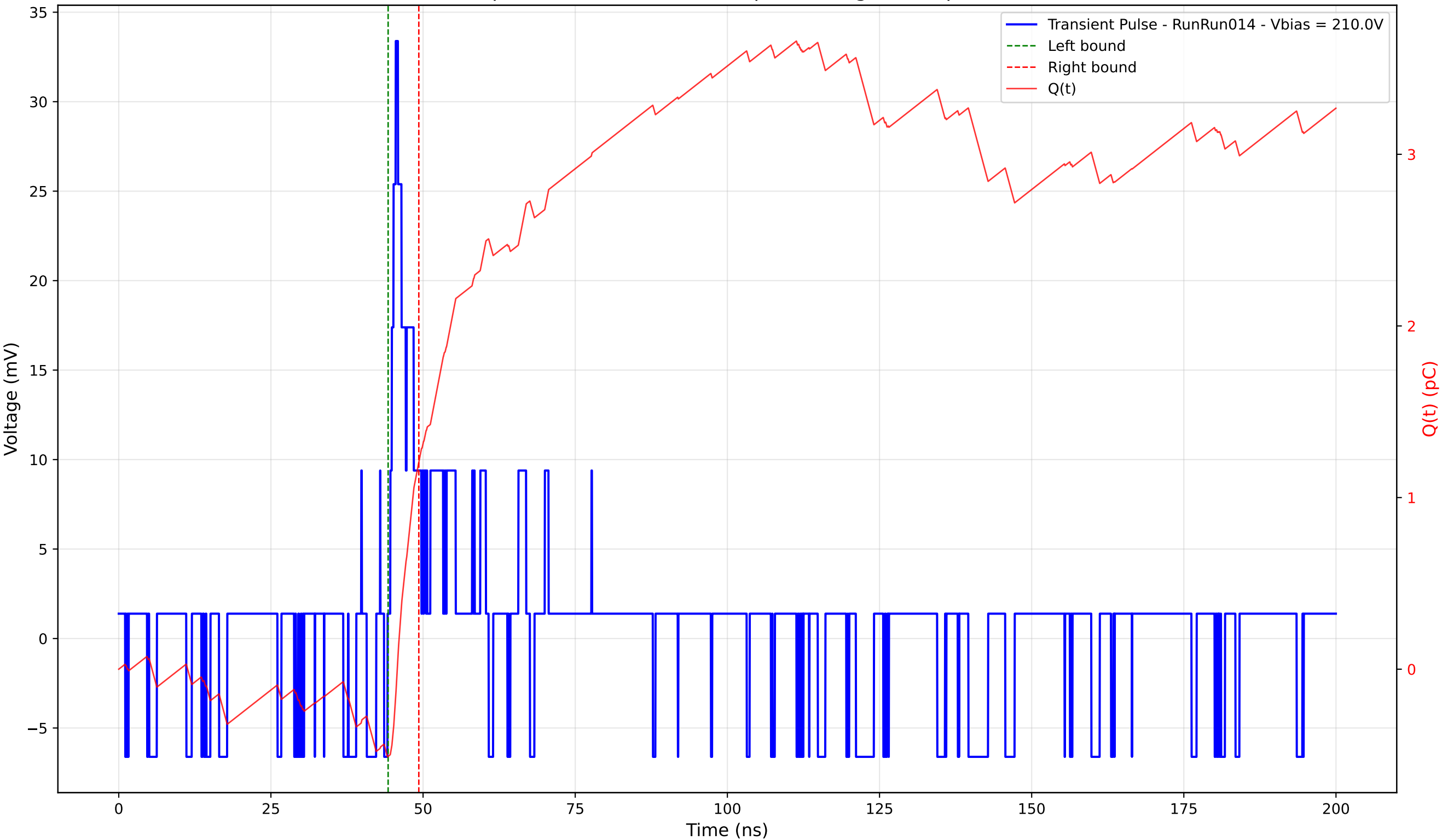
Transient Pulse - Sample: 4003 - Position: 40.0 \mu\text{m} - Charge: 1.72 pC - Rise Time: 0.90 ns
