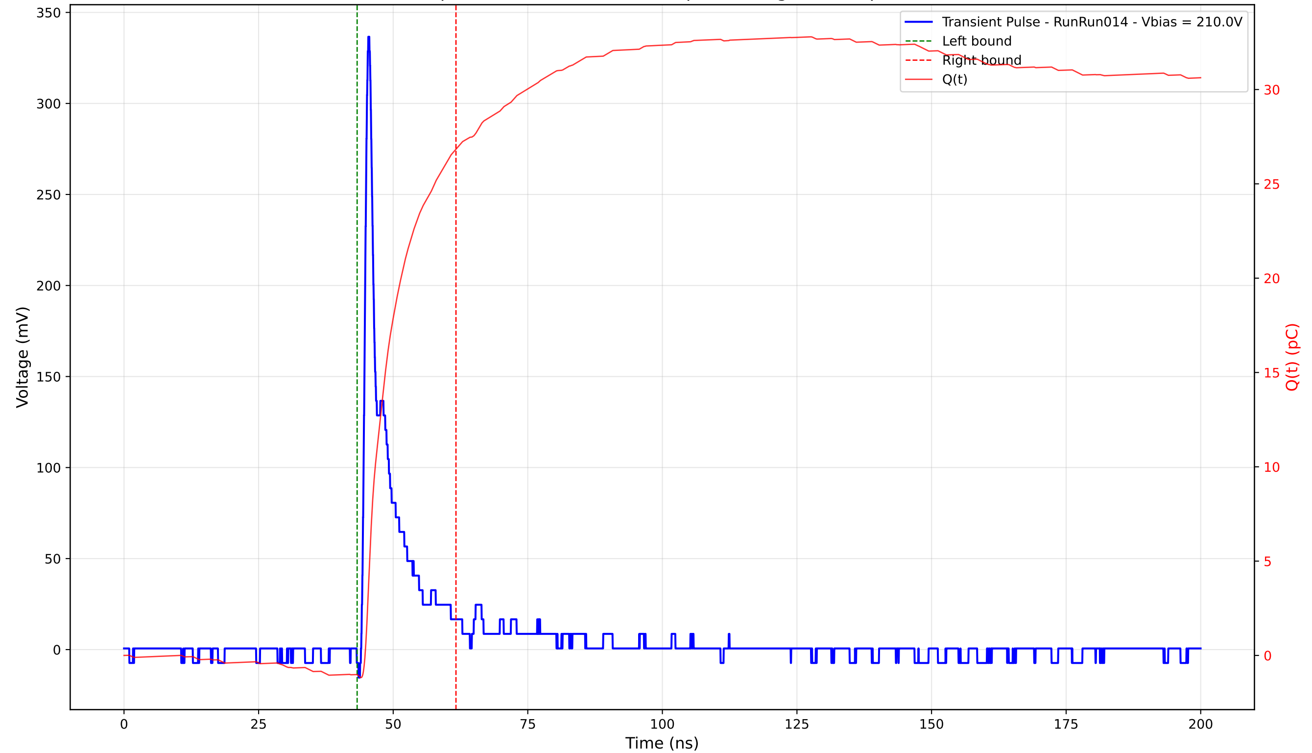
Transient Pulse - Sample: 4003 - Position: 105.0 \mu\text{m} - Charge: 27.86 pC - Rise Time: 0.88 ns
