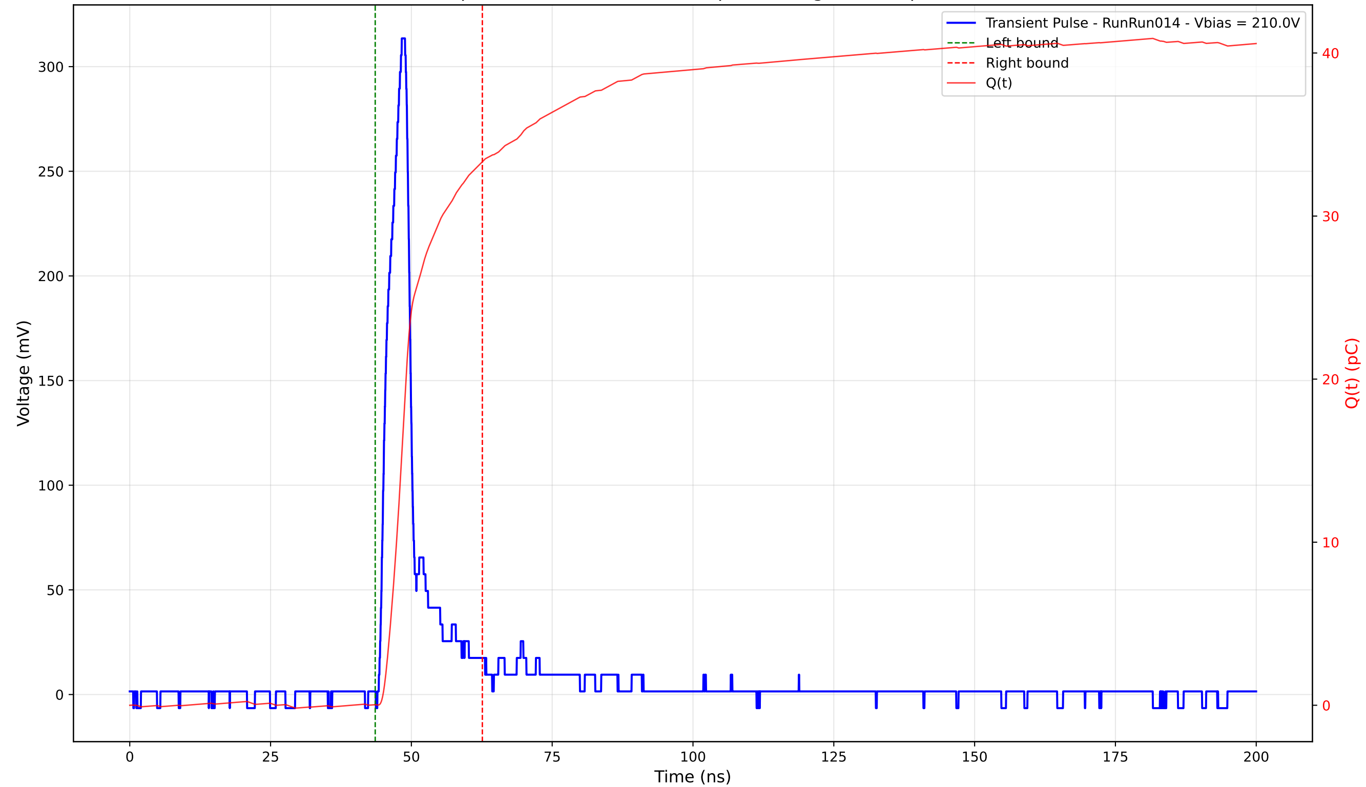
Transient Pulse - Sample: 4003 - Position: 325.0 \mu\text{m} - Charge: 33.30 pC - Rise Time: 3.29 ns
