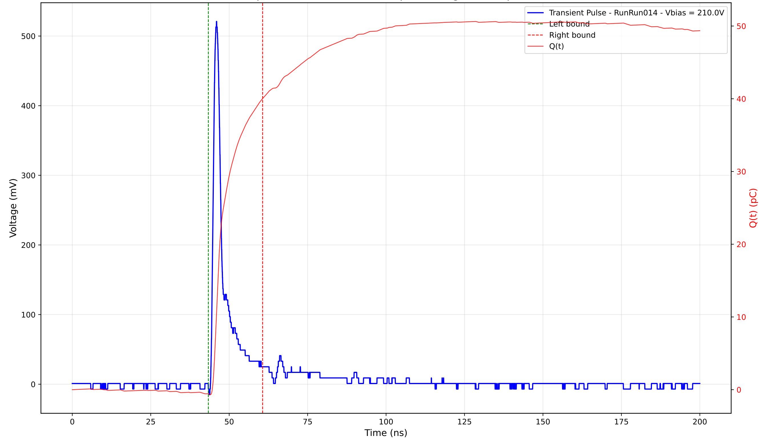
Transient Pulse - Sample: 4003 - Position: 225.0 \mu\text{m} - Charge: 40.58 pC - Rise Time: 1.15 ns
