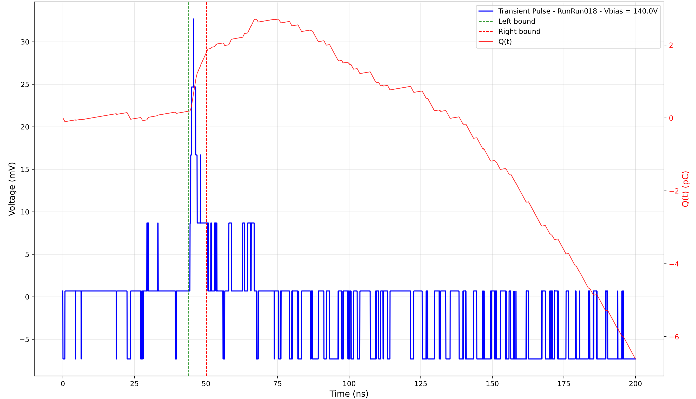
Transient Pulse - Sample: 4003 - Position: 35.0 \mu\text{m} - Charge: 1.62 pC - Rise Time: 1.21 ns
