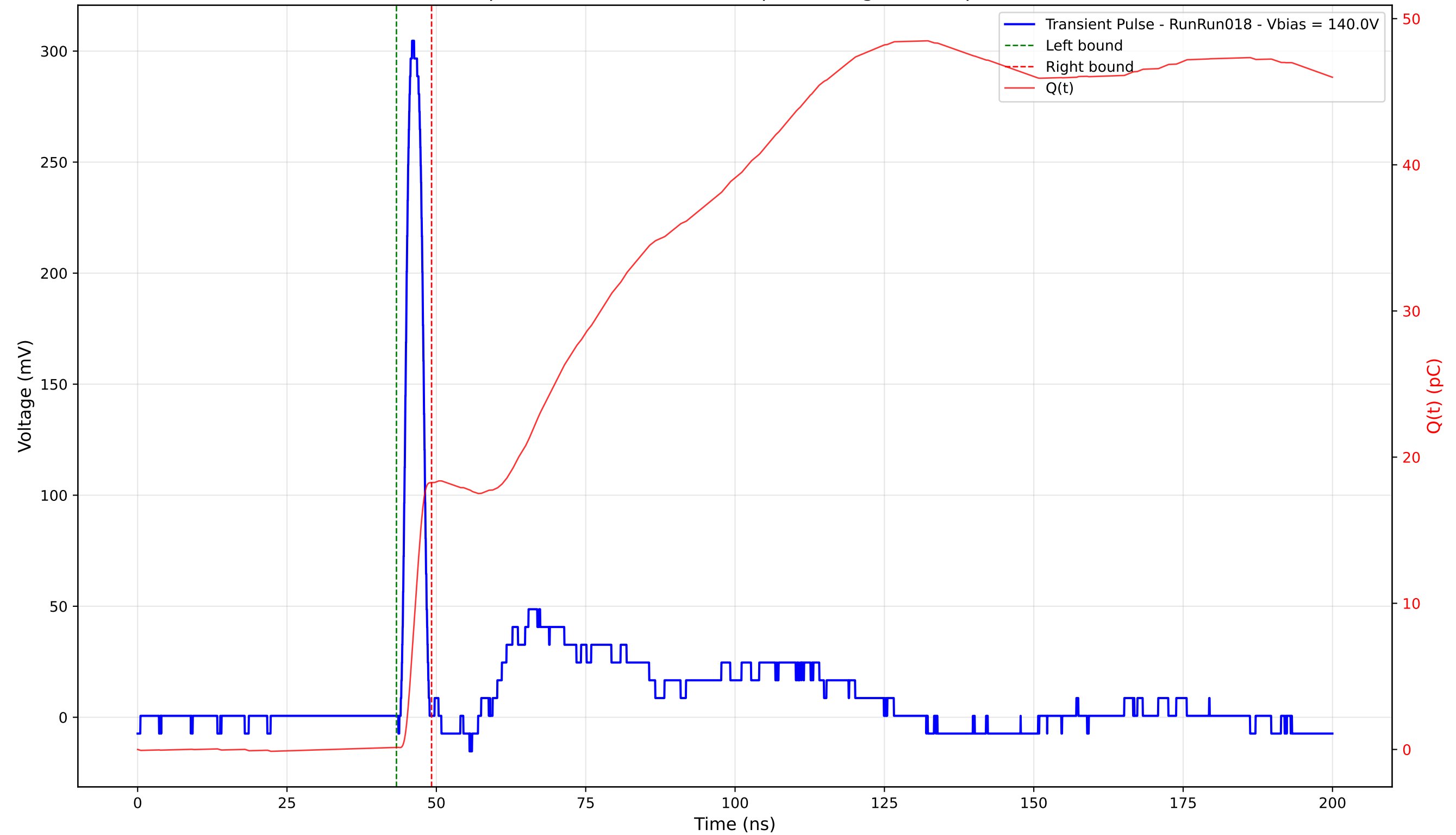
Transient Pulse - Sample: 4003 - Position: 240.0 \mu\text{m} - Charge: 18.11 pC - Rise Time: 1.23 ns
