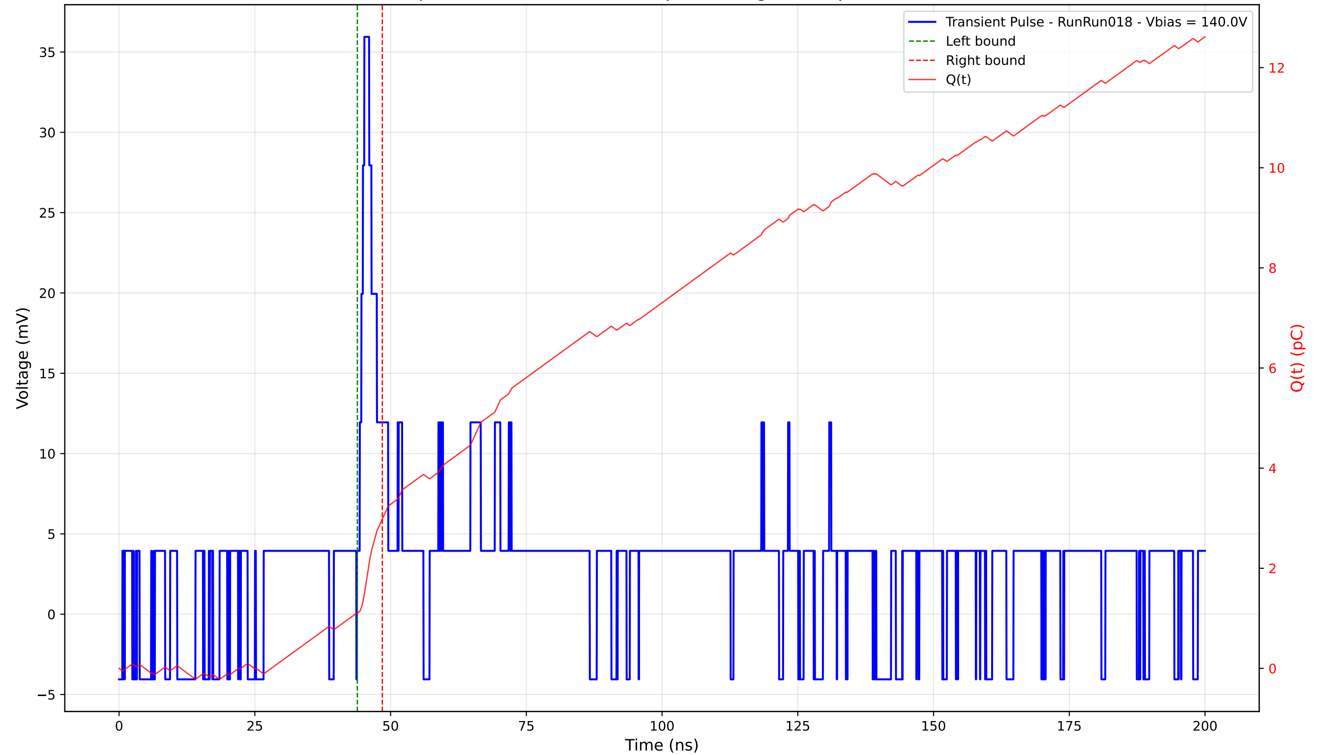
Transient Pulse - Sample: 4003 - Position: 365.0 \mu\text{m} - Charge: 1.88 pC - Rise Time: 0.00 ns (N/A)
