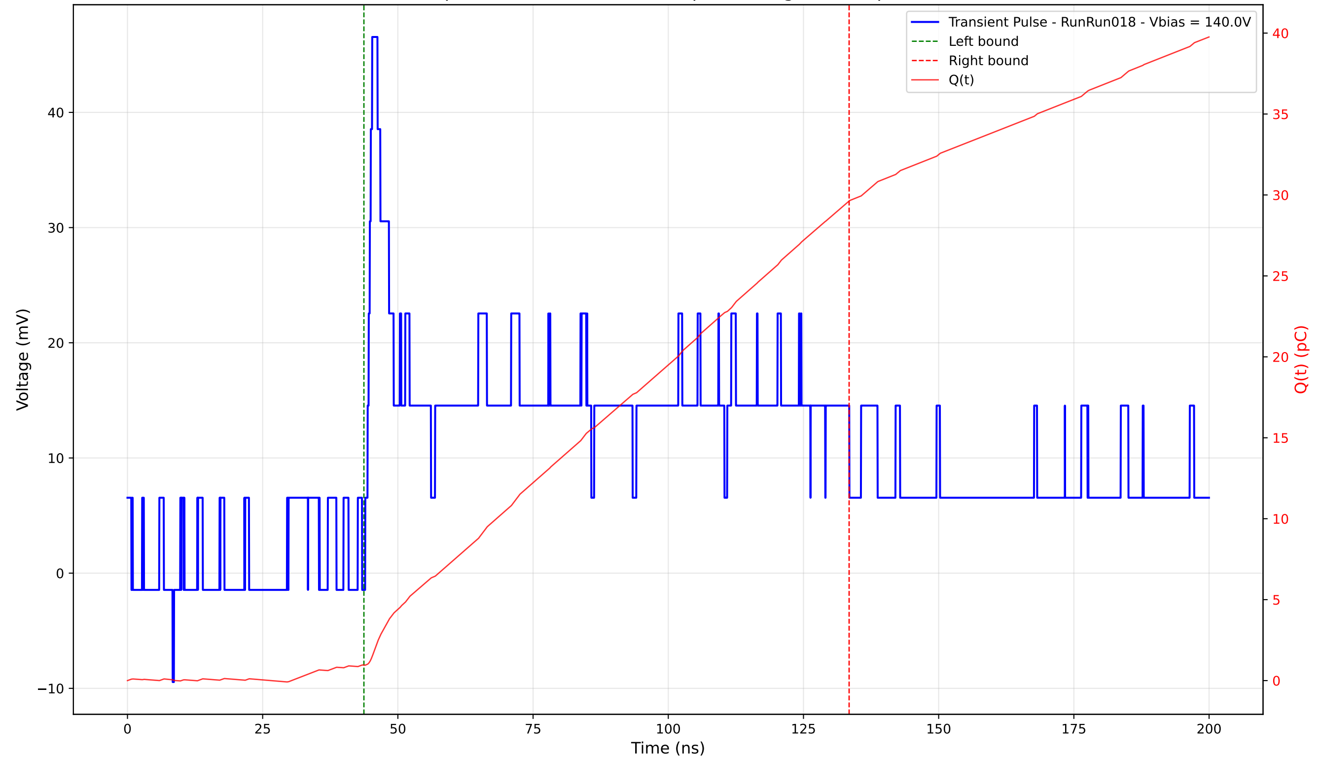
Transient Pulse - Sample: 4003 - Position: 305.0 \mu\text{m} - Charge: 28.68 pC - Rise Time: 1.29 ns
