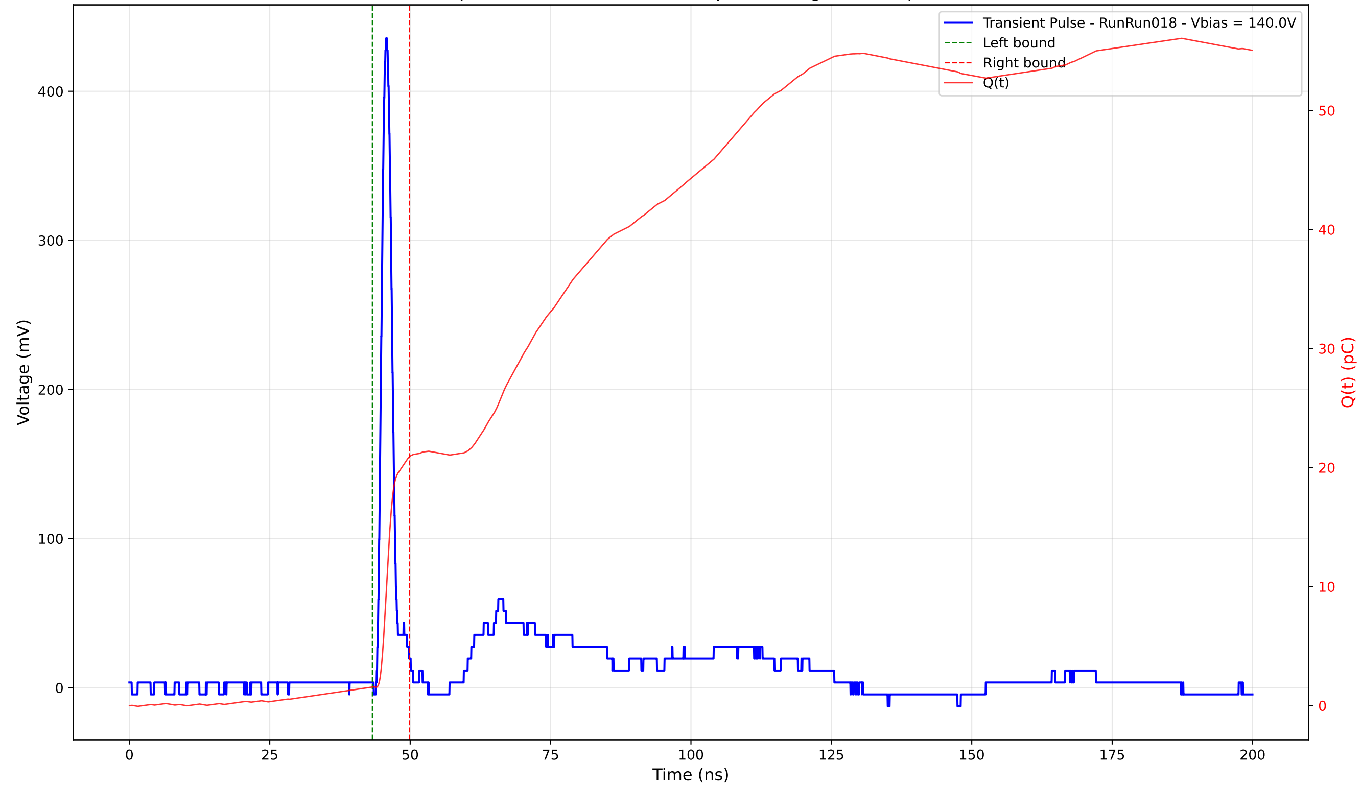
Transient Pulse - Sample: 4003 - Position: 195.0 \mu\text{m} - Charge: 19.35 pC - Rise Time: 1.10 ns
