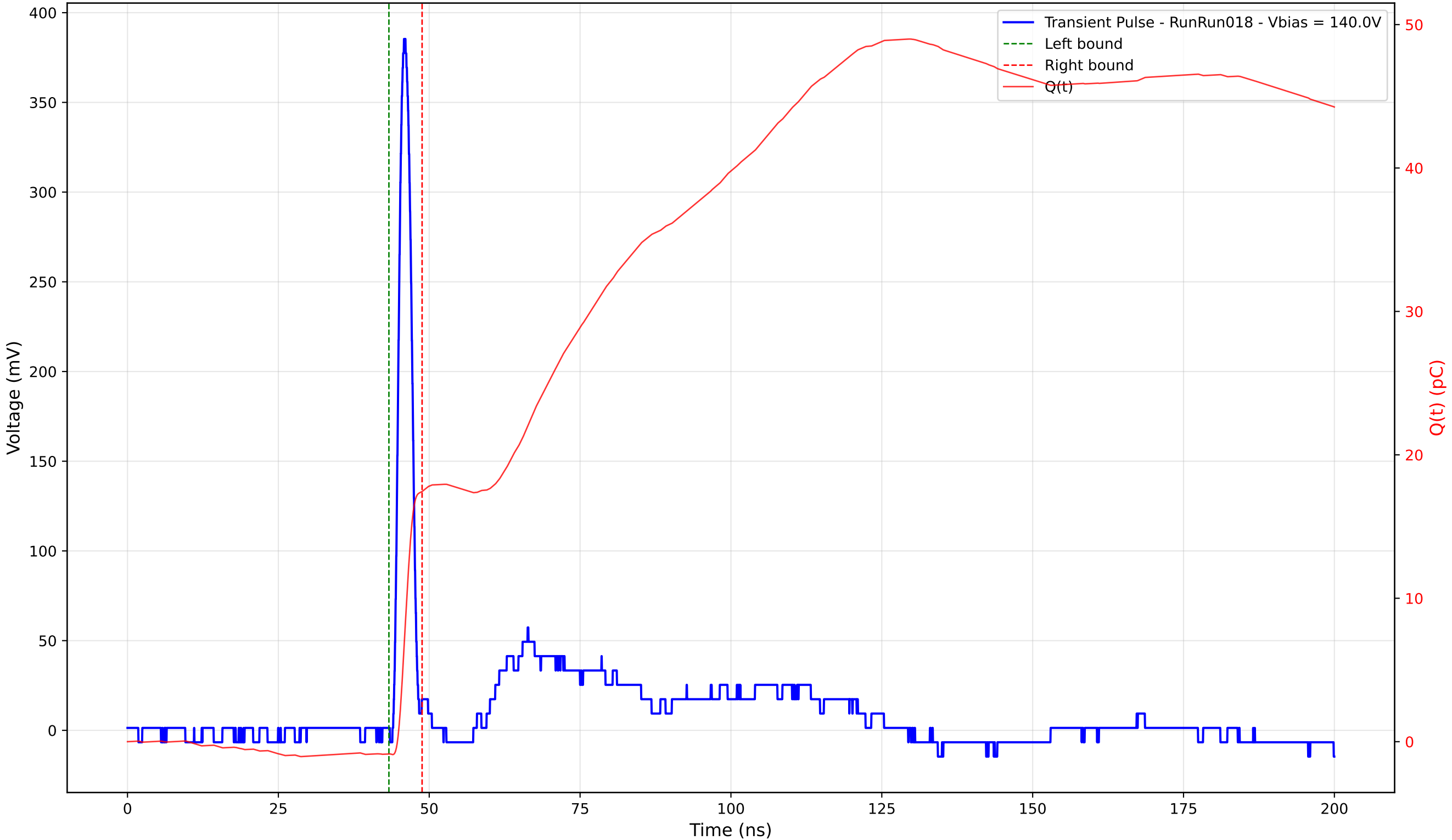
Transient Pulse - Sample: 4003 - Position: 215.0 \mu\text{m} - Charge: 18.29 pC - Rise Time: 1.17 ns
