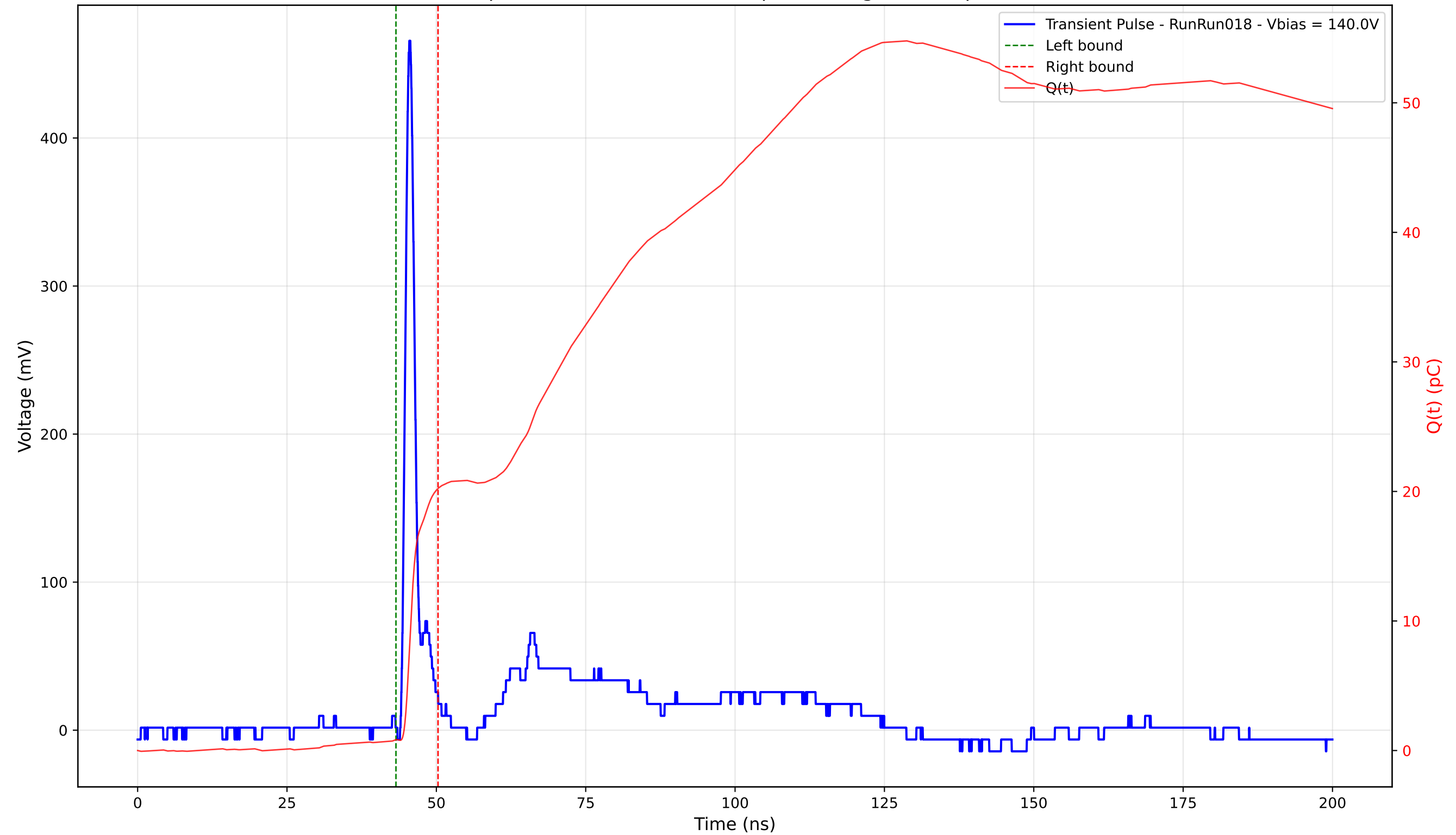
Transient Pulse - Sample: 4003 - Position: 155.0 \mu\text{m} - Charge: 19.40 pC - Rise Time: 0.97 ns
