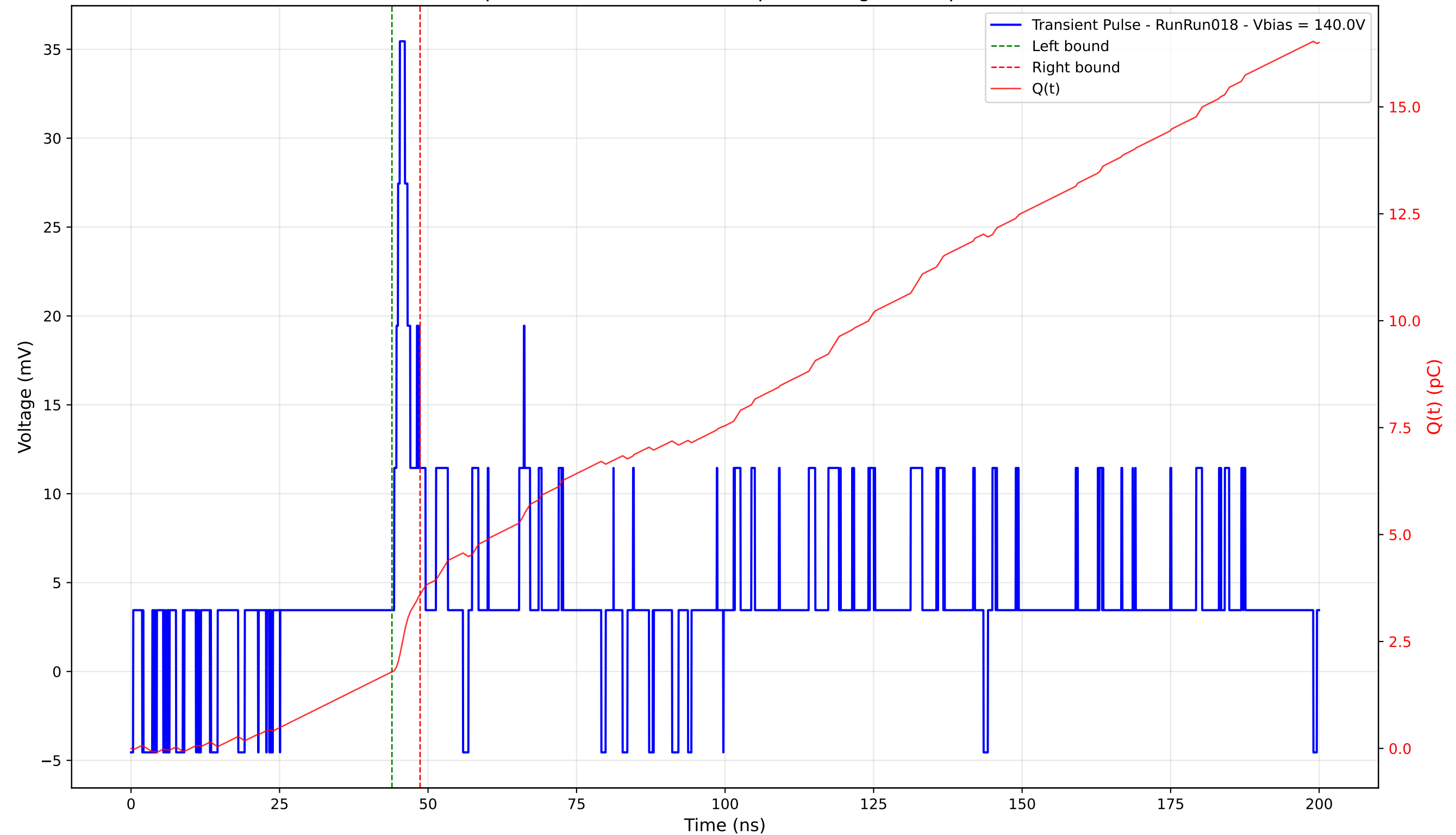
Transient Pulse - Sample: 4003 - Position: 345.0 \mu\text{m} - Charge: 1.82 pC - Rise Time: 0.96 ns
