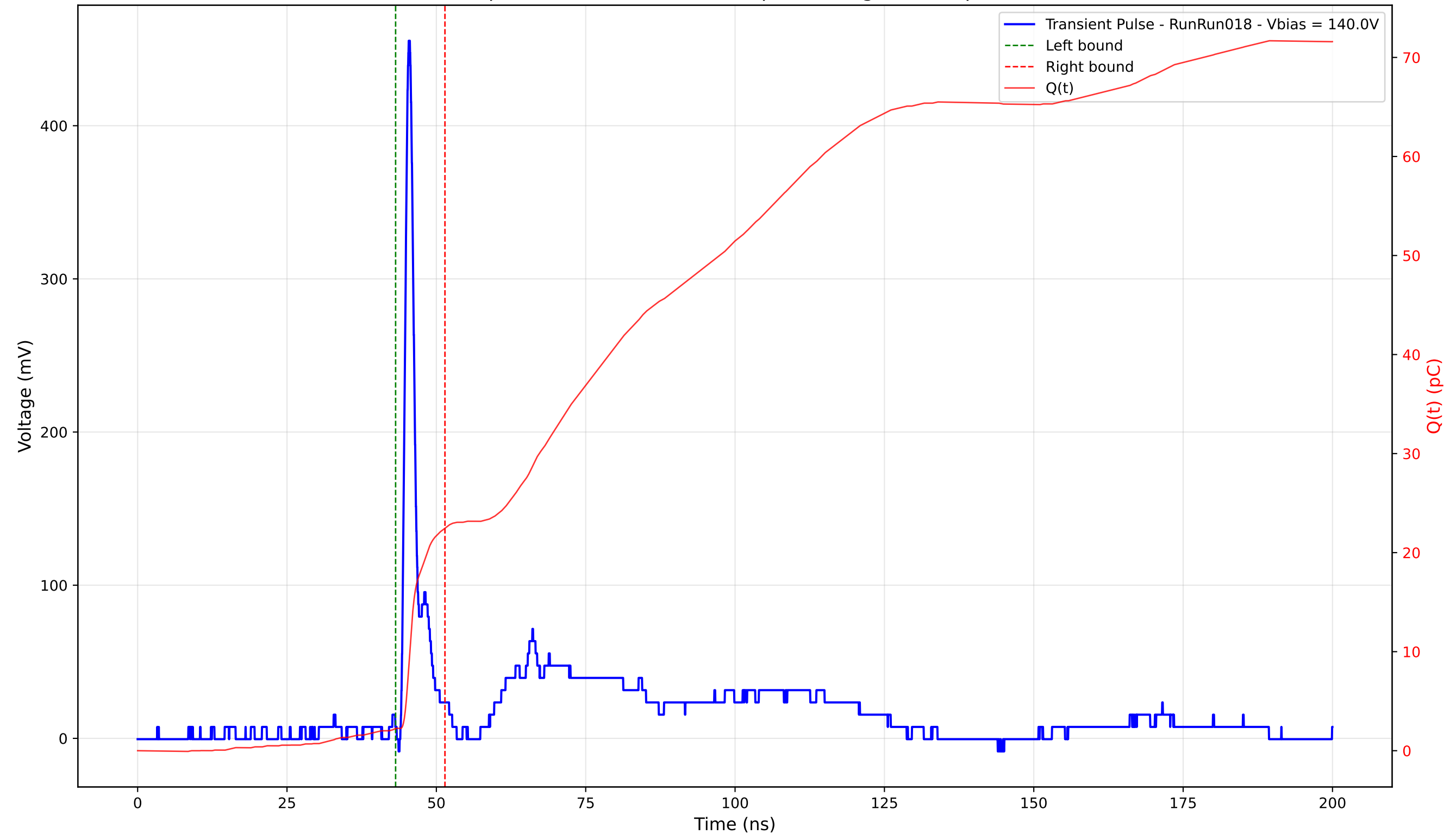
Transient Pulse - Sample: 4003 - Position: 135.0 \mu\text{m} - Charge: 20.22 pC - Rise Time: 0.91 ns
