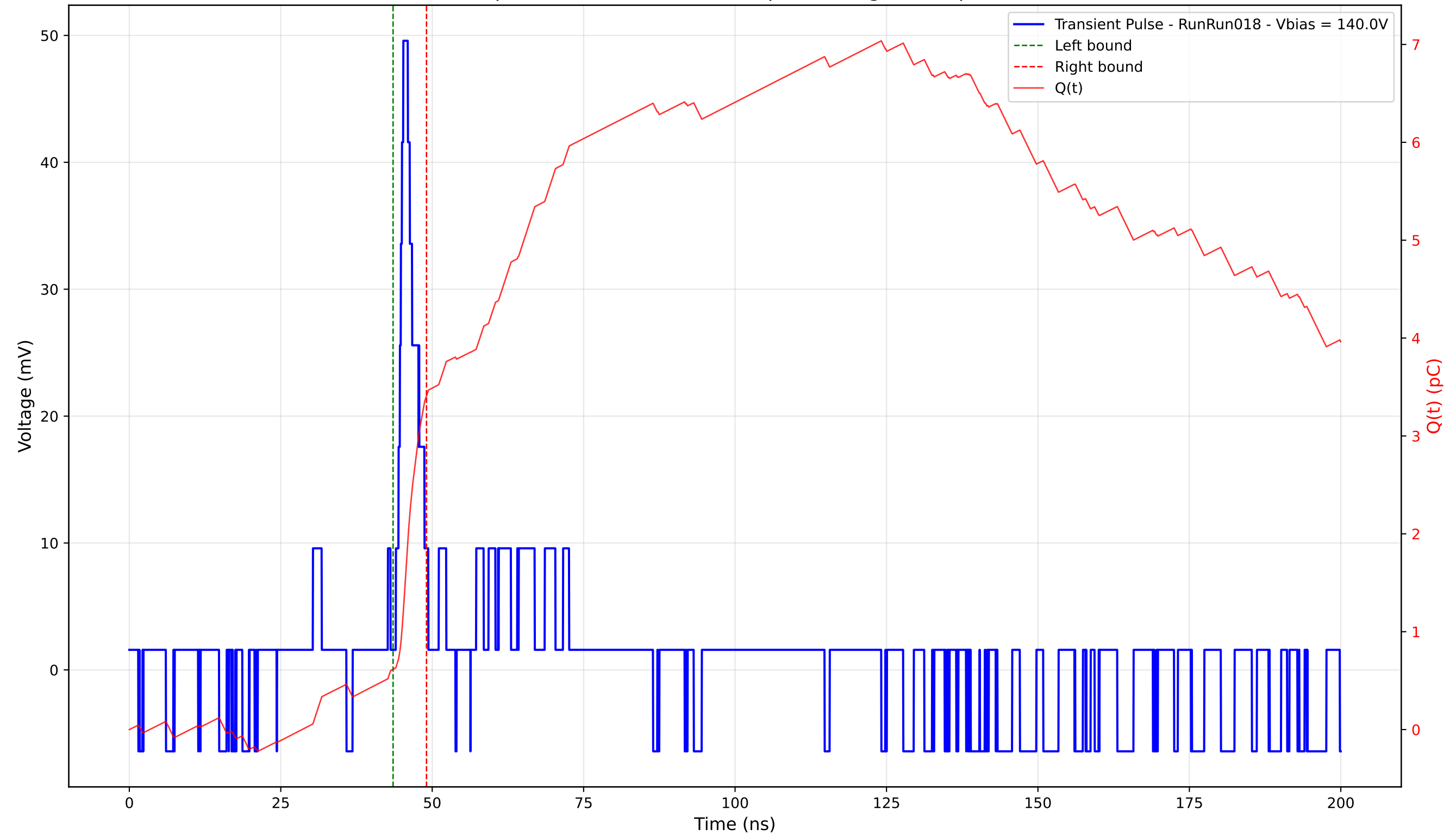
Transient Pulse - Sample: 4003 - Position: 390.0 \mu\text{m} - Charge: 2.80 pC - Rise Time: 1.23 ns
