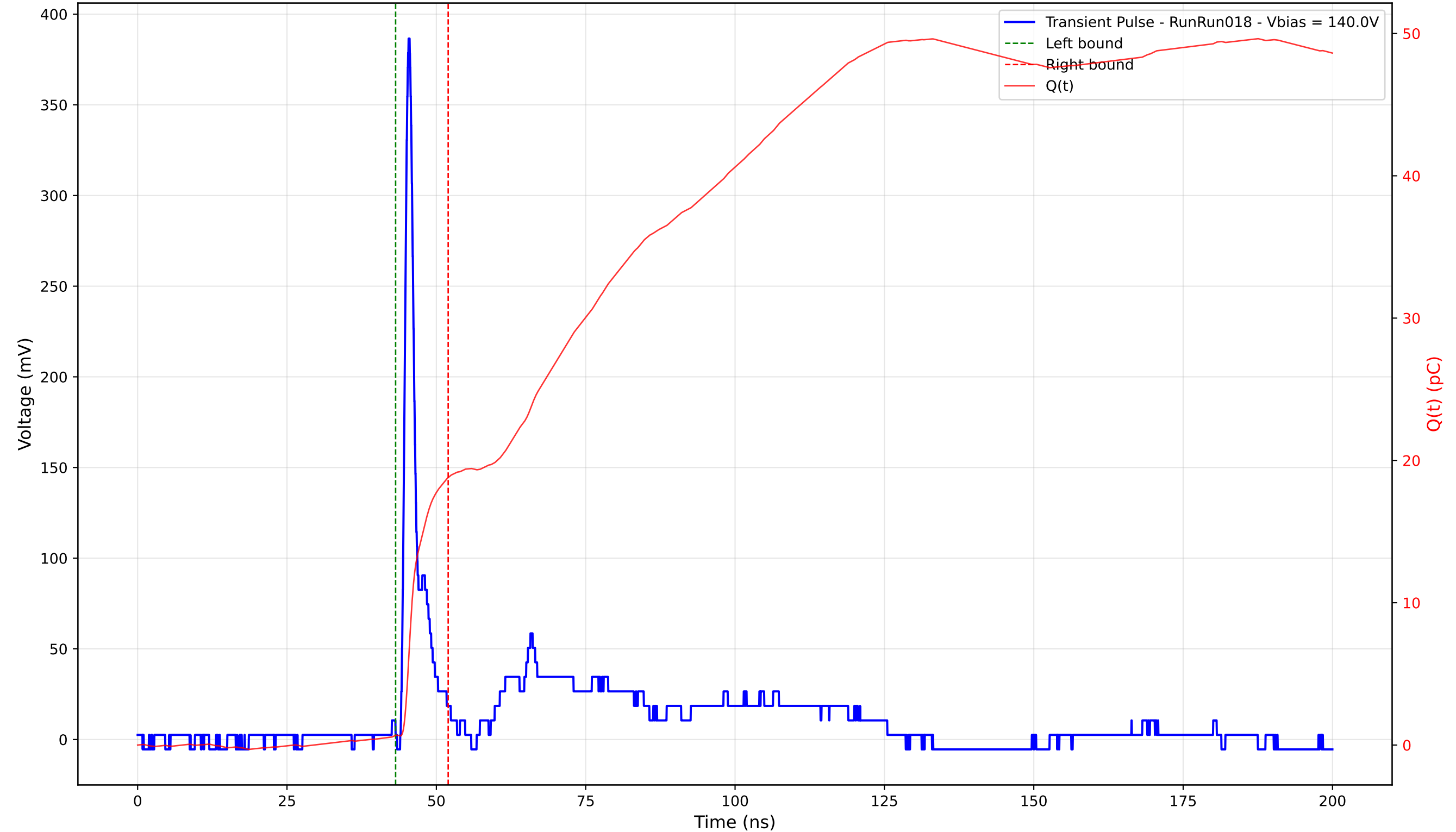
Transient Pulse - Sample: 4003 - Position: 115.0 \mu\text{m} - Charge: 18.11 pC - Rise Time: 0.93 ns
