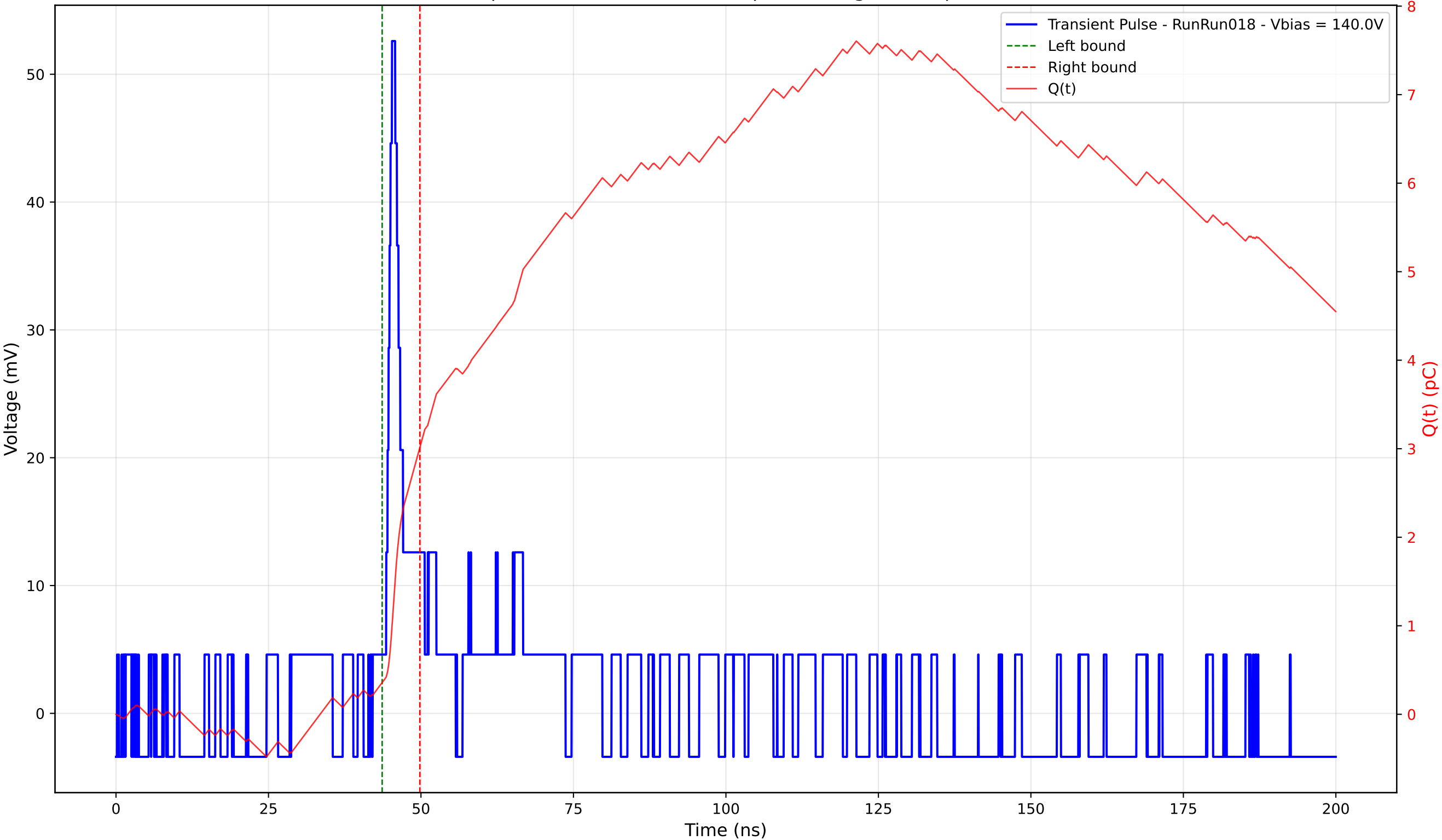
Transient Pulse - Sample: 4003 - Position: 85.0 \mu\text{m} - Charge: 2.66 pC - Rise Time: 0.96 ns
