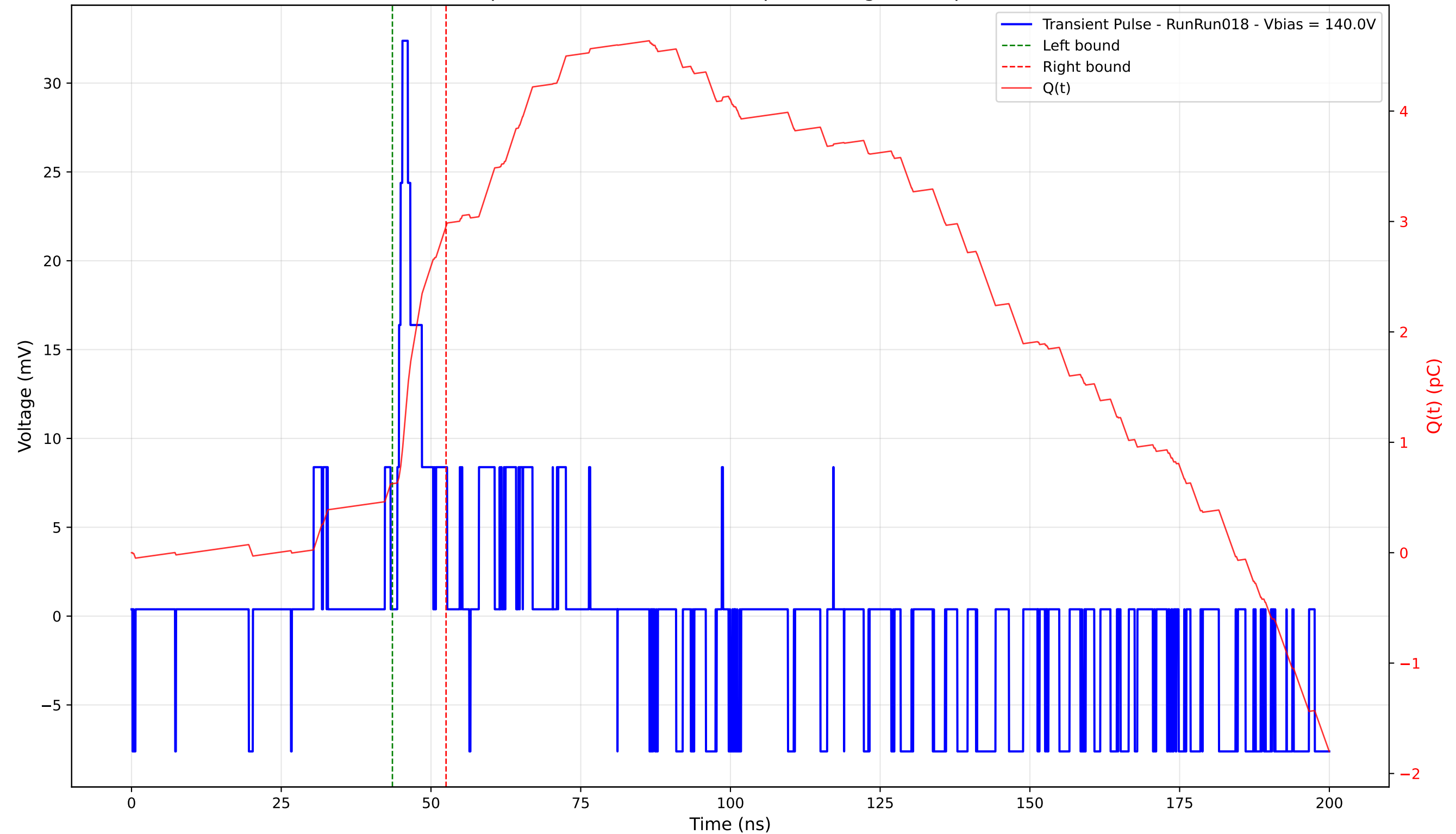
Transient Pulse - Sample: 4003 - Position: 370.0 \mu\text{m} - Charge: 2.33 pC - Rise Time: 0.85 ns
