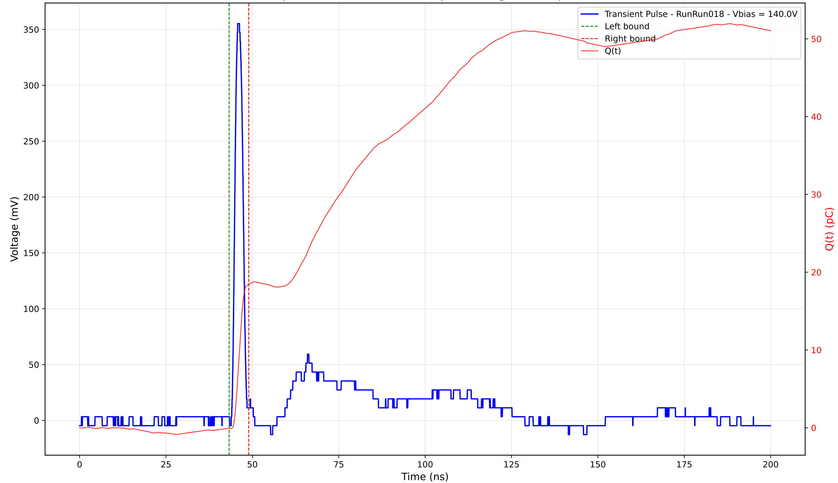
Transient Pulse - Sample: 4003 - Position: 225.0 \mu\text{m} - Charge: 18.50 pC - Rise Time: 1.16 ns
