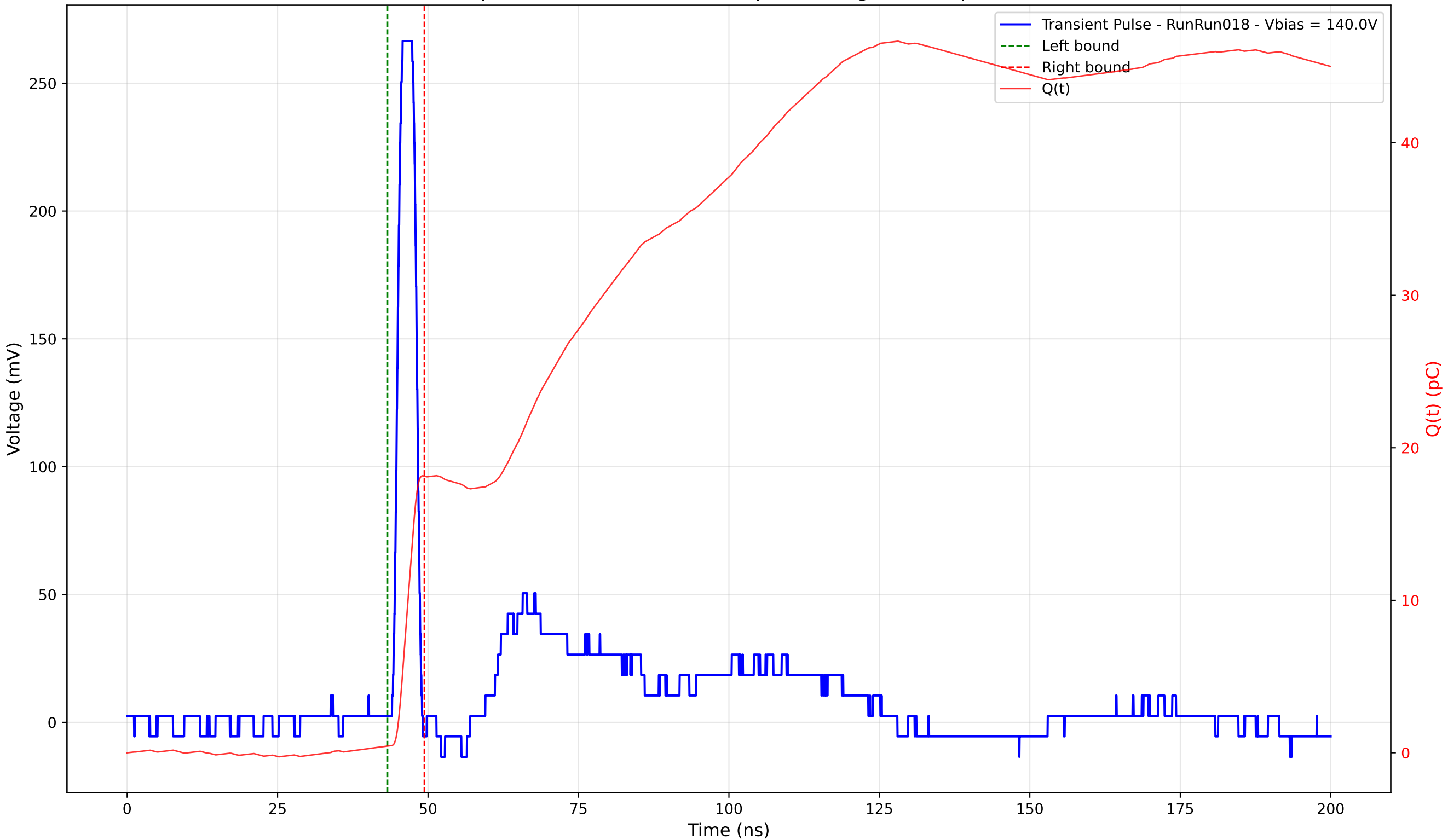
Transient Pulse - Sample: 4003 - Position: 250.0 \mu\text{m} - Charge: 17.70 pC - Rise Time: 1.16 ns
