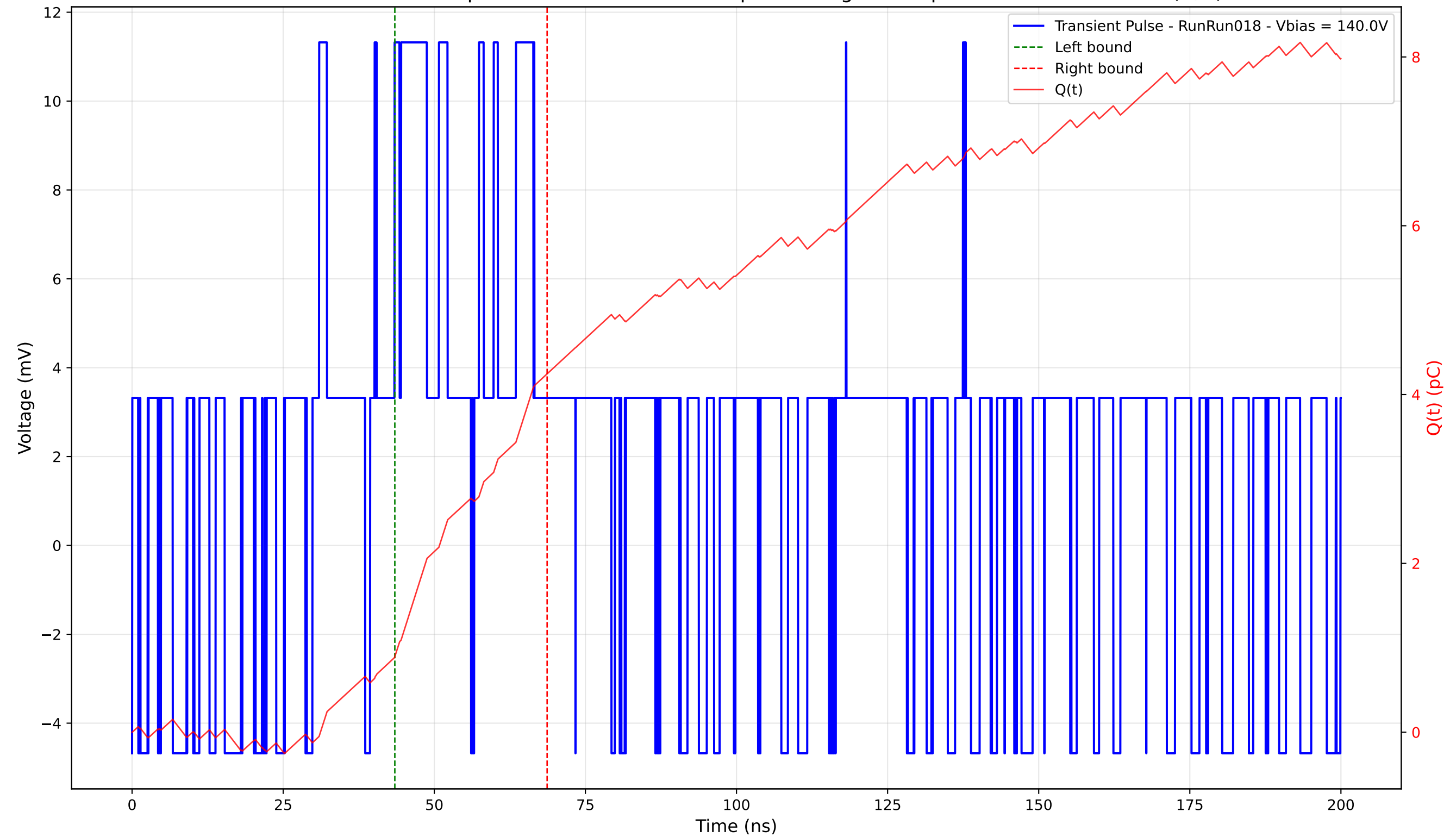
Transient Pulse - Sample: 4003 - Position: 425.0 \mu\text{m} - Charge: 3.35 pC - Rise Time: 0.00 ns (N/A)
