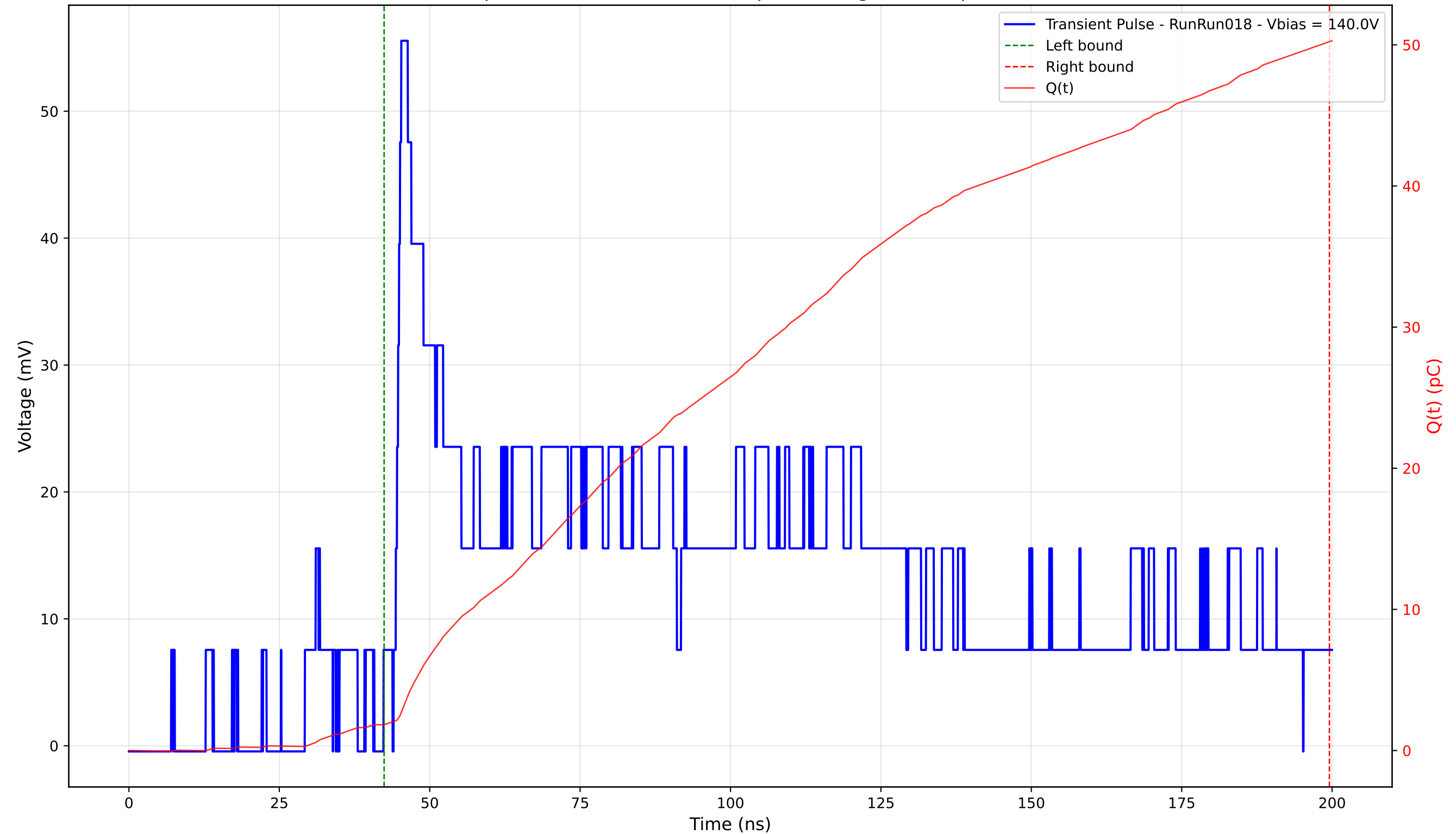
Transient Pulse - Sample: 4003 - Position: 300.0 \mu\text{m} - Charge: 48.39 pC - Rise Time: 1.27 ns
