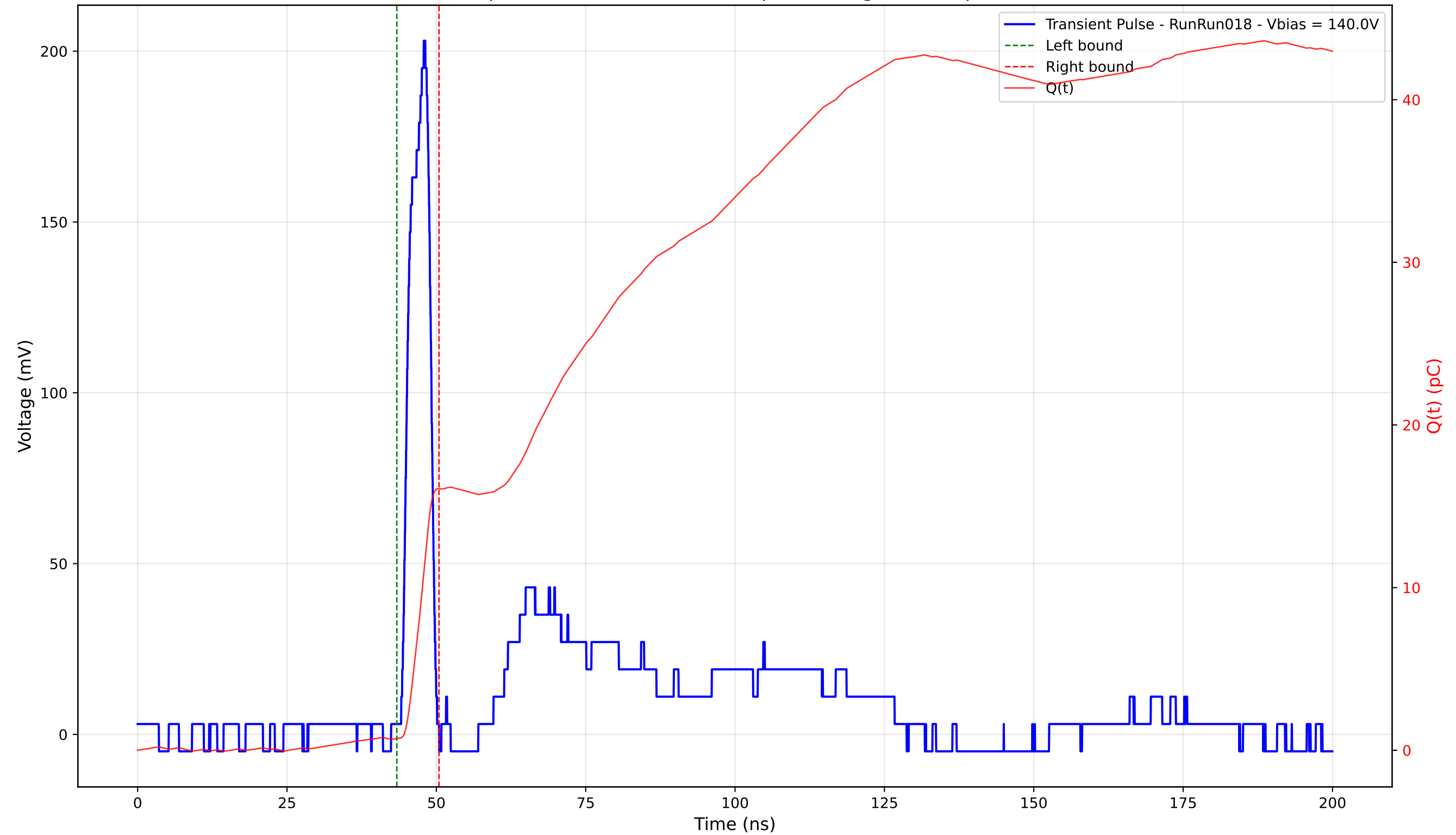
Transient Pulse - Sample: 4003 - Position: 275.0 \mu\text{m} - Charge: 15.37 pC - Rise Time: 2.96 ns
