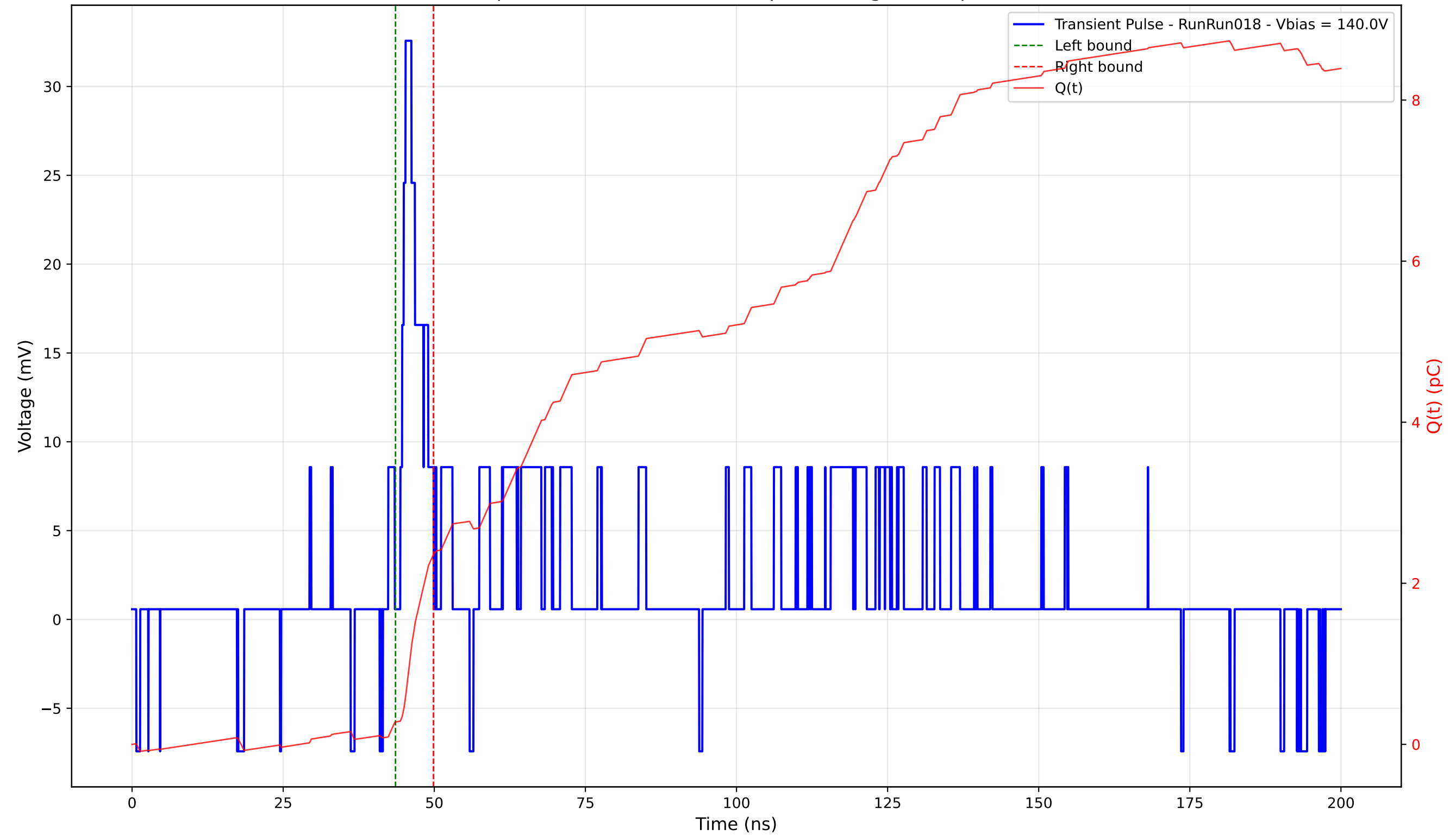
Transient Pulse - Sample: 4003 - Position: 325.0 \mu\text{m} - Charge: 2.08 pC - Rise Time: 0.87 ns
