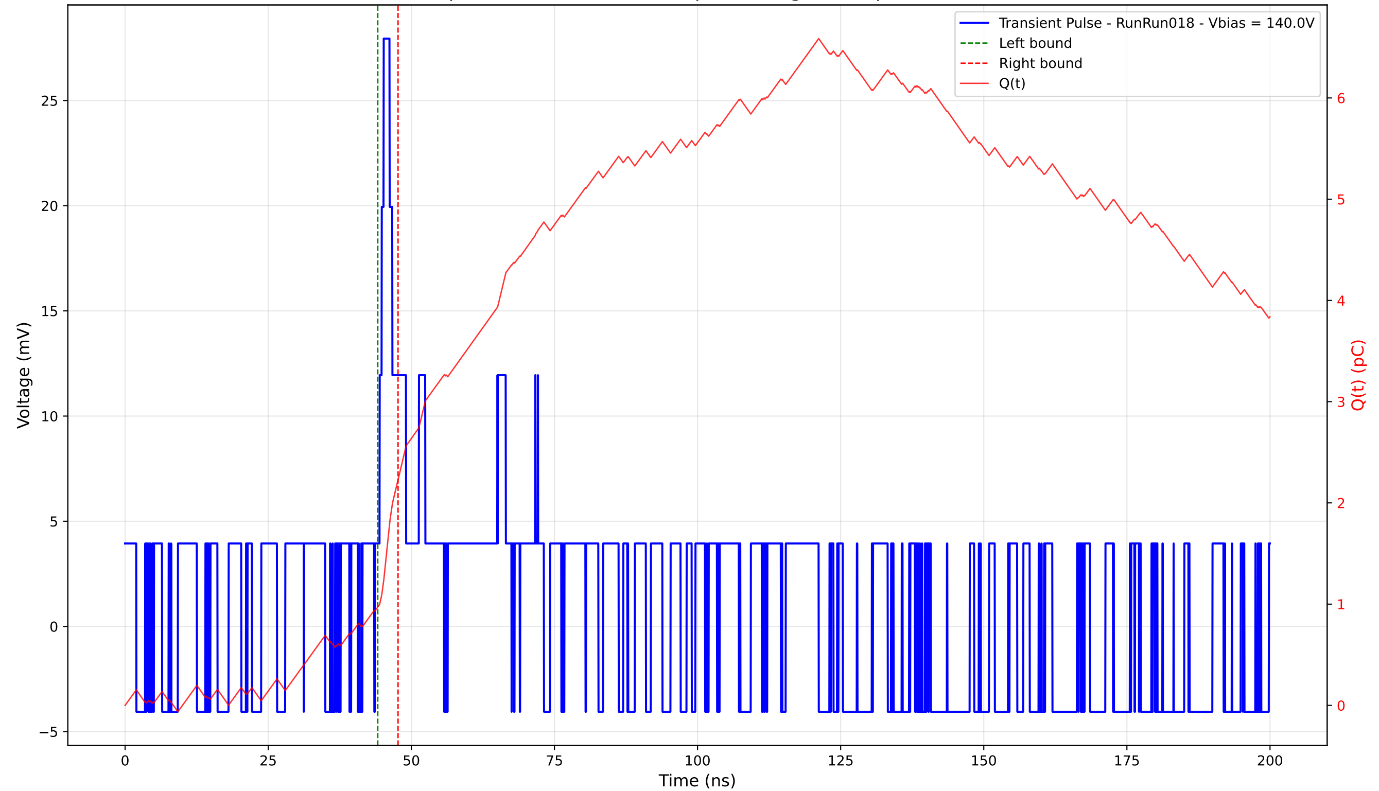
Transient Pulse - Sample: 4003 - Position: 30.0 \mu\text{m} - Charge: 1.26 pC - Rise Time: 0.00 ns (N/A)
