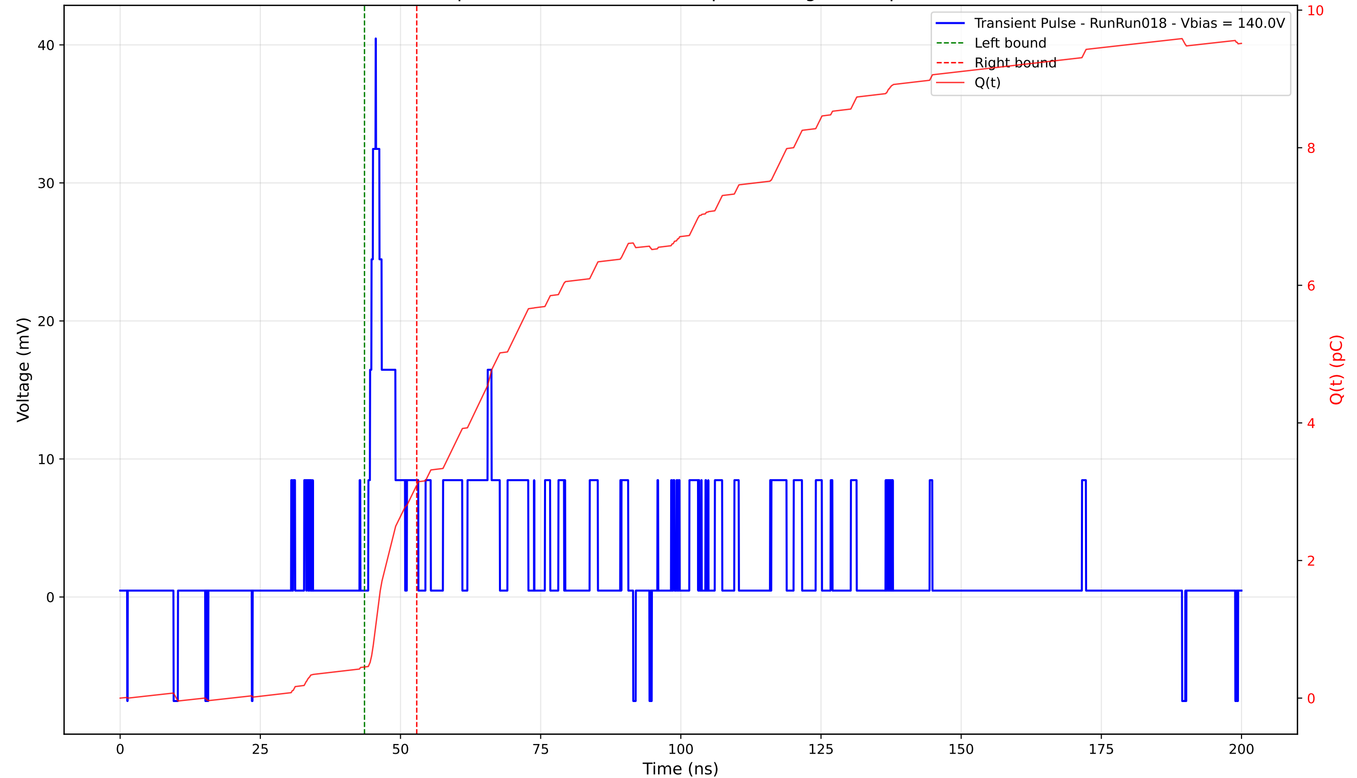
Transient Pulse - Sample: 4003 - Position: 340.0 \mu\text{m} - Charge: 2.65 pC - Rise Time: 1.31 ns
