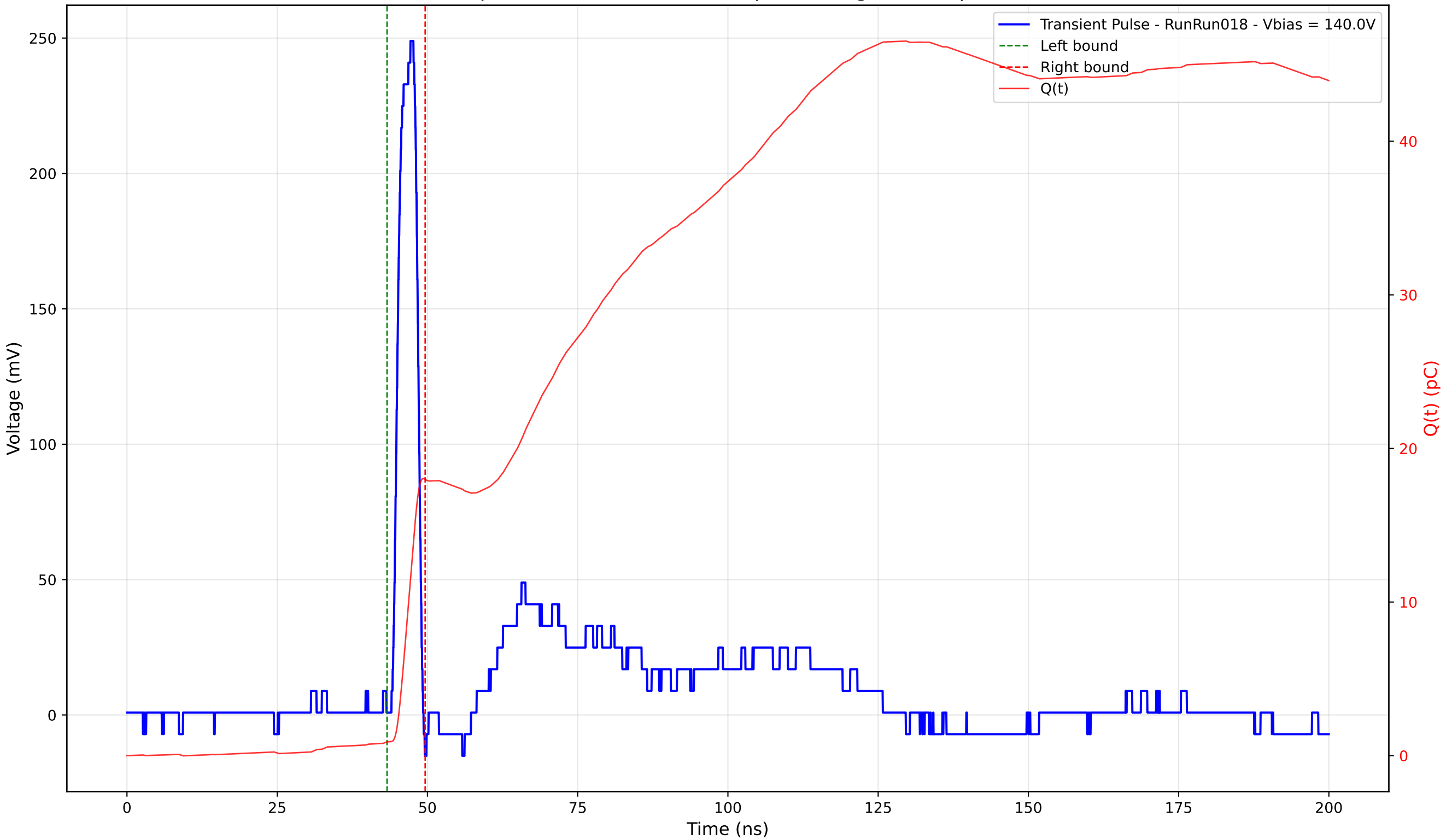
Transient Pulse - Sample: 4003 - Position: 260.0 \mu\text{m} - Charge: 17.09 pC - Rise Time: 1.48 ns
