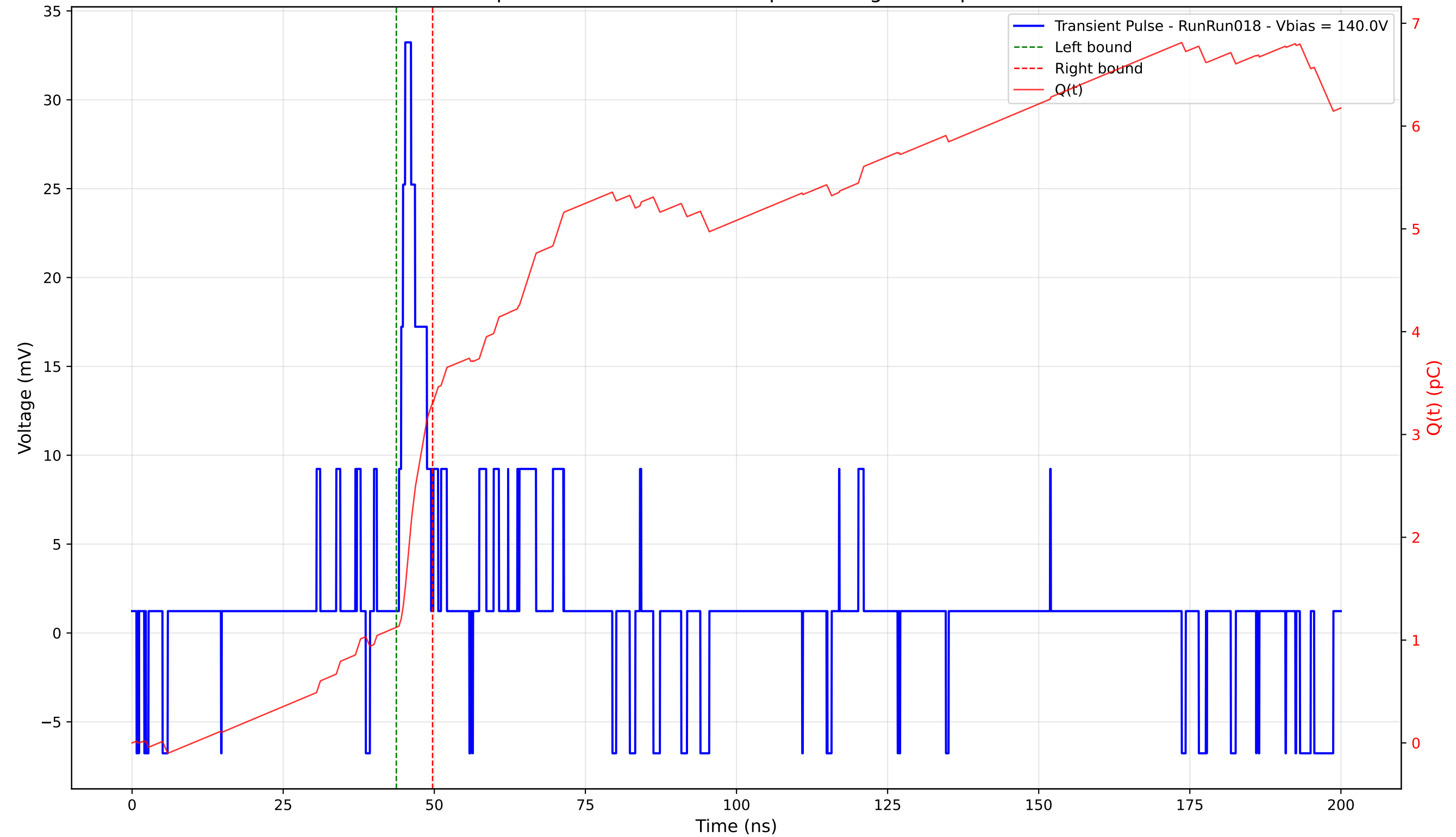
Transient Pulse - Sample: 4003 - Position: 360.0 \mu\text{m} - Charge: 2.19 pC - Rise Time: 1.03 ns
