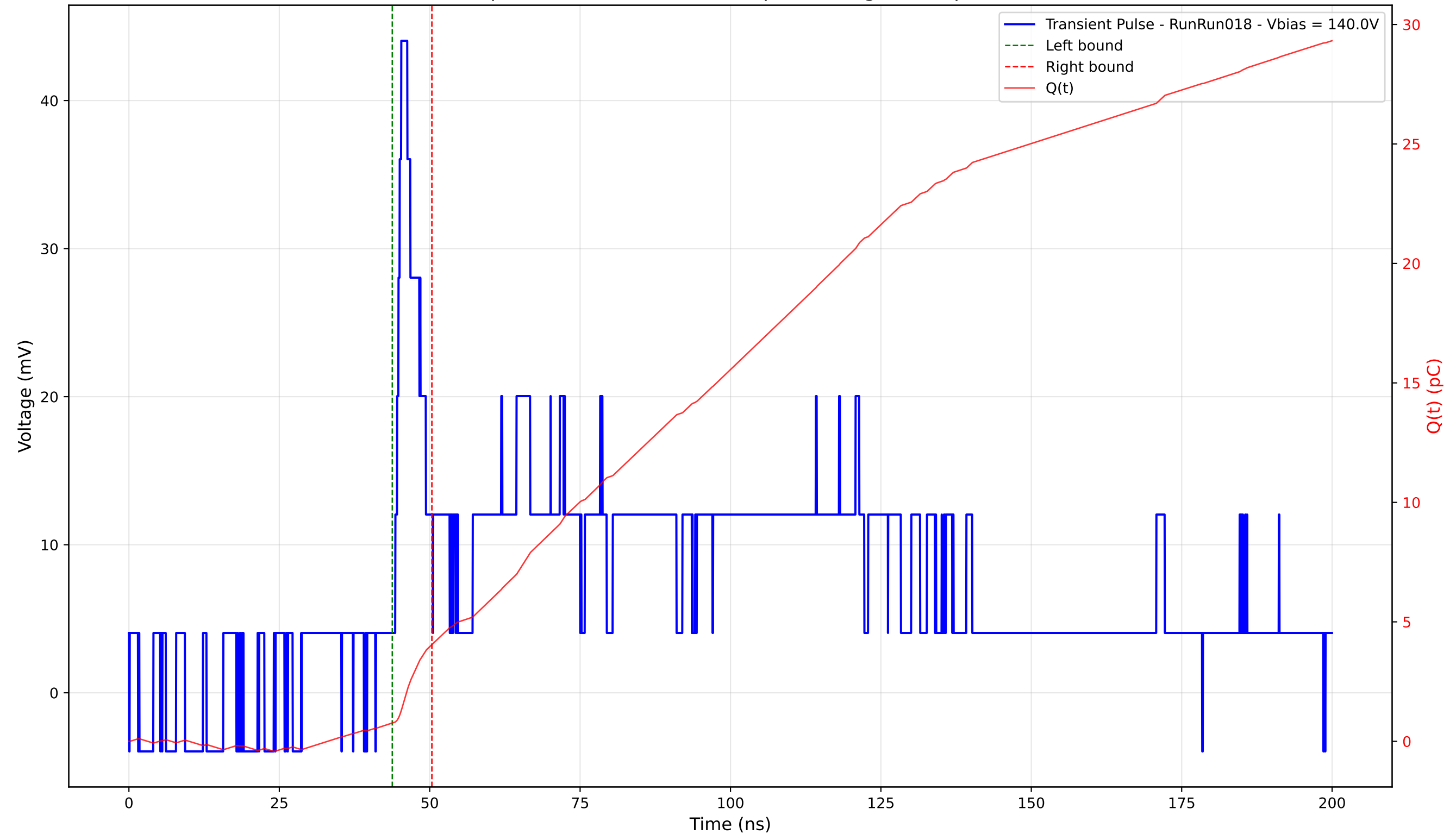
Transient Pulse - Sample: 4003 - Position: 310.0 \mu\text{m} - Charge: 3.29 pC - Rise Time: 1.00 ns
