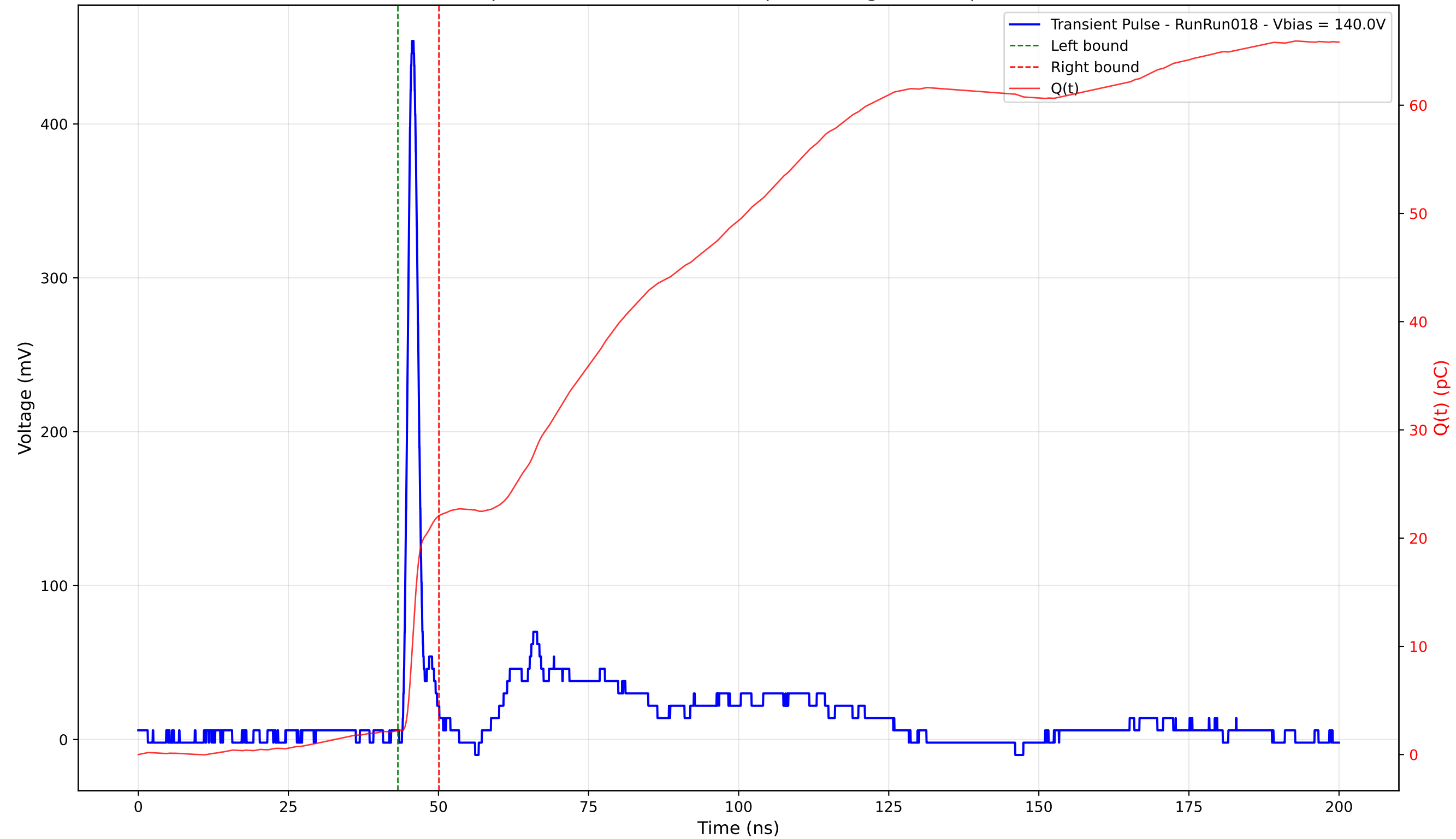
Transient Pulse - Sample: 4003 - Position: 185.0 \mu\text{m} - Charge: 19.84 pC - Rise Time: 1.06 ns
