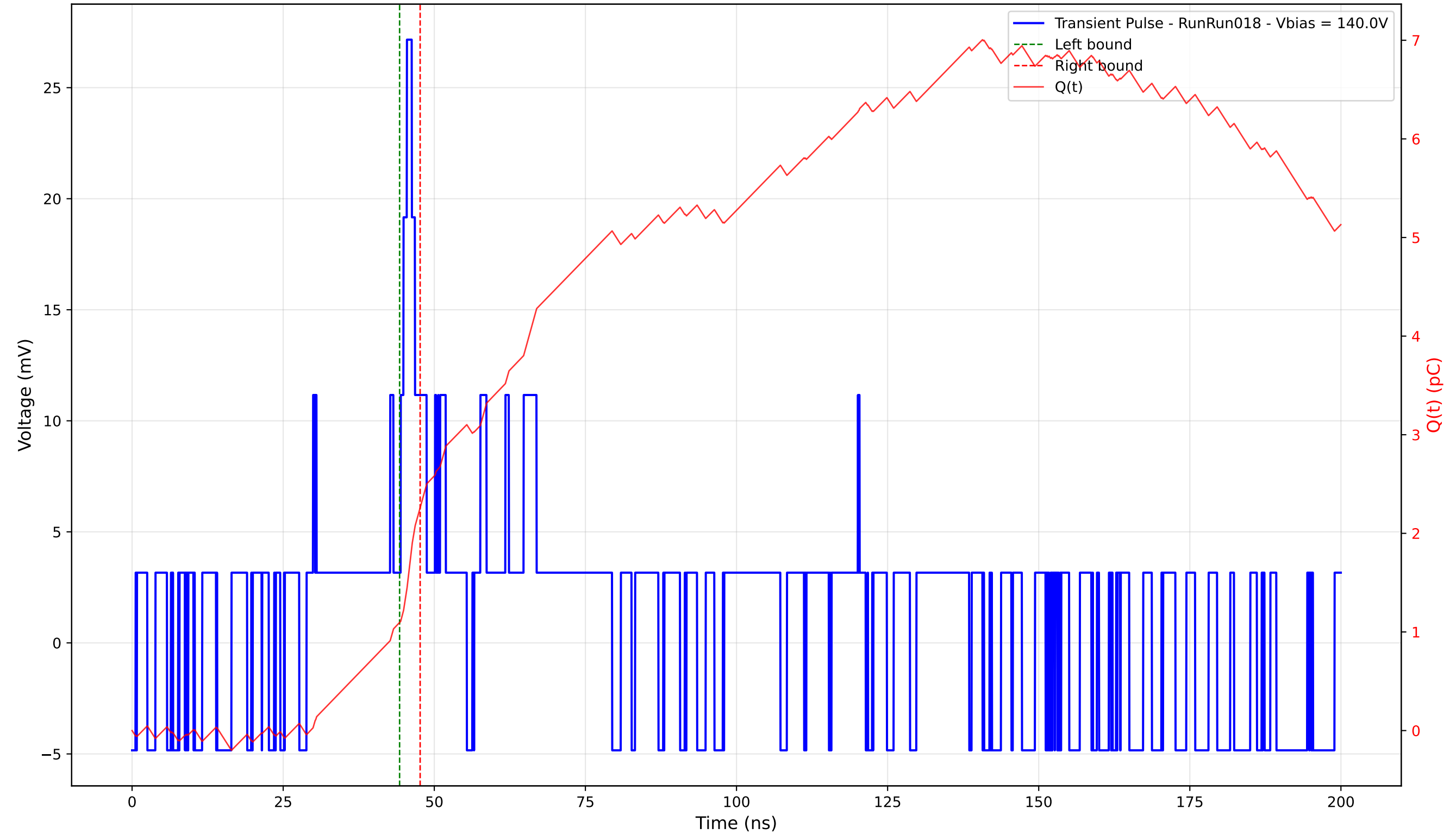
Transient Pulse - Sample: 4003 - Position: 415.0 \mu\text{m} - Charge: 1.17 pC - Rise Time: 0.00 ns (N/A)
