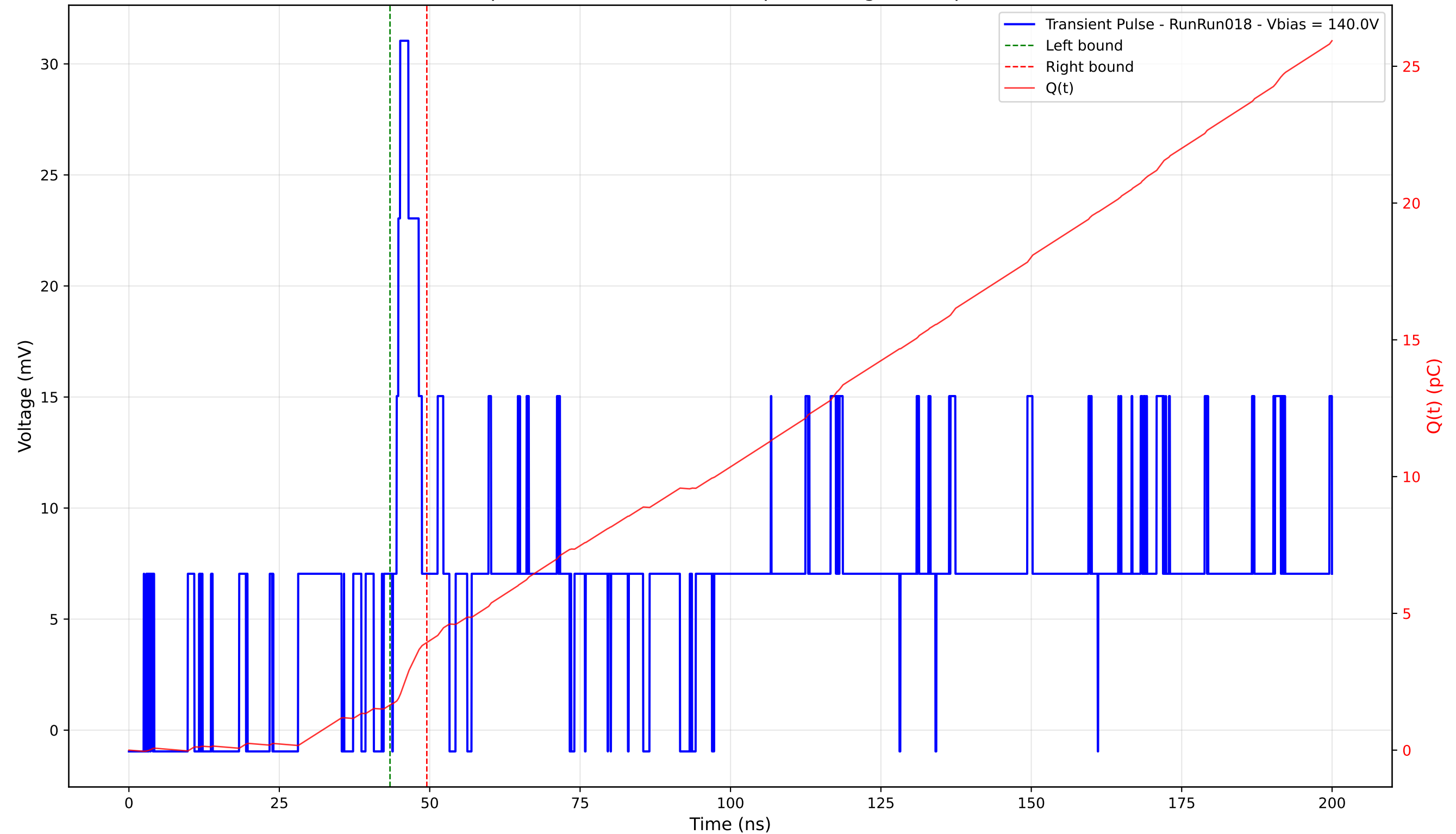
Transient Pulse - Sample: 4003 - Position: 335.0 \mu\text{m} - Charge: 2.28 pC - Rise Time: 1.21 ns
