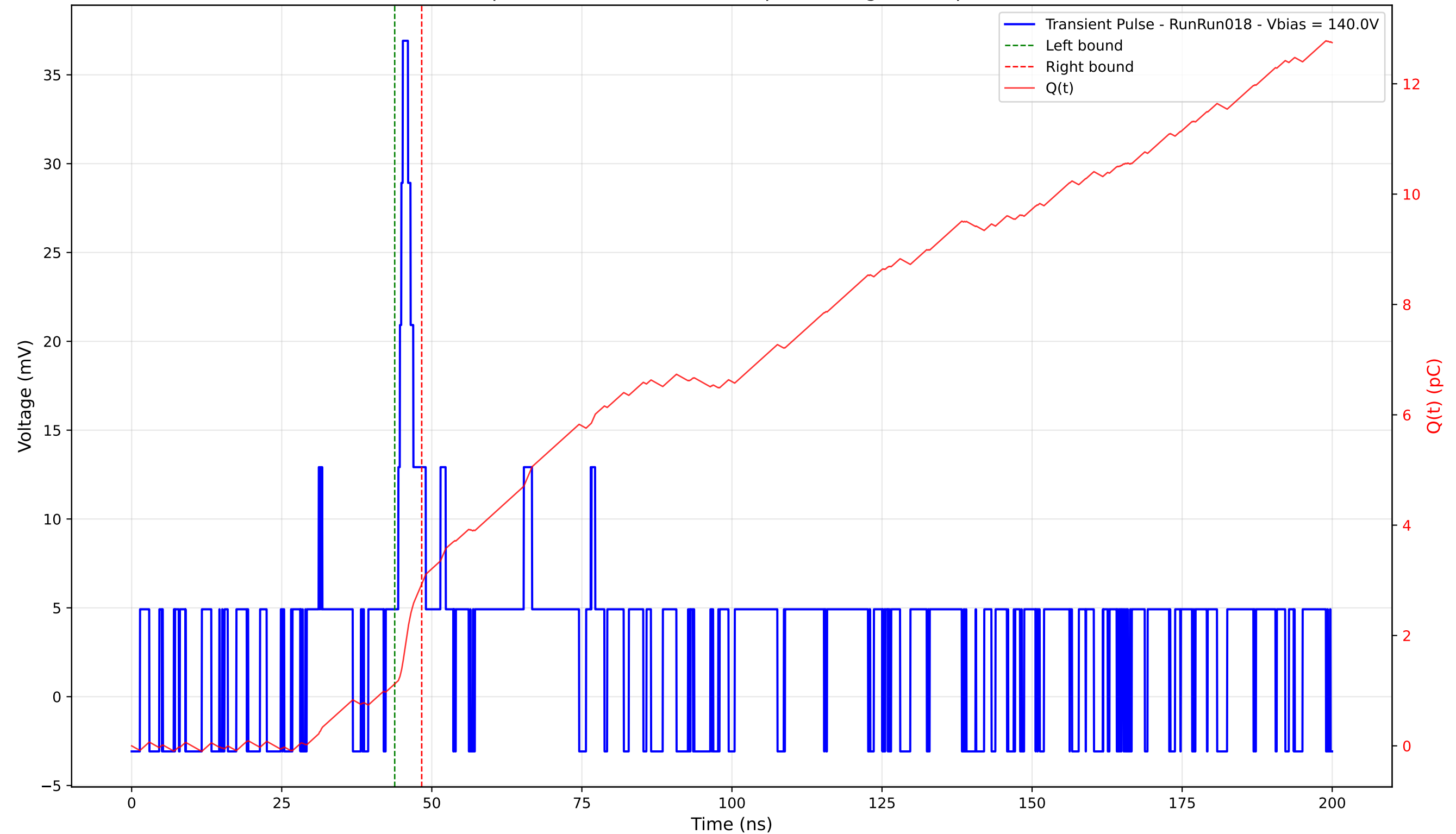
Transient Pulse - Sample: 4003 - Position: 410.0 \mu\text{m} - Charge: 1.81 pC - Rise Time: 2.85 ns
