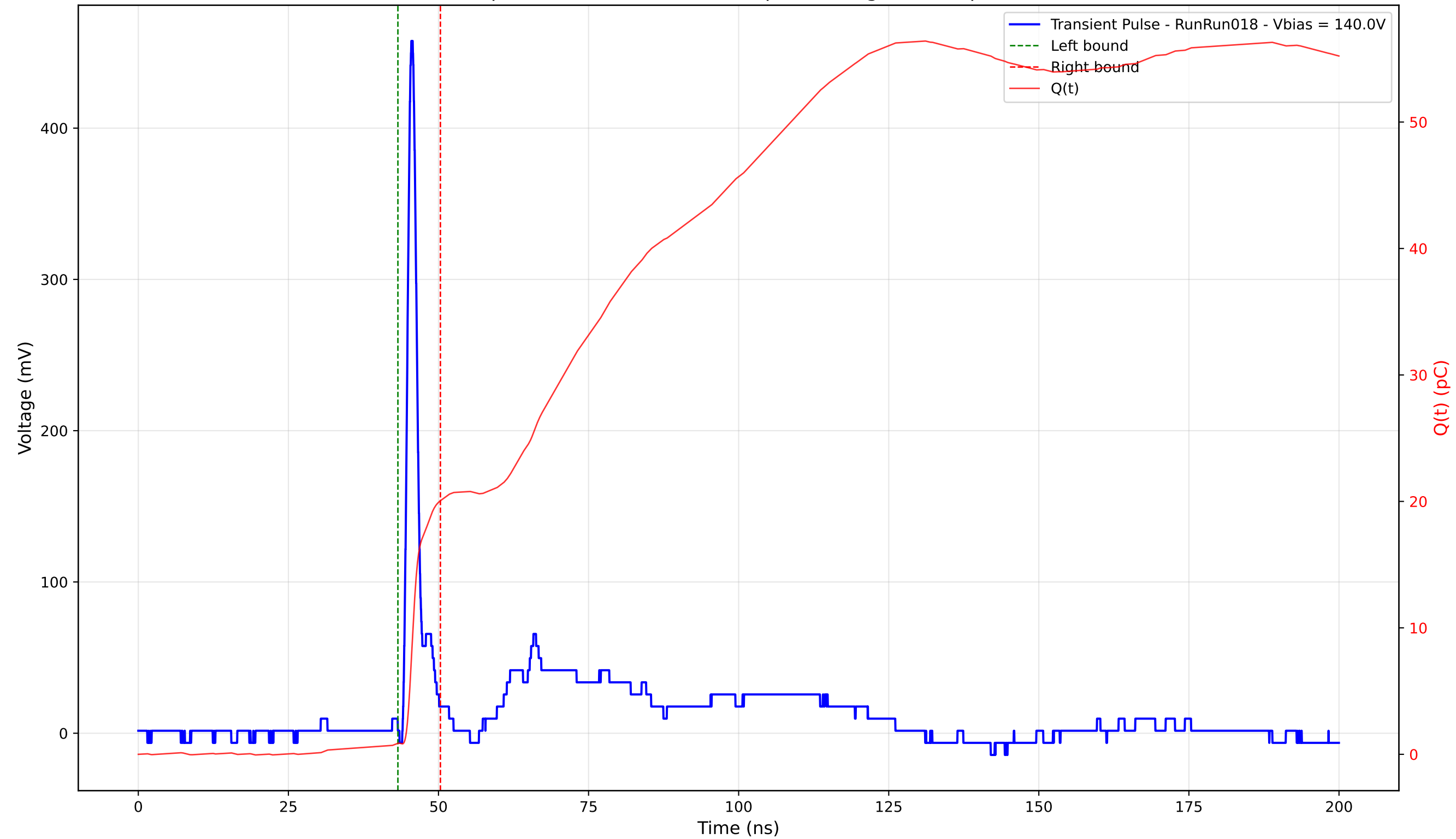
Transient Pulse - Sample: 4003 - Position: 160.0 \mu\text{m} - Charge: 19.18 pC - Rise Time: 0.97 ns
