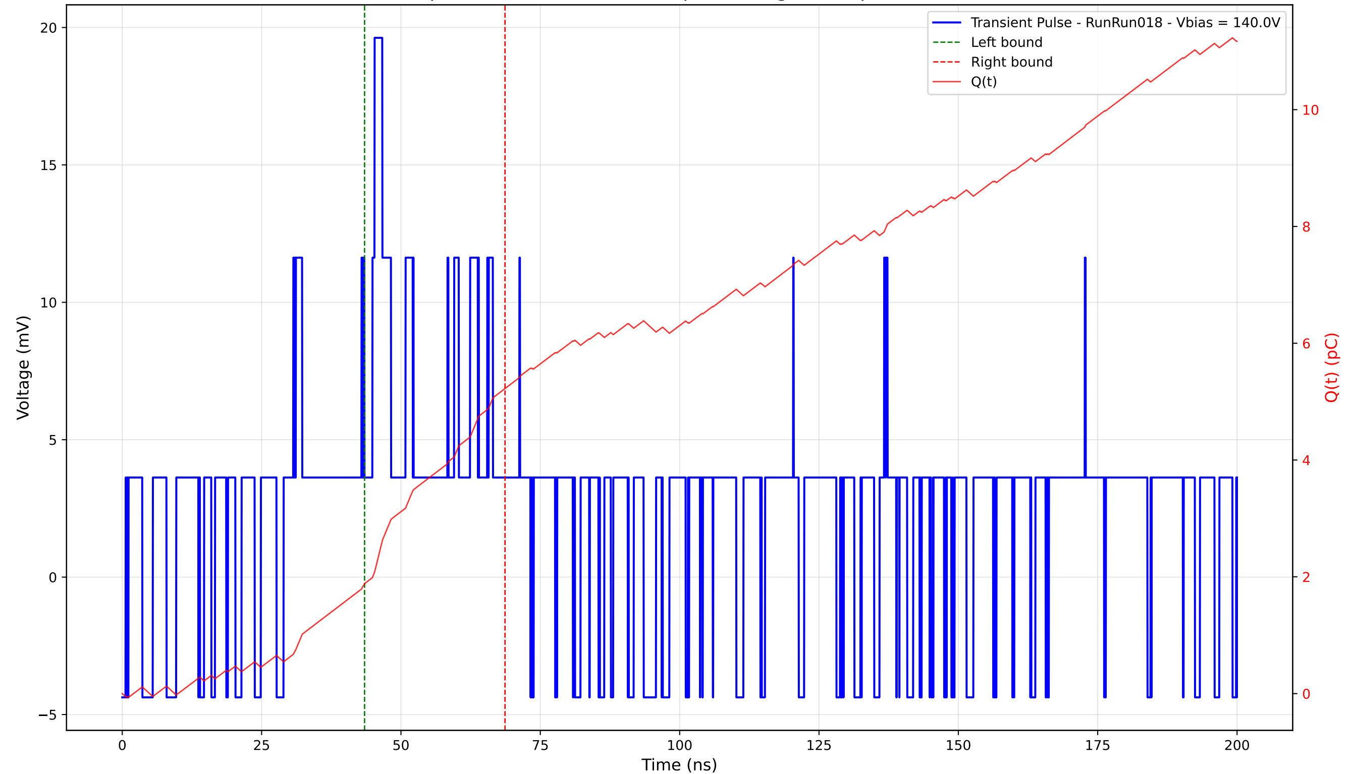
Transient Pulse - Sample: 4003 - Position: 420.0 \mu\text{m} - Charge: 3.34 pC - Rise Time: 0.00 ns (N/A)
