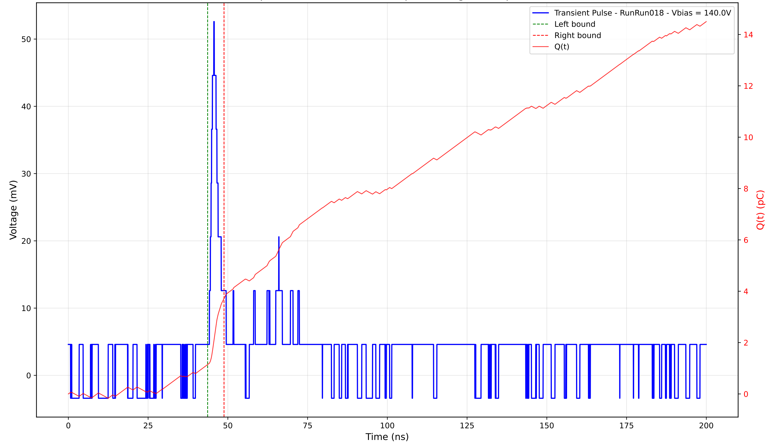
Transient Pulse - Sample: 4003 - Position: 400.0 \mu\text{m} - Charge: 2.58 pC - Rise Time: 1.40 ns
