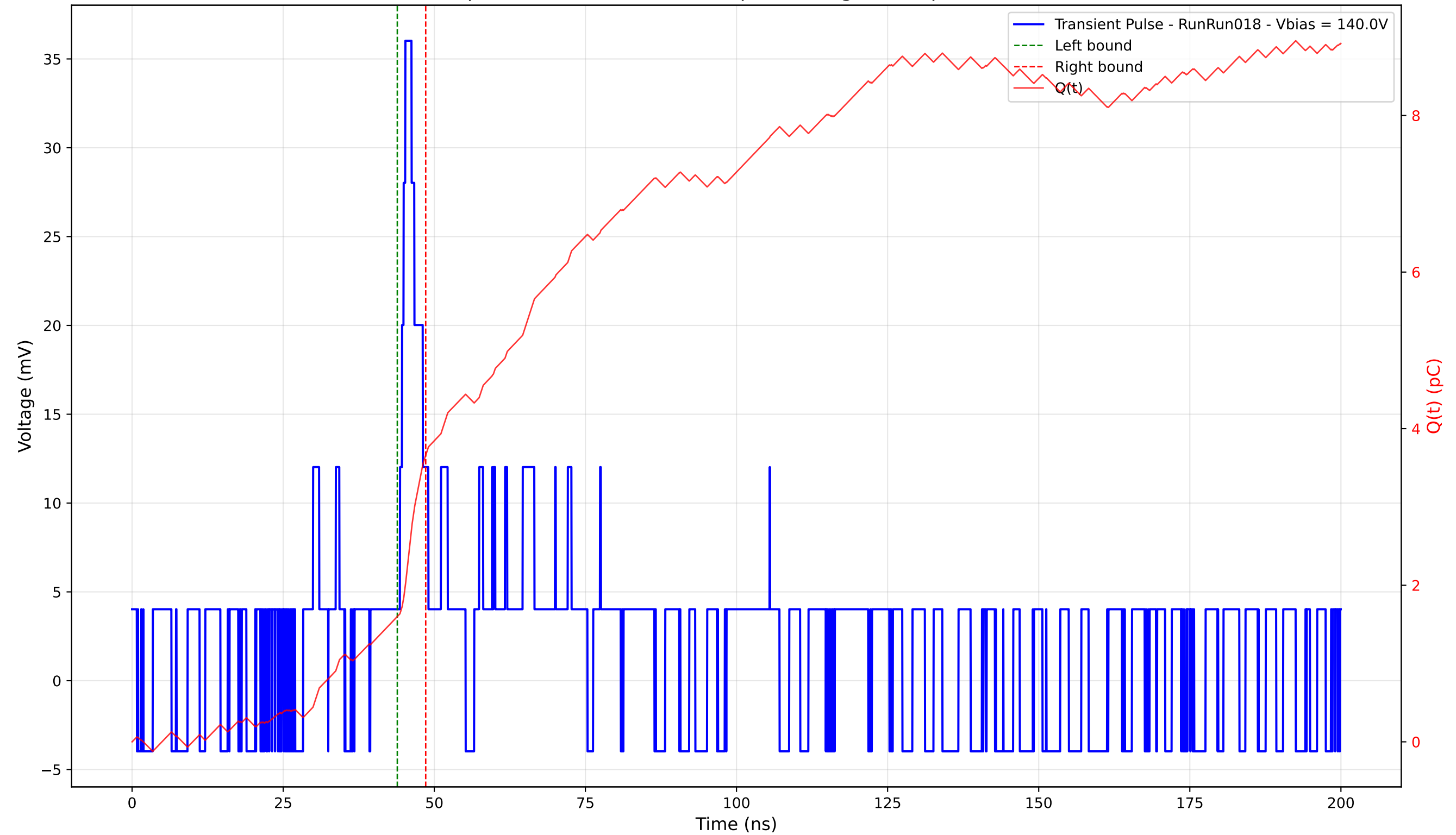
Transient Pulse - Sample: 4003 - Position: 380.0 \mu\text{m} - Charge: 2.06 pC - Rise Time: 0.00 ns (N/A)
