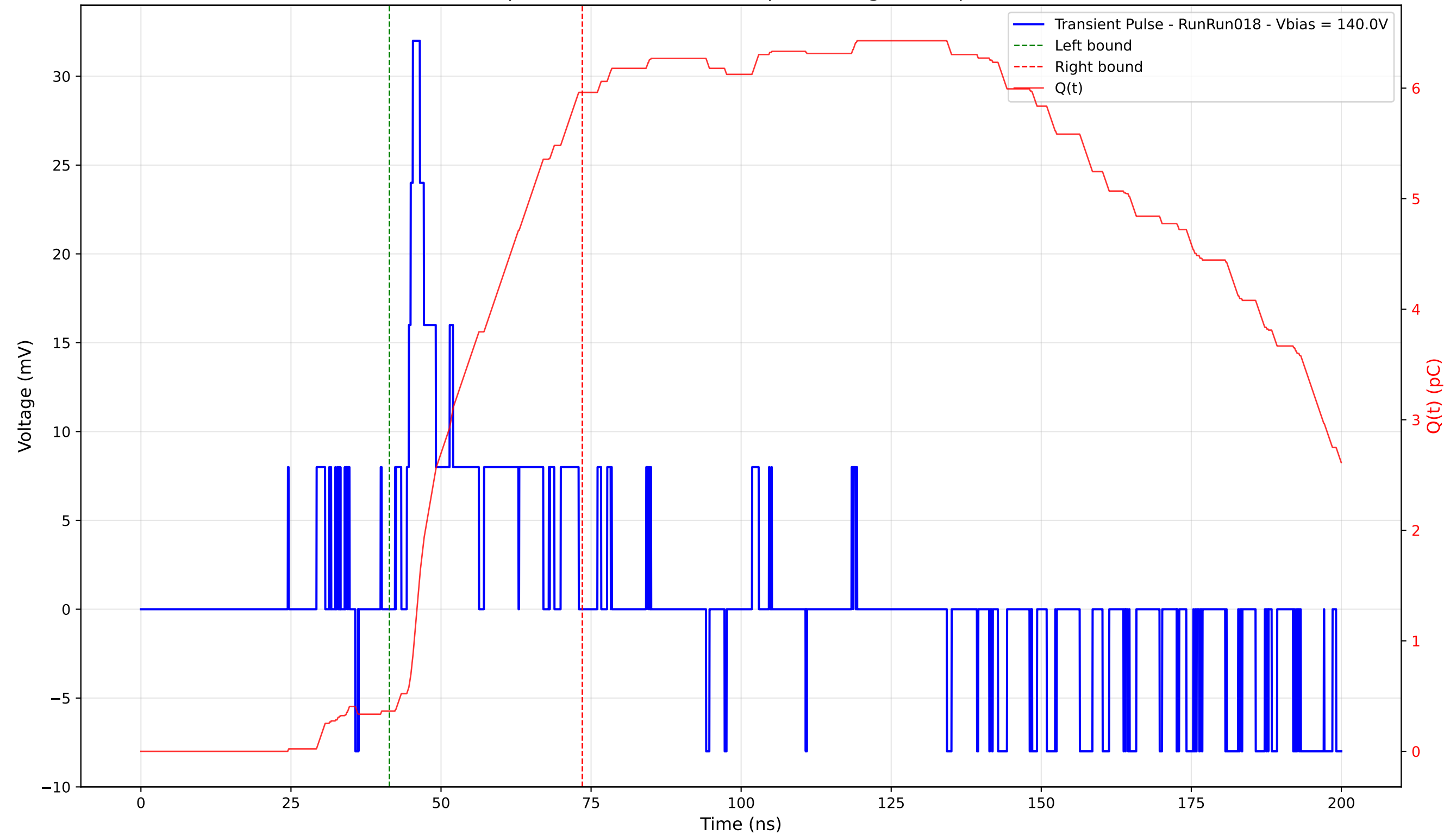
Transient Pulse - Sample: 4003 - Position: 45.0 \mu\text{m} - Charge: 5.60 pC - Rise Time: 1.01 ns
