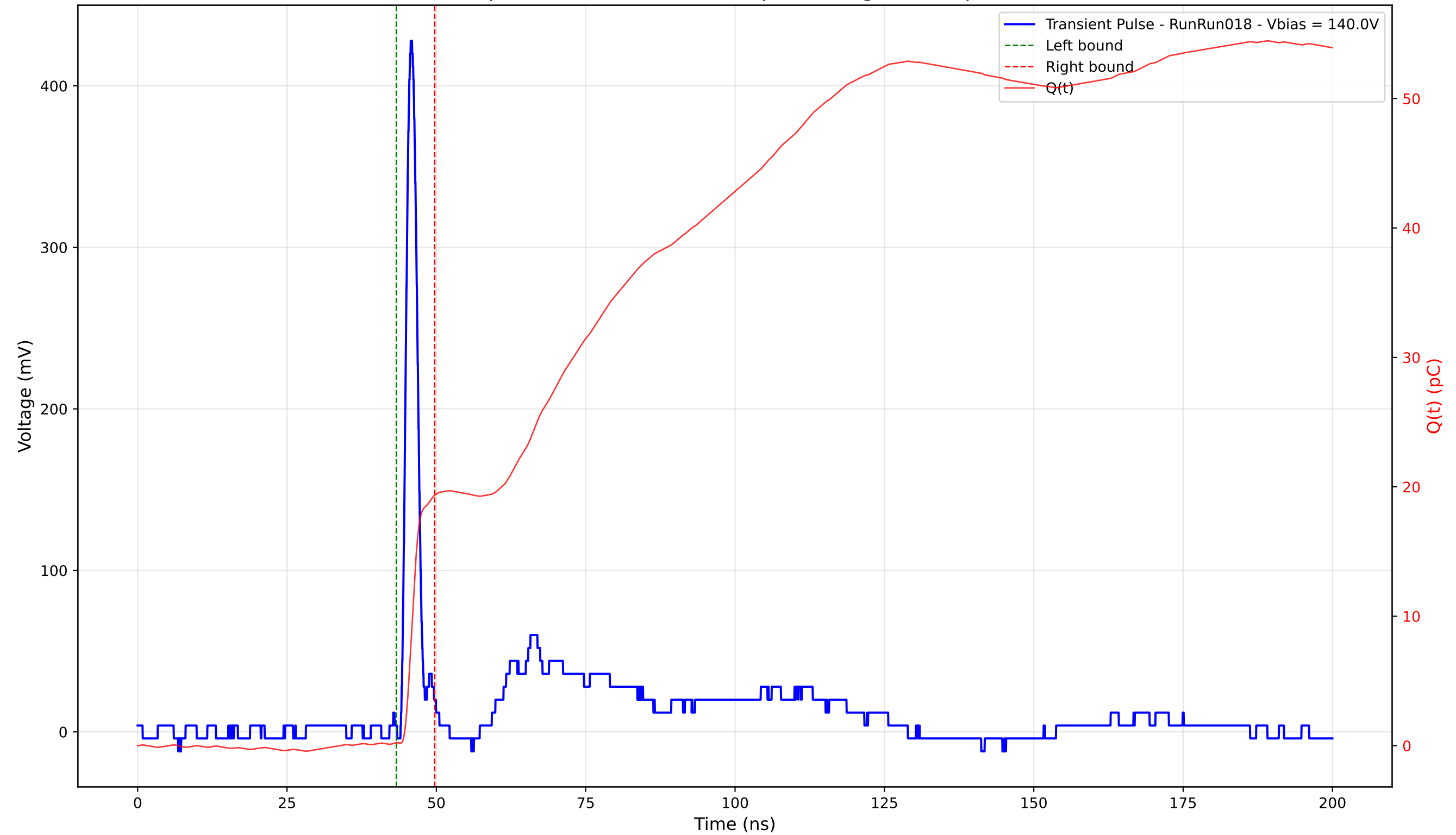
Transient Pulse - Sample: 4003 - Position: 200.0 \mu\text{m} - Charge: 19.13 pC - Rise Time: 1.10 ns
