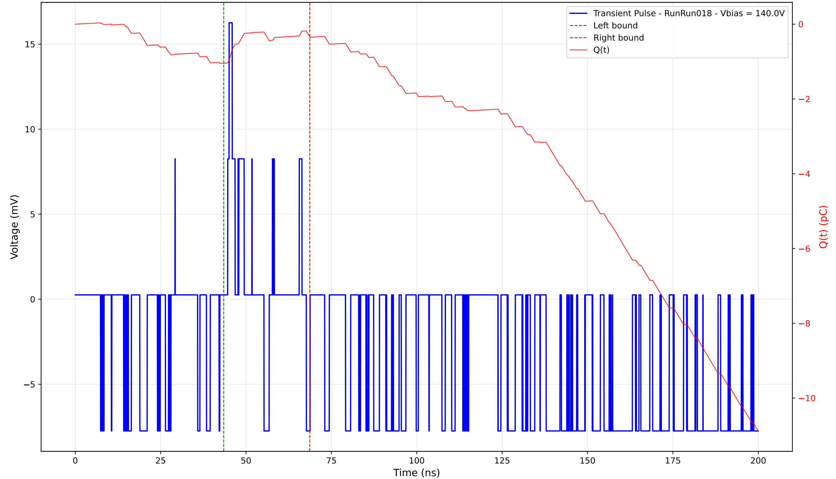
Transient Pulse - Sample: 4003 - Position: 15.0 \mu\text{m} - Charge: 0.71 pC - Rise Time: 0.42 ns
