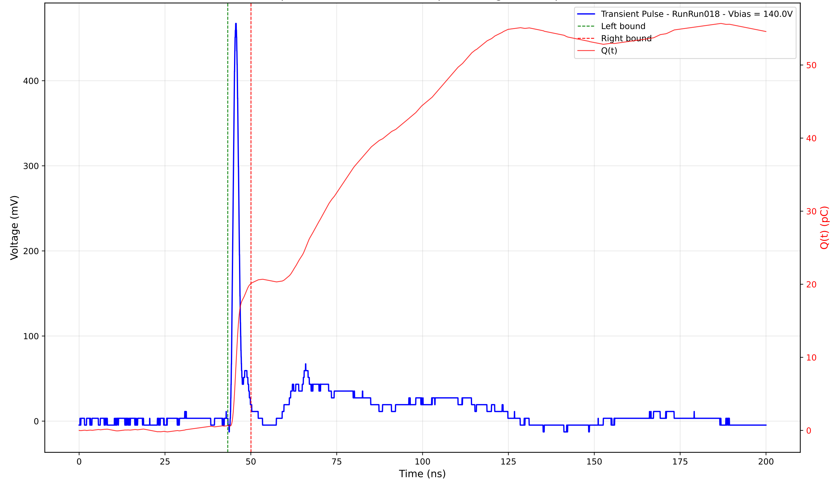
Transient Pulse - Sample: 4003 - Position: 175.0 \mu\text{m} - Charge: 19.44 pC - Rise Time: 1.03 ns
