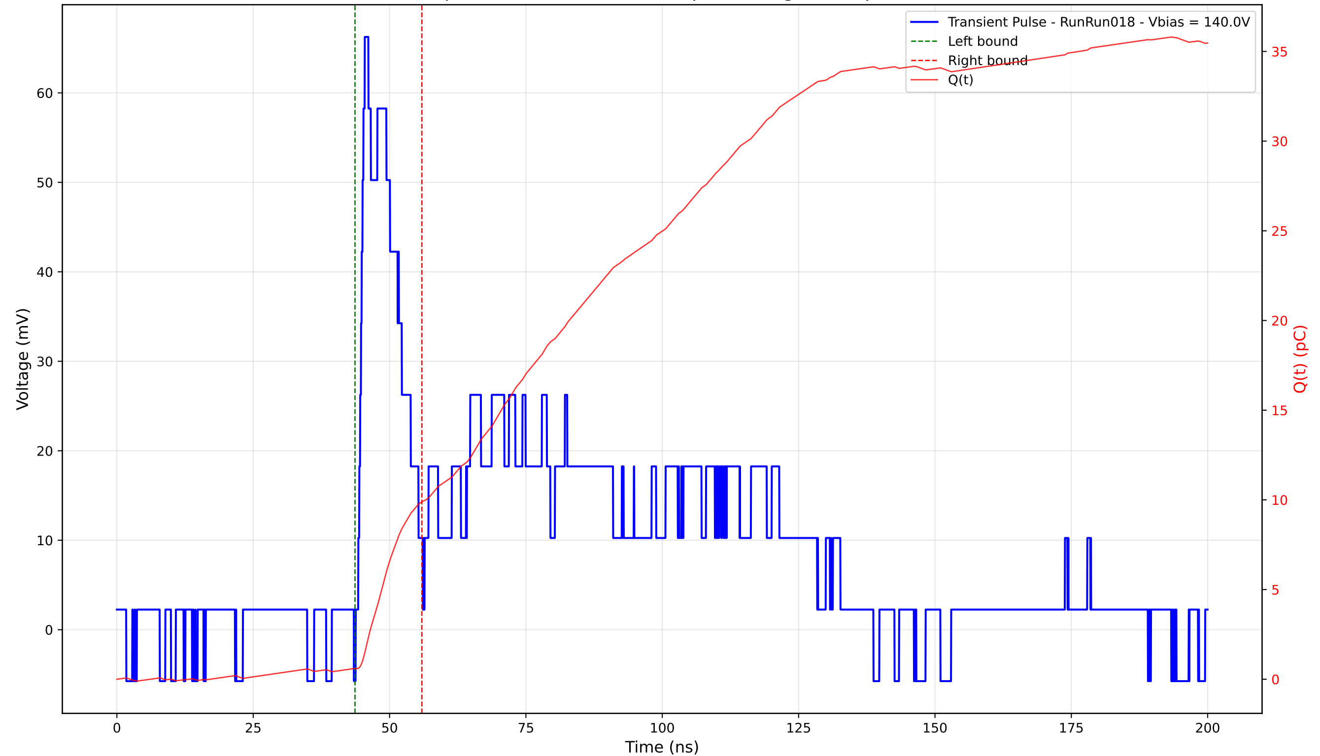
Transient Pulse - Sample: 4003 - Position: 295.0 \mu\text{m} - Charge: 9.30 pC - Rise Time: 1.19 ns
