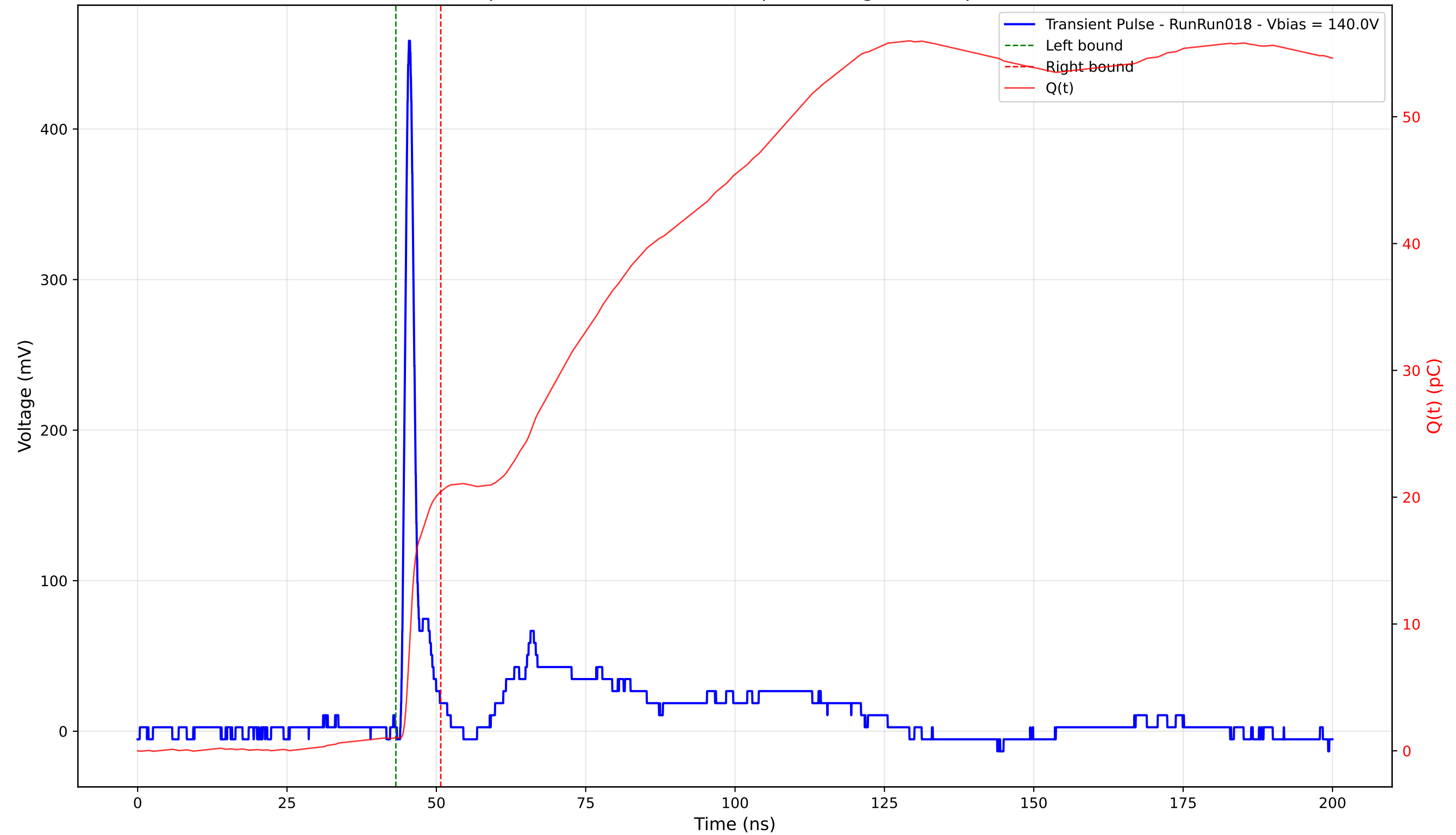
Transient Pulse - Sample: 4003 - Position: 145.0 \mu\text{m} - Charge: 19.40 pC - Rise Time: 0.95 ns
