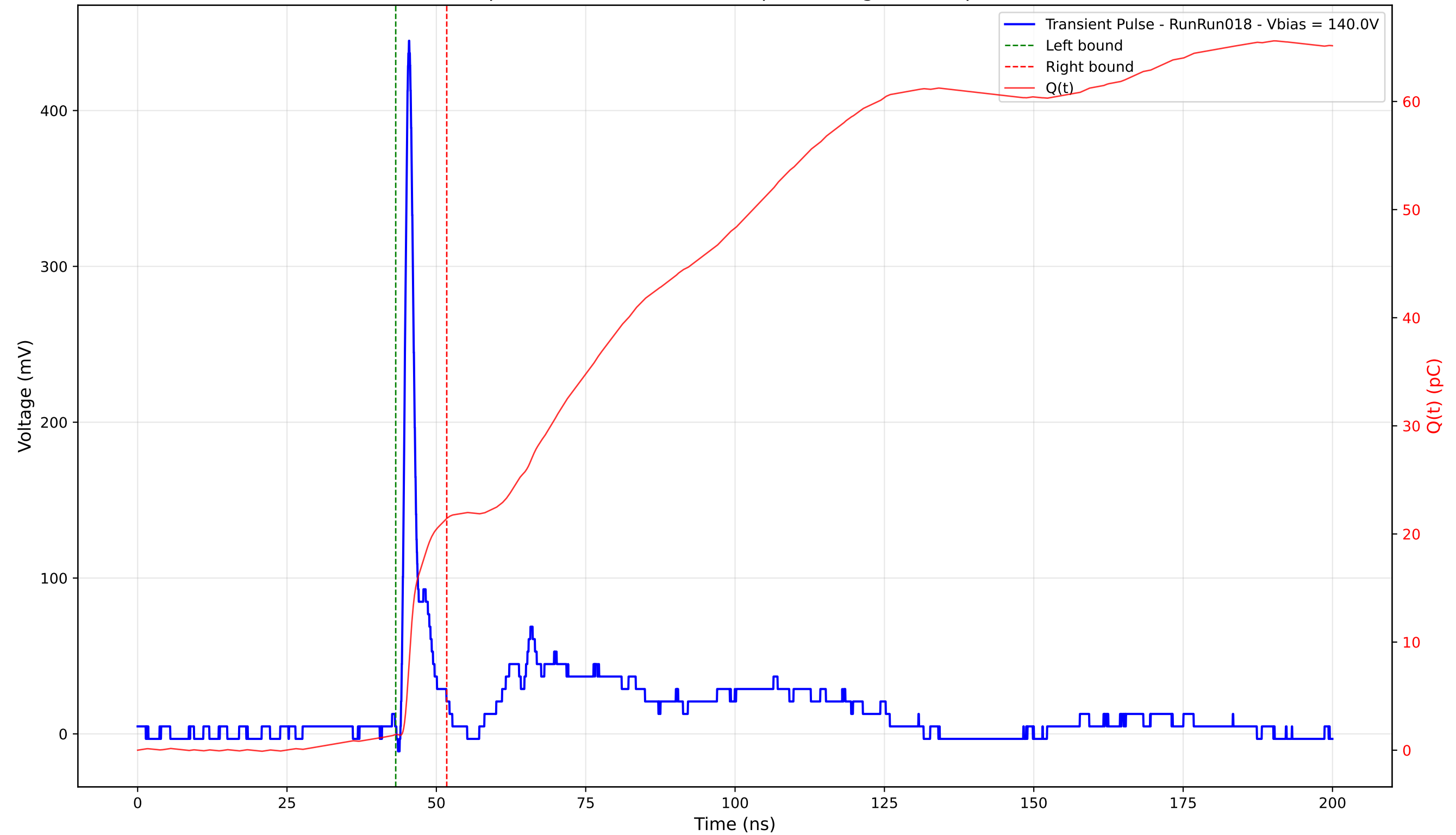
Transient Pulse - Sample: 4003 - Position: 125.0 \mu\text{m} - Charge: 19.98 pC - Rise Time: 0.92 ns
