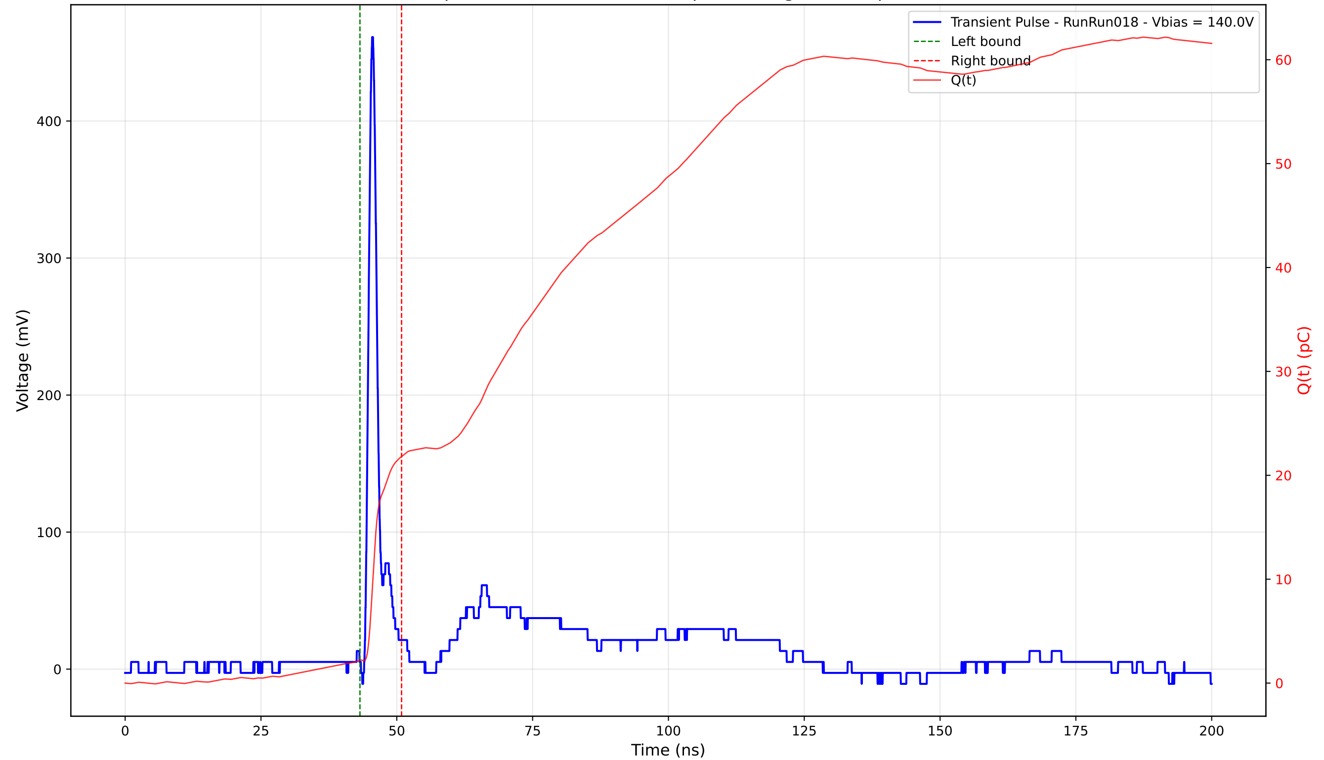
Transient Pulse - Sample: 4003 - Position: 150.0 \mu\text{m} - Charge: 19.61 pC - Rise Time: 0.96 ns
