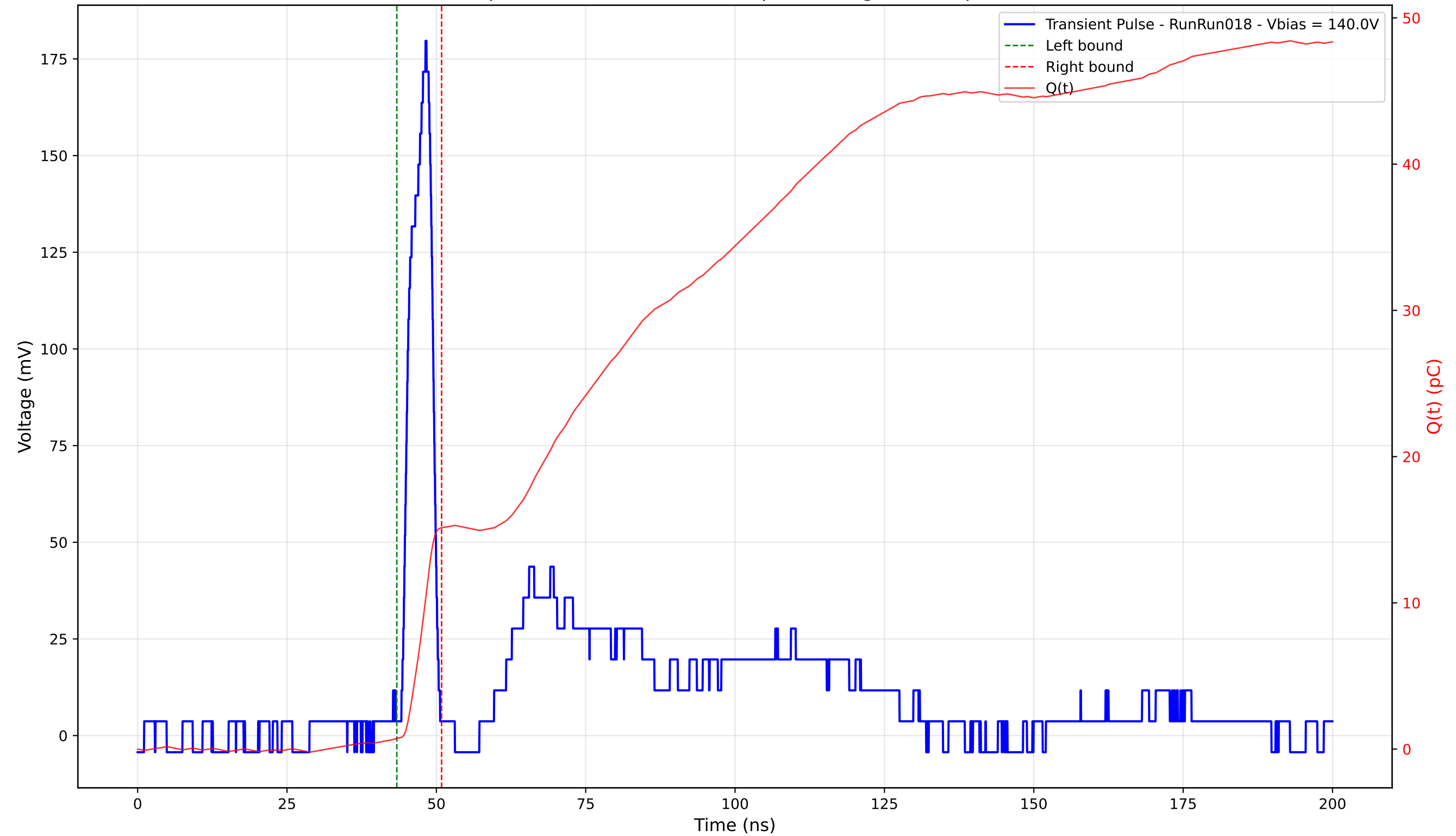
Transient Pulse - Sample: 4003 - Position: 280.0 \mu\text{m} - Charge: 14.40 pC - Rise Time: 3.20 ns
