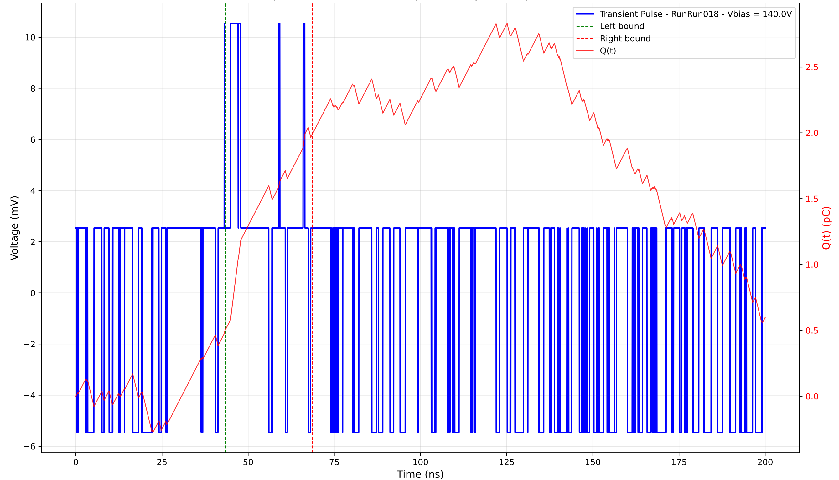
Transient Pulse - Sample: 4003 - Position: 0.0 \mu\text{m} - Charge: 1.48 pC - Rise Time: 0.00 ns (N/A)
