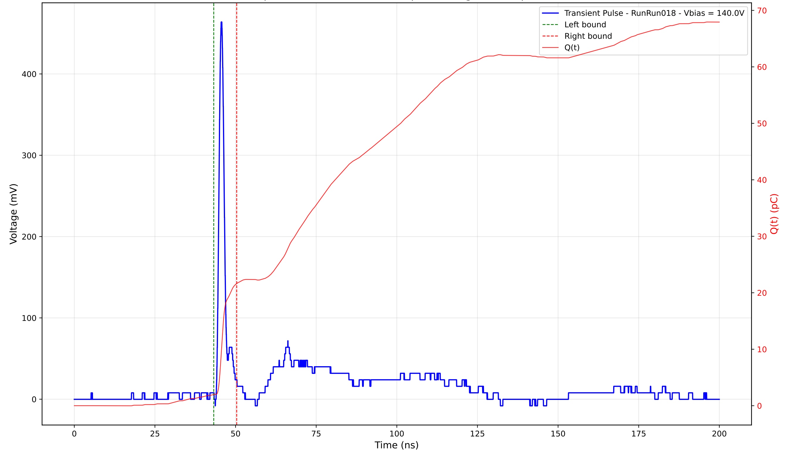
Transient Pulse - Sample: 4003 - Position: 170.0 \mu\text{m} - Charge: 19.64 pC - Rise Time: 1.03 ns
