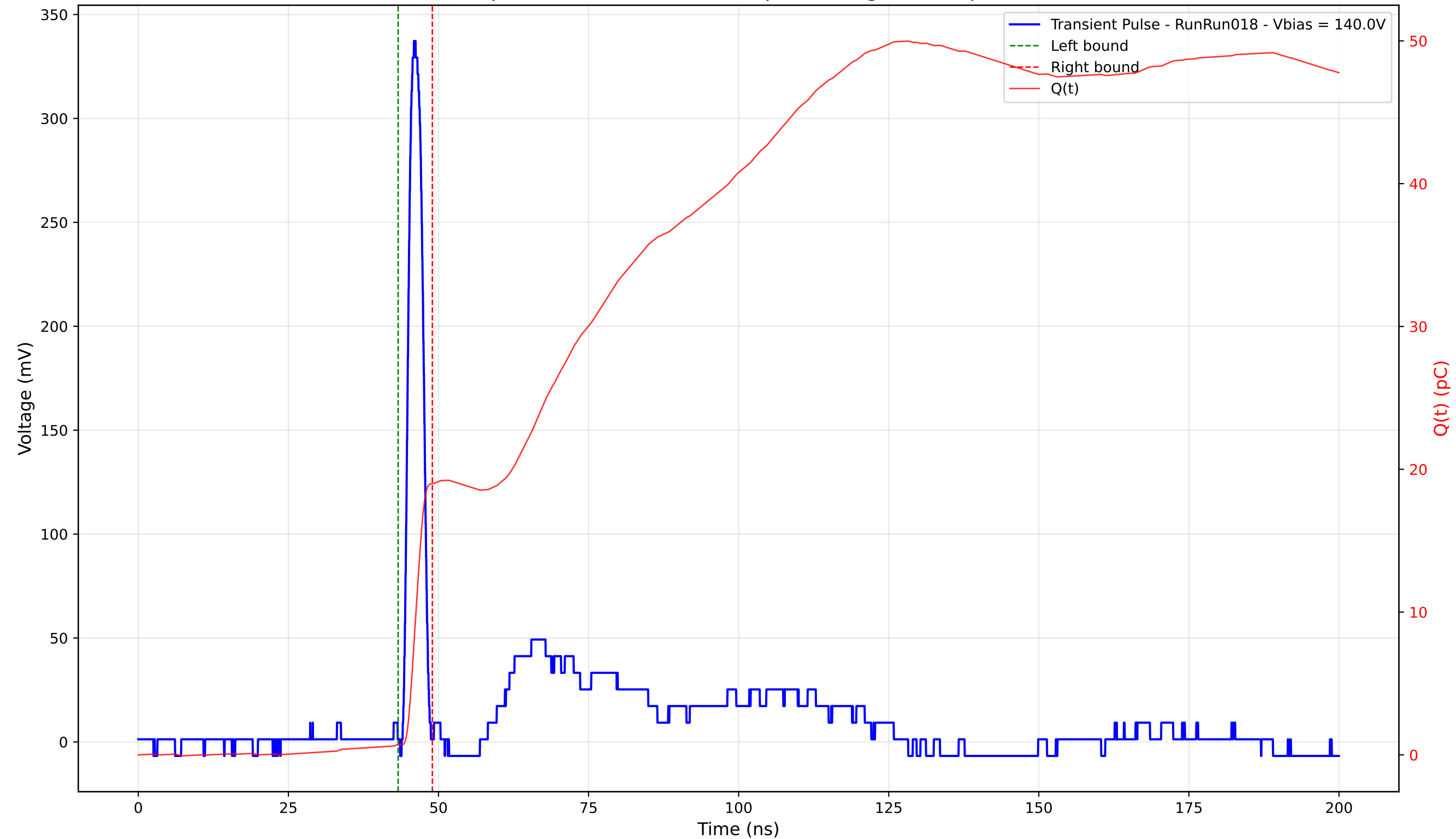
Transient Pulse - Sample: 4003 - Position: 230.0 \mu\text{m} - Charge: 18.26 pC - Rise Time: 1.14 ns
