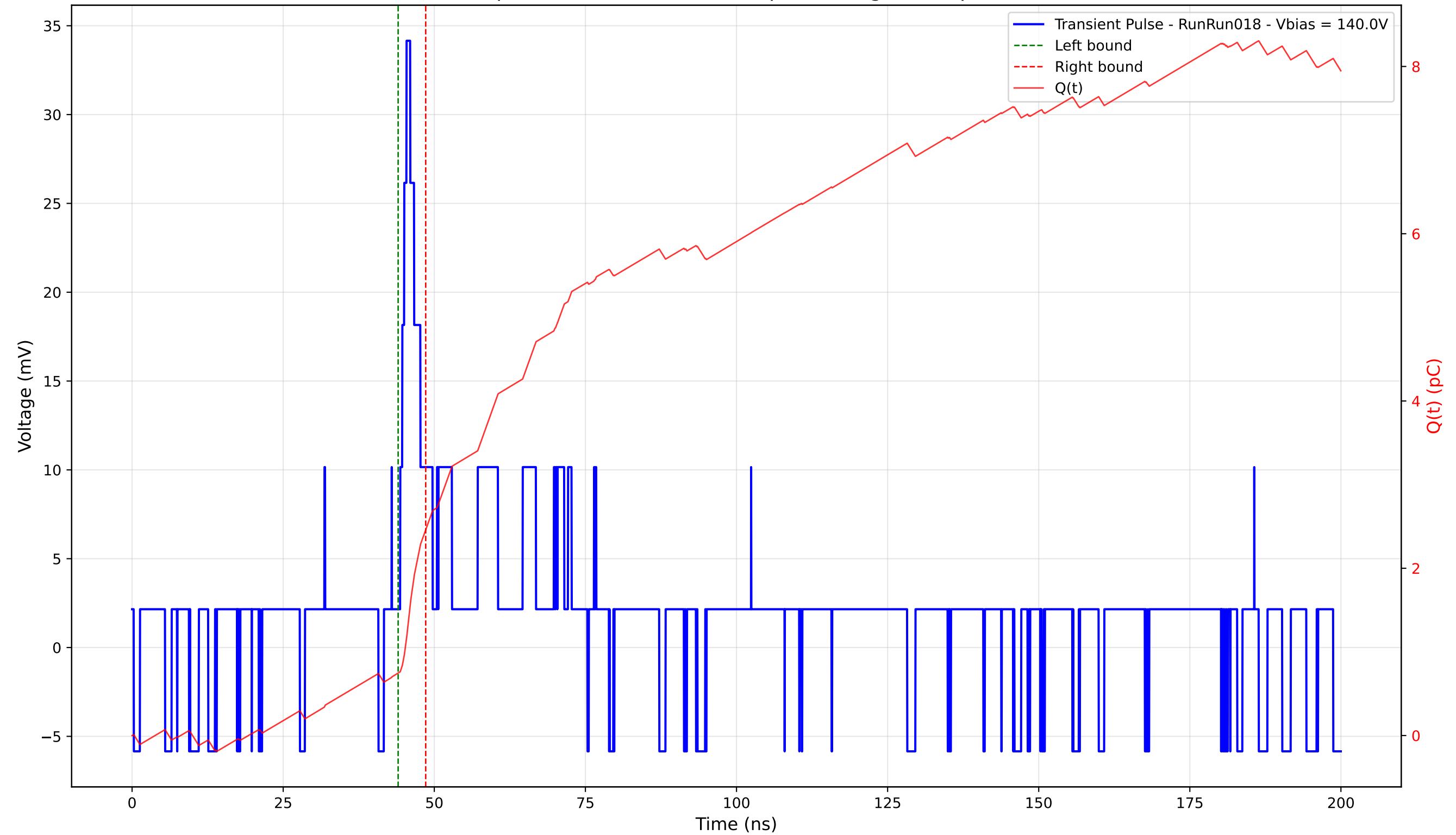
Transient Pulse - Sample: 4003 - Position: 355.0 \mu\text{m} - Charge: 1.71 pC - Rise Time: 1.06 ns
