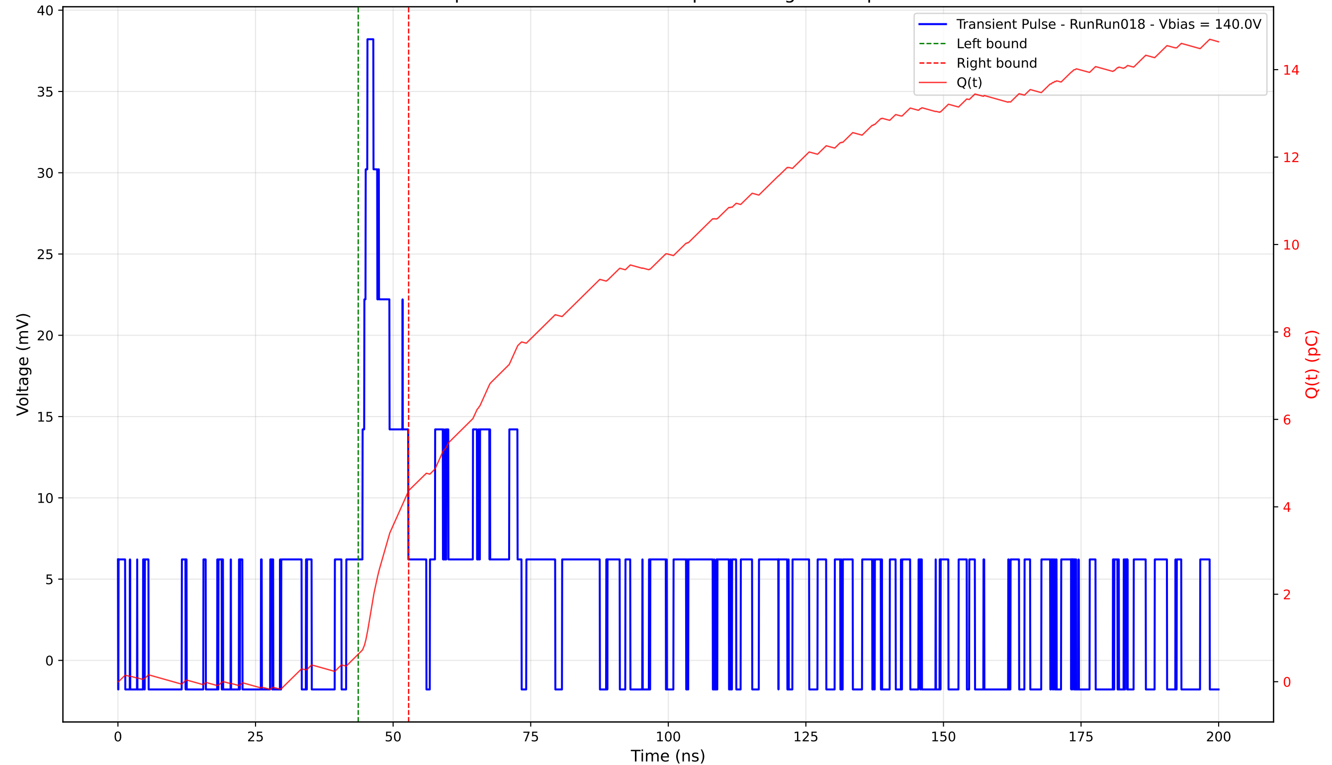
Transient Pulse - Sample: 4003 - Position: 50.0 \mu\text{m} - Charge: 3.74 pC - Rise Time: 3.85 ns
