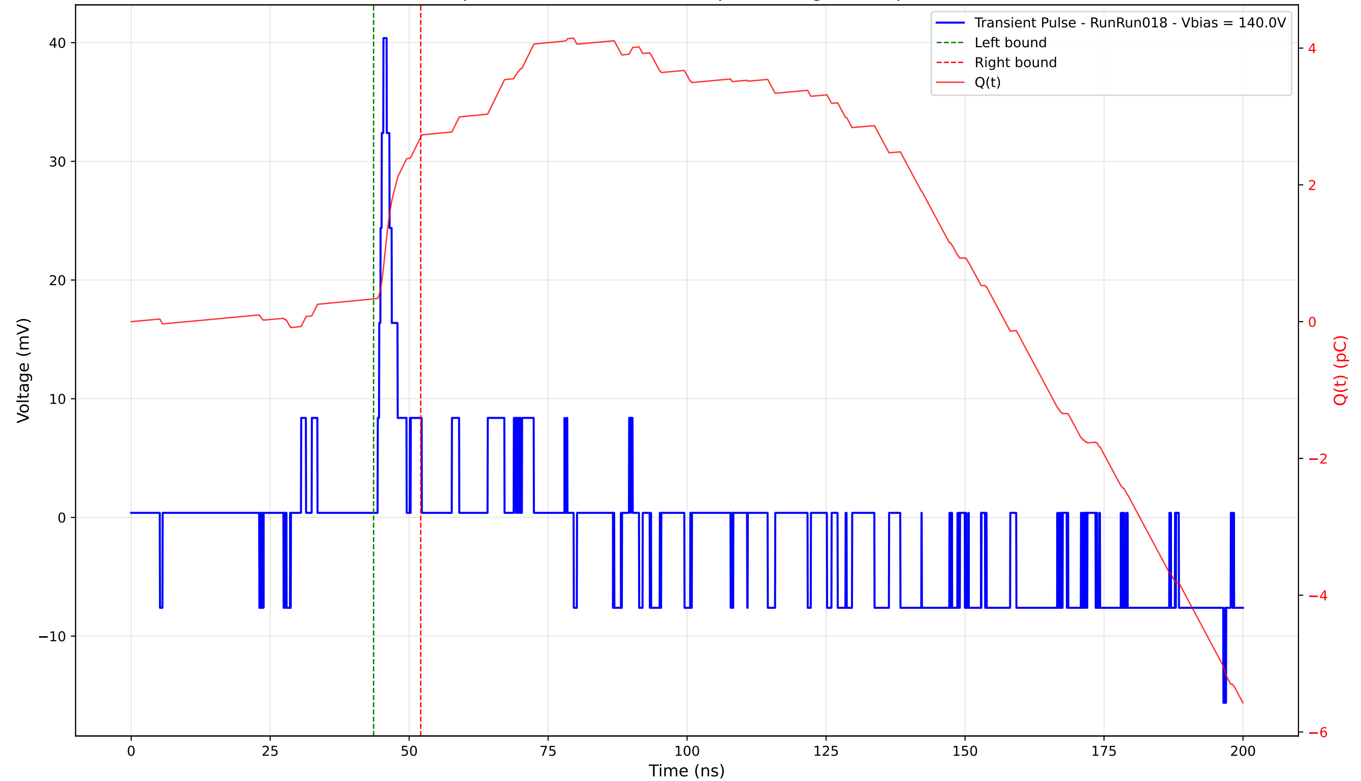
Transient Pulse - Sample: 4003 - Position: 405.0 \mu\text{m} - Charge: 2.37 pC - Rise Time: 1.03 ns
