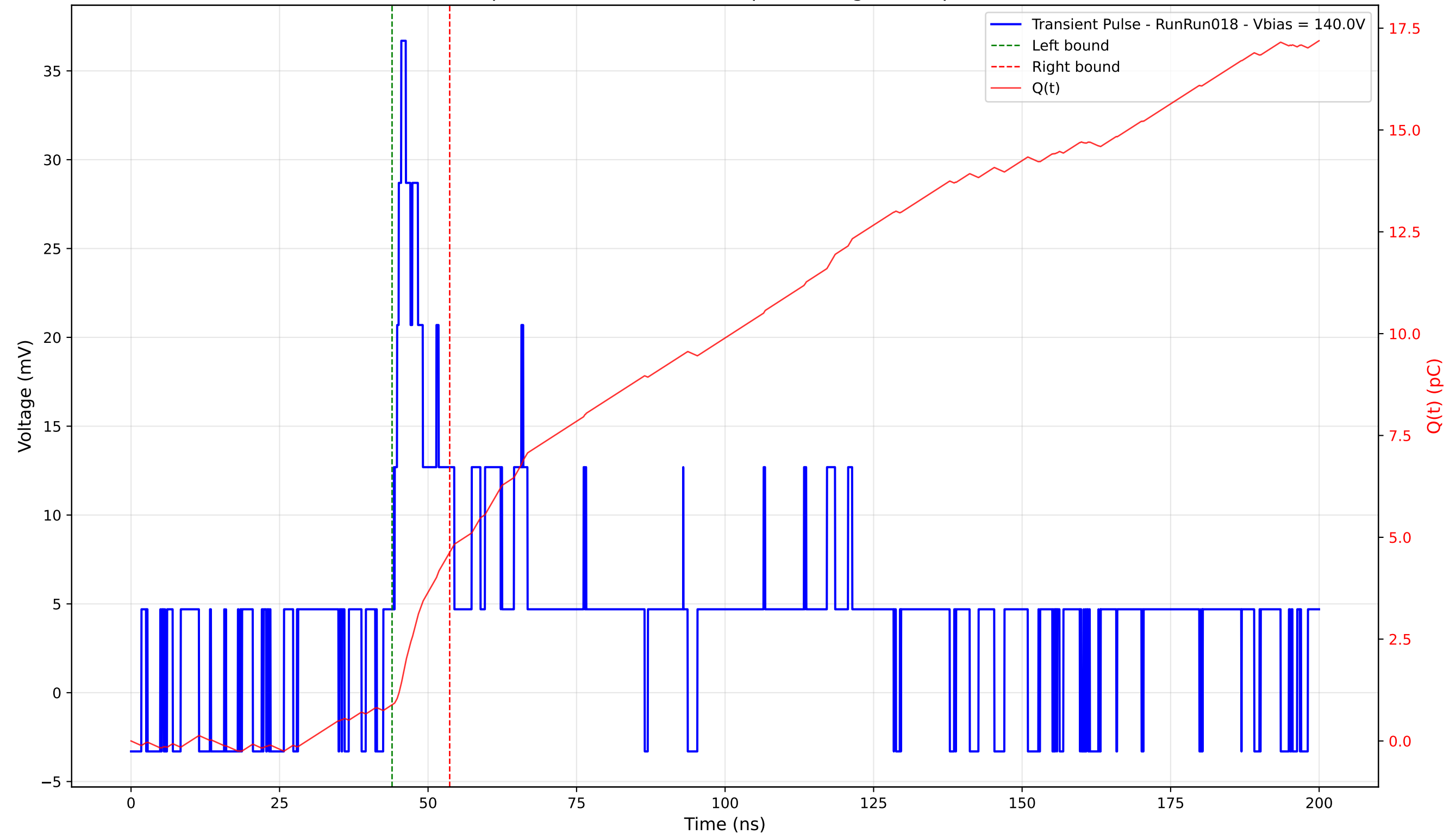
Transient Pulse - Sample: 4003 - Position: 60.0 \mu\text{m} - Charge: 3.75 pC - Rise Time: 3.03 ns
