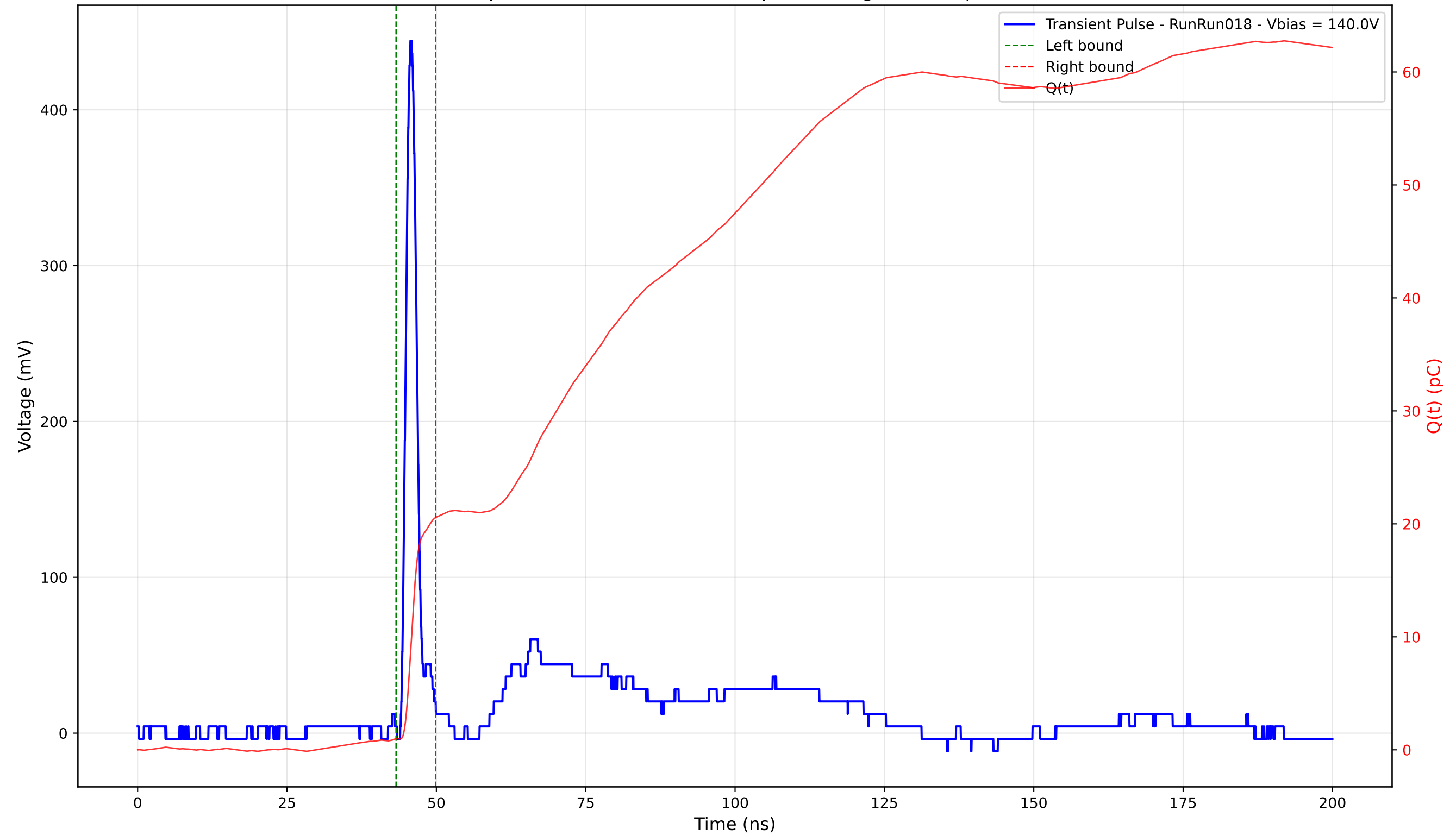
Transient Pulse - Sample: 4003 - Position: 190.0 \mu\text{m} - Charge: 19.58 pC - Rise Time: 1.08 ns
