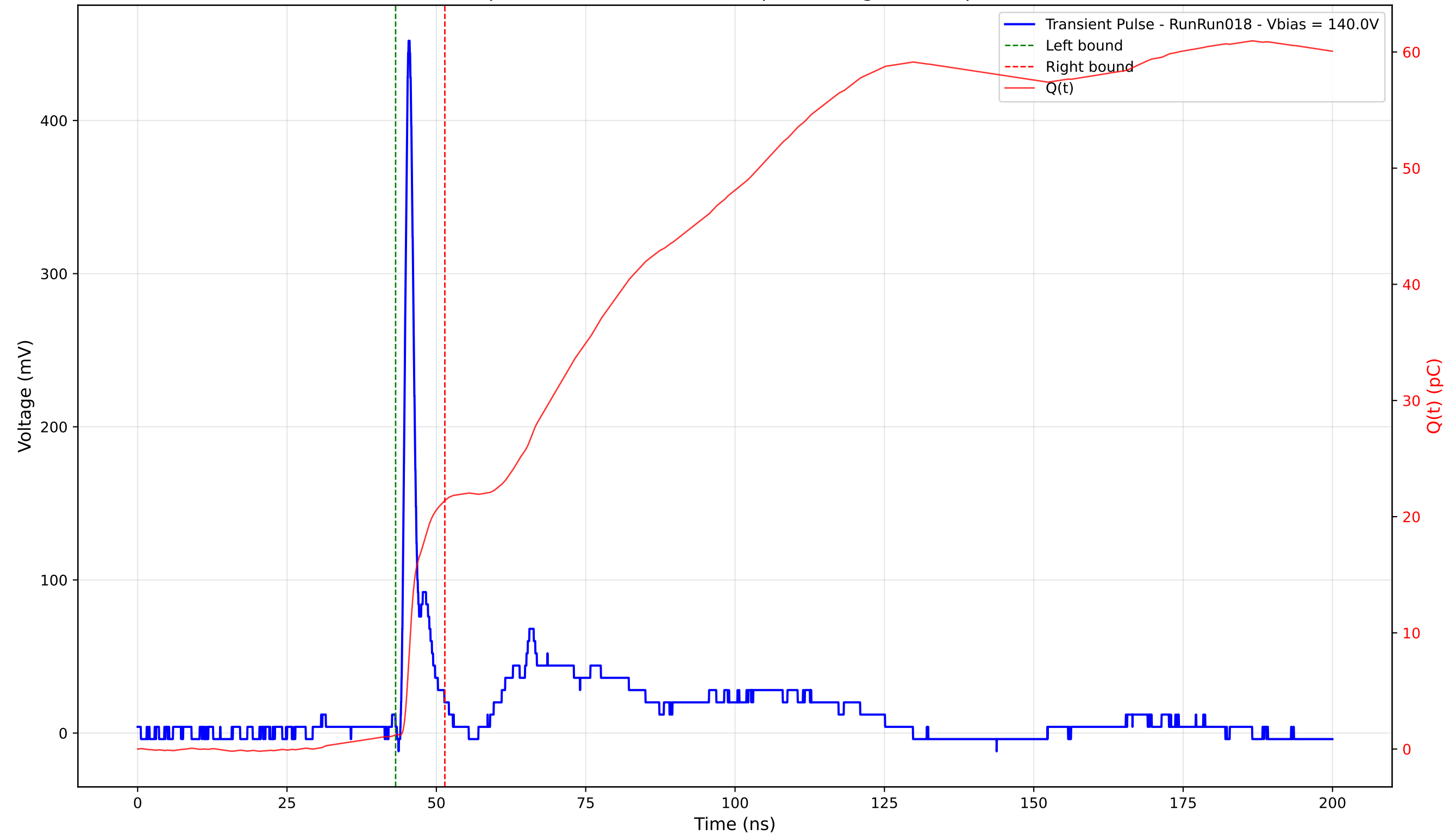
Transient Pulse - Sample: 4003 - Position: 130.0 \mu\text{m} - Charge: 20.16 pC - Rise Time: 0.92 ns
