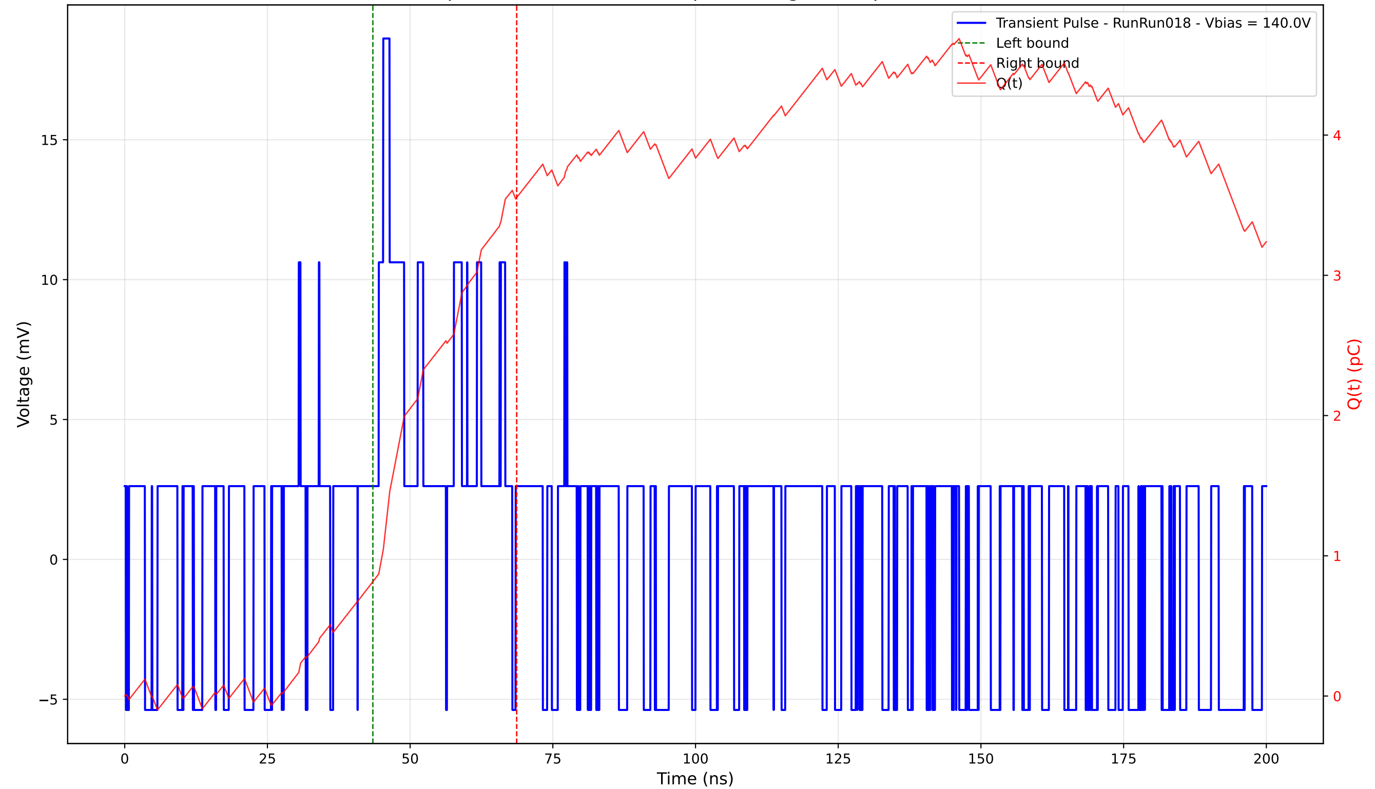
Transient Pulse - Sample: 4003 - Position: 10.0 \mu\text{m} - Charge: 2.74 pC - Rise Time: 0.00 ns (N/A)
