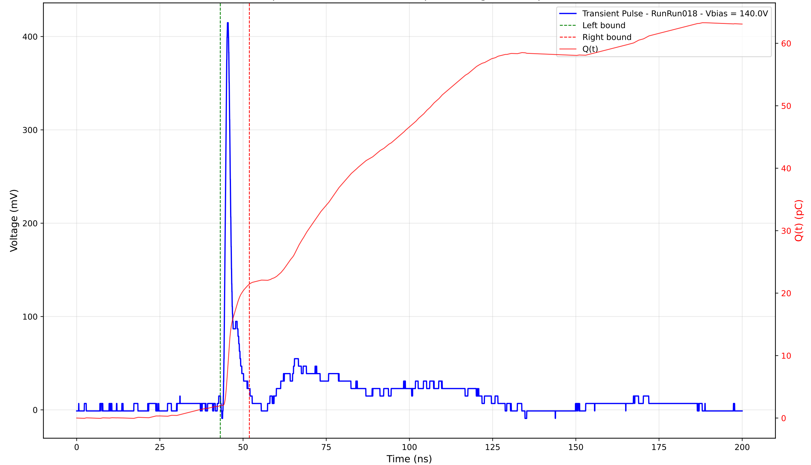
Transient Pulse - Sample: 4003 - Position: 120.0 \mu\text{m} - Charge: 19.41 pC - Rise Time: 0.87 ns
