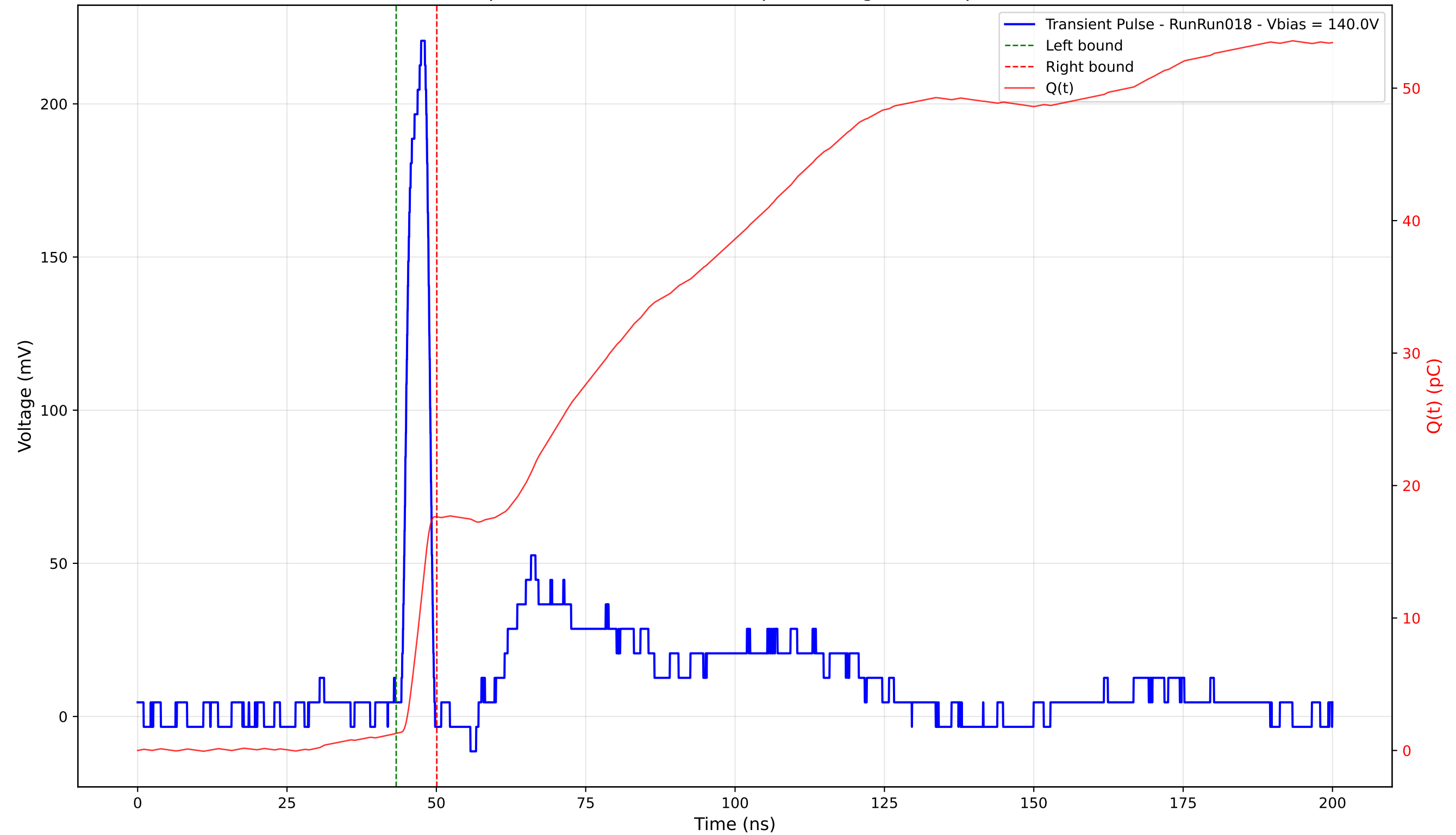
Transient Pulse - Sample: 4003 - Position: 270.0 \mu\text{m} - Charge: 16.34 pC - Rise Time: 2.48 ns
