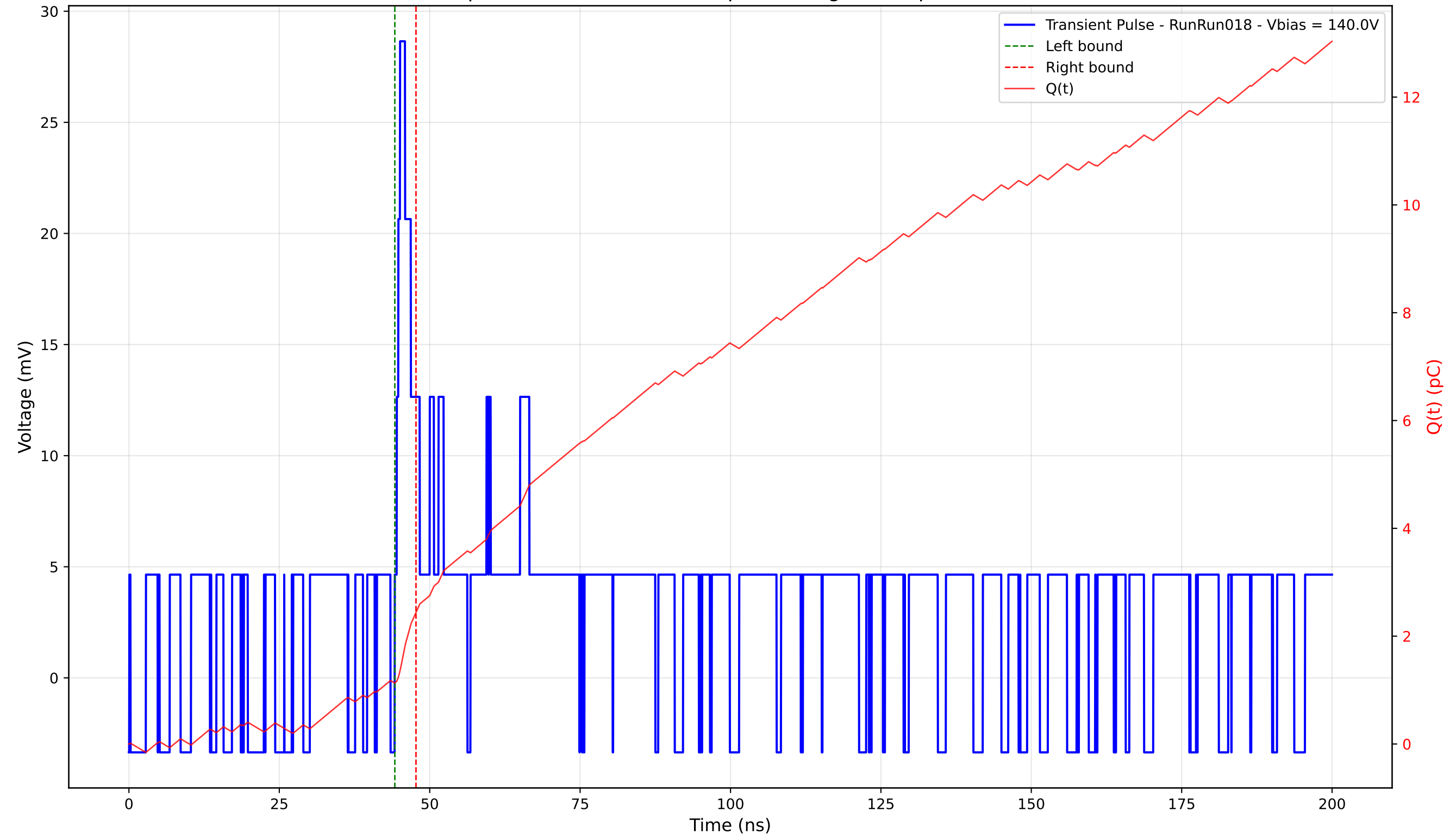
Transient Pulse - Sample: 4003 - Position: 25.0 \mu\text{m} - Charge: 1.31 pC - Rise Time: 0.00 ns (N/A)
