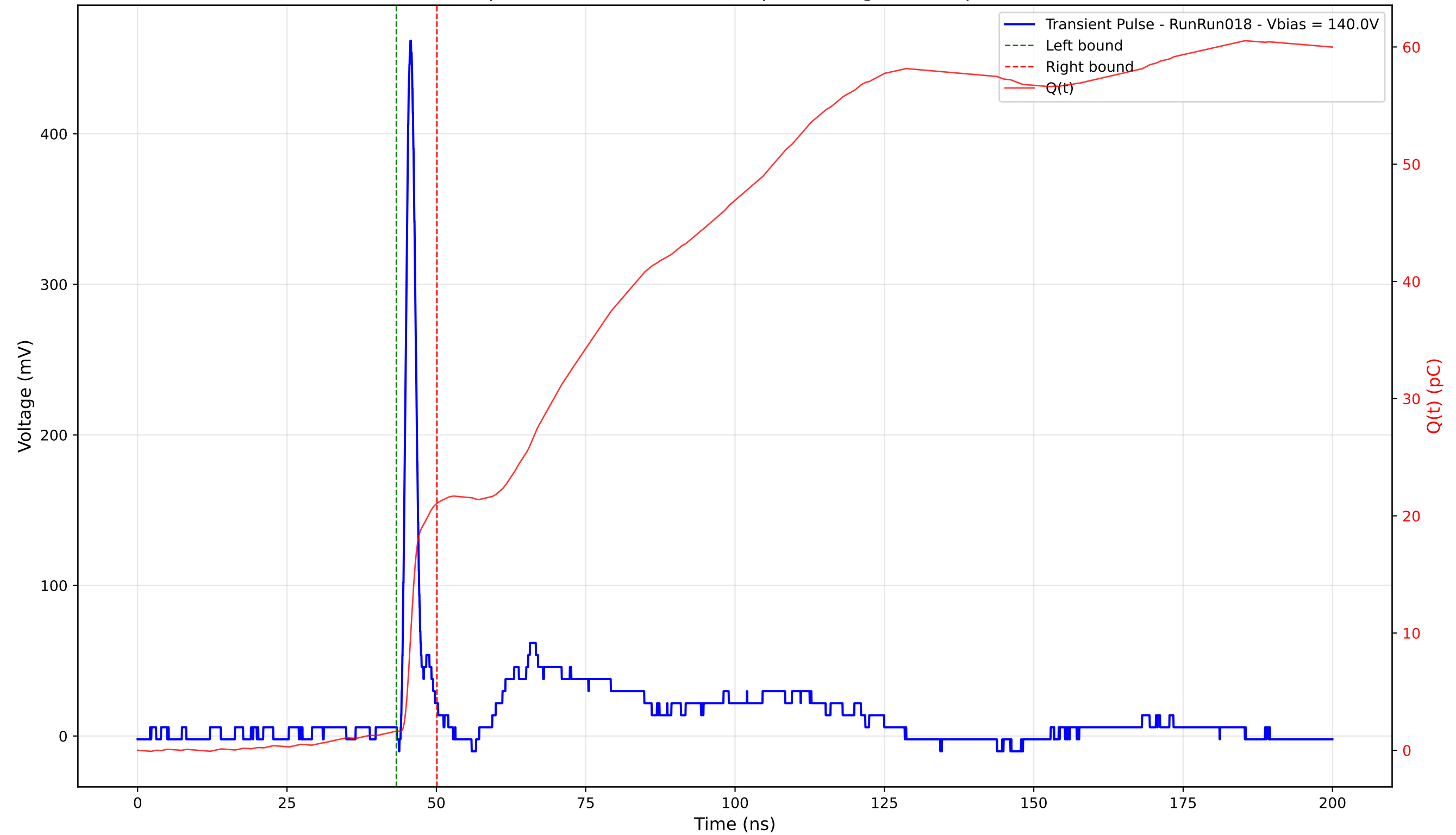
Transient Pulse - Sample: 4003 - Position: 180.0 \mu\text{m} - Charge: 19.43 pC - Rise Time: 1.04 ns
