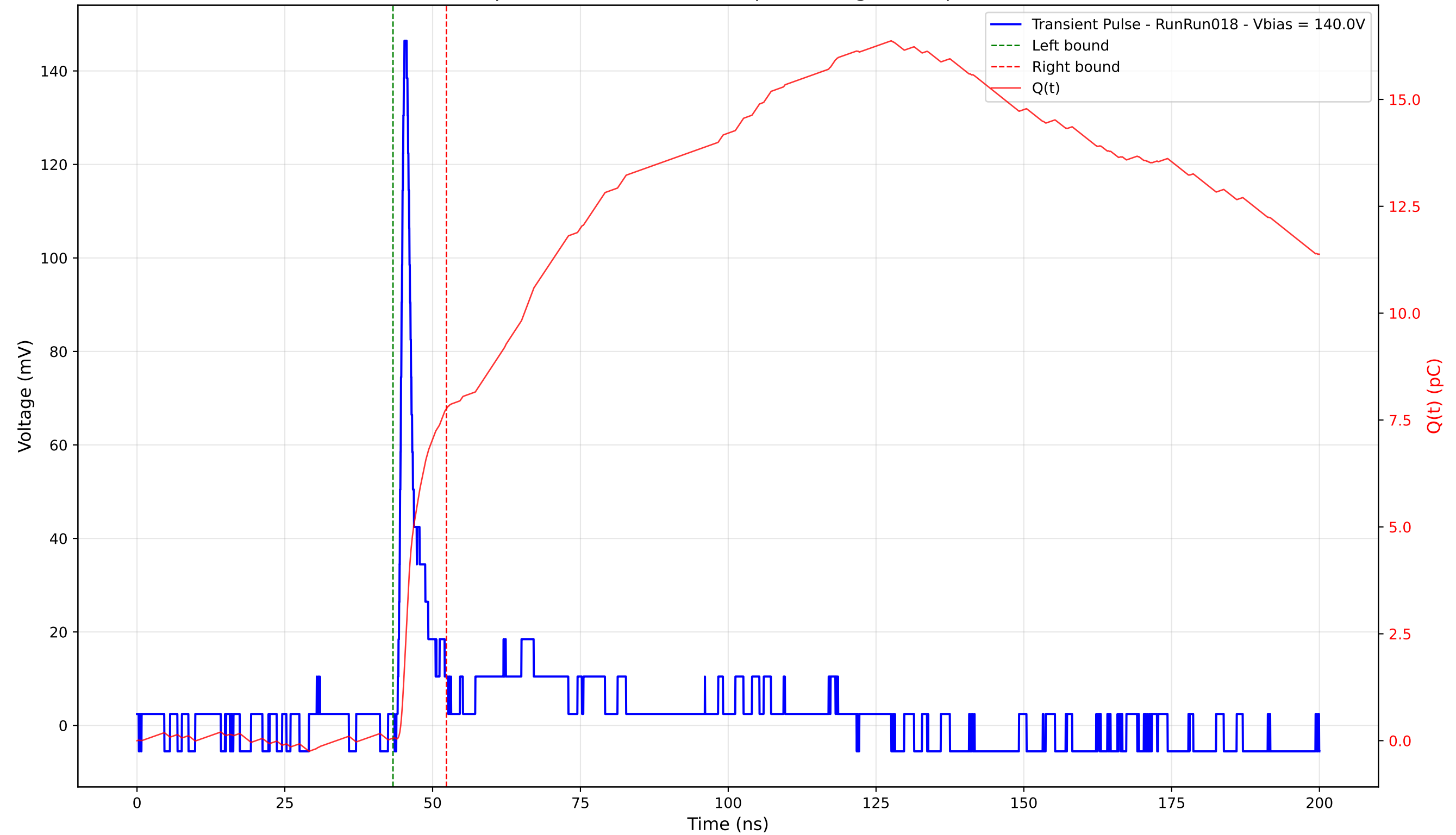
Transient Pulse - Sample: 4003 - Position: 95.0 \mu\text{m} - Charge: 7.71 pC - Rise Time: 0.91 ns
