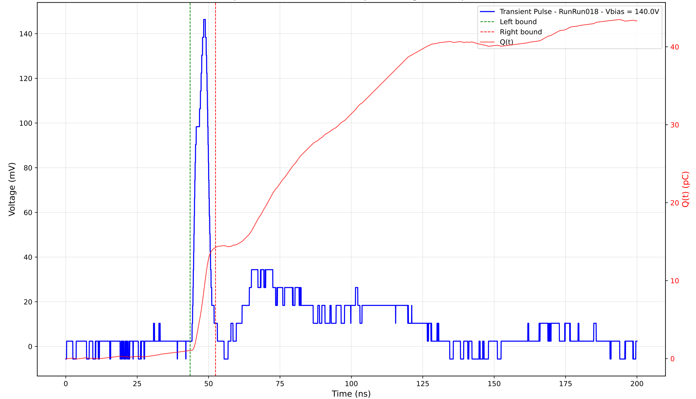
Transient Pulse - Sample: 4003 - Position: 285.0 \mu\text{m} - Charge: 13.24 pC - Rise Time: 3.49 ns
