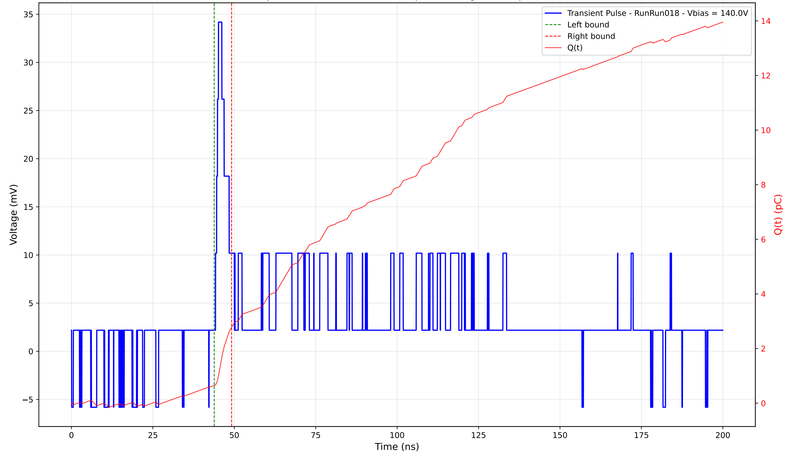
Transient Pulse - Sample: 4003 - Position: 320.0 \mu\text{m} - Charge: 2.13 pC - Rise Time: 0.92 ns
