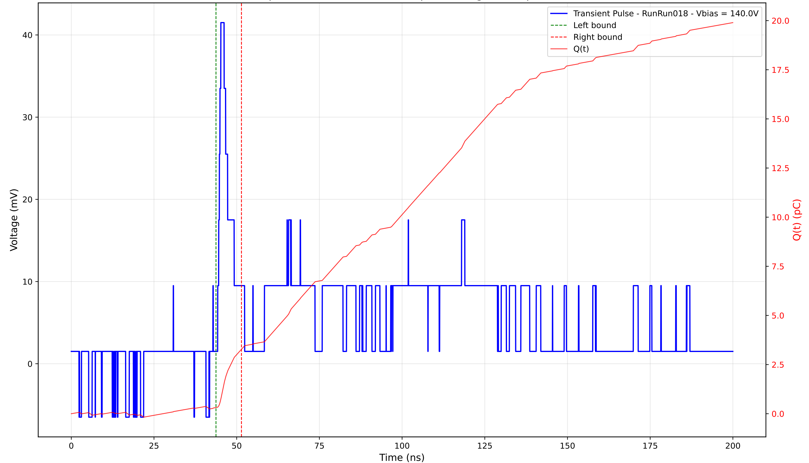
Transient Pulse - Sample: 4003 - Position: 315.0 \mu\text{m} - Charge: 2.97 pC - Rise Time: 0.95 ns
