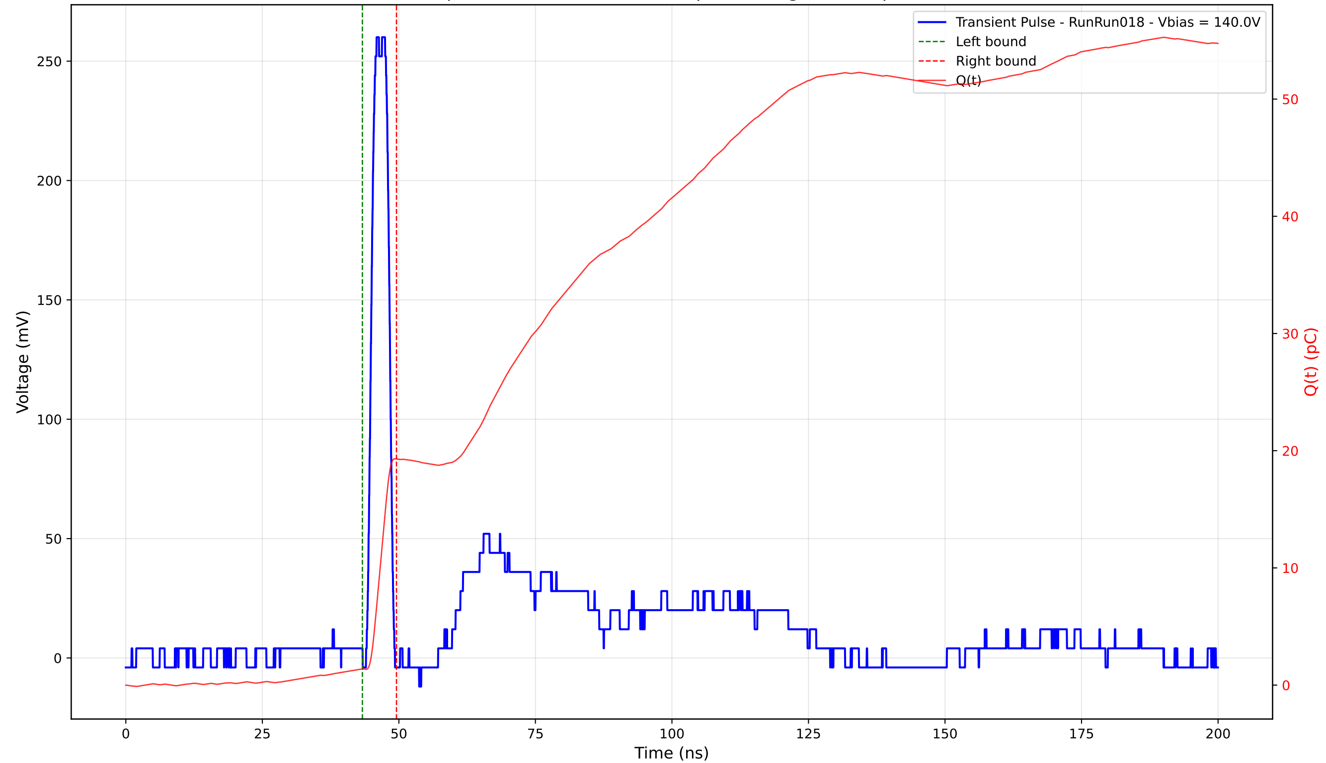
Transient Pulse - Sample: 4003 - Position: 255.0 \mu\text{m} - Charge: 17.91 pC - Rise Time: 1.21 ns
