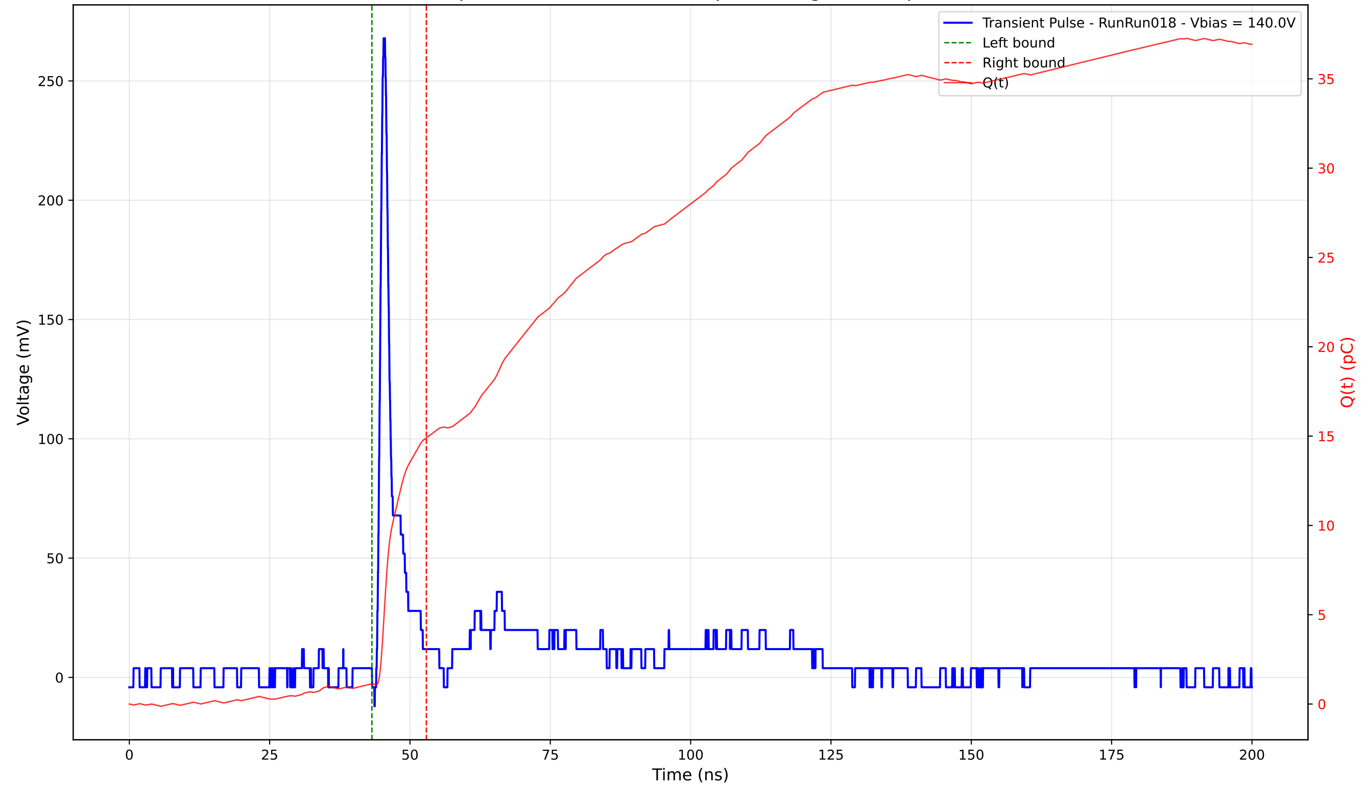
Transient Pulse - Sample: 4003 - Position: 105.0 \mu\text{m} - Charge: 13.76 pC - Rise Time: 0.90 ns
