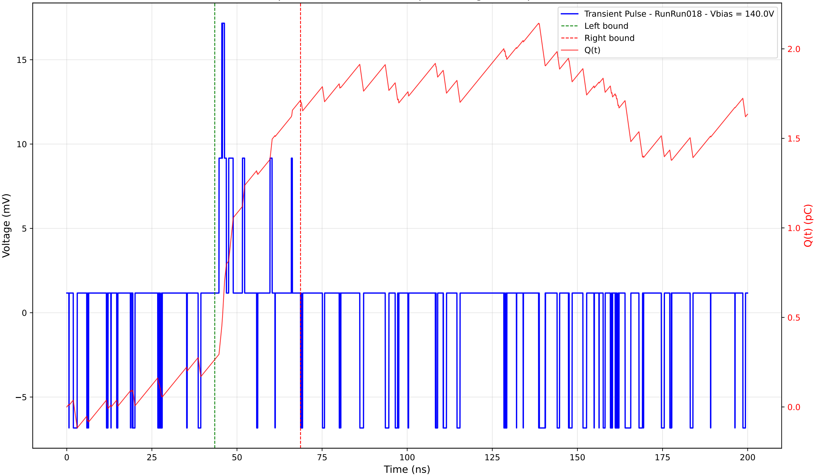
Transient Pulse - Sample: 4003 - Position: 5.0 \mu\text{m} - Charge: 1.45 pC - Rise Time: 0.84 ns
