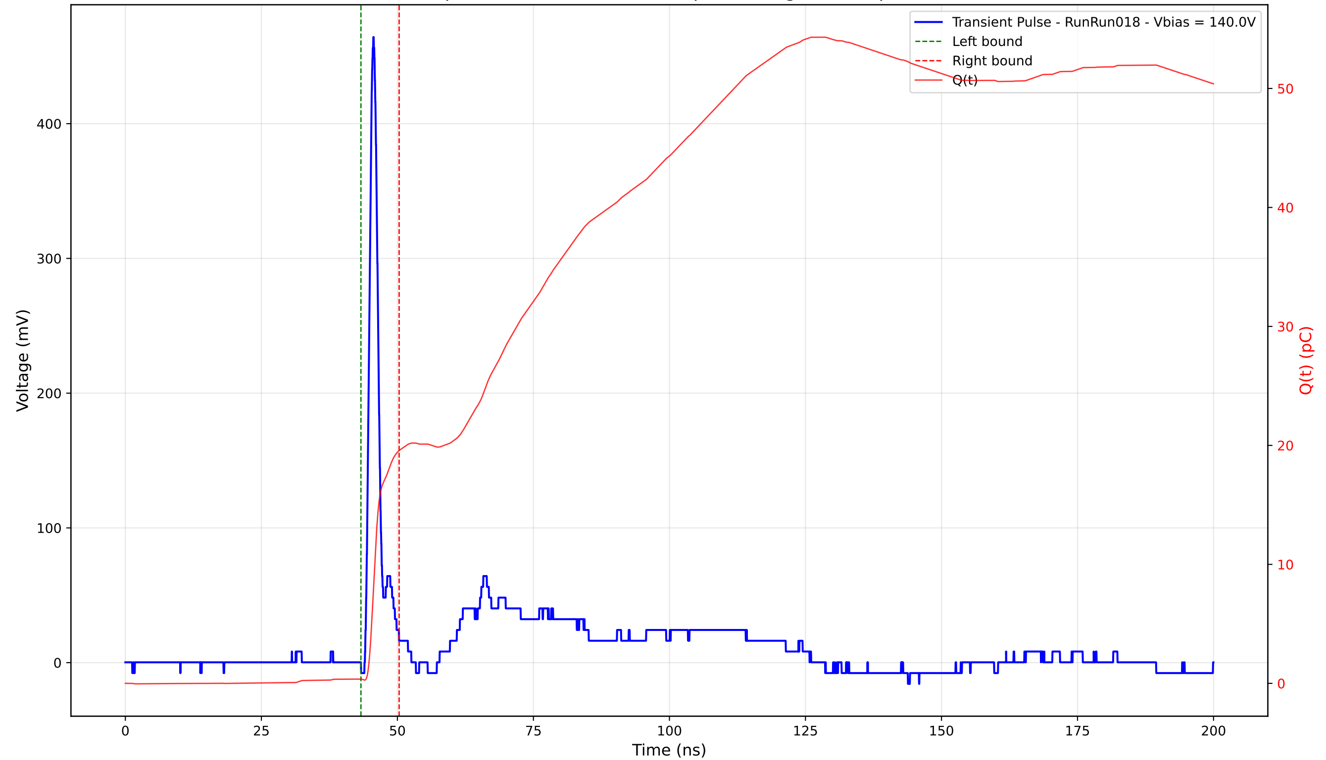
Transient Pulse - Sample: 4003 - Position: 165.0 \mu\text{m} - Charge: 19.20 pC - Rise Time: 1.02 ns
