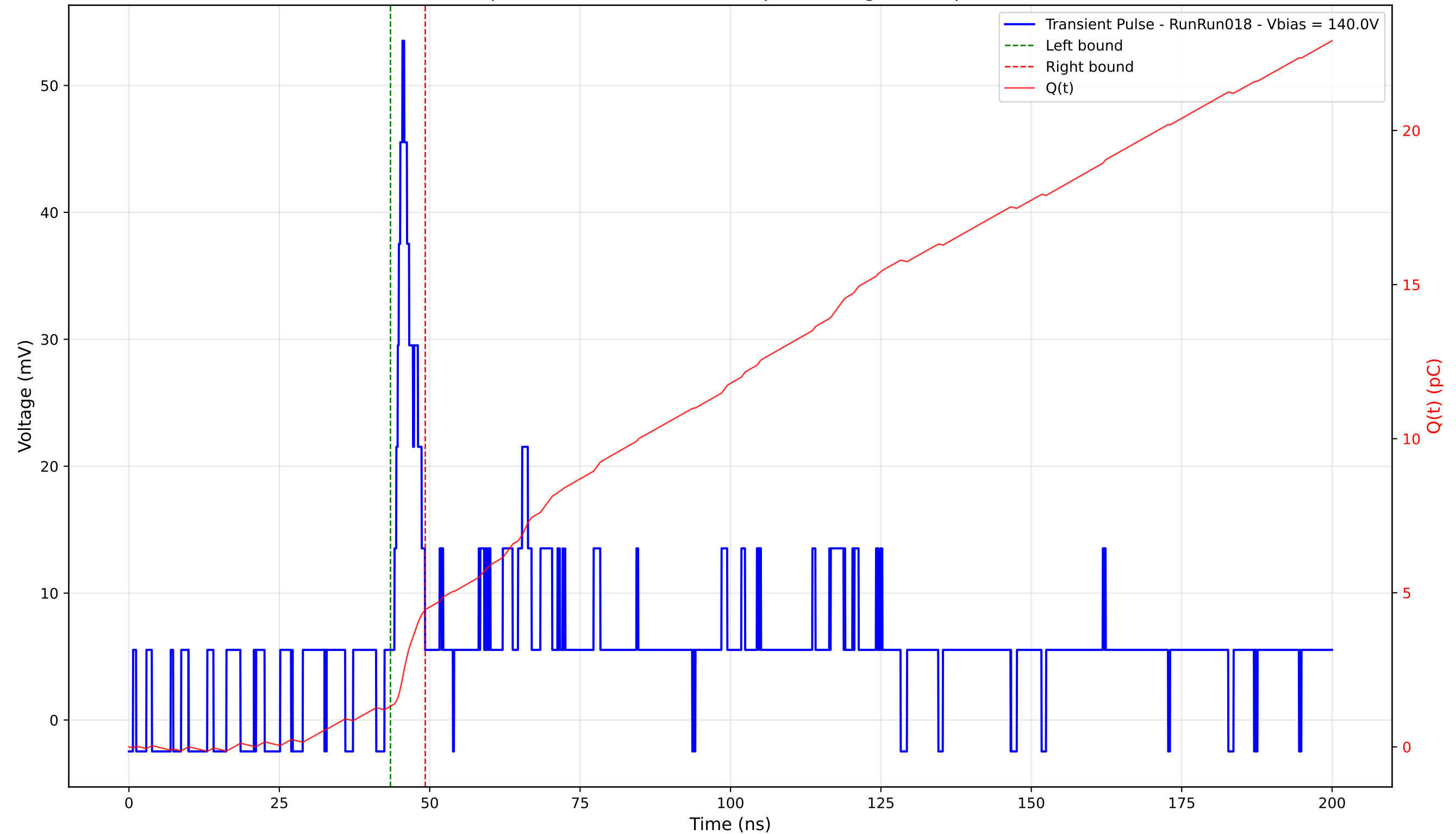
Transient Pulse - Sample: 4003 - Position: 395.0 \mu\text{m} - Charge: 3.14 pC - Rise Time: 2.98 ns
