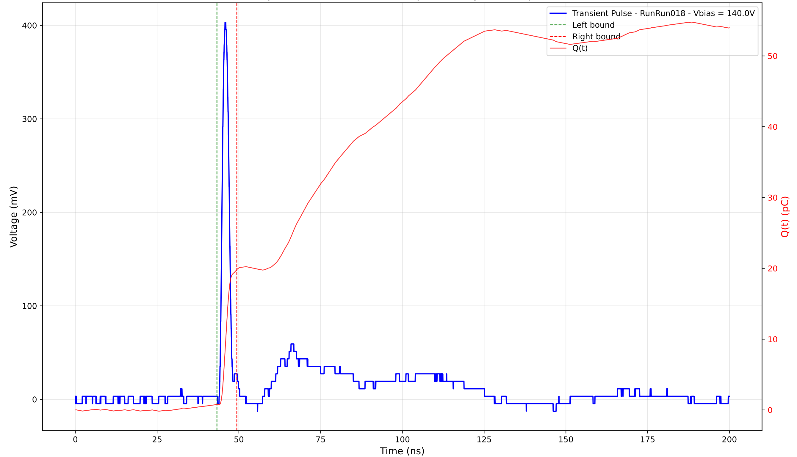
Transient Pulse - Sample: 4003 - Position: 210.0 \mu\text{m} - Charge: 19.05 pC - Rise Time: 1.11 ns
