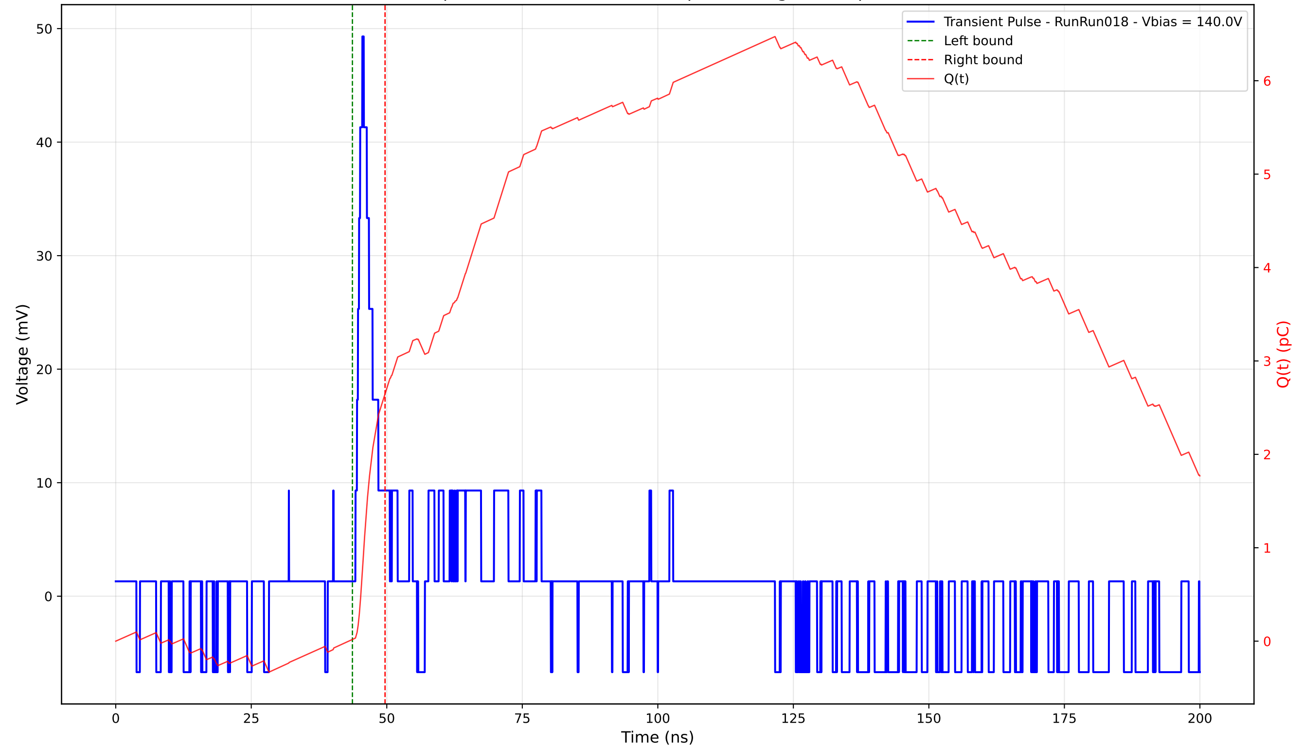
Transient Pulse - Sample: 4003 - Position: 385.0 \mu\text{m} - Charge: 2.63 pC - Rise Time: 1.27 ns
