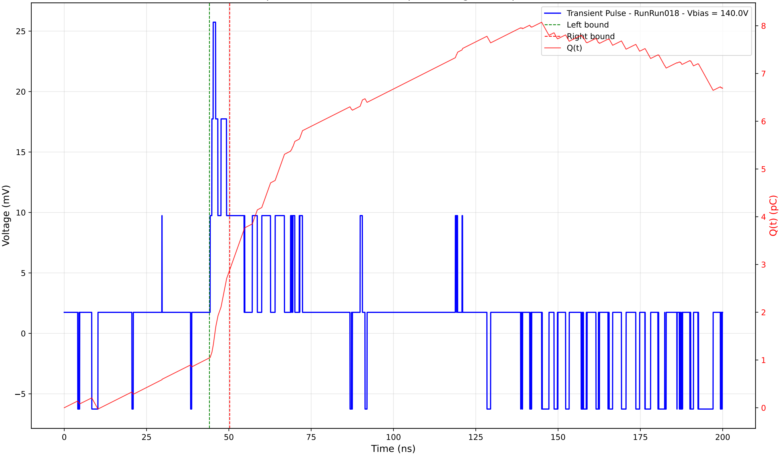
Transient Pulse - Sample: 4003 - Position: 65.0 \mu\text{m} - Charge: 1.84 pC - Rise Time: 0.94 ns
