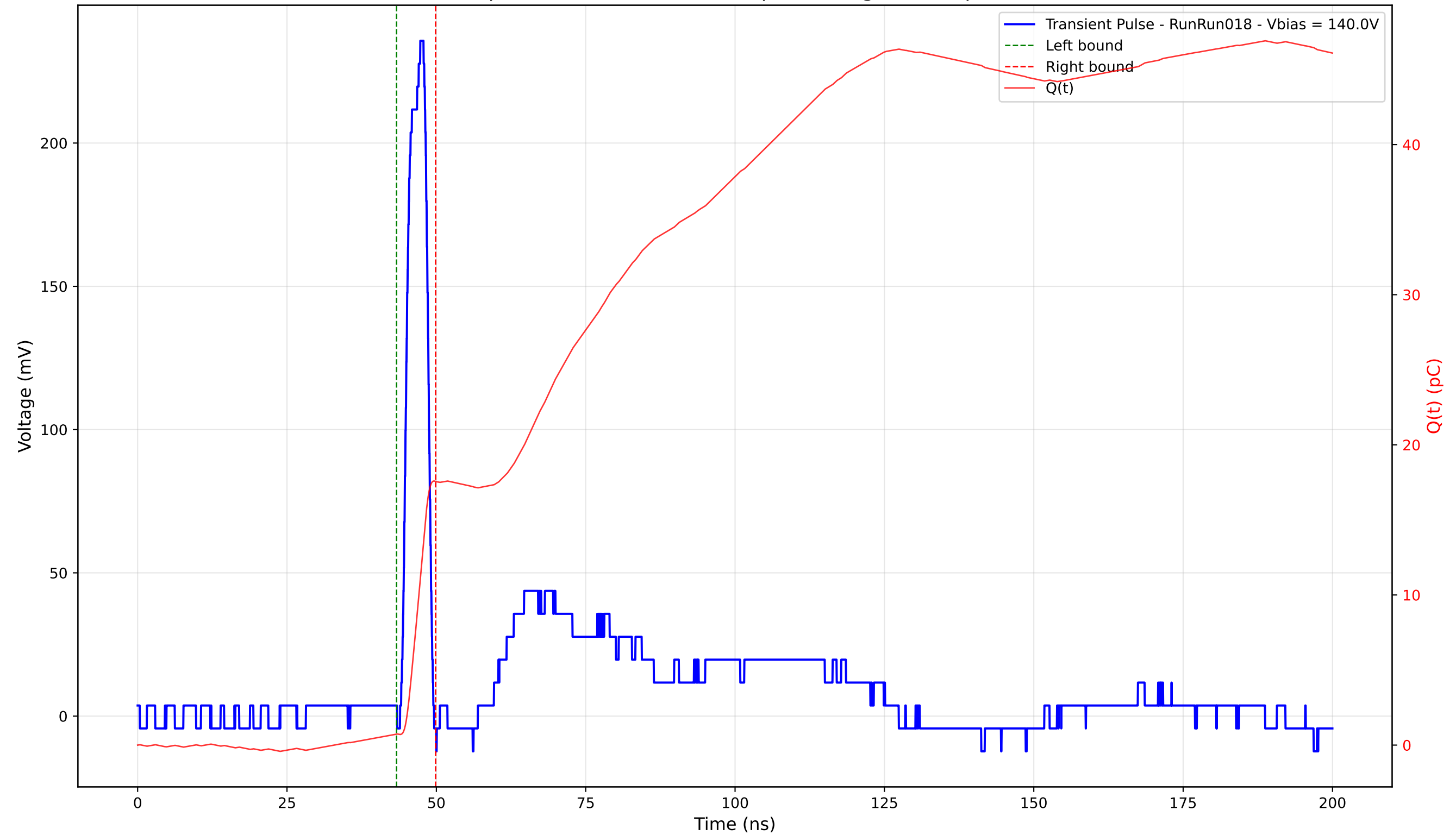
Transient Pulse - Sample: 4003 - Position: 265.0 \mu\text{m} - Charge: 16.83 pC - Rise Time: 2.45 ns
