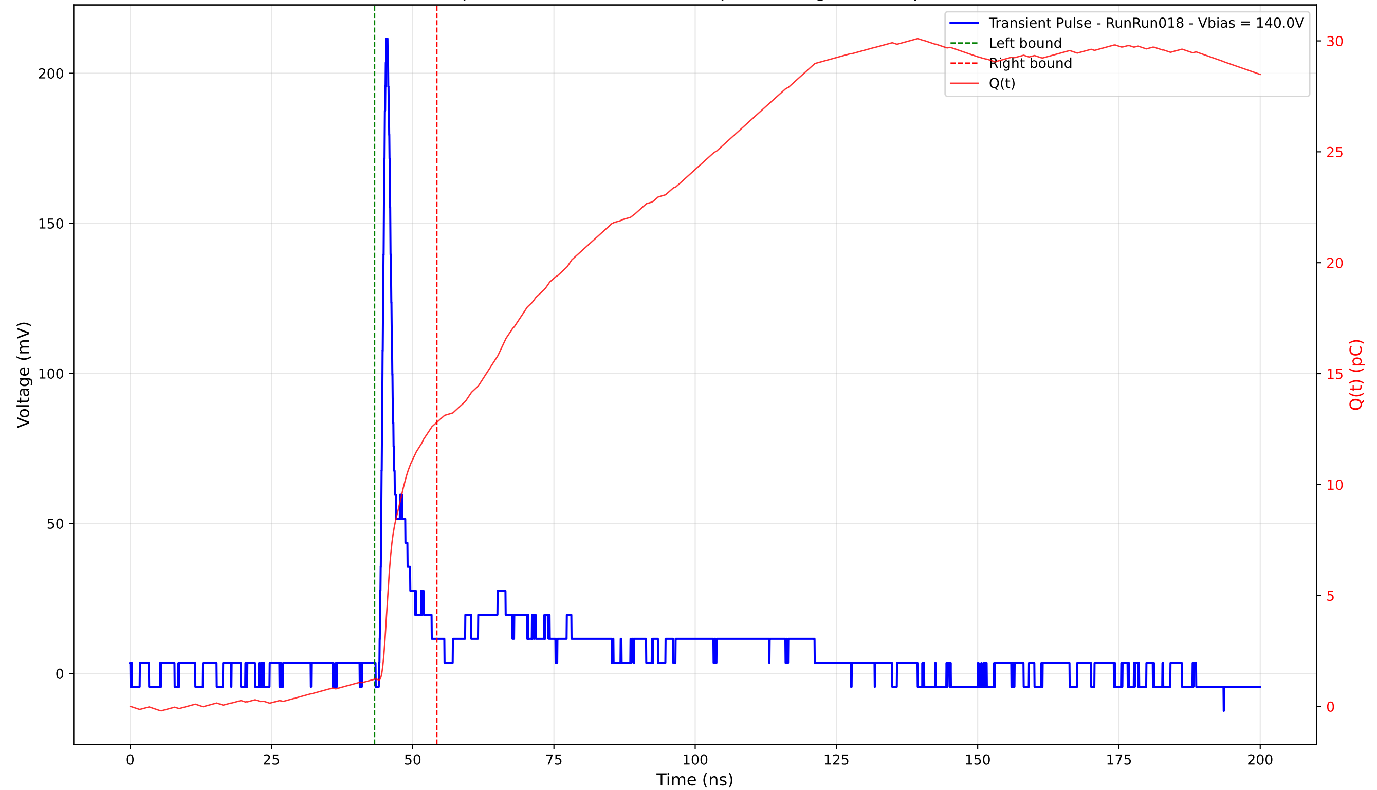
Transient Pulse - Sample: 4003 - Position: 100.0 \mu\text{m} - Charge: 11.58 pC - Rise Time: 0.90 ns
