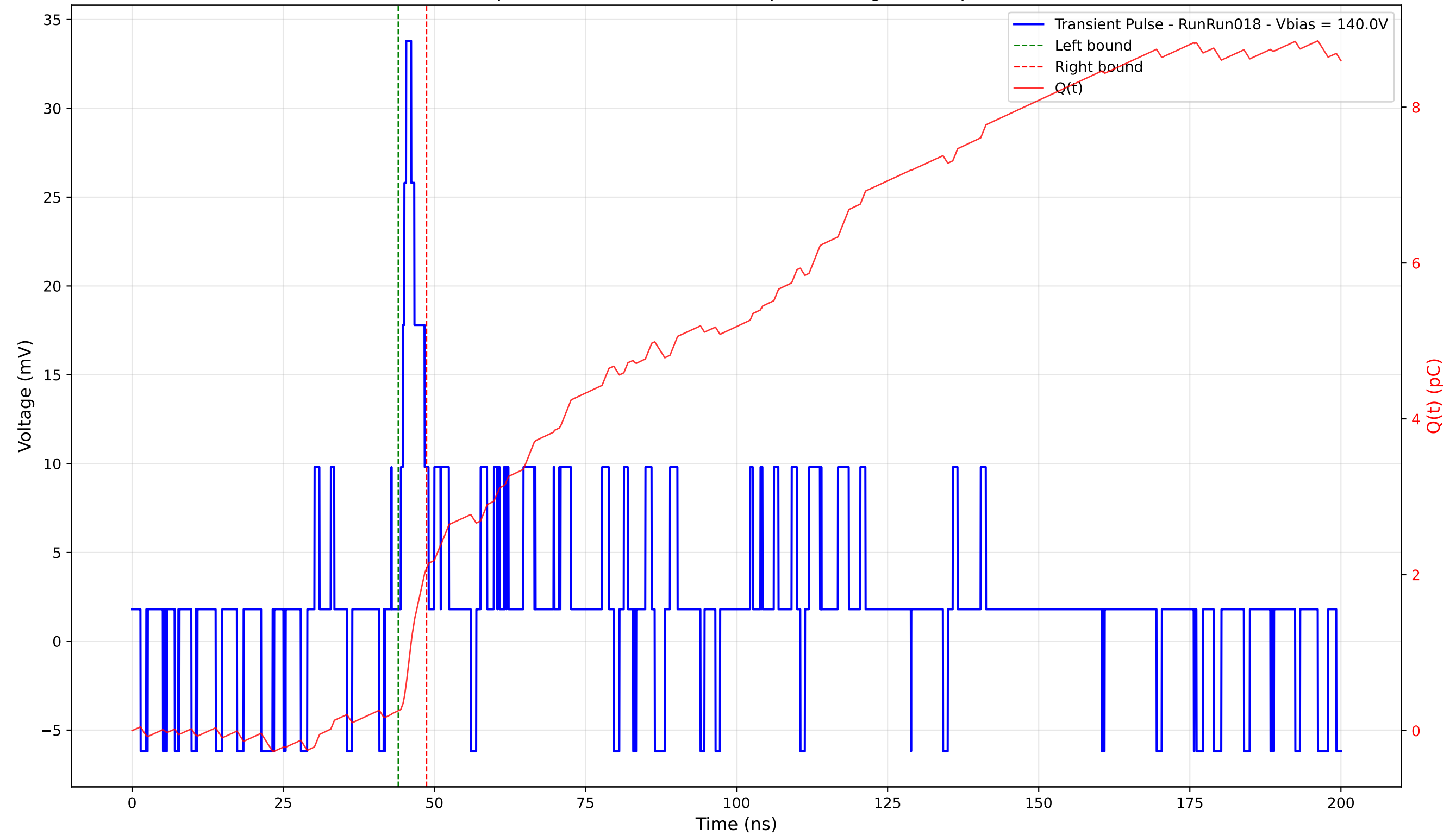
Transient Pulse - Sample: 4003 - Position: 330.0 \mu\text{m} - Charge: 1.83 pC - Rise Time: 0.90 ns
