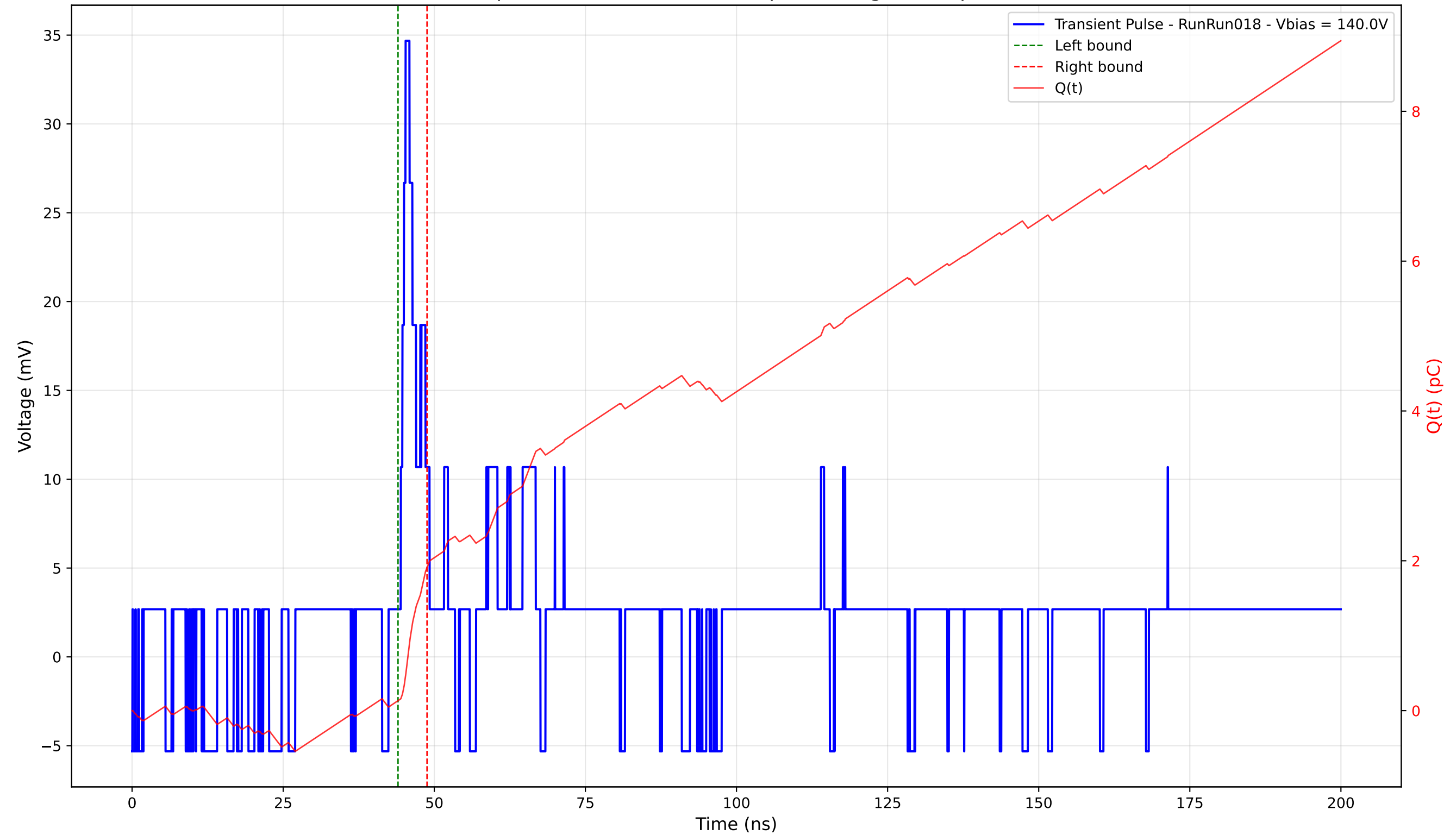
Transient Pulse - Sample: 4003 - Position: 350.0 \mu\text{m} - Charge: 1.78 pC - Rise Time: 0.80 ns
