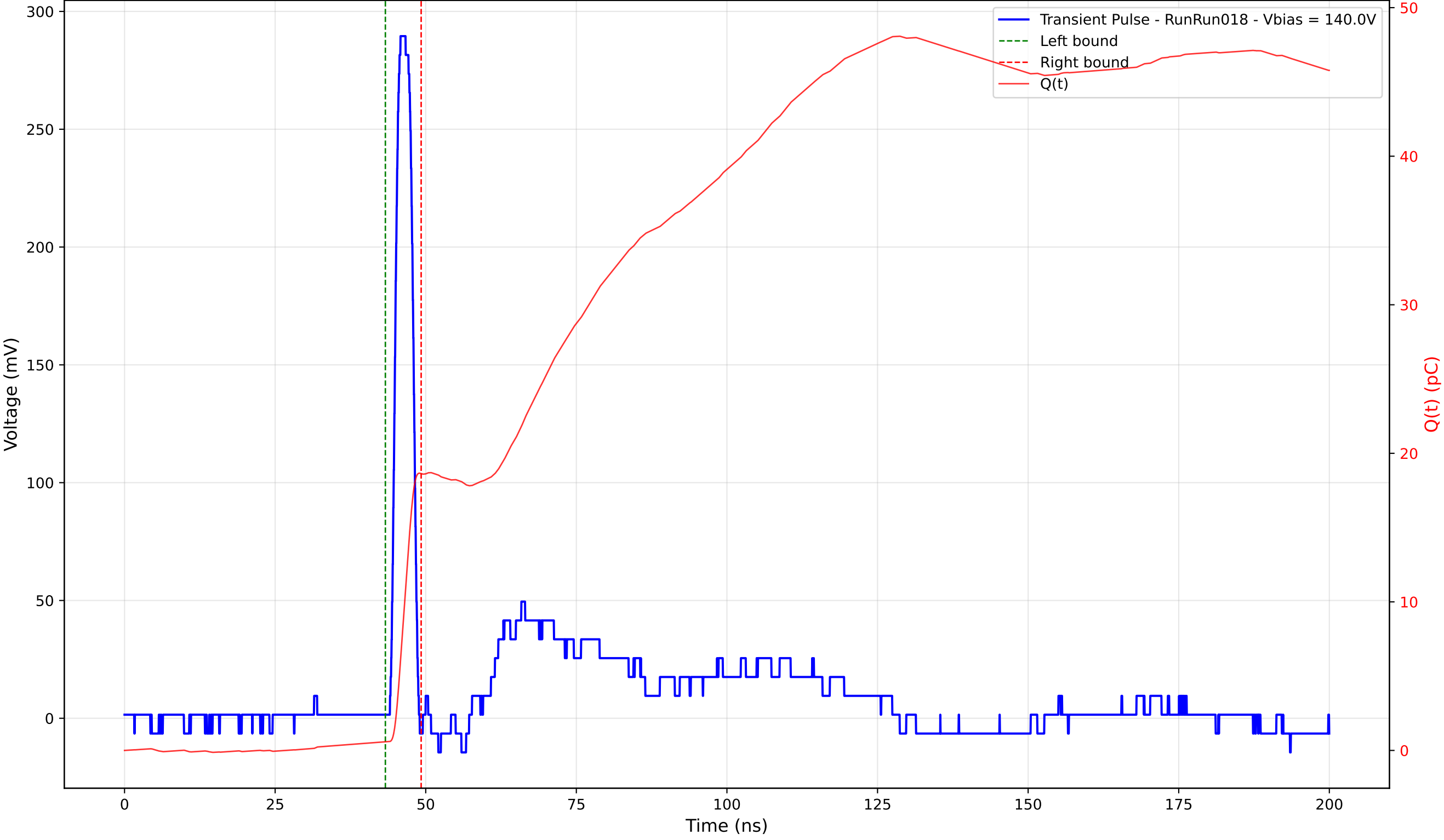
Transient Pulse - Sample: 4003 - Position: 245.0 \mu\text{m} - Charge: 18.06 pC - Rise Time: 1.15 ns
