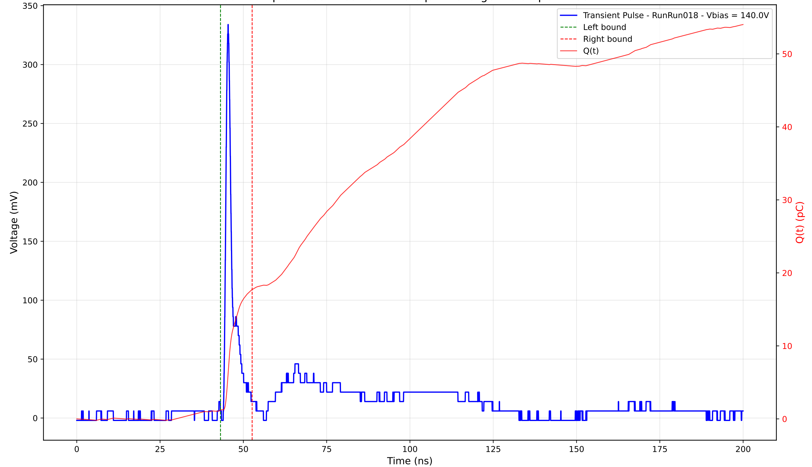
Transient Pulse - Sample: 4003 - Position: 110.0 \mu\text{m} - Charge: 16.50 pC - Rise Time: 0.91 ns
