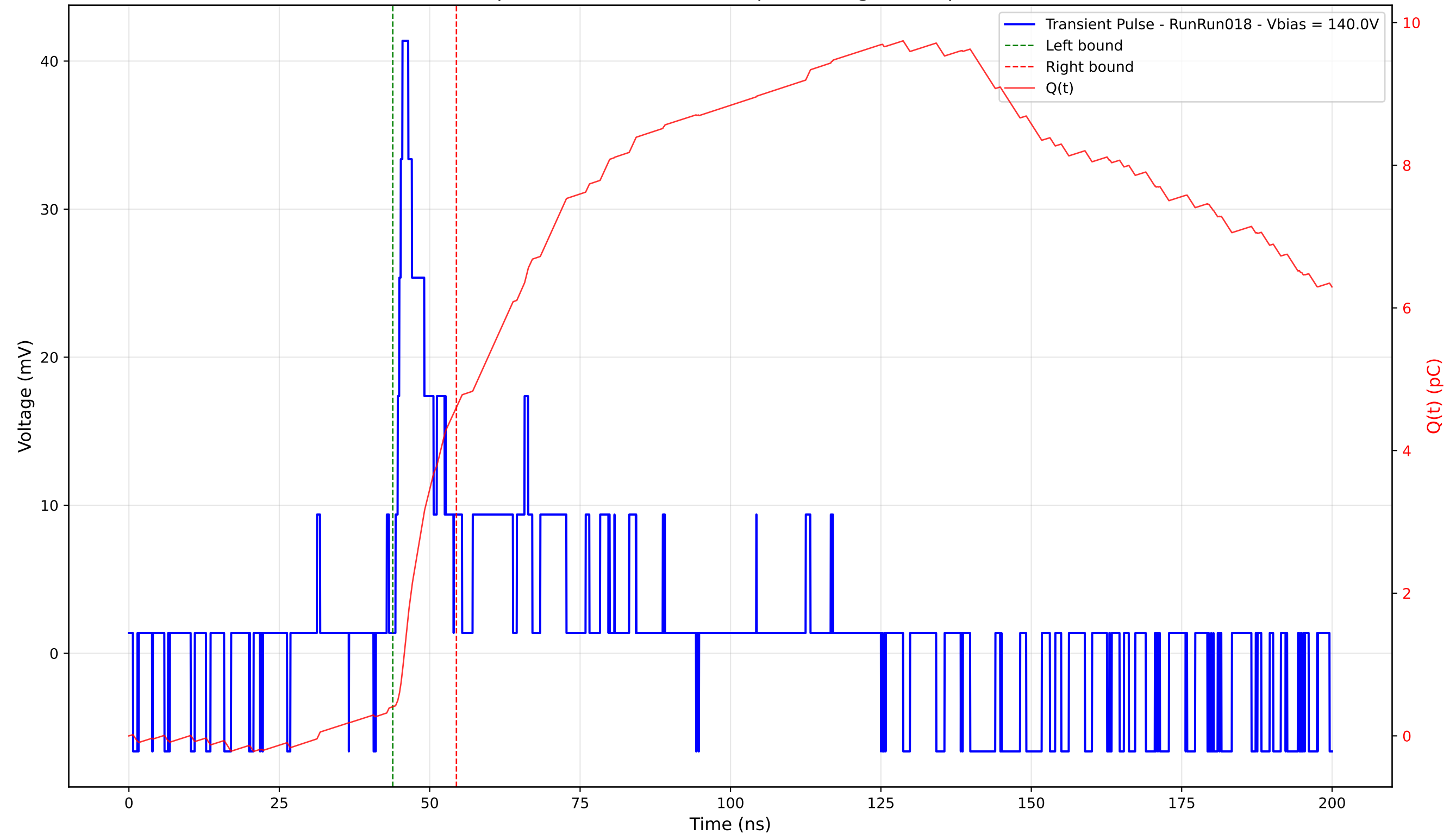
Transient Pulse - Sample: 4003 - Position: 55.0 \mu\text{m} - Charge: 4.20 pC - Rise Time: 1.15 ns
