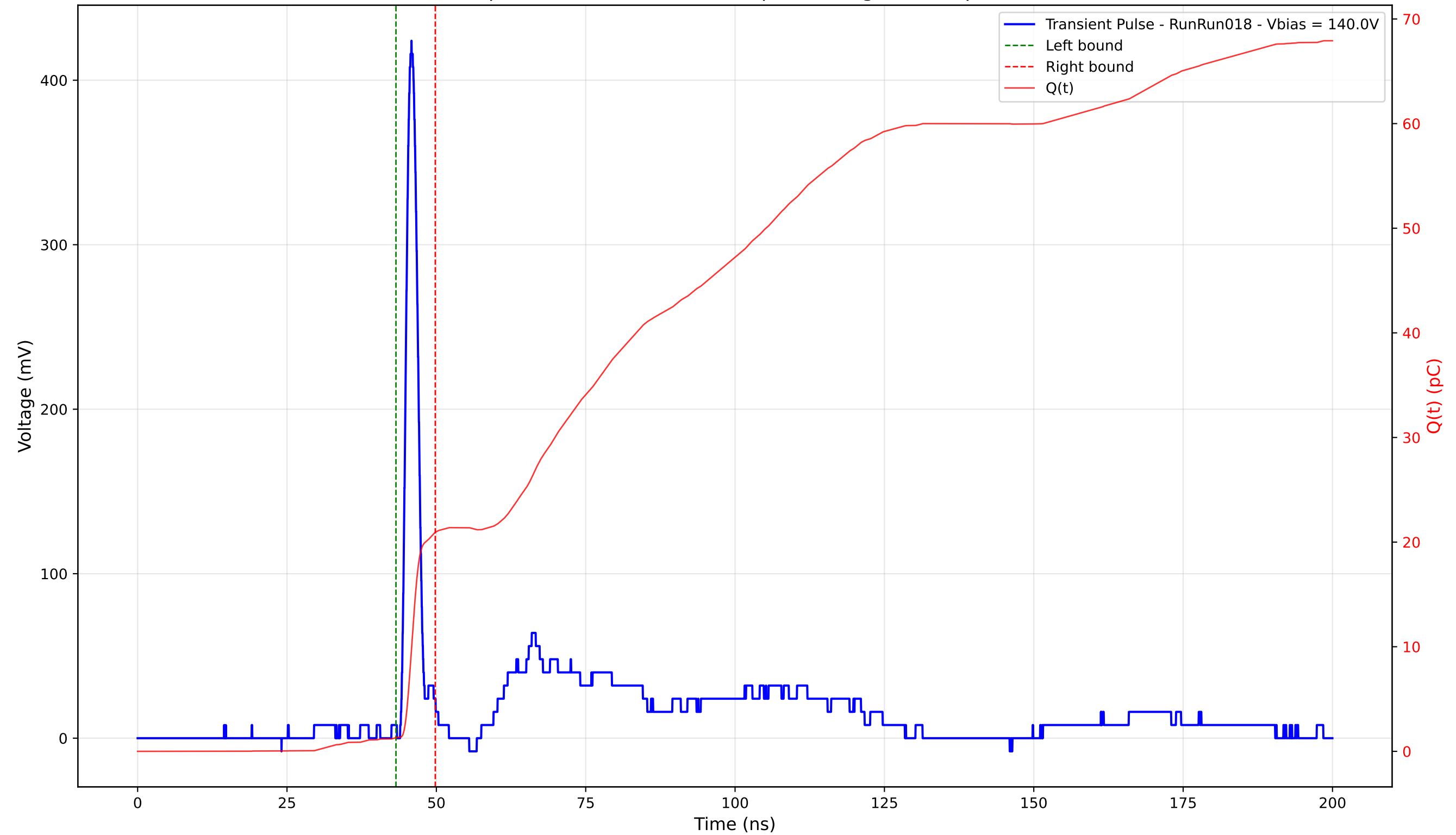
Transient Pulse - Sample: 4003 - Position: 205.0 \mu\text{m} - Charge: 19.62 pC - Rise Time: 1.13 ns
