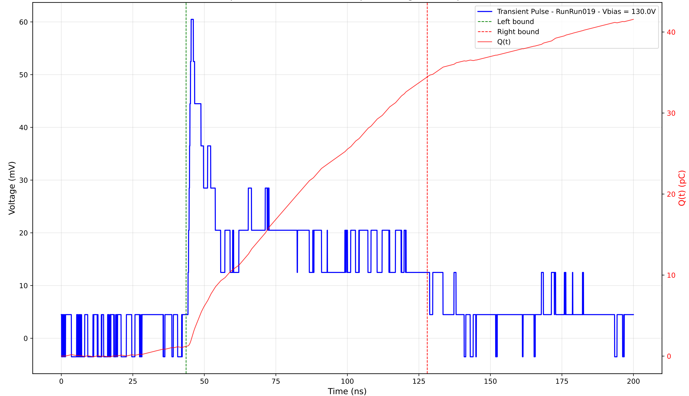
Transient Pulse - Sample: 4003 - Position: 290.0 \mu\text{m} - Charge: 33.27 pC - Rise Time: 1.10 ns
