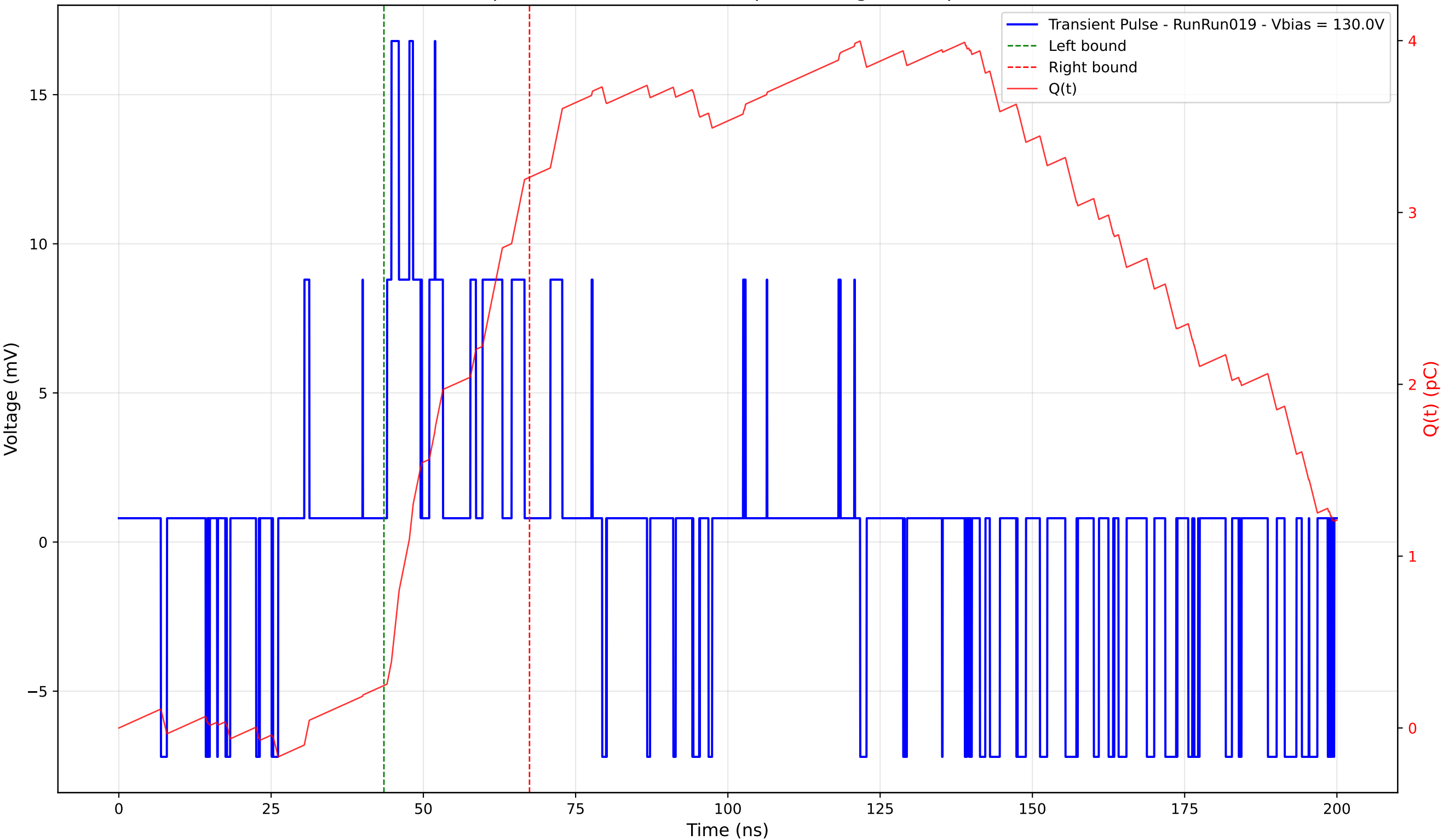
Transient Pulse - Sample: 4003 - Position: 70.0 \mu\text{m} - Charge: 2.96 pC - Rise Time: 0.74 ns
