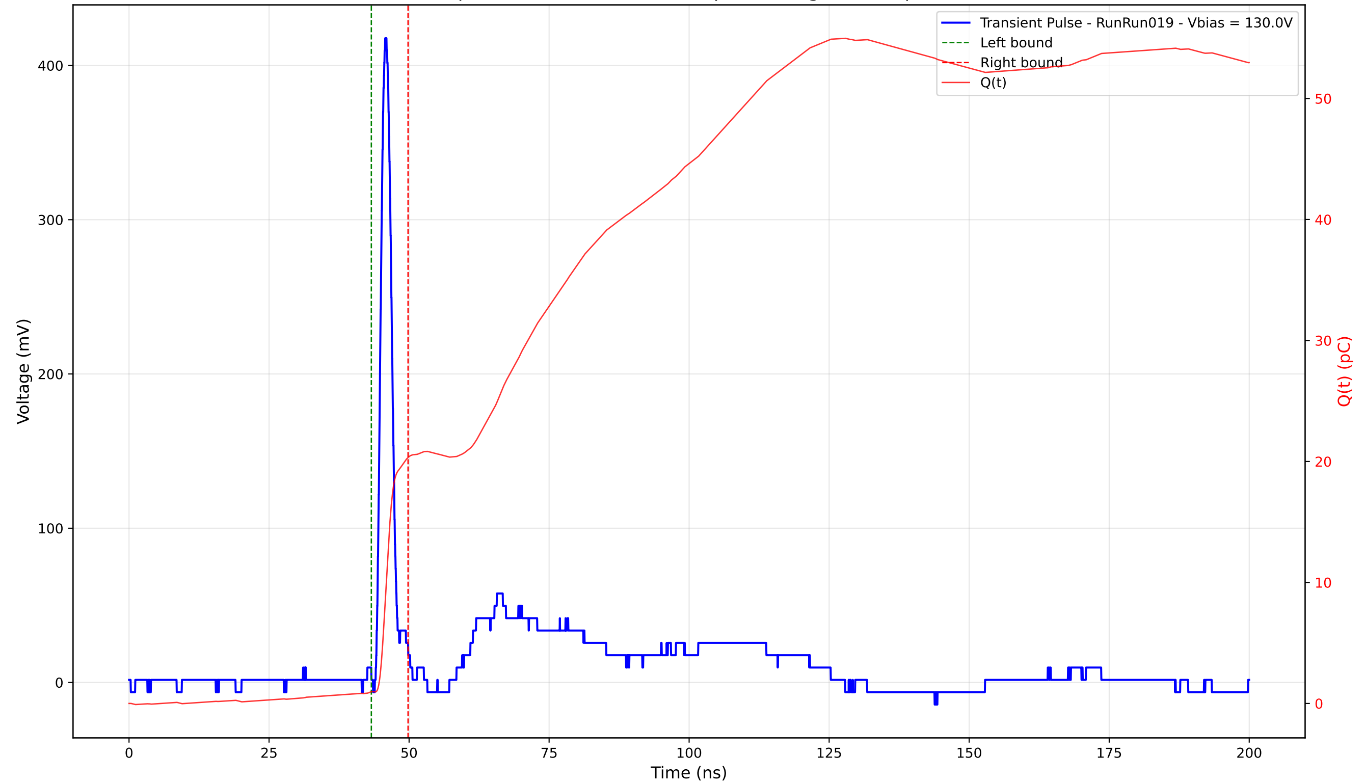
Transient Pulse - Sample: 4003 - Position: 200.0 \mu\text{m} - Charge: 19.36 pC - Rise Time: 1.10 ns
