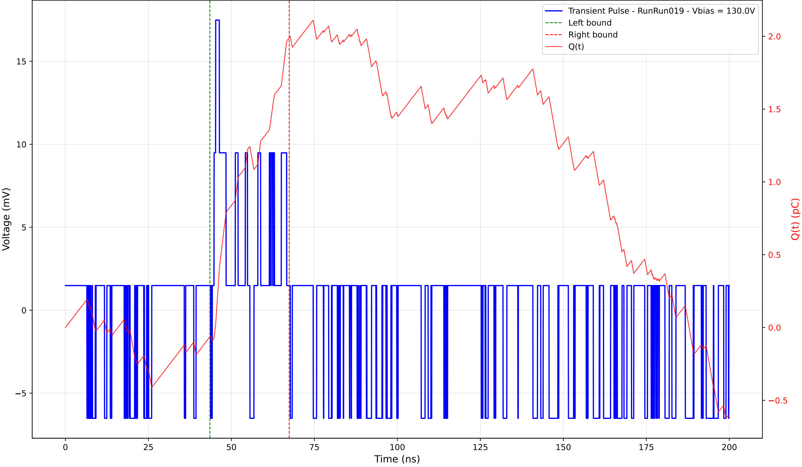
Transient Pulse - Sample: 4003 - Position: 10.0 \mu\text{m} - Charge: 2.05 pC - Rise Time: 0.50 ns
