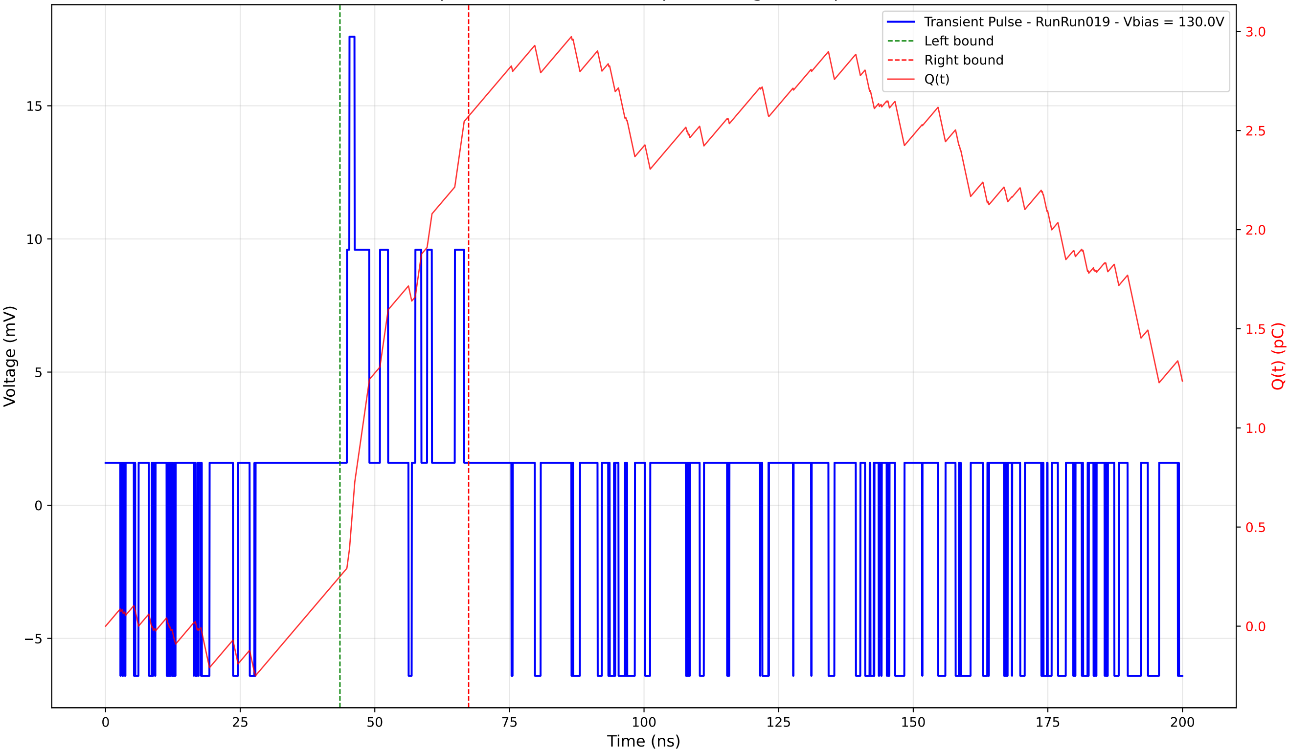
Transient Pulse - Sample: 4003 - Position: 0.0 \mu\text{m} - Charge: 2.32 pC - Rise Time: 0.48 ns
