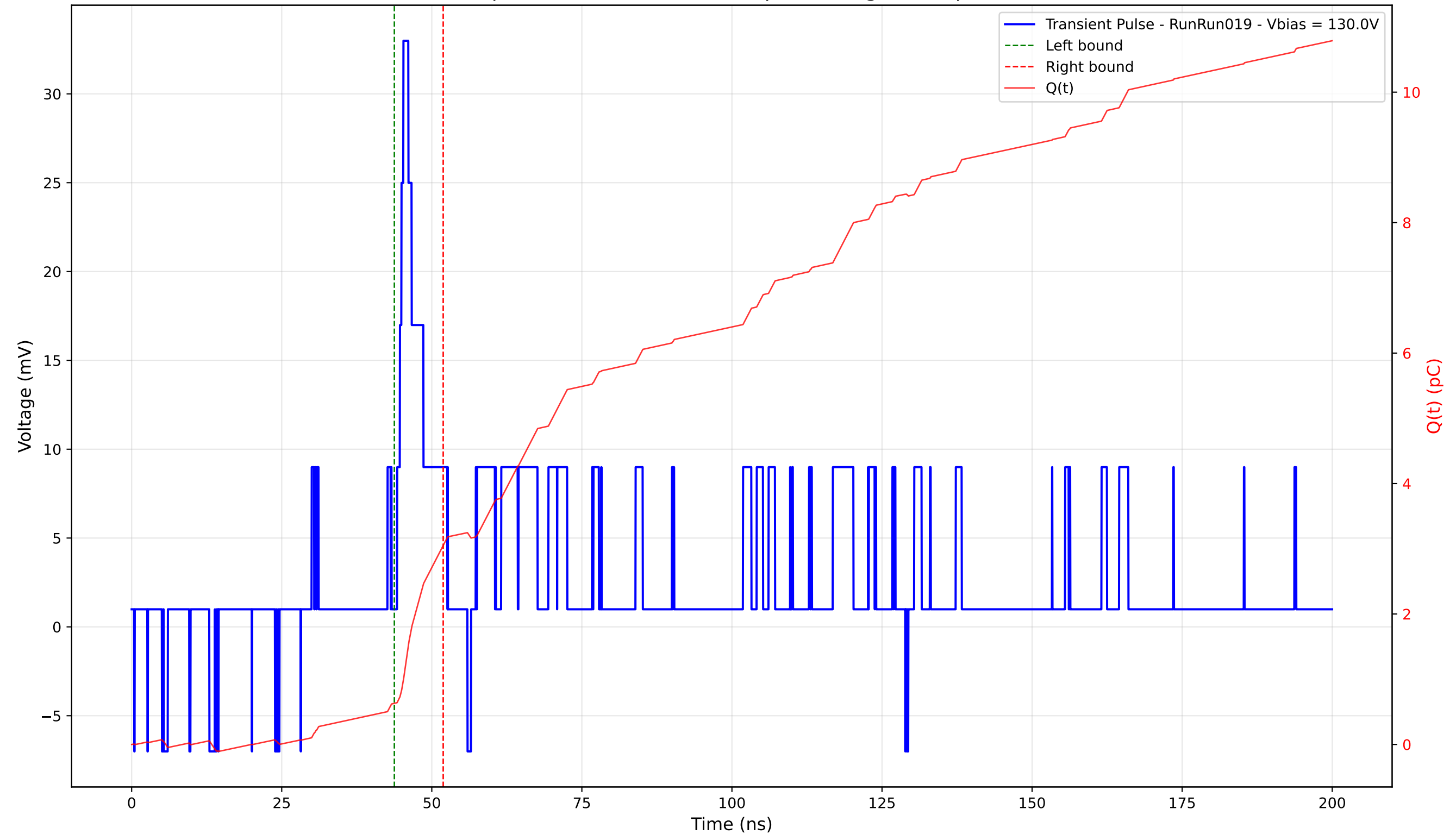
Transient Pulse - Sample: 4003 - Position: 330.0 \mu\text{m} - Charge: 2.43 pC - Rise Time: 1.05 ns
