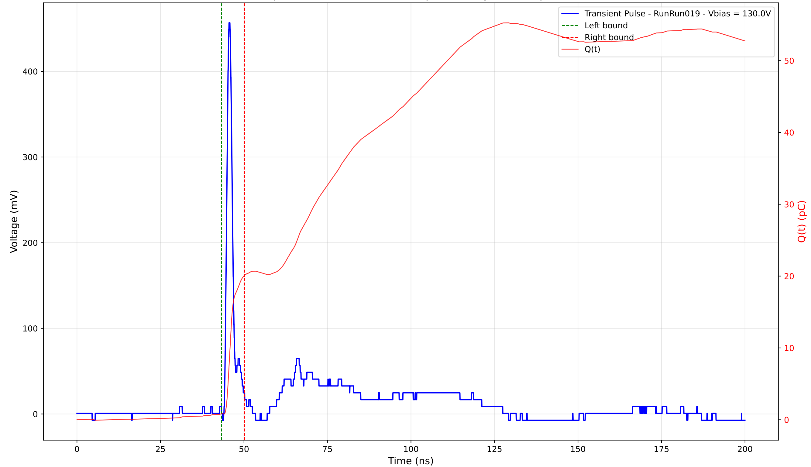
Transient Pulse - Sample: 4003 - Position: 170.0 \mu\text{m} - Charge: 19.28 pC - Rise Time: 1.01 ns
