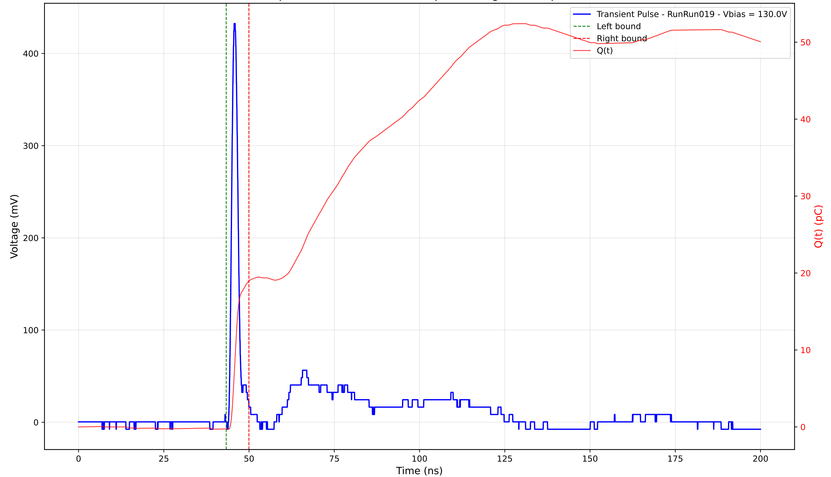
Transient Pulse - Sample: 4003 - Position: 190.0 \mu\text{m} - Charge: 19.23 pC - Rise Time: 1.07 ns
