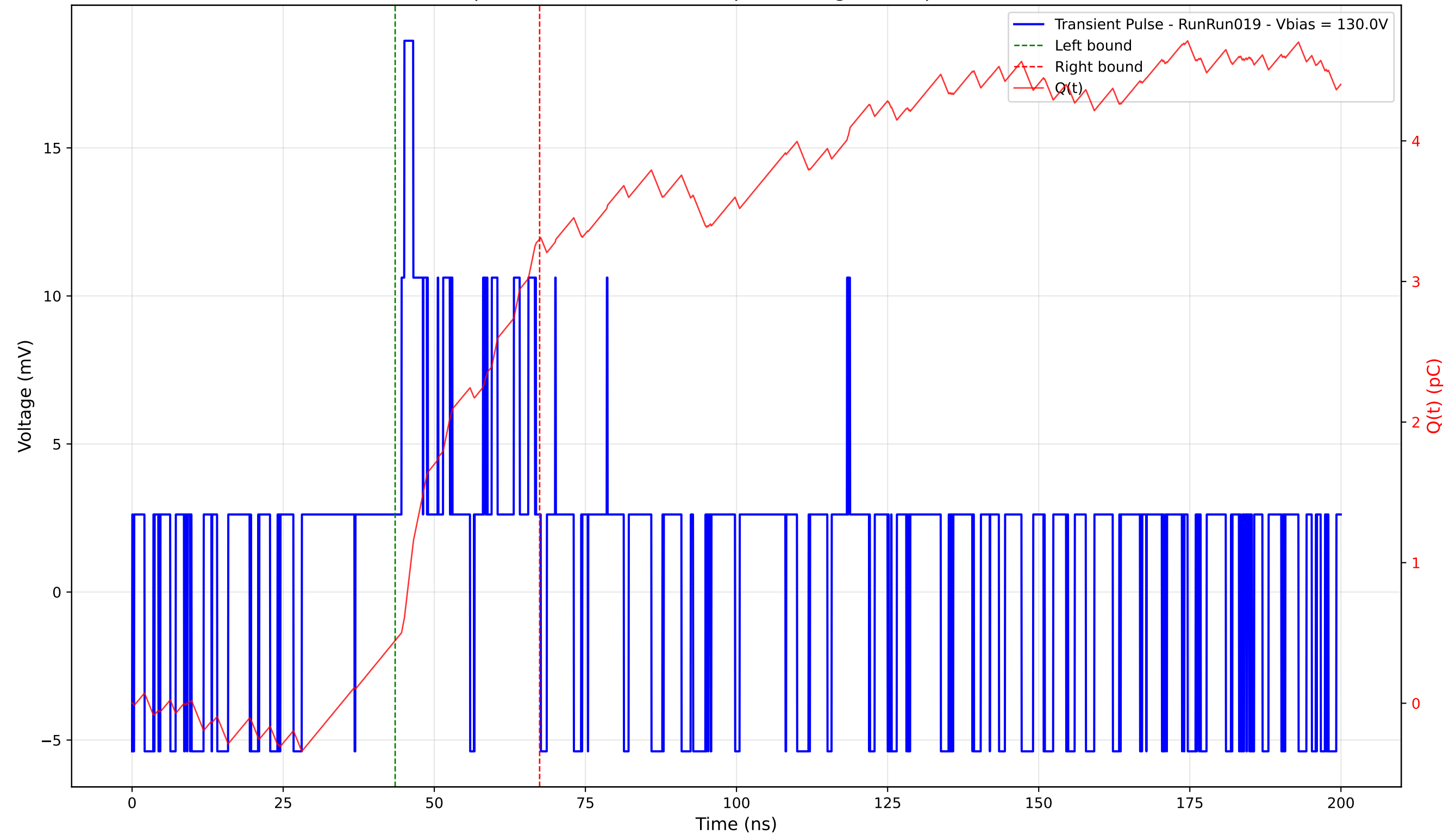
Transient Pulse - Sample: 4003 - Position: 15.0 \mu\text{m} - Charge: 2.86 pC - Rise Time: 0.00 ns (N/A)
