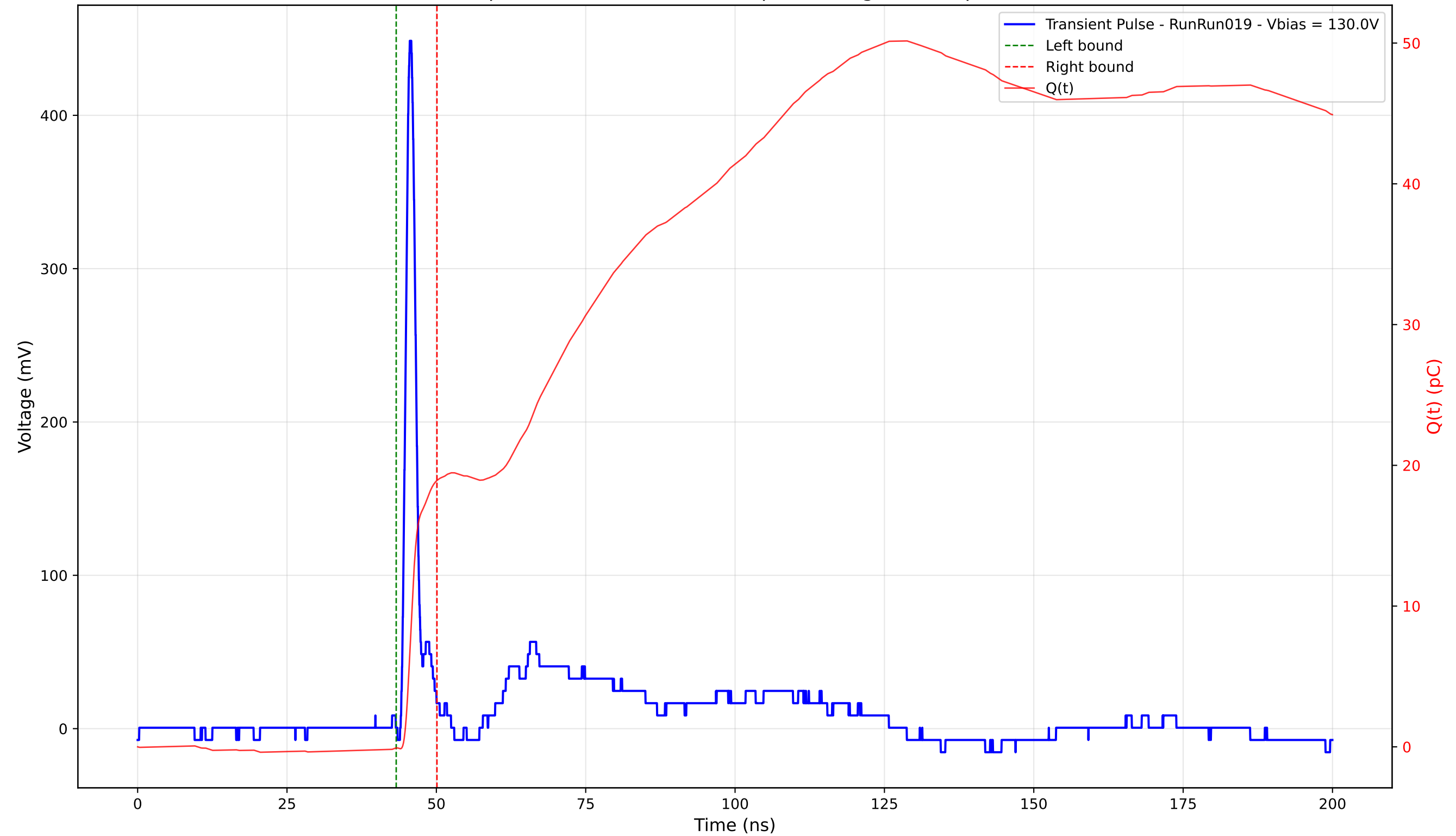
Transient Pulse - Sample: 4003 - Position: 175.0 \mu\text{m} - Charge: 19.00 pC - Rise Time: 1.02 ns
