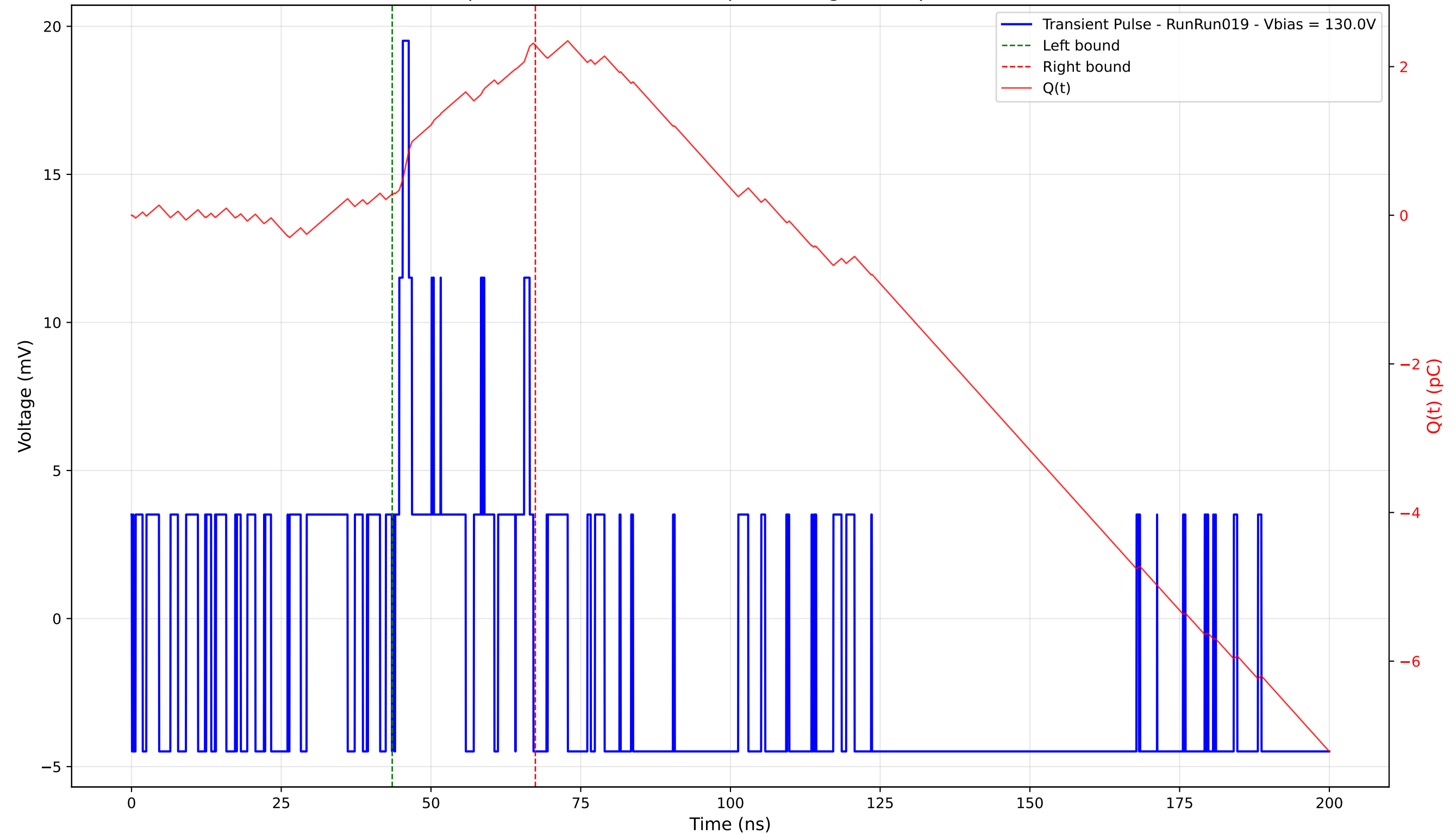
Transient Pulse - Sample: 4003 - Position: 75.0 \mu\text{m} - Charge: 2.01 pC - Rise Time: 0.00 ns (N/A)
