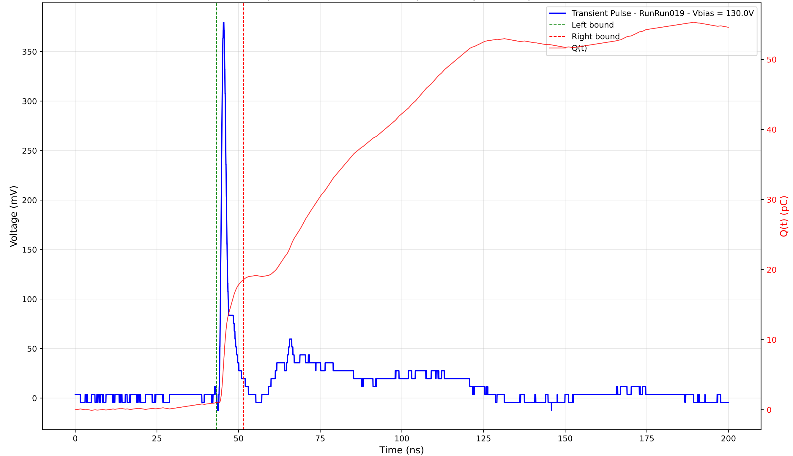
Transient Pulse - Sample: 4003 - Position: 115.0 \mu\text{m} - Charge: 17.53 pC - Rise Time: 0.91 ns
