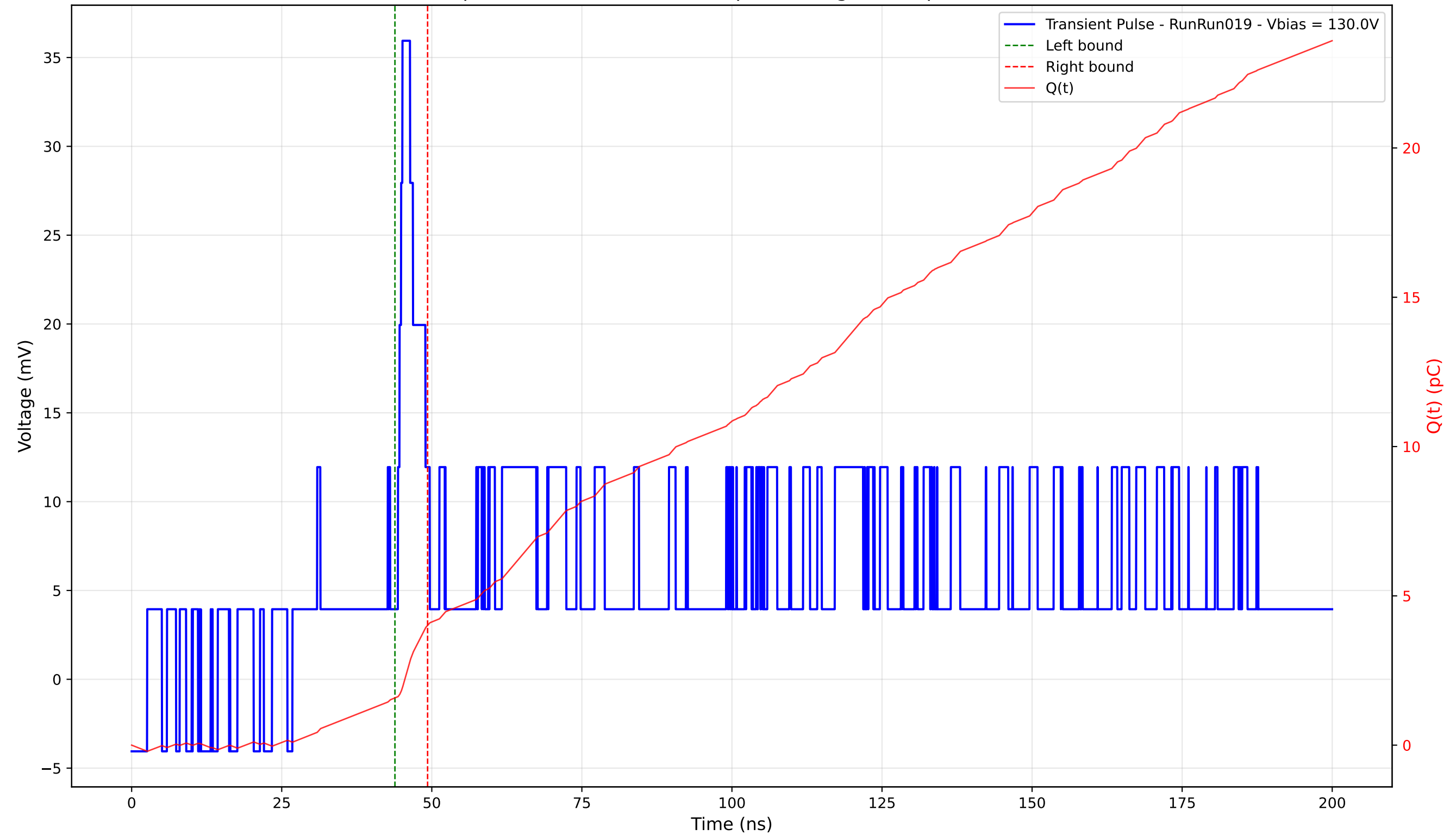
Transient Pulse - Sample: 4003 - Position: 320.0 \mu\text{m} - Charge: 2.43 pC - Rise Time: 0.00 ns (N/A)
