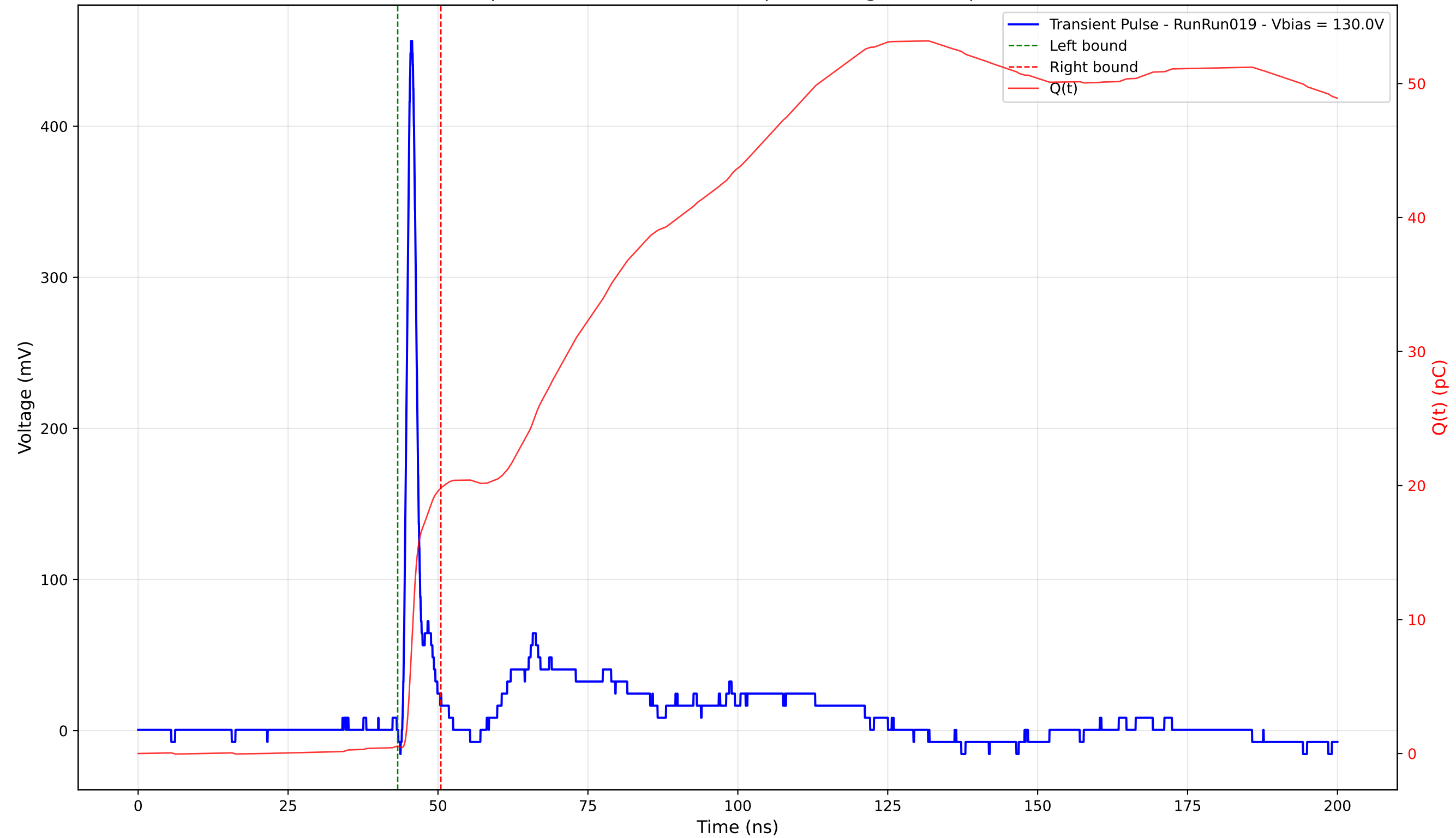
Transient Pulse - Sample: 4003 - Position: 160.0 \mu\text{m} - Charge: 19.27 pC - Rise Time: 0.99 ns
