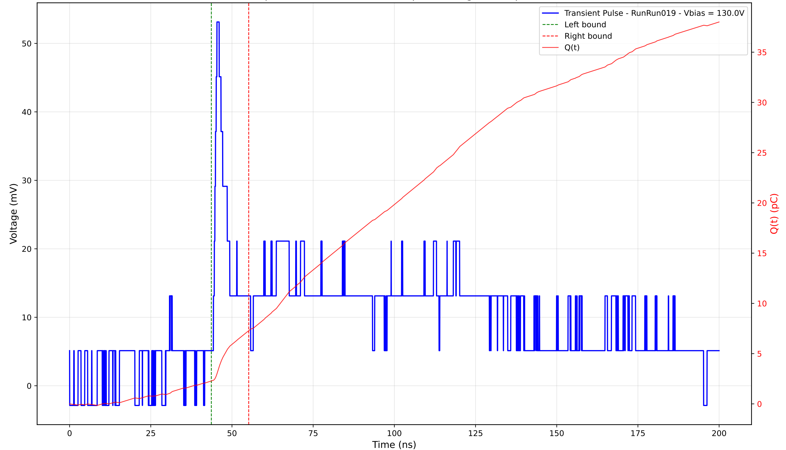
Transient Pulse - Sample: 4003 - Position: 300.0 \mu\text{m} - Charge: 5.02 pC - Rise Time: 1.10 ns
