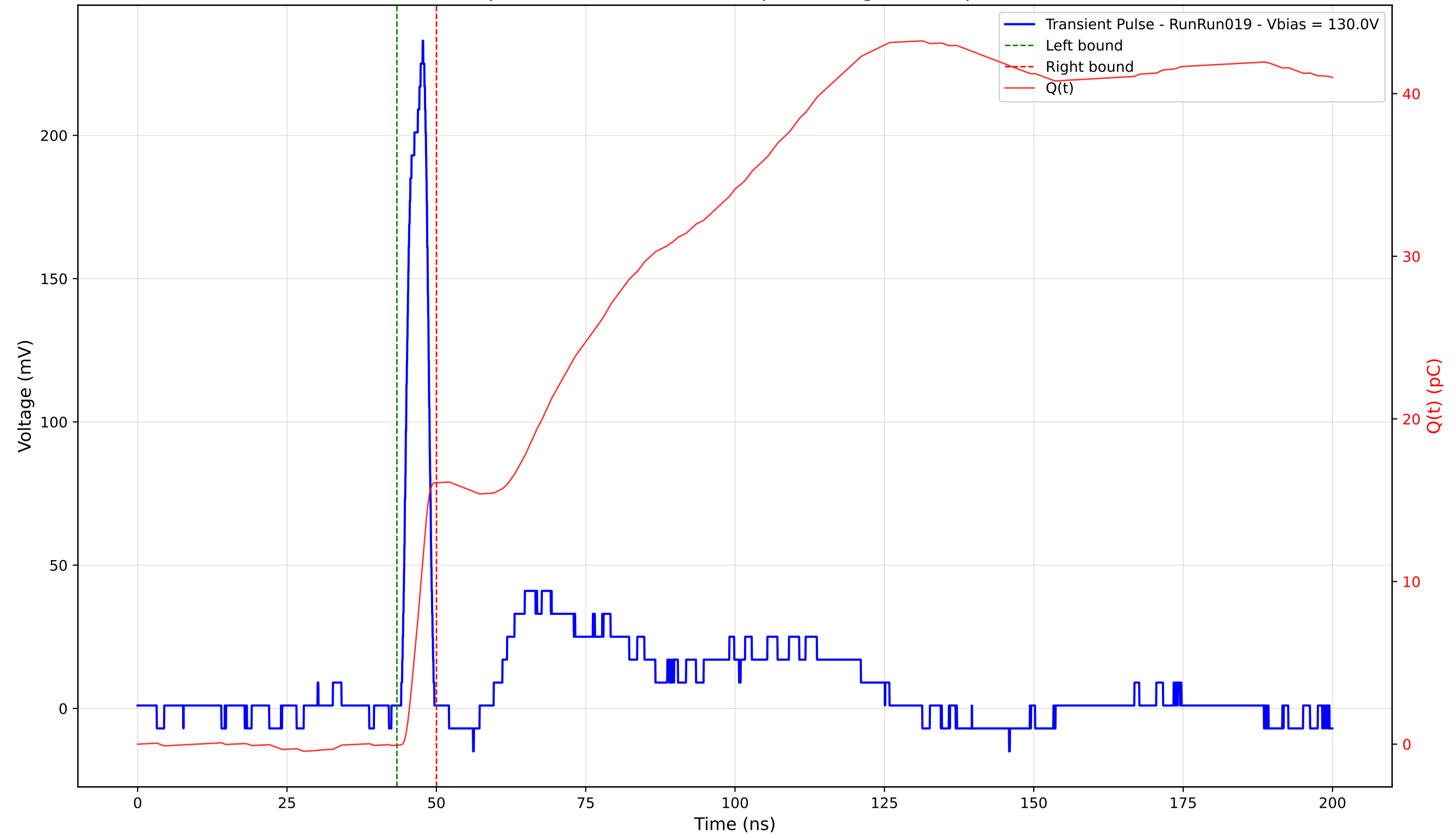
Transient Pulse - Sample: 4003 - Position: 260.0 \mu\text{m} - Charge: 16.14 pC - Rise Time: 2.80 ns
