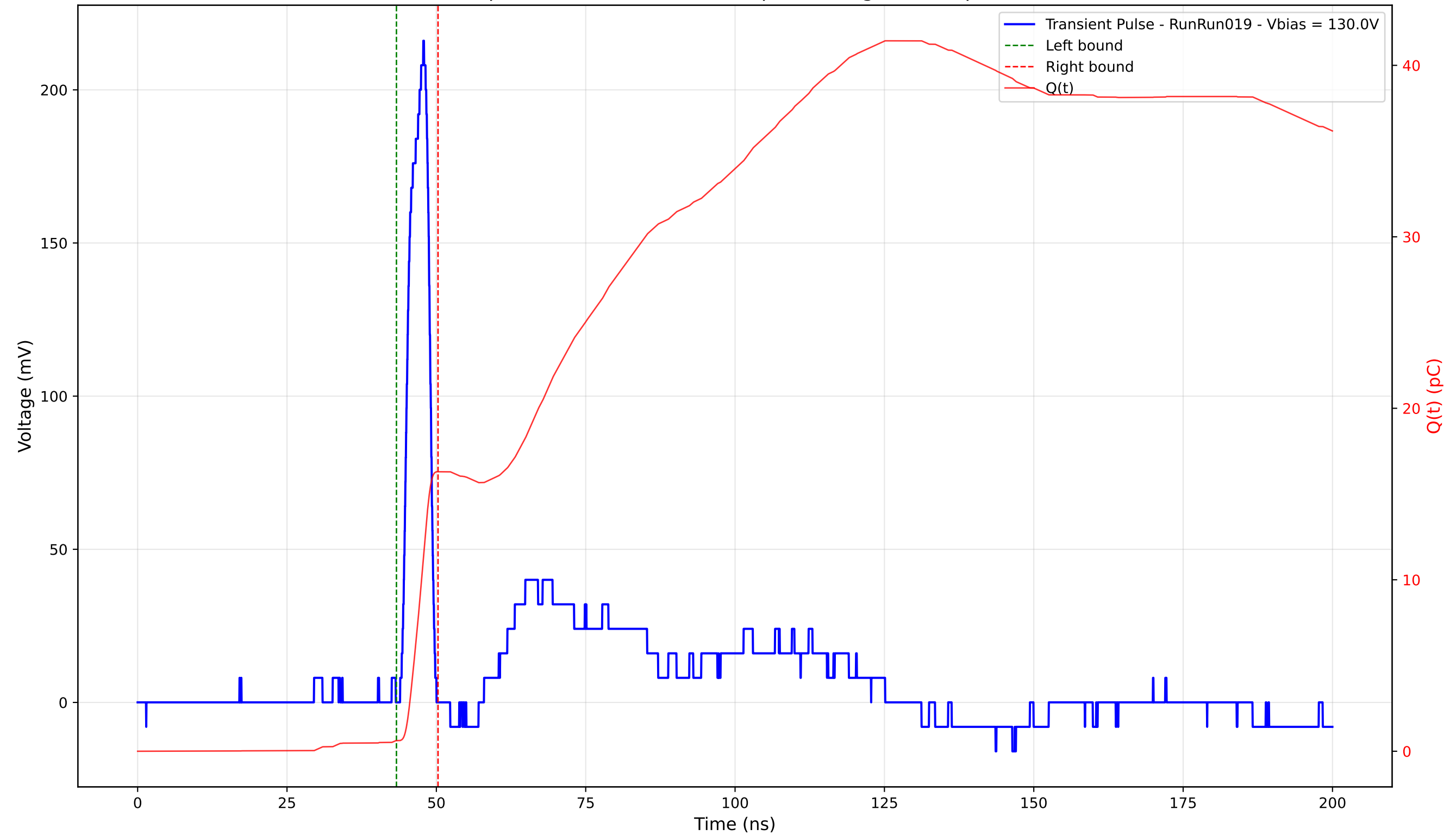
Transient Pulse - Sample: 4003 - Position: 265.0 \mu\text{m} - Charge: 15.68 pC - Rise Time: 2.85 ns
