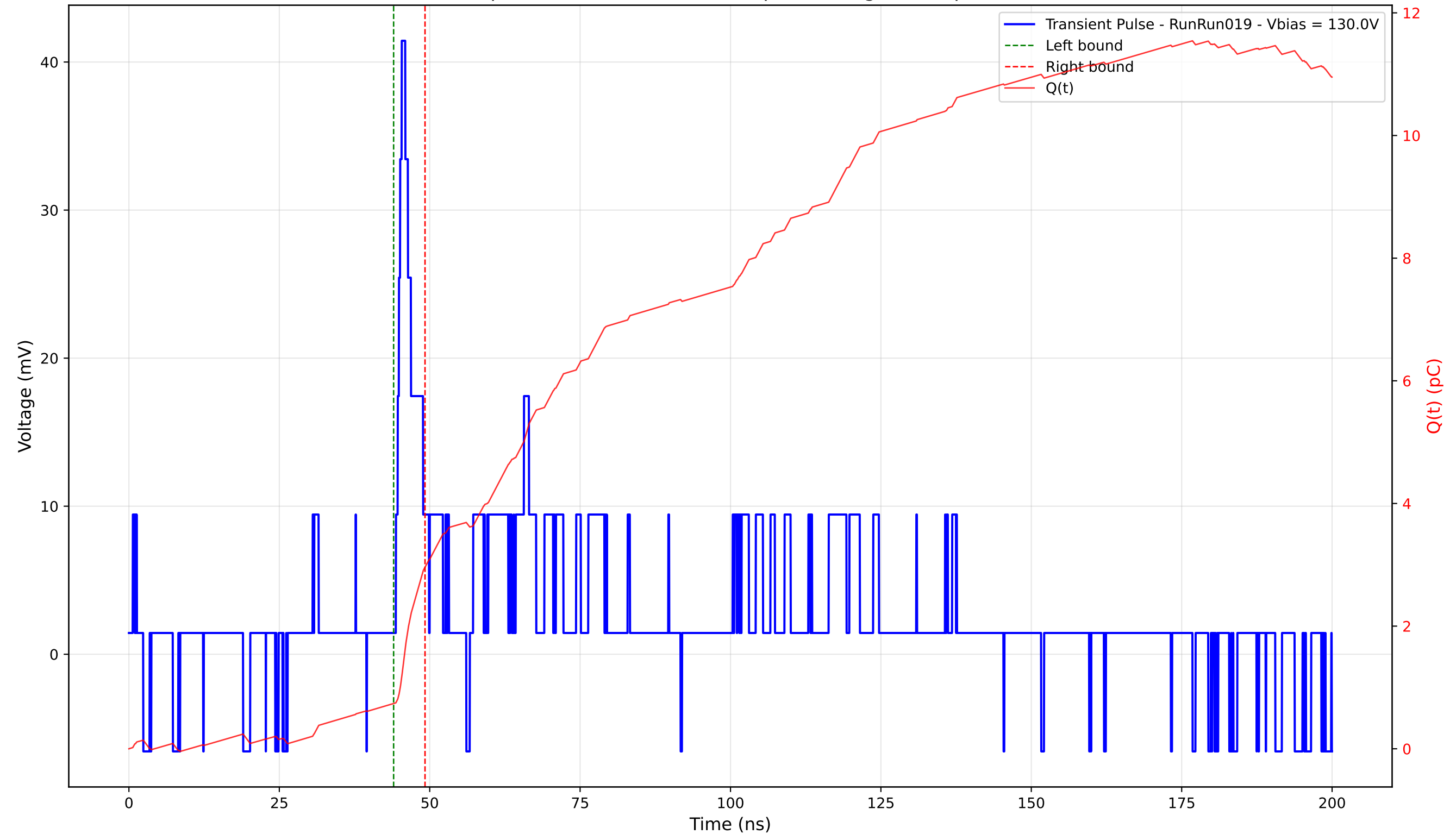
Transient Pulse - Sample: 4003 - Position: 315.0 \mu\text{m} - Charge: 2.23 pC - Rise Time: 0.97 ns
