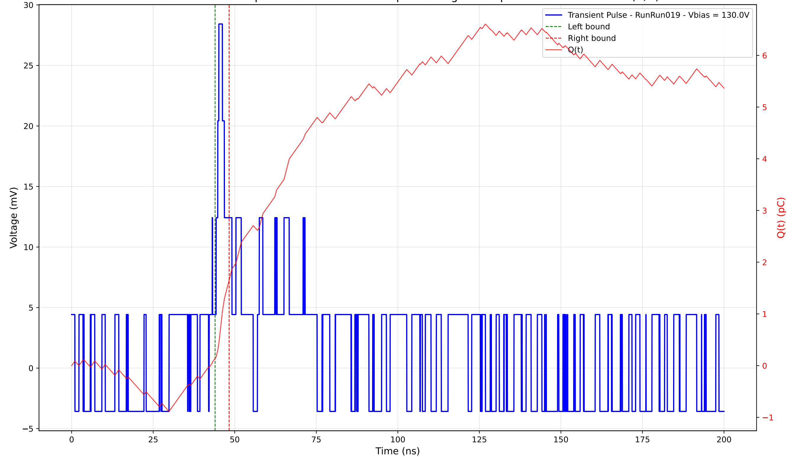
Transient Pulse - Sample: 4003 - Position: 80.0 \mu\text{m} - Charge: 1.52 pC - Rise Time: 0.00 ns (N/A)
