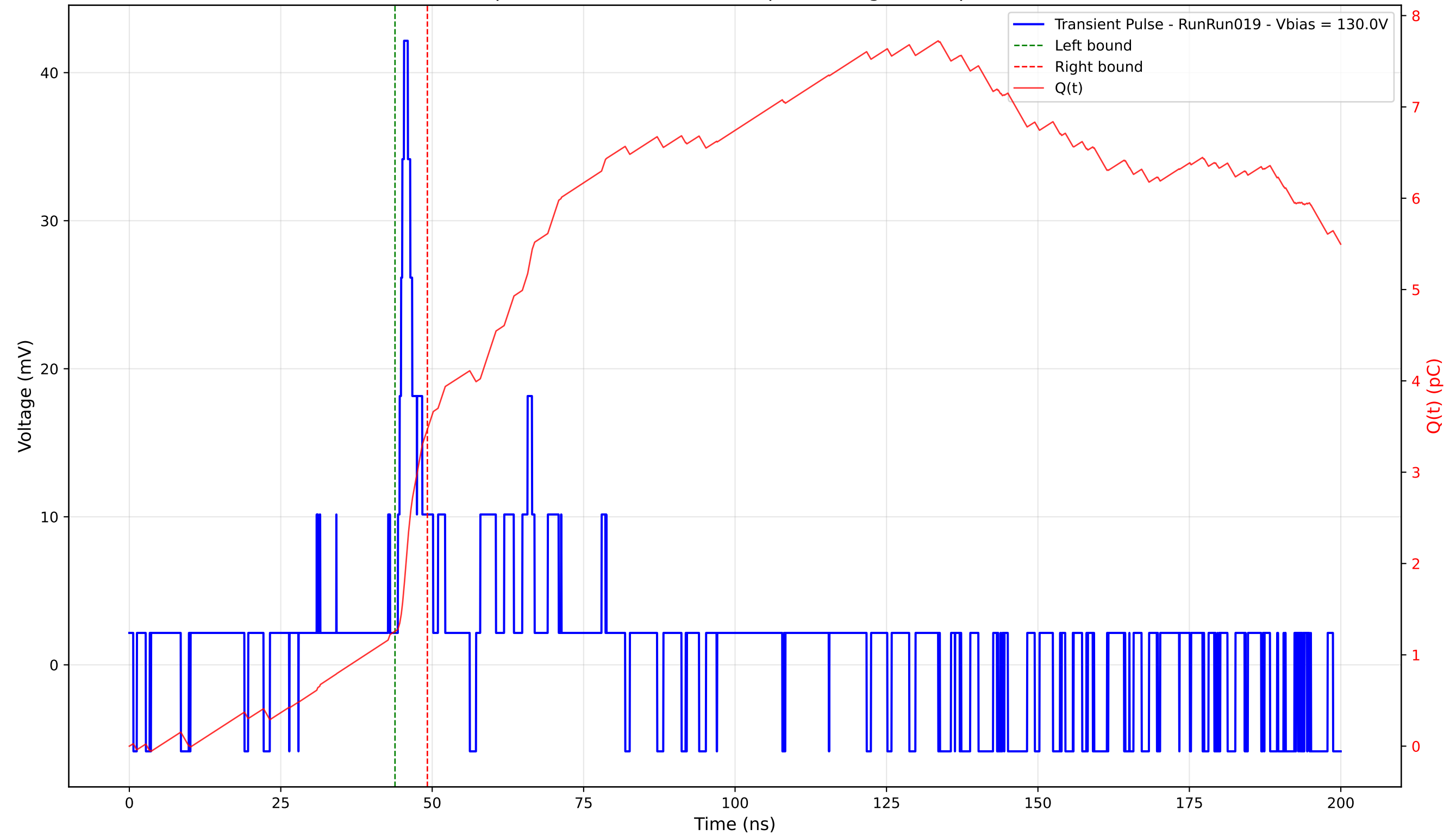
Transient Pulse - Sample: 4003 - Position: 405.0 \mu\text{m} - Charge: 2.21 pC - Rise Time: 1.01 ns
