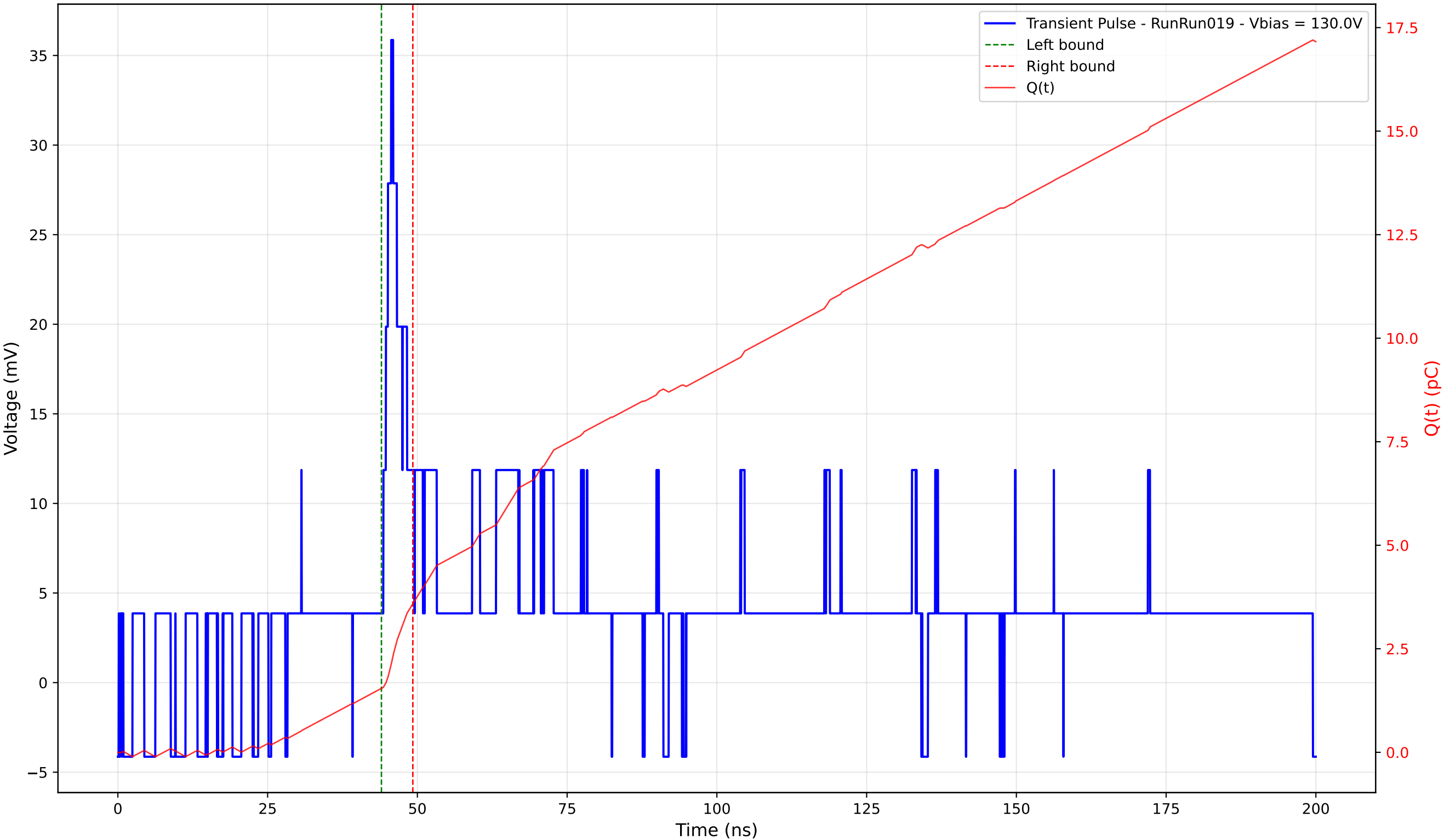
Transient Pulse - Sample: 4003 - Position: 335.0 \mu\text{m} - Charge: 2.04 pC - Rise Time: 0.00 ns (N/A)
