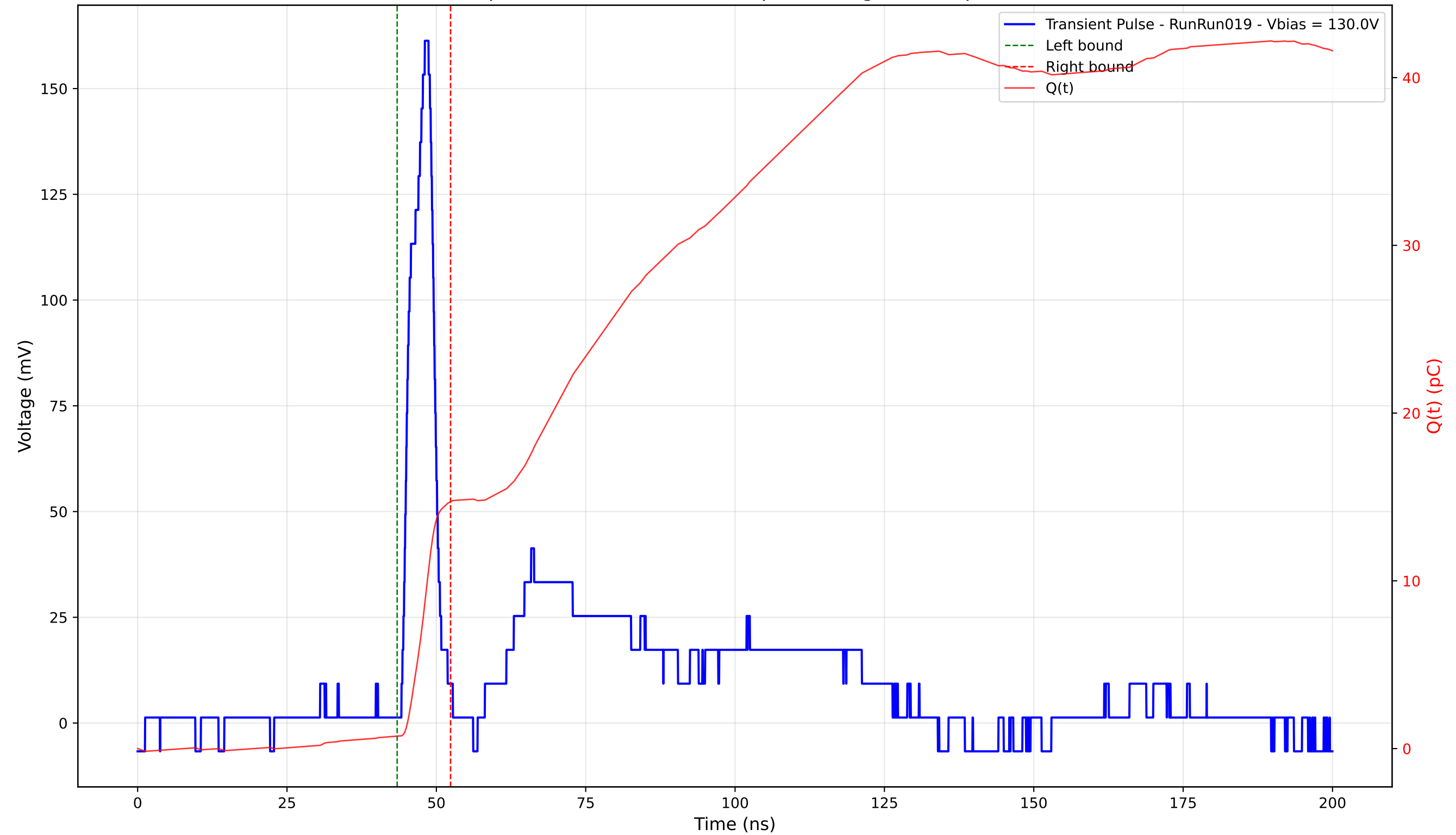
Transient Pulse - Sample: 4003 - Position: 275.0 \mu\text{m} - Charge: 13.98 pC - Rise Time: 3.18 ns
