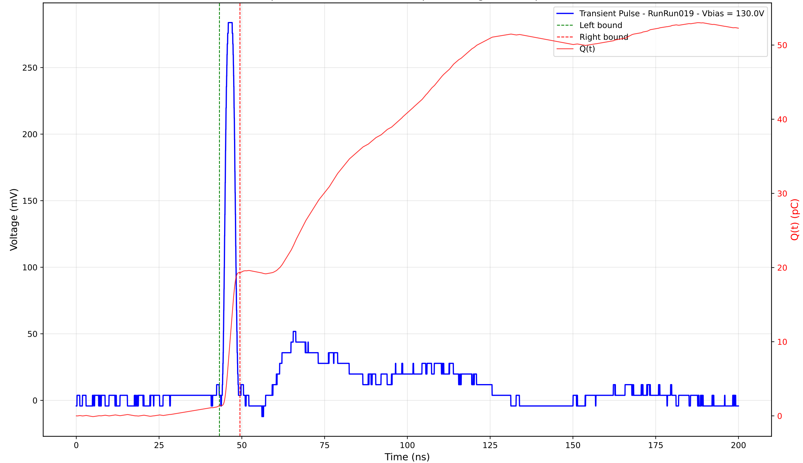
Transient Pulse - Sample: 4003 - Position: 240.0 \mu\text{m} - Charge: 17.96 pC - Rise Time: 1.18 ns
