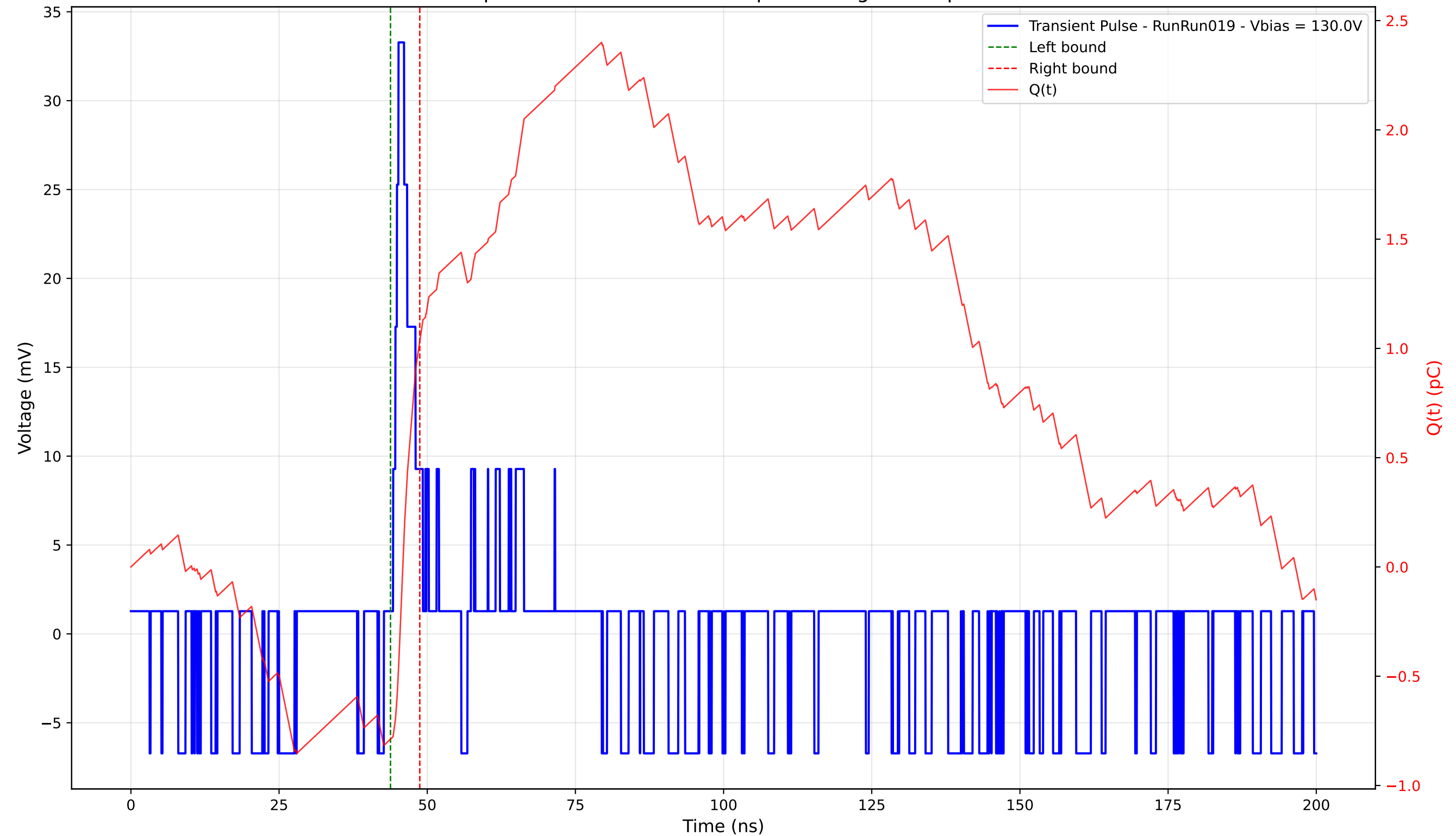
Transient Pulse - Sample: 4003 - Position: 380.0 \mu\text{m} - Charge: 1.82 pC - Rise Time: 0.91 ns
