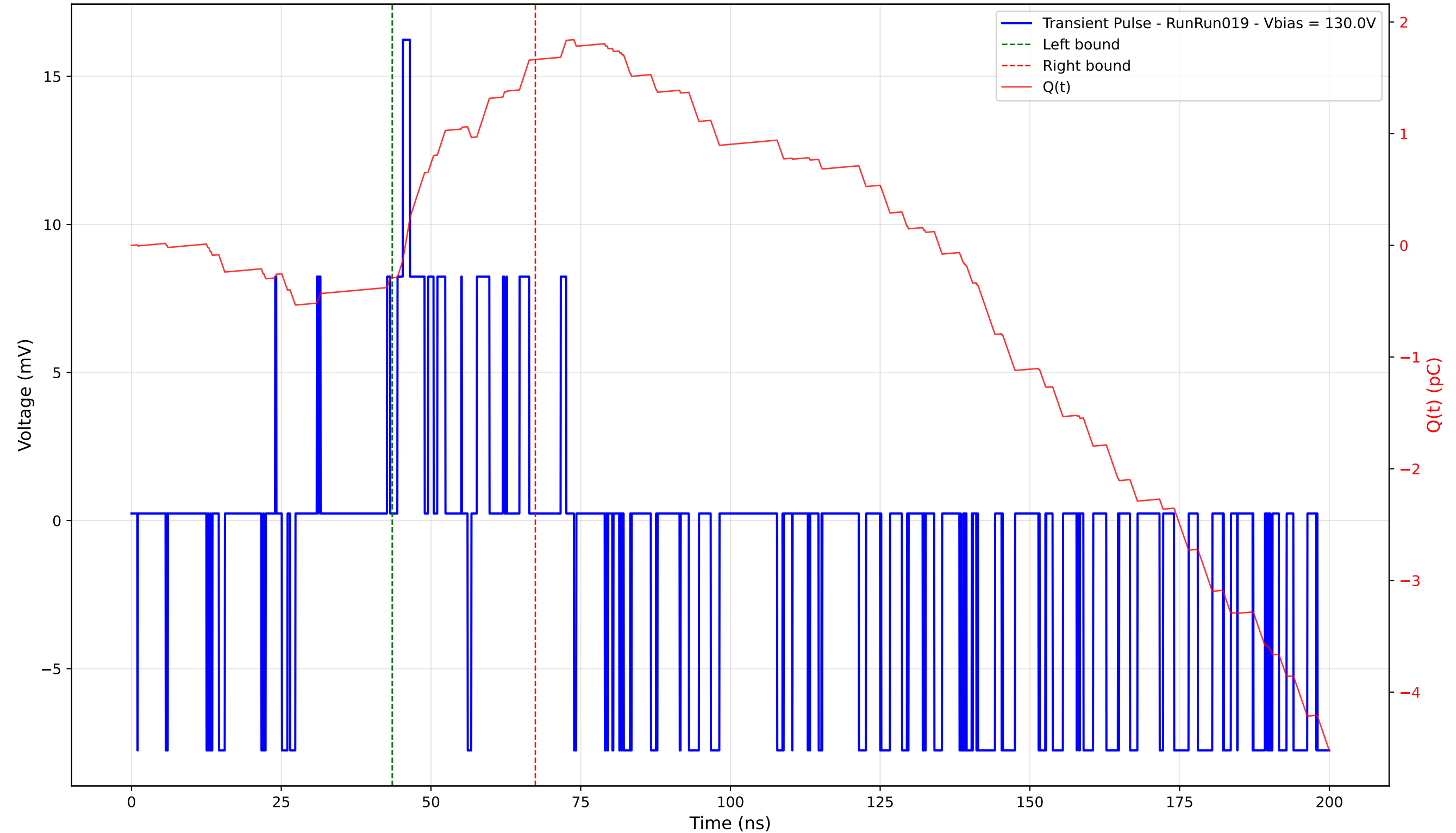
Transient Pulse - Sample: 4003 - Position: 425.0 \mu\text{m} - Charge: 1.95 pC - Rise Time: 0.92 ns
