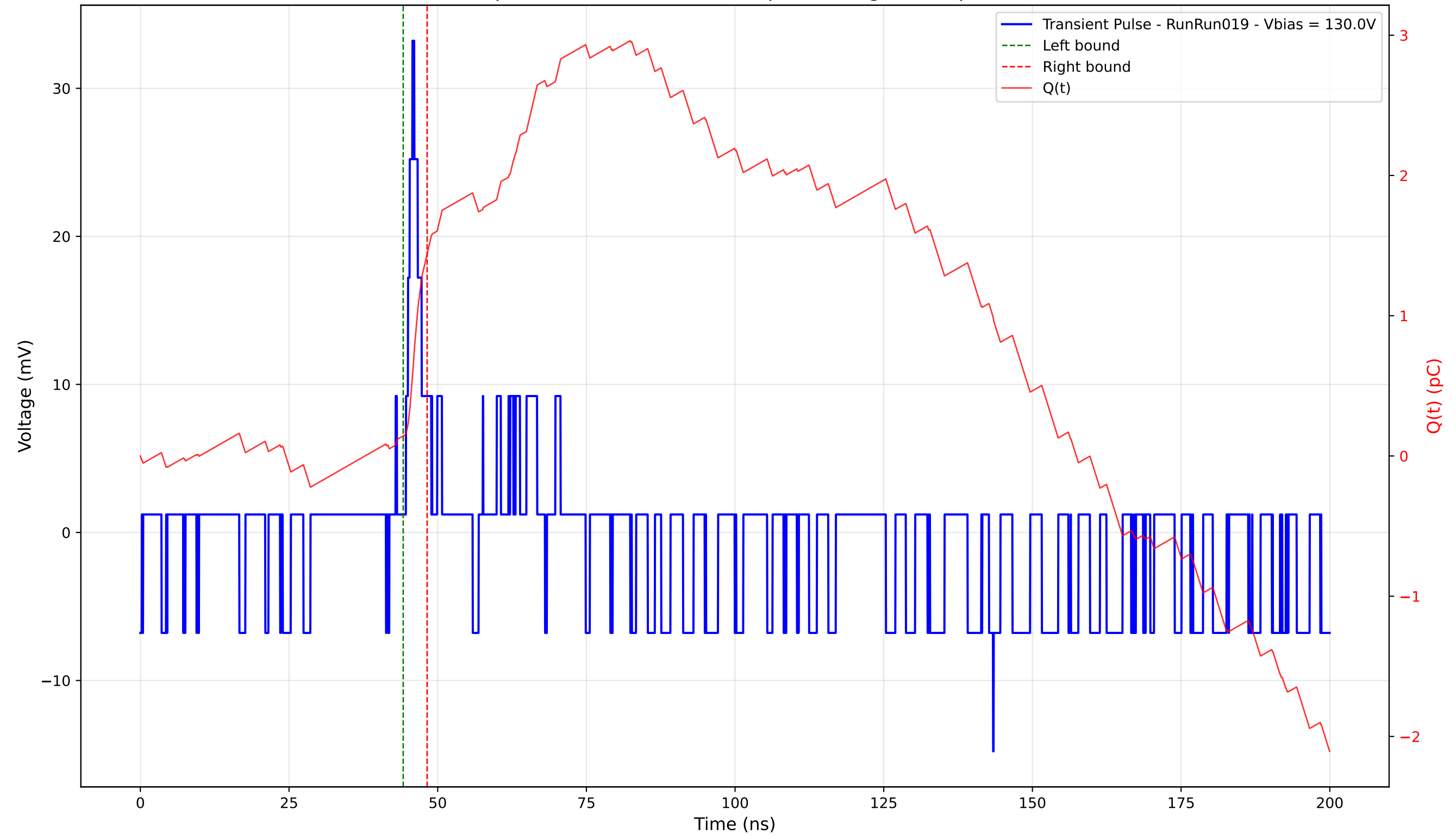
Transient Pulse - Sample: 4003 - Position: 345.0 \mu\text{m} - Charge: 1.30 pC - Rise Time: 1.09 ns
