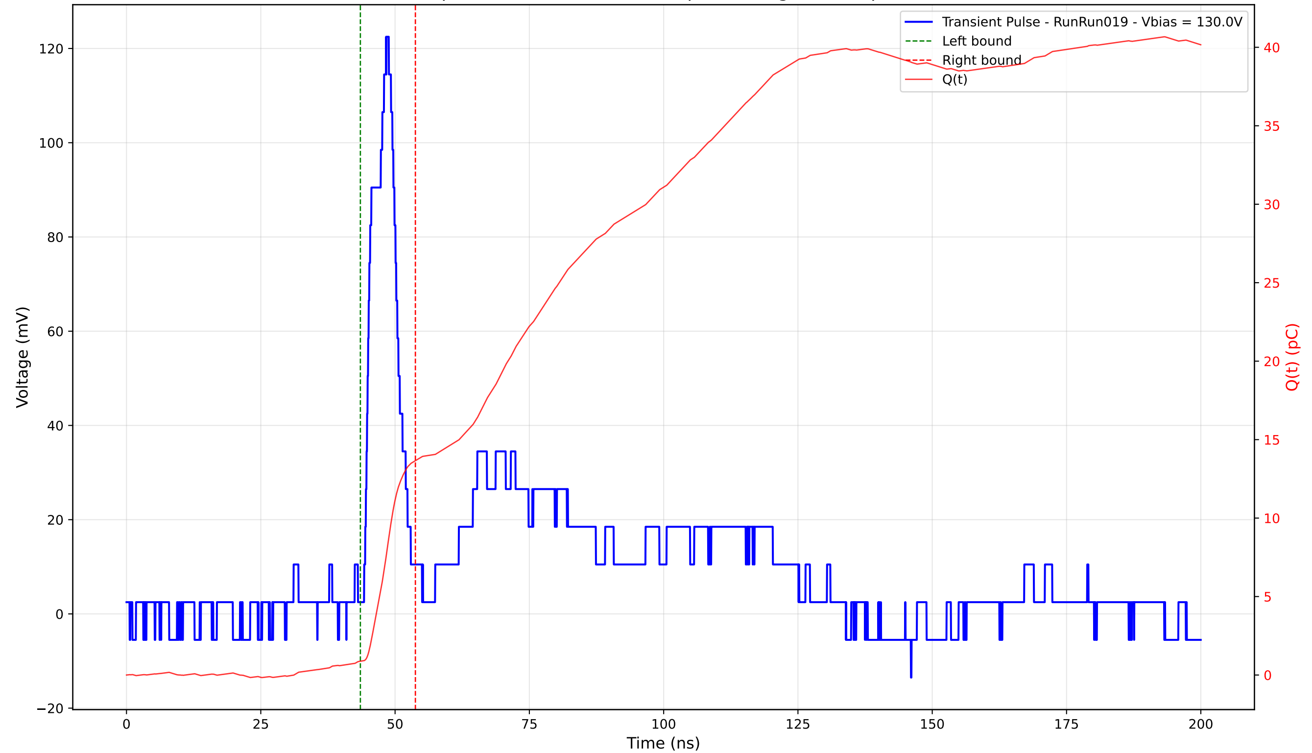
Transient Pulse - Sample: 4003 - Position: 280.0 \mu\text{m} - Charge: 12.78 pC - Rise Time: 3.52 ns
