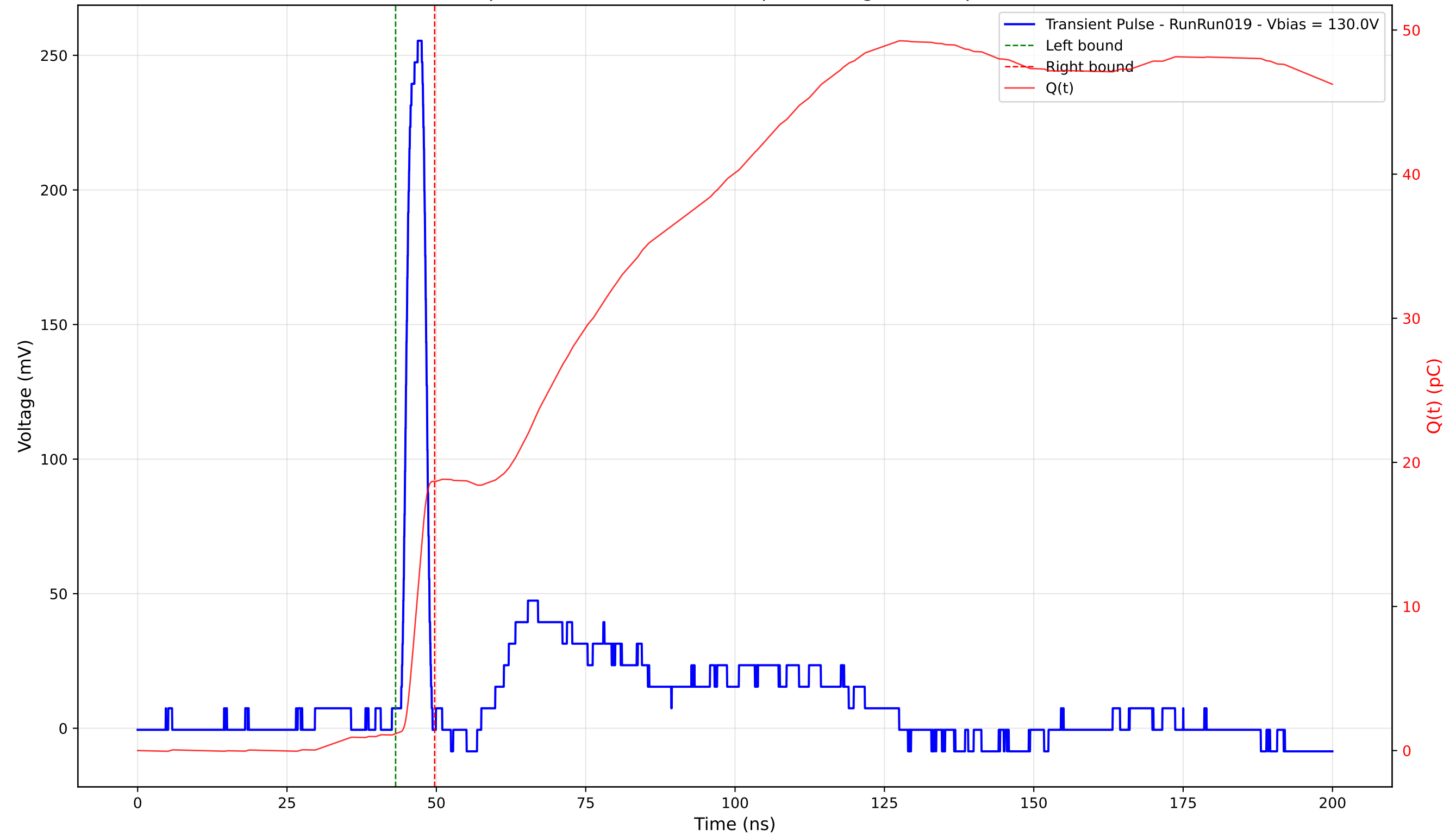
Transient Pulse - Sample: 4003 - Position: 250.0 \mu\text{m} - Charge: 17.51 pC - Rise Time: 1.37 ns
