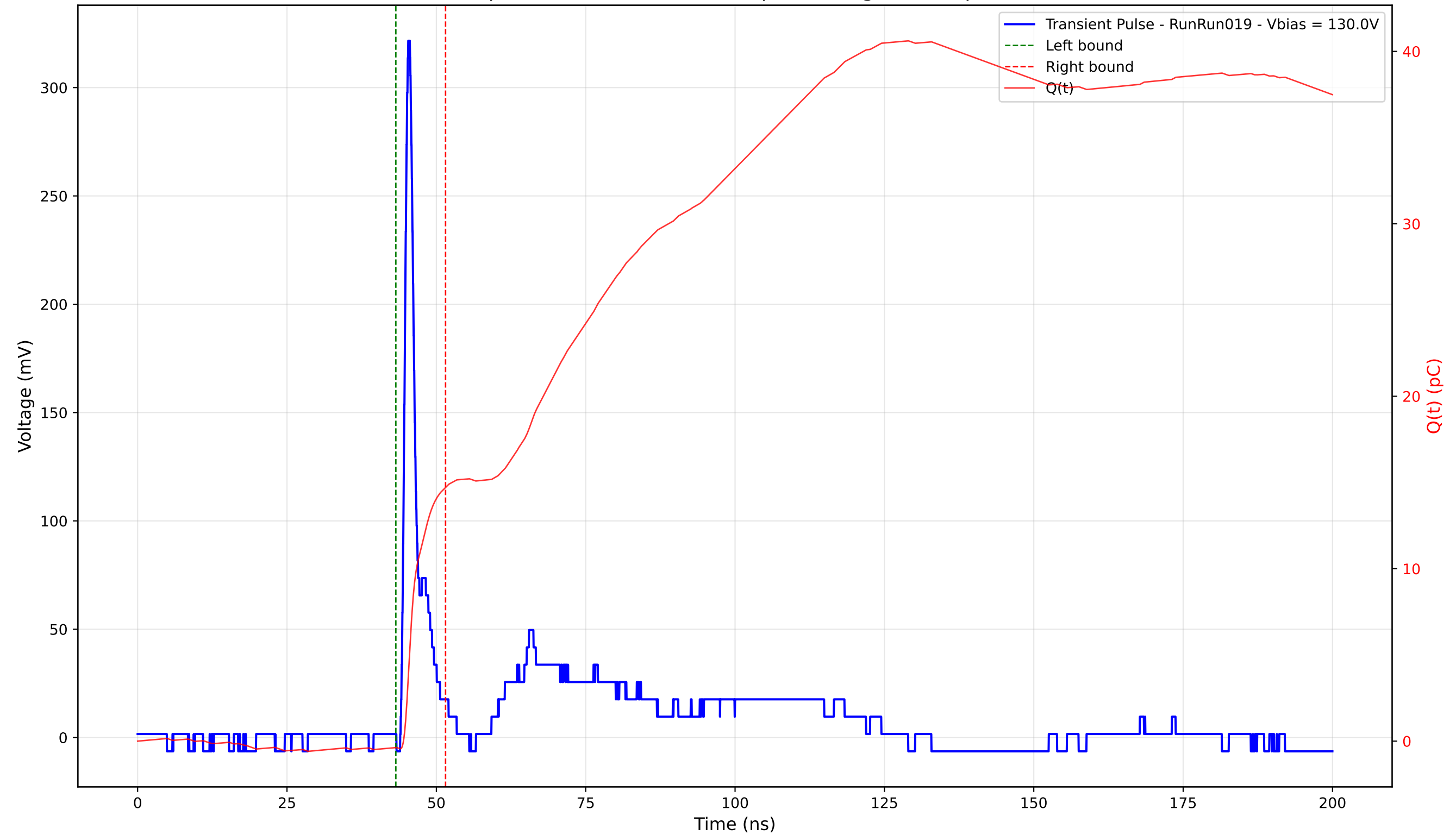
Transient Pulse - Sample: 4003 - Position: 110.0 \mu\text{m} - Charge: 15.08 pC - Rise Time: 0.88 ns
