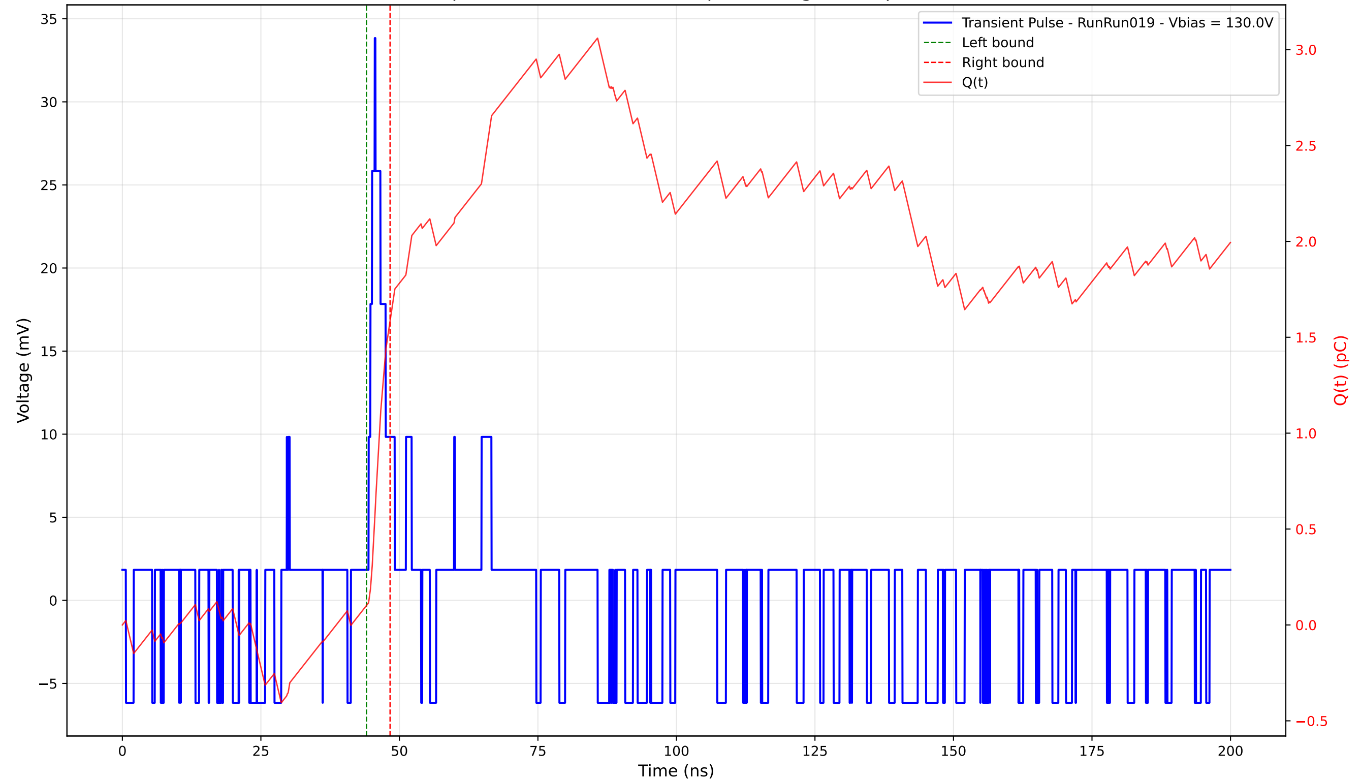
Transient Pulse - Sample: 4003 - Position: 355.0 \mu\text{m} - Charge: 1.49 pC - Rise Time: 1.12 ns
