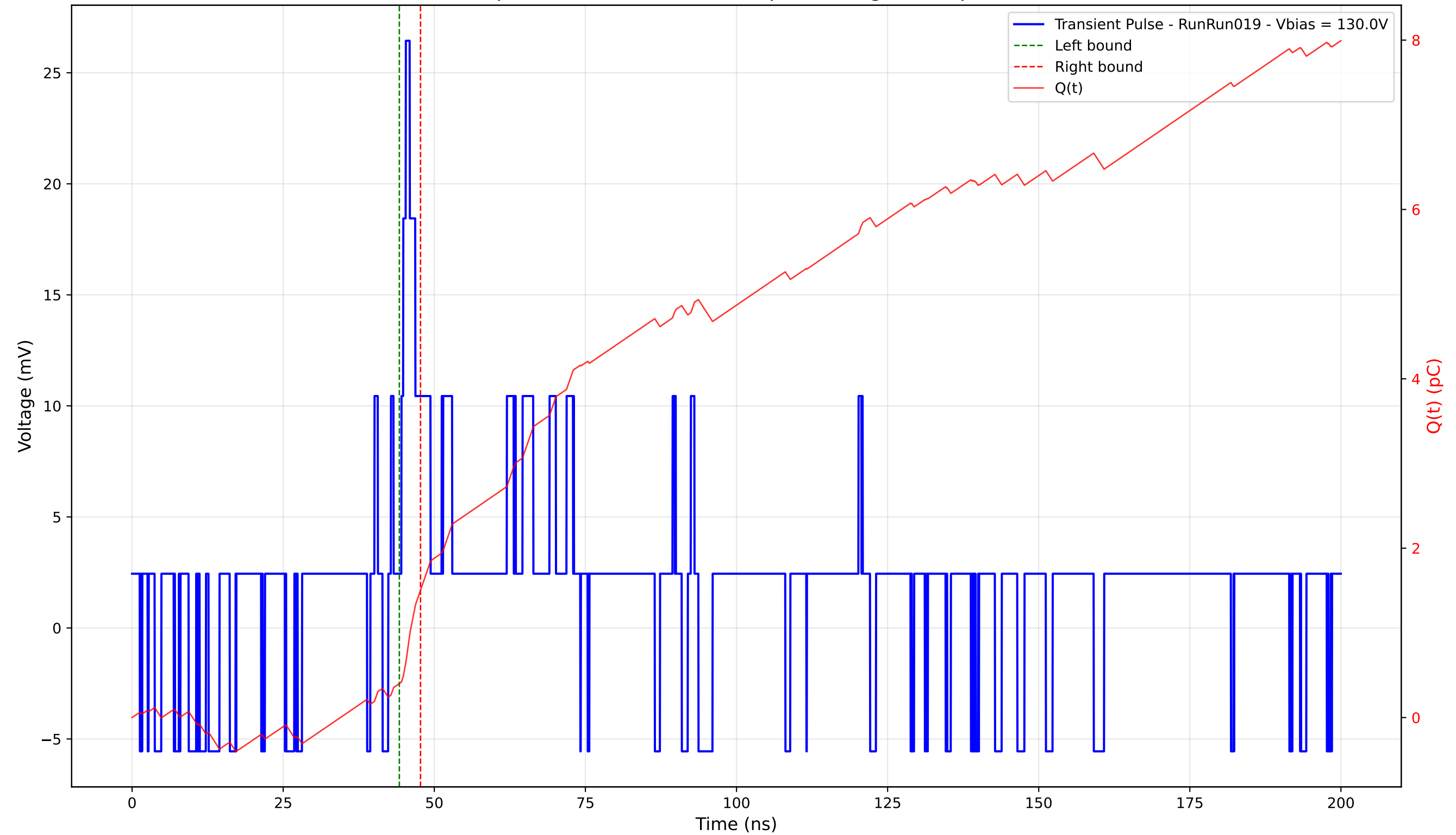
Transient Pulse - Sample: 4003 - Position: 415.0 \mu\text{m} - Charge: 1.10 pC - Rise Time: 0.74 ns
