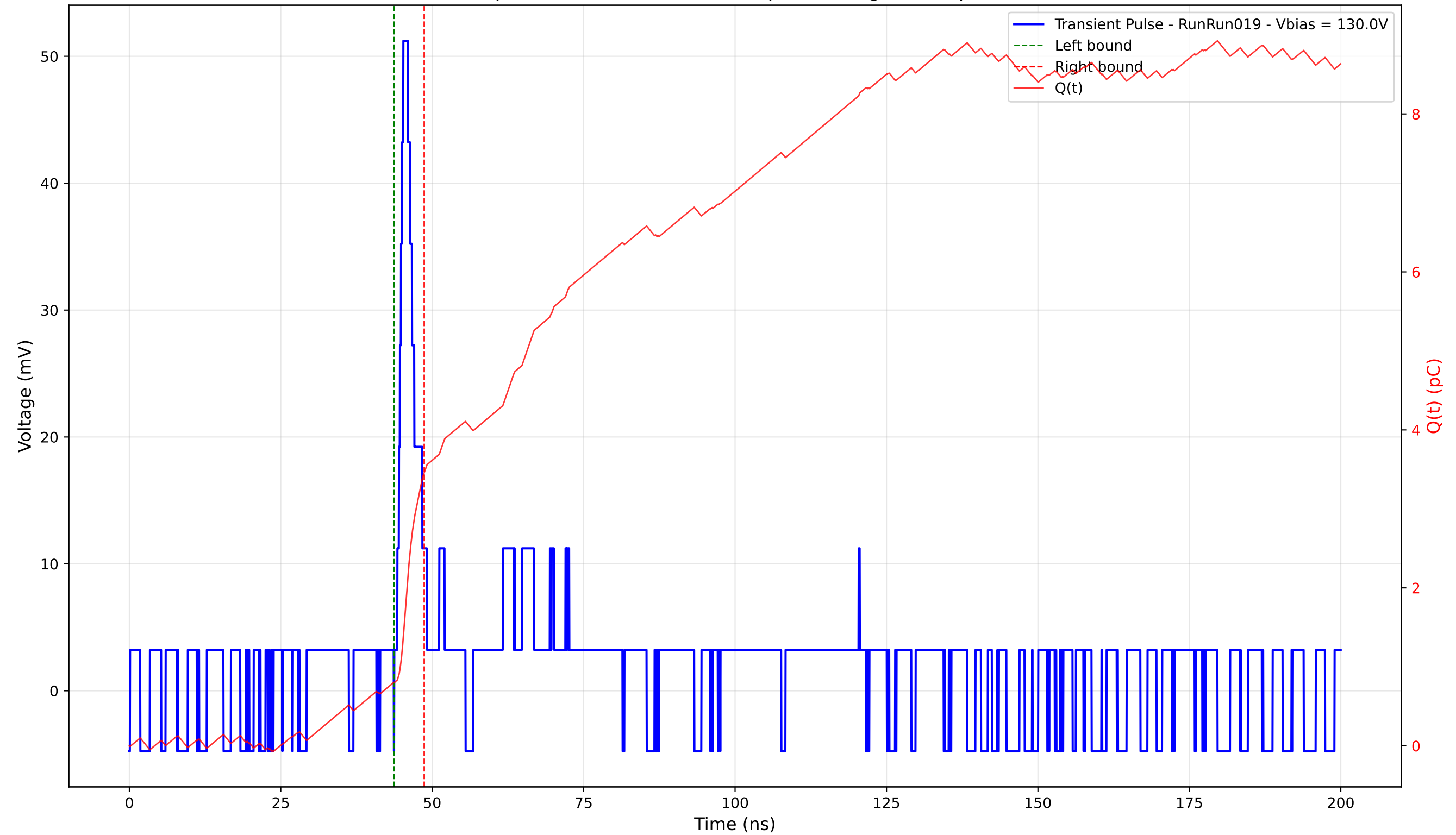
Transient Pulse - Sample: 4003 - Position: 390.0 \mu\text{m} - Charge: 2.66 pC - Rise Time: 1.00 ns
