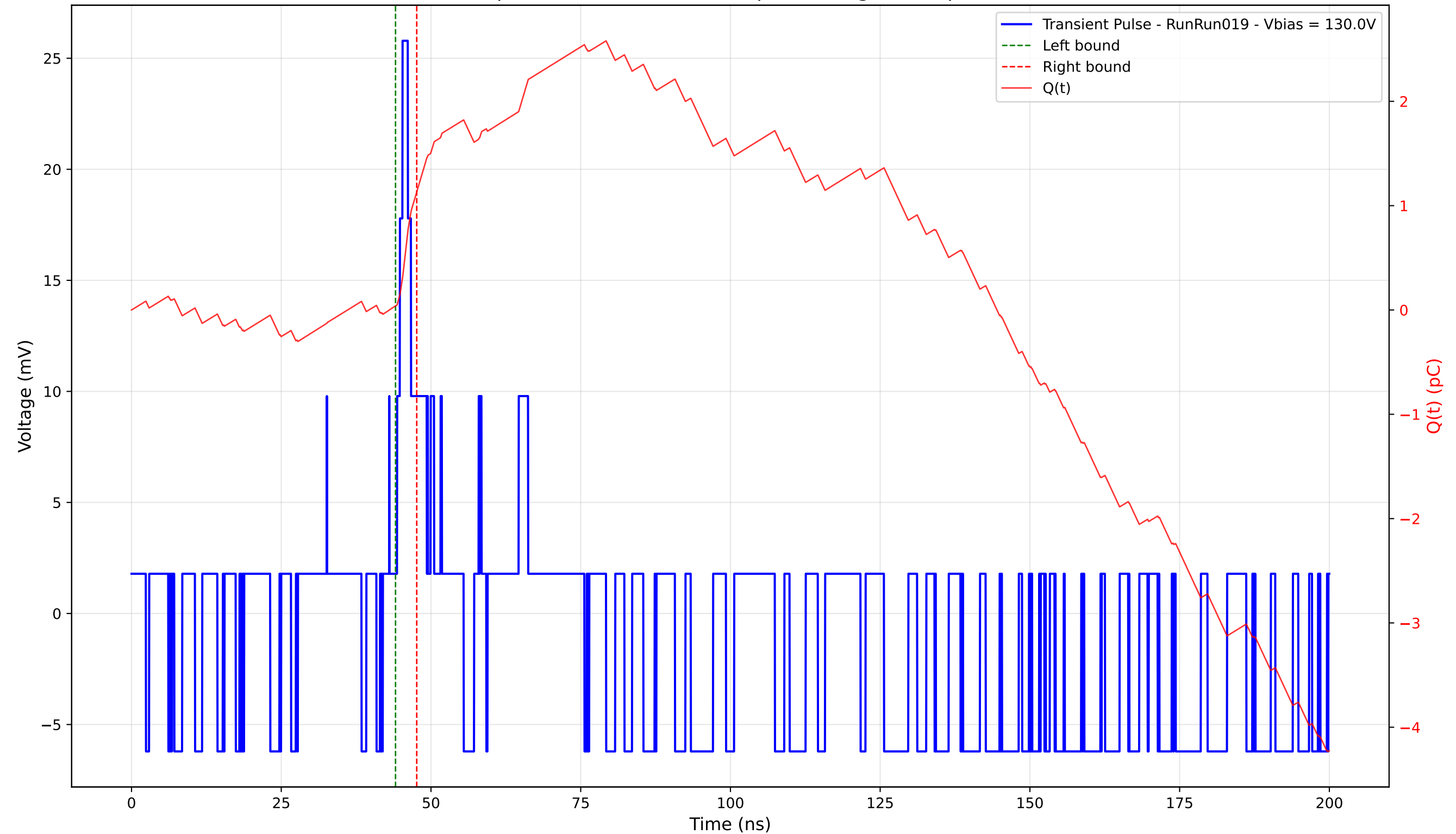
Transient Pulse - Sample: 4003 - Position: 30.0 \mu\text{m} - Charge: 1.09 pC - Rise Time: 0.92 ns
