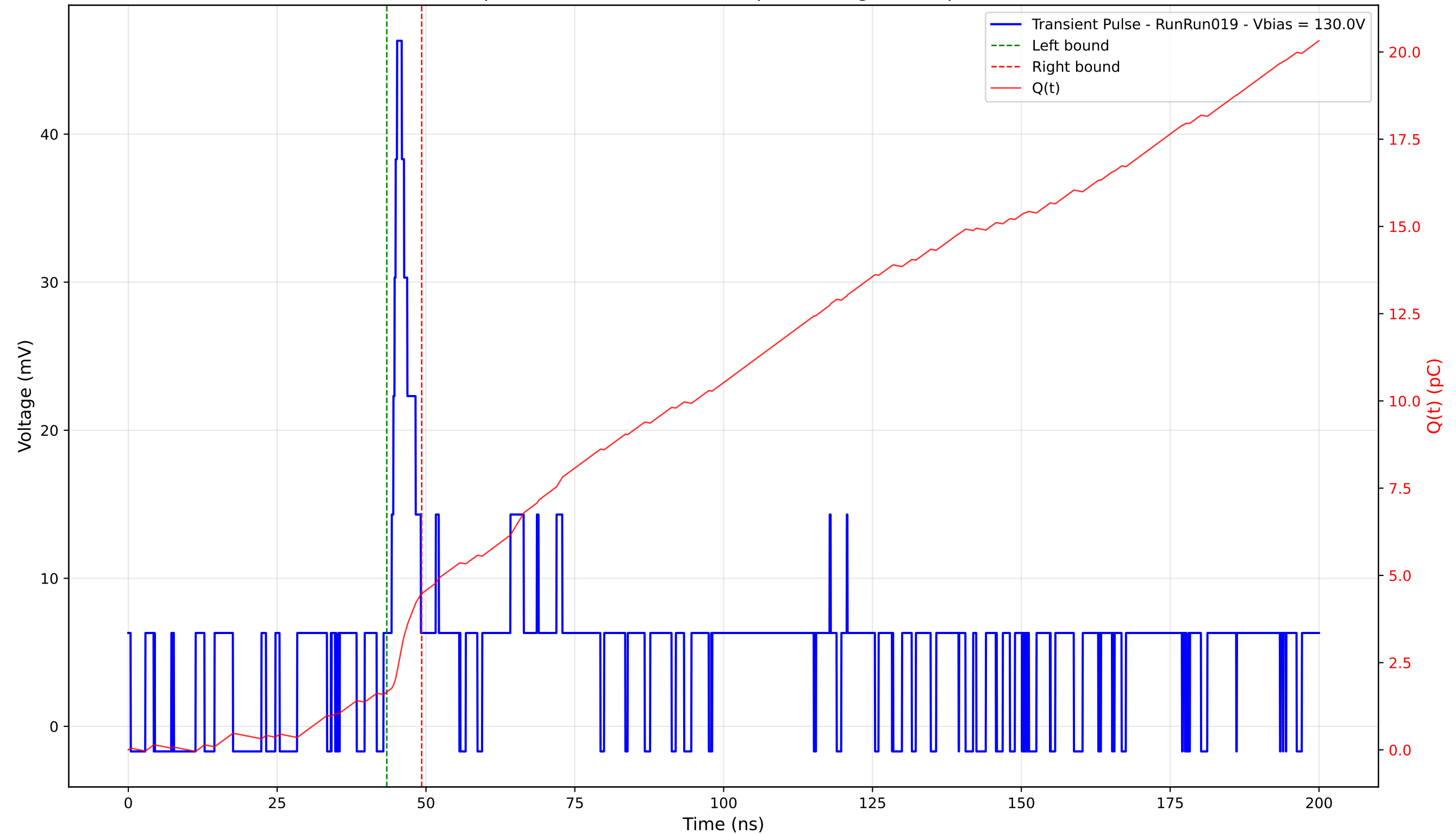
Transient Pulse - Sample: 4003 - Position: 385.0 \mu\text{m} - Charge: 2.82 pC - Rise Time: 2.29 ns
