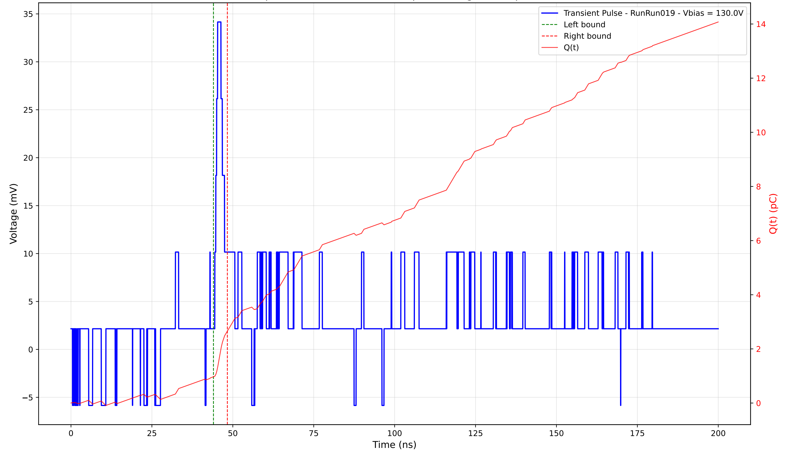
Transient Pulse - Sample: 4003 - Position: 325.0 \mu\text{m} - Charge: 1.69 pC - Rise Time: 0.88 ns
