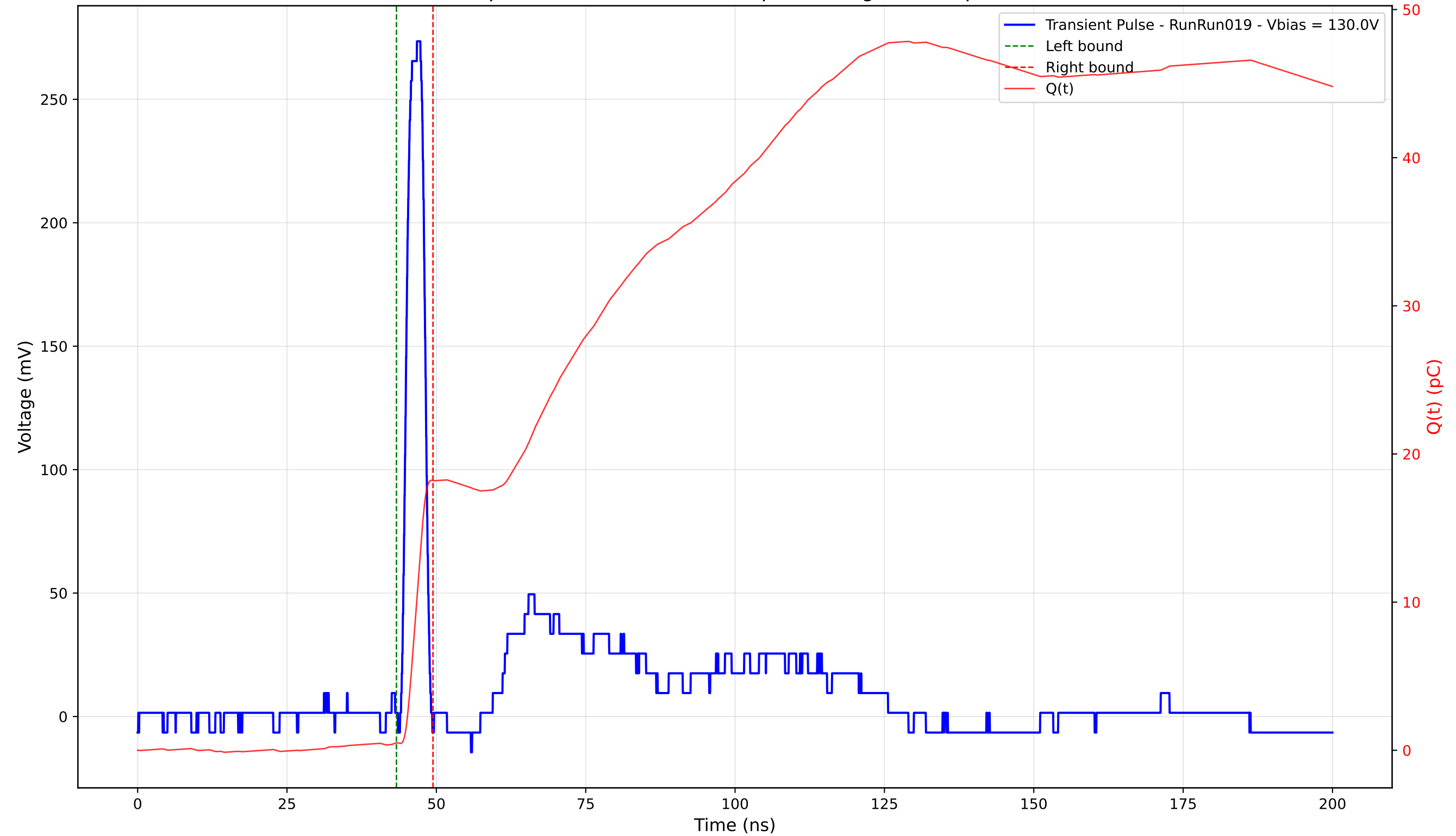
Transient Pulse - Sample: 4003 - Position: 245.0 \mu\text{m} - Charge: 17.71 pC - Rise Time: 1.28 ns
