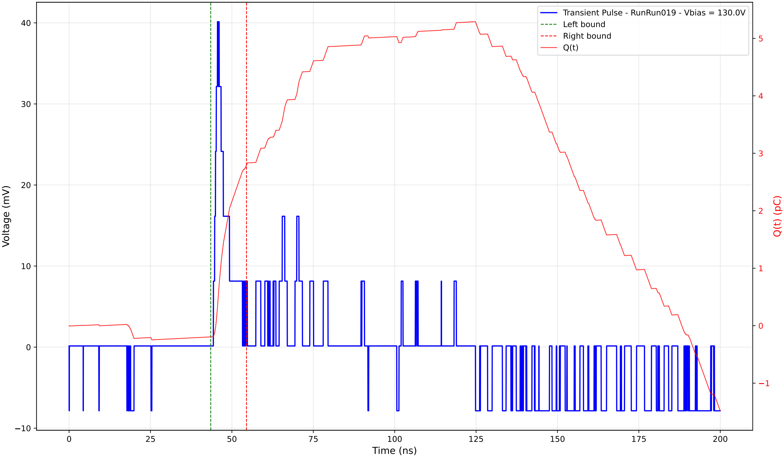
Transient Pulse - Sample: 4003 - Position: 50.0 \mu\text{m} - Charge: 2.99 pC - Rise Time: 1.25 ns
