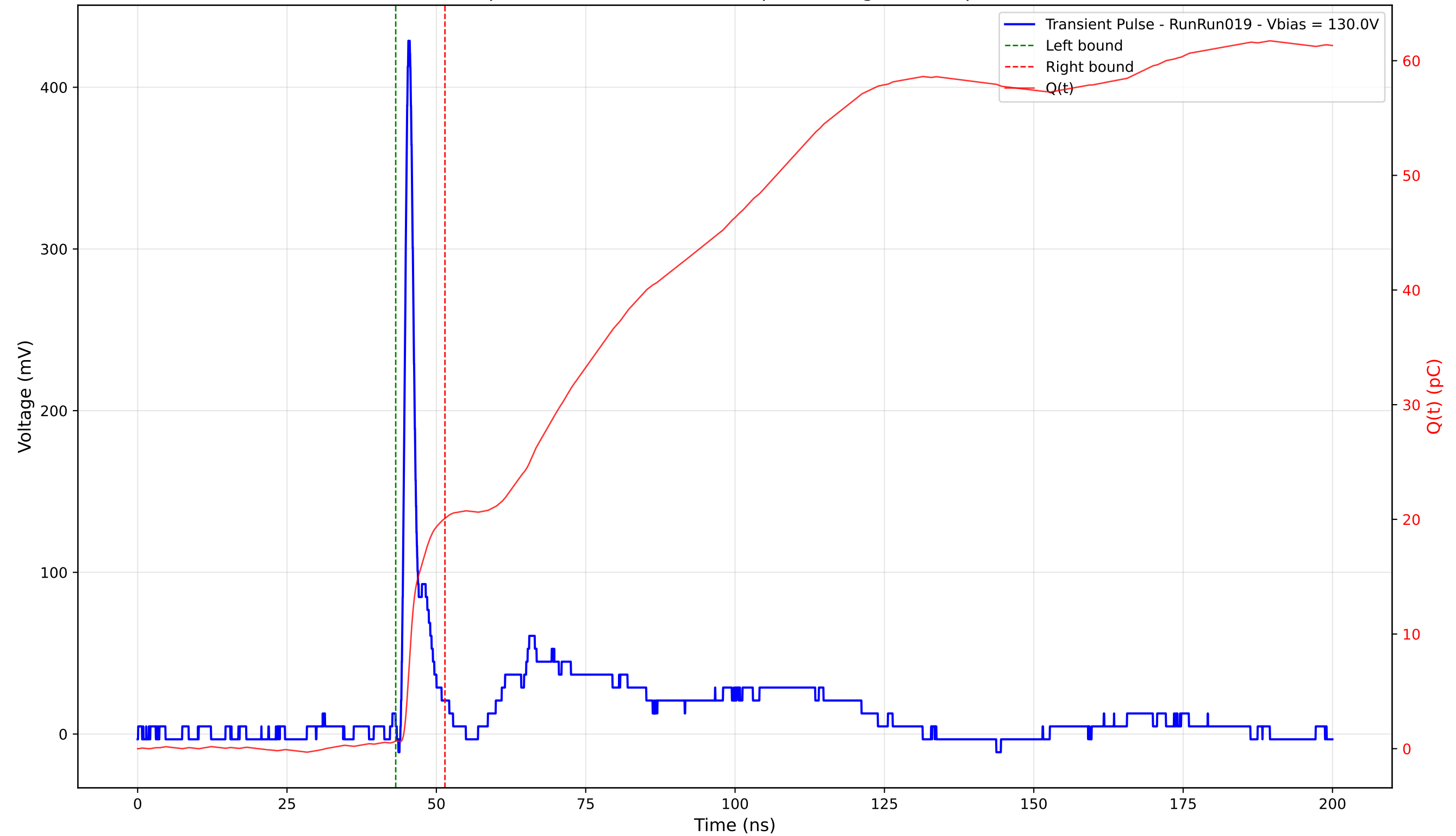
Transient Pulse - Sample: 4003 - Position: 125.0 \mu\text{m} - Charge: 19.42 pC - Rise Time: 0.90 ns
