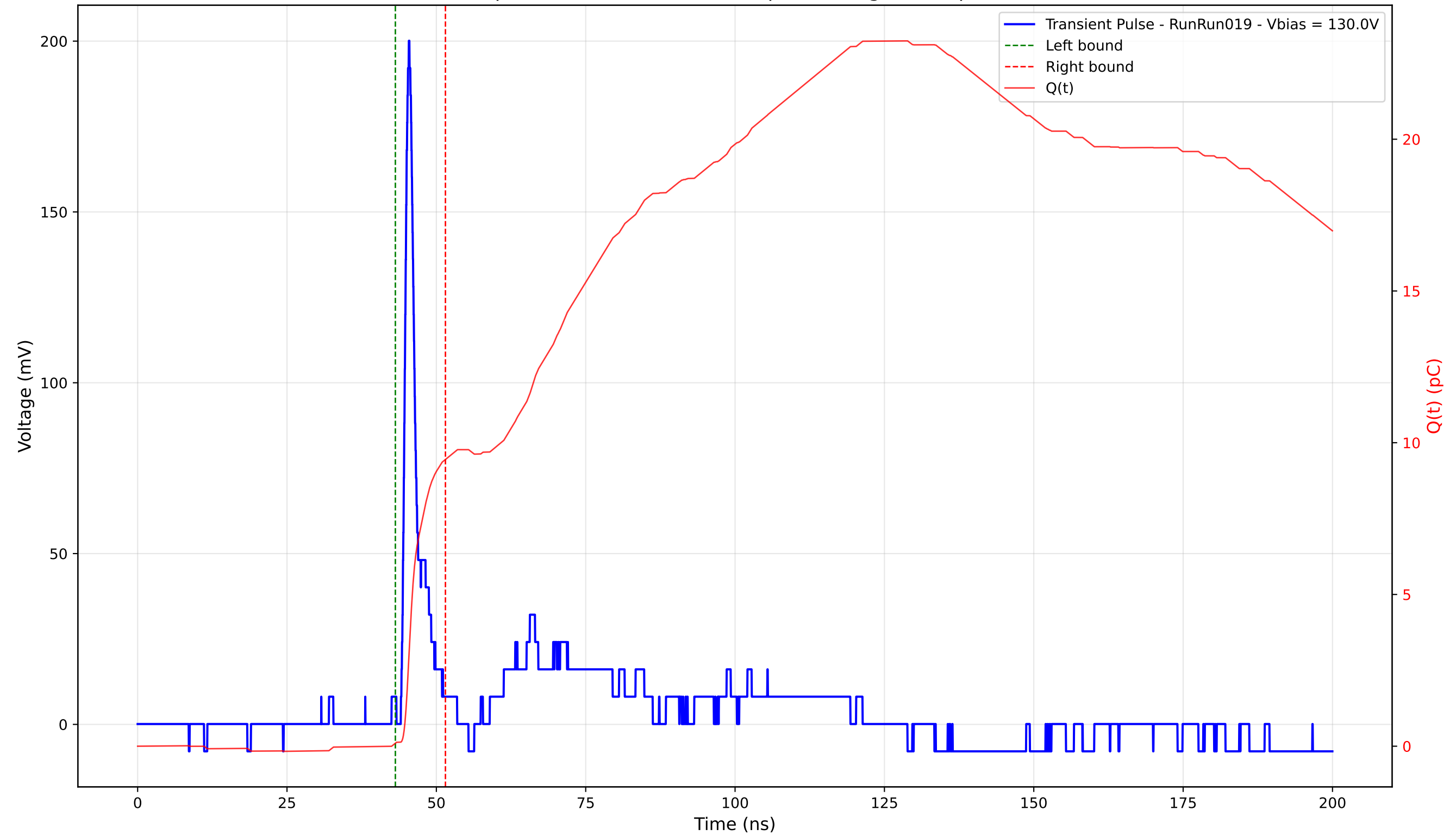
Transient Pulse - Sample: 4003 - Position: 100.0 \mu\text{m} - Charge: 9.35 pC - Rise Time: 0.93 ns
