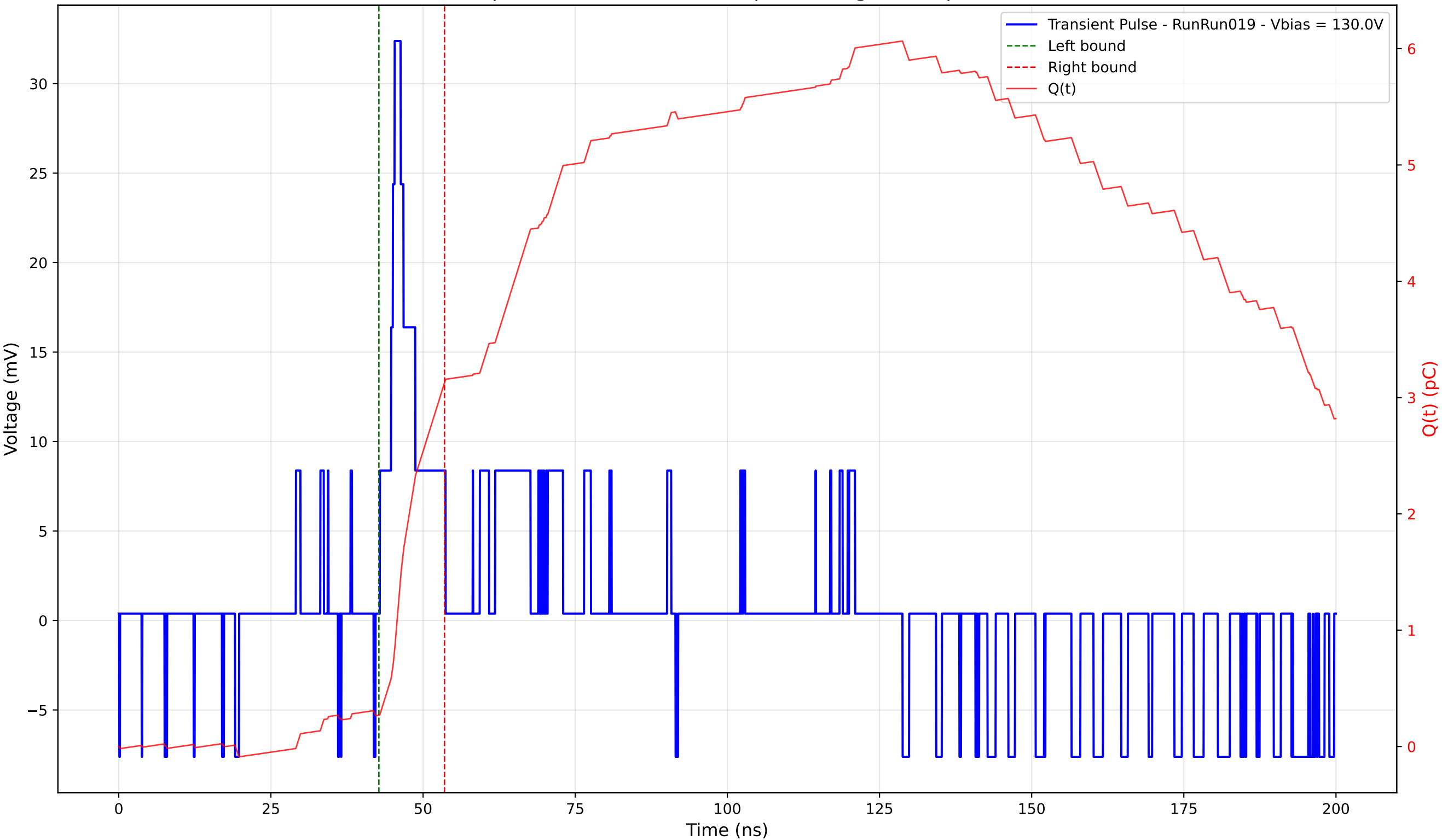
Transient Pulse - Sample: 4003 - Position: 45.0 \mu\text{m} - Charge: 2.86 pC - Rise Time: 2.43 ns
