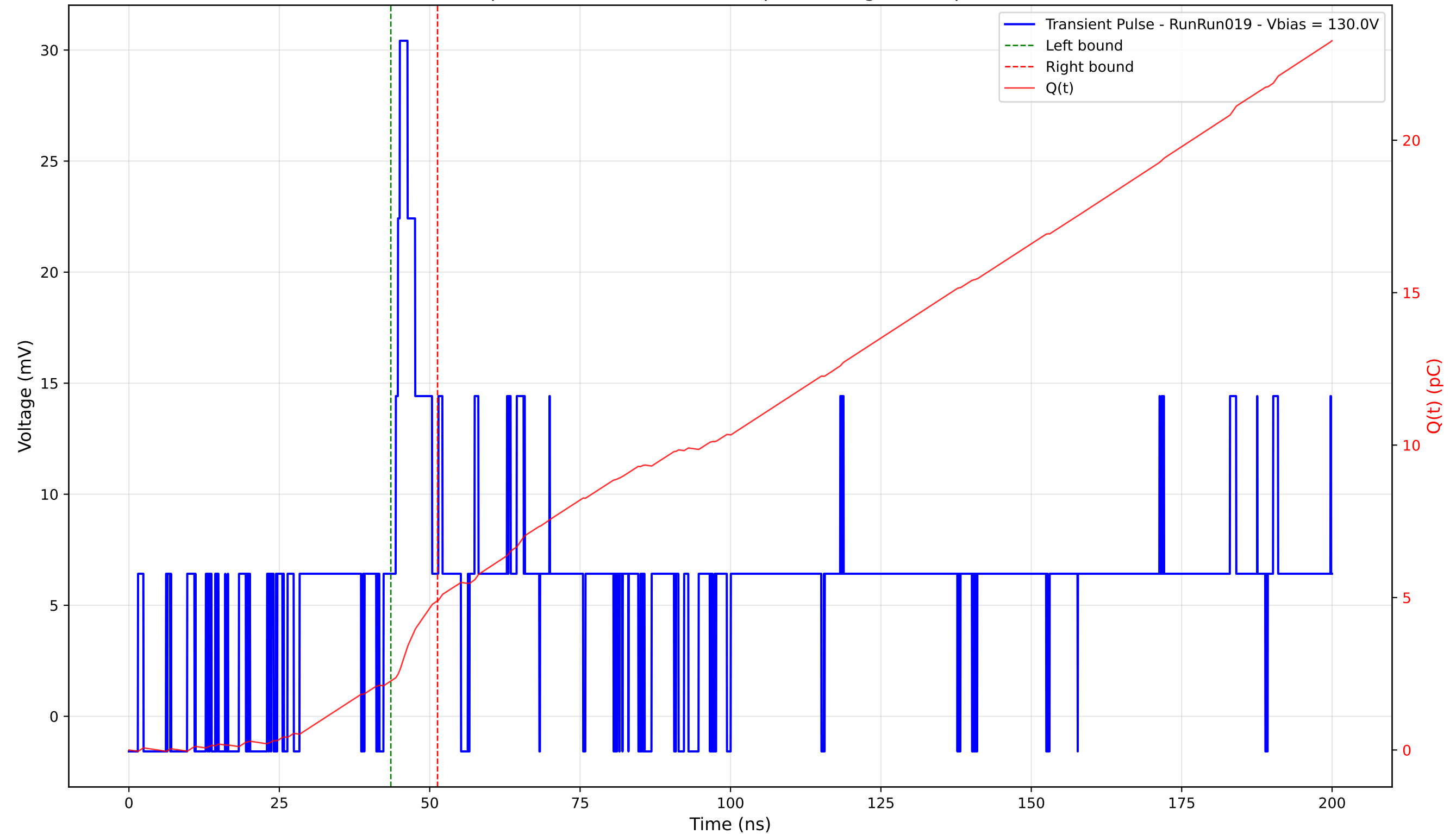
Transient Pulse - Sample: 4003 - Position: 340.0 \mu\text{m} - Charge: 2.63 pC - Rise Time: 2.71 ns
