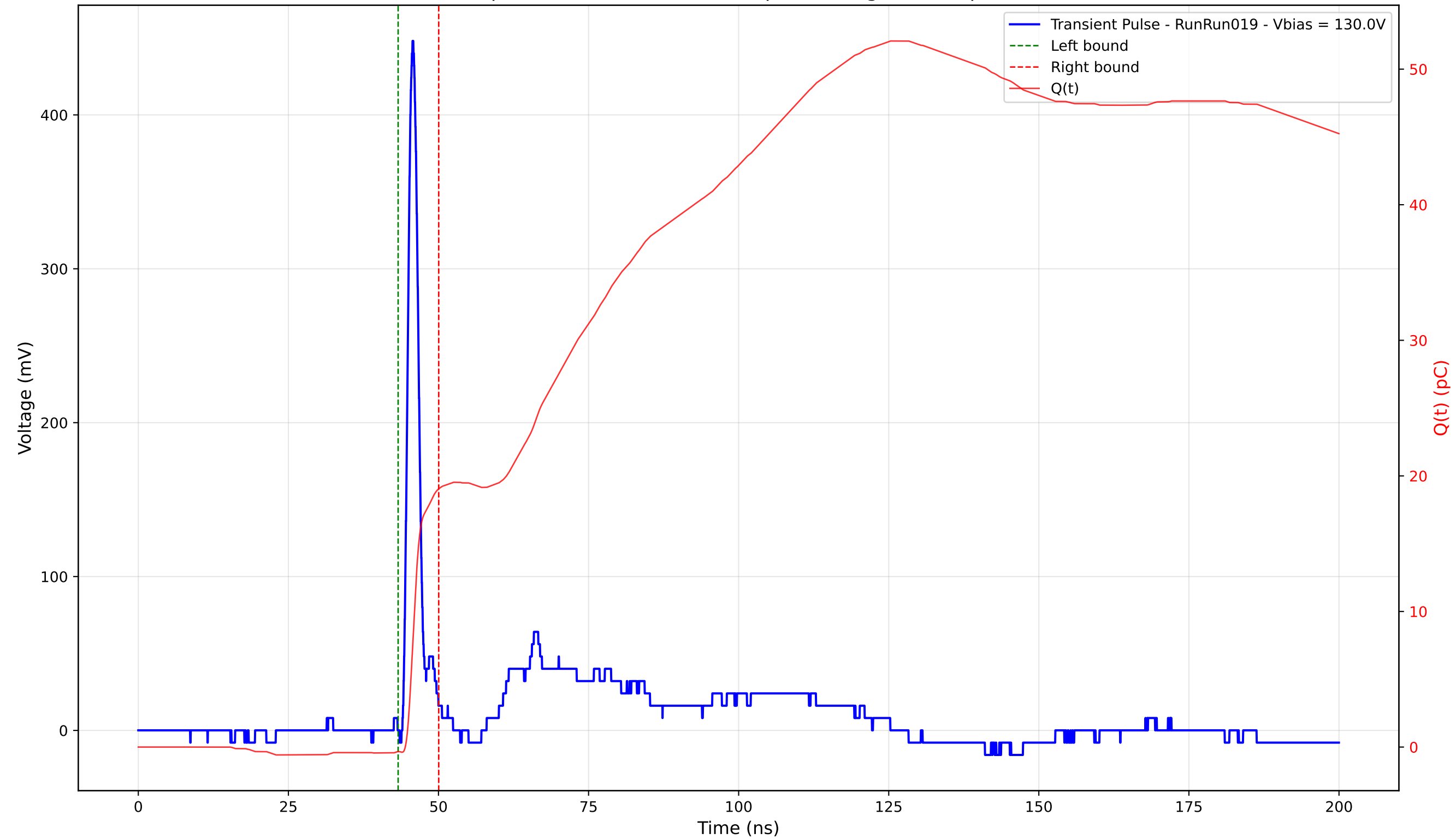
Transient Pulse - Sample: 4003 - Position: 185.0 \mu\text{m} - Charge: 19.38 pC - Rise Time: 1.09 ns
