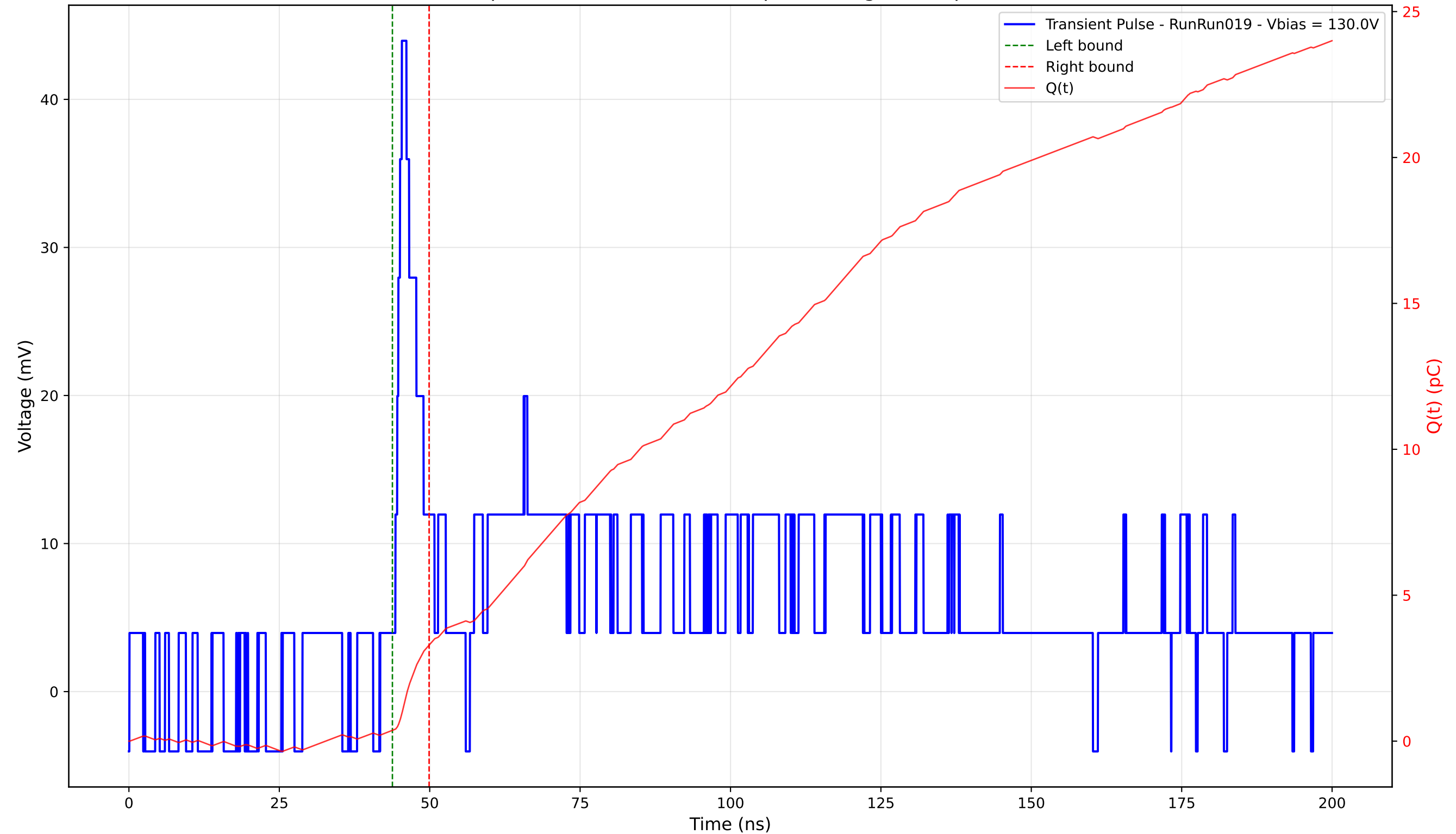
Transient Pulse - Sample: 4003 - Position: 310.0 \mu\text{m} - Charge: 2.93 pC - Rise Time: 1.08 ns
