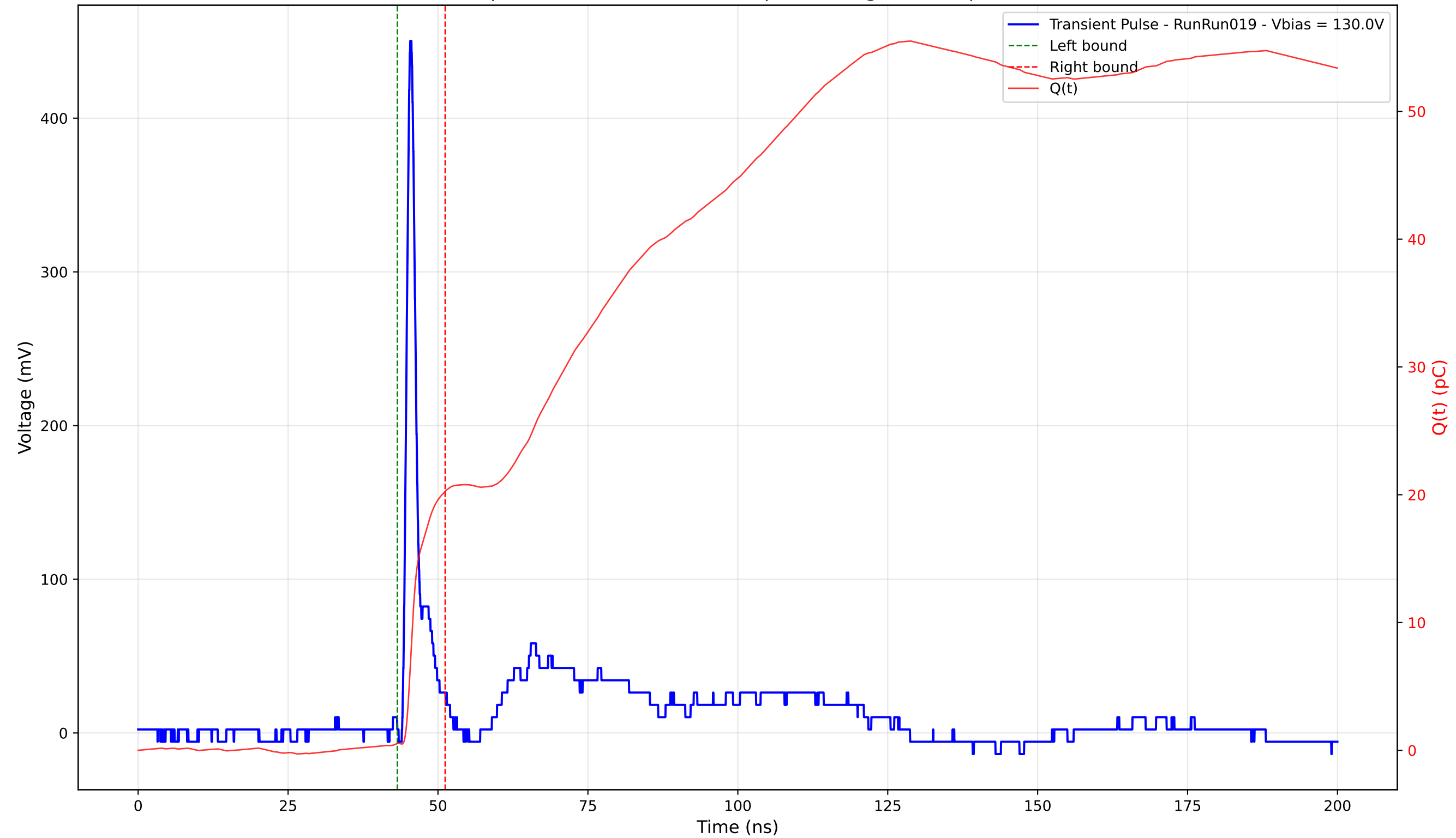
Transient Pulse - Sample: 4003 - Position: 135.0 \mu\text{m} - Charge: 19.74 pC - Rise Time: 0.91 ns
