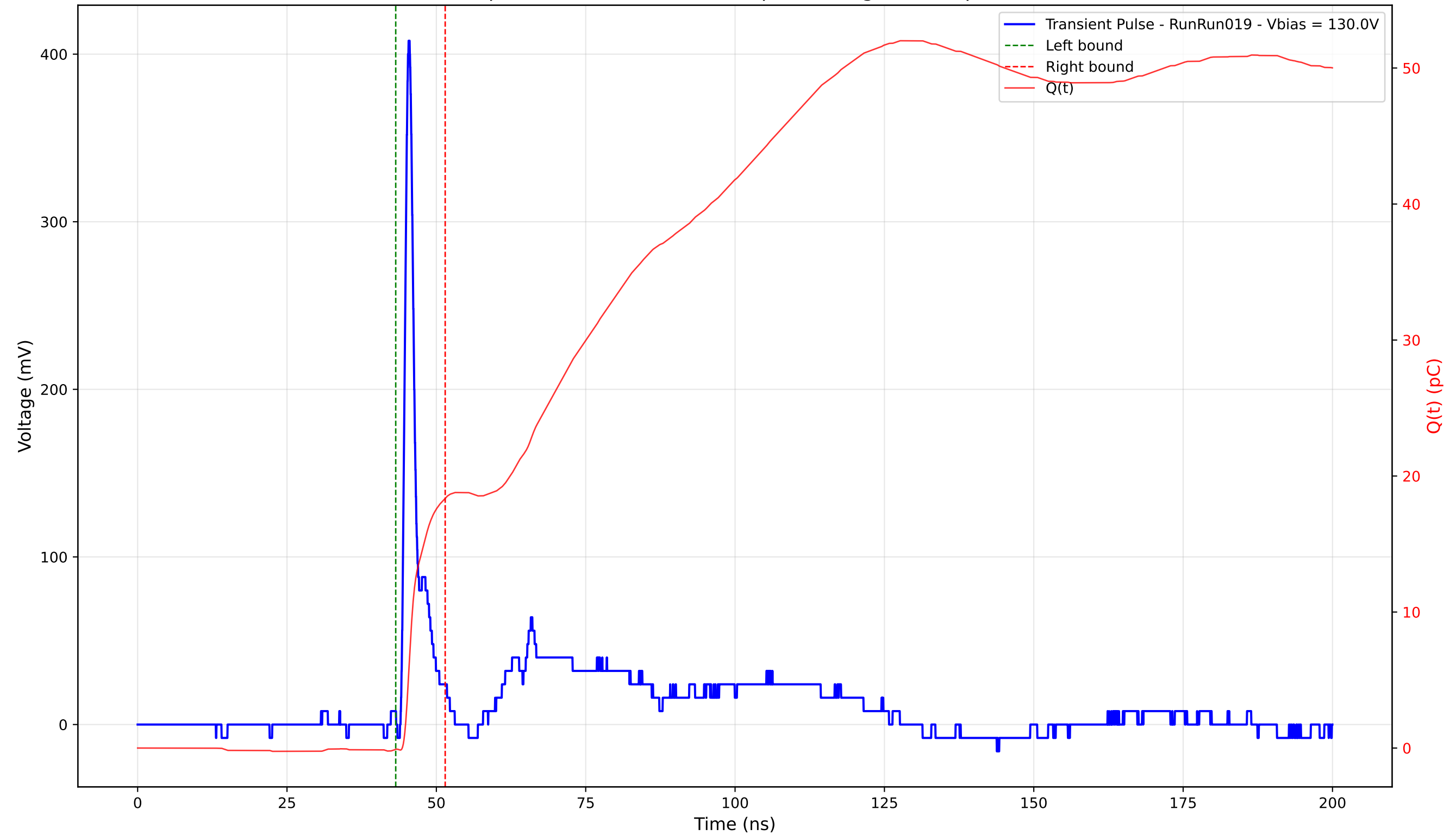
Transient Pulse - Sample: 4003 - Position: 120.0 \mu\text{m} - Charge: 18.45 pC - Rise Time: 0.90 ns
