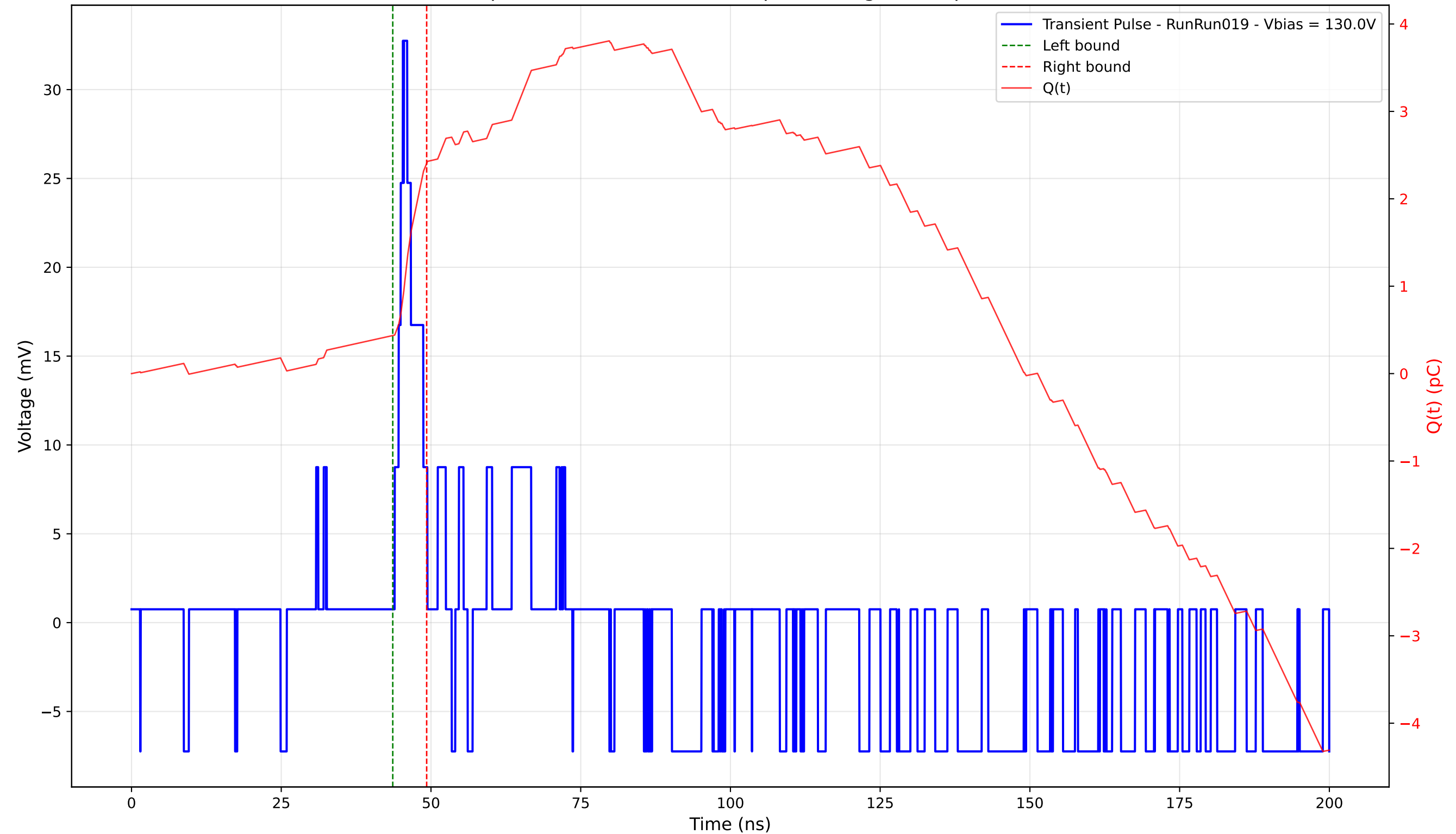
Transient Pulse - Sample: 4003 - Position: 410.0 \mu\text{m} - Charge: 1.97 pC - Rise Time: 1.37 ns
