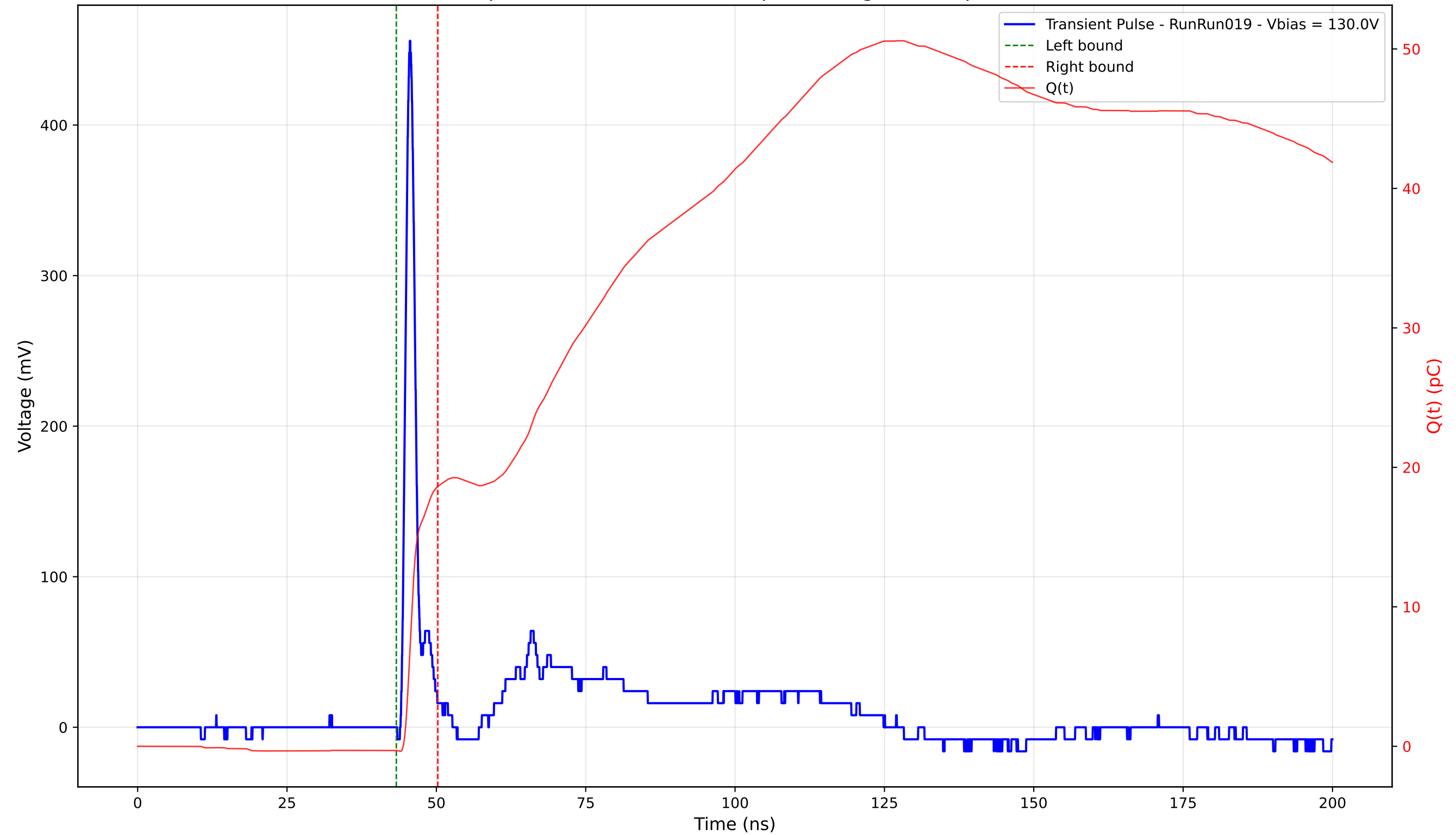
Transient Pulse - Sample: 4003 - Position: 165.0 \mu\text{m} - Charge: 18.93 pC - Rise Time: 1.05 ns
