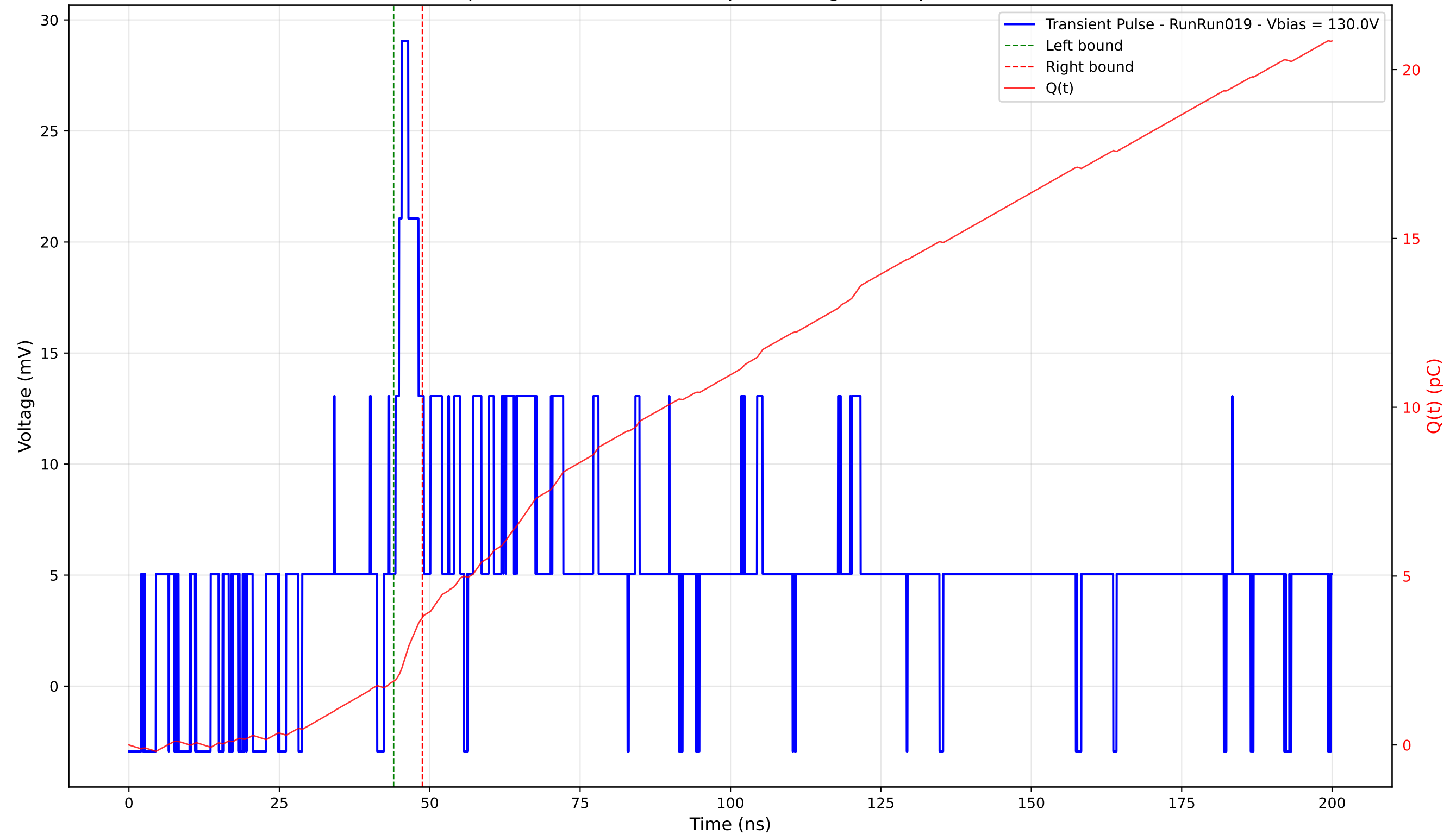
Transient Pulse - Sample: 4003 - Position: 40.0 \mu\text{m} - Charge: 1.89 pC - Rise Time: 0.00 ns (N/A)
