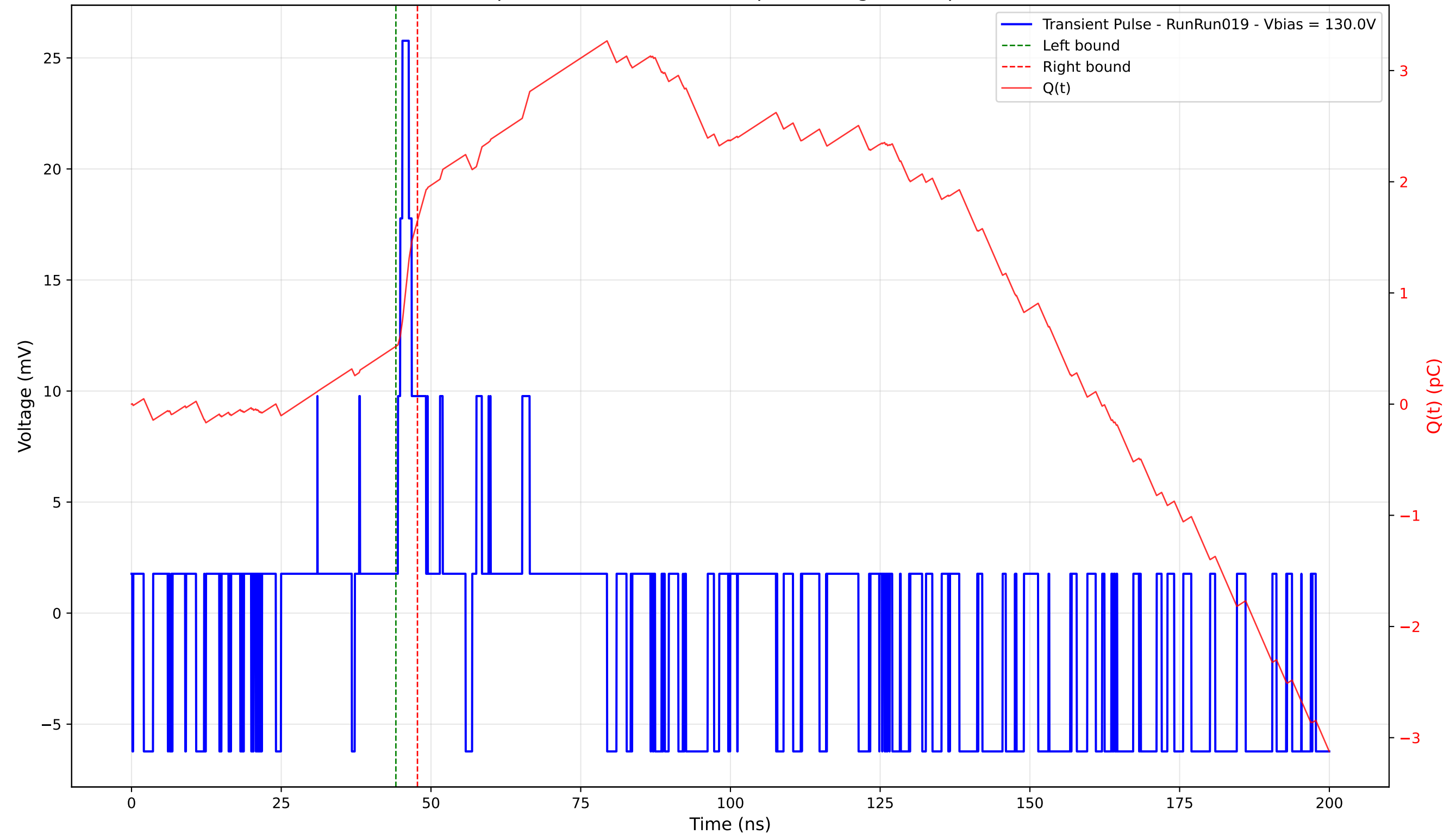
Transient Pulse - Sample: 4003 - Position: 35.0 \mu\text{m} - Charge: 1.13 pC - Rise Time: 0.76 ns
