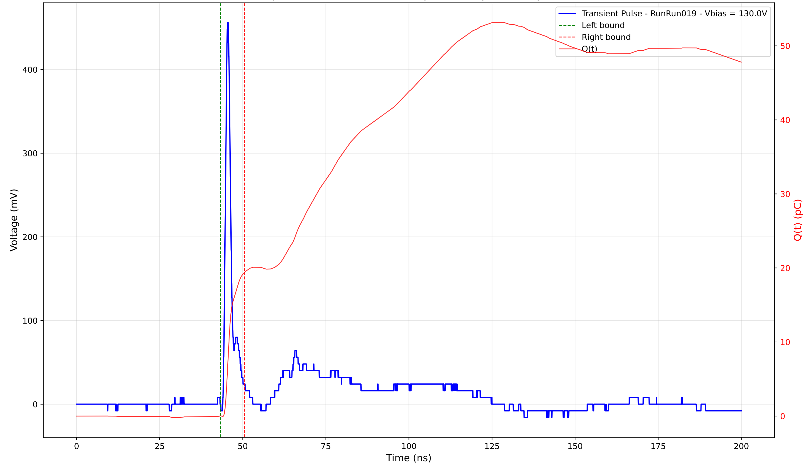
Transient Pulse - Sample: 4003 - Position: 145.0 \mu\text{m} - Charge: 19.42 pC - Rise Time: 0.95 ns
