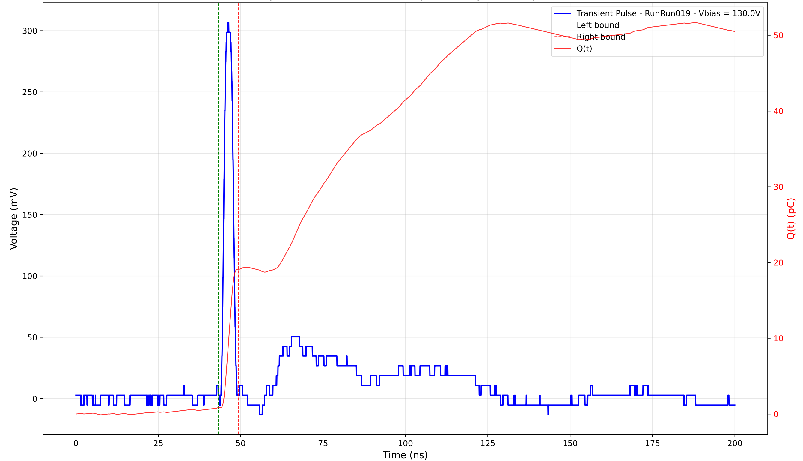
Transient Pulse - Sample: 4003 - Position: 235.0 \mu\text{m} - Charge: 18.22 pC - Rise Time: 1.23 ns
