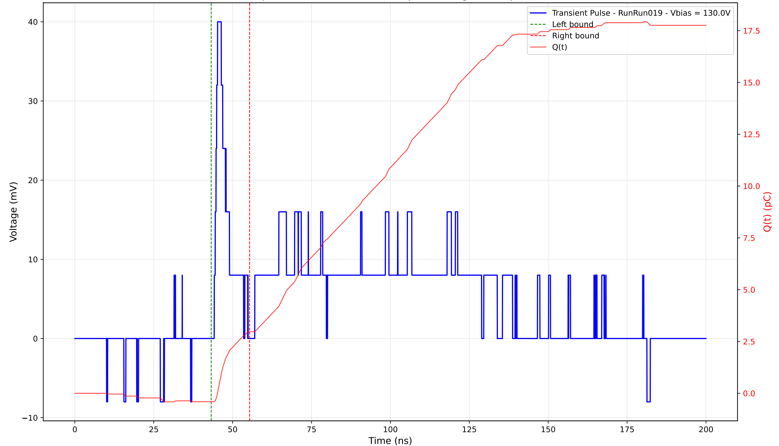
Transient Pulse - Sample: 4003 - Position: 305.0 \mu\text{m} - Charge: 3.38 pC - Rise Time: 1.05 ns
