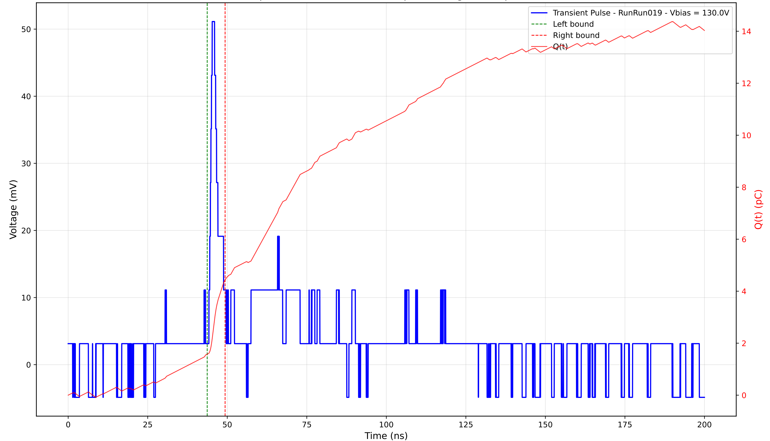
Transient Pulse - Sample: 4003 - Position: 395.0 \mu\text{m} - Charge: 2.86 pC - Rise Time: 1.04 ns
