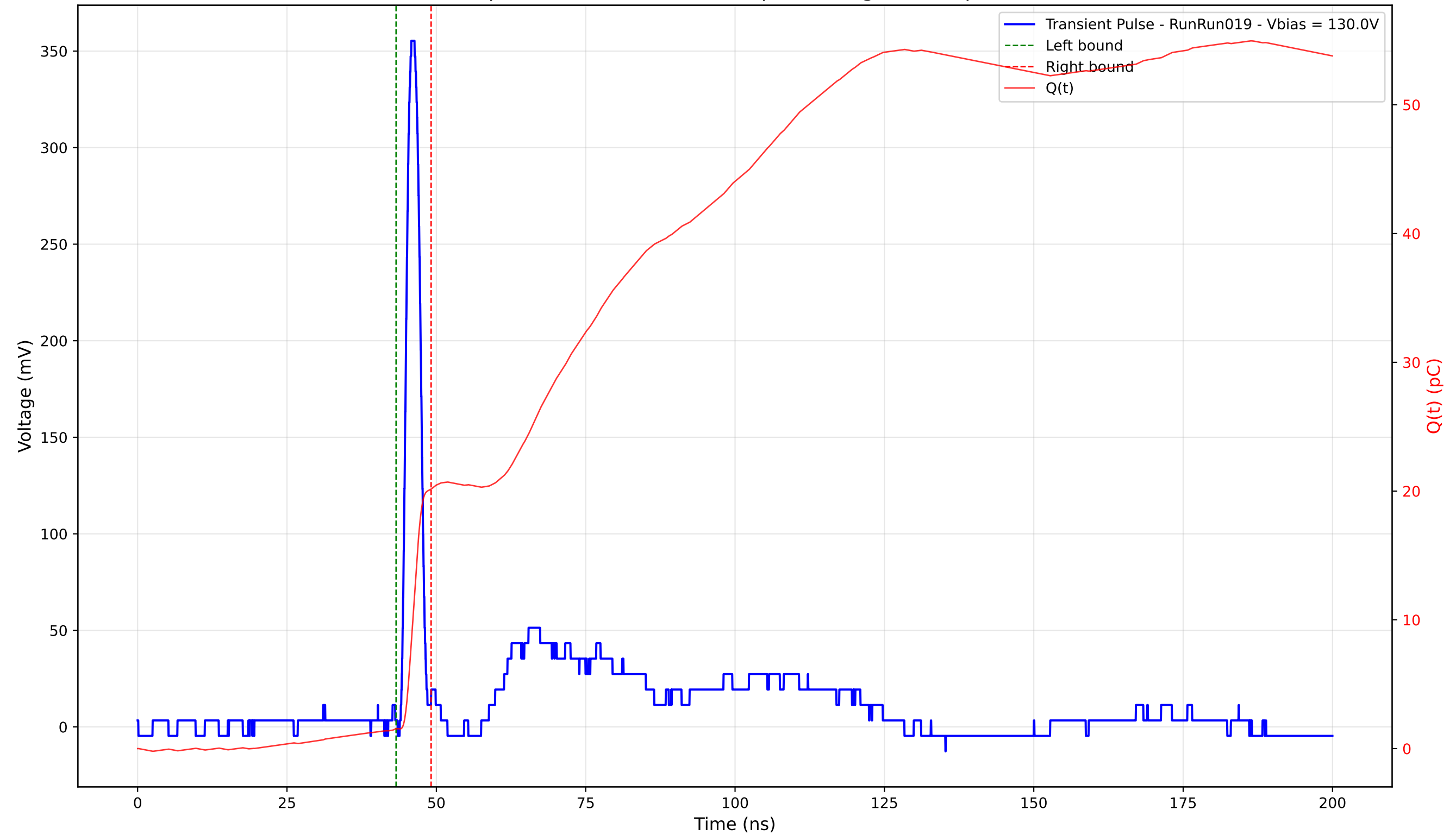
Transient Pulse - Sample: 4003 - Position: 220.0 \mu\text{m} - Charge: 18.61 pC - Rise Time: 1.16 ns
