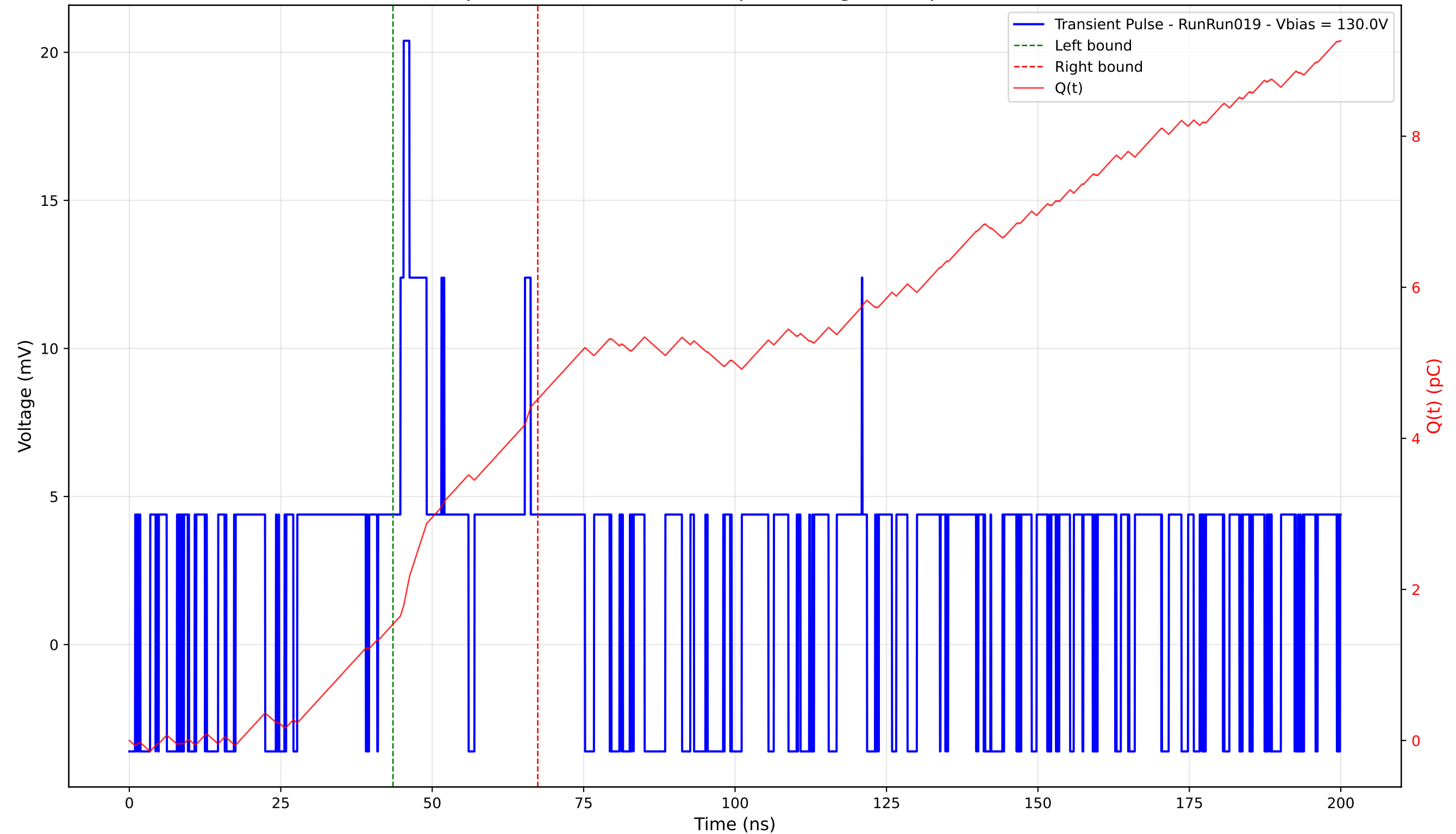
Transient Pulse - Sample: 4003 - Position: 420.0 \mu\text{m} - Charge: 2.98 pC - Rise Time: 0.00 ns (N/A)
