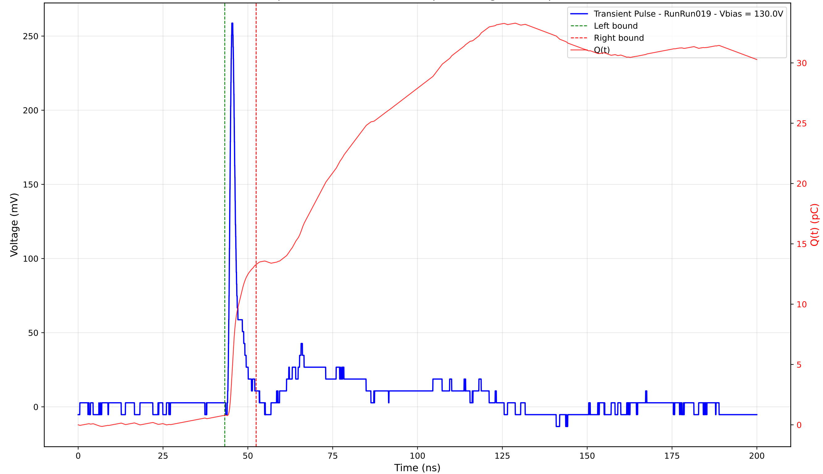
Transient Pulse - Sample: 4003 - Position: 105.0 \mu\text{m} - Charge: 12.49 pC - Rise Time: 0.90 ns
