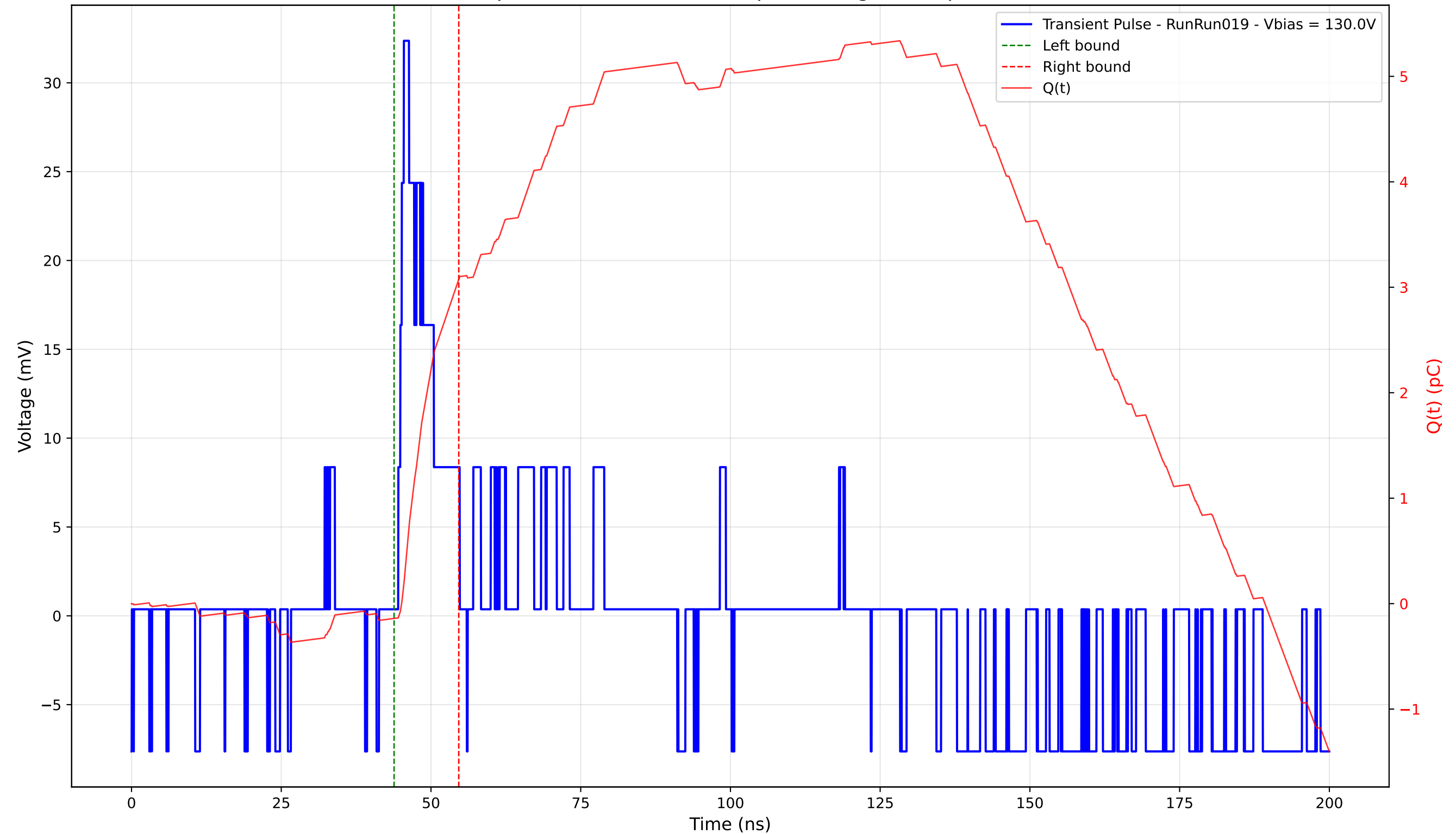
Transient Pulse - Sample: 4003 - Position: 60.0 \mu\text{m} - Charge: 3.22 pC - Rise Time: 0.93 ns
