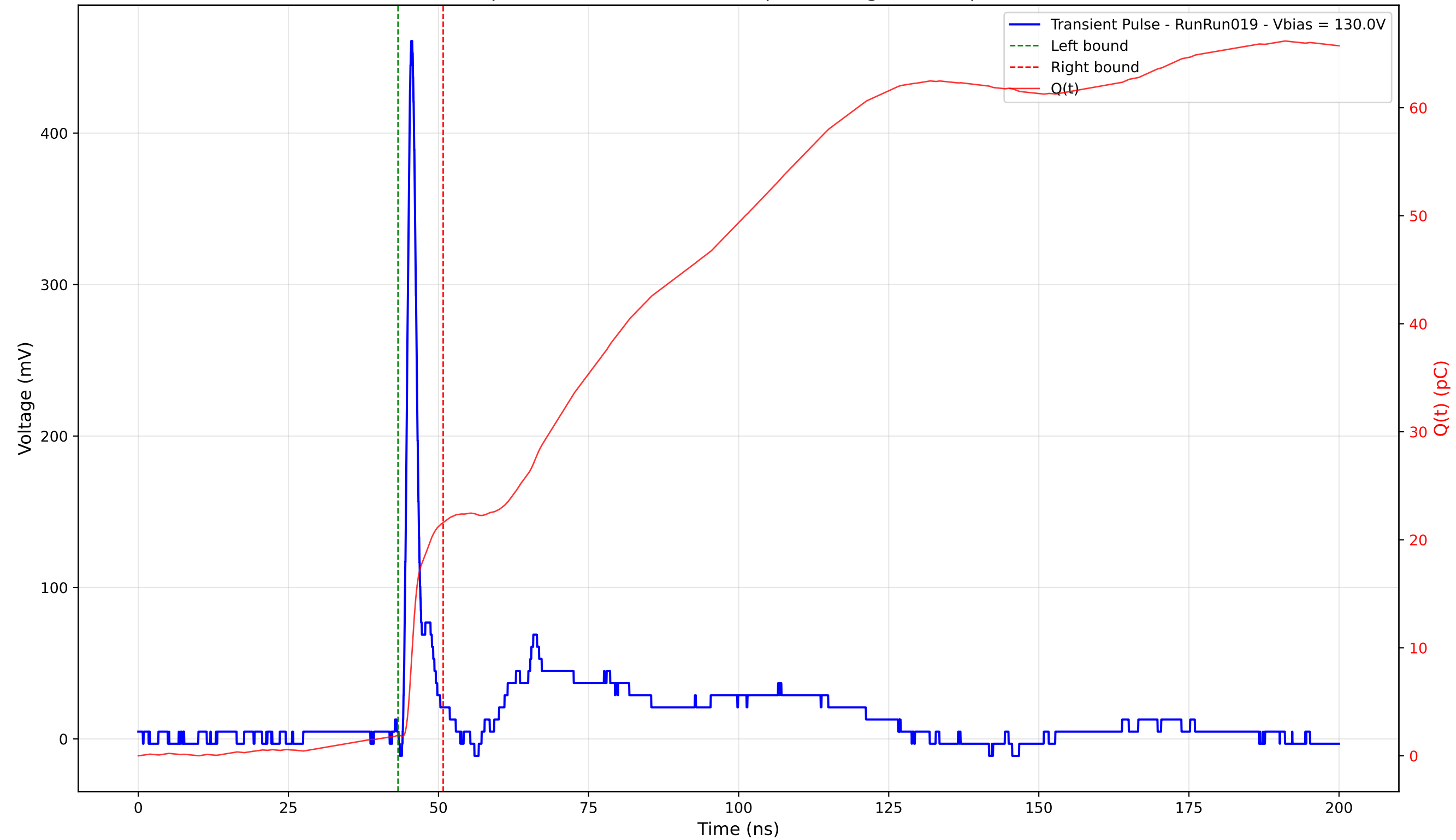
Transient Pulse - Sample: 4003 - Position: 150.0 \mu\text{m} - Charge: 19.70 pC - Rise Time: 0.94 ns
