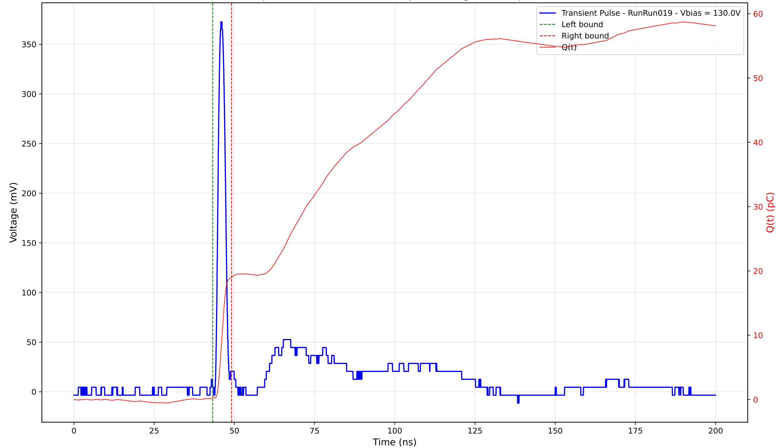
Transient Pulse - Sample: 4003 - Position: 215.0 \mu\text{m} - Charge: 18.76 pC - Rise Time: 1.14 ns
