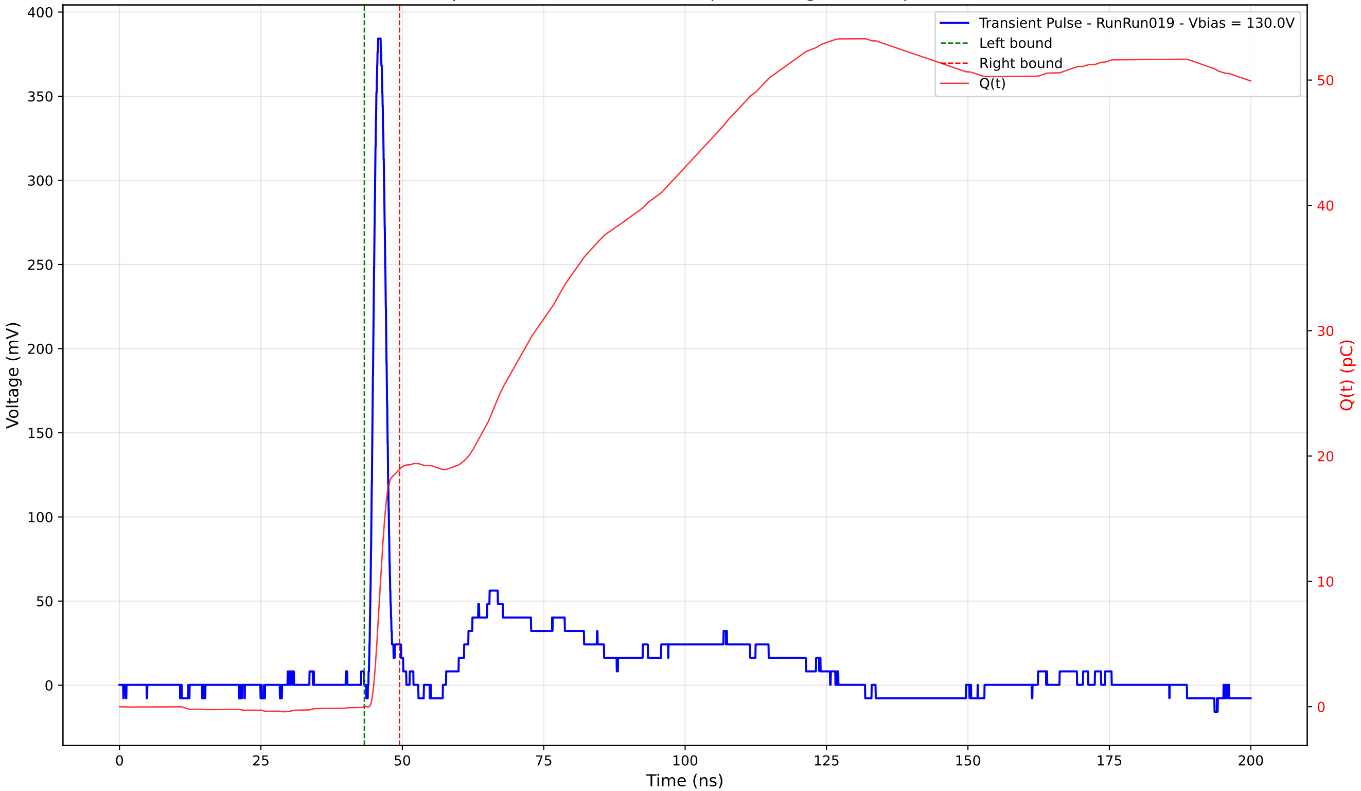
Transient Pulse - Sample: 4003 - Position: 210.0 \mu\text{m} - Charge: 18.94 pC - Rise Time: 1.14 ns
