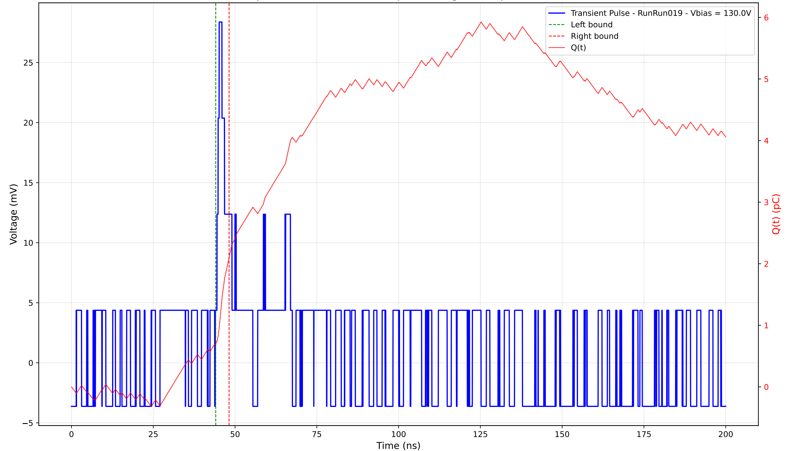
Transient Pulse - Sample: 4003 - Position: 25.0 \mu\text{m} - Charge: 1.40 pC - Rise Time: 0.00 ns (N/A)
