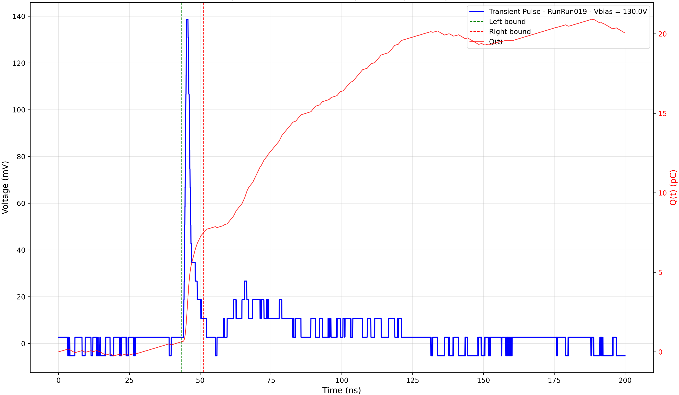
Transient Pulse - Sample: 4003 - Position: 95.0 \mu\text{m} - Charge: 6.85 pC - Rise Time: 0.93 ns
