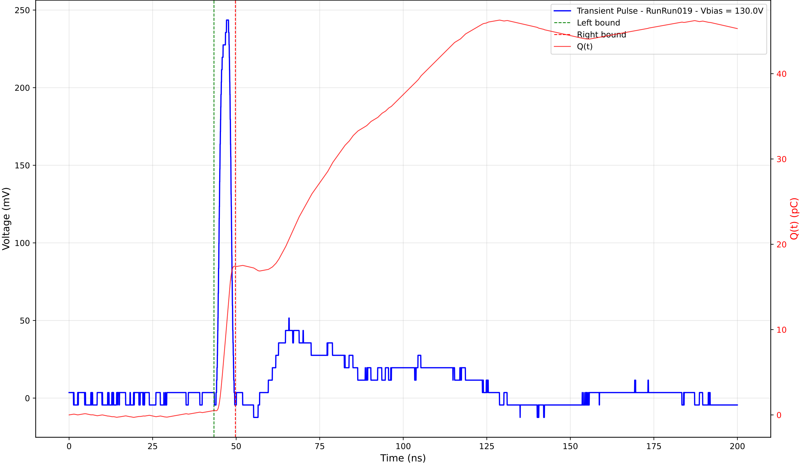
Transient Pulse - Sample: 4003 - Position: 255.0 \mu\text{m} - Charge: 16.90 pC - Rise Time: 1.45 ns
