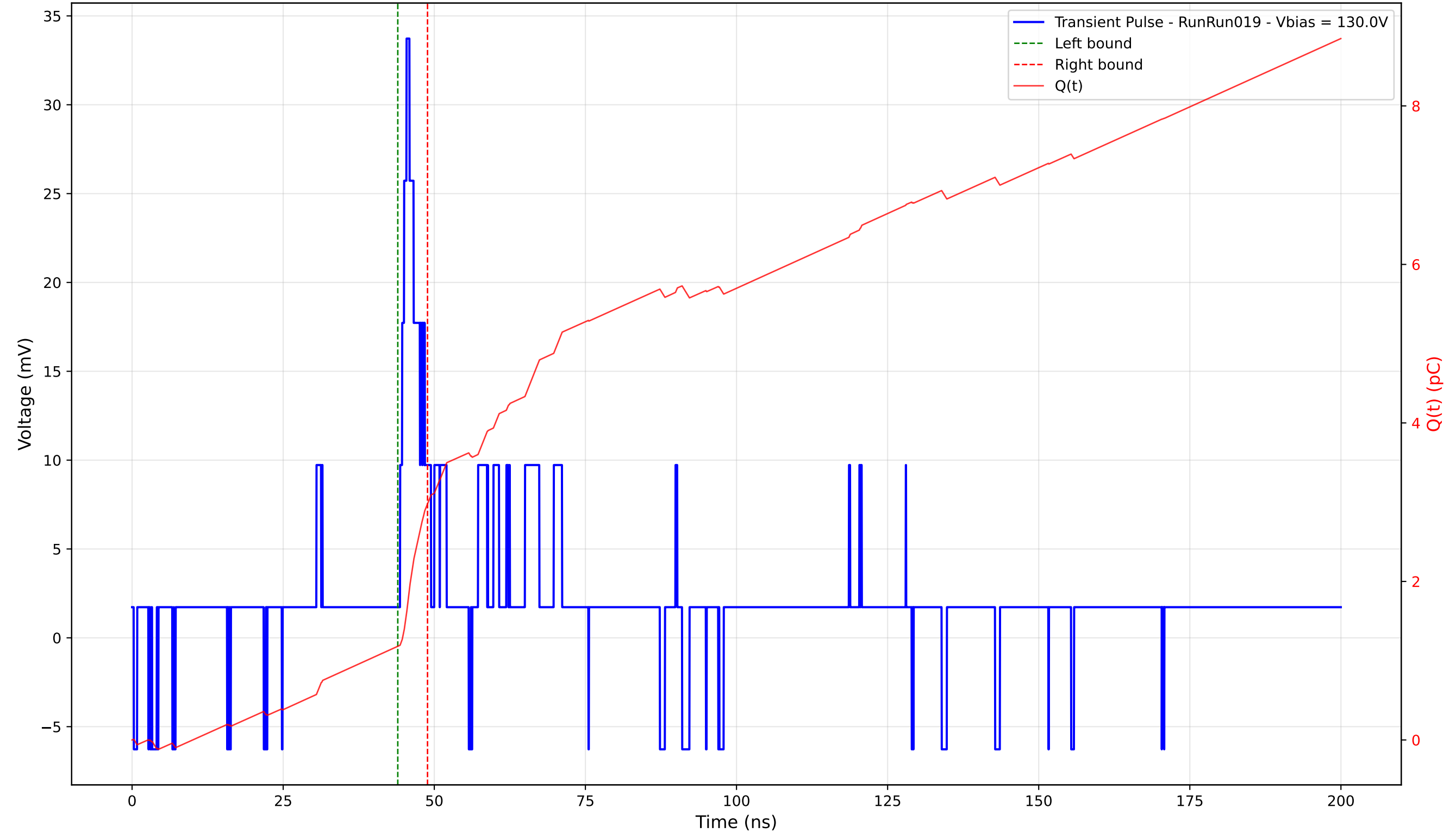
Transient Pulse - Sample: 4003 - Position: 350.0 \mu\text{m} - Charge: 1.80 pC - Rise Time: 1.08 ns
