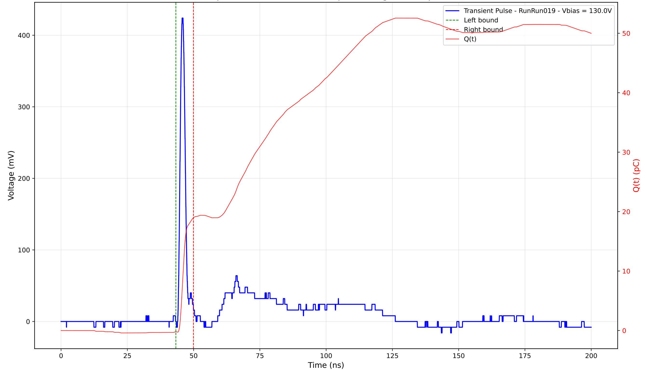
Transient Pulse - Sample: 4003 - Position: 195.0 \mu\text{m} - Charge: 19.17 pC - Rise Time: 1.09 ns
