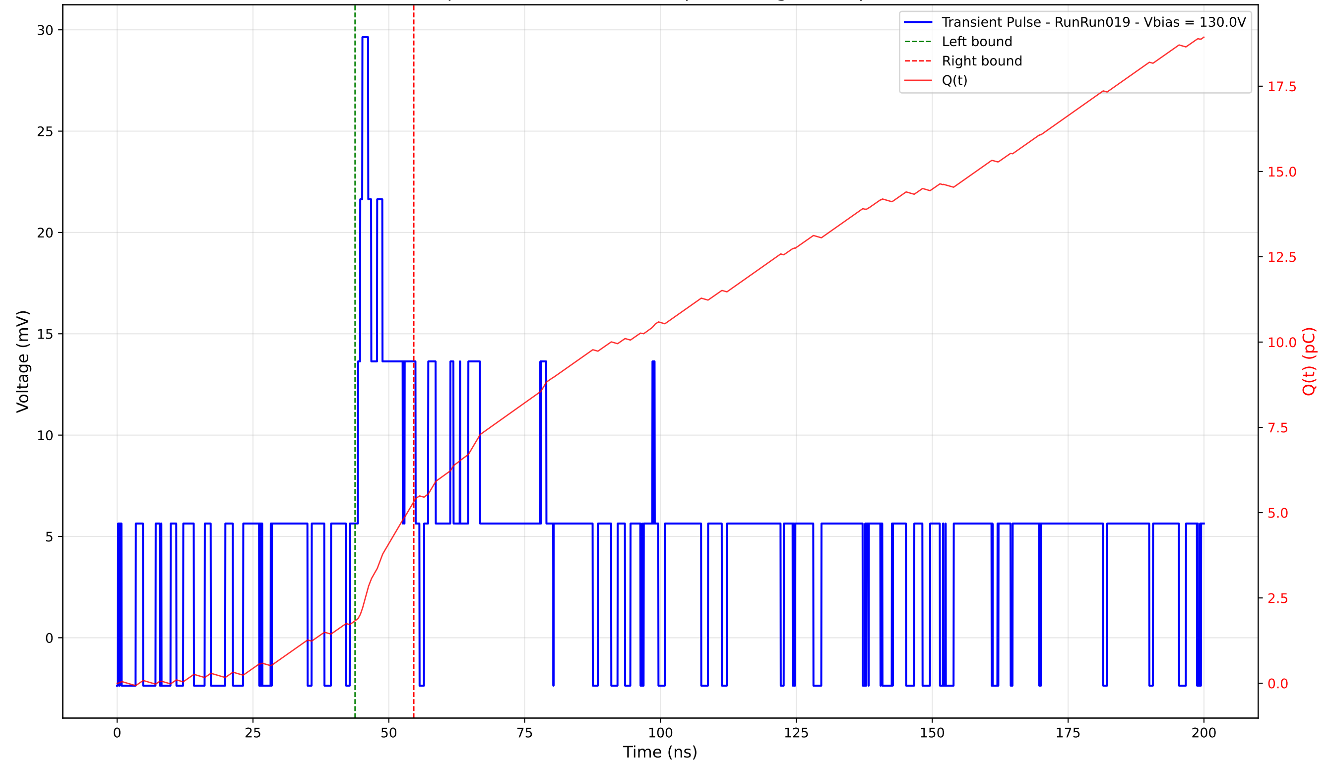
Transient Pulse - Sample: 4003 - Position: 65.0 \mu\text{m} - Charge: 3.50 pC - Rise Time: 2.32 ns
