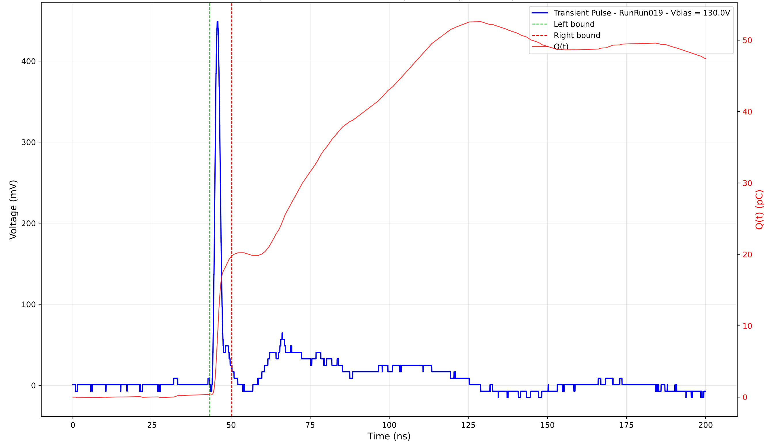
Transient Pulse - Sample: 4003 - Position: 180.0 \mu\text{m} - Charge: 19.32 pC - Rise Time: 1.05 ns
