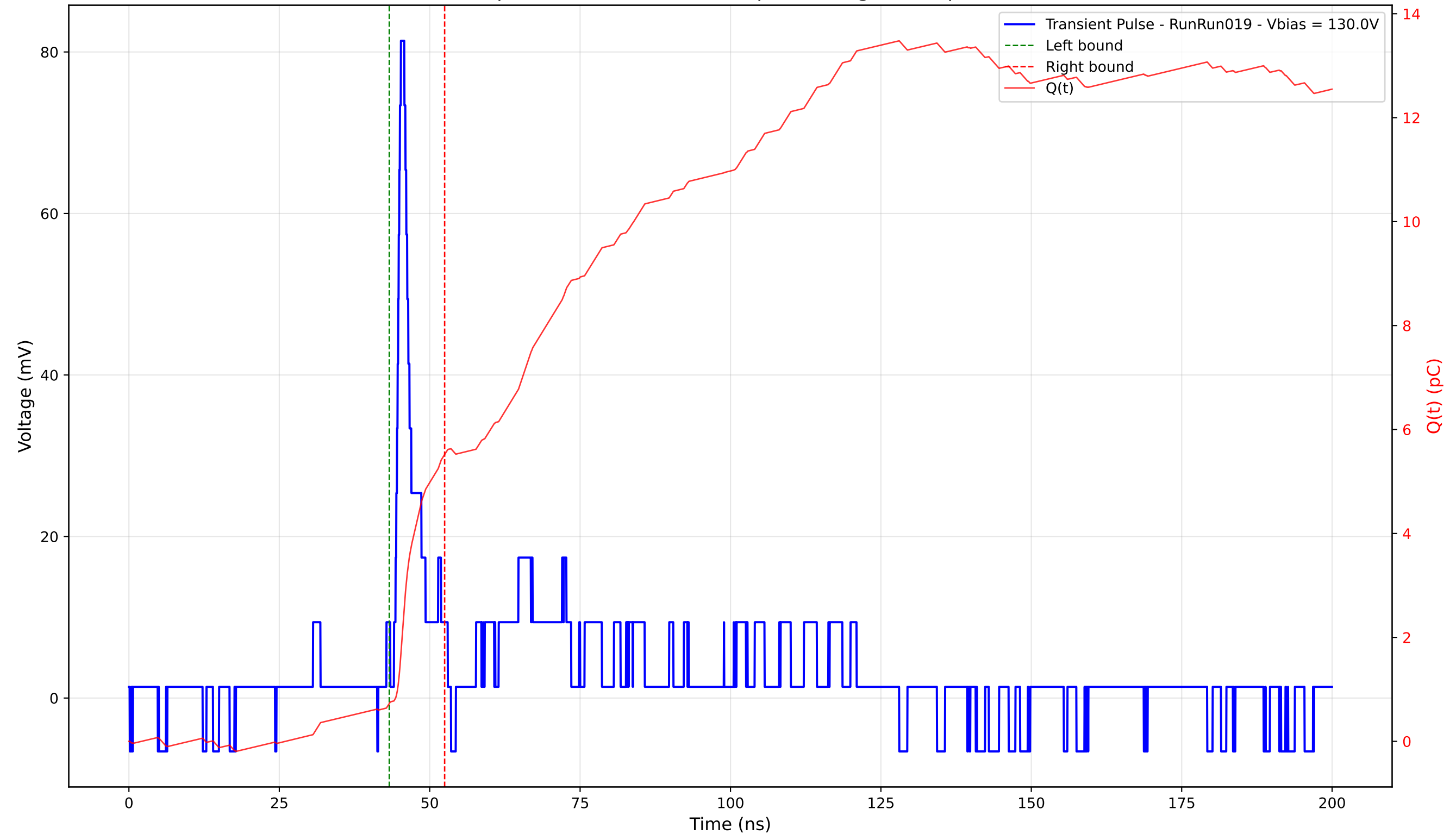
Transient Pulse - Sample: 4003 - Position: 90.0 \mu\text{m} - Charge: 4.79 pC - Rise Time: 0.98 ns
