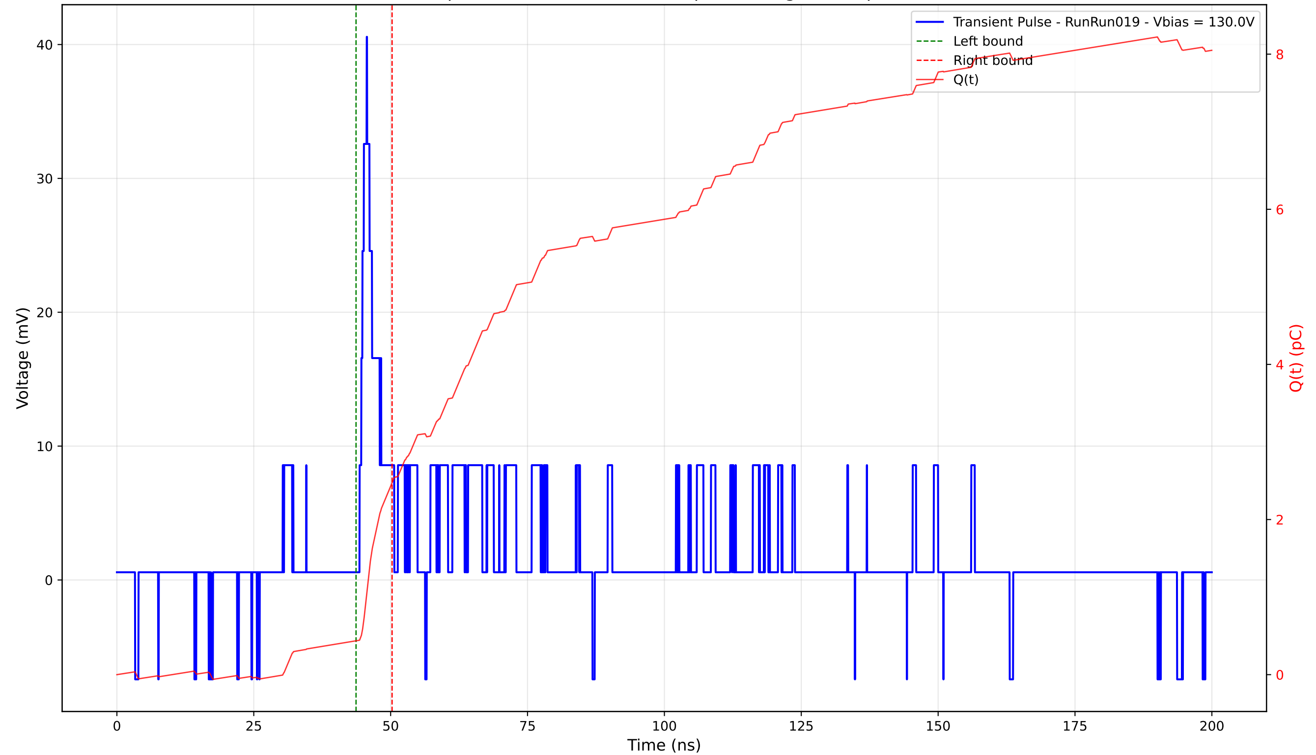
Transient Pulse - Sample: 4003 - Position: 375.0 \mu\text{m} - Charge: 2.04 pC - Rise Time: 1.31 ns
