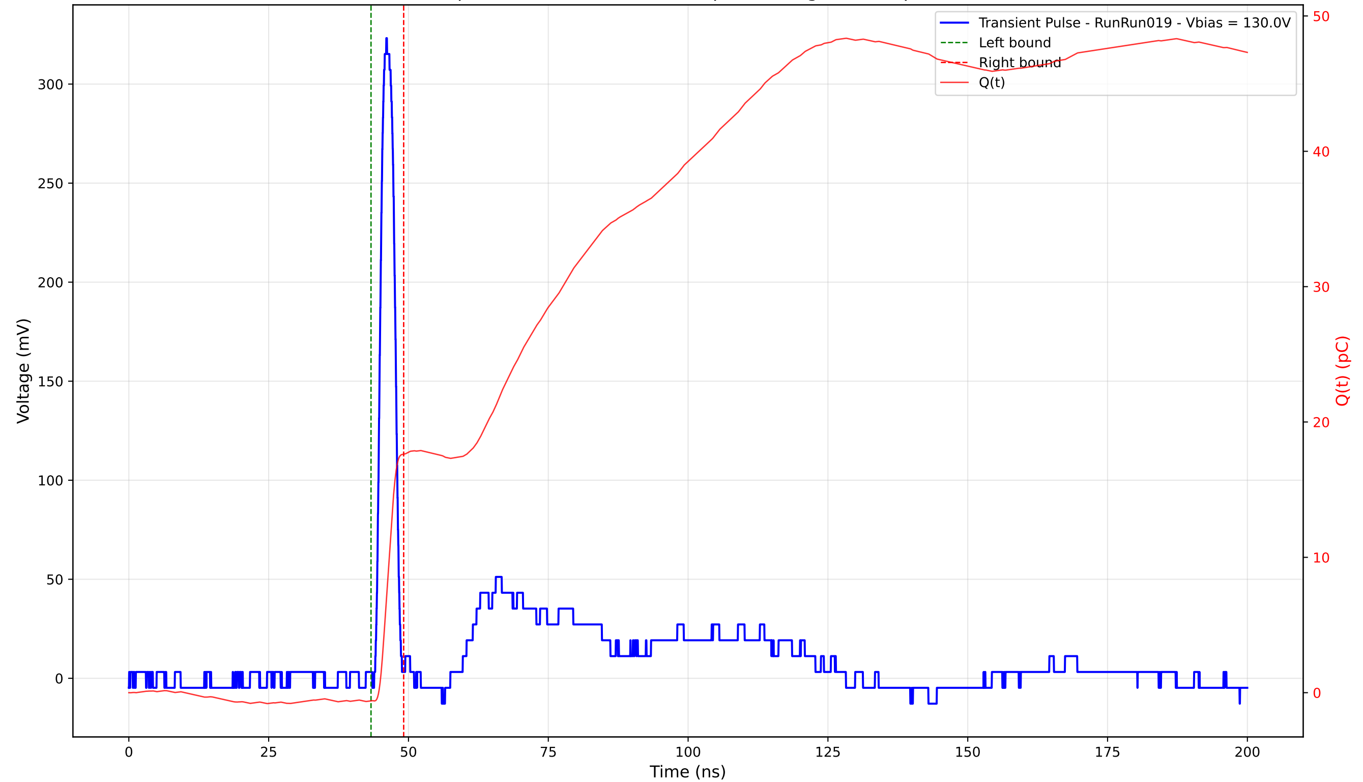
Transient Pulse - Sample: 4003 - Position: 230.0 \mu\text{m} - Charge: 18.22 pC - Rise Time: 1.21 ns
