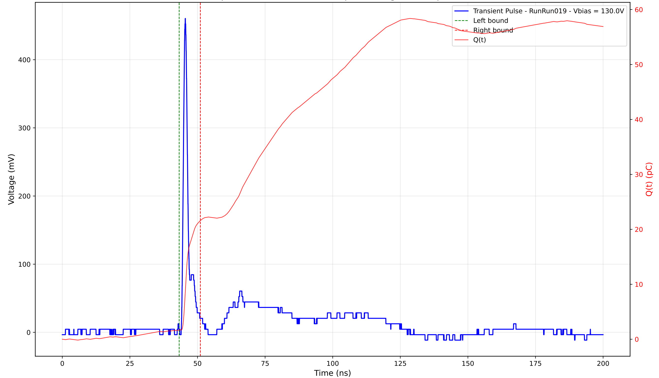
Transient Pulse - Sample: 4003 - Position: 140.0 \mu\text{m} - Charge: 19.91 pC - Rise Time: 0.94 ns
