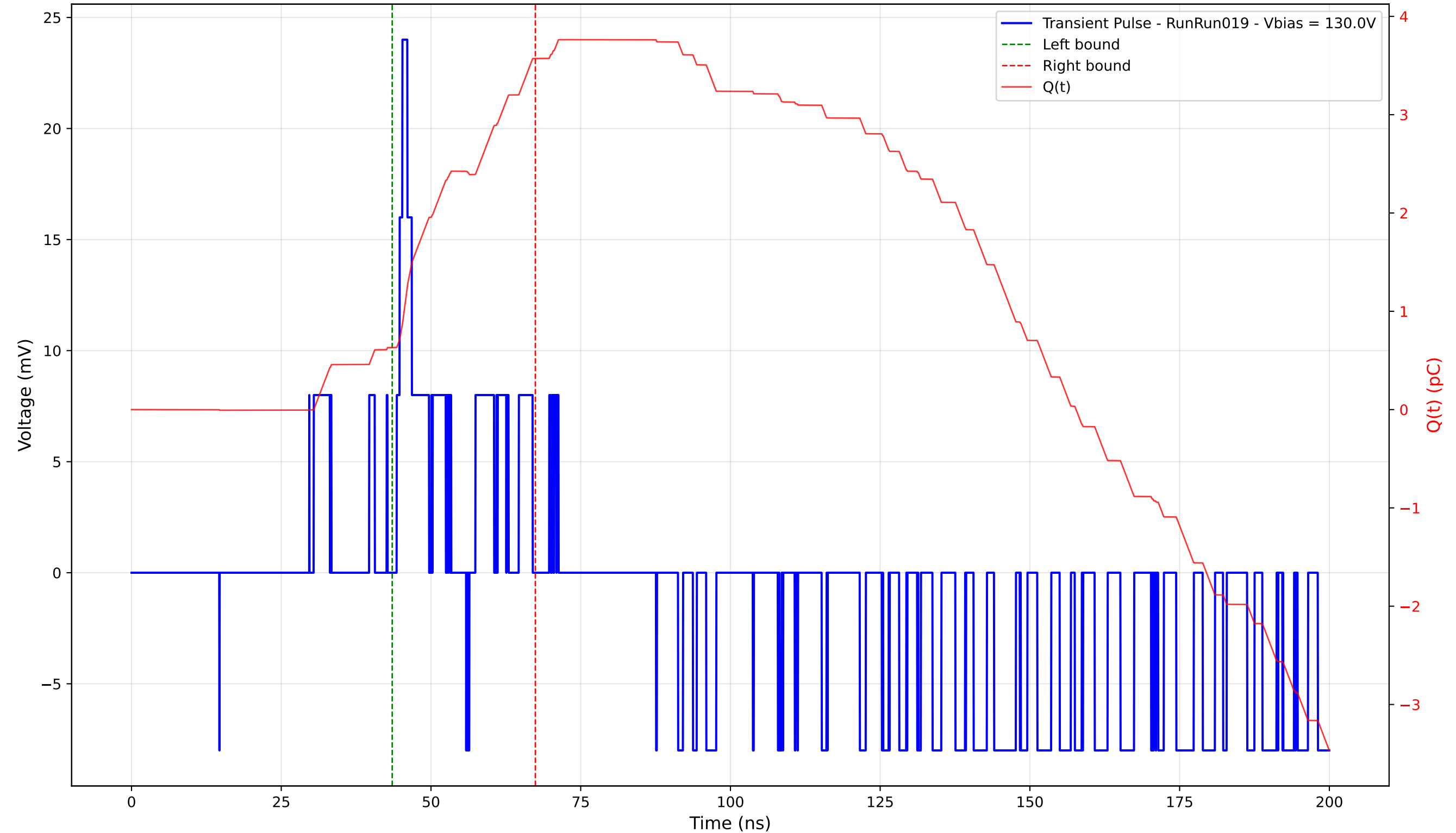
Transient Pulse - Sample: 4003 - Position: 20.0 \mu\text{m} - Charge: 2.94 pC - Rise Time: 0.95 ns
