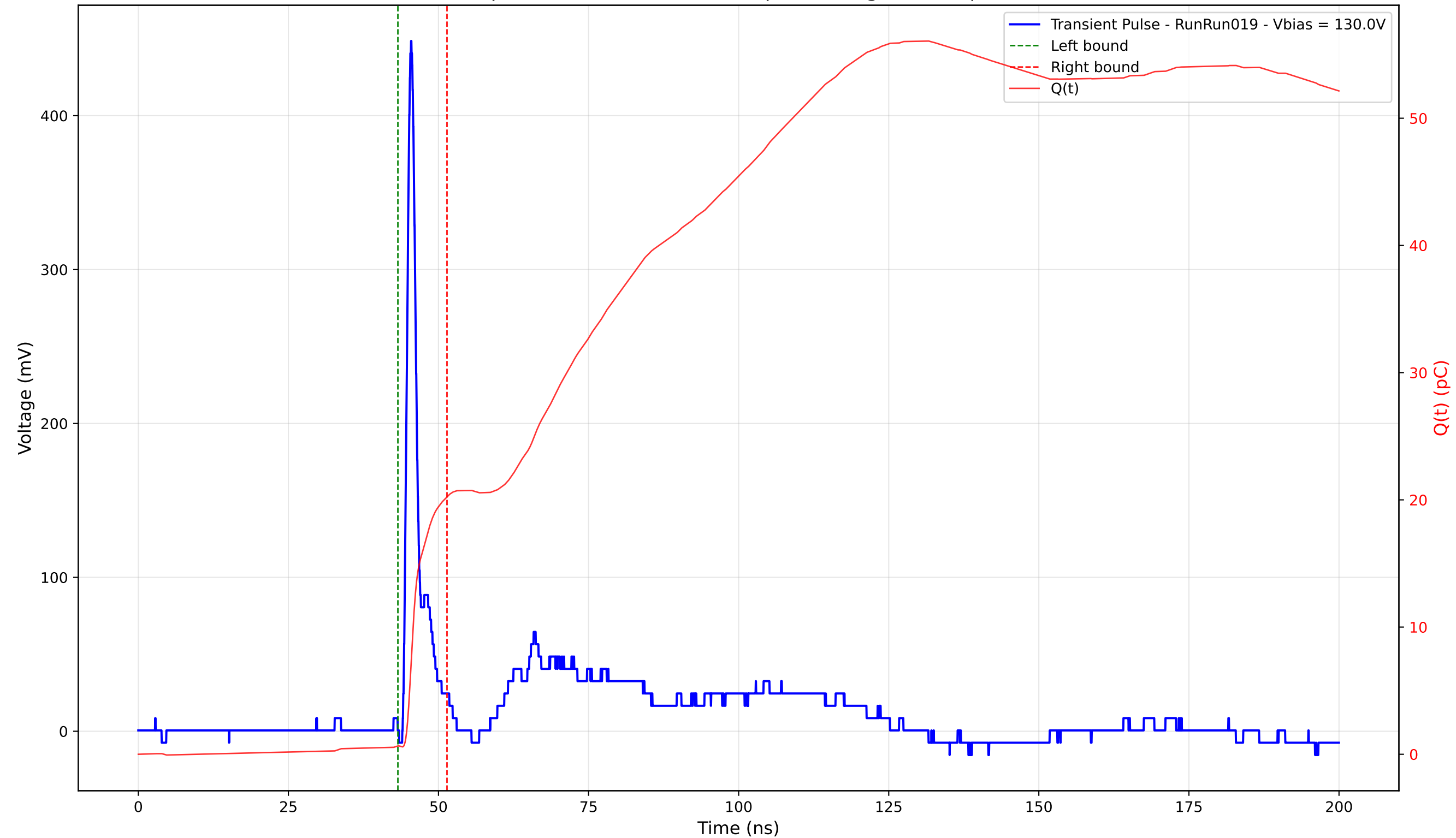
Transient Pulse - Sample: 4003 - Position: 130.0 \mu\text{m} - Charge: 19.58 pC - Rise Time: 0.92 ns
