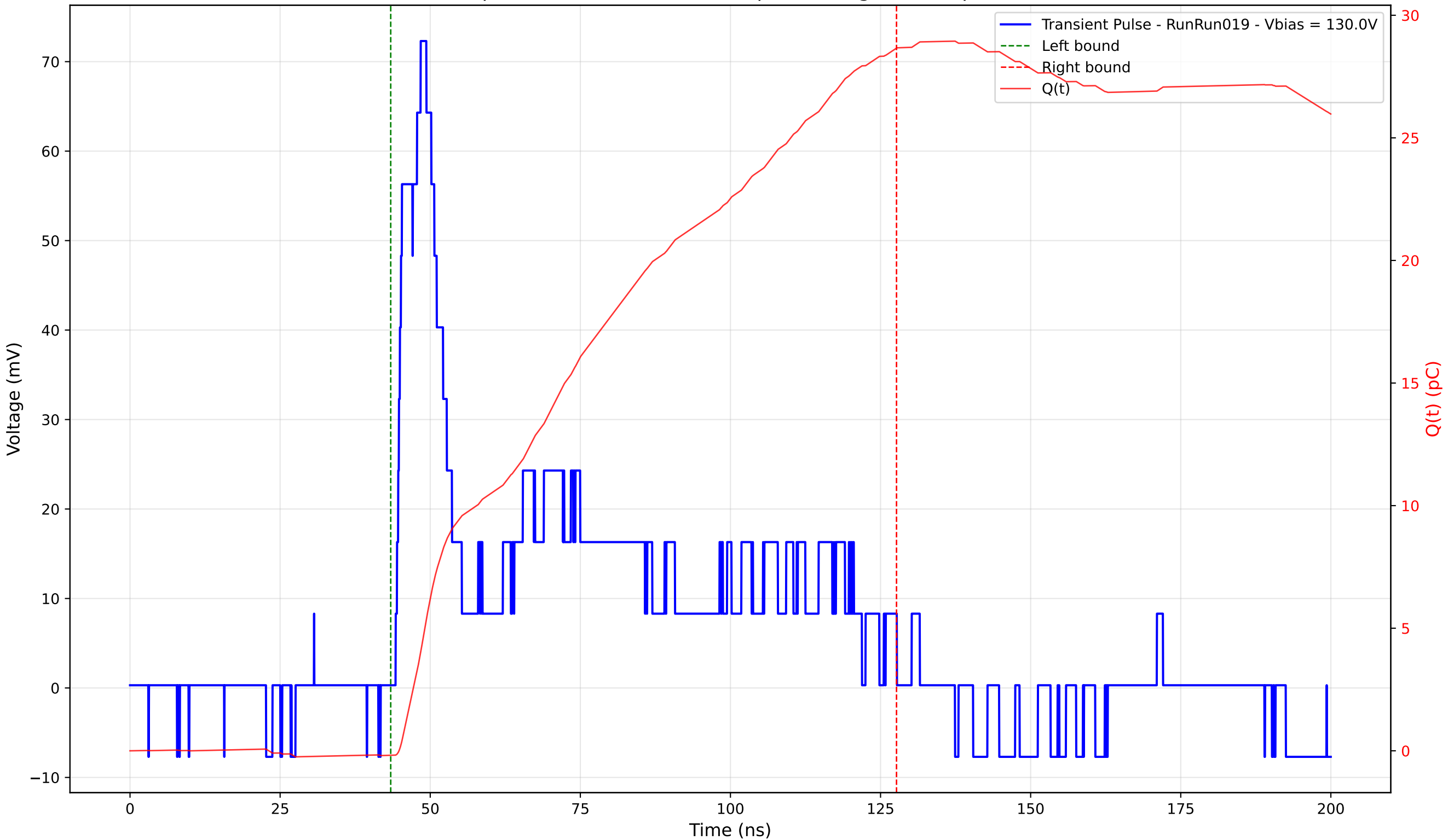
Transient Pulse - Sample: 4003 - Position: 285.0 \mu\text{m} - Charge: 28.85 pC - Rise Time: 4.16 ns
