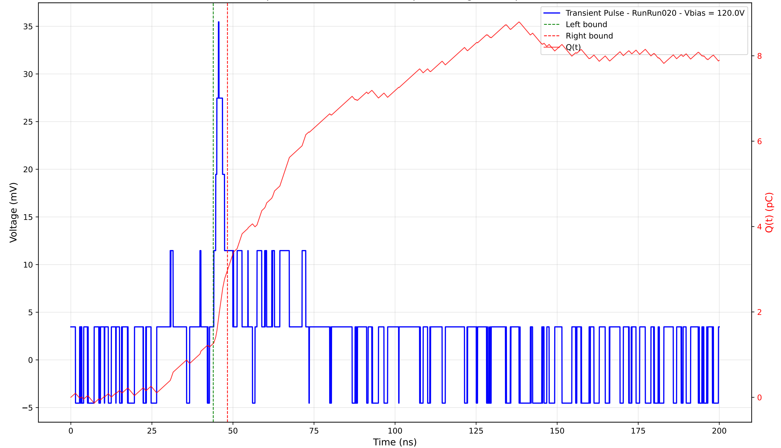
Transient Pulse - Sample: 4003 - Position: 355.0 \mu\text{m} - Charge: 1.72 pC - Rise Time: 1.44 ns
