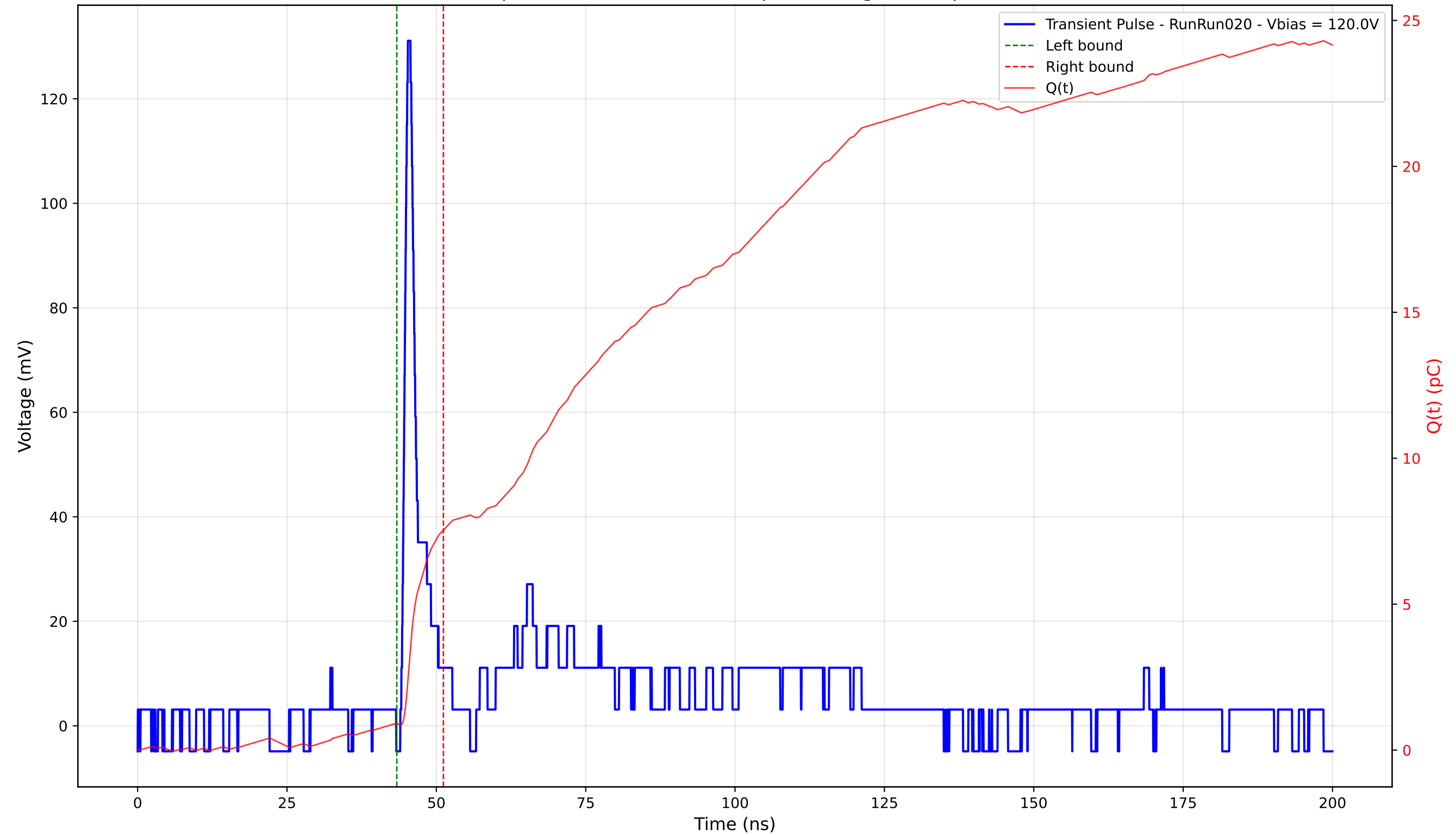
Transient Pulse - Sample: 4003 - Position: 95.0 \mu\text{m} - Charge: 6.63 pC - Rise Time: 0.88 ns
