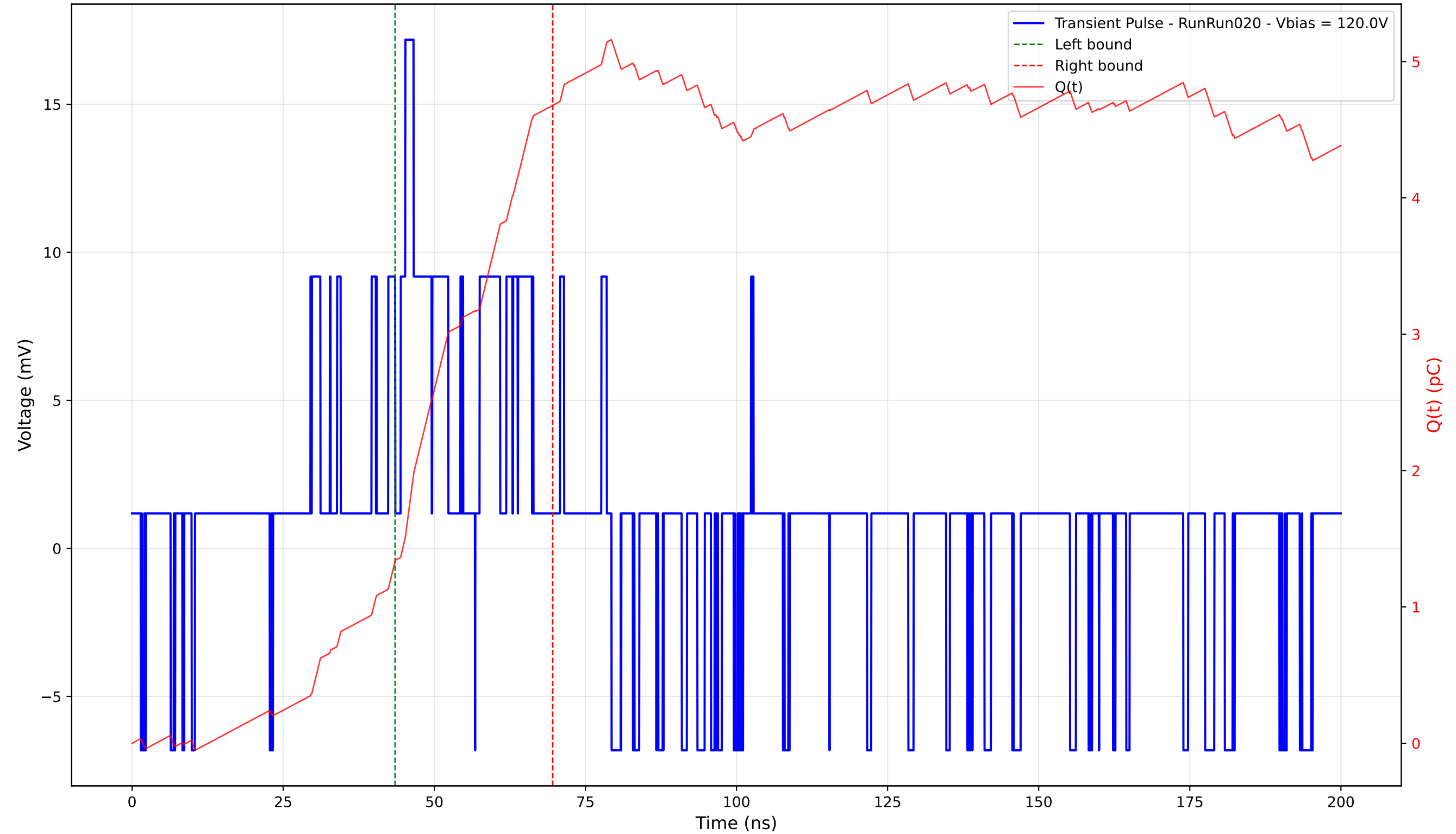
Transient Pulse - Sample: 4003 - Position: 5.0 \mu\text{m} - Charge: 3.34 pC - Rise Time: 0.78 ns
