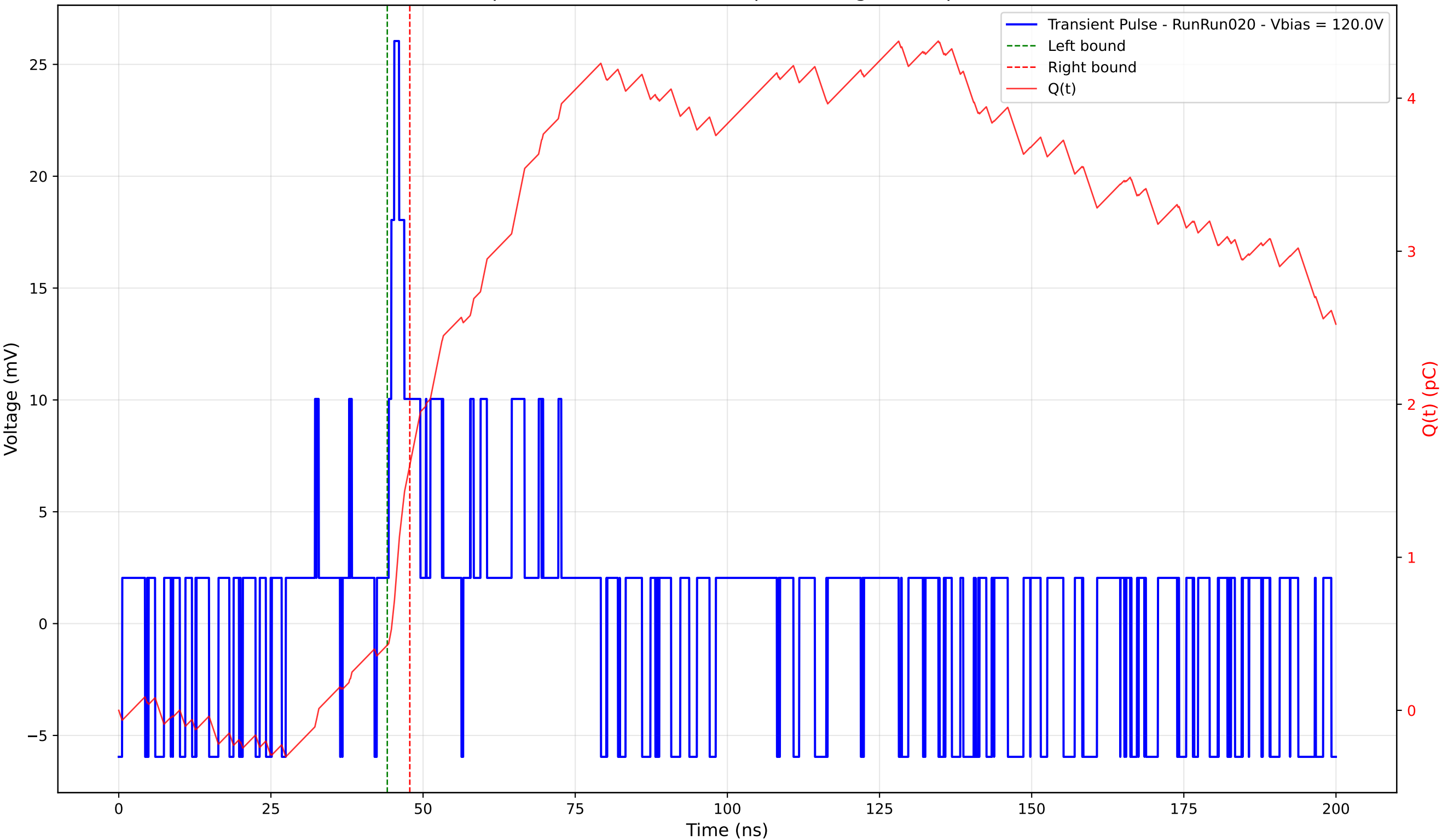
Transient Pulse - Sample: 4003 - Position: 25.0 \mu\text{m} - Charge: 1.18 pC - Rise Time: 0.92 ns
