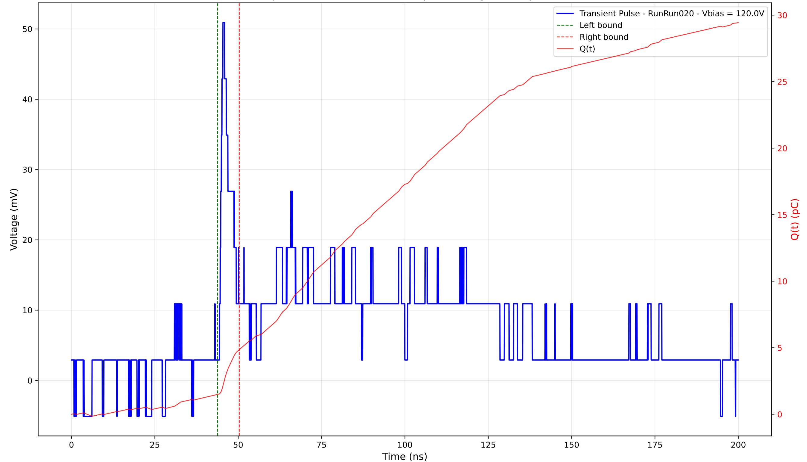
Transient Pulse - Sample: 4003 - Position: 295.0 \mu\text{m} - Charge: 3.36 pC - Rise Time: 1.05 ns
