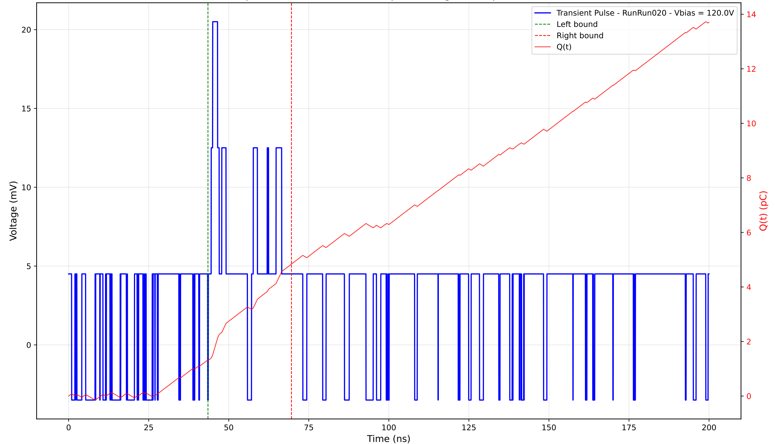
Transient Pulse - Sample: 4003 - Position: 420.0 \mu\text{m} - Charge: 3.53 pC - Rise Time: 0.00 ns (N/A)
