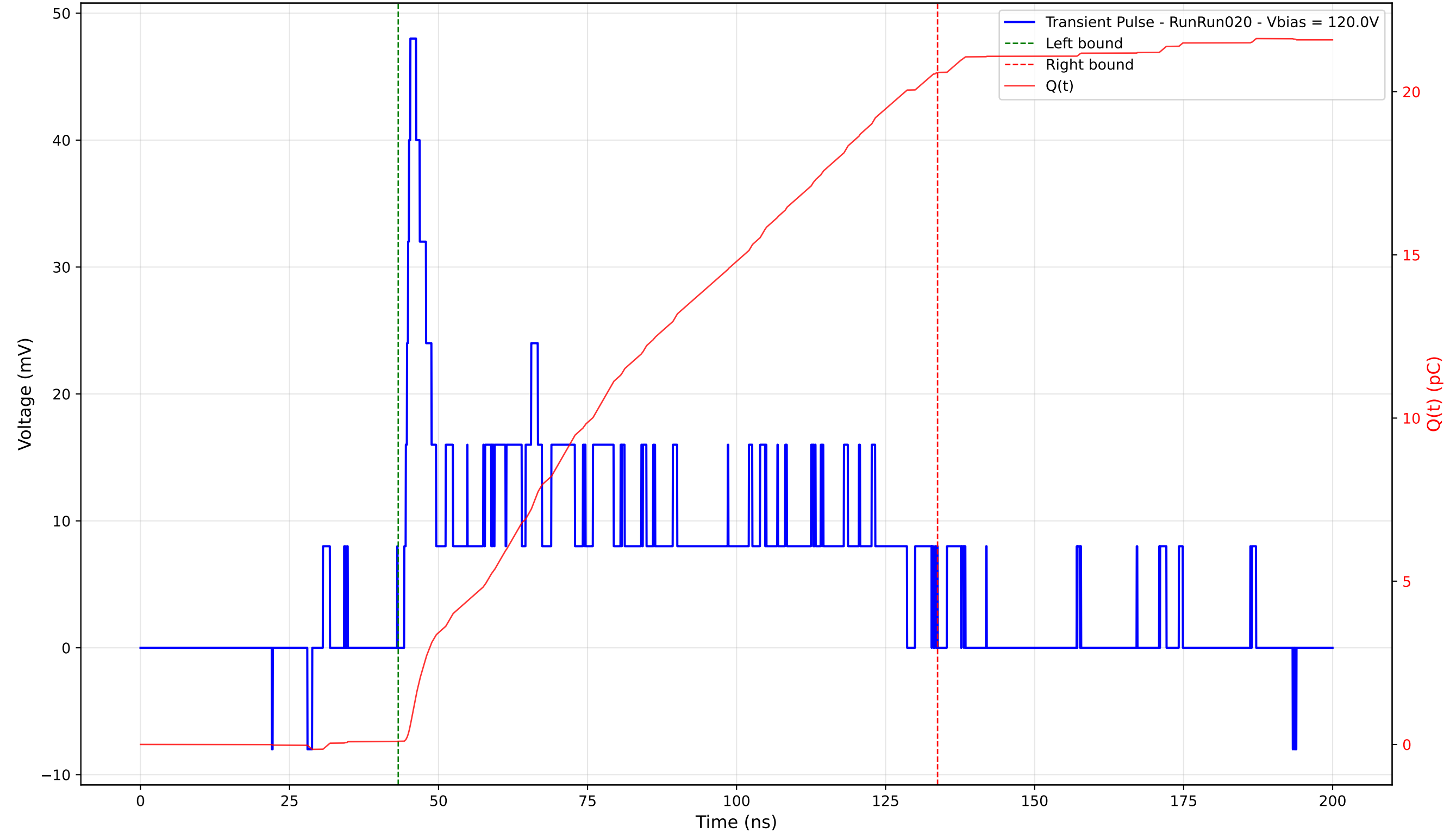
Transient Pulse - Sample: 4003 - Position: 290.0 \mu\text{m} - Charge: 20.49 pC - Rise Time: 1.03 ns
