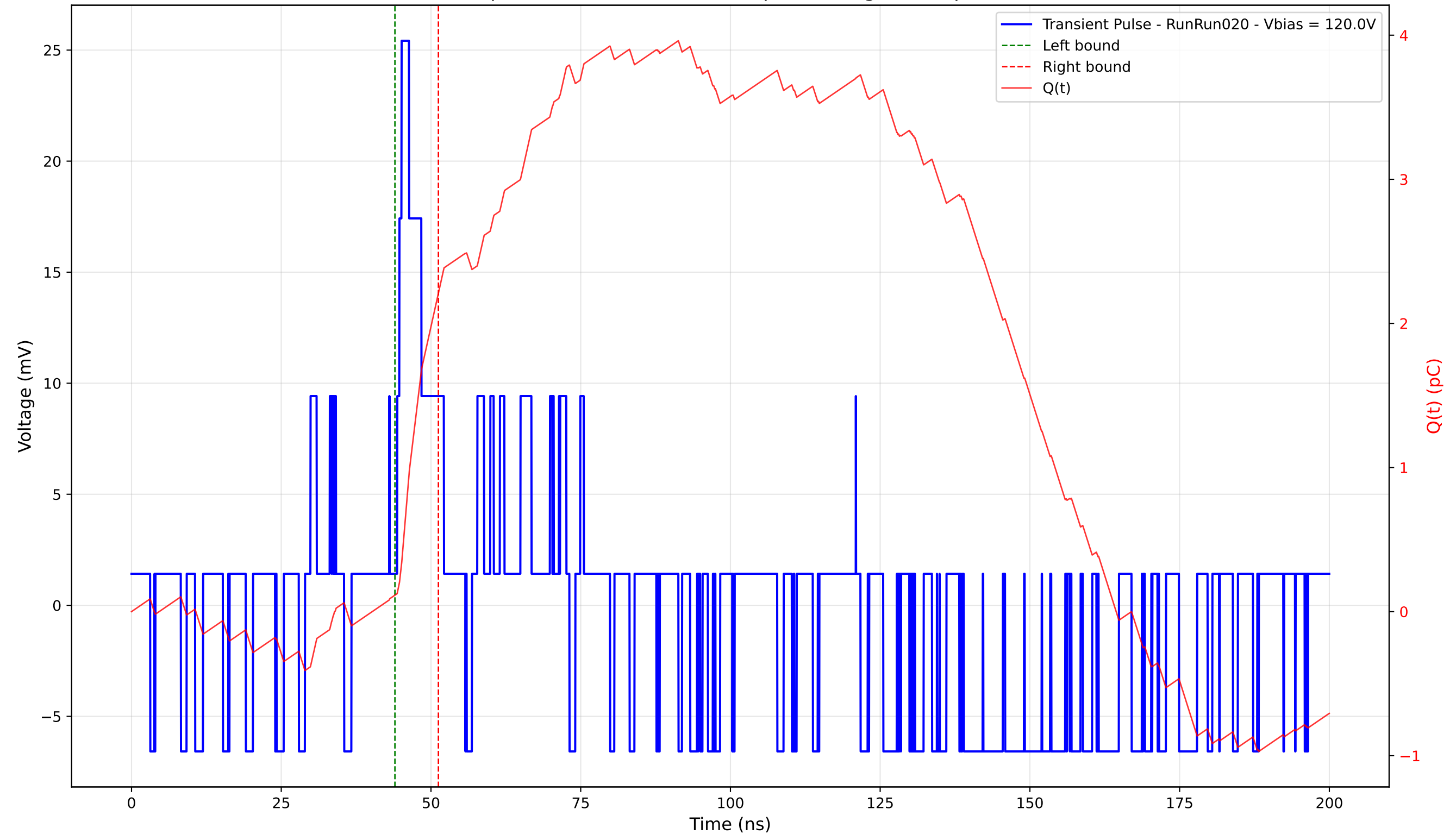
Transient Pulse - Sample: 4003 - Position: 330.0 \mu\text{m} - Charge: 2.10 pC - Rise Time: 0.74 ns
