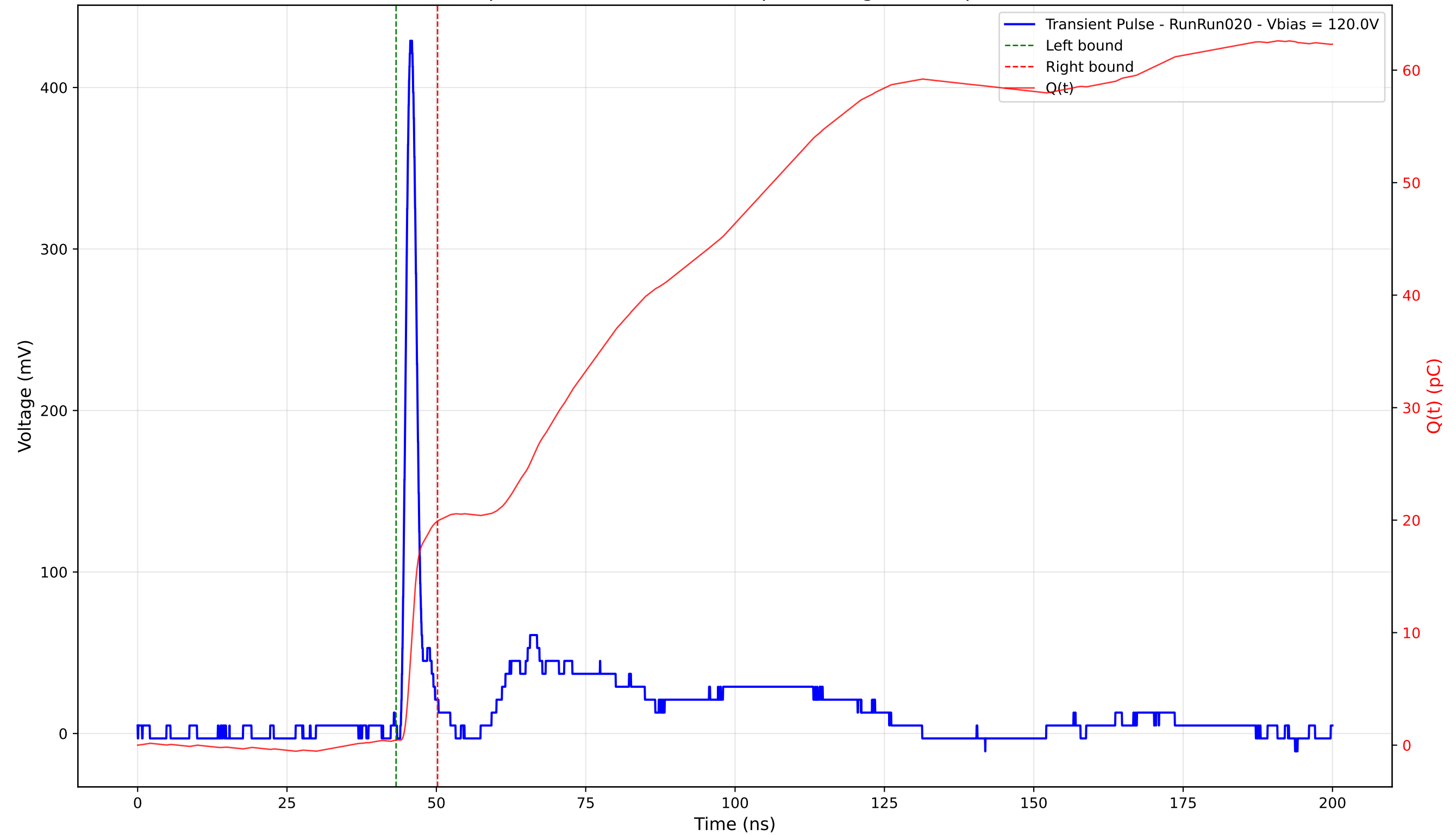
Transient Pulse - Sample: 4003 - Position: 185.0 \mu\text{m} - Charge: 19.46 pC - Rise Time: 1.09 ns
