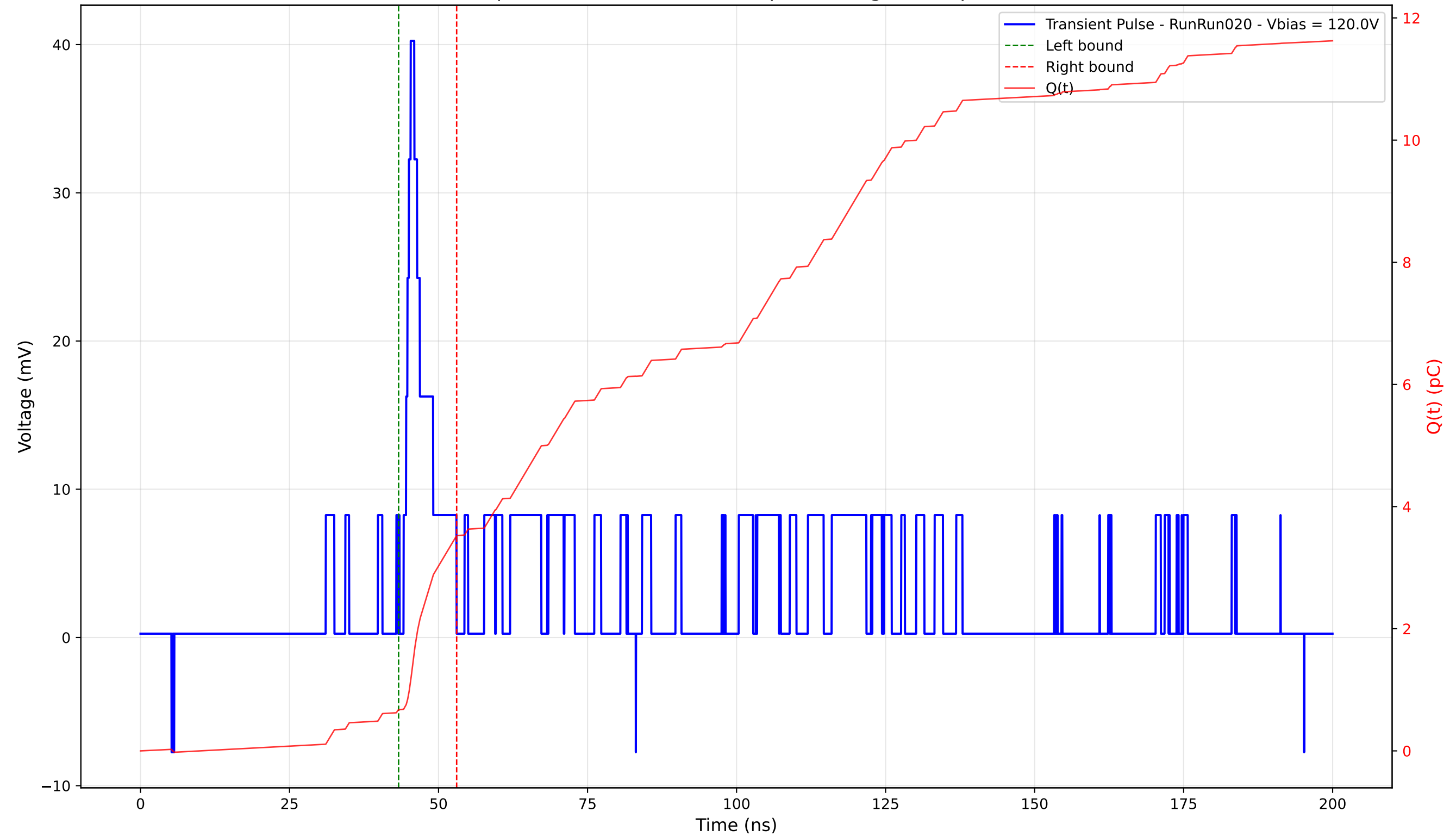
Transient Pulse - Sample: 4003 - Position: 305.0 \mu\text{m} - Charge: 2.86 pC - Rise Time: 1.19 ns
