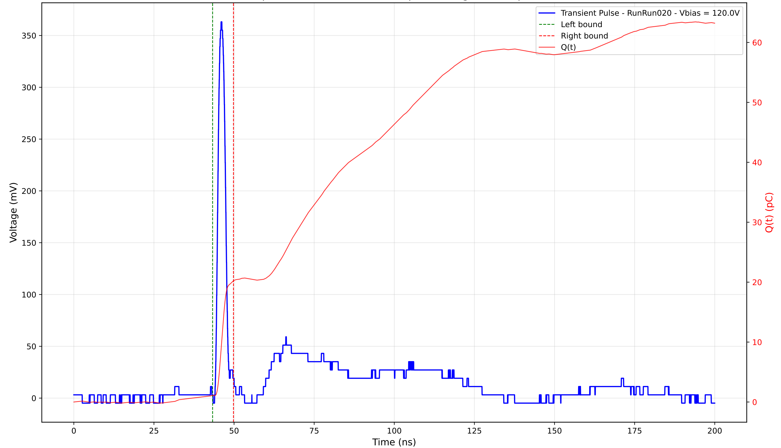
Transient Pulse - Sample: 4003 - Position: 215.0 \mu\text{m} - Charge: 19.11 pC - Rise Time: 1.20 ns
