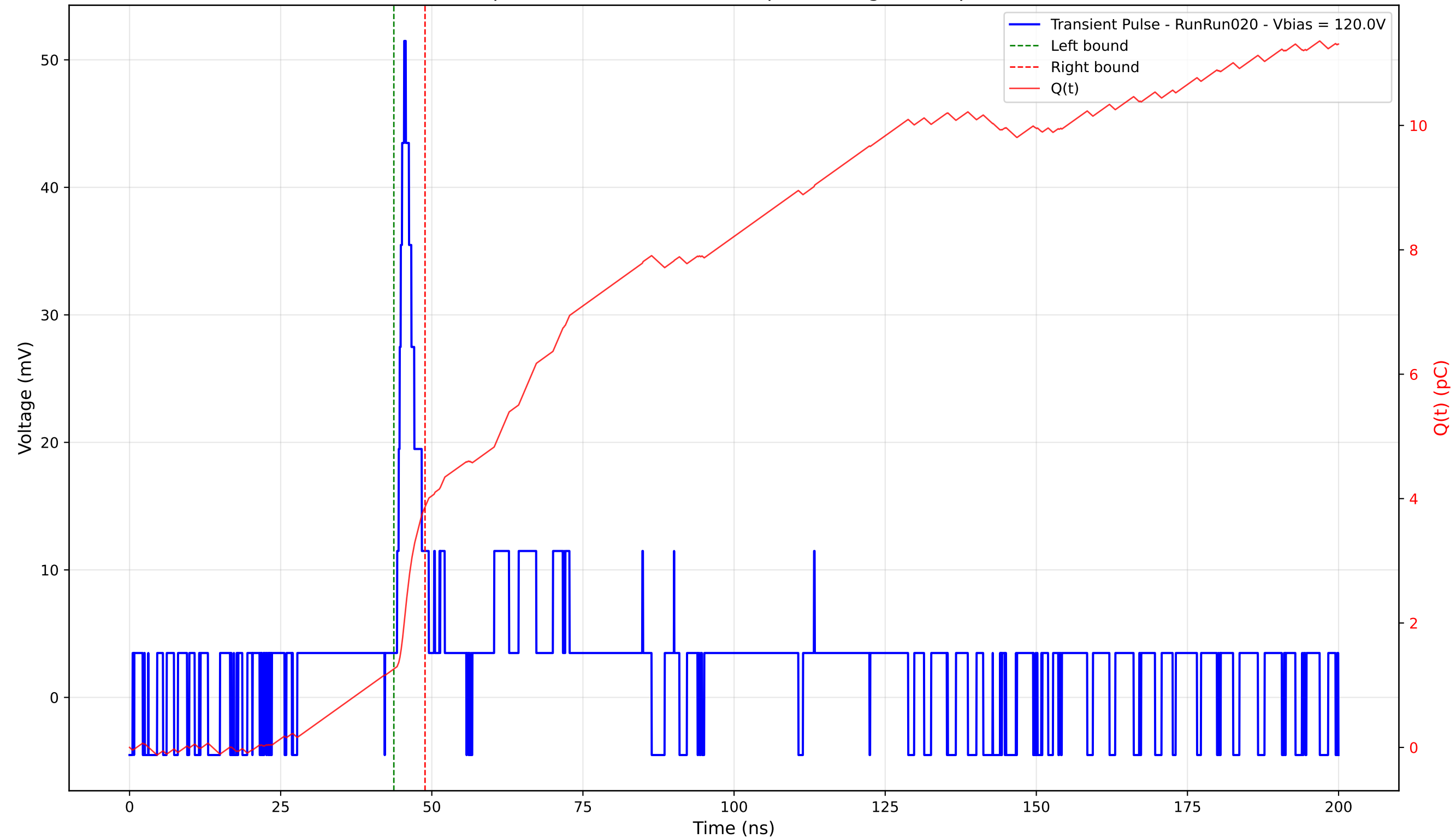
Transient Pulse - Sample: 4003 - Position: 390.0 \mu\text{m} - Charge: 2.61 pC - Rise Time: 1.18 ns
