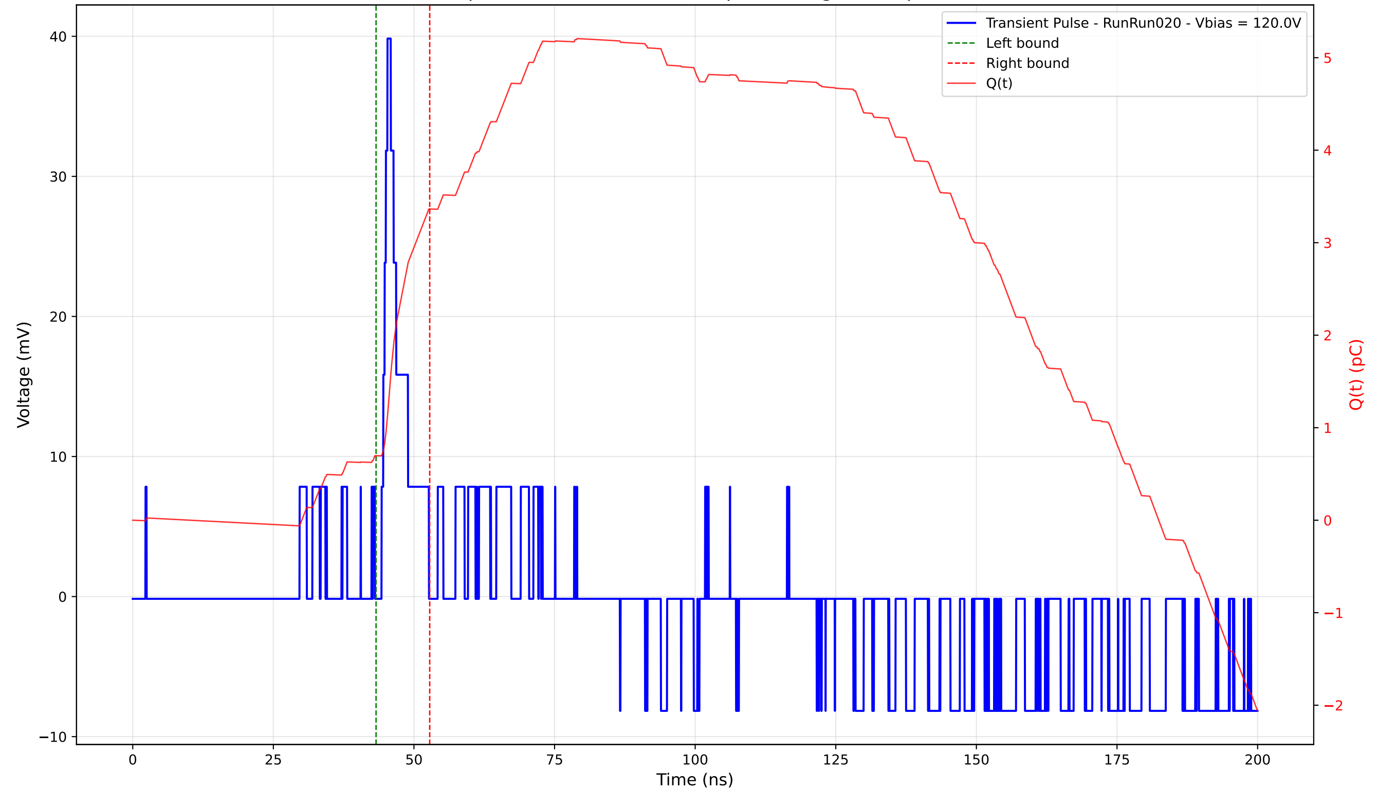
Transient Pulse - Sample: 4003 - Position: 405.0 \mu\text{m} - Charge: 2.67 pC - Rise Time: 1.05 ns
