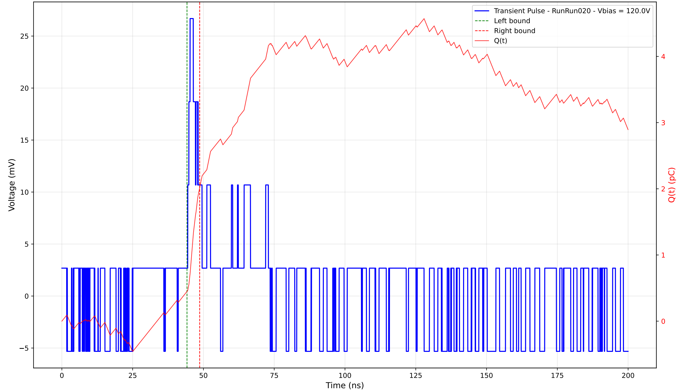
Transient Pulse - Sample: 4003 - Position: 40.0 \mu\text{m} - Charge: 1.57 pC - Rise Time: 0.00 ns (N/A)
