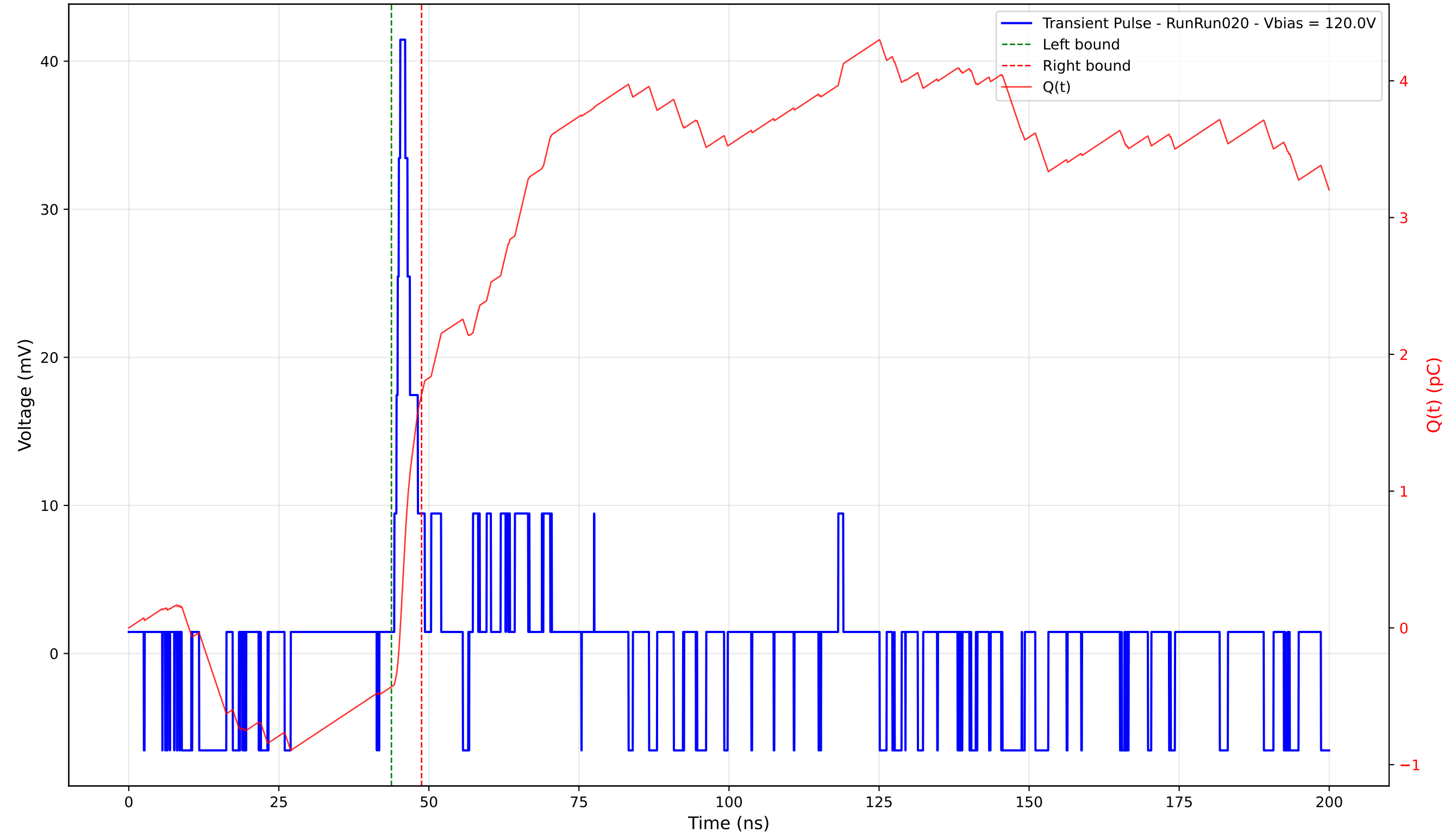
Transient Pulse - Sample: 4003 - Position: 400.0 \mu\text{m} - Charge: 2.14 pC - Rise Time: 0.99 ns
