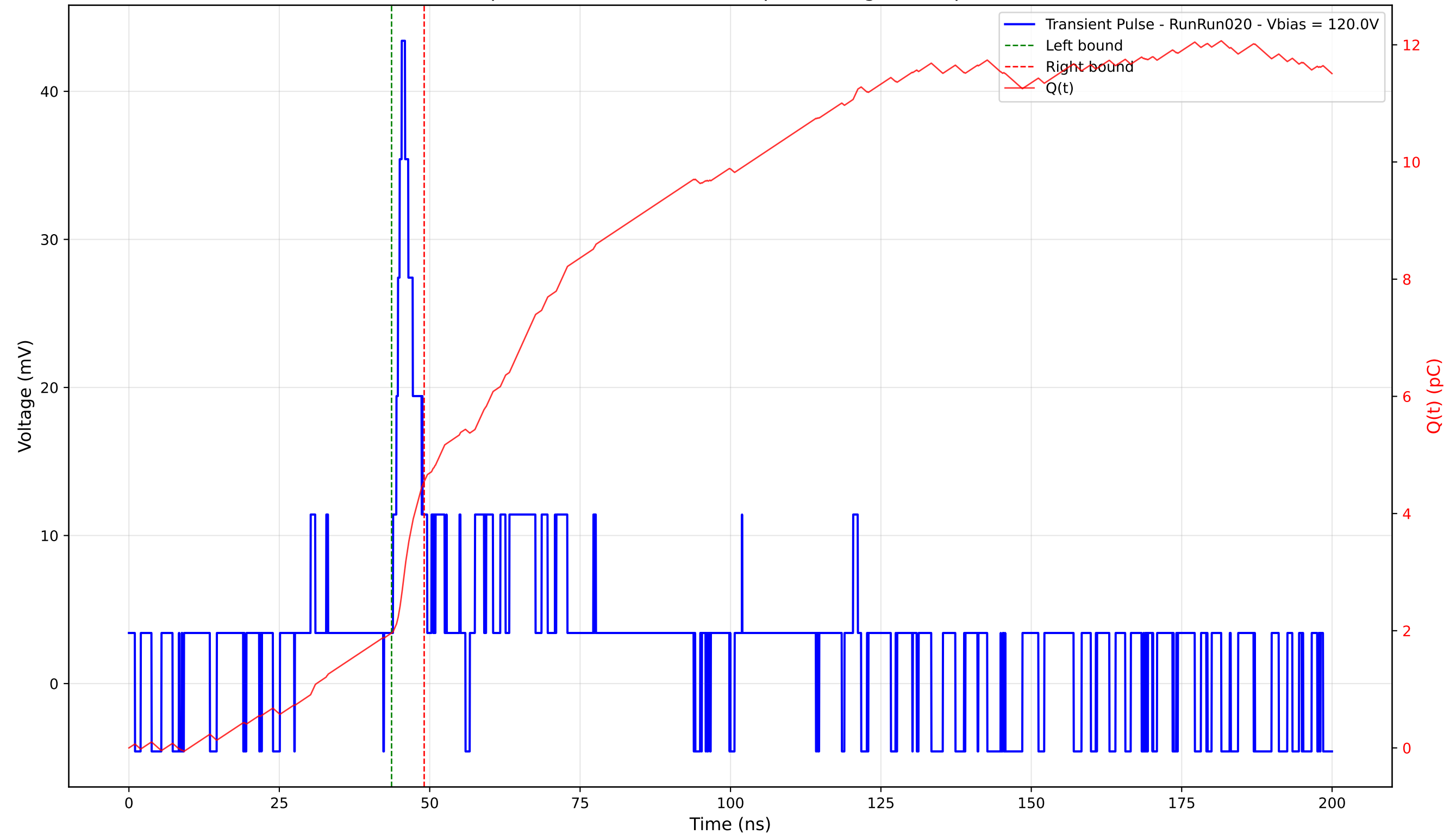
Transient Pulse - Sample: 4003 - Position: 385.0 \mu\text{m} - Charge: 2.59 pC - Rise Time: 1.46 ns
