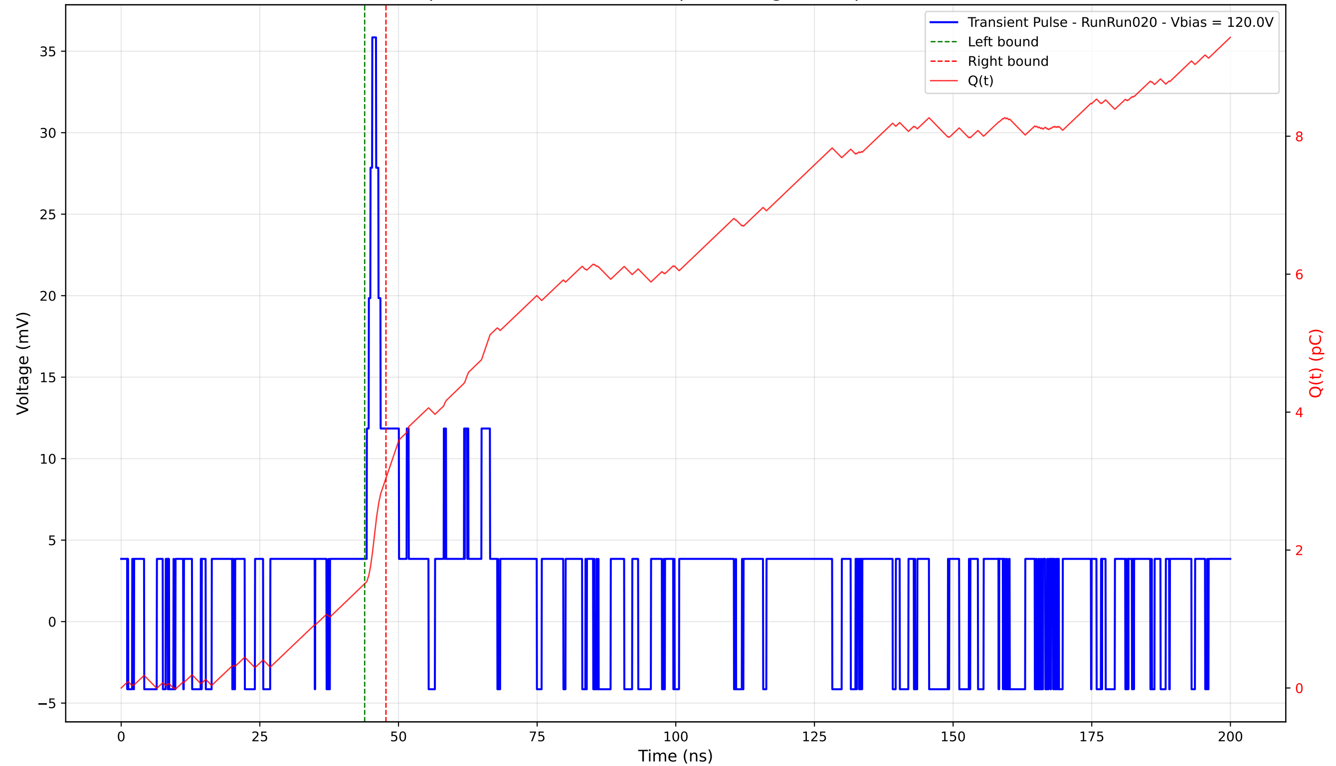
Transient Pulse - Sample: 4003 - Position: 325.0 \mu\text{m} - Charge: 1.53 pC - Rise Time: 0.00 ns (N/A)
