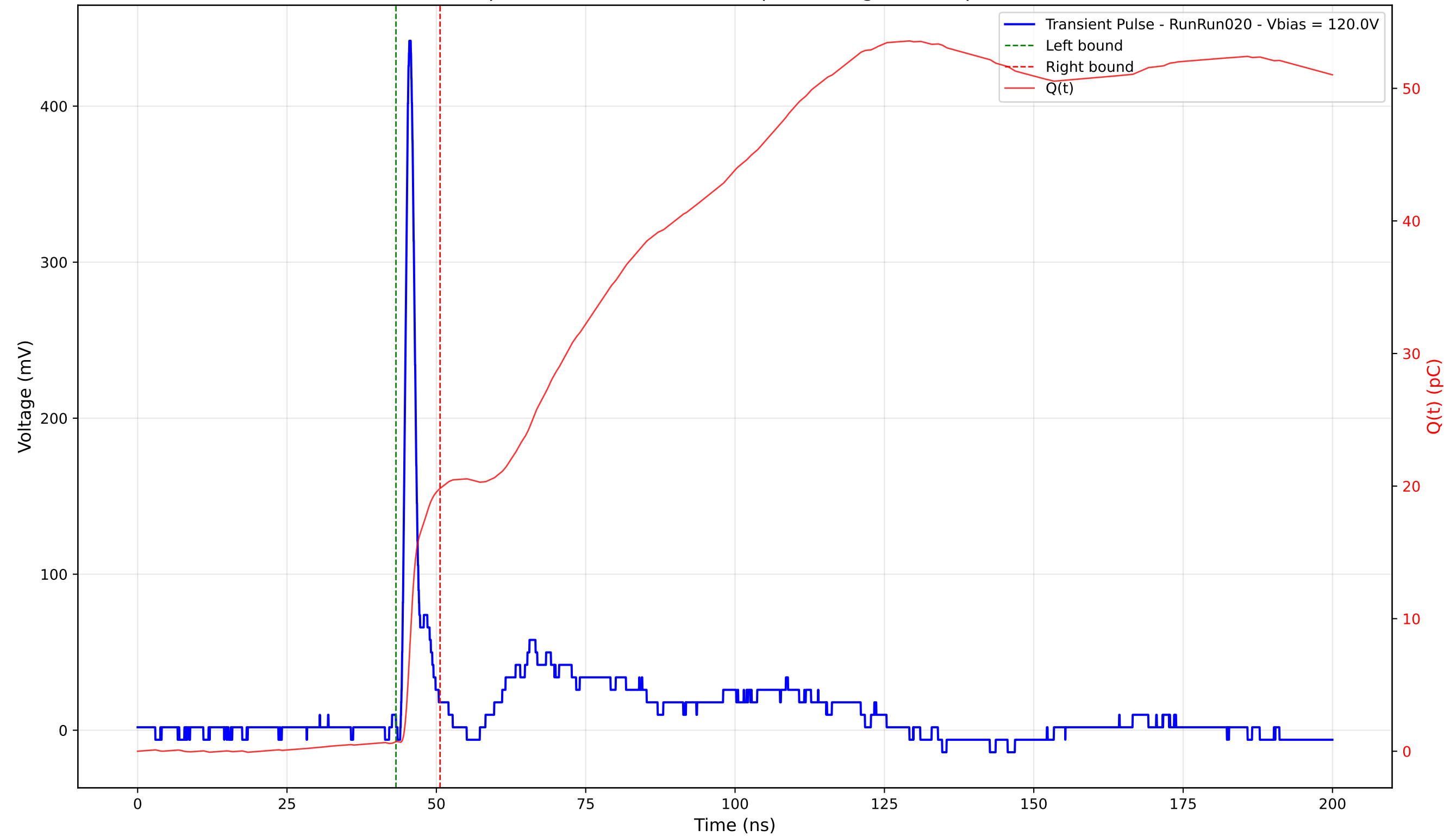
Transient Pulse - Sample: 4003 - Position: 155.0 \mu\text{m} - Charge: 19.10 pC - Rise Time: 0.97 ns
