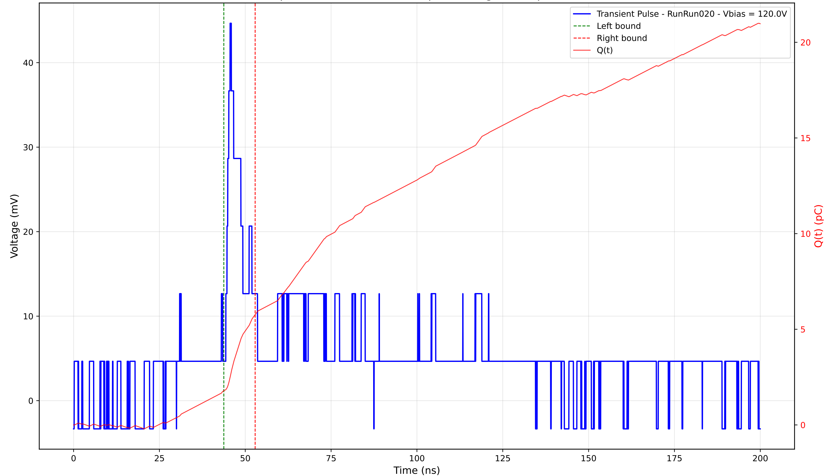
Transient Pulse - Sample: 4003 - Position: 55.0 \mu\text{m} - Charge: 3.98 pC - Rise Time: 15.58 ns
