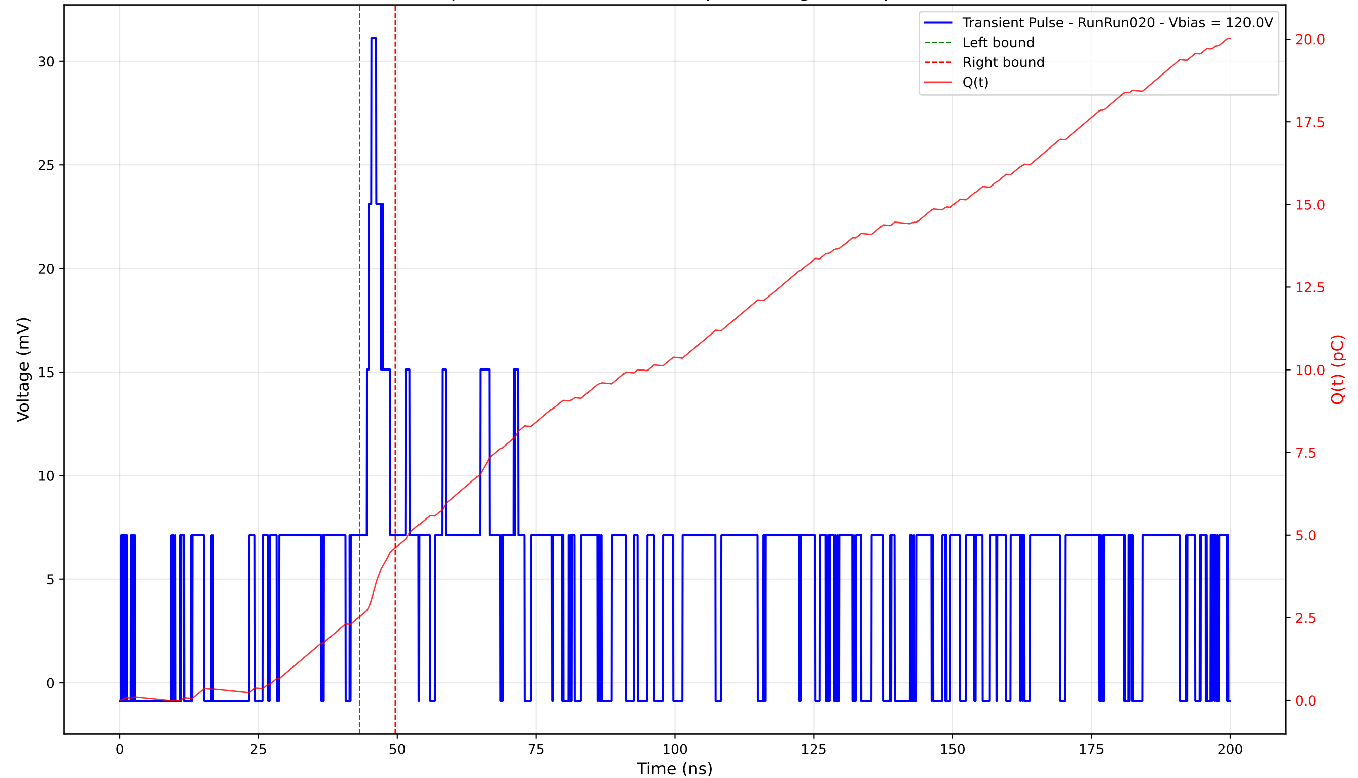
Transient Pulse - Sample: 4003 - Position: 345.0 \mu\text{m} - Charge: 2.08 pC - Rise Time: 3.73 ns
