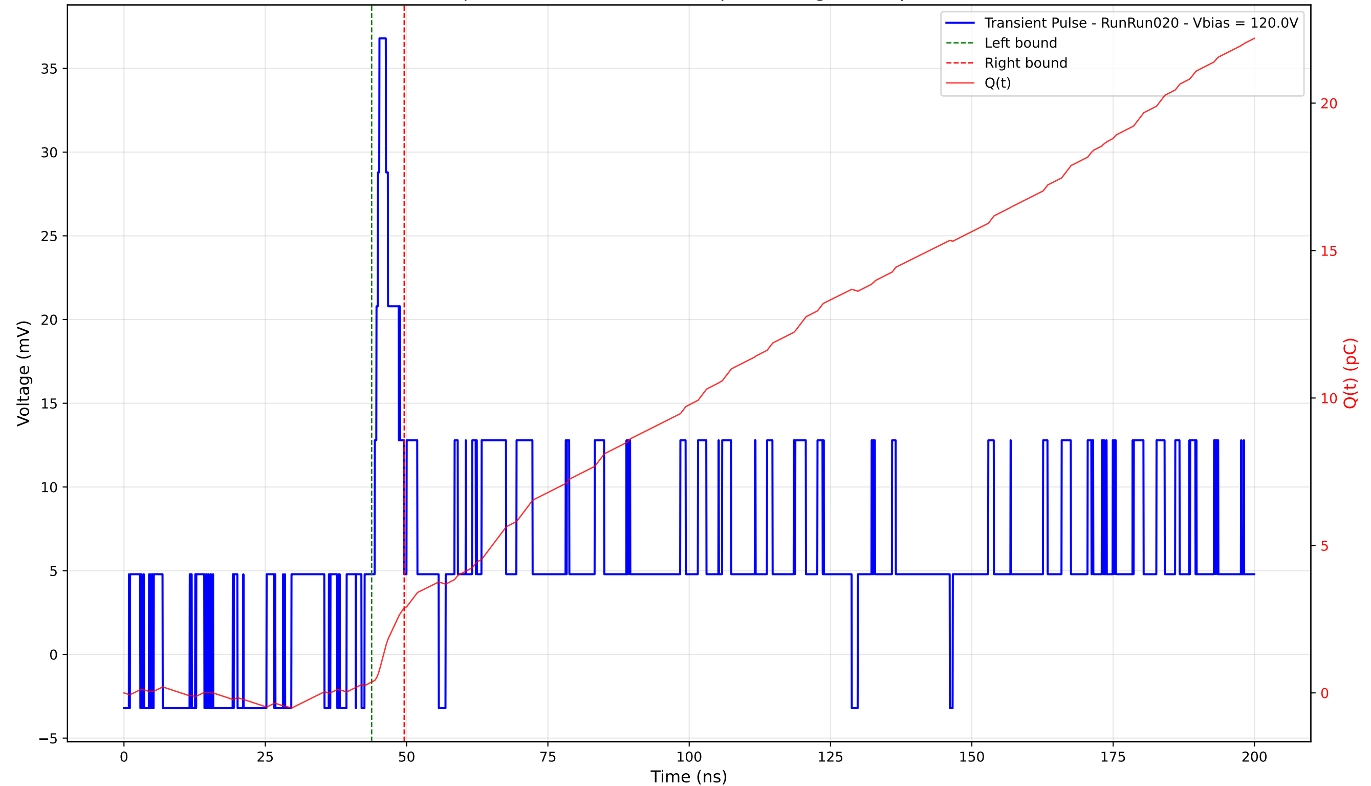
Transient Pulse - Sample: 4003 - Position: 315.0 \mu\text{m} - Charge: 2.51 pC - Rise Time: 2.63 ns
