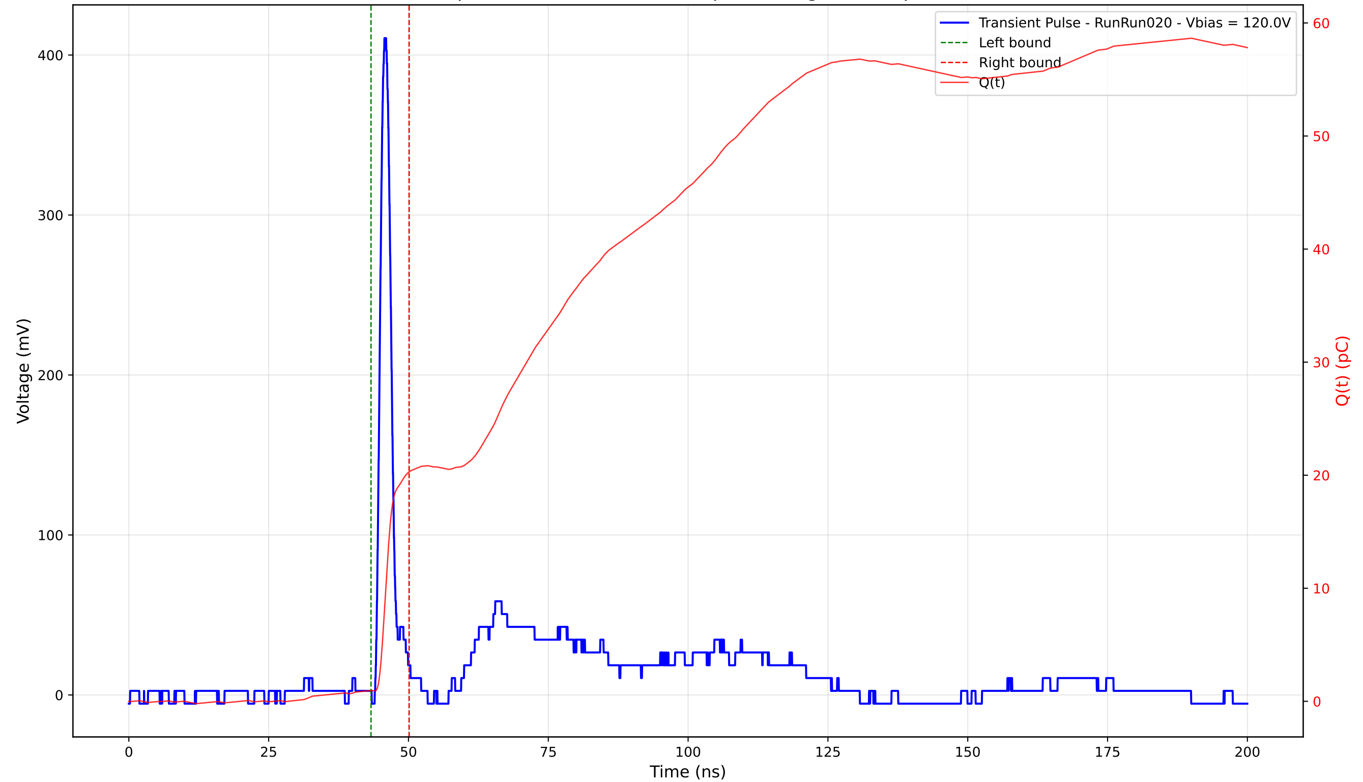
Transient Pulse - Sample: 4003 - Position: 195.0 \mu\text{m} - Charge: 19.34 pC - Rise Time: 1.08 ns
