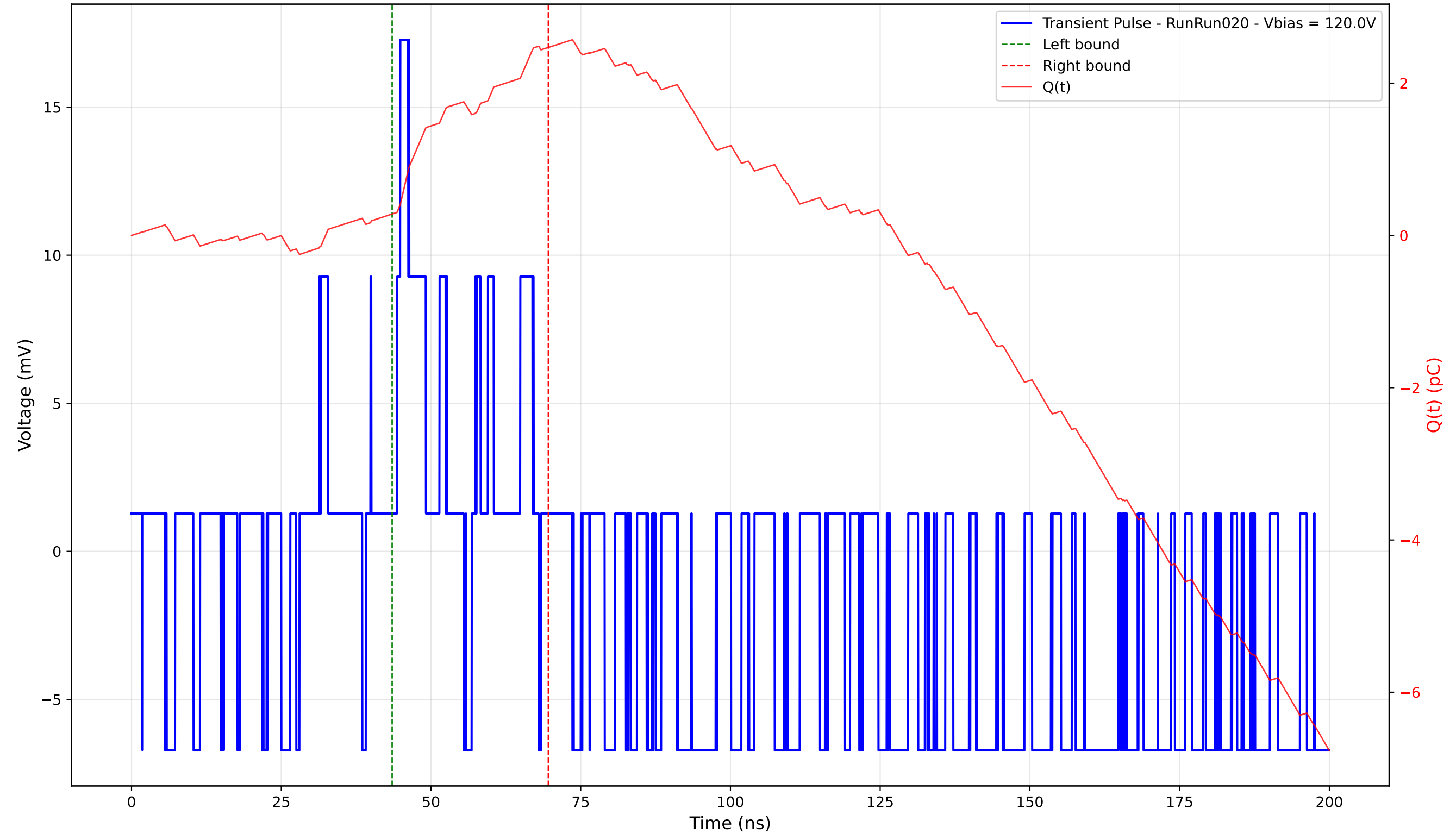
Transient Pulse - Sample: 4003 - Position: 15.0 \mu\text{m} - Charge: 2.19 pC - Rise Time: 0.54 ns
