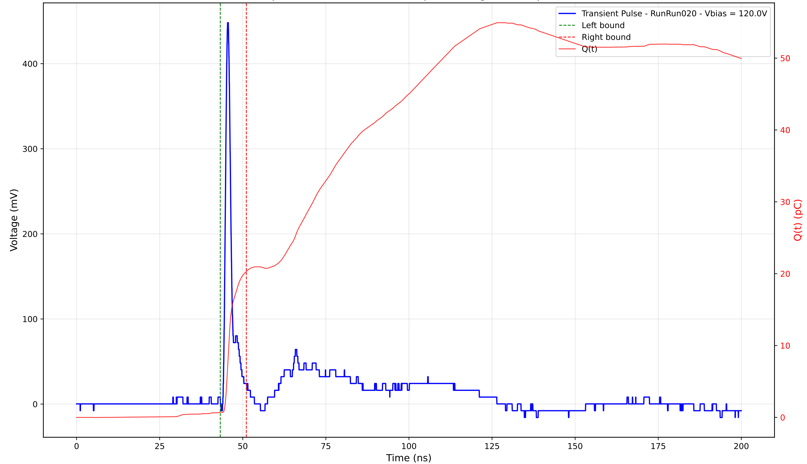
Transient Pulse - Sample: 4003 - Position: 145.0 \mu\text{m} - Charge: 19.57 pC - Rise Time: 0.96 ns
