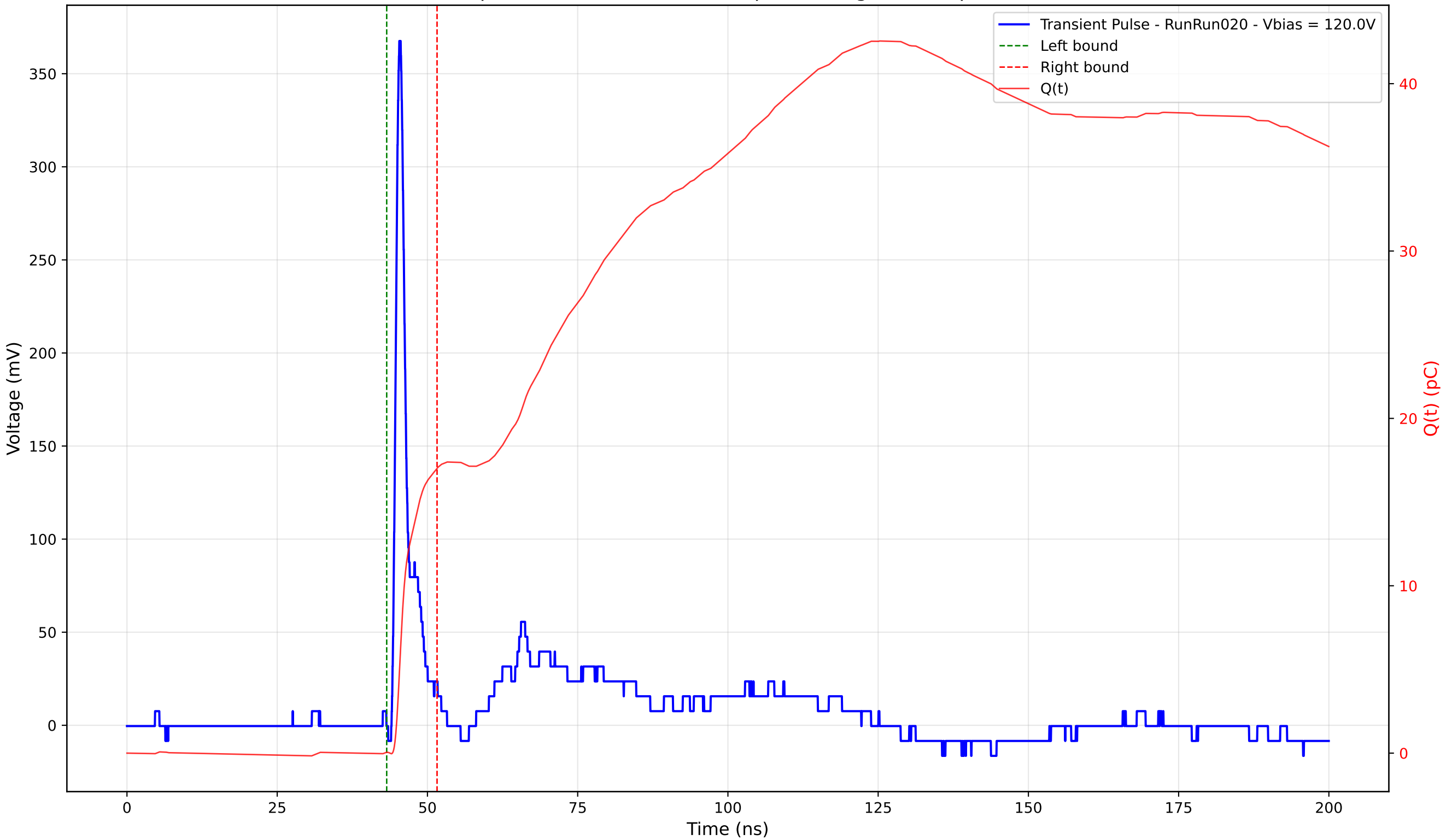
Transient Pulse - Sample: 4003 - Position: 115.0 \mu\text{m} - Charge: 16.97 pC - Rise Time: 0.89 ns
