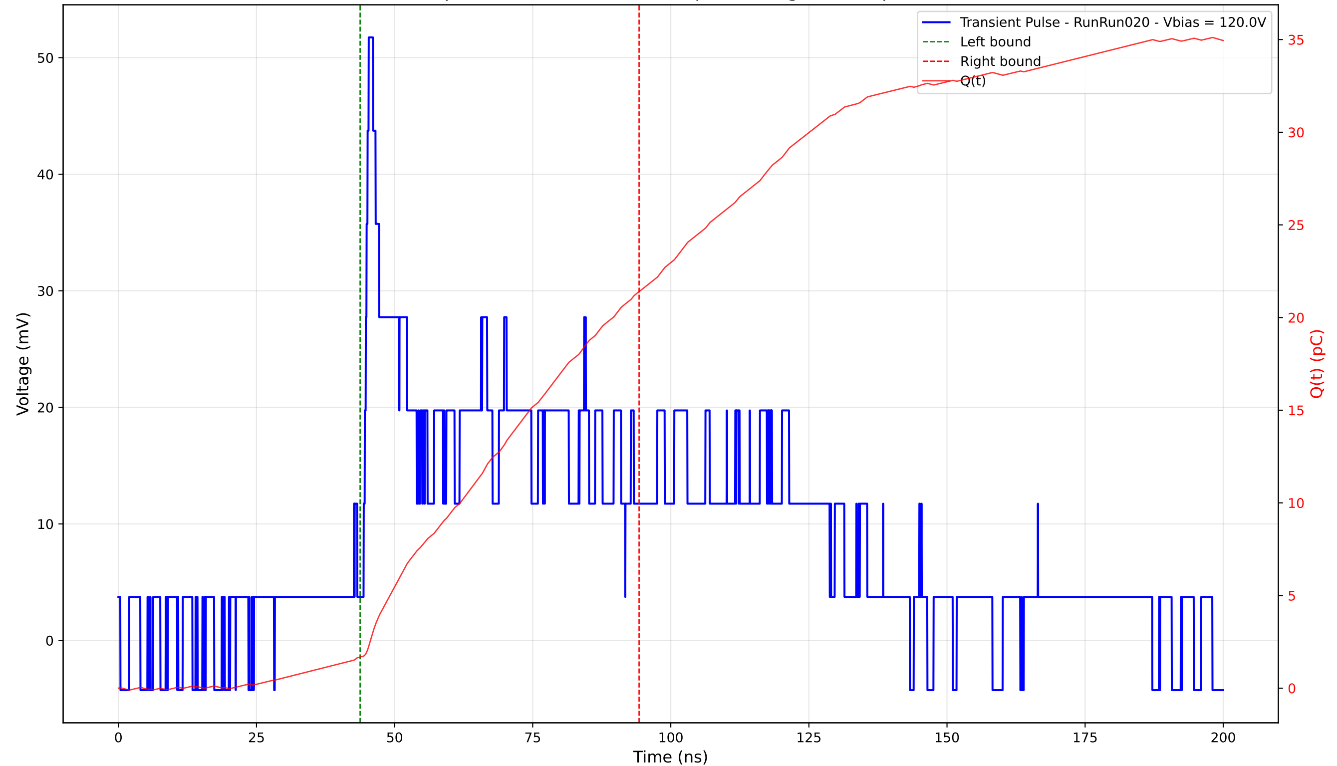
Transient Pulse - Sample: 4003 - Position: 285.0 \mu\text{m} - Charge: 19.72 pC - Rise Time: 0.92 ns
