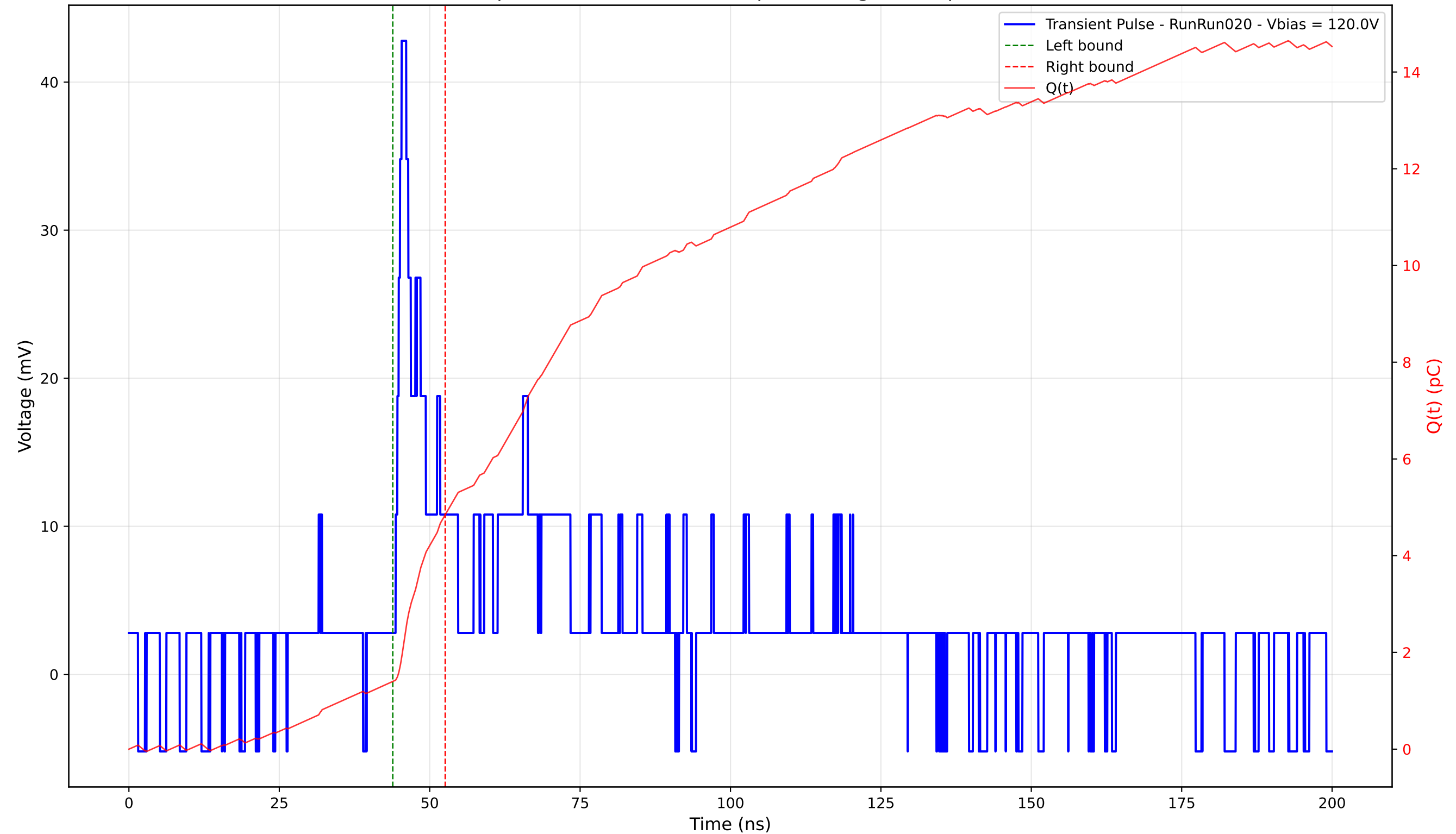
Transient Pulse - Sample: 4003 - Position: 50.0 \mu\text{m} - Charge: 3.45 pC - Rise Time: 1.00 ns
