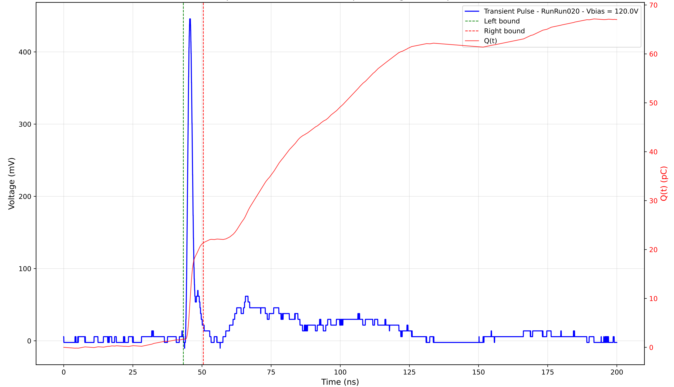
Transient Pulse - Sample: 4003 - Position: 170.0 \mu\text{m} - Charge: 19.66 pC - Rise Time: 1.02 ns
