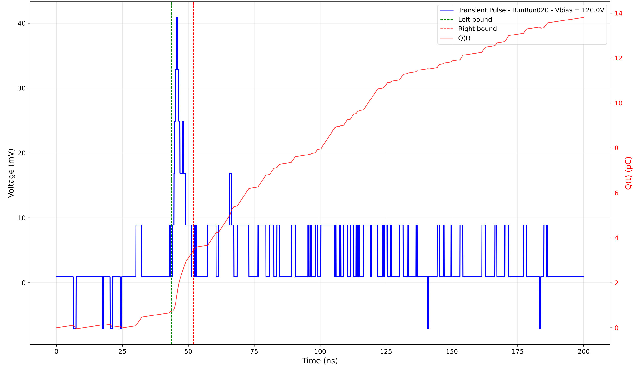
Transient Pulse - Sample: 4003 - Position: 310.0 \mu\text{m} - Charge: 2.70 pC - Rise Time: 1.39 ns
