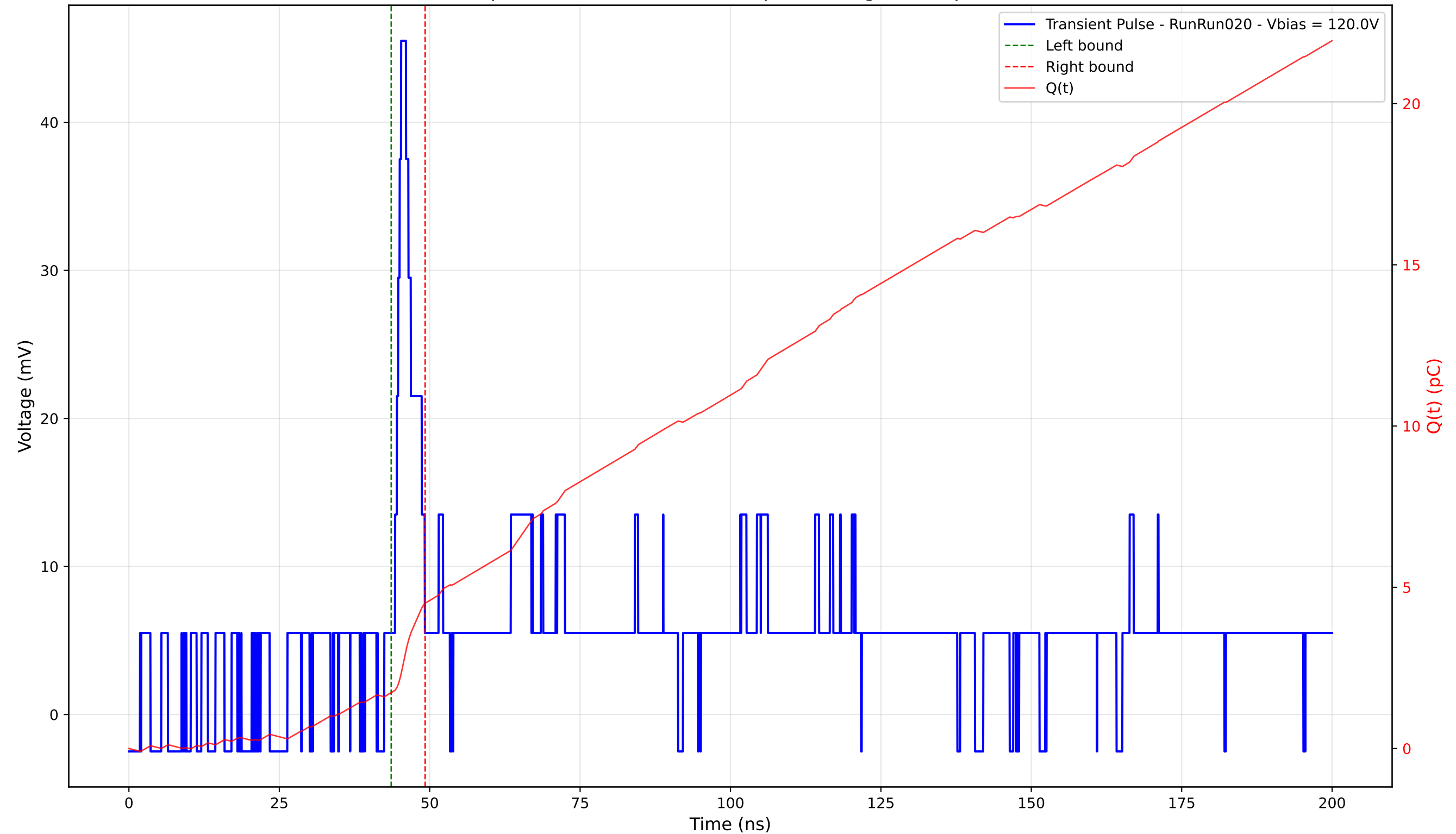
Transient Pulse - Sample: 4003 - Position: 395.0 \mu\text{m} - Charge: 2.78 pC - Rise Time: 2.81 ns
