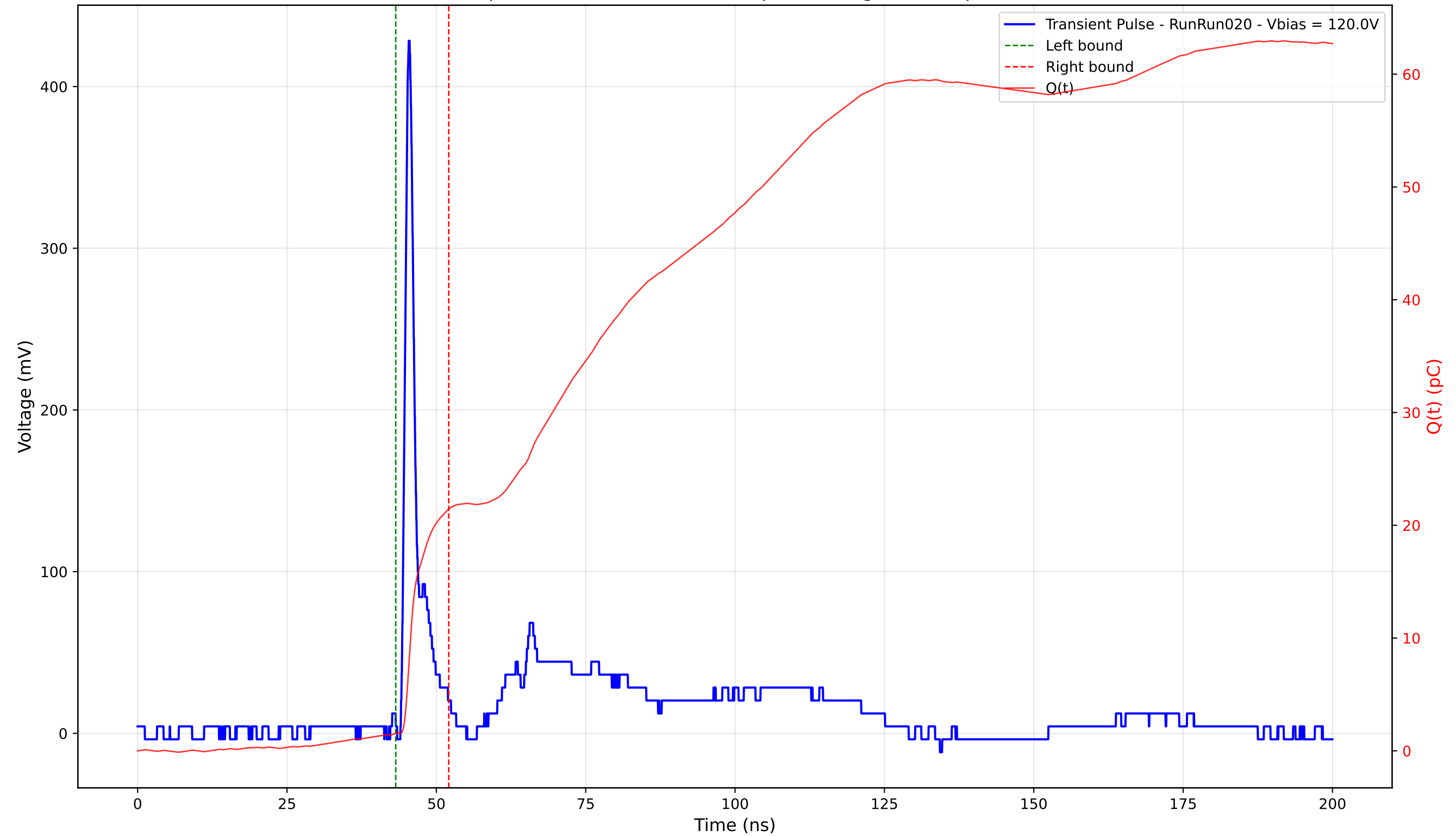
Transient Pulse - Sample: 4003 - Position: 125.0 \mu\text{m} - Charge: 19.88 pC - Rise Time: 0.90 ns
