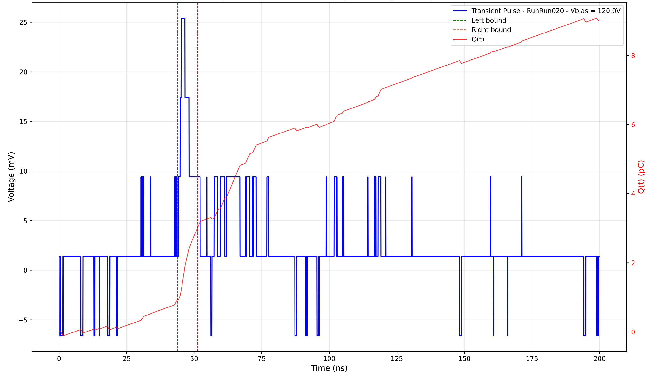
Transient Pulse - Sample: 4003 - Position: 350.0 \mu\text{m} - Charge: 2.10 pC - Rise Time: 0.86 ns
