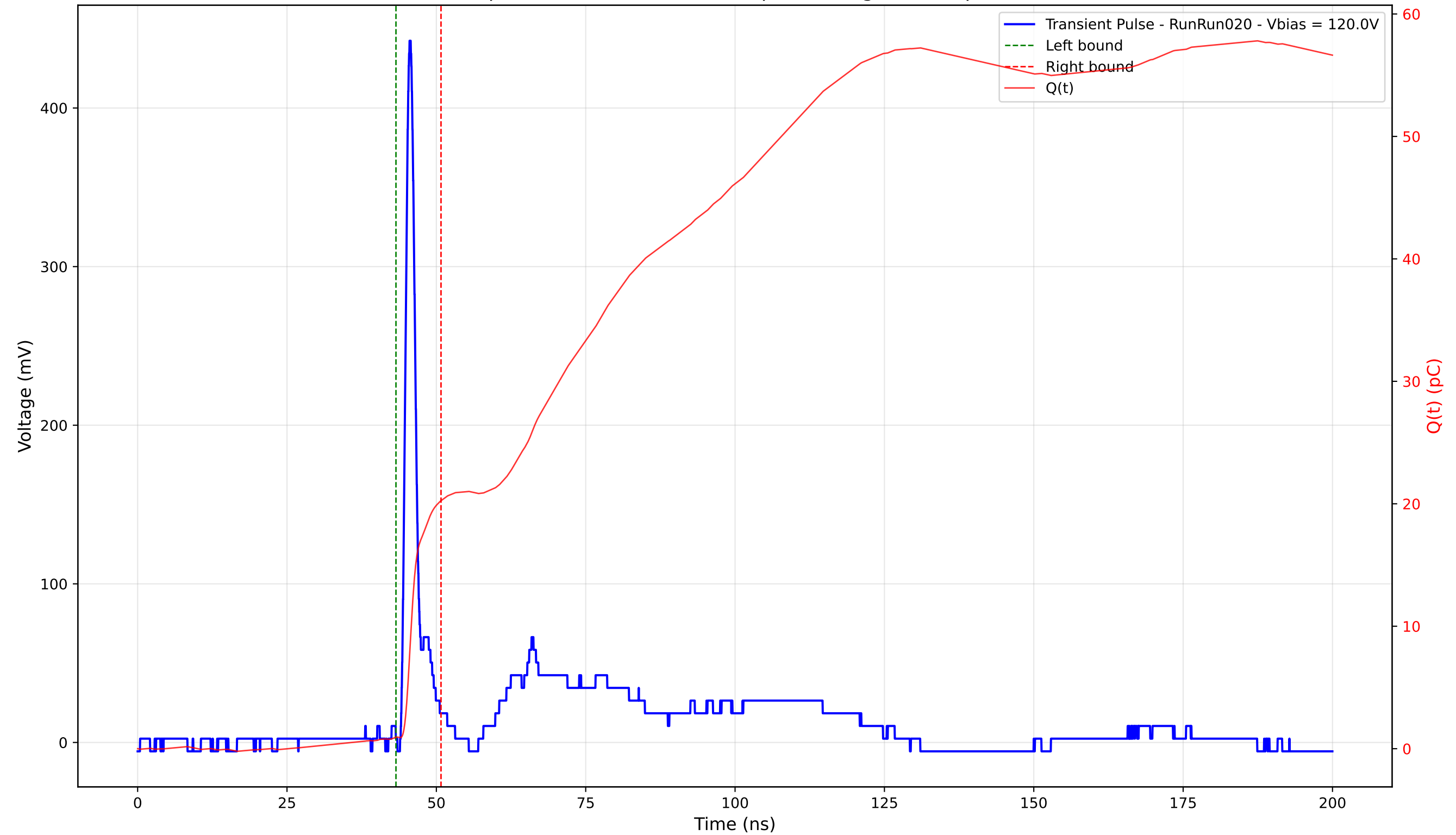
Transient Pulse - Sample: 4003 - Position: 160.0 \mu\text{m} - Charge: 19.31 pC - Rise Time: 1.00 ns
