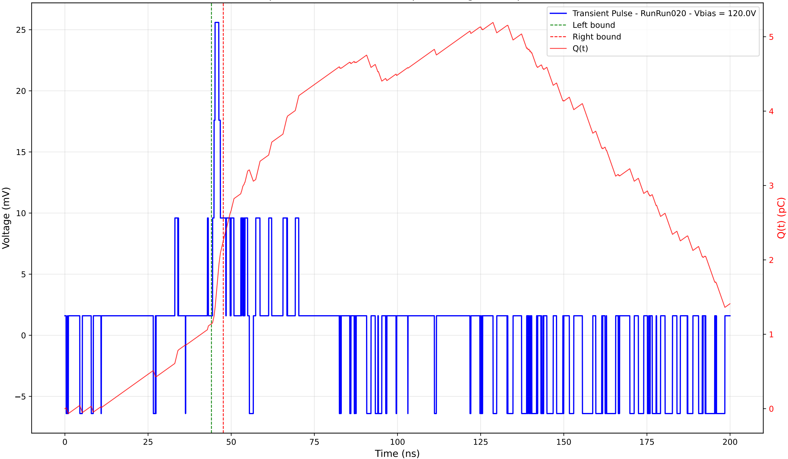
Transient Pulse - Sample: 4003 - Position: 80.0 \mu\text{m} - Charge: 1.12 pC - Rise Time: 0.76 ns
