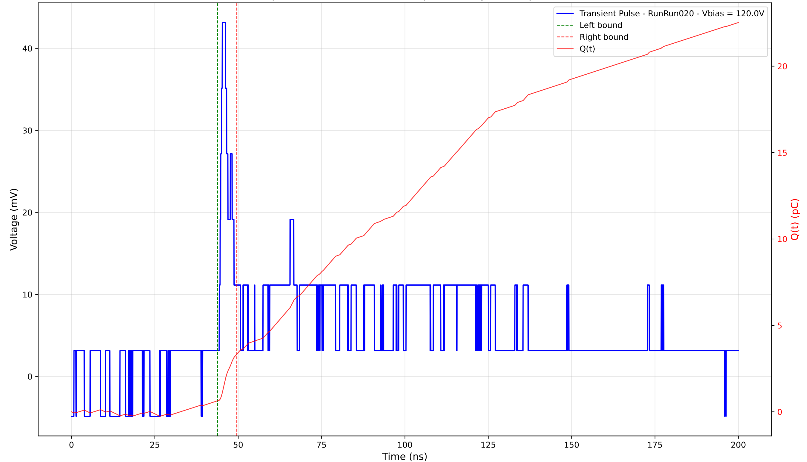
Transient Pulse - Sample: 4003 - Position: 300.0 \mu\text{m} - Charge: 2.70 pC - Rise Time: 0.92 ns
