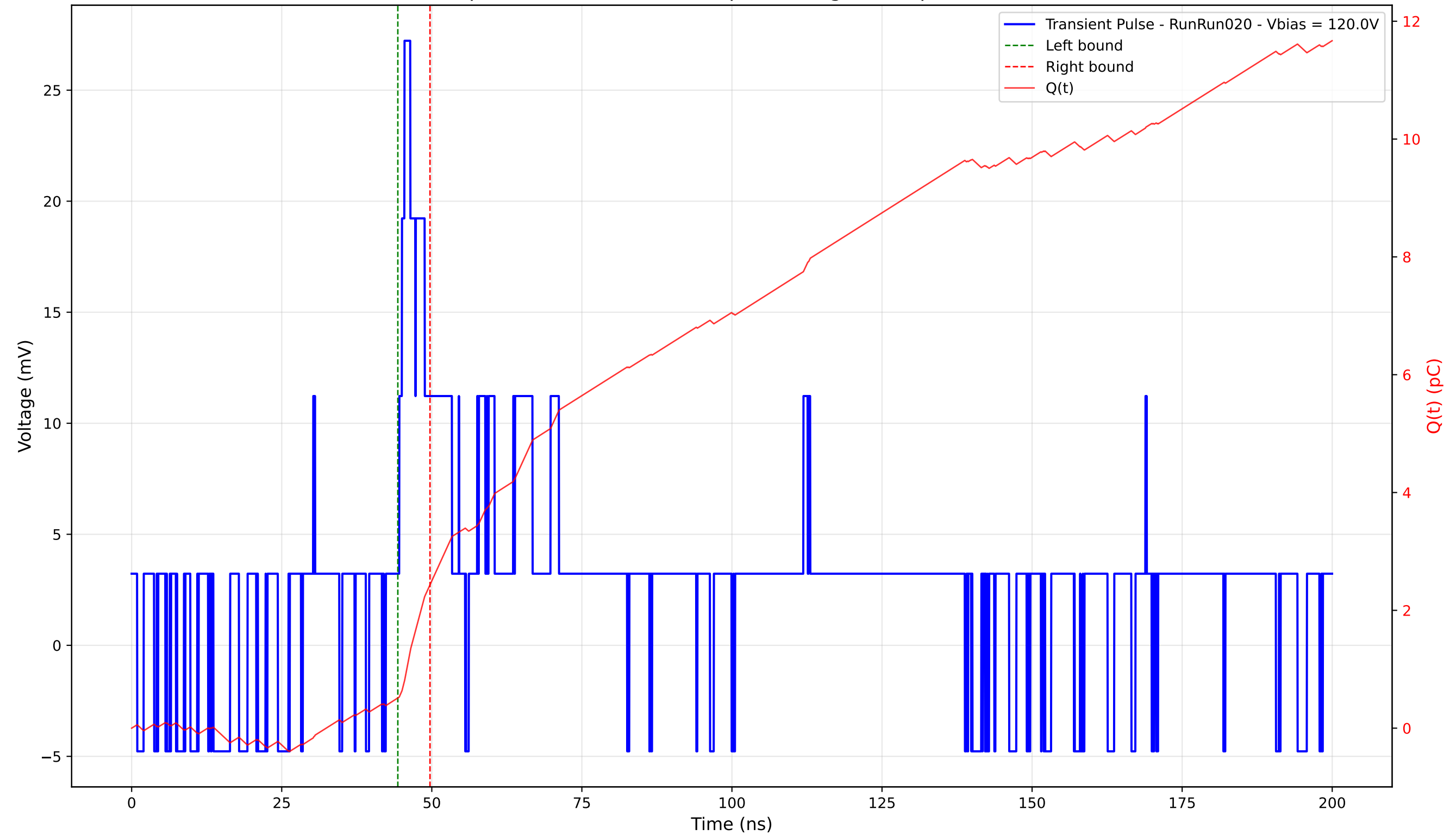
Transient Pulse - Sample: 4003 - Position: 65.0 \mu\text{m} - Charge: 1.92 pC - Rise Time: 0.00 ns (N/A)
