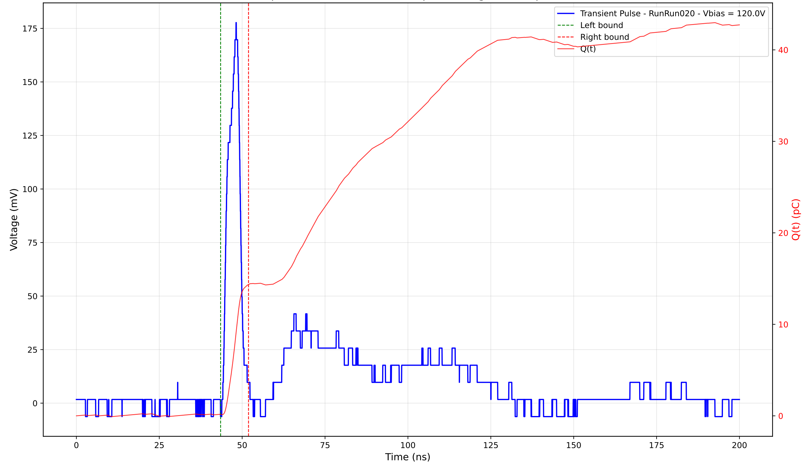
Transient Pulse - Sample: 4003 - Position: 265.0 \mu\text{m} - Charge: 14.18 pC - Rise Time: 3.12 ns
