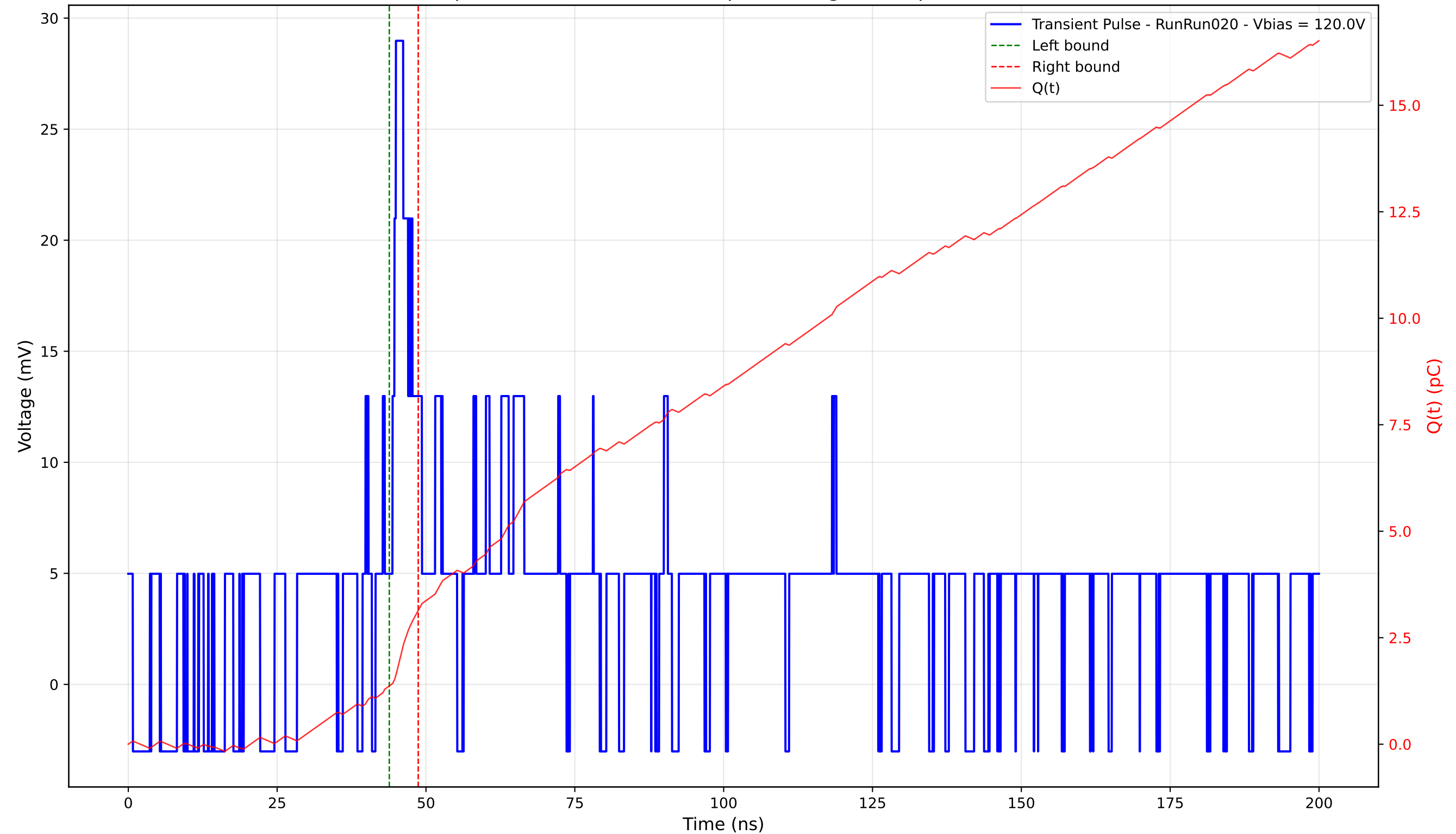
Transient Pulse - Sample: 4003 - Position: 335.0 \mu\text{m} - Charge: 1.78 pC - Rise Time: 0.00 ns (N/A)
