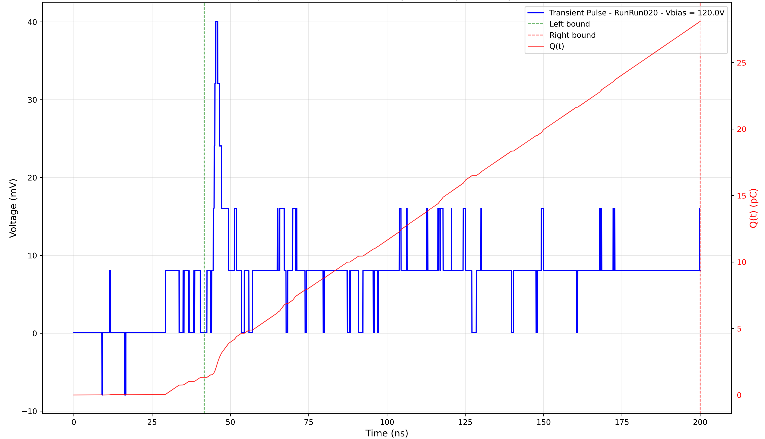
Transient Pulse - Sample: 4003 - Position: 320.0 \mu\text{m} - Charge: 26.78 pC - Rise Time: 1.33 ns
