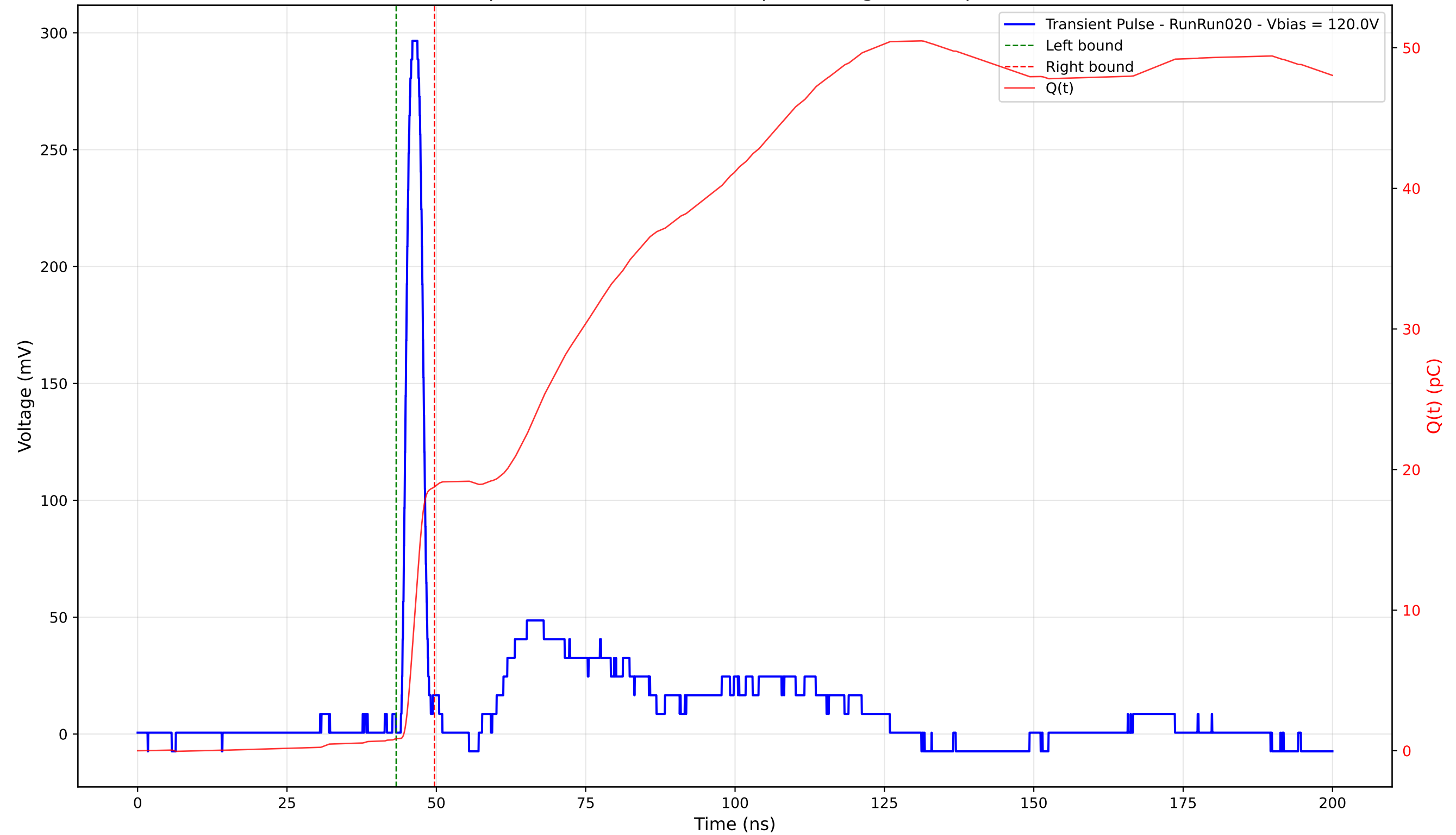
Transient Pulse - Sample: 4003 - Position: 230.0 \mu\text{m} - Charge: 17.91 pC - Rise Time: 1.25 ns
