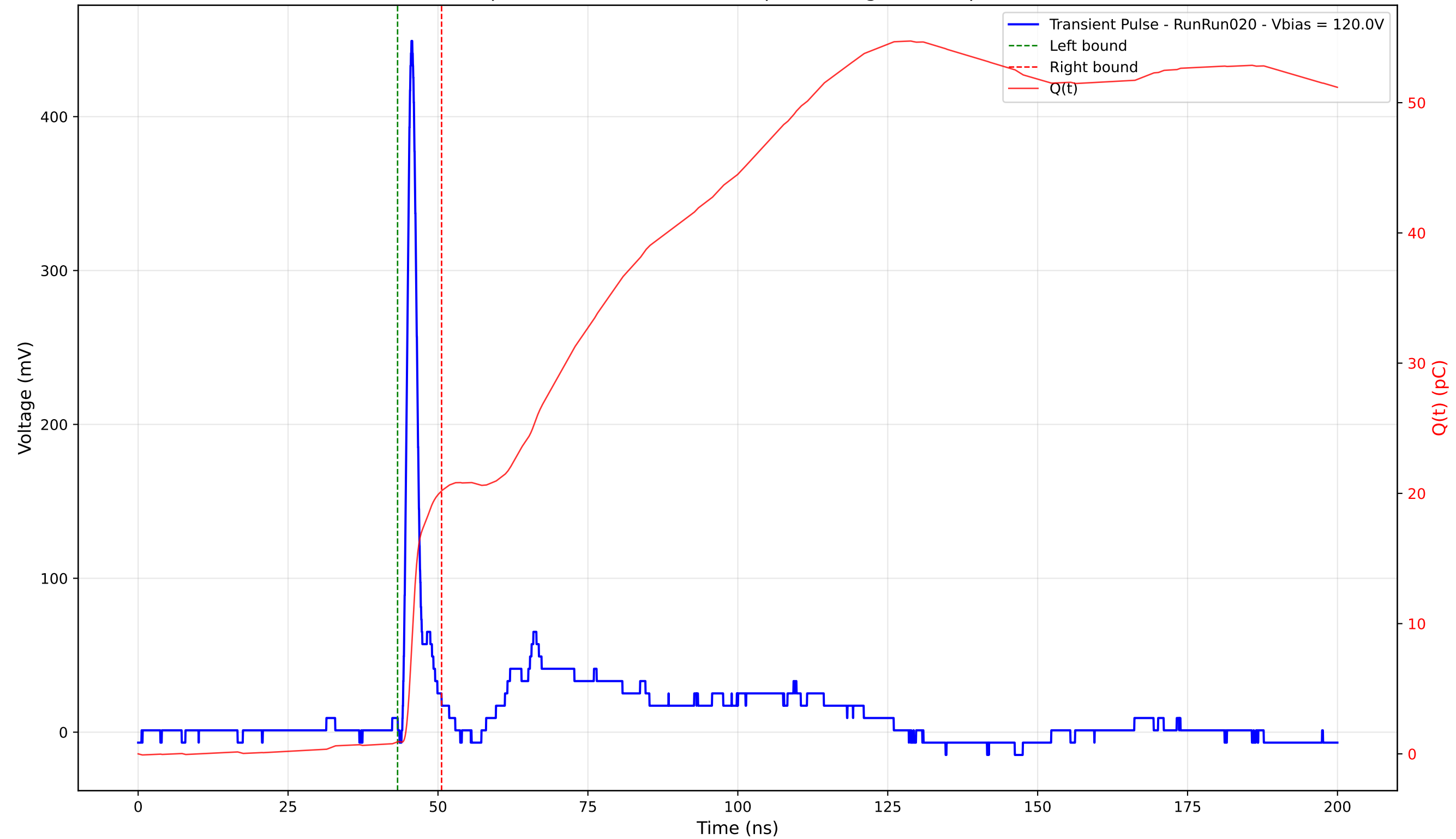
Transient Pulse - Sample: 4003 - Position: 165.0 \mu\text{m} - Charge: 19.27 pC - Rise Time: 1.01 ns
