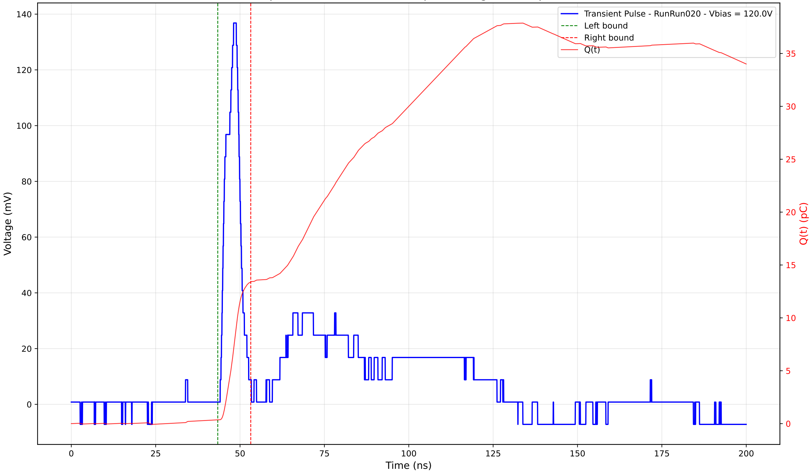
Transient Pulse - Sample: 4003 - Position: 270.0 \mu\text{m} - Charge: 13.05 pC - Rise Time: 3.43 ns
