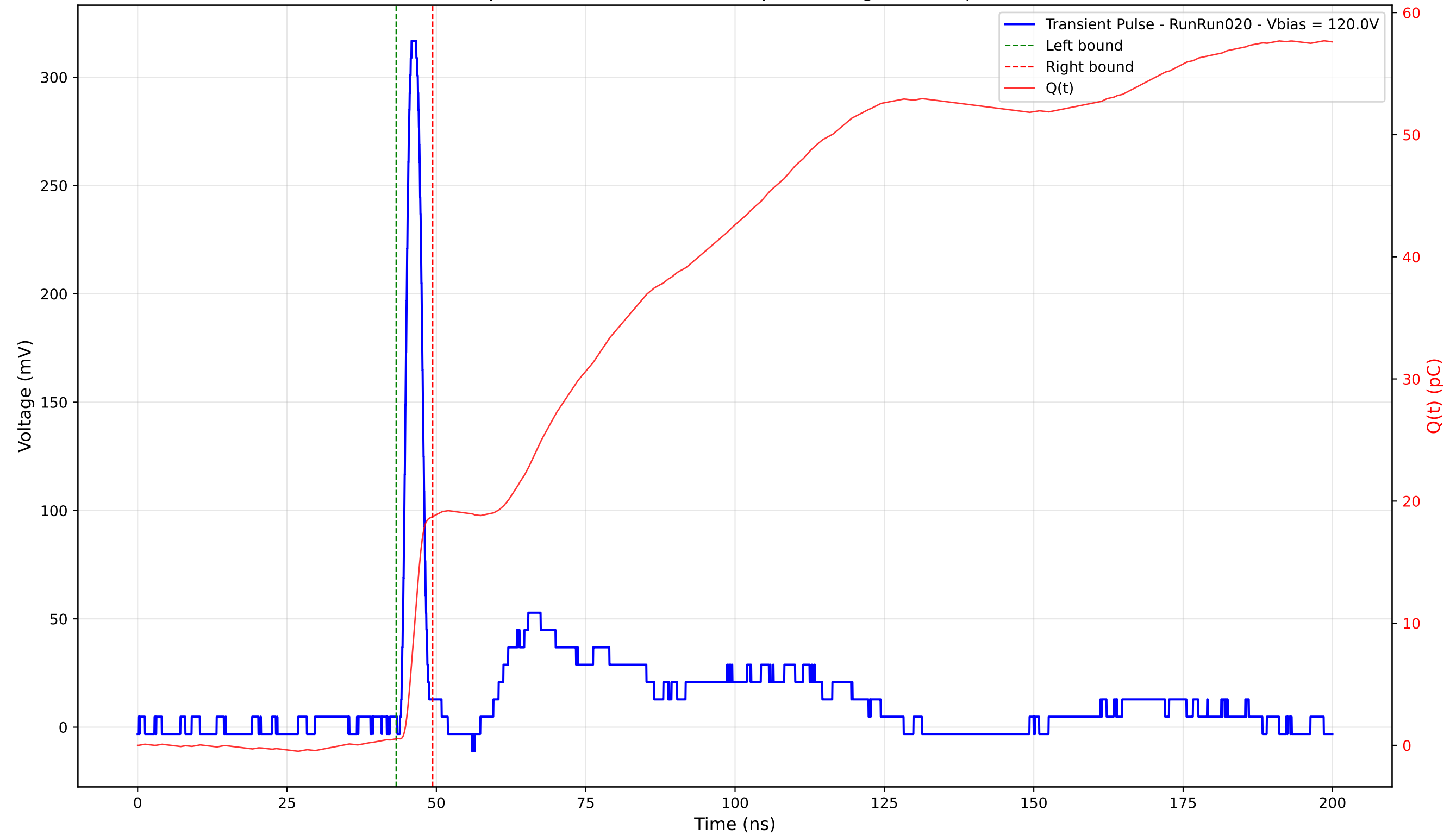
Transient Pulse - Sample: 4003 - Position: 225.0 \mu\text{m} - Charge: 18.20 pC - Rise Time: 1.23 ns
