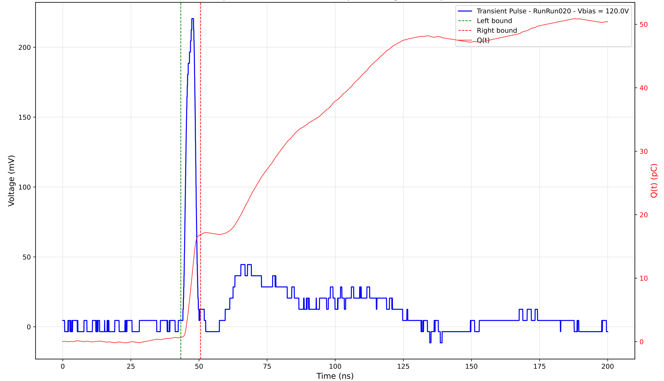
Transient Pulse - Sample: 4003 - Position: 255.0 \mu\text{m} - Charge: 16.15 pC - Rise Time: 2.52 ns
