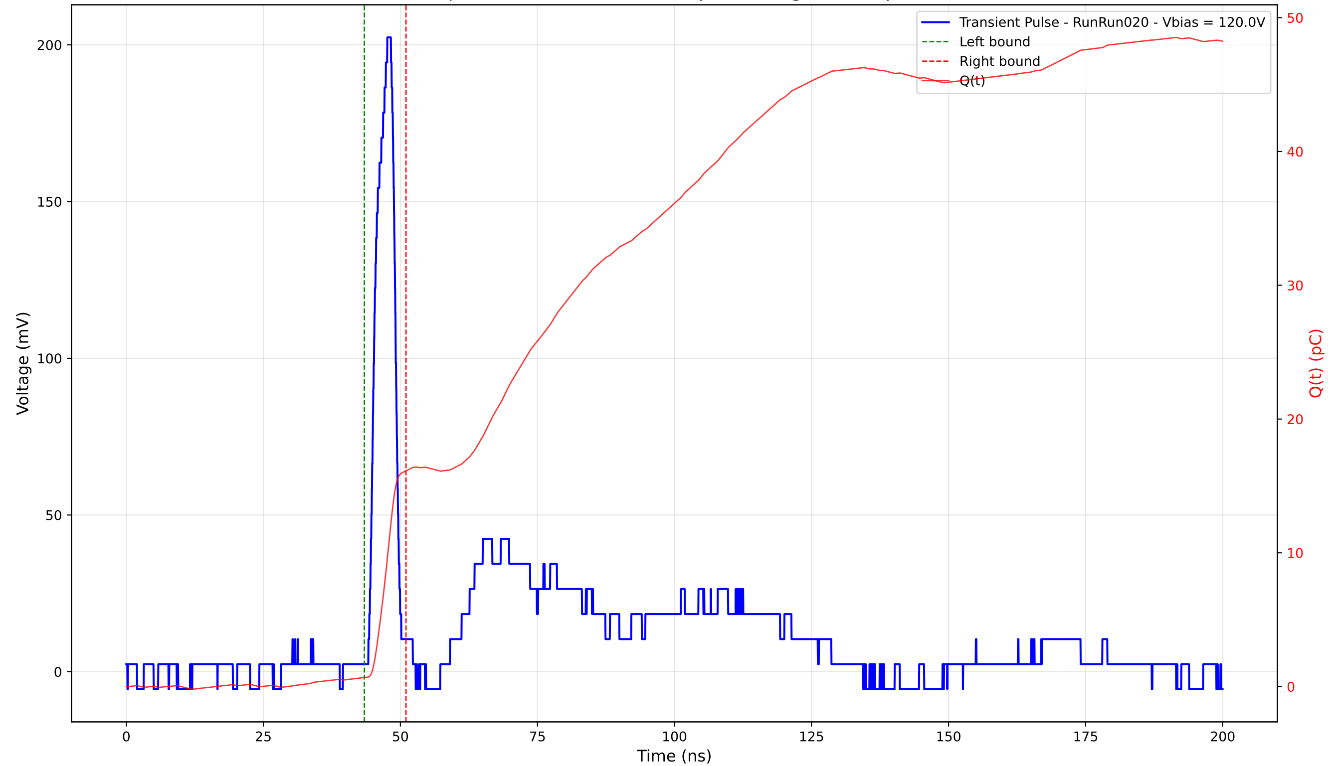
Transient Pulse - Sample: 4003 - Position: 260.0 \mu\text{m} - Charge: 15.46 pC - Rise Time: 2.68 ns
