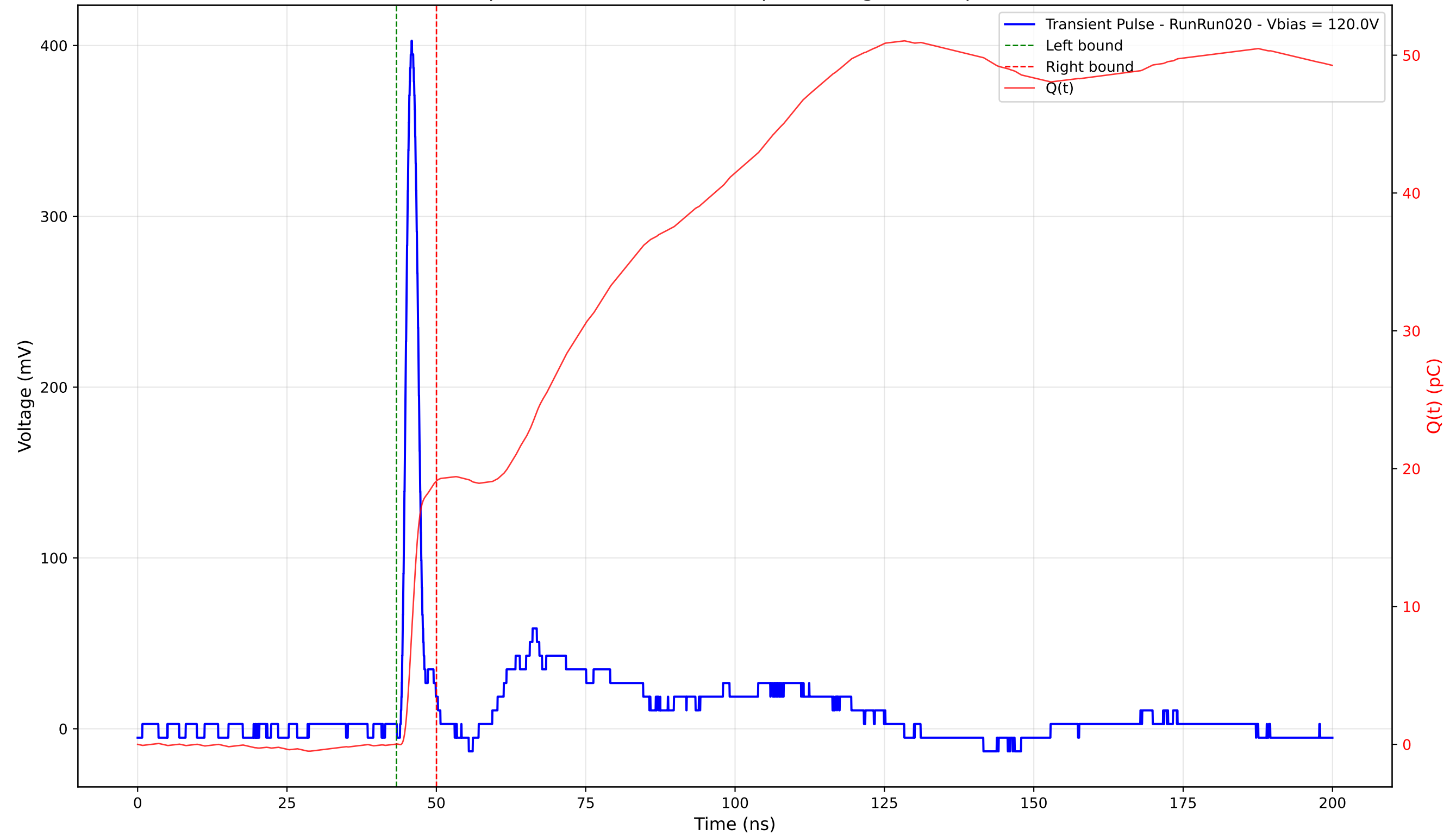
Transient Pulse - Sample: 4003 - Position: 200.0 \mu\text{m} - Charge: 19.08 pC - Rise Time: 1.15 ns
