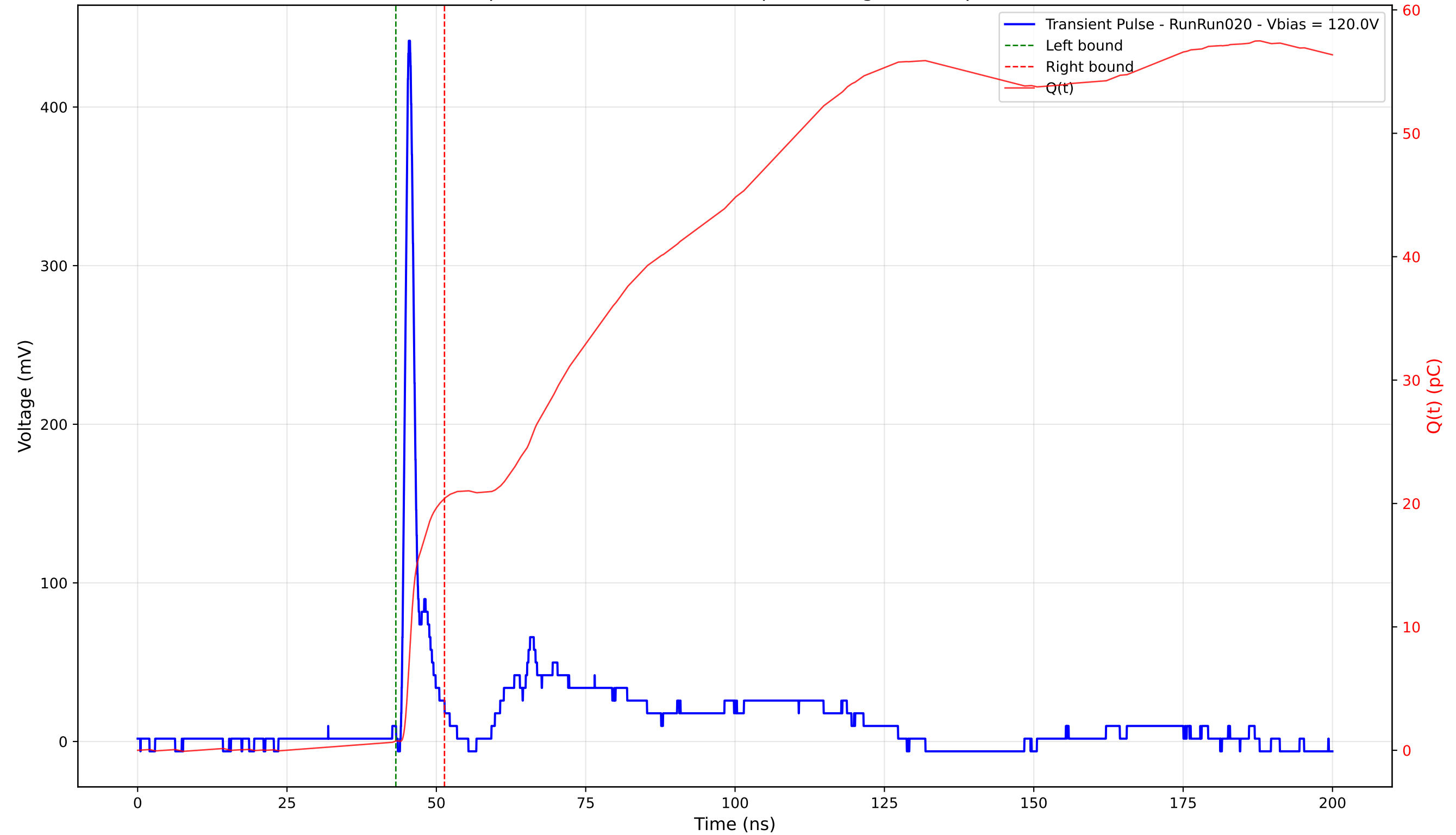
Transient Pulse - Sample: 4003 - Position: 135.0 \mu\text{m} - Charge: 19.66 pC - Rise Time: 0.92 ns
