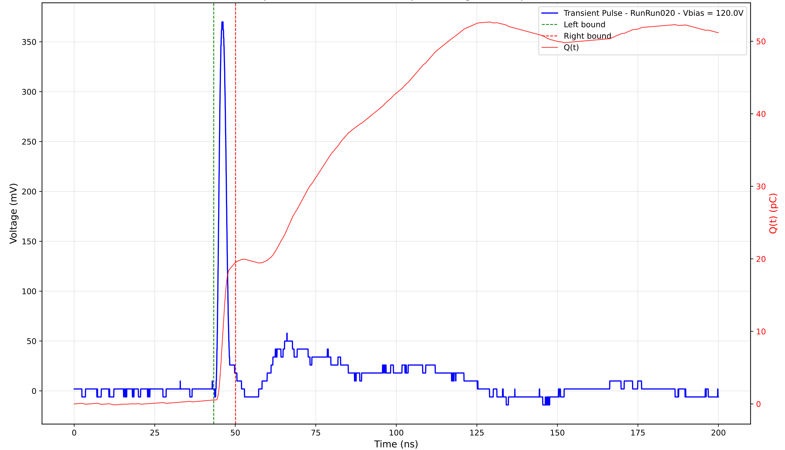
Transient Pulse - Sample: 4003 - Position: 210.0 \mu\text{m} - Charge: 18.94 pC - Rise Time: 1.19 ns
