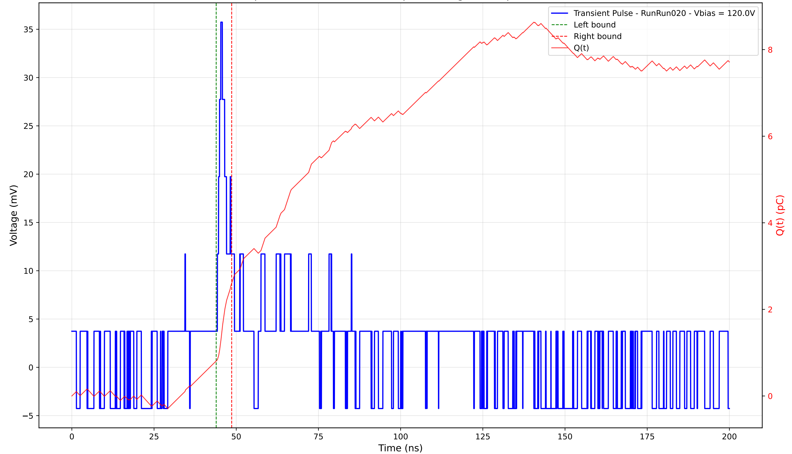
Transient Pulse - Sample: 4003 - Position: 365.0 \mu\text{m} - Charge: 1.80 pC - Rise Time: 0.00 ns (N/A)
