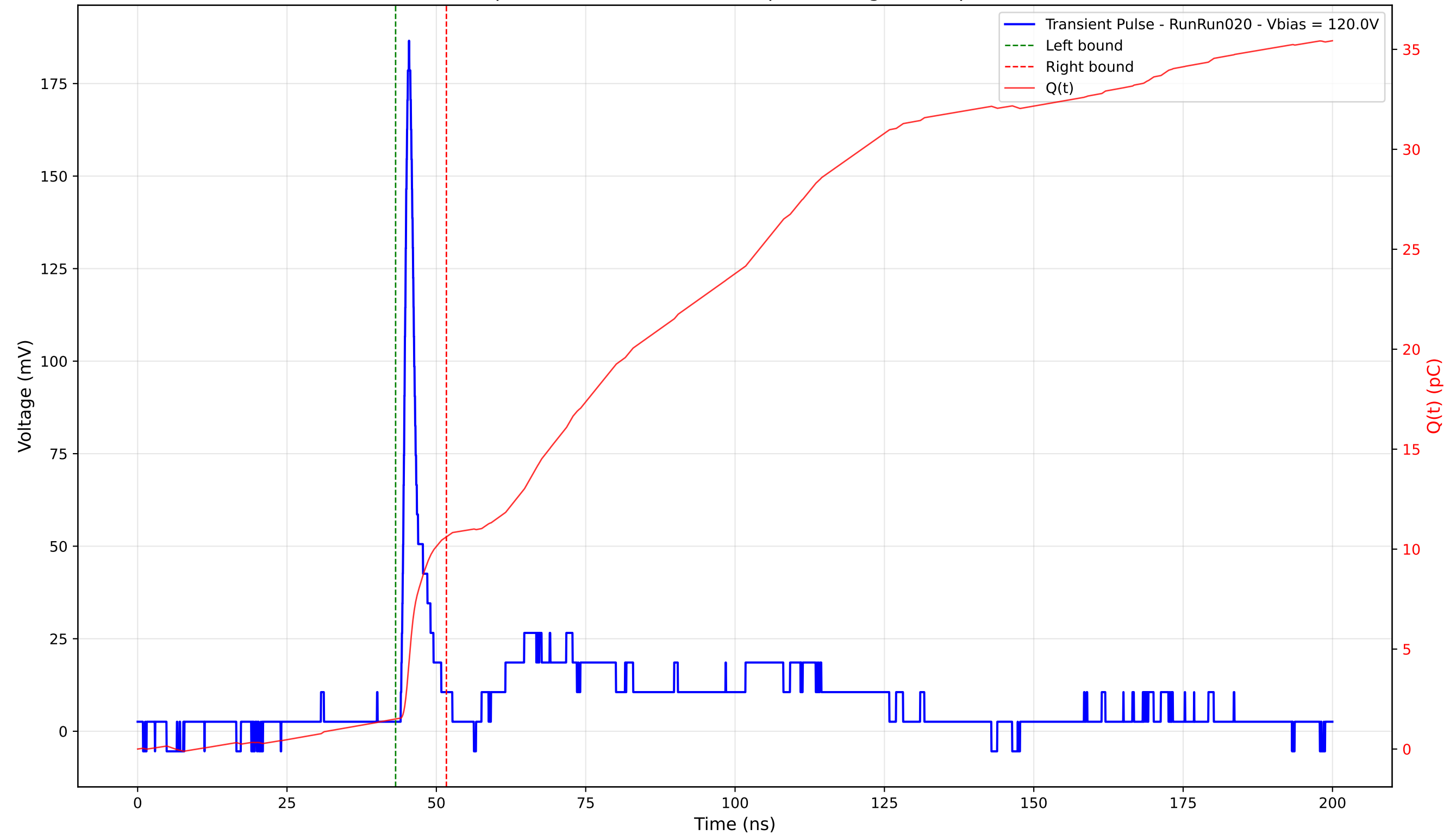
Transient Pulse - Sample: 4003 - Position: 100.0 \mu\text{m} - Charge: 9.12 pC - Rise Time: 0.94 ns
