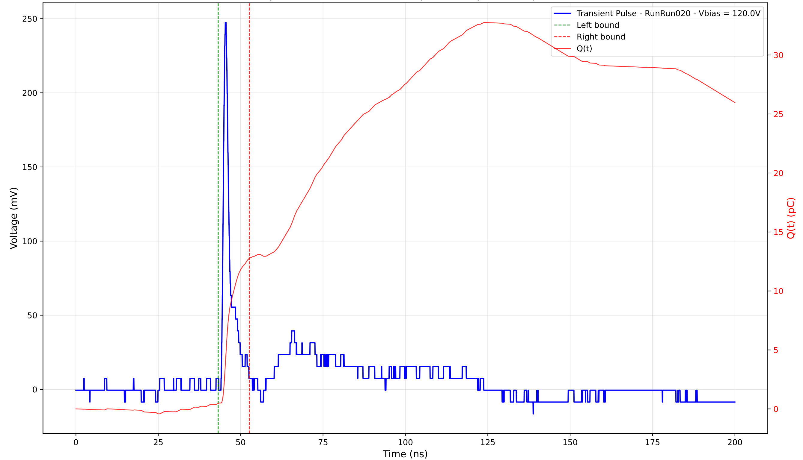
Transient Pulse - Sample: 4003 - Position: 105.0 \mu\text{m} - Charge: 12.29 pC - Rise Time: 0.88 ns
