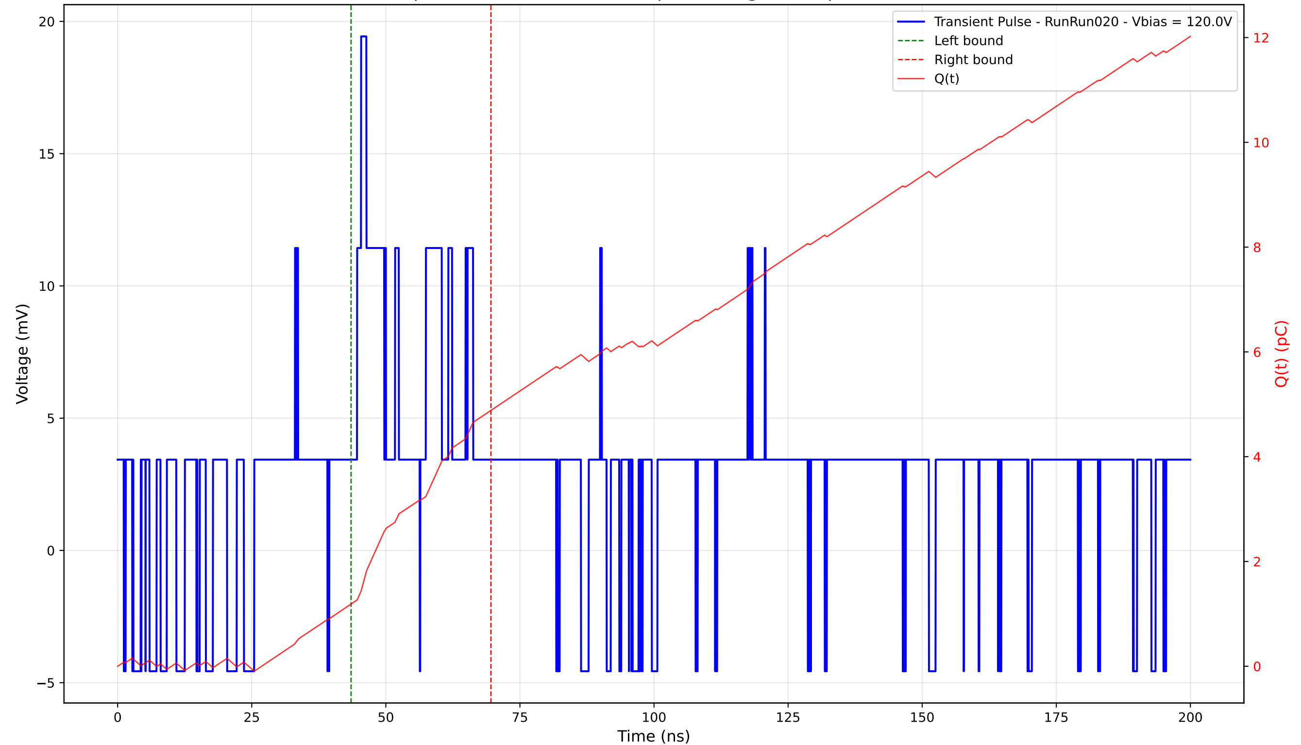
Transient Pulse - Sample: 4003 - Position: 425.0 \mu\text{m} - Charge: 3.70 pC - Rise Time: 0.00 ns (N/A)
