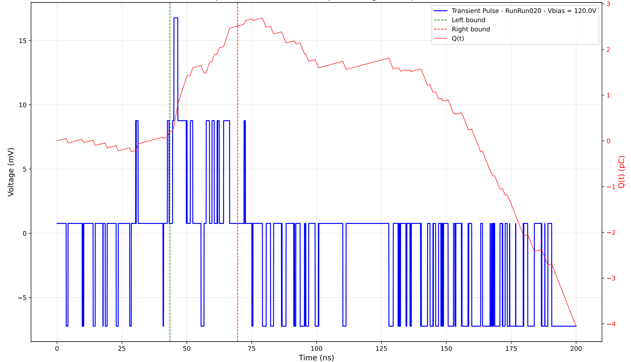
Transient Pulse - Sample: 4003 - Position: 75.0 \mu\text{m} - Charge: 2.31 pC - Rise Time: 0.52 ns
