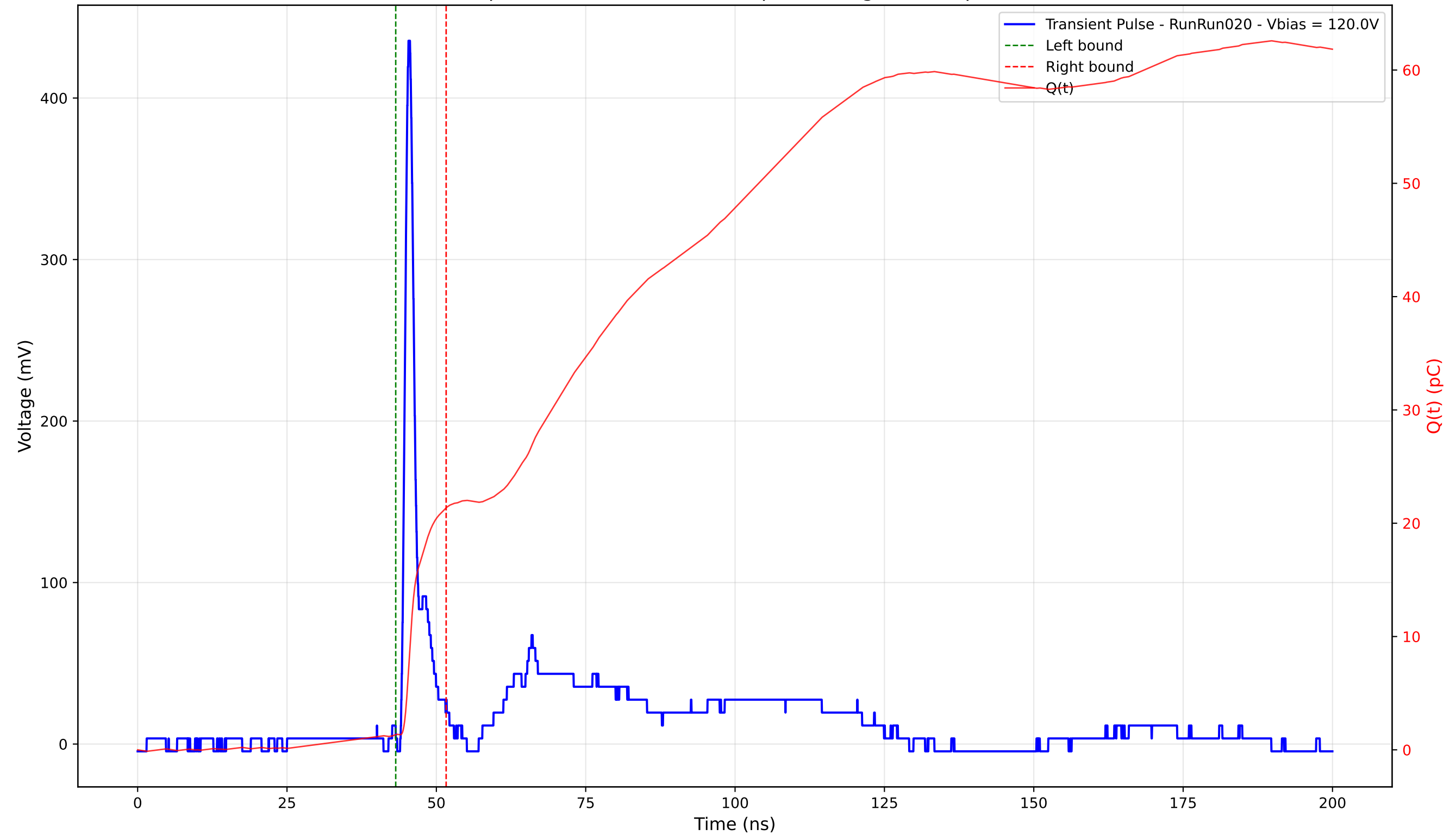
Transient Pulse - Sample: 4003 - Position: 130.0 \mu\text{m} - Charge: 20.00 pC - Rise Time: 0.90 ns
