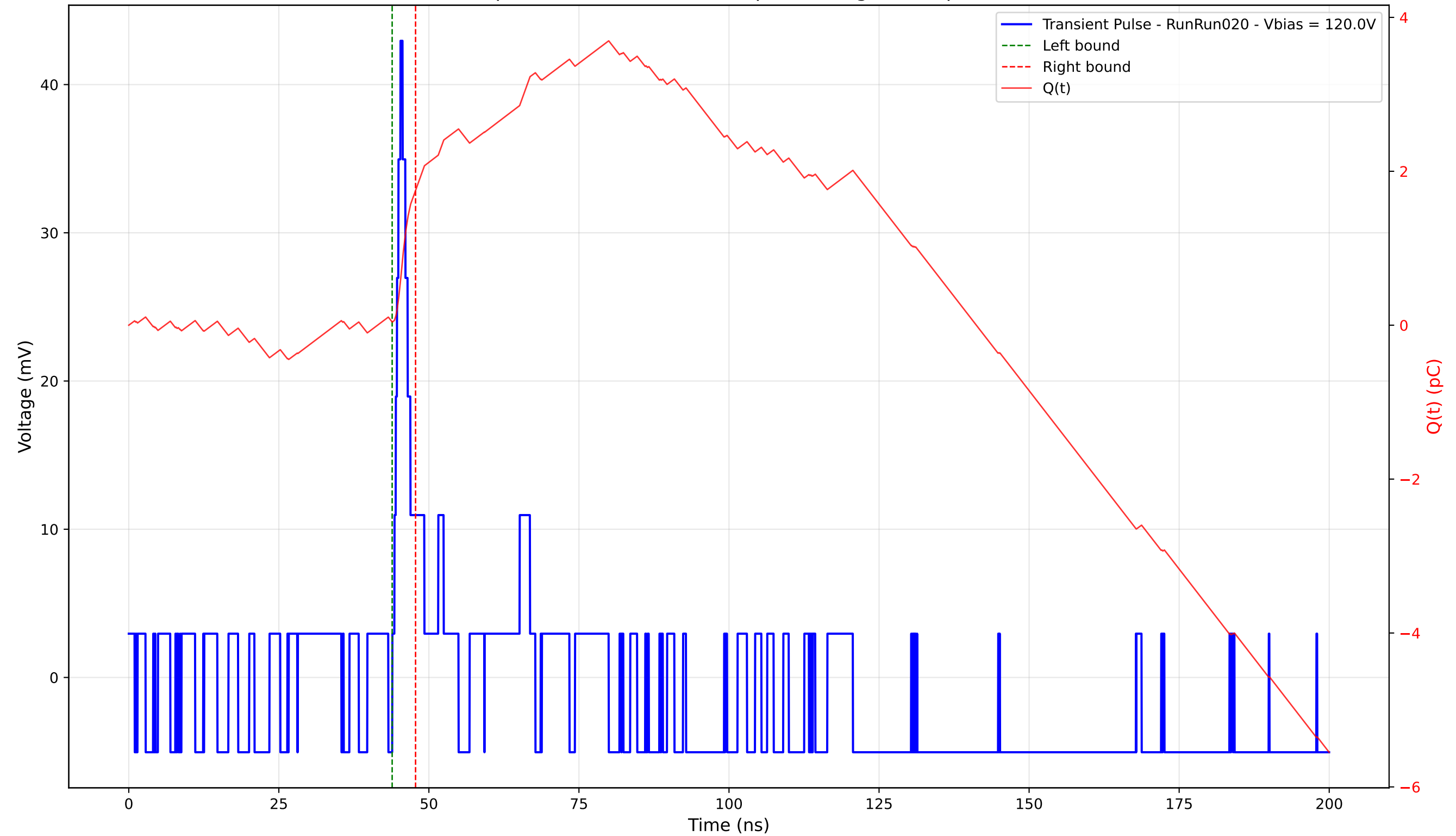
Transient Pulse - Sample: 4003 - Position: 85.0 \mu\text{m} - Charge: 1.71 pC - Rise Time: 1.02 ns
