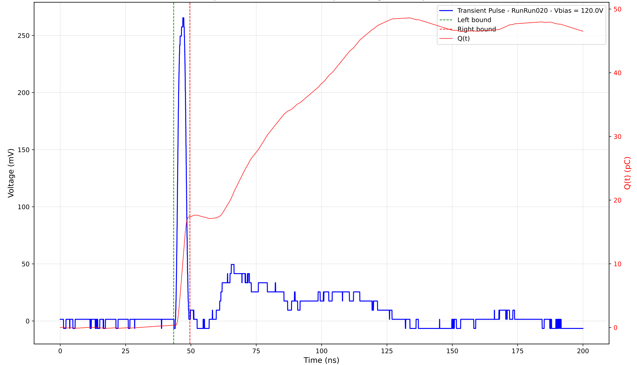
Transient Pulse - Sample: 4003 - Position: 240.0 \mu\text{m} - Charge: 17.00 pC - Rise Time: 1.30 ns
