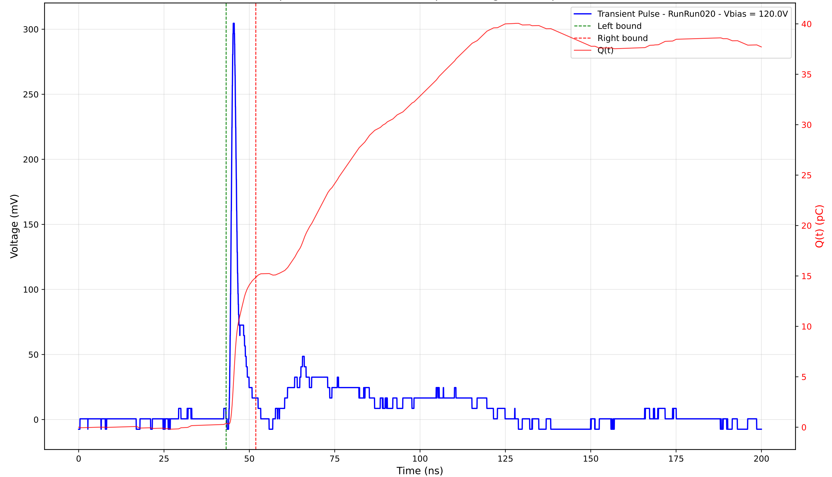
Transient Pulse - Sample: 4003 - Position: 110.0 \mu\text{m} - Charge: 14.49 pC - Rise Time: 0.89 ns
