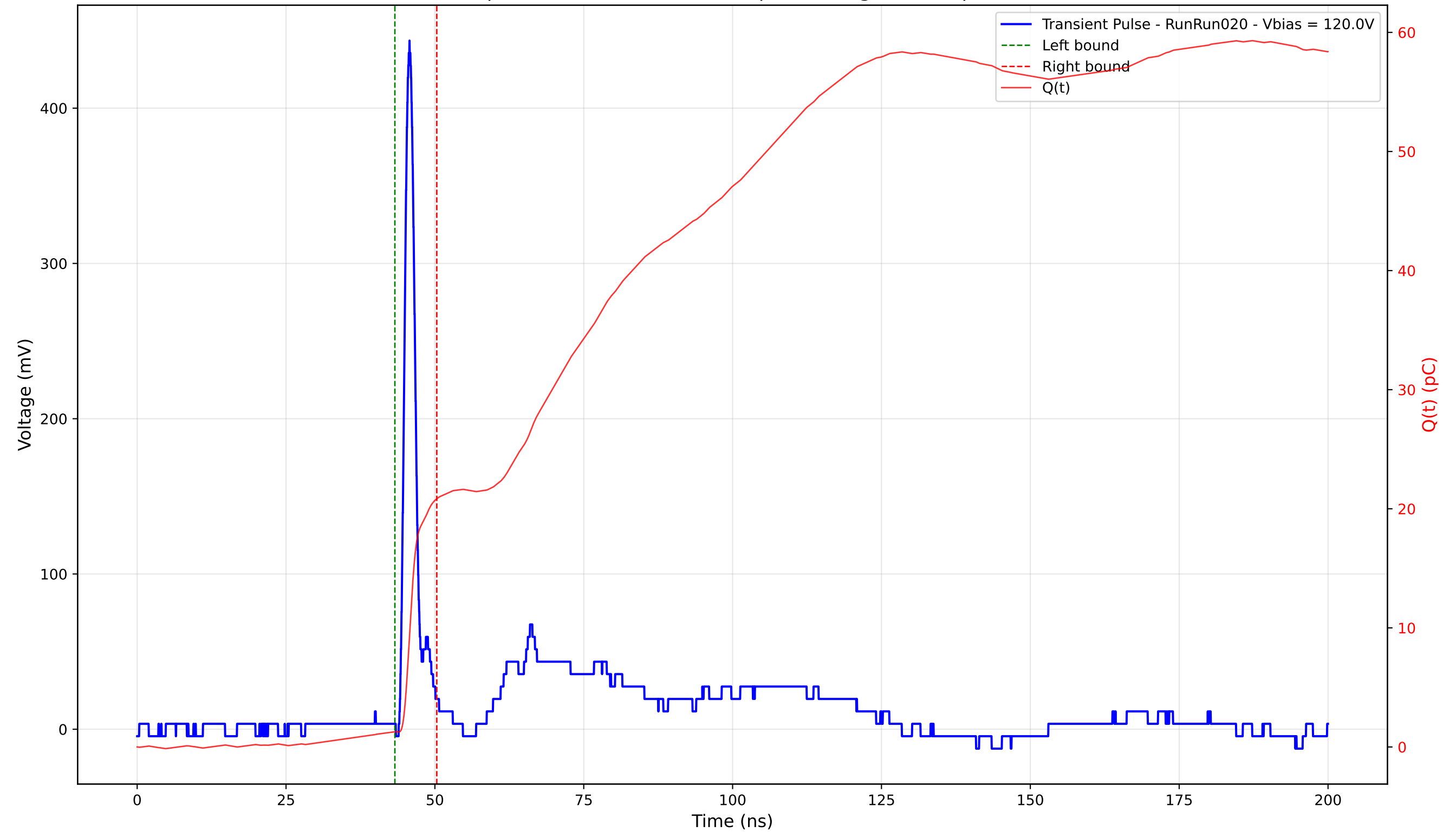
Transient Pulse - Sample: 4003 - Position: 180.0 \mu\text{m} - Charge: 19.56 pC - Rise Time: 1.10 ns
