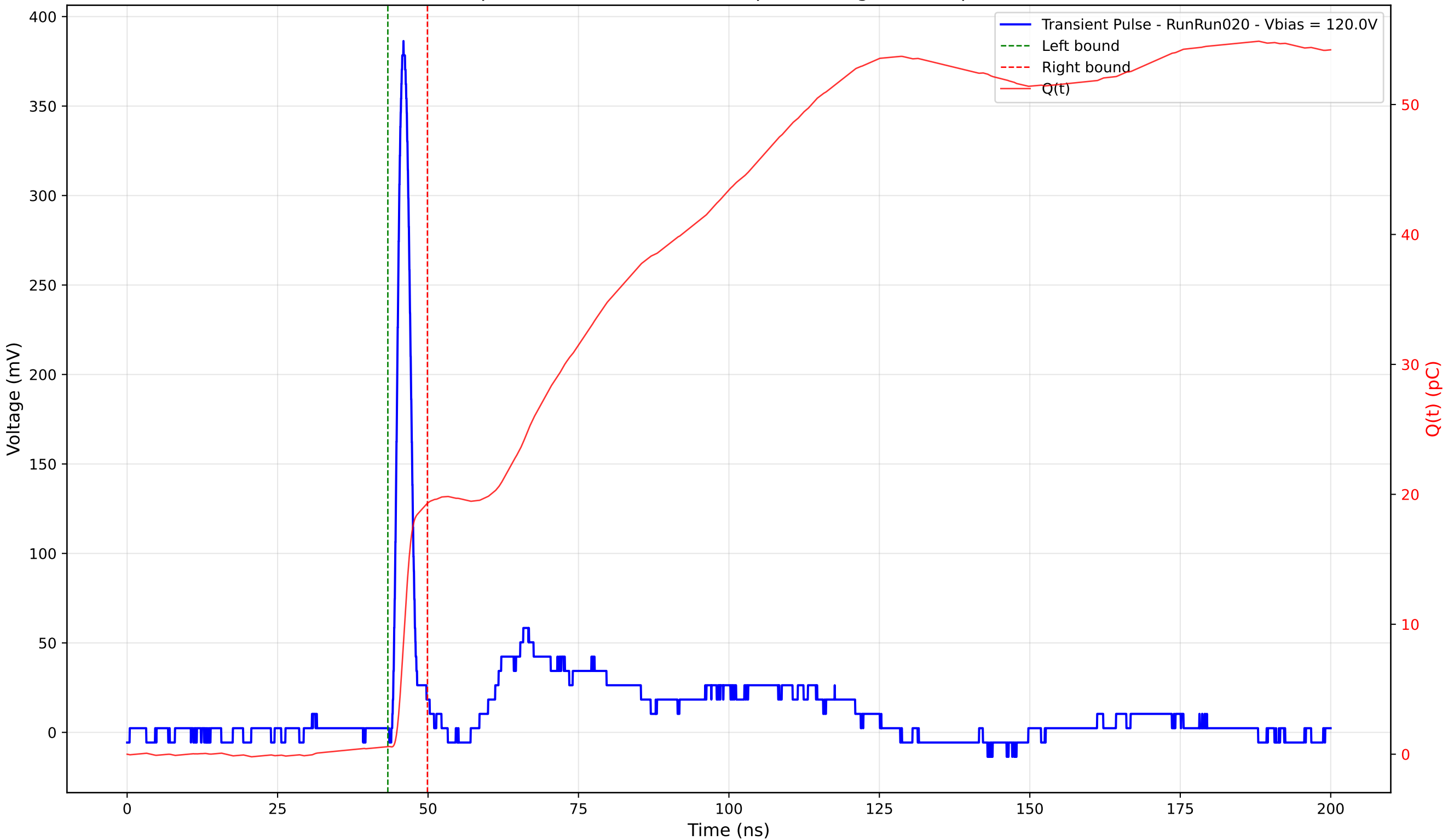
Transient Pulse - Sample: 4003 - Position: 205.0 \mu\text{m} - Charge: 18.72 pC - Rise Time: 1.19 ns
