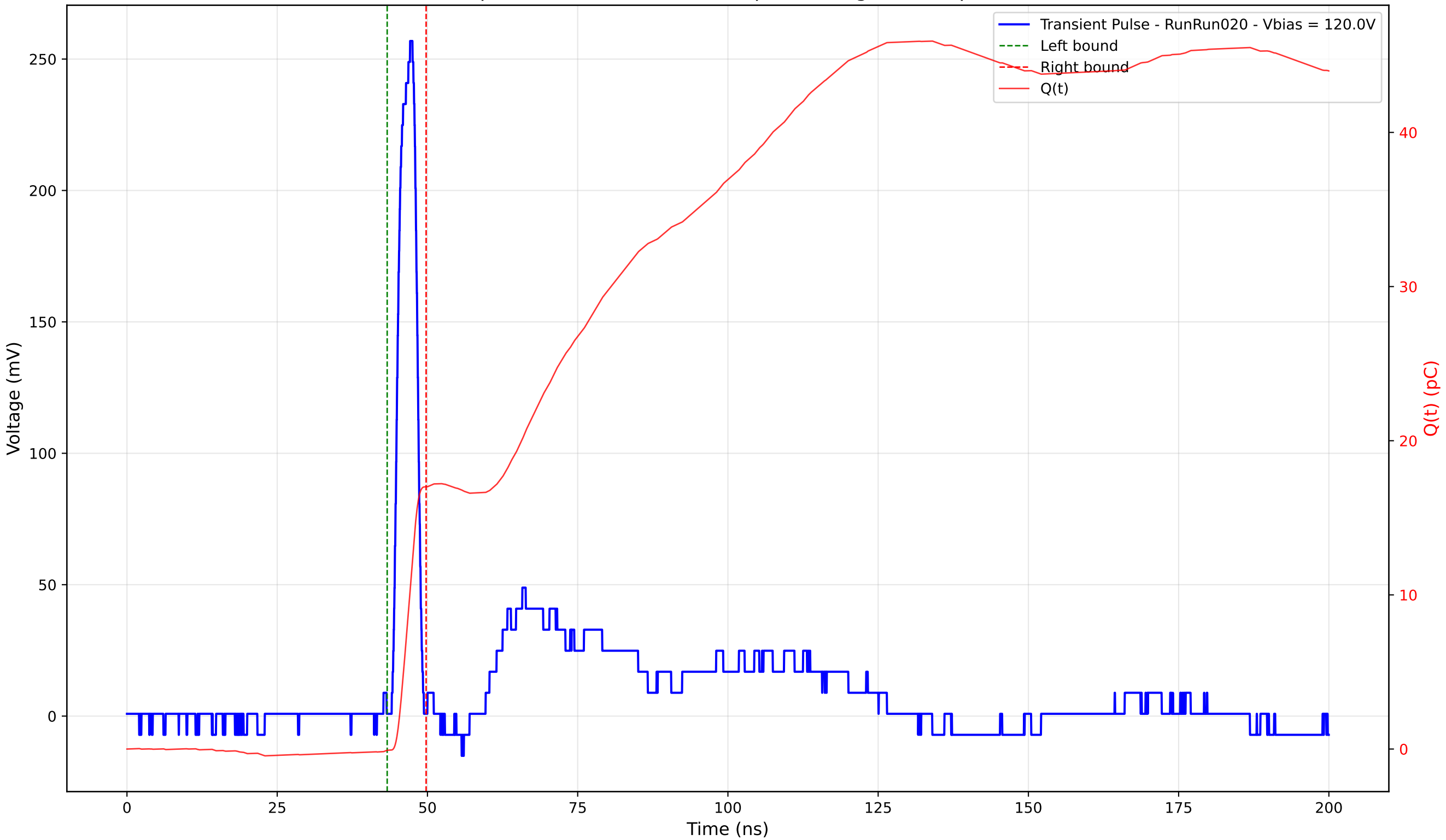
Transient Pulse - Sample: 4003 - Position: 245.0 \mu\text{m} - Charge: 17.09 pC - Rise Time: 1.58 ns
