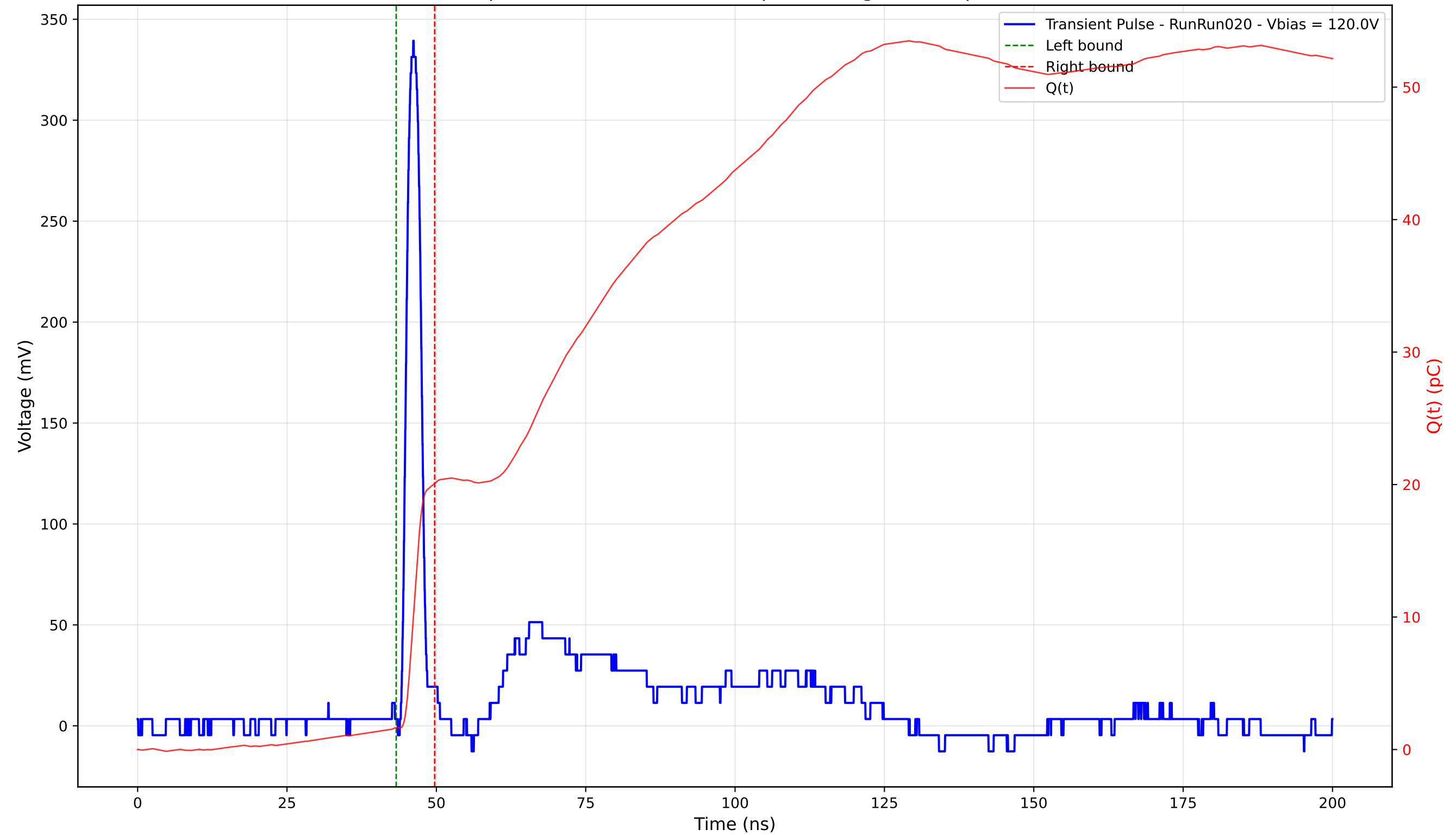
Transient Pulse - Sample: 4003 - Position: 220.0 \mu\text{m} - Charge: 18.45 pC - Rise Time: 1.24 ns
