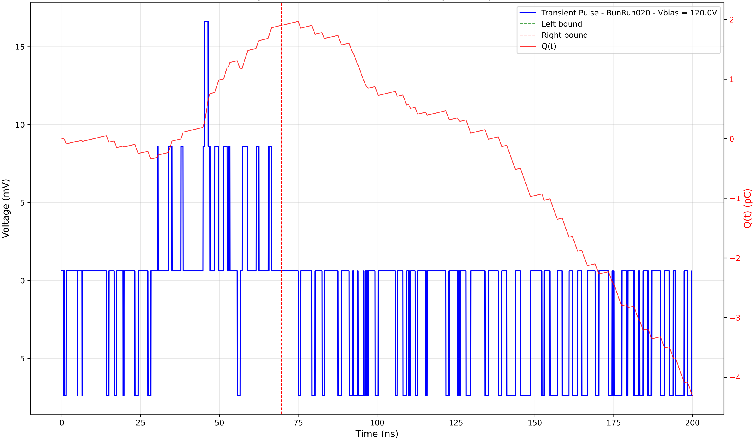
Transient Pulse - Sample: 4003 - Position: 0.0 \mu\text{m} - Charge: 1.73 pC - Rise Time: 0.48 ns
