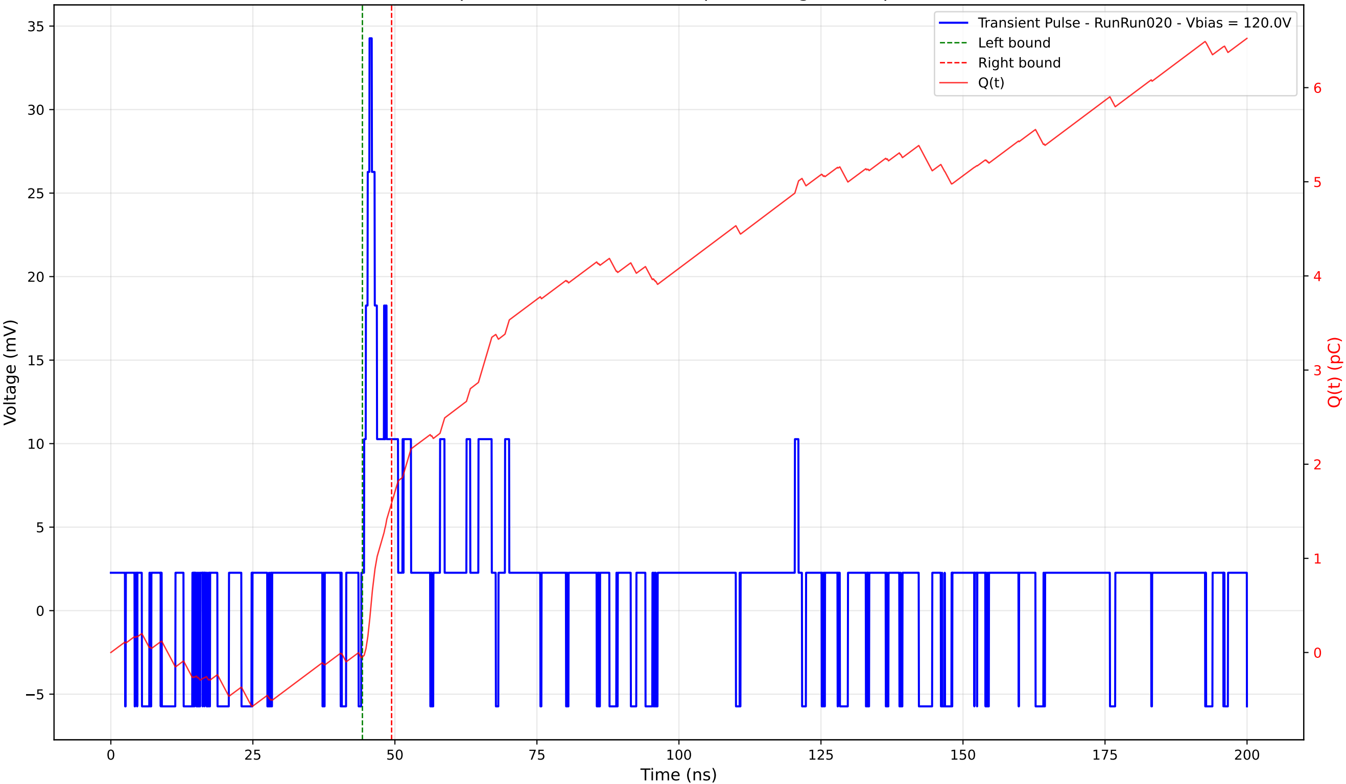
Transient Pulse - Sample: 4003 - Position: 35.0 \mu\text{m} - Charge: 1.64 pC - Rise Time: 0.96 ns
