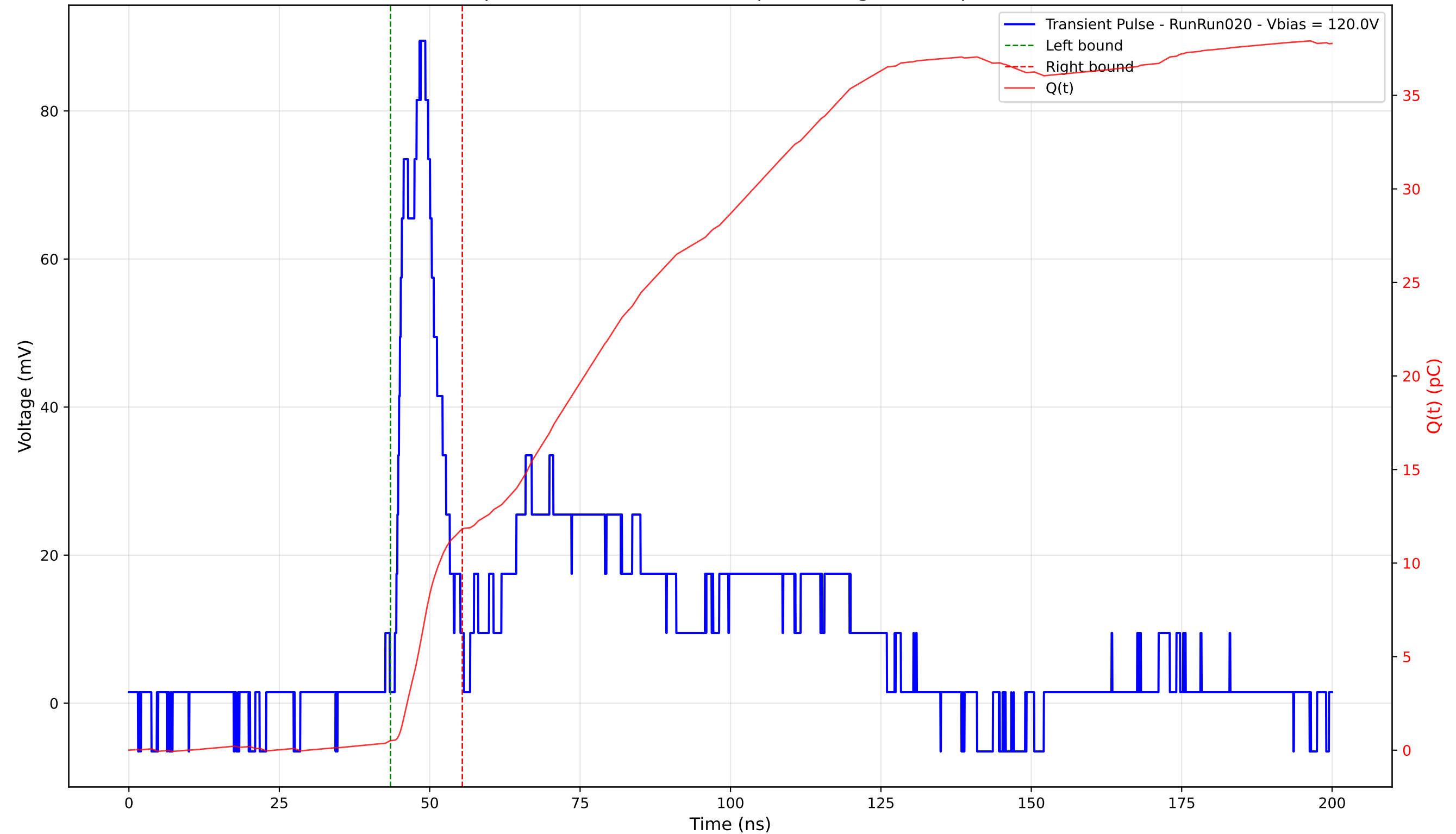
Transient Pulse - Sample: 4003 - Position: 275.0 \mu\text{m} - Charge: 11.30 pC - Rise Time: 3.62 ns
