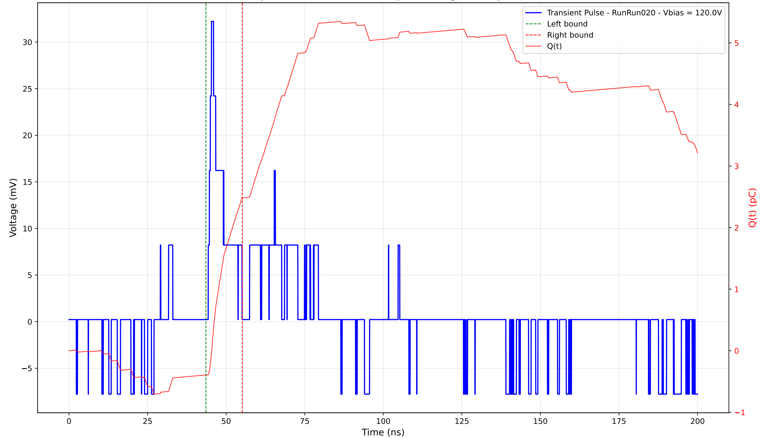
Transient Pulse - Sample: 4003 - Position: 45.0 \mu\text{m} - Charge: 2.88 pC - Rise Time: 1.03 ns
