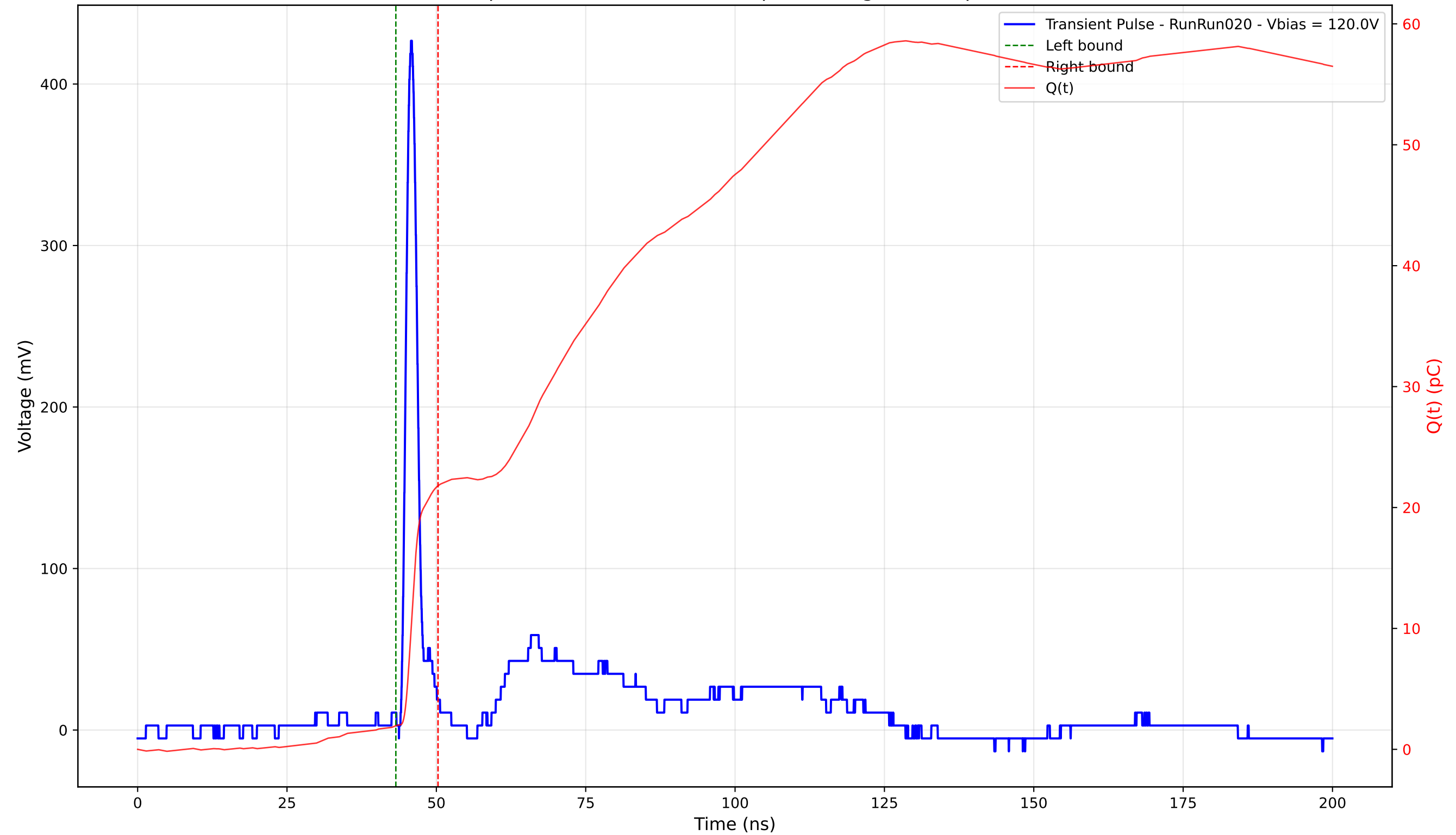
Transient Pulse - Sample: 4003 - Position: 190.0 \mu\text{m} - Charge: 19.84 pC - Rise Time: 1.14 ns
