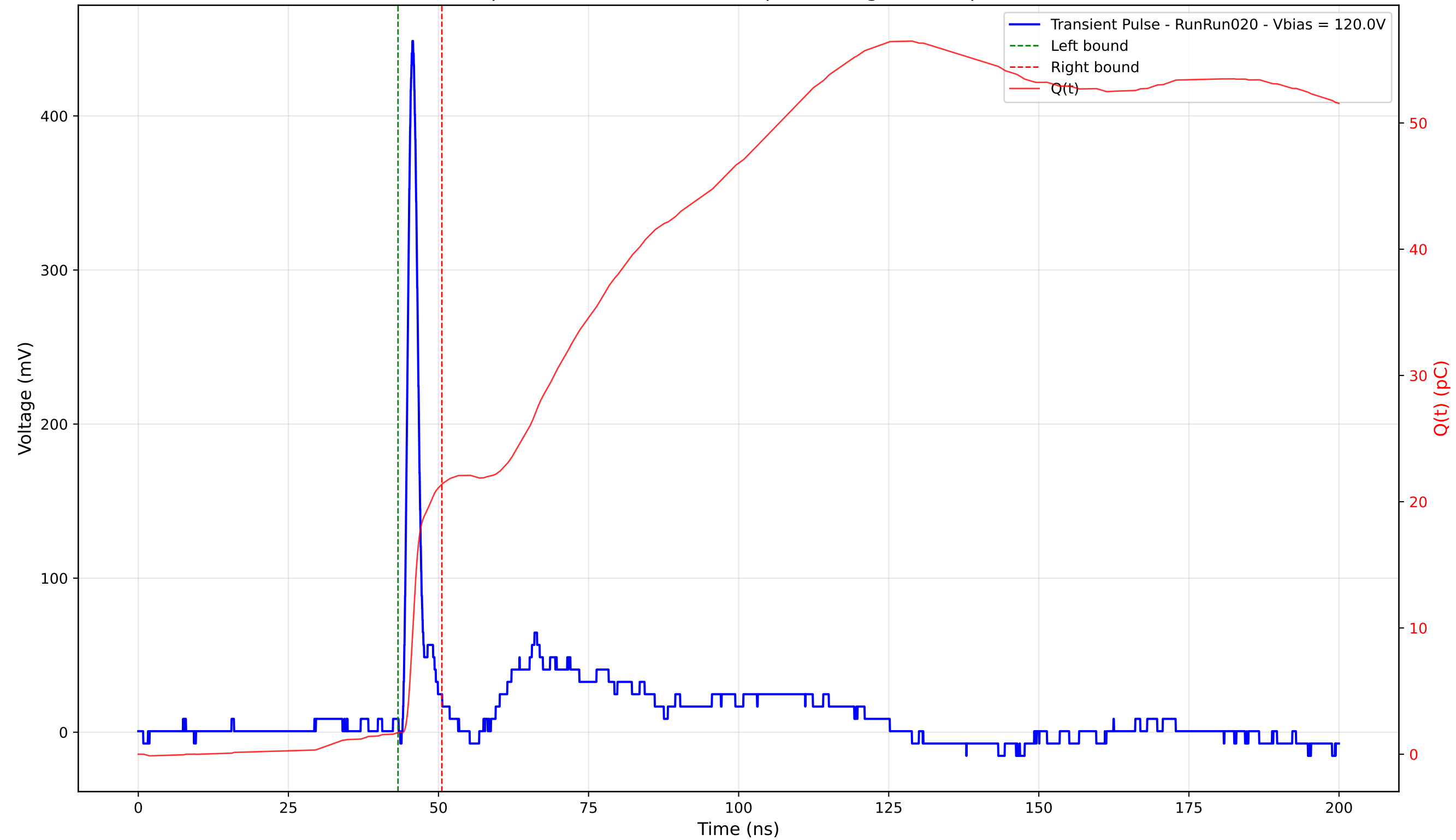
Transient Pulse - Sample: 4003 - Position: 175.0 \mu\text{m} - Charge: 19.66 pC - Rise Time: 1.05 ns
