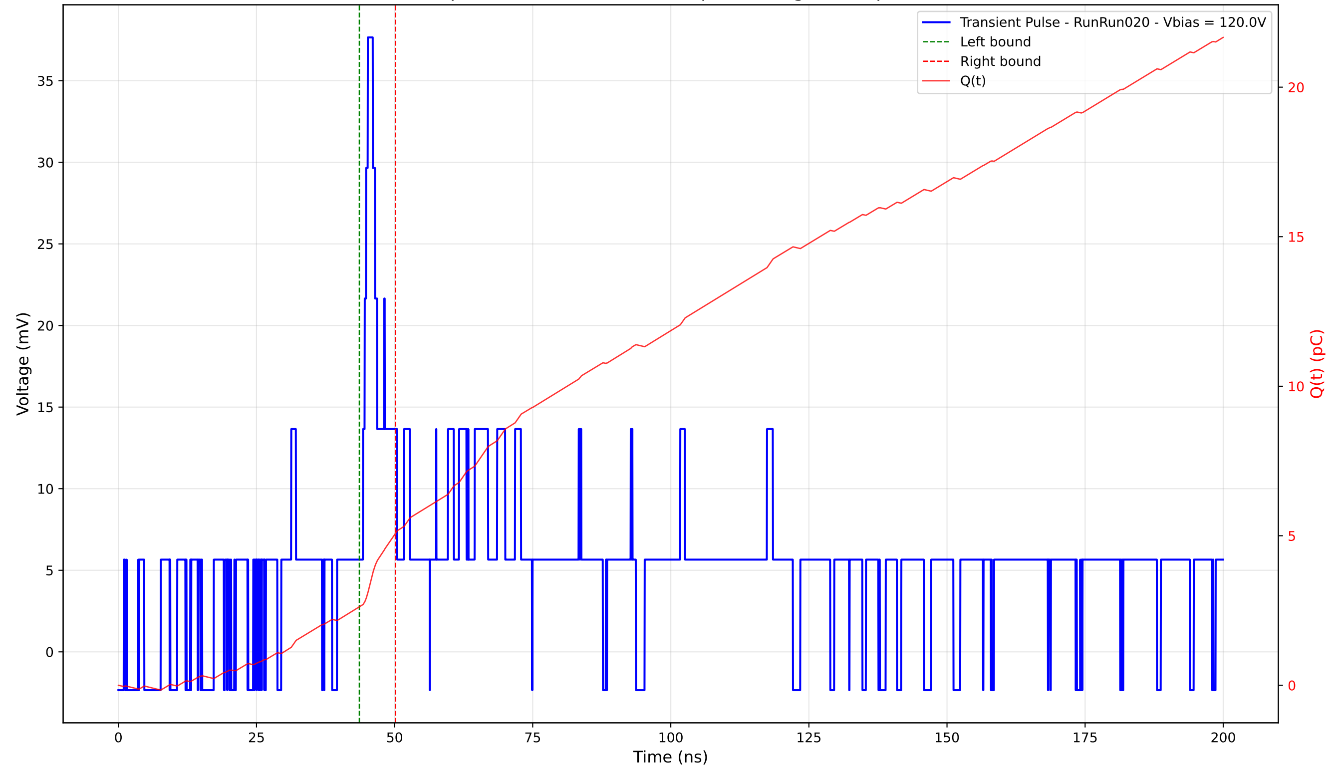
Transient Pulse - Sample: 4003 - Position: 380.0 \mu\text{m} - Charge: 2.47 pC - Rise Time: 5.57 ns
