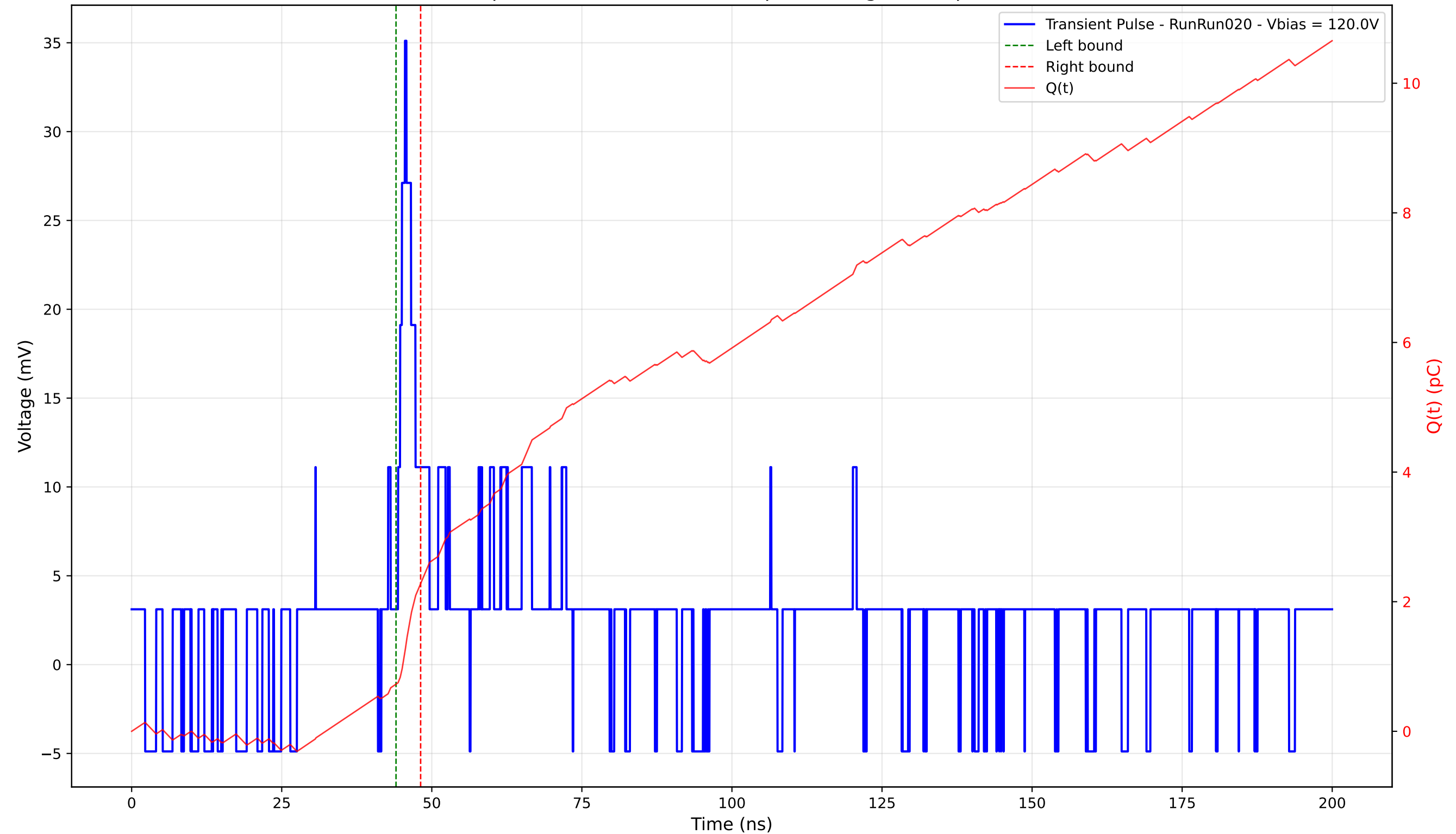
Transient Pulse - Sample: 4003 - Position: 375.0 \mu\text{m} - Charge: 1.55 pC - Rise Time: 1.16 ns
