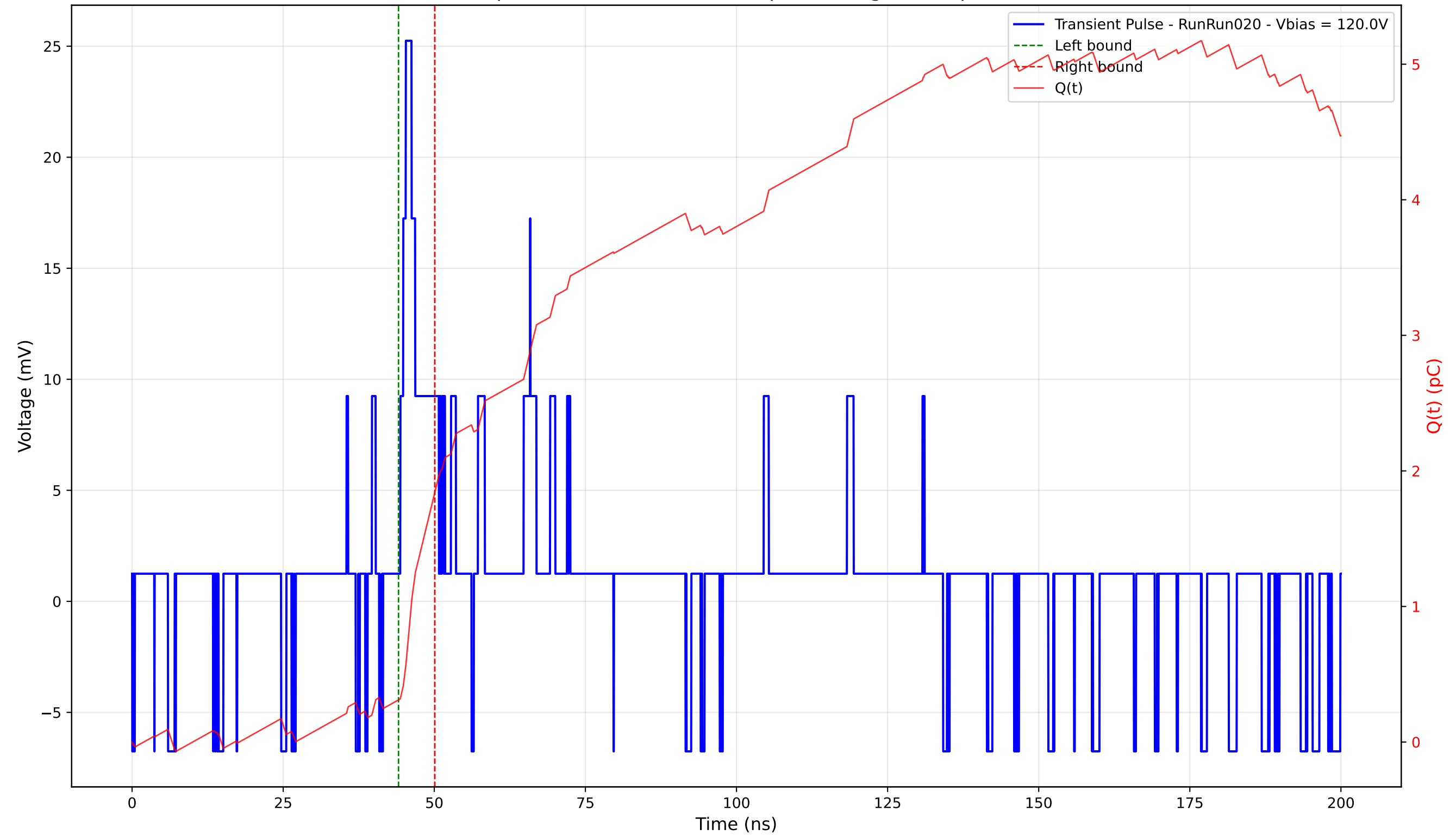
Transient Pulse - Sample: 4003 - Position: 415.0 \mu\text{m} - Charge: 1.53 pC - Rise Time: 0.92 ns
