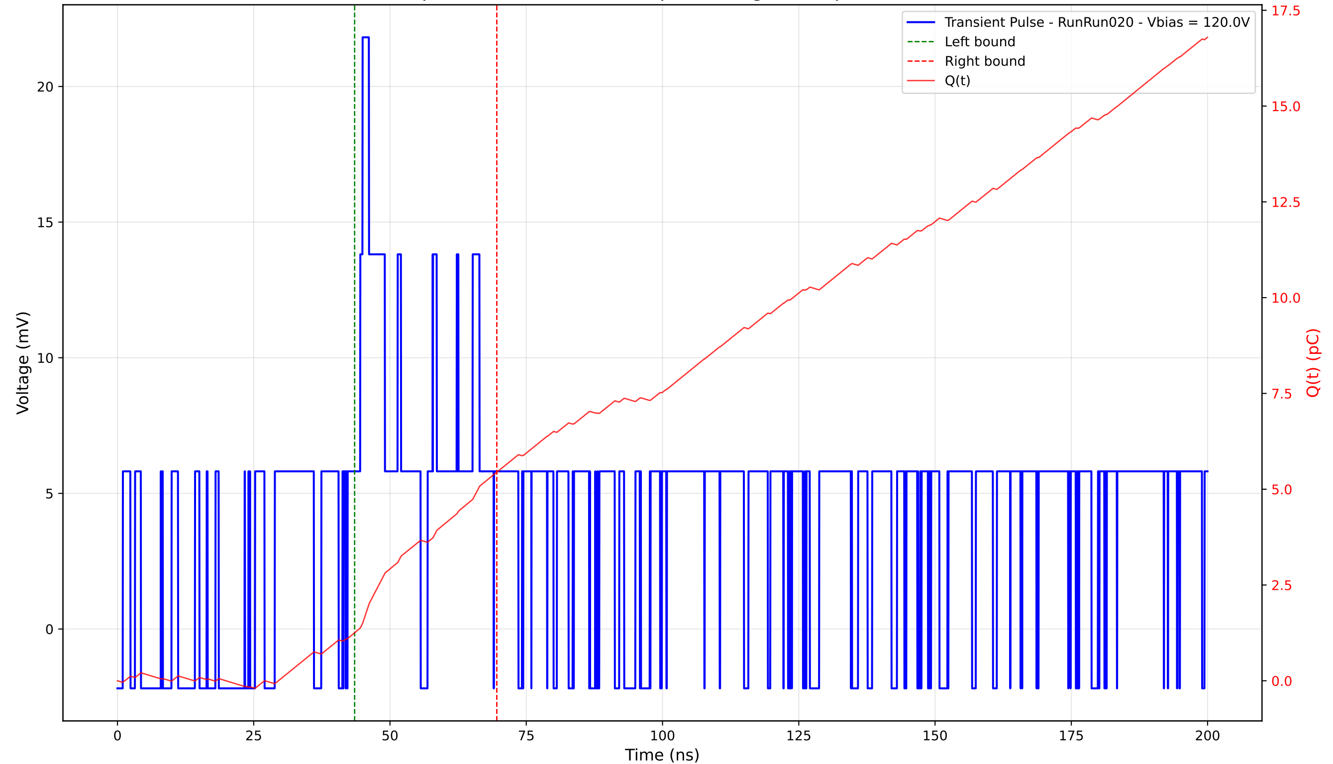
Transient Pulse - Sample: 4003 - Position: 20.0 \mu\text{m} - Charge: 4.19 pC - Rise Time: 0.00 ns (N/A)
