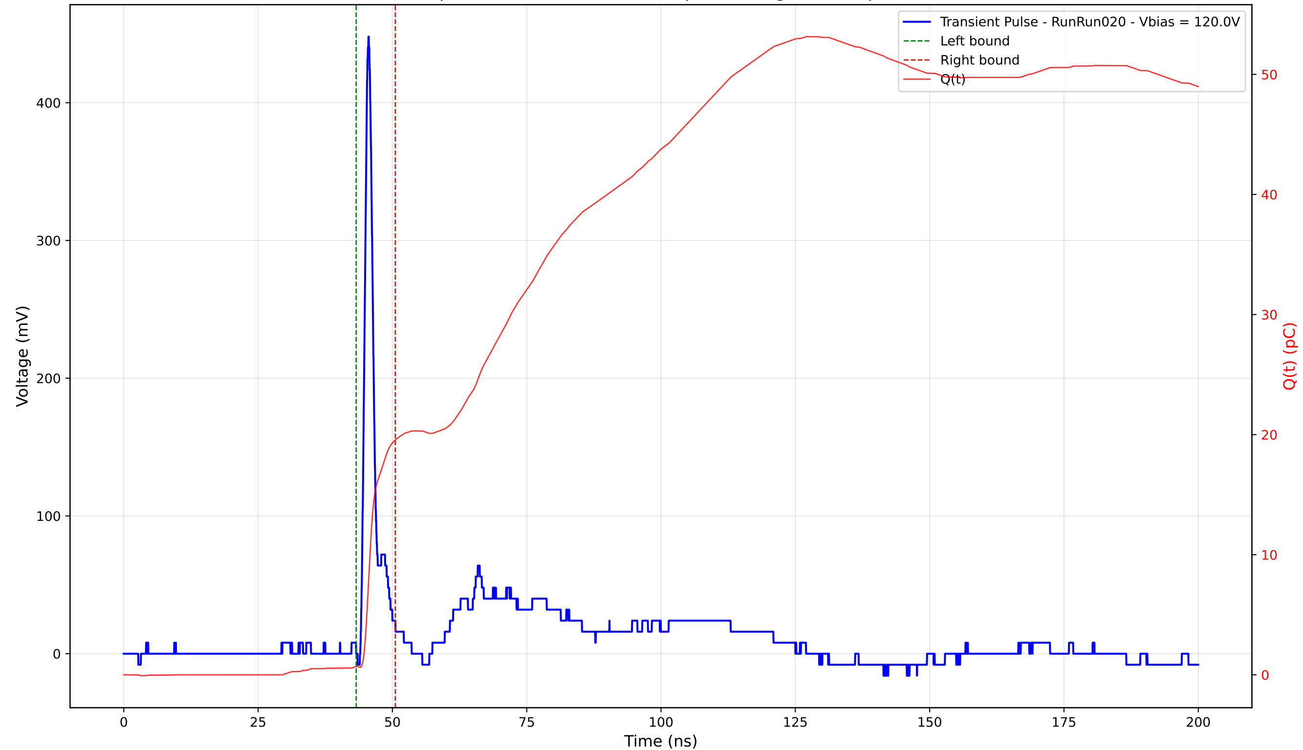
Transient Pulse - Sample: 4003 - Position: 150.0 \mu\text{m} - Charge: 18.88 pC - Rise Time: 0.97 ns
