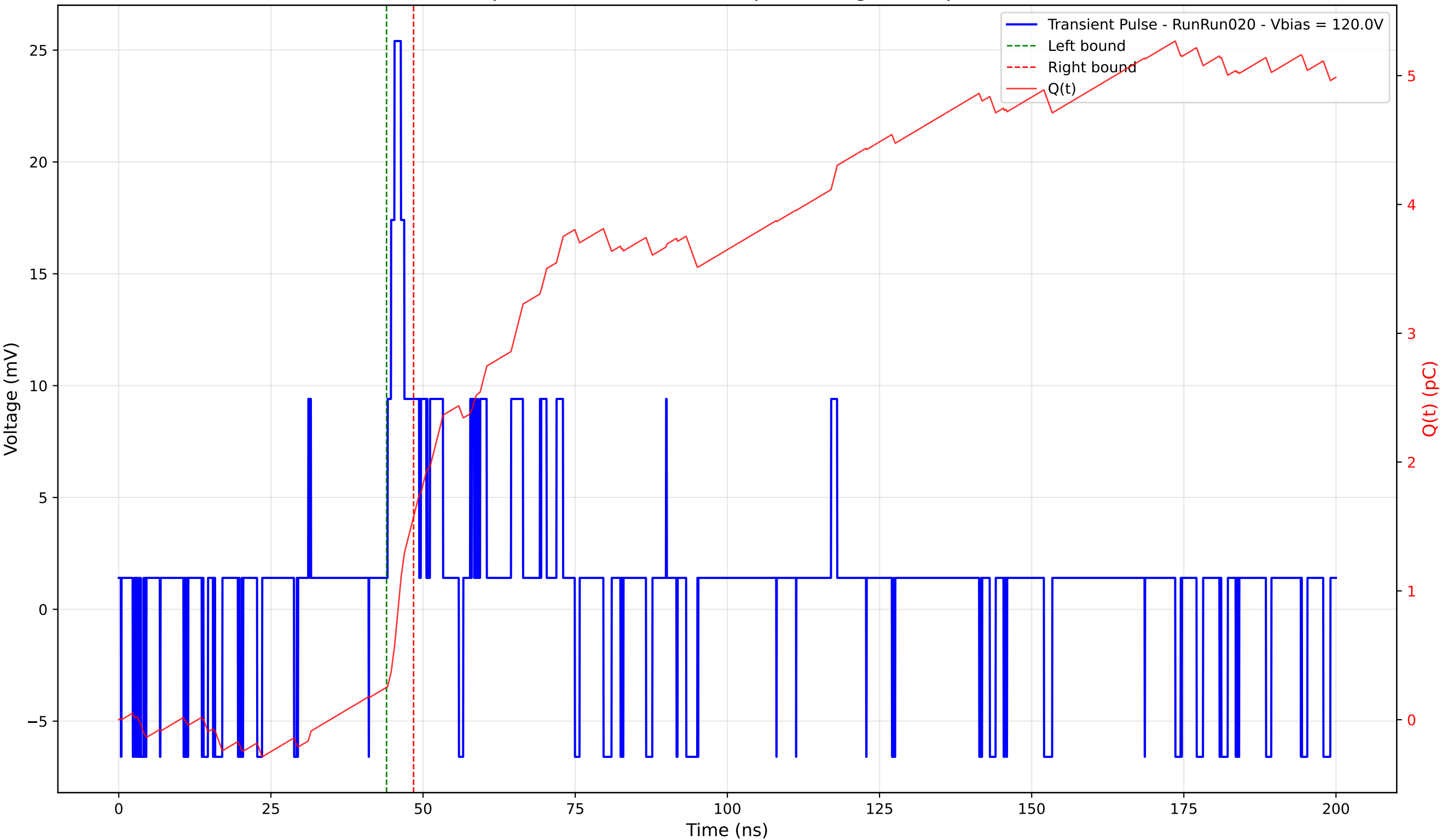
Transient Pulse - Sample: 4003 - Position: 30.0 \mu\text{m} - Charge: 1.33 pC - Rise Time: 1.14 ns
