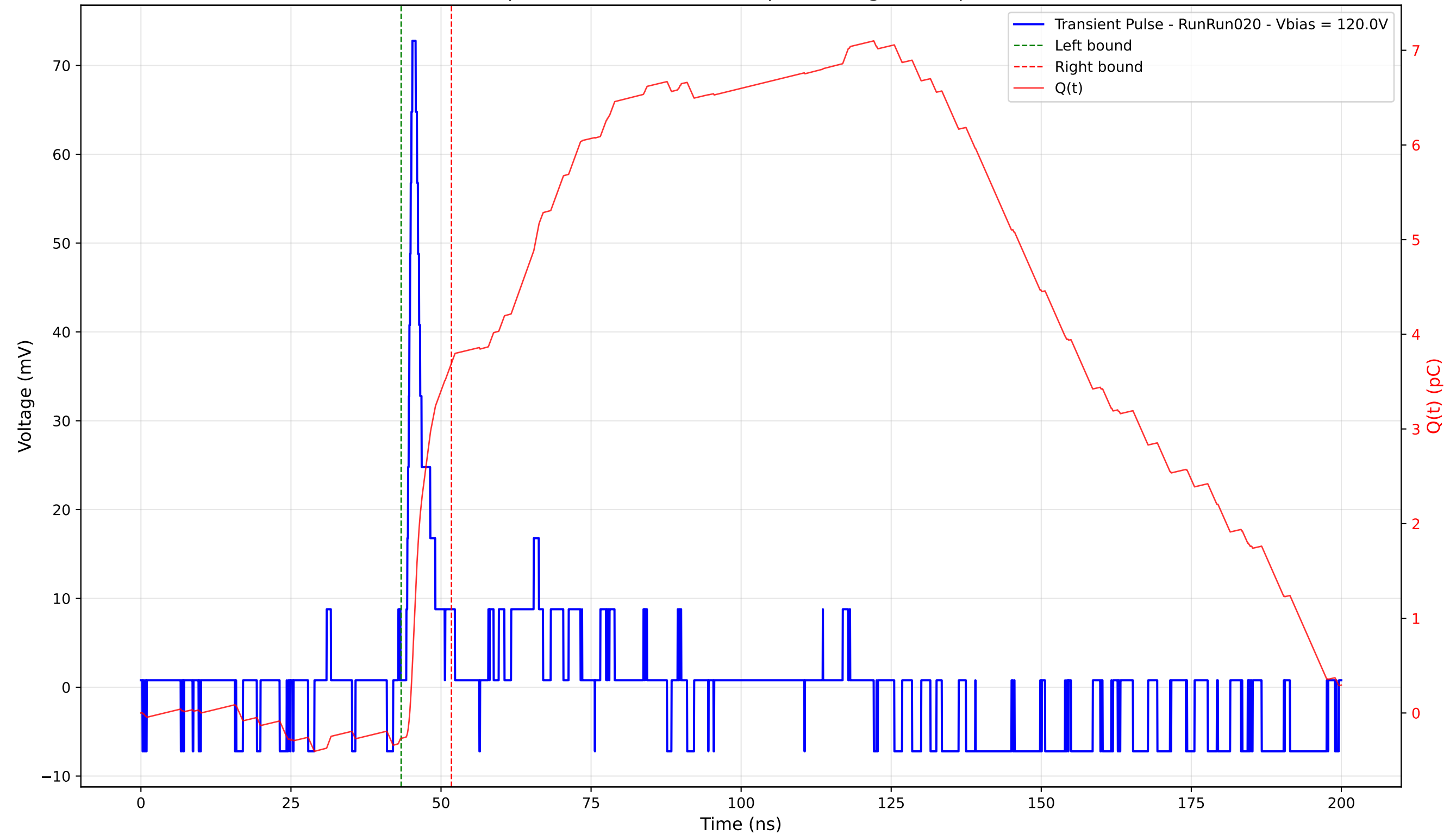
Transient Pulse - Sample: 4003 - Position: 90.0 \mu\text{m} - Charge: 3.97 pC - Rise Time: 1.00 ns
