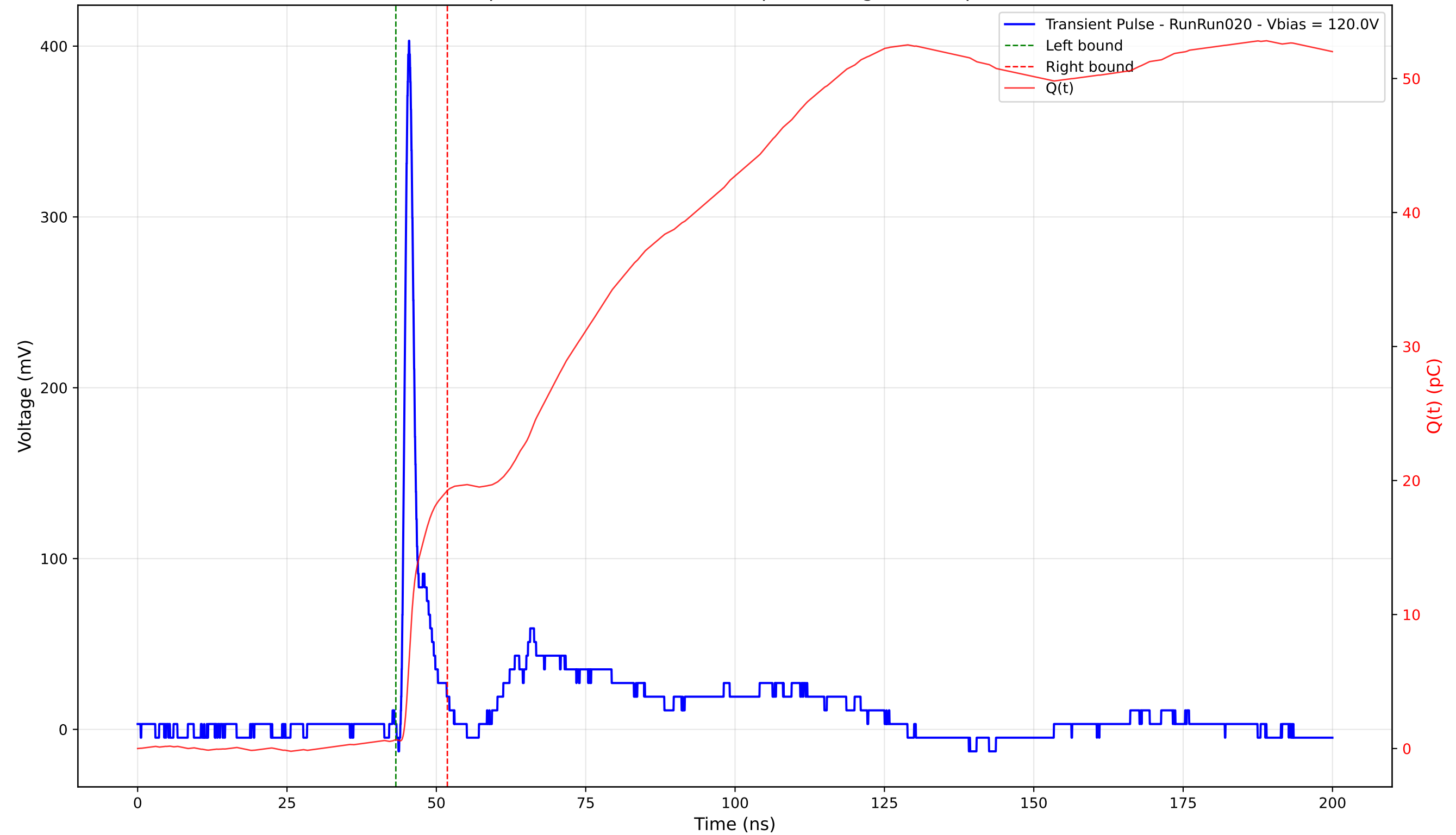
Transient Pulse - Sample: 4003 - Position: 120.0 \mu\text{m} - Charge: 18.61 pC - Rise Time: 0.91 ns
