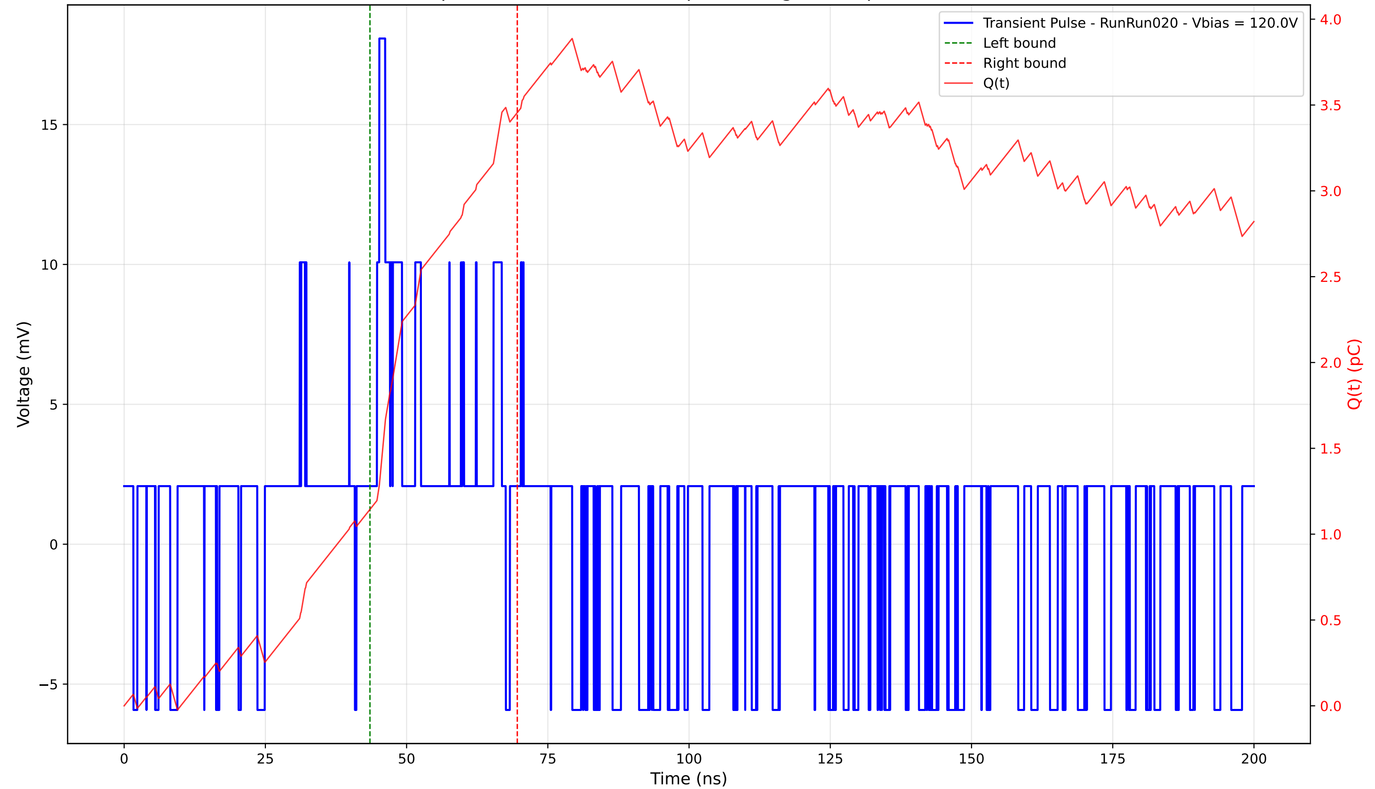
Transient Pulse - Sample: 4003 - Position: 10.0 \mu\text{m} - Charge: 2.31 pC - Rise Time: 0.00 ns (N/A)
